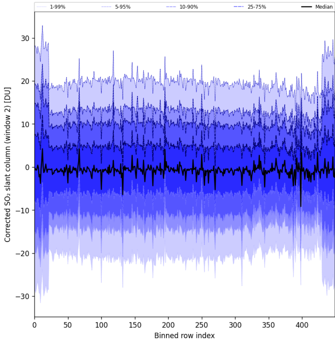
Figure 95: Along track statistics of “Corrected SO 2 slant column (window 2)” for 2025-10-18 to 2025-10-20
