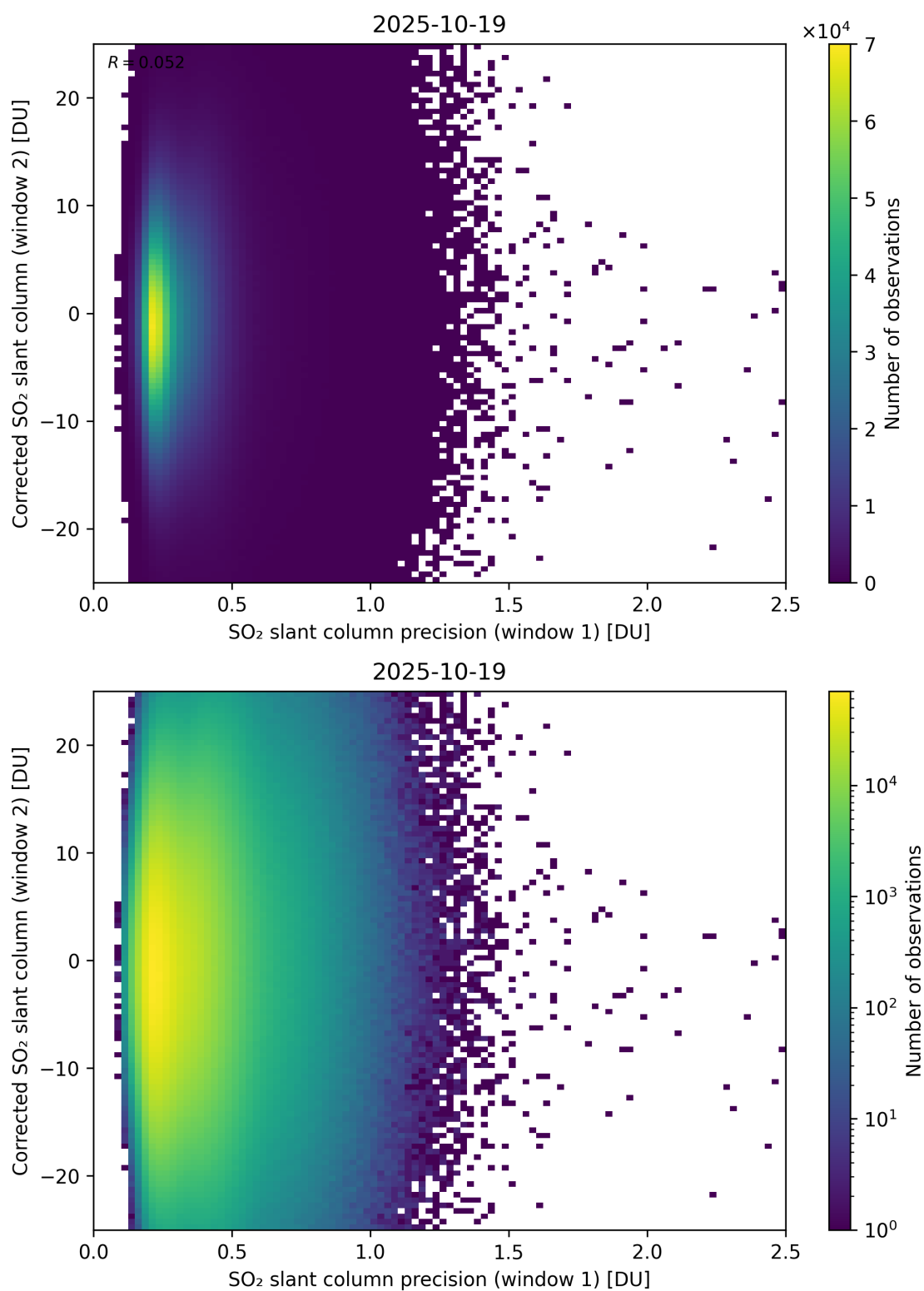
Figure 275: Scatter density plot of “SO 2 slant column precision (window 1)” against “Corrected SO 2 slant column (window 2)” for 2025-10-18 to 2025-10-20.
