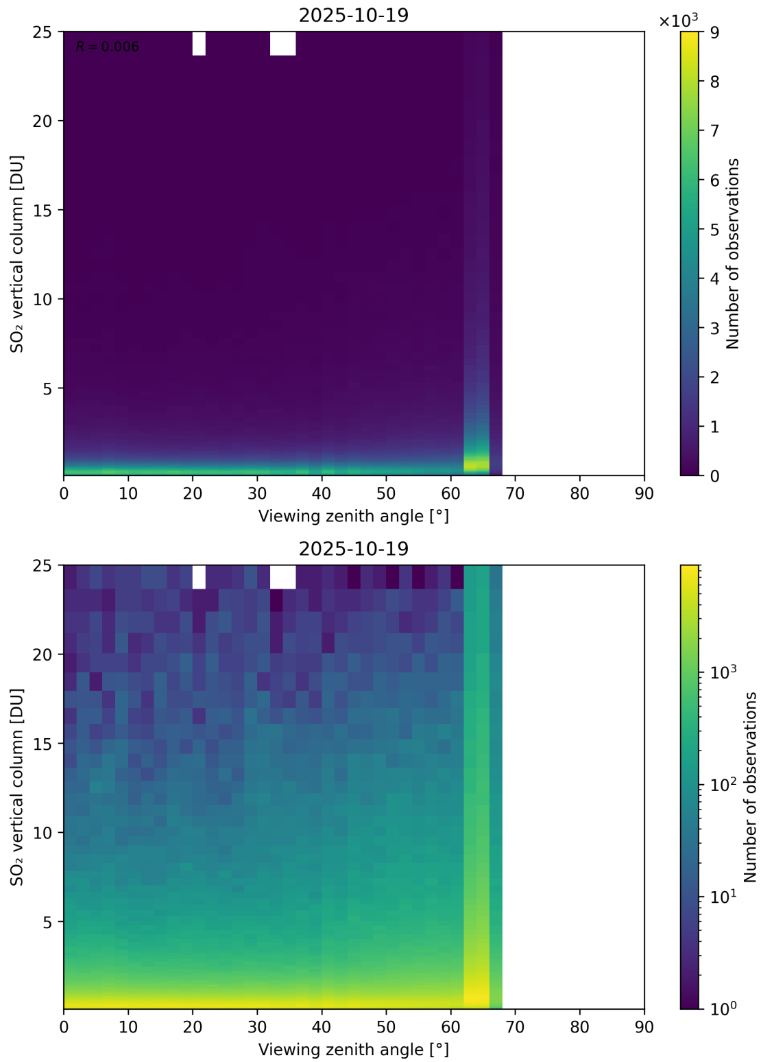
Figure 383: Scatter density plot of “Viewing zenith angle” against “SO 2 vertical column” for 2025-10-18 to 2025-10-20.
