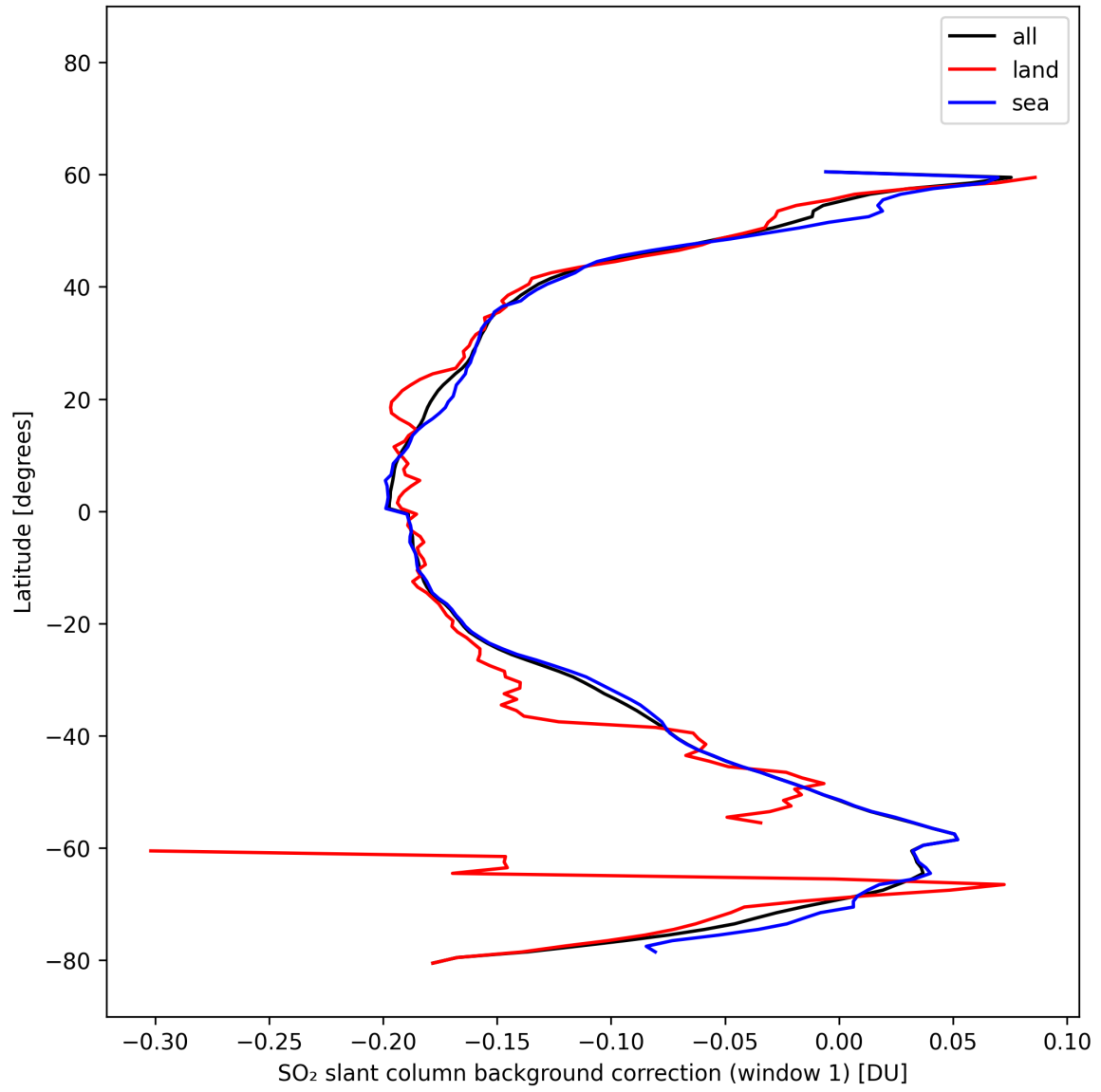
Figure 40: Zonal average of “SO 2 slant column background correction (window 1)” for 2025-10-18 to 2025-10-20.
