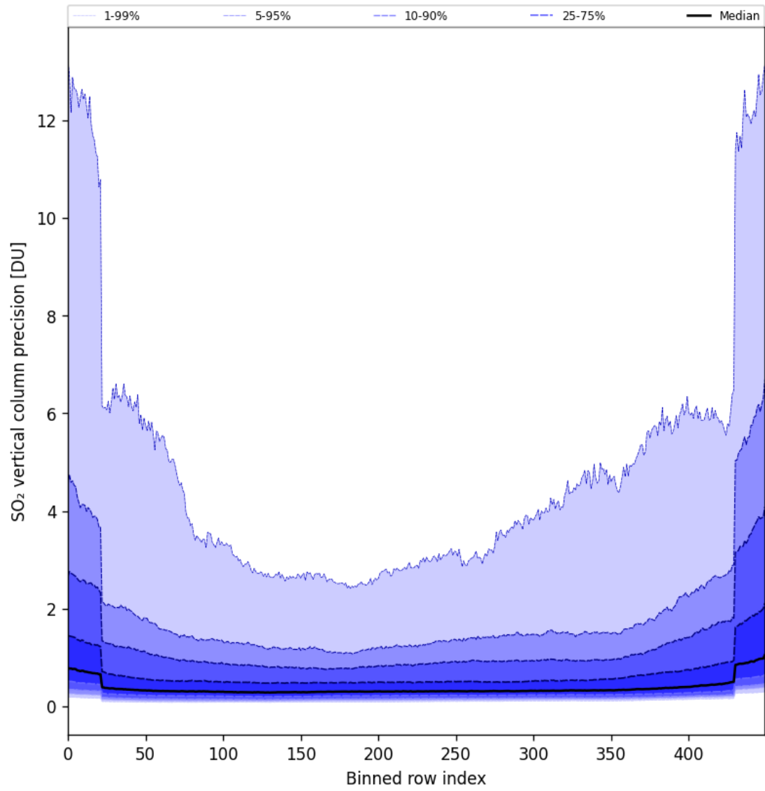
Figure 85: Along track statistics of “SO 2 vertical column precision” for 2025-10-18 to 2025-10-20
