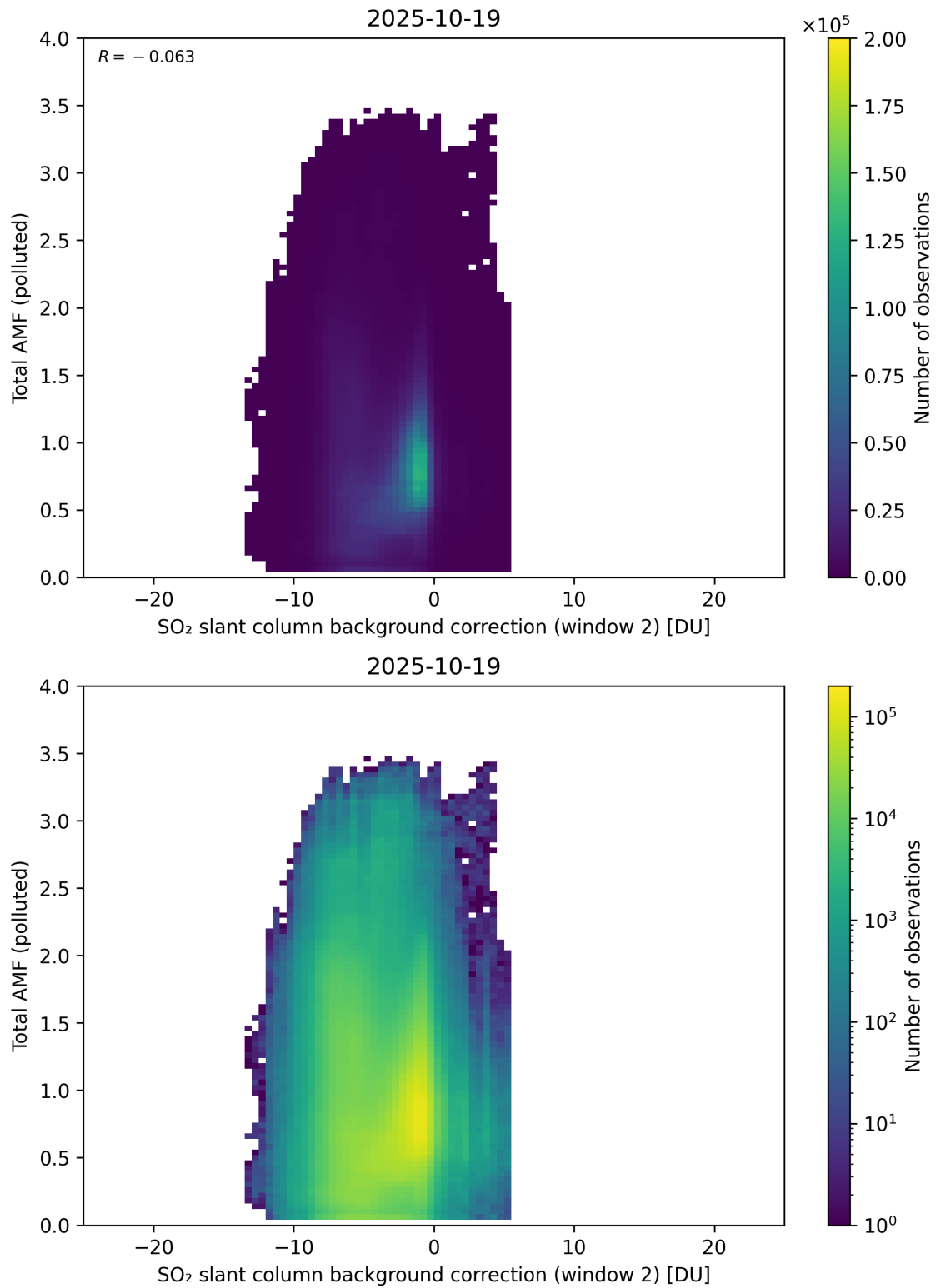
Figure 130: Scatter density plot of “SO 2 slant column background correction (window 2)” against “Total AMF (polluted)” for 2025-10-18 to 2025-10-20.
