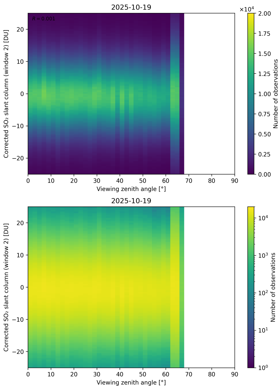
Figure 374: Scatter density plot of “Viewing zenith angle” against “Corrected SO 2 slant column (window 2)” for 2025-10-18 to 2025-10-20.
