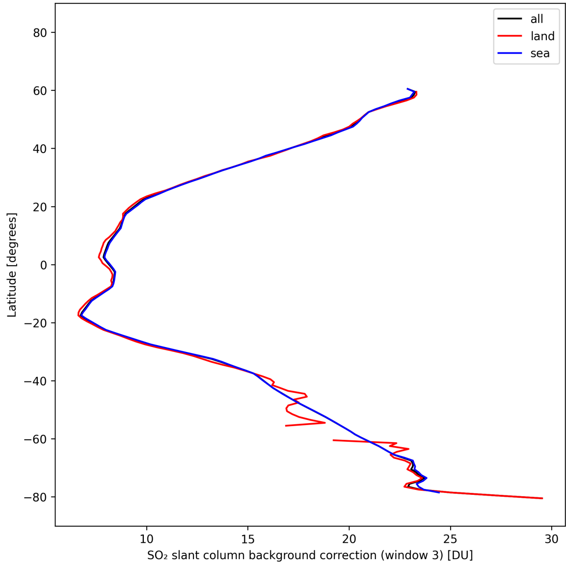
Figure 48: Zonal average of “SO 2 slant column background correction (window 3)” for 2025-10-18 to 2025-10-20.
