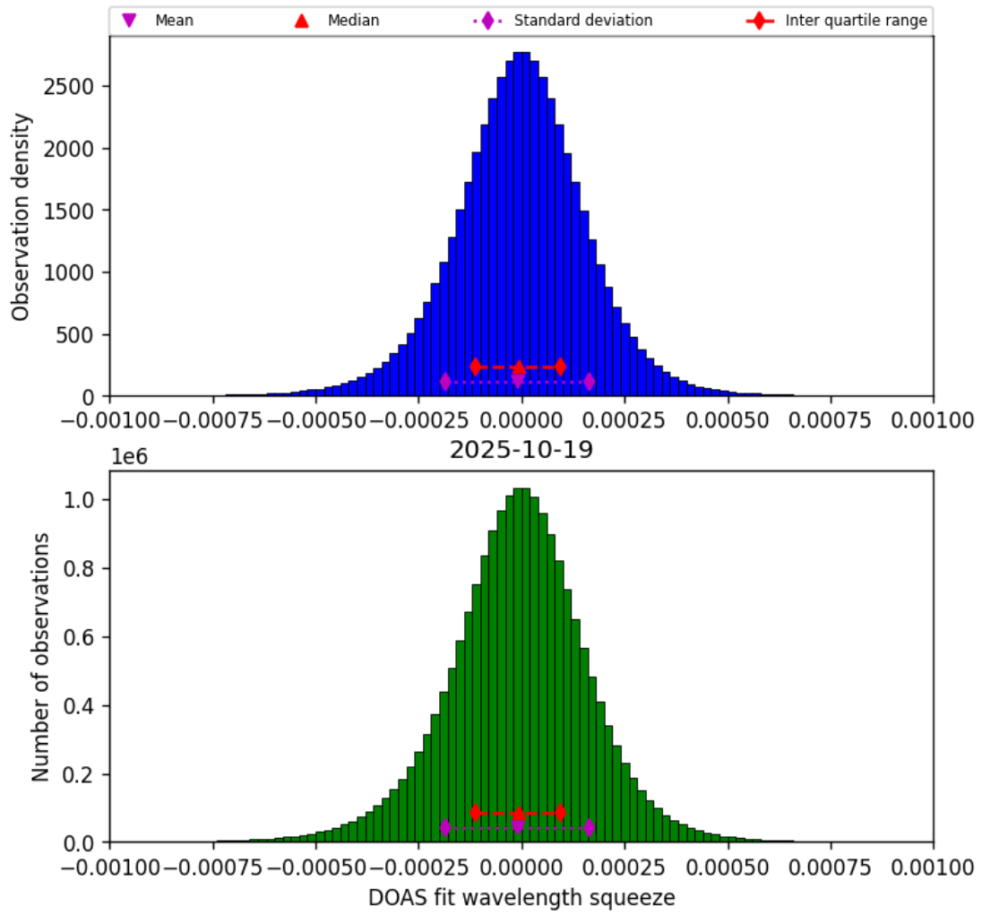
Figure 77: Histogram of “DOAS fit wavelength squeeze” for 2025-10-18 to 2025-10-20
