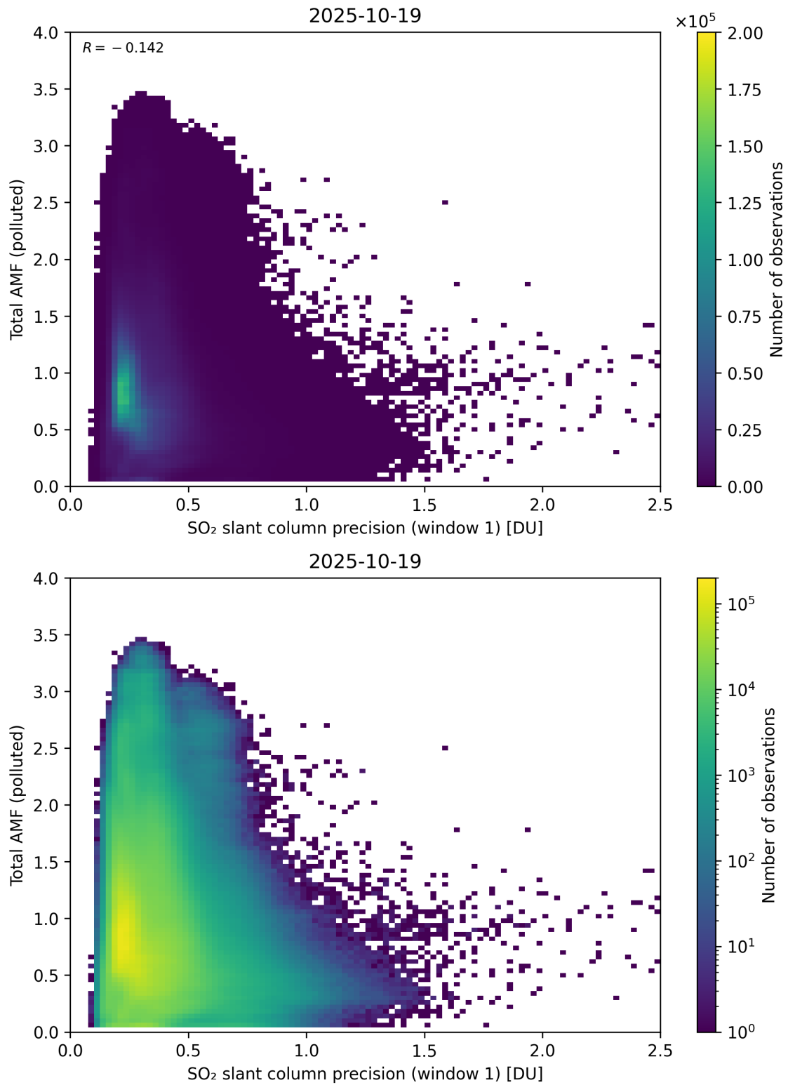
Figure 280: Scatter density plot of “SO 2 slant column precision (window 1)” against “Total AMF (polluted)” for 2025-10-18 to 2025-10-20.
