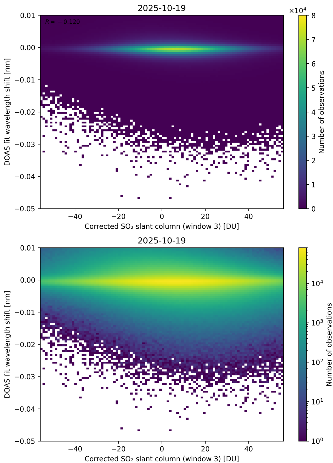
Figure 256: Scatter density plot of “Corrected SO 2 slant column (window 3)” against “DOAS fit wavelength shift” for 2025-10-18 to 2025-10-20.
