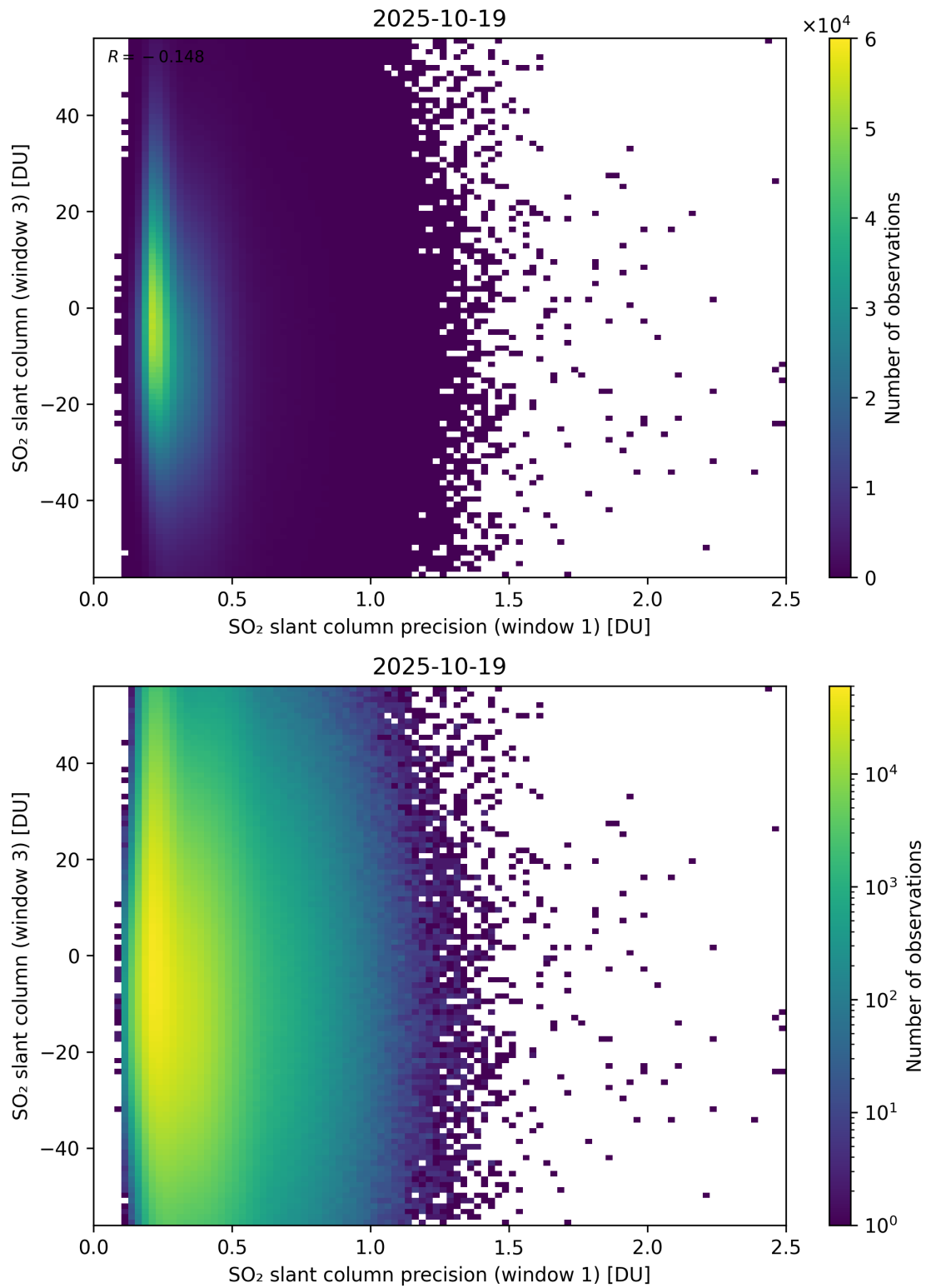
Figure 278: Scatter density plot of “SO 2 slant column precision (window 1)” against “SO 2 slant column (window 3)” for 2025-10-18 to 2025-10-20.
