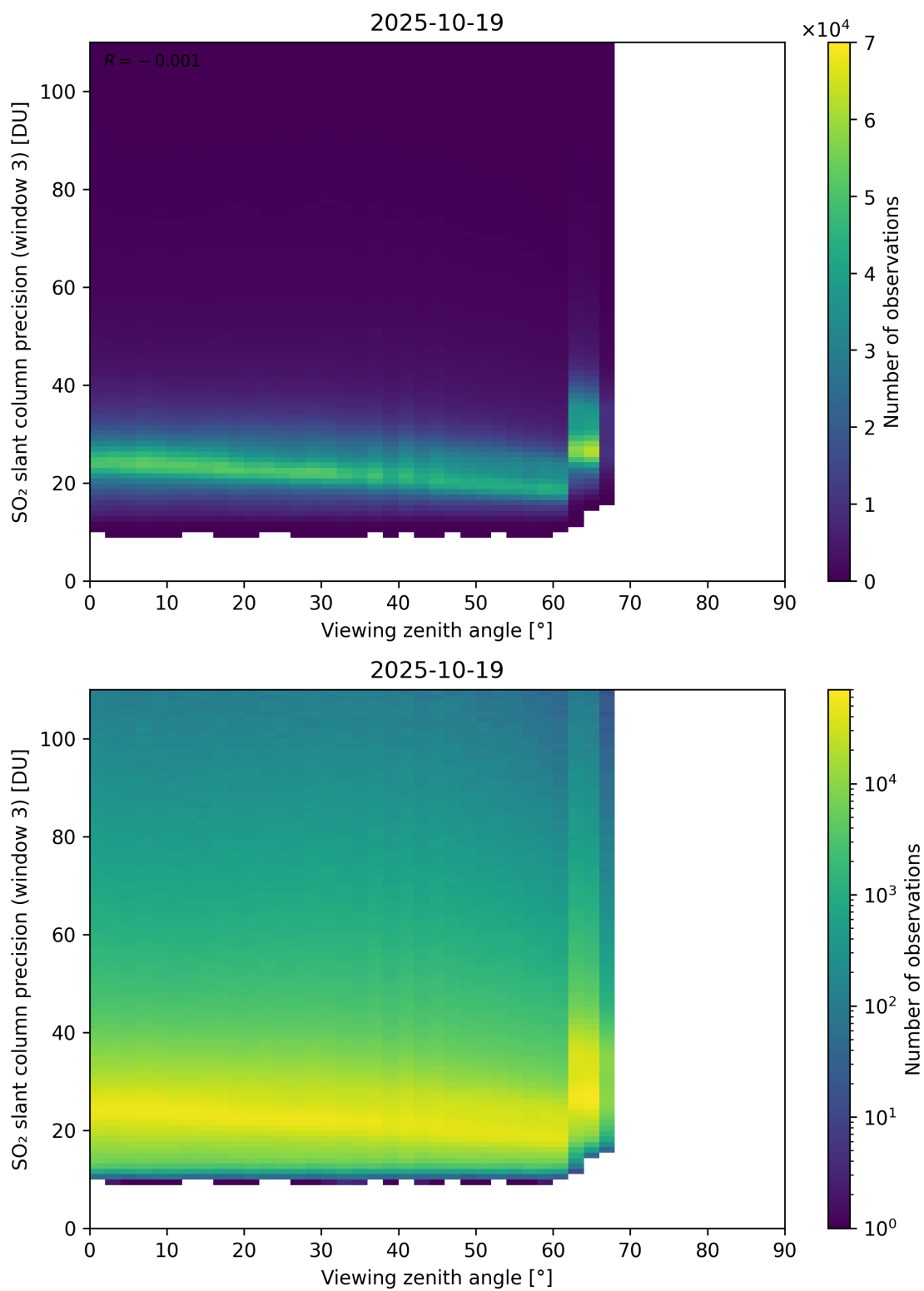
Figure 380: Scatter density plot of “Viewing zenith angle” against “SO 2 slant column precision (window 3)” for 2025-10-18 to 2025-10-20.
