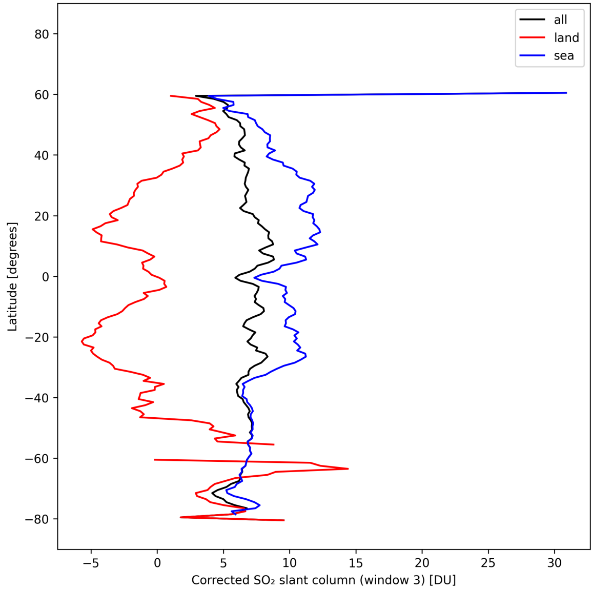
Figure 47: Zonal average of “Corrected SO 2 slant column (window 3)” for 2025-10-18 to 2025-10-20.
