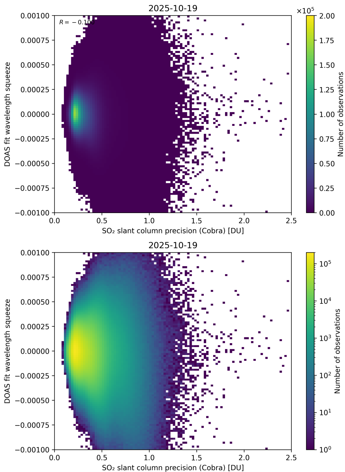
Figure 203: Scatter density plot of “SO 2 slant column precision (Cobra)” against “DOAS fit wavelength squeeze” for 2025-10-18 to 2025-10-20.
