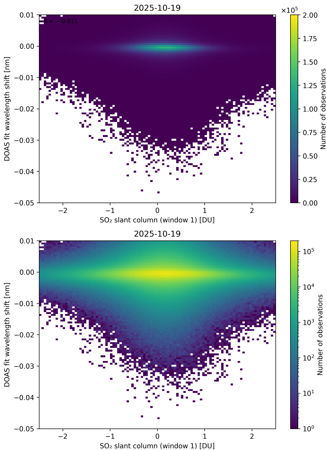
Figure 265: Scatter density plot of “SO 2 slant column (window 1)” against “DOAS fit wavelength shift” for 2025-10-18 to 2025-10-20.
