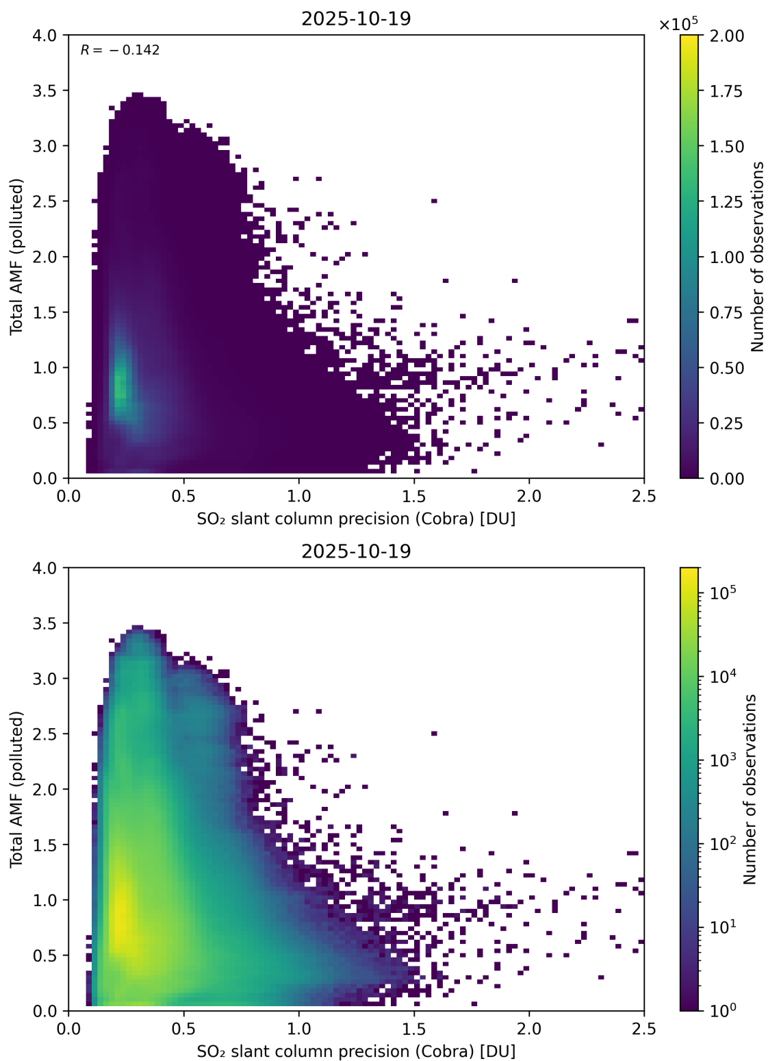
Figure 213: Scatter density plot of “SO 2 slant column precision (Cobra)” against “Total AMF (polluted)” for 2025-10-18 to 2025-10-20.
