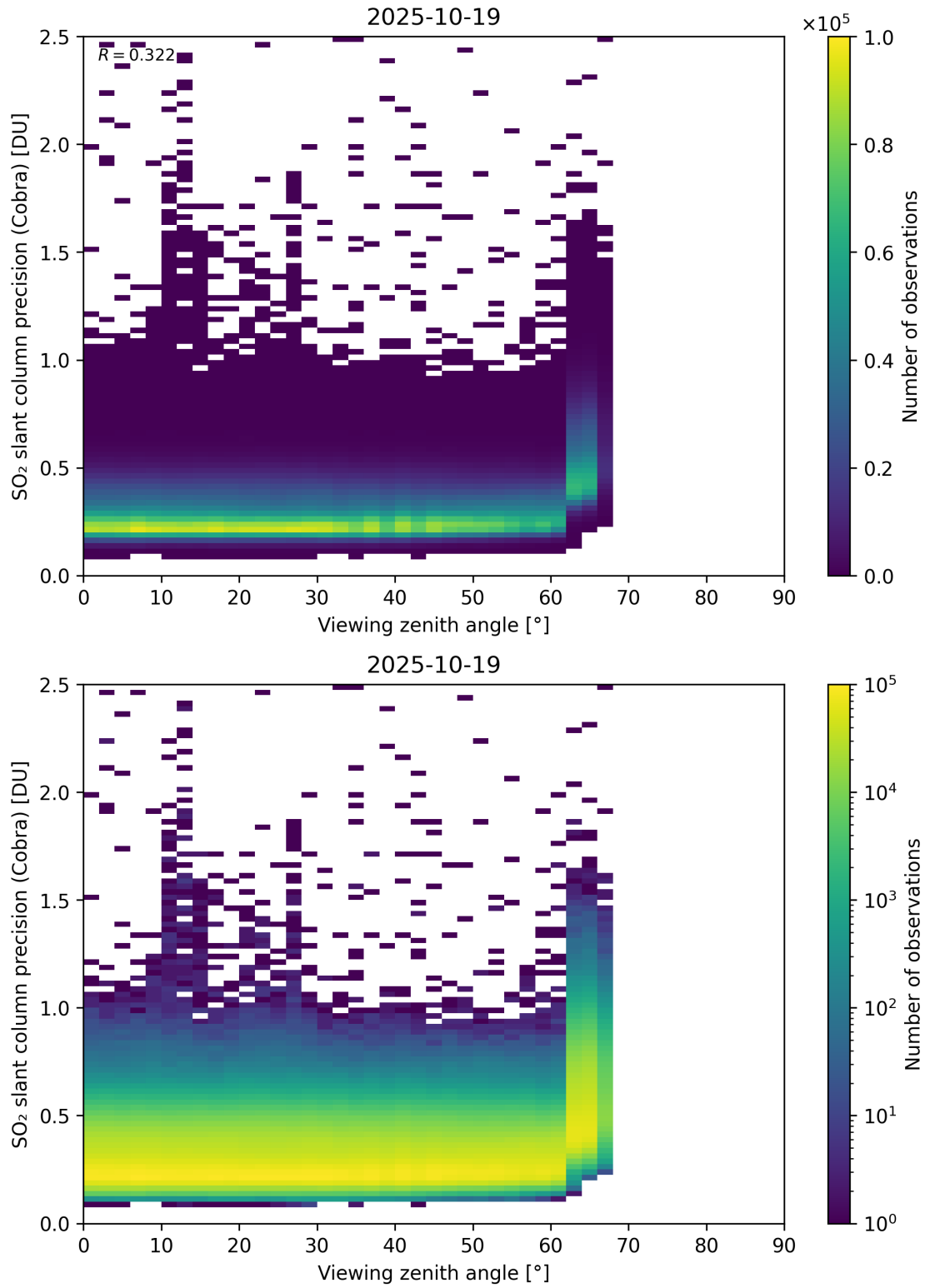
Figure 372: Scatter density plot of “Viewing zenith angle” against “SO 2 slant column precision (Cobra)” for 2025-10-18 to 2025-10-20.
