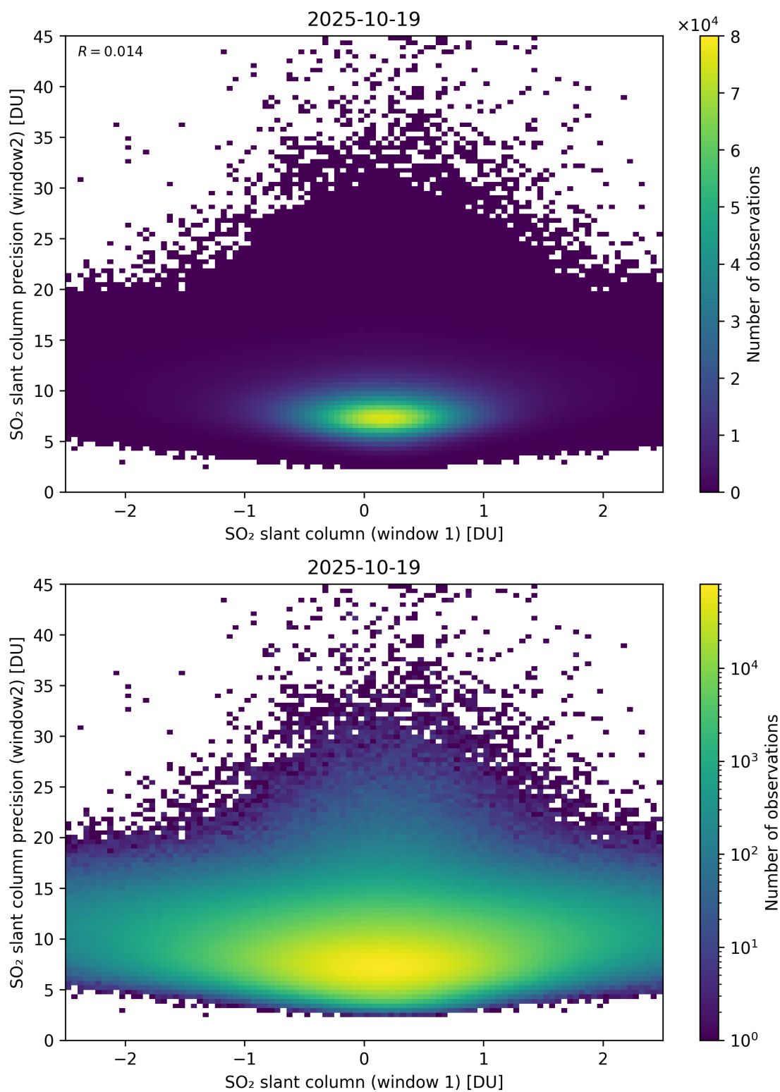
Figure 286: Scatter density plot of “SO 2 slant column (window 1)” against “SO 2 slant column precision (window2)” for 2025-10-18 to 2025-10-20.
