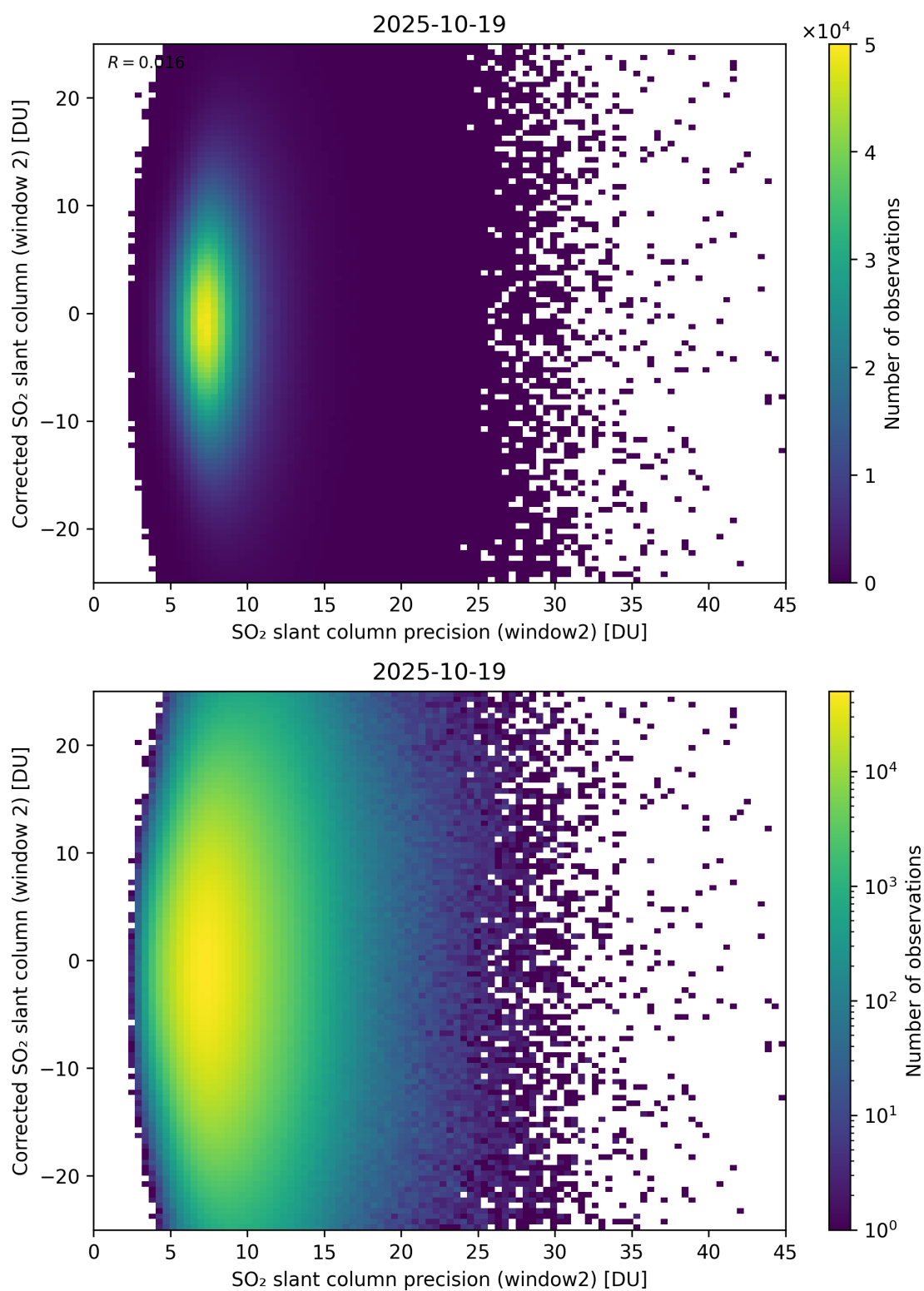
Figure 297: Scatter density plot of “SO 2 slant column precision (window2)” against “Corrected SO 2 slant column (window 2)” for 2025-10-18 to 2025-10-20.
