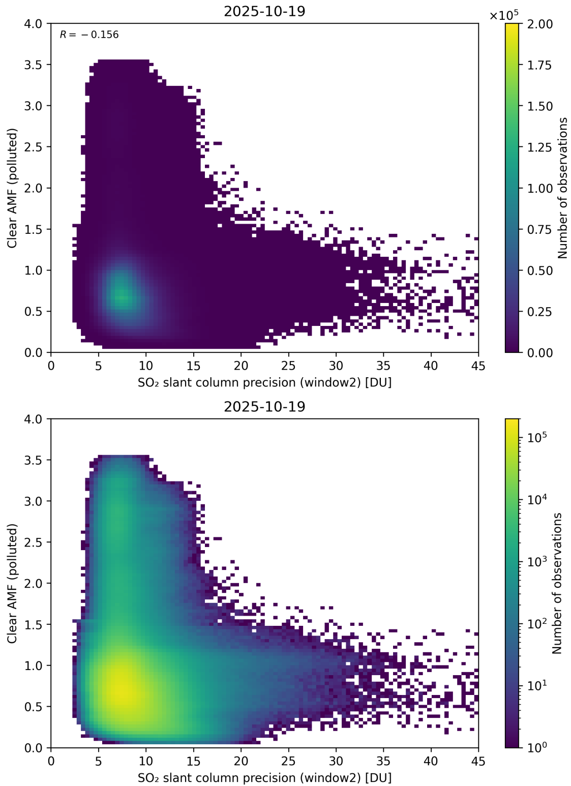
Figure 296: Scatter density plot of “SO 2 slant column precision (window2)” against “Clear AMF (polluted)” for 2025-10-18 to 2025-10-20.
