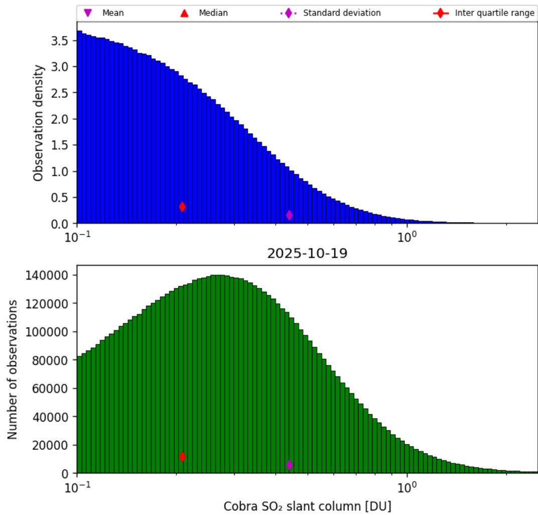
Figure 61: Histogram of “Cobra SO 2 slant column” for 2025-10-18 to 2025-10-20
