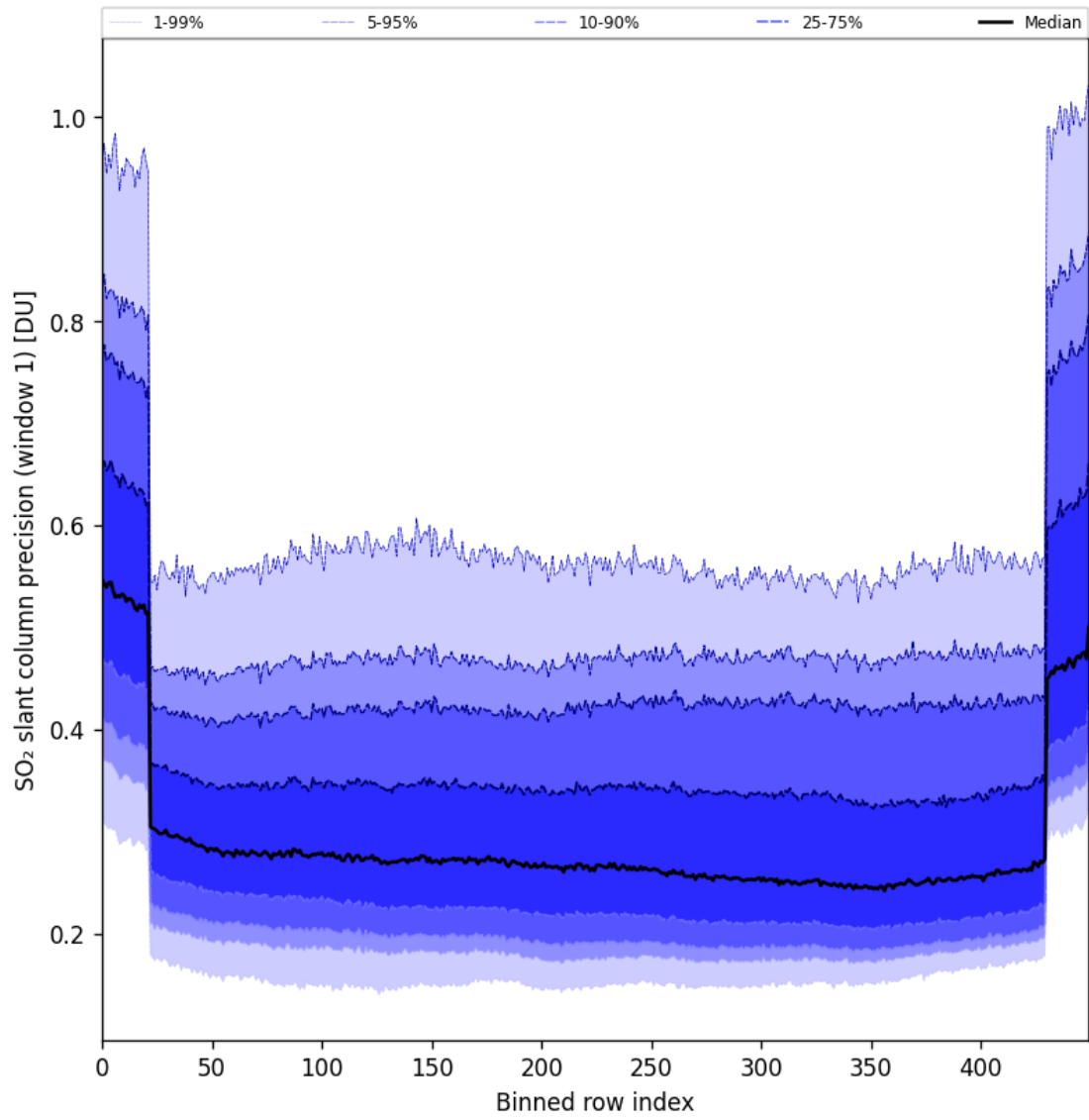
Figure 90: Along track statistics of “SO 2 slant column precision (window 1)” for 2025-10-18 to 2025-10-20
