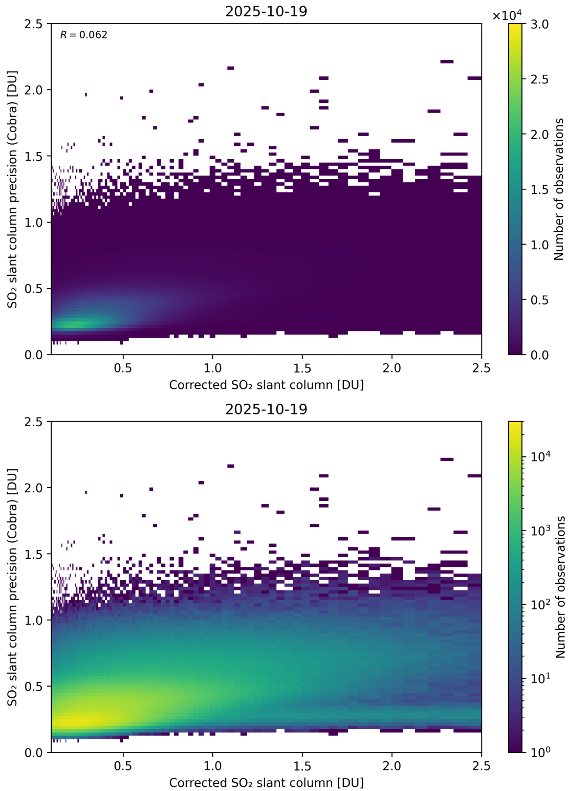
Figure 234: Scatter density plot of “Corrected SO 2 slant column” against “SO 2 slant column precision (Cobra)” for 2025-10-18 to 2025-10-20.
