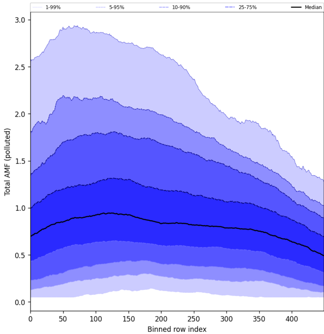
Figure 105: Along track statistics of “Total AMF (polluted)” for 2025-10-18 to 2025-10-20
