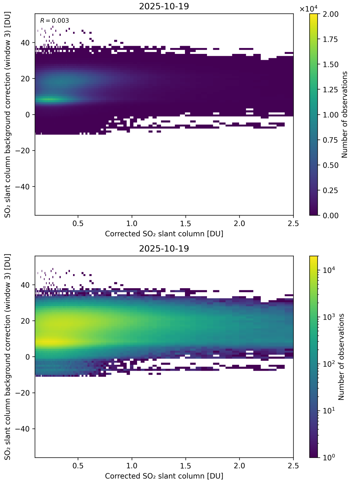
Figure 228: Scatter density plot of “Corrected SO 2 slant column” against “SO 2 slant column background correction (window 3)” for 2025-10-18 to 2025-10-20.
