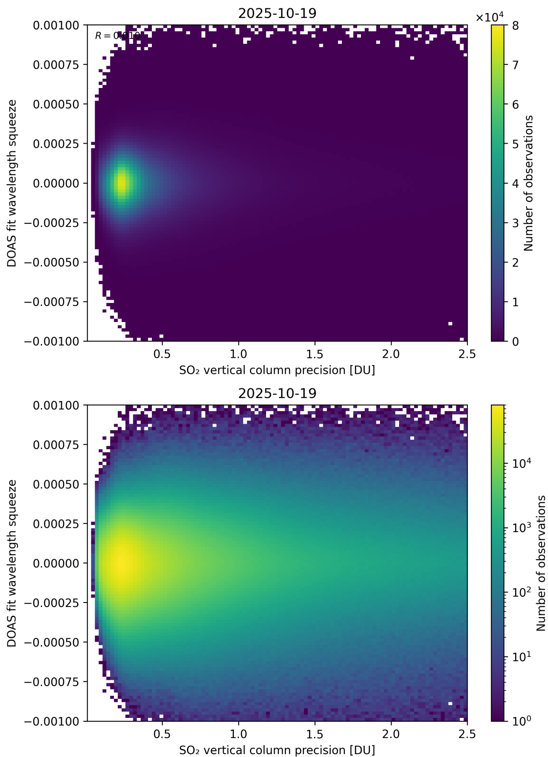
Figure 333: Scatter density plot of “SO 2 vertical column precision” against “DOAS fit wavelength squeeze” for 2025-10-18 to 2025-10-20.
