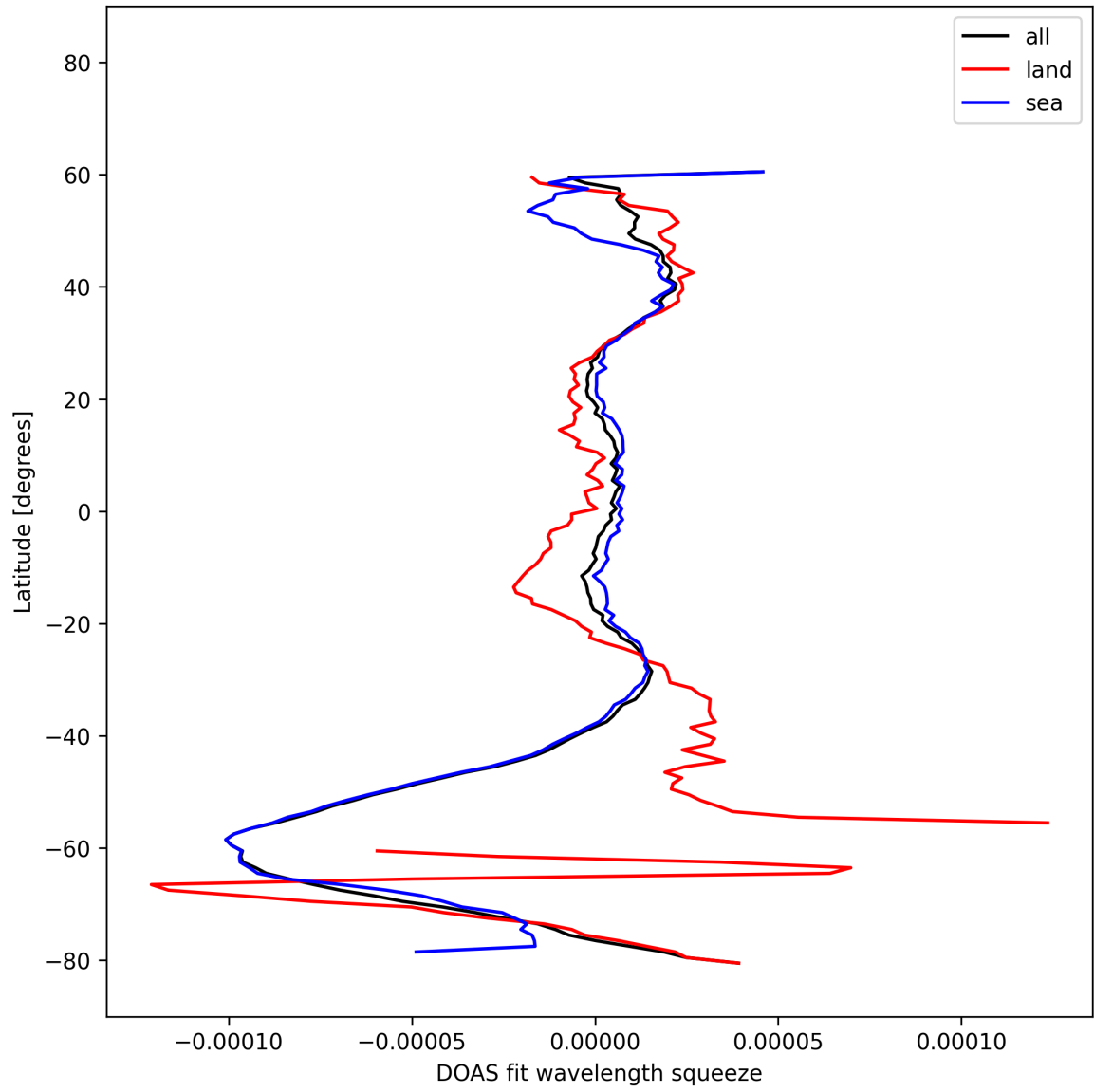
Figure 51: Zonal average of “DOAS fit wavelength squeeze” for 2025-10-18 to 2025-10-20.
