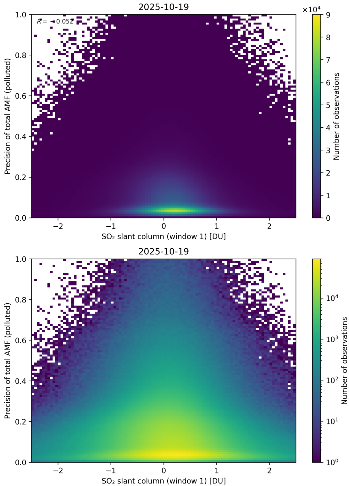
Figure 290: Scatter density plot of “SO 2 slant column (window 1)” against “Precision of total AMF (polluted)” for 2025-10-18 to 2025-10-20.
