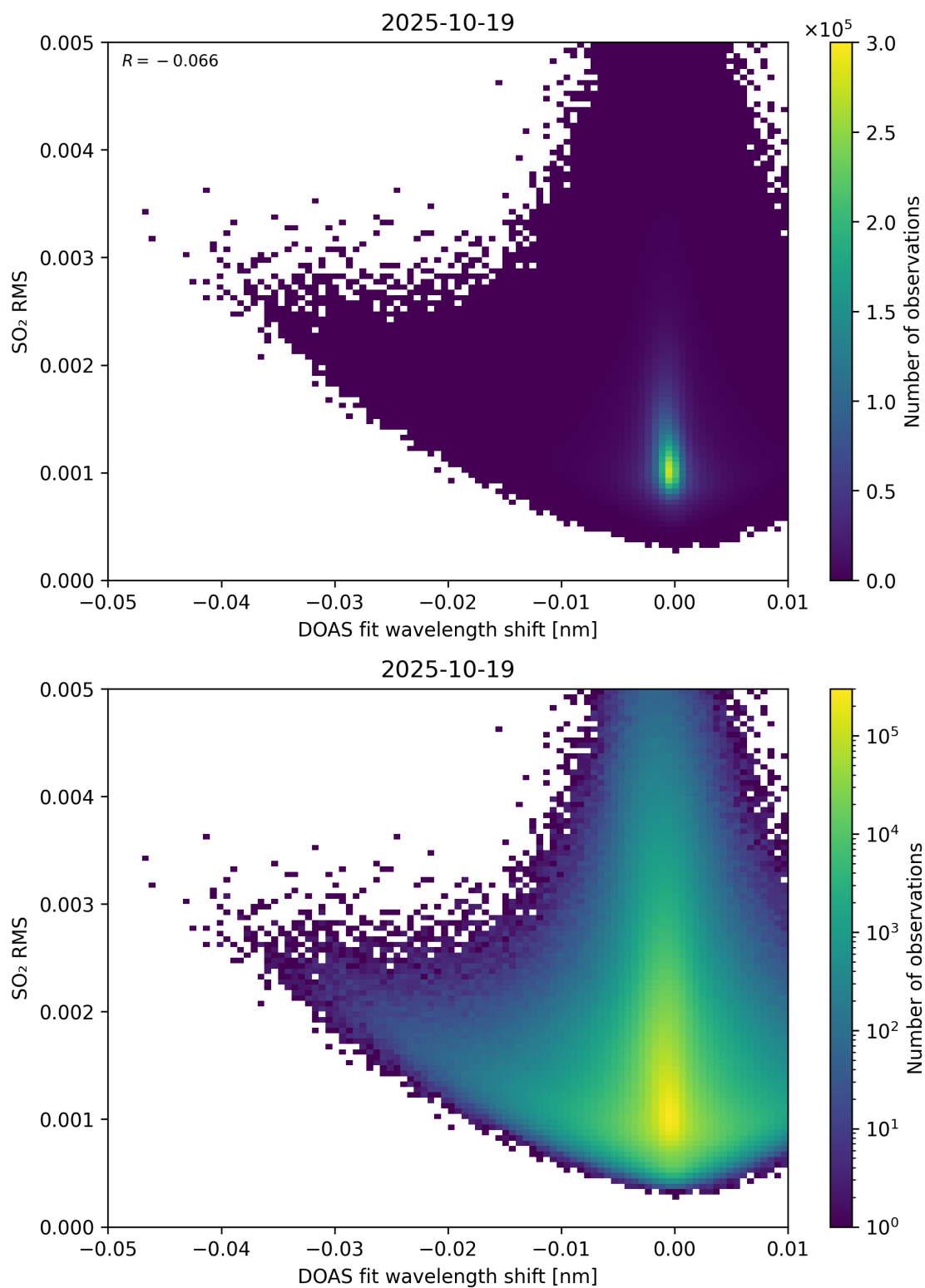
Figure 139: Scatter density plot of “DOAS fit wavelength shift” against “SO 2 RMS” for 2025-10-18 to 2025-10-20.
