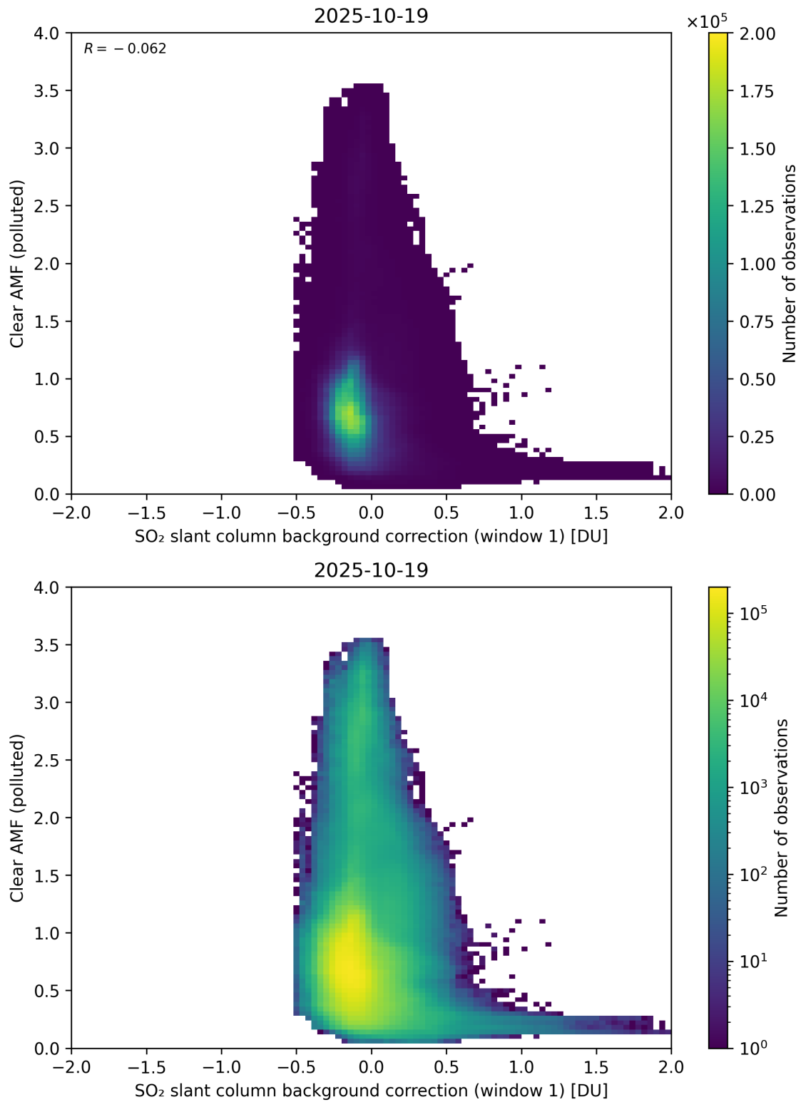
Figure 114: Scatter density plot of “SO 2 slant column background correction (window 1)” against “Clear AMF (polluted)” for 2025-10-18 to 2025-10-20.
