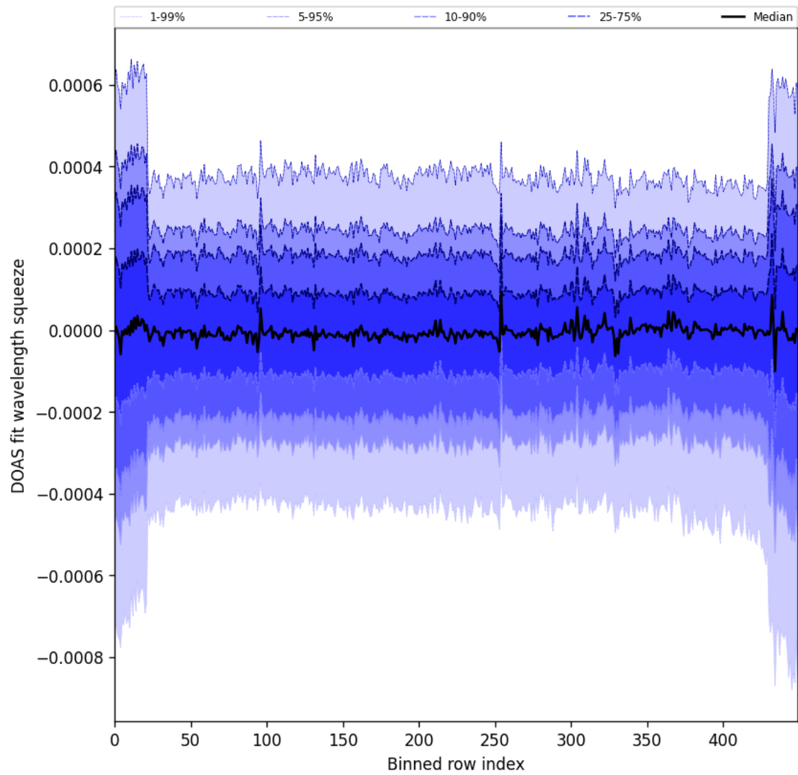
Figure 103: Along track statistics of “DOAS fit wavelength squeeze” for 2025-10-18 to 2025-10-20
