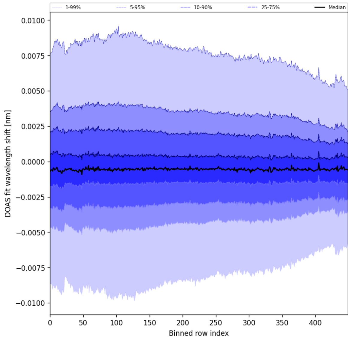
Figure 102: Along track statistics of “DOAS fit wavelength shift” for 2025-10-18 to 2025-10-20
