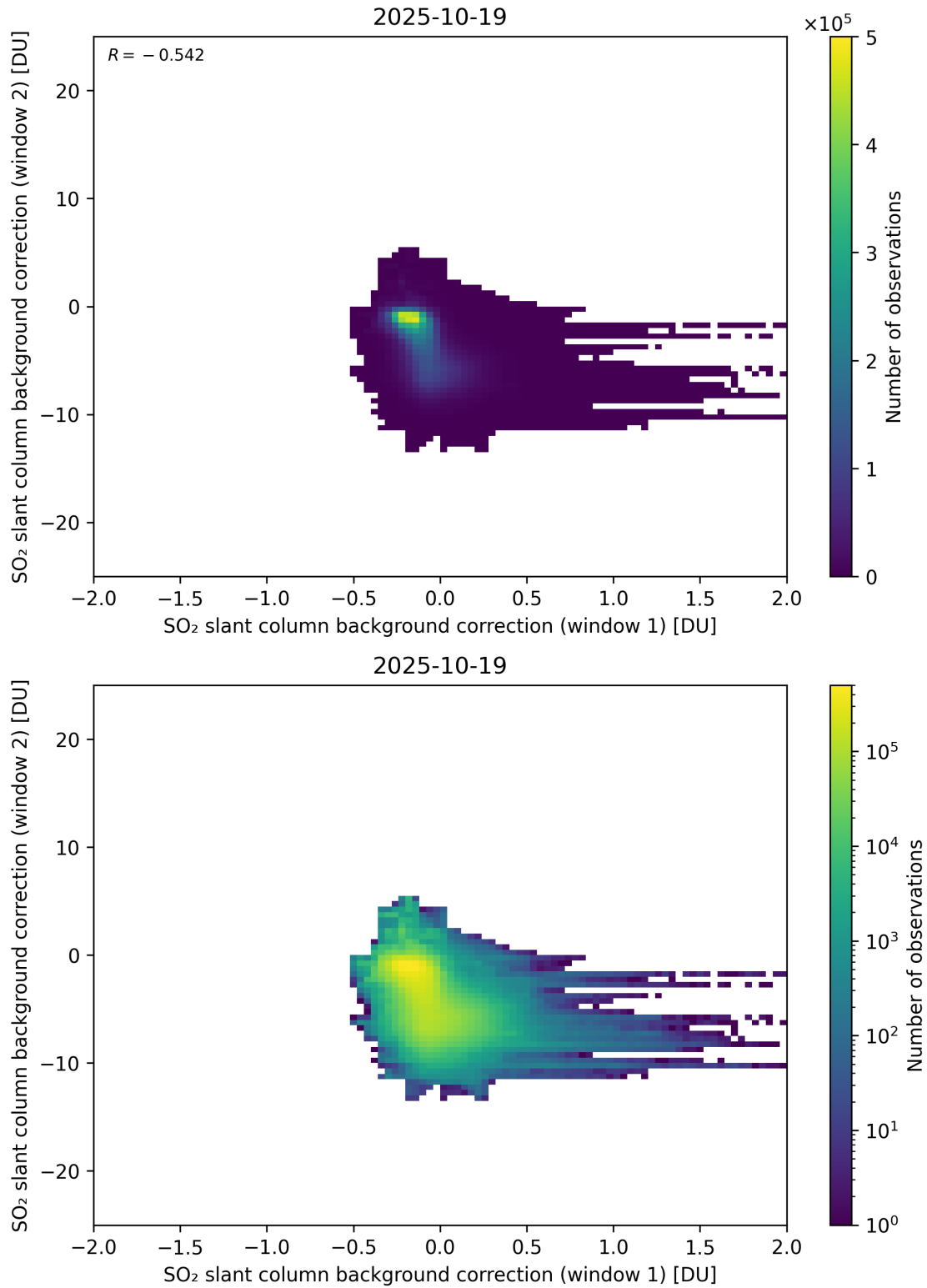
Figure 109: Scatter density plot of “SO 2 slant column background correction (window 1)” against “SO 2 slant column background correction (window 2)” for 2025-10-18 to 2025-10-20.
