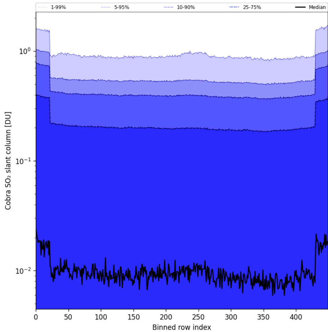
Figure 87: Along track statistics of “Cobra SO 2 slant column” for 2025-10-18 to 2025-10-20
