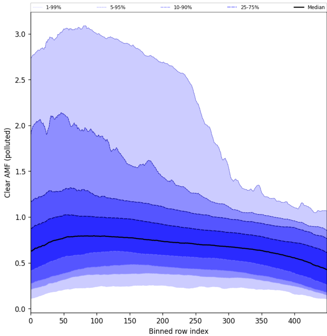
Figure 107: Along track statistics of “Clear AMF (polluted)” for 2025-10-18 to 2025-10-20
