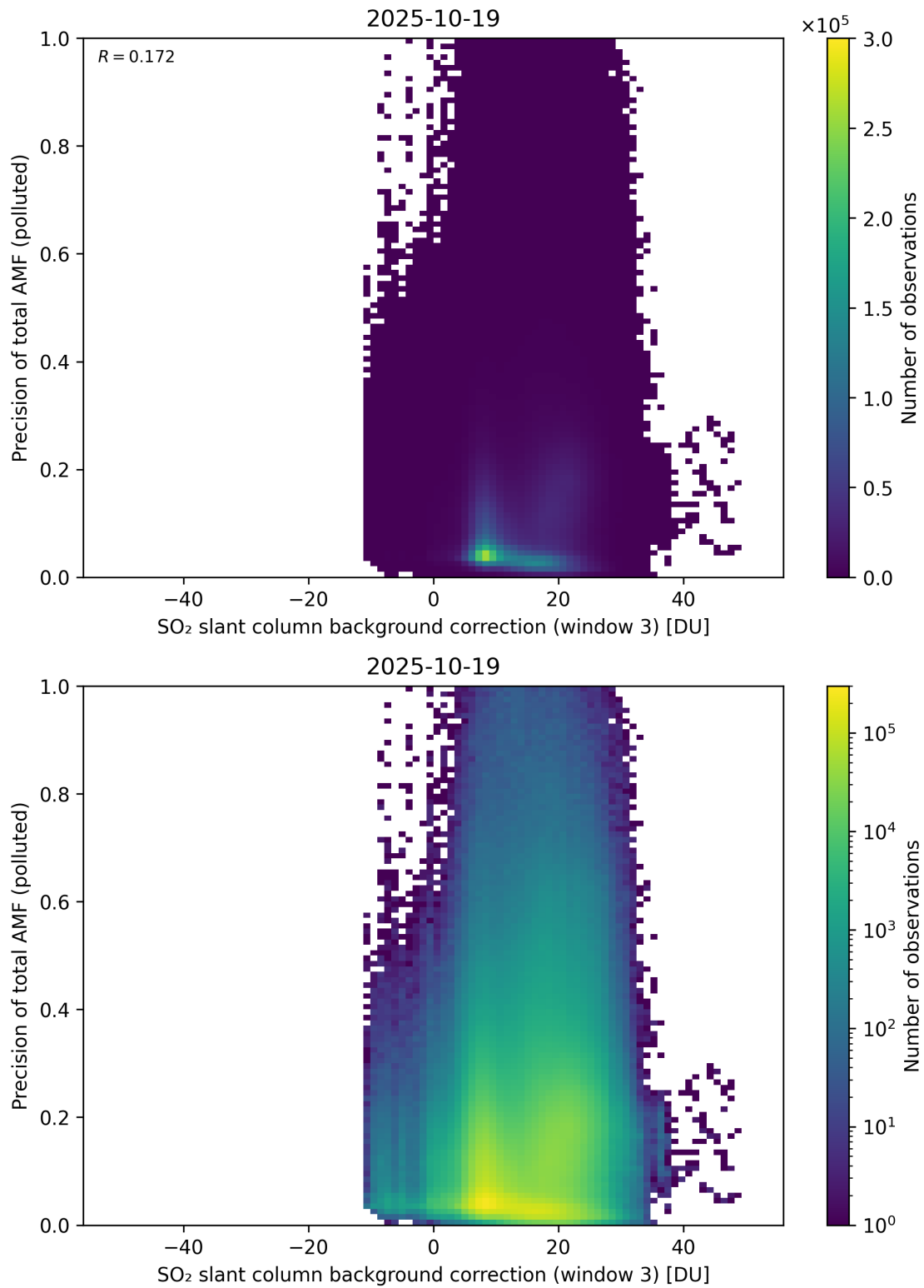
Figure 137: Scatter density plot of “SO 2 slant column background correction (window 3)” against “Precision of total AMF (polluted)” for 2025-10-18 to 2025-10-20.
