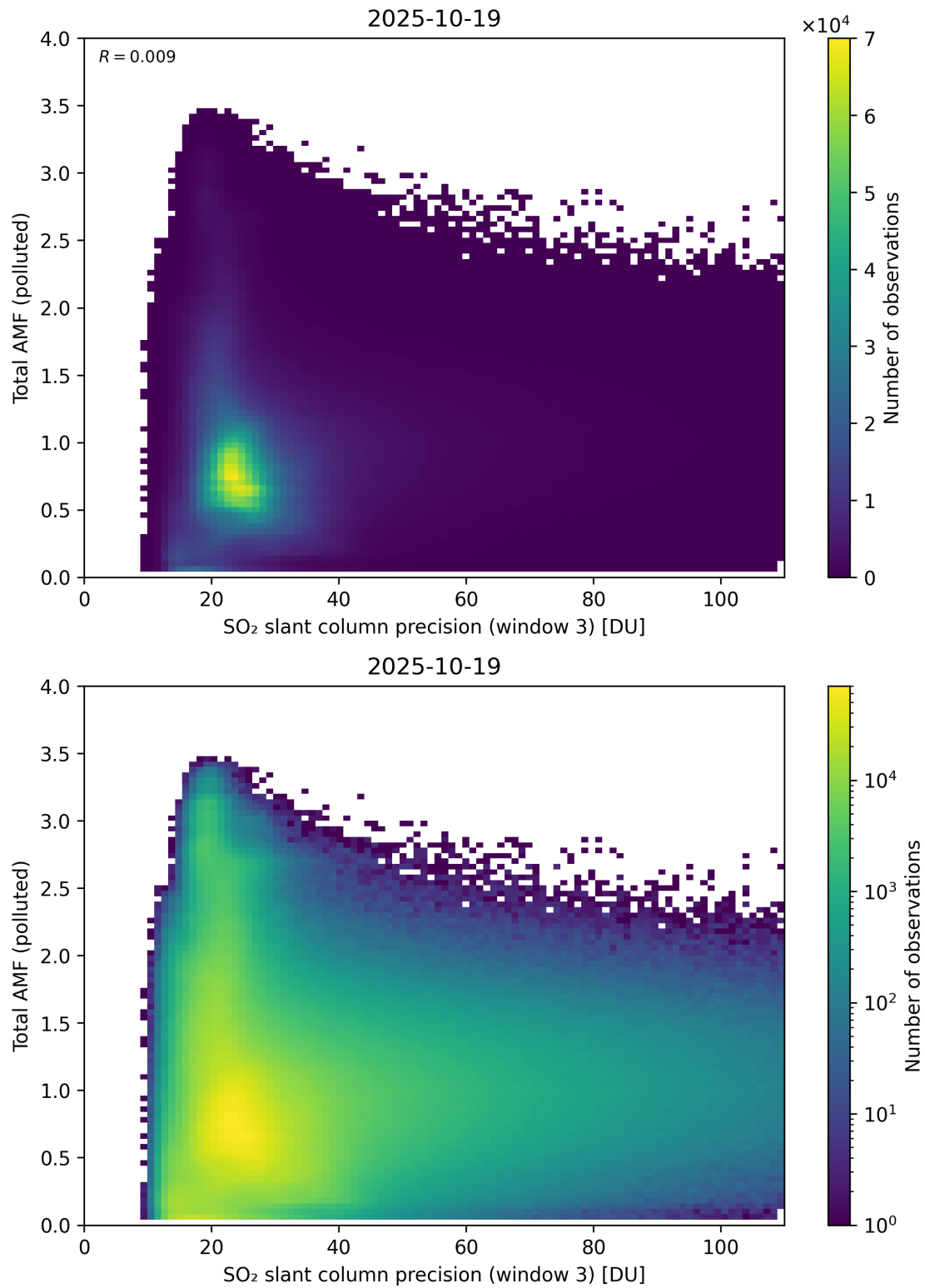
Figure 313: Scatter density plot of “SO 2 slant column precision (window 3)” against “Total AMF (polluted)” for 2025-10-18 to 2025-10-20.
