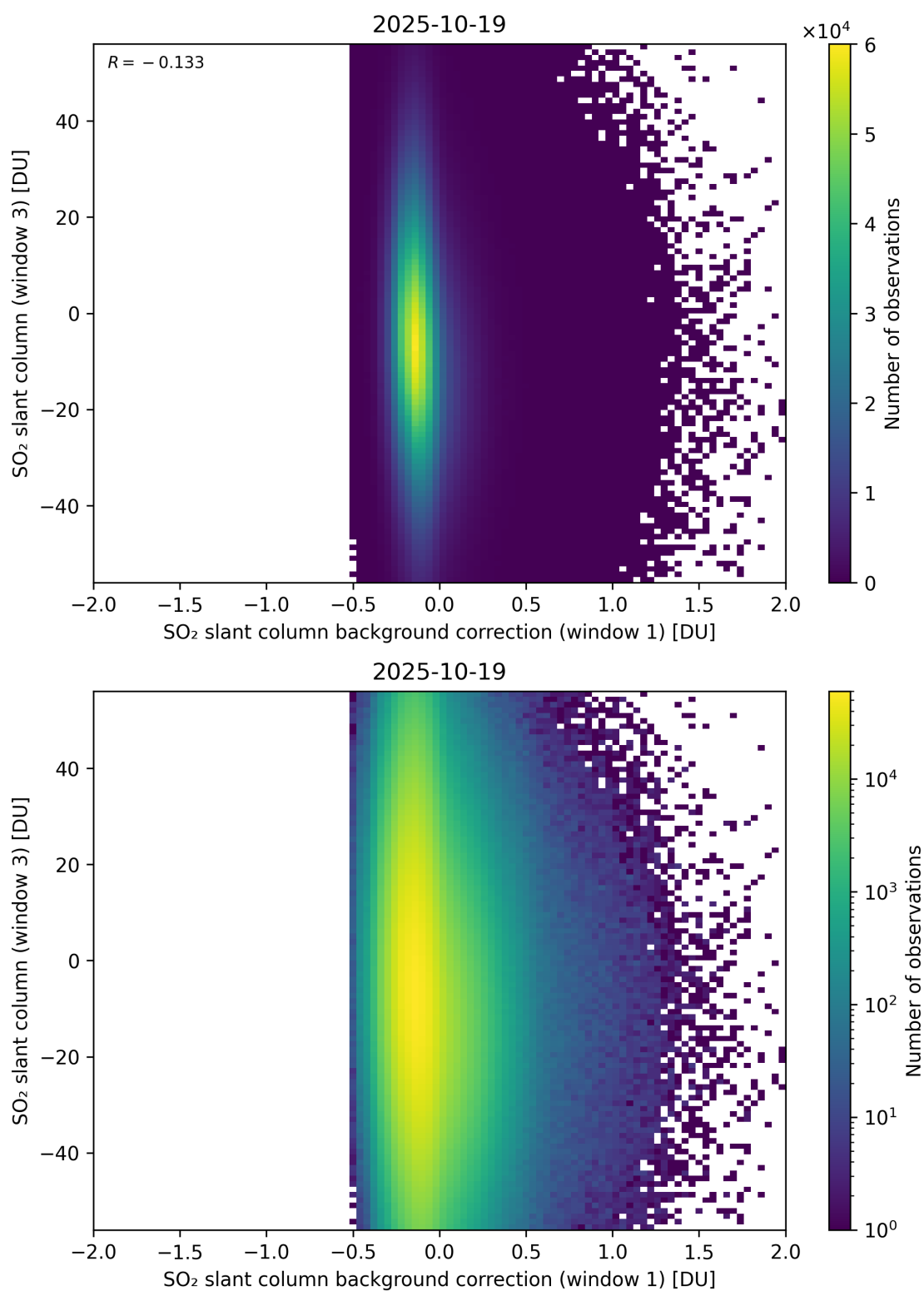
Figure 118: Scatter density plot of “SO 2 slant column background correction (window 1)” against “SO 2 slant column (window 3)” for 2025-10-18 to 2025-10-20.
