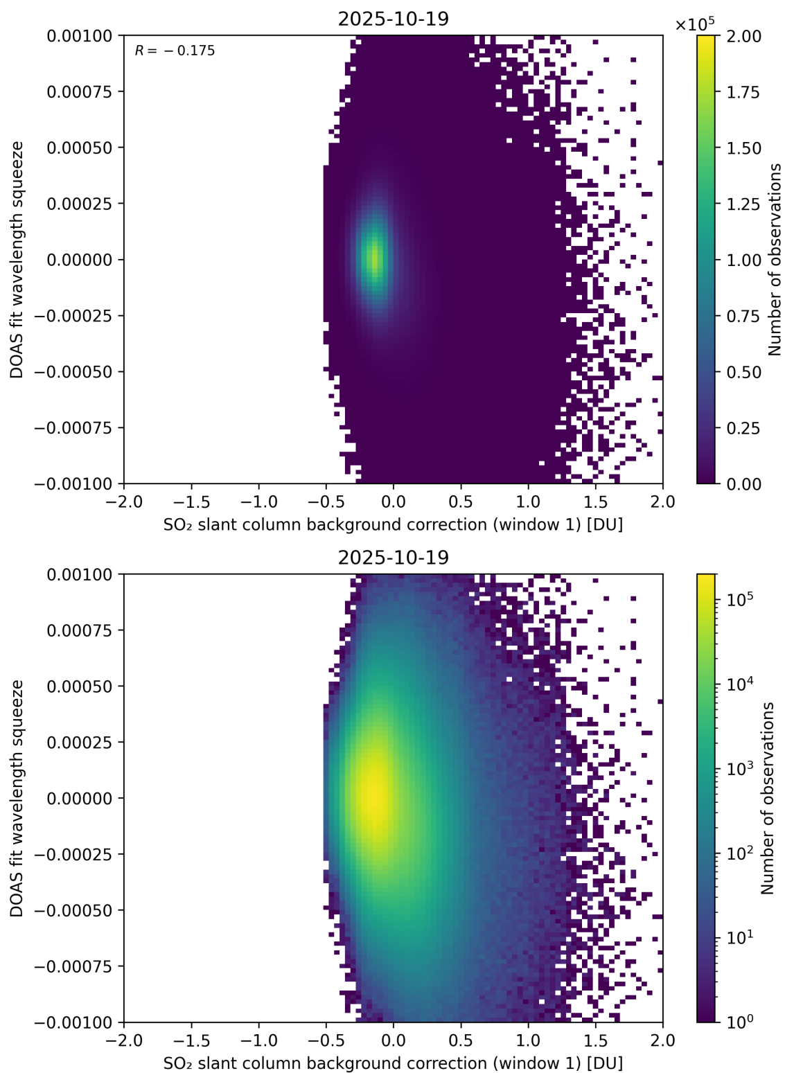
Figure 112: Scatter density plot of “SO 2 slant column background correction (window 1)” against “DOAS fit wavelength squeeze” for 2025-10-18 to 2025-10-20.
