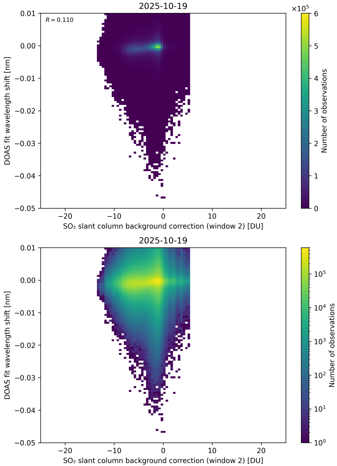
Figure 123: Scatter density plot of “SO 2 slant column background correction (window 2)” against “DOAS fit wavelength shift” for 2025-10-18 to 2025-10-20.
