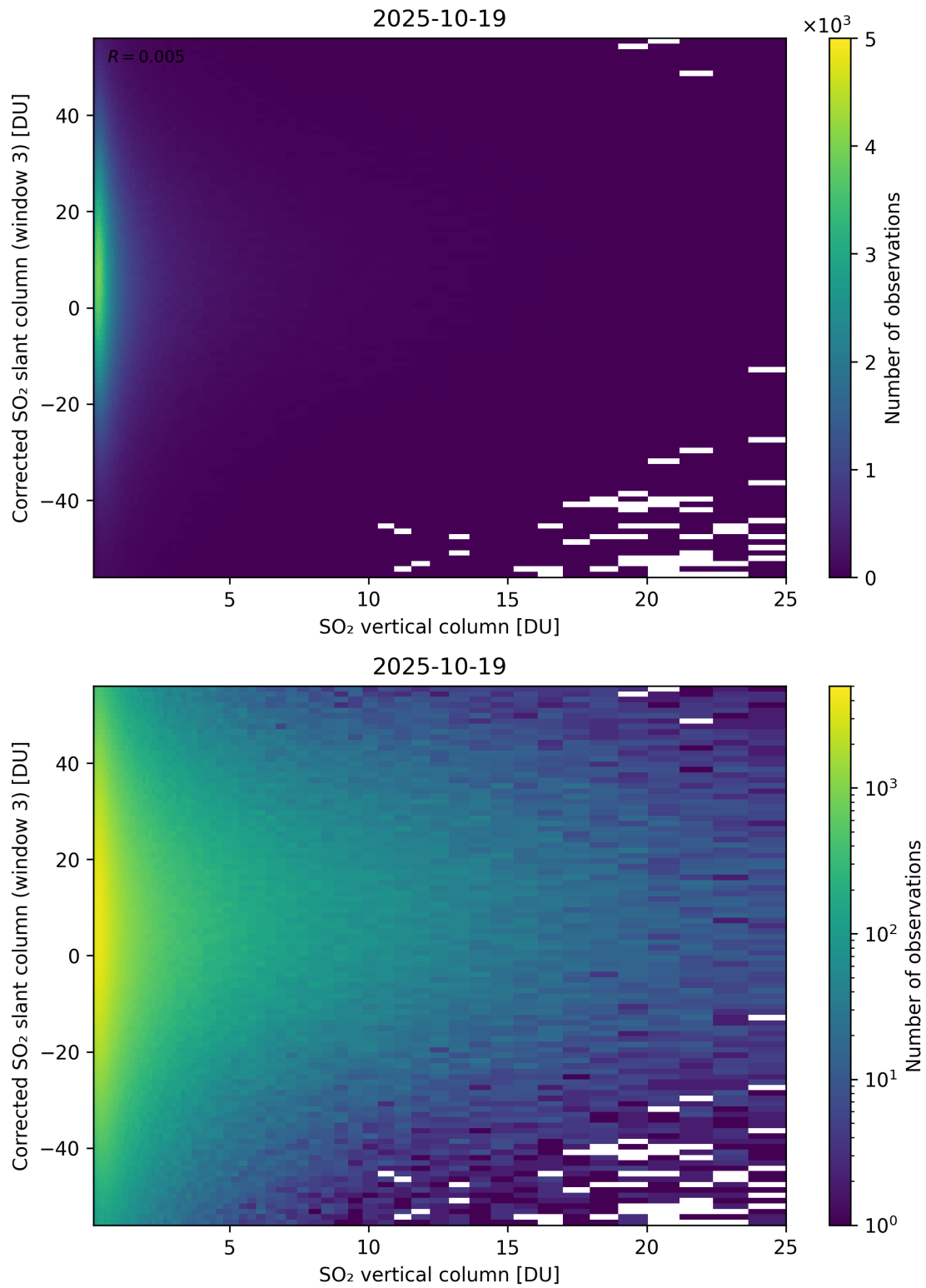
Figure 353: Scatter density plot of “SO 2 vertical column” against “Corrected SO 2 slant column (window 3)” for 2025-10-18 to 2025-10-20.
