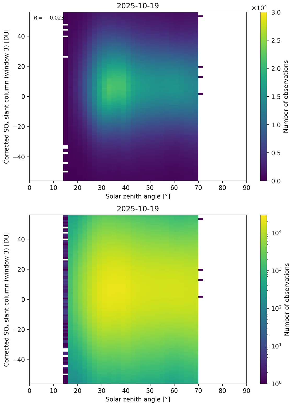
Figure 183: Scatter density plot of “Solar zenith angle” against “Corrected SO 2 slant column (window 3)” for 2025-10-18 to 2025-10-20.
