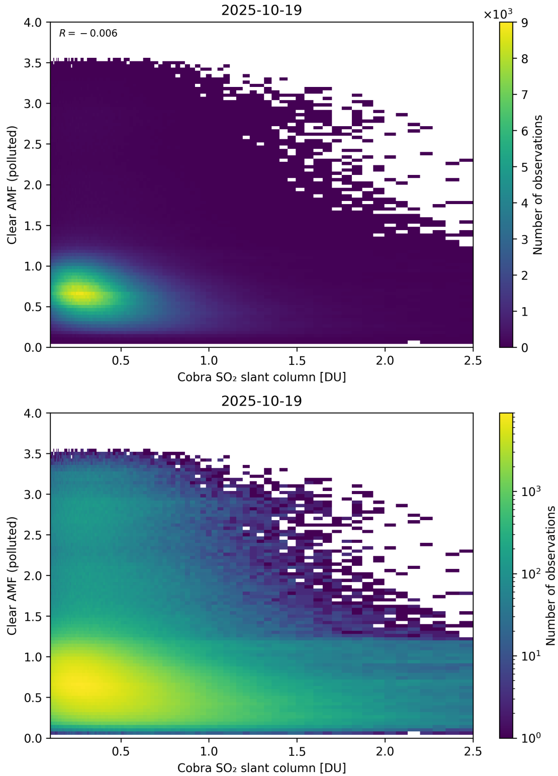
Figure 215: Scatter density plot of “Cobra SO 2 slant column” against “Clear AMF (polluted)” for 2025-10-18 to 2025-10-20.
