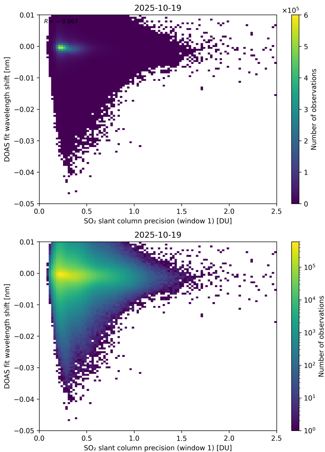
Figure 271: Scatter density plot of “SO 2 slant column precision (window 1)” against “DOAS fit wavelength shift” for 2025-10-18 to 2025-10-20.
