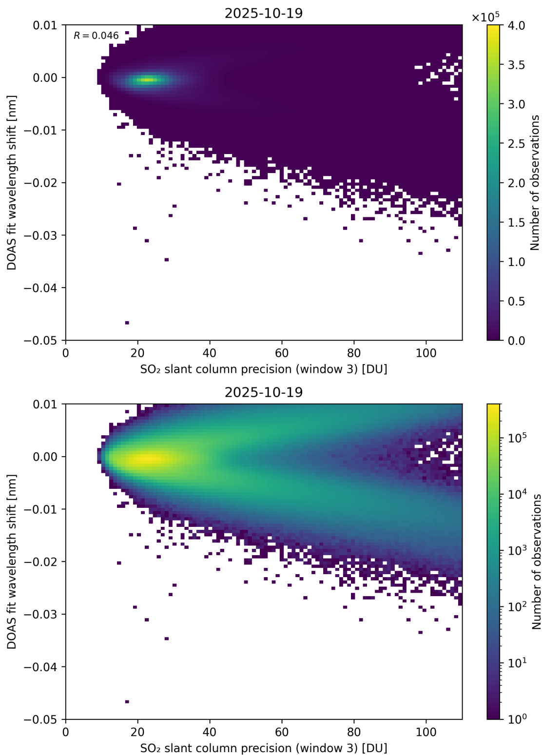
Figure 308: Scatter density plot of “SO 2 slant column precision (window 3)” against “DOAS fit wavelength shift” for 2025-10-18 to 2025-10-20.
