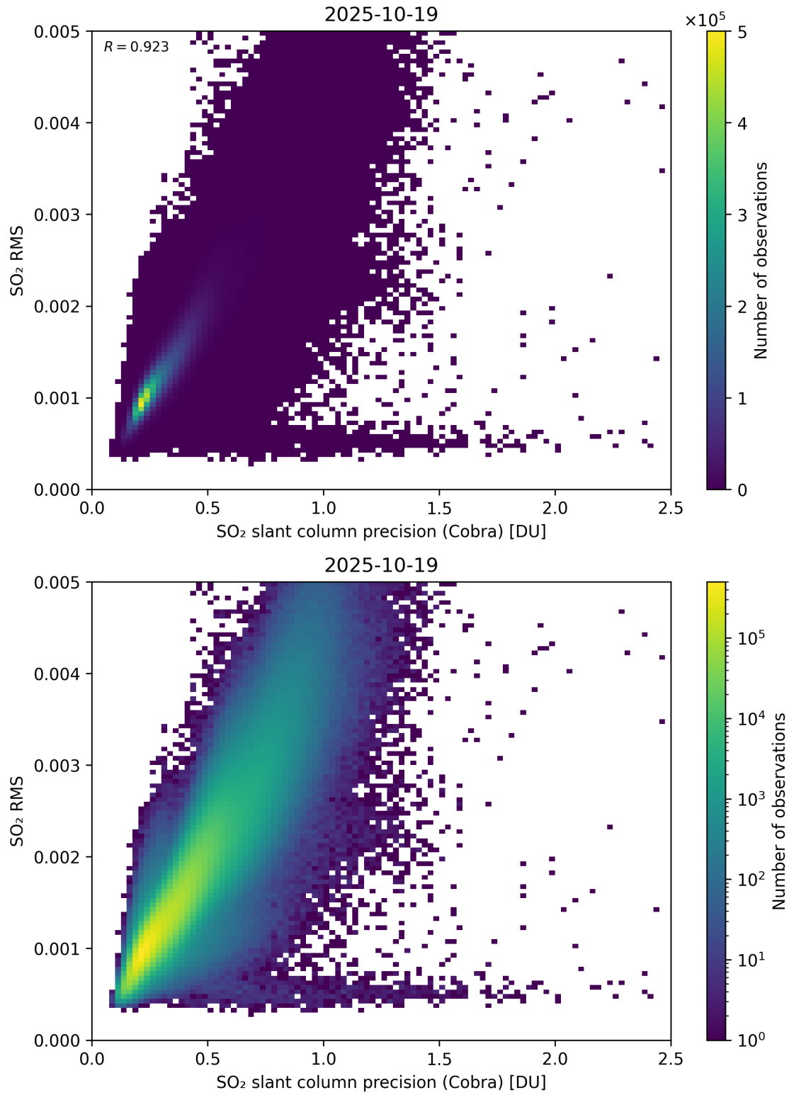
Figure 204: Scatter density plot of “SO 2 slant column precision (Cobra)” against “SO 2 RMS” for 2025-10-18 to 2025-10-20.
