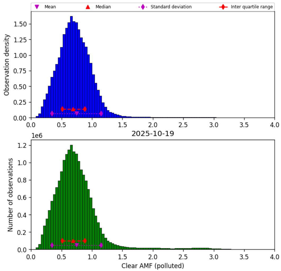
Figure 81: Histogram of “Clear AMF (polluted)” for 2025-10-18 to 2025-10-20
