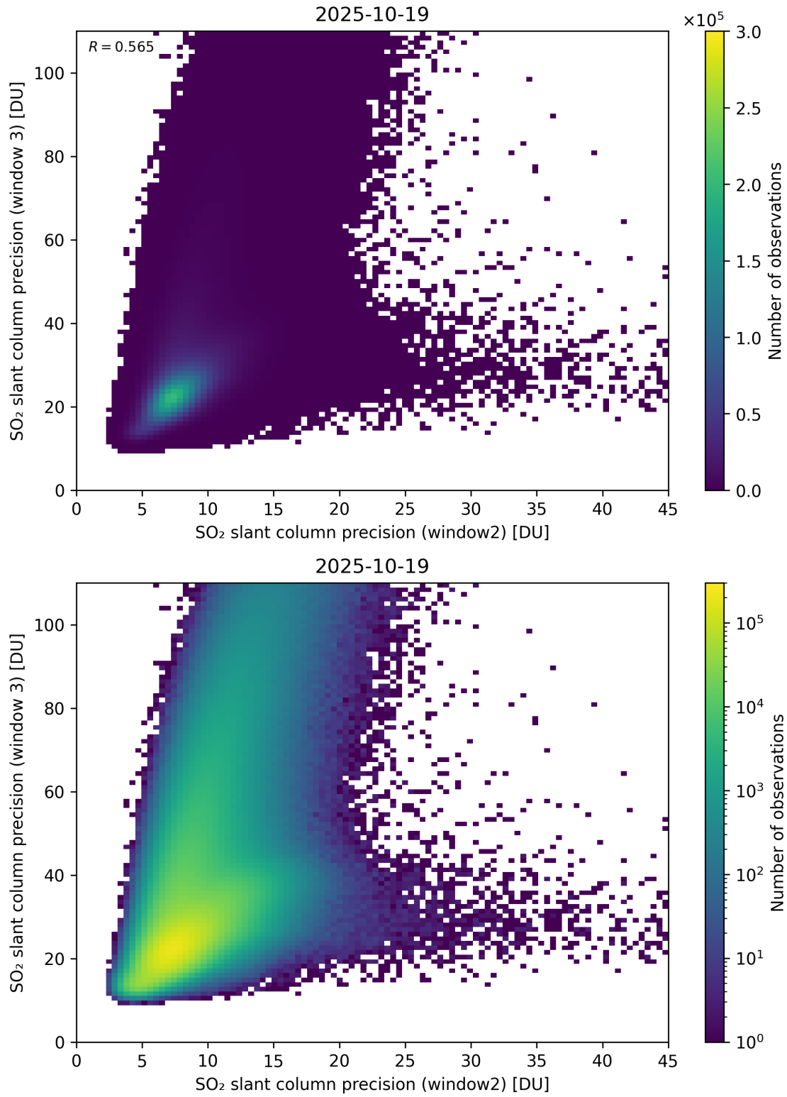
Figure 300: Scatter density plot of “SO 2 slant column precision (window2)” against “SO 2 slant column precision (window 3)” for 2025-10-18 to 2025-10-20.
