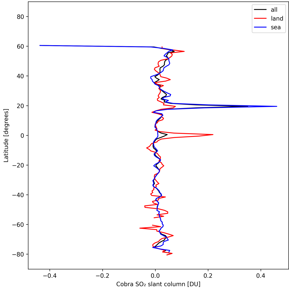
Figure 35: Zonal average of “Cobra SO 2 slant column” for 2025-10-18 to 2025-10-20.
