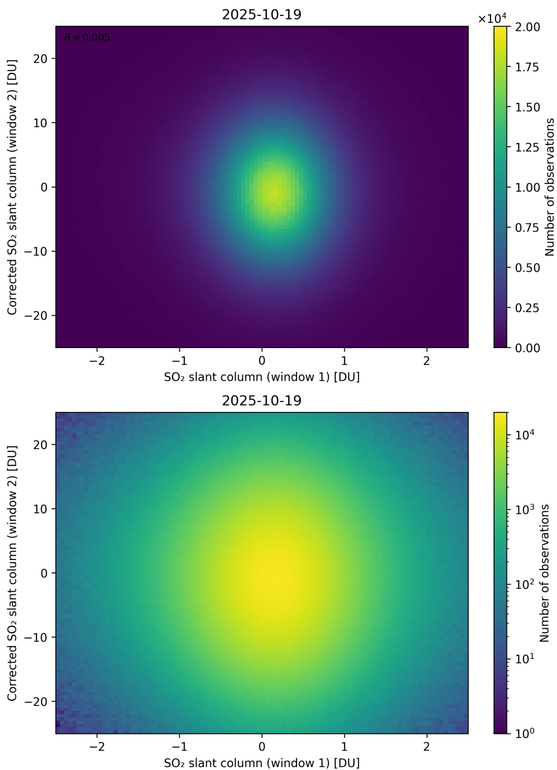
Figure 283: Scatter density plot of “SO 2 slant column (window 1)” against “Corrected SO 2 slant column (window 2)” for 2025-10-18 to 2025-10-20.
