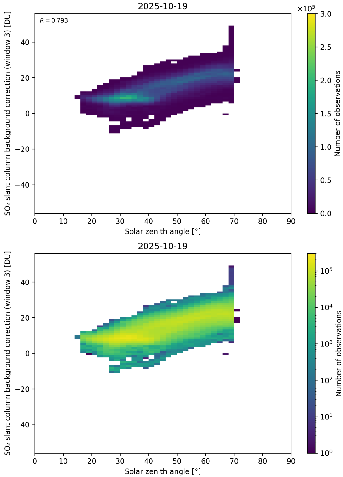
Figure 173: Scatter density plot of “Solar zenith angle” against “SO 2 slant column background correction (window 3)” for 2025-10-18 to 2025-10-20.
