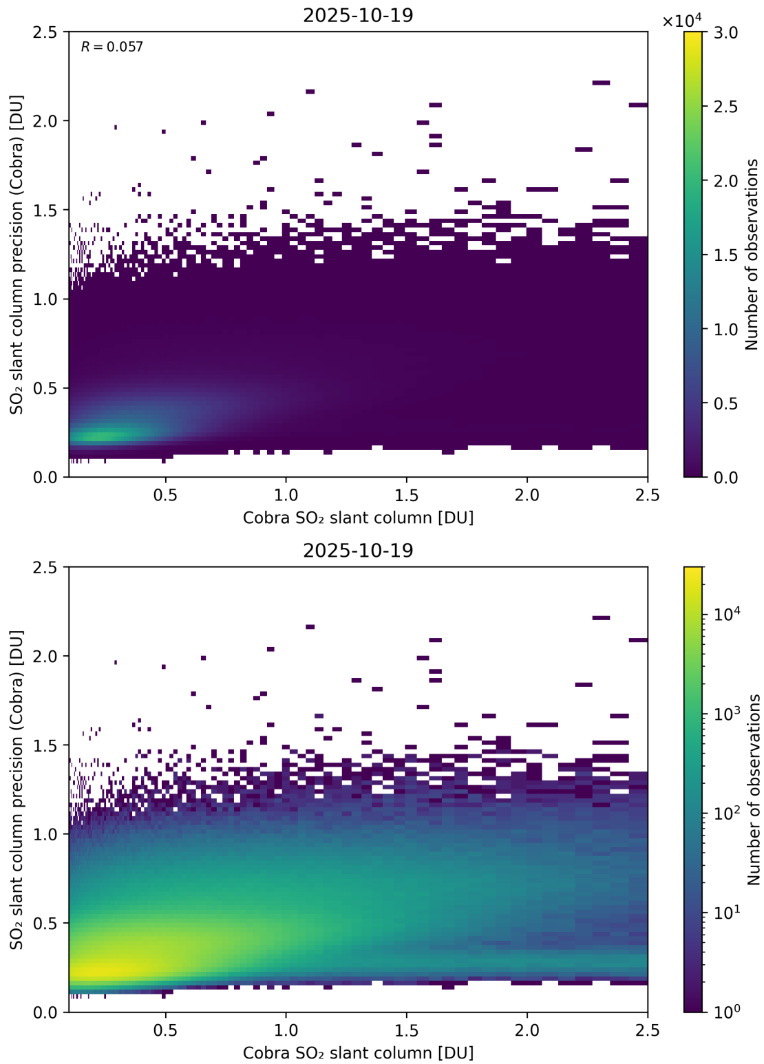
Figure 216: Scatter density plot of “Cobra SO 2 slant column” against “SO 2 slant column precision (Cobra)” for 2025-10-18 to 2025-10-20.
