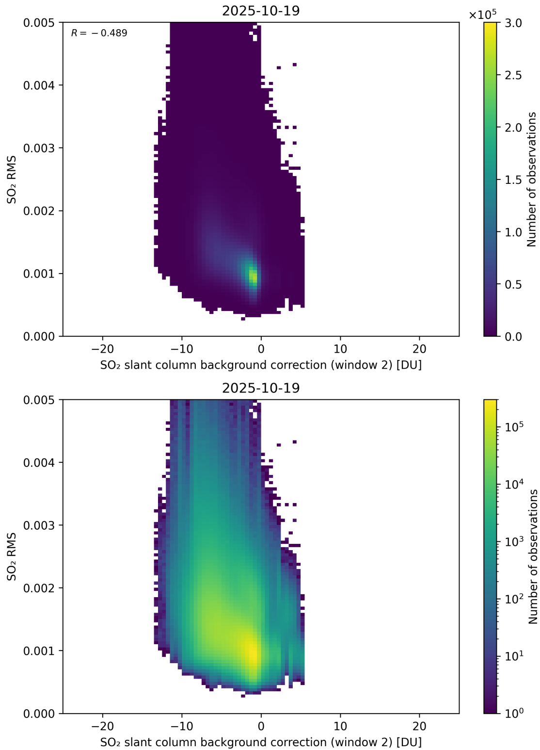
Figure 125: Scatter density plot of “SO 2 slant column background correction (window 2)” against “SO 2 RMS” for 2025-10-18 to 2025-10-20.
