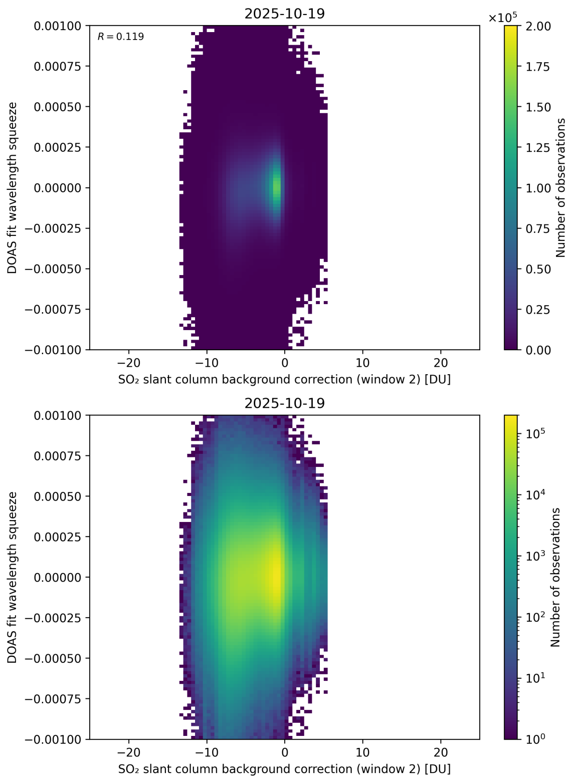
Figure 124: Scatter density plot of “SO 2 slant column background correction (window 2)” against “DOAS fit wavelength squeeze” for 2025-10-18 to 2025-10-20.
