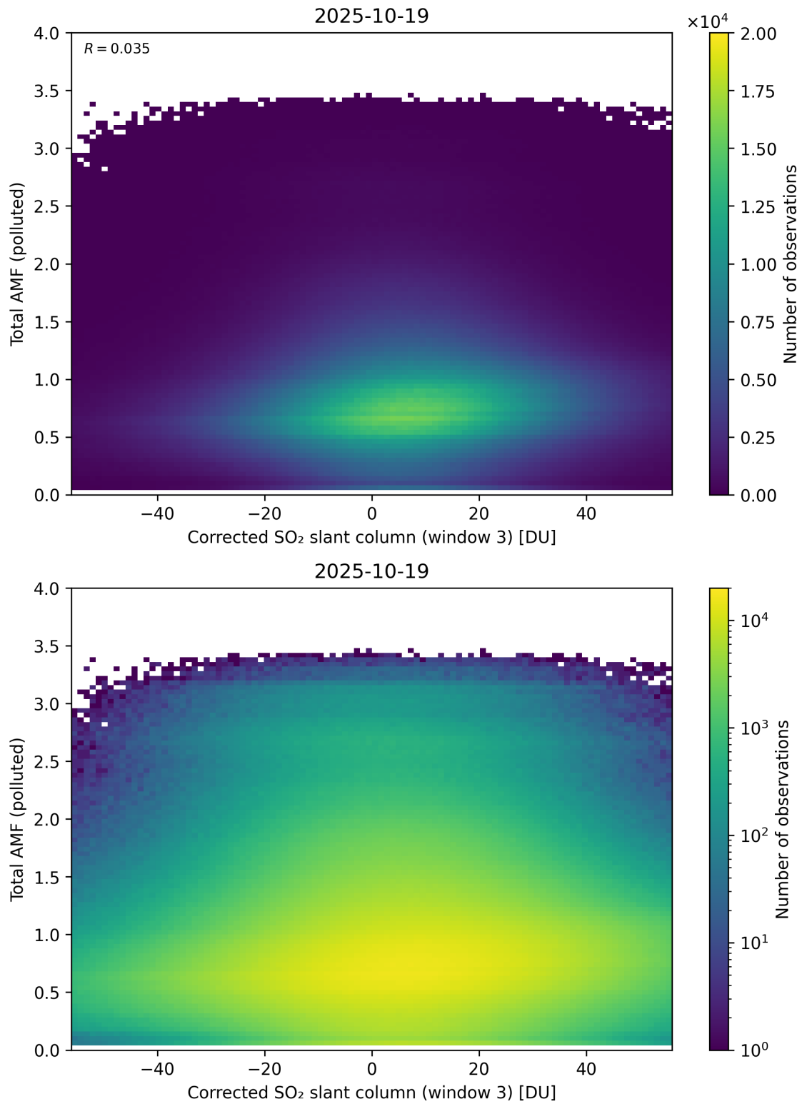
Figure 260: Scatter density plot of “Corrected SO 2 slant column (window 3)” against “Total AMF (polluted)” for 2025-10-18 to 2025-10-20.
