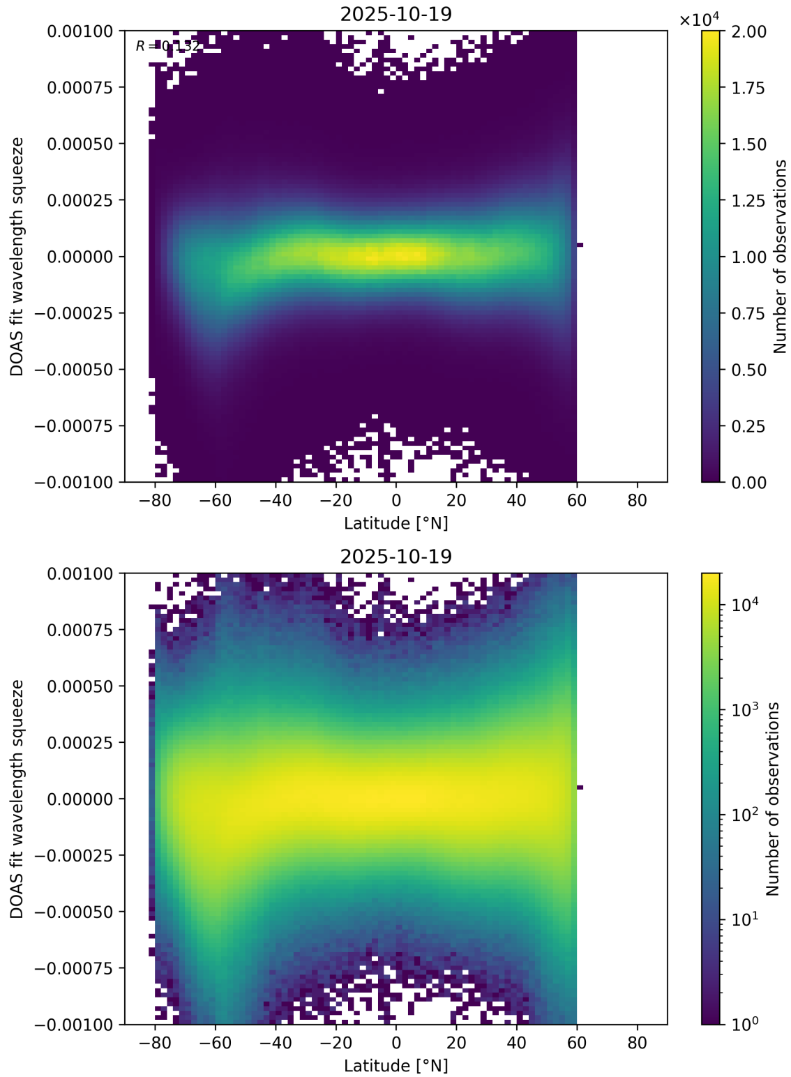
Figure 154: Scatter density plot of “Latitude” against “DOAS fit wavelength squeeze” for 2025-10-18 to 2025-10-20.
