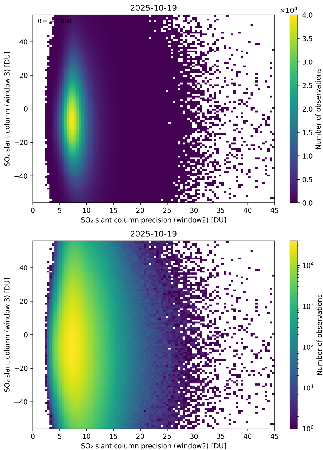
Figure 299: Scatter density plot of “SO 2 slant column precision (window2)” against “SO 2 slant column (window 3)” for 2025-10-18 to 2025-10-20.
