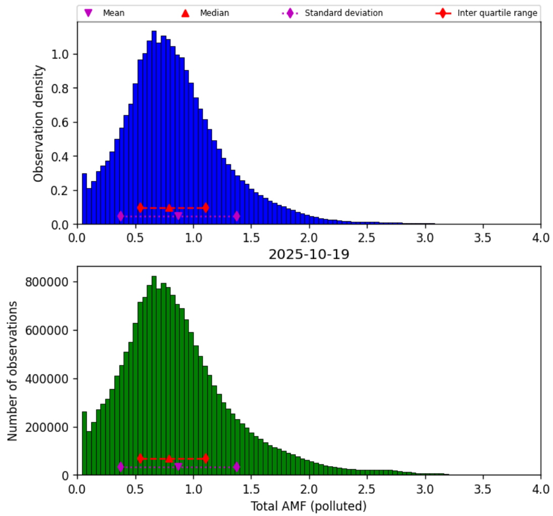
Figure 79: Histogram of “Total AMF (polluted)” for 2025-10-18 to 2025-10-20
