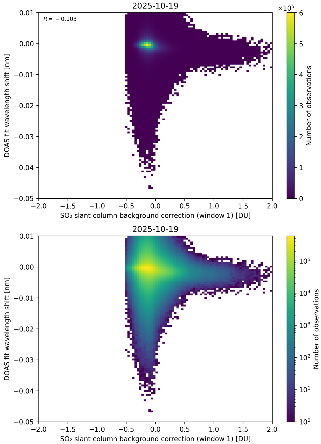
Figure 111: Scatter density plot of “SO 2 slant column background correction (window 1)” against “DOAS fit wavelength shift” for 2025-10-18 to 2025-10-20.
