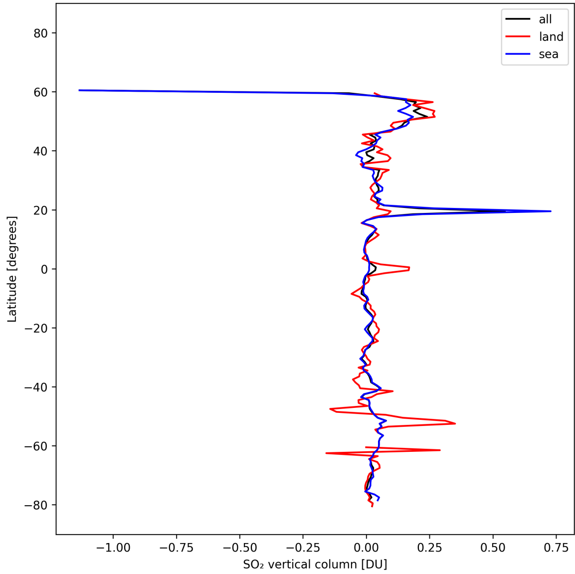
Figure 32: Zonal average of “SO 2 vertical column” for 2025-10-18 to 2025-10-20.
