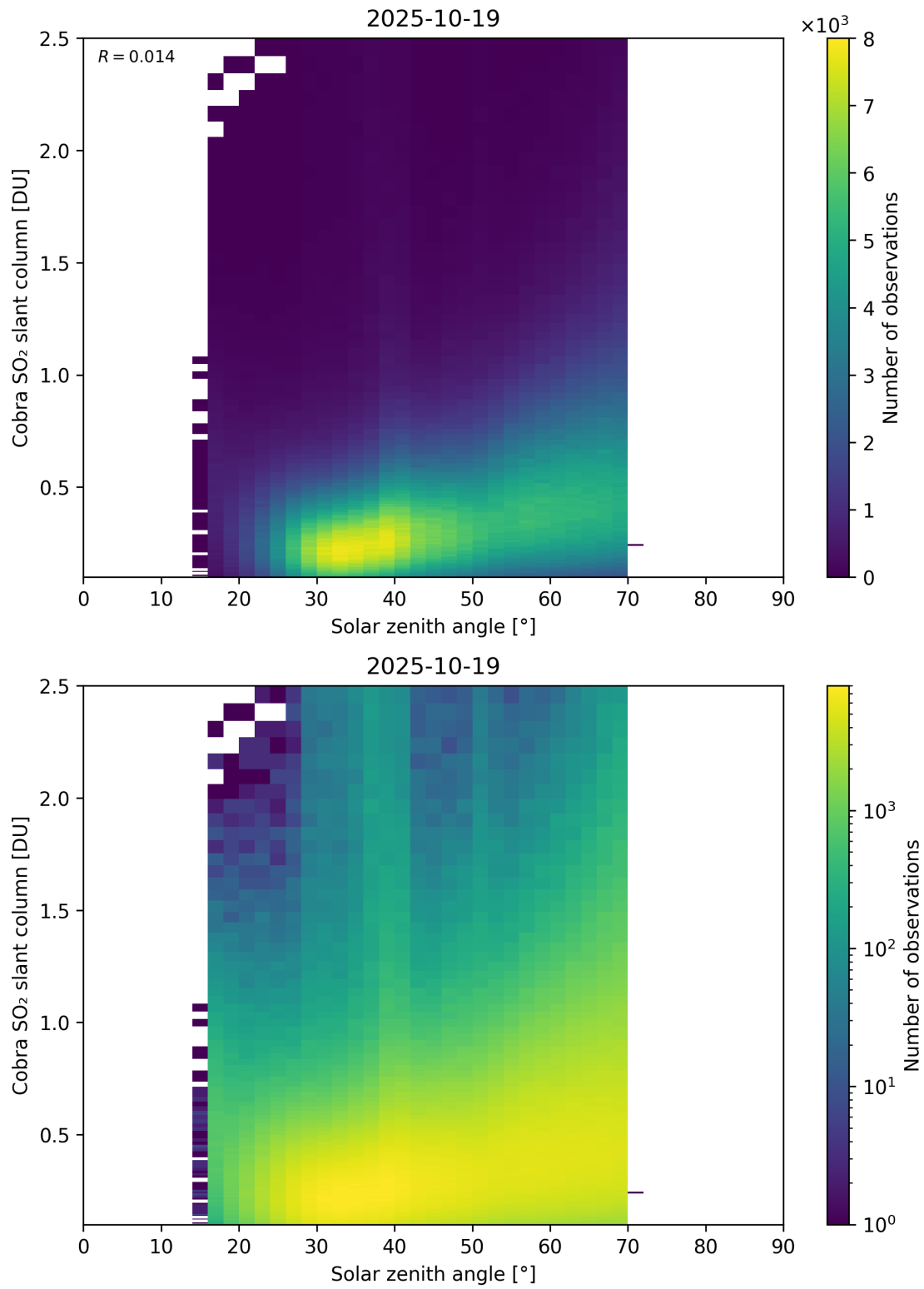
Figure 179: Scatter density plot of “Solar zenith angle” against “Cobra SO 2 slant column” for 2025-10-18 to 2025-10-20.
