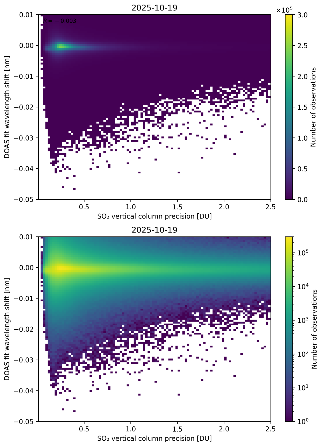
Figure 332: Scatter density plot of “SO 2 vertical column precision” against “DOAS fit wavelength shift” for 2025-10-18 to 2025-10-20.
