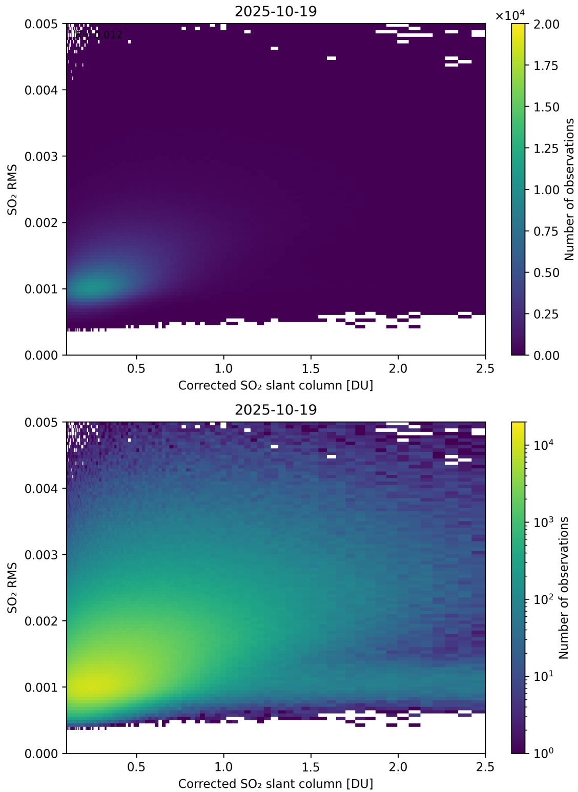
Figure 231: Scatter density plot of “Corrected SO 2 slant column” against “SO 2 RMS” for 2025-10-18 to 2025-10-20.
