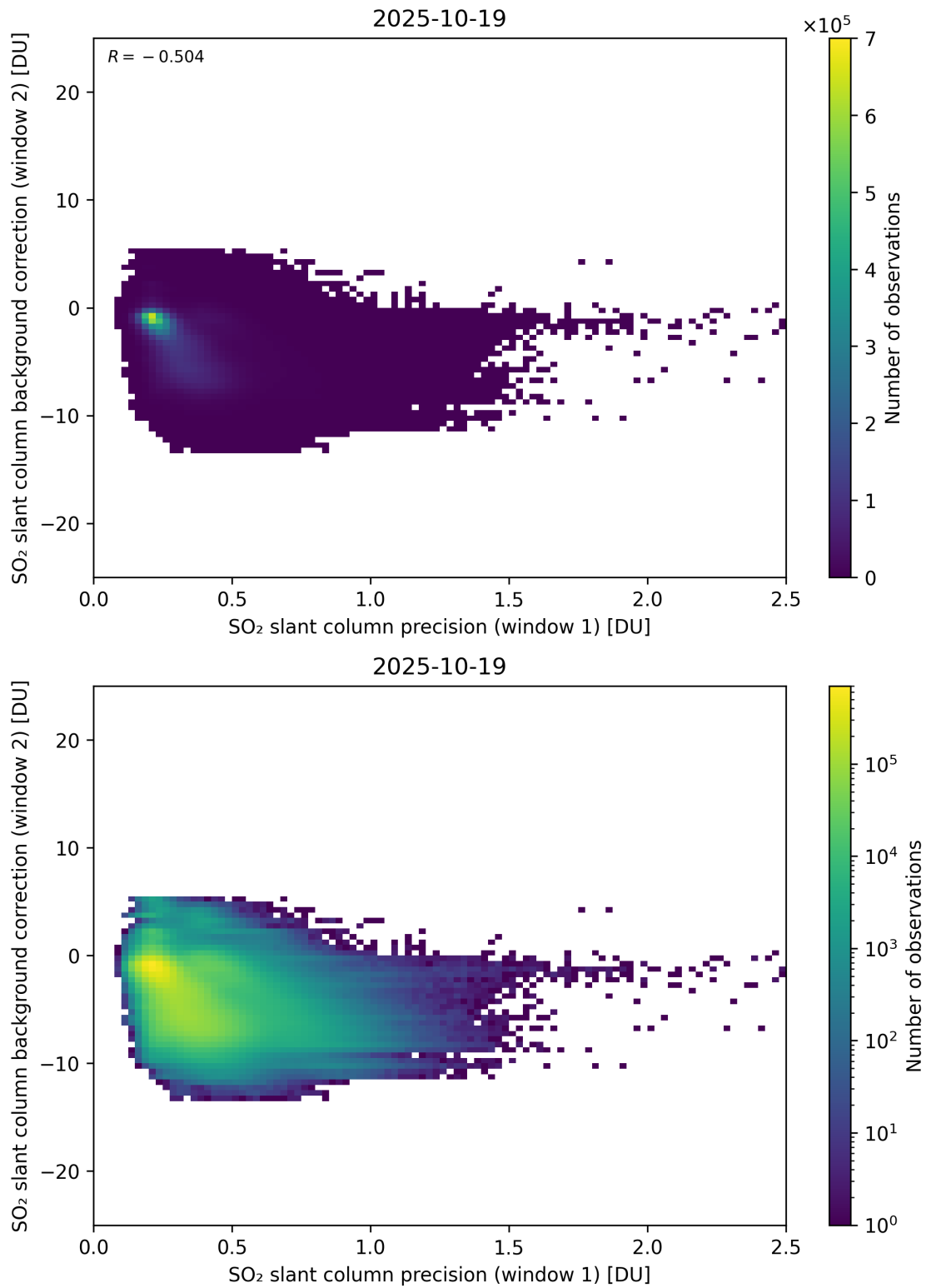
Figure 269: Scatter density plot of “SO 2 slant column precision (window 1)” against “SO 2 slant column background correction (window 2)” for 2025-10-18 to 2025-10-20.
