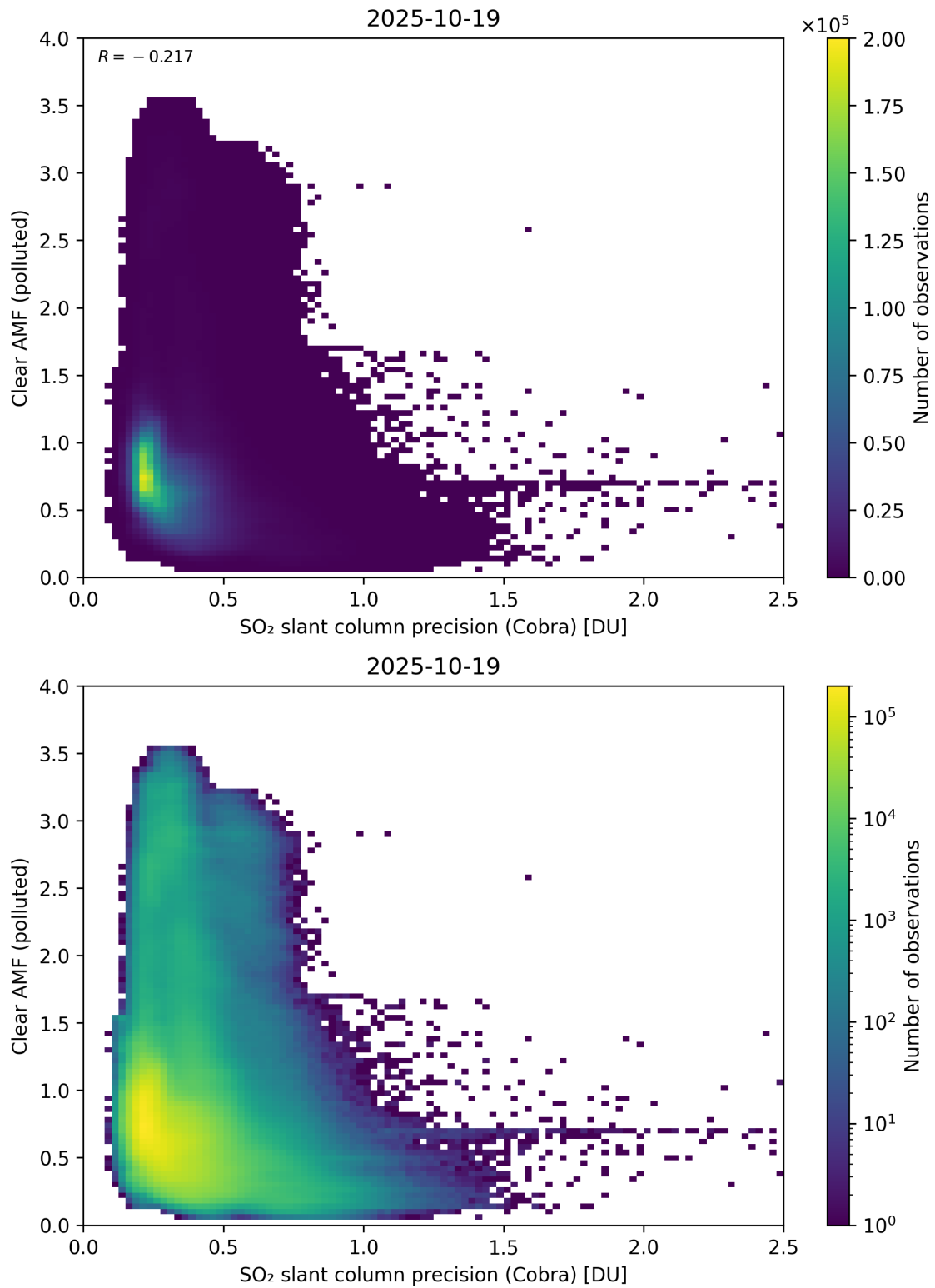
Figure 205: Scatter density plot of “SO 2 slant column precision (Cobra)” against “Clear AMF (polluted)” for 2025-10-18 to 2025-10-20.
