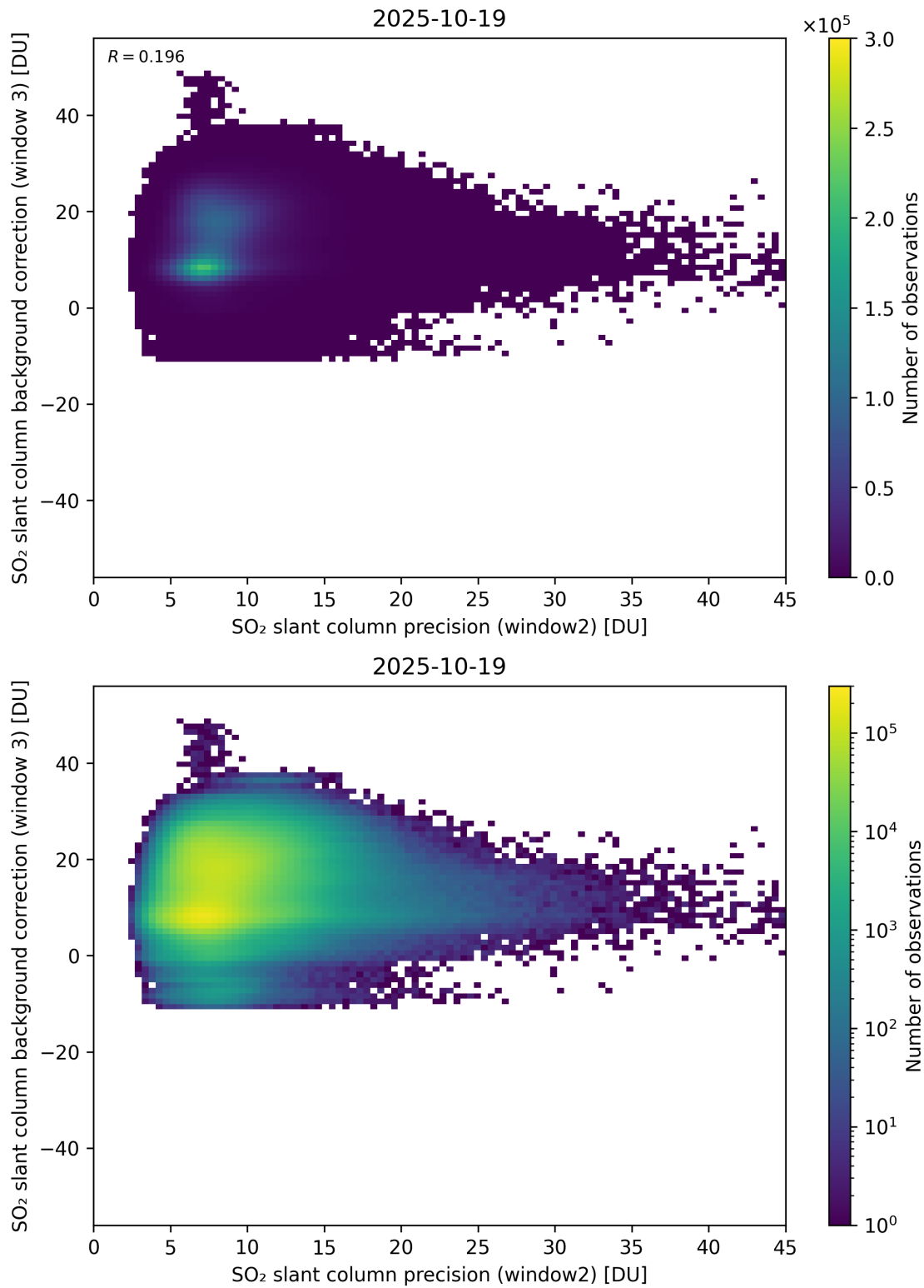
Figure 292: Scatter density plot of “SO 2 slant column precision (window2)” against “SO 2 slant column background correction (window 3)” for 2025-10-18 to 2025-10-20.
