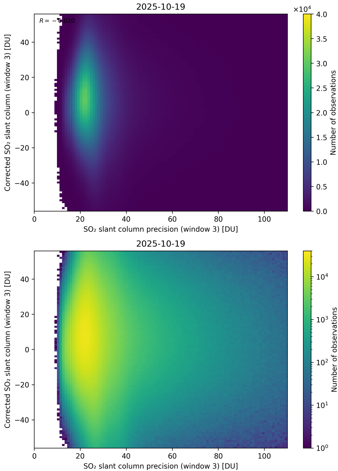
Figure 312: Scatter density plot of “SO 2 slant column precision (window 3)” against “Corrected SO 2 slant column (window 3)” for 2025-10-18 to 2025-10-20.
