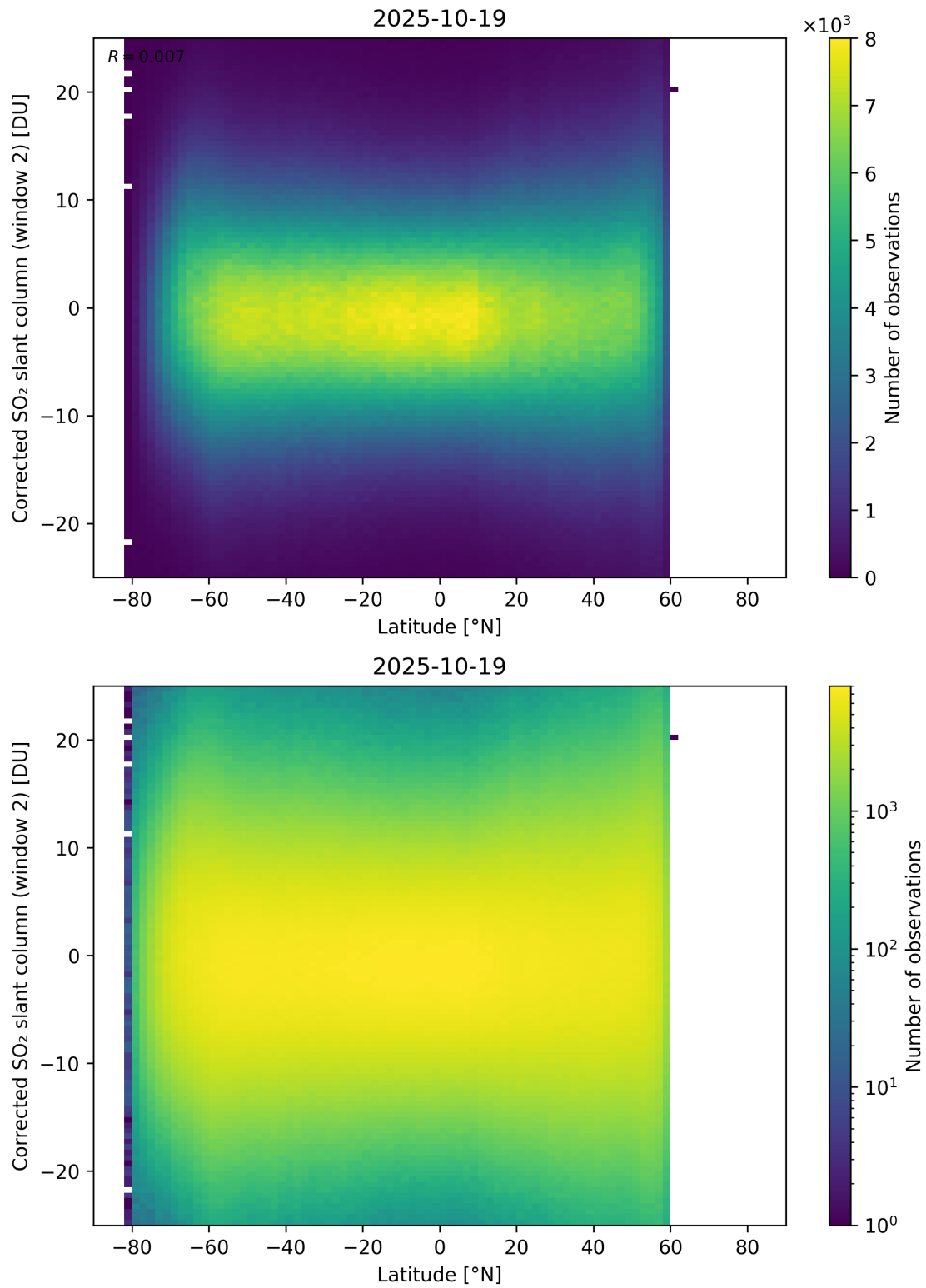
Figure 160: Scatter density plot of “Latitude” against “Corrected SO 2 slant column (window 2)” for 2025-10-18 to 2025-10-20.
