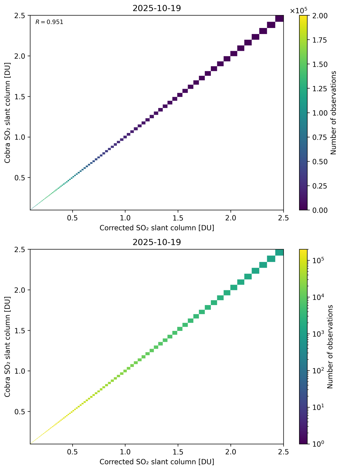
Figure 233: Scatter density plot of “Corrected SO 2 slant column” against “Cobra SO 2 slant column” for 2025-10-18 to 2025-10-20.
