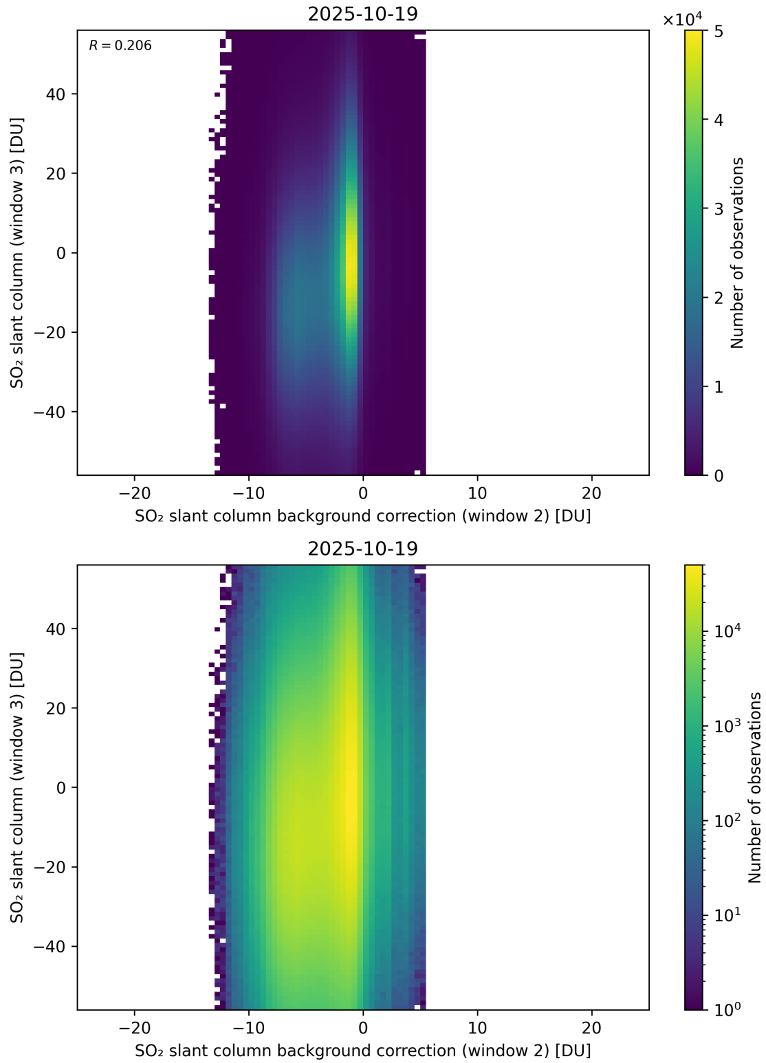
Figure 128: Scatter density plot of “SO 2 slant column background correction (window 2)” against “SO 2 slant column (window 3)” for 2025-10-18 to 2025-10-20.
