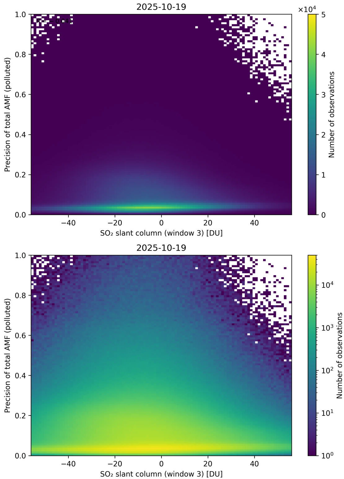
Figure 319: Scatter density plot of “SO 2 slant column (window 3)” against “Precision of total AMF (polluted)” for 2025-10-18 to 2025-10-20.
