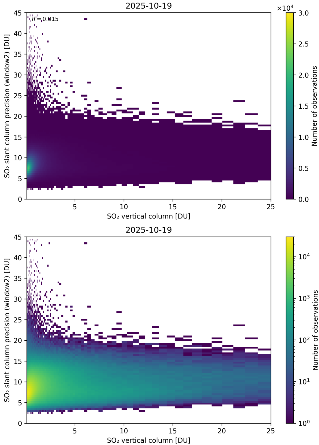
Figure 356: Scatter density plot of “SO 2 vertical column” against “SO 2 slant column precision (window2)” for 2025-10-18 to 2025-10-20.
