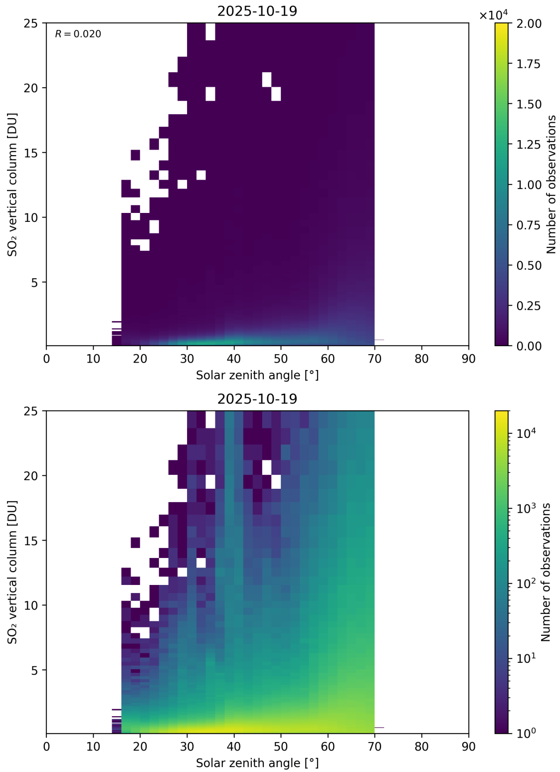
Figure 191: Scatter density plot of “Solar zenith angle” against “SO 2 vertical column” for 2025-10-18 to 2025-10-20.
