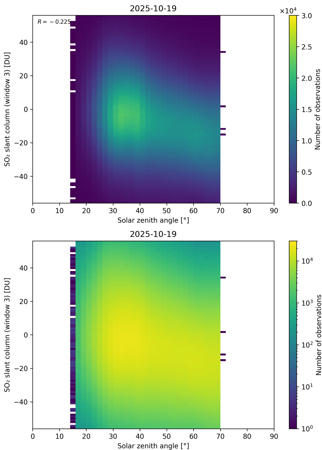
Figure 187: Scatter density plot of “Solar zenith angle” against “SO 2 slant column (window 3)” for 2025-10-18 to 2025-10-20.
