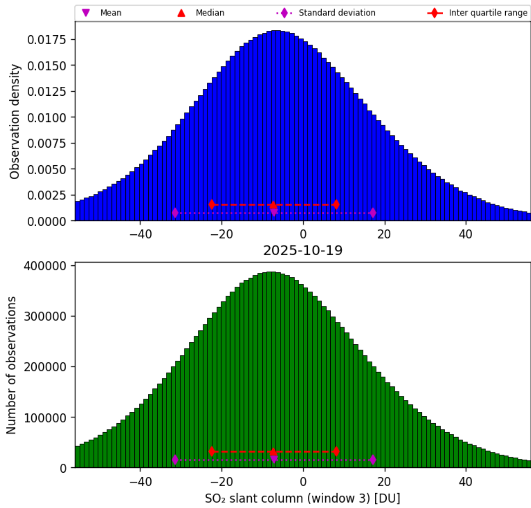
Figure 71: Histogram of “SO 2 slant column (window 3)” for 2025-10-18 to 2025-10-20
