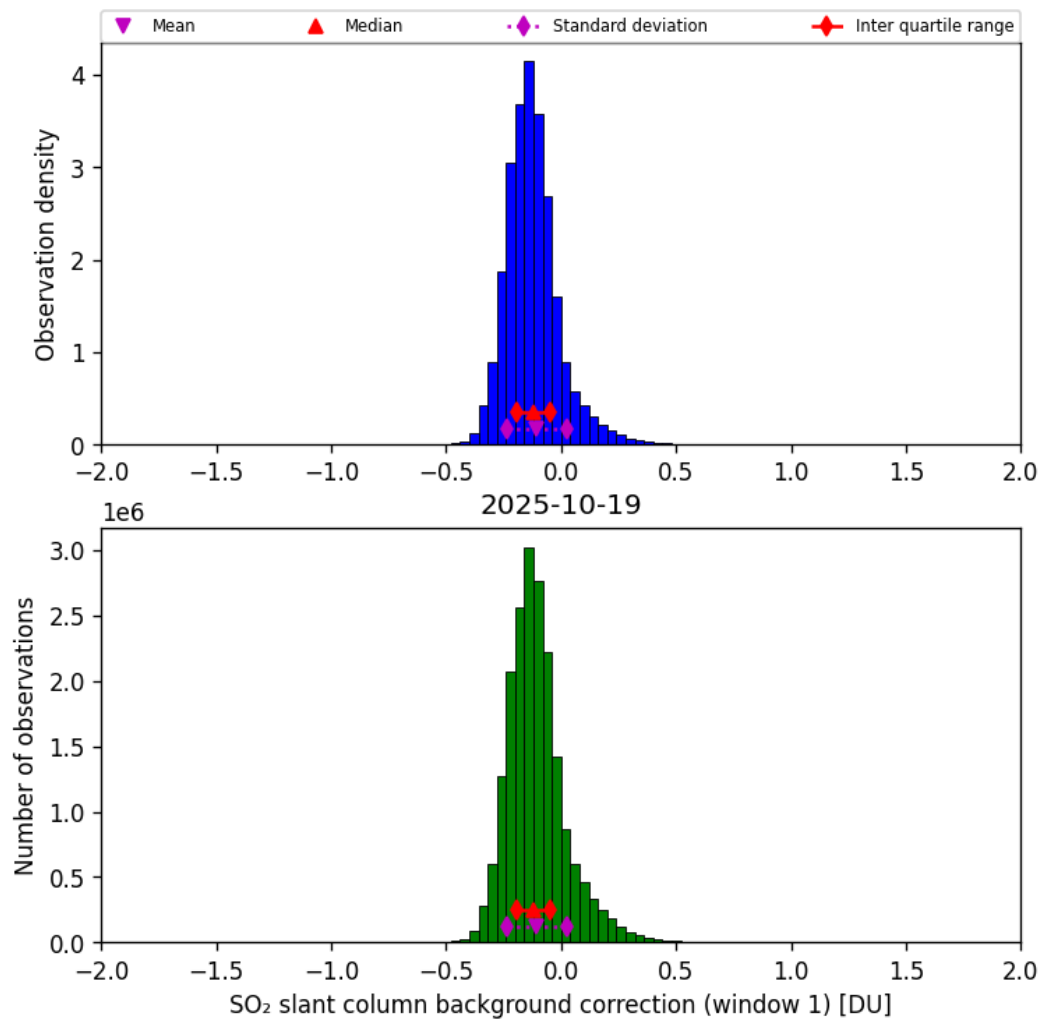
Figure 66: Histogram of “SO 2 slant column background correction (window 1)” for 2025-10-18 to 2025-10-20
