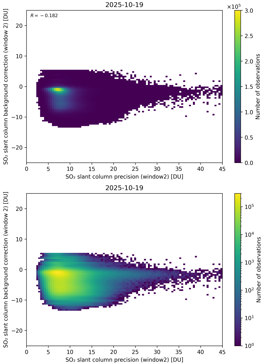
Figure 291: Scatter density plot of “SO 2 slant column precision (window2)” against “SO 2 slant column background correction (window 2)” for 2025-10-18 to 2025-10-20.
