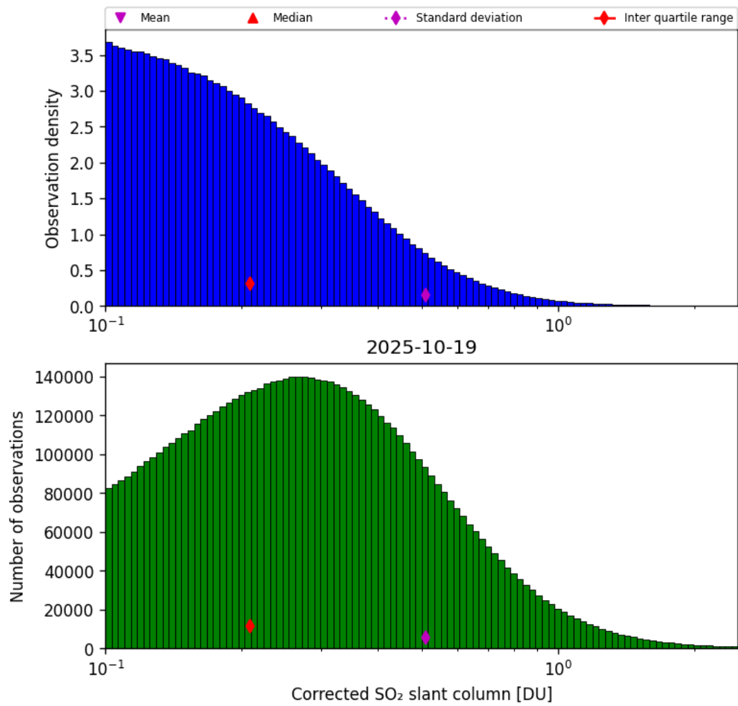
Figure 60: Histogram of "Corrected SO 2 slant column" for 2025-10-18 to 2025-10-20
