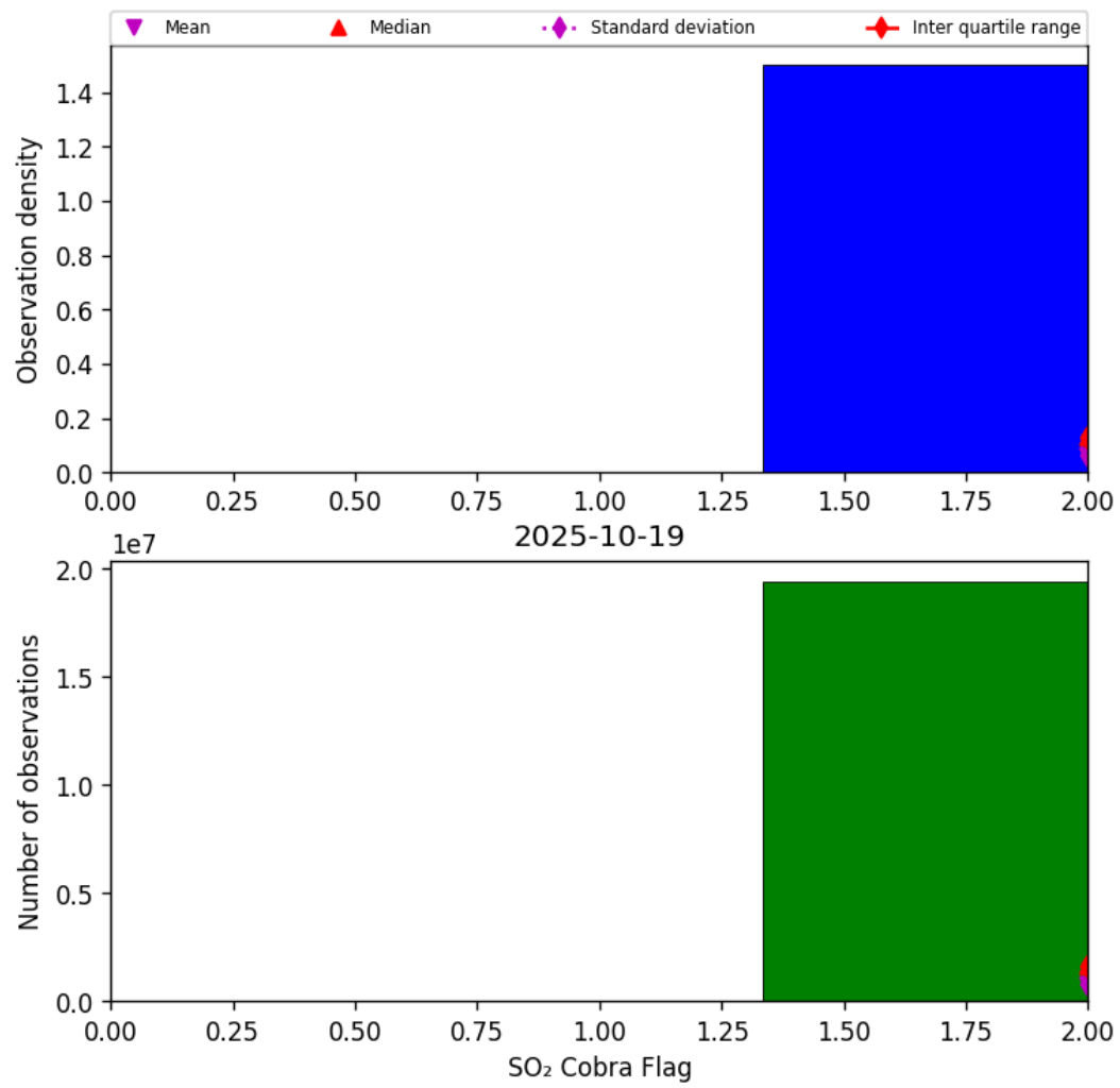
Figure 75: Histogram of “SO 2 Cobra Flag” for 2025-10-18 to 2025-10-20
