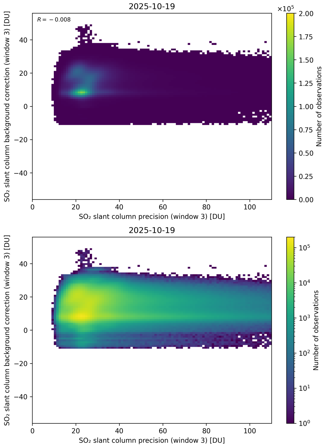
Figure 307: Scatter density plot of “SO 2 slant column precision (window 3)” against “SO 2 slant column background correction (window 3)” for 2025-10-18 to 2025-10-20.
