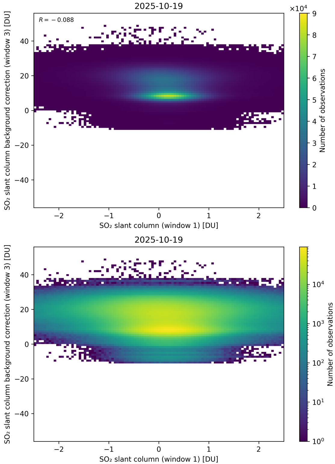
Figure 264: Scatter density plot of “SO 2 slant column (window 1)” against “SO 2 slant column background correction (window 3)” for 2025-10-18 to 2025-10-20.
