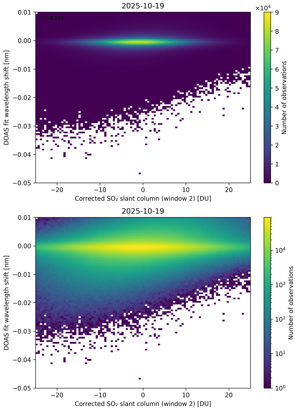
Figure 246: Scatter density plot of “Corrected SO 2 slant column (window 2)” against “DOAS fit wavelength shift” for 2025-10-18 to 2025-10-20.
