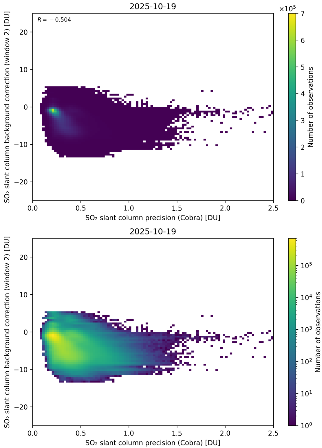
Figure 200: Scatter density plot of “SO 2 slant column precision (Cobra)” against “SO 2 slant column background correction (window 2)” for 2025-10-18 to 2025-10-20.
