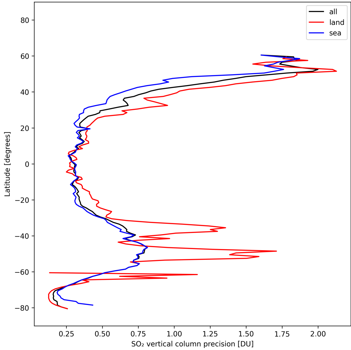
Figure 33: Zonal average of “SO 2 vertical column precision” for 2025-10-18 to 2025-10-20.
