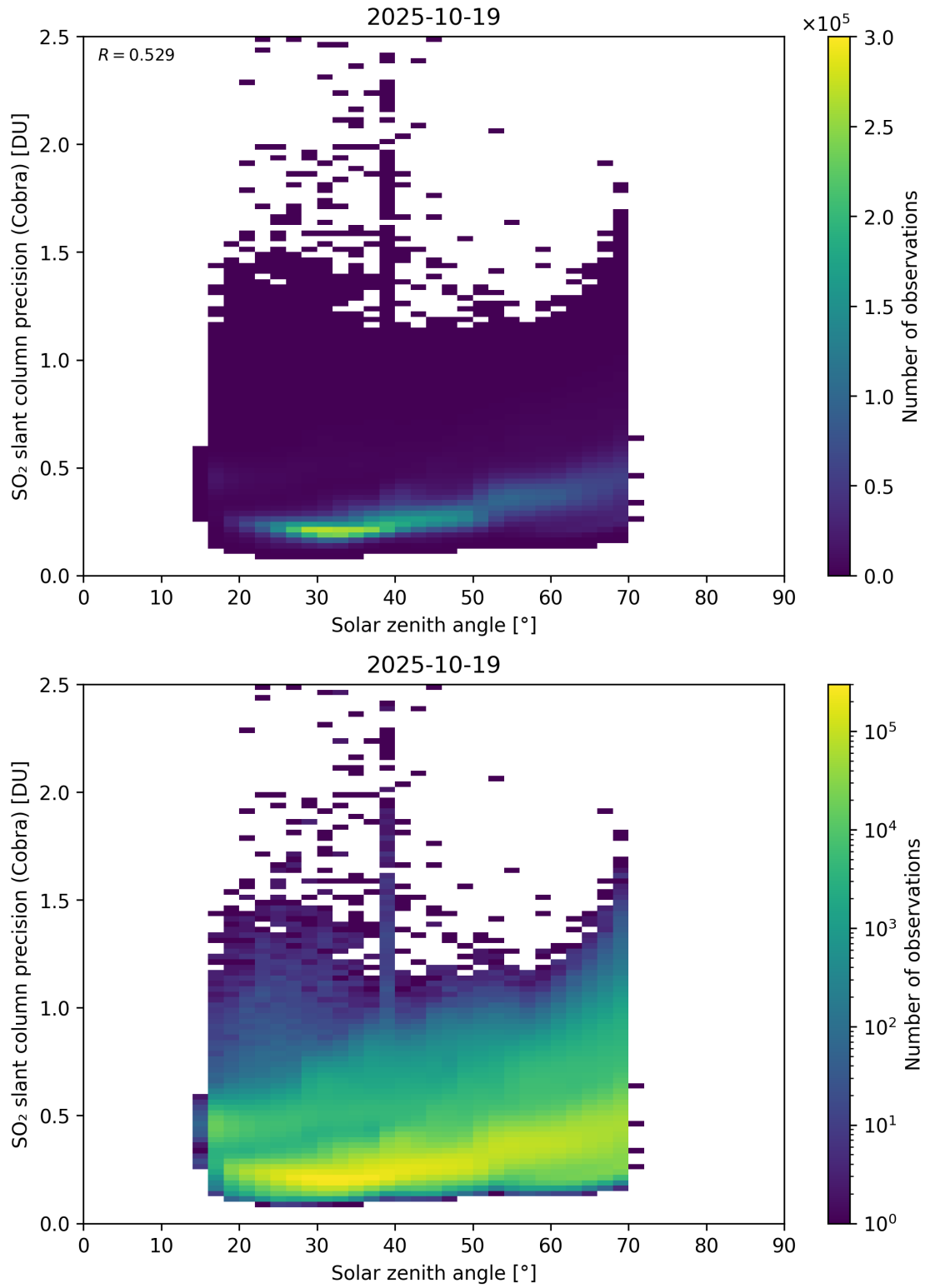
Figure 180: Scatter density plot of “Solar zenith angle” against “SO 2 slant column precision (Cobra)” for 2025-10-18 to 2025-10-20.
