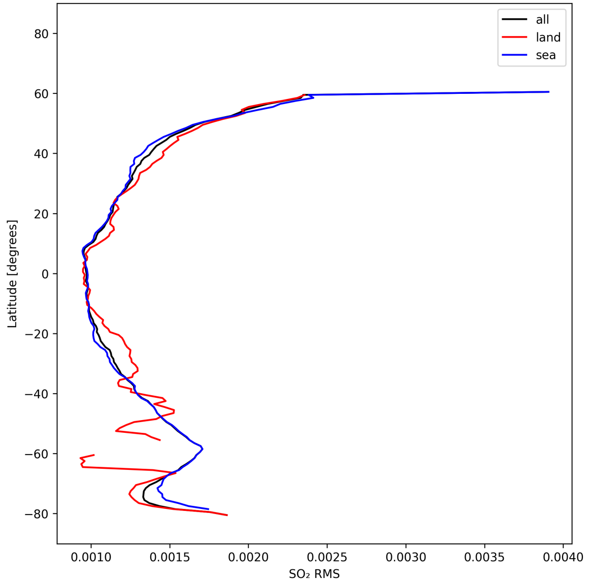
Figure 52: Zonal average of “SO 2 RMS” for 2025-10-18 to 2025-10-20.
