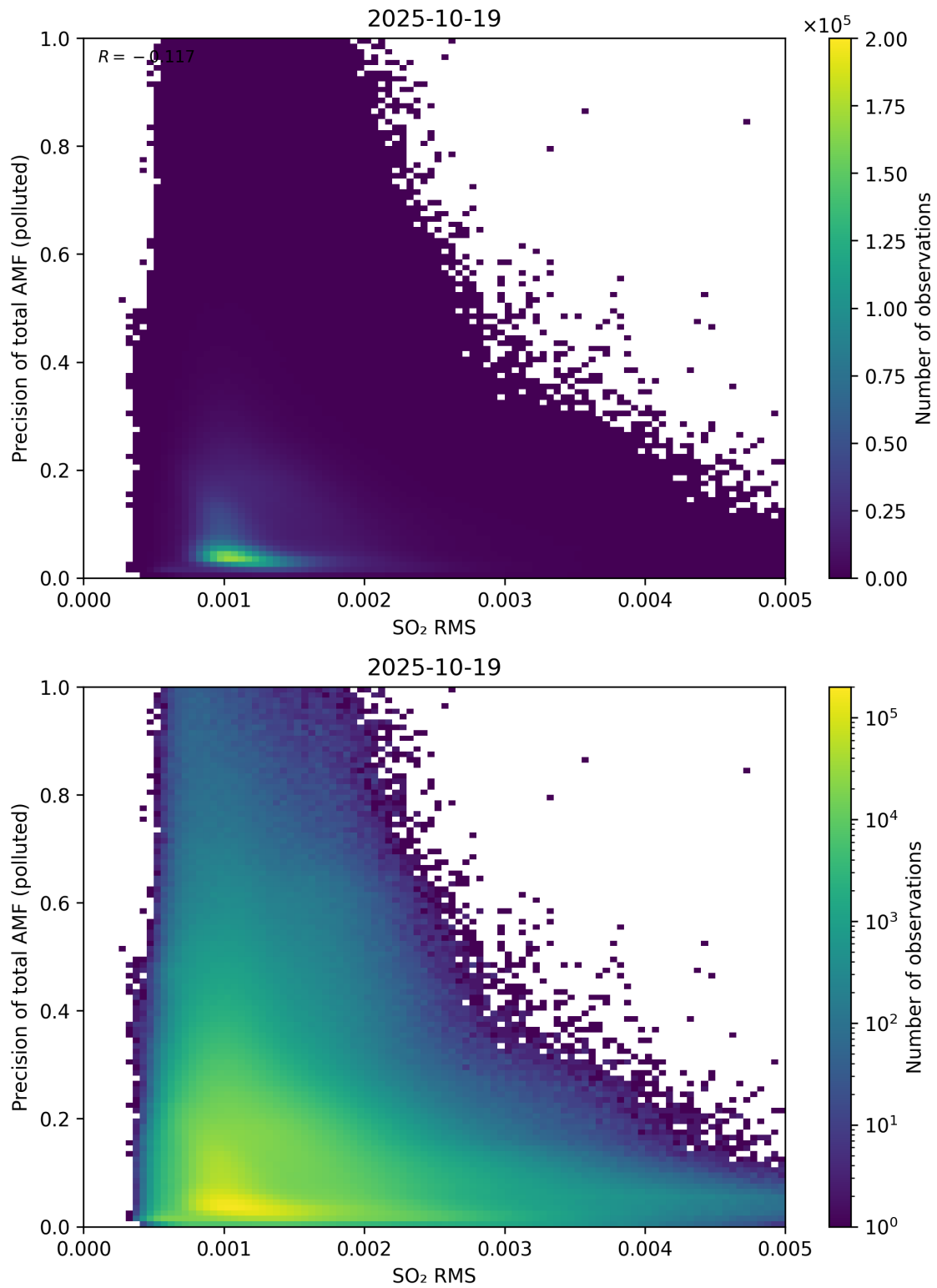
Figure 149: Scatter density plot of “SO 2 RMS” against “Precision of total AMF (polluted)” for 2025-10-18 to 2025-10-20.
