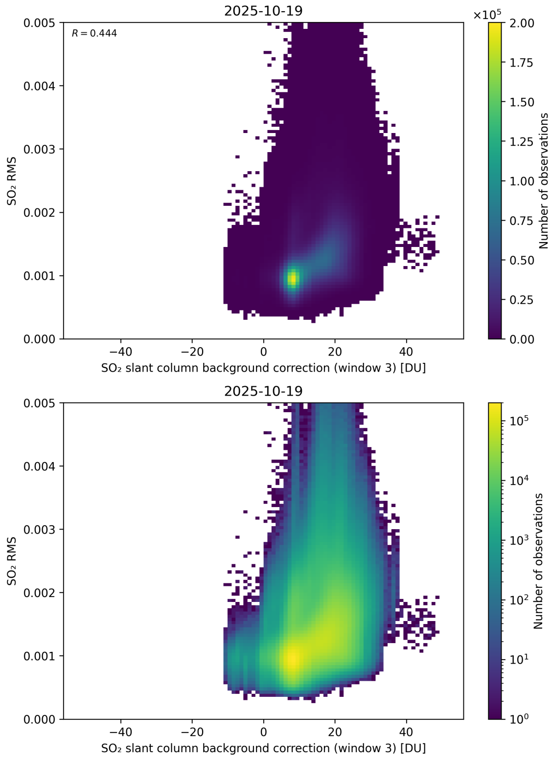
Figure 134: Scatter density plot of “SO 2 slant column background correction (window 3)” against “SO 2 RMS” for 2025-10-18 to 2025-10-20.
