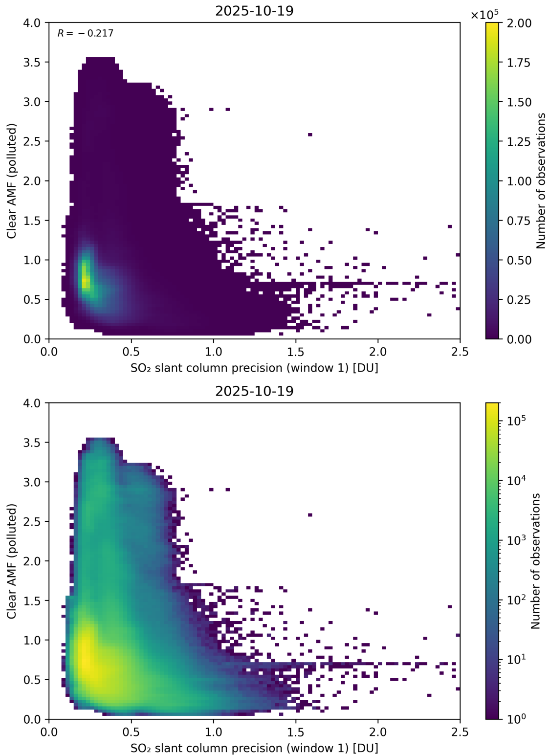
Figure 274: Scatter density plot of “SO 2 slant column precision (window 1)” against “Clear AMF (polluted)” for 2025-10-18 to 2025-10-20.
