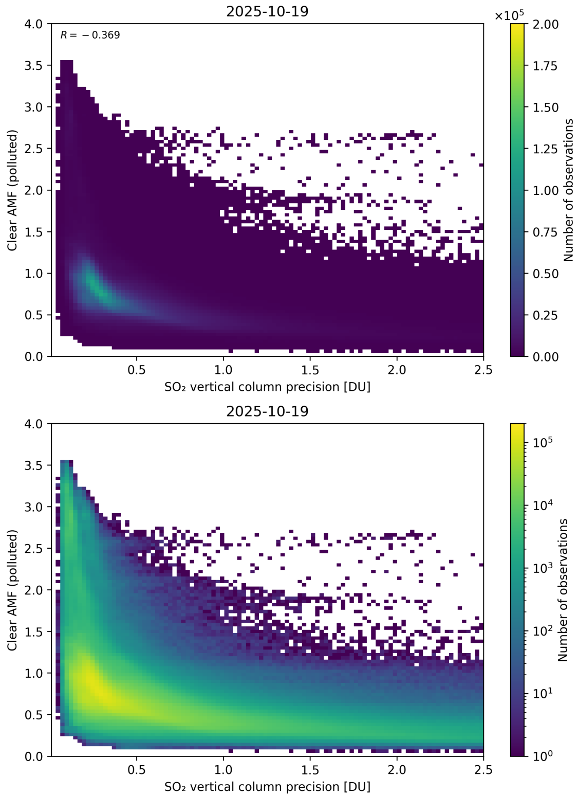
Figure 335: Scatter density plot of “SO 2 vertical column precision” against “Clear AMF (polluted)” for 2025-10-18 to 2025-10-20.
