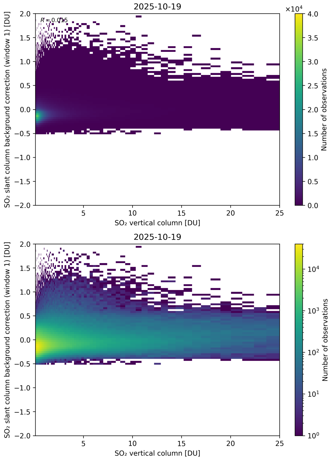
Figure 323: Scatter density plot of “SO 2 vertical column” against “SO 2 slant column background correction (window 1)” for 2025-10-18 to 2025-10-20.
