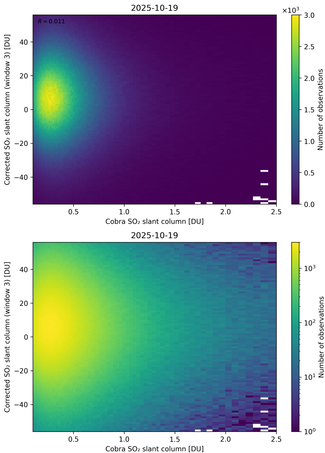
Figure 218: Scatter density plot of “Cobra SO 2 slant column” against “Corrected SO 2 slant column (window 3)” for 2025-10-18 to 2025-10-20.
