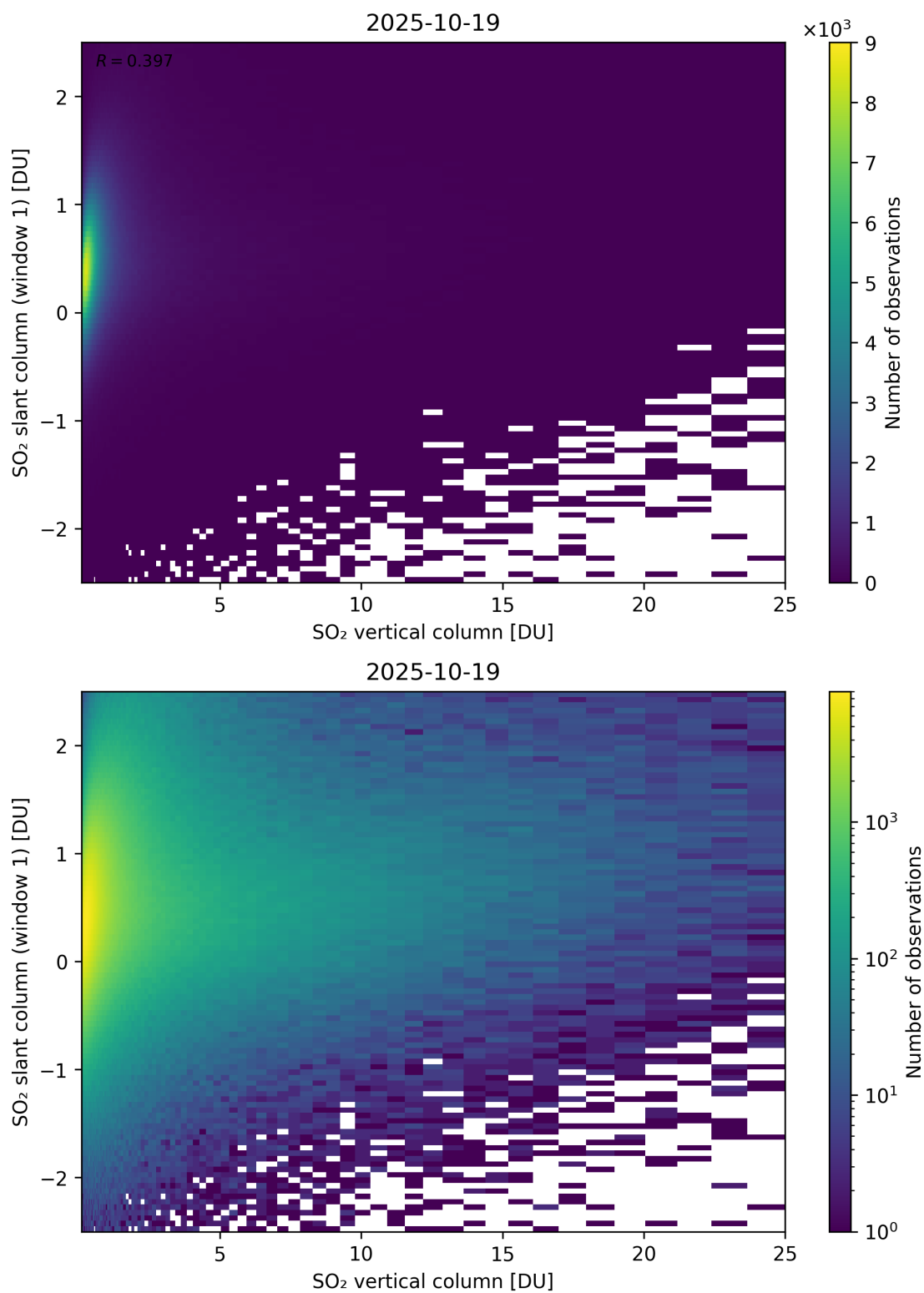
Figure 354: Scatter density plot of “SO 2 vertical column” against “SO 2 slant column (window 1)” for 2025-10-18 to 2025-10-20.
