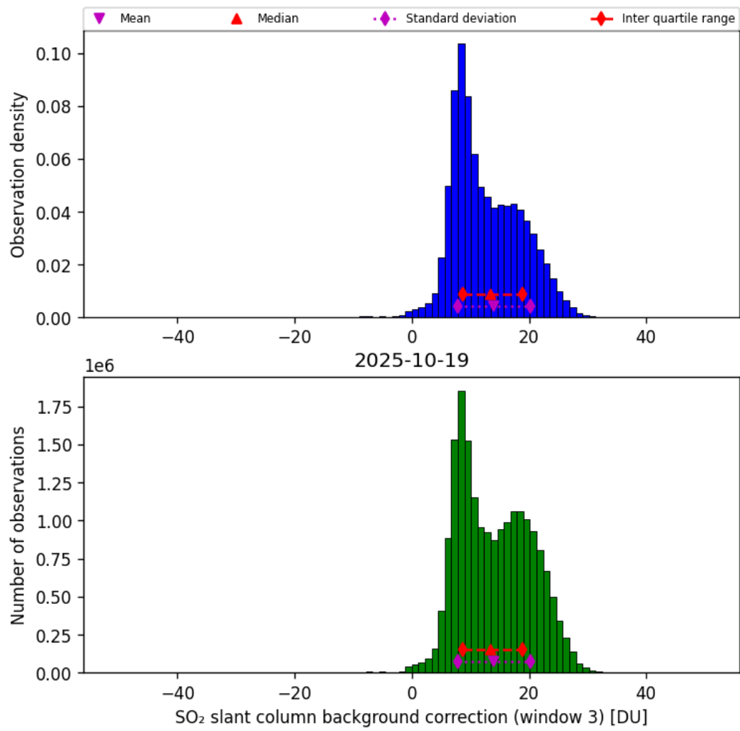
Figure 74: Histogram of “SO 2 slant column background correction (window 3)” for 2025-10-18 to 2025-10-20
