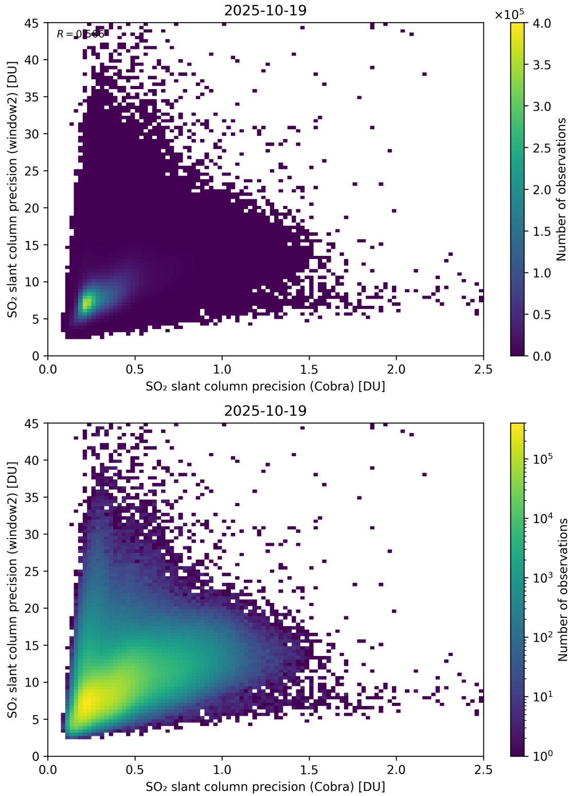
Figure 210: Scatter density plot of “SO 2 slant column precision (Cobra)” against “SO 2 slant column precision (window2)” for 2025-10-18 to 2025-10-20.
