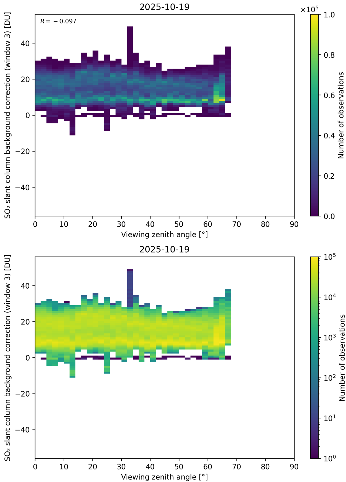
Figure 364: Scatter density plot of “Viewing zenith angle” against “SO 2 slant column background correction (window 3)” for 2025-10-18 to 2025-10-20.
