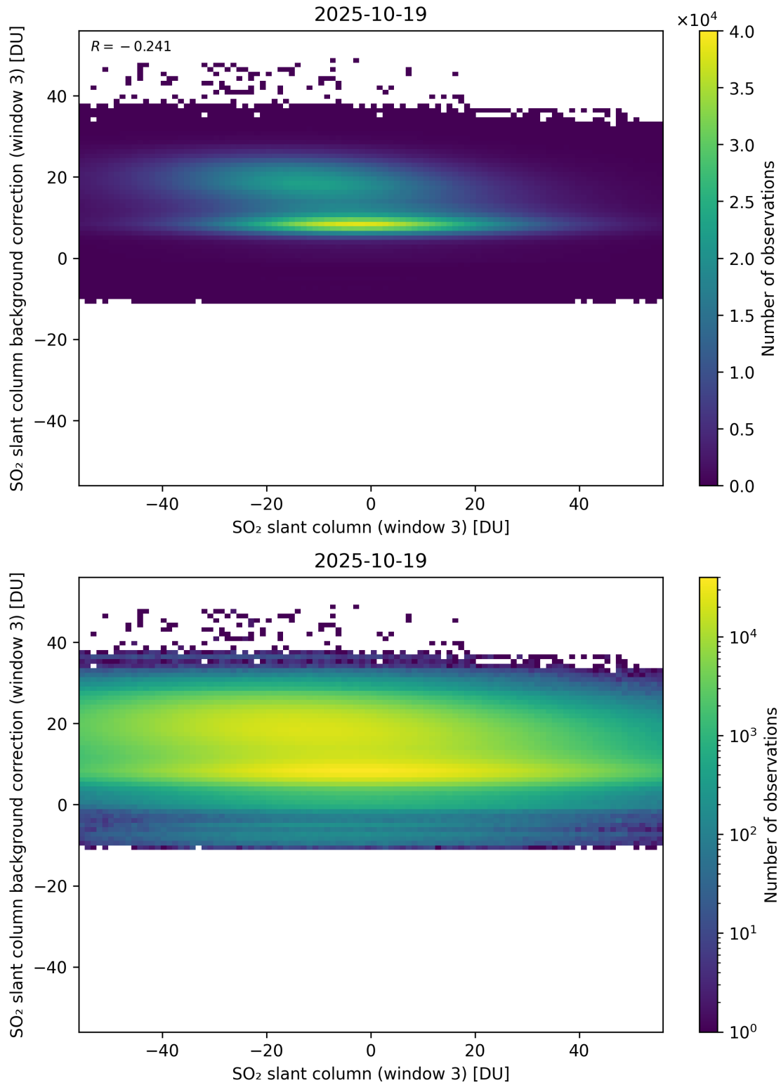
Figure 303: Scatter density plot of “SO 2 slant column (window 3)” against “SO 2 slant column background correction (window 3)” for 2025-10-18 to 2025-10-20.
