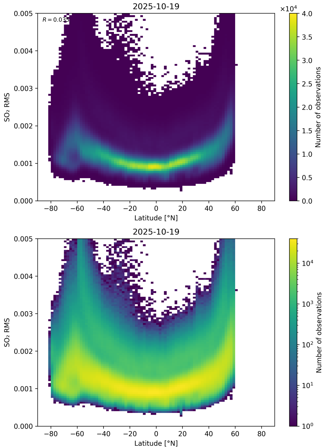
Figure 155: Scatter density plot of “Latitude” against “SO 2 RMS” for 2025-10-18 to 2025-10-20.
