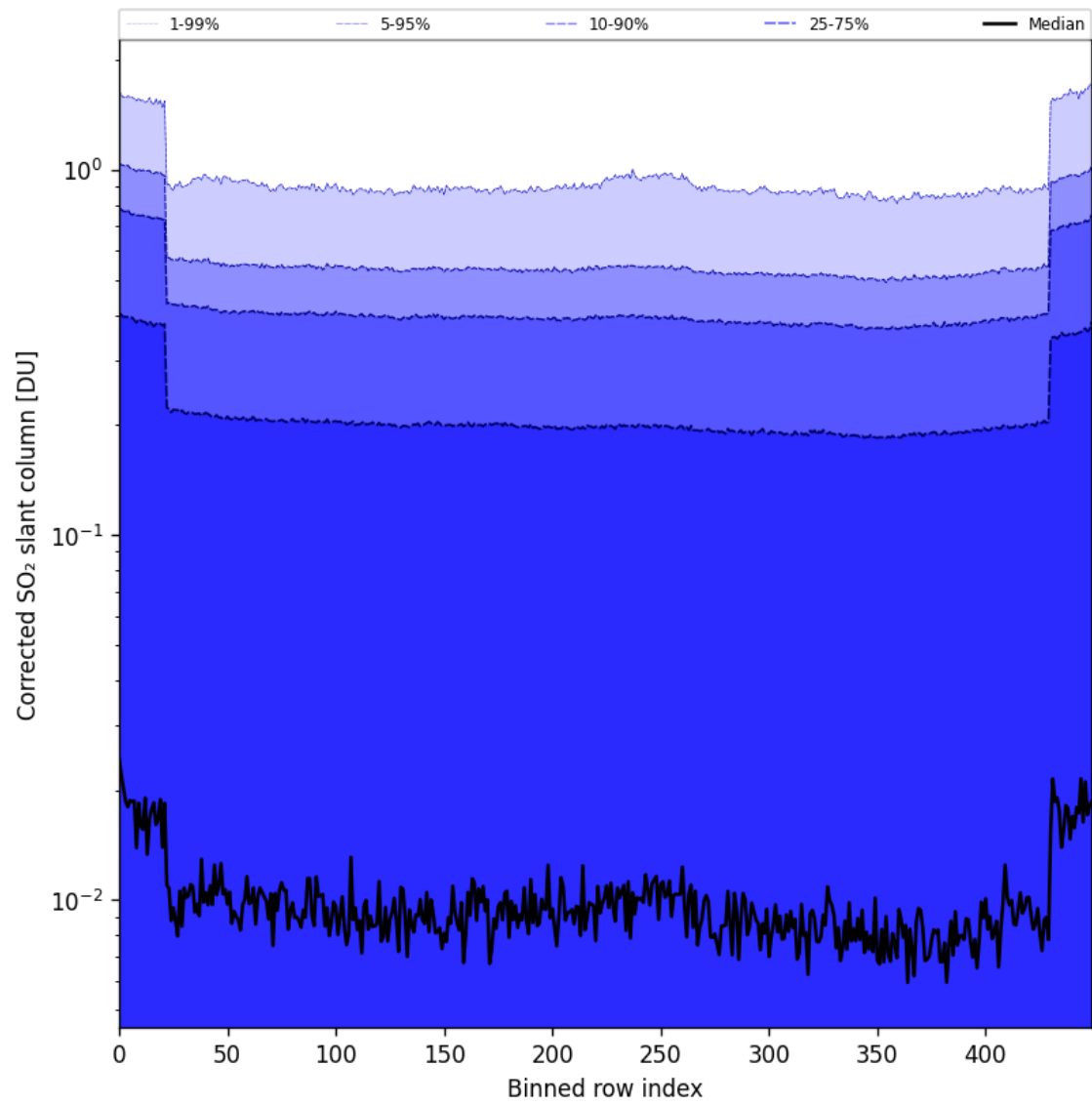
Figure 86: Along track statistics of "Corrected SO 2 slant column" for 2025-10-18 to 2025-10-20
