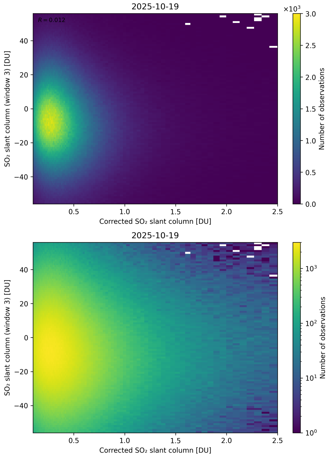
Figure 240: Scatter density plot of “Corrected SO 2 slant column” against “SO 2 slant column (window 3)” for 2025-10-18 to 2025-10-20.
