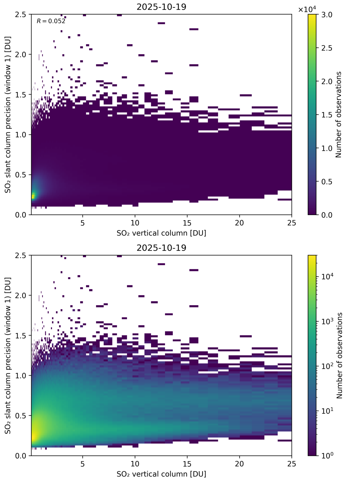
Figure 355: Scatter density plot of “SO 2 vertical column” against “SO 2 slant column precision (window 1)” for 2025-10-18 to 2025-10-20.
