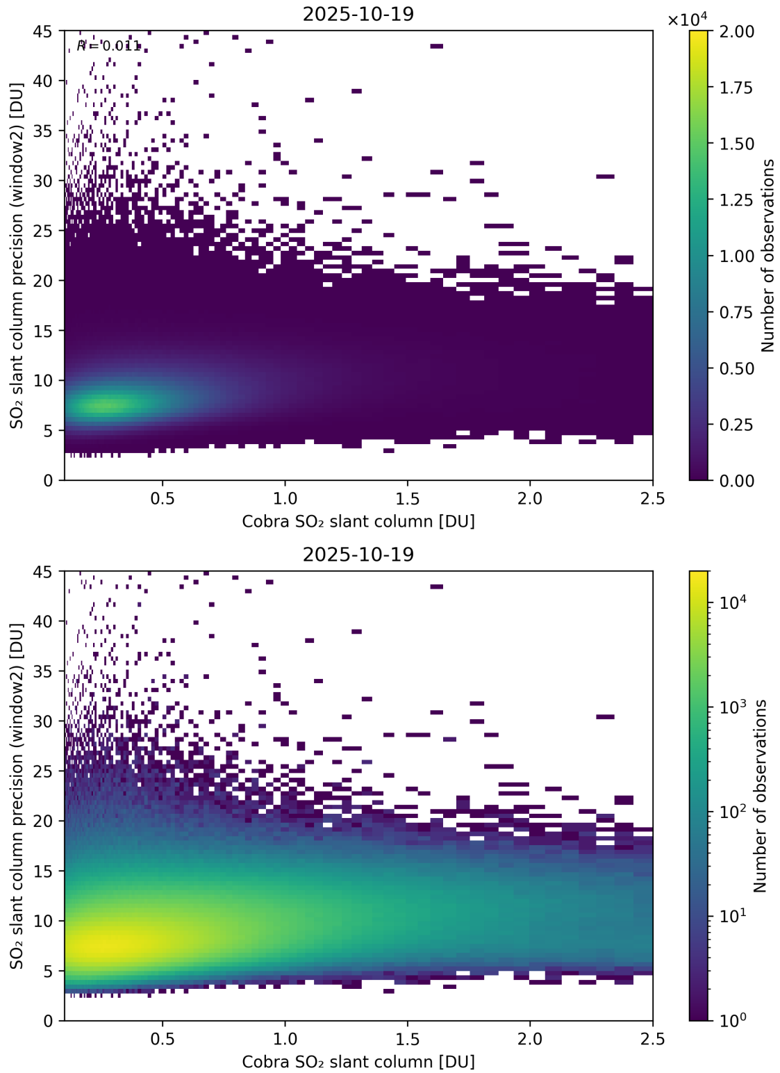
Figure 221: Scatter density plot of “Cobra SO 2 slant column” against “SO 2 slant column precision (window2)” for 2025-10-18 to 2025-10-20.
