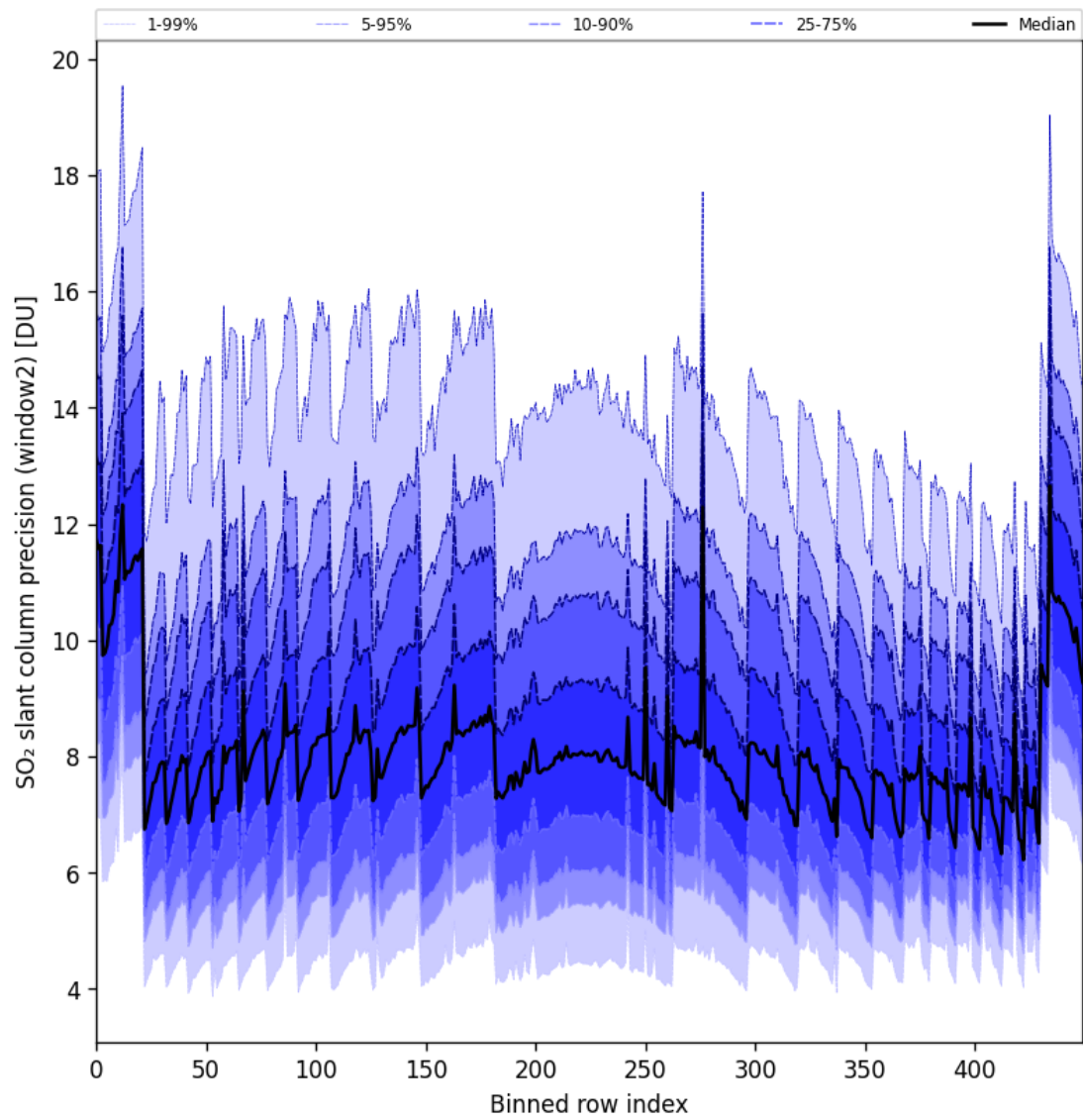
Figure 94: Along track statistics of “SO 2 slant column precision (window2)” for 2025-10-18 to 2025-10-20
