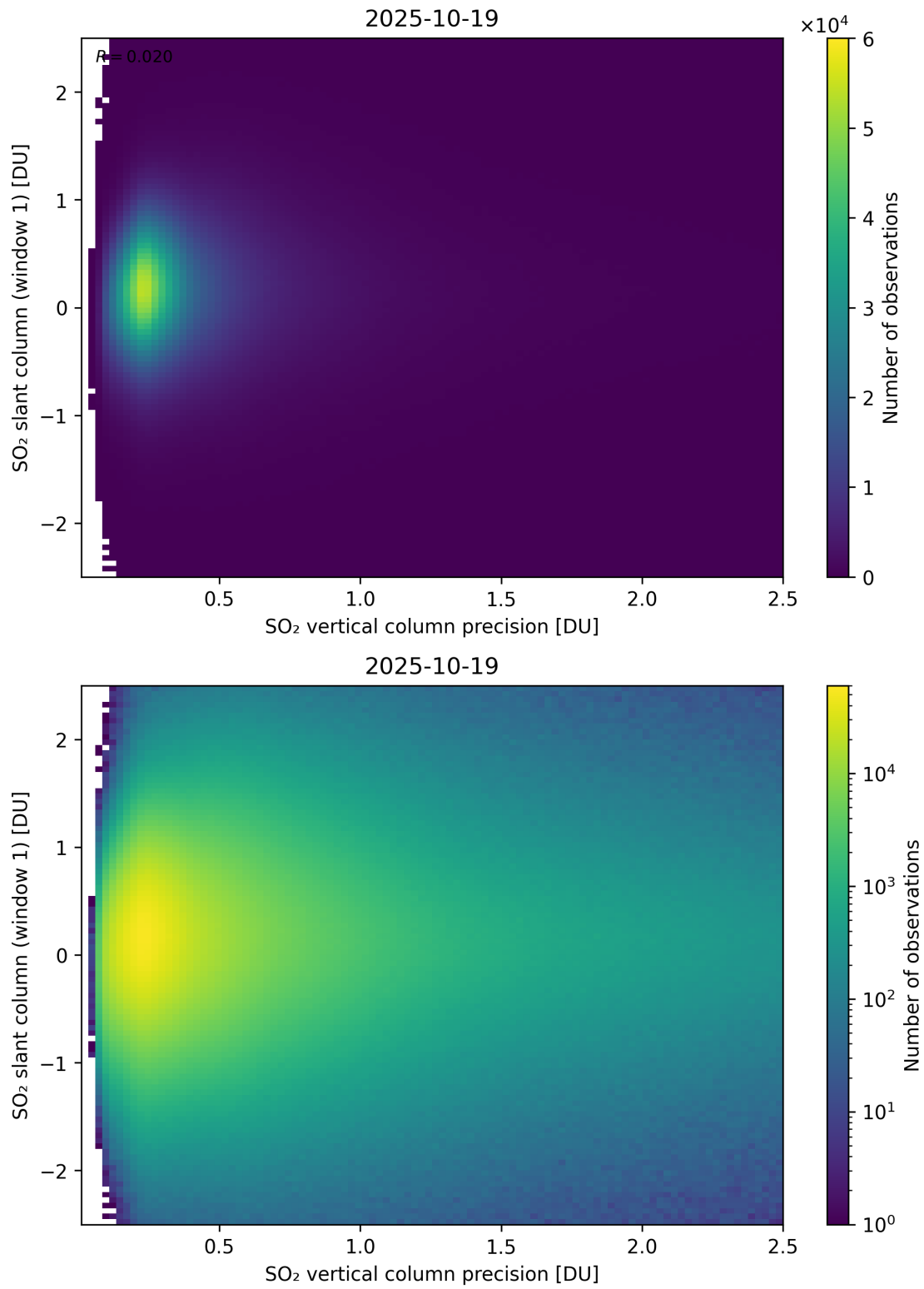
Figure 341: Scatter density plot of “SO 2 vertical column precision” against “SO 2 slant column (window 1)” for 2025-10-18 to 2025-10-20.
