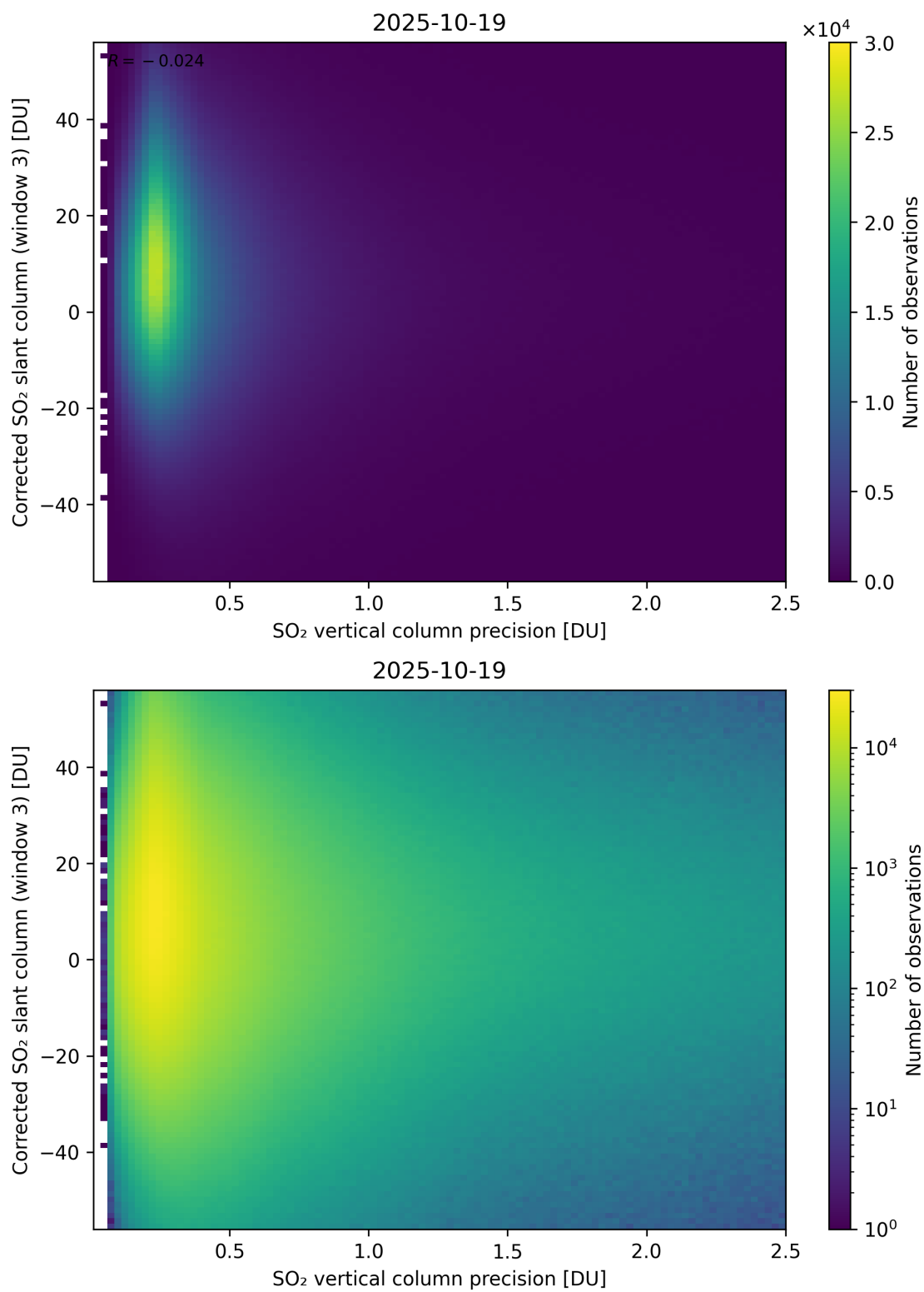
Figure 340: Scatter density plot of “SO 2 vertical column precision” against “Corrected SO 2 slant column (window 3)” for 2025-10-18 to 2025-10-20.
