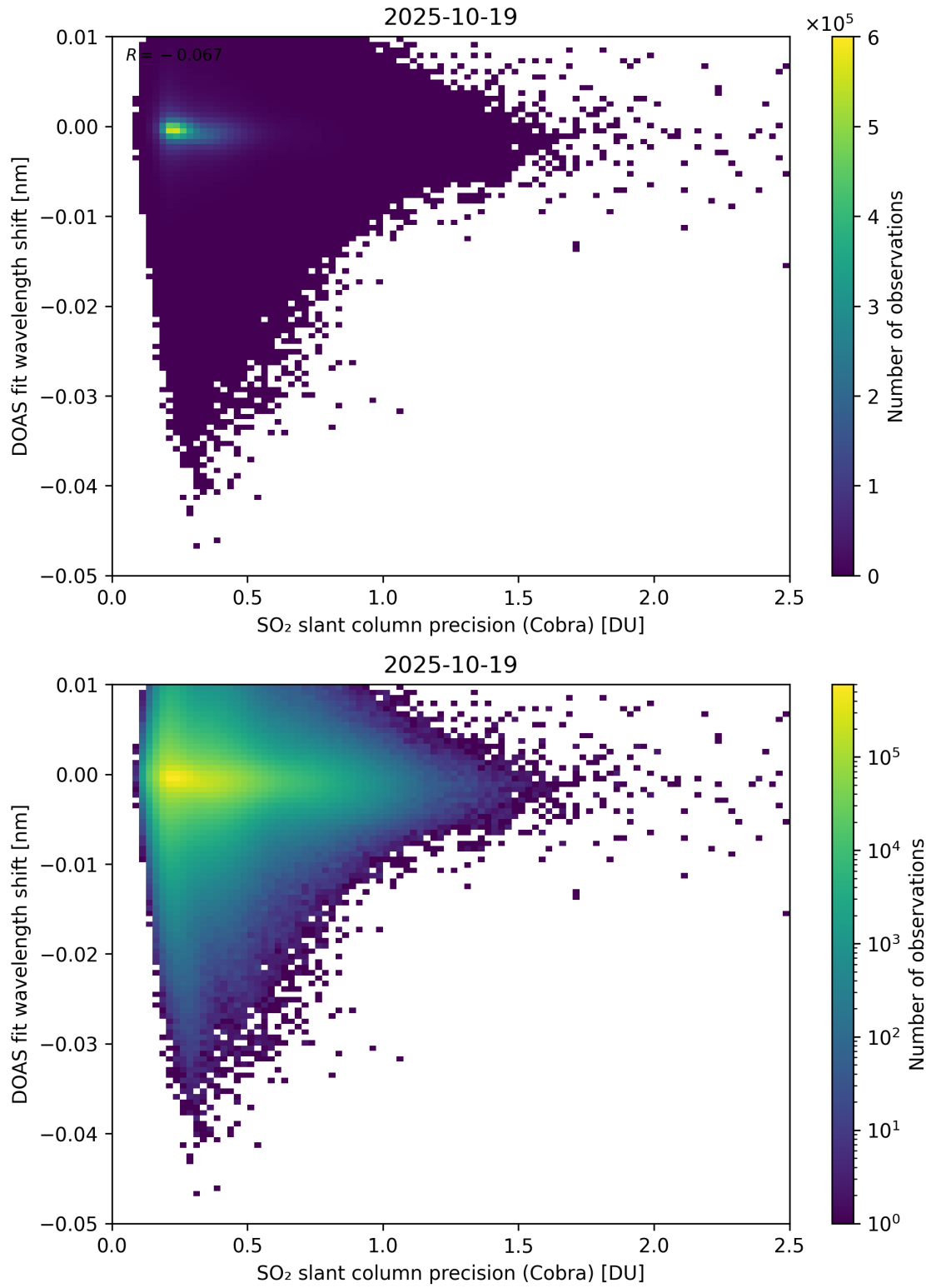
Figure 202: Scatter density plot of “SO 2 slant column precision (Cobra)” against “DOAS fit wavelength shift” for 2025-10-18 to 2025-10-20.
