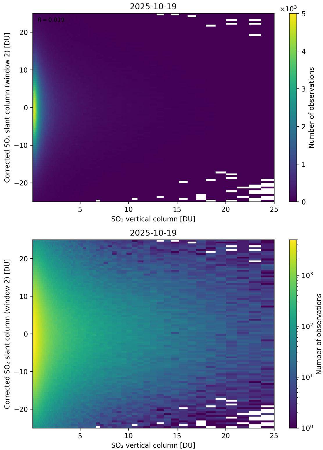
Figure 352: Scatter density plot of “SO 2 vertical column” against “Corrected SO 2 slant column (window 2)” for 2025-10-18 to 2025-10-20.
