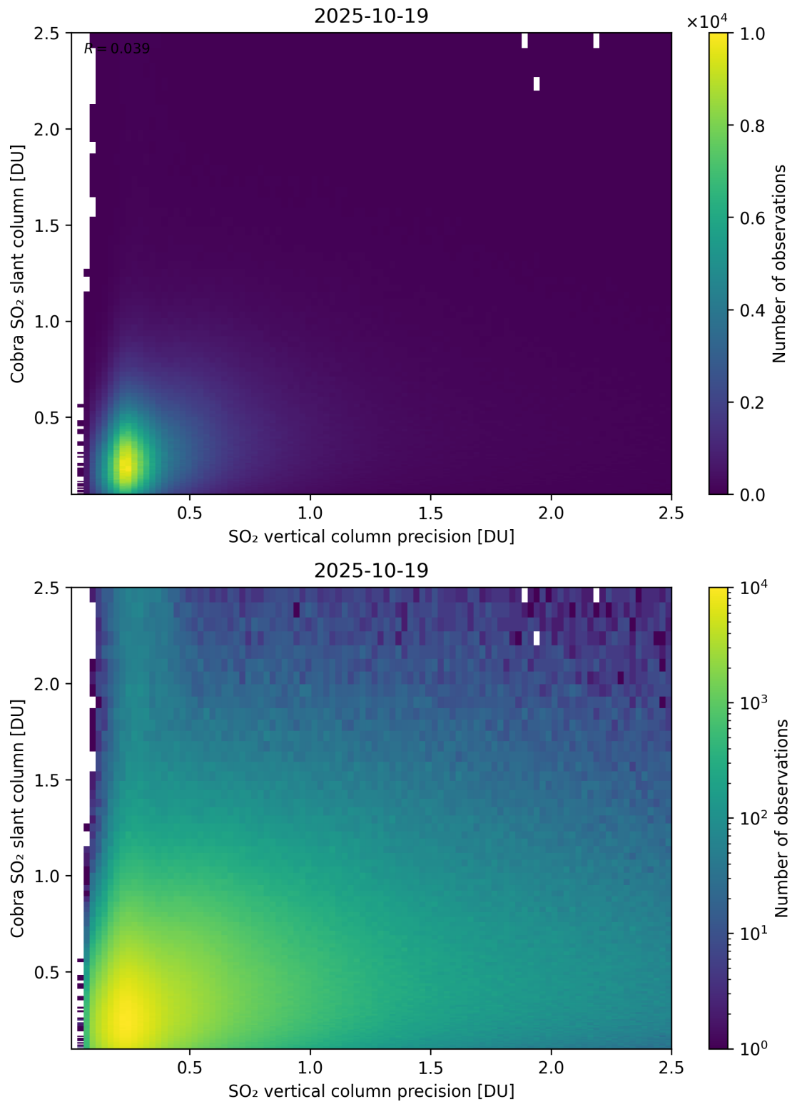
Figure 336: Scatter density plot of “SO 2 vertical column precision” against “Cobra SO 2 slant column” for 2025-10-18 to 2025-10-20.
