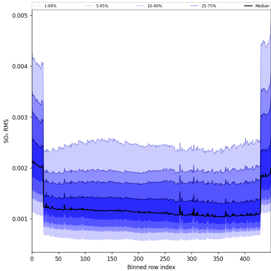
Figure 104: Along track statistics of “SO 2 RMS” for 2025-10-18 to 2025-10-20
