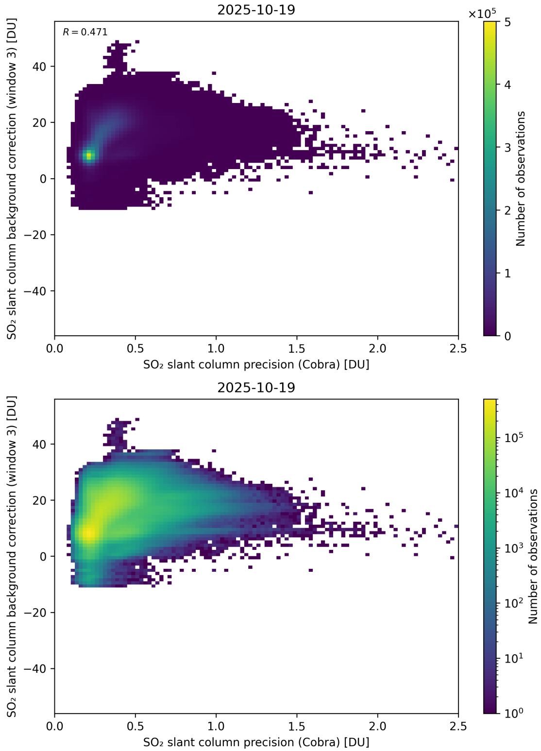
Figure 201: Scatter density plot of “SO 2 slant column precision (Cobra)” against “SO 2 slant column background correction (window 3)” for 2025-10-18 to 2025-10-20.
