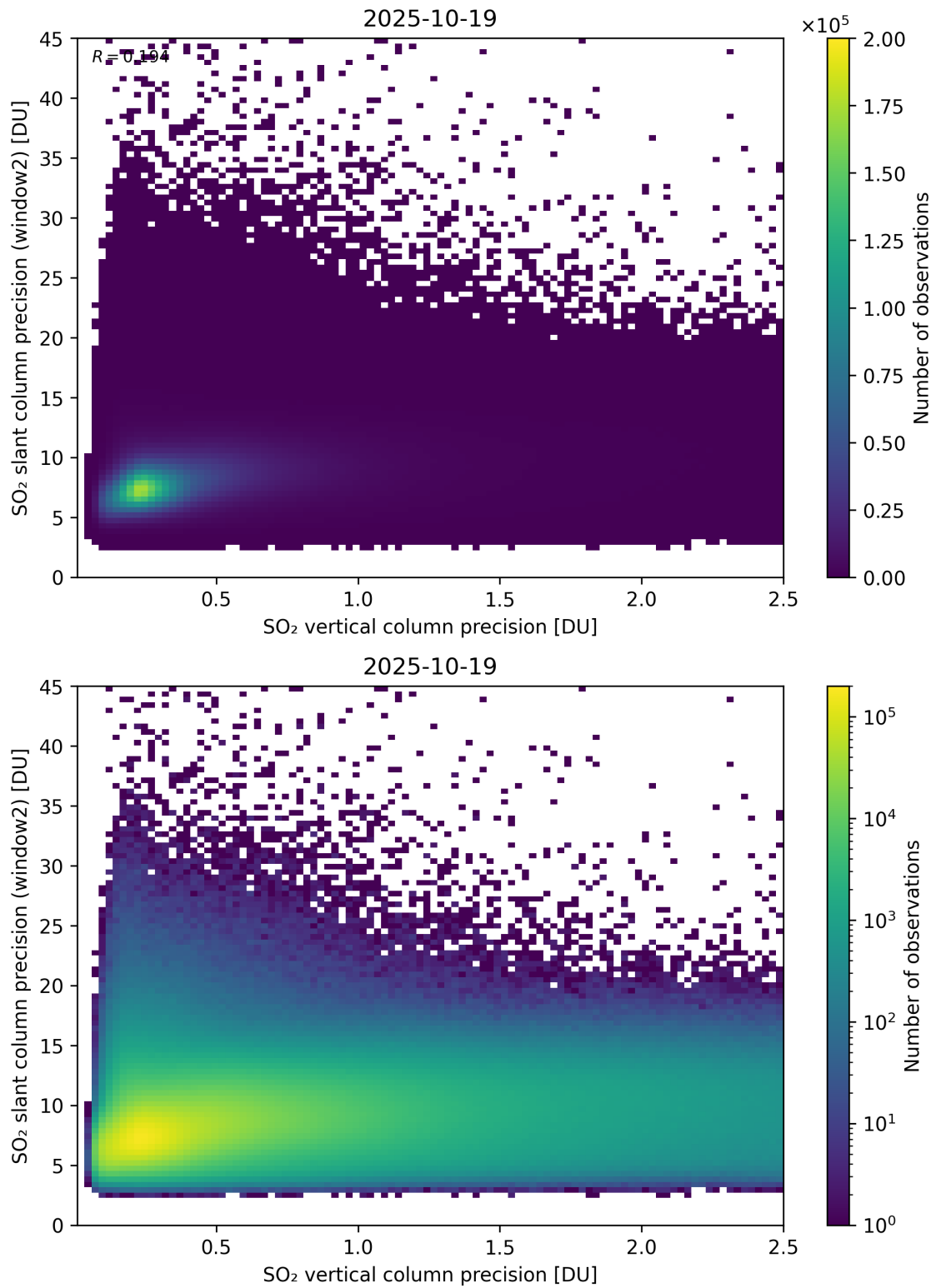
Figure 343: Scatter density plot of “SO 2 vertical column precision” against “SO 2 slant column precision (window2)” for 2025-10-18 to 2025-10-20.
