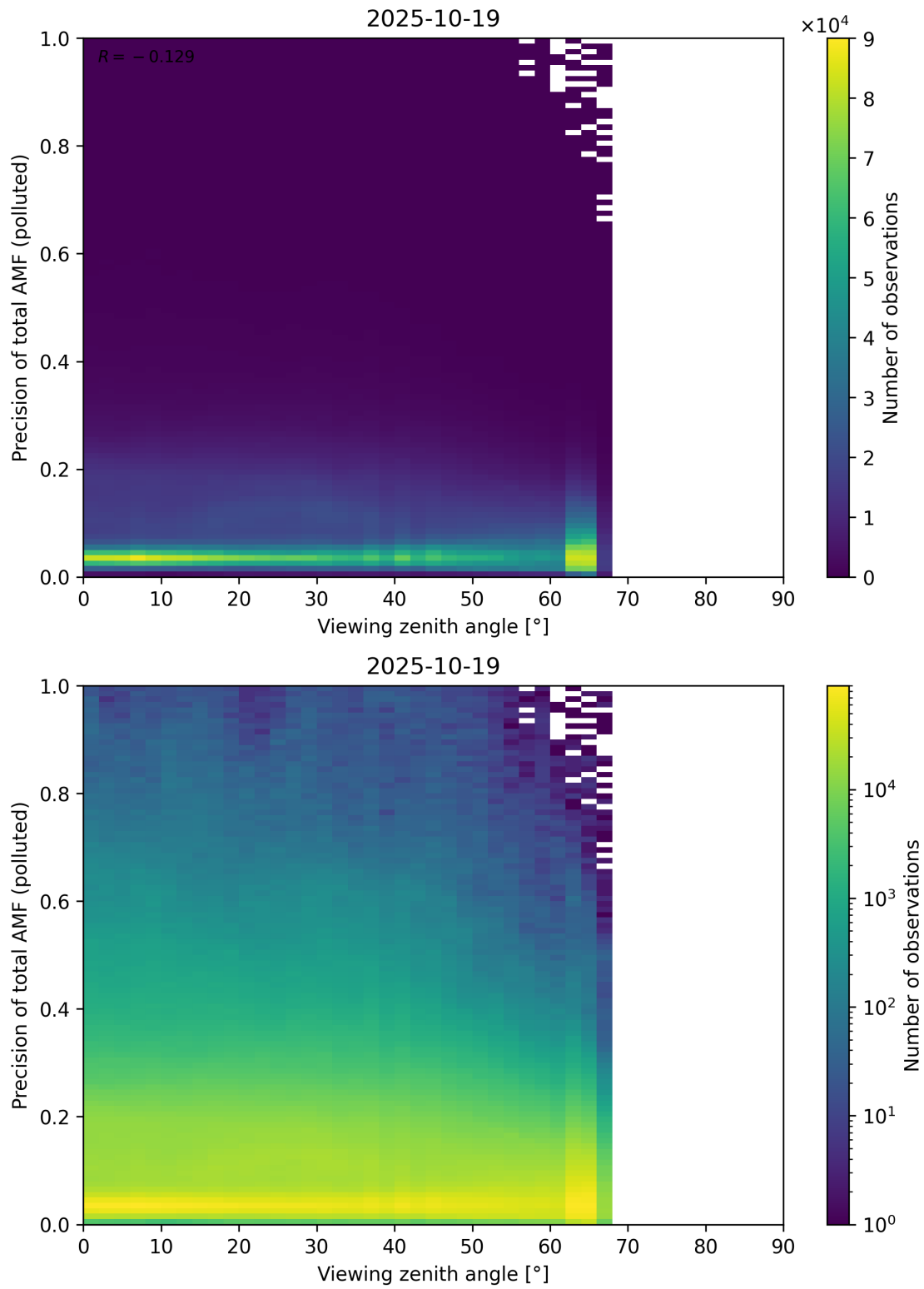
Figure 382: Scatter density plot of “Viewing zenith angle” against “Precision of total AMF (polluted)” for 2025-10-18 to 2025-10-20.
