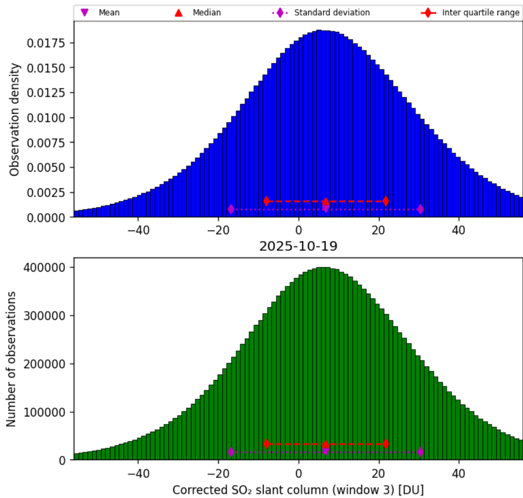
Figure 73: Histogram of “Corrected SO 2 slant column (window 3)” for 2025-10-18 to 2025-10-20
