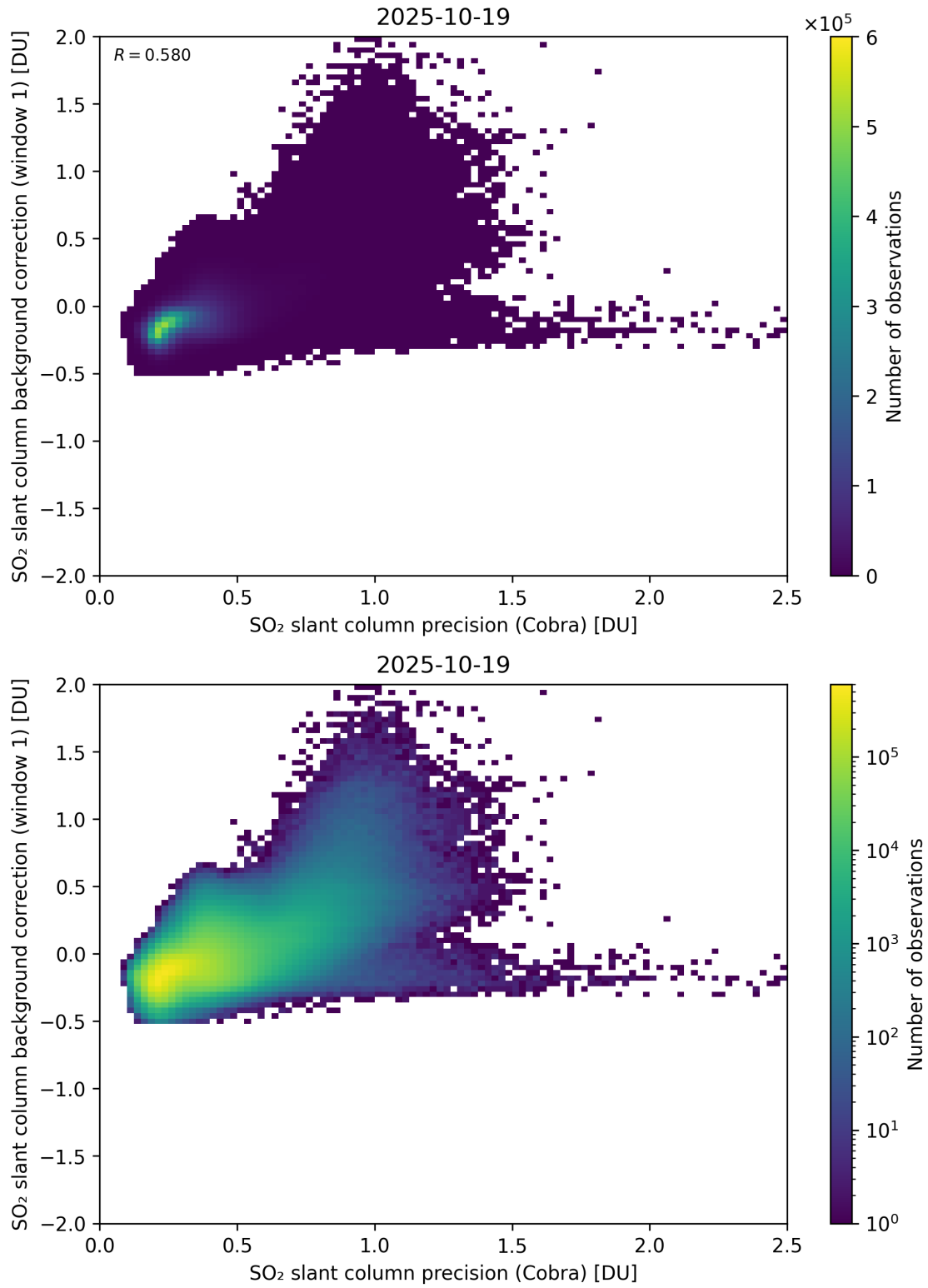
Figure 199: Scatter density plot of “SO 2 slant column precision (Cobra)” against “SO 2 slant column background correction (window 1)” for 2025-10-18 to 2025-10-20.
