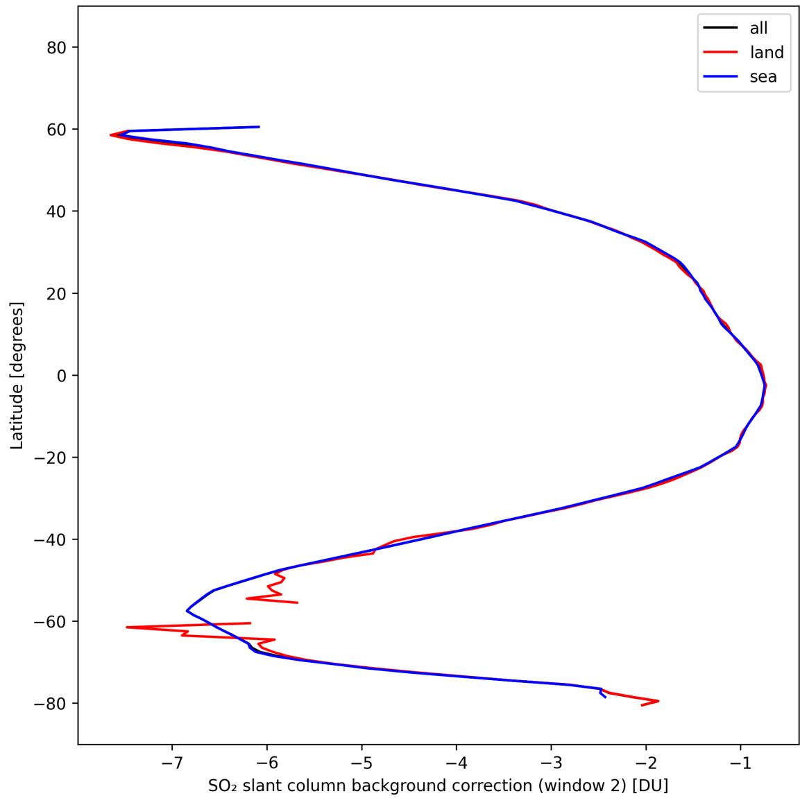
Figure 44: Zonal average of “SO 2 slant column background correction (window 2)” for 2025-10-18 to 2025-10-20.
