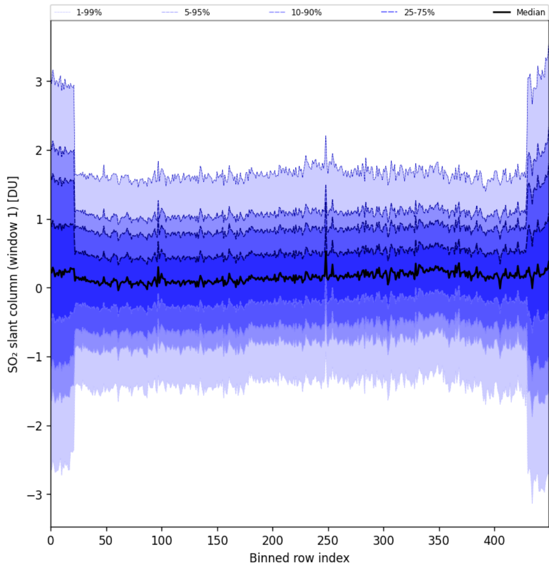
Figure 89: Along track statistics of “SO 2 slant column (window 1)” for 2025-10-18 to 2025-10-20
