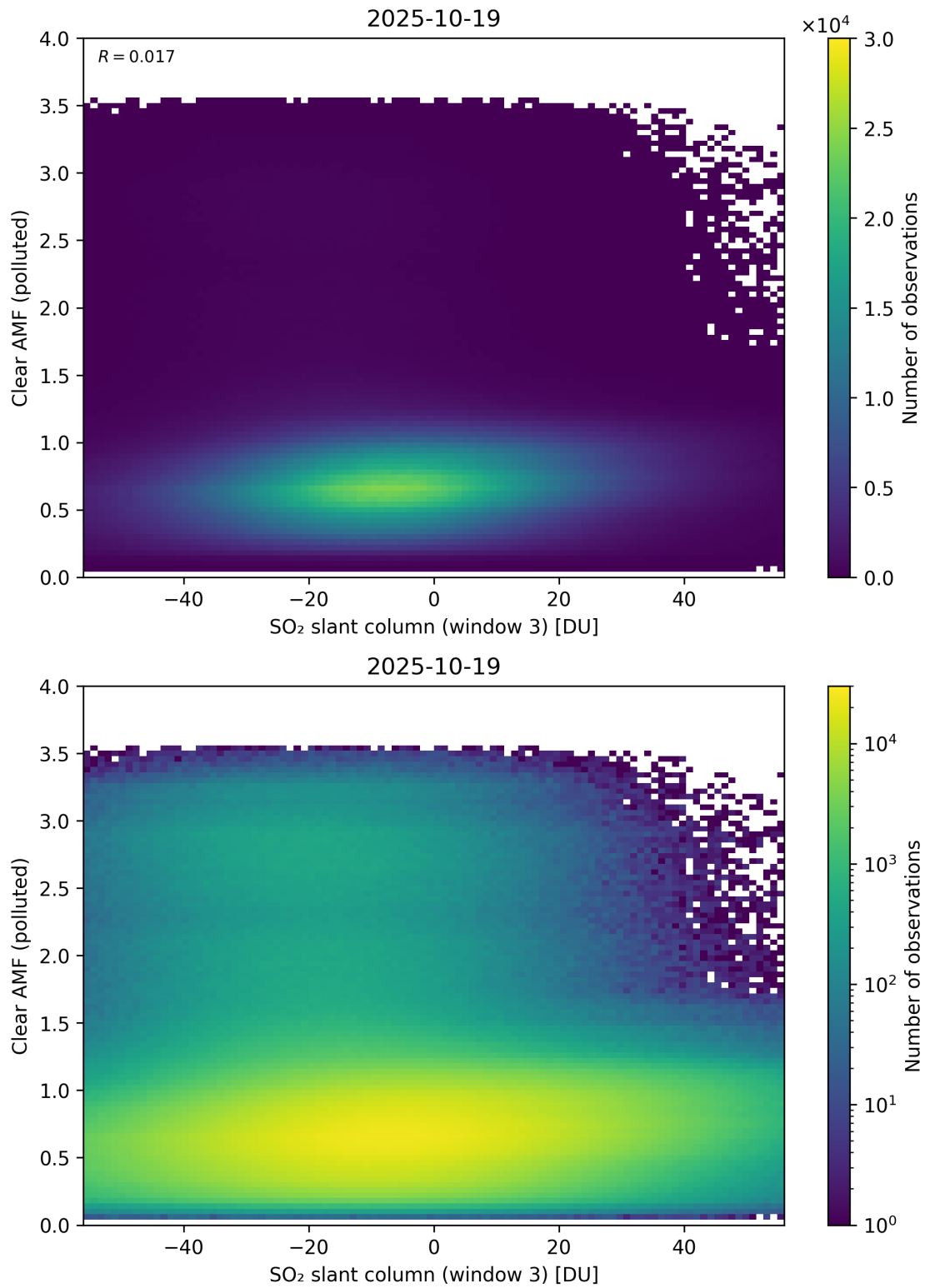
Figure 315: Scatter density plot of “SO 2 slant column (window 3)” against “Clear AMF (polluted)” for 2025-10-18 to 2025-10-20.
