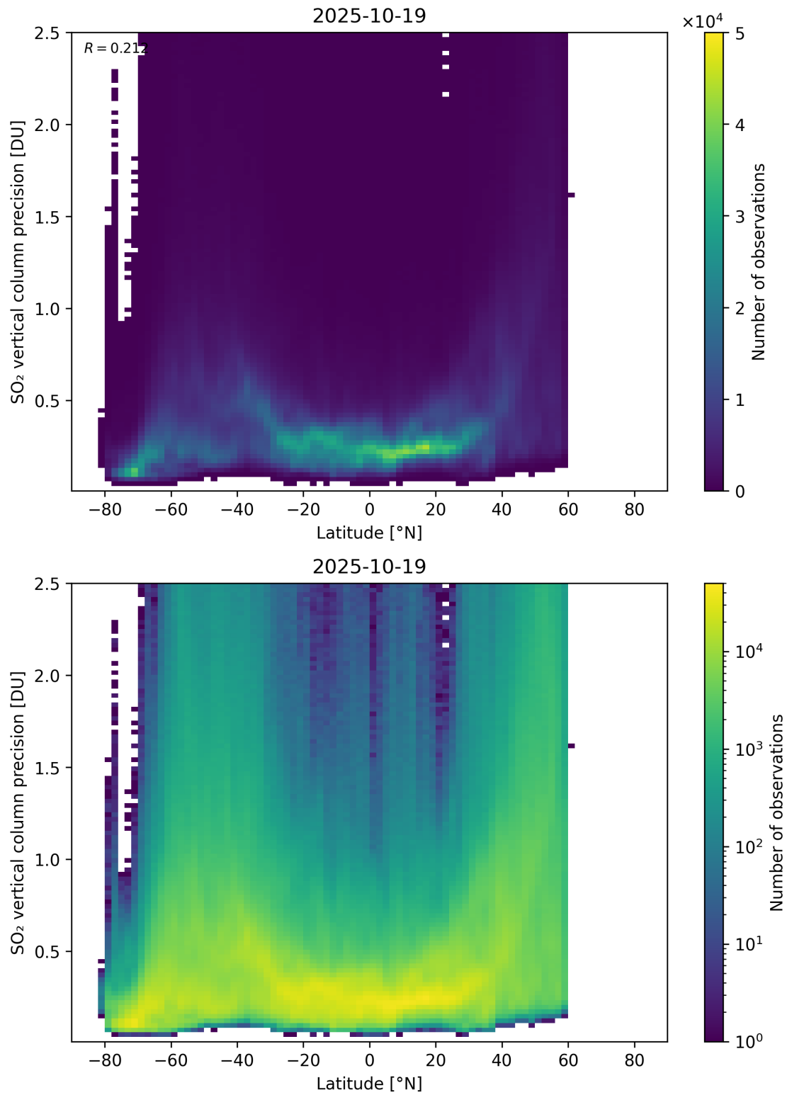
Figure 170: Scatter density plot of “Latitude” against “SO 2 vertical column precision” for 2025-10-18 to 2025-10-20.
