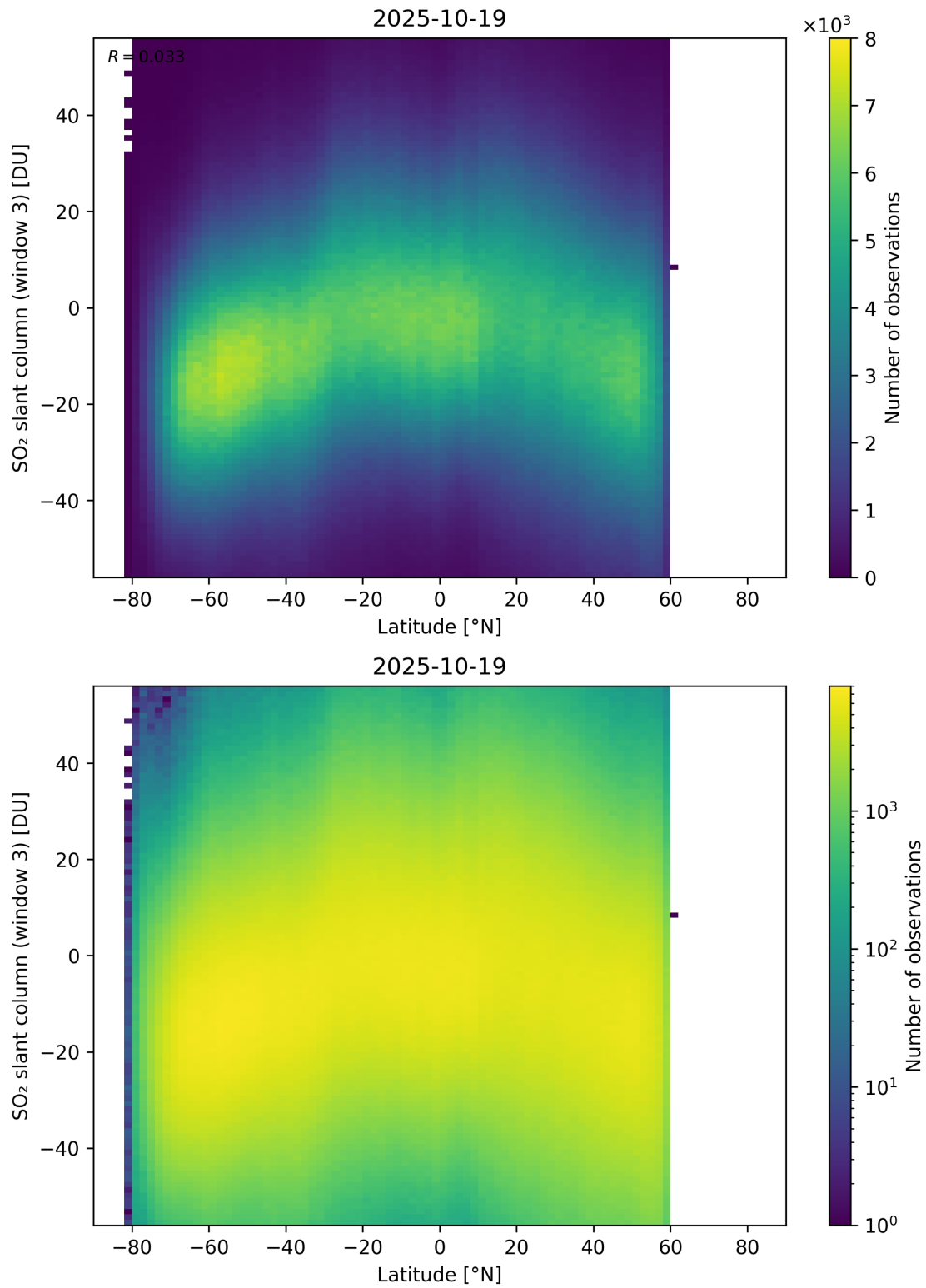
Figure 165: Scatter density plot of “Latitude” against “SO 2 slant column (window 3)” for 2025-10-18 to 2025-10-20.
