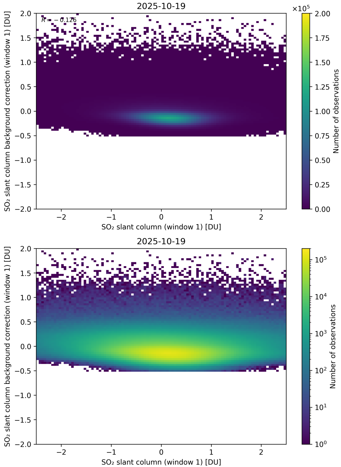
Figure 262: Scatter density plot of “SO 2 slant column (window 1)” against “SO 2 slant column background correction (window 1)” for 2025-10-18 to 2025-10-20.
