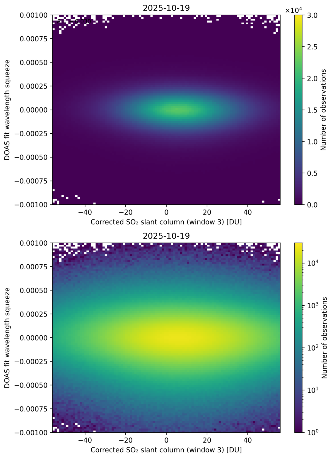
Figure 257: Scatter density plot of “Corrected SO 2 slant column (window 3)” against “DOAS fit wavelength squeeze” for 2025-10-18 to 2025-10-20.
