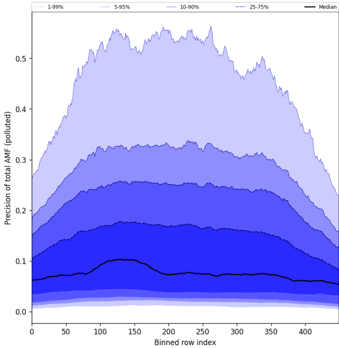
Figure 106: Along track statistics of “Precision of total AMF (polluted)” for 2025-10-18 to 2025-10-20
