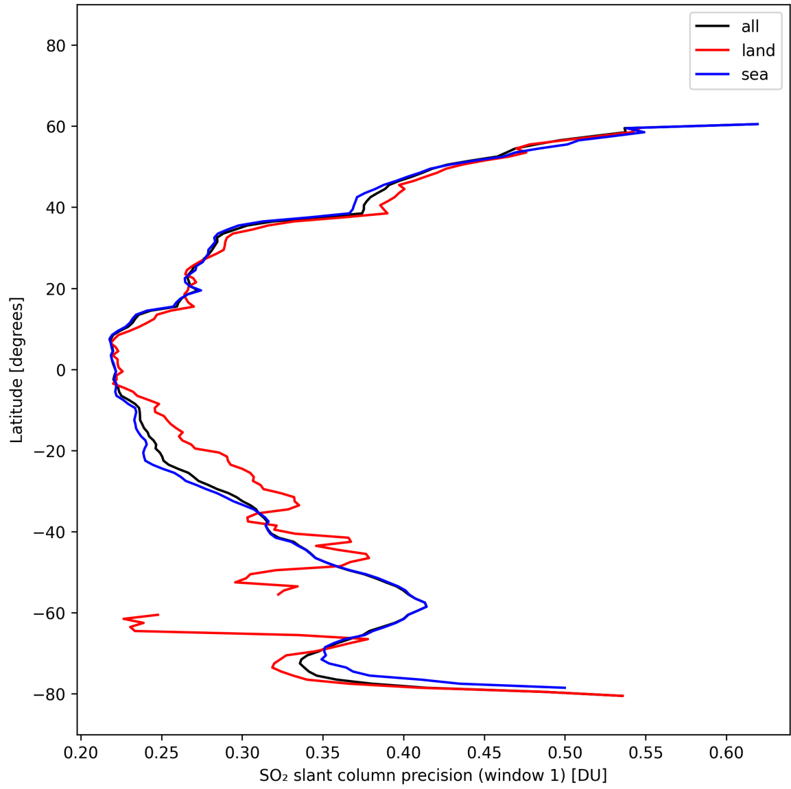
Figure 38: Zonal average of “SO 2 slant column precision (window 1)” for 2025-10-18 to 2025-10-20.
