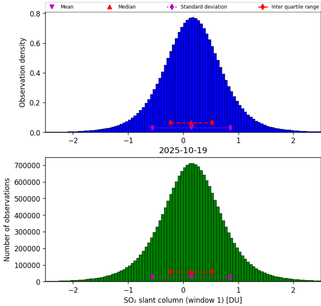
Figure 63: Histogram of “SO 2 slant column (window 1)” for 2025-10-18 to 2025-10-20
