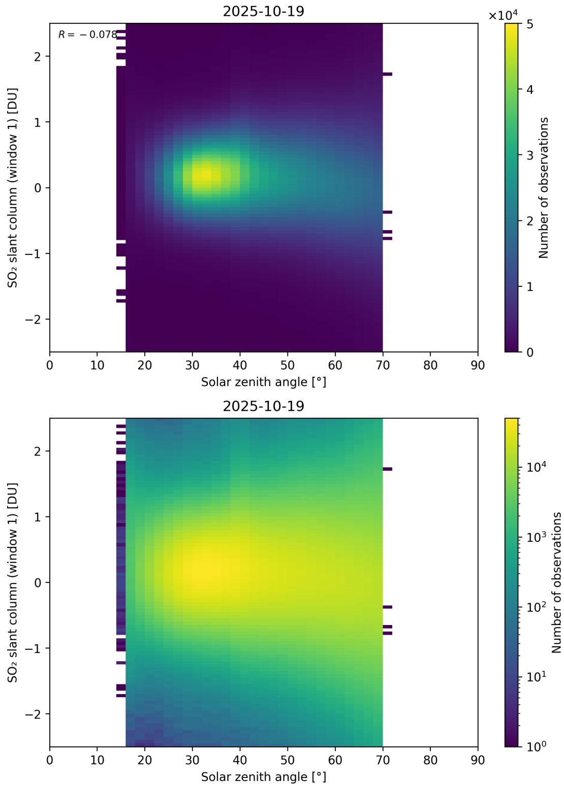
Figure 184: Scatter density plot of “Solar zenith angle” against “SO 2 slant column (window 1)” for 2025-10-18 to 2025-10-20.
