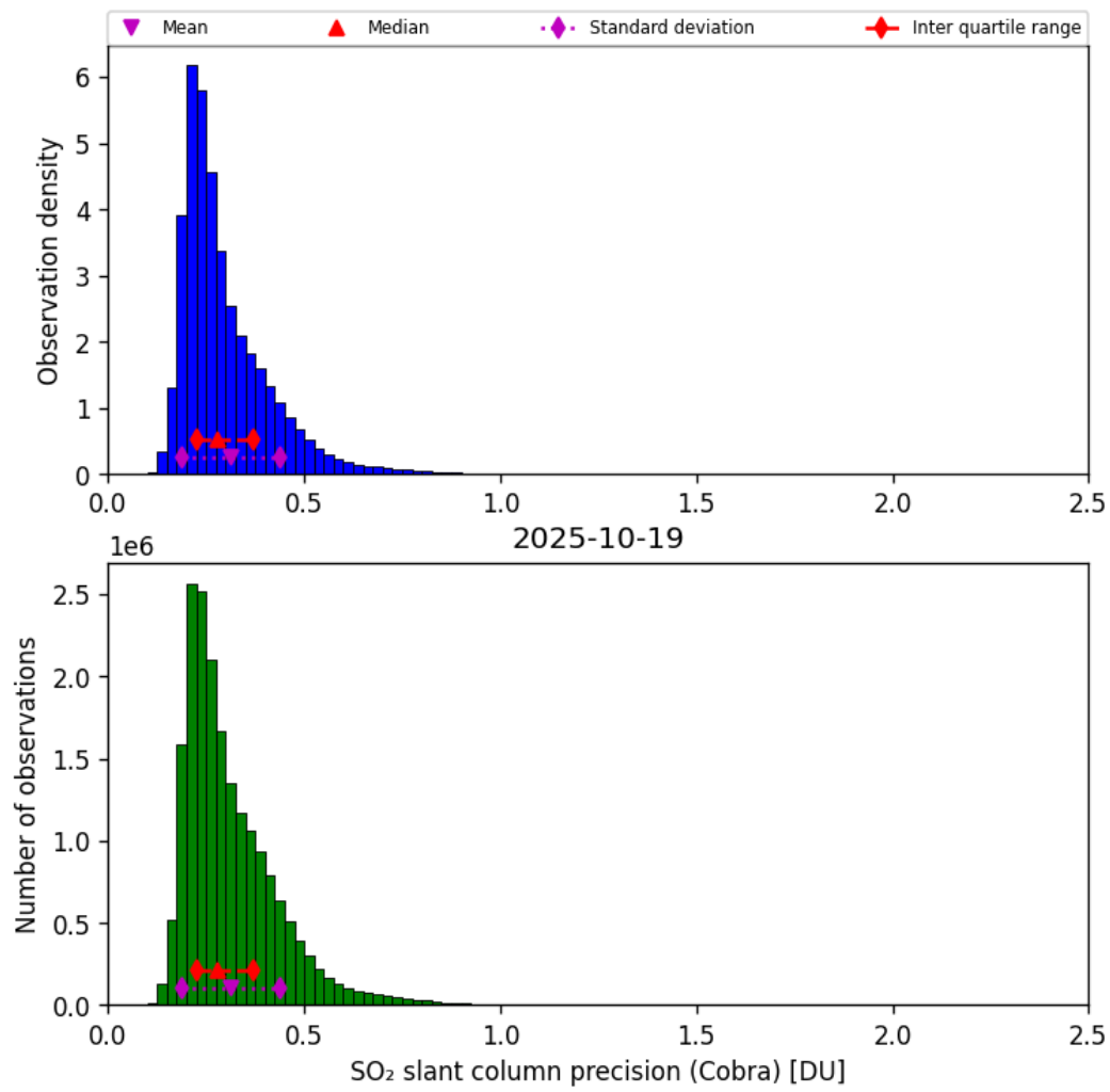
Figure 62: Histogram of “SO 2 slant column precision (Cobra)” for 2025-10-18 to 2025-10-20
