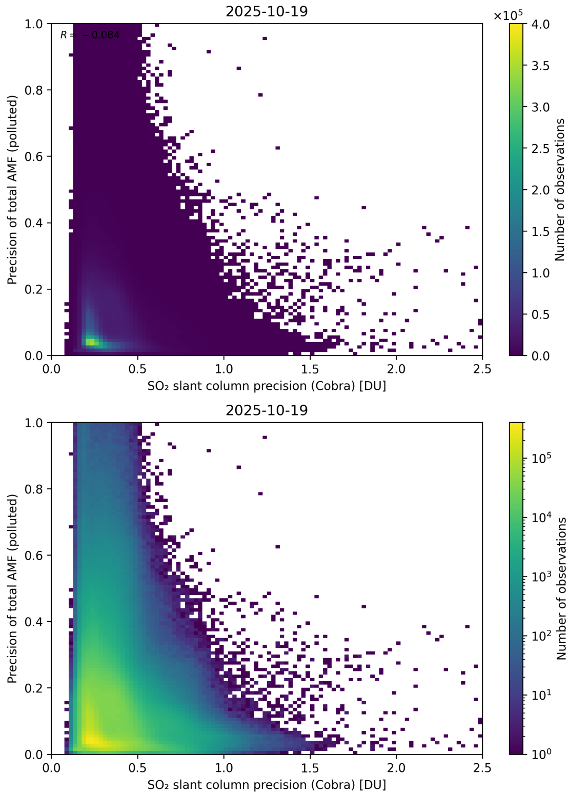
Figure 214: Scatter density plot of “SO 2 slant column precision (Cobra)” against “Precision of total AMF (polluted)” for 2025-10-18 to 2025-10-20.
