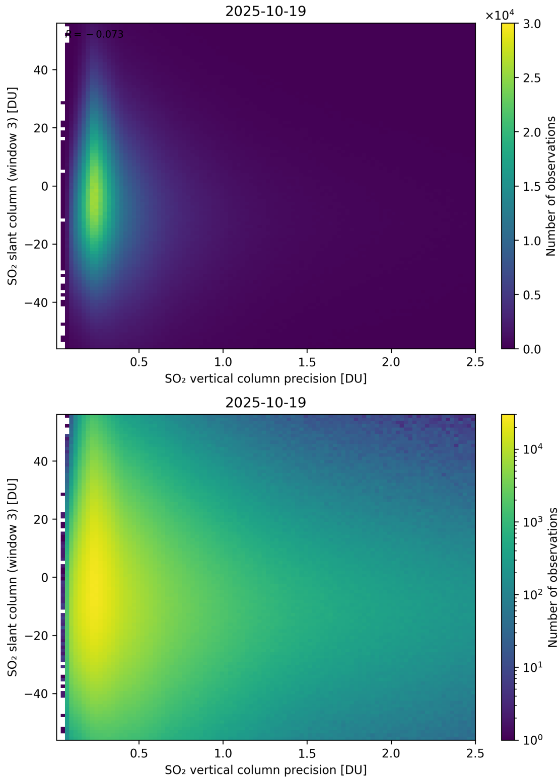
Figure 344: Scatter density plot of “SO 2 vertical column precision” against “SO 2 slant column (window 3)” for 2025-10-18 to 2025-10-20.
