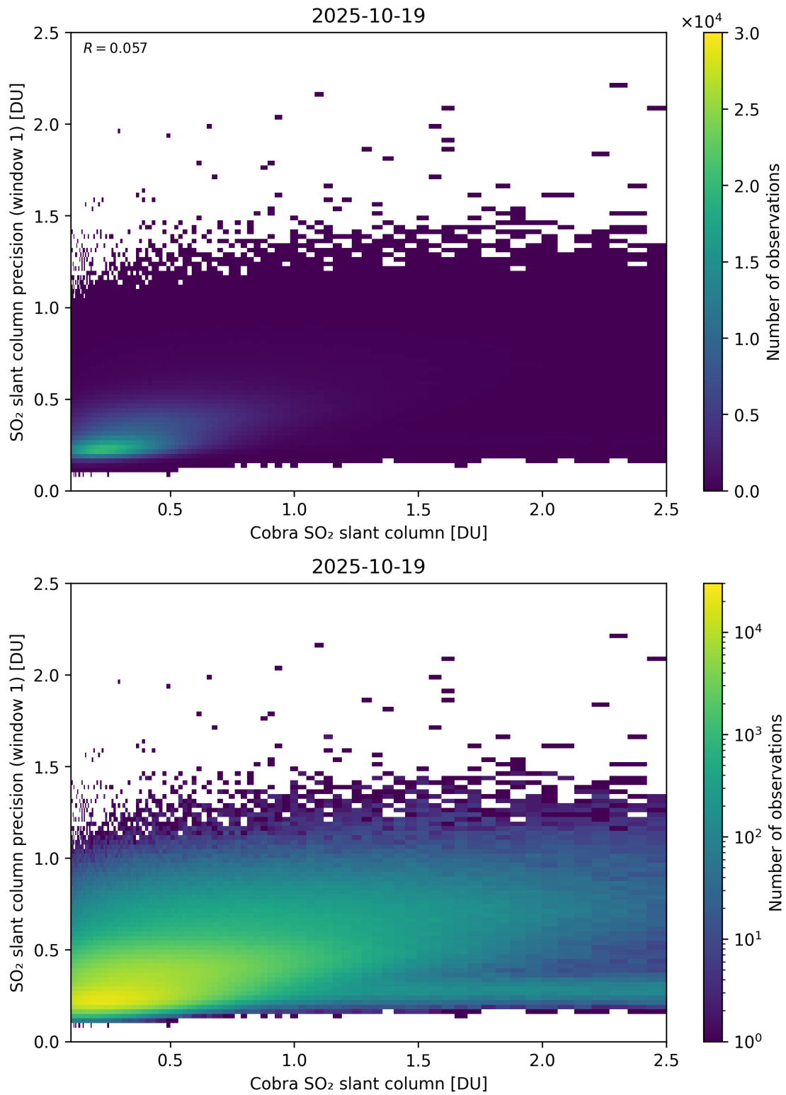
Figure 220: Scatter density plot of “Cobra SO 2 slant column” against “SO 2 slant column precision (window 1)” for 2025-10-18 to 2025-10-20.
