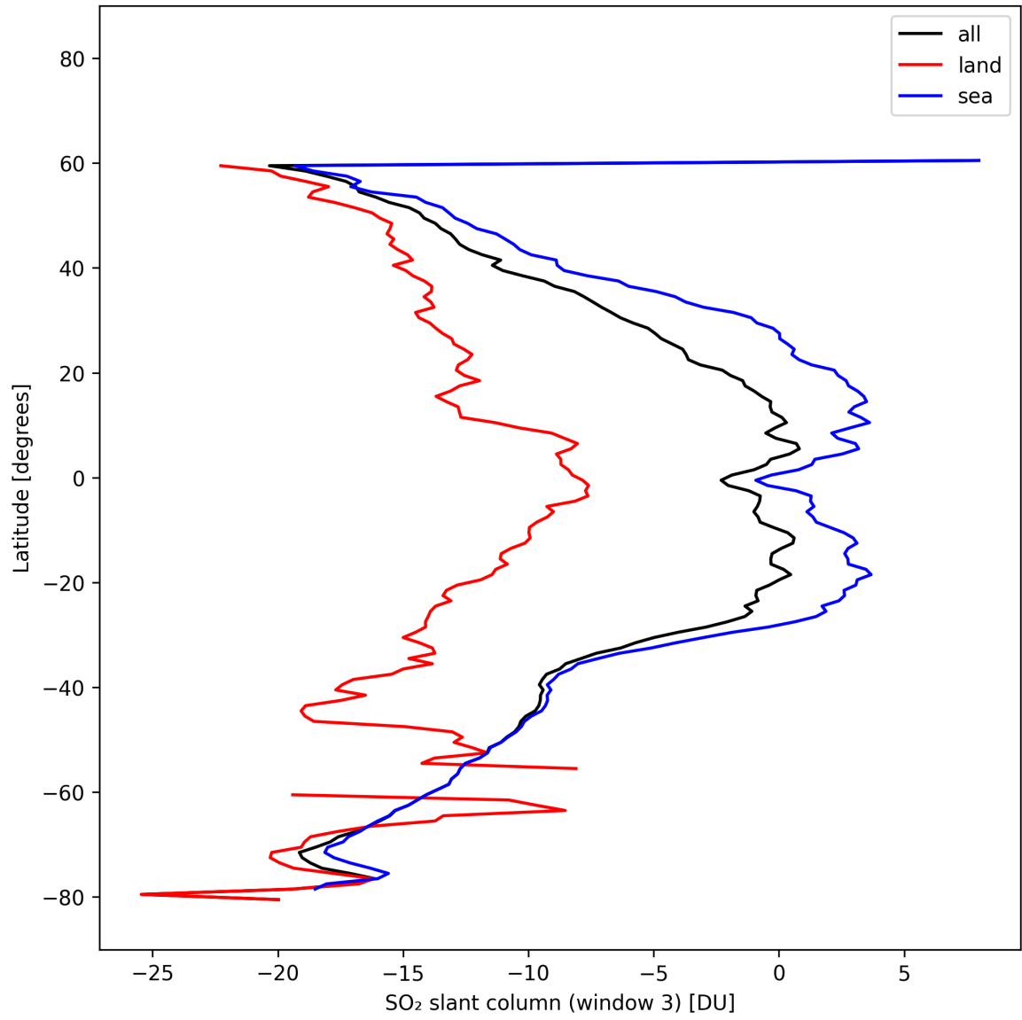
Figure 45: Zonal average of “SO 2 slant column (window 3)” for 2025-10-18 to 2025-10-20.
