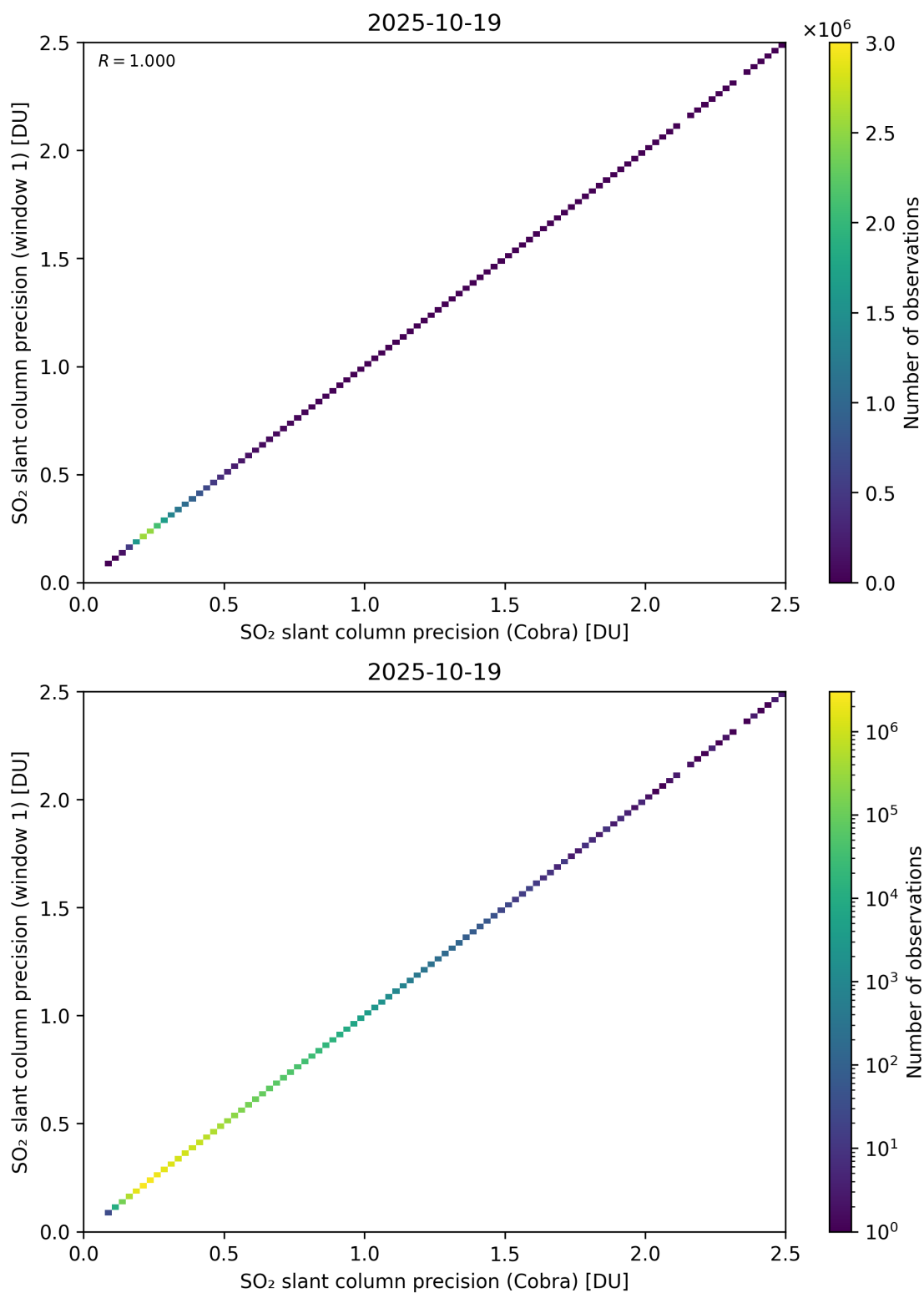
Figure 209: Scatter density plot of “SO 2 slant column precision (Cobra)” against “SO 2 slant column precision (window 1)” for 2025-10-18 to 2025-10-20.
