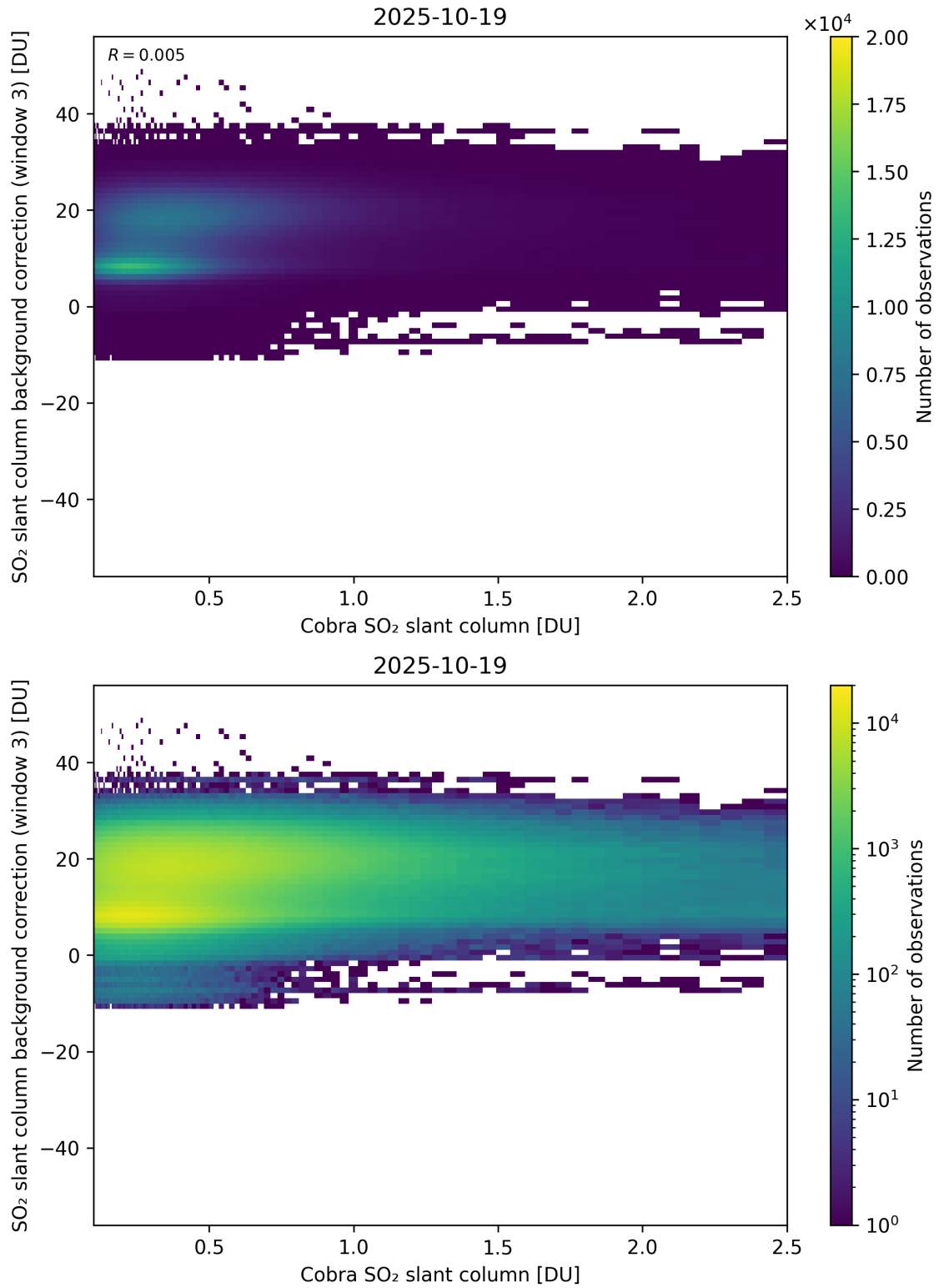
Figure 195: Scatter density plot of “Cobra SO 2 slant column” against “SO 2 slant column background correction (window 3)” for 2025-10-18 to 2025-10-20.
