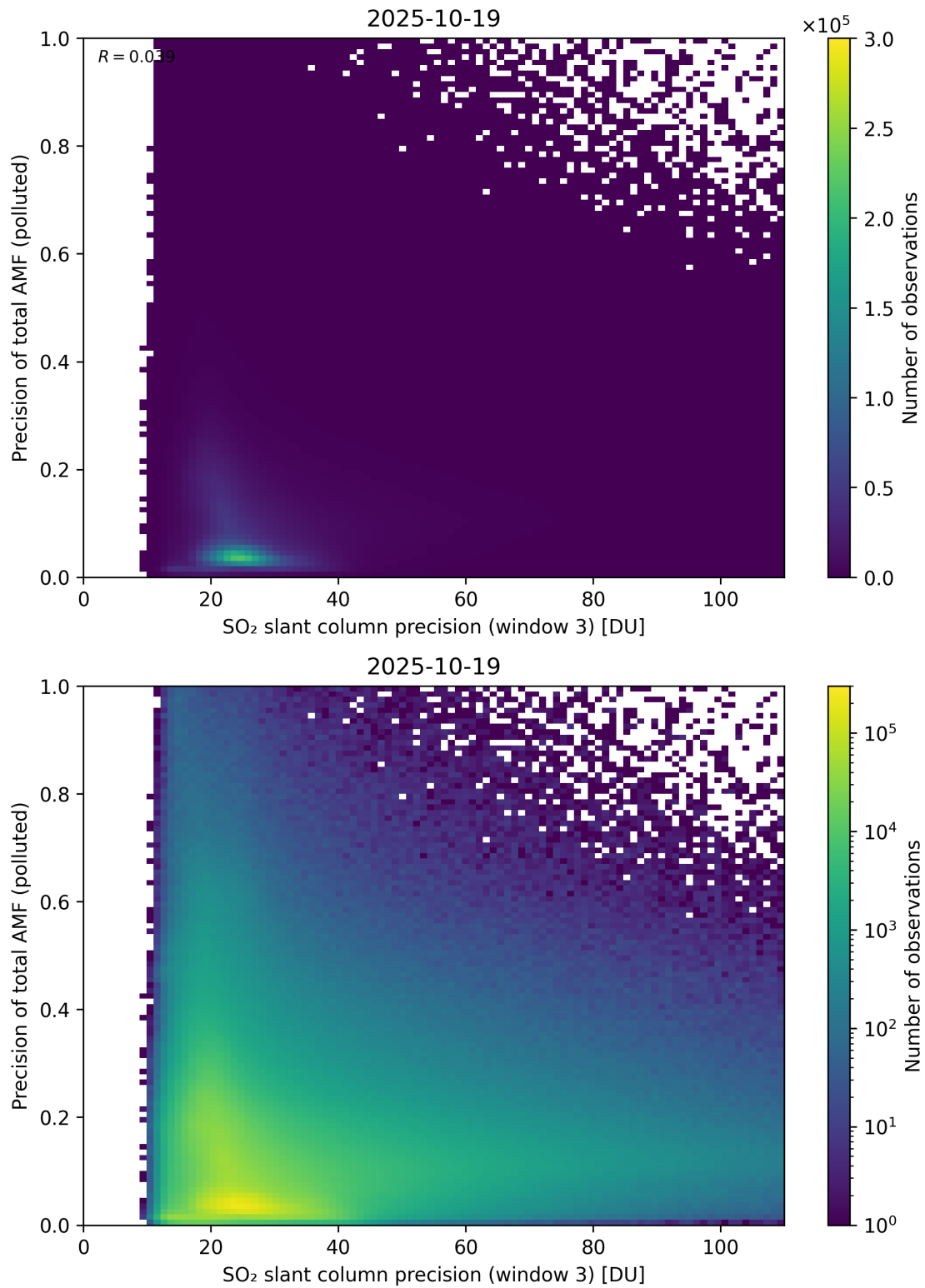
Figure 314: Scatter density plot of “SO 2 slant column precision (window 3)” against “Precision of total AMF (polluted)” for 2025-10-18 to 2025-10-20.
