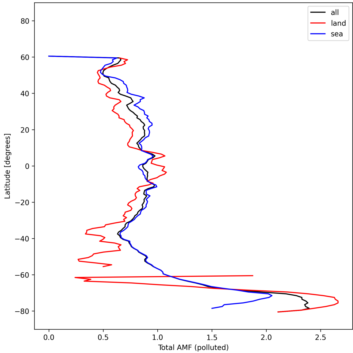
Figure 53: Zonal average of “Total AMF (polluted)” for 2025-10-18 to 2025-10-20.
