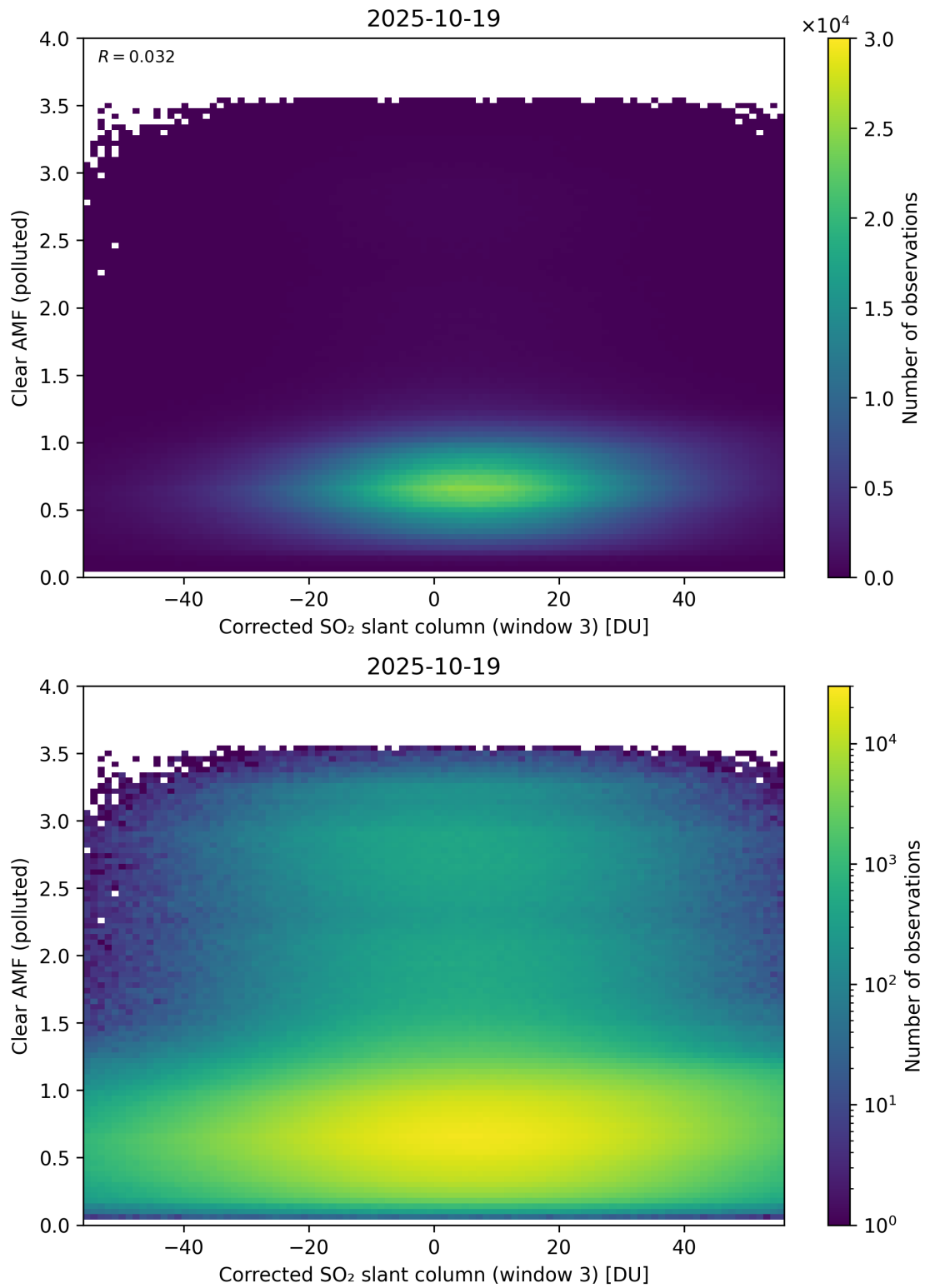
Figure 259: Scatter density plot of “Corrected SO 2 slant column (window 3)” against “Clear AMF (polluted)” for 2025-10-18 to 2025-10-20.
