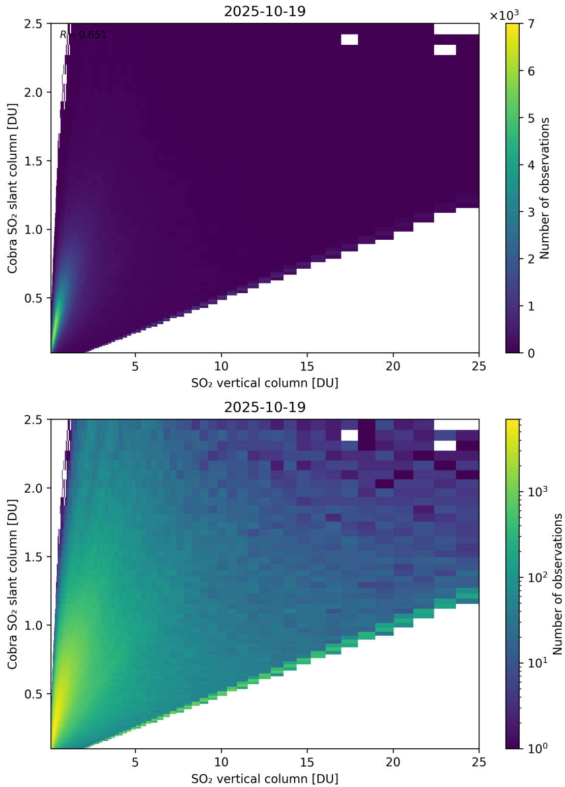
Figure 349: Scatter density plot of “SO 2 vertical column” against “Cobra SO 2 slant column” for 2025-10-18 to 2025-10-20.
