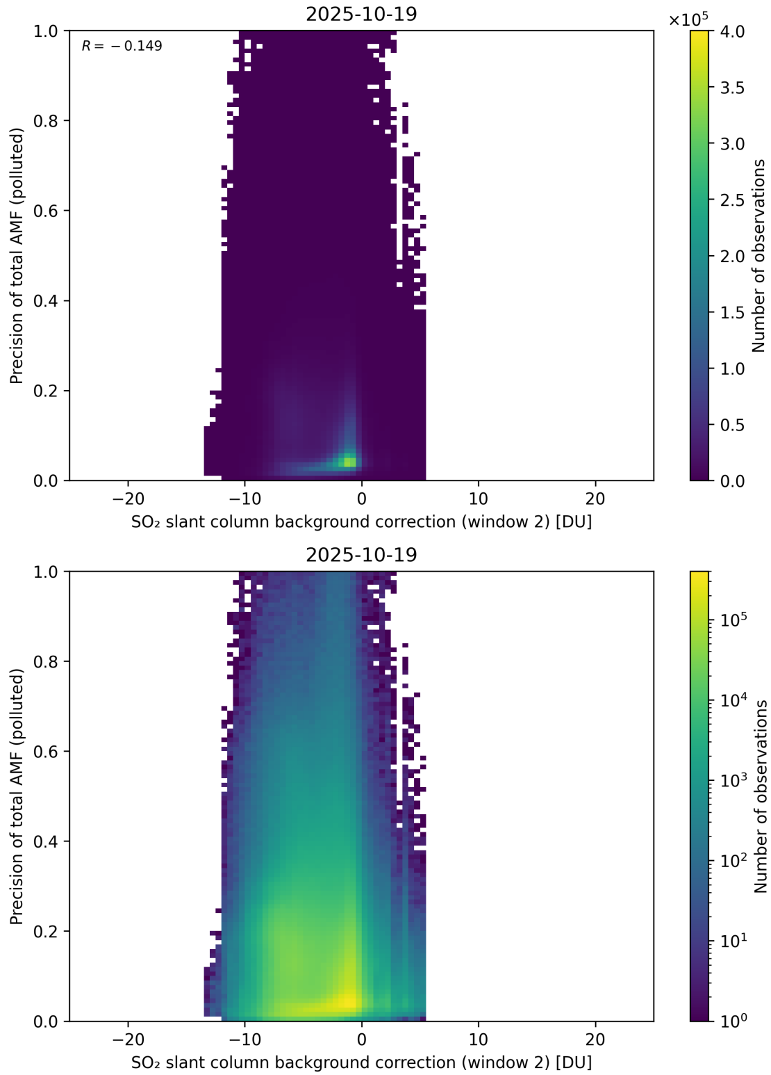
Figure 131: Scatter density plot of “SO 2 slant column background correction (window 2)” against “Precision of total AMF (polluted)” for 2025-10-18 to 2025-10-20.
