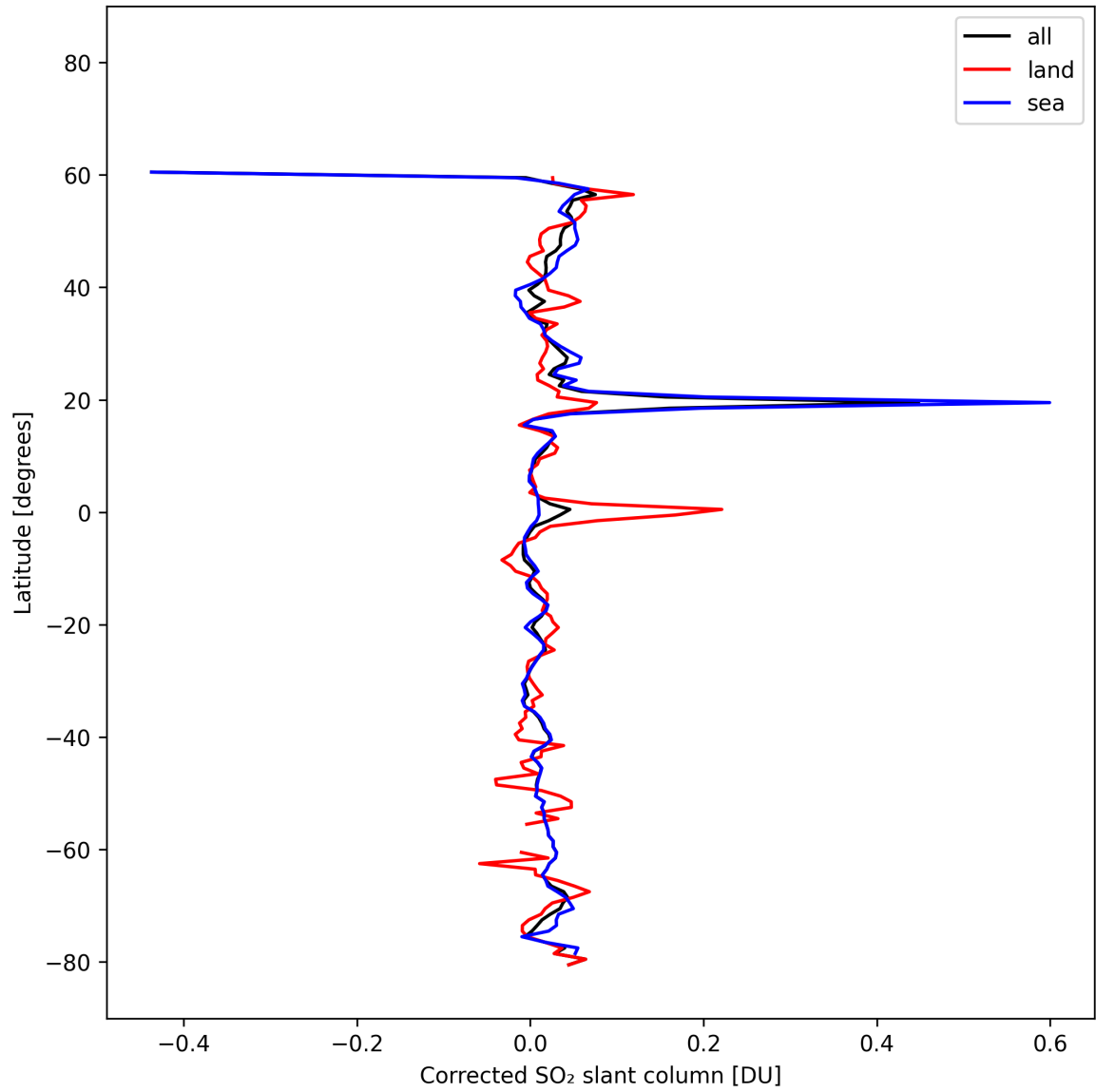
Figure 34: Zonal average of “Corrected SO 2 slant column” for 2025-10-18 to 2025-10-20.
