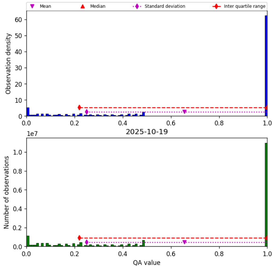
Figure 57: Histogram of “QA value” for 2025-10-18 to 2025-10-20
