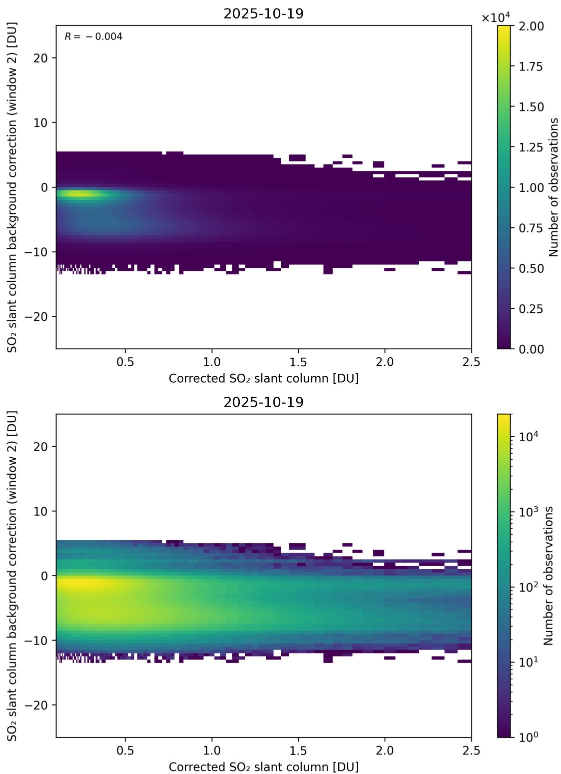
Figure 227: Scatter density plot of “Corrected SO 2 slant column” against “SO 2 slant column background correction (window 2)” for 2025-10-18 to 2025-10-20.
