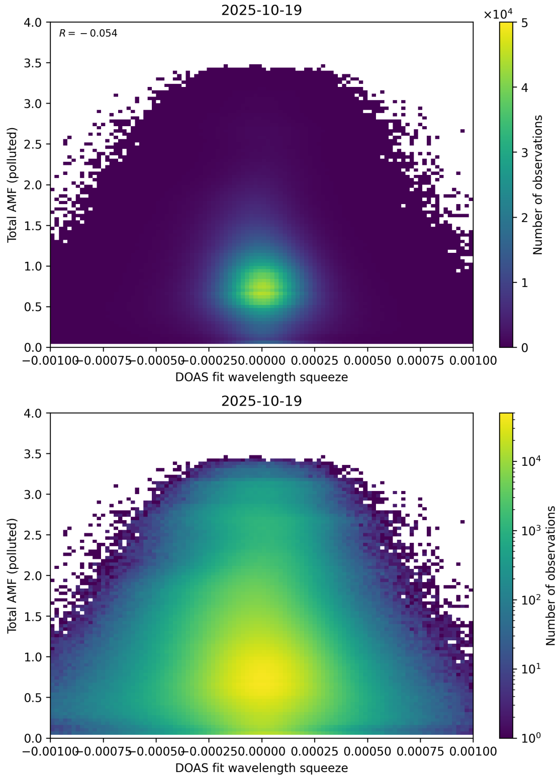
Figure 145: Scatter density plot of “DOAS fit wavelength squeeze” against “Total AMF (polluted)” for 2025-10-18 to 2025-10-20.
