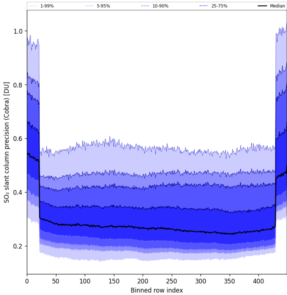
Figure 88: Along track statistics of “SO 2 slant column precision (Cobra)” for 2025-10-18 to 2025-10-20
