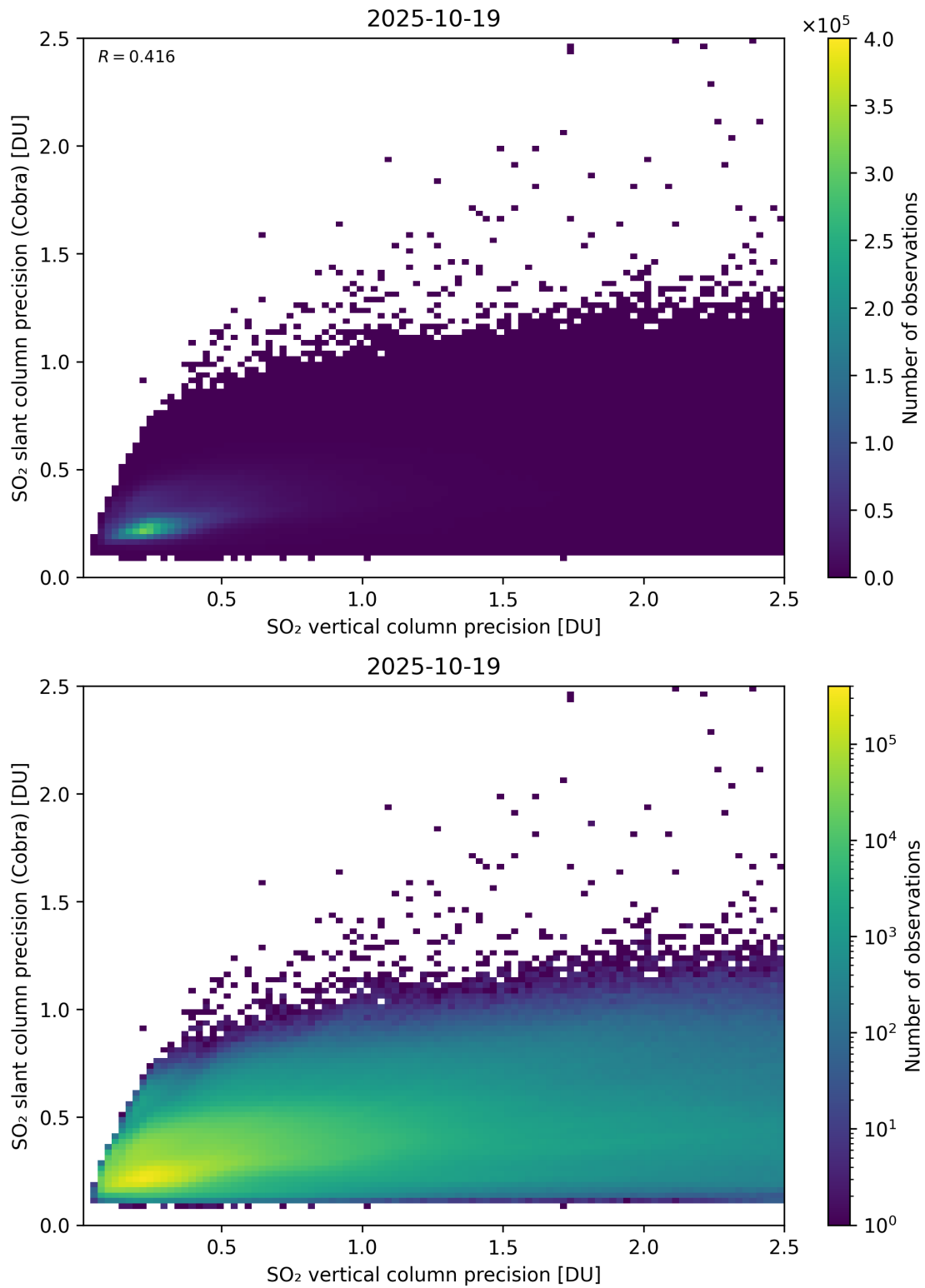
Figure 337: Scatter density plot of “SO 2 vertical column precision” against “SO 2 slant column precision (Cobra)” for 2025-10-18 to 2025-10-20.
