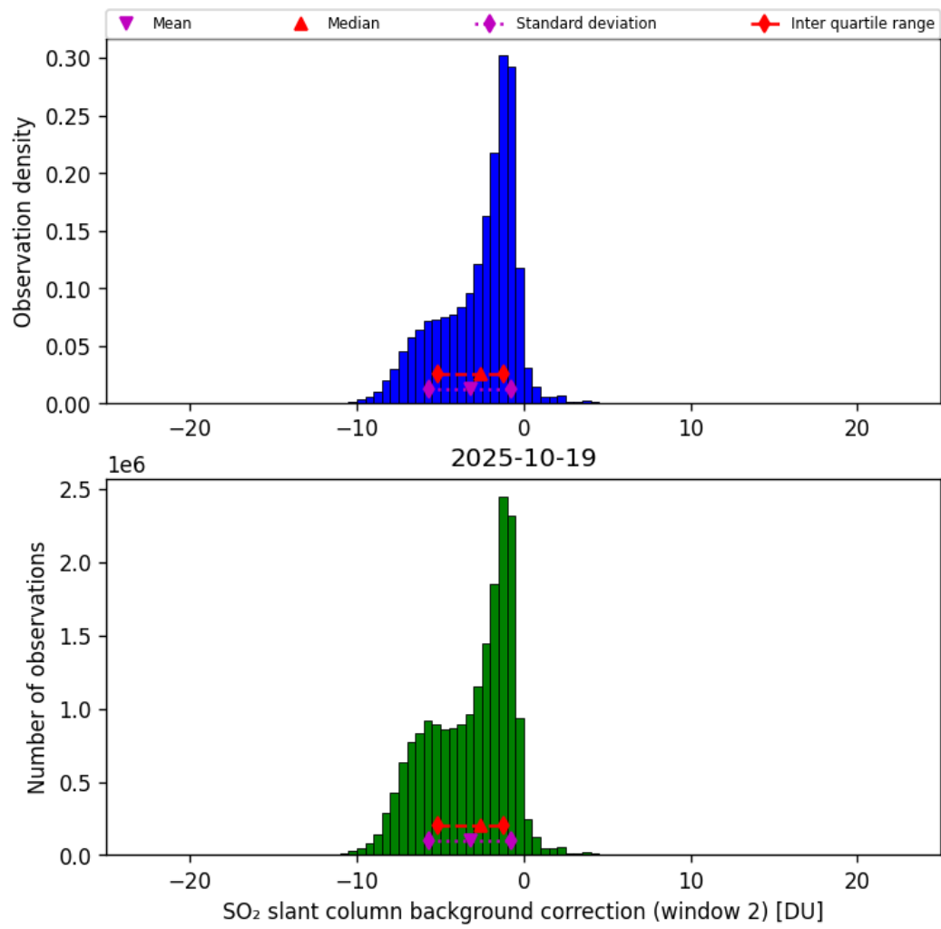
Figure 70: Histogram of “SO 2 slant column background correction (window 2)” for 2025-10-18 to 2025-10-20
