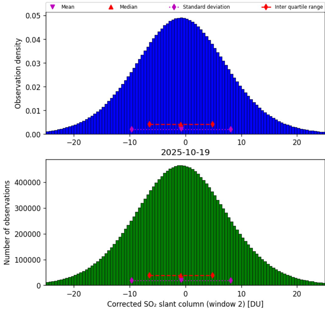
Figure 69: Histogram of “Corrected SO 2 slant column (window 2)” for 2025-10-18 to 2025-10-20
