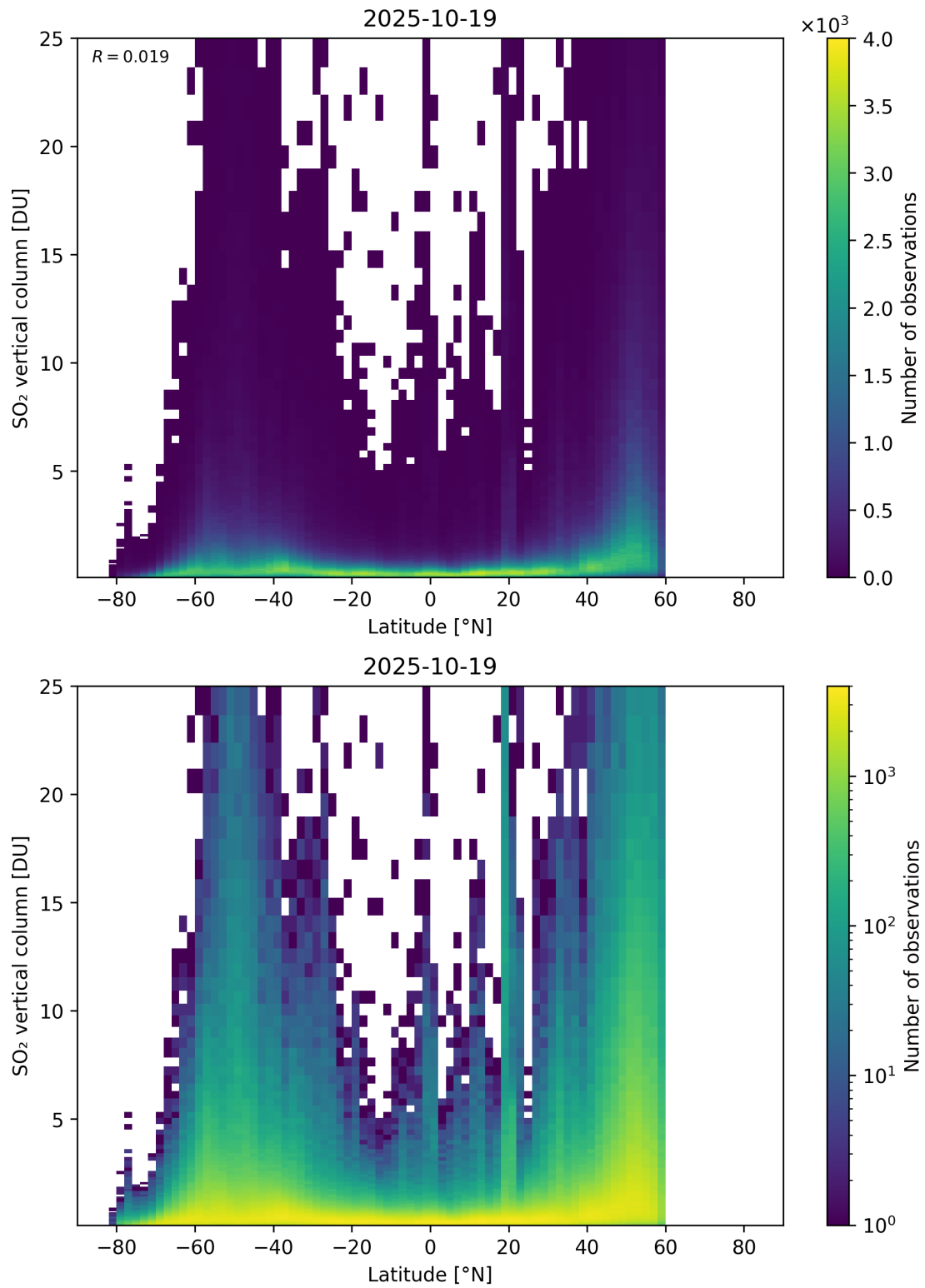
Figure 169: Scatter density plot of “Latitude” against “SO 2 vertical column” for 2025-10-18 to 2025-10-20.
