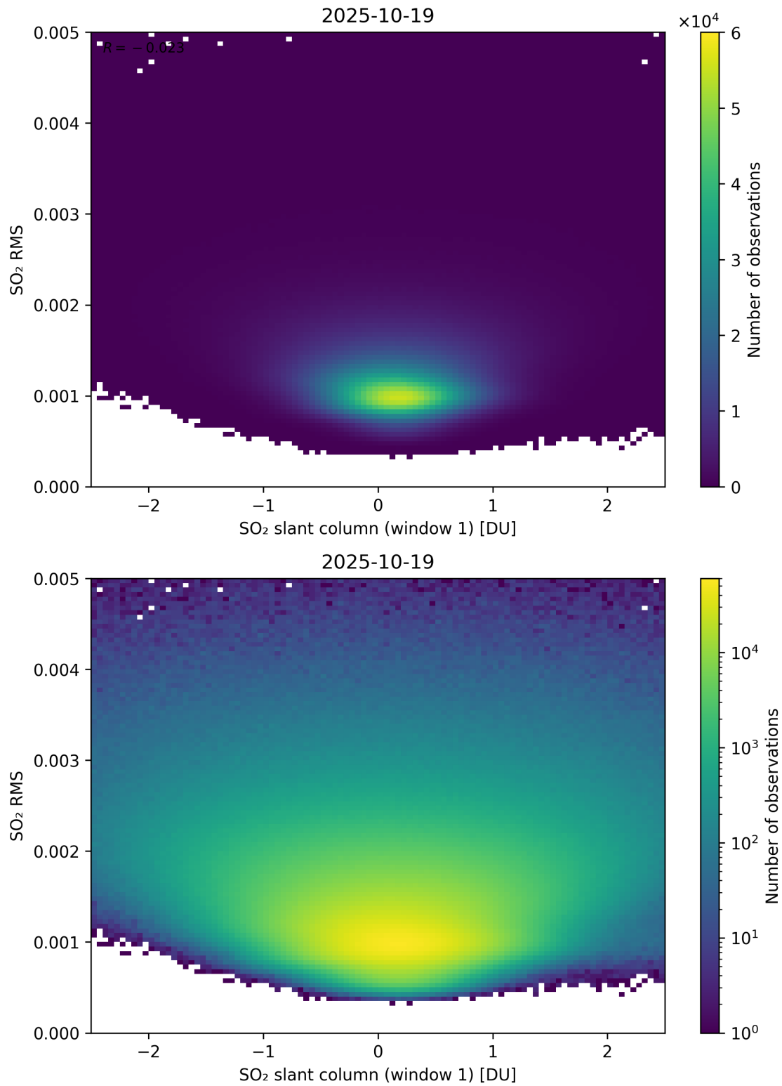
Figure 267: Scatter density plot of “SO 2 slant column (window 1)” against “SO 2 RMS” for 2025-10-18 to 2025-10-20.
