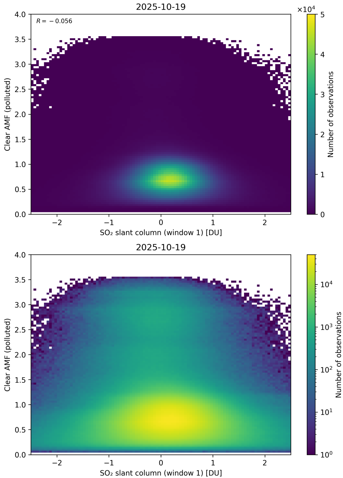
Figure 282: Scatter density plot of “SO 2 slant column (window 1)” against “Clear AMF (polluted)” for 2025-10-18 to 2025-10-20.
