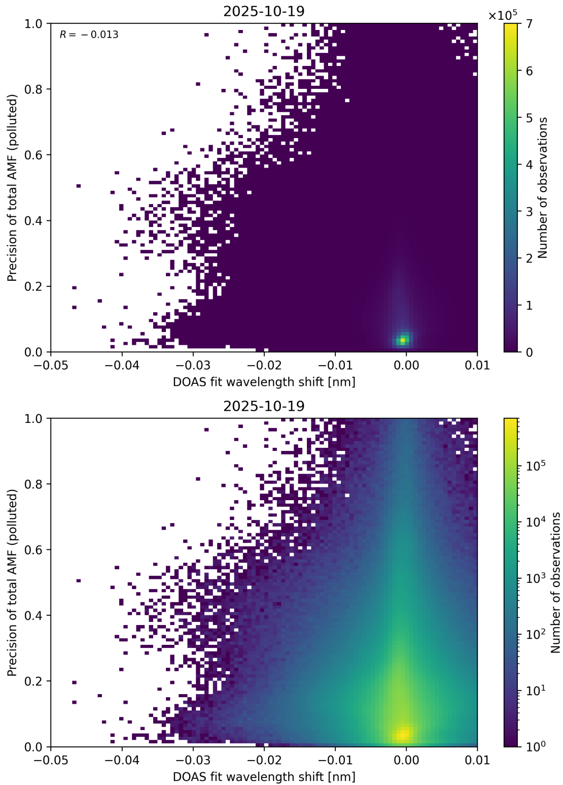
Figure 142: Scatter density plot of “DOAS fit wavelength shift” against “Precision of total AMF (polluted)” for 2025-10-18 to 2025-10-20.
