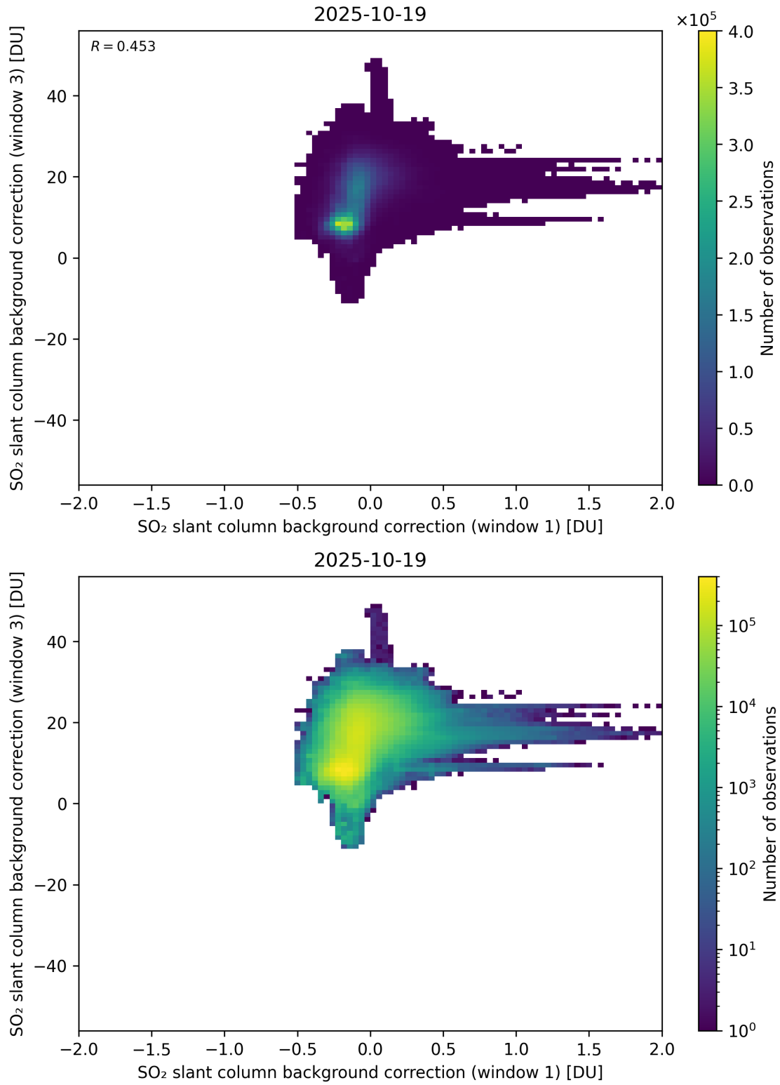
Figure 110: Scatter density plot of “SO 2 slant column background correction (window 1)” against “SO 2 slant column background correction (window 3)” for 2025-10-18 to 2025-10-20.
