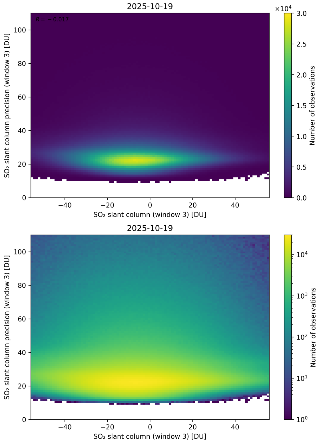
Figure 317: Scatter density plot of “SO 2 slant column (window 3)” against “SO 2 slant column precision (window 3)” for 2025-10-18 to 2025-10-20.
