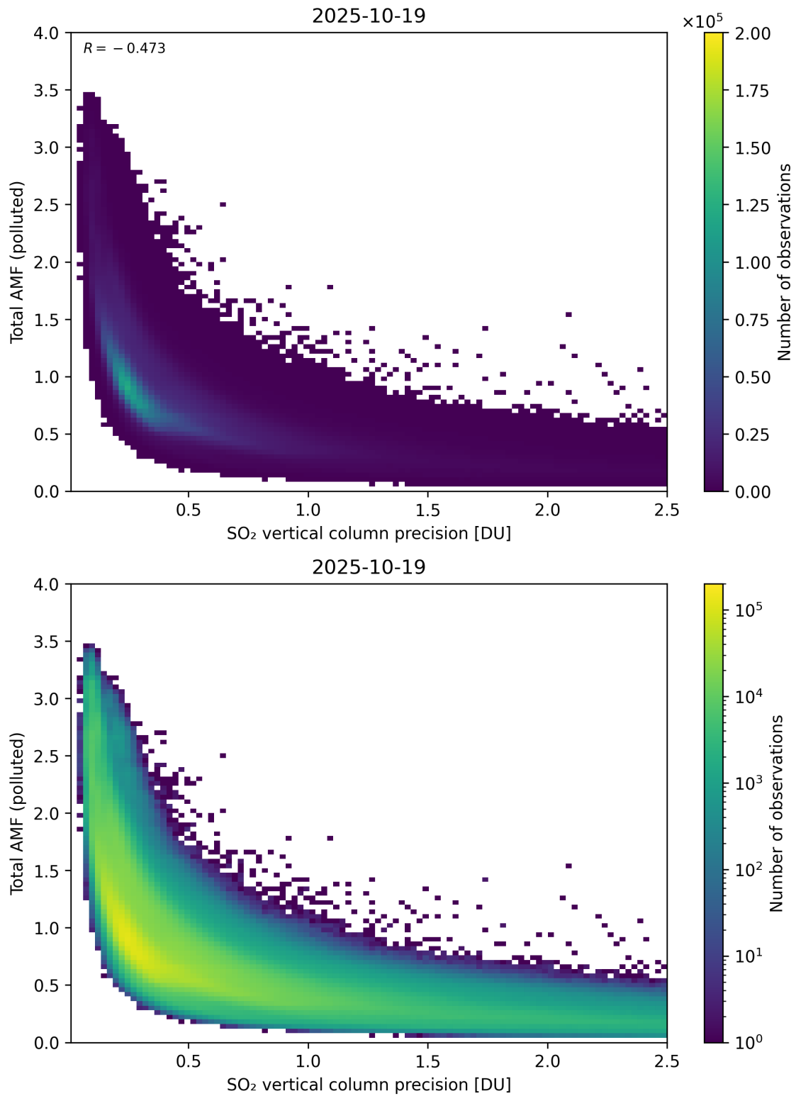
Figure 346: Scatter density plot of “SO 2 vertical column precision” against “Total AMF (polluted)” for 2025-10-18 to 2025-10-20.
