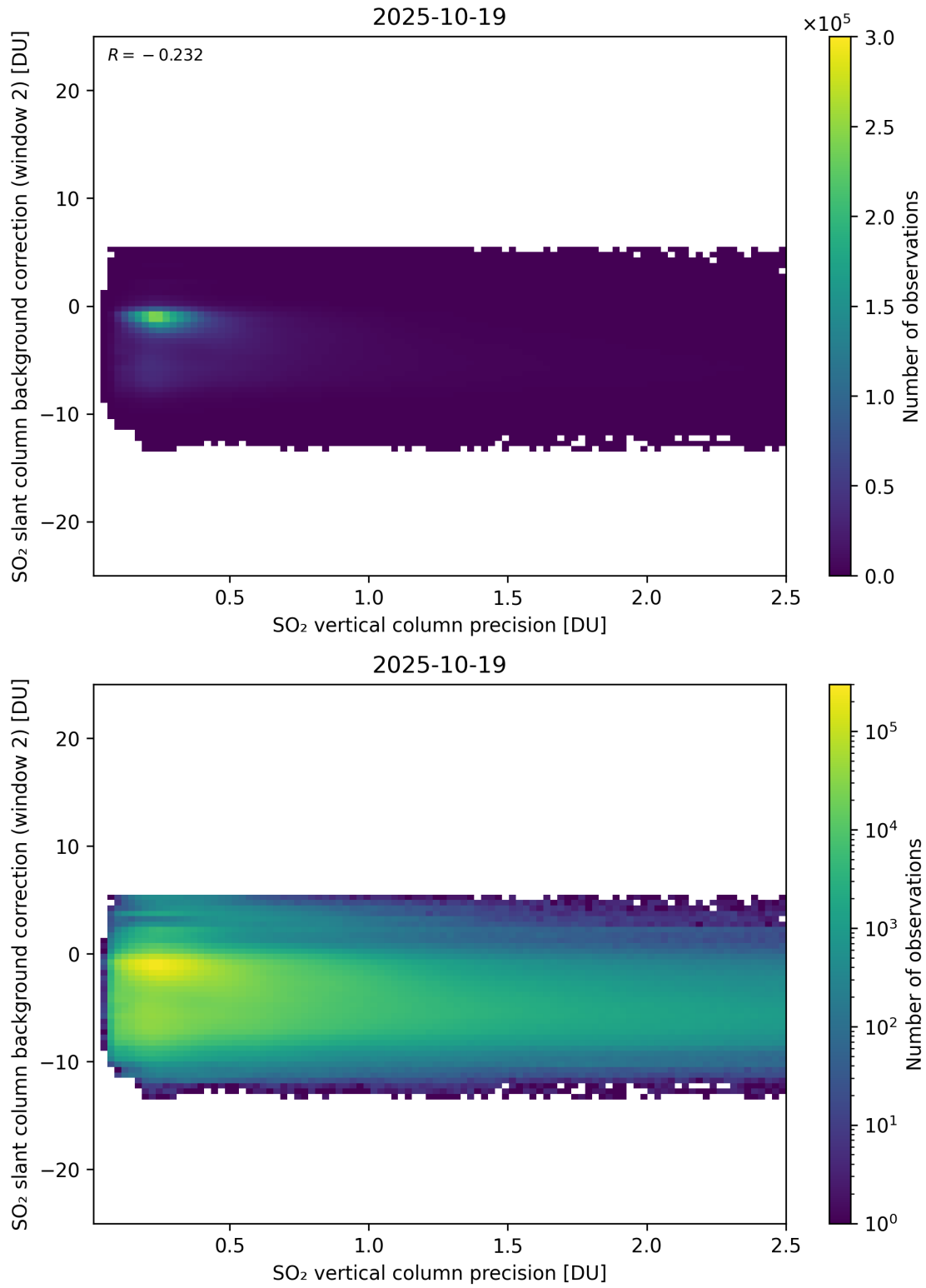
Figure 330: Scatter density plot of “SO 2 vertical column precision” against “SO 2 slant column background correction (window 2)” for 2025-10-18 to 2025-10-20.
