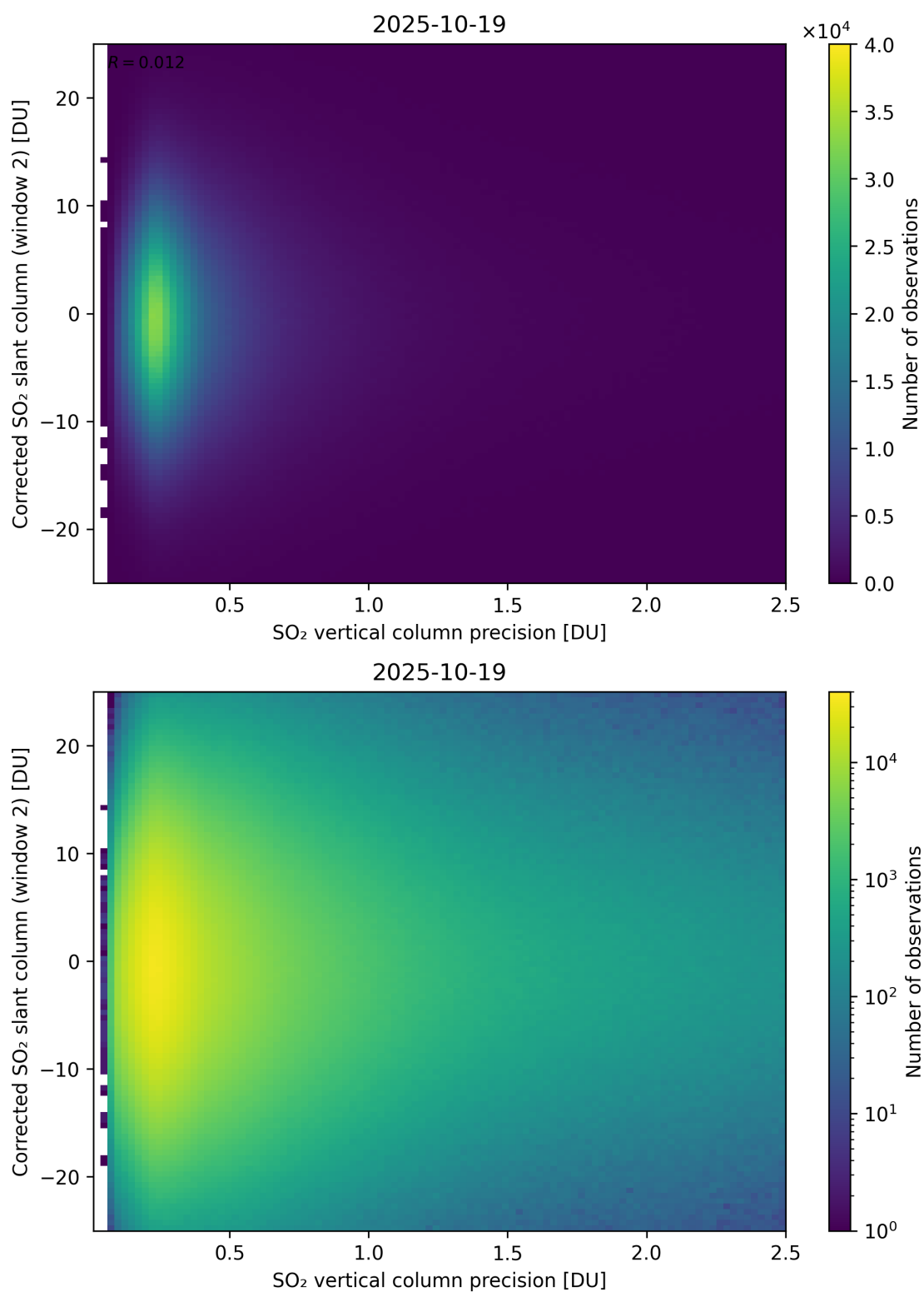
Figure 339: Scatter density plot of “SO 2 vertical column precision” against “Corrected SO 2 slant column (window 2)” for 2025-10-18 to 2025-10-20.
