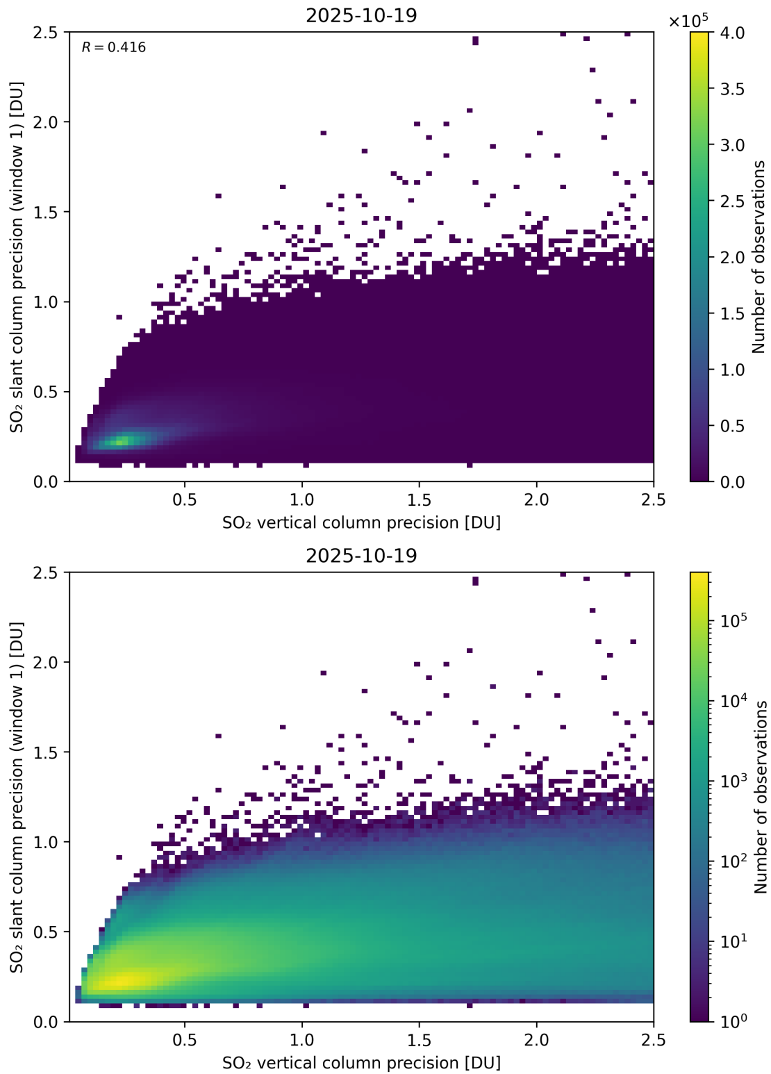
Figure 342: Scatter density plot of “SO 2 vertical column precision” against “SO 2 slant column precision (window 1)” for 2025-10-18 to 2025-10-20.
