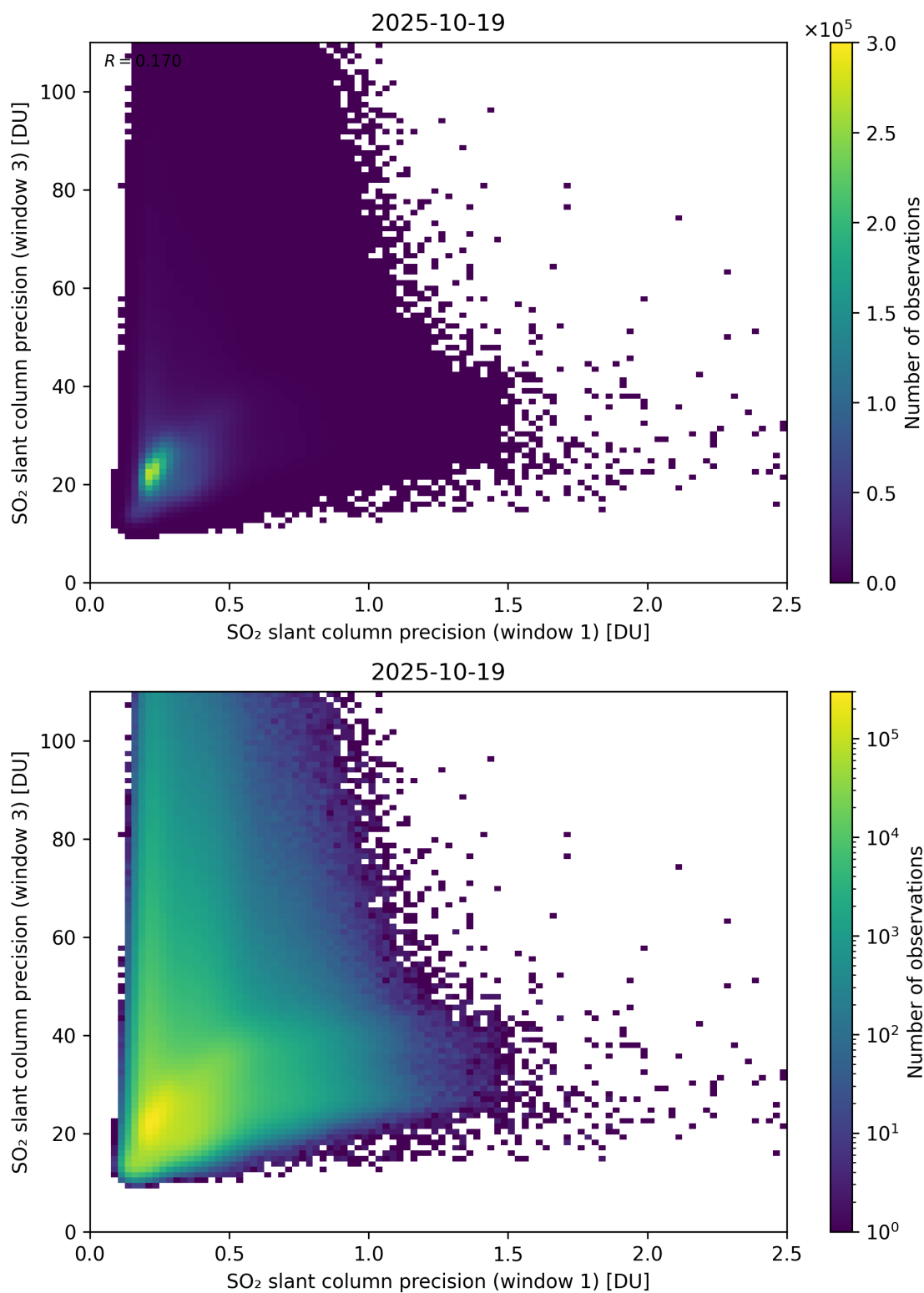
Figure 279: Scatter density plot of “SO 2 slant column precision (window 1)” against “SO 2 slant column precision (window 3)” for 2025-10-18 to 2025-10-20.
