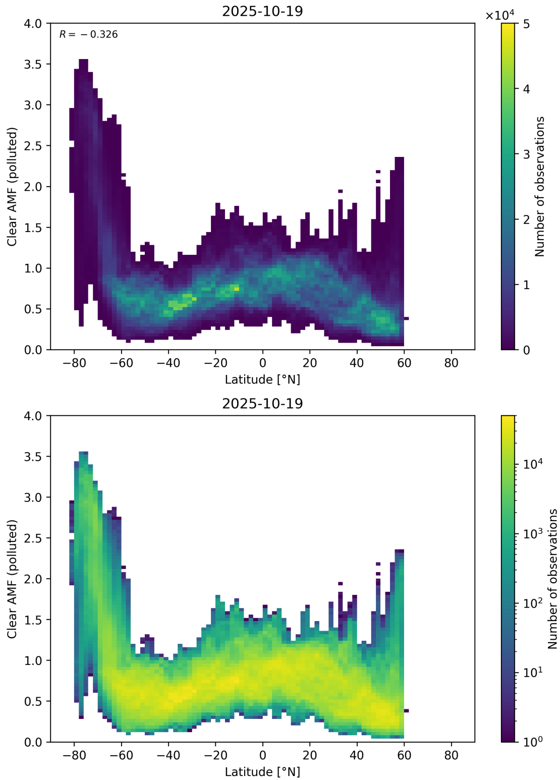
Figure 156: Scatter density plot of “Latitude” against “Clear AMF (polluted)” for 2025-10-18 to 2025-10-20.
