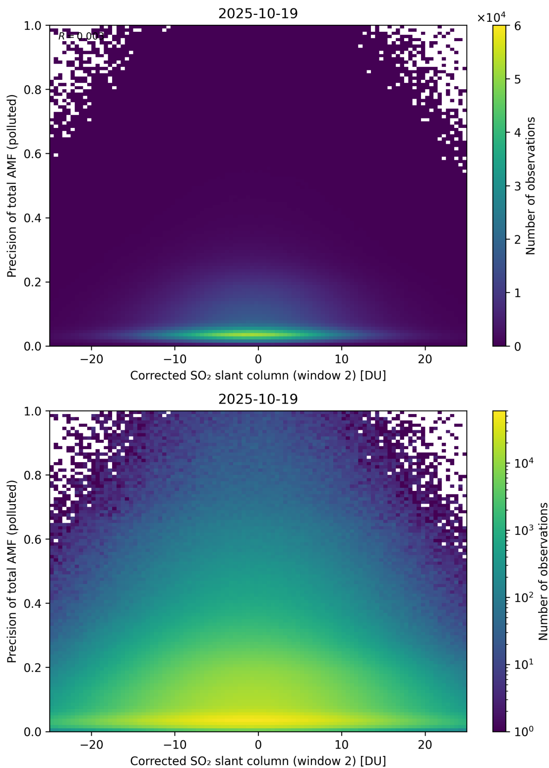
Figure 254: Scatter density plot of “Corrected SO 2 slant column (window 2)” against “Precision of total AMF (polluted)” for 2025-10-18 to 2025-10-20.
