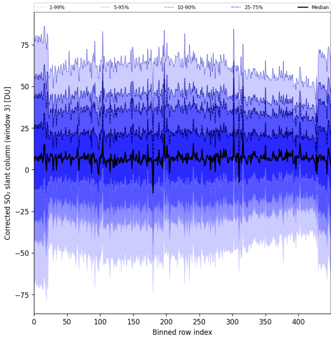
Figure 99: Along track statistics of “Corrected SO 2 slant column (window 3)” for 2025-10-18 to 2025-10-20
