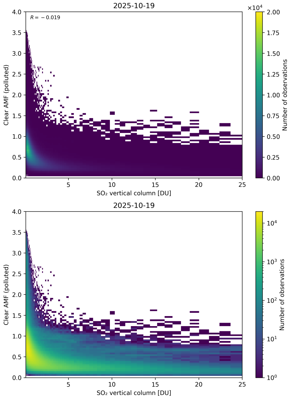
Figure 348: Scatter density plot of “SO 2 vertical column” against “Clear AMF (polluted)” for 2025-10-18 to 2025-10-20.
