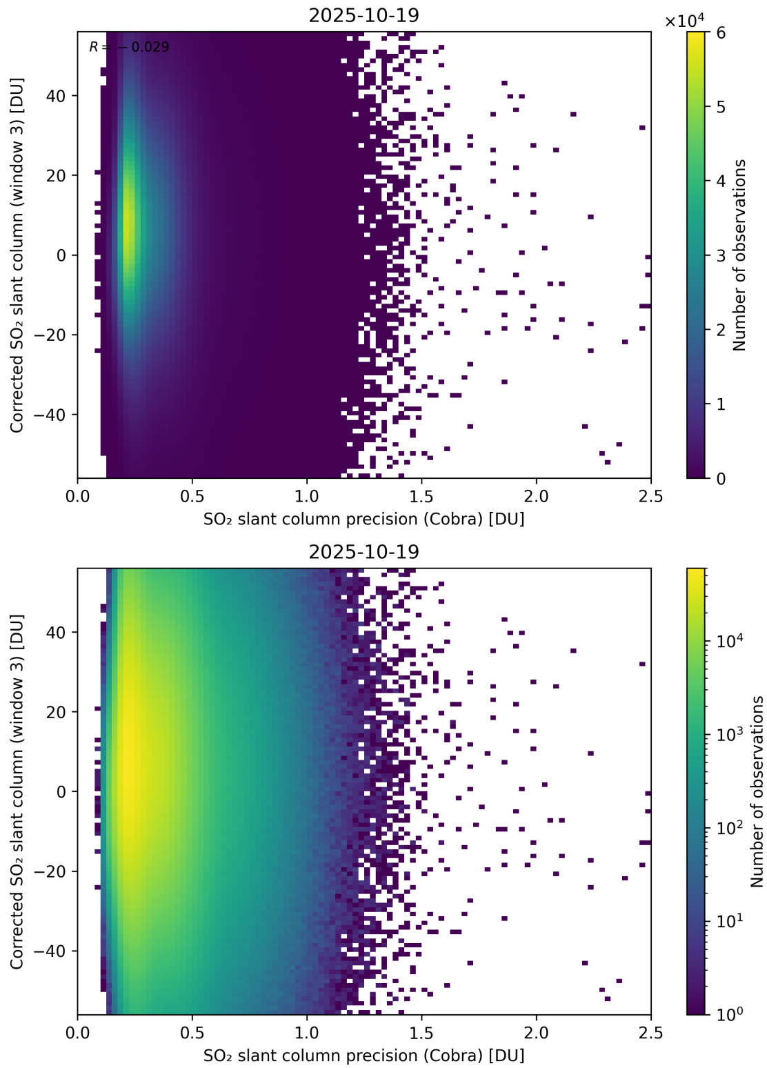
Figure 207: Scatter density plot of “SO 2 slant column precision (Cobra)” against “Corrected SO 2 slant column (window 3)” for 2025-10-18 to 2025-10-20.
