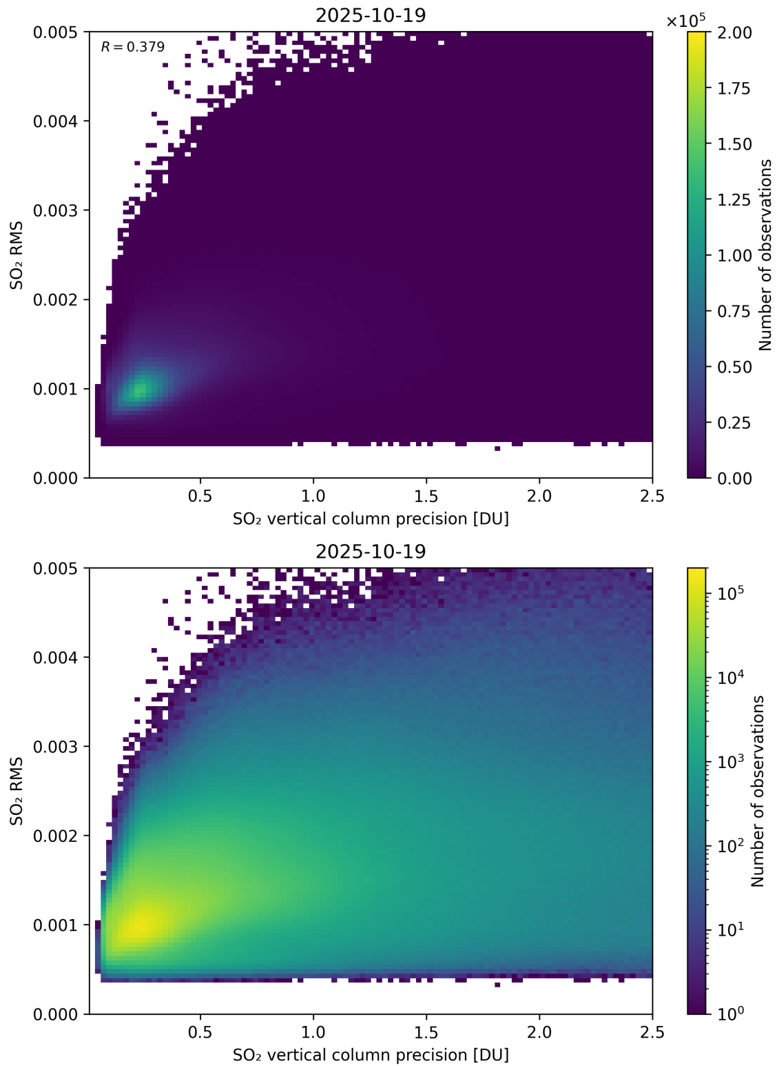
Figure 334: Scatter density plot of “SO 2 vertical column precision” against “SO 2 RMS” for 2025-10-18 to 2025-10-20.
