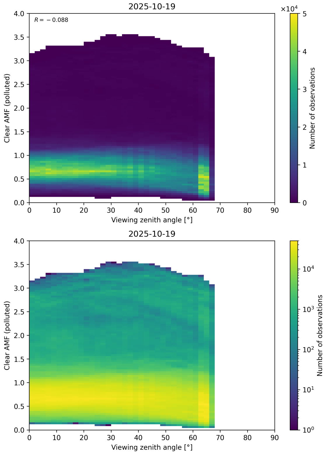
Figure 370: Scatter density plot of “Viewing zenith angle” against “Clear AMF (polluted)” for 2025-10-18 to 2025-10-20.
