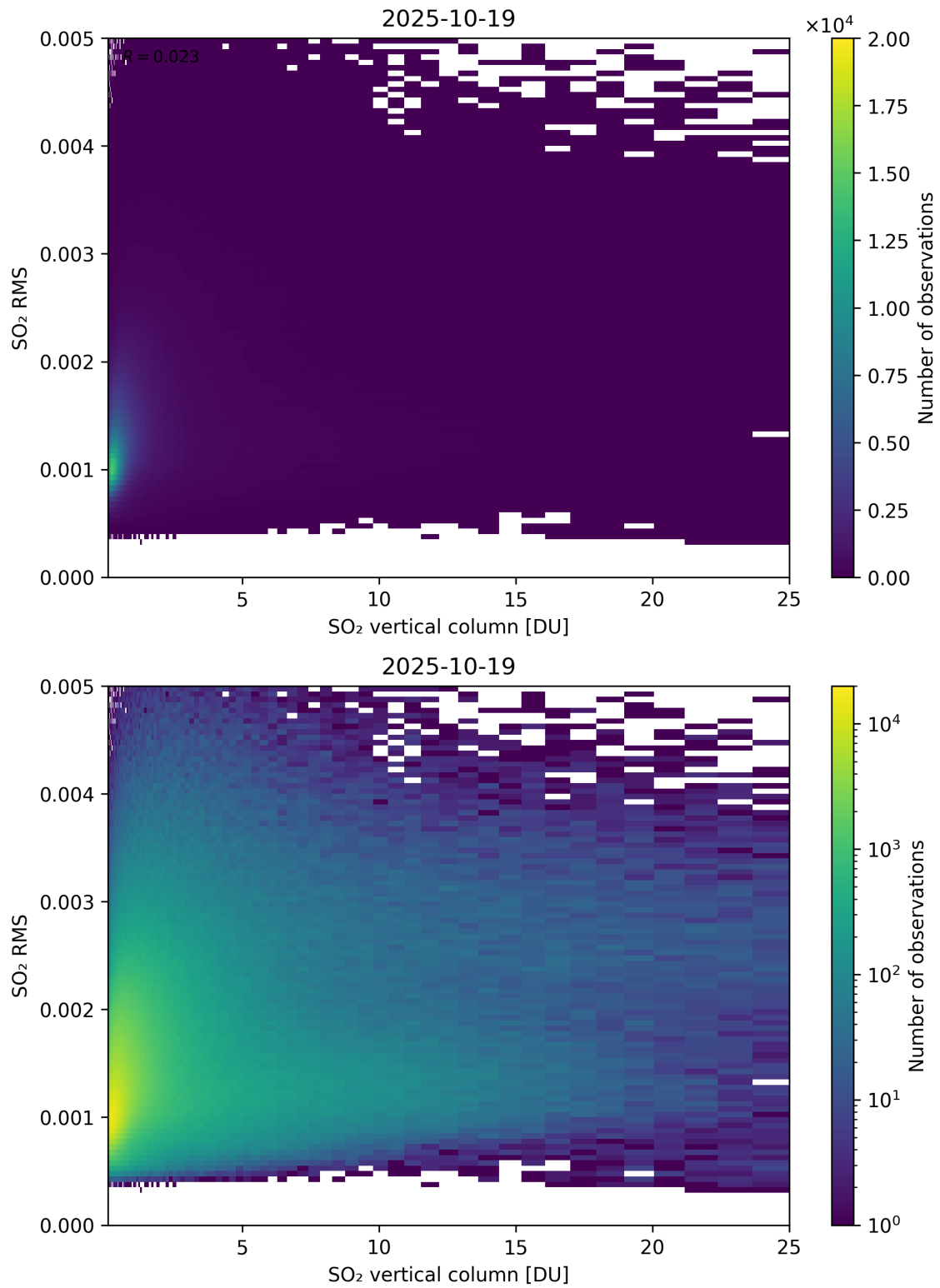
Figure 328: Scatter density plot of “SO 2 vertical column” against “SO 2 RMS” for 2025-10-18 to 2025-10-20.
