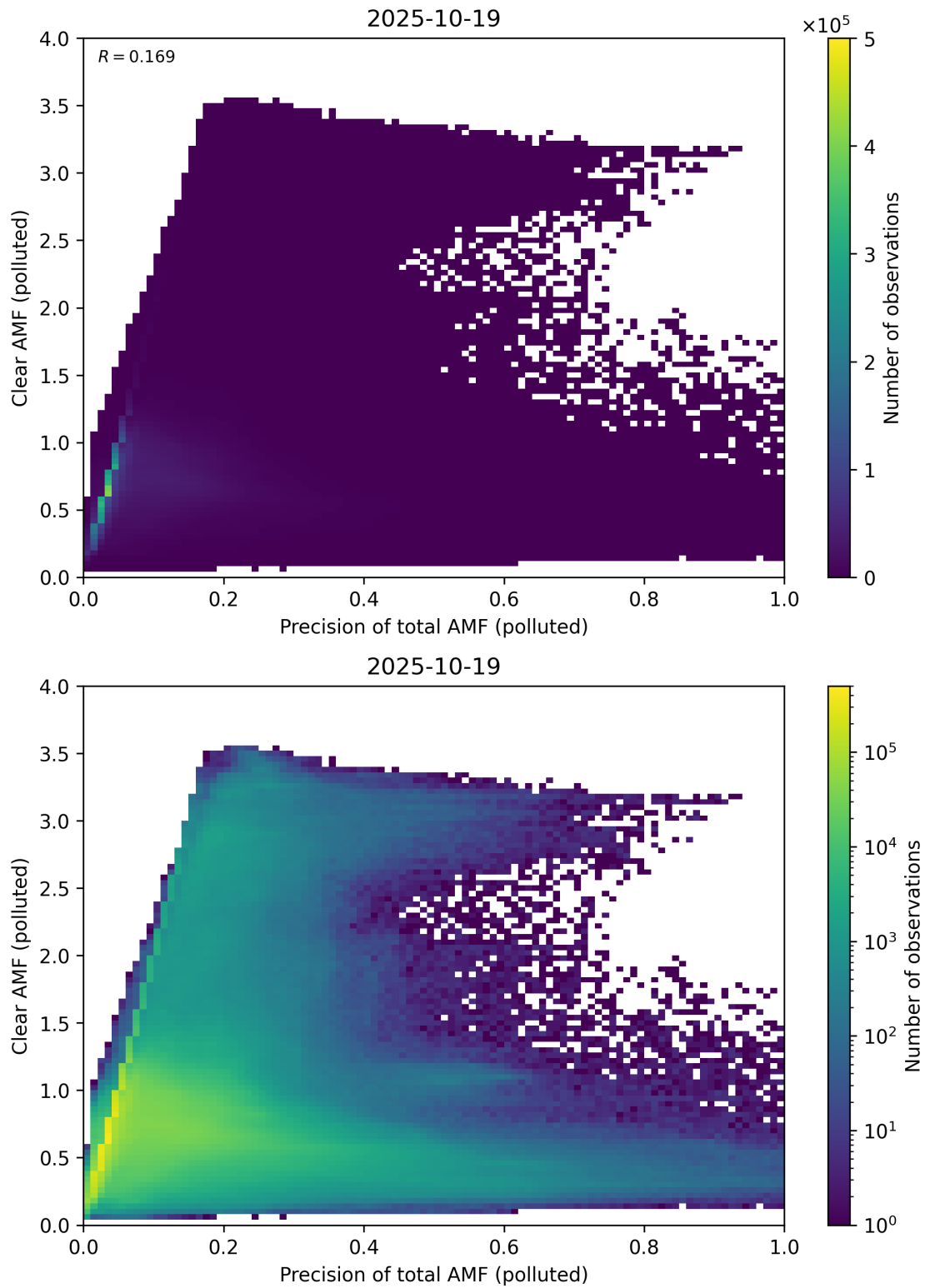
Figure 320: Scatter density plot of “Precision of total AMF (polluted)” against “Clear AMF (polluted)” for 2025-10-18 to 2025-10-20.
