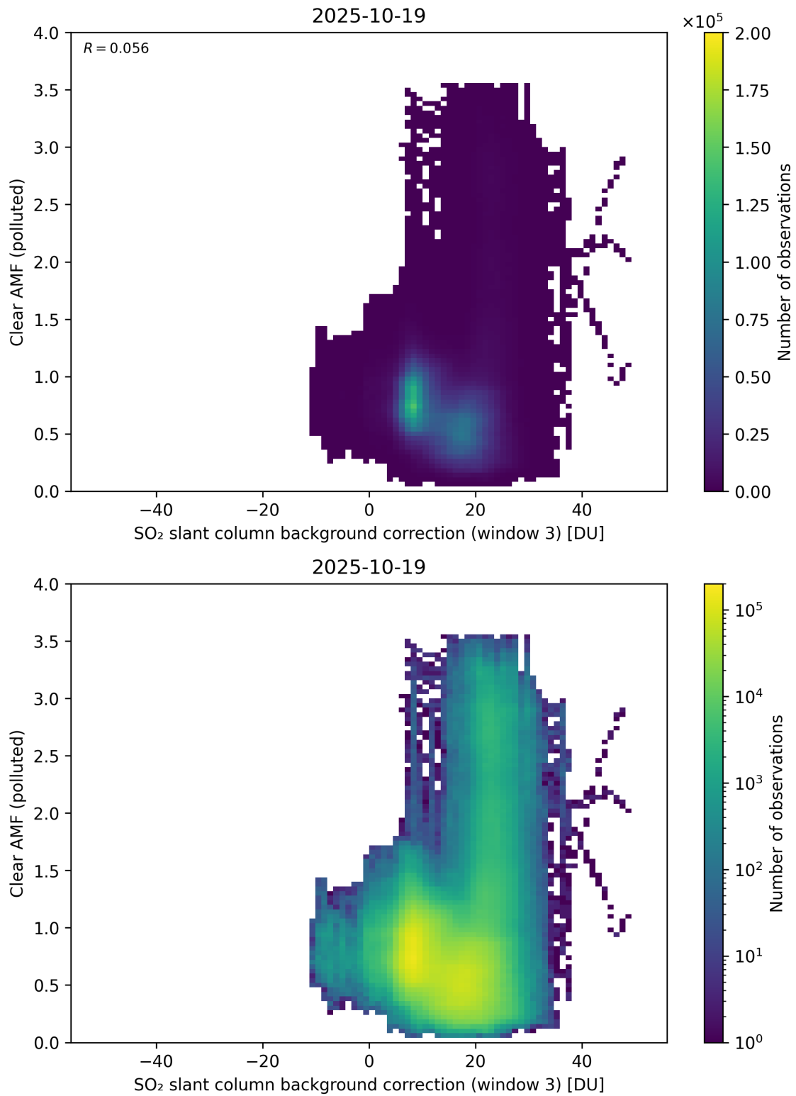
Figure 135: Scatter density plot of “SO 2 slant column background correction (window 3)” against “Clear AMF (polluted)” for 2025-10-18 to 2025-10-20.
