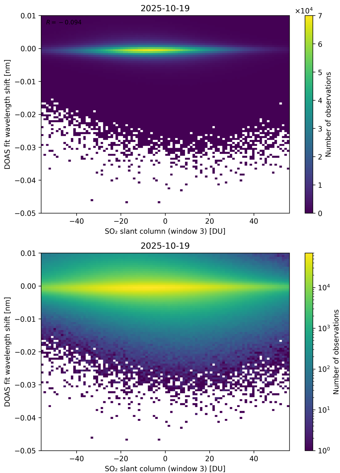
Figure 304: Scatter density plot of “SO 2 slant column (window 3)” against “DOAS fit wavelength shift” for 2025-10-18 to 2025-10-20.
