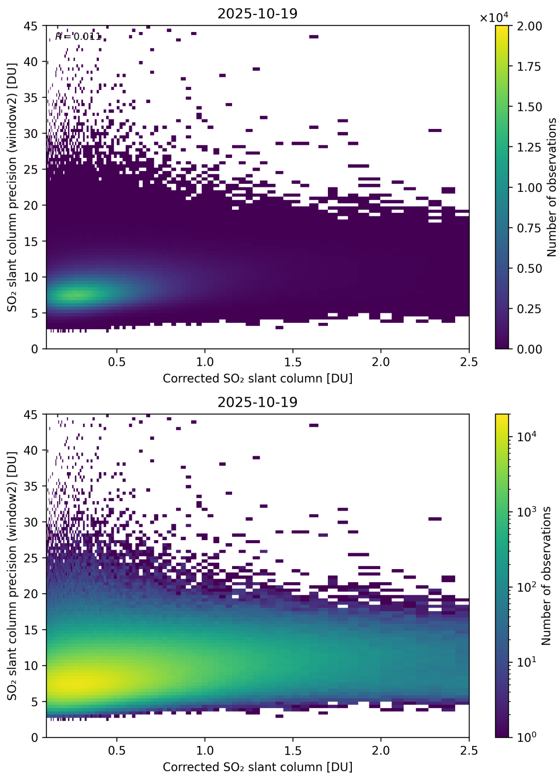
Figure 239: Scatter density plot of “Corrected SO 2 slant column” against “SO 2 slant column precision (window2)” for 2025-10-18 to 2025-10-20.
