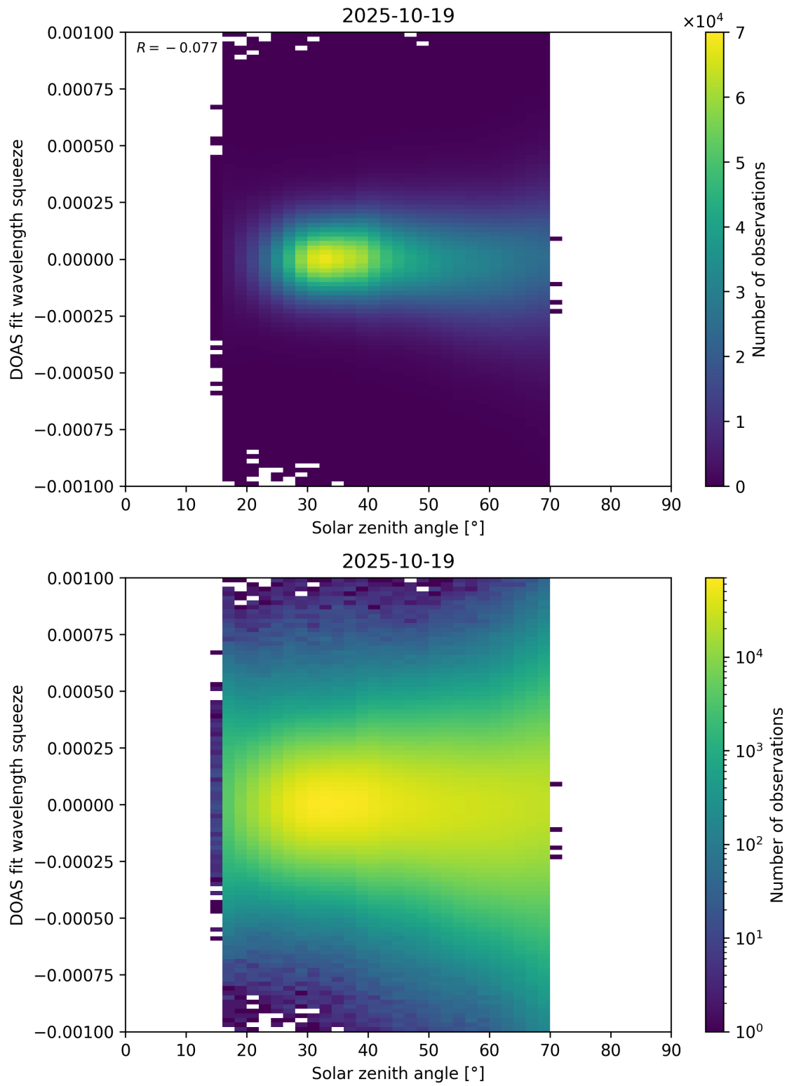
Figure 175: Scatter density plot of “Solar zenith angle” against “DOAS fit wavelength squeeze” for 2025-10-18 to 2025-10-20.
