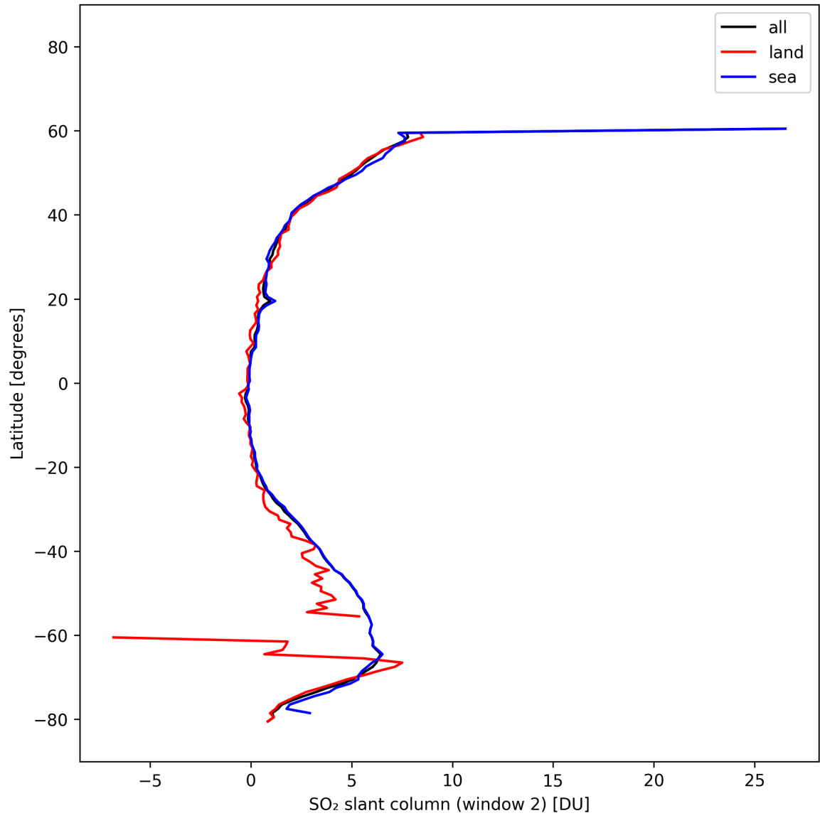
Figure 41: Zonal average of “SO 2 slant column (window 2)” for 2025-10-18 to 2025-10-20.
