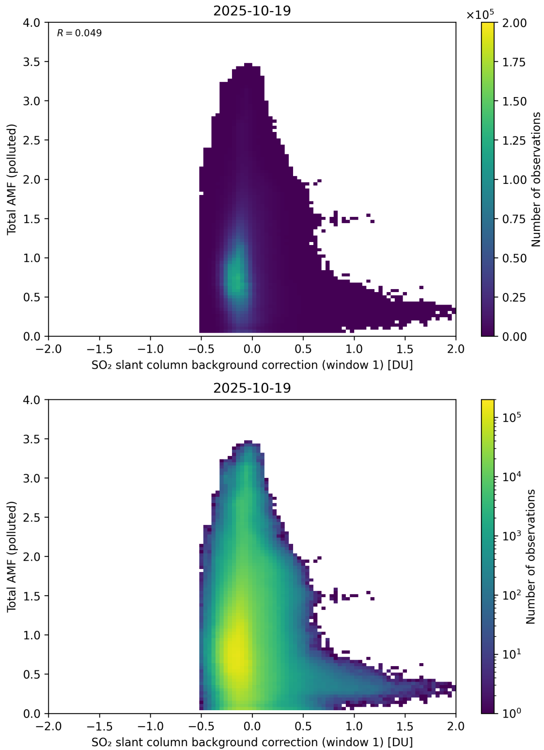
Figure 120: Scatter density plot of “SO 2 slant column background correction (window 1)” against “Total AMF (polluted)” for 2025-10-18 to 2025-10-20.
