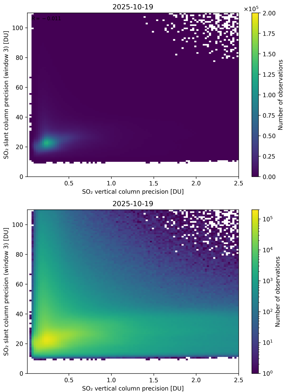
Figure 345: Scatter density plot of “SO 2 vertical column precision” against “SO 2 slant column precision (window 3)” for 2025-10-18 to 2025-10-20.
