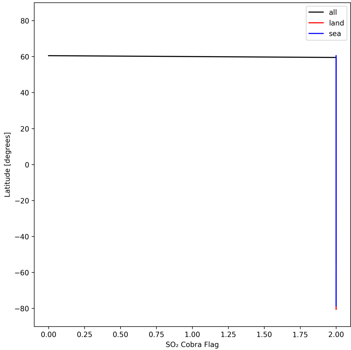
Figure 49: Zonal average of “SO 2 Cobra Flag” for 2025-10-18 to 2025-10-20.
