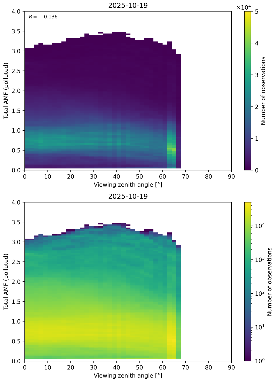
Figure 381: Scatter density plot of “Viewing zenith angle” against “Total AMF (polluted)” for 2025-10-18 to 2025-10-20.
