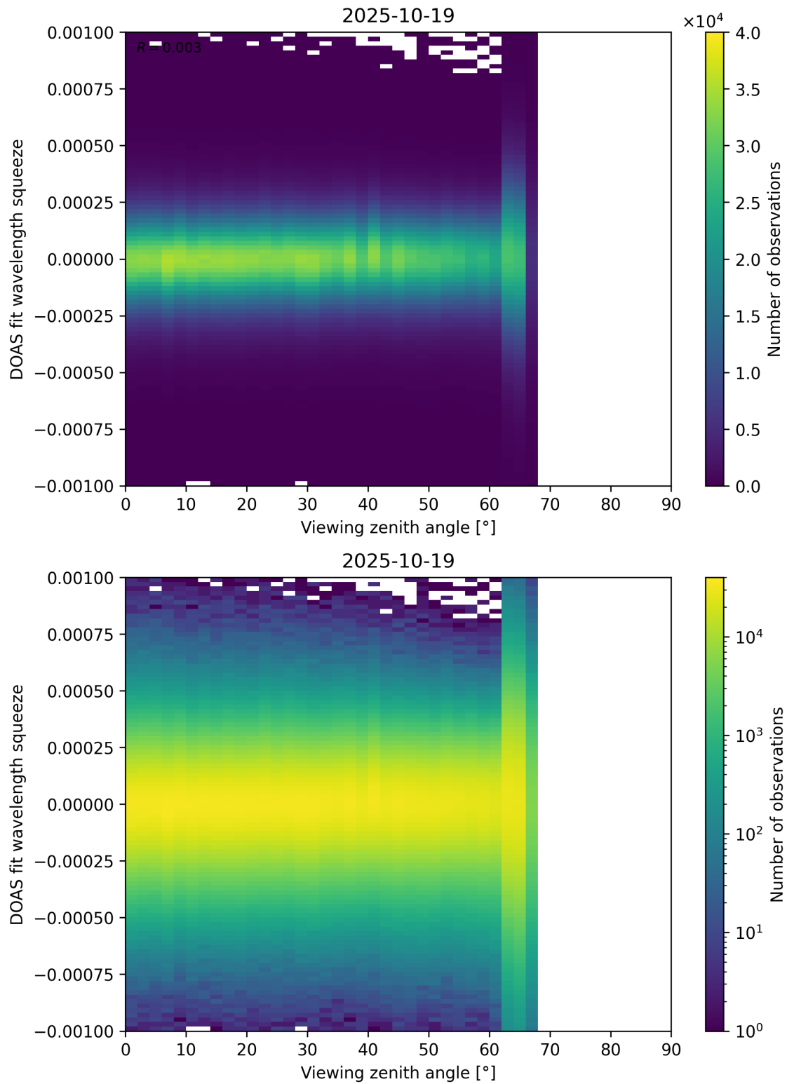
Figure 366: Scatter density plot of “Viewing zenith angle” against “DOAS fit wavelength squeeze” for 2025-10-18 to 2025-10-20.
