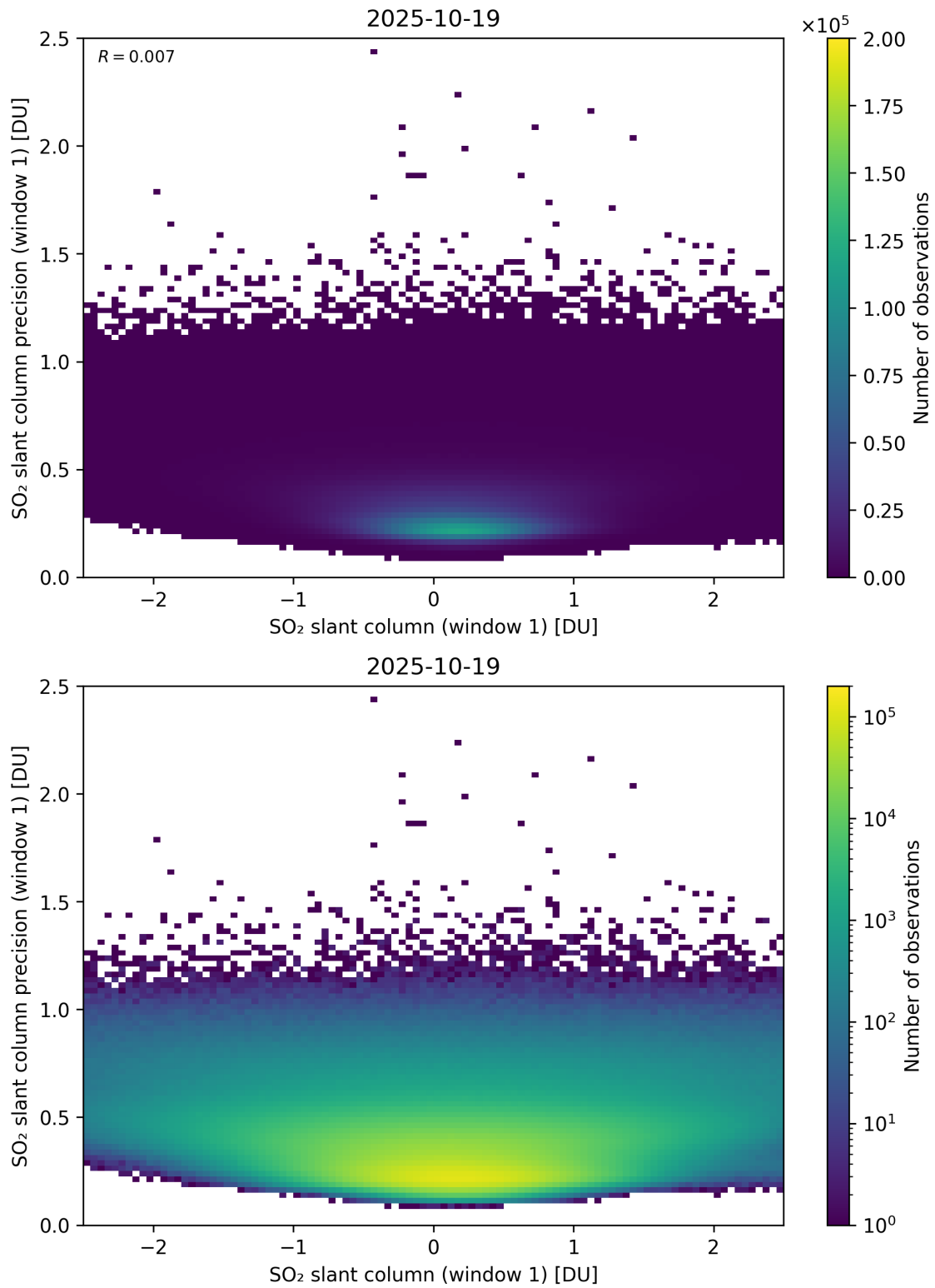
Figure 285: Scatter density plot of “SO 2 slant column (window 1)” against “SO 2 slant column precision (window 1)” for 2025-10-18 to 2025-10-20.
