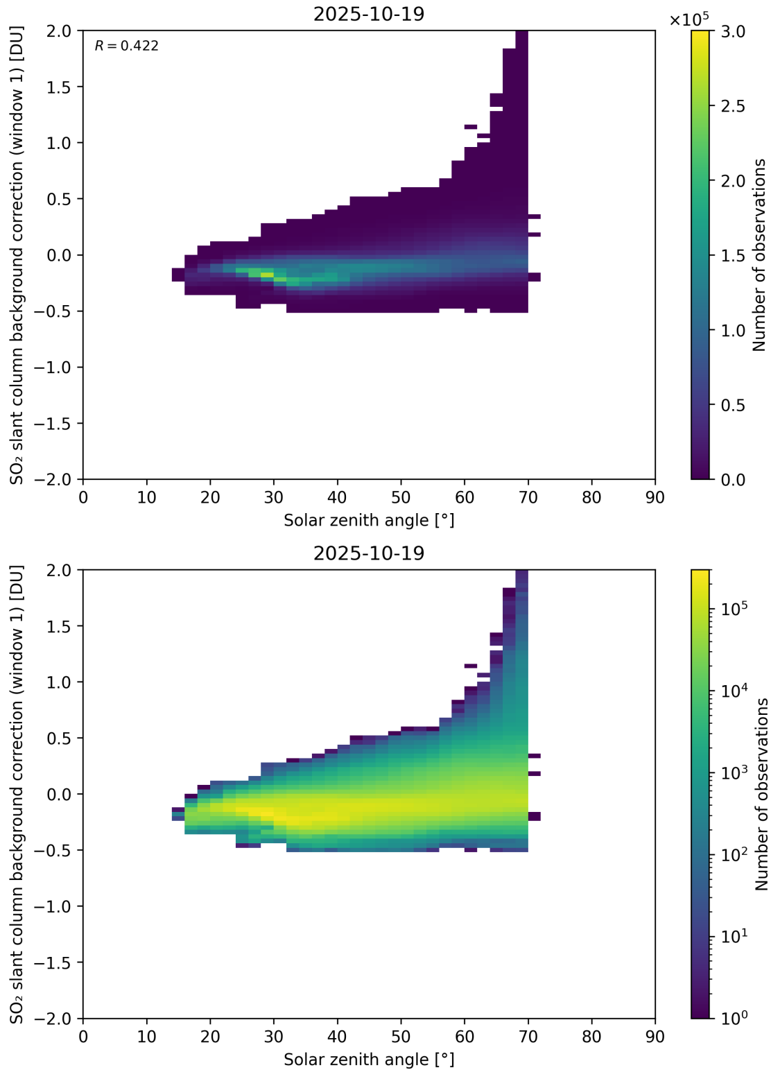
Figure 171: Scatter density plot of “Solar zenith angle” against “SO 2 slant column background correction (window 1)” for 2025-10-18 to 2025-10-20.
