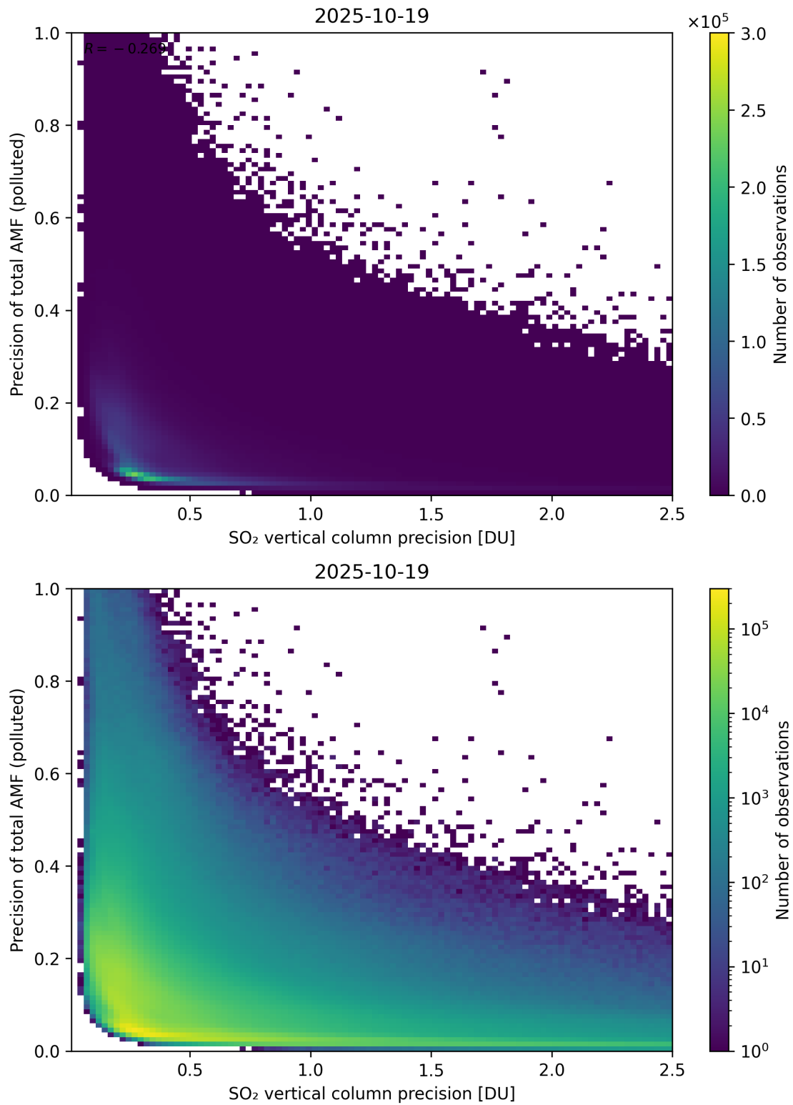
Figure 347: Scatter density plot of “SO 2 vertical column precision” against “Precision of total AMF (polluted)” for 2025-10-18 to 2025-10-20.
