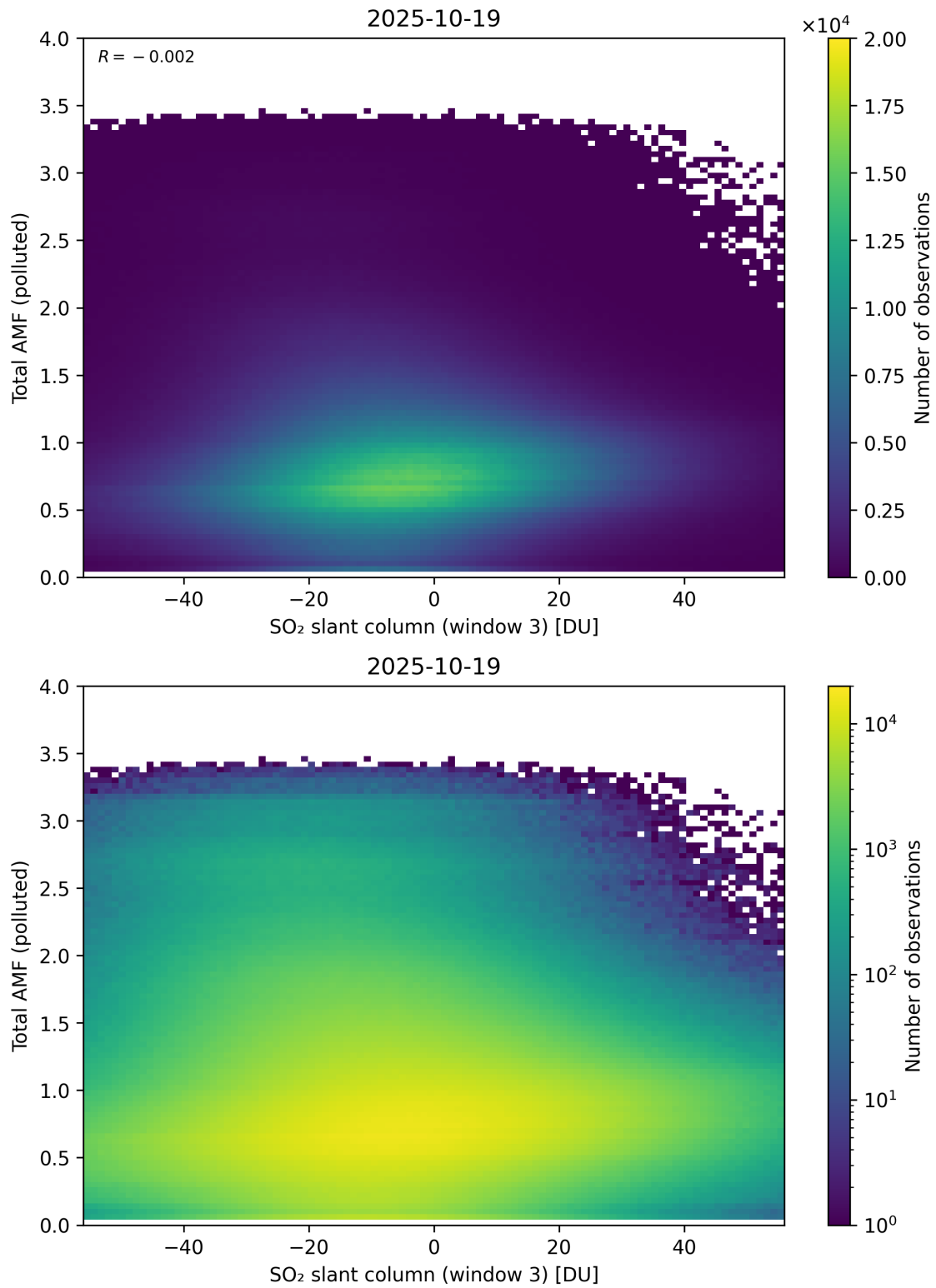
Figure 318: Scatter density plot of “SO 2 slant column (window 3)” against “Total AMF (polluted)” for 2025-10-18 to 2025-10-20.
