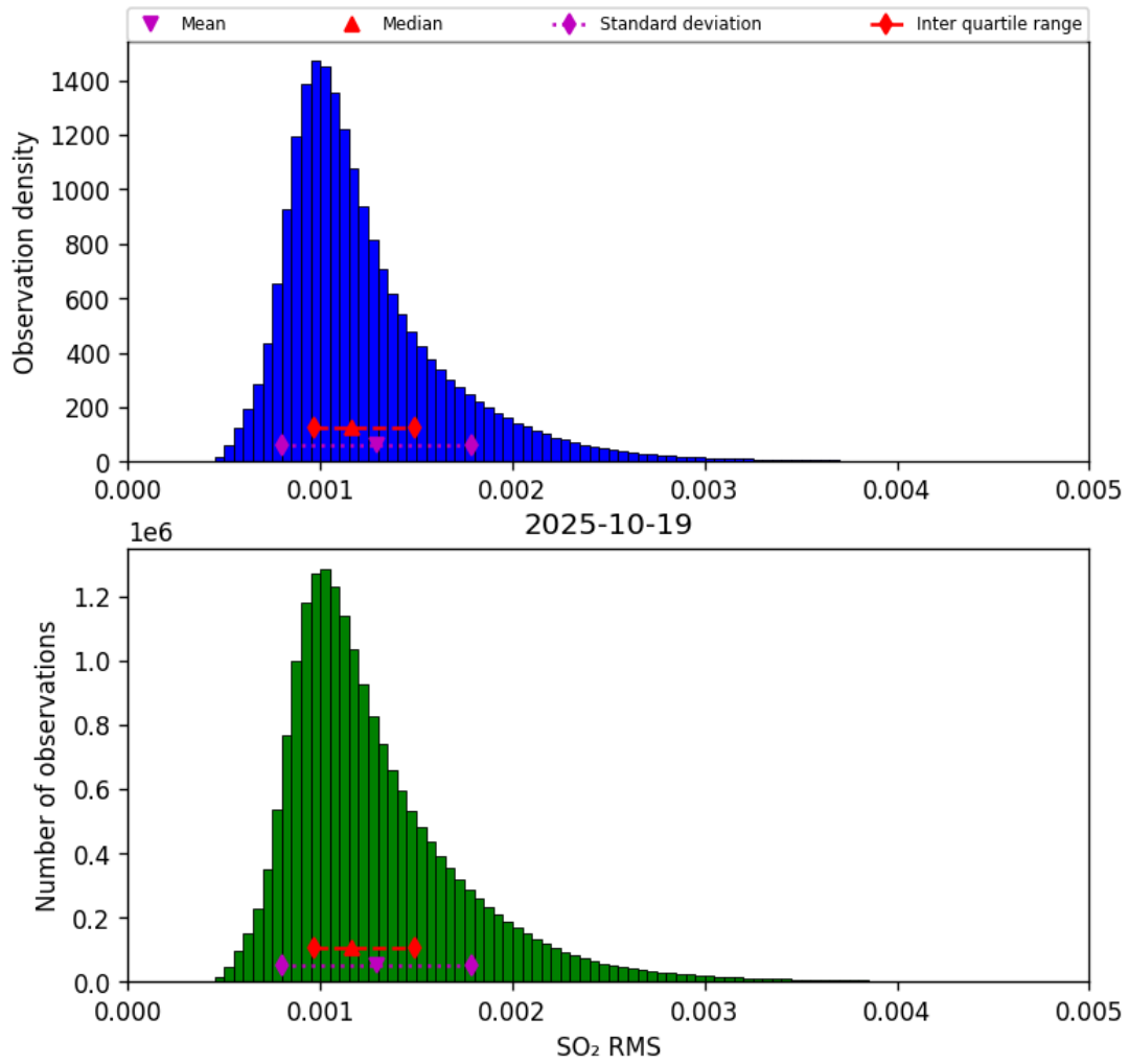
Figure 78: Histogram of “SO 2 RMS” for 2025-10-18 to 2025-10-20
