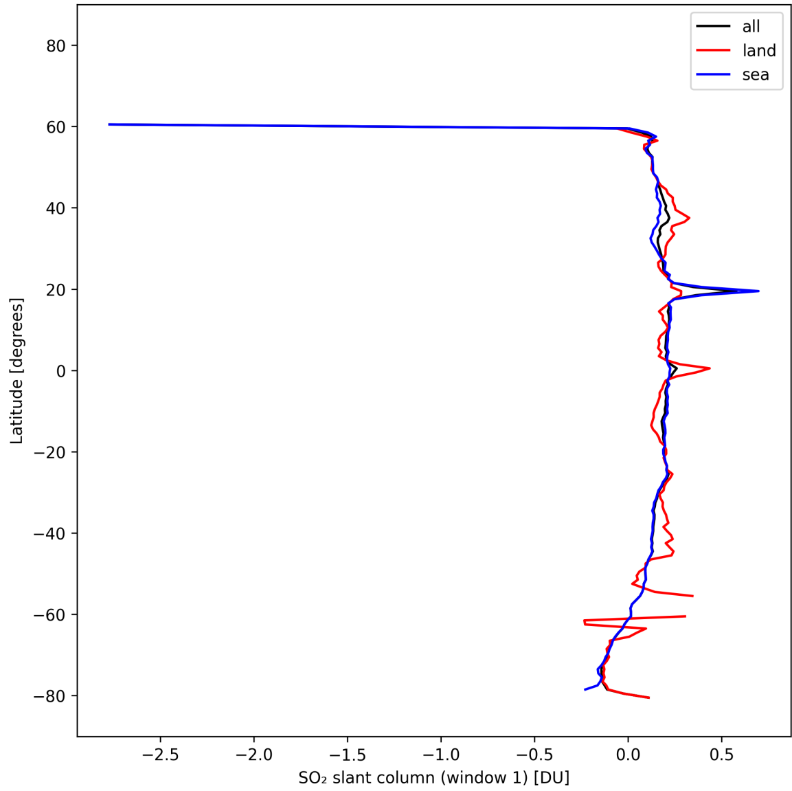
Figure 37: Zonal average of “SO 2 slant column (window 1)” for 2025-10-18 to 2025-10-20.
