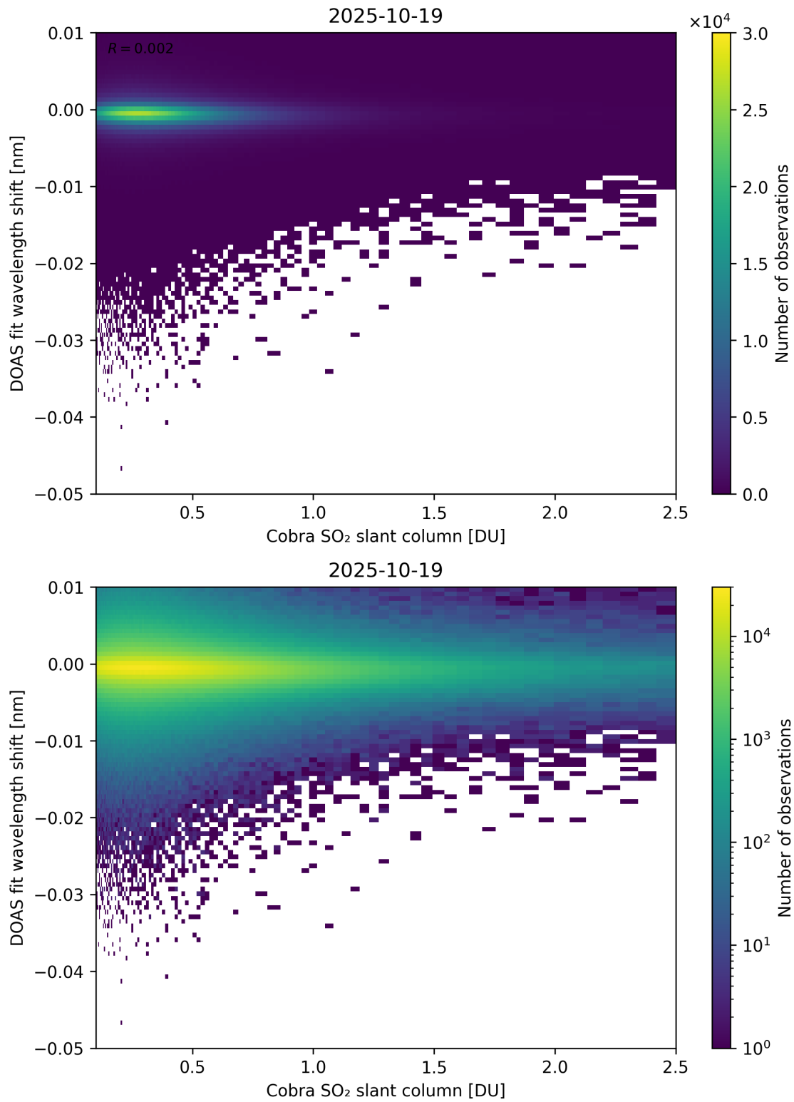
Figure 196: Scatter density plot of “Cobra SO 2 slant column” against “DOAS fit wavelength shift” for 2025-10-18 to 2025-10-20.
