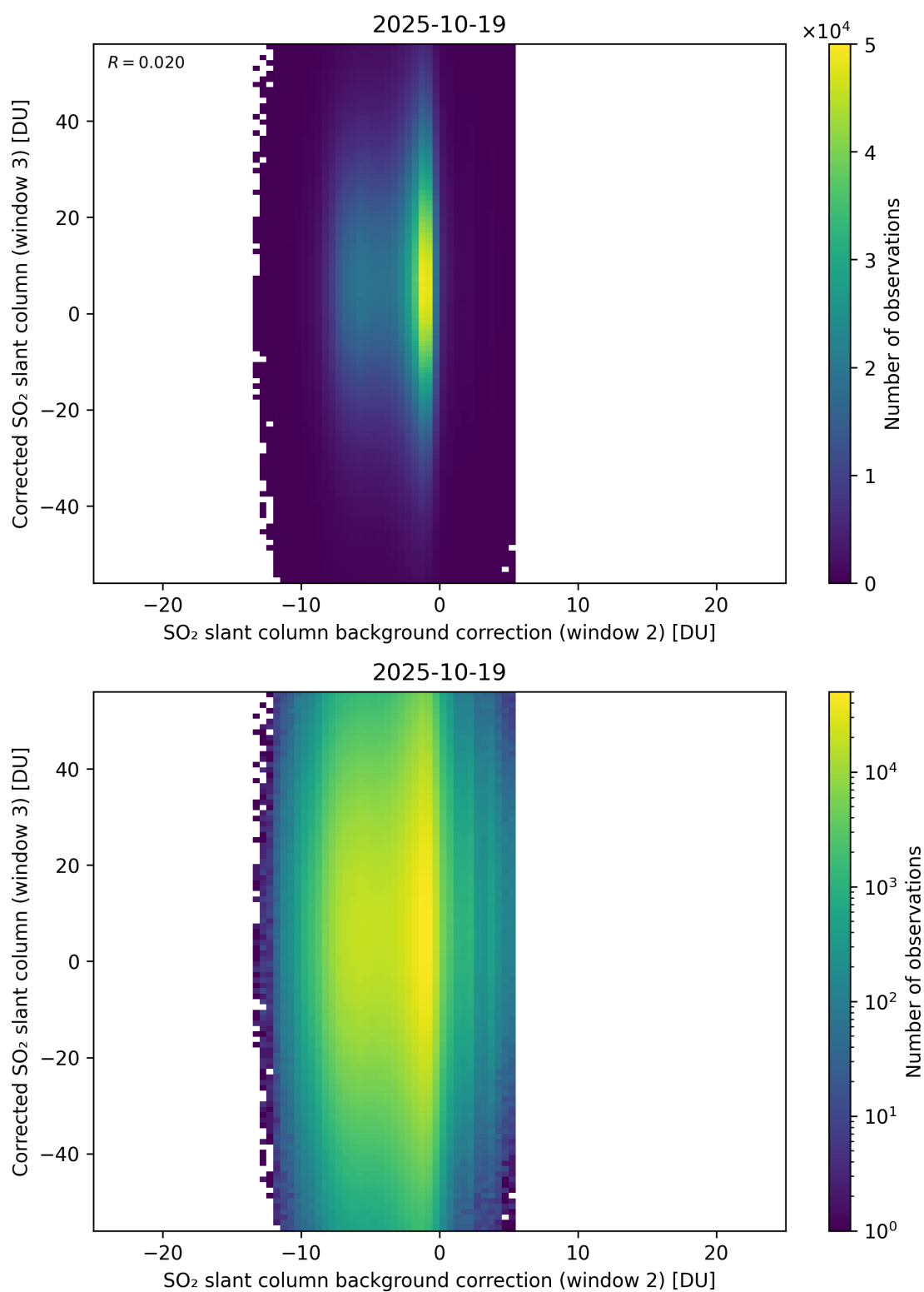
Figure 127: Scatter density plot of “SO 2 slant column background correction (window 2)” against “Corrected SO 2 slant column (window 3)” for 2025-10-18 to 2025-10-20.
