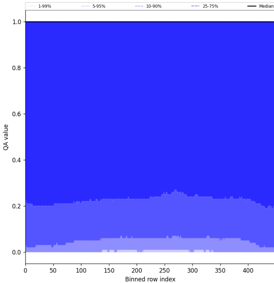
Figure 83: Along track statistics of “QA value” for 2025-10-18 to 2025-10-20
