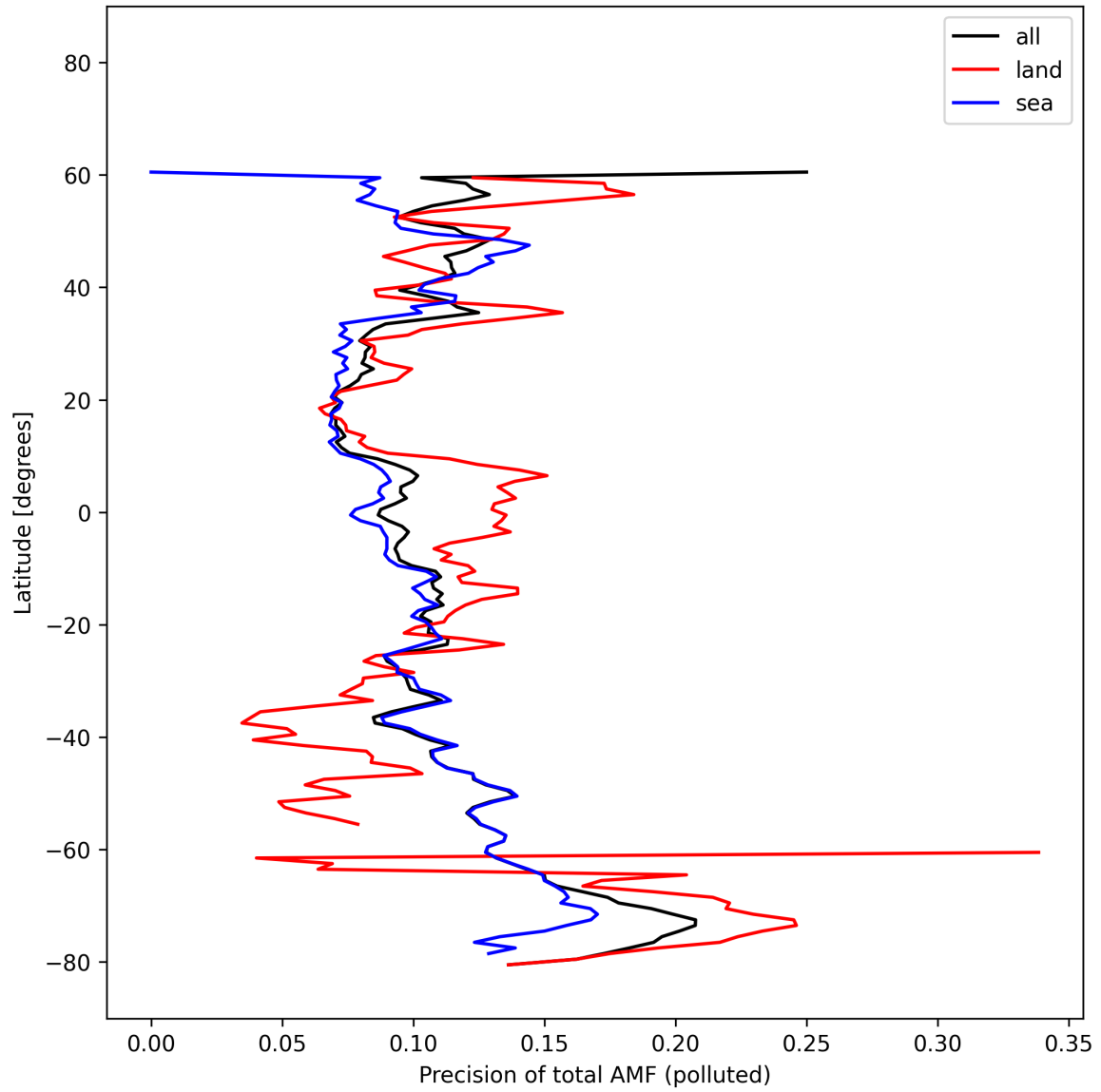
Figure 54: Zonal average of “Precision of total AMF (polluted)” for 2025-10-18 to 2025-10-20.
