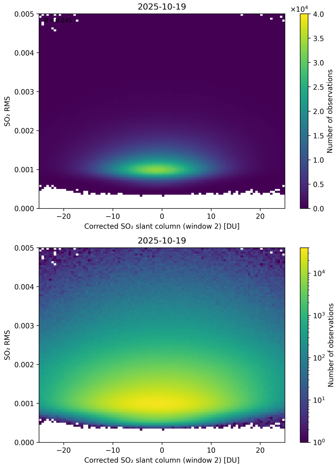
Figure 248: Scatter density plot of “Corrected SO 2 slant column (window 2)” against “SO 2 RMS” for 2025-10-18 to 2025-10-20.
