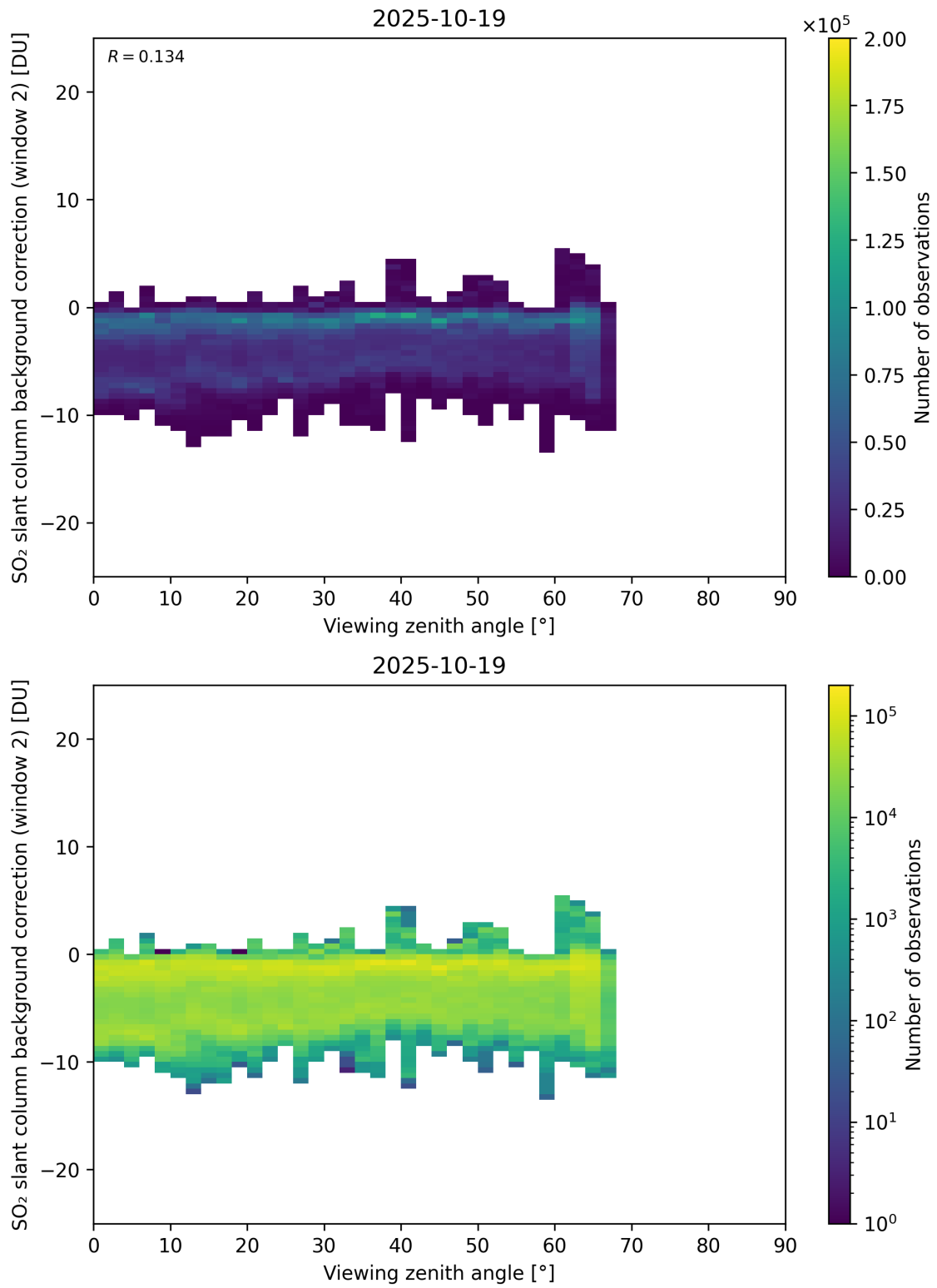
Figure 363: Scatter density plot of “Viewing zenith angle” against “SO 2 slant column background correction (window 2)” for 2025-10-18 to 2025-10-20.
