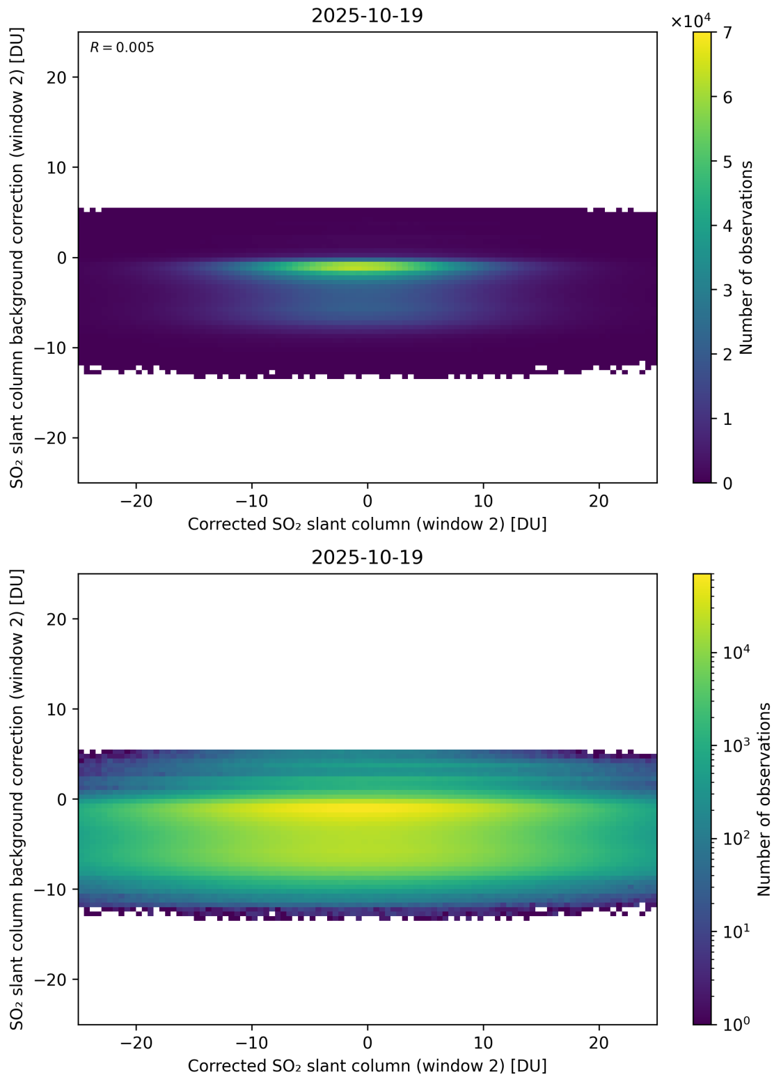
Figure 244: Scatter density plot of “Corrected SO 2 slant column (window 2)” against “SO 2 slant column background correction (window 2)” for 2025-10-18 to 2025-10-20.
