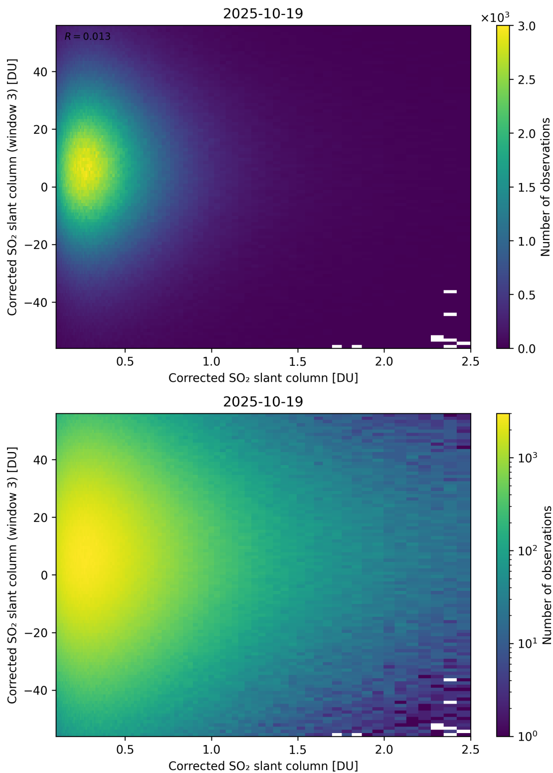
Figure 236: Scatter density plot of “Corrected SO 2 slant column” against “Corrected SO 2 slant column (window 3)” for 2025-10-18 to 2025-10-20.
