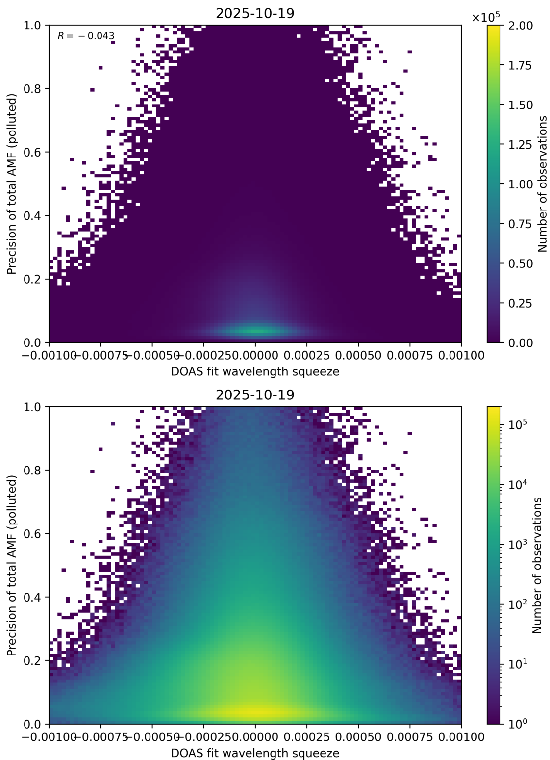
Figure 146: Scatter density plot of “DOAS fit wavelength squeeze” against “Precision of total AMF (polluted)” for 2025-10-18 to 2025-10-20.
