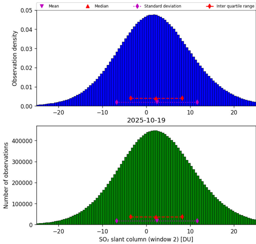
Figure 67: Histogram of “SO 2 slant column (window 2)” for 2025-10-18 to 2025-10-20
