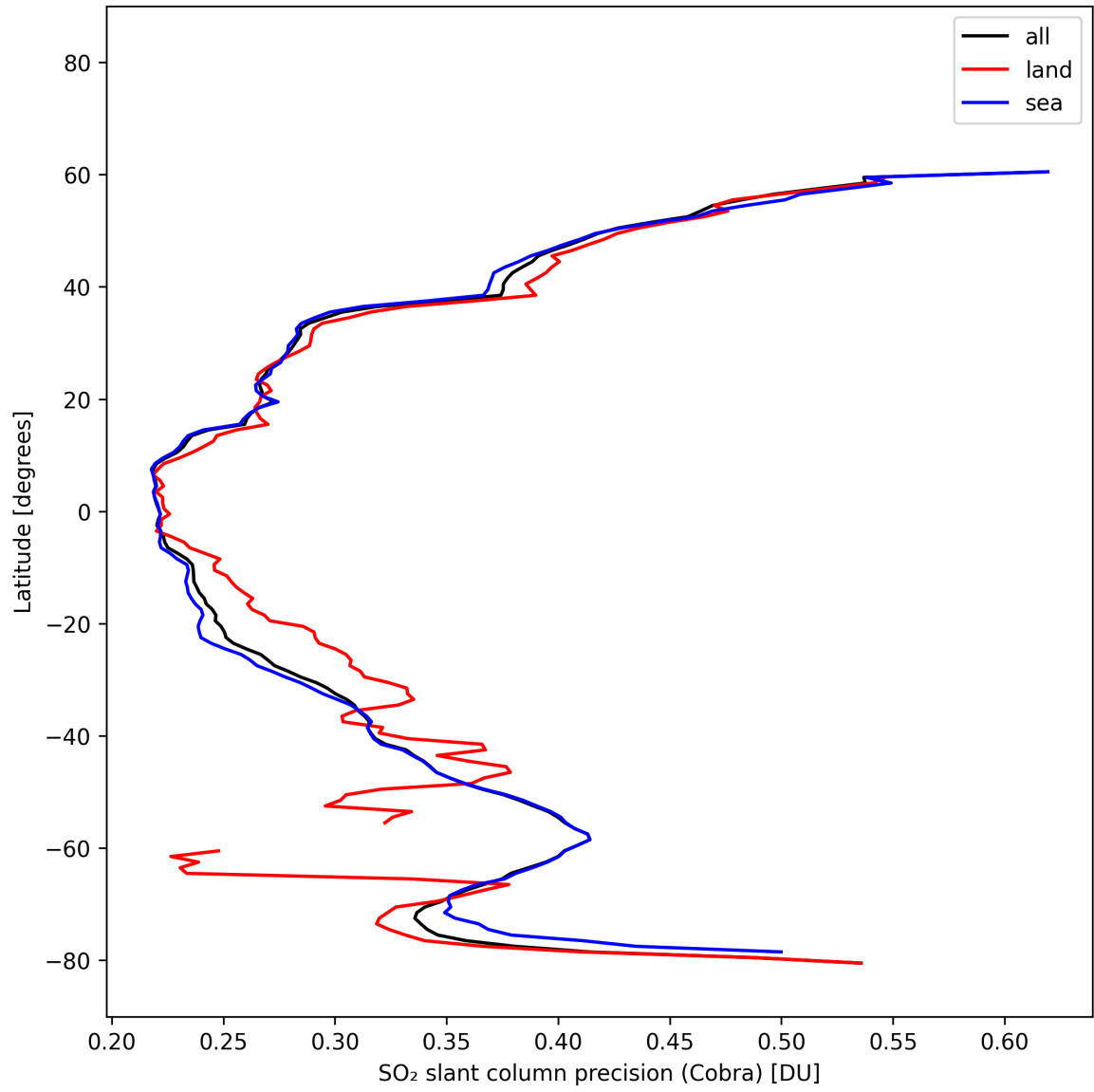
Figure 36: Zonal average of "SO 2 slant column precision (Cobra)" for 2025-10-18 to 2025-10-20.
