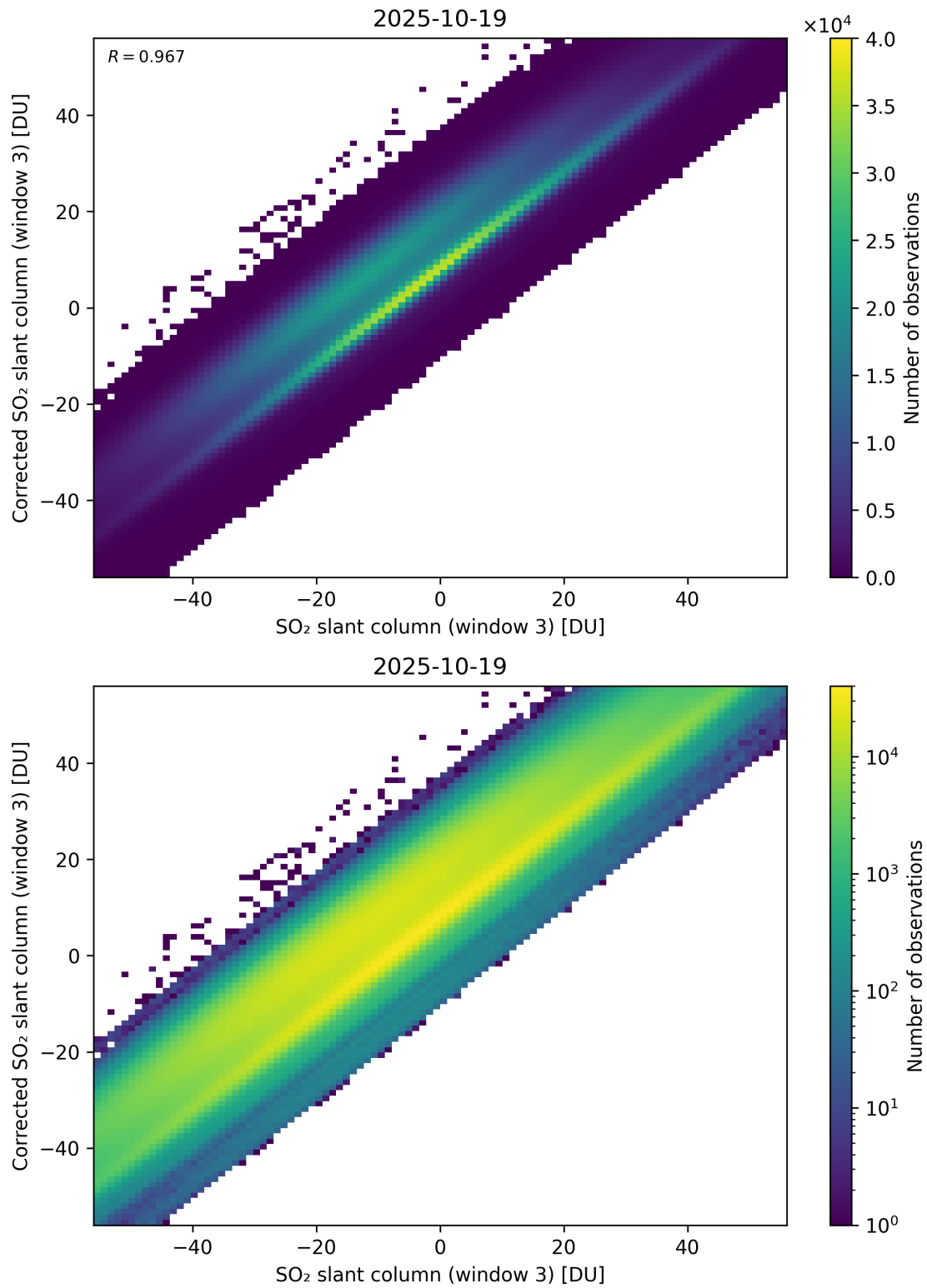
Figure 316: Scatter density plot of “SO 2 slant column (window 3)” against “Corrected SO 2 slant column (window 3)” for 2025-10-18 to 2025-10-20.
