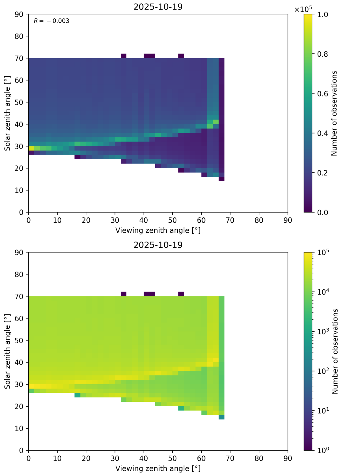
Figure 369: Scatter density plot of “Viewing zenith angle” against “Solar zenith angle” for 2025-10-18 to 2025-10-20.
