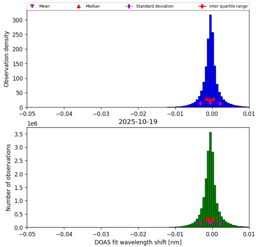
Figure 76: Histogram of “DOAS fit wavelength shift” for 2025-10-18 to 2025-10-20
