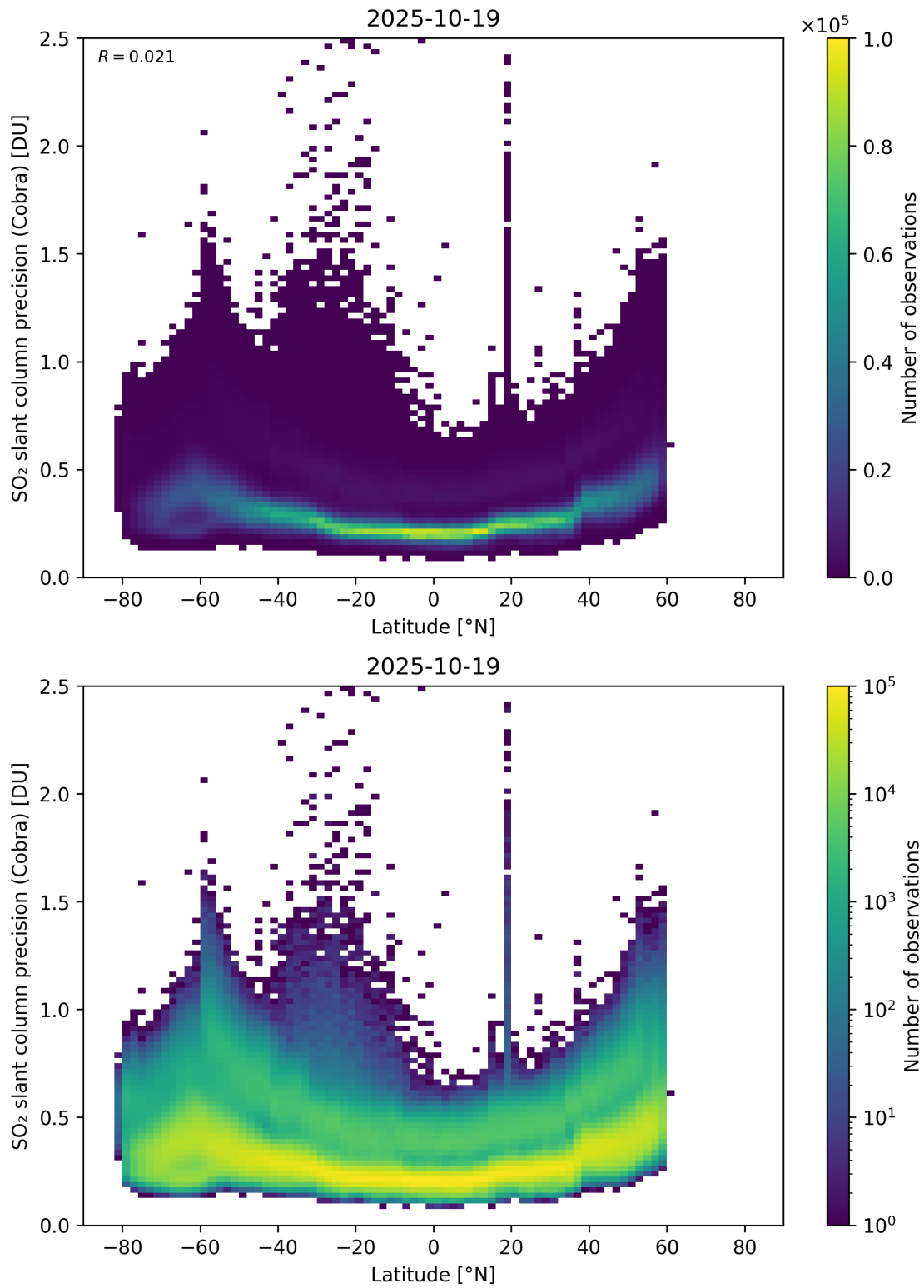
Figure 158: Scatter density plot of “Latitude” against “SO 2 slant column precision (Cobra)” for 2025-10-18 to 2025-10-20.
