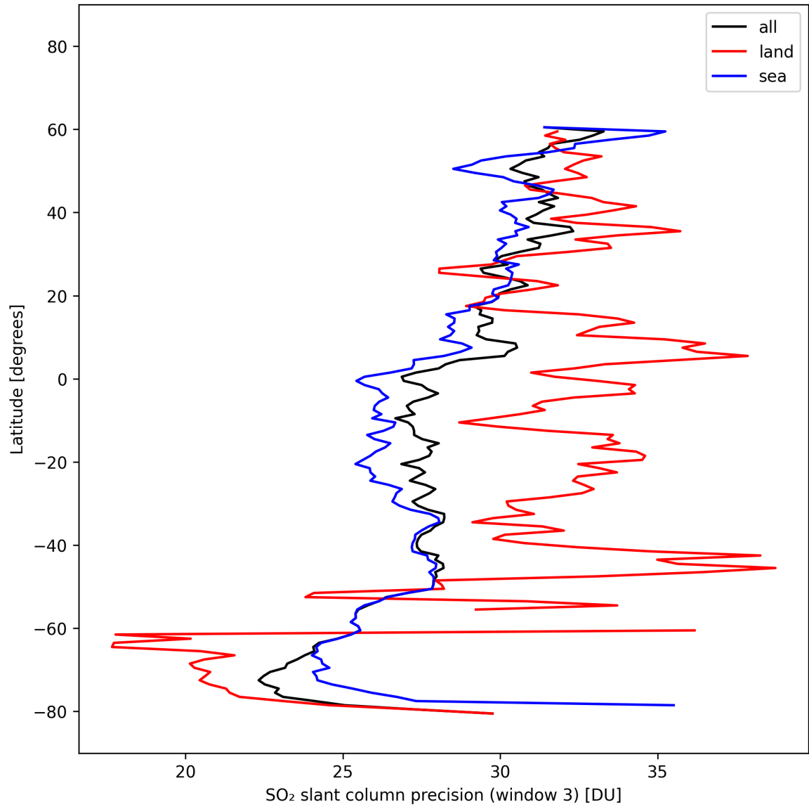
Figure 46: Zonal average of “SO 2 slant column precision (window 3)” for 2025-10-18 to 2025-10-20.
