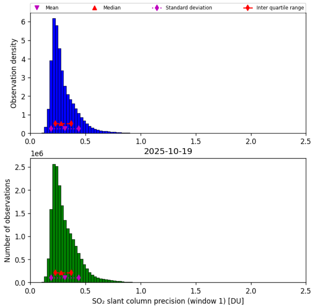
Figure 64: Histogram of “SO 2 slant column precision (window 1)” for 2025-10-18 to 2025-10-20
