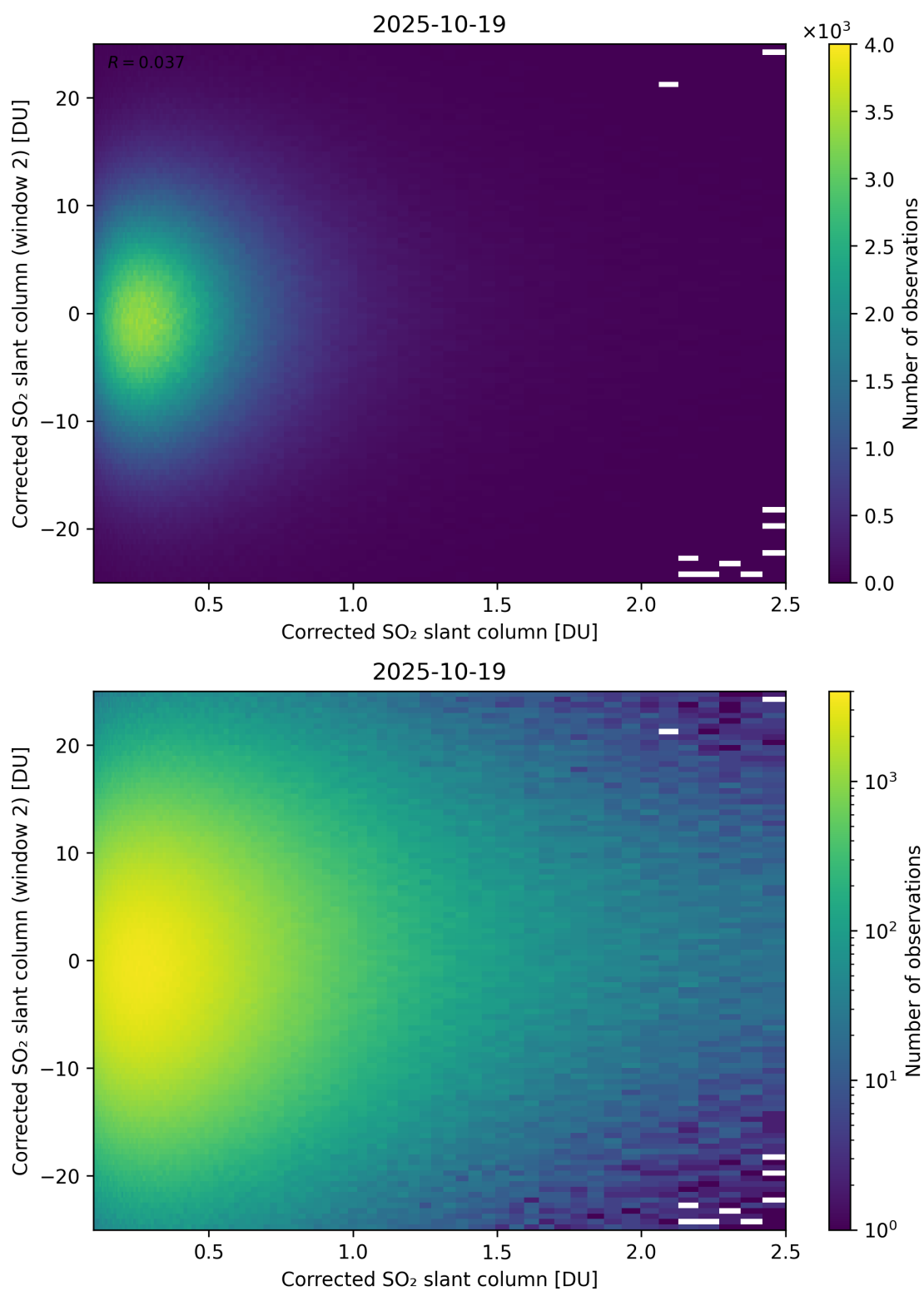
Figure 235: Scatter density plot of “Corrected SO 2 slant column” against “Corrected SO 2 slant column (window 2)” for 2025-10-18 to 2025-10-20.
