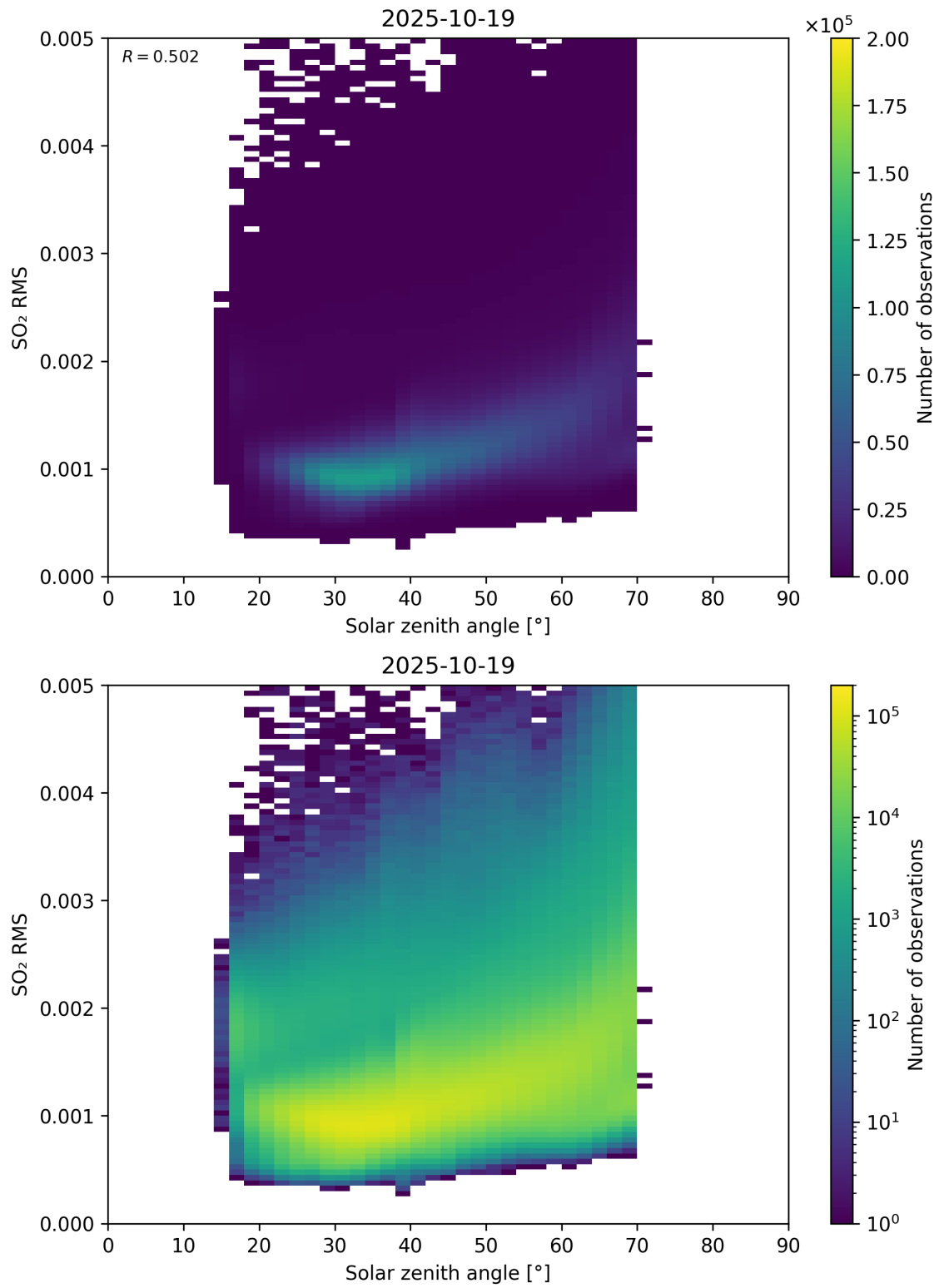
Figure 176: Scatter density plot of “Solar zenith angle” against “SO 2 RMS” for 2025-10-18 to 2025-10-20.
