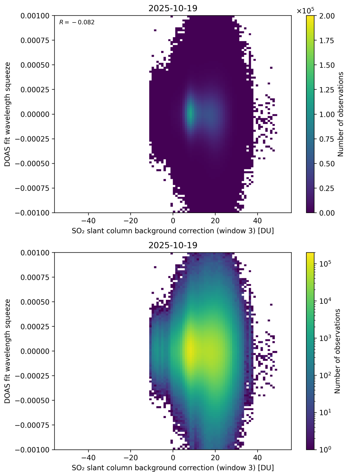
Figure 133: Scatter density plot of “SO 2 slant column background correction (window 3)” against “DOAS fit wavelength squeeze” for 2025-10-18 to 2025-10-20.
