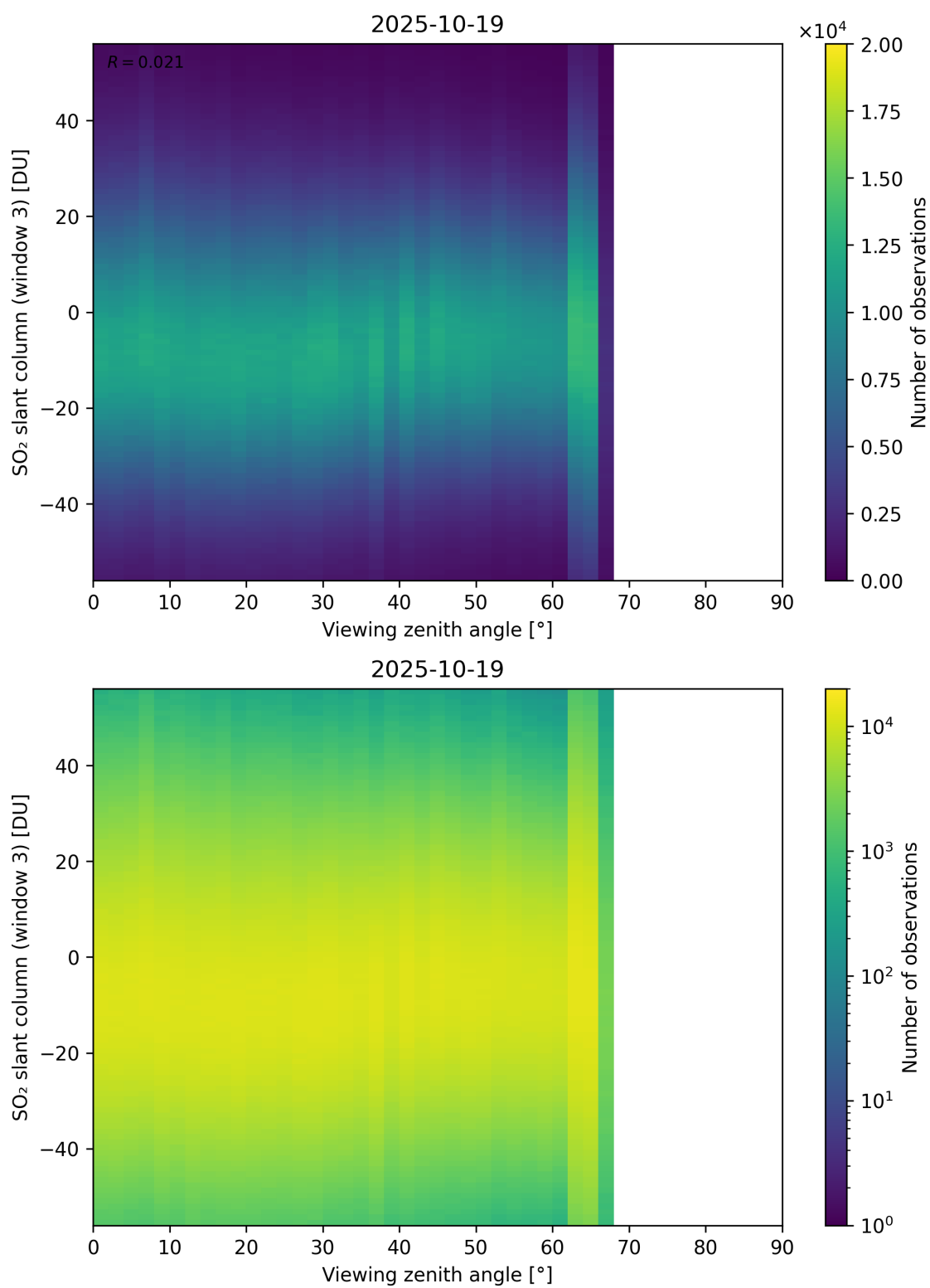
Figure 379: Scatter density plot of “Viewing zenith angle” against “SO 2 slant column (window 3)” for 2025-10-18 to 2025-10-20.
