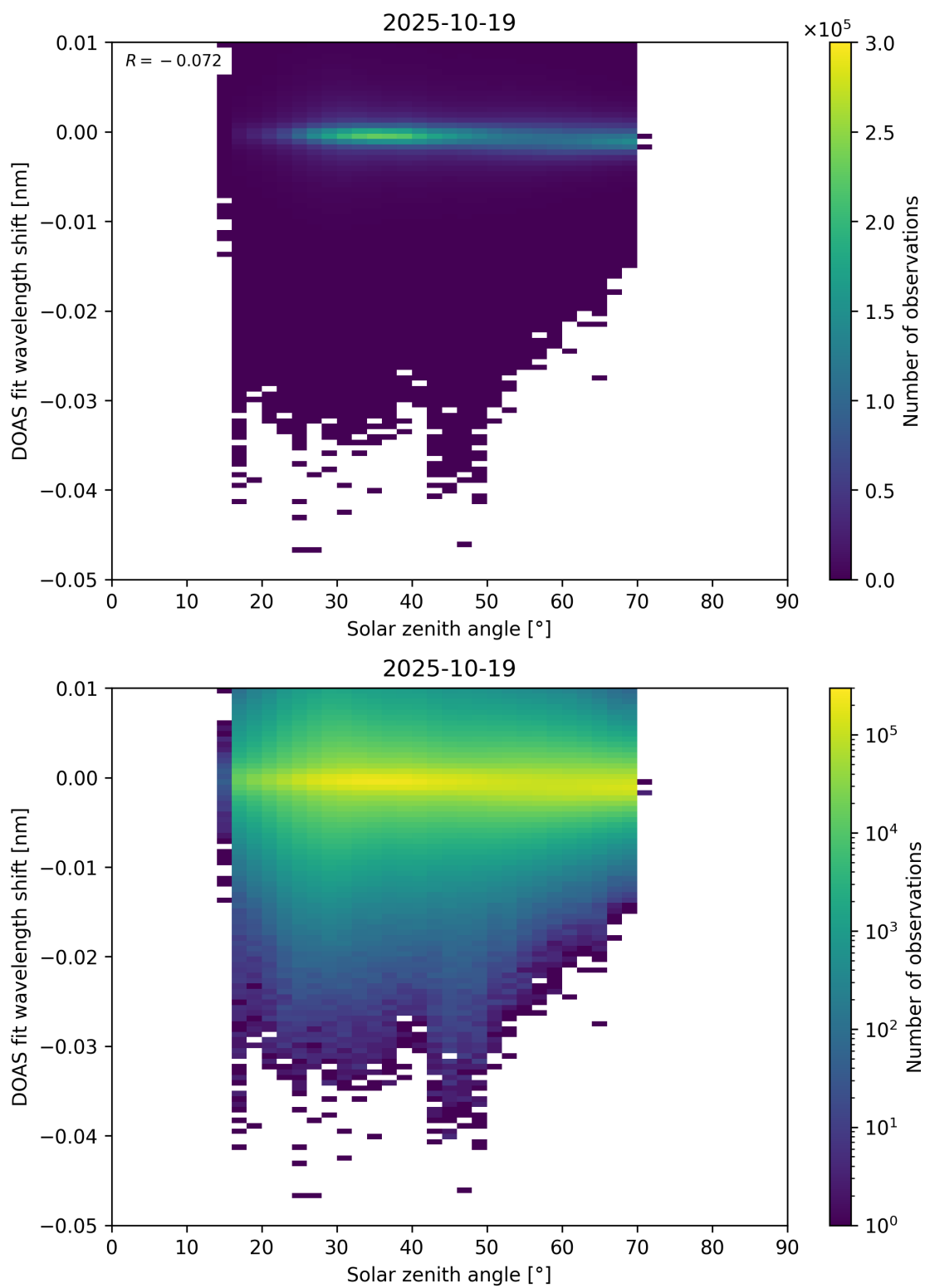
Figure 174: Scatter density plot of “Solar zenith angle” against “DOAS fit wavelength shift” for 2025-10-18 to 2025-10-20.
