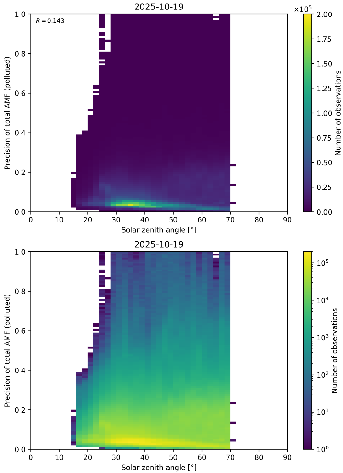
Figure 190: Scatter density plot of “Solar zenith angle” against “Precision of total AMF (polluted)” for 2025-10-18 to 2025-10-20.
