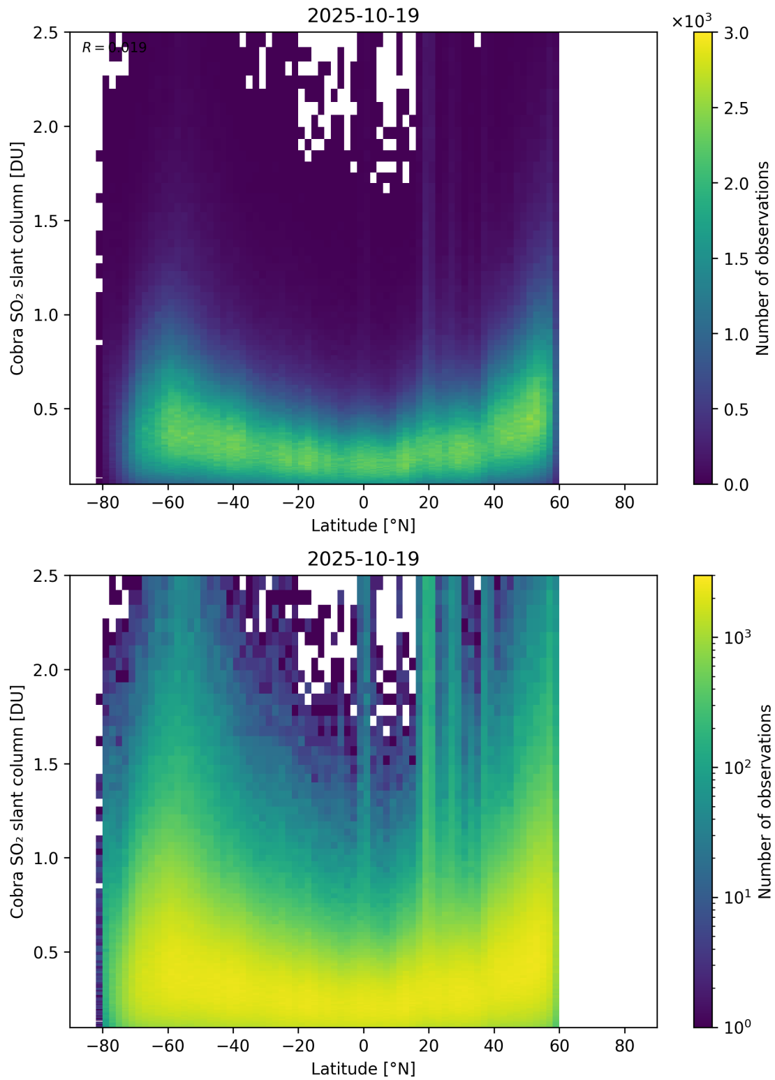
Figure 157: Scatter density plot of “Latitude” against “Cobra SO 2 slant column” for 2025-10-18 to 2025-10-20.
