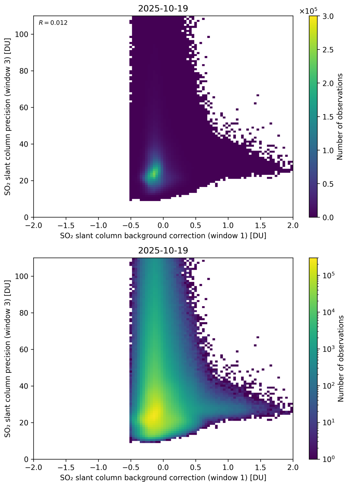
Figure 119: Scatter density plot of “SO 2 slant column background correction (window 1)” against “SO 2 slant column precision (window 3)” for 2025-10-18 to 2025-10-20.
