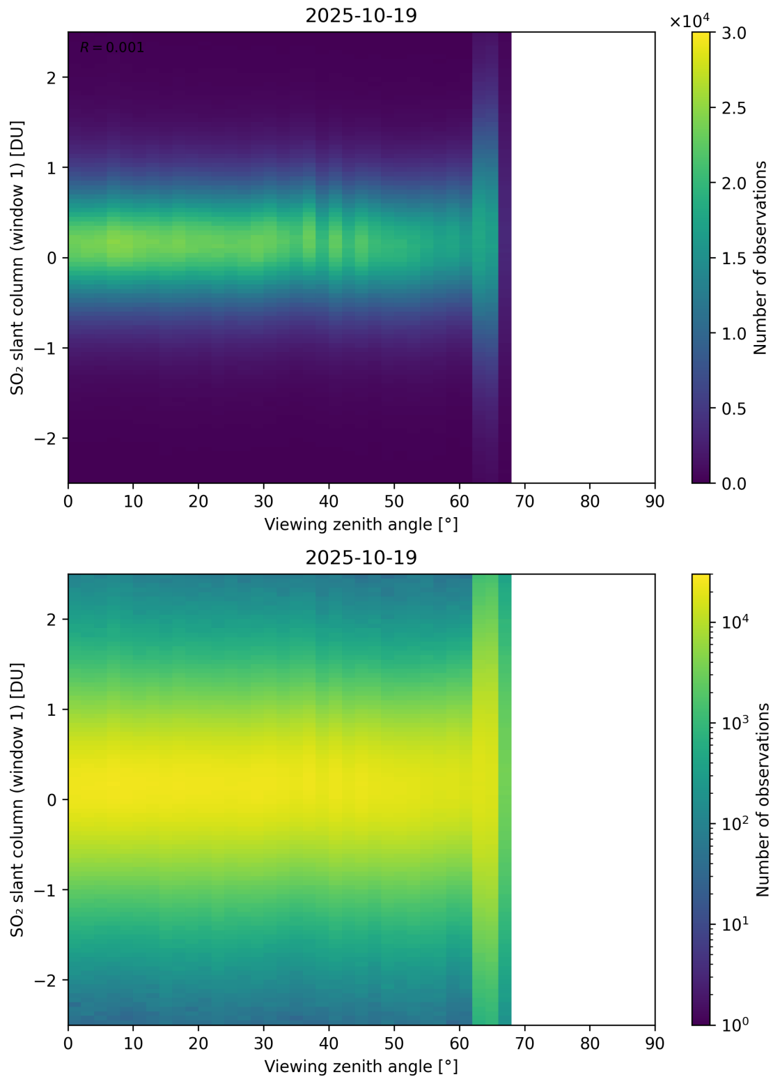
Figure 376: Scatter density plot of “Viewing zenith angle” against “SO 2 slant column (window 1)” for 2025-10-18 to 2025-10-20.
