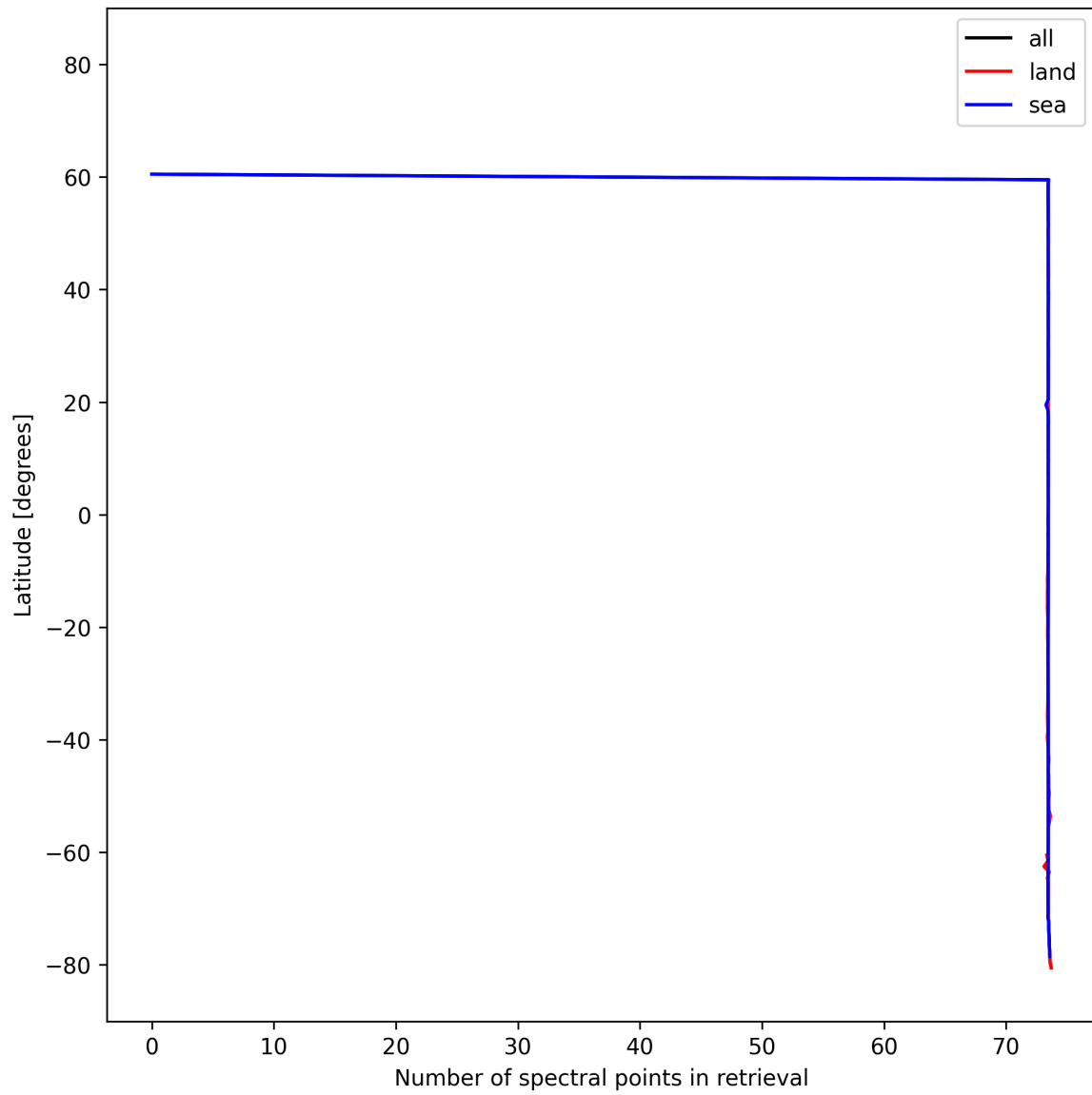
Figure 56: Zonal average of “Number of spectral points in retrieval” for 2025-10-18 to 2025-10-20.
