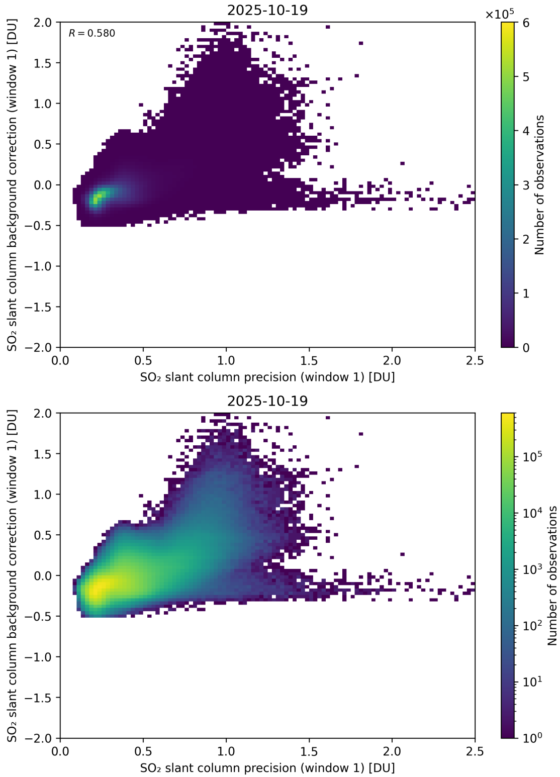
Figure 268: Scatter density plot of “SO 2 slant column precision (window 1)” against “SO 2 slant column background correction (window 1)” for 2025-10-18 to 2025-10-20.
