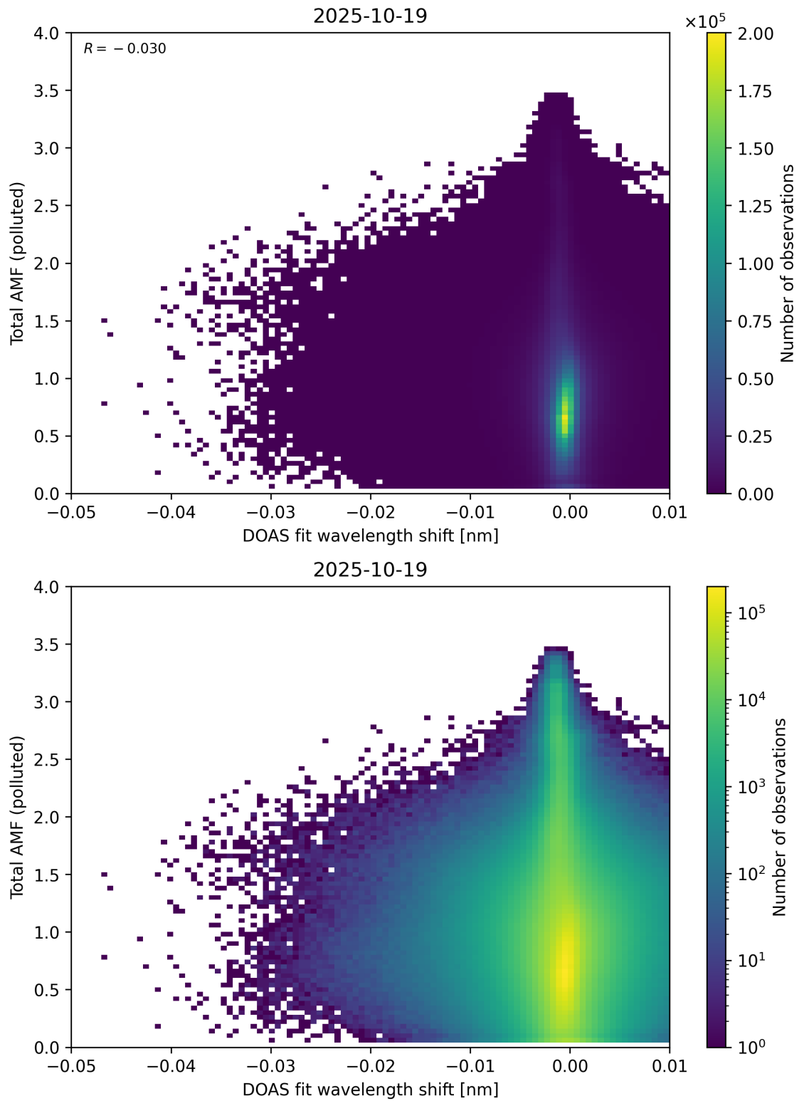
Figure 141: Scatter density plot of “DOAS fit wavelength shift” against “Total AMF (polluted)” for 2025-10-18 to 2025-10-20.
