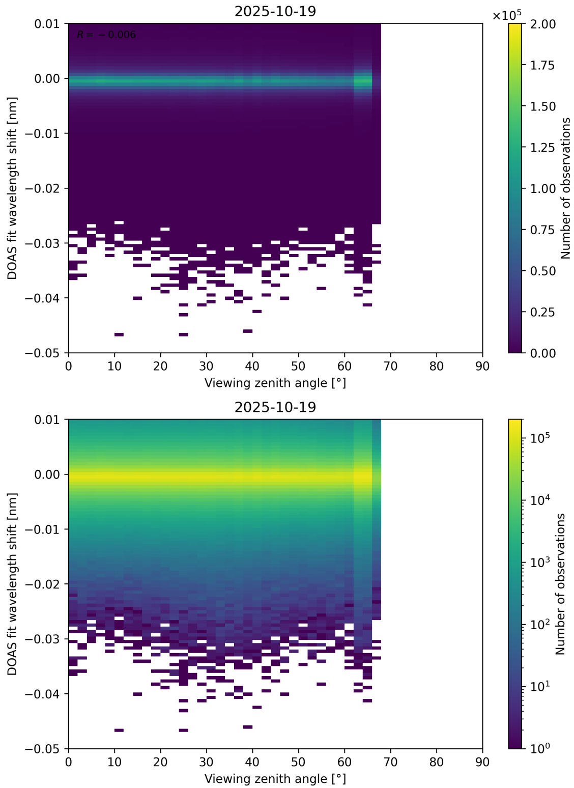
Figure 365: Scatter density plot of “Viewing zenith angle” against “DOAS fit wavelength shift” for 2025-10-18 to 2025-10-20.
