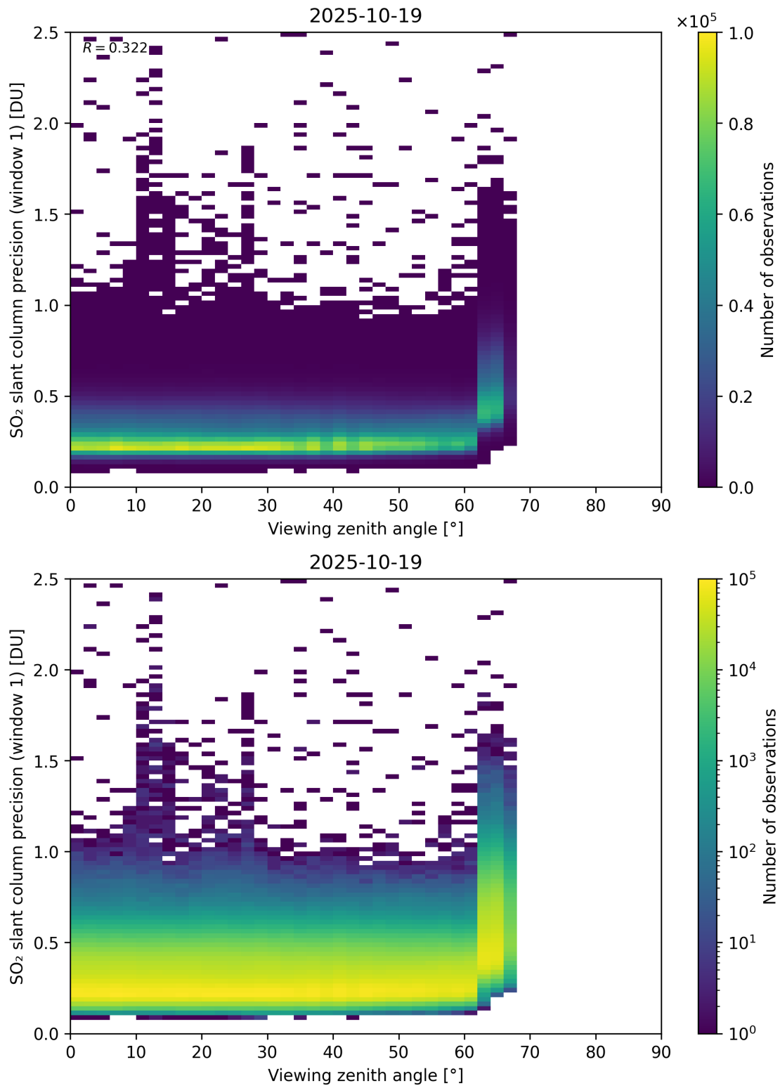
Figure 377: Scatter density plot of “Viewing zenith angle” against “SO 2 slant column precision (window 1)” for 2025-10-18 to 2025-10-20.
