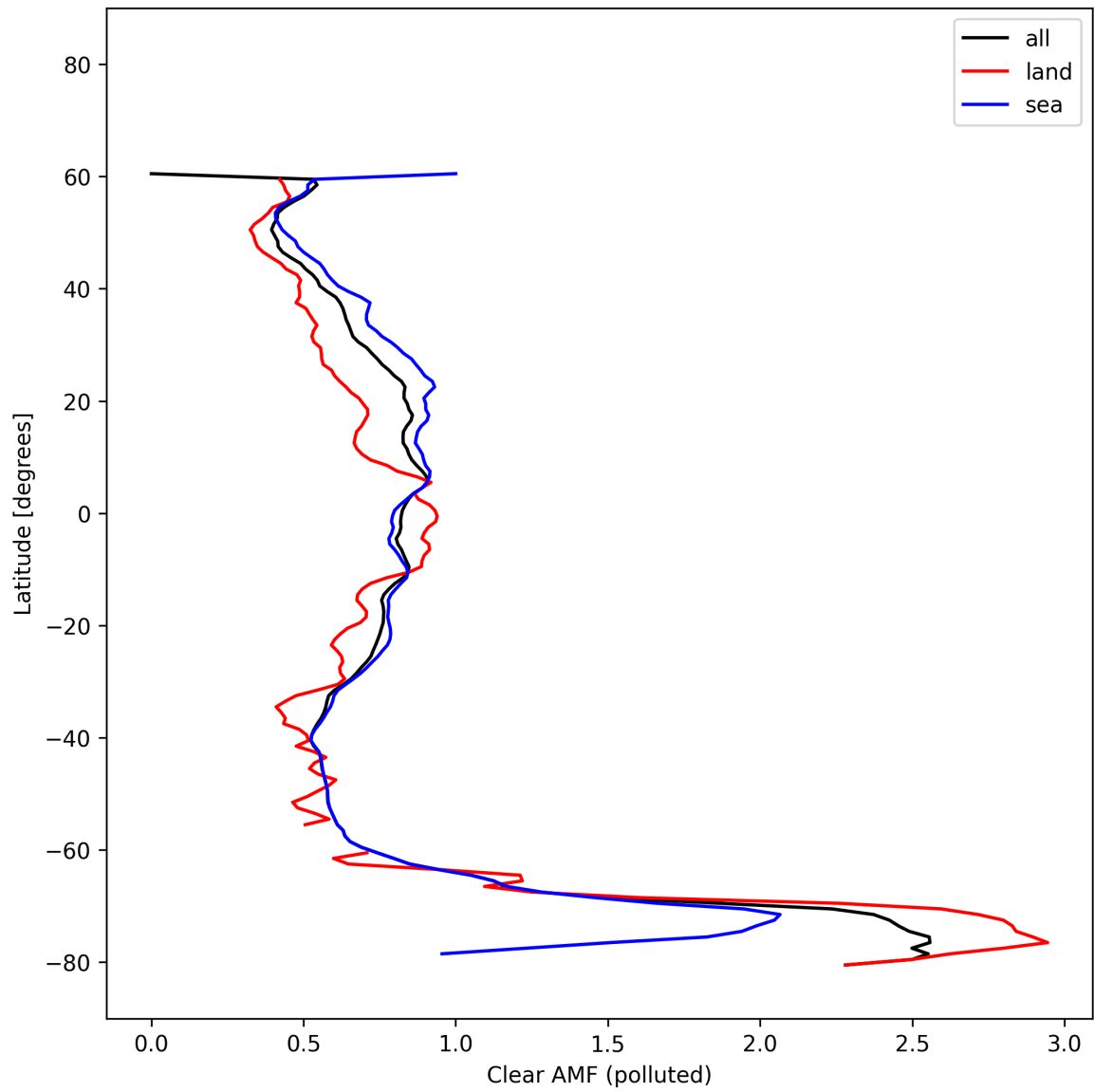
Figure 55: Zonal average of “Clear AMF (polluted)” for 2025-10-18 to 2025-10-20.
