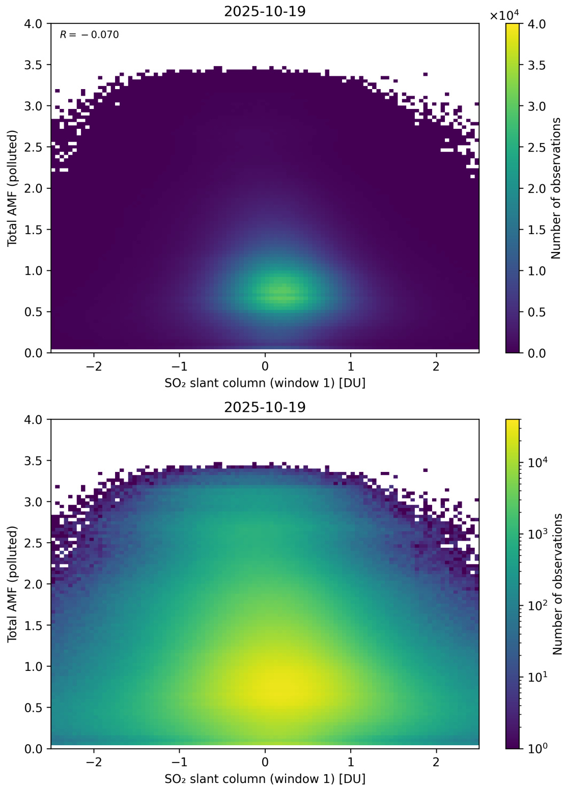
Figure 289: Scatter density plot of “SO 2 slant column (window 1)” against “Total AMF (polluted)” for 2025-10-18 to 2025-10-20.
