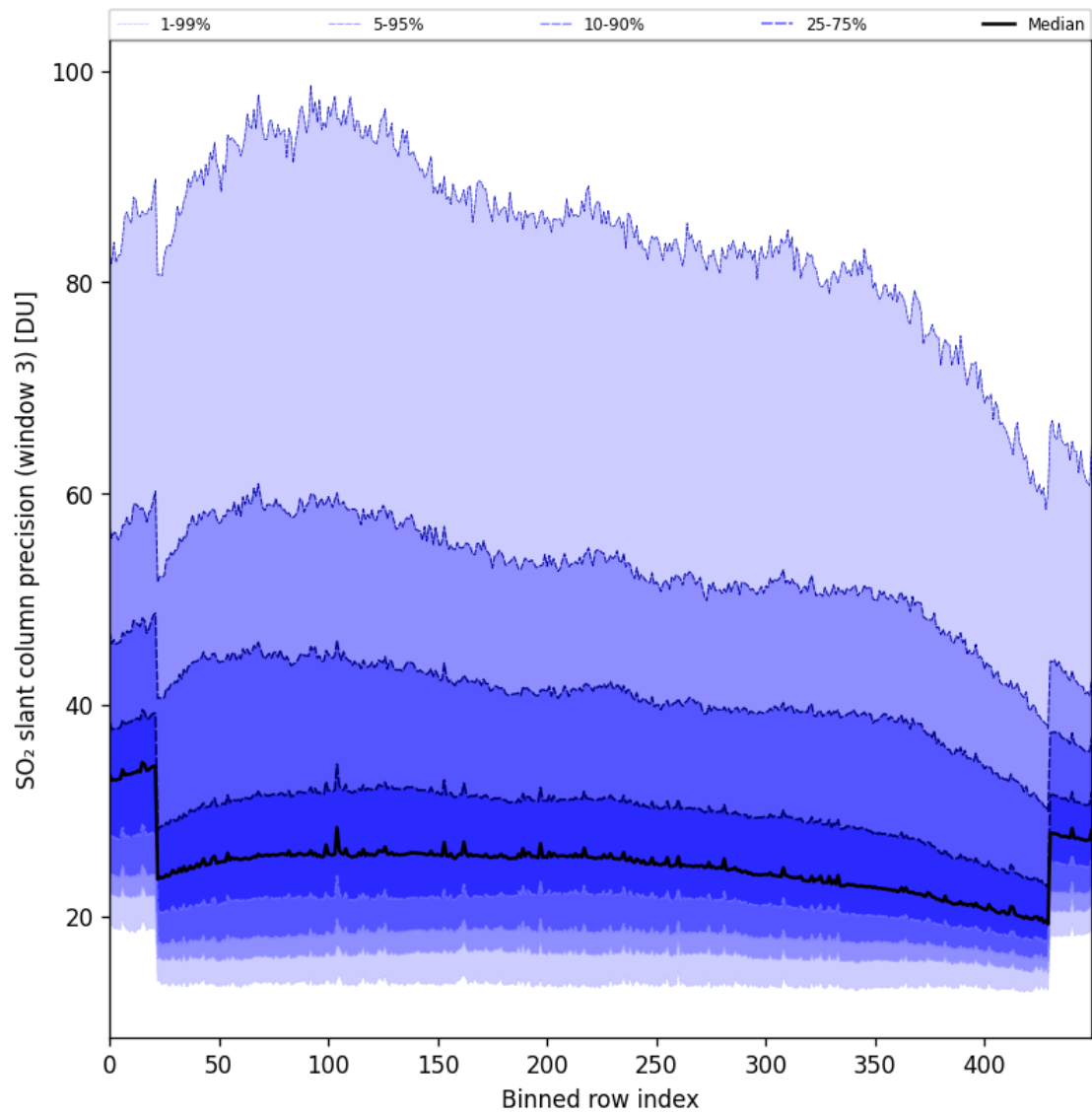
Figure 98: Along track statistics of “SO 2 slant column precision (window 3)” for 2025-10-18 to 2025-10-20
