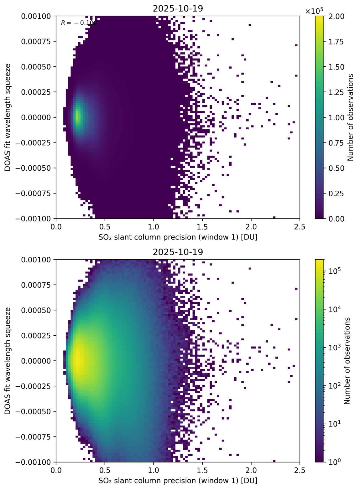
Figure 272: Scatter density plot of “SO 2 slant column precision (window 1)” against “DOAS fit wavelength squeeze” for 2025-10-18 to 2025-10-20.
