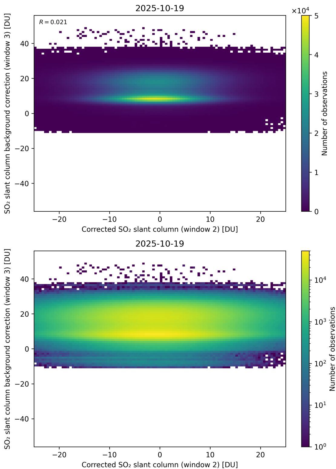
Figure 245: Scatter density plot of “Corrected SO 2 slant column (window 2)” against “SO 2 slant column background correction (window 3)” for 2025-10-18 to 2025-10-20.
