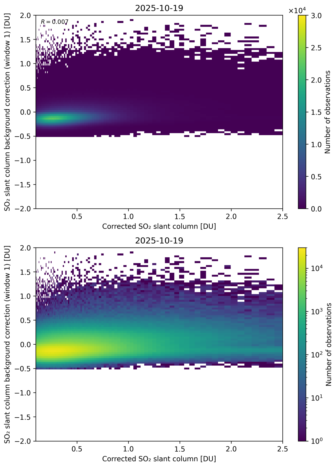
Figure 226: Scatter density plot of “Corrected SO 2 slant column” against “SO 2 slant column background correction (window 1)” for 2025-10-18 to 2025-10-20.
