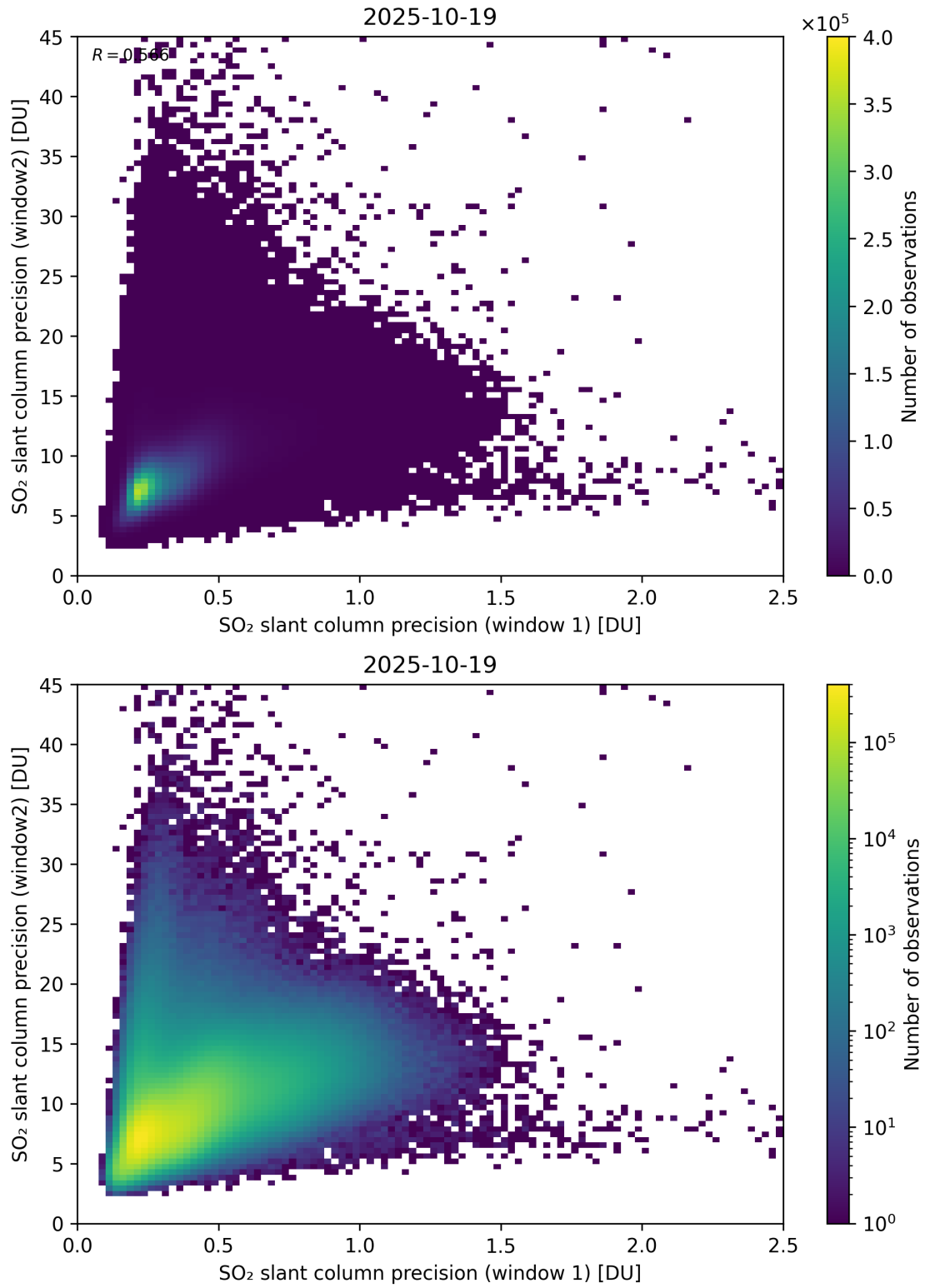
Figure 277: Scatter density plot of “SO 2 slant column precision (window 1)” against “SO 2 slant column precision (window 2)” for 2025-10-18 to 2025-10-20.
