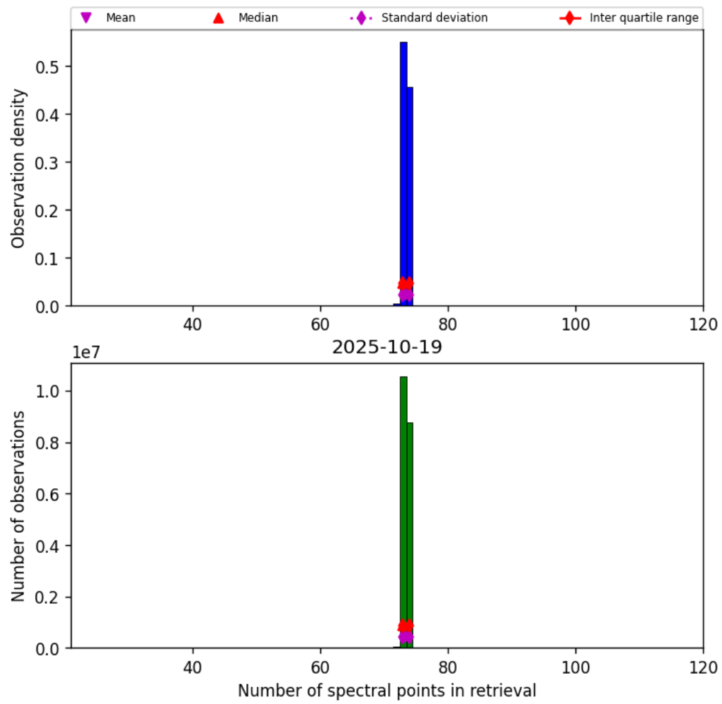
Figure 82: Histogram of “Number of spectral points in retrieval” for 2025-10-18 to 2025-10-20
