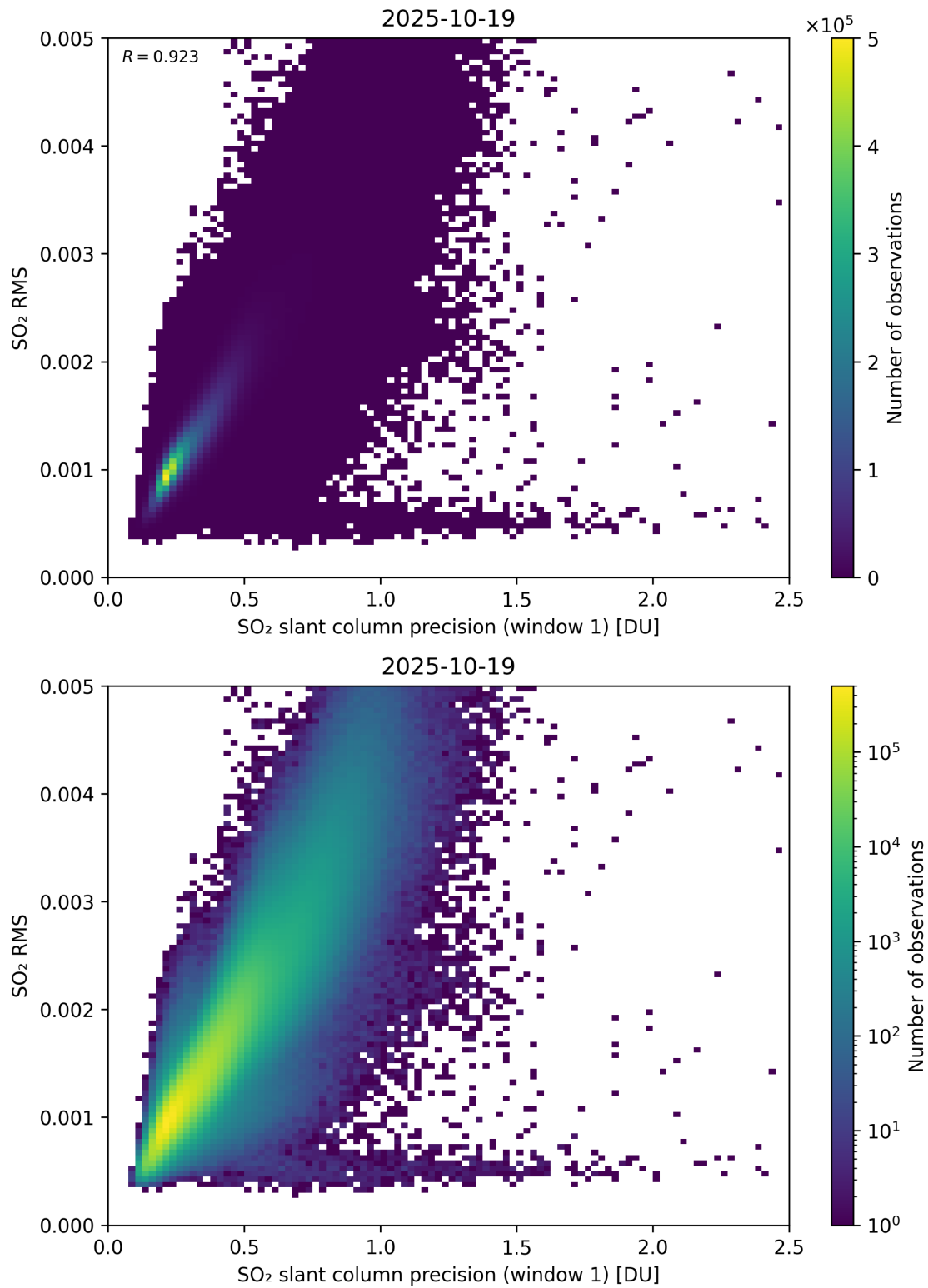
Figure 273: Scatter density plot of “SO 2 slant column precision (window 1)” against “SO 2 RMS” for 2025-10-18 to 2025-10-20.
