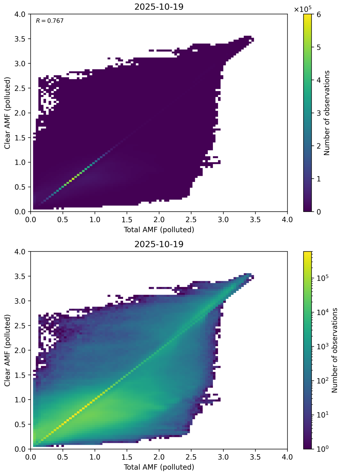
Figure 321: Scatter density plot of “Total AMF (polluted)” against “Clear AMF (polluted)” for 2025-10-18 to 2025-10-20.
