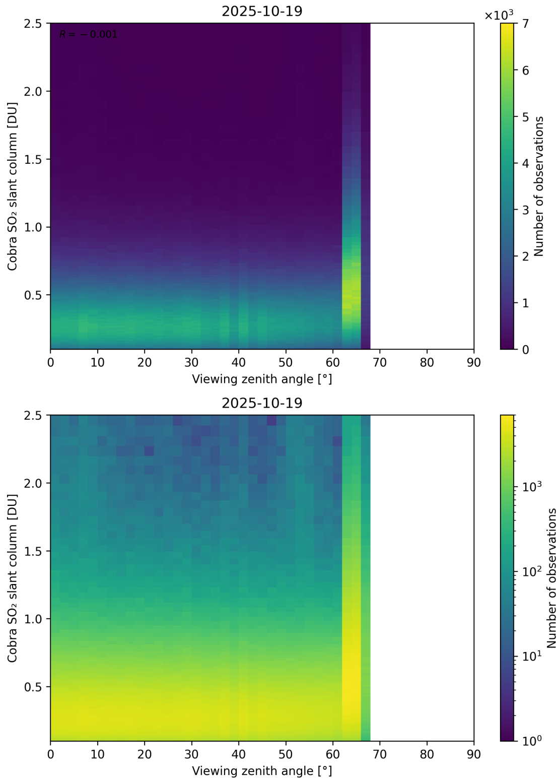
Figure 371: Scatter density plot of “Viewing zenith angle” against “Cobra SO 2 slant column” for 2025-10-18 to 2025-10-20.
