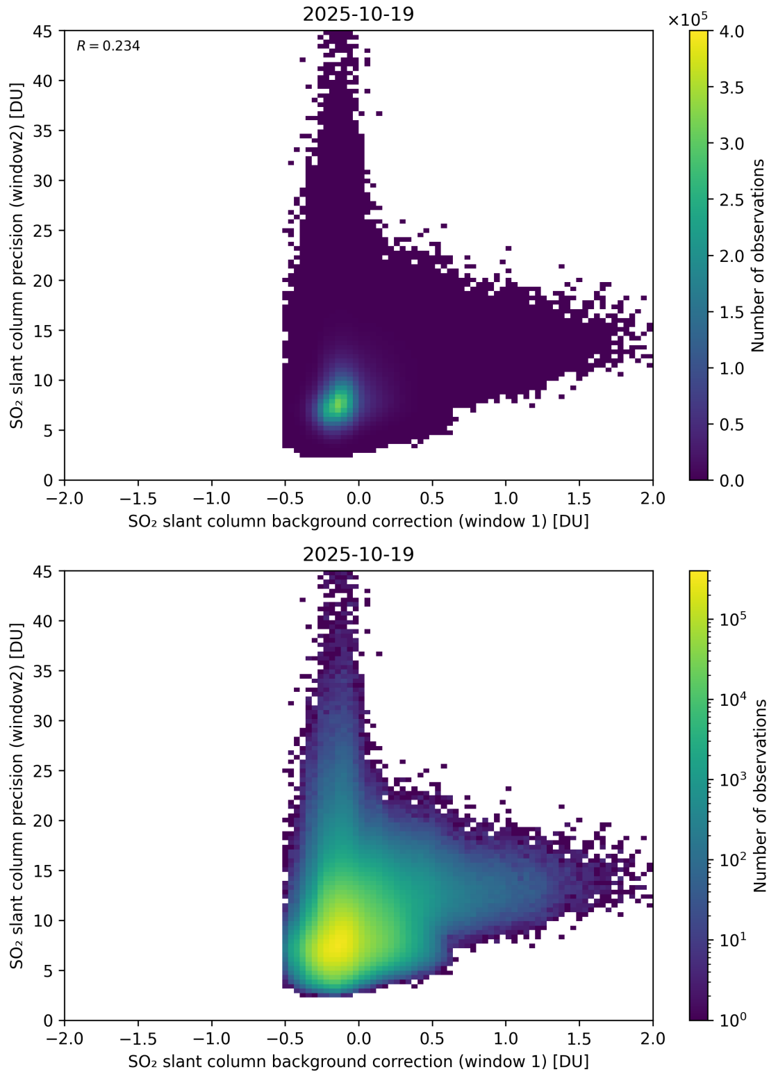
Figure 117: Scatter density plot of “SO 2 slant column background correction (window 1)” against “SO 2 slant column precision (window2)” for 2025-10-18 to 2025-10-20.
