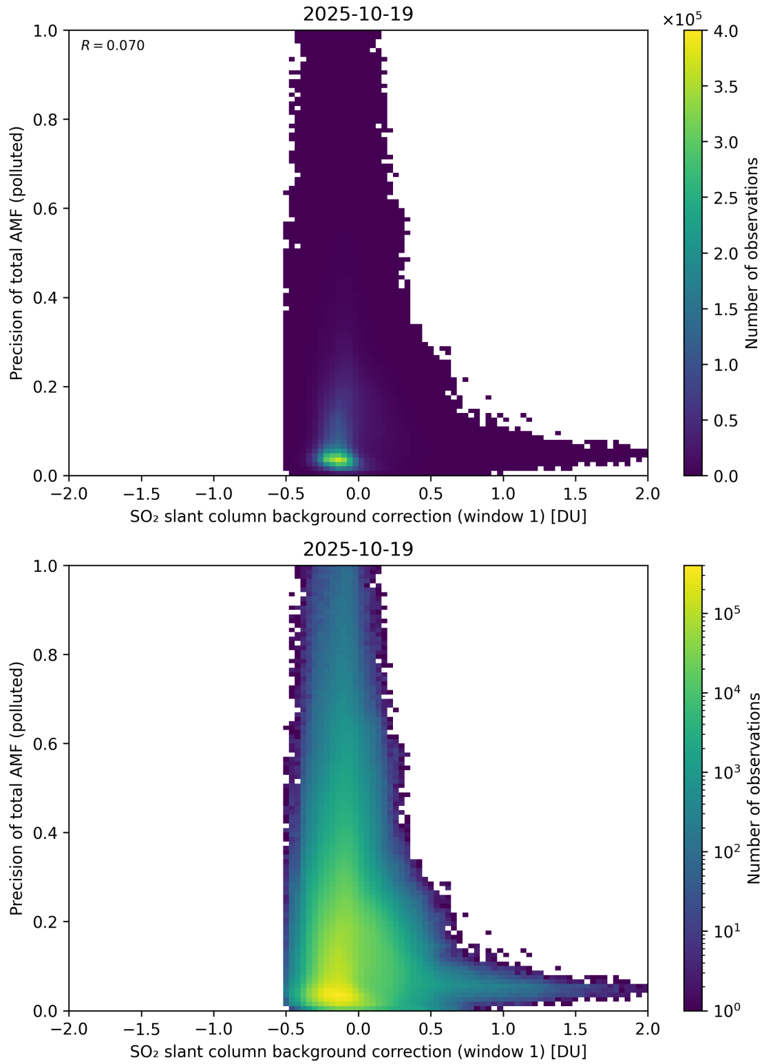
Figure 121: Scatter density plot of “SO 2 slant column background correction (window 1)” against “Precision of total AMF (polluted)” for 2025-10-18 to 2025-10-20.
