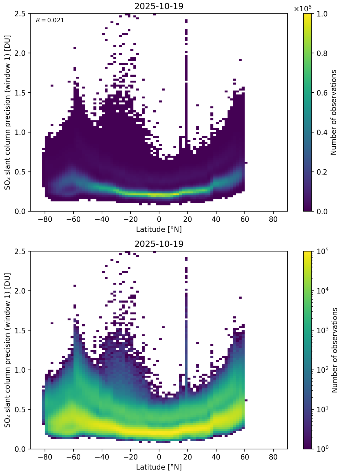
Figure 163: Scatter density plot of “Latitude” against “SO 2 slant column precision (window 1)” for 2025-10-18 to 2025-10-20.
