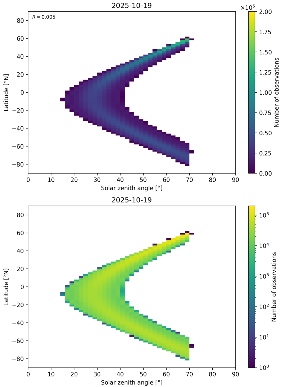
Figure 177: Scatter density plot of “Solar zenith angle” against “Latitude” for 2025-10-18 to 2025-10-20.
