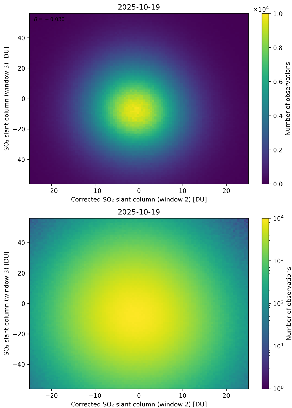
Figure 251: Scatter density plot of “Corrected SO 2 slant column (window 2)” against “SO 2 slant column (window 3)” for 2025-10-18 to 2025-10-20.
