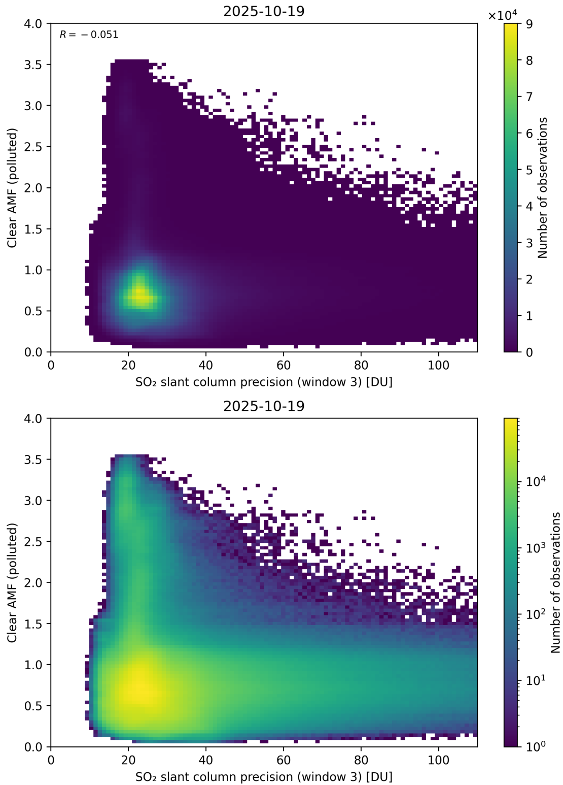
Figure 311: Scatter density plot of “SO 2 slant column precision (window 3)” against “Clear AMF (polluted)” for 2025-10-18 to 2025-10-20.
