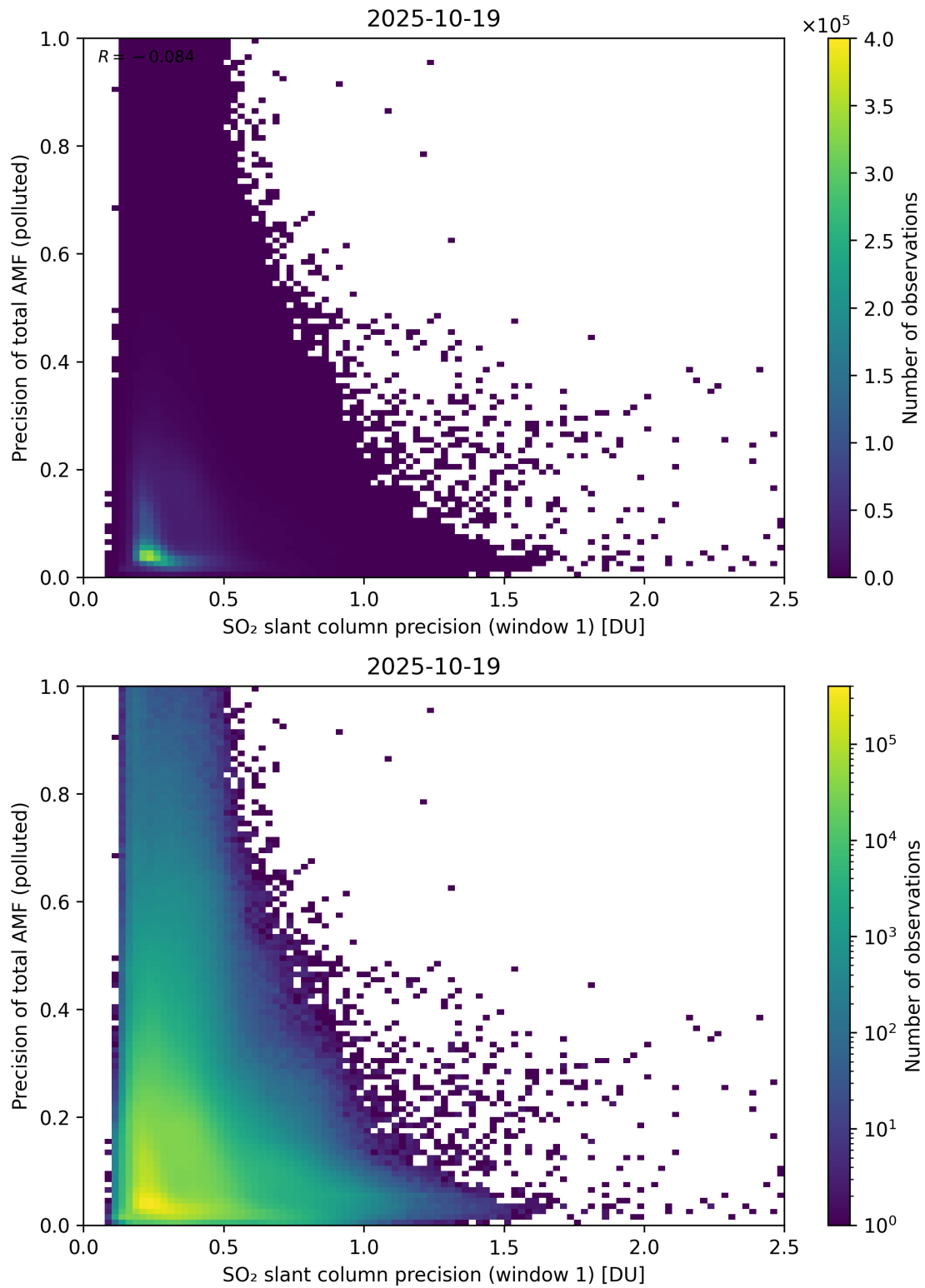
Figure 281: Scatter density plot of “SO 2 slant column precision (window 1)” against “Precision of total AMF (polluted)” for 2025-10-18 to 2025-10-20.
