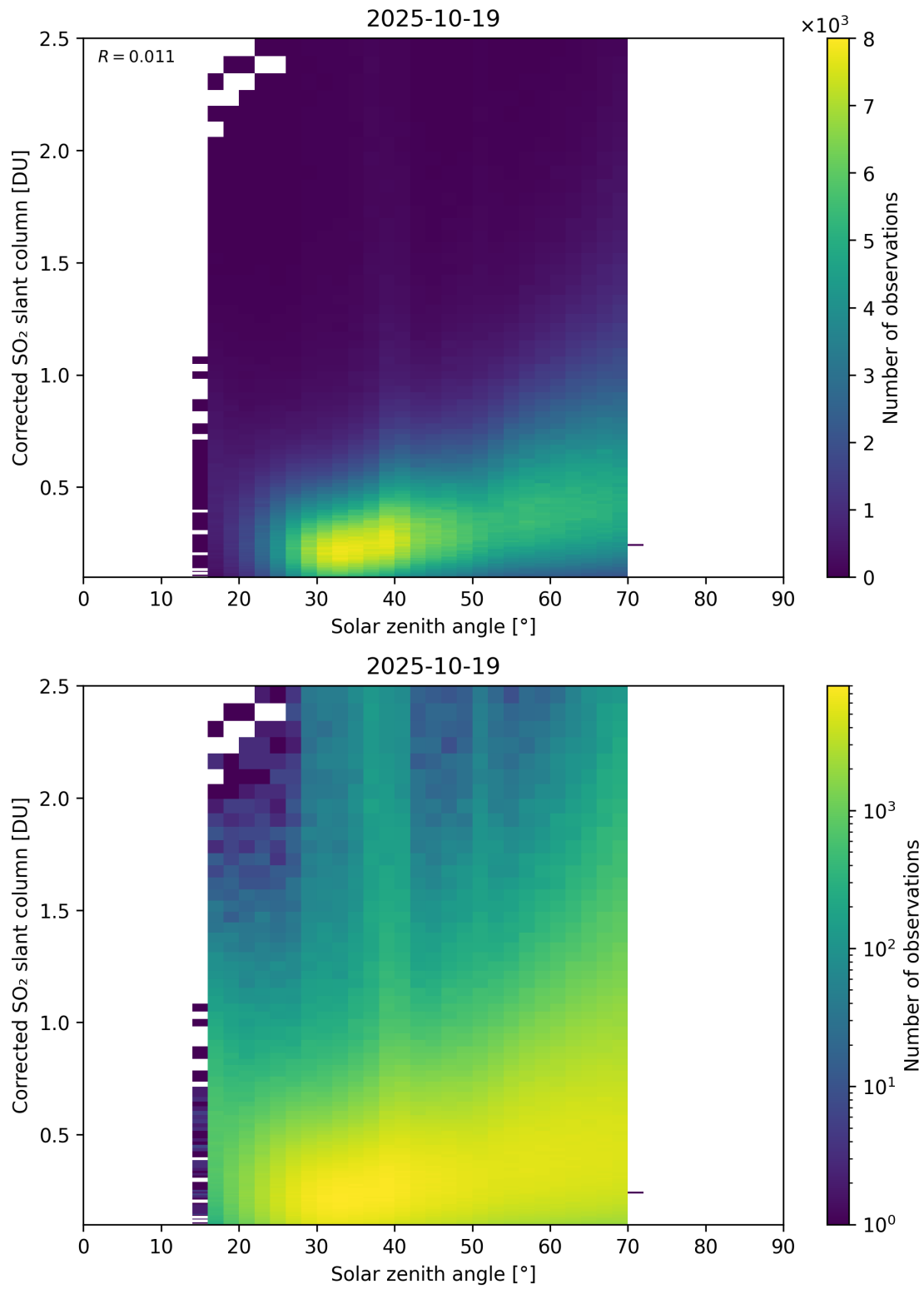
Figure 181: Scatter density plot of “Solar zenith angle” against “Corrected SO 2 slant column” for 2025-10-18 to 2025-10-20.
