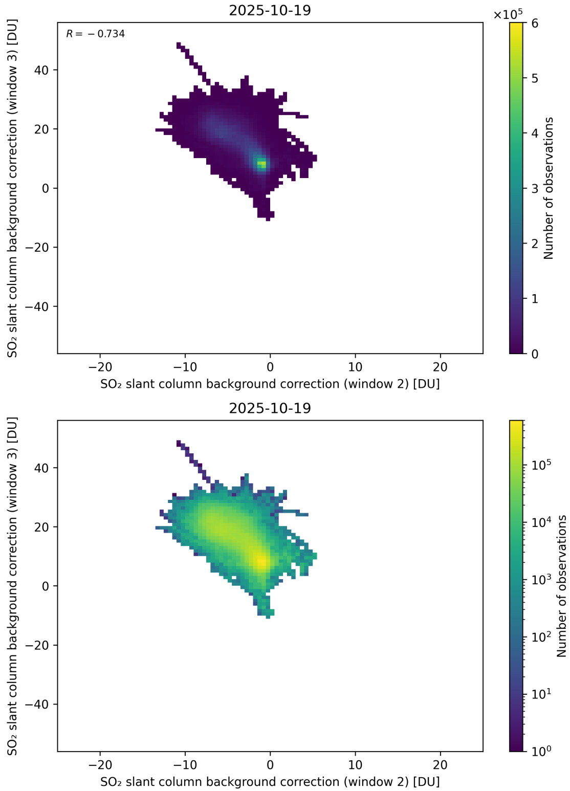
Figure 122: Scatter density plot of “SO 2 slant column background correction (window 2)” against “SO 2 slant column background correction (window 3)” for 2025-10-18 to 2025-10-20.
