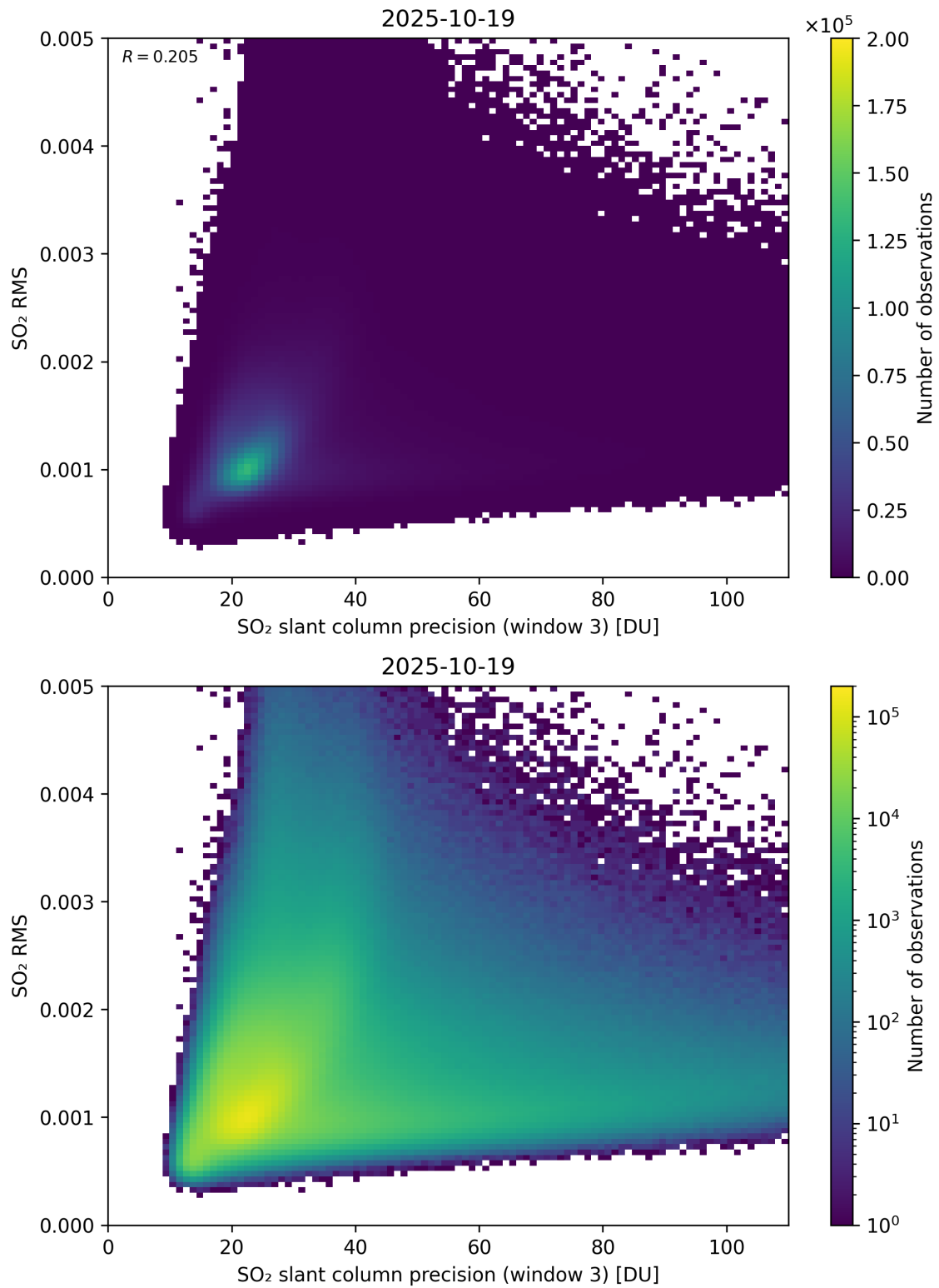
Figure 310: Scatter density plot of “SO 2 slant column precision (window 3)” against “SO 2 RMS” for 2025-10-18 to 2025-10-20.
