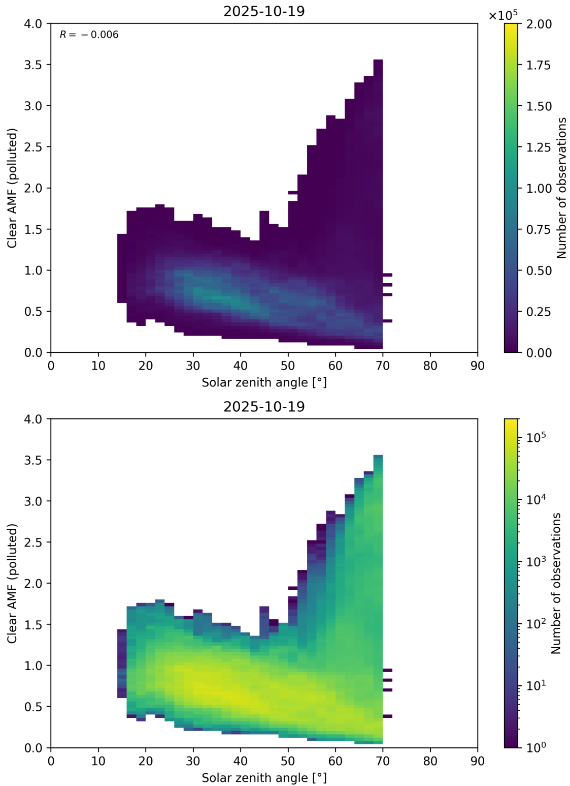
Figure 178: Scatter density plot of “Solar zenith angle” against “Clear AMF (polluted)” for 2025-10-18 to 2025-10-20.
