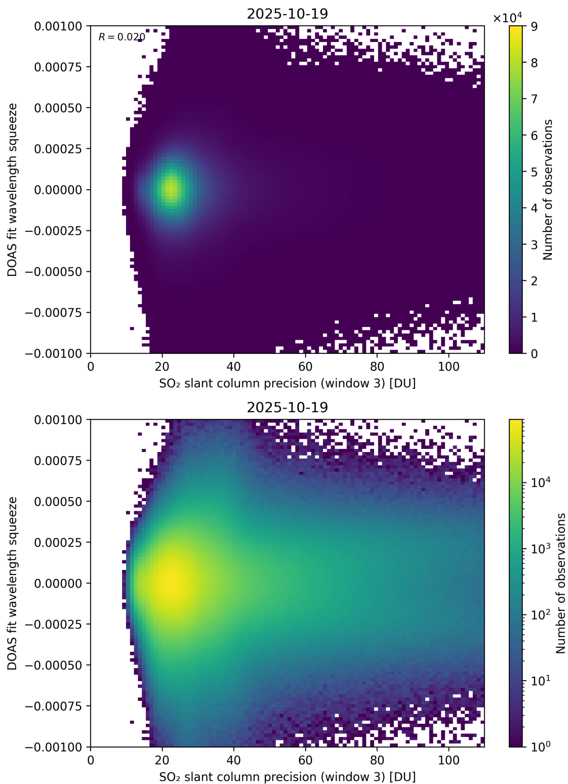
Figure 309: Scatter density plot of “SO 2 slant column precision (window 3)” against “DOAS fit wavelength squeeze” for 2025-10-18 to 2025-10-20.
