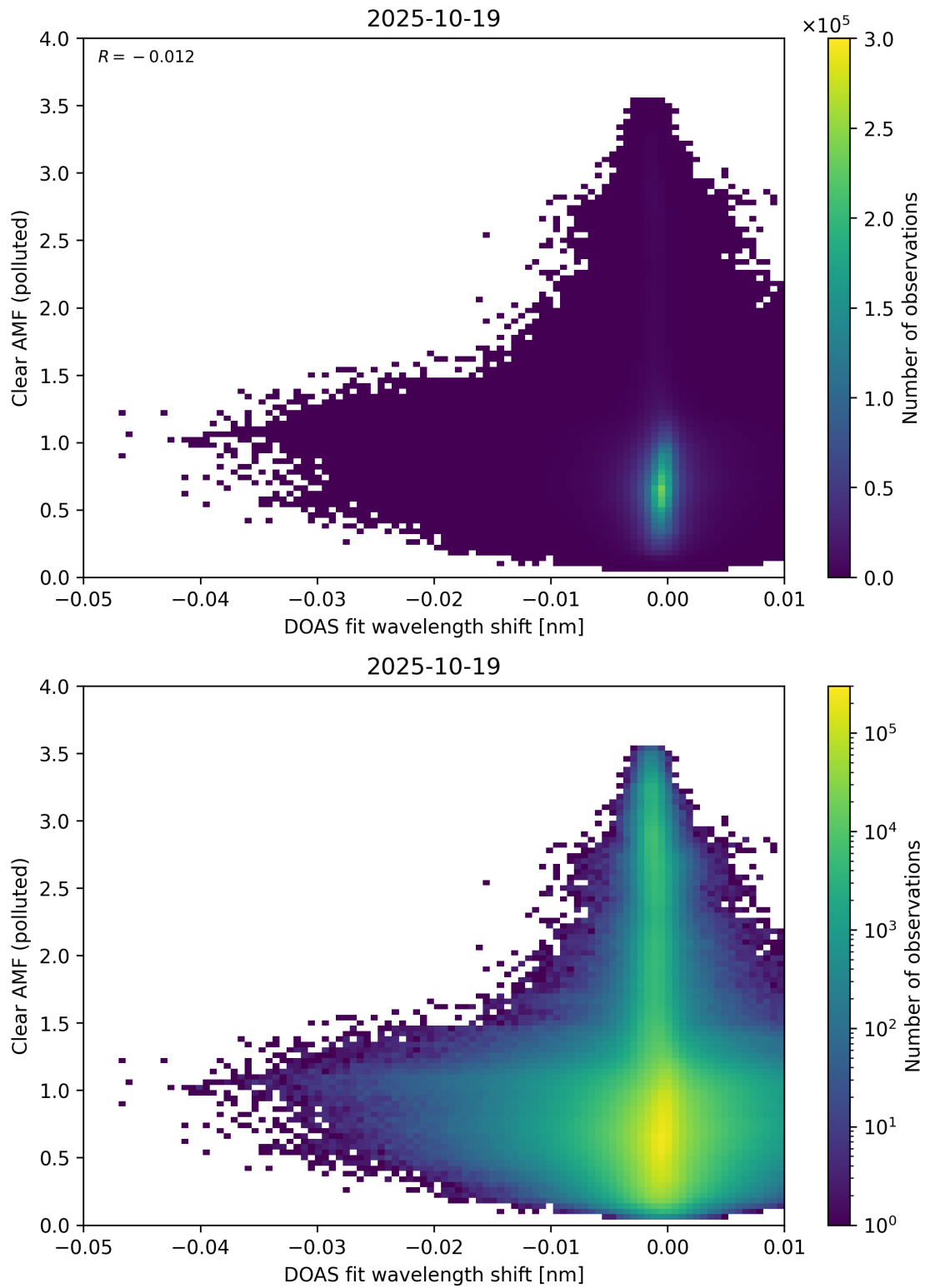
Figure 140: Scatter density plot of “DOAS fit wavelength shift” against “Clear AMF (polluted)” for 2025-10-18 to 2025-10-20.
