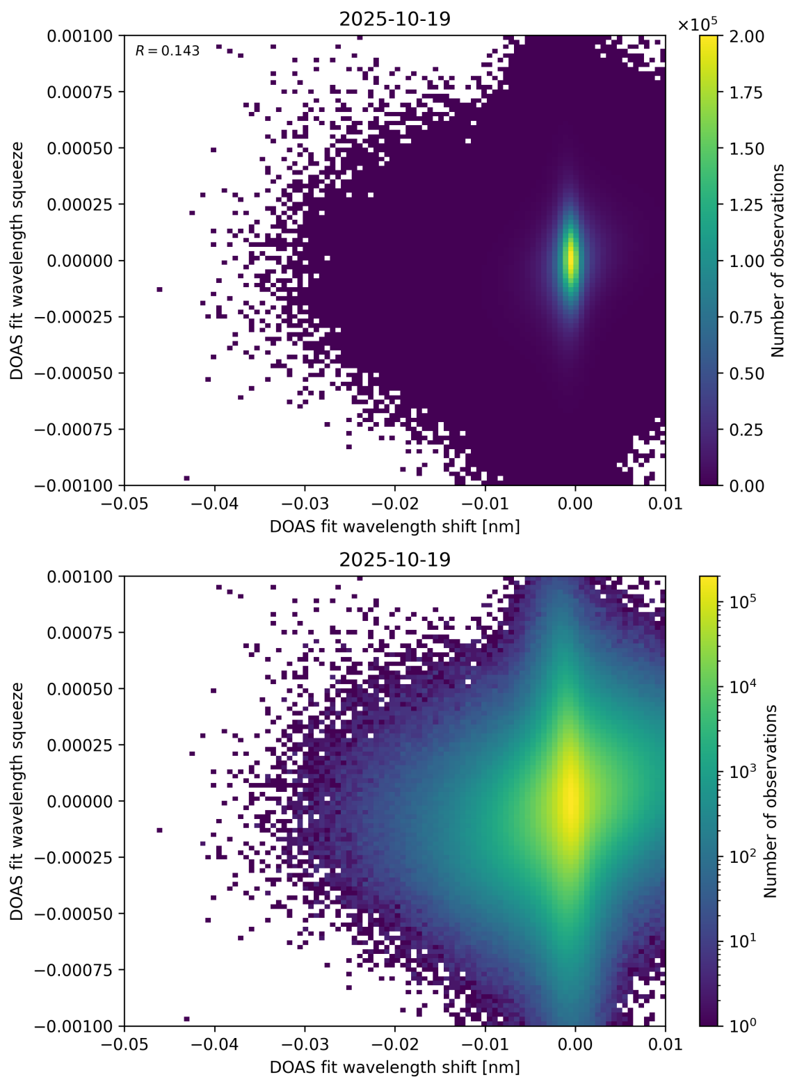
Figure 138: Scatter density plot of “DOAS fit wavelength shift” against “DOAS fit wavelength squeeze” for 2025-10-18 to 2025-10-20.
