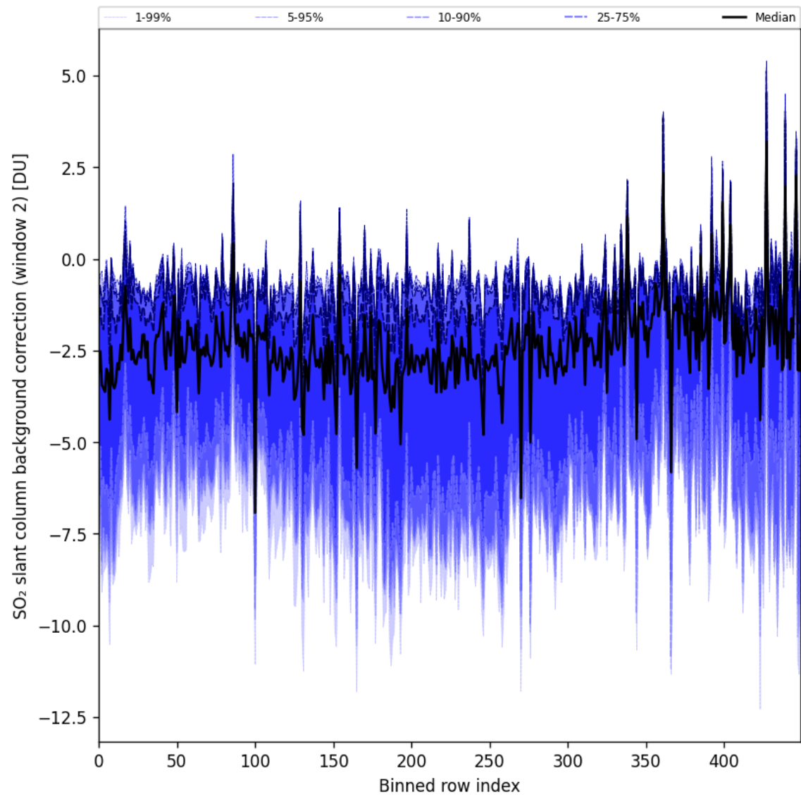
Figure 96: Along track statistics of “SO 2 slant column background correction (window 2)” for 2025-10-18 to 2025-10-20
