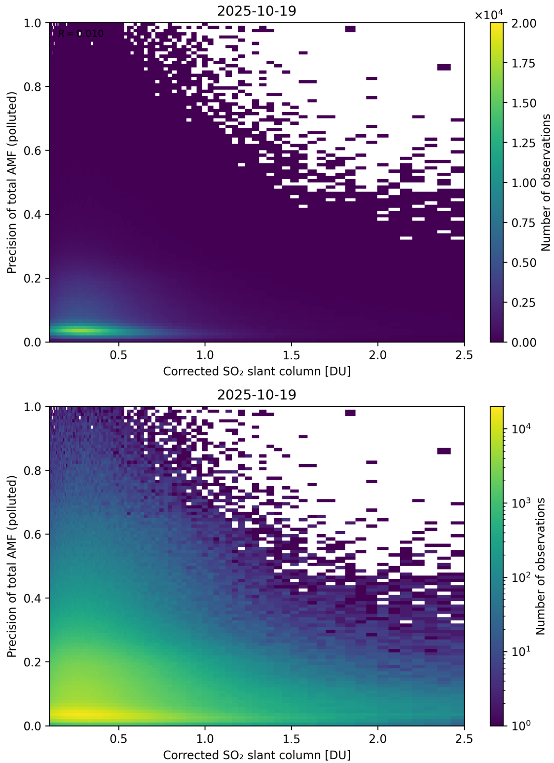
Figure 243: Scatter density plot of “Corrected SO 2 slant column” against “Precision of total AMF (polluted)” for 2025-10-18 to 2025-10-20.
