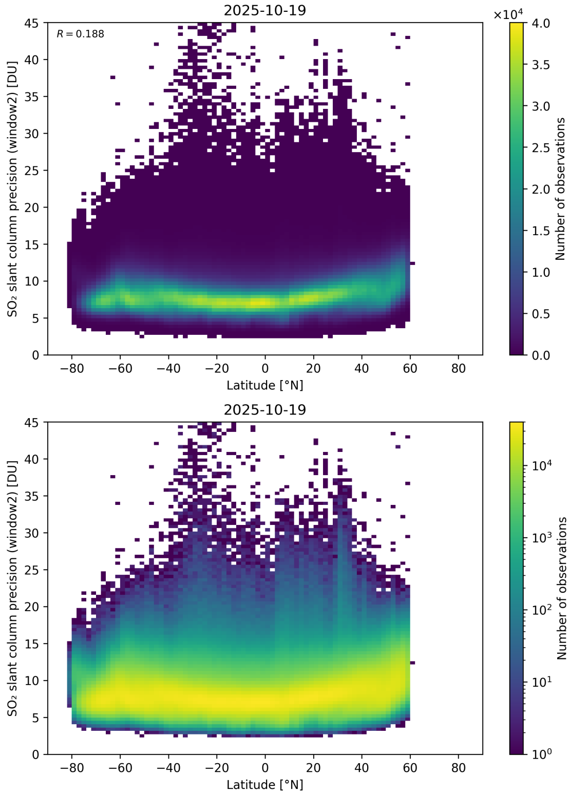
Figure 164: Scatter density plot of “Latitude” against “SO 2 slant column precision (window2)” for 2025-10-18 to 2025-10-20.
