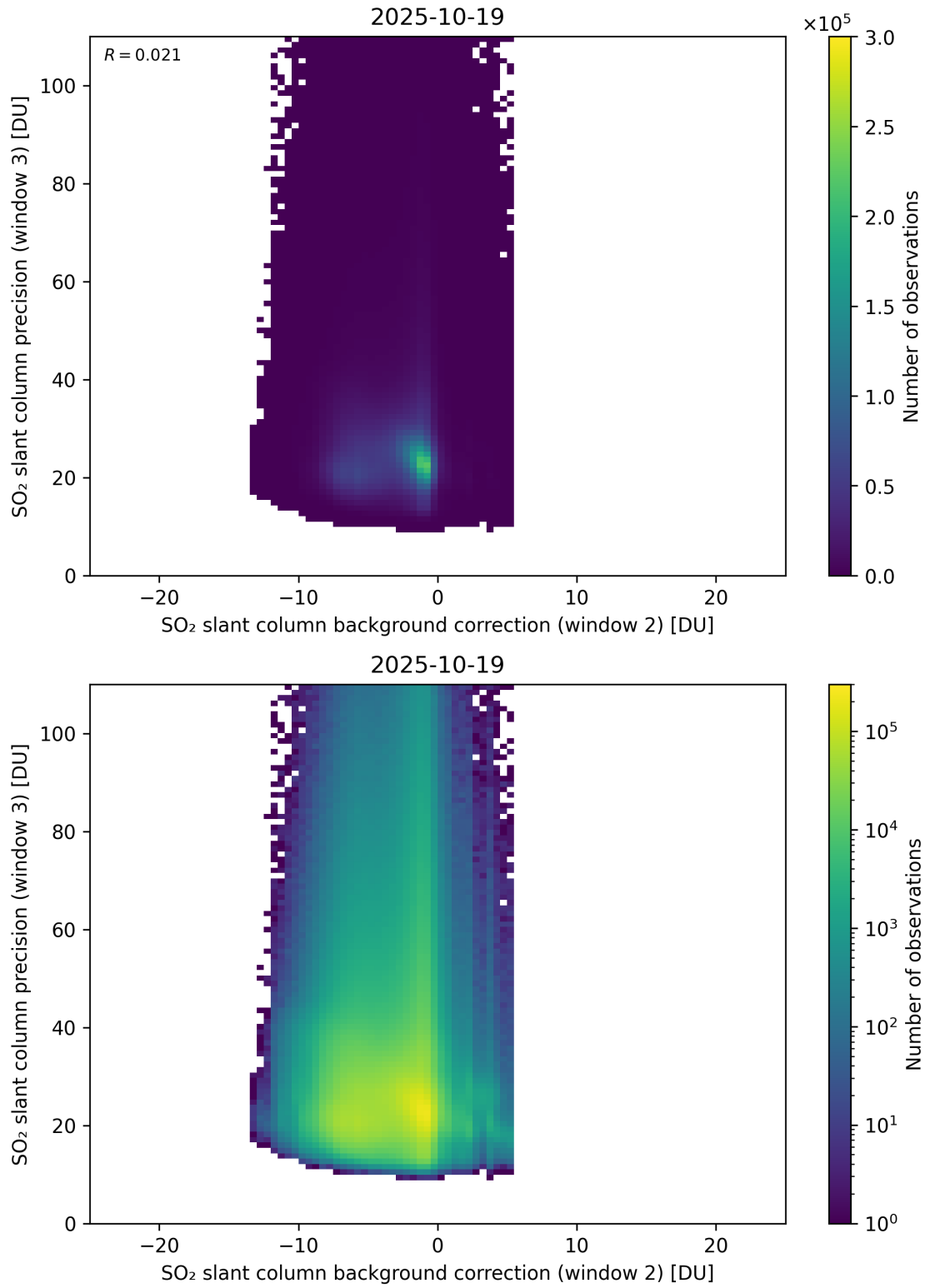
Figure 129: Scatter density plot of “SO 2 slant column background correction (window 2)” against “SO 2 slant column precision (window 3)” for 2025-10-18 to 2025-10-20.
