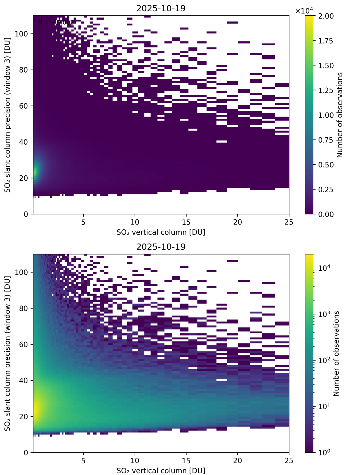
Figure 358: Scatter density plot of “SO 2 vertical column” against “SO 2 slant column precision (window 3)” for 2025-10-18 to 2025-10-20.
