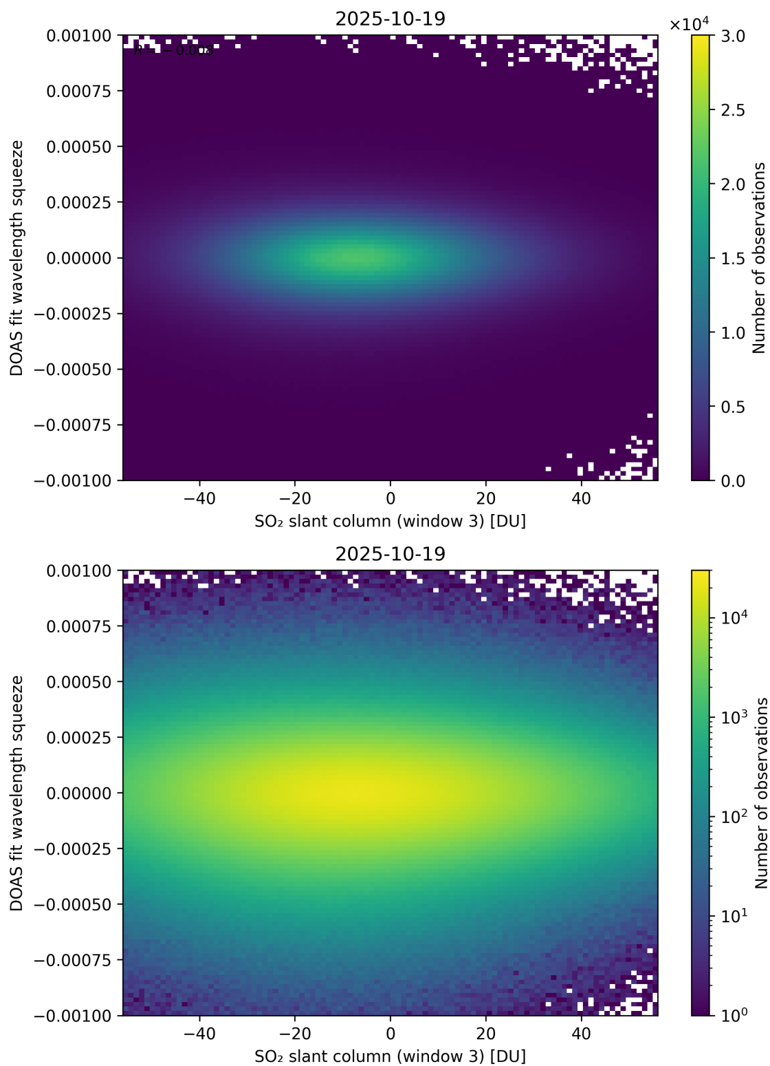
Figure 305: Scatter density plot of “SO 2 slant column (window 3)” against “DOAS fit wavelength squeeze” for 2025-10-18 to 2025-10-20.
