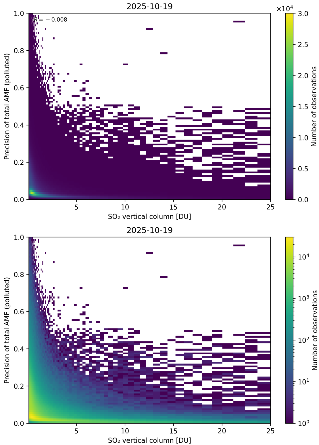
Figure 360: Scatter density plot of “SO 2 vertical column” against “Precision of total AMF (polluted)” for 2025-10-18 to 2025-10-20.
