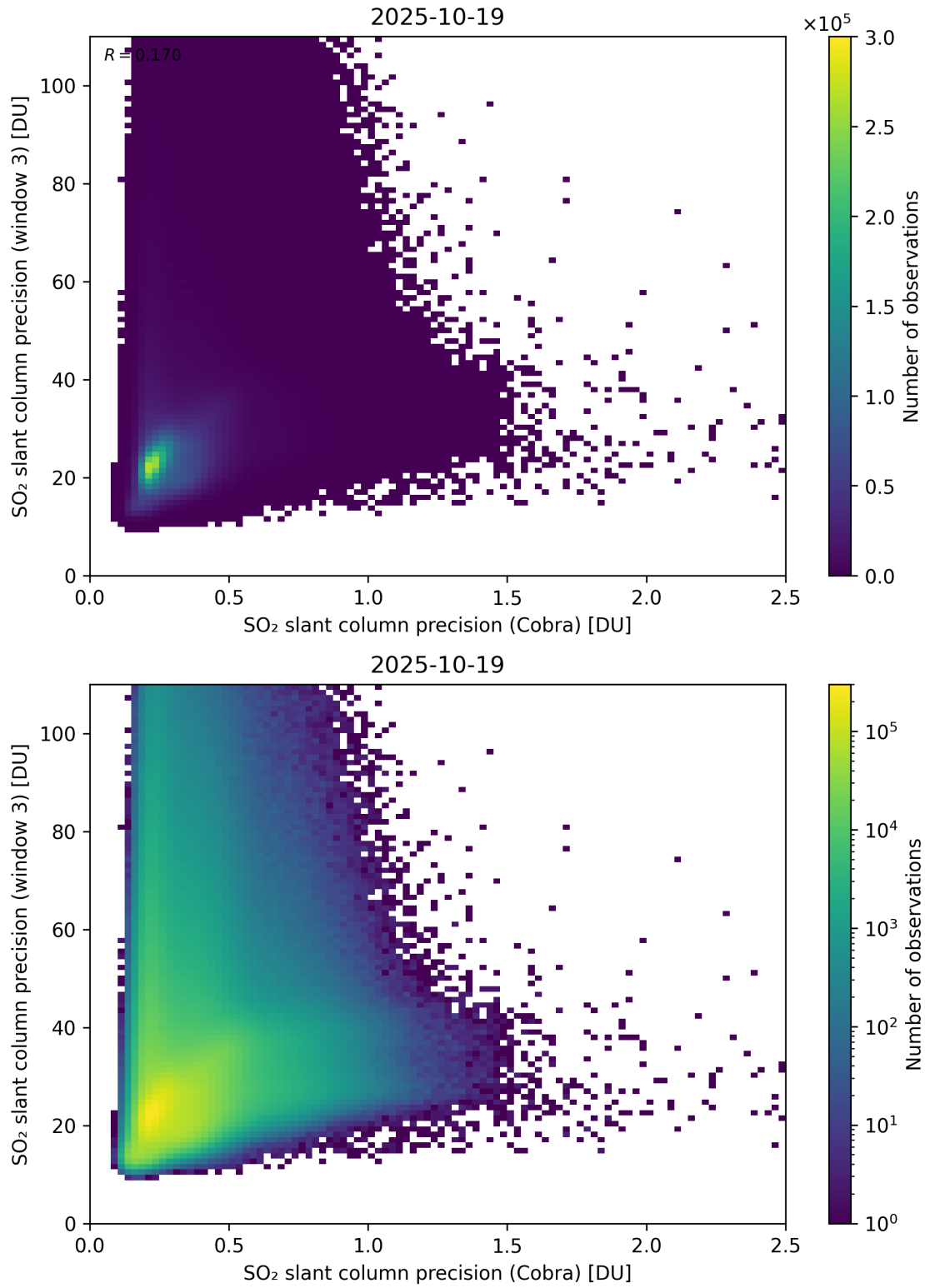
Figure 212: Scatter density plot of “SO 2 slant column precision (Cobra)” against “SO 2 slant column precision (window 3)” for 2025-10-18 to 2025-10-20.
