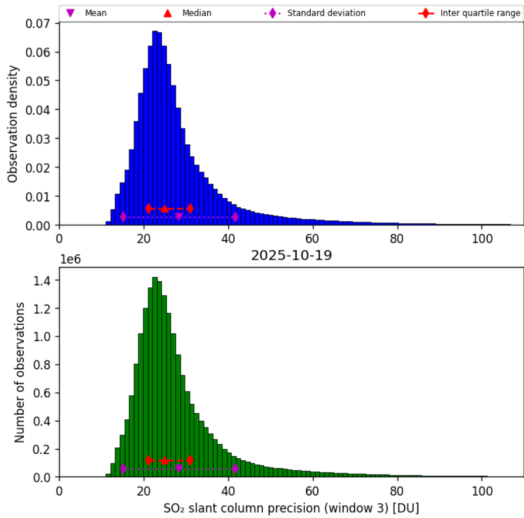
Figure 72: Histogram of “SO 2 slant column precision (window 3)” for 2025-10-18 to 2025-10-20
