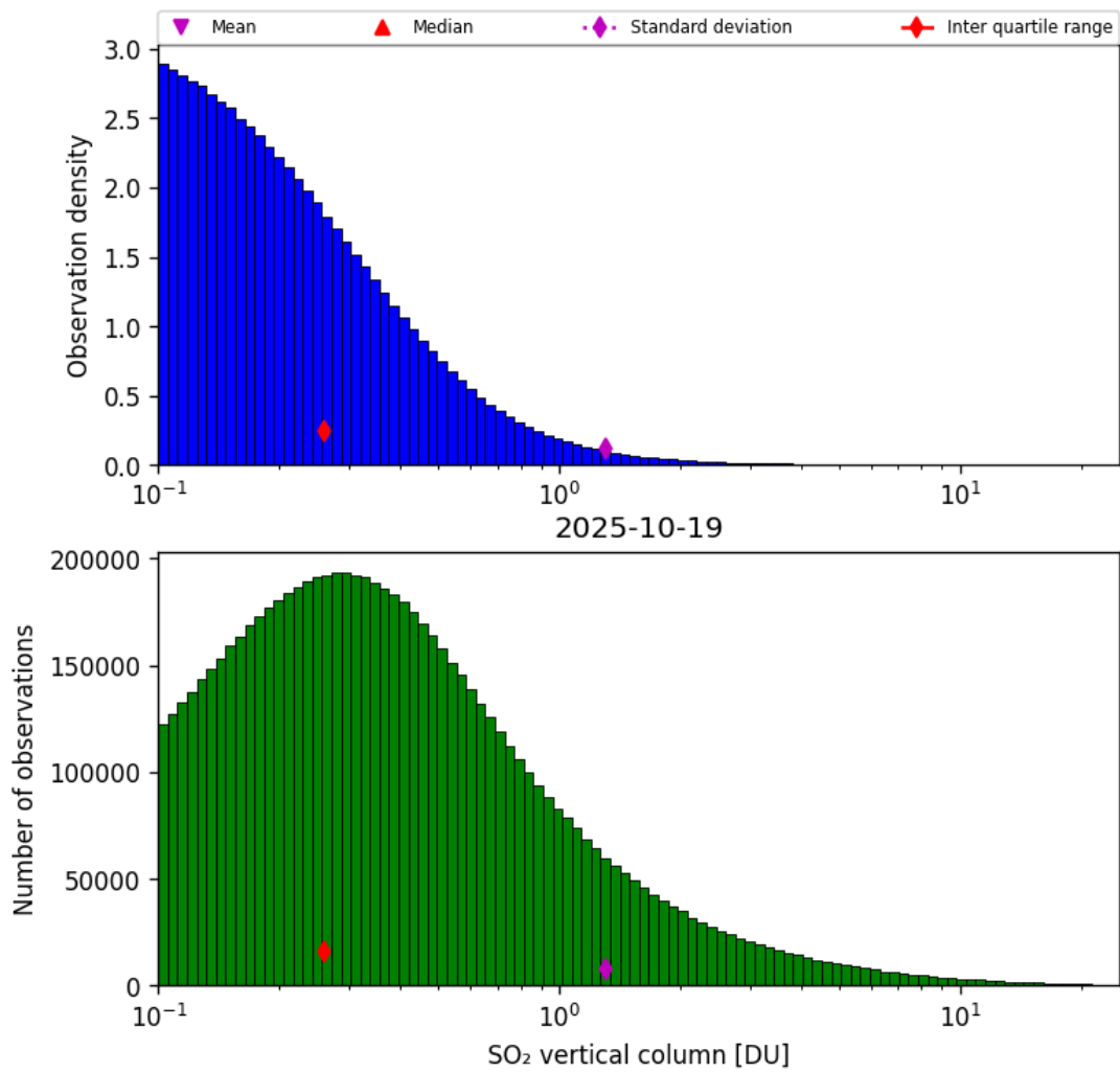
Figure 58: Histogram of “SO 2 vertical column” for 2025-10-18 to 2025-10-20
