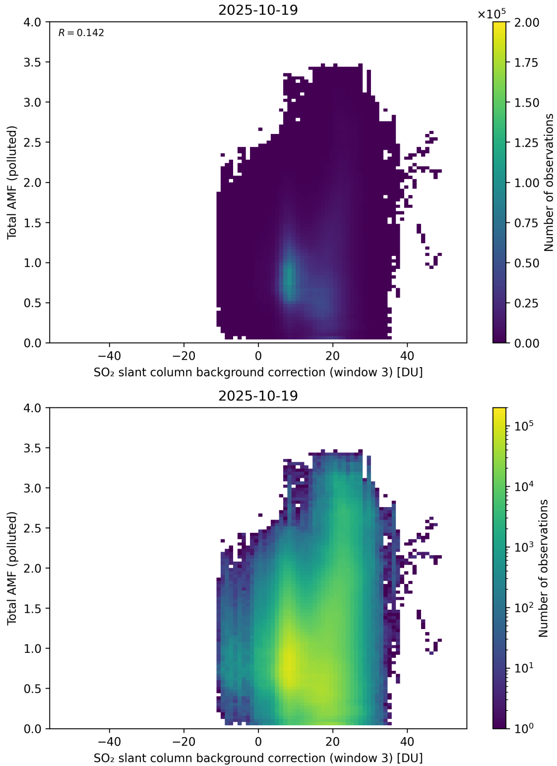
Figure 136: Scatter density plot of “SO 2 slant column background correction (window 3)” against “Total AMF (polluted)” for 2025-10-18 to 2025-10-20.
