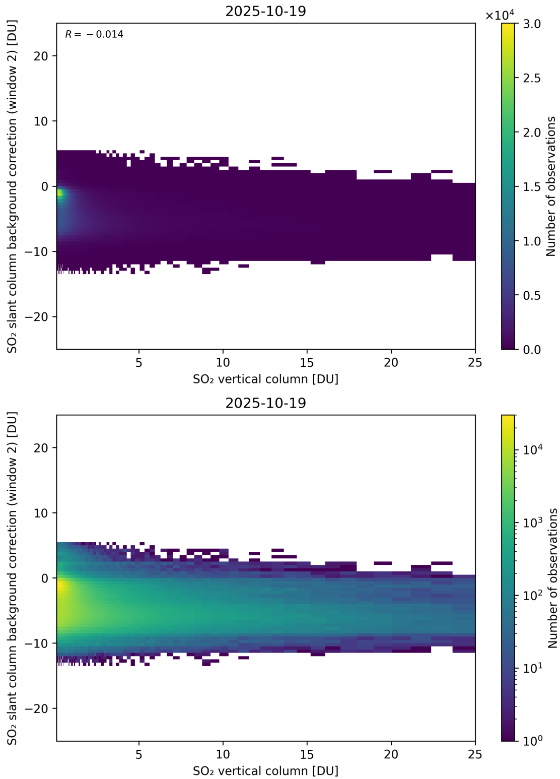
Figure 324: Scatter density plot of “SO 2 vertical column” against “SO 2 slant column background correction (window 2)” for 2025-10-18 to 2025-10-20.
