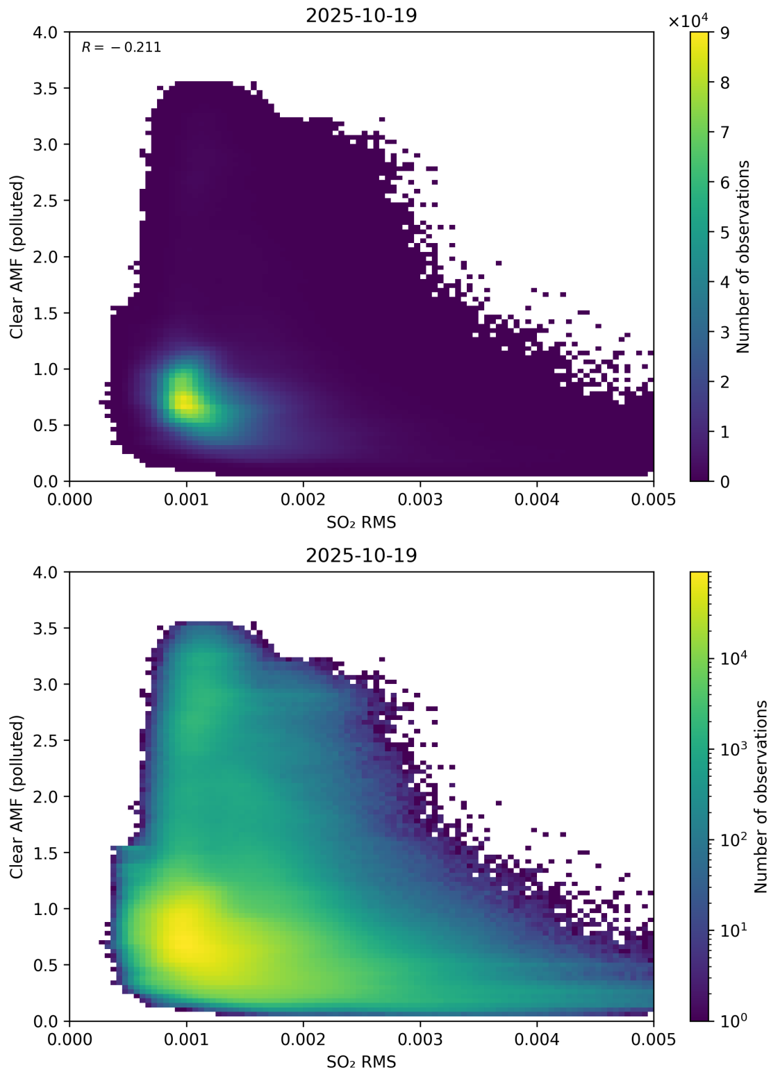
Figure 147: Scatter density plot of “SO 2 RMS” against “Clear AMF (polluted)” for 2025-10-18 to 2025-10-20.
