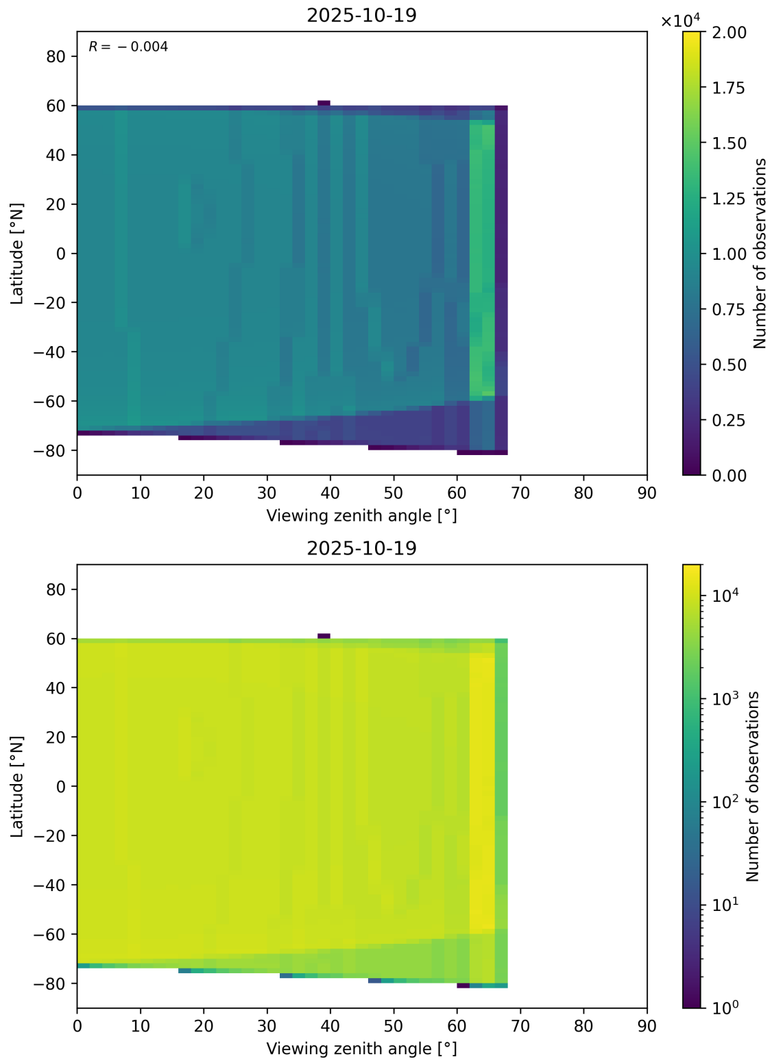
Figure 368: Scatter density plot of “Viewing zenith angle” against “Latitude” for 2025-10-18 to 2025-10-20.
