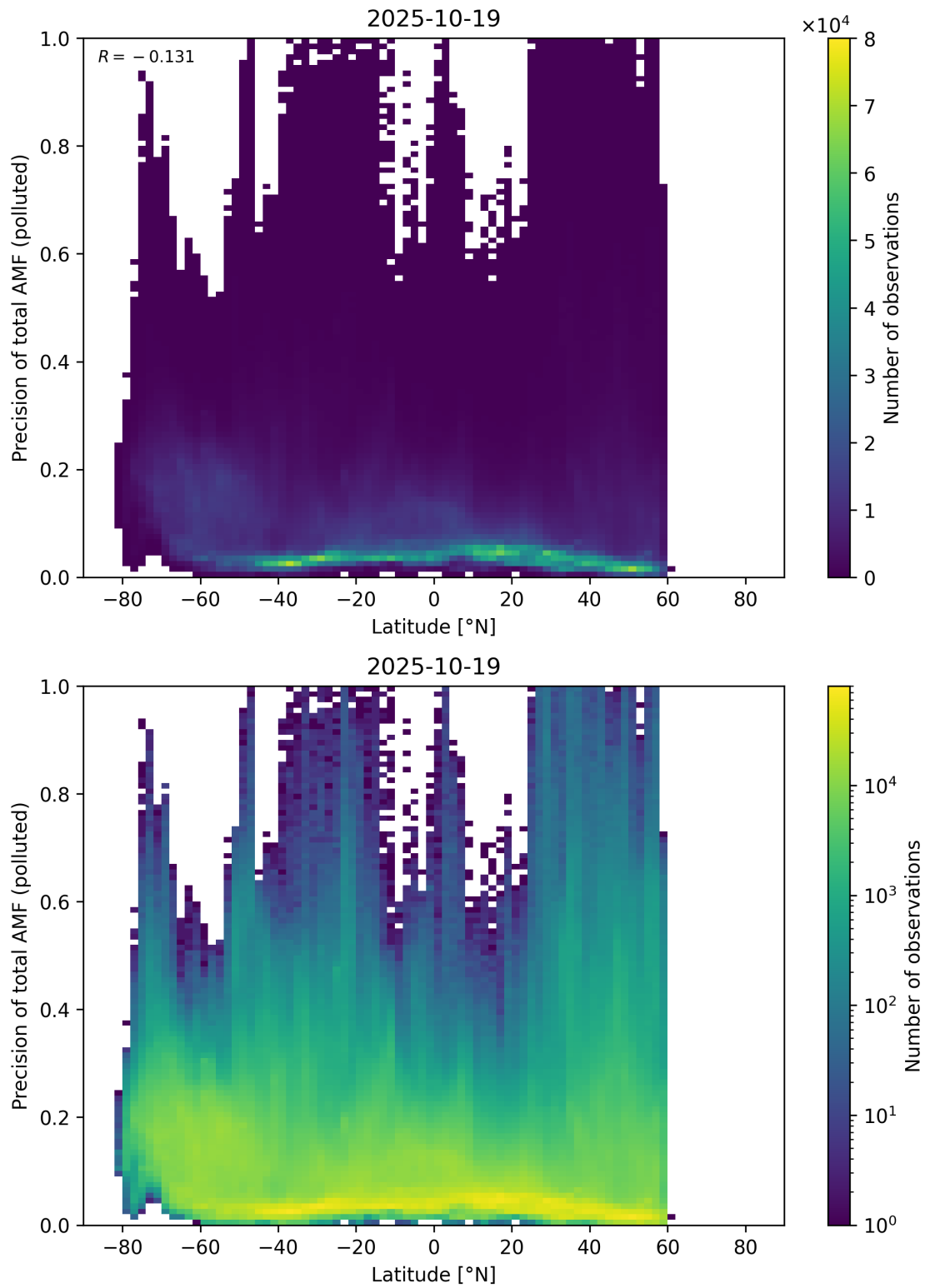
Figure 168: Scatter density plot of “Latitude” against “Precision of total AMF (polluted)” for 2025-10-18 to 2025-10-20.
