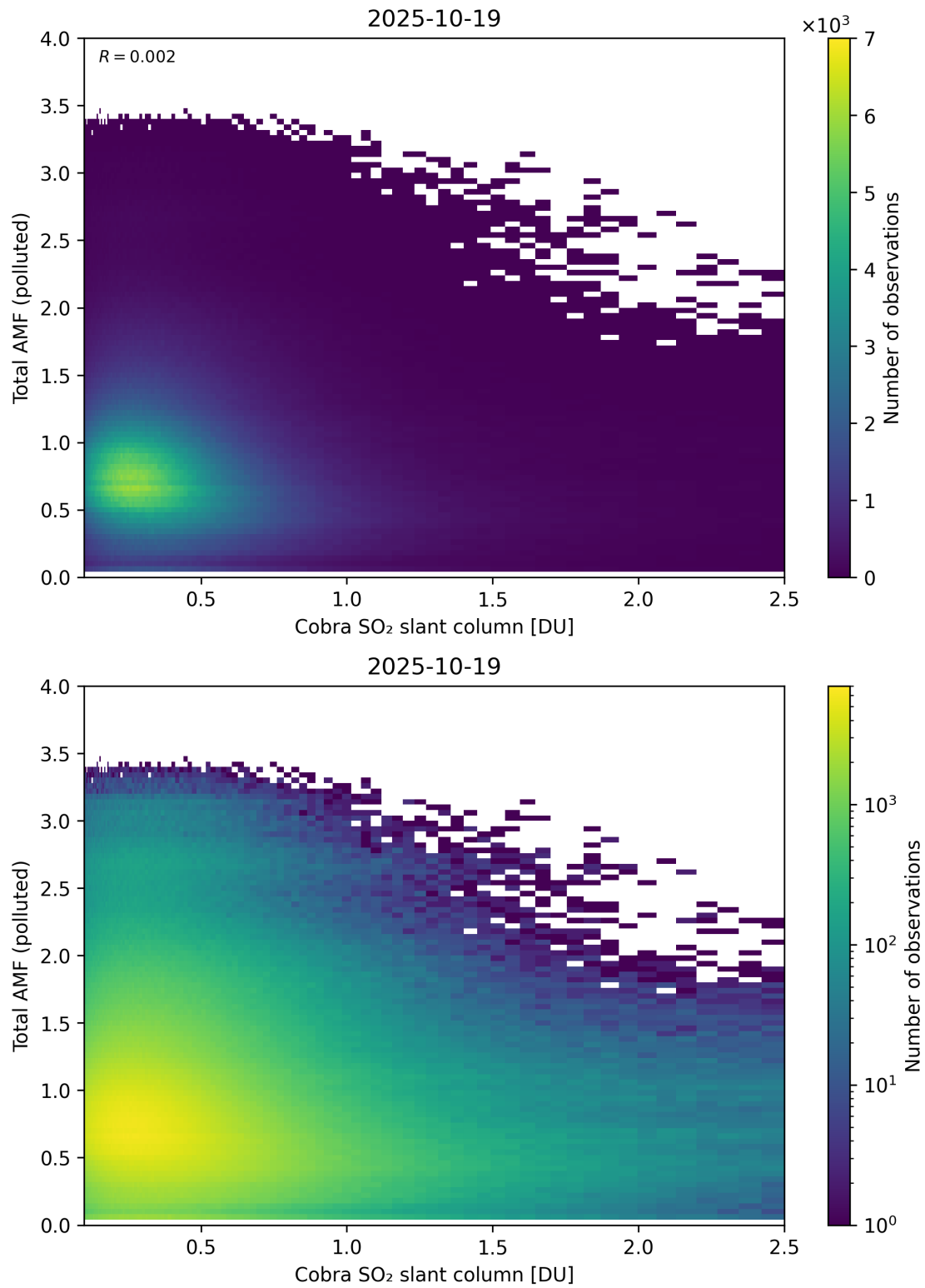
Figure 224: Scatter density plot of “Cobra SO 2 slant column” against “Total AMF (polluted)” for 2025-10-18 to 2025-10-20.
