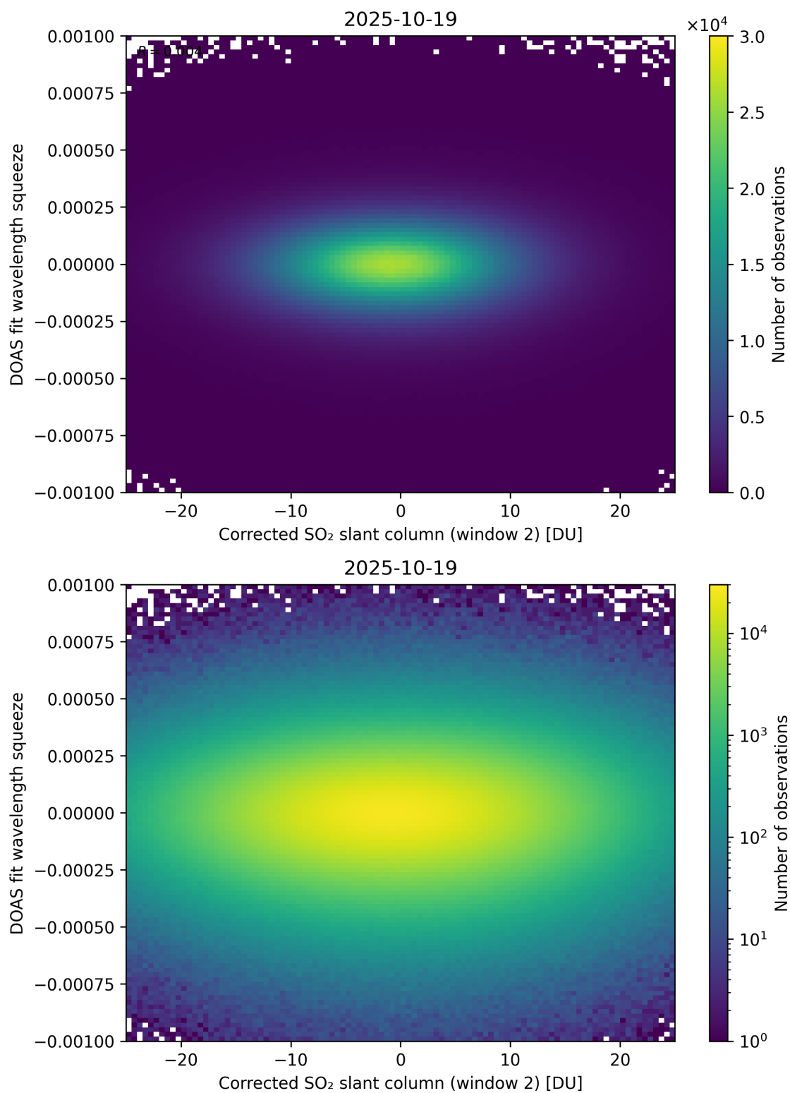
Figure 247: Scatter density plot of “Corrected SO 2 slant column (window 2)” against “DOAS fit wavelength squeeze” for 2025-10-18 to 2025-10-20.
