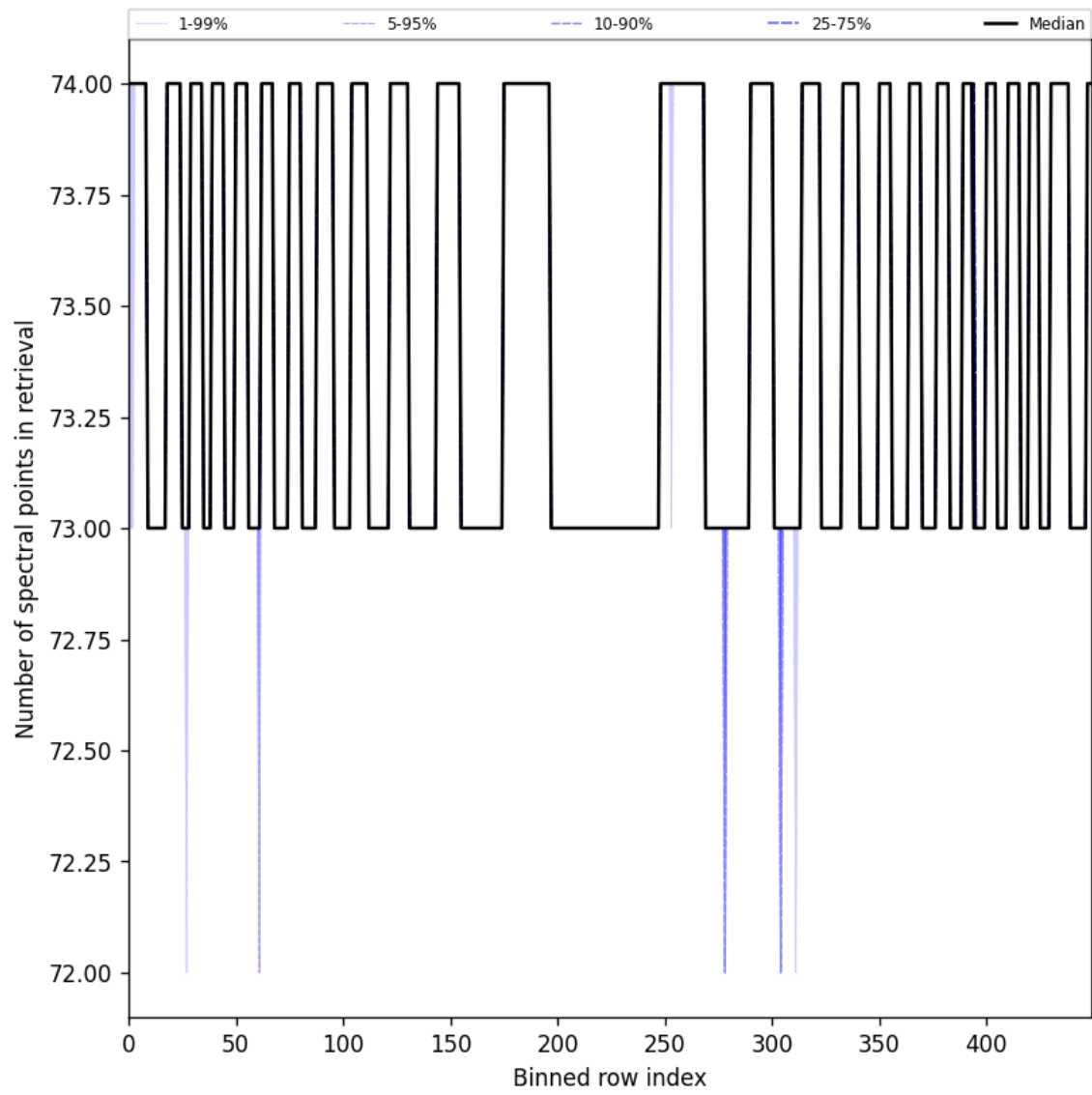
Figure 108: Along track statistics of “Number of spectral points in retrieval” for 2025-10-18 to 2025-10-20
