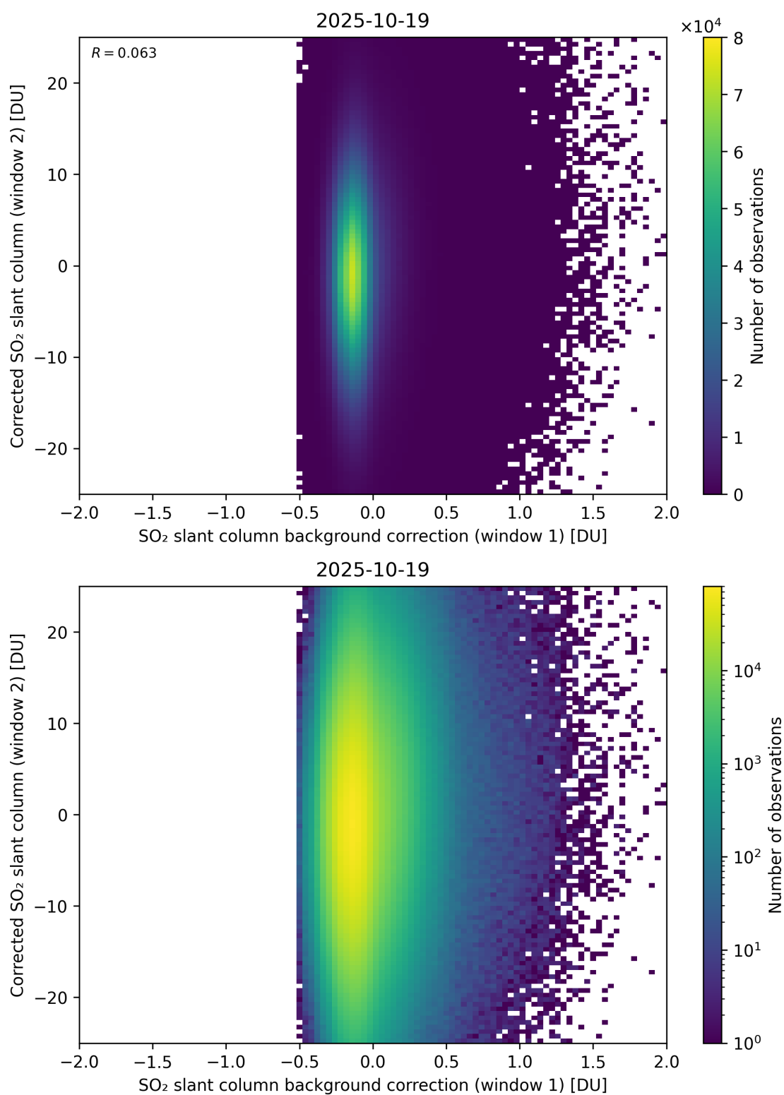
Figure 115: Scatter density plot of “SO 2 slant column background correction (window 1)” against “Corrected SO 2 slant column (window 2)” for 2025-10-18 to 2025-10-20.
