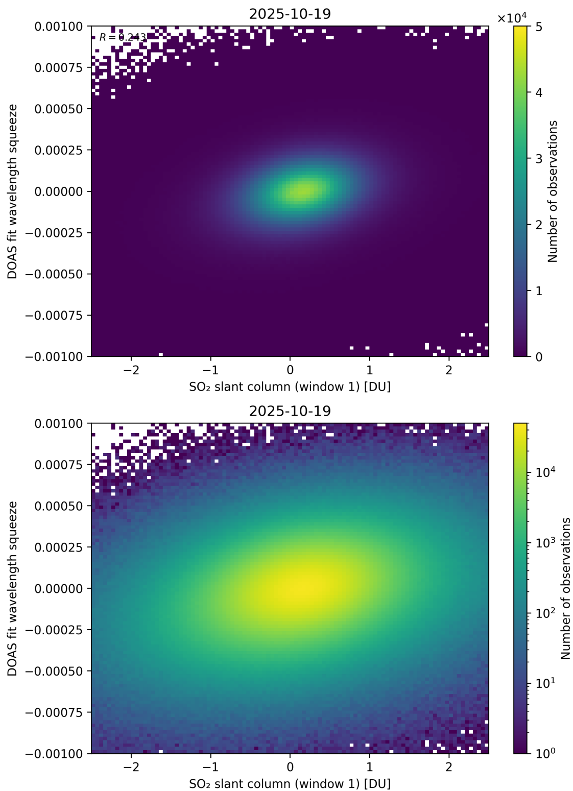
Figure 266: Scatter density plot of “SO 2 slant column (window 1)” against “DOAS fit wavelength squeeze” for 2025-10-18 to 2025-10-20.
