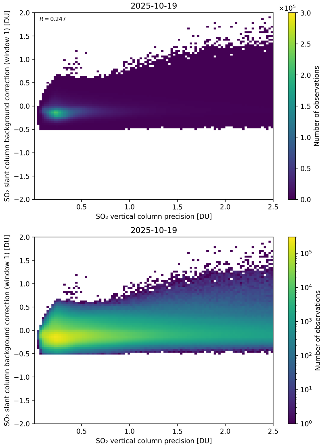
Figure 329: Scatter density plot of “SO 2 vertical column precision” against “SO 2 slant column background correction (window 1)” for 2025-10-18 to 2025-10-20.
