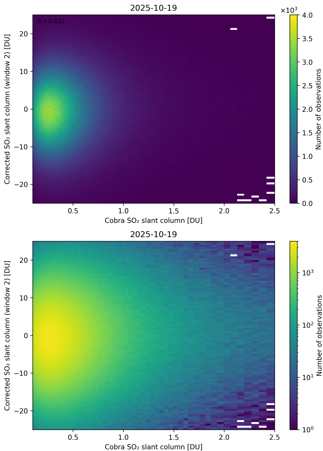
Figure 217: Scatter density plot of “Cobra SO 2 slant column” against “Corrected SO 2 slant column (window 2)” for 2025-10-18 to 2025-10-20.
