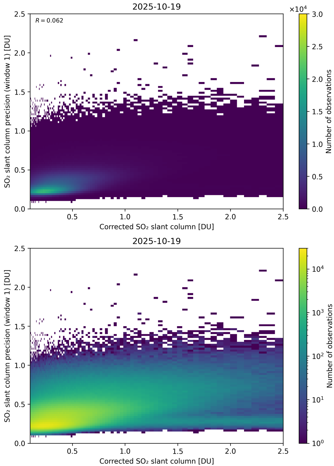
Figure 238: Scatter density plot of “Corrected SO 2 slant column” against “SO 2 slant column precision (window 1)” for 2025-10-18 to 2025-10-20.
