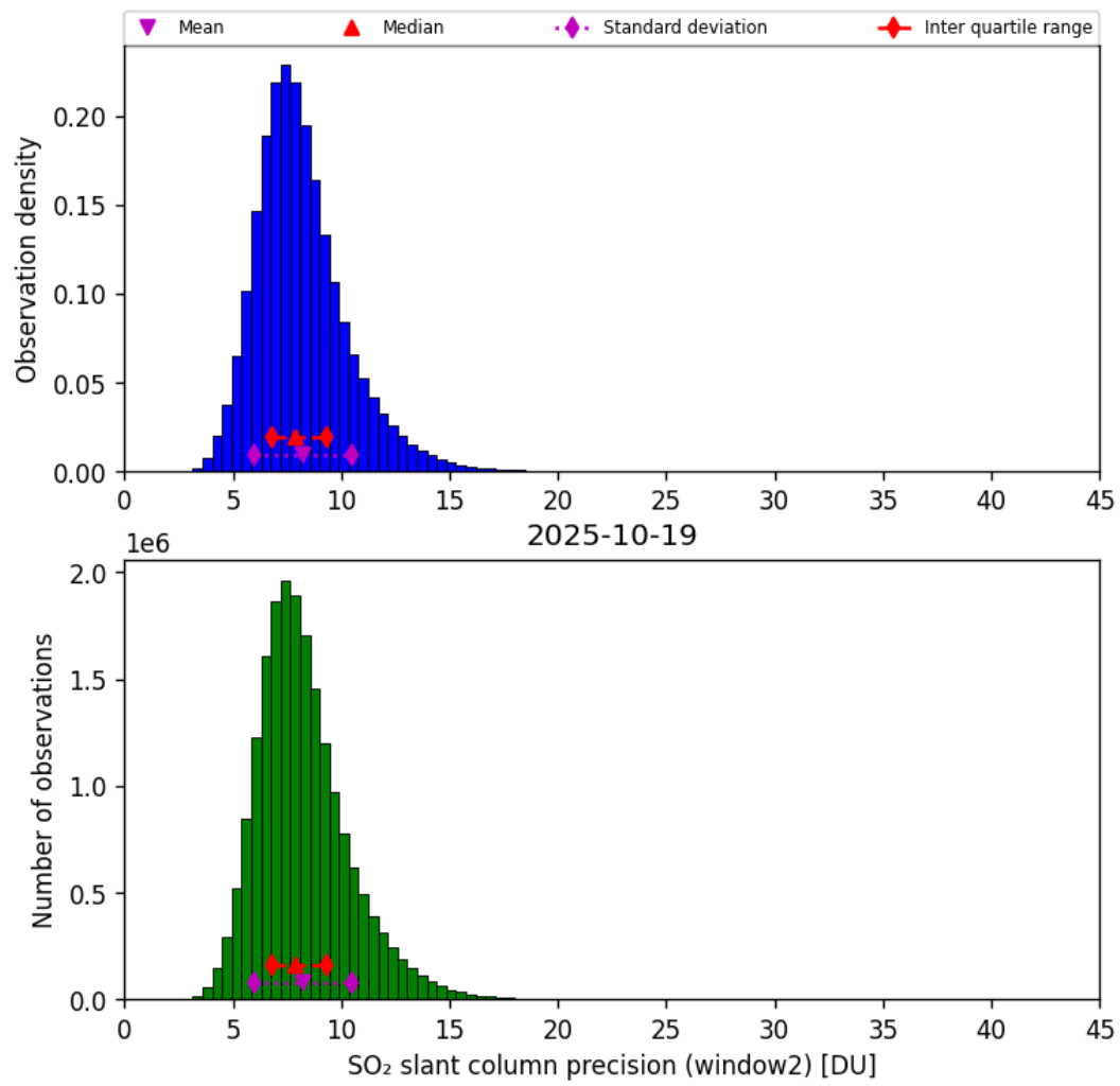
Figure 68: Histogram of “SO 2 slant column precision (window2)” for 2025-10-18 to 2025-10-20
