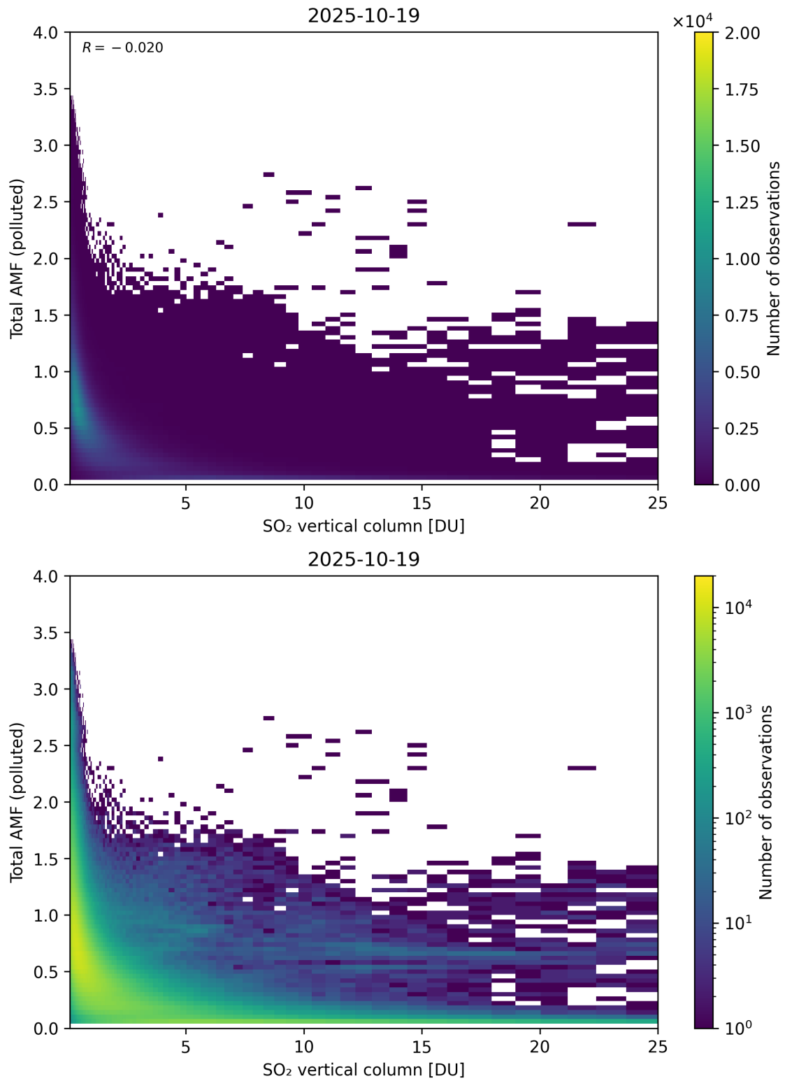
Figure 359: Scatter density plot of “SO 2 vertical column” against “Total AMF (polluted)” for 2025-10-18 to 2025-10-20.
