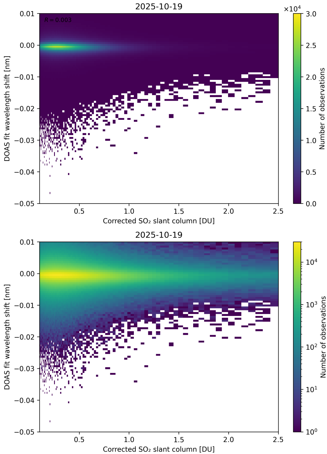
Figure 229: Scatter density plot of “Corrected SO 2 slant column” against “DOAS fit wavelength shift” for 2025-10-18 to 2025-10-20.
