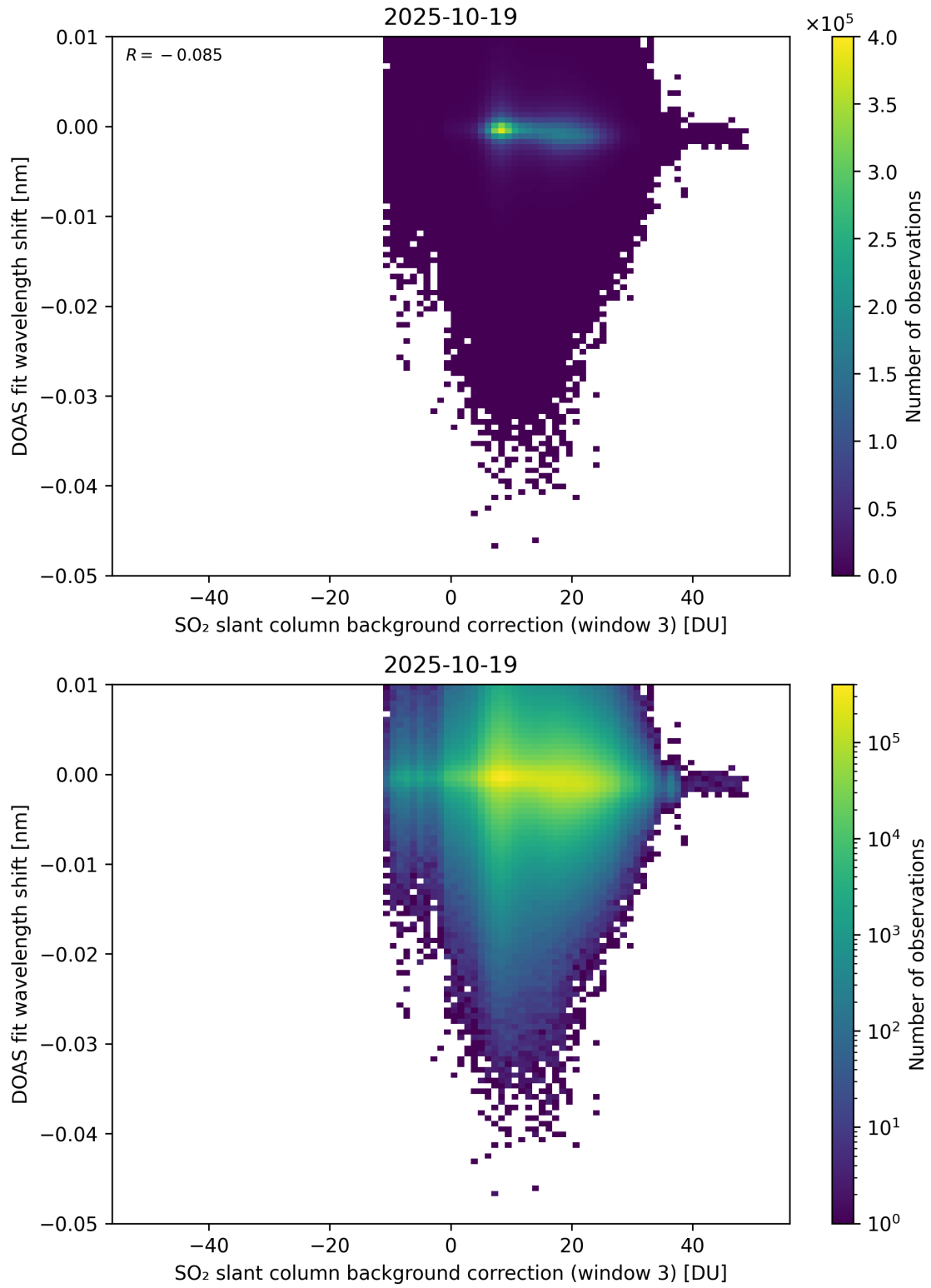
Figure 132: Scatter density plot of “SO 2 slant column background correction (window 3)” against “DOAS fit wavelength shift” for 2025-10-18 to 2025-10-20.
