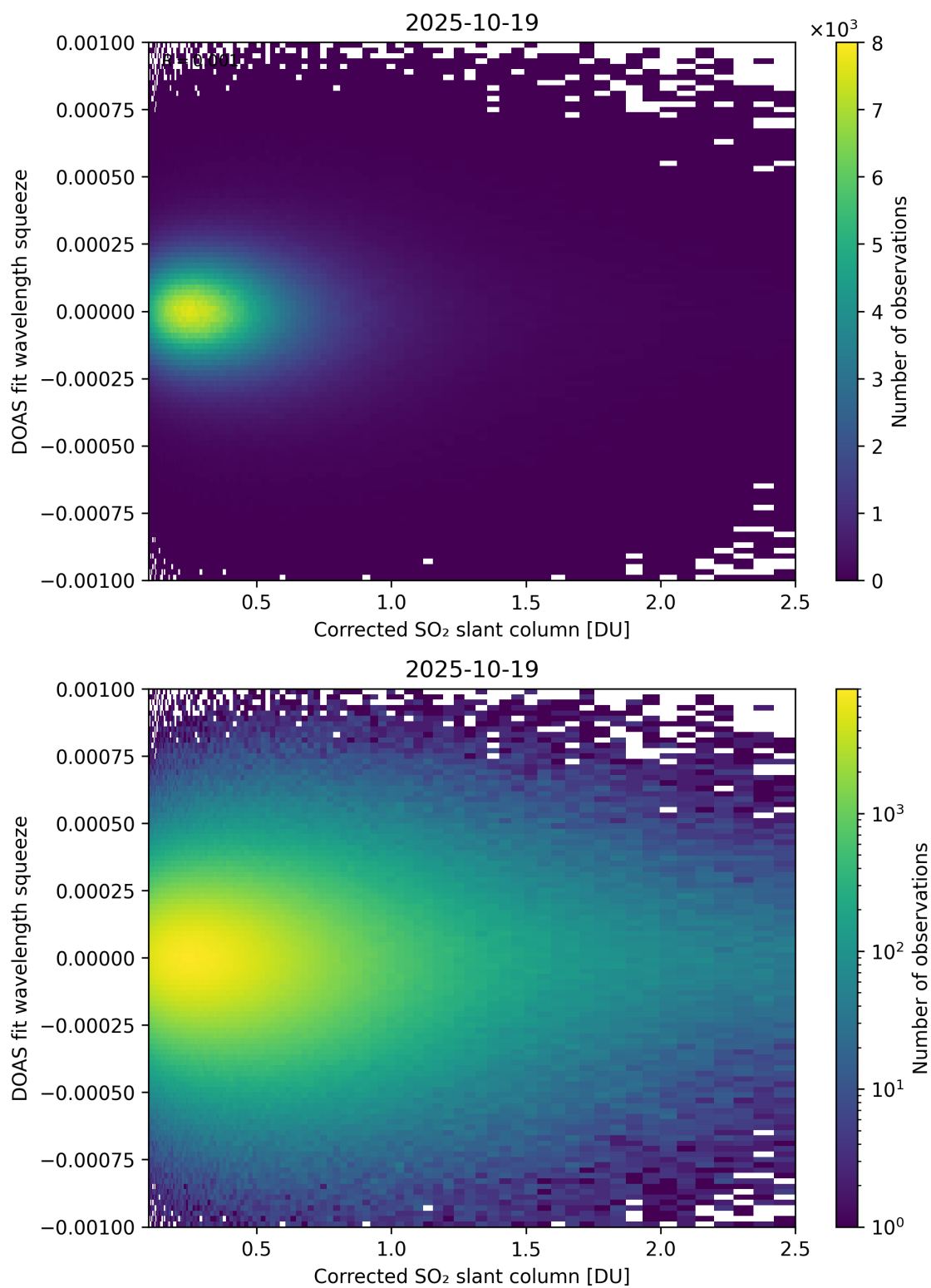
Figure 230: Scatter density plot of "Corrected SO 2 slant column" against "DOAS fit wavelength squeeze" for 2025-10-18 to 2025-10-20.
