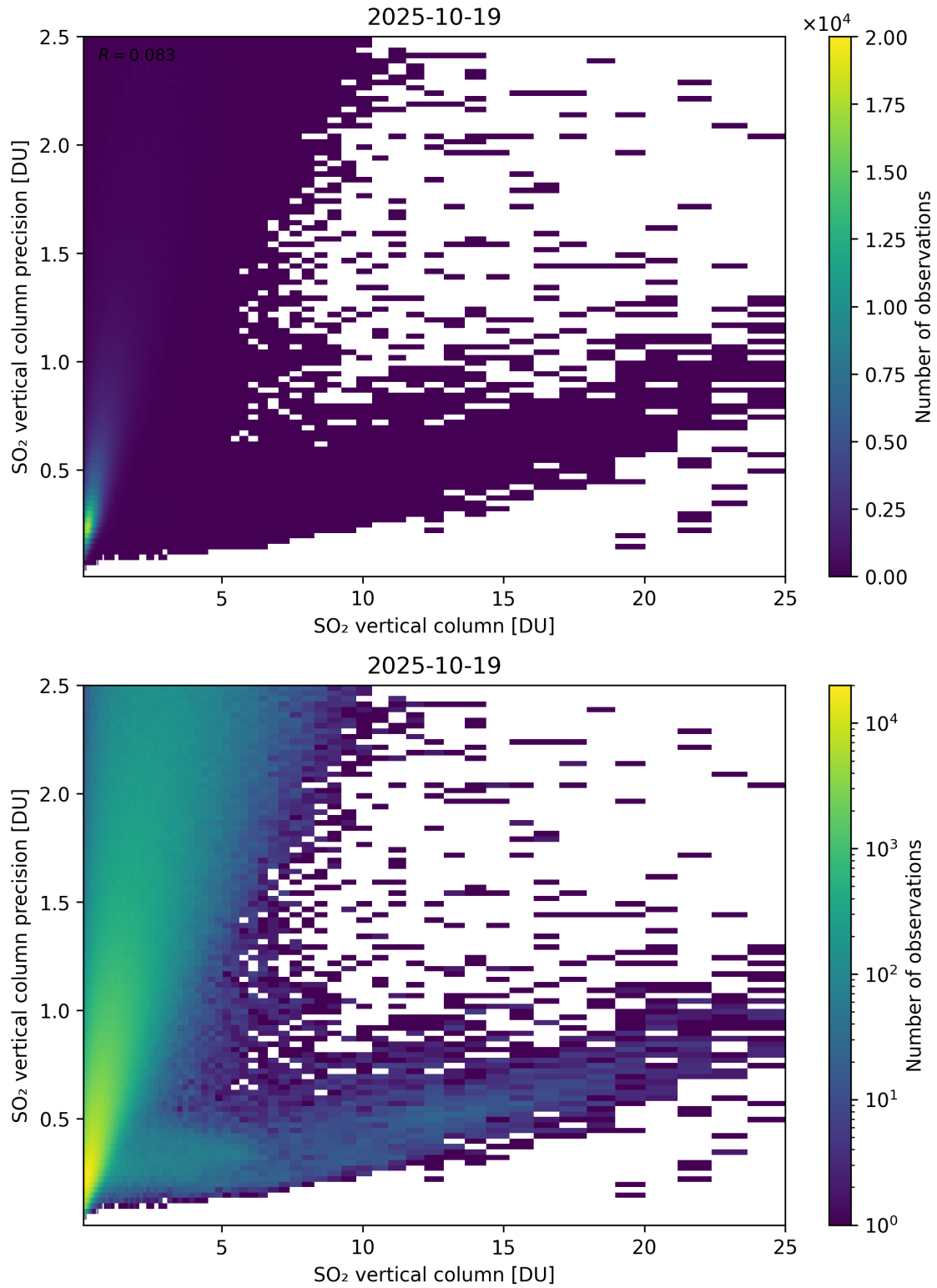
Figure 361: Scatter density plot of “SO 2 vertical column” against “SO 2 vertical column precision” for 2025-10-18 to 2025-10-20.
