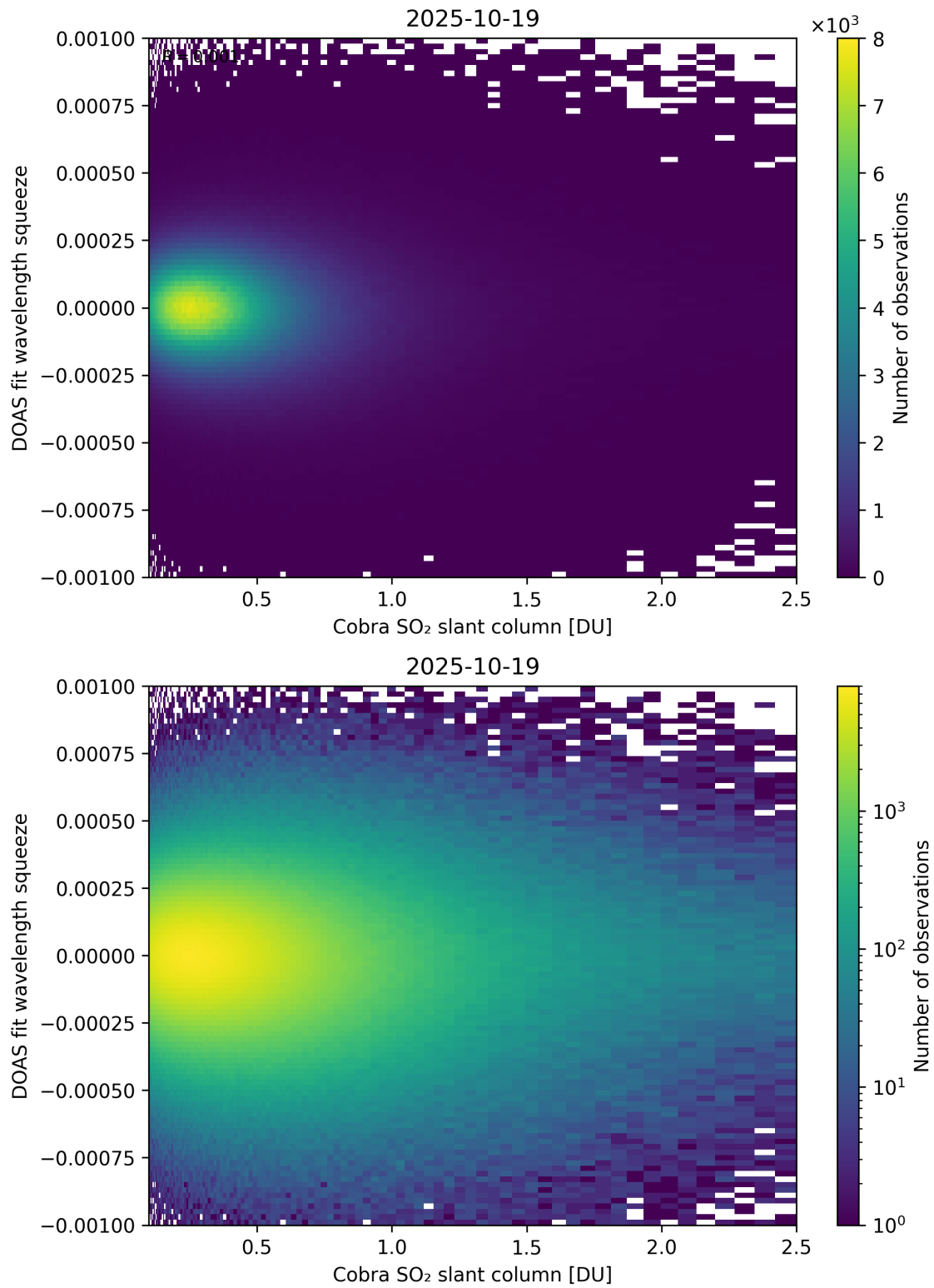
Figure 197: Scatter density plot of “Cobra SO 2 slant column” against “DOAS fit wavelength squeeze” for 2025-10-18 to 2025-10-20.
