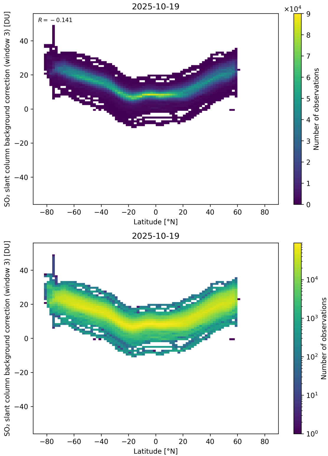
Figure 152: Scatter density plot of “Latitude” against “SO 2 slant column background correction (window 3)” for 2025-10-18 to 2025-10-20.
