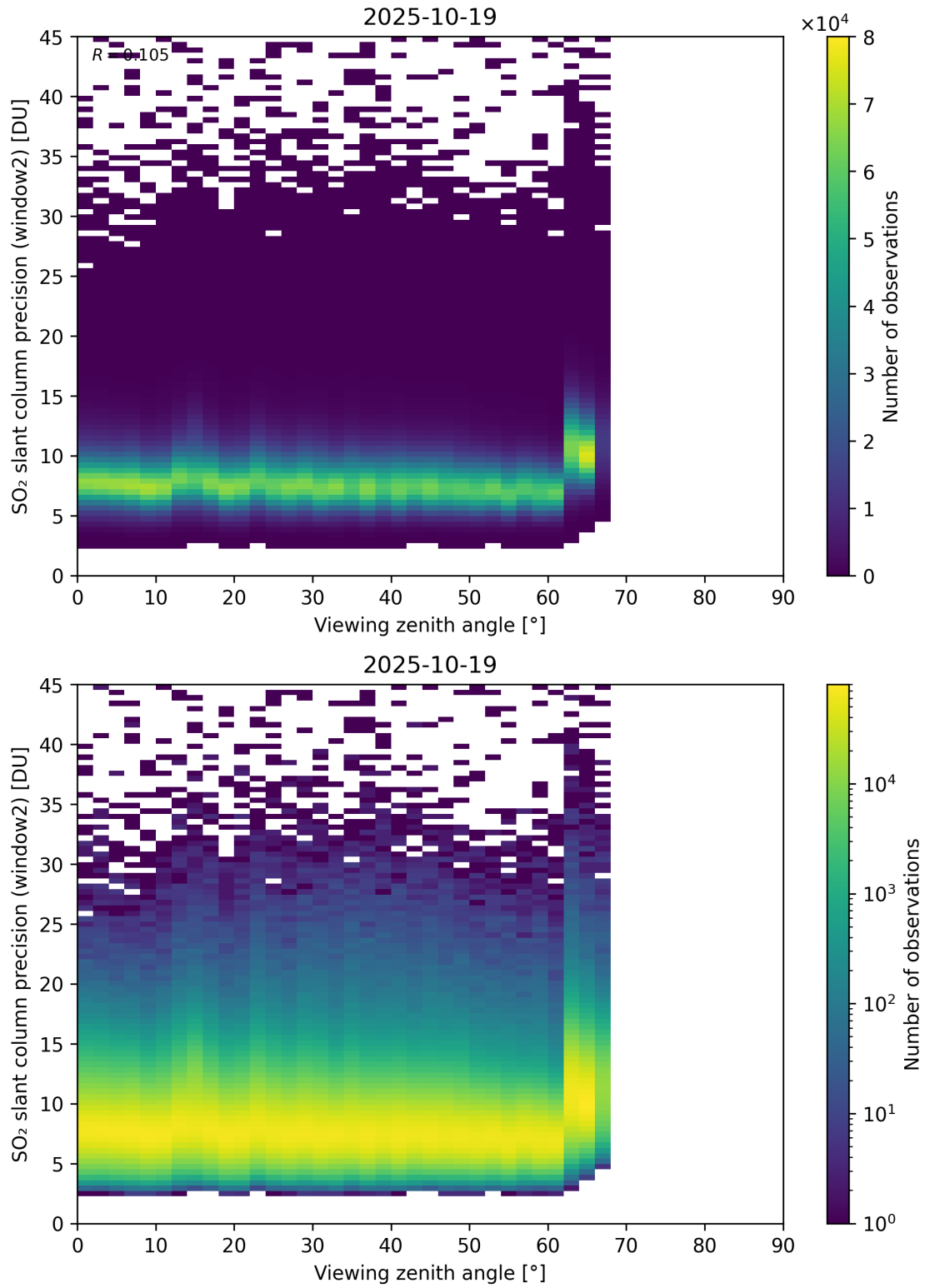
Figure 378: Scatter density plot of “Viewing zenith angle” against “SO 2 slant column precision (window2)” for 2025-10-18 to 2025-10-20.
