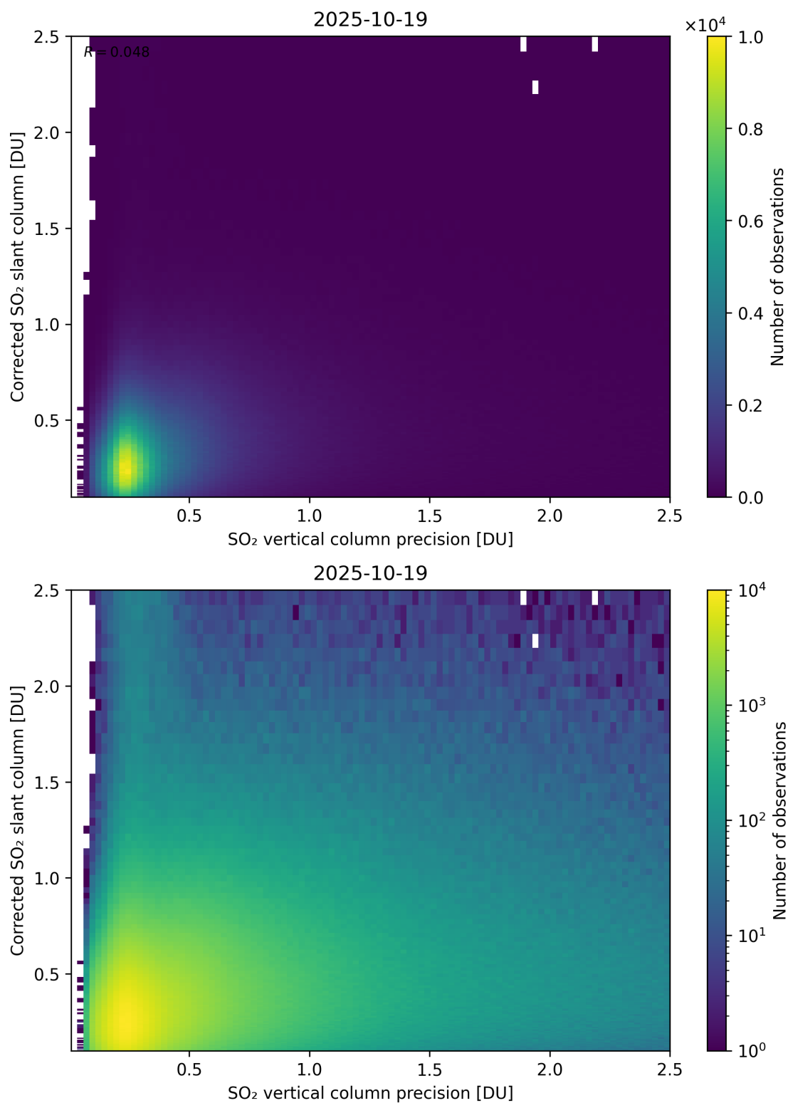
Figure 338: Scatter density plot of “SO 2 vertical column precision” against “Corrected SO 2 slant column” for 2025-10-18 to 2025-10-20.
