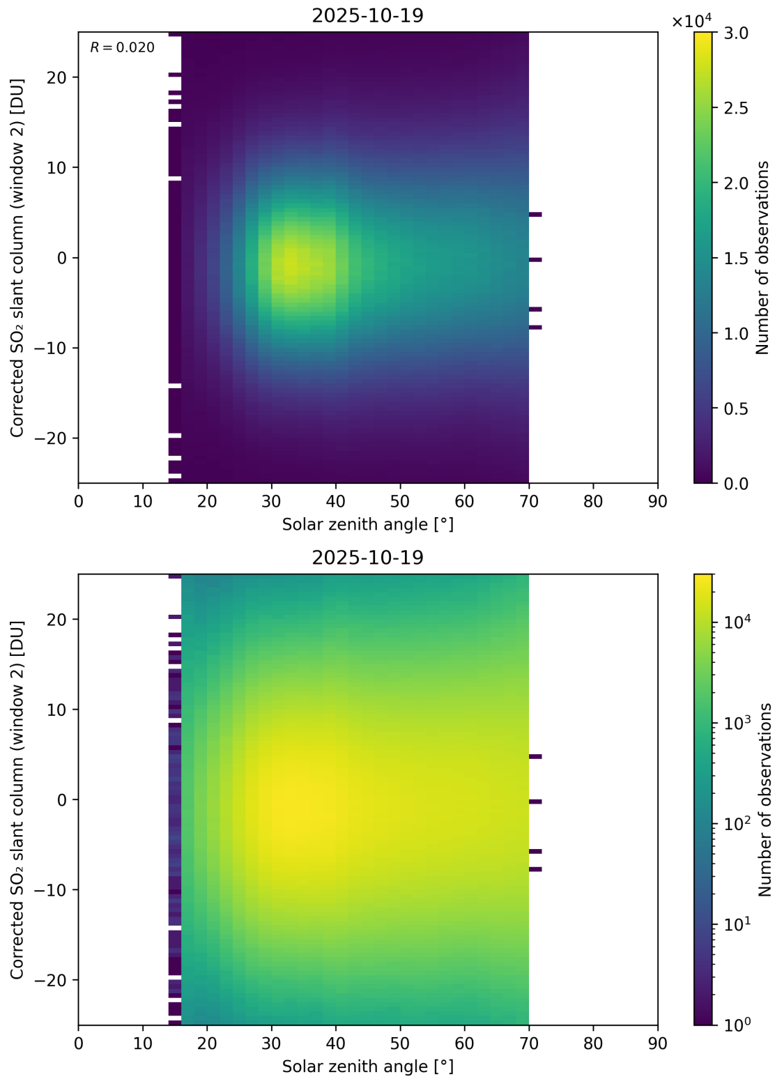
Figure 182: Scatter density plot of “Solar zenith angle” against “Corrected SO 2 slant column (window 2)” for 2025-10-18 to 2025-10-20.
