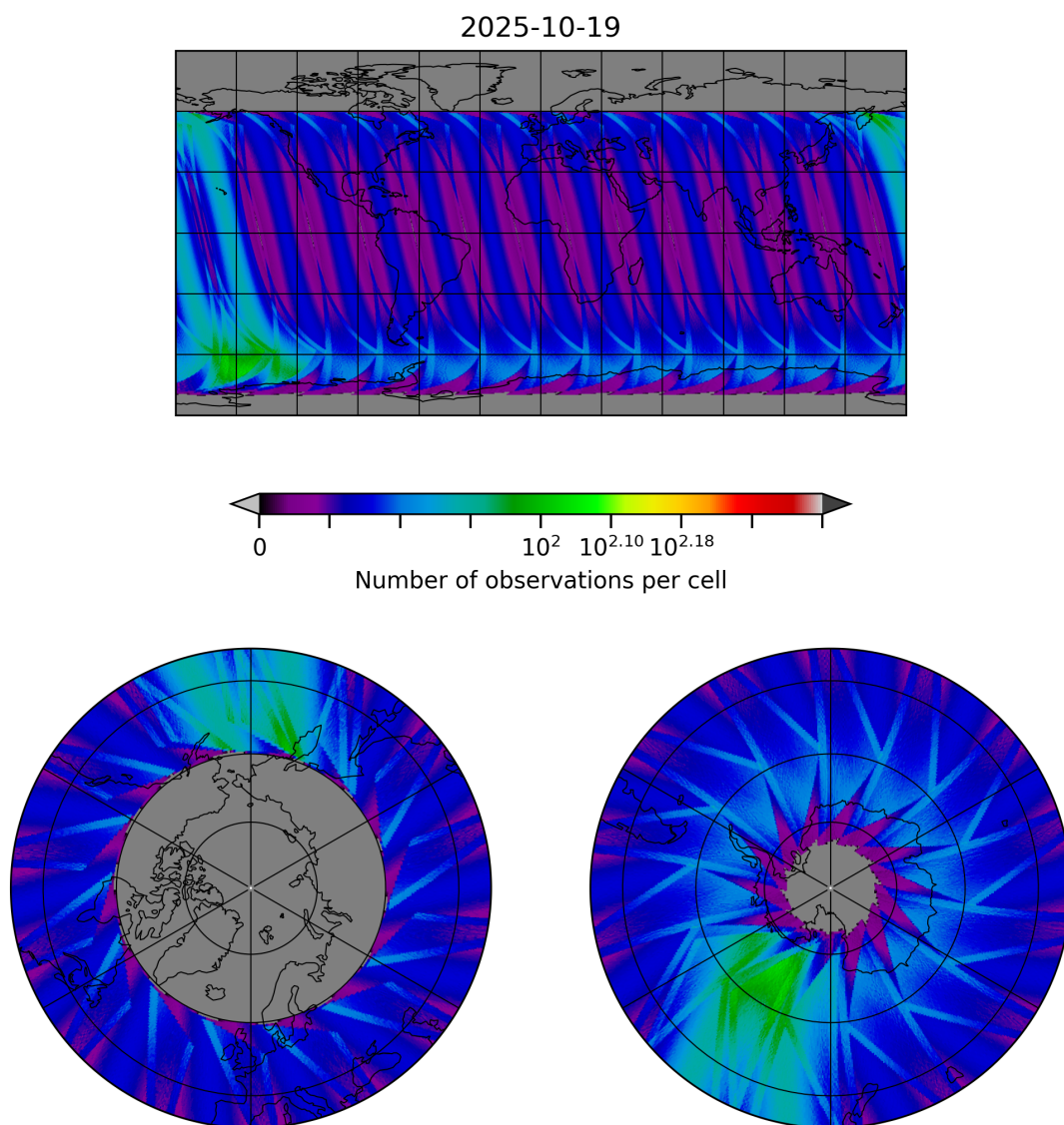
Figure 30: Map of the number of observations for 2025-10-18 to 2025-10-20
