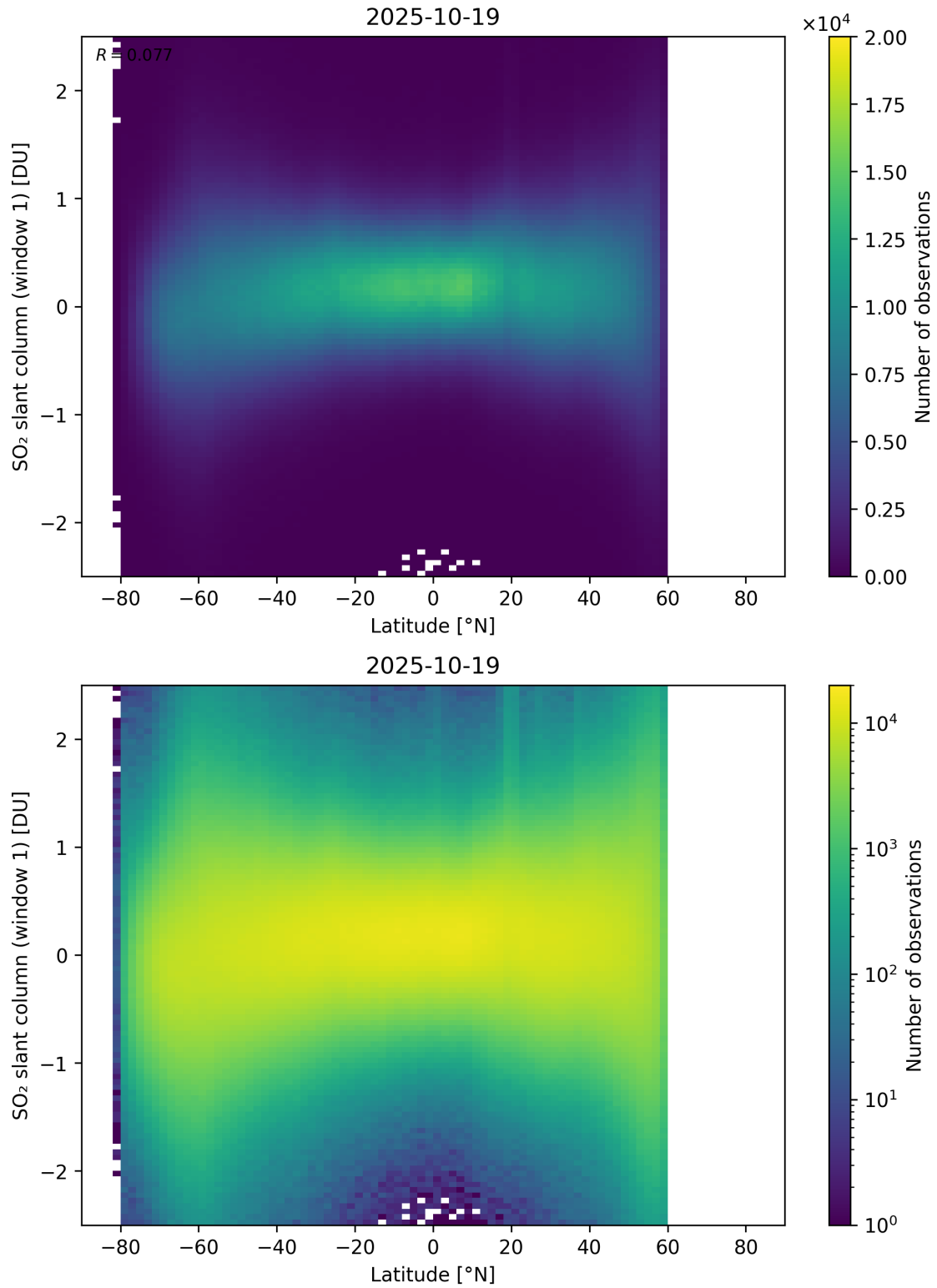
Figure 162: Scatter density plot of “Latitude” against “SO 2 slant column (window 1)” for 2025-10-18 to 2025-10-20.
