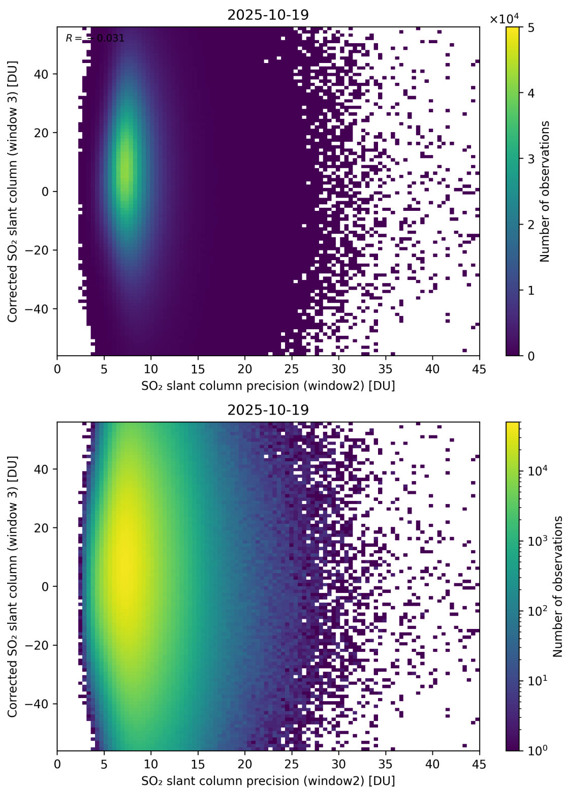
Figure 298: Scatter density plot of “SO 2 slant column precision (window2)” against “Corrected SO 2 slant column (window 3)” for 2025-10-18 to 2025-10-20.
