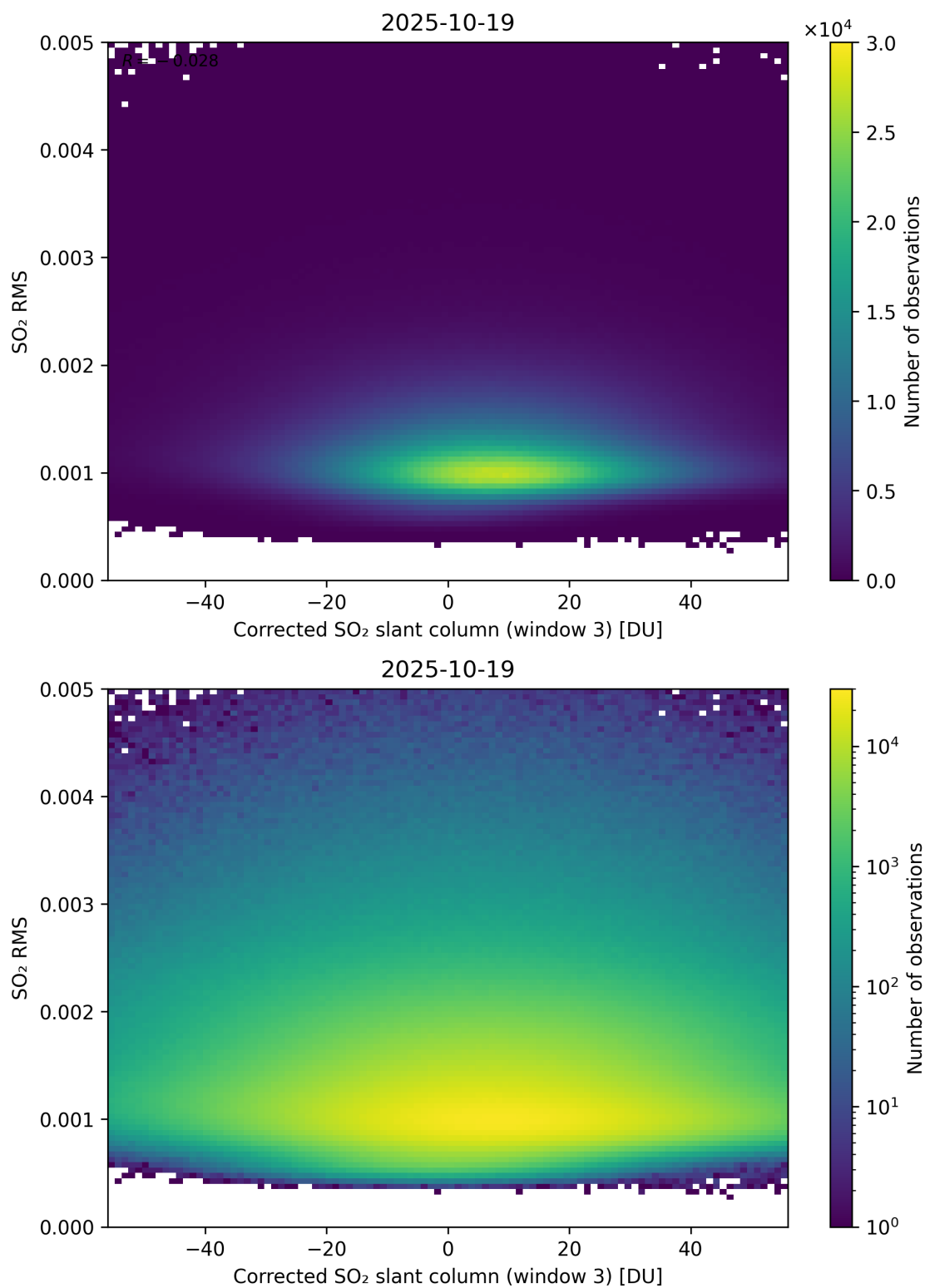
Figure 258: Scatter density plot of “Corrected SO 2 slant column (window 3)” against “SO 2 RMS” for 2025-10-18 to 2025-10-20.
