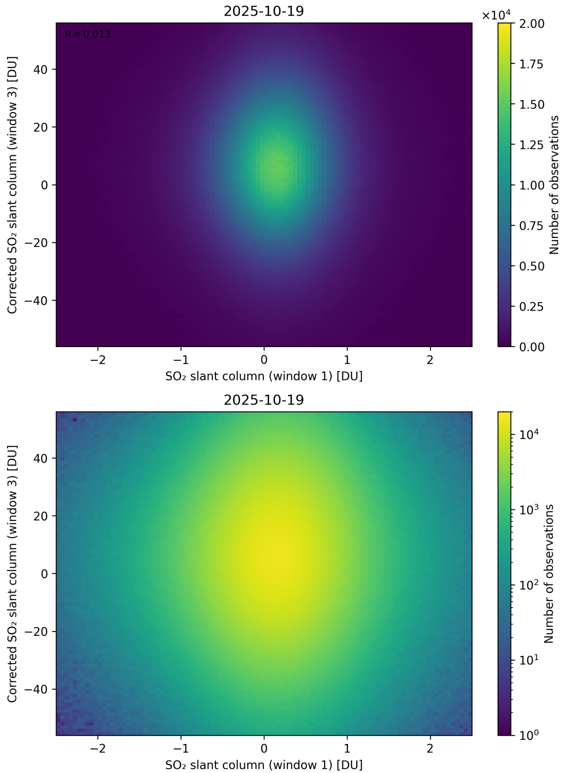
Figure 284: Scatter density plot of “SO 2 slant column (window 1)” against “Corrected SO 2 slant column (window 3)” for 2025-10-18 to 2025-10-20.
