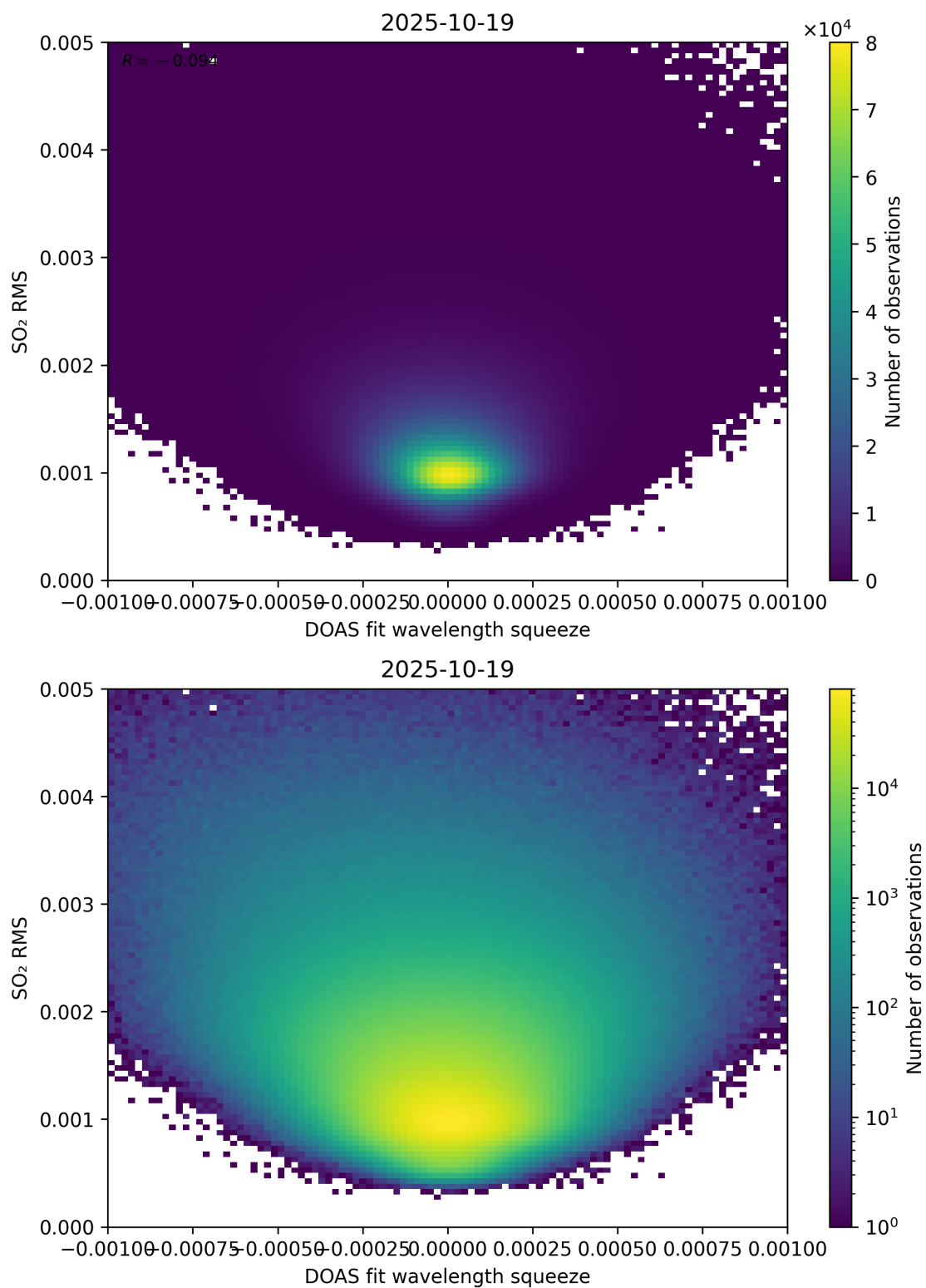
Figure 143: Scatter density plot of “DOAS fit wavelength squeeze” against “SO 2 RMS” for 2025-10-18 to 2025-10-20.
