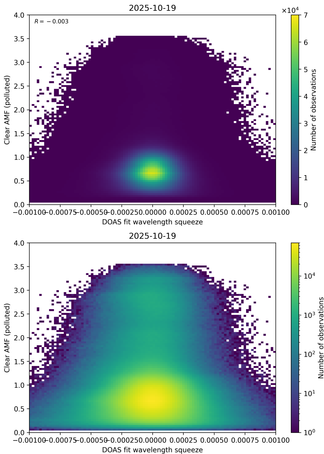
Figure 144: Scatter density plot of “DOAS fit wavelength squeeze” against “Clear AMF (polluted)” for 2025-10-18 to 2025-10-20.
