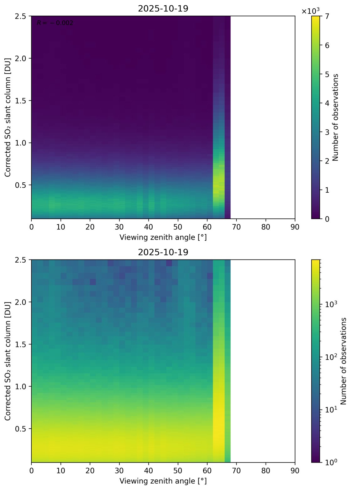
Figure 373: Scatter density plot of “Viewing zenith angle” against “Corrected SO 2 slant column” for 2025-10-18 to 2025-10-20.
