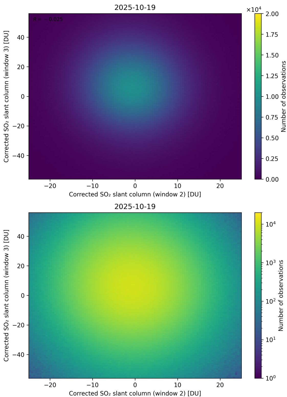
Figure 250: Scatter density plot of “Corrected SO 2 slant column (window 2)” against “Corrected SO 2 slant column (window 3)” for 2025-10-18 to 2025-10-20.
