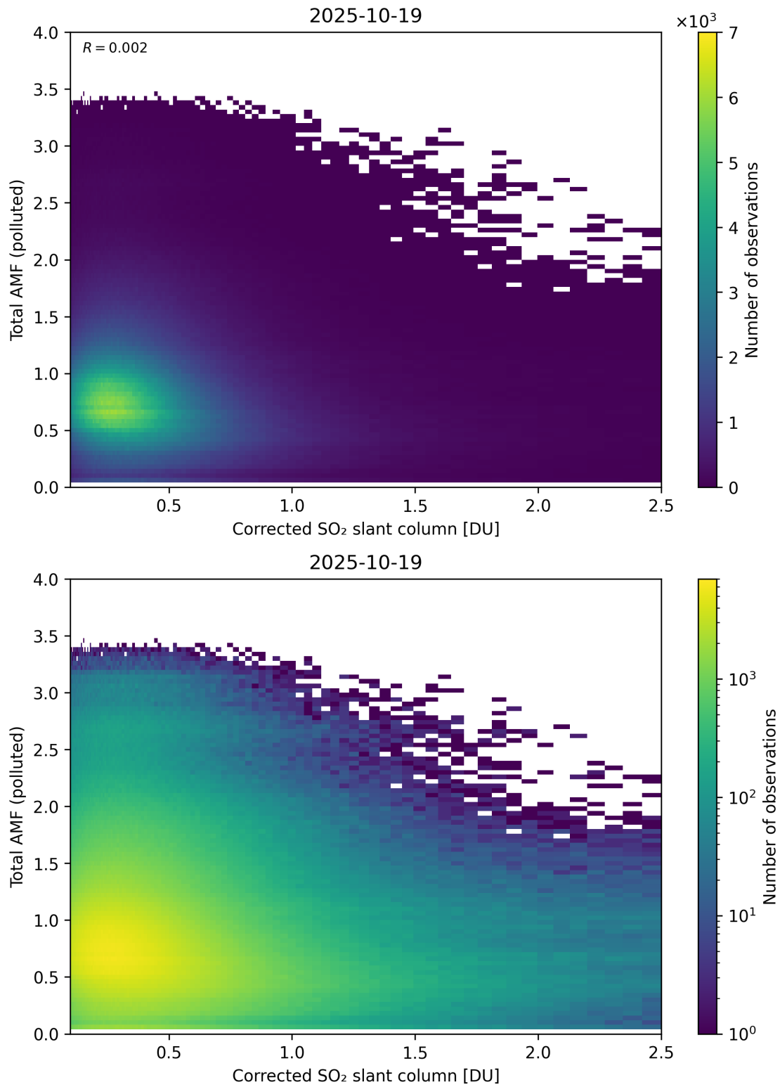
Figure 242: Scatter density plot of “Corrected SO 2 slant column” against “Total AMF (polluted)” for 2025-10-18 to 2025-10-20.
