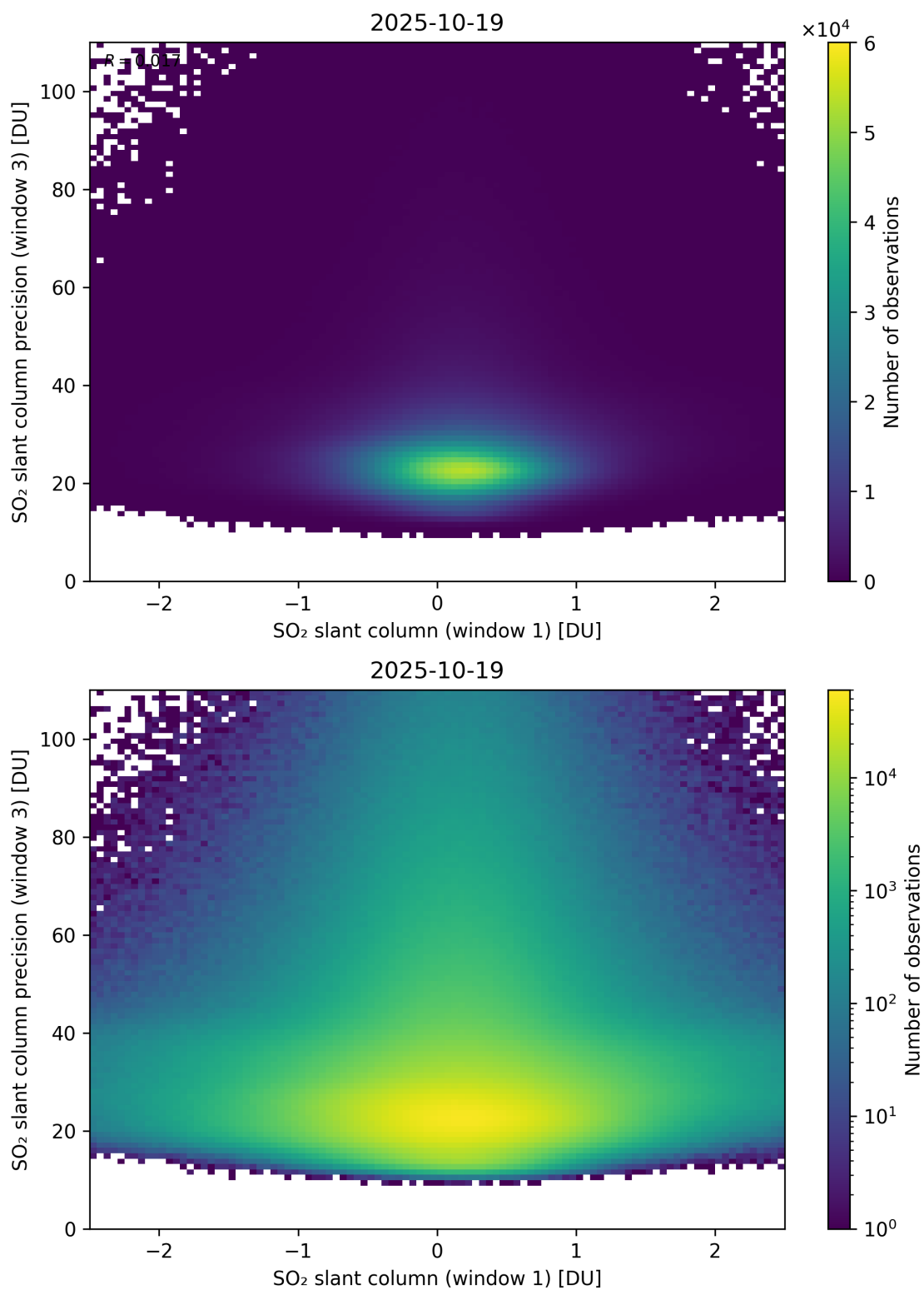
Figure 288: Scatter density plot of “SO 2 slant column (window 1)” against “SO 2 slant column precision (window 3)” for 2025-10-18 to 2025-10-20.
