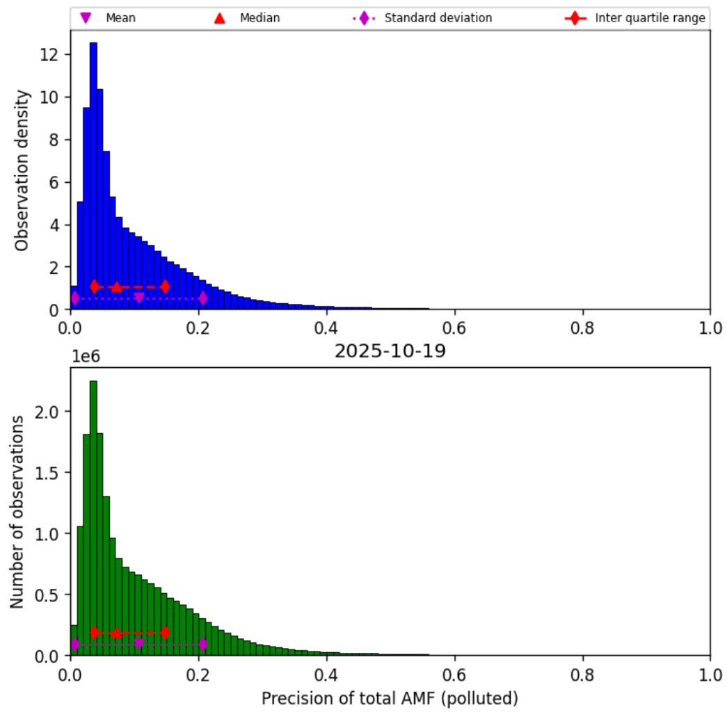
Figure 80: Histogram of “Precision of total AMF (polluted)” for 2025-10-18 to 2025-10-20
