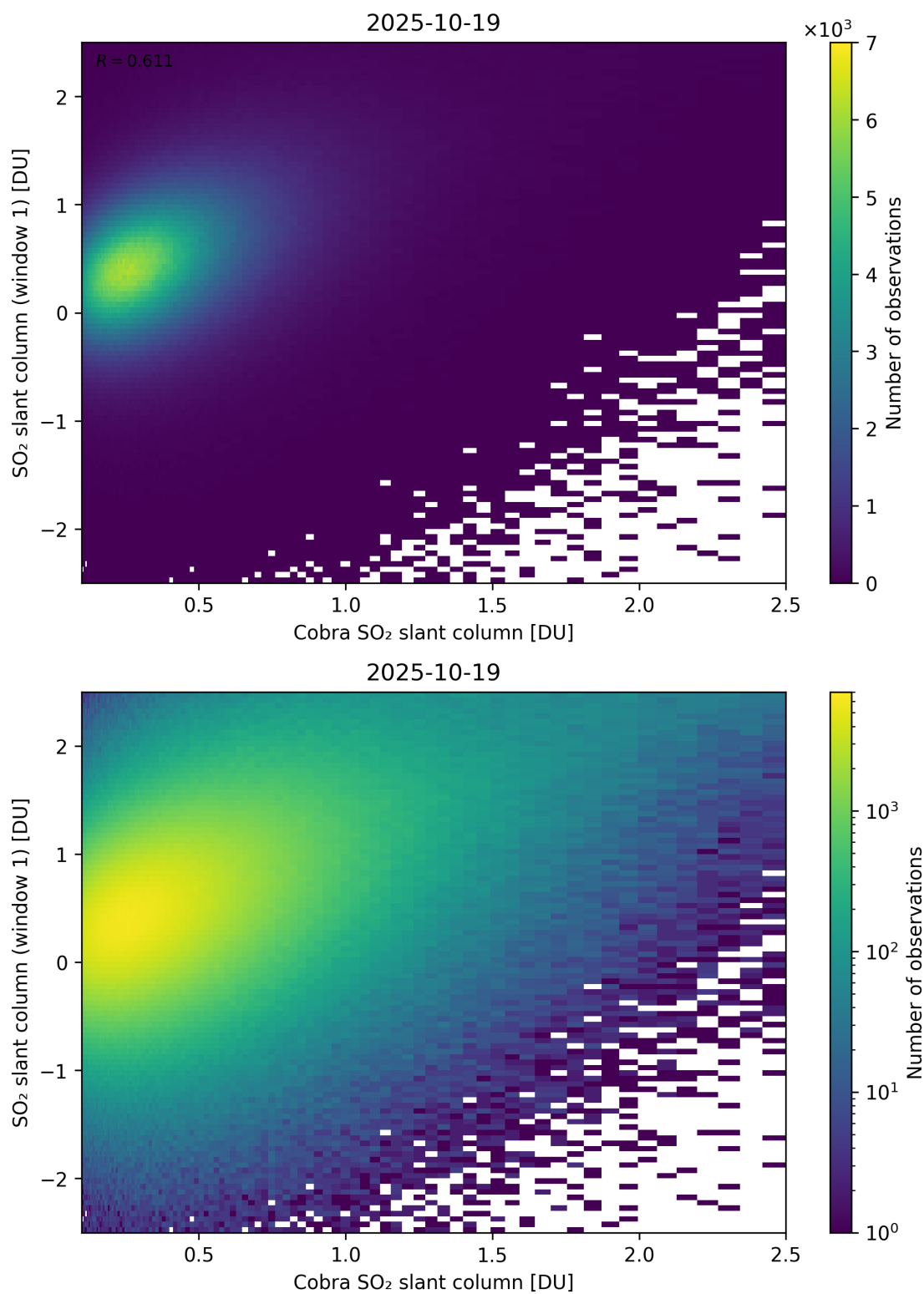
Figure 219: Scatter density plot of “Cobra SO 2 slant column” against “SO 2 slant column (window 1)” for 2025-10-18 to 2025-10-20.
