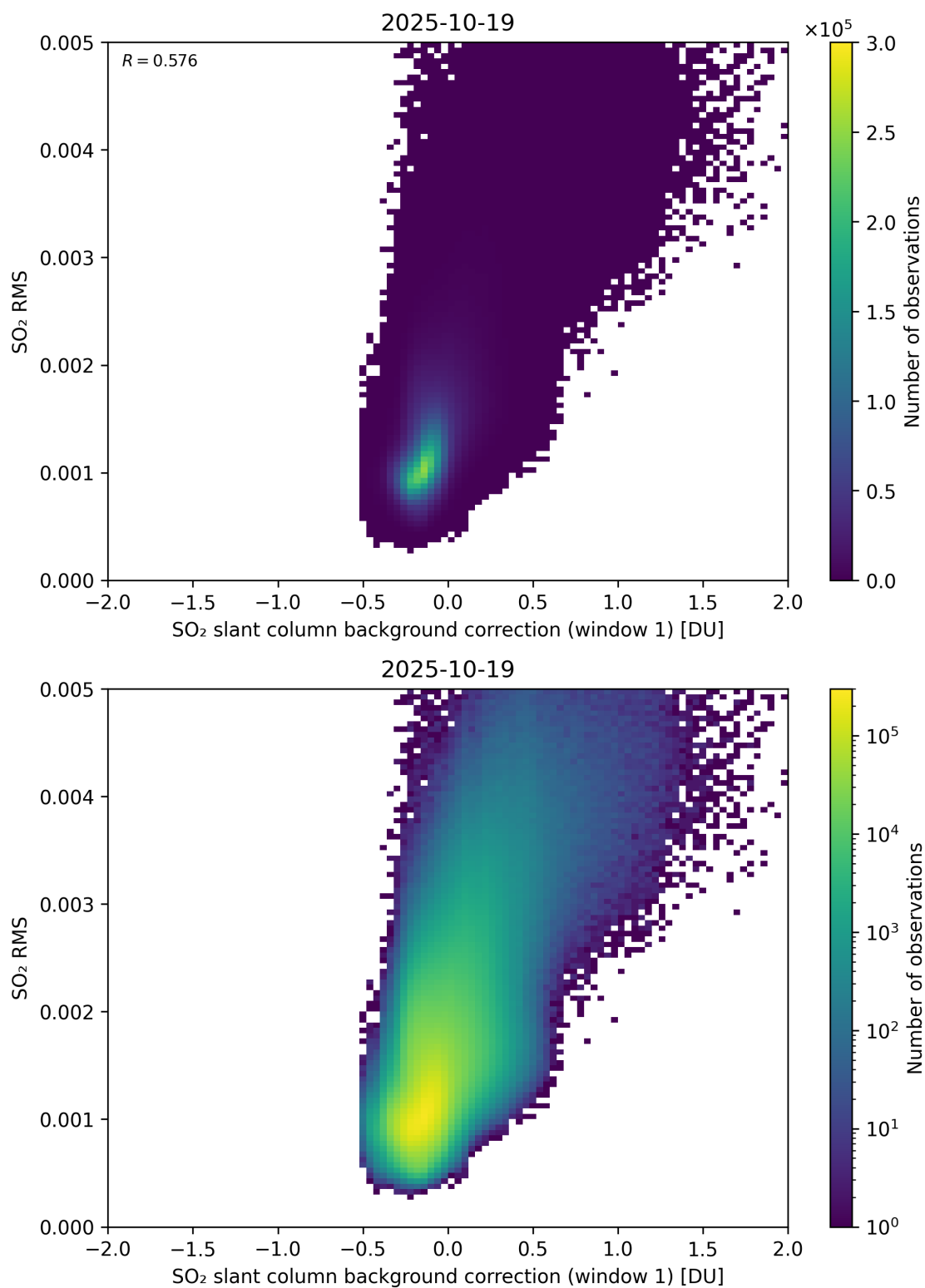
Figure 113: Scatter density plot of “SO 2 slant column background correction (window 1)” against “SO 2 RMS” for 2025-10-18 to 2025-10-20.
