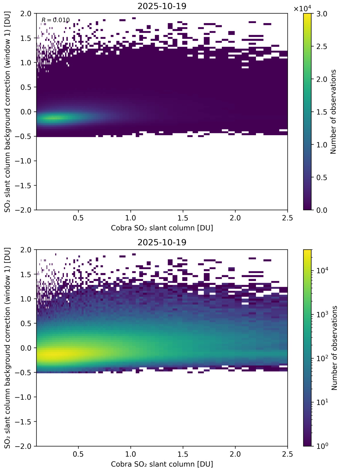
Figure 193: Scatter density plot of “Cobra SO 2 slant column” against “SO 2 slant column background correction (window 1)” for 2025-10-18 to 2025-10-20.
