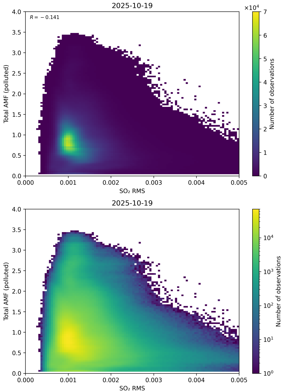
Figure 148: Scatter density plot of “SO 2 RMS” against “Total AMF (polluted)” for 2025-10-18 to 2025-10-20.
