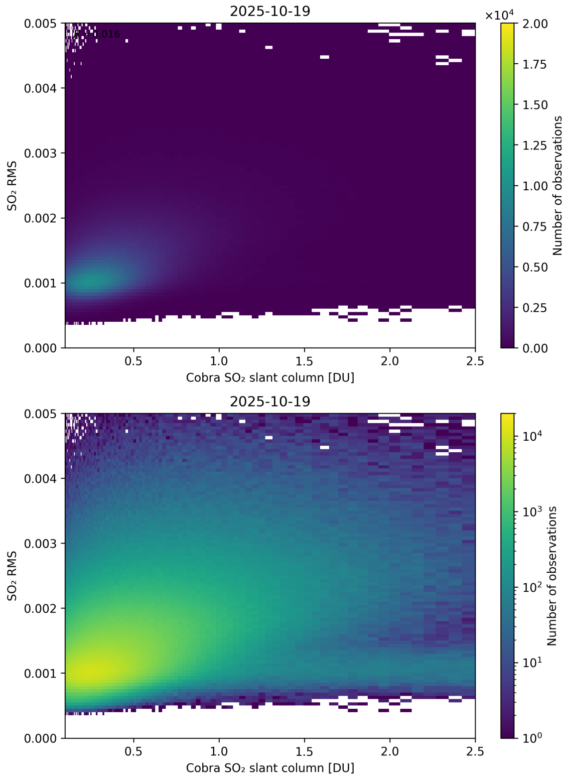
Figure 198: Scatter density plot of “Cobra SO 2 slant column” against “SO 2 RMS” for 2025-10-18 to 2025-10-20.
