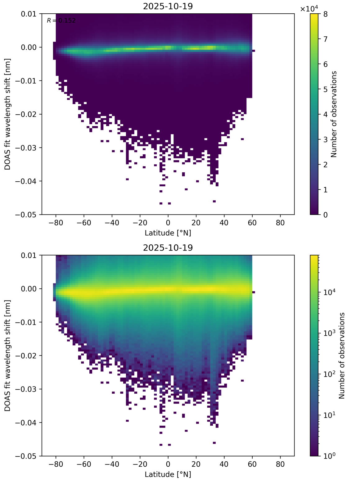
Figure 153: Scatter density plot of “Latitude” against “DOAS fit wavelength shift” for 2025-10-18 to 2025-10-20.
