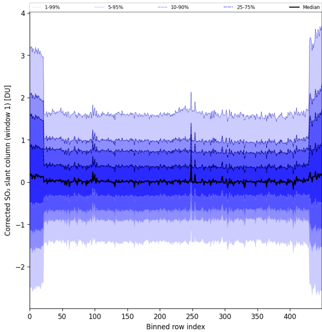
Figure 91: Along track statistics of “Corrected SO 2 slant column (window 1)” for 2025-10-18 to 2025-10-20
