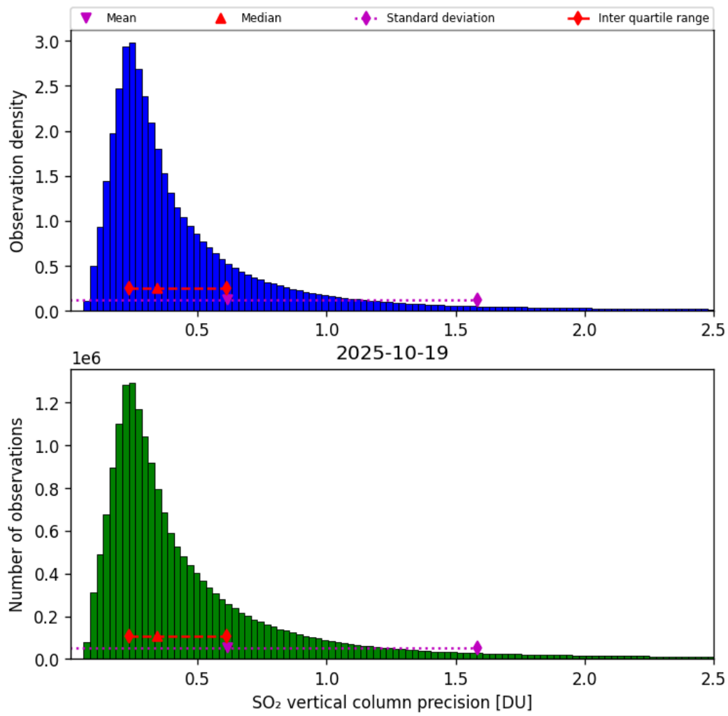
Figure 59: Histogram of “SO 2 vertical column precision” for 2025-10-18 to 2025-10-20
