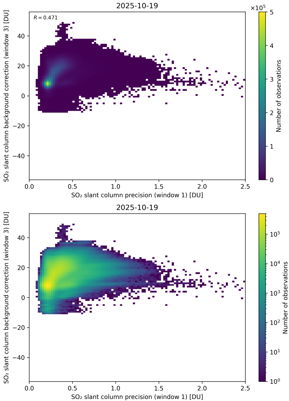
Figure 270: Scatter density plot of “SO 2 slant column precision (window 1)” against “SO 2 slant column background correction (window 3)” for 2025-10-18 to 2025-10-20.
