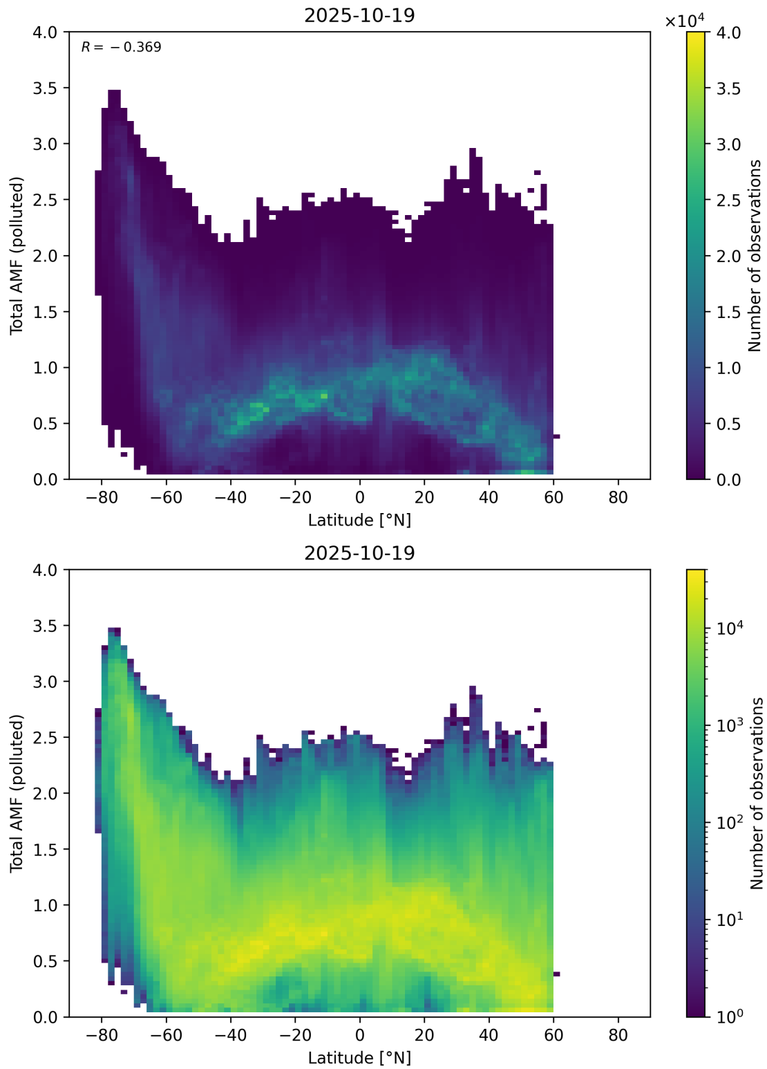
Figure 167: Scatter density plot of “Latitude” against “Total AMF (polluted)” for 2025-10-18 to 2025-10-20.
