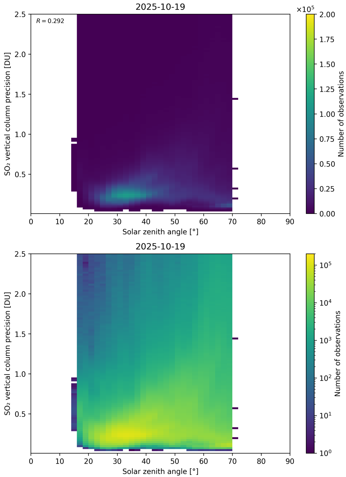
Figure 192: Scatter density plot of “Solar zenith angle” against “SO 2 vertical column precision” for 2025-10-18 to 2025-10-20.
