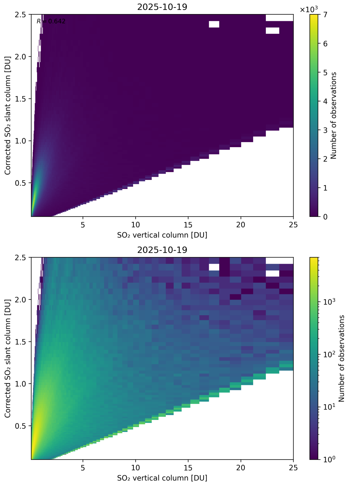
Figure 351: Scatter density plot of “SO 2 vertical column” against “Corrected SO 2 slant column” for 2025-10-18 to 2025-10-20.
