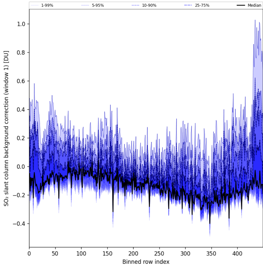
Figure 92: Along track statistics of “SO 2 slant column background correction (window 1)” for 2025-10-18 to 2025-10-20
