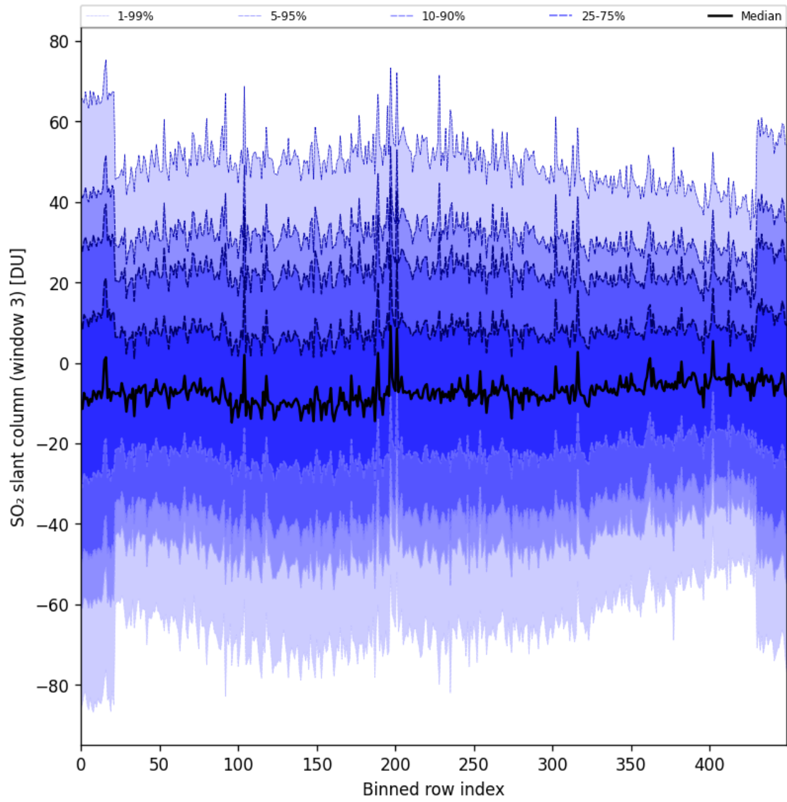
Figure 97: Along track statistics of “SO 2 slant column (window 3)” for 2025-10-18 to 2025-10-20
