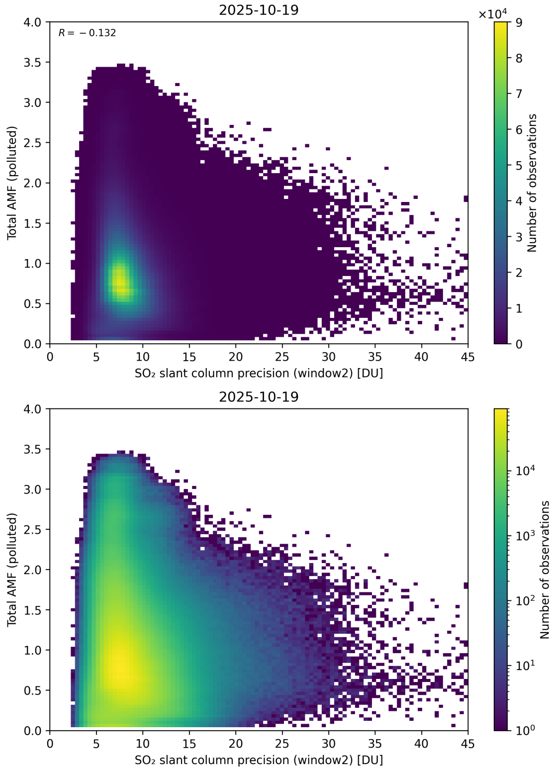
Figure 301: Scatter density plot of “SO 2 slant column precision (window2)” against “Total AMF (polluted)” for 2025-10-18 to 2025-10-20.
