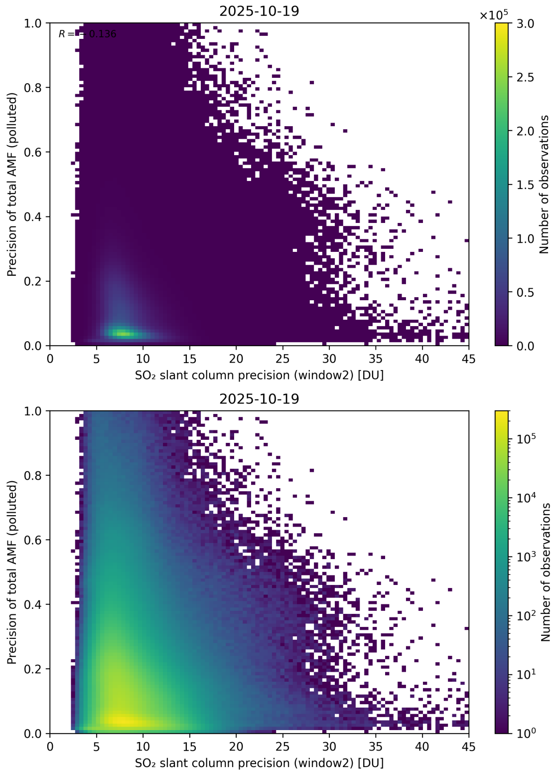
Figure 302: Scatter density plot of “SO 2 slant column precision (window2)” against “Precision of total AMF (polluted)” for 2025-10-18 to 2025-10-20.
