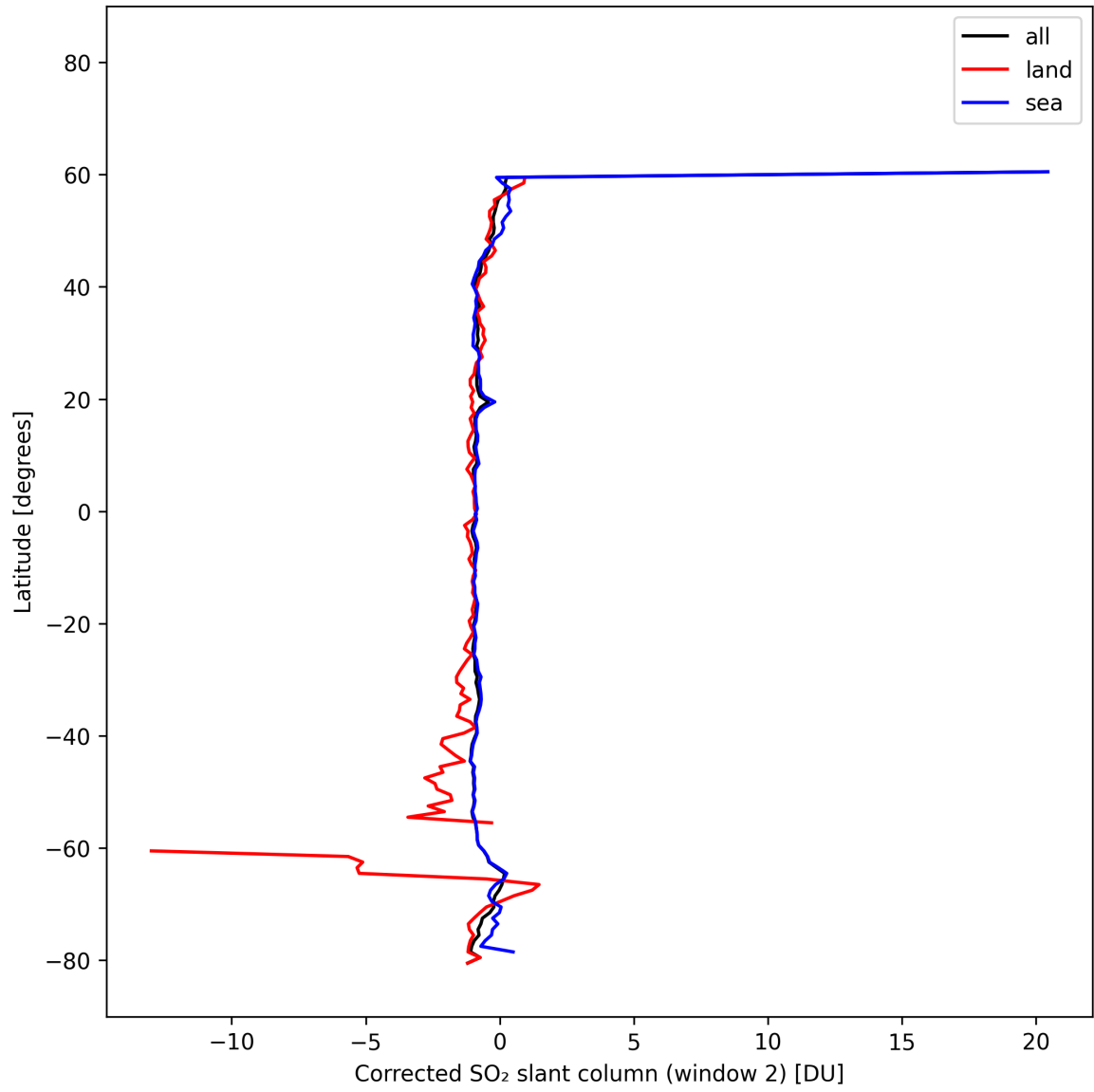
Figure 43: Zonal average of “Corrected SO 2 slant column (window 2)” for 2025-10-18 to 2025-10-20.
