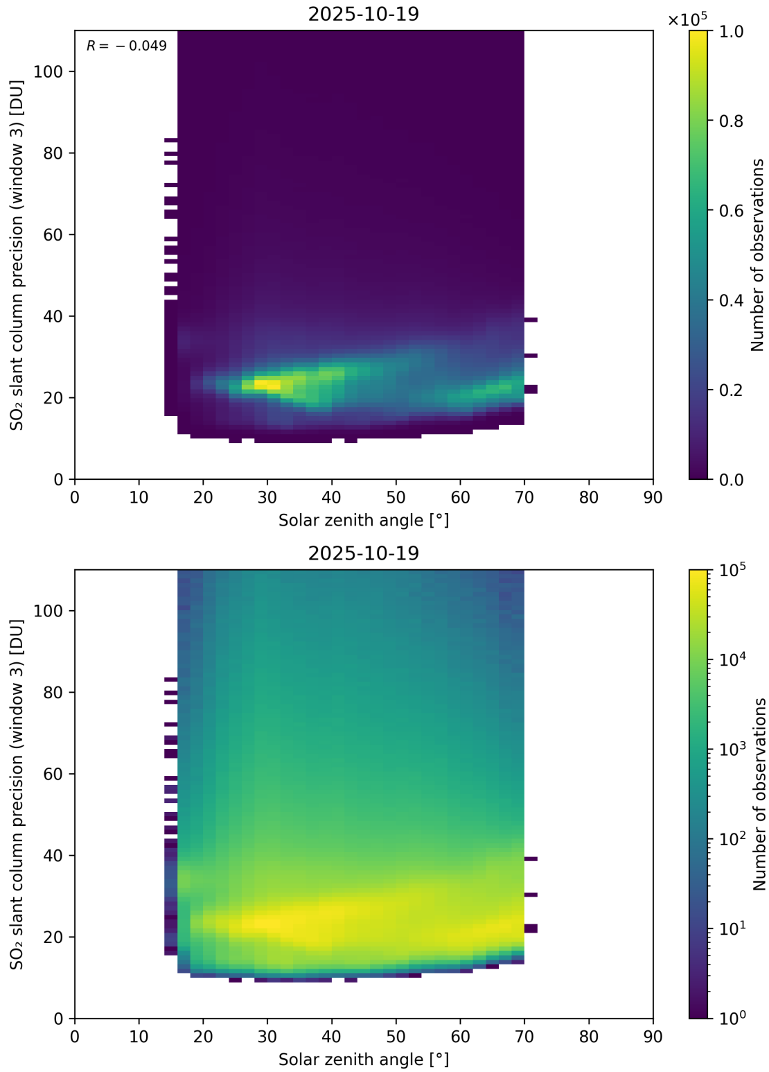
Figure 188: Scatter density plot of “Solar zenith angle” against “SO 2 slant column precision (window 3)” for 2025-10-18 to 2025-10-20.
