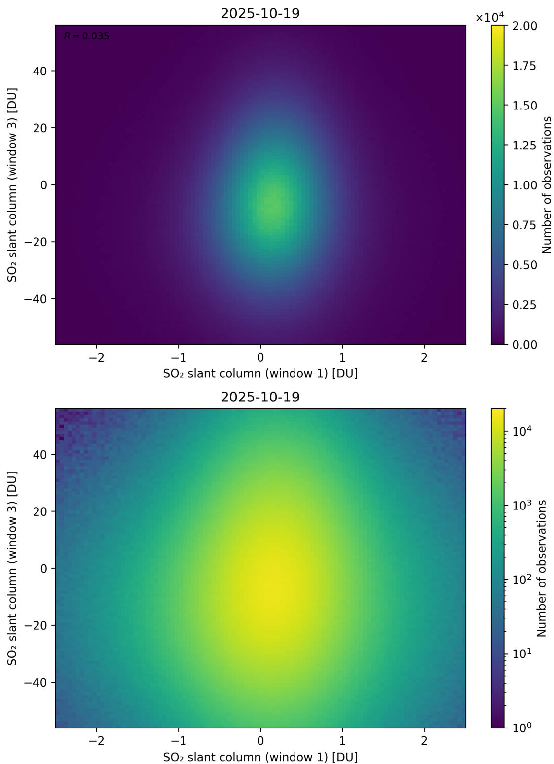
Figure 287: Scatter density plot of “SO 2 slant column (window 1)” against “SO 2 slant column (window 3)” for 2025-10-18 to 2025-10-20.
