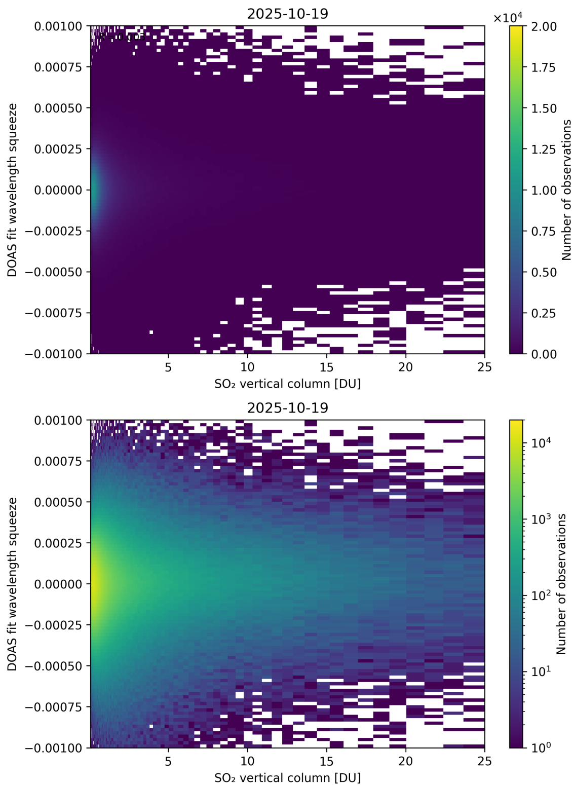
Figure 327: Scatter density plot of “SO 2 vertical column” against “DOAS fit wavelength squeeze” for 2025-10-18 to 2025-10-20.
