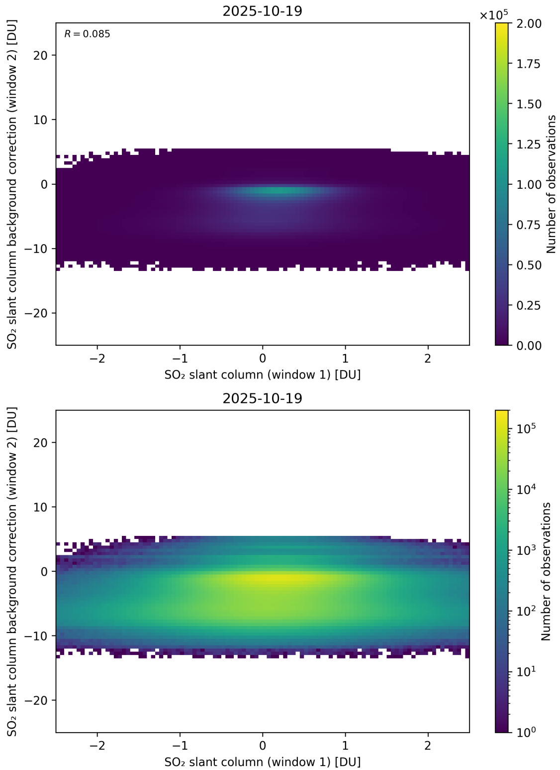
Figure 263: Scatter density plot of “SO 2 slant column (window 1)” against “SO 2 slant column background correction (window 2)” for 2025-10-18 to 2025-10-20.
