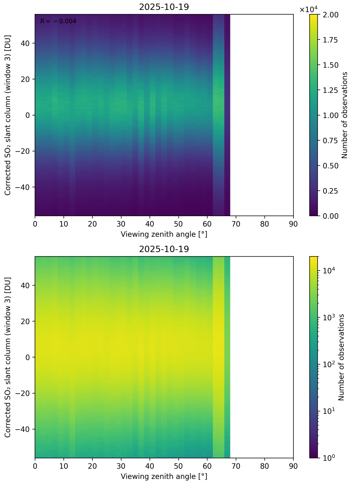
Figure 375: Scatter density plot of “Viewing zenith angle” against “Corrected SO 2 slant column (window 3)” for 2025-10-18 to 2025-10-20.
