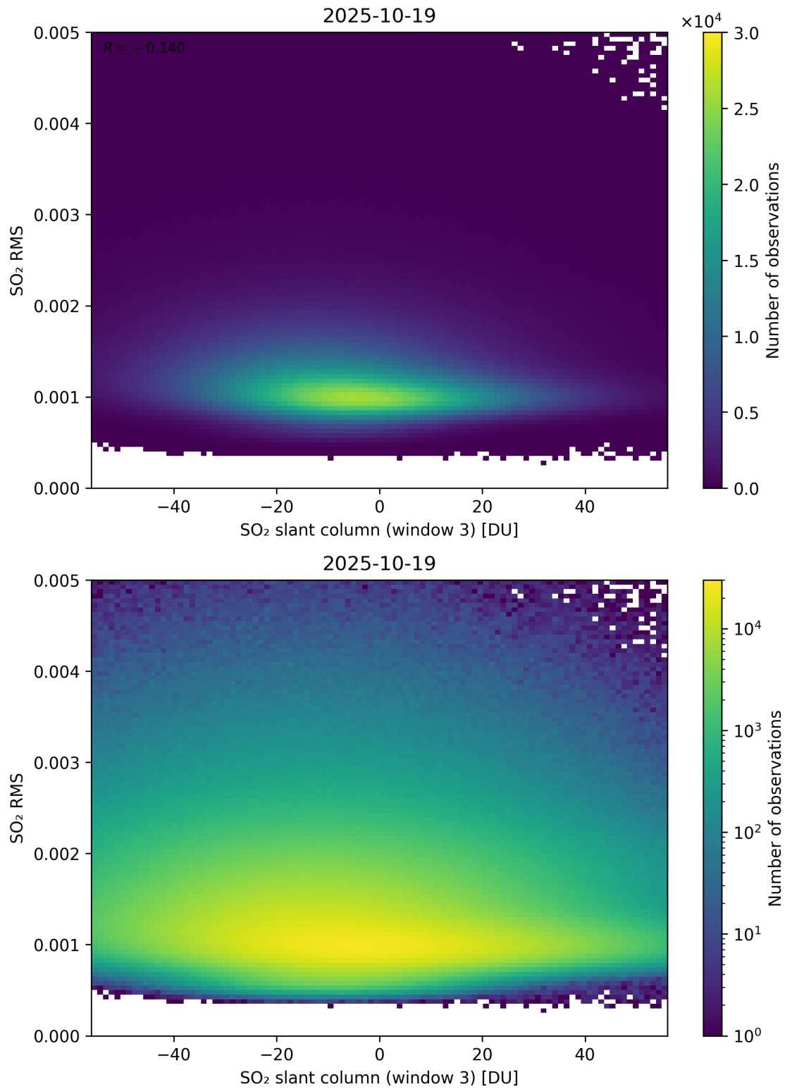
Figure 306: Scatter density plot of “SO 2 slant column (window 3)” against “SO 2 RMS” for 2025-10-18 to 2025-10-20.
