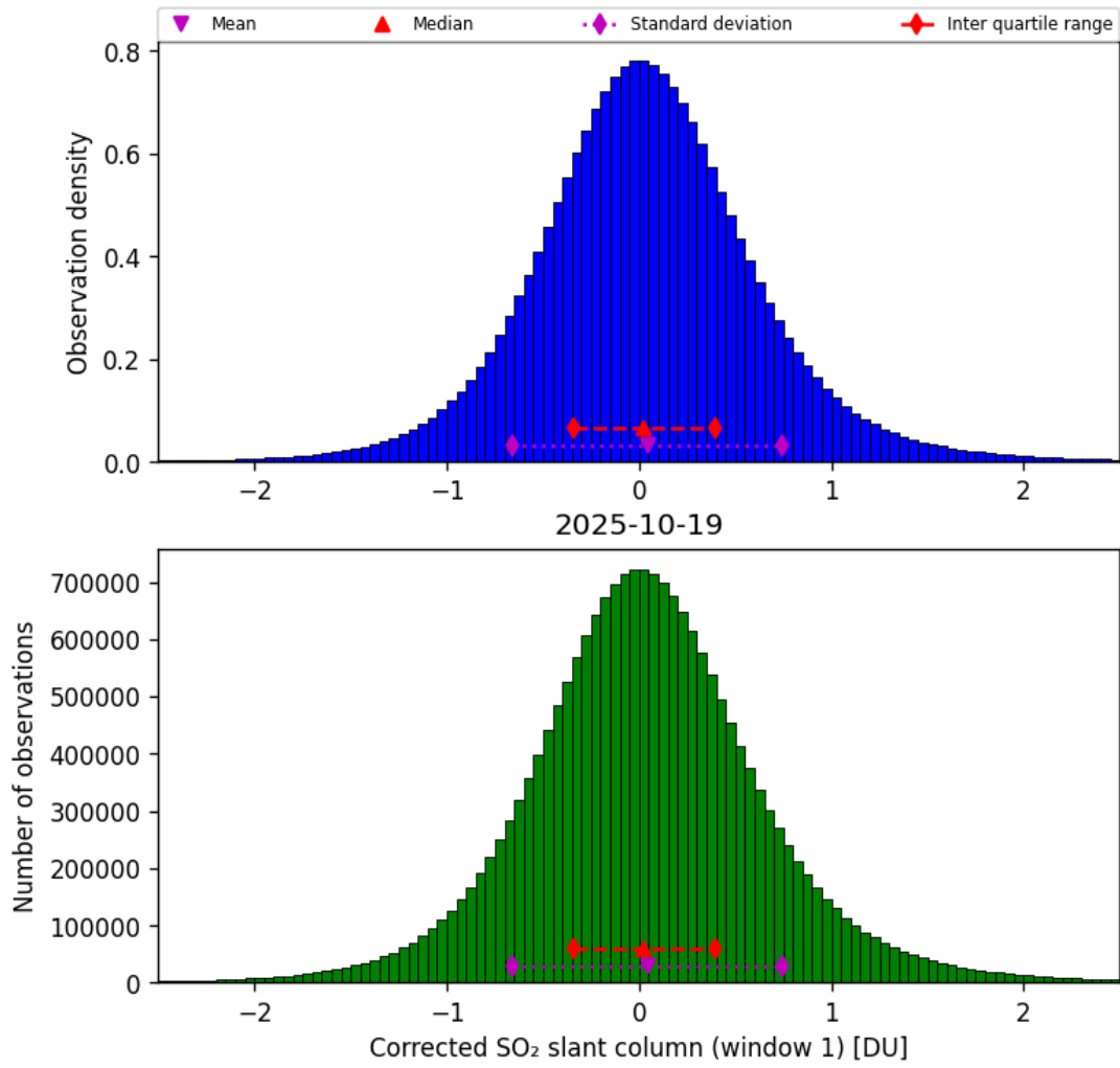
Figure 65: Histogram of “Corrected SO 2 slant column (window 1)” for 2025-10-18 to 2025-10-20
