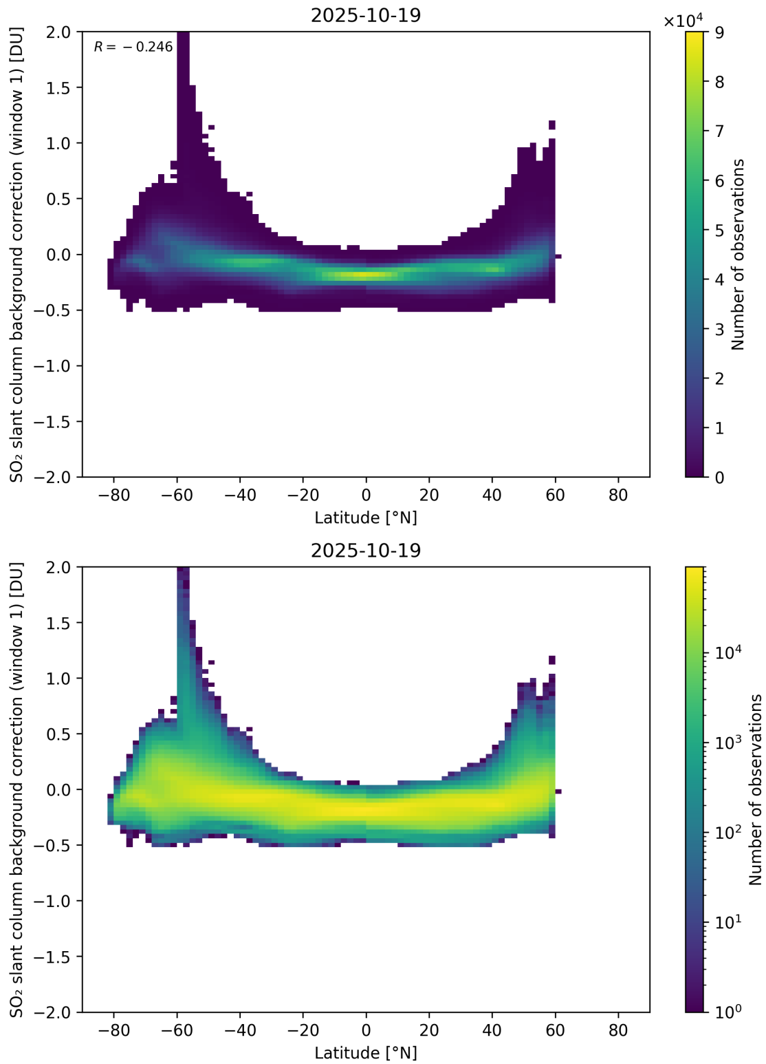
Figure 150: Scatter density plot of “Latitude” against “SO 2 slant column background correction (window 1)” for 2025-10-18 to 2025-10-20.
