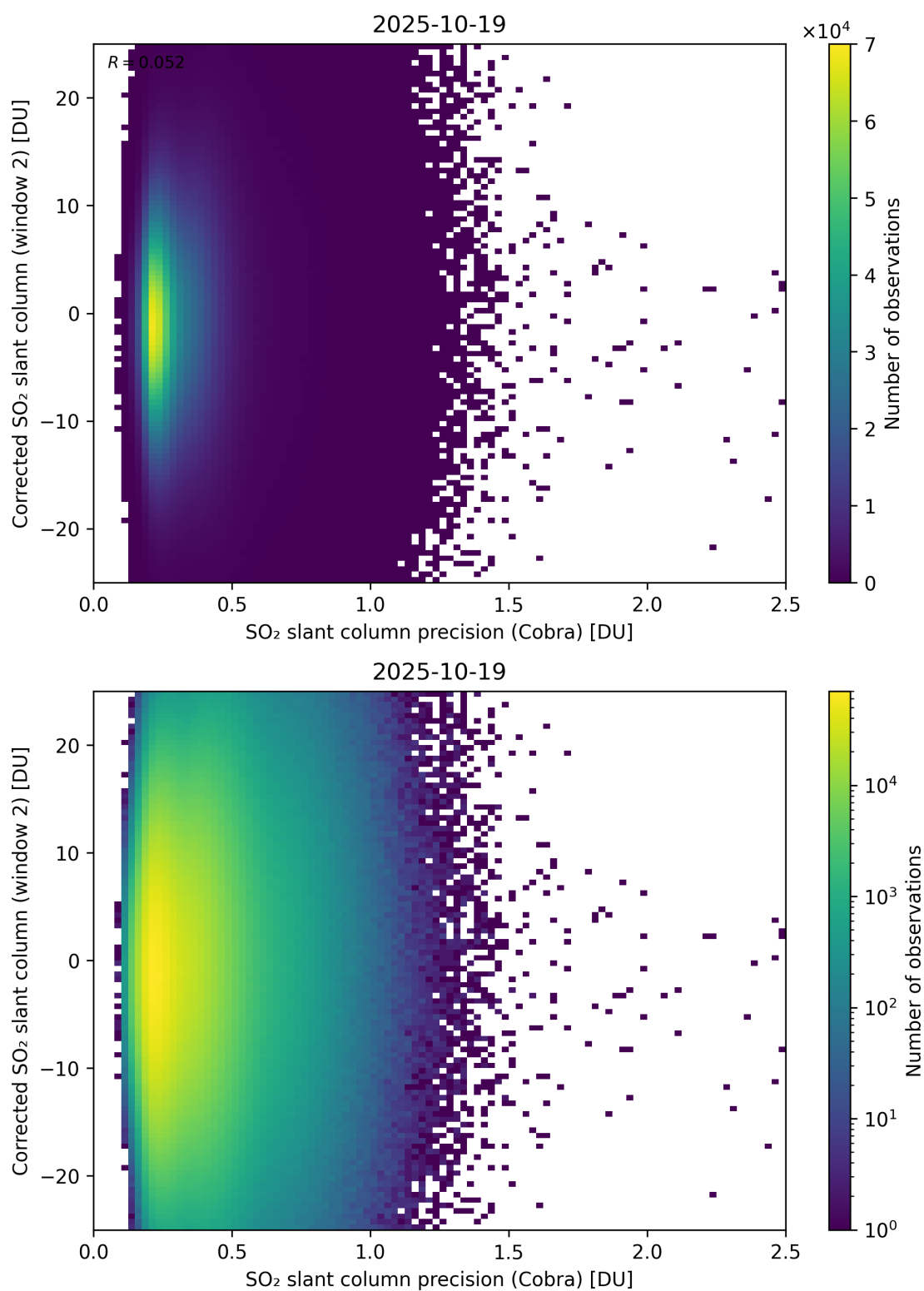
Figure 206: Scatter density plot of “SO 2 slant column precision (Cobra)” against “Corrected SO 2 slant column (window 2)” for 2025-10-18 to 2025-10-20.
