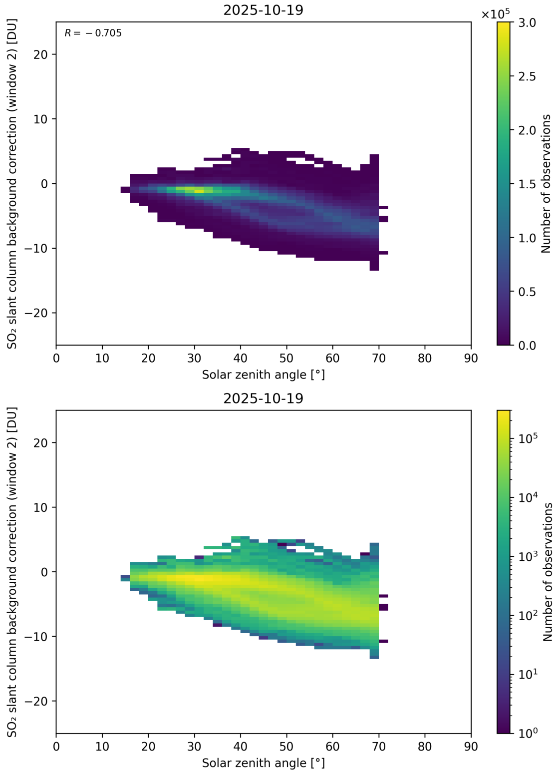
Figure 172: Scatter density plot of “Solar zenith angle” against “SO 2 slant column background correction (window 2)” for 2025-10-18 to 2025-10-20.
