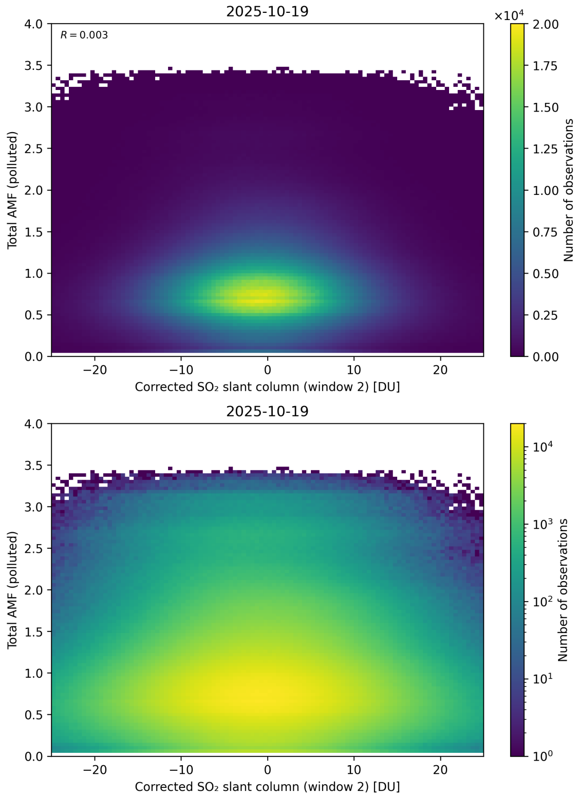
Figure 253: Scatter density plot of “Corrected SO 2 slant column (window 2)” against “Total AMF (polluted)” for 2025-10-18 to 2025-10-20.
