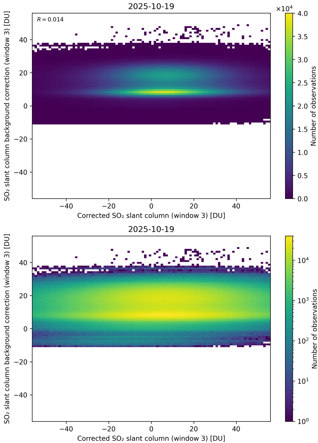
Figure 255: Scatter density plot of “Corrected SO 2 slant column (window 3)” against “SO 2 slant column background correction (window 3)” for 2025-10-18 to 2025-10-20.
