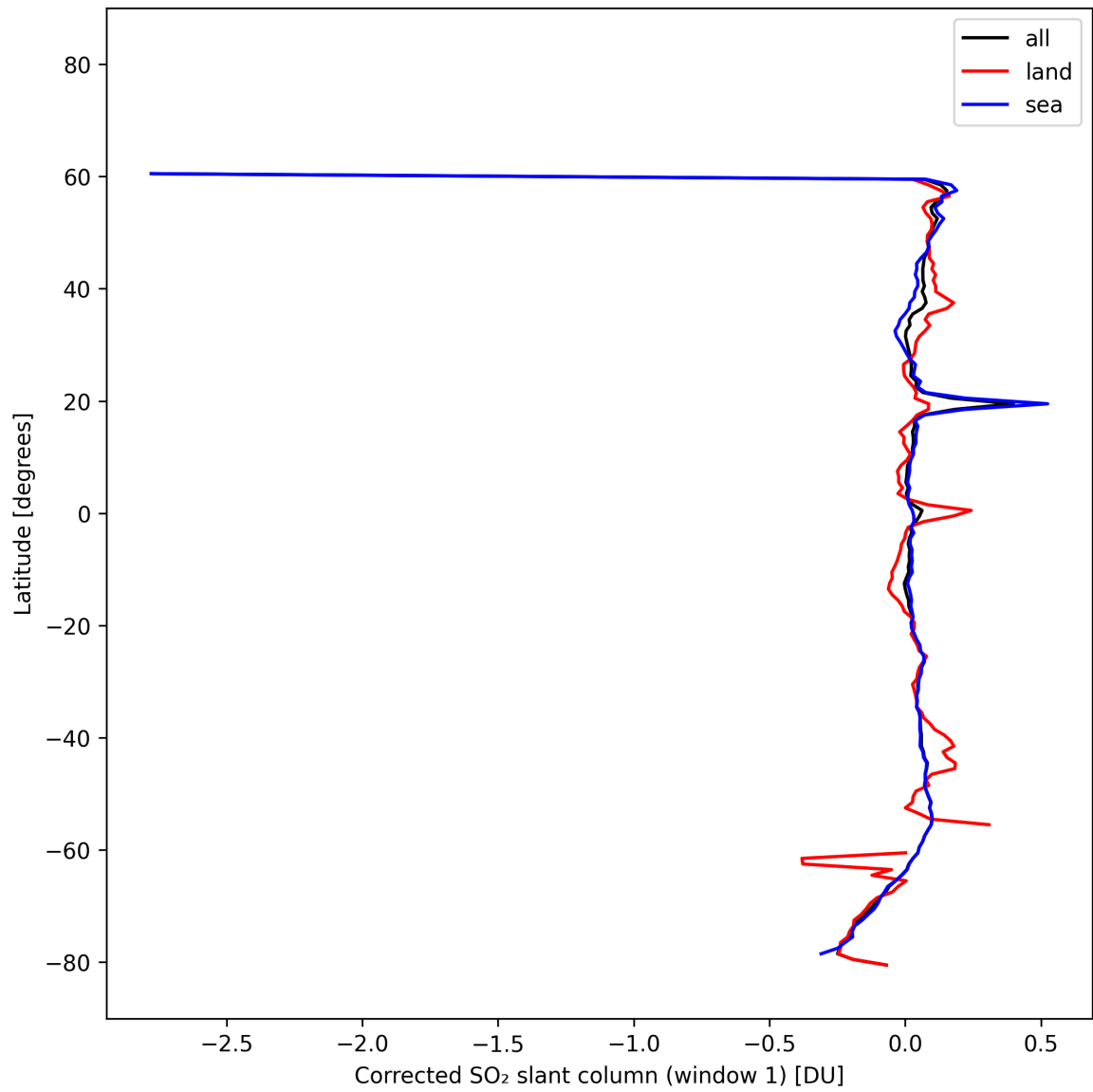
Figure 39: Zonal average of “Corrected SO 2 slant column (window 1)” for 2025-10-18 to 2025-10-20.
