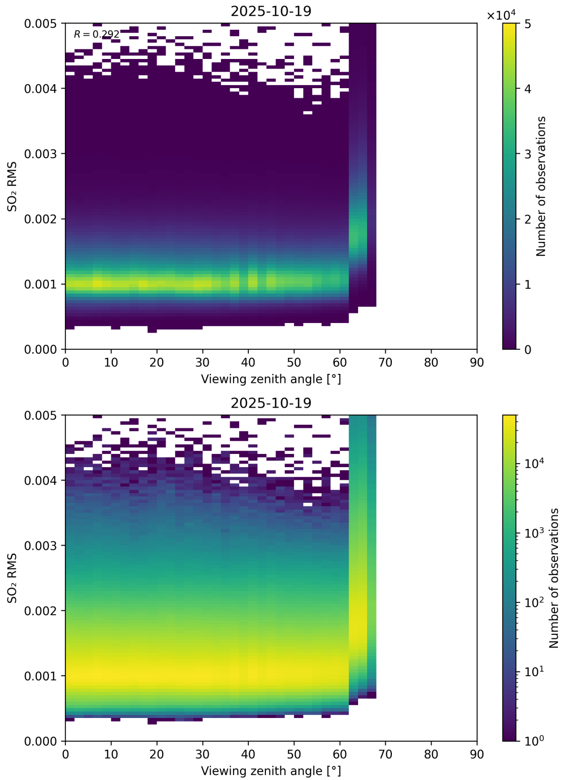
Figure 367: Scatter density plot of “Viewing zenith angle” against “SO 2 RMS” for 2025-10-18 to 2025-10-20.
