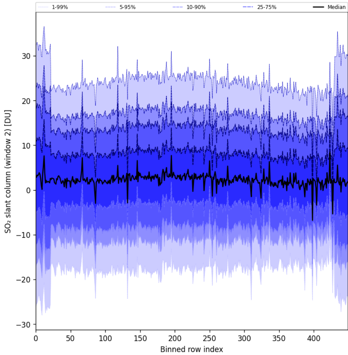
Figure 93: Along track statistics of “SO 2 slant column (window 2)” for 2025-10-18 to 2025-10-20
