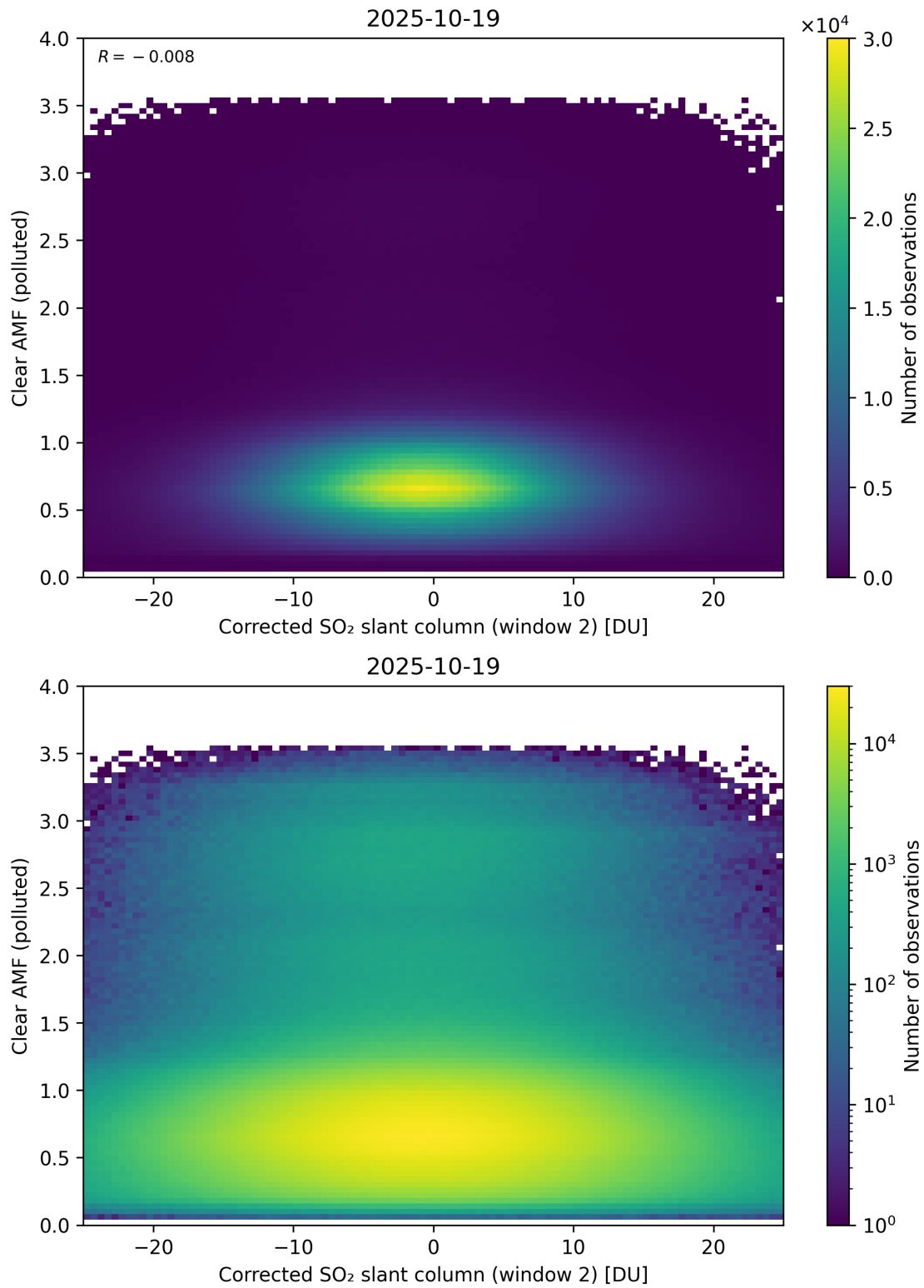
Figure 249: Scatter density plot of “Corrected SO 2 slant column (window 2)” against “Clear AMF (polluted)” for 2025-10-18 to 2025-10-20.
