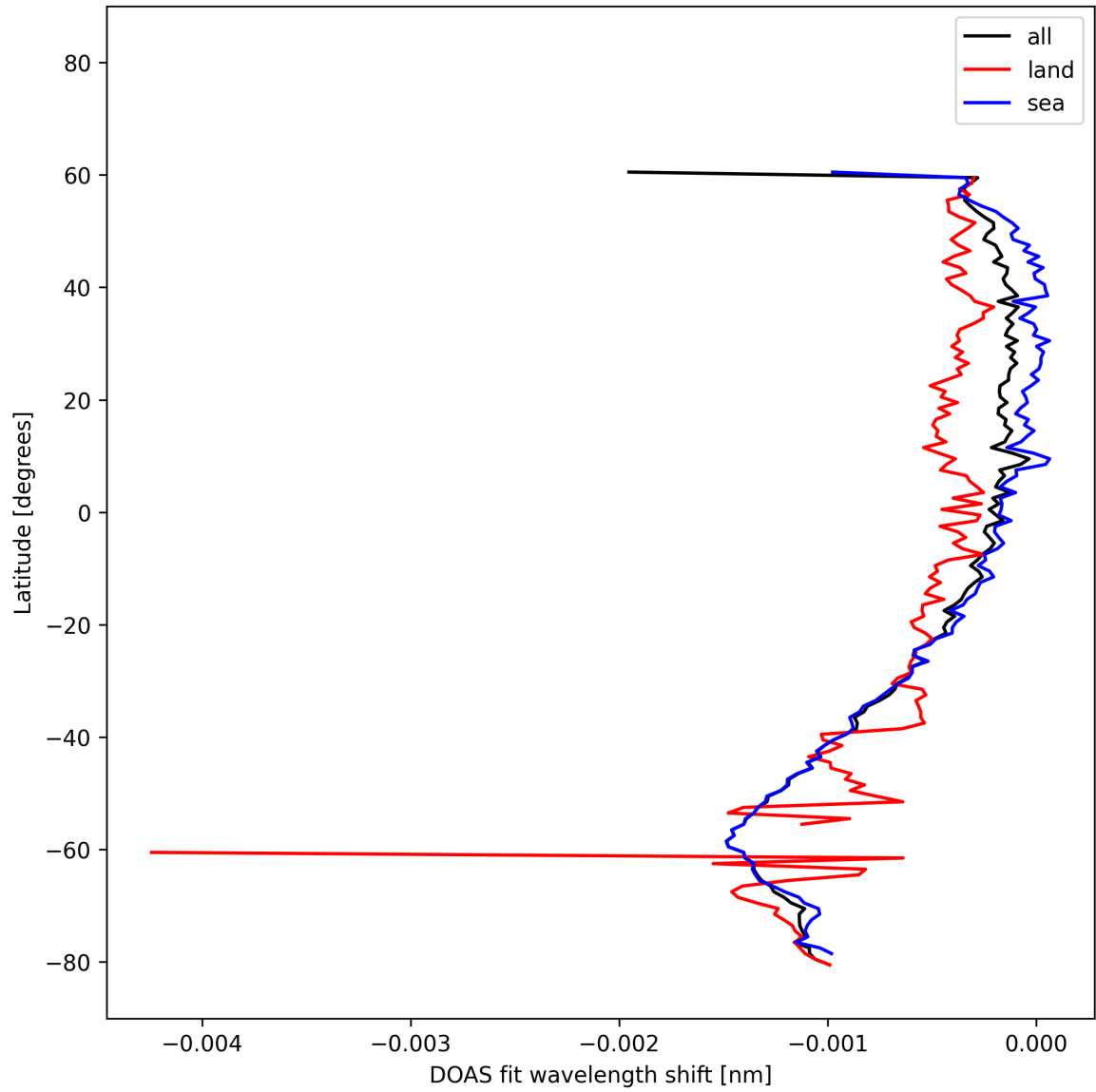
Figure 50: Zonal average of “DOAS fit wavelength shift” for 2025-10-18 to 2025-10-20.
