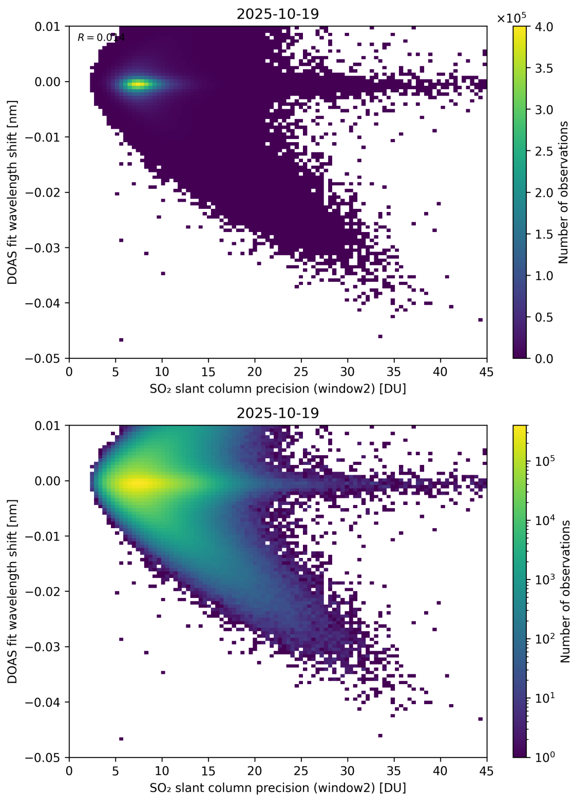
Figure 293: Scatter density plot of “SO 2 slant column precision (window2)” against “DOAS fit wavelength shift” for 2025-10-18 to 2025-10-20.
