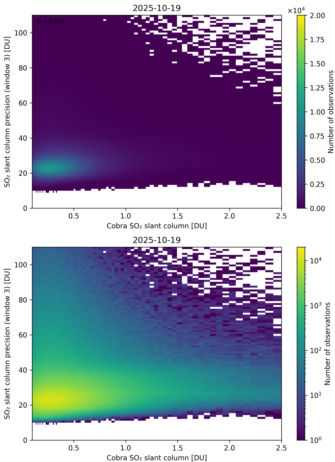
Figure 223: Scatter density plot of “Cobra SO 2 slant column” against “SO 2 slant column precision (window 3)” for 2025-10-18 to 2025-10-20.
