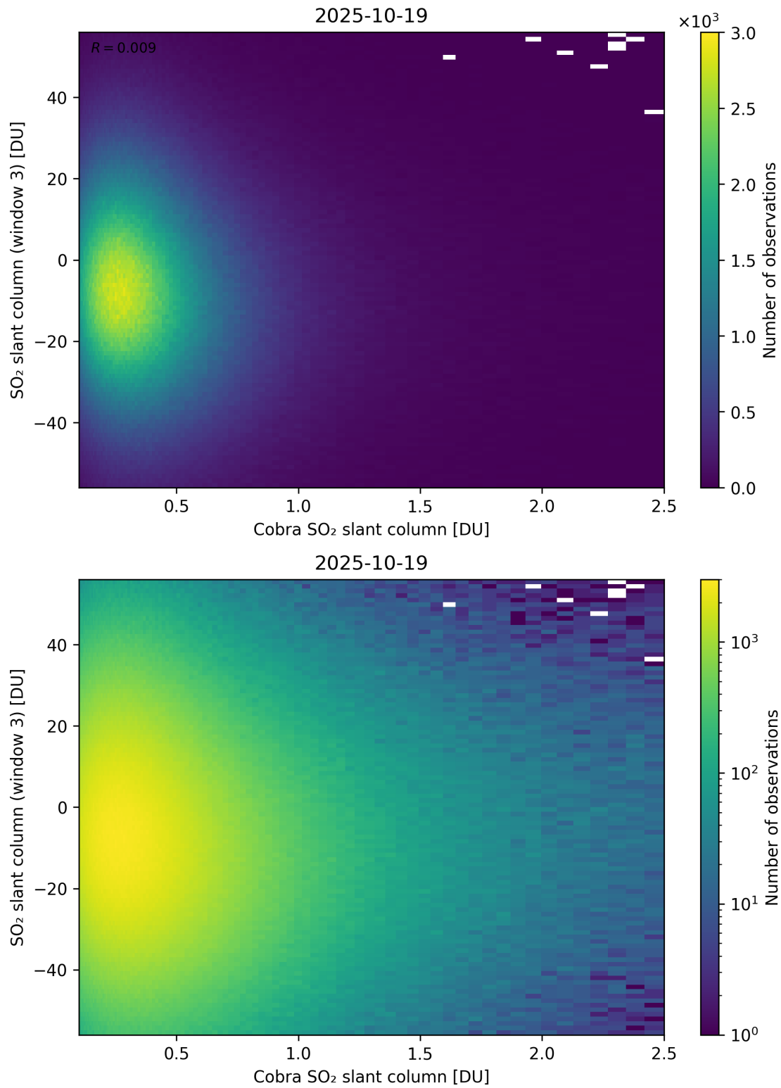
Figure 222: Scatter density plot of “Cobra SO 2 slant column” against “SO 2 slant column (window 3)” for 2025-10-18 to 2025-10-20.
