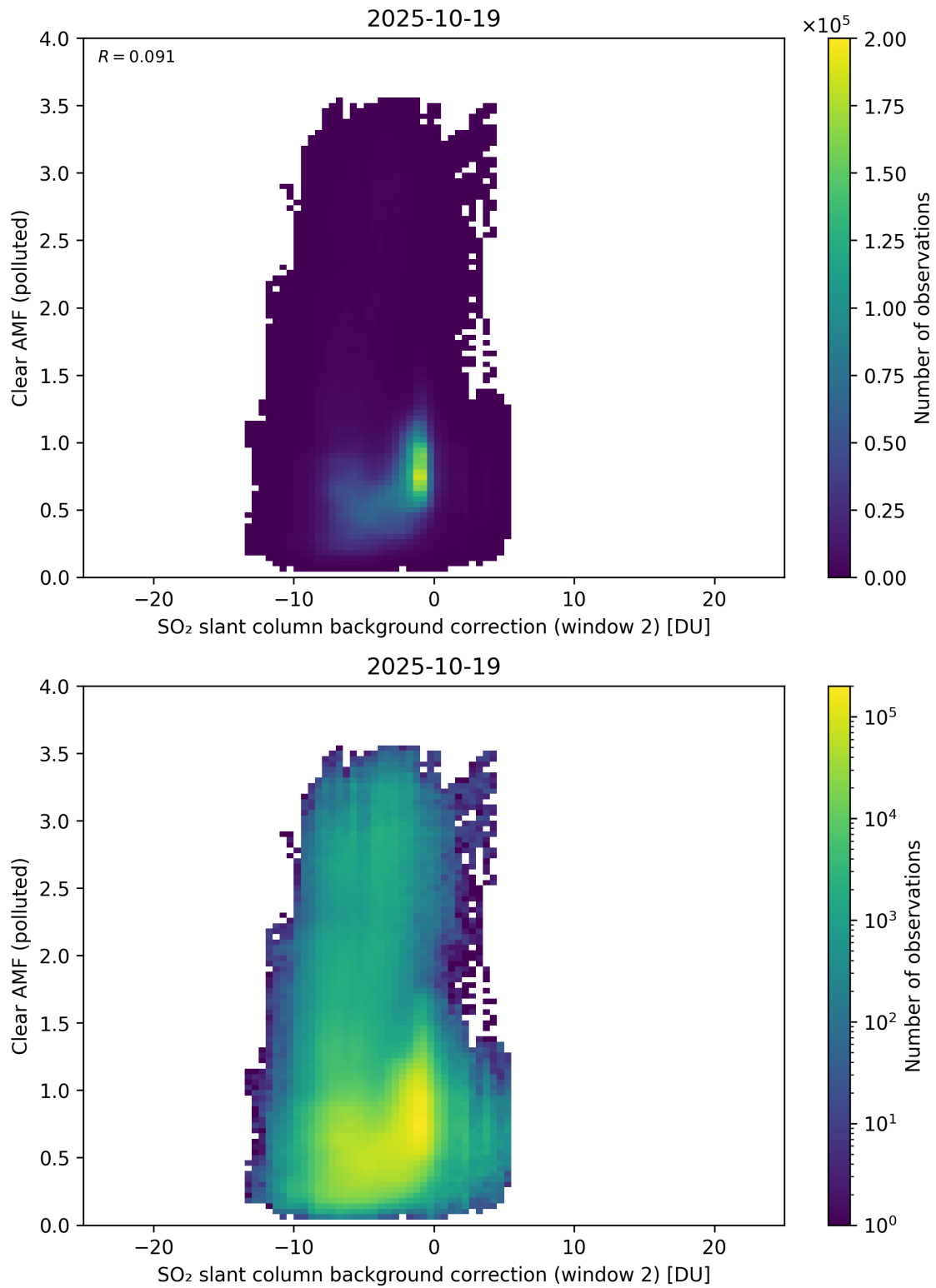
Figure 126: Scatter density plot of “SO 2 slant column background correction (window 2)” against “Clear AMF (polluted)” for 2025-10-18 to 2025-10-20.
