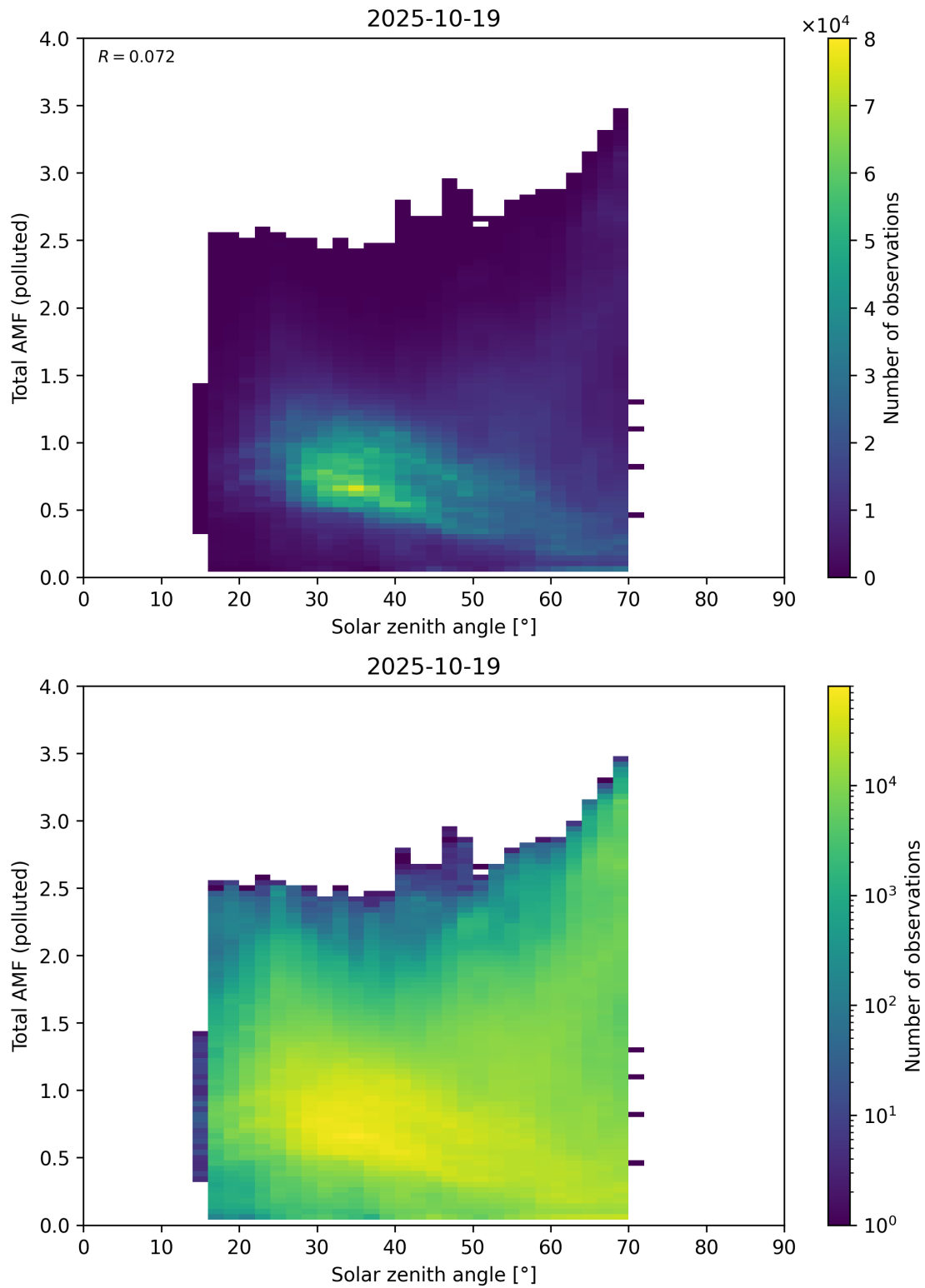
Figure 189: Scatter density plot of “Solar zenith angle” against “Total AMF (polluted)” for 2025-10-18 to 2025-10-20.
