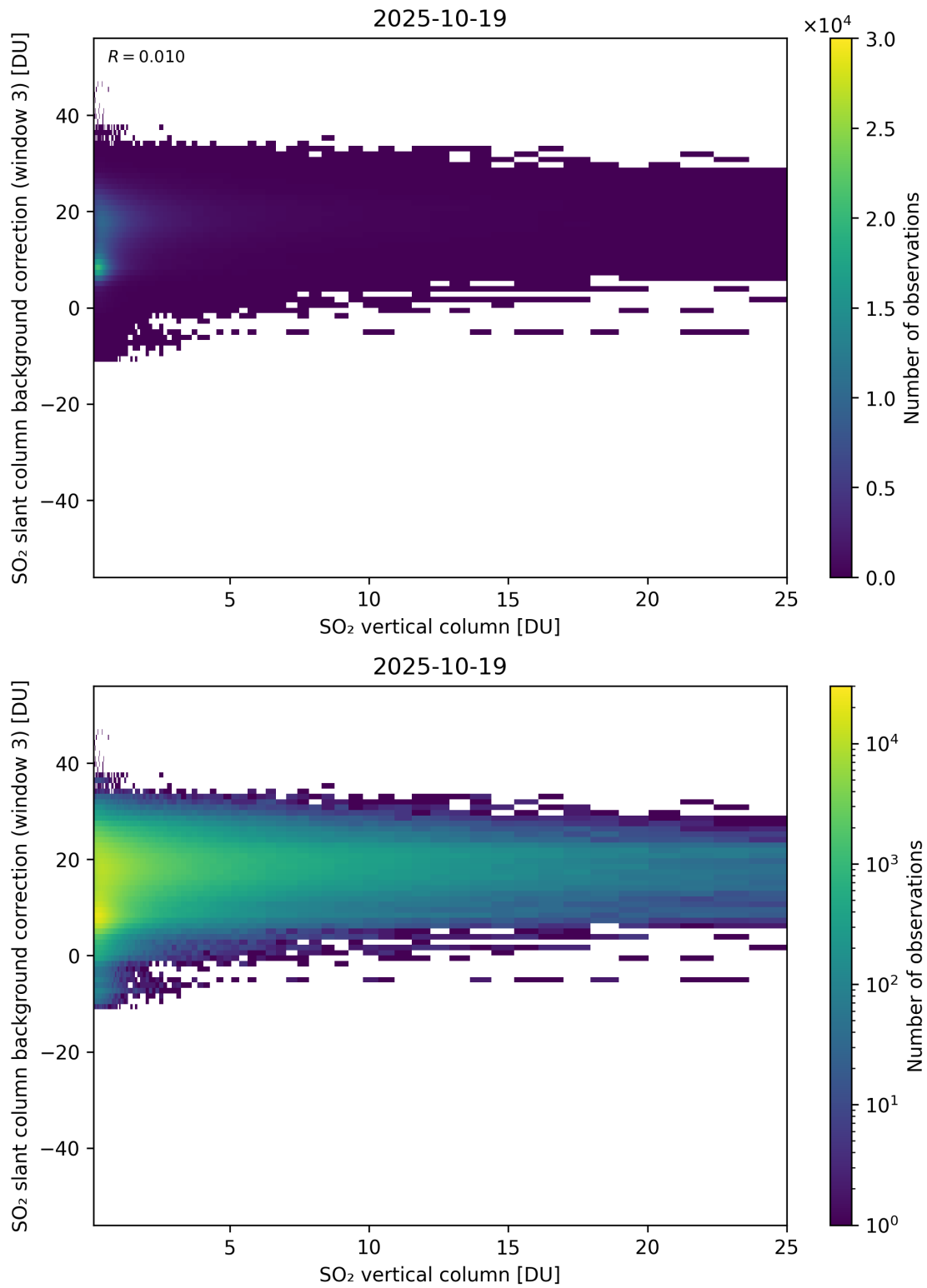
Figure 325: Scatter density plot of “SO 2 vertical column” against “SO 2 slant column background correction (window 3)” for 2025-10-18 to 2025-10-20.
