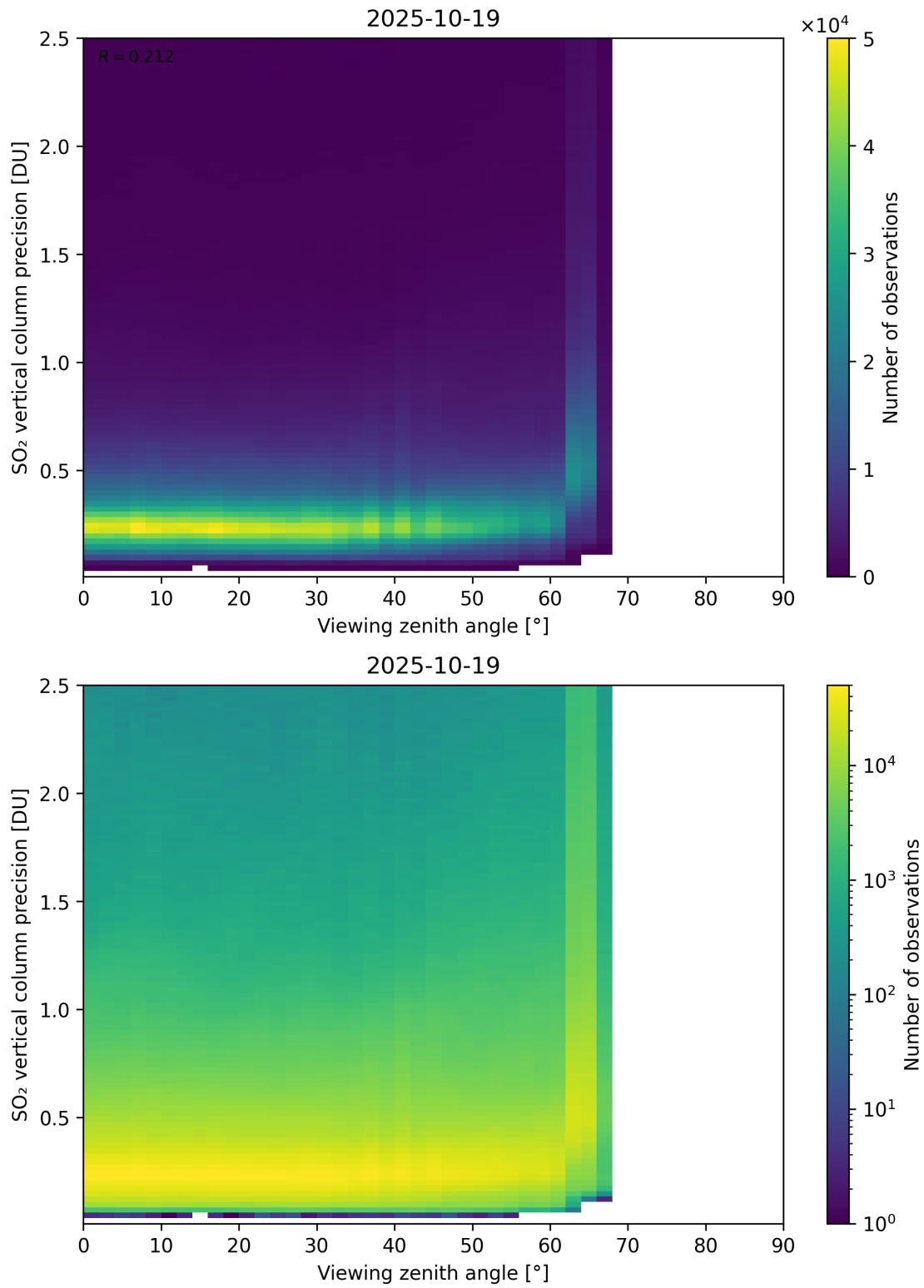
Figure 384: Scatter density plot of “Viewing zenith angle” against “SO 2 vertical column precision” for 2025-10-18 to 2025-10-20.
