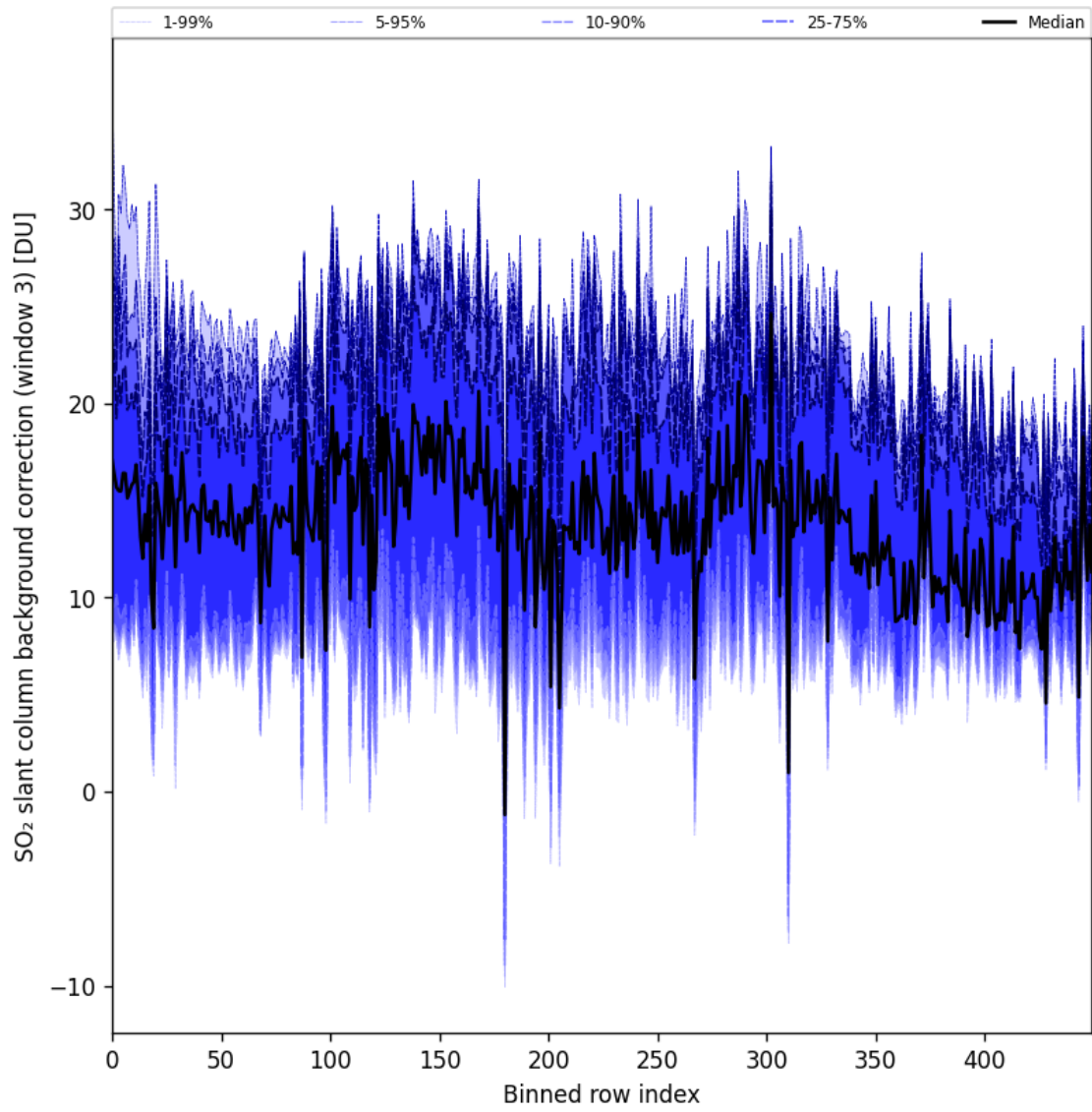
Figure 100: Along track statistics of “SO 2 slant column background correction (window 3)” for 2025-10-18 to 2025-10-20
