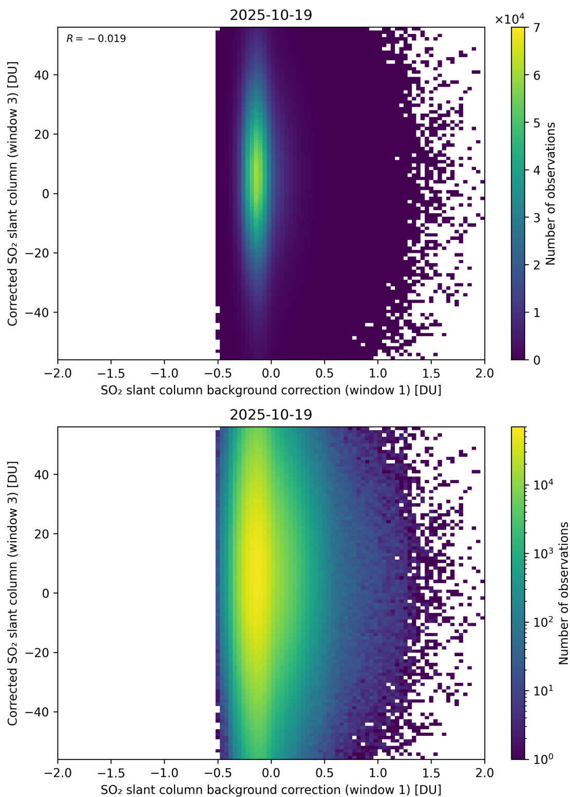
Figure 116: Scatter density plot of “SO 2 slant column background correction (window 1)” against “Corrected SO 2 slant column (window 3)” for 2025-10-18 to 2025-10-20.
