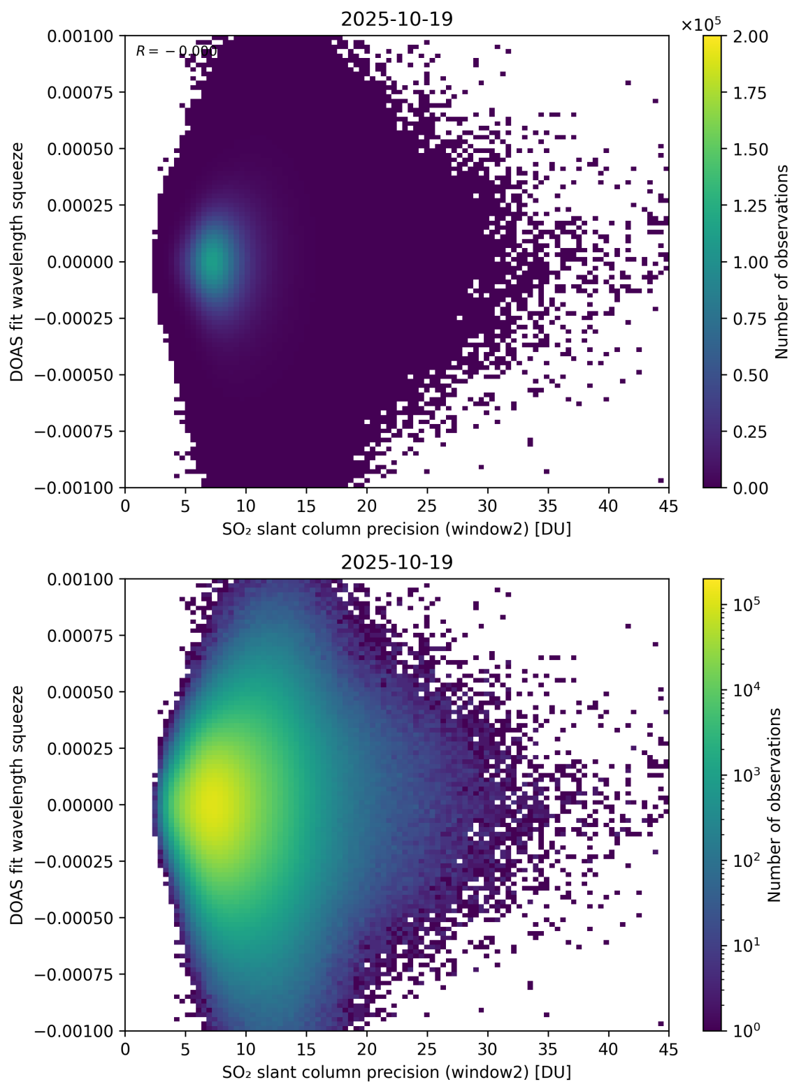
Figure 294: Scatter density plot of “SO 2 slant column precision (window2)” against “DOAS fit wavelength squeeze” for 2025-10-18 to 2025-10-20.
