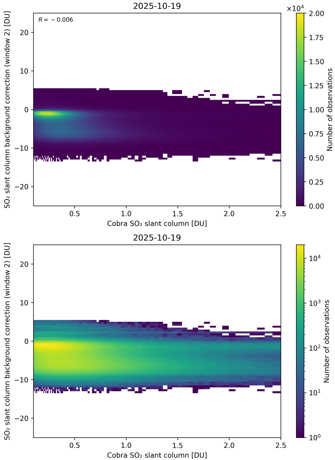
Figure 194: Scatter density plot of “Cobra SO 2 slant column” against “SO 2 slant column background correction (window 2)” for 2025-10-18 to 2025-10-20.
