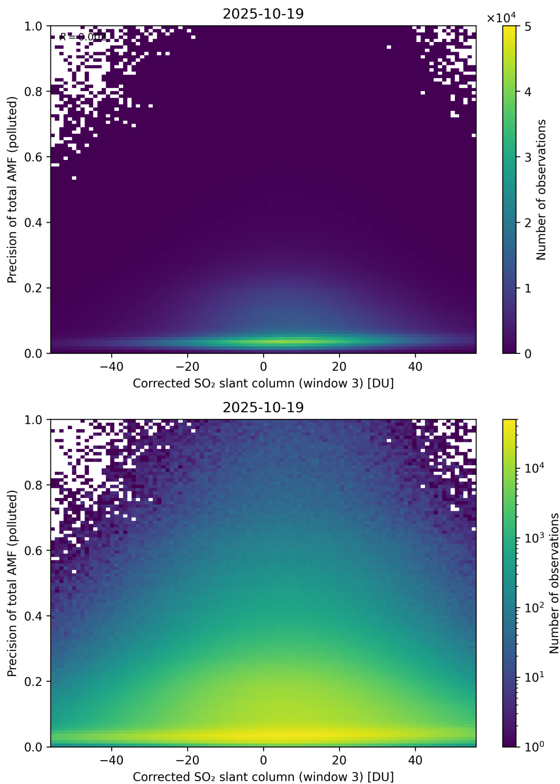
Figure 261: Scatter density plot of “Corrected SO 2 slant column (window 3)” against “Precision of total AMF (polluted)” for 2025-10-18 to 2025-10-20.
