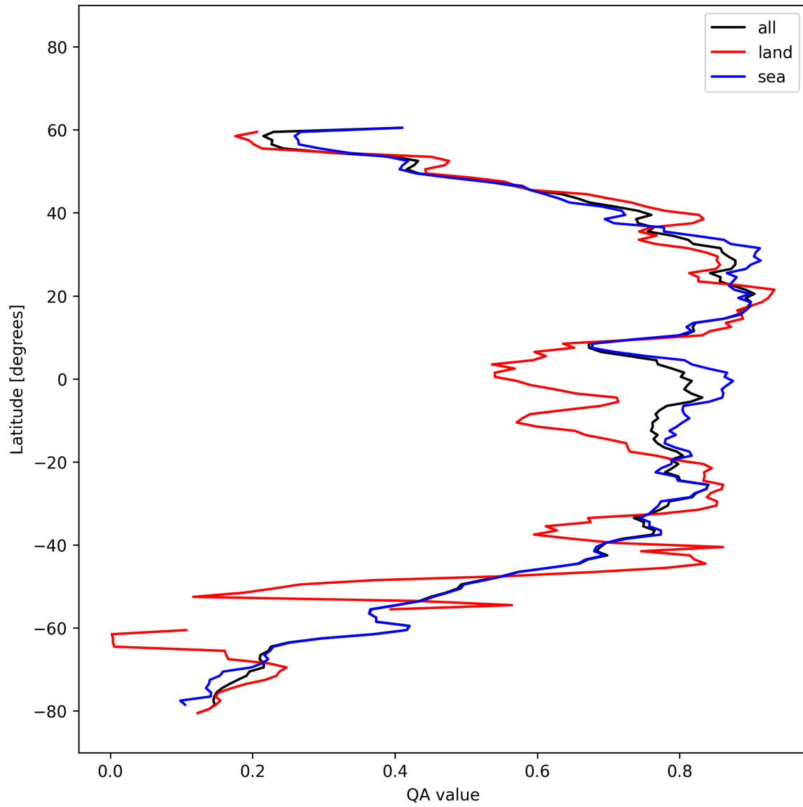
Figure 31: Zonal average of “QA value” for 2025-10-18 to 2025-10-20.
