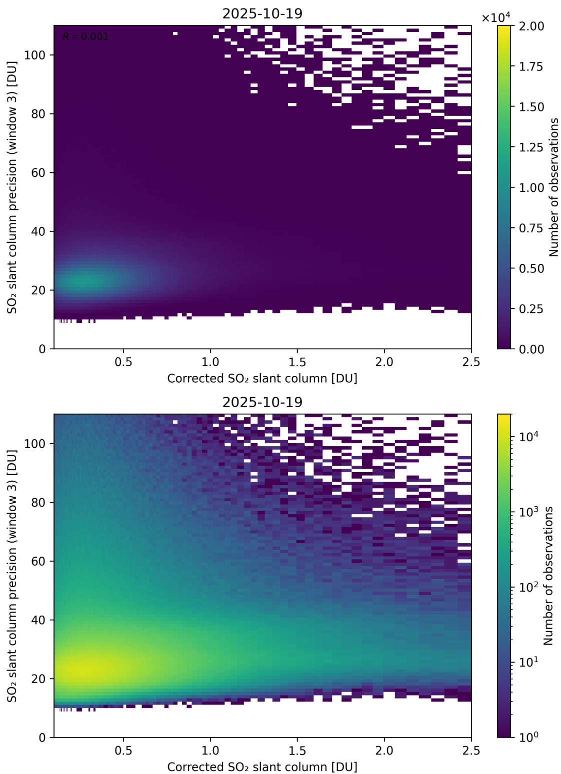
Figure 241: Scatter density plot of “Corrected SO 2 slant column” against “SO 2 slant column precision (window 3)” for 2025-10-18 to 2025-10-20.
