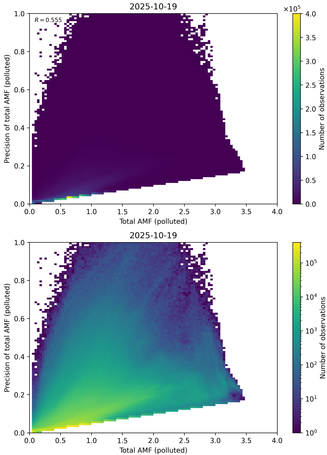
Figure 322: Scatter density plot of “Total AMF (polluted)” against “Precision of total AMF (polluted)” for 2025-10-18 to 2025-10-20.
