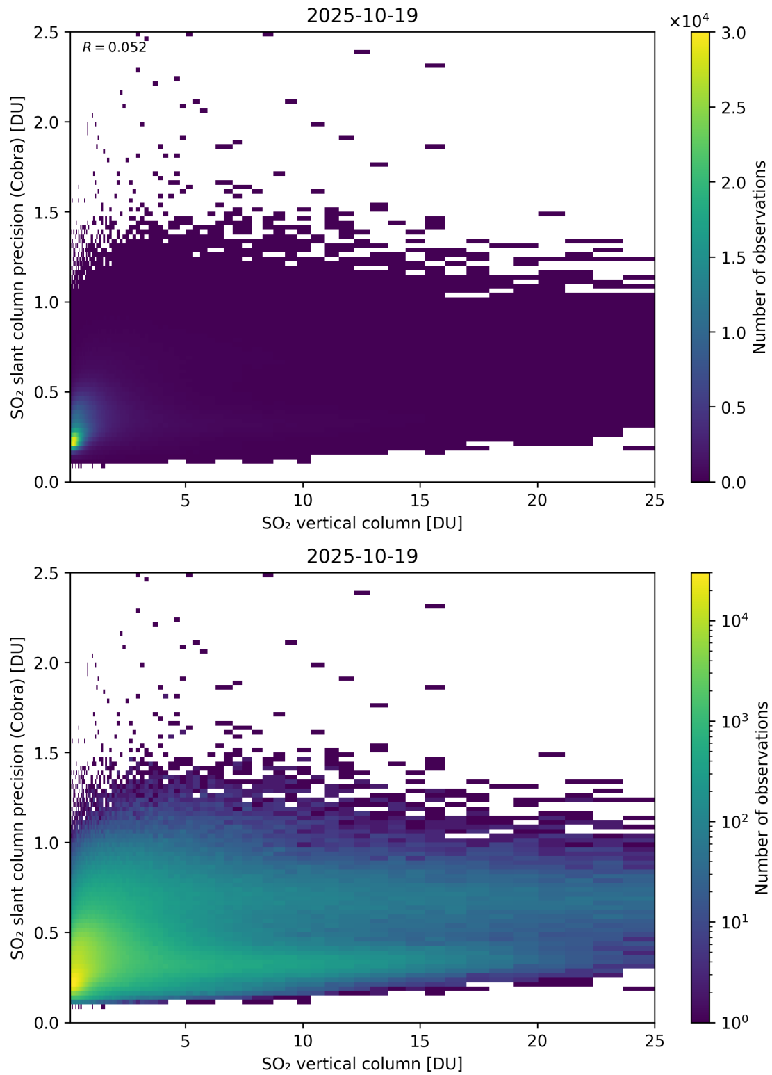
Figure 350: Scatter density plot of “SO 2 vertical column” against “SO 2 slant column precision (Cobra)” for 2025-10-18 to 2025-10-20.
