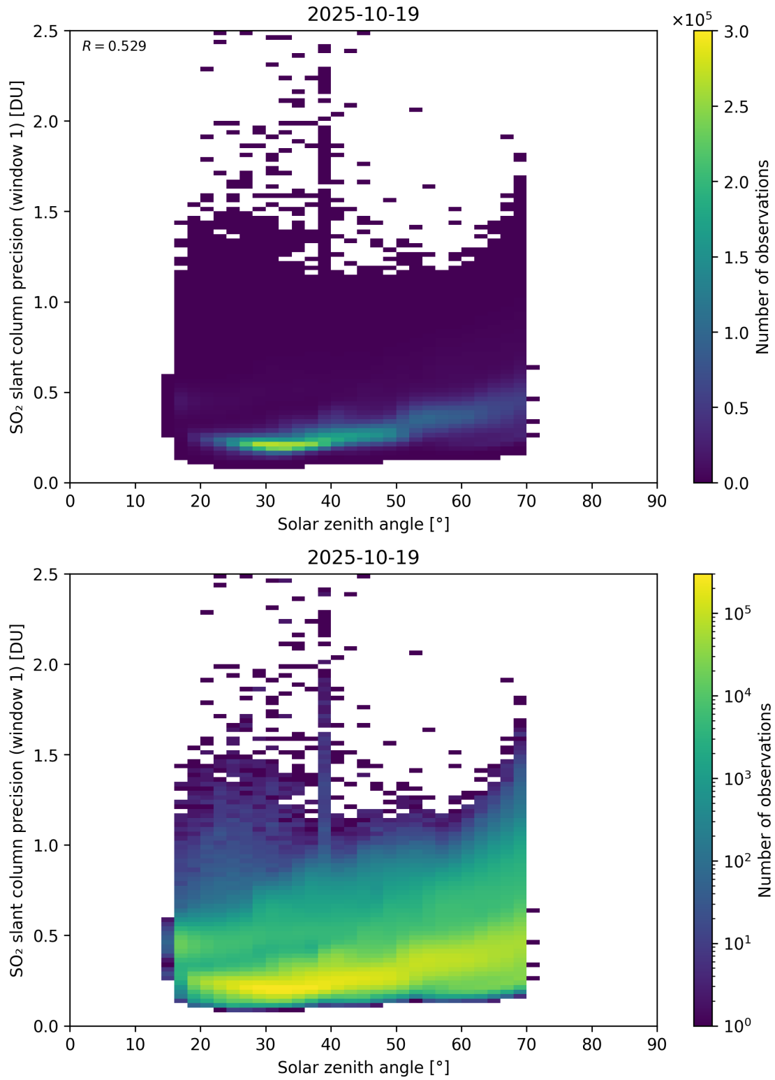
Figure 185: Scatter density plot of “Solar zenith angle” against “SO 2 slant column precision (window 1)” for 2025-10-18 to 2025-10-20.
