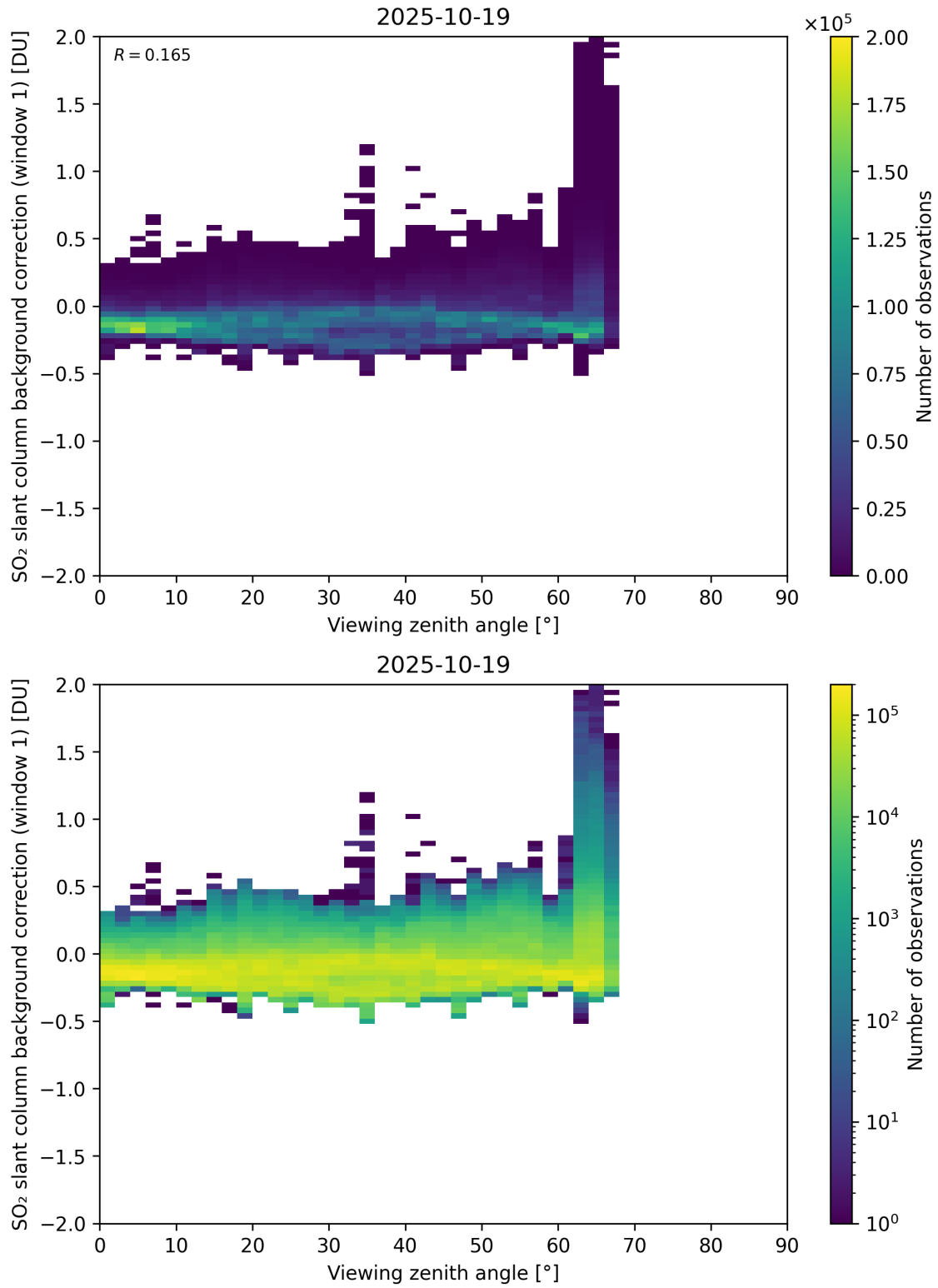
Figure 362: Scatter density plot of “Viewing zenith angle” against “SO 2 slant column background correction (window 1)” for 2025-10-18 to 2025-10-20.
