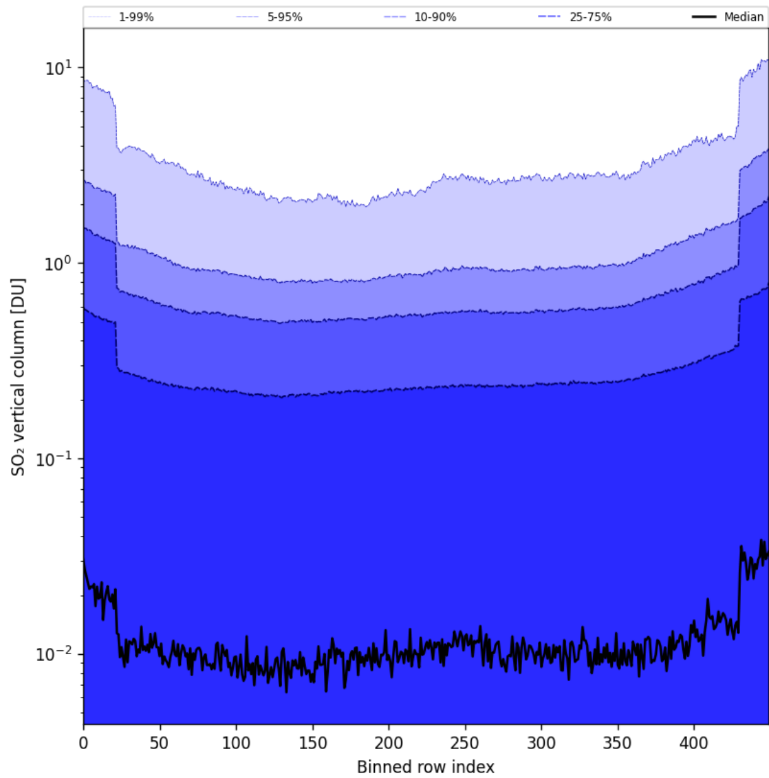
Figure 84: Along track statistics of “SO 2 vertical column” for 2025-10-18 to 2025-10-20
