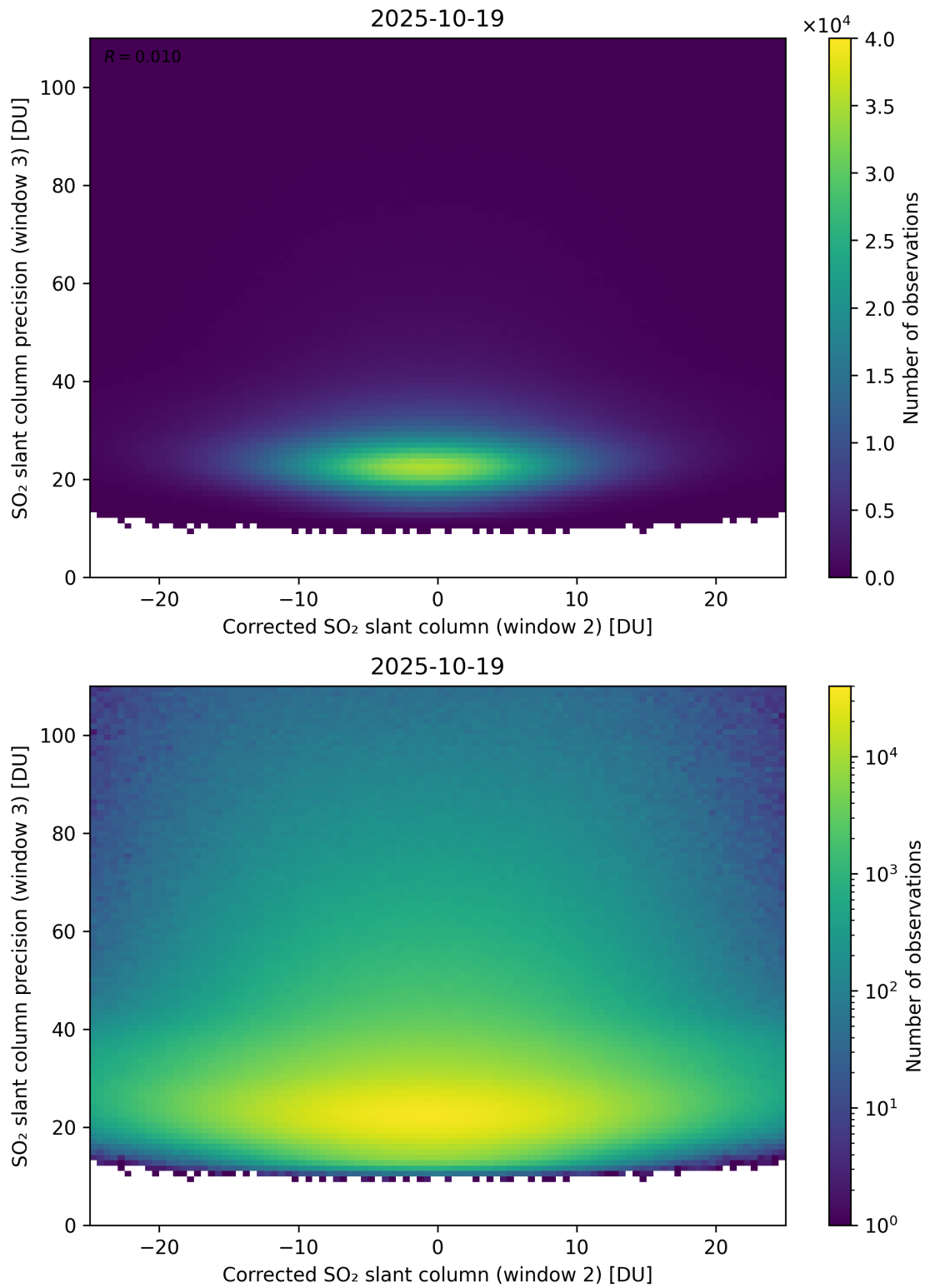
Figure 252: Scatter density plot of “Corrected SO 2 slant column (window 2)” against “SO 2 slant column precision (window 3)” for 2025-10-18 to 2025-10-20.
