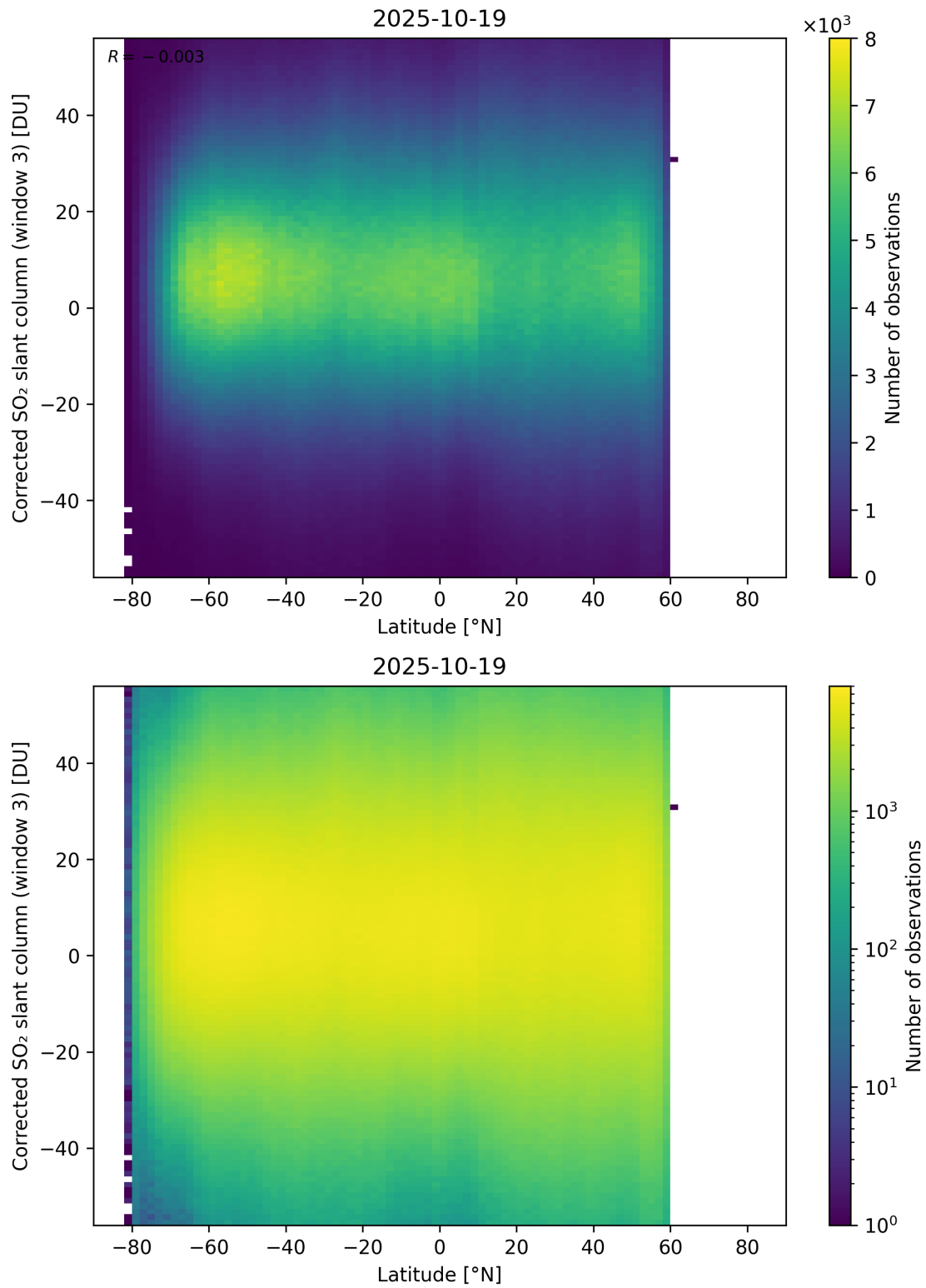
Figure 161: Scatter density plot of “Latitude” against “Corrected SO 2 slant column (window 3)” for 2025-10-18 to 2025-10-20.
