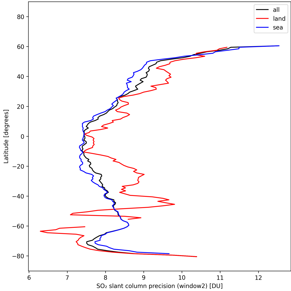
Figure 42: Zonal average of “SO 2 slant column precision (window2)” for 2025-10-18 to 2025-10-20.
