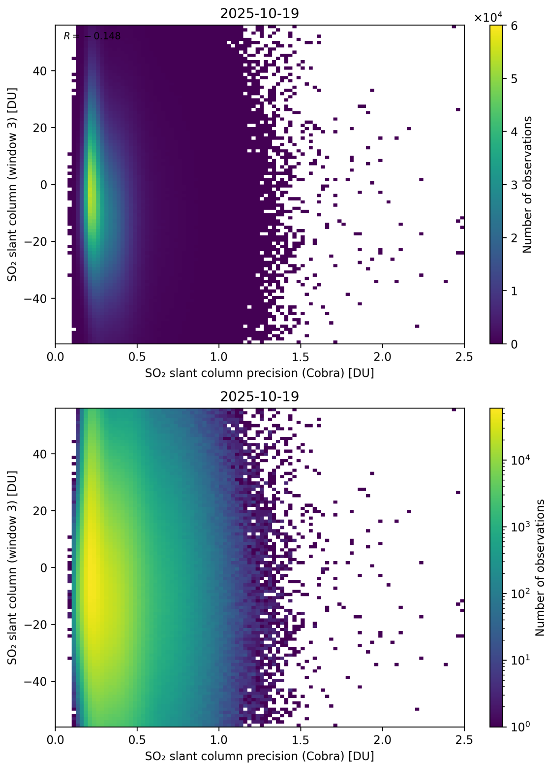
Figure 211: Scatter density plot of “SO 2 slant column precision (Cobra)” against “SO 2 slant column (window 3)” for 2025-10-18 to 2025-10-20.
