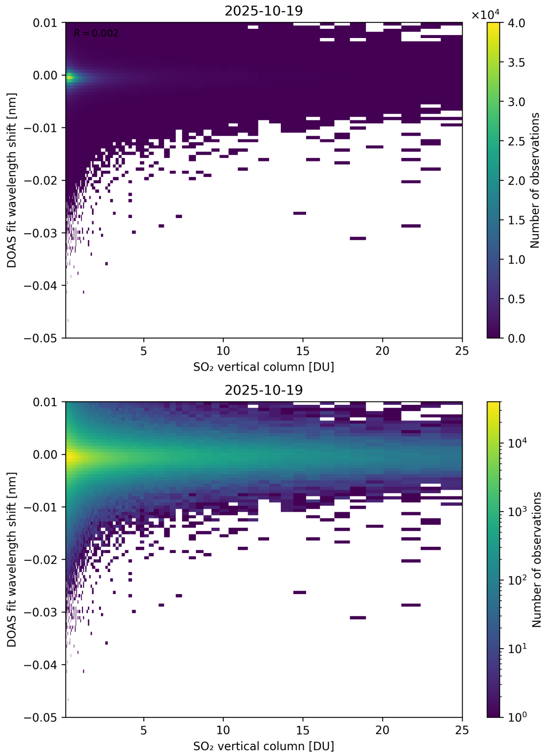
Figure 326: Scatter density plot of “SO 2 vertical column” against “DOAS fit wavelength shift” for 2025-10-18 to 2025-10-20.
