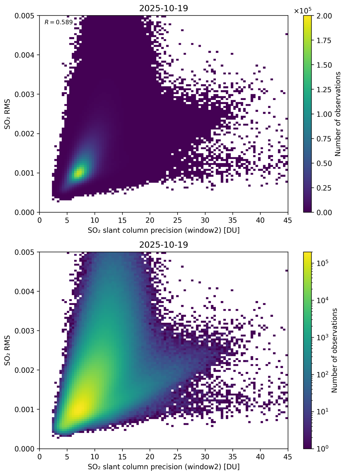
Figure 295: Scatter density plot of “SO 2 slant column precision (window2)” against “SO 2 RMS” for 2025-10-18 to 2025-10-20.
