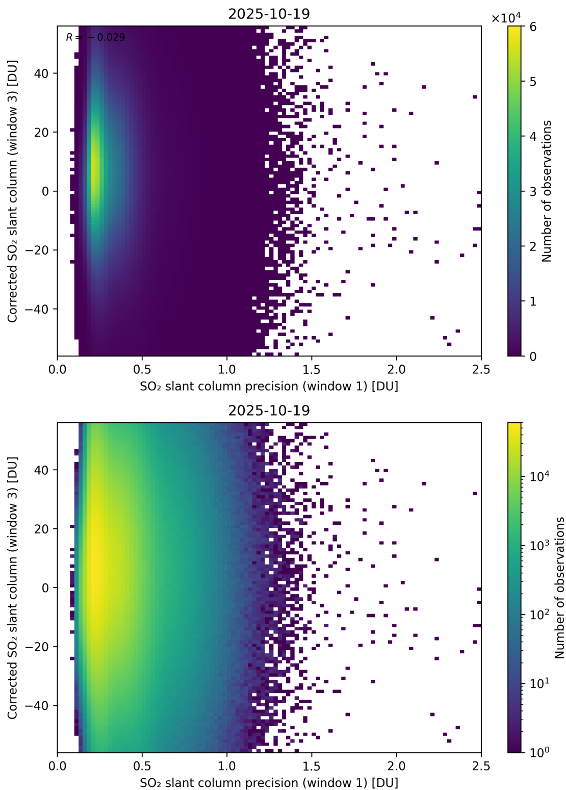
Figure 276: Scatter density plot of “SO 2 slant column precision (window 1)” against “Corrected SO 2 slant column (window 3)” for 2025-10-18 to 2025-10-20.
