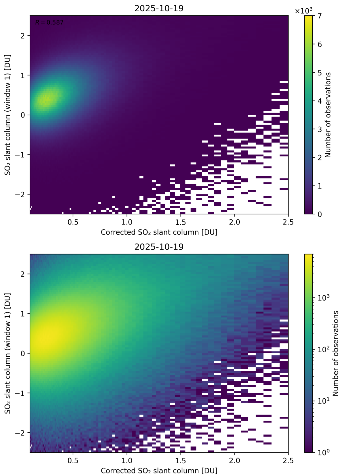
Figure 237: Scatter density plot of “Corrected SO 2 slant column” against “SO 2 slant column (window 1)” for 2025-10-18 to 2025-10-20.
