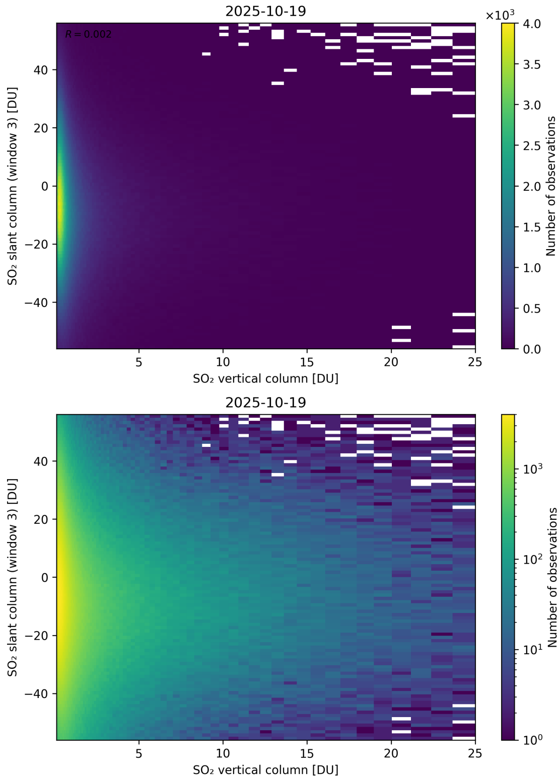
Figure 357: Scatter density plot of “SO 2 vertical column” against “SO 2 slant column (window 3)” for 2025-10-18 to 2025-10-20.
