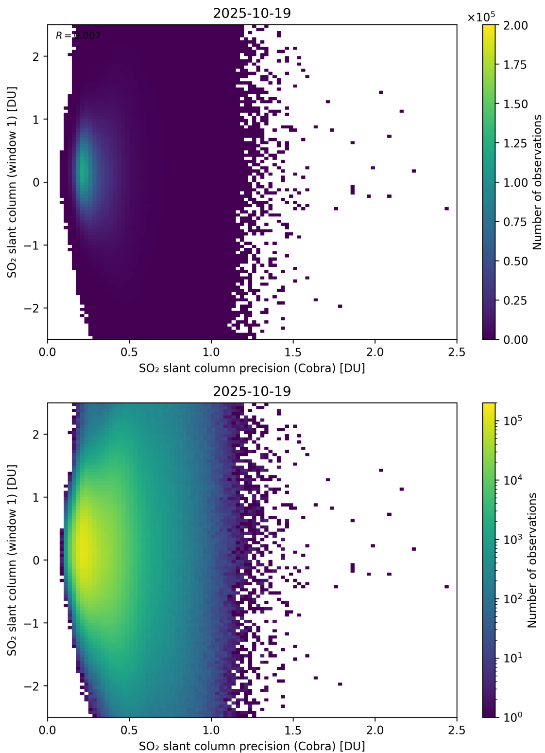
Figure 208: Scatter density plot of “SO 2 slant column precision (Cobra)” against “SO 2 slant column (window 1)” for 2025-10-18 to 2025-10-20.
