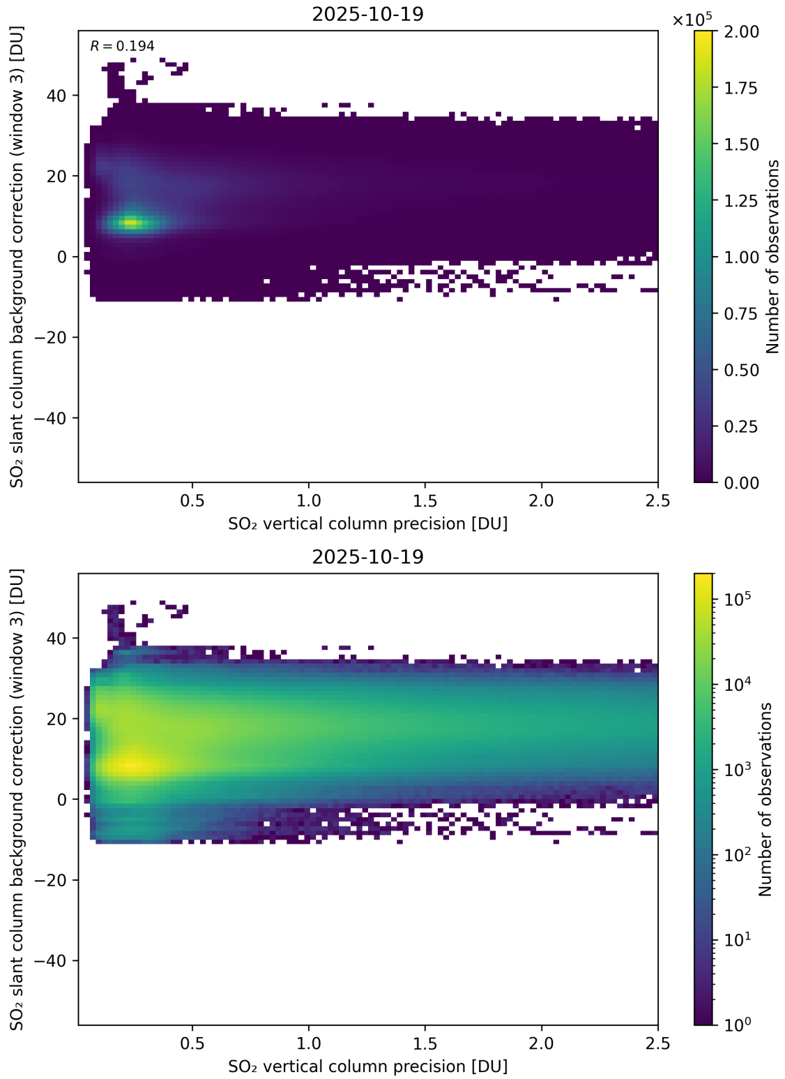
Figure 331: Scatter density plot of “SO 2 vertical column precision” against “SO 2 slant column background correction (window 3)” for 2025-10-18 to 2025-10-20.
