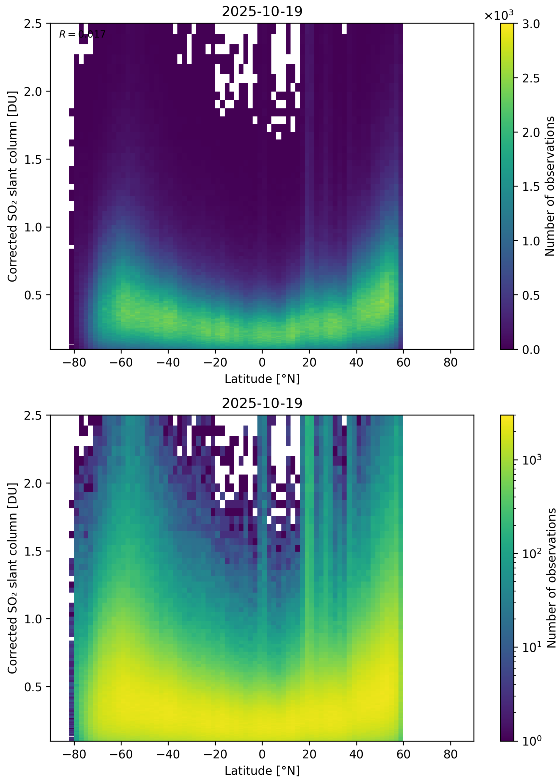
Figure 159: Scatter density plot of “Latitude” against “Corrected SO 2 slant column” for 2025-10-18 to 2025-10-20.
