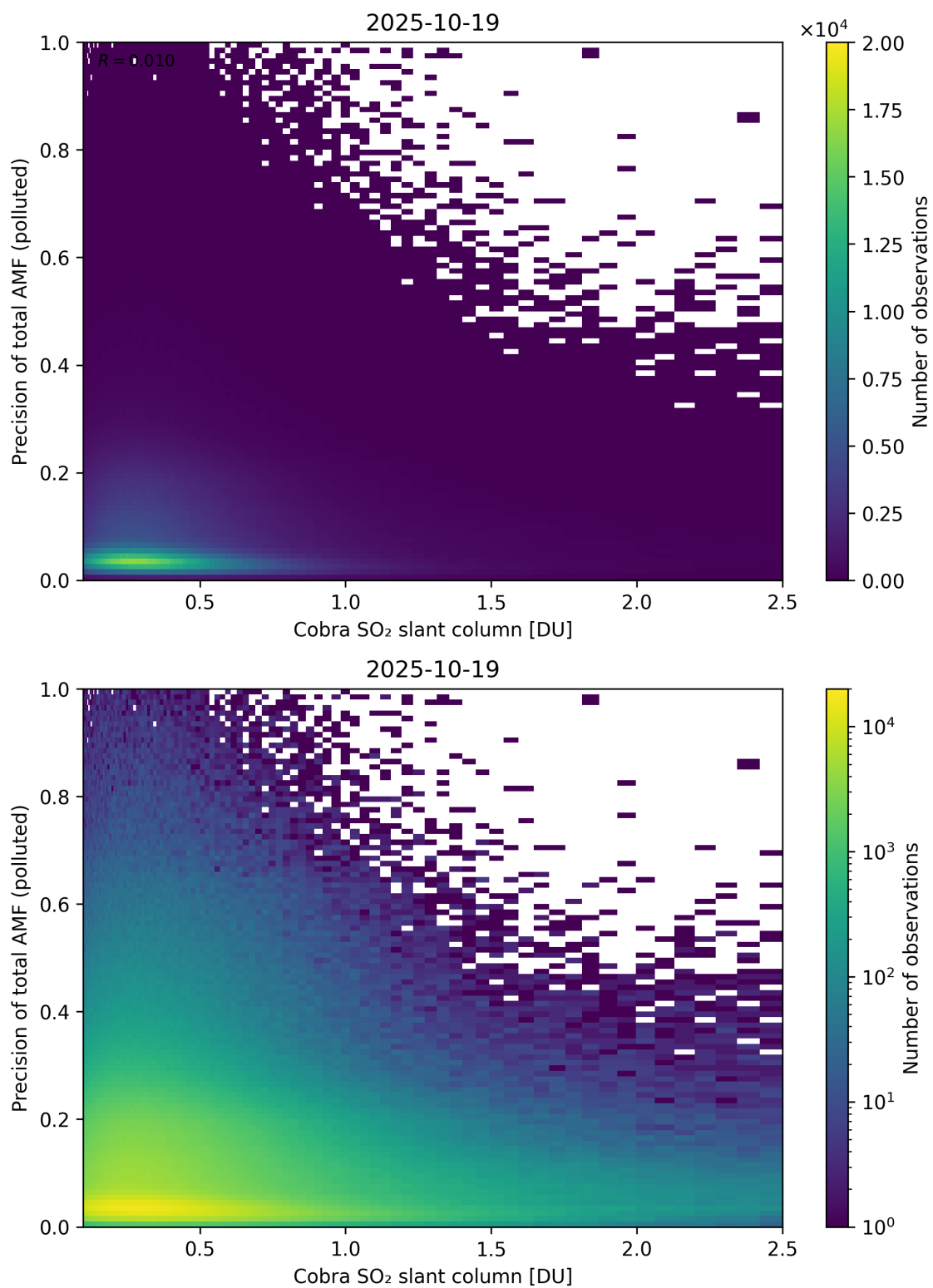
Figure 225: Scatter density plot of “Cobra SO 2 slant column” against “Precision of total AMF (polluted)” for 2025-10-18 to 2025-10-20.
