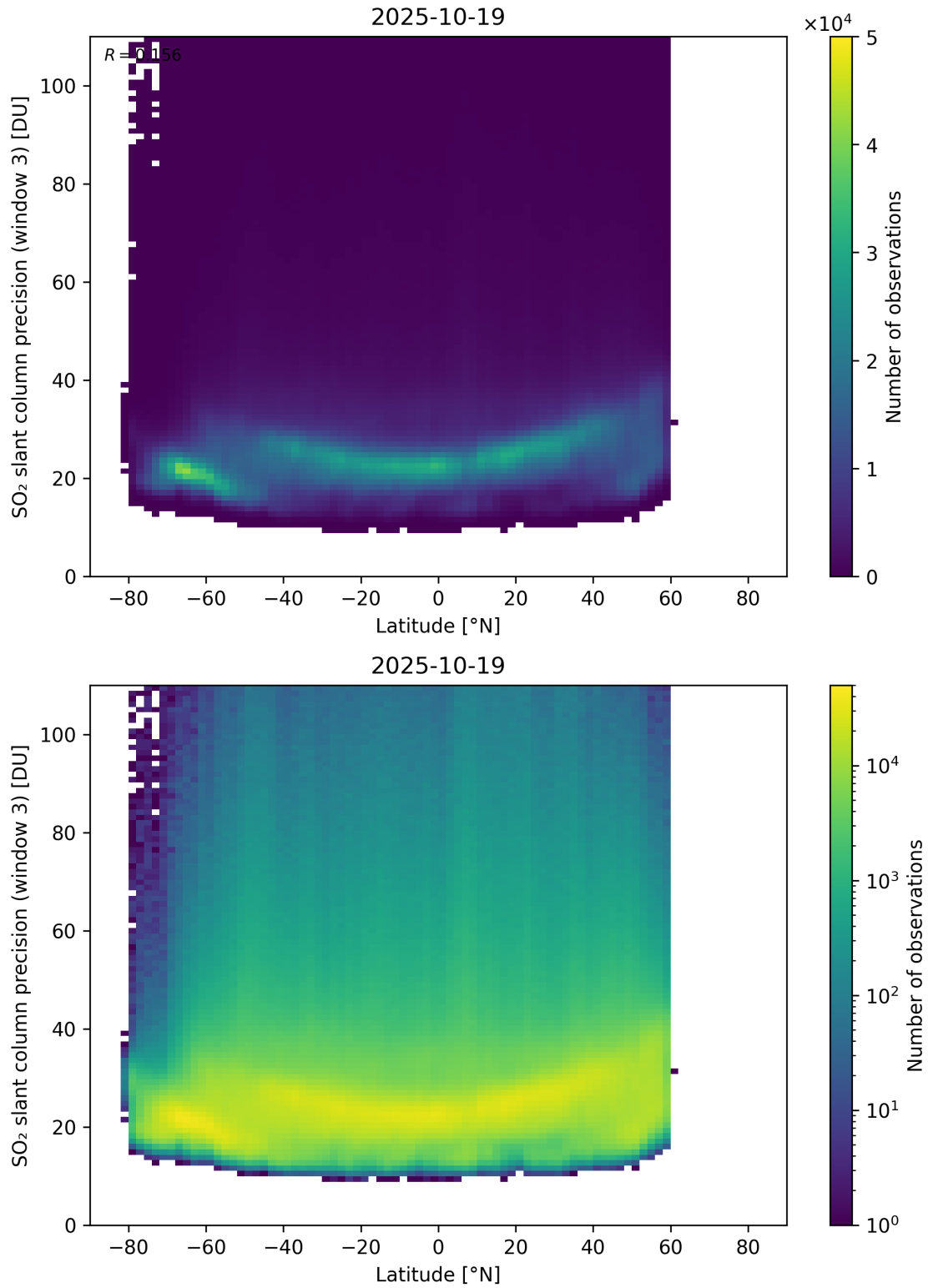
Figure 166: Scatter density plot of “Latitude” against “SO 2 slant column precision (window 3)” for 2025-10-18 to 2025-10-20.
