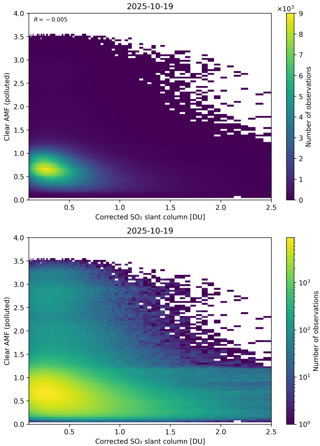
Figure 232: Scatter density plot of “Corrected SO 2 slant column” against “Clear AMF (polluted)” for 2025-10-18 to 2025-10-20.
