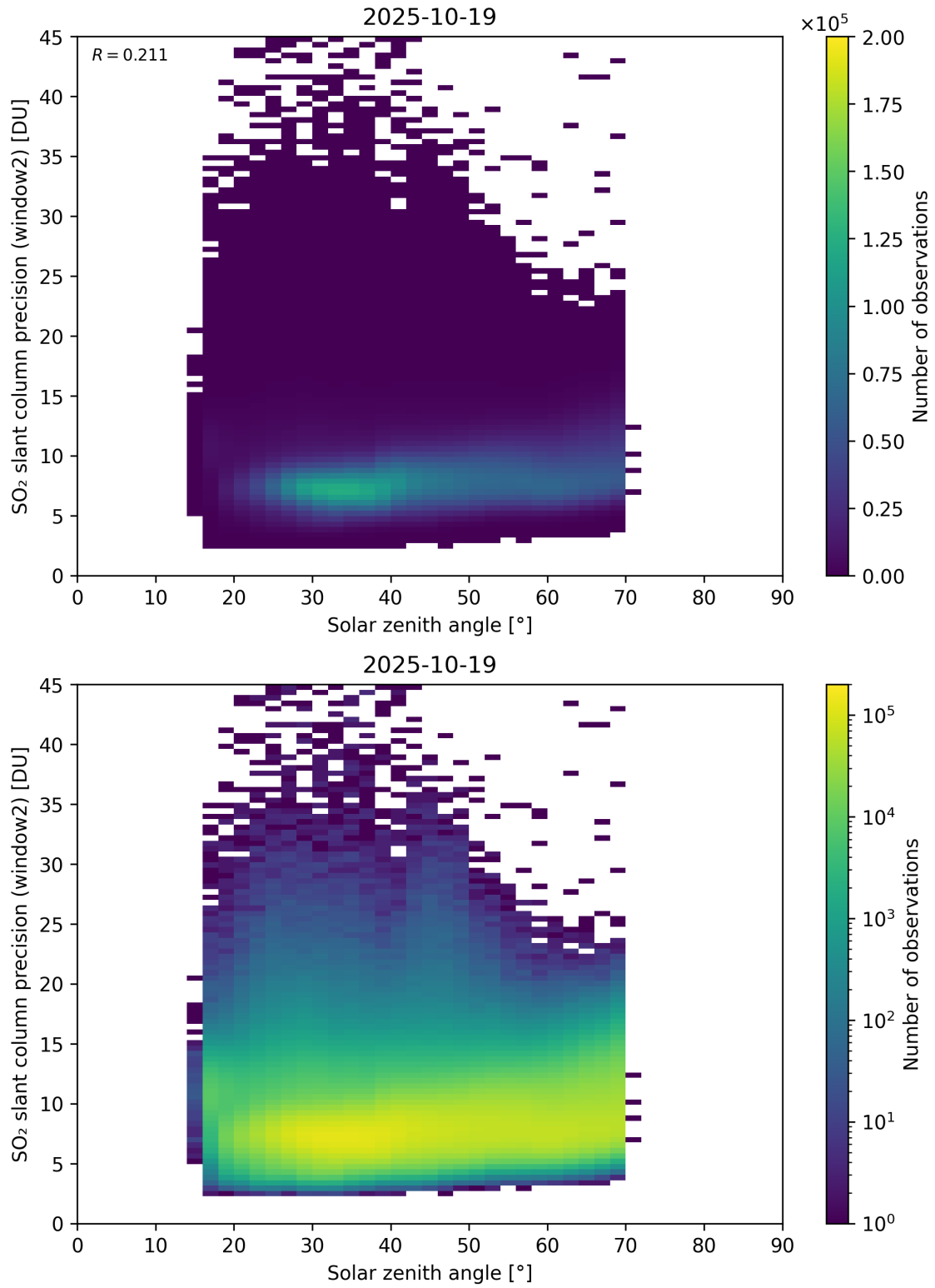
Figure 186: Scatter density plot of “Solar zenith angle” against “SO 2 slant column precision (window2)” for 2025-10-18 to 2025-10-20.
