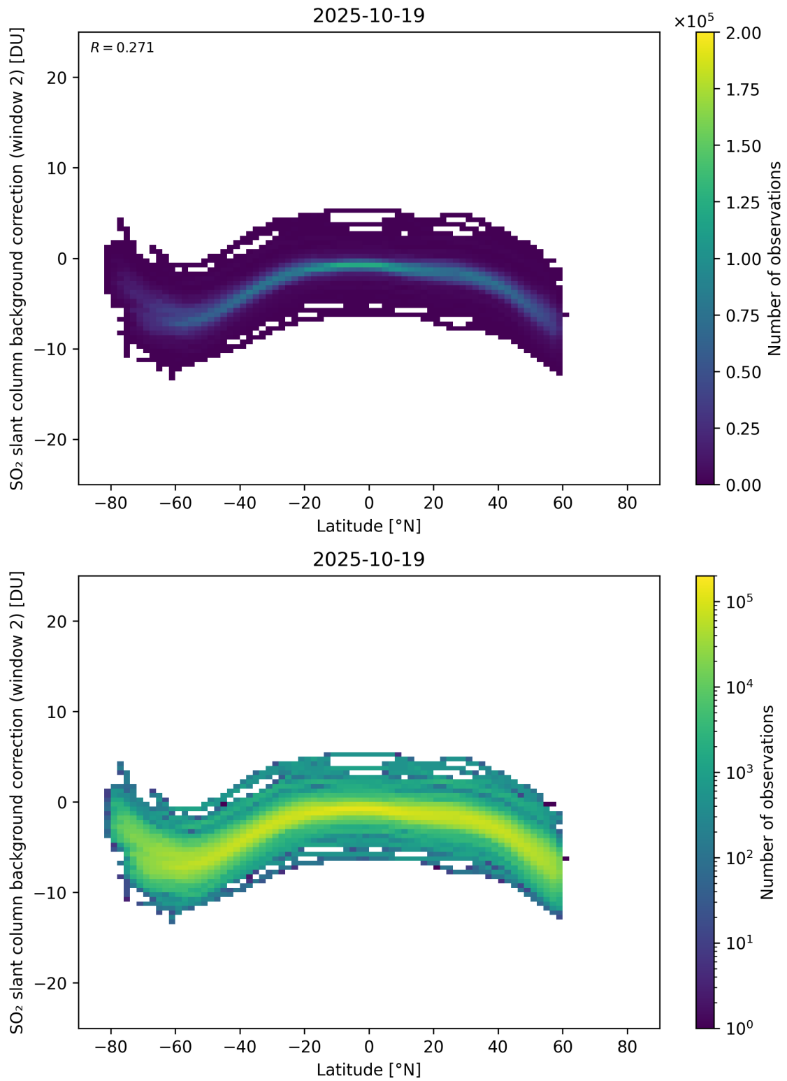
Figure 151: Scatter density plot of “Latitude” against “SO 2 slant column background correction (window 2)” for 2025-10-18 to 2025-10-20.
