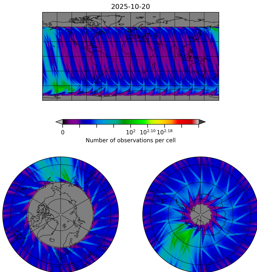
Figure 30: Map of the number of observations for 2025-10-19 to 2025-10-21
