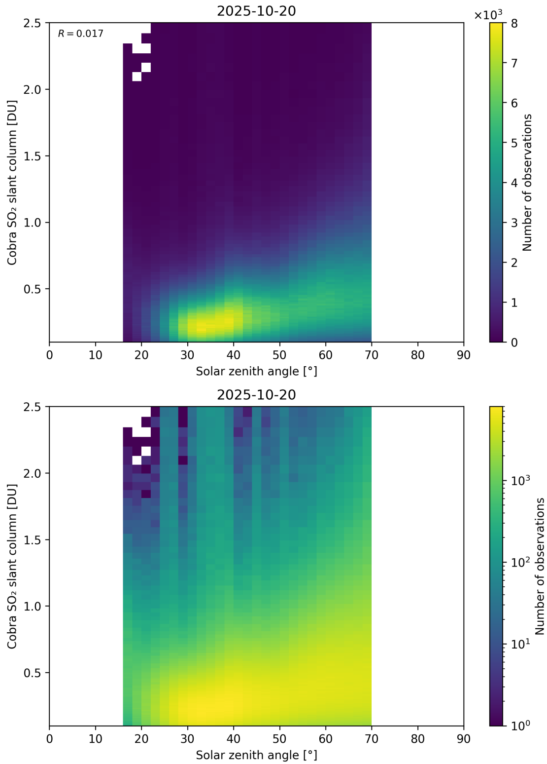
Figure 179: Scatter density plot of “Solar zenith angle” against “Cobra SO 2 slant column” for 2025-10-19 to 2025-10-21.
