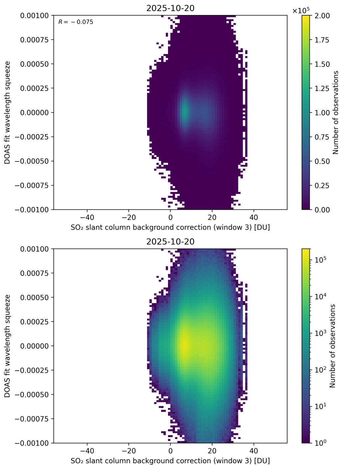
Figure 133: Scatter density plot of “SO 2 slant column background correction (window 3)” against “DOAS fit wavelength squeeze” for 2025-10-19 to 2025-10-21.
