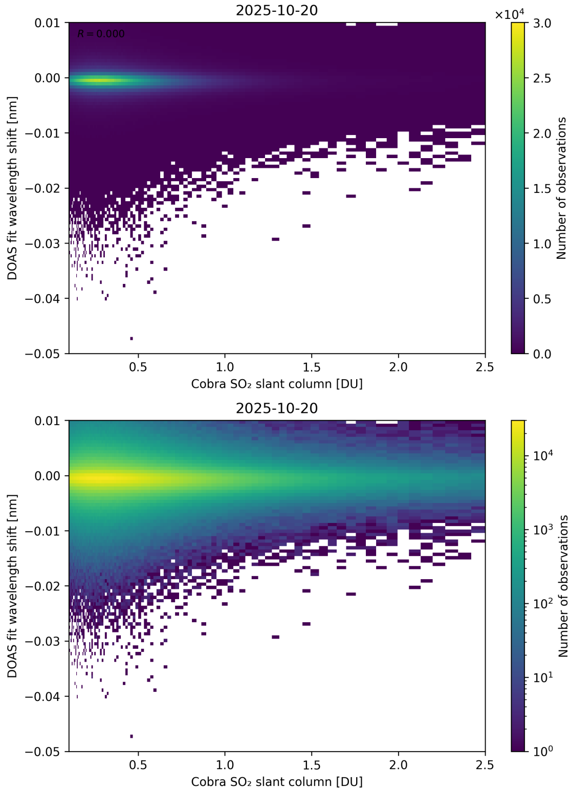
Figure 196: Scatter density plot of “Cobra SO 2 slant column” against “DOAS fit wavelength shift” for 2025-10-19 to 2025-10-21.
