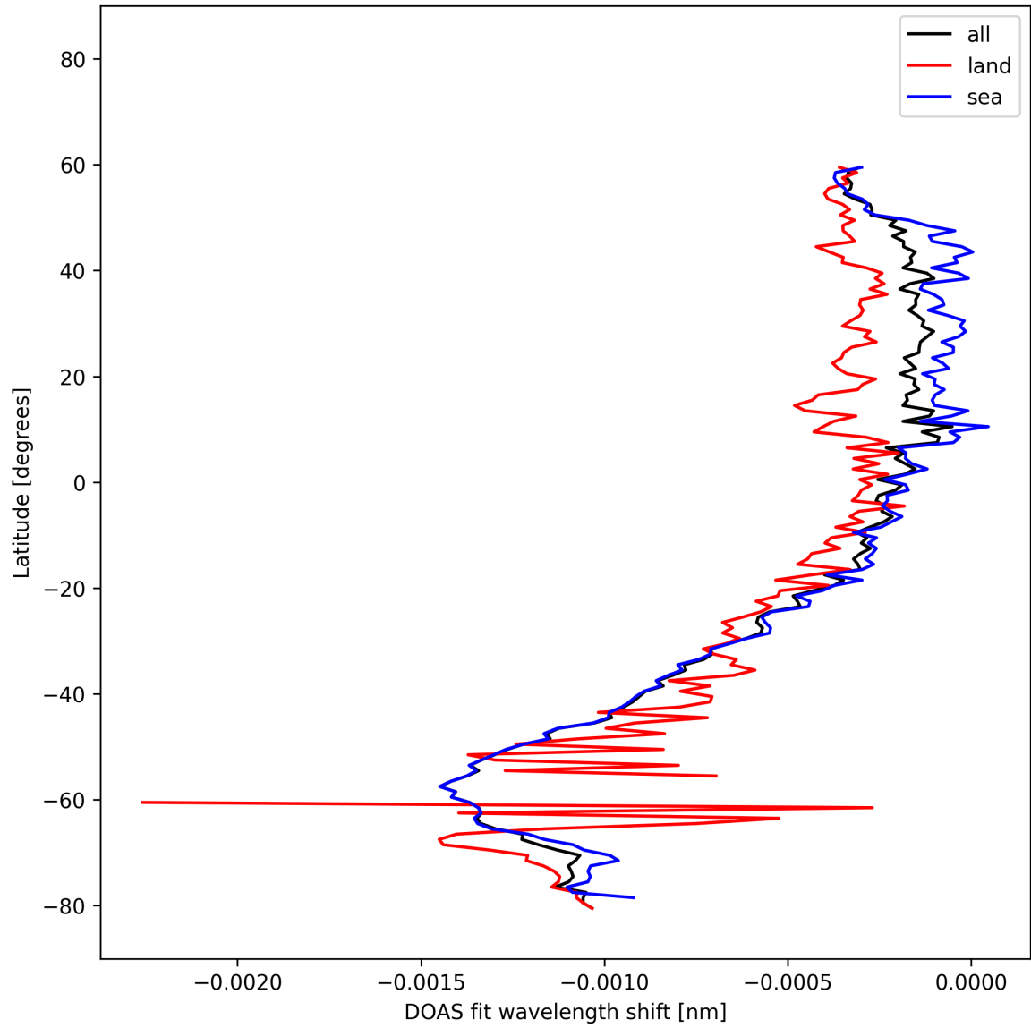
Figure 50: Zonal average of “DOAS fit wavelength shift” for 2025-10-19 to 2025-10-21.
