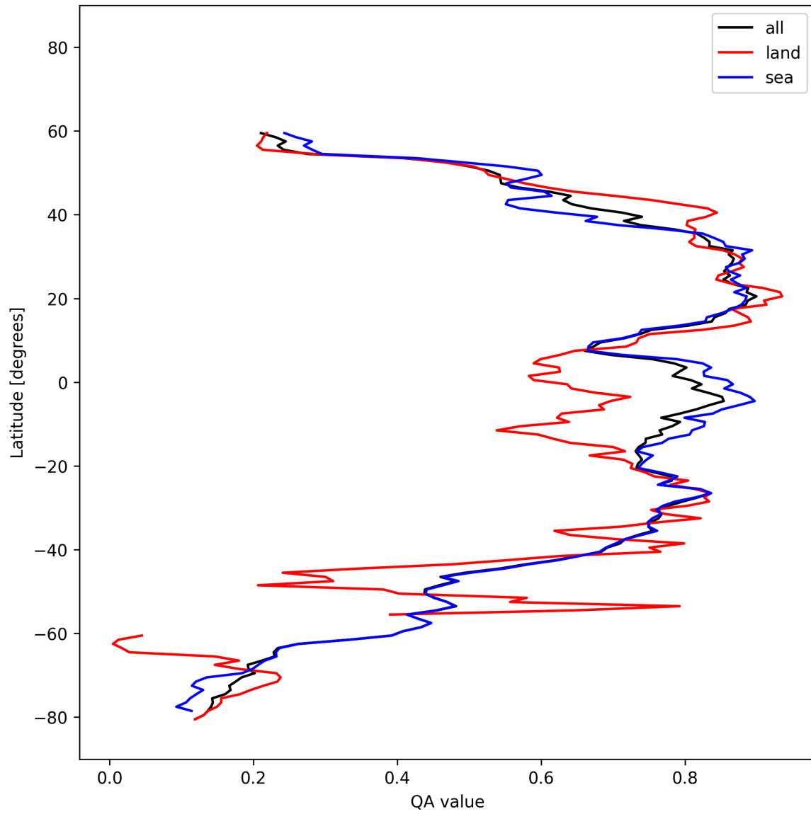
Figure 31: Zonal average of “QA value” for 2025-10-19 to 2025-10-21.
