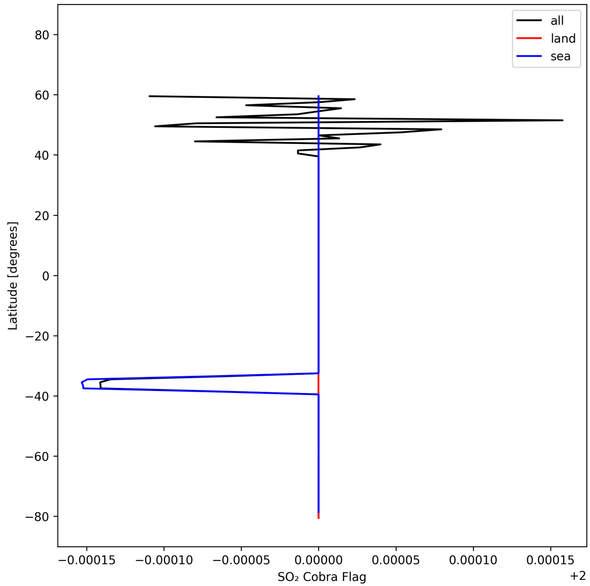
Figure 49: Zonal average of “SO 2 Cobra Flag” for 2025-10-19 to 2025-10-21.
