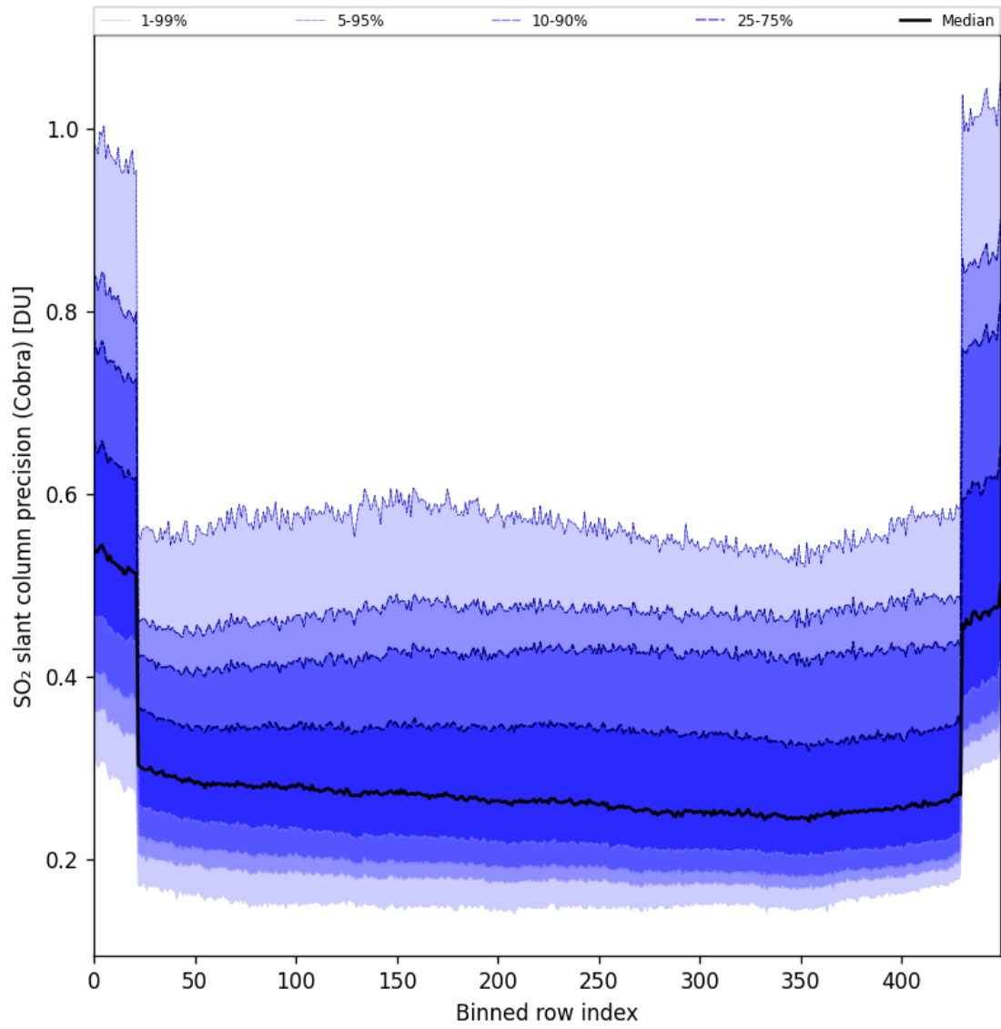
Figure 88: Along track statistics of “SO 2 slant column precision (Cobra)” for 2025-10-19 to 2025-10-21
