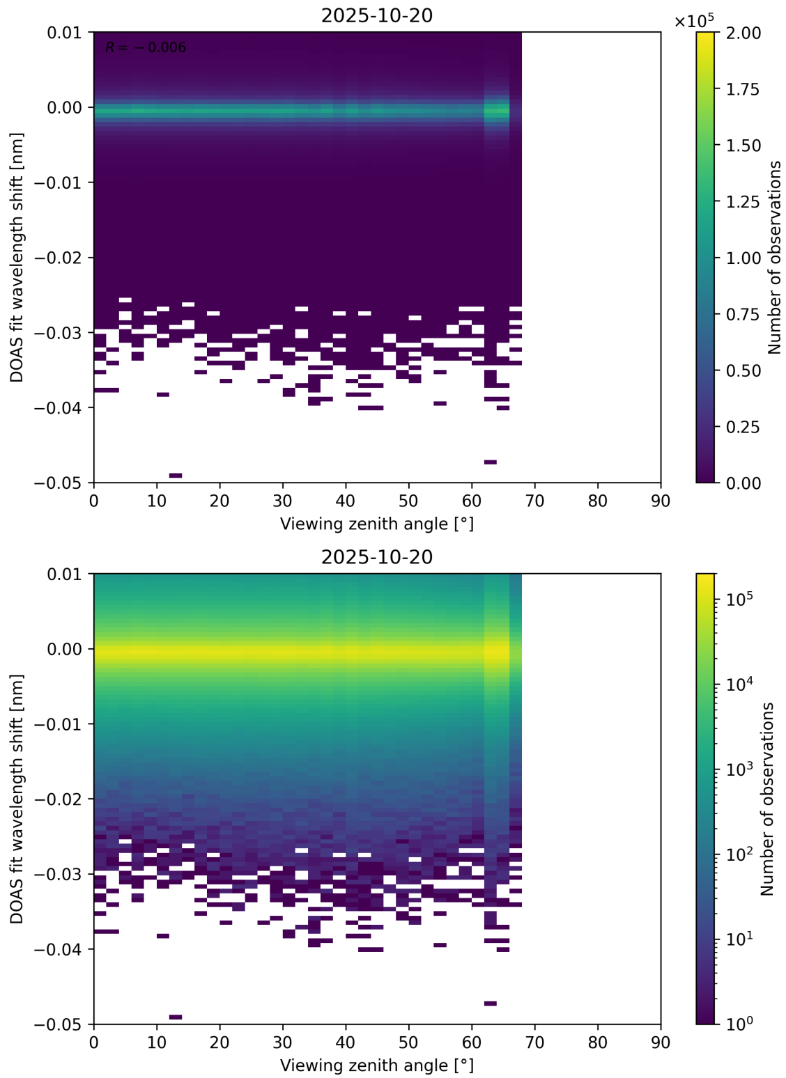
Figure 365: Scatter density plot of “Viewing zenith angle” against “DOAS fit wavelength shift” for 2025-10-19 to 2025-10-21.
