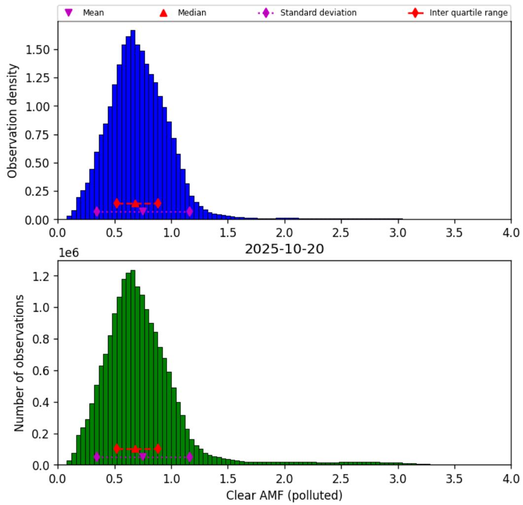
Figure 81: Histogram of “Clear AMF (polluted)” for 2025-10-19 to 2025-10-21
