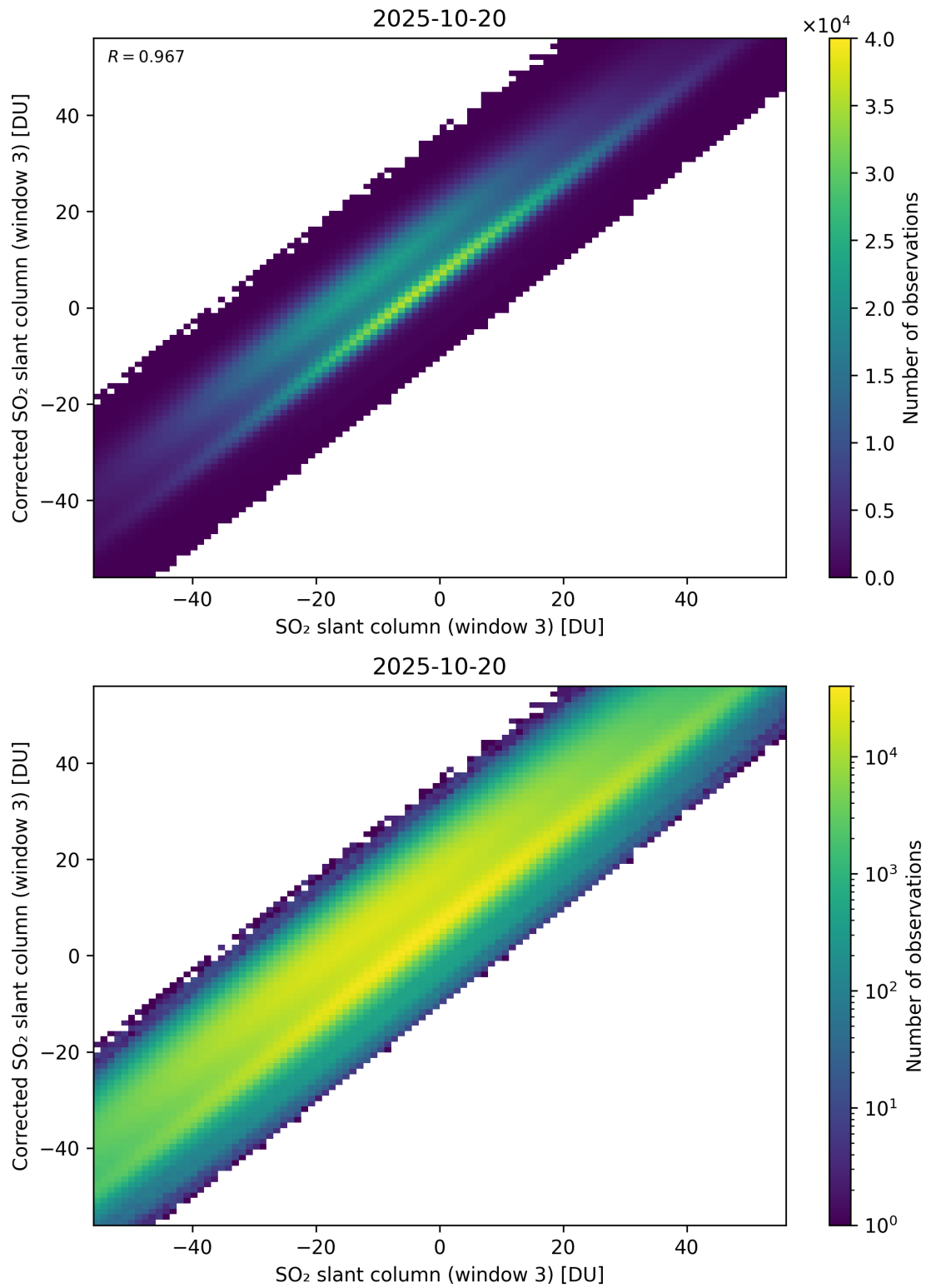
Figure 316: Scatter density plot of “SO 2 slant column (window 3)” against “Corrected SO 2 slant column (window 3)” for 2025-10-19 to 2025-10-21.
