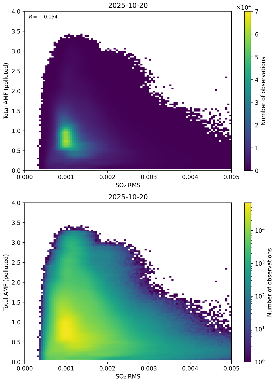
Figure 148: Scatter density plot of “SO 2 RMS” against “Total AMF (polluted)” for 2025-10-19 to 2025-10-21.
