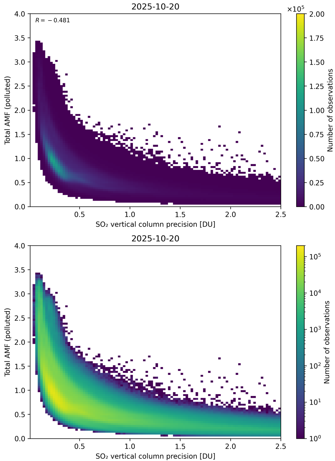
Figure 346: Scatter density plot of “SO 2 vertical column precision” against “Total AMF (polluted)” for 2025-10-19 to 2025-10-21.
