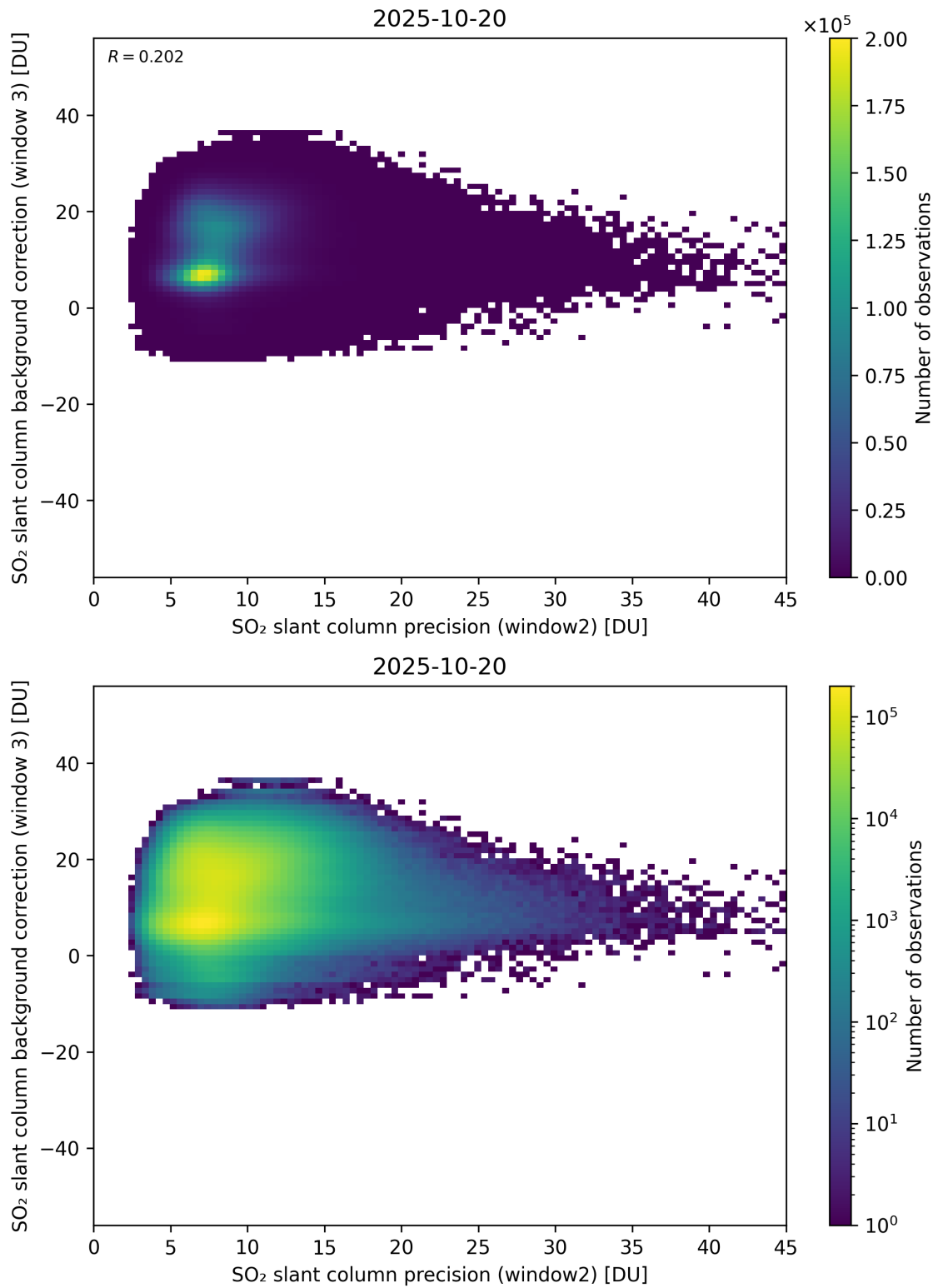
Figure 292: Scatter density plot of “SO 2 slant column precision (window2)” against “SO 2 slant column background correction (window 3)” for 2025-10-19 to 2025-10-21.
