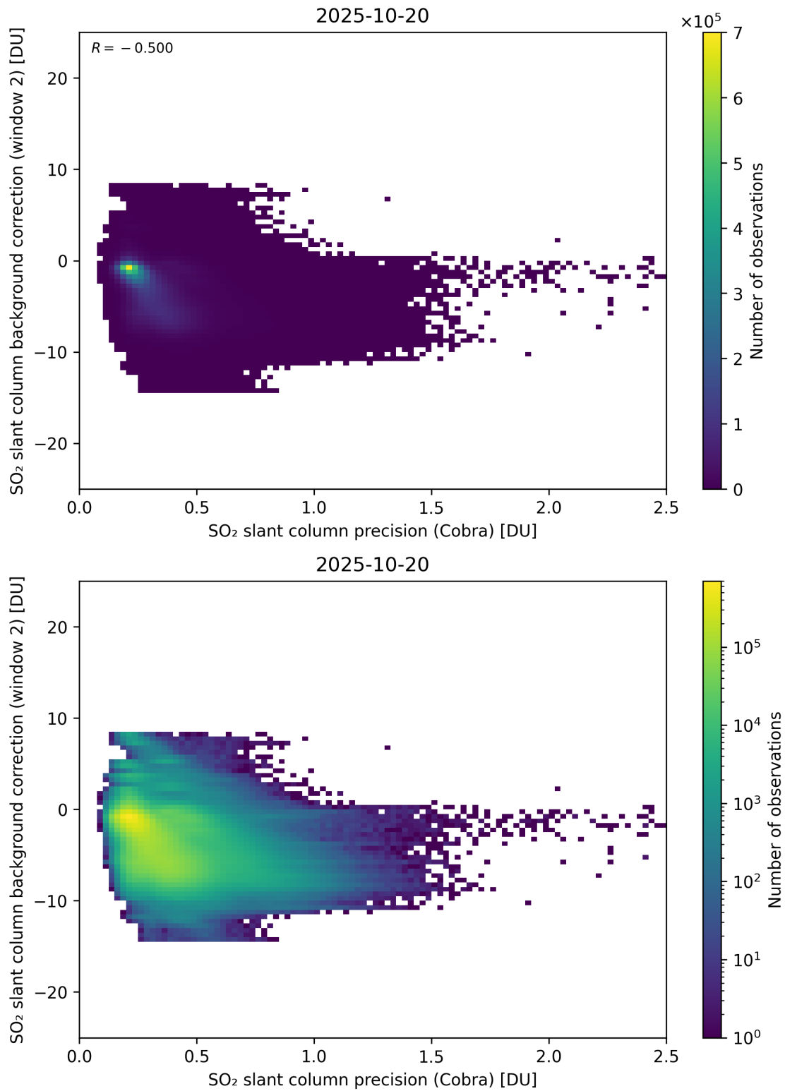
Figure 200: Scatter density plot of “SO 2 slant column precision (Cobra)” against “SO 2 slant column background correction (window 2)” for 2025-10-19 to 2025-10-21.
