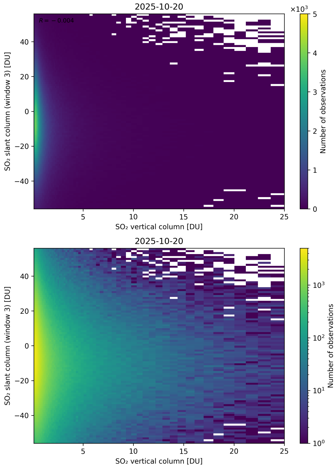
Figure 357: Scatter density plot of “SO 2 vertical column” against “SO 2 slant column (window 3)” for 2025-10-19 to 2025-10-21.
