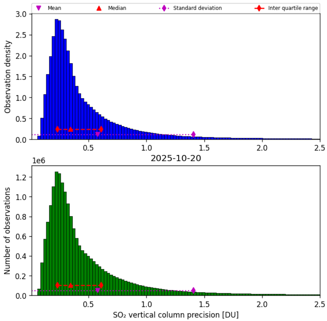
Figure 59: Histogram of “SO 2 vertical column precision” for 2025-10-19 to 2025-10-21
