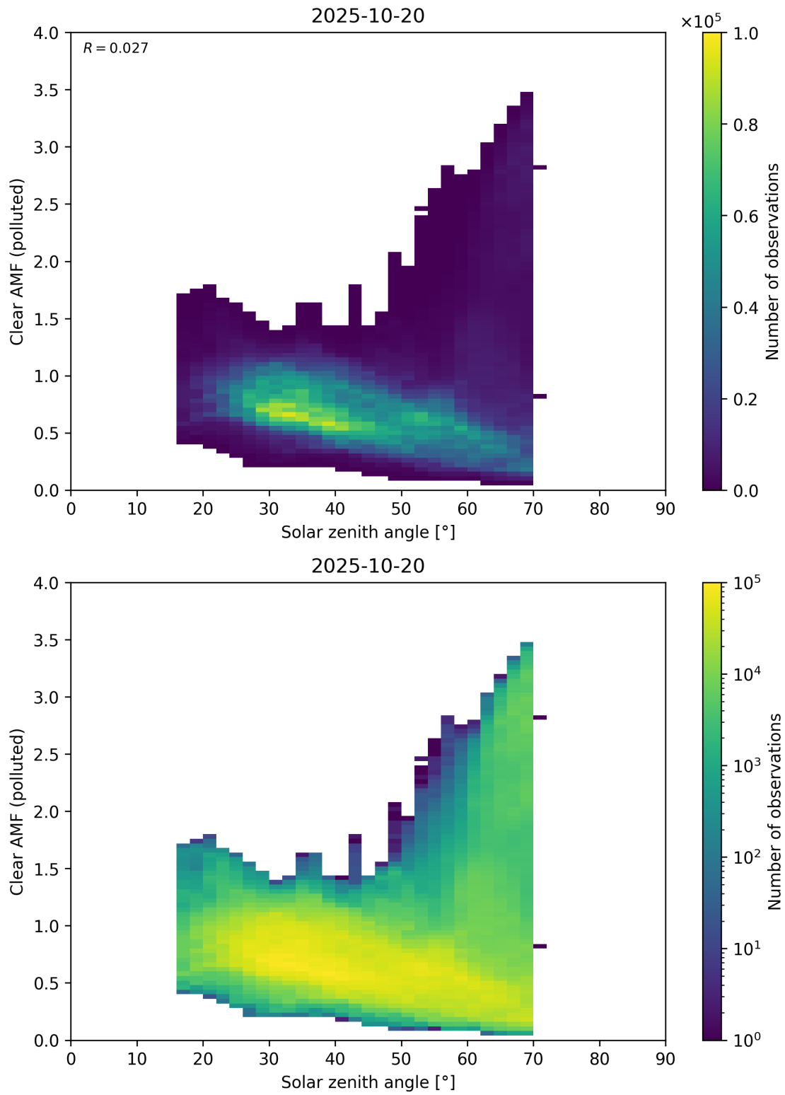
Figure 178: Scatter density plot of “Solar zenith angle” against “Clear AMF (polluted)” for 2025-10-19 to 2025-10-21.
