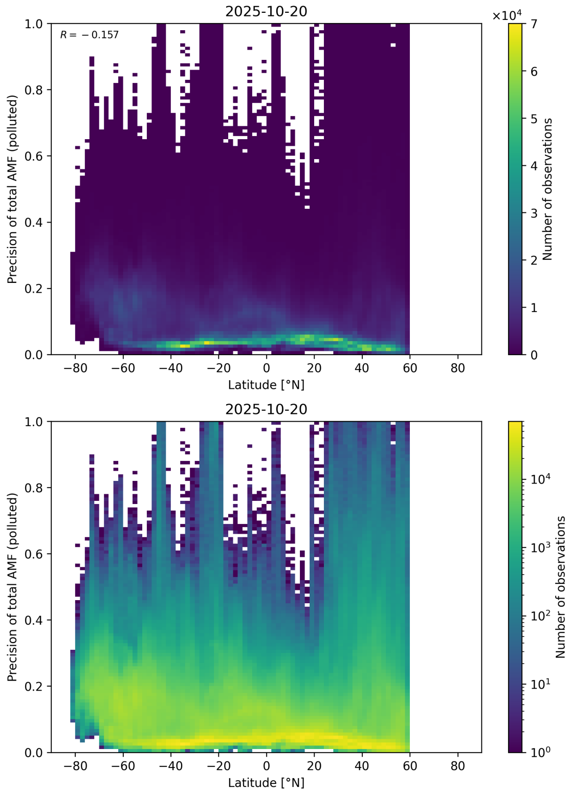
Figure 168: Scatter density plot of “Latitude” against “Precision of total AMF (polluted)” for 2025-10-19 to 2025-10-21.
