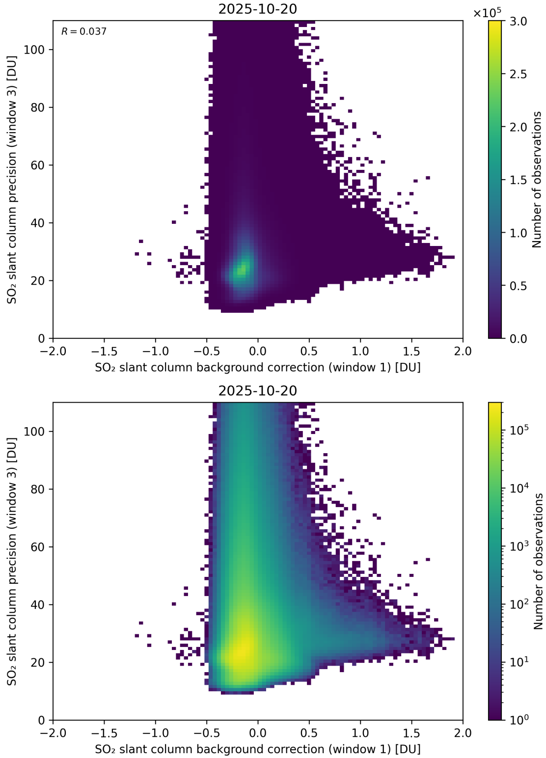
Figure 119: Scatter density plot of “SO 2 slant column background correction (window 1)” against “SO 2 slant column precision (window 3)” for 2025-10-19 to 2025-10-21.
