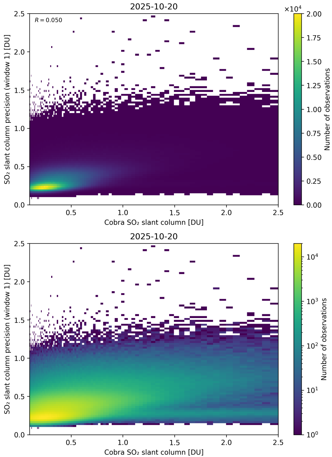
Figure 220: Scatter density plot of “Cobra SO 2 slant column” against “SO 2 slant column precision (window 1)” for 2025-10-19 to 2025-10-21.
