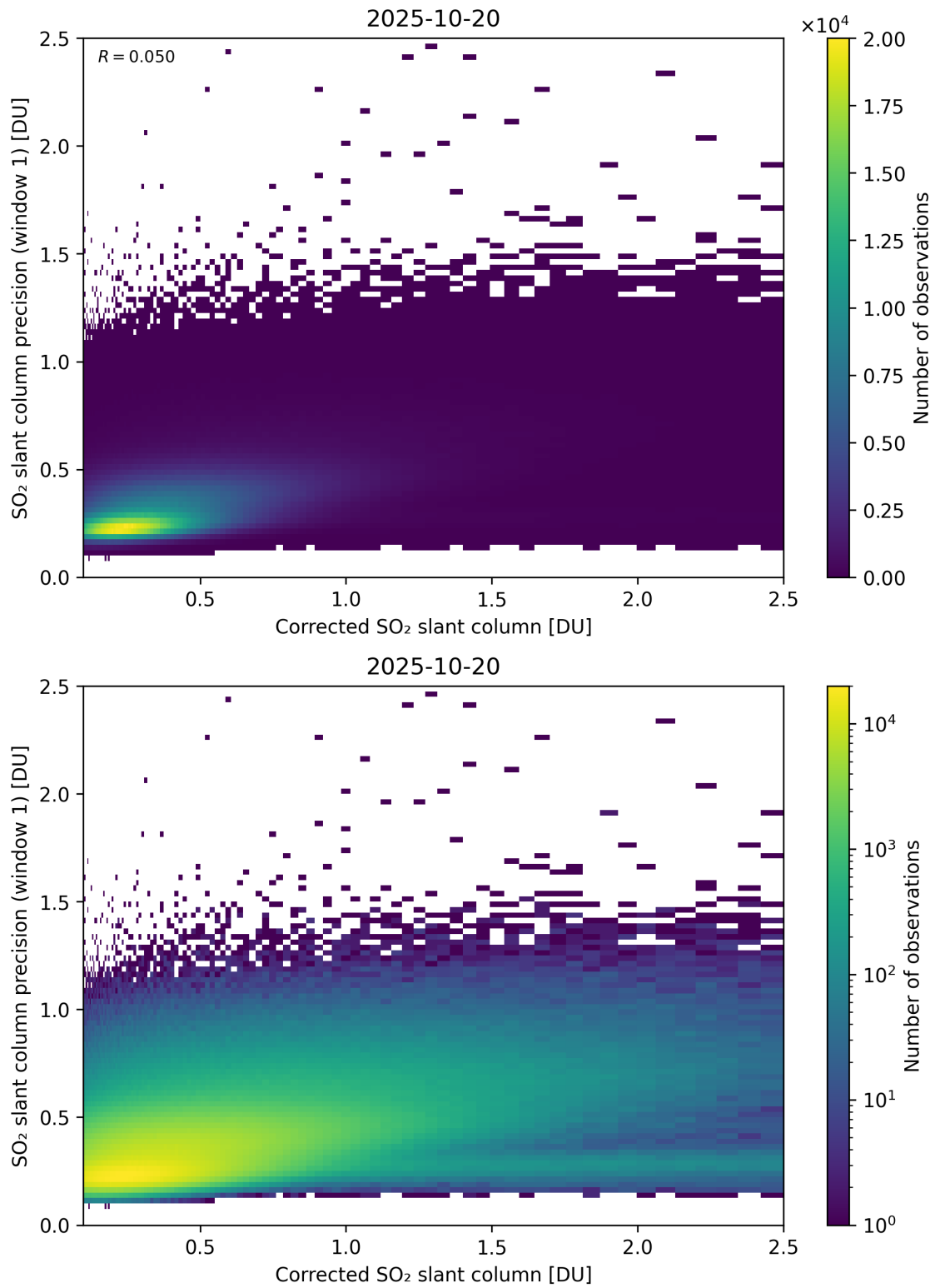
Figure 238: Scatter density plot of “Corrected SO 2 slant column” against “SO 2 slant column precision (window 1)” for 2025-10-19 to 2025-10-21.
