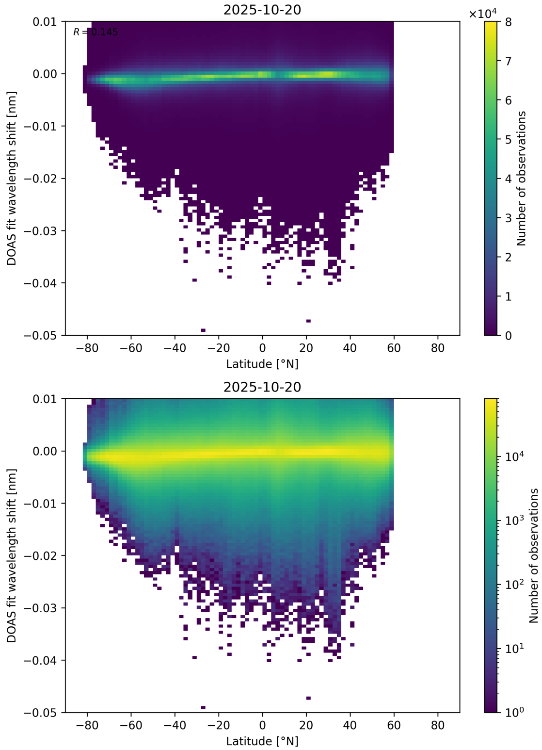
Figure 153: Scatter density plot of “Latitude” against “DOAS fit wavelength shift” for 2025-10-19 to 2025-10-21.
