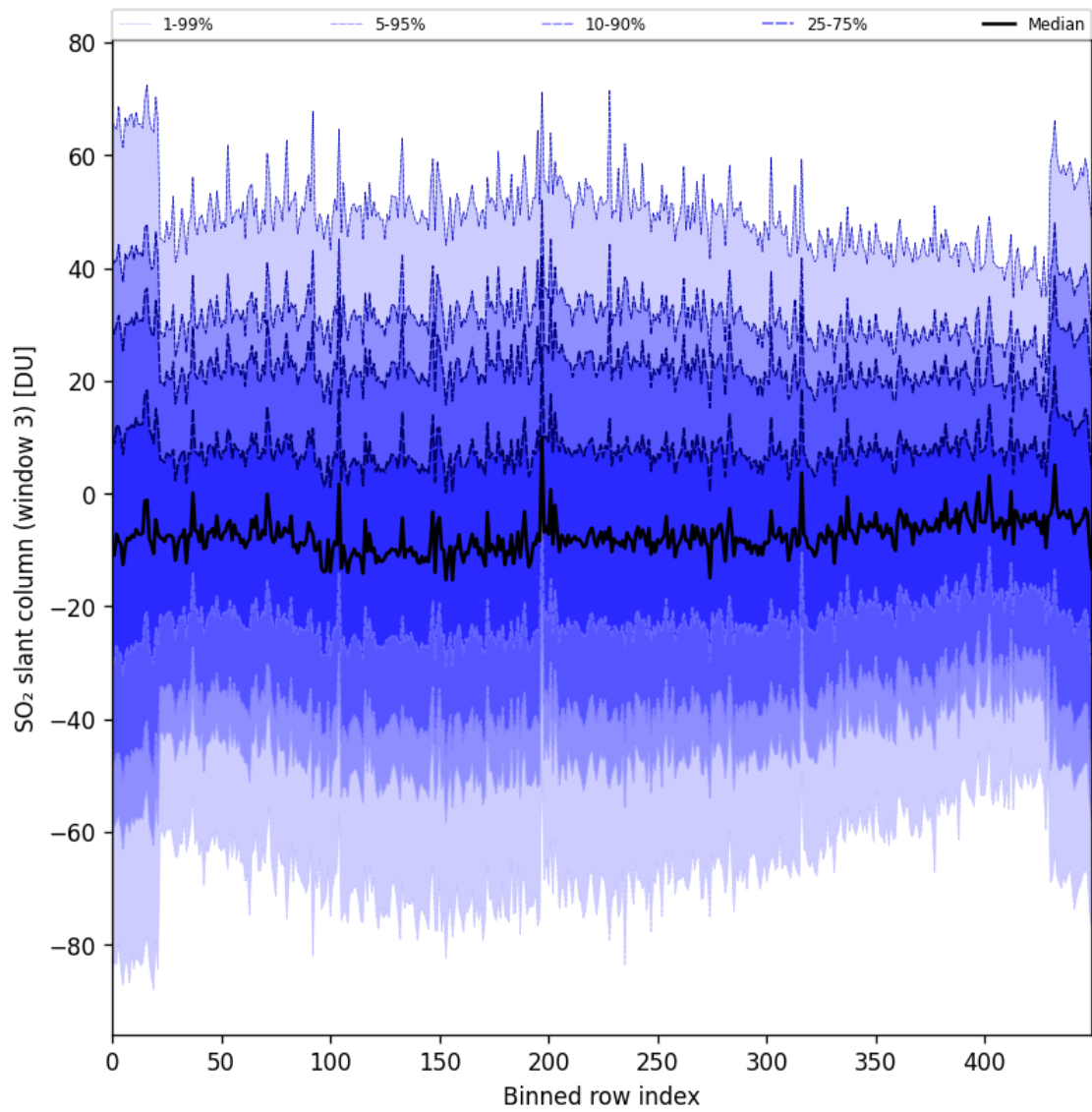
Figure 97: Along track statistics of “SO 2 slant column (window 3)” for 2025-10-19 to 2025-10-21
