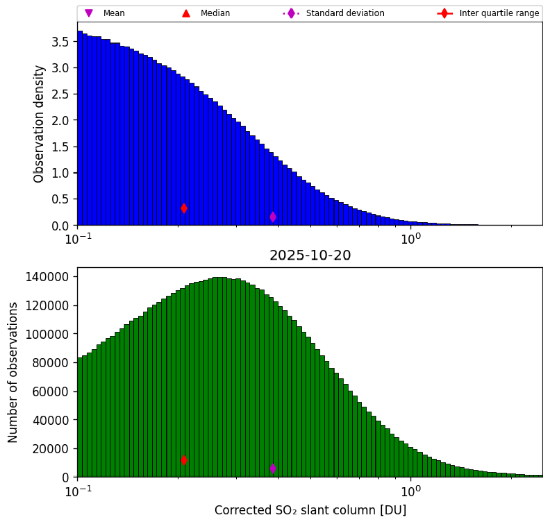
Figure 60: Histogram of “Corrected SO 2 slant column” for 2025-10-19 to 2025-10-21
