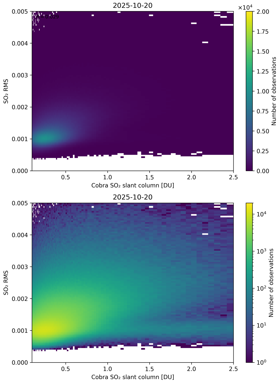
Figure 198: Scatter density plot of “Cobra SO 2 slant column” against “SO 2 RMS” for 2025-10-19 to 2025-10-21.
