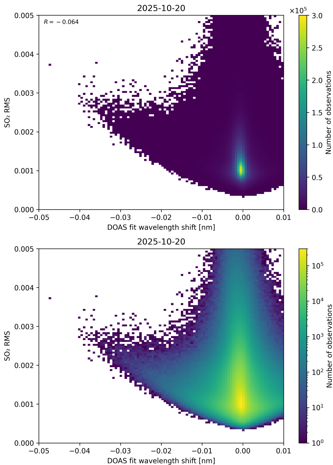
Figure 139: Scatter density plot of “DOAS fit wavelength shift” against “SO 2 RMS” for 2025-10-19 to 2025-10-21.
