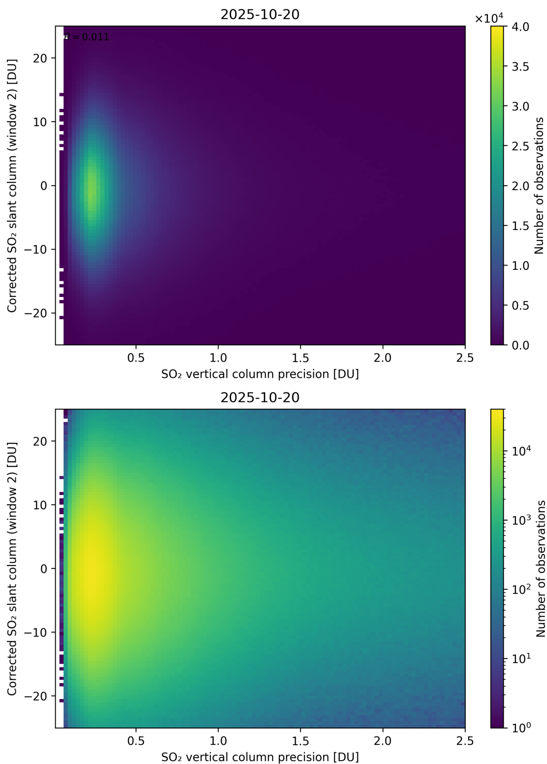
Figure 339: Scatter density plot of “SO 2 vertical column precision” against “Corrected SO 2 slant column (window 2)” for 2025-10-19 to 2025-10-21.
