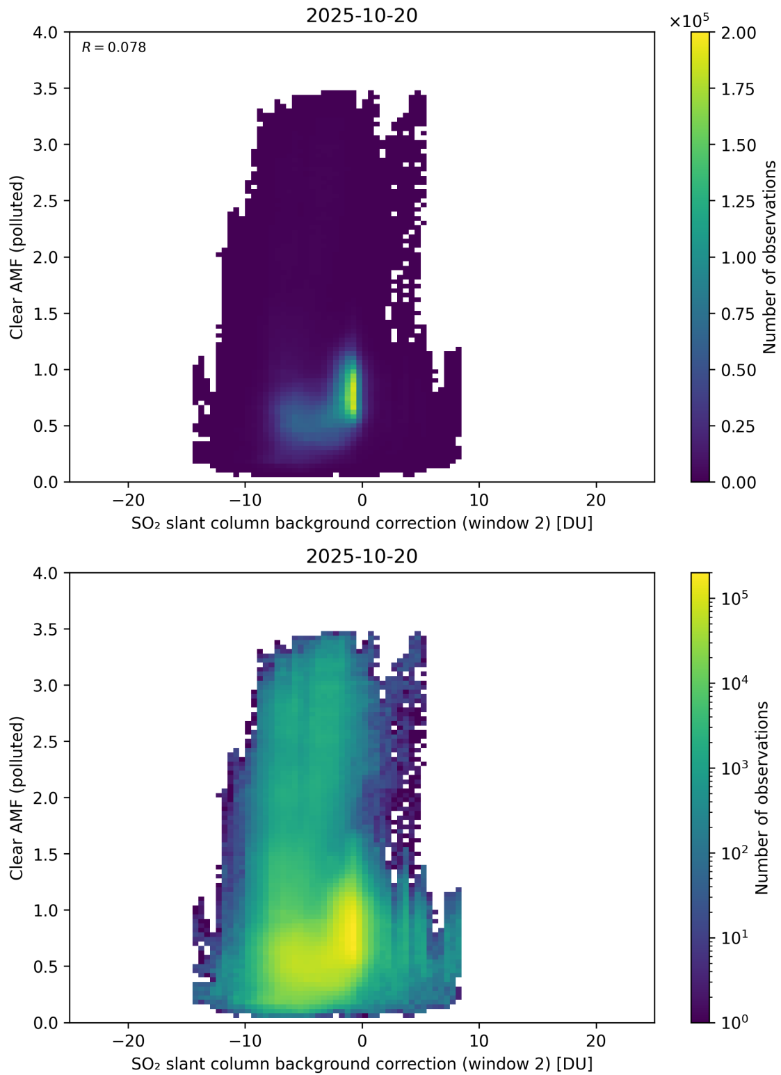
Figure 126: Scatter density plot of “SO 2 slant column background correction (window 2)” against “Clear AMF (polluted)” for 2025-10-19 to 2025-10-21.
