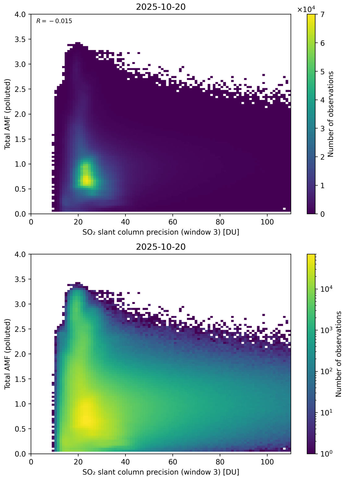
Figure 313: Scatter density plot of “SO 2 slant column precision (window 3)” against “Total AMF (polluted)” for 2025-10-19 to 2025-10-21.
