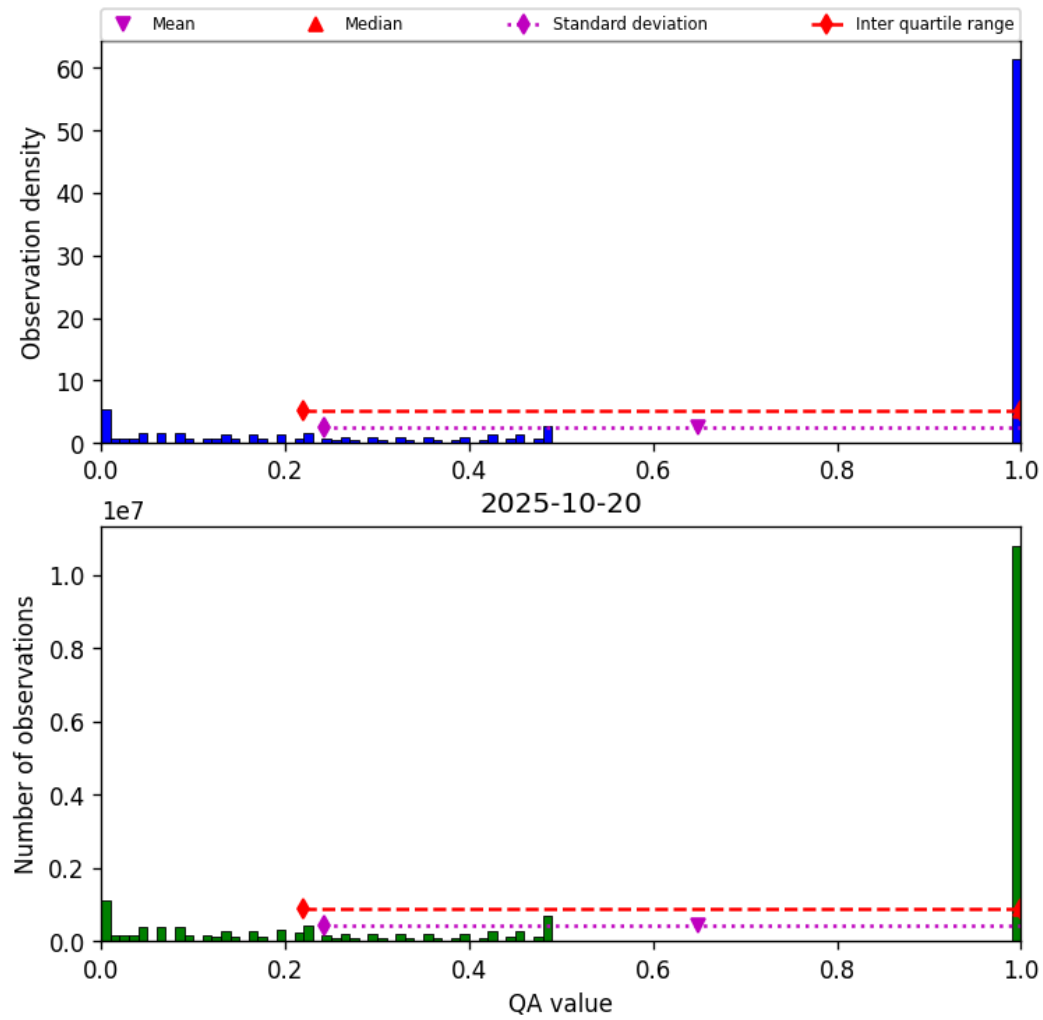
Figure 57: Histogram of “QA value” for 2025-10-19 to 2025-10-21
