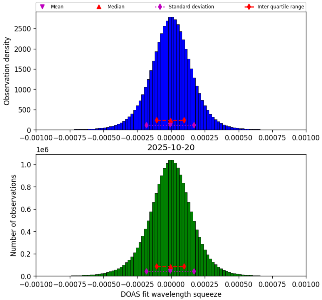
Figure 77: Histogram of “DOAS fit wavelength squeeze” for 2025-10-19 to 2025-10-21
