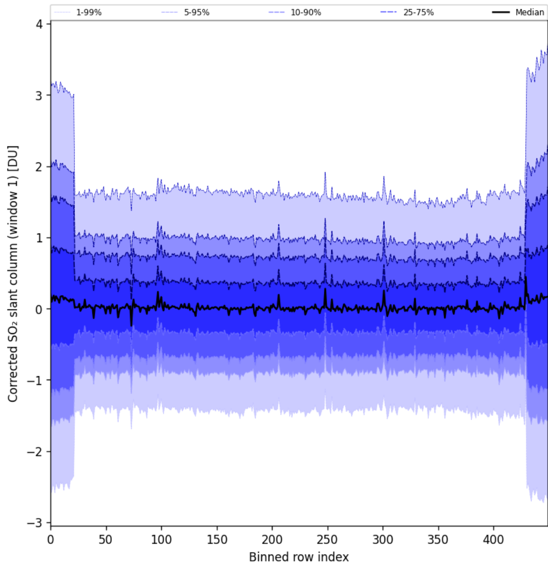
Figure 91: Along track statistics of “Corrected SO 2 slant column (window 1)” for 2025-10-19 to 2025-10-21
