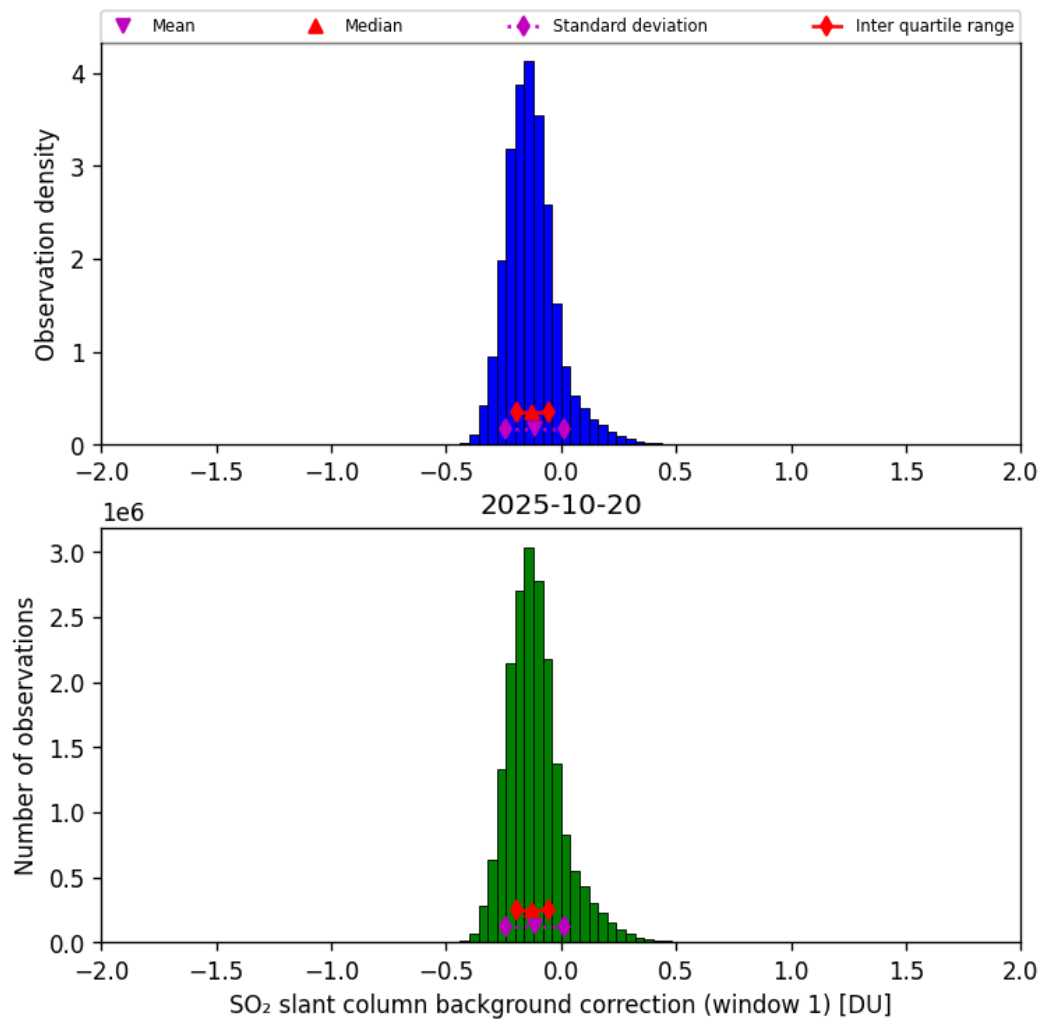
Figure 66: Histogram of “SO 2 slant column background correction (window 1)” for 2025-10-19 to 2025-10-21
