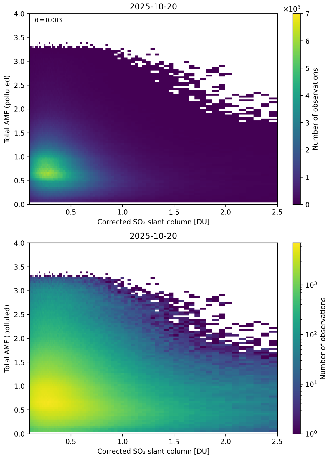
Figure 242: Scatter density plot of “Corrected SO 2 slant column” against “Total AMF (polluted)” for 2025-10-19 to 2025-10-21.
