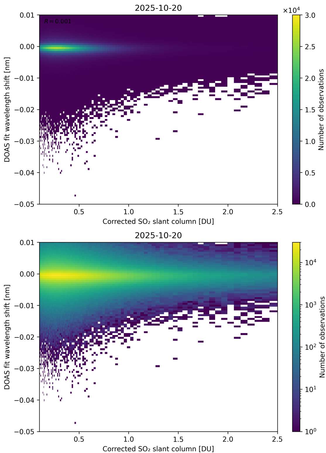
Figure 229: Scatter density plot of “Corrected SO 2 slant column” against “DOAS fit wavelength shift” for 2025-10-19 to 2025-10-21.
