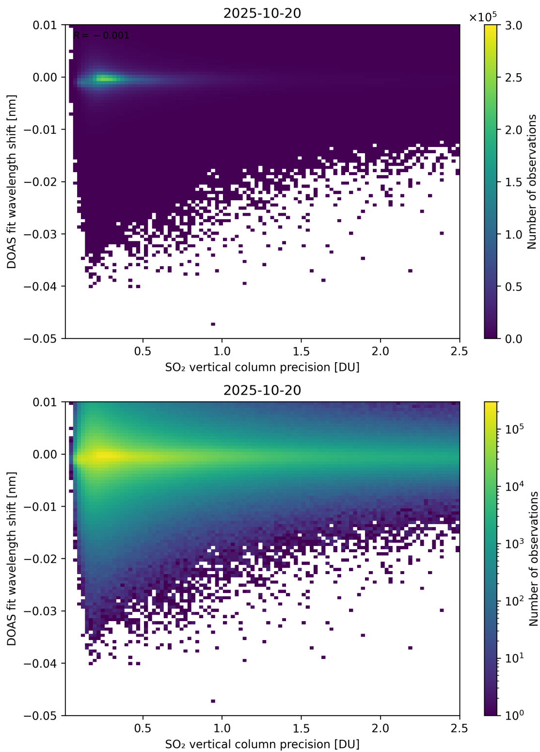
Figure 332: Scatter density plot of “SO 2 vertical column precision” against “DOAS fit wavelength shift” for 2025-10-19 to 2025-10-21.
