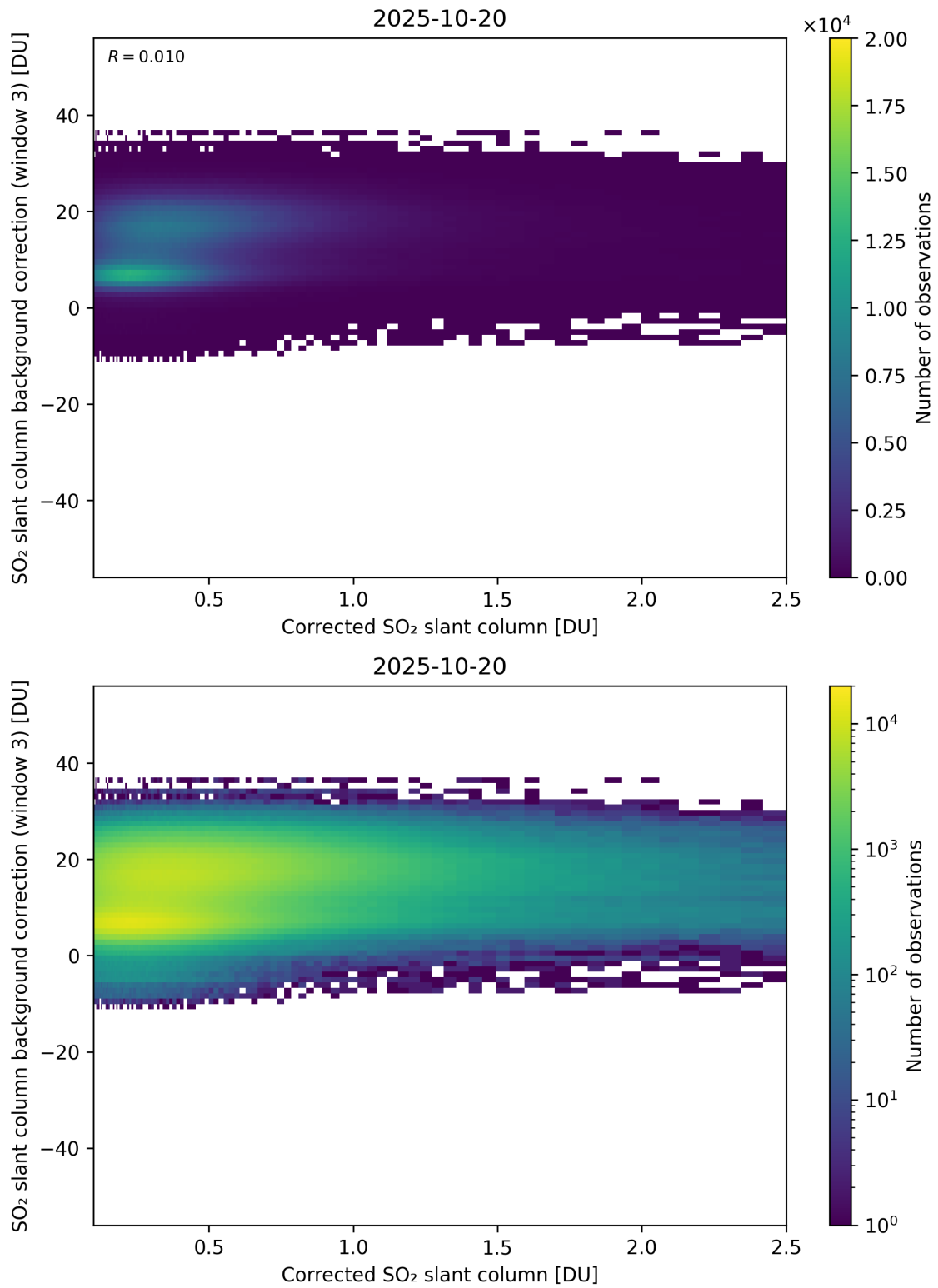
Figure 228: Scatter density plot of “Corrected SO 2 slant column” against “SO 2 slant column background correction (window 3)” for 2025-10-19 to 2025-10-21.
