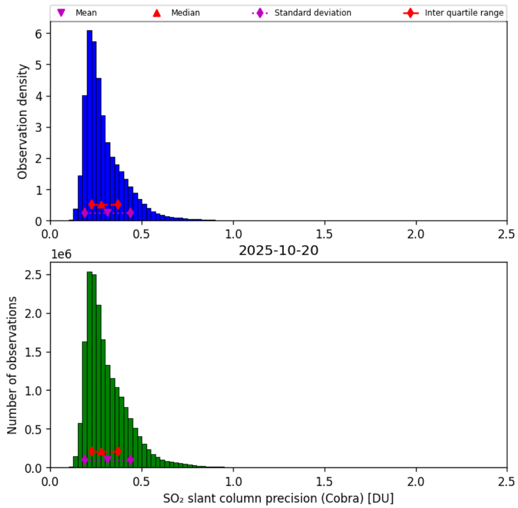
Figure 62: Histogram of “SO 2 slant column precision (Cobra)” for 2025-10-19 to 2025-10-21
