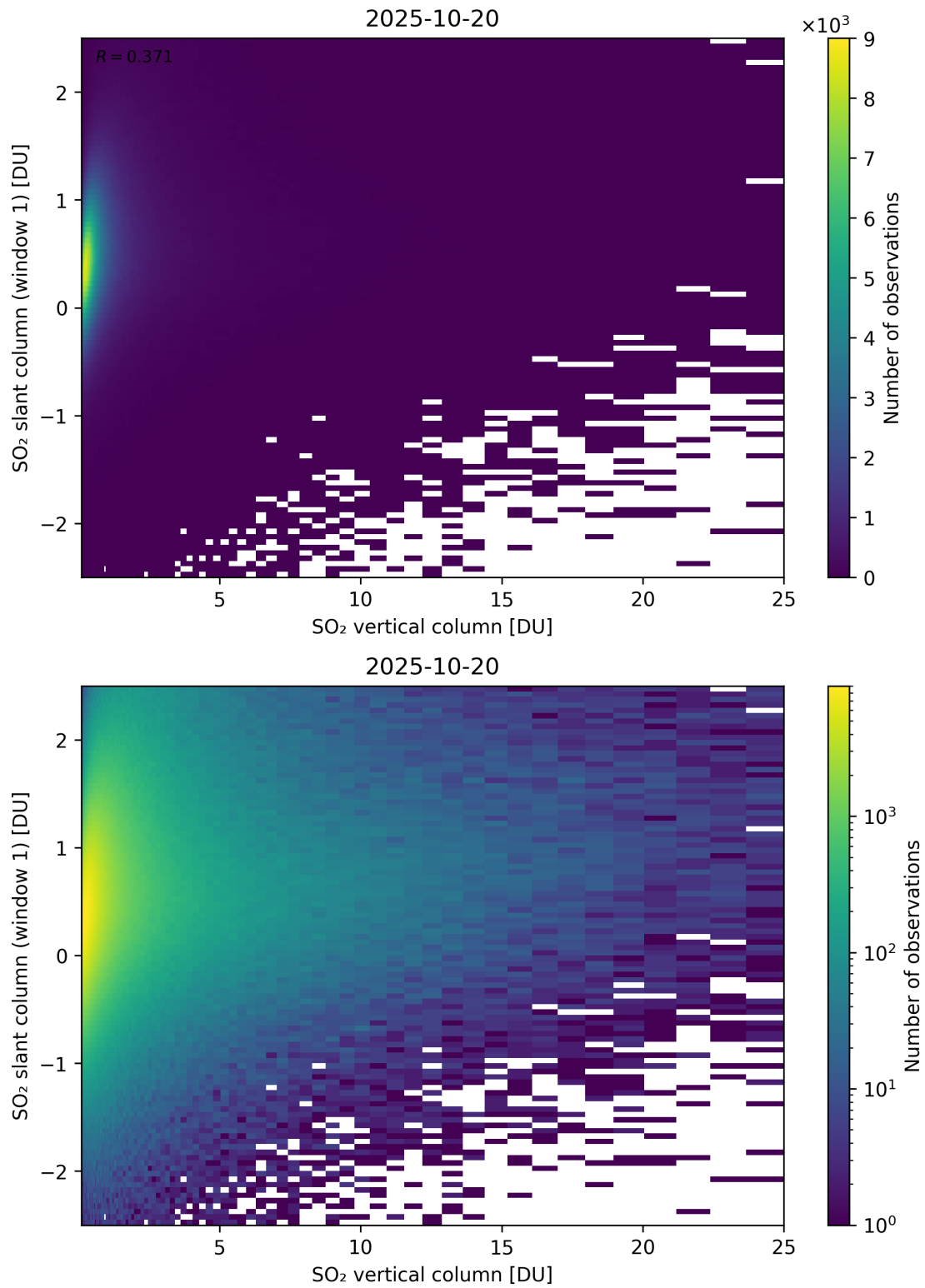
Figure 354: Scatter density plot of “SO 2 vertical column” against “SO 2 slant column (window 1)” for 2025-10-19 to 2025-10-21.
