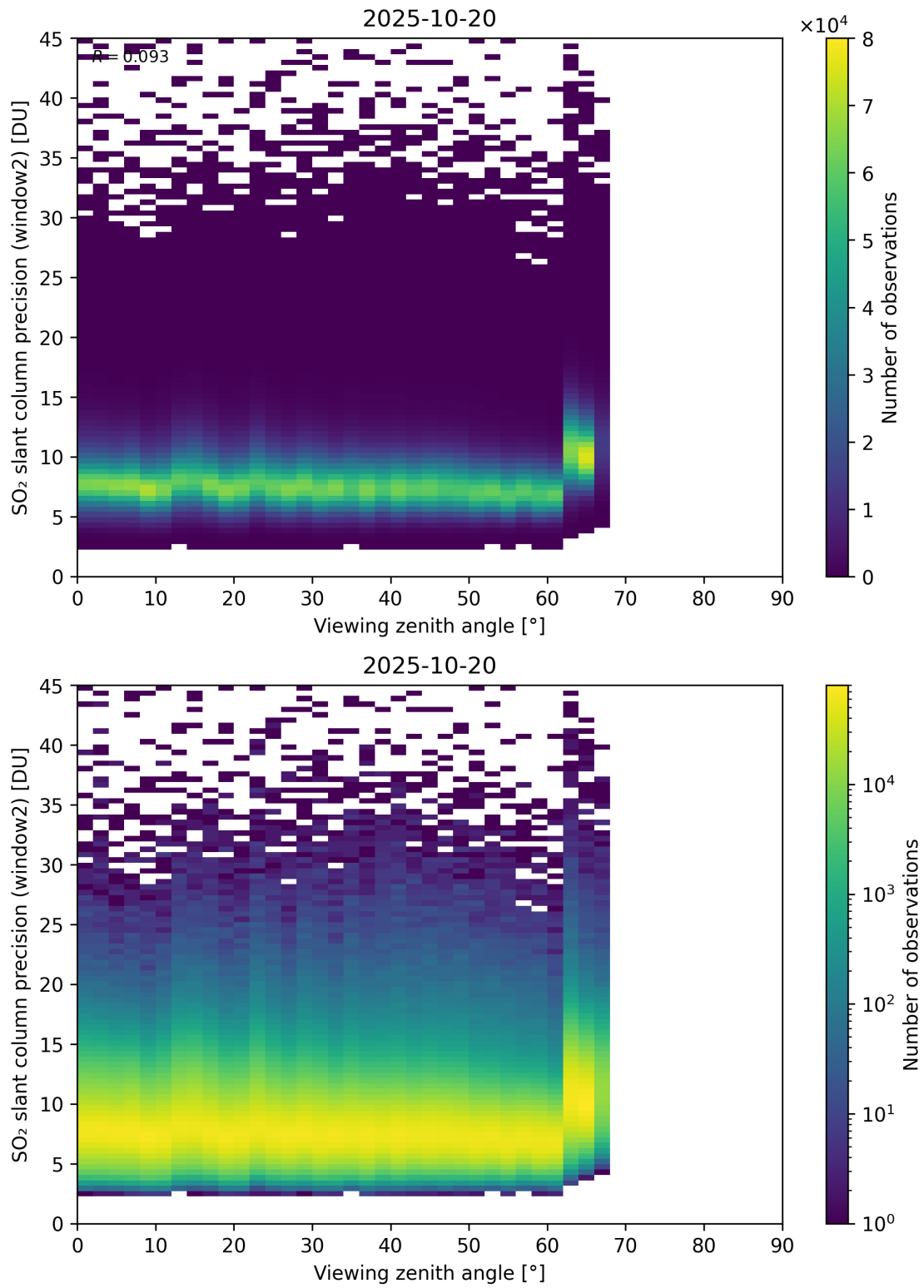
Figure 378: Scatter density plot of “Viewing zenith angle” against “SO 2 slant column precision (window2)” for 2025-10-19 to 2025-10-21.
