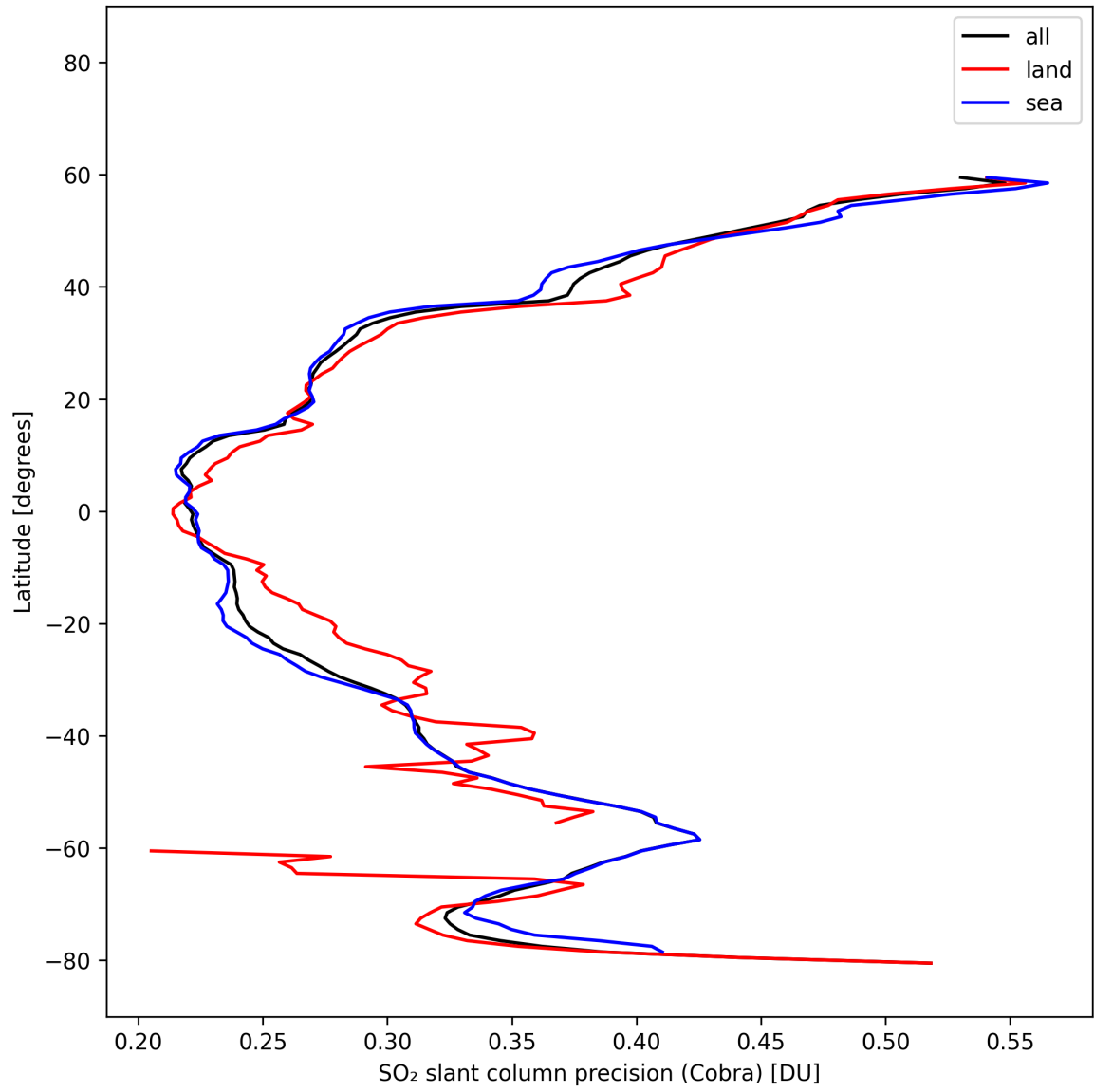
Figure 36: Zonal average of “SO 2 slant column precision (Cobra)” for 2025-10-19 to 2025-10-21.
