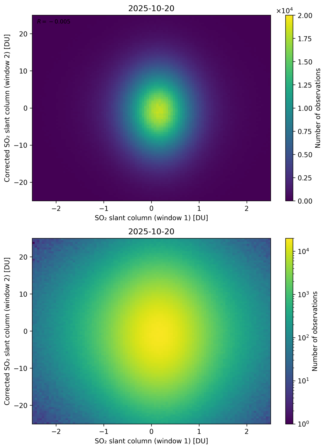
Figure 283: Scatter density plot of “SO 2 slant column (window 1)” against “Corrected SO 2 slant column (window 2)” for 2025-10-19 to 2025-10-21.
