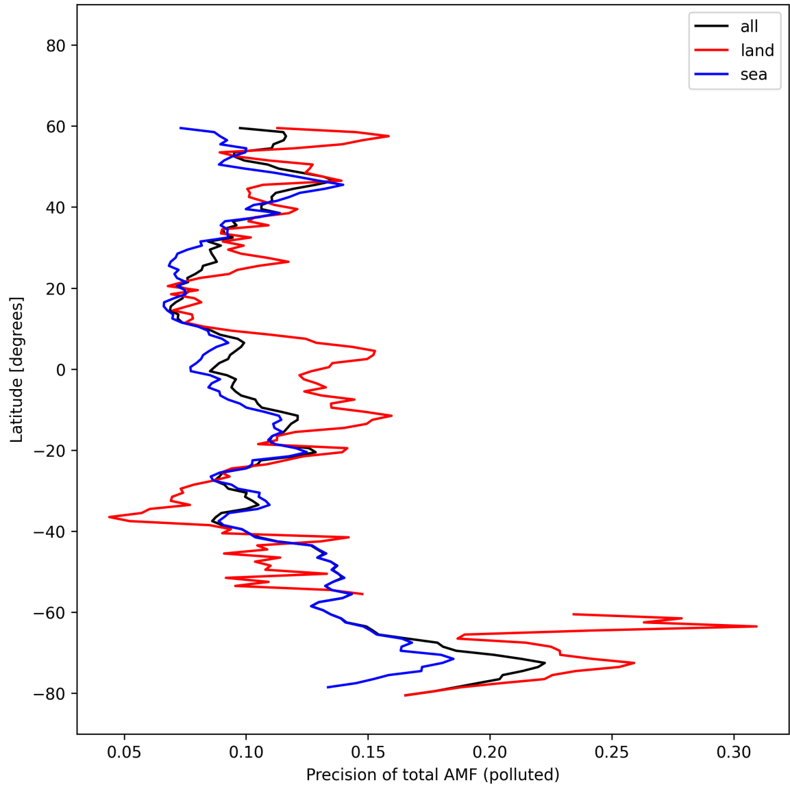
Figure 54: Zonal average of “Precision of total AMF (polluted)” for 2025-10-19 to 2025-10-21.
