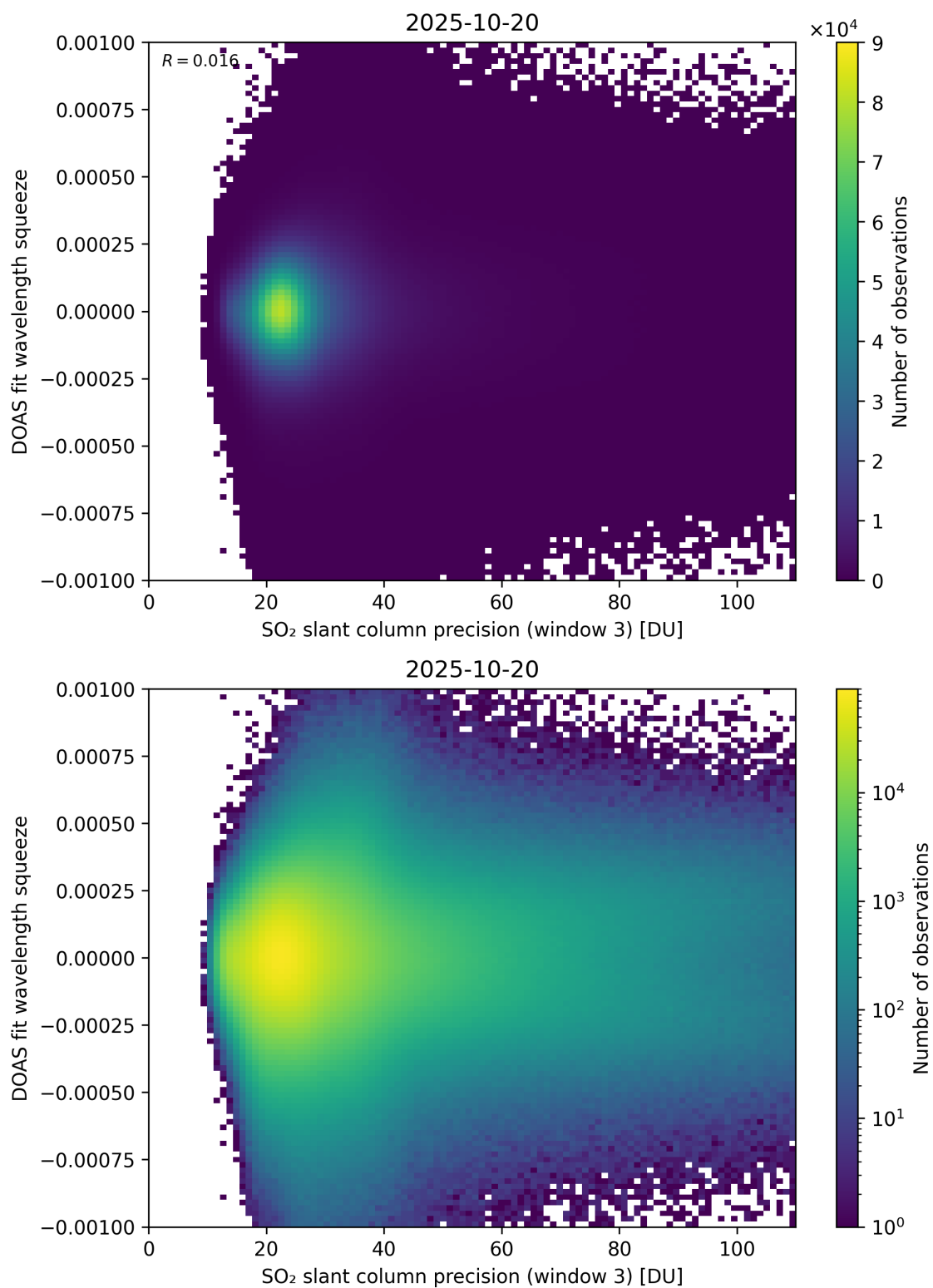
Figure 309: Scatter density plot of “SO 2 slant column precision (window 3)” against “DOAS fit wavelength squeeze” for 2025-10-19 to 2025-10-21.
