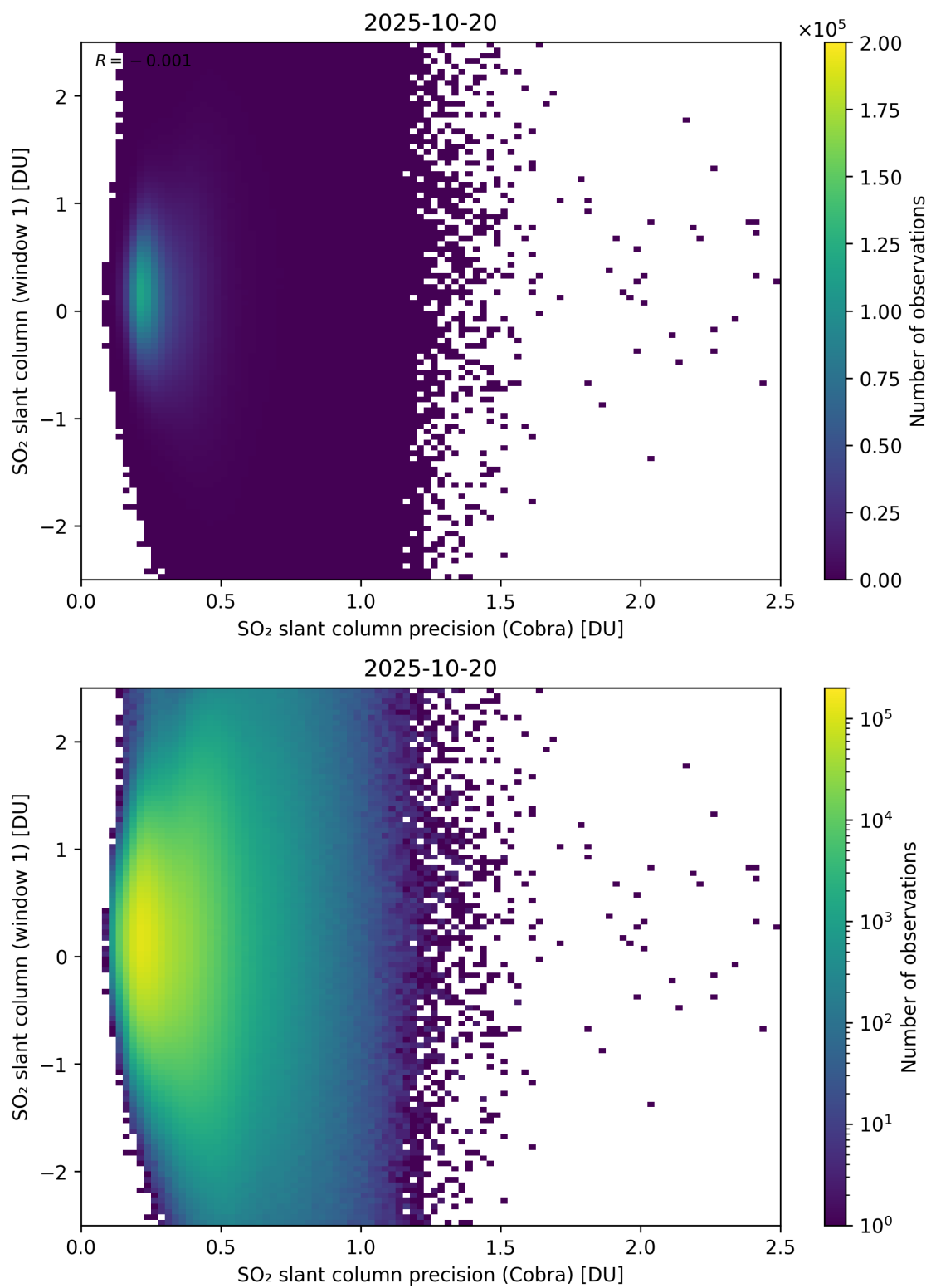
Figure 208: Scatter density plot of “SO 2 slant column precision (Cobra)” against “SO 2 slant column (window 1)” for 2025-10-19 to 2025-10-21.
