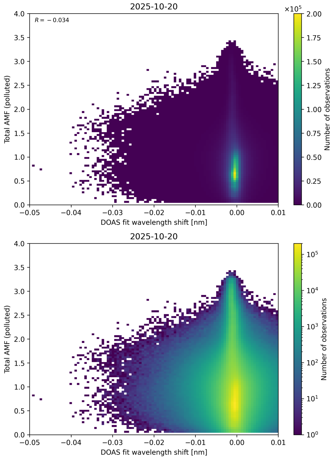
Figure 141: Scatter density plot of “DOAS fit wavelength shift” against “Total AMF (polluted)” for 2025-10-19 to 2025-10-21.
