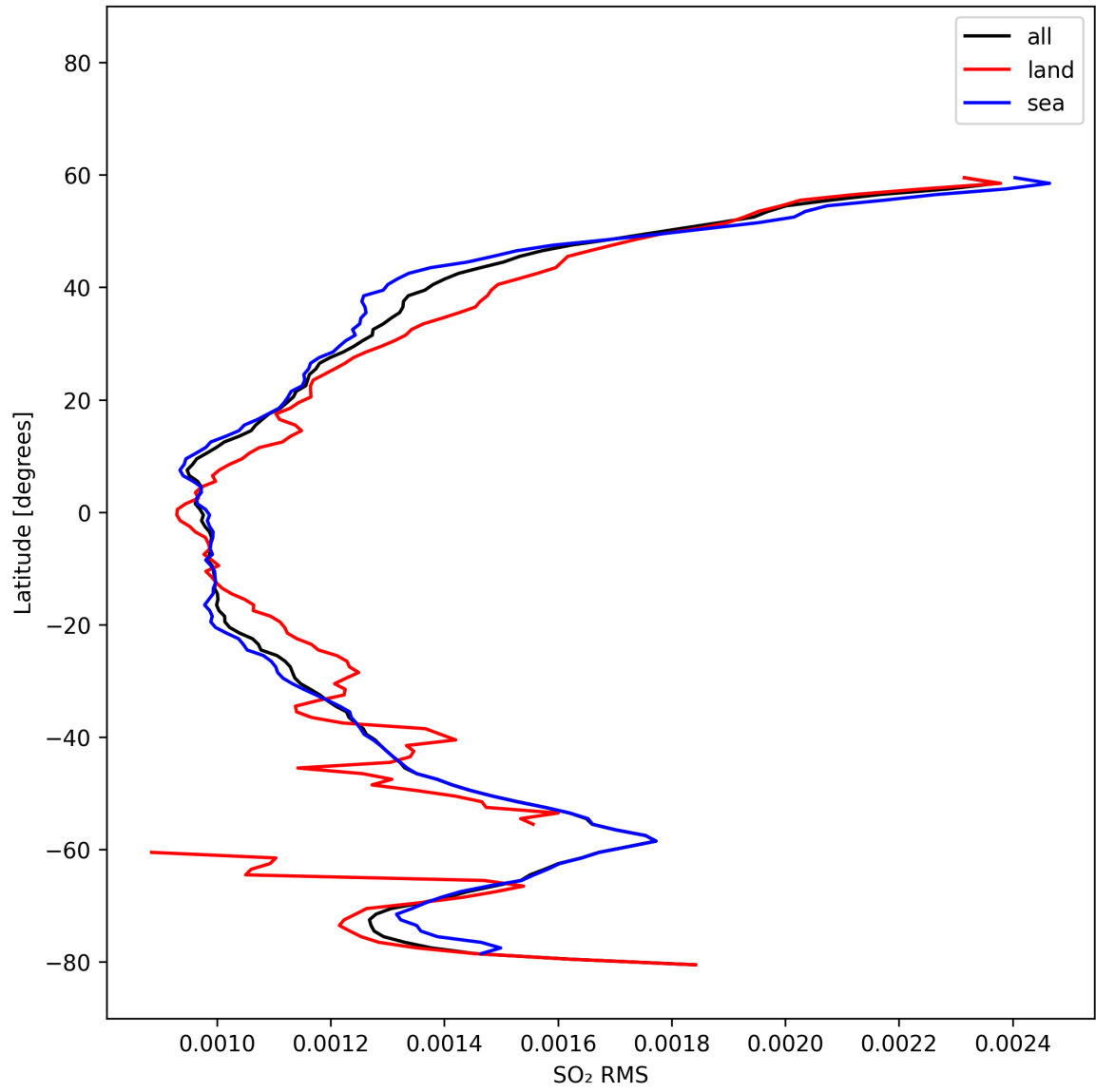
Figure 52: Zonal average of “SO 2 RMS” for 2025-10-19 to 2025-10-21.
