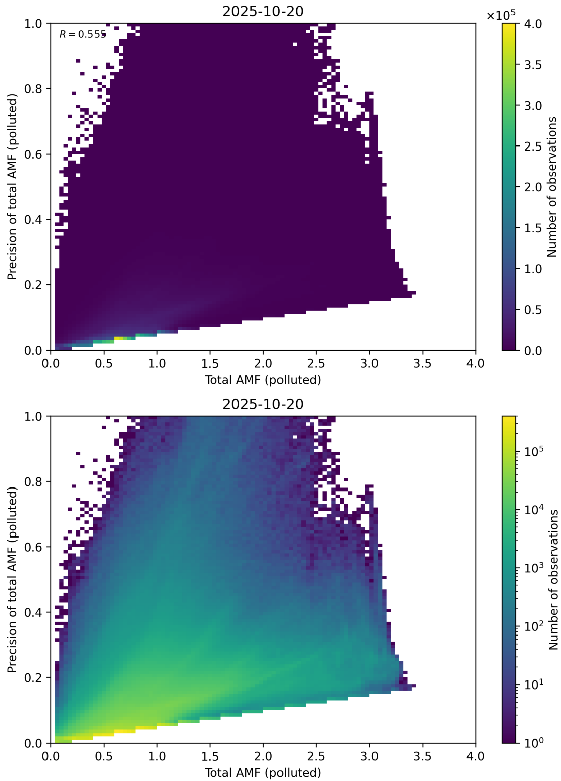
Figure 322: Scatter density plot of “Total AMF (polluted)” against “Precision of total AMF (polluted)” for 2025-10-19 to 2025-10-21.
