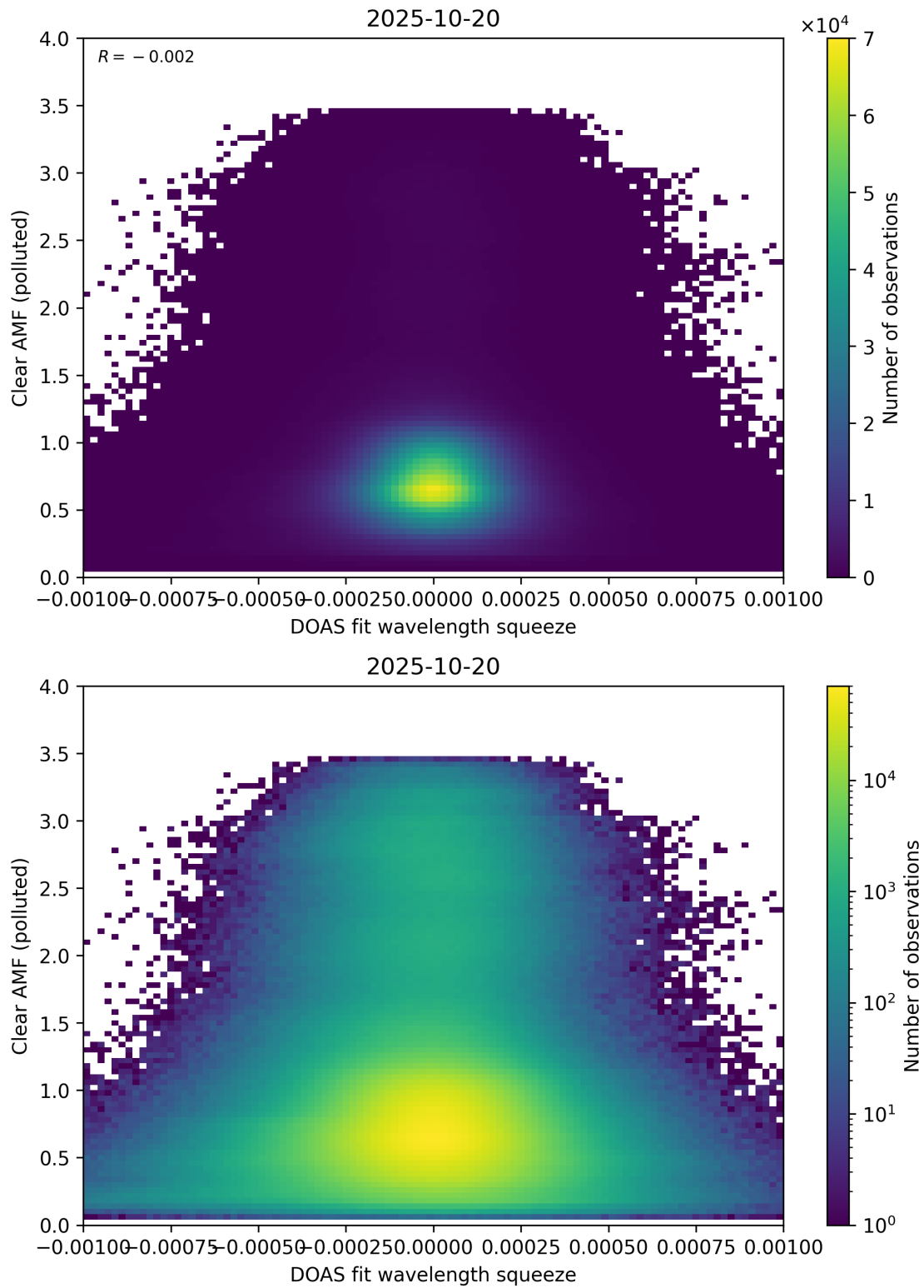
Figure 144: Scatter density plot of “DOAS fit wavelength squeeze” against “Clear AMF (polluted)” for 2025-10-19 to 2025-10-21.
