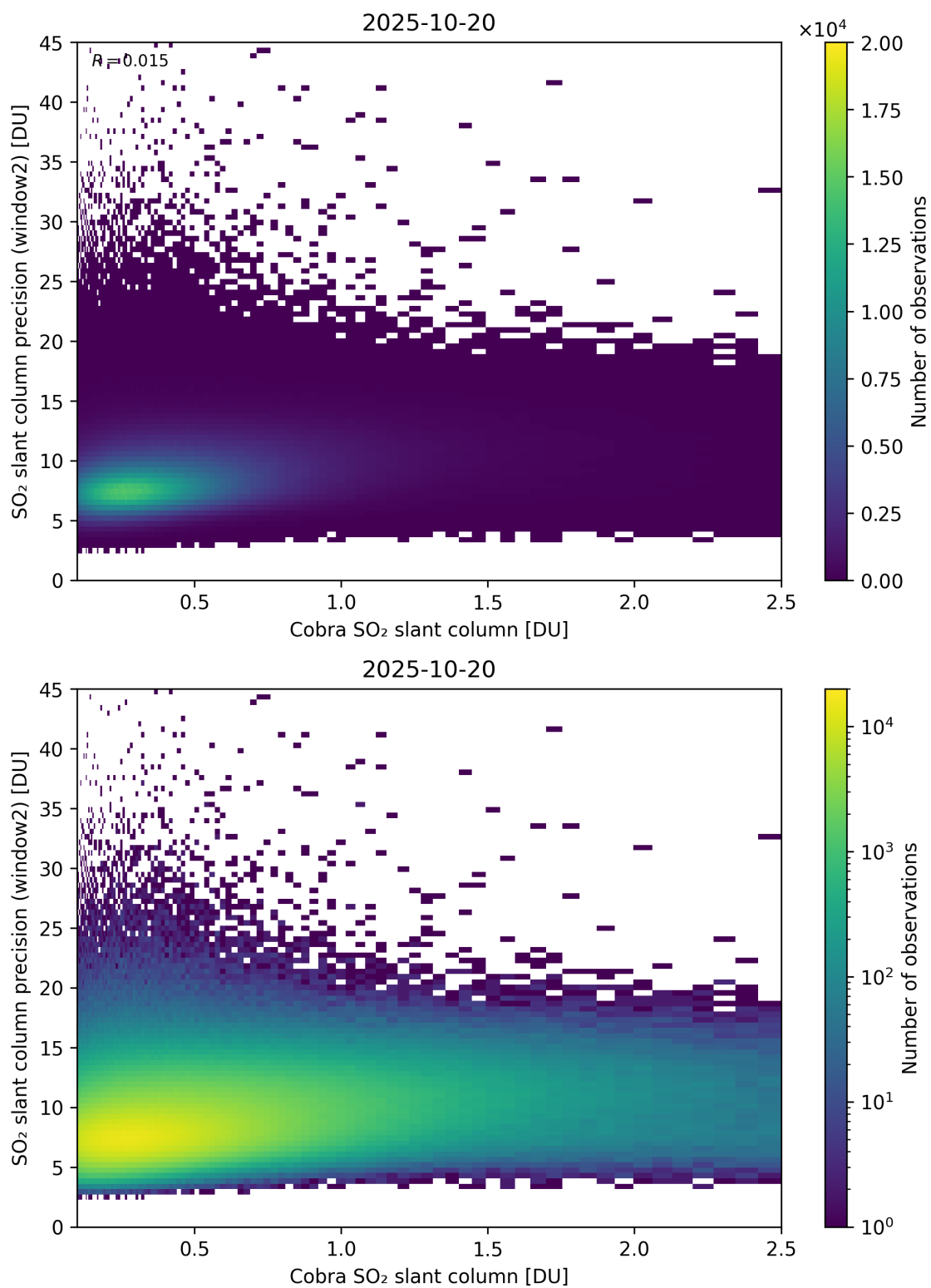
Figure 221: Scatter density plot of “Cobra SO 2 slant column” against “SO 2 slant column precision (window2)” for 2025-10-19 to 2025-10-21.
