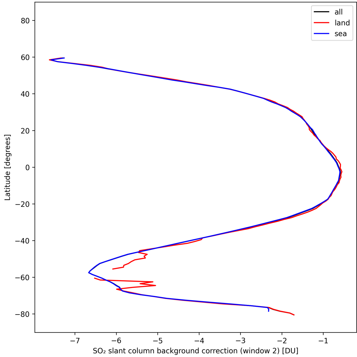
Figure 44: Zonal average of “SO 2 slant column background correction (window 2)” for 2025-10-19 to 2025-10-21.
