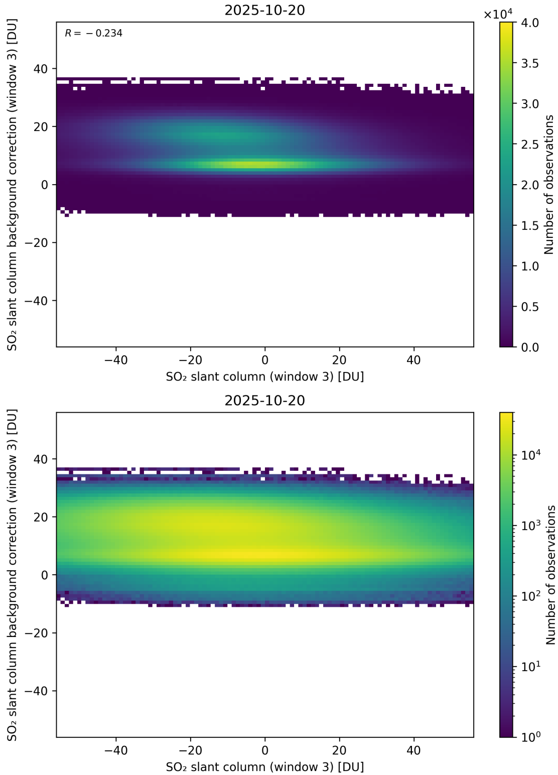
Figure 303: Scatter density plot of “SO 2 slant column (window 3)” against “SO 2 slant column background correction (window 3)” for 2025-10-19 to 2025-10-21.
