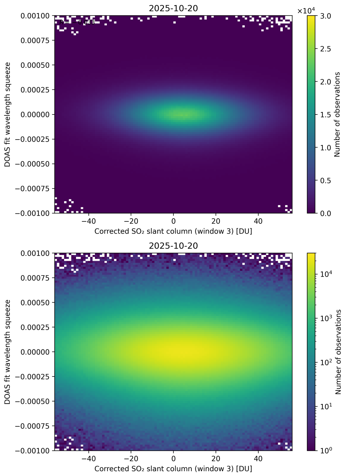
Figure 257: Scatter density plot of “Corrected SO 2 slant column (window 3)” against “DOAS fit wavelength squeeze” for 2025-10-19 to 2025-10-21.
