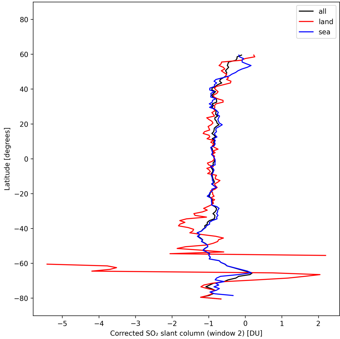
Figure 43: Zonal average of “Corrected SO 2 slant column (window 2)” for 2025-10-19 to 2025-10-21.
