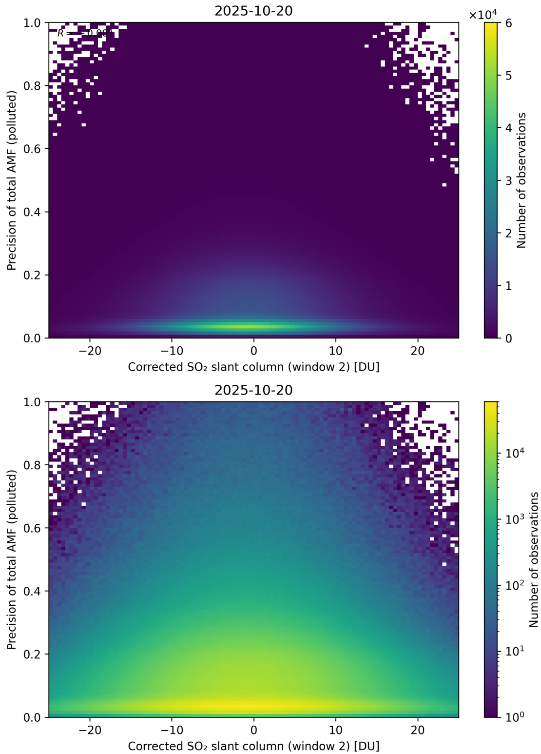
Figure 254: Scatter density plot of “Corrected SO 2 slant column (window 2)” against “Precision of total AMF (polluted)” for 2025-10-19 to 2025-10-21.
