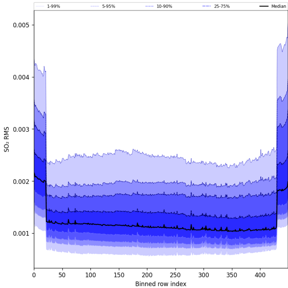
Figure 104: Along track statistics of “SO 2 RMS” for 2025-10-19 to 2025-10-21
