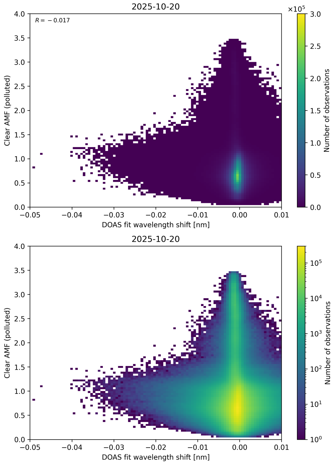
Figure 140: Scatter density plot of “DOAS fit wavelength shift” against “Clear AMF (polluted)” for 2025-10-19 to 2025-10-21.
