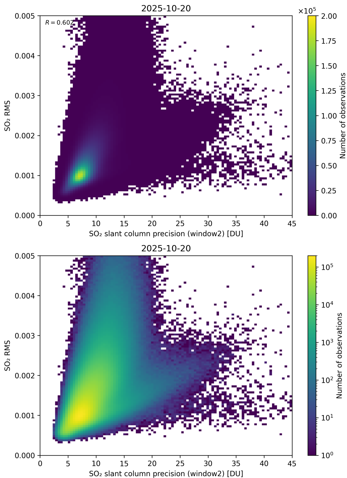
Figure 295: Scatter density plot of “SO 2 slant column precision (window2)” against “SO 2 RMS” for 2025-10-19 to 2025-10-21.
