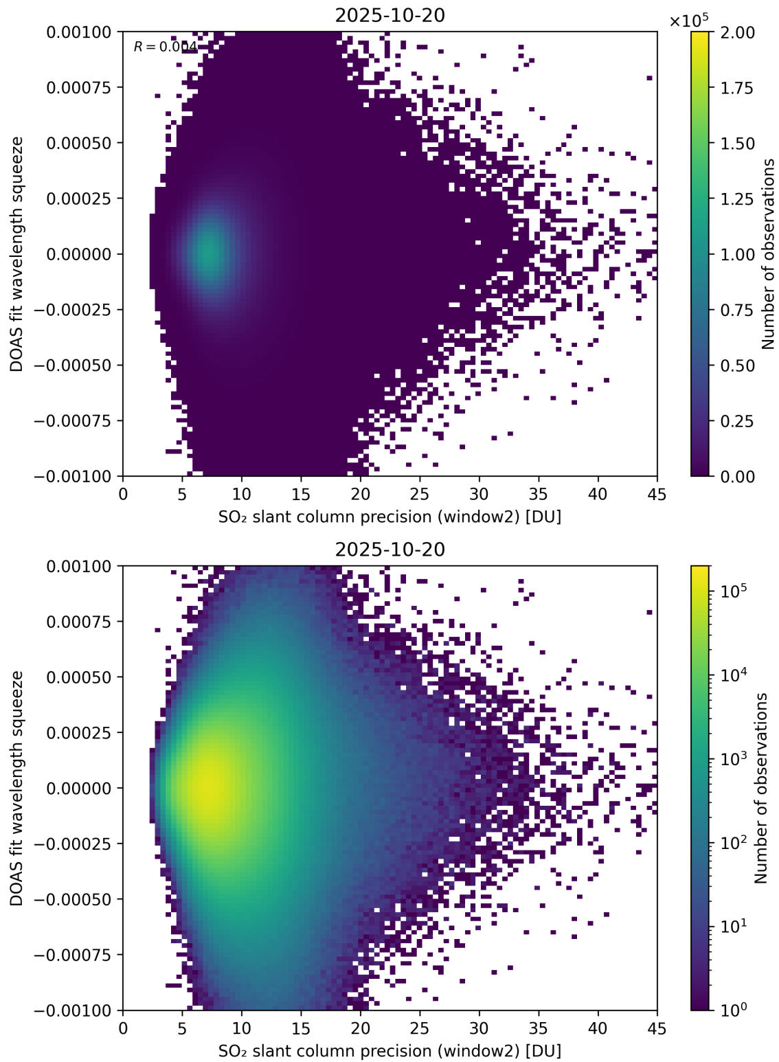
Figure 294: Scatter density plot of “SO 2 slant column precision (window2)” against “DOAS fit wavelength squeeze” for 2025-10-19 to 2025-10-21.
