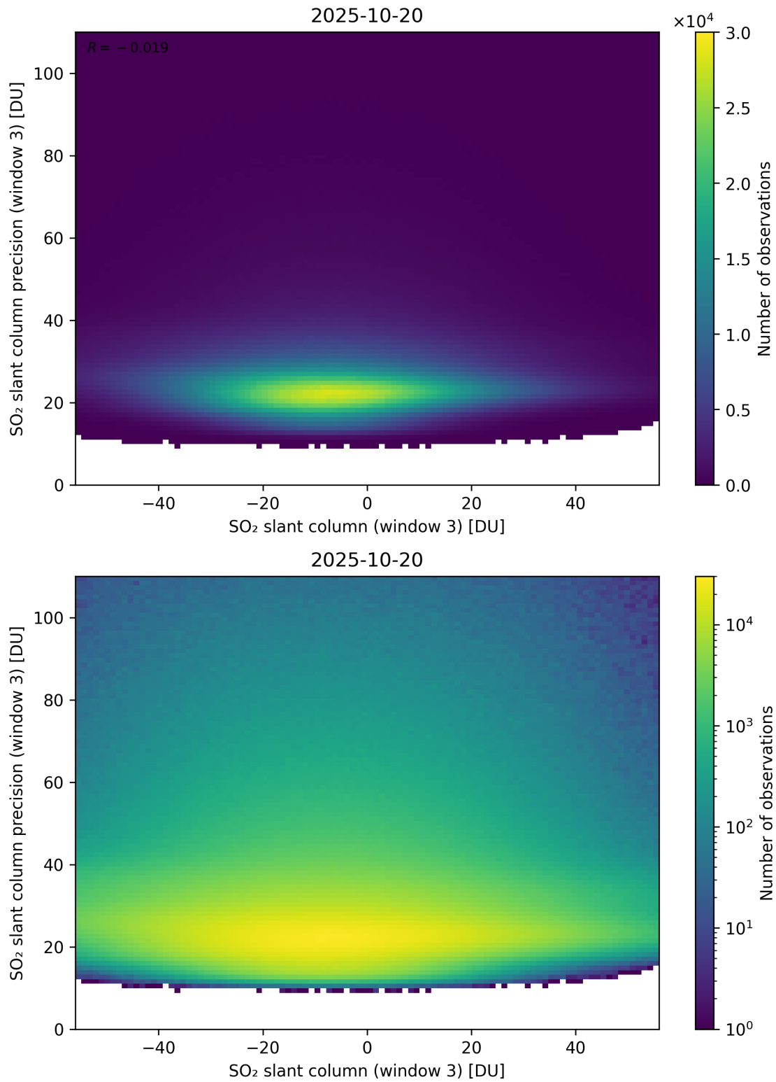
Figure 317: Scatter density plot of “SO 2 slant column (window 3)” against “SO 2 slant column precision (window 3)” for 2025-10-19 to 2025-10-21.
