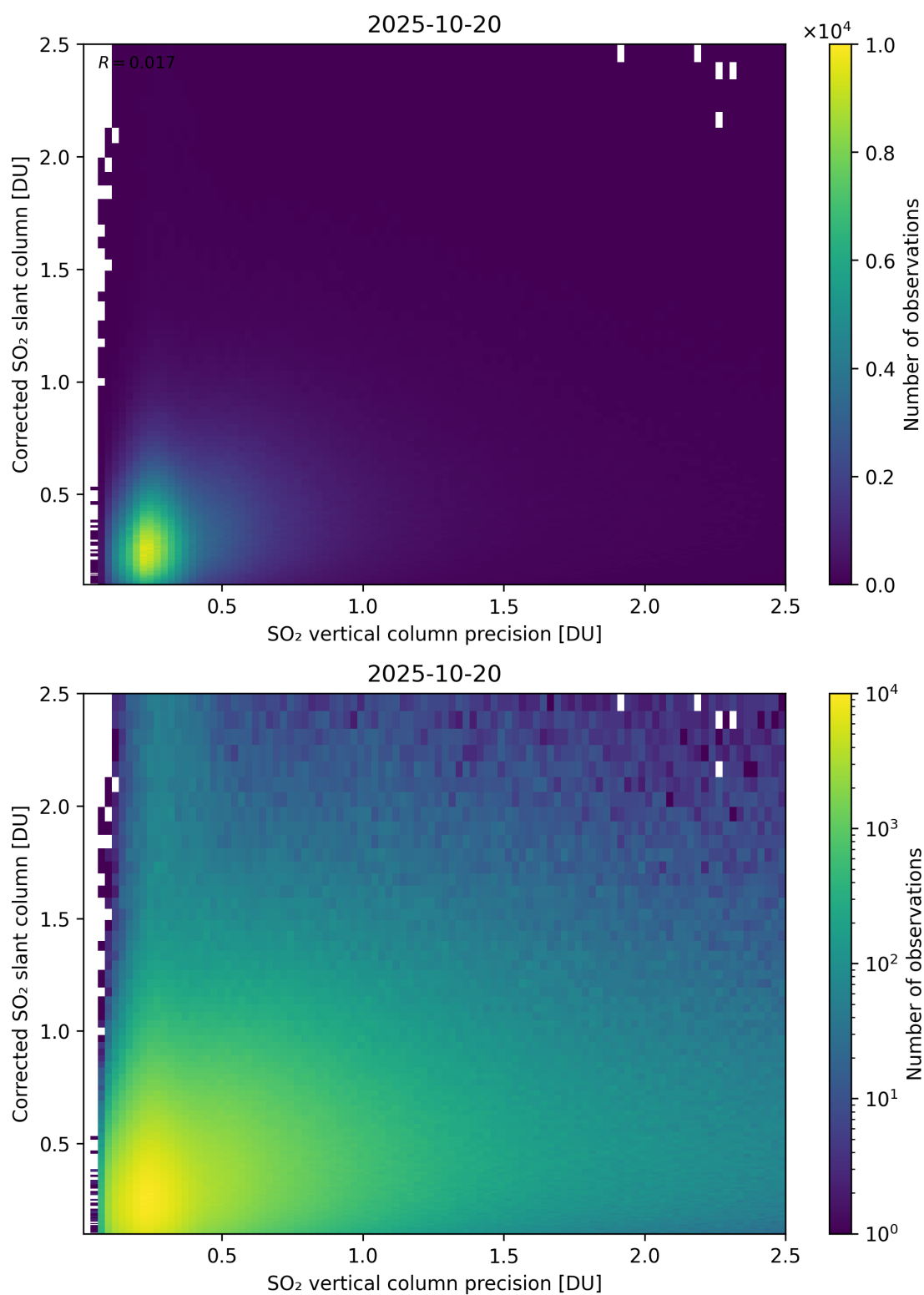
Figure 338: Scatter density plot of “SO 2 vertical column precision” against “Corrected SO 2 slant column” for 2025-10-19 to 2025-10-21.
