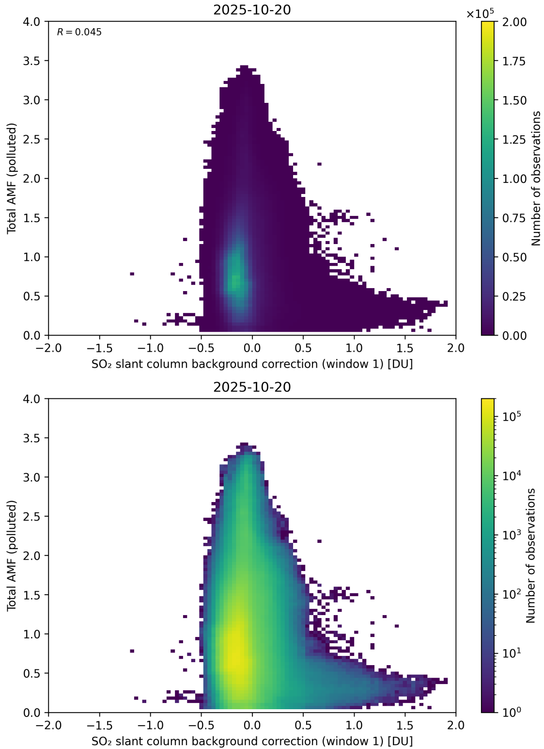
Figure 120: Scatter density plot of “SO 2 slant column background correction (window 1)” against “Total AMF (polluted)” for 2025-10-19 to 2025-10-21.
