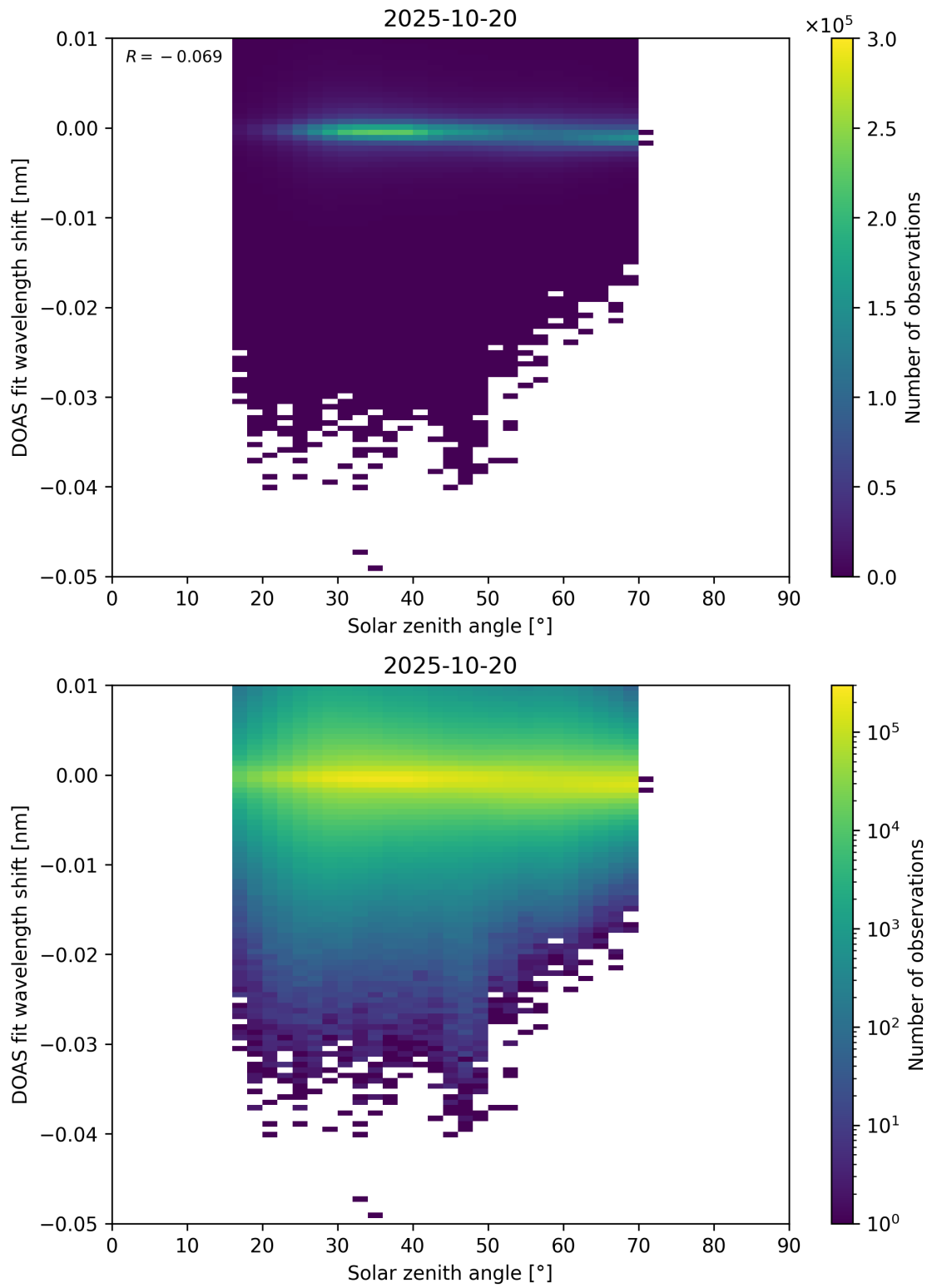
Figure 174: Scatter density plot of “Solar zenith angle” against “DOAS fit wavelength shift” for 2025-10-19 to 2025-10-21.
