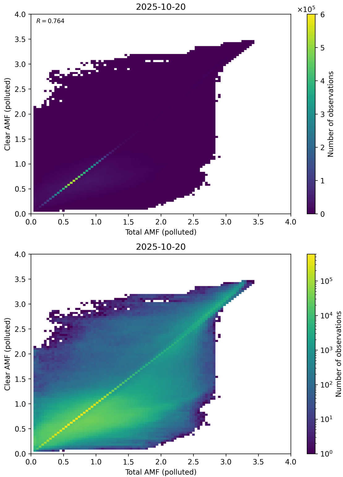
Figure 321: Scatter density plot of “Total AMF (polluted)” against “Clear AMF (polluted)” for 2025-10-19 to 2025-10-21.
