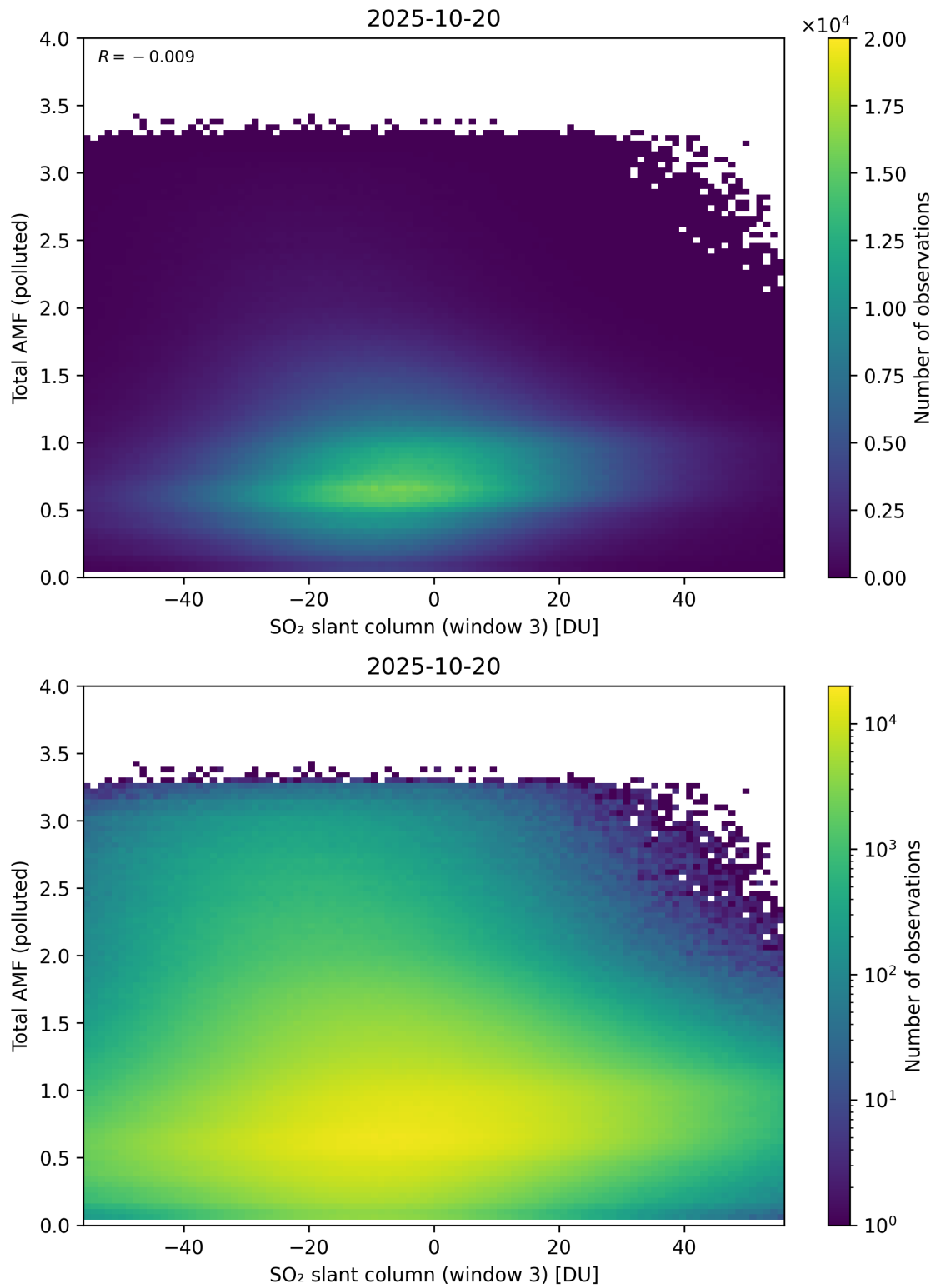
Figure 318: Scatter density plot of “SO 2 slant column (window 3)” against “Total AMF (polluted)” for 2025-10-19 to 2025-10-21.
