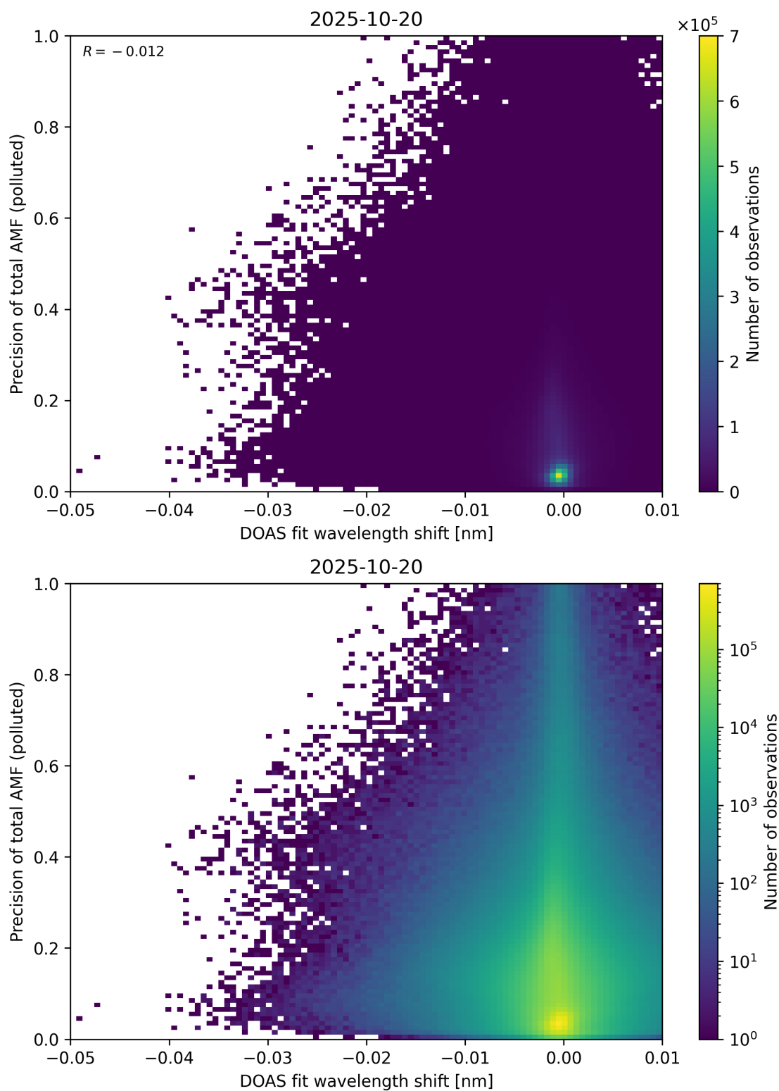
Figure 142: Scatter density plot of “DOAS fit wavelength shift” against “Precision of total AMF (polluted)” for 2025-10-19 to 2025-10-21.
