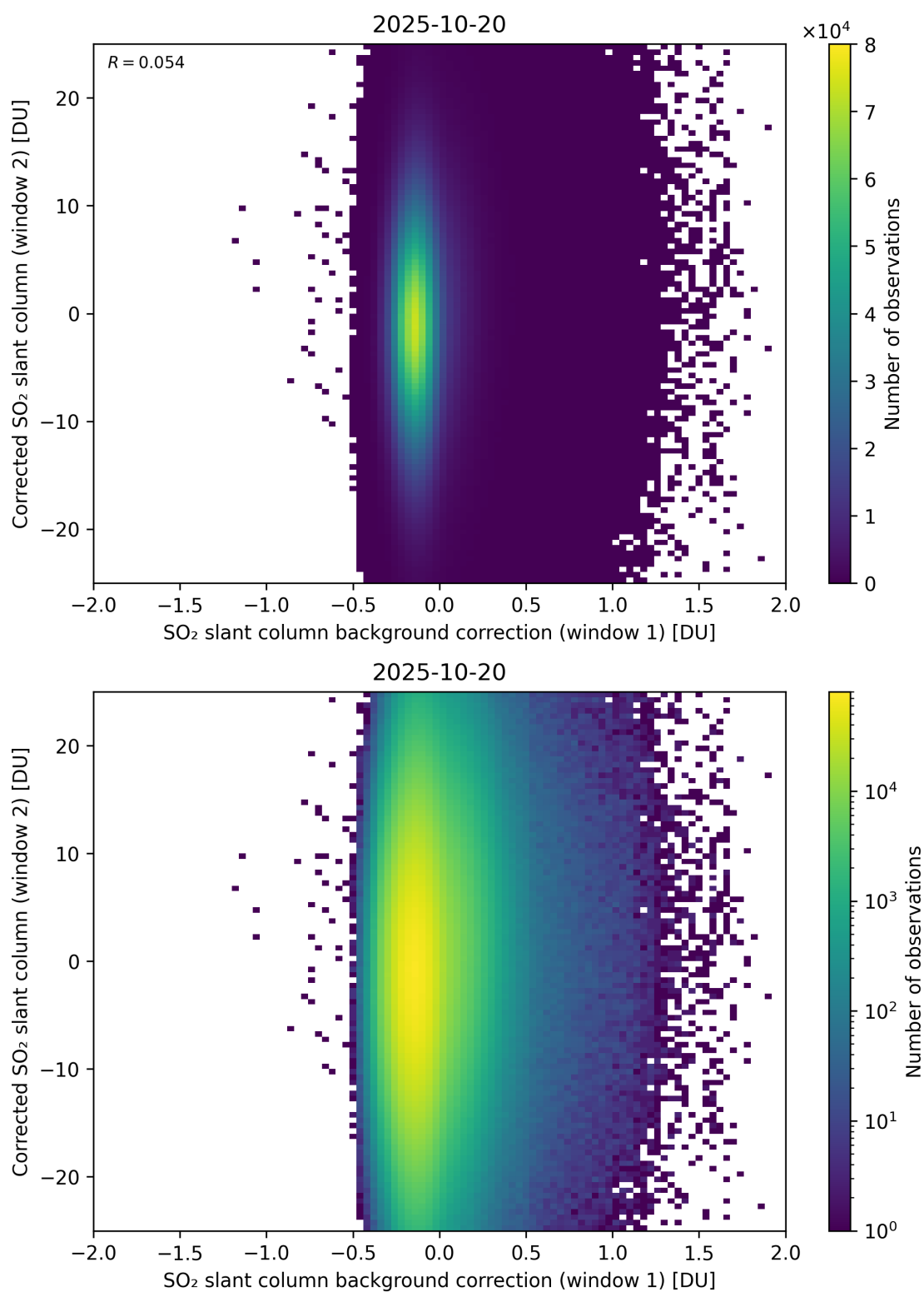
Figure 115: Scatter density plot of “SO 2 slant column background correction (window 1)” against “Corrected SO 2 slant column (window 2)” for 2025-10-19 to 2025-10-21.
