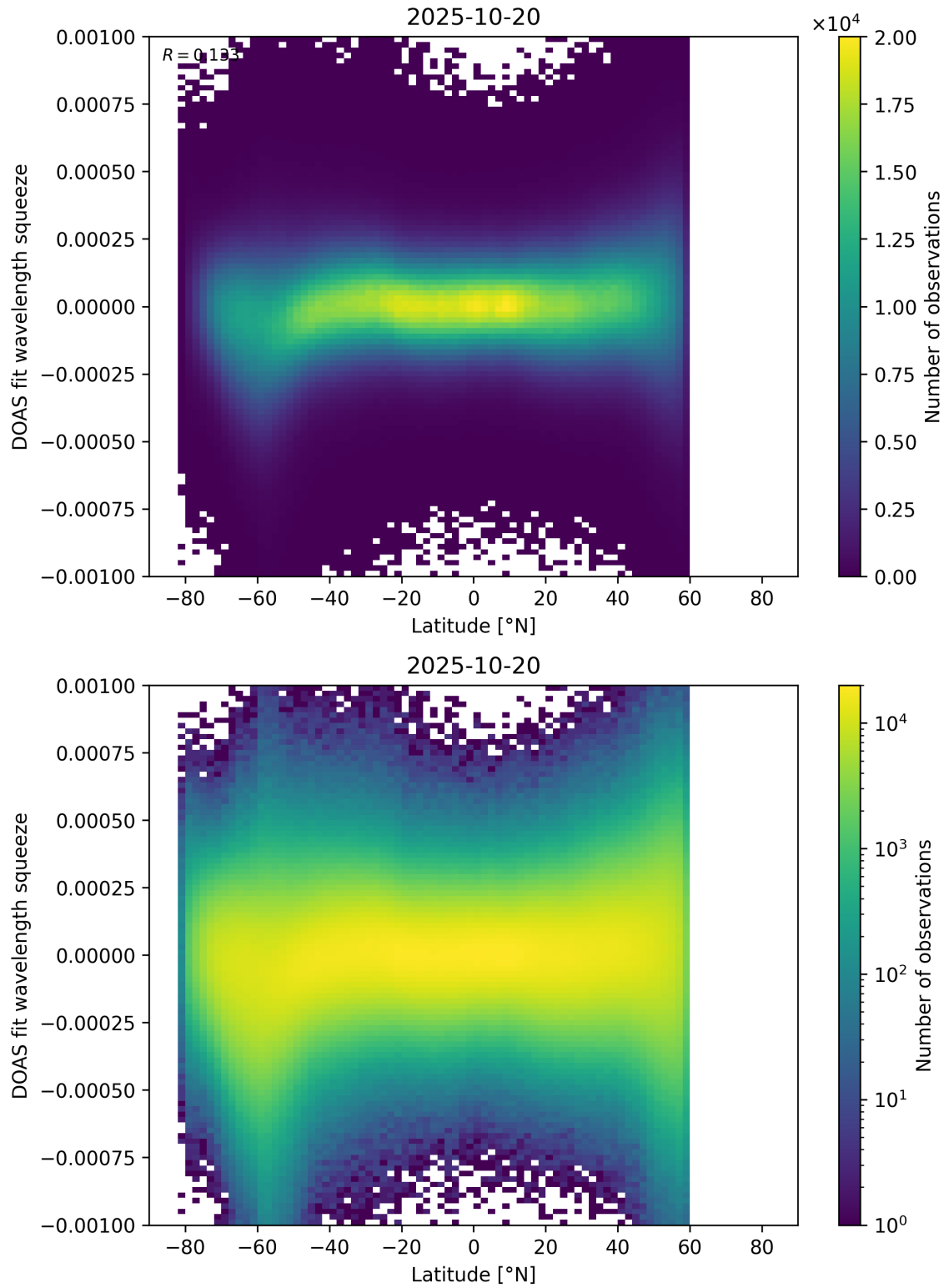
Figure 154: Scatter density plot of “Latitude” against “DOAS fit wavelength squeeze” for 2025-10-19 to 2025-10-21.
