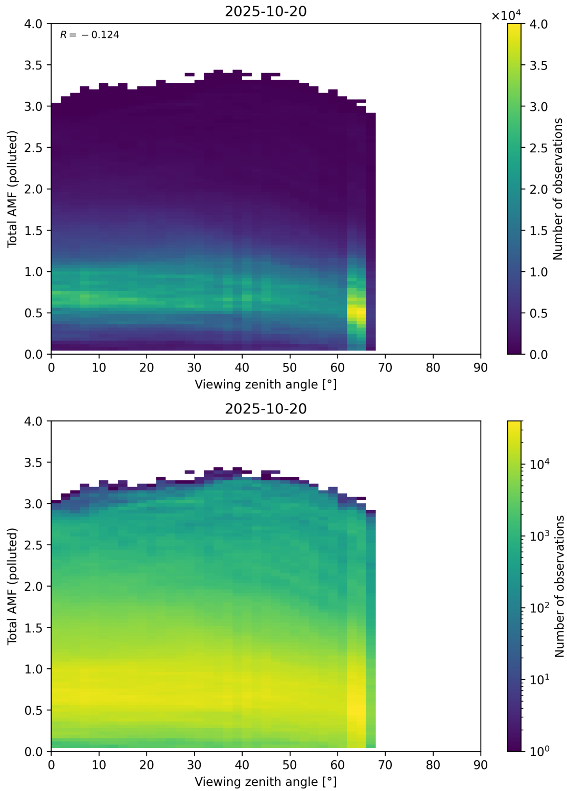
Figure 381: Scatter density plot of “Viewing zenith angle” against “Total AMF (polluted)” for 2025-10-19 to 2025-10-21.
