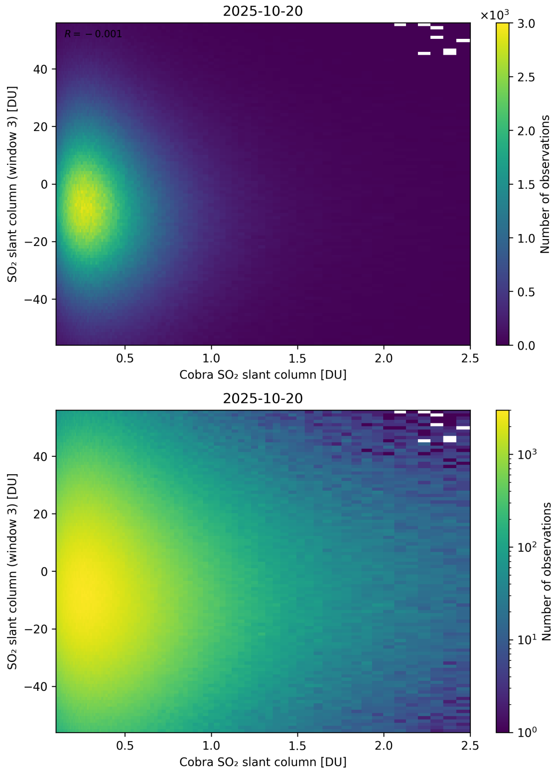
Figure 222: Scatter density plot of “Cobra SO 2 slant column” against “SO 2 slant column (window 3)” for 2025-10-19 to 2025-10-21.
