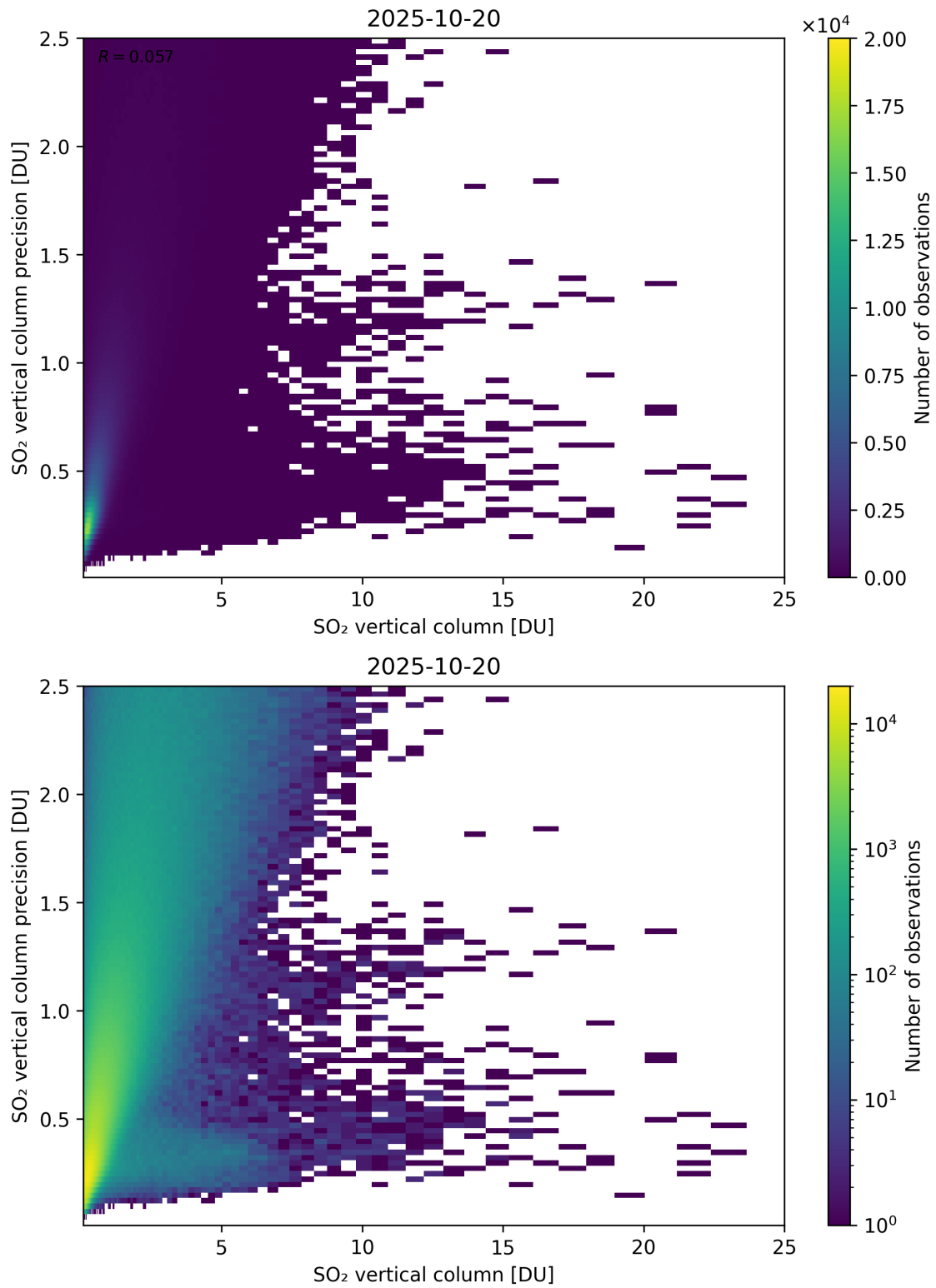
Figure 361: Scatter density plot of “SO 2 vertical column” against “SO 2 vertical column precision” for 2025-10-19 to 2025-10-21.
