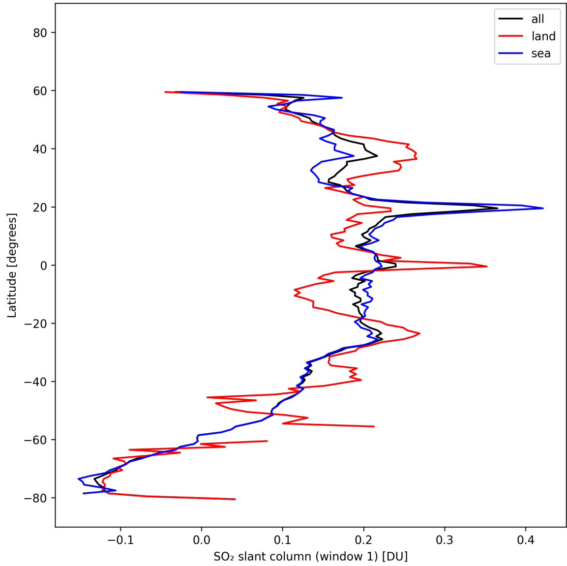
Figure 37: Zonal average of “SO 2 slant column (window 1)” for 2025-10-19 to 2025-10-21.
