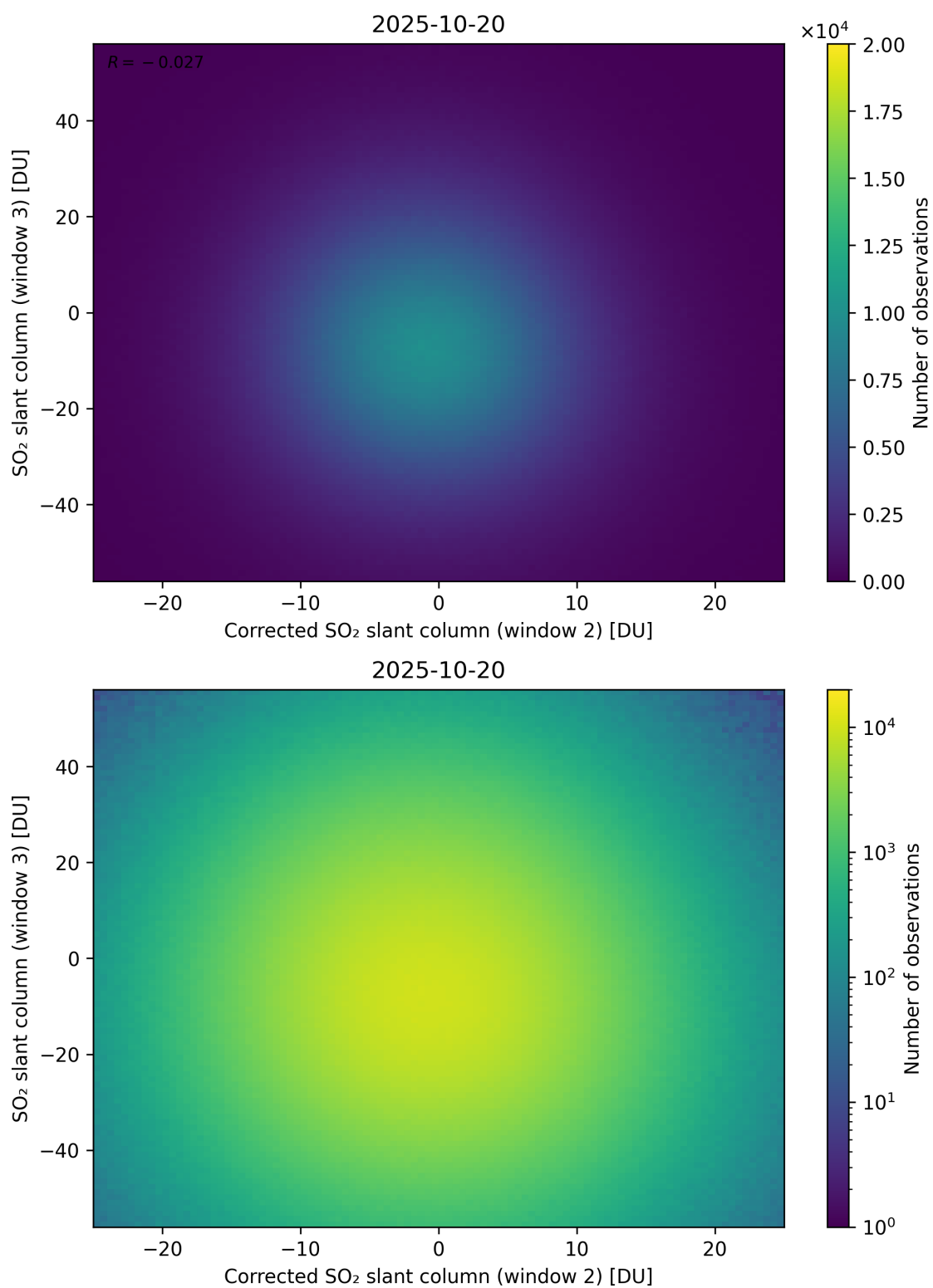
Figure 251: Scatter density plot of “Corrected SO 2 slant column (window 2)” against “SO 2 slant column (window 3)” for 2025-10-19 to 2025-10-21.
