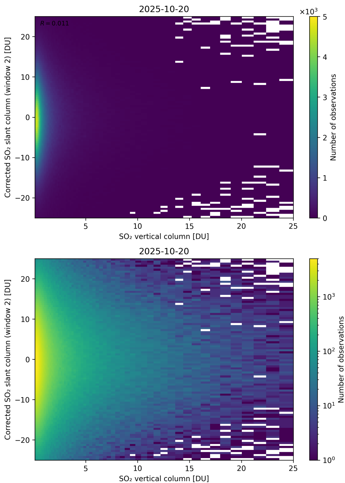
Figure 352: Scatter density plot of “SO 2 vertical column” against “Corrected SO 2 slant column (window 2)” for 2025-10-19 to 2025-10-21.
