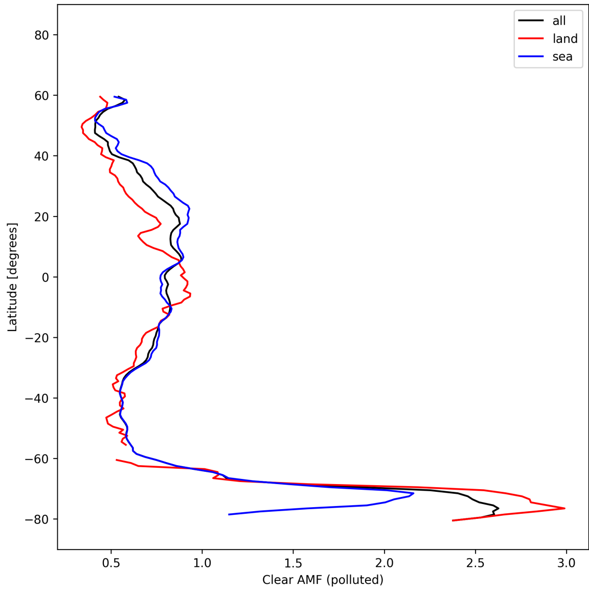
Figure 55: Zonal average of “Clear AMF (polluted)” for 2025-10-19 to 2025-10-21.
