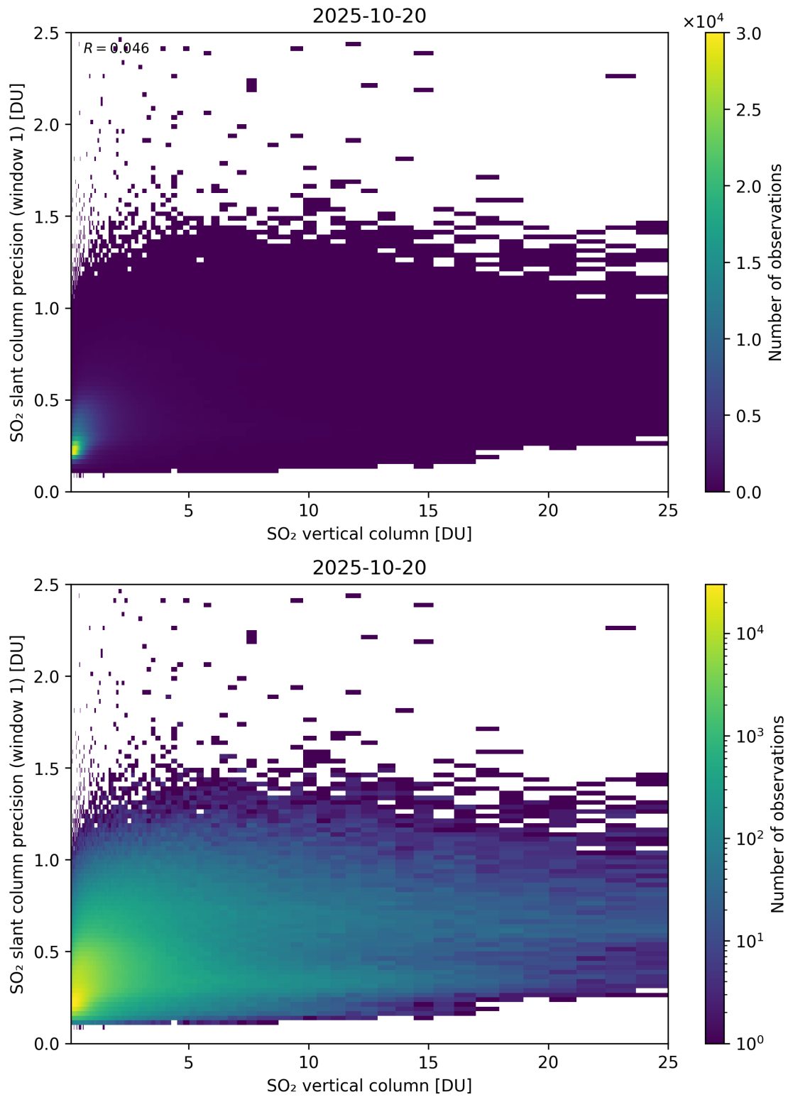
Figure 355: Scatter density plot of “SO 2 vertical column” against “SO 2 slant column precision (window 1)” for 2025-10-19 to 2025-10-21.
