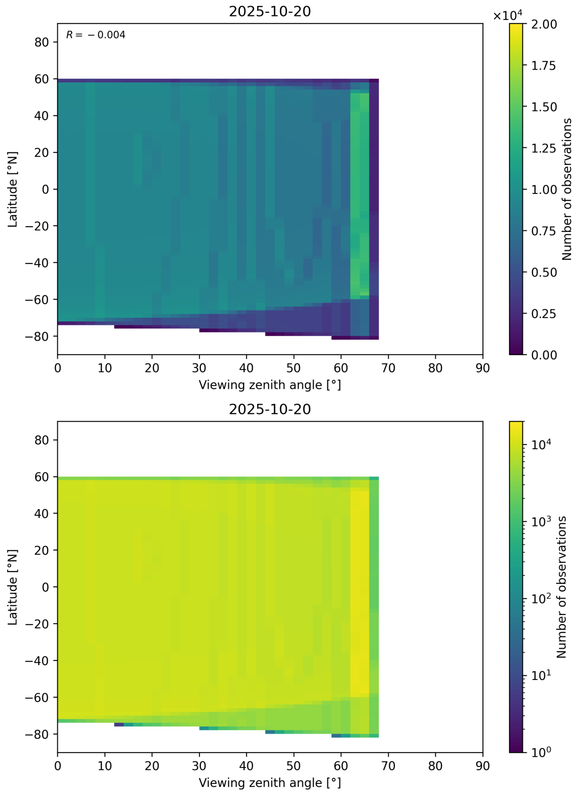
Figure 368: Scatter density plot of “Viewing zenith angle” against “Latitude” for 2025-10-19 to 2025-10-21.
