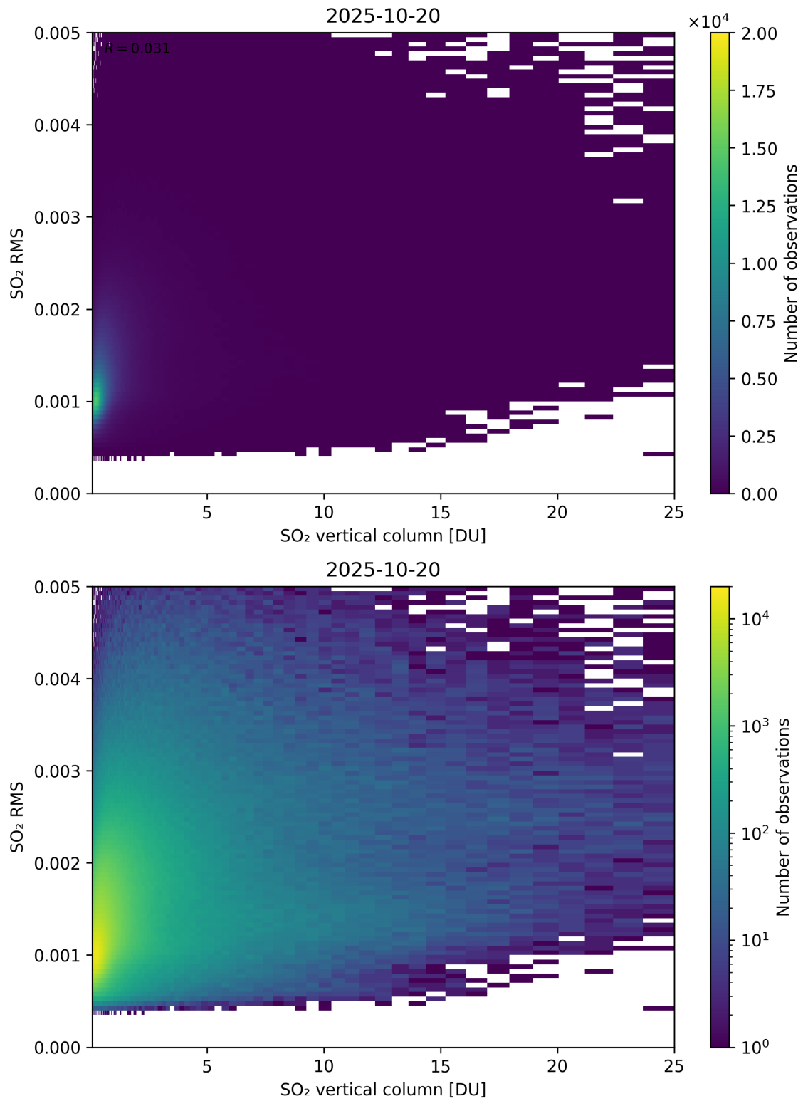
Figure 328: Scatter density plot of “SO 2 vertical column” against “SO 2 RMS” for 2025-10-19 to 2025-10-21.
