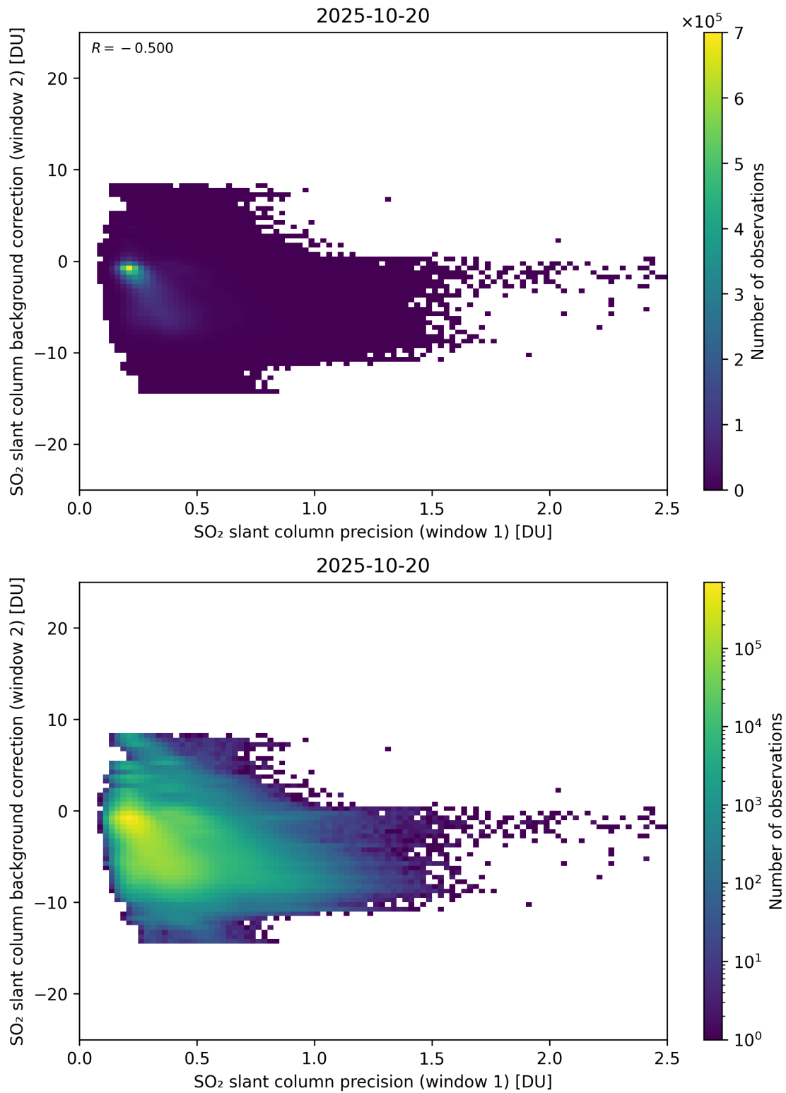
Figure 269: Scatter density plot of “SO 2 slant column precision (window 1)” against “SO 2 slant column background correction (window 2)” for 2025-10-19 to 2025-10-21.
