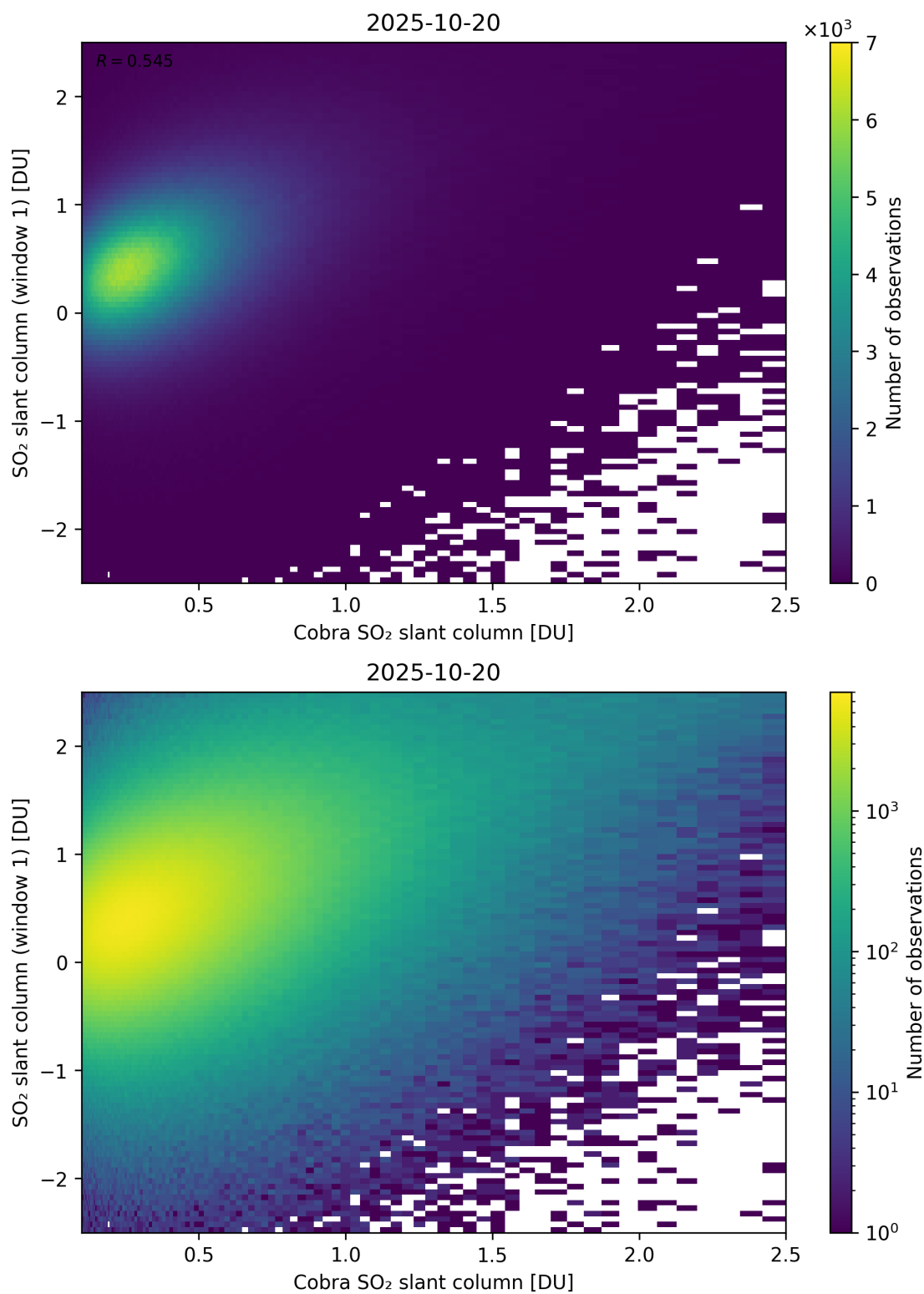
Figure 219: Scatter density plot of “Cobra SO 2 slant column” against “SO 2 slant column (window 1)” for 2025-10-19 to 2025-10-21.
