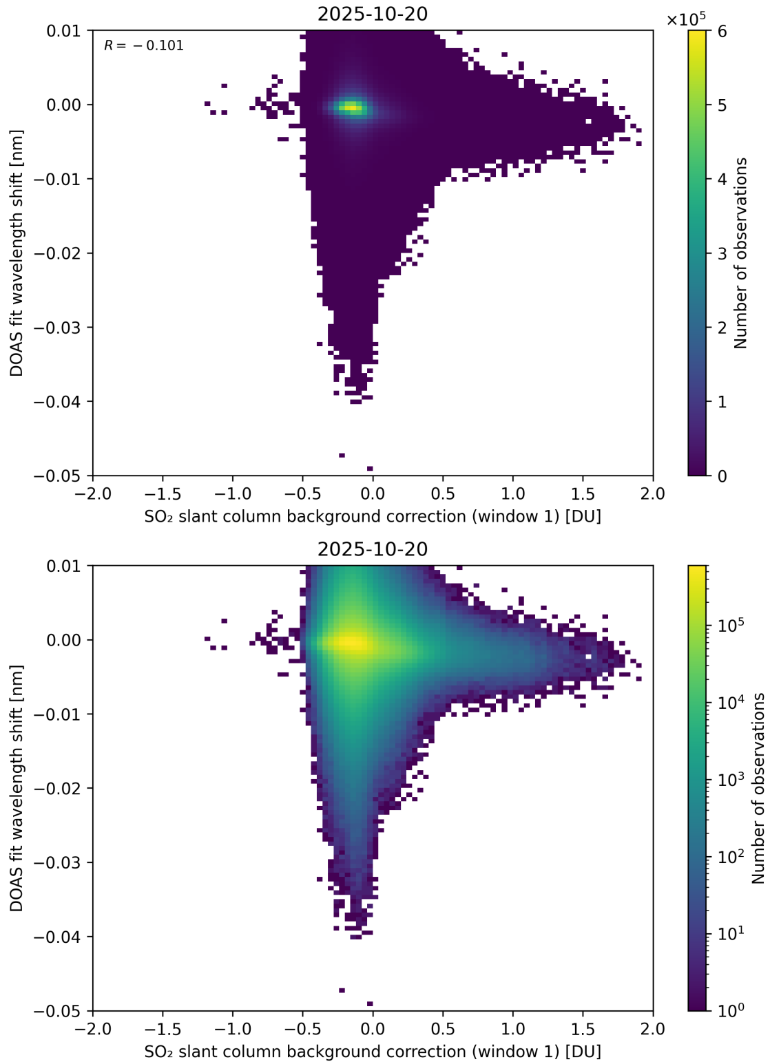
Figure 111: Scatter density plot of “SO 2 slant column background correction (window 1)” against “DOAS fit wavelength shift” for 2025-10-19 to 2025-10-21.
