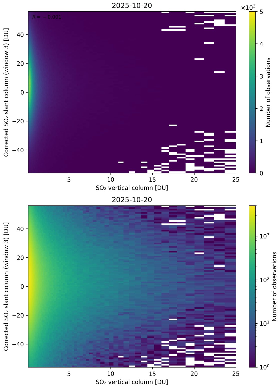
Figure 353: Scatter density plot of “SO 2 vertical column” against “Corrected SO 2 slant column (window 3)” for 2025-10-19 to 2025-10-21.
