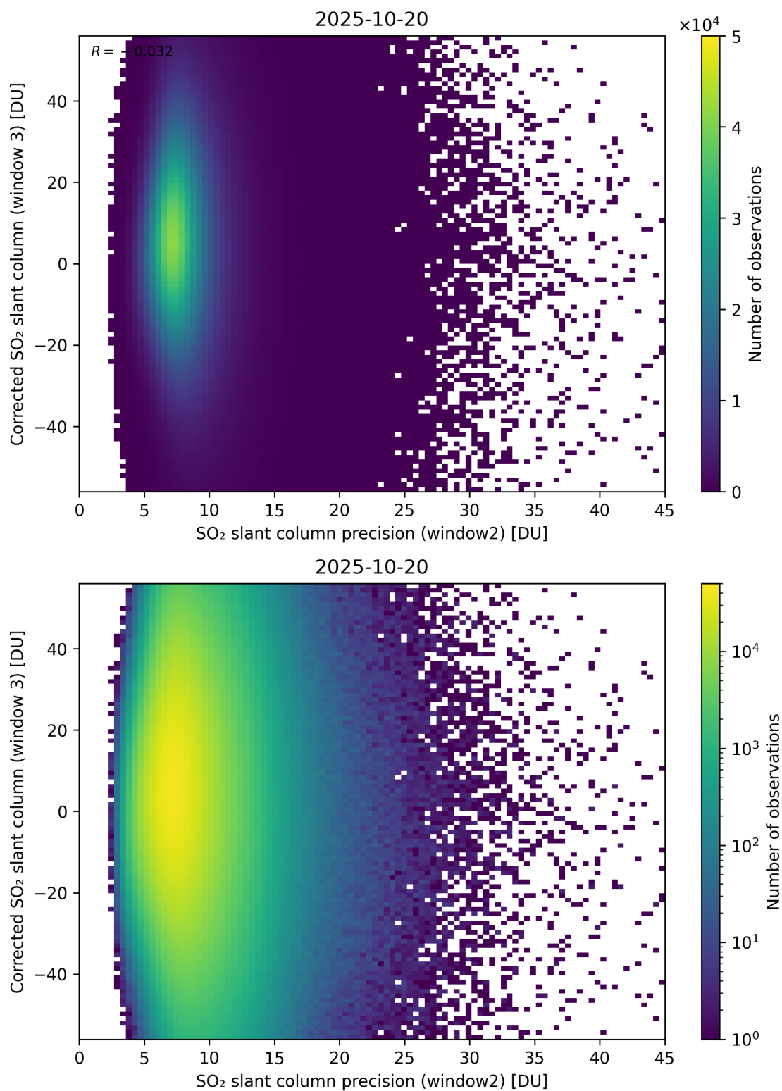
Figure 298: Scatter density plot of “SO 2 slant column precision (window2)” against “Corrected SO 2 slant column (window 3)” for 2025-10-19 to 2025-10-21.
