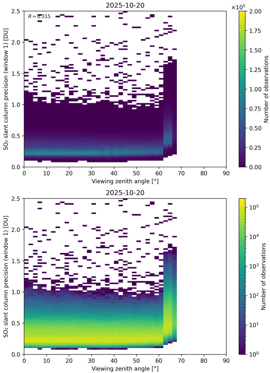
Figure 377: Scatter density plot of “Viewing zenith angle” against “SO 2 slant column precision (window 1)” for 2025-10-19 to 2025-10-21.
