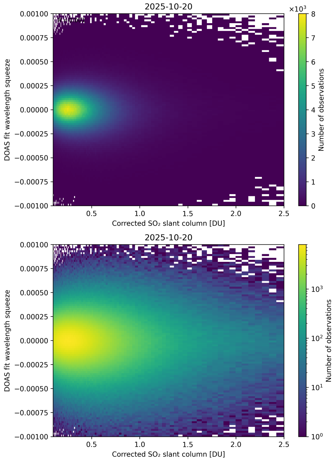
Figure 230: Scatter density plot of "Corrected SO 2 slant column" against "DOAS fit wavelength squeeze" for 2025-10-19 to 2025-10-21.
