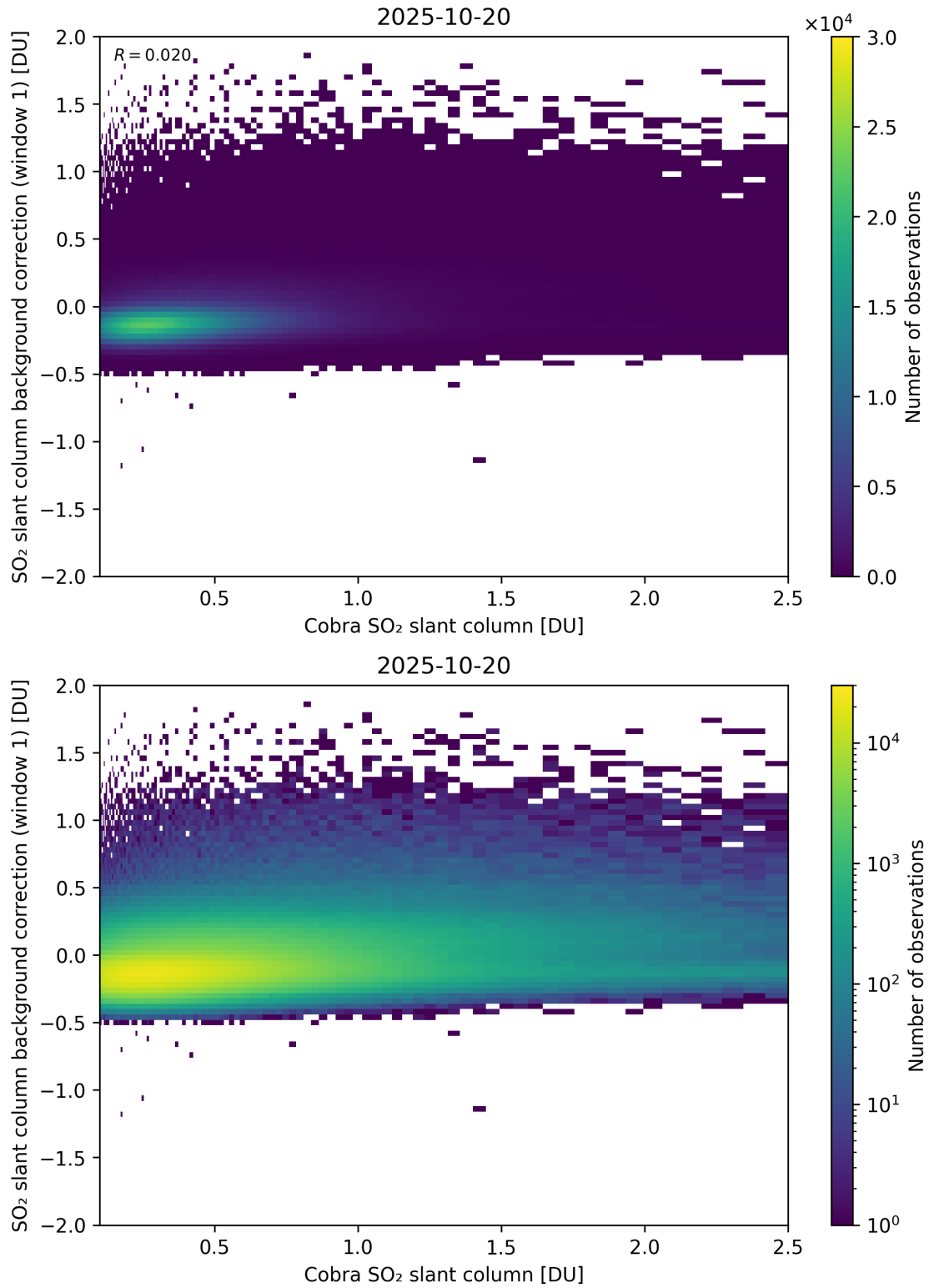
Figure 193: Scatter density plot of “Cobra SO 2 slant column” against “SO 2 slant column background correction (window 1)” for 2025-10-19 to 2025-10-21.
