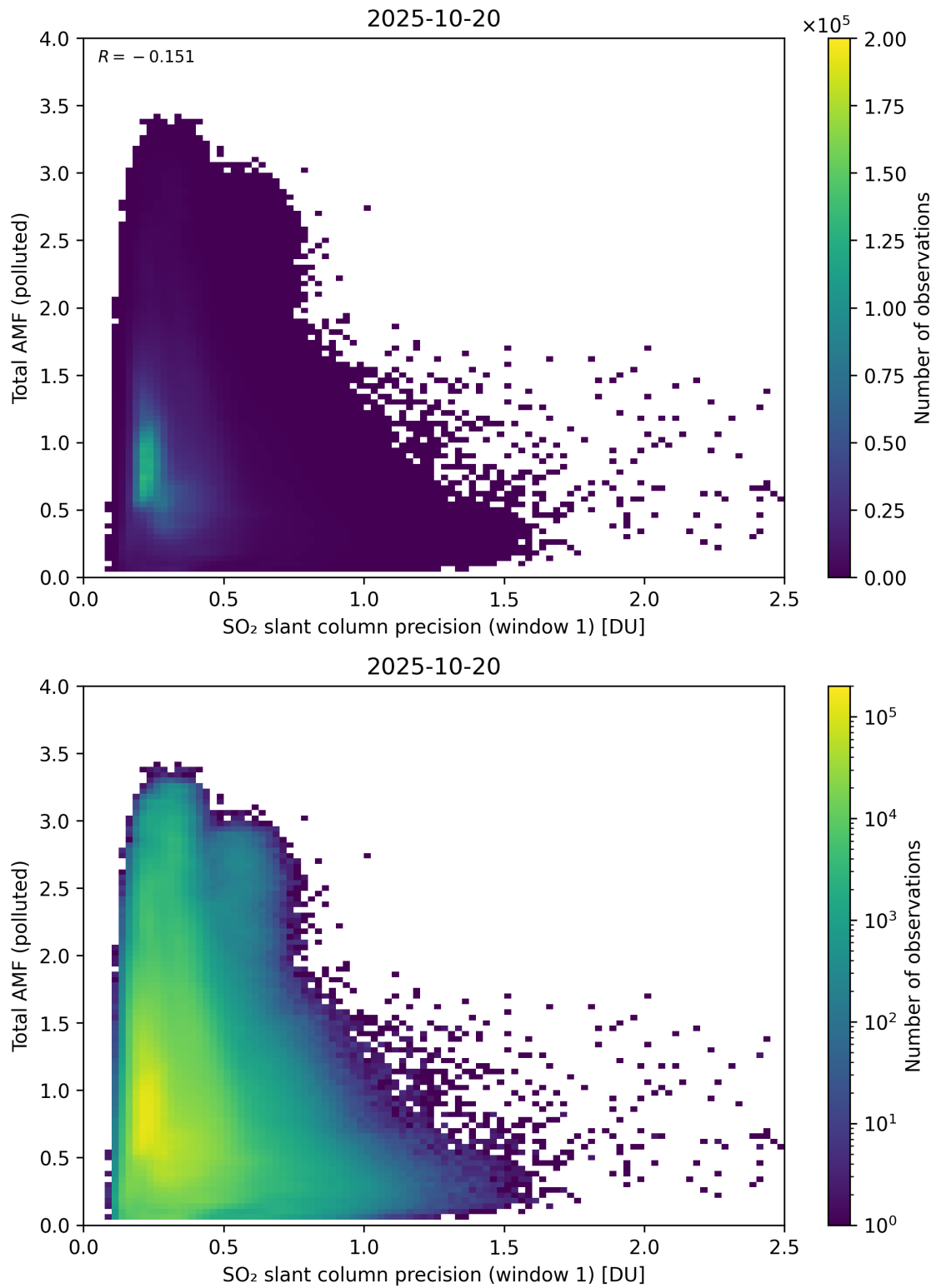
Figure 280: Scatter density plot of “SO 2 slant column precision (window 1)” against “Total AMF (polluted)” for 2025-10-19 to 2025-10-21.
