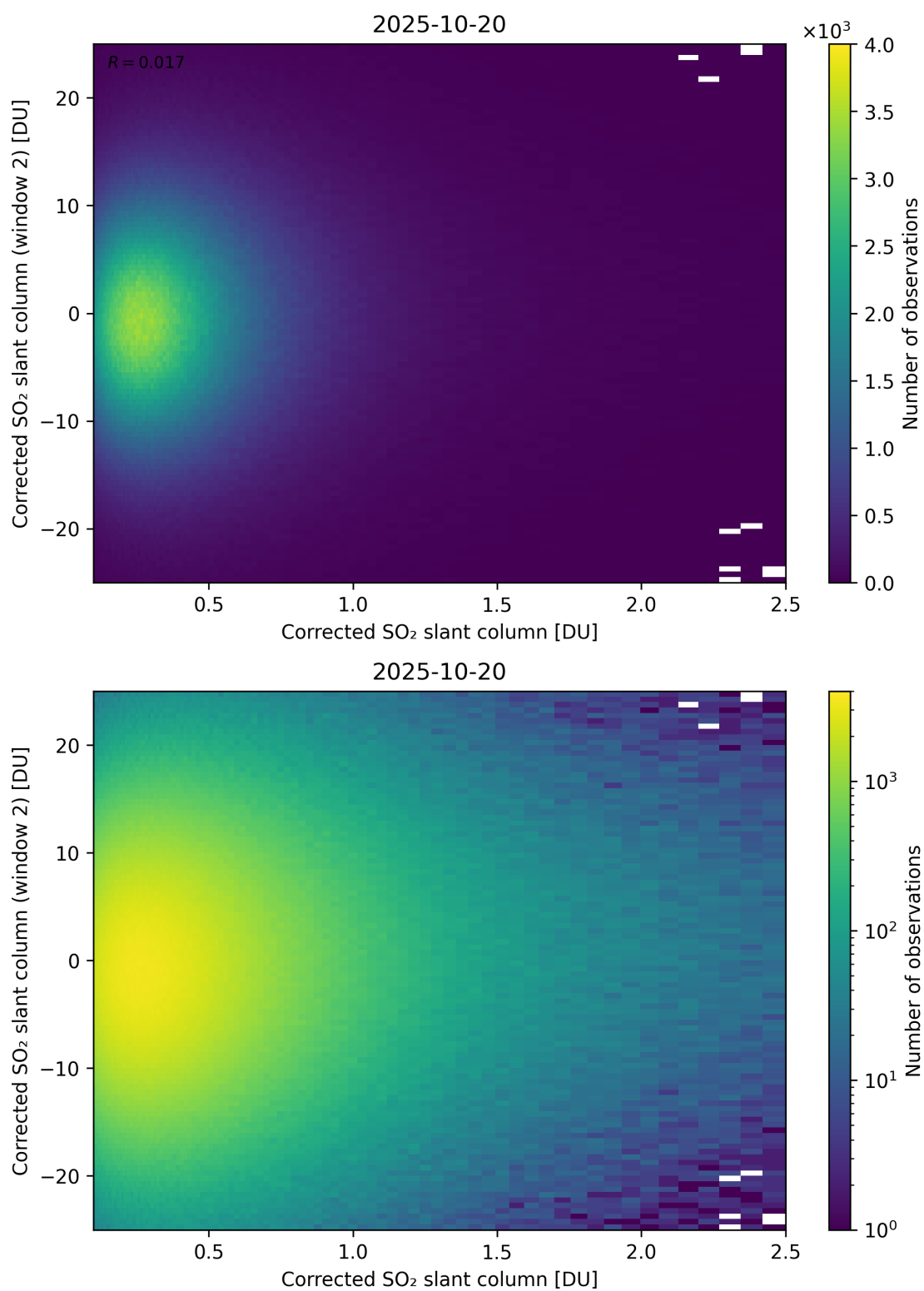
Figure 235: Scatter density plot of “Corrected SO 2 slant column” against “Corrected SO 2 slant column (window 2)” for 2025-10-19 to 2025-10-21.
