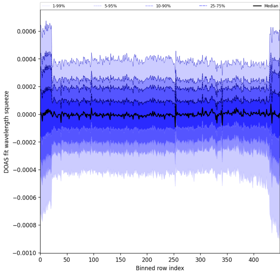
Figure 103: Along track statistics of “DOAS fit wavelength squeeze” for 2025-10-19 to 2025-10-21
