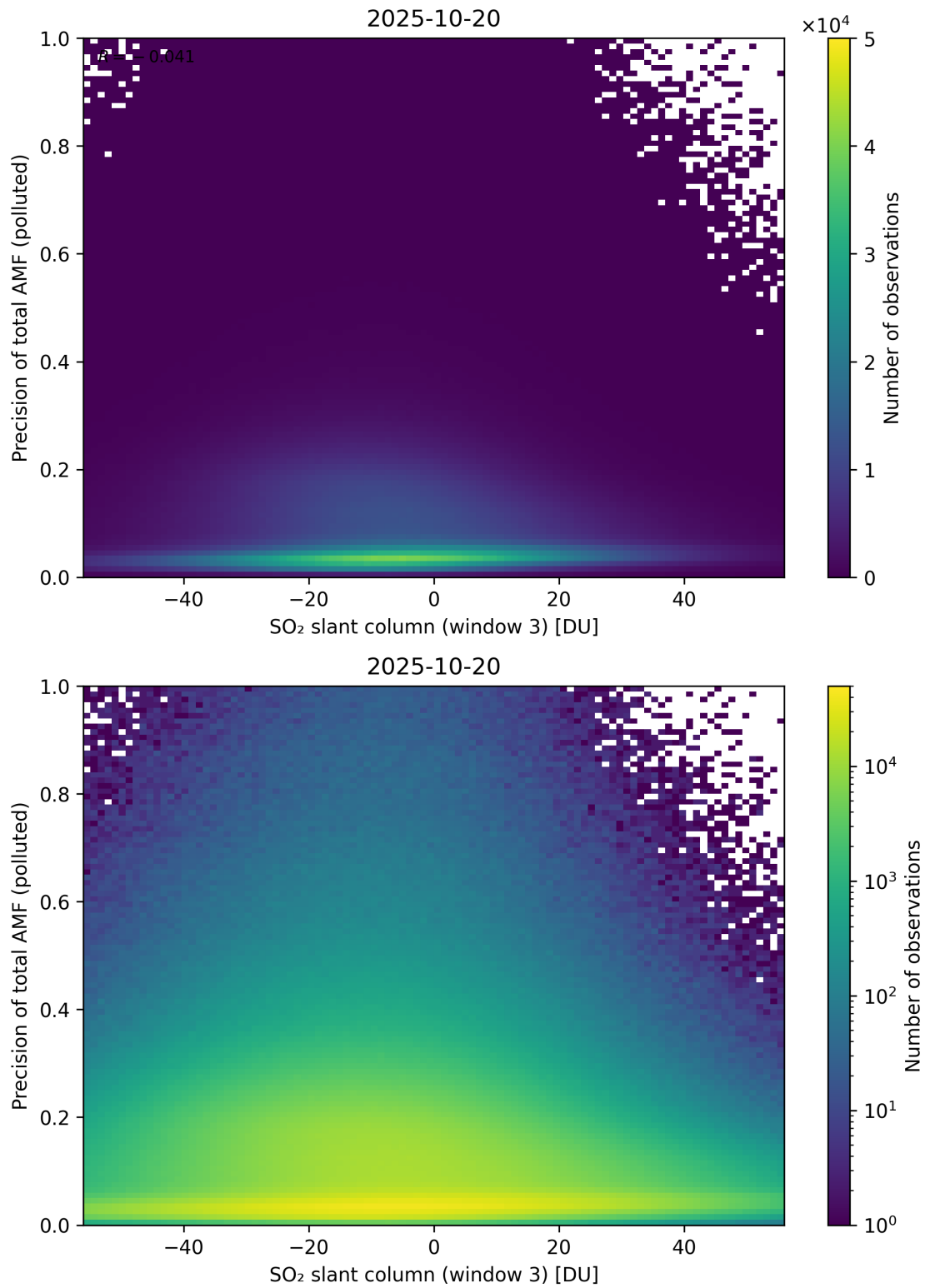
Figure 319: Scatter density plot of “SO 2 slant column (window 3)” against “Precision of total AMF (polluted)” for 2025-10-19 to 2025-10-21.
