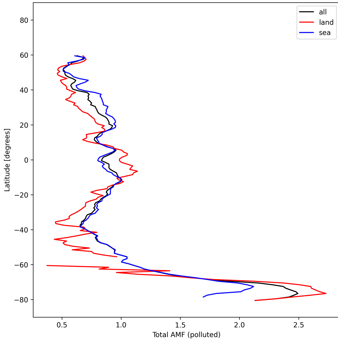
Figure 53: Zonal average of “Total AMF (polluted)” for 2025-10-19 to 2025-10-21.
