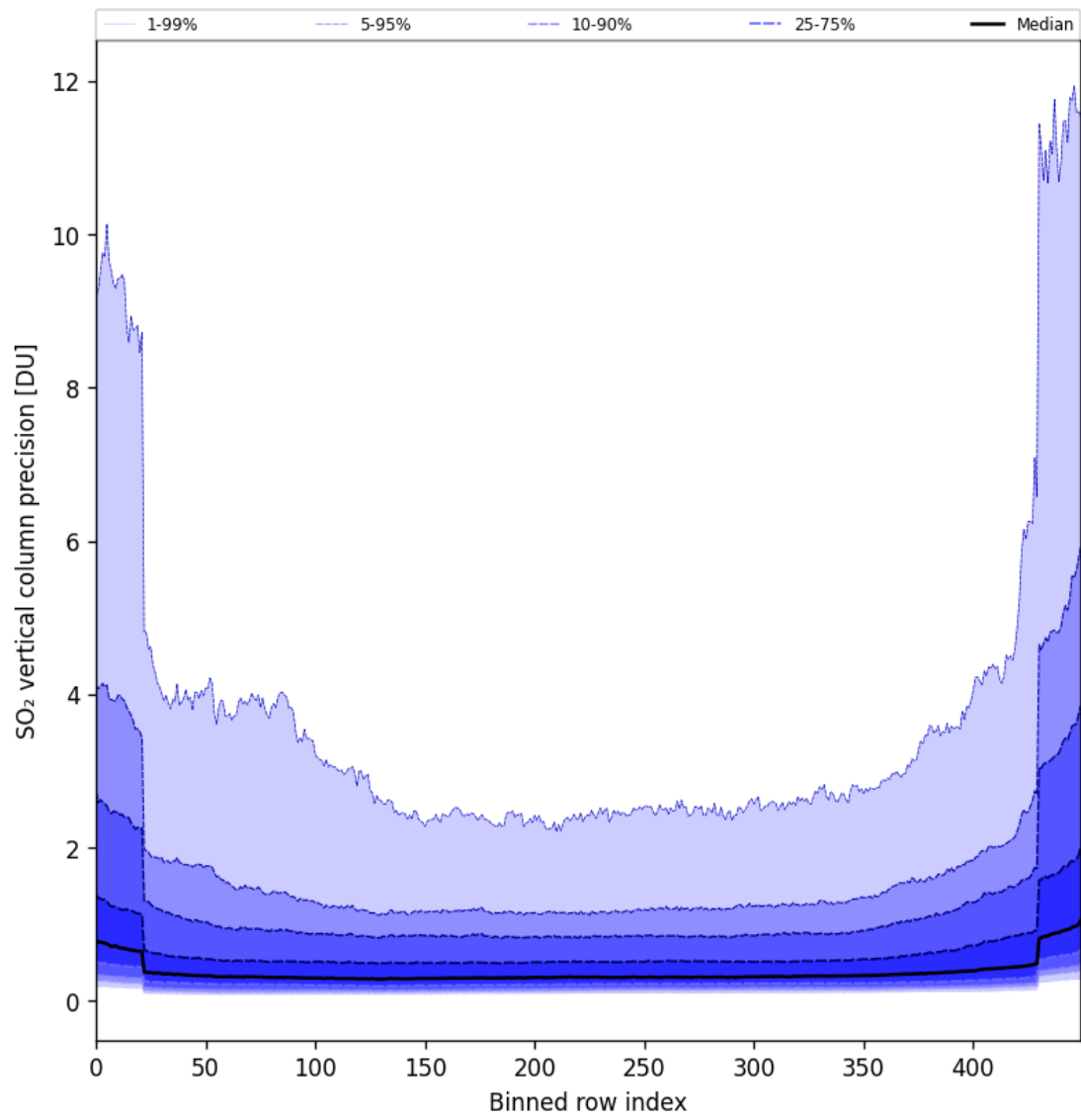
Figure 85: Along track statistics of “SO 2 vertical column precision” for 2025-10-19 to 2025-10-21
