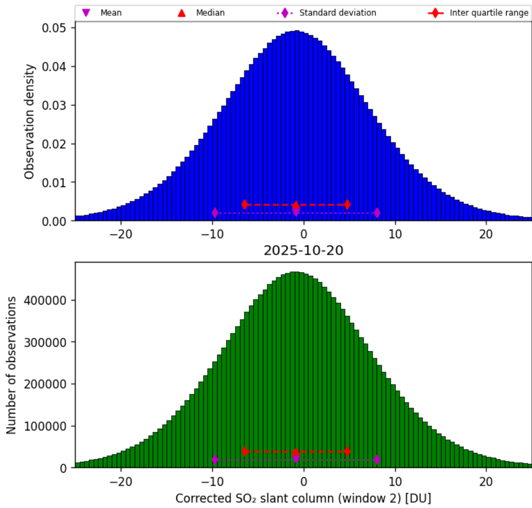
Figure 69: Histogram of “Corrected SO 2 slant column (window 2)” for 2025-10-19 to 2025-10-21
