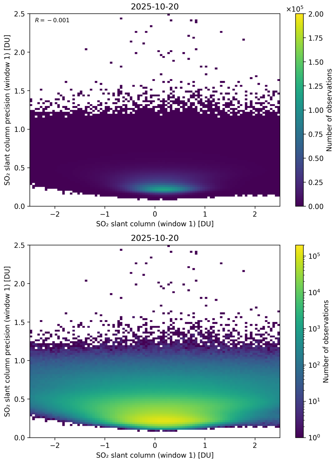
Figure 285: Scatter density plot of “SO 2 slant column (window 1)” against “SO 2 slant column precision (window 1)” for 2025-10-19 to 2025-10-21.
