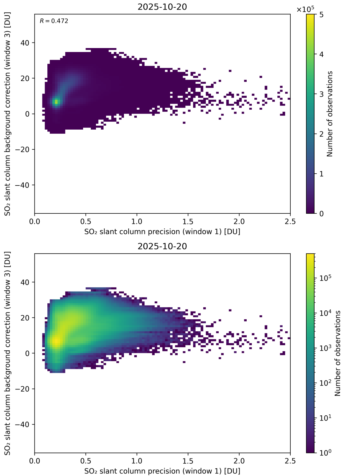
Figure 270: Scatter density plot of “SO 2 slant column precision (window 1)” against “SO 2 slant column background correction (window 3)” for 2025-10-19 to 2025-10-21.
