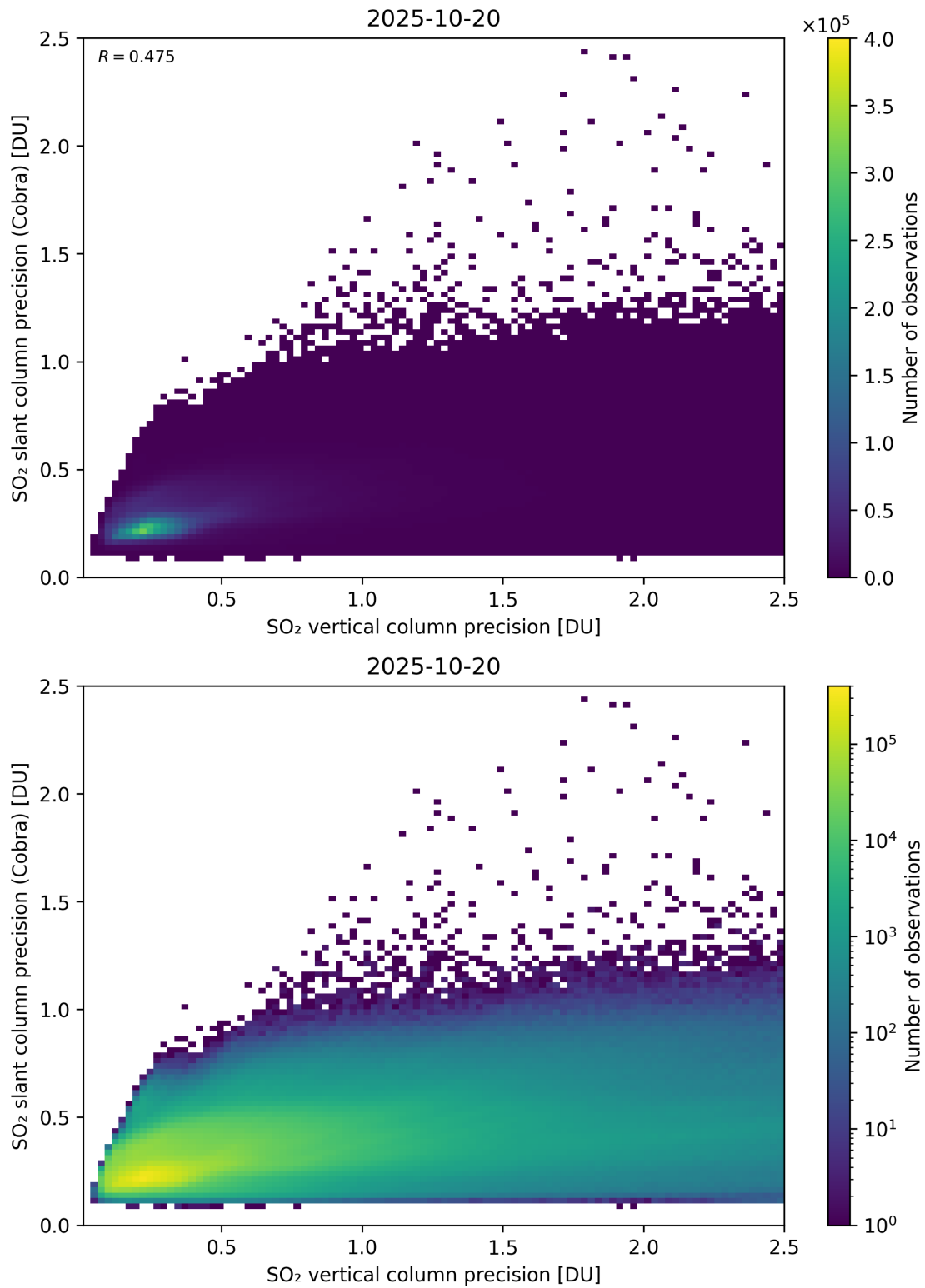
Figure 337: Scatter density plot of “SO 2 vertical column precision” against “SO 2 slant column precision (Cobra)” for 2025-10-19 to 2025-10-21.
