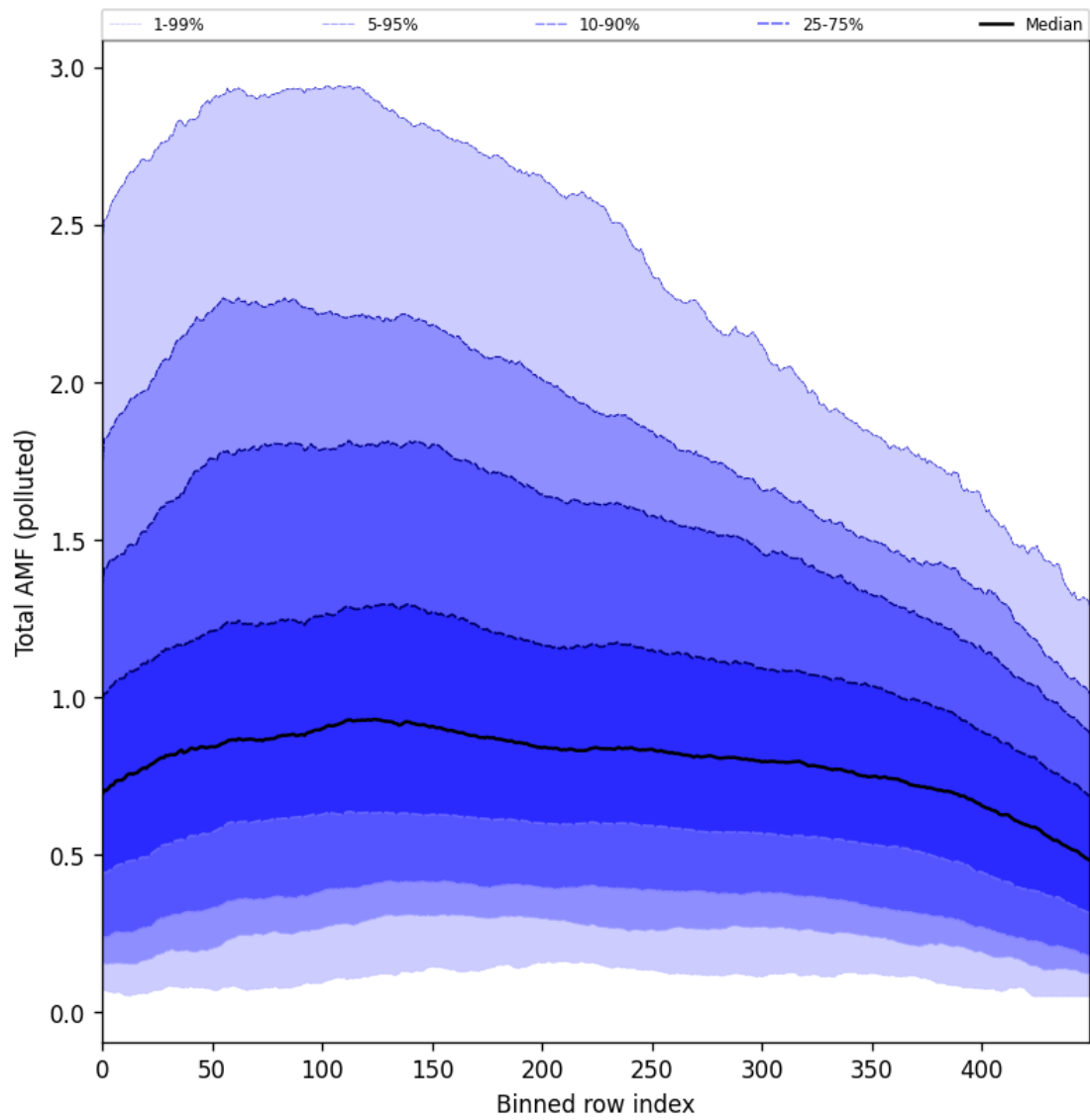
Figure 105: Along track statistics of “Total AMF (polluted)” for 2025-10-19 to 2025-10-21
