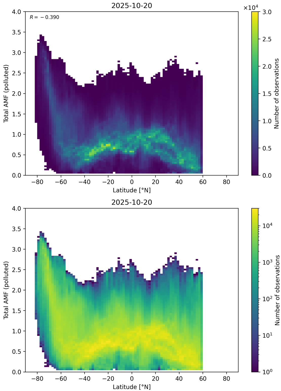
Figure 167: Scatter density plot of “Latitude” against “Total AMF (polluted)” for 2025-10-19 to 2025-10-21.
