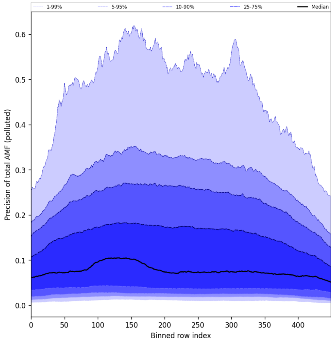
Figure 106: Along track statistics of “Precision of total AMF (polluted)” for 2025-10-19 to 2025-10-21
