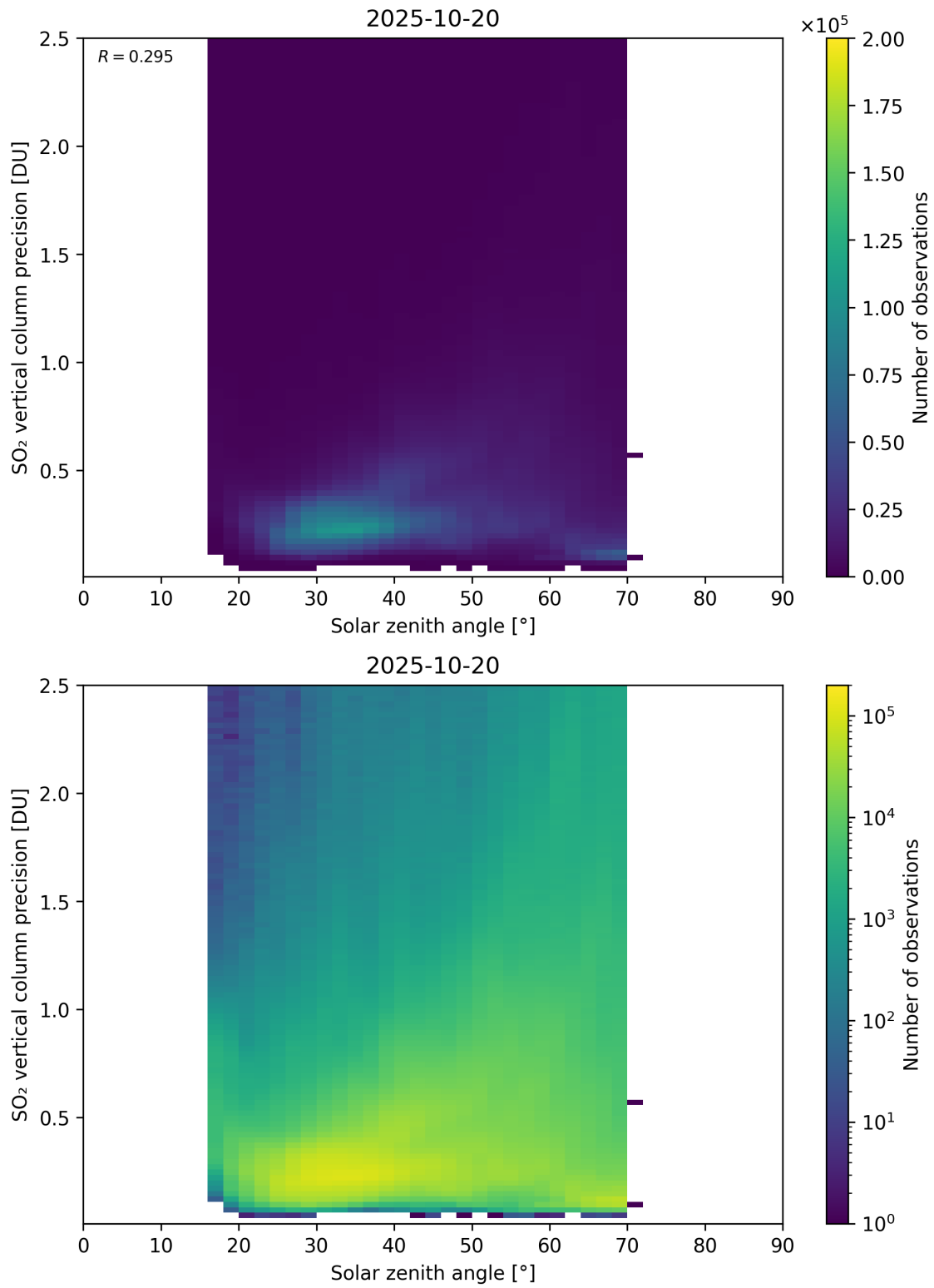
Figure 192: Scatter density plot of “Solar zenith angle” against “SO 2 vertical column precision” for 2025-10-19 to 2025-10-21.
