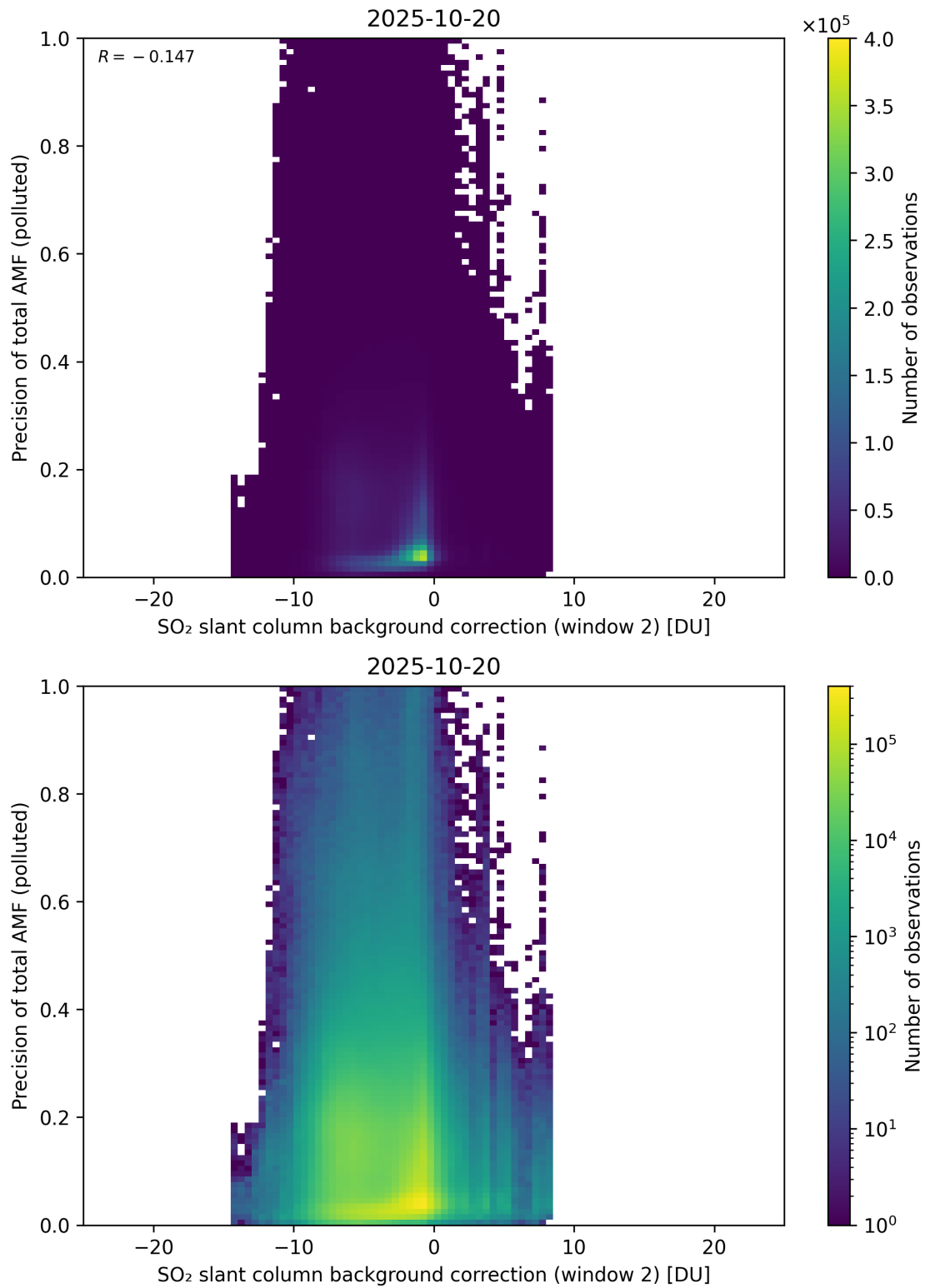
Figure 131: Scatter density plot of “SO 2 slant column background correction (window 2)” against “Precision of total AMF (polluted)” for 2025-10-19 to 2025-10-21.
