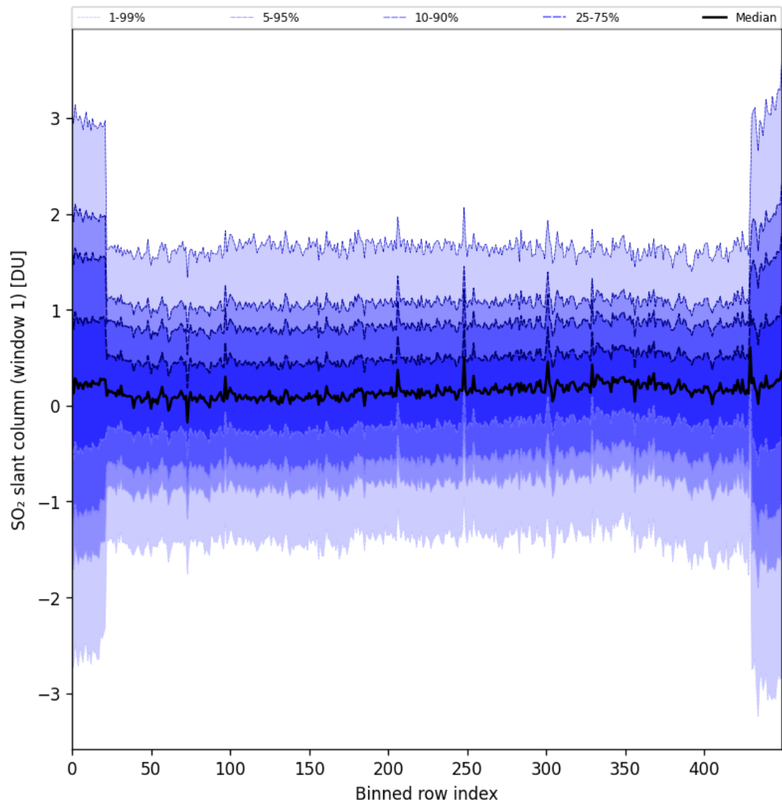
Figure 89: Along track statistics of “SO 2 slant column (window 1)” for 2025-10-19 to 2025-10-21
