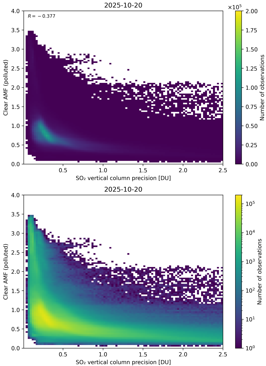
Figure 335: Scatter density plot of “SO 2 vertical column precision” against “Clear AMF (polluted)” for 2025-10-19 to 2025-10-21.
