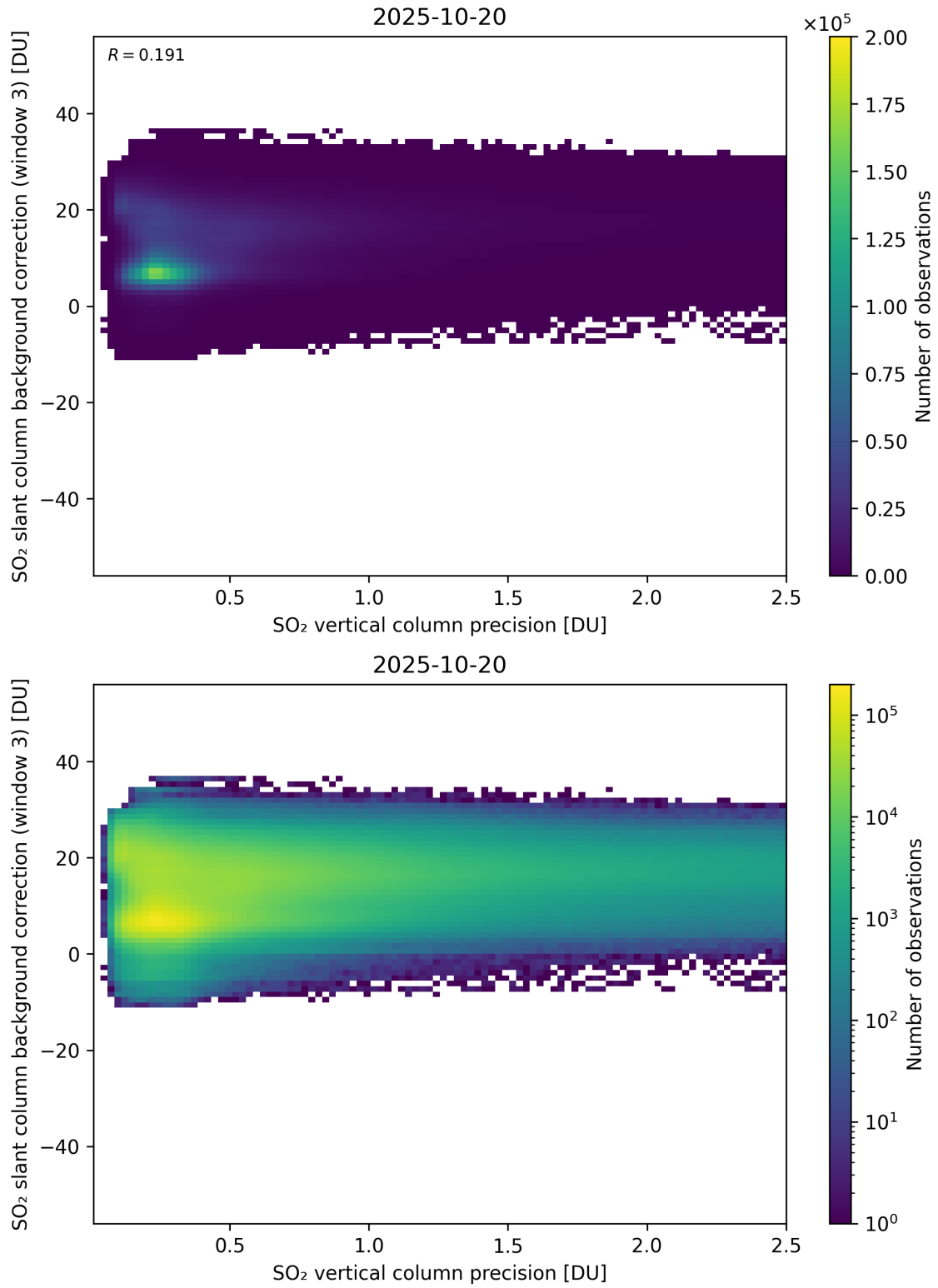
Figure 331: Scatter density plot of “SO 2 vertical column precision” against “SO 2 slant column background correction (window 3)” for 2025-10-19 to 2025-10-21.
