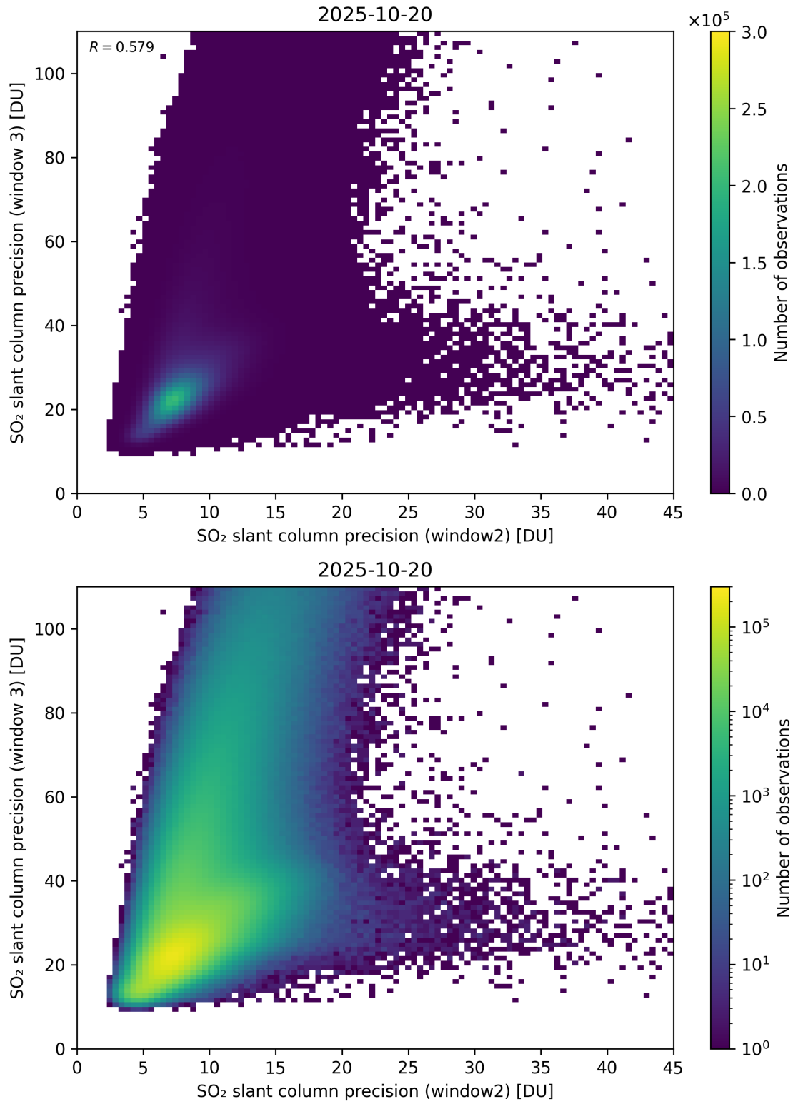
Figure 300: Scatter density plot of “SO 2 slant column precision (window2)” against “SO 2 slant column precision (window 3)” for 2025-10-19 to 2025-10-21.
