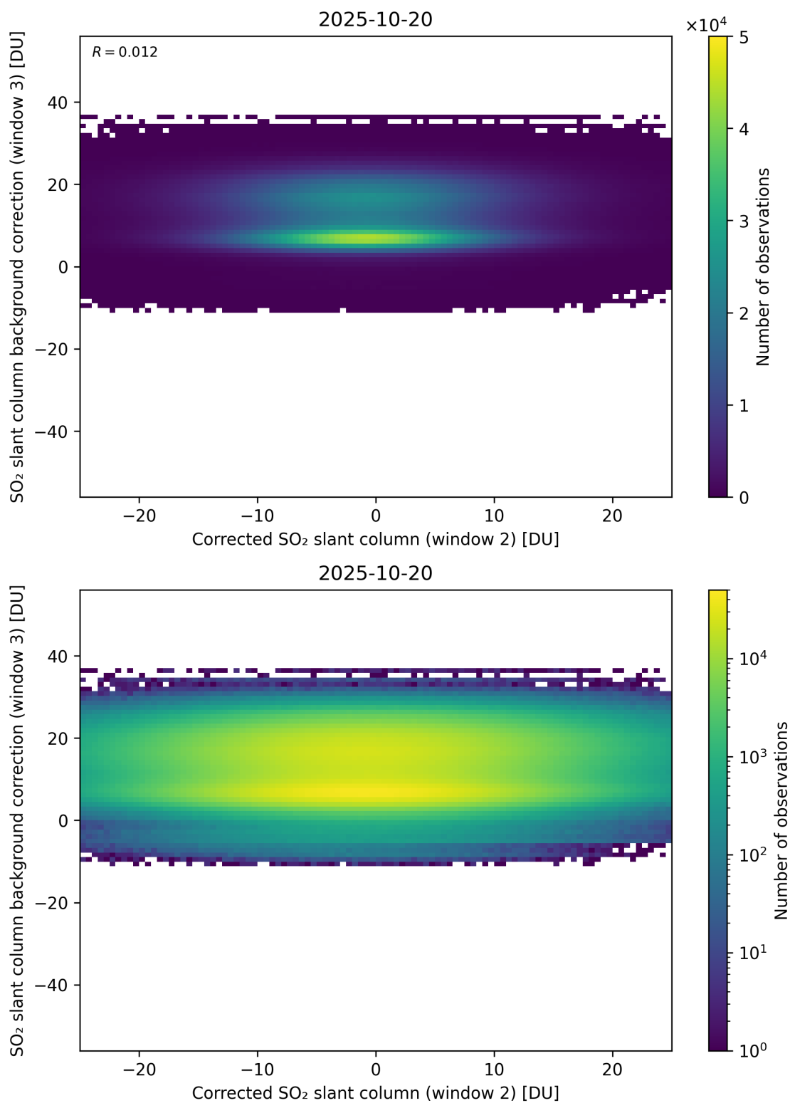
Figure 245: Scatter density plot of “Corrected SO 2 slant column (window 2)” against “SO 2 slant column background correction (window 3)” for 2025-10-19 to 2025-10-21.
