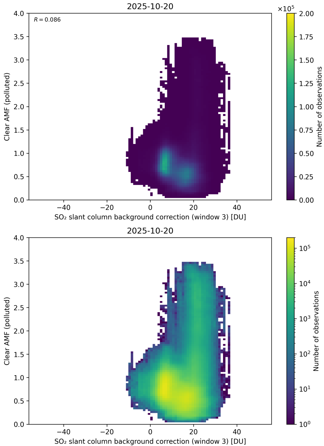
Figure 135: Scatter density plot of “SO 2 slant column background correction (window 3)” against “Clear AMF (polluted)” for 2025-10-19 to 2025-10-21.
