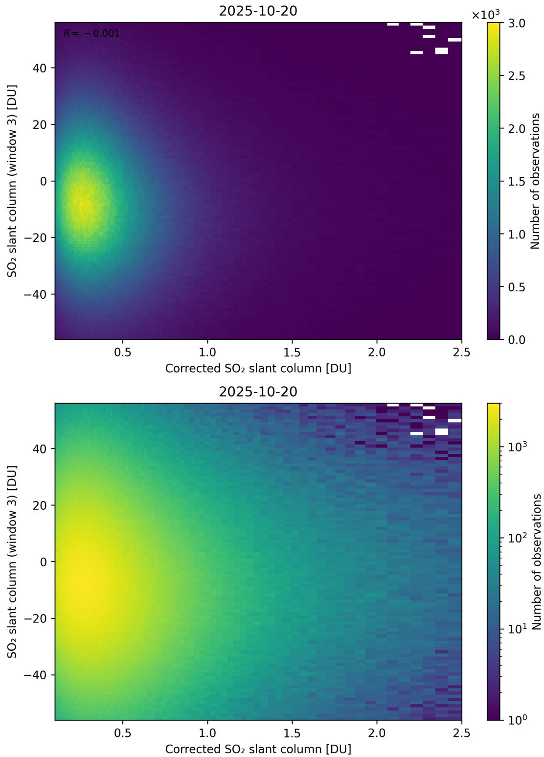
Figure 240: Scatter density plot of “Corrected SO 2 slant column” against “SO 2 slant column (window 3)” for 2025-10-19 to 2025-10-21.
