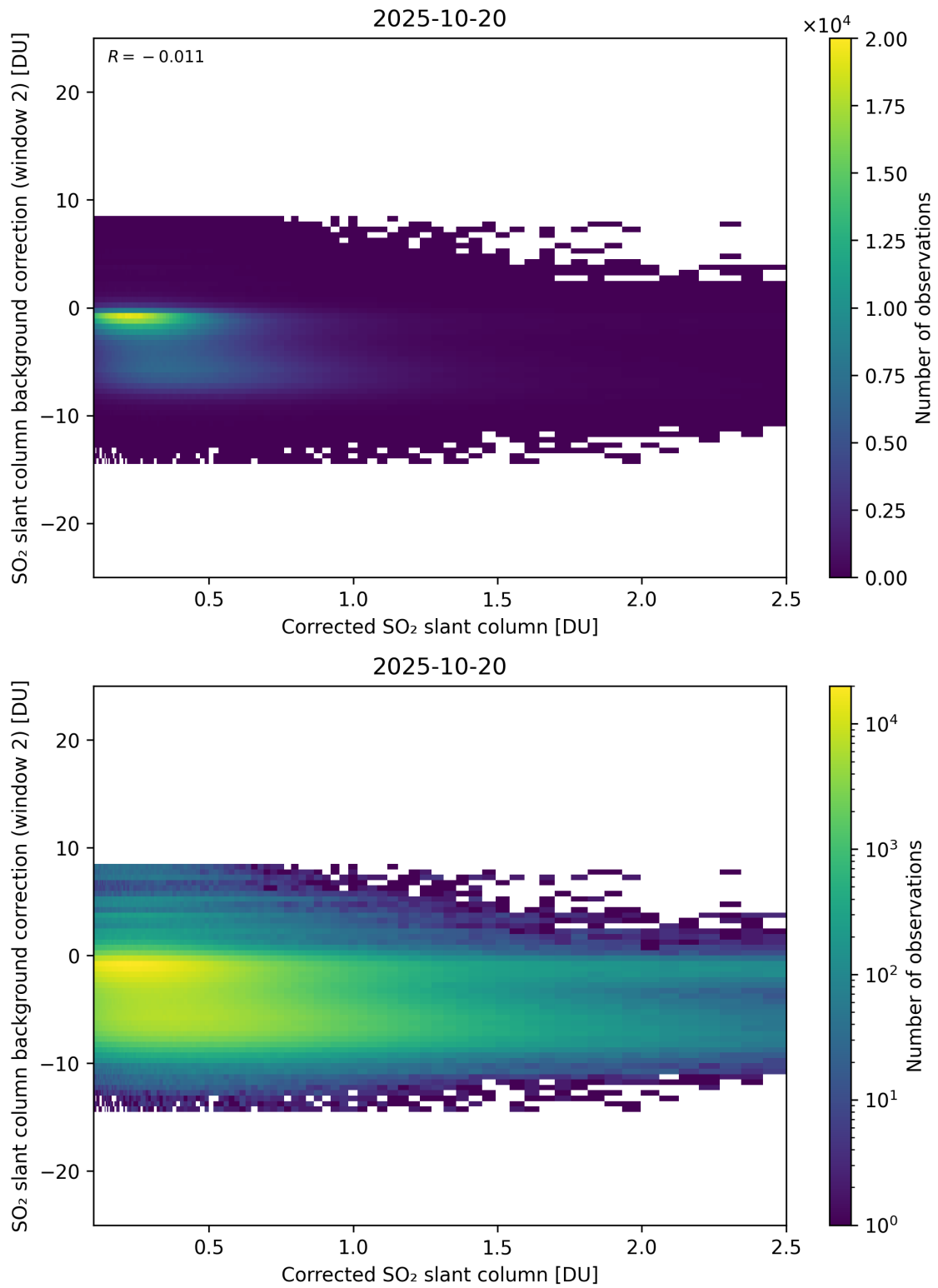
Figure 227: Scatter density plot of “Corrected SO 2 slant column” against “SO 2 slant column background correction (window 2)” for 2025-10-19 to 2025-10-21.
