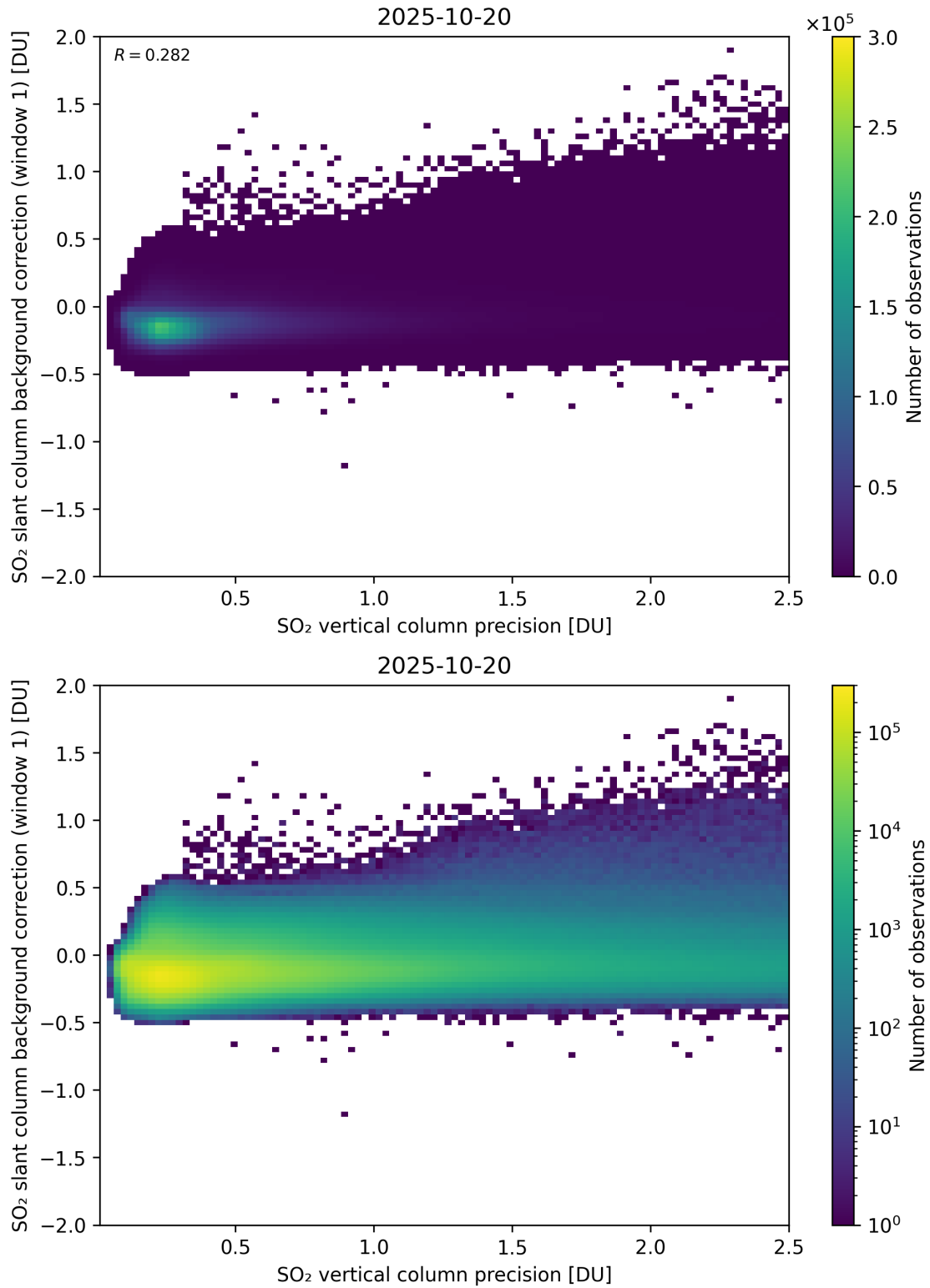
Figure 329: Scatter density plot of “SO 2 vertical column precision” against “SO 2 slant column background correction (window 1)” for 2025-10-19 to 2025-10-21.
