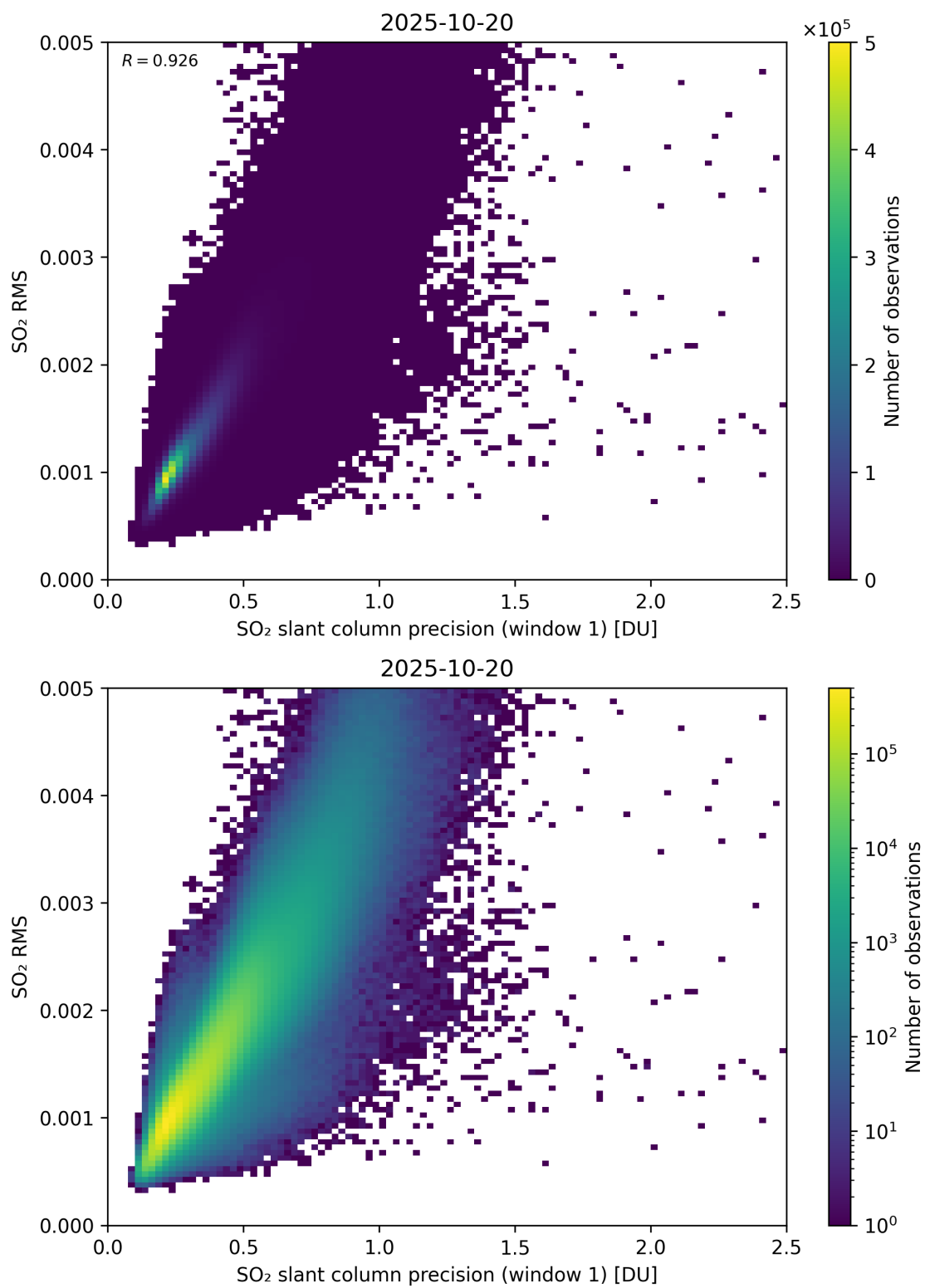
Figure 273: Scatter density plot of “SO 2 slant column precision (window 1)” against “SO 2 RMS” for 2025-10-19 to 2025-10-21.
