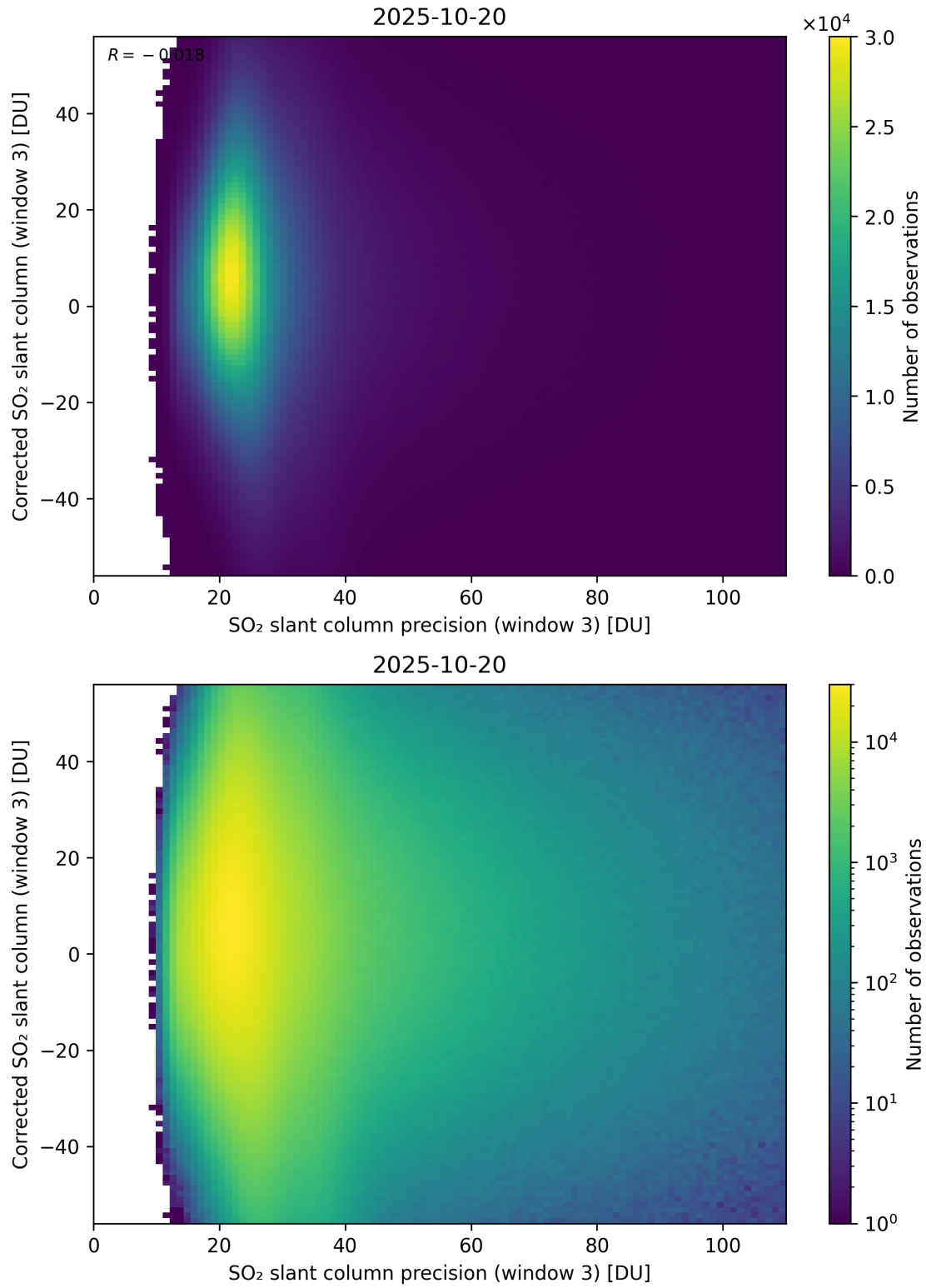
Figure 312: Scatter density plot of “SO 2 slant column precision (window 3)” against “Corrected SO 2 slant column (window 3)” for 2025-10-19 to 2025-10-21.
