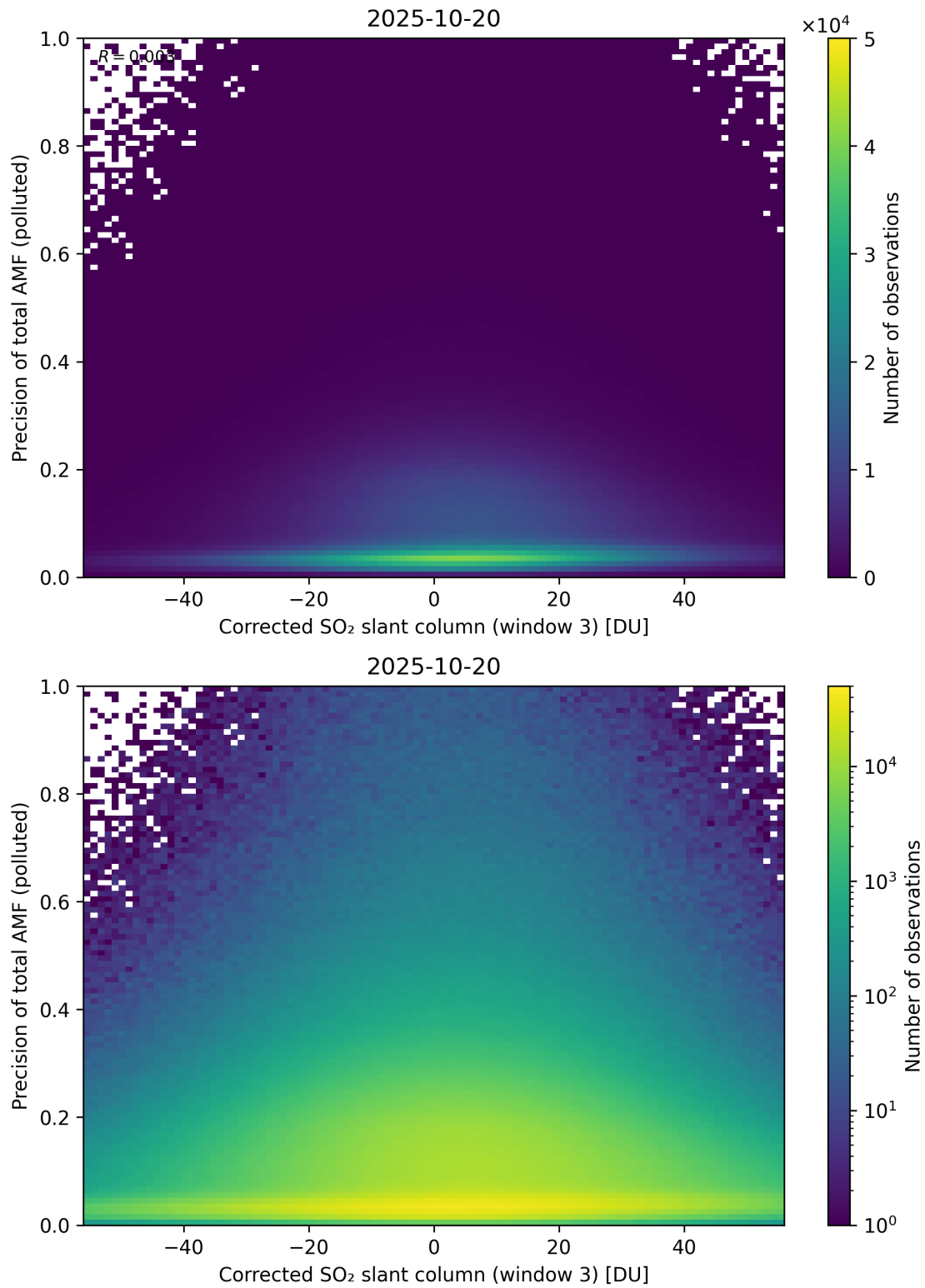
Figure 261: Scatter density plot of “Corrected SO 2 slant column (window 3)” against “Precision of total AMF (polluted)” for 2025-10-19 to 2025-10-21.
