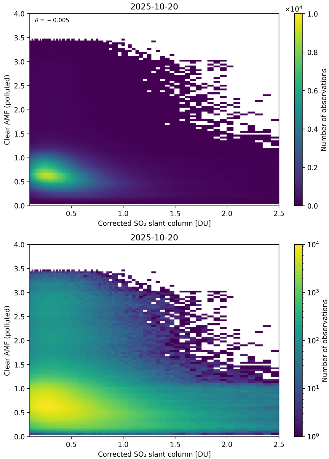
Figure 232: Scatter density plot of “Corrected SO 2 slant column” against “Clear AMF (polluted)” for 2025-10-19 to 2025-10-21.
