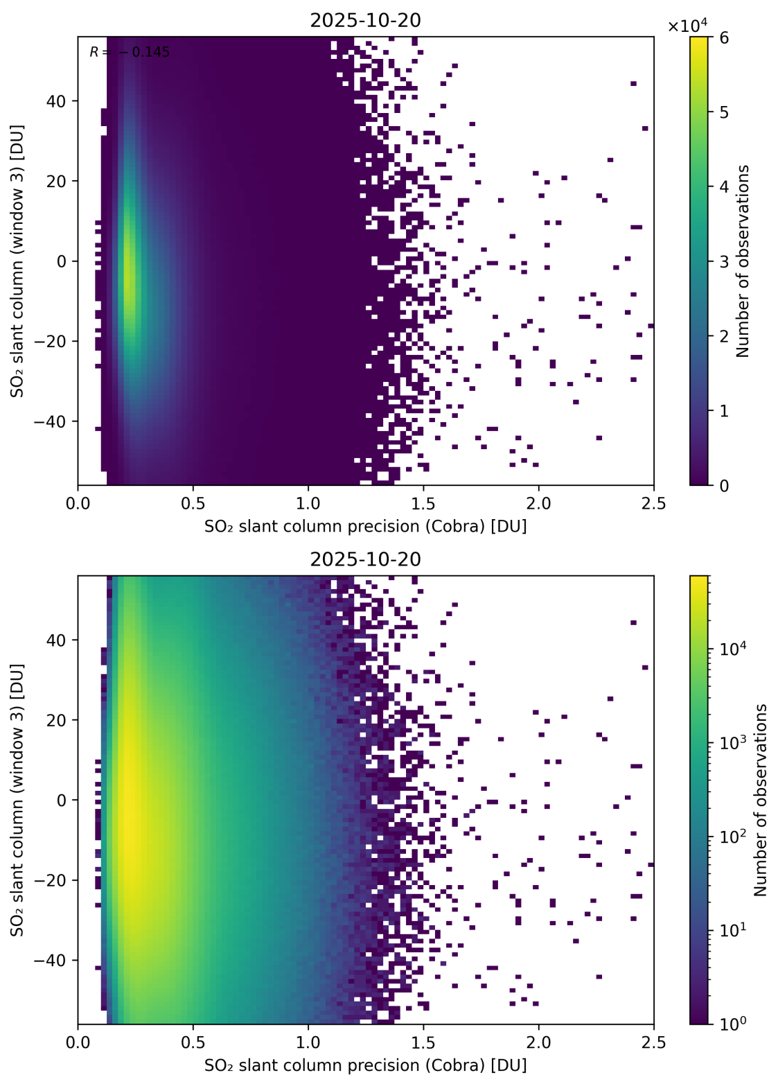
Figure 211: Scatter density plot of “SO 2 slant column precision (Cobra)” against “SO 2 slant column (window 3)” for 2025-10-19 to 2025-10-21.
