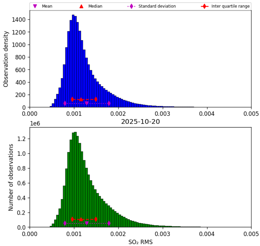
Figure 78: Histogram of “SO 2 RMS” for 2025-10-19 to 2025-10-21
