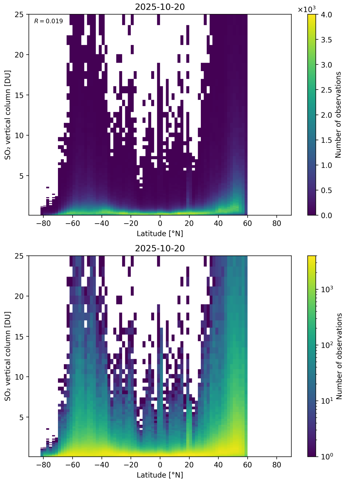
Figure 169: Scatter density plot of “Latitude” against “SO 2 vertical column” for 2025-10-19 to 2025-10-21.
