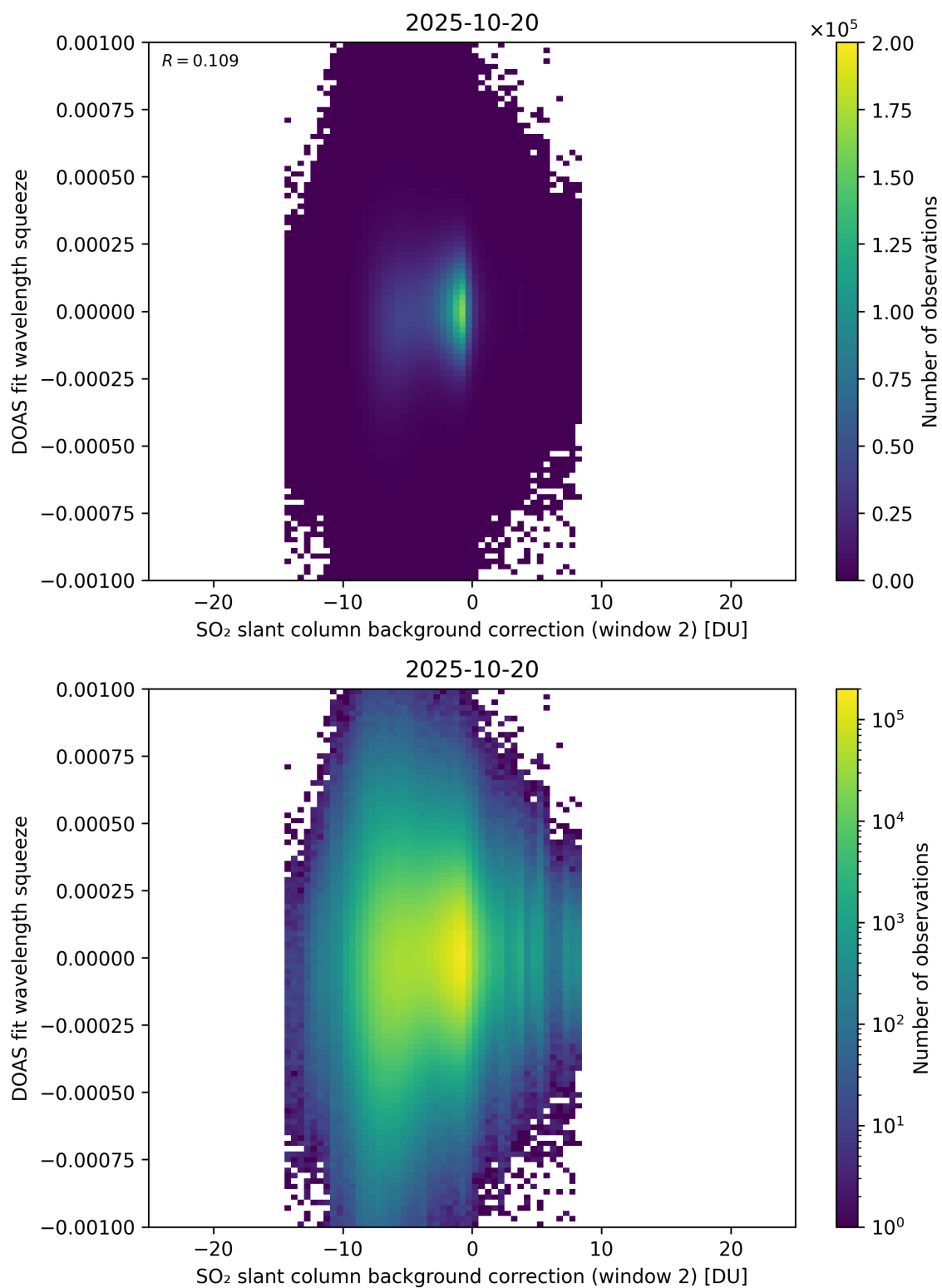
Figure 124: Scatter density plot of “SO 2 slant column background correction (window 2)” against “DOAS fit wavelength squeeze” for 2025-10-19 to 2025-10-21.
