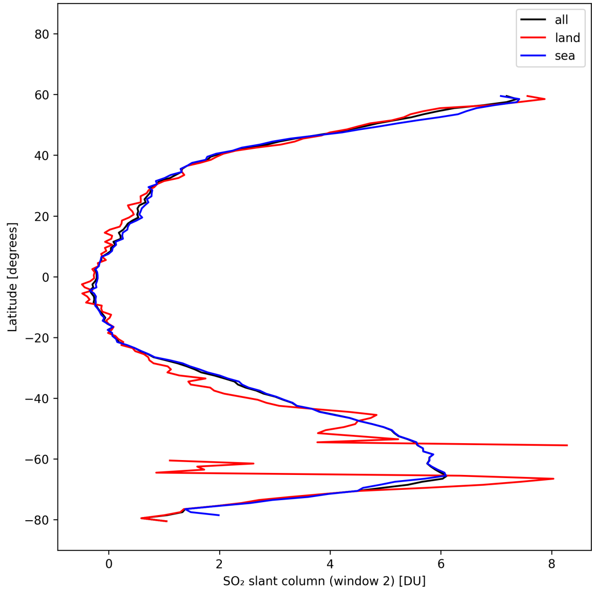
Figure 41: Zonal average of “SO 2 slant column (window 2)” for 2025-10-19 to 2025-10-21.
