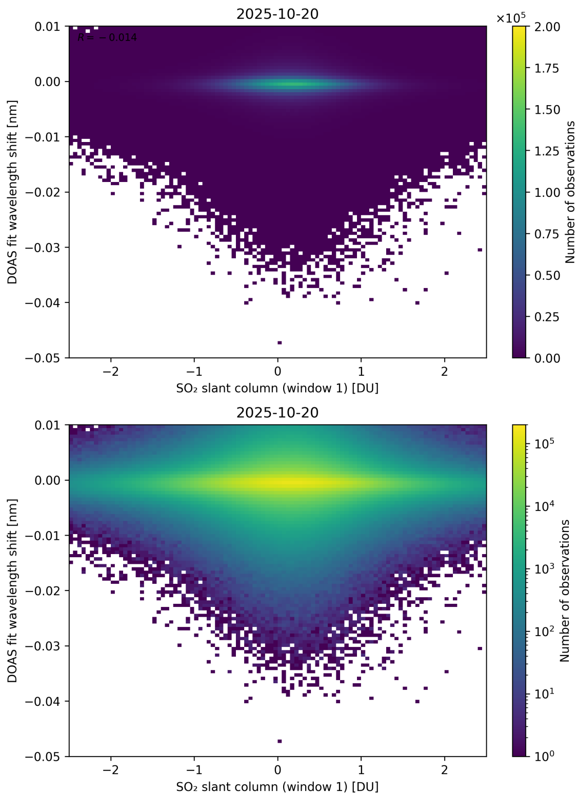
Figure 265: Scatter density plot of “SO 2 slant column (window 1)” against “DOAS fit wavelength shift” for 2025-10-19 to 2025-10-21.
