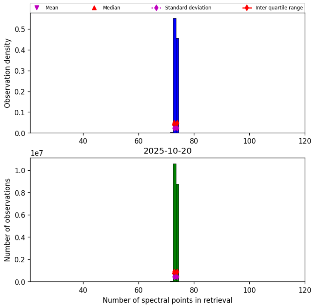
Figure 82: Histogram of “Number of spectral points in retrieval” for 2025-10-19 to 2025-10-21
