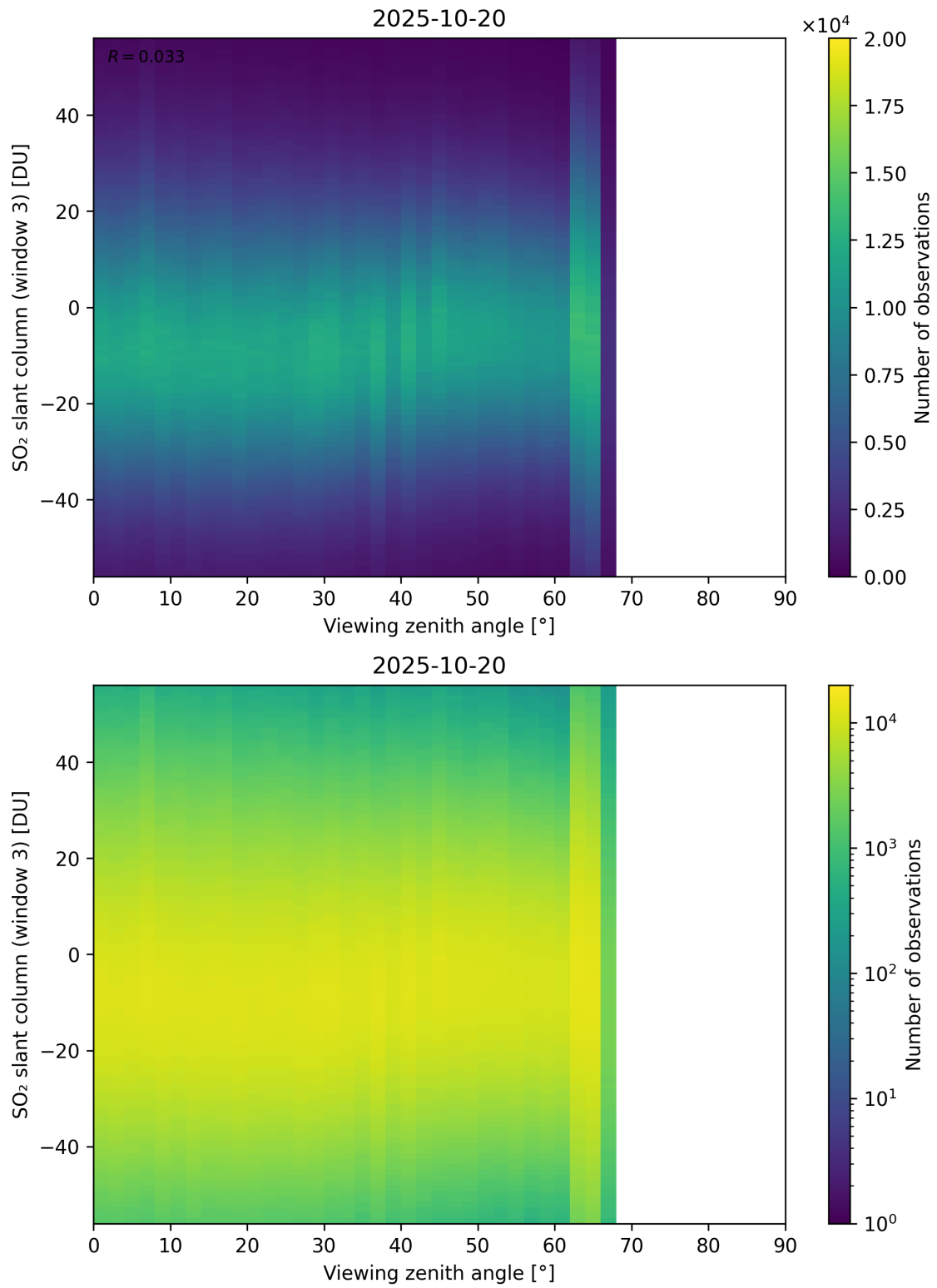
Figure 379: Scatter density plot of “Viewing zenith angle” against “SO 2 slant column (window 3)” for 2025-10-19 to 2025-10-21.
