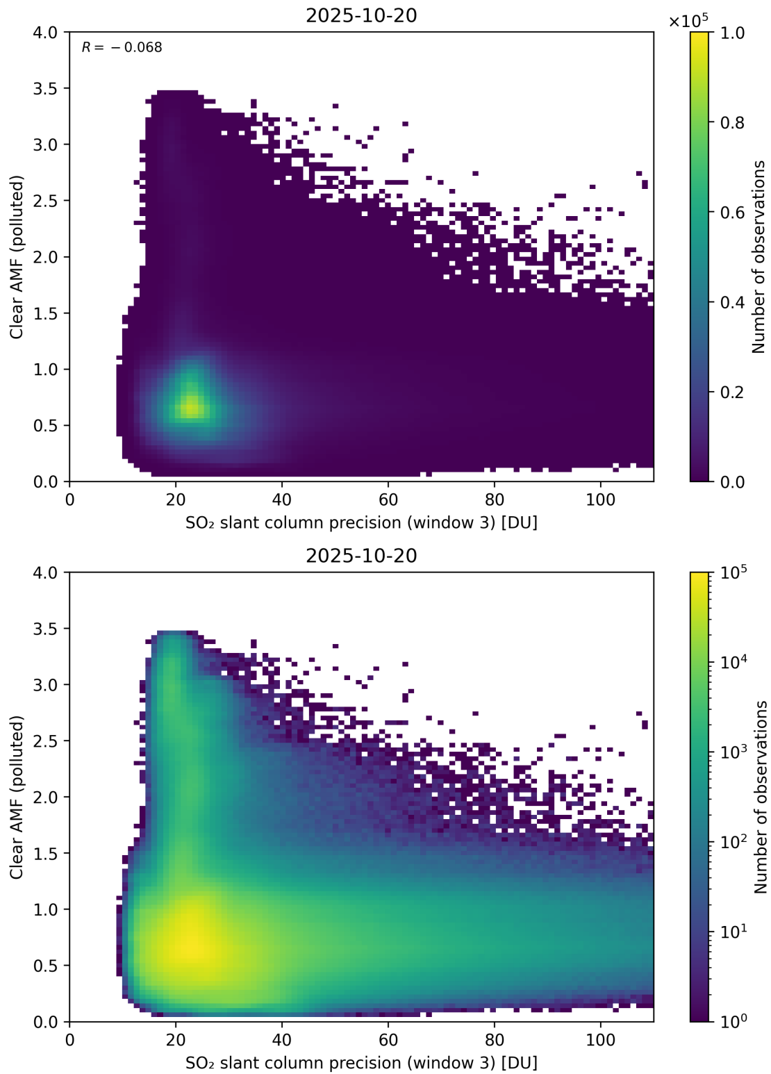
Figure 311: Scatter density plot of “SO 2 slant column precision (window 3)” against “Clear AMF (polluted)” for 2025-10-19 to 2025-10-21.
