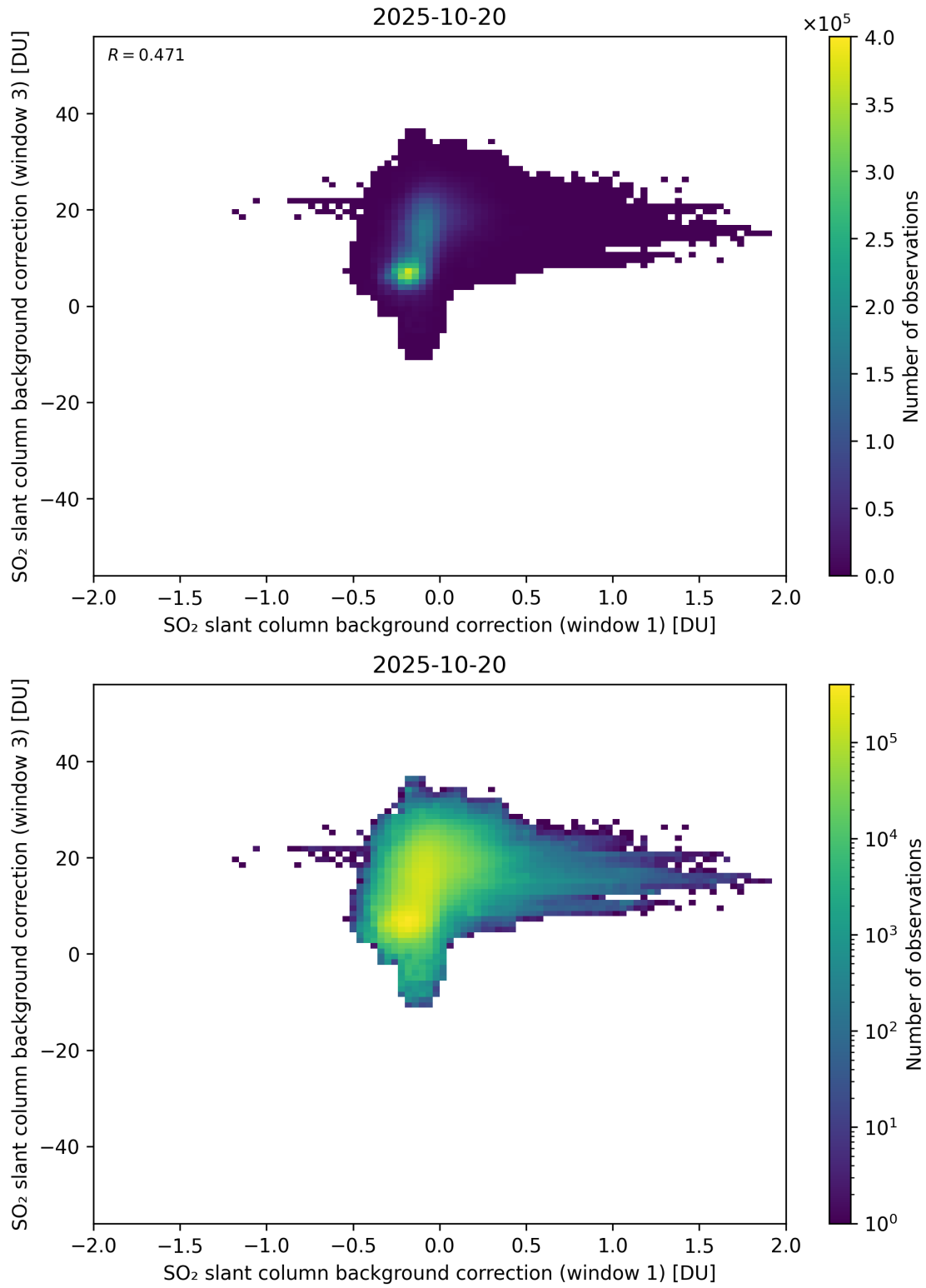
Figure 110: Scatter density plot of “SO 2 slant column background correction (window 1)” against “SO 2 slant column background correction (window 3)” for 2025-10-19 to 2025-10-21.
