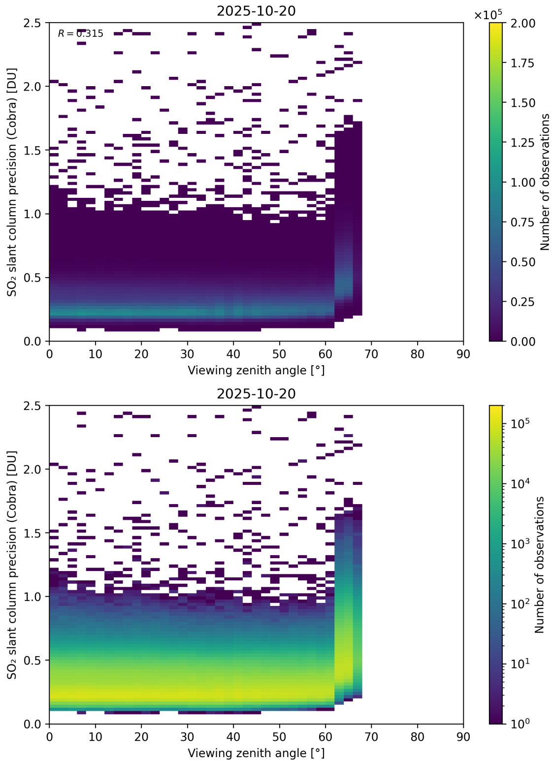
Figure 372: Scatter density plot of “Viewing zenith angle” against “SO 2 slant column precision (Cobra)” for 2025-10-19 to 2025-10-21.
