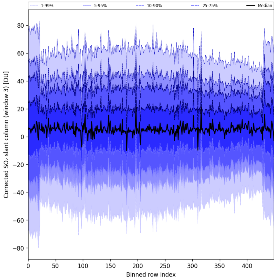
Figure 99: Along track statistics of “Corrected SO 2 slant column (window 3)” for 2025-10-19 to 2025-10-21
