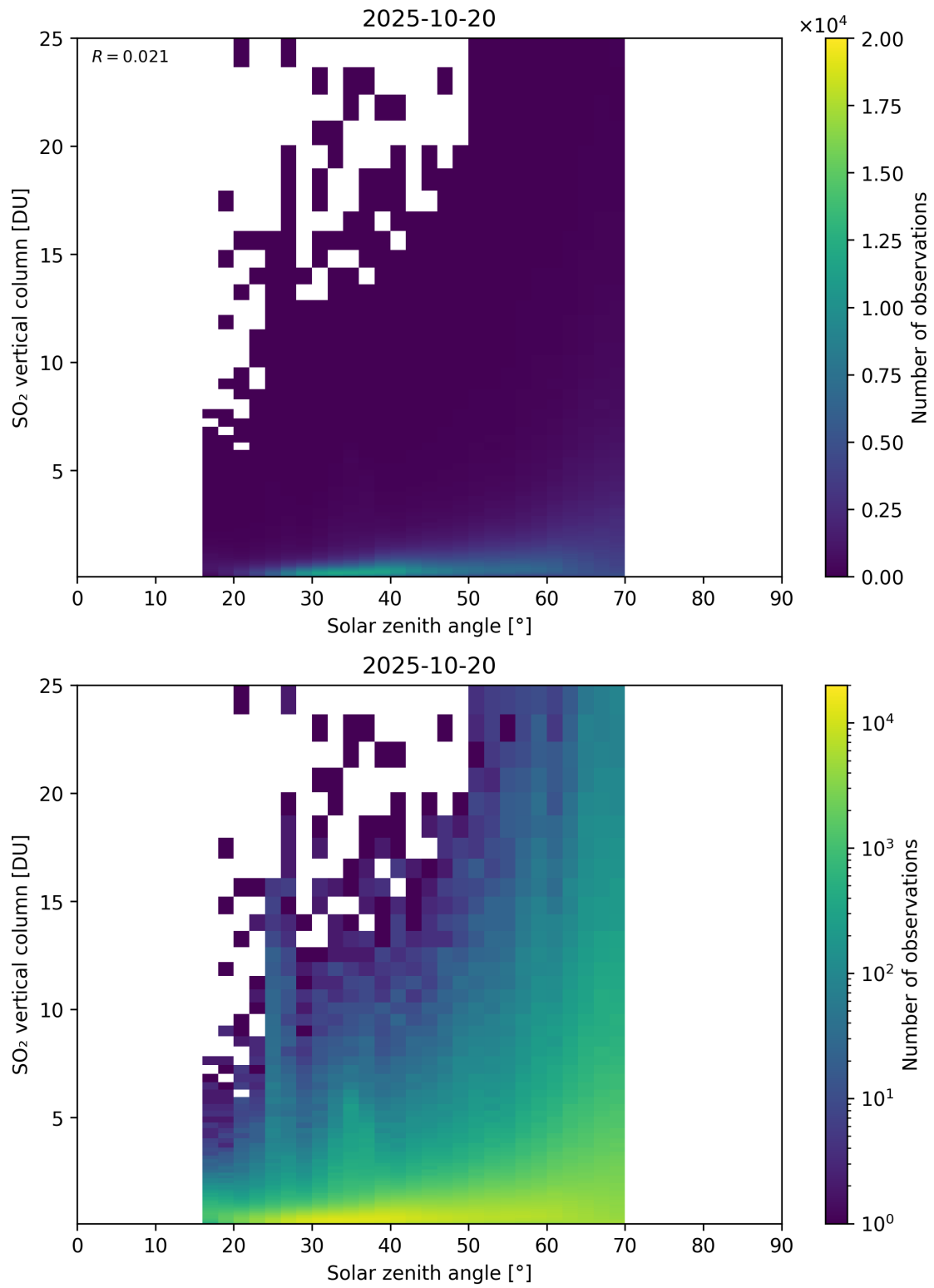
Figure 191: Scatter density plot of “Solar zenith angle” against “SO 2 vertical column” for 2025-10-19 to 2025-10-21.
