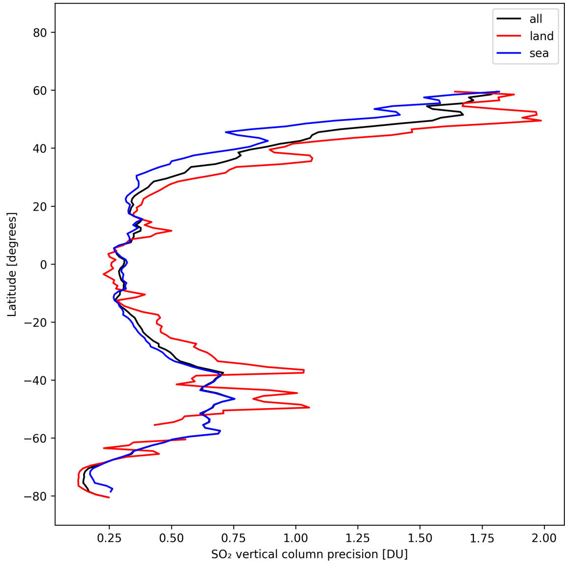
Figure 33: Zonal average of “SO 2 vertical column precision” for 2025-10-19 to 2025-10-21.
