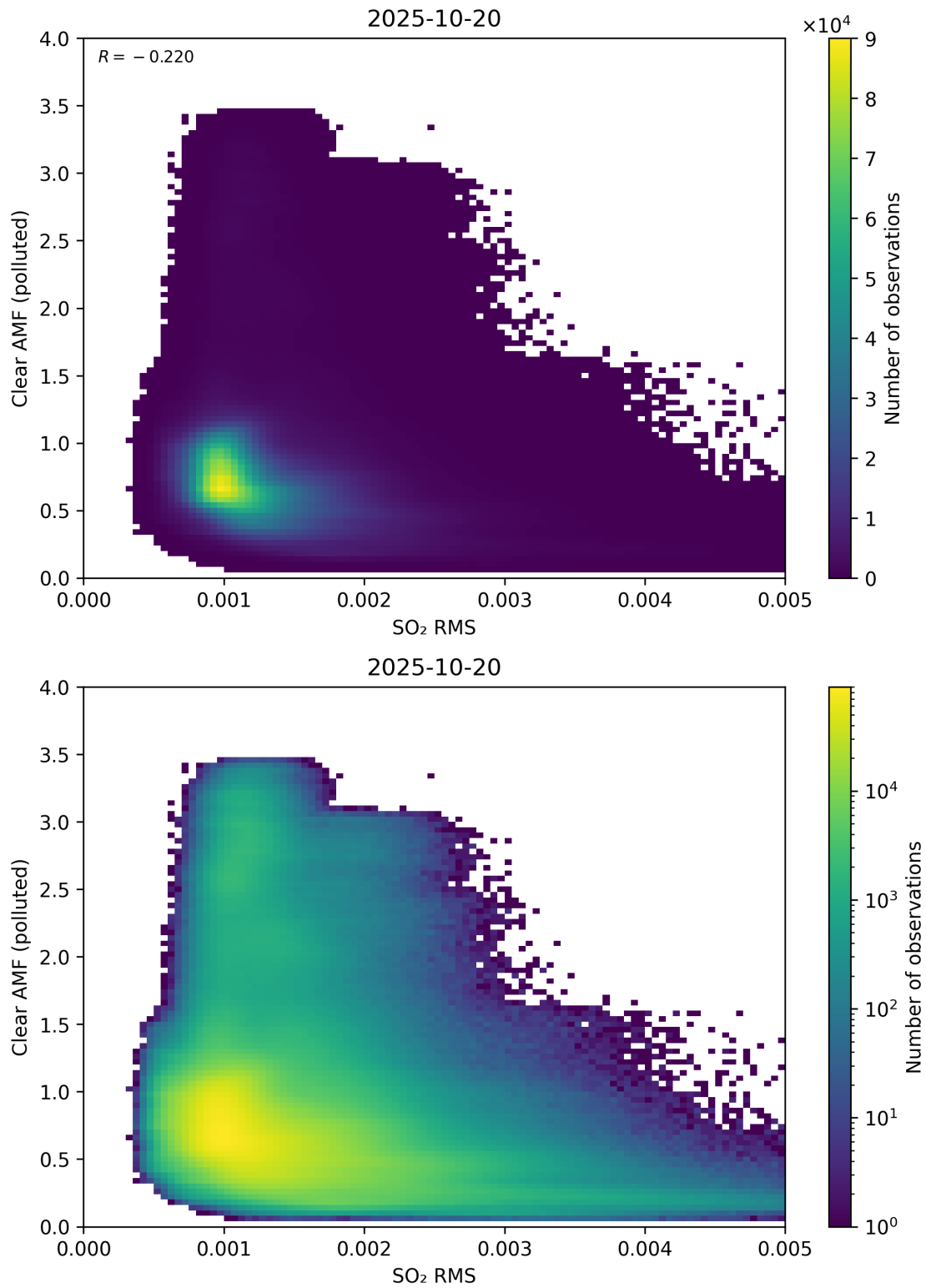
Figure 147: Scatter density plot of “SO 2 RMS” against “Clear AMF (polluted)” for 2025-10-19 to 2025-10-21.
