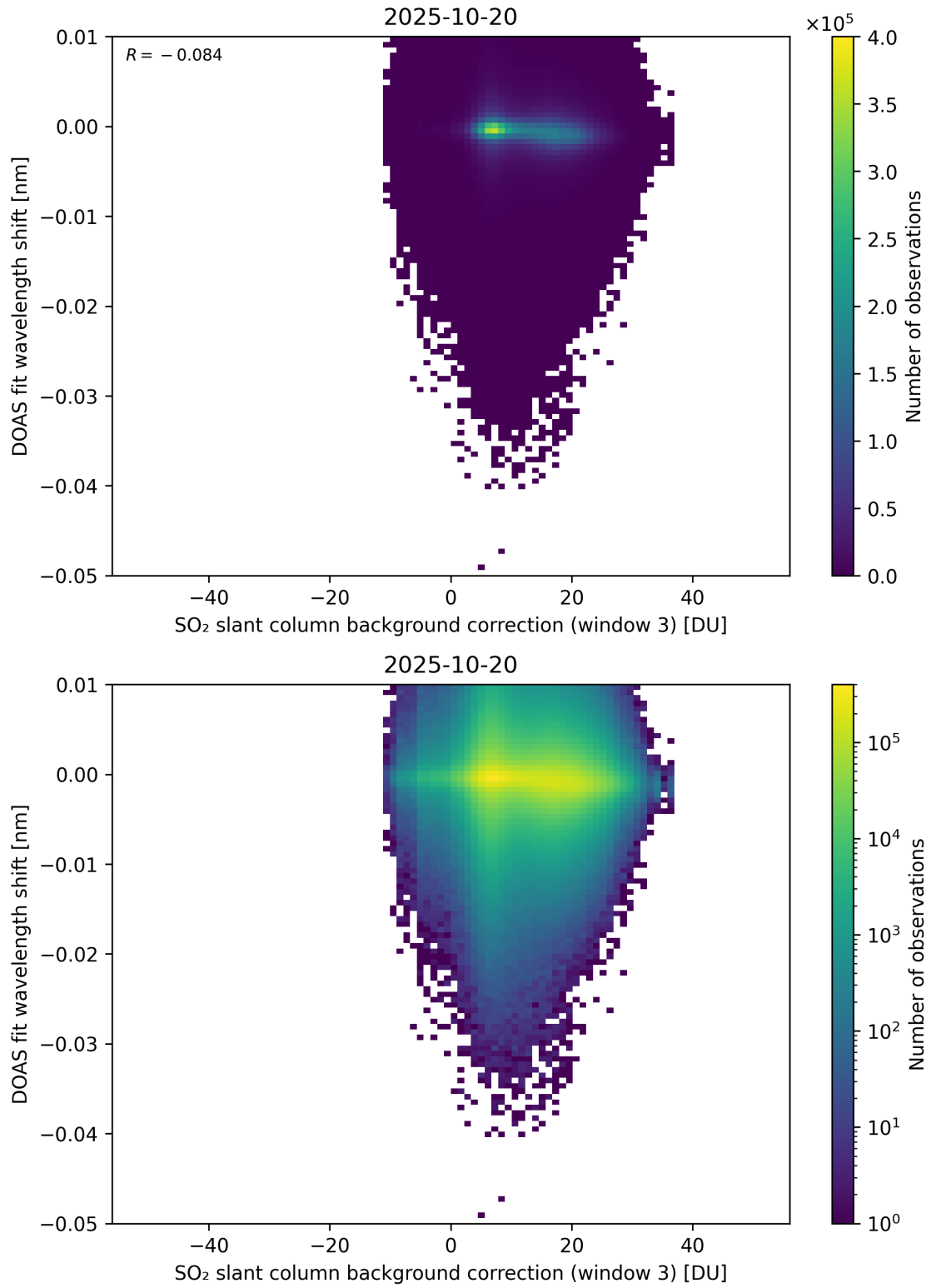
Figure 132: Scatter density plot of “SO 2 slant column background correction (window 3)” against “DOAS fit wavelength shift” for 2025-10-19 to 2025-10-21.
