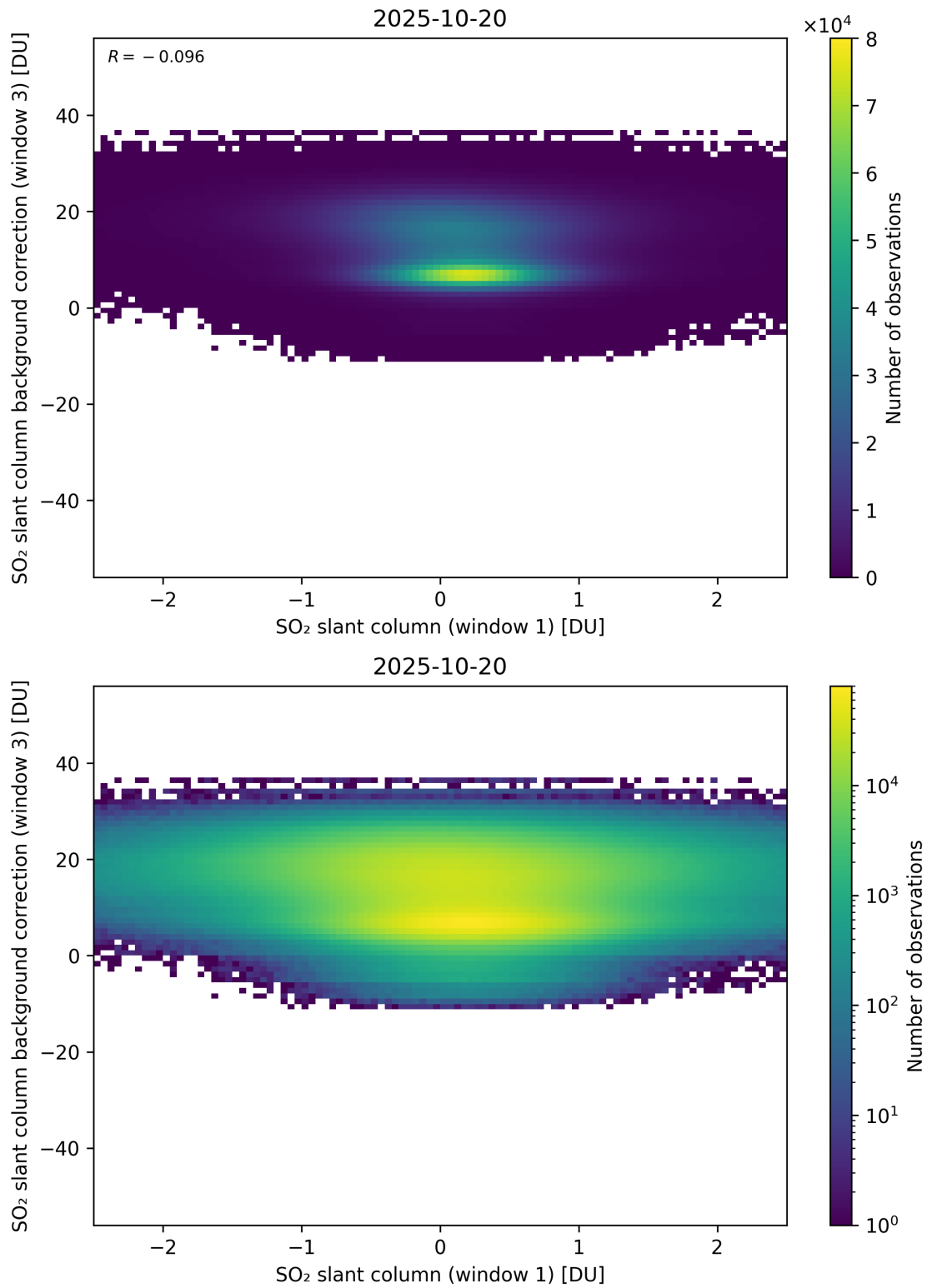
Figure 264: Scatter density plot of “SO 2 slant column (window 1)” against “SO 2 slant column background correction (window 3)” for 2025-10-19 to 2025-10-21.
