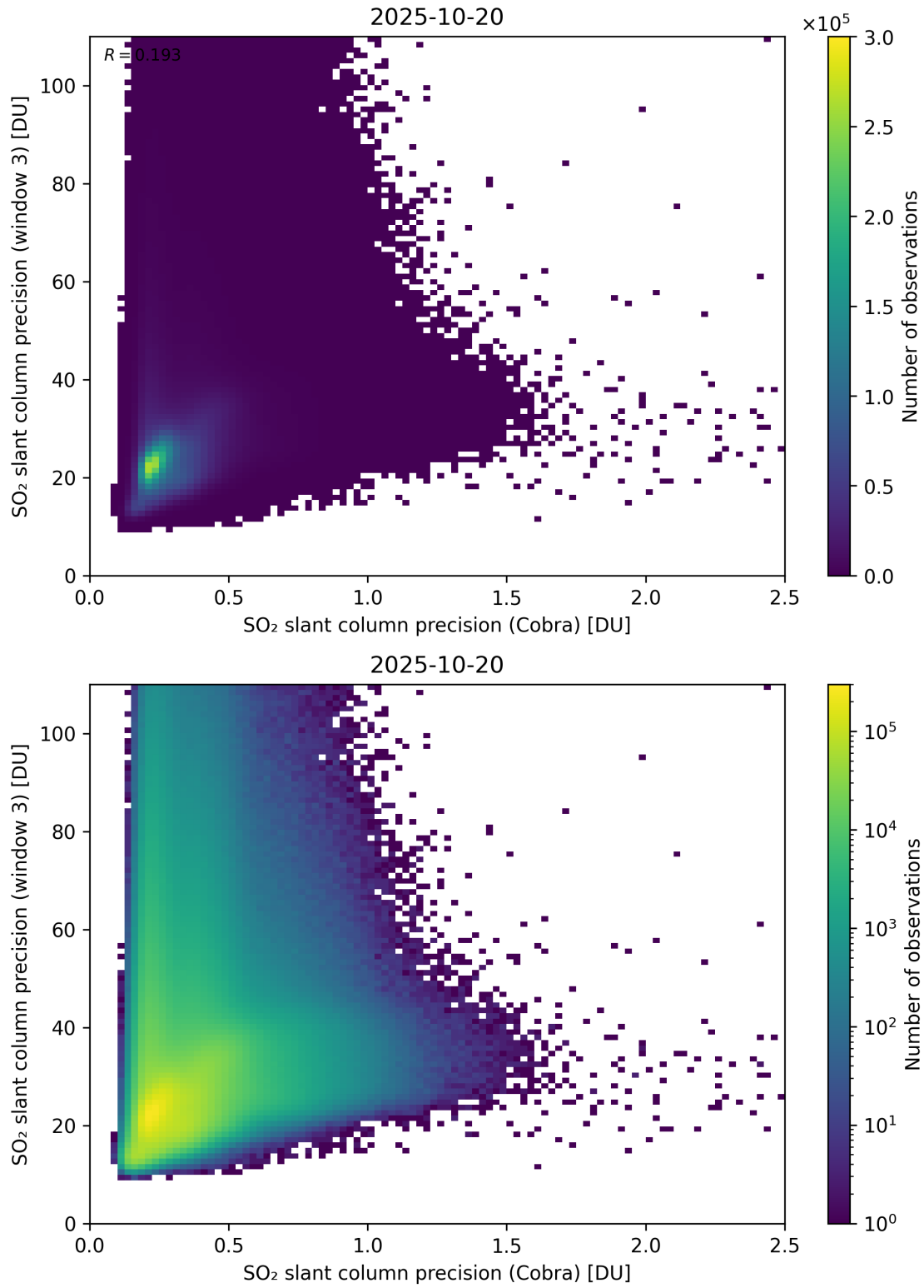
Figure 212: Scatter density plot of “SO 2 slant column precision (Cobra)” against “SO 2 slant column precision (window 3)” for 2025-10-19 to 2025-10-21.
