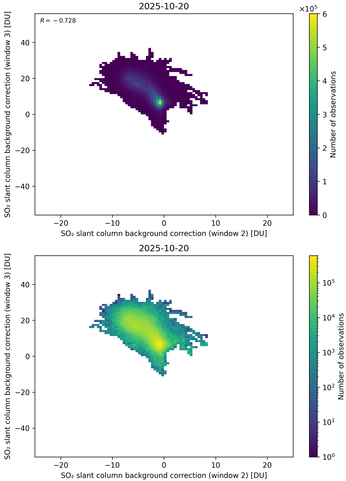
Figure 122: Scatter density plot of “SO 2 slant column background correction (window 2)” against “SO 2 slant column background correction (window 3)” for 2025-10-19 to 2025-10-21.
