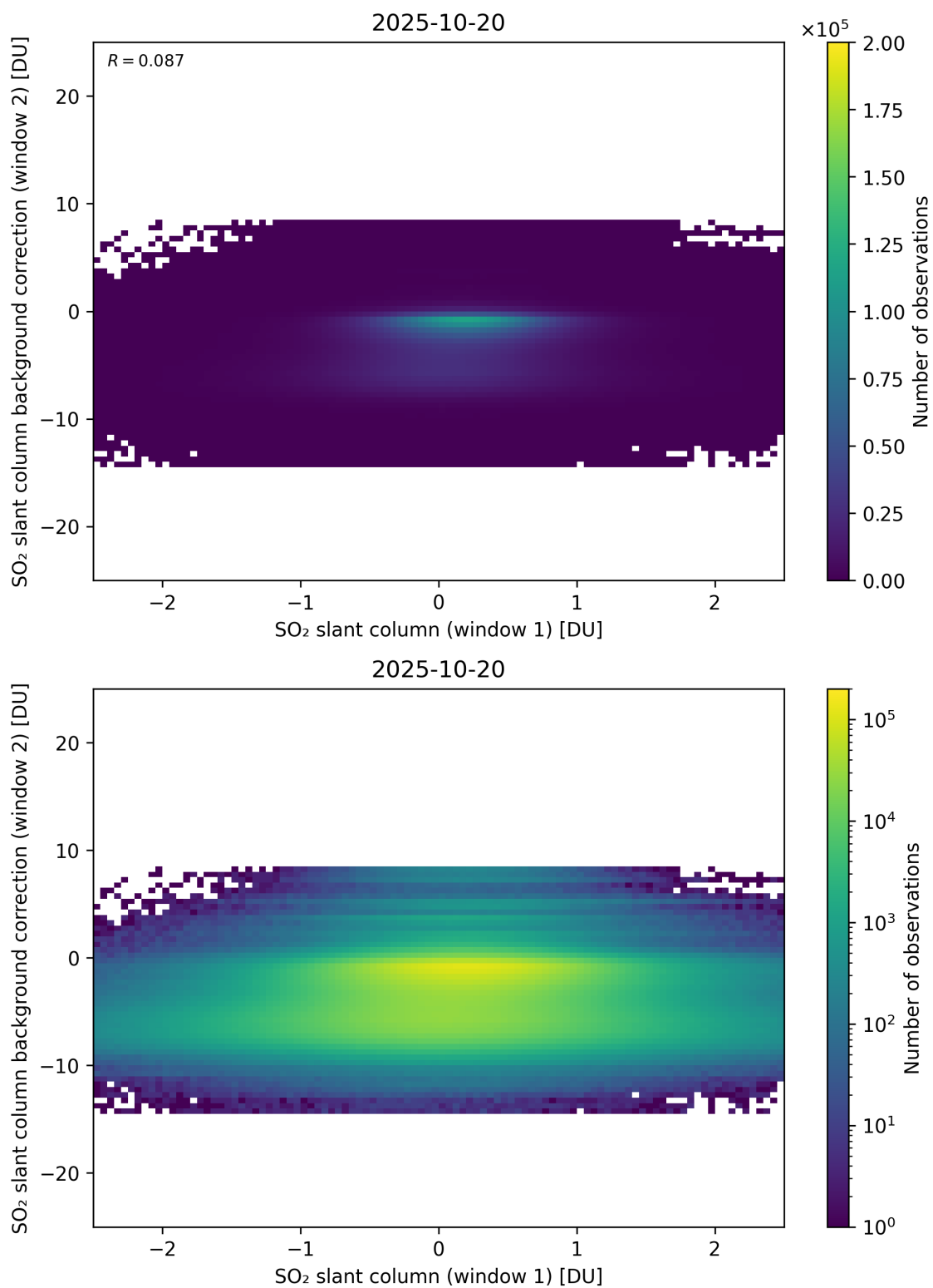
Figure 263: Scatter density plot of “SO 2 slant column (window 1)” against “SO 2 slant column background correction (window 2)” for 2025-10-19 to 2025-10-21.
