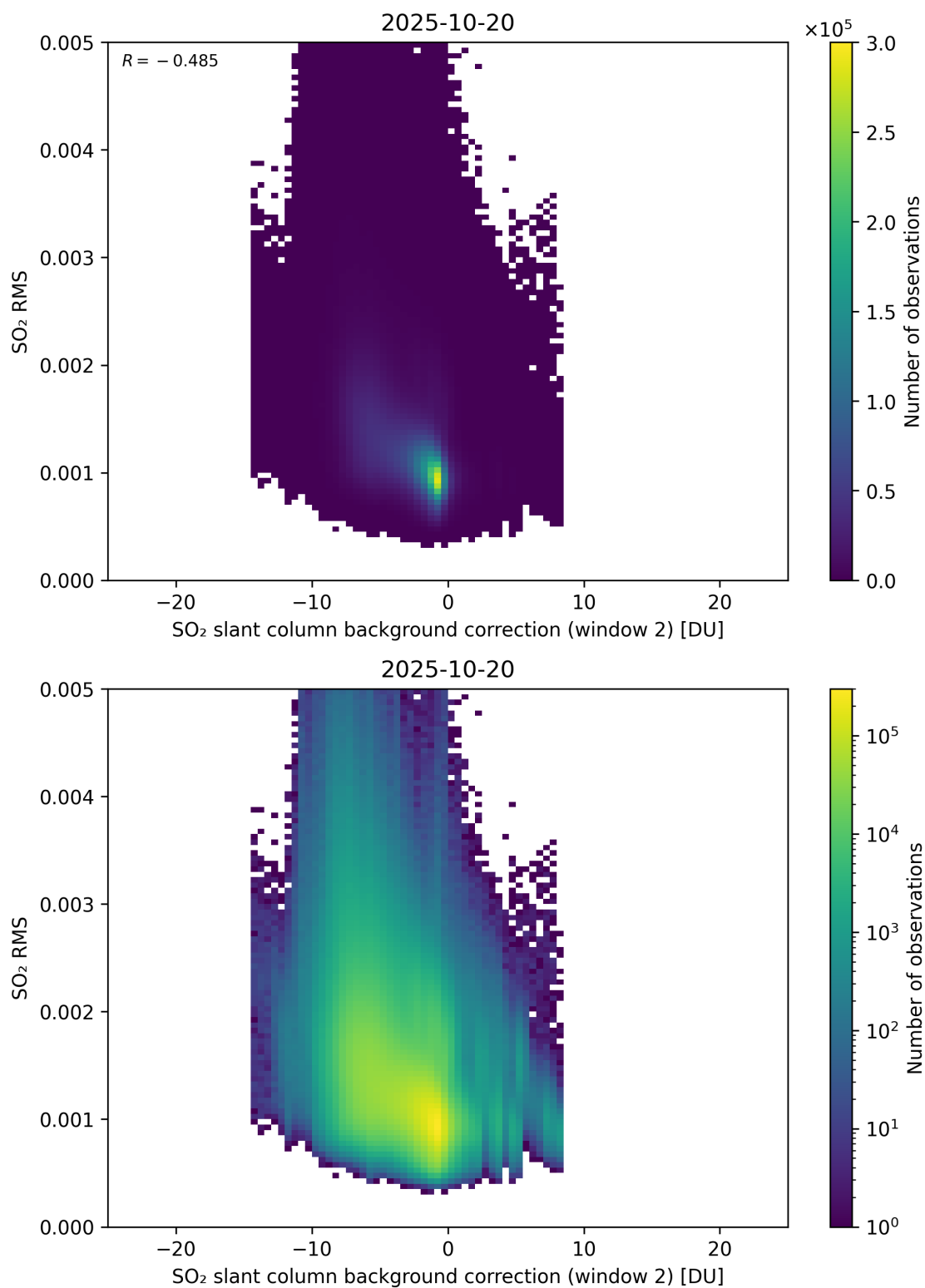
Figure 125: Scatter density plot of “SO 2 slant column background correction (window 2)” against “SO 2 RMS” for 2025-10-19 to 2025-10-21.
