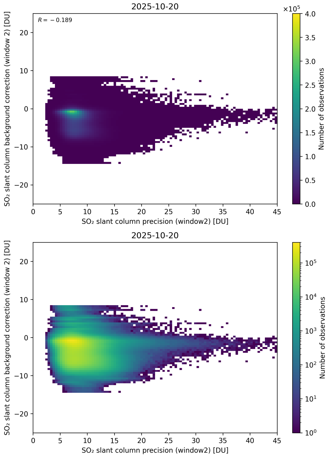
Figure 291: Scatter density plot of “SO 2 slant column precision (window2)” against “SO 2 slant column background correction (window 2)” for 2025-10-19 to 2025-10-21.
