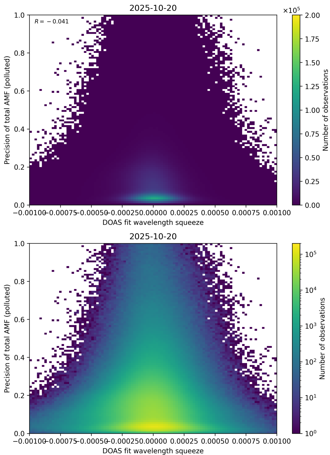
Figure 146: Scatter density plot of “DOAS fit wavelength squeeze” against “Precision of total AMF (polluted)” for 2025-10-19 to 2025-10-21.
