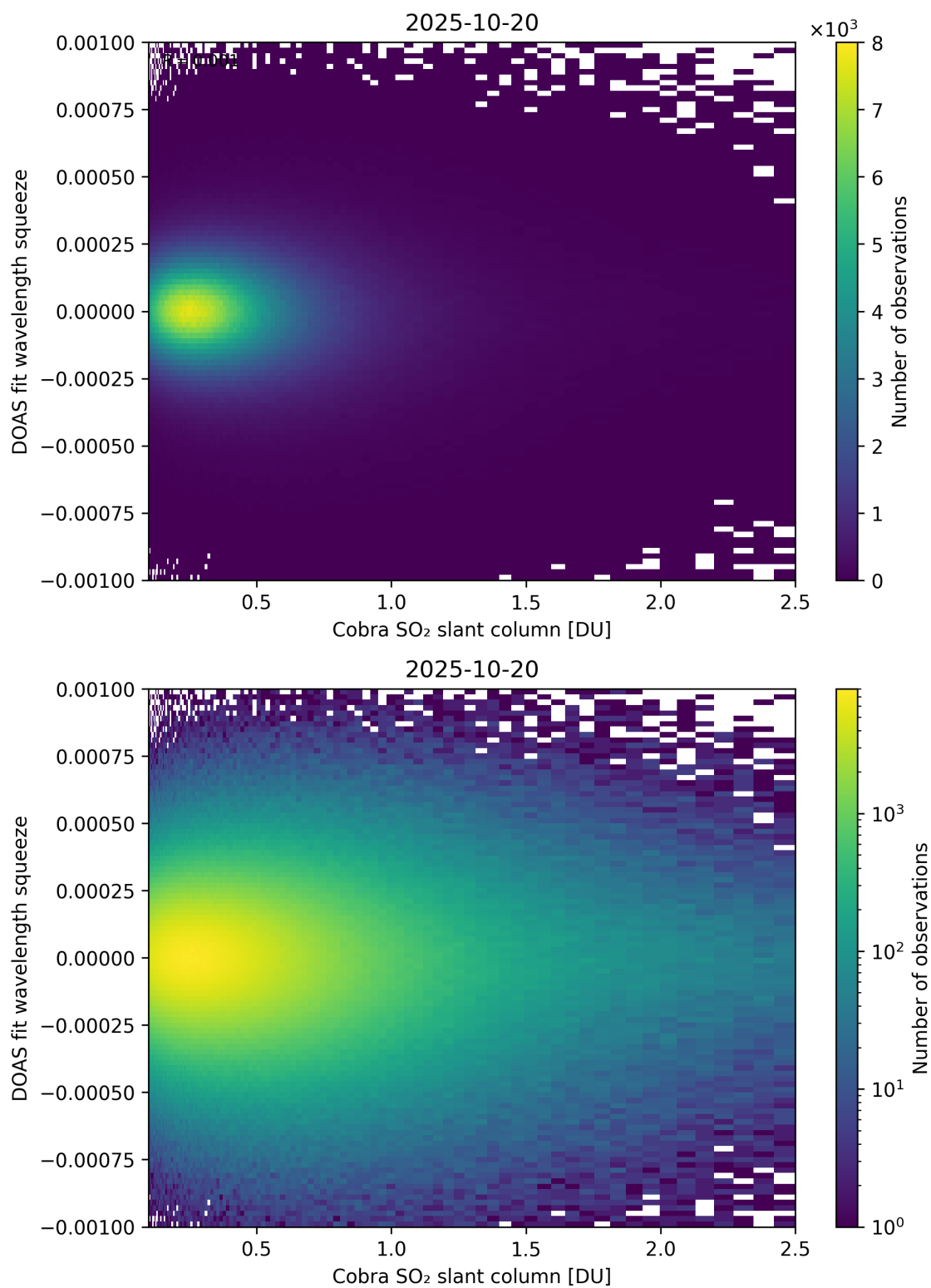
Figure 197: Scatter density plot of “Cobra SO 2 slant column” against “DOAS fit wavelength squeeze” for 2025-10-19 to 2025-10-21.
