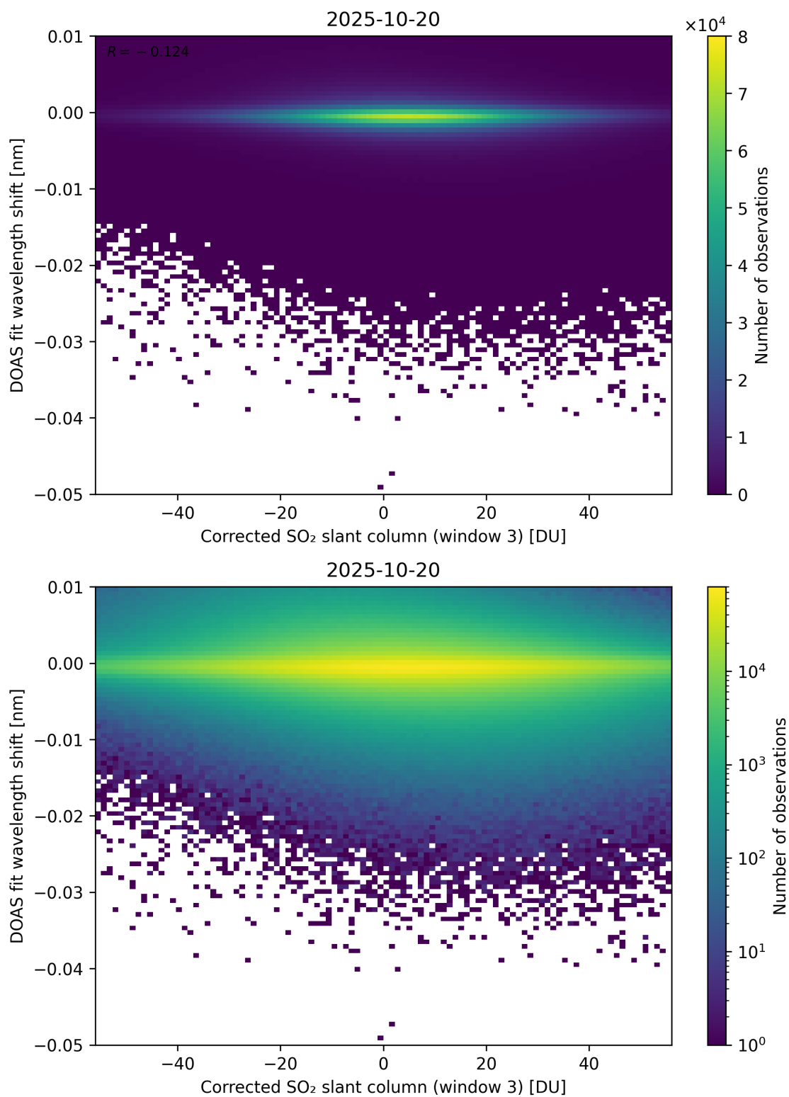
Figure 256: Scatter density plot of “Corrected SO 2 slant column (window 3)” against “DOAS fit wavelength shift” for 2025-10-19 to 2025-10-21.
