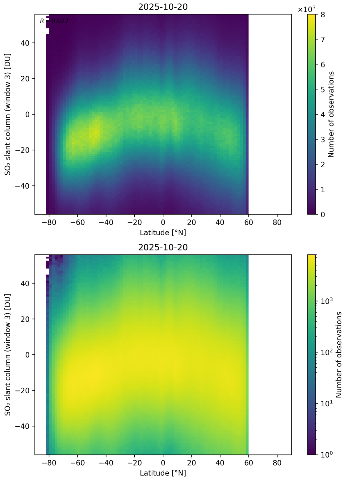
Figure 165: Scatter density plot of “Latitude” against “SO 2 slant column (window 3)” for 2025-10-19 to 2025-10-21.
