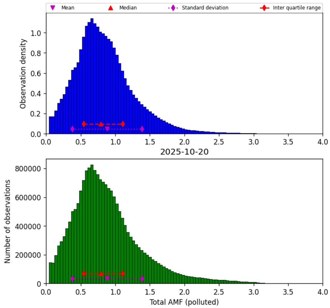
Figure 79: Histogram of “Total AMF (polluted)” for 2025-10-19 to 2025-10-21
