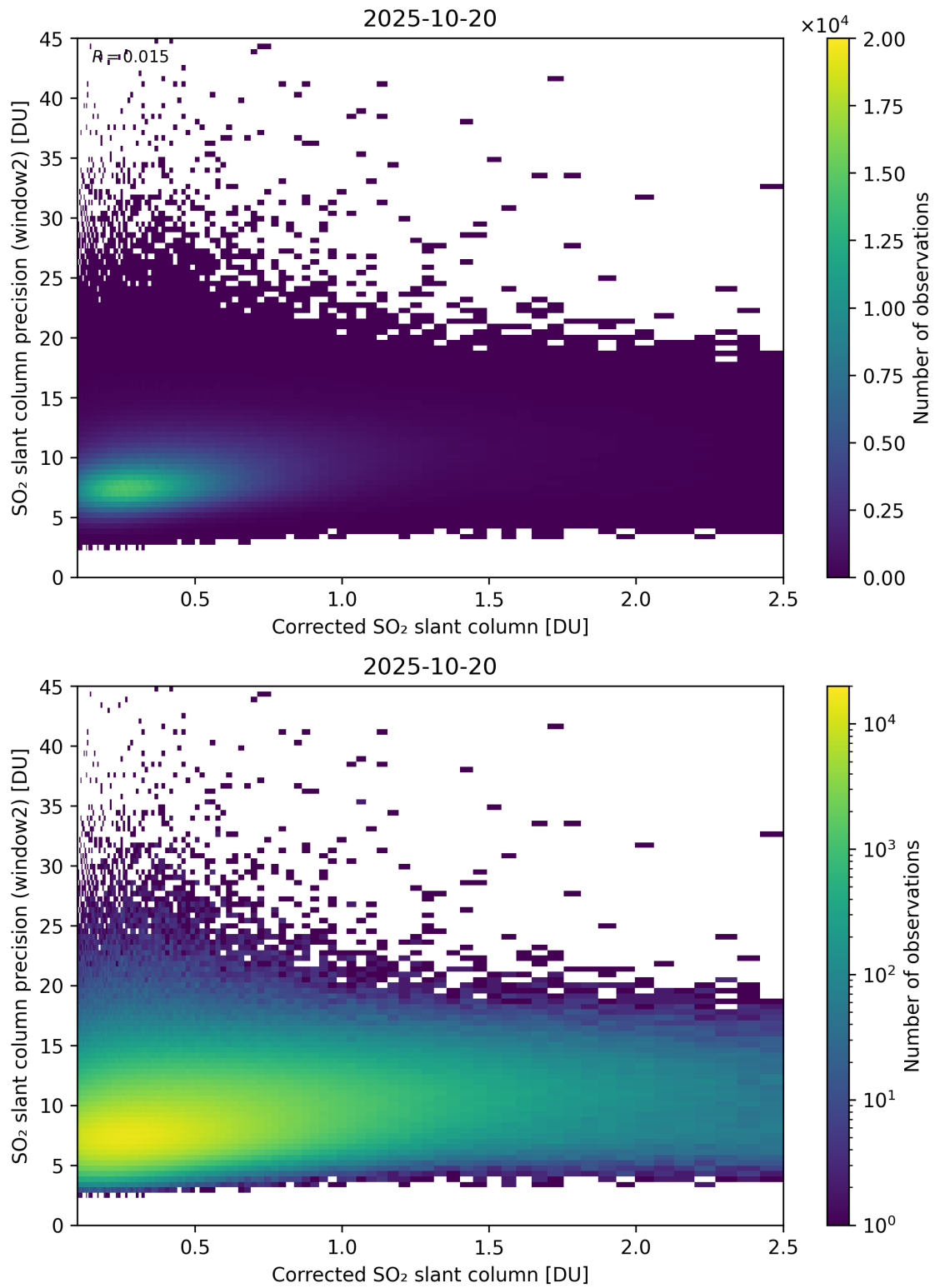
Figure 239: Scatter density plot of “Corrected SO 2 slant column” against “SO 2 slant column precision (window2)” for 2025-10-19 to 2025-10-21.
