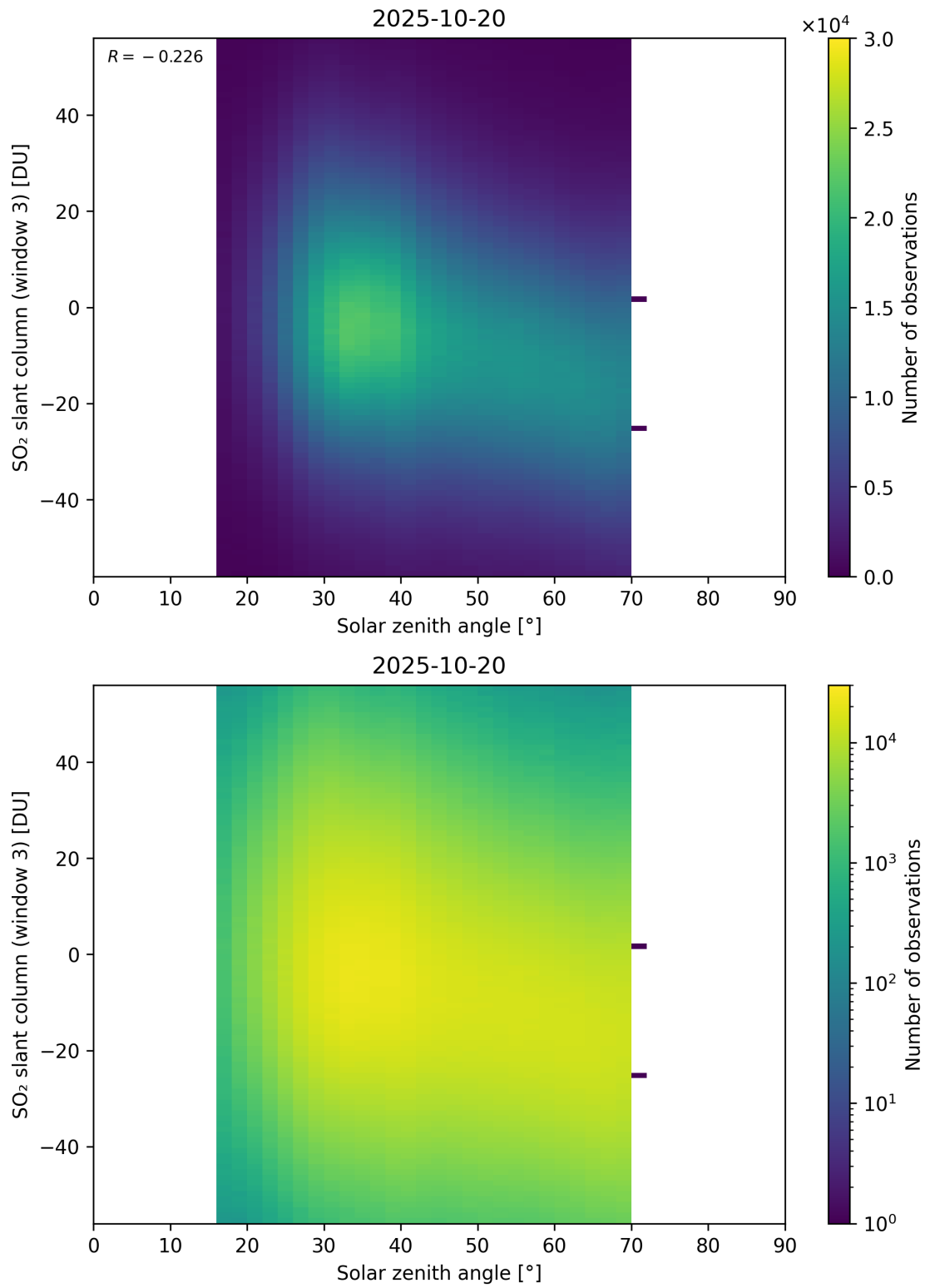
Figure 187: Scatter density plot of “Solar zenith angle” against “SO 2 slant column (window 3)” for 2025-10-19 to 2025-10-21.
