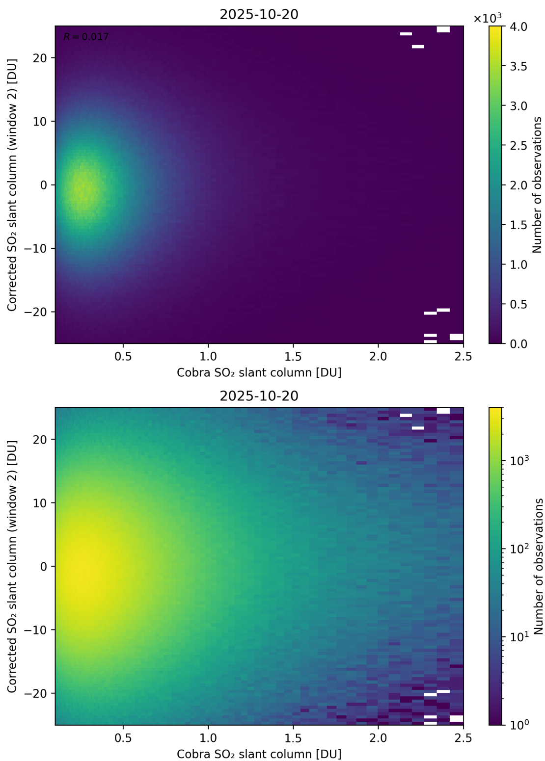
Figure 217: Scatter density plot of “Cobra SO 2 slant column” against “Corrected SO 2 slant column (window 2)” for 2025-10-19 to 2025-10-21.
