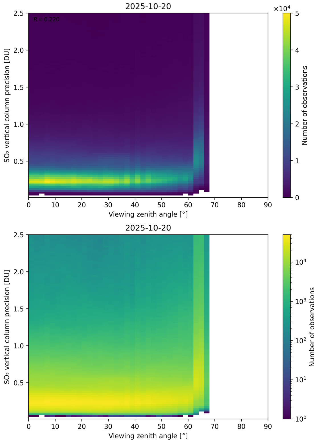
Figure 384: Scatter density plot of “Viewing zenith angle” against “SO 2 vertical column precision” for 2025-10-19 to 2025-10-21.
