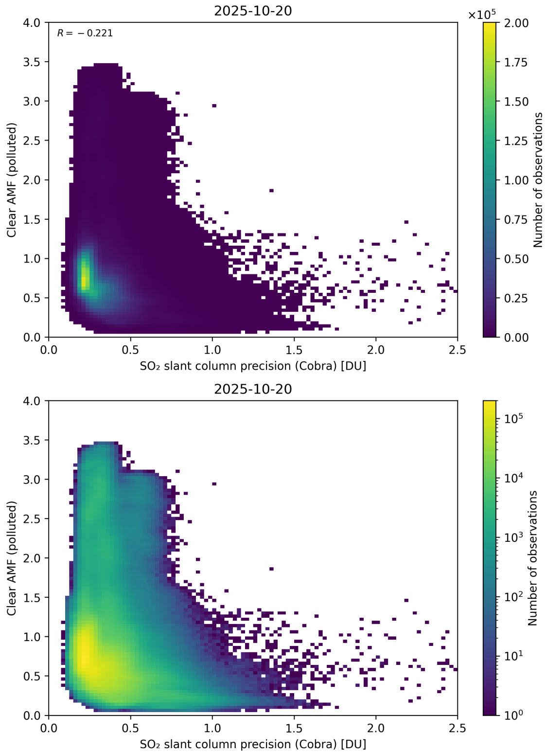
Figure 205: Scatter density plot of “SO 2 slant column precision (Cobra)” against “Clear AMF (polluted)” for 2025-10-19 to 2025-10-21.
