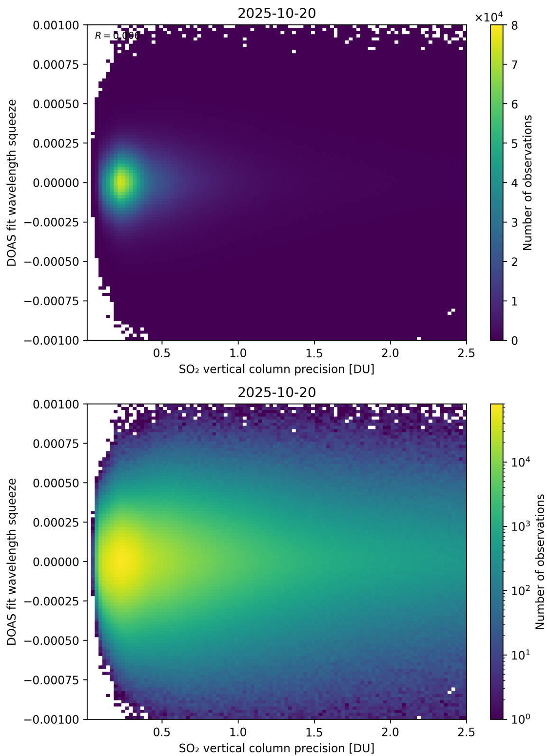
Figure 333: Scatter density plot of “SO 2 vertical column precision” against “DOAS fit wavelength squeeze” for 2025-10-19 to 2025-10-21.
