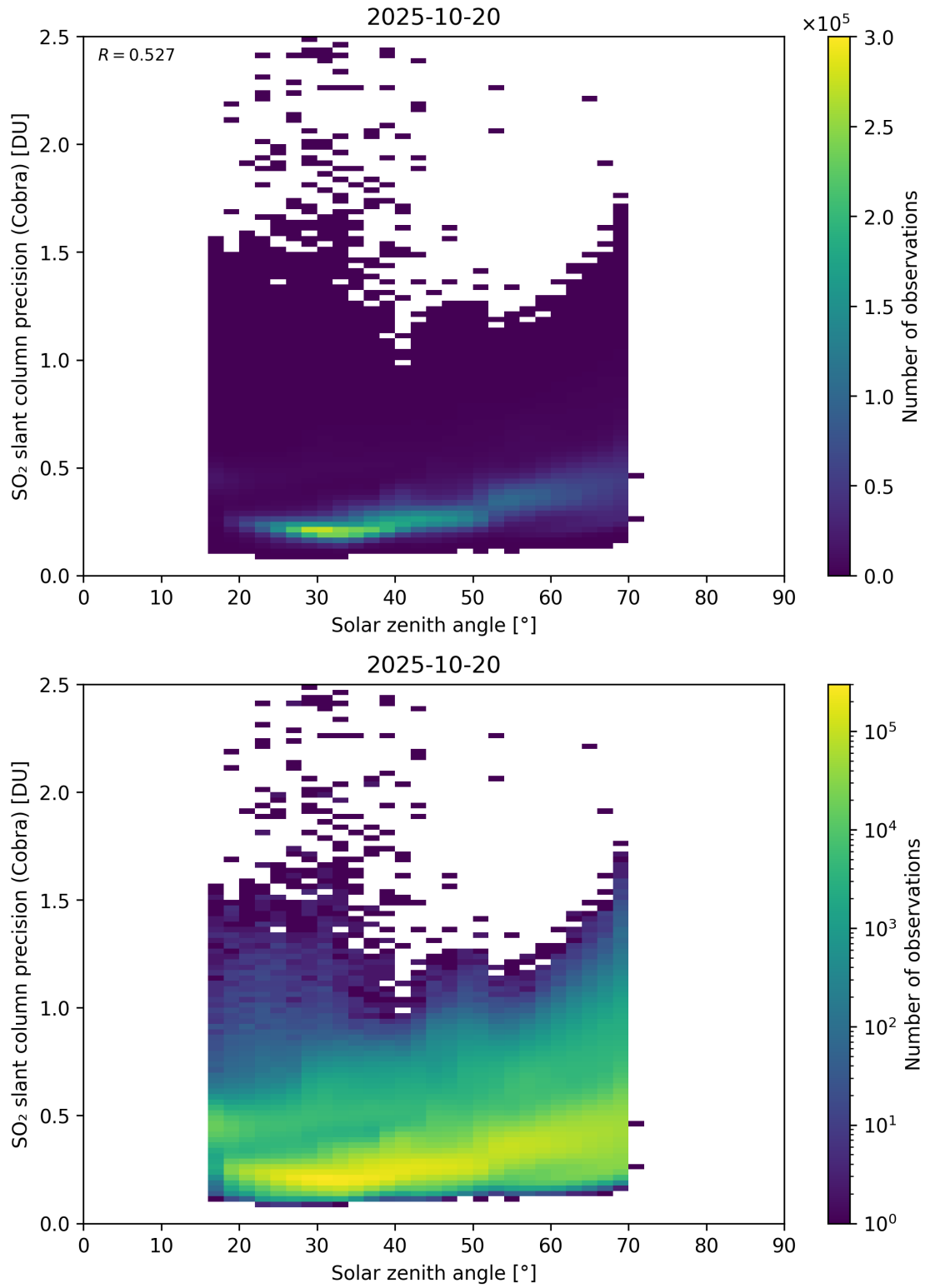
Figure 180: Scatter density plot of “Solar zenith angle” against “SO 2 slant column precision (Cobra)” for 2025-10-19 to 2025-10-21.
