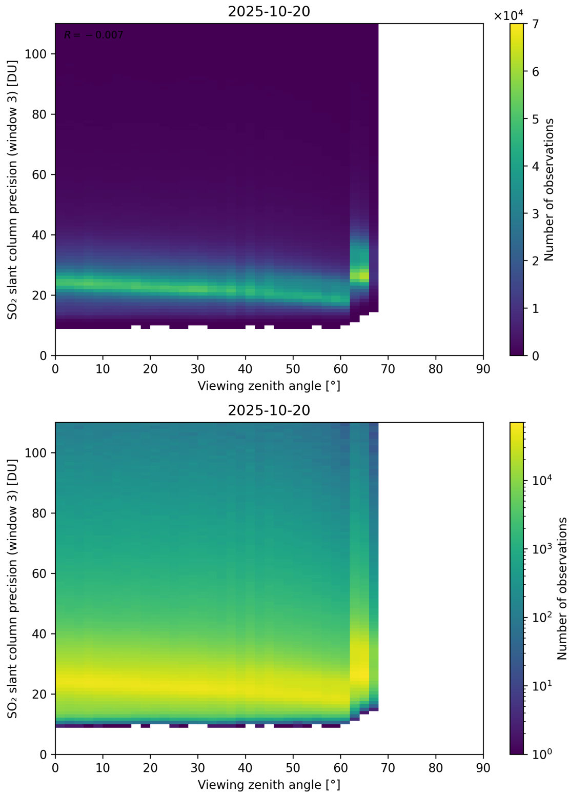
Figure 380: Scatter density plot of “Viewing zenith angle” against “SO 2 slant column precision (window 3)” for 2025-10-19 to 2025-10-21.
