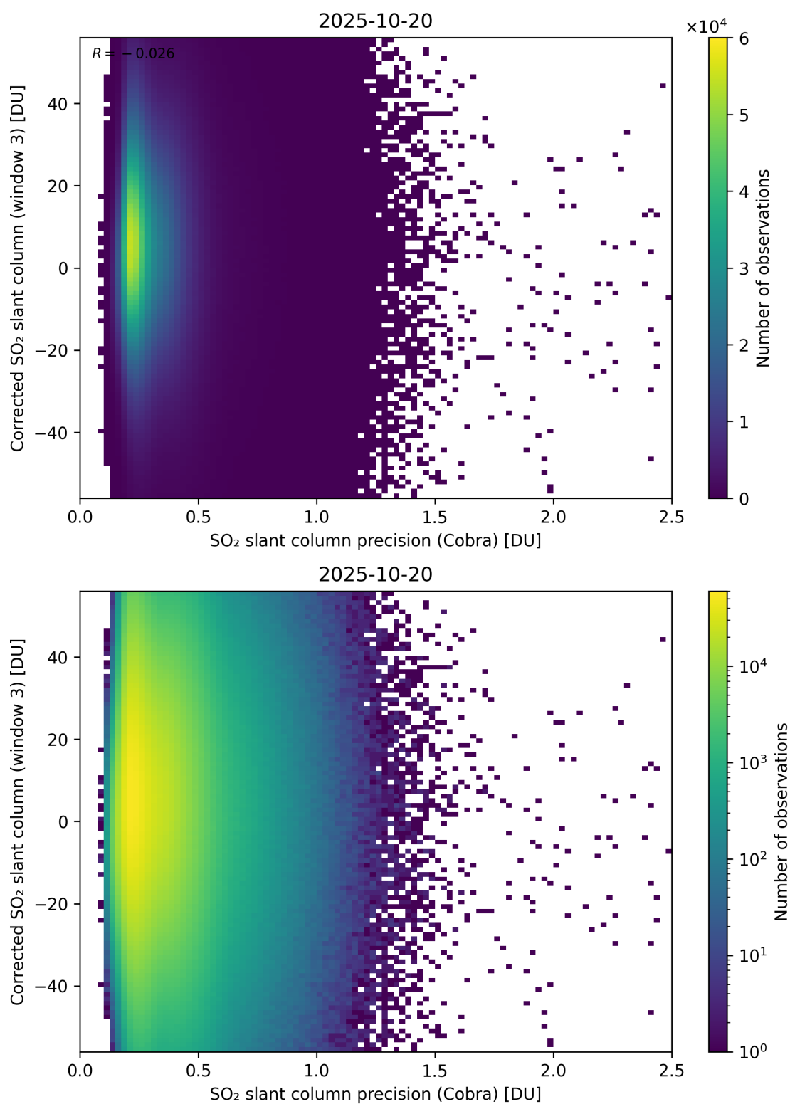
Figure 207: Scatter density plot of “SO 2 slant column precision (Cobra)” against “Corrected SO 2 slant column (window 3)” for 2025-10-19 to 2025-10-21.
