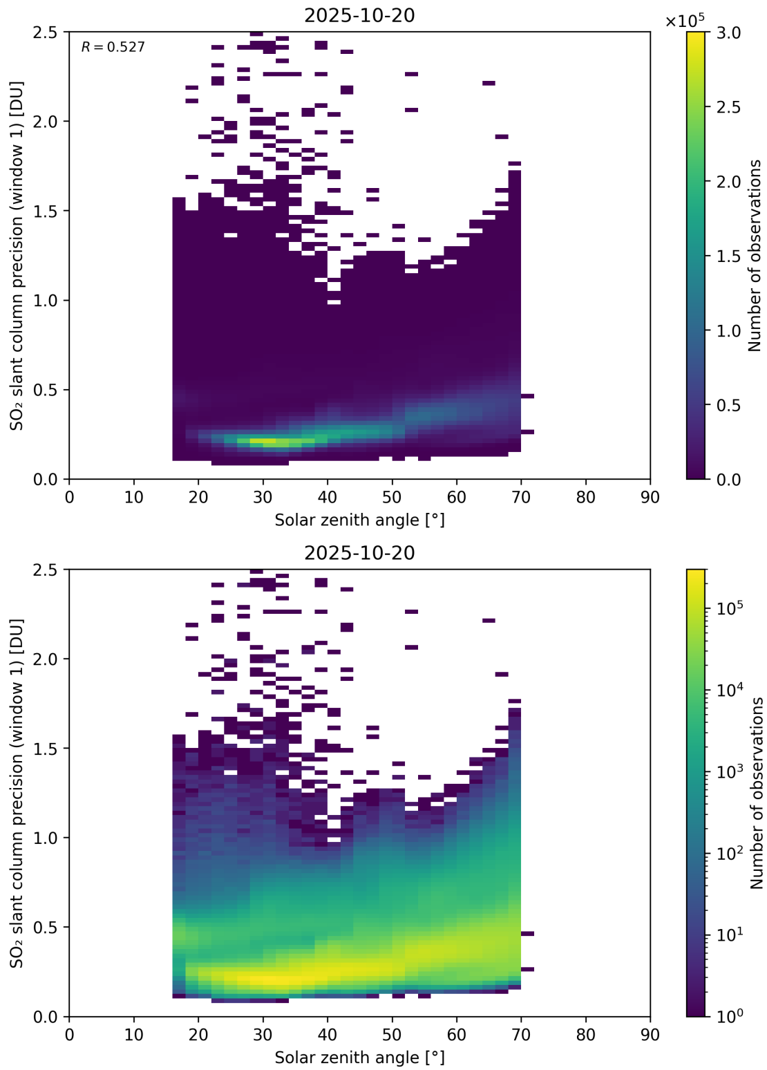
Figure 185: Scatter density plot of “Solar zenith angle” against “SO 2 slant column precision (window 1)” for 2025-10-19 to 2025-10-21.
