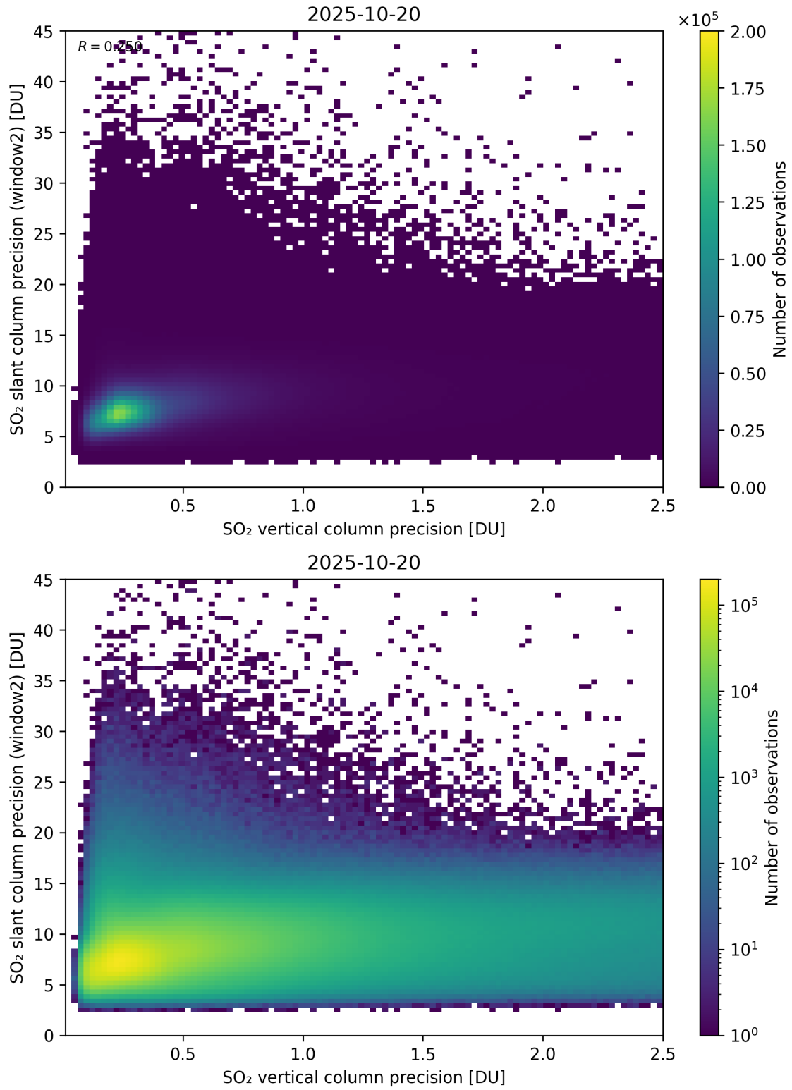
Figure 343: Scatter density plot of “SO 2 vertical column precision” against “SO 2 slant column precision (window2)” for 2025-10-19 to 2025-10-21.
