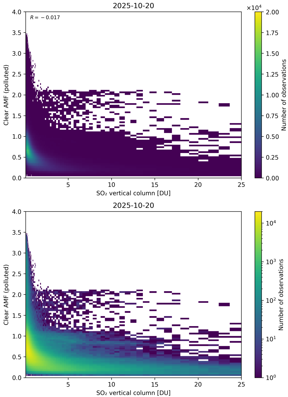
Figure 348: Scatter density plot of “SO 2 vertical column” against “Clear AMF (polluted)” for 2025-10-19 to 2025-10-21.
