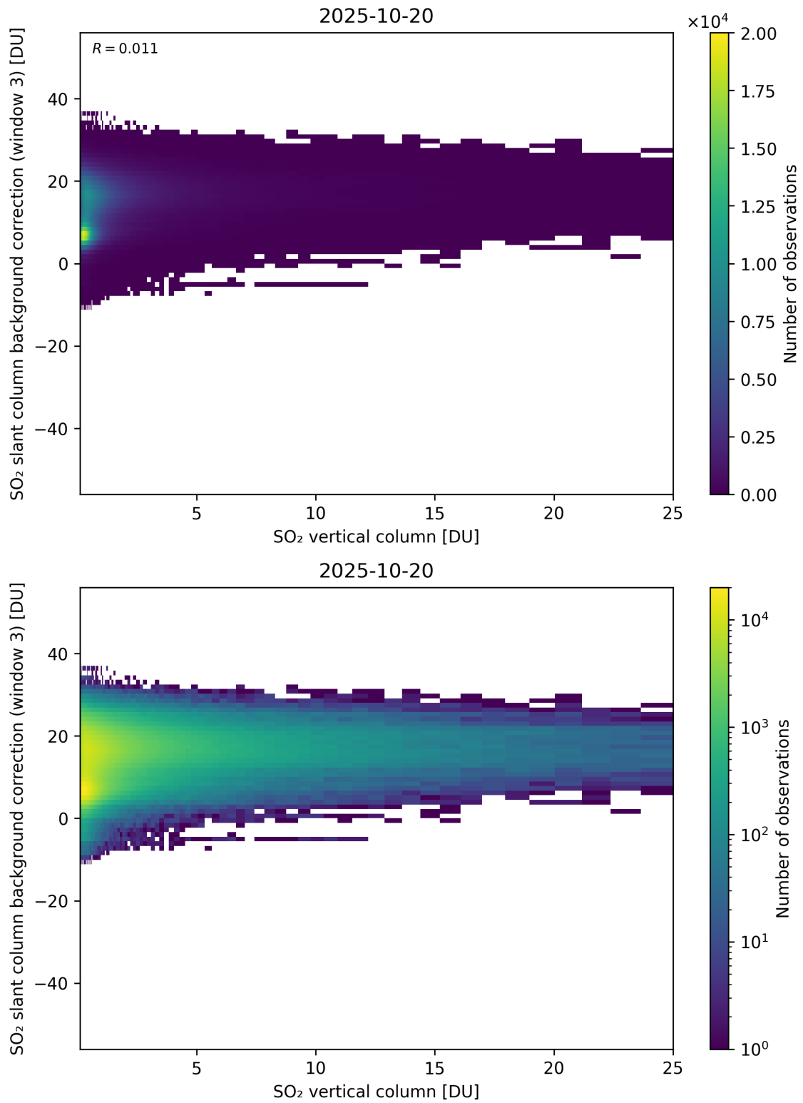
Figure 325: Scatter density plot of “SO 2 vertical column” against “SO 2 slant column background correction (window 3)” for 2025-10-19 to 2025-10-21.
