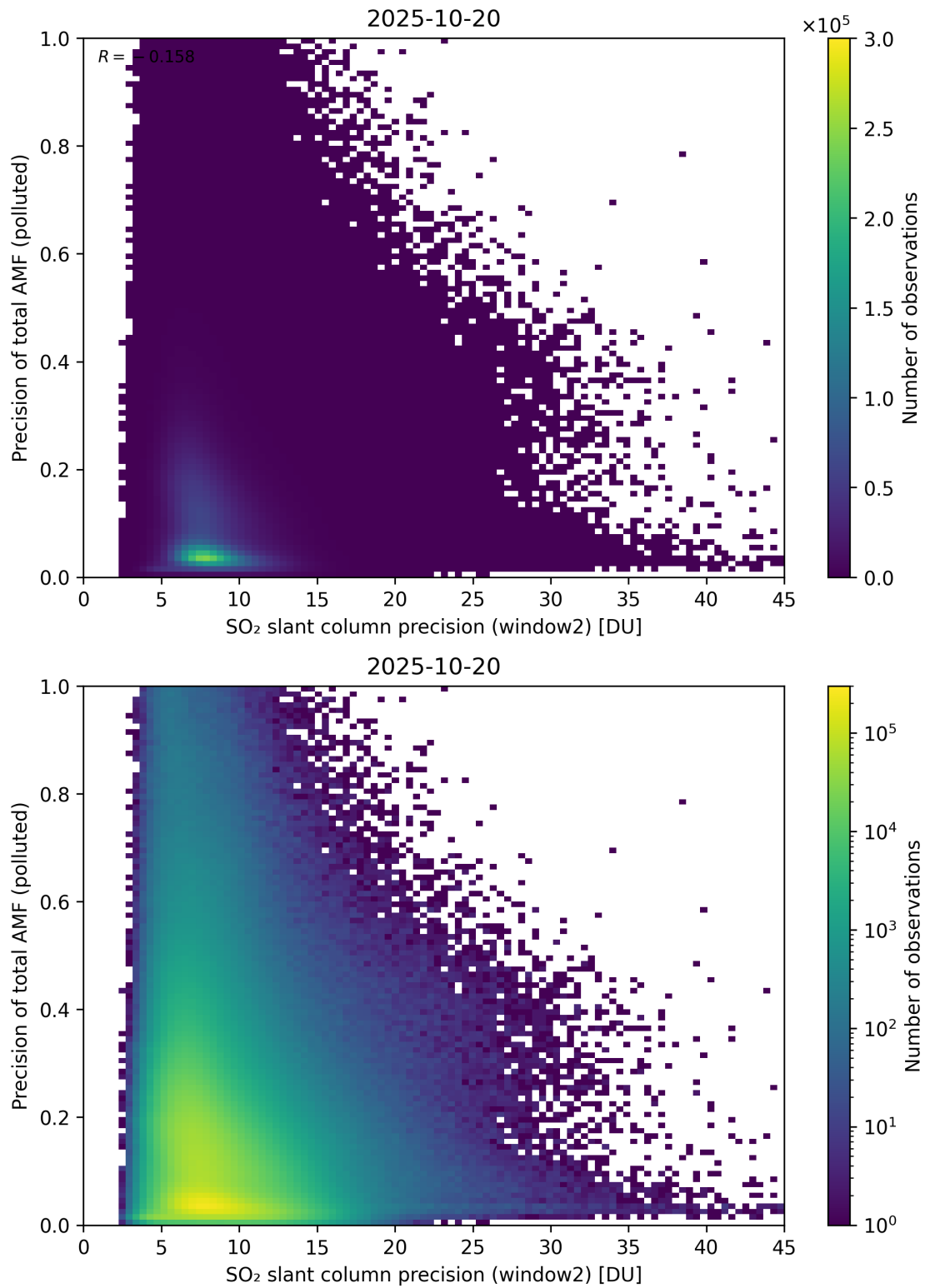
Figure 302: Scatter density plot of “SO 2 slant column precision (window2)” against “Precision of total AMF (polluted)” for 2025-10-19 to 2025-10-21.
