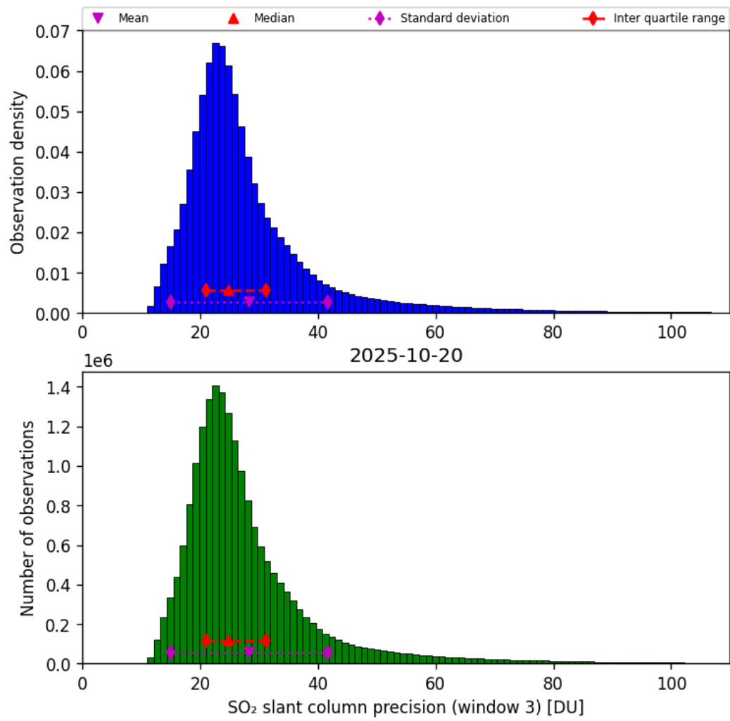
Figure 72: Histogram of “SO 2 slant column precision (window 3)” for 2025-10-19 to 2025-10-21
