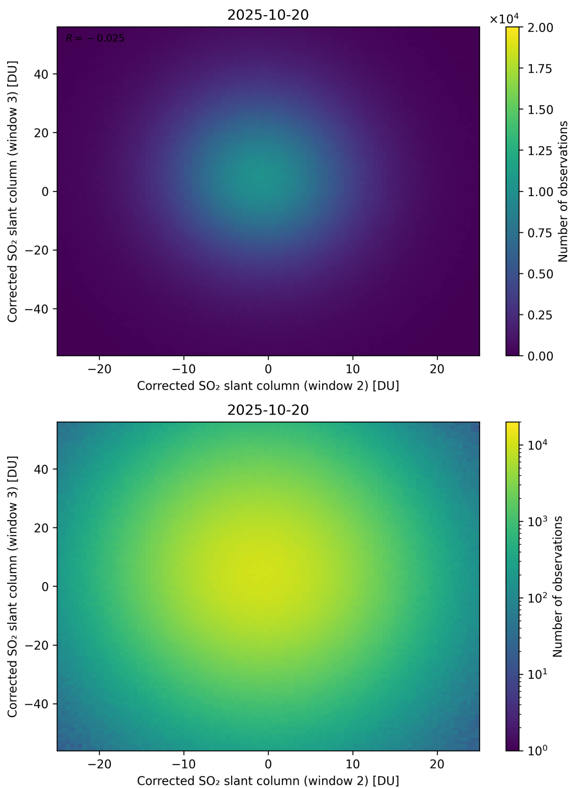
Figure 250: Scatter density plot of “Corrected SO 2 slant column (window 2)” against “Corrected SO 2 slant column (window 3)” for 2025-10-19 to 2025-10-21.
