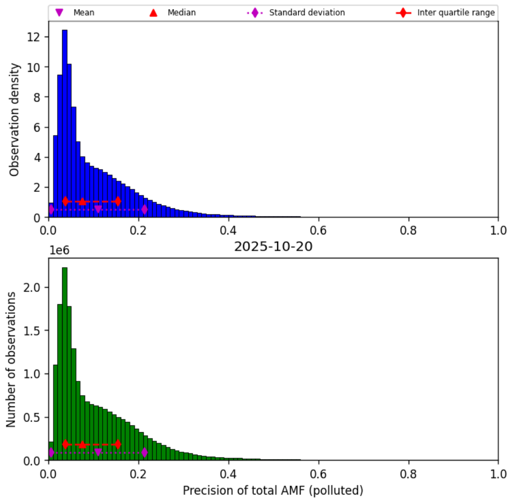
Figure 80: Histogram of “Precision of total AMF (polluted)” for 2025-10-19 to 2025-10-21
