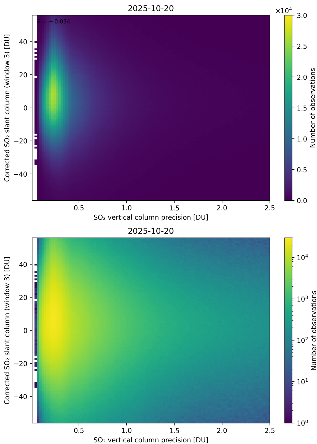
Figure 340: Scatter density plot of “SO 2 vertical column precision” against “Corrected SO 2 slant column (window 3)” for 2025-10-19 to 2025-10-21.
