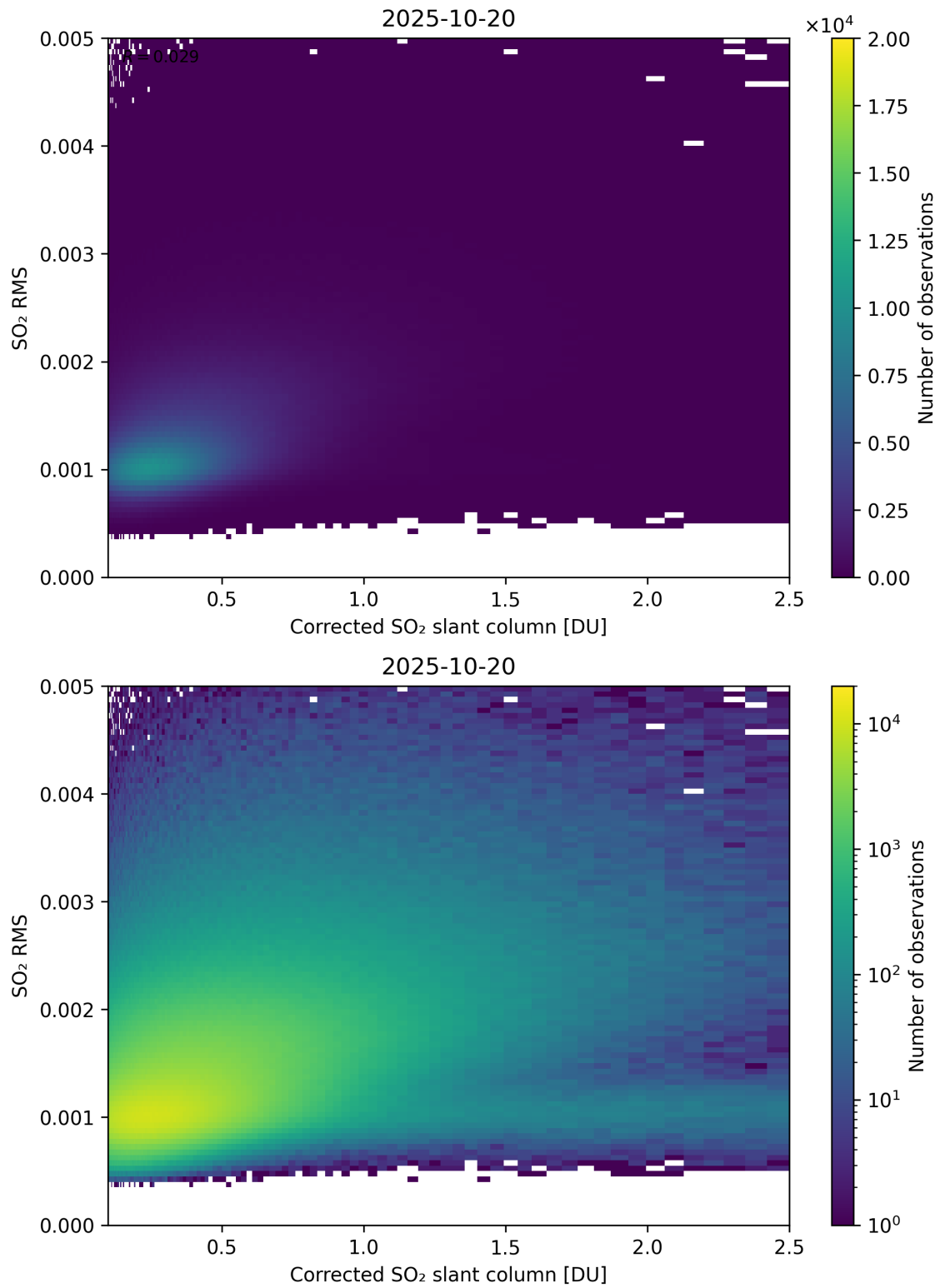
Figure 231: Scatter density plot of “Corrected SO 2 slant column” against “SO 2 RMS” for 2025-10-19 to 2025-10-21.
