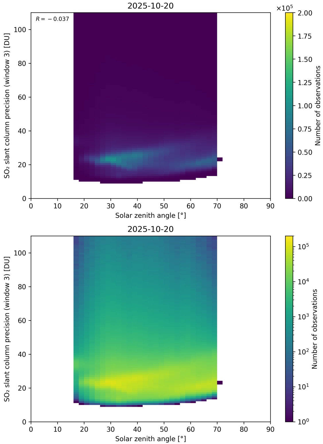
Figure 188: Scatter density plot of “Solar zenith angle” against “SO 2 slant column precision (window 3)” for 2025-10-19 to 2025-10-21.
