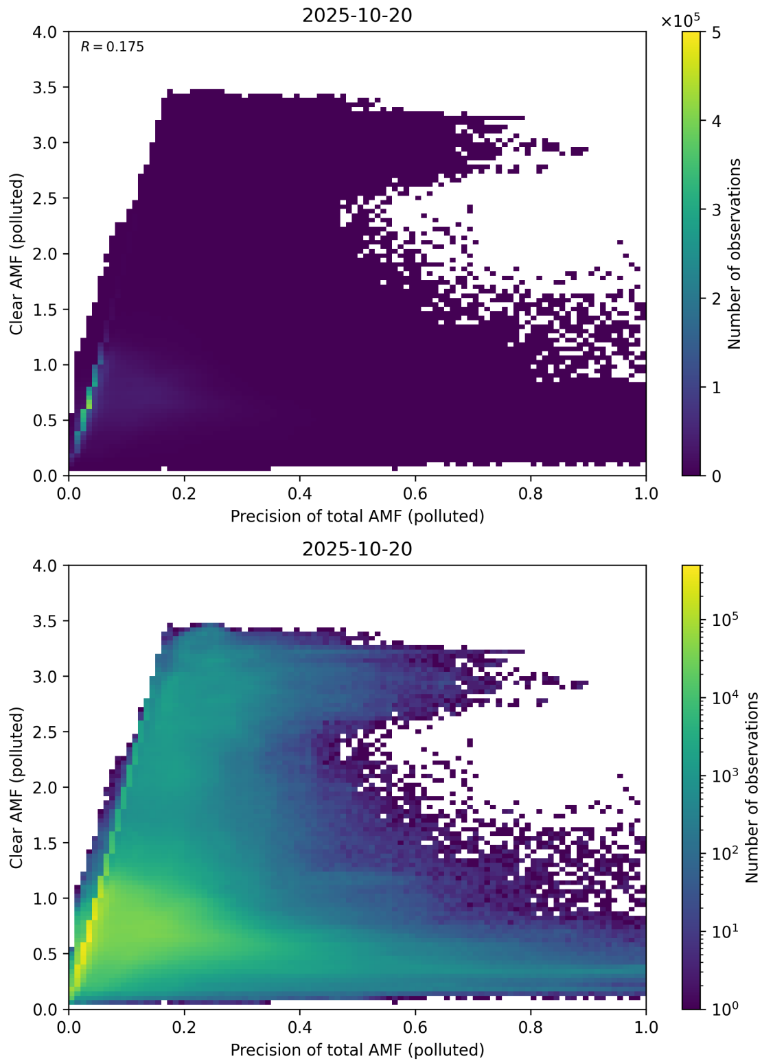
Figure 320: Scatter density plot of “Precision of total AMF (polluted)” against “Clear AMF (polluted)” for 2025-10-19 to 2025-10-21.
