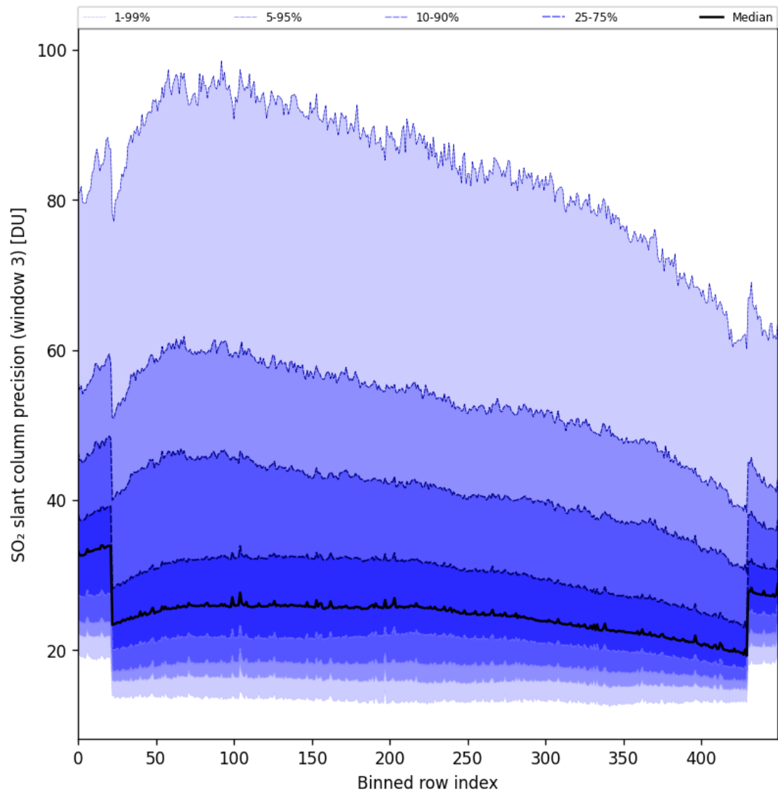
Figure 98: Along track statistics of “SO 2 slant column precision (window 3)” for 2025-10-19 to 2025-10-21
