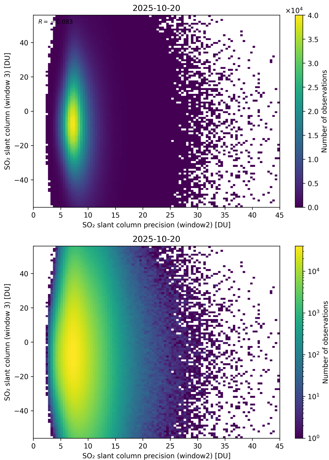
Figure 299: Scatter density plot of “SO 2 slant column precision (window2)” against “SO 2 slant column (window 3)” for 2025-10-19 to 2025-10-21.
