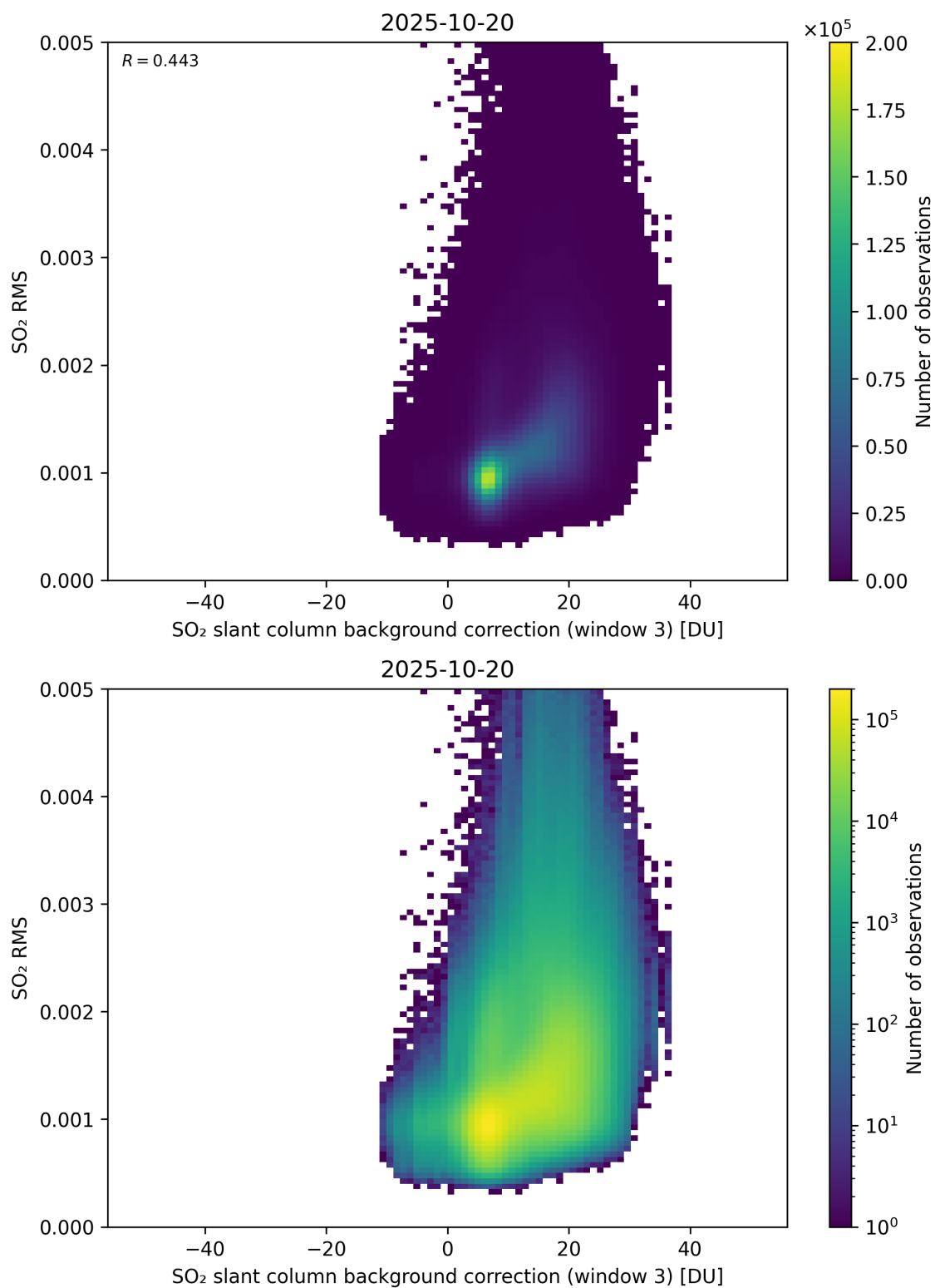
Figure 134: Scatter density plot of “SO 2 slant column background correction (window 3)” against “SO 2 RMS” for 2025-10-19 to 2025-10-21.
