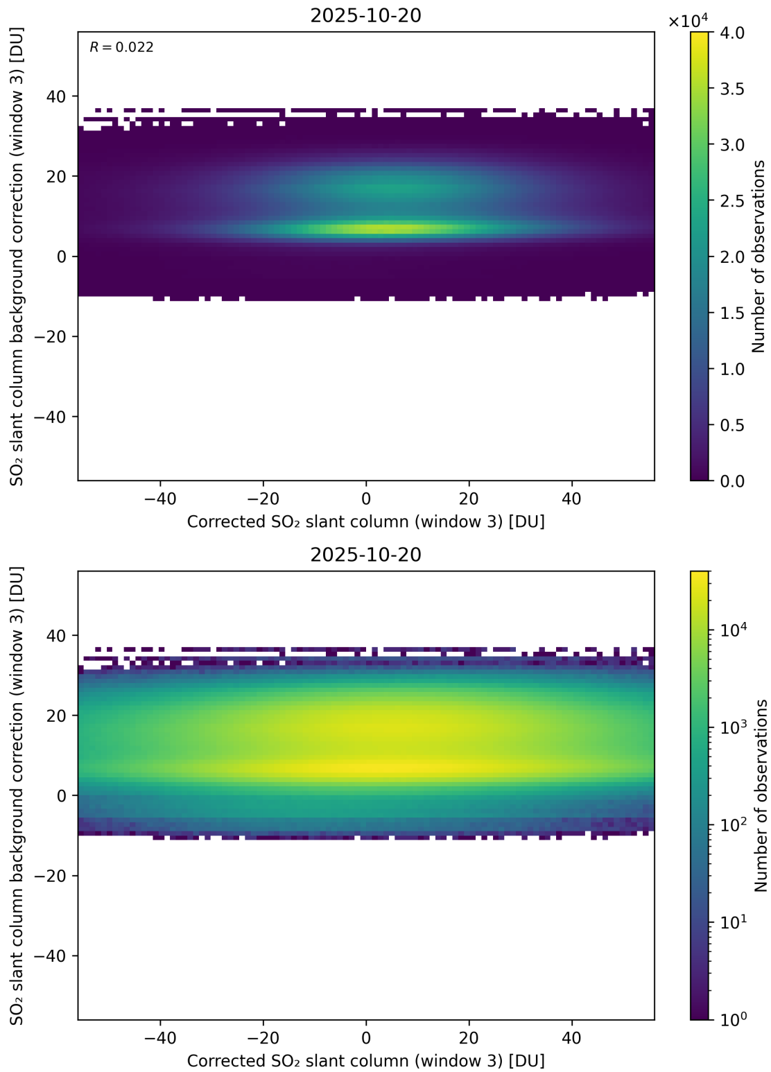
Figure 255: Scatter density plot of “Corrected SO 2 slant column (window 3)” against “SO 2 slant column background correction (window 3)” for 2025-10-19 to 2025-10-21.
