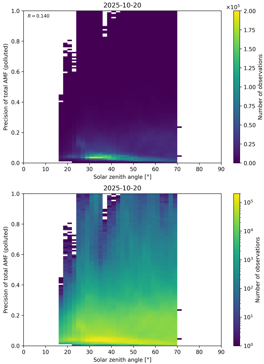
Figure 190: Scatter density plot of “Solar zenith angle” against “Precision of total AMF (polluted)” for 2025-10-19 to 2025-10-21.
