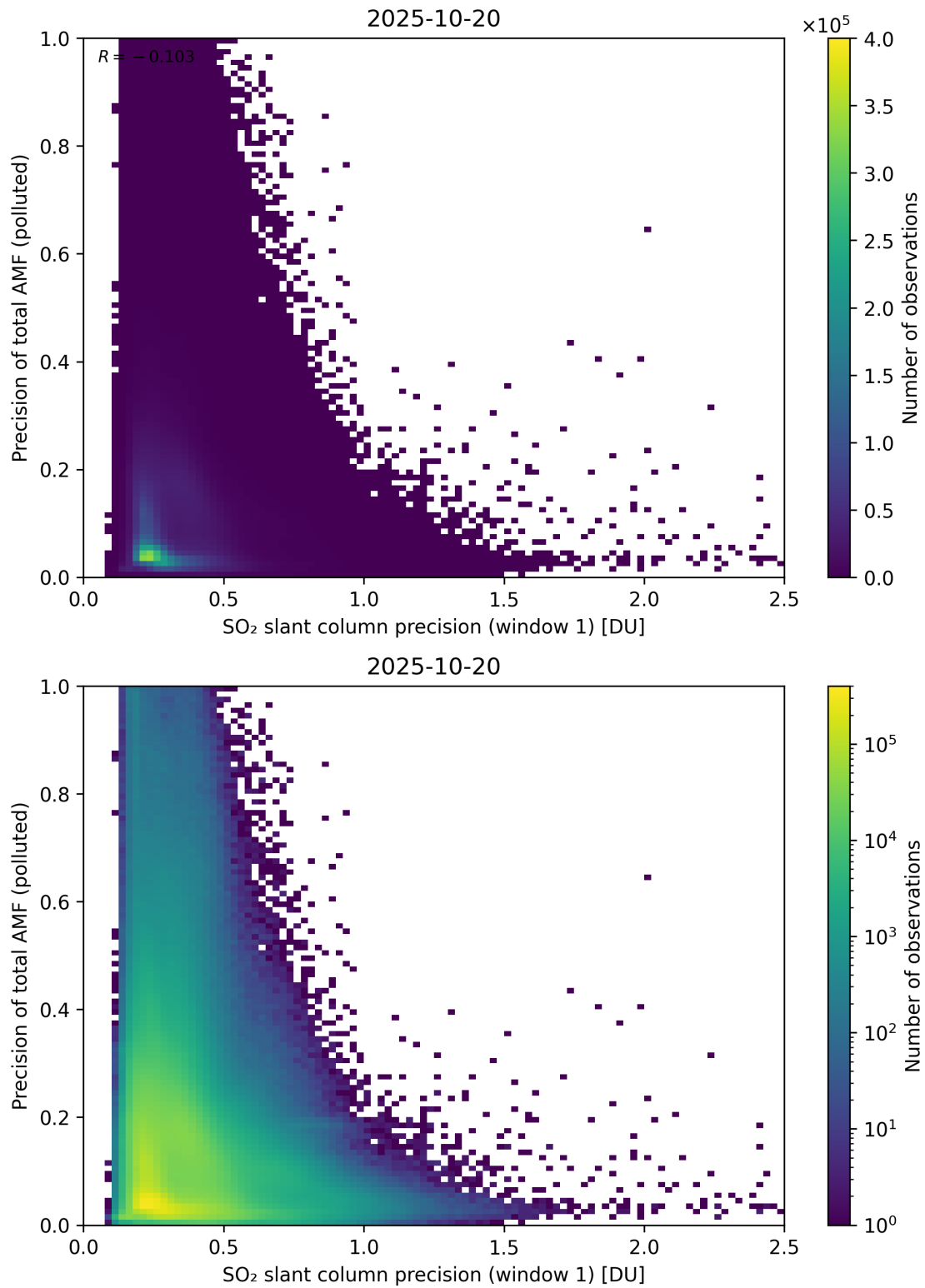
Figure 281: Scatter density plot of “SO 2 slant column precision (window 1)” against “Precision of total AMF (polluted)” for 2025-10-19 to 2025-10-21.
