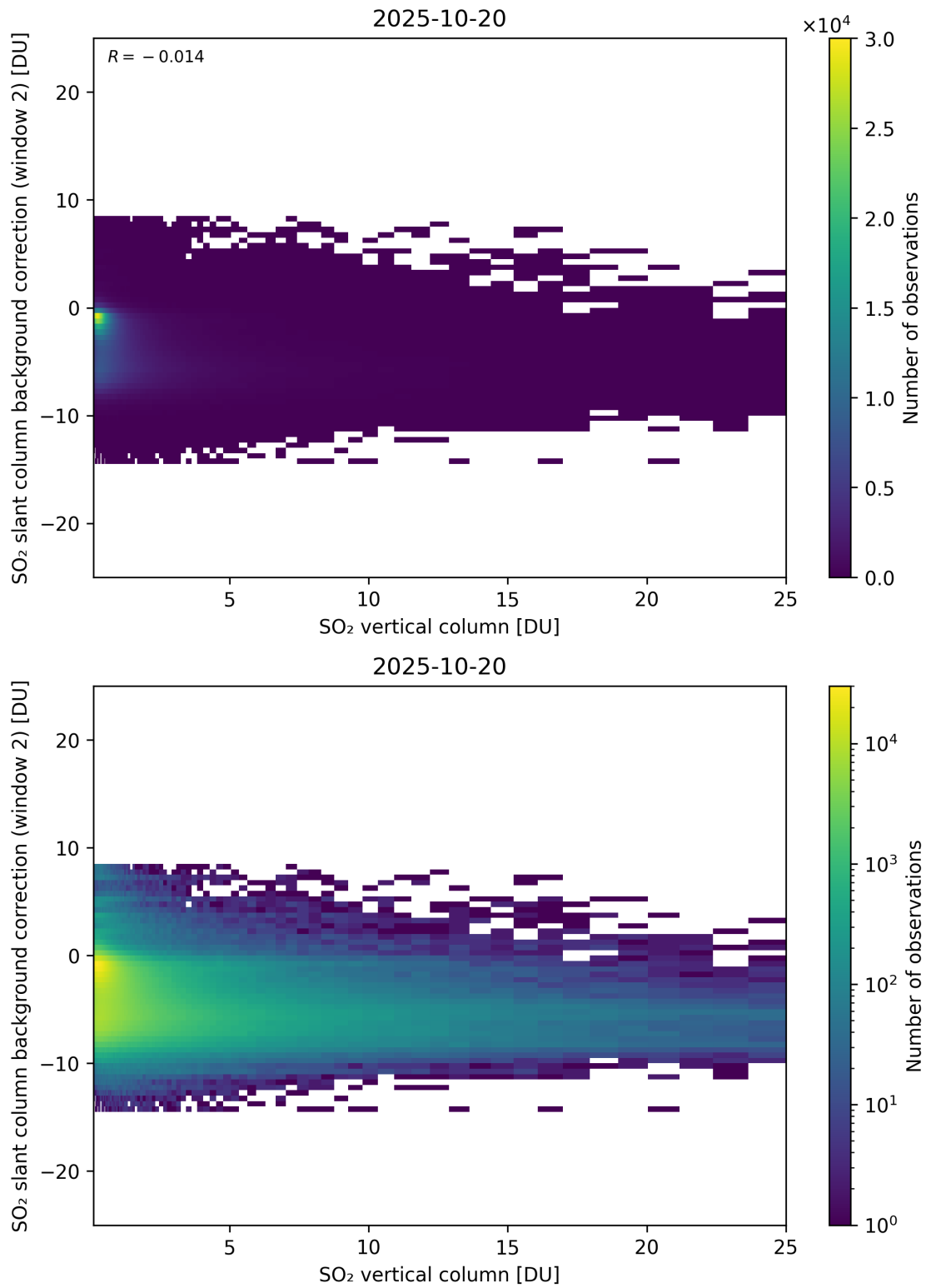
Figure 324: Scatter density plot of “SO 2 vertical column” against “SO 2 slant column background correction (window 2)” for 2025-10-19 to 2025-10-21.
