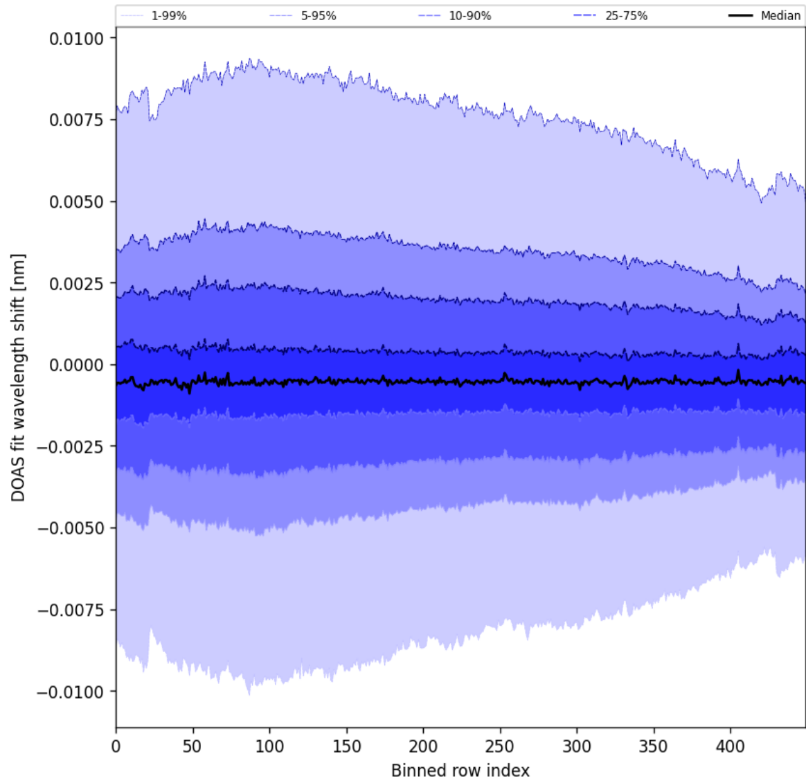
Figure 102: Along track statistics of “DOAS fit wavelength shift” for 2025-10-19 to 2025-10-21
