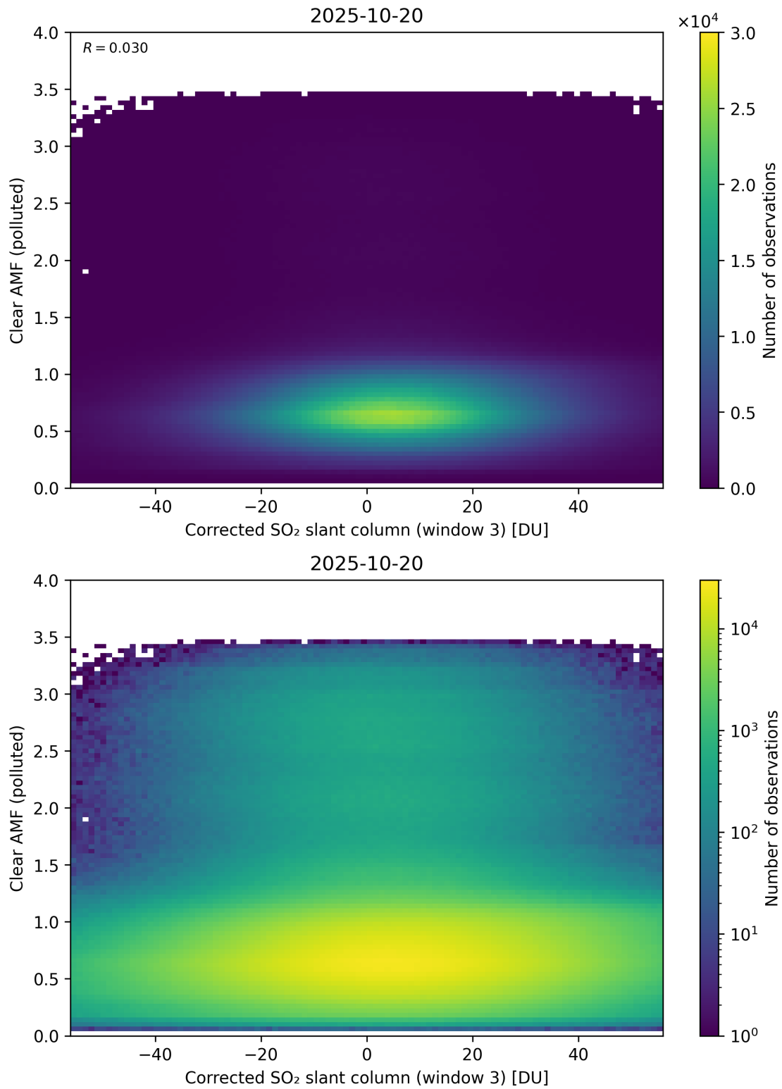
Figure 259: Scatter density plot of “Corrected SO 2 slant column (window 3)” against “Clear AMF (polluted)” for 2025-10-19 to 2025-10-21.
