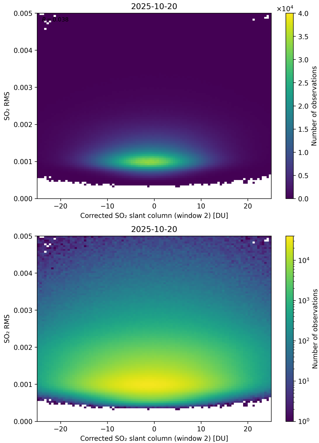
Figure 248: Scatter density plot of “Corrected SO 2 slant column (window 2)” against “SO 2 RMS” for 2025-10-19 to 2025-10-21.
