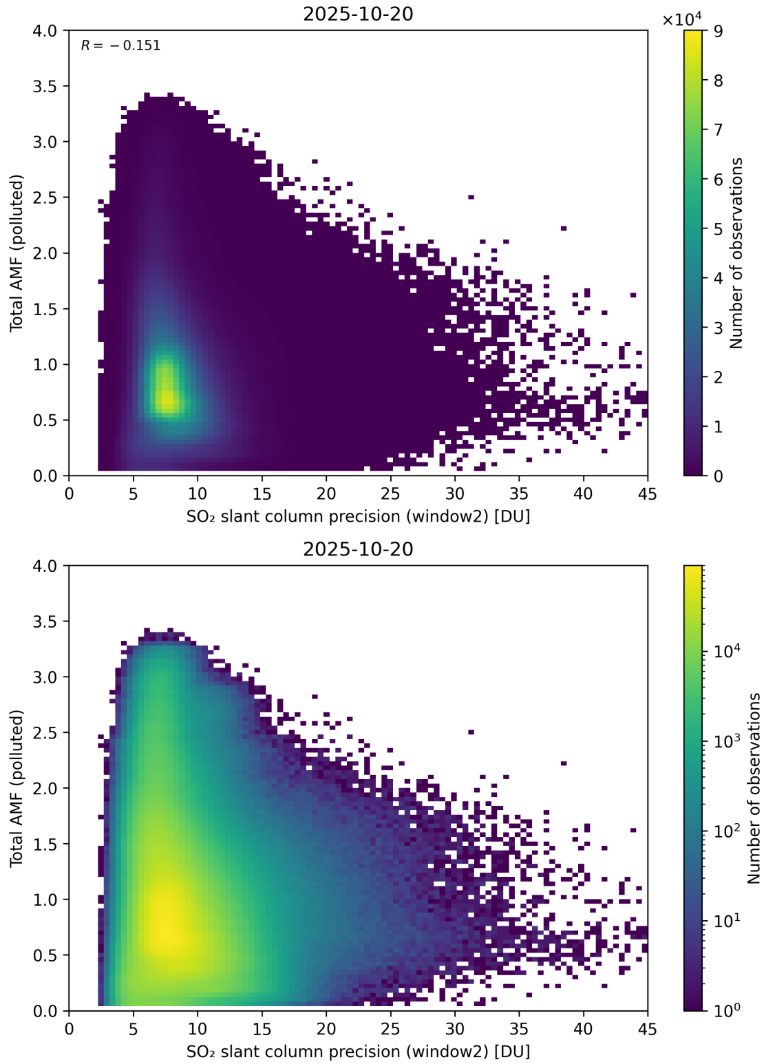
Figure 301: Scatter density plot of “SO 2 slant column precision (window2)” against “Total AMF (polluted)” for 2025-10-19 to 2025-10-21.
