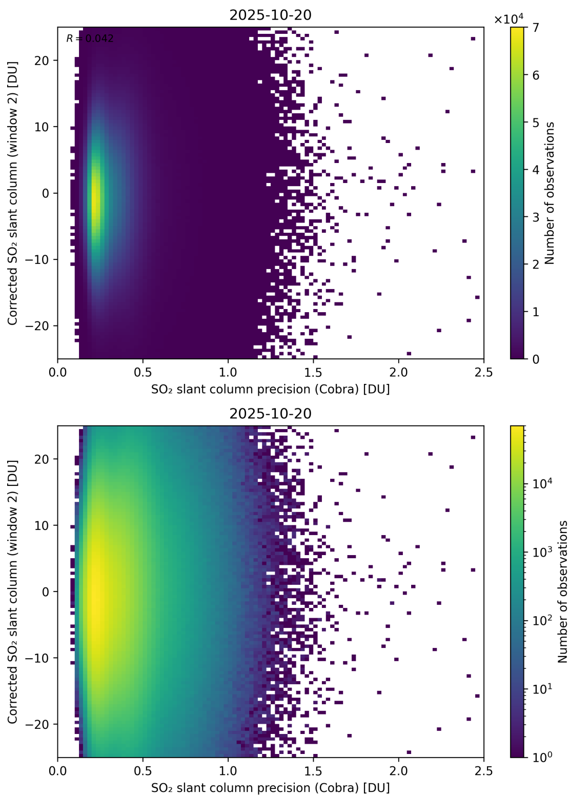
Figure 206: Scatter density plot of “SO 2 slant column precision (Cobra)” against “Corrected SO 2 slant column (window 2)” for 2025-10-19 to 2025-10-21.
