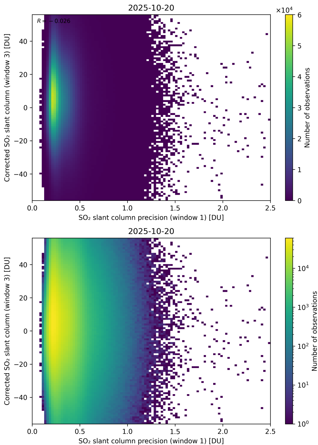
Figure 276: Scatter density plot of “SO 2 slant column precision (window 1)” against “Corrected SO 2 slant column (window 3)” for 2025-10-19 to 2025-10-21.
