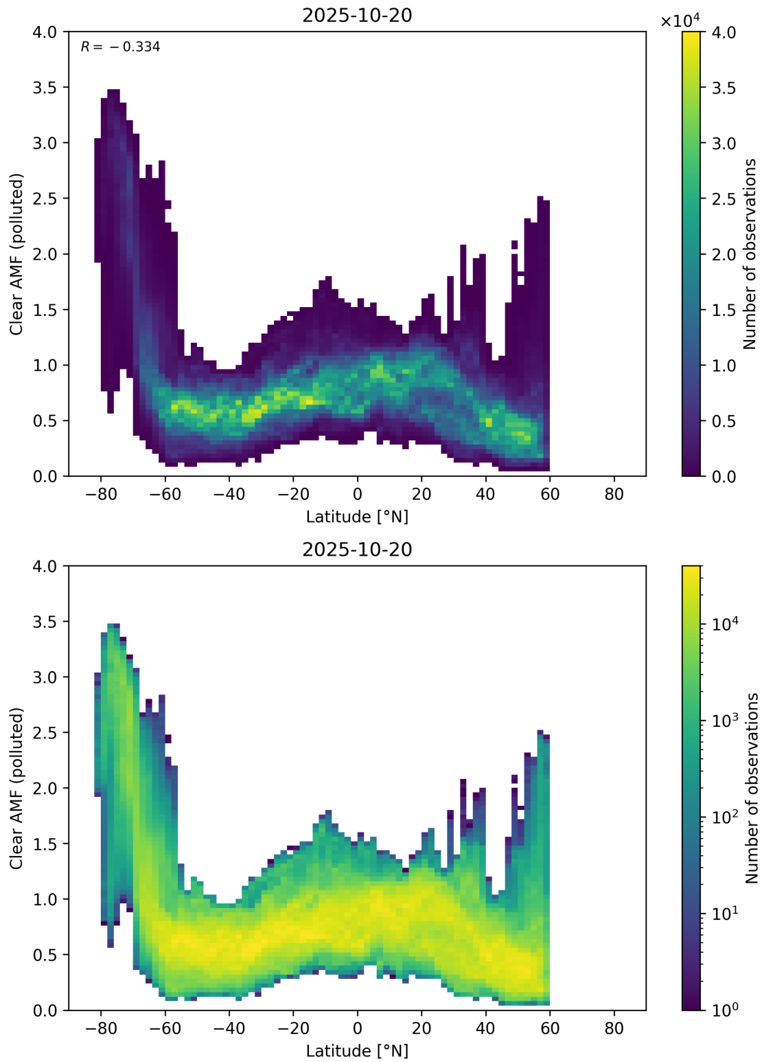
Figure 156: Scatter density plot of “Latitude” against “Clear AMF (polluted)” for 2025-10-19 to 2025-10-21.
