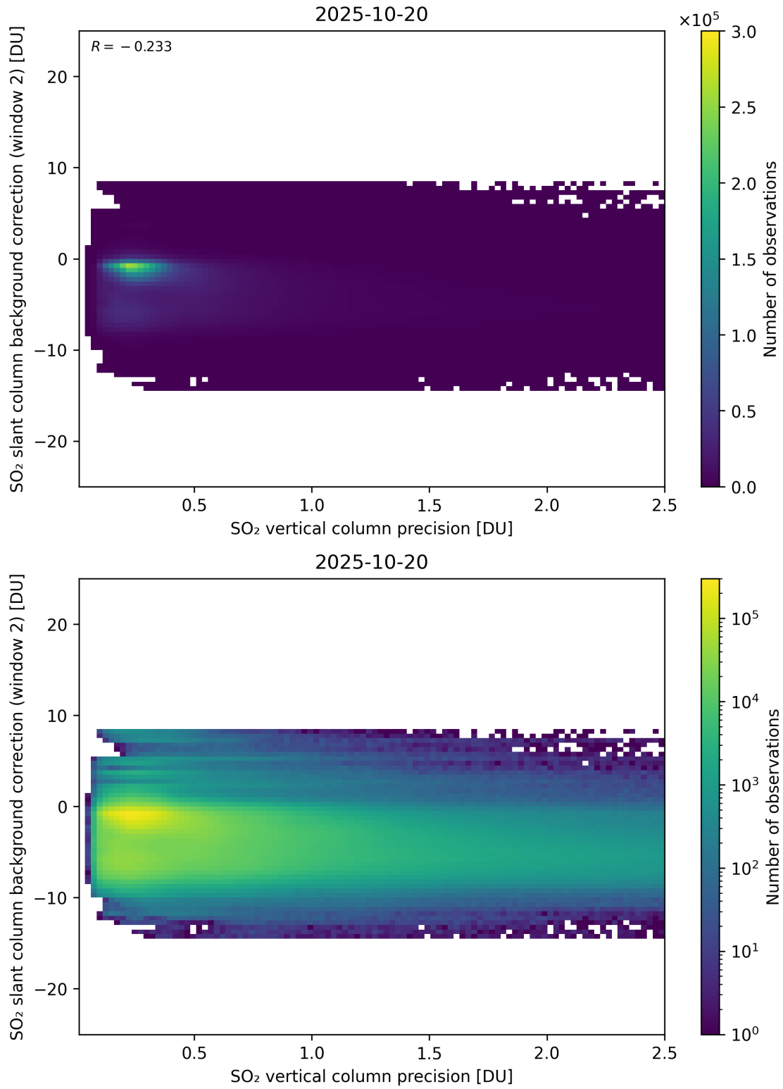
Figure 330: Scatter density plot of “SO 2 vertical column precision” against “SO 2 slant column background correction (window 2)” for 2025-10-19 to 2025-10-21.
