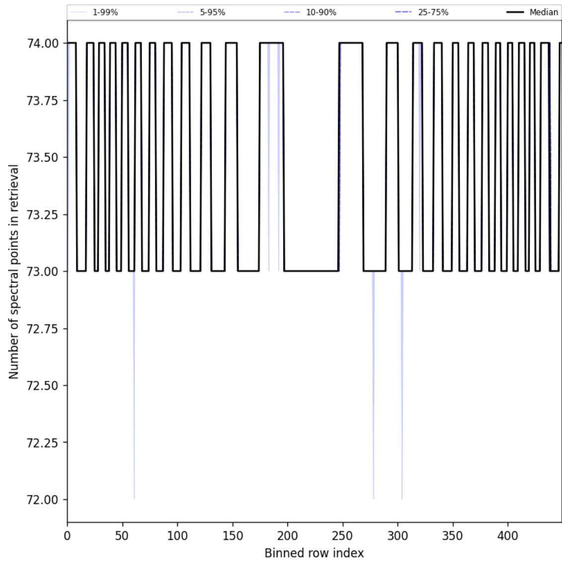
Figure 108: Along track statistics of “Number of spectral points in retrieval” for 2025-10-19 to 2025-10-21
