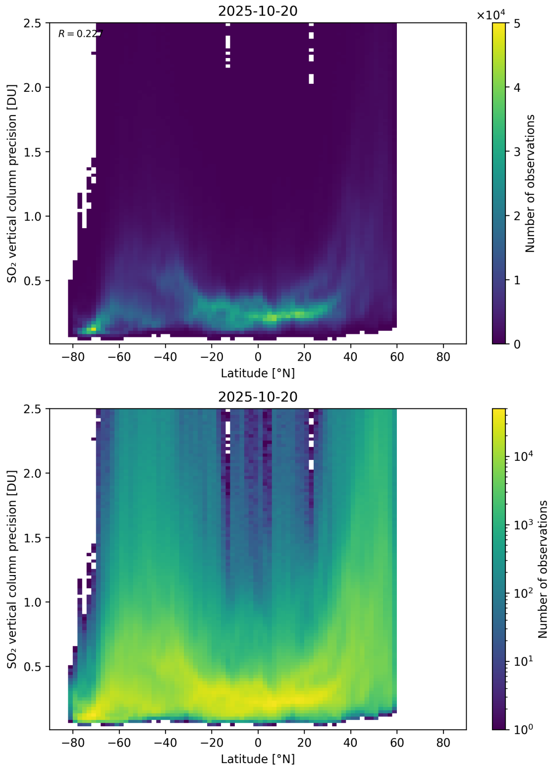
Figure 170: Scatter density plot of “Latitude” against “SO 2 vertical column precision” for 2025-10-19 to 2025-10-21.
