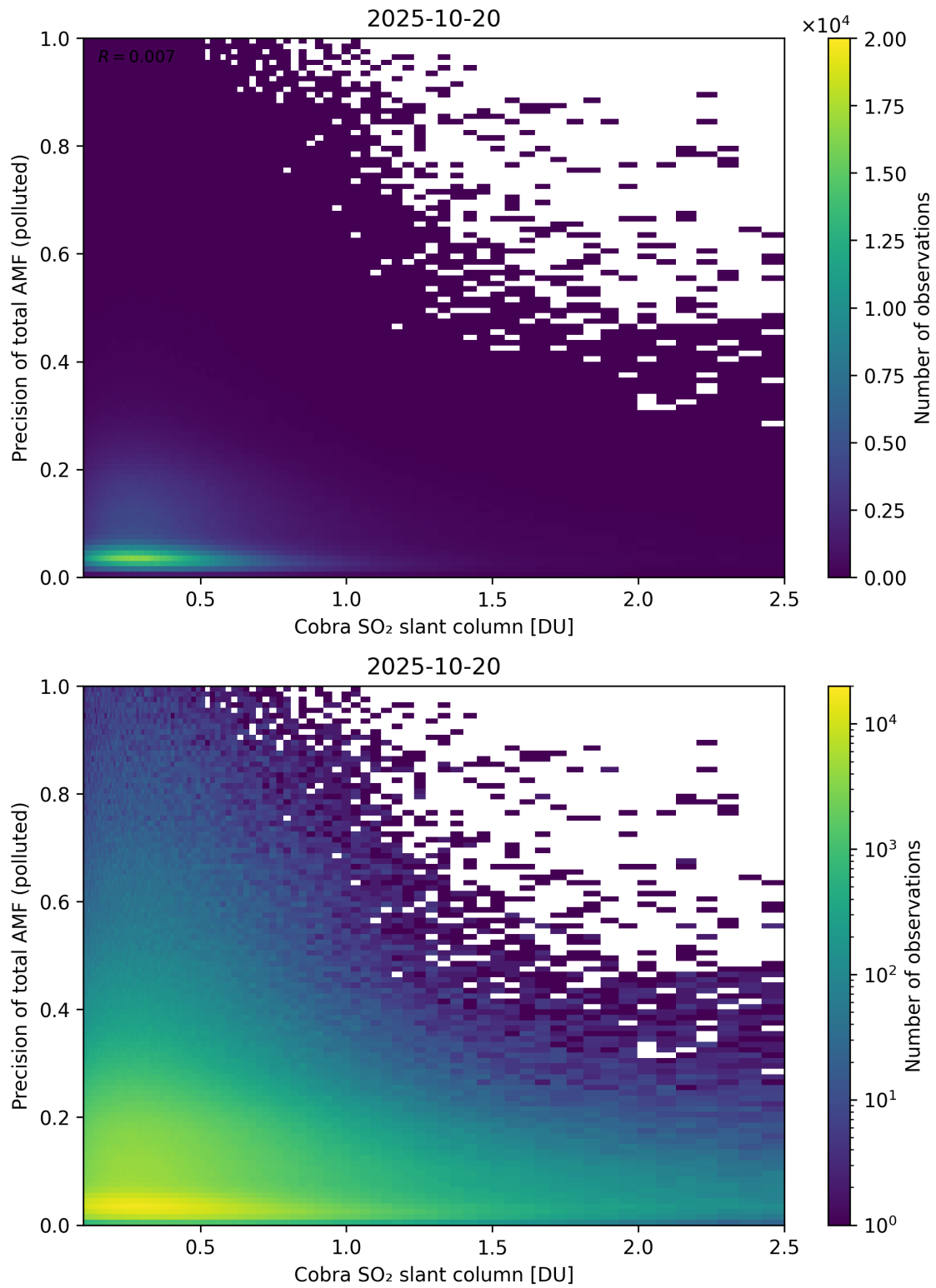
Figure 225: Scatter density plot of “Cobra SO 2 slant column” against “Precision of total AMF (polluted)” for 2025-10-19 to 2025-10-21.
