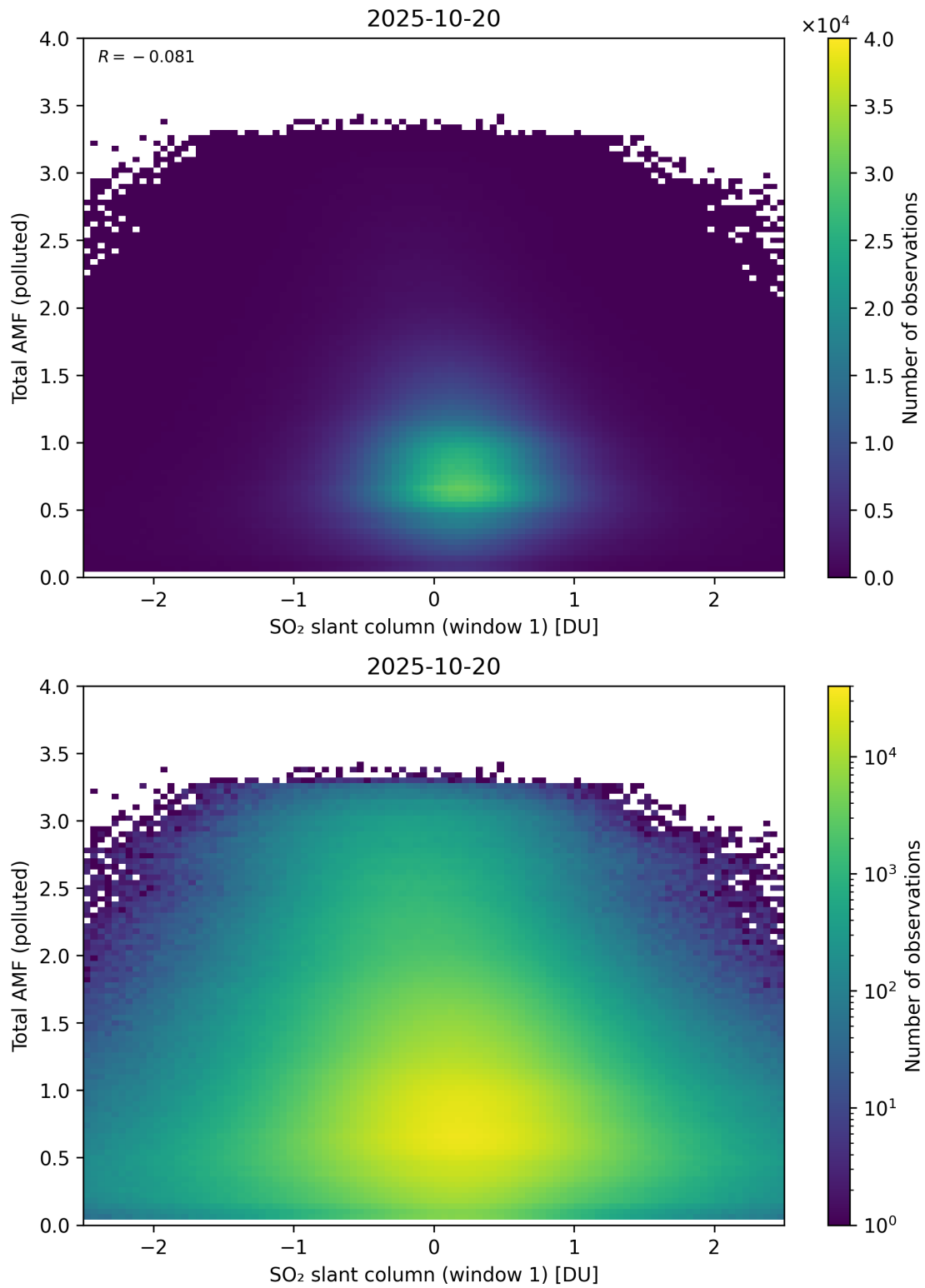
Figure 289: Scatter density plot of “SO 2 slant column (window 1)” against “Total AMF (polluted)” for 2025-10-19 to 2025-10-21.
