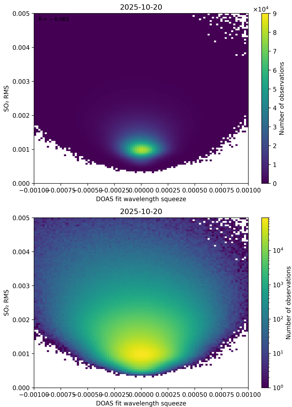
Figure 143: Scatter density plot of “DOAS fit wavelength squeeze” against “SO 2 RMS” for 2025-10-19 to 2025-10-21.
