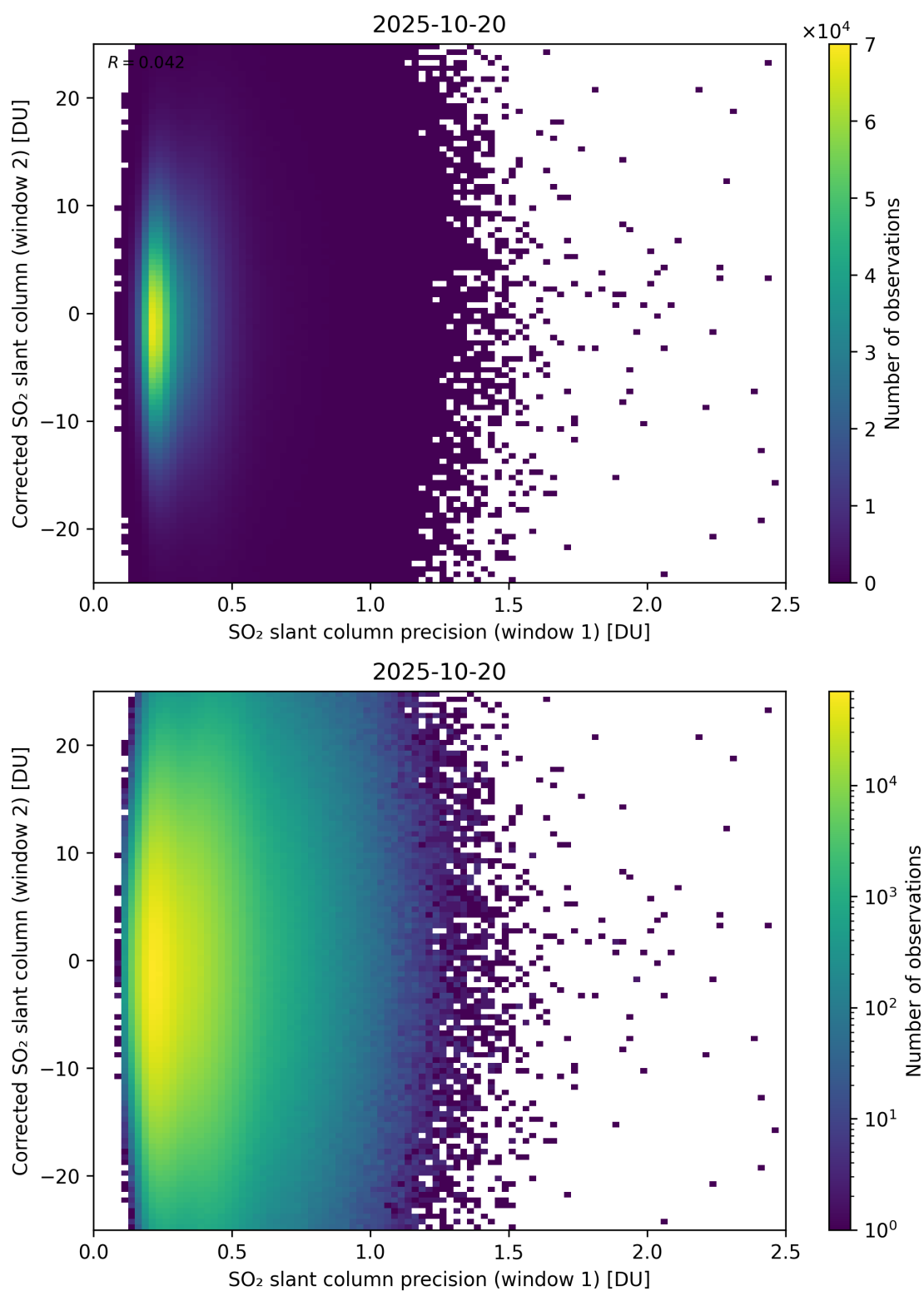
Figure 275: Scatter density plot of “SO 2 slant column precision (window 1)” against “Corrected SO 2 slant column (window 2)” for 2025-10-19 to 2025-10-21.
