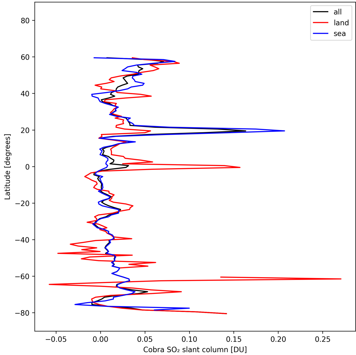
Figure 35: Zonal average of “Cobra SO 2 slant column” for 2025-10-19 to 2025-10-21.
