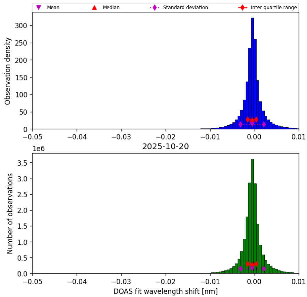
Figure 76: Histogram of “DOAS fit wavelength shift” for 2025-10-19 to 2025-10-21
