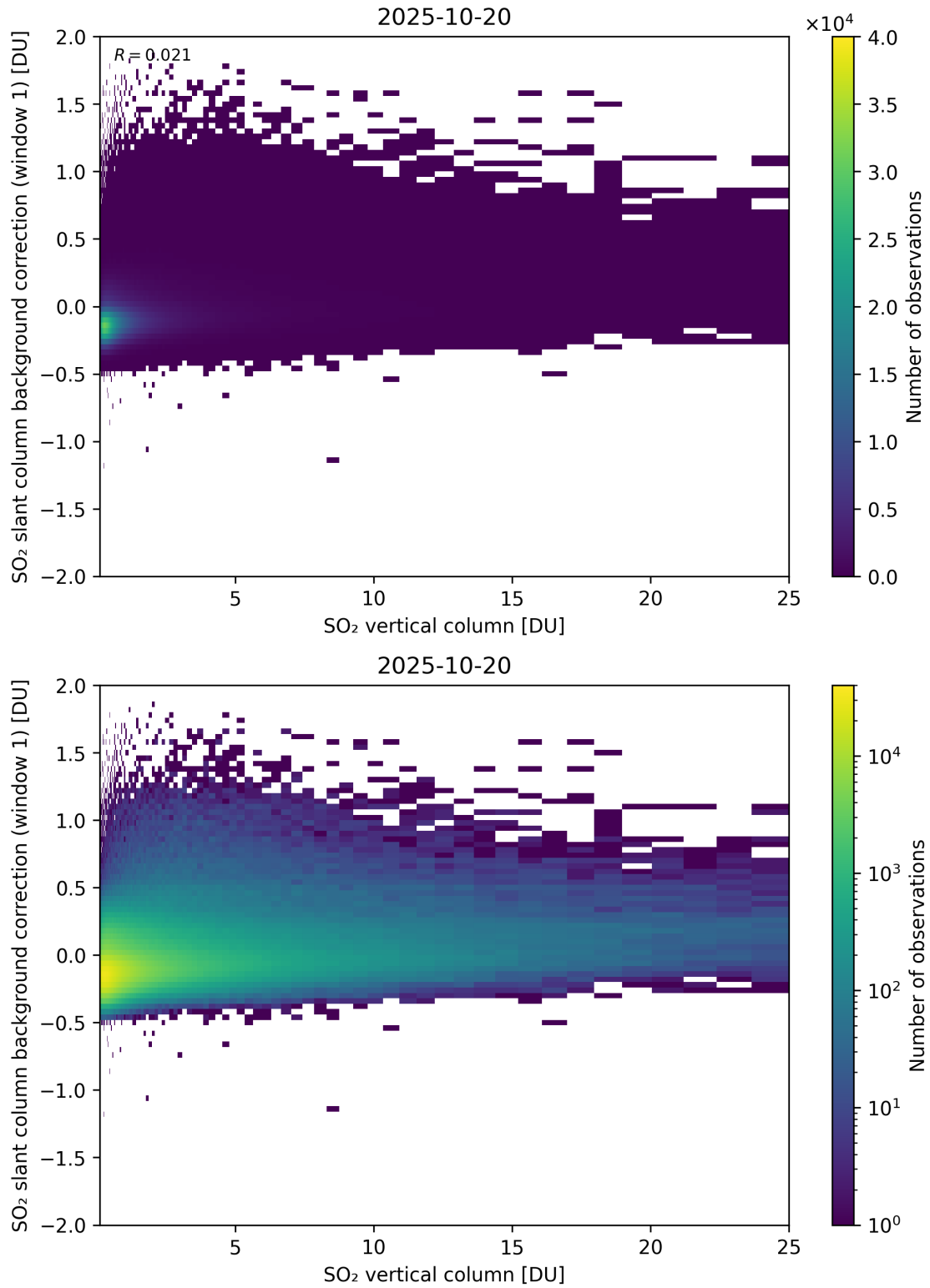
Figure 323: Scatter density plot of “SO 2 vertical column” against “SO 2 slant column background correction (window 1)” for 2025-10-19 to 2025-10-21.
