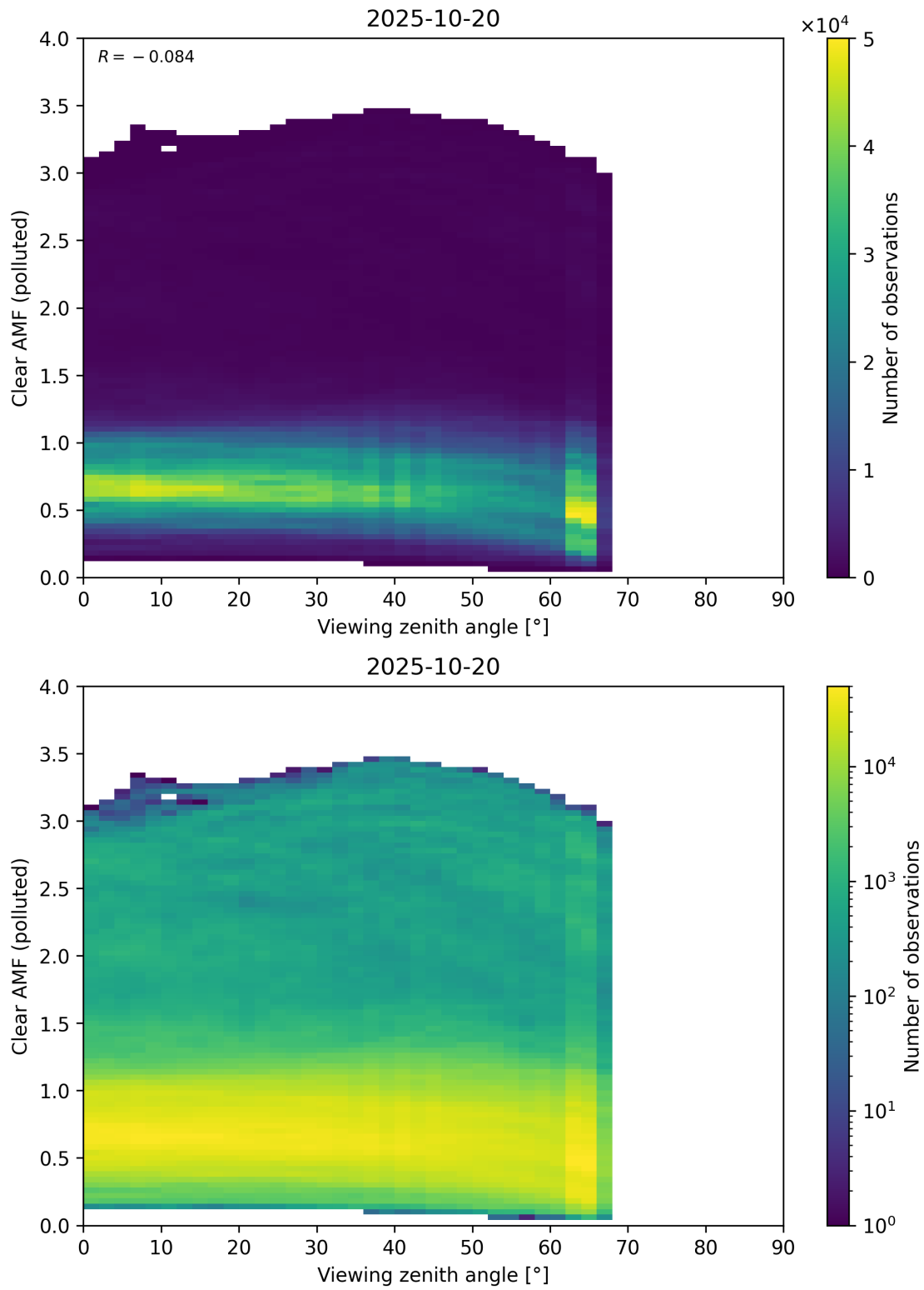
Figure 370: Scatter density plot of “Viewing zenith angle” against “Clear AMF (polluted)” for 2025-10-19 to 2025-10-21.
