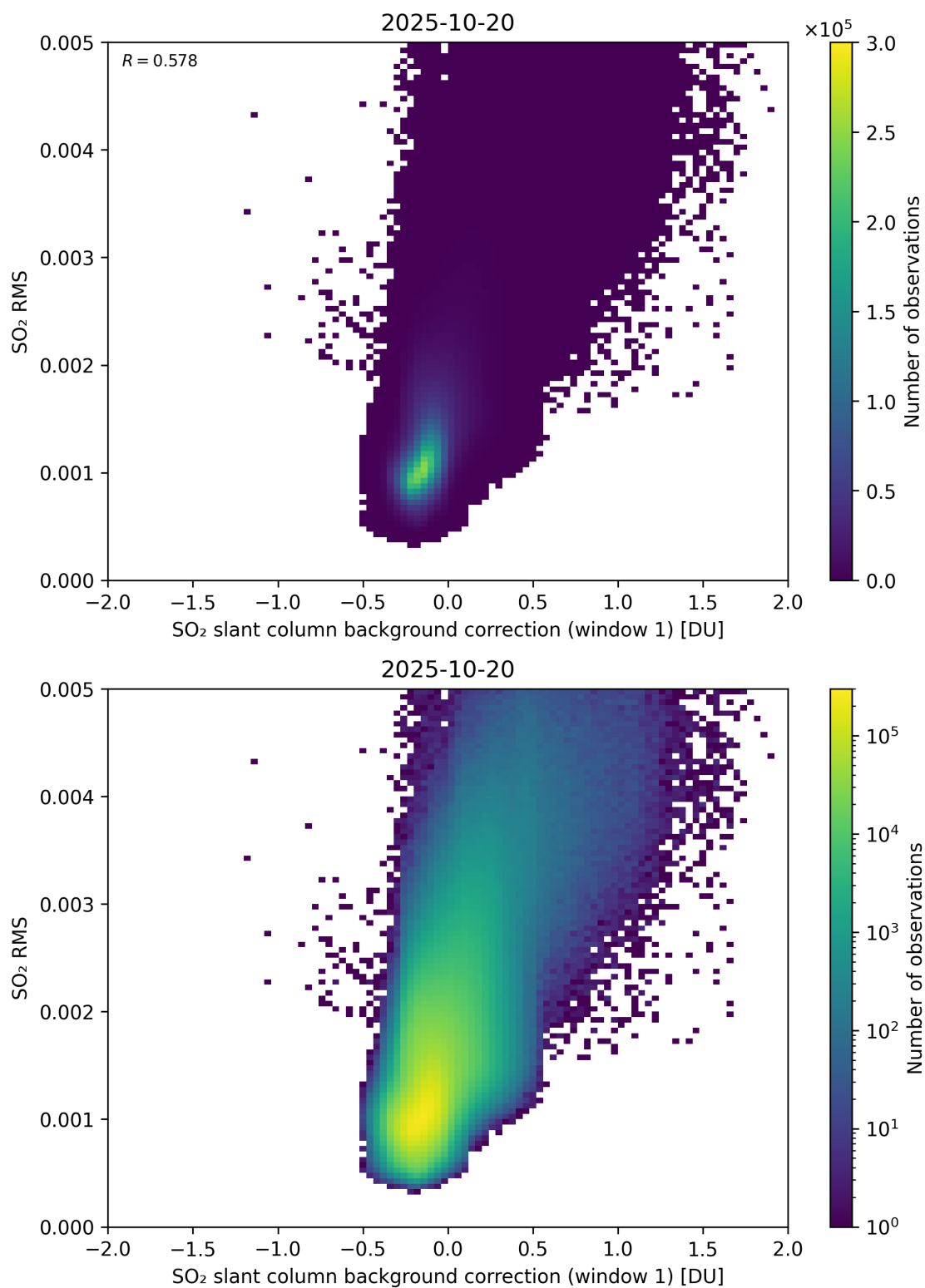
Figure 113: Scatter density plot of “SO 2 slant column background correction (window 1)” against “SO 2 RMS” for 2025-10-19 to 2025-10-21.
