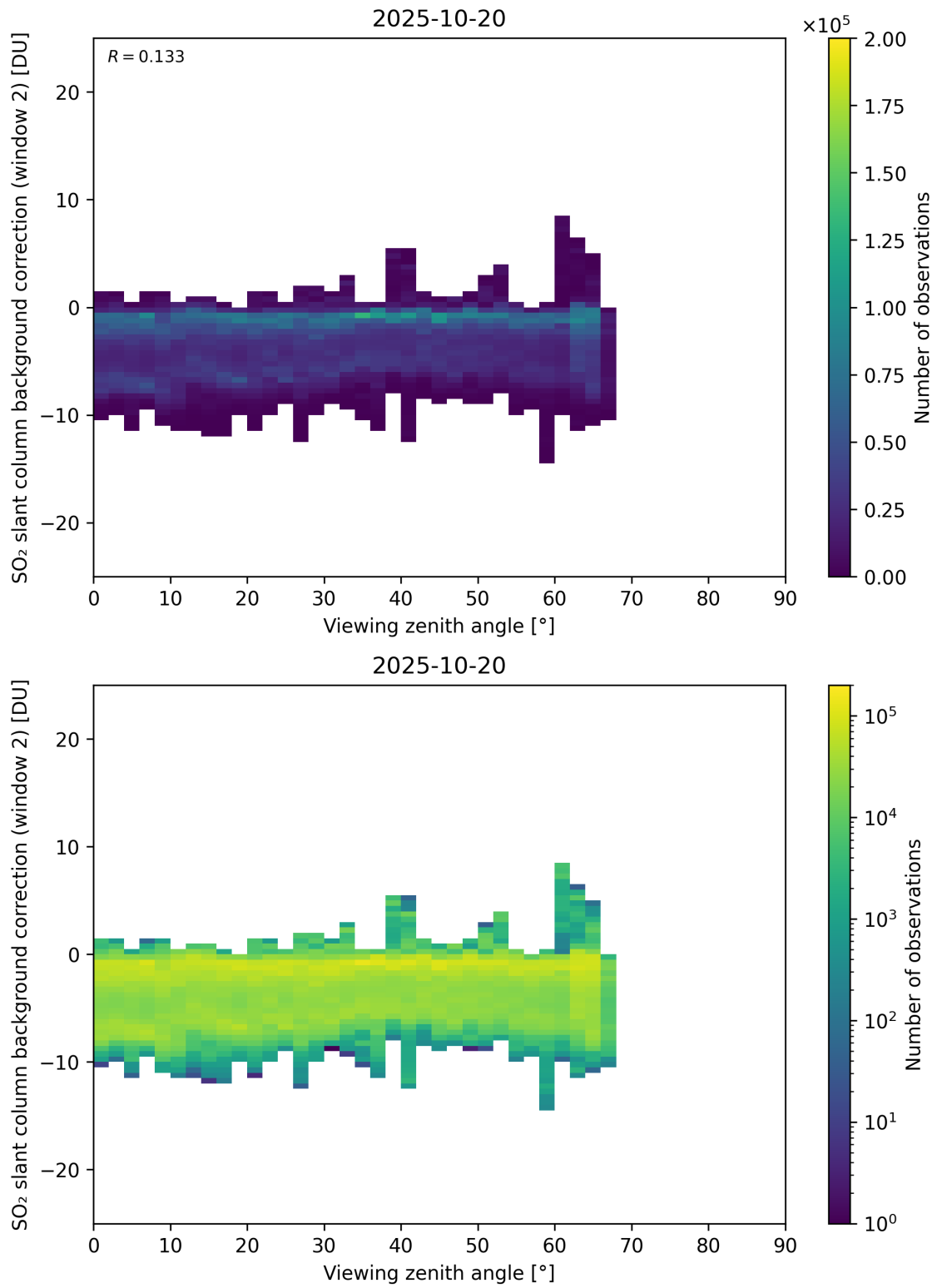
Figure 363: Scatter density plot of “Viewing zenith angle” against “SO 2 slant column background correction (window 2)” for 2025-10-19 to 2025-10-21.
