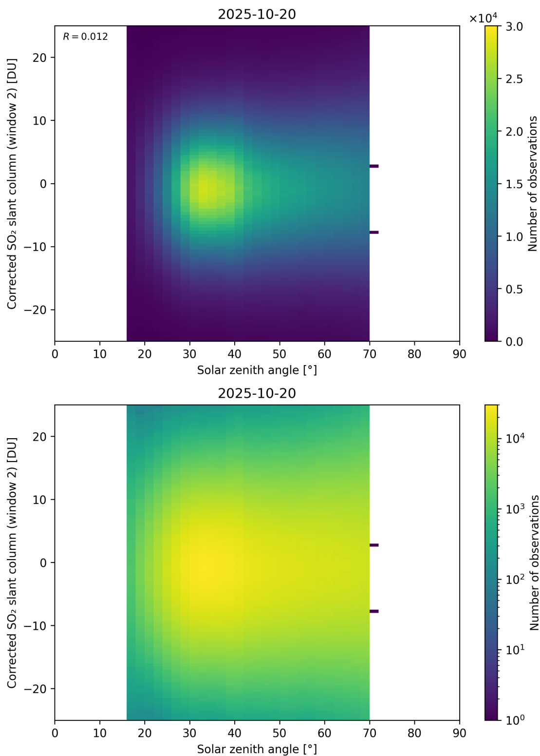
Figure 182: Scatter density plot of “Solar zenith angle” against “Corrected SO 2 slant column (window 2)” for 2025-10-19 to 2025-10-21.
