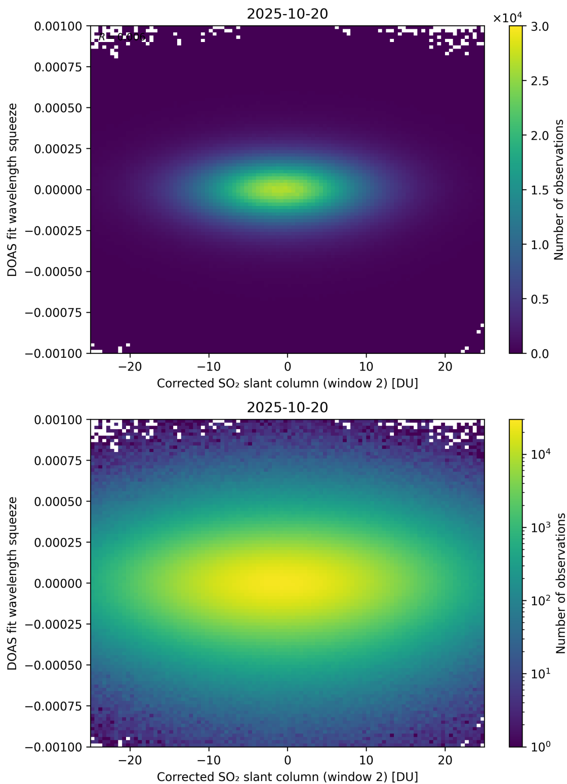
Figure 247: Scatter density plot of “Corrected SO 2 slant column (window 2)” against “DOAS fit wavelength squeeze” for 2025-10-19 to 2025-10-21.
