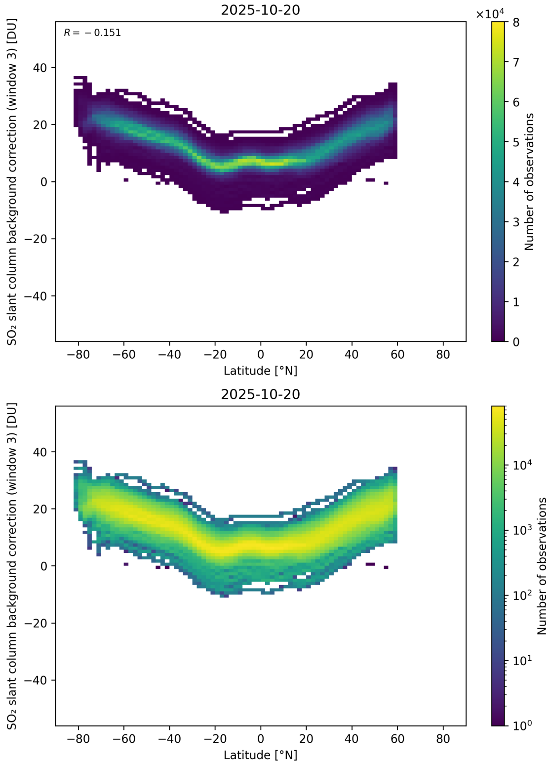
Figure 152: Scatter density plot of “Latitude” against “SO 2 slant column background correction (window 3)” for 2025-10-19 to 2025-10-21.
