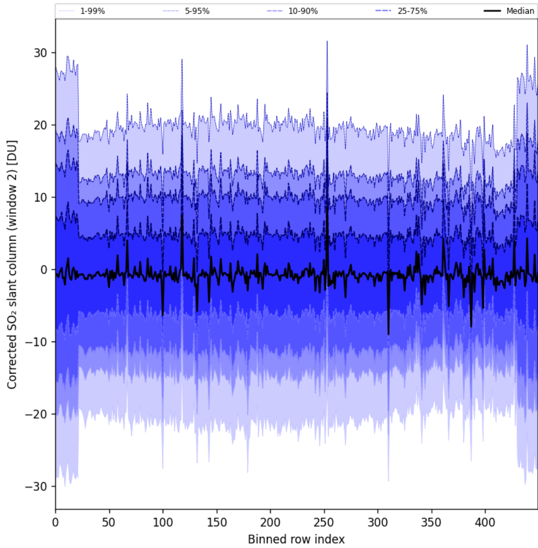
Figure 95: Along track statistics of “Corrected SO 2 slant column (window 2)” for 2025-10-19 to 2025-10-21
