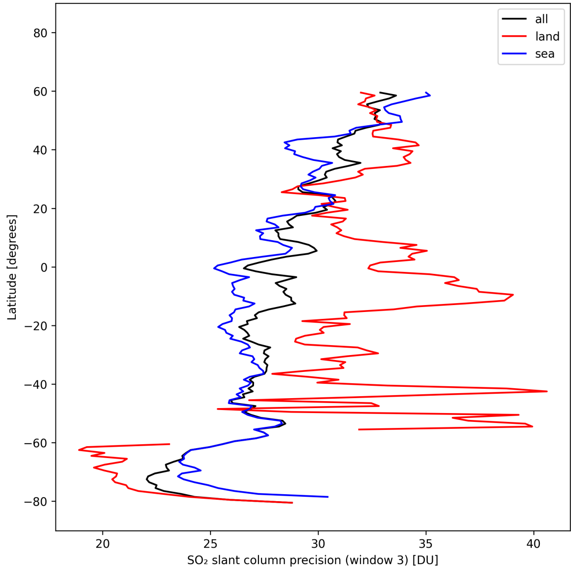
Figure 46: Zonal average of “SO 2 slant column precision (window 3)” for 2025-10-19 to 2025-10-21.
