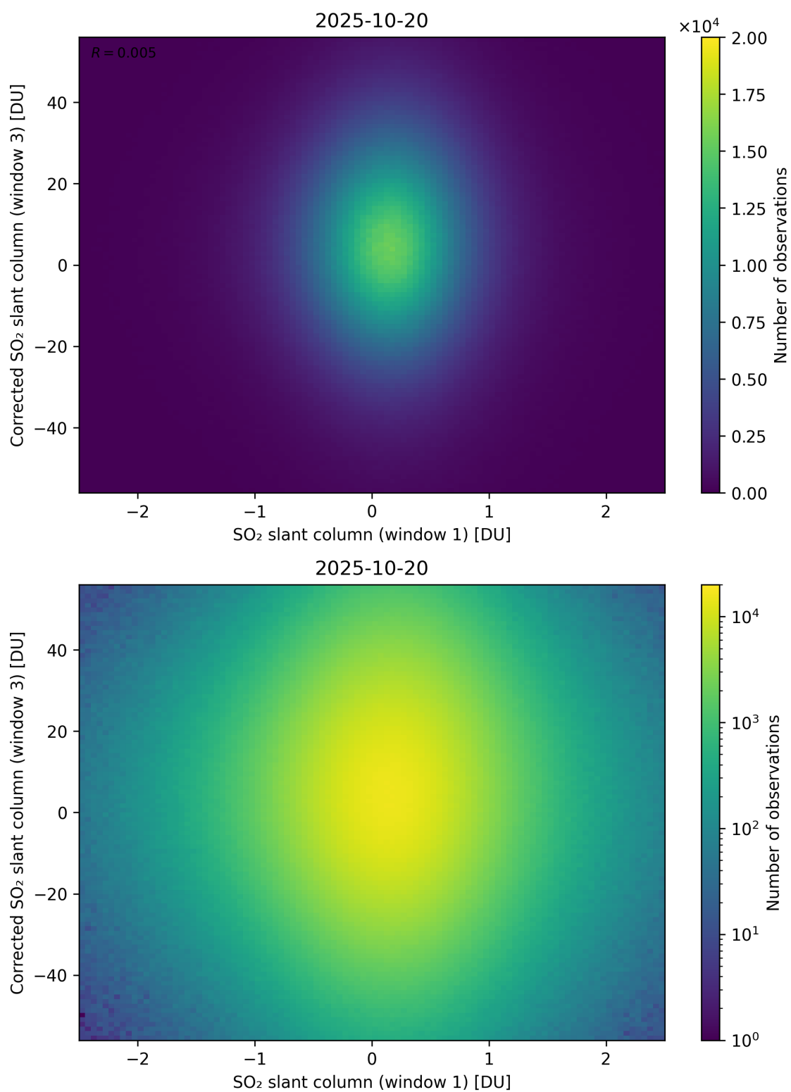
Figure 284: Scatter density plot of “SO 2 slant column (window 1)” against “Corrected SO 2 slant column (window 3)” for 2025-10-19 to 2025-10-21.
