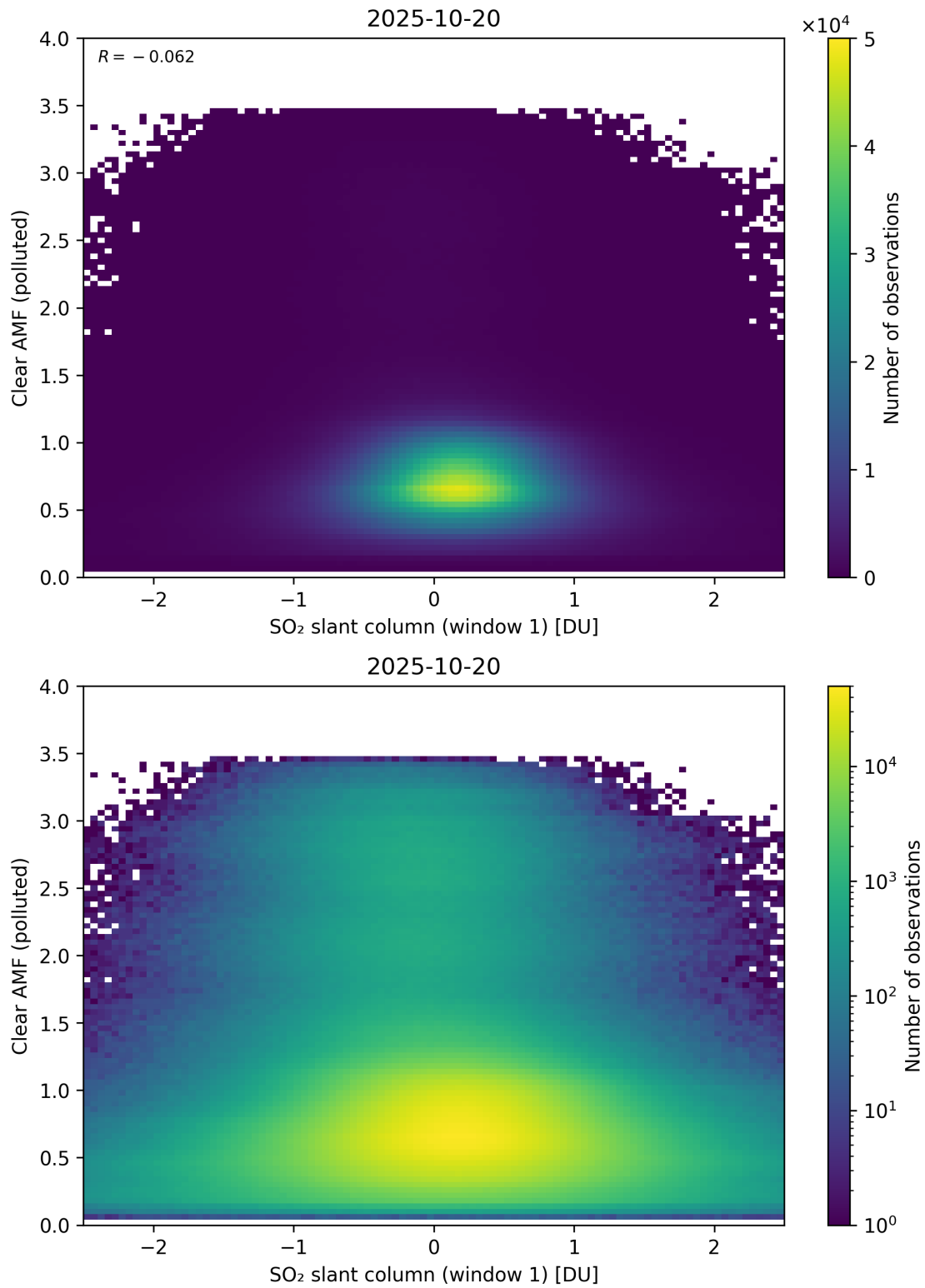
Figure 282: Scatter density plot of “SO 2 slant column (window 1)” against “Clear AMF (polluted)” for 2025-10-19 to 2025-10-21.
