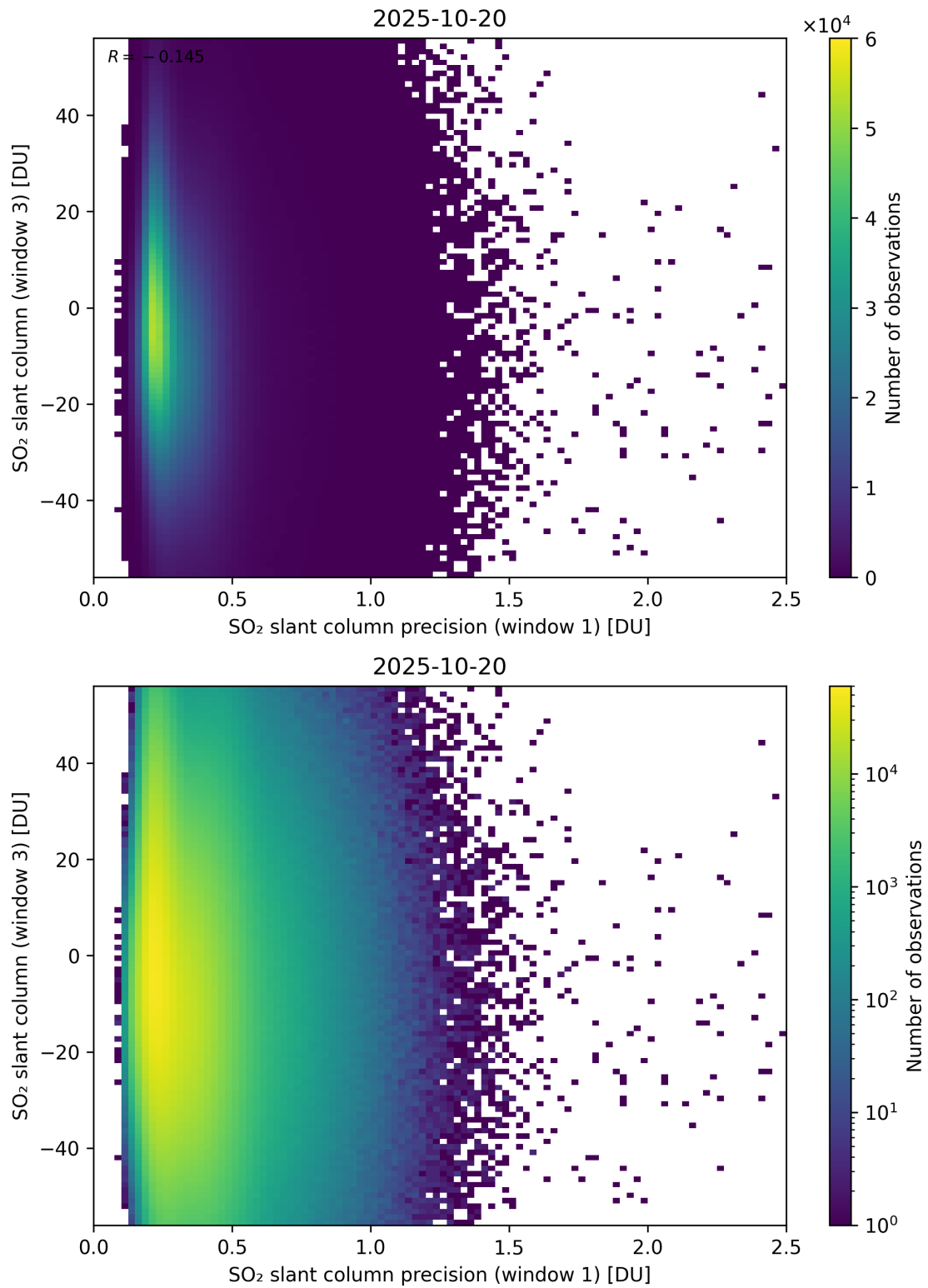
Figure 278: Scatter density plot of “SO 2 slant column precision (window 1)” against “SO 2 slant column (window 3)” for 2025-10-19 to 2025-10-21.
