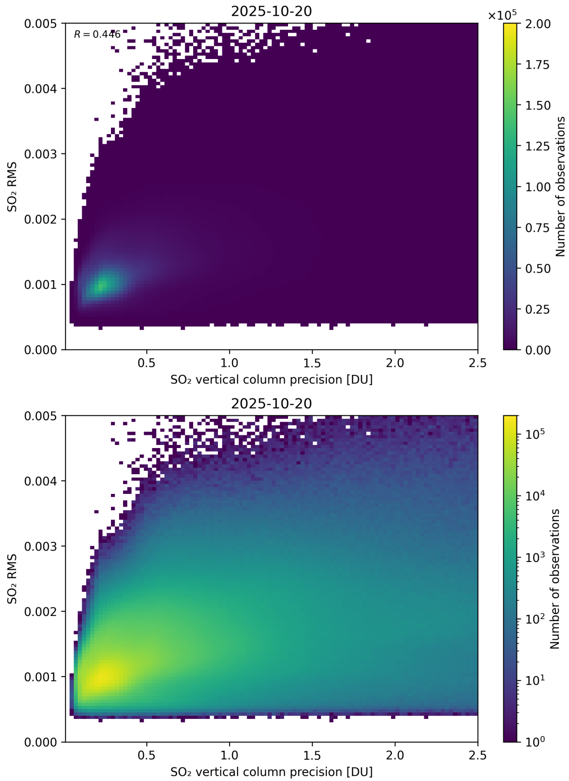
Figure 334: Scatter density plot of “SO 2 vertical column precision” against “SO 2 RMS” for 2025-10-19 to 2025-10-21.
