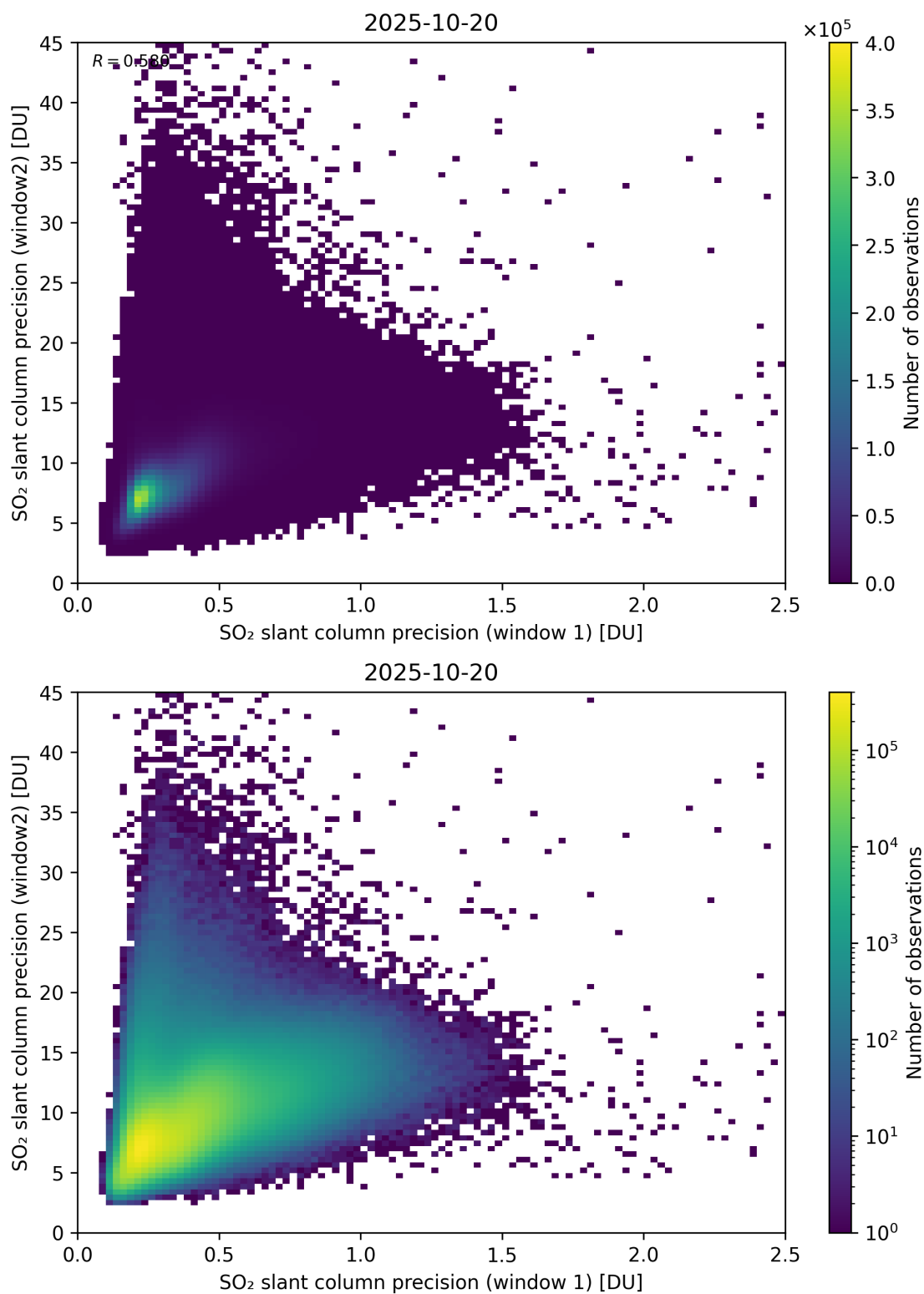
Figure 277: Scatter density plot of “SO 2 slant column precision (window 1)” against “SO 2 slant column precision (window2)” for 2025-10-19 to 2025-10-21.
