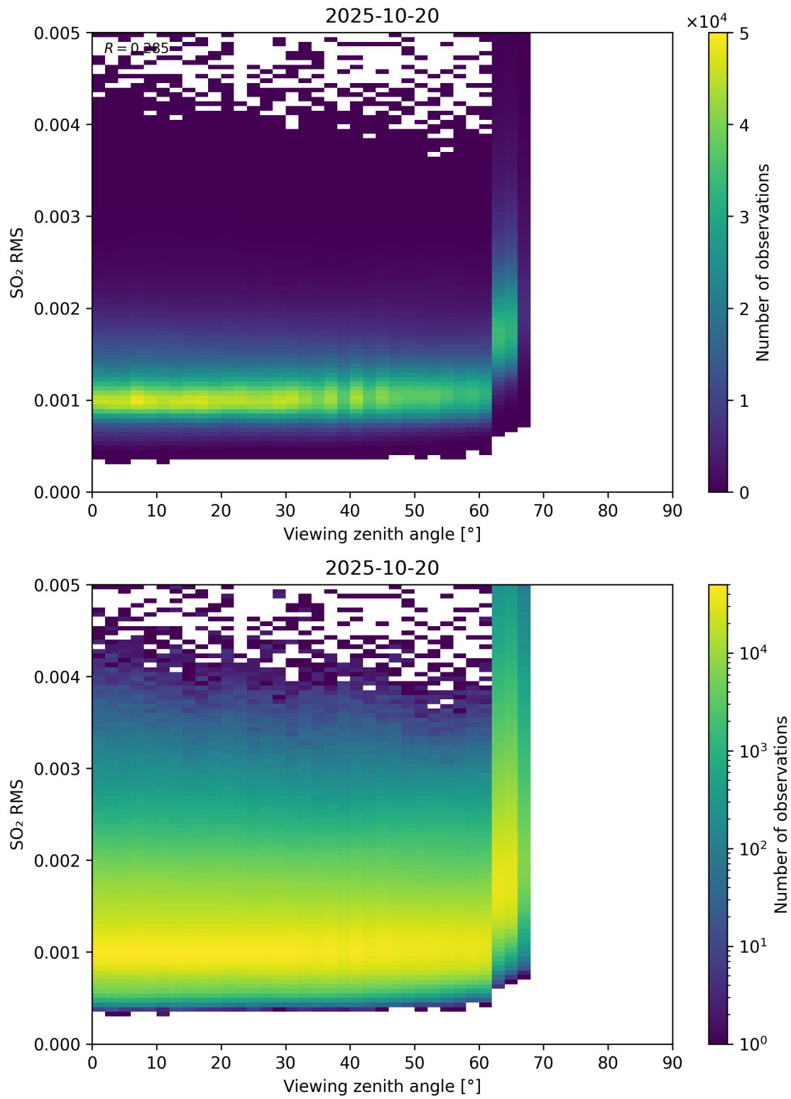
Figure 367: Scatter density plot of “Viewing zenith angle” against “SO 2 RMS” for 2025-10-19 to 2025-10-21.
