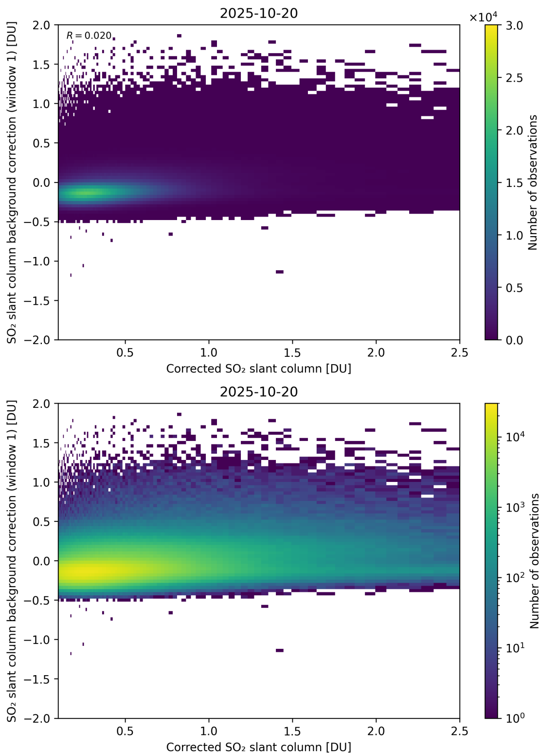
Figure 226: Scatter density plot of “Corrected SO 2 slant column” against “SO 2 slant column background correction (window 1)” for 2025-10-19 to 2025-10-21.
