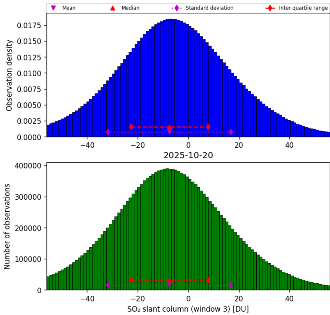
Figure 71: Histogram of “SO 2 slant column (window 3)” for 2025-10-19 to 2025-10-21
