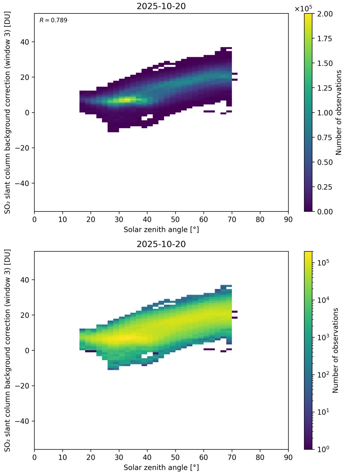
Figure 173: Scatter density plot of “Solar zenith angle” against “SO 2 slant column background correction (window 3)” for 2025-10-19 to 2025-10-21.
