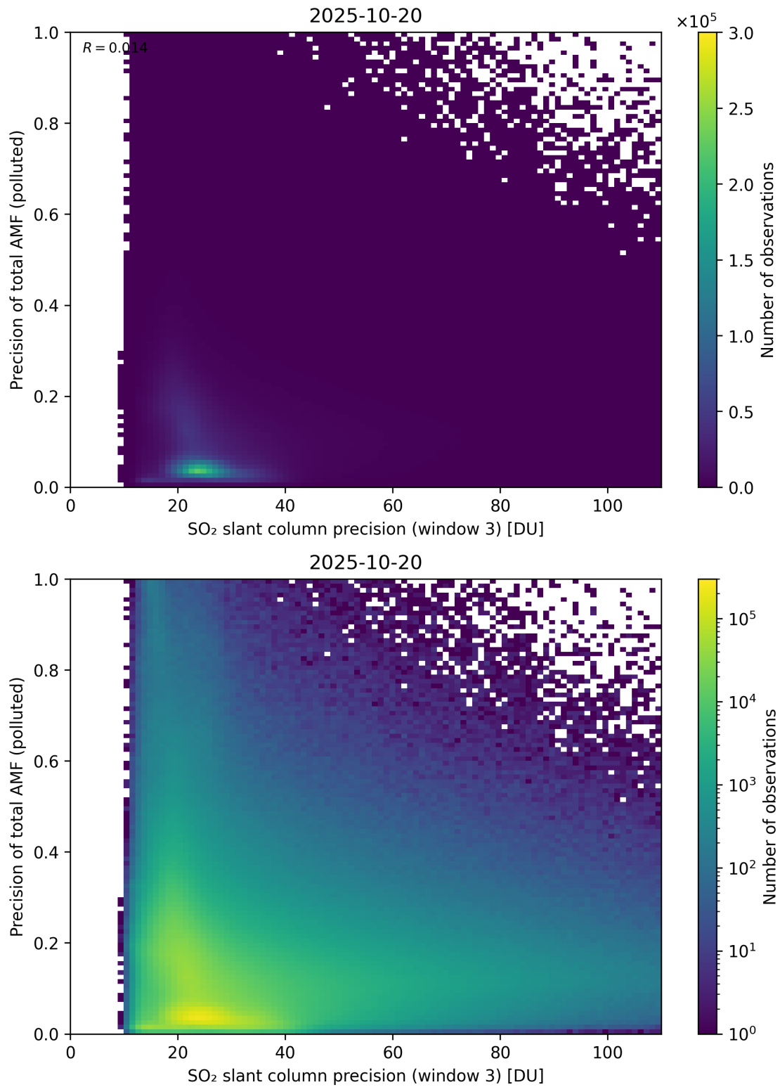
Figure 314: Scatter density plot of “SO 2 slant column precision (window 3)” against “Precision of total AMF (polluted)” for 2025-10-19 to 2025-10-21.
