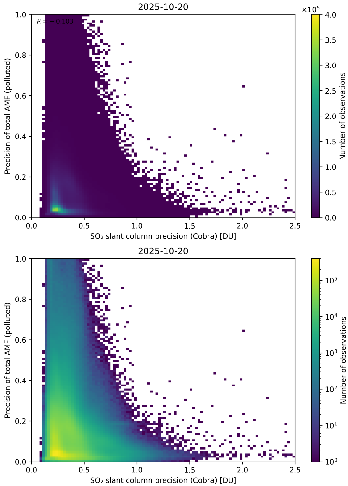
Figure 214: Scatter density plot of “SO 2 slant column precision (Cobra)” against “Precision of total AMF (polluted)” for 2025-10-19 to 2025-10-21.
