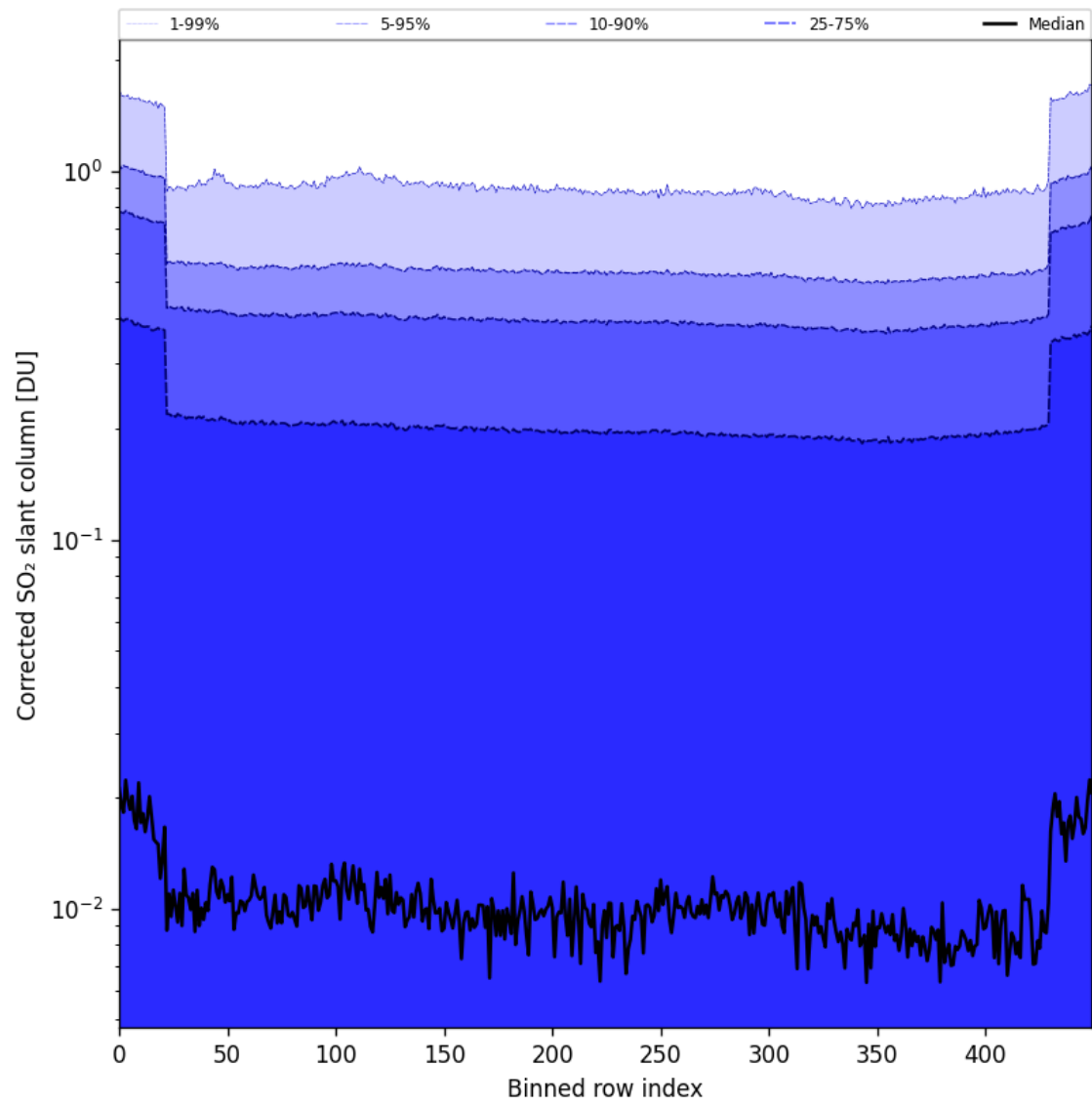
Figure 86: Along track statistics of “Corrected SO 2 slant column” for 2025-10-19 to 2025-10-21
