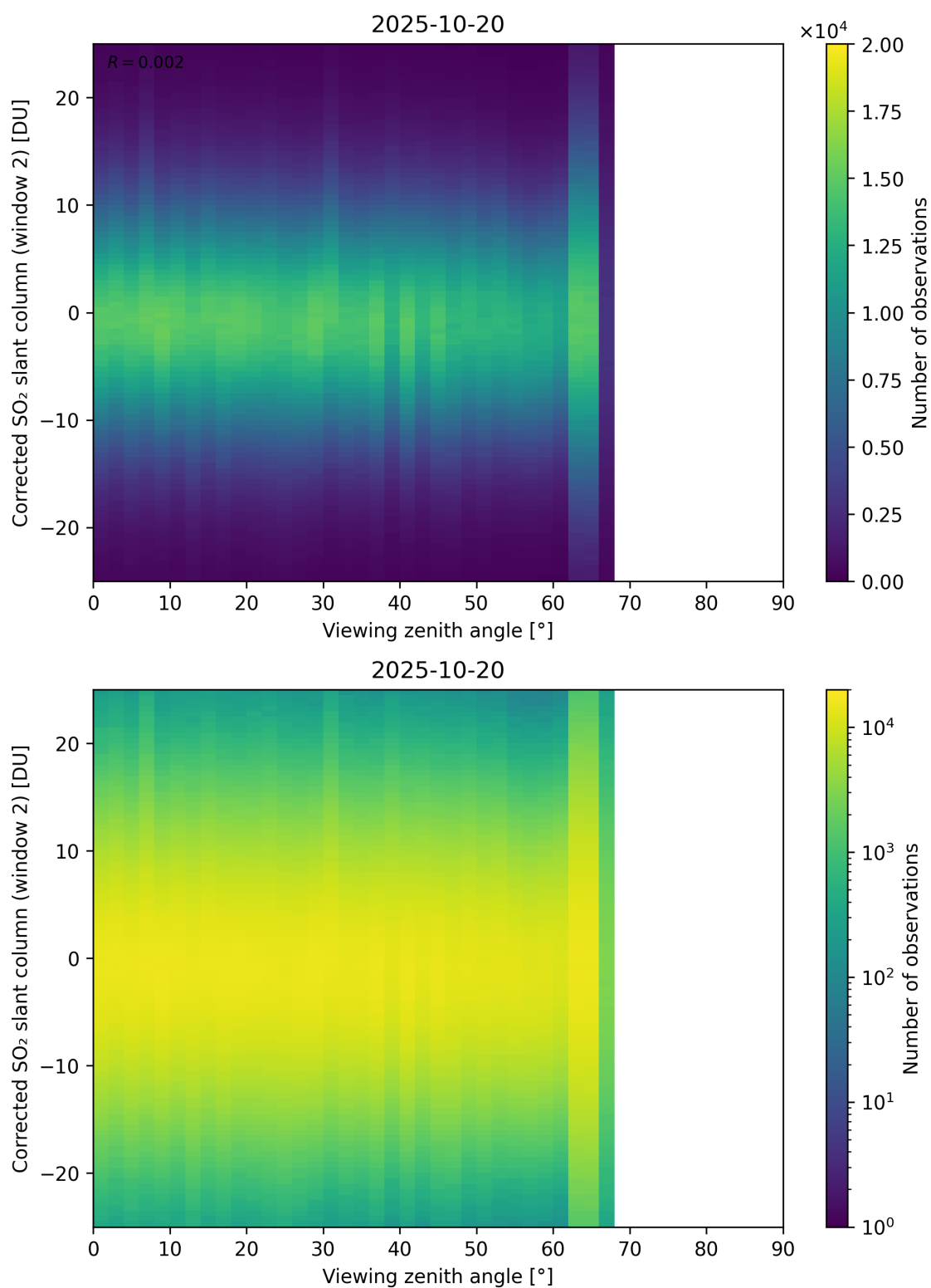
Figure 374: Scatter density plot of “Viewing zenith angle” against “Corrected SO 2 slant column (window 2)” for 2025-10-19 to 2025-10-21.
