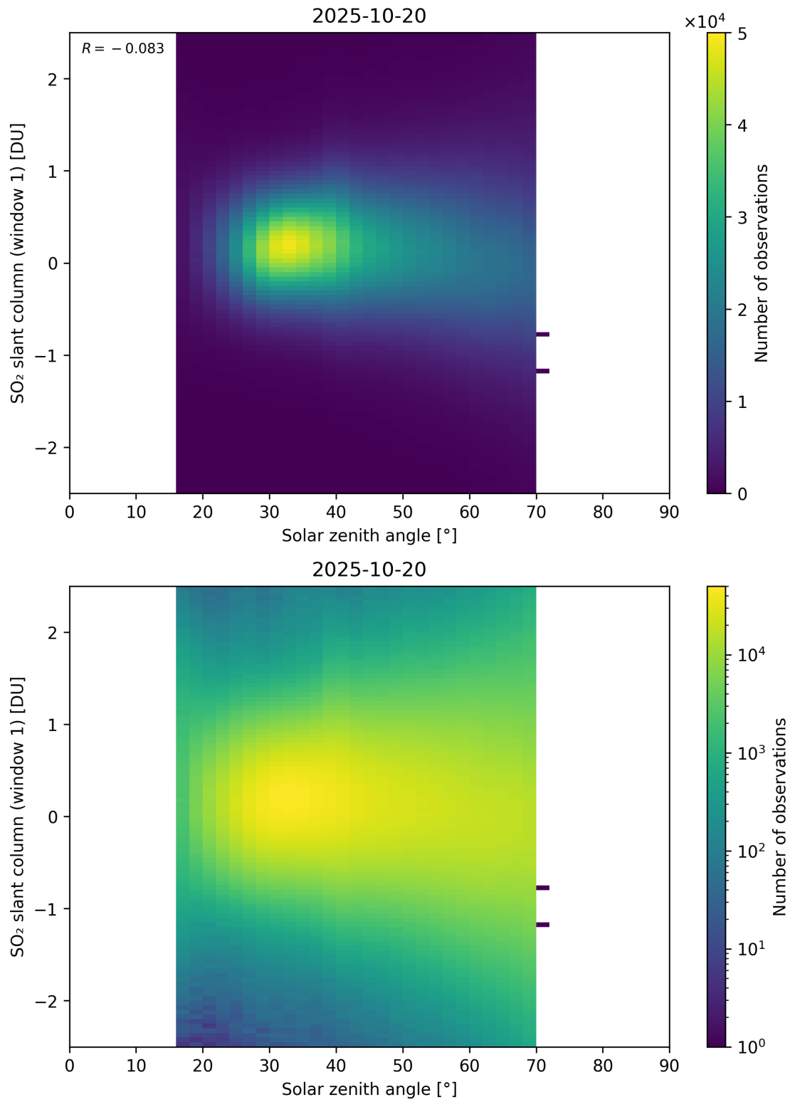
Figure 184: Scatter density plot of “Solar zenith angle” against “SO 2 slant column (window 1)” for 2025-10-19 to 2025-10-21.
