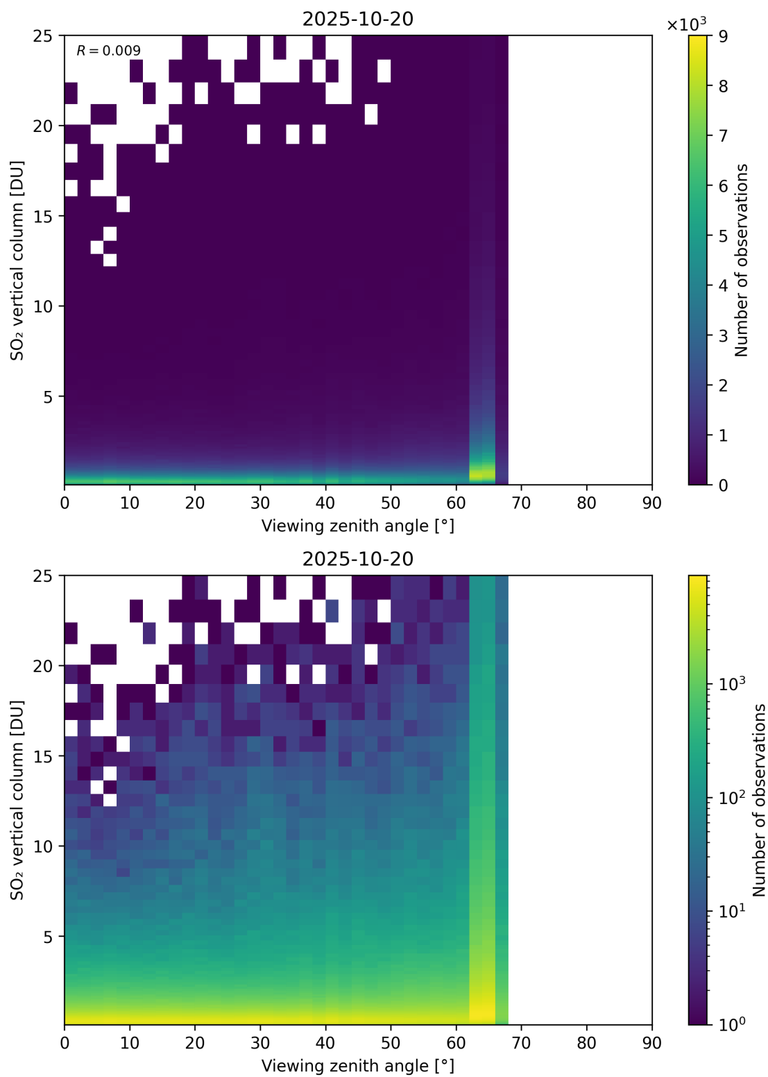
Figure 383: Scatter density plot of “Viewing zenith angle” against “SO 2 vertical column” for 2025-10-19 to 2025-10-21.
