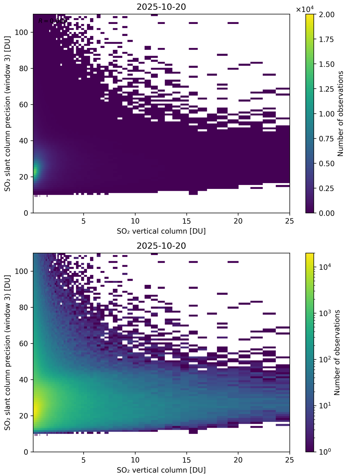
Figure 358: Scatter density plot of “SO 2 vertical column” against “SO 2 slant column precision (window 3)” for 2025-10-19 to 2025-10-21.
