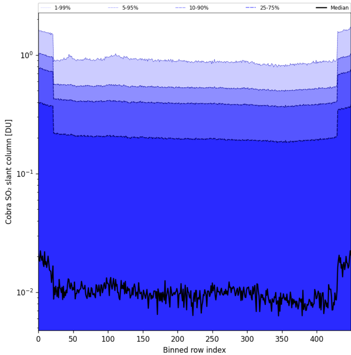
Figure 87: Along track statistics of "Cobra SO 2 slant column" for 2025-10-19 to 2025-10-21
