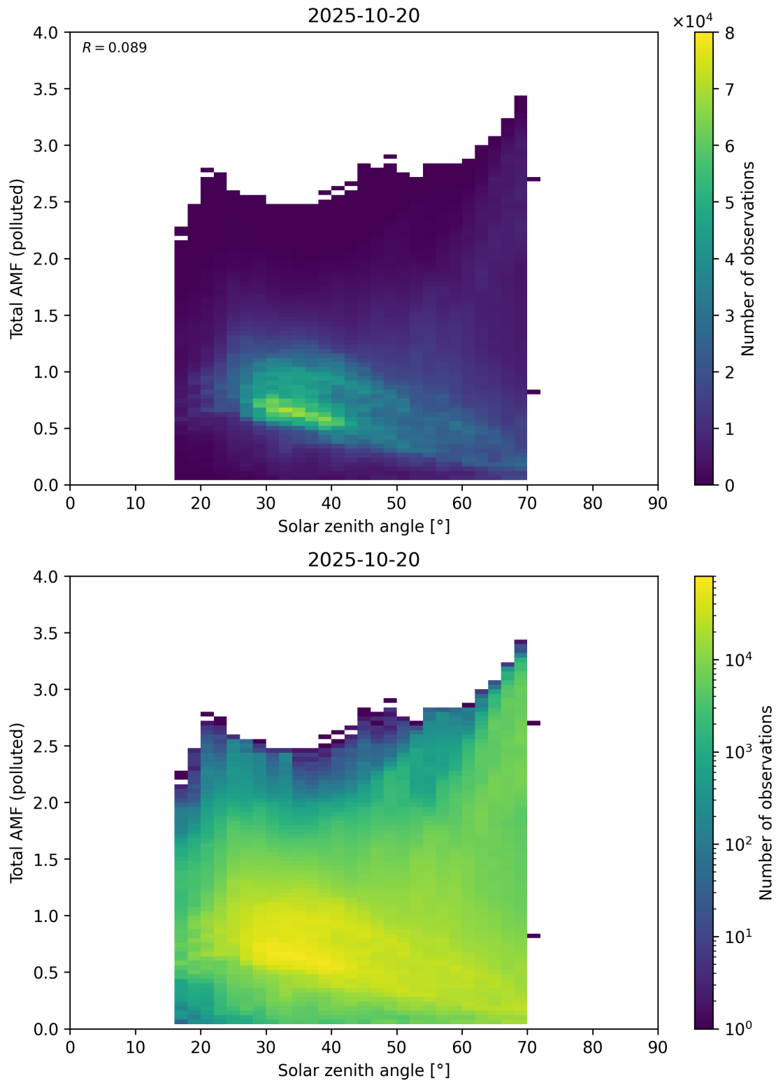
Figure 189: Scatter density plot of “Solar zenith angle” against “Total AMF (polluted)” for 2025-10-19 to 2025-10-21.
