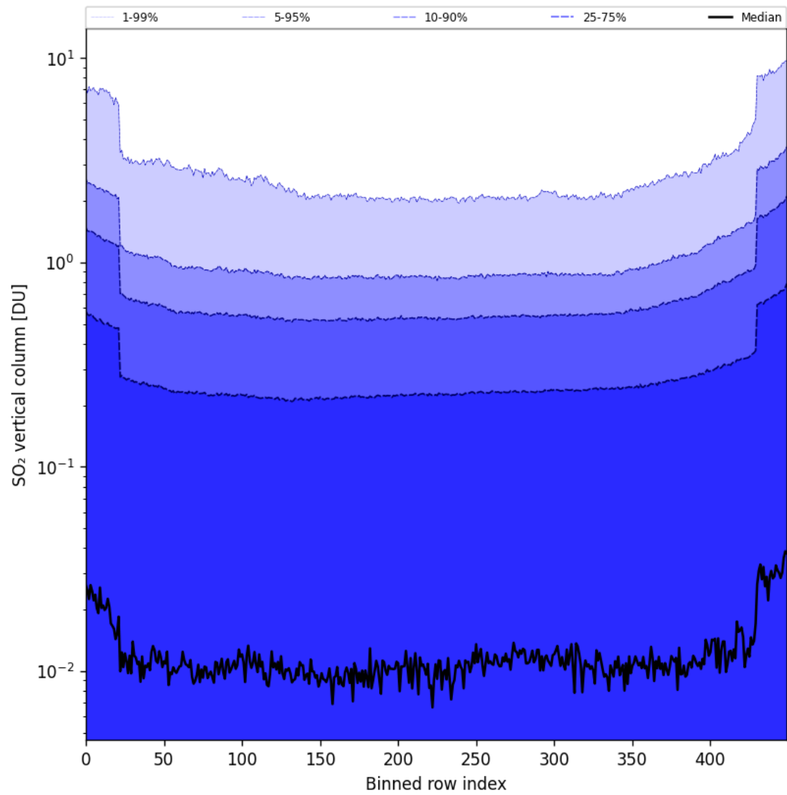
Figure 84: Along track statistics of “SO 2 vertical column” for 2025-10-19 to 2025-10-21
