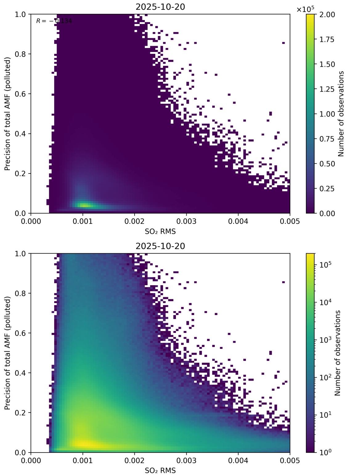
Figure 149: Scatter density plot of “SO 2 RMS” against “Precision of total AMF (polluted)” for 2025-10-19 to 2025-10-21.
