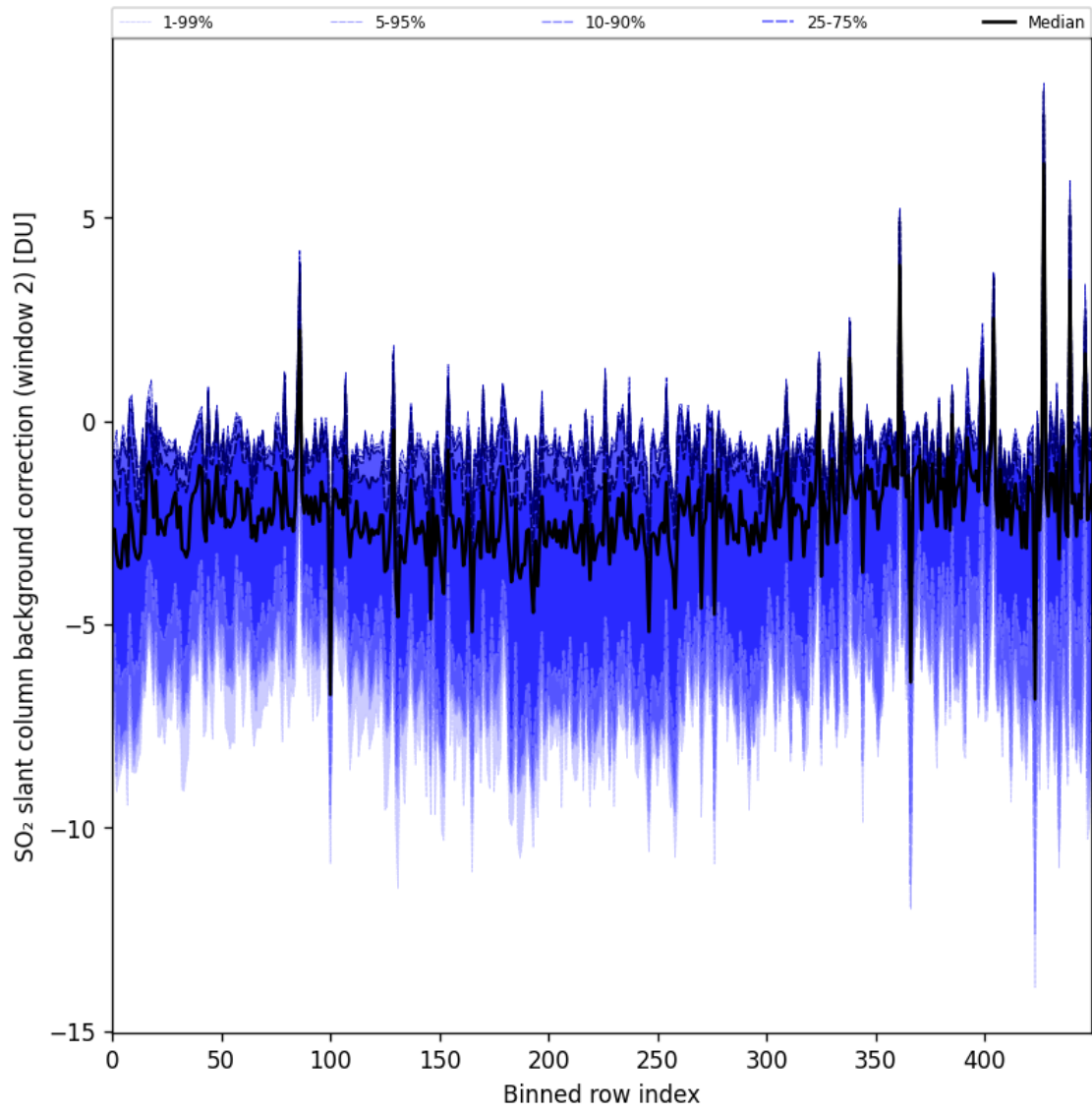
Figure 96: Along track statistics of “SO 2 slant column background correction (window 2)” for 2025-10-19 to 2025-10-21
