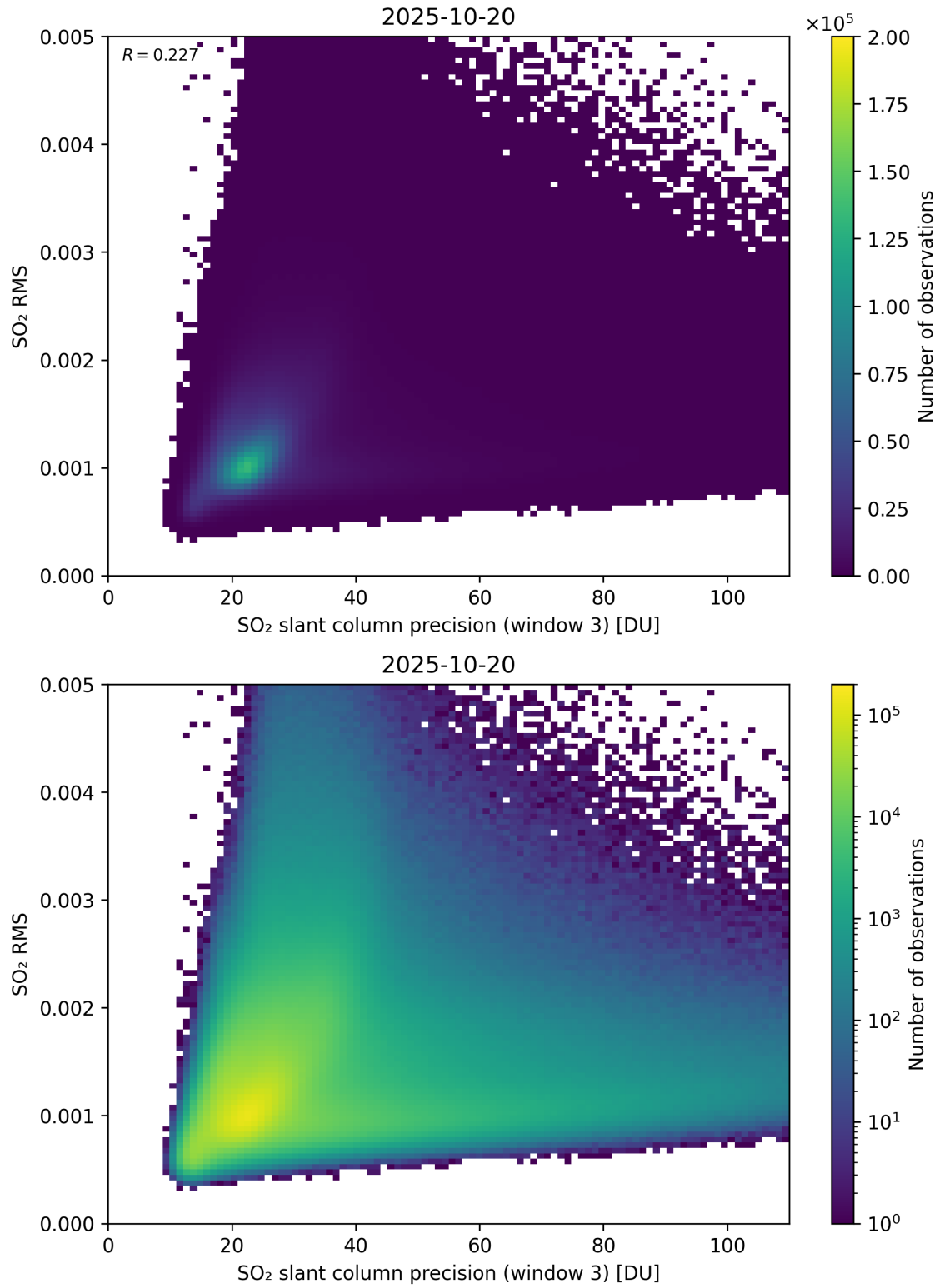
Figure 310: Scatter density plot of “SO 2 slant column precision (window 3)” against “SO 2 RMS” for 2025-10-19 to 2025-10-21.
