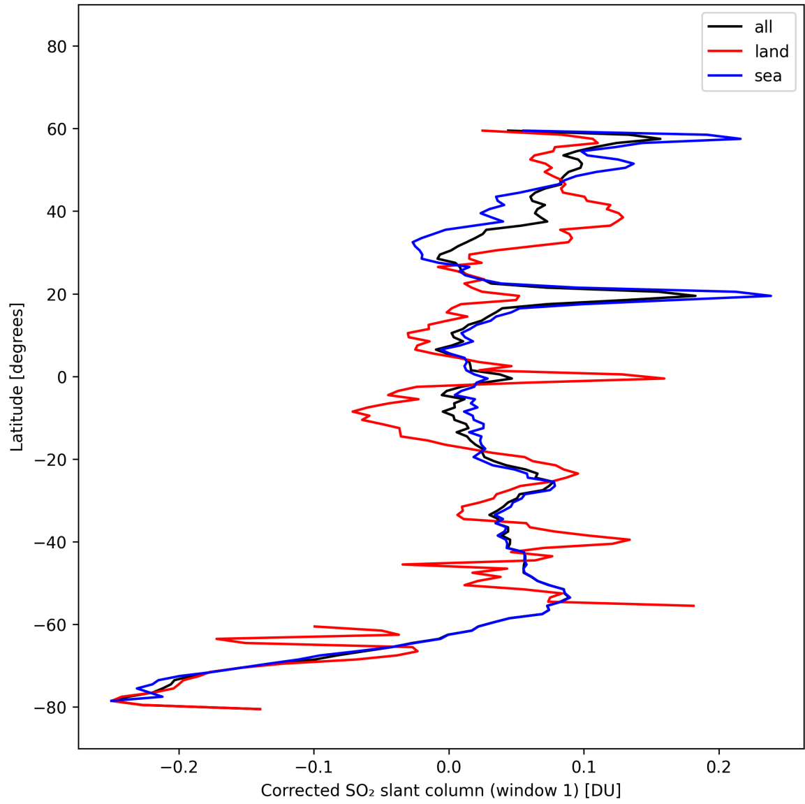
Figure 39: Zonal average of “Corrected SO 2 slant column (window 1)” for 2025-10-19 to 2025-10-21.
