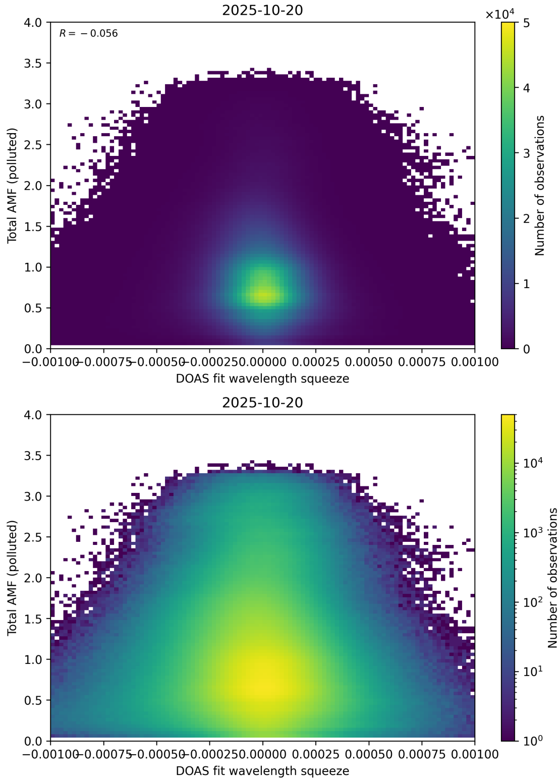
Figure 145: Scatter density plot of “DOAS fit wavelength squeeze” against “Total AMF (polluted)” for 2025-10-19 to 2025-10-21.
