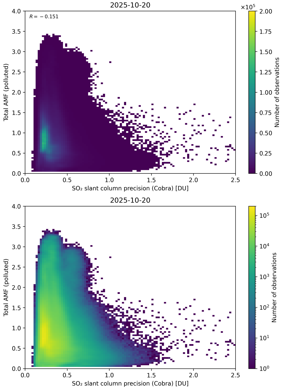
Figure 213: Scatter density plot of “SO 2 slant column precision (Cobra)” against “Total AMF (polluted)” for 2025-10-19 to 2025-10-21.
