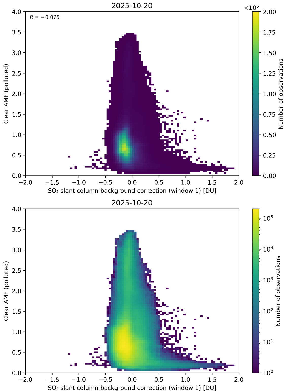
Figure 114: Scatter density plot of “SO 2 slant column background correction (window 1)” against “Clear AMF (polluted)” for 2025-10-19 to 2025-10-21.
