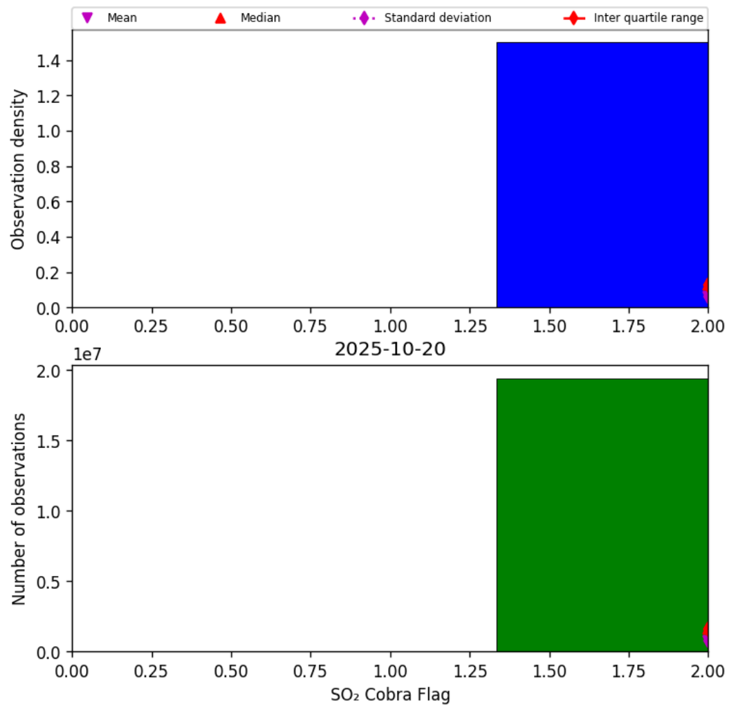
Figure 75: Histogram of “SO 2 Cobra Flag” for 2025-10-19 to 2025-10-21
