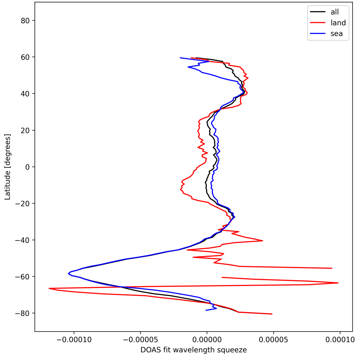
Figure 51: Zonal average of “DOAS fit wavelength squeeze” for 2025-10-19 to 2025-10-21.
