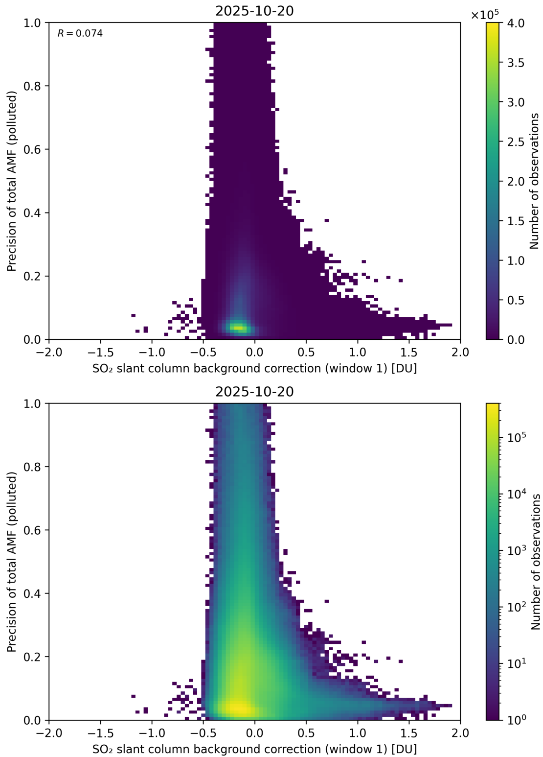
Figure 121: Scatter density plot of “SO 2 slant column background correction (window 1)” against “Precision of total AMF (polluted)” for 2025-10-19 to 2025-10-21.
