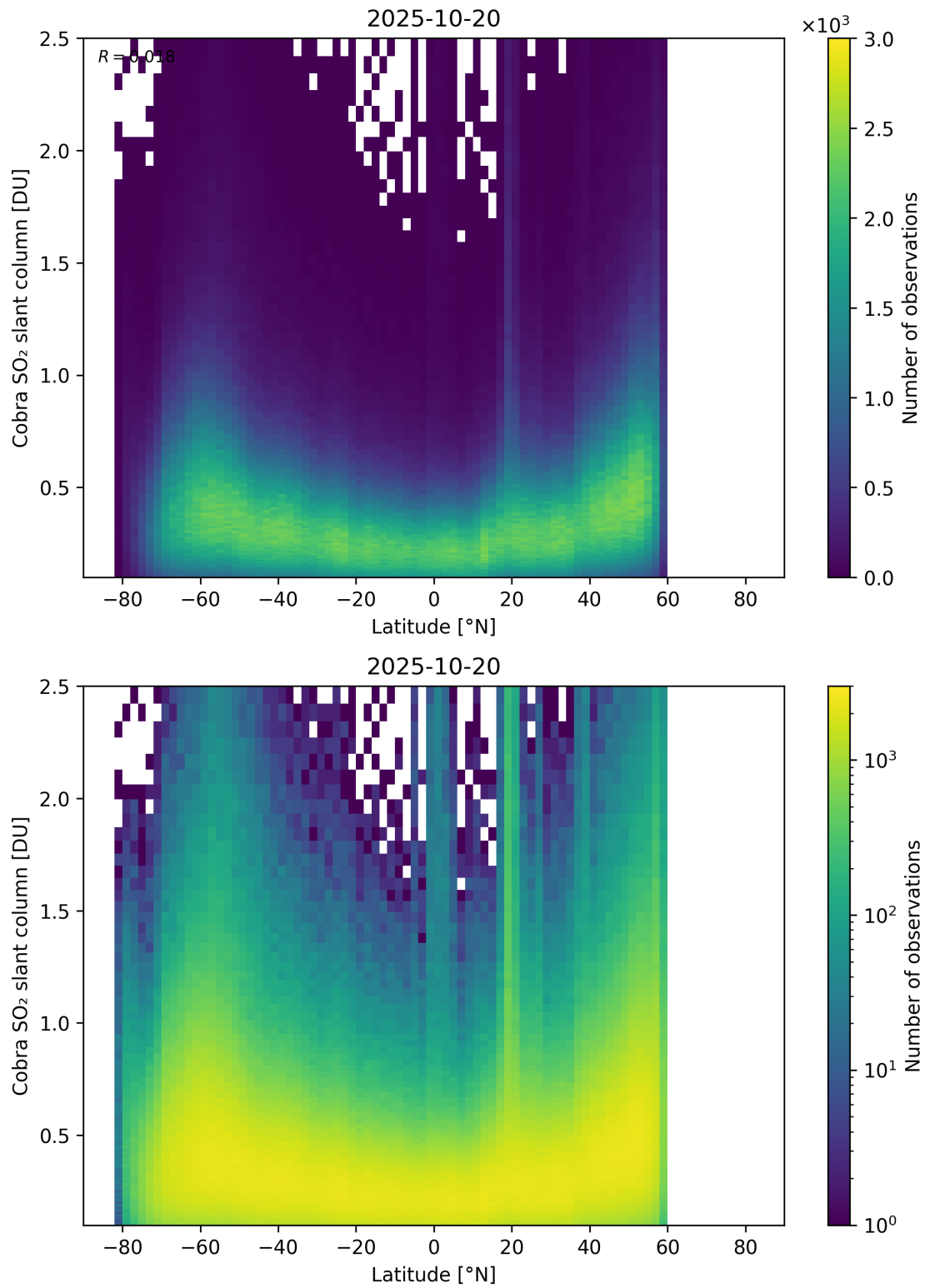
Figure 157: Scatter density plot of “Latitude” against “Cobra SO 2 slant column” for 2025-10-19 to 2025-10-21.
