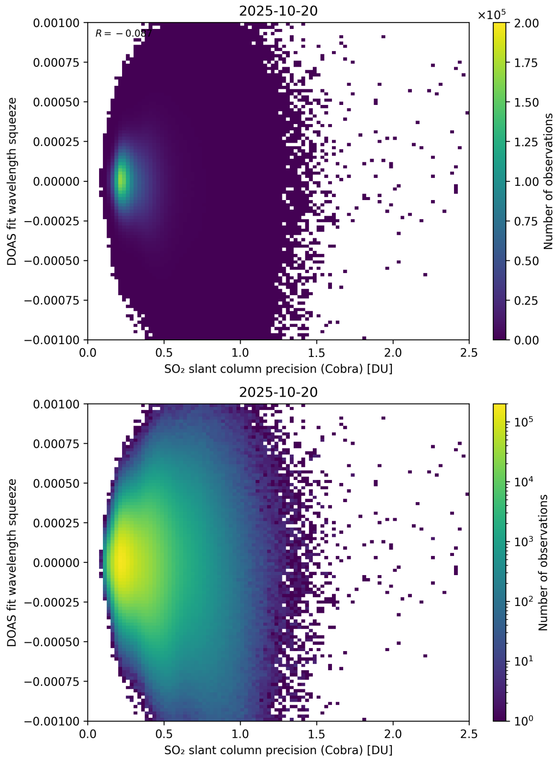
Figure 203: Scatter density plot of “SO 2 slant column precision (Cobra)” against “DOAS fit wavelength squeeze” for 2025-10-19 to 2025-10-21.
