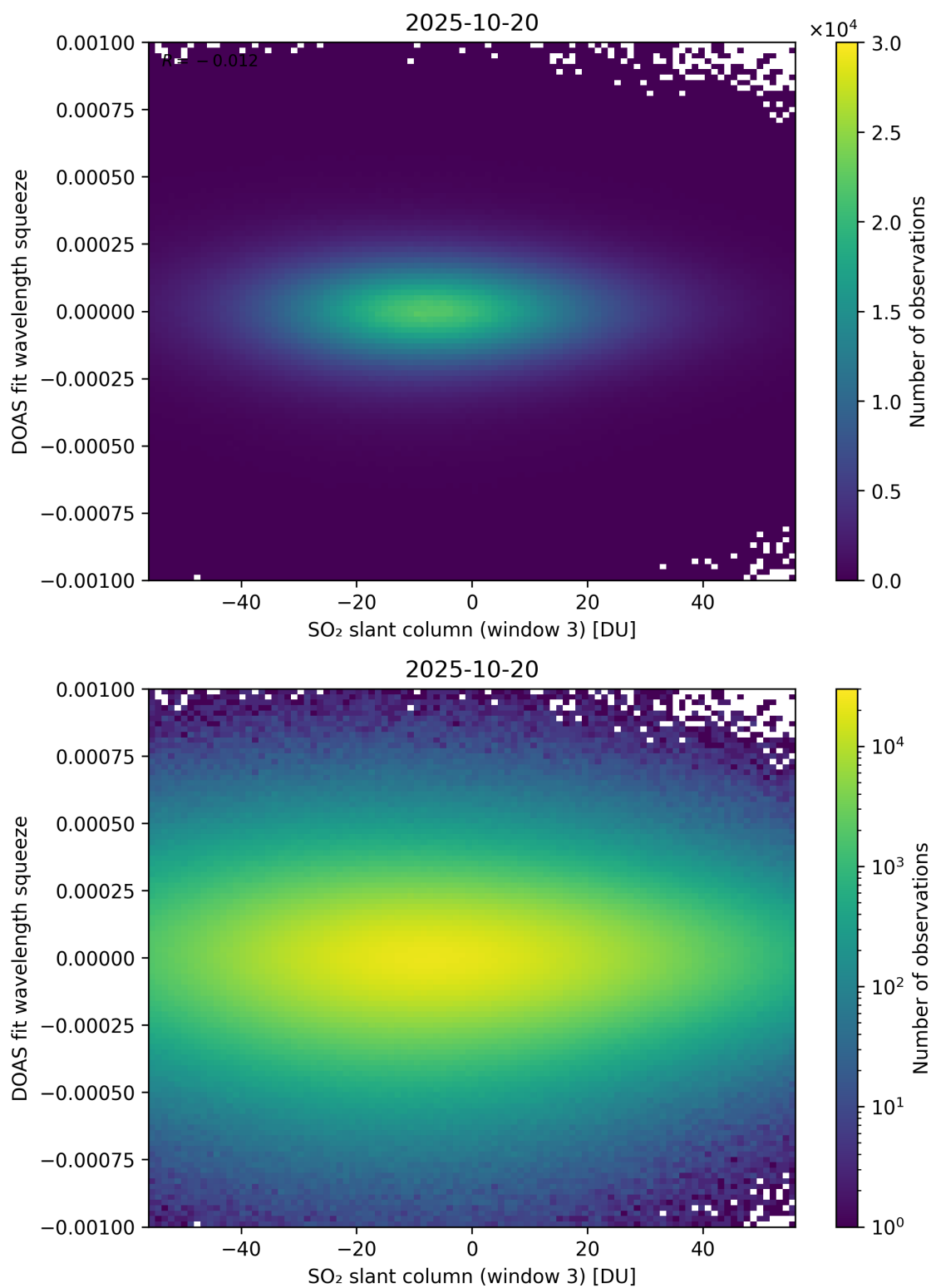
Figure 305: Scatter density plot of “SO 2 slant column (window 3)” against “DOAS fit wavelength squeeze” for 2025-10-19 to 2025-10-21.
