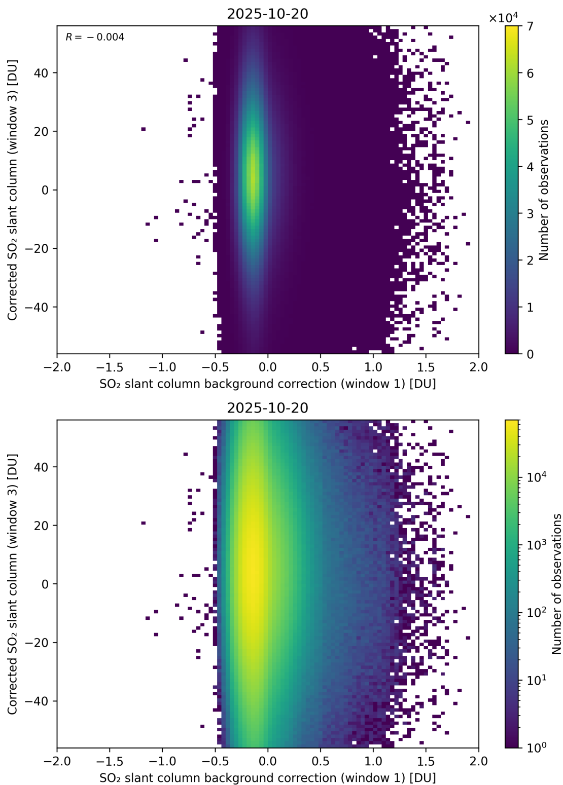
Figure 116: Scatter density plot of “SO 2 slant column background correction (window 1)” against “Corrected SO 2 slant column (window 3)” for 2025-10-19 to 2025-10-21.
