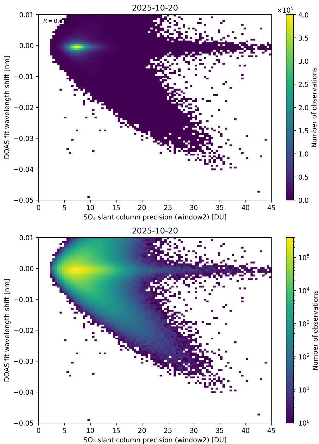
Figure 293: Scatter density plot of “SO 2 slant column precision (window2)” against “DOAS fit wavelength shift” for 2025-10-19 to 2025-10-21.
