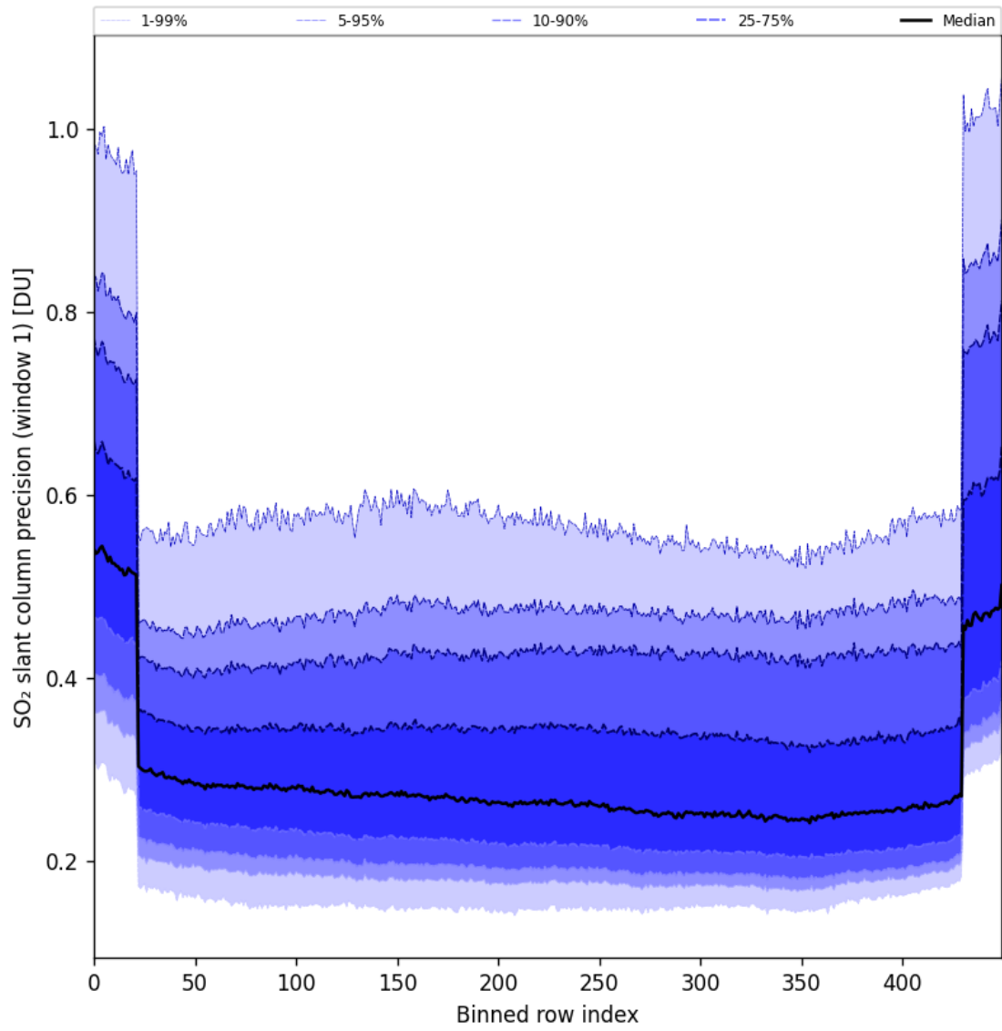
Figure 90: Along track statistics of “SO 2 slant column precision (window 1)” for 2025-10-19 to 2025-10-21
