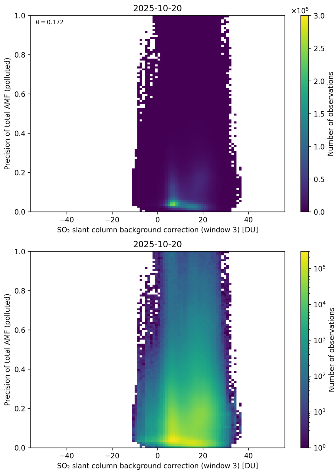
Figure 137: Scatter density plot of “SO 2 slant column background correction (window 3)” against “Precision of total AMF (polluted)” for 2025-10-19 to 2025-10-21.
