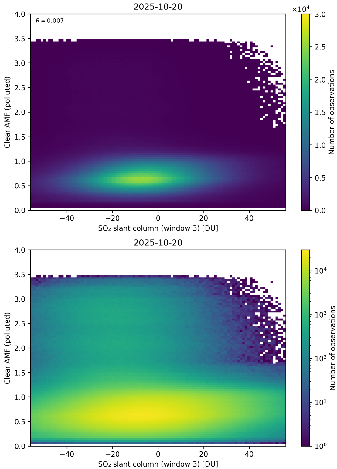
Figure 315: Scatter density plot of “SO 2 slant column (window 3)” against “Clear AMF (polluted)” for 2025-10-19 to 2025-10-21.
