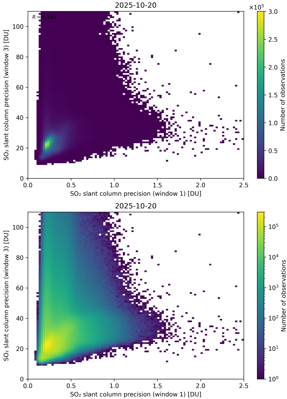
Figure 279: Scatter density plot of “SO 2 slant column precision (window 1)” against “SO 2 slant column precision (window 3)” for 2025-10-19 to 2025-10-21.
