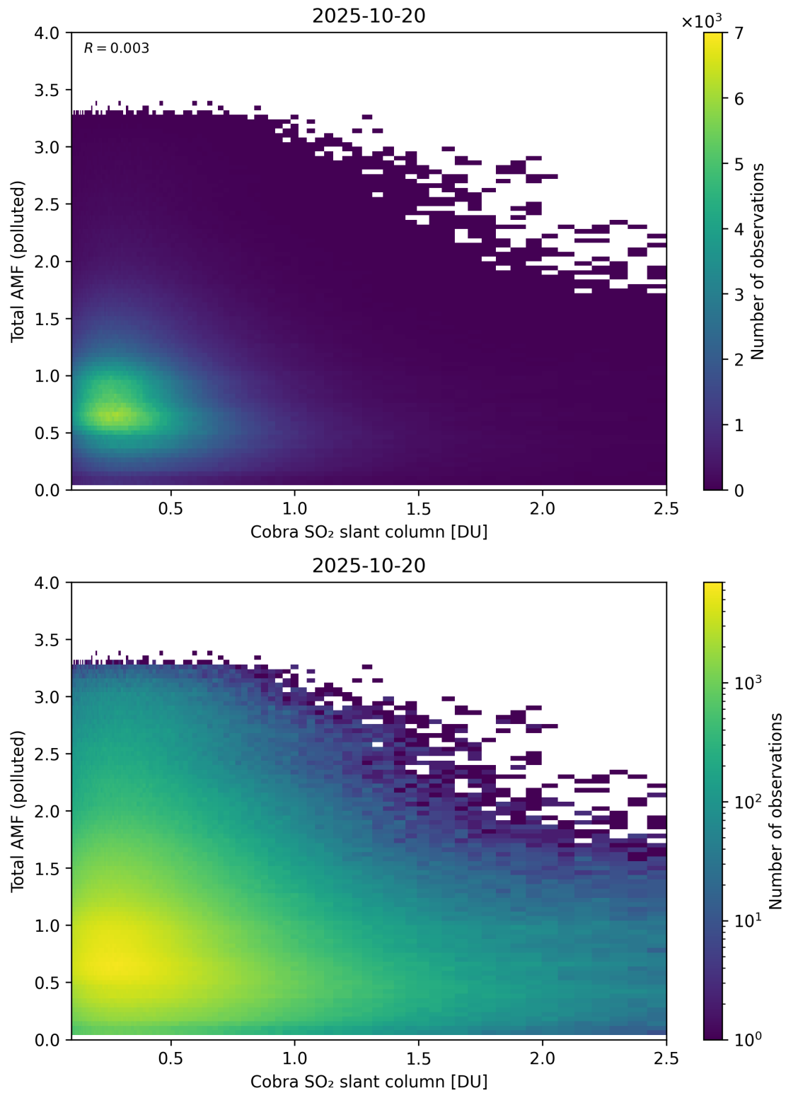
Figure 224: Scatter density plot of “Cobra SO 2 slant column” against “Total AMF (polluted)” for 2025-10-19 to 2025-10-21.
