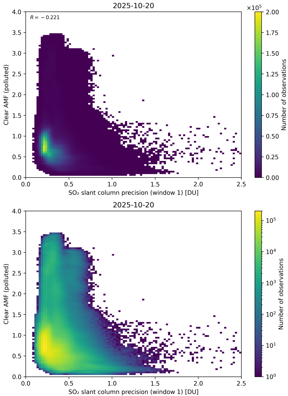
Figure 274: Scatter density plot of “SO 2 slant column precision (window 1)” against “Clear AMF (polluted)” for 2025-10-19 to 2025-10-21.
