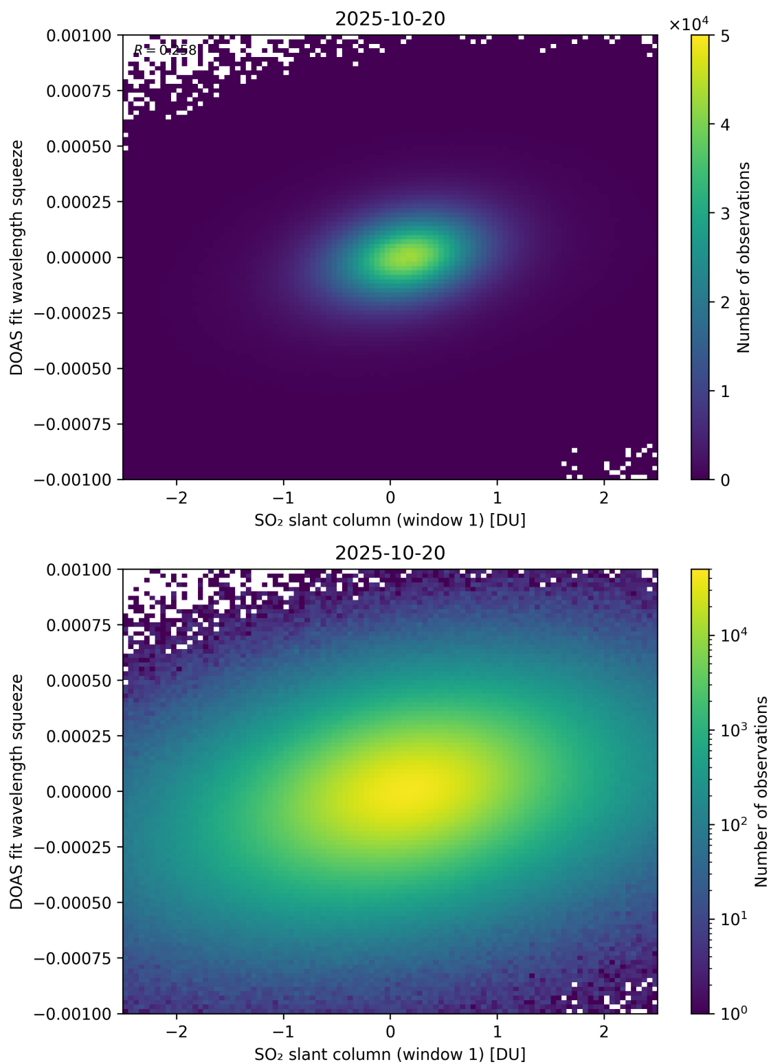
Figure 266: Scatter density plot of “SO 2 slant column (window 1)” against “DOAS fit wavelength squeeze” for 2025-10-19 to 2025-10-21.
