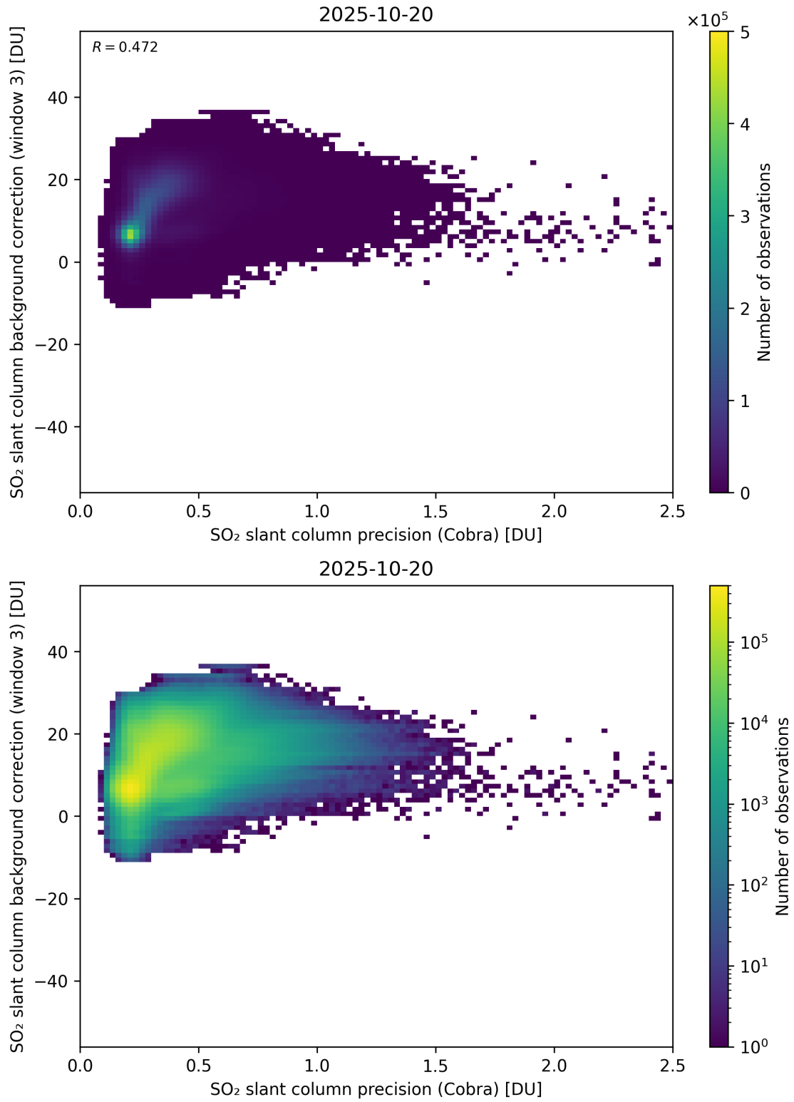
Figure 201: Scatter density plot of “SO 2 slant column precision (Cobra)” against “SO 2 slant column background correction (window 3)” for 2025-10-19 to 2025-10-21.
