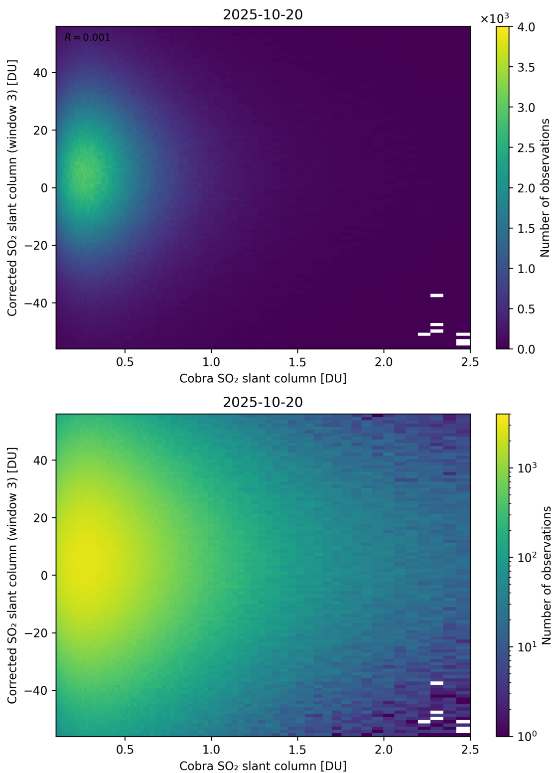
Figure 218: Scatter density plot of “Cobra SO 2 slant column” against “Corrected SO 2 slant column (window 3)” for 2025-10-19 to 2025-10-21.
