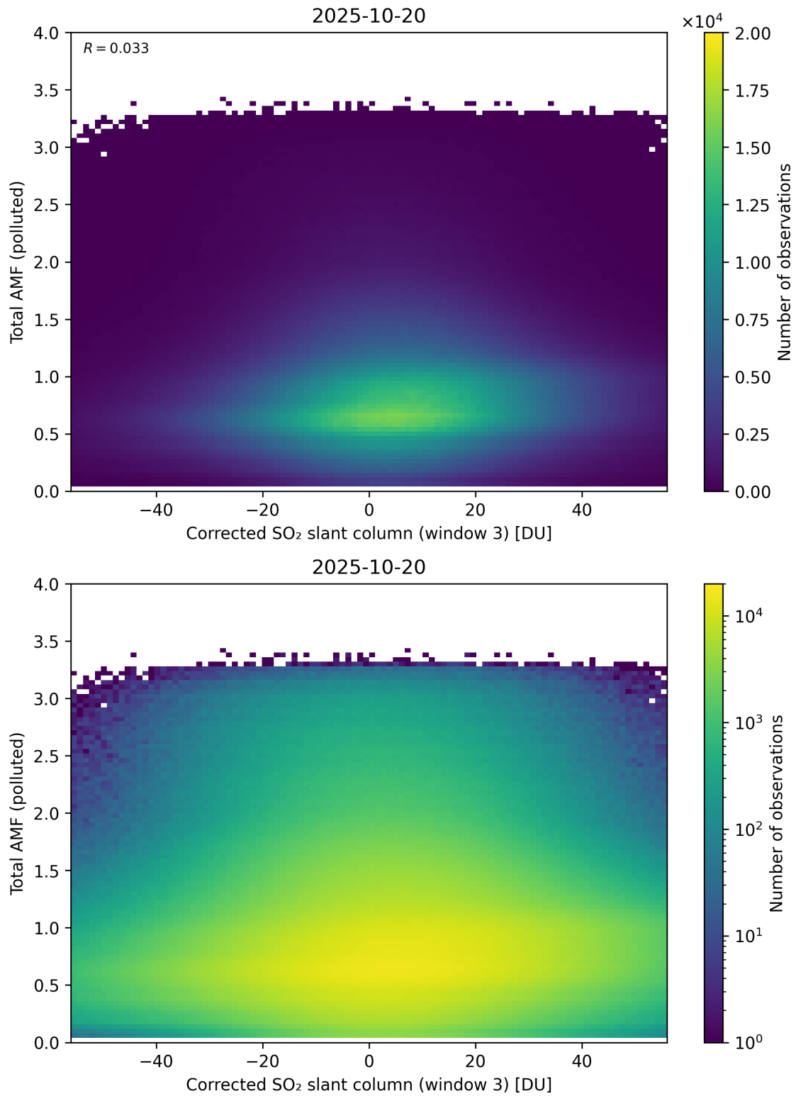
Figure 260: Scatter density plot of “Corrected SO 2 slant column (window 3)” against “Total AMF (polluted)” for 2025-10-19 to 2025-10-21.
