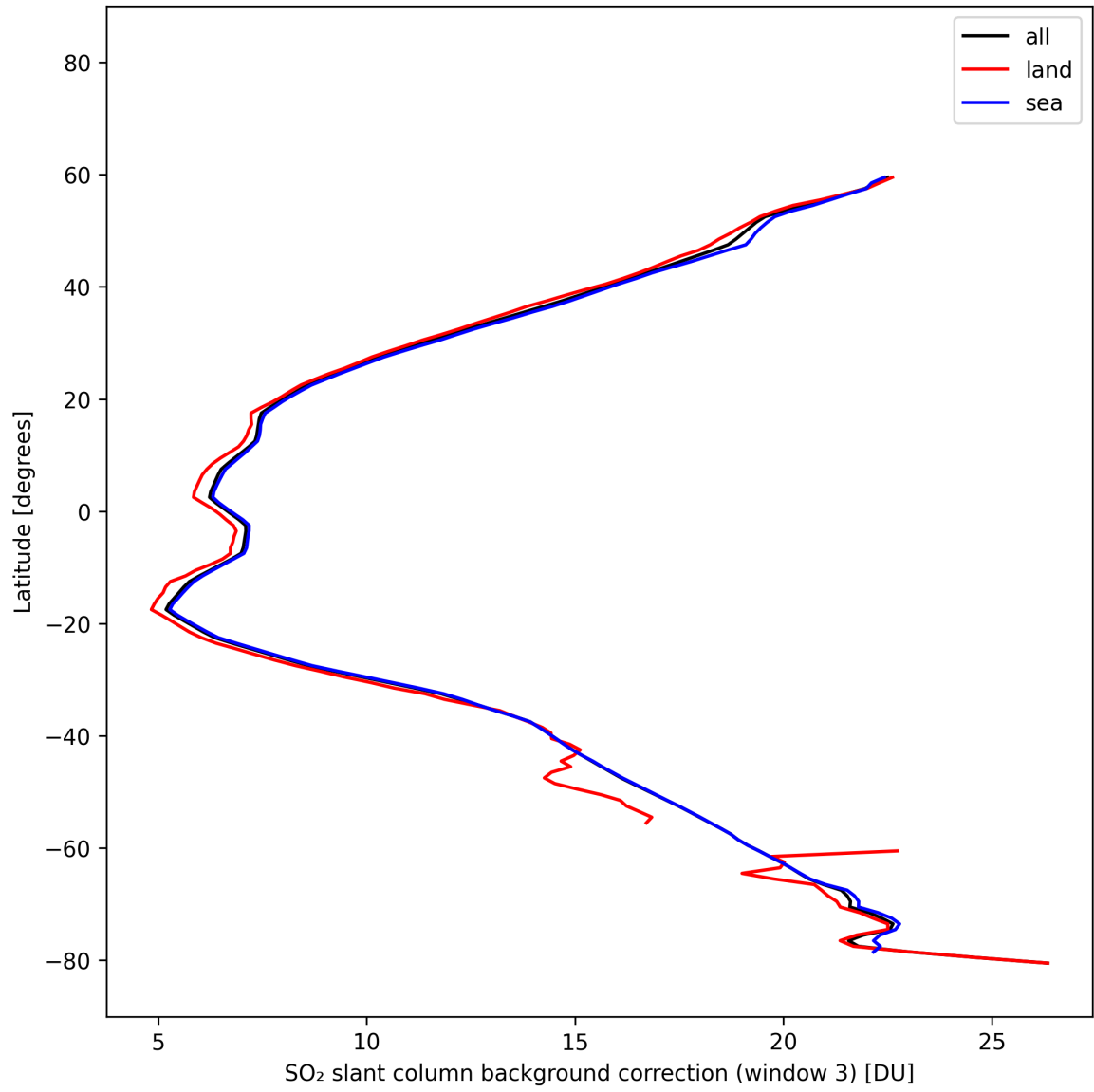
Figure 48: Zonal average of “SO 2 slant column background correction (window 3)” for 2025-10-19 to 2025-10-21.
