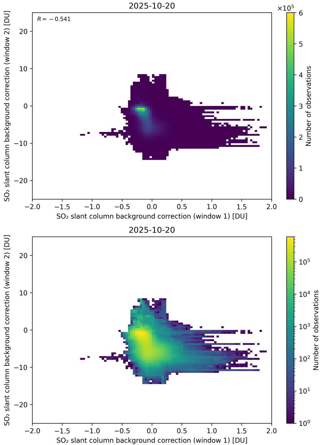
Figure 109: Scatter density plot of “SO 2 slant column background correction (window 1)” against “SO 2 slant column background correction (window 2)” for 2025-10-19 to 2025-10-21.
