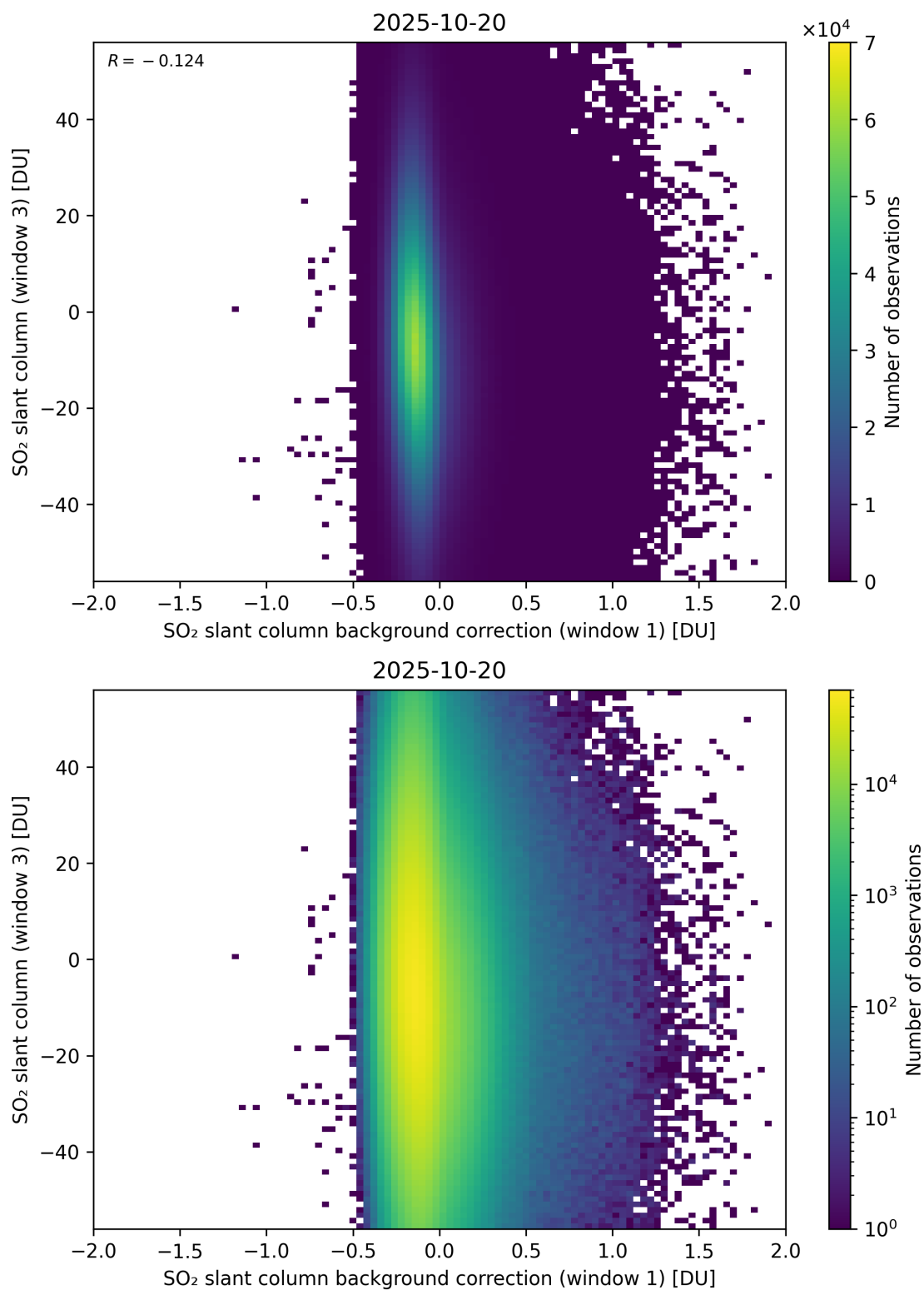
Figure 118: Scatter density plot of “SO 2 slant column background correction (window 1)” against “SO 2 slant column (window 3)” for 2025-10-19 to 2025-10-21.
