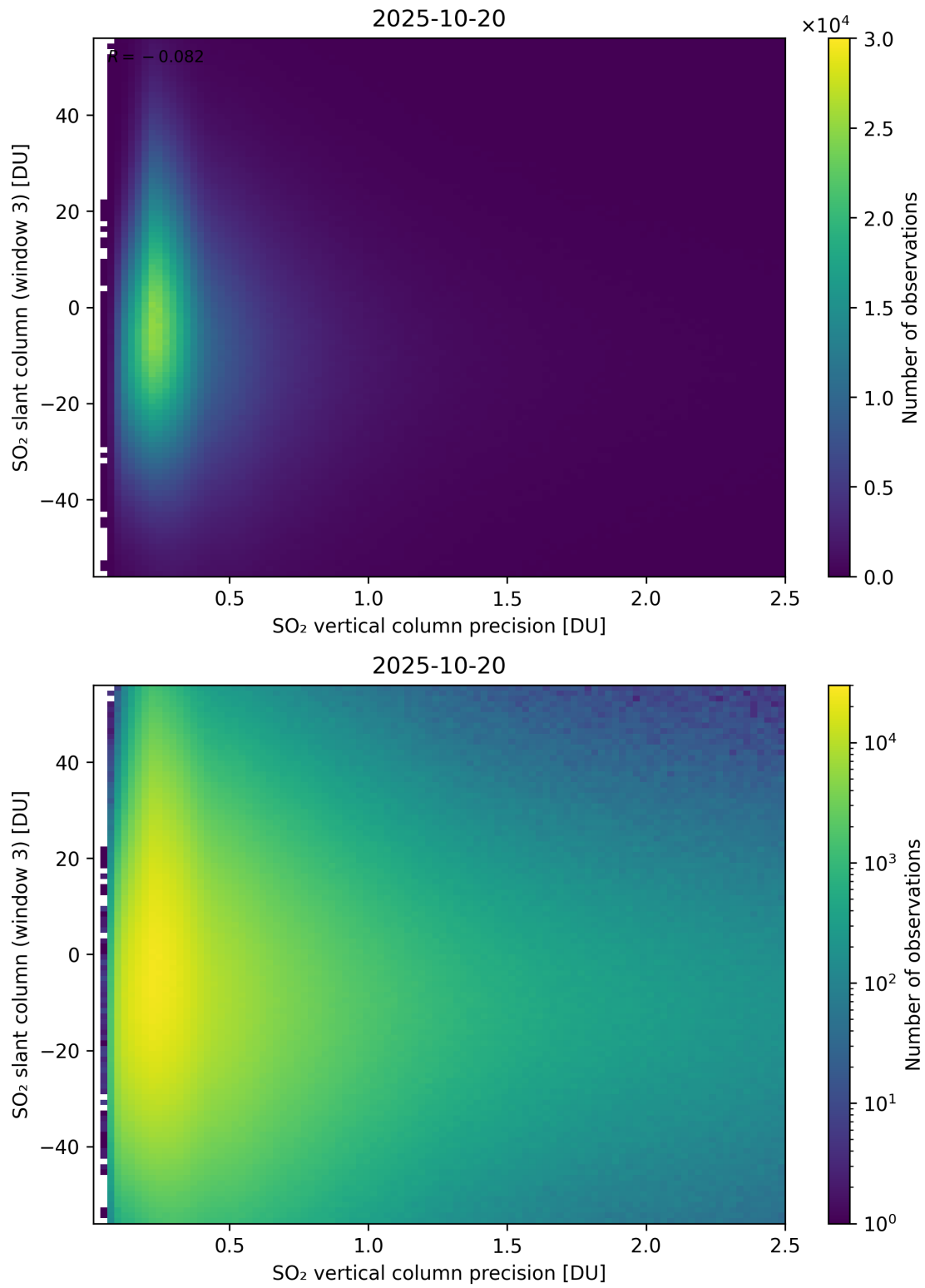
Figure 344: Scatter density plot of “SO 2 vertical column precision” against “SO 2 slant column (window 3)” for 2025-10-19 to 2025-10-21.
