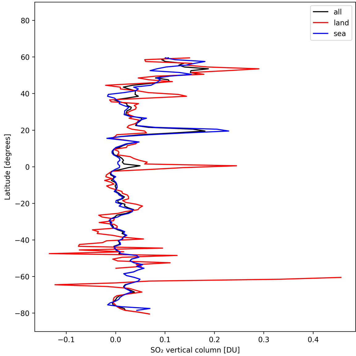
Figure 32: Zonal average of “SO 2 vertical column” for 2025-10-19 to 2025-10-21.
