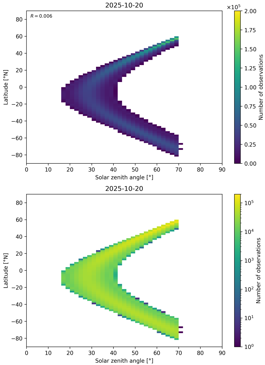
Figure 177: Scatter density plot of “Solar zenith angle” against “Latitude” for 2025-10-19 to 2025-10-21.
