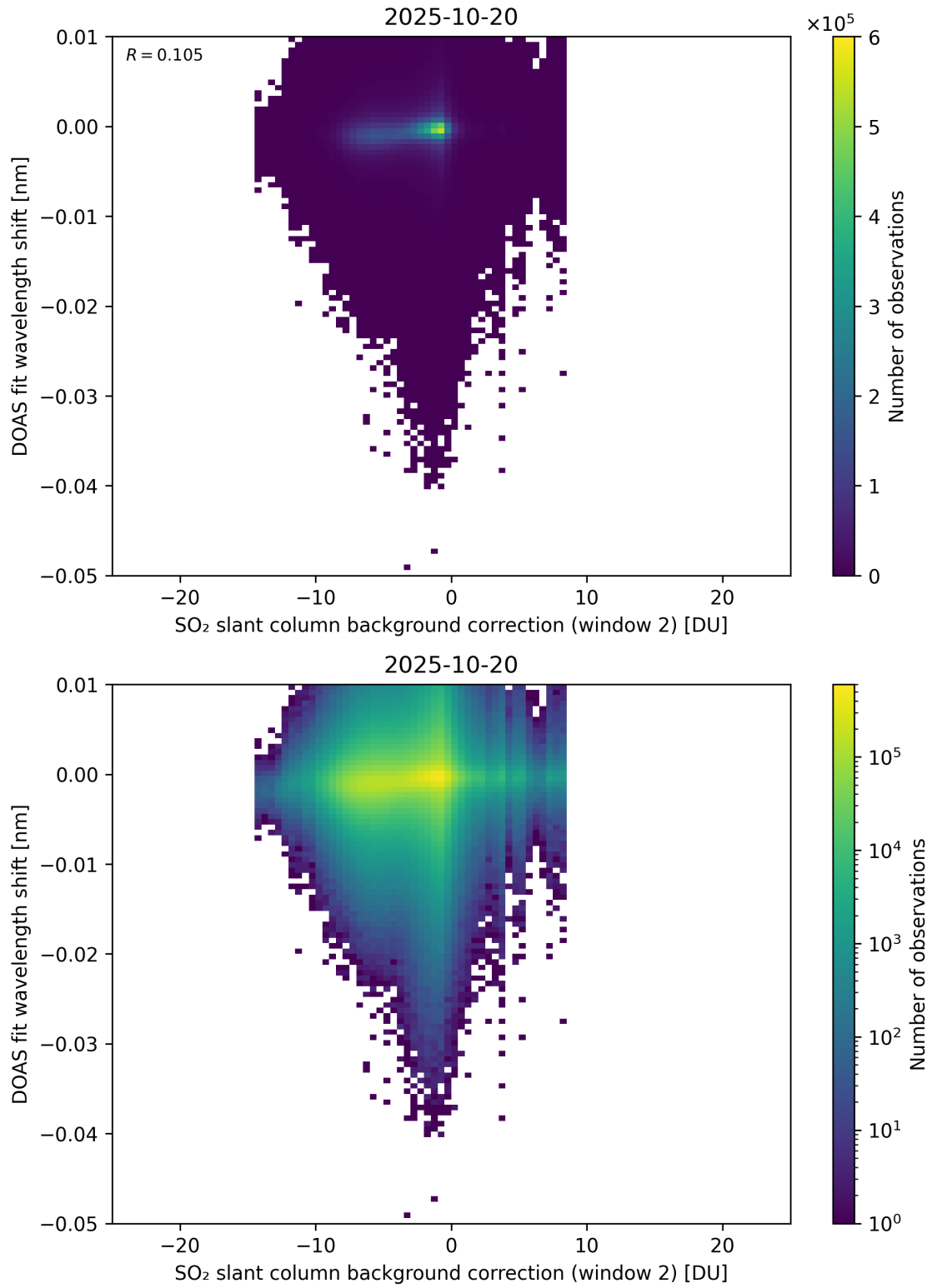
Figure 123: Scatter density plot of “SO 2 slant column background correction (window 2)” against “DOAS fit wavelength shift” for 2025-10-19 to 2025-10-21.
