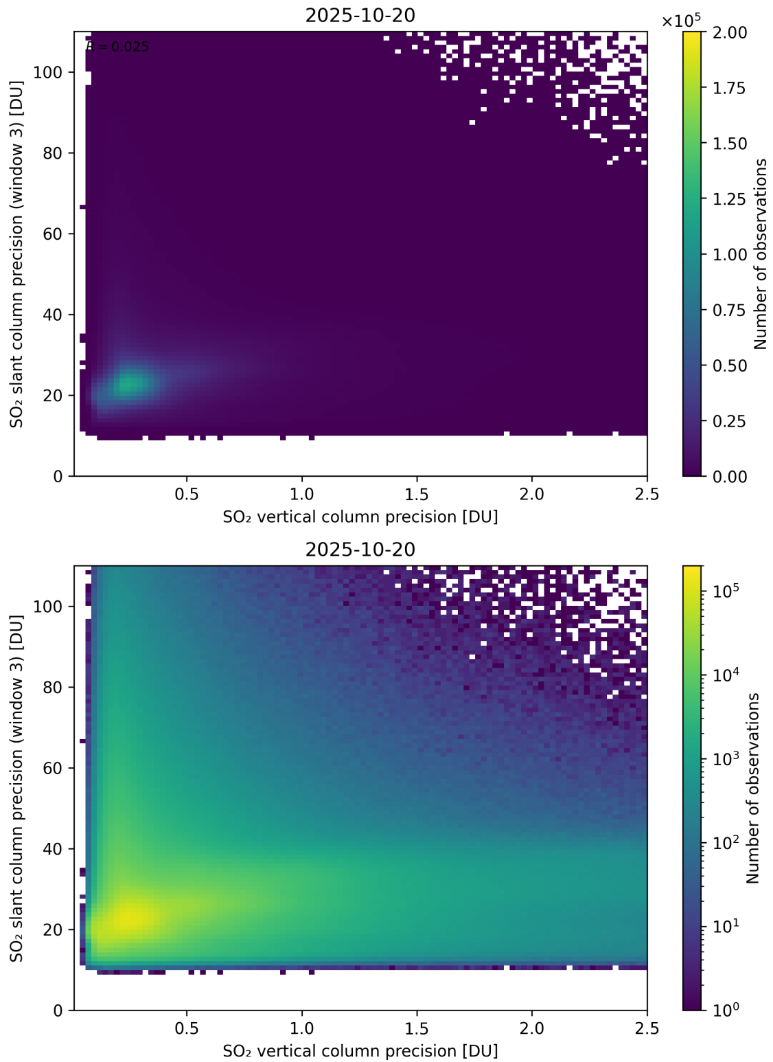
Figure 345: Scatter density plot of “SO 2 vertical column precision” against “SO 2 slant column precision (window 3)” for 2025-10-19 to 2025-10-21.
