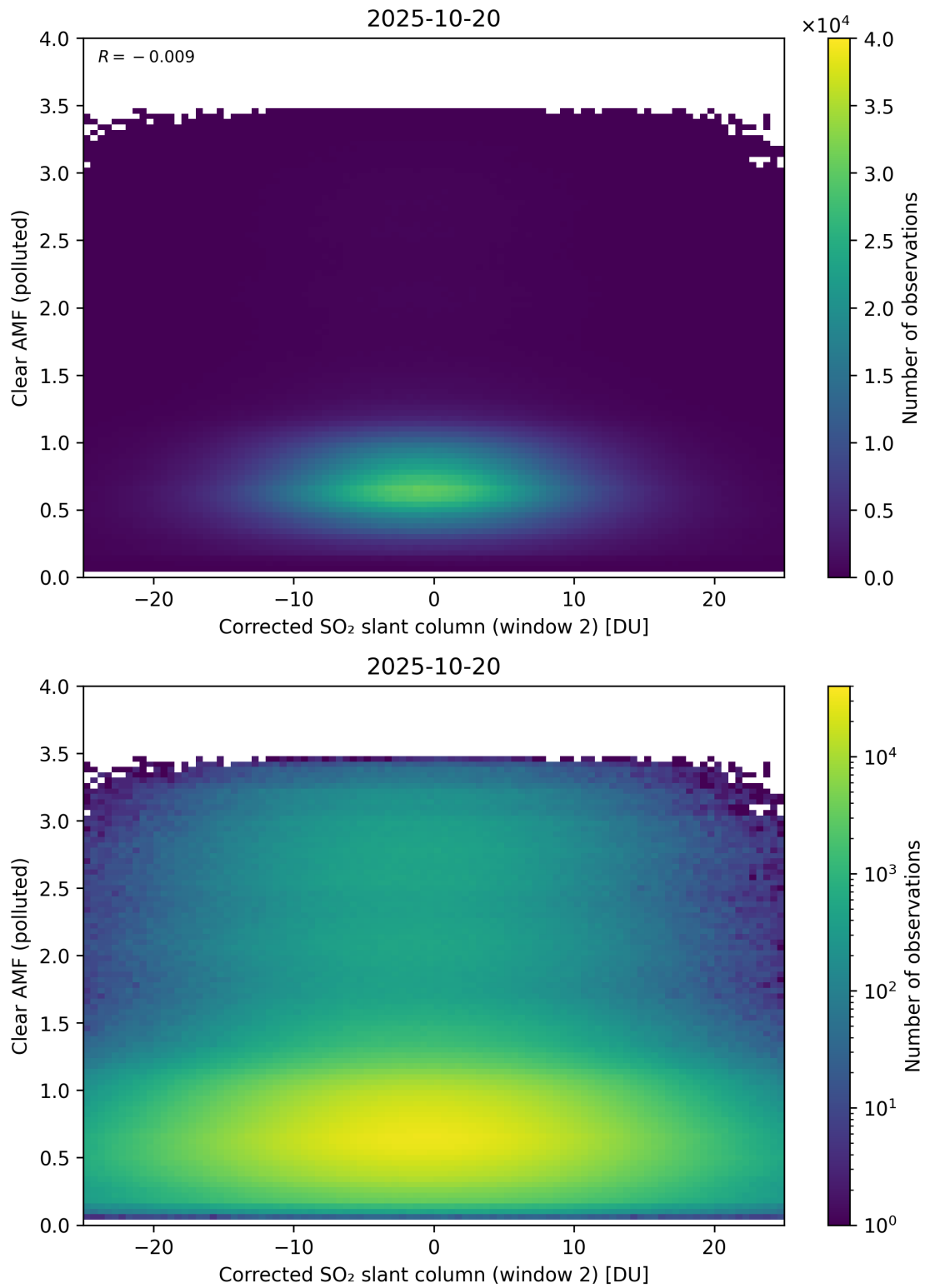
Figure 249: Scatter density plot of “Corrected SO 2 slant column (window 2)” against “Clear AMF (polluted)” for 2025-10-19 to 2025-10-21.
