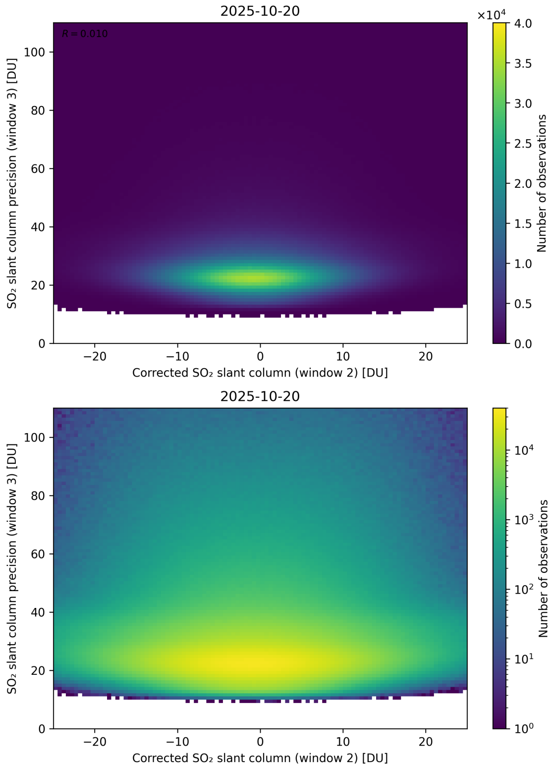
Figure 252: Scatter density plot of “Corrected SO 2 slant column (window 2)” against “SO 2 slant column precision (window 3)” for 2025-10-19 to 2025-10-21.
