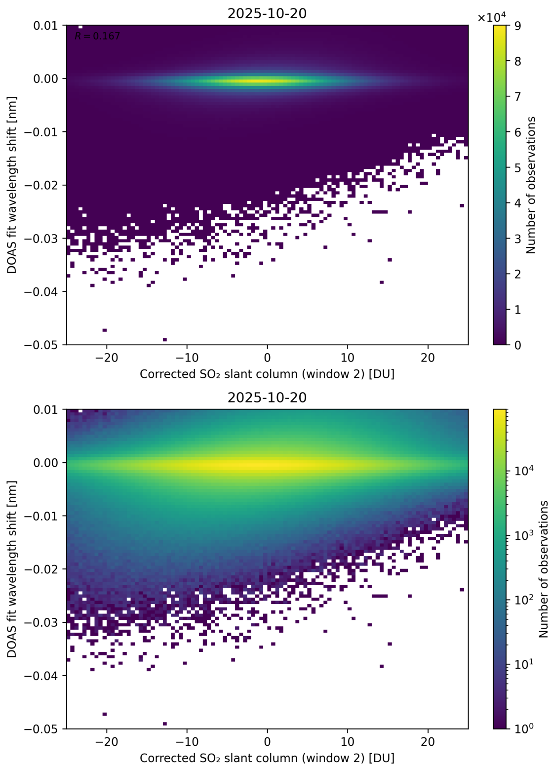
Figure 246: Scatter density plot of “Corrected SO 2 slant column (window 2)” against “DOAS fit wavelength shift” for 2025-10-19 to 2025-10-21.
