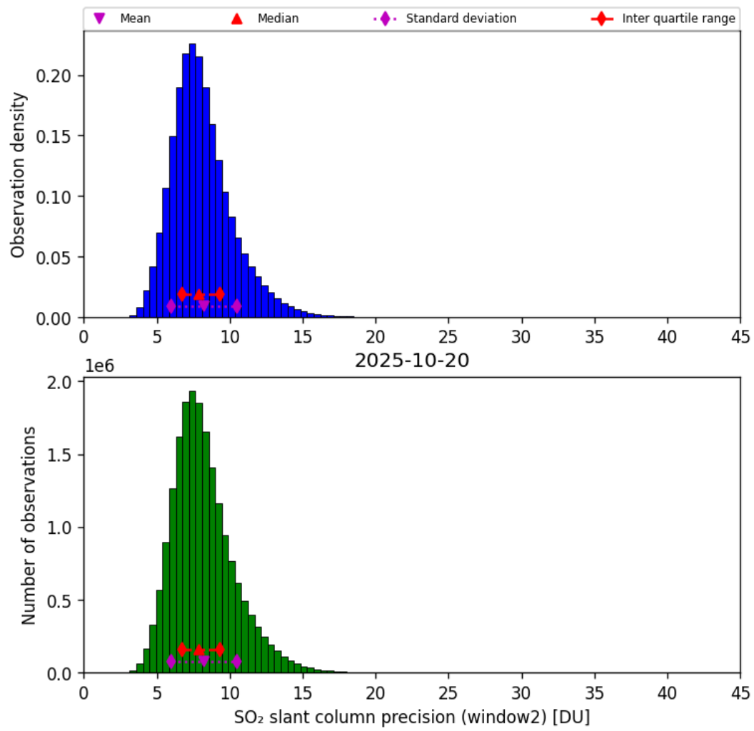
Figure 68: Histogram of “SO 2 slant column precision (window2)” for 2025-10-19 to 2025-10-21
