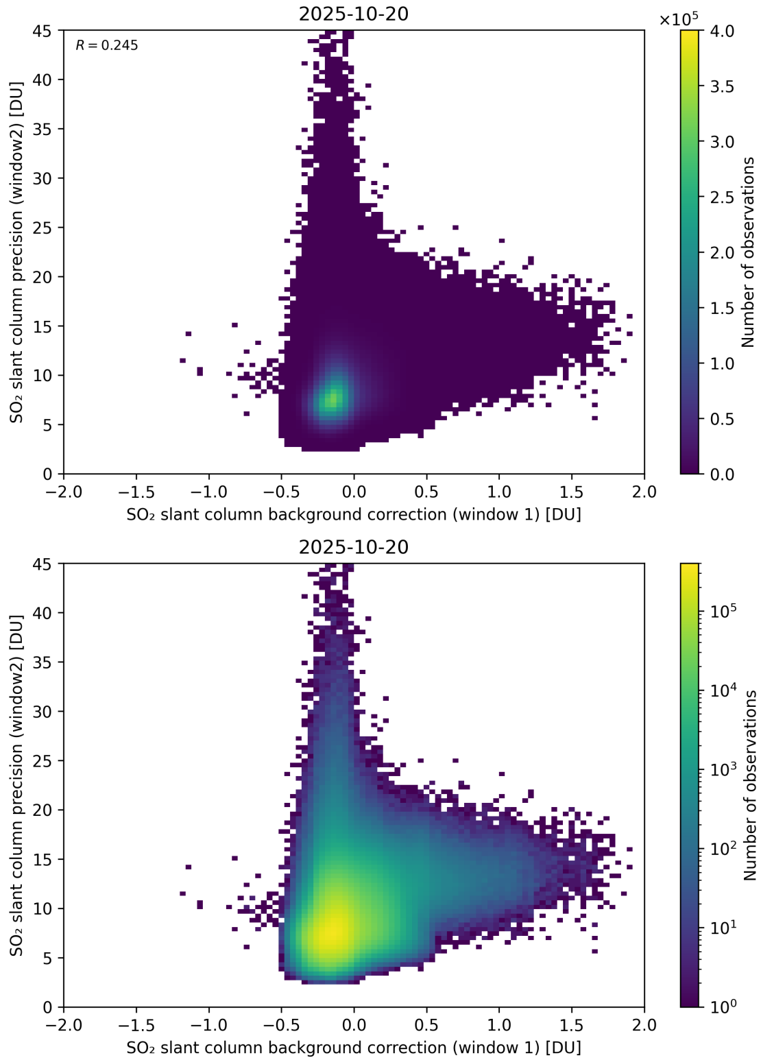
Figure 117: Scatter density plot of “SO 2 slant column background correction (window 1)” against “SO 2 slant column precision (window2)” for 2025-10-19 to 2025-10-21.
