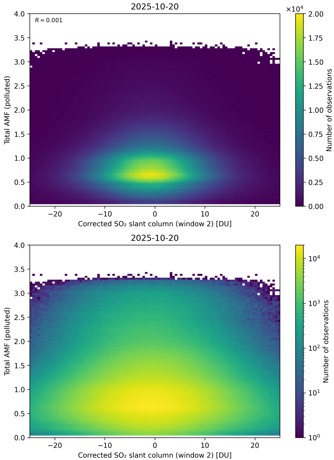
Figure 253: Scatter density plot of “Corrected SO 2 slant column (window 2)” against “Total AMF (polluted)” for 2025-10-19 to 2025-10-21.
