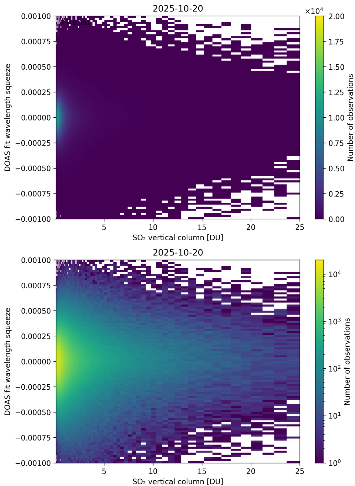
Figure 327: Scatter density plot of “SO 2 vertical column” against “DOAS fit wavelength squeeze” for 2025-10-19 to 2025-10-21.
