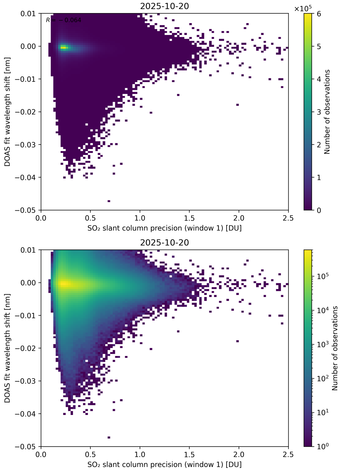
Figure 271: Scatter density plot of “SO 2 slant column precision (window 1)” against “DOAS fit wavelength shift” for 2025-10-19 to 2025-10-21.
