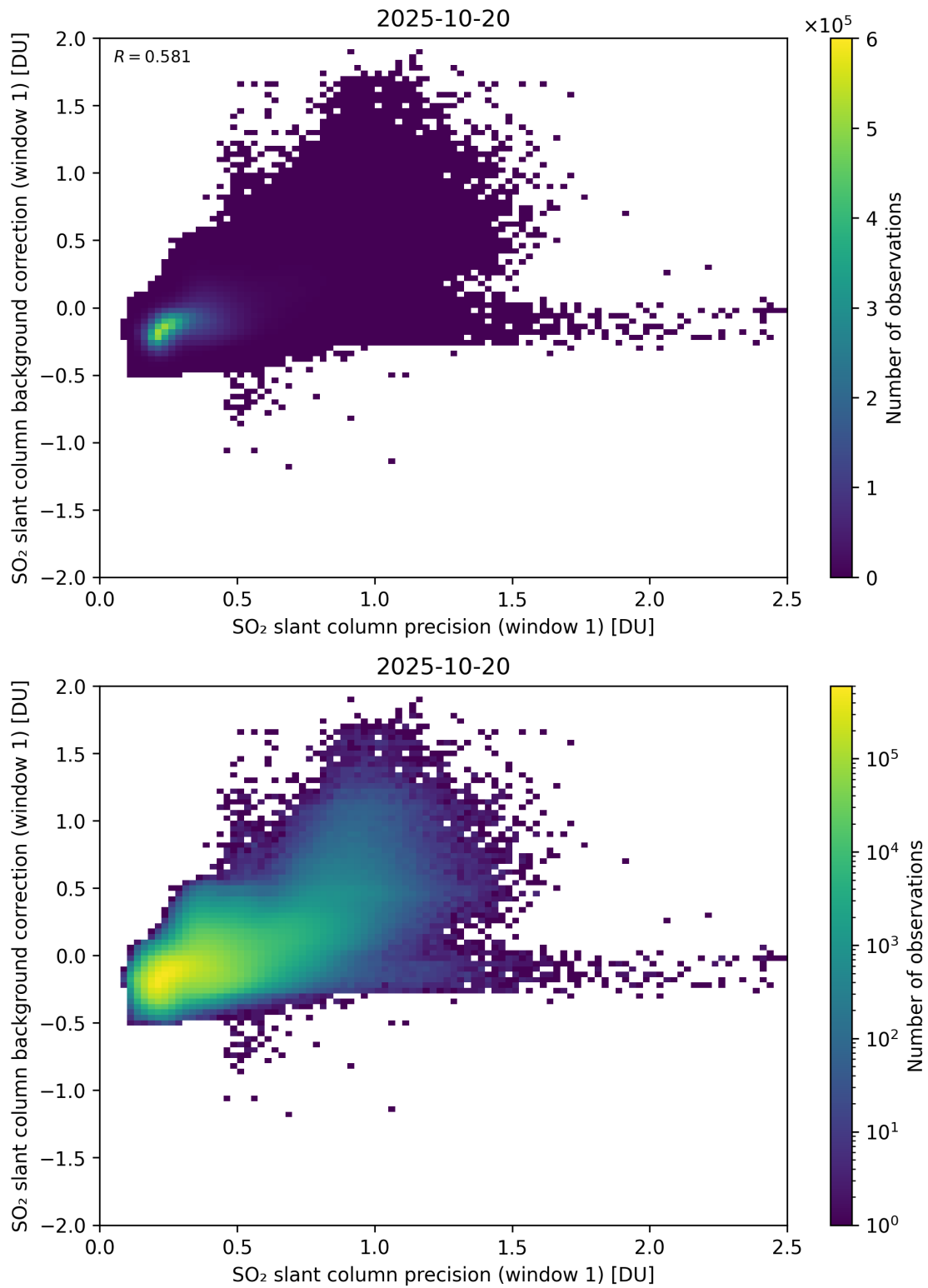
Figure 268: Scatter density plot of “SO 2 slant column precision (window 1)” against “SO 2 slant column background correction (window 1)” for 2025-10-19 to 2025-10-21.
