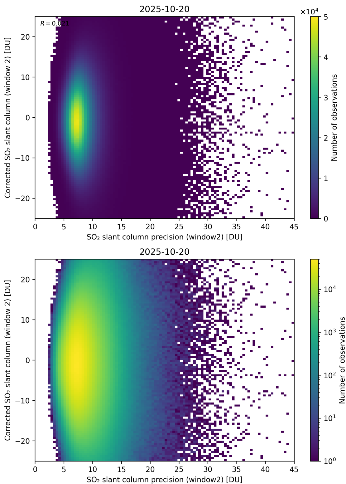
Figure 297: Scatter density plot of “SO 2 slant column precision (window2)” against “Corrected SO 2 slant column (window 2)” for 2025-10-19 to 2025-10-21.
