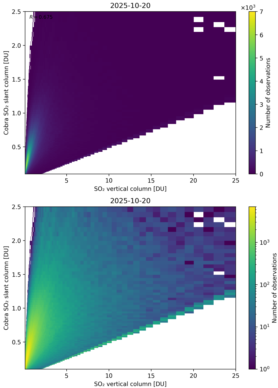
Figure 349: Scatter density plot of “SO 2 vertical column” against “Cobra SO 2 slant column” for 2025-10-19 to 2025-10-21.
