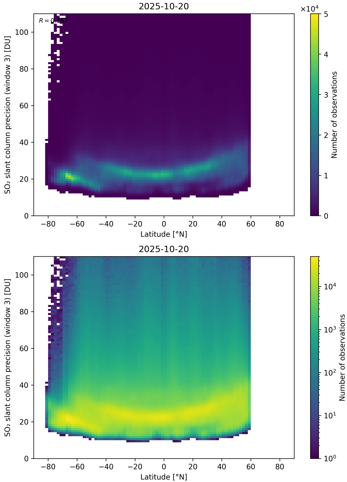
Figure 166: Scatter density plot of “Latitude” against “SO 2 slant column precision (window 3)” for 2025-10-19 to 2025-10-21.
