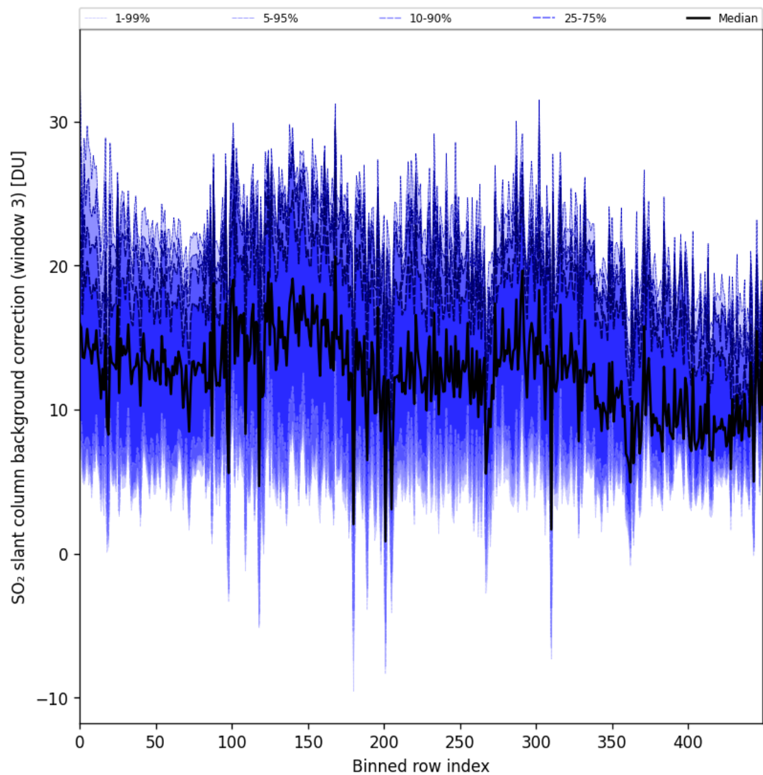
Figure 100: Along track statistics of “SO 2 slant column background correction (window 3)” for 2025-10-19 to 2025-10-21
