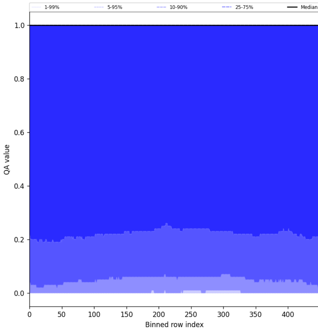
Figure 83: Along track statistics of “QA value” for 2025-10-19 to 2025-10-21
