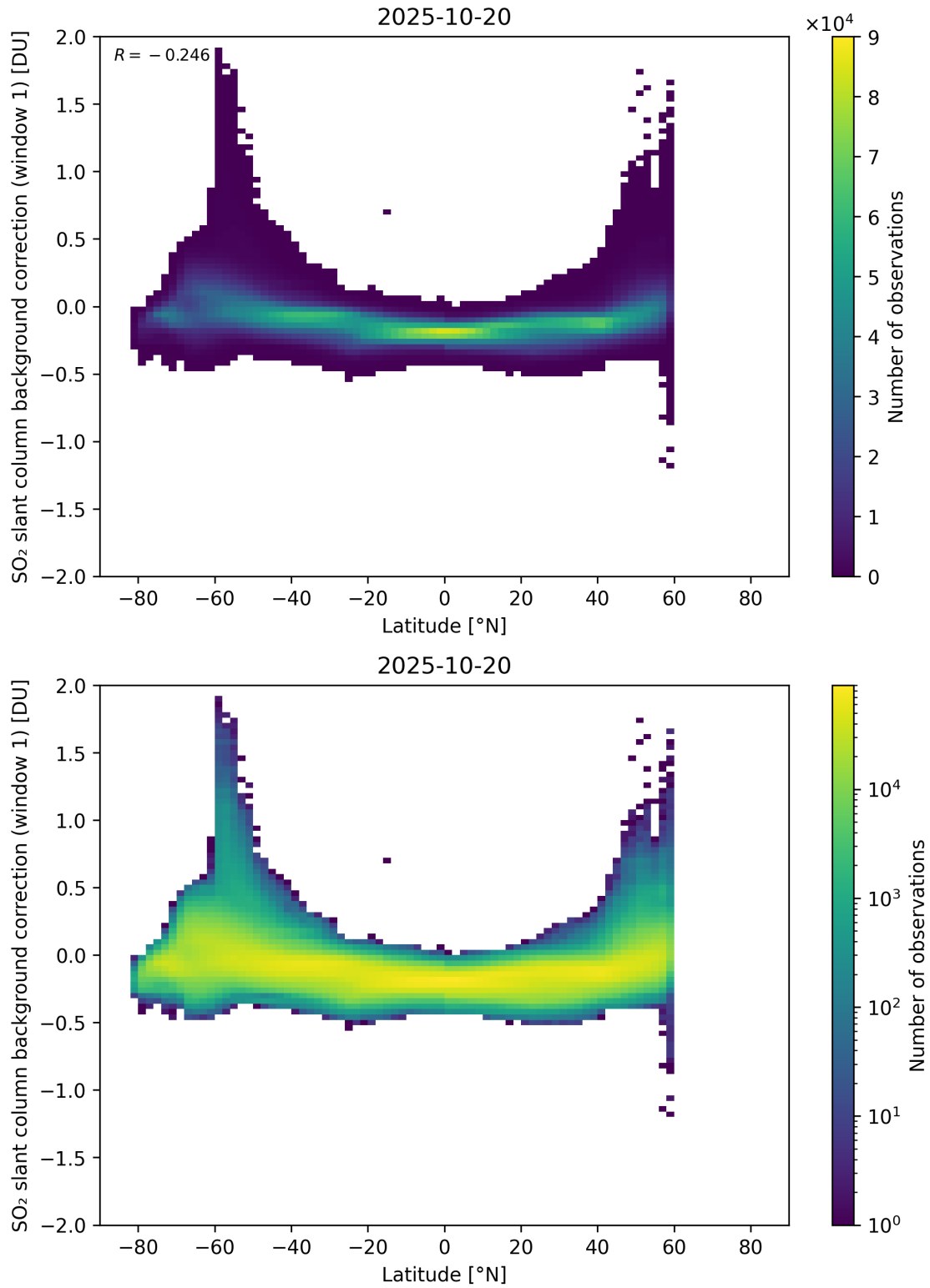
Figure 150: Scatter density plot of “Latitude” against “SO 2 slant column background correction (window 1)” for 2025-10-19 to 2025-10-21.
