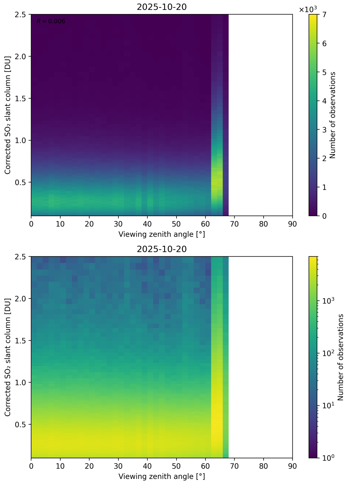
Figure 373: Scatter density plot of “Viewing zenith angle” against “Corrected SO 2 slant column” for 2025-10-19 to 2025-10-21.
