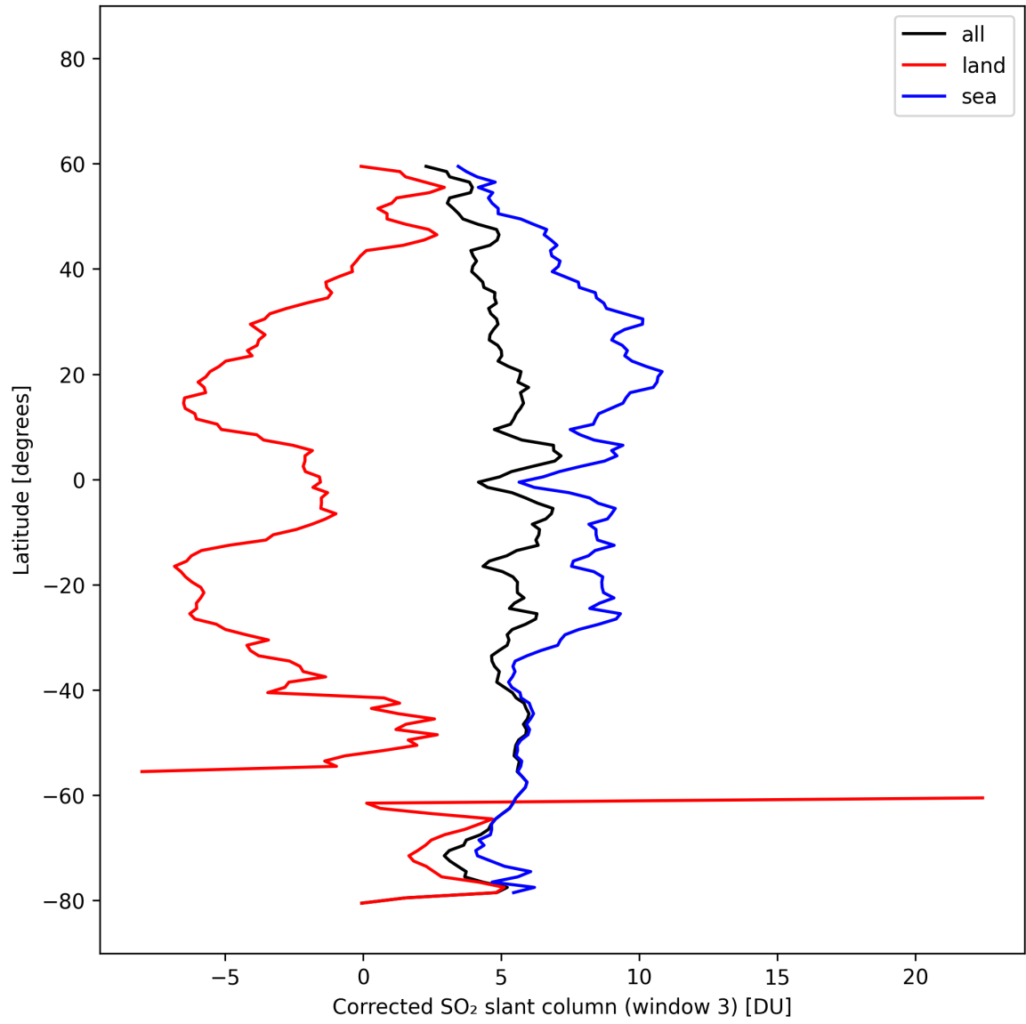
Figure 47: Zonal average of “Corrected SO 2 slant column (window 3)” for 2025-10-19 to 2025-10-21.
