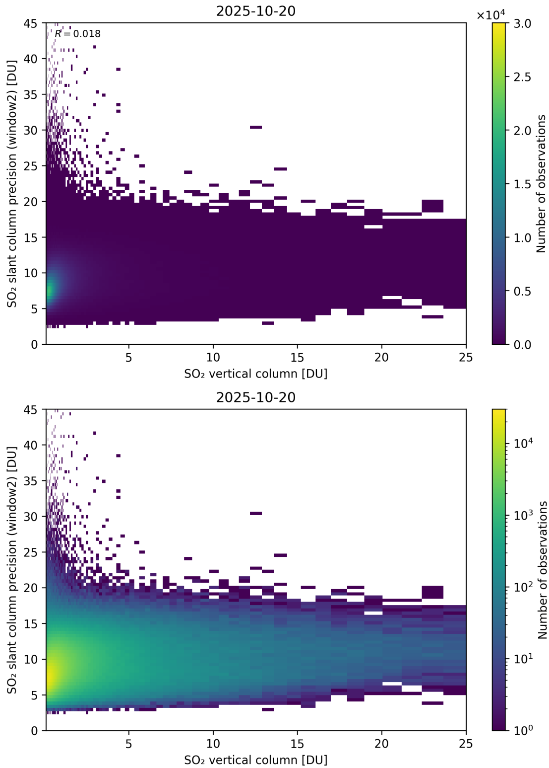
Figure 356: Scatter density plot of “SO 2 vertical column” against “SO 2 slant column precision (window2)” for 2025-10-19 to 2025-10-21.
