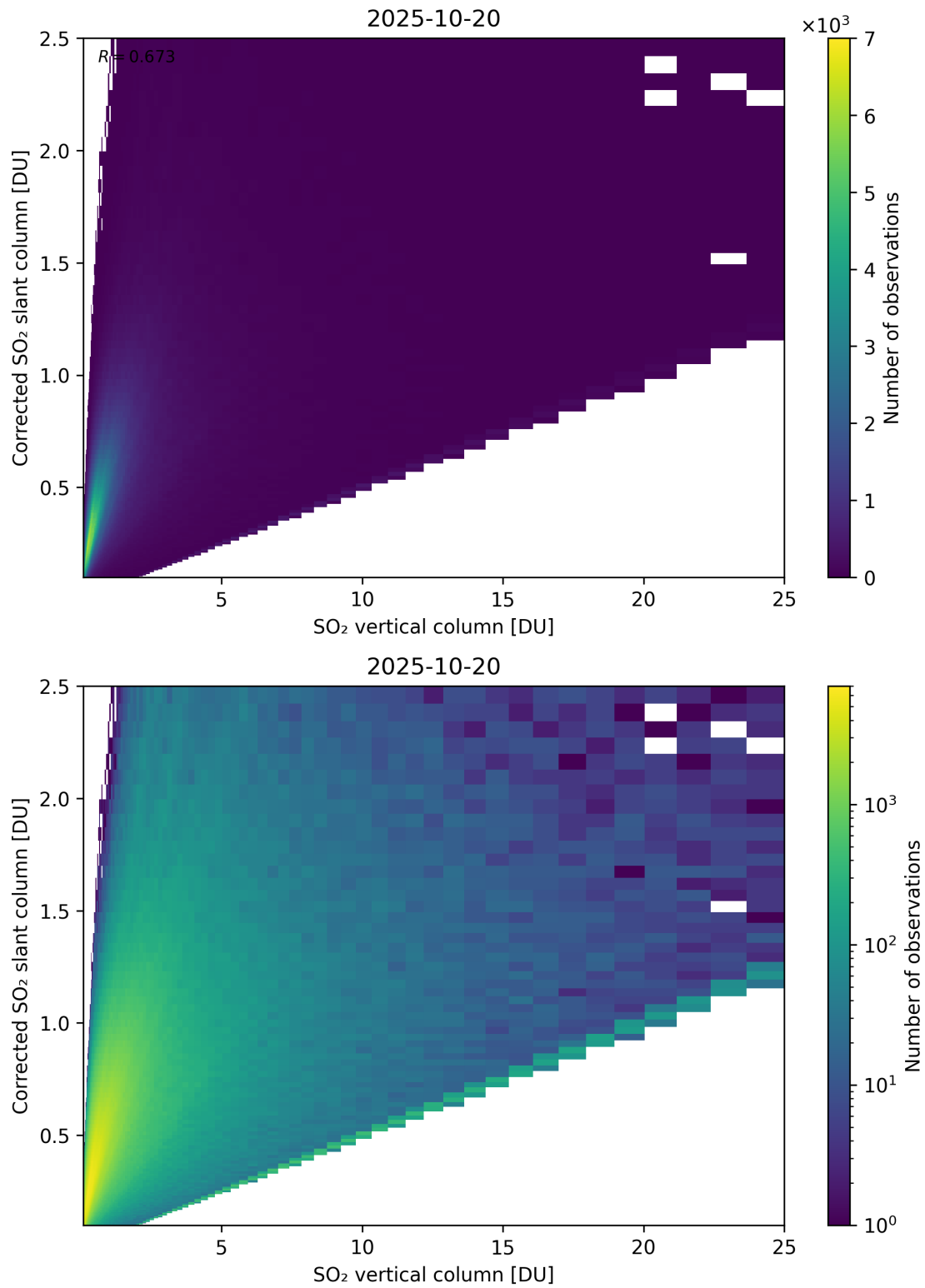
Figure 351: Scatter density plot of “SO 2 vertical column” against “Corrected SO 2 slant column” for 2025-10-19 to 2025-10-21.
