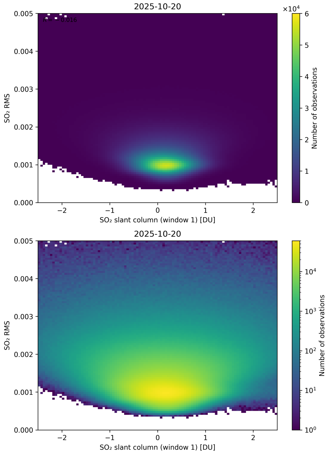
Figure 267: Scatter density plot of “SO 2 slant column (window 1)” against “SO 2 RMS” for 2025-10-19 to 2025-10-21.
