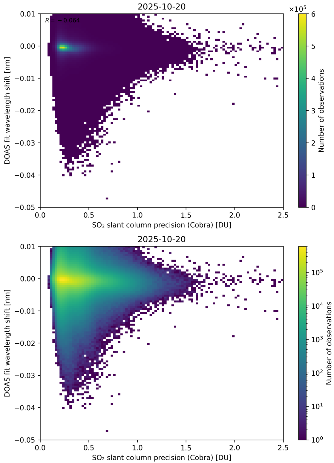
Figure 202: Scatter density plot of “SO 2 slant column precision (Cobra)” against “DOAS fit wavelength shift” for 2025-10-19 to 2025-10-21.
