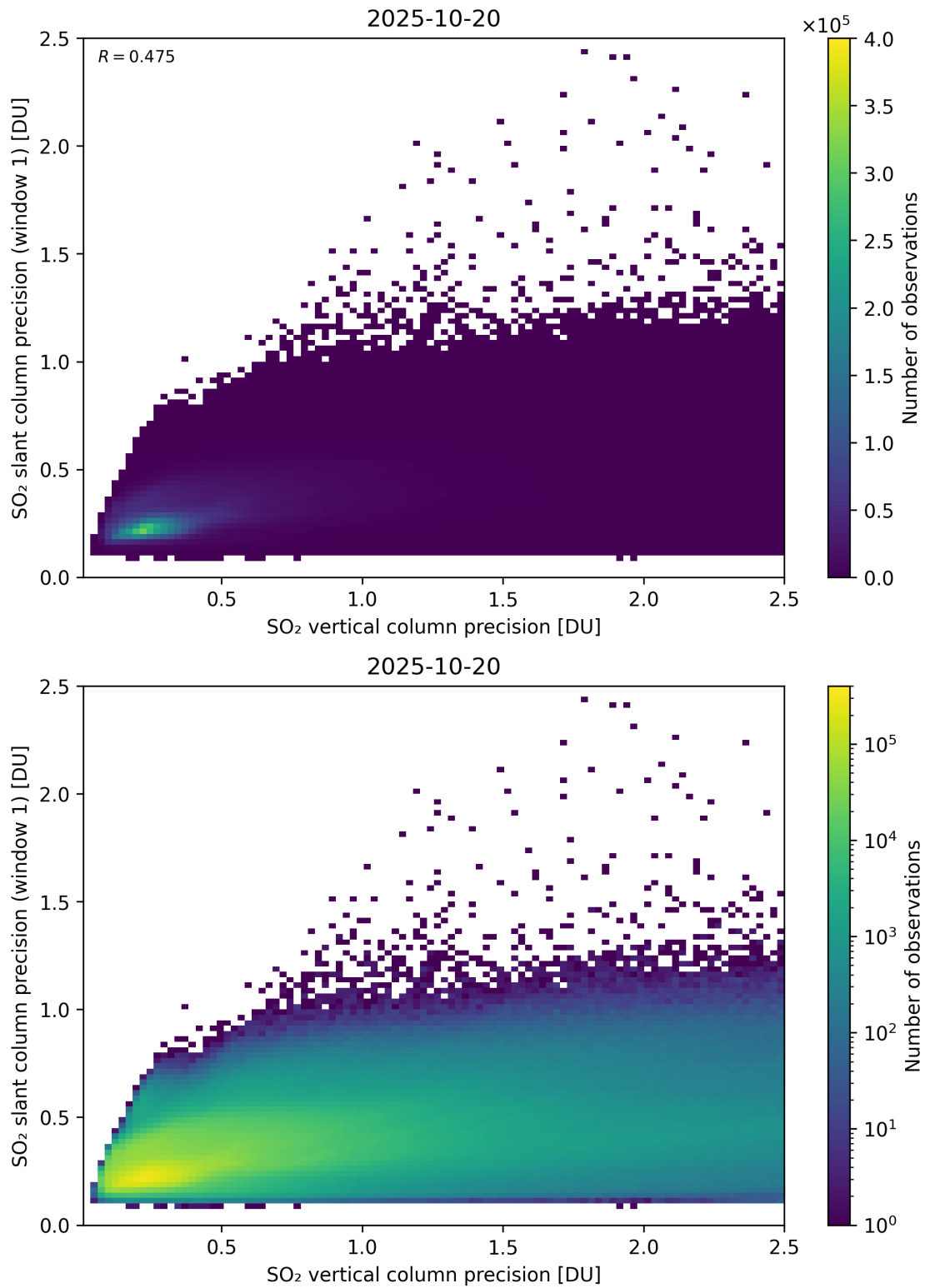
Figure 342: Scatter density plot of “SO 2 vertical column precision” against “SO 2 slant column precision (window 1)” for 2025-10-19 to 2025-10-21.
