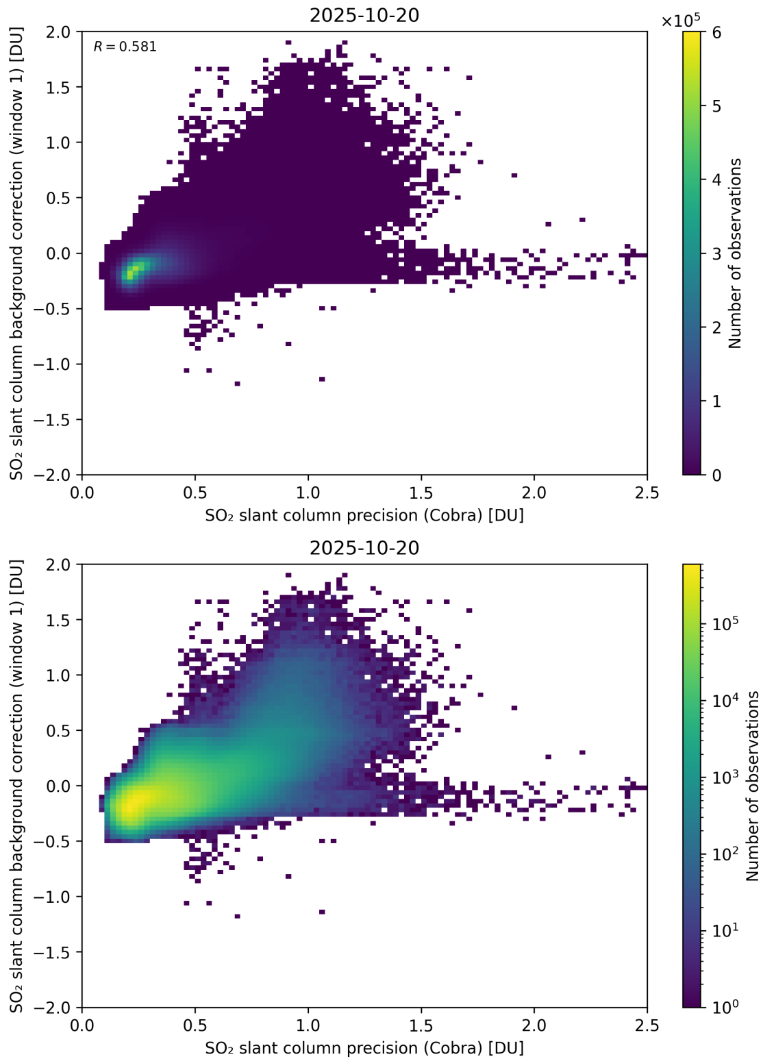
Figure 199: Scatter density plot of “SO 2 slant column precision (Cobra)” against “SO 2 slant column background correction (window 1)” for 2025-10-19 to 2025-10-21.
