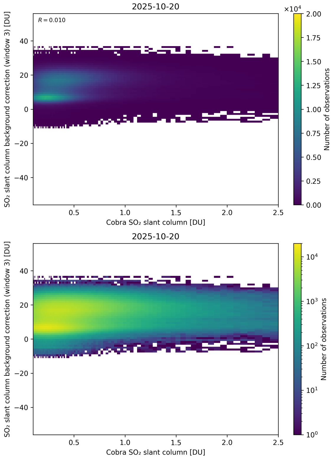
Figure 195: Scatter density plot of “Cobra SO 2 slant column” against “SO 2 slant column background correction (window 3)” for 2025-10-19 to 2025-10-21.
