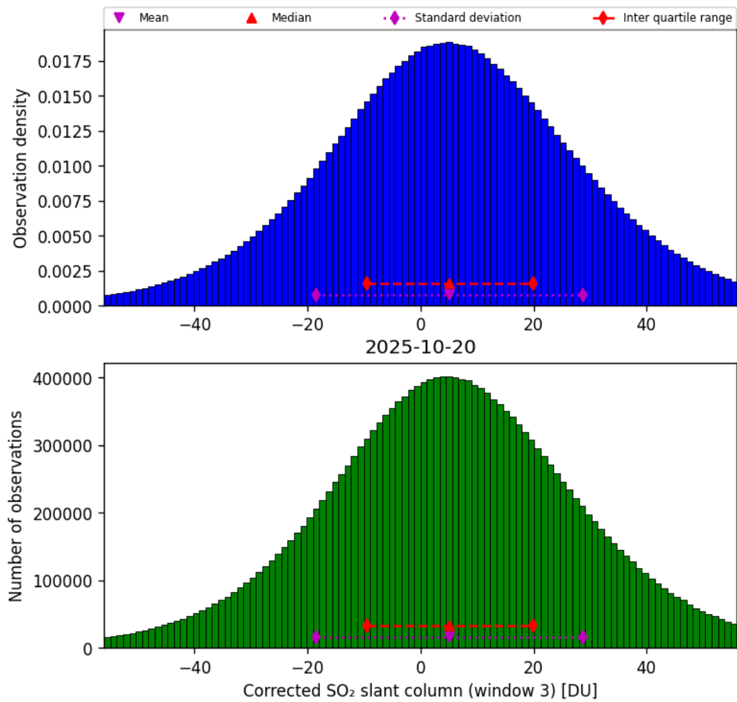
Figure 73: Histogram of "Corrected SO 2 slant column (window 3)" for 2025-10-19 to 2025-10-21
