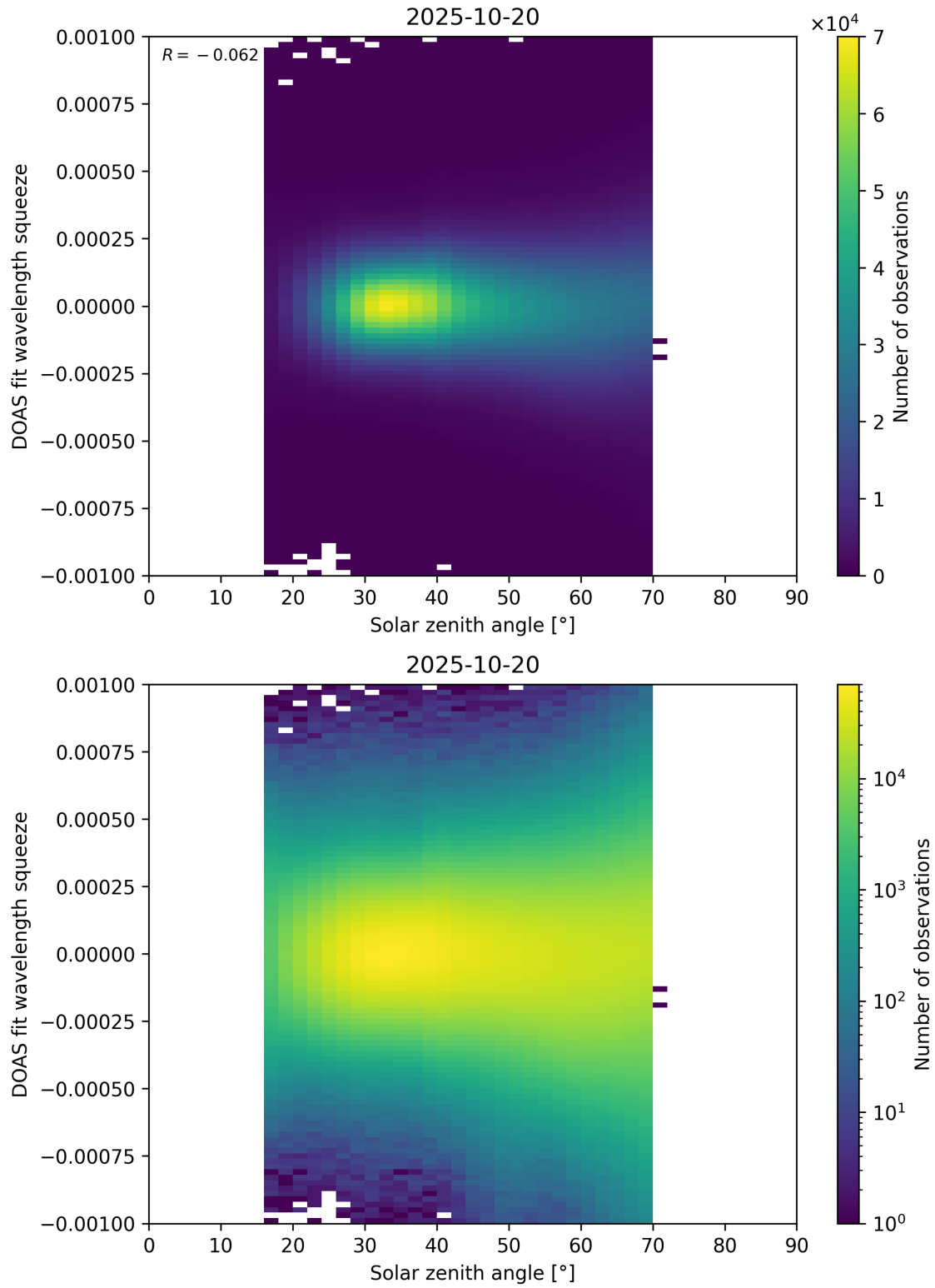
Figure 175: Scatter density plot of “Solar zenith angle” against “DOAS fit wavelength squeeze” for 2025-10-19 to 2025-10-21.
