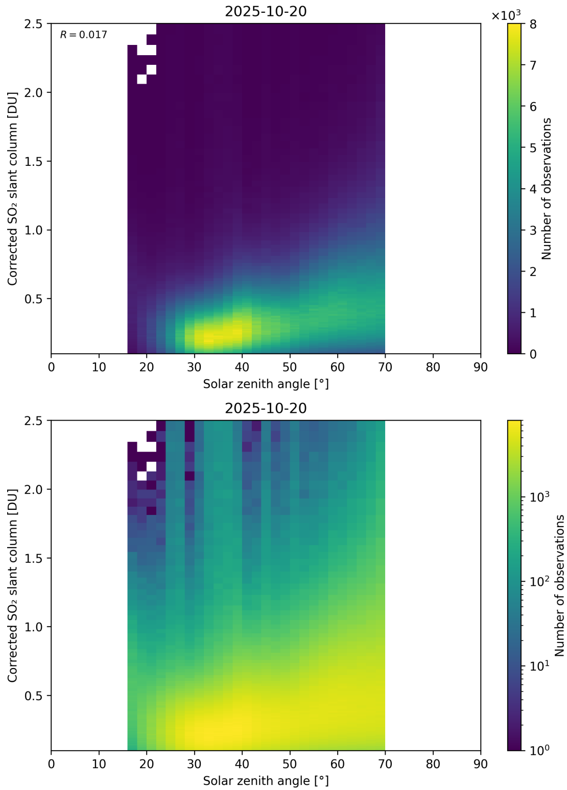
Figure 181: Scatter density plot of “Solar zenith angle” against “Corrected SO 2 slant column” for 2025-10-19 to 2025-10-21.
