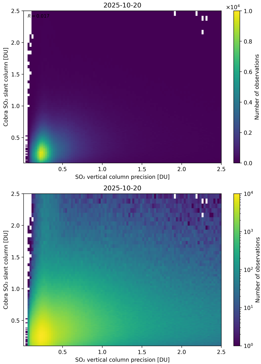
Figure 336: Scatter density plot of “SO 2 vertical column precision” against “Cobra SO 2 slant column” for 2025-10-19 to 2025-10-21.
