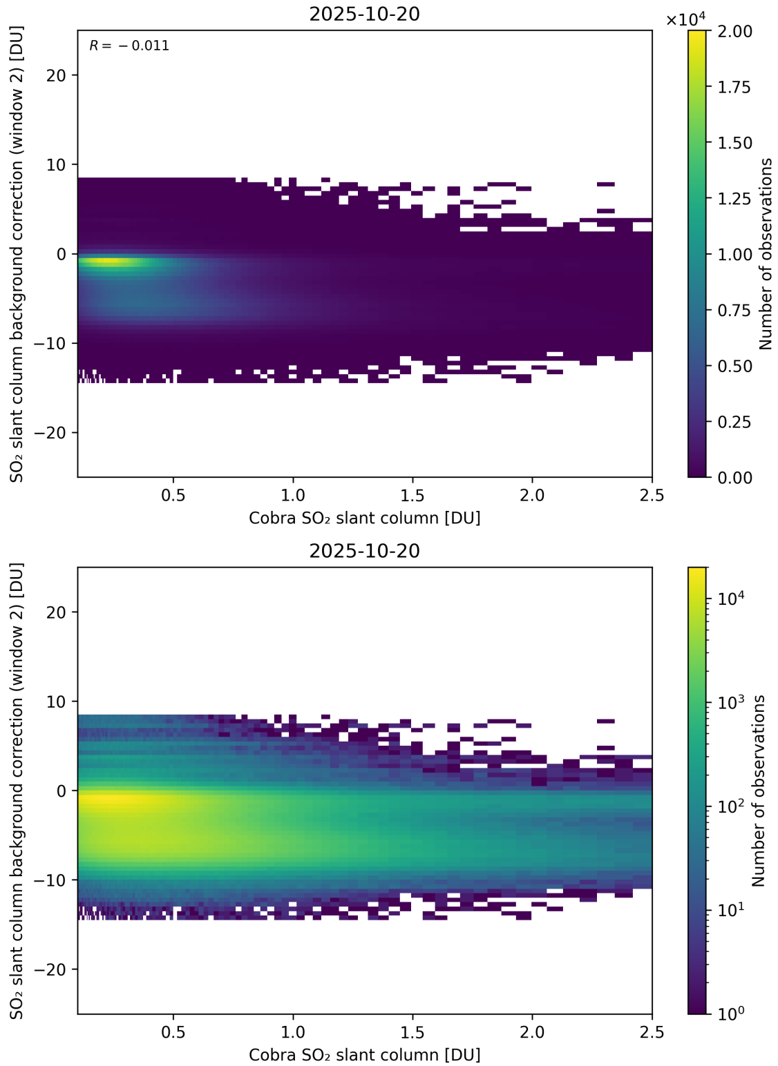
Figure 194: Scatter density plot of “Cobra SO 2 slant column” against “SO 2 slant column background correction (window 2)” for 2025-10-19 to 2025-10-21.
