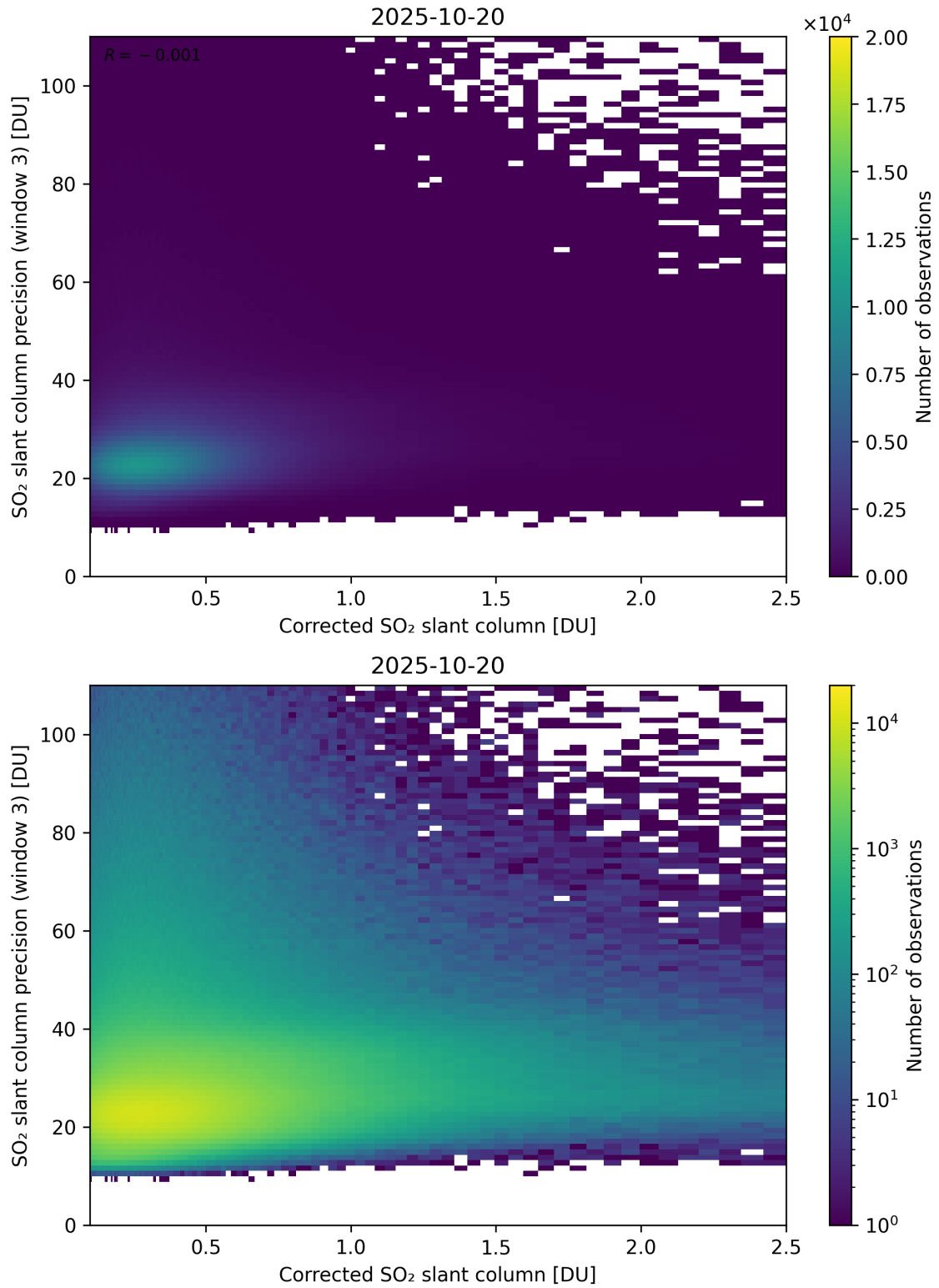
Figure 241: Scatter density plot of “Corrected SO 2 slant column” against “SO 2 slant column precision (window 3)” for 2025-10-19 to 2025-10-21.
