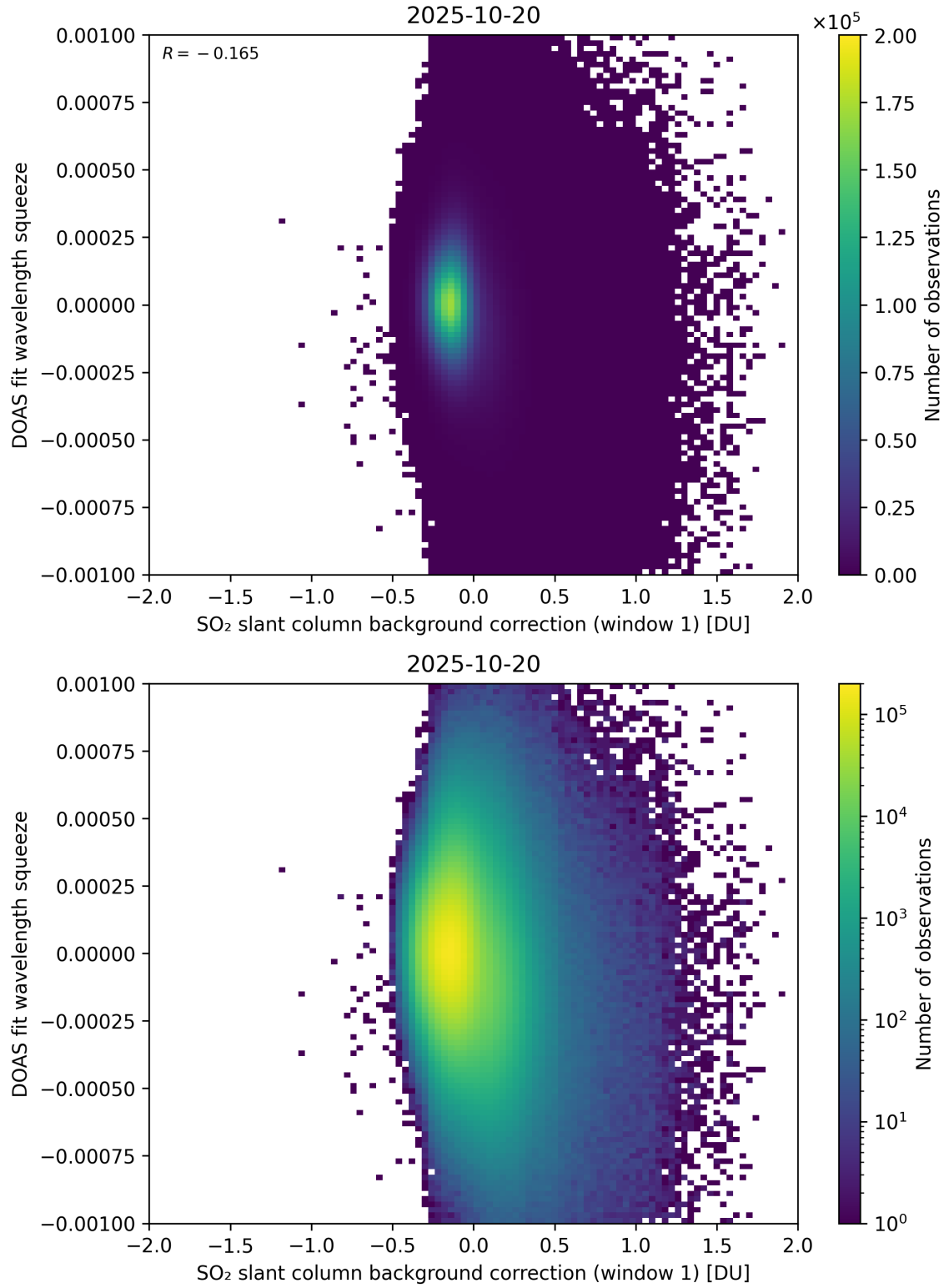
Figure 112: Scatter density plot of “SO 2 slant column background correction (window 1)” against “DOAS fit wavelength squeeze” for 2025-10-19 to 2025-10-21.
