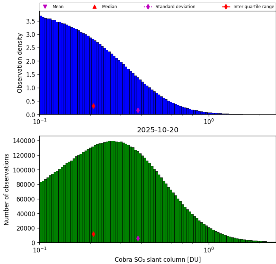
Figure 61: Histogram of “Cobra SO 2 slant column” for 2025-10-19 to 2025-10-21
