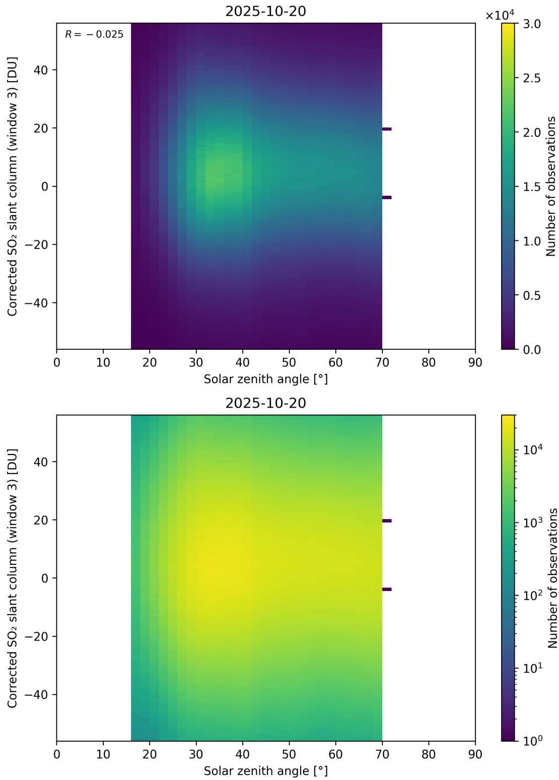
Figure 183: Scatter density plot of “Solar zenith angle” against “Corrected SO 2 slant column (window 3)” for 2025-10-19 to 2025-10-21.
