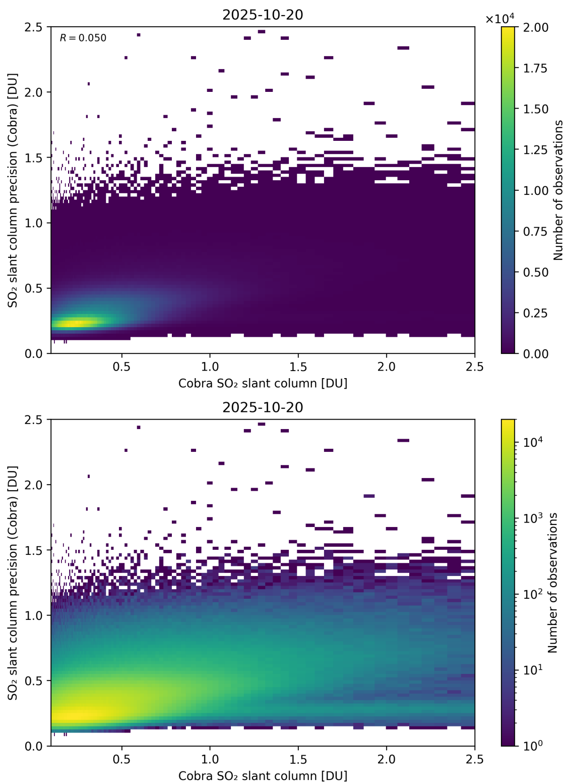
Figure 216: Scatter density plot of “Cobra SO 2 slant column” against “SO 2 slant column precision (Cobra)” for 2025-10-19 to 2025-10-21.
