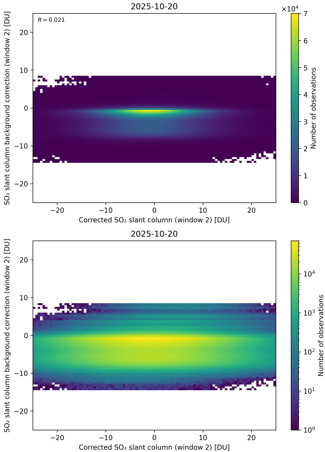
Figure 244: Scatter density plot of “Corrected SO 2 slant column (window 2)” against “SO 2 slant column background correction (window 2)” for 2025-10-19 to 2025-10-21.
