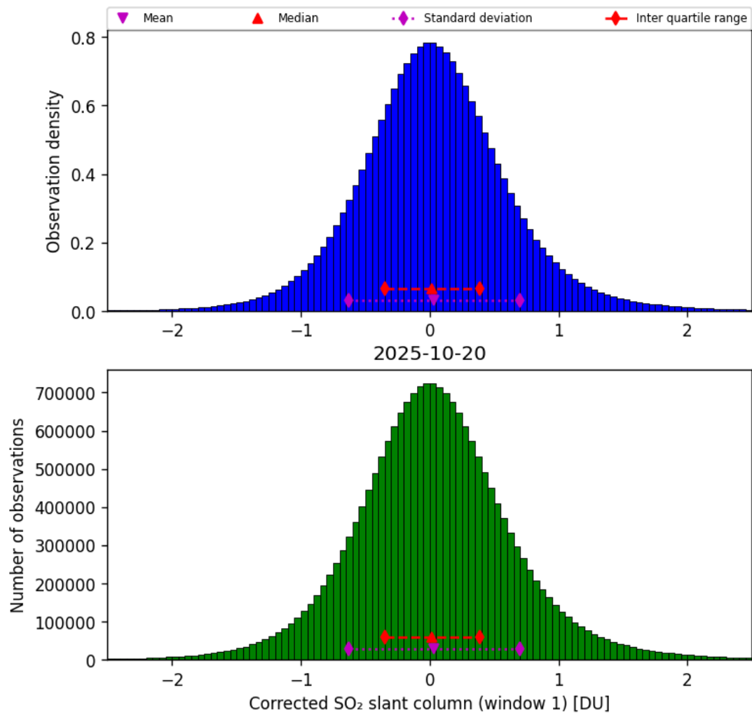
Figure 65: Histogram of “Corrected SO 2 slant column (window 1)” for 2025-10-19 to 2025-10-21
