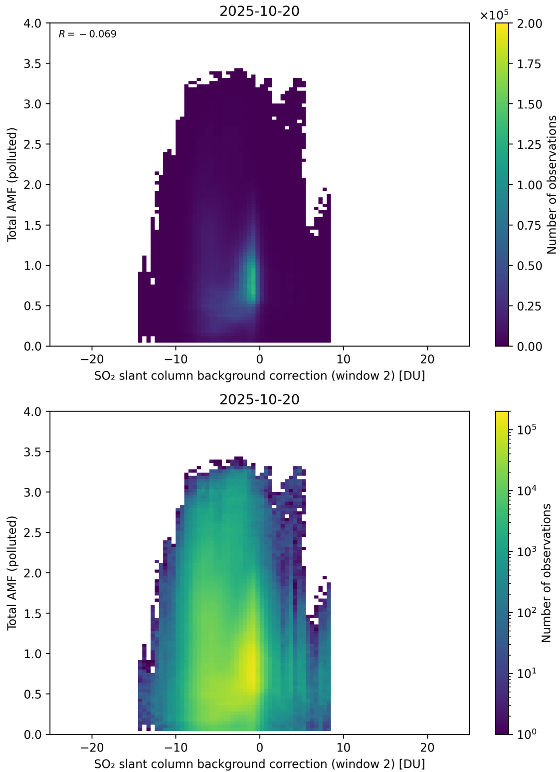
Figure 130: Scatter density plot of “SO 2 slant column background correction (window 2)” against “Total AMF (polluted)” for 2025-10-19 to 2025-10-21.
