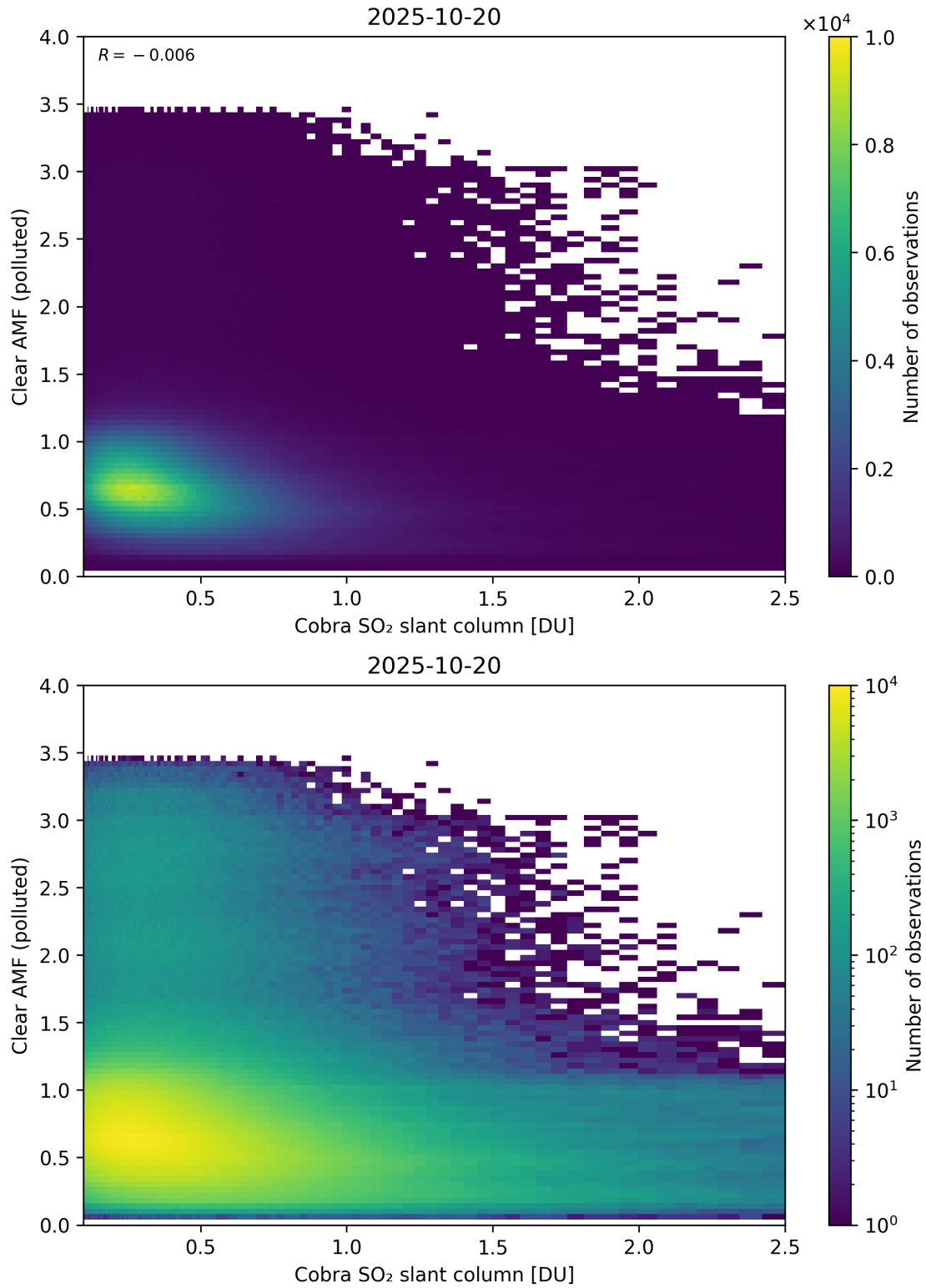
Figure 215: Scatter density plot of “Cobra SO 2 slant column” against “Clear AMF (polluted)” for 2025-10-19 to 2025-10-21.
