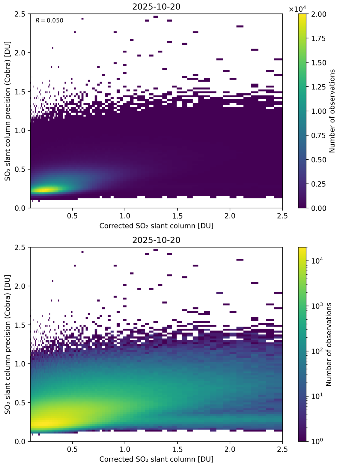
Figure 234: Scatter density plot of “Corrected SO 2 slant column” against “SO 2 slant column precision (Cobra)” for 2025-10-19 to 2025-10-21.
