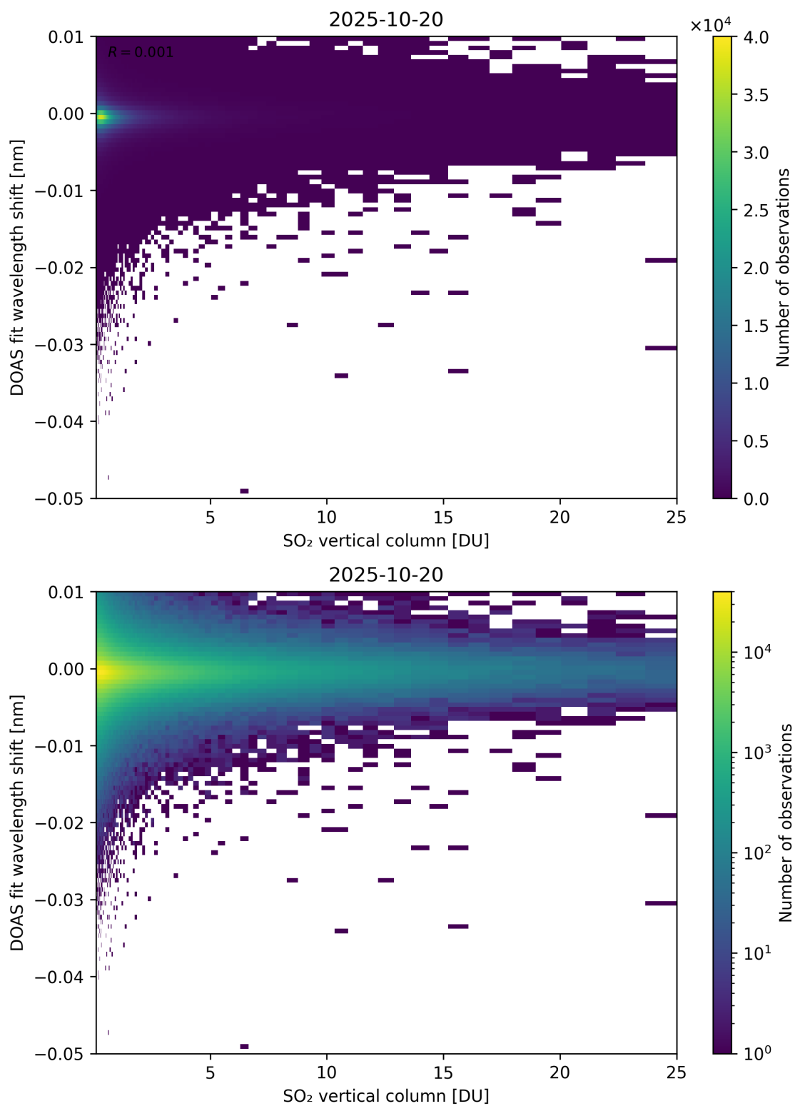
Figure 326: Scatter density plot of “SO 2 vertical column” against “DOAS fit wavelength shift” for 2025-10-19 to 2025-10-21.
