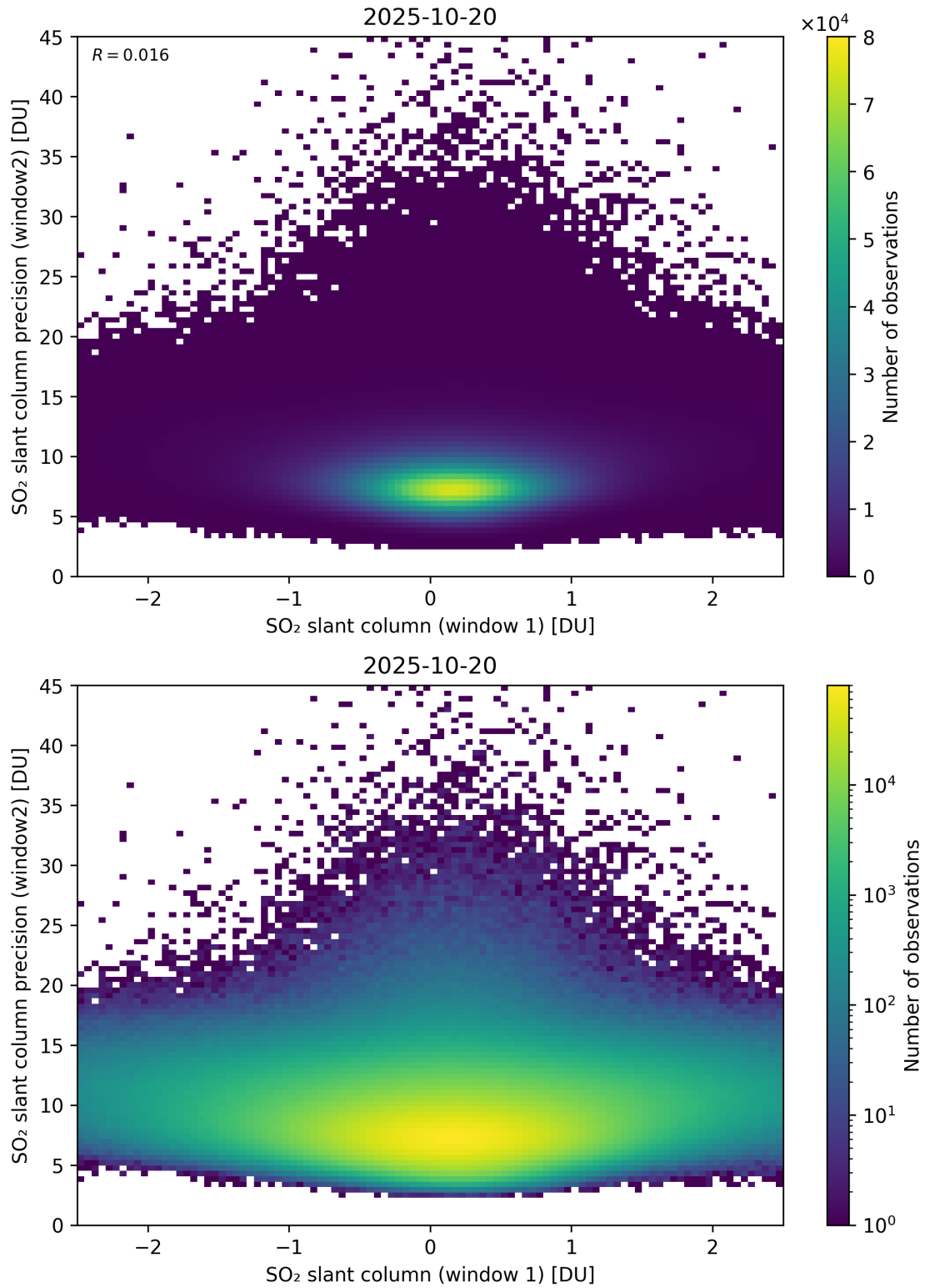
Figure 286: Scatter density plot of “SO 2 slant column (window 1)” against “SO 2 slant column precision (window2)” for 2025-10-19 to 2025-10-21.
