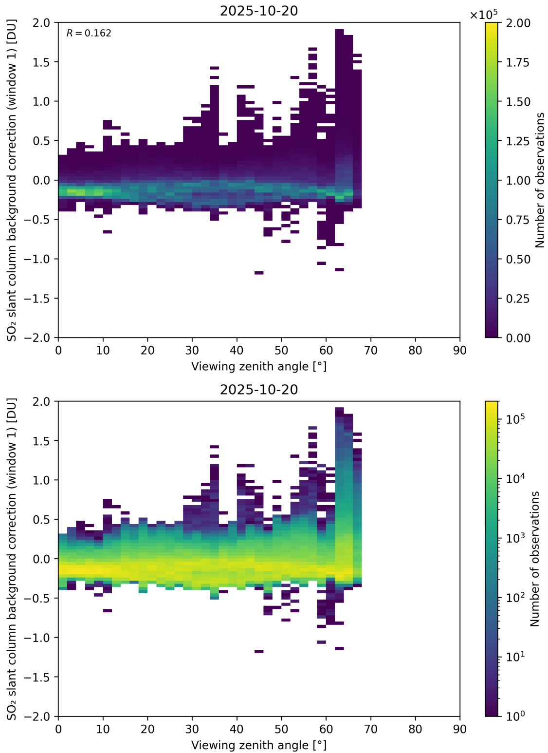
Figure 362: Scatter density plot of “Viewing zenith angle” against “SO 2 slant column background correction (window 1)” for 2025-10-19 to 2025-10-21.
