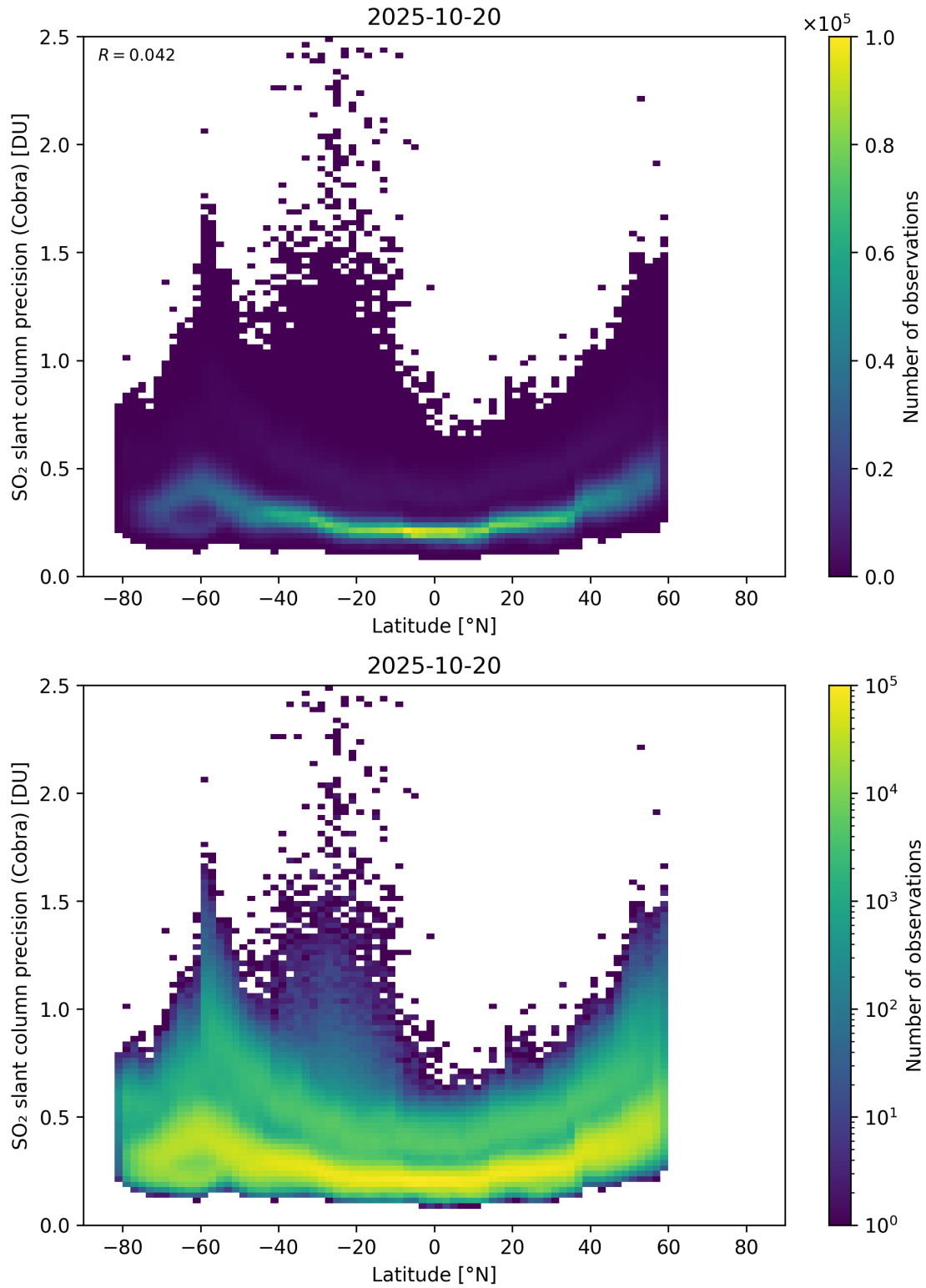
Figure 158: Scatter density plot of “Latitude” against “SO 2 slant column precision (Cobra)” for 2025-10-19 to 2025-10-21.
