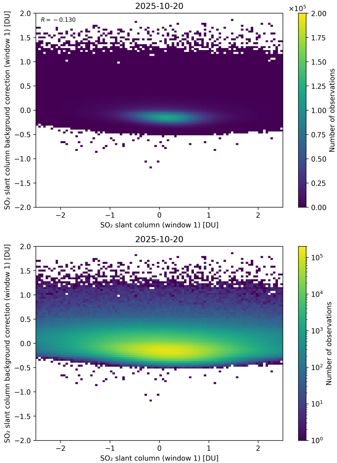
Figure 262: Scatter density plot of “SO 2 slant column (window 1)” against “SO 2 slant column background correction (window 1)” for 2025-10-19 to 2025-10-21.
