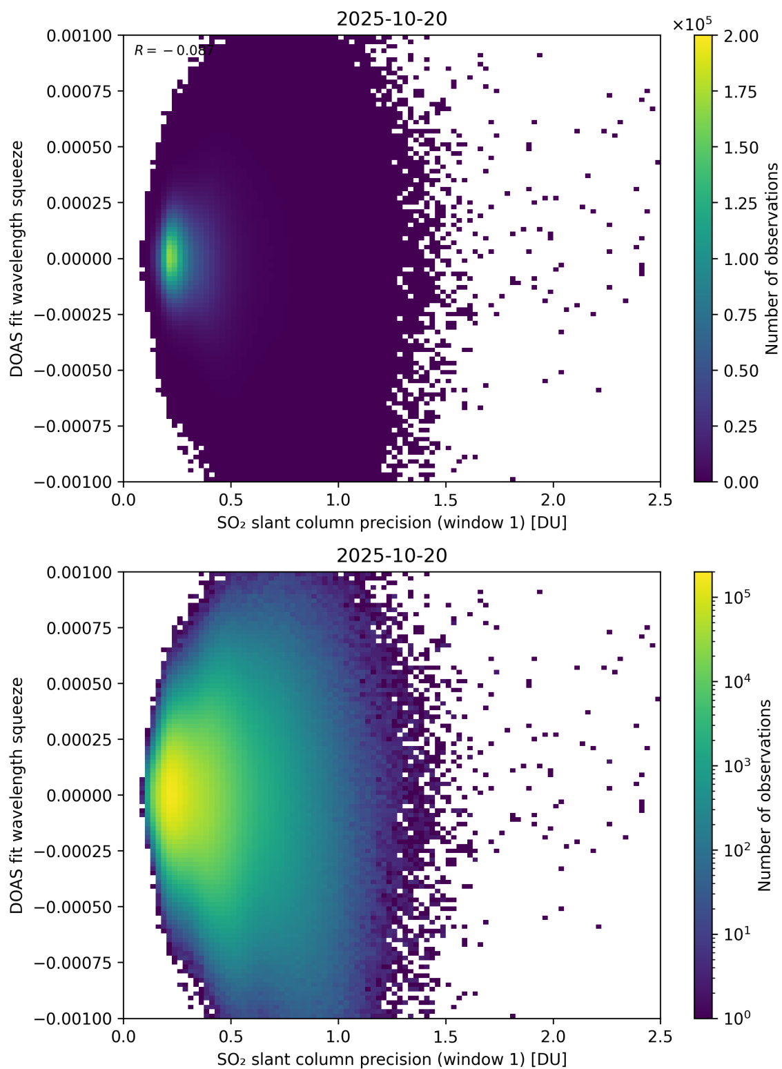
Figure 272: Scatter density plot of “SO 2 slant column precision (window 1)” against “DOAS fit wavelength squeeze” for 2025-10-19 to 2025-10-21.
