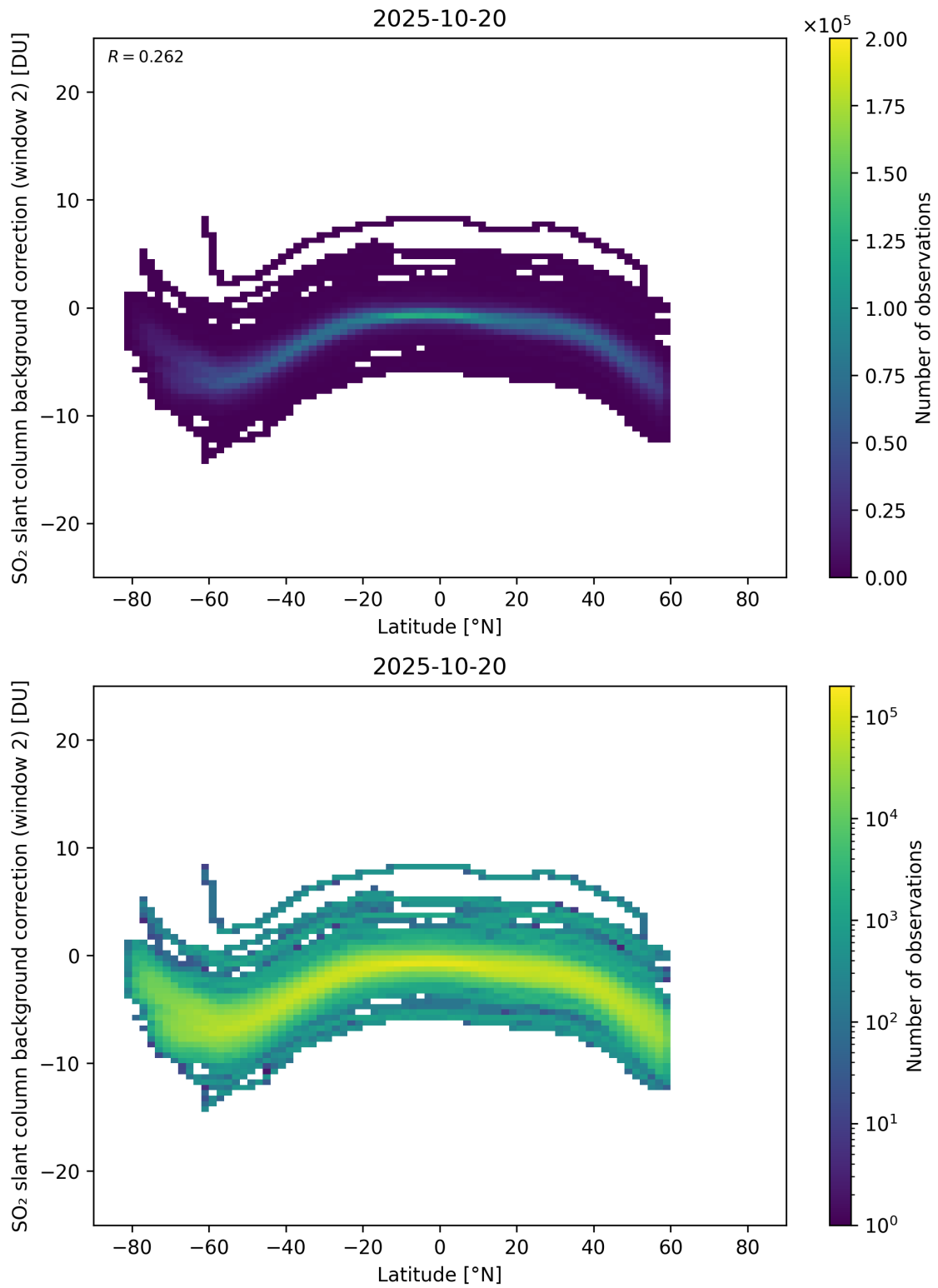
Figure 151: Scatter density plot of “Latitude” against “SO 2 slant column background correction (window 2)” for 2025-10-19 to 2025-10-21.
