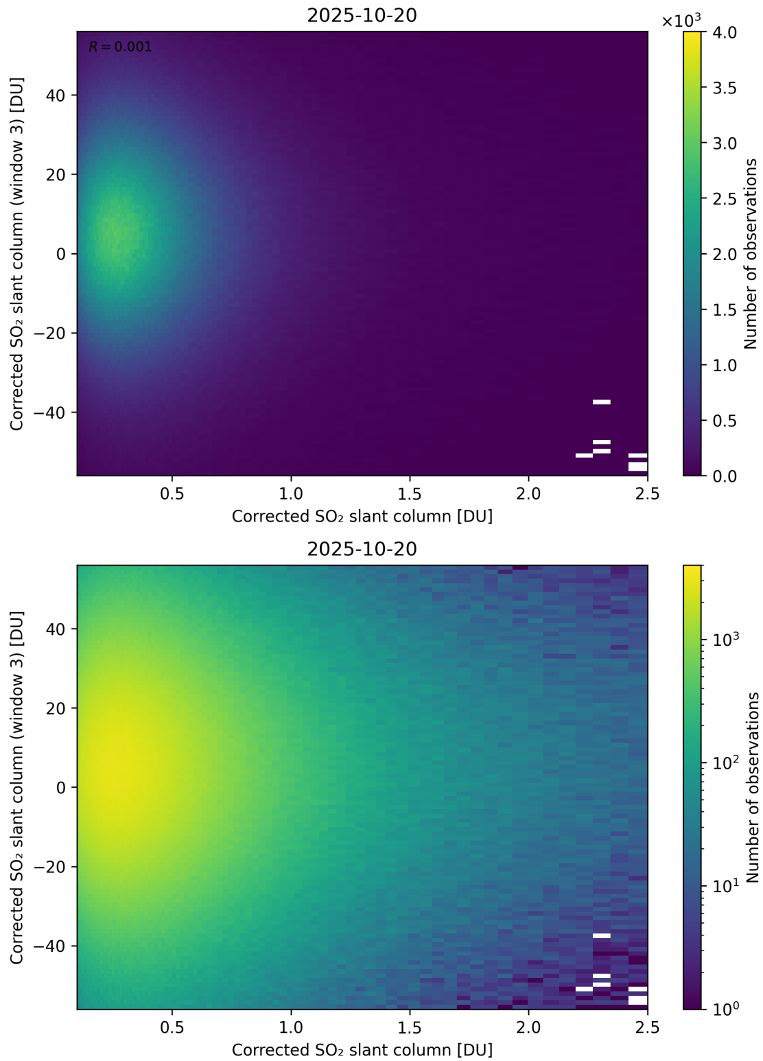
Figure 236: Scatter density plot of “Corrected SO 2 slant column” against “Corrected SO 2 slant column (window 3)” for 2025-10-19 to 2025-10-21.
