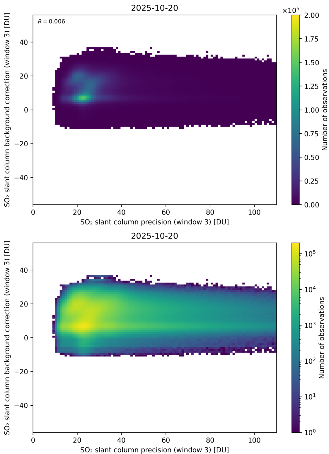
Figure 307: Scatter density plot of “SO 2 slant column precision (window 3)” against “SO 2 slant column background correction (window 3)” for 2025-10-19 to 2025-10-21.
