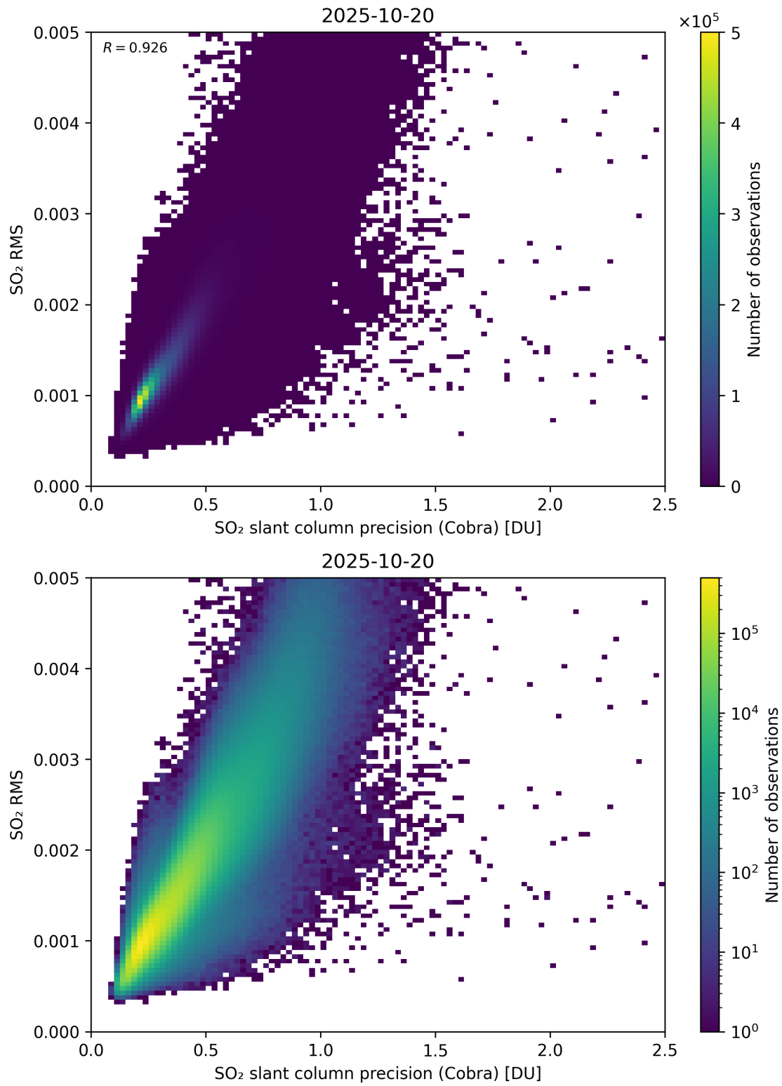
Figure 204: Scatter density plot of “SO 2 slant column precision (Cobra)” against “SO 2 RMS” for 2025-10-19 to 2025-10-21.
