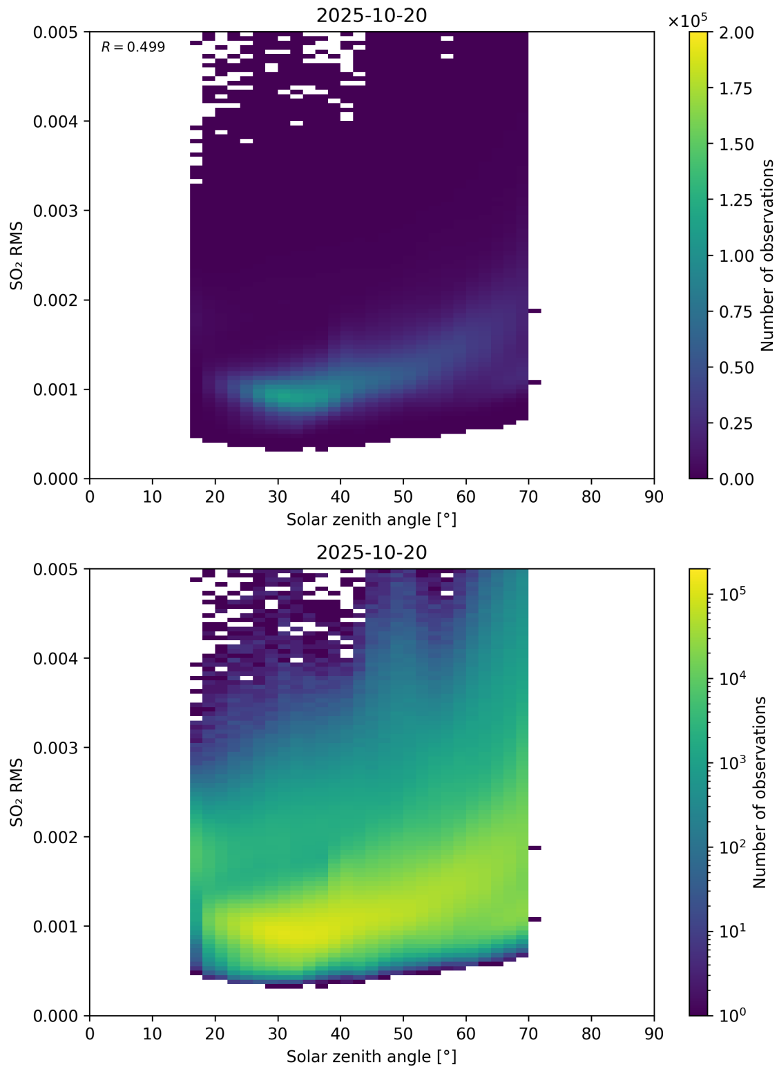
Figure 176: Scatter density plot of “Solar zenith angle” against “SO 2 RMS” for 2025-10-19 to 2025-10-21.
