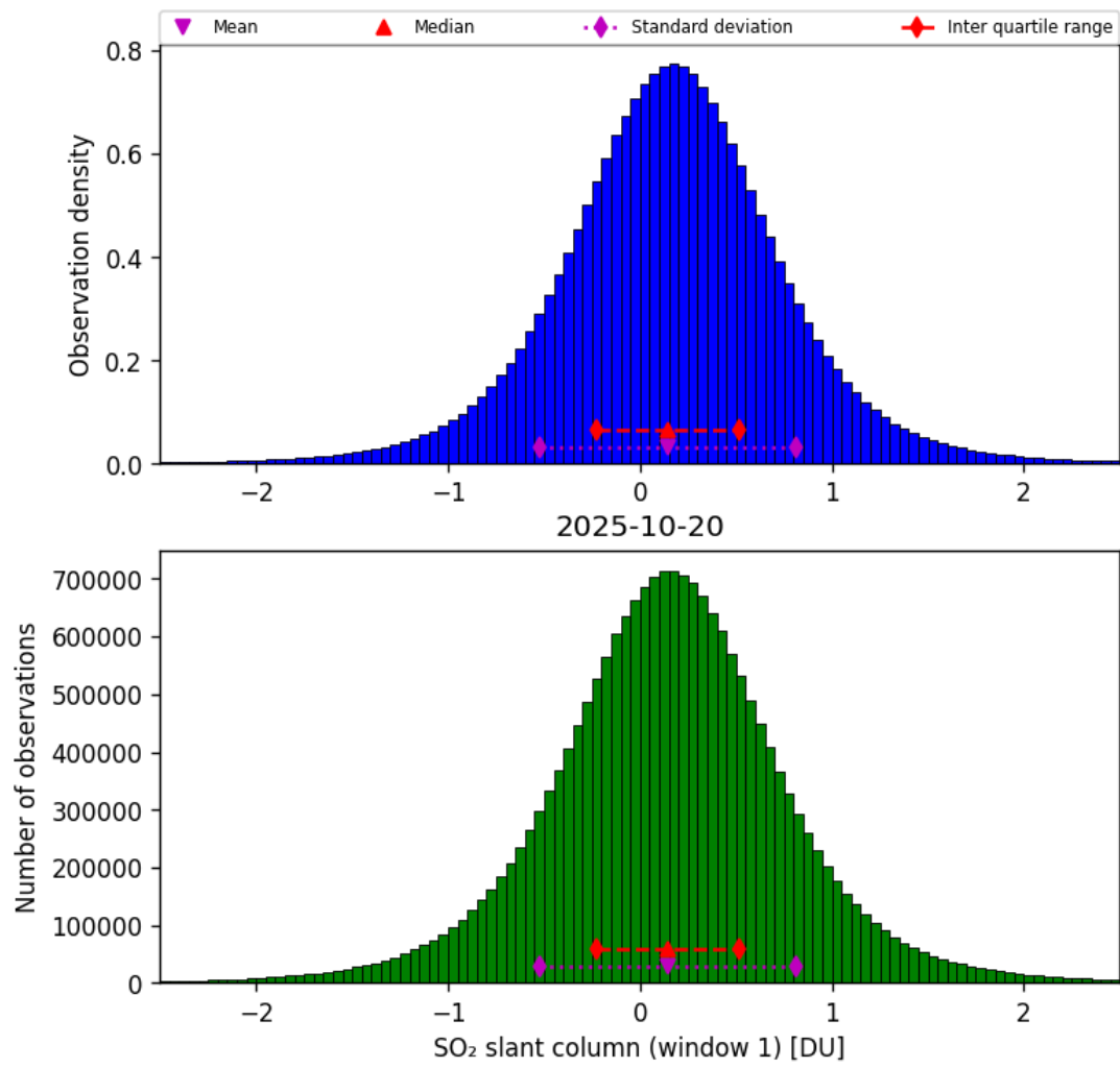
Figure 63: Histogram of “SO 2 slant column (window 1)” for 2025-10-19 to 2025-10-21
