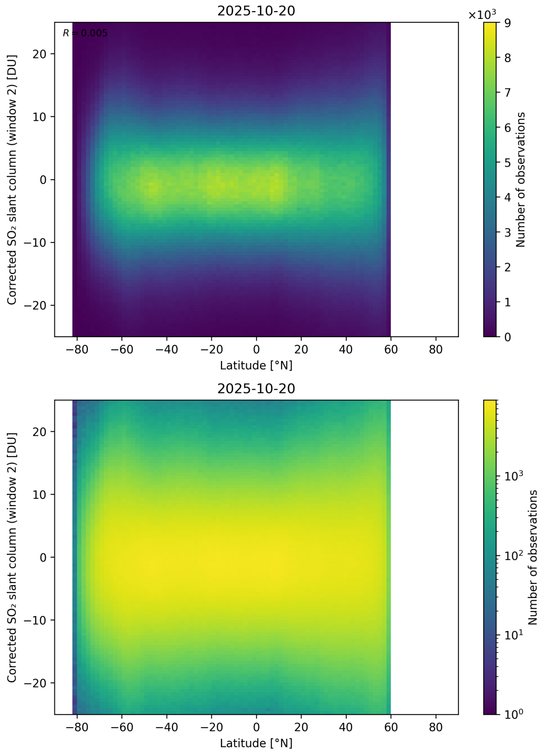
Figure 160: Scatter density plot of “Latitude” against “Corrected SO 2 slant column (window 2)” for 2025-10-19 to 2025-10-21.
