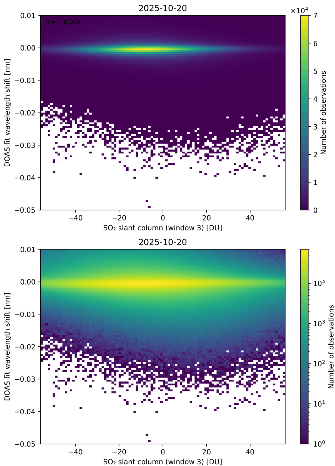
Figure 304: Scatter density plot of “SO 2 slant column (window 3)” against “DOAS fit wavelength shift” for 2025-10-19 to 2025-10-21.
