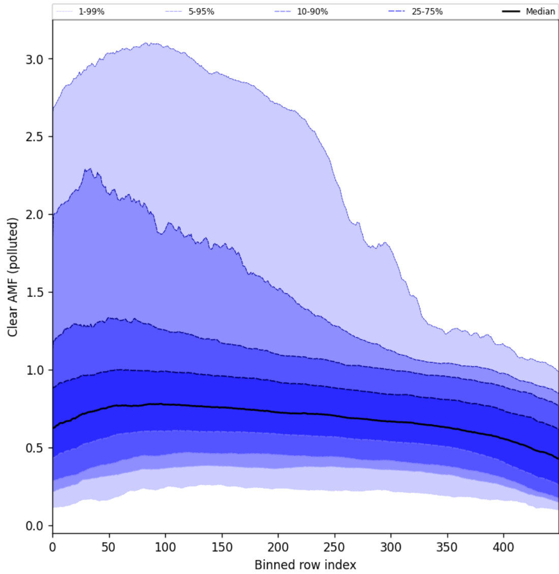
Figure 107: Along track statistics of “Clear AMF (polluted)” for 2025-10-19 to 2025-10-21
