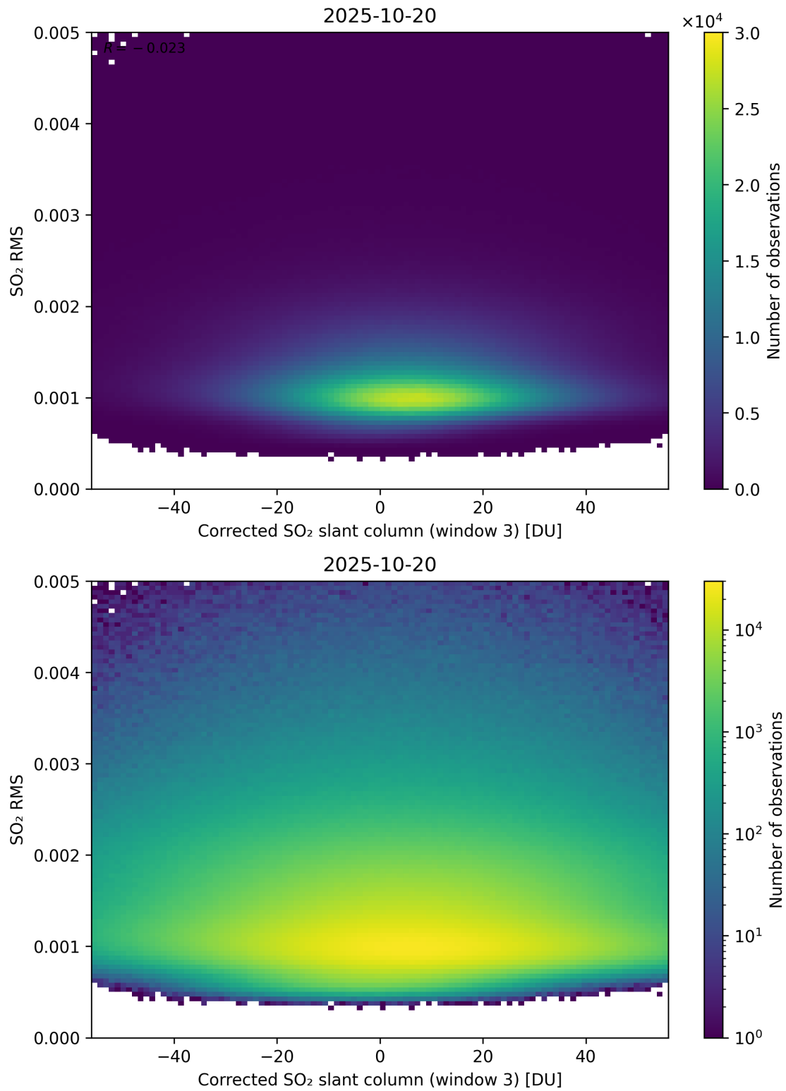
Figure 258: Scatter density plot of “Corrected SO 2 slant column (window 3)” against “SO 2 RMS” for 2025-10-19 to 2025-10-21.
