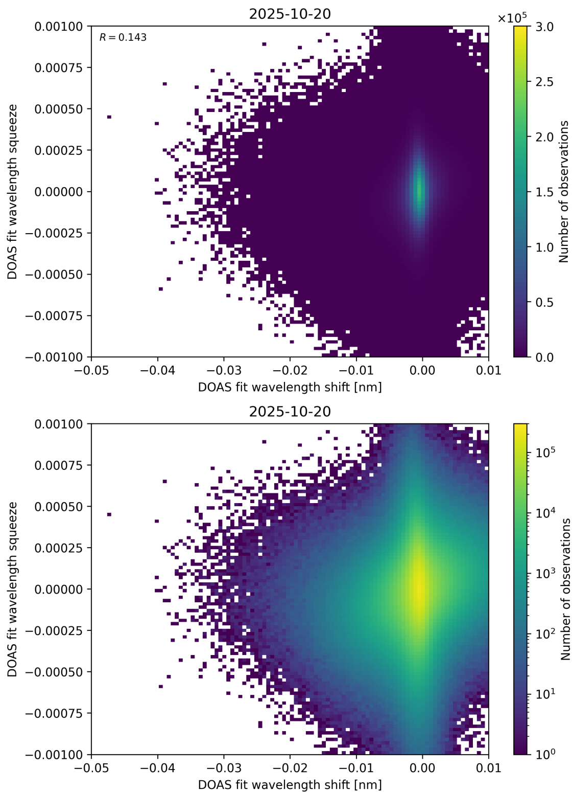
Figure 138: Scatter density plot of “DOAS fit wavelength shift” against “DOAS fit wavelength squeeze” for 2025-10-19 to 2025-10-21.
