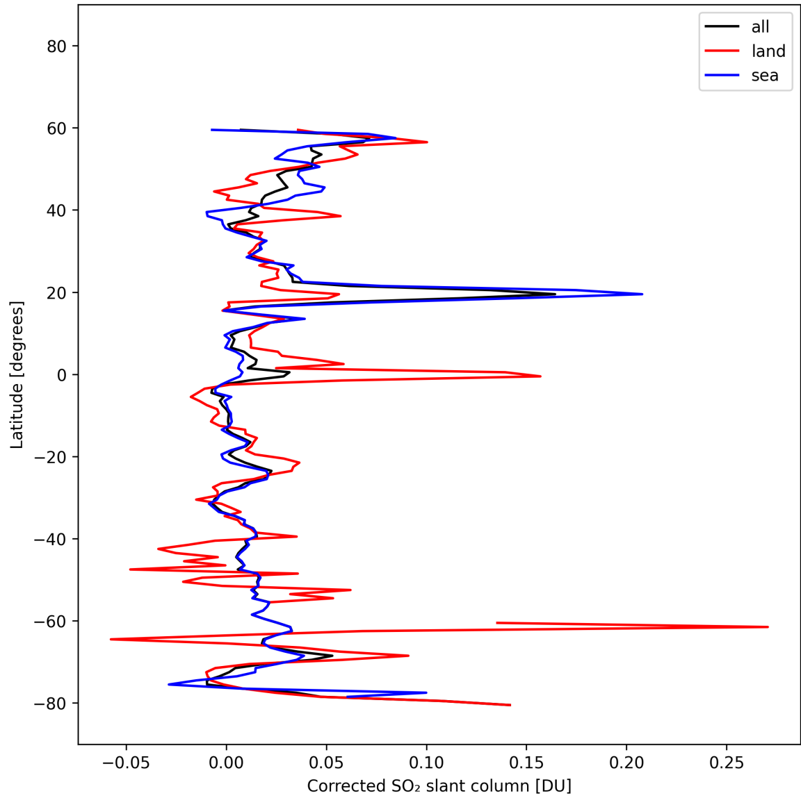
Figure 34: Zonal average of “Corrected SO 2 slant column” for 2025-10-19 to 2025-10-21.
