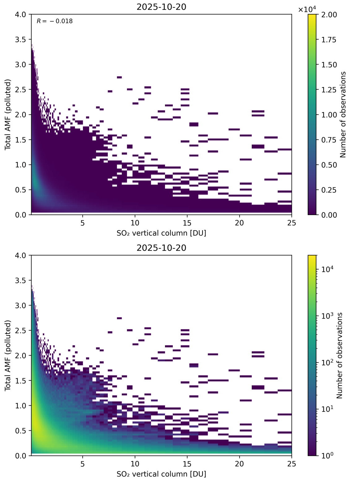
Figure 359: Scatter density plot of “SO 2 vertical column” against “Total AMF (polluted)” for 2025-10-19 to 2025-10-21.
