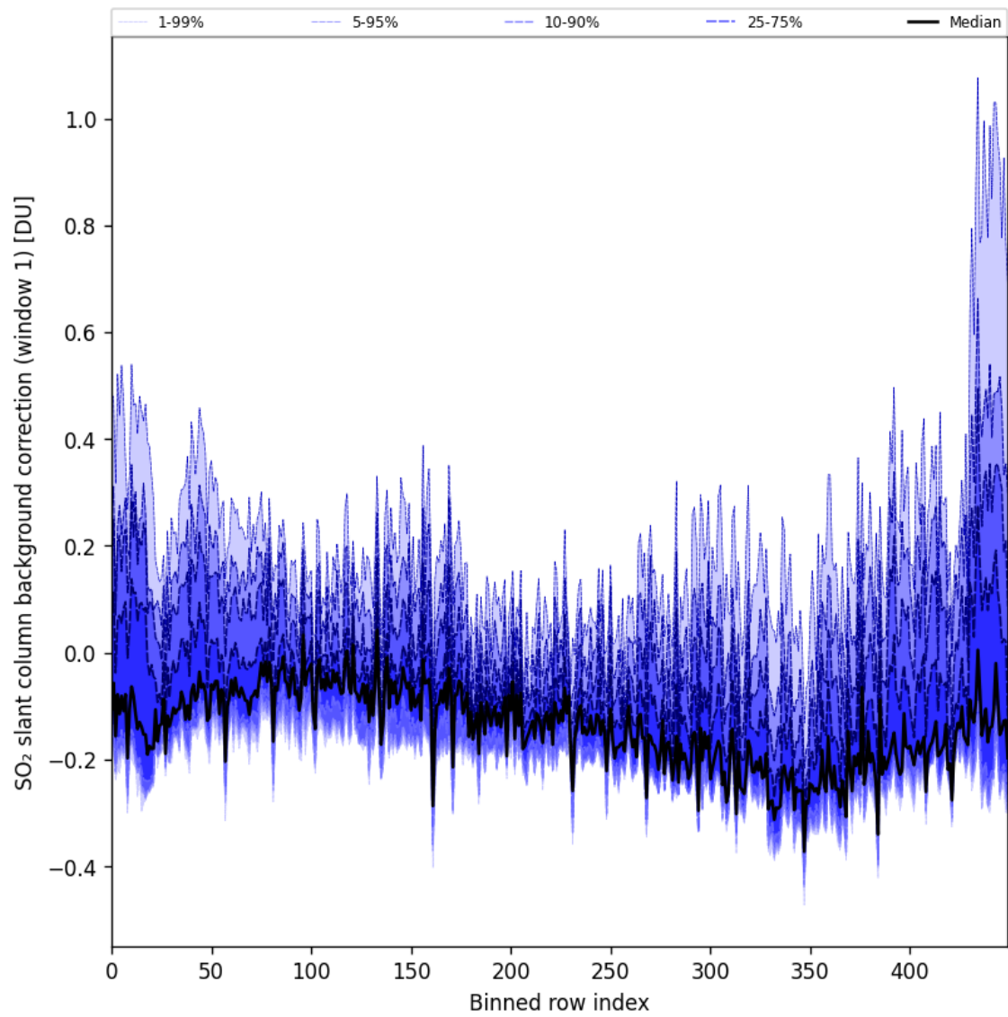
Figure 92: Along track statistics of “SO 2 slant column background correction (window 1)” for 2025-10-19 to 2025-10-21
