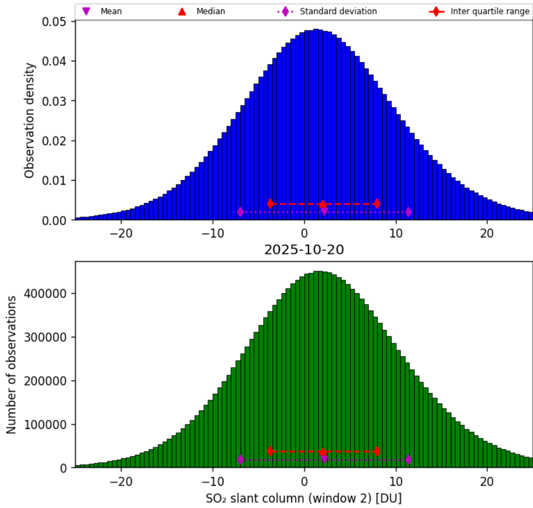
Figure 67: Histogram of “SO 2 slant column (window 2)” for 2025-10-19 to 2025-10-21
