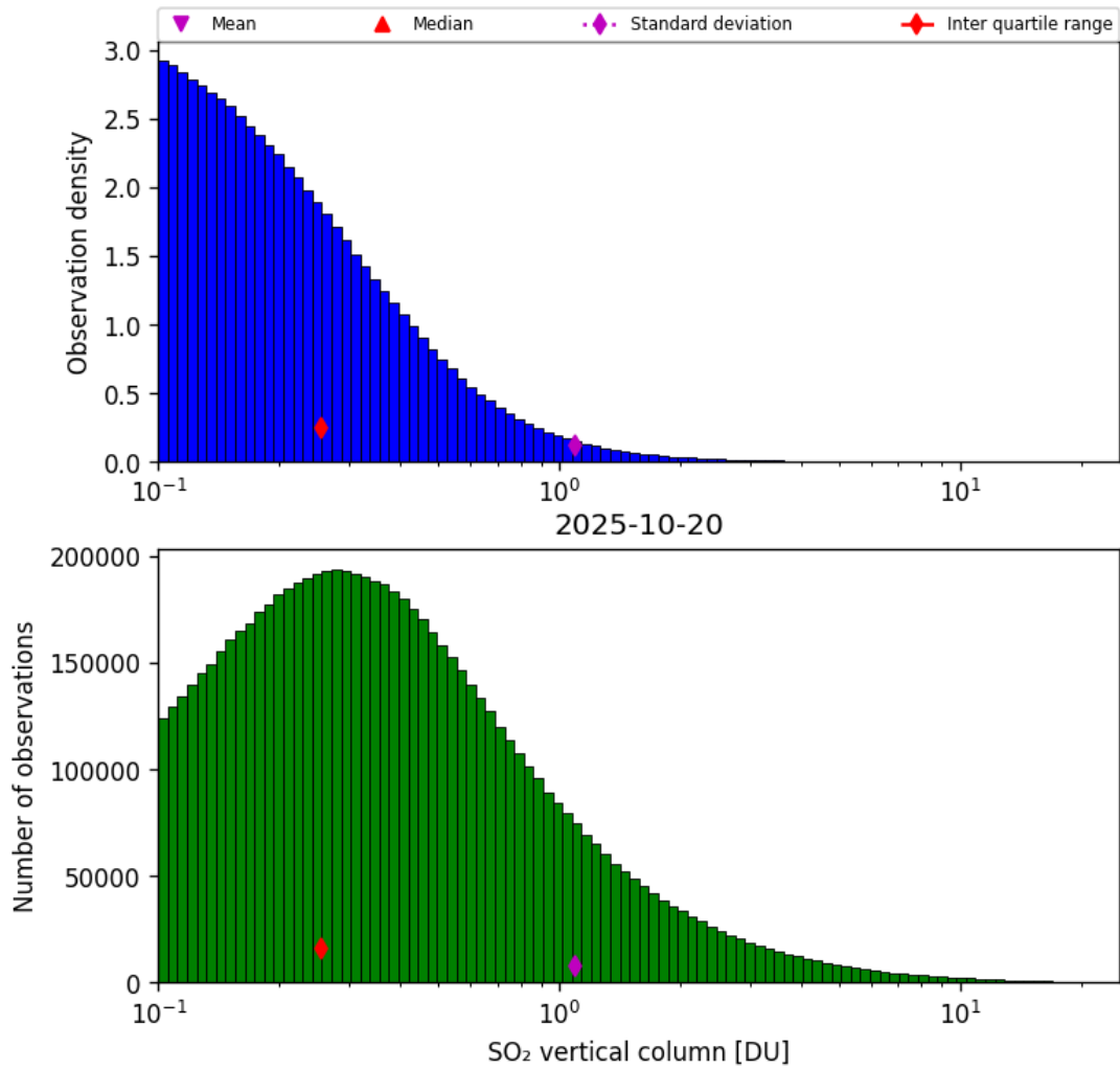
Figure 58: Histogram of “SO 2 vertical column” for 2025-10-19 to 2025-10-21
