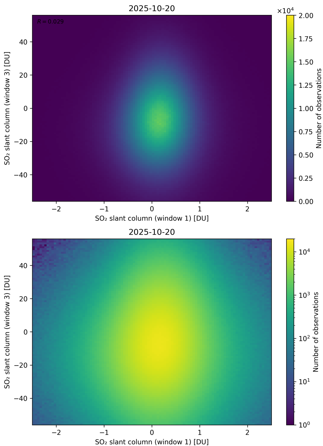
Figure 287: Scatter density plot of “SO 2 slant column (window 1)” against “SO 2 slant column (window 3)” for 2025-10-19 to 2025-10-21.
