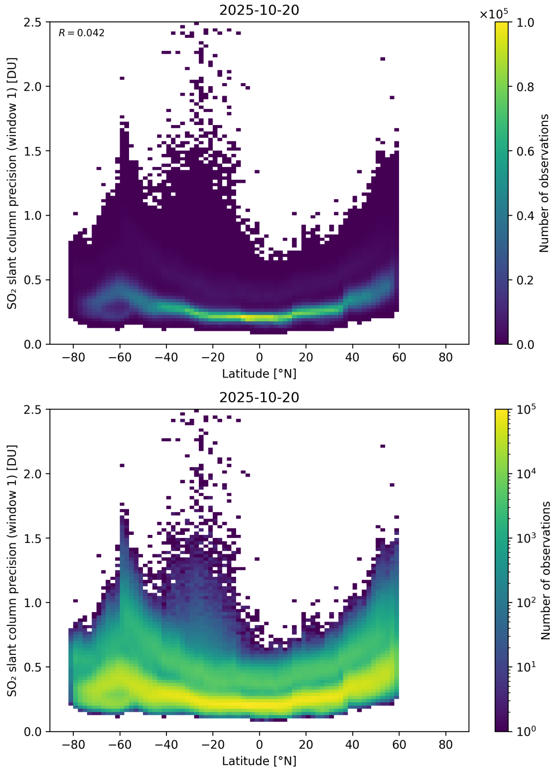
Figure 163: Scatter density plot of “Latitude” against “SO 2 slant column precision (window 1)” for 2025-10-19 to 2025-10-21.
