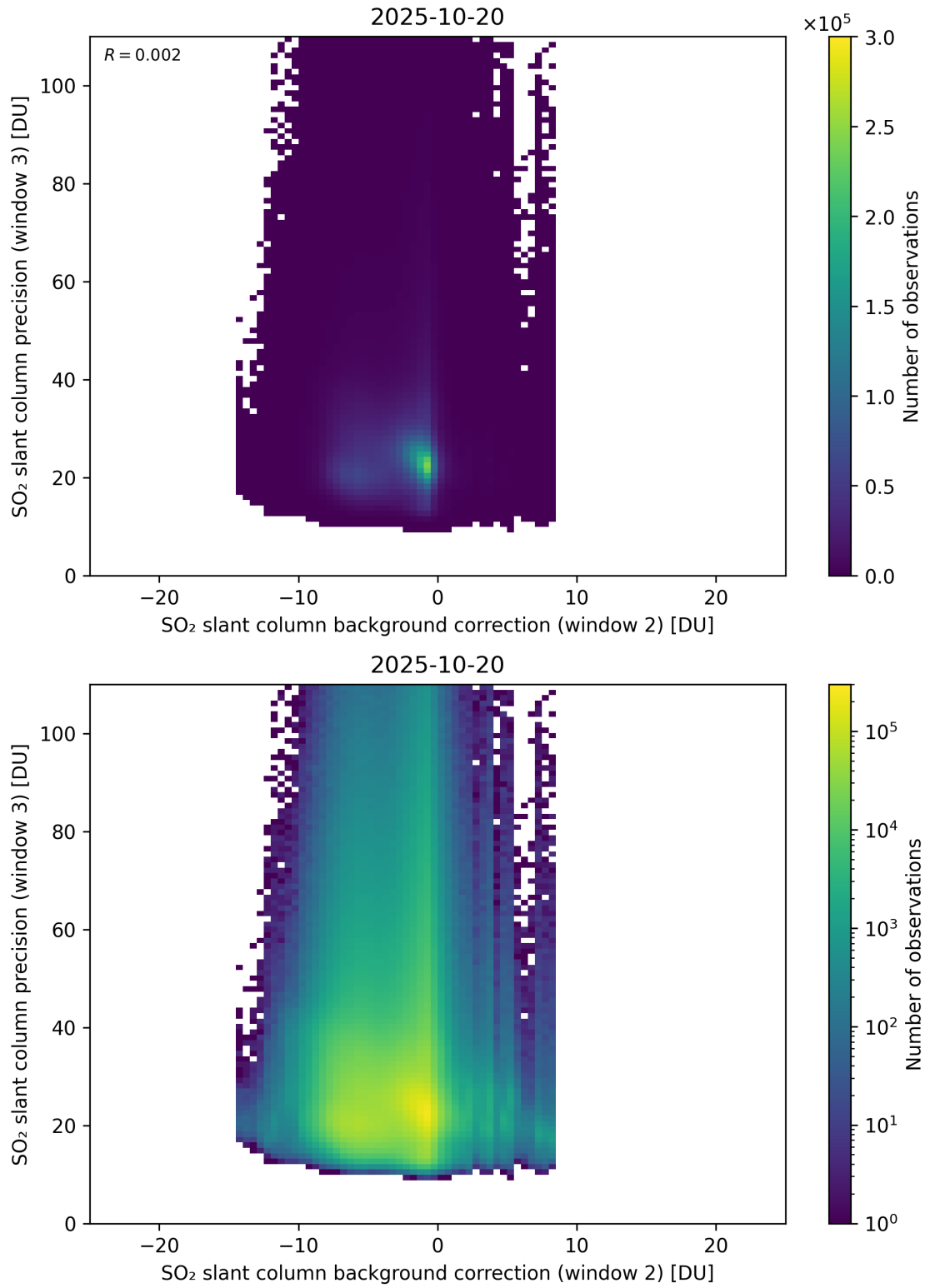
Figure 129: Scatter density plot of “SO 2 slant column background correction (window 2)” against “SO 2 slant column precision (window 3)” for 2025-10-19 to 2025-10-21.
