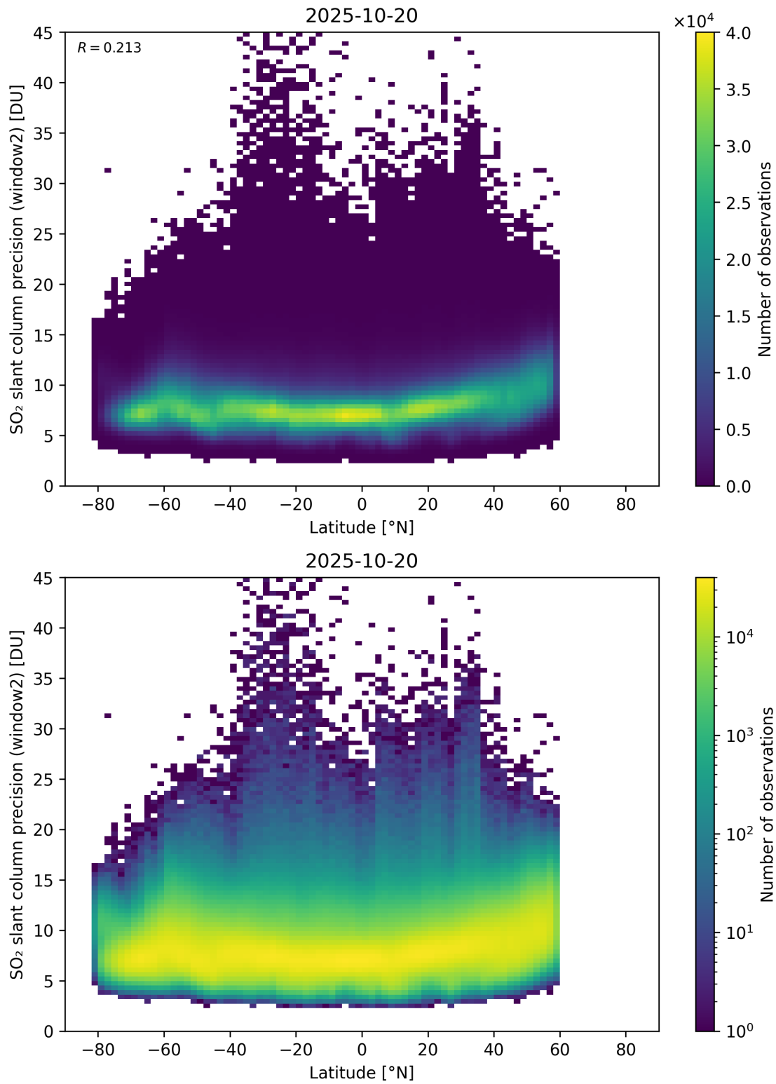
Figure 164: Scatter density plot of “Latitude” against “SO 2 slant column precision (window2)” for 2025-10-19 to 2025-10-21.
