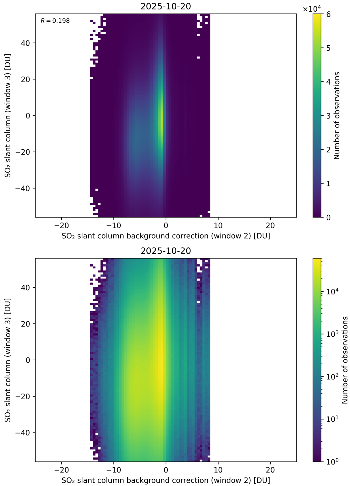
Figure 128: Scatter density plot of “SO 2 slant column background correction (window 2)” against “SO 2 slant column (window 3)” for 2025-10-19 to 2025-10-21.
