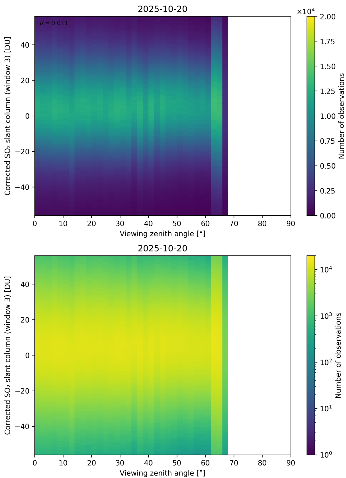
Figure 375: Scatter density plot of “Viewing zenith angle” against “Corrected SO 2 slant column (window 3)” for 2025-10-19 to 2025-10-21.
