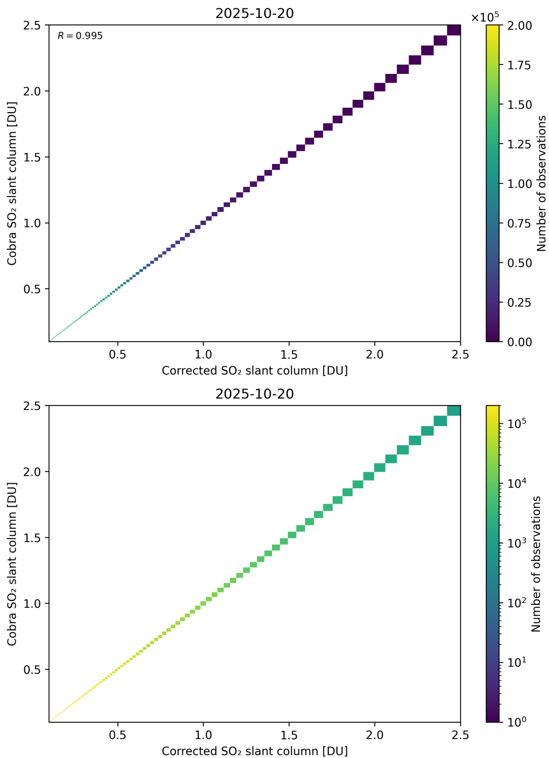
Figure 233: Scatter density plot of “Corrected SO 2 slant column” against “Cobra SO 2 slant column” for 2025-10-19 to 2025-10-21.
