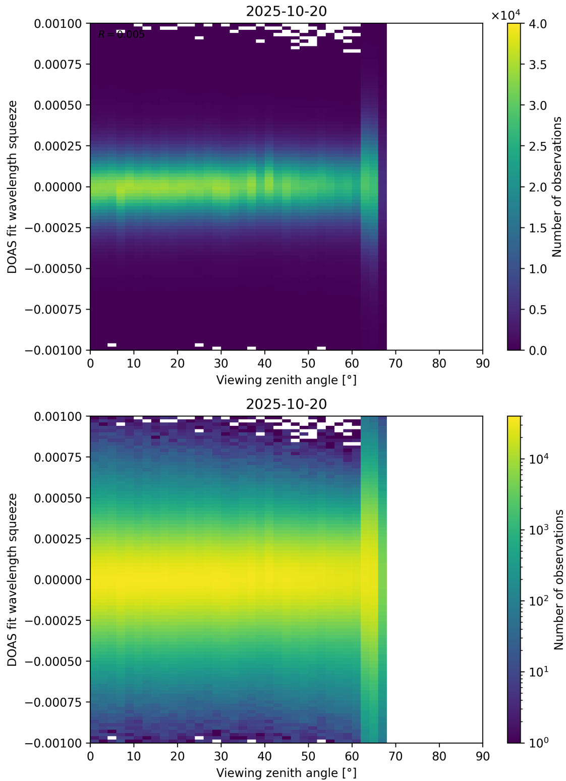
Figure 366: Scatter density plot of “Viewing zenith angle” against “DOAS fit wavelength squeeze” for 2025-10-19 to 2025-10-21.
