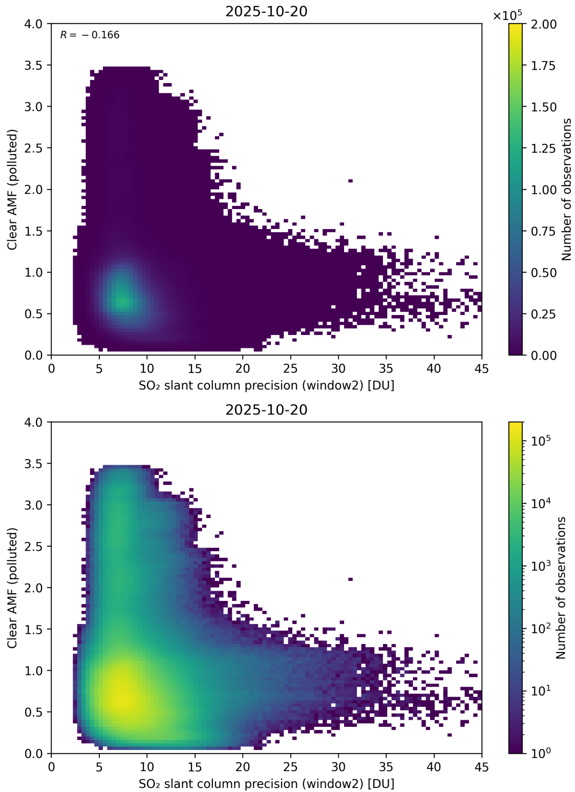
Figure 296: Scatter density plot of “SO 2 slant column precision (window2)” against “Clear AMF (polluted)” for 2025-10-19 to 2025-10-21.
