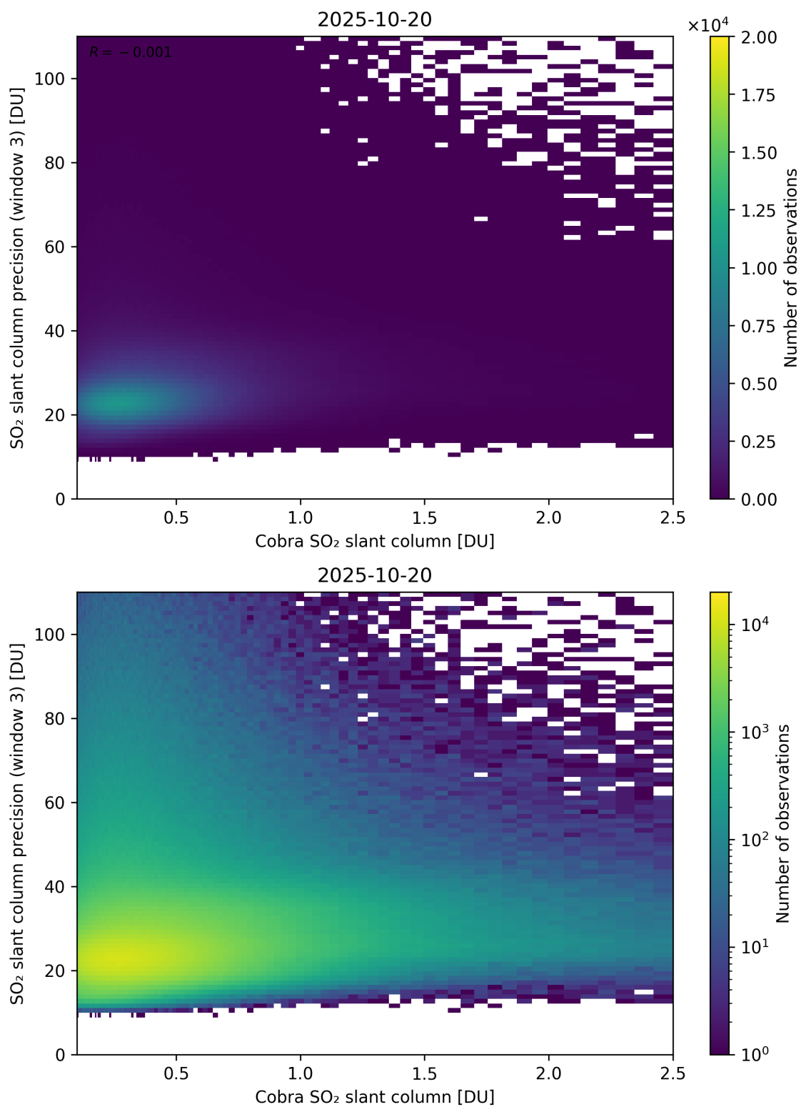
Figure 223: Scatter density plot of “Cobra SO 2 slant column” against “SO 2 slant column precision (window 3)” for 2025-10-19 to 2025-10-21.
