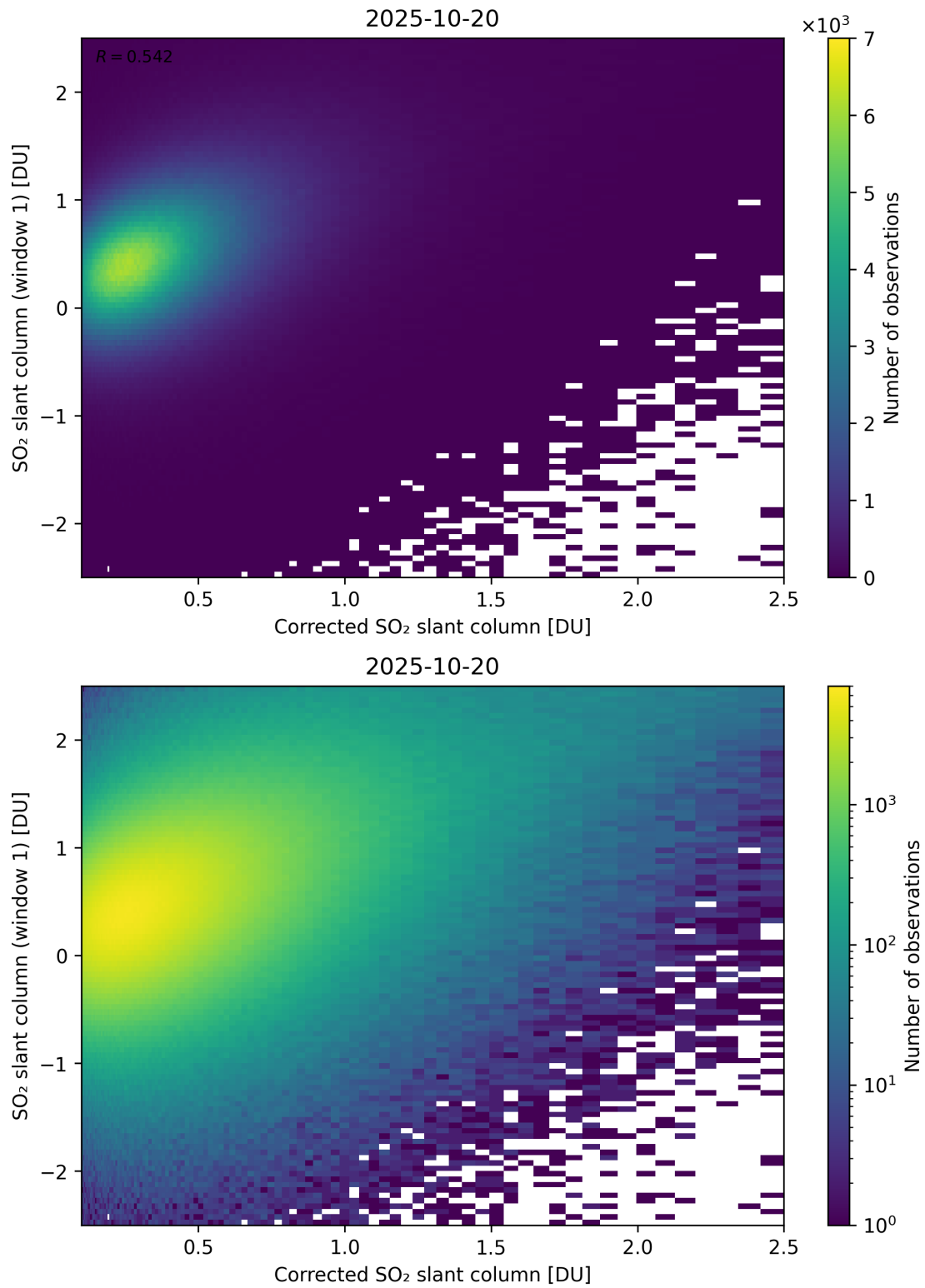
Figure 237: Scatter density plot of “Corrected SO 2 slant column” against “SO 2 slant column (window 1)” for 2025-10-19 to 2025-10-21.
