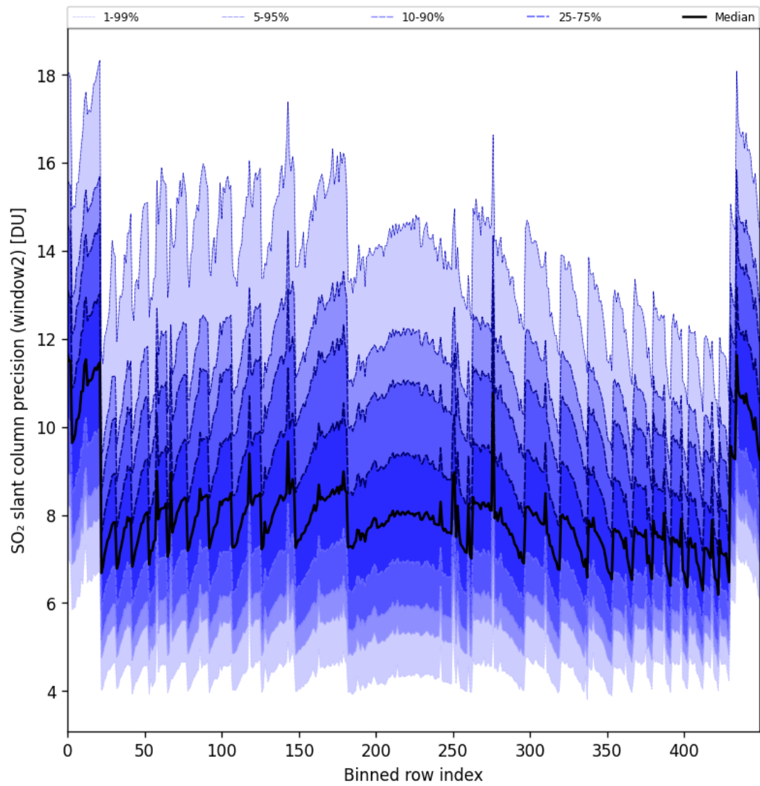
Figure 94: Along track statistics of “SO 2 slant column precision (window2)” for 2025-10-19 to 2025-10-21
