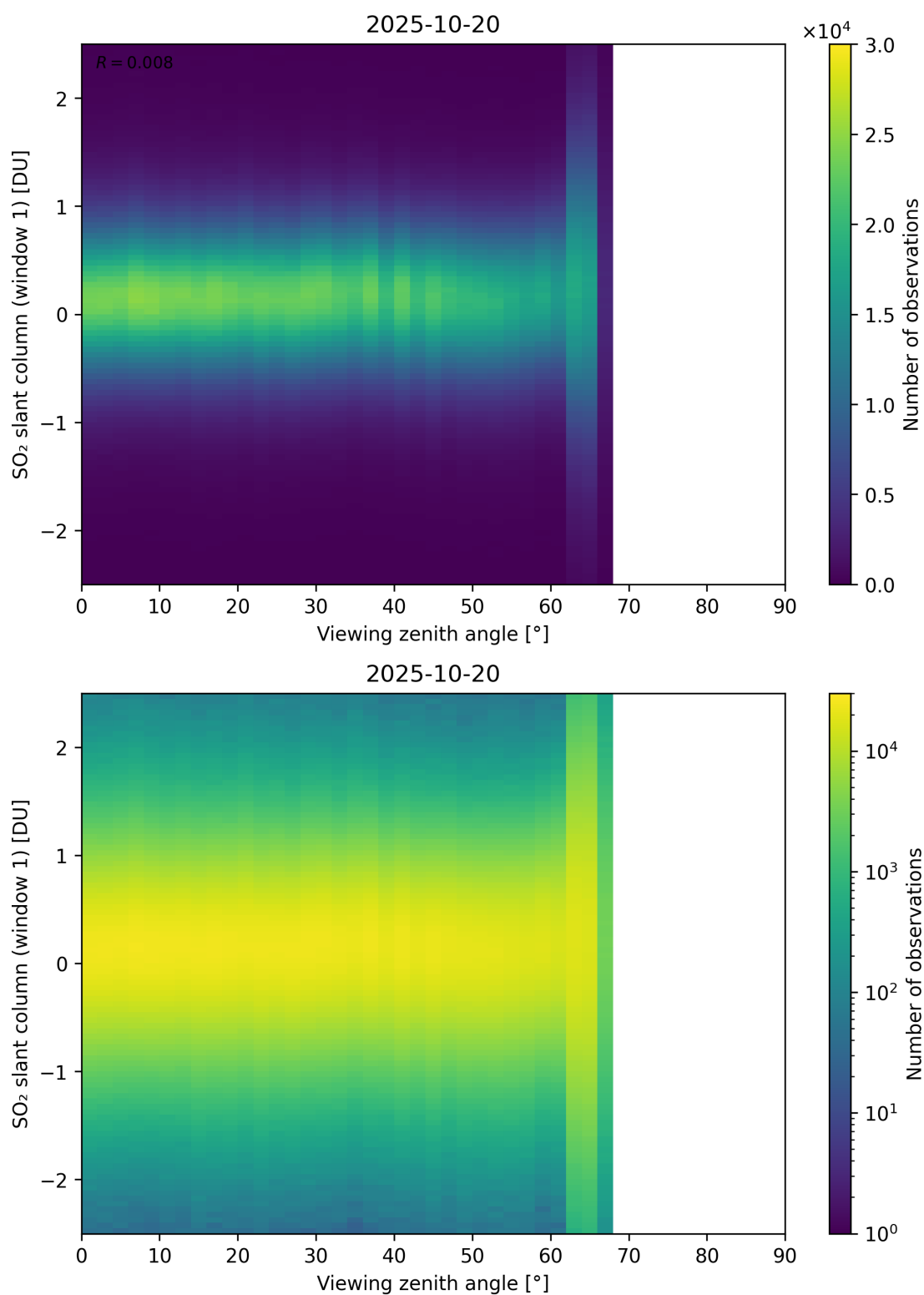
Figure 376: Scatter density plot of “Viewing zenith angle” against “SO 2 slant column (window 1)” for 2025-10-19 to 2025-10-21.
