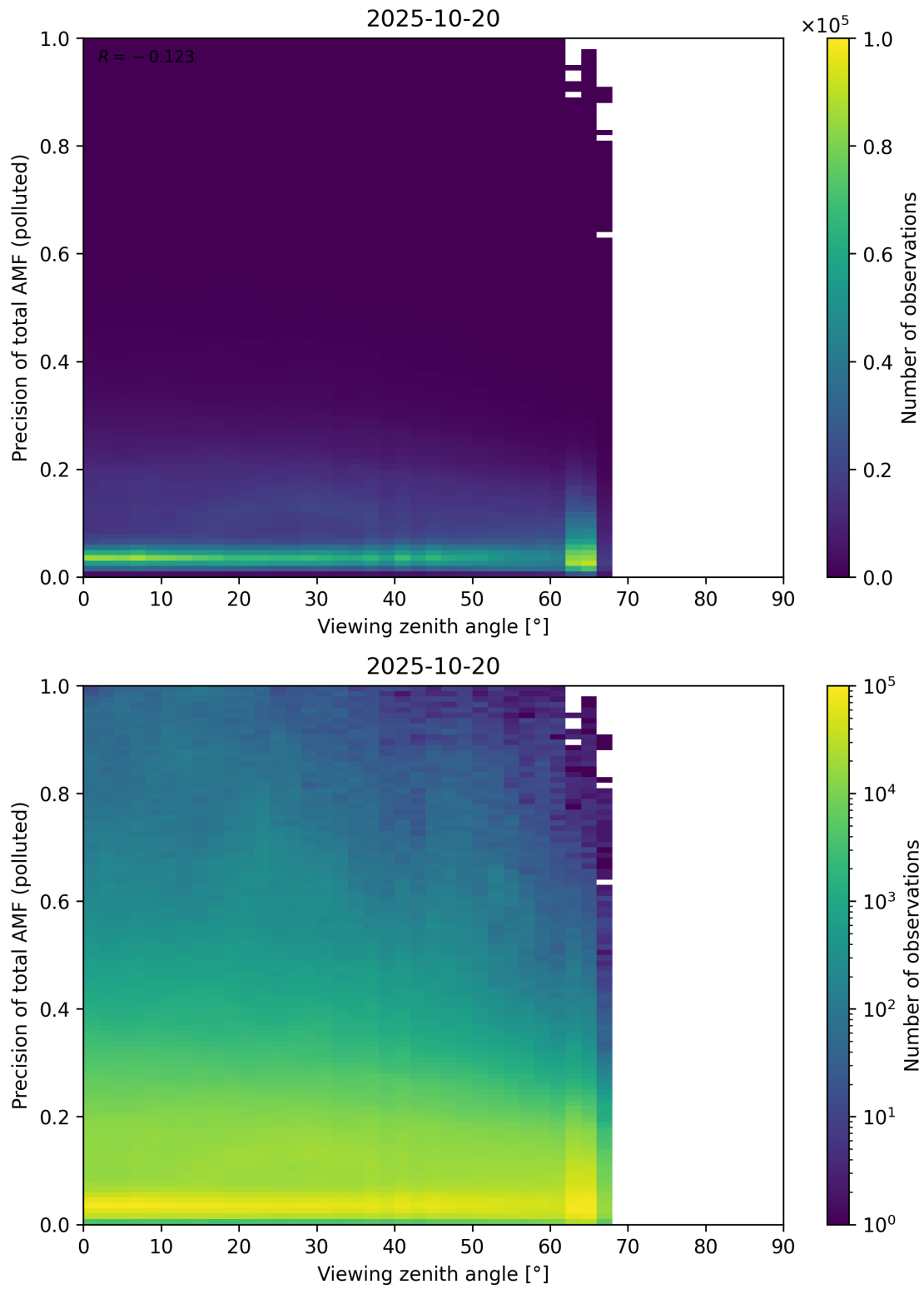
Figure 382: Scatter density plot of “Viewing zenith angle” against “Precision of total AMF (polluted)” for 2025-10-19 to 2025-10-21.
