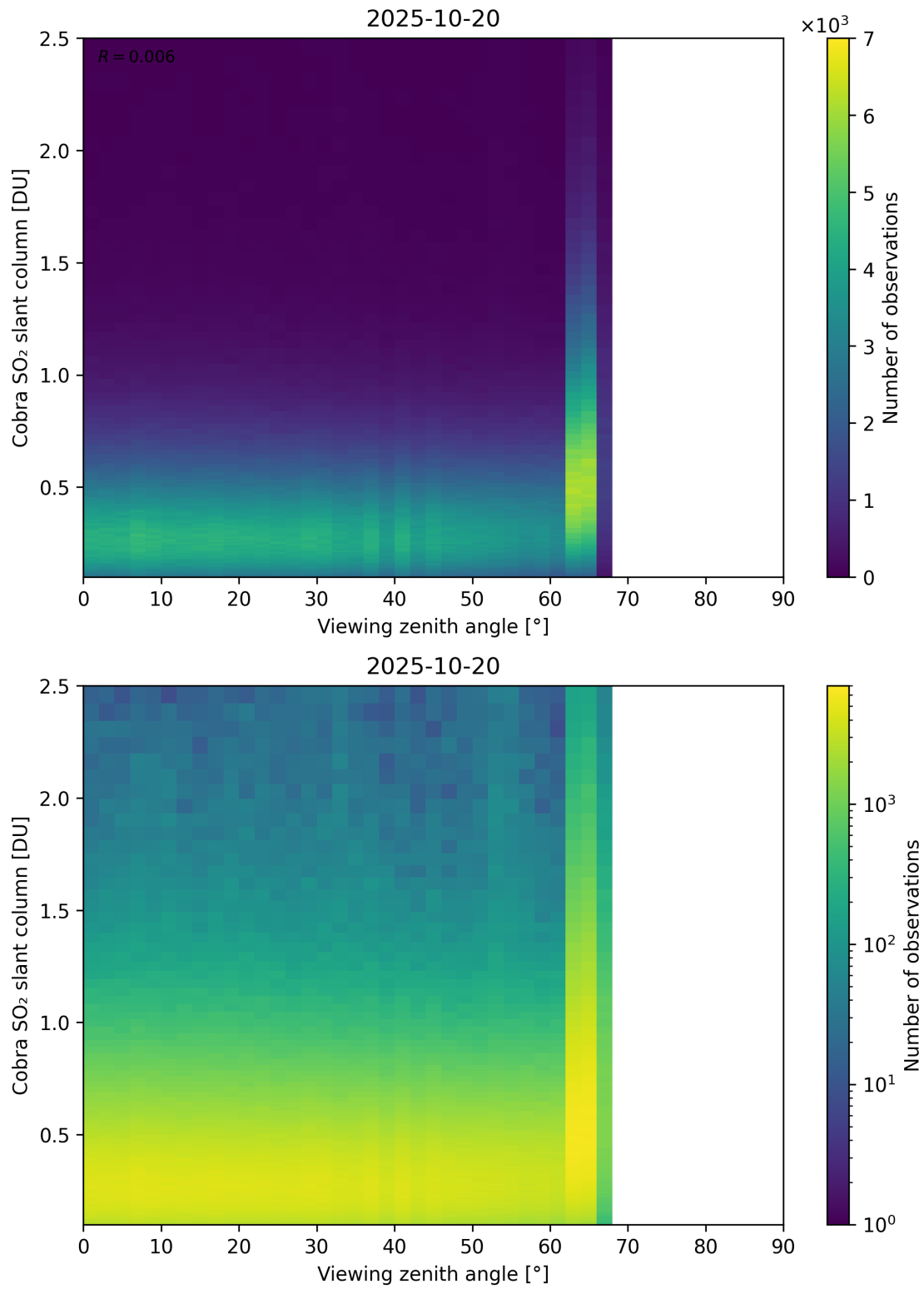
Figure 371: Scatter density plot of “Viewing zenith angle” against “Cobra SO 2 slant column” for 2025-10-19 to 2025-10-21.
