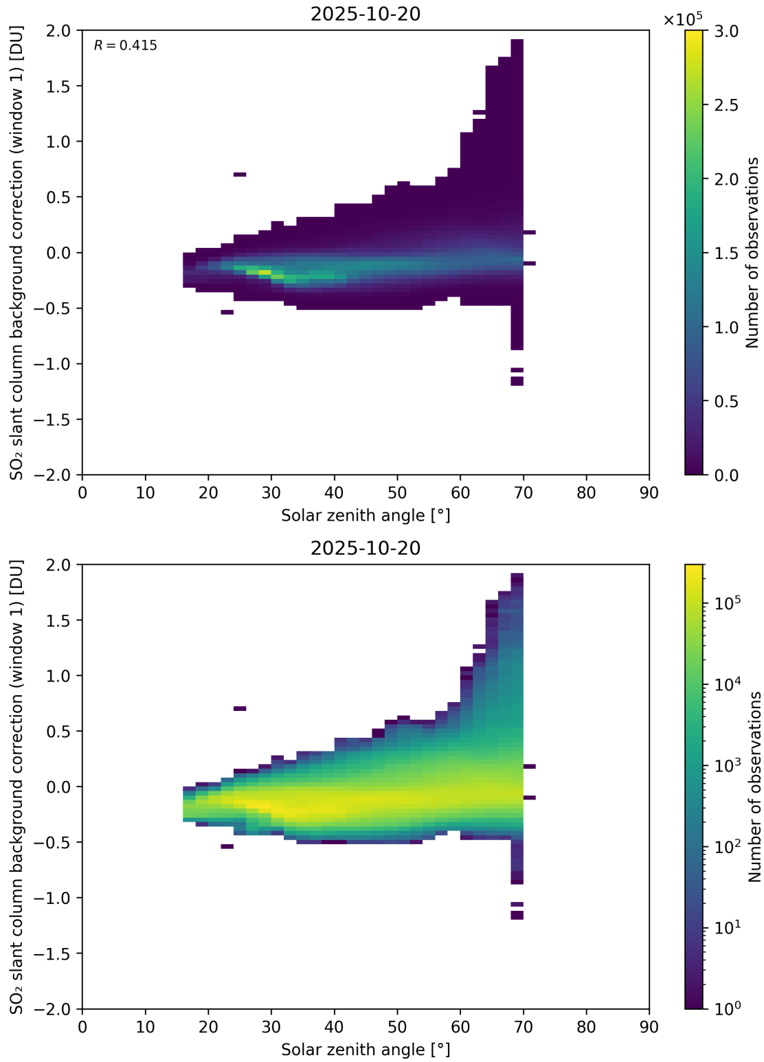
Figure 171: Scatter density plot of “Solar zenith angle” against “SO 2 slant column background correction (window 1)” for 2025-10-19 to 2025-10-21.
