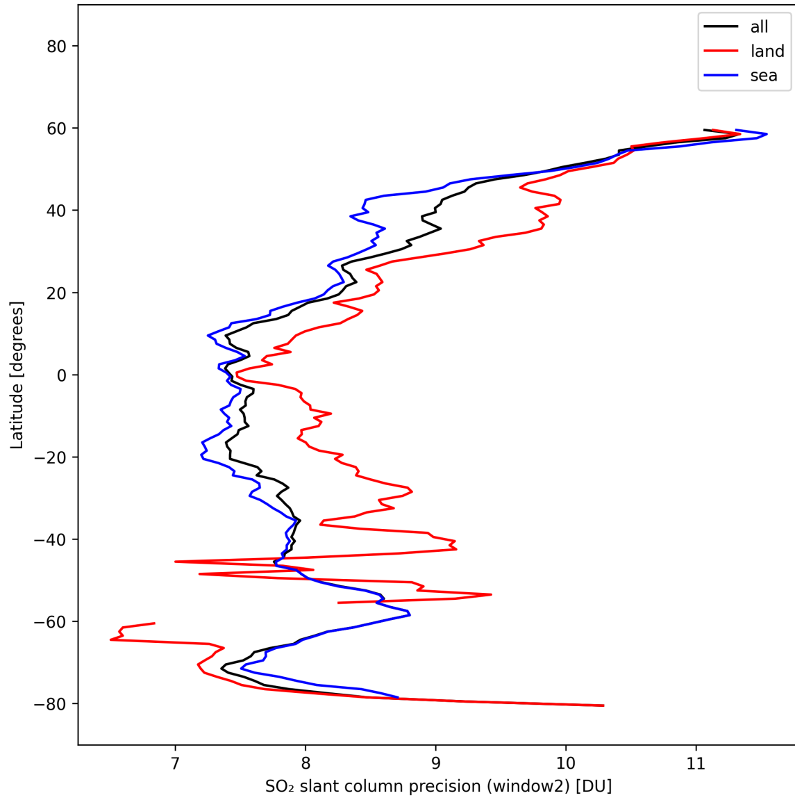
Figure 42: Zonal average of “SO 2 slant column precision (window2)” for 2025-10-19 to 2025-10-21.
