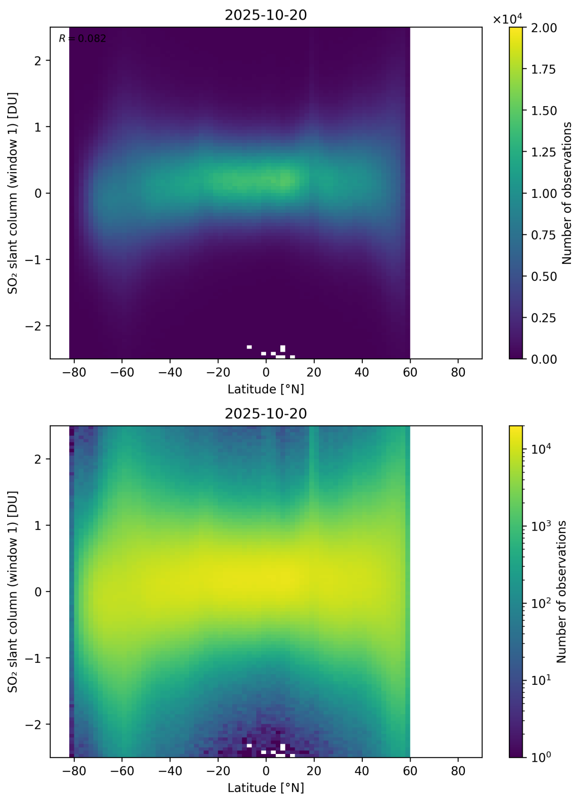
Figure 162: Scatter density plot of “Latitude” against “SO 2 slant column (window 1)” for 2025-10-19 to 2025-10-21.
