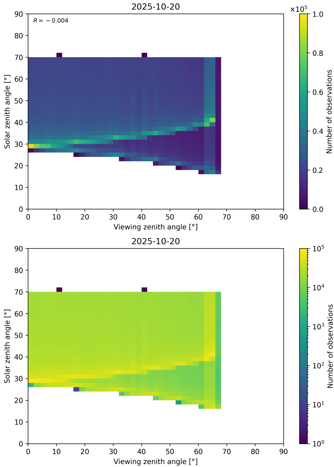
Figure 369: Scatter density plot of “Viewing zenith angle” against “Solar zenith angle” for 2025-10-19 to 2025-10-21.
