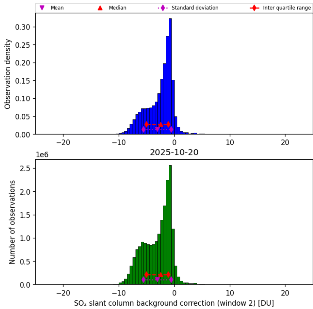
Figure 70: Histogram of “SO 2 slant column background correction (window 2)” for 2025-10-19 to 2025-10-21
