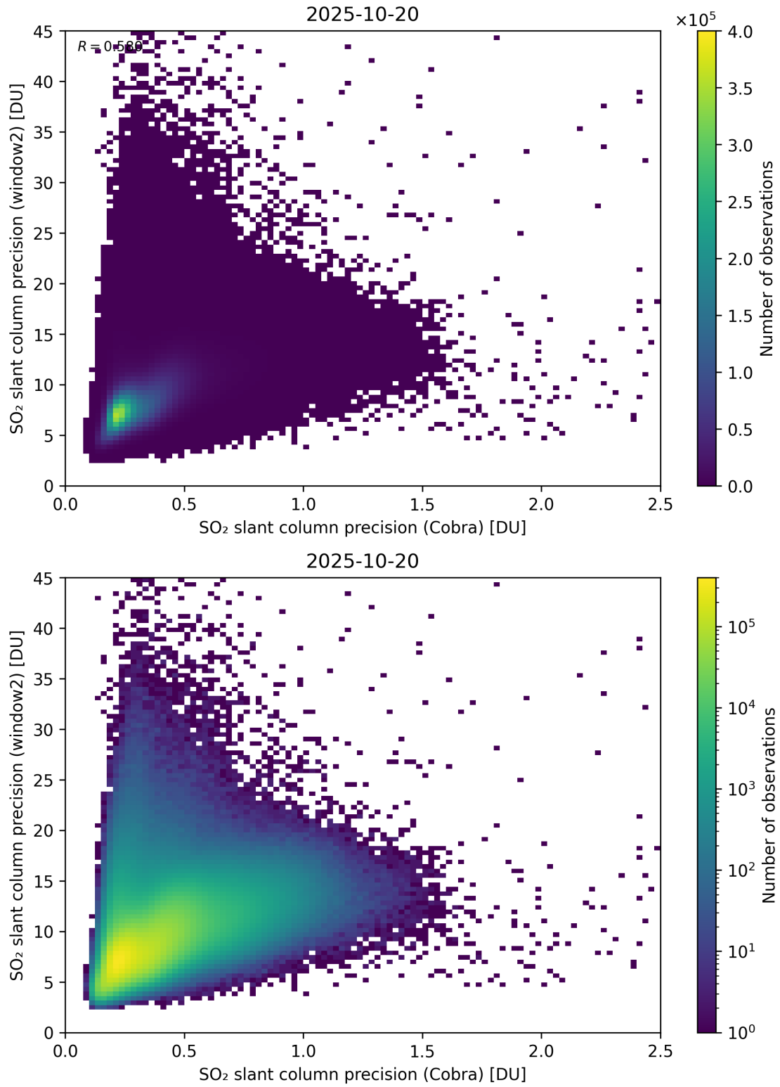
Figure 210: Scatter density plot of “SO 2 slant column precision (Cobra)” against “SO 2 slant column precision (window2)” for 2025-10-19 to 2025-10-21.
