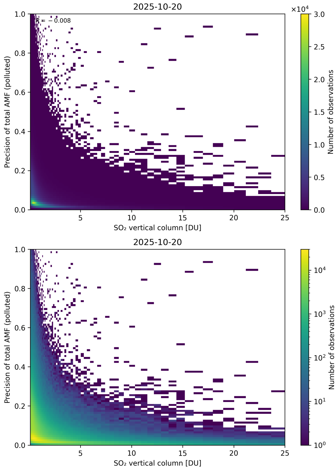
Figure 360: Scatter density plot of “SO 2 vertical column” against “Precision of total AMF (polluted)” for 2025-10-19 to 2025-10-21.
