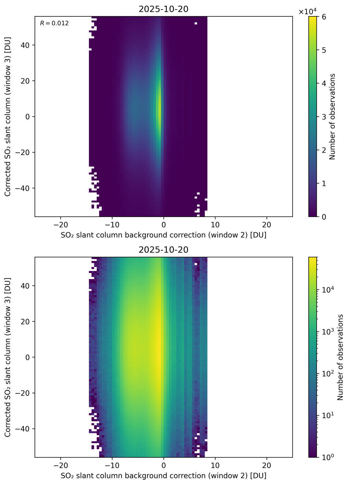
Figure 127: Scatter density plot of “SO 2 slant column background correction (window 2)” against “Corrected SO 2 slant column (window 3)” for 2025-10-19 to 2025-10-21.
