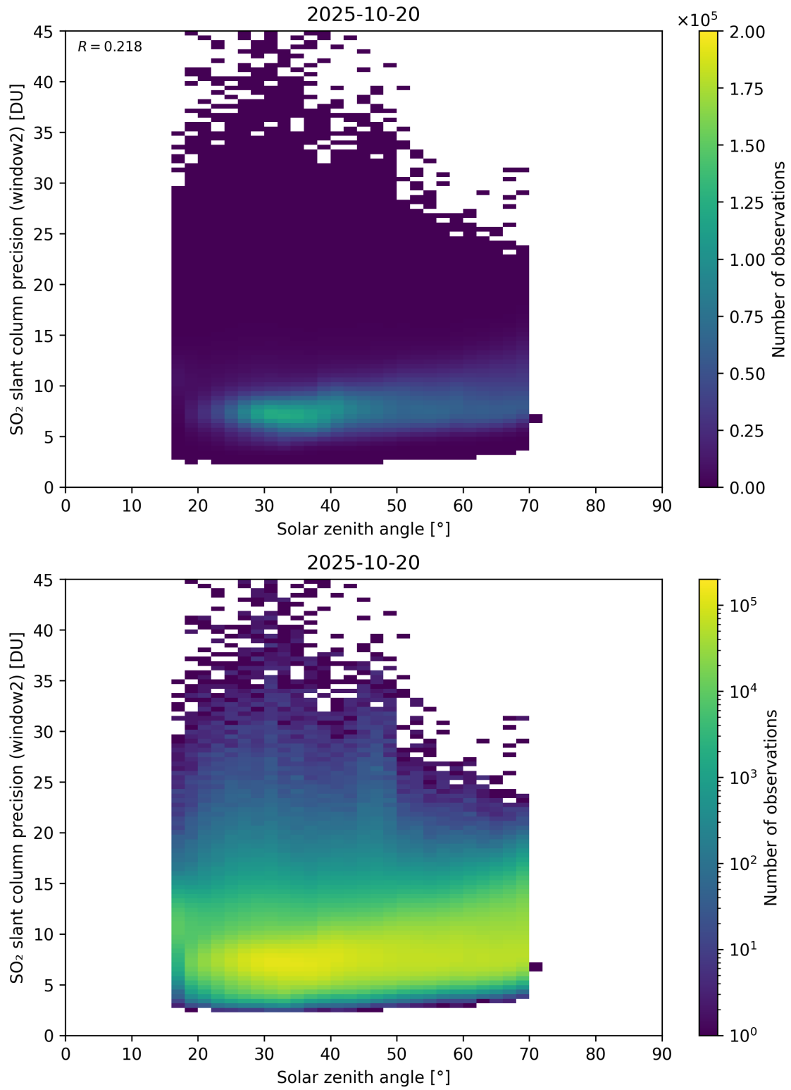
Figure 186: Scatter density plot of “Solar zenith angle” against “SO 2 slant column precision (window2)” for 2025-10-19 to 2025-10-21.
