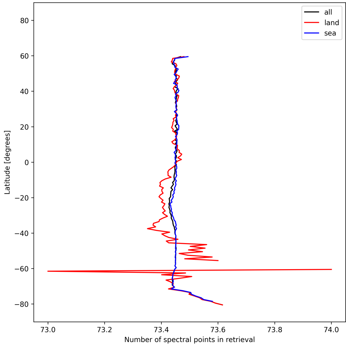
Figure 56: Zonal average of “Number of spectral points in retrieval” for 2025-10-19 to 2025-10-21.
