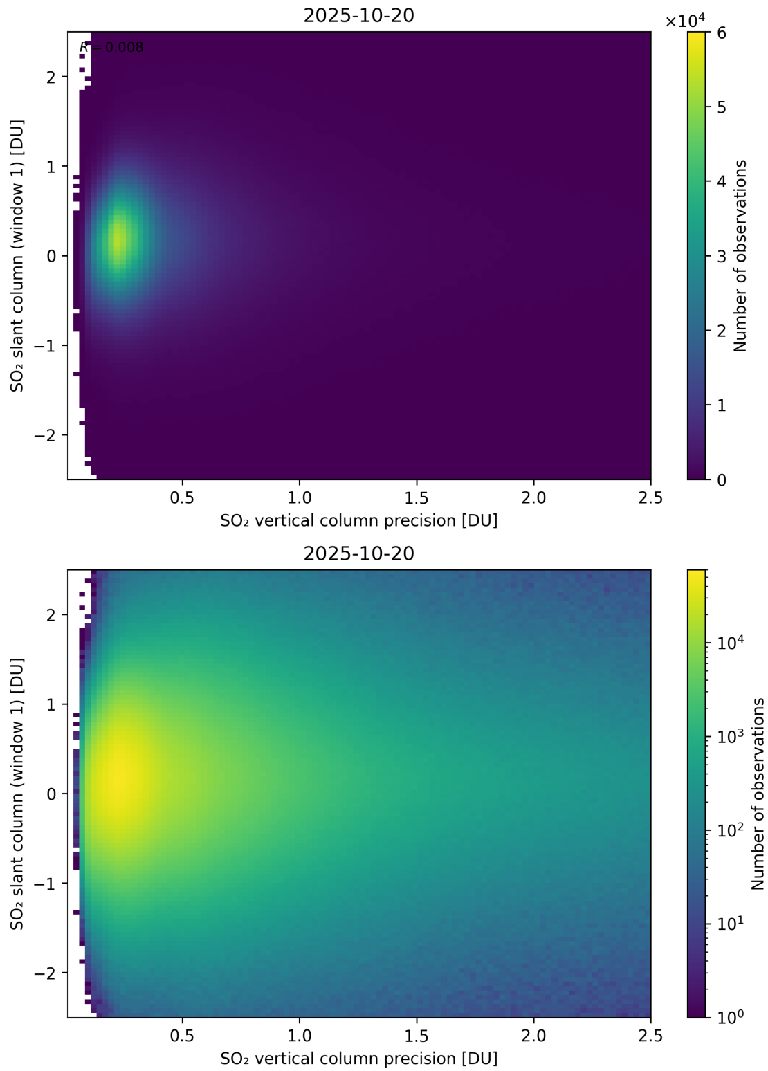
Figure 341: Scatter density plot of “SO 2 vertical column precision” against “SO 2 slant column (window 1)” for 2025-10-19 to 2025-10-21.
