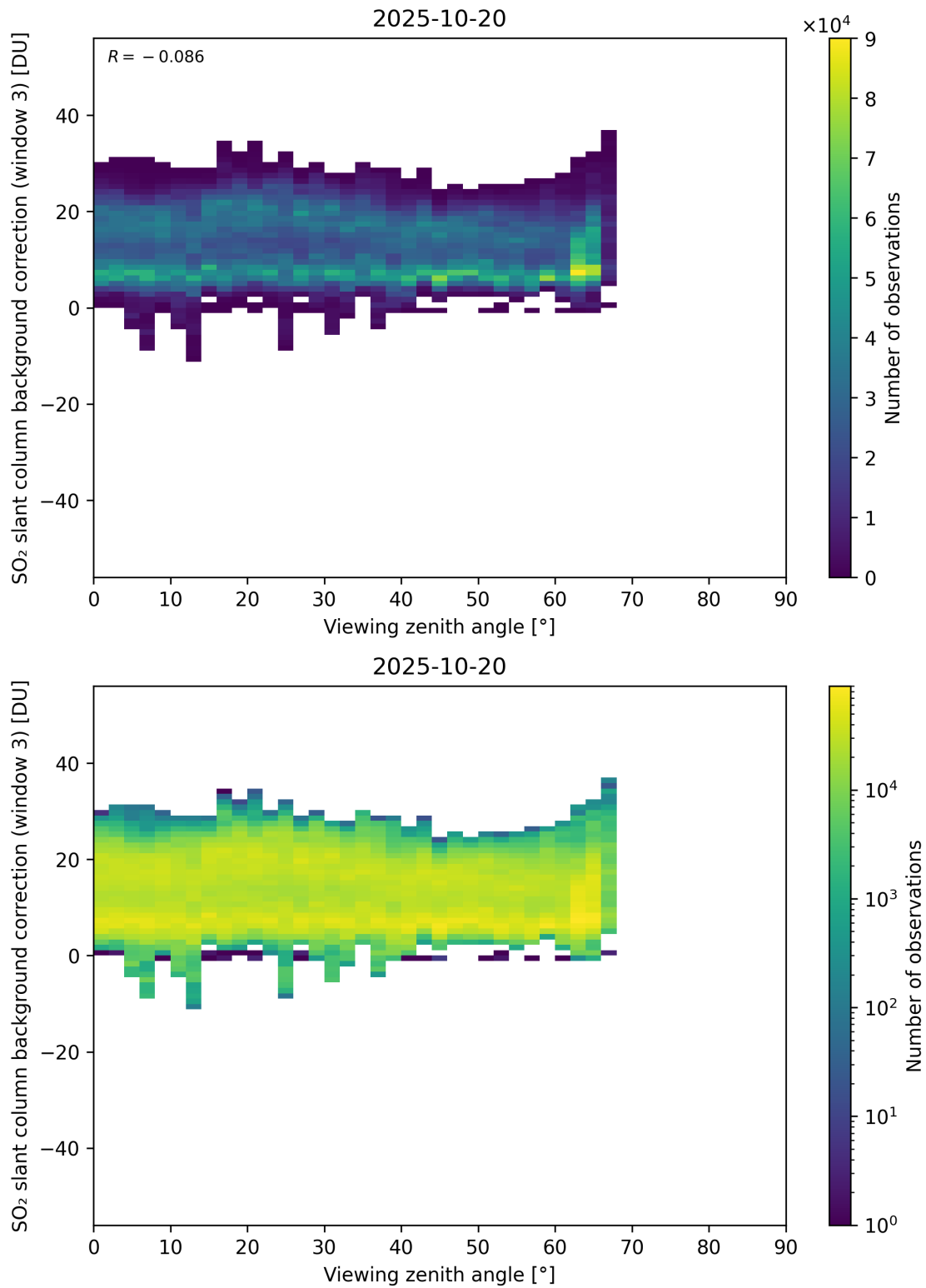
Figure 364: Scatter density plot of “Viewing zenith angle” against “SO 2 slant column background correction (window 3)” for 2025-10-19 to 2025-10-21.
