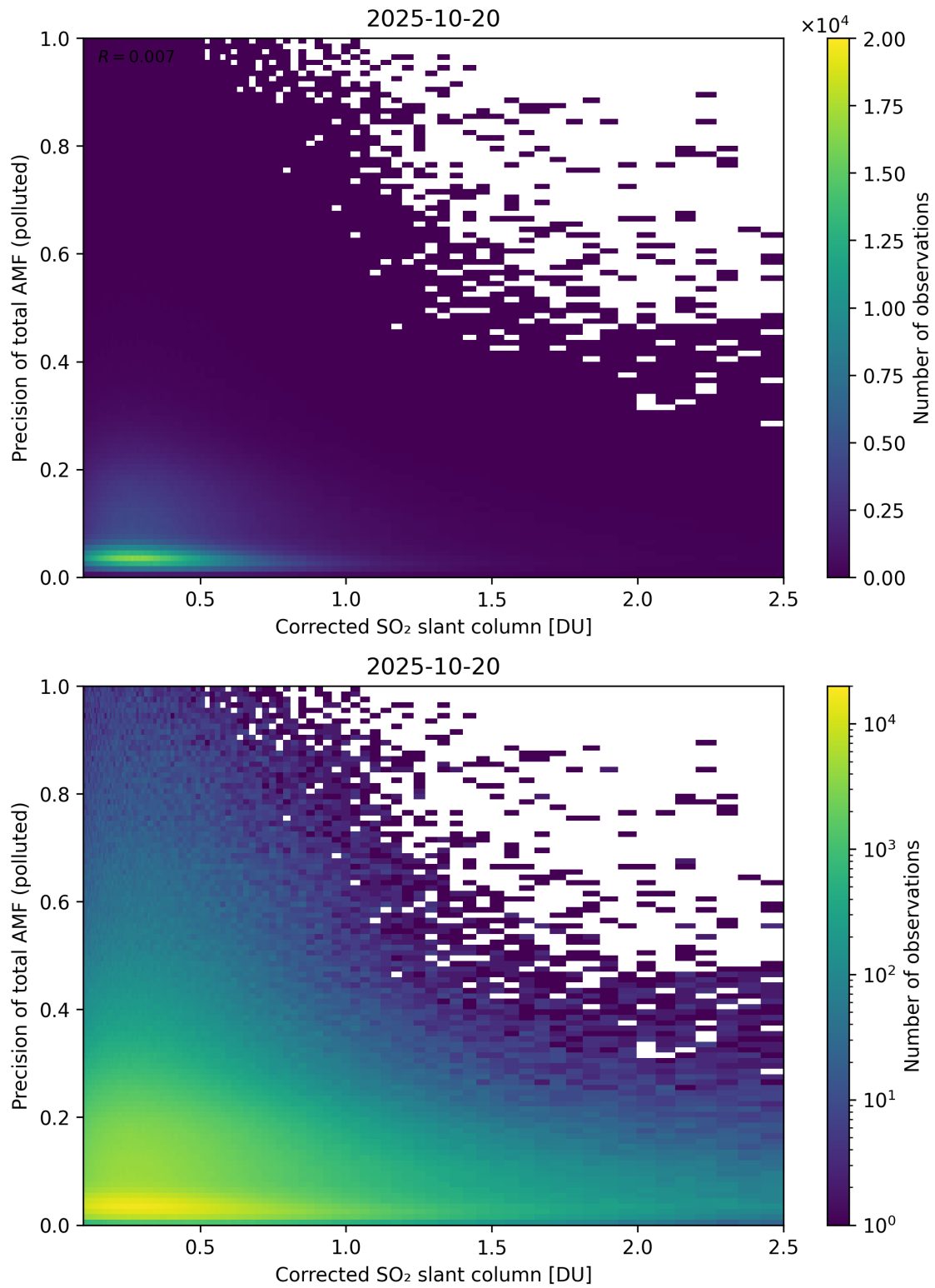
Figure 243: Scatter density plot of “Corrected SO 2 slant column” against “Precision of total AMF (polluted)” for 2025-10-19 to 2025-10-21.
