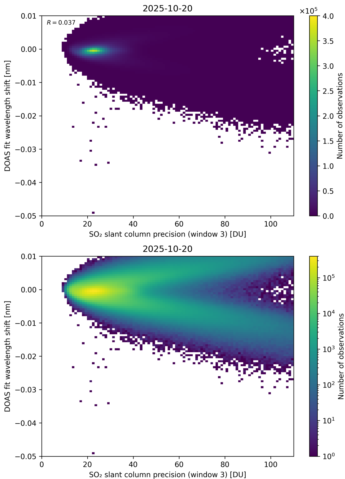
Figure 308: Scatter density plot of “SO 2 slant column precision (window 3)” against “DOAS fit wavelength shift” for 2025-10-19 to 2025-10-21.
