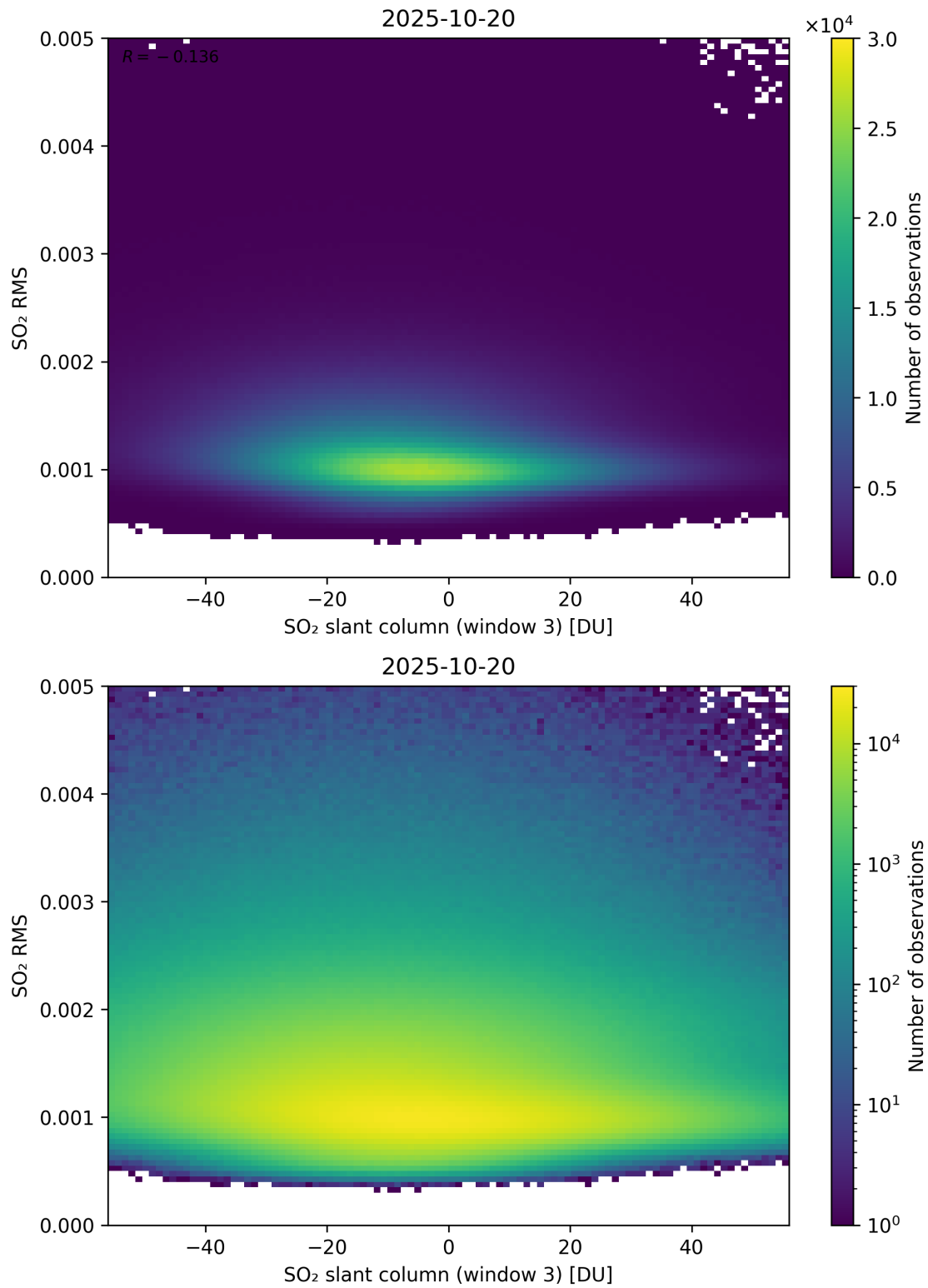
Figure 306: Scatter density plot of “SO 2 slant column (window 3)” against “SO 2 RMS” for 2025-10-19 to 2025-10-21.
