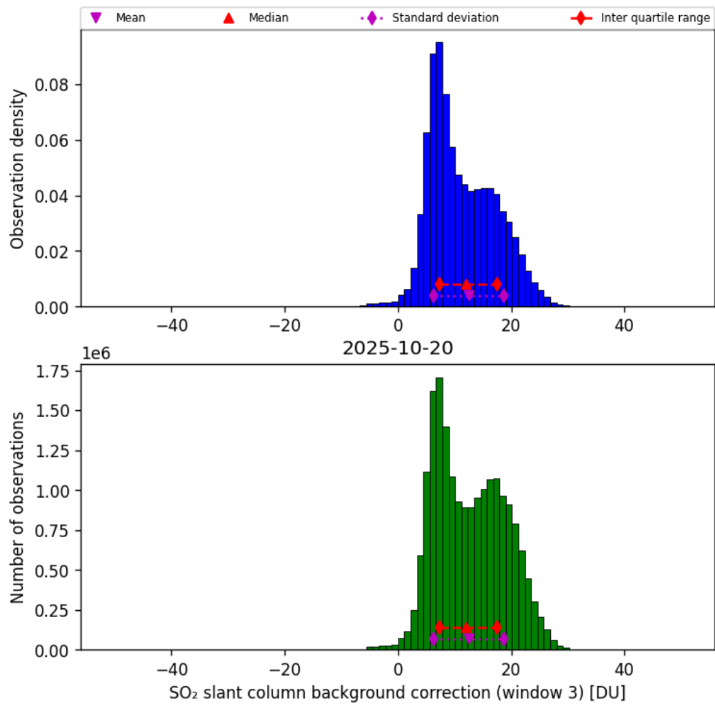
Figure 74: Histogram of “SO 2 slant column background correction (window 3)” for 2025-10-19 to 2025-10-21
