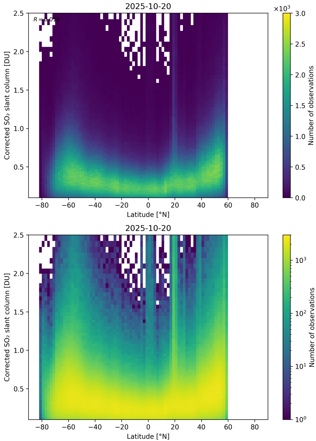
Figure 159: Scatter density plot of “Latitude” against “Corrected SO 2 slant column” for 2025-10-19 to 2025-10-21.
