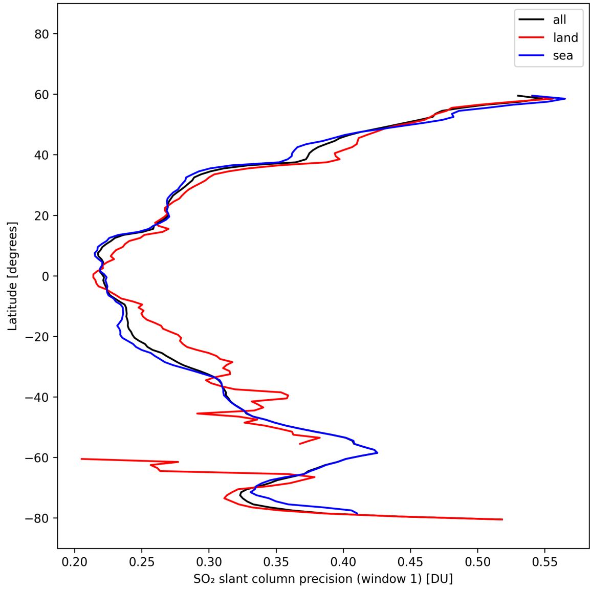
Figure 38: Zonal average of “SO 2 slant column precision (window 1)” for 2025-10-19 to 2025-10-21.
