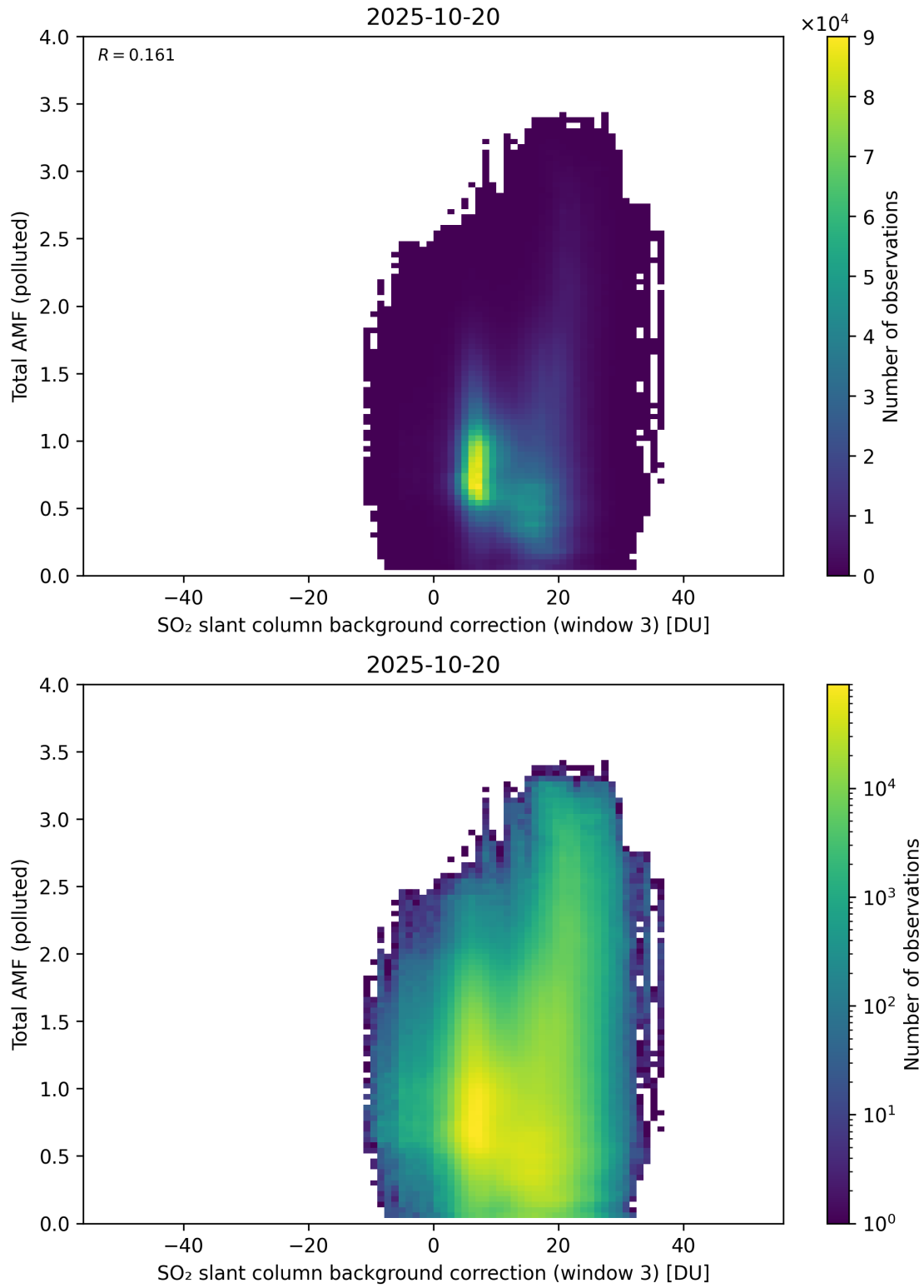
Figure 136: Scatter density plot of “SO 2 slant column background correction (window 3)” against “Total AMF (polluted)” for 2025-10-19 to 2025-10-21.
