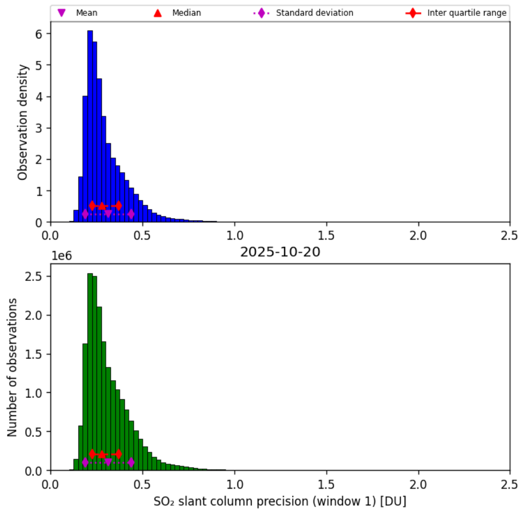
Figure 64: Histogram of “SO 2 slant column precision (window 1)” for 2025-10-19 to 2025-10-21
