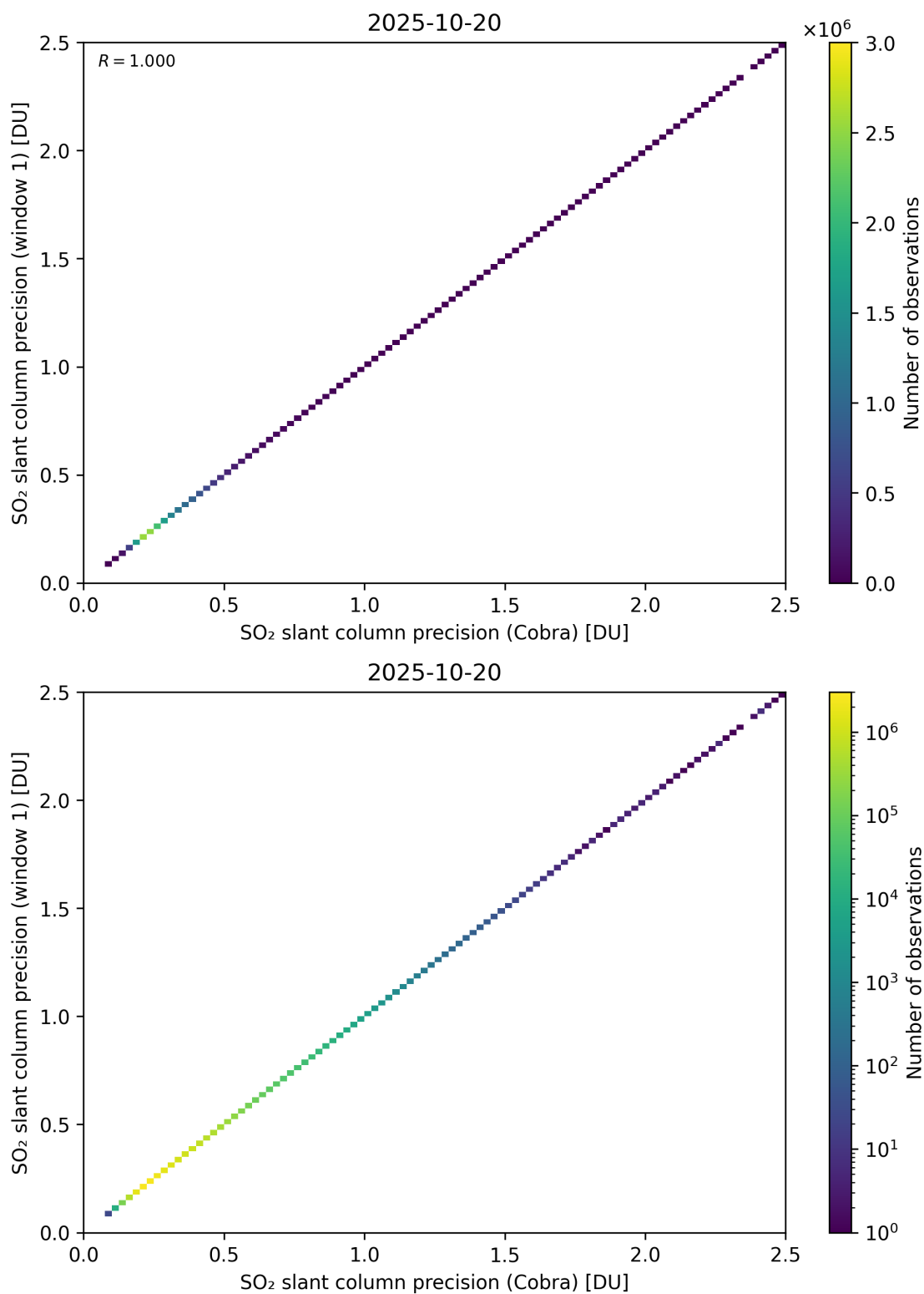
Figure 209: Scatter density plot of “SO 2 slant column precision (Cobra)” against “SO 2 slant column precision (window 1)” for 2025-10-19 to 2025-10-21.
