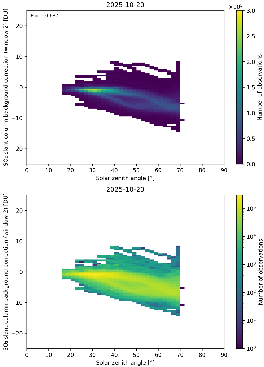
Figure 172: Scatter density plot of “Solar zenith angle” against “SO 2 slant column background correction (window 2)” for 2025-10-19 to 2025-10-21.
