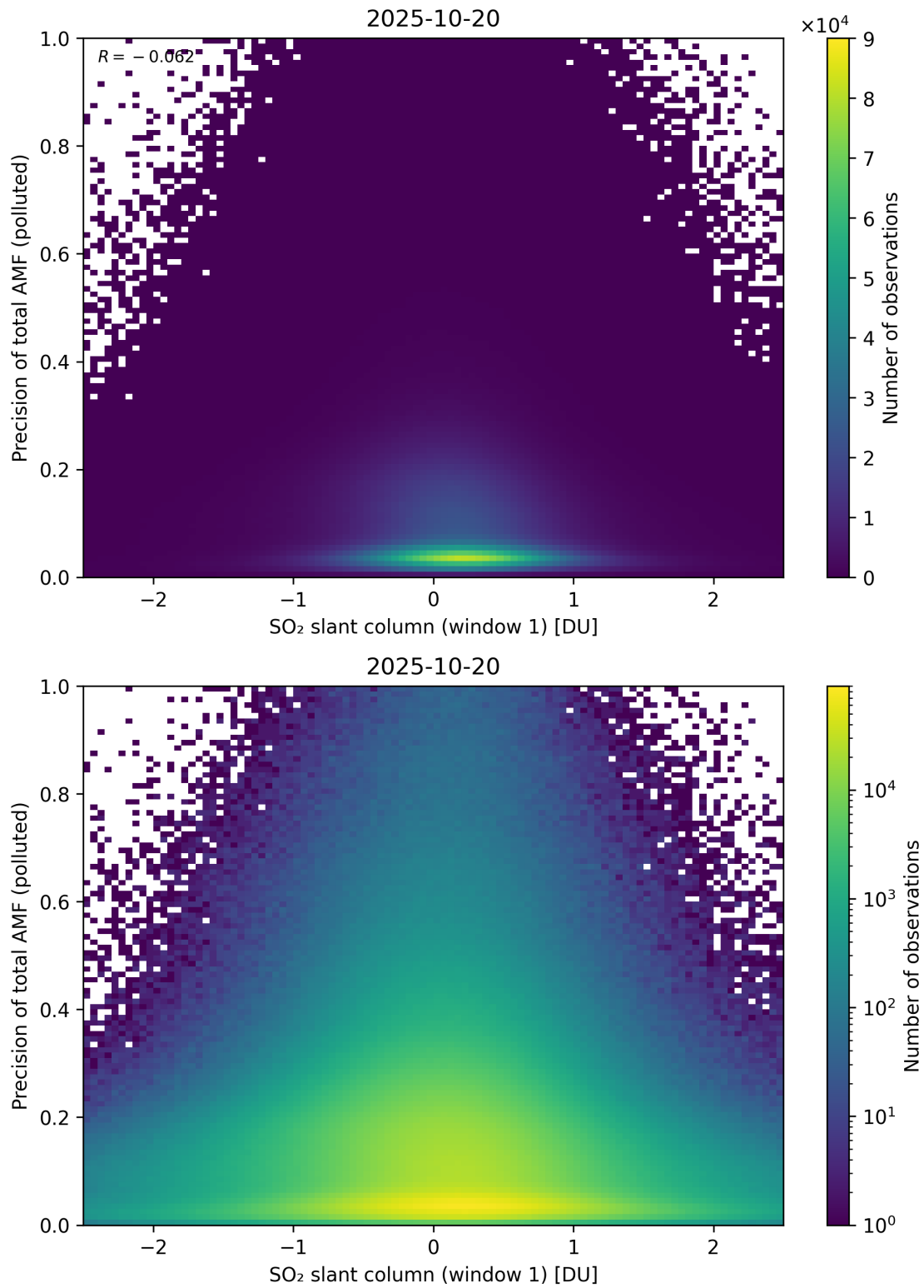
Figure 290: Scatter density plot of “SO 2 slant column (window 1)” against “Precision of total AMF (polluted)” for 2025-10-19 to 2025-10-21.
