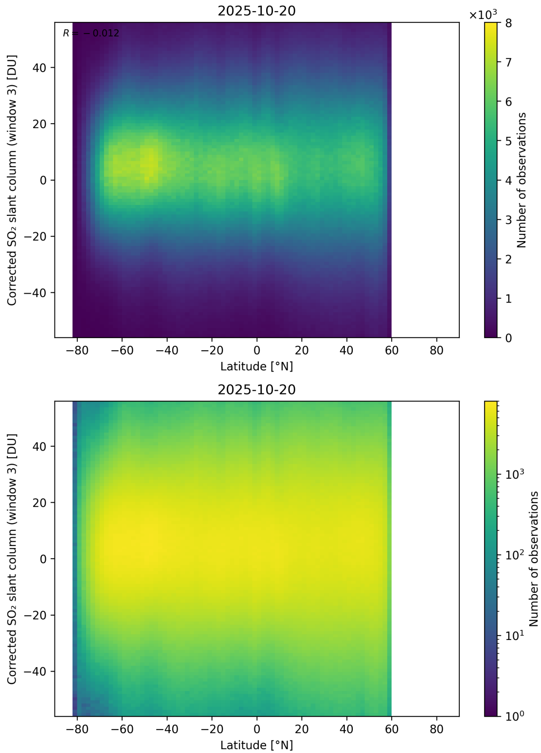
Figure 161: Scatter density plot of “Latitude” against “Corrected SO 2 slant column (window 3)” for 2025-10-19 to 2025-10-21.
