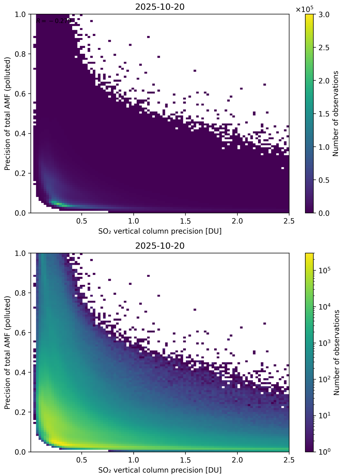
Figure 347: Scatter density plot of “SO 2 vertical column precision” against “Precision of total AMF (polluted)” for 2025-10-19 to 2025-10-21.
