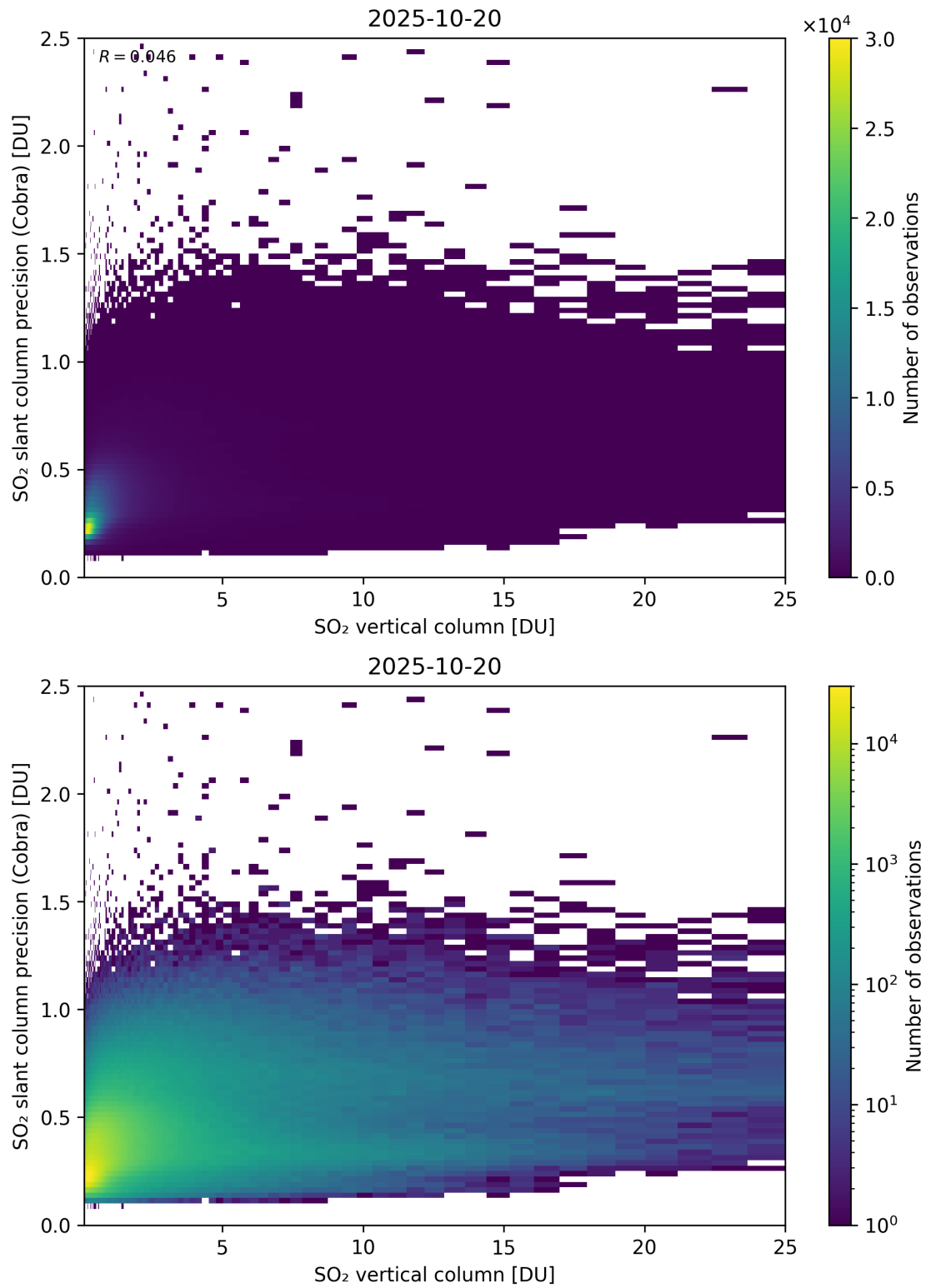
Figure 350: Scatter density plot of “SO 2 vertical column” against “SO 2 slant column precision (Cobra)” for 2025-10-19 to 2025-10-21.
