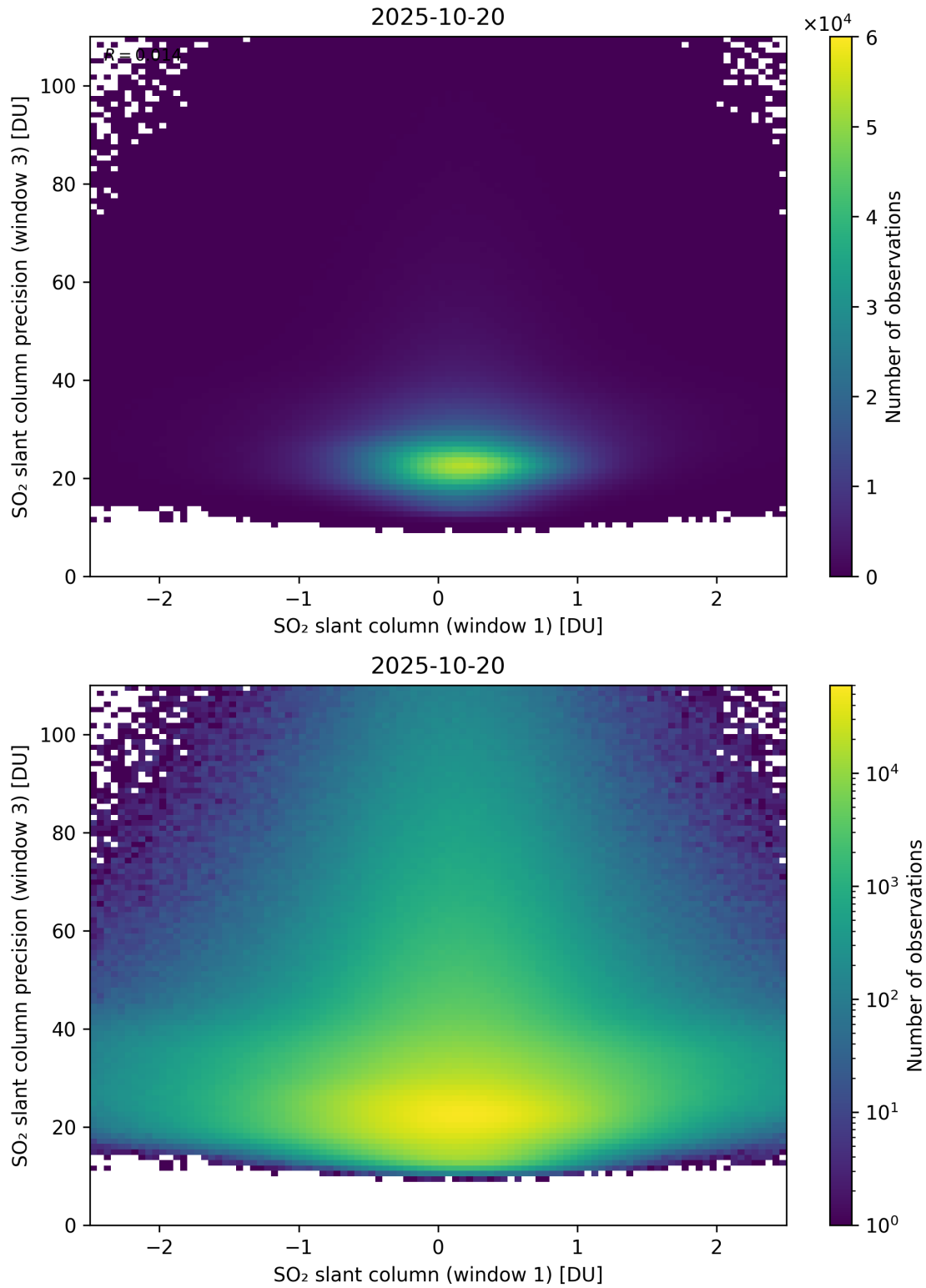
Figure 288: Scatter density plot of “SO 2 slant column (window 1)” against “SO 2 slant column precision (window 3)” for 2025-10-19 to 2025-10-21.
