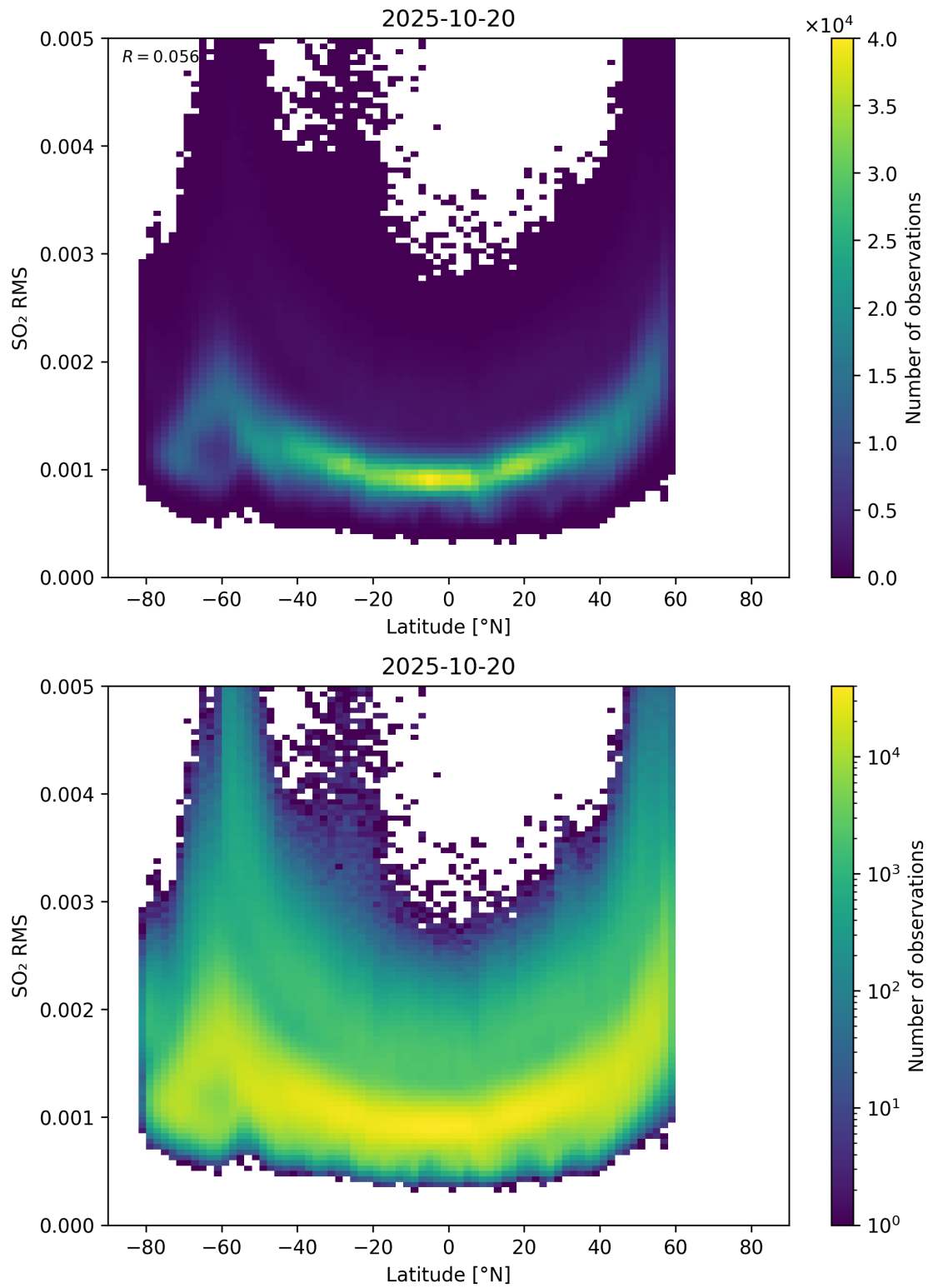
Figure 155: Scatter density plot of “Latitude” against “SO 2 RMS” for 2025-10-19 to 2025-10-21.
