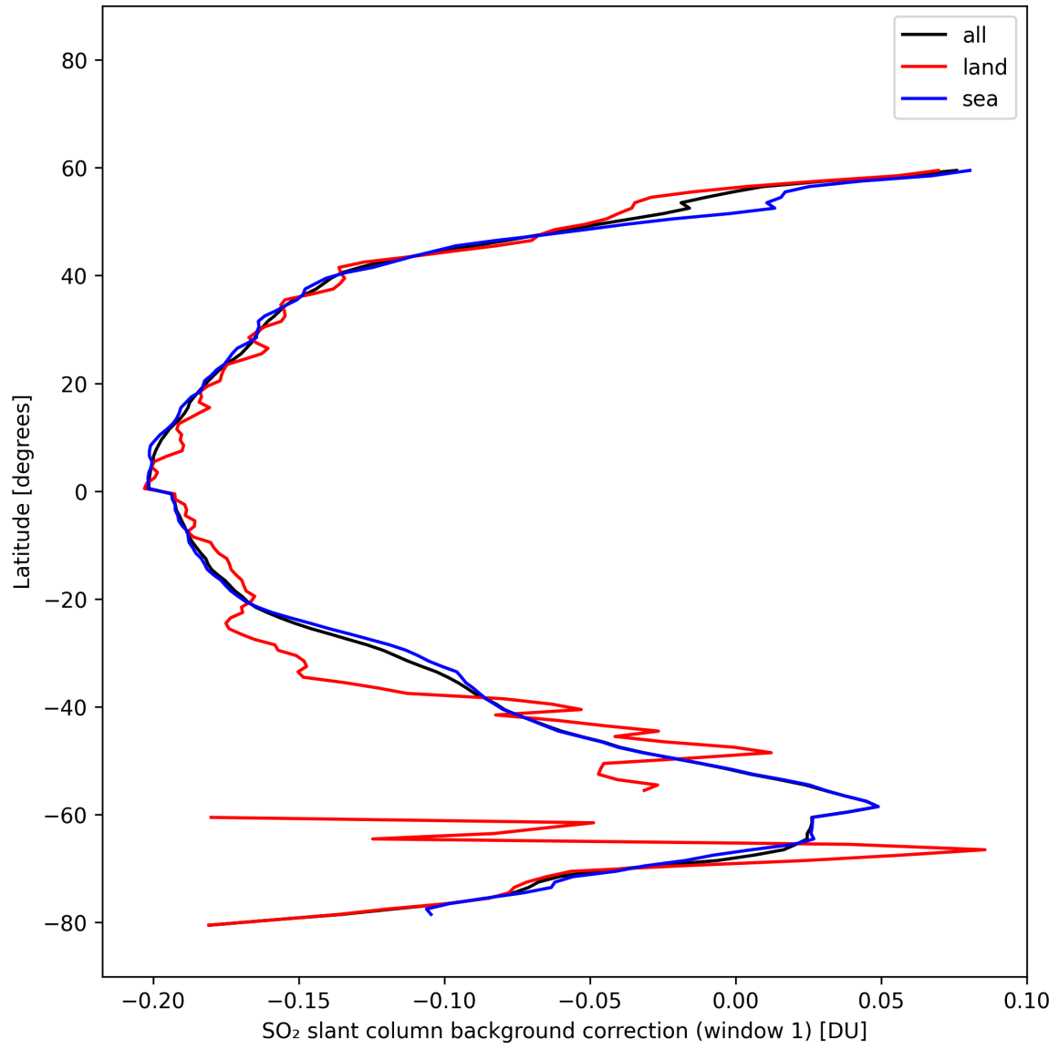
Figure 40: Zonal average of “SO 2 slant column background correction (window 1)” for 2025-10-19 to 2025-10-21.
