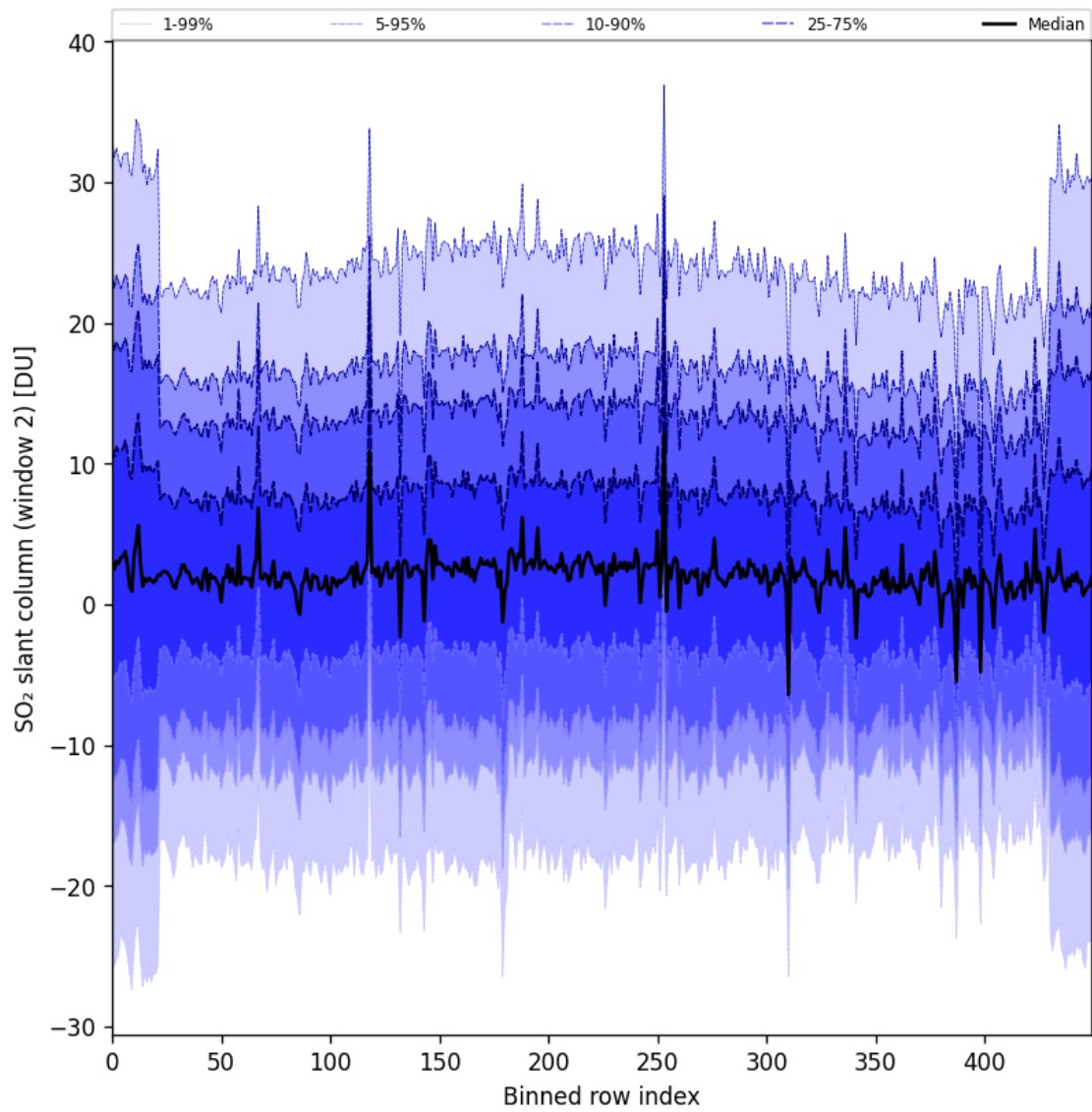
Figure 93: Along track statistics of “SO 2 slant column (window 2)” for 2025-10-19 to 2025-10-21
