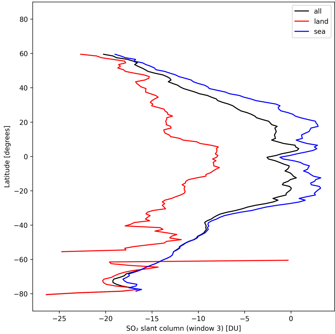
Figure 45: Zonal average of “SO 2 slant column (window 3)” for 2025-10-19 to 2025-10-21.
