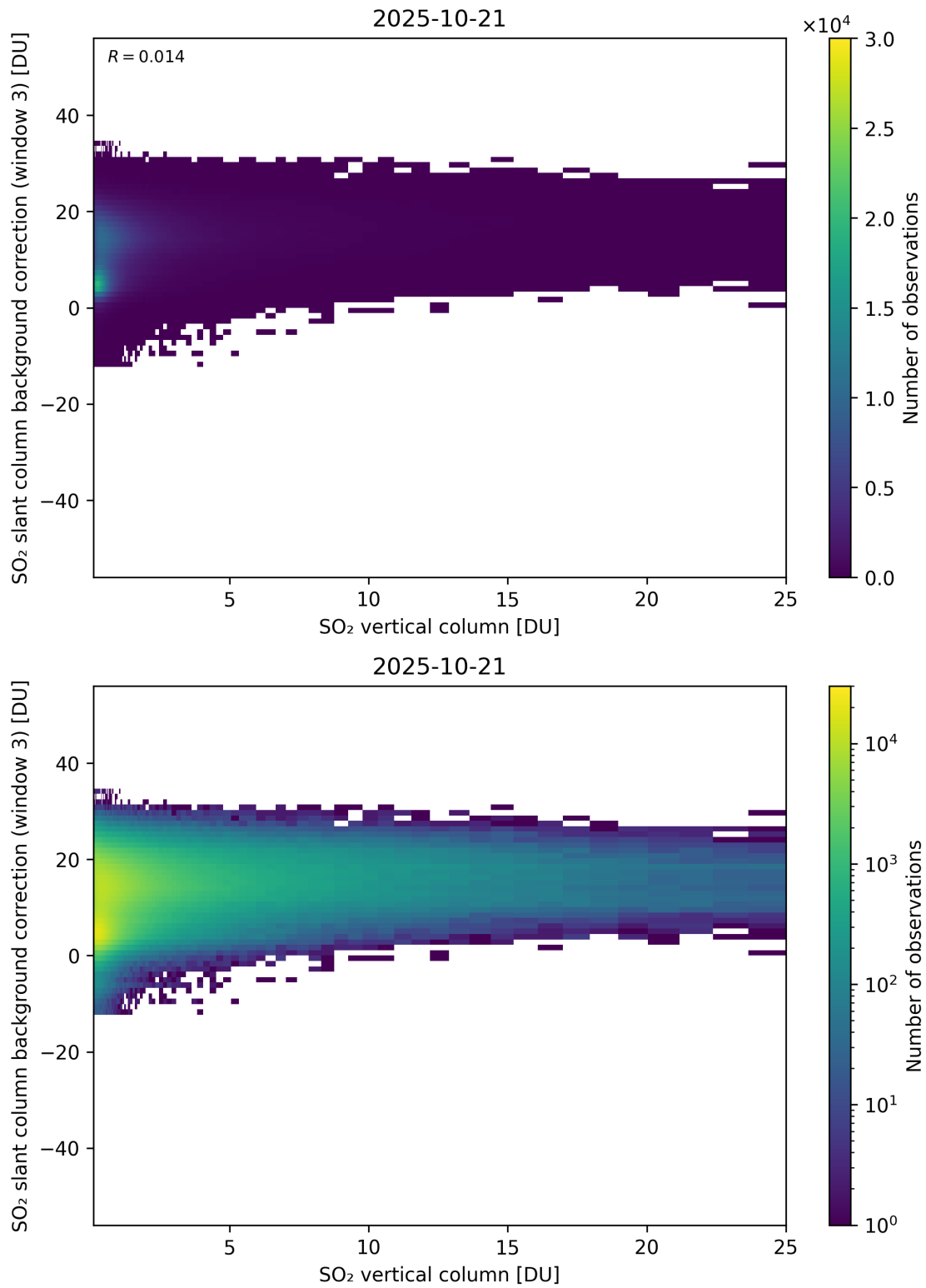
Figure 325: Scatter density plot of “SO 2 vertical column” against “SO 2 slant column background correction (window 3)” for 2025-10-20 to 2025-10-22.
