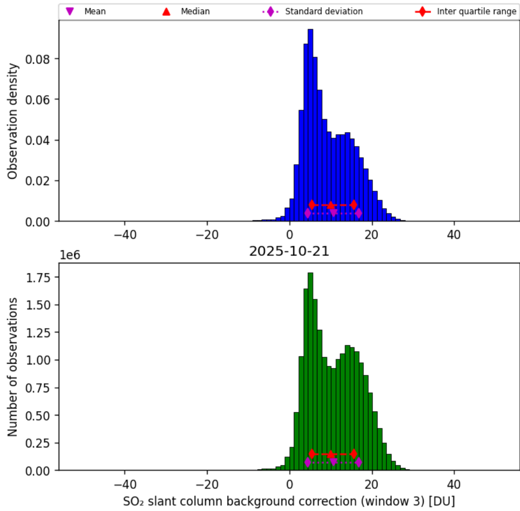
Figure 74: Histogram of “SO 2 slant column background correction (window 3)” for 2025-10-20 to 2025-10-22
