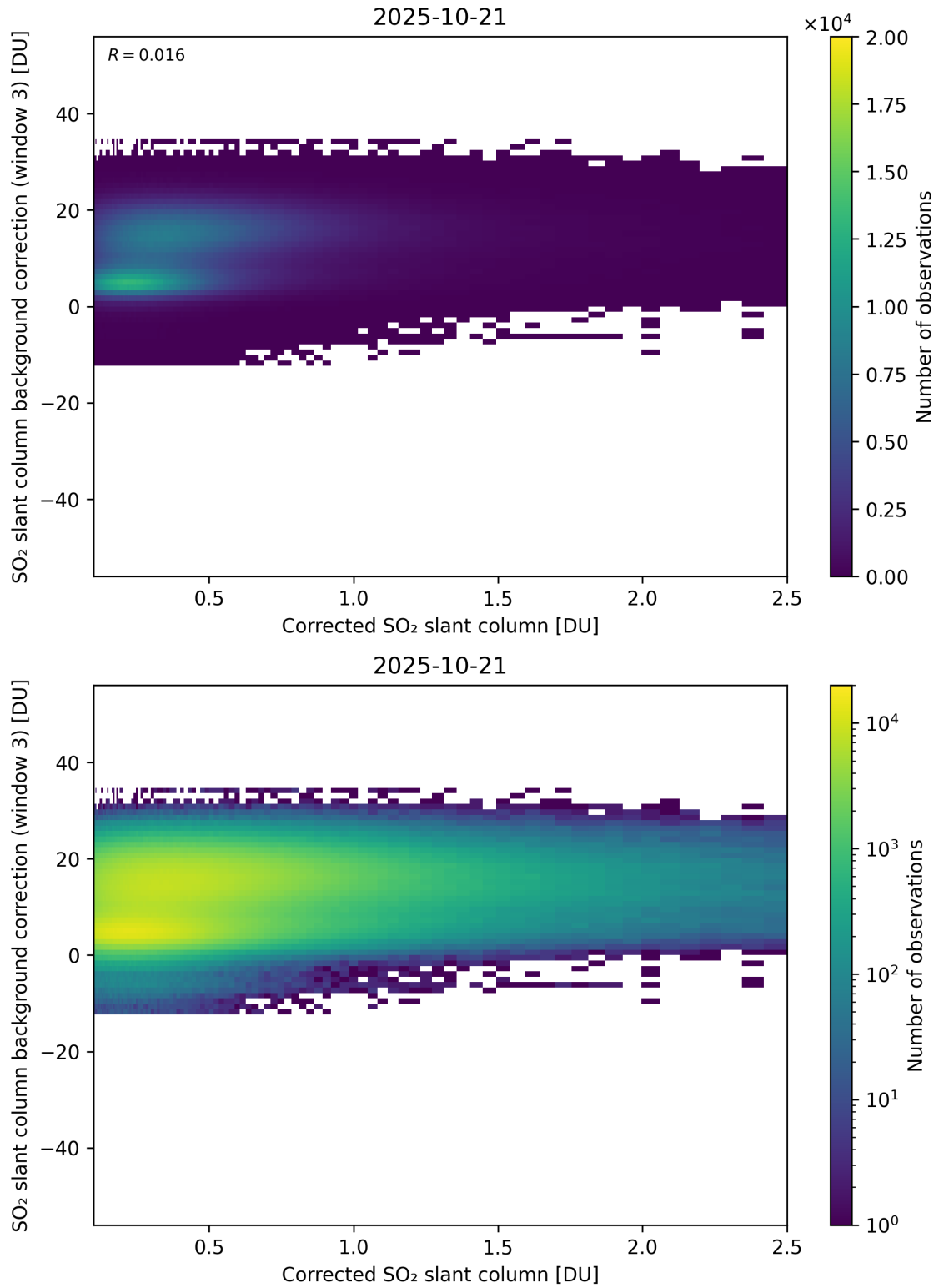
Figure 228: Scatter density plot of “Corrected SO 2 slant column” against “SO 2 slant column background correction (window 3)” for 2025-10-20 to 2025-10-22.
