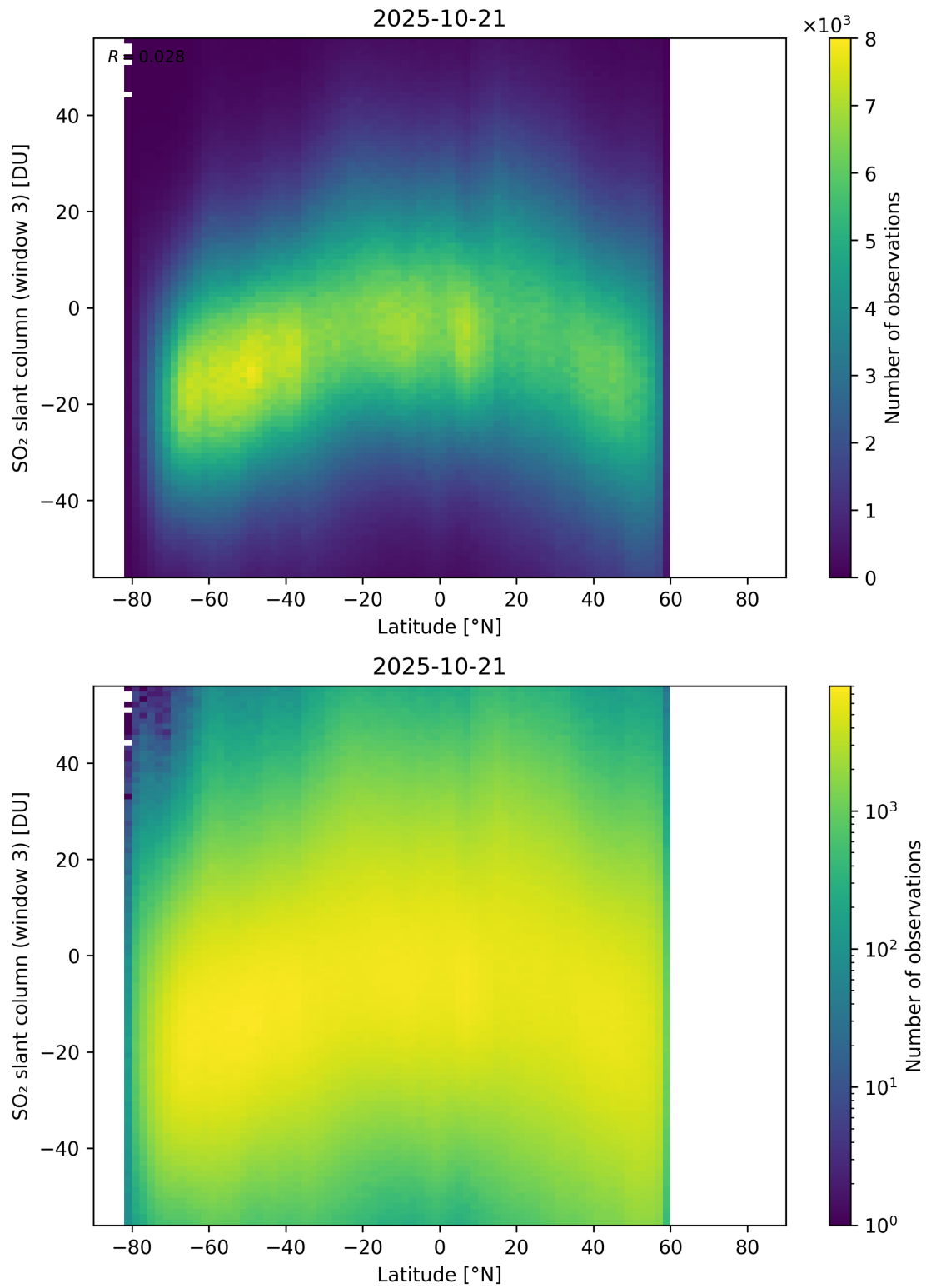
Figure 165: Scatter density plot of “Latitude” against “SO 2 slant column (window 3)” for 2025-10-20 to 2025-10-22.
