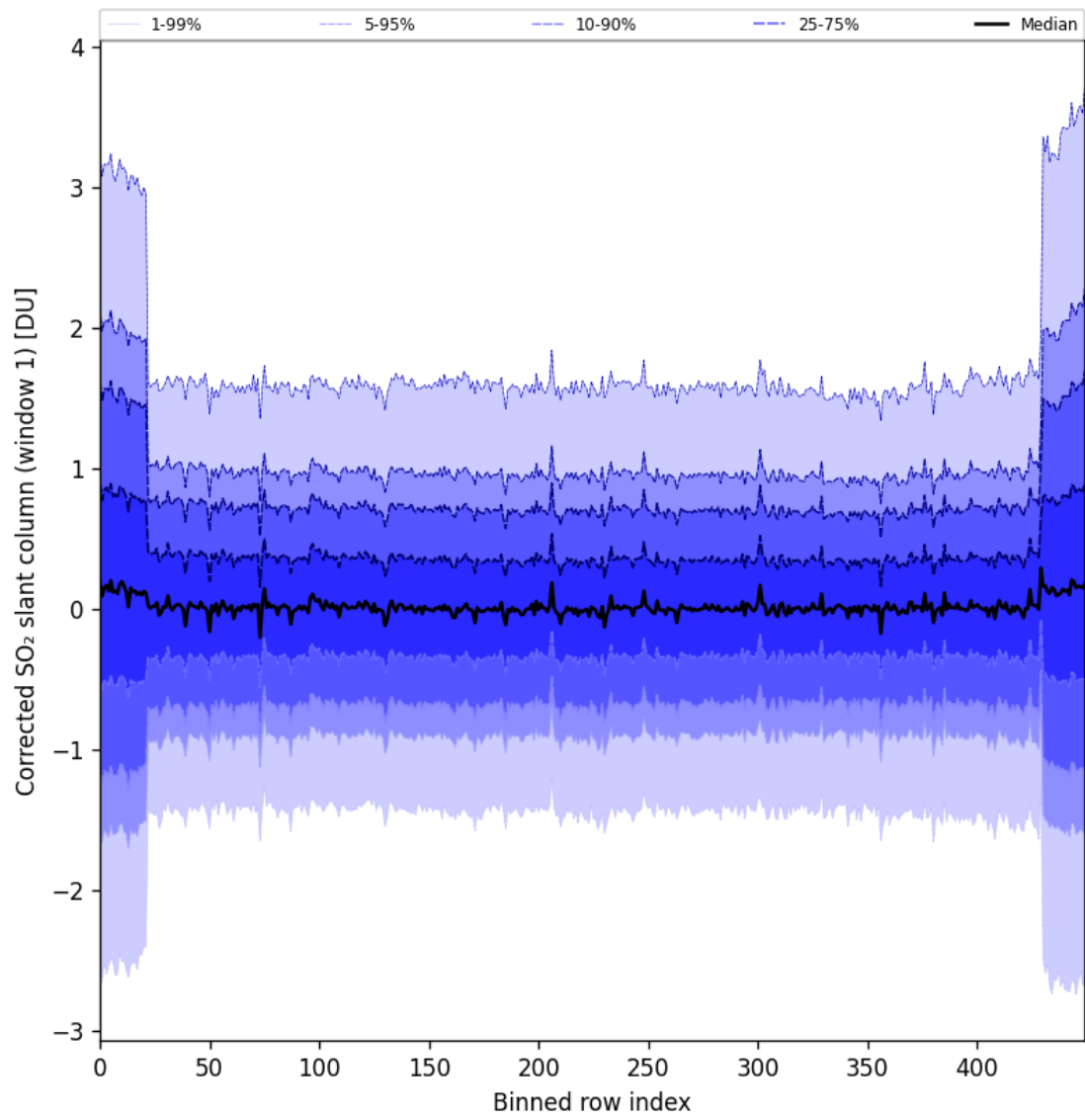
Figure 91: Along track statistics of “Corrected SO 2 slant column (window 1)” for 2025-10-20 to 2025-10-22
