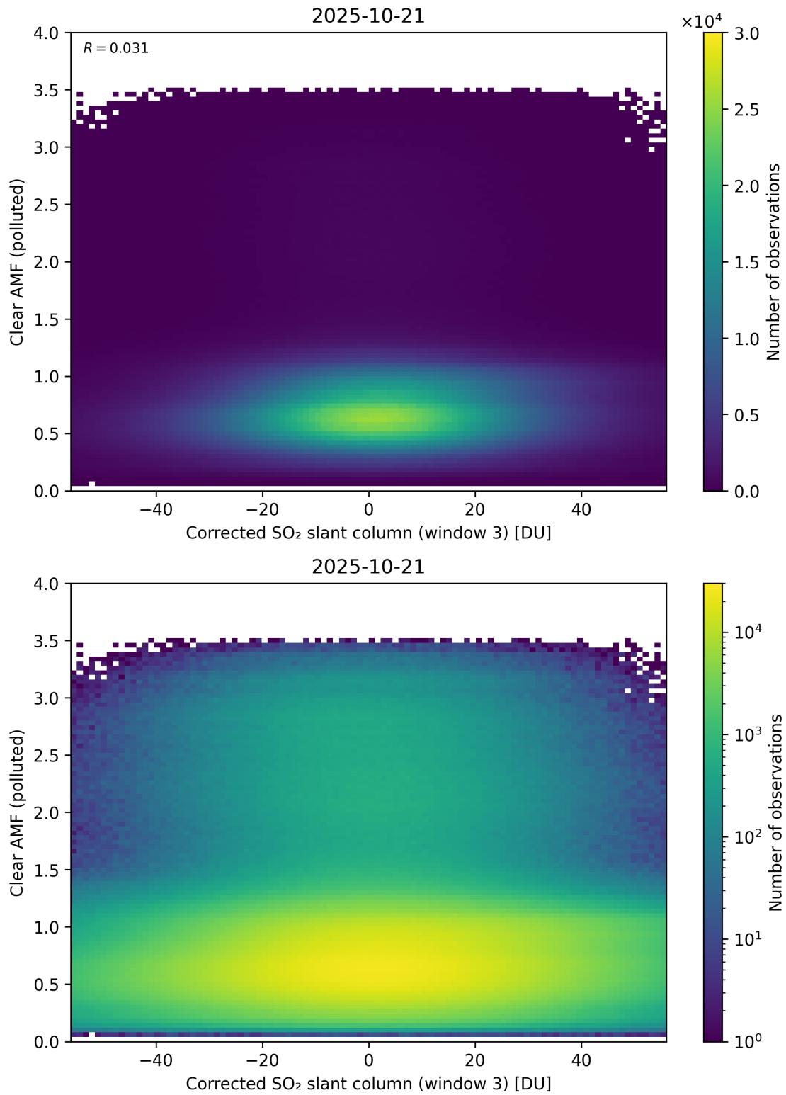
Figure 259: Scatter density plot of “Corrected SO 2 slant column (window 3)” against “Clear AMF (polluted)” for 2025-10-20 to 2025-10-22.
