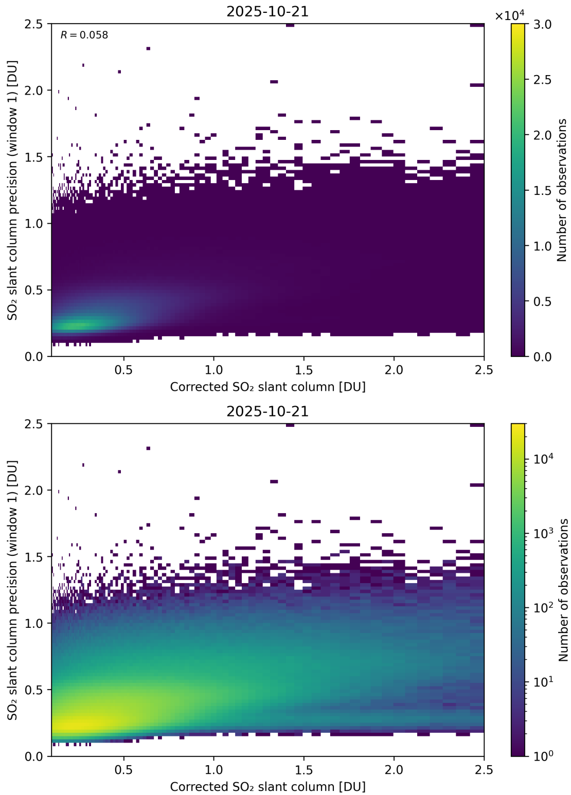
Figure 238: Scatter density plot of “Corrected SO 2 slant column” against “SO 2 slant column precision (window 1)” for 2025-10-20 to 2025-10-22.
