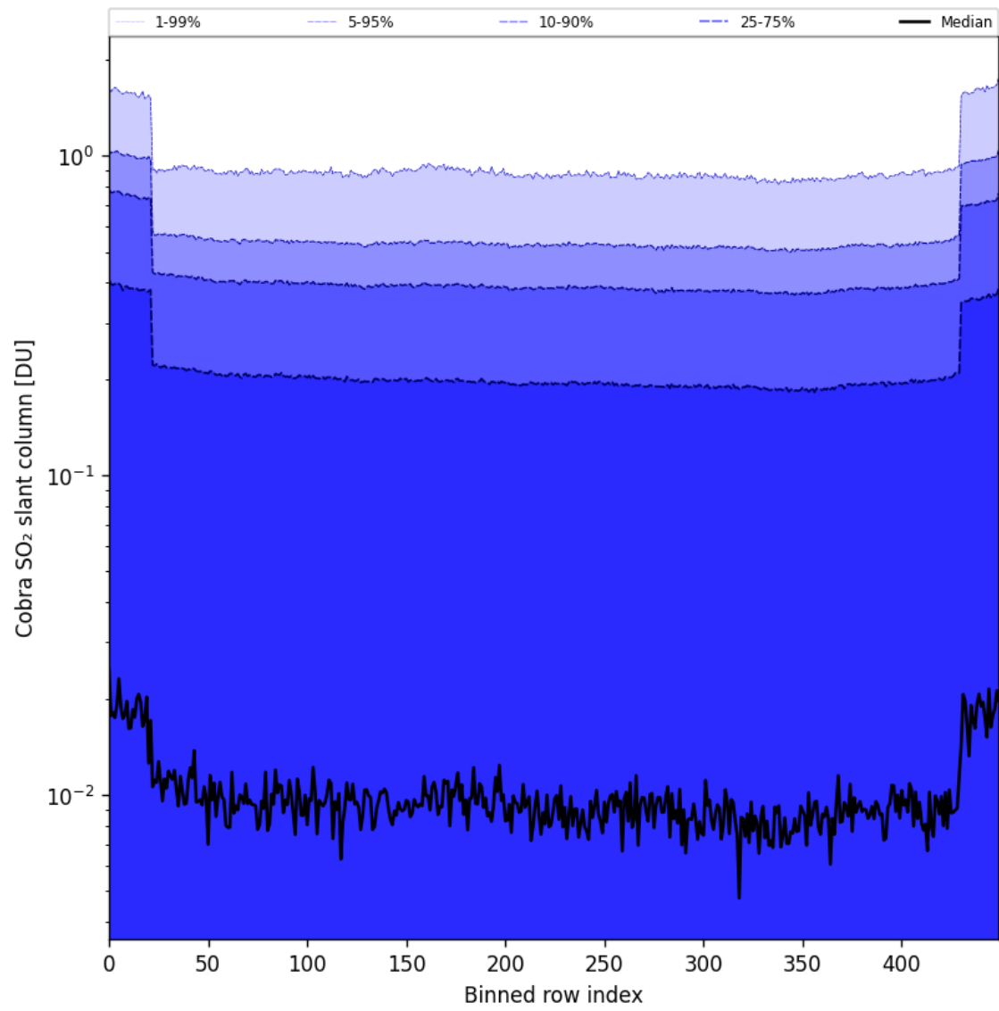
Figure 87: Along track statistics of “Cobra SO 2 slant column” for 2025-10-20 to 2025-10-22
