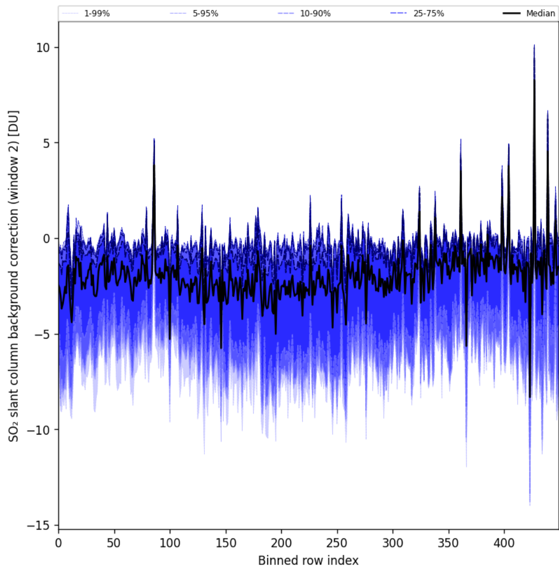
Figure 96: Along track statistics of “SO 2 slant column background correction (window 2)” for 2025-10-20 to 2025-10-22
