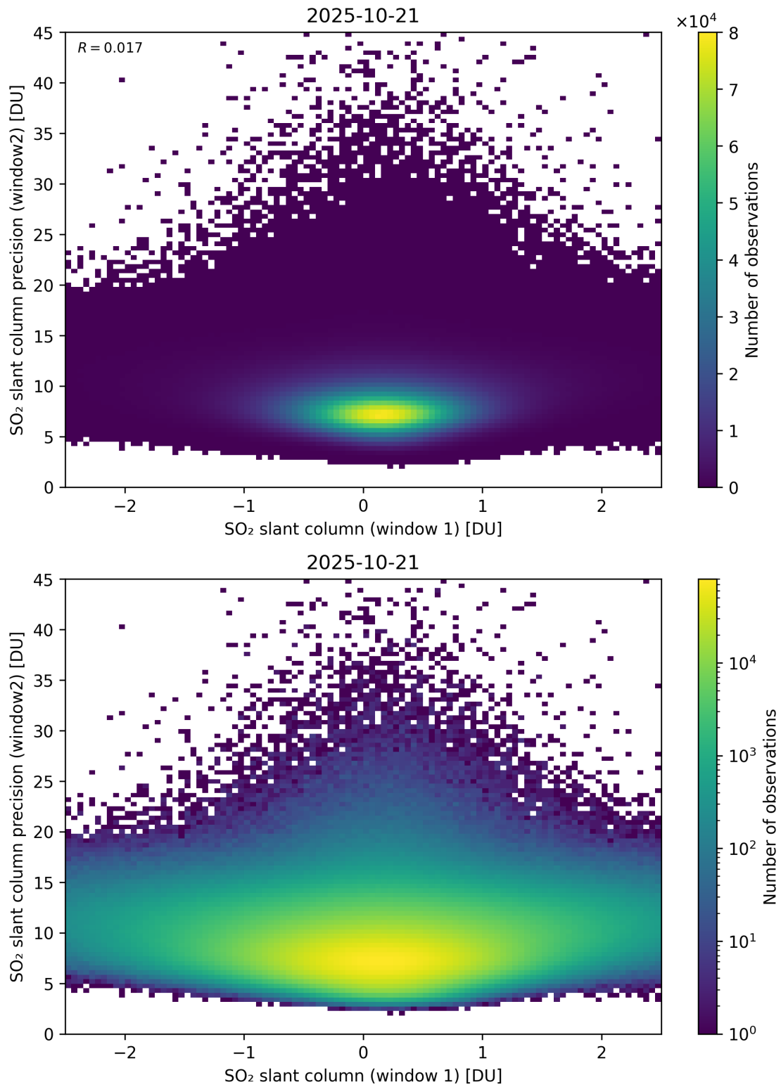
Figure 286: Scatter density plot of “SO 2 slant column (window 1)” against “SO 2 slant column precision (window2)” for 2025-10-20 to 2025-10-22.
