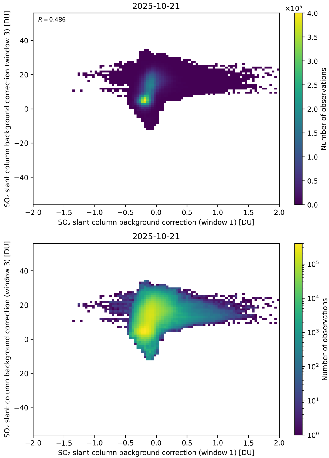
Figure 110: Scatter density plot of “SO 2 slant column background correction (window 1)” against “SO 2 slant column background correction (window 3)” for 2025-10-20 to 2025-10-22.
