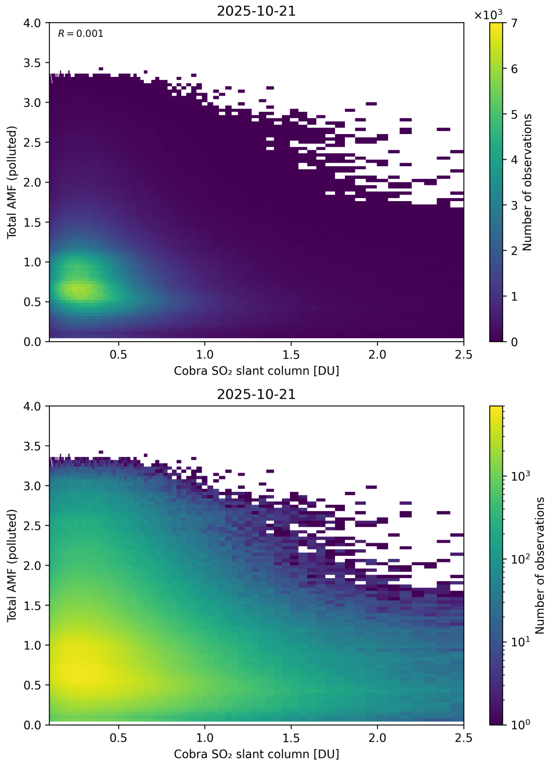
Figure 224: Scatter density plot of “Cobra SO 2 slant column” against “Total AMF (polluted)” for 2025-10-20 to 2025-10-22.
