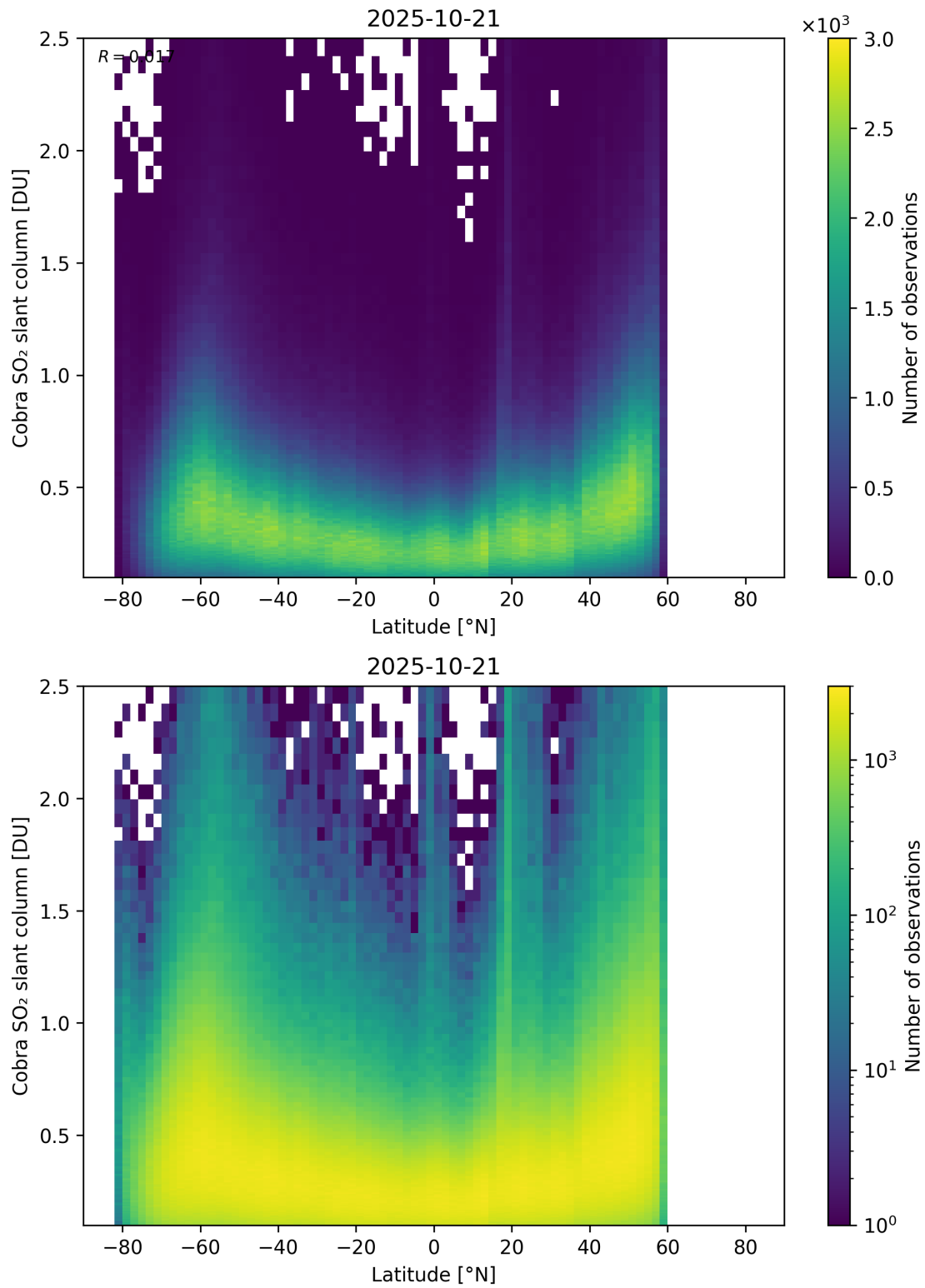
Figure 157: Scatter density plot of “Latitude” against “Cobra SO 2 slant column” for 2025-10-20 to 2025-10-22.
