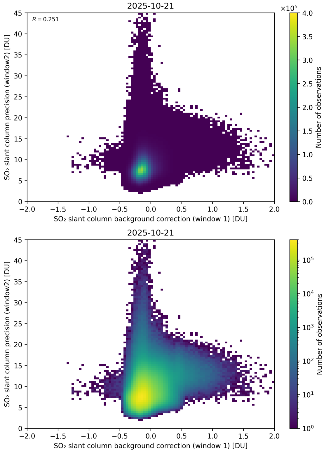
Figure 117: Scatter density plot of “SO 2 slant column background correction (window 1)” against “SO 2 slant column precision (window2)” for 2025-10-20 to 2025-10-22.
