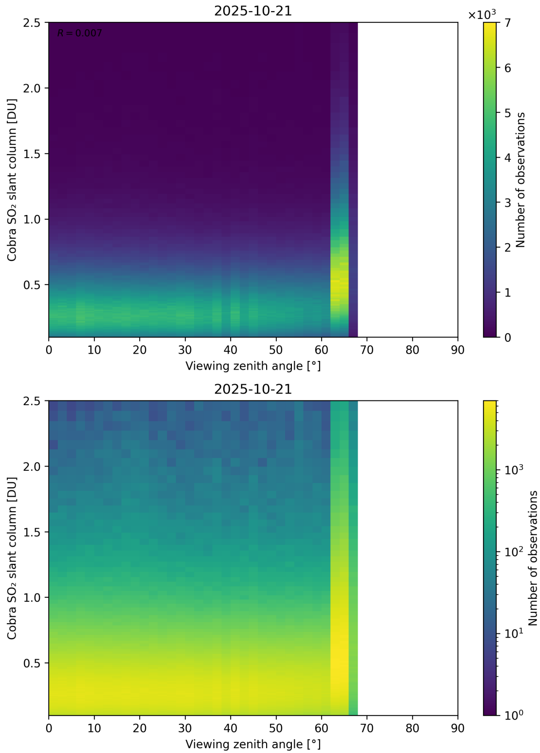
Figure 371: Scatter density plot of “Viewing zenith angle” against “Cobra SO 2 slant column” for 2025-10-20 to 2025-10-22.
