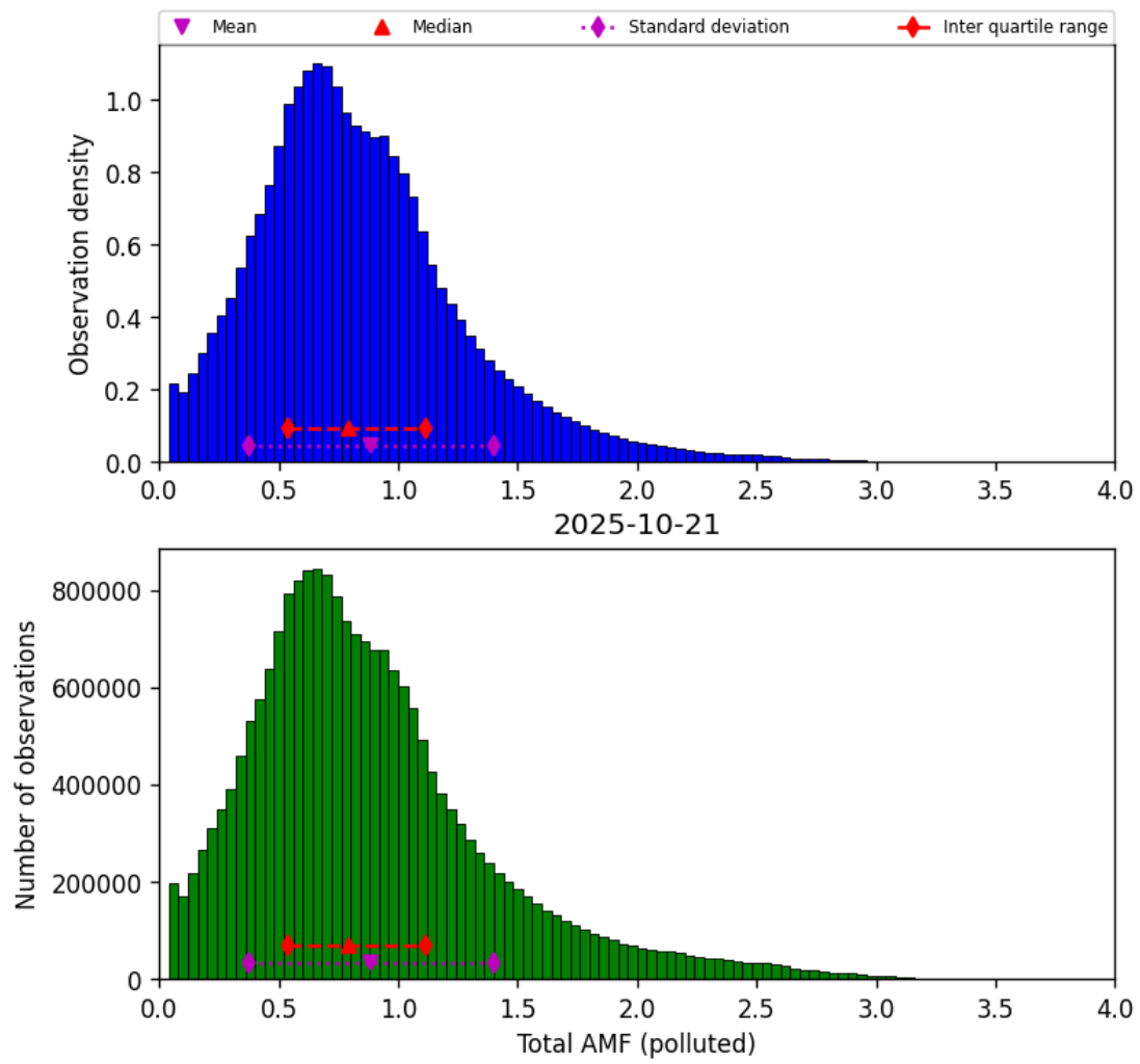
Figure 79: Histogram of “Total AMF (polluted)” for 2025-10-20 to 2025-10-22
