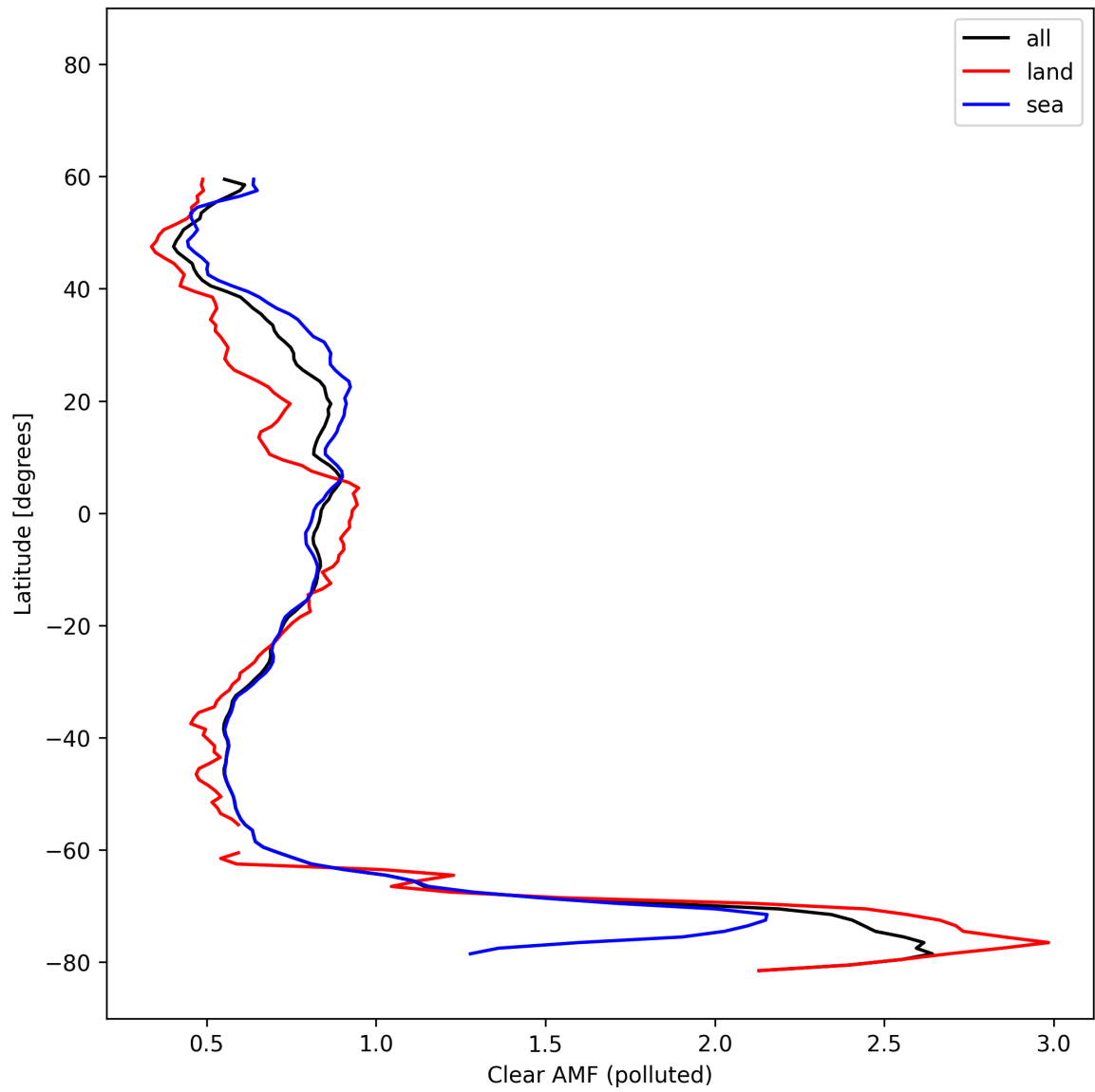
Figure 55: Zonal average of “Clear AMF (polluted)” for 2025-10-20 to 2025-10-22.
