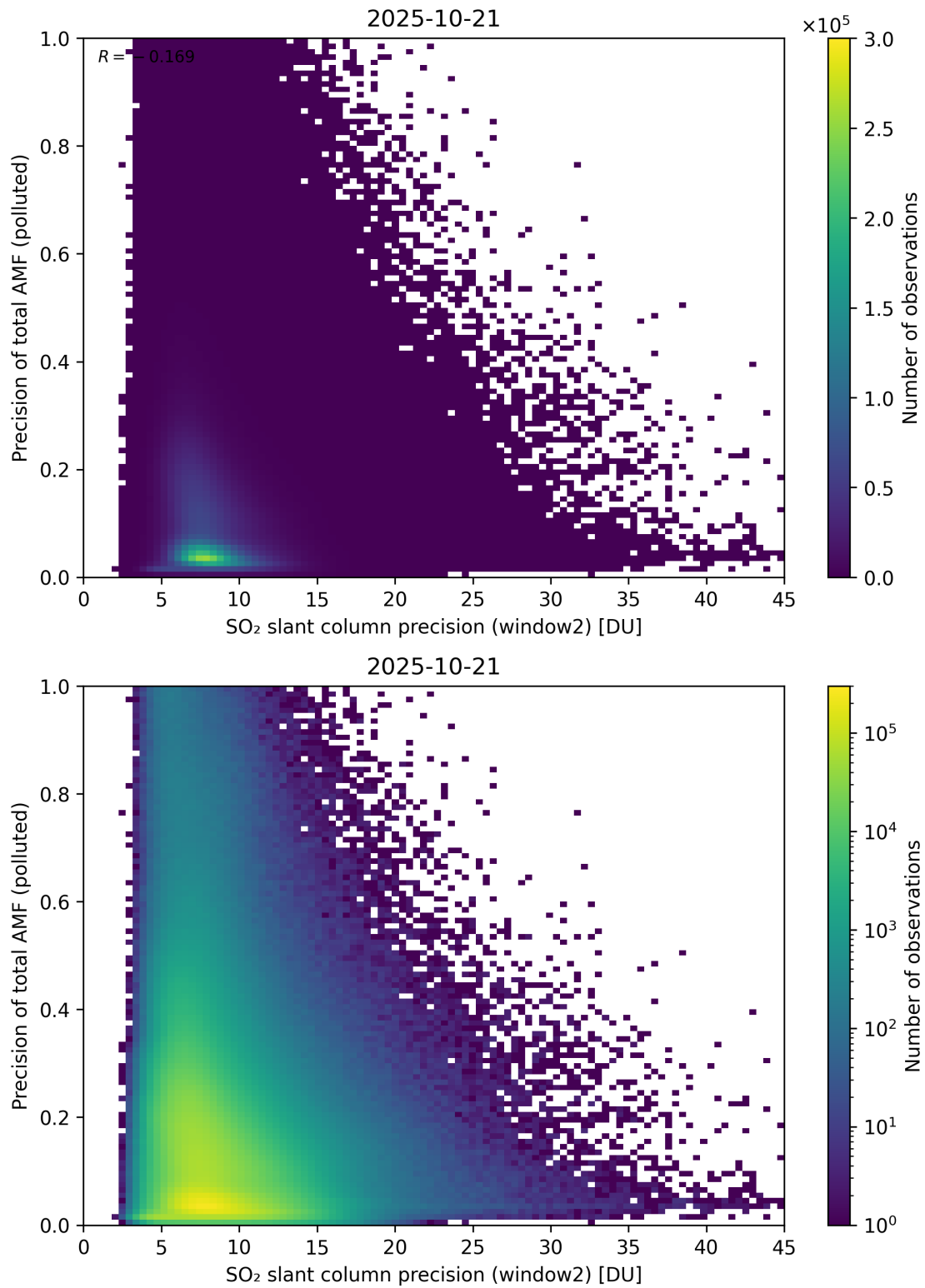
Figure 302: Scatter density plot of “SO 2 slant column precision (window2)” against “Precision of total AMF (polluted)” for 2025-10-20 to 2025-10-22.
