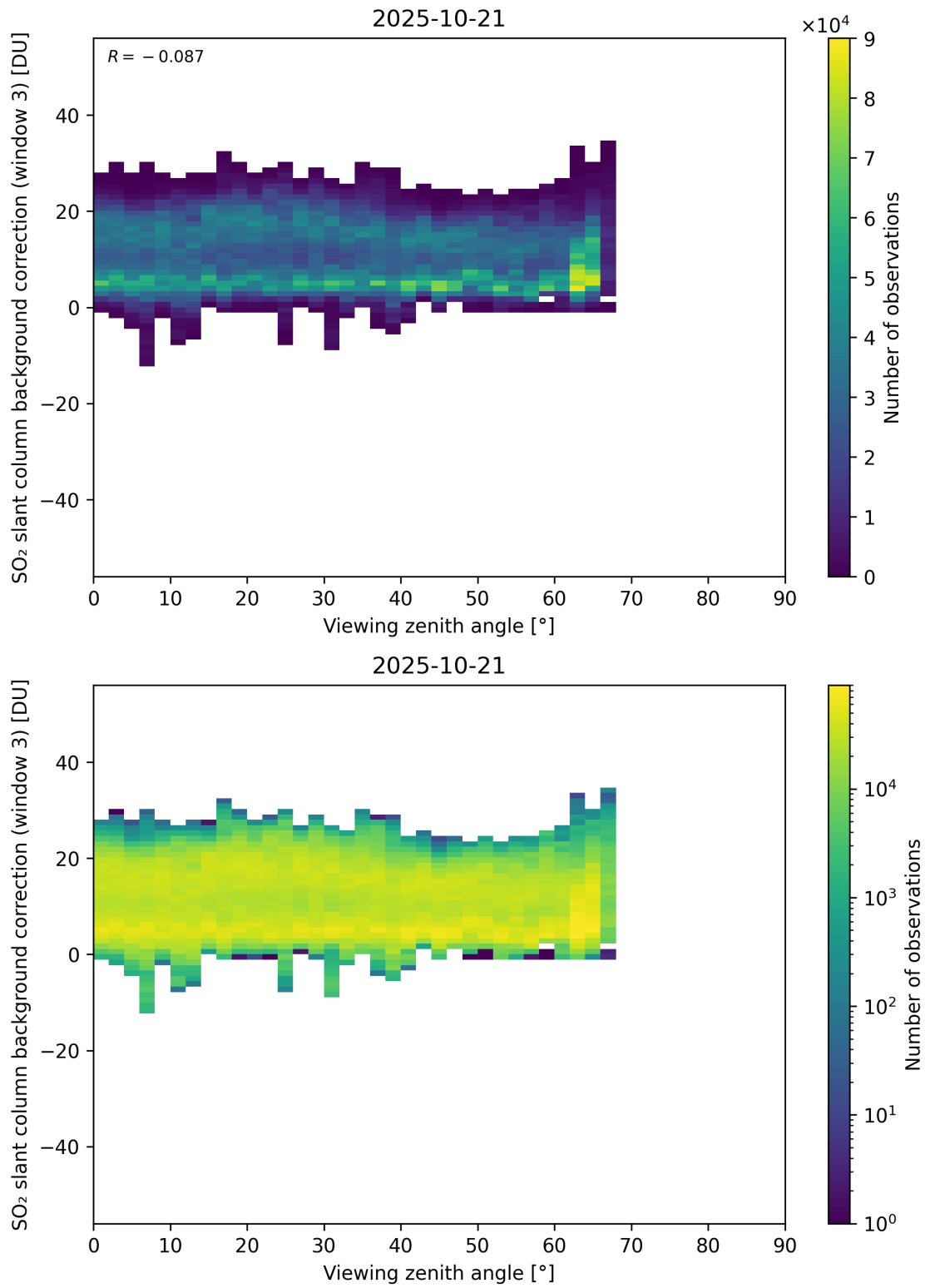
Figure 364: Scatter density plot of “Viewing zenith angle” against “SO 2 slant column background correction (window 3)” for 2025-10-20 to 2025-10-22.
