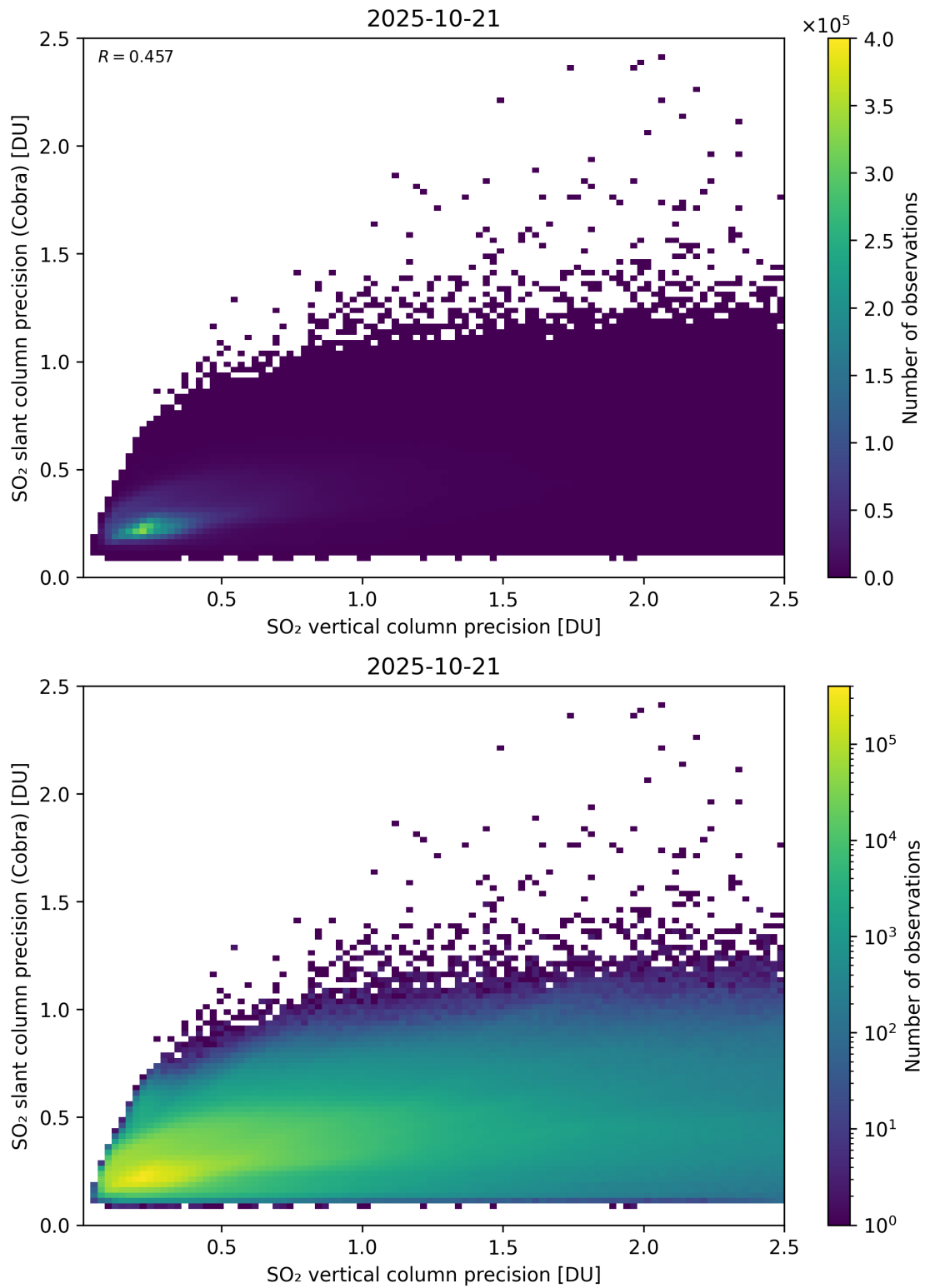
Figure 337: Scatter density plot of “SO 2 vertical column precision” against “SO 2 slant column precision (Cobra)” for 2025-10-20 to 2025-10-22.
