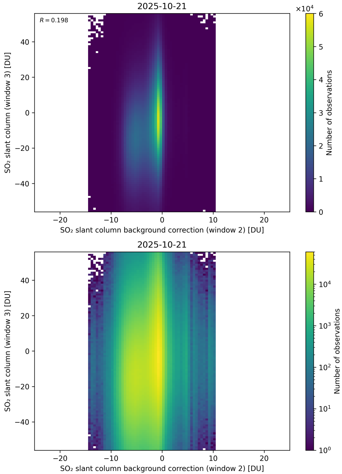
Figure 128: Scatter density plot of “SO 2 slant column background correction (window 2)” against “SO 2 slant column (window 3)” for 2025-10-20 to 2025-10-22.
