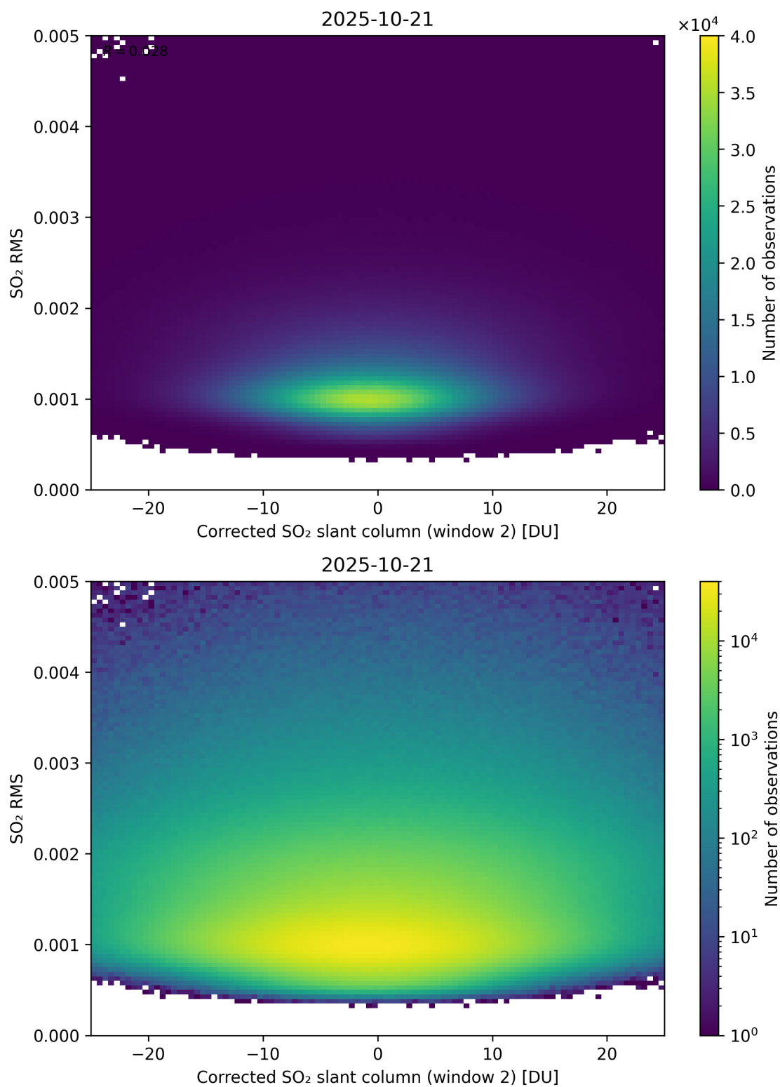
Figure 248: Scatter density plot of “Corrected SO 2 slant column (window 2)” against “SO 2 RMS” for 2025-10-20 to 2025-10-22.
