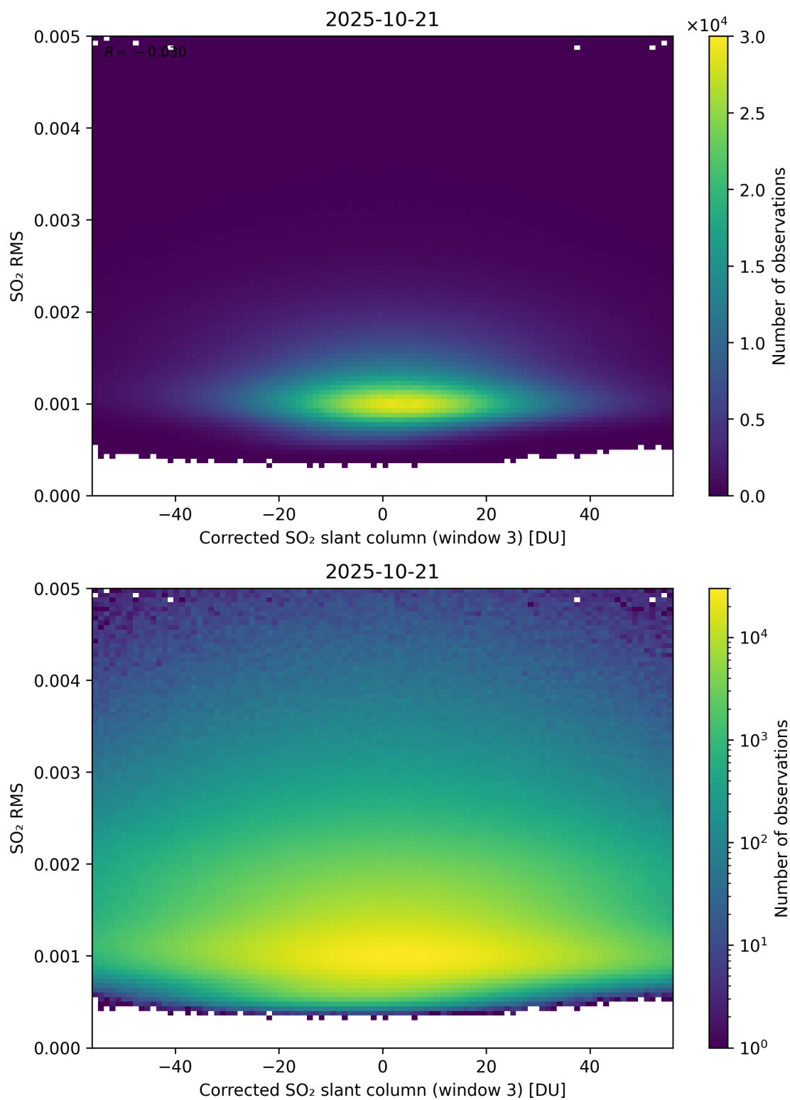
Figure 258: Scatter density plot of “Corrected SO 2 slant column (window 3)” against “SO 2 RMS” for 2025-10-20 to 2025-10-22.
