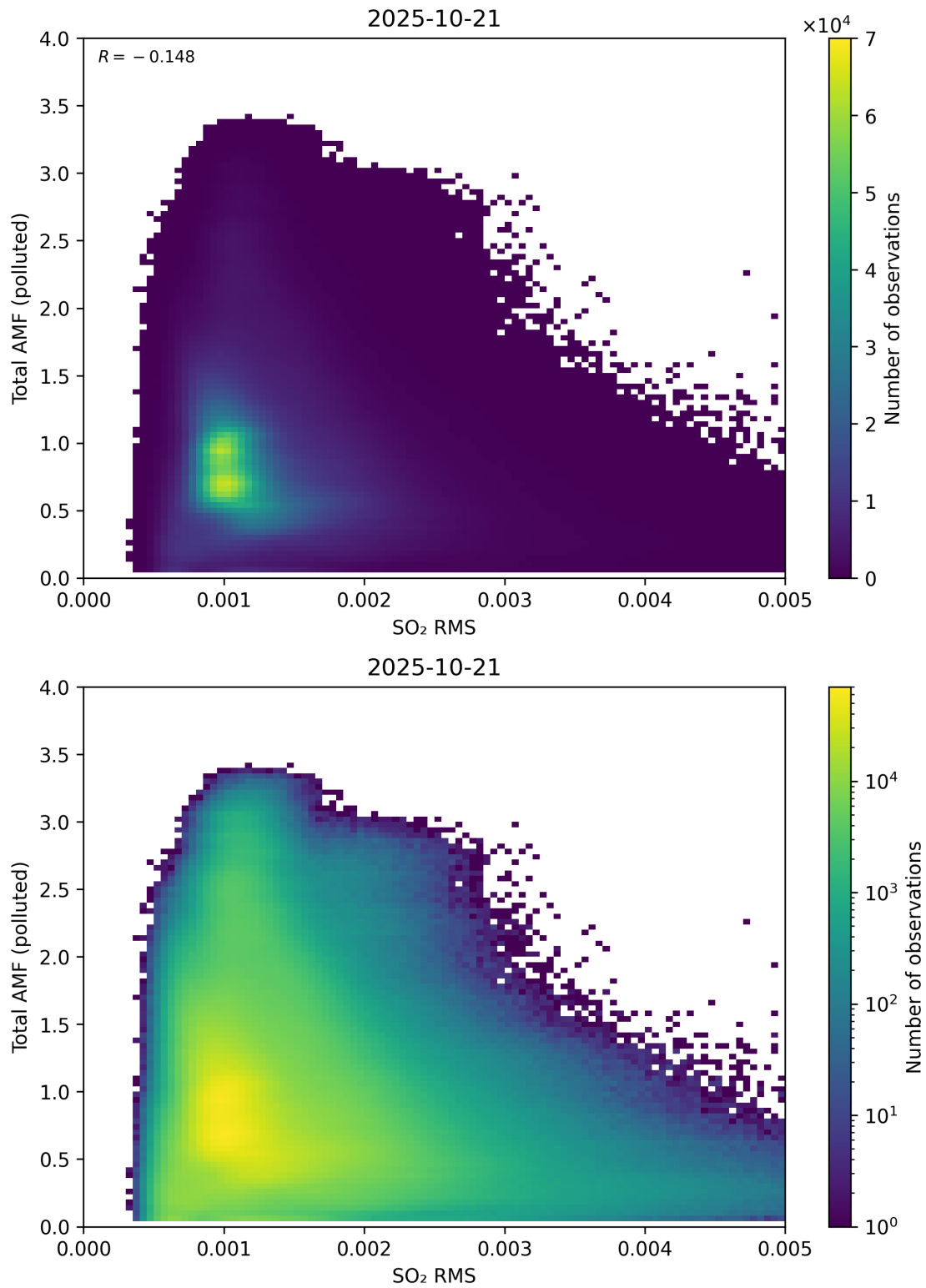
Figure 148: Scatter density plot of “SO 2 RMS” against “Total AMF (polluted)” for 2025-10-20 to 2025-10-22.
