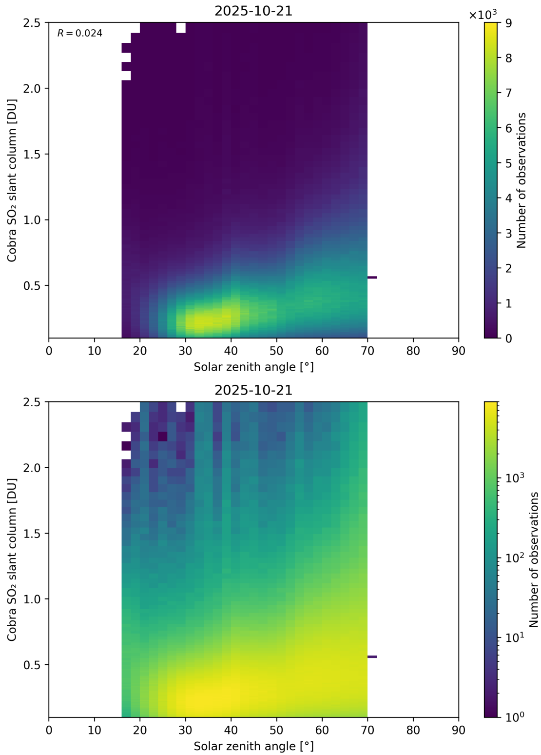
Figure 179: Scatter density plot of “Solar zenith angle” against “Cobra SO 2 slant column” for 2025-10-20 to 2025-10-22.
