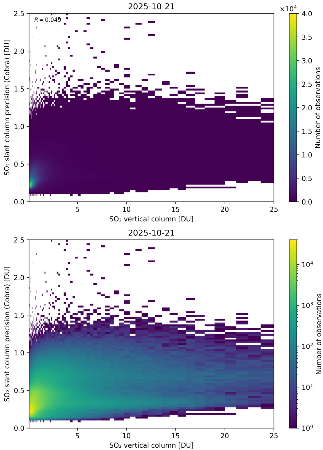
Figure 350: Scatter density plot of “SO 2 vertical column” against “SO 2 slant column precision (Cobra)” for 2025-10-20 to 2025-10-22.
