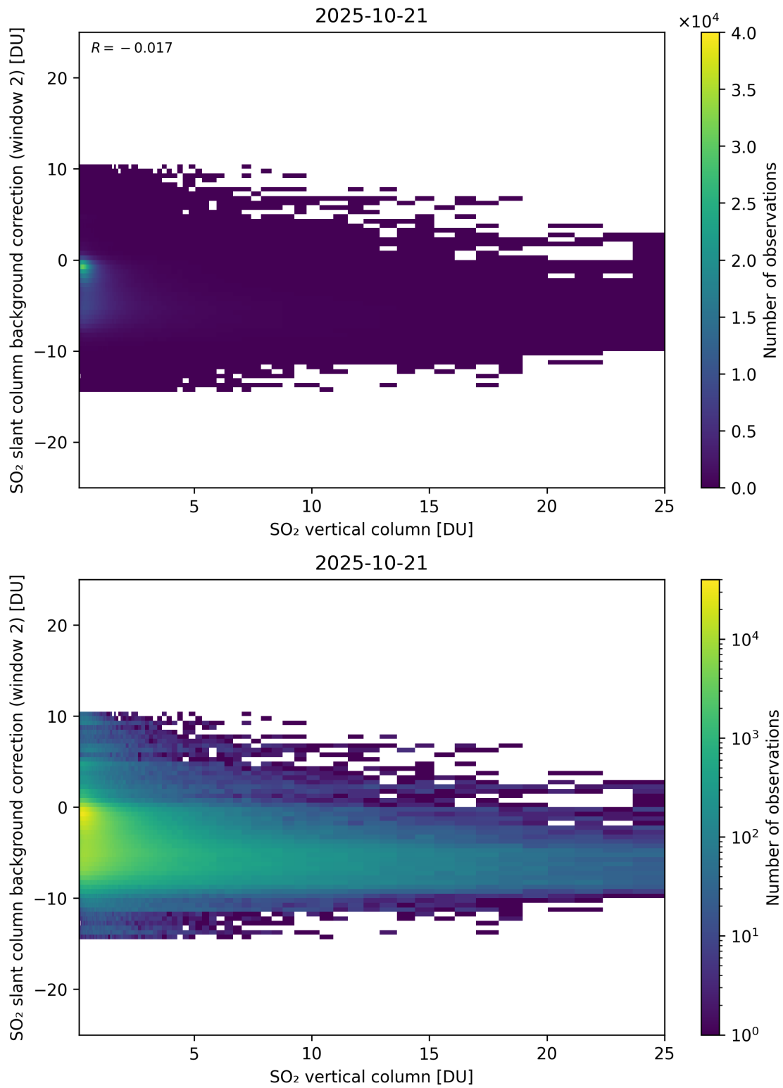
Figure 324: Scatter density plot of “SO 2 vertical column” against “SO 2 slant column background correction (window 2)” for 2025-10-20 to 2025-10-22.
