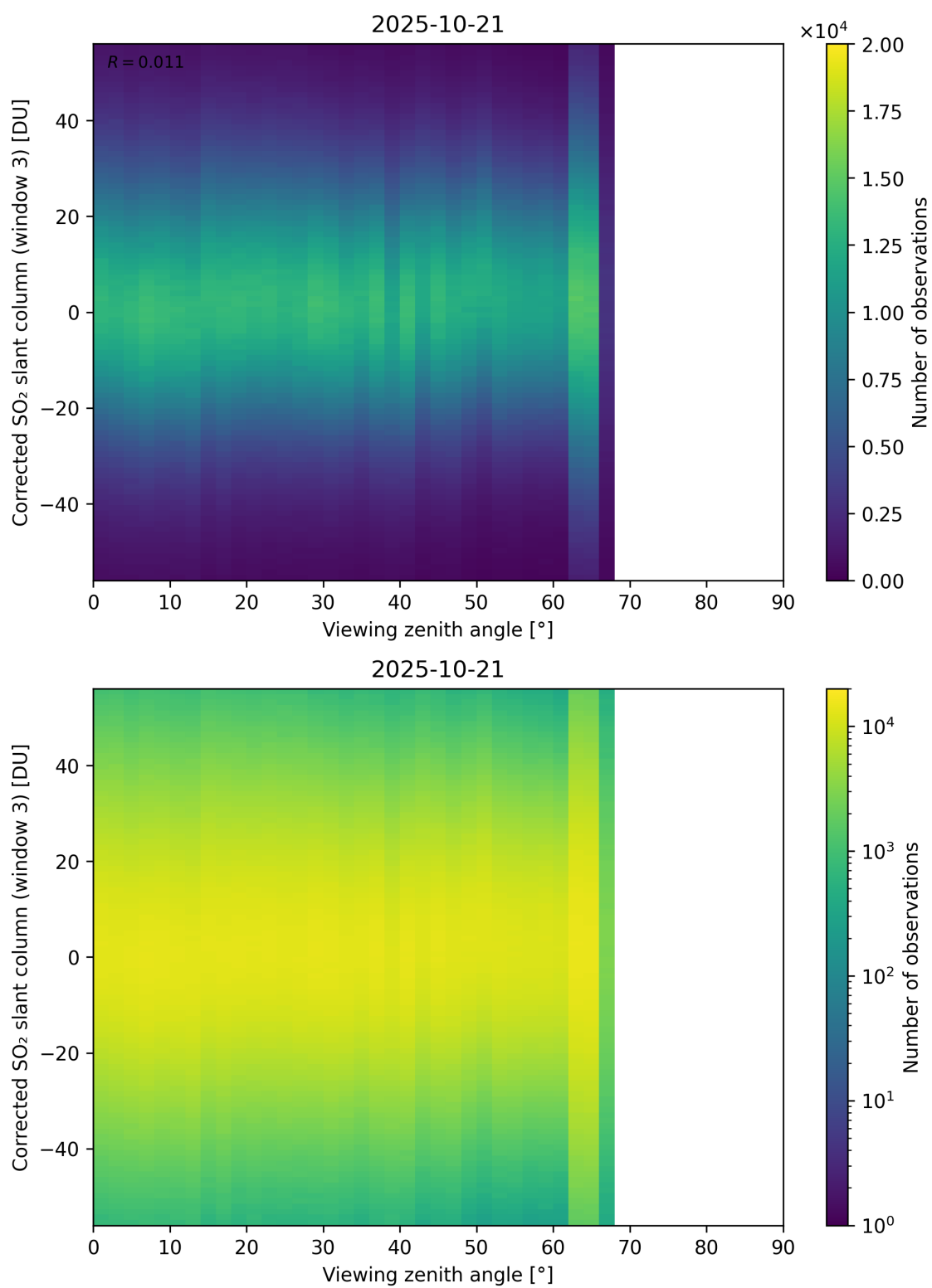
Figure 375: Scatter density plot of “Viewing zenith angle” against “Corrected SO 2 slant column (window 3)” for 2025-10-20 to 2025-10-22.
