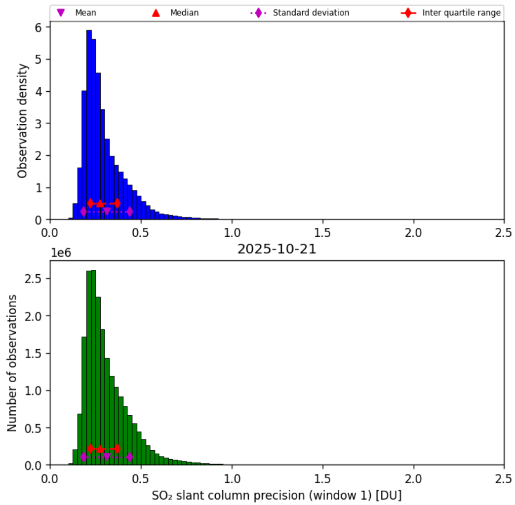
Figure 64: Histogram of “SO 2 slant column precision (window 1)” for 2025-10-20 to 2025-10-22
