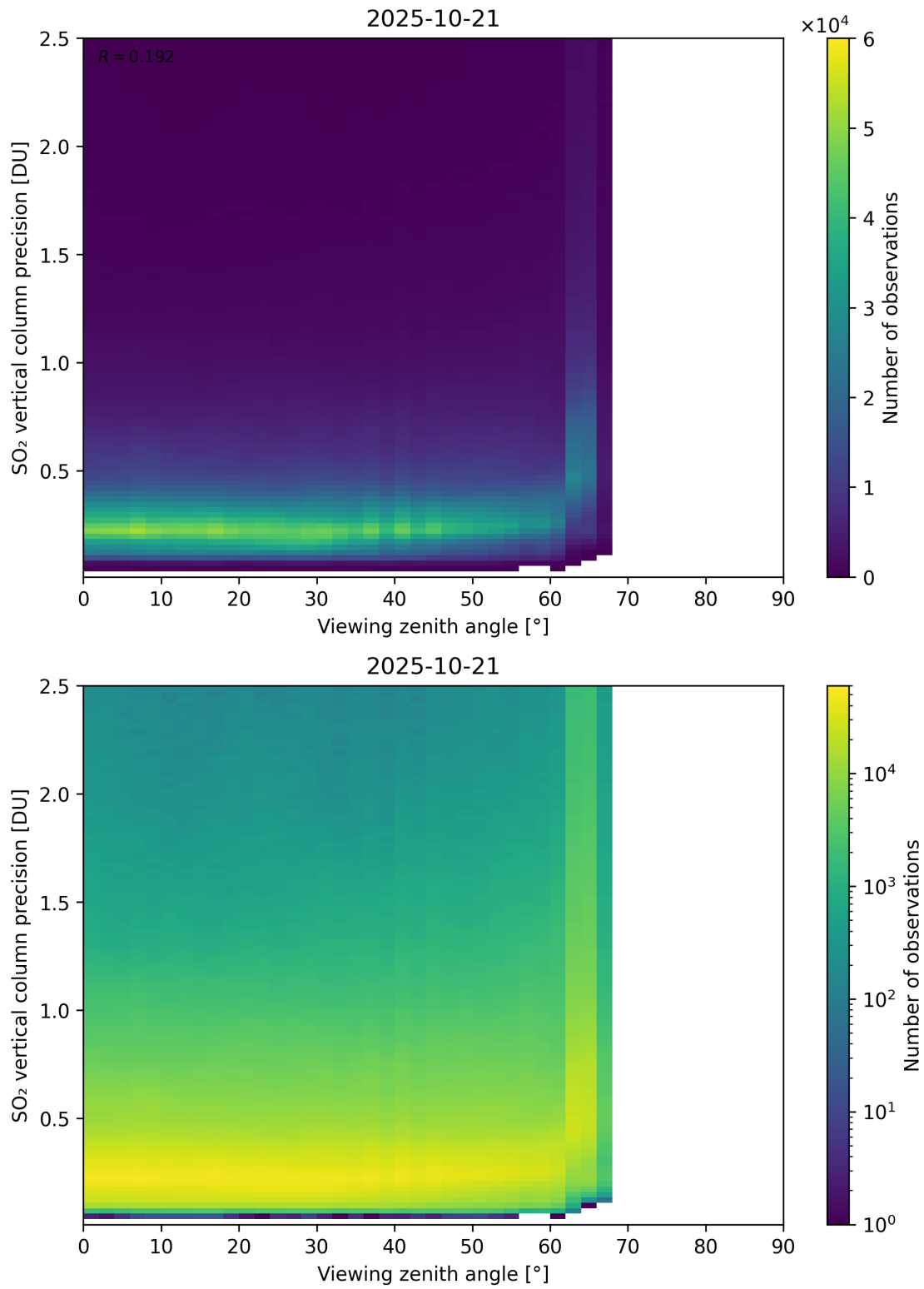
Figure 384: Scatter density plot of “Viewing zenith angle” against “SO 2 vertical column precision” for 2025-10-20 to 2025-10-22.
