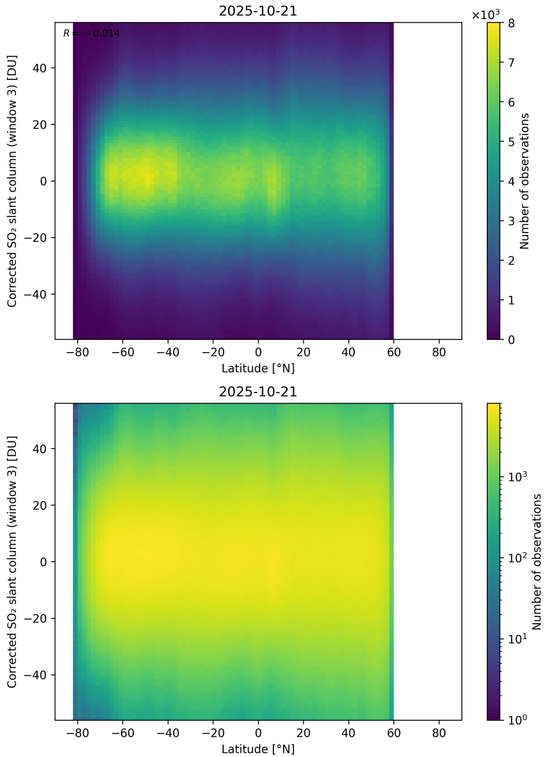
Figure 161: Scatter density plot of “Latitude” against “Corrected SO 2 slant column (window 3)” for 2025-10-20 to 2025-10-22.
