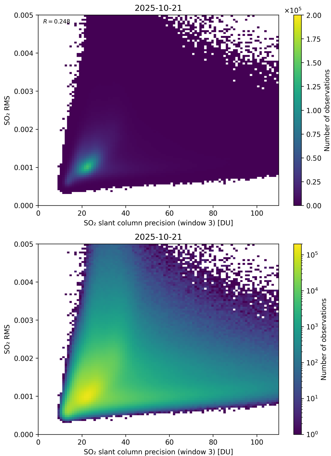
Figure 310: Scatter density plot of “SO 2 slant column precision (window 3)” against “SO 2 RMS” for 2025-10-20 to 2025-10-22.
