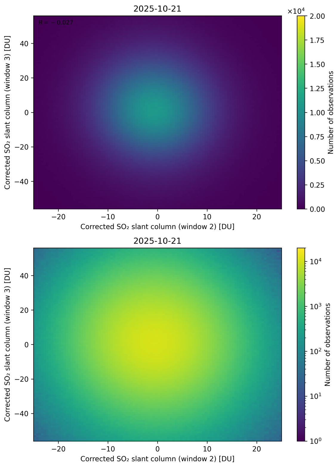
Figure 250: Scatter density plot of “Corrected SO 2 slant column (window 2)” against “Corrected SO 2 slant column (window 3)” for 2025-10-20 to 2025-10-22.
