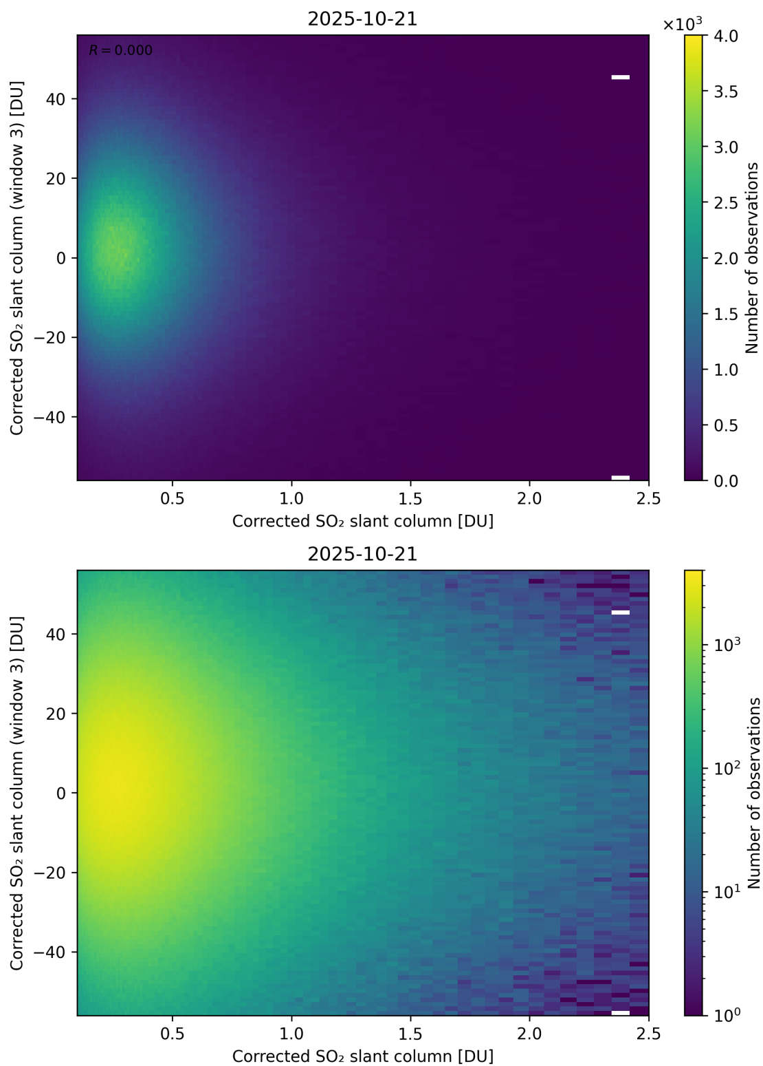
Figure 236: Scatter density plot of “Corrected SO 2 slant column” against “Corrected SO 2 slant column (window 3)” for 2025-10-20 to 2025-10-22.
