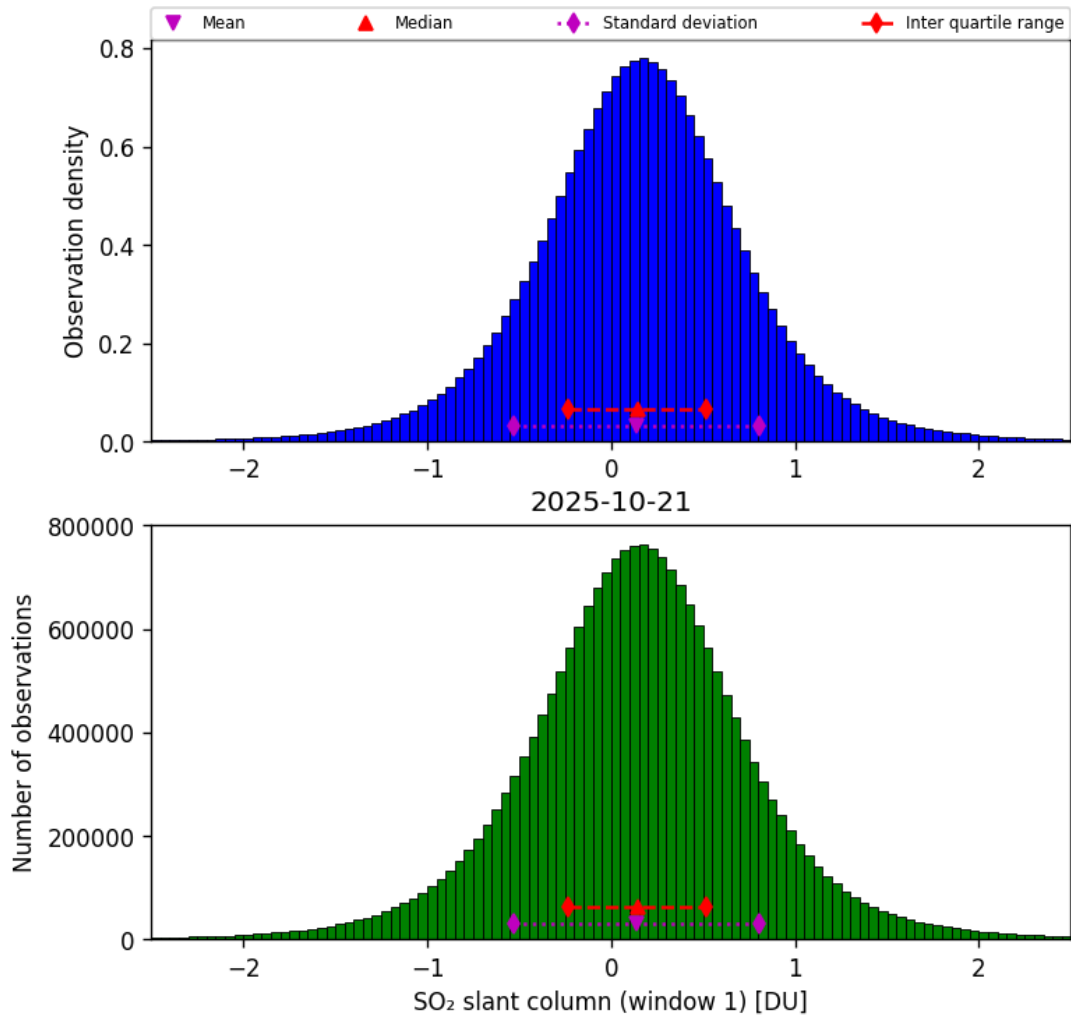
Figure 63: Histogram of “SO 2 slant column (window 1)” for 2025-10-20 to 2025-10-22
