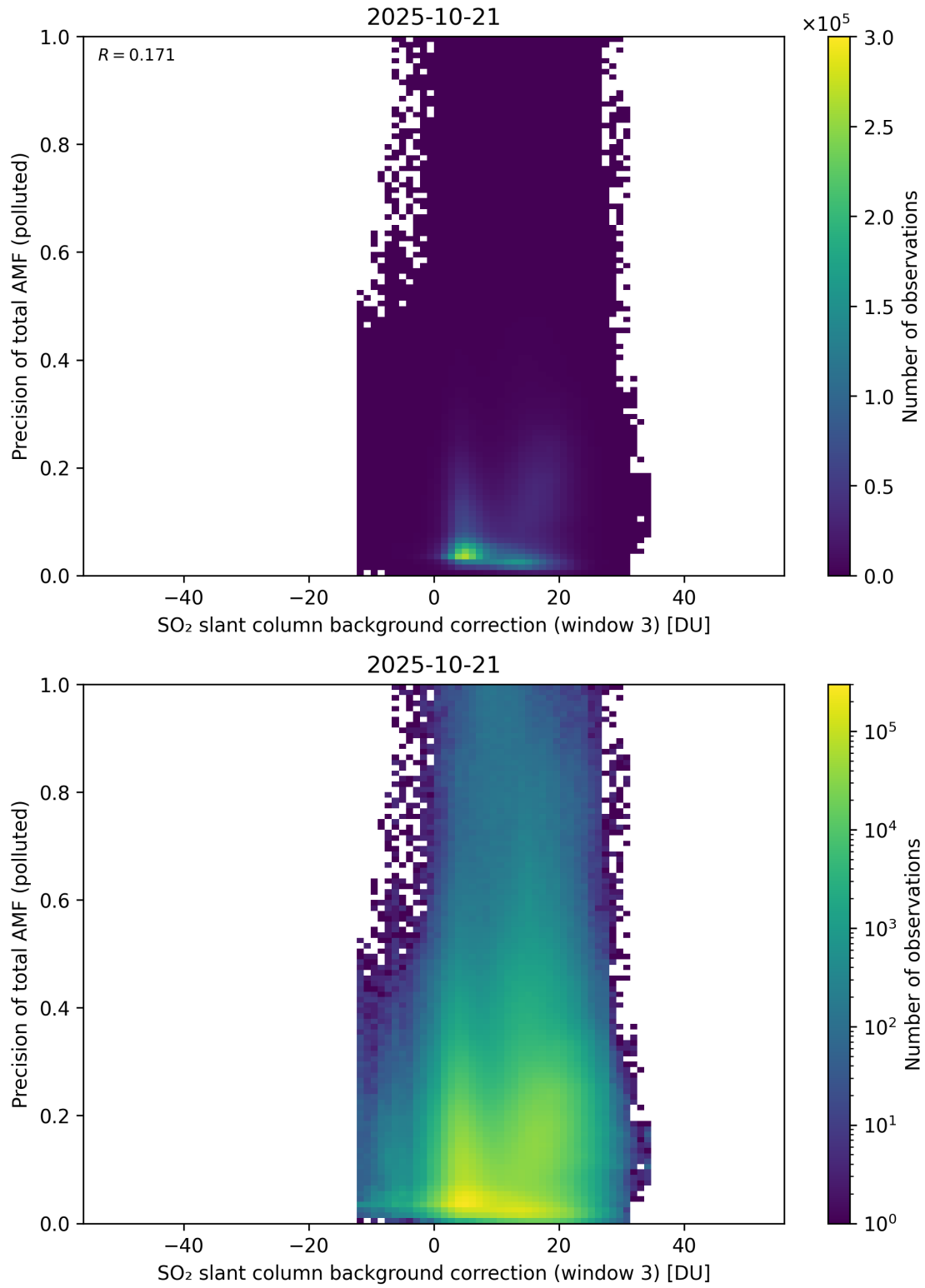
Figure 137: Scatter density plot of “SO 2 slant column background correction (window 3)” against “Precision of total AMF (polluted)” for 2025-10-20 to 2025-10-22.
