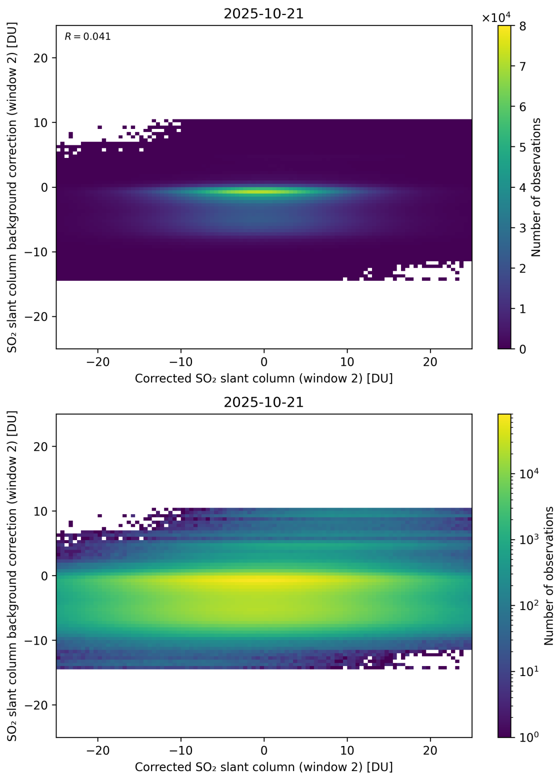
Figure 244: Scatter density plot of “Corrected SO 2 slant column (window 2)” against “SO 2 slant column background correction (window 2)” for 2025-10-20 to 2025-10-22.
