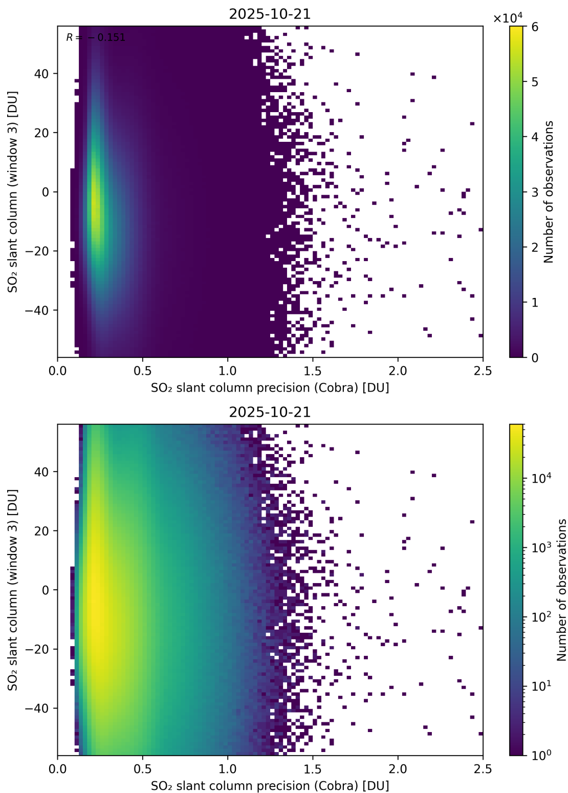
Figure 211: Scatter density plot of “SO 2 slant column precision (Cobra)” against “SO 2 slant column (window 3)” for 2025-10-20 to 2025-10-22.
