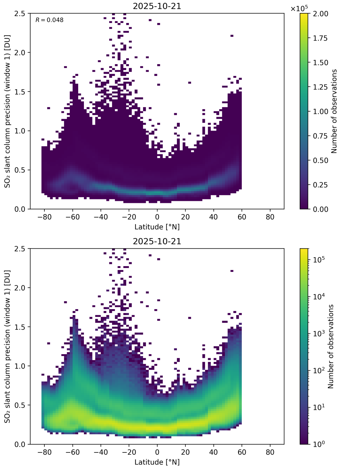
Figure 163: Scatter density plot of “Latitude” against “SO 2 slant column precision (window 1)” for 2025-10-20 to 2025-10-22.
