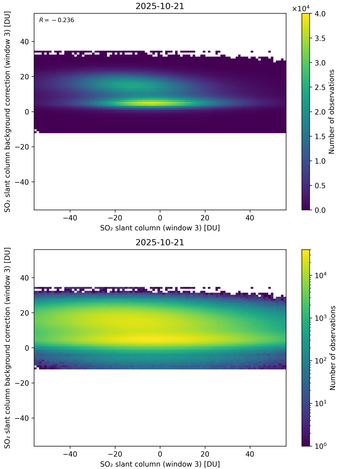
Figure 303: Scatter density plot of “SO 2 slant column (window 3)” against “SO 2 slant column background correction (window 3)” for 2025-10-20 to 2025-10-22.
