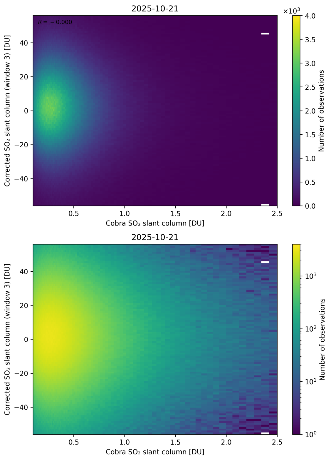
Figure 218: Scatter density plot of “Cobra SO 2 slant column” against “Corrected SO 2 slant column (window 3)” for 2025-10-20 to 2025-10-22.
