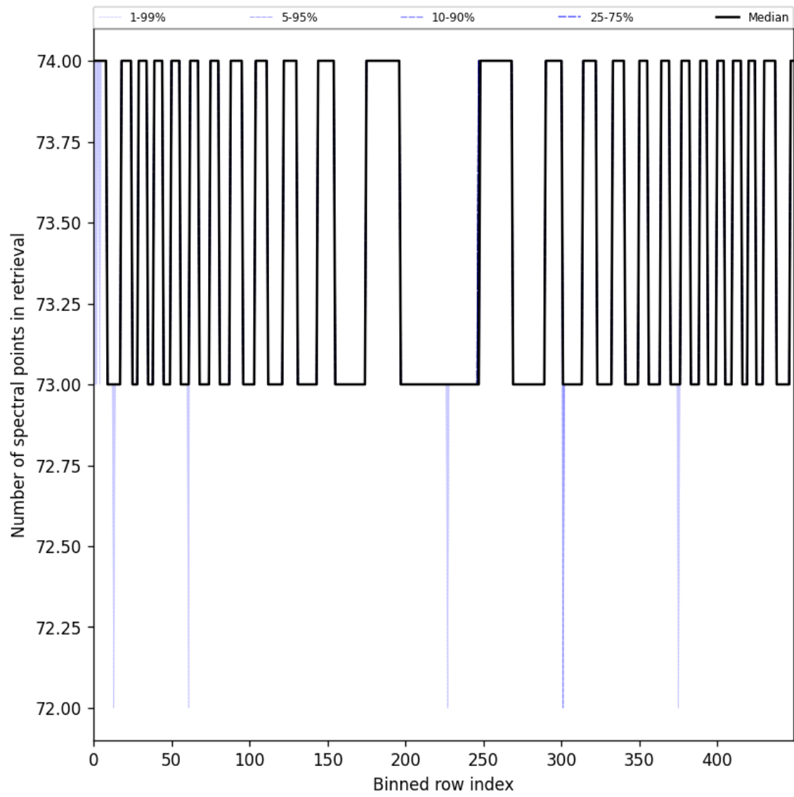
Figure 108: Along track statistics of “Number of spectral points in retrieval” for 2025-10-20 to 2025-10-22
