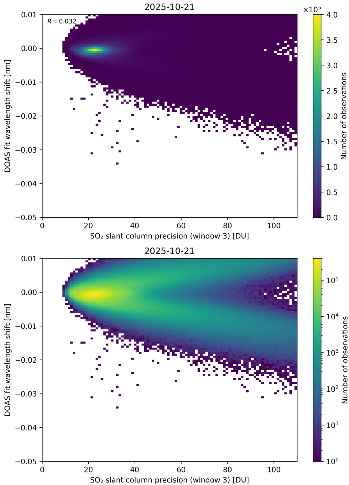
Figure 308: Scatter density plot of “SO 2 slant column precision (window 3)” against “DOAS fit wavelength shift” for 2025-10-20 to 2025-10-22.
