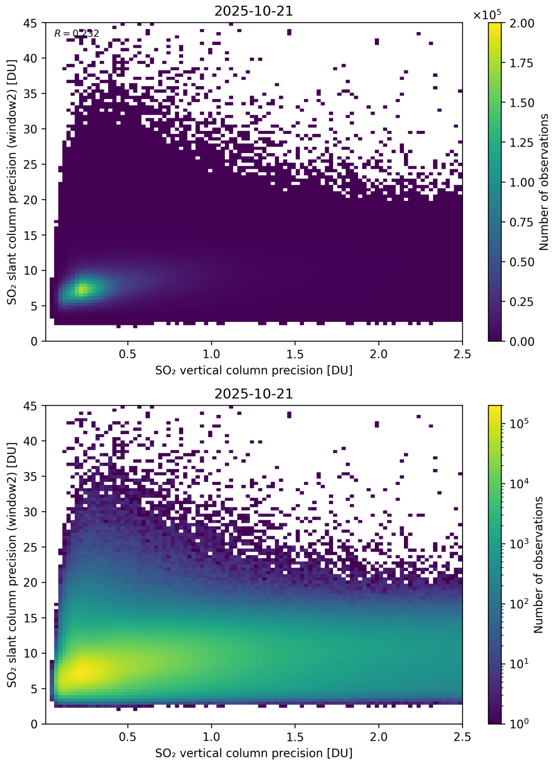
Figure 343: Scatter density plot of “SO 2 vertical column precision” against “SO 2 slant column precision (window2)” for 2025-10-20 to 2025-10-22.
