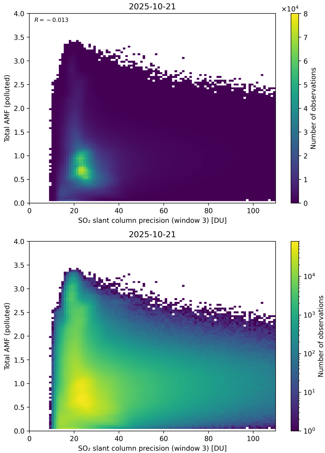
Figure 313: Scatter density plot of “SO 2 slant column precision (window 3)” against “Total AMF (polluted)” for 2025-10-20 to 2025-10-22.
