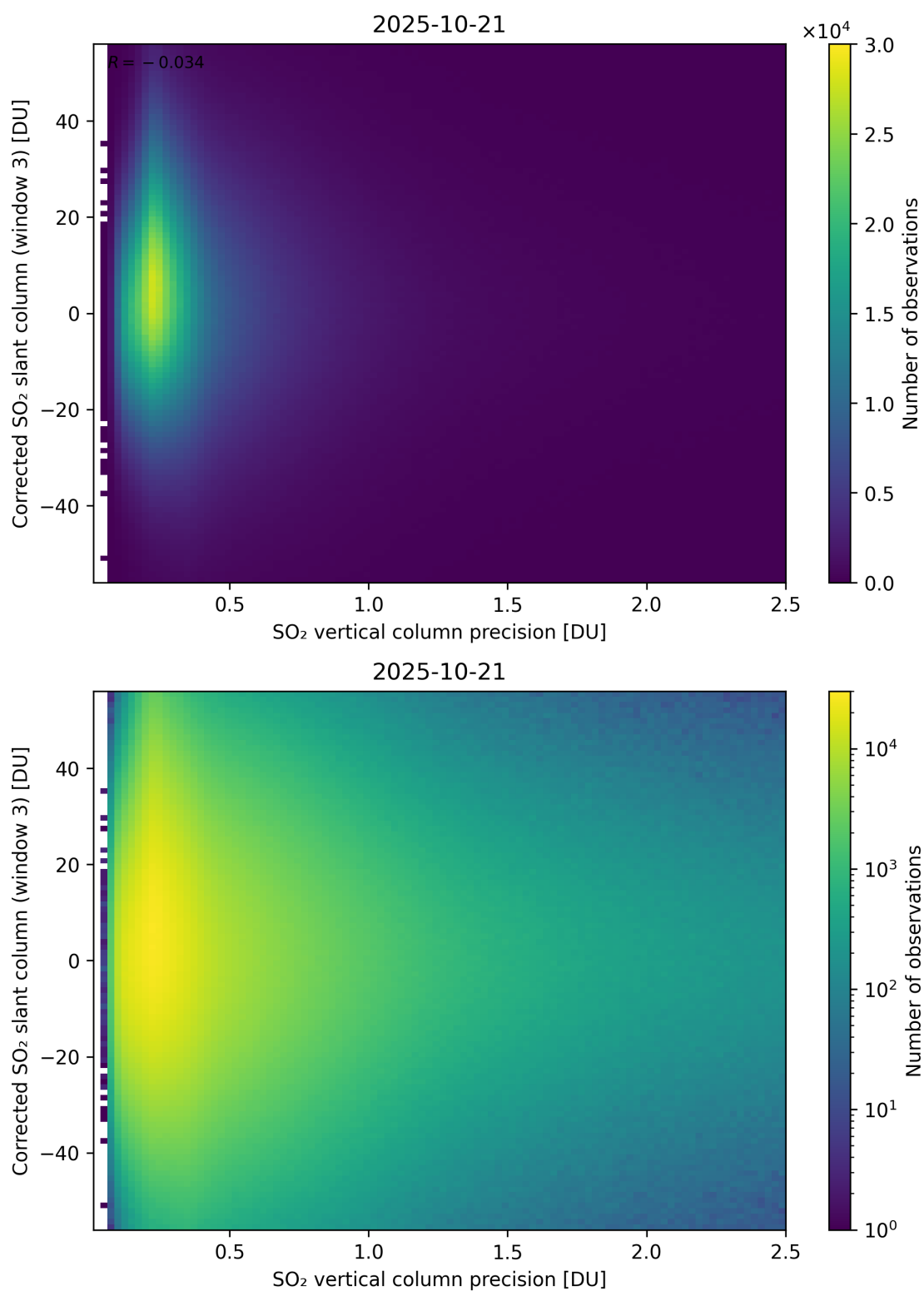
Figure 340: Scatter density plot of “SO 2 vertical column precision” against “Corrected SO 2 slant column (window 3)” for 2025-10-20 to 2025-10-22.
