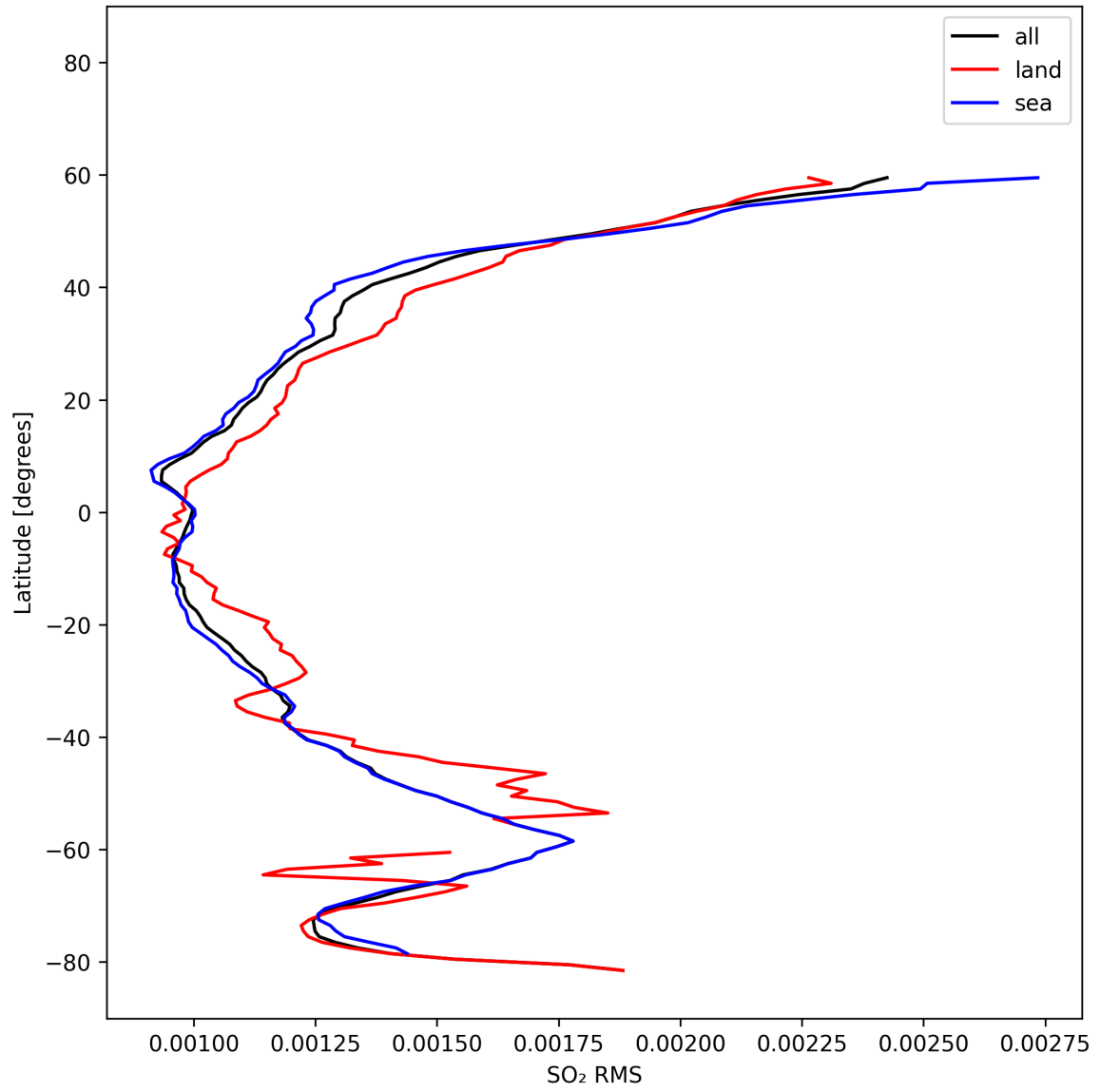
Figure 52: Zonal average of “SO 2 RMS” for 2025-10-20 to 2025-10-22.
