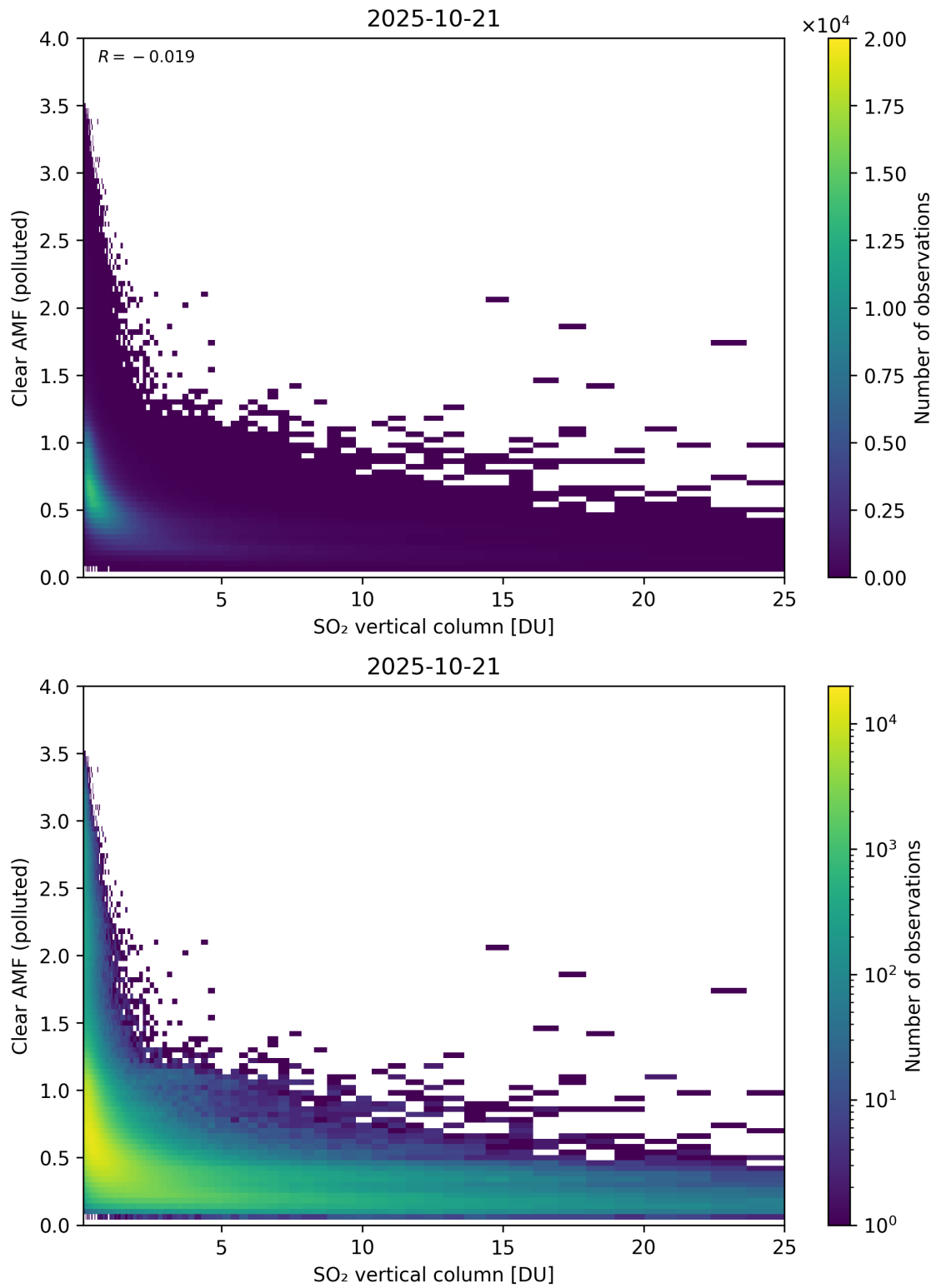
Figure 348: Scatter density plot of “SO 2 vertical column” against “Clear AMF (polluted)” for 2025-10-20 to 2025-10-22.
