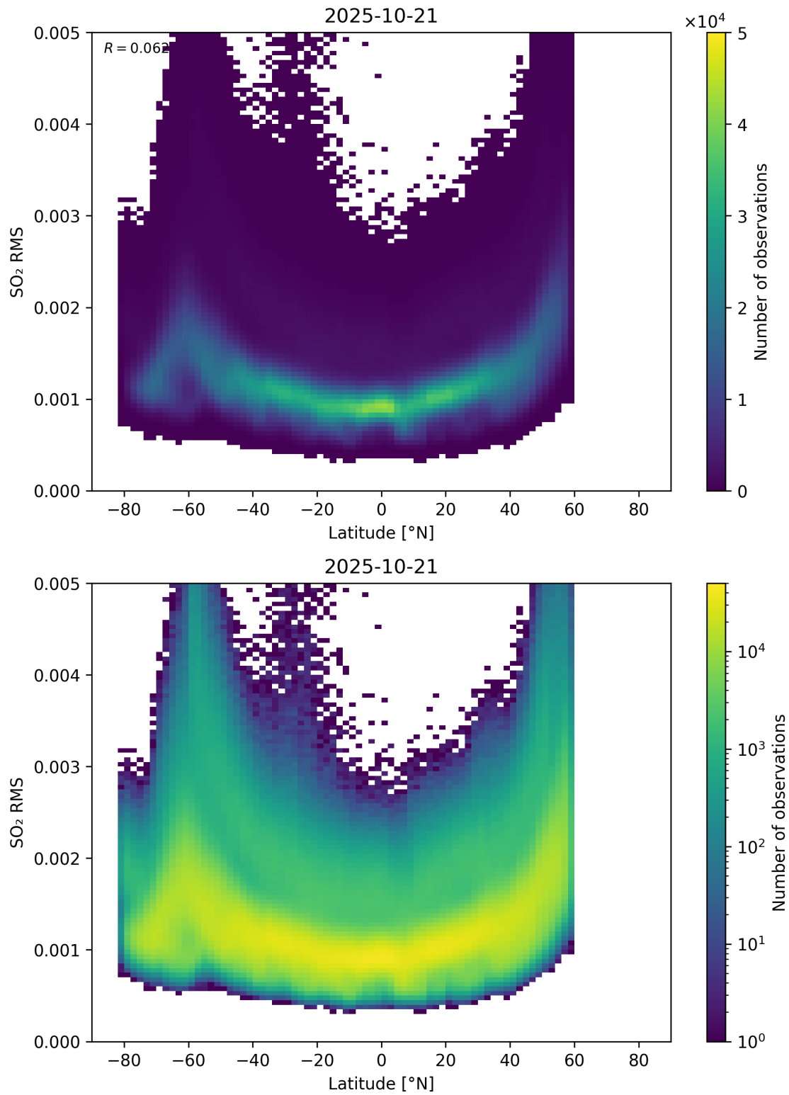
Figure 155: Scatter density plot of “Latitude” against “SO 2 RMS” for 2025-10-20 to 2025-10-22.
