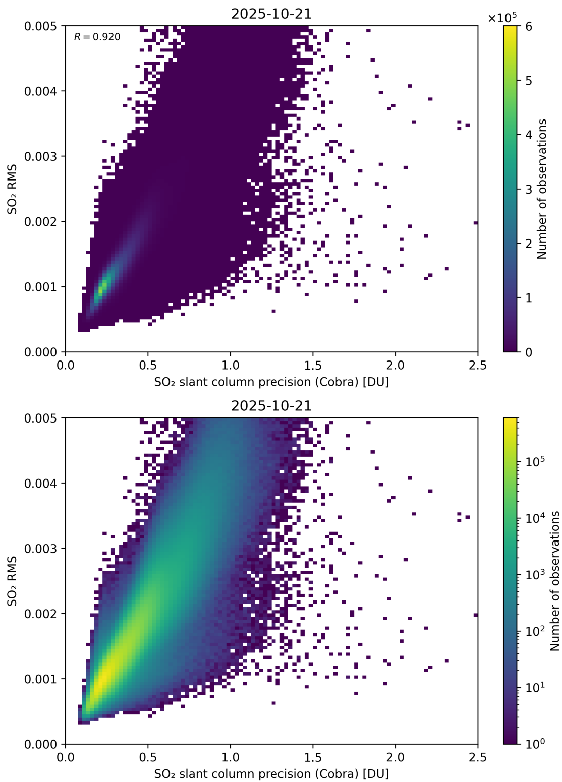
Figure 204: Scatter density plot of “SO 2 slant column precision (Cobra)” against “SO 2 RMS” for 2025-10-20 to 2025-10-22.
