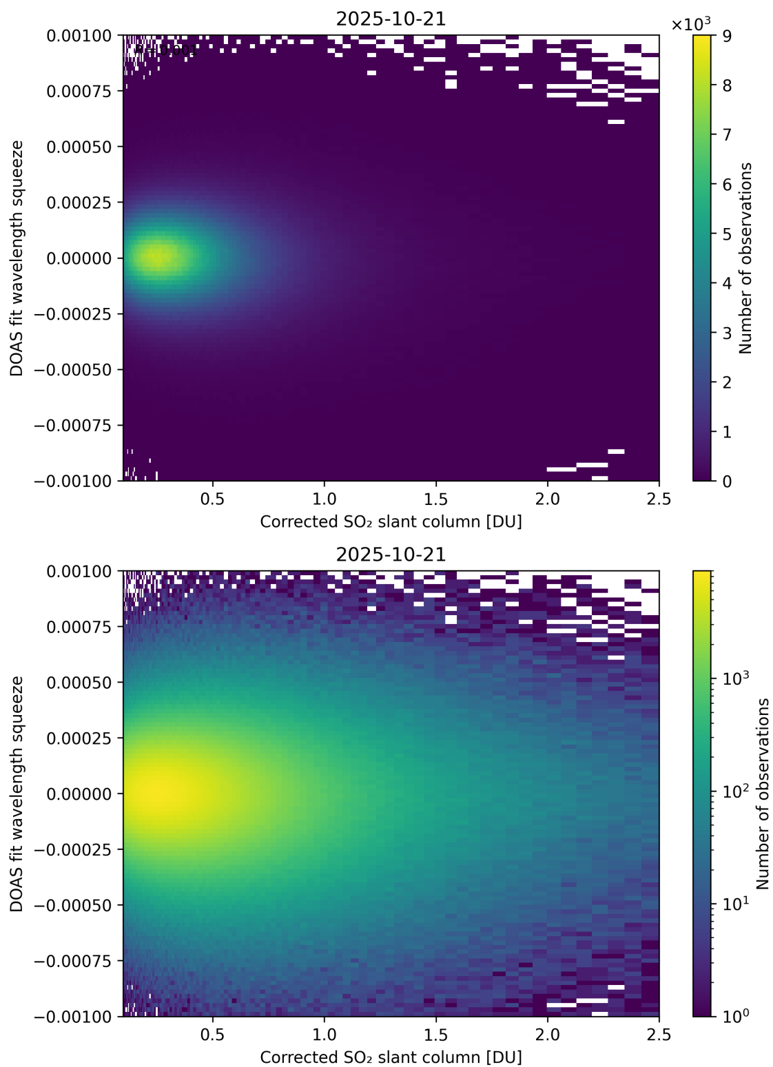
Figure 230: Scatter density plot of “Corrected SO 2 slant column” against “DOAS fit wavelength squeeze” for 2025-10-20 to 2025-10-22.
