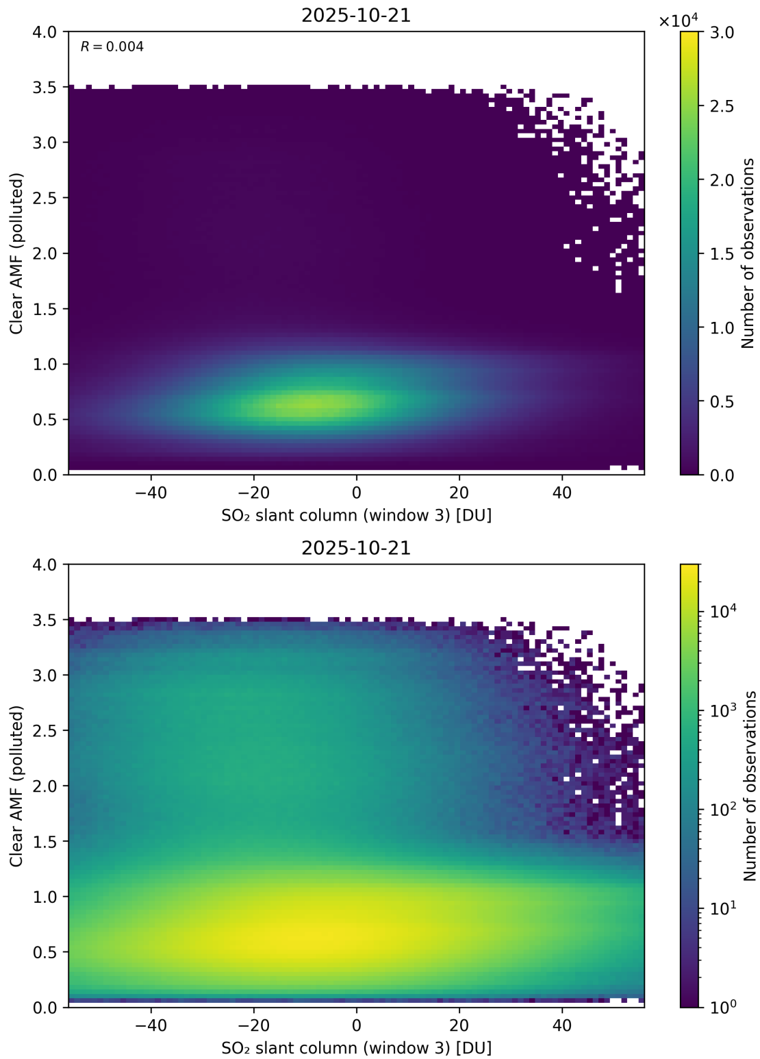
Figure 315: Scatter density plot of “SO 2 slant column (window 3)” against “Clear AMF (polluted)” for 2025-10-20 to 2025-10-22.
