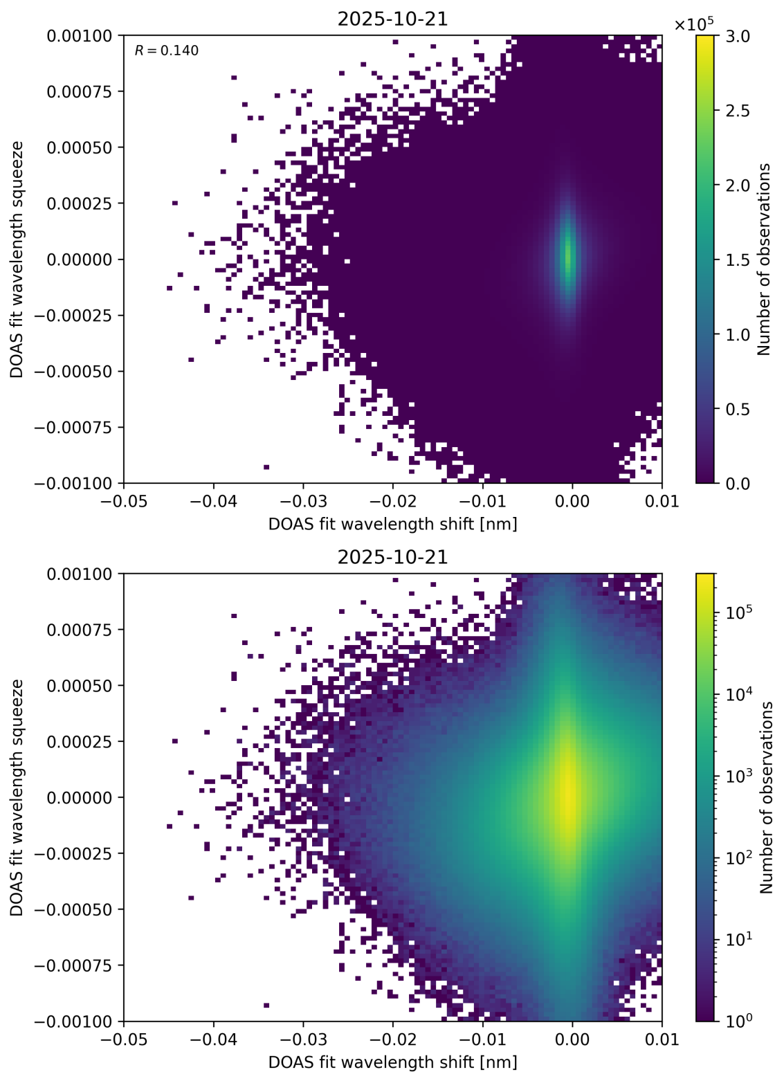
Figure 138: Scatter density plot of “DOAS fit wavelength shift” against “DOAS fit wavelength squeeze” for 2025-10-20 to 2025-10-22.
