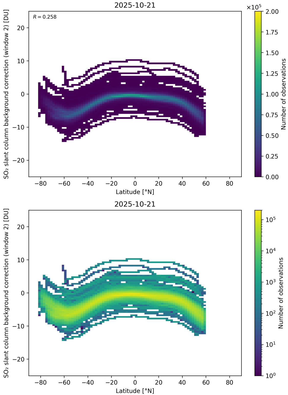
Figure 151: Scatter density plot of “Latitude” against “SO 2 slant column background correction (window 2)” for 2025-10-20 to 2025-10-22.
