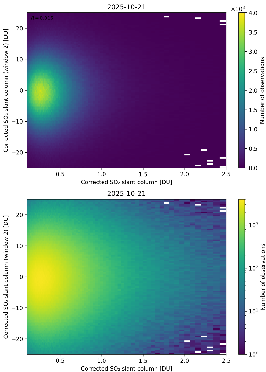
Figure 235: Scatter density plot of “Corrected SO 2 slant column” against “Corrected SO 2 slant column (window 2)” for 2025-10-20 to 2025-10-22.
