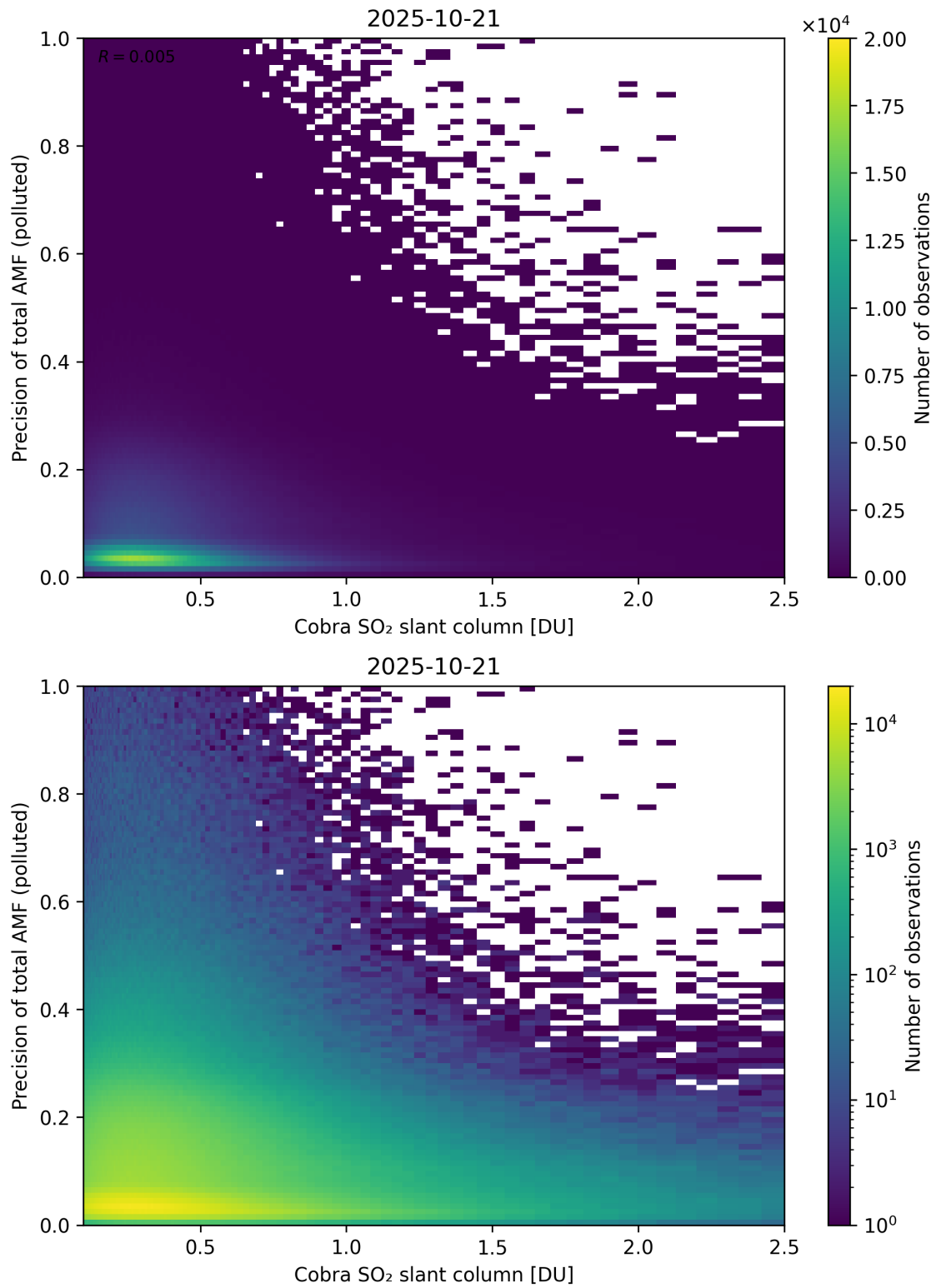
Figure 225: Scatter density plot of “Cobra SO 2 slant column” against “Precision of total AMF (polluted)” for 2025-10-20 to 2025-10-22.
