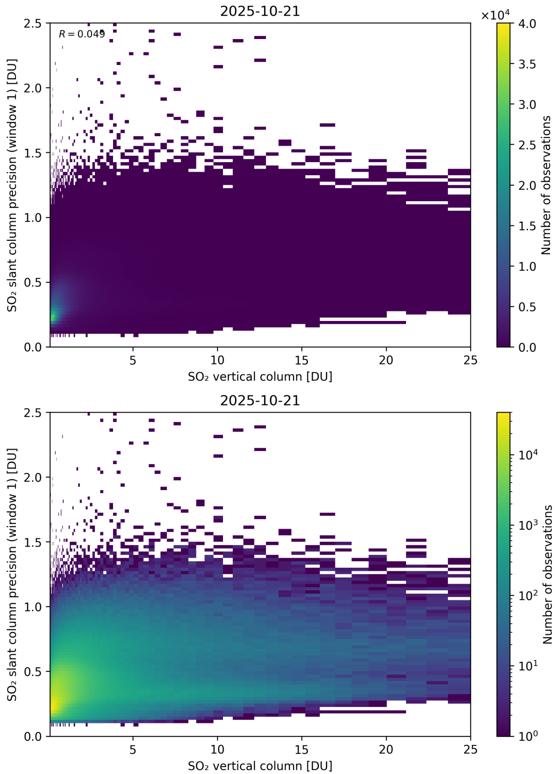
Figure 355: Scatter density plot of “SO 2 vertical column” against “SO 2 slant column precision (window 1)” for 2025-10-20 to 2025-10-22.
