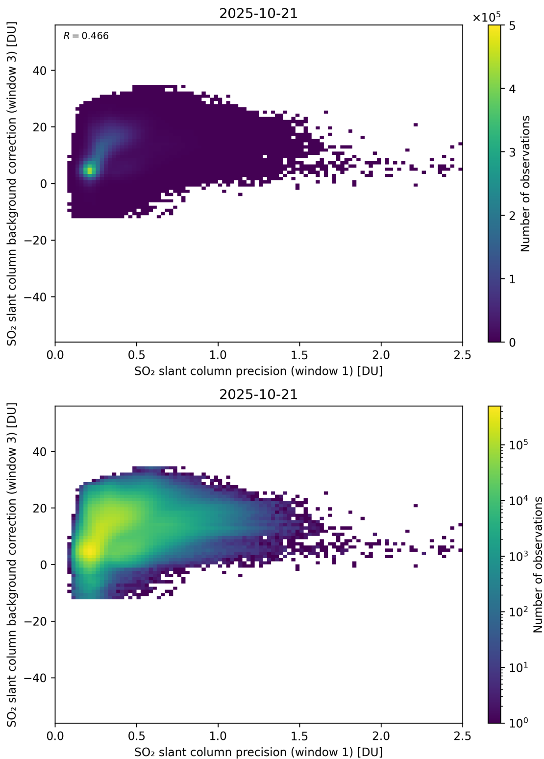
Figure 270: Scatter density plot of “SO 2 slant column precision (window 1)” against “SO 2 slant column background correction (window 3)” for 2025-10-20 to 2025-10-22.
