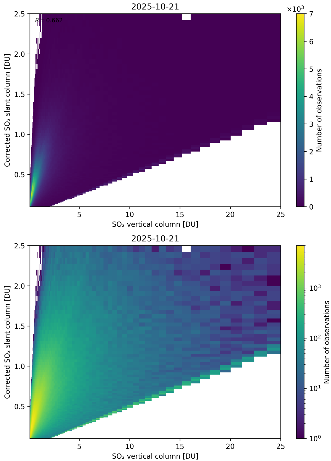
Figure 351: Scatter density plot of “SO 2 vertical column” against “Corrected SO 2 slant column” for 2025-10-20 to 2025-10-22.
