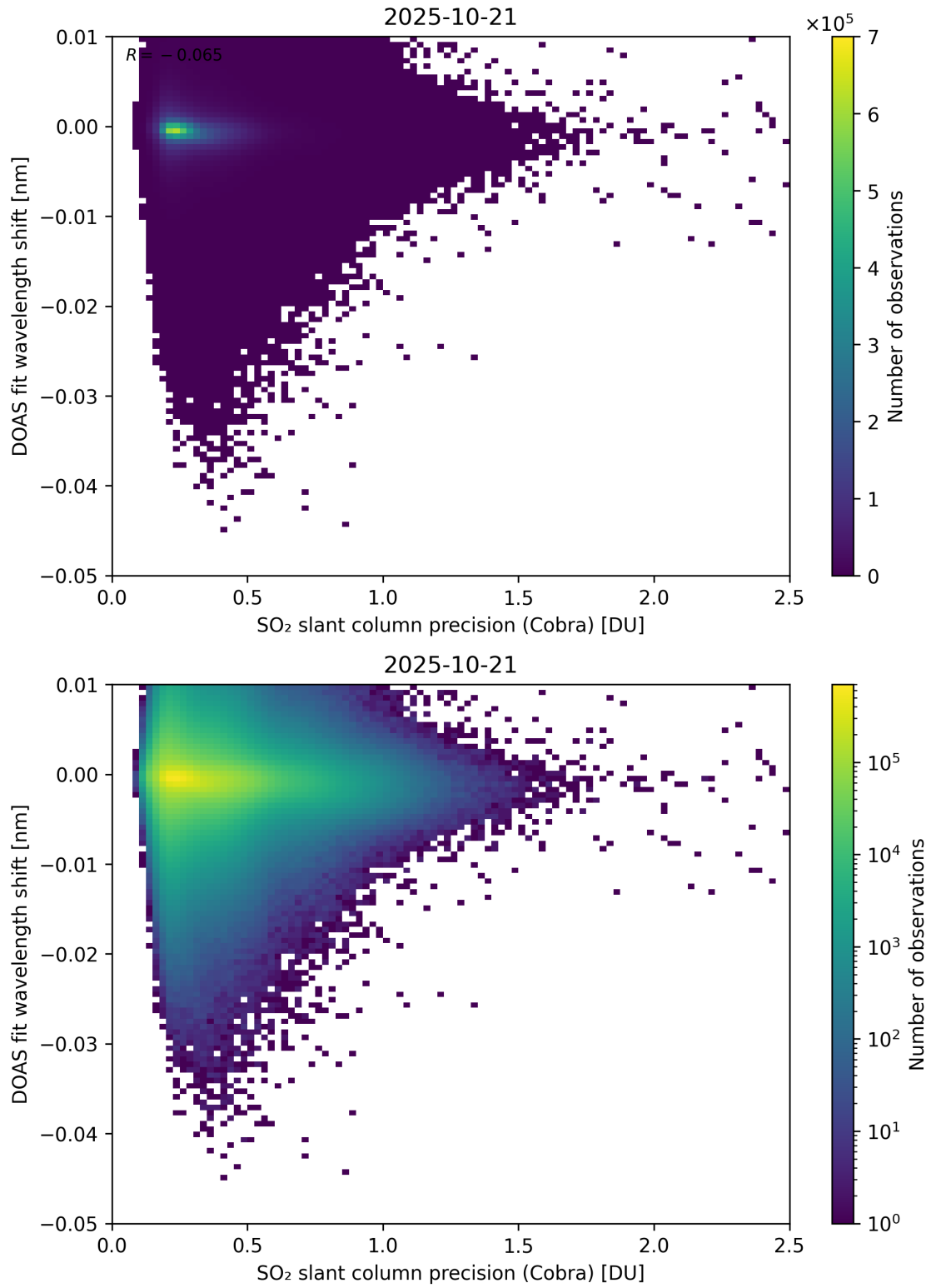
Figure 202: Scatter density plot of “SO 2 slant column precision (Cobra)” against “DOAS fit wavelength shift” for 2025-10-20 to 2025-10-22.
