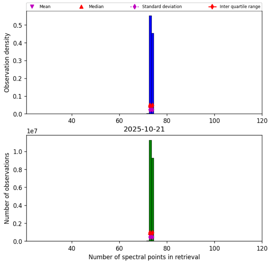
Figure 82: Histogram of “Number of spectral points in retrieval” for 2025-10-20 to 2025-10-22
