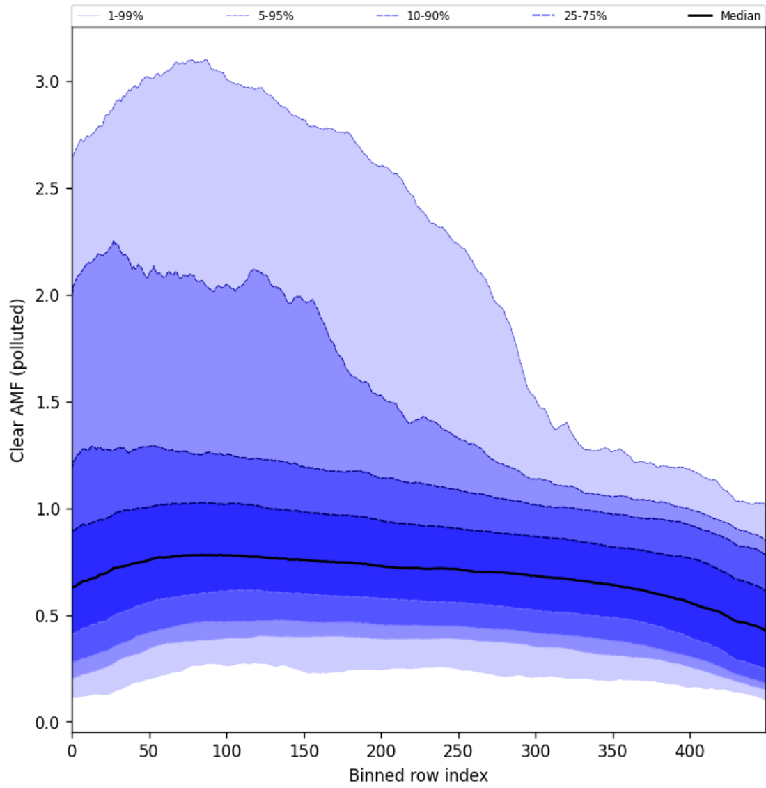
Figure 107: Along track statistics of “Clear AMF (polluted)” for 2025-10-20 to 2025-10-22
