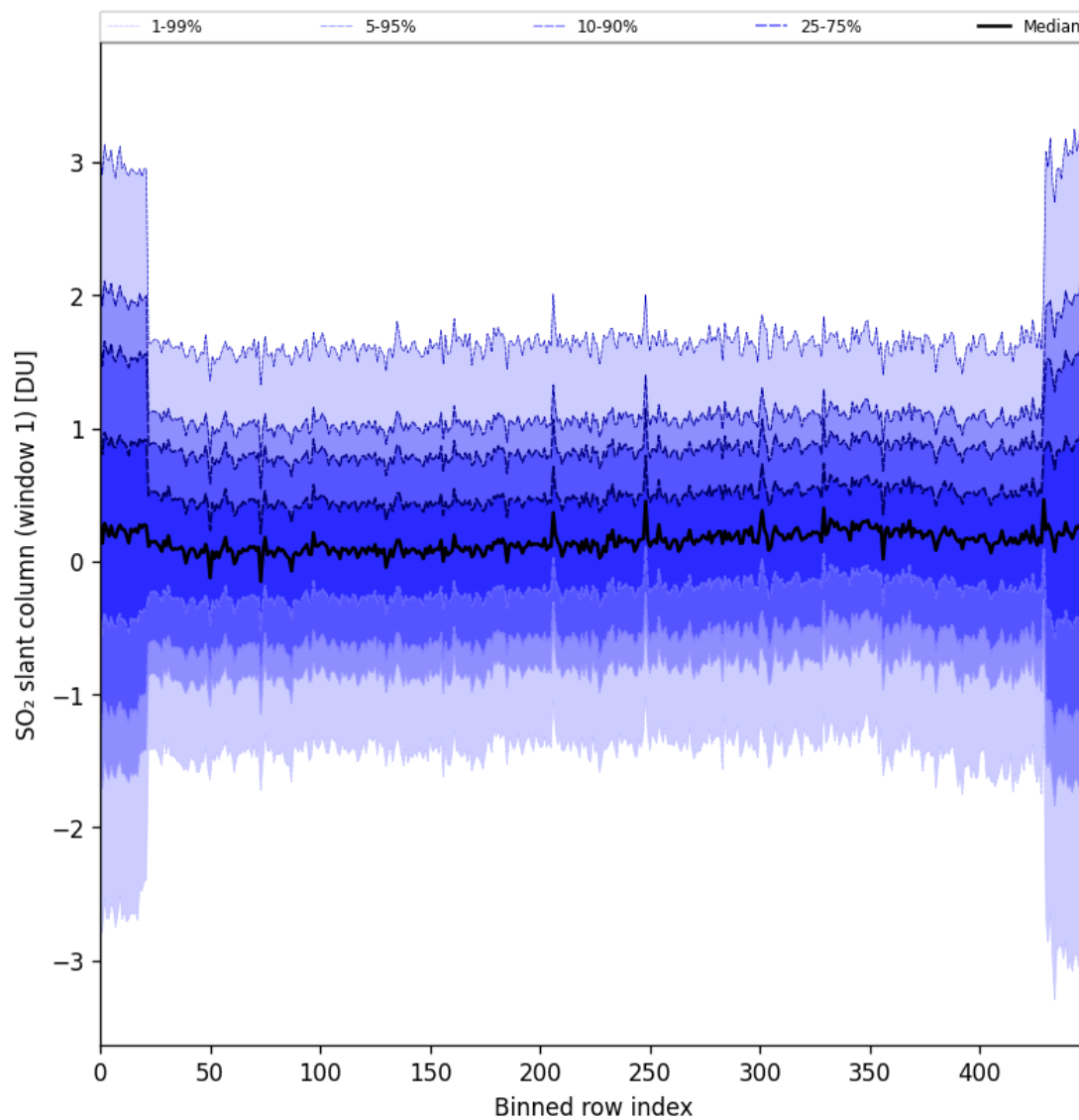
Figure 89: Along track statistics of “SO 2 slant column (window 1)” for 2025-10-20 to 2025-10-22
