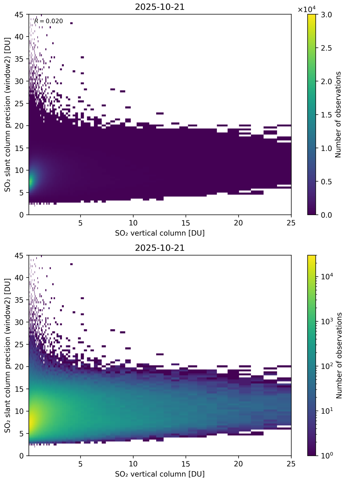
Figure 356: Scatter density plot of “SO 2 vertical column” against “SO 2 slant column precision (window2)” for 2025-10-20 to 2025-10-22.
