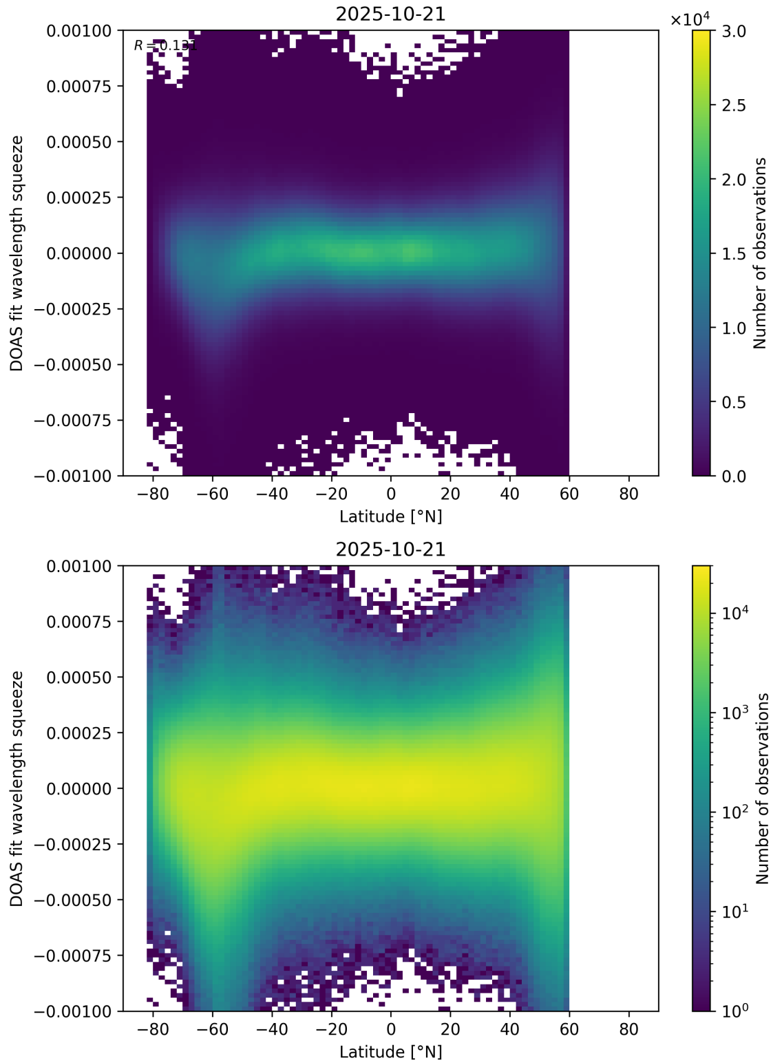
Figure 154: Scatter density plot of “Latitude” against “DOAS fit wavelength squeeze” for 2025-10-20 to 2025-10-22.
