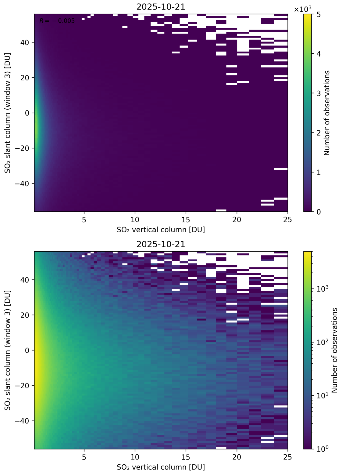
Figure 357: Scatter density plot of “SO 2 vertical column” against “SO 2 slant column (window 3)” for 2025-10-20 to 2025-10-22.
