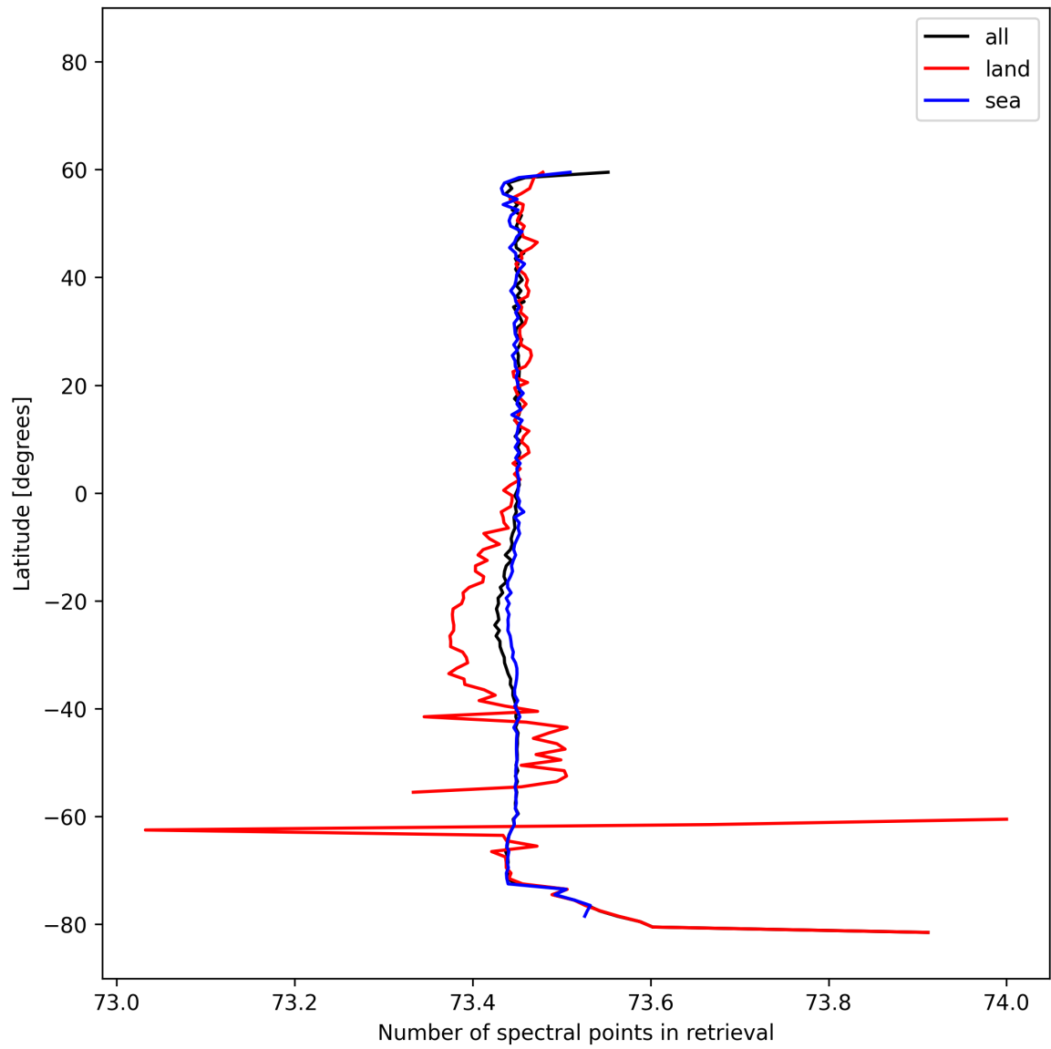
Figure 56: Zonal average of “Number of spectral points in retrieval” for 2025-10-20 to 2025-10-22.
