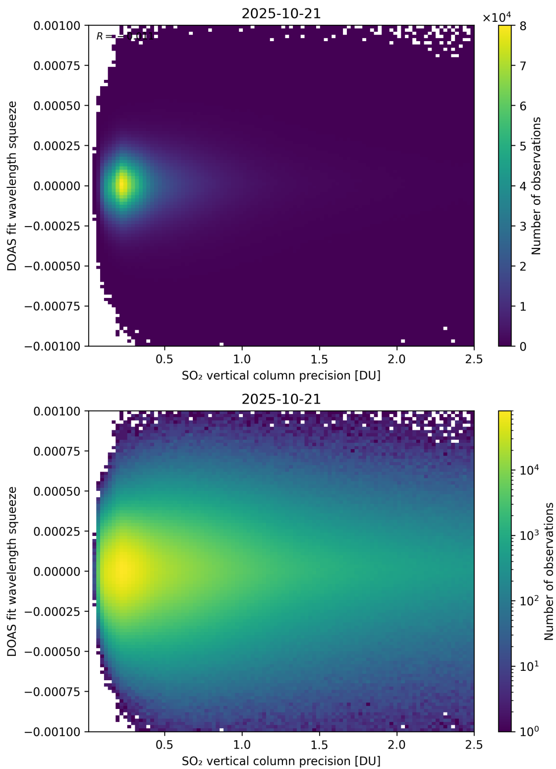
Figure 333: Scatter density plot of “SO 2 vertical column precision” against “DOAS fit wavelength squeeze” for 2025-10-20 to 2025-10-22.
