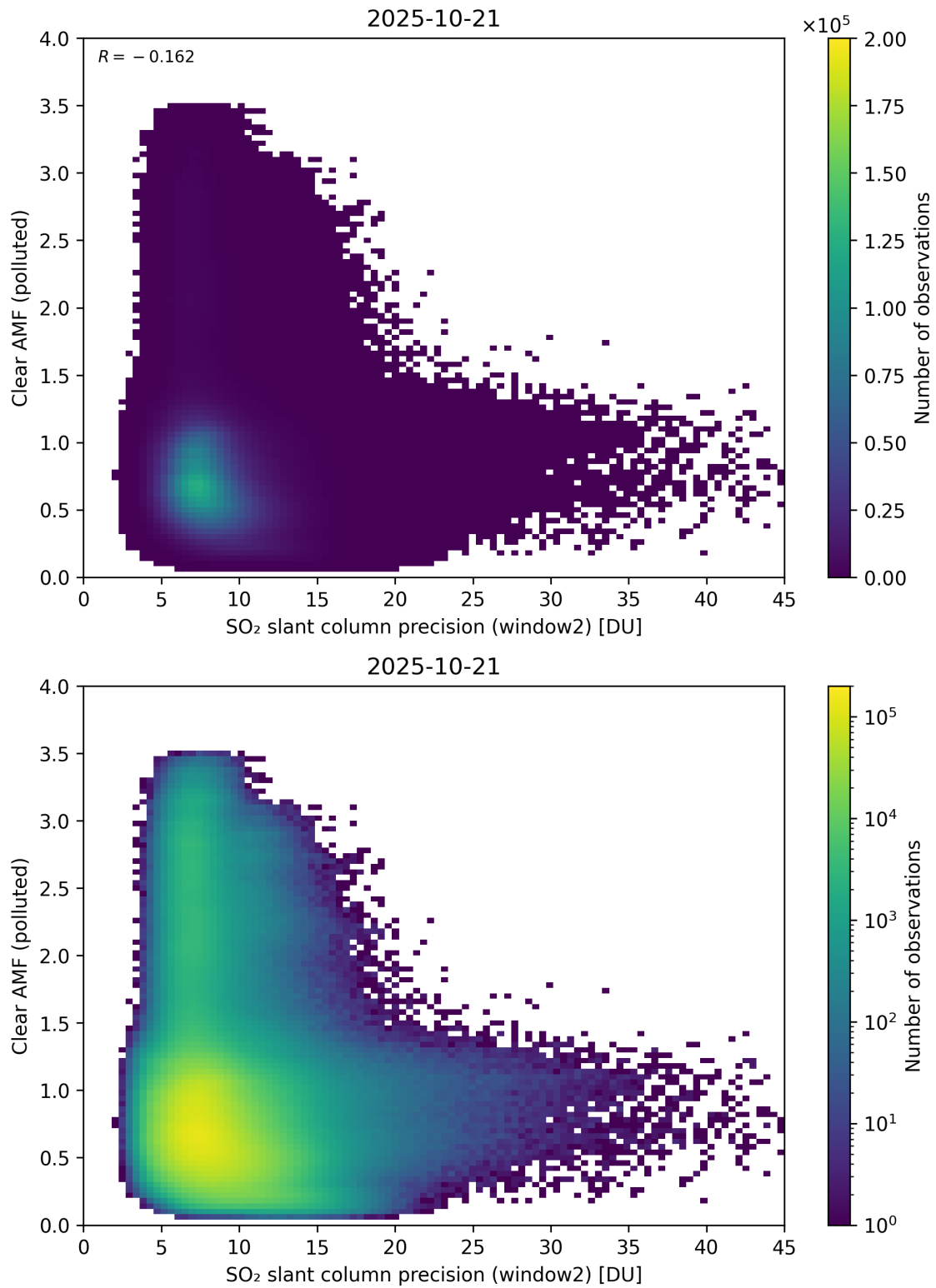
Figure 296: Scatter density plot of “SO 2 slant column precision (window2)” against “Clear AMF (polluted)” for 2025-10-20 to 2025-10-22.
