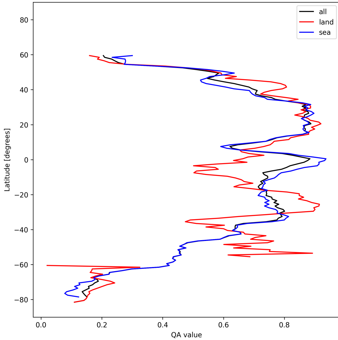
Figure 31: Zonal average of “QA value” for 2025-10-20 to 2025-10-22.
