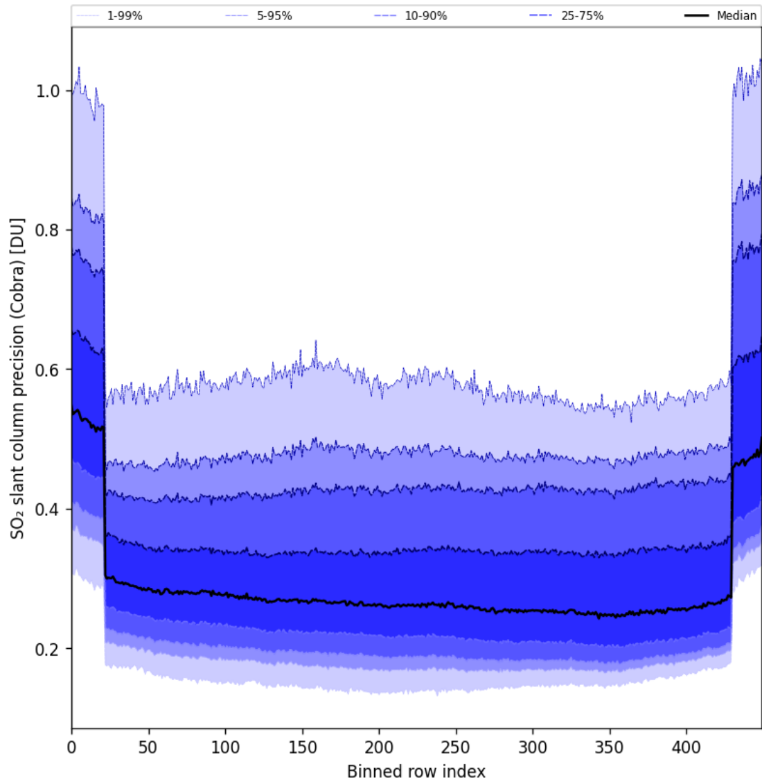
Figure 88: Along track statistics of “SO 2 slant column precision (Cobra)” for 2025-10-20 to 2025-10-22
