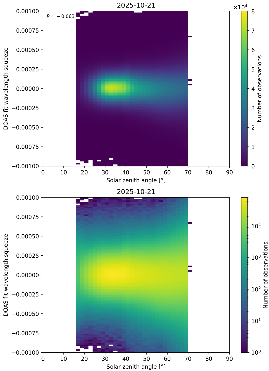
Figure 175: Scatter density plot of “Solar zenith angle” against “DOAS fit wavelength squeeze” for 2025-10-20 to 2025-10-22.
