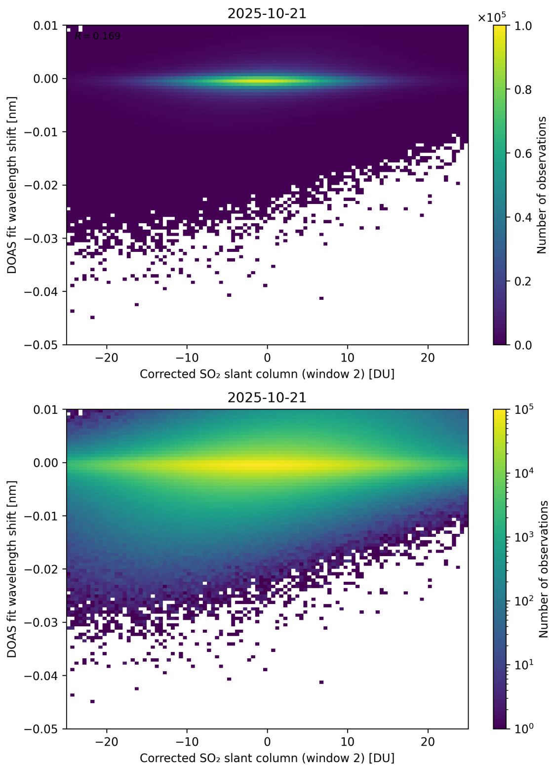
Figure 246: Scatter density plot of “Corrected SO 2 slant column (window 2)” against “DOAS fit wavelength shift” for 2025-10-20 to 2025-10-22.
