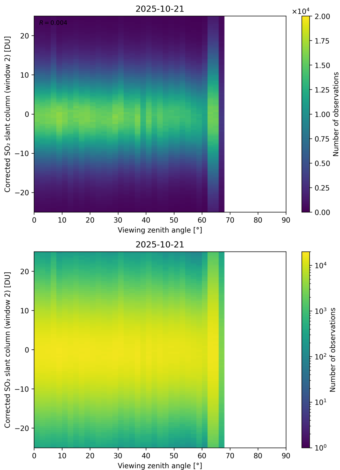
Figure 374: Scatter density plot of “Viewing zenith angle” against “Corrected SO 2 slant column (window 2)” for 2025-10-20 to 2025-10-22.
