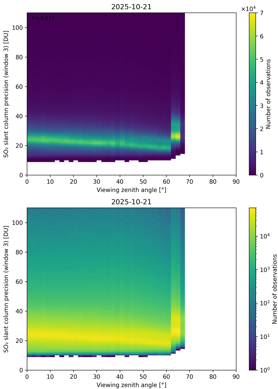
Figure 380: Scatter density plot of “Viewing zenith angle” against “SO 2 slant column precision (window 3)” for 2025-10-20 to 2025-10-22.
