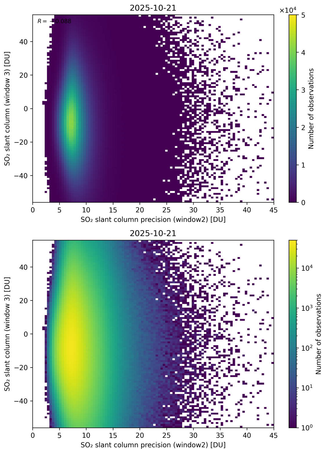
Figure 299: Scatter density plot of “SO 2 slant column precision (window2)” against “SO 2 slant column (window 3)” for 2025-10-20 to 2025-10-22.
