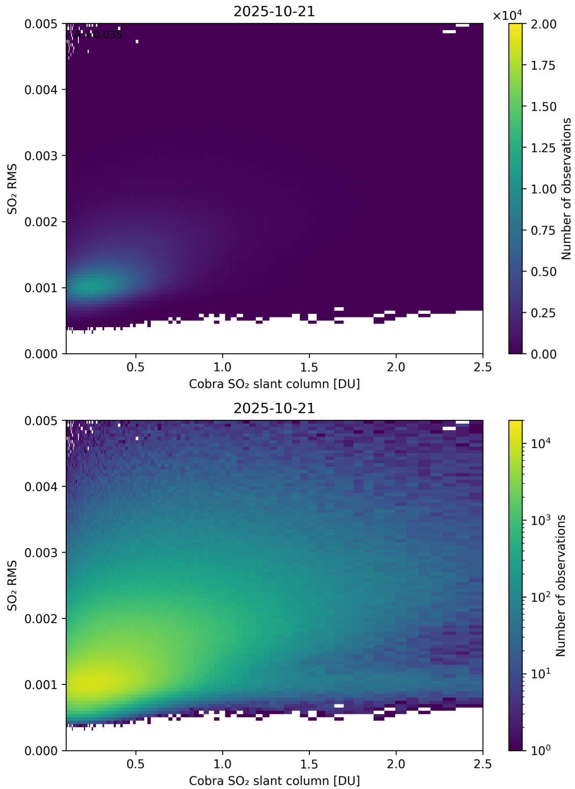
Figure 198: Scatter density plot of “Cobra SO 2 slant column” against “SO 2 RMS” for 2025-10-20 to 2025-10-22.
