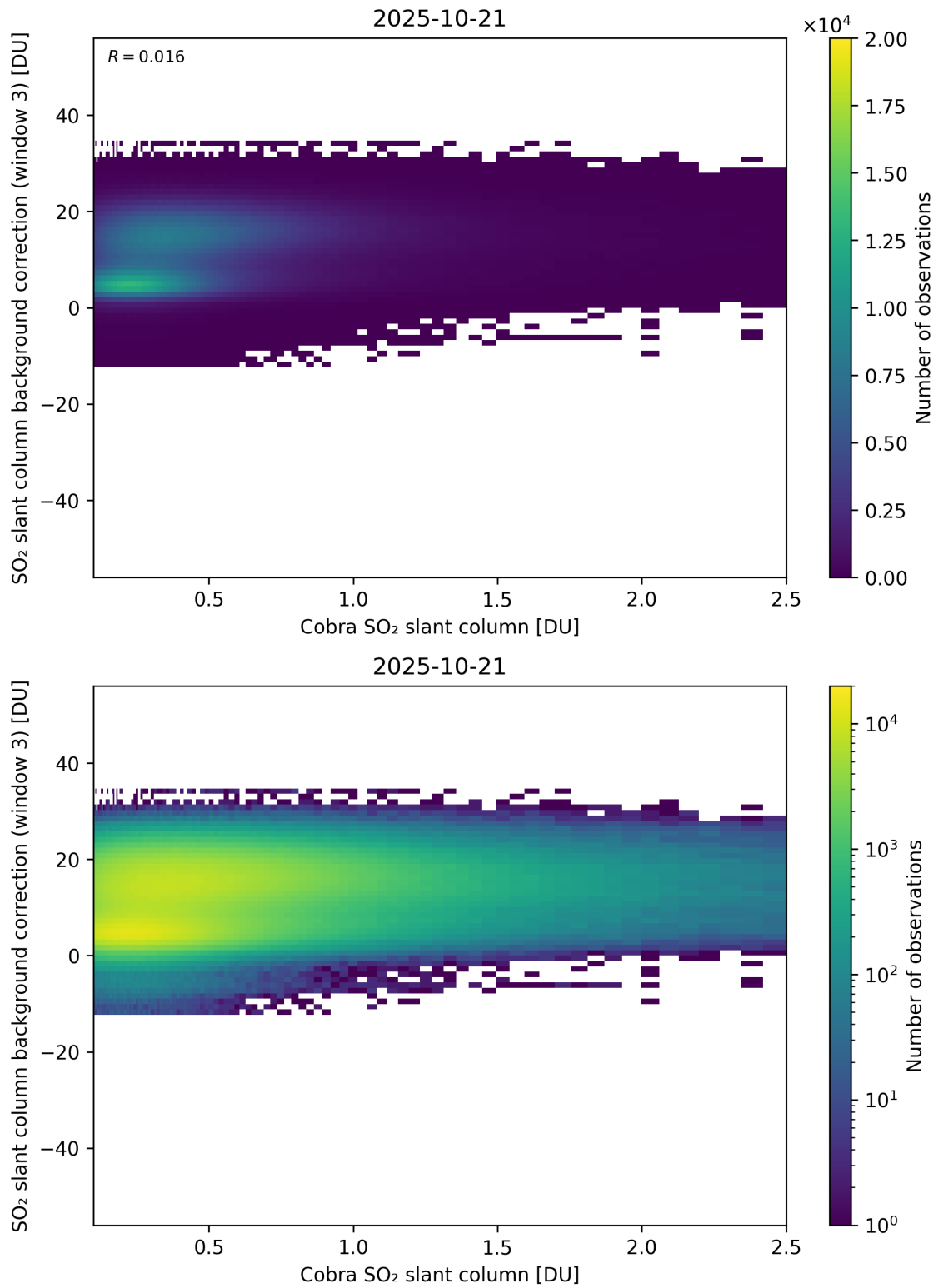
Figure 195: Scatter density plot of “Cobra SO 2 slant column” against “SO 2 slant column background correction (window 3)” for 2025-10-20 to 2025-10-22.
