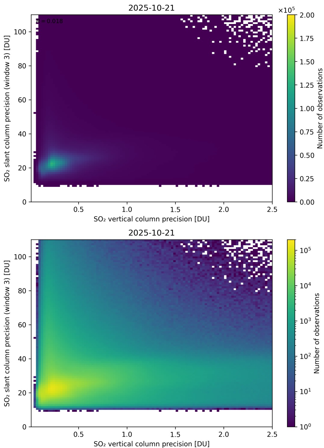
Figure 345: Scatter density plot of “SO 2 vertical column precision” against “SO 2 slant column precision (window 3)” for 2025-10-20 to 2025-10-22.
