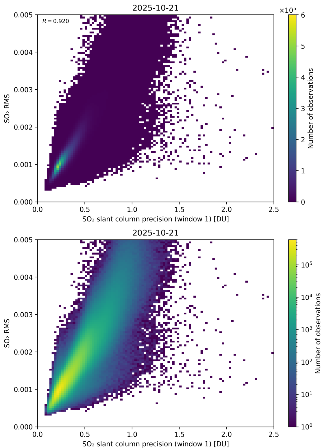
Figure 273: Scatter density plot of “SO 2 slant column precision (window 1)” against “SO 2 RMS” for 2025-10-20 to 2025-10-22.
