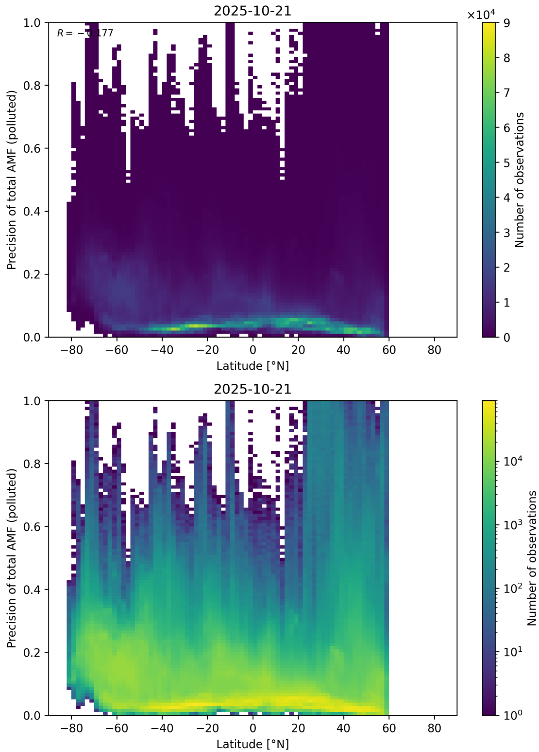
Figure 168: Scatter density plot of “Latitude” against “Precision of total AMF (polluted)” for 2025-10-20 to 2025-10-22.
