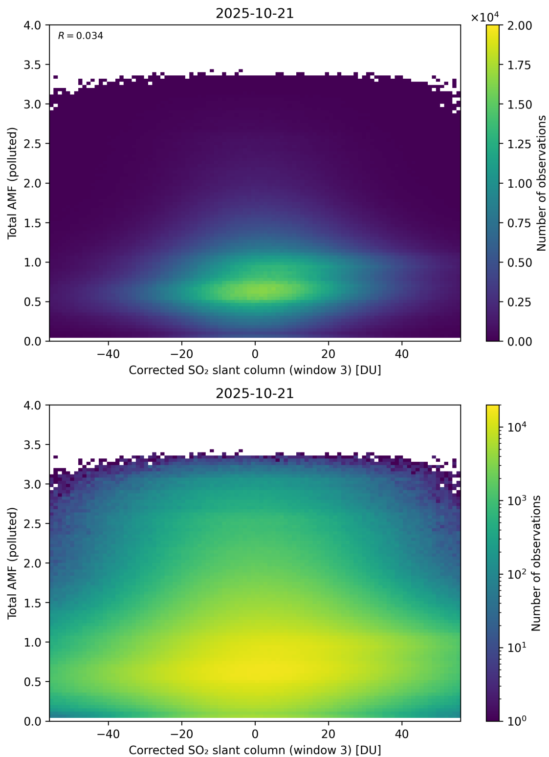
Figure 260: Scatter density plot of “Corrected SO 2 slant column (window 3)” against “Total AMF (polluted)” for 2025-10-20 to 2025-10-22.
