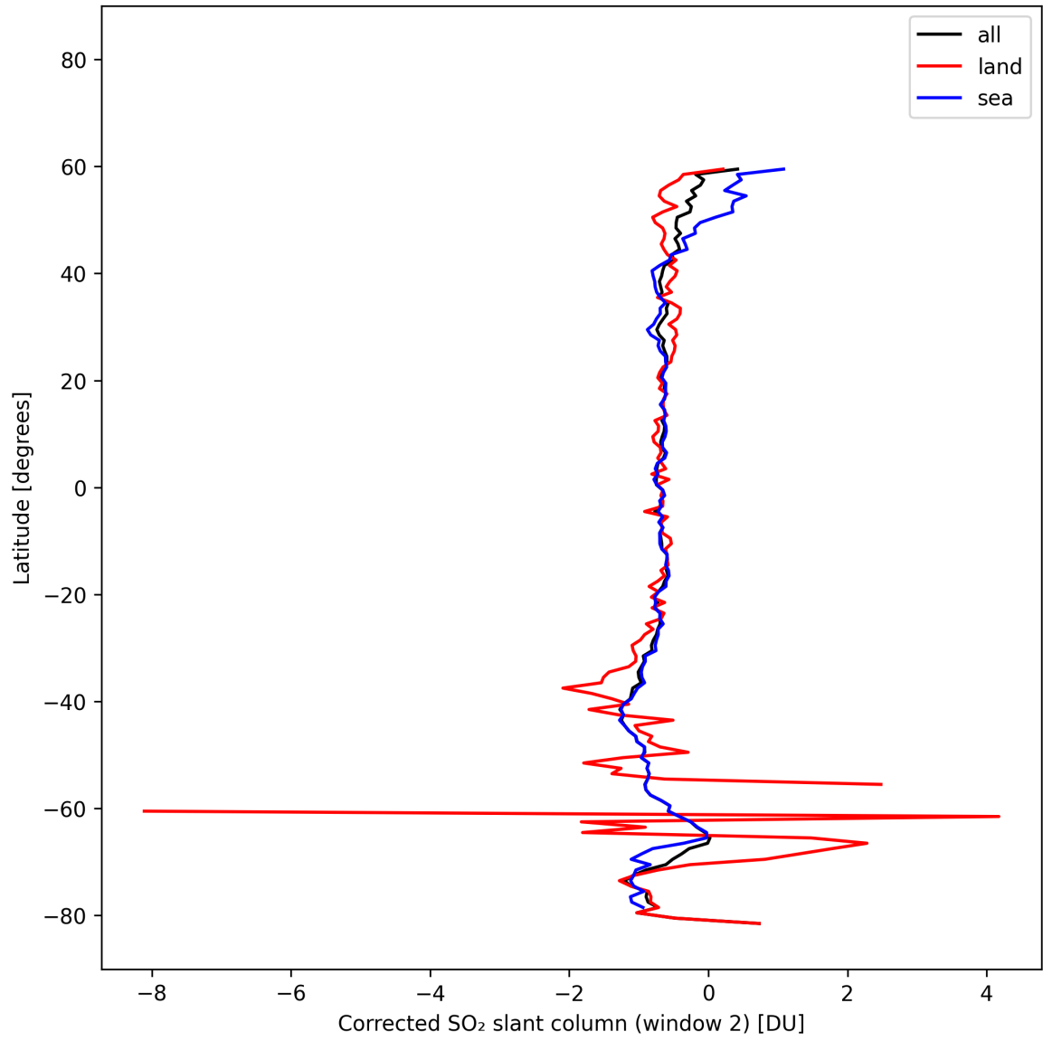
Figure 43: Zonal average of “Corrected SO 2 slant column (window 2)” for 2025-10-20 to 2025-10-22.
