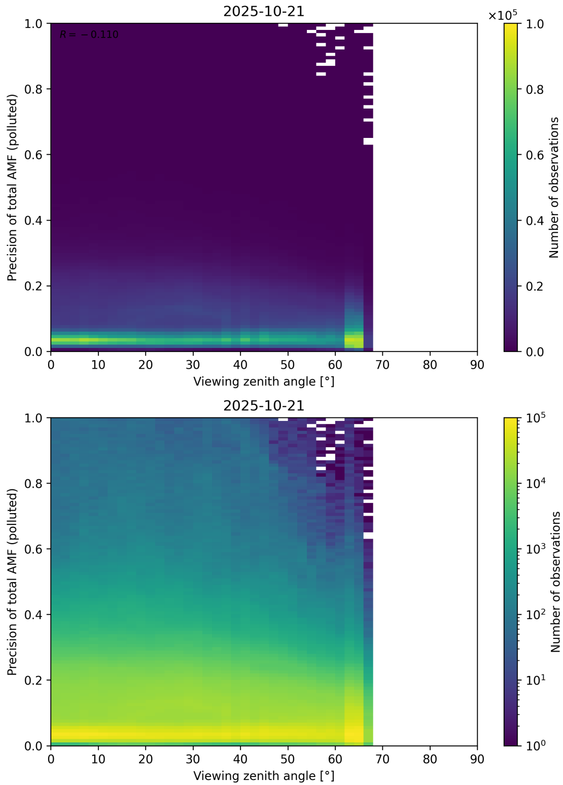
Figure 382: Scatter density plot of “Viewing zenith angle” against “Precision of total AMF (polluted)” for 2025-10-20 to 2025-10-22.
