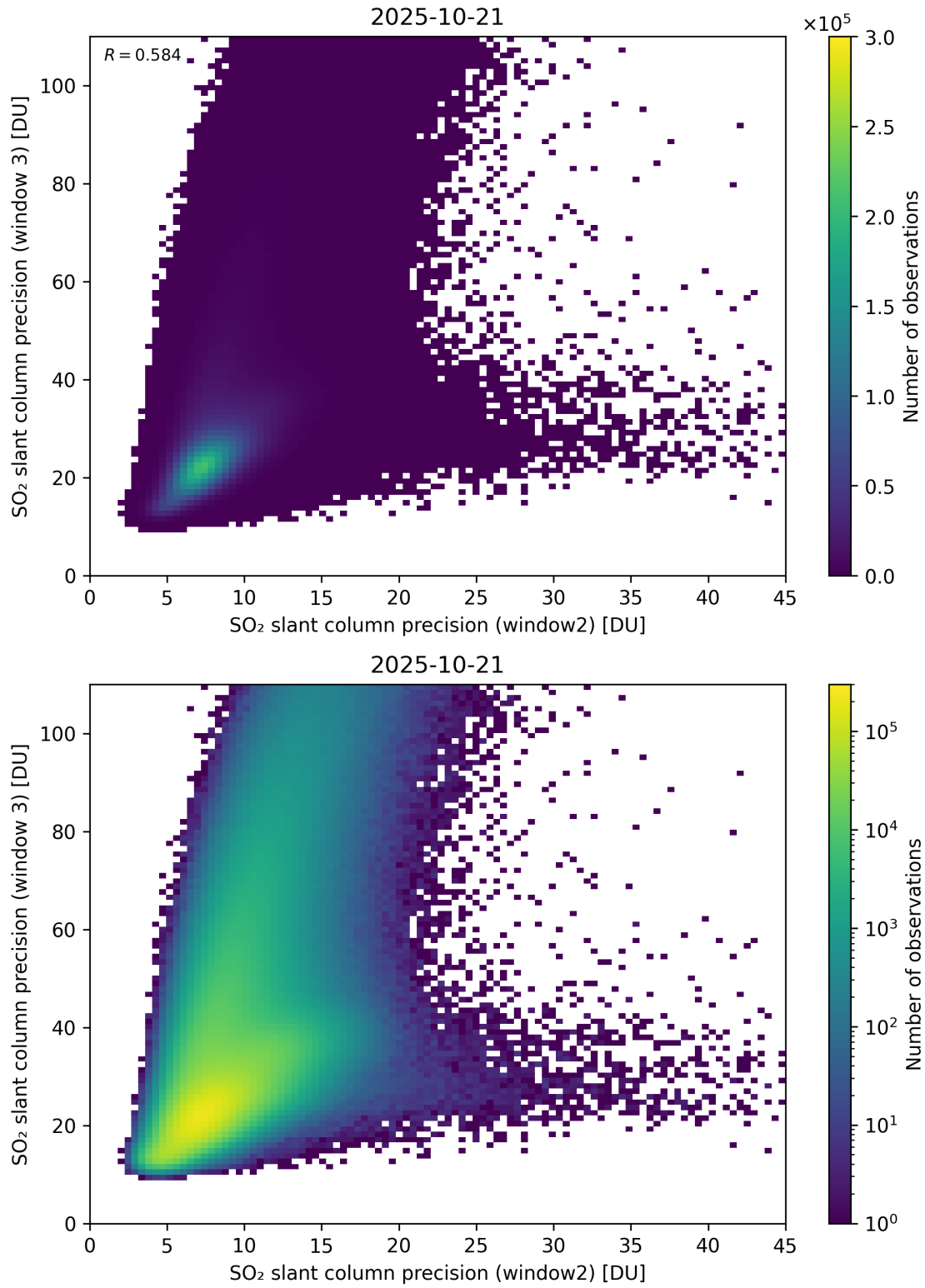
Figure 300: Scatter density plot of “SO 2 slant column precision (window2)” against “SO 2 slant column precision (window 3)” for 2025-10-20 to 2025-10-22.
