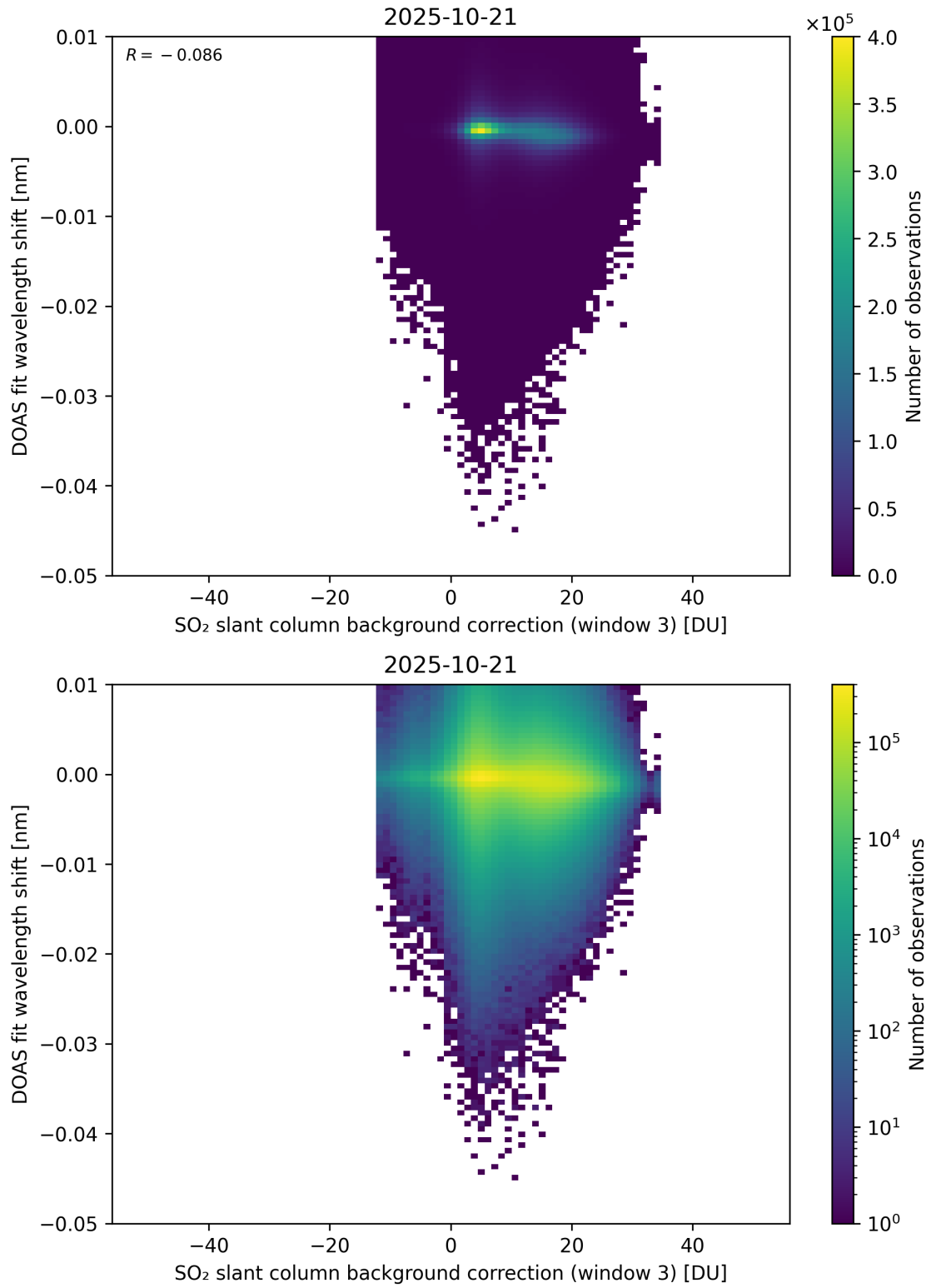
Figure 132: Scatter density plot of “SO 2 slant column background correction (window 3)” against “DOAS fit wavelength shift” for 2025-10-20 to 2025-10-22.
