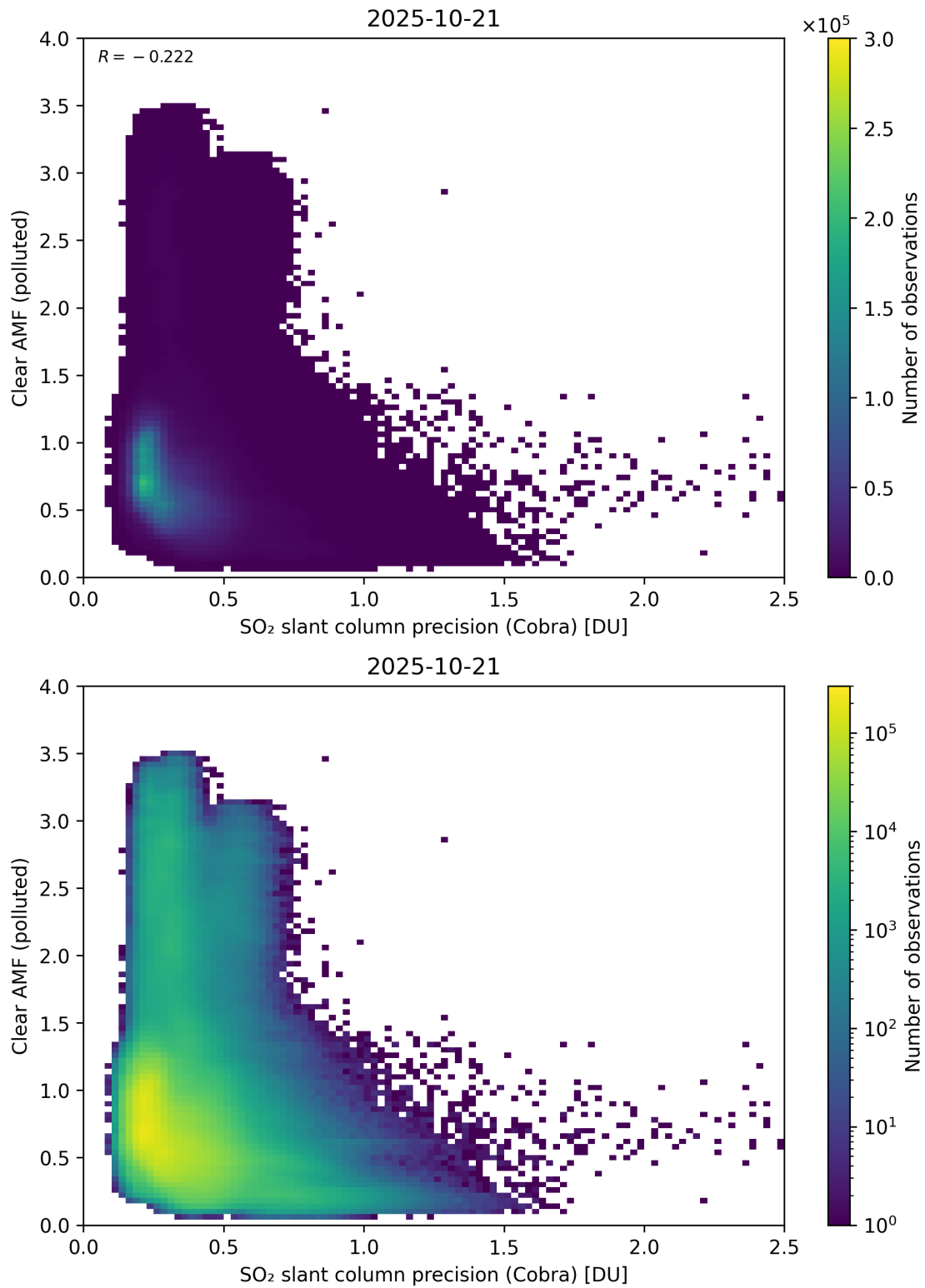
Figure 205: Scatter density plot of “SO 2 slant column precision (Cobra)” against “Clear AMF (polluted)” for 2025-10-20 to 2025-10-22.
