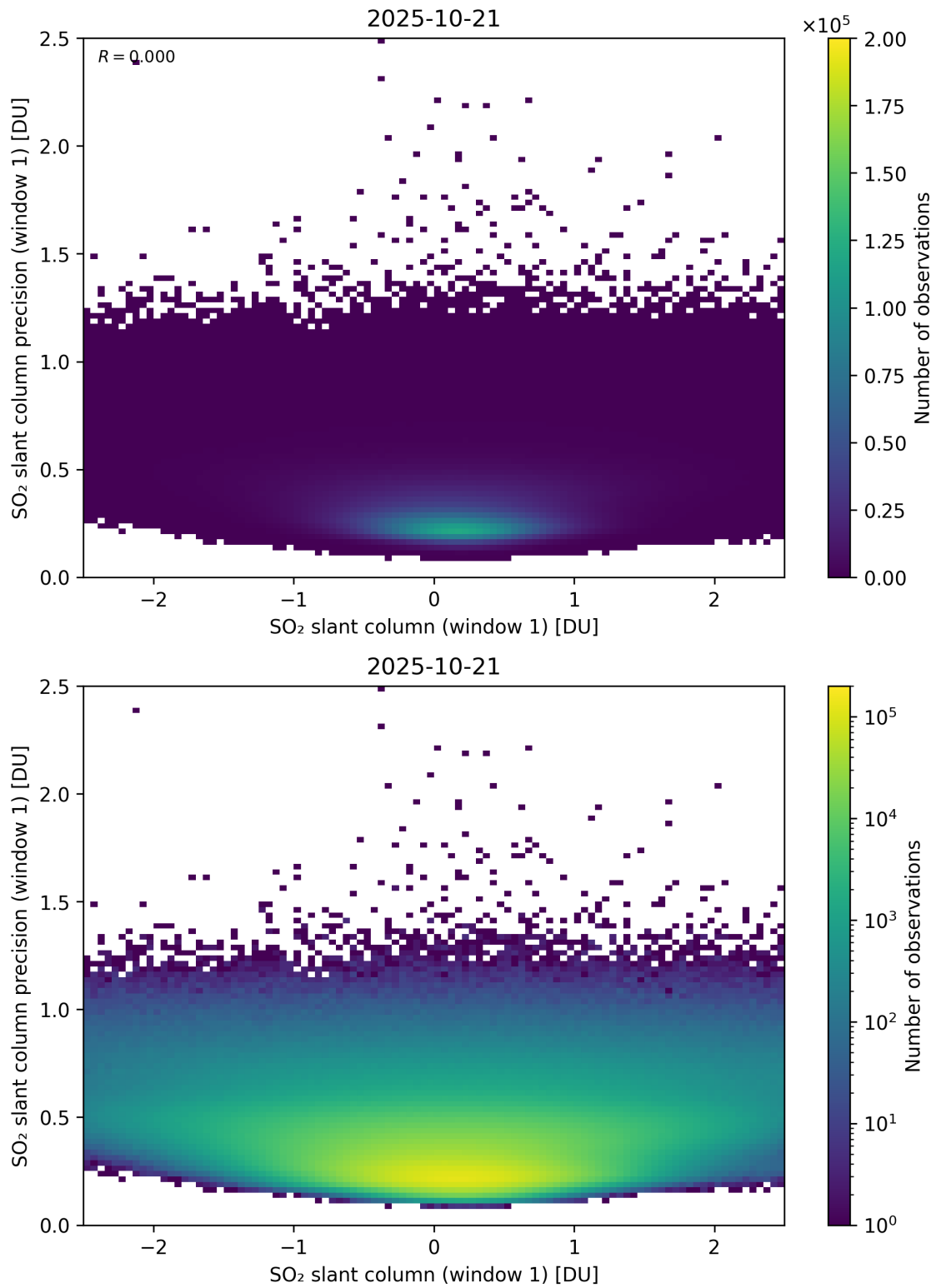
Figure 285: Scatter density plot of “SO 2 slant column (window 1)” against “SO 2 slant column precision (window 1)” for 2025-10-20 to 2025-10-22.
