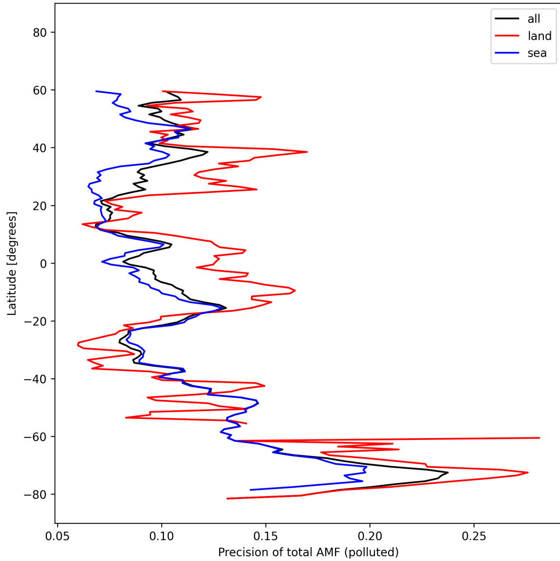
Figure 54: Zonal average of “Precision of total AMF (polluted)” for 2025-10-20 to 2025-10-22.
