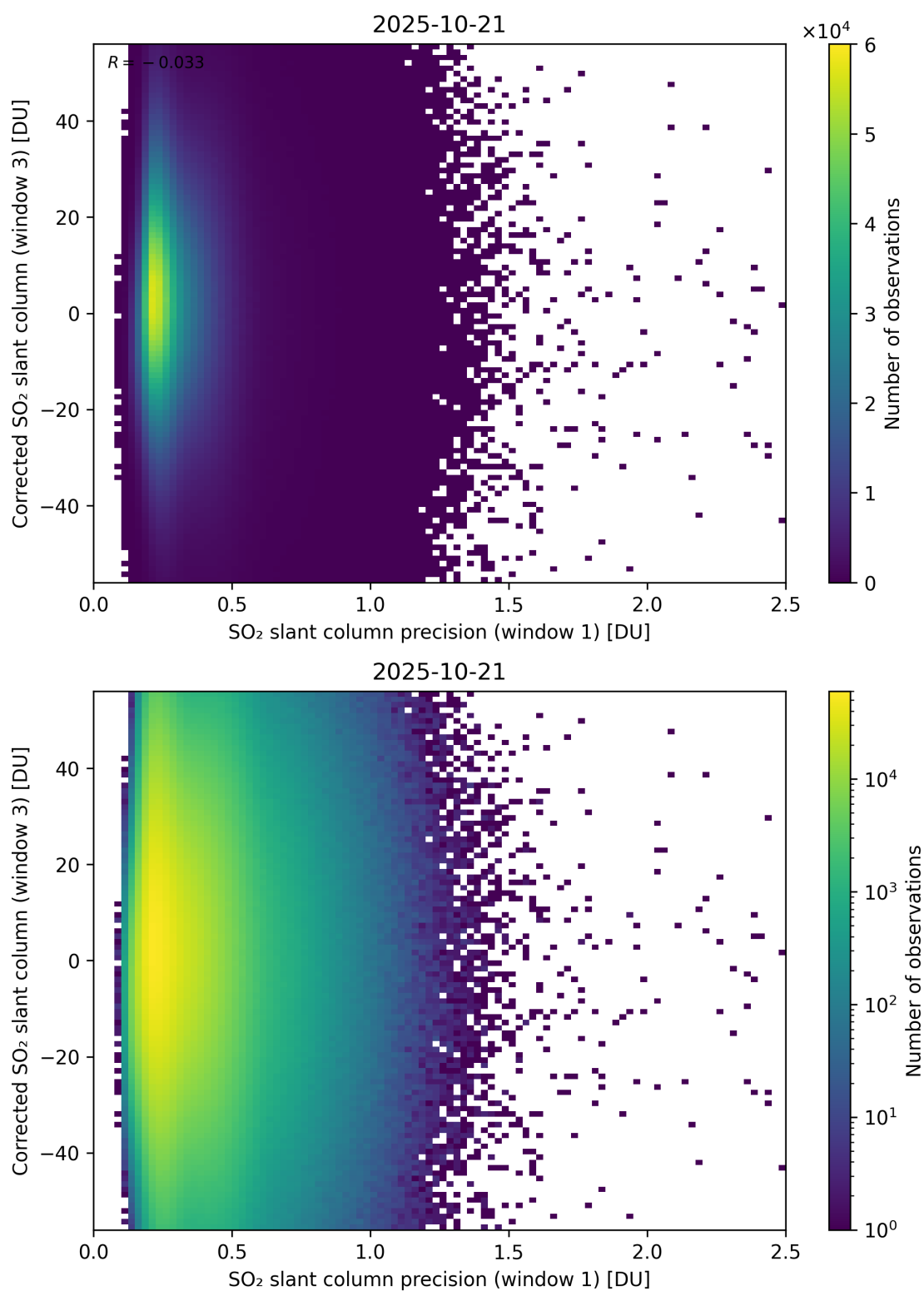
Figure 276: Scatter density plot of “SO 2 slant column precision (window 1)” against “Corrected SO 2 slant column (window 3)” for 2025-10-20 to 2025-10-22.
