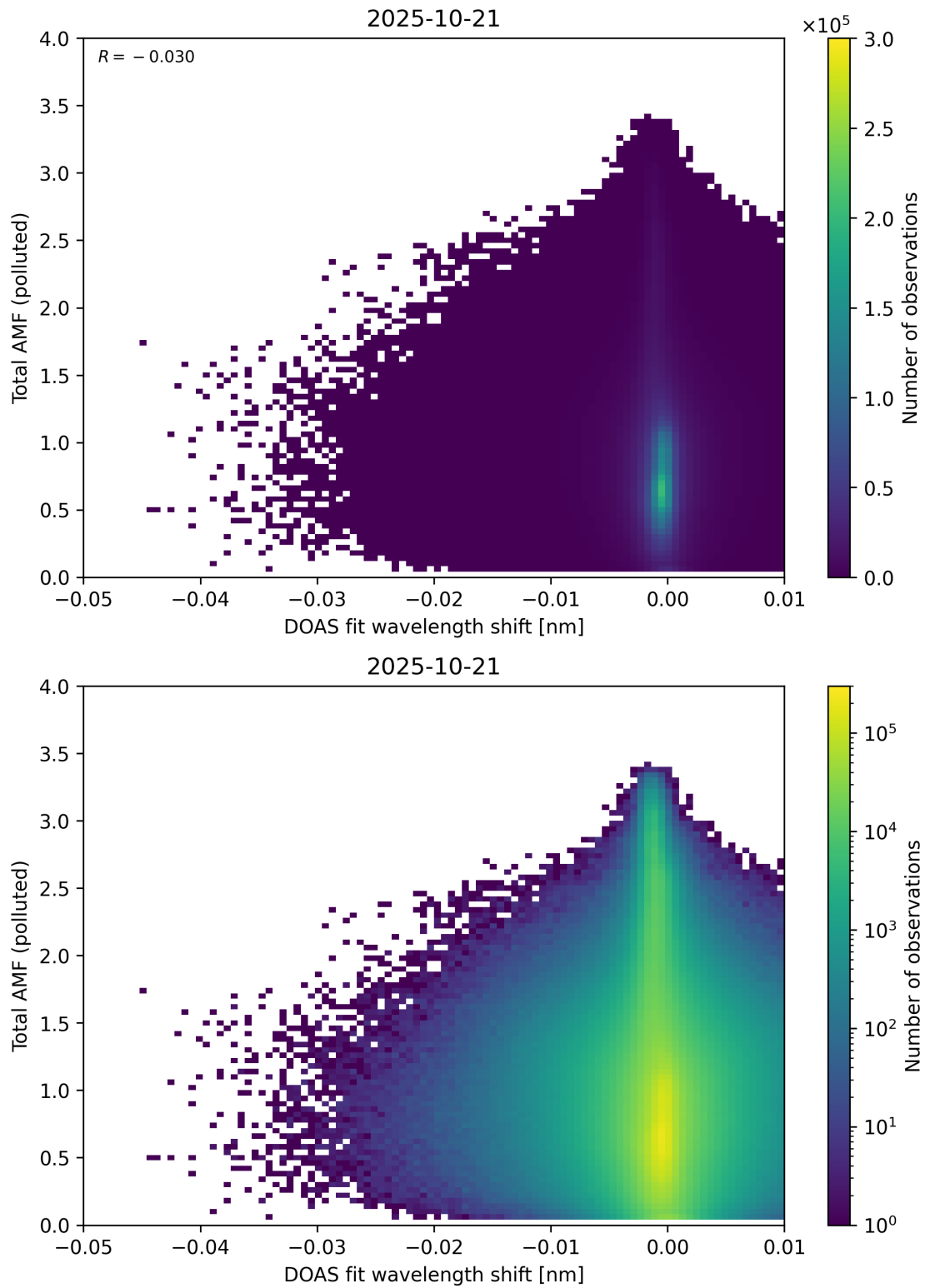
Figure 141: Scatter density plot of “DOAS fit wavelength shift” against “Total AMF (polluted)” for 2025-10-20 to 2025-10-22.
