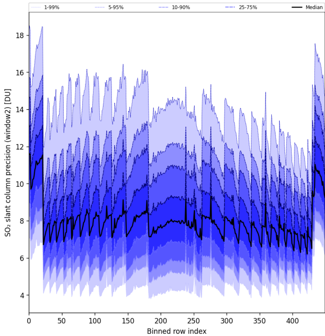
Figure 94: Along track statistics of “SO 2 slant column precision (window2)” for 2025-10-20 to 2025-10-22
