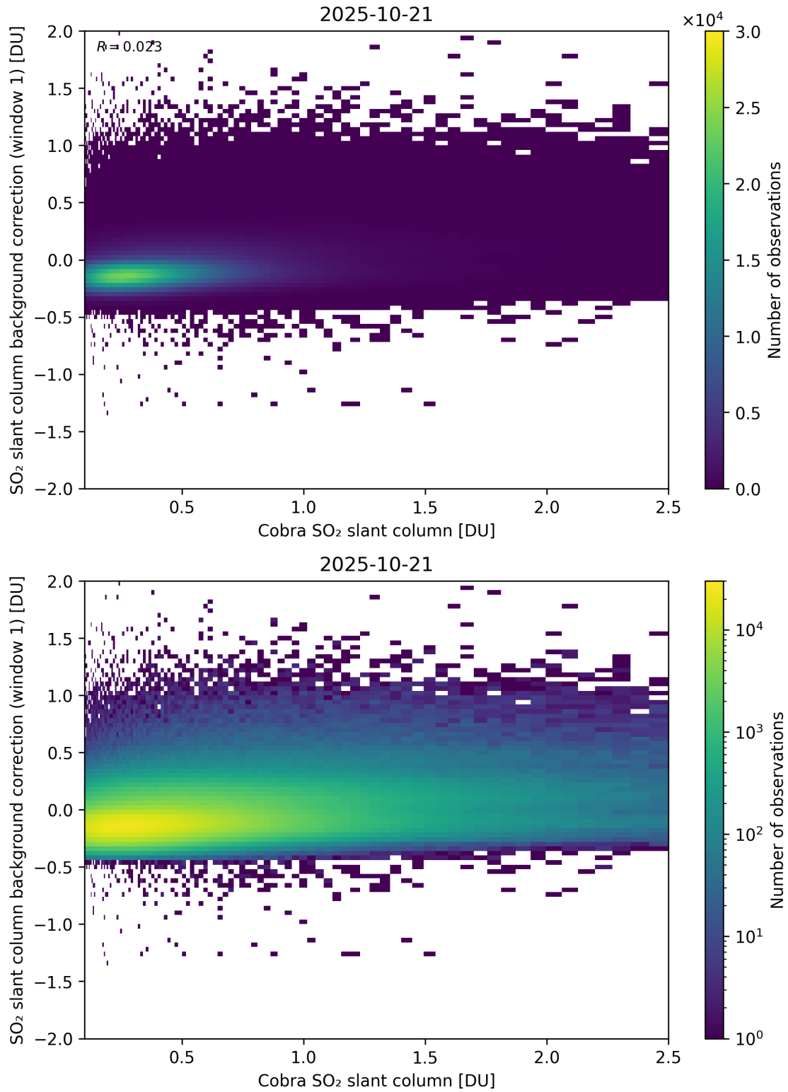
Figure 193: Scatter density plot of “Cobra SO 2 slant column” against “SO 2 slant column background correction (window 1)” for 2025-10-20 to 2025-10-22.
