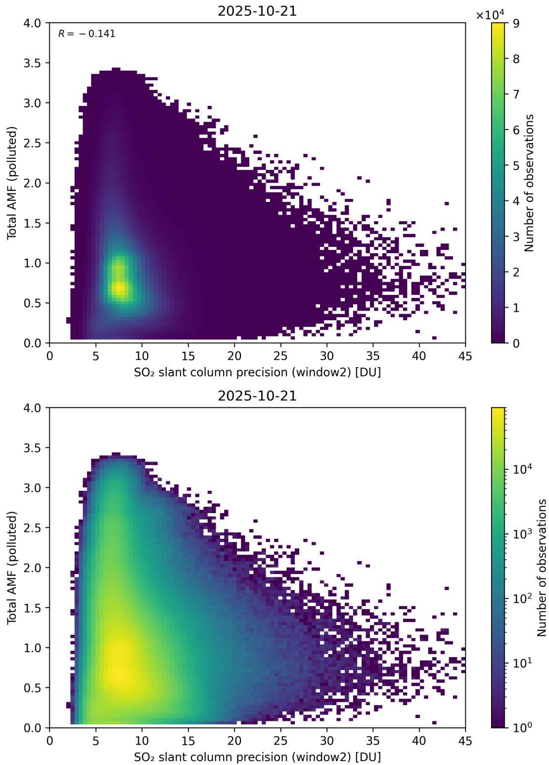
Figure 301: Scatter density plot of “SO 2 slant column precision (window2)” against “Total AMF (polluted)” for 2025-10-20 to 2025-10-22.
