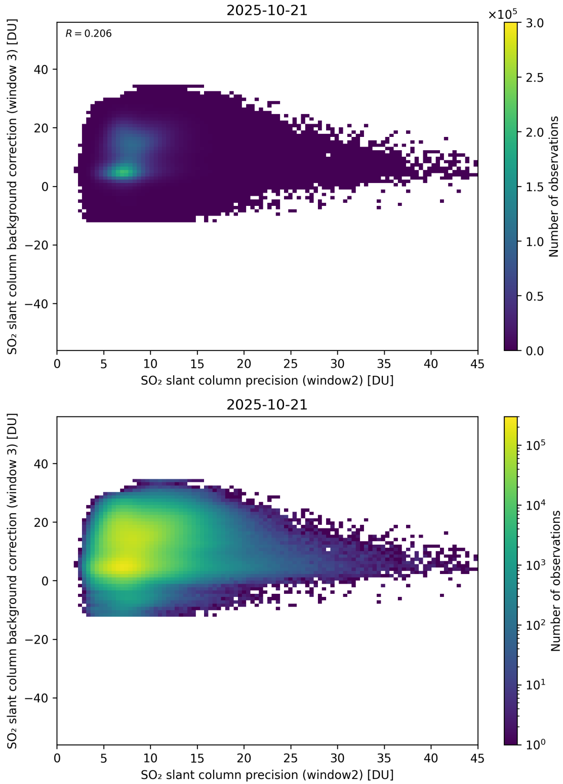
Figure 292: Scatter density plot of “SO 2 slant column precision (window2)” against “SO 2 slant column background correction (window 3)” for 2025-10-20 to 2025-10-22.
