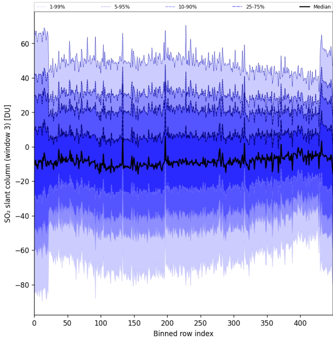
Figure 97: Along track statistics of “SO 2 slant column (window 3)” for 2025-10-20 to 2025-10-22
