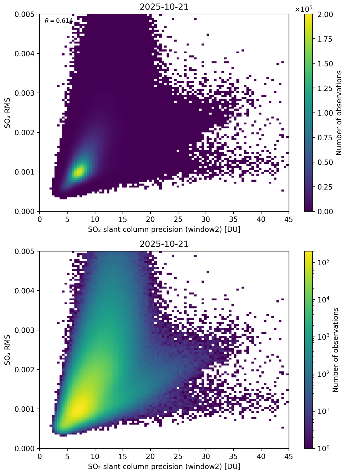
Figure 295: Scatter density plot of “SO 2 slant column precision (window2)” against “SO 2 RMS” for 2025-10-20 to 2025-10-22.
