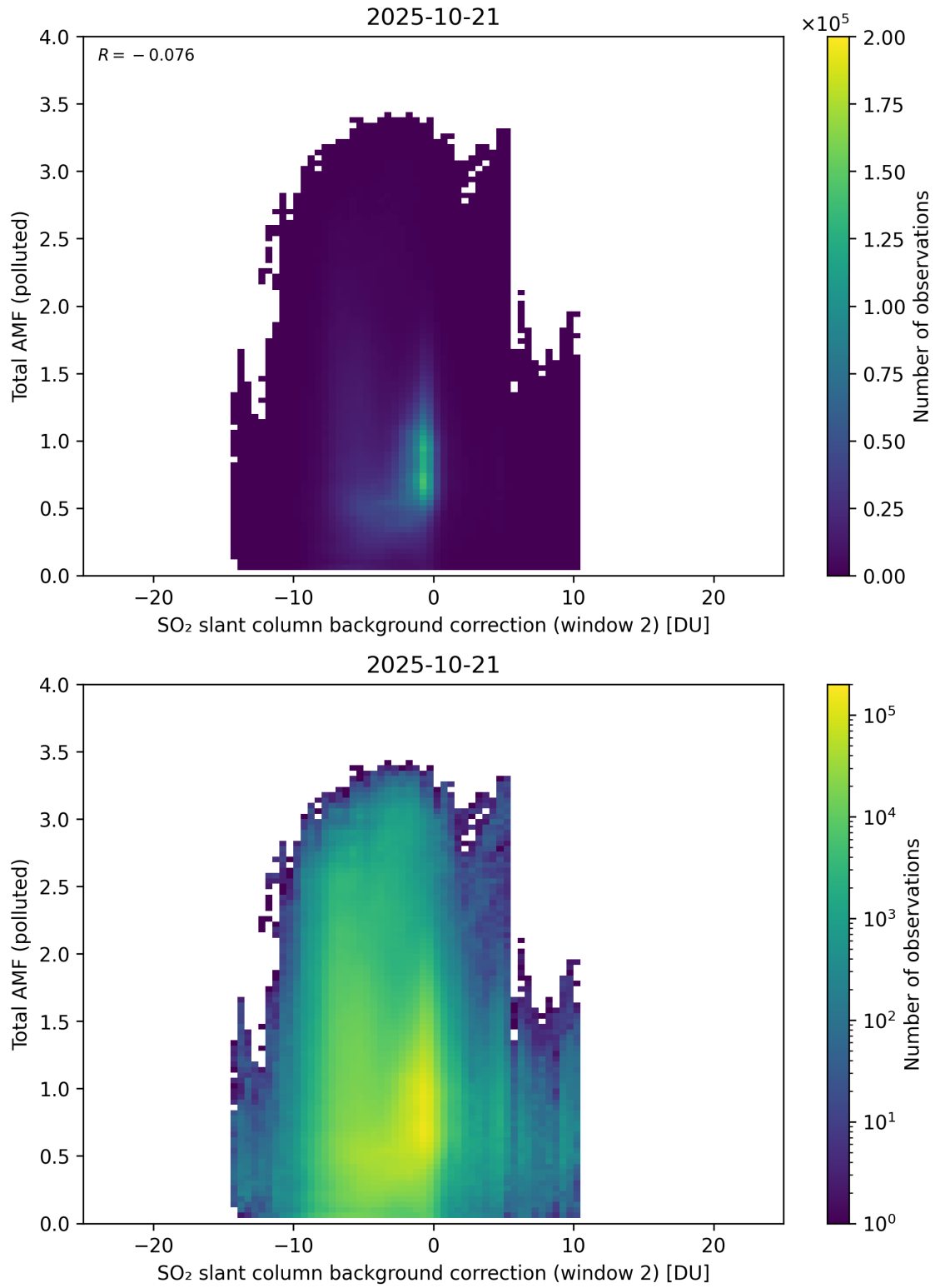
Figure 130: Scatter density plot of “SO 2 slant column background correction (window 2)” against “Total AMF (polluted)” for 2025-10-20 to 2025-10-22.
