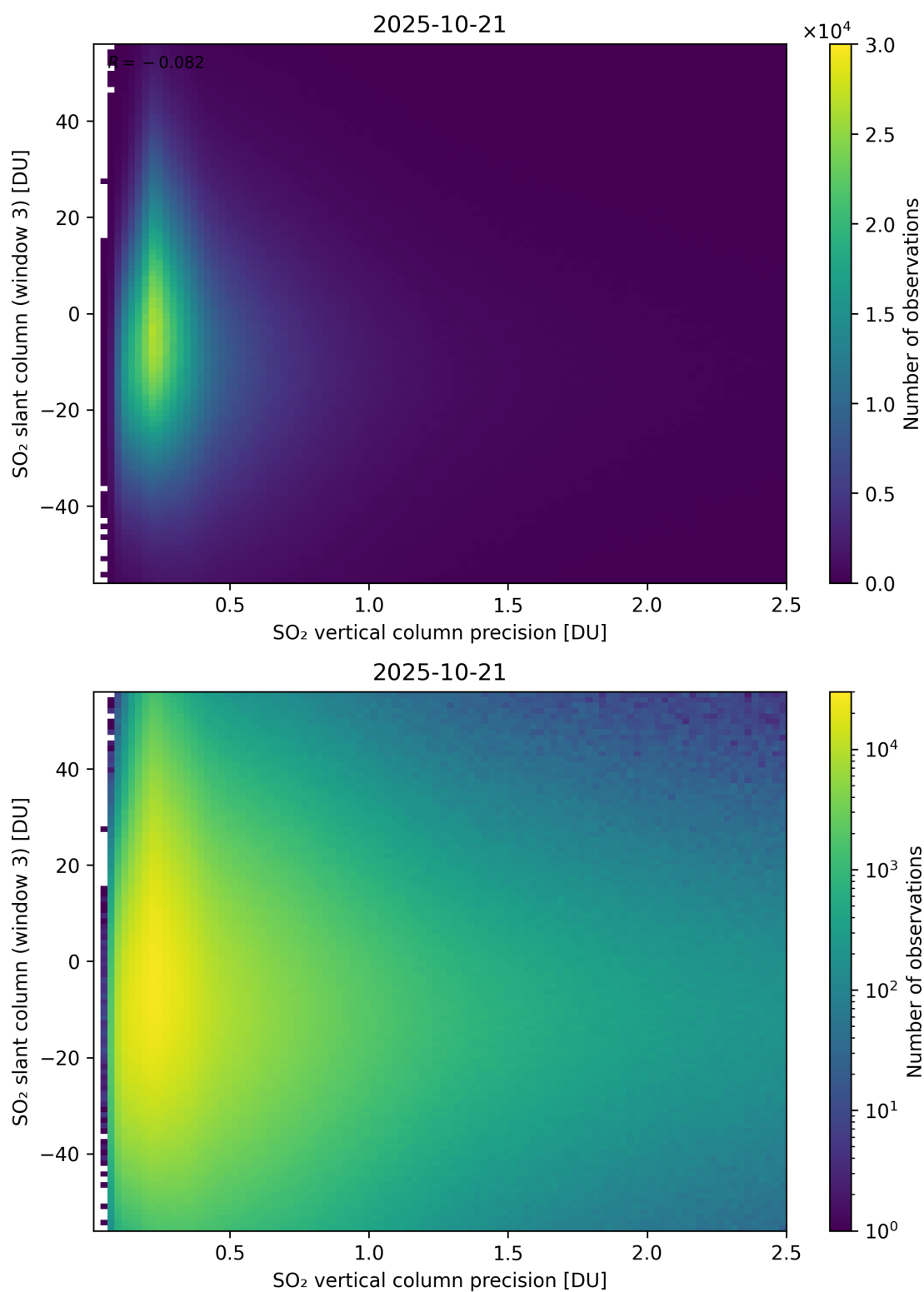
Figure 344: Scatter density plot of “SO 2 vertical column precision” against “SO 2 slant column (window 3)” for 2025-10-20 to 2025-10-22.
