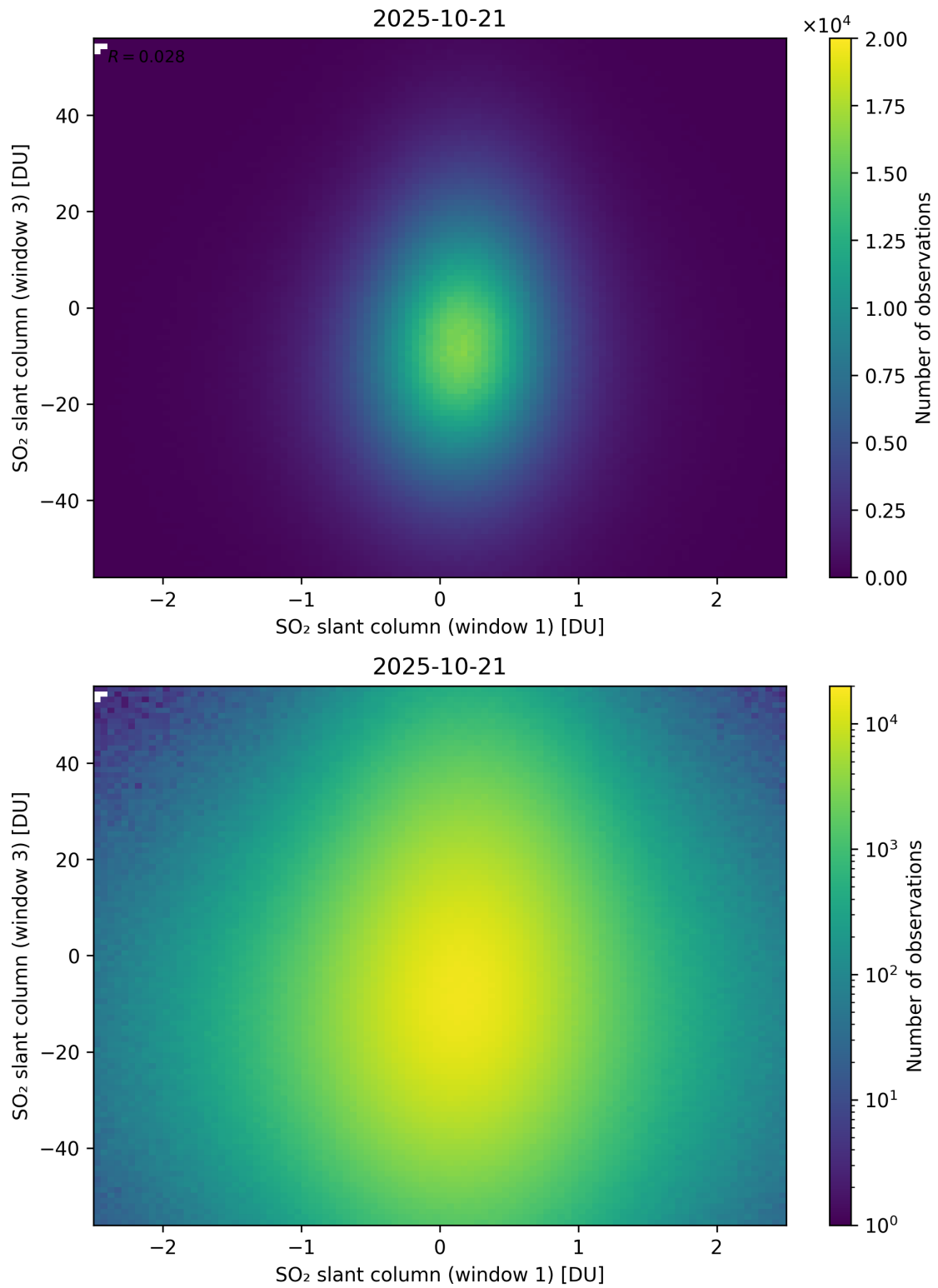
Figure 287: Scatter density plot of “SO 2 slant column (window 1)” against “SO 2 slant column (window 3)” for 2025-10-20 to 2025-10-22.
