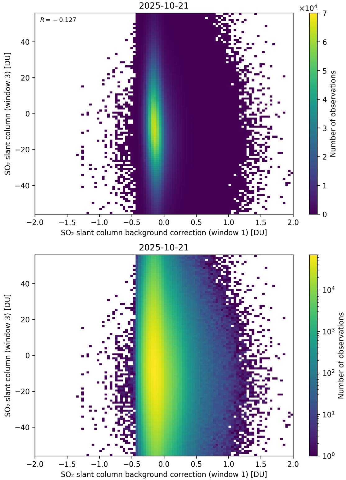
Figure 118: Scatter density plot of “SO 2 slant column background correction (window 1)” against “SO 2 slant column (window 3)” for 2025-10-20 to 2025-10-22.
