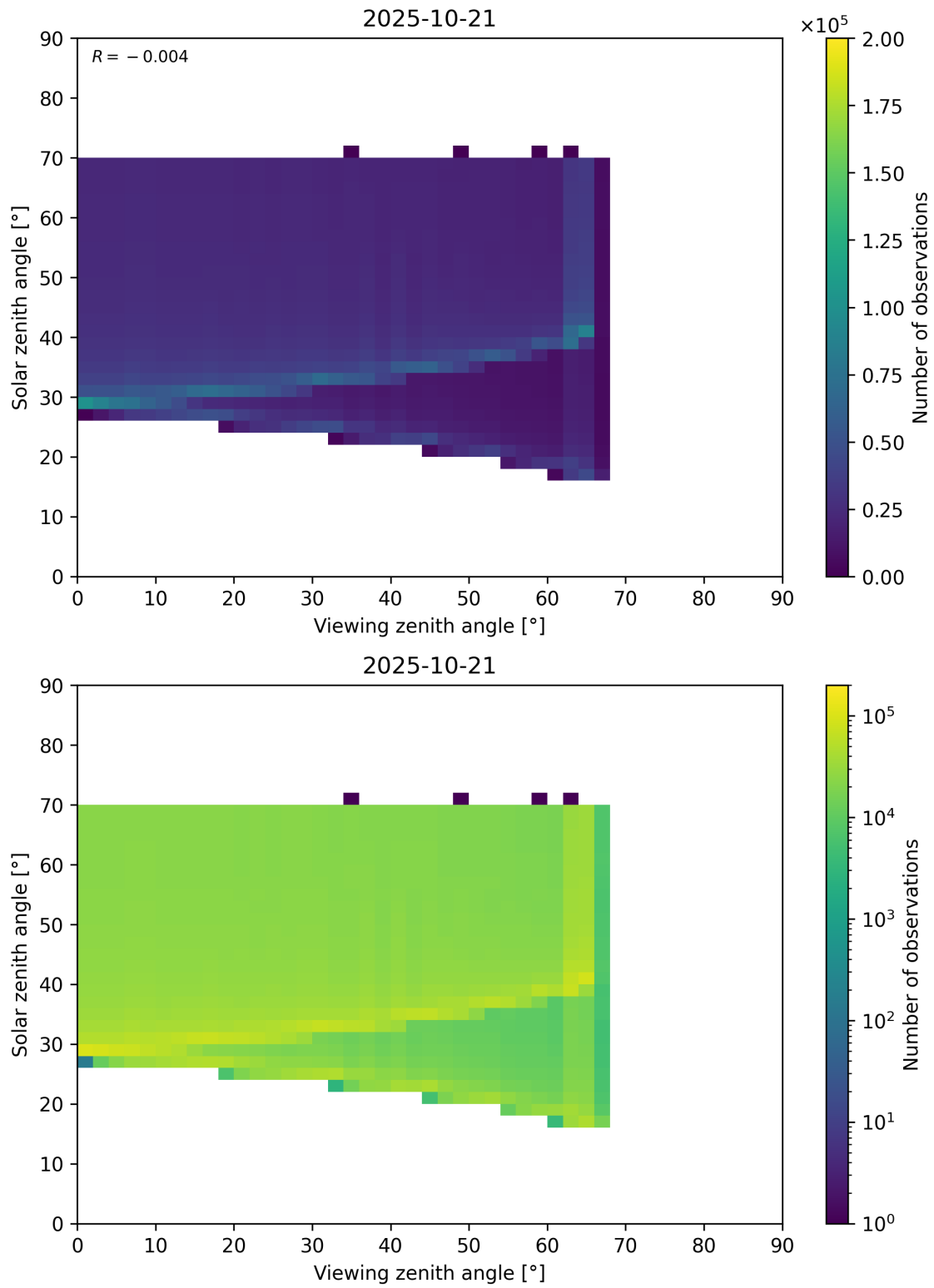
Figure 369: Scatter density plot of “Viewing zenith angle” against “Solar zenith angle” for 2025-10-20 to 2025-10-22.
