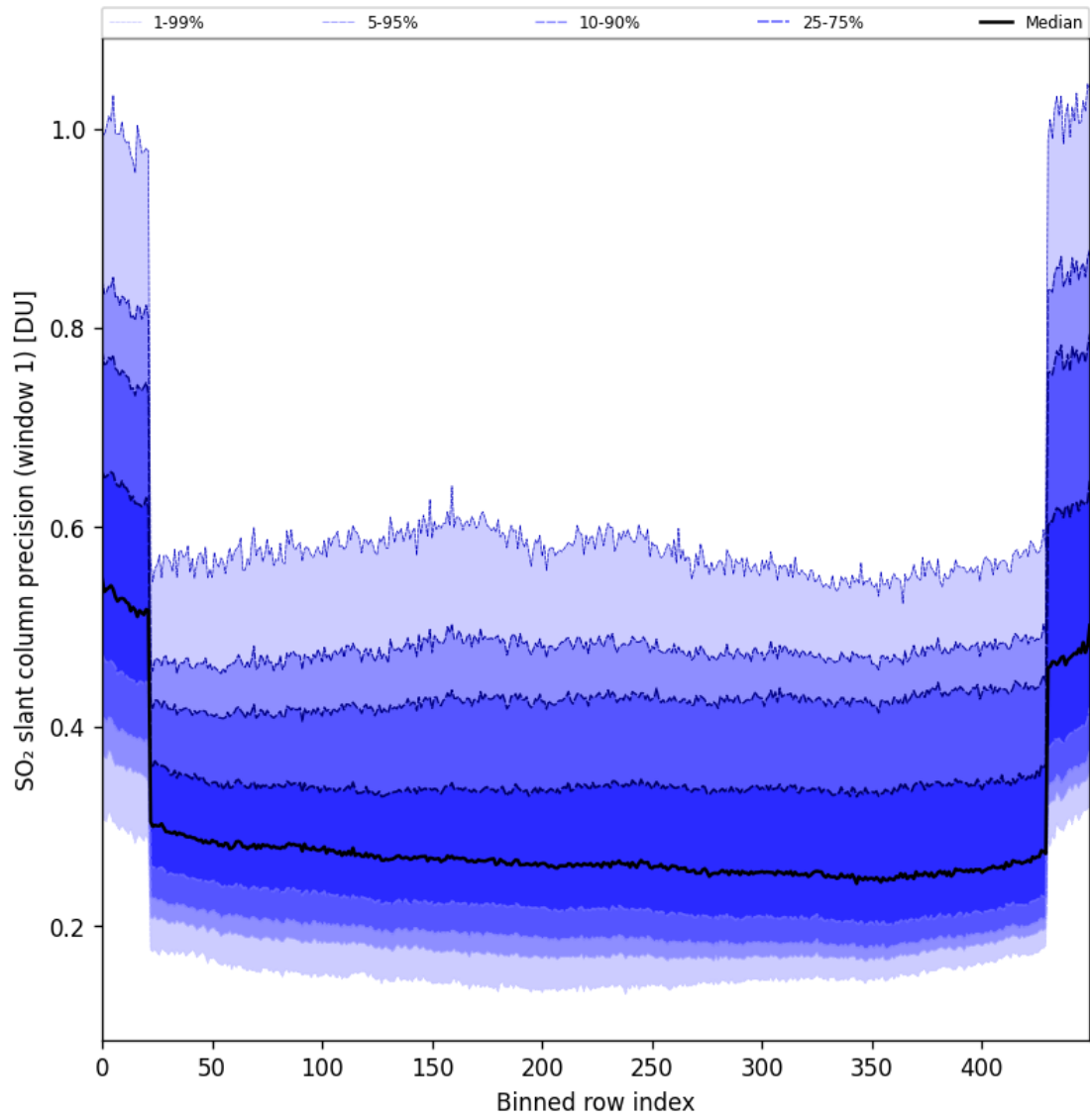
Figure 90: Along track statistics of “SO 2 slant column precision (window 1)” for 2025-10-20 to 2025-10-22
