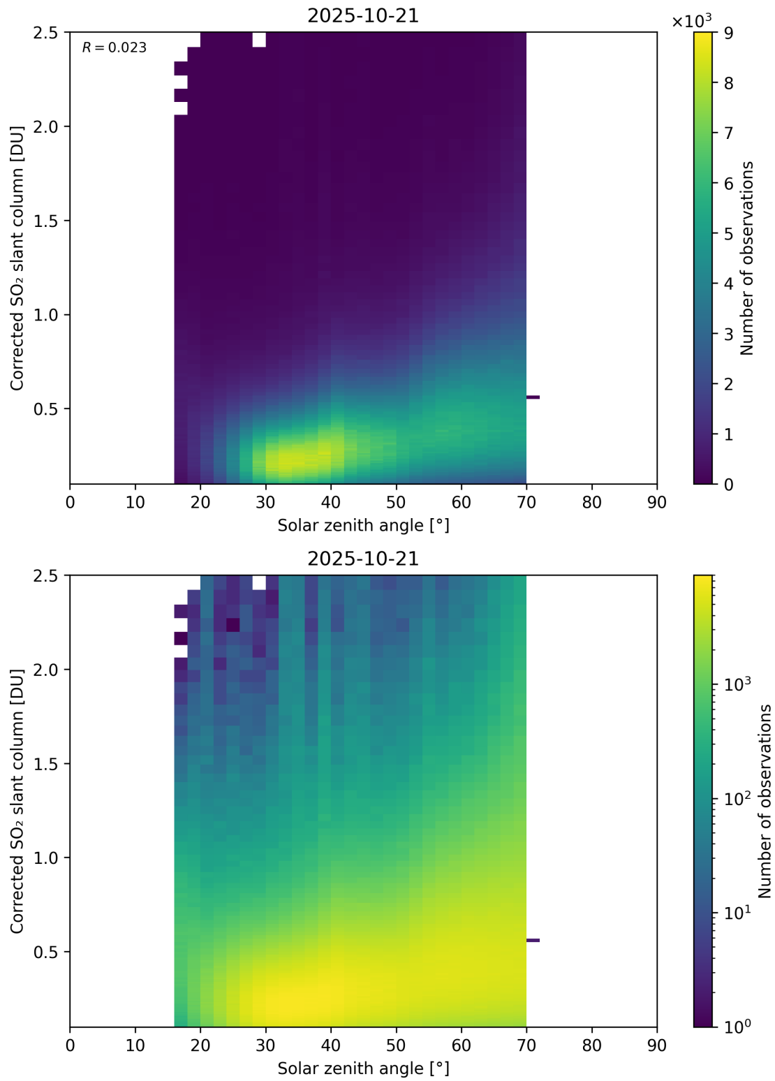
Figure 181: Scatter density plot of “Solar zenith angle” against “Corrected SO 2 slant column” for 2025-10-20 to 2025-10-22.
