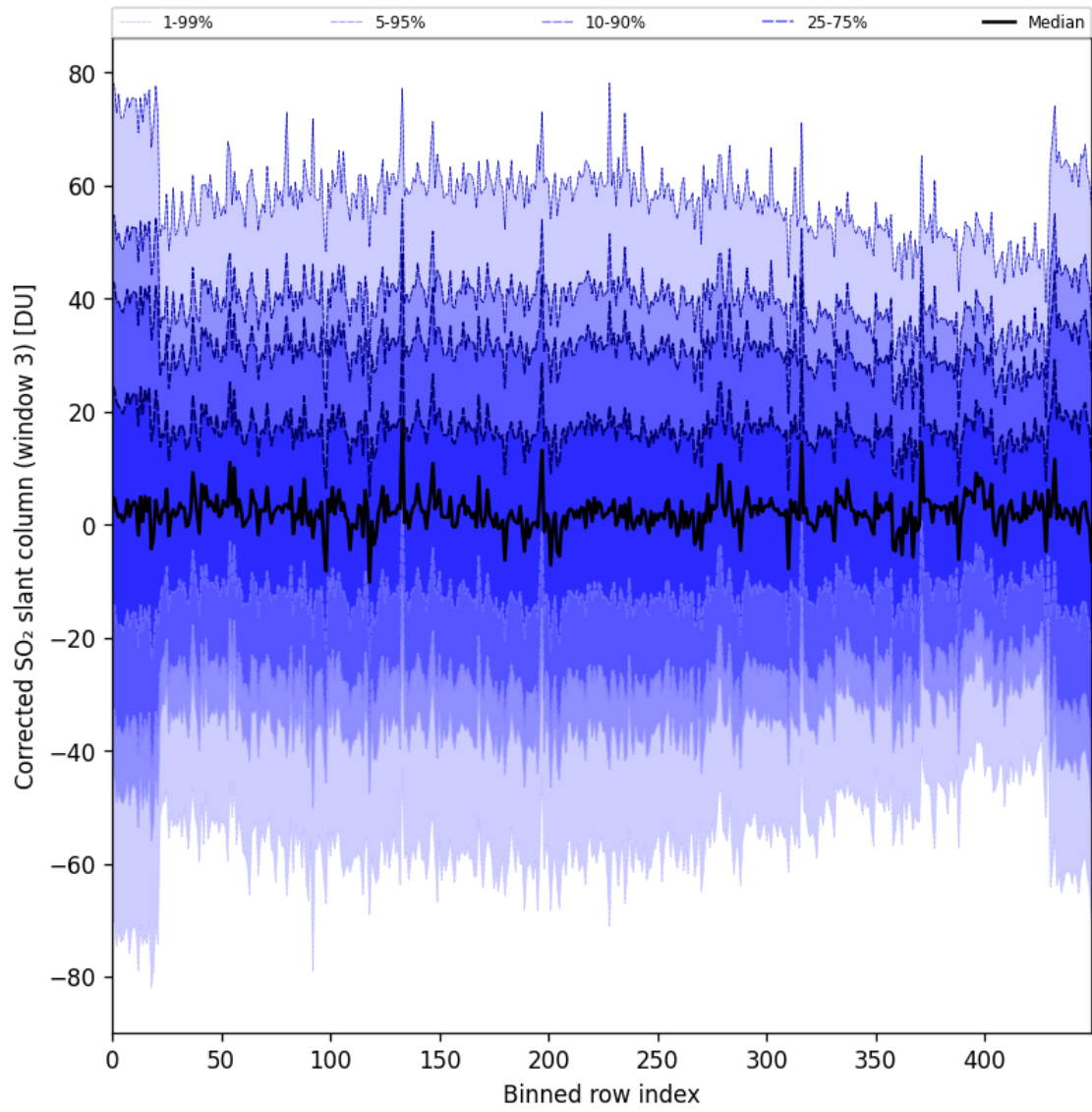
Figure 99: Along track statistics of “Corrected SO 2 slant column (window 3)” for 2025-10-20 to 2025-10-22
