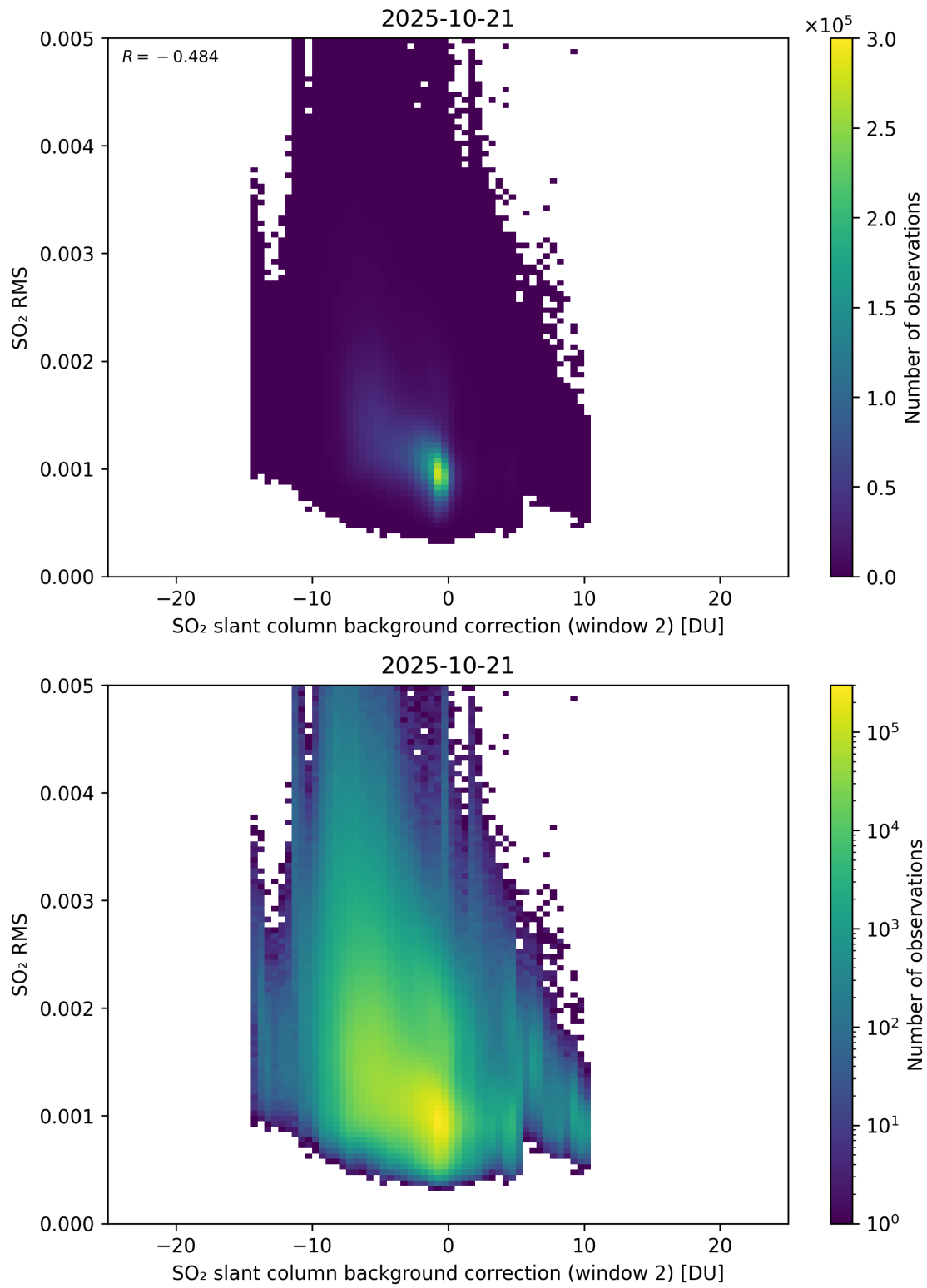
Figure 125: Scatter density plot of “SO 2 slant column background correction (window 2)” against “SO 2 RMS” for 2025-10-20 to 2025-10-22.
