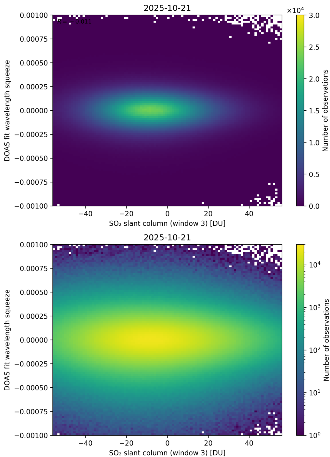
Figure 305: Scatter density plot of “SO 2 slant column (window 3)” against “DOAS fit wavelength squeeze” for 2025-10-20 to 2025-10-22.
