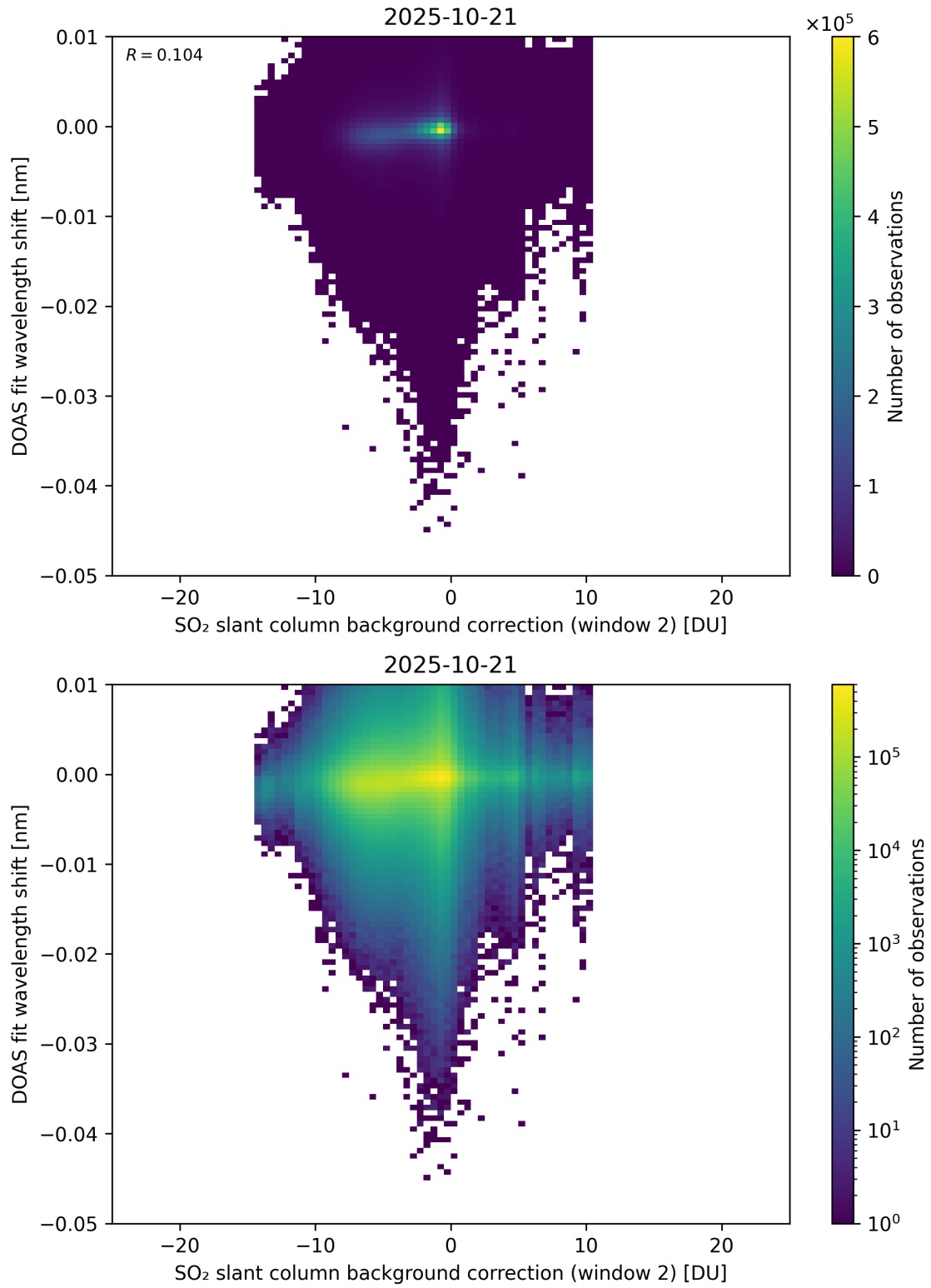
Figure 123: Scatter density plot of “SO 2 slant column background correction (window 2)” against “DOAS fit wavelength shift” for 2025-10-20 to 2025-10-22.
