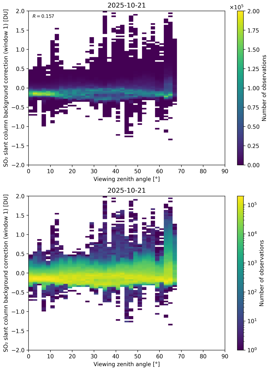
Figure 362: Scatter density plot of “Viewing zenith angle” against “SO 2 slant column background correction (window 1)” for 2025-10-20 to 2025-10-22.
