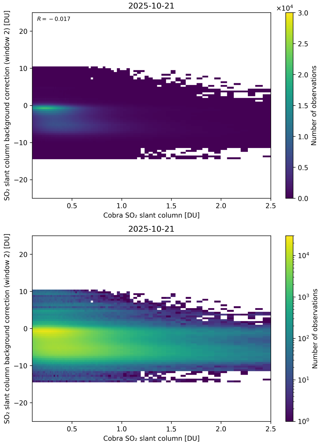
Figure 194: Scatter density plot of “Cobra SO 2 slant column” against “SO 2 slant column background correction (window 2)” for 2025-10-20 to 2025-10-22.
