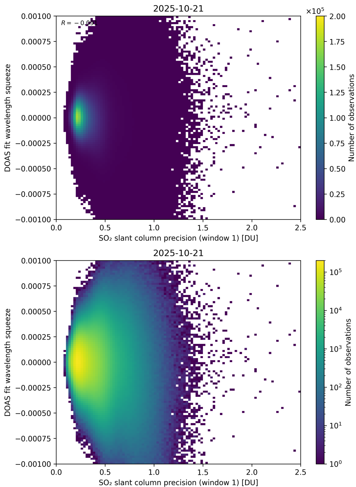
Figure 272: Scatter density plot of “SO 2 slant column precision (window 1)” against “DOAS fit wavelength squeeze” for 2025-10-20 to 2025-10-22.
