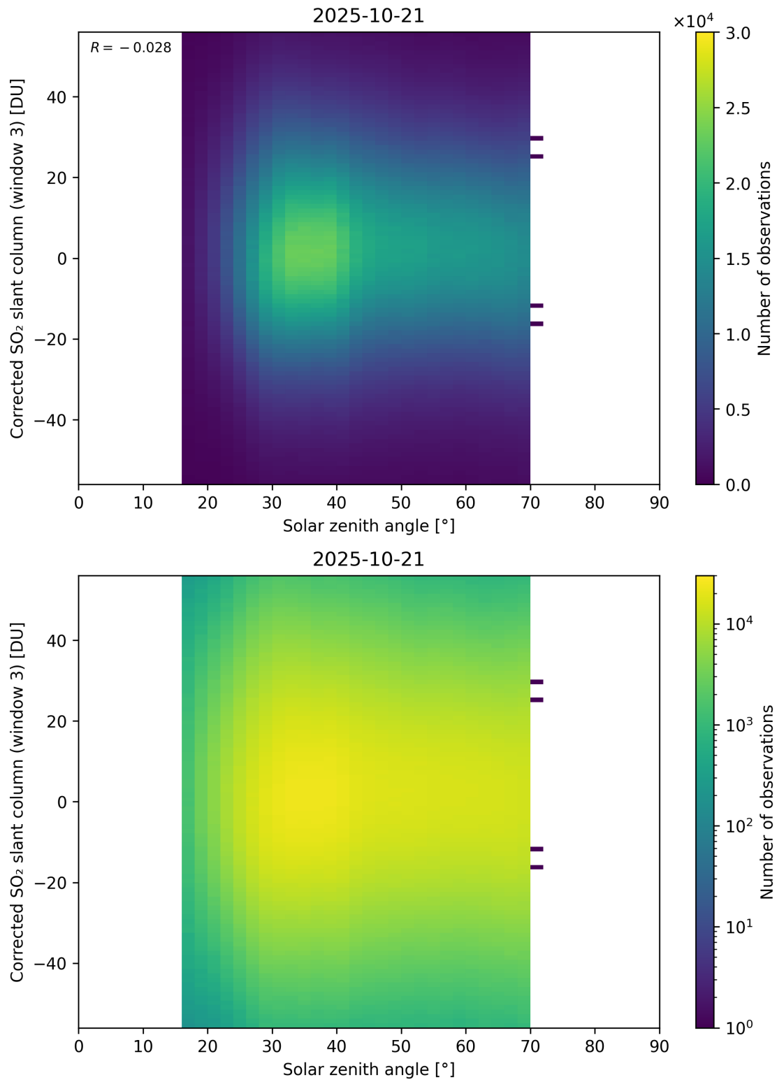
Figure 183: Scatter density plot of “Solar zenith angle” against “Corrected SO 2 slant column (window 3)” for 2025-10-20 to 2025-10-22.
