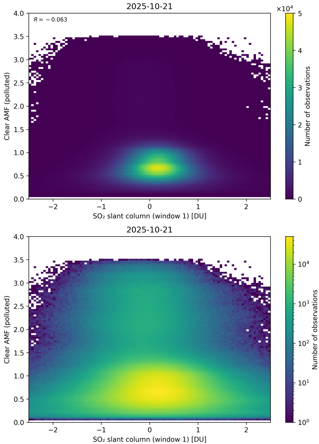
Figure 282: Scatter density plot of “SO 2 slant column (window 1)” against “Clear AMF (polluted)” for 2025-10-20 to 2025-10-22.
