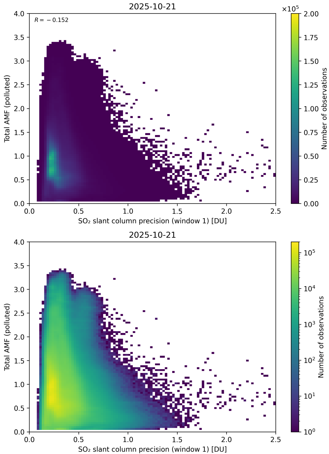
Figure 280: Scatter density plot of “SO 2 slant column precision (window 1)” against “Total AMF (polluted)” for 2025-10-20 to 2025-10-22.
