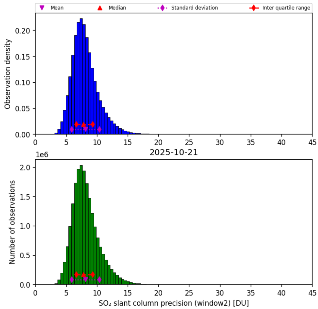
Figure 68: Histogram of “SO 2 slant column precision (window2)” for 2025-10-20 to 2025-10-22
