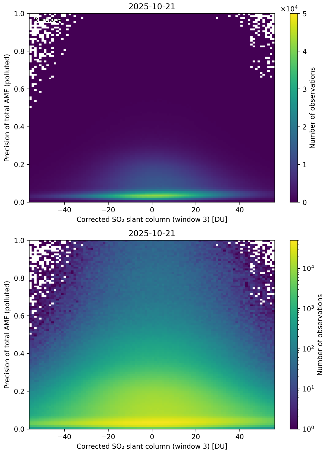
Figure 261: Scatter density plot of “Corrected SO 2 slant column (window 3)” against “Precision of total AMF (polluted)” for 2025-10-20 to 2025-10-22.
