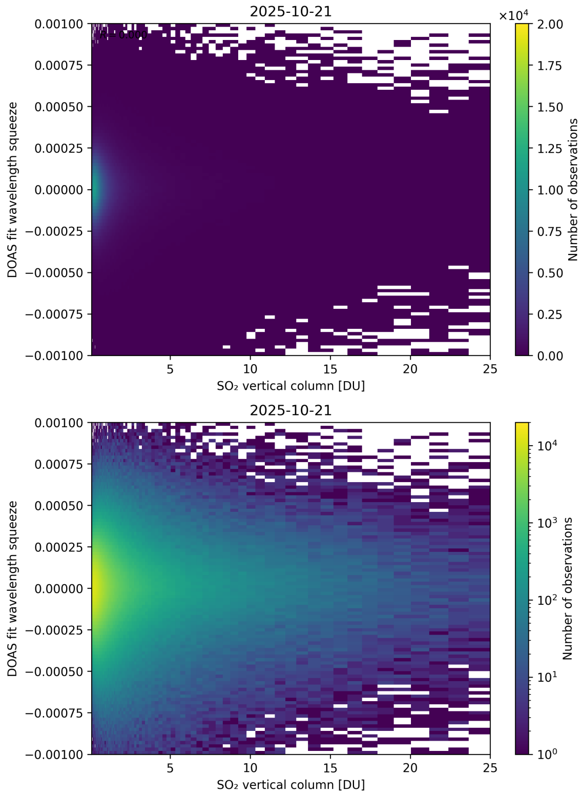
Figure 327: Scatter density plot of “SO 2 vertical column” against “DOAS fit wavelength squeeze” for 2025-10-20 to 2025-10-22.
