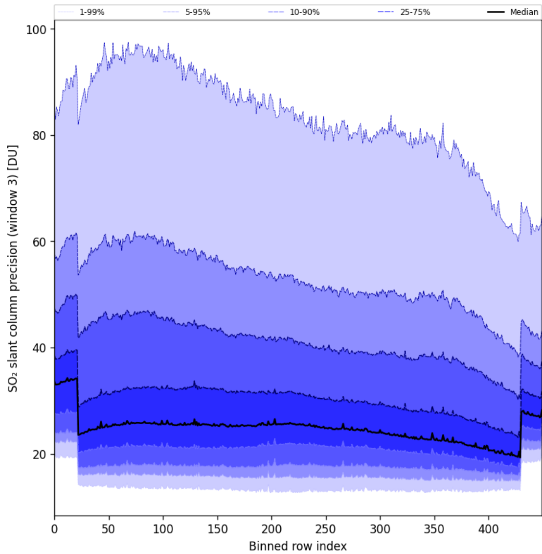
Figure 98: Along track statistics of “SO 2 slant column precision (window 3)” for 2025-10-20 to 2025-10-22
