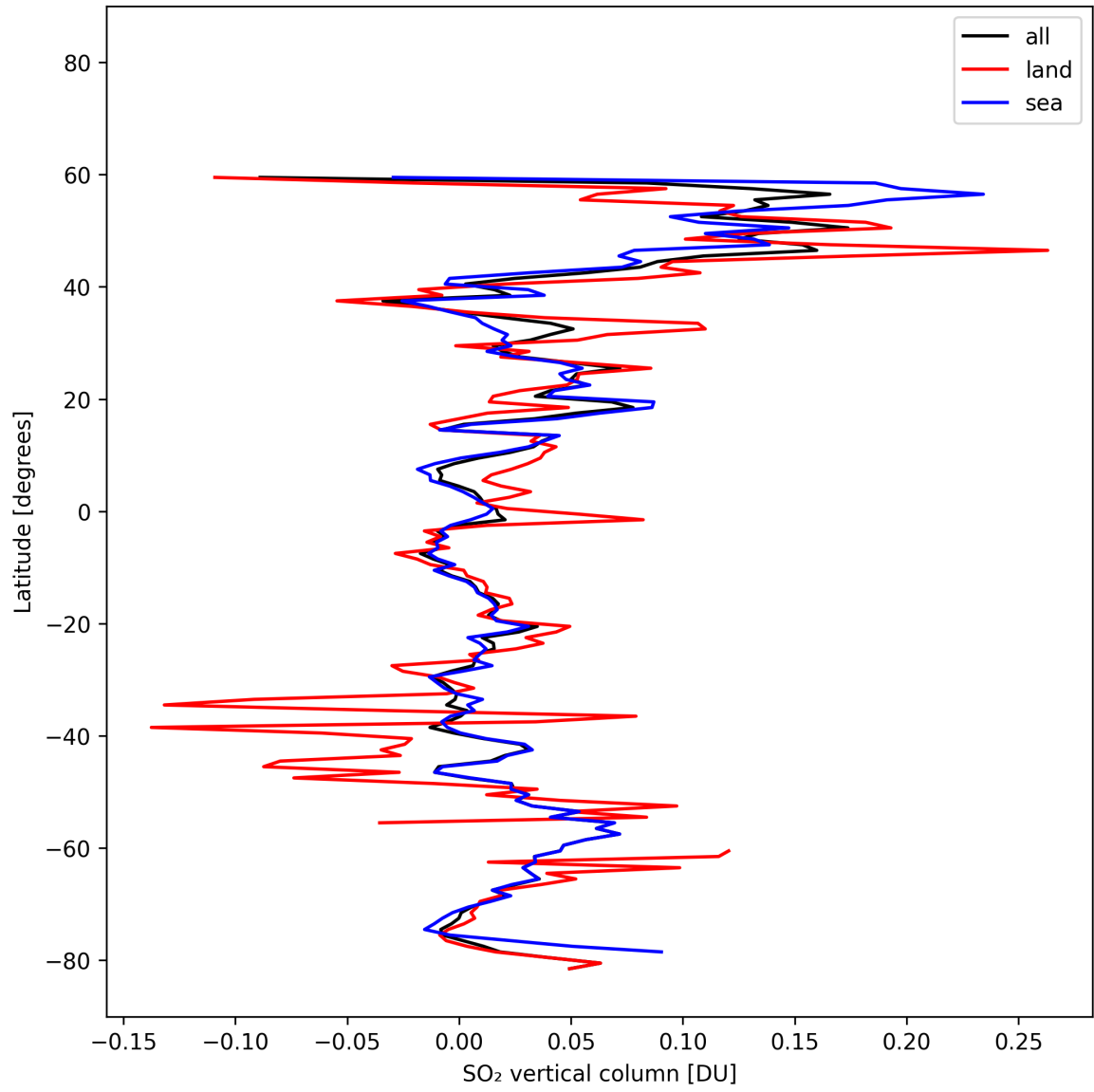
Figure 32: Zonal average of “SO 2 vertical column” for 2025-10-20 to 2025-10-22.
