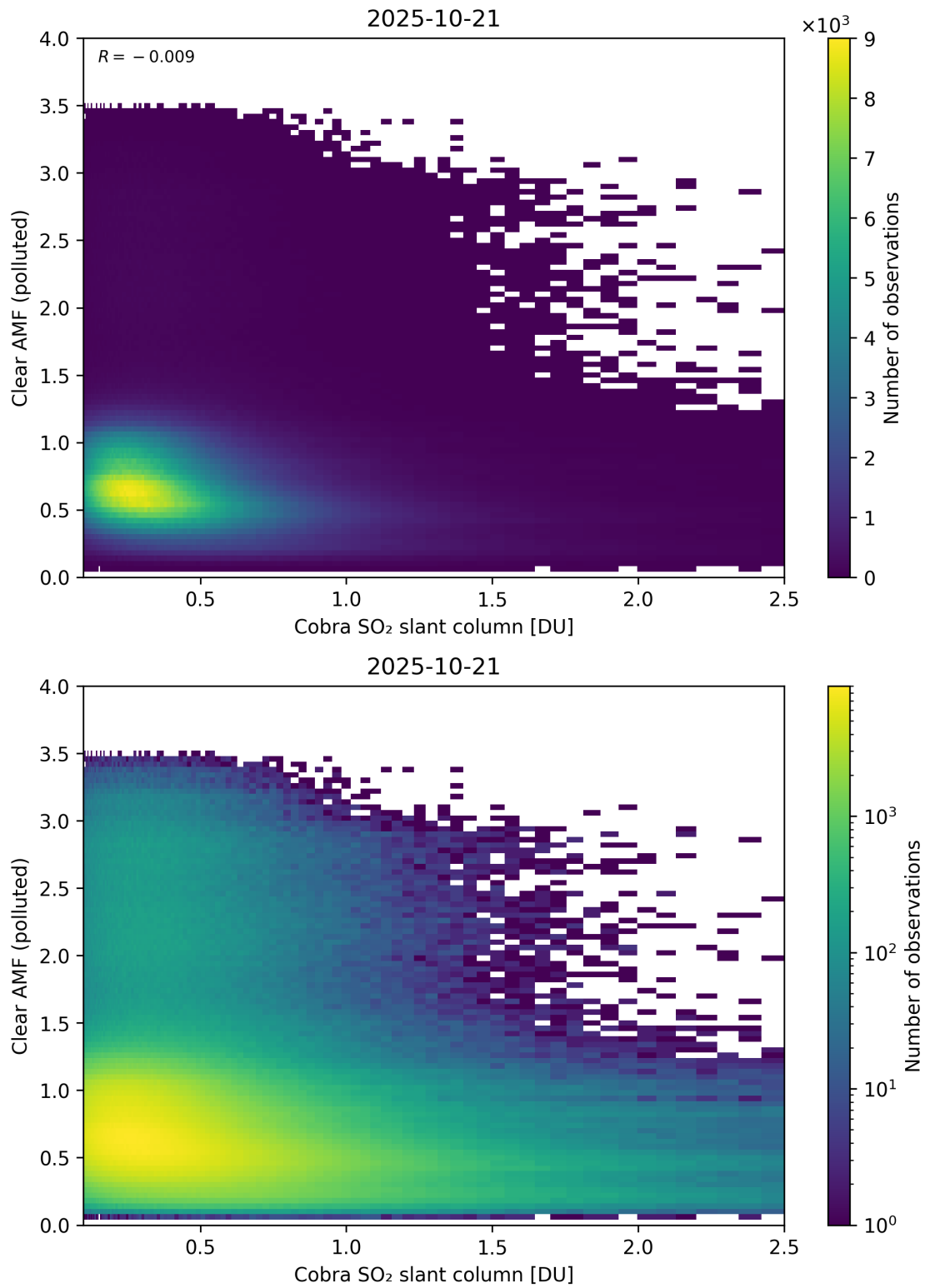
Figure 215: Scatter density plot of “Cobra SO 2 slant column” against “Clear AMF (polluted)” for 2025-10-20 to 2025-10-22.
