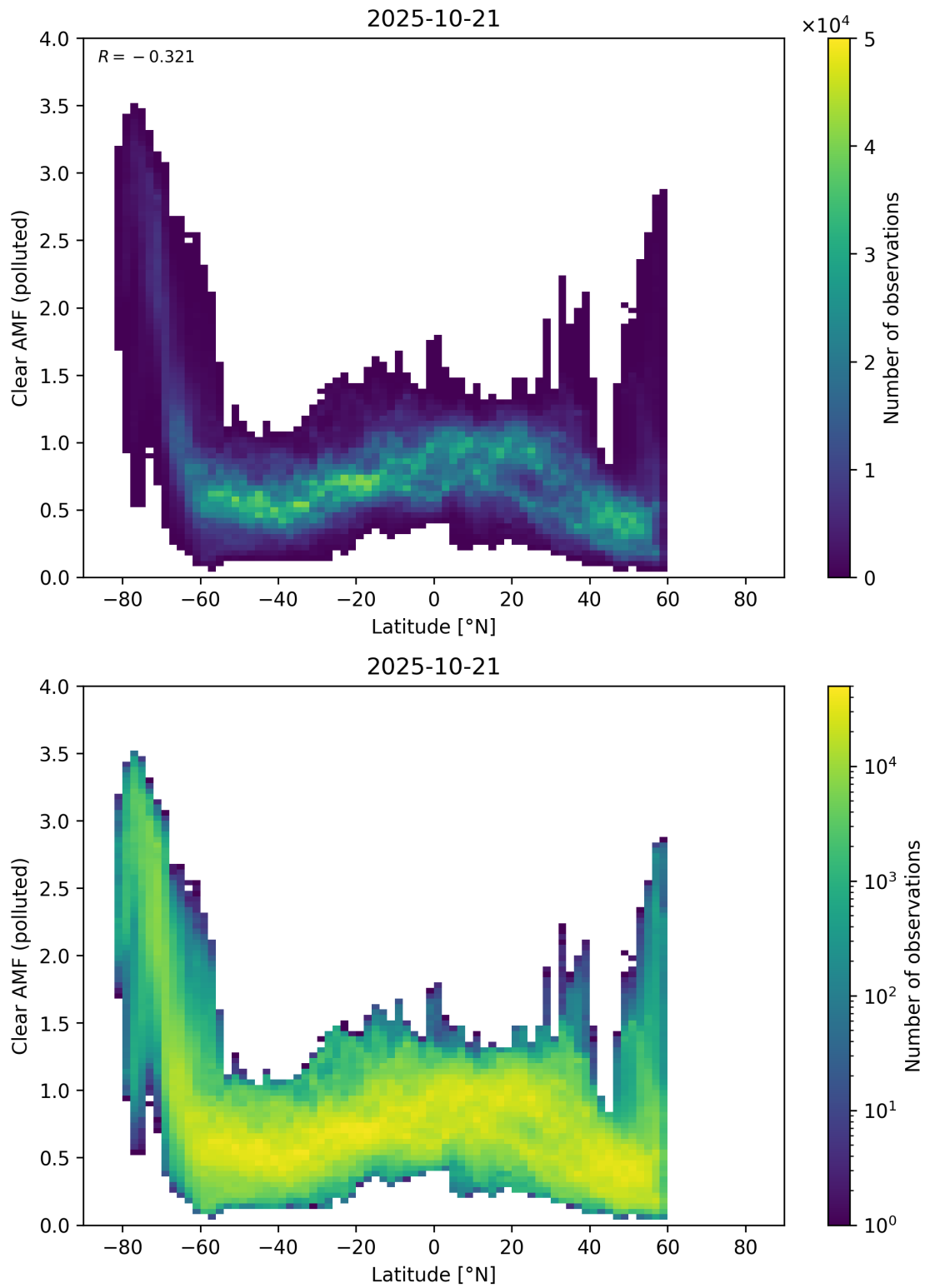
Figure 156: Scatter density plot of “Latitude” against “Clear AMF (polluted)” for 2025-10-20 to 2025-10-22.
