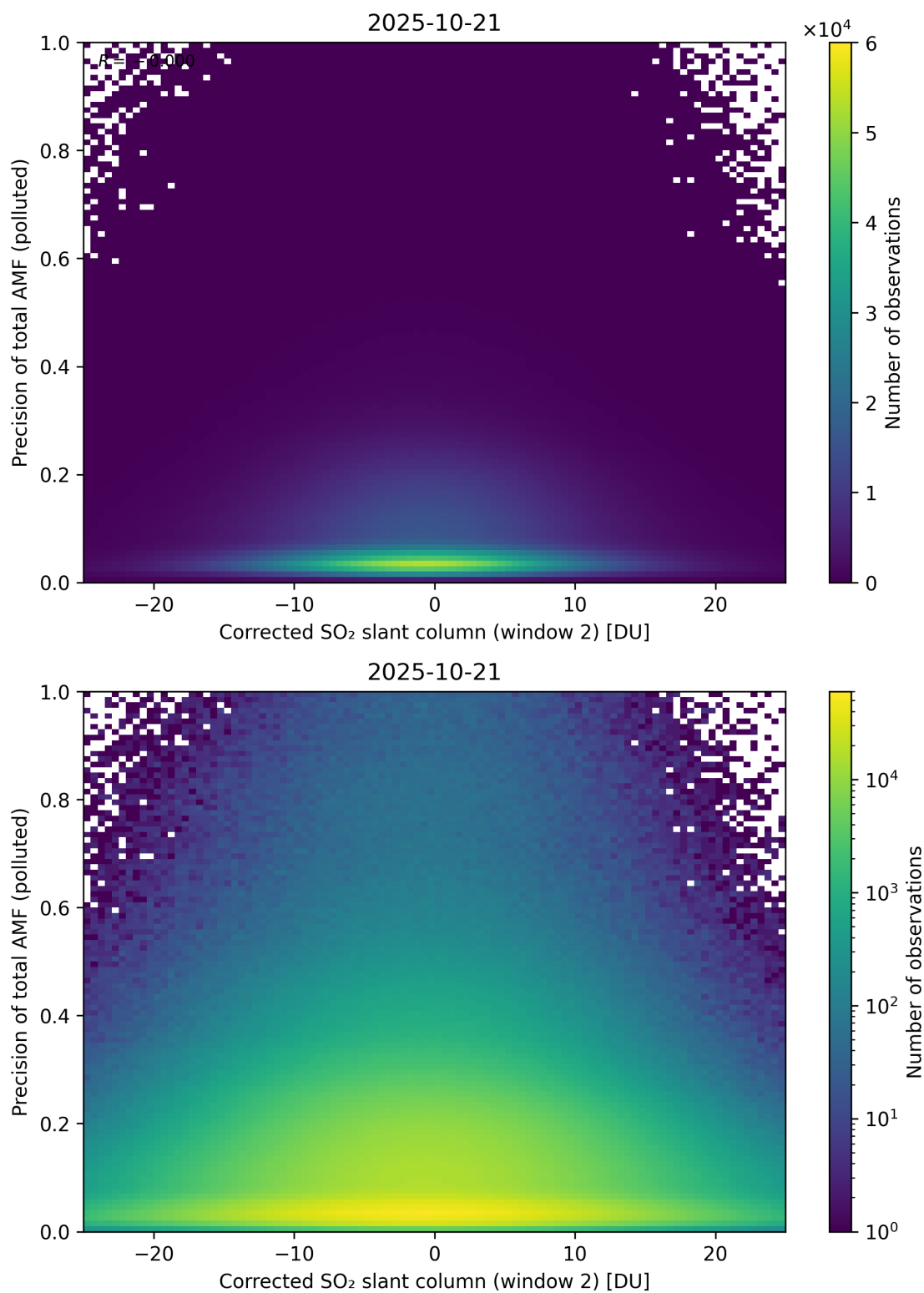
Figure 254: Scatter density plot of “Corrected SO 2 slant column (window 2)” against “Precision of total AMF (polluted)” for 2025-10-20 to 2025-10-22.
