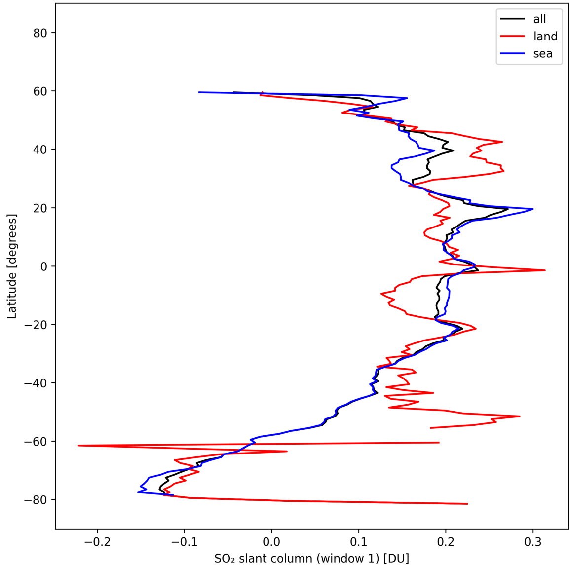
Figure 37: Zonal average of “SO 2 slant column (window 1)” for 2025-10-20 to 2025-10-22.
