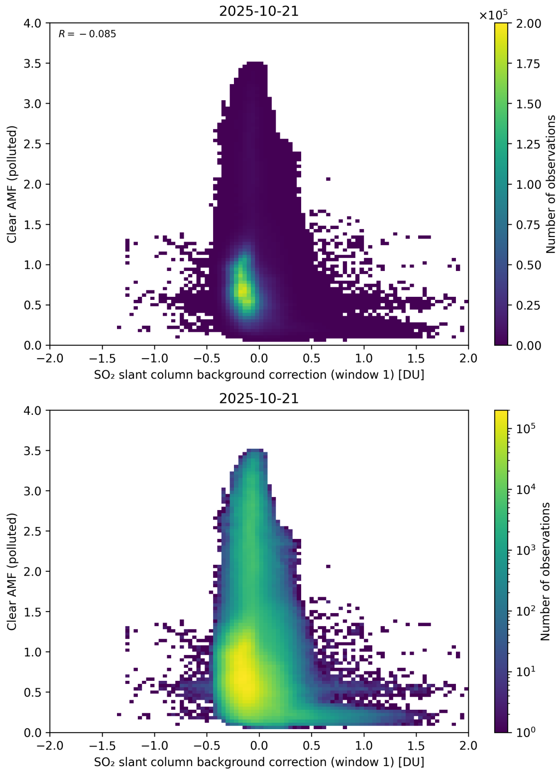
Figure 114: Scatter density plot of “SO 2 slant column background correction (window 1)” against “Clear AMF (polluted)” for 2025-10-20 to 2025-10-22.
