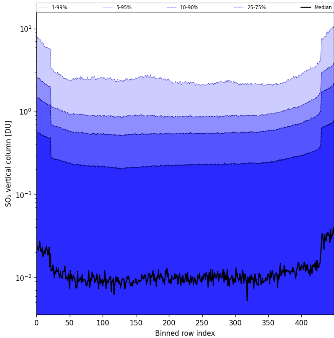
Figure 84: Along track statistics of “SO 2 vertical column” for 2025-10-20 to 2025-10-22
