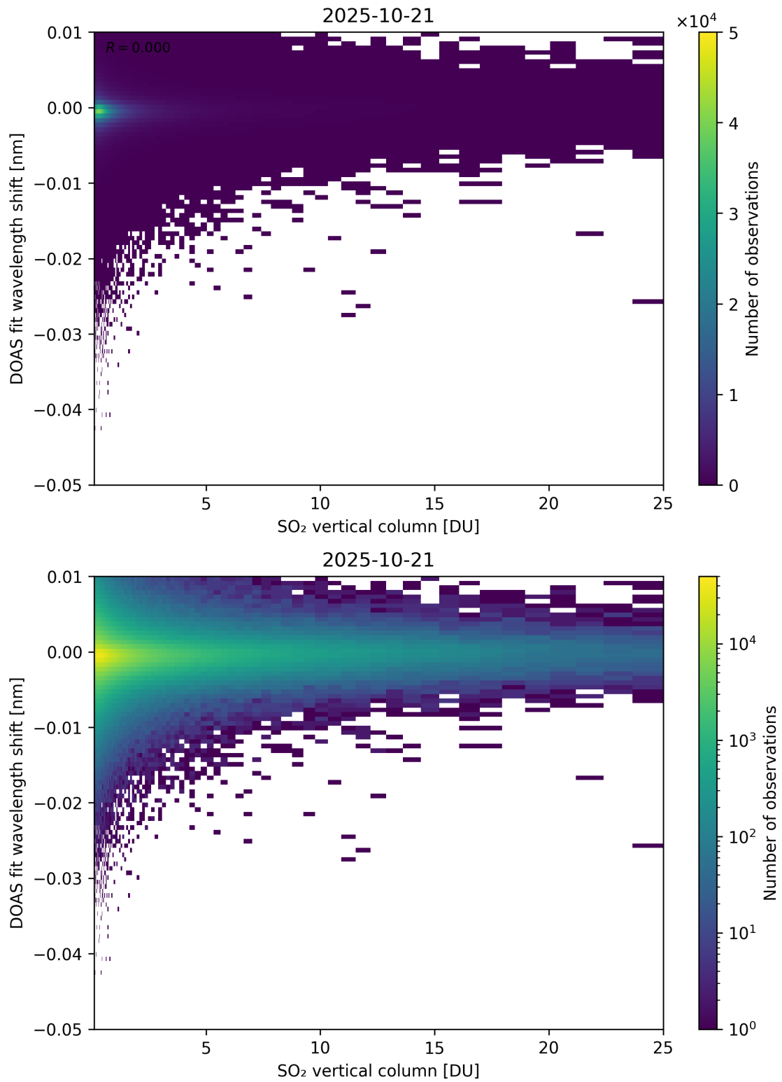
Figure 326: Scatter density plot of “SO 2 vertical column” against “DOAS fit wavelength shift” for 2025-10-20 to 2025-10-22.
