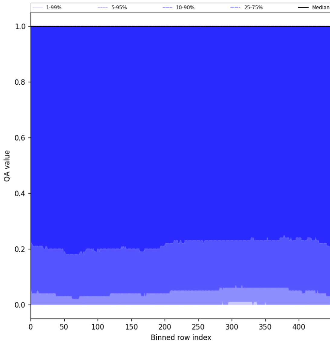
Figure 83: Along track statistics of “QA value” for 2025-10-20 to 2025-10-22
