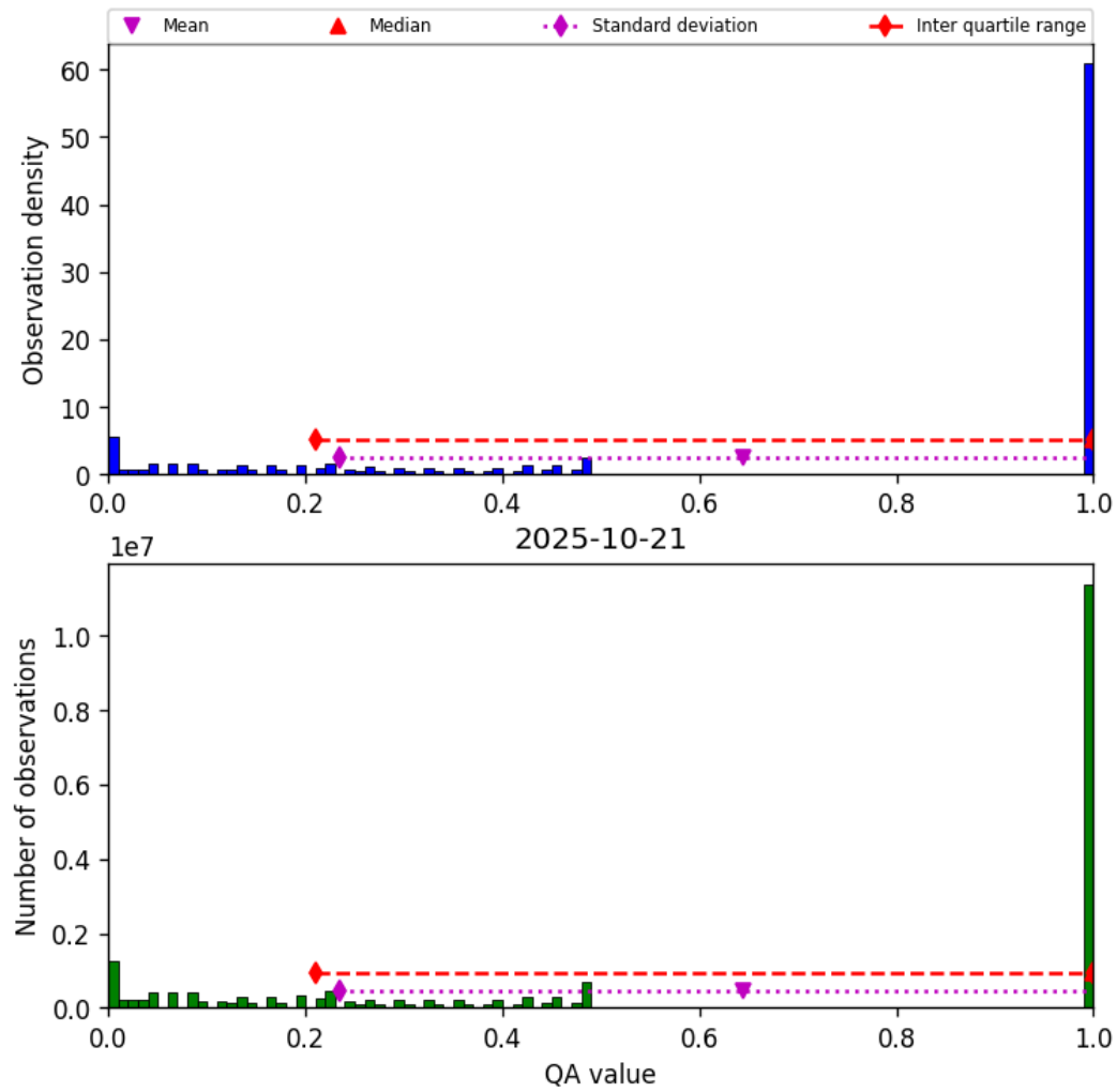
Figure 57: Histogram of “QA value” for 2025-10-20 to 2025-10-22
