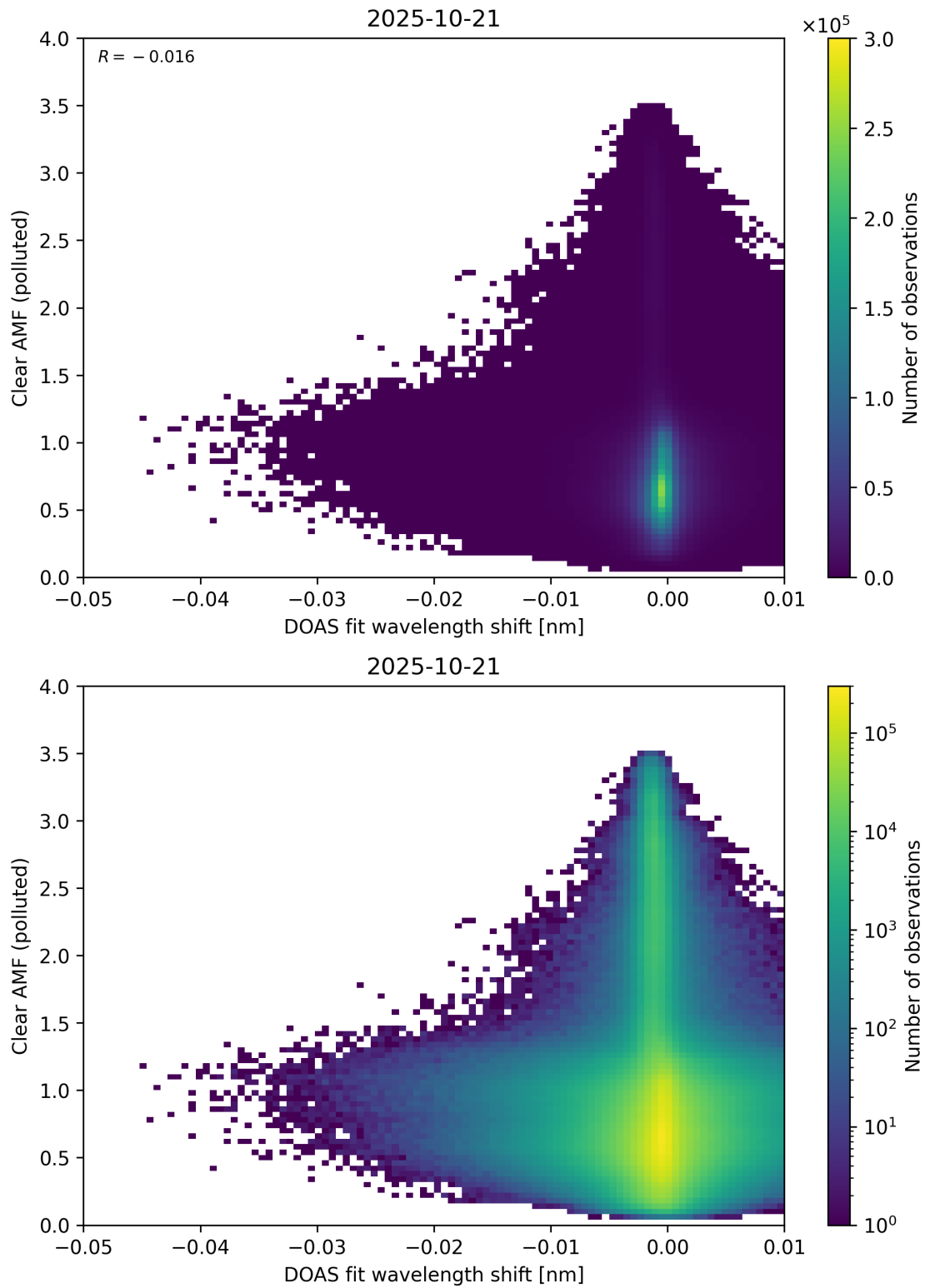
Figure 140: Scatter density plot of “DOAS fit wavelength shift” against “Clear AMF (polluted)” for 2025-10-20 to 2025-10-22.
