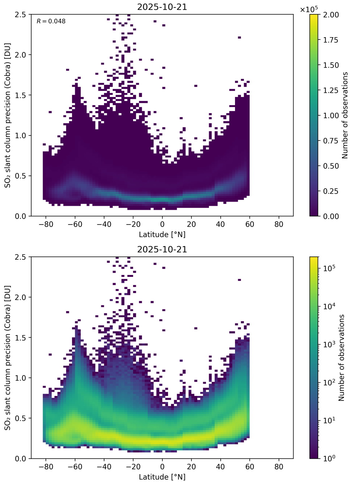
Figure 158: Scatter density plot of “Latitude” against “SO 2 slant column precision (Cobra)” for 2025-10-20 to 2025-10-22.
