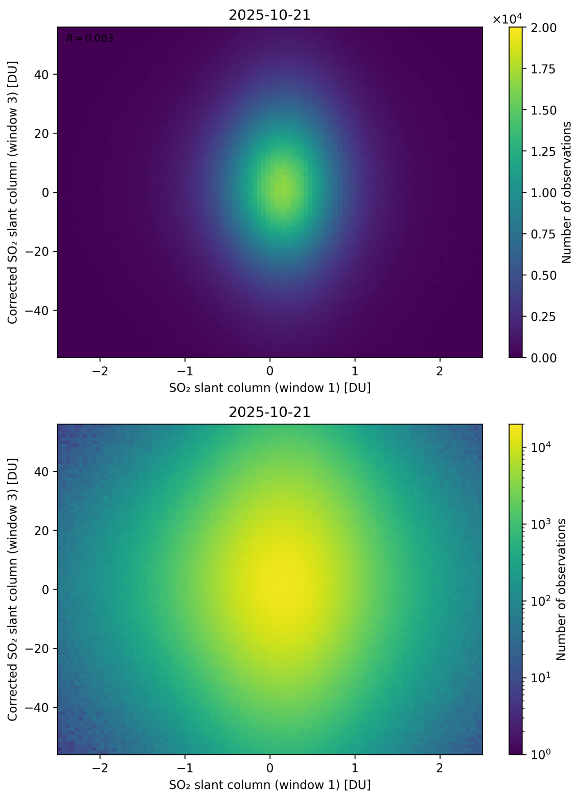
Figure 284: Scatter density plot of “SO 2 slant column (window 1)” against “Corrected SO 2 slant column (window 3)” for 2025-10-20 to 2025-10-22.
