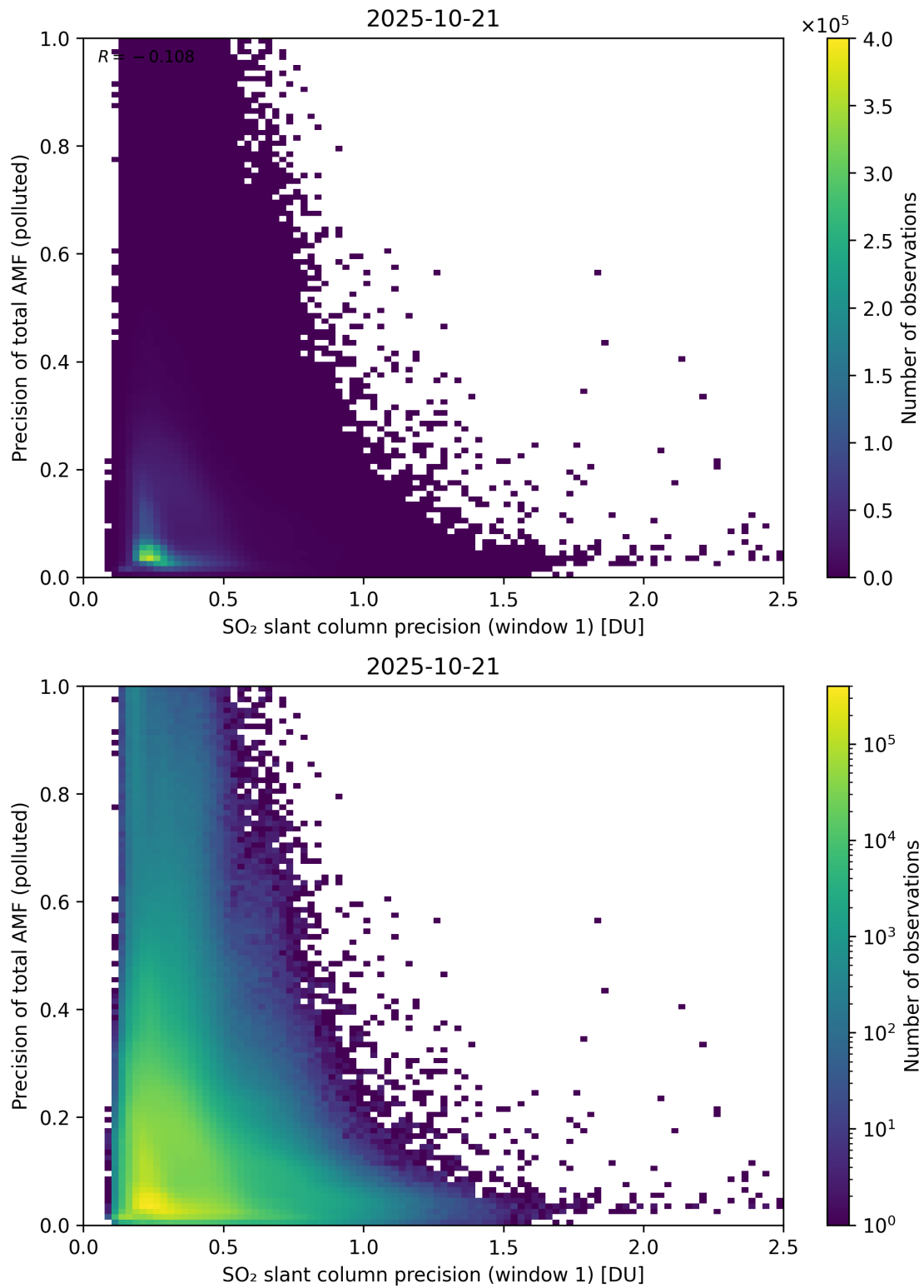
Figure 281: Scatter density plot of “SO 2 slant column precision (window 1)” against “Precision of total AMF (polluted)” for 2025-10-20 to 2025-10-22.
