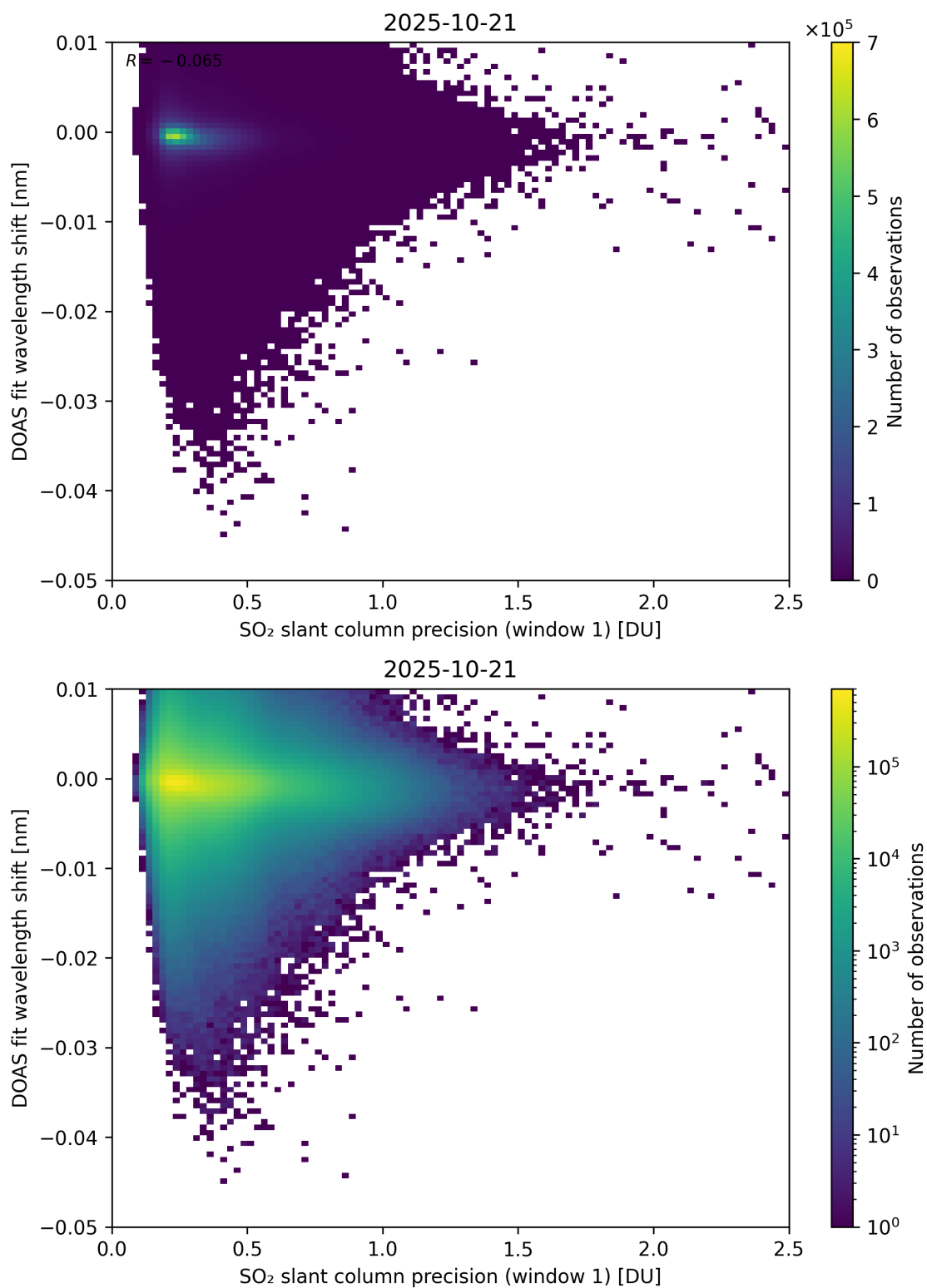
Figure 271: Scatter density plot of “SO 2 slant column precision (window 1)” against “DOAS fit wavelength shift” for 2025-10-20 to 2025-10-22.
