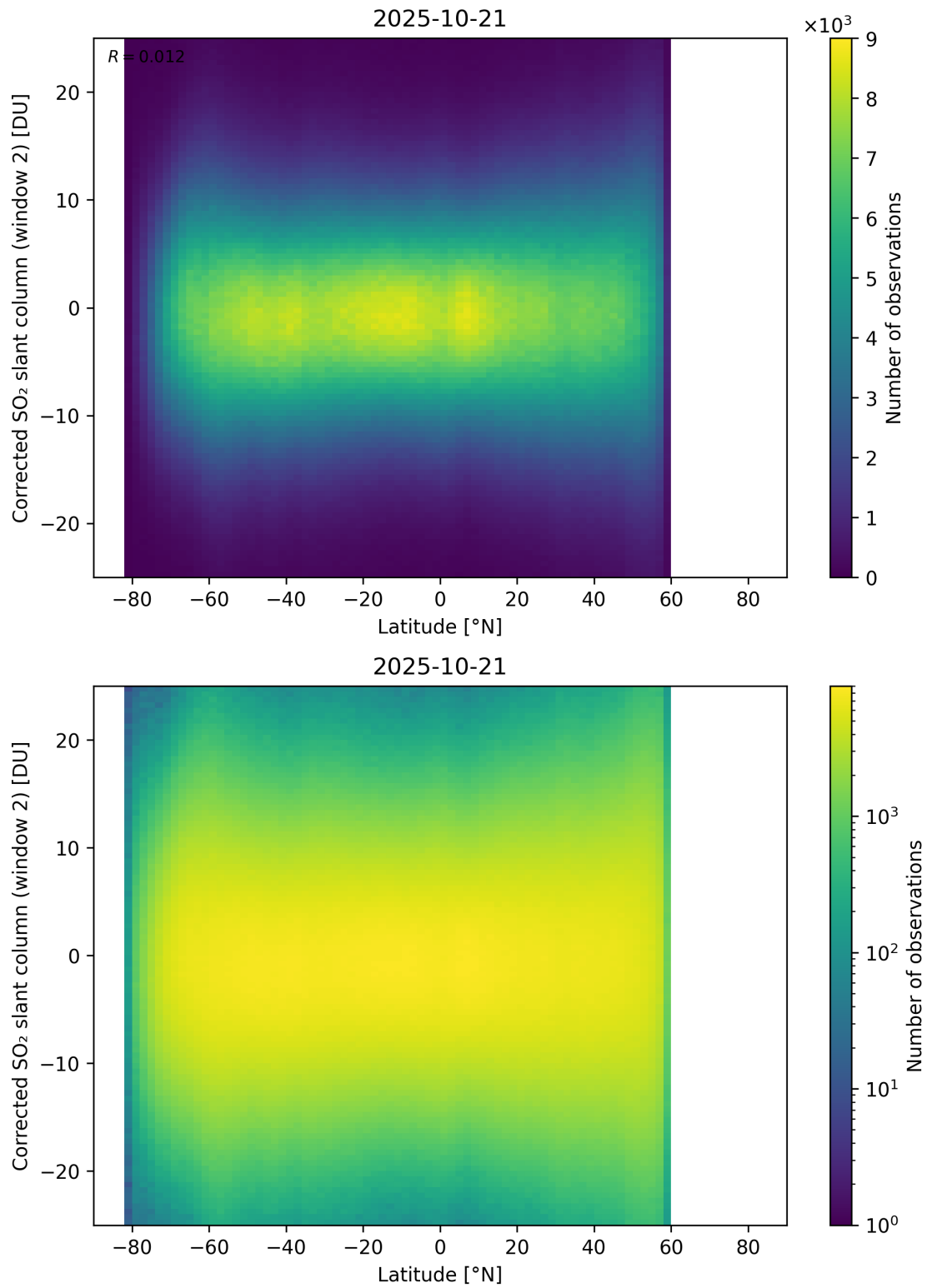
Figure 160: Scatter density plot of “Latitude” against “Corrected SO 2 slant column (window 2)” for 2025-10-20 to 2025-10-22.
