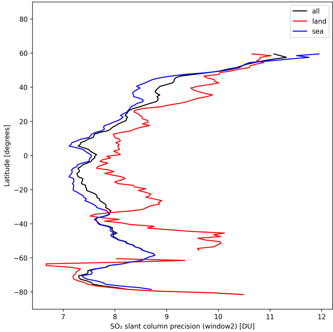
Figure 42: Zonal average of “SO 2 slant column precision (window2)” for 2025-10-20 to 2025-10-22.
