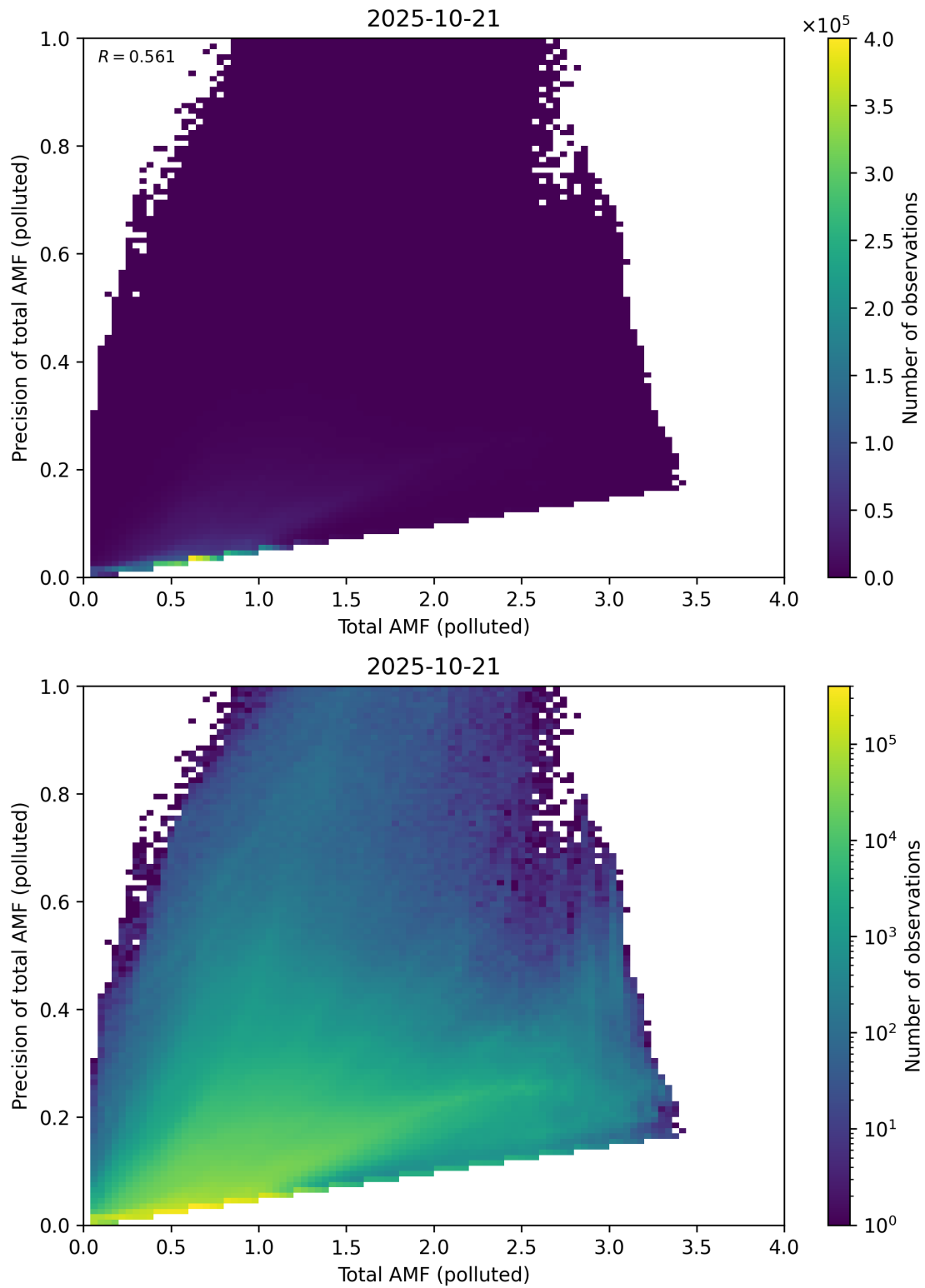
Figure 322: Scatter density plot of “Total AMF (polluted)” against “Precision of total AMF (polluted)” for 2025-10-20 to 2025-10-22.
