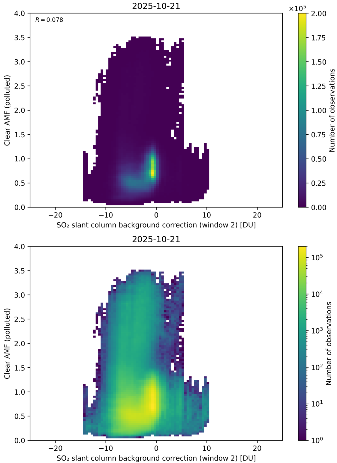
Figure 126: Scatter density plot of “SO 2 slant column background correction (window 2)” against “Clear AMF (polluted)” for 2025-10-20 to 2025-10-22.
