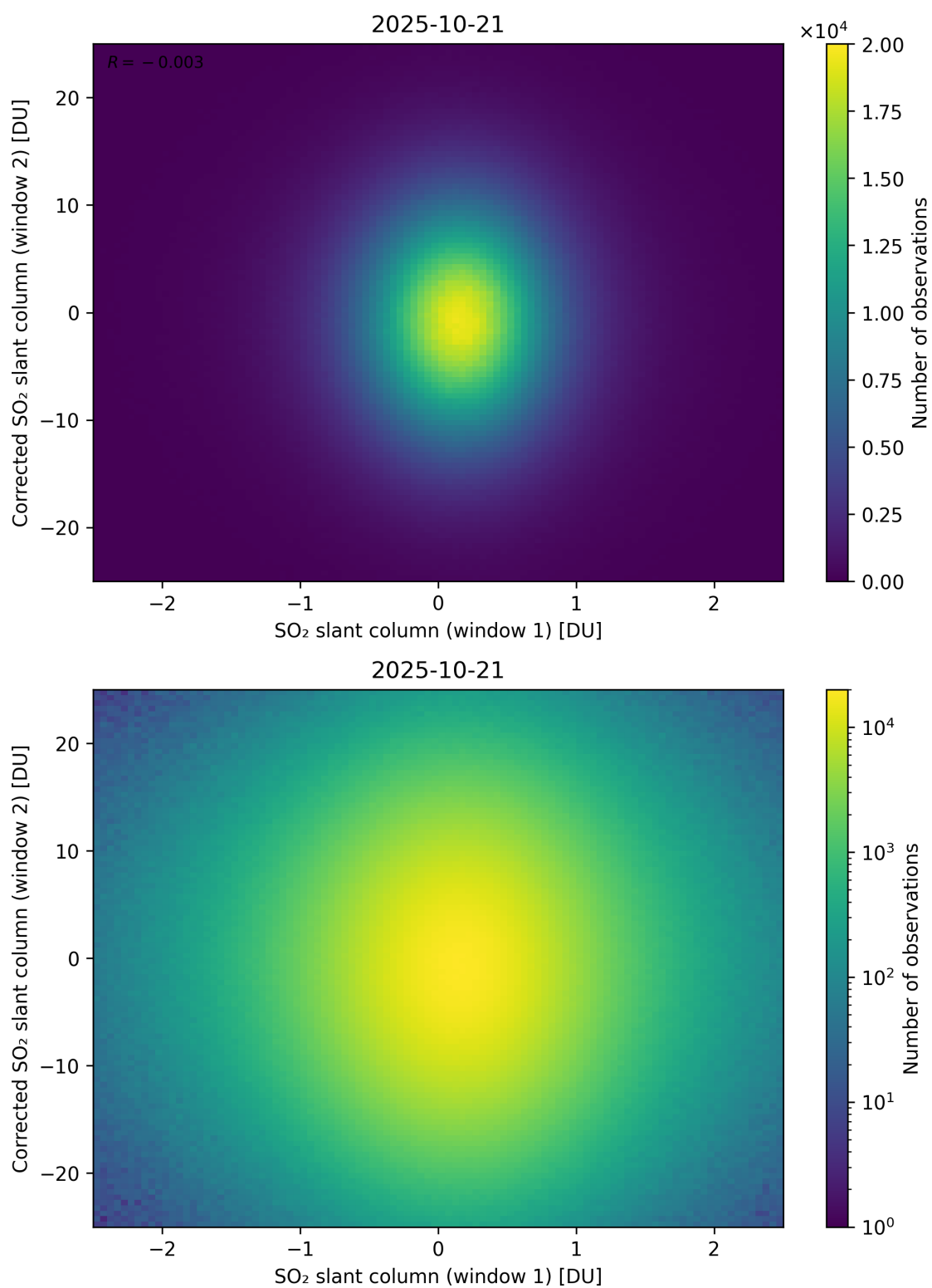
Figure 283: Scatter density plot of “SO 2 slant column (window 1)” against “Corrected SO 2 slant column (window 2)” for 2025-10-20 to 2025-10-22.
