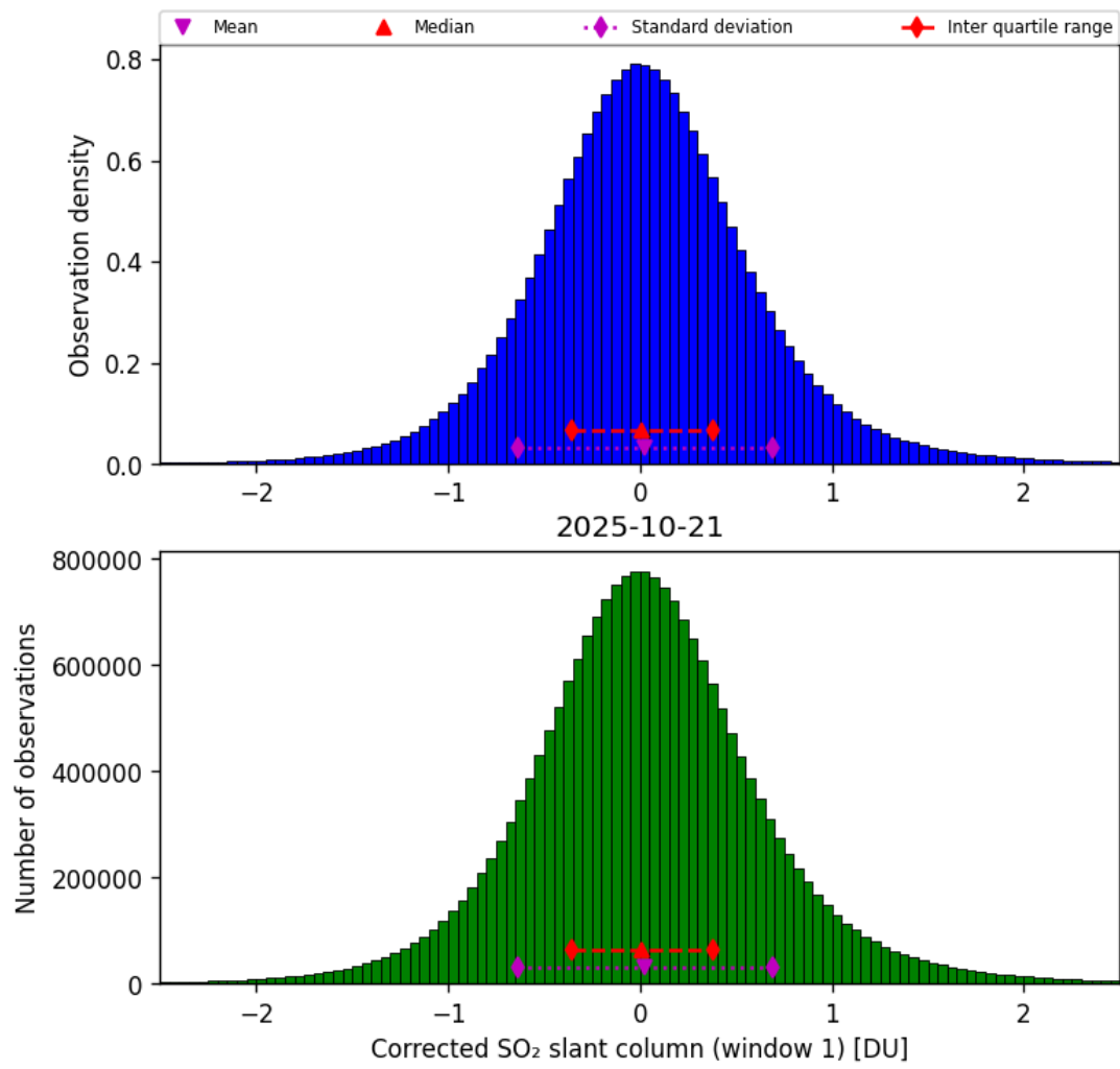
Figure 65: Histogram of “Corrected SO 2 slant column (window 1)” for 2025-10-20 to 2025-10-22
