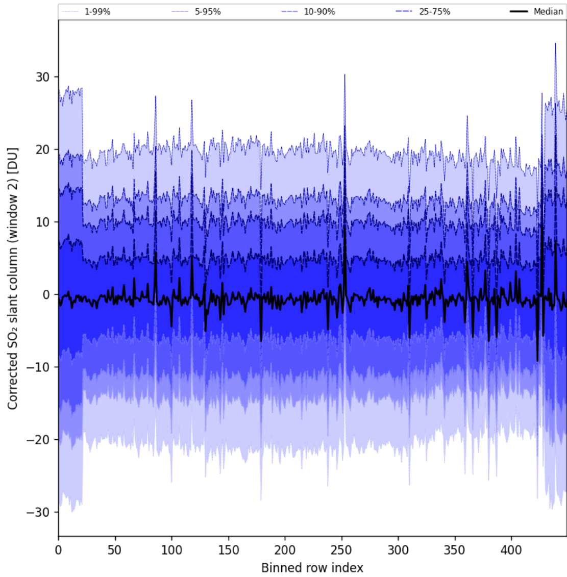
Figure 95: Along track statistics of “Corrected SO 2 slant column (window 2)” for 2025-10-20 to 2025-10-22
