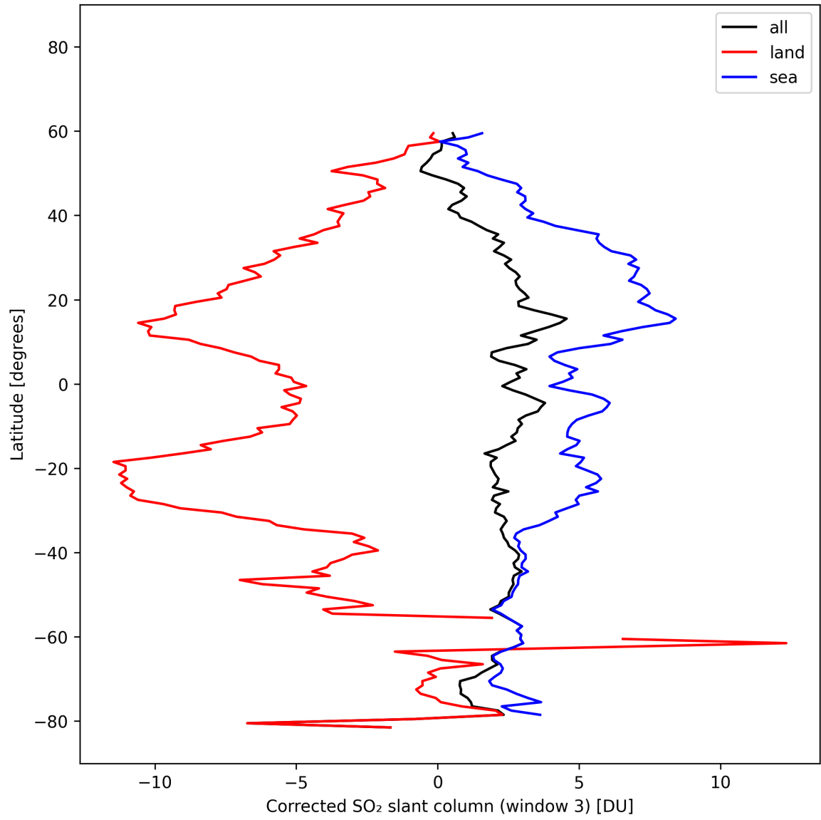
Figure 47: Zonal average of “Corrected SO 2 slant column (window 3)” for 2025-10-20 to 2025-10-22.
