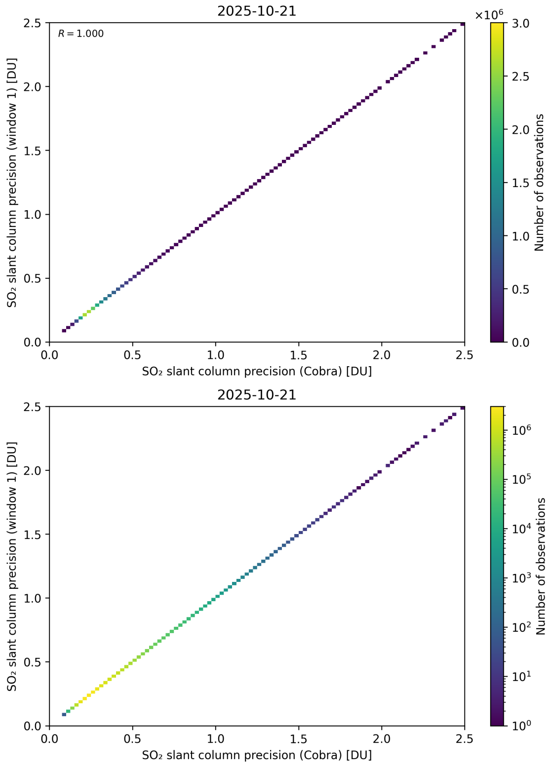
Figure 209: Scatter density plot of “SO 2 slant column precision (Cobra)” against “SO 2 slant column precision (window 1)” for 2025-10-20 to 2025-10-22.
