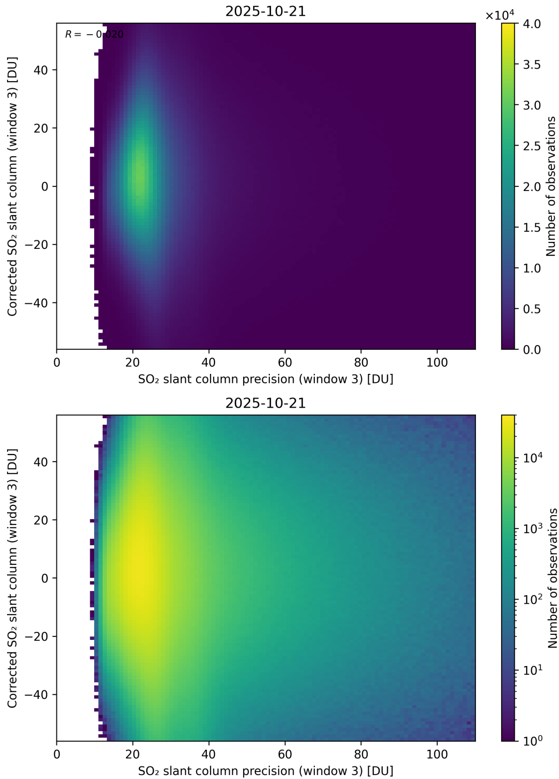
Figure 312: Scatter density plot of “SO 2 slant column precision (window 3)” against “Corrected SO 2 slant column (window 3)” for 2025-10-20 to 2025-10-22.
