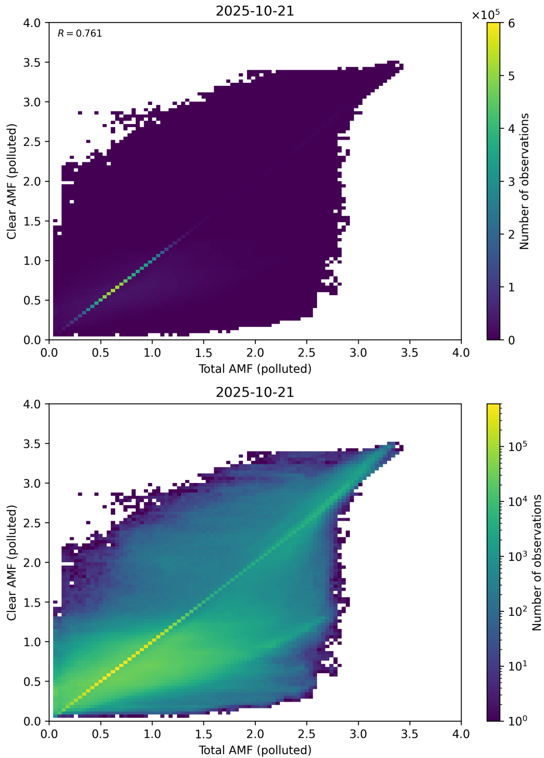
Figure 321: Scatter density plot of “Total AMF (polluted)” against “Clear AMF (polluted)” for 2025-10-20 to 2025-10-22.
