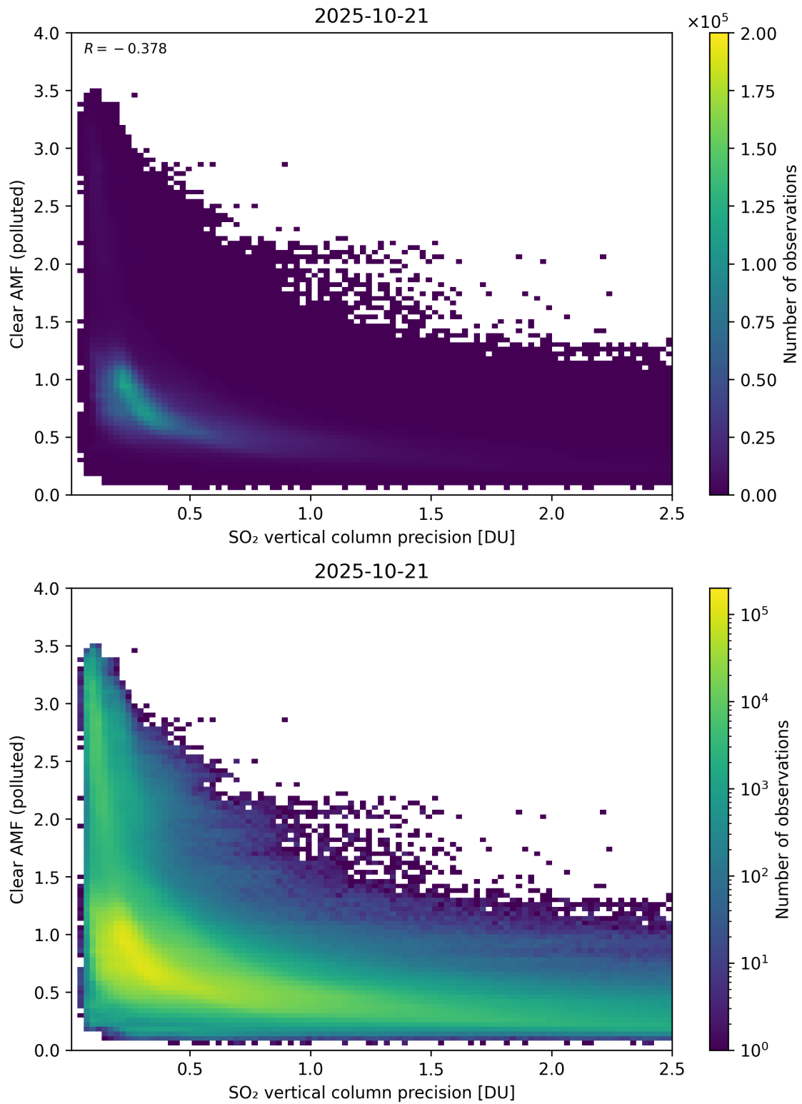
Figure 335: Scatter density plot of “SO 2 vertical column precision” against “Clear AMF (polluted)” for 2025-10-20 to 2025-10-22.
