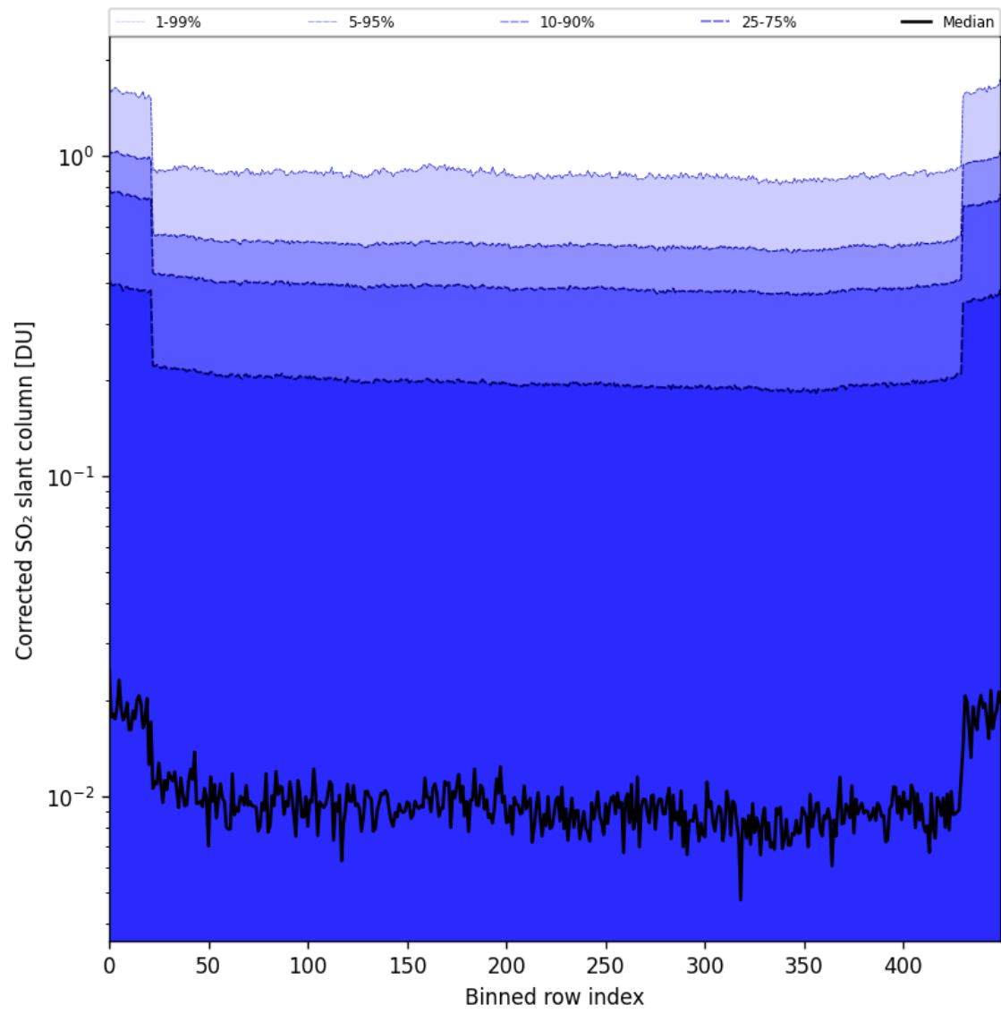
Figure 86: Along track statistics of "Corrected SO 2 slant column" for 2025-10-20 to 2025-10-22
