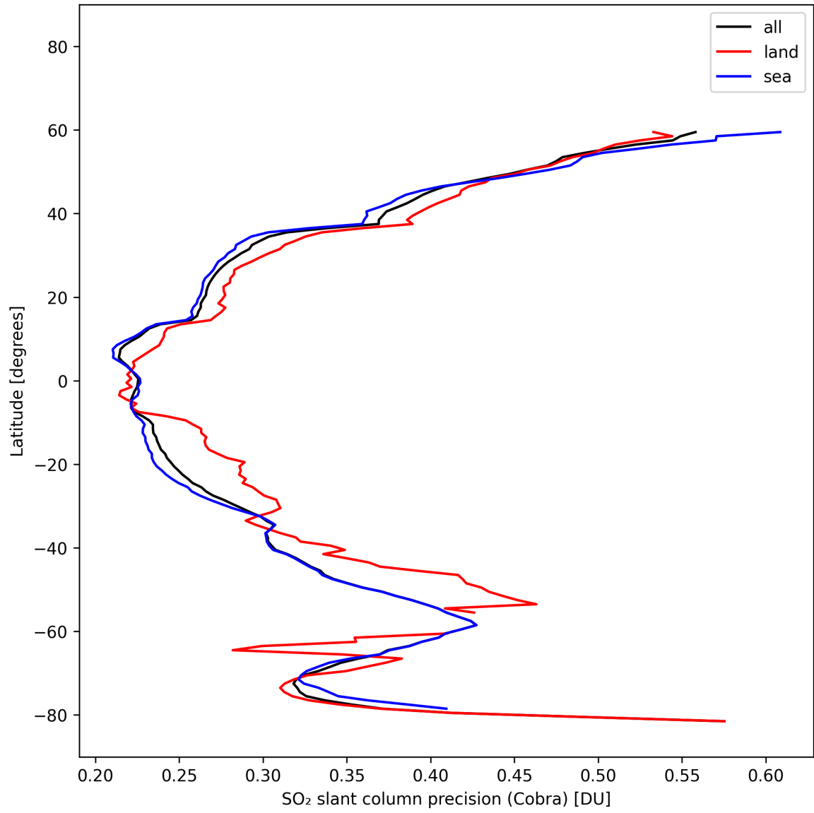
Figure 36: Zonal average of “SO 2 slant column precision (Cobra)” for 2025-10-20 to 2025-10-22.
