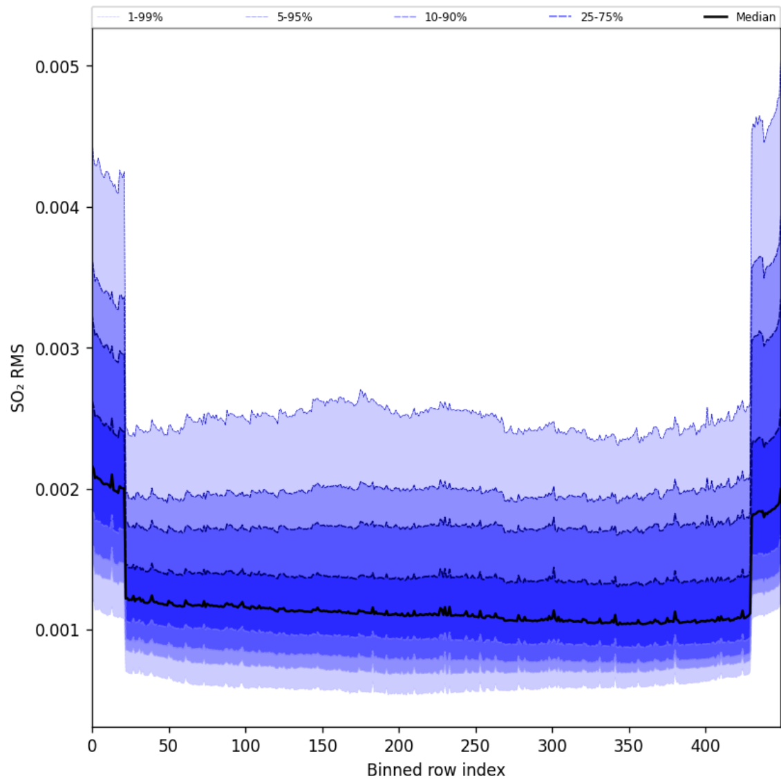
Figure 104: Along track statistics of “SO 2 RMS” for 2025-10-20 to 2025-10-22
