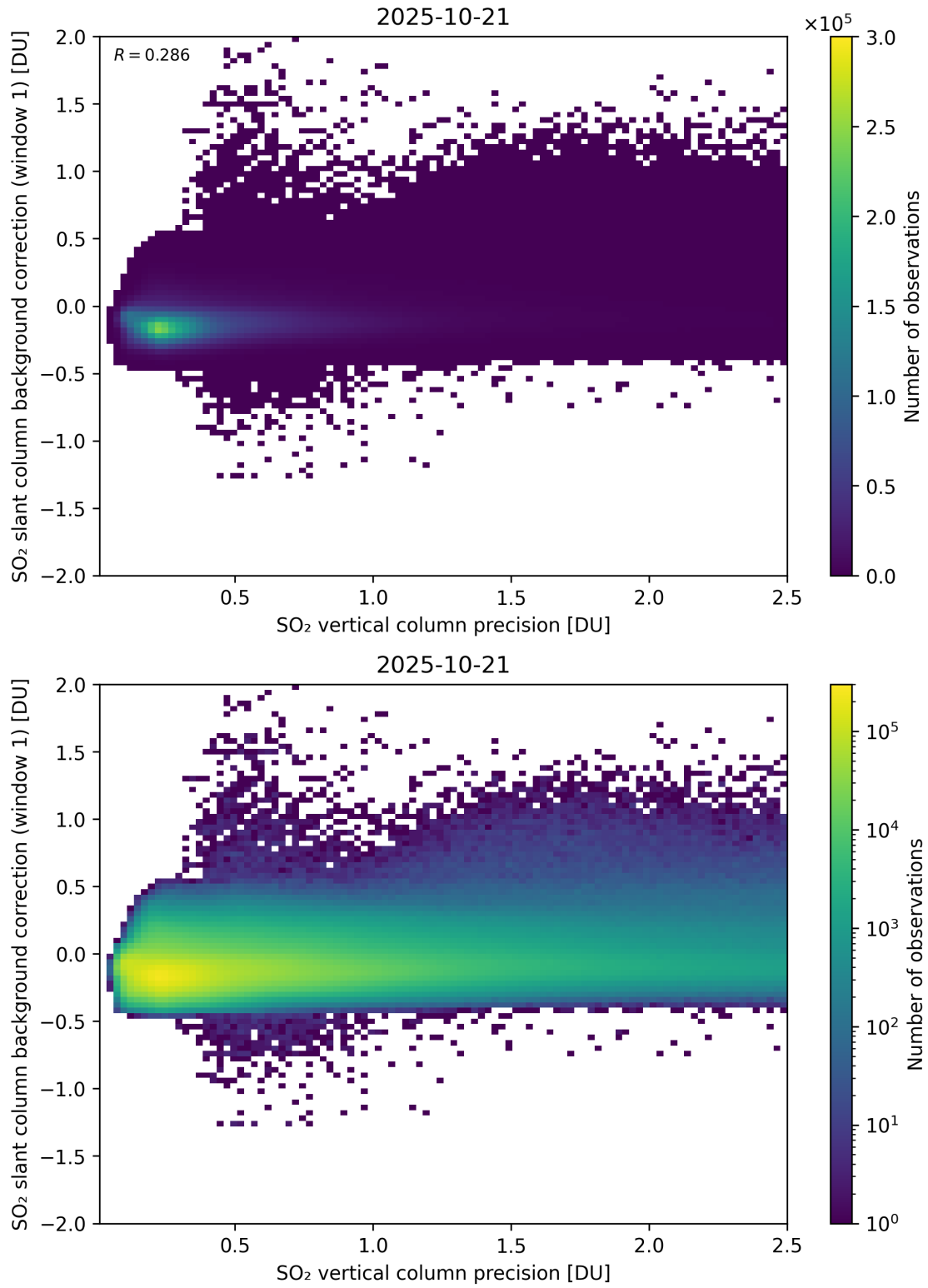
Figure 329: Scatter density plot of “SO 2 vertical column precision” against “SO 2 slant column background correction (window 1)” for 2025-10-20 to 2025-10-22.
