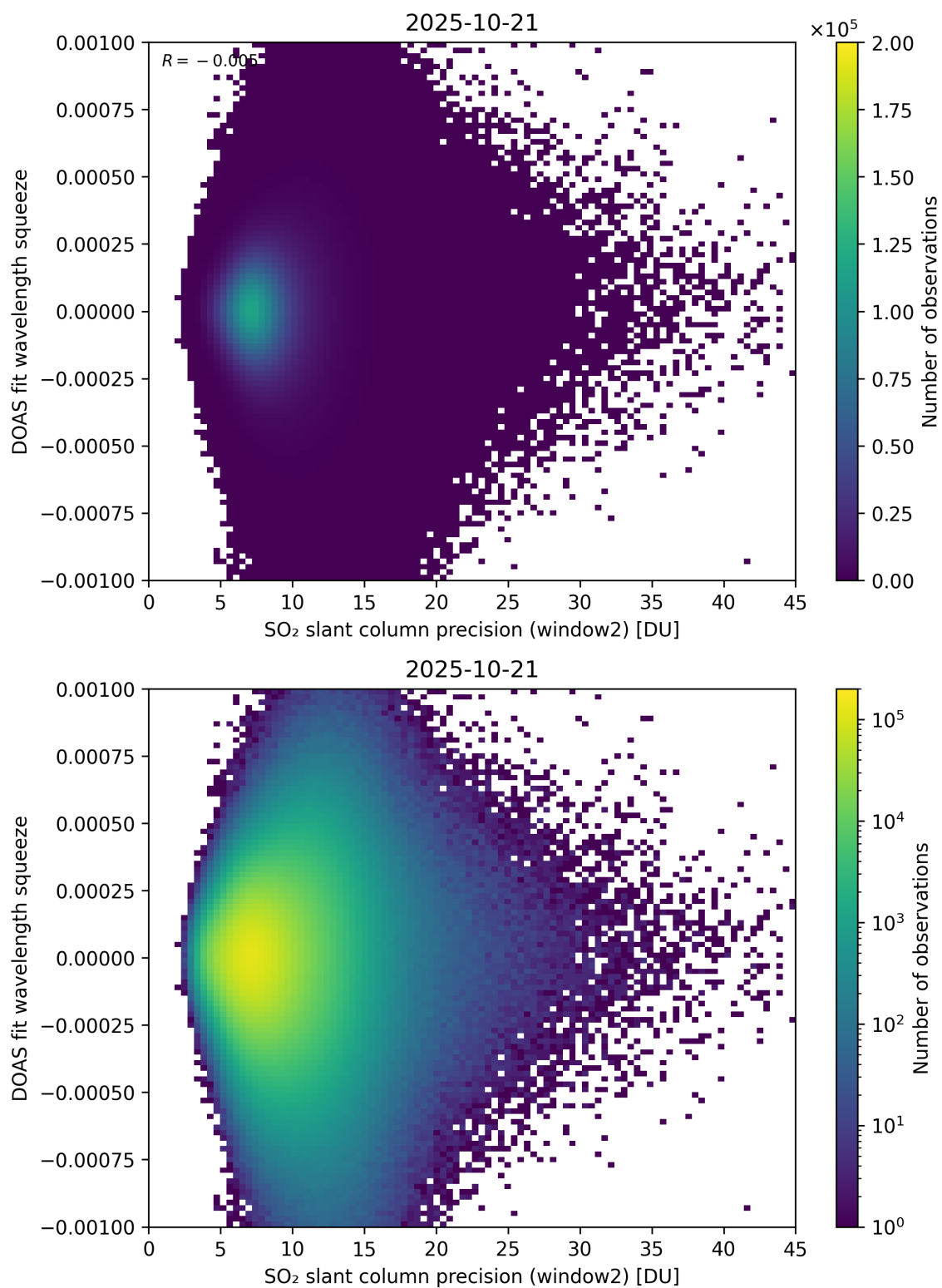
Figure 294: Scatter density plot of “SO 2 slant column precision (window2)” against “DOAS fit wavelength squeeze” for 2025-10-20 to 2025-10-22.
