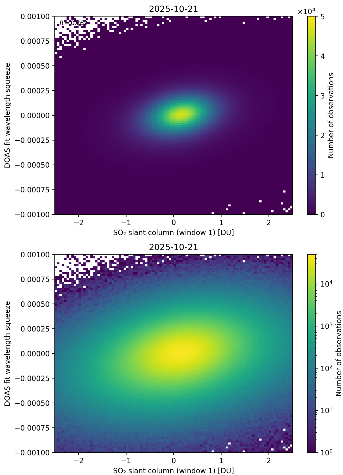
Figure 266: Scatter density plot of “SO 2 slant column (window 1)” against “DOAS fit wavelength squeeze” for 2025-10-20 to 2025-10-22.
