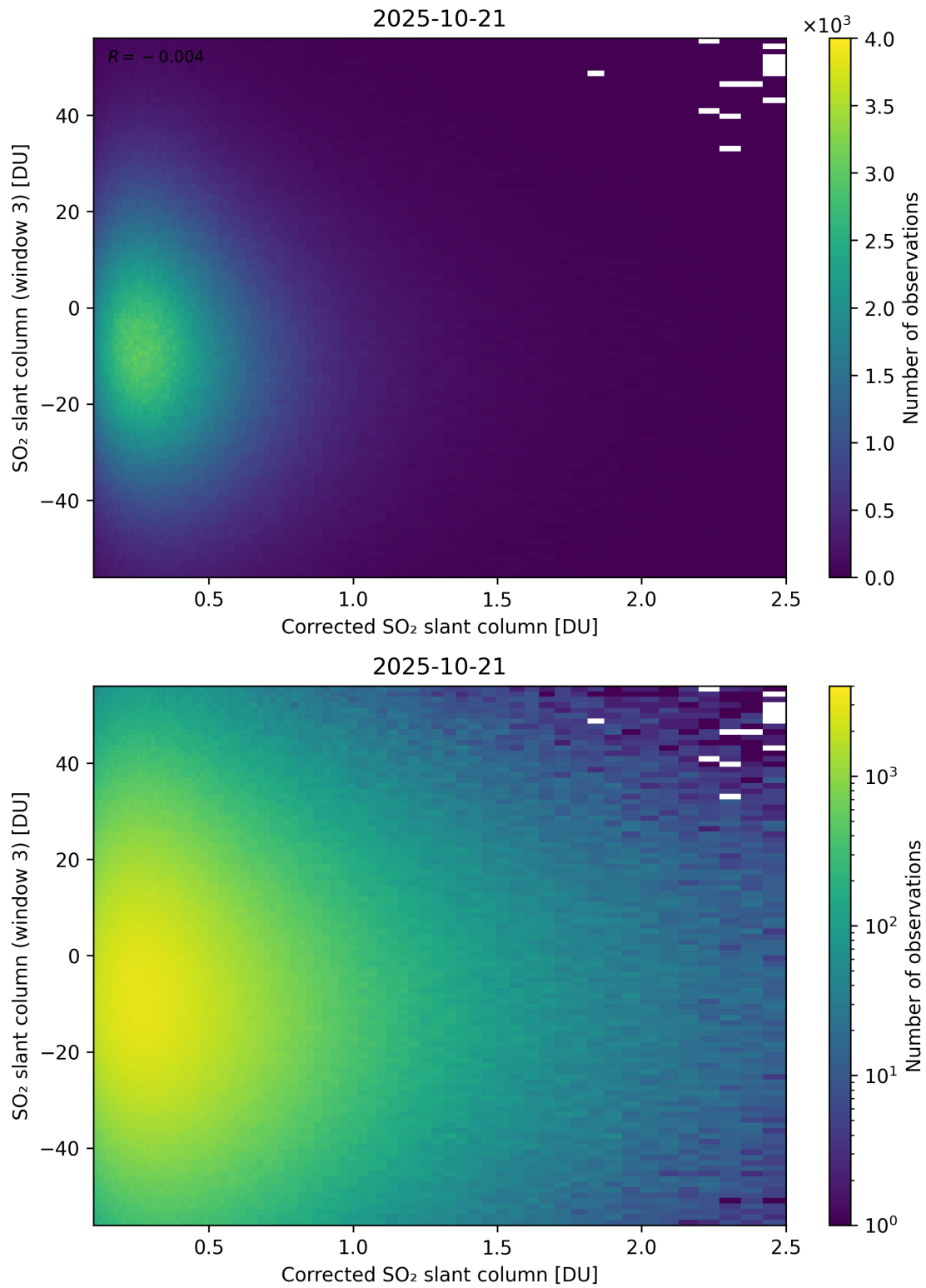
Figure 240: Scatter density plot of “Corrected SO 2 slant column” against “SO 2 slant column (window 3)” for 2025-10-20 to 2025-10-22.
