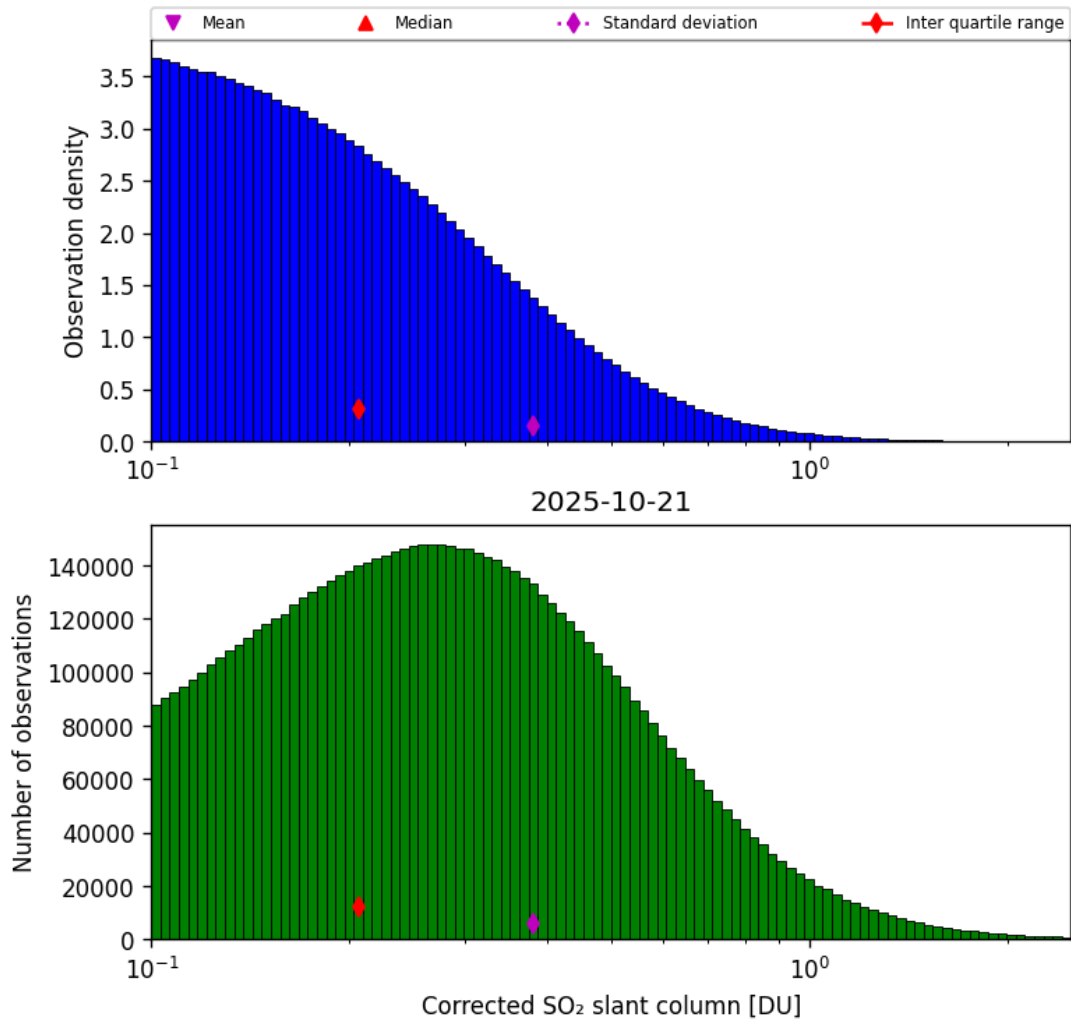
Figure 60: Histogram of "Corrected SO 2 slant column" for 2025-10-20 to 2025-10-22
