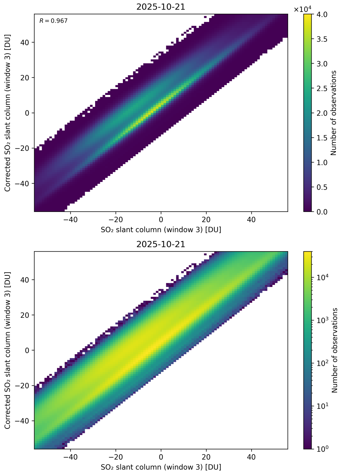
Figure 316: Scatter density plot of “SO 2 slant column (window 3)” against “Corrected SO 2 slant column (window 3)” for 2025-10-20 to 2025-10-22.
