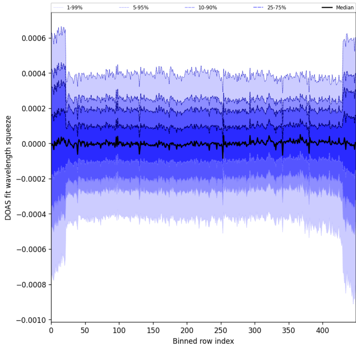
Figure 103: Along track statistics of “DOAS fit wavelength squeeze” for 2025-10-20 to 2025-10-22
