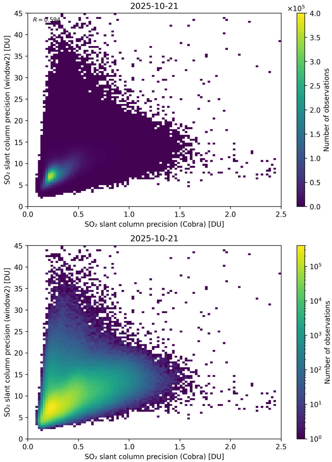
Figure 210: Scatter density plot of “SO 2 slant column precision (Cobra)” against “SO 2 slant column precision (window2)” for 2025-10-20 to 2025-10-22.
