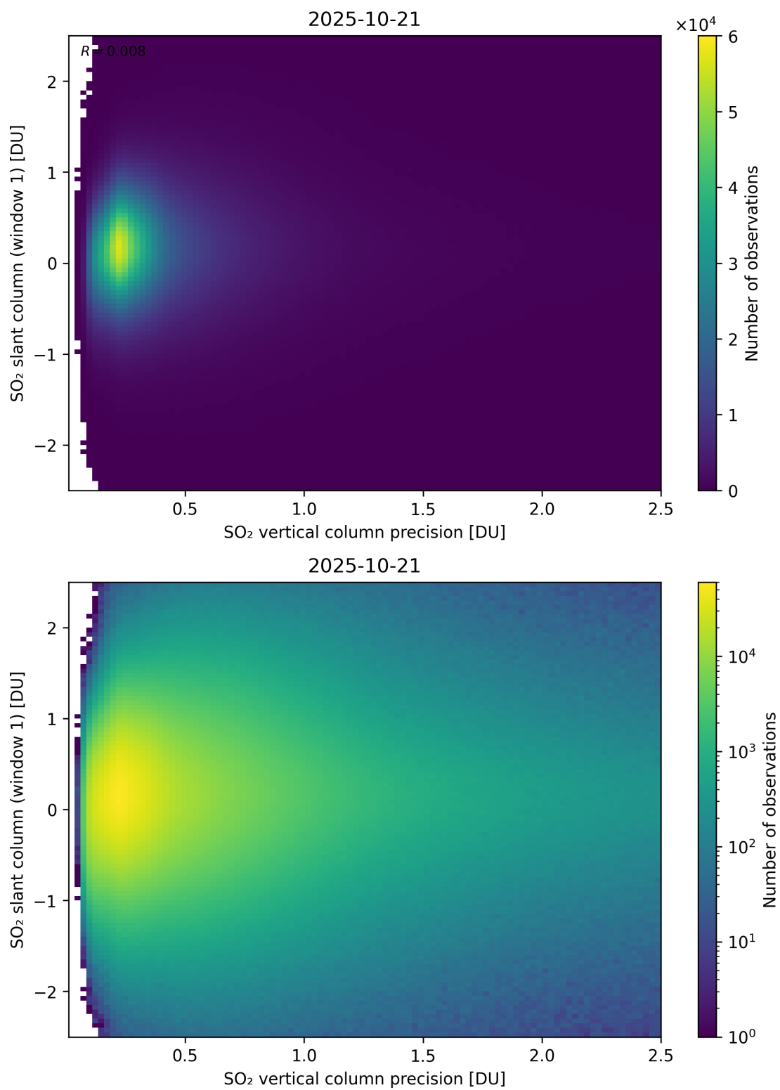
Figure 341: Scatter density plot of “SO 2 vertical column precision” against “SO 2 slant column (window 1)” for 2025-10-20 to 2025-10-22.
