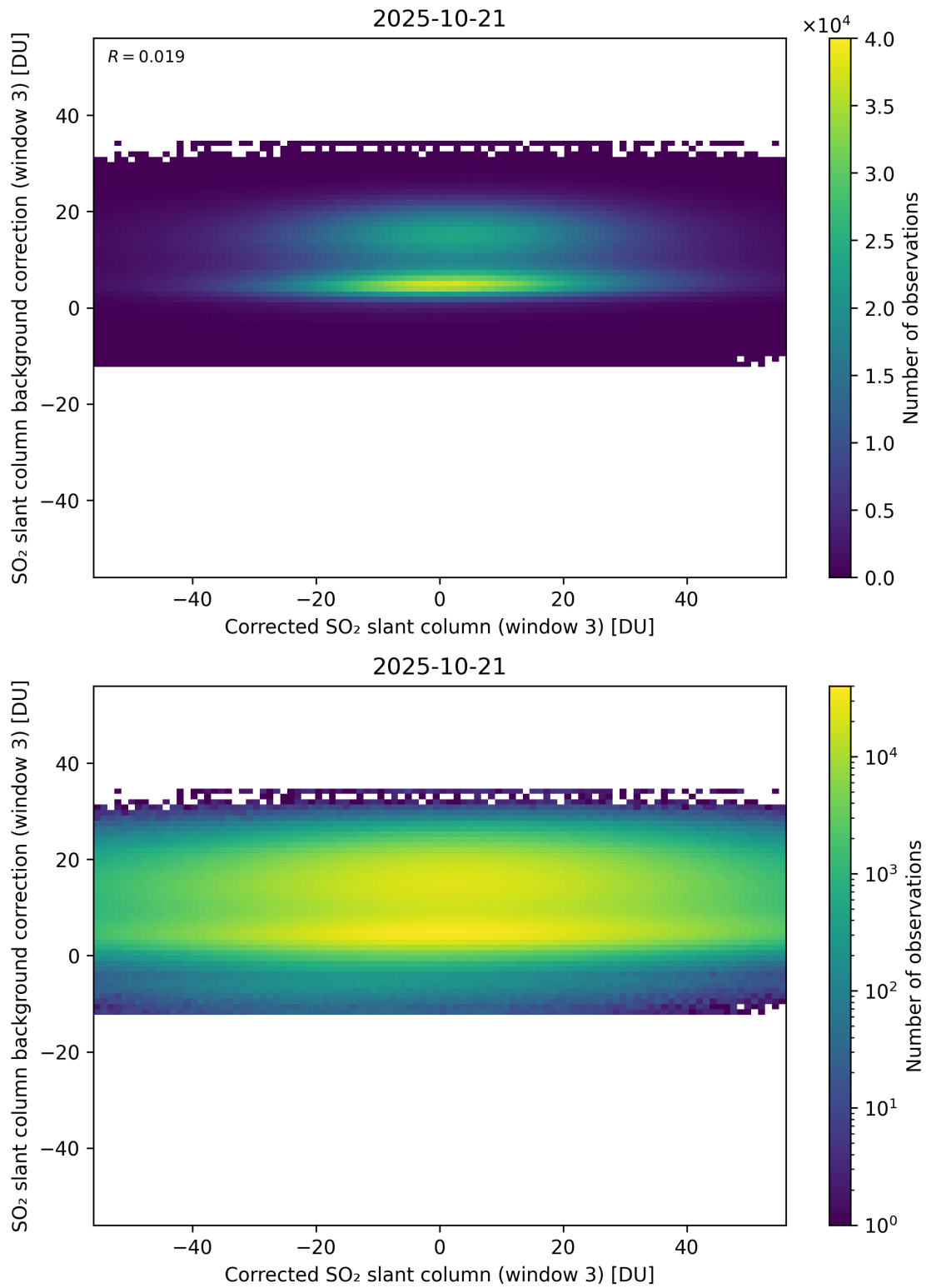
Figure 255: Scatter density plot of “Corrected SO 2 slant column (window 3)” against “SO 2 slant column background correction (window 3)” for 2025-10-20 to 2025-10-22.
