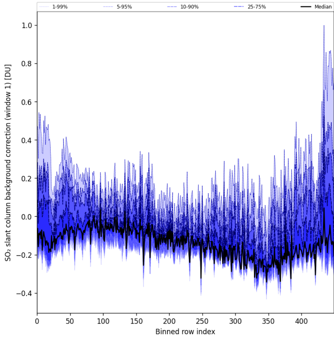
Figure 92: Along track statistics of “SO 2 slant column background correction (window 1)” for 2025-10-20 to 2025-10-22
