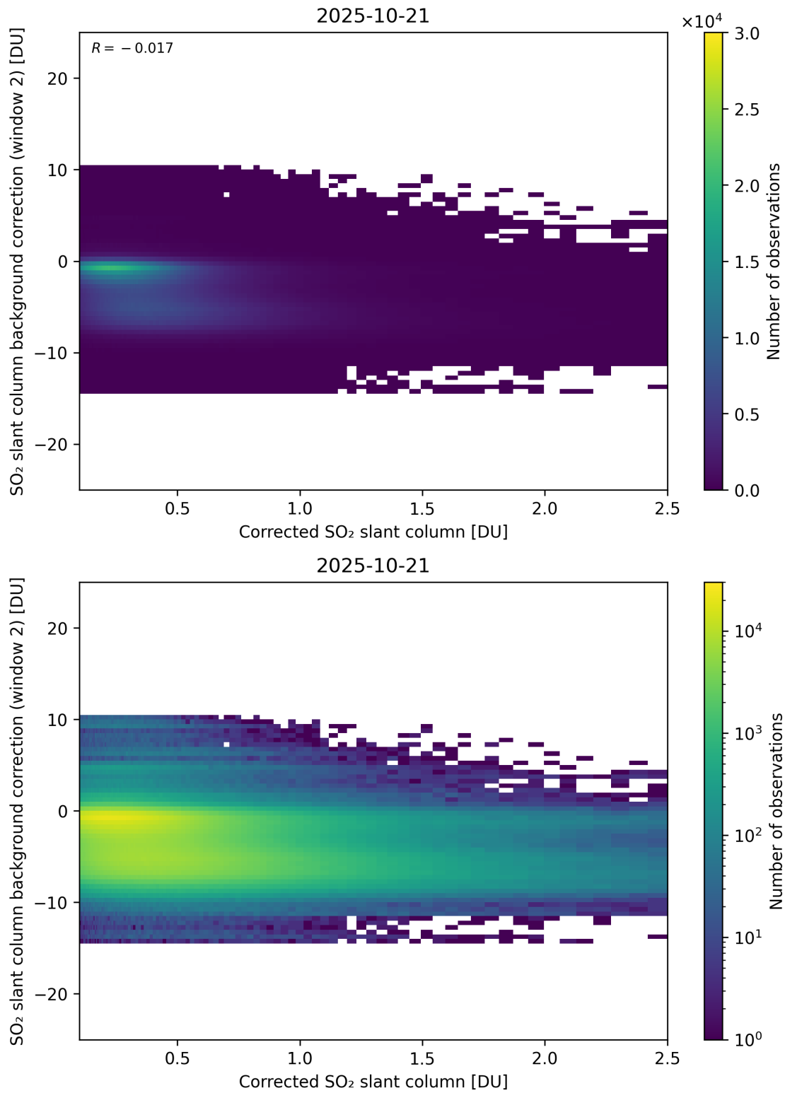
Figure 227: Scatter density plot of “Corrected SO 2 slant column” against “SO 2 slant column background correction (window 2)” for 2025-10-20 to 2025-10-22.
