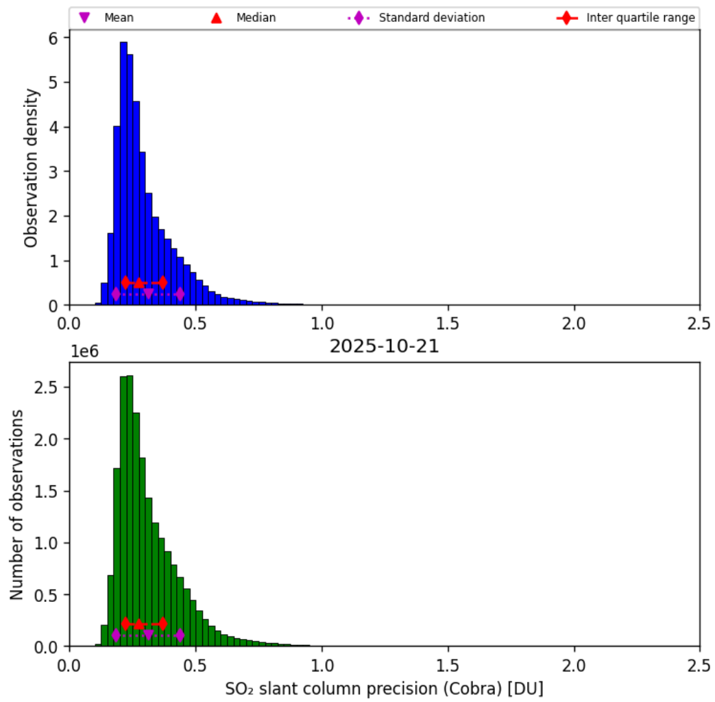
Figure 62: Histogram of “SO 2 slant column precision (Cobra)” for 2025-10-20 to 2025-10-22
