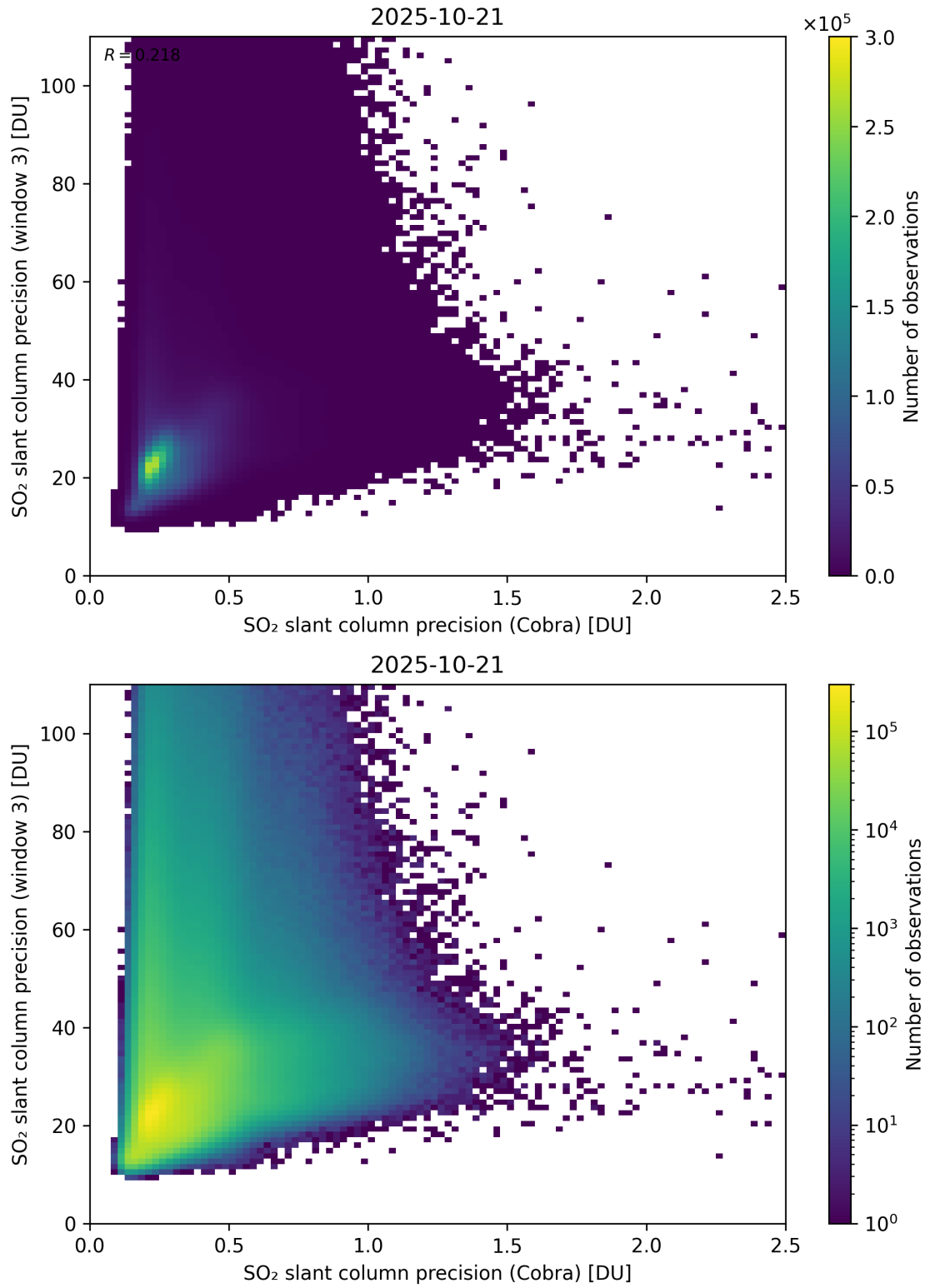
Figure 212: Scatter density plot of “SO 2 slant column precision (Cobra)” against “SO 2 slant column precision (window 3)” for 2025-10-20 to 2025-10-22.
