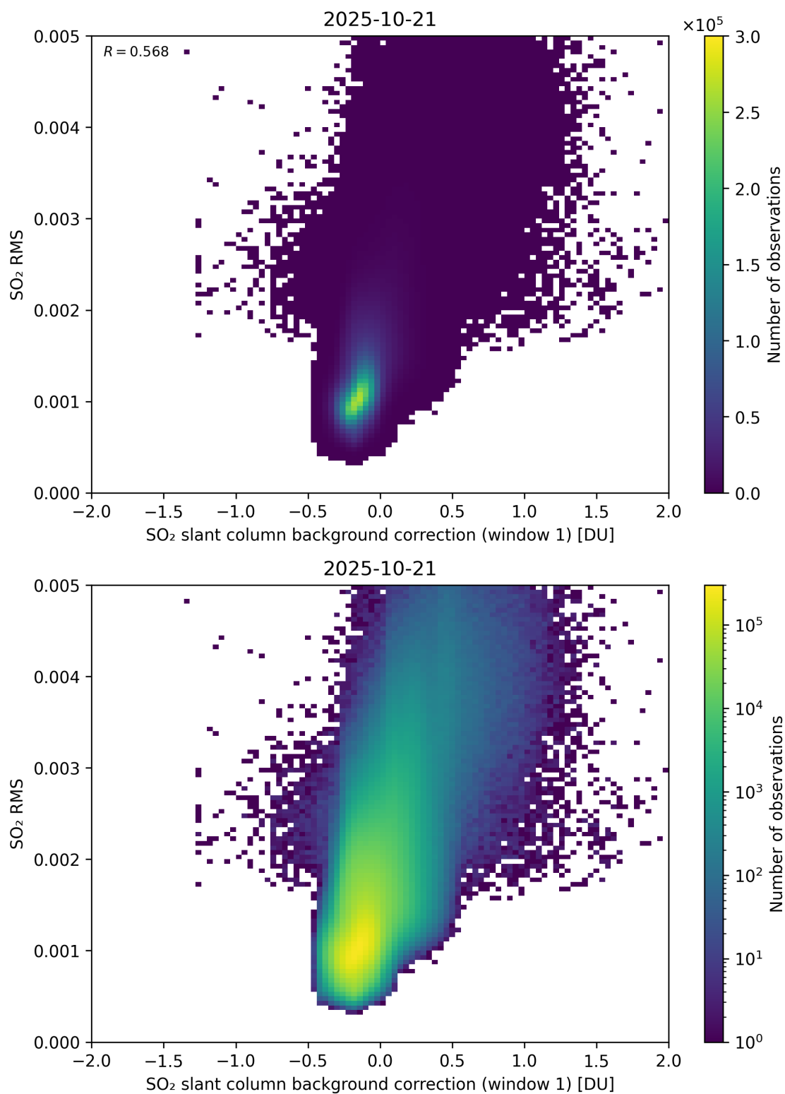
Figure 113: Scatter density plot of “SO 2 slant column background correction (window 1)” against “SO 2 RMS” for 2025-10-20 to 2025-10-22.
