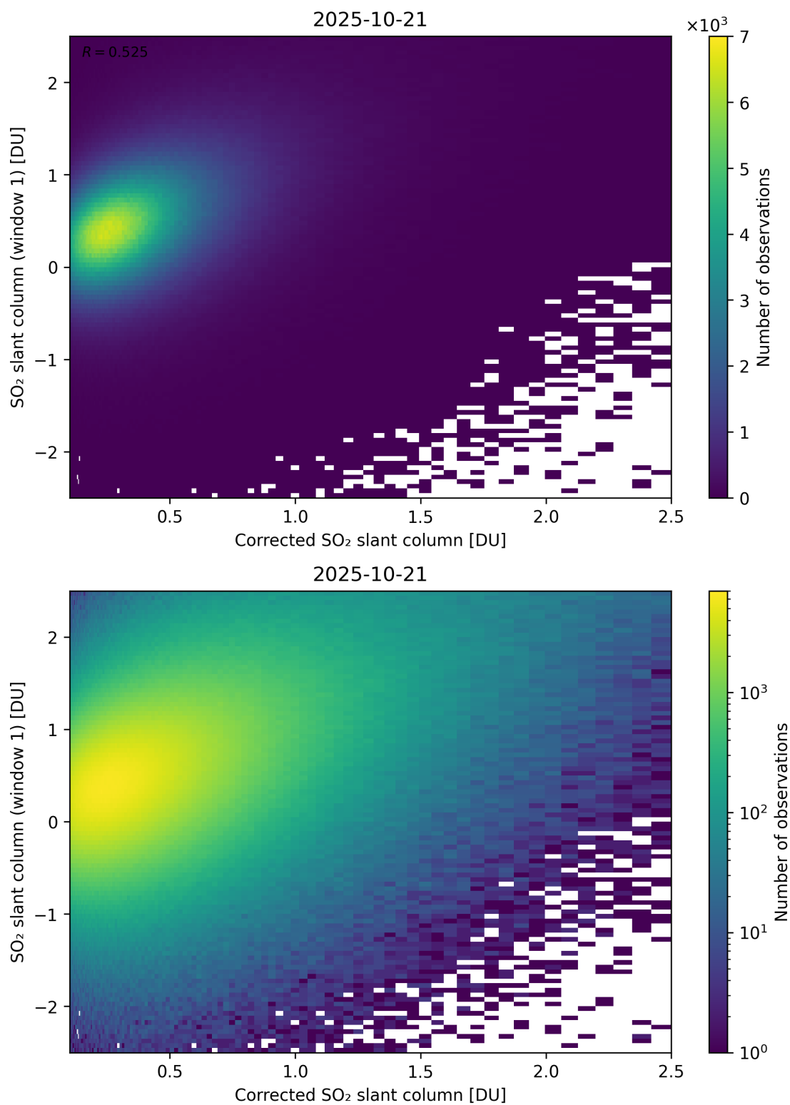
Figure 237: Scatter density plot of “Corrected SO 2 slant column” against “SO 2 slant column (window 1)” for 2025-10-20 to 2025-10-22.
