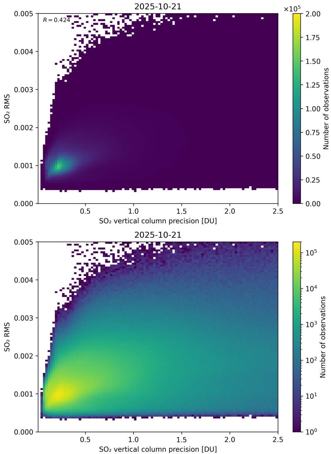
Figure 334: Scatter density plot of “SO 2 vertical column precision” against “SO 2 RMS” for 2025-10-20 to 2025-10-22.
