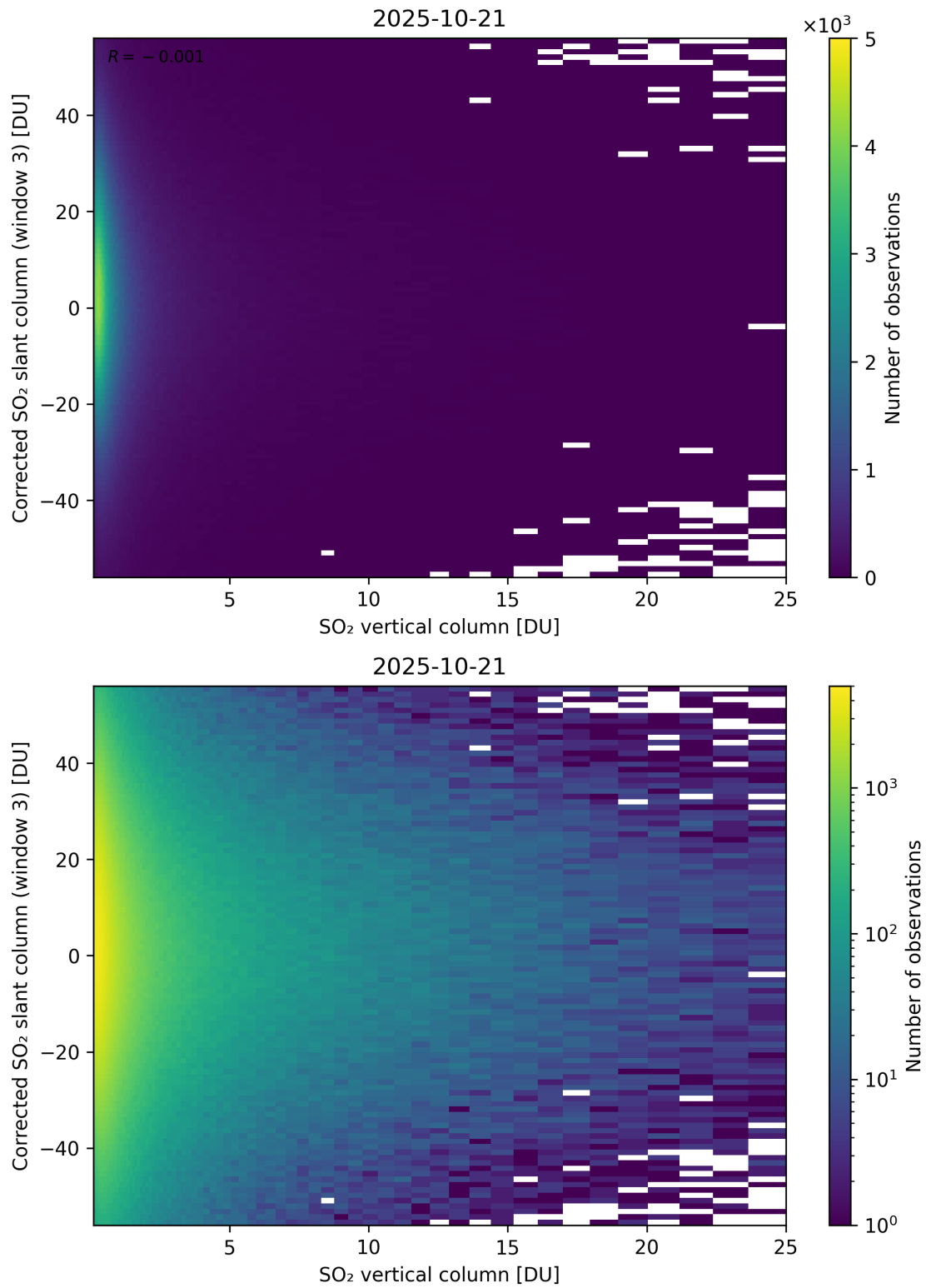
Figure 353: Scatter density plot of “SO 2 vertical column” against “Corrected SO 2 slant column (window 3)” for 2025-10-20 to 2025-10-22.
