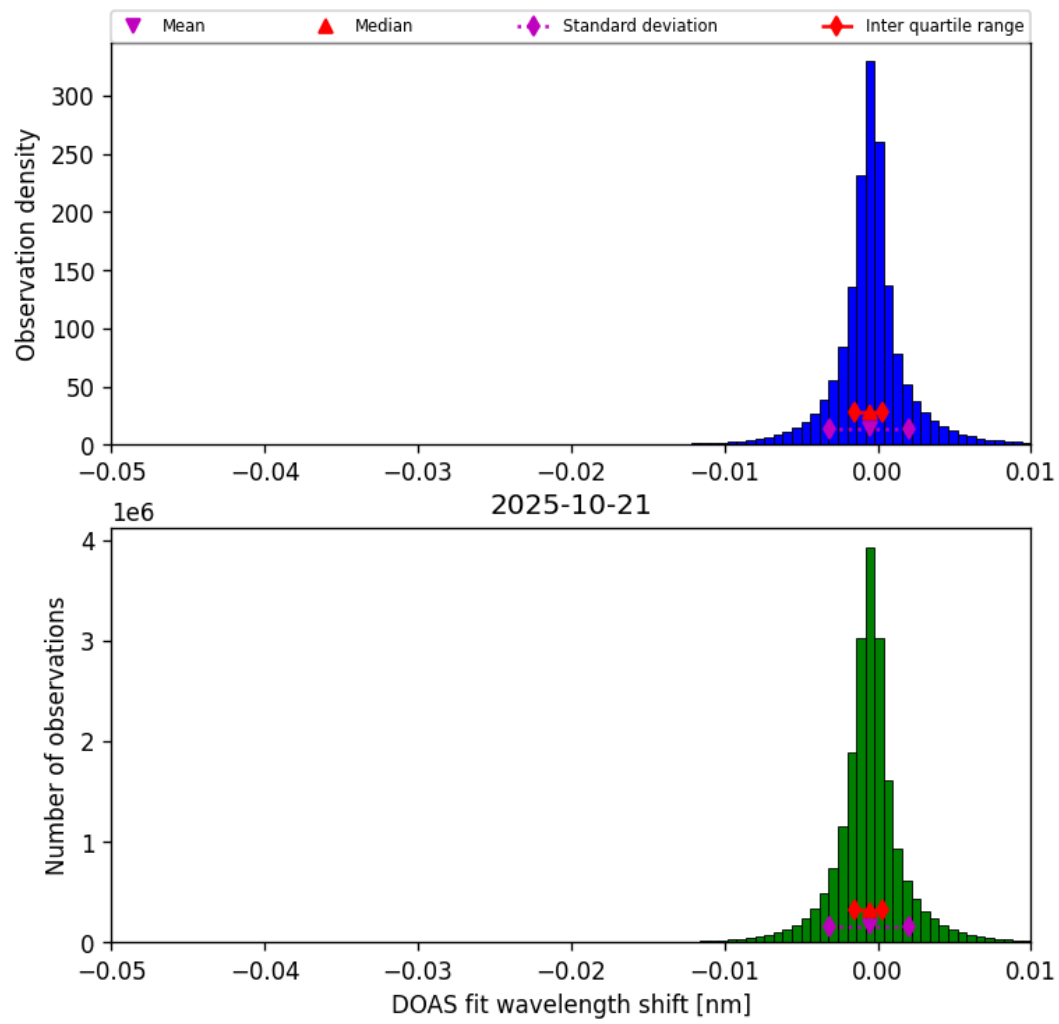
Figure 76: Histogram of “DOAS fit wavelength shift” for 2025-10-20 to 2025-10-22
