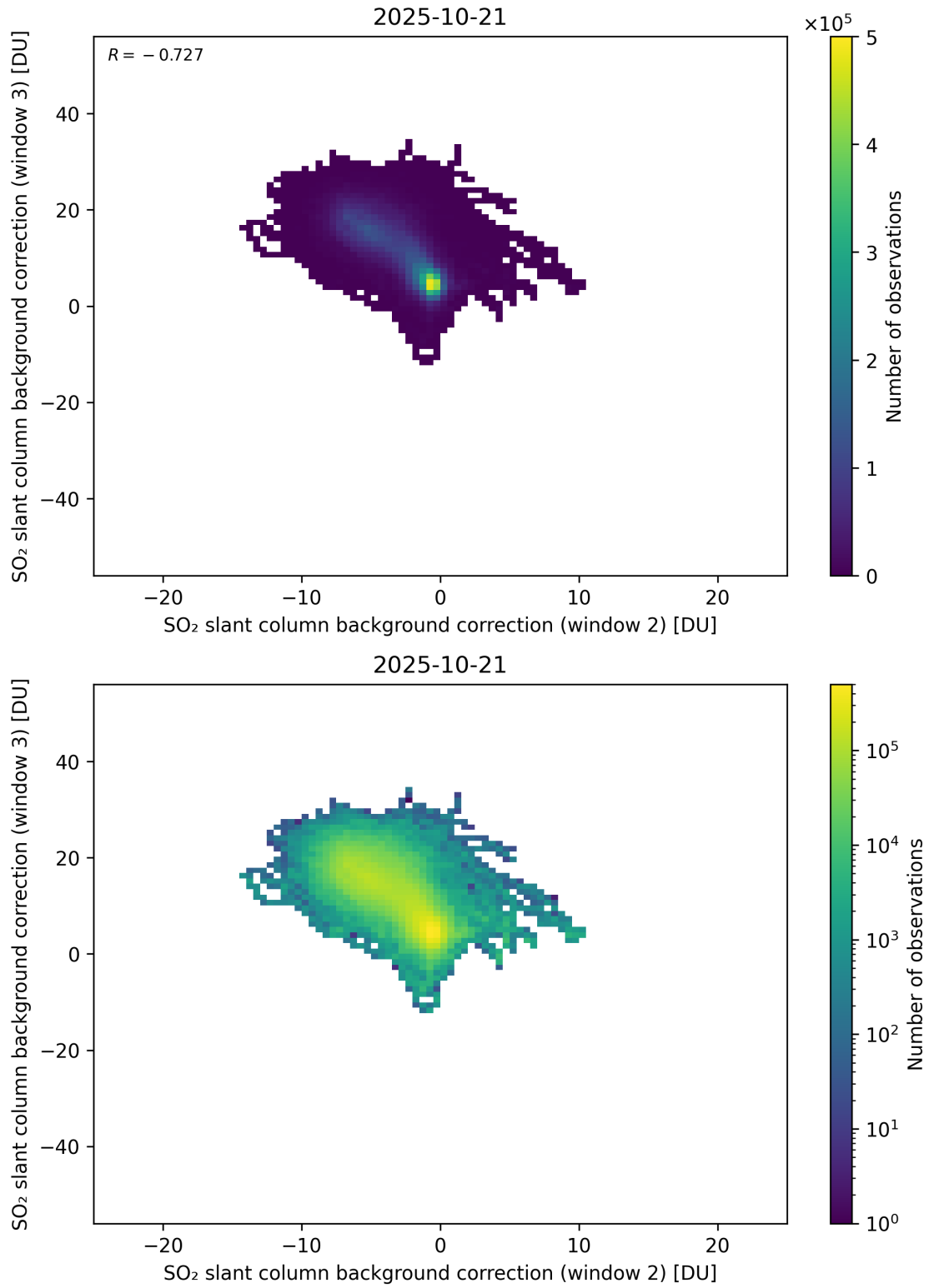
Figure 122: Scatter density plot of “SO 2 slant column background correction (window 2)” against “SO 2 slant column background correction (window 3)” for 2025-10-20 to 2025-10-22.
