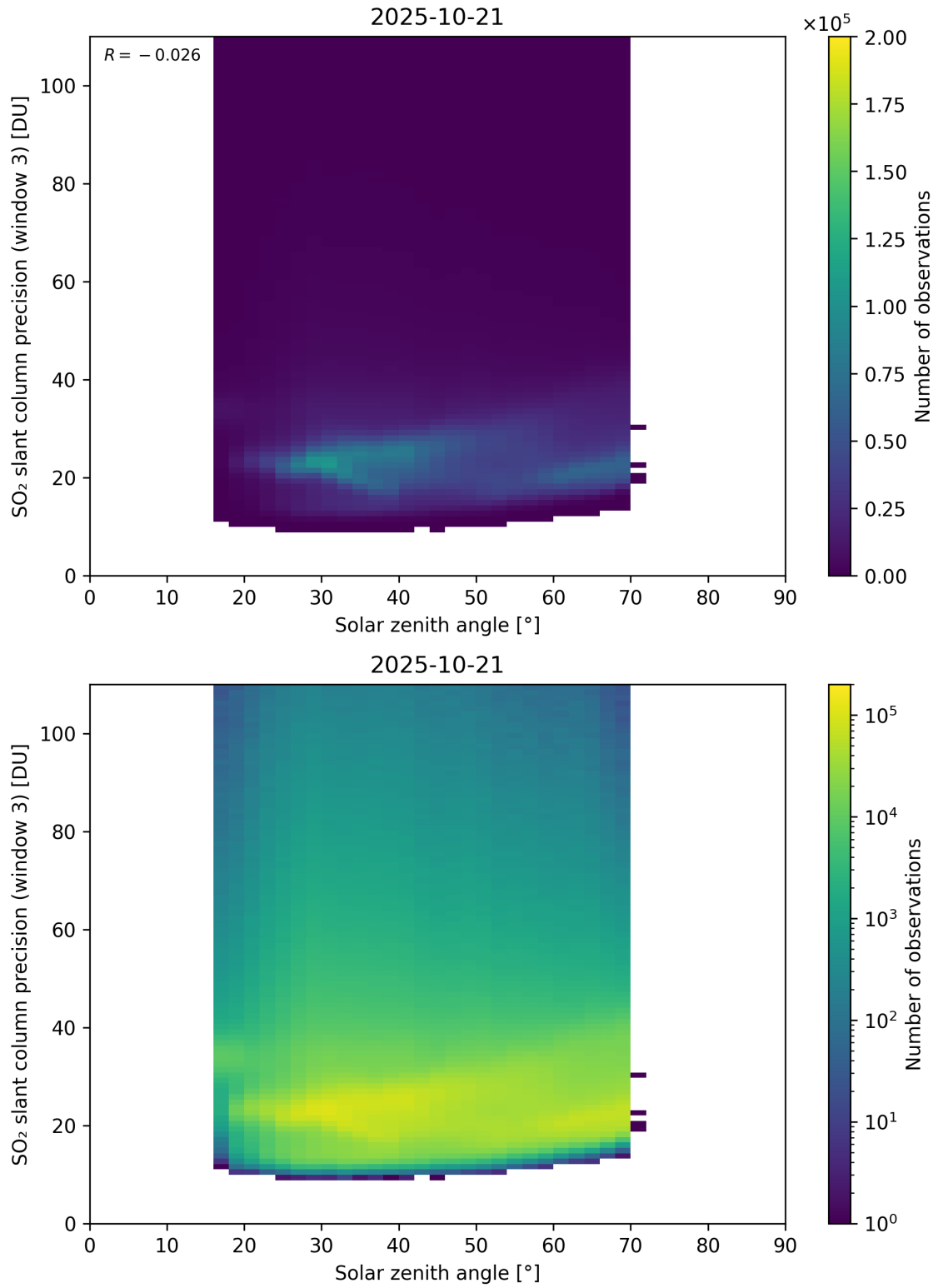
Figure 188: Scatter density plot of “Solar zenith angle” against “SO 2 slant column precision (window 3)” for 2025-10-20 to 2025-10-22.
