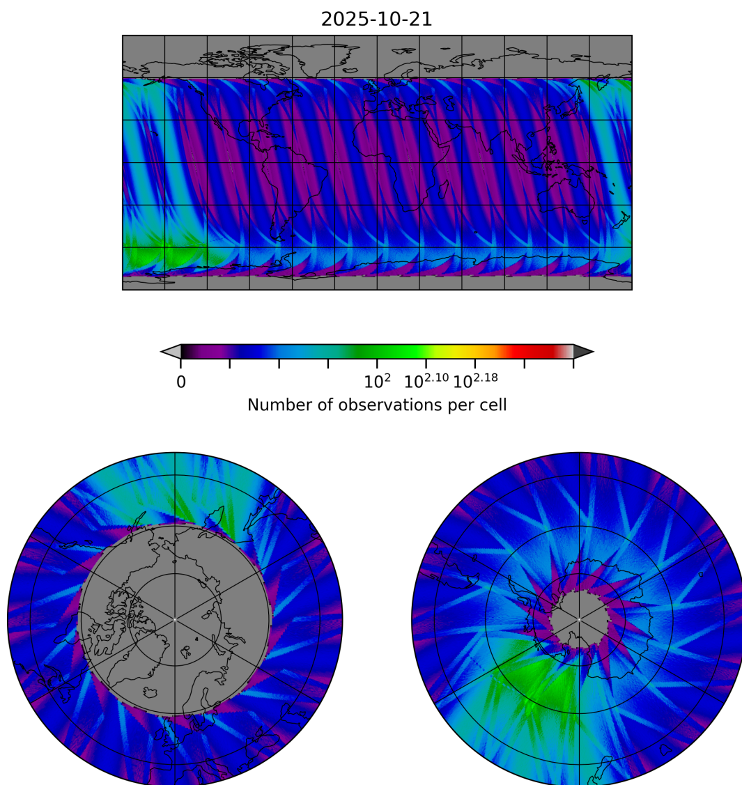
Figure 30: Map of the number of observations for 2025-10-20 to 2025-10-22
