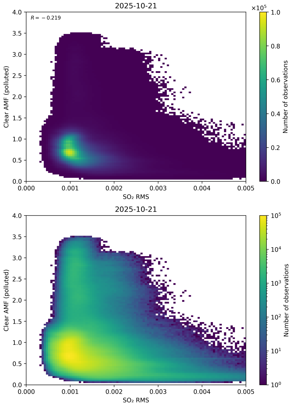
Figure 147: Scatter density plot of “SO 2 RMS” against “Clear AMF (polluted)” for 2025-10-20 to 2025-10-22.
