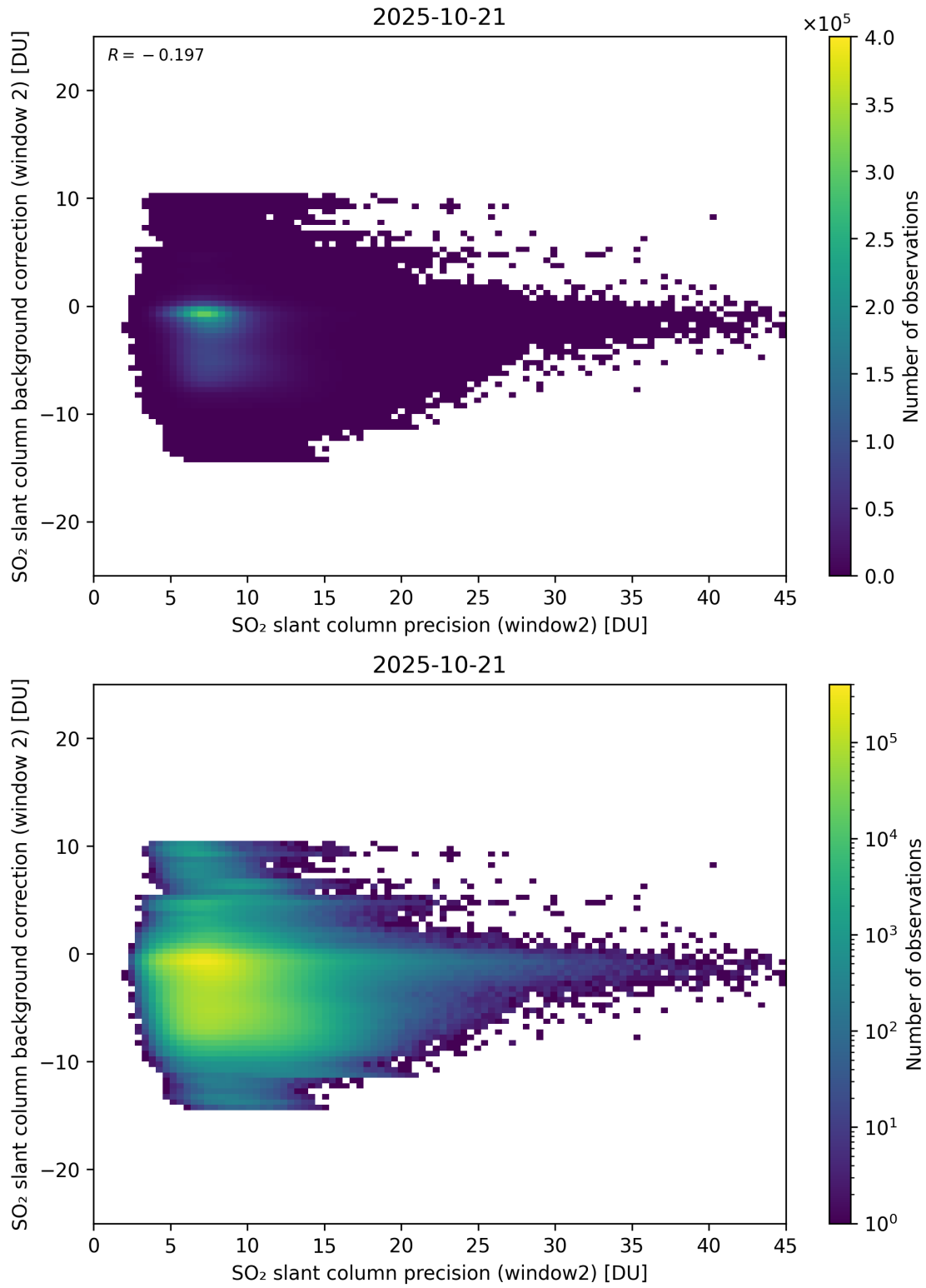
Figure 291: Scatter density plot of “SO 2 slant column precision (window2)” against “SO 2 slant column background correction (window 2)” for 2025-10-20 to 2025-10-22.
