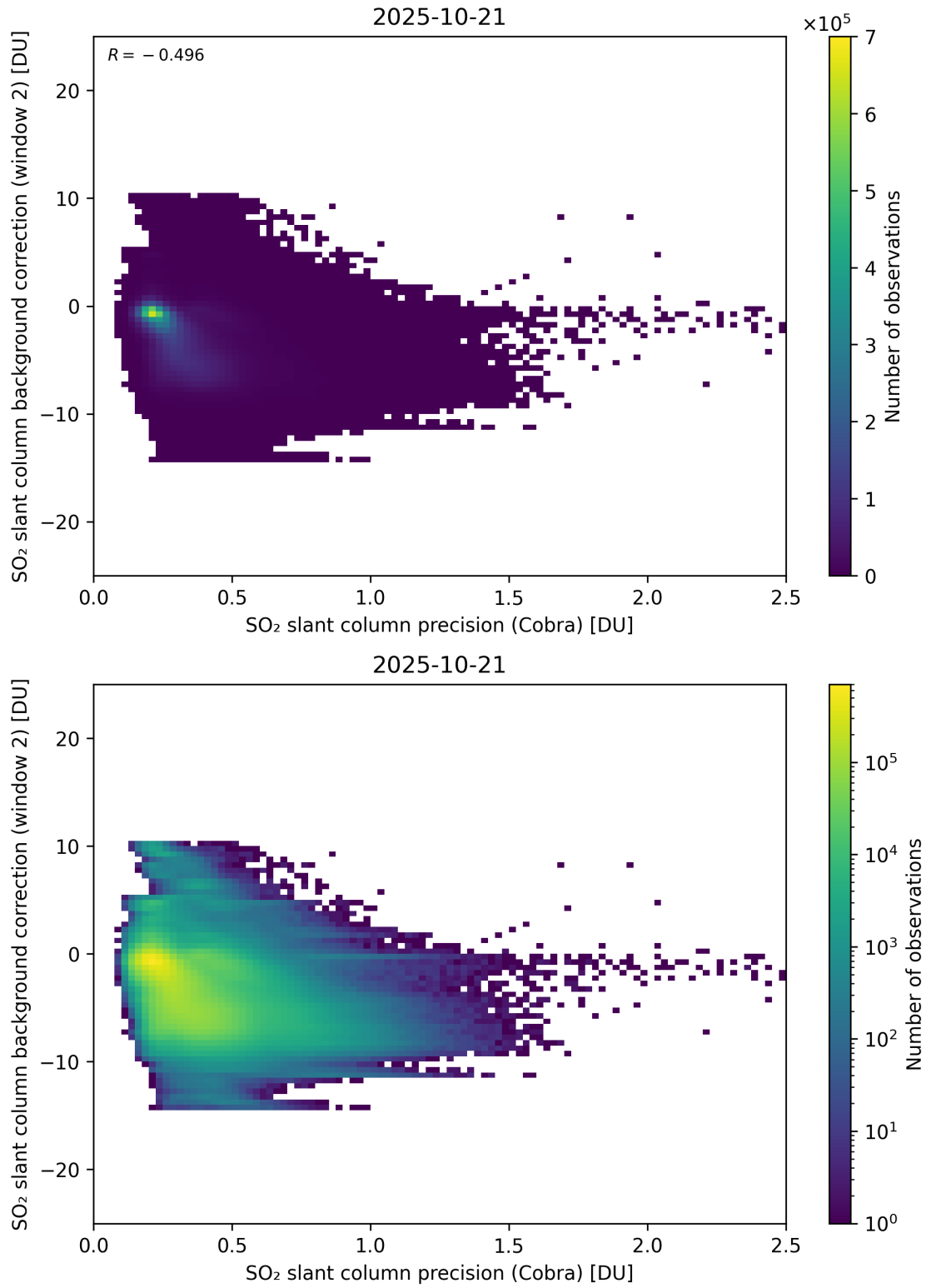
Figure 200: Scatter density plot of “SO 2 slant column precision (Cobra)” against “SO 2 slant column background correction (window 2)” for 2025-10-20 to 2025-10-22.
