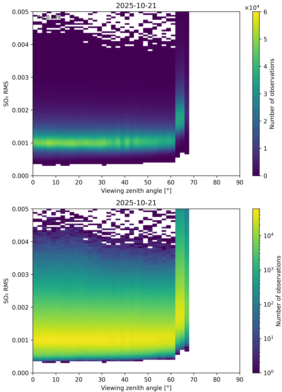
Figure 367: Scatter density plot of “Viewing zenith angle” against “SO 2 RMS” for 2025-10-20 to 2025-10-22.
