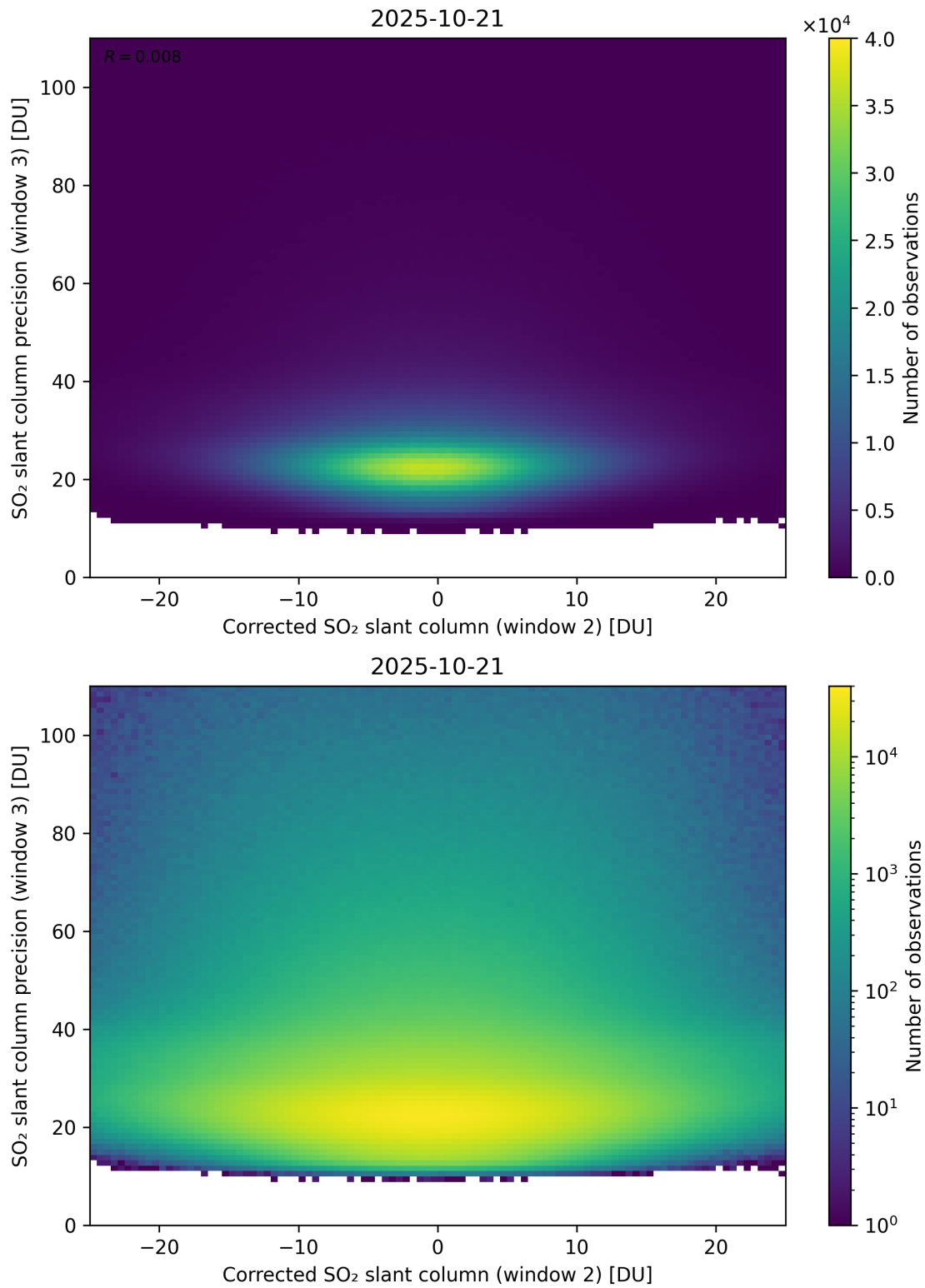
Figure 252: Scatter density plot of “Corrected SO 2 slant column (window 2)” against “SO 2 slant column precision (window 3)” for 2025-10-20 to 2025-10-22.
