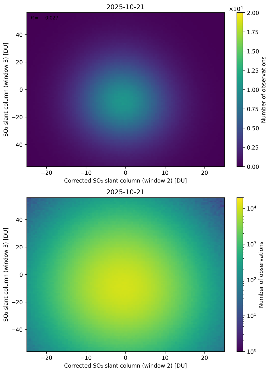
Figure 251: Scatter density plot of “Corrected SO 2 slant column (window 2)” against “SO 2 slant column (window 3)” for 2025-10-20 to 2025-10-22.
