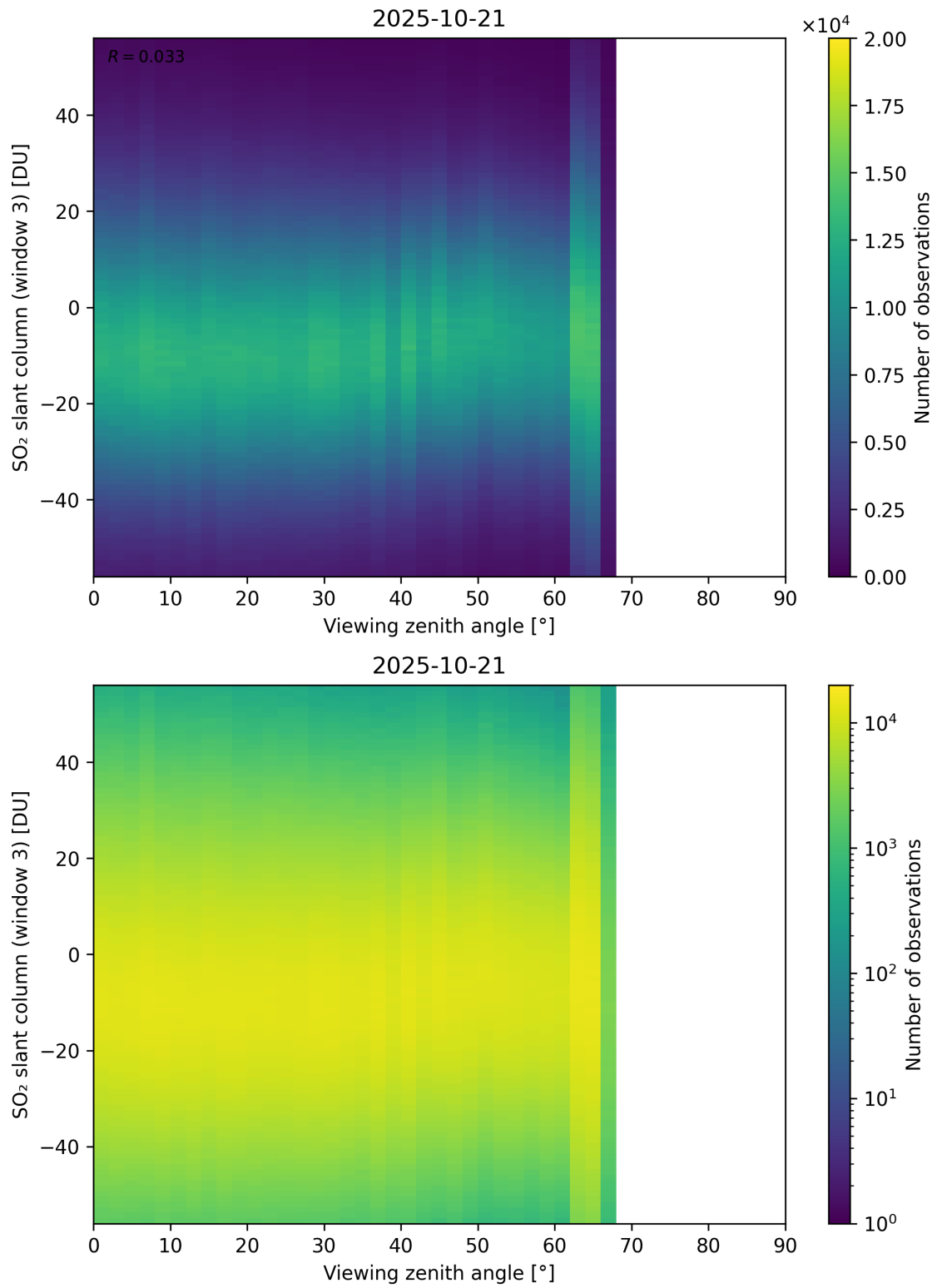
Figure 379: Scatter density plot of “Viewing zenith angle” against “SO 2 slant column (window 3)” for 2025-10-20 to 2025-10-22.
