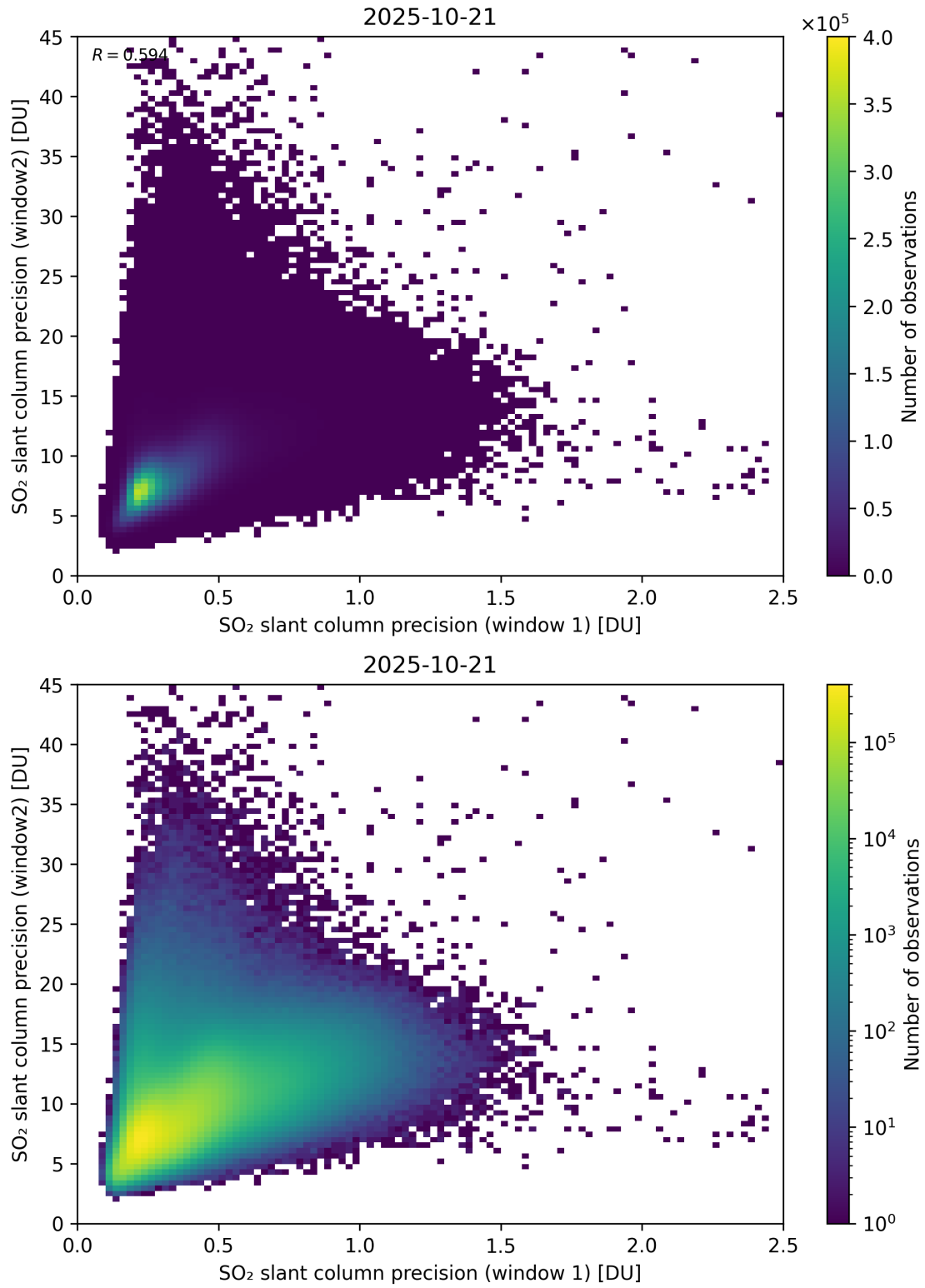
Figure 277: Scatter density plot of “SO 2 slant column precision (window 1)” against “SO 2 slant column precision (window2)” for 2025-10-20 to 2025-10-22.
