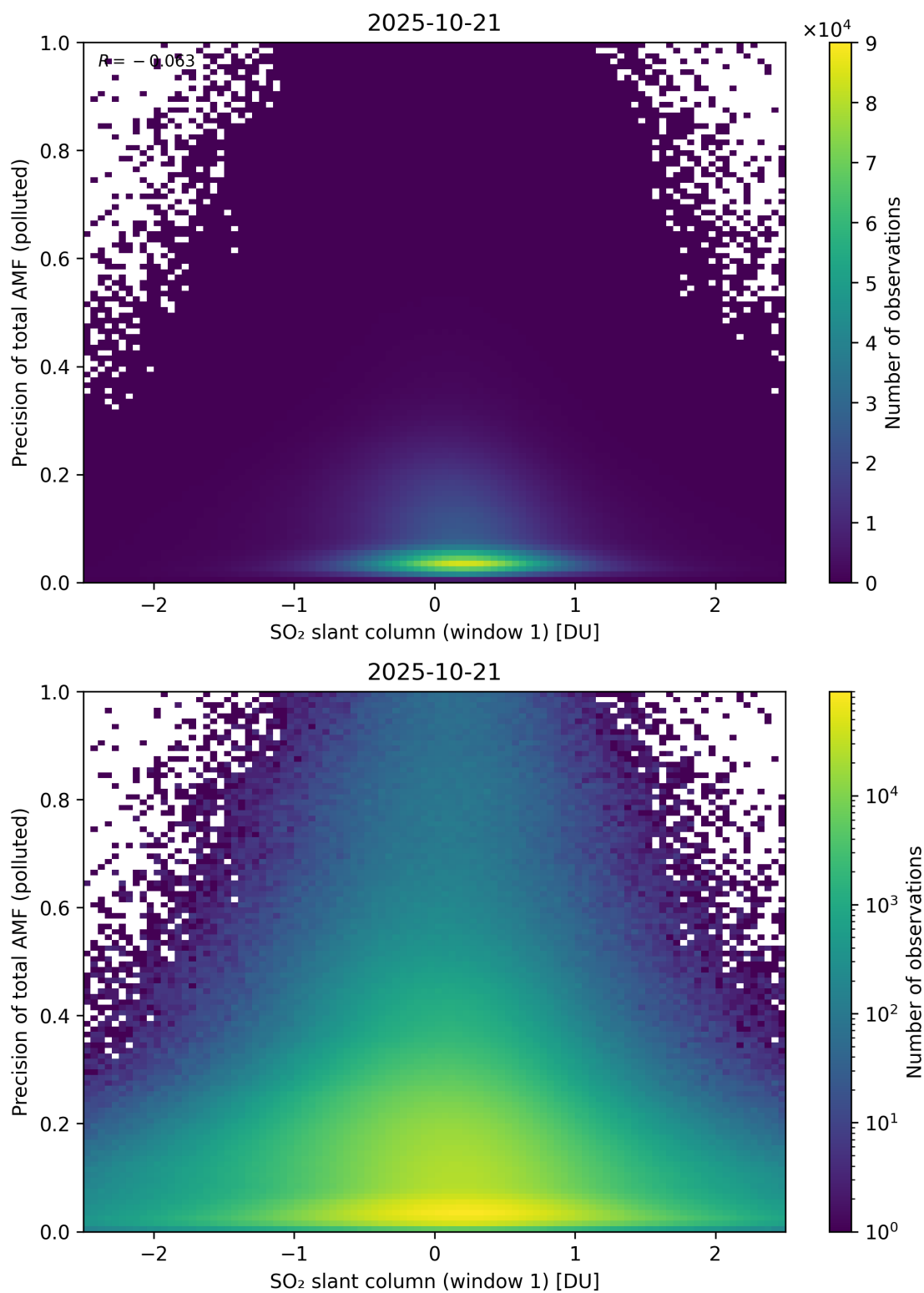
Figure 290: Scatter density plot of “SO 2 slant column (window 1)” against “Precision of total AMF (polluted)” for 2025-10-20 to 2025-10-22.
