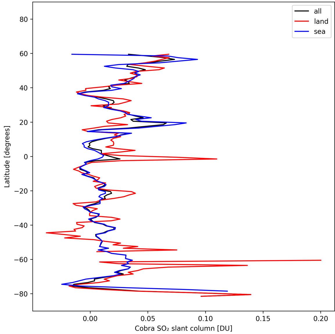
Figure 35: Zonal average of “Cobra SO 2 slant column” for 2025-10-20 to 2025-10-22.
