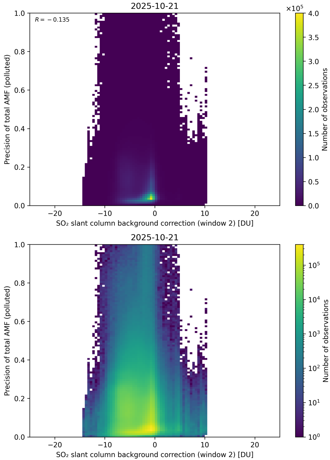
Figure 131: Scatter density plot of “SO 2 slant column background correction (window 2)” against “Precision of total AMF (polluted)” for 2025-10-20 to 2025-10-22.
