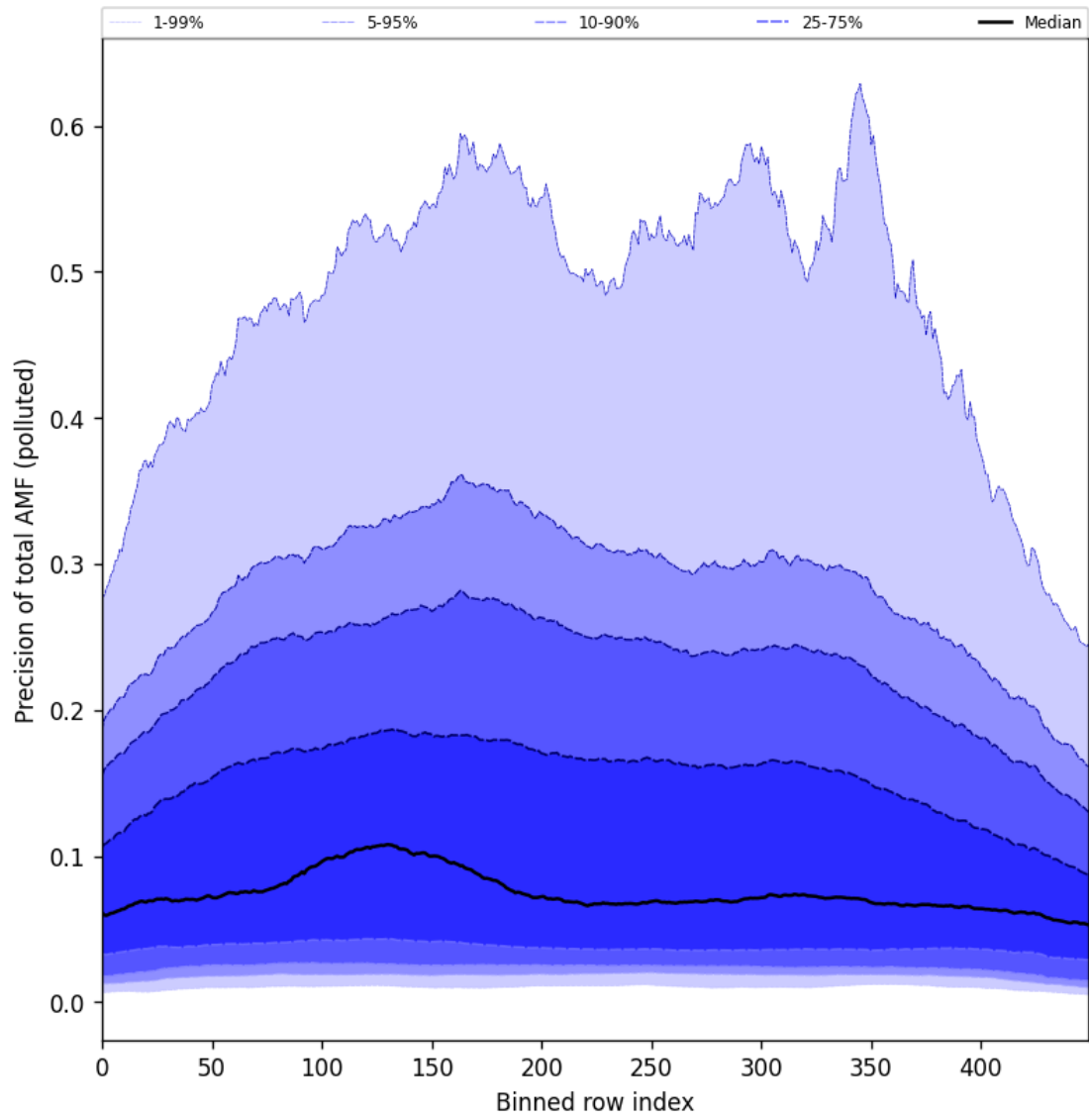
Figure 106: Along track statistics of “Precision of total AMF (polluted)” for 2025-10-20 to 2025-10-22
