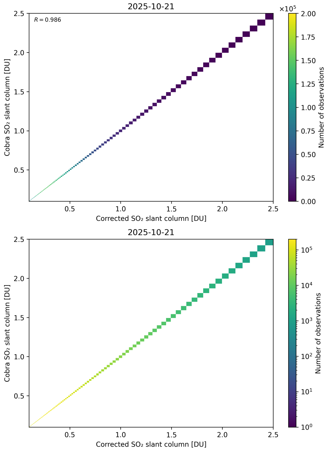
Figure 233: Scatter density plot of “Corrected SO 2 slant column” against “Cobra SO 2 slant column” for 2025-10-20 to 2025-10-22.
