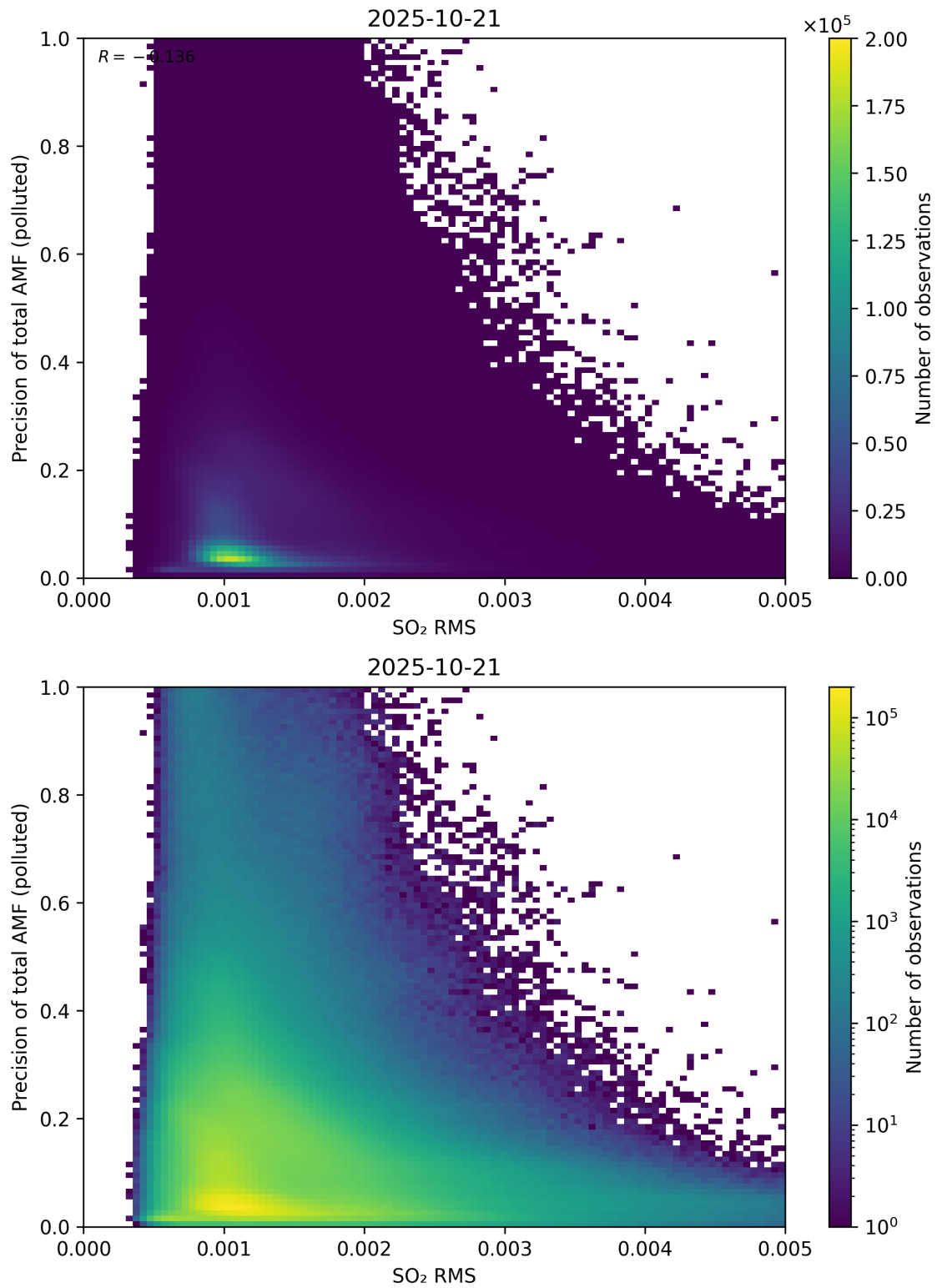
Figure 149: Scatter density plot of “SO 2 RMS” against “Precision of total AMF (polluted)” for 2025-10-20 to 2025-10-22.
