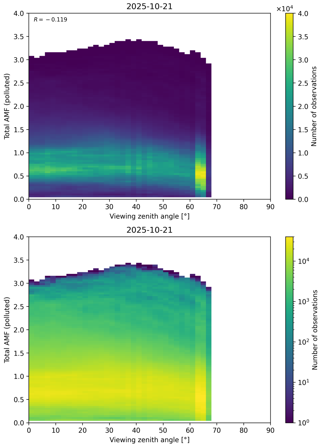
Figure 381: Scatter density plot of “Viewing zenith angle” against “Total AMF (polluted)” for 2025-10-20 to 2025-10-22.
