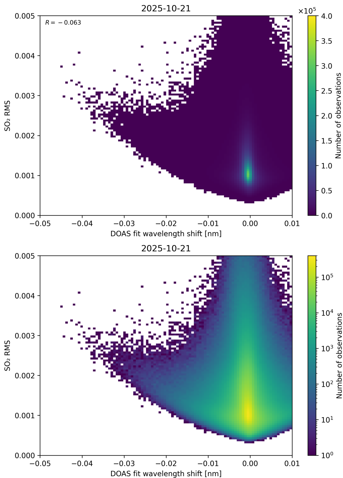
Figure 139: Scatter density plot of “DOAS fit wavelength shift” against “SO 2 RMS” for 2025-10-20 to 2025-10-22.
