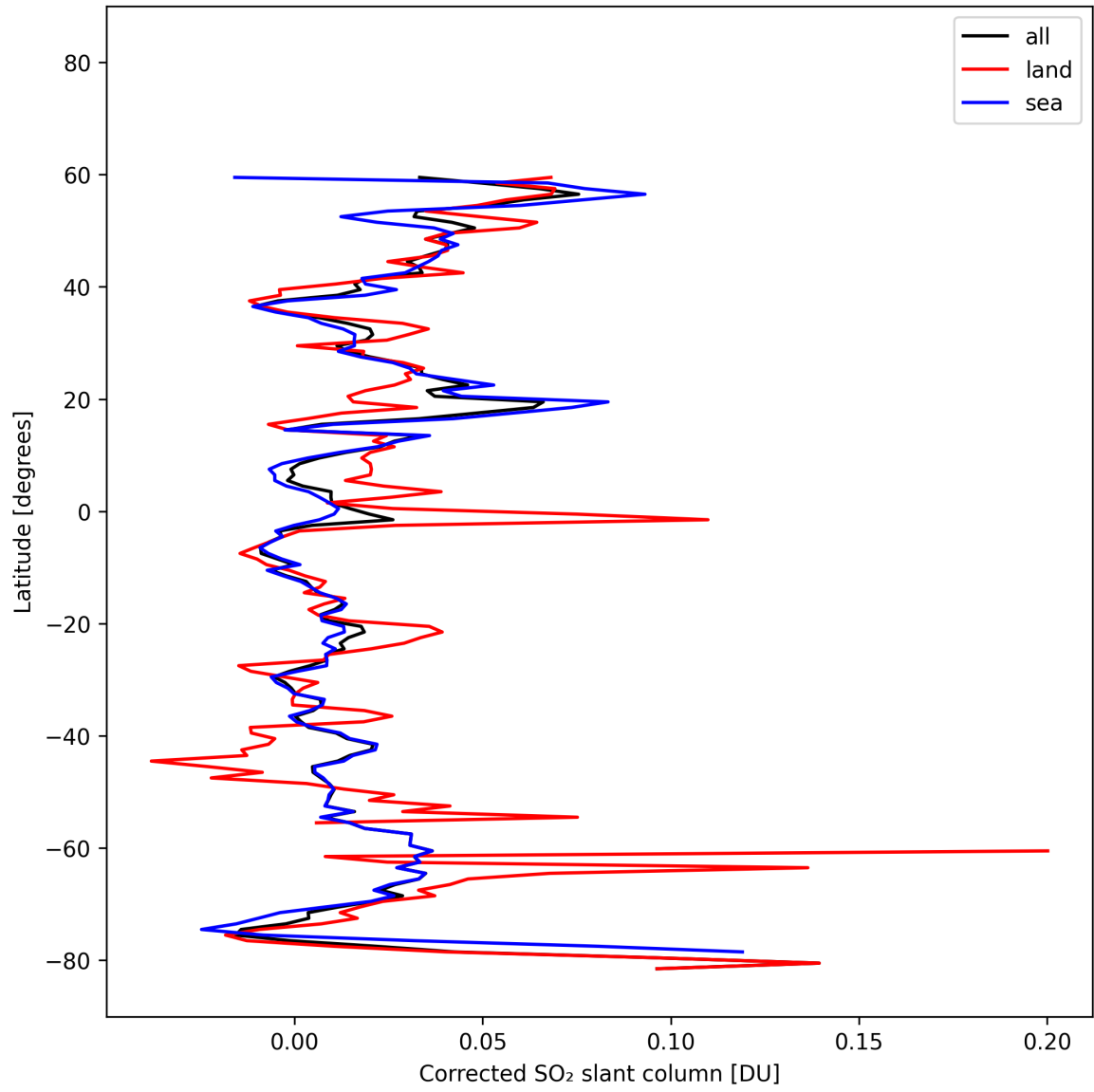
Figure 34: Zonal average of “Corrected SO 2 slant column” for 2025-10-20 to 2025-10-22.
