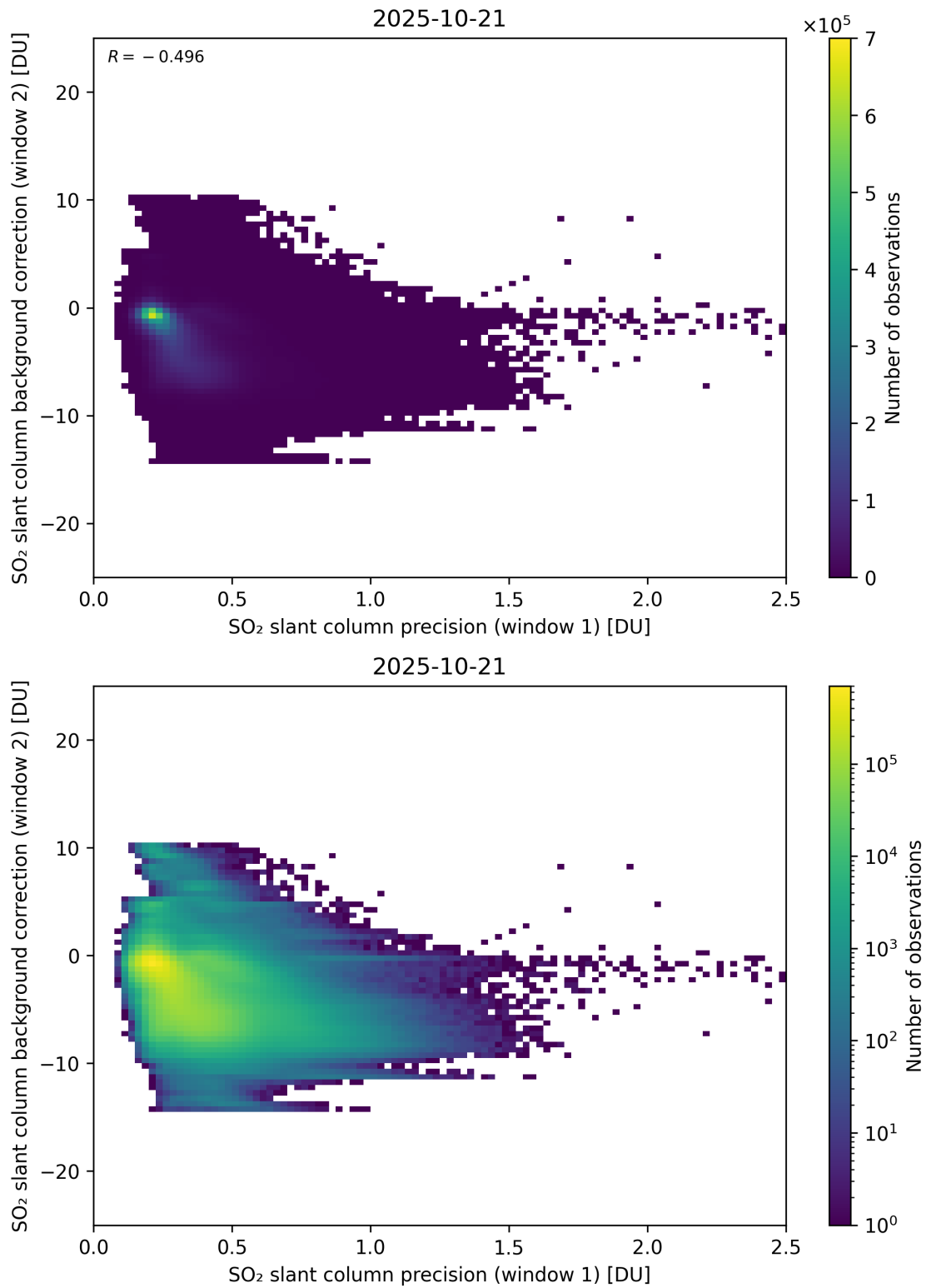
Figure 269: Scatter density plot of “SO 2 slant column precision (window 1)” against “SO 2 slant column background correction (window 2)” for 2025-10-20 to 2025-10-22.
