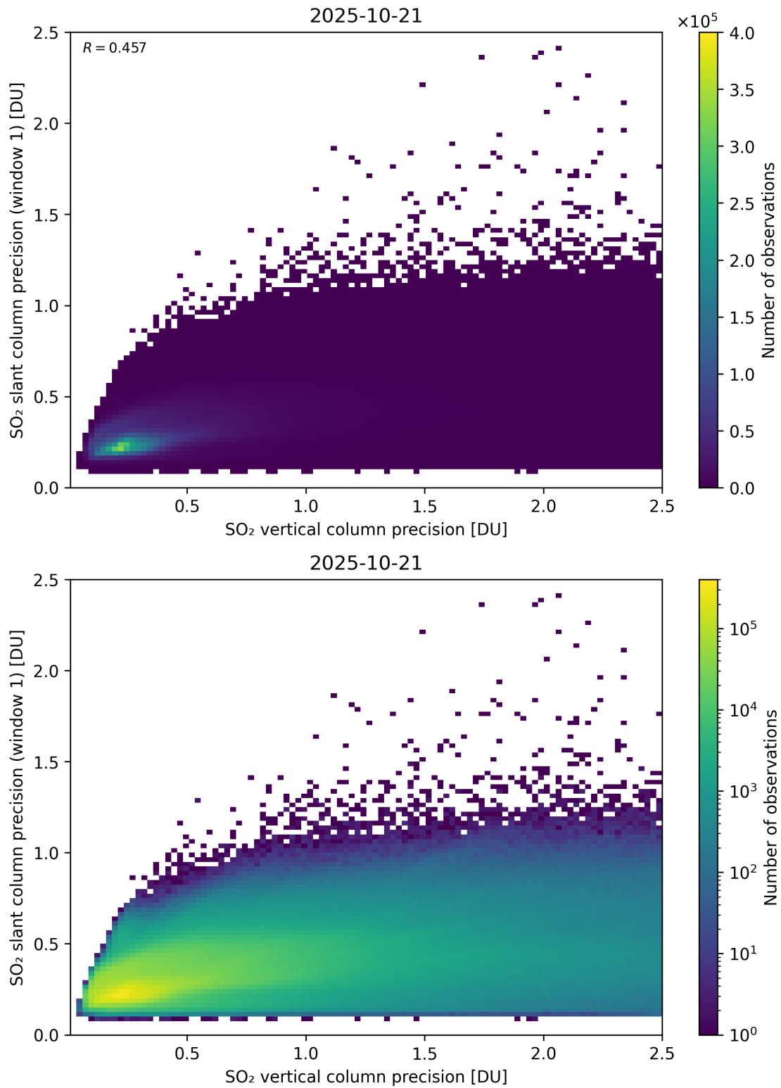
Figure 342: Scatter density plot of “SO 2 vertical column precision” against “SO 2 slant column precision (window 1)” for 2025-10-20 to 2025-10-22.
