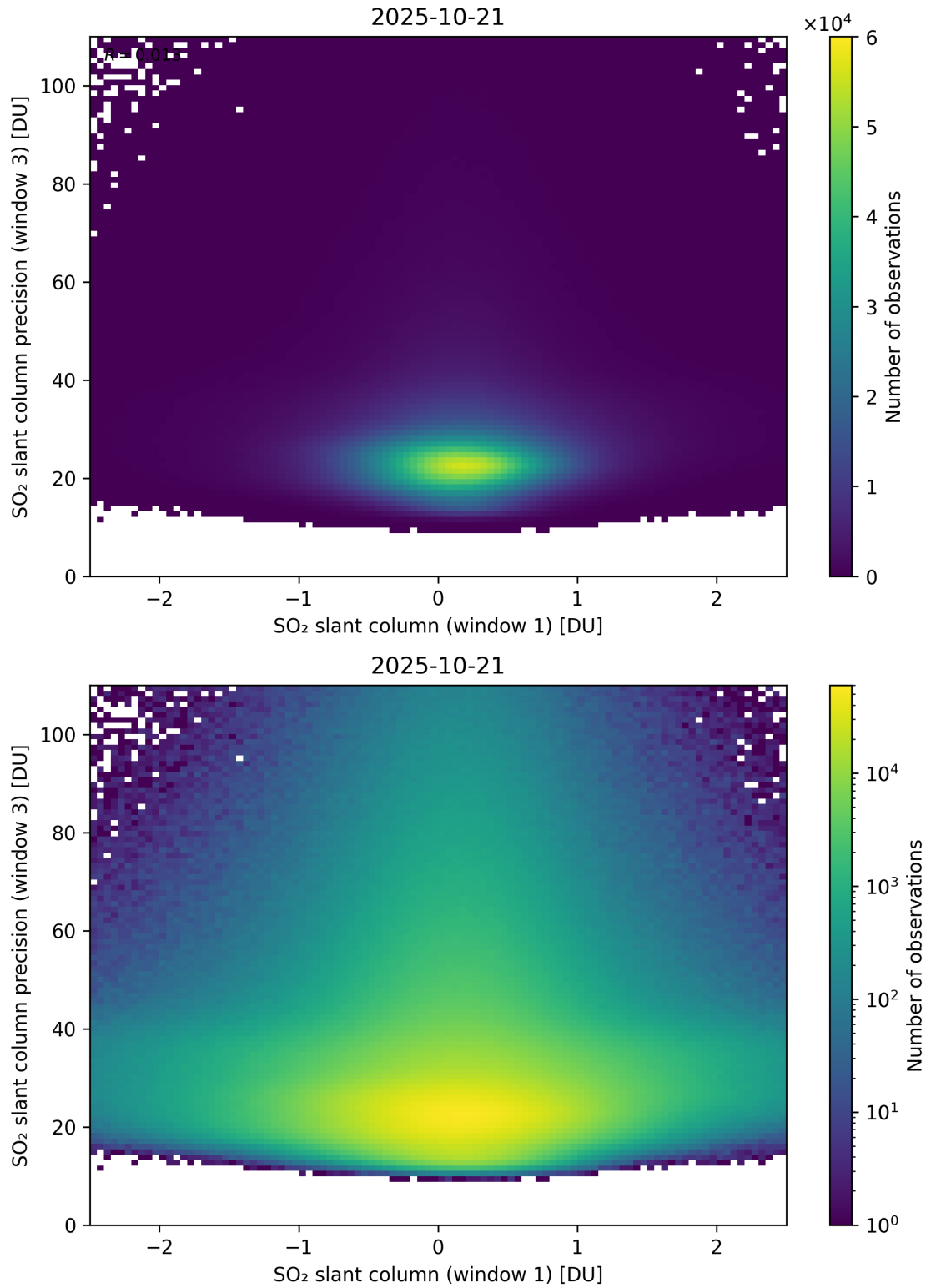
Figure 288: Scatter density plot of “SO 2 slant column (window 1)” against “SO 2 slant column precision (window 3)” for 2025-10-20 to 2025-10-22.
