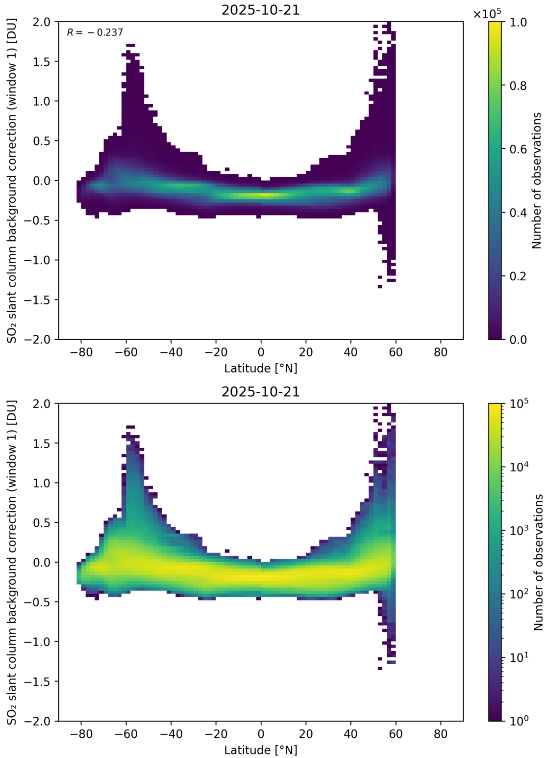
Figure 150: Scatter density plot of “Latitude” against “SO 2 slant column background correction (window 1)” for 2025-10-20 to 2025-10-22.
