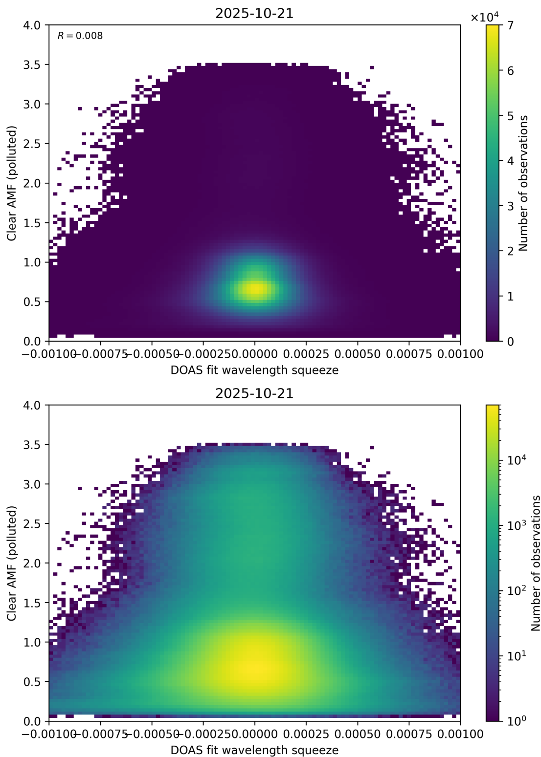
Figure 144: Scatter density plot of “DOAS fit wavelength squeeze” against “Clear AMF (polluted)” for 2025-10-20 to 2025-10-22.
