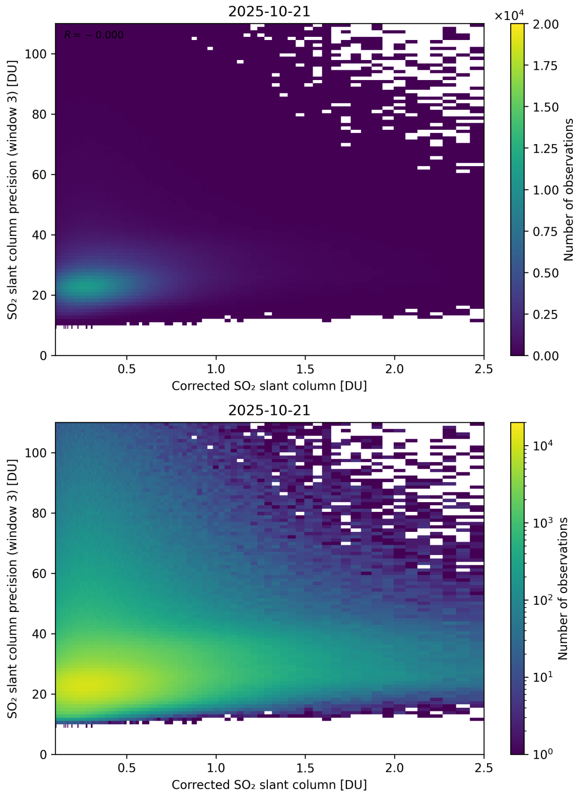
Figure 241: Scatter density plot of “Corrected SO 2 slant column” against “SO 2 slant column precision (window 3)” for 2025-10-20 to 2025-10-22.
