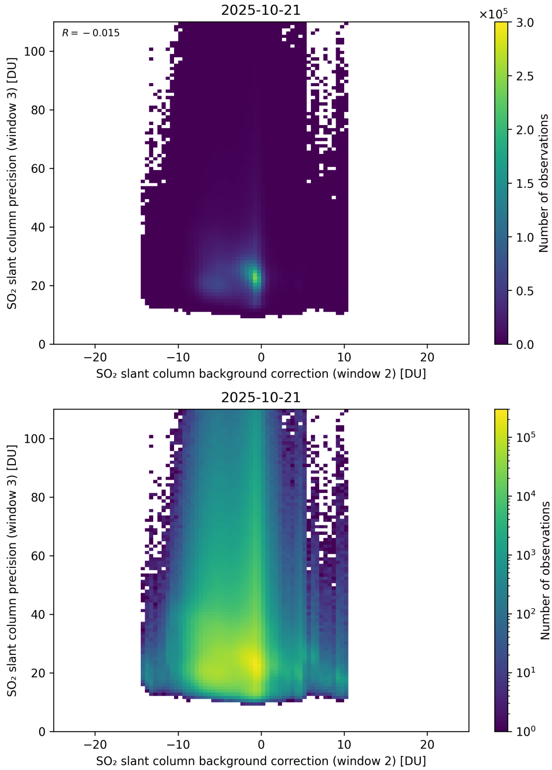
Figure 129: Scatter density plot of “SO 2 slant column background correction (window 2)” against “SO 2 slant column precision (window 3)” for 2025-10-20 to 2025-10-22.
