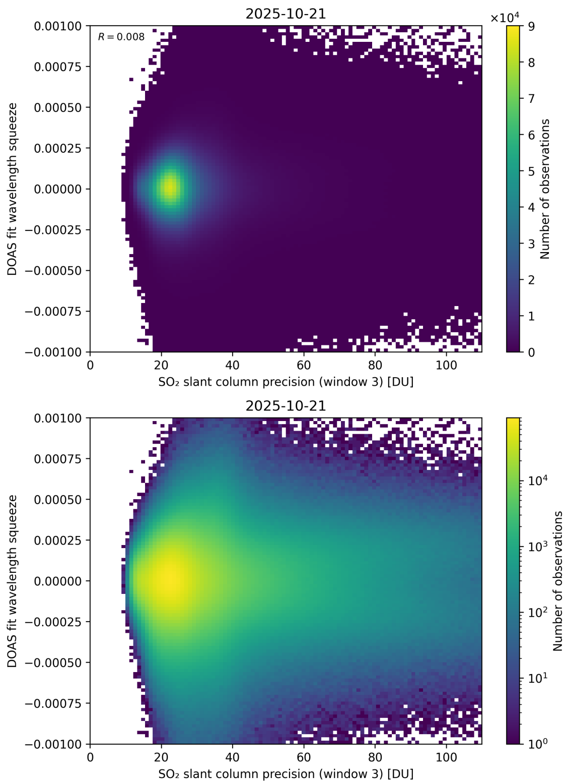
Figure 309: Scatter density plot of “SO 2 slant column precision (window 3)” against “DOAS fit wavelength squeeze” for 2025-10-20 to 2025-10-22.
