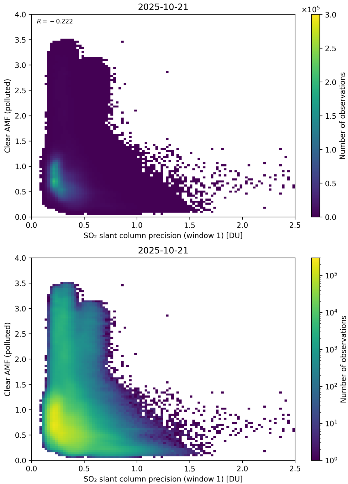
Figure 274: Scatter density plot of “SO 2 slant column precision (window 1)” against “Clear AMF (polluted)” for 2025-10-20 to 2025-10-22.
