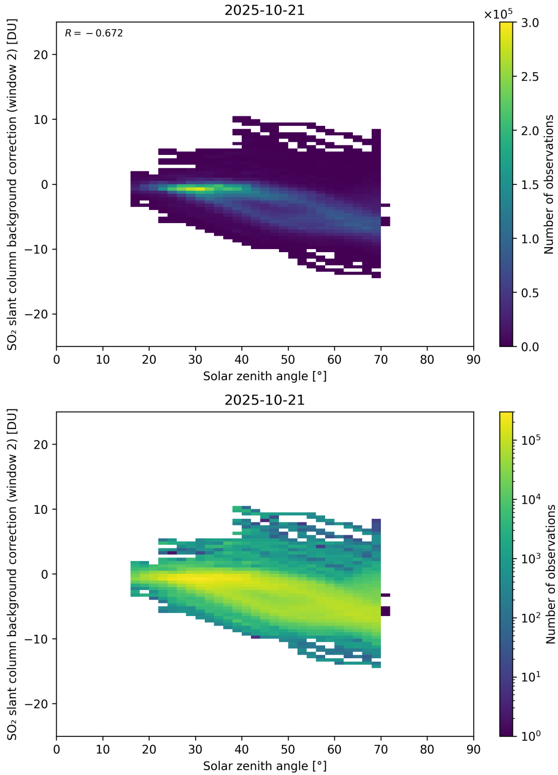
Figure 172: Scatter density plot of “Solar zenith angle” against “SO 2 slant column background correction (window 2)” for 2025-10-20 to 2025-10-22.
