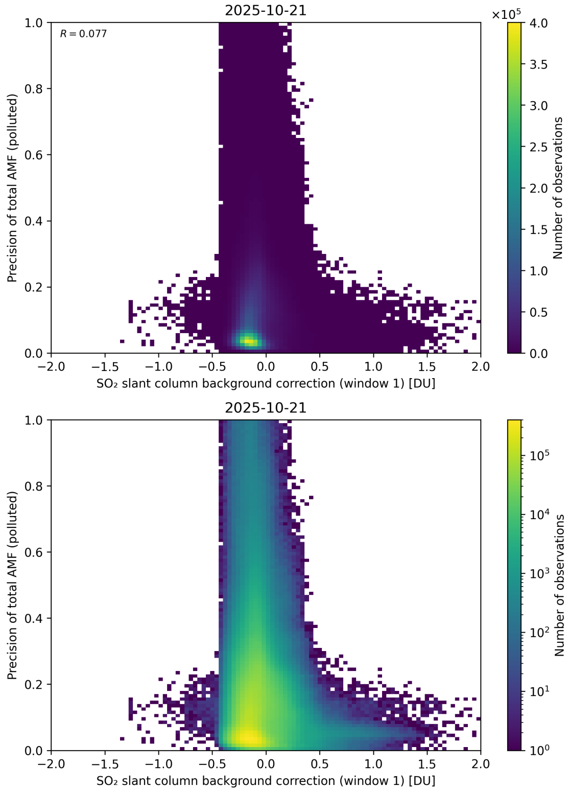
Figure 121: Scatter density plot of “SO 2 slant column background correction (window 1)” against “Precision of total AMF (polluted)” for 2025-10-20 to 2025-10-22.
