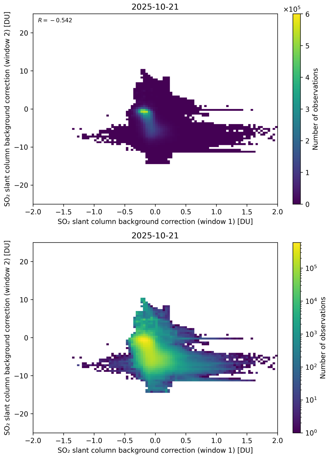
Figure 109: Scatter density plot of “SO 2 slant column background correction (window 1)” against “SO 2 slant column background correction (window 2)” for 2025-10-20 to 2025-10-22.
