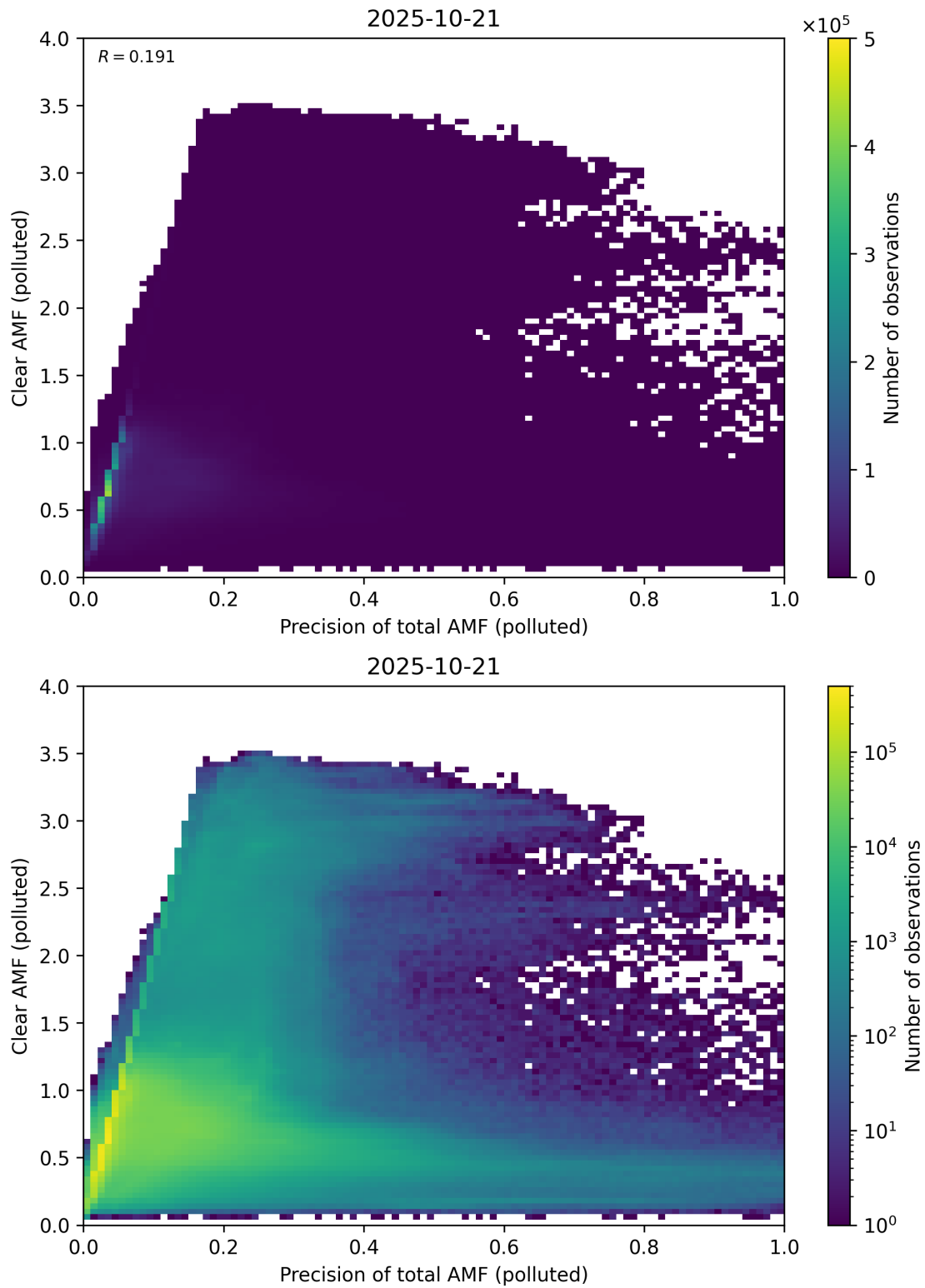
Figure 320: Scatter density plot of “Precision of total AMF (polluted)” against “Clear AMF (polluted)” for 2025-10-20 to 2025-10-22.
