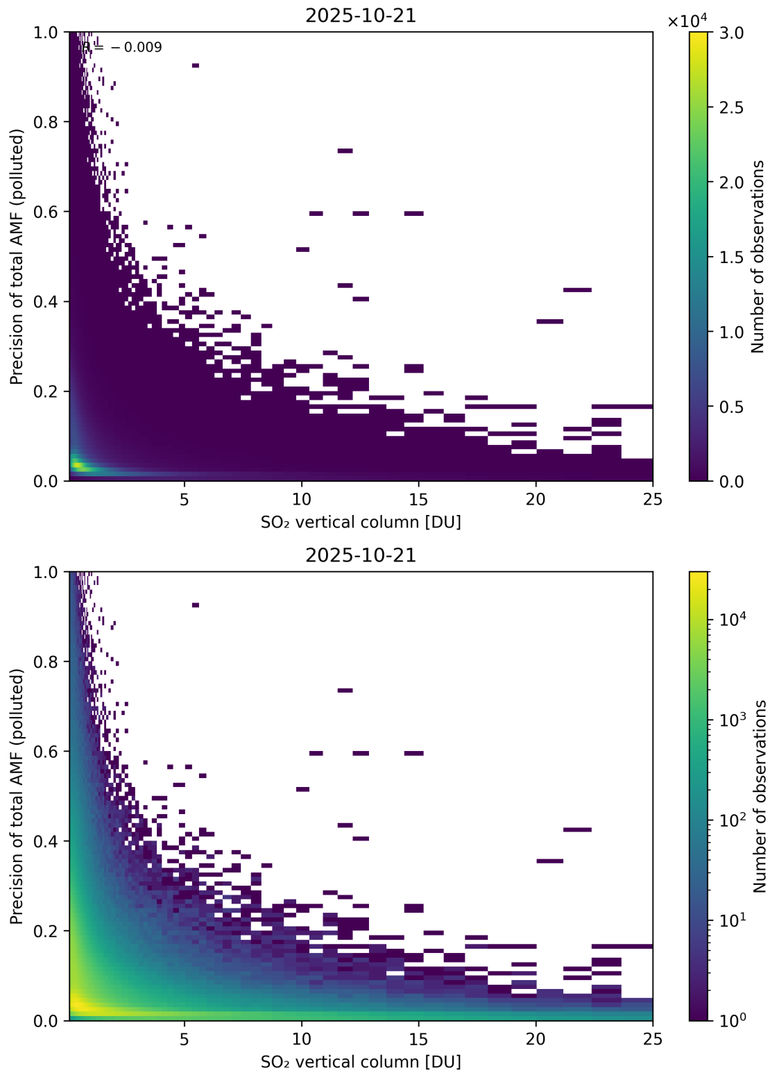
Figure 360: Scatter density plot of “SO 2 vertical column” against “Precision of total AMF (polluted)” for 2025-10-20 to 2025-10-22.
