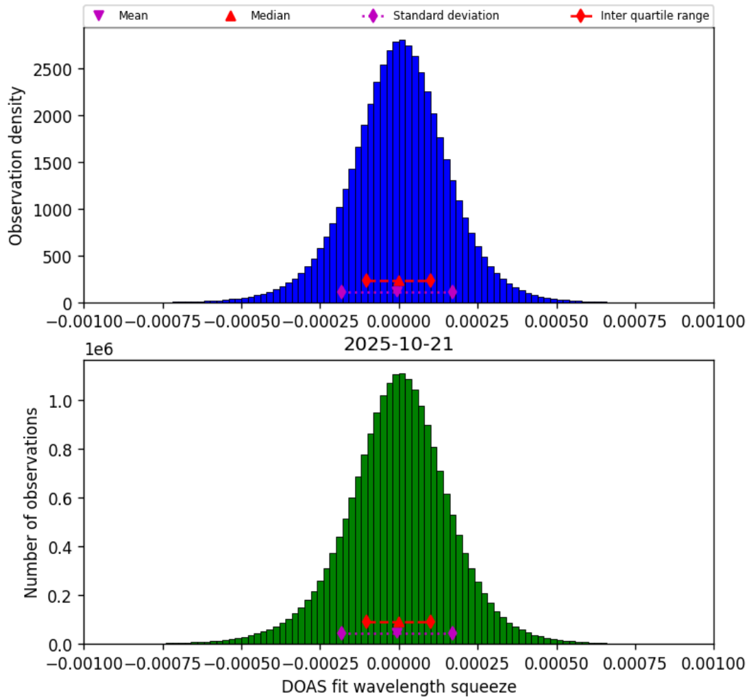
Figure 77: Histogram of “DOAS fit wavelength squeeze” for 2025-10-20 to 2025-10-22
