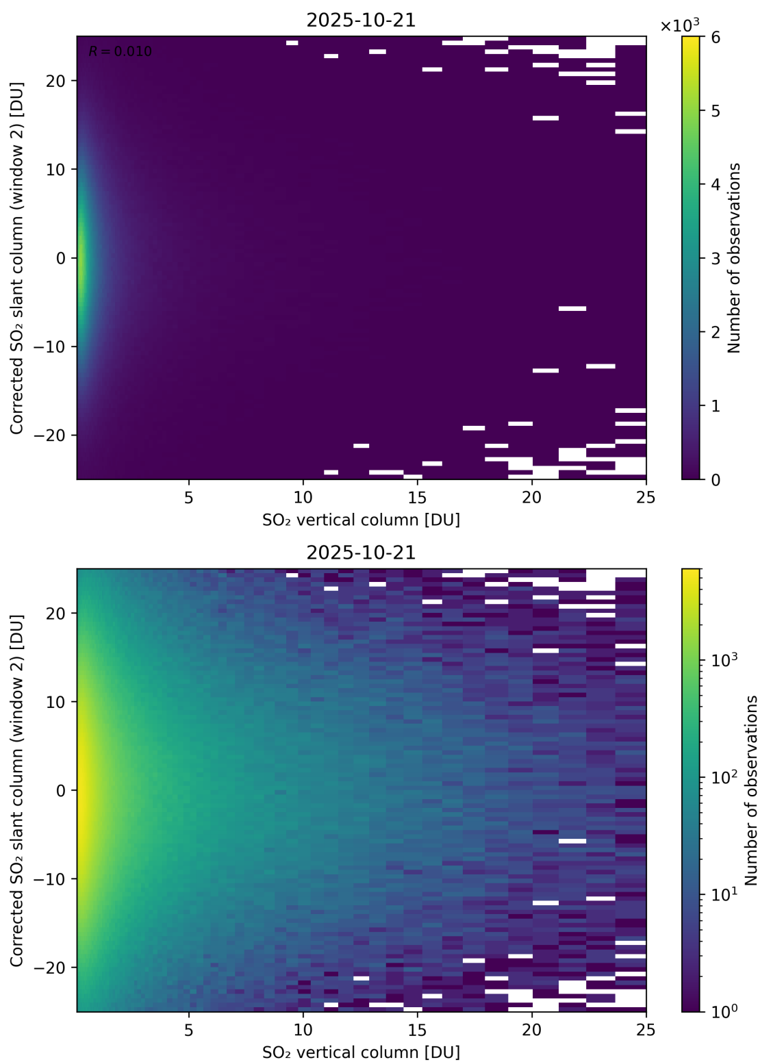
Figure 352: Scatter density plot of “SO 2 vertical column” against “Corrected SO 2 slant column (window 2)” for 2025-10-20 to 2025-10-22.
