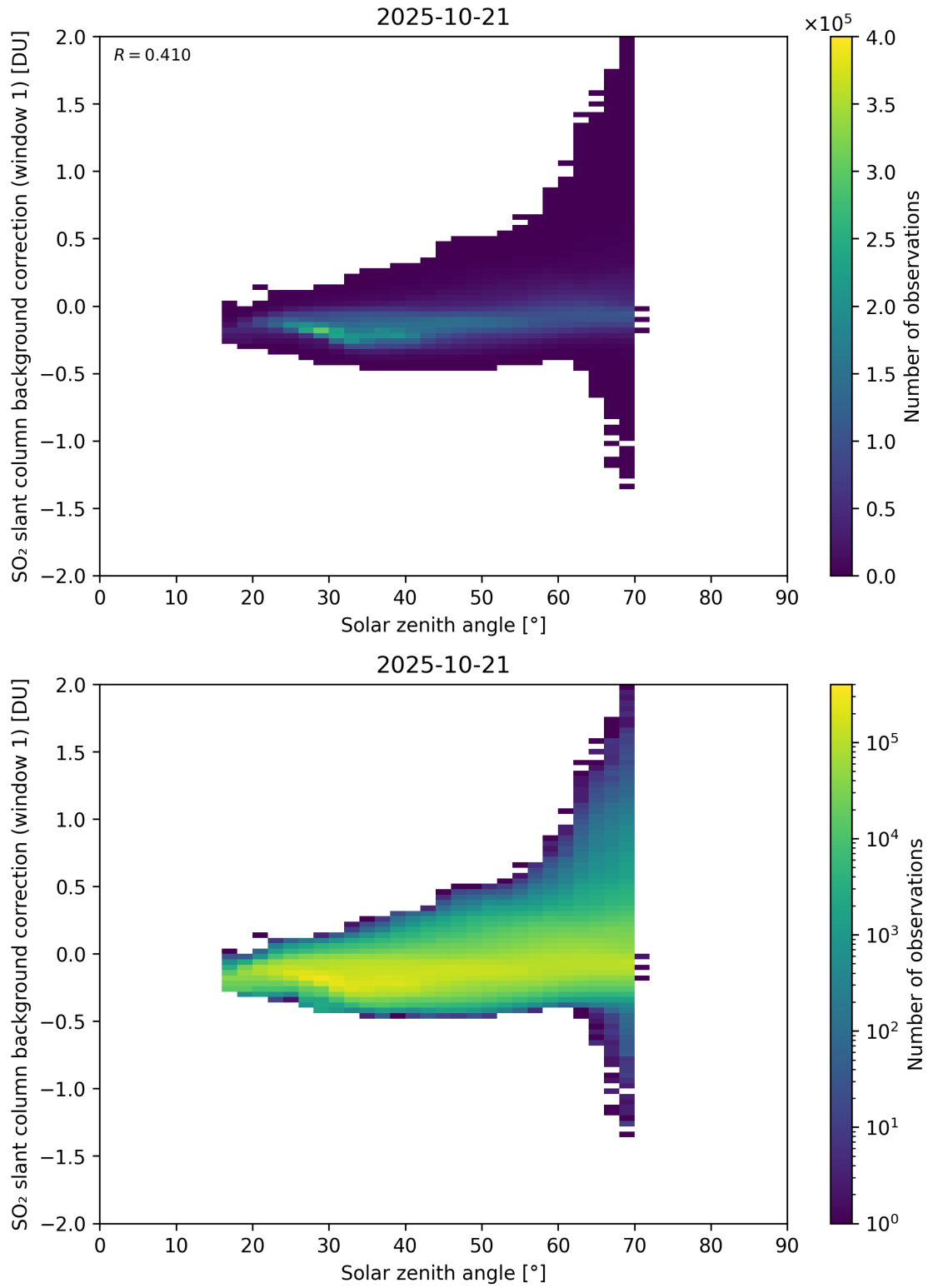
Figure 171: Scatter density plot of “Solar zenith angle” against “SO 2 slant column background correction (window 1)” for 2025-10-20 to 2025-10-22.
