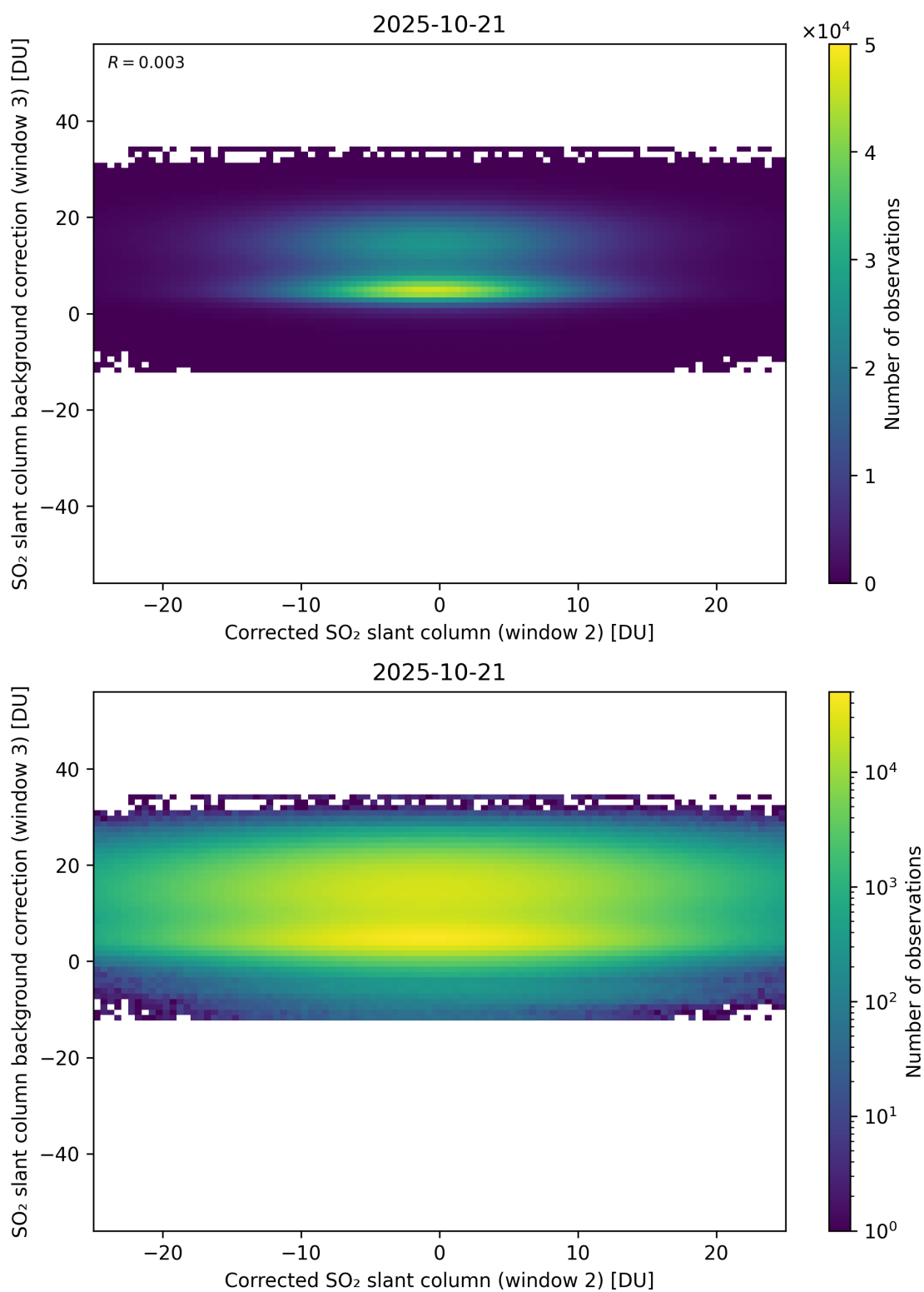
Figure 245: Scatter density plot of “Corrected SO 2 slant column (window 2)” against “SO 2 slant column background correction (window 3)” for 2025-10-20 to 2025-10-22.
