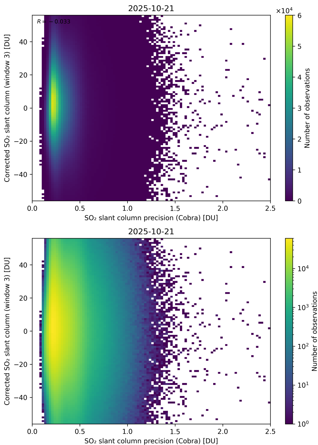
Figure 207: Scatter density plot of “SO 2 slant column precision (Cobra)” against “Corrected SO 2 slant column (window 3)” for 2025-10-20 to 2025-10-22.
