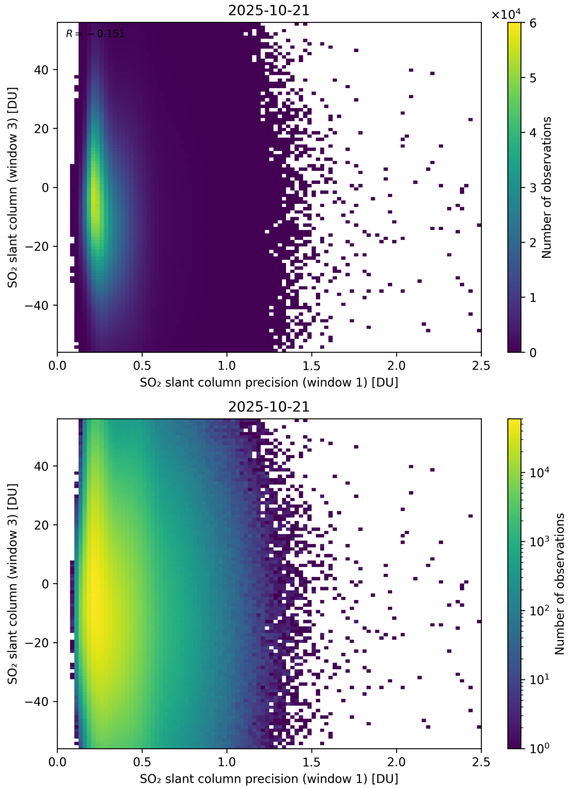
Figure 278: Scatter density plot of “SO 2 slant column precision (window 1)” against “SO 2 slant column (window 3)” for 2025-10-20 to 2025-10-22.
