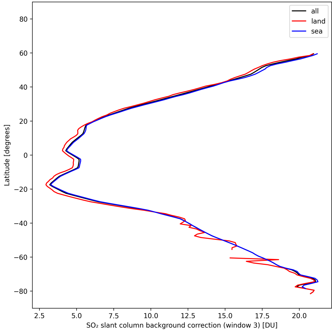
Figure 48: Zonal average of “SO 2 slant column background correction (window 3)” for 2025-10-20 to 2025-10-22.
