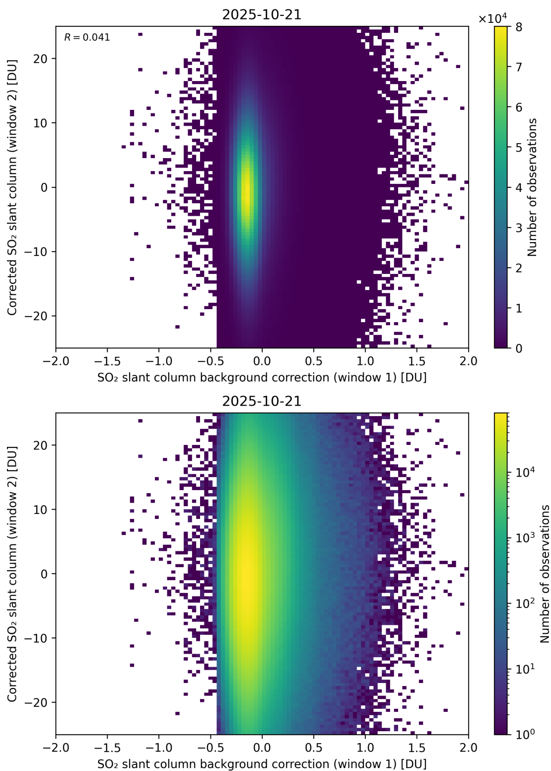
Figure 115: Scatter density plot of “SO 2 slant column background correction (window 1)” against “Corrected SO 2 slant column (window 2)” for 2025-10-20 to 2025-10-22.
