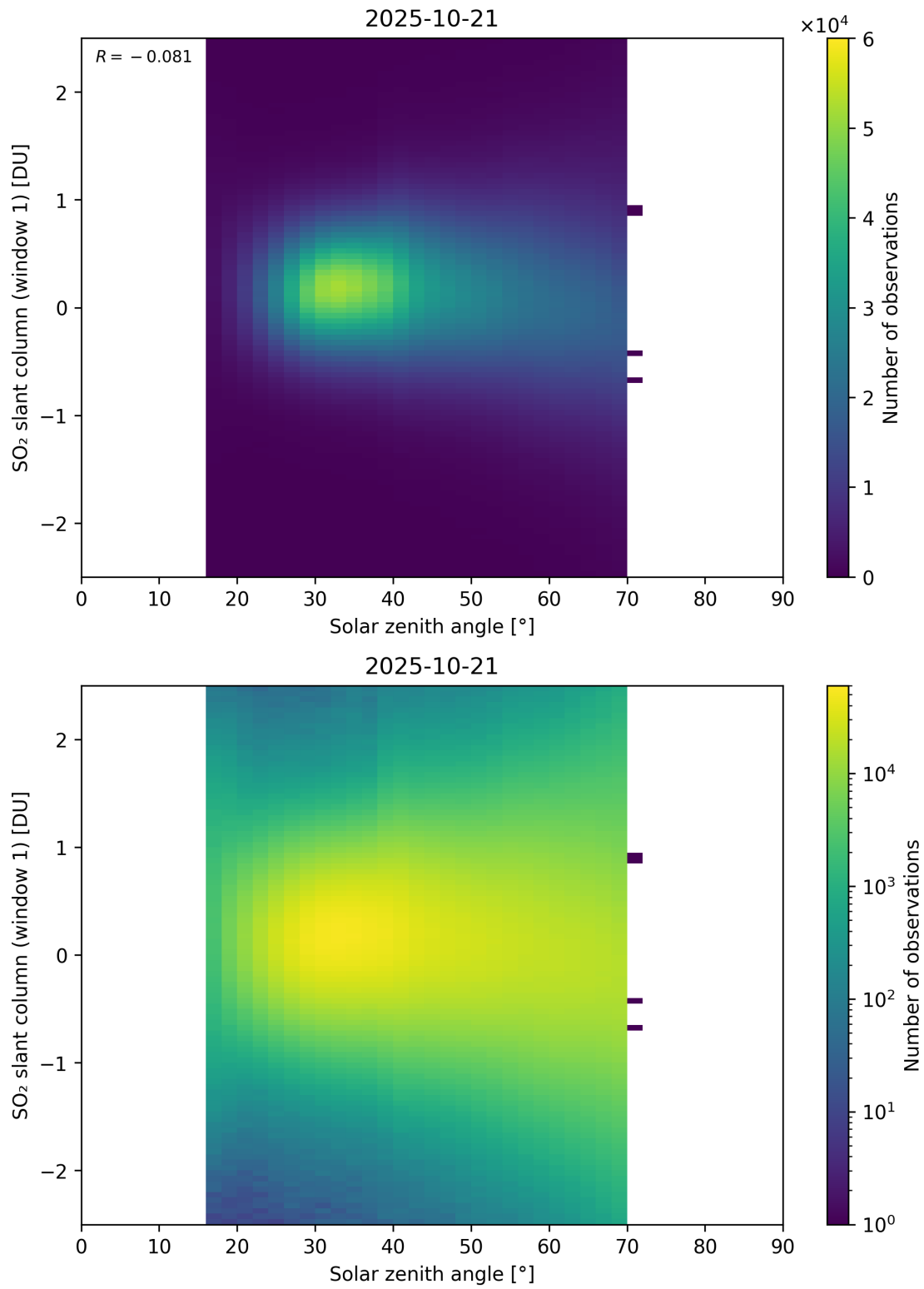
Figure 184: Scatter density plot of “Solar zenith angle” against “SO 2 slant column (window 1)” for 2025-10-20 to 2025-10-22.
