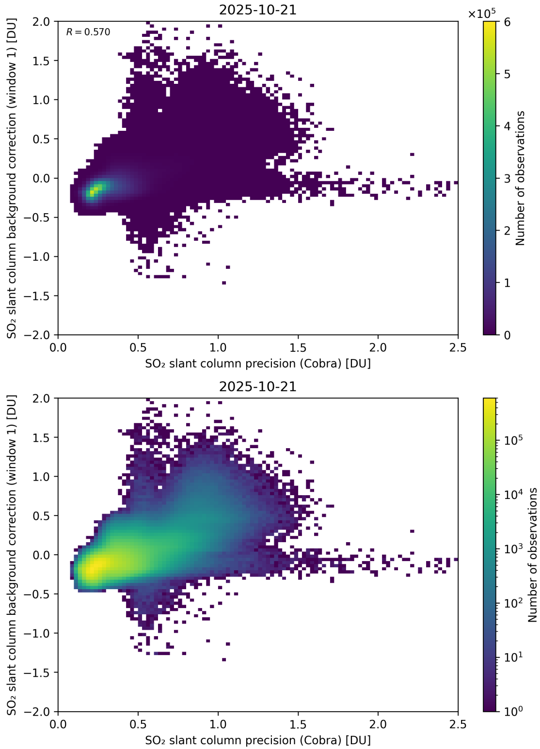
Figure 199: Scatter density plot of “SO 2 slant column precision (Cobra)” against “SO 2 slant column background correction (window 1)” for 2025-10-20 to 2025-10-22.
