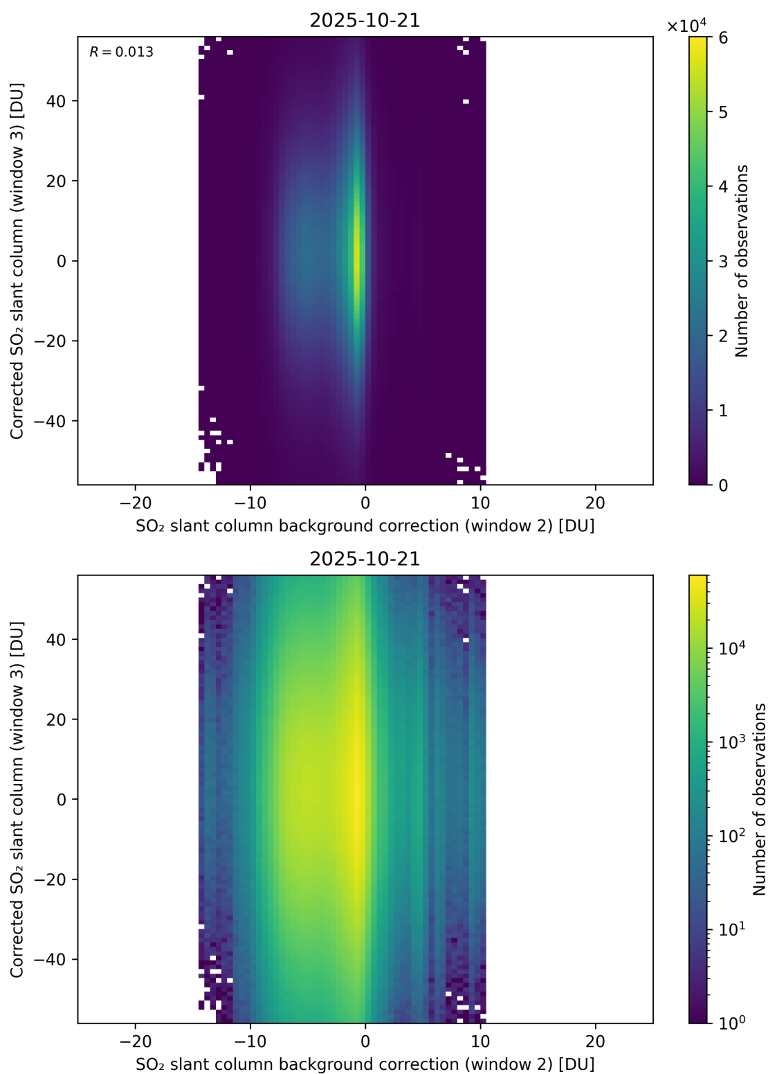
Figure 127: Scatter density plot of “SO 2 slant column background correction (window 2)” against “Corrected SO 2 slant column (window 3)” for 2025-10-20 to 2025-10-22.
