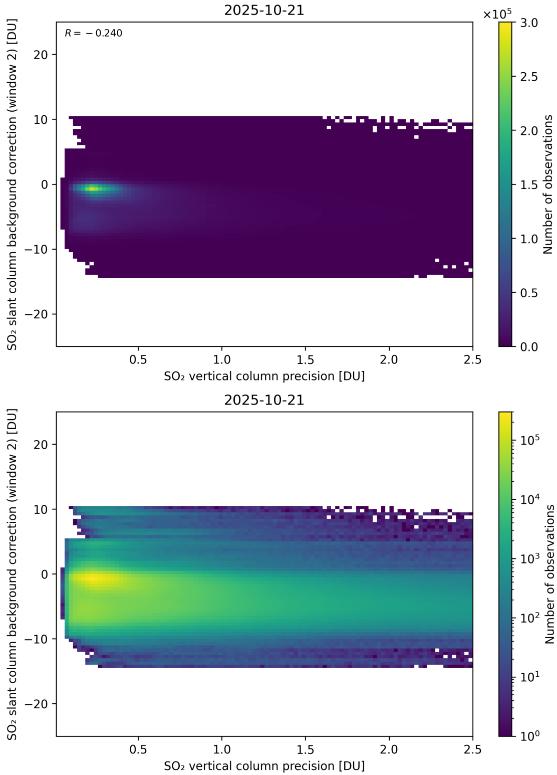
Figure 330: Scatter density plot of “SO 2 vertical column precision” against “SO 2 slant column background correction (window 2)” for 2025-10-20 to 2025-10-22.
