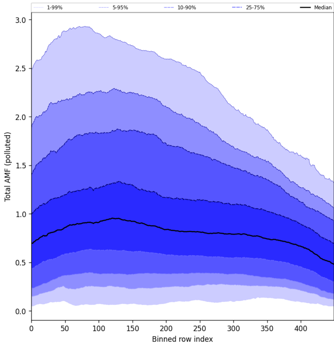
Figure 105: Along track statistics of “Total AMF (polluted)” for 2025-10-20 to 2025-10-22
