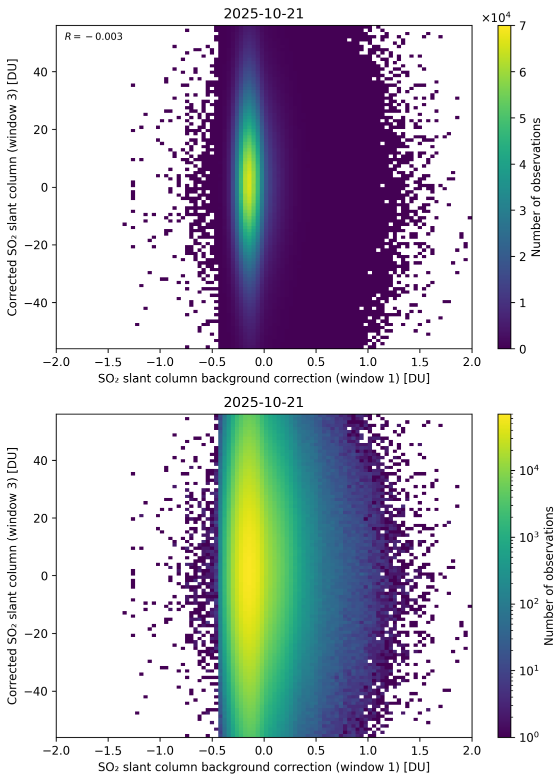
Figure 116: Scatter density plot of “SO 2 slant column background correction (window 1)” against “Corrected SO 2 slant column (window 3)” for 2025-10-20 to 2025-10-22.
