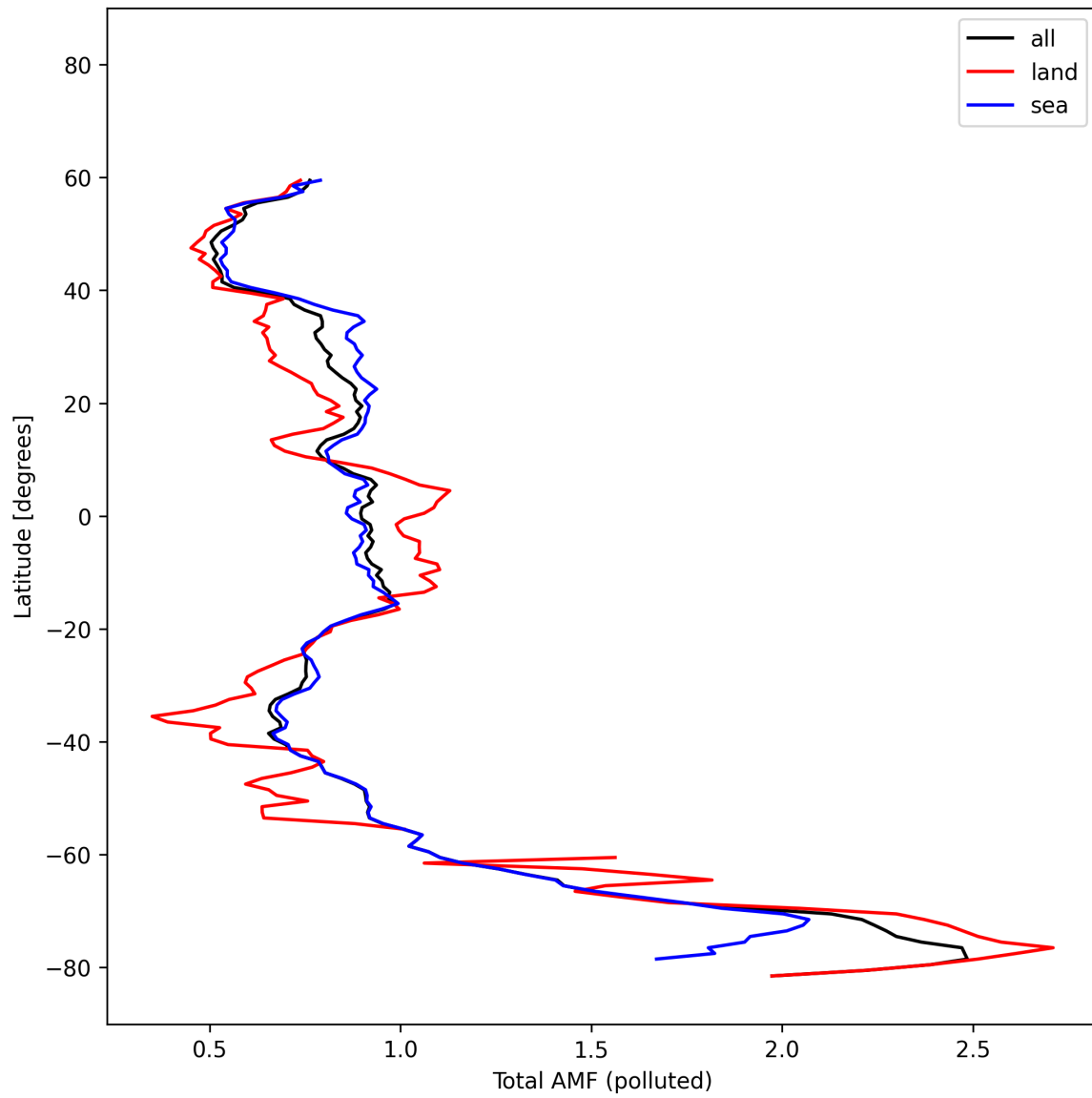
Figure 53: Zonal average of “Total AMF (polluted)” for 2025-10-20 to 2025-10-22.
