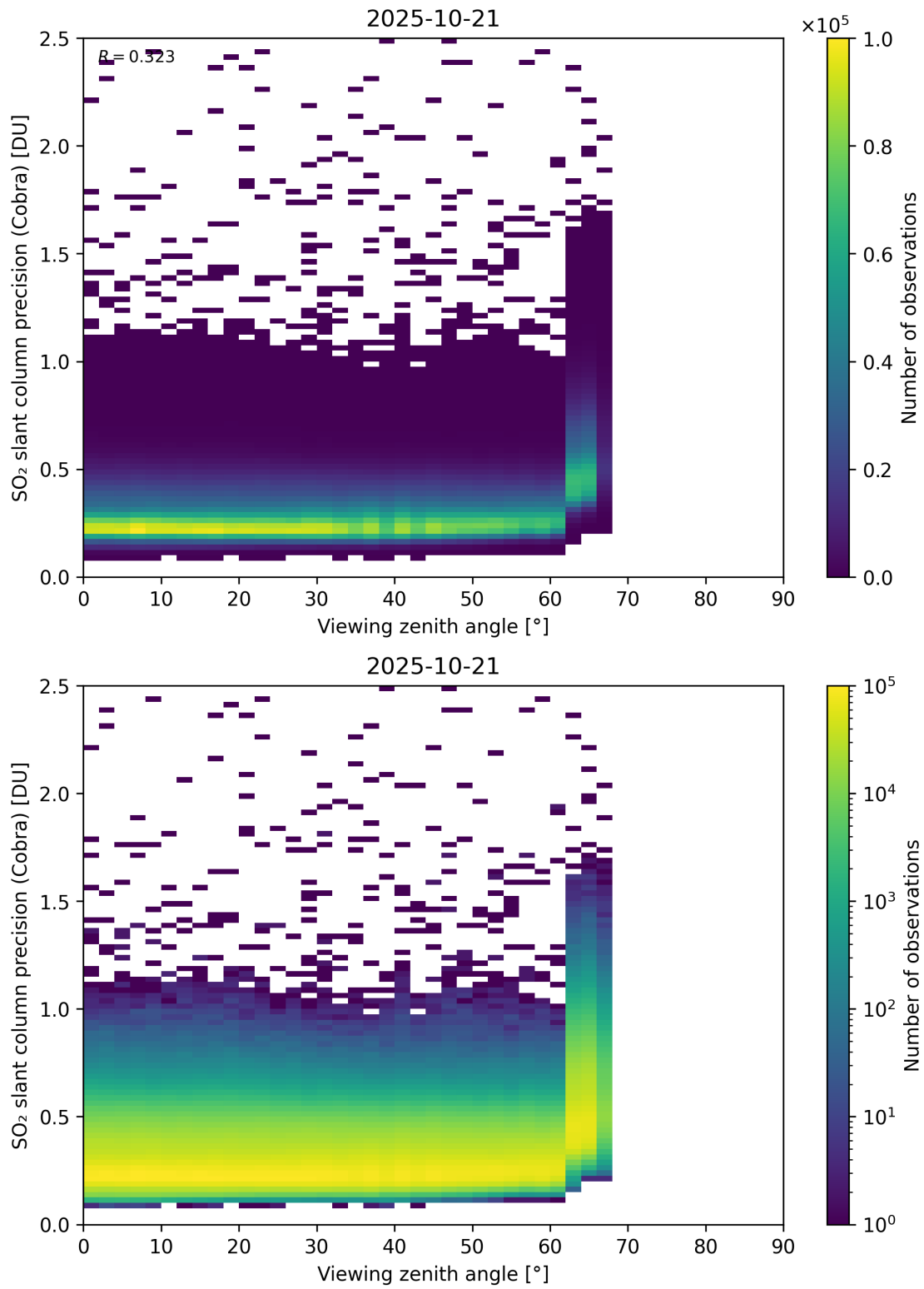
Figure 372: Scatter density plot of “Viewing zenith angle” against “SO 2 slant column precision (Cobra)” for 2025-10-20 to 2025-10-22.
