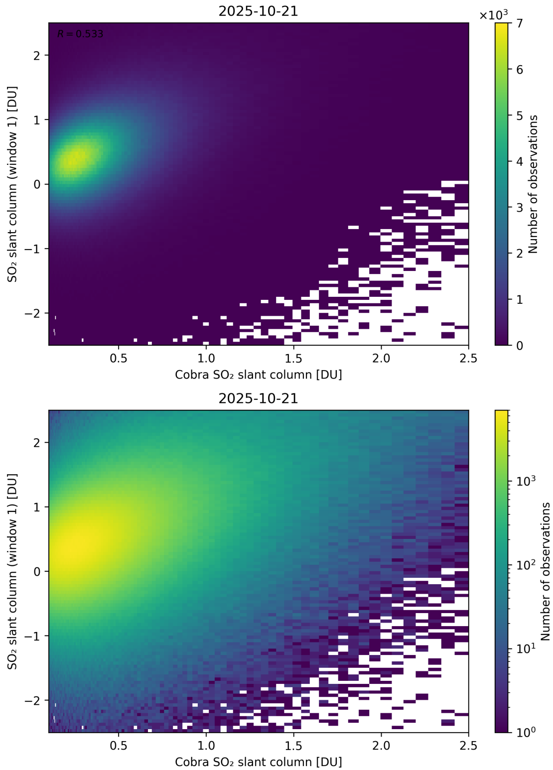
Figure 219: Scatter density plot of “Cobra SO 2 slant column” against “SO 2 slant column (window 1)” for 2025-10-20 to 2025-10-22.
