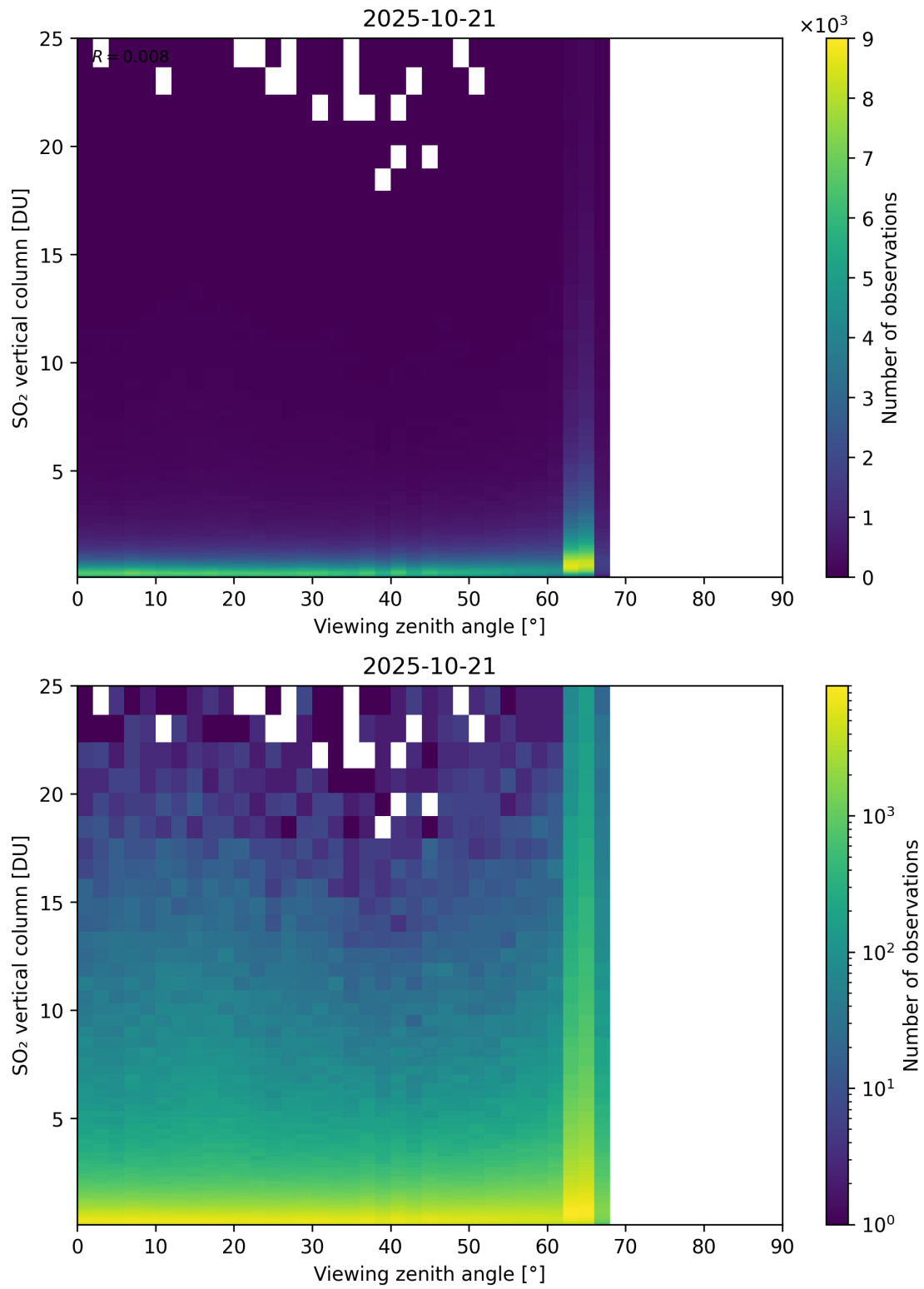
Figure 383: Scatter density plot of “Viewing zenith angle” against “SO 2 vertical column” for 2025-10-20 to 2025-10-22.
