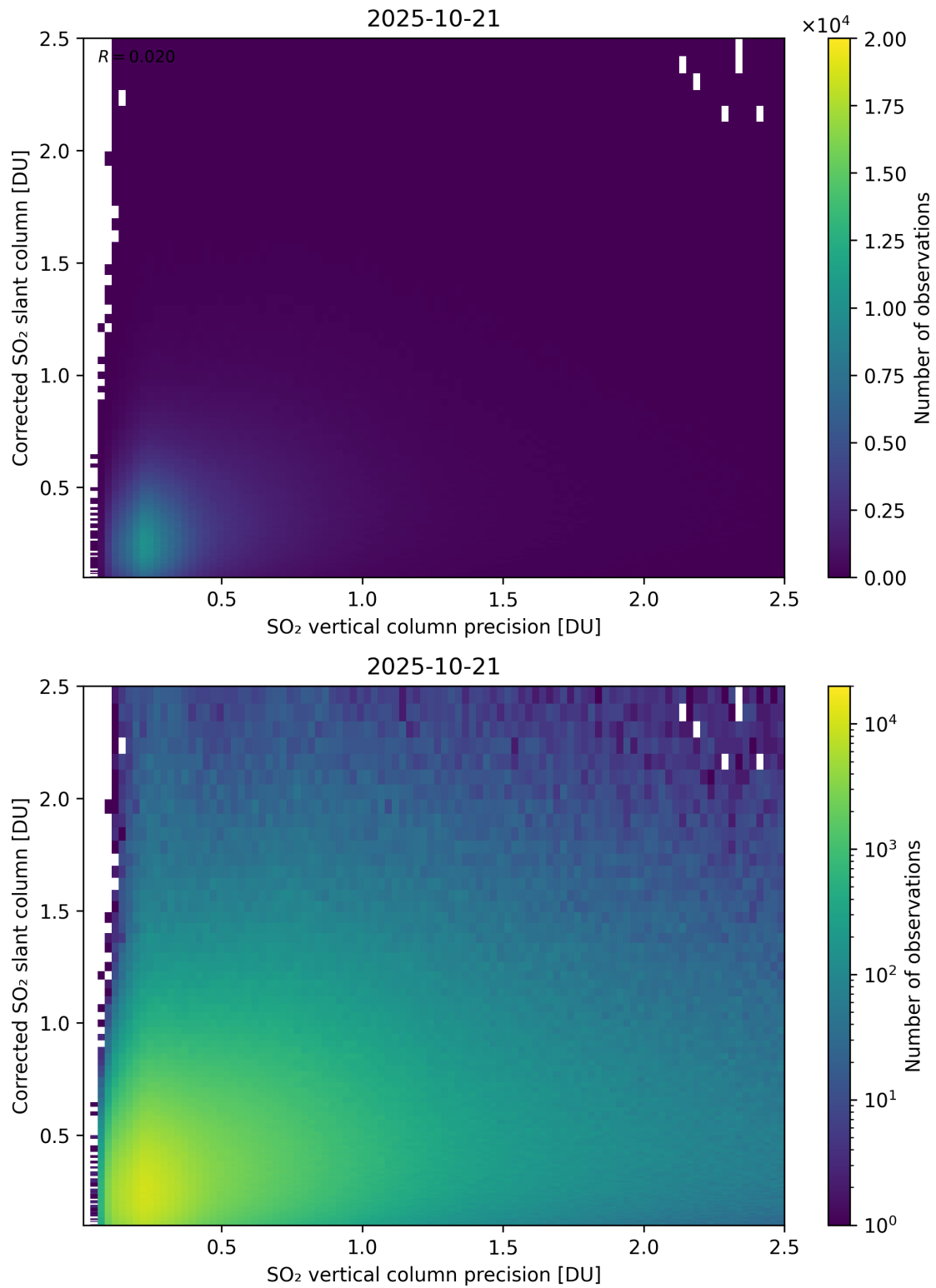
Figure 338: Scatter density plot of “SO 2 vertical column precision” against “Corrected SO 2 slant column” for 2025-10-20 to 2025-10-22.
