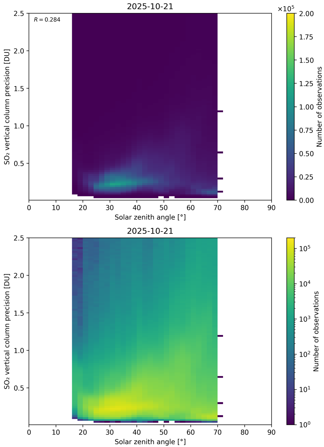
Figure 192: Scatter density plot of “Solar zenith angle” against “SO 2 vertical column precision” for 2025-10-20 to 2025-10-22.
