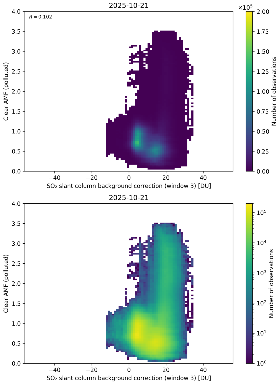
Figure 135: Scatter density plot of “SO 2 slant column background correction (window 3)” against “Clear AMF (polluted)” for 2025-10-20 to 2025-10-22.
