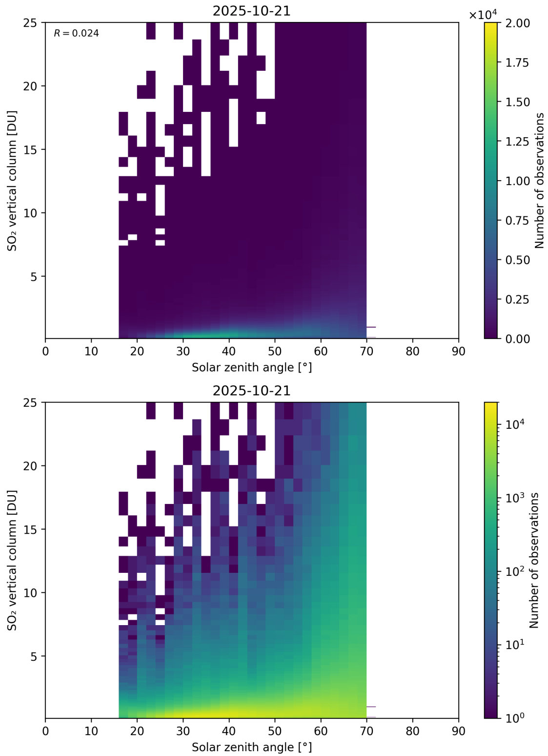
Figure 191: Scatter density plot of “Solar zenith angle” against “SO 2 vertical column” for 2025-10-20 to 2025-10-22.
