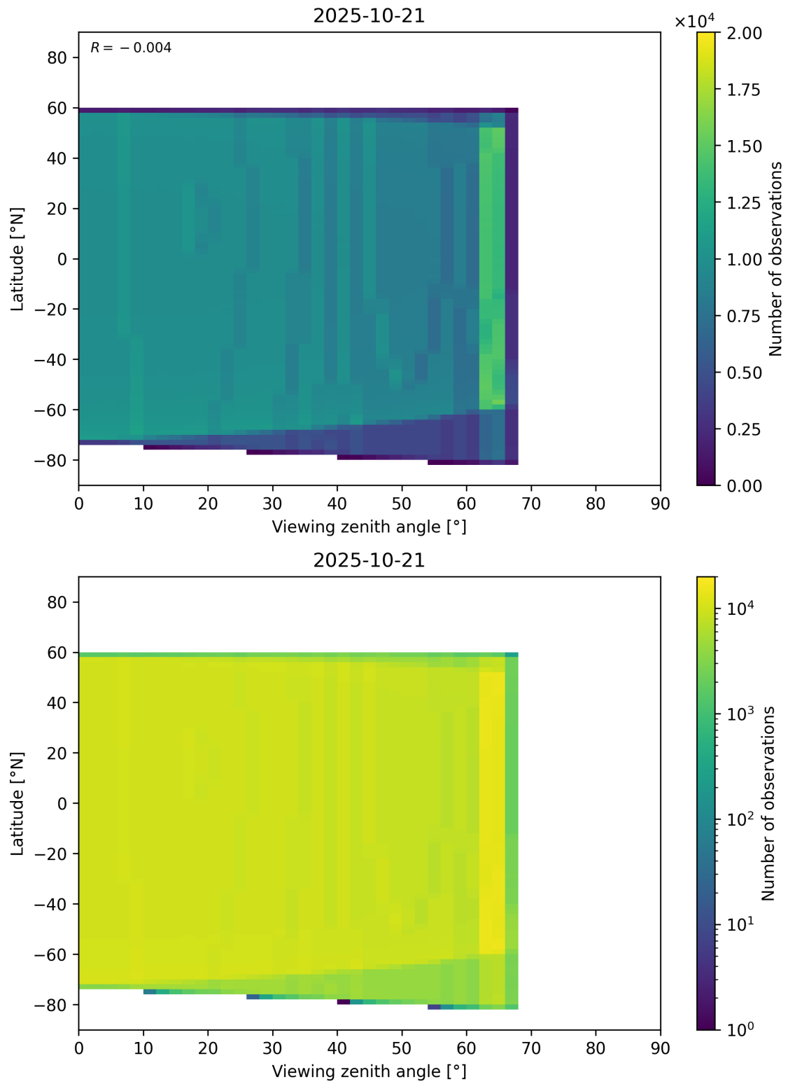
Figure 368: Scatter density plot of “Viewing zenith angle” against “Latitude” for 2025-10-20 to 2025-10-22.
