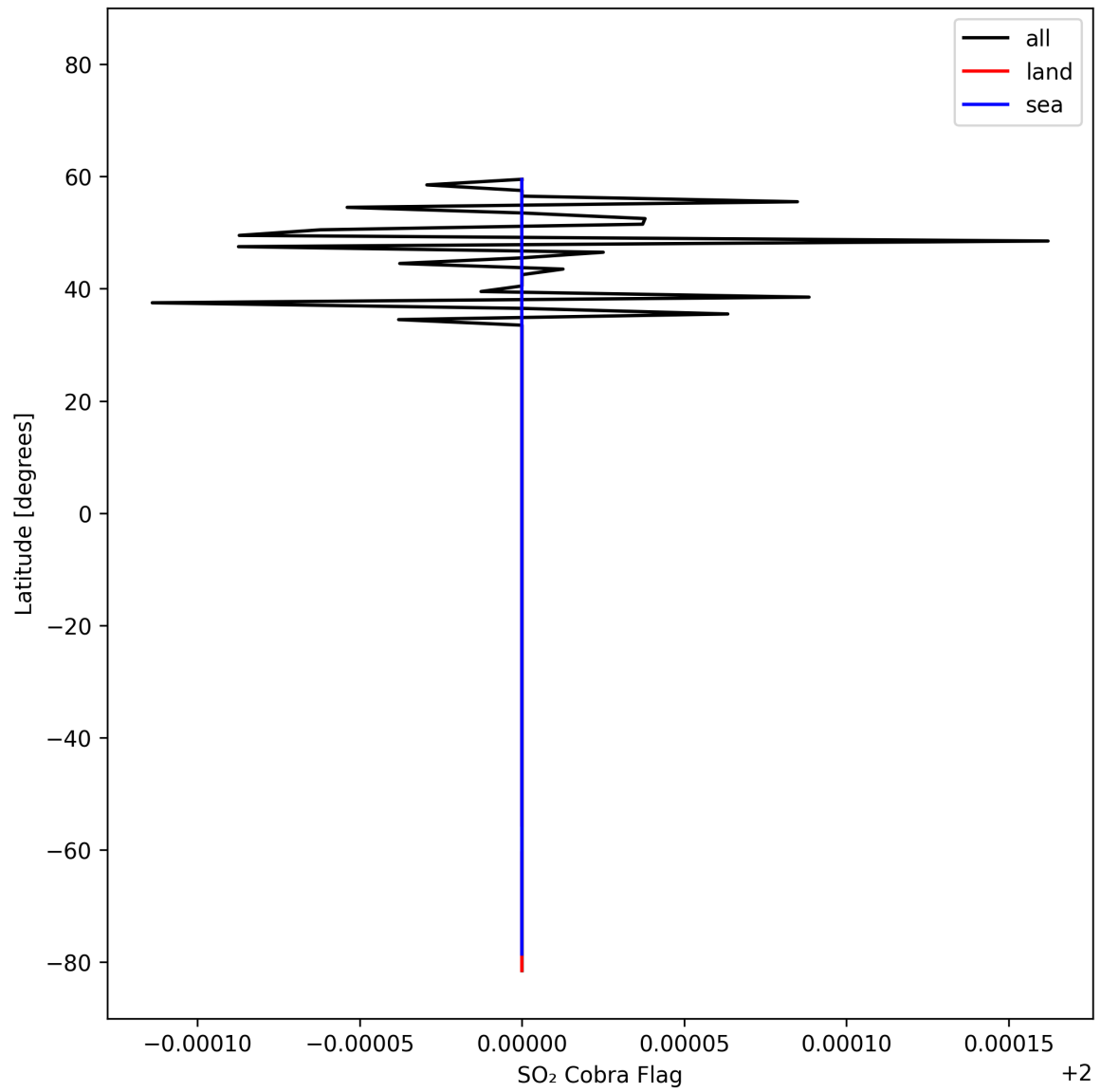
Figure 49: Zonal average of "SO 2 Cobra Flag" for 2025-10-20 to 2025-10-22.
