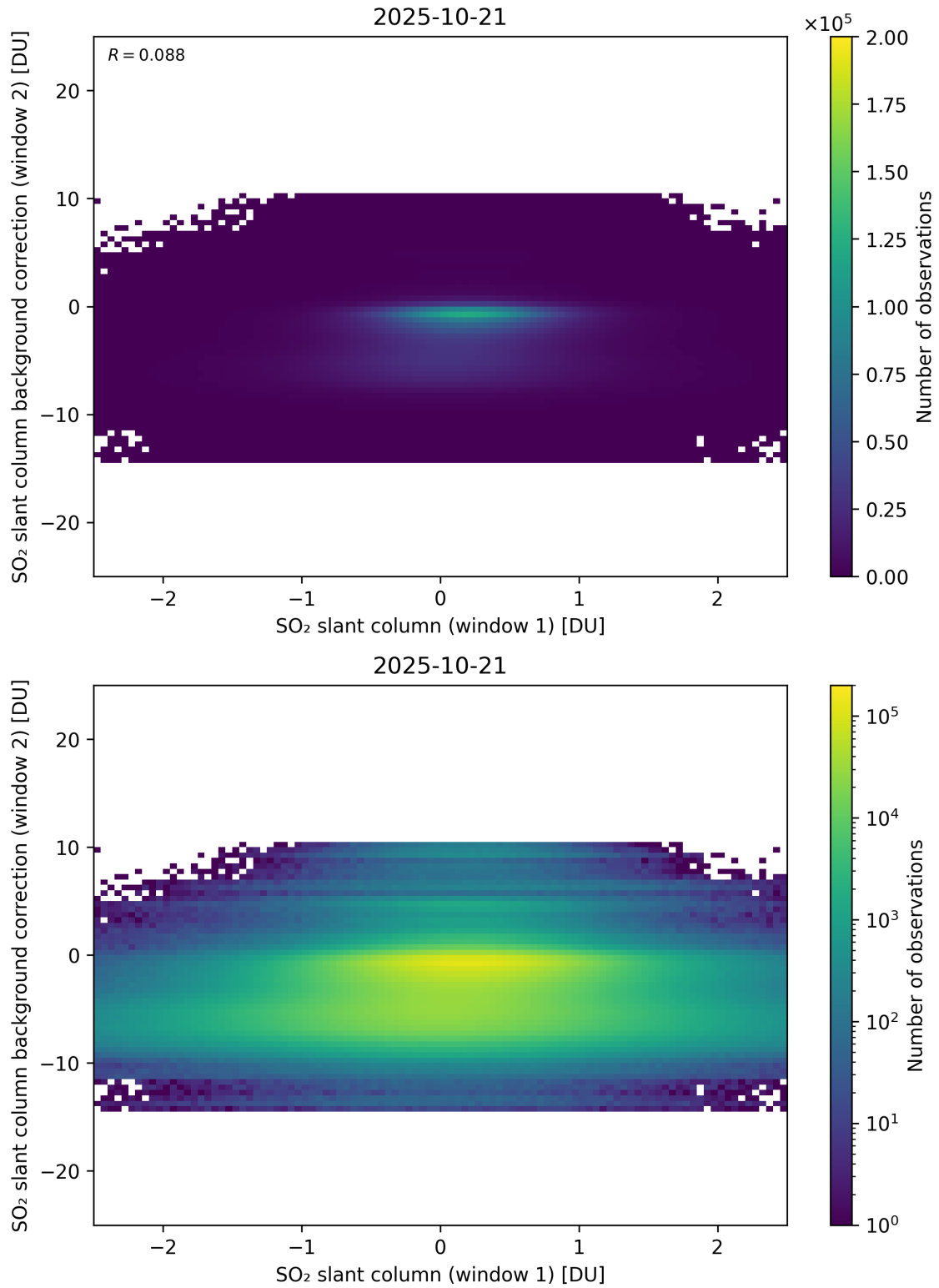
Figure 263: Scatter density plot of “SO 2 slant column (window 1)” against “SO 2 slant column background correction (window 2)” for 2025-10-20 to 2025-10-22.
