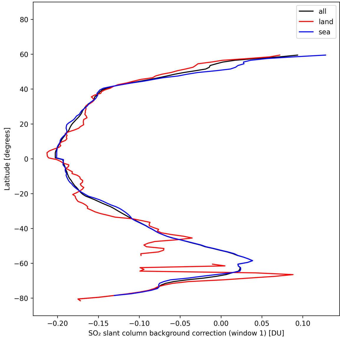
Figure 40: Zonal average of “SO 2 slant column background correction (window 1)” for 2025-10-20 to 2025-10-22.
