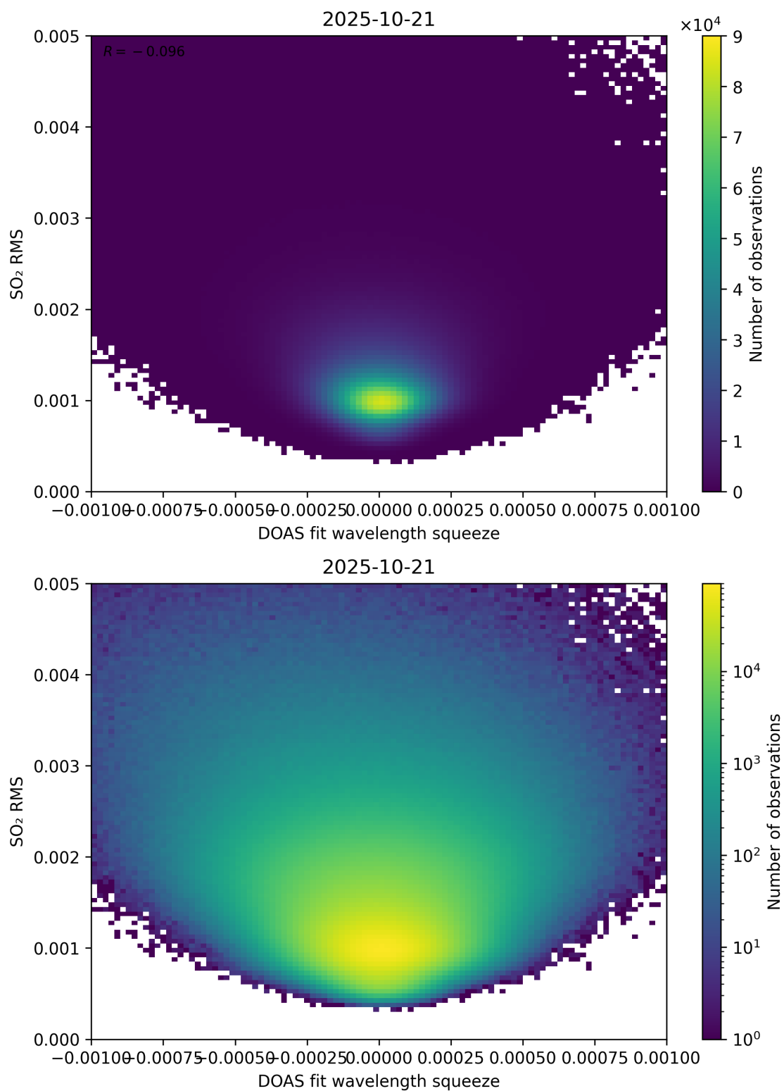
Figure 143: Scatter density plot of “DOAS fit wavelength squeeze” against “SO 2 RMS” for 2025-10-20 to 2025-10-22.
