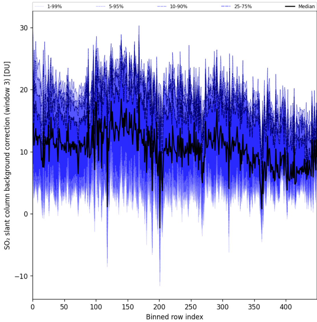
Figure 100: Along track statistics of “SO 2 slant column background correction (window 3)” for 2025-10-20 to 2025-10-22
