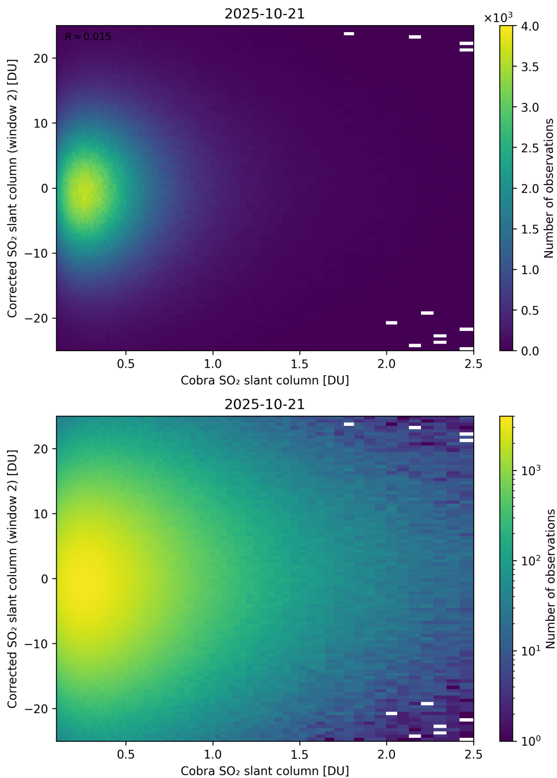
Figure 217: Scatter density plot of “Cobra SO 2 slant column” against “Corrected SO 2 slant column (window 2)” for 2025-10-20 to 2025-10-22.
