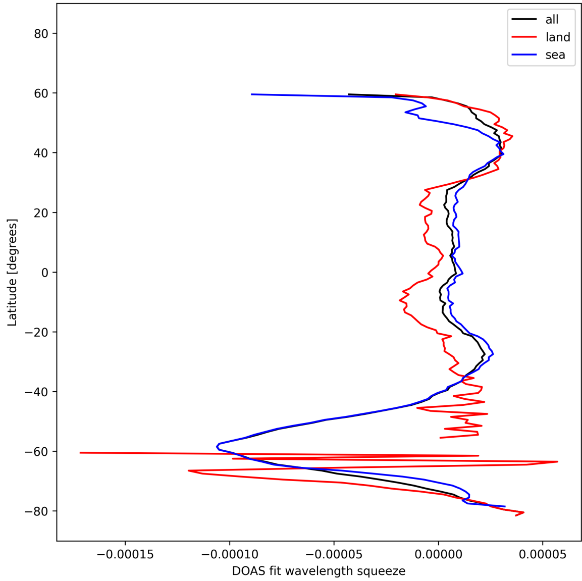
Figure 51: Zonal average of “DOAS fit wavelength squeeze” for 2025-10-20 to 2025-10-22.
