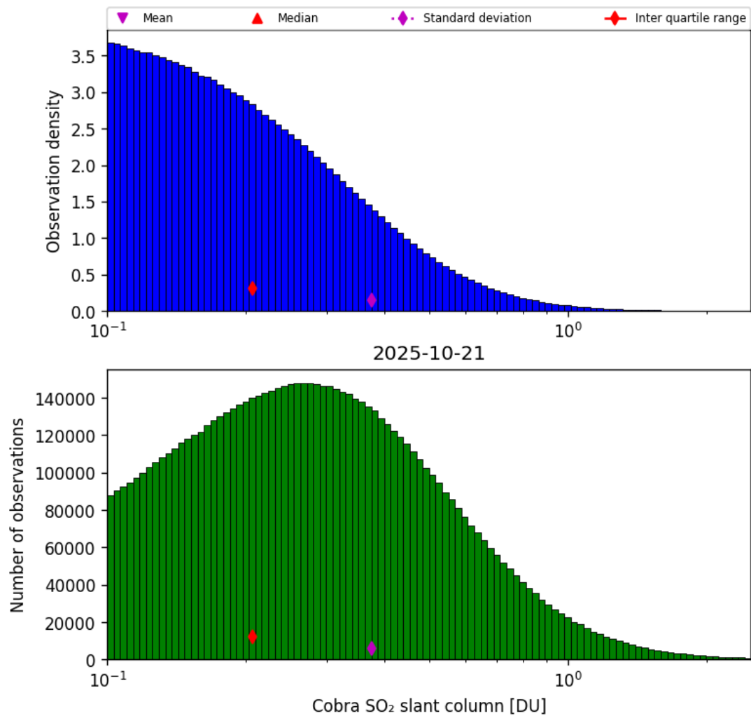
Figure 61: Histogram of “Cobra SO 2 slant column” for 2025-10-20 to 2025-10-22
