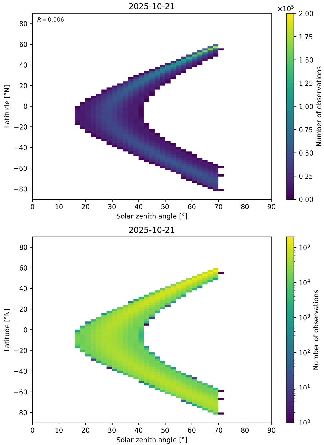
Figure 177: Scatter density plot of “Solar zenith angle” against “Latitude” for 2025-10-20 to 2025-10-22.
