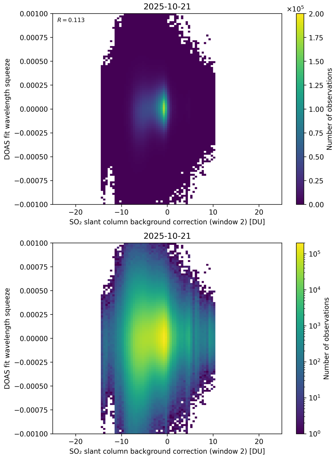
Figure 124: Scatter density plot of “SO 2 slant column background correction (window 2)” against “DOAS fit wavelength squeeze” for 2025-10-20 to 2025-10-22.
