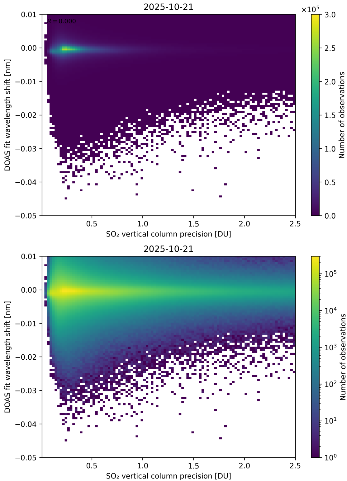
Figure 332: Scatter density plot of “SO 2 vertical column precision” against “DOAS fit wavelength shift” for 2025-10-20 to 2025-10-22.
