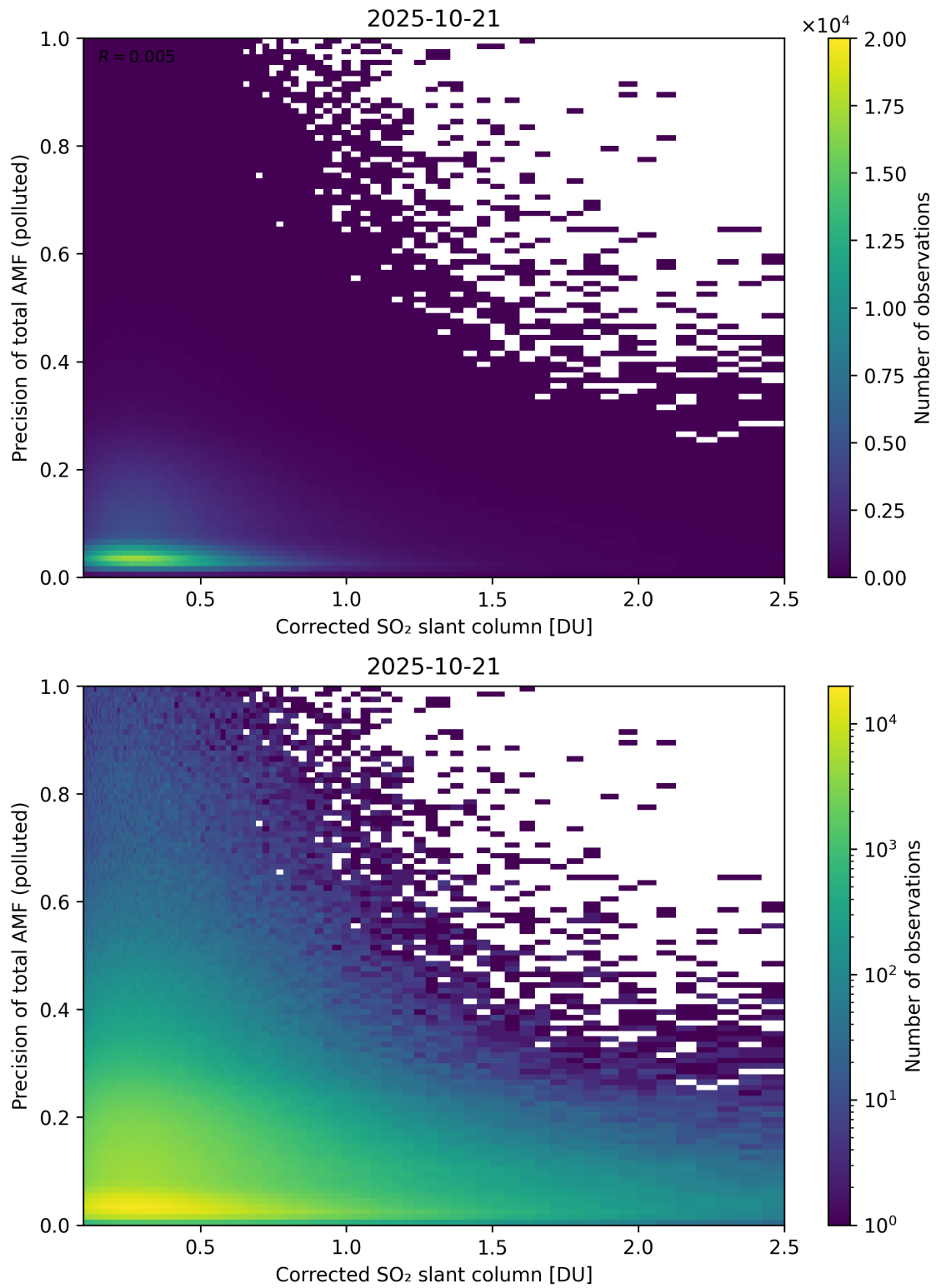
Figure 243: Scatter density plot of “Corrected SO 2 slant column” against “Precision of total AMF (polluted)” for 2025-10-20 to 2025-10-22.
