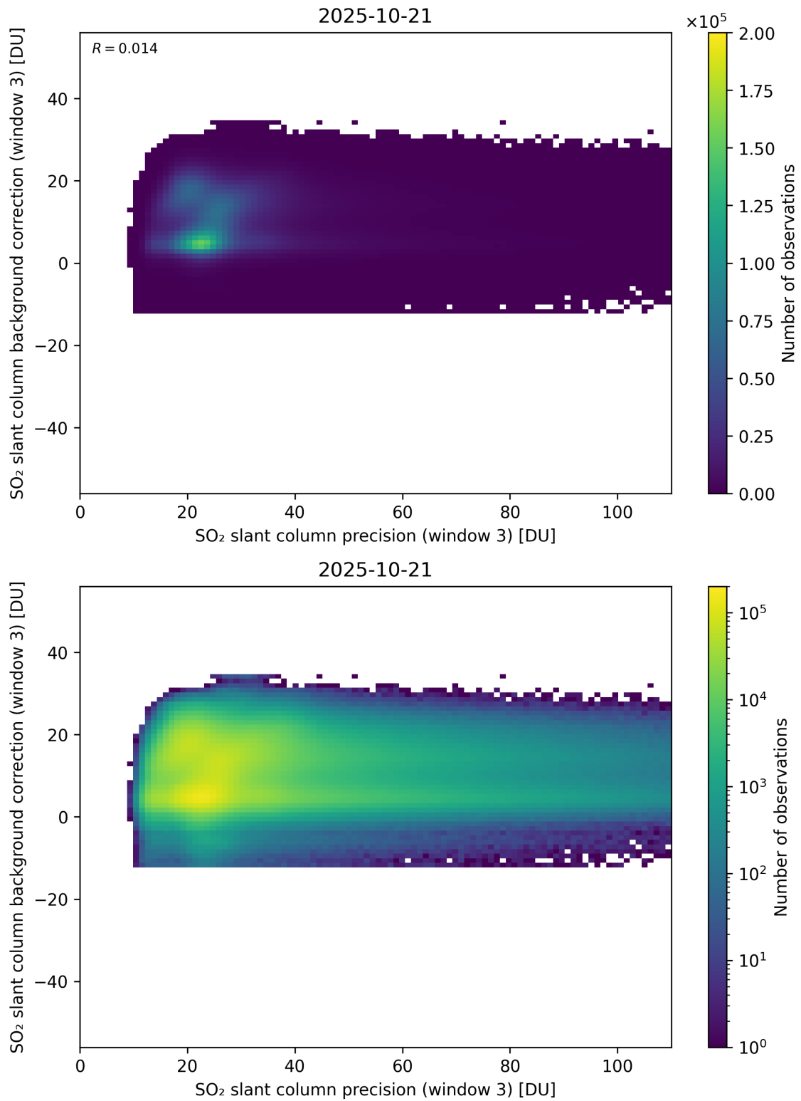
Figure 307: Scatter density plot of “SO 2 slant column precision (window 3)” against “SO 2 slant column background correction (window 3)” for 2025-10-20 to 2025-10-22.
