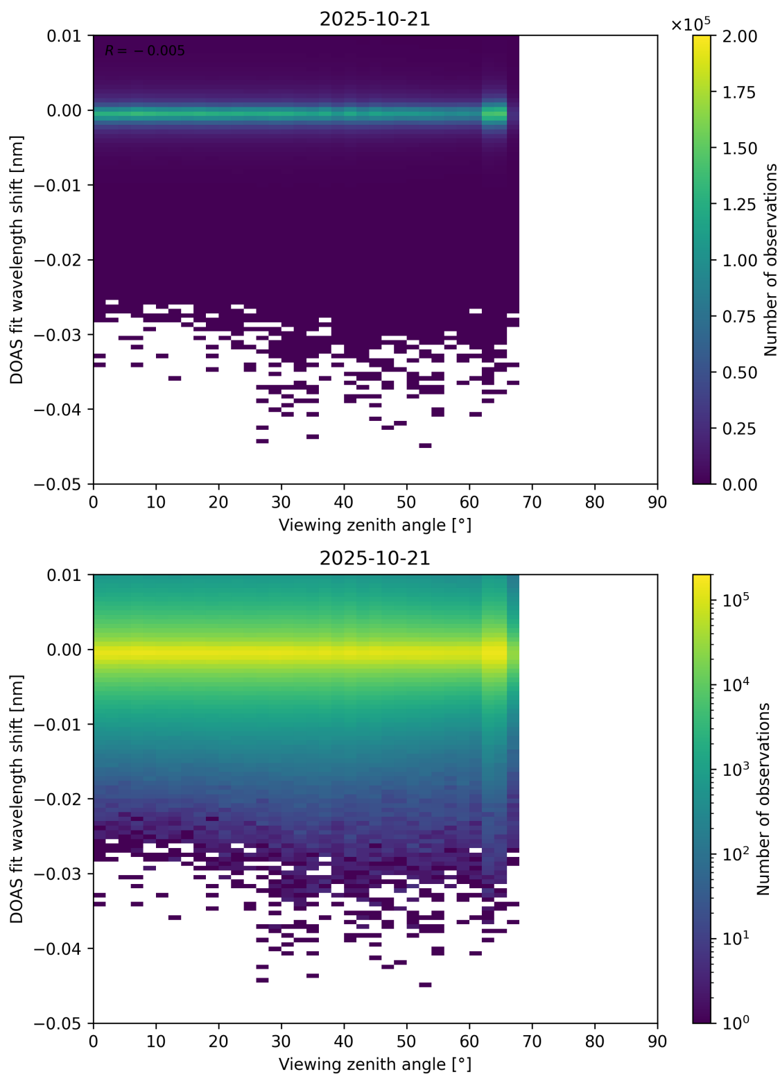
Figure 365: Scatter density plot of “Viewing zenith angle” against “DOAS fit wavelength shift” for 2025-10-20 to 2025-10-22.
