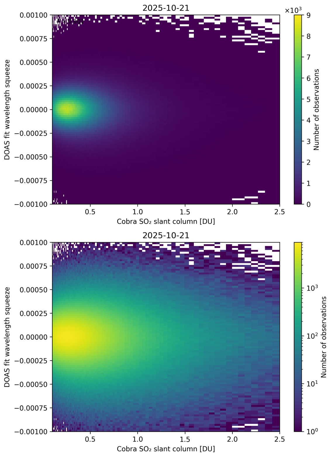
Figure 197: Scatter density plot of “Cobra SO 2 slant column” against “DOAS fit wavelength squeeze” for 2025-10-20 to 2025-10-22.
