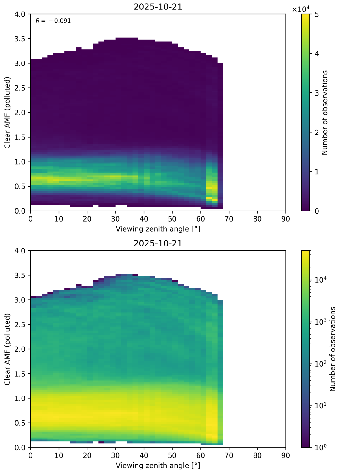
Figure 370: Scatter density plot of “Viewing zenith angle” against “Clear AMF (polluted)” for 2025-10-20 to 2025-10-22.
