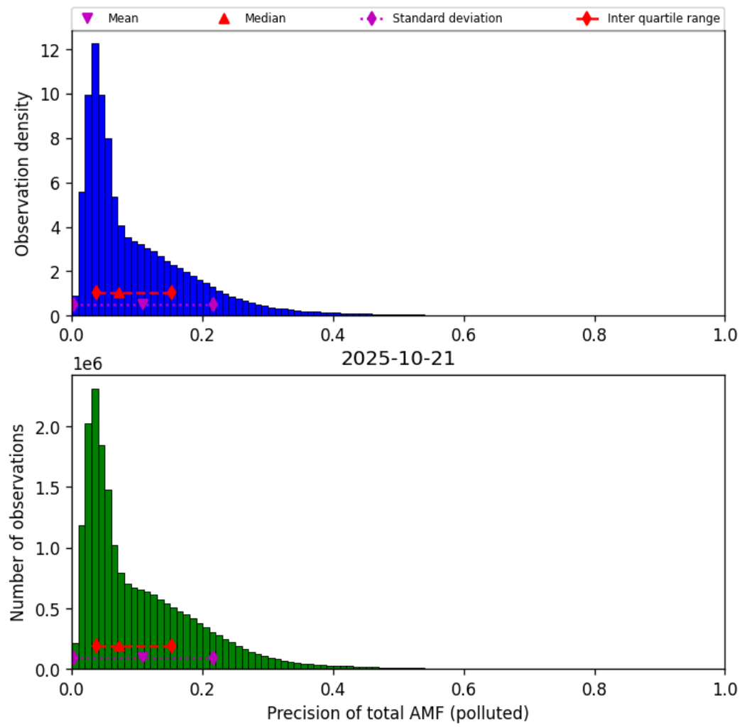
Figure 80: Histogram of “Precision of total AMF (polluted)” for 2025-10-20 to 2025-10-22
