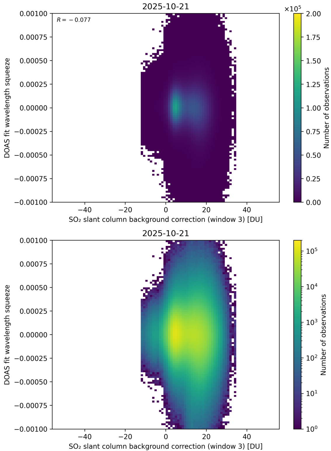
Figure 133: Scatter density plot of “SO 2 slant column background correction (window 3)” against “DOAS fit wavelength squeeze” for 2025-10-20 to 2025-10-22.
