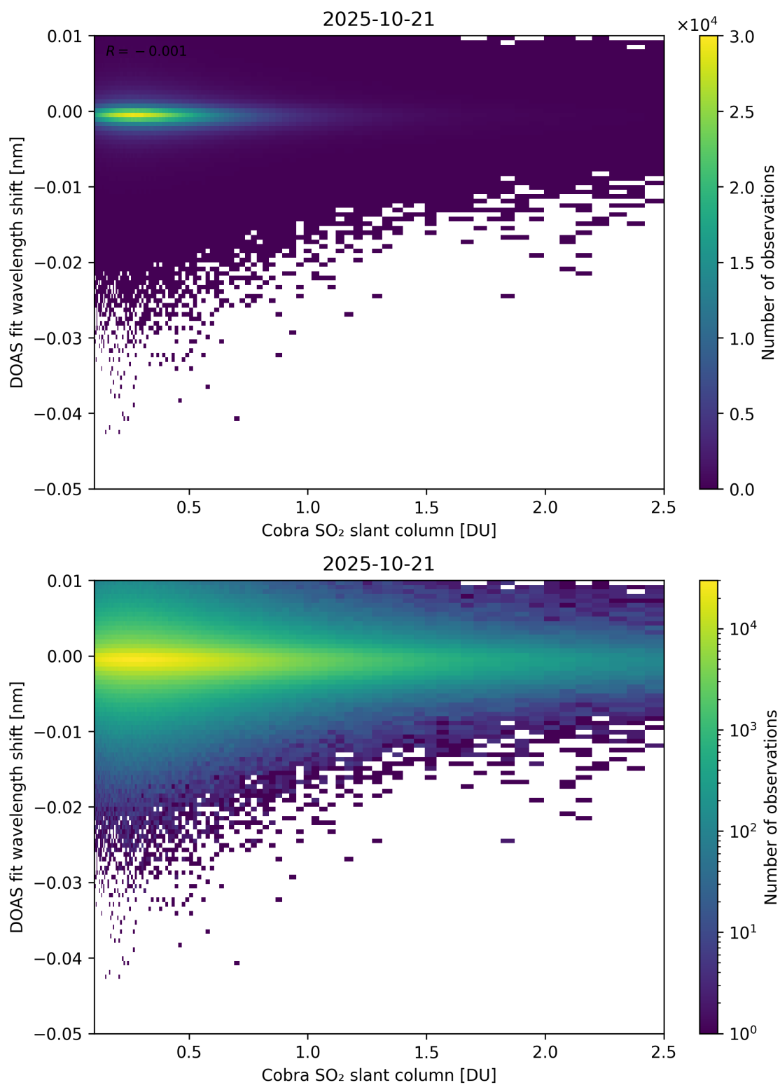
Figure 196: Scatter density plot of “Cobra SO 2 slant column” against “DOAS fit wavelength shift” for 2025-10-20 to 2025-10-22.
