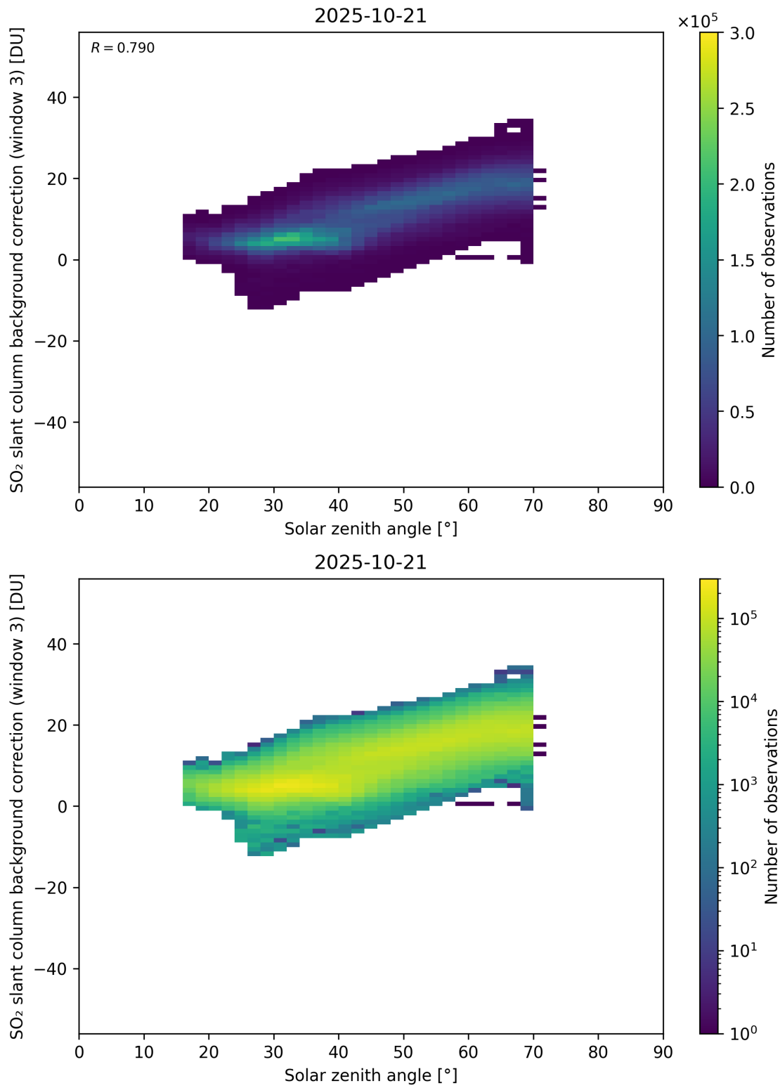
Figure 173: Scatter density plot of “Solar zenith angle” against “SO 2 slant column background correction (window 3)” for 2025-10-20 to 2025-10-22.
