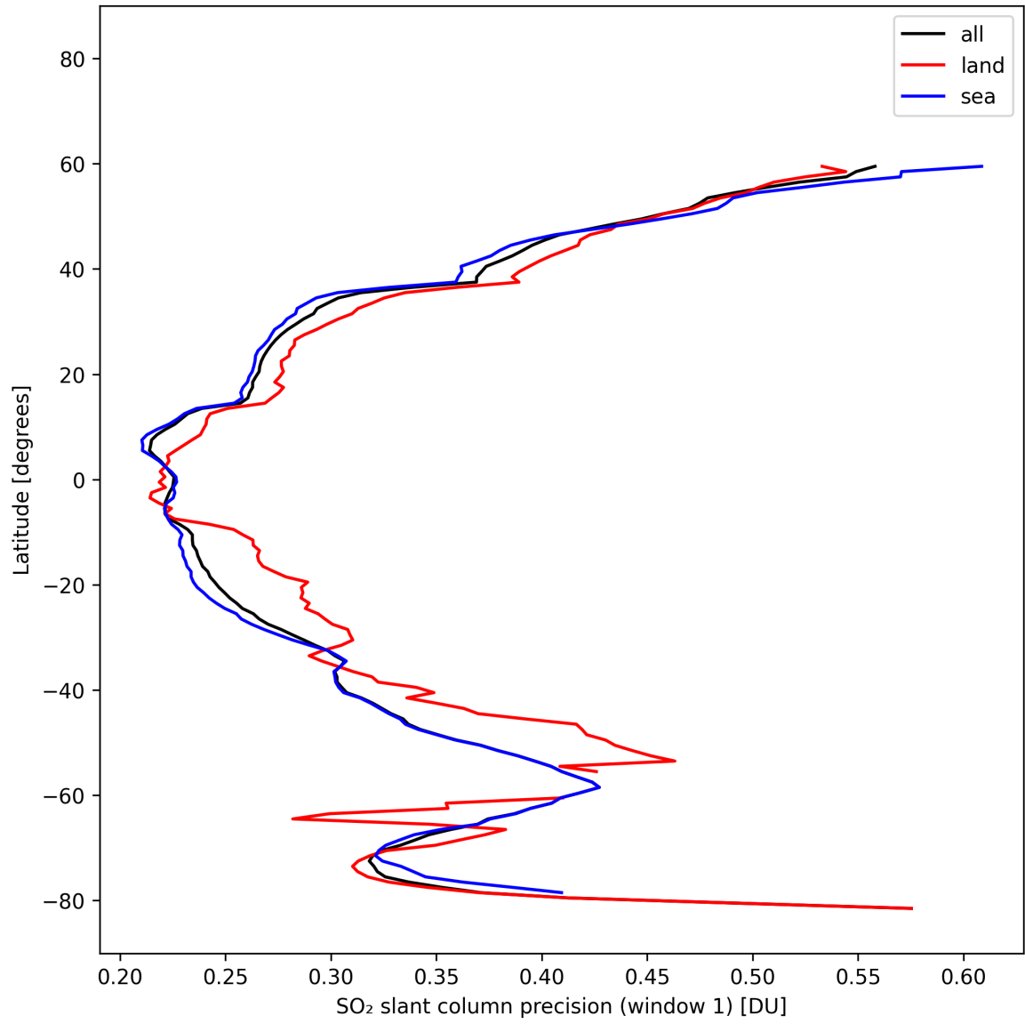
Figure 38: Zonal average of “SO 2 slant column precision (window 1)” for 2025-10-20 to 2025-10-22.
