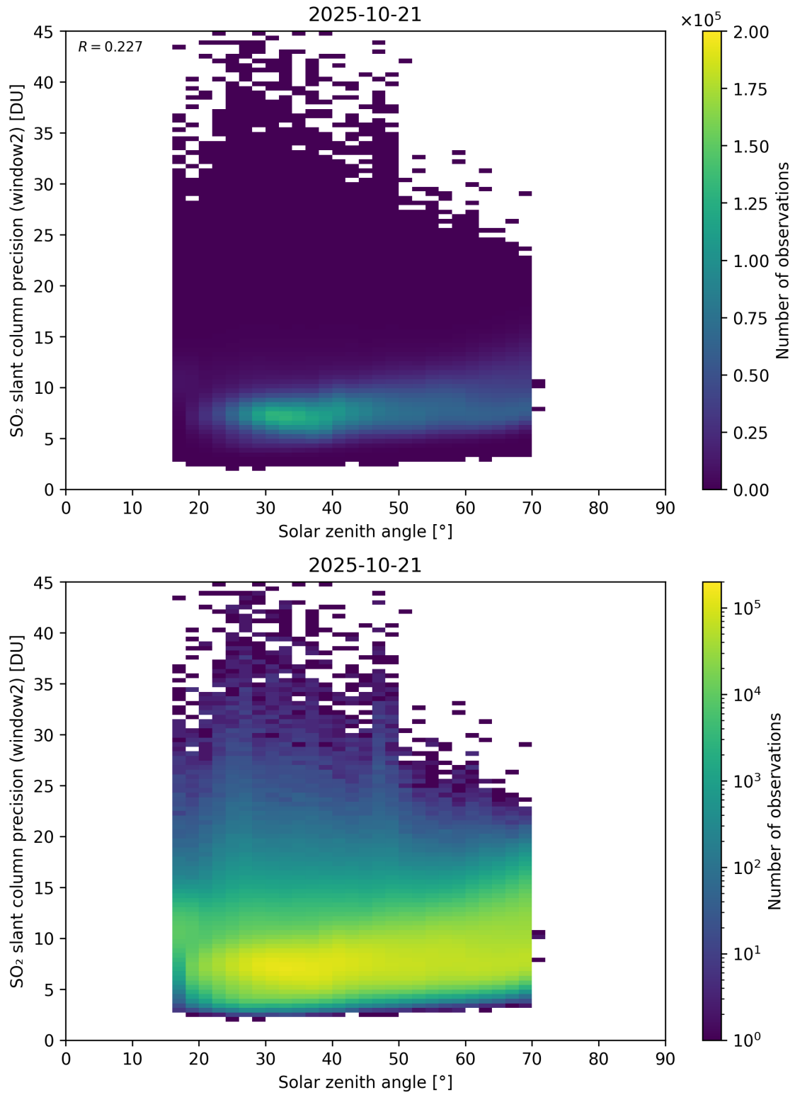
Figure 186: Scatter density plot of “Solar zenith angle” against “SO 2 slant column precision (window2)” for 2025-10-20 to 2025-10-22.
