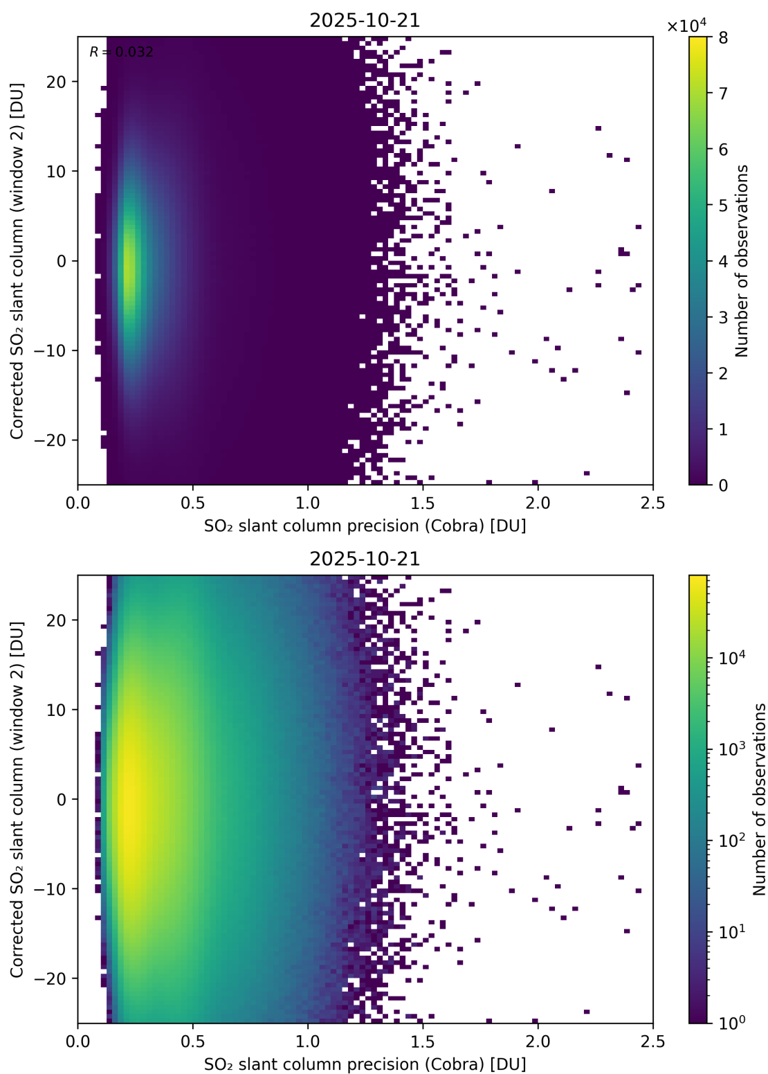
Figure 206: Scatter density plot of “SO 2 slant column precision (Cobra)” against “Corrected SO 2 slant column (window 2)” for 2025-10-20 to 2025-10-22.
