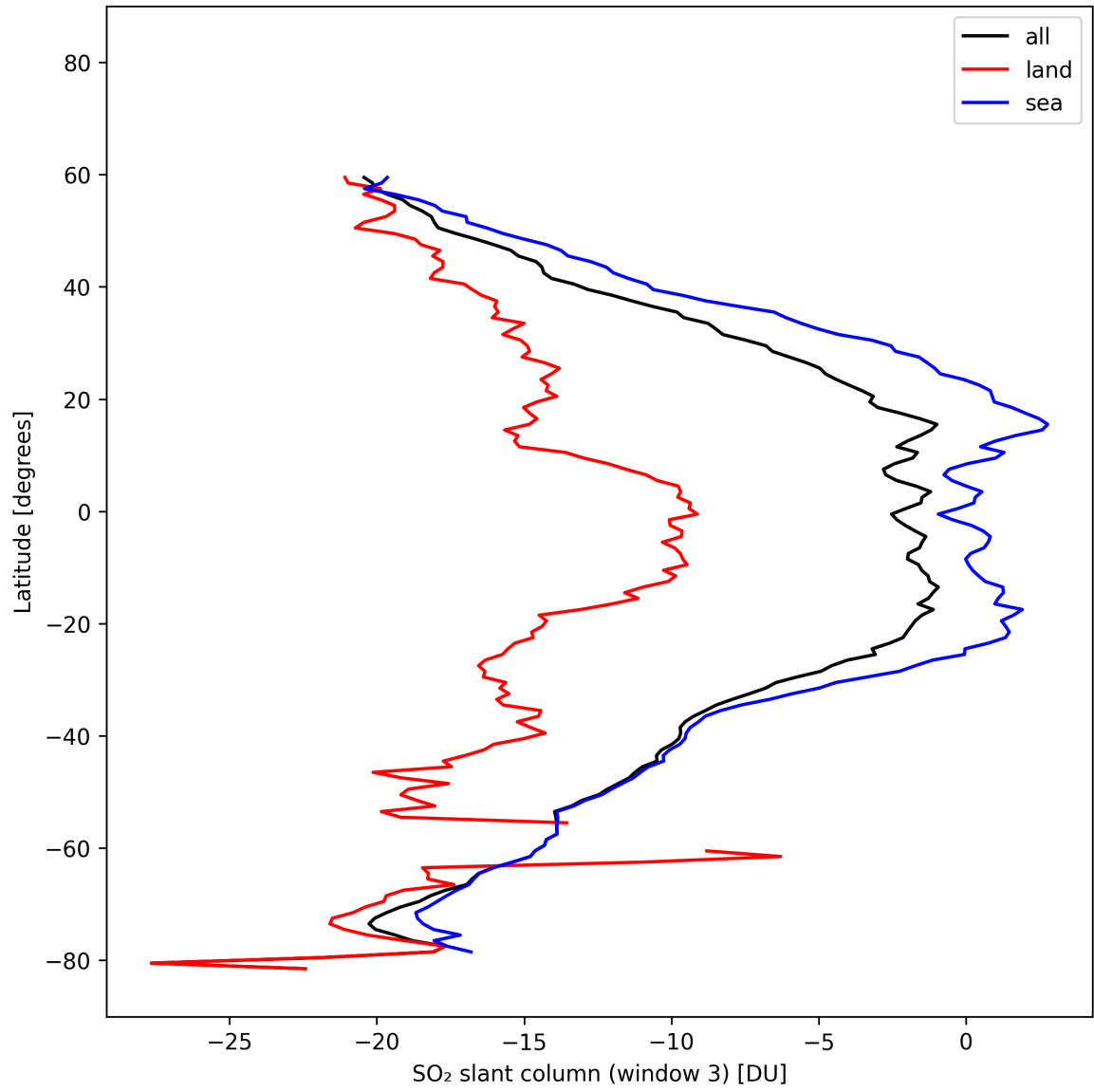
Figure 45: Zonal average of “SO 2 slant column (window 3)” for 2025-10-20 to 2025-10-22.
