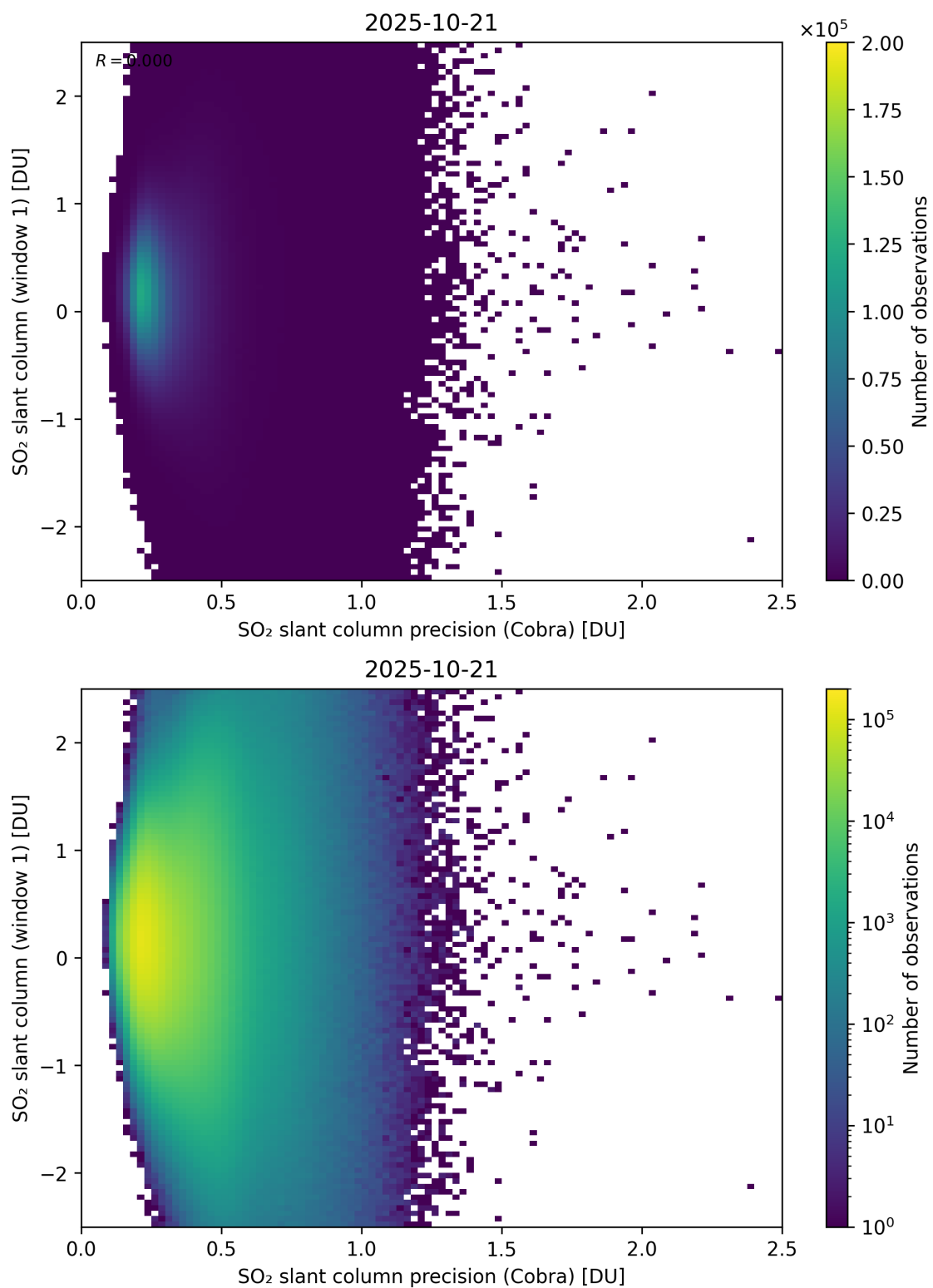
Figure 208: Scatter density plot of “SO 2 slant column precision (Cobra)” against “SO 2 slant column (window 1)” for 2025-10-20 to 2025-10-22.
