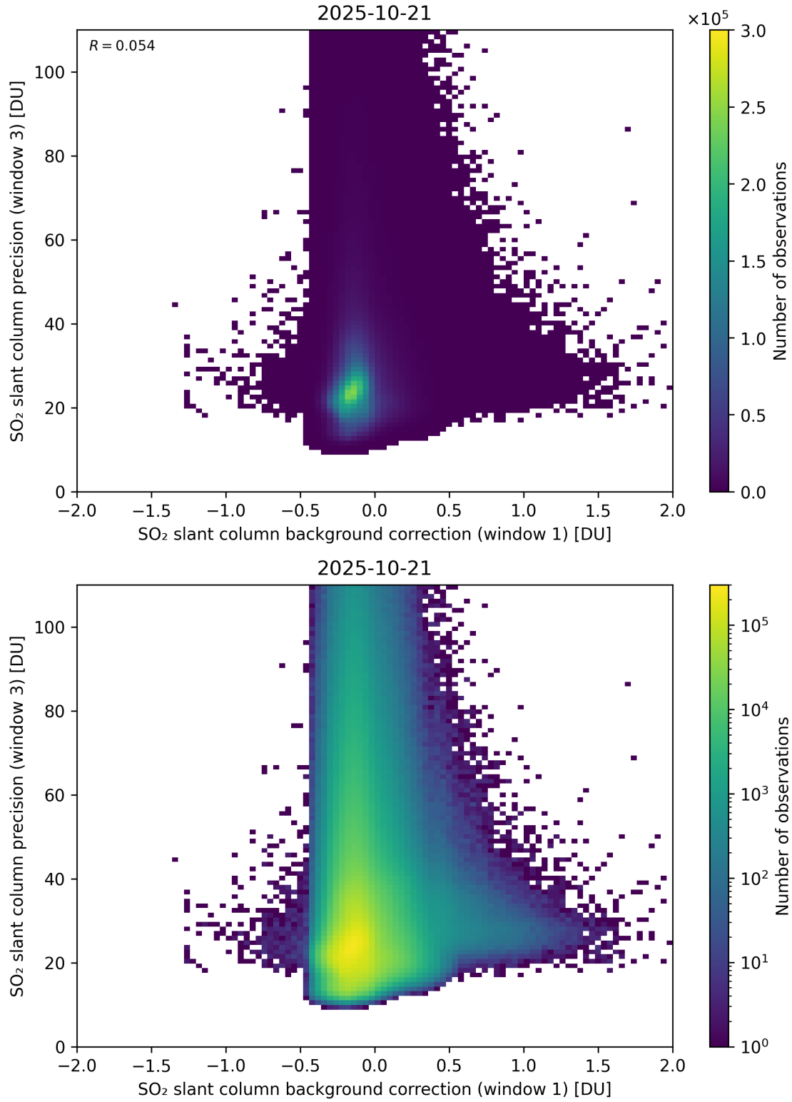
Figure 119: Scatter density plot of “SO 2 slant column background correction (window 1)” against “SO 2 slant column precision (window 3)” for 2025-10-20 to 2025-10-22.
