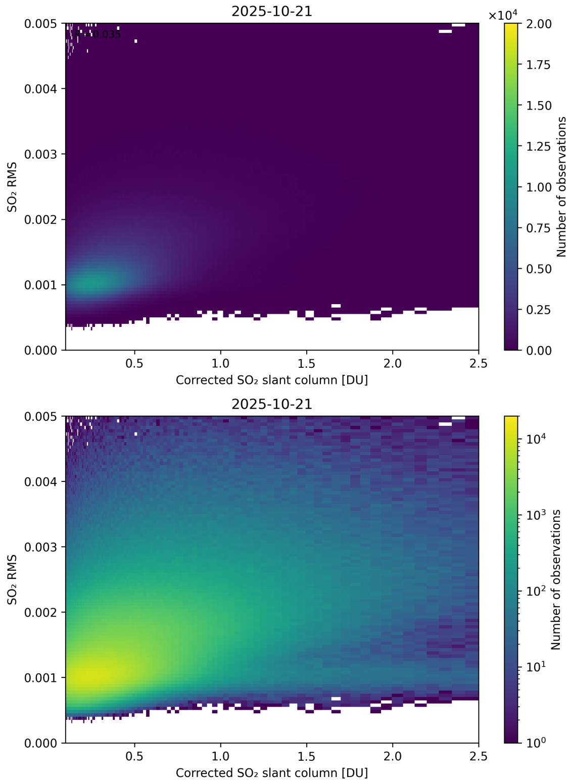
Figure 231: Scatter density plot of “Corrected SO 2 slant column” against “SO 2 RMS” for 2025-10-20 to 2025-10-22.
