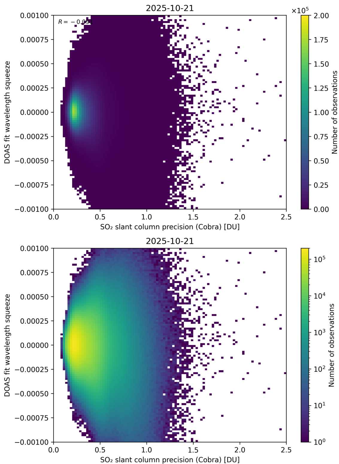
Figure 203: Scatter density plot of “SO 2 slant column precision (Cobra)” against “DOAS fit wavelength squeeze” for 2025-10-20 to 2025-10-22.
