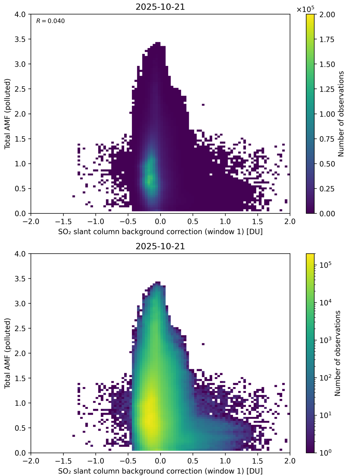
Figure 120: Scatter density plot of “SO 2 slant column background correction (window 1)” against “Total AMF (polluted)” for 2025-10-20 to 2025-10-22.
