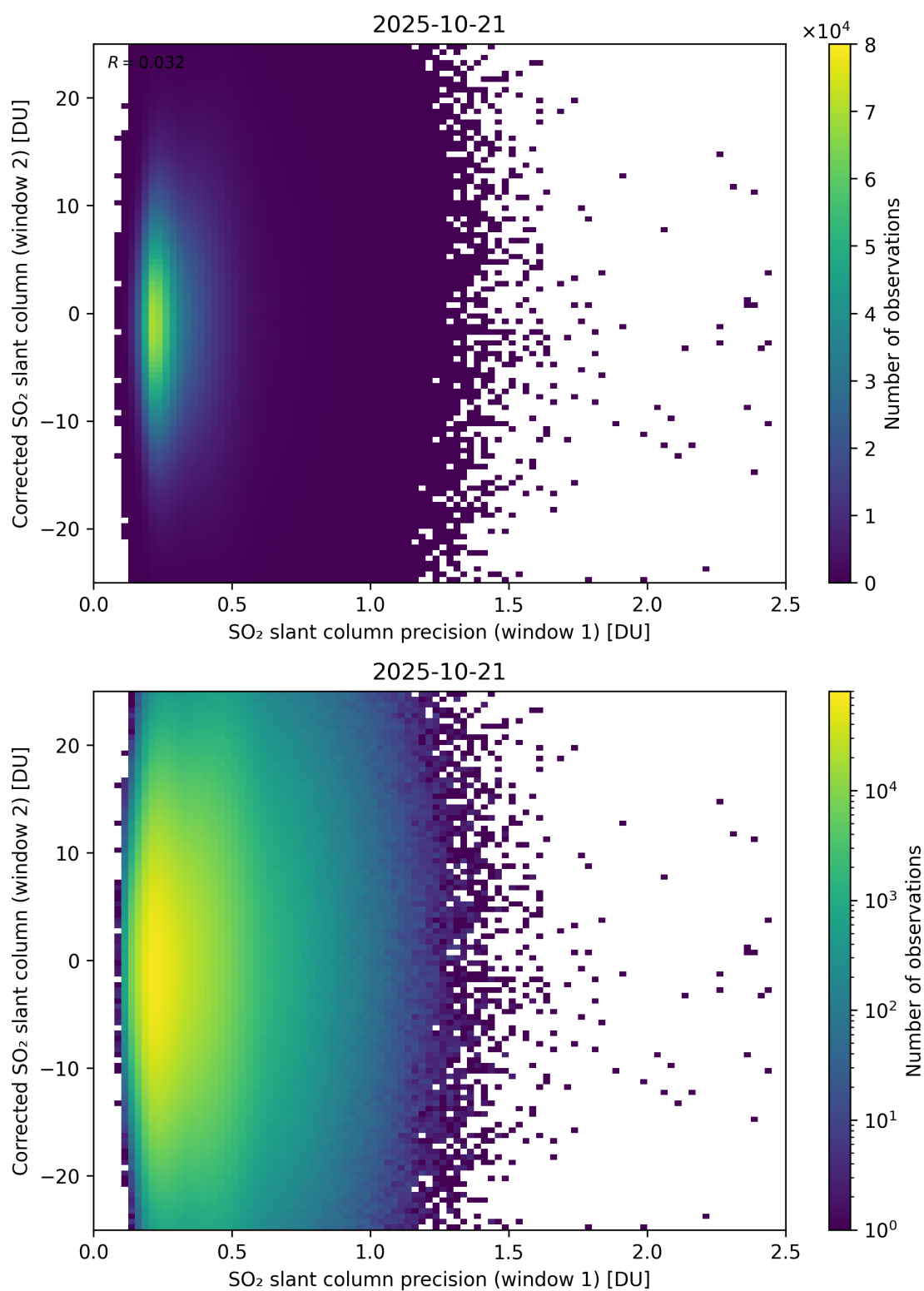
Figure 275: Scatter density plot of “SO 2 slant column precision (window 1)” against “Corrected SO 2 slant column (window 2)” for 2025-10-20 to 2025-10-22.
