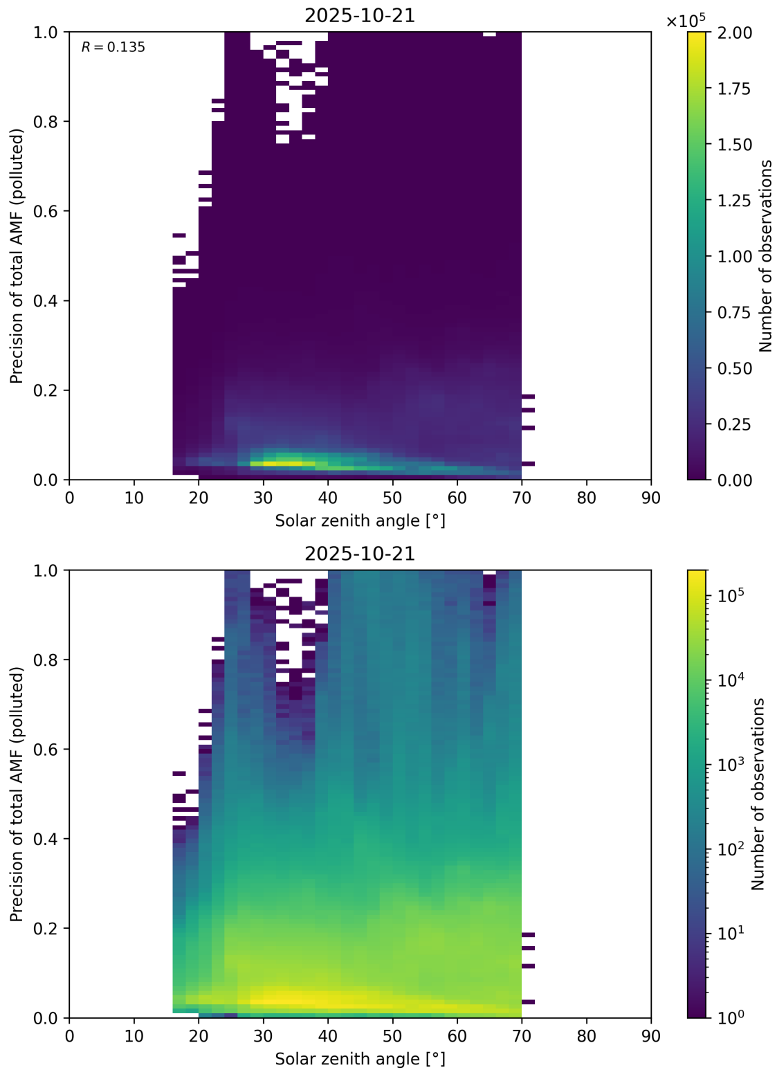
Figure 190: Scatter density plot of “Solar zenith angle” against “Precision of total AMF (polluted)” for 2025-10-20 to 2025-10-22.
