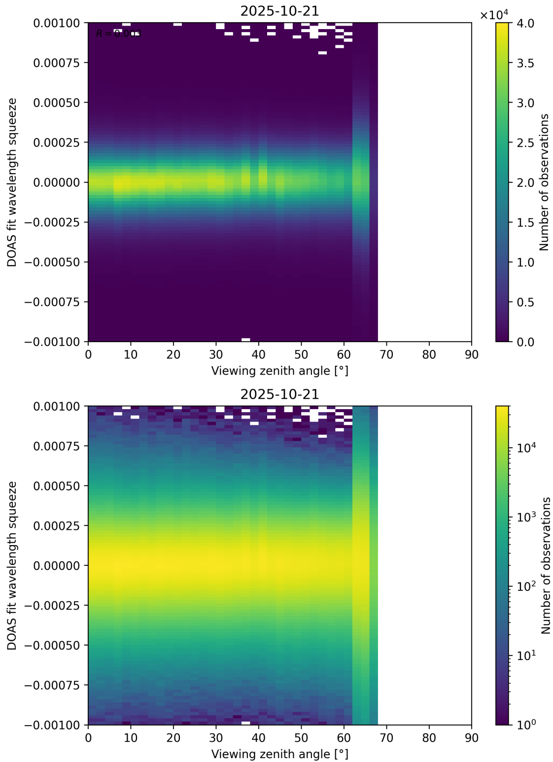
Figure 366: Scatter density plot of “Viewing zenith angle” against “DOAS fit wavelength squeeze” for 2025-10-20 to 2025-10-22.
