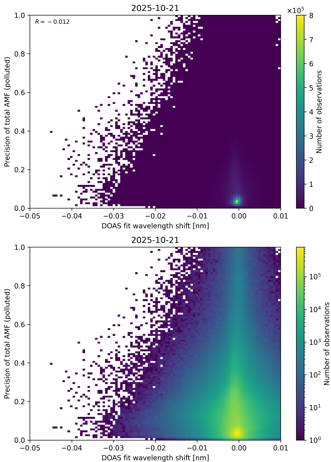
Figure 142: Scatter density plot of “DOAS fit wavelength shift” against “Precision of total AMF (polluted)” for 2025-10-20 to 2025-10-22.
