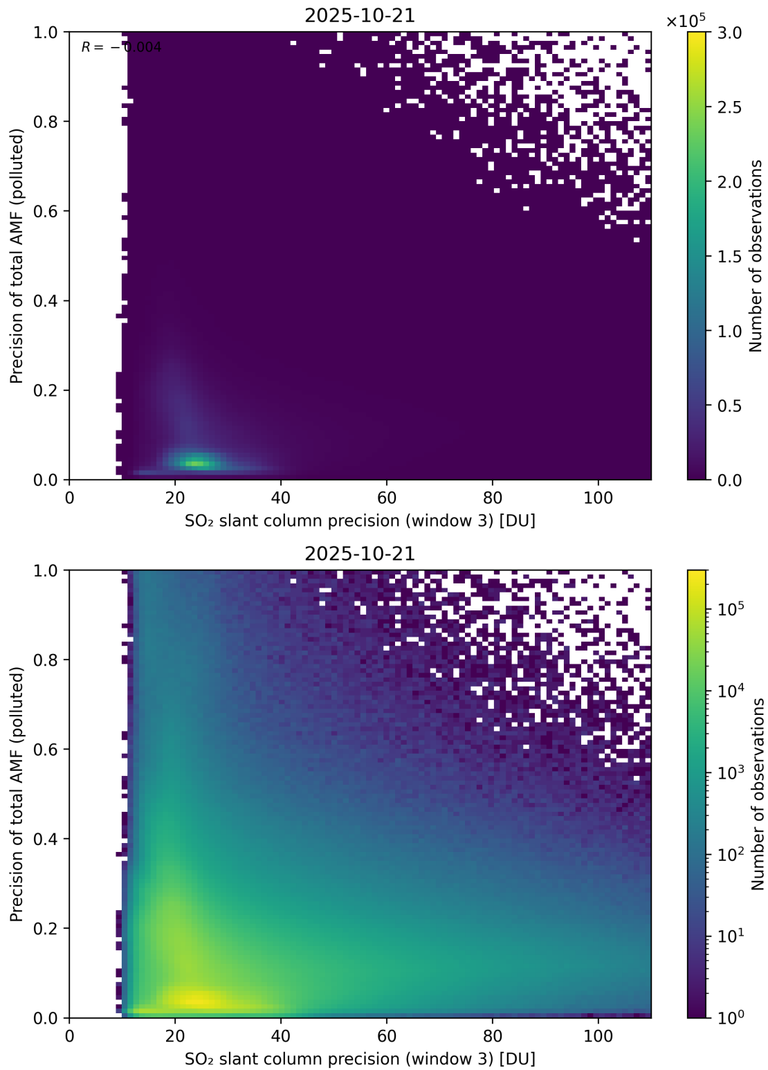
Figure 314: Scatter density plot of “SO 2 slant column precision (window 3)” against “Precision of total AMF (polluted)” for 2025-10-20 to 2025-10-22.
