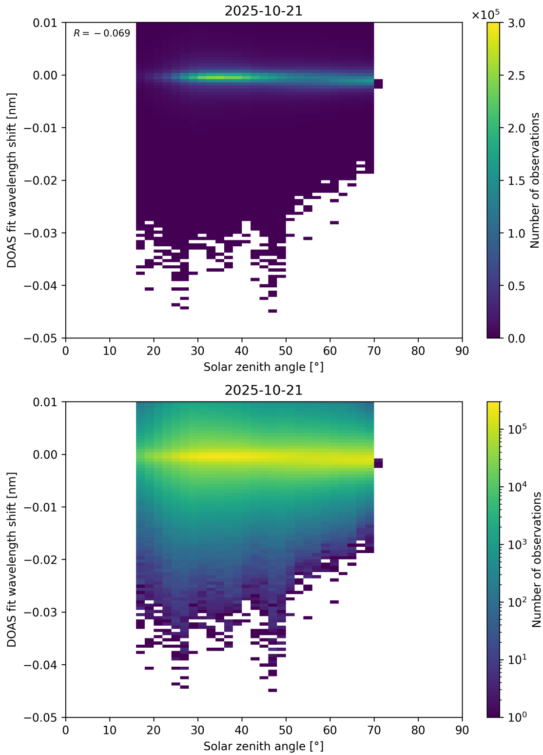
Figure 174: Scatter density plot of “Solar zenith angle” against “DOAS fit wavelength shift” for 2025-10-20 to 2025-10-22.
