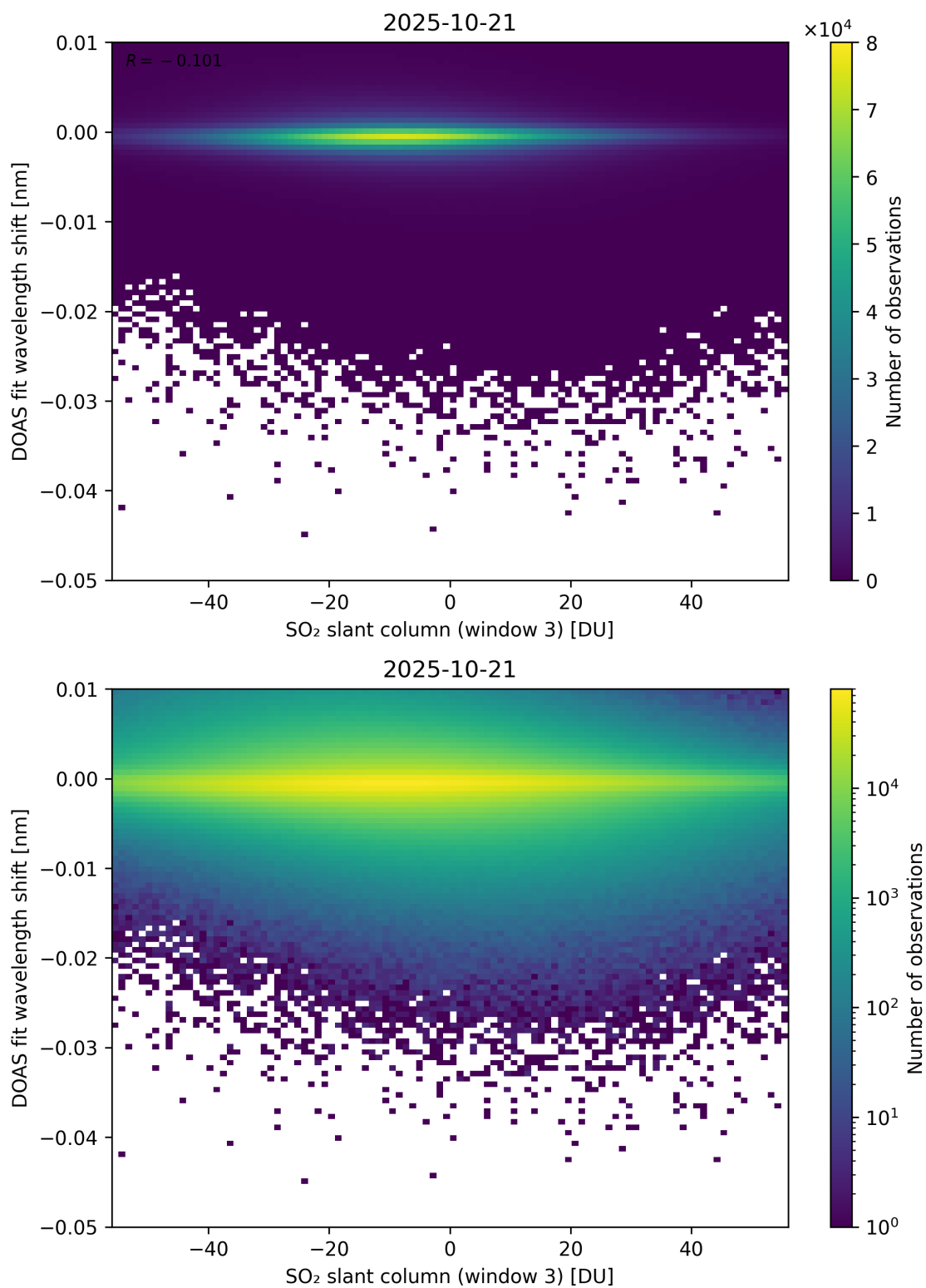
Figure 304: Scatter density plot of “SO 2 slant column (window 3)” against “DOAS fit wavelength shift” for 2025-10-20 to 2025-10-22.
