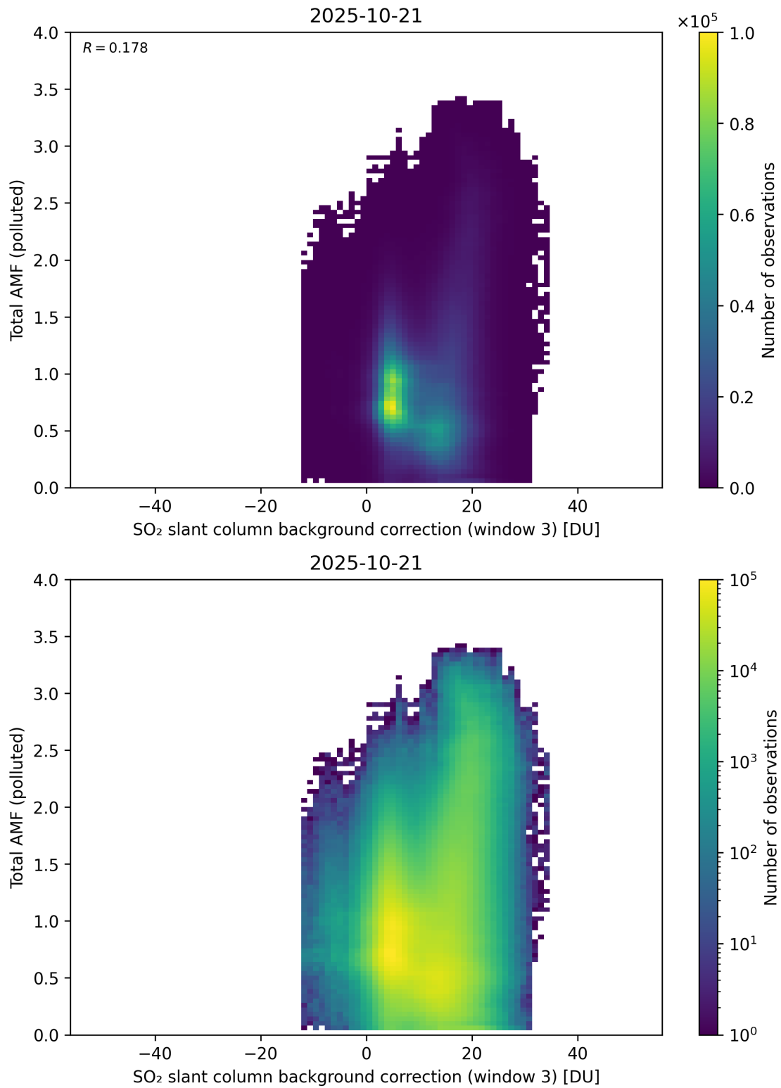
Figure 136: Scatter density plot of “SO 2 slant column background correction (window 3)” against “Total AMF (polluted)” for 2025-10-20 to 2025-10-22.
