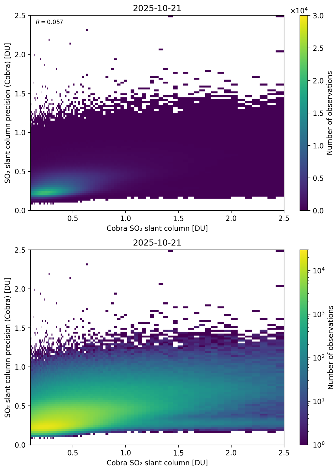
Figure 216: Scatter density plot of “Cobra SO 2 slant column” against “SO 2 slant column precision (Cobra)” for 2025-10-20 to 2025-10-22.
