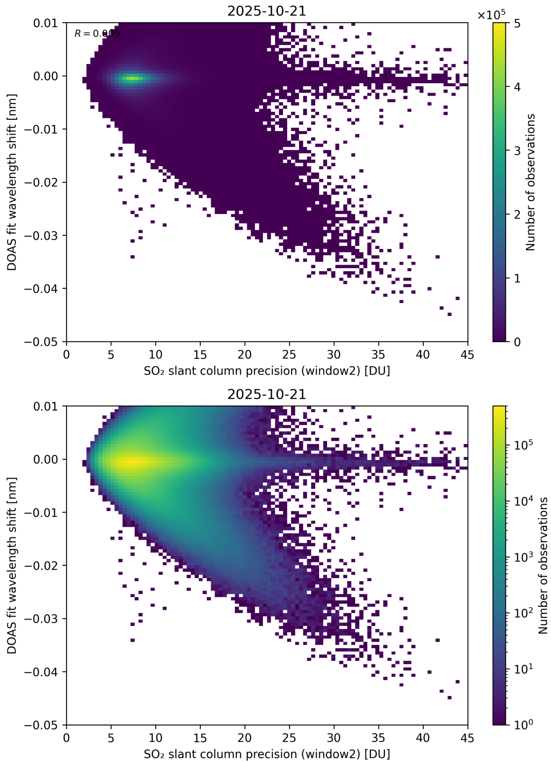
Figure 293: Scatter density plot of “SO 2 slant column precision (window2)” against “DOAS fit wavelength shift” for 2025-10-20 to 2025-10-22.
