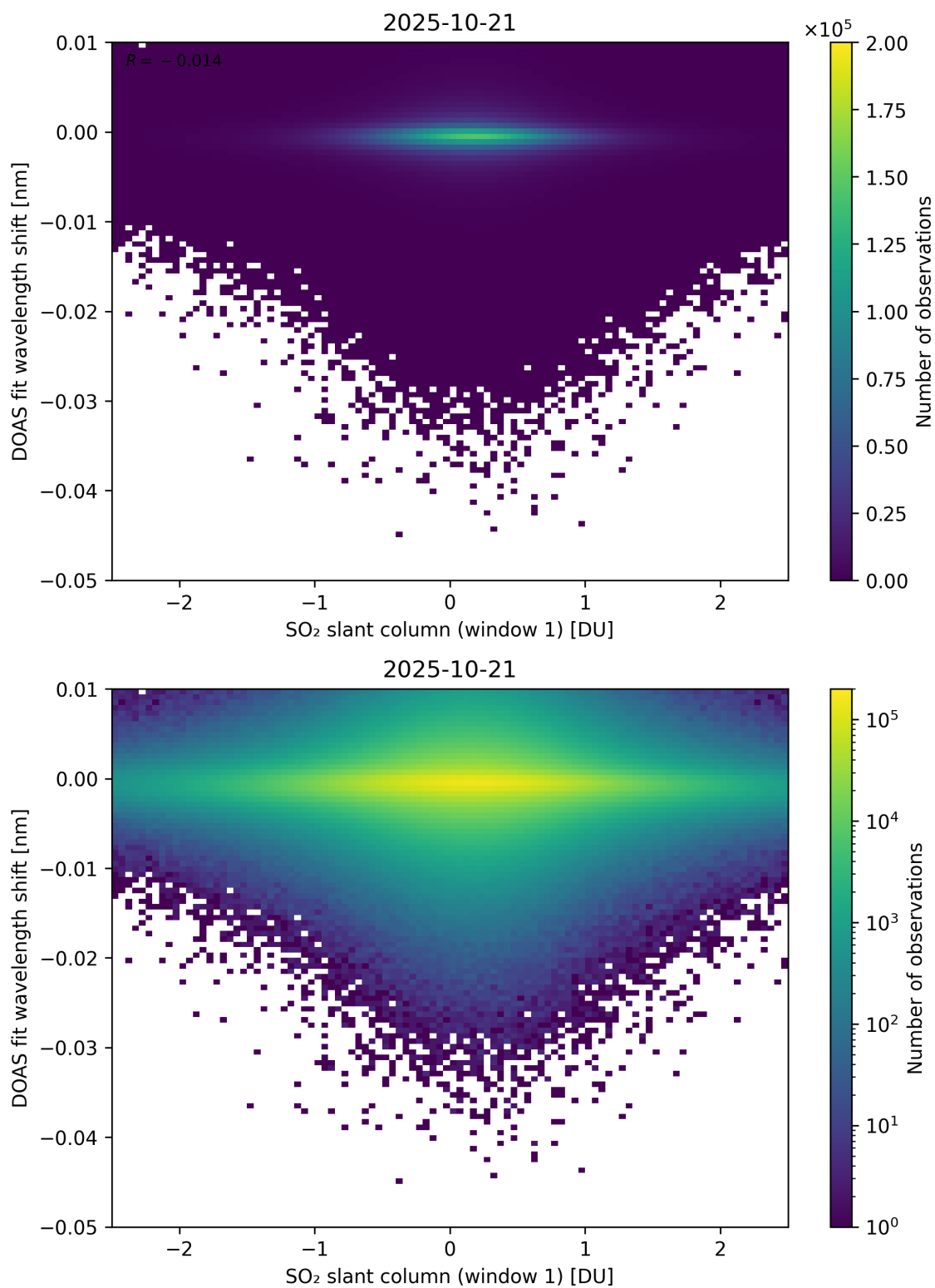
Figure 265: Scatter density plot of “SO 2 slant column (window 1)” against “DOAS fit wavelength shift” for 2025-10-20 to 2025-10-22.
