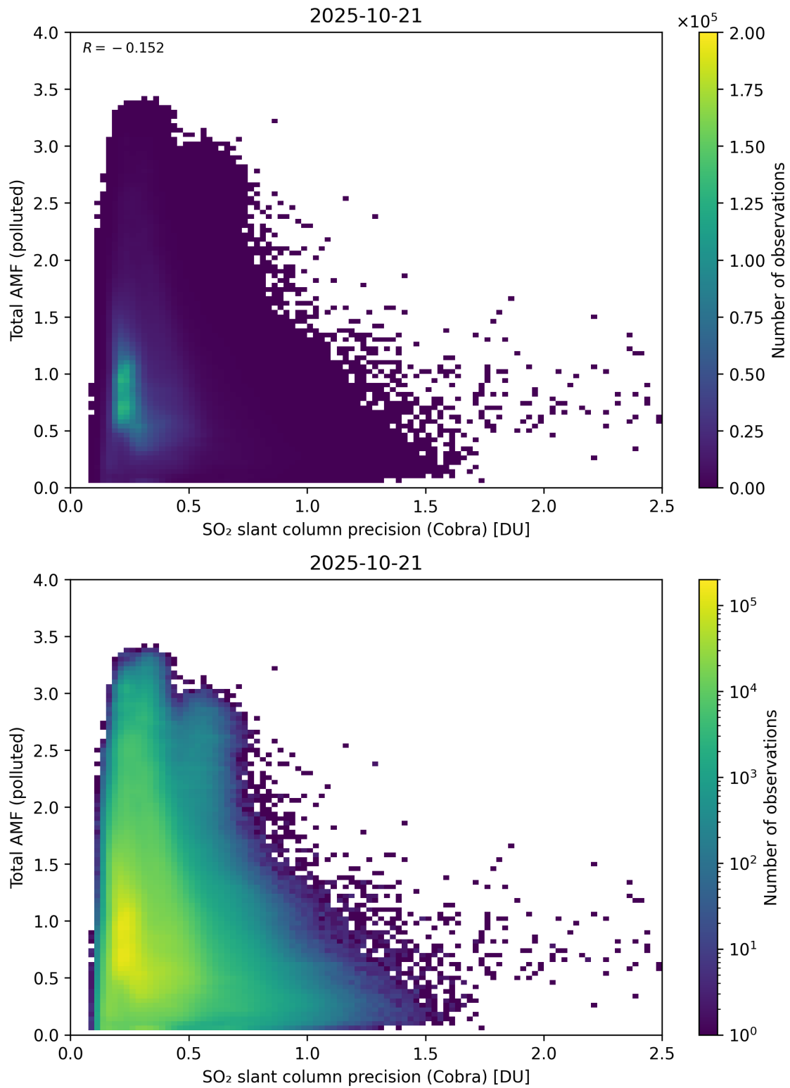
Figure 213: Scatter density plot of “SO 2 slant column precision (Cobra)” against “Total AMF (polluted)” for 2025-10-20 to 2025-10-22.
