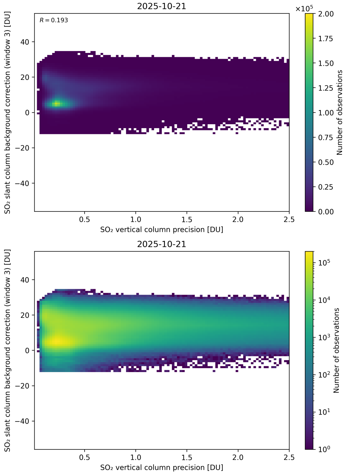
Figure 331: Scatter density plot of “SO 2 vertical column precision” against “SO 2 slant column background correction (window 3)” for 2025-10-20 to 2025-10-22.
