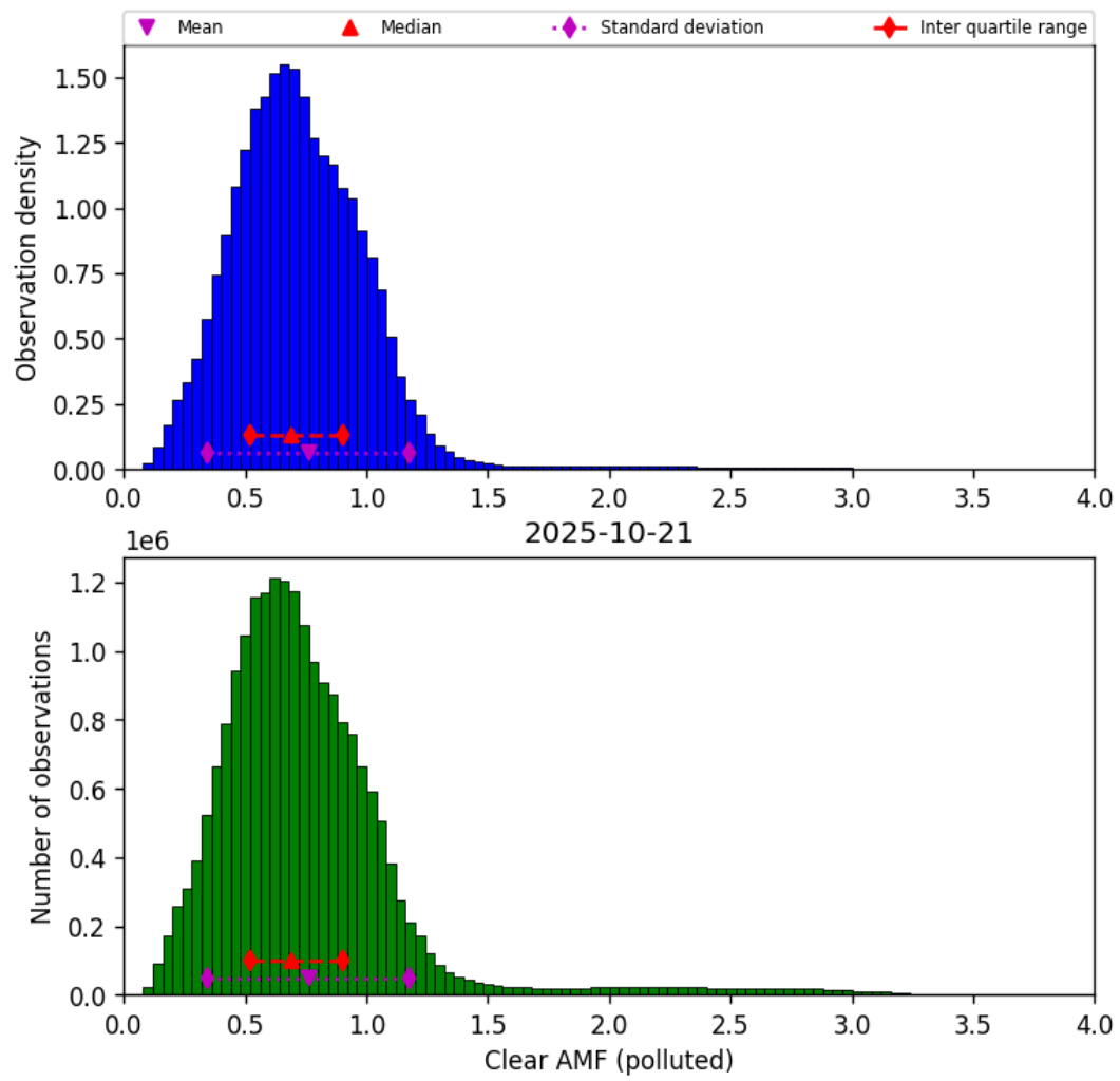
Figure 81: Histogram of “Clear AMF (polluted)” for 2025-10-20 to 2025-10-22
