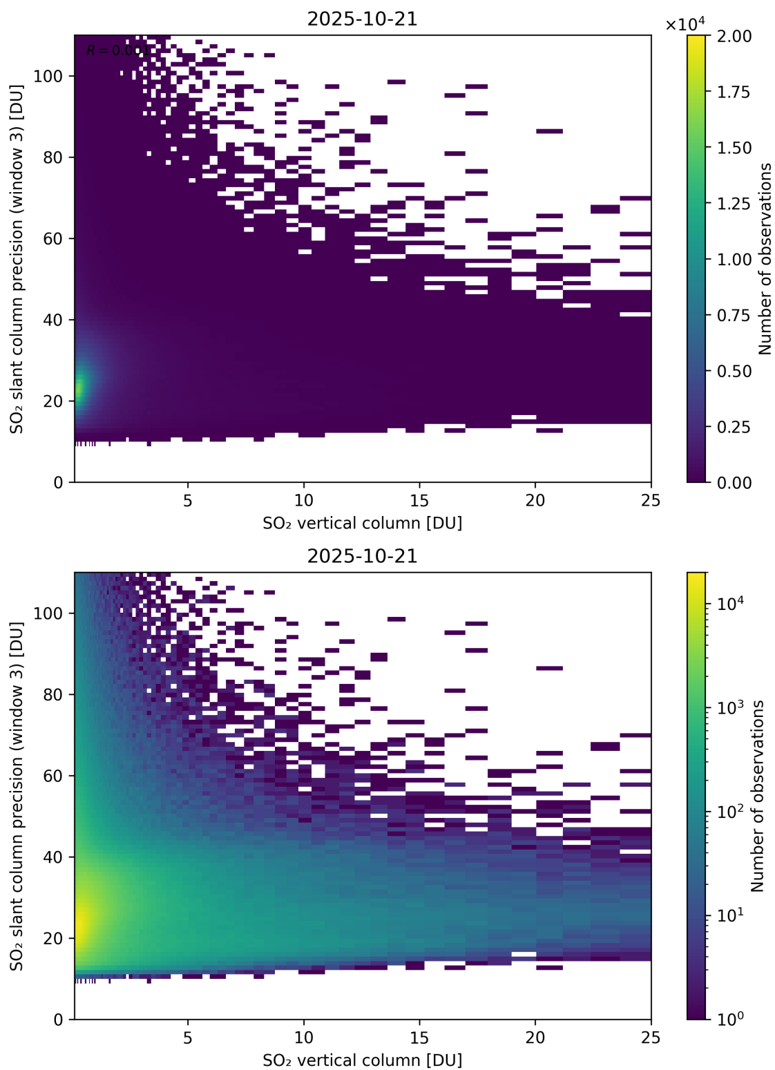
Figure 358: Scatter density plot of “SO 2 vertical column” against “SO 2 slant column precision (window 3)” for 2025-10-20 to 2025-10-22.
