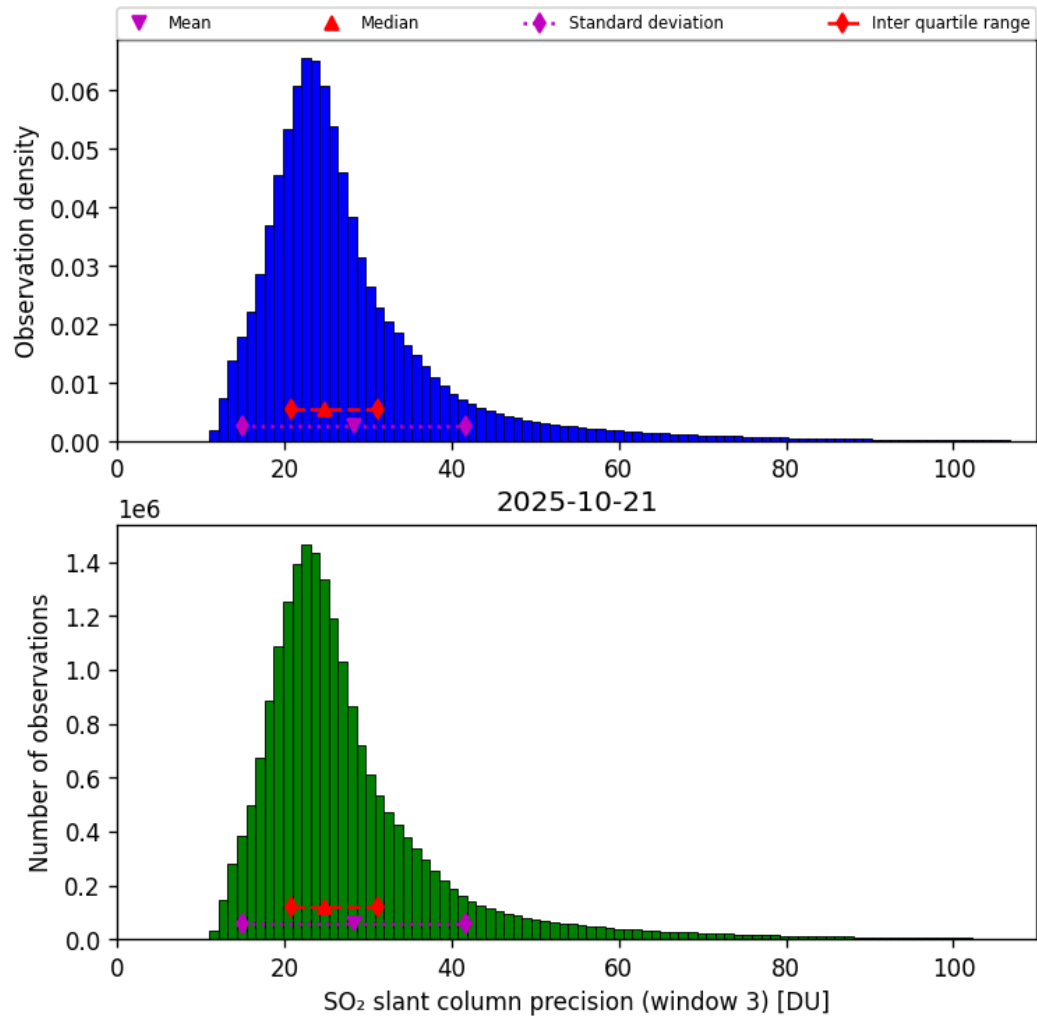
Figure 72: Histogram of “SO 2 slant column precision (window 3)” for 2025-10-20 to 2025-10-22
