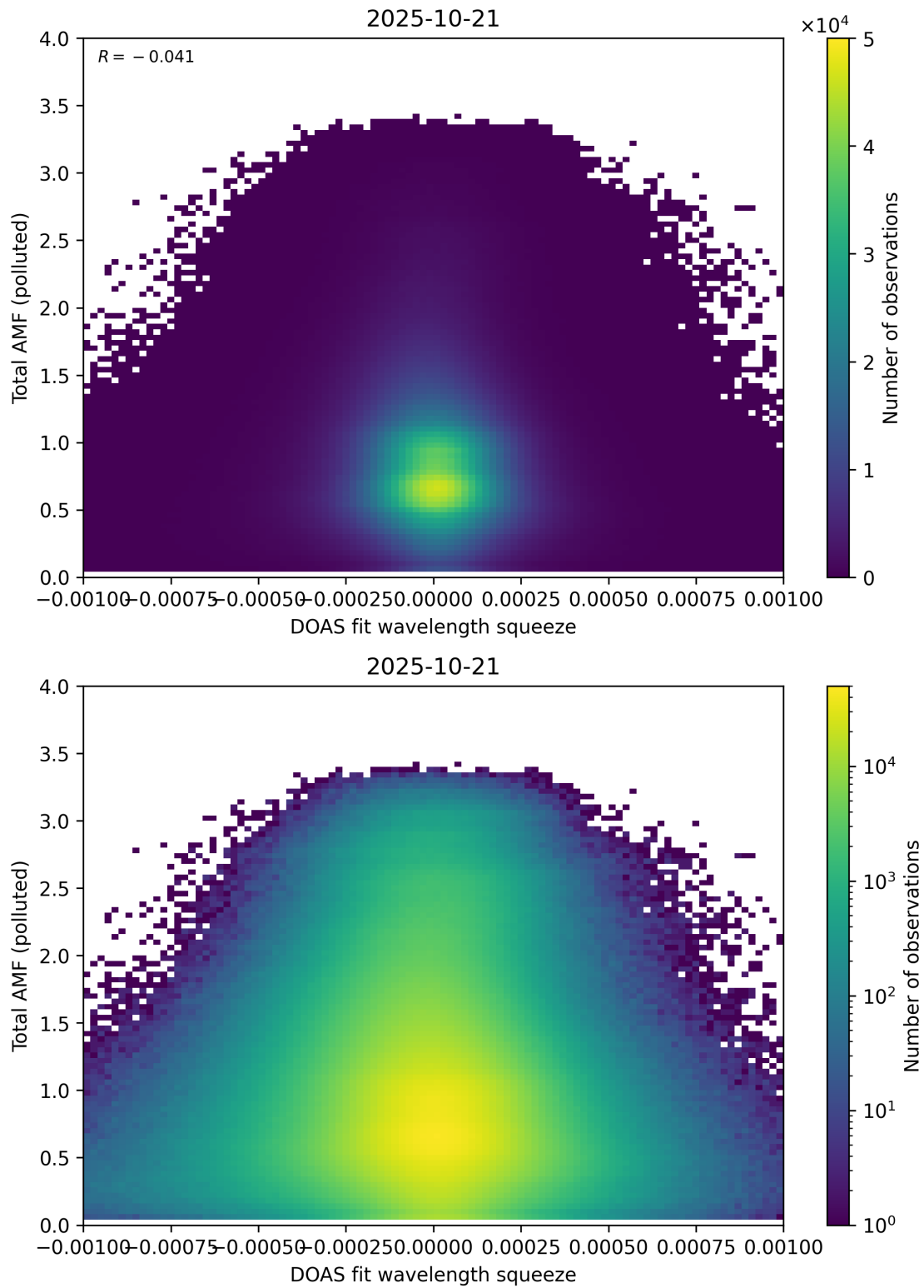
Figure 145: Scatter density plot of “DOAS fit wavelength squeeze” against “Total AMF (polluted)” for 2025-10-20 to 2025-10-22.
