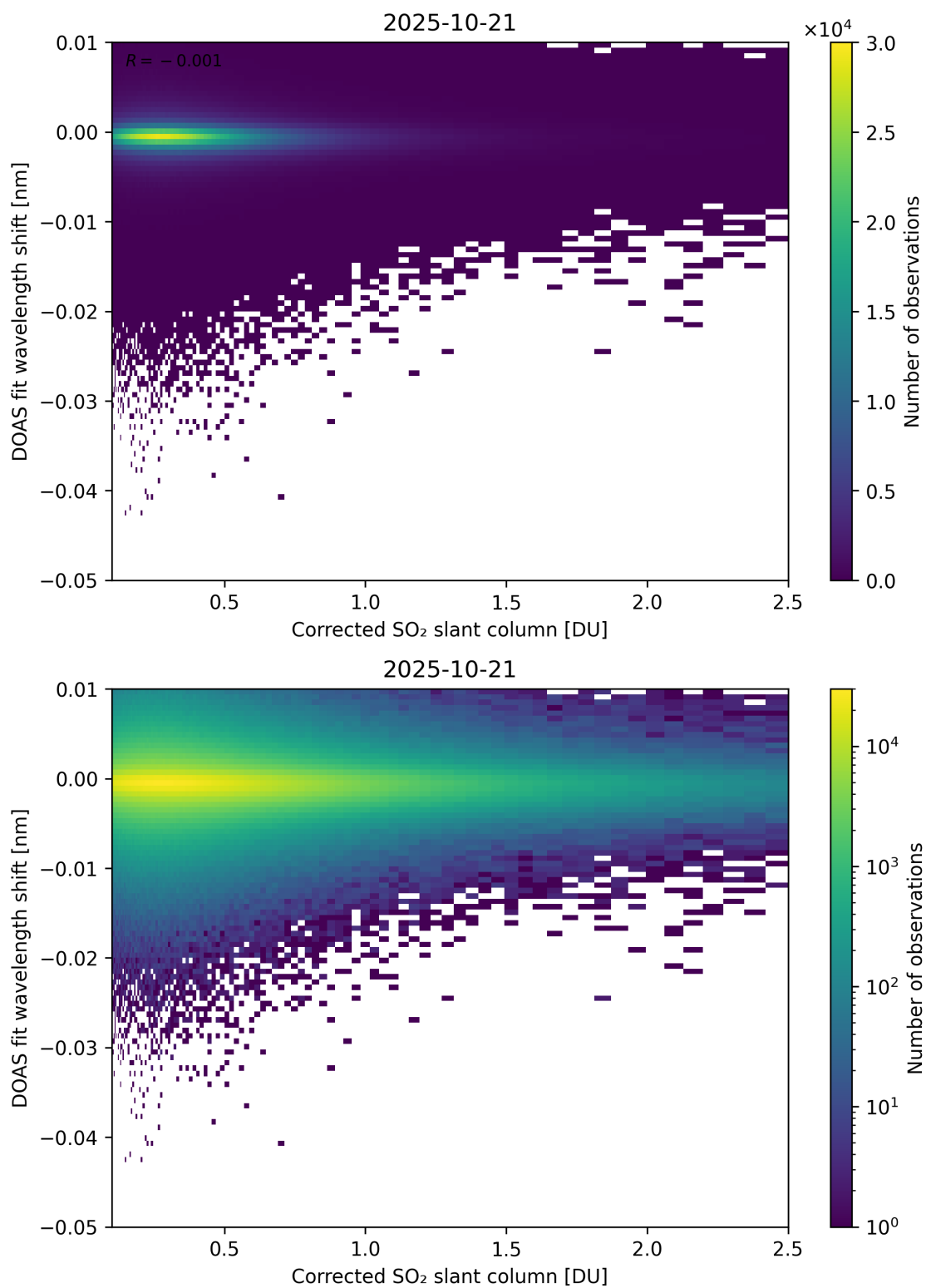
Figure 229: Scatter density plot of “Corrected SO 2 slant column” against “DOAS fit wavelength shift” for 2025-10-20 to 2025-10-22.
