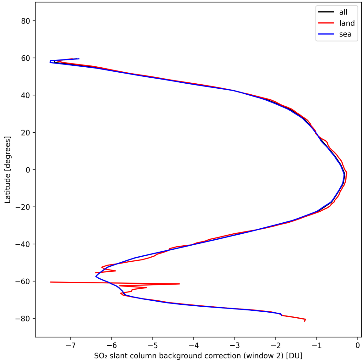
Figure 44: Zonal average of “SO 2 slant column background correction (window 2)” for 2025-10-20 to 2025-10-22.
