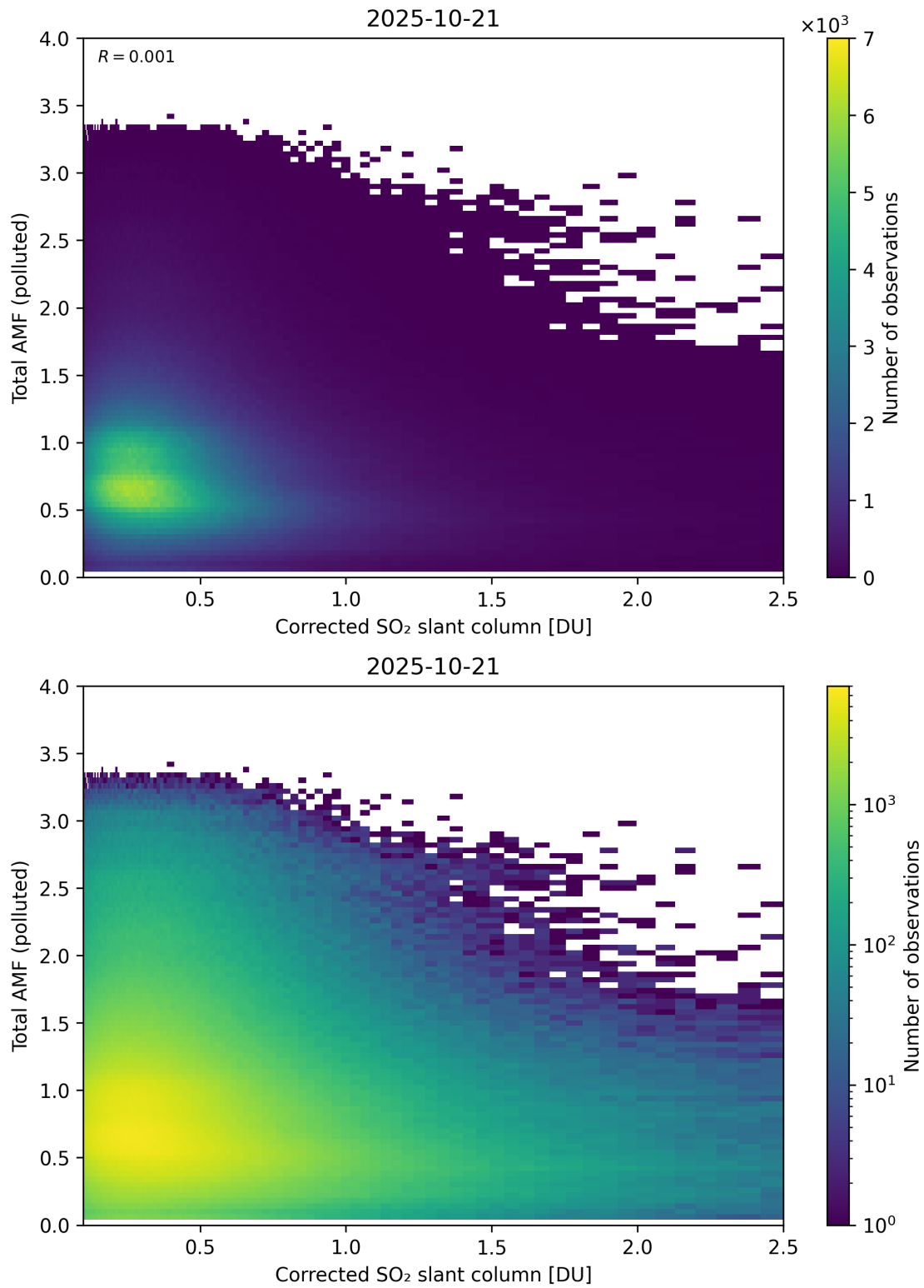
Figure 242: Scatter density plot of “Corrected SO 2 slant column” against “Total AMF (polluted)” for 2025-10-20 to 2025-10-22.
