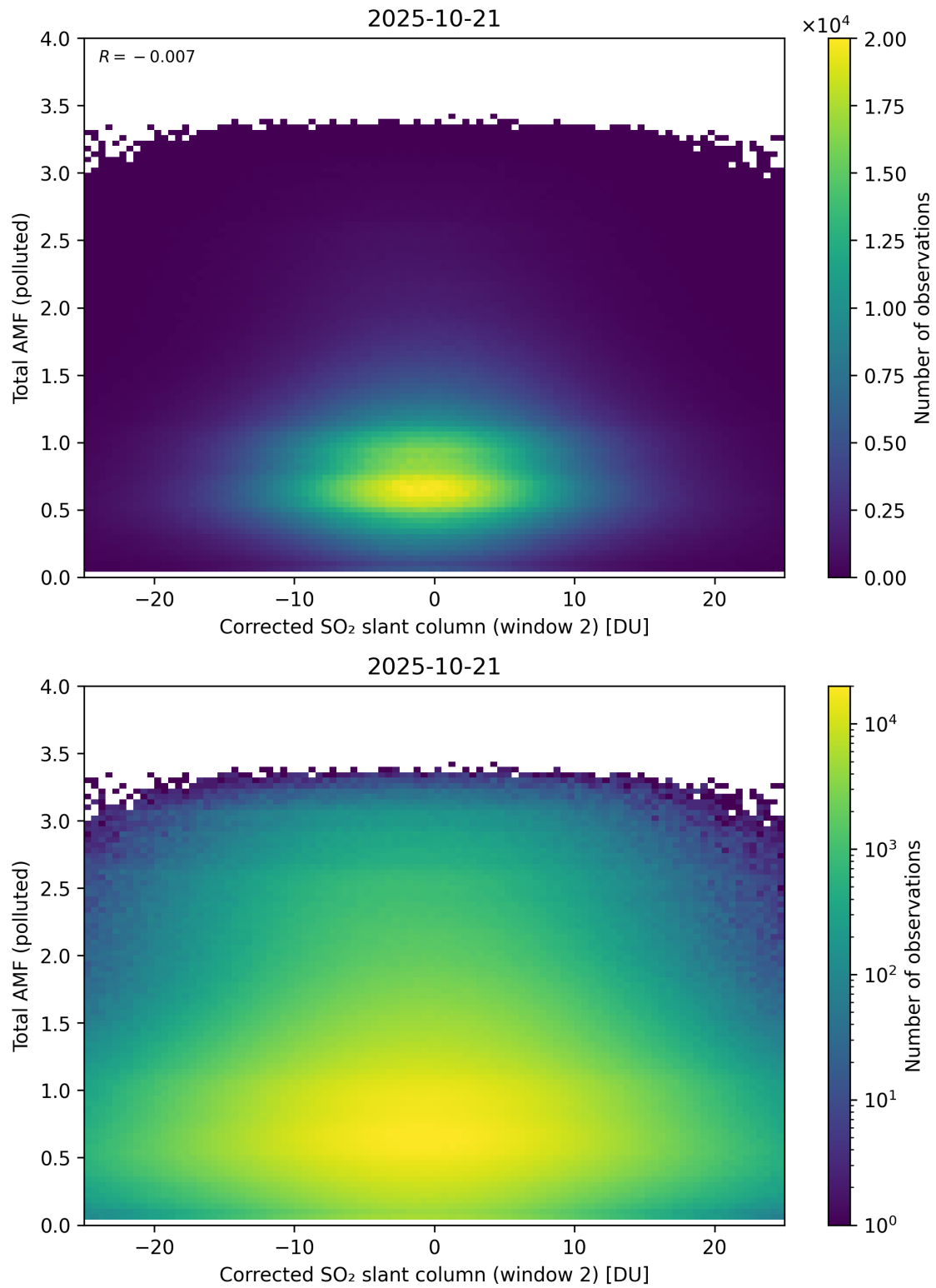
Figure 253: Scatter density plot of “Corrected SO 2 slant column (window 2)” against “Total AMF (polluted)” for 2025-10-20 to 2025-10-22.
