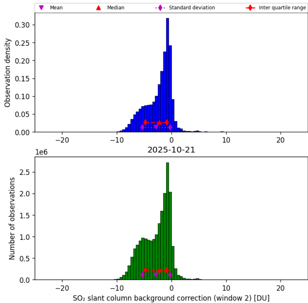
Figure 70: Histogram of “SO 2 slant column background correction (window 2)” for 2025-10-20 to 2025-10-22
