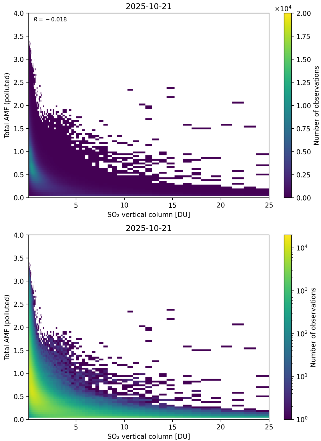
Figure 359: Scatter density plot of “SO 2 vertical column” against “Total AMF (polluted)” for 2025-10-20 to 2025-10-22.
