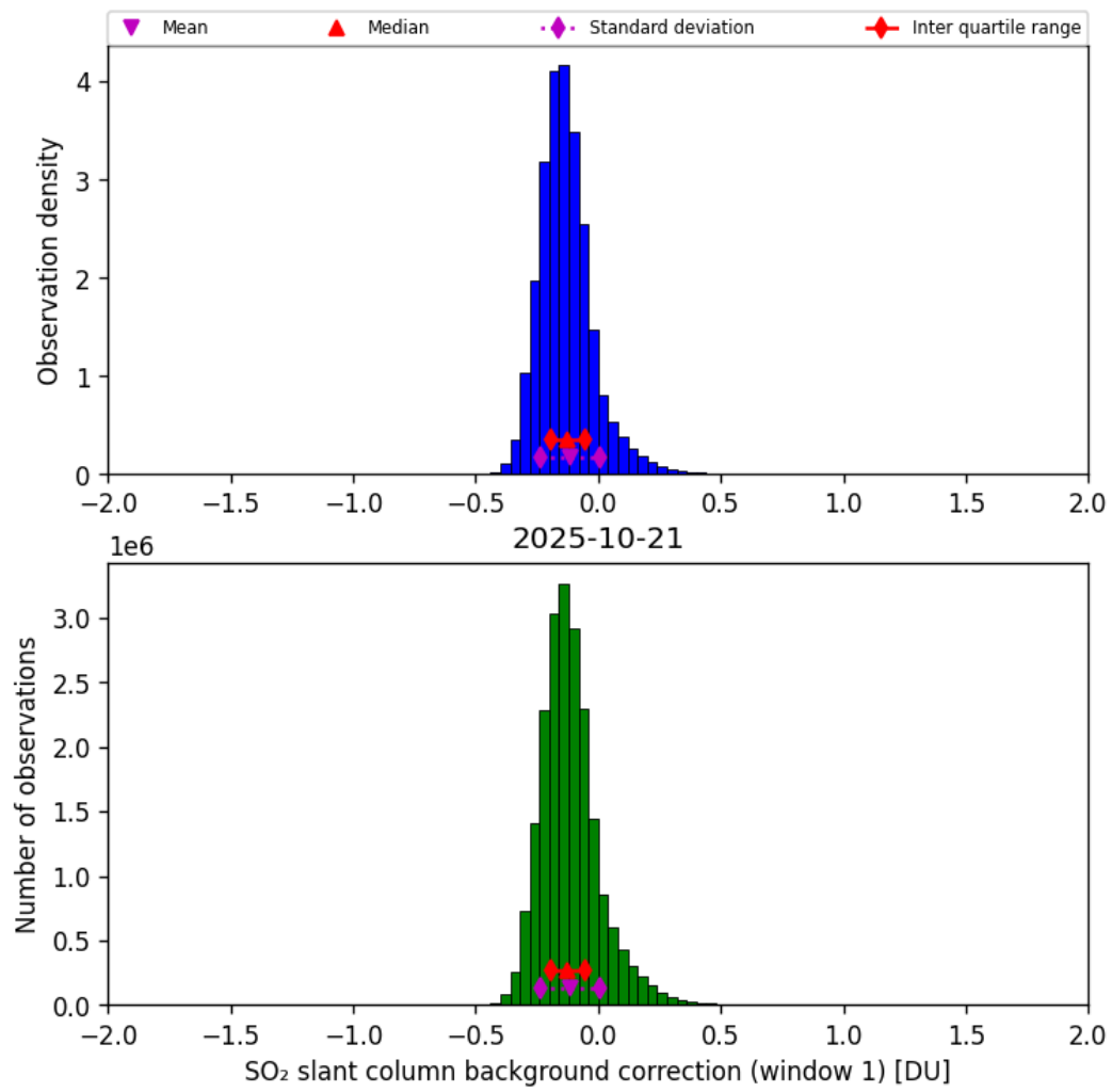
Figure 66: Histogram of “SO 2 slant column background correction (window 1)” for 2025-10-20 to 2025-10-22
