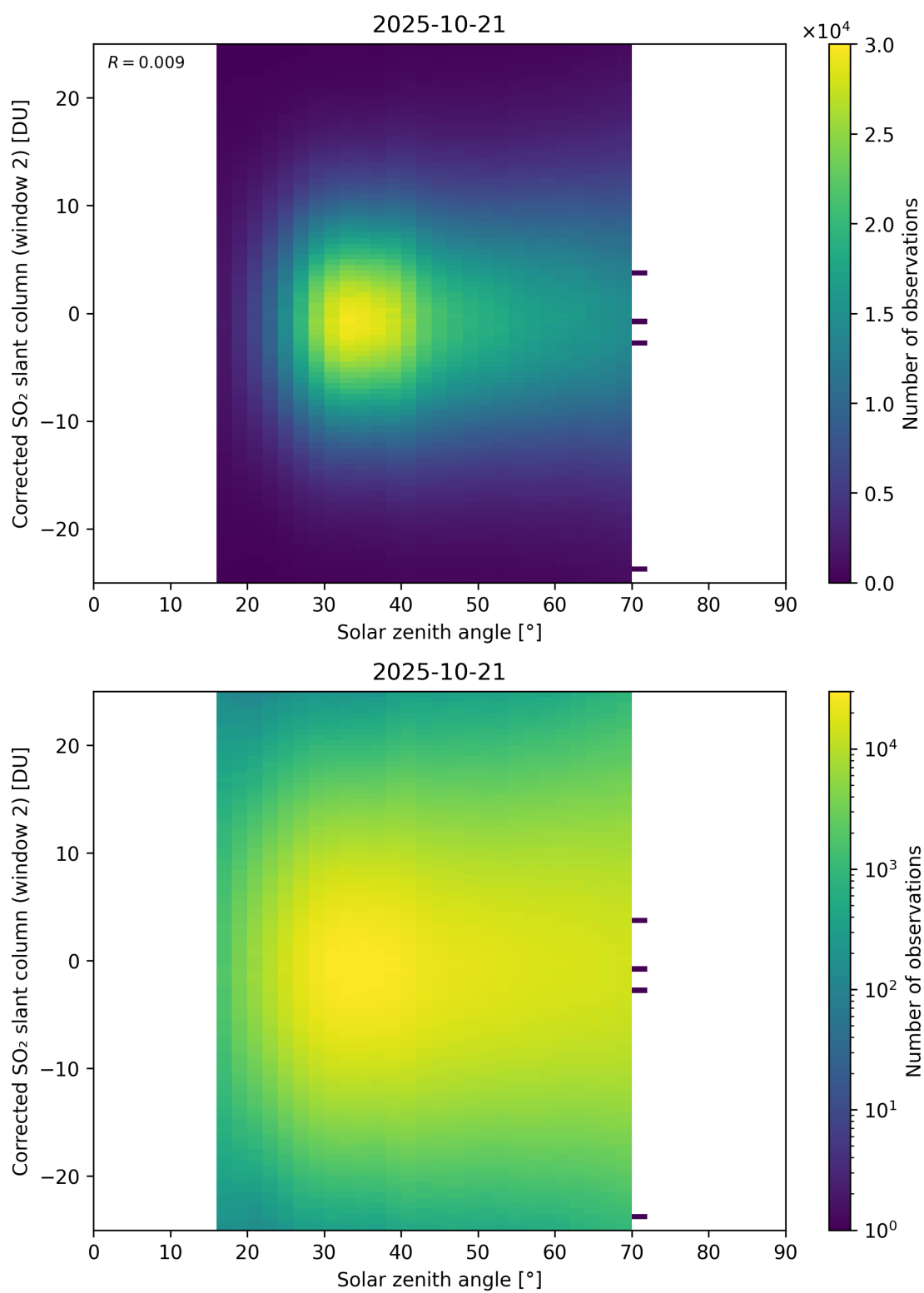
Figure 182: Scatter density plot of “Solar zenith angle” against “Corrected SO 2 slant column (window 2)” for 2025-10-20 to 2025-10-22.
