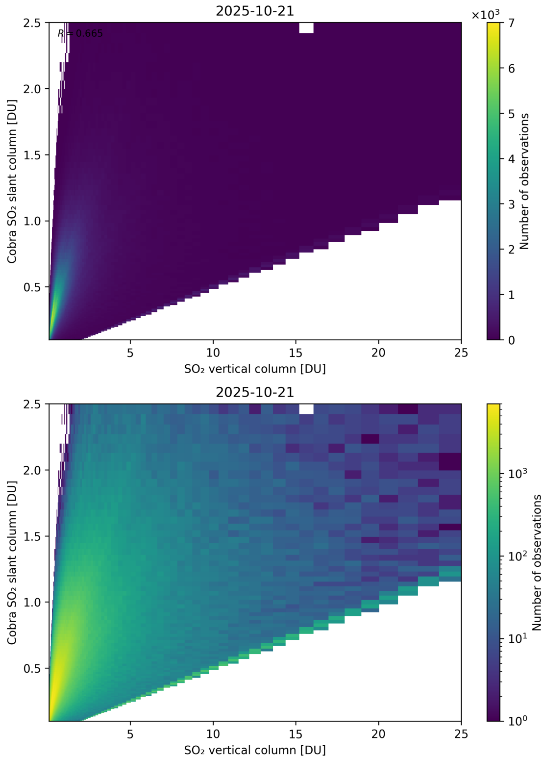
Figure 349: Scatter density plot of “SO 2 vertical column” against “Cobra SO 2 slant column” for 2025-10-20 to 2025-10-22.
