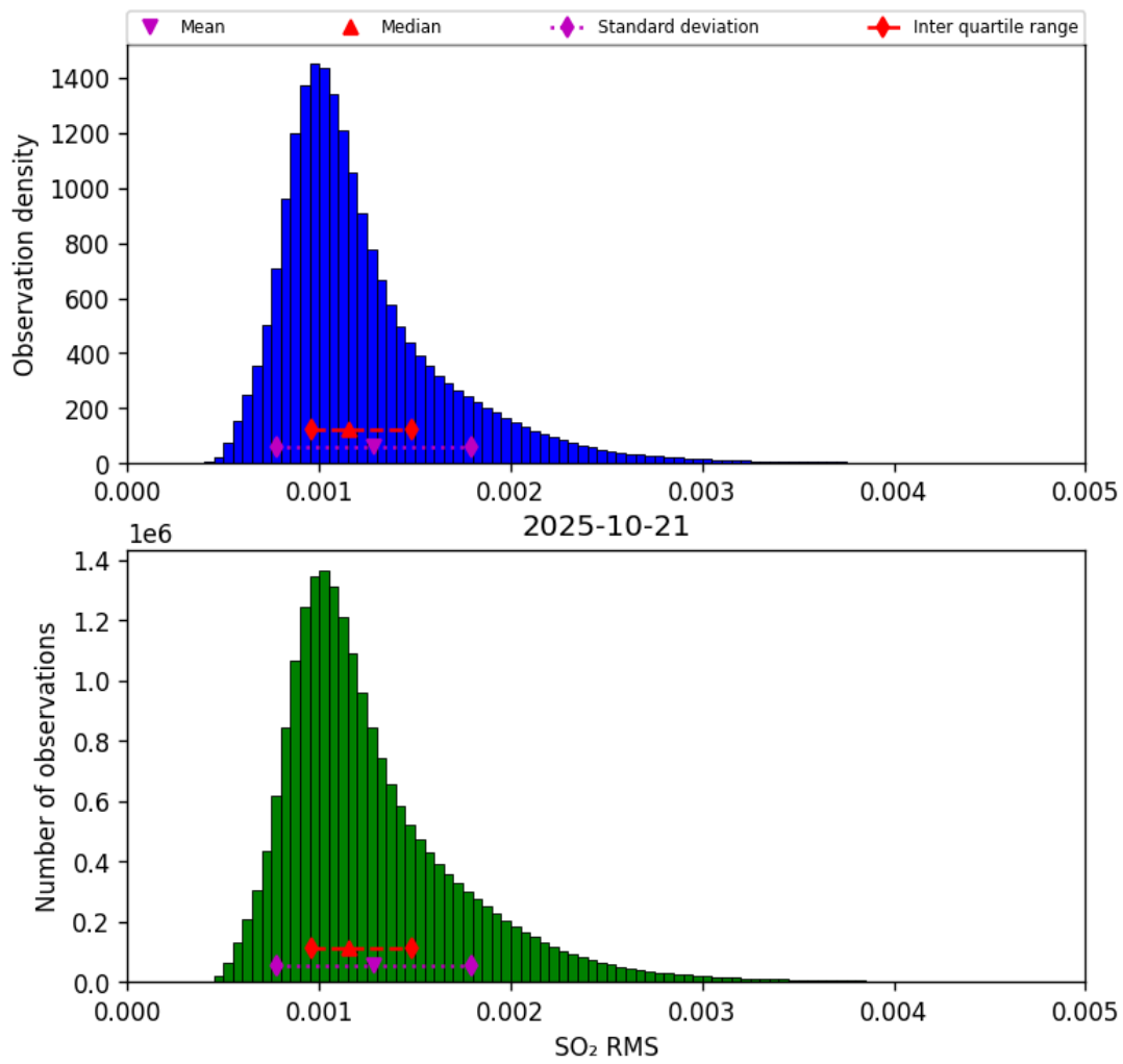
Figure 78: Histogram of “SO 2 RMS” for 2025-10-20 to 2025-10-22
