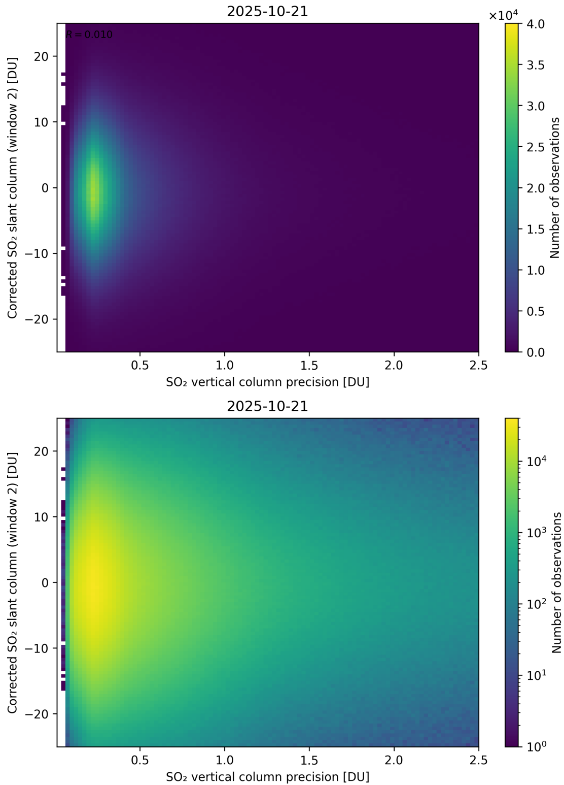
Figure 339: Scatter density plot of “SO 2 vertical column precision” against “Corrected SO 2 slant column (window 2)” for 2025-10-20 to 2025-10-22.
