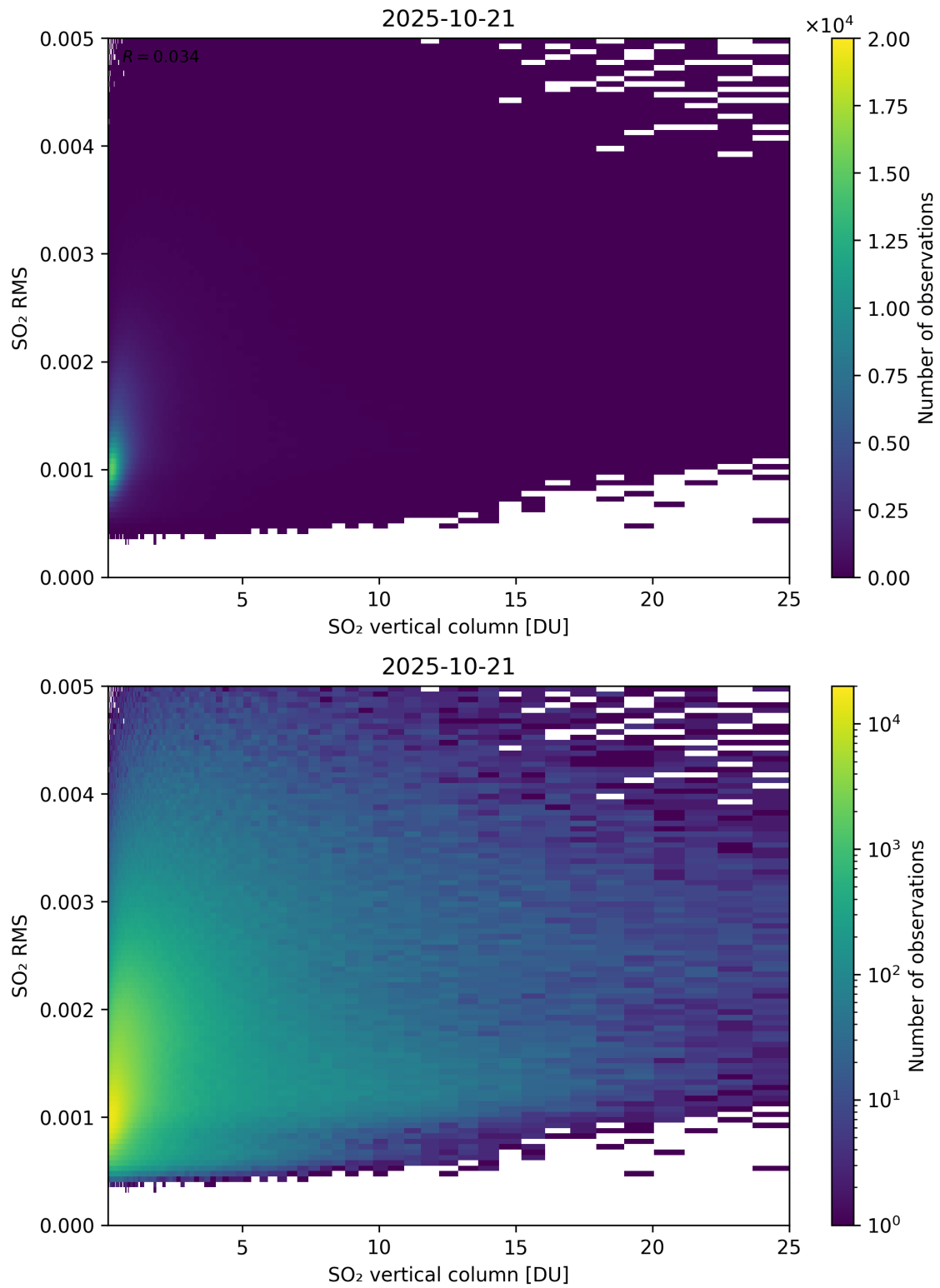
Figure 328: Scatter density plot of “SO 2 vertical column” against “SO 2 RMS” for 2025-10-20 to 2025-10-22.
