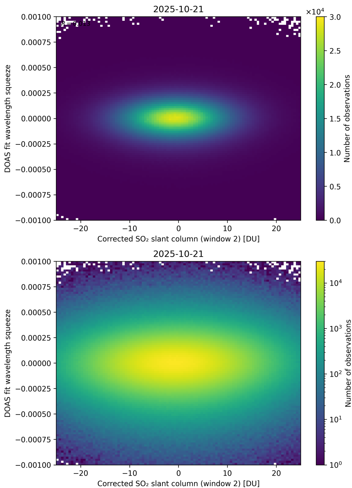
Figure 247: Scatter density plot of “Corrected SO 2 slant column (window 2)” against “DOAS fit wavelength squeeze” for 2025-10-20 to 2025-10-22.
