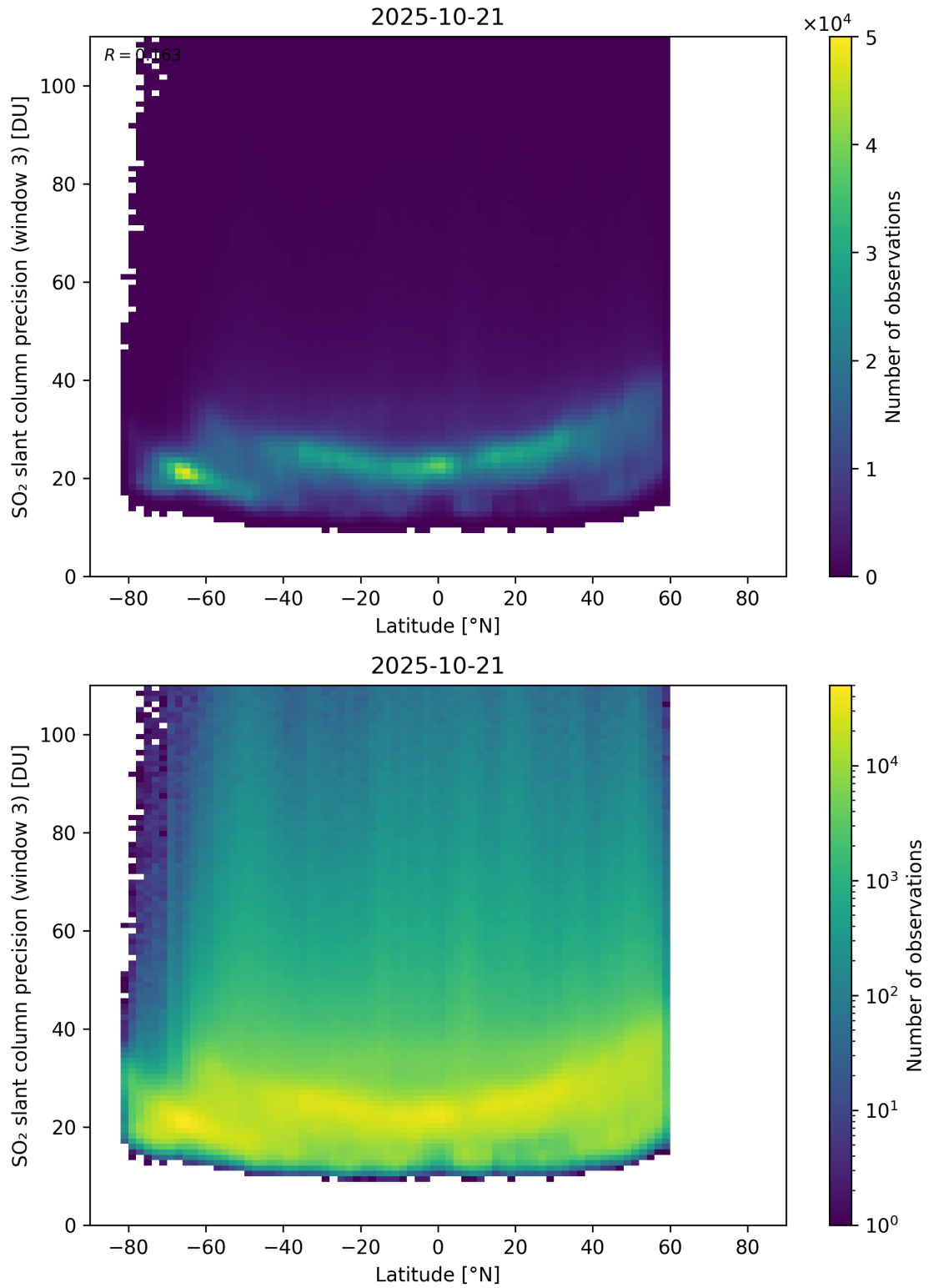
Figure 166: Scatter density plot of “Latitude” against “SO 2 slant column precision (window 3)” for 2025-10-20 to 2025-10-22.
