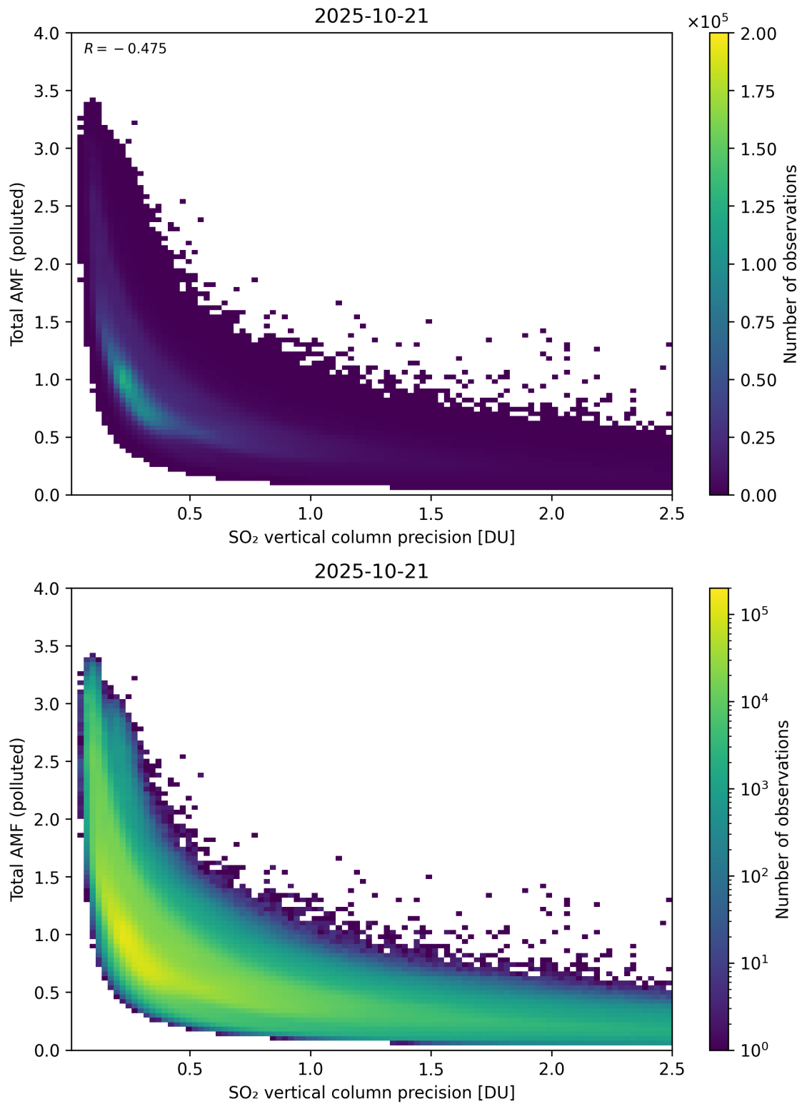
Figure 346: Scatter density plot of “SO 2 vertical column precision” against “Total AMF (polluted)” for 2025-10-20 to 2025-10-22.
