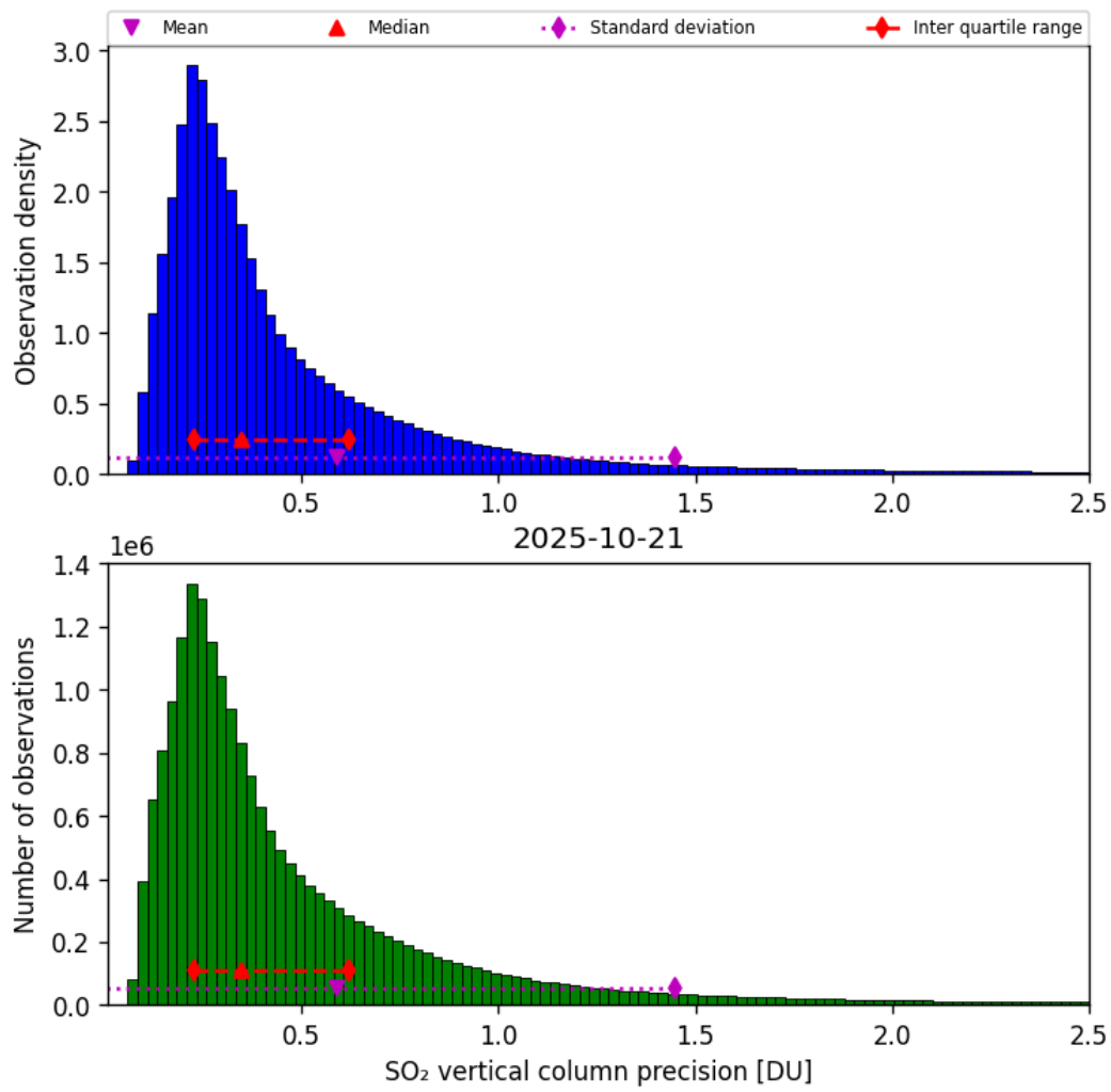
Figure 59: Histogram of “SO 2 vertical column precision” for 2025-10-20 to 2025-10-22
