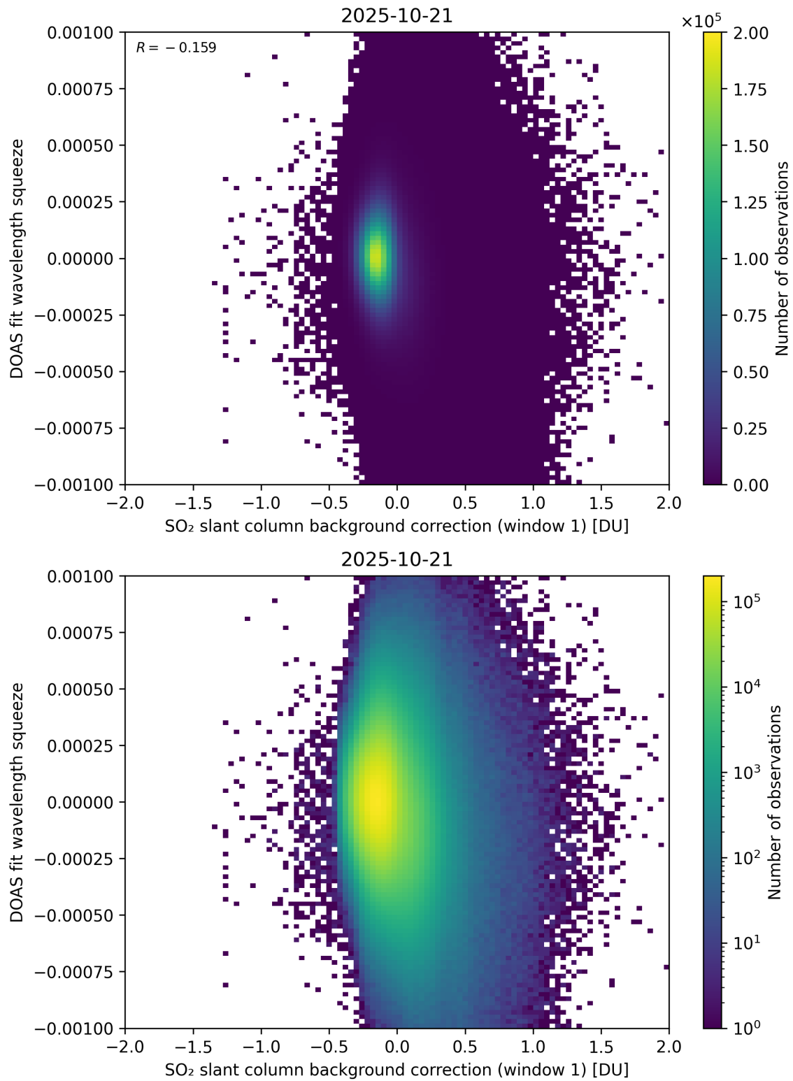
Figure 112: Scatter density plot of “SO 2 slant column background correction (window 1)” against “DOAS fit wavelength squeeze” for 2025-10-20 to 2025-10-22.
