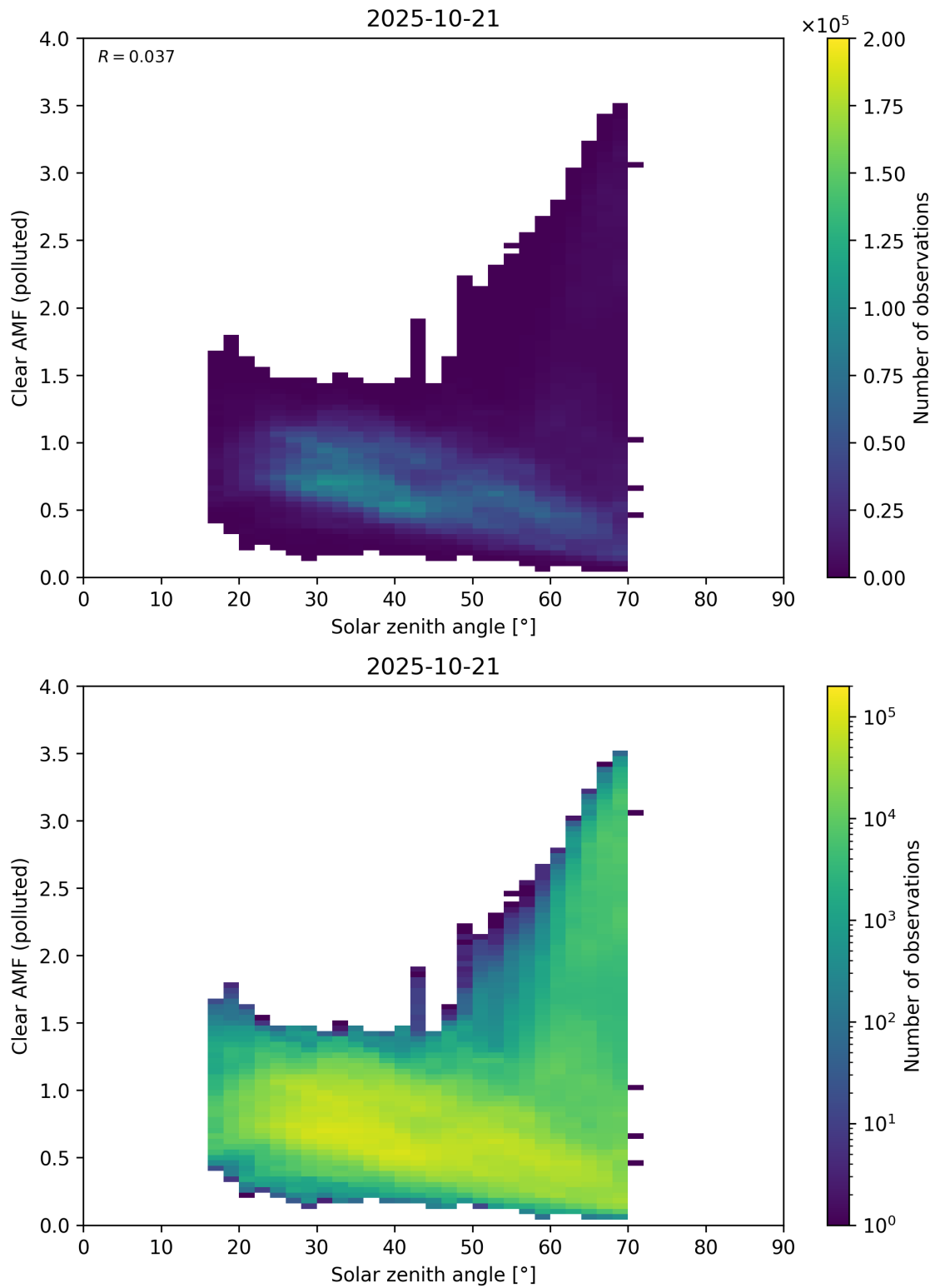
Figure 178: Scatter density plot of “Solar zenith angle” against “Clear AMF (polluted)” for 2025-10-20 to 2025-10-22.
