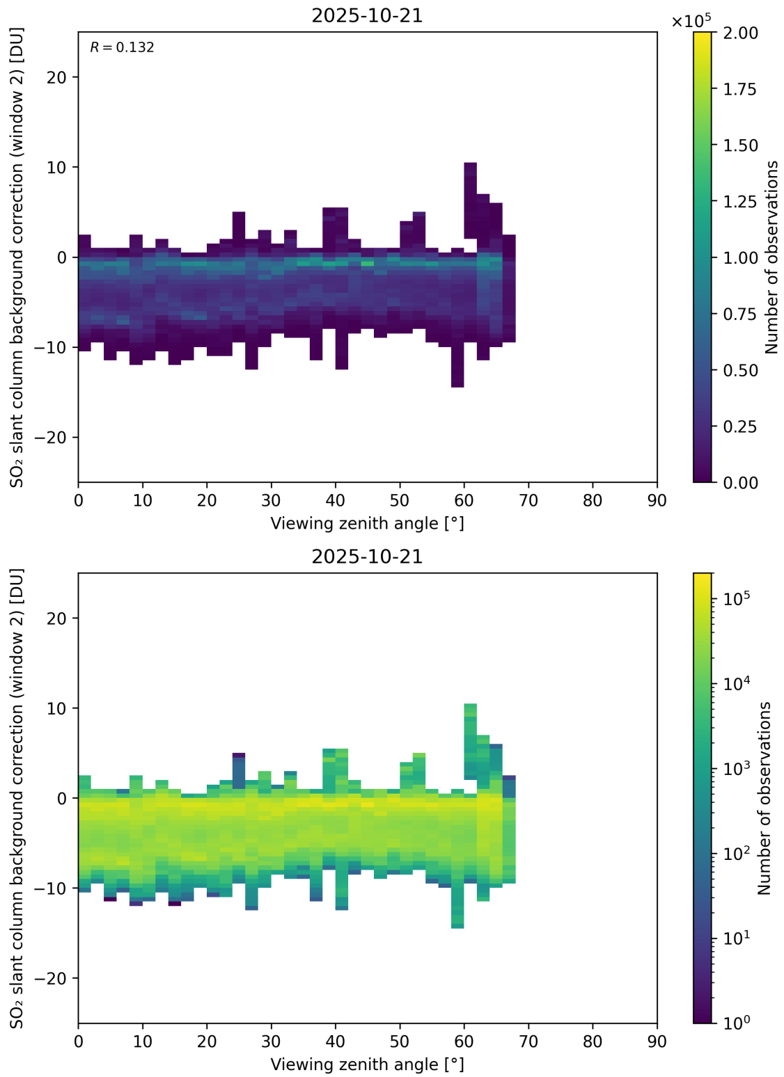
Figure 363: Scatter density plot of “Viewing zenith angle” against “SO 2 slant column background correction (window 2)” for 2025-10-20 to 2025-10-22.
