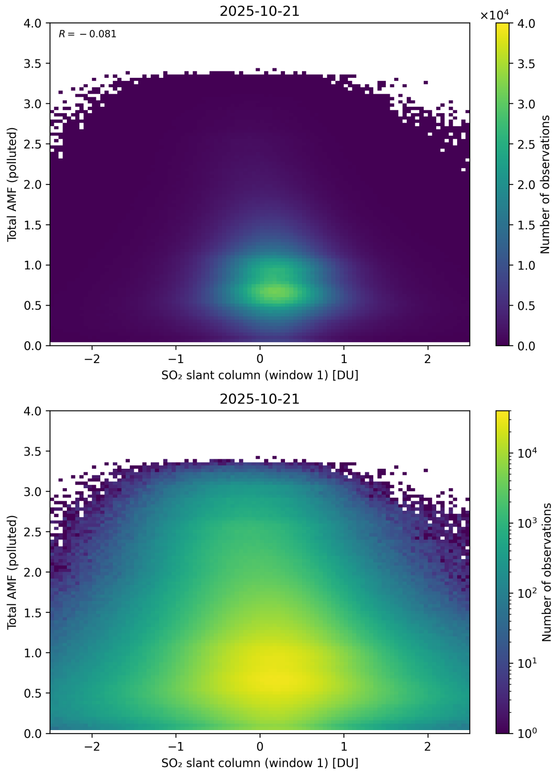
Figure 289: Scatter density plot of “SO 2 slant column (window 1)” against “Total AMF (polluted)” for 2025-10-20 to 2025-10-22.
