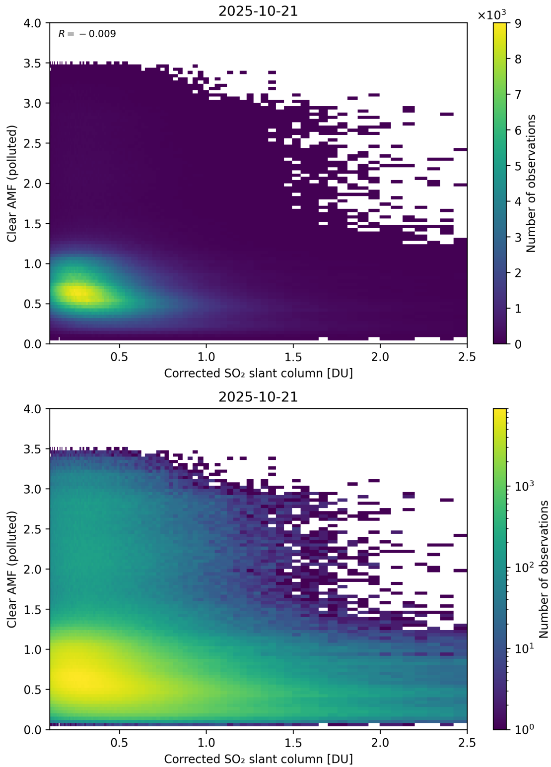
Figure 232: Scatter density plot of “Corrected SO 2 slant column” against “Clear AMF (polluted)” for 2025-10-20 to 2025-10-22.
