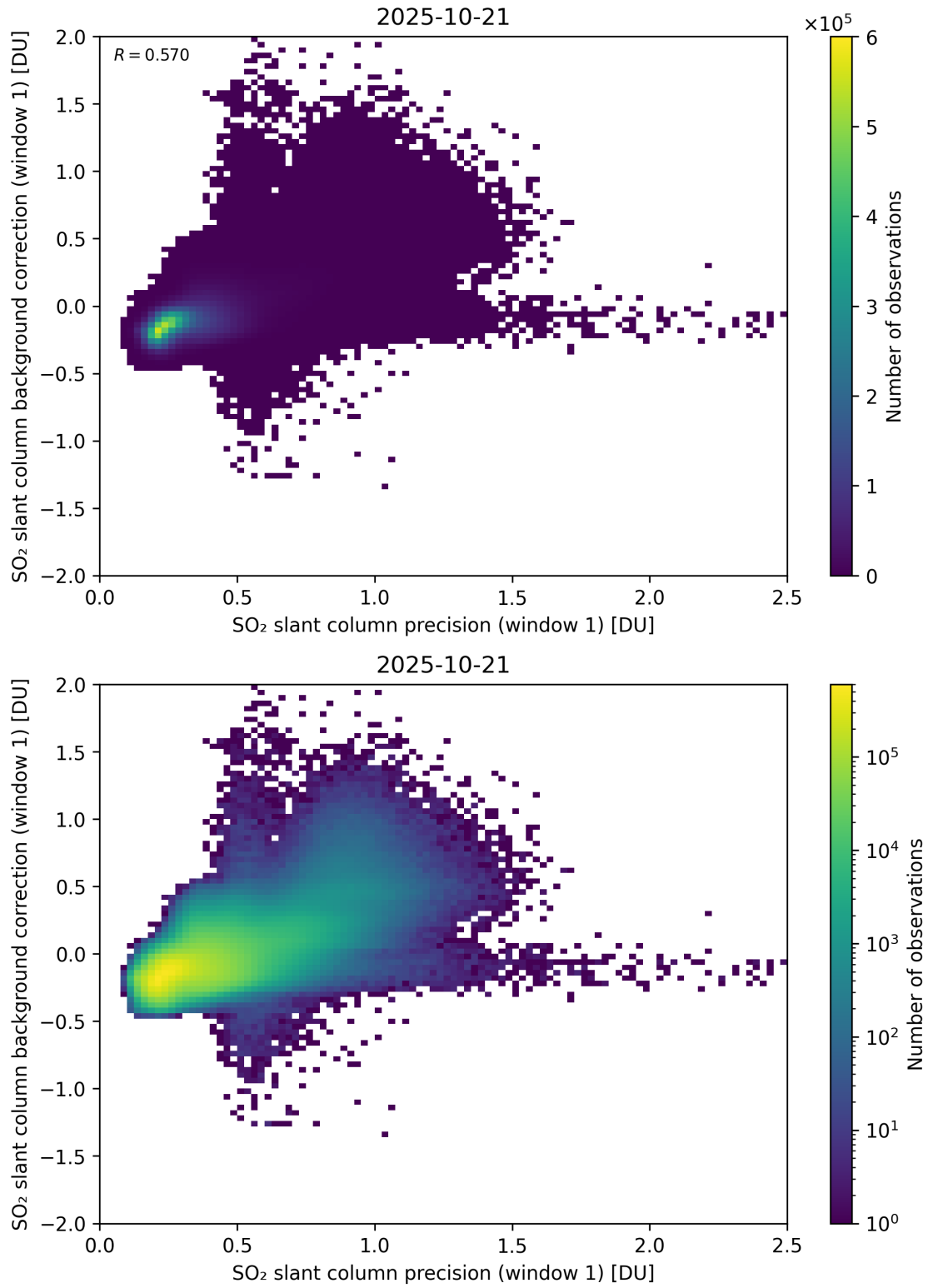
Figure 268: Scatter density plot of “SO 2 slant column precision (window 1)” against “SO 2 slant column background correction (window 1)” for 2025-10-20 to 2025-10-22.
