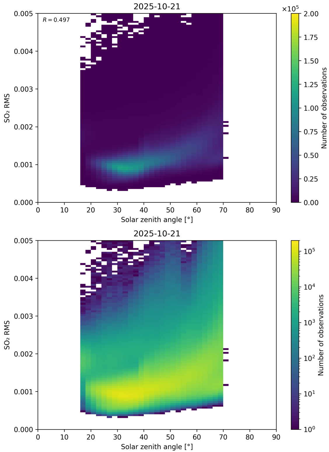
Figure 176: Scatter density plot of “Solar zenith angle” against “SO 2 RMS” for 2025-10-20 to 2025-10-22.
