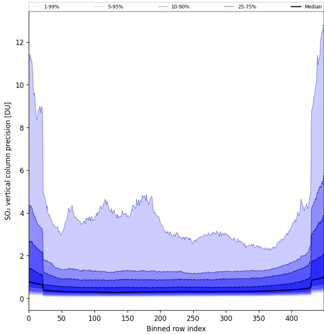
Figure 85: Along track statistics of “SO 2 vertical column precision” for 2025-10-20 to 2025-10-22
