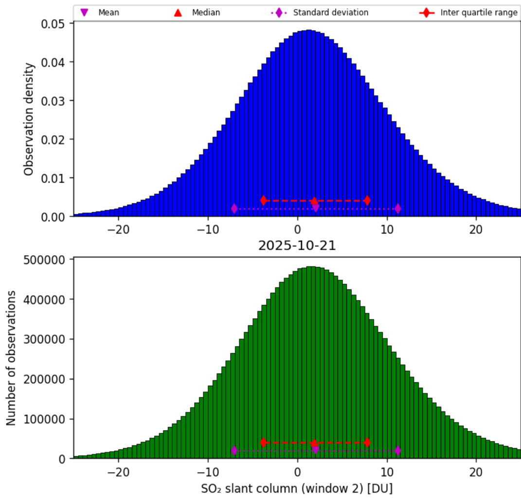
Figure 67: Histogram of “SO 2 slant column (window 2)” for 2025-10-20 to 2025-10-22
