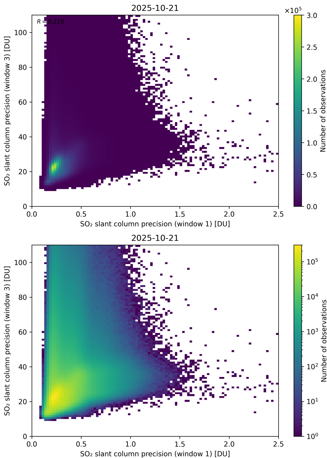
Figure 279: Scatter density plot of “SO 2 slant column precision (window 1)” against “SO 2 slant column precision (window 3)” for 2025-10-20 to 2025-10-22.
