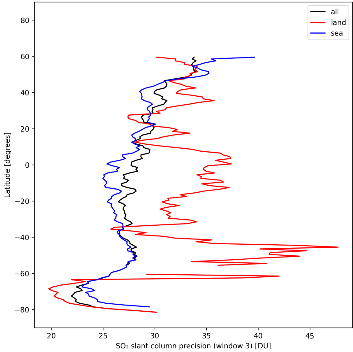
Figure 46: Zonal average of “SO 2 slant column precision (window 3)” for 2025-10-20 to 2025-10-22.
