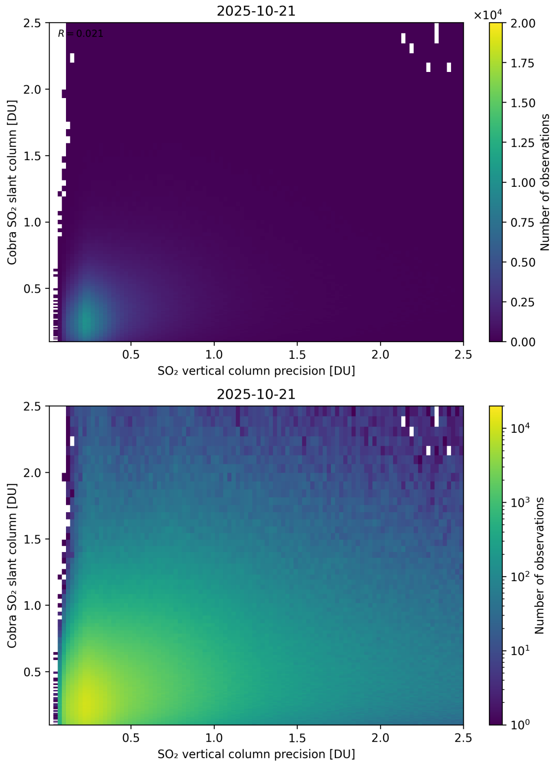
Figure 336: Scatter density plot of “SO 2 vertical column precision” against “Cobra SO 2 slant column” for 2025-10-20 to 2025-10-22.
