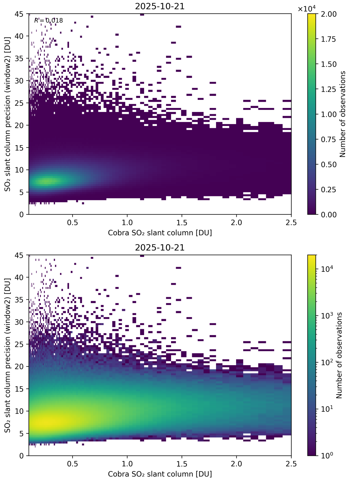
Figure 221: Scatter density plot of “Cobra SO 2 slant column” against “SO 2 slant column precision (window2)” for 2025-10-20 to 2025-10-22.
