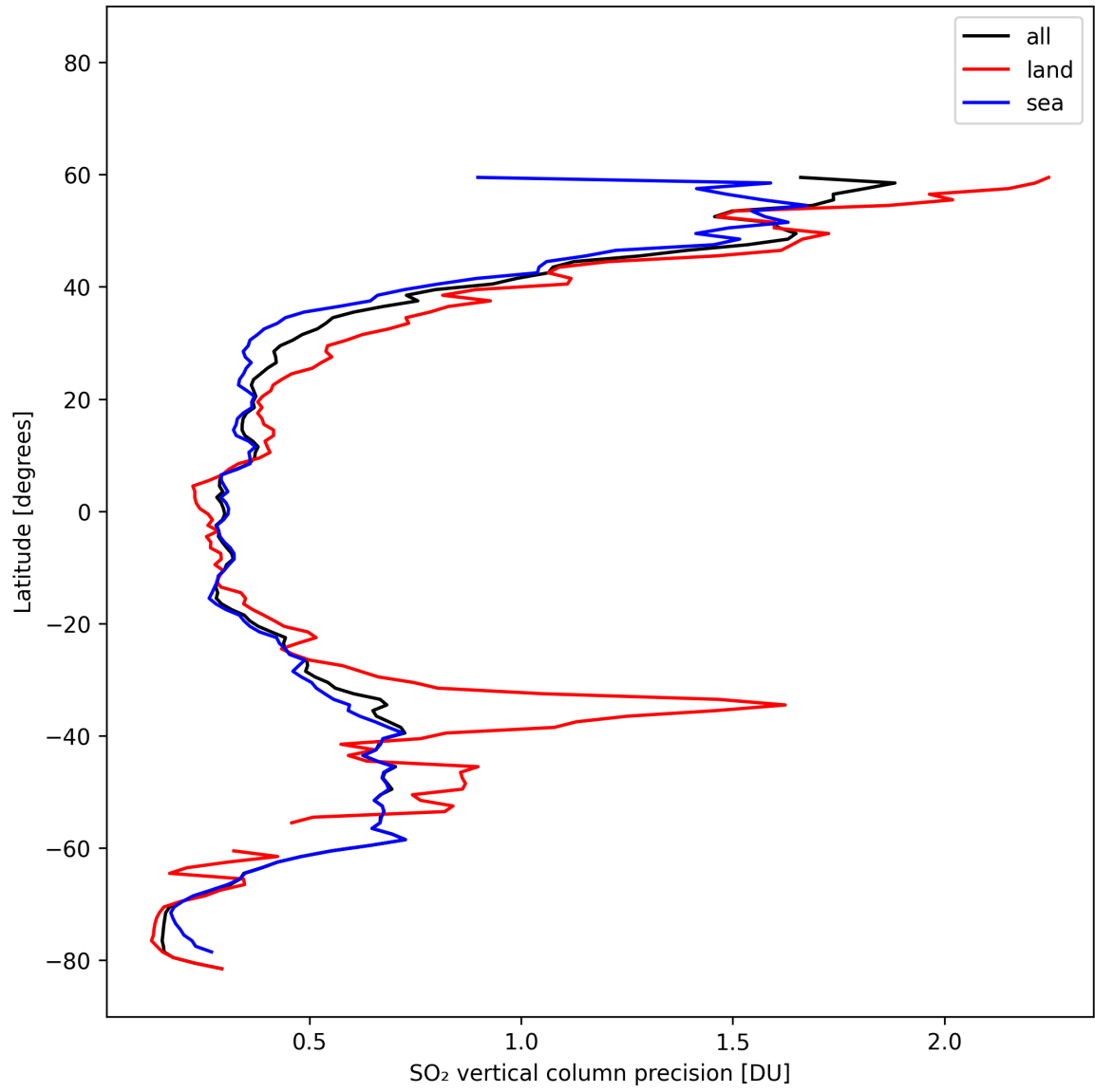
Figure 33: Zonal average of “SO 2 vertical column precision” for 2025-10-20 to 2025-10-22.
