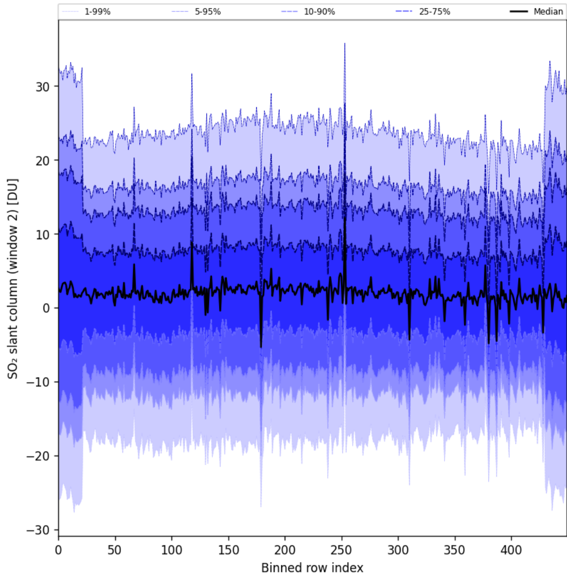
Figure 93: Along track statistics of “SO 2 slant column (window 2)” for 2025-10-20 to 2025-10-22
