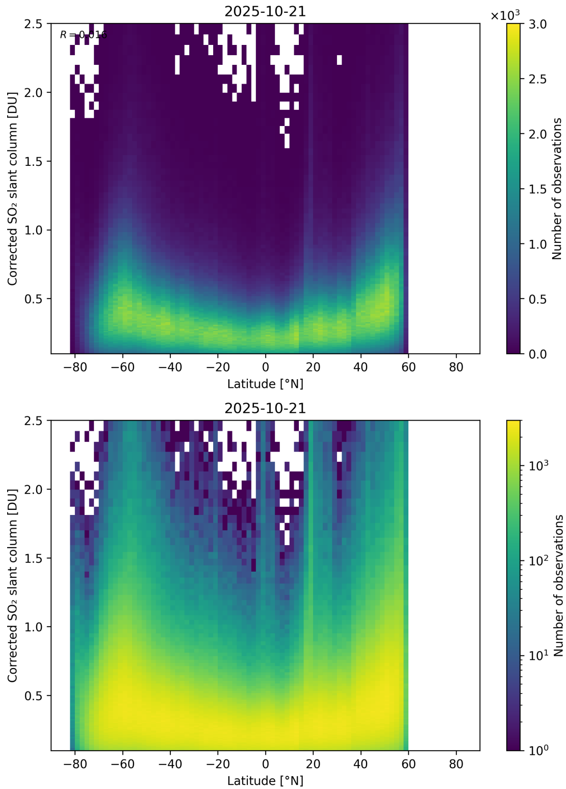
Figure 159: Scatter density plot of “Latitude” against “Corrected SO 2 slant column” for 2025-10-20 to 2025-10-22.
