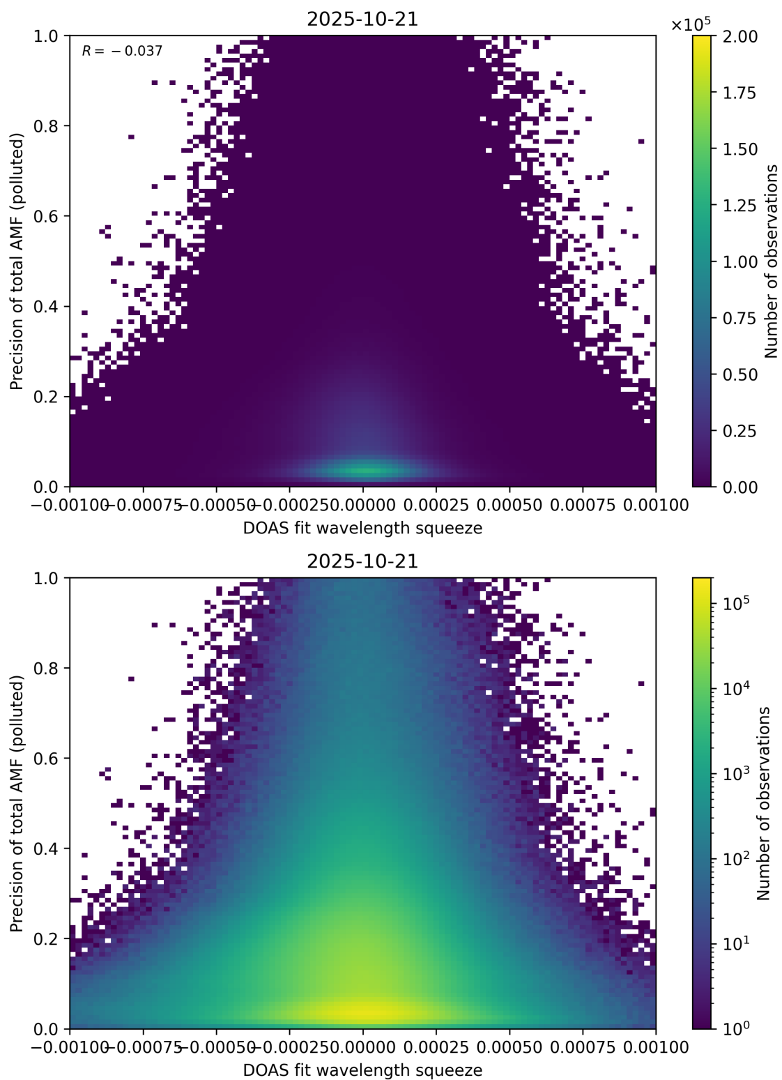
Figure 146: Scatter density plot of “DOAS fit wavelength squeeze” against “Precision of total AMF (polluted)” for 2025-10-20 to 2025-10-22.
