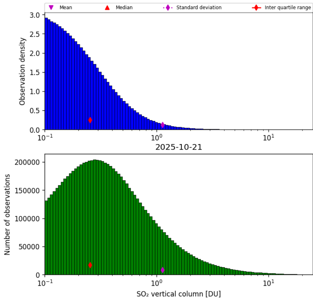
Figure 58: Histogram of “SO 2 vertical column” for 2025-10-20 to 2025-10-22
