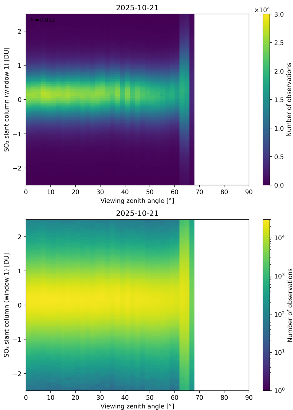
Figure 376: Scatter density plot of “Viewing zenith angle” against “SO 2 slant column (window 1)” for 2025-10-20 to 2025-10-22.
