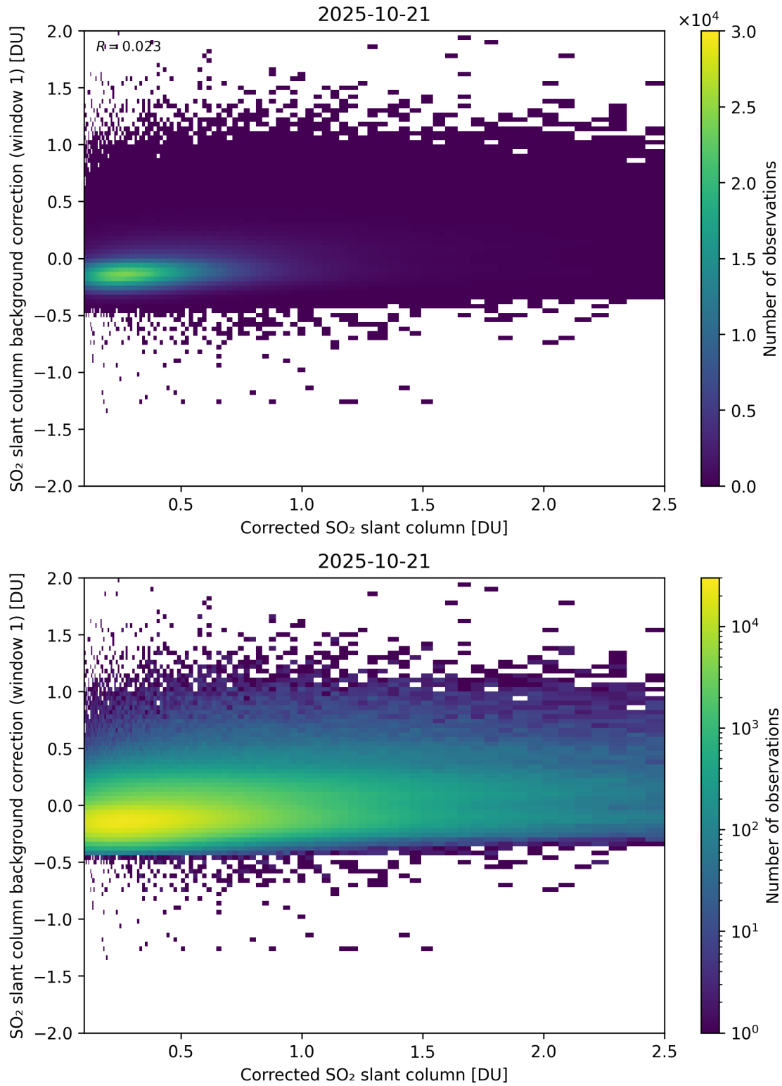
Figure 226: Scatter density plot of “Corrected SO 2 slant column” against “SO 2 slant column background correction (window 1)” for 2025-10-20 to 2025-10-22.
