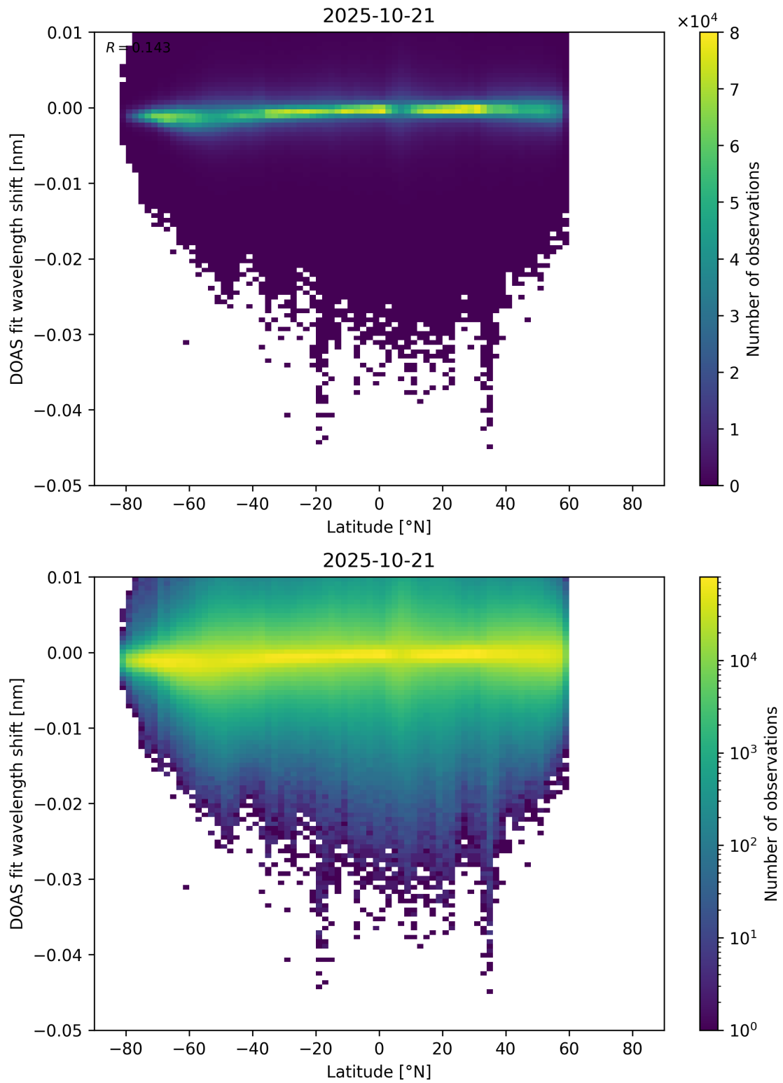
Figure 153: Scatter density plot of “Latitude” against “DOAS fit wavelength shift” for 2025-10-20 to 2025-10-22.
