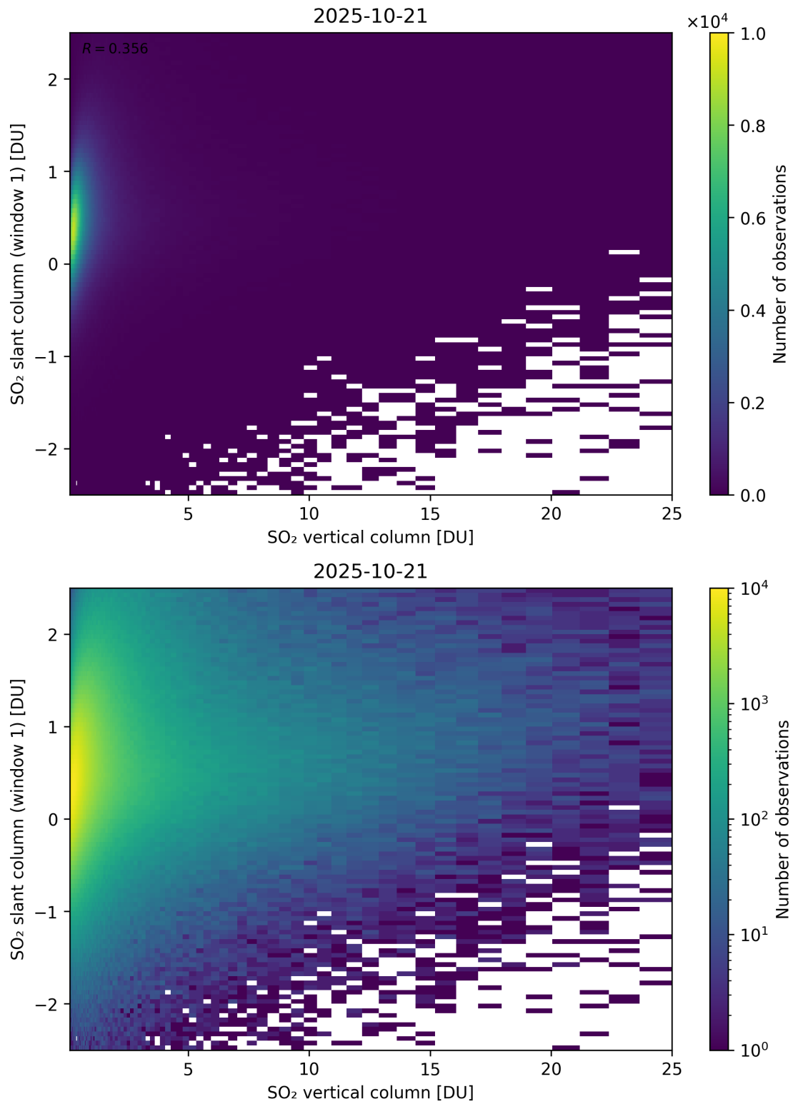
Figure 354: Scatter density plot of “SO 2 vertical column” against “SO 2 slant column (window 1)” for 2025-10-20 to 2025-10-22.
