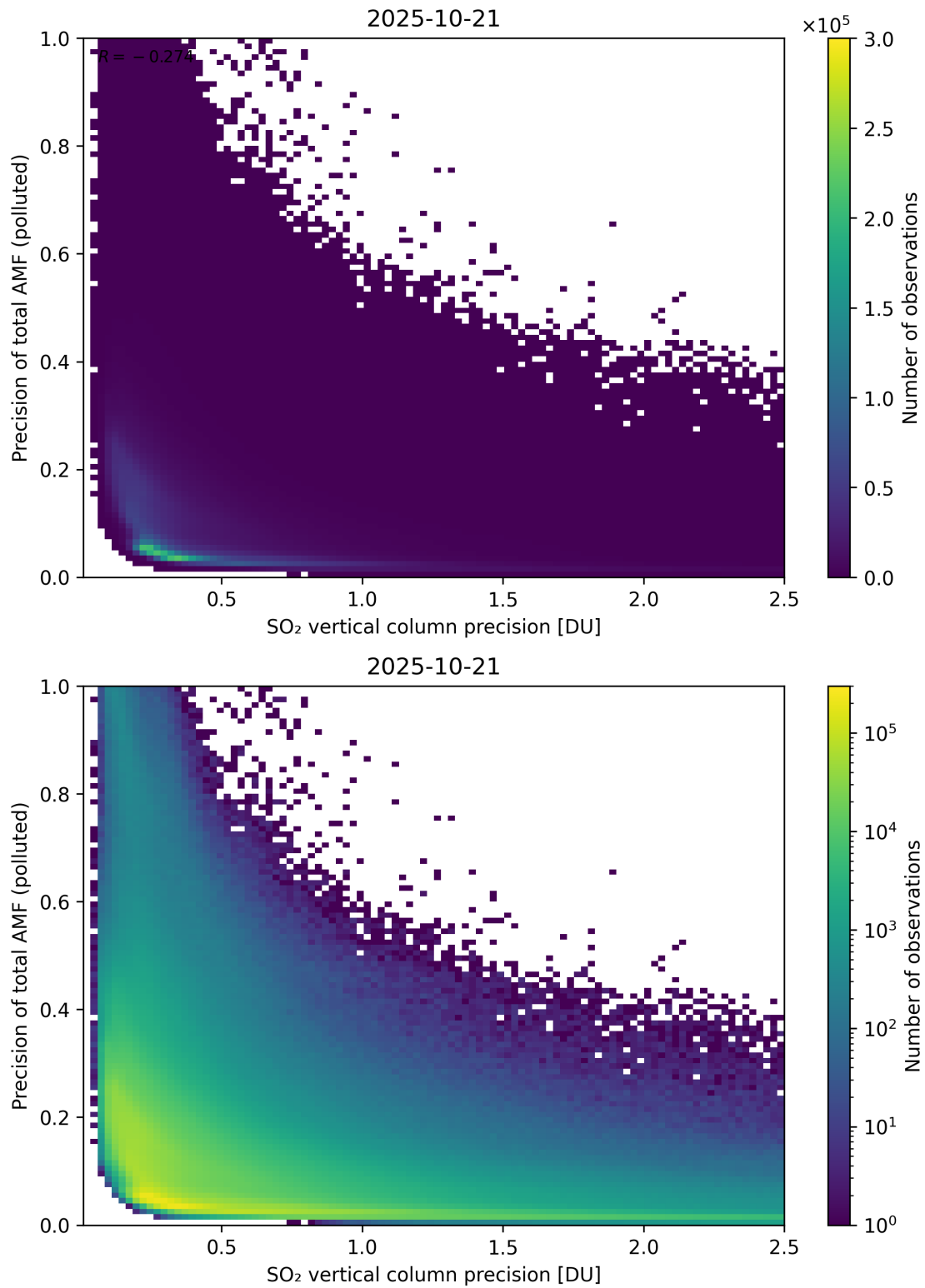
Figure 347: Scatter density plot of “SO 2 vertical column precision” against “Precision of total AMF (polluted)” for 2025-10-20 to 2025-10-22.
