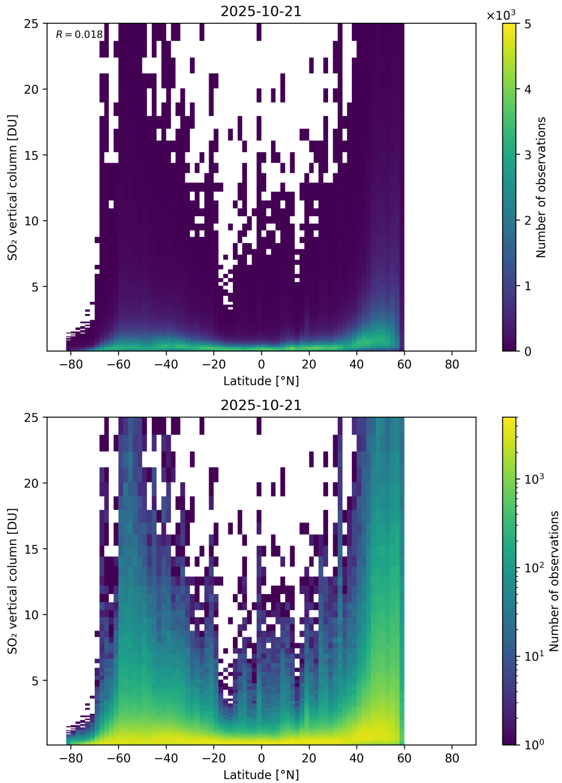
Figure 169: Scatter density plot of “Latitude” against “SO 2 vertical column” for 2025-10-20 to 2025-10-22.
