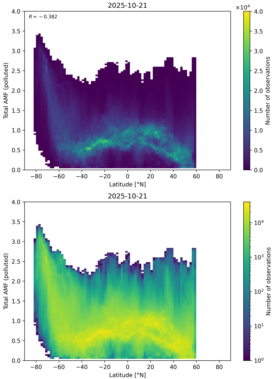
Figure 167: Scatter density plot of “Latitude” against “Total AMF (polluted)” for 2025-10-20 to 2025-10-22.
