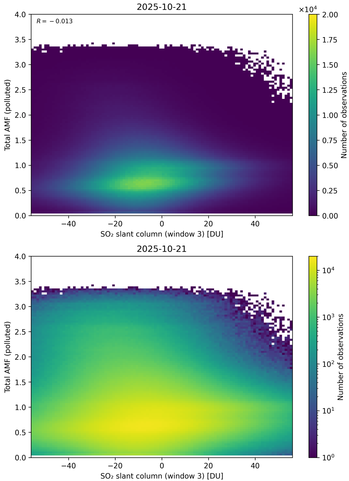
Figure 318: Scatter density plot of “SO 2 slant column (window 3)” against “Total AMF (polluted)” for 2025-10-20 to 2025-10-22.
