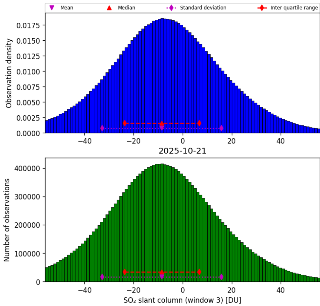
Figure 71: Histogram of “SO 2 slant column (window 3)” for 2025-10-20 to 2025-10-22
