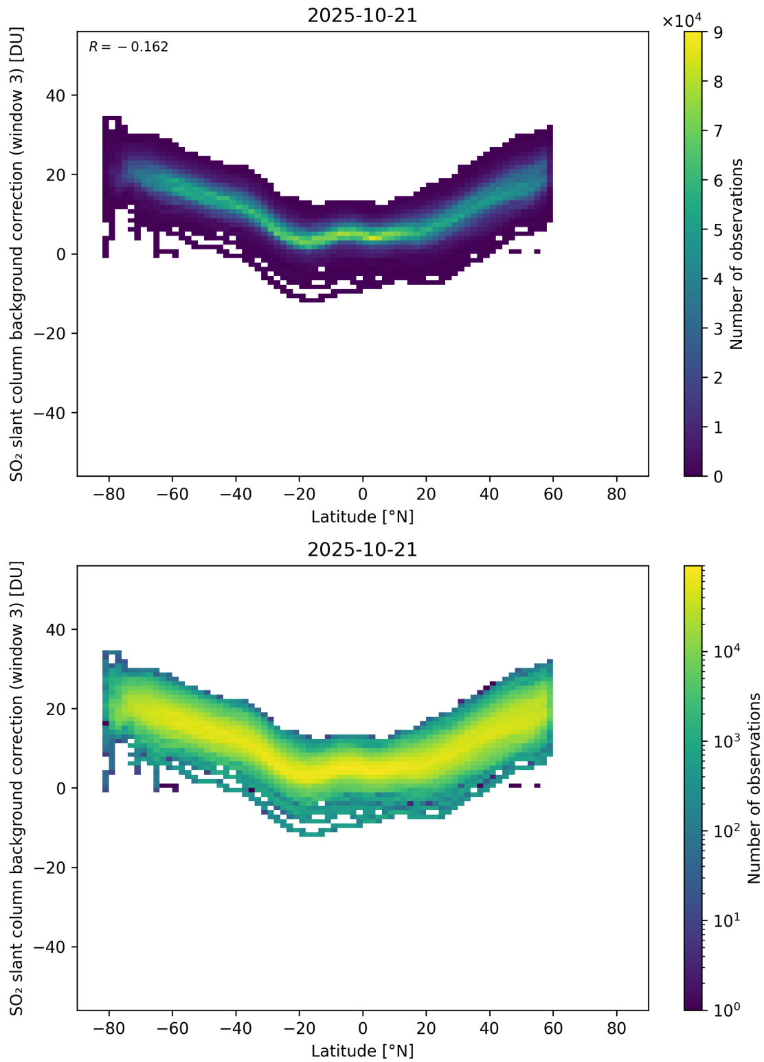
Figure 152: Scatter density plot of “Latitude” against “SO 2 slant column background correction (window 3)” for 2025-10-20 to 2025-10-22.
