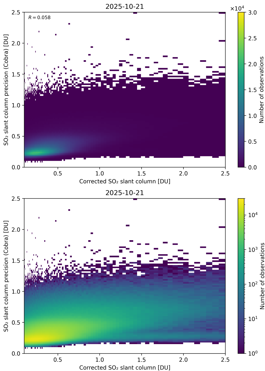
Figure 234: Scatter density plot of “Corrected SO 2 slant column” against “SO 2 slant column precision (Cobra)” for 2025-10-20 to 2025-10-22.
