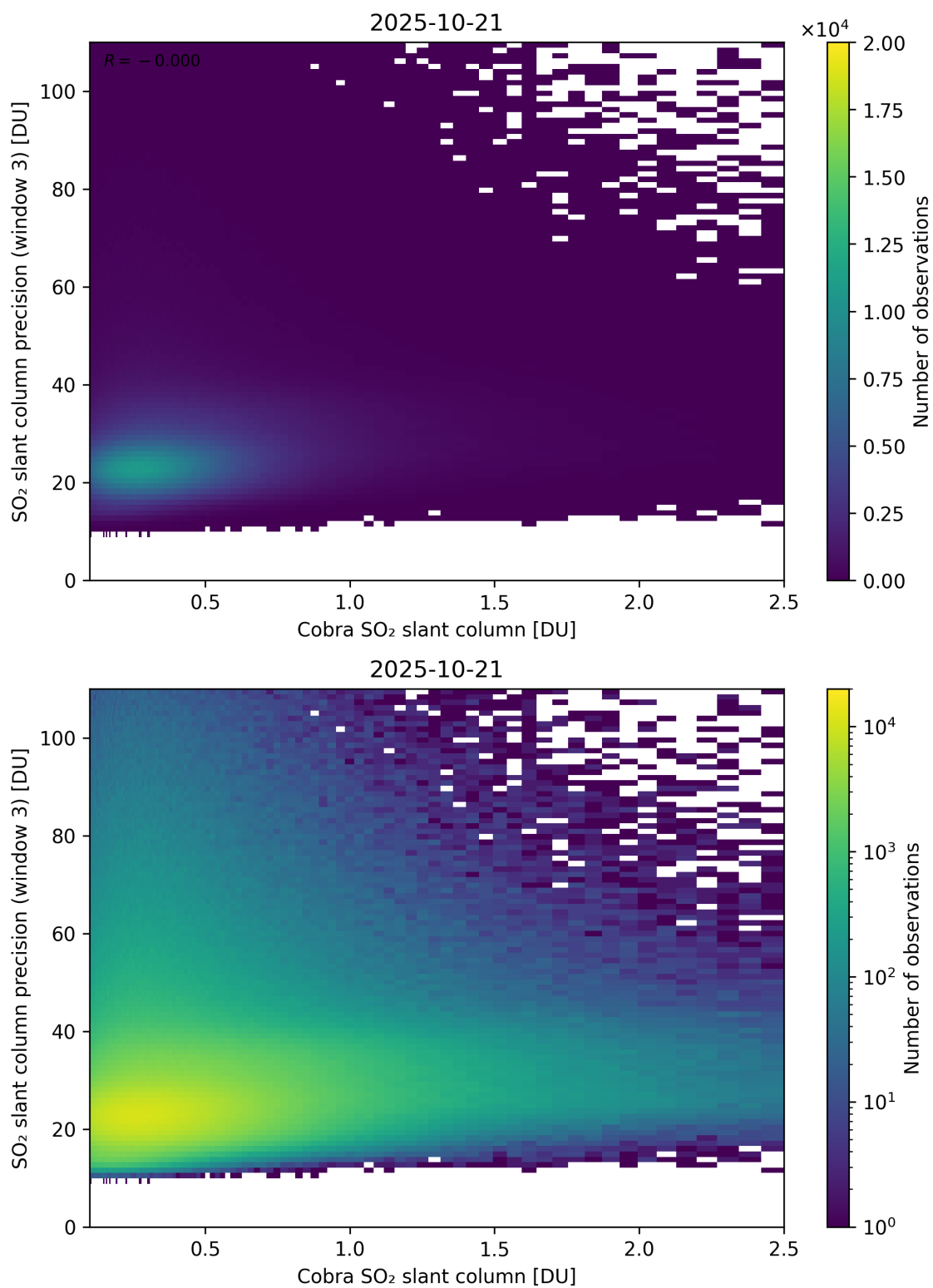
Figure 223: Scatter density plot of “Cobra SO 2 slant column” against “SO 2 slant column precision (window 3)” for 2025-10-20 to 2025-10-22.
