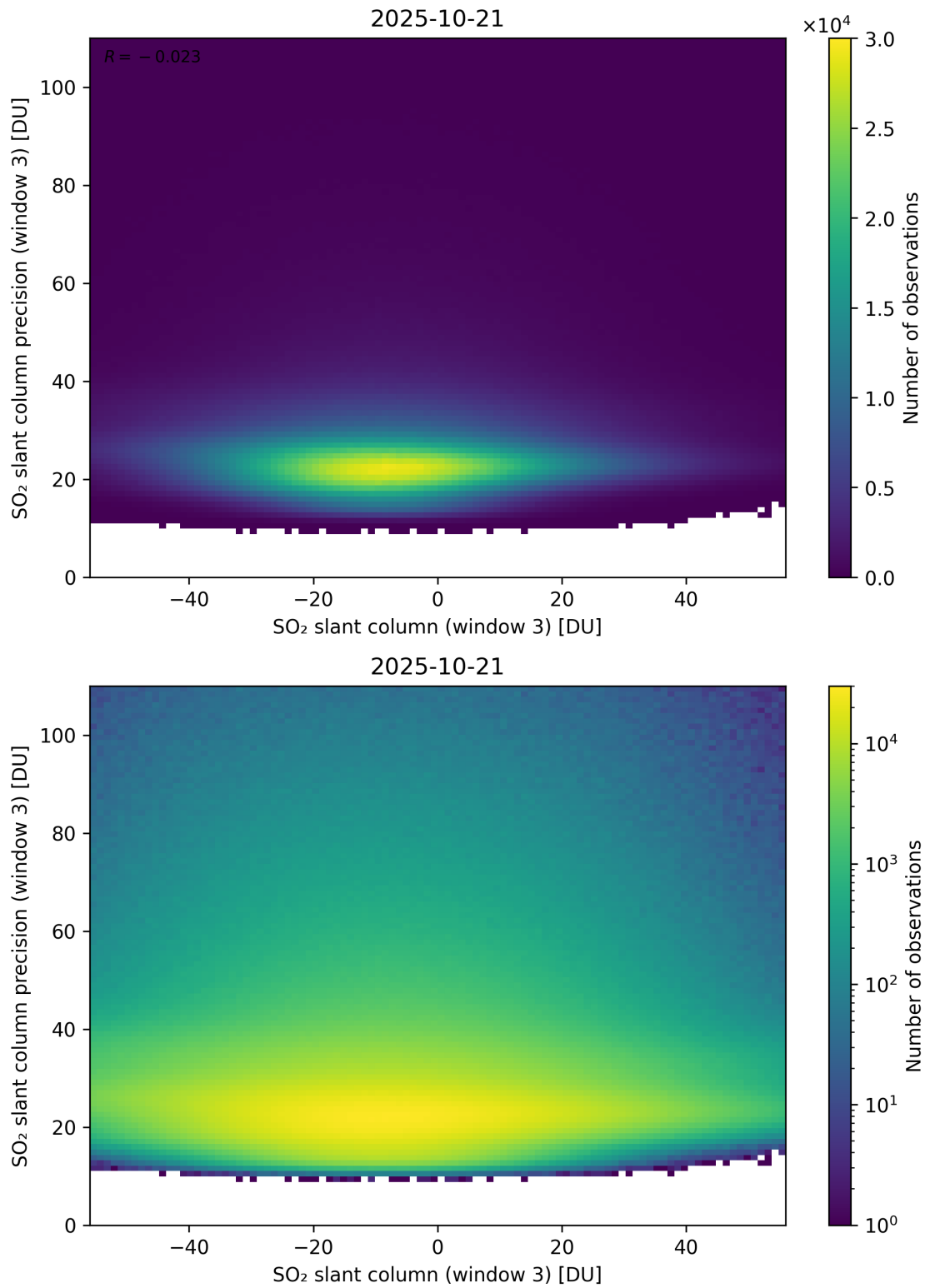
Figure 317: Scatter density plot of “SO 2 slant column (window 3)” against “SO 2 slant column precision (window 3)” for 2025-10-20 to 2025-10-22.
