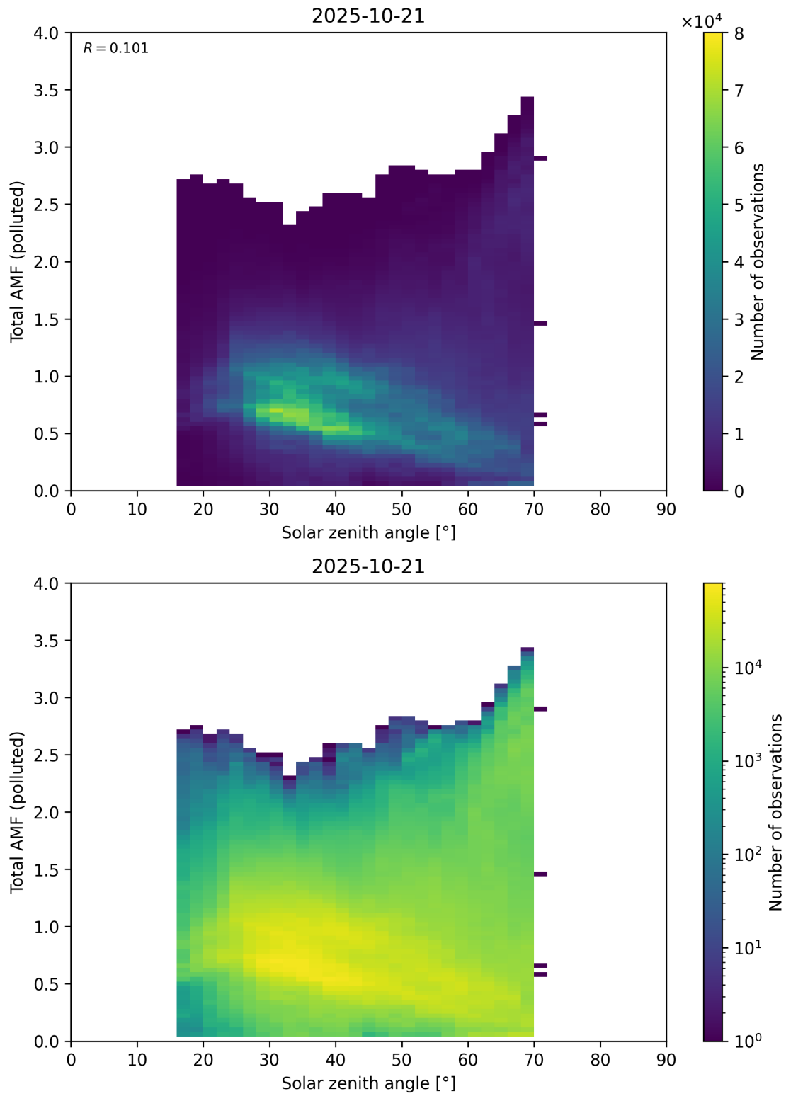
Figure 189: Scatter density plot of “Solar zenith angle” against “Total AMF (polluted)” for 2025-10-20 to 2025-10-22.
