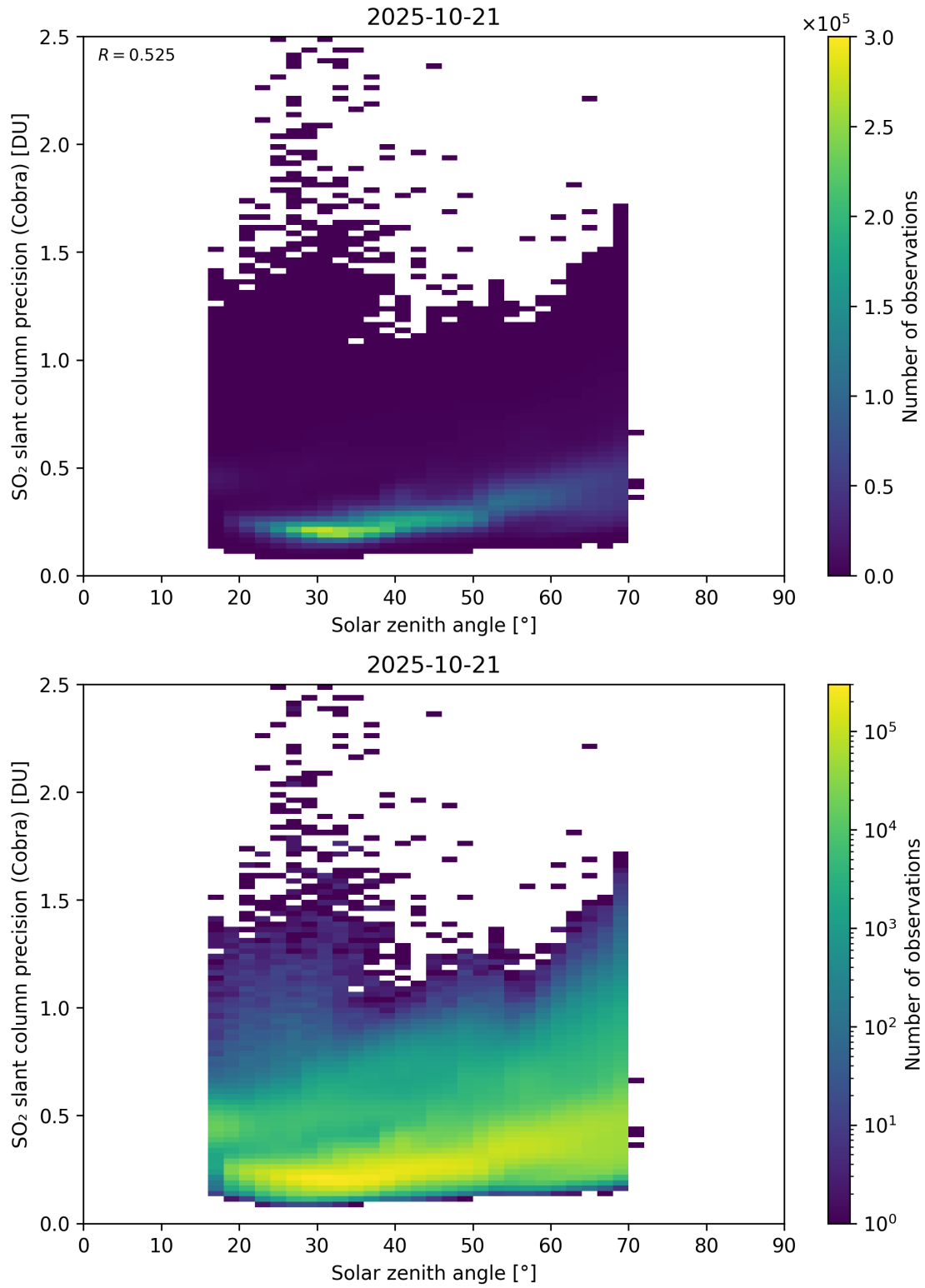
Figure 180: Scatter density plot of “Solar zenith angle” against “SO 2 slant column precision (Cobra)” for 2025-10-20 to 2025-10-22.
