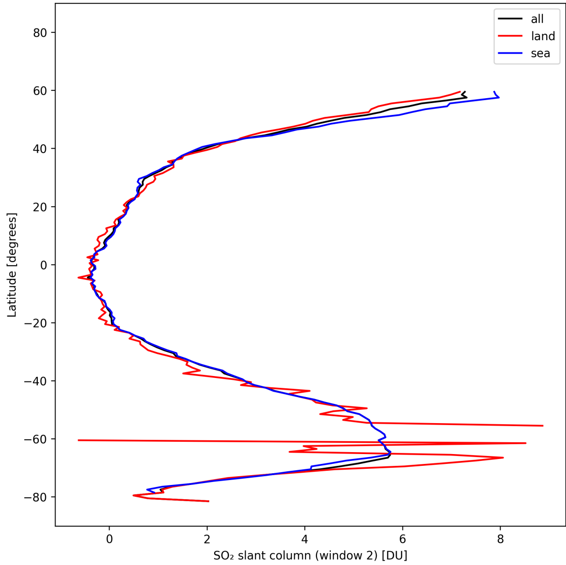
Figure 41: Zonal average of “SO 2 slant column (window 2)” for 2025-10-20 to 2025-10-22.
