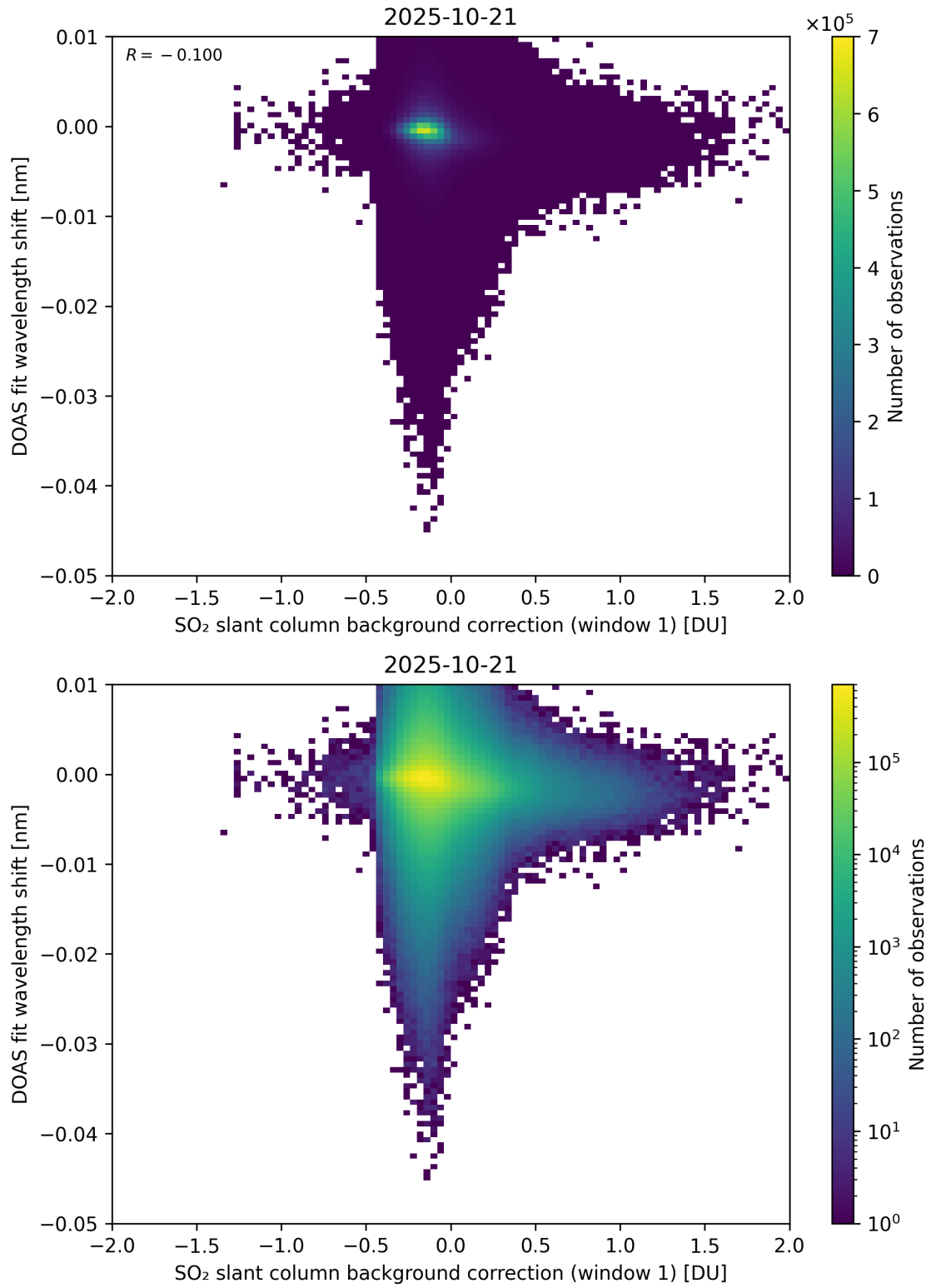
Figure 111: Scatter density plot of “SO 2 slant column background correction (window 1)” against “DOAS fit wavelength shift” for 2025-10-20 to 2025-10-22.
