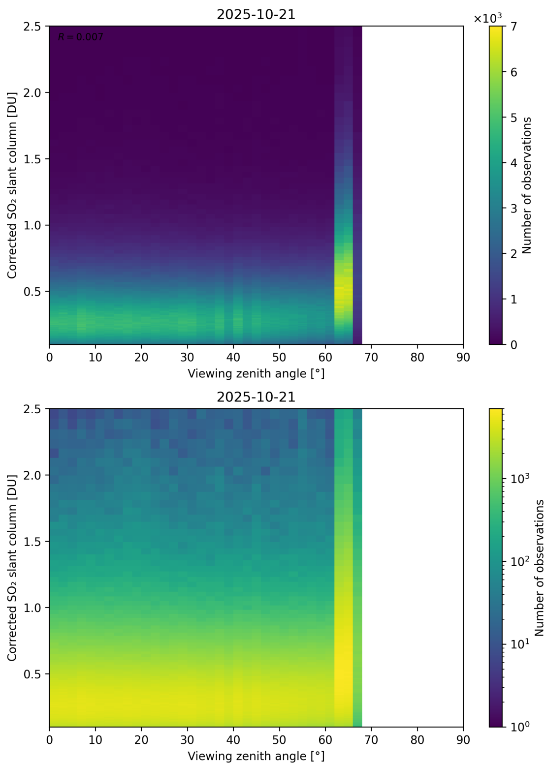
Figure 373: Scatter density plot of “Viewing zenith angle” against “Corrected SO 2 slant column” for 2025-10-20 to 2025-10-22.
