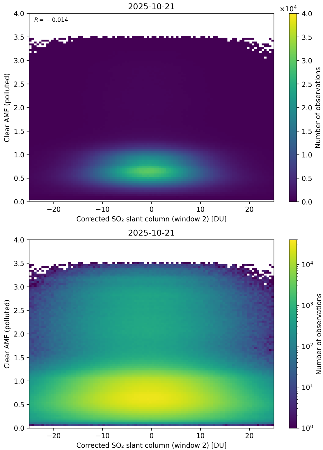
Figure 249: Scatter density plot of “Corrected SO 2 slant column (window 2)” against “Clear AMF (polluted)” for 2025-10-20 to 2025-10-22.
