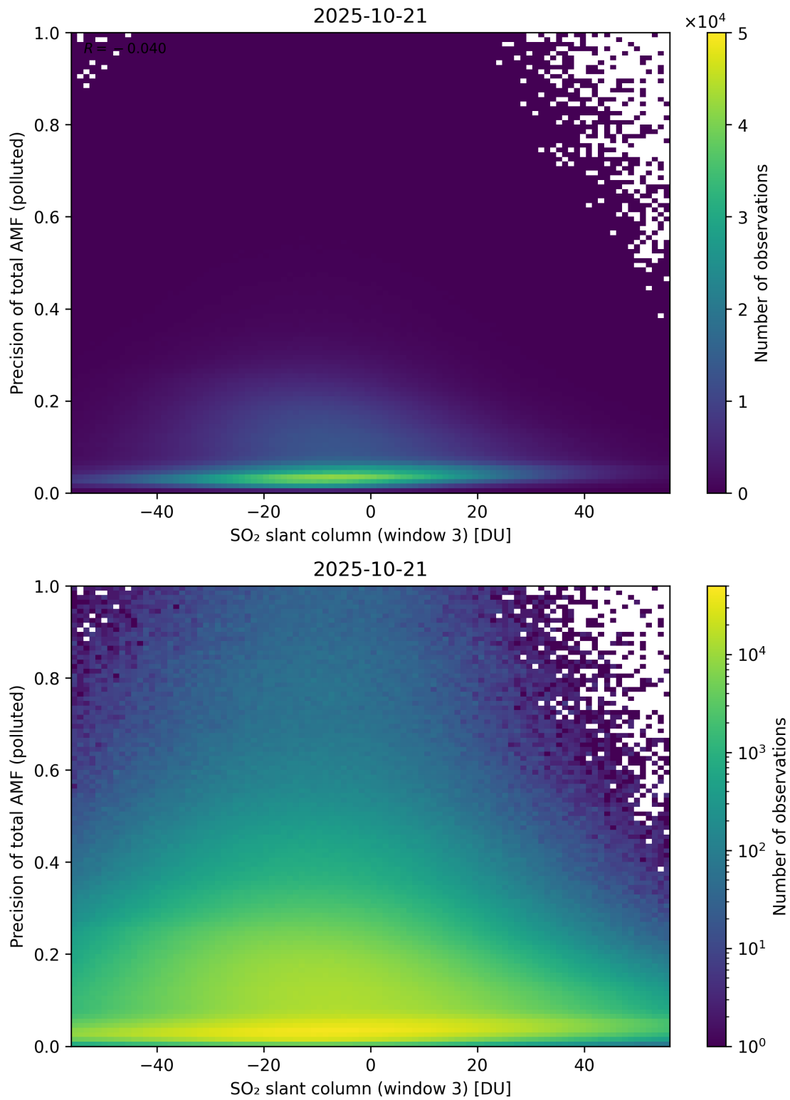
Figure 319: Scatter density plot of “SO 2 slant column (window 3)” against “Precision of total AMF (polluted)” for 2025-10-20 to 2025-10-22.
