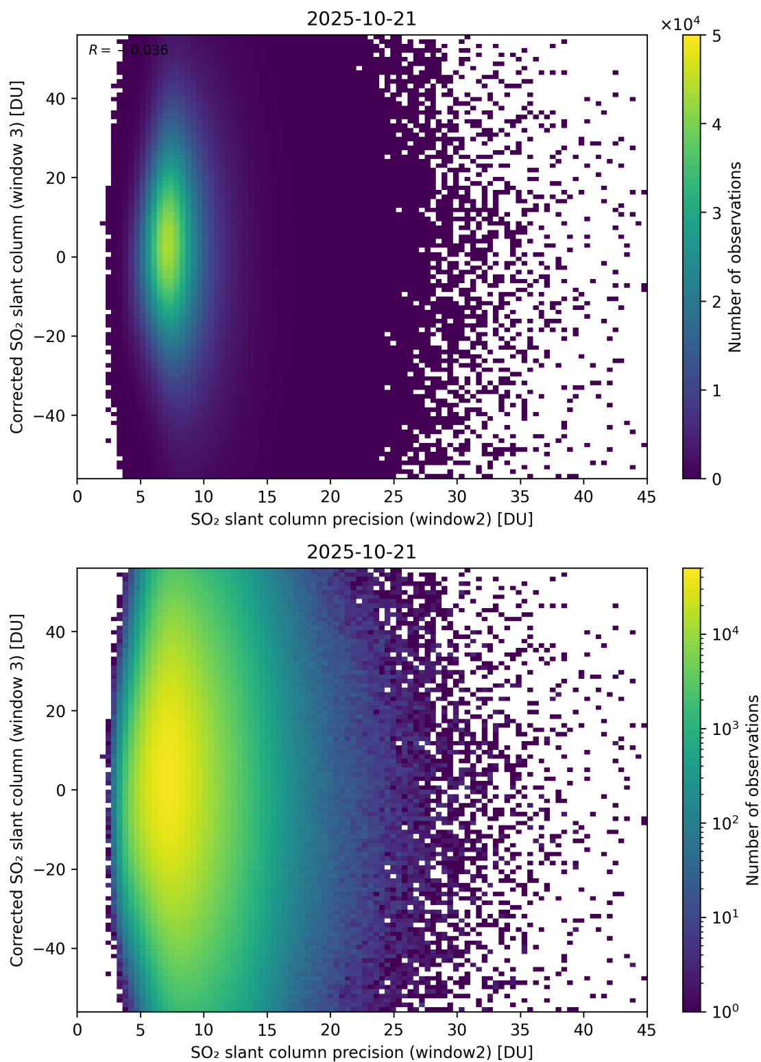
Figure 298: Scatter density plot of “SO 2 slant column precision (window2)” against “Corrected SO 2 slant column (window 3)” for 2025-10-20 to 2025-10-22.
