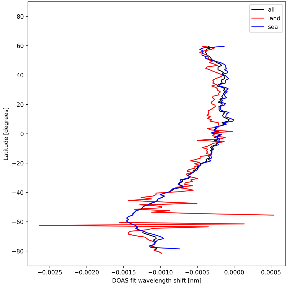
Figure 50: Zonal average of “DOAS fit wavelength shift” for 2025-10-20 to 2025-10-22.
