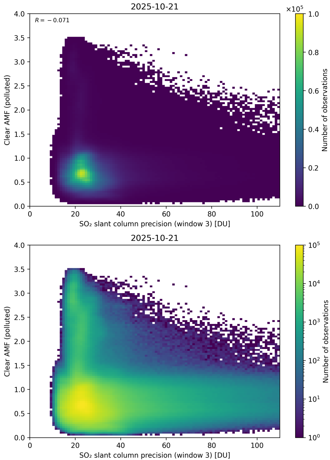
Figure 311: Scatter density plot of “SO 2 slant column precision (window 3)” against “Clear AMF (polluted)” for 2025-10-20 to 2025-10-22.
