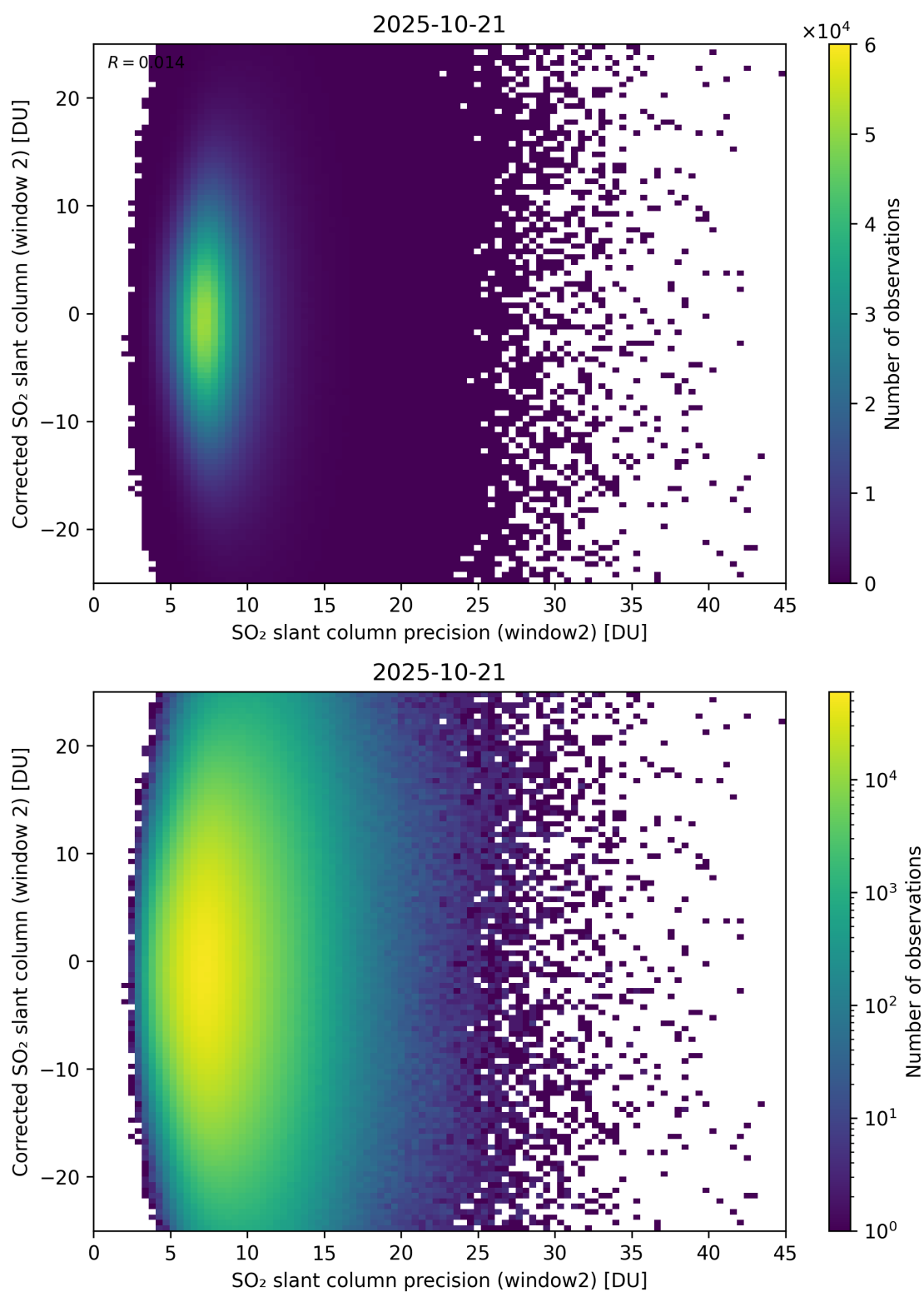
Figure 297: Scatter density plot of “SO 2 slant column precision (window2)” against “Corrected SO 2 slant column (window 2)” for 2025-10-20 to 2025-10-22.
