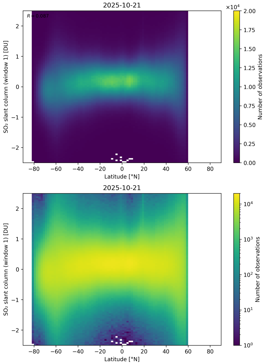
Figure 162: Scatter density plot of “Latitude” against “SO 2 slant column (window 1)” for 2025-10-20 to 2025-10-22.
