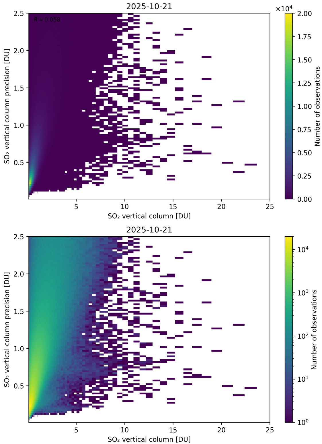
Figure 361: Scatter density plot of “SO 2 vertical column” against “SO 2 vertical column precision” for 2025-10-20 to 2025-10-22.
