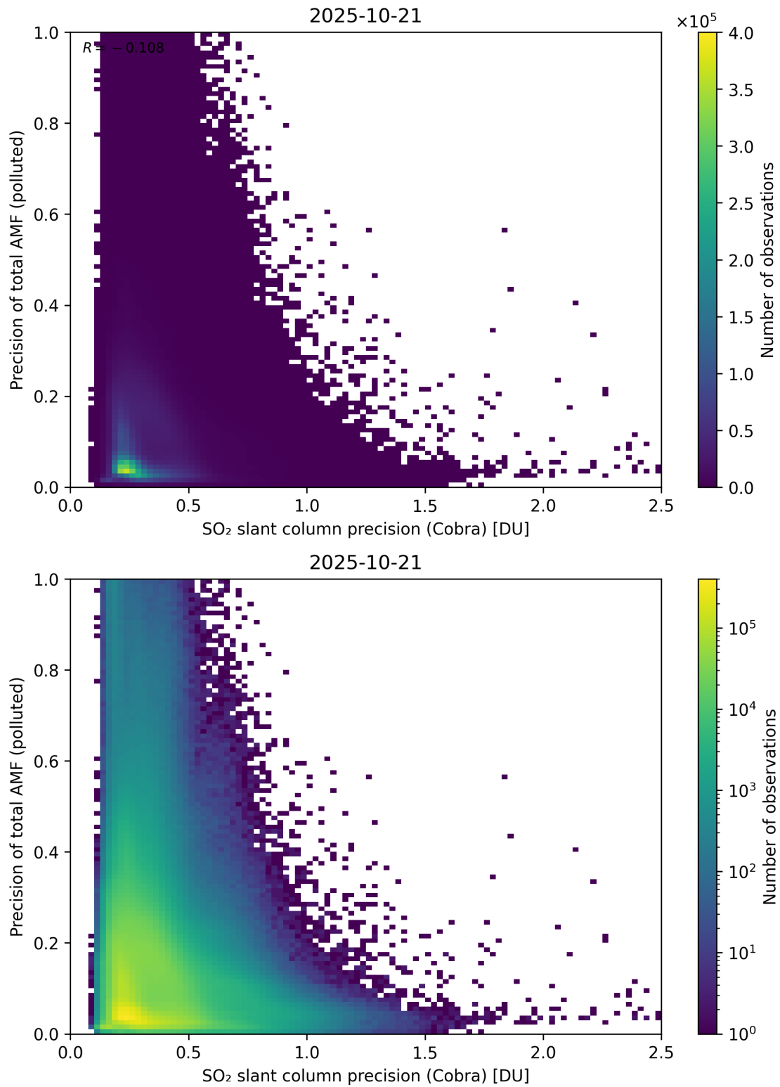
Figure 214: Scatter density plot of “SO 2 slant column precision (Cobra)” against “Precision of total AMF (polluted)” for 2025-10-20 to 2025-10-22.
