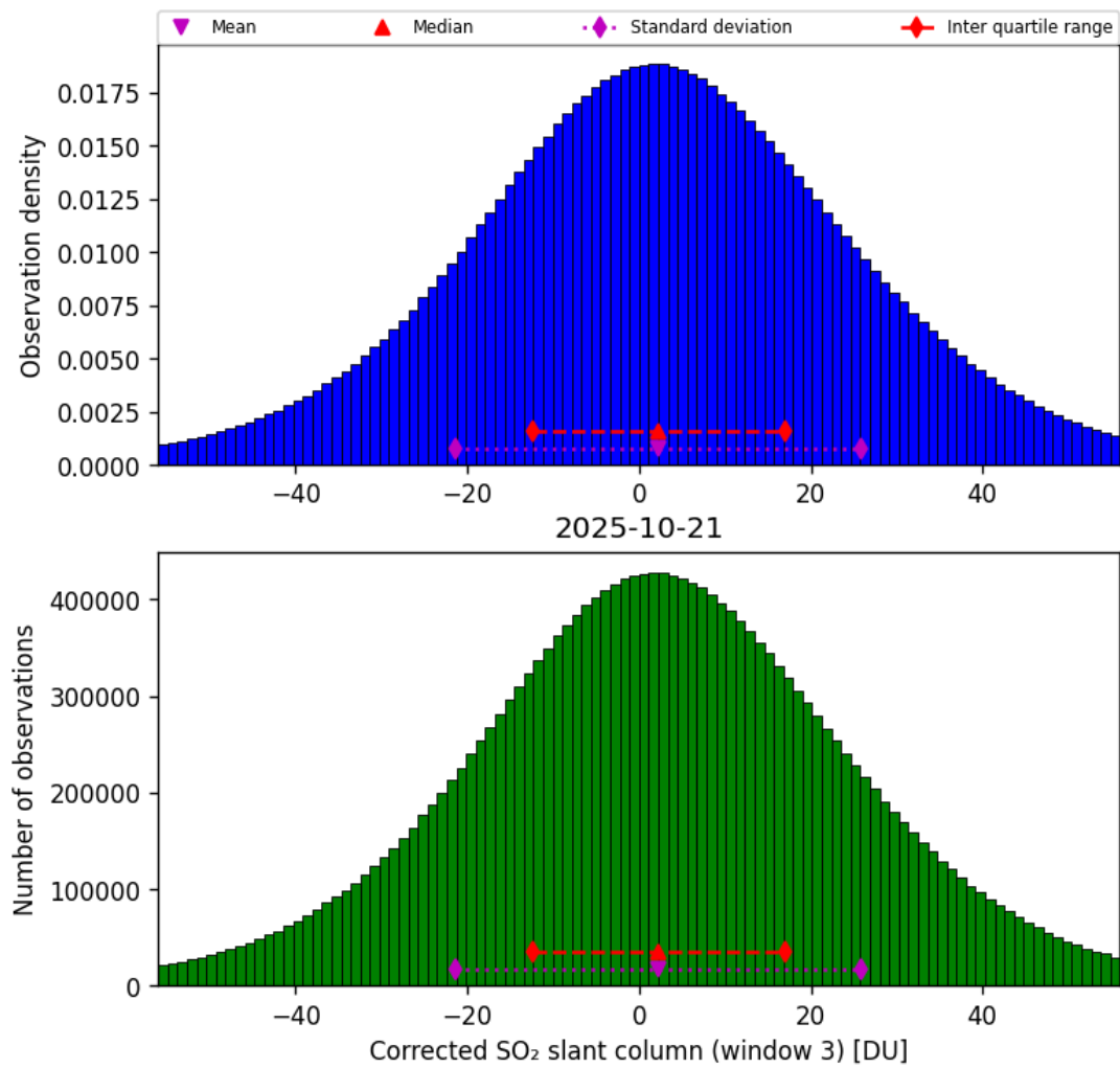
Figure 73: Histogram of “Corrected SO 2 slant column (window 3)” for 2025-10-20 to 2025-10-22
