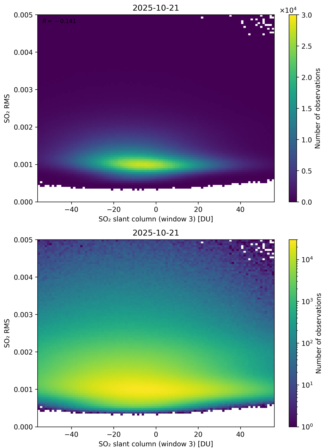
Figure 306: Scatter density plot of “SO 2 slant column (window 3)” against “SO 2 RMS” for 2025-10-20 to 2025-10-22.
