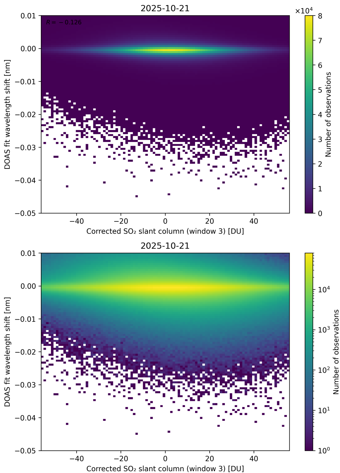
Figure 256: Scatter density plot of “Corrected SO 2 slant column (window 3)” against “DOAS fit wavelength shift” for 2025-10-20 to 2025-10-22.
