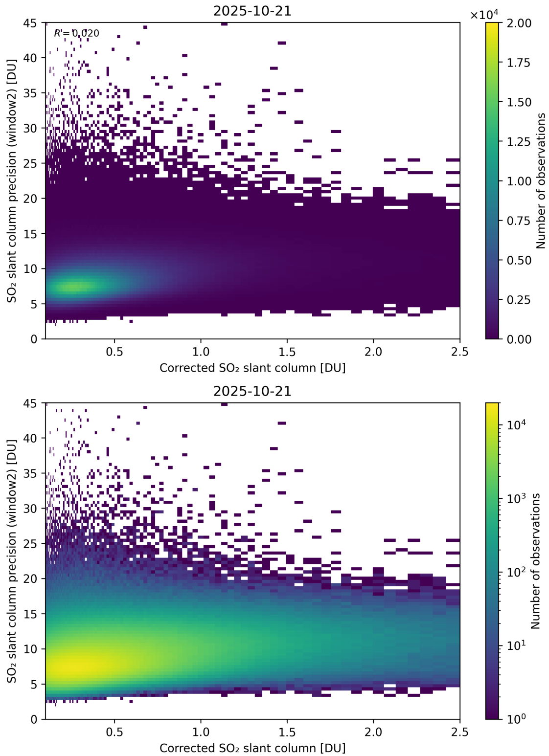
Figure 239: Scatter density plot of “Corrected SO 2 slant column” against “SO 2 slant column precision (window2)” for 2025-10-20 to 2025-10-22.
