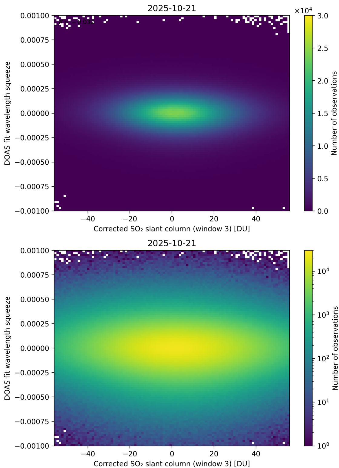
Figure 257: Scatter density plot of “Corrected SO 2 slant column (window 3)” against “DOAS fit wavelength squeeze” for 2025-10-20 to 2025-10-22.
