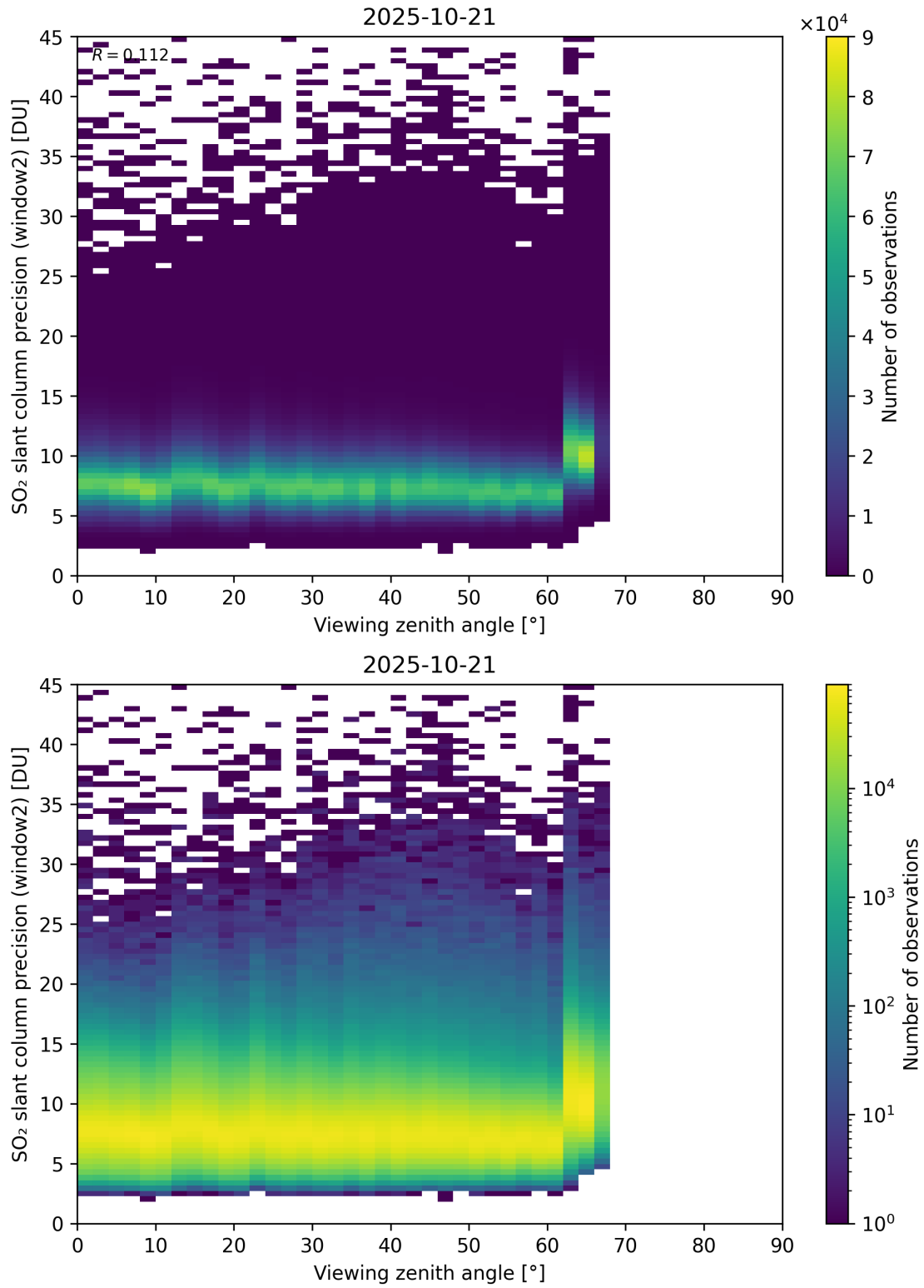
Figure 378: Scatter density plot of “Viewing zenith angle” against “SO 2 slant column precision (window2)” for 2025-10-20 to 2025-10-22.
