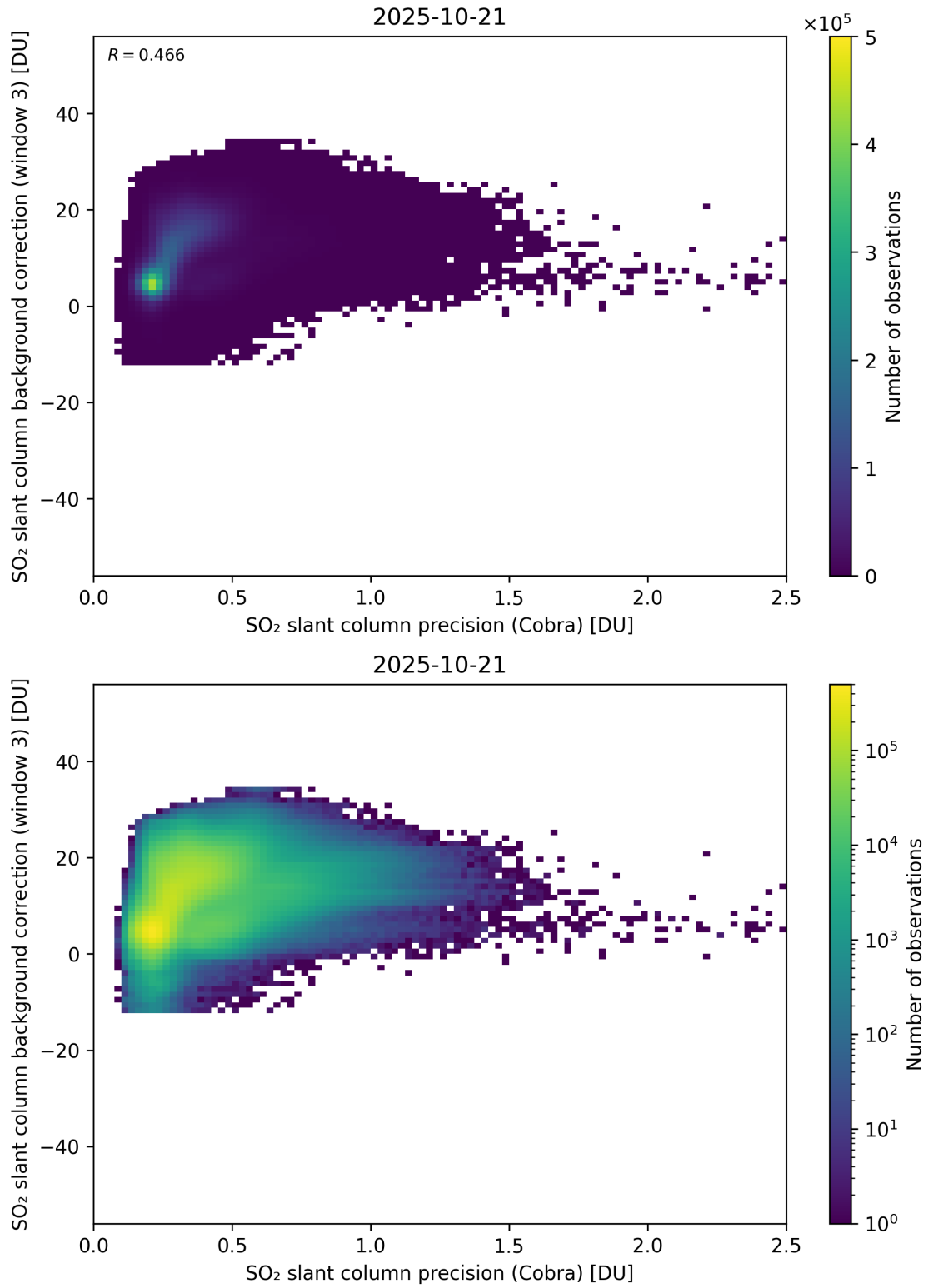
Figure 201: Scatter density plot of “SO 2 slant column precision (Cobra)” against “SO 2 slant column background correction (window 3)” for 2025-10-20 to 2025-10-22.
