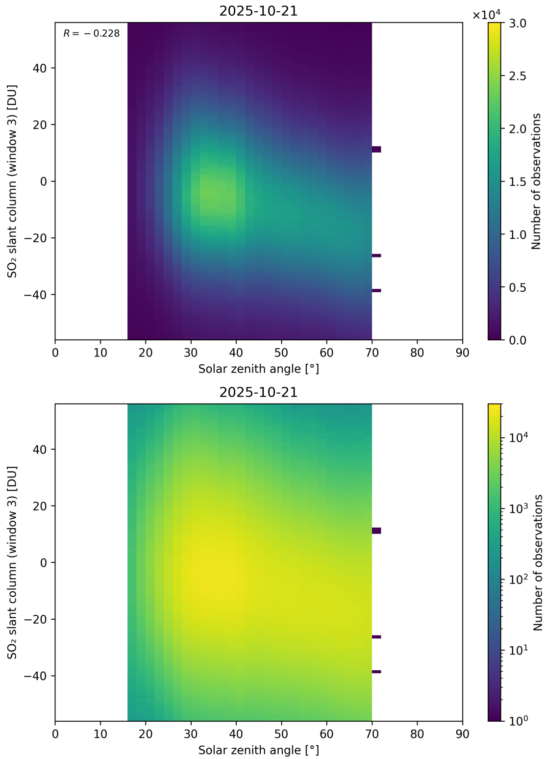
Figure 187: Scatter density plot of “Solar zenith angle” against “SO 2 slant column (window 3)” for 2025-10-20 to 2025-10-22.
