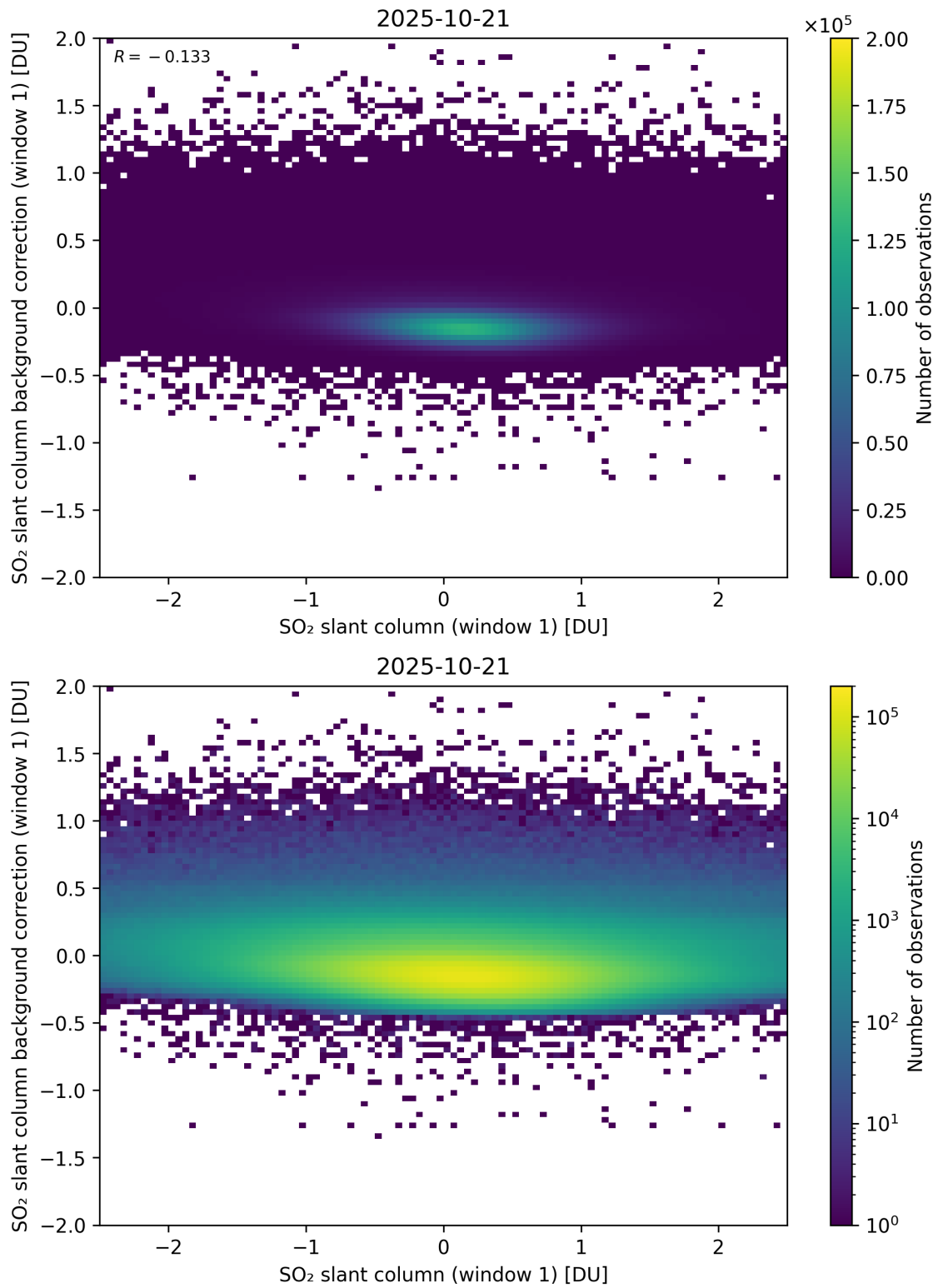
Figure 262: Scatter density plot of “SO 2 slant column (window 1)” against “SO 2 slant column background correction (window 1)” for 2025-10-20 to 2025-10-22.
