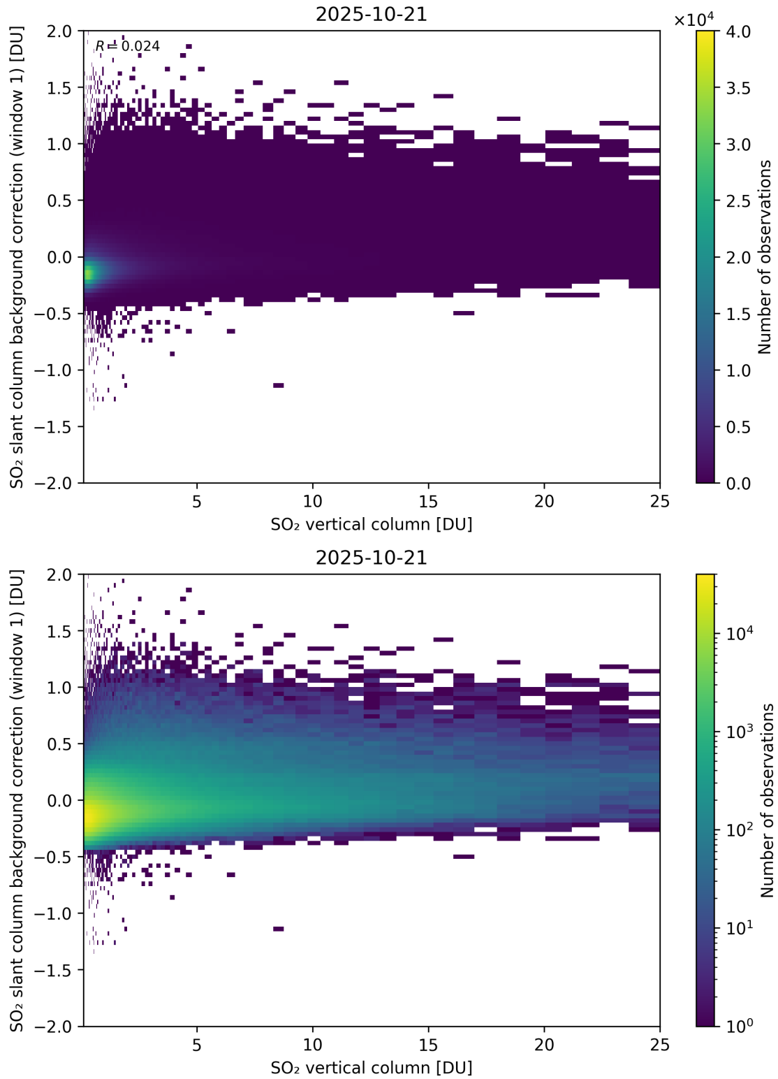
Figure 323: Scatter density plot of “SO 2 vertical column” against “SO 2 slant column background correction (window 1)” for 2025-10-20 to 2025-10-22.
