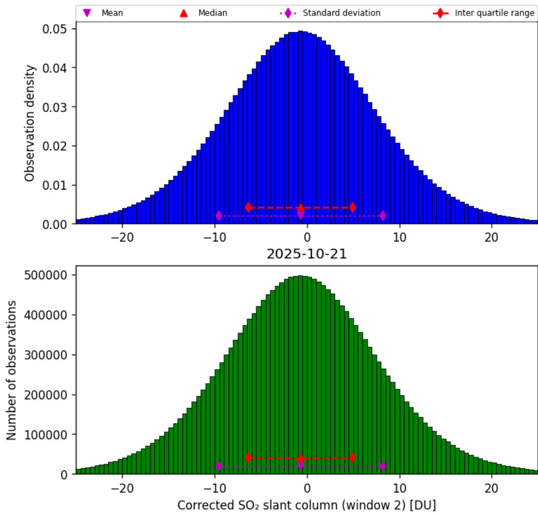
Figure 69: Histogram of “Corrected SO 2 slant column (window 2)” for 2025-10-20 to 2025-10-22
