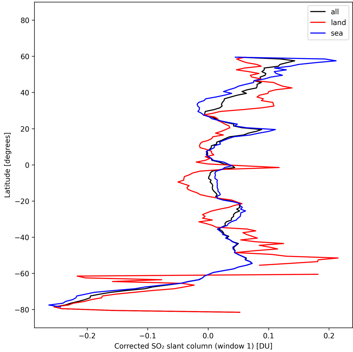
Figure 39: Zonal average of “Corrected SO 2 slant column (window 1)” for 2025-10-20 to 2025-10-22.
