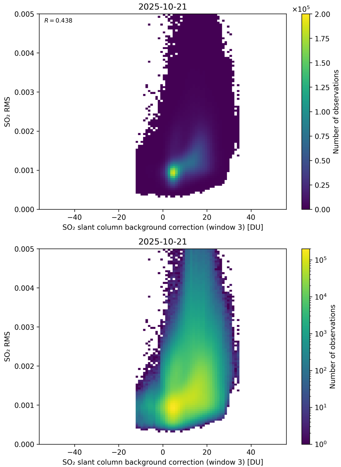
Figure 134: Scatter density plot of “SO 2 slant column background correction (window 3)” against “SO 2 RMS” for 2025-10-20 to 2025-10-22.
