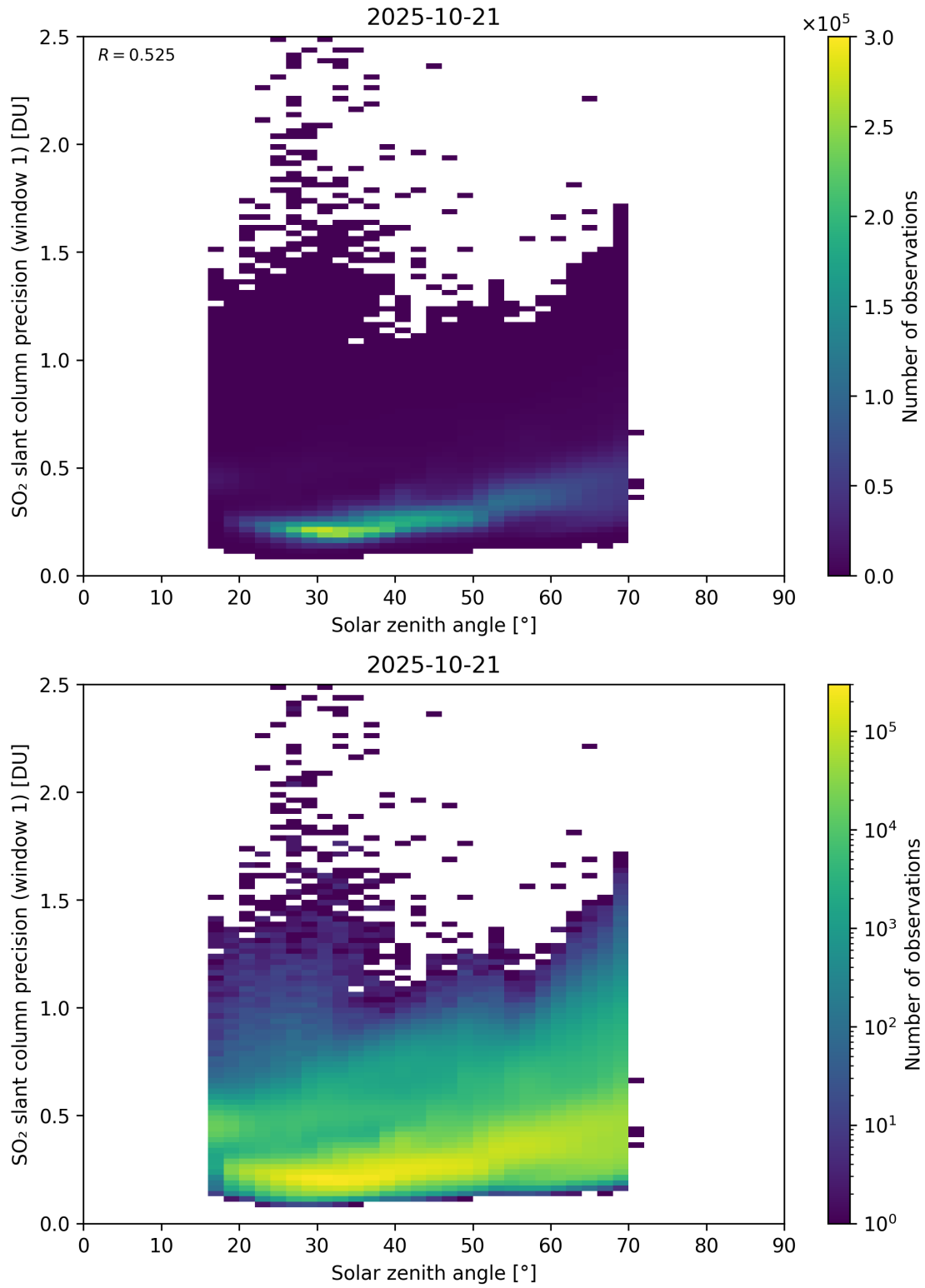
Figure 185: Scatter density plot of “Solar zenith angle” against “SO 2 slant column precision (window 1)” for 2025-10-20 to 2025-10-22.
