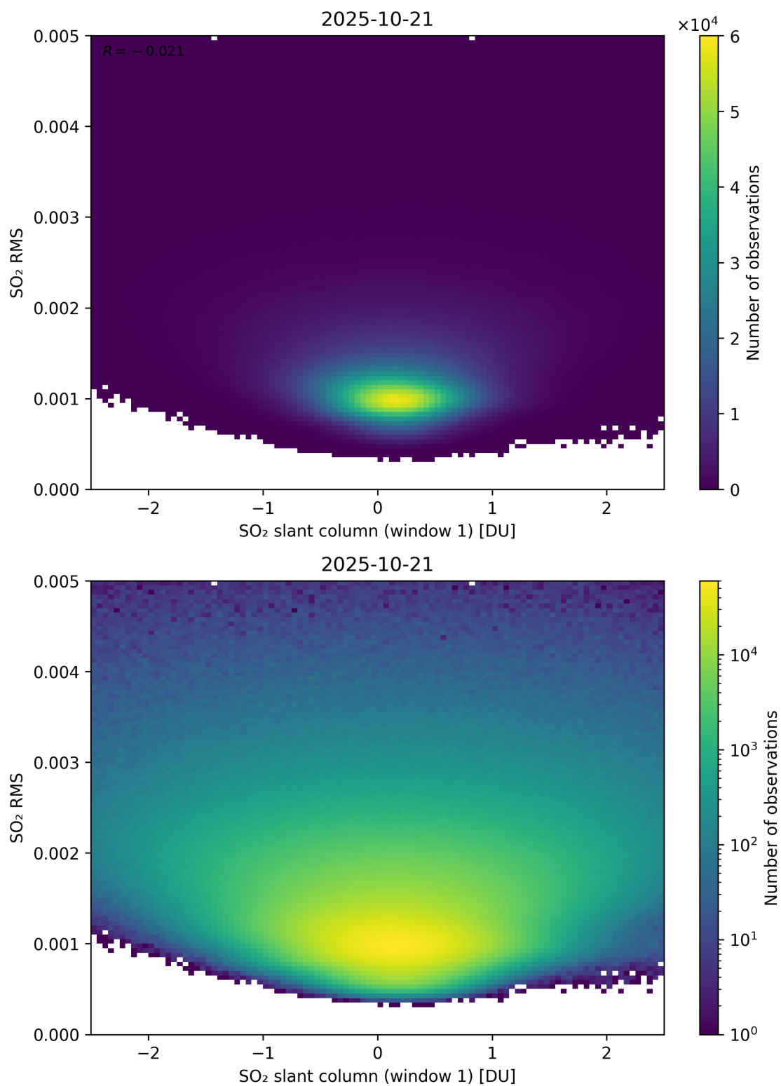
Figure 267: Scatter density plot of “SO 2 slant column (window 1)” against “SO 2 RMS” for 2025-10-20 to 2025-10-22.
