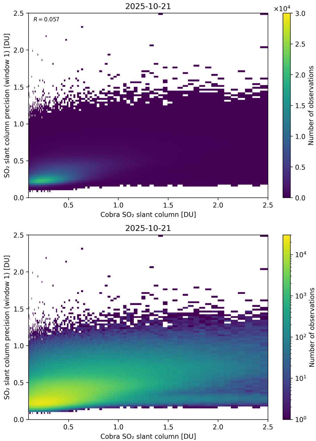
Figure 220: Scatter density plot of “Cobra SO 2 slant column” against “SO 2 slant column precision (window 1)” for 2025-10-20 to 2025-10-22.
