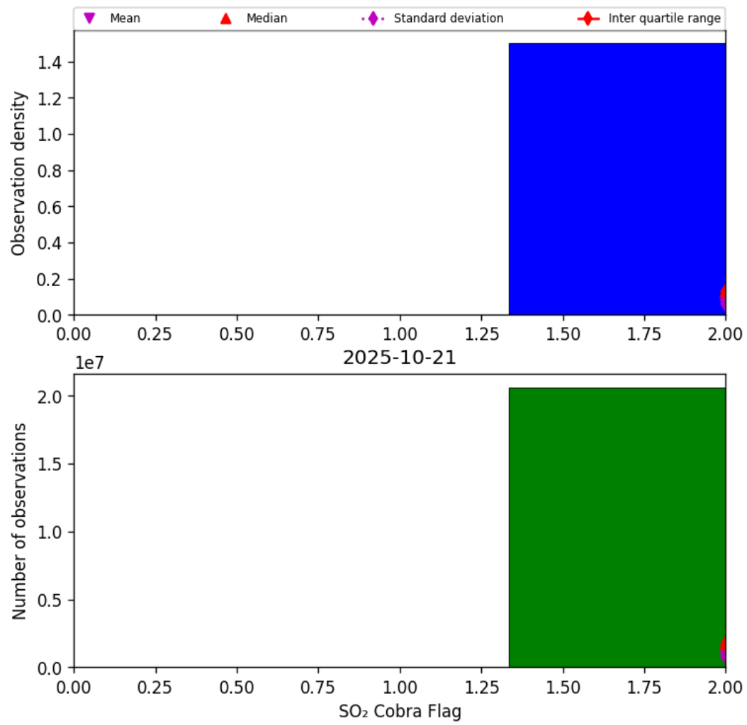
Figure 75: Histogram of “SO 2 Cobra Flag” for 2025-10-20 to 2025-10-22
