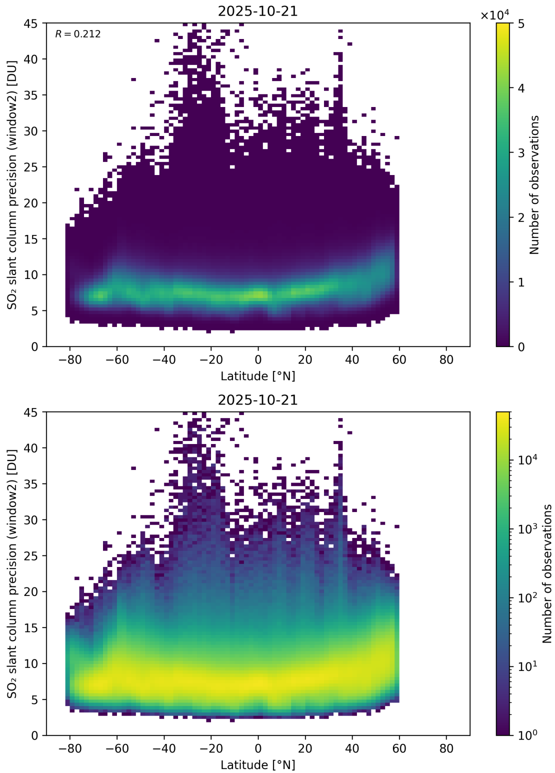
Figure 164: Scatter density plot of “Latitude” against “SO 2 slant column precision (window2)” for 2025-10-20 to 2025-10-22.
