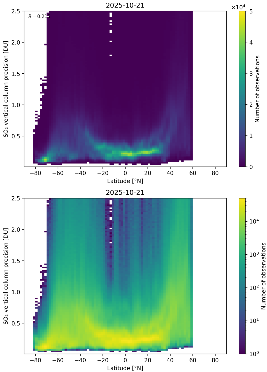
Figure 170: Scatter density plot of “Latitude” against “SO 2 vertical column precision” for 2025-10-20 to 2025-10-22.
