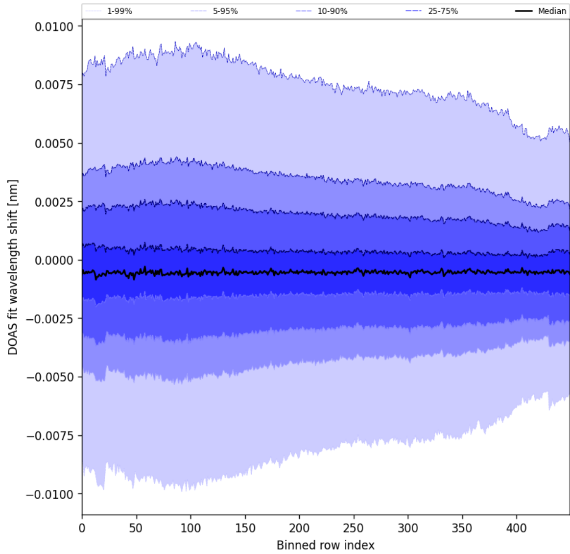
Figure 102: Along track statistics of “DOAS fit wavelength shift” for 2025-10-20 to 2025-10-22
