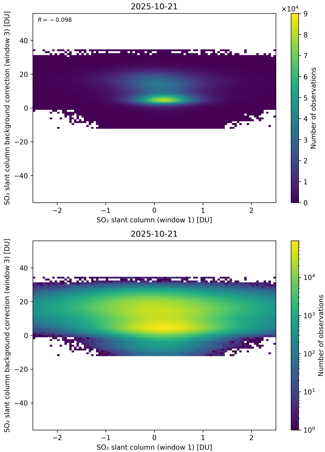
Figure 264: Scatter density plot of “SO 2 slant column (window 1)” against “SO 2 slant column background correction (window 3)” for 2025-10-20 to 2025-10-22.
