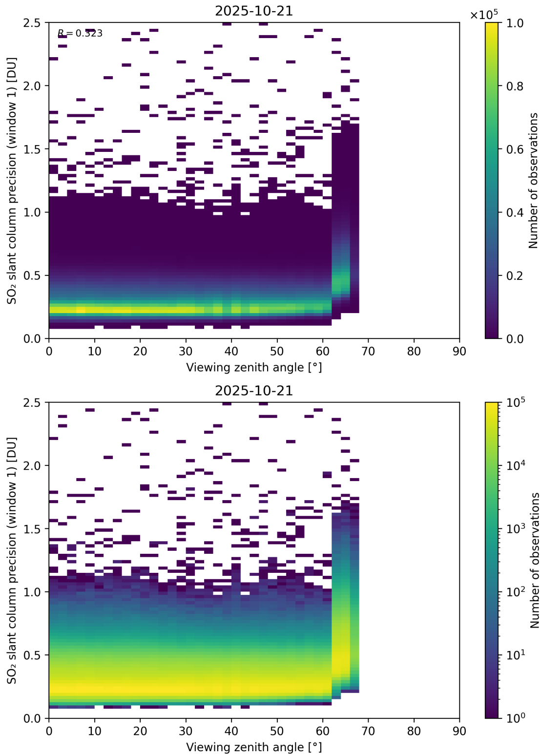
Figure 377: Scatter density plot of “Viewing zenith angle” against “SO 2 slant column precision (window 1)” for 2025-10-20 to 2025-10-22.
