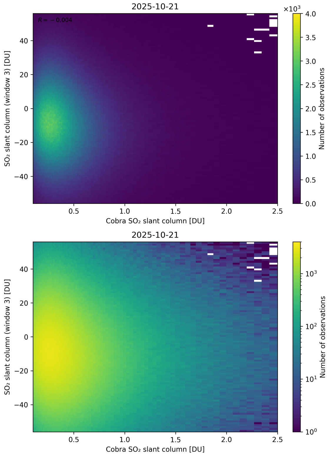
Figure 222: Scatter density plot of “Cobra SO 2 slant column” against “SO 2 slant column (window 3)” for 2025-10-20 to 2025-10-22.
