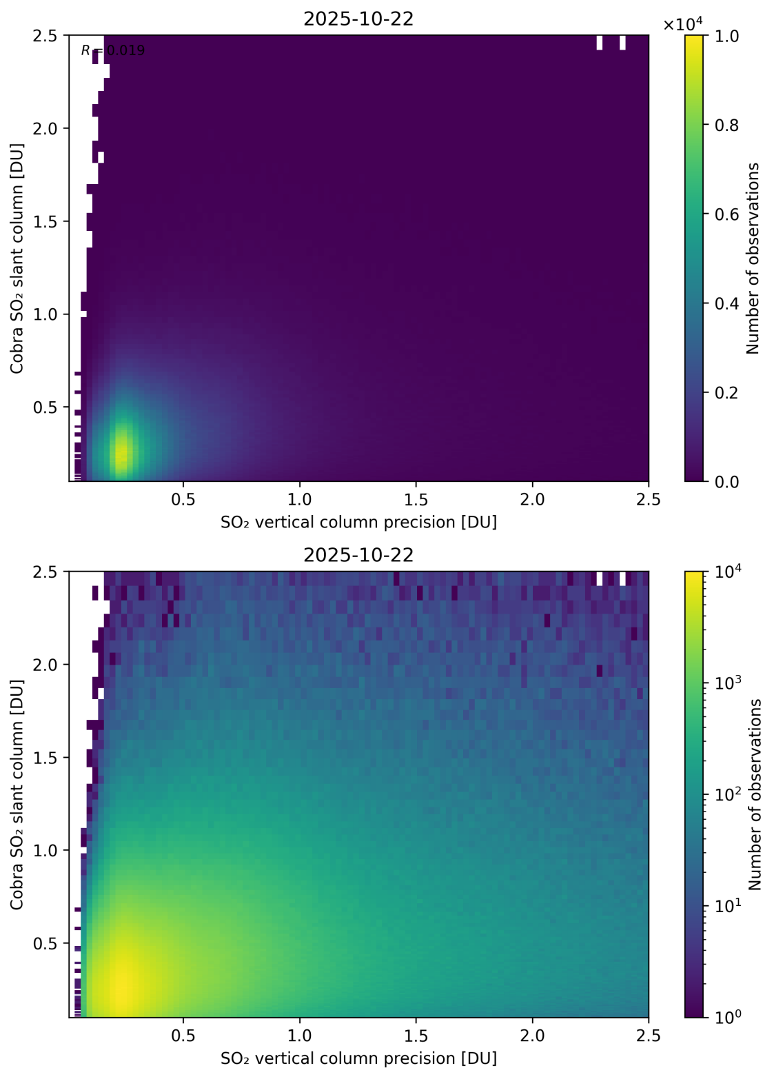
Figure 336: Scatter density plot of “SO 2 vertical column precision” against “Cobra SO 2 slant column” for 2025-10-22 to 2025-10-23.
