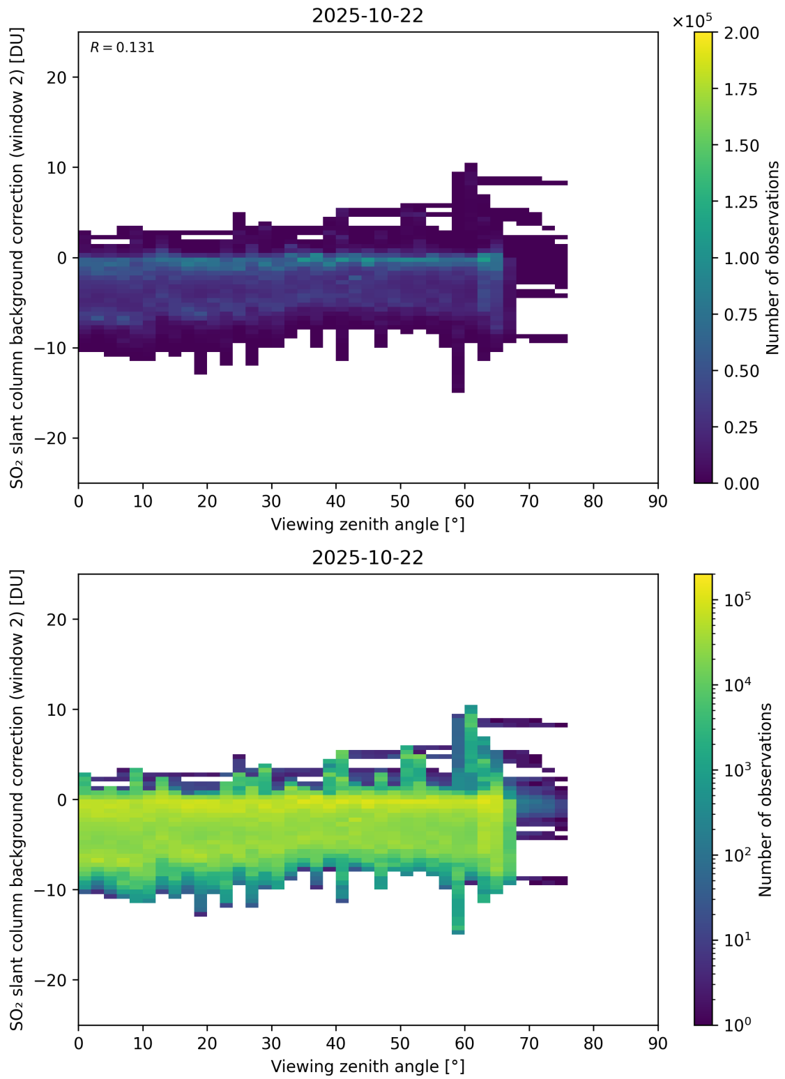
Figure 363: Scatter density plot of “Viewing zenith angle” against “SO 2 slant column background correction (window 2)” for 2025-10-22 to 2025-10-23.
