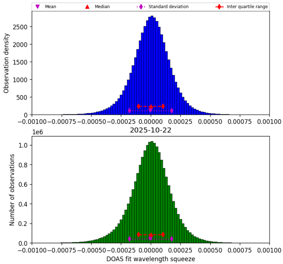
Figure 77: Histogram of “DOAS fit wavelength squeeze” for 2025-10-22 to 2025-10-23
