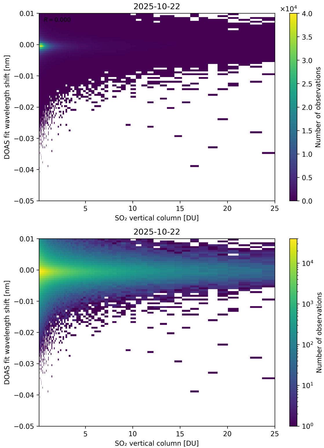
Figure 326: Scatter density plot of “SO 2 vertical column” against “DOAS fit wavelength shift” for 2025-10-22 to 2025-10-23.
