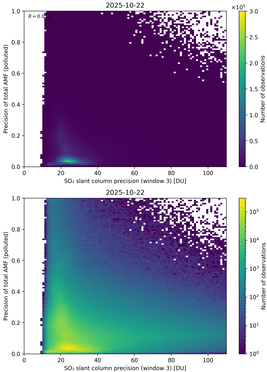
Figure 314: Scatter density plot of “SO 2 slant column precision (window 3)” against “Precision of total AMF (polluted)” for 2025-10-22 to 2025-10-23.
