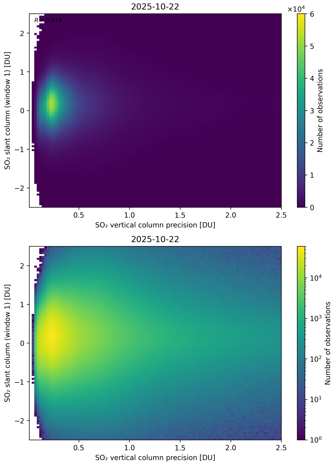
Figure 341: Scatter density plot of “SO 2 vertical column precision” against “SO 2 slant column (window 1)” for 2025-10-22 to 2025-10-23.
