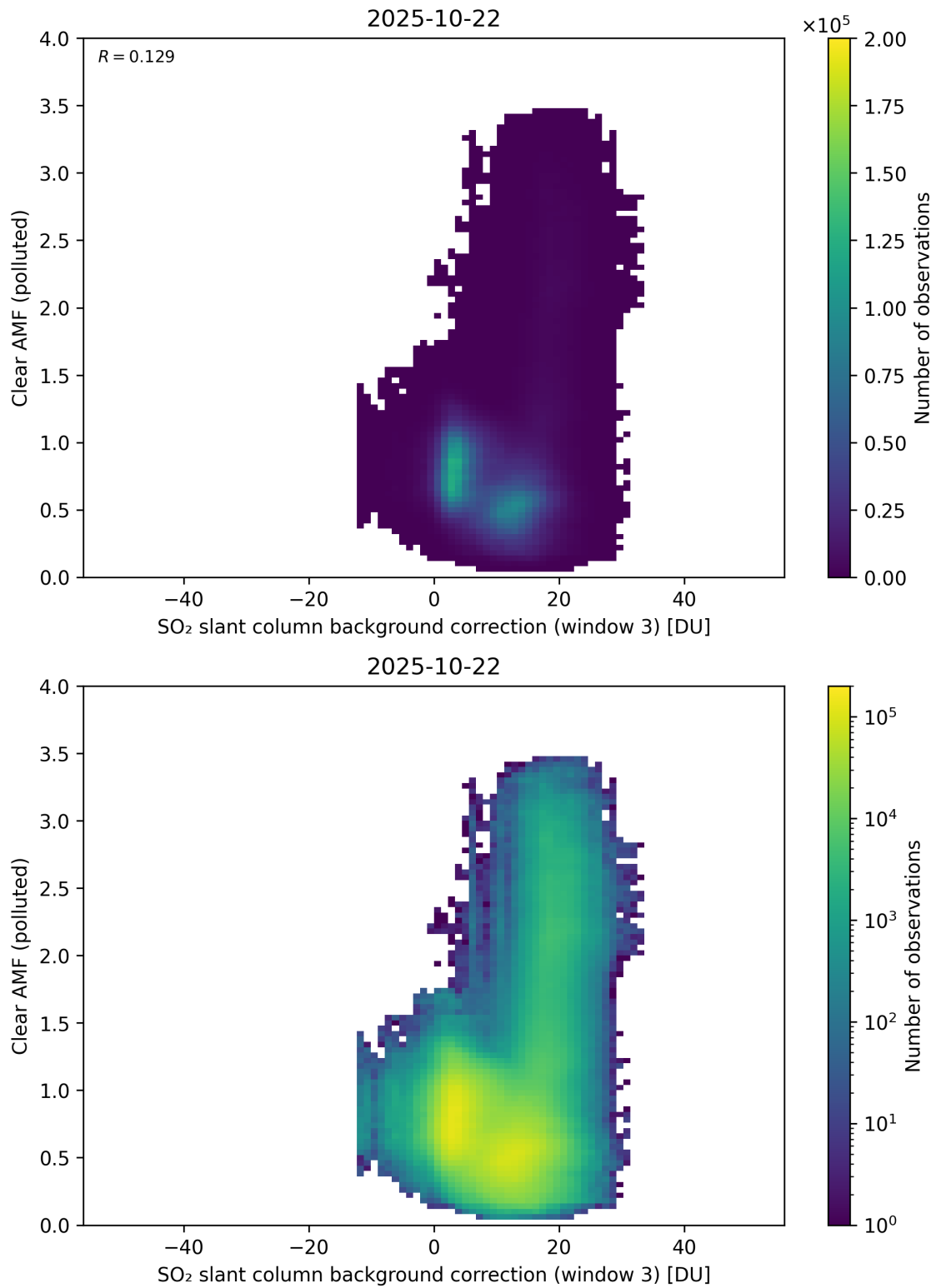
Figure 135: Scatter density plot of “SO 2 slant column background correction (window 3)” against “Clear AMF (polluted)” for 2025-10-22 to 2025-10-23.
