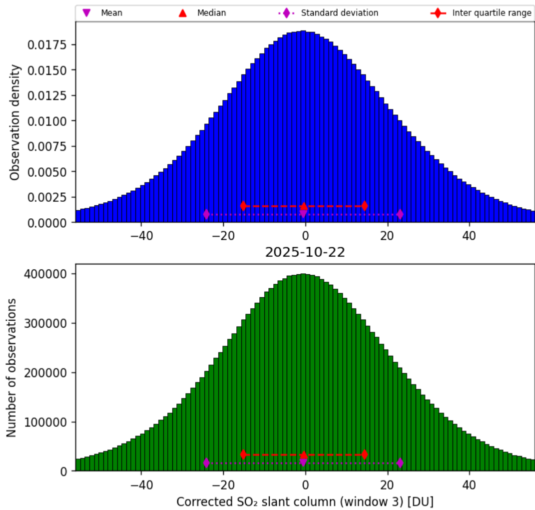
Figure 73: Histogram of “Corrected SO 2 slant column (window 3)” for 2025-10-22 to 2025-10-23
