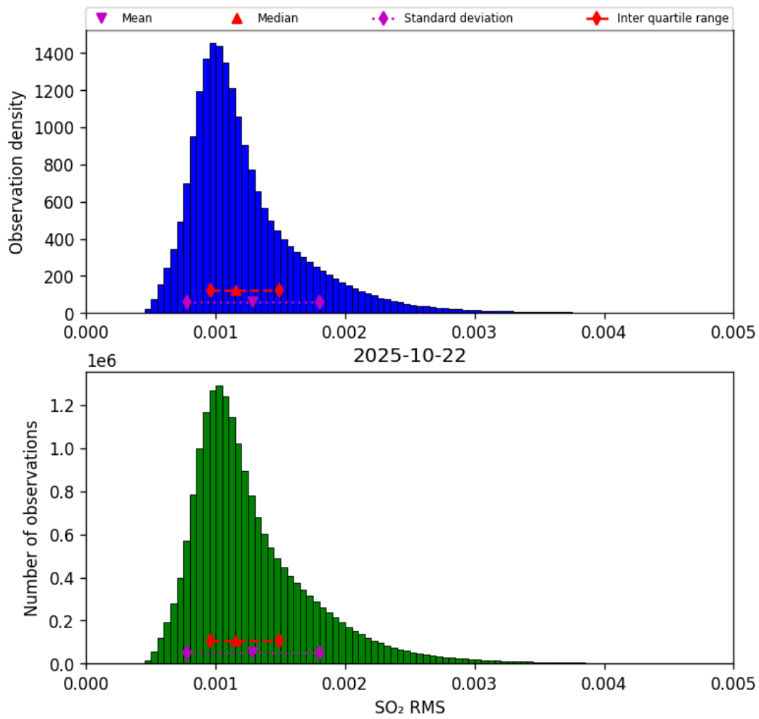
Figure 78: Histogram of “SO 2 RMS” for 2025-10-22 to 2025-10-23
