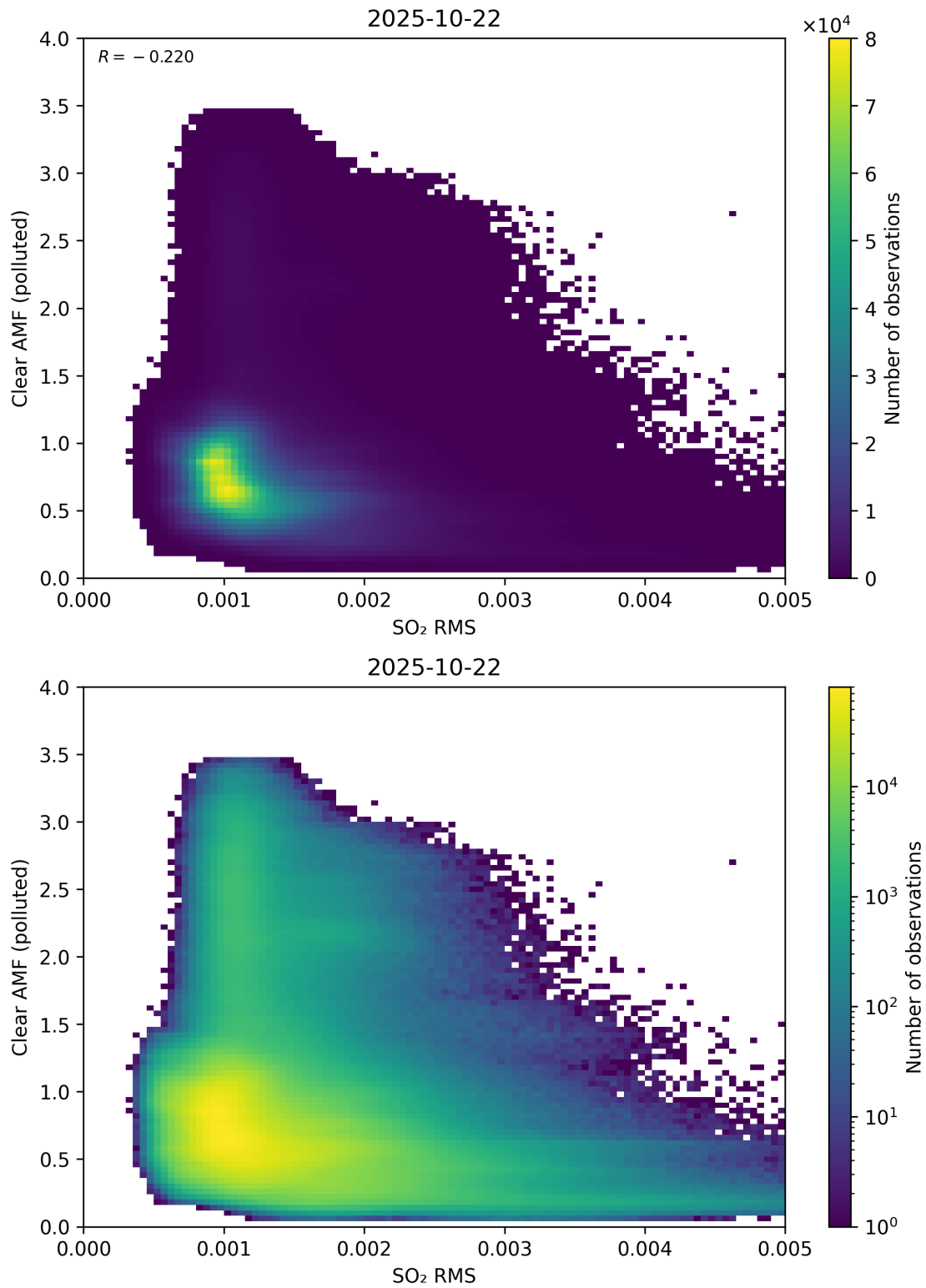
Figure 147: Scatter density plot of “SO 2 RMS” against “Clear AMF (polluted)” for 2025-10-22 to 2025-10-23.
