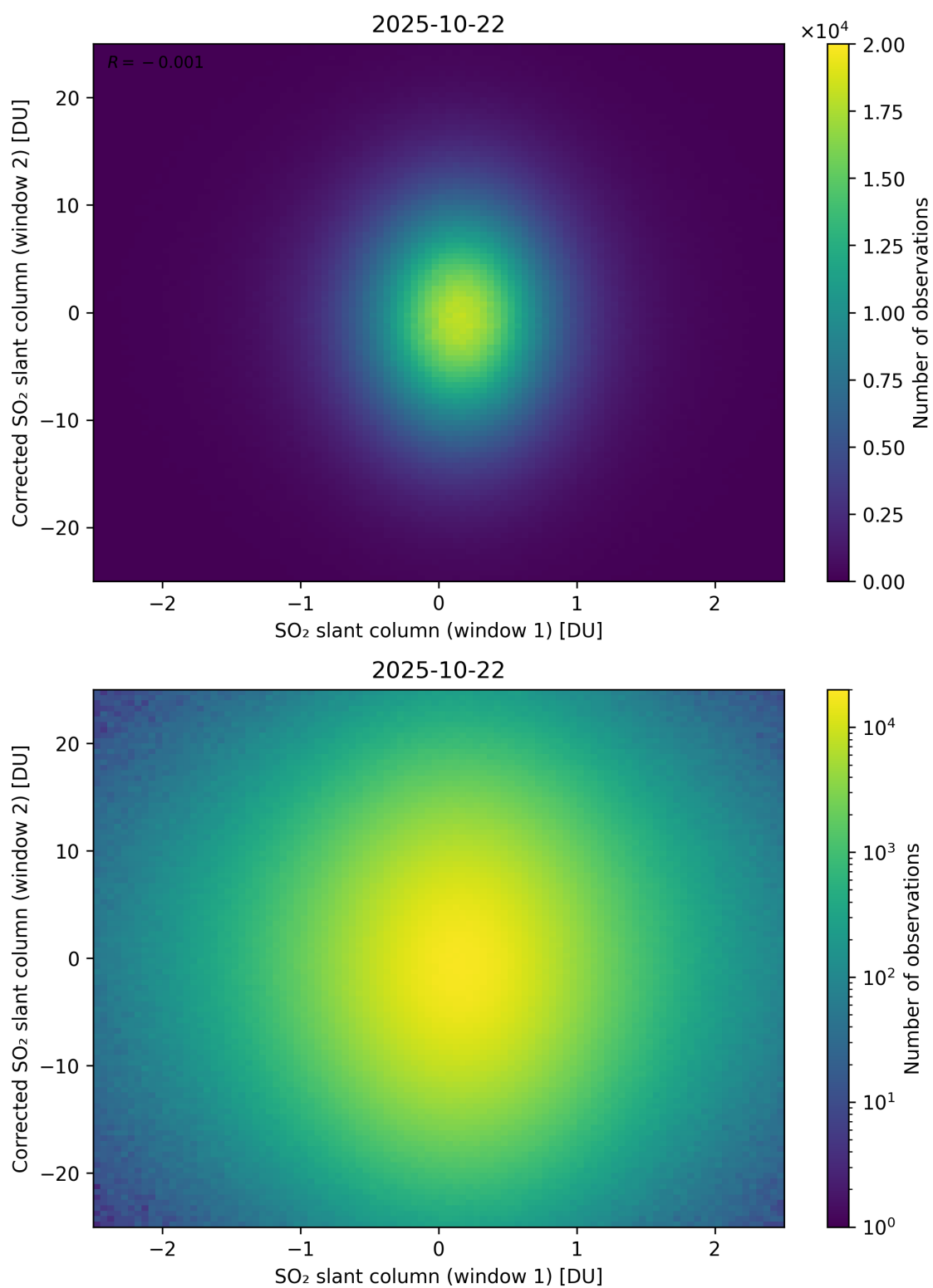
Figure 283: Scatter density plot of “SO 2 slant column (window 1)” against “Corrected SO 2 slant column (window 2)” for 2025-10-22 to 2025-10-23.
