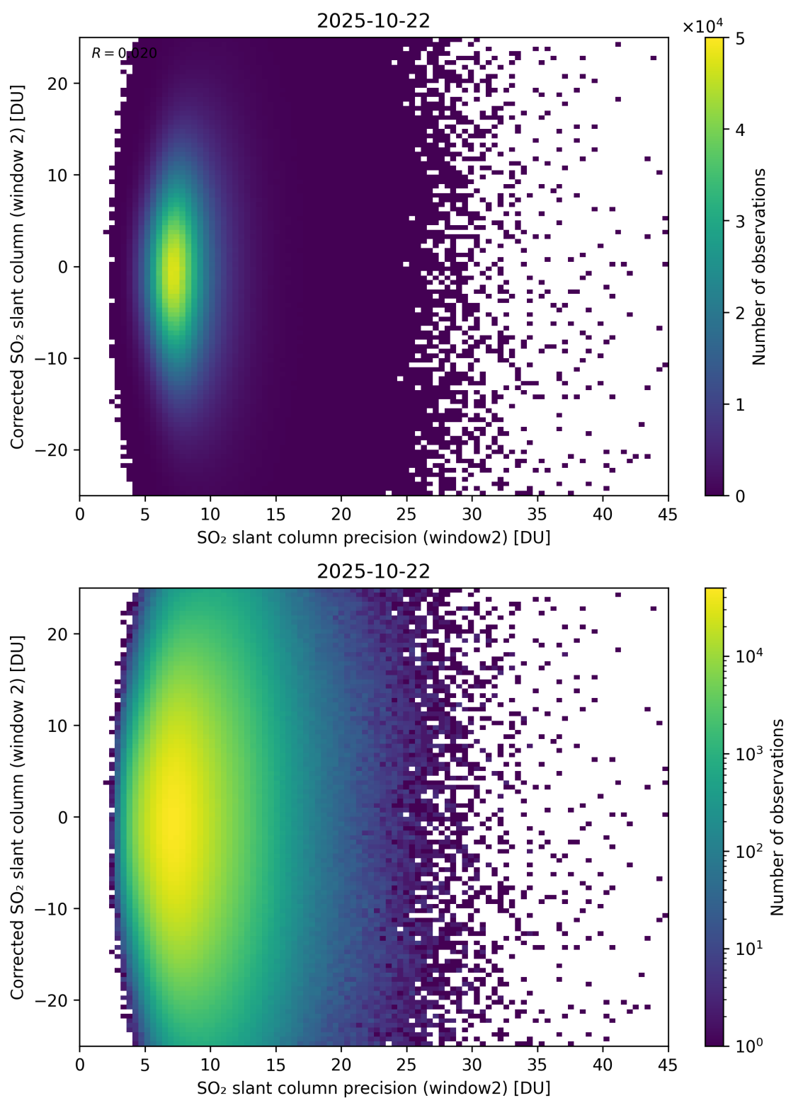
Figure 297: Scatter density plot of “SO 2 slant column precision (window2)” against “Corrected SO 2 slant column (window 2)” for 2025-10-22 to 2025-10-23.
