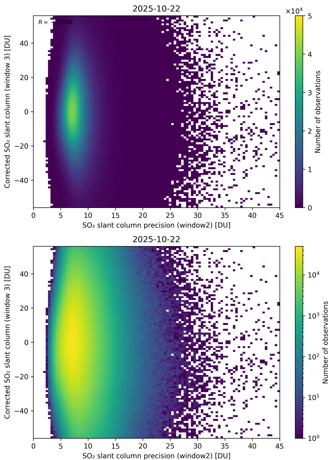
Figure 298: Scatter density plot of “SO 2 slant column precision (window2)” against “Corrected SO 2 slant column (window 3)” for 2025-10-22 to 2025-10-23.
