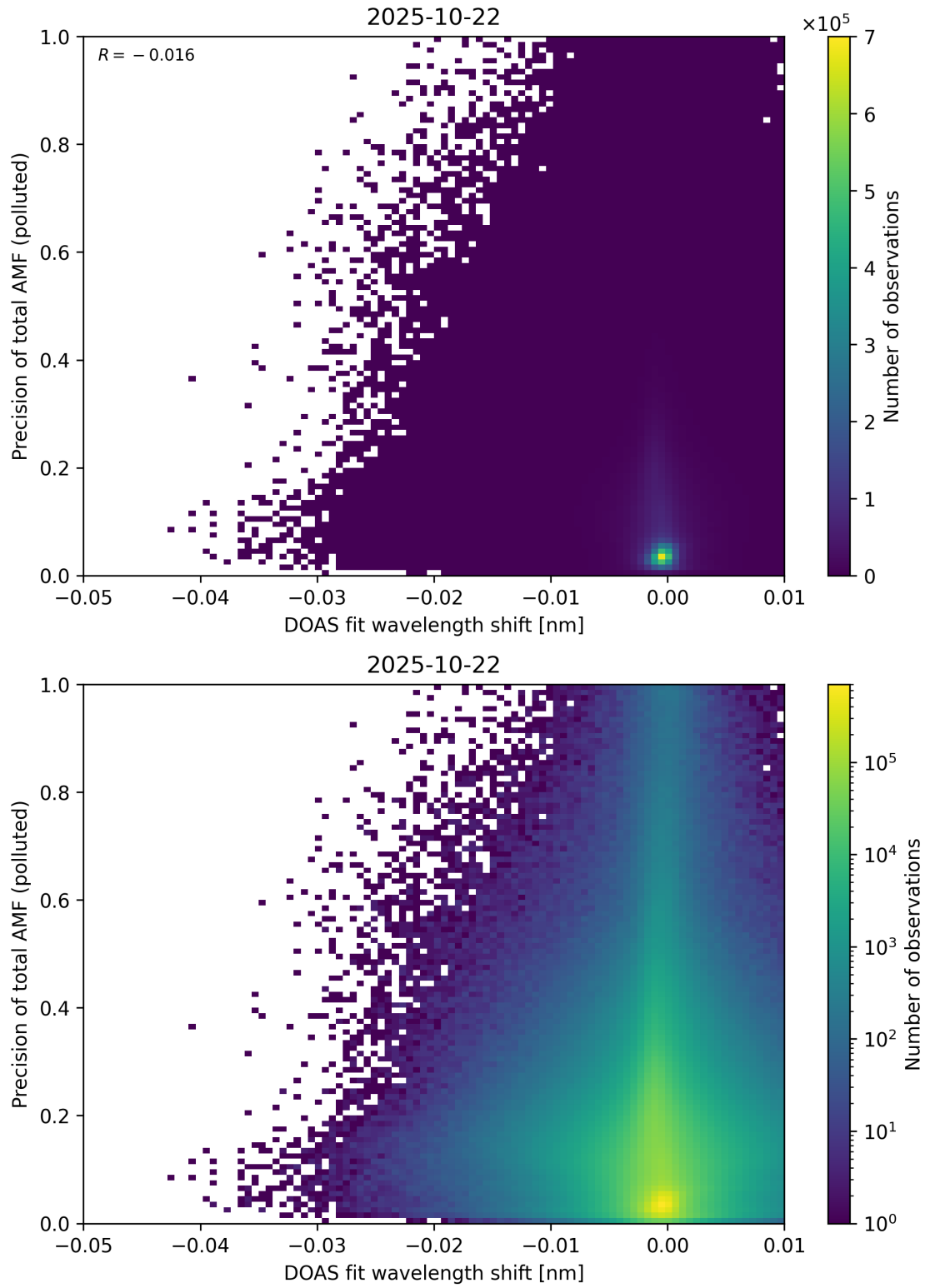
Figure 142: Scatter density plot of “DOAS fit wavelength shift” against “Precision of total AMF (polluted)” for 2025-10-22 to 2025-10-23.
