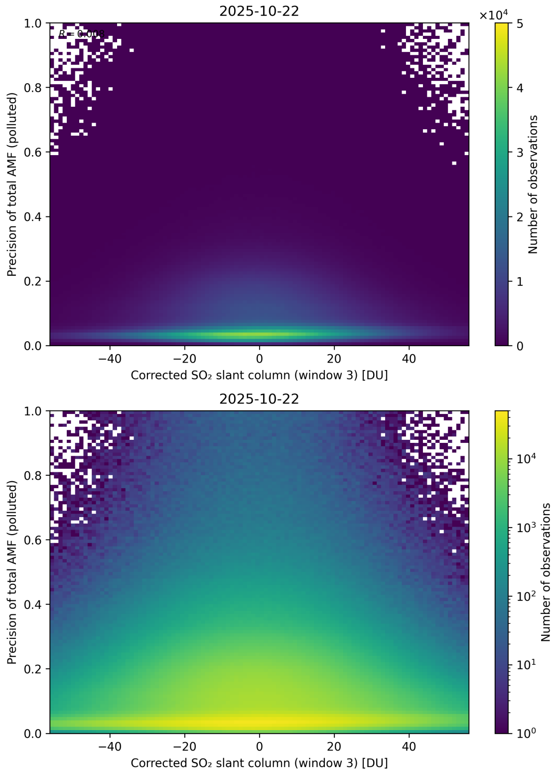
Figure 261: Scatter density plot of “Corrected SO 2 slant column (window 3)” against “Precision of total AMF (polluted)” for 2025-10-22 to 2025-10-23.
