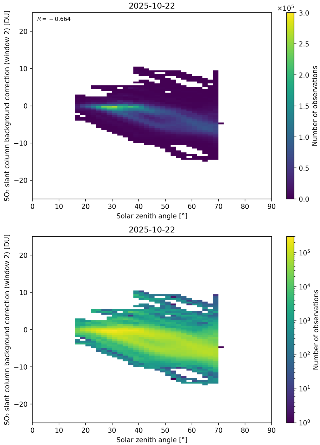
Figure 172: Scatter density plot of “Solar zenith angle” against “SO 2 slant column background correction (window 2)” for 2025-10-22 to 2025-10-23.
