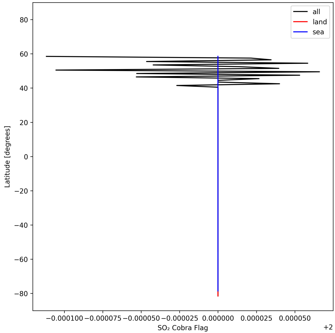
Figure 49: Zonal average of "SO 2 Cobra Flag" for 2025-10-22 to 2025-10-23.
