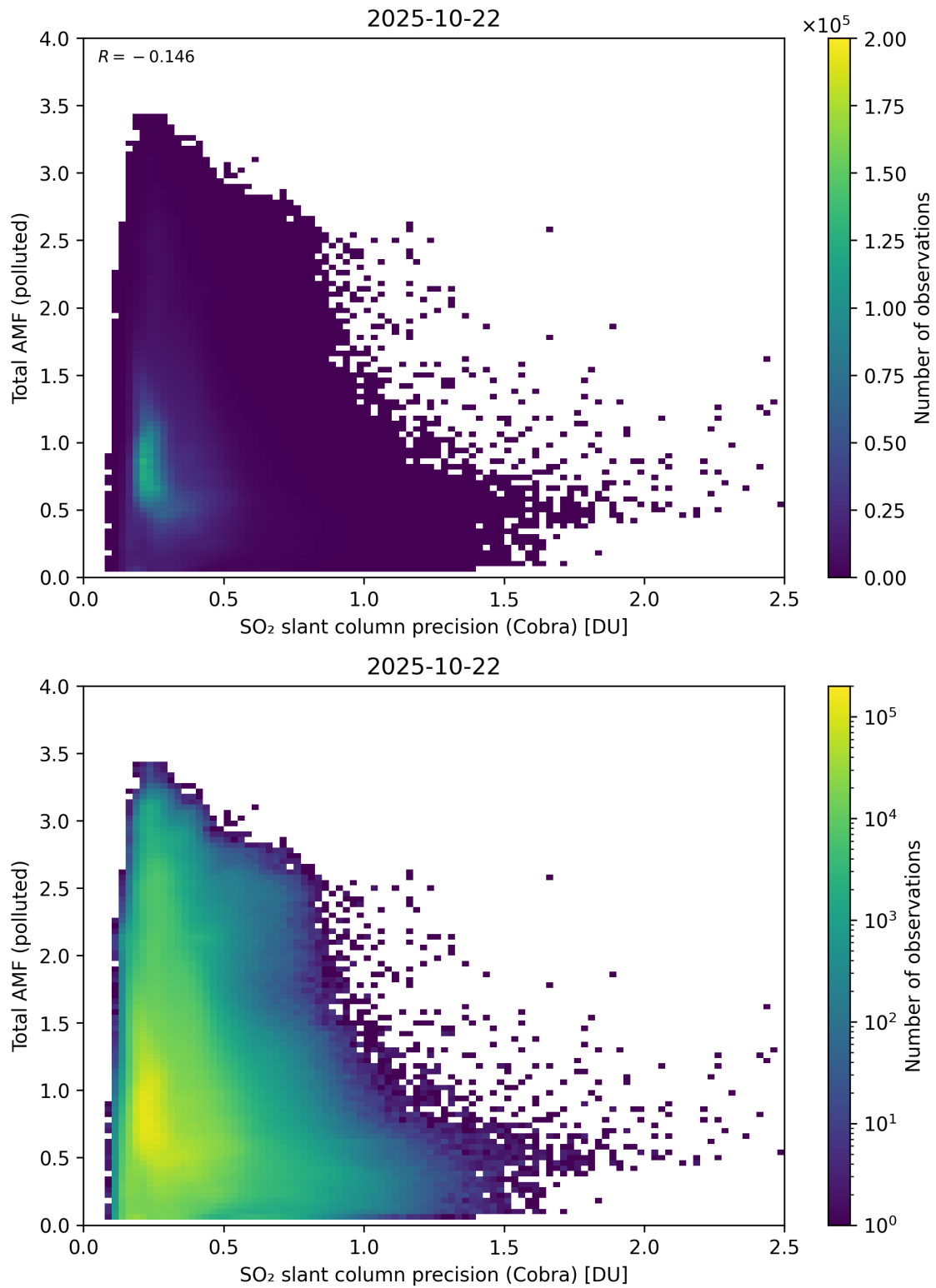
Figure 213: Scatter density plot of “SO 2 slant column precision (Cobra)” against “Total AMF (polluted)” for 2025-10-22 to 2025-10-23.
