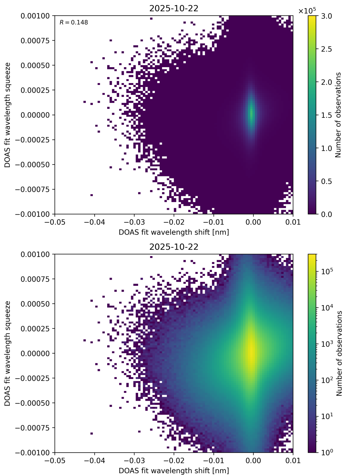
Figure 138: Scatter density plot of “DOAS fit wavelength shift” against “DOAS fit wavelength squeeze” for 2025-10-22 to 2025-10-23.
