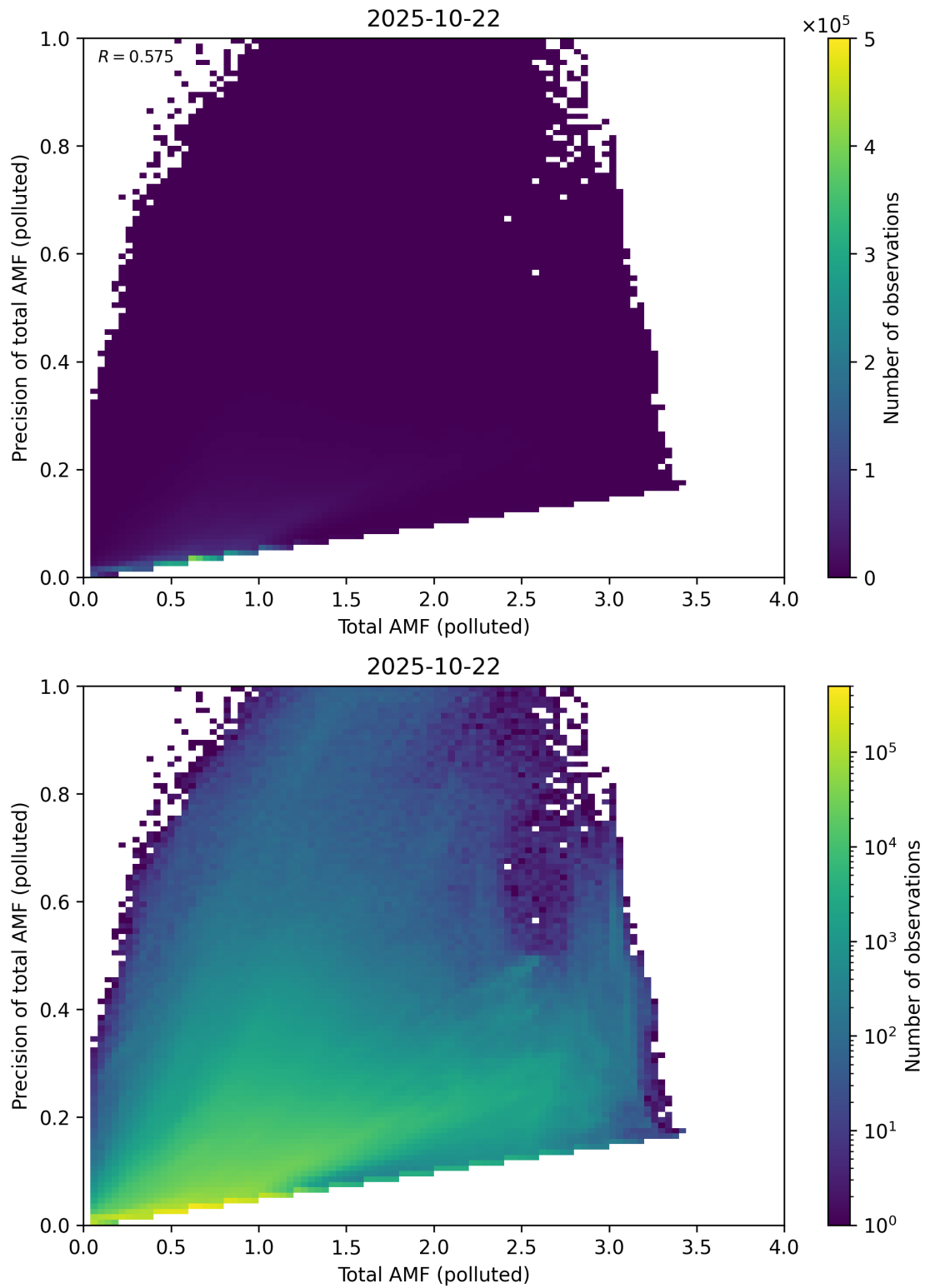
Figure 322: Scatter density plot of “Total AMF (polluted)” against “Precision of total AMF (polluted)” for 2025-10-22 to 2025-10-23.
