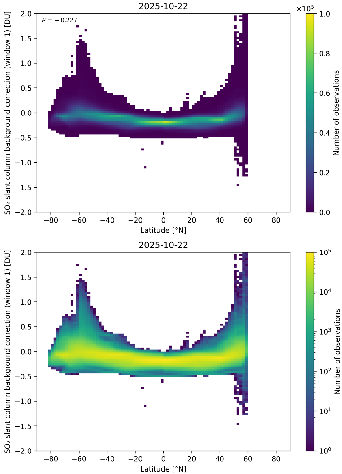
Figure 150: Scatter density plot of “Latitude” against “SO 2 slant column background correction (window 1)” for 2025-10-22 to 2025-10-23.
