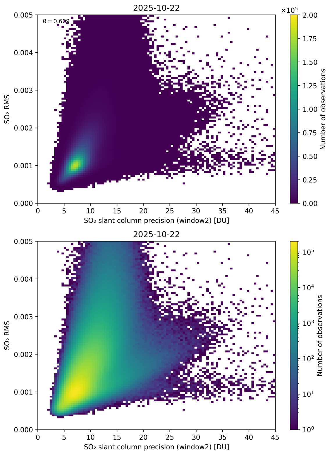
Figure 295: Scatter density plot of “SO 2 slant column precision (window2)” against “SO 2 RMS” for 2025-10-22 to 2025-10-23.
