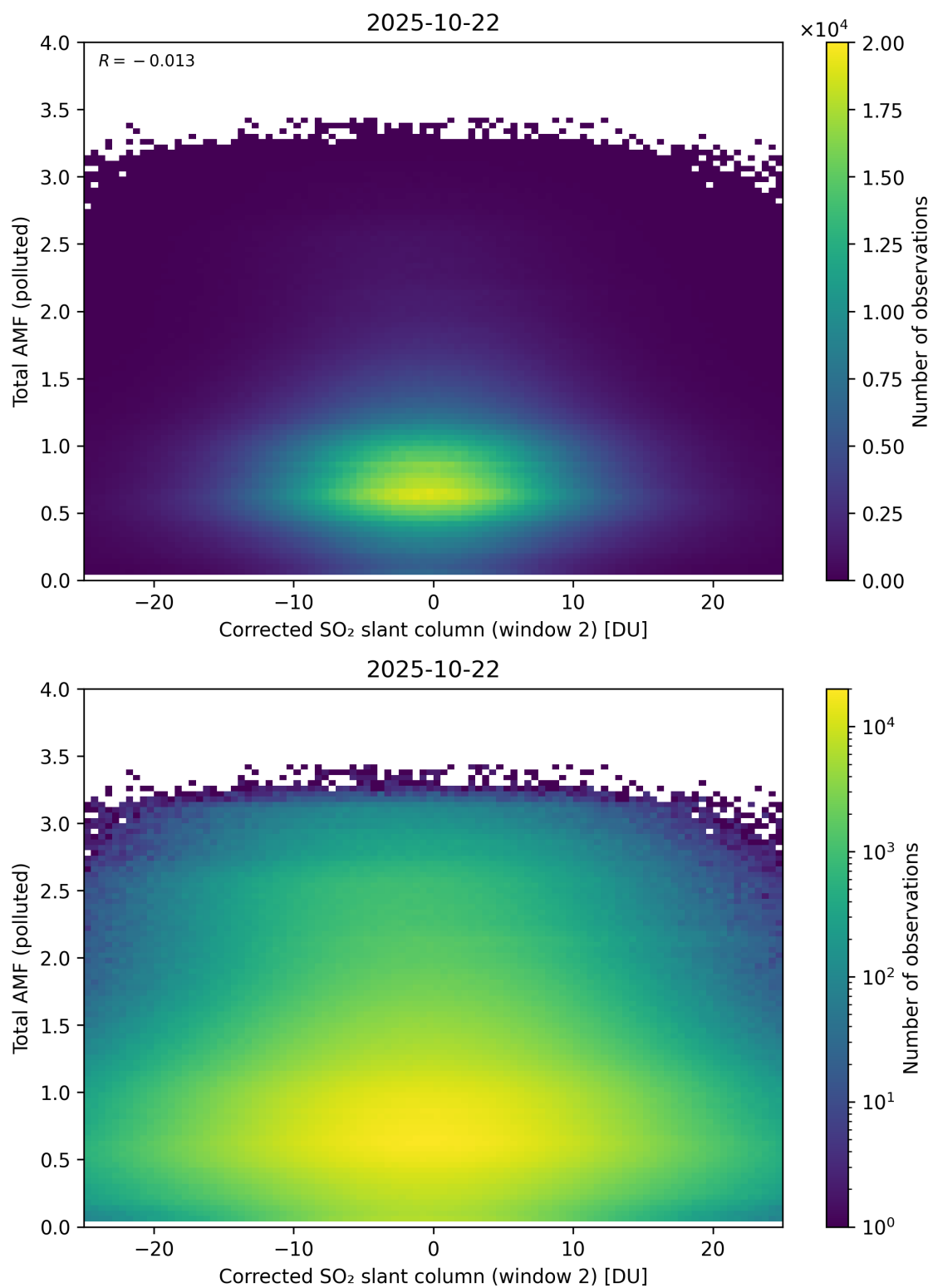
Figure 253: Scatter density plot of “Corrected SO 2 slant column (window 2)” against “Total AMF (polluted)” for 2025-10-22 to 2025-10-23.
