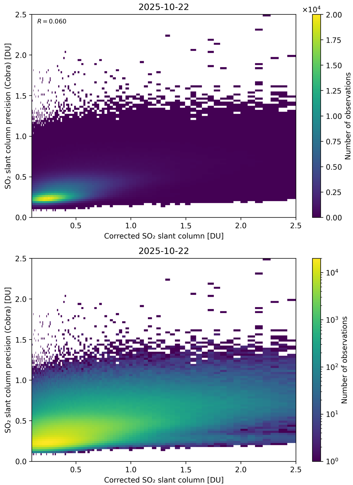
Figure 234: Scatter density plot of “Corrected SO 2 slant column” against “SO 2 slant column precision (Cobra)” for 2025-10-22 to 2025-10-23.
