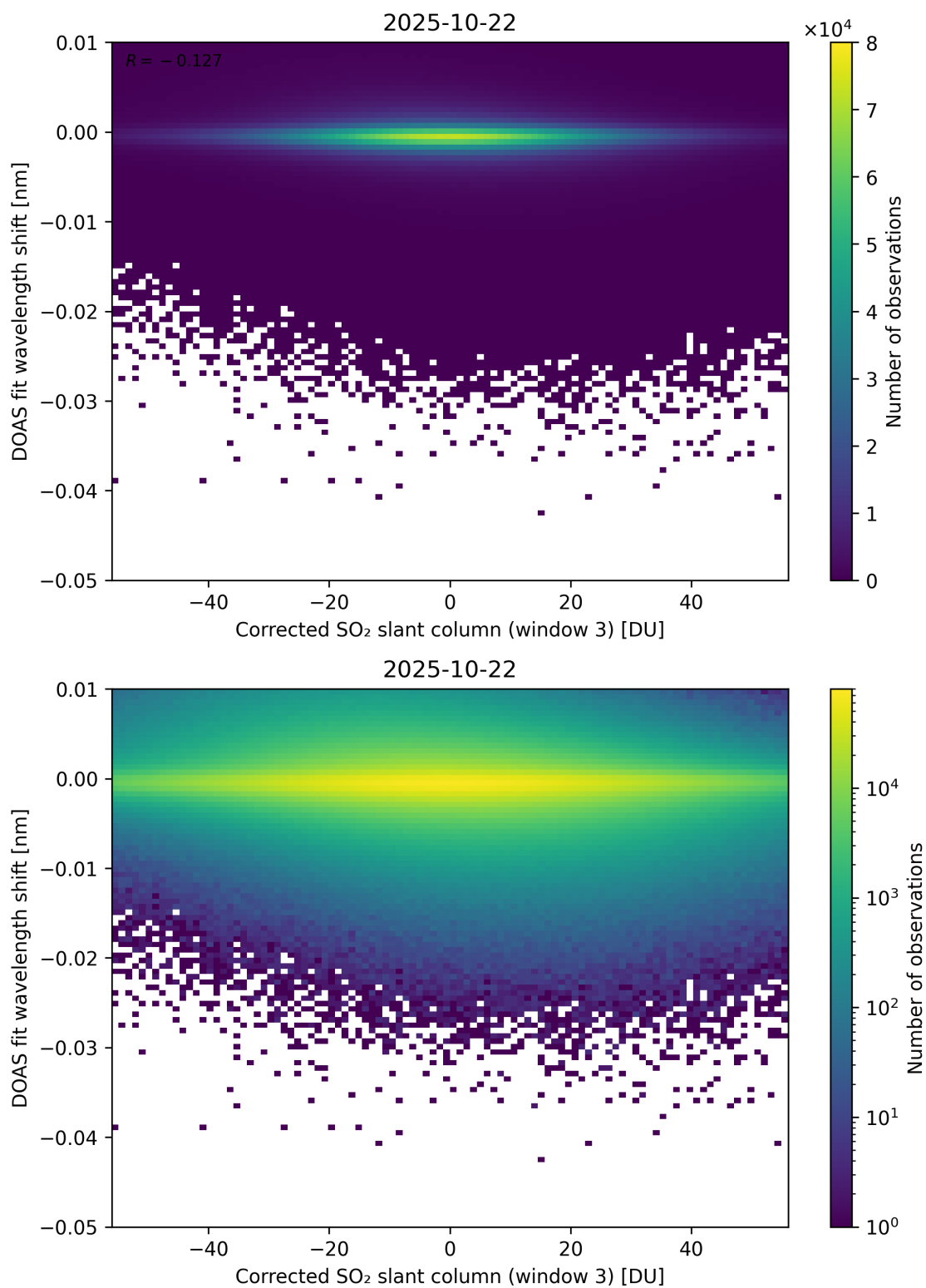
Figure 256: Scatter density plot of “Corrected SO 2 slant column (window 3)” against “DOAS fit wavelength shift” for 2025-10-22 to 2025-10-23.
