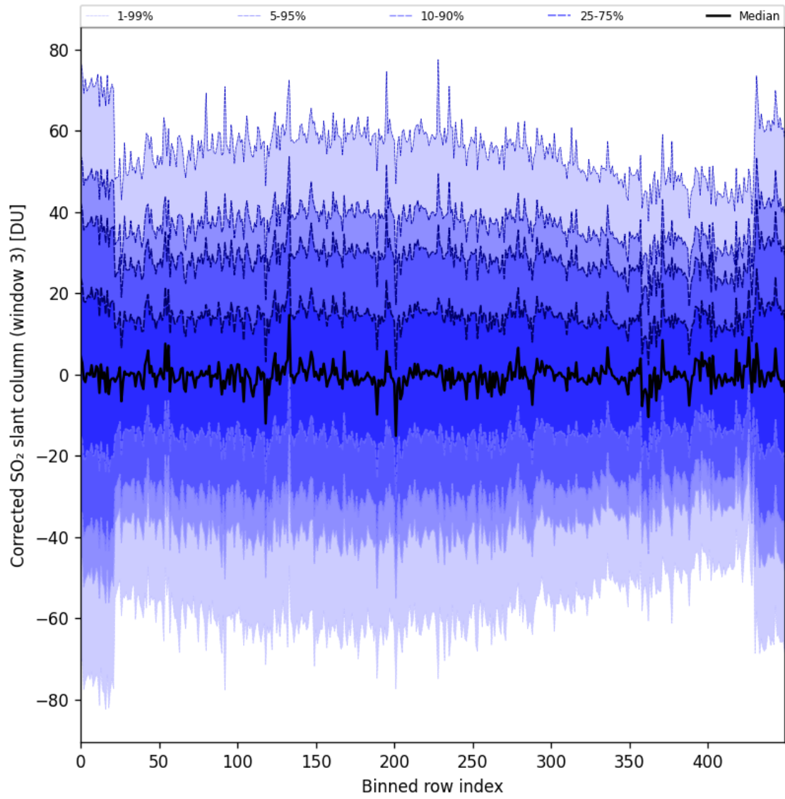
Figure 99: Along track statistics of “Corrected SO 2 slant column (window 3)” for 2025-10-22 to 2025-10-23
