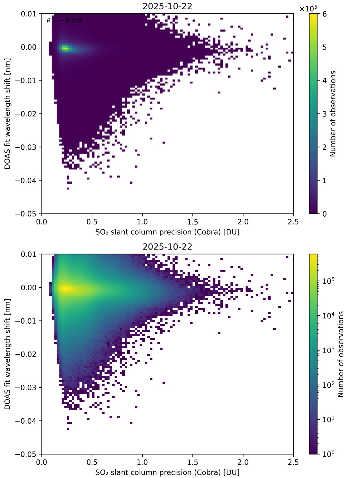
Figure 202: Scatter density plot of “SO 2 slant column precision (Cobra)” against “DOAS fit wavelength shift” for 2025-10-22 to 2025-10-23.
