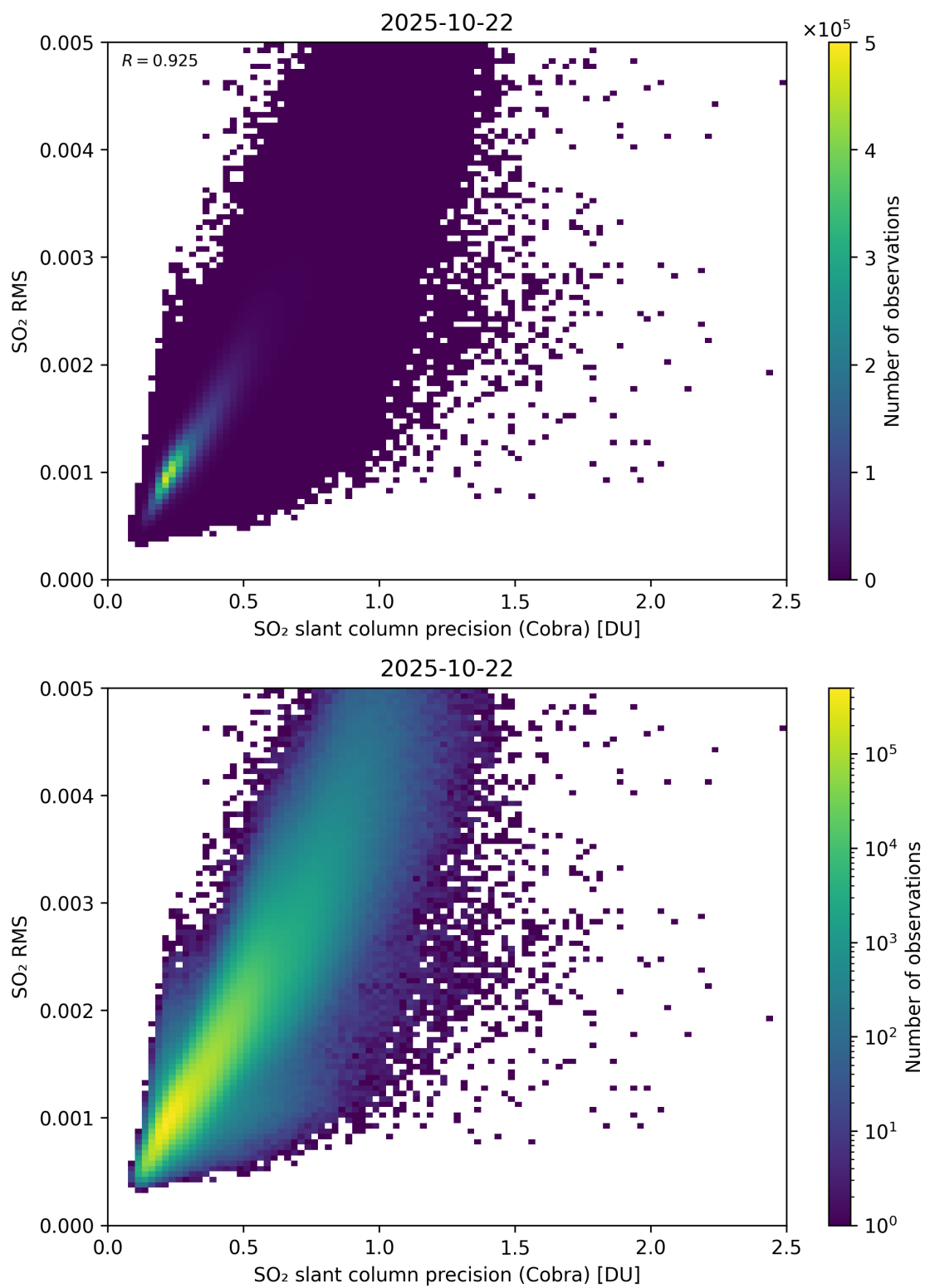
Figure 204: Scatter density plot of “SO 2 slant column precision (Cobra)” against “SO 2 RMS” for 2025-10-22 to 2025-10-23.
