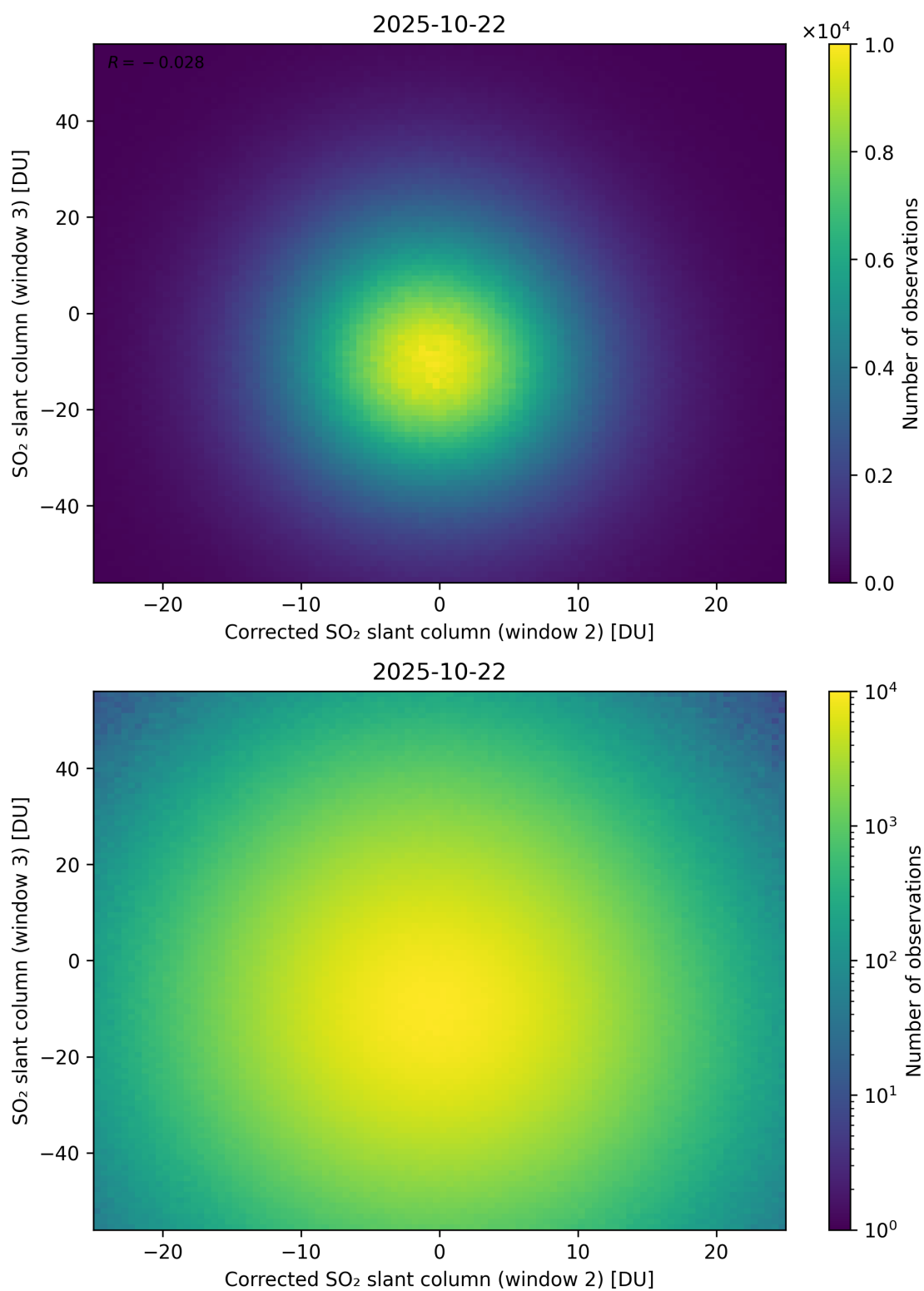
Figure 251: Scatter density plot of “Corrected SO 2 slant column (window 2)” against “SO 2 slant column (window 3)” for 2025-10-22 to 2025-10-23.
