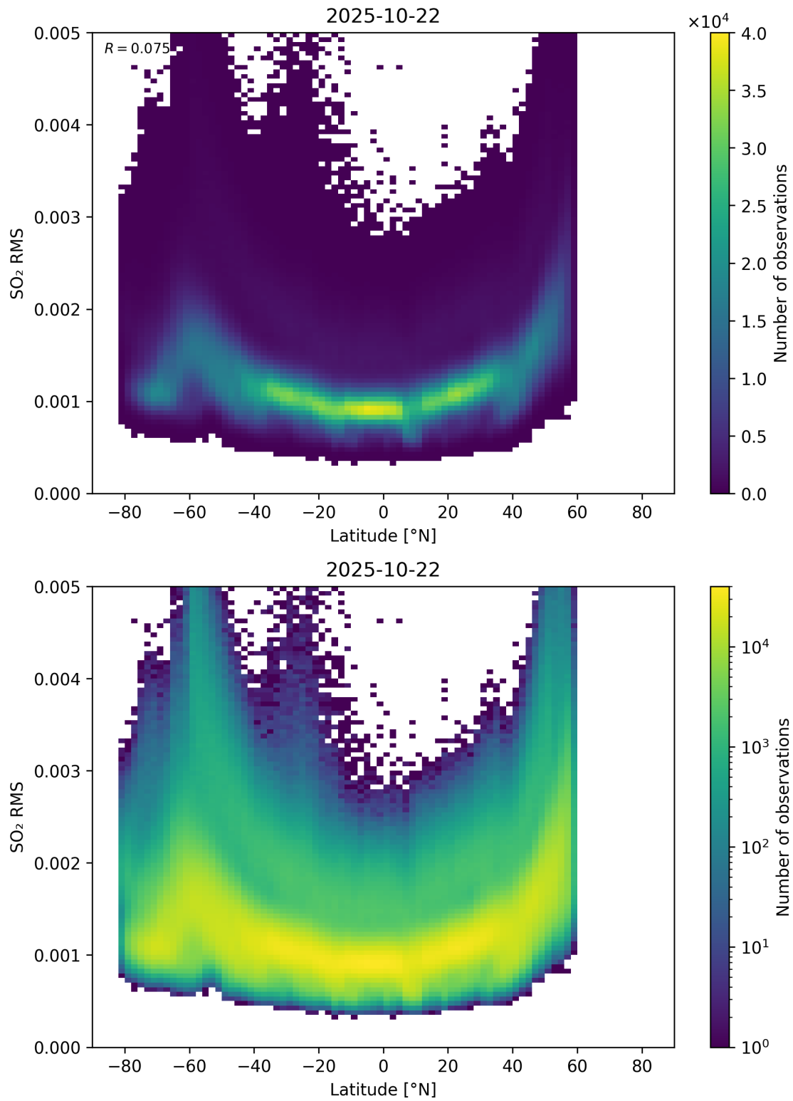
Figure 155: Scatter density plot of “Latitude” against “SO 2 RMS” for 2025-10-22 to 2025-10-23.
