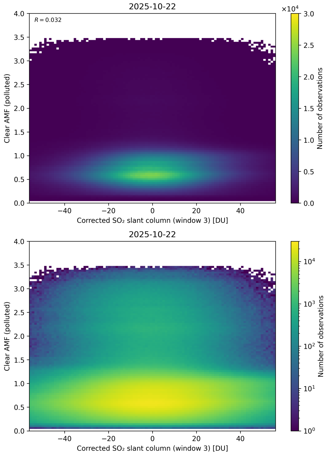
Figure 259: Scatter density plot of “Corrected SO 2 slant column (window 3)” against “Clear AMF (polluted)” for 2025-10-22 to 2025-10-23.
