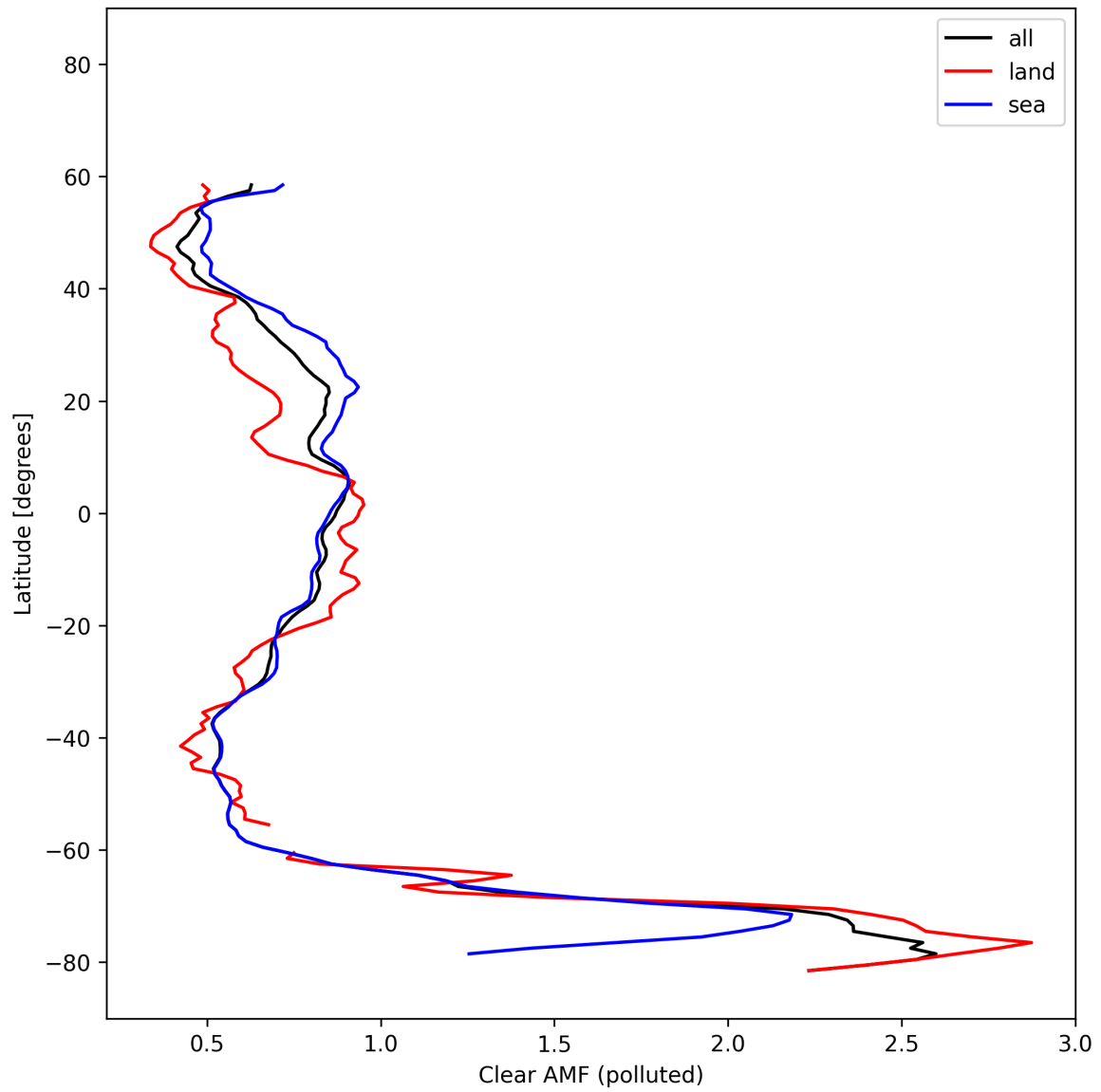
Figure 55: Zonal average of “Clear AMF (polluted)” for 2025-10-22 to 2025-10-23.
