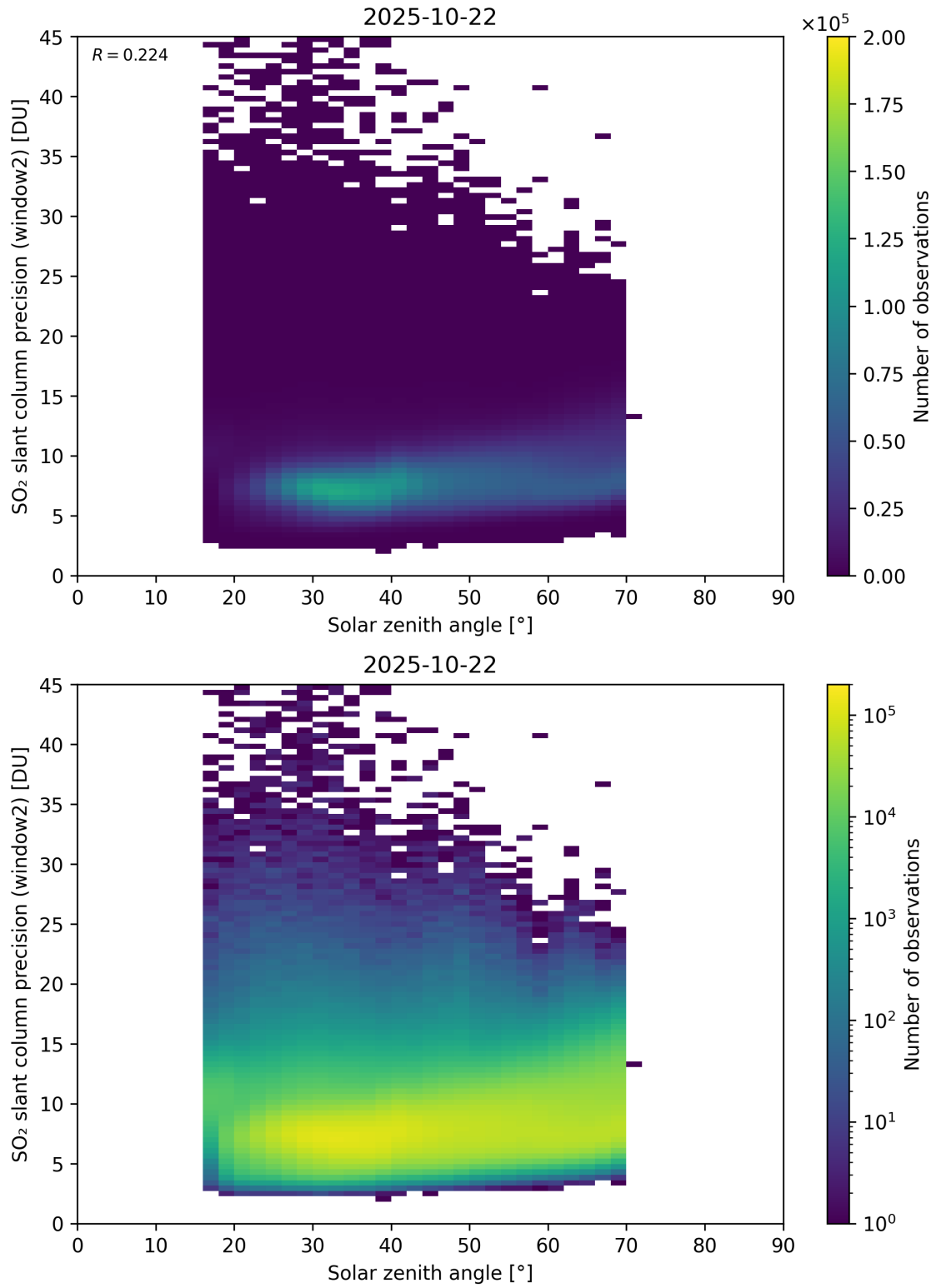
Figure 186: Scatter density plot of “Solar zenith angle” against “SO 2 slant column precision (window2)” for 2025-10-22 to 2025-10-23.
