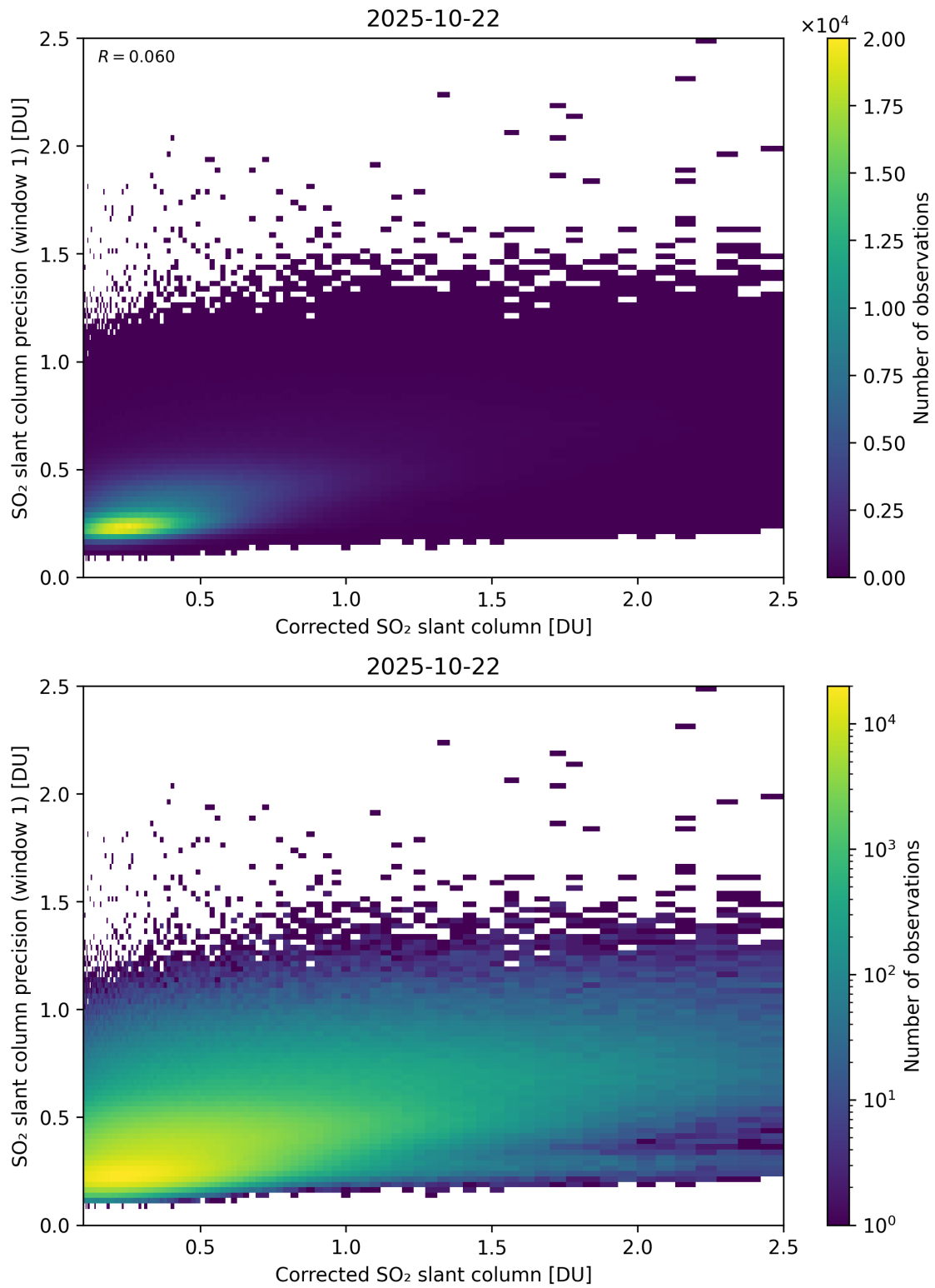
Figure 238: Scatter density plot of “Corrected SO 2 slant column” against “SO 2 slant column precision (window 1)” for 2025-10-22 to 2025-10-23.
