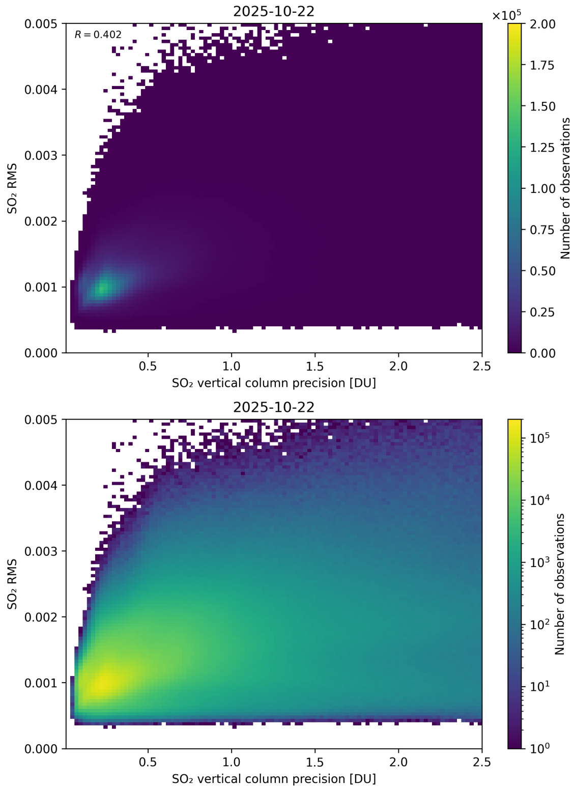
Figure 334: Scatter density plot of “SO 2 vertical column precision” against “SO 2 RMS” for 2025-10-22 to 2025-10-23.
