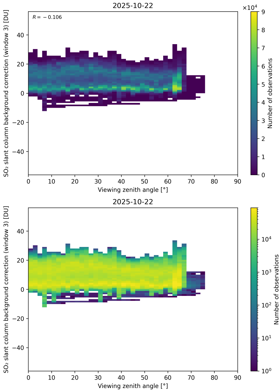
Figure 364: Scatter density plot of “Viewing zenith angle” against “SO 2 slant column background correction (window 3)” for 2025-10-22 to 2025-10-23.
