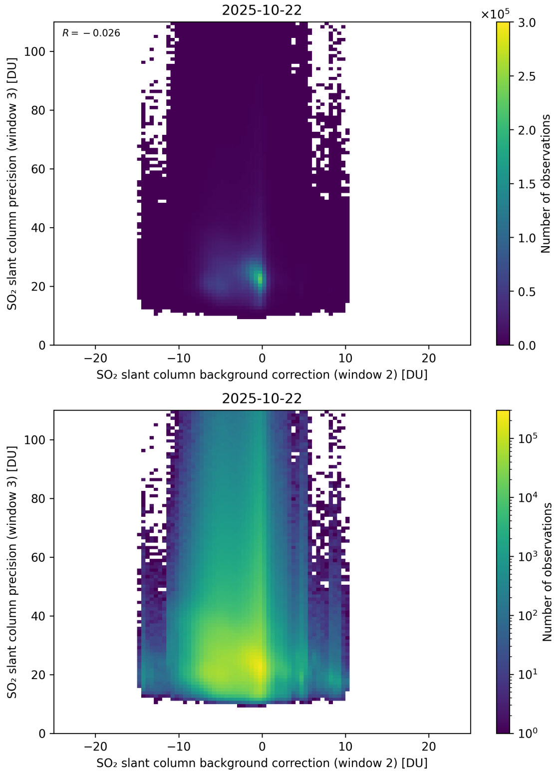
Figure 129: Scatter density plot of “SO 2 slant column background correction (window 2)” against “SO 2 slant column precision (window 3)” for 2025-10-22 to 2025-10-23.
