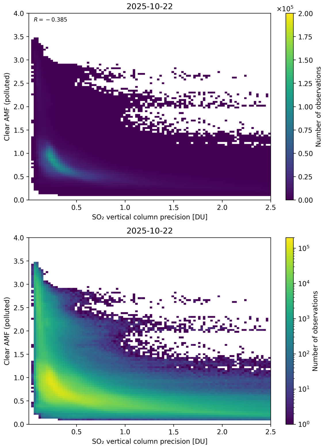
Figure 335: Scatter density plot of “SO 2 vertical column precision” against “Clear AMF (polluted)” for 2025-10-22 to 2025-10-23.
