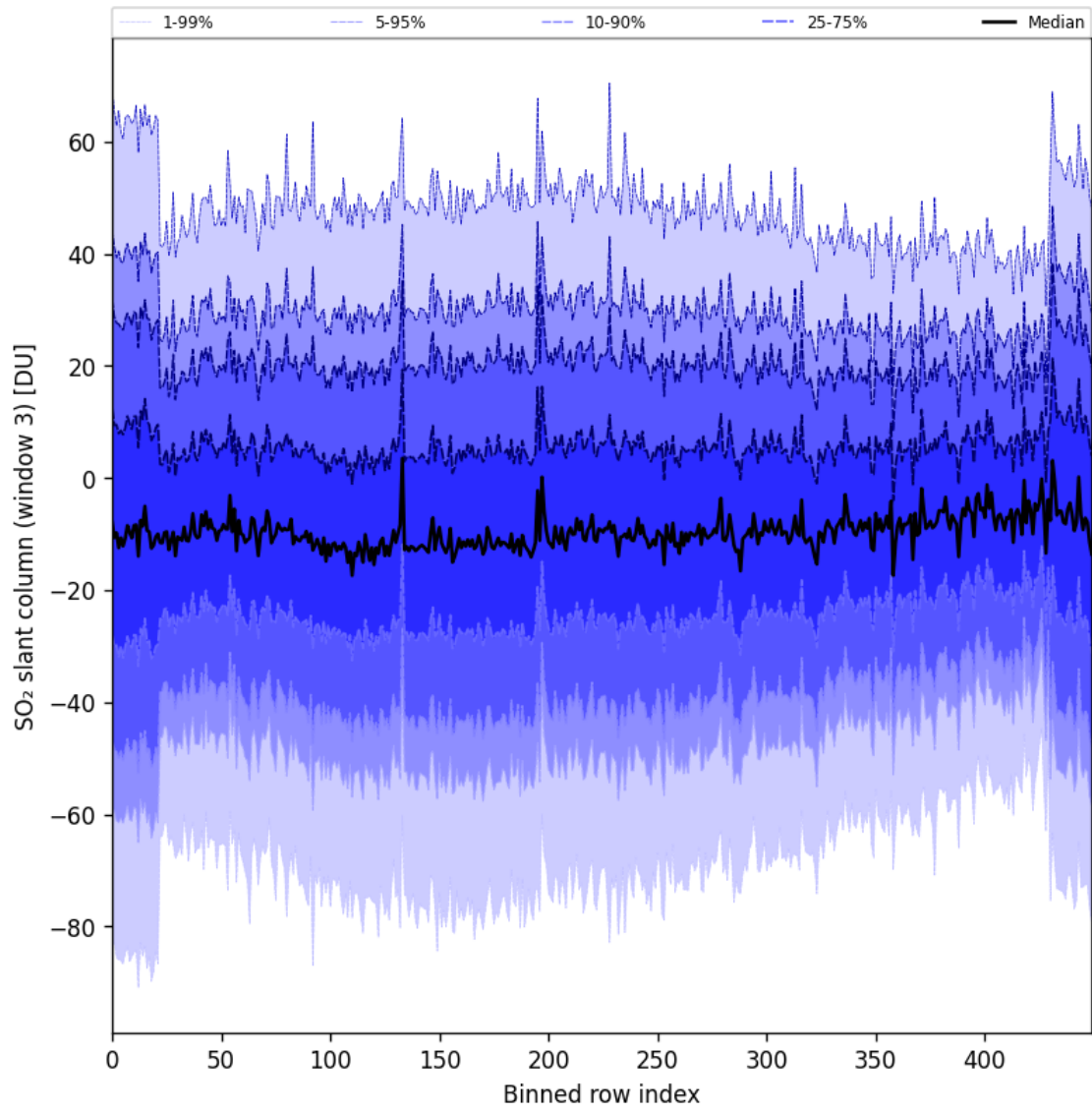
Figure 97: Along track statistics of “SO 2 slant column (window 3)” for 2025-10-22 to 2025-10-23
