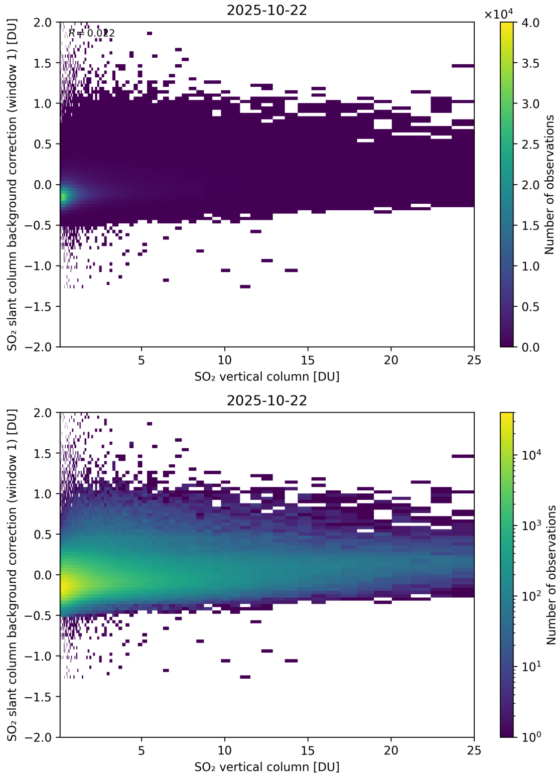
Figure 323: Scatter density plot of “SO 2 vertical column” against “SO 2 slant column background correction (window 1)” for 2025-10-22 to 2025-10-23.
