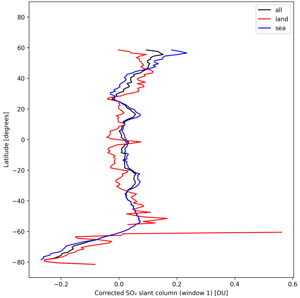
Figure 39: Zonal average of “Corrected SO 2 slant column (window 1)” for 2025-10-22 to 2025-10-23.
