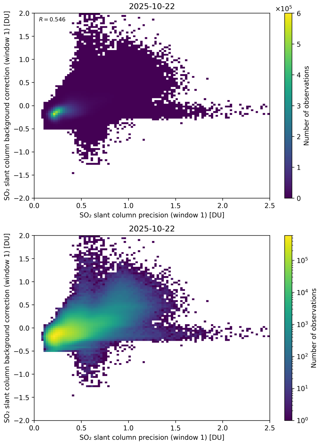
Figure 268: Scatter density plot of “SO 2 slant column precision (window 1)” against “SO 2 slant column background correction (window 1)” for 2025-10-22 to 2025-10-23.
