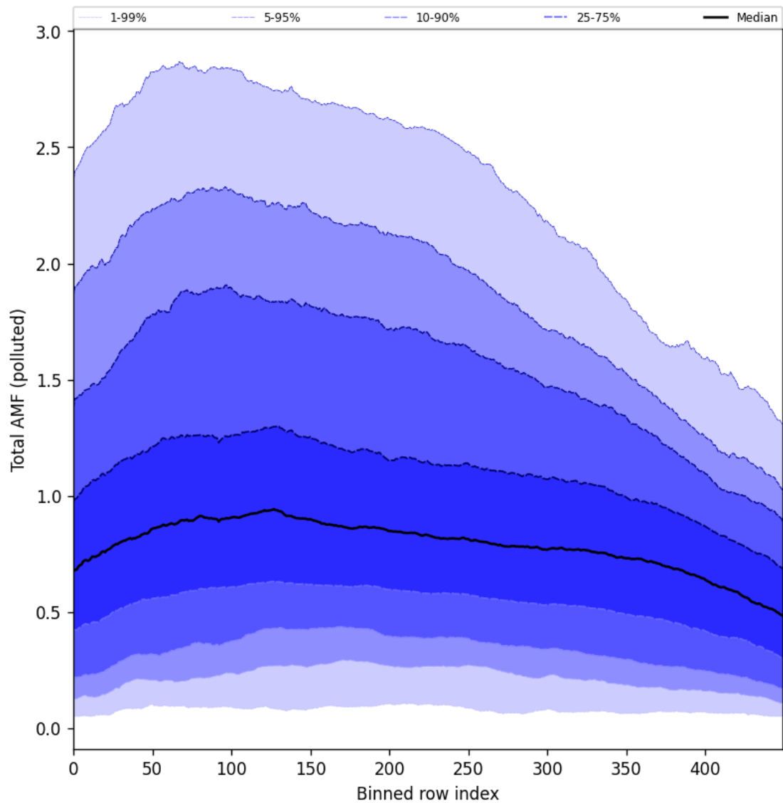
Figure 105: Along track statistics of “Total AMF (polluted)” for 2025-10-22 to 2025-10-23
