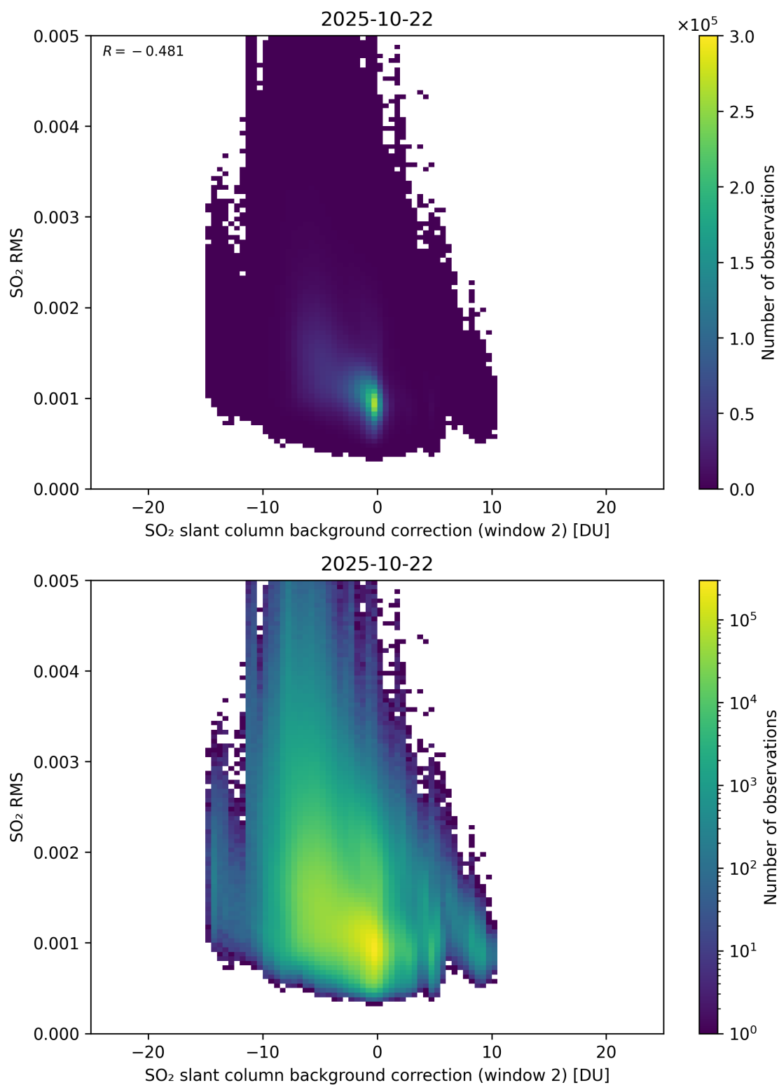
Figure 125: Scatter density plot of “SO 2 slant column background correction (window 2)” against “SO 2 RMS” for 2025-10-22 to 2025-10-23.
