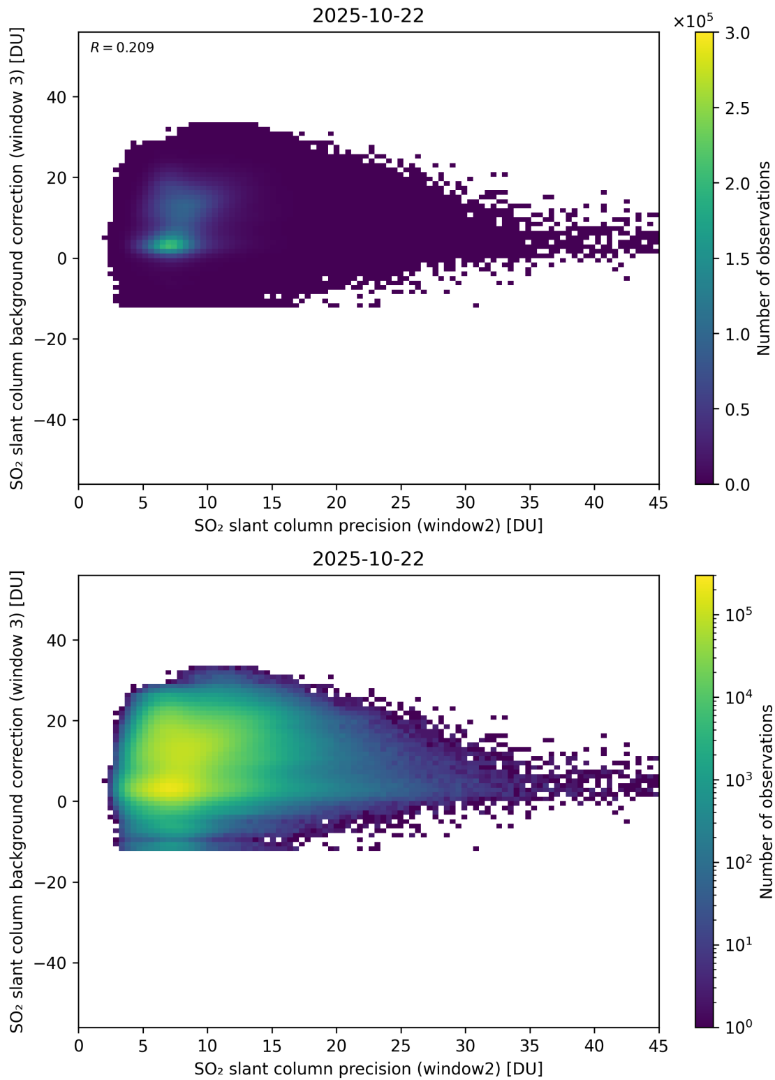
Figure 292: Scatter density plot of “SO 2 slant column precision (window2)” against “SO 2 slant column background correction (window 3)” for 2025-10-22 to 2025-10-23.
