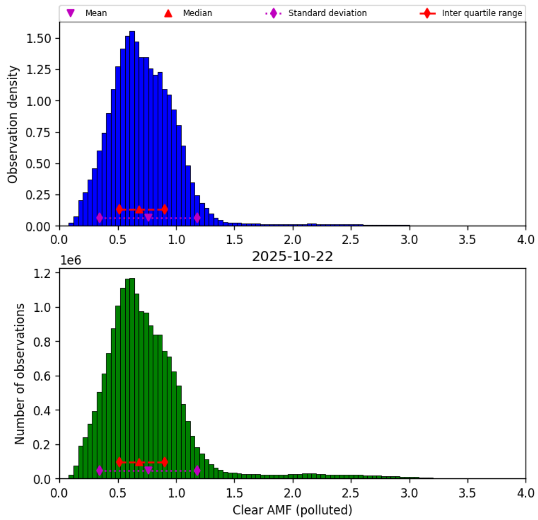
Figure 81: Histogram of “Clear AMF (polluted)” for 2025-10-22 to 2025-10-23
