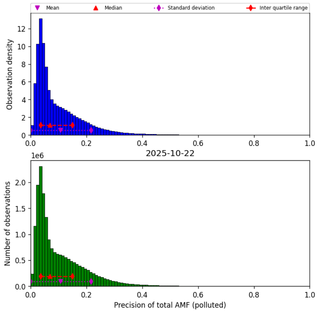
Figure 80: Histogram of “Precision of total AMF (polluted)” for 2025-10-22 to 2025-10-23
