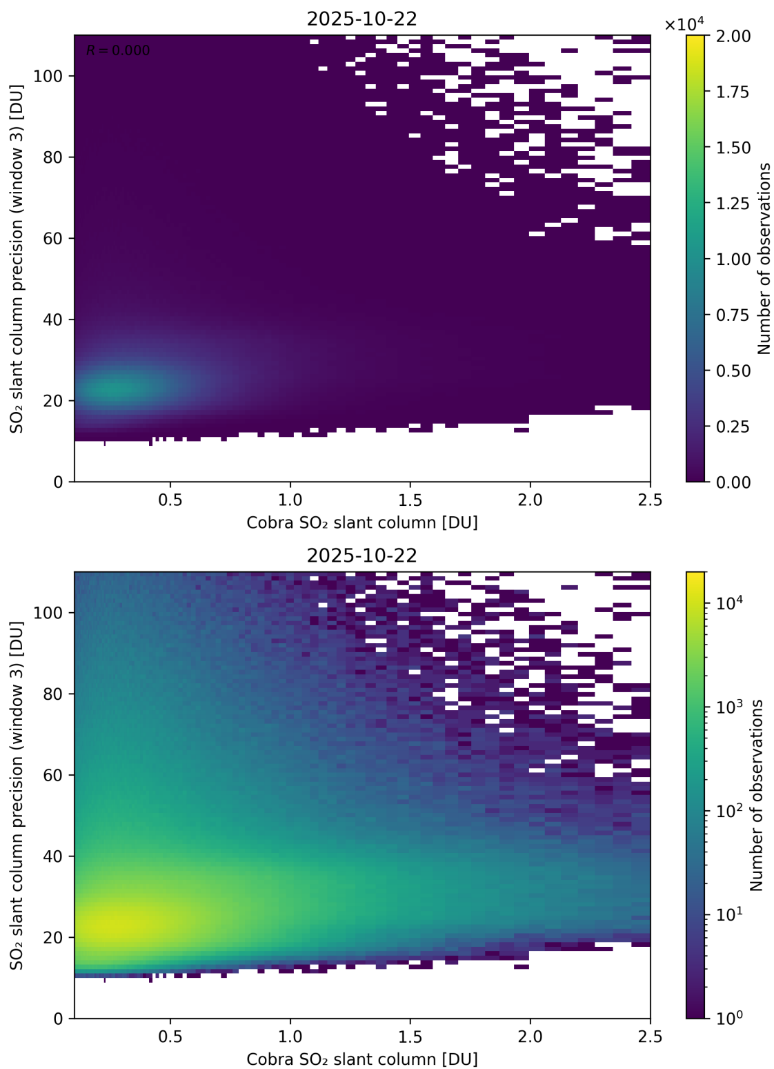
Figure 223: Scatter density plot of “Cobra SO 2 slant column” against “SO 2 slant column precision (window 3)” for 2025-10-22 to 2025-10-23.
