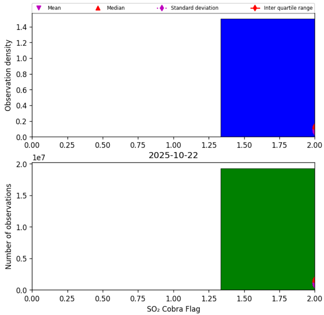
Figure 75: Histogram of “SO 2 Cobra Flag” for 2025-10-22 to 2025-10-23
