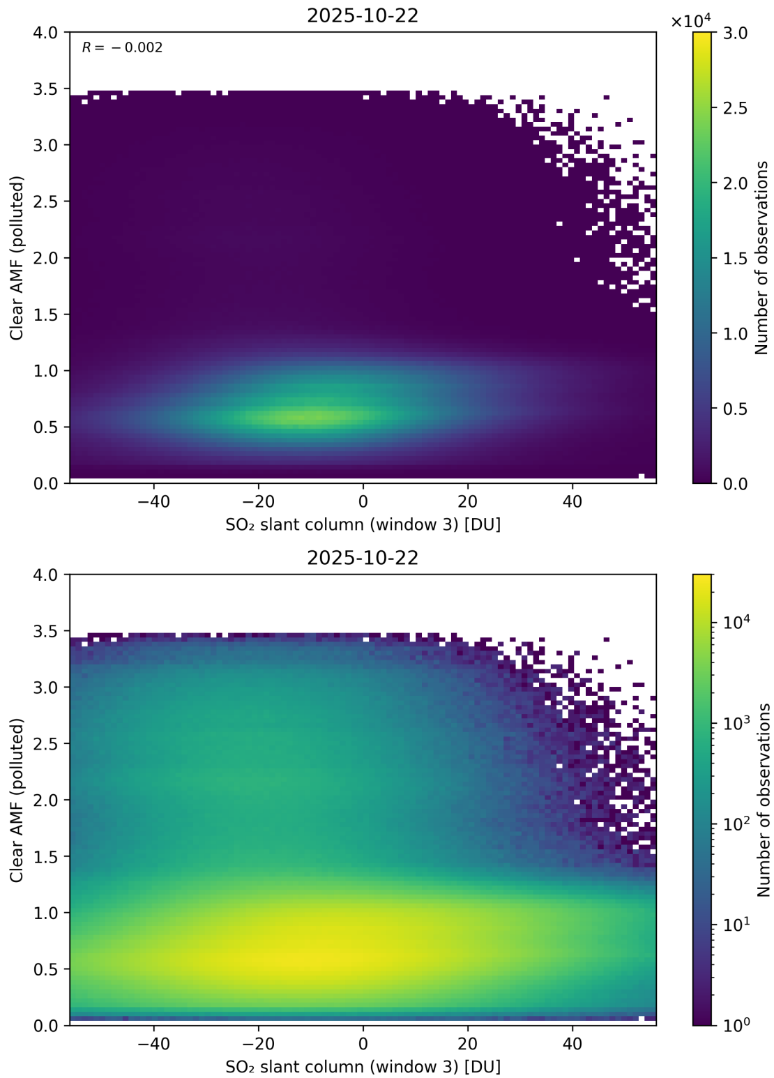
Figure 315: Scatter density plot of “SO 2 slant column (window 3)” against “Clear AMF (polluted)” for 2025-10-22 to 2025-10-23.
