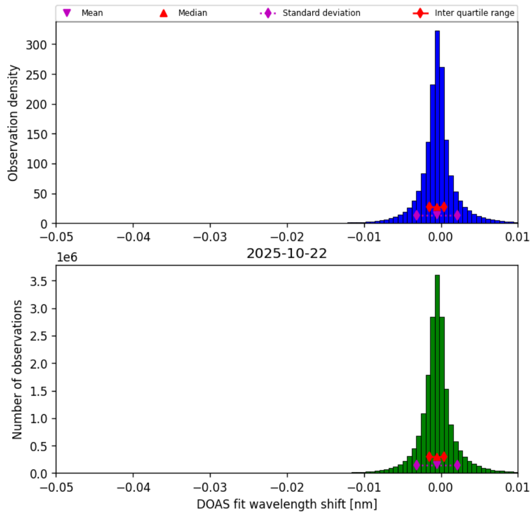
Figure 76: Histogram of “DOAS fit wavelength shift” for 2025-10-22 to 2025-10-23
