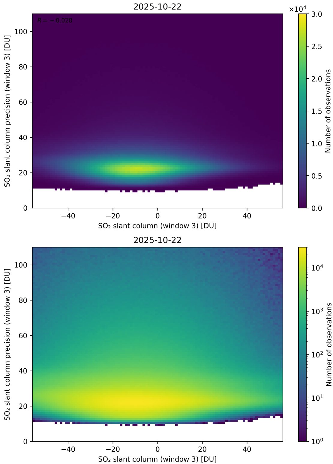
Figure 317: Scatter density plot of “SO 2 slant column (window 3)” against “SO 2 slant column precision (window 3)” for 2025-10-22 to 2025-10-23.
