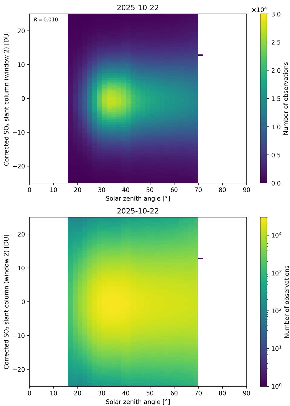
Figure 182: Scatter density plot of “Solar zenith angle” against “Corrected SO 2 slant column (window 2)” for 2025-10-22 to 2025-10-23.
