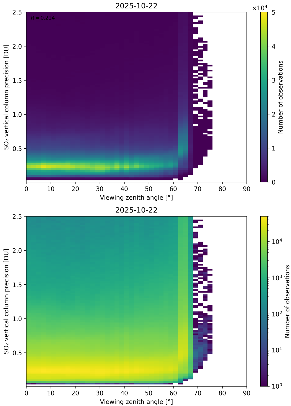
Figure 384: Scatter density plot of “Viewing zenith angle” against “SO 2 vertical column precision” for 2025-10-22 to 2025-10-23.
