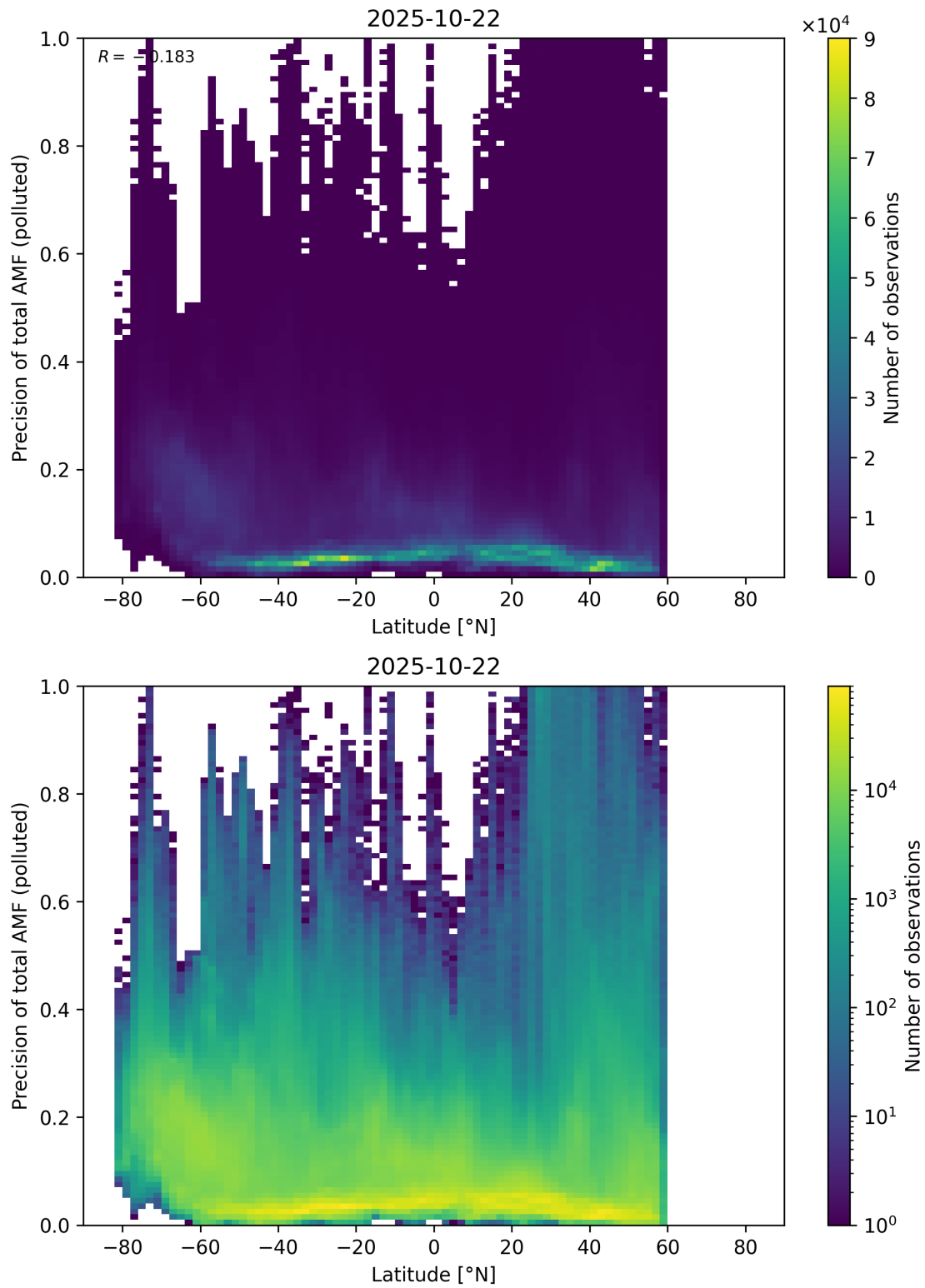
Figure 168: Scatter density plot of “Latitude” against “Precision of total AMF (polluted)” for 2025-10-22 to 2025-10-23.
