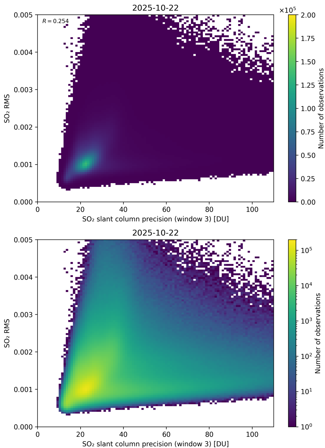
Figure 310: Scatter density plot of “SO 2 slant column precision (window 3)” against “SO 2 RMS” for 2025-10-22 to 2025-10-23.
