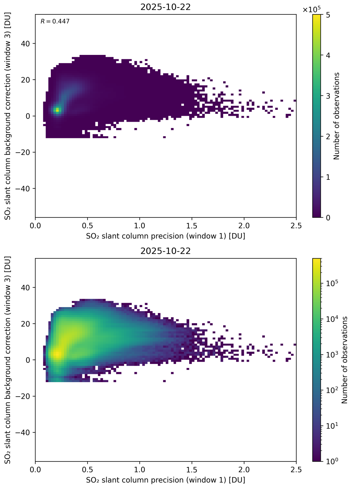
Figure 270: Scatter density plot of “SO 2 slant column precision (window 1)” against “SO 2 slant column background correction (window 3)” for 2025-10-22 to 2025-10-23.
