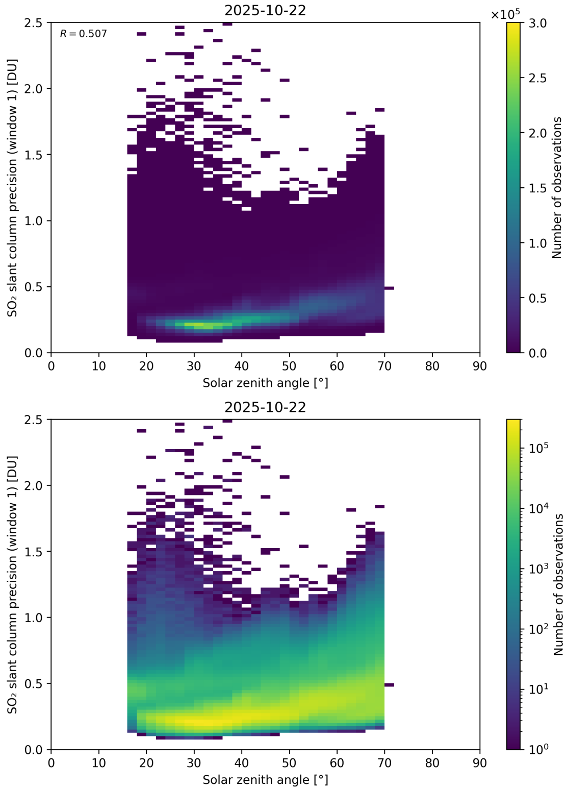
Figure 185: Scatter density plot of “Solar zenith angle” against “SO 2 slant column precision (window 1)” for 2025-10-22 to 2025-10-23.
