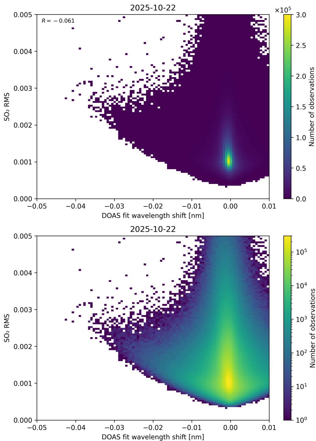
Figure 139: Scatter density plot of “DOAS fit wavelength shift” against “SO 2 RMS” for 2025-10-22 to 2025-10-23.
