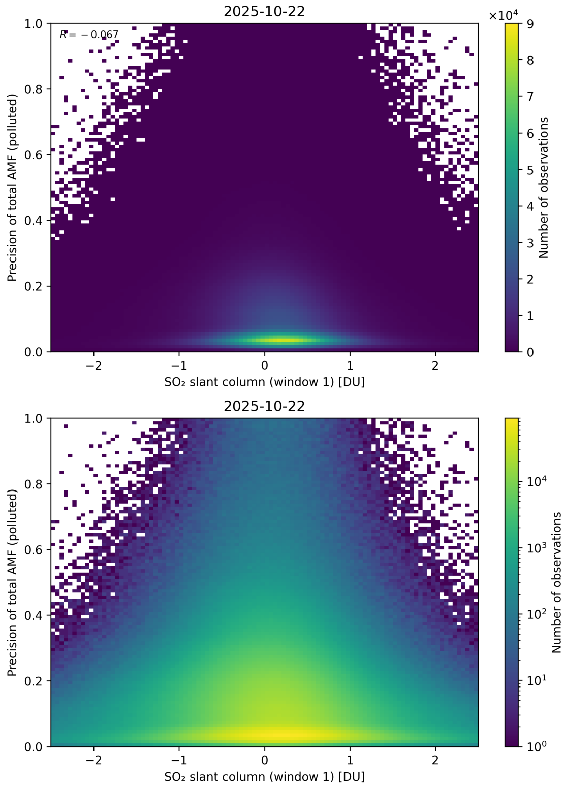
Figure 290: Scatter density plot of “SO 2 slant column (window 1)” against “Precision of total AMF (polluted)” for 2025-10-22 to 2025-10-23.
