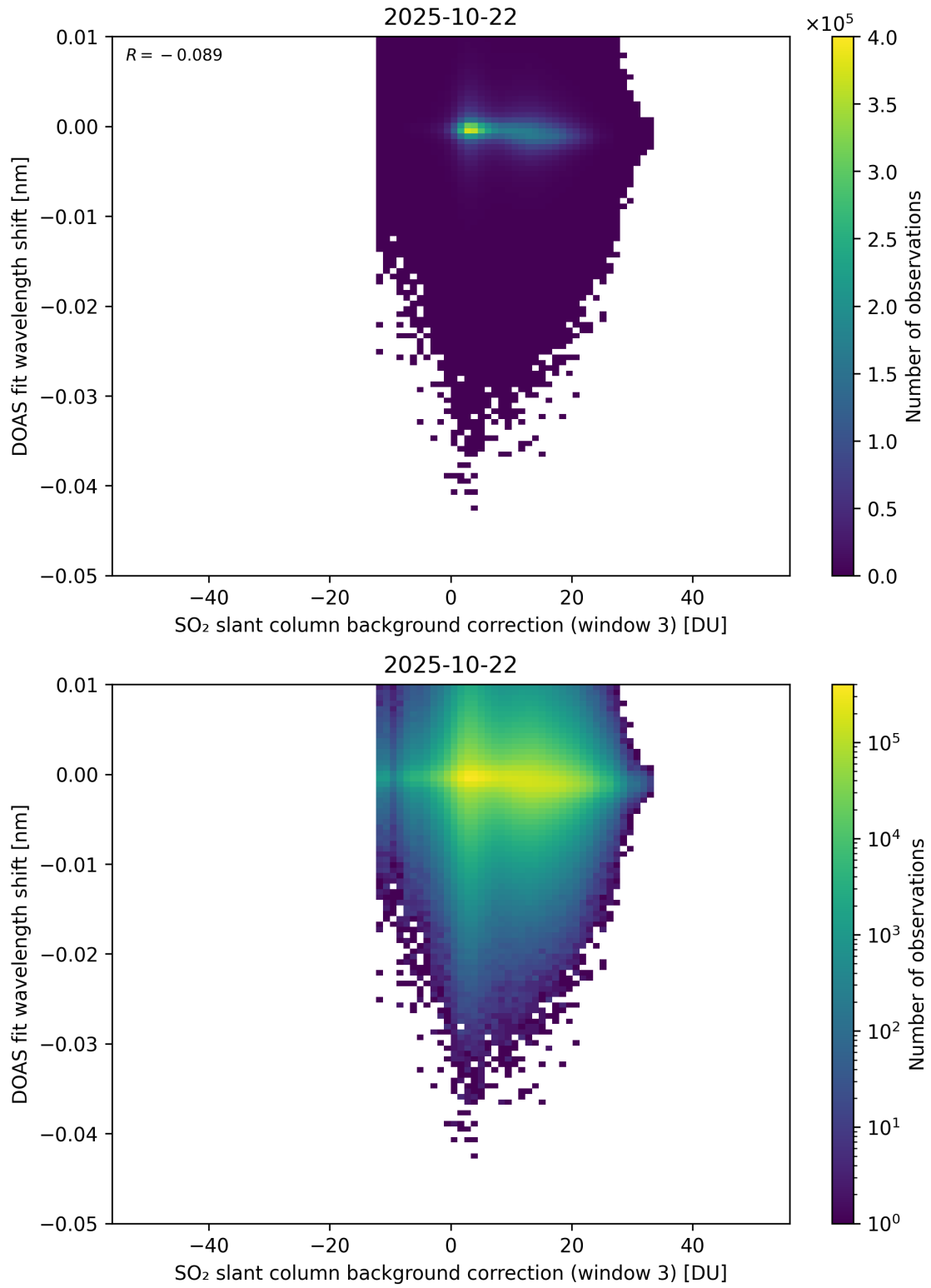
Figure 132: Scatter density plot of “SO 2 slant column background correction (window 3)” against “DOAS fit wavelength shift” for 2025-10-22 to 2025-10-23.
