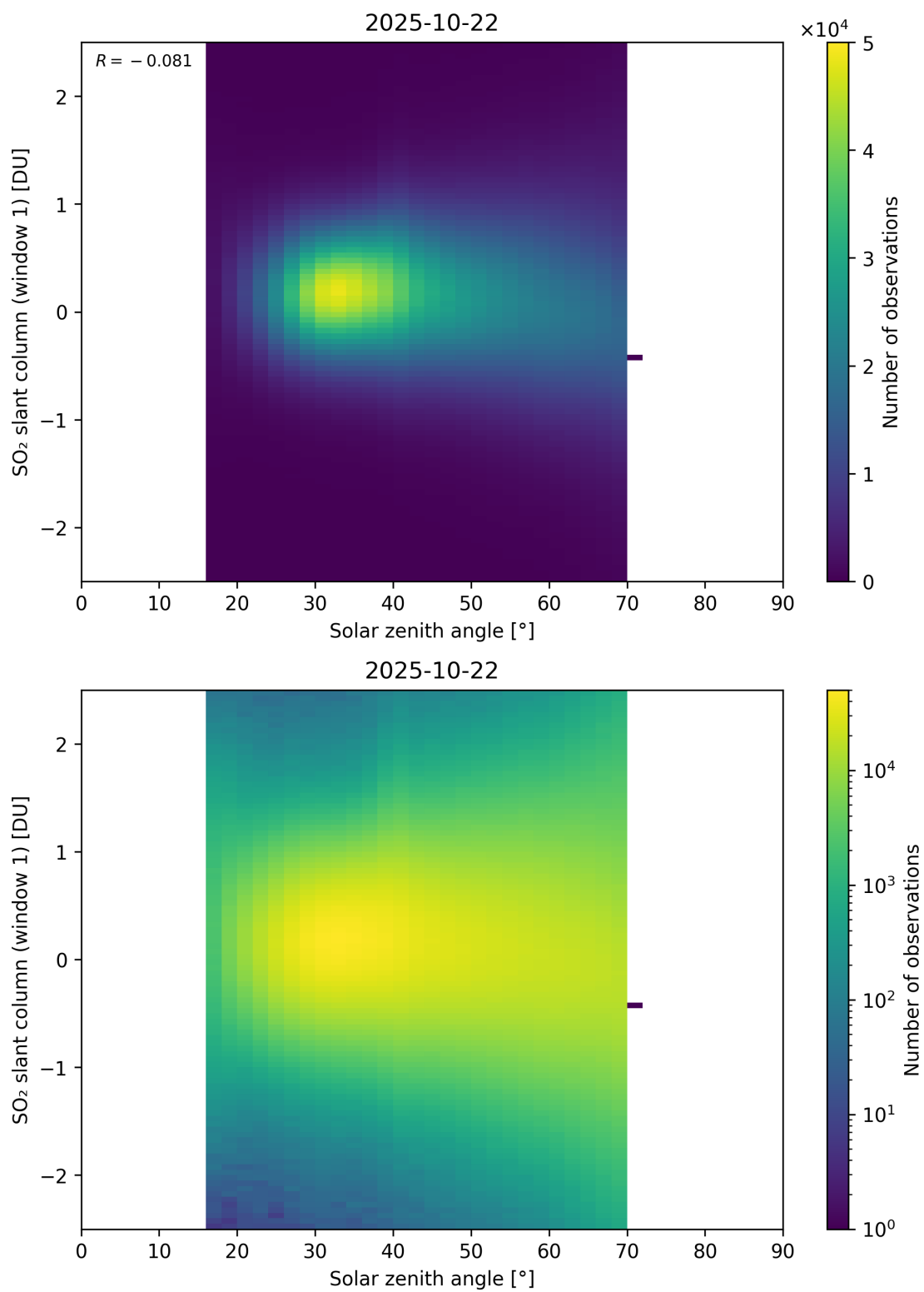
Figure 184: Scatter density plot of “Solar zenith angle” against “SO 2 slant column (window 1)” for 2025-10-22 to 2025-10-23.
