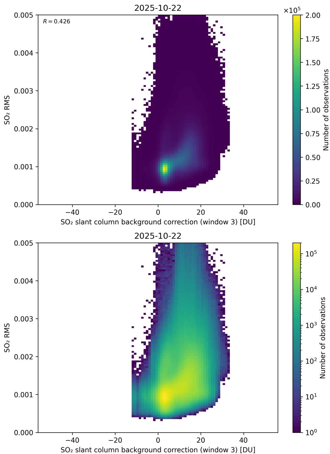
Figure 134: Scatter density plot of “SO 2 slant column background correction (window 3)” against “SO 2 RMS” for 2025-10-22 to 2025-10-23.
