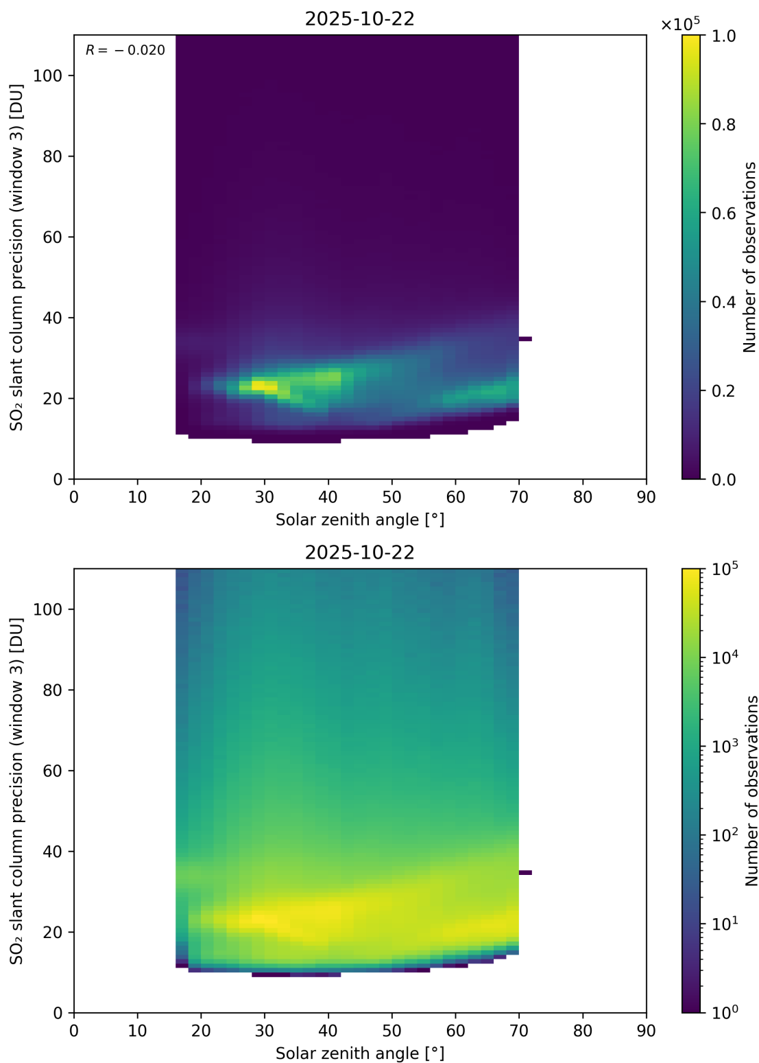
Figure 188: Scatter density plot of “Solar zenith angle” against “SO 2 slant column precision (window 3)” for 2025-10-22 to 2025-10-23.
