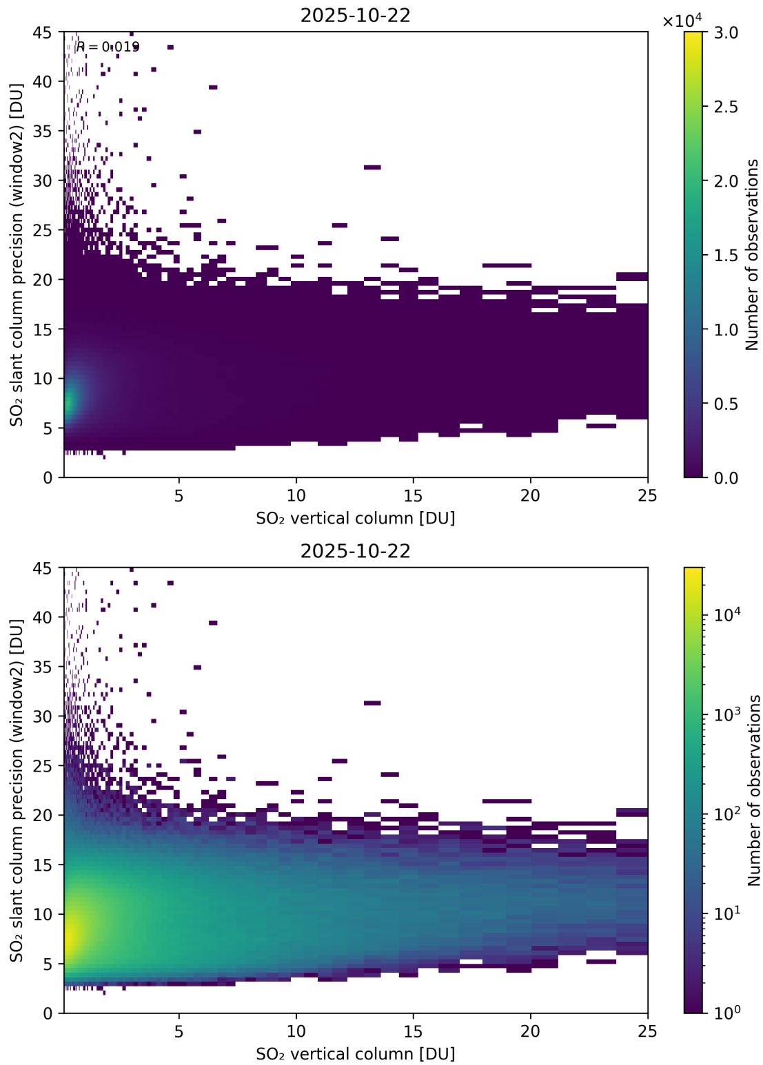
Figure 356: Scatter density plot of “SO 2 vertical column” against “SO 2 slant column precision (window2)” for 2025-10-22 to 2025-10-23.
