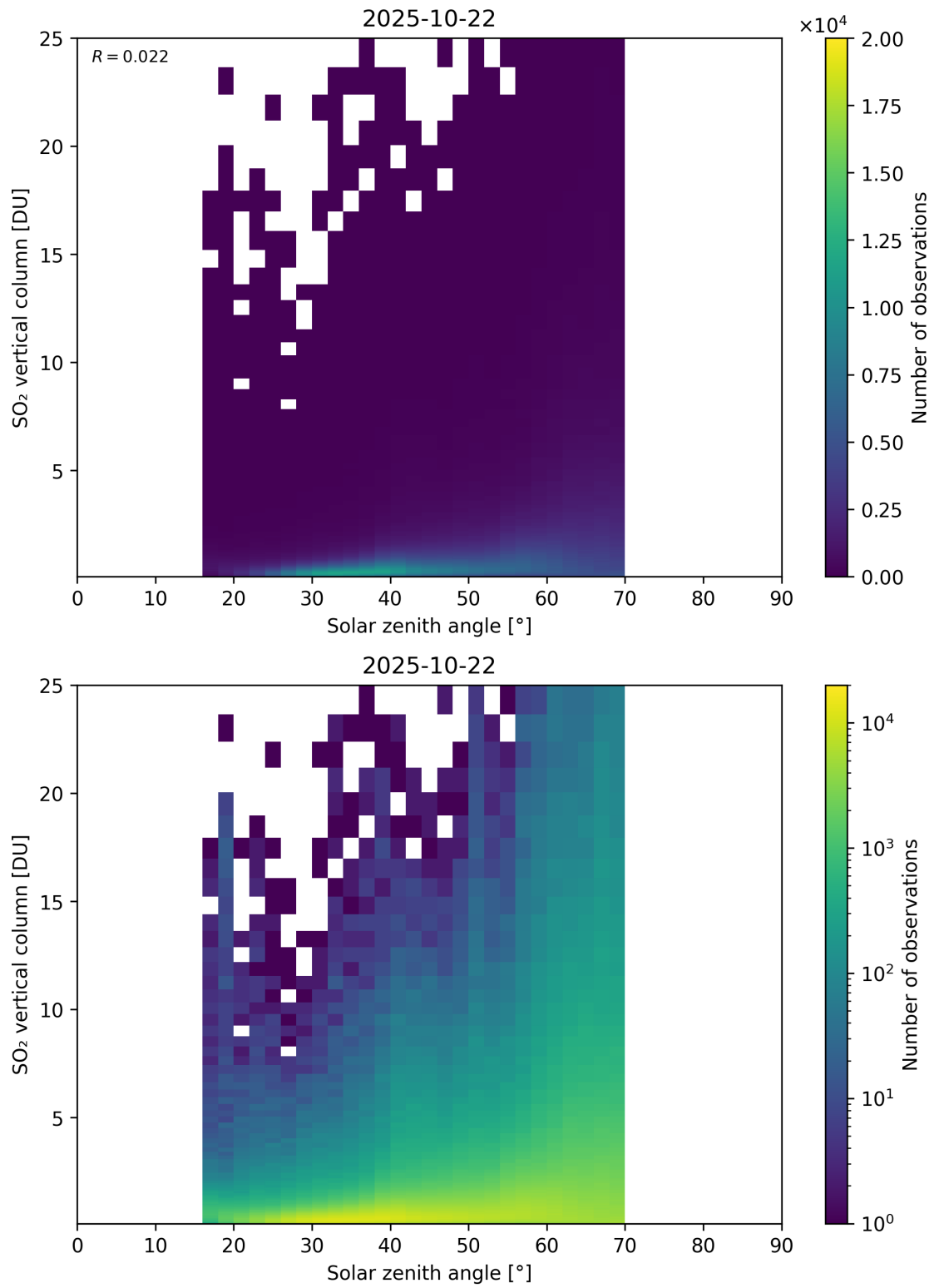
Figure 191: Scatter density plot of “Solar zenith angle” against “SO 2 vertical column” for 2025-10-22 to 2025-10-23.
