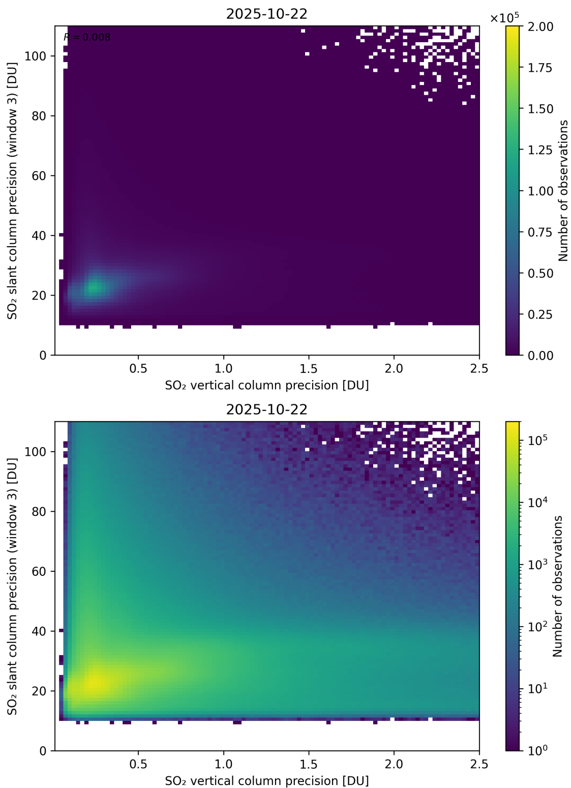
Figure 345: Scatter density plot of “SO 2 vertical column precision” against “SO 2 slant column precision (window 3)” for 2025-10-22 to 2025-10-23.
