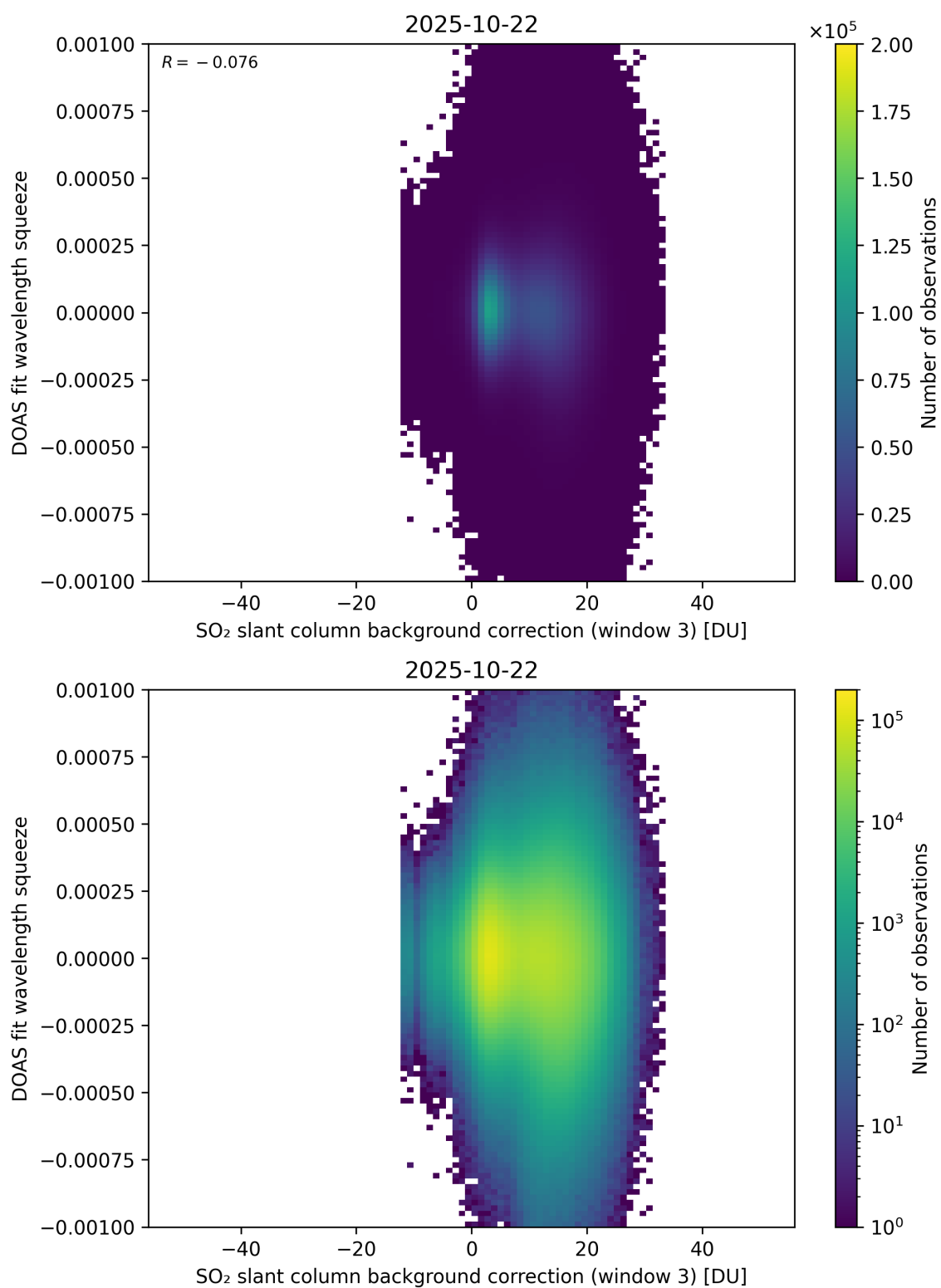
Figure 133: Scatter density plot of “SO 2 slant column background correction (window 3)” against “DOAS fit wavelength squeeze” for 2025-10-22 to 2025-10-23.
