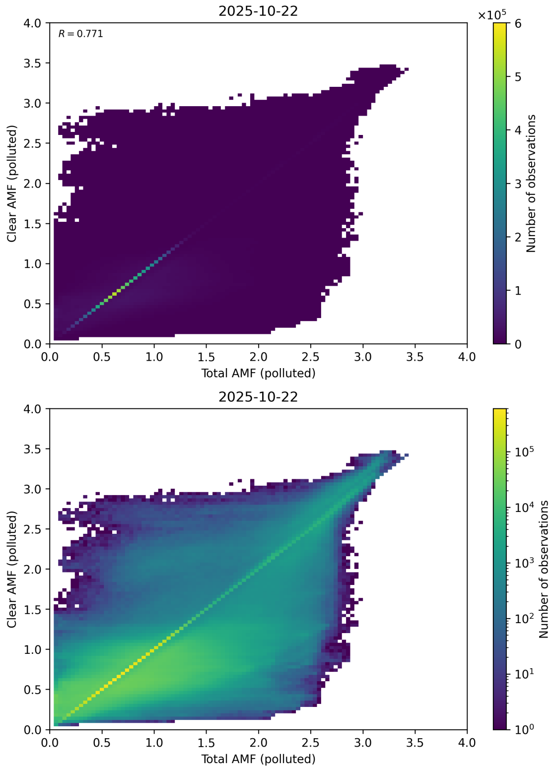
Figure 321: Scatter density plot of “Total AMF (polluted)” against “Clear AMF (polluted)” for 2025-10-22 to 2025-10-23.
