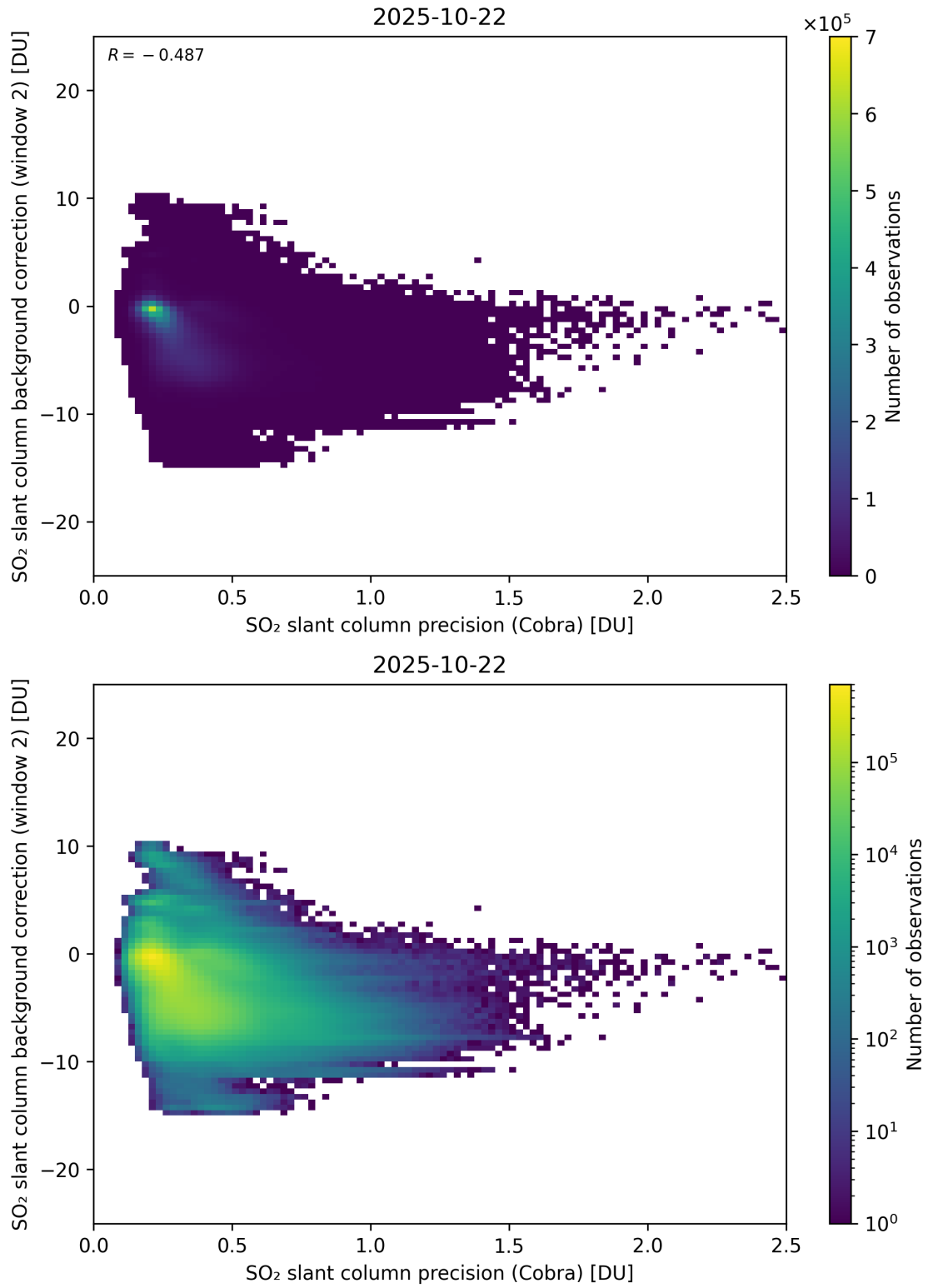
Figure 200: Scatter density plot of “SO 2 slant column precision (Cobra)” against “SO 2 slant column background correction (window 2)” for 2025-10-22 to 2025-10-23.
