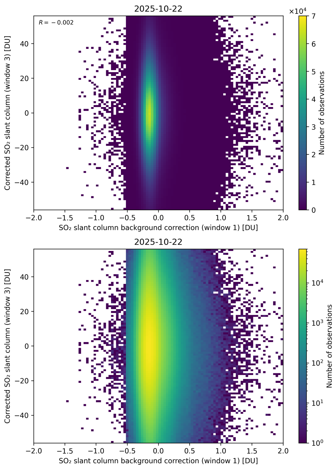
Figure 116: Scatter density plot of “SO 2 slant column background correction (window 1)” against “Corrected SO 2 slant column (window 3)” for 2025-10-22 to 2025-10-23.
