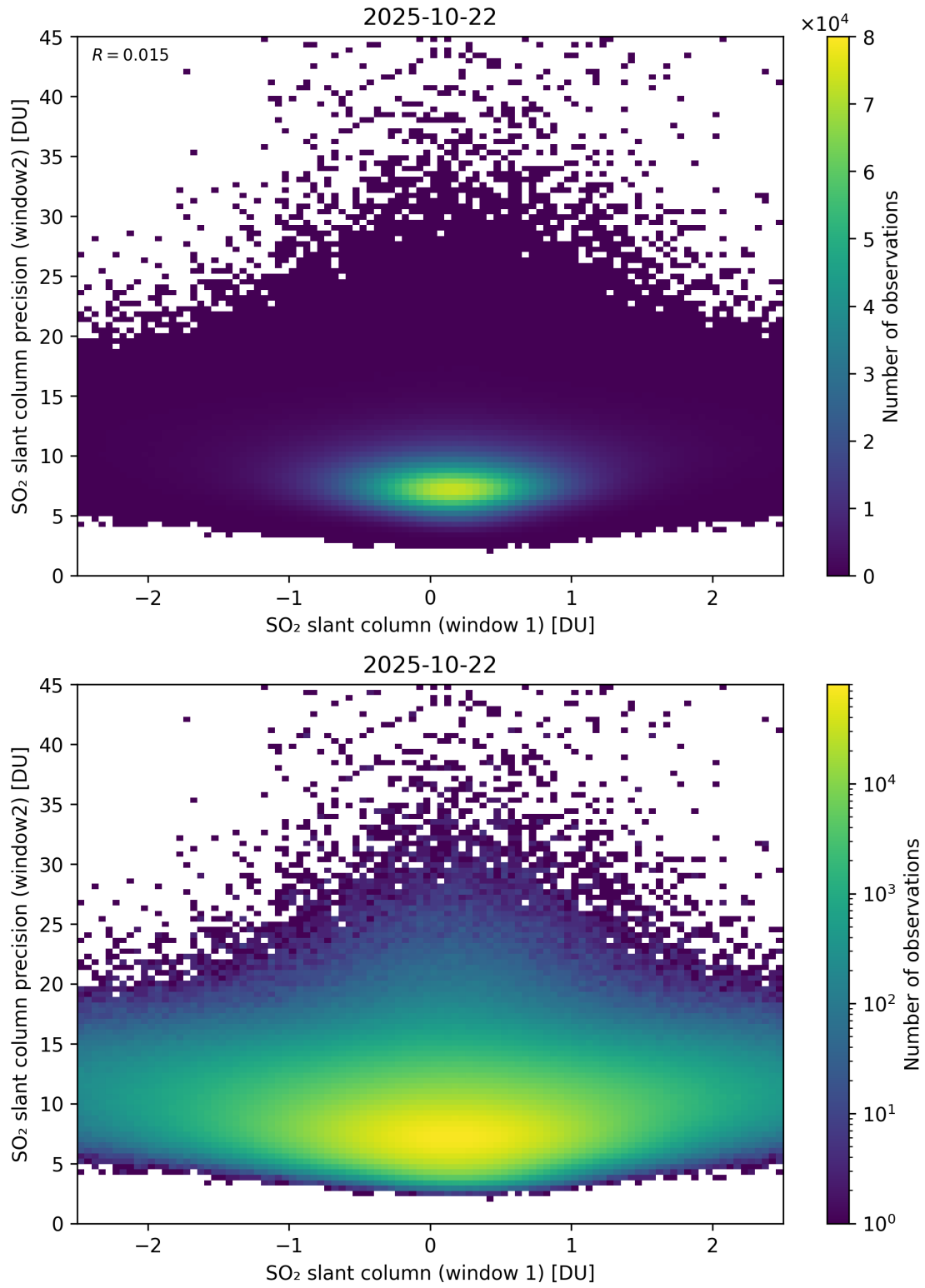
Figure 286: Scatter density plot of “SO 2 slant column (window 1)” against “SO 2 slant column precision (window2)” for 2025-10-22 to 2025-10-23.
