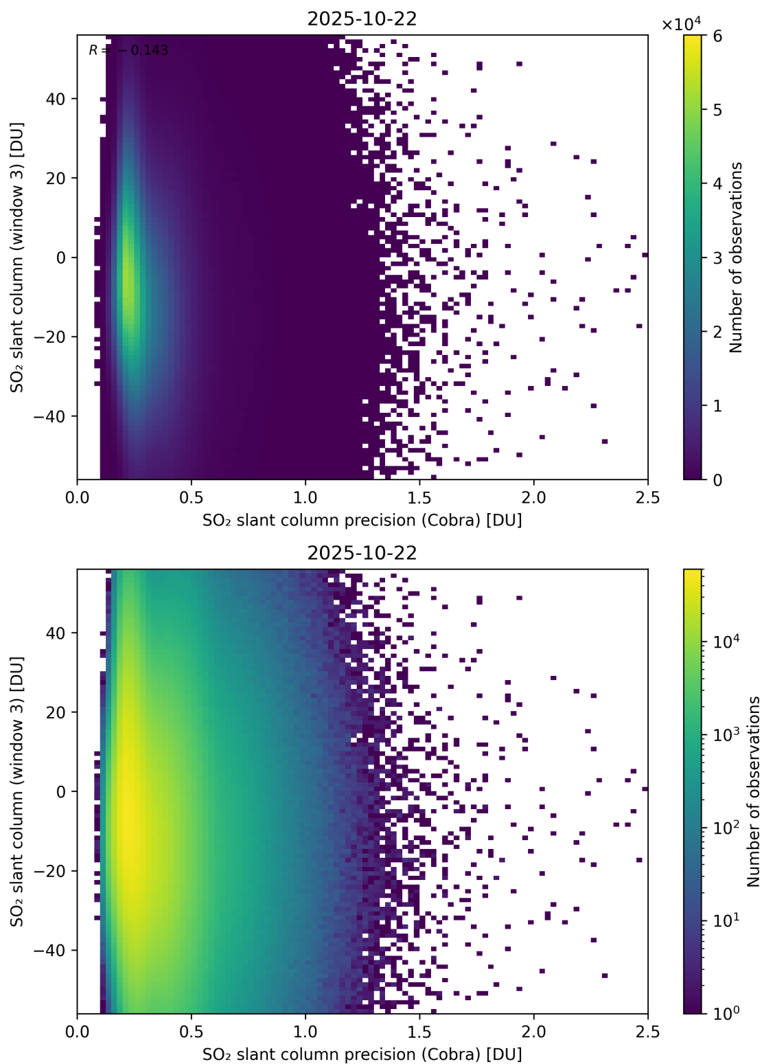
Figure 211: Scatter density plot of “SO 2 slant column precision (Cobra)” against “SO 2 slant column (window 3)” for 2025-10-22 to 2025-10-23.
