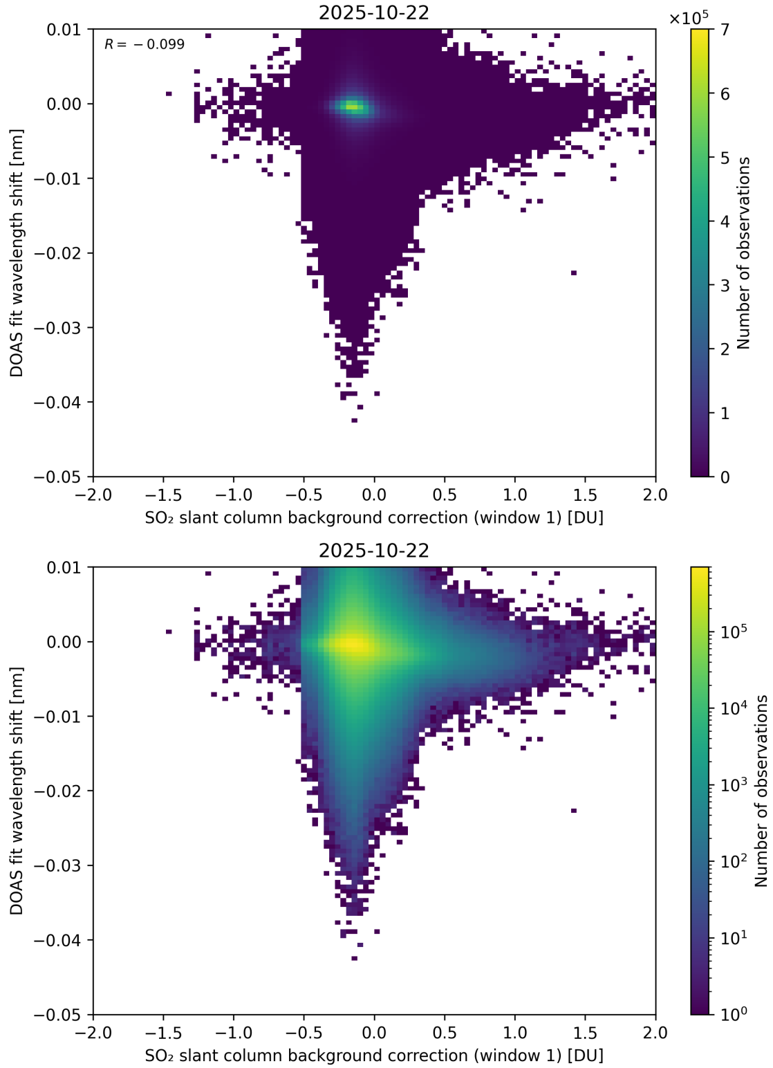
Figure 111: Scatter density plot of “SO 2 slant column background correction (window 1)” against “DOAS fit wavelength shift” for 2025-10-22 to 2025-10-23.
