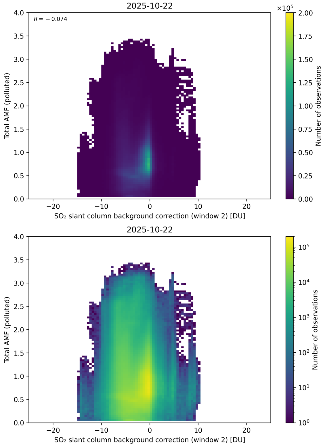
Figure 130: Scatter density plot of “SO 2 slant column background correction (window 2)” against “Total AMF (polluted)” for 2025-10-22 to 2025-10-23.
