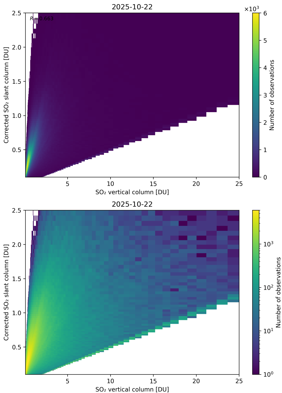
Figure 351: Scatter density plot of “SO 2 vertical column” against “Corrected SO 2 slant column” for 2025-10-22 to 2025-10-23.
