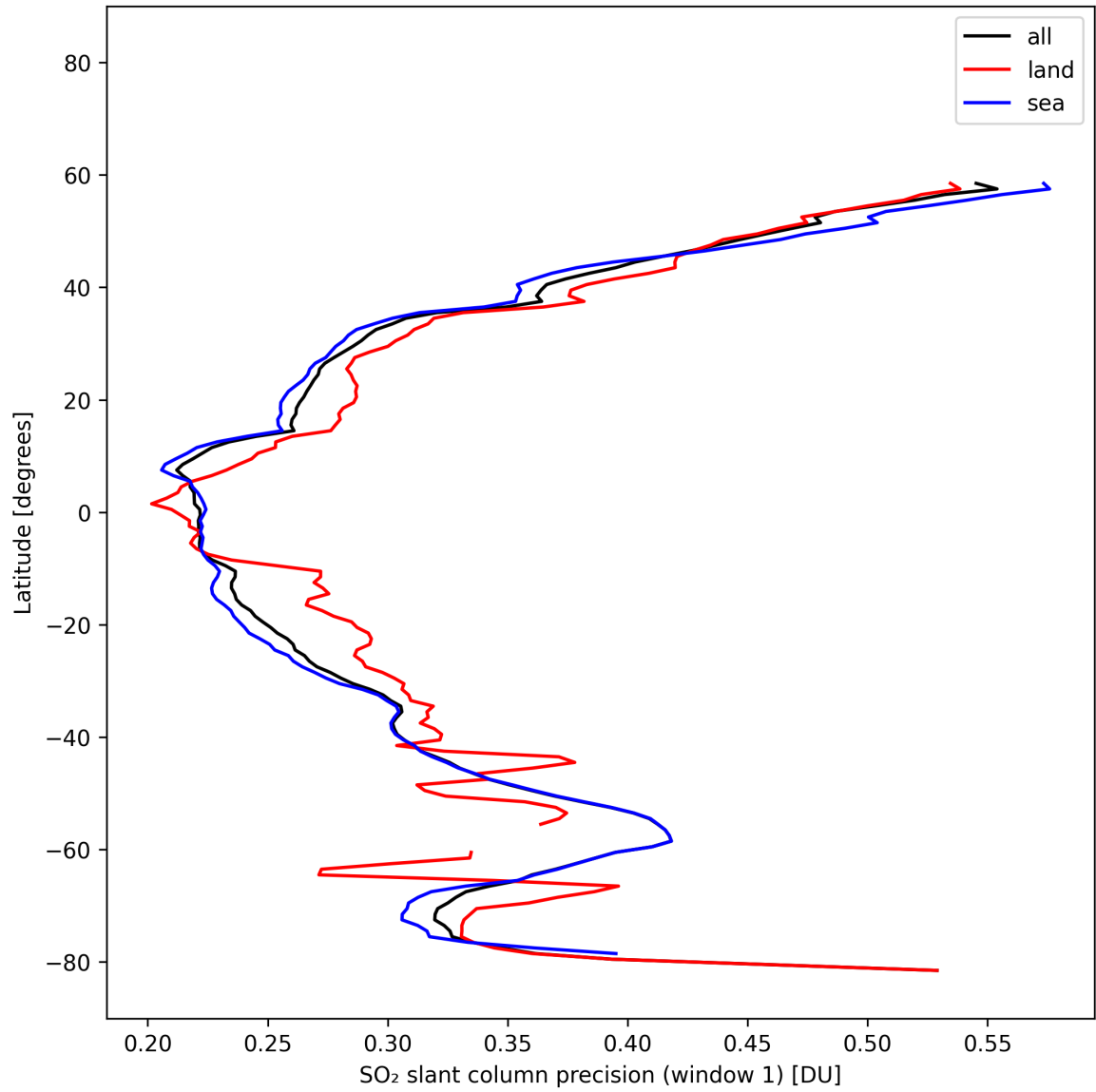
Figure 38: Zonal average of “SO 2 slant column precision (window 1)” for 2025-10-22 to 2025-10-23.
