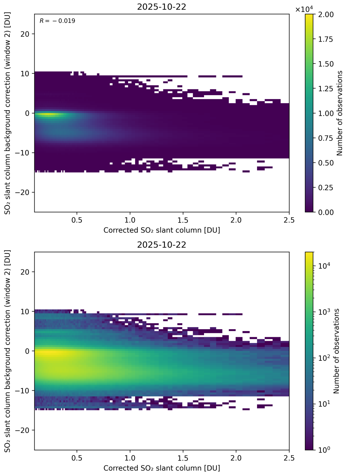
Figure 227: Scatter density plot of “Corrected SO 2 slant column” against “SO 2 slant column background correction (window 2)” for 2025-10-22 to 2025-10-23.
