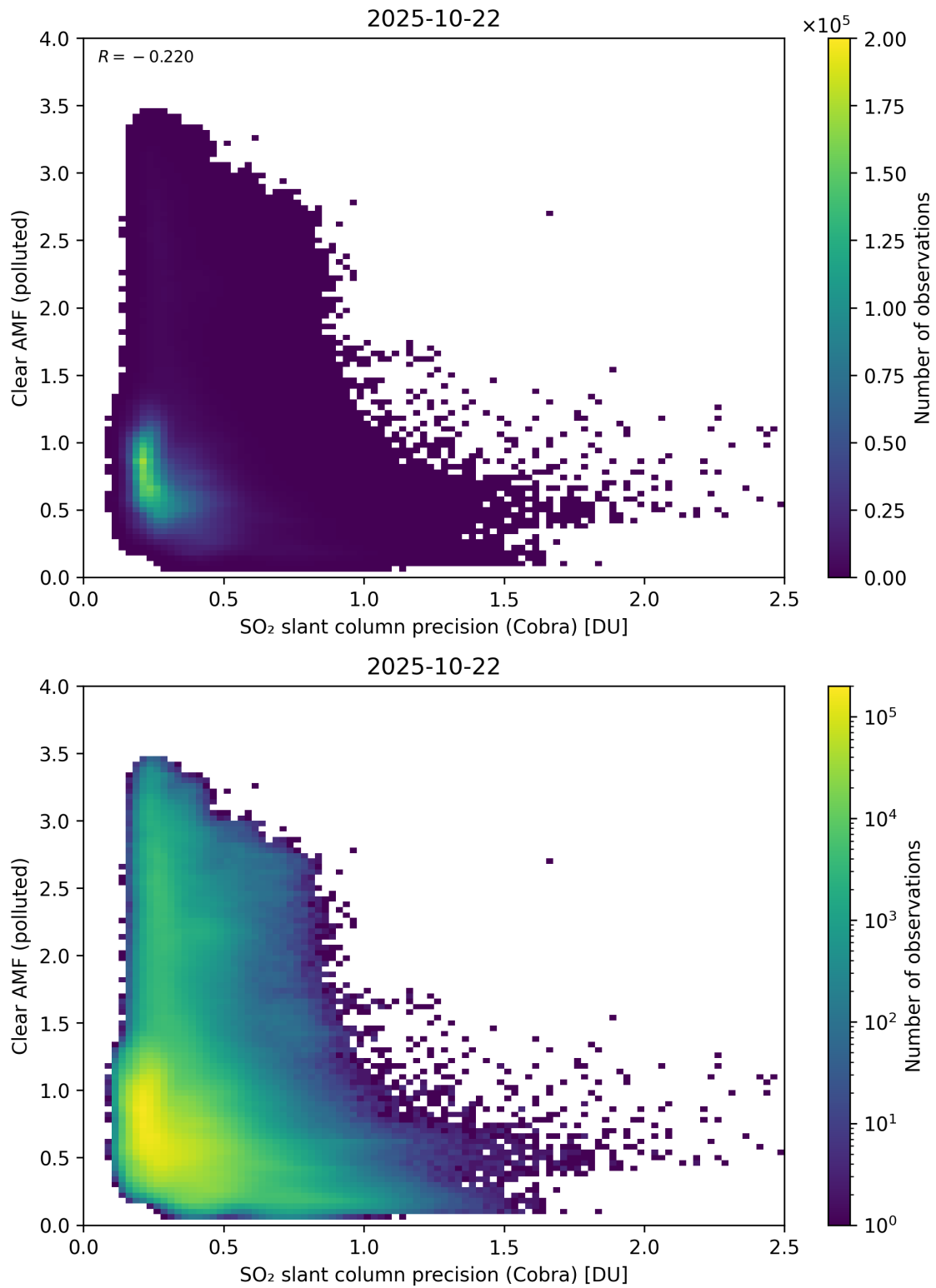
Figure 205: Scatter density plot of “SO 2 slant column precision (Cobra)” against “Clear AMF (polluted)” for 2025-10-22 to 2025-10-23.
