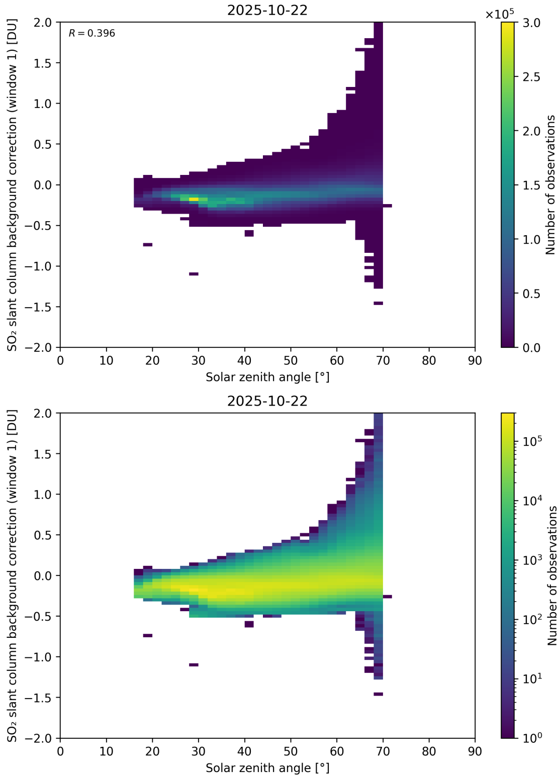
Figure 171: Scatter density plot of “Solar zenith angle” against “SO 2 slant column background correction (window 1)” for 2025-10-22 to 2025-10-23.
