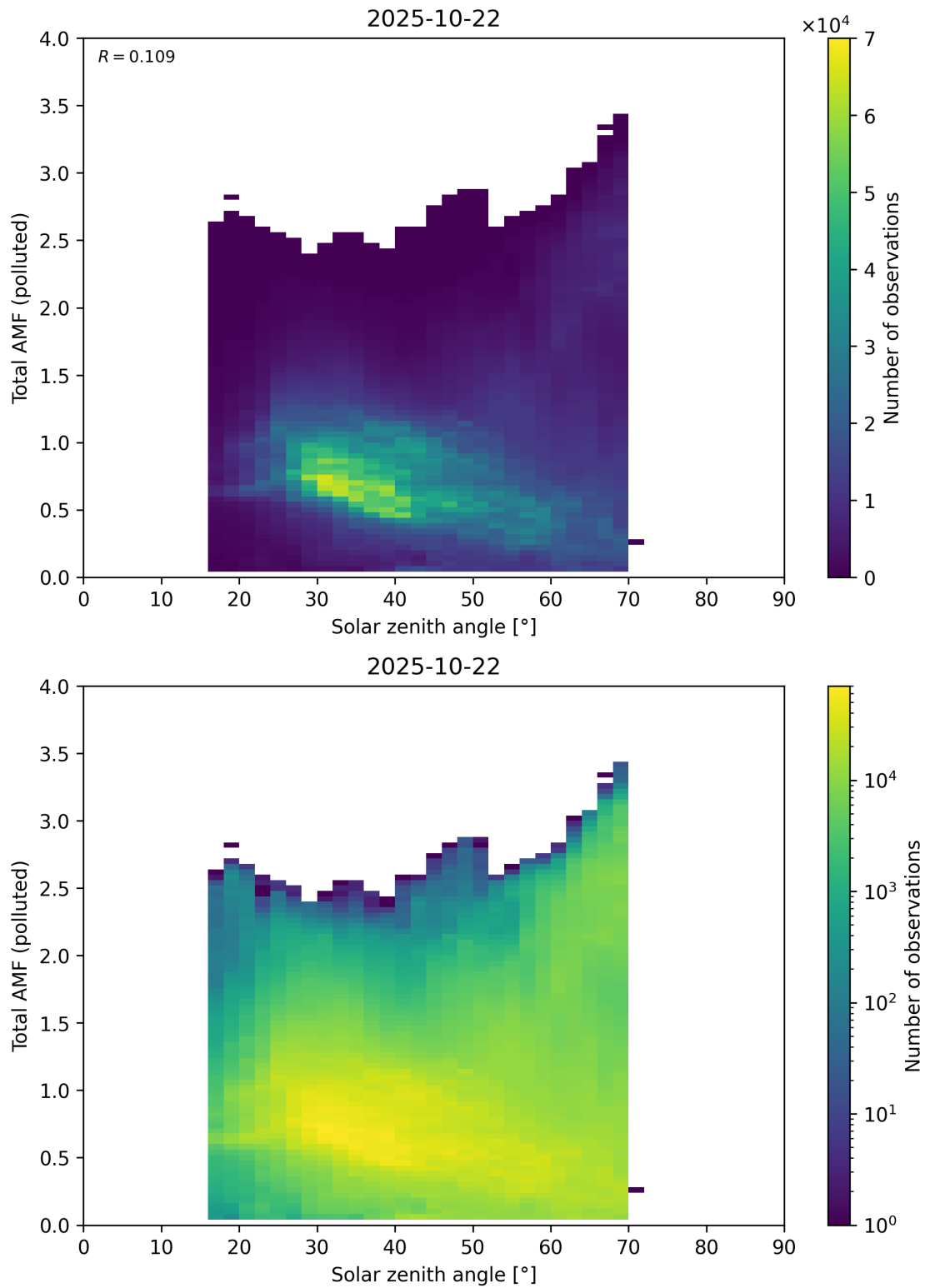
Figure 189: Scatter density plot of “Solar zenith angle” against “Total AMF (polluted)” for 2025-10-22 to 2025-10-23.
