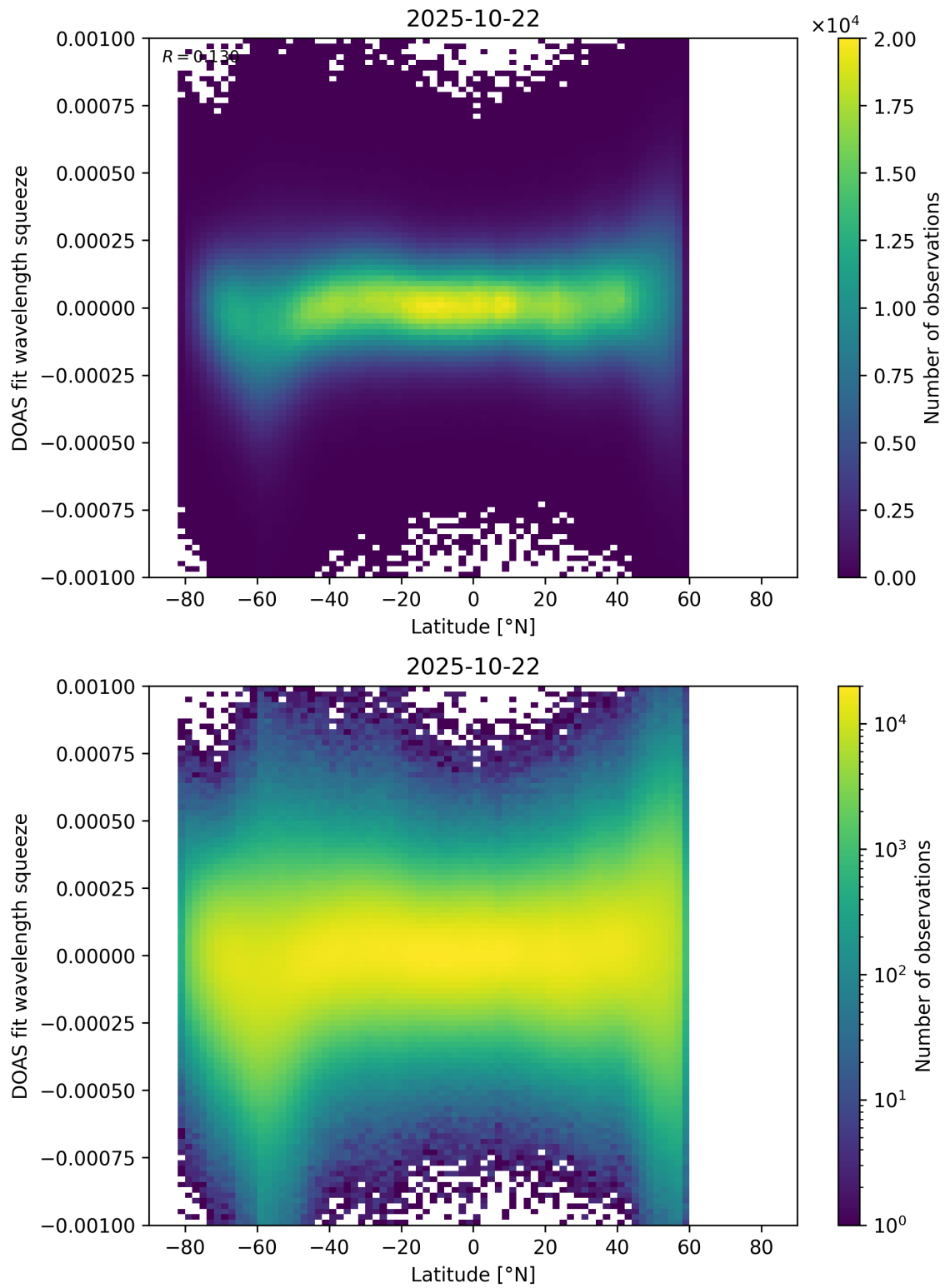
Figure 154: Scatter density plot of “Latitude” against “DOAS fit wavelength squeeze” for 2025-10-22 to 2025-10-23.
