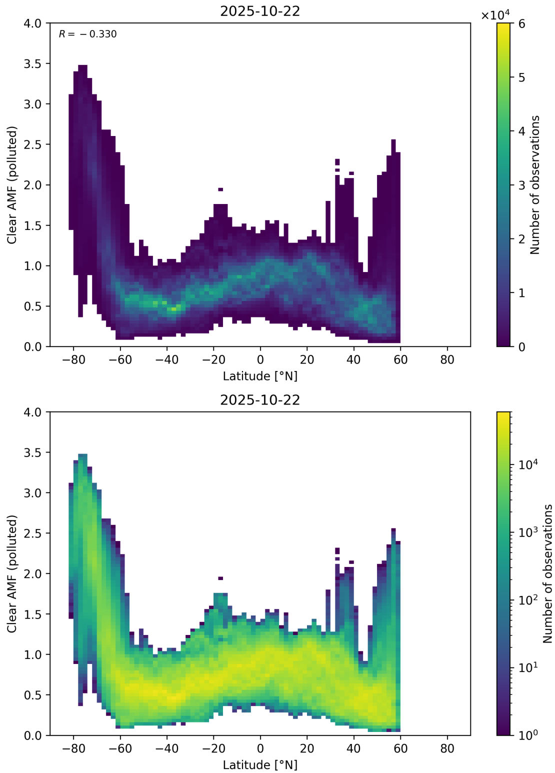
Figure 156: Scatter density plot of “Latitude” against “Clear AMF (polluted)” for 2025-10-22 to 2025-10-23.
