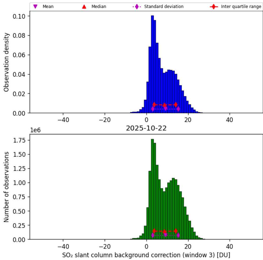
Figure 74: Histogram of “SO 2 slant column background correction (window 3)” for 2025-10-22 to 2025-10-23
