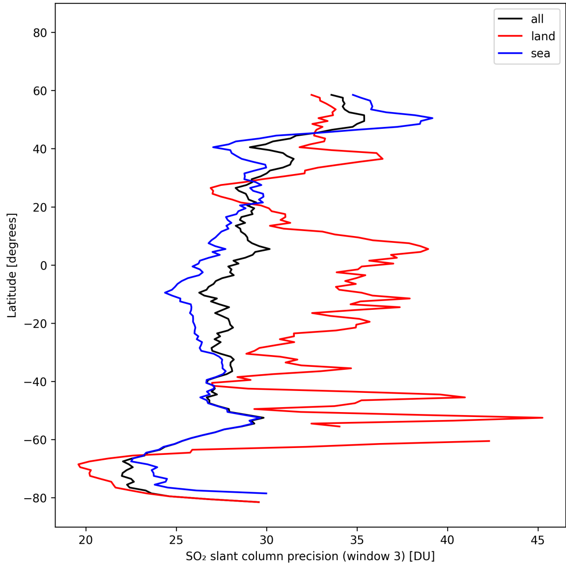
Figure 46: Zonal average of “SO 2 slant column precision (window 3)” for 2025-10-22 to 2025-10-23.
