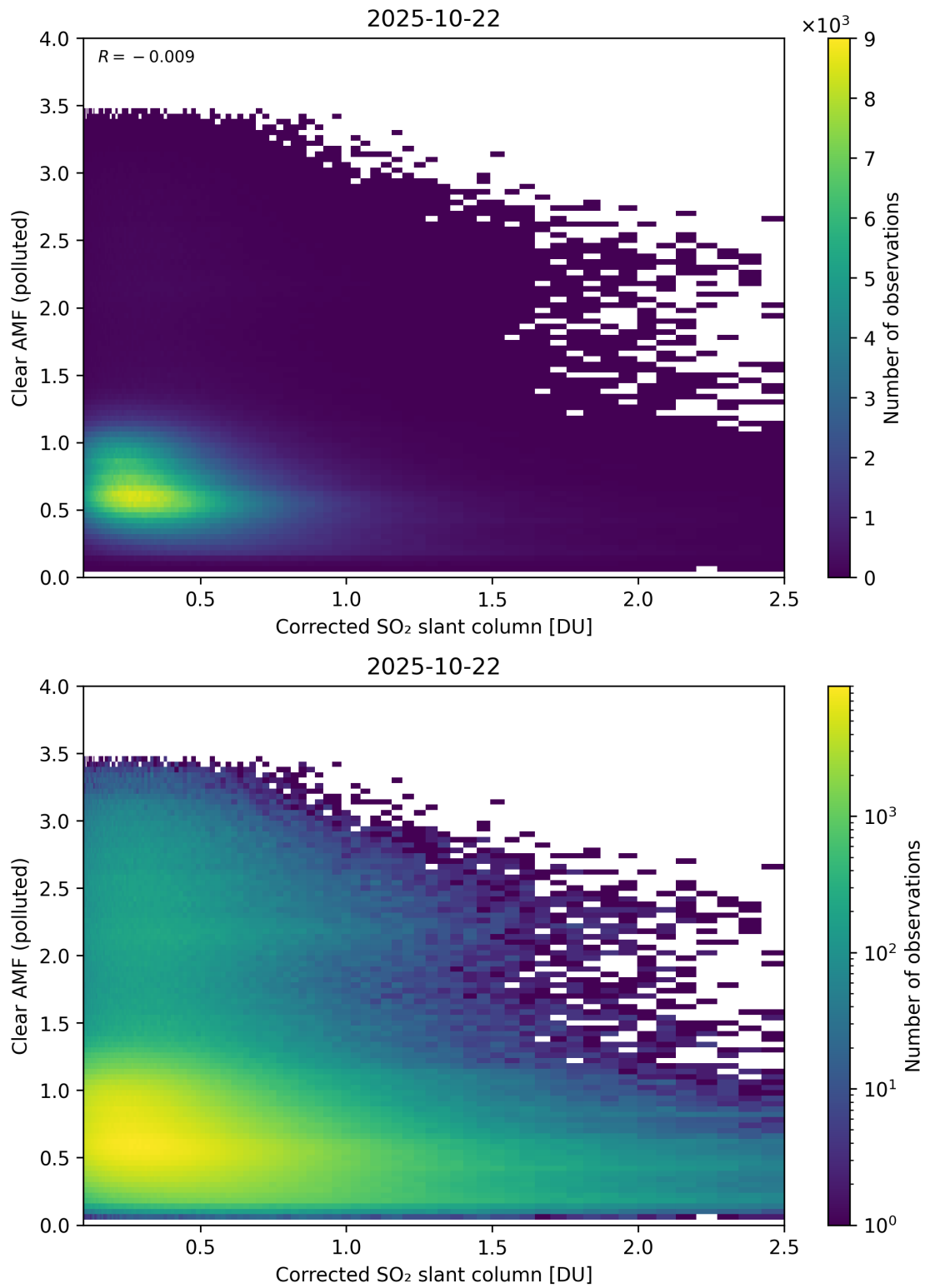
Figure 232: Scatter density plot of “Corrected SO 2 slant column” against “Clear AMF (polluted)” for 2025-10-22 to 2025-10-23.
