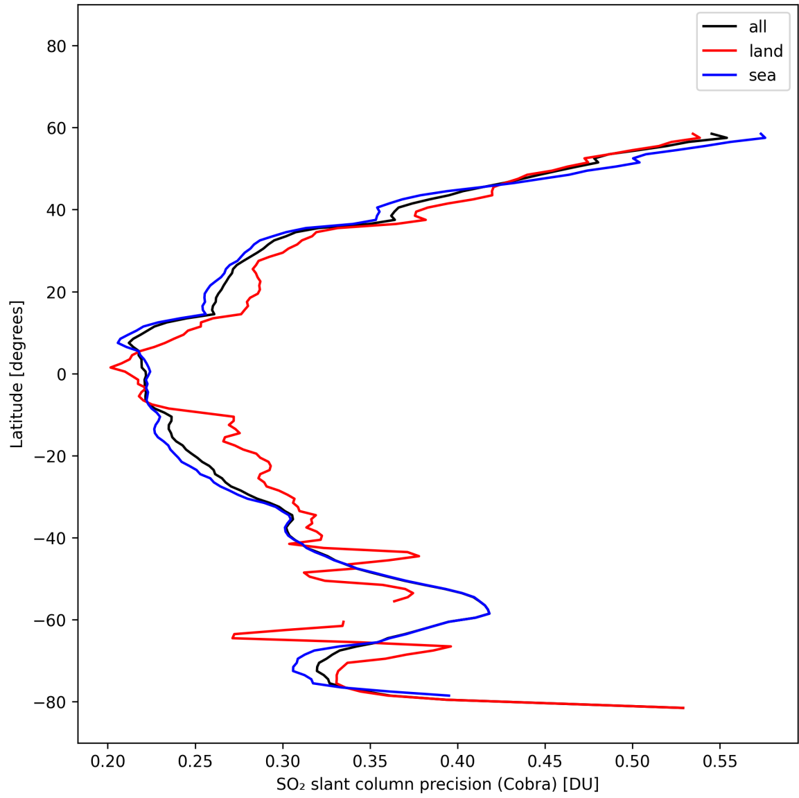
Figure 36: Zonal average of “SO 2 slant column precision (Cobra)” for 2025-10-22 to 2025-10-23.
