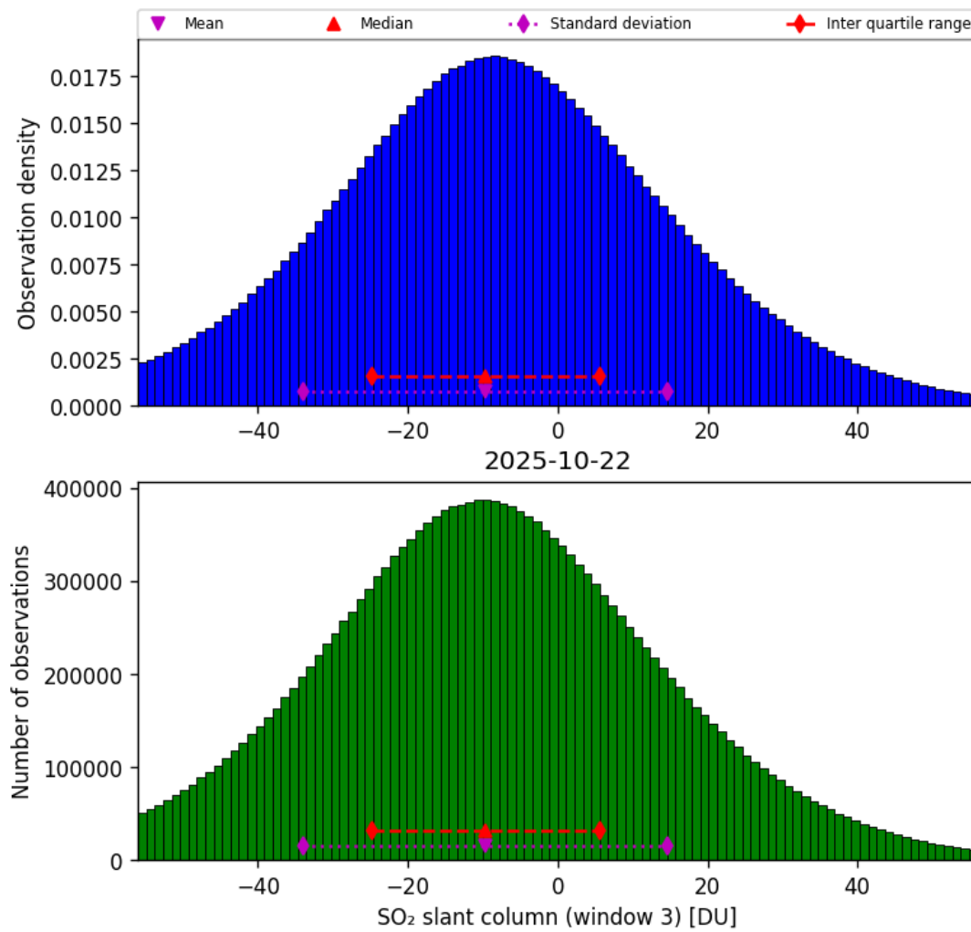
Figure 71: Histogram of “SO 2 slant column (window 3)” for 2025-10-22 to 2025-10-23
