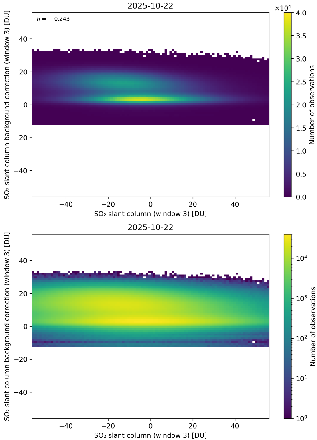
Figure 303: Scatter density plot of “SO 2 slant column (window 3)” against “SO 2 slant column background correction (window 3)” for 2025-10-22 to 2025-10-23.
