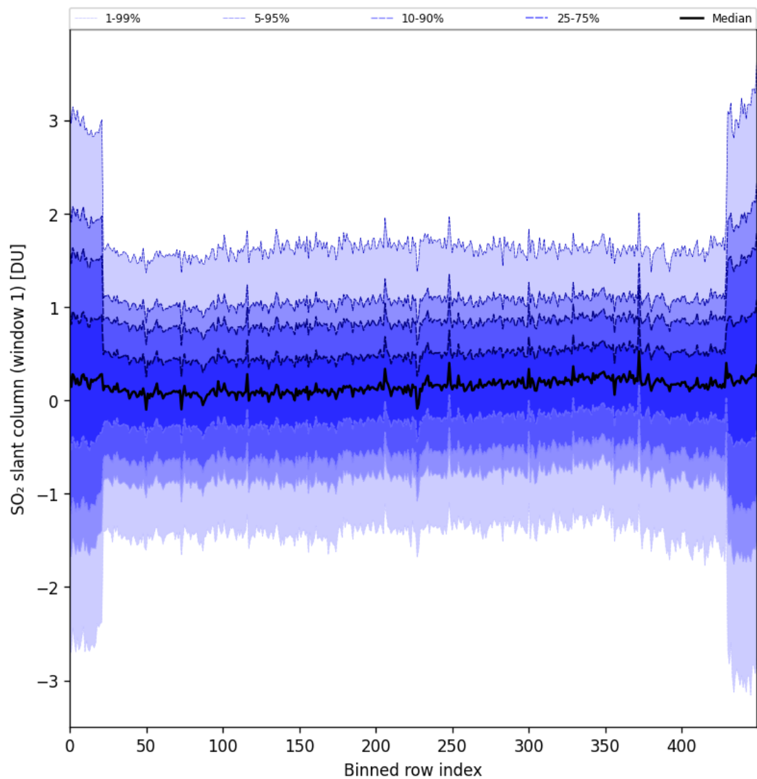
Figure 89: Along track statistics of “SO 2 slant column (window 1)” for 2025-10-22 to 2025-10-23
