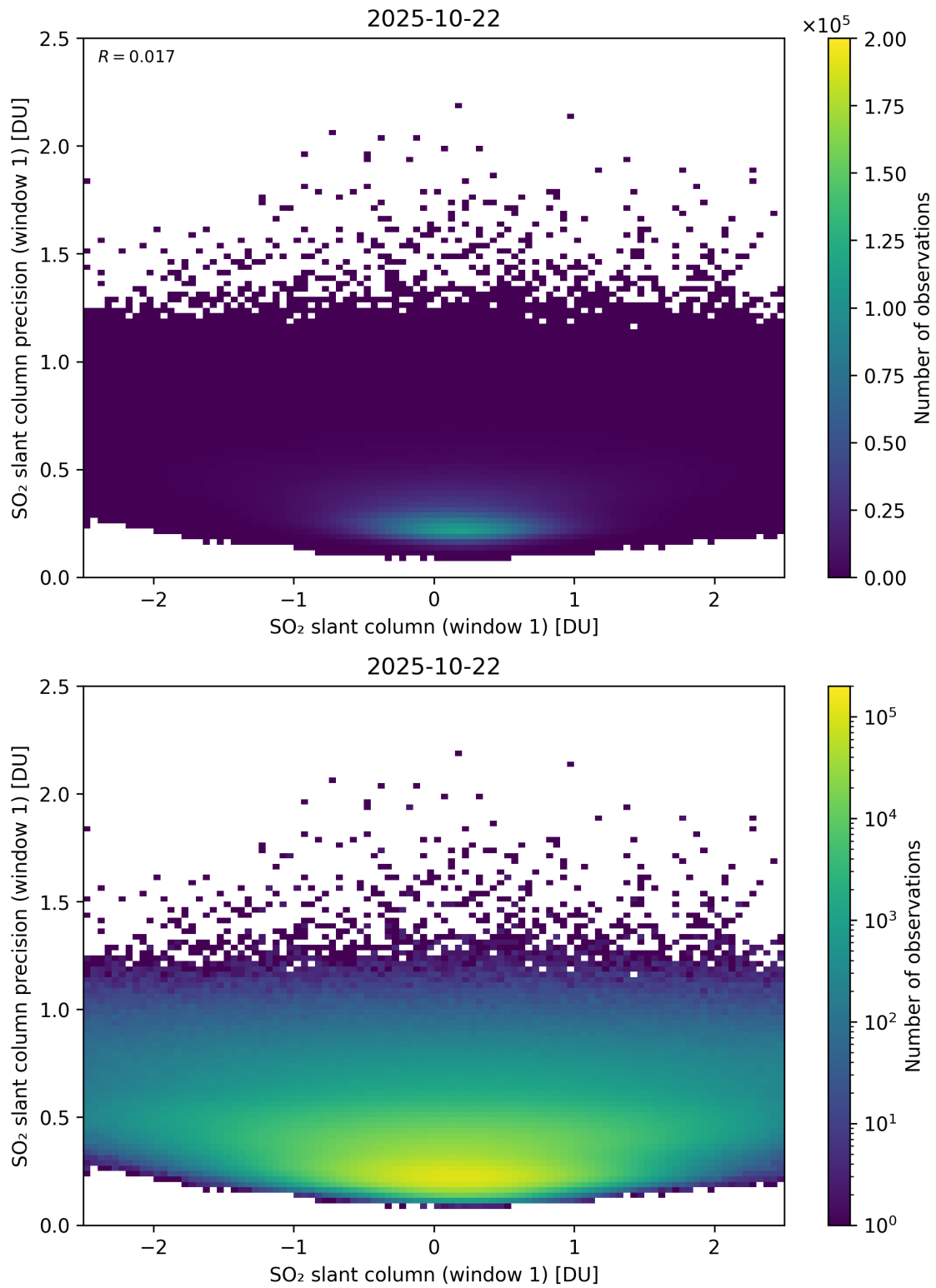
Figure 285: Scatter density plot of “SO 2 slant column (window 1)” against “SO 2 slant column precision (window 1)” for 2025-10-22 to 2025-10-23.
