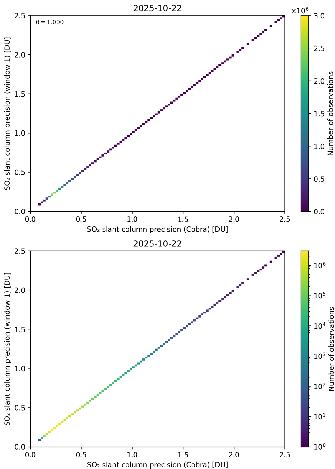
Figure 209: Scatter density plot of “SO 2 slant column precision (Cobra)” against “SO 2 slant column precision (window 1)” for 2025-10-22 to 2025-10-23.
