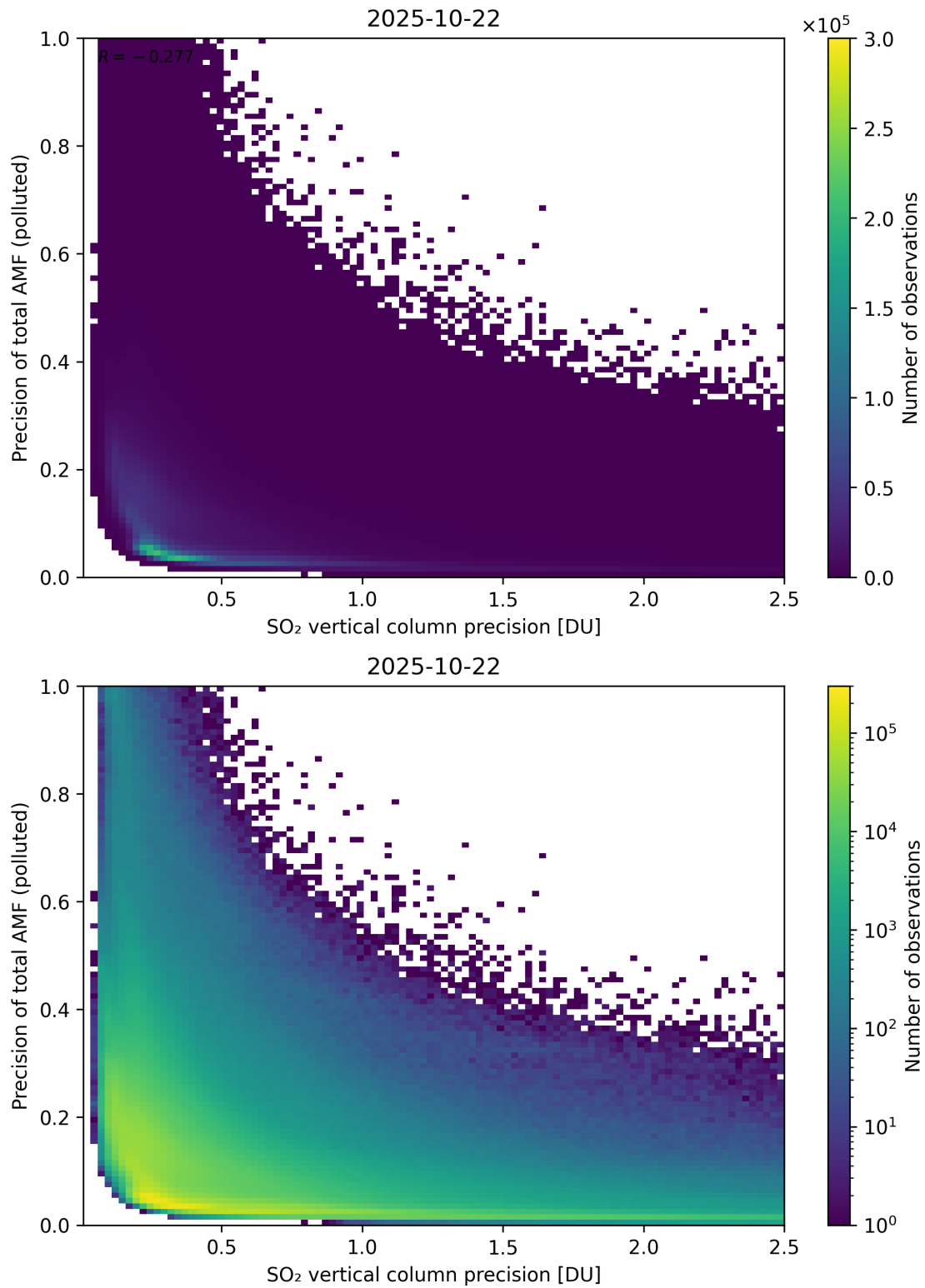
Figure 347: Scatter density plot of “SO 2 vertical column precision” against “Precision of total AMF (polluted)” for 2025-10-22 to 2025-10-23.
