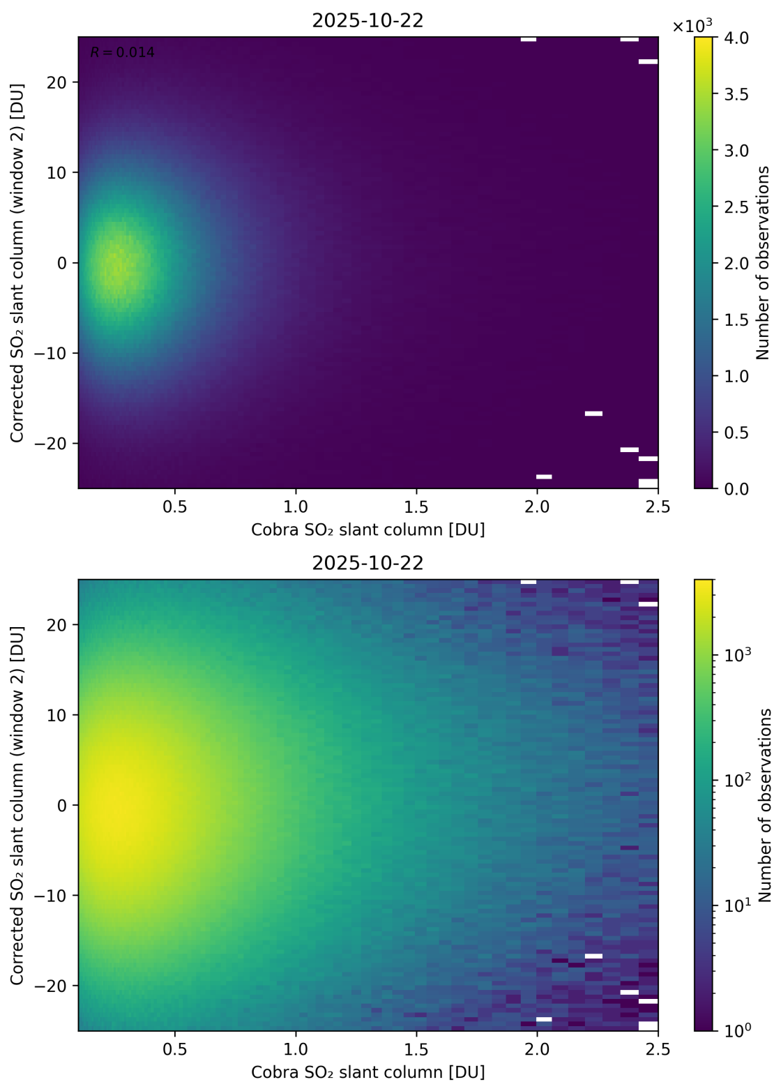
Figure 217: Scatter density plot of “Cobra SO 2 slant column” against “Corrected SO 2 slant column (window 2)” for 2025-10-22 to 2025-10-23.
