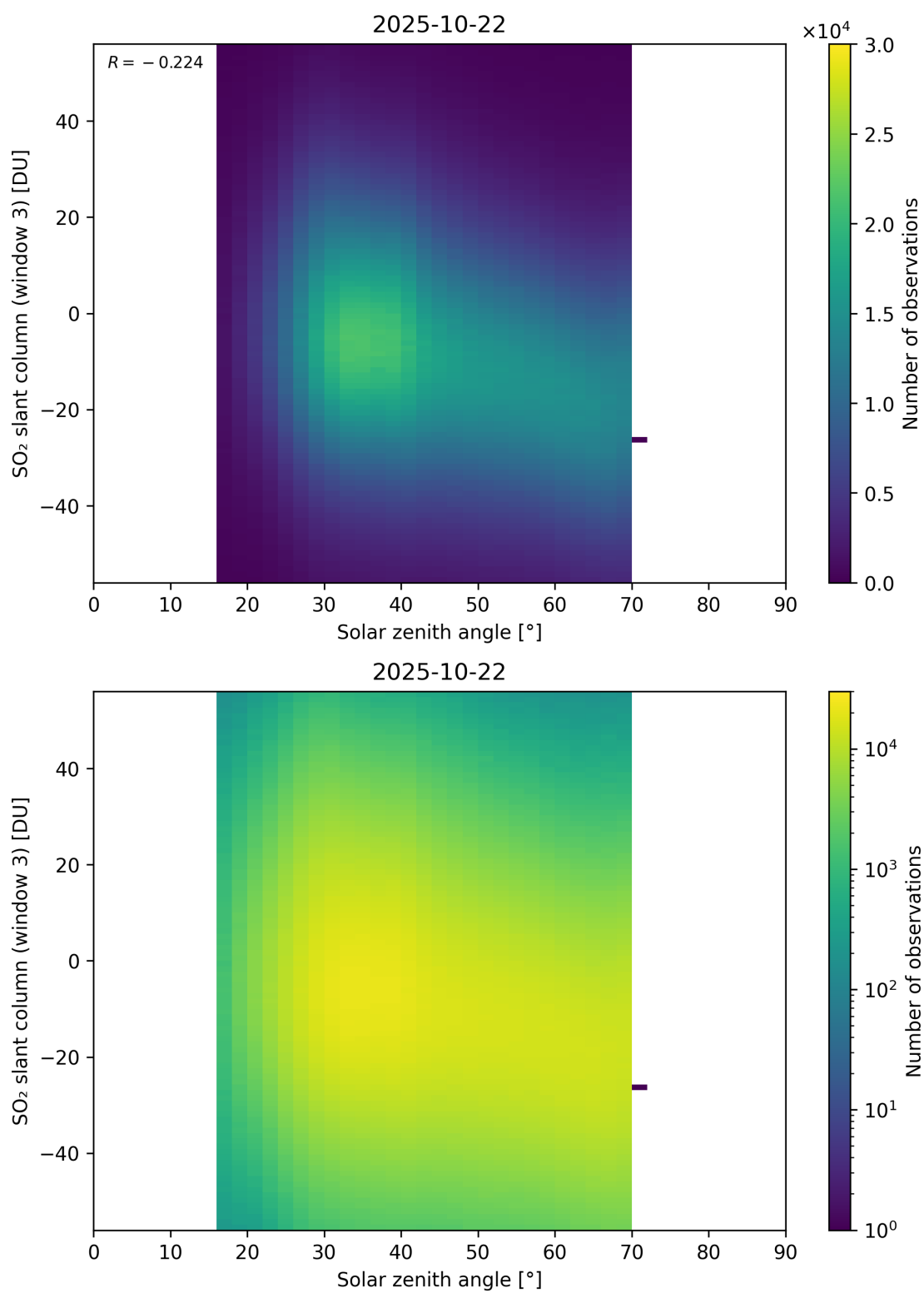
Figure 187: Scatter density plot of “Solar zenith angle” against “SO 2 slant column (window 3)” for 2025-10-22 to 2025-10-23.
