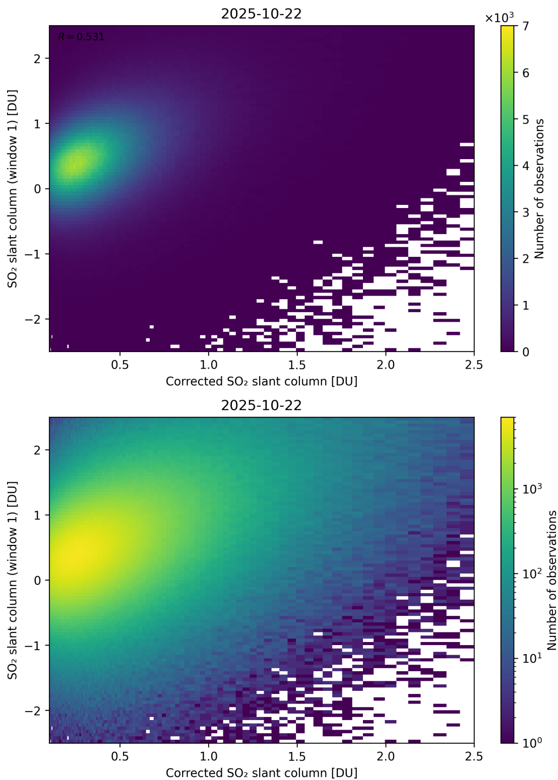
Figure 237: Scatter density plot of “Corrected SO 2 slant column” against “SO 2 slant column (window 1)” for 2025-10-22 to 2025-10-23.
