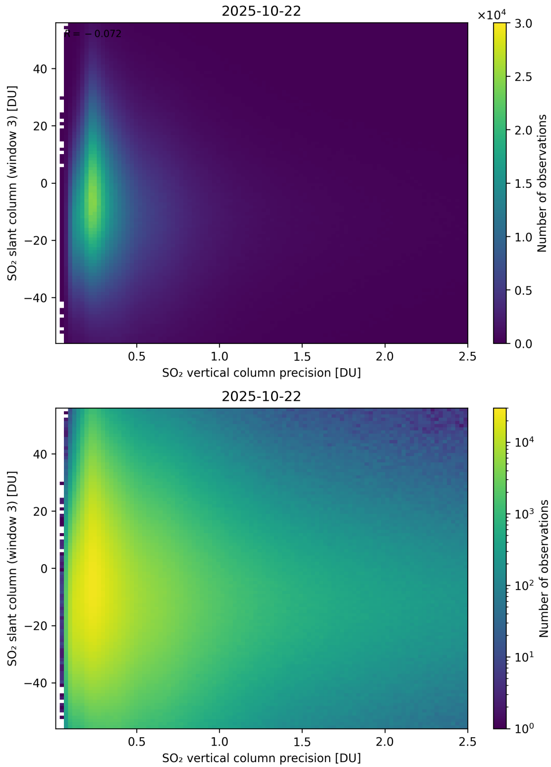
Figure 344: Scatter density plot of “SO 2 vertical column precision” against “SO 2 slant column (window 3)” for 2025-10-22 to 2025-10-23.
