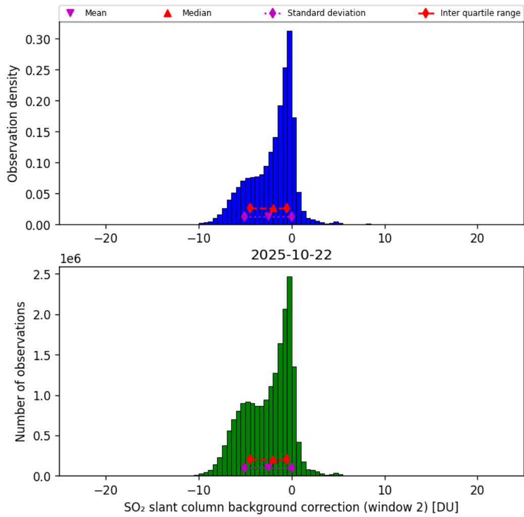
Figure 70: Histogram of “SO 2 slant column background correction (window 2)” for 2025-10-22 to 2025-10-23
