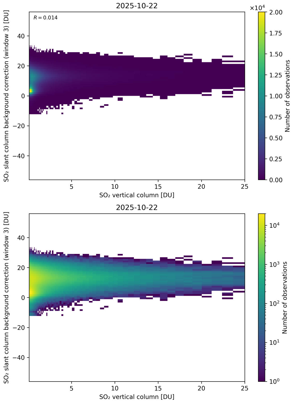
Figure 325: Scatter density plot of “SO 2 vertical column” against “SO 2 slant column background correction (window 3)” for 2025-10-22 to 2025-10-23.
