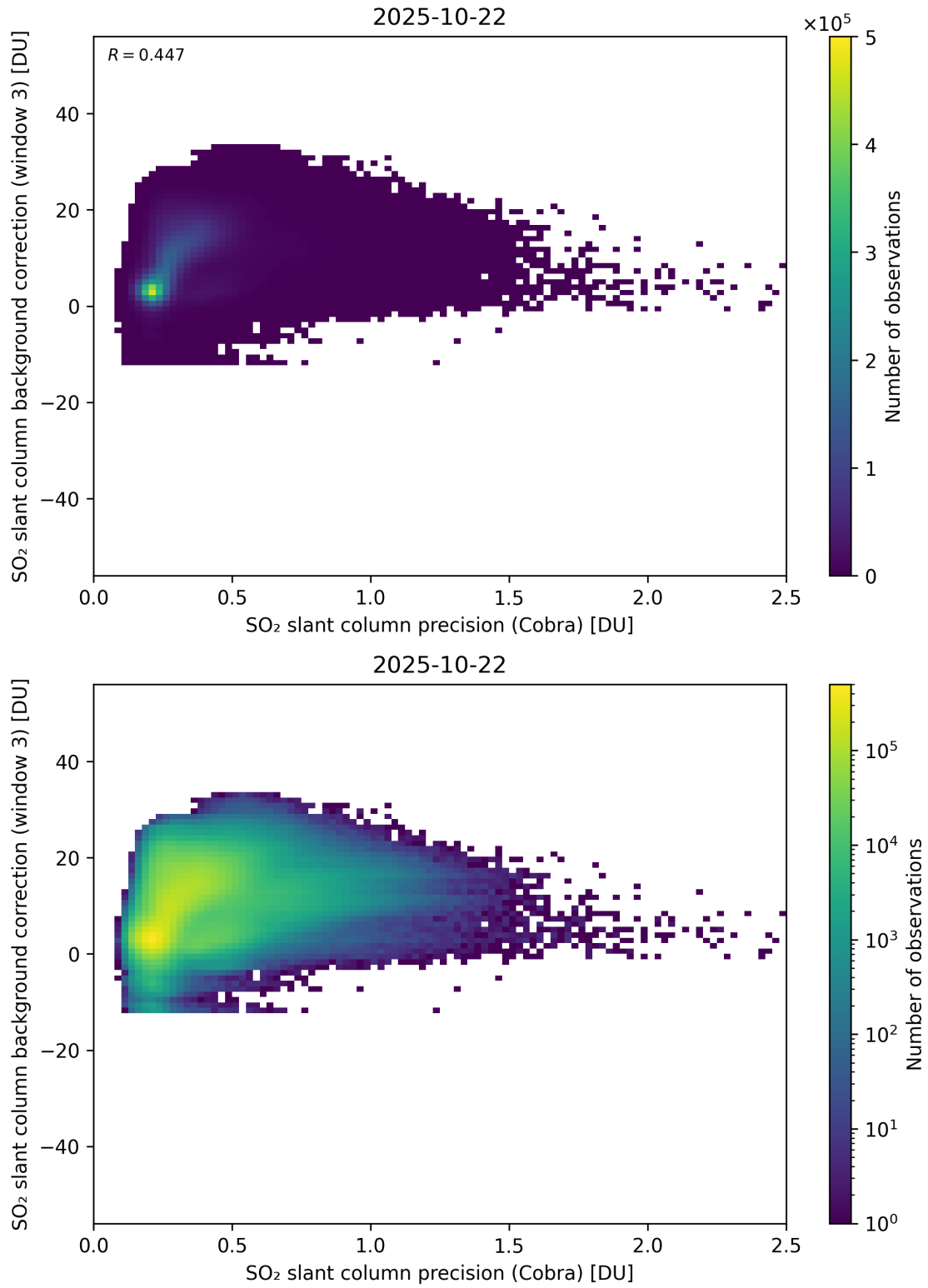
Figure 201: Scatter density plot of “SO 2 slant column precision (Cobra)” against “SO 2 slant column background correction (window 3)” for 2025-10-22 to 2025-10-23.
