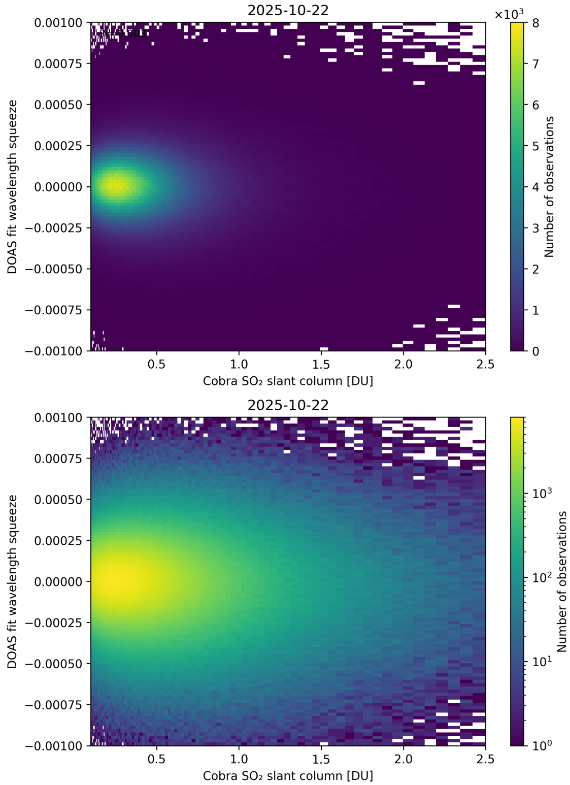
Figure 197: Scatter density plot of “Cobra SO 2 slant column” against “DOAS fit wavelength squeeze” for 2025-10-22 to 2025-10-23.
