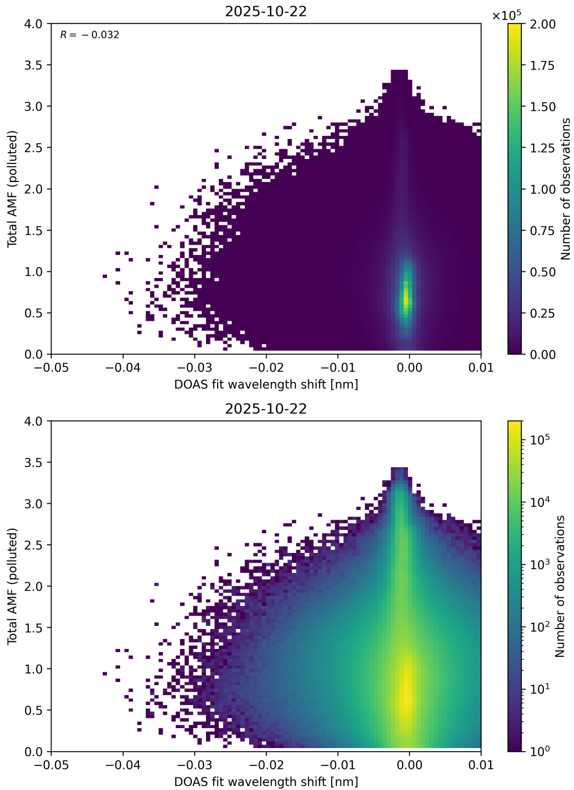
Figure 141: Scatter density plot of “DOAS fit wavelength shift” against “Total AMF (polluted)” for 2025-10-22 to 2025-10-23.
