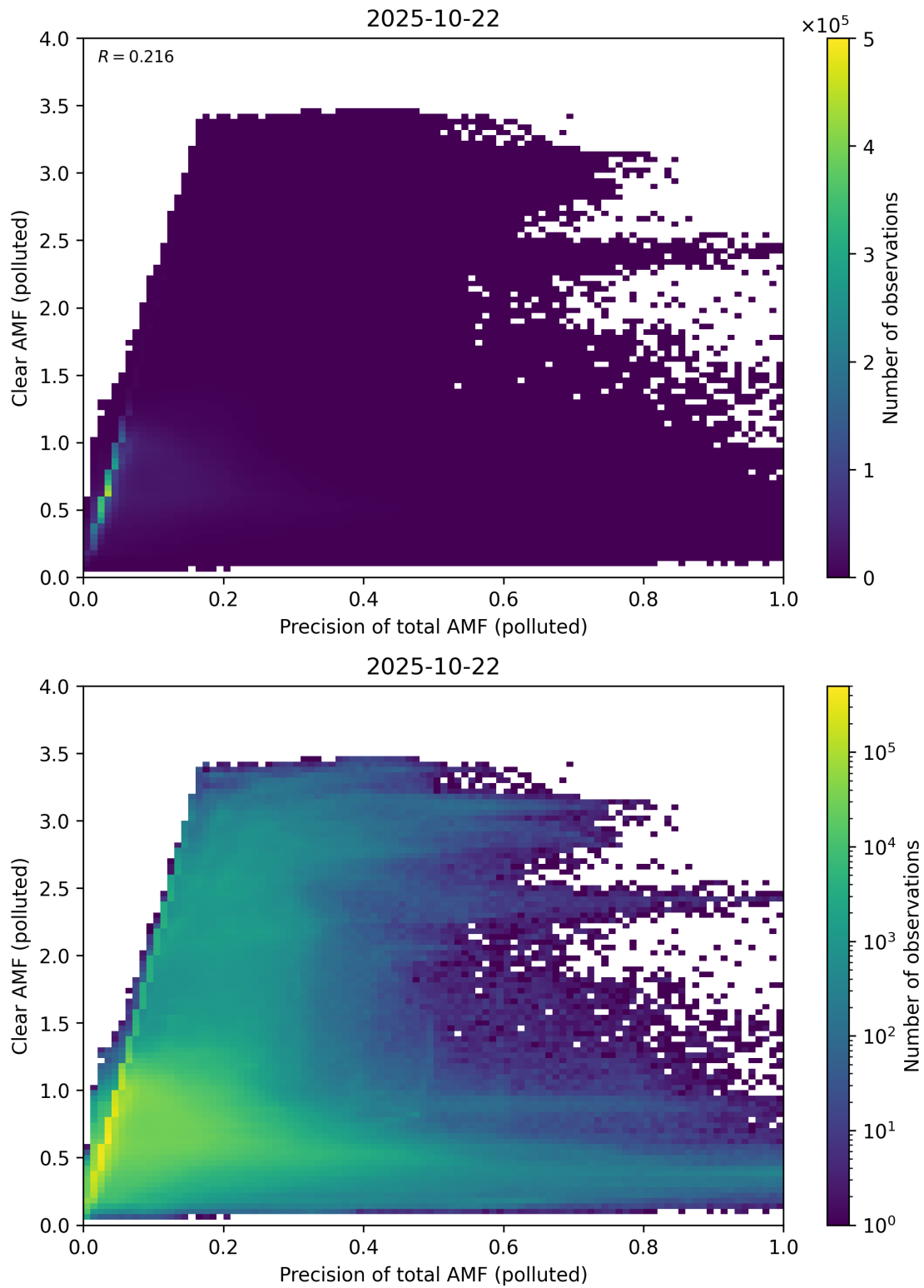
Figure 320: Scatter density plot of “Precision of total AMF (polluted)” against “Clear AMF (polluted)” for 2025-10-22 to 2025-10-23.
