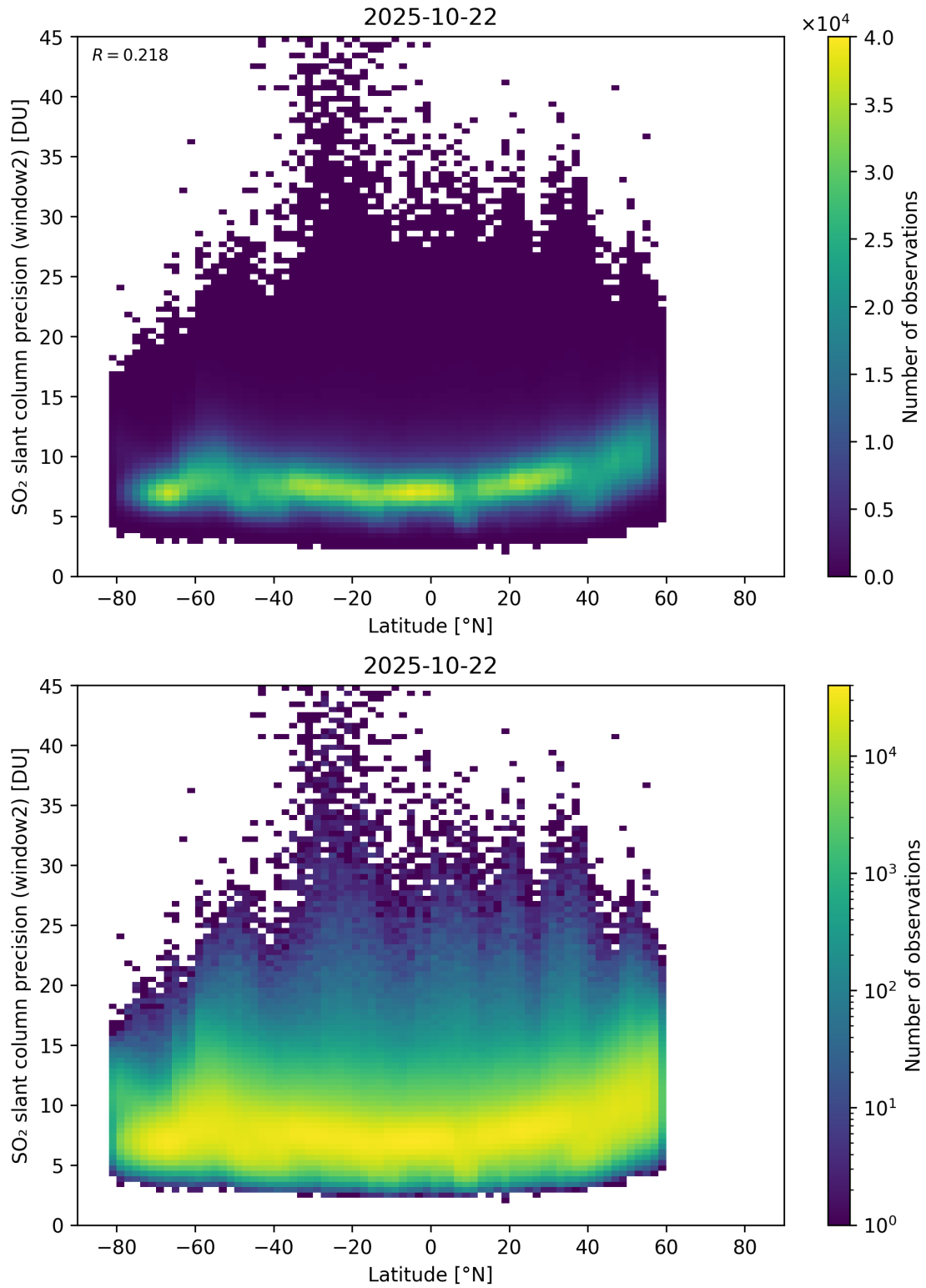
Figure 164: Scatter density plot of “Latitude” against “SO 2 slant column precision (window2)” for 2025-10-22 to 2025-10-23.
