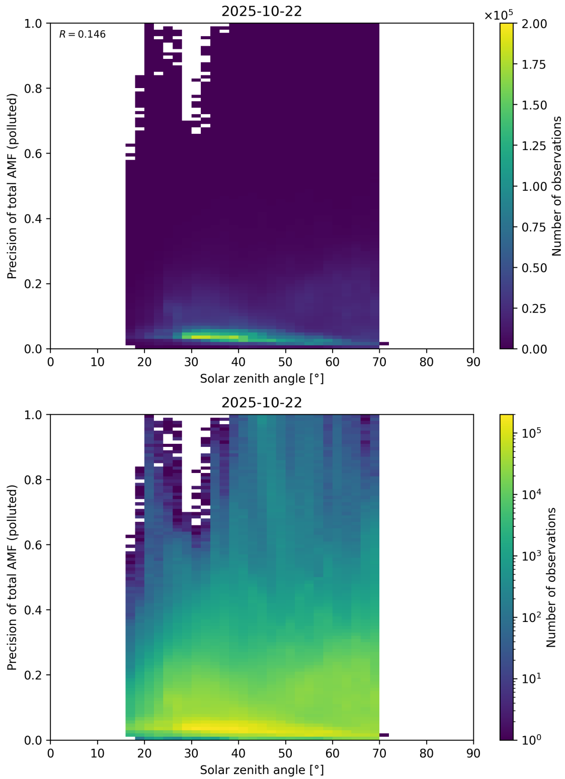
Figure 190: Scatter density plot of “Solar zenith angle” against “Precision of total AMF (polluted)” for 2025-10-22 to 2025-10-23.
