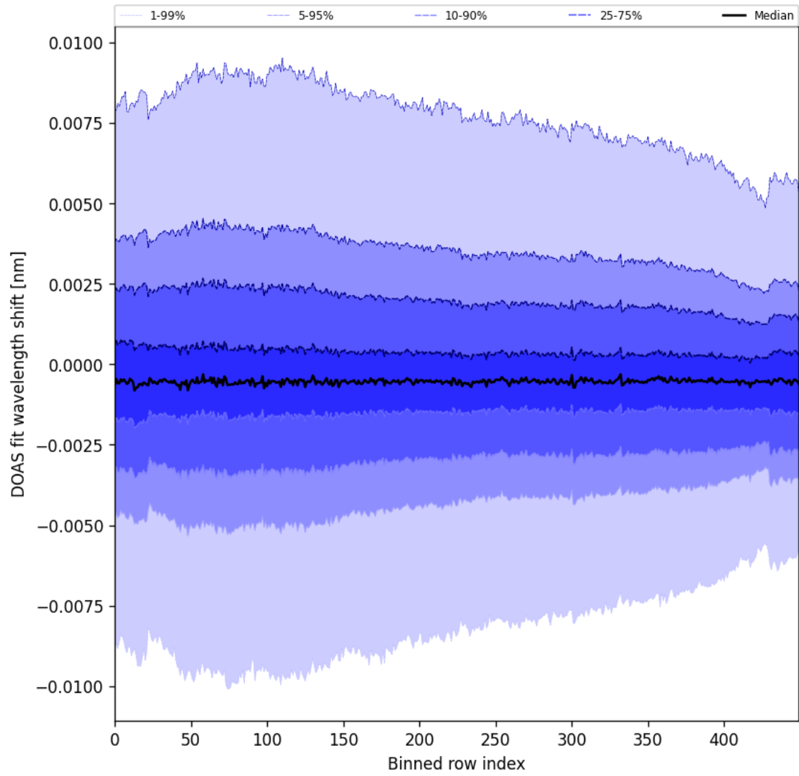
Figure 102: Along track statistics of “DOAS fit wavelength shift” for 2025-10-22 to 2025-10-23
