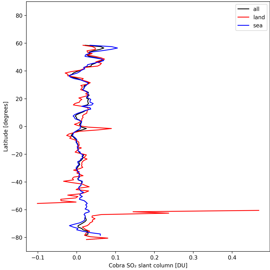
Figure 35: Zonal average of “Cobra SO 2 slant column” for 2025-10-22 to 2025-10-23.
