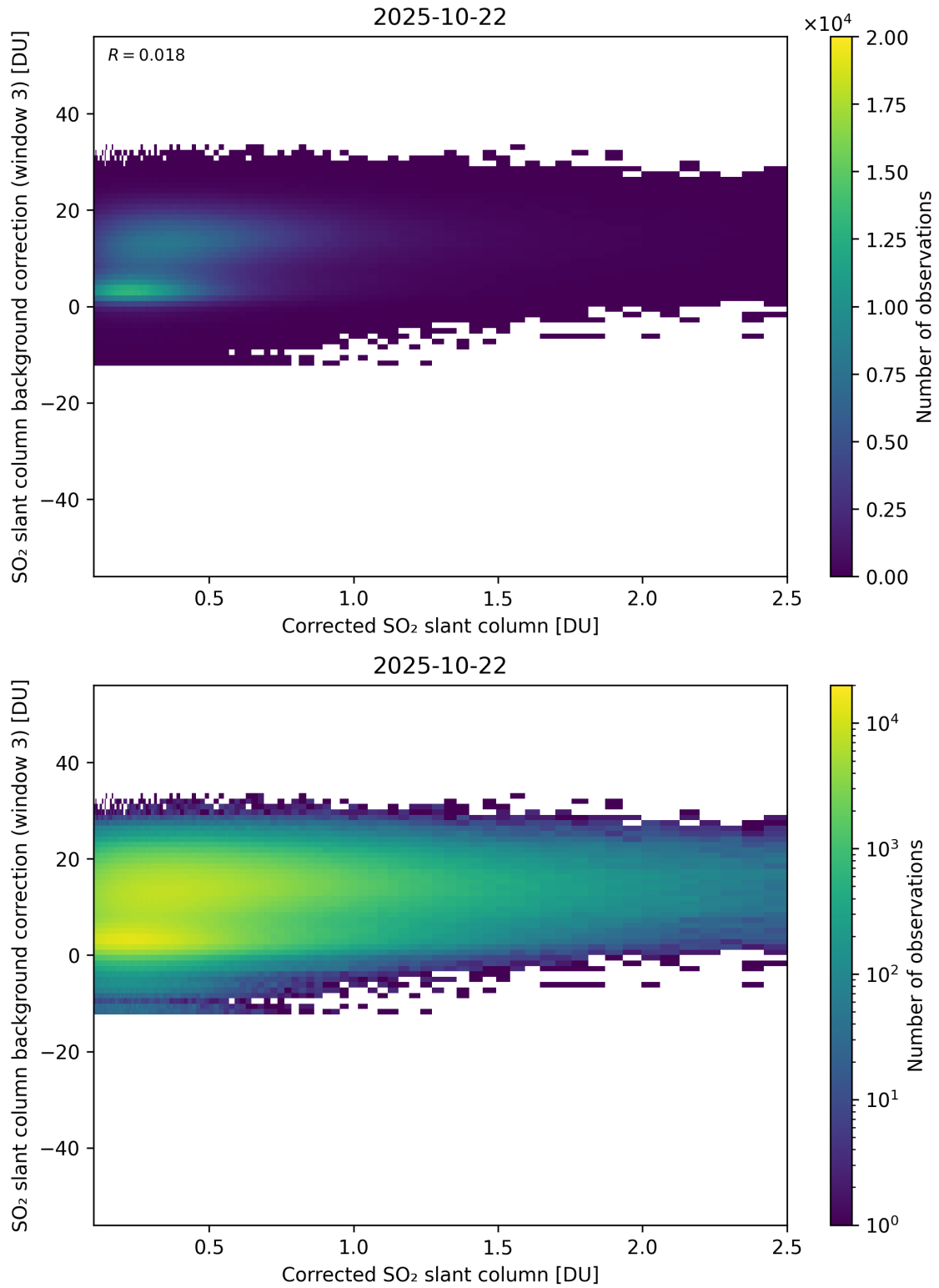
Figure 228: Scatter density plot of “Corrected SO 2 slant column” against “SO 2 slant column background correction (window 3)” for 2025-10-22 to 2025-10-23.
