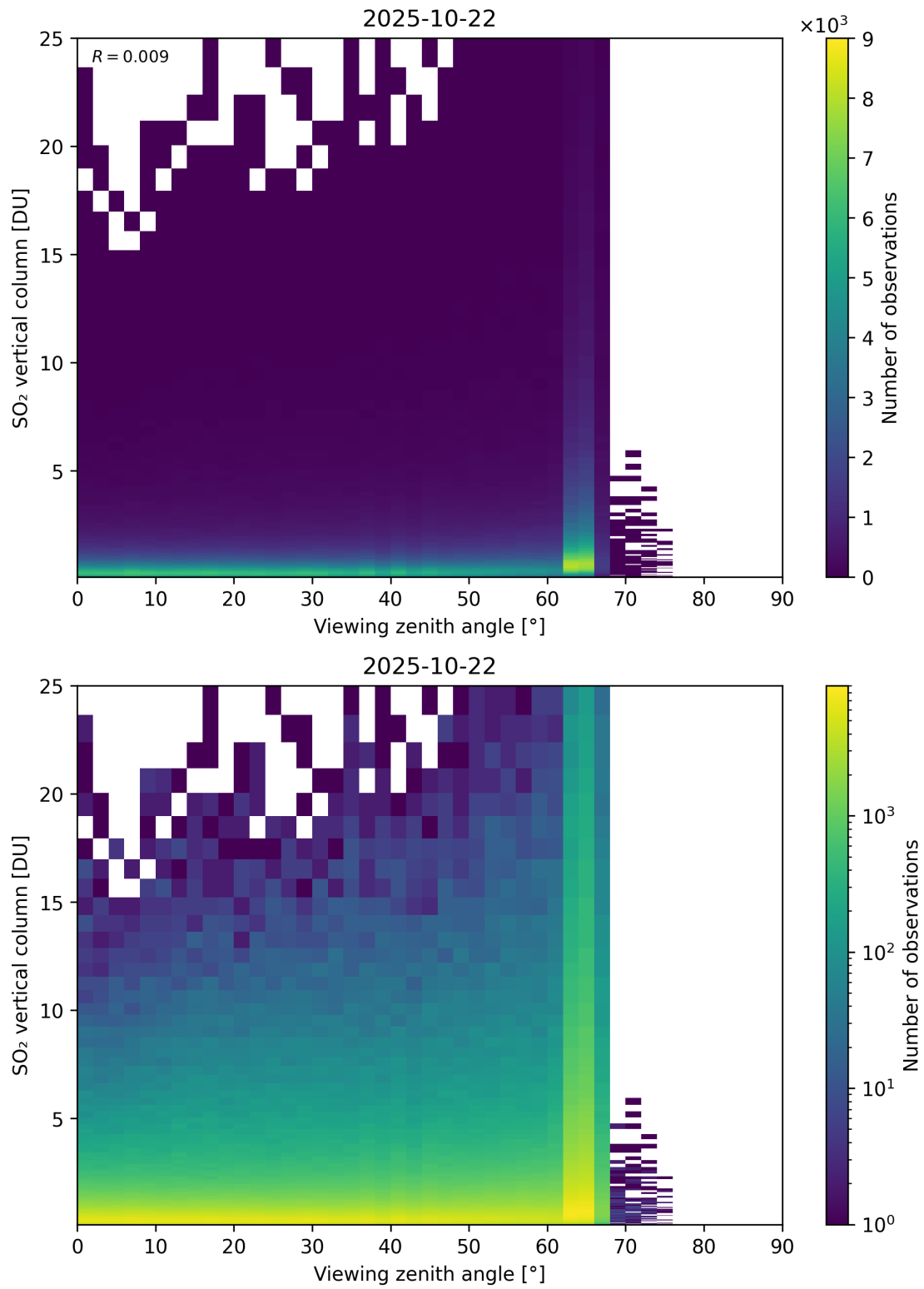
Figure 383: Scatter density plot of “Viewing zenith angle” against “SO 2 vertical column” for 2025-10-22 to 2025-10-23.
