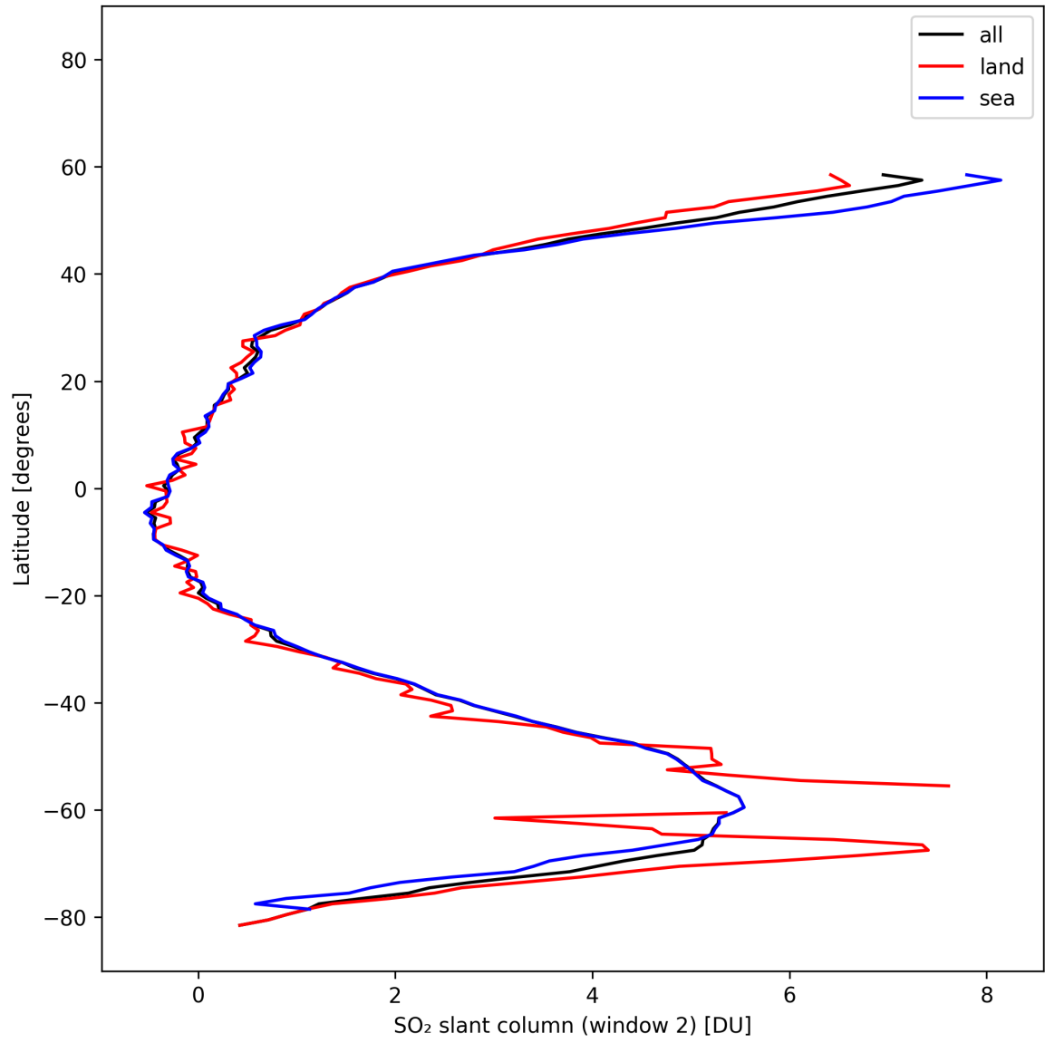
Figure 41: Zonal average of “SO 2 slant column (window 2)” for 2025-10-22 to 2025-10-23.
