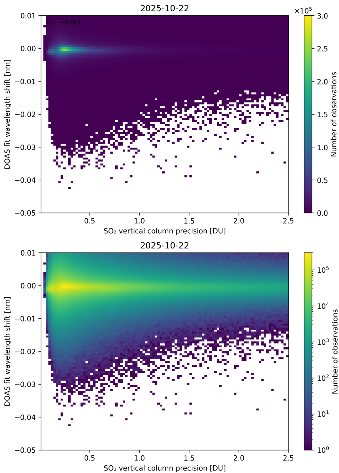
Figure 332: Scatter density plot of “SO 2 vertical column precision” against “DOAS fit wavelength shift” for 2025-10-22 to 2025-10-23.
