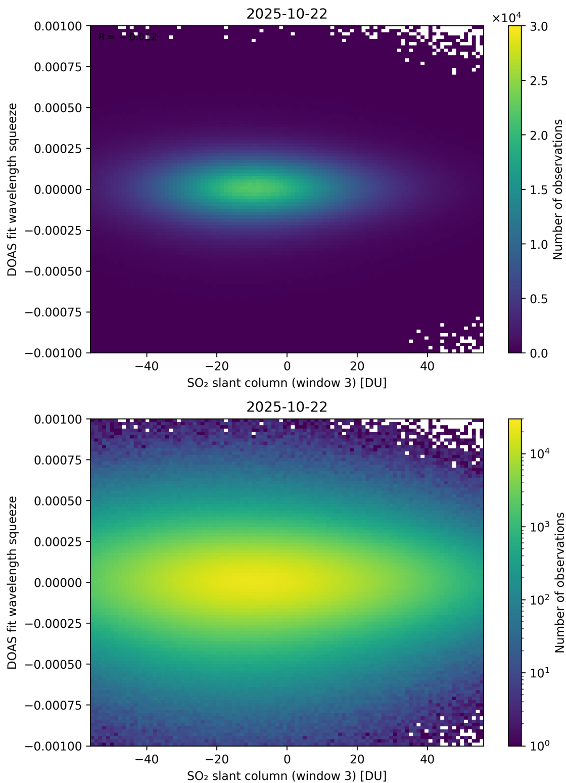
Figure 305: Scatter density plot of “SO 2 slant column (window 3)” against “DOAS fit wavelength squeeze” for 2025-10-22 to 2025-10-23.
