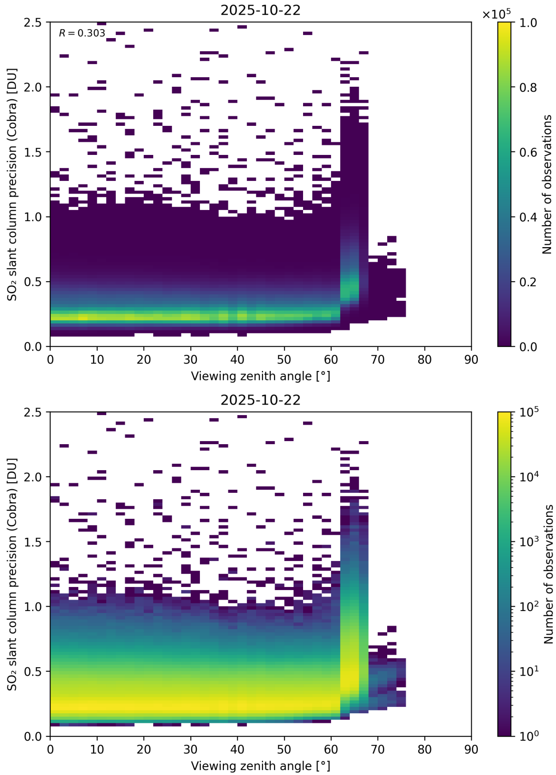
Figure 372: Scatter density plot of “Viewing zenith angle” against “SO 2 slant column precision (Cobra)” for 2025-10-22 to 2025-10-23.
