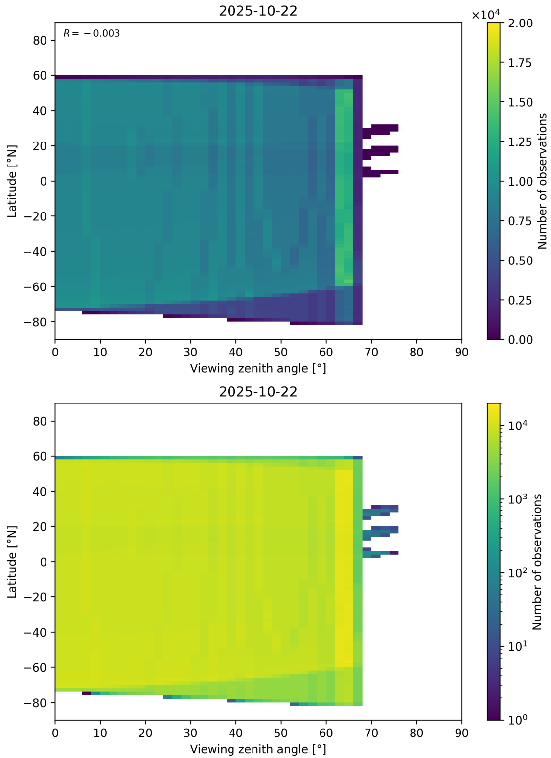
Figure 368: Scatter density plot of “Viewing zenith angle” against “Latitude” for 2025-10-22 to 2025-10-23.
