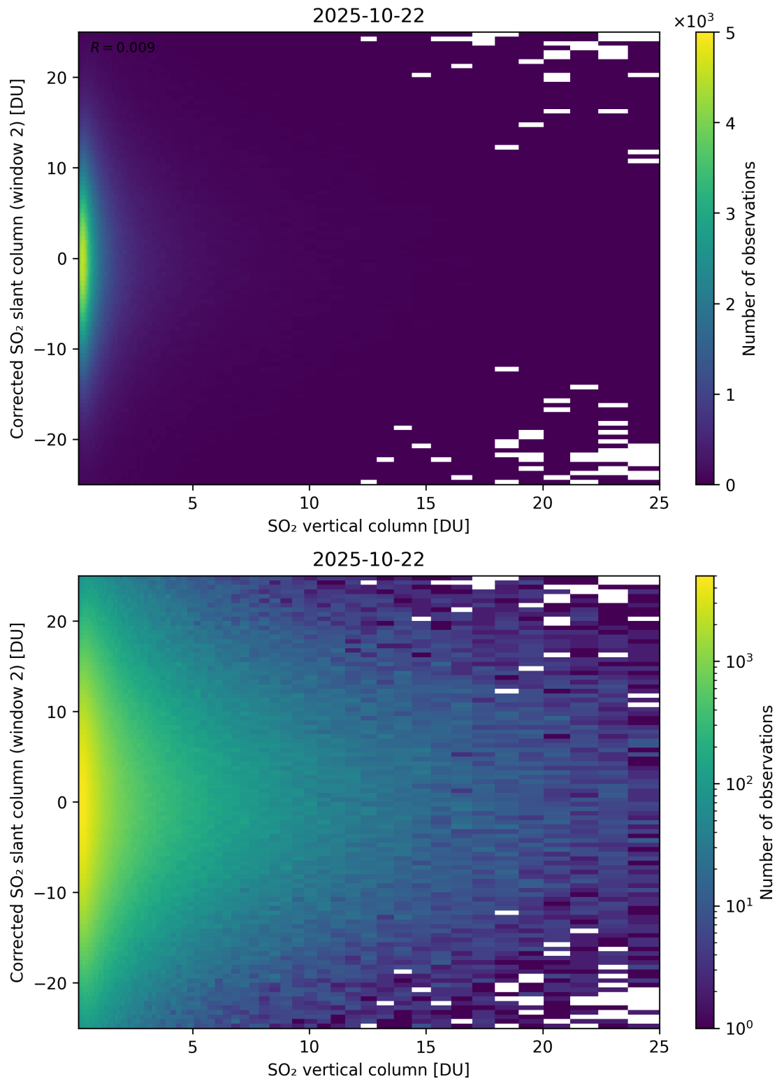
Figure 352: Scatter density plot of “SO 2 vertical column” against “Corrected SO 2 slant column (window 2)” for 2025-10-22 to 2025-10-23.
