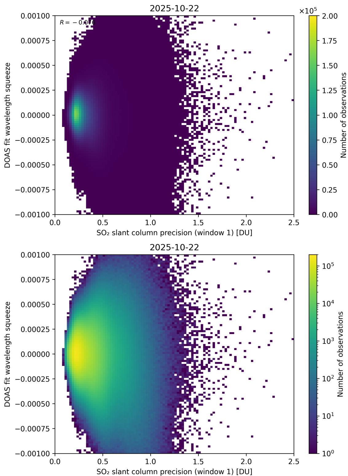
Figure 272: Scatter density plot of “SO 2 slant column precision (window 1)” against “DOAS fit wavelength squeeze” for 2025-10-22 to 2025-10-23.
