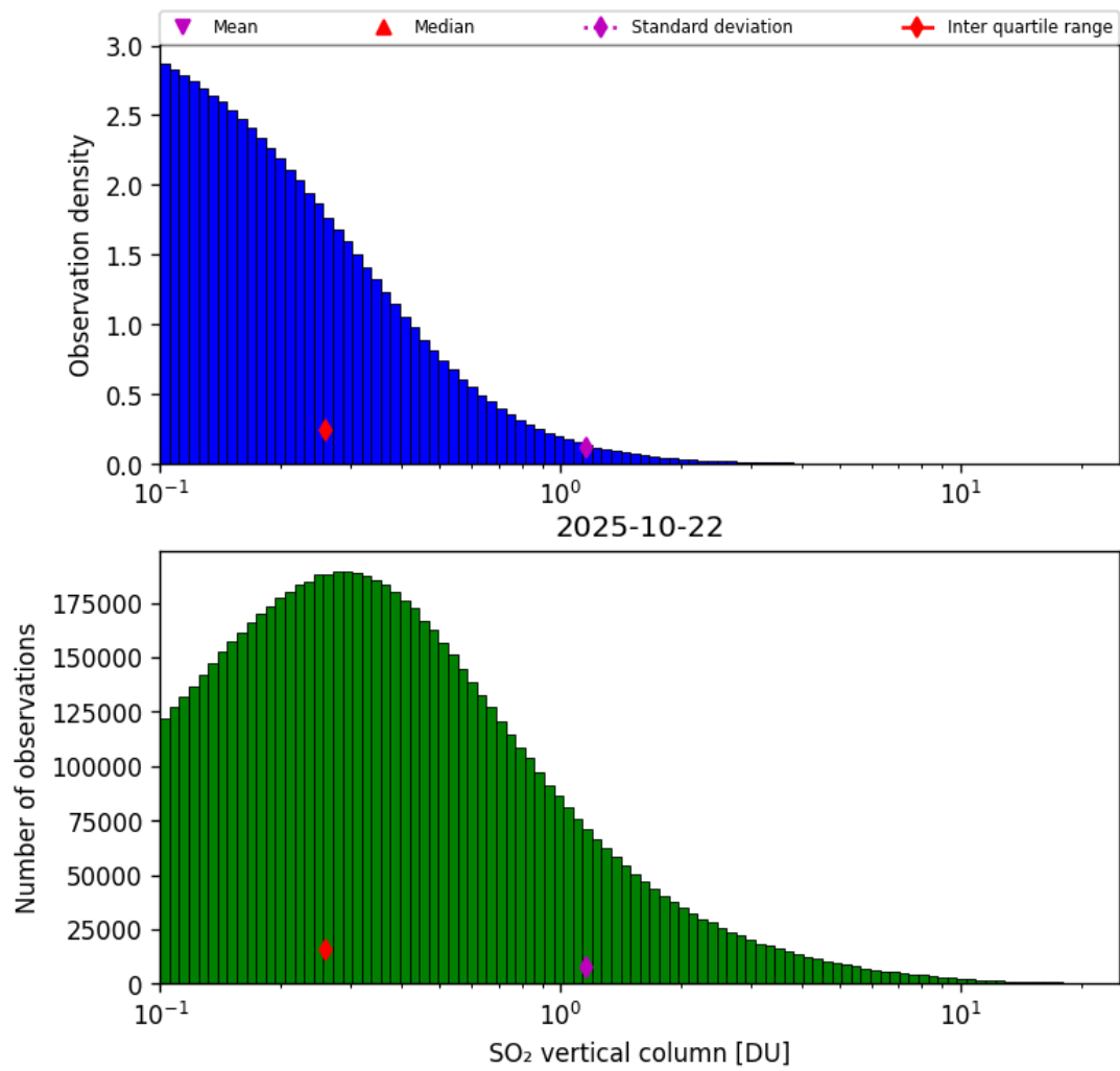
Figure 58: Histogram of “SO 2 vertical column” for 2025-10-22 to 2025-10-23
