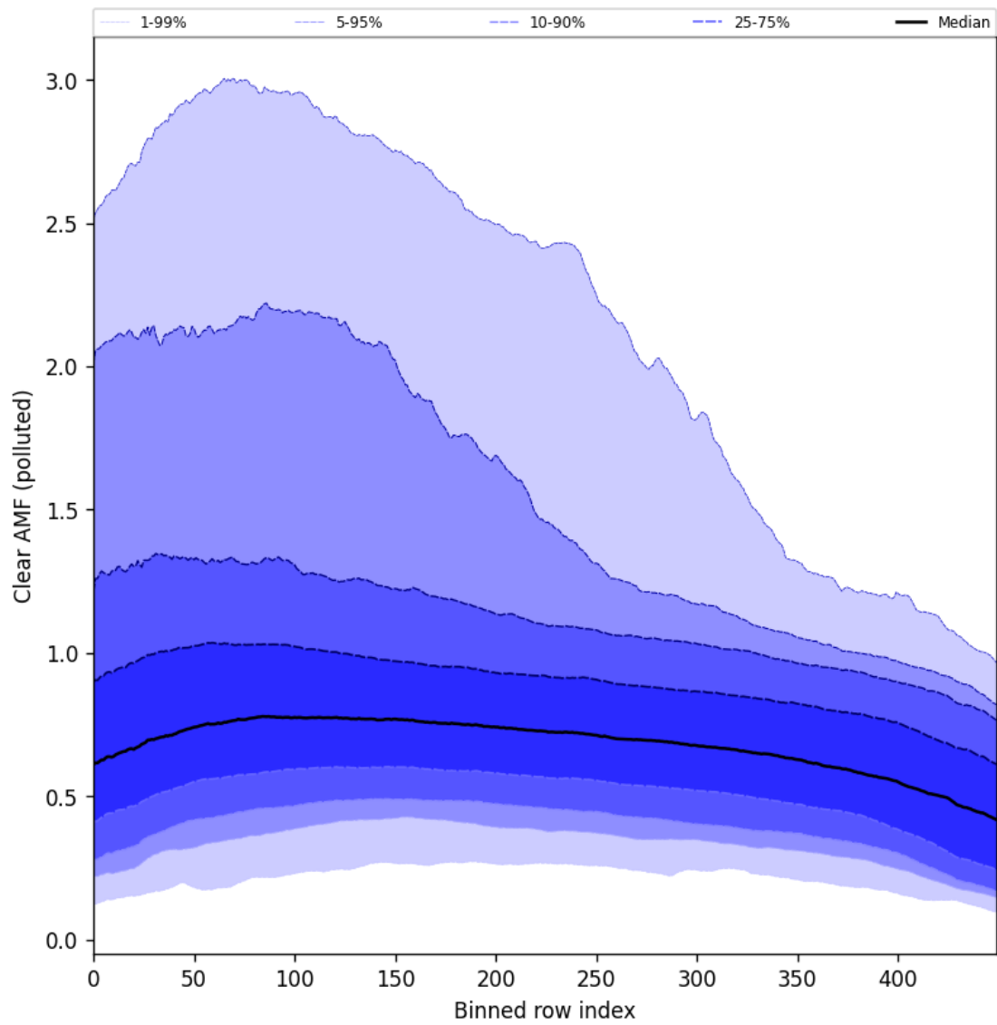
Figure 107: Along track statistics of “Clear AMF (polluted)” for 2025-10-22 to 2025-10-23
