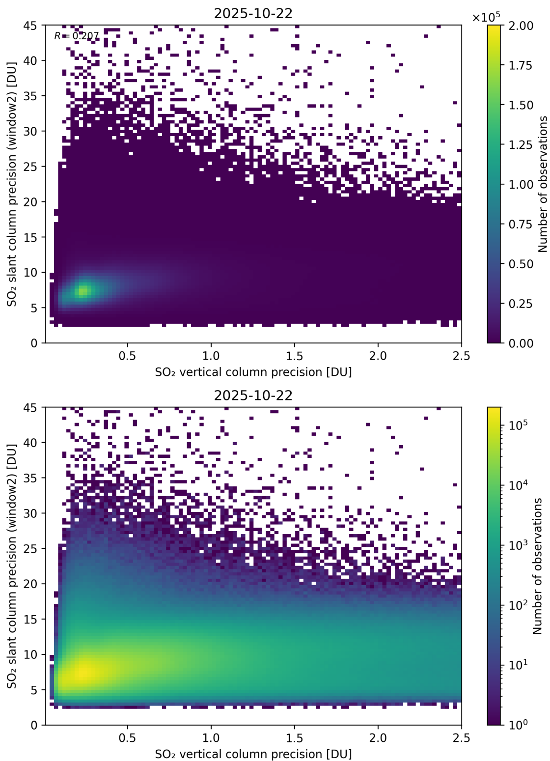
Figure 343: Scatter density plot of “SO 2 vertical column precision” against “SO 2 slant column precision (window2)” for 2025-10-22 to 2025-10-23.
