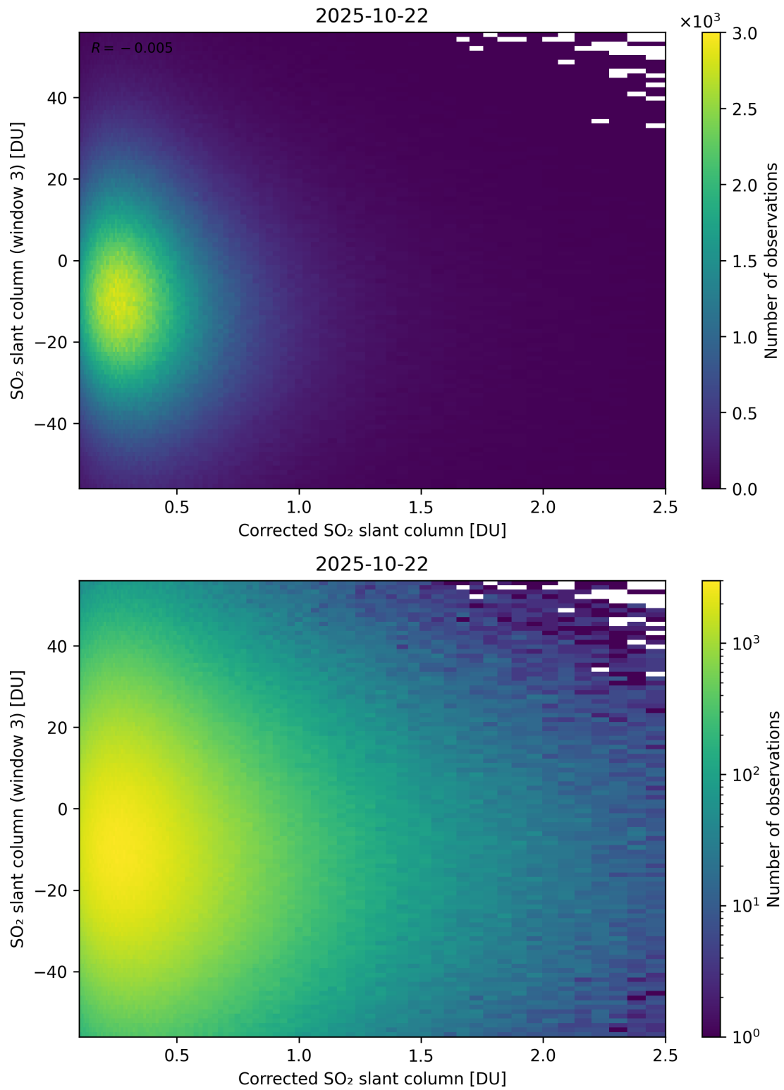
Figure 240: Scatter density plot of “Corrected SO 2 slant column” against “SO 2 slant column (window 3)” for 2025-10-22 to 2025-10-23.
