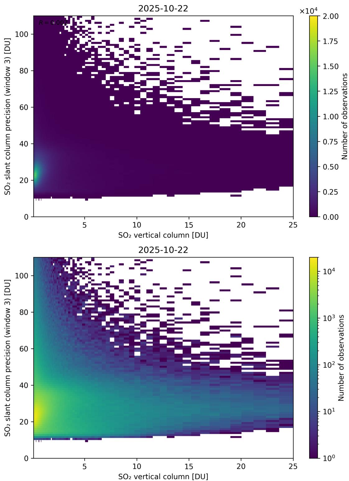
Figure 358: Scatter density plot of “SO 2 vertical column” against “SO 2 slant column precision (window 3)” for 2025-10-22 to 2025-10-23.
