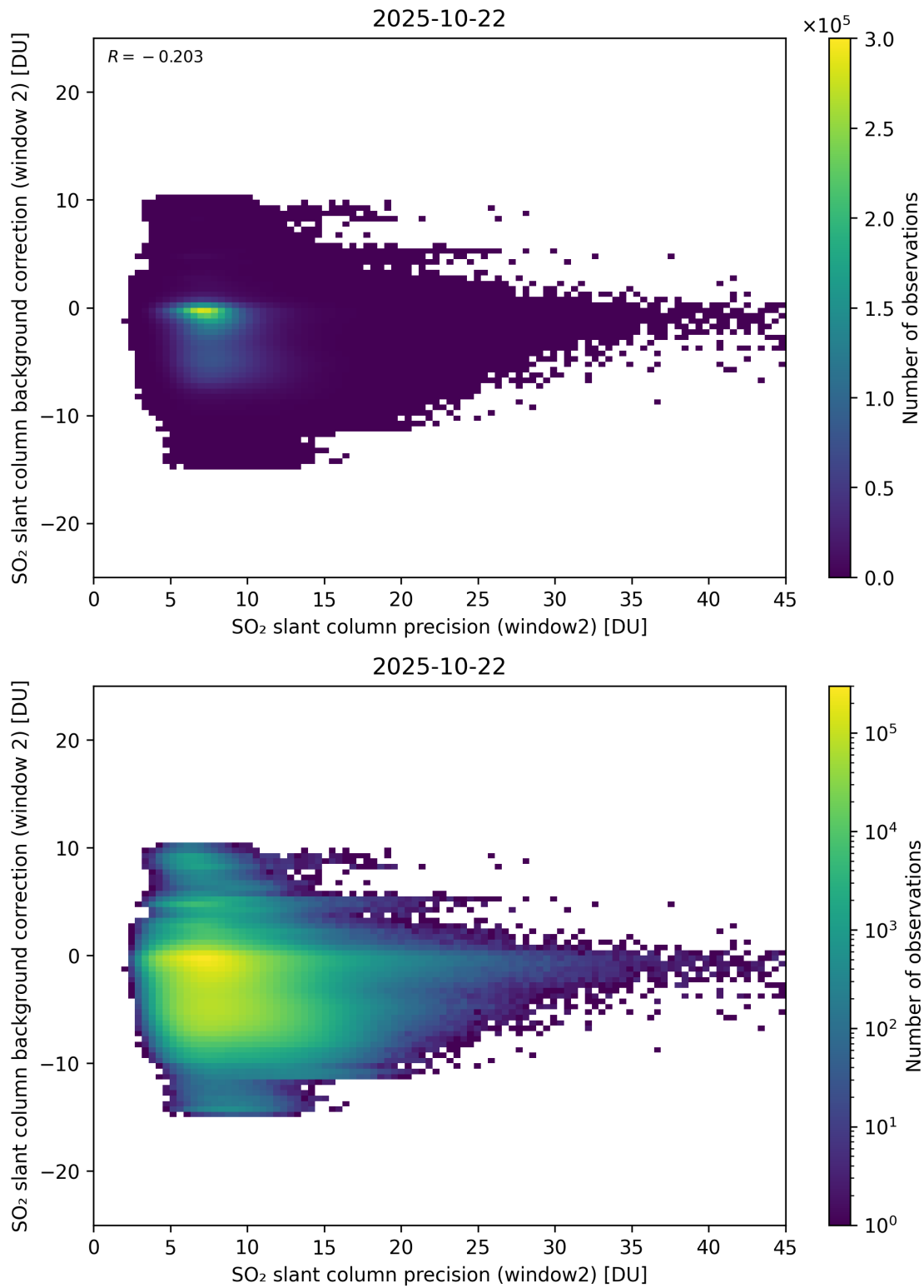
Figure 291: Scatter density plot of “SO 2 slant column precision (window2)” against “SO 2 slant column background correction (window 2)” for 2025-10-22 to 2025-10-23.
