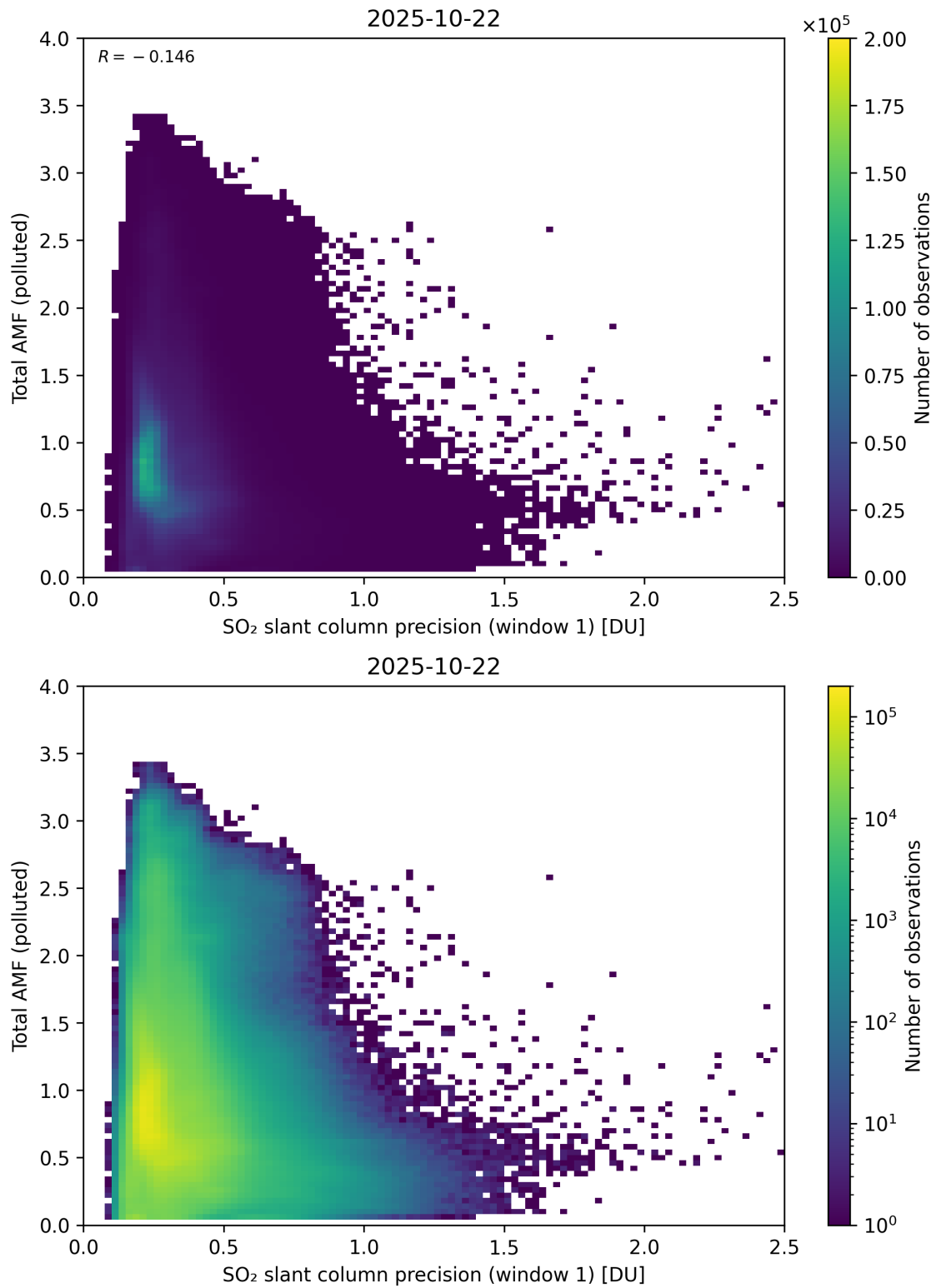
Figure 280: Scatter density plot of “SO 2 slant column precision (window 1)” against “Total AMF (polluted)” for 2025-10-22 to 2025-10-23.
