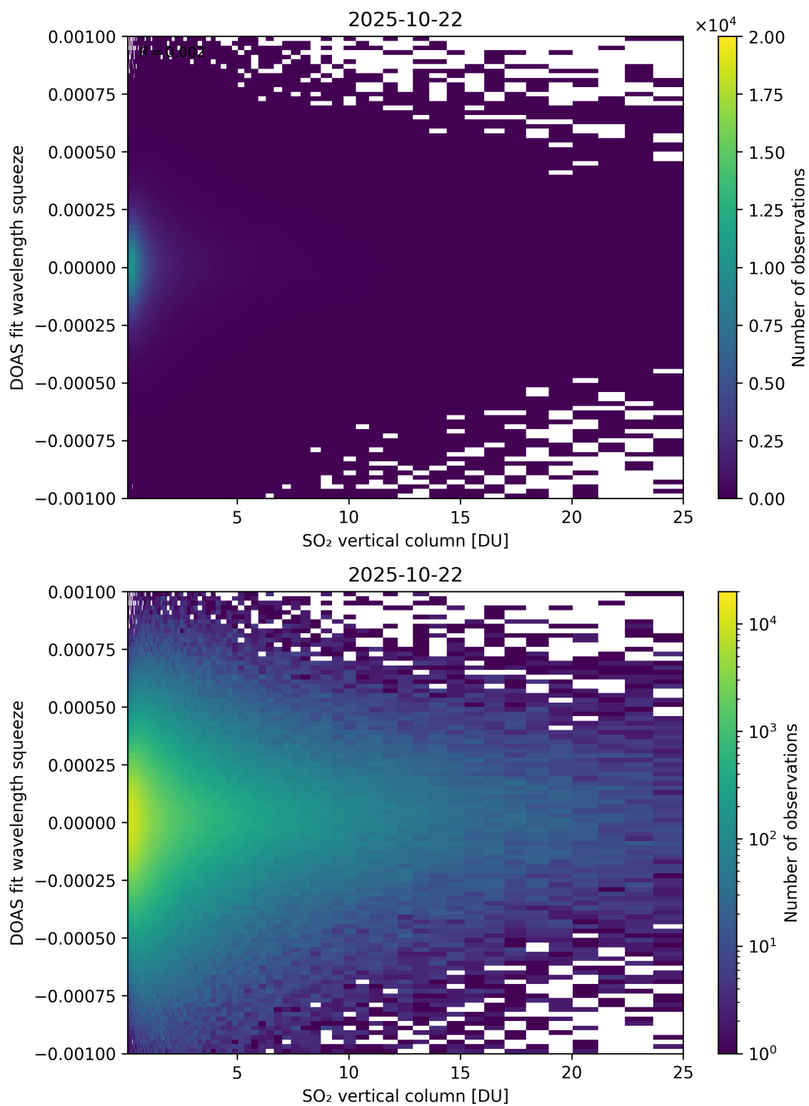
Figure 327: Scatter density plot of “SO 2 vertical column” against “DOAS fit wavelength squeeze” for 2025-10-22 to 2025-10-23.
