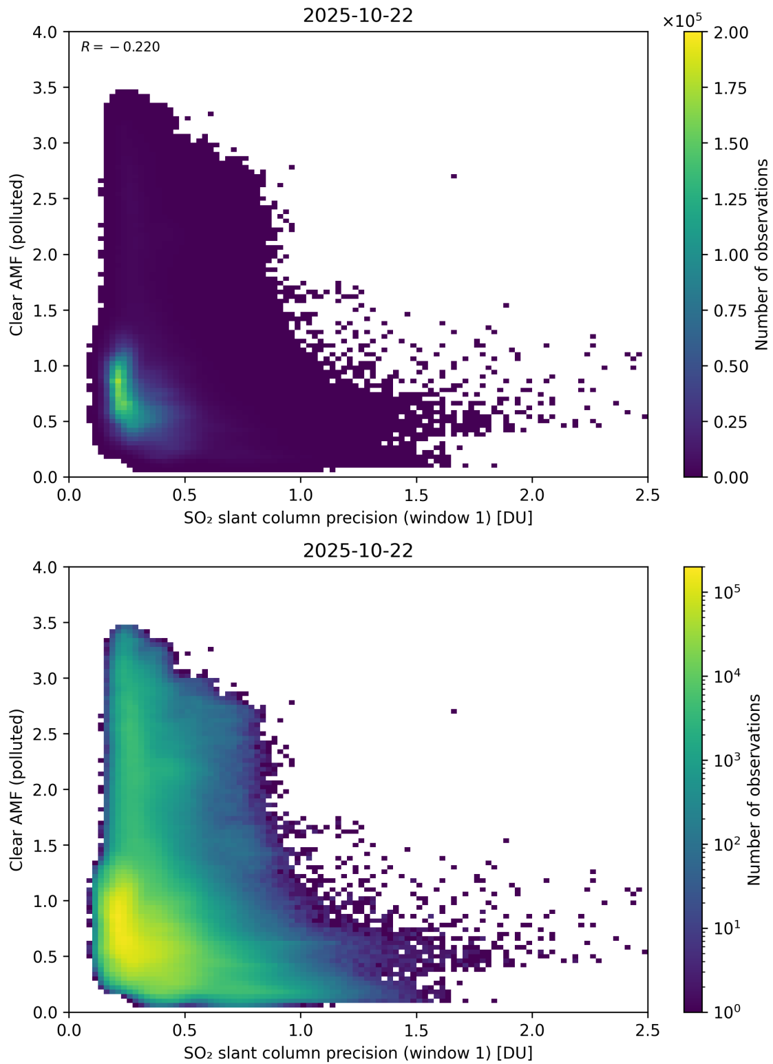
Figure 274: Scatter density plot of “SO 2 slant column precision (window 1)” against “Clear AMF (polluted)” for 2025-10-22 to 2025-10-23.
