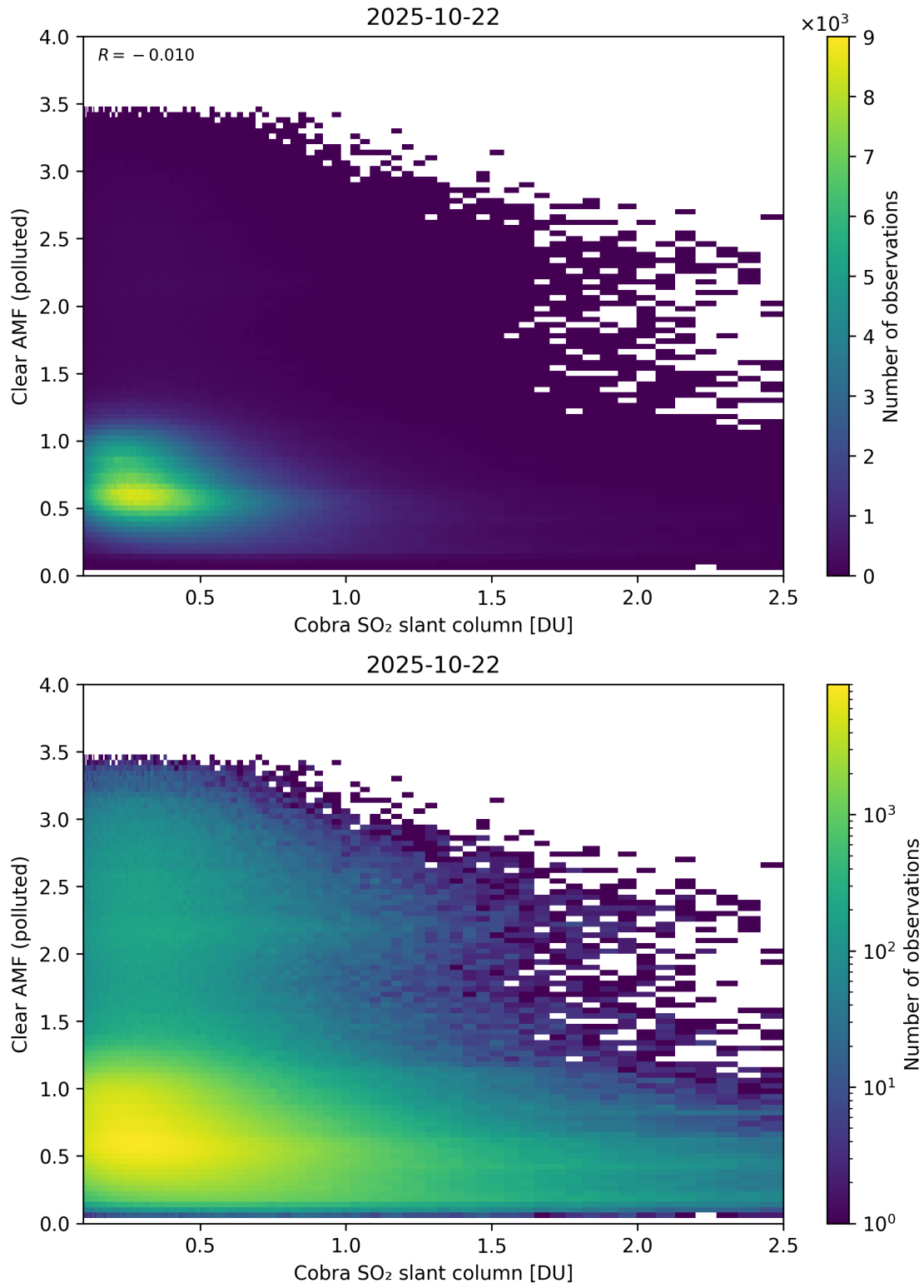
Figure 215: Scatter density plot of “Cobra SO 2 slant column” against “Clear AMF (polluted)” for 2025-10-22 to 2025-10-23.
