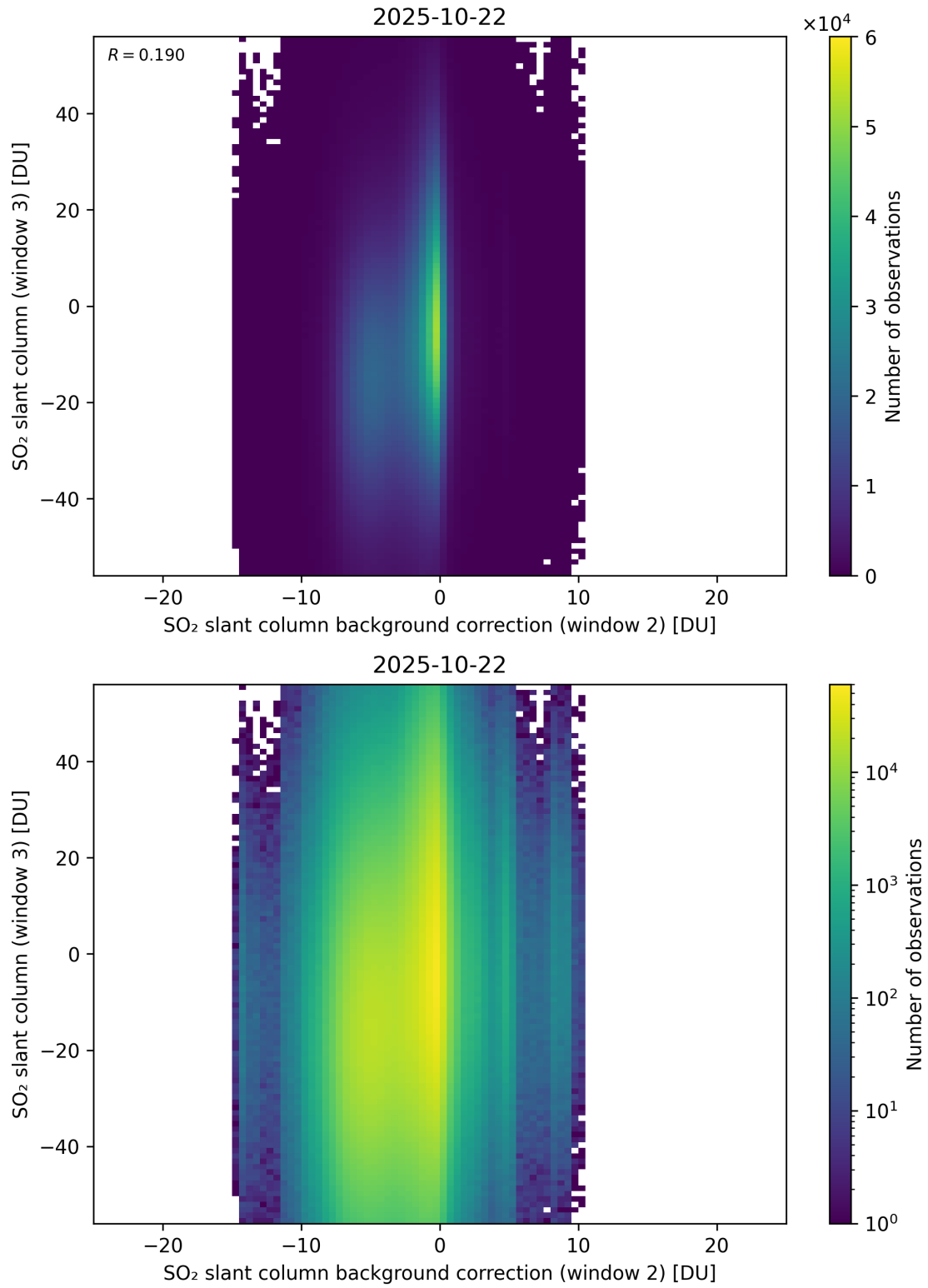
Figure 128: Scatter density plot of “SO 2 slant column background correction (window 2)” against “SO 2 slant column (window 3)” for 2025-10-22 to 2025-10-23.
