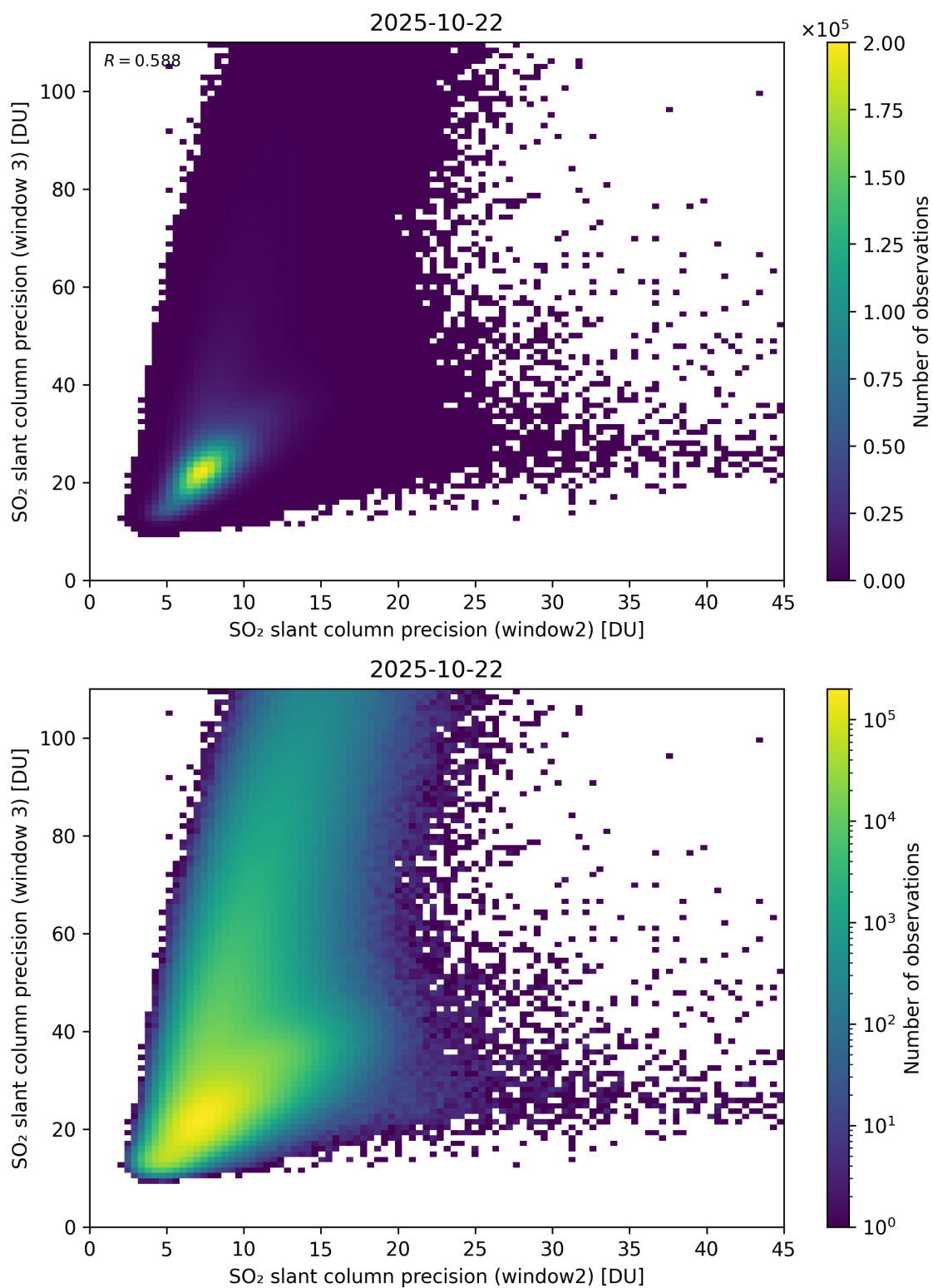
Figure 300: Scatter density plot of “SO 2 slant column precision (window2)” against “SO 2 slant column precision (window 3)” for 2025-10-22 to 2025-10-23.
