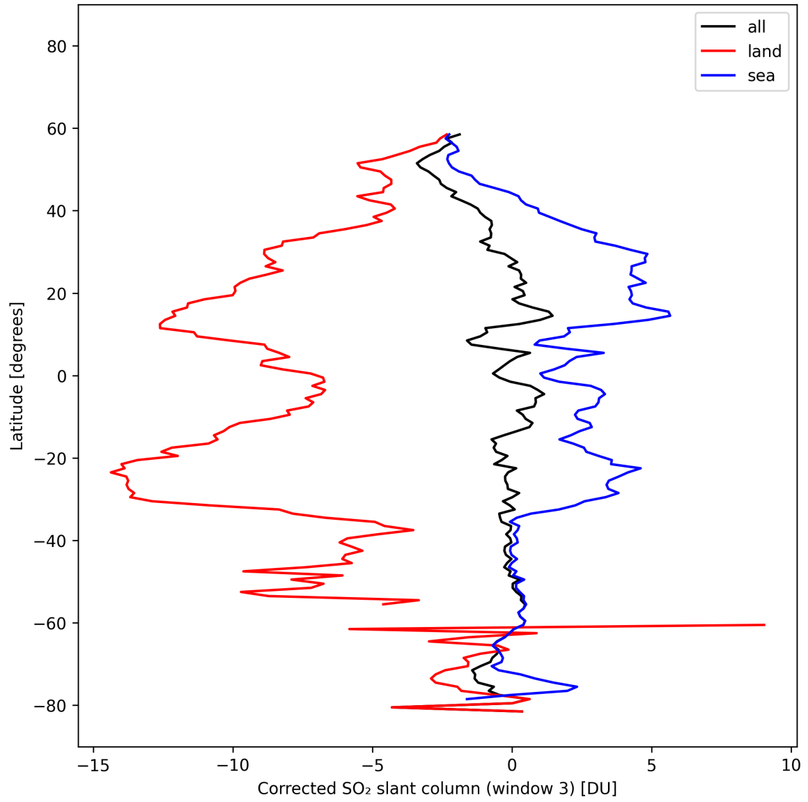
Figure 47: Zonal average of “Corrected SO 2 slant column (window 3)” for 2025-10-22 to 2025-10-23.
