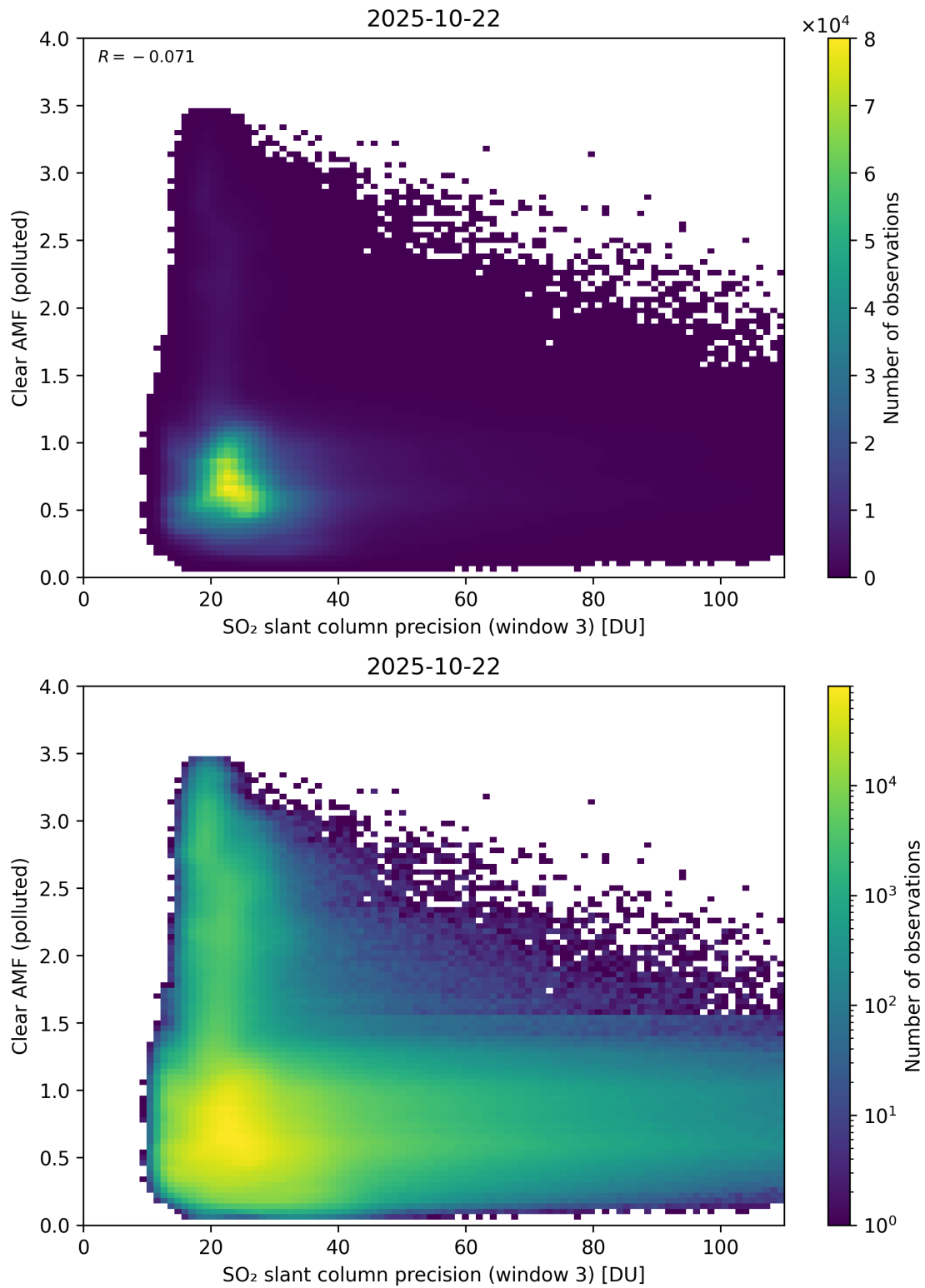
Figure 311: Scatter density plot of “SO 2 slant column precision (window 3)” against “Clear AMF (polluted)” for 2025-10-22 to 2025-10-23.
