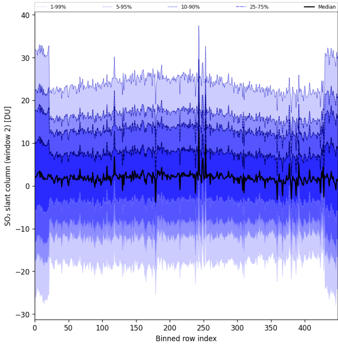
Figure 93: Along track statistics of “SO 2 slant column (window 2)” for 2025-10-22 to 2025-10-23
