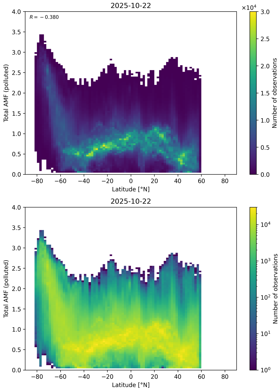
Figure 167: Scatter density plot of “Latitude” against “Total AMF (polluted)” for 2025-10-22 to 2025-10-23.
