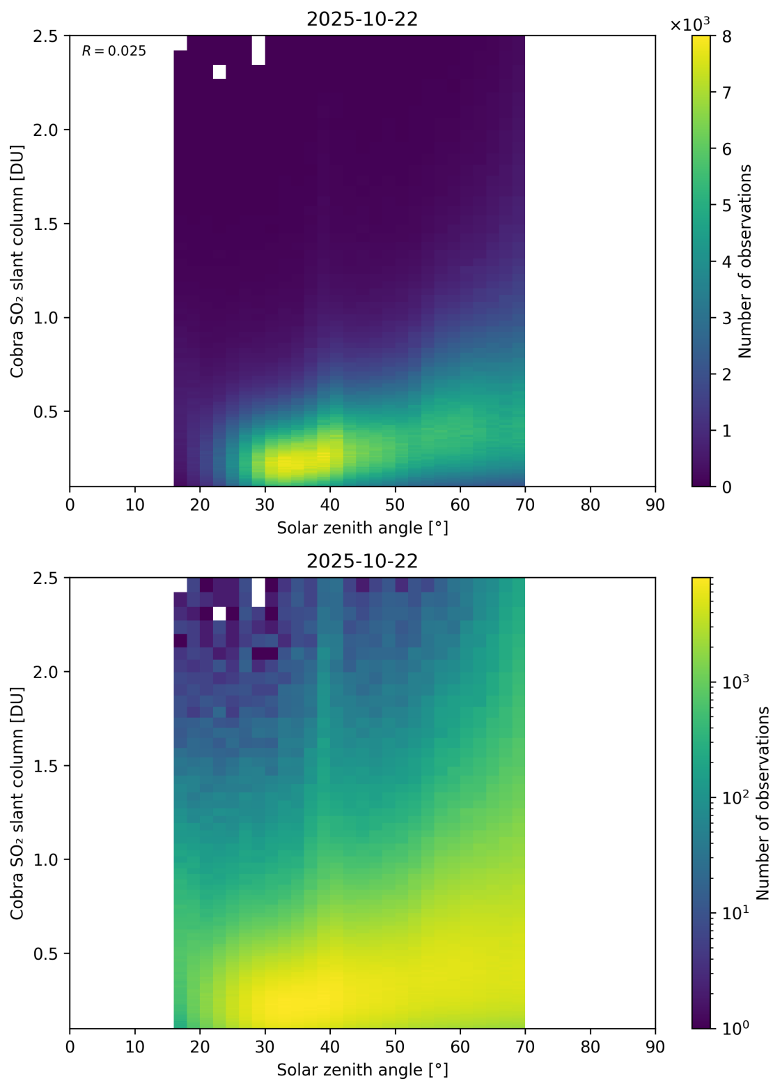
Figure 179: Scatter density plot of “Solar zenith angle” against “Cobra SO 2 slant column” for 2025-10-22 to 2025-10-23.
