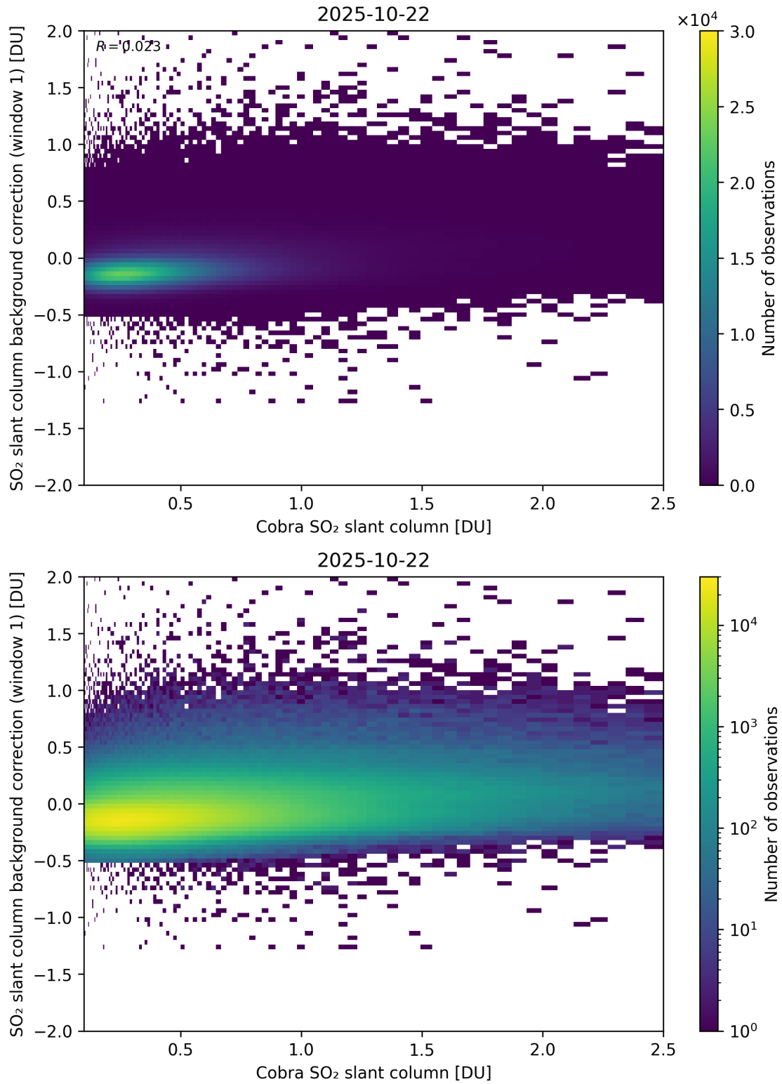
Figure 193: Scatter density plot of “Cobra SO 2 slant column” against “SO 2 slant column background correction (window 1)” for 2025-10-22 to 2025-10-23.
