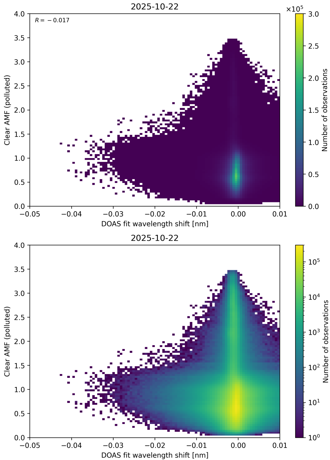
Figure 140: Scatter density plot of “DOAS fit wavelength shift” against “Clear AMF (polluted)” for 2025-10-22 to 2025-10-23.
