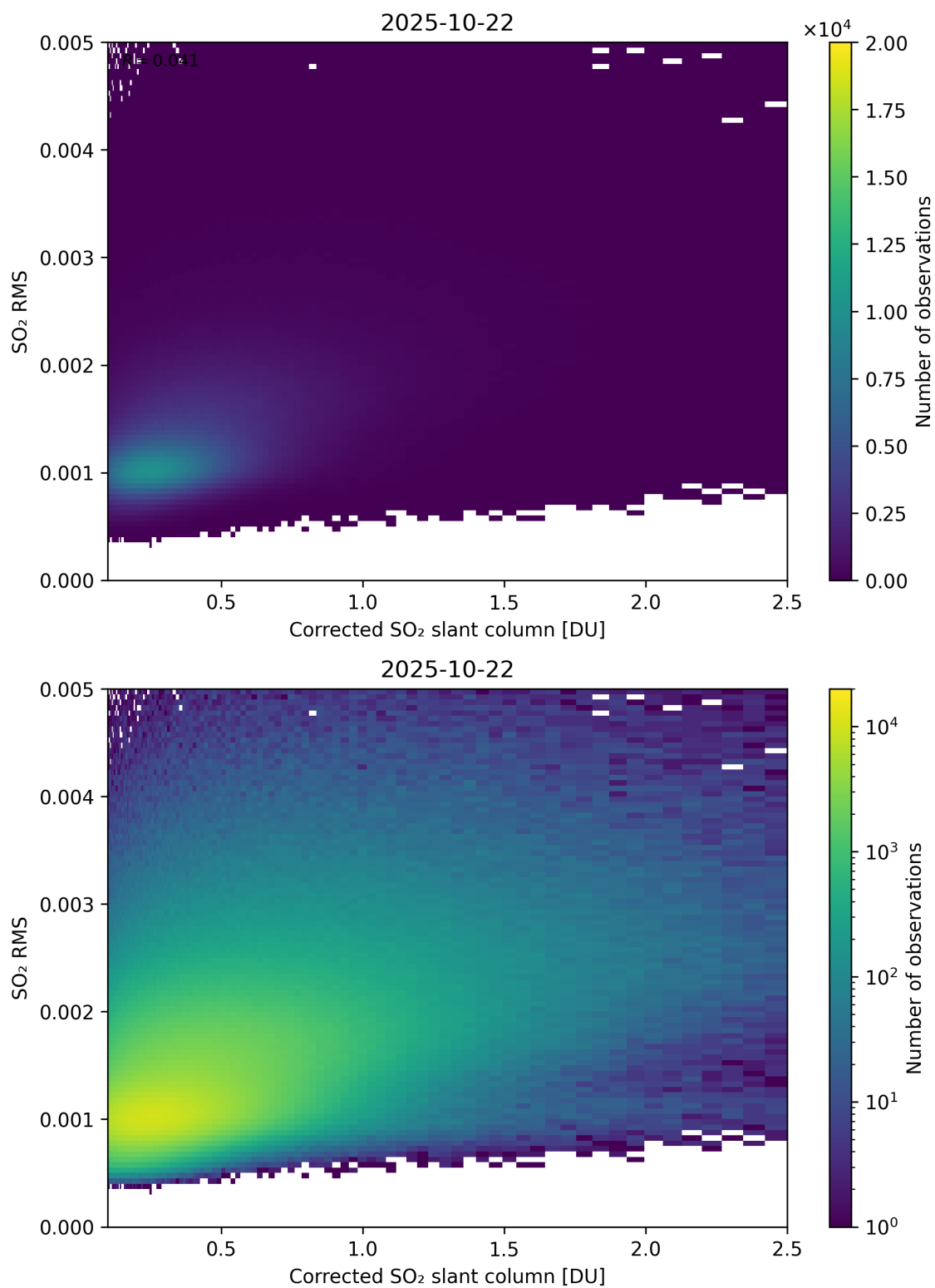
Figure 231: Scatter density plot of “Corrected SO 2 slant column” against “SO 2 RMS” for 2025-10-22 to 2025-10-23.
