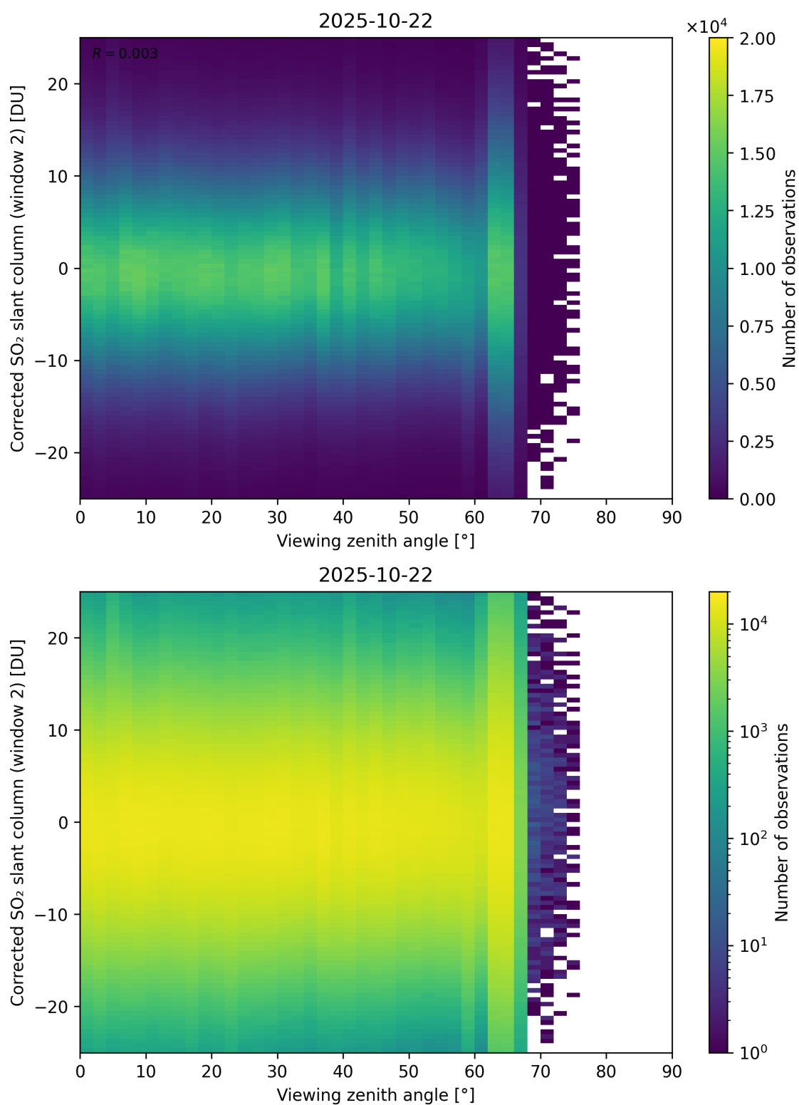
Figure 374: Scatter density plot of “Viewing zenith angle” against “Corrected SO 2 slant column (window 2)” for 2025-10-22 to 2025-10-23.
