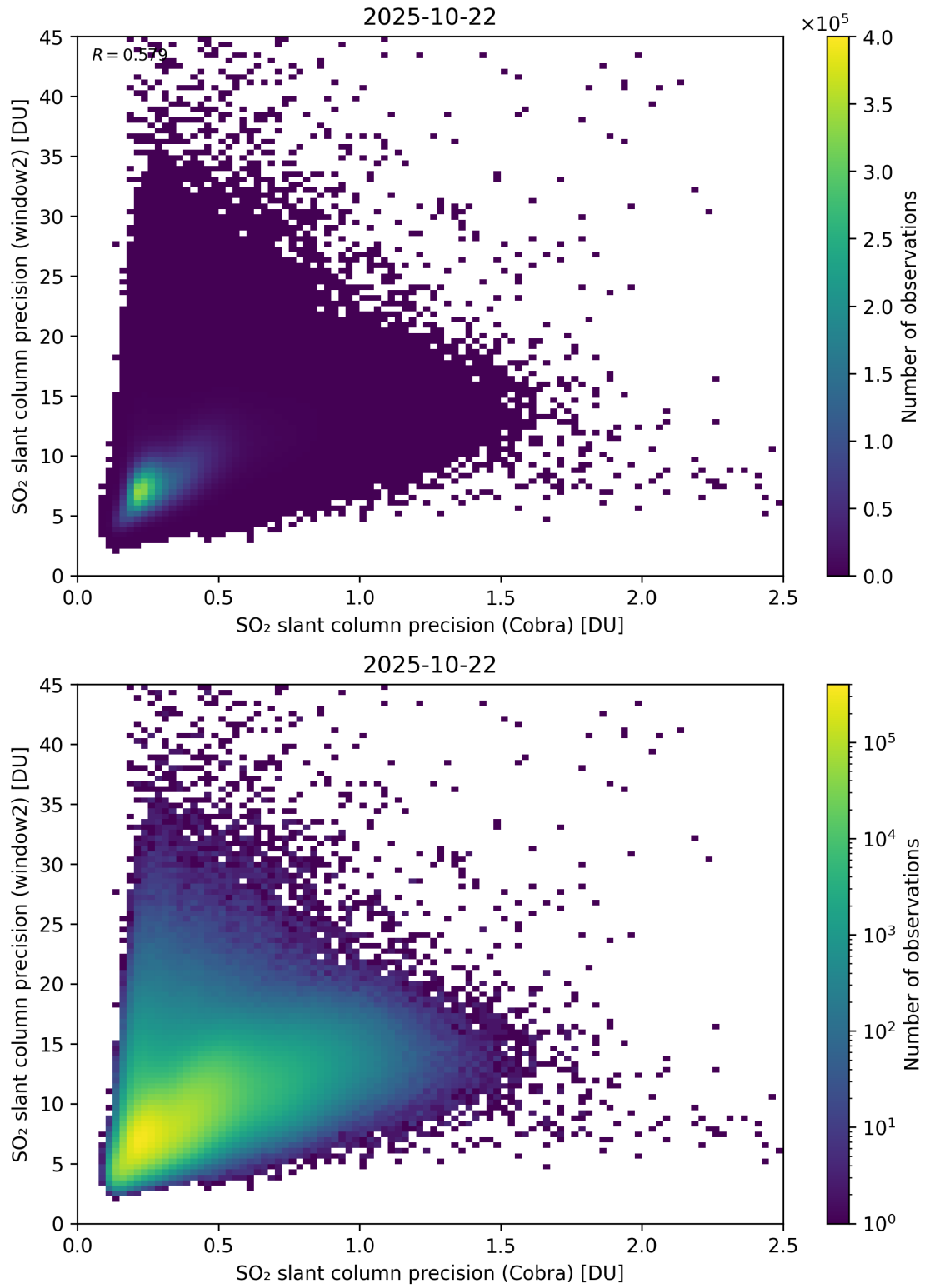
Figure 210: Scatter density plot of “SO 2 slant column precision (Cobra)” against “SO 2 slant column precision (window2)” for 2025-10-22 to 2025-10-23.
