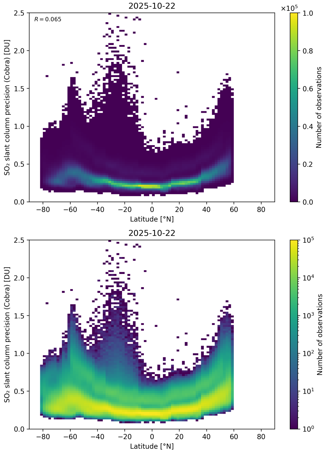
Figure 158: Scatter density plot of “Latitude” against “SO 2 slant column precision (Cobra)” for 2025-10-22 to 2025-10-23.
