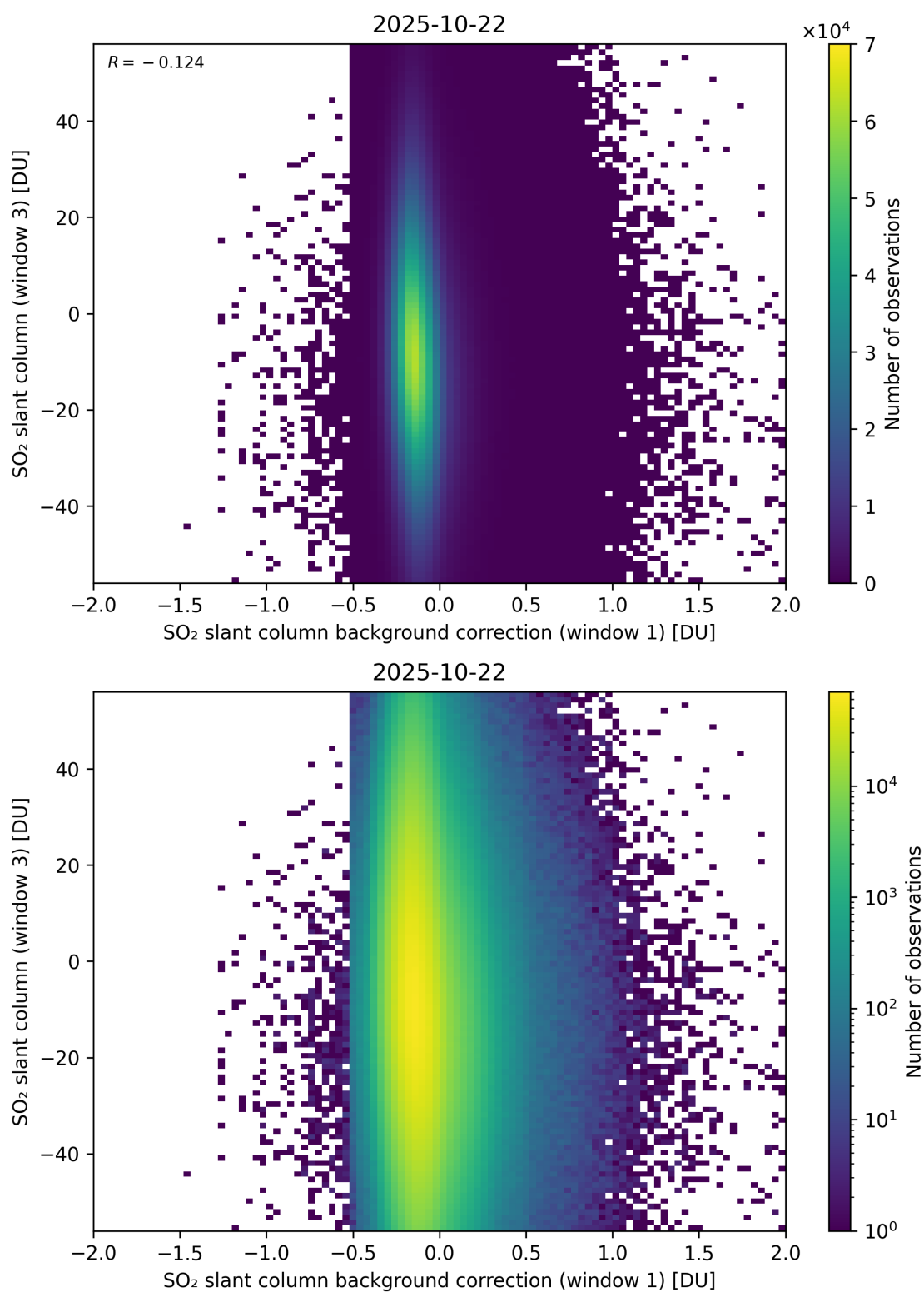
Figure 118: Scatter density plot of “SO 2 slant column background correction (window 1)” against “SO 2 slant column (window 3)” for 2025-10-22 to 2025-10-23.
