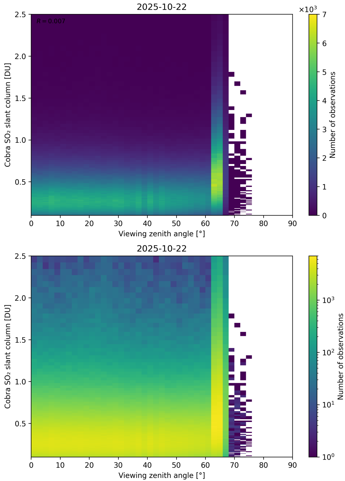
Figure 371: Scatter density plot of “Viewing zenith angle” against “Cobra SO 2 slant column” for 2025-10-22 to 2025-10-23.
