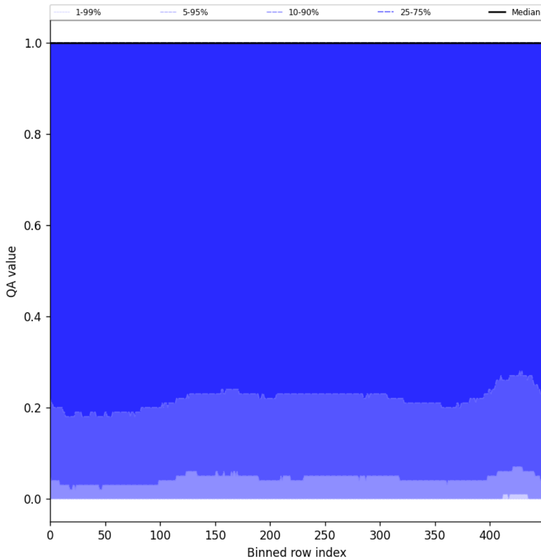
Figure 83: Along track statistics of “QA value” for 2025-10-22 to 2025-10-23
