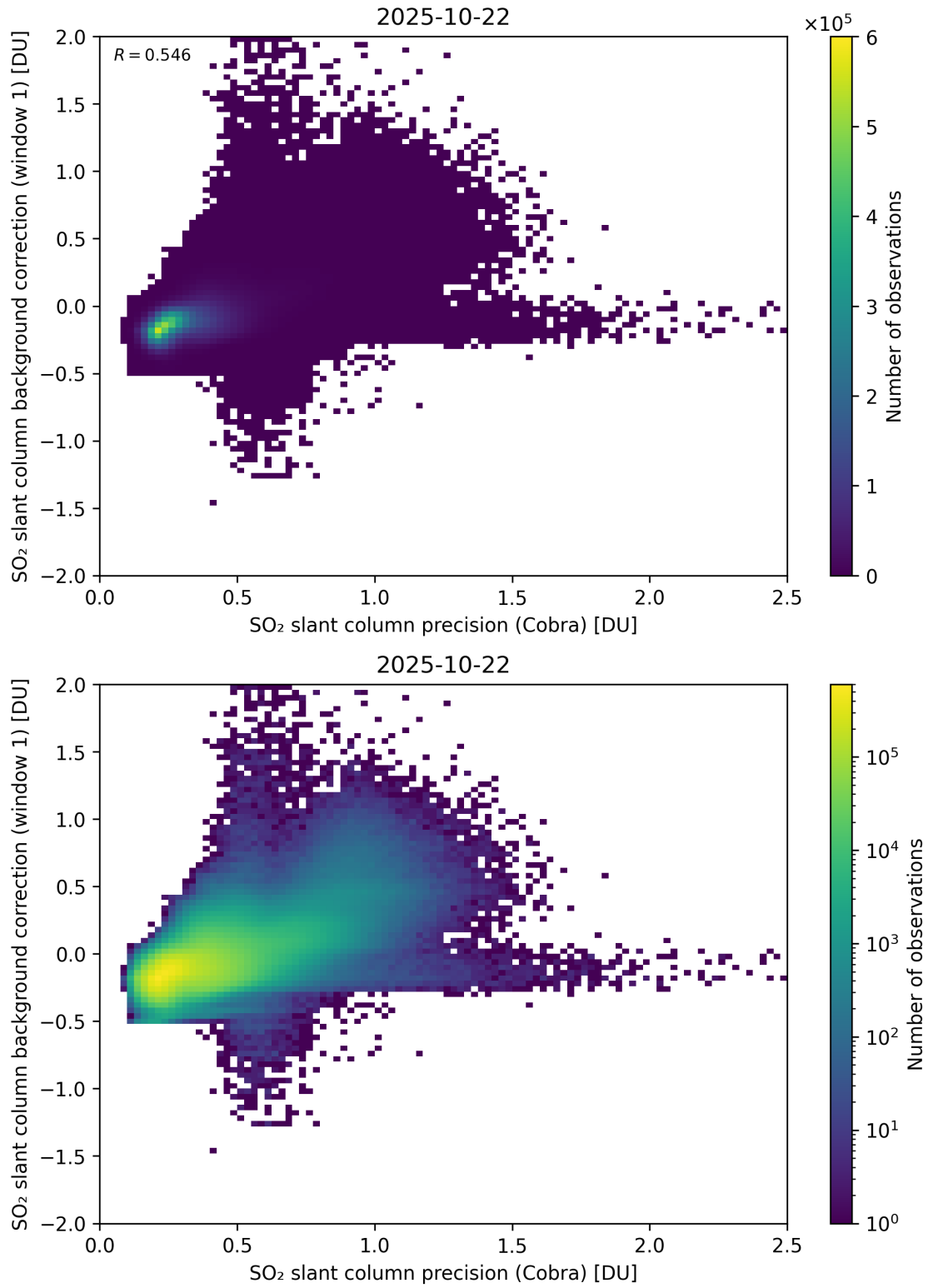
Figure 199: Scatter density plot of “SO 2 slant column precision (Cobra)” against “SO 2 slant column background correction (window 1)” for 2025-10-22 to 2025-10-23.
