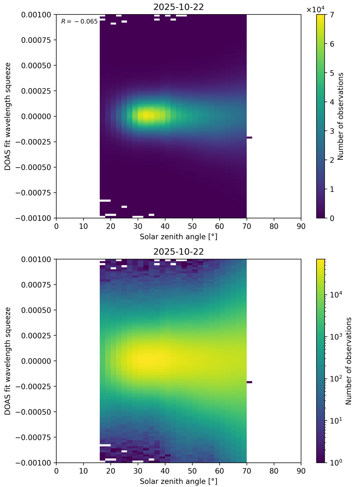
Figure 175: Scatter density plot of “Solar zenith angle” against “DOAS fit wavelength squeeze” for 2025-10-22 to 2025-10-23.
