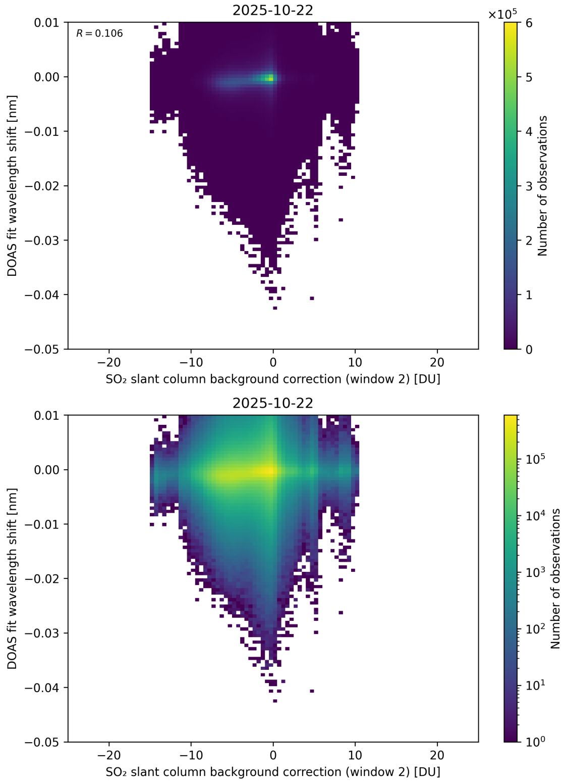
Figure 123: Scatter density plot of “SO 2 slant column background correction (window 2)” against “DOAS fit wavelength shift” for 2025-10-22 to 2025-10-23.
