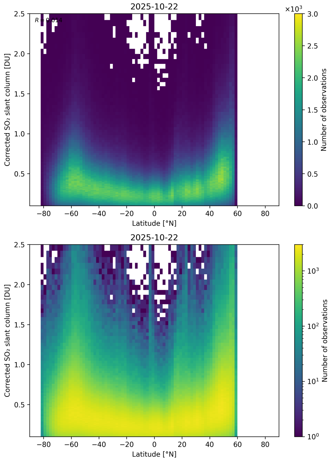
Figure 159: Scatter density plot of “Latitude” against “Corrected SO 2 slant column” for 2025-10-22 to 2025-10-23.
