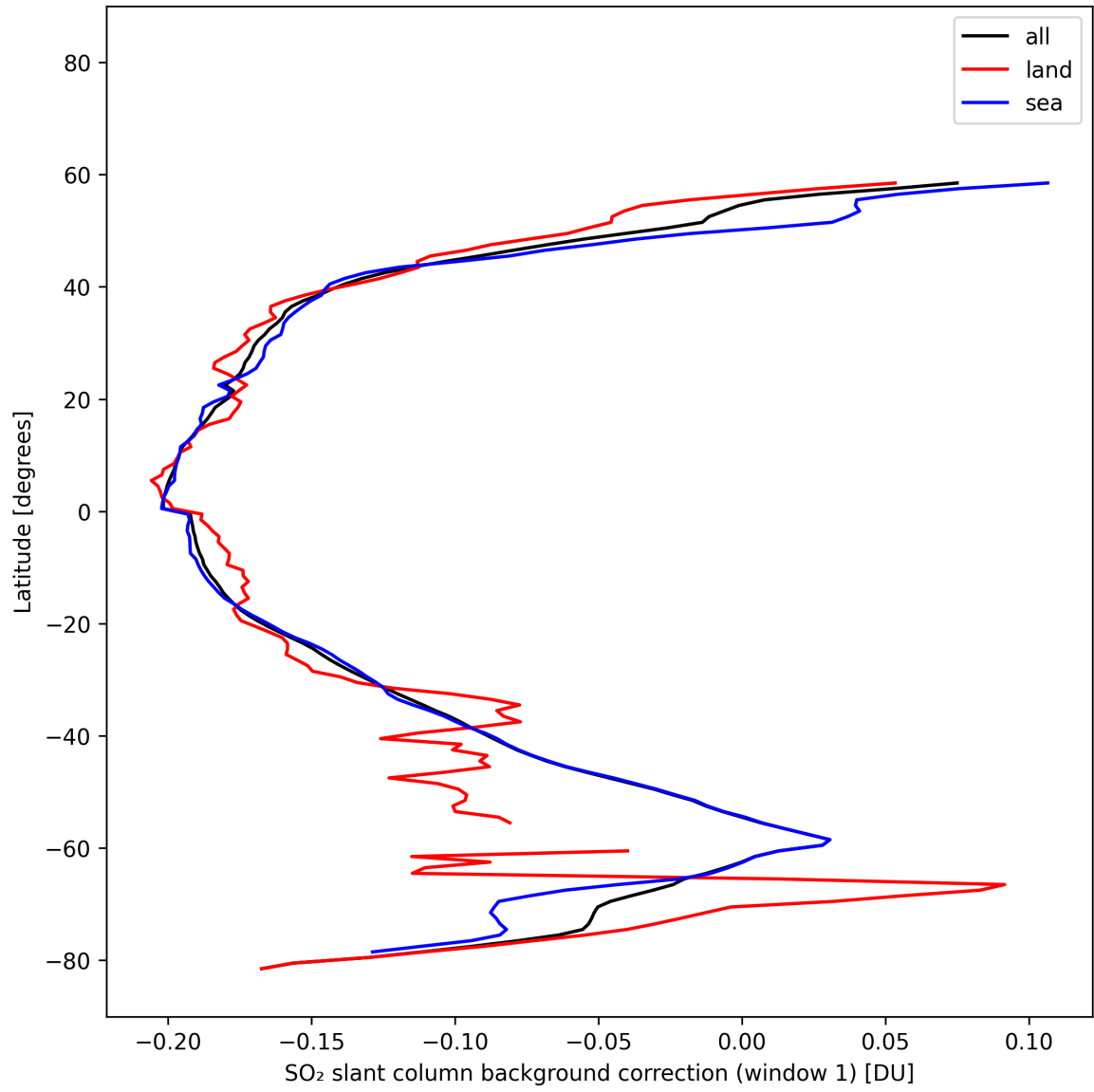
Figure 40: Zonal average of “SO 2 slant column background correction (window 1)” for 2025-10-22 to 2025-10-23.
