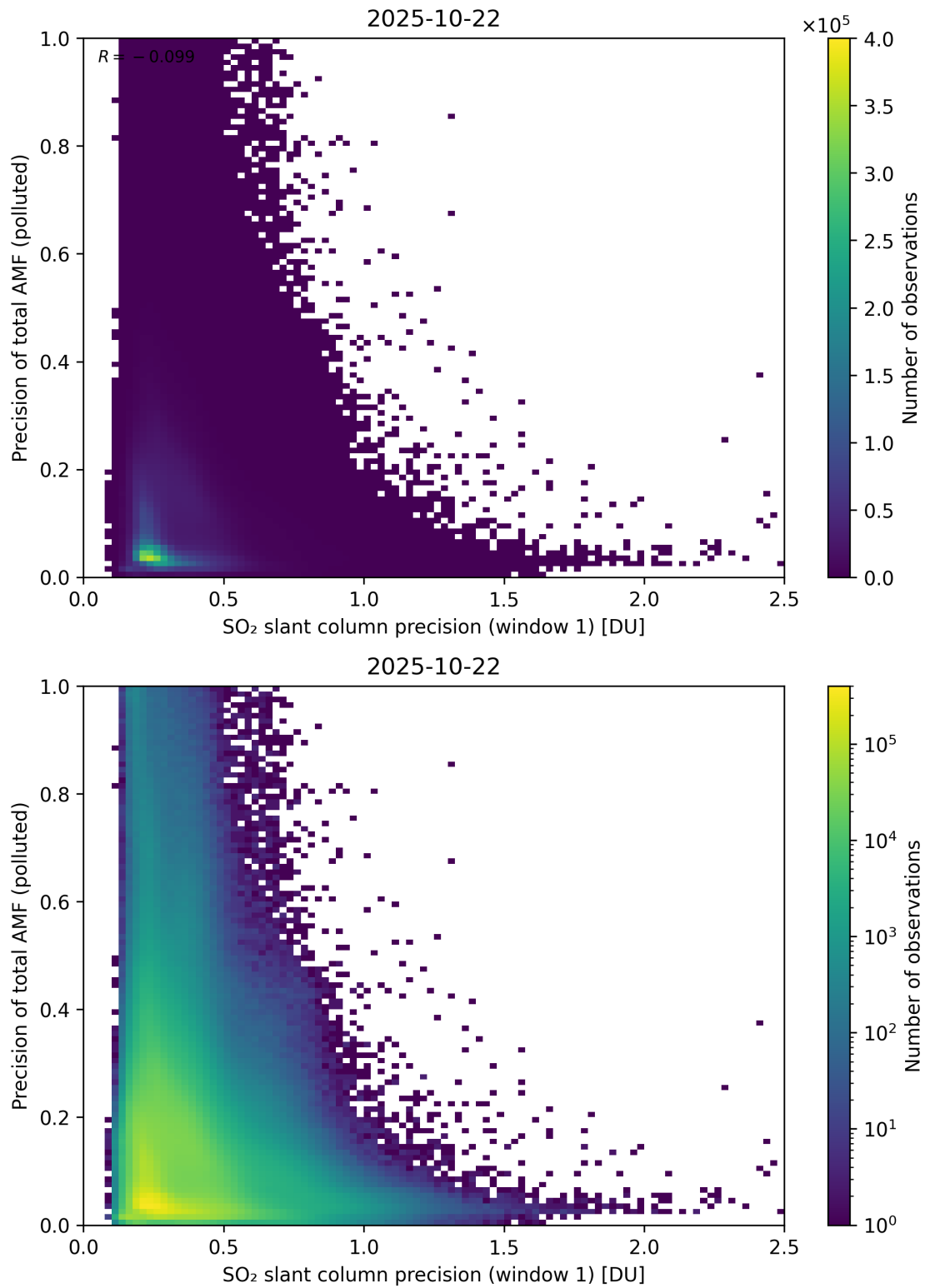
Figure 281: Scatter density plot of “SO 2 slant column precision (window 1)” against “Precision of total AMF (polluted)” for 2025-10-22 to 2025-10-23.
