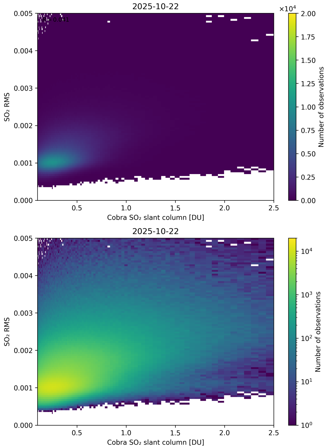
Figure 198: Scatter density plot of “Cobra SO 2 slant column” against “SO 2 RMS” for 2025-10-22 to 2025-10-23.
