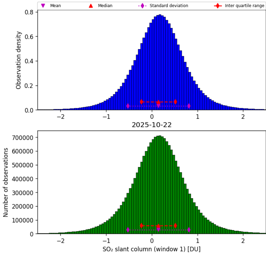
Figure 63: Histogram of “SO 2 slant column (window 1)” for 2025-10-22 to 2025-10-23
