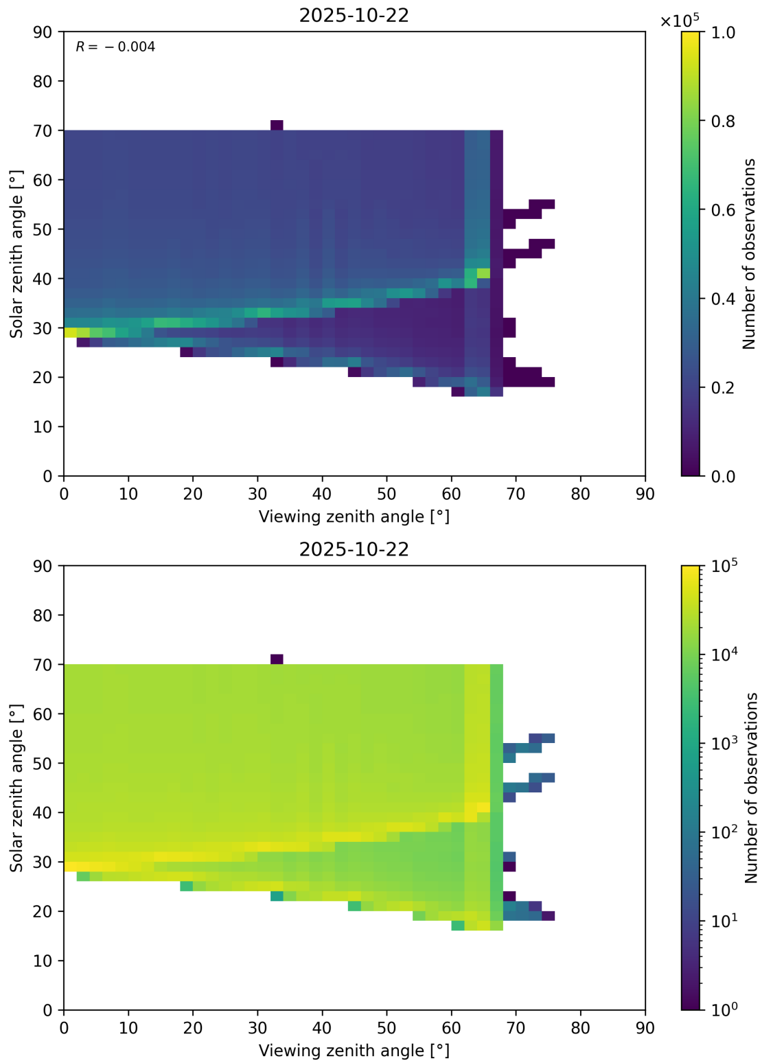
Figure 369: Scatter density plot of “Viewing zenith angle” against “Solar zenith angle” for 2025-10-22 to 2025-10-23.
