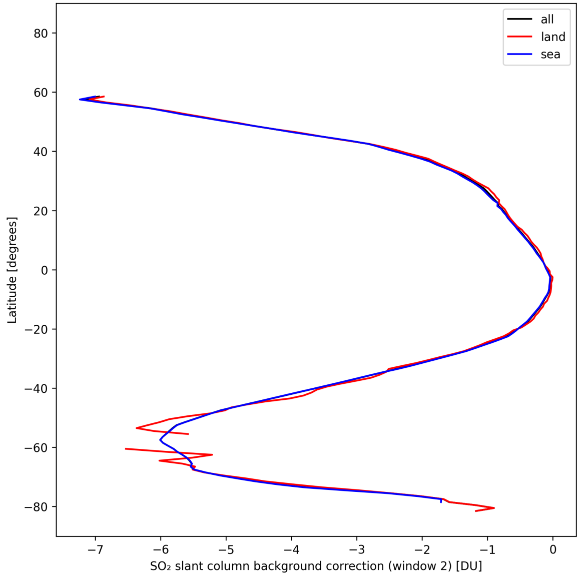
Figure 44: Zonal average of “SO 2 slant column background correction (window 2)” for 2025-10-22 to 2025-10-23.
