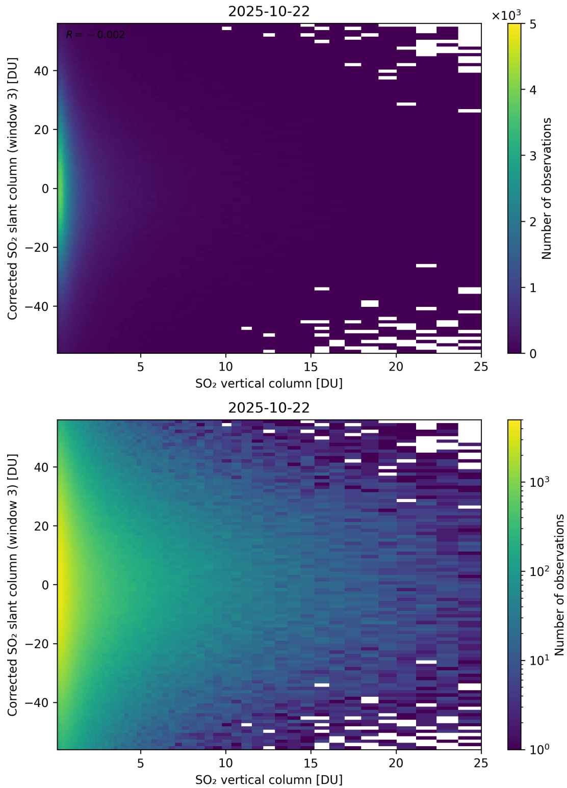
Figure 353: Scatter density plot of “SO 2 vertical column” against “Corrected SO 2 slant column (window 3)” for 2025-10-22 to 2025-10-23.
