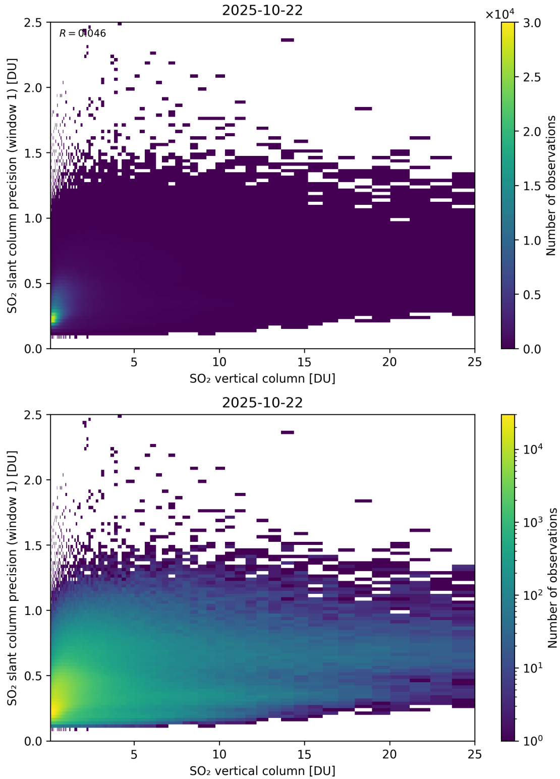
Figure 355: Scatter density plot of “SO 2 vertical column” against “SO 2 slant column precision (window 1)” for 2025-10-22 to 2025-10-23.
