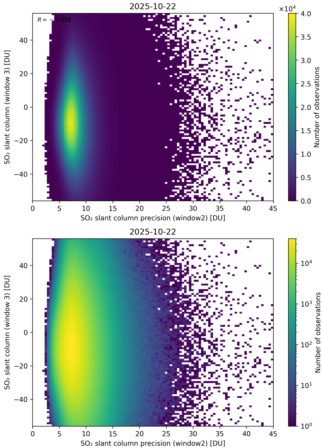
Figure 299: Scatter density plot of “SO 2 slant column precision (window2)” against “SO 2 slant column (window 3)” for 2025-10-22 to 2025-10-23.
