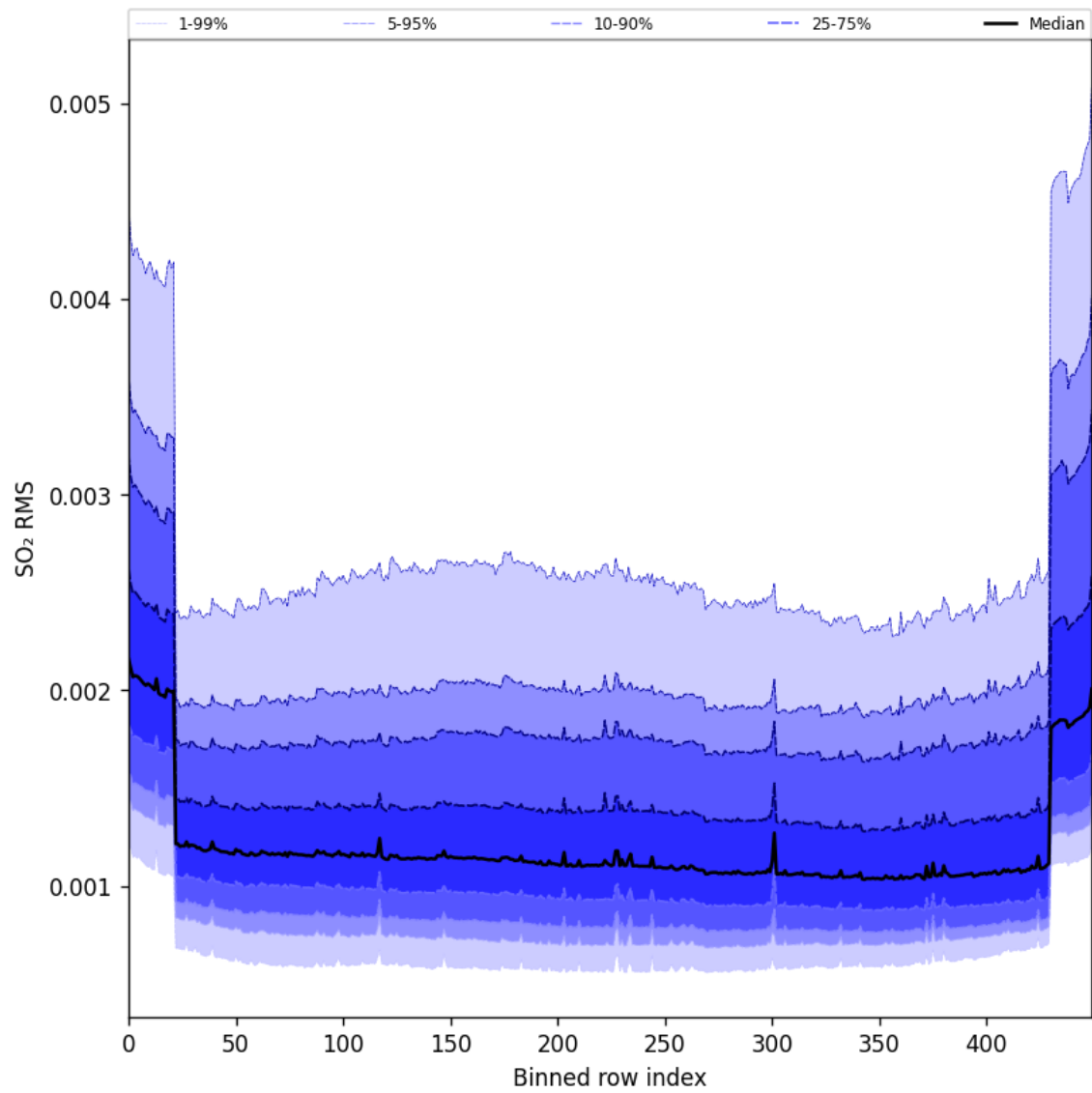
Figure 104: Along track statistics of “SO 2 RMS” for 2025-10-22 to 2025-10-23
