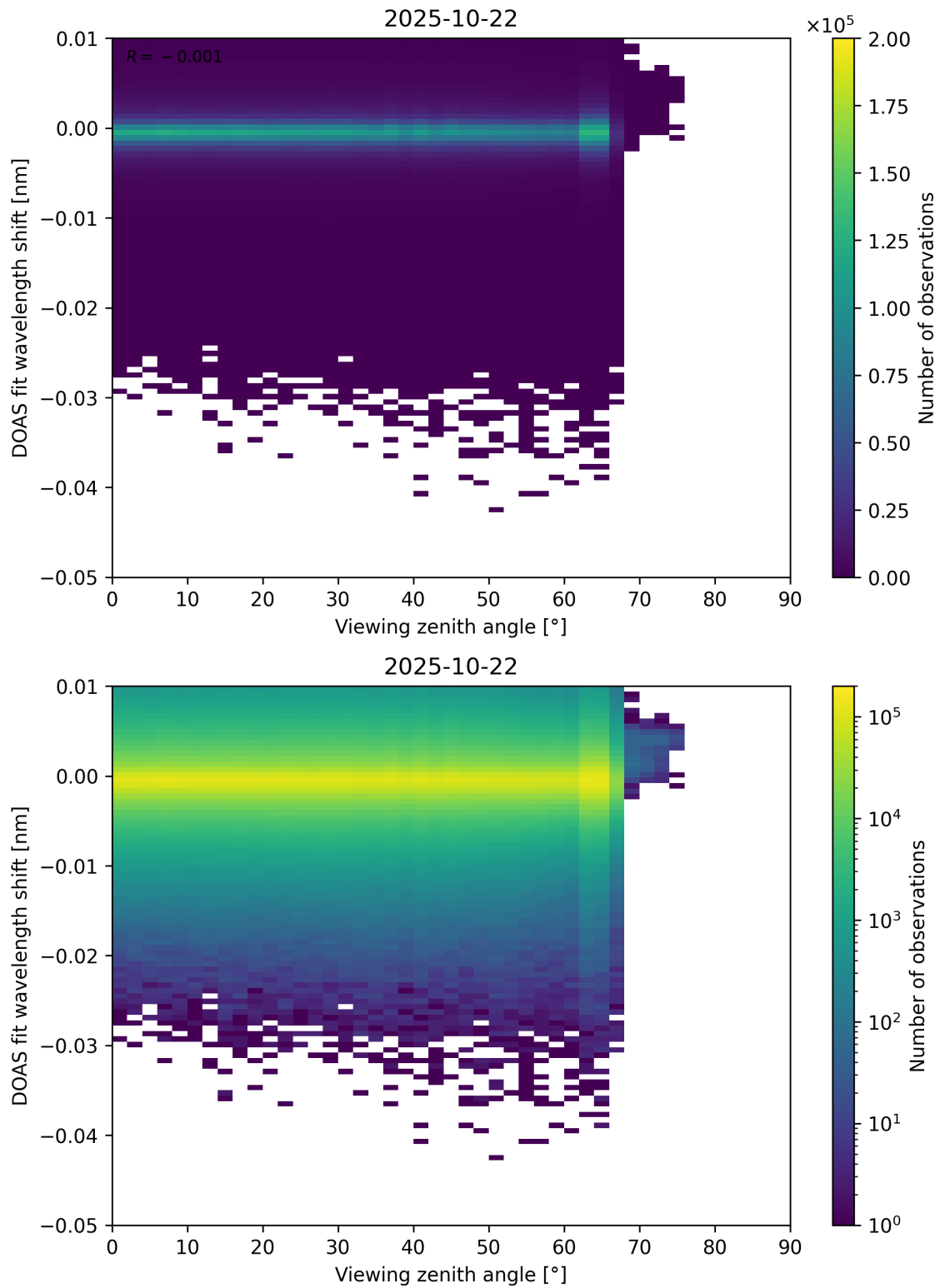
Figure 365: Scatter density plot of “Viewing zenith angle” against “DOAS fit wavelength shift” for 2025-10-22 to 2025-10-23.
