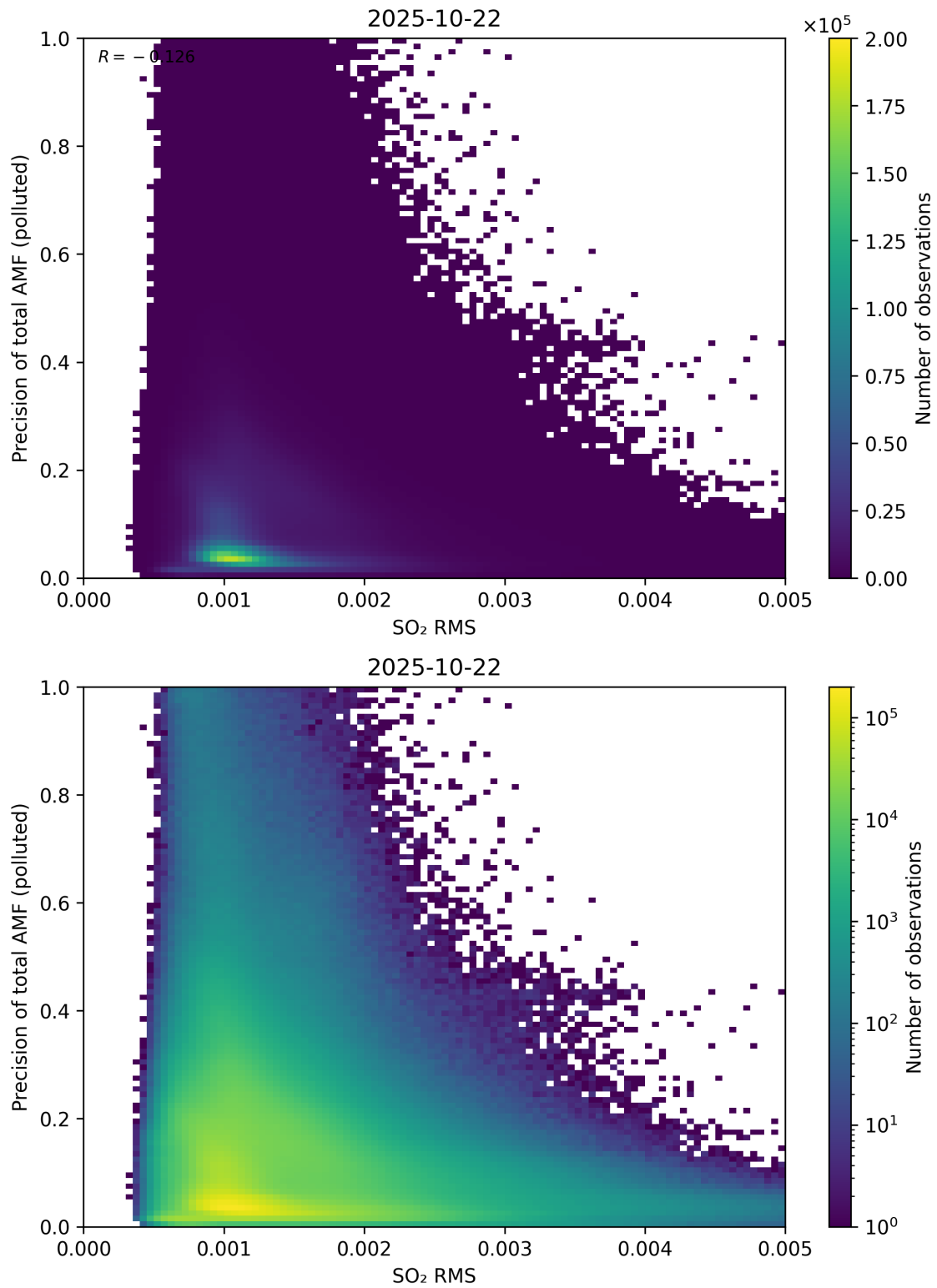
Figure 149: Scatter density plot of “SO 2 RMS” against “Precision of total AMF (polluted)” for 2025-10-22 to 2025-10-23.
