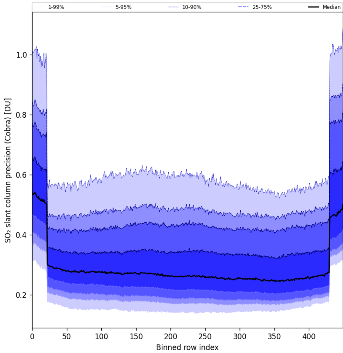
Figure 88: Along track statistics of “SO 2 slant column precision (Cobra)” for 2025-10-22 to 2025-10-23
