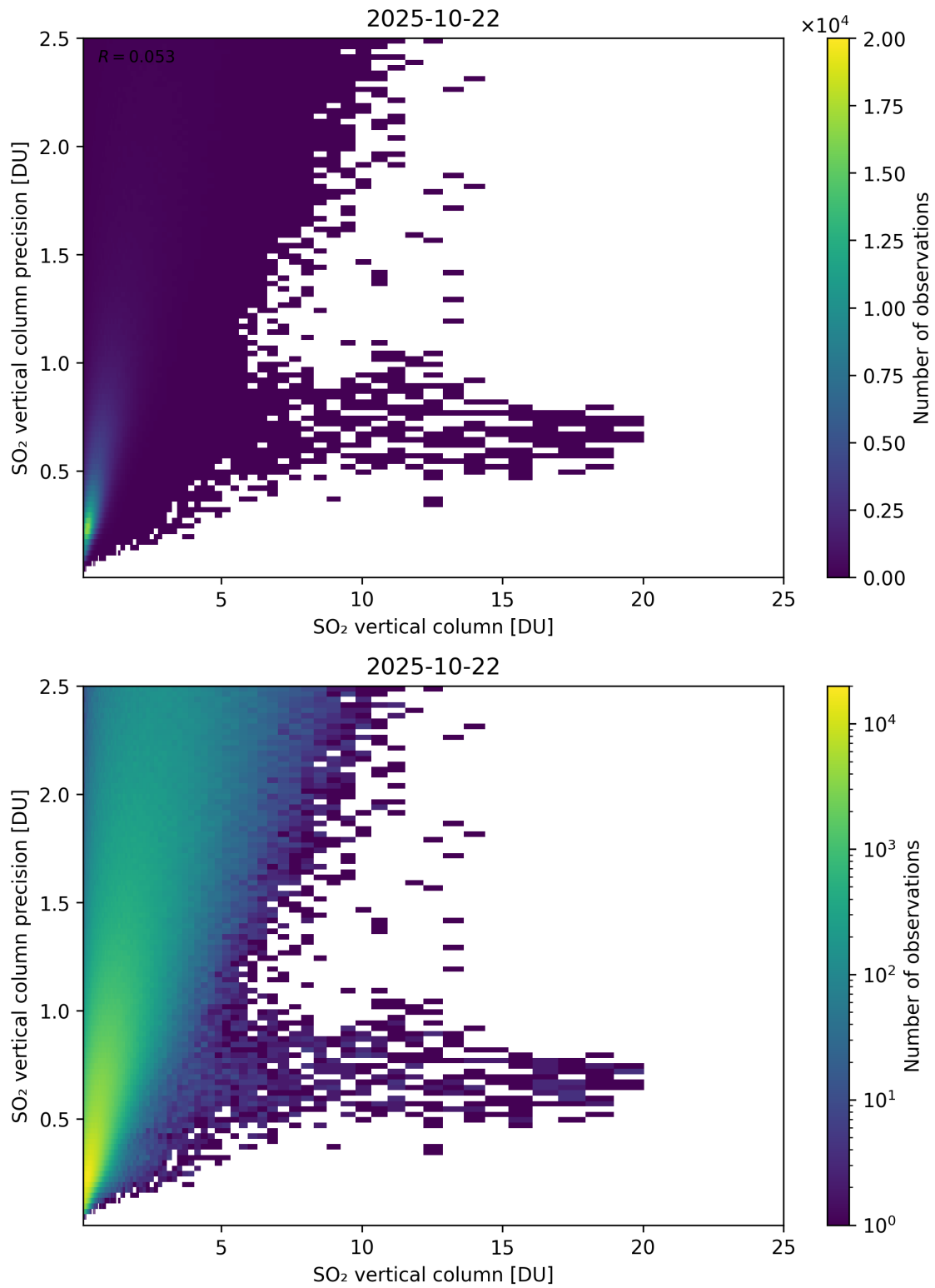
Figure 361: Scatter density plot of “SO 2 vertical column” against “SO 2 vertical column precision” for 2025-10-22 to 2025-10-23.
