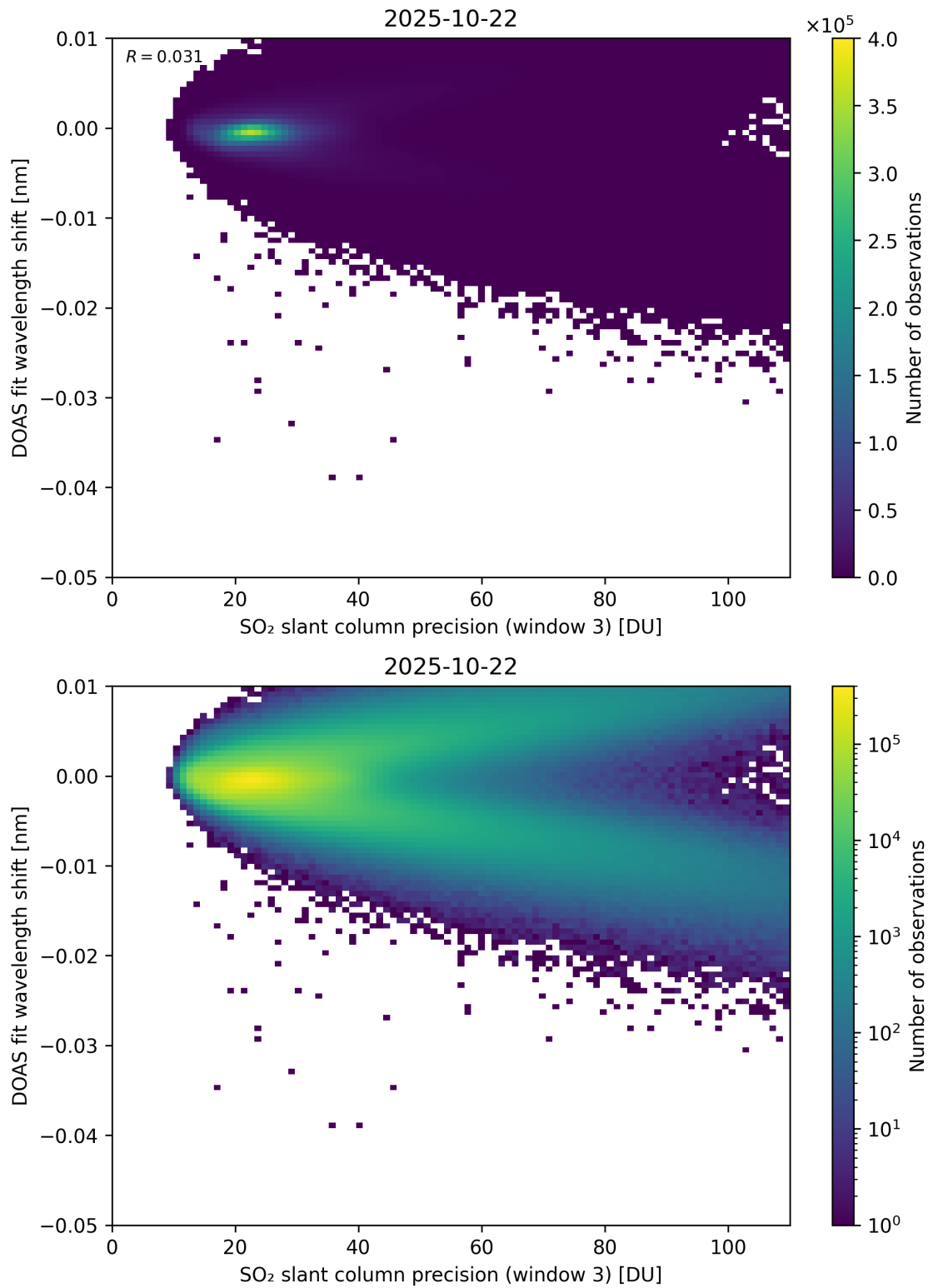
Figure 308: Scatter density plot of “SO 2 slant column precision (window 3)” against “DOAS fit wavelength shift” for 2025-10-22 to 2025-10-23.
