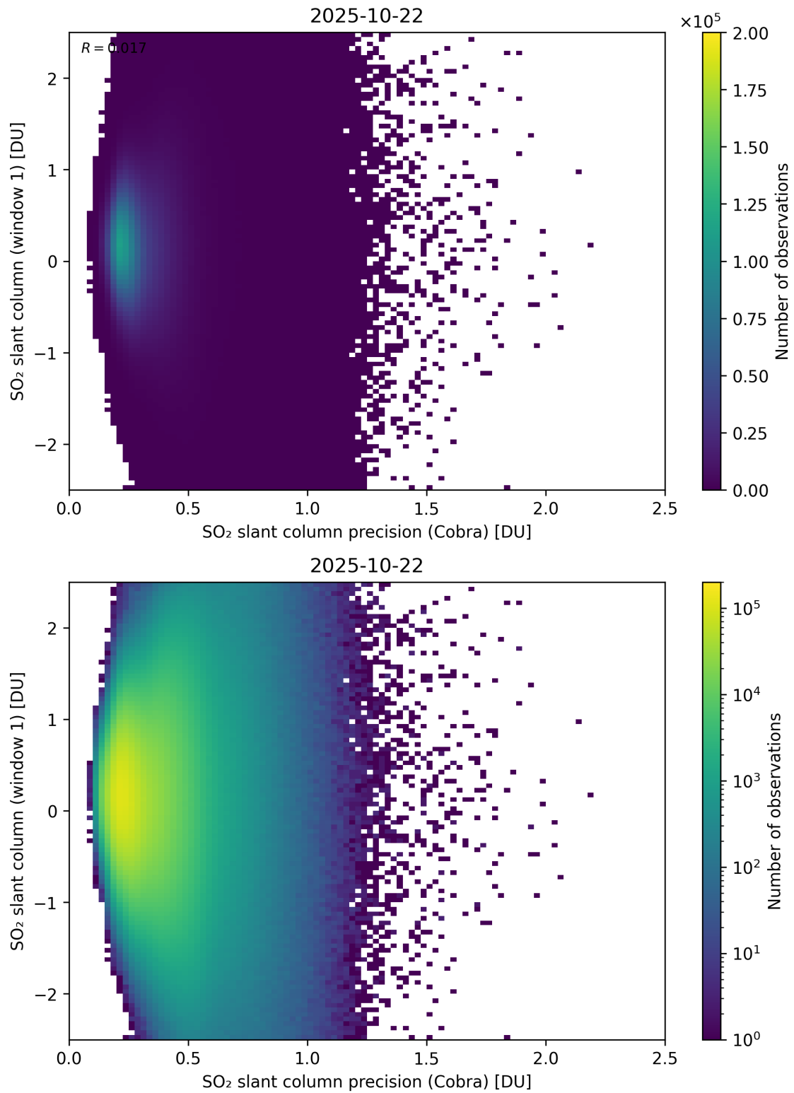
Figure 208: Scatter density plot of “SO 2 slant column precision (Cobra)” against “SO 2 slant column (window 1)” for 2025-10-22 to 2025-10-23.
