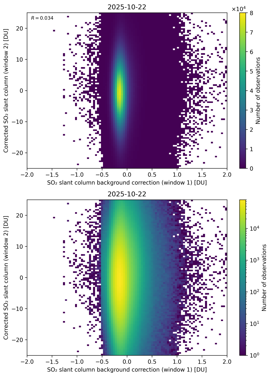
Figure 115: Scatter density plot of “SO 2 slant column background correction (window 1)” against “Corrected SO 2 slant column (window 2)” for 2025-10-22 to 2025-10-23.
