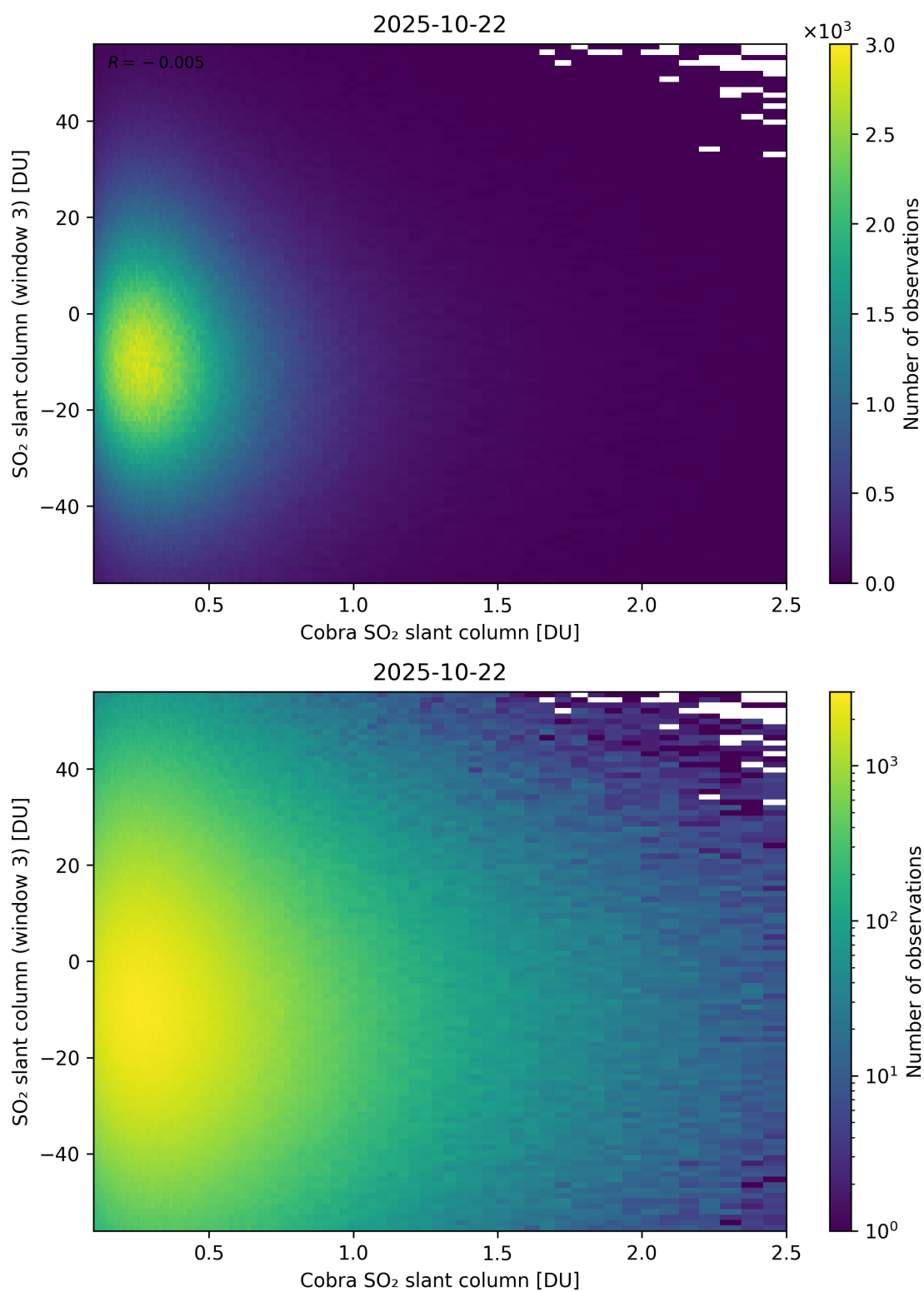
Figure 222: Scatter density plot of “Cobra SO 2 slant column” against “SO 2 slant column (window 3)” for 2025-10-22 to 2025-10-23.
