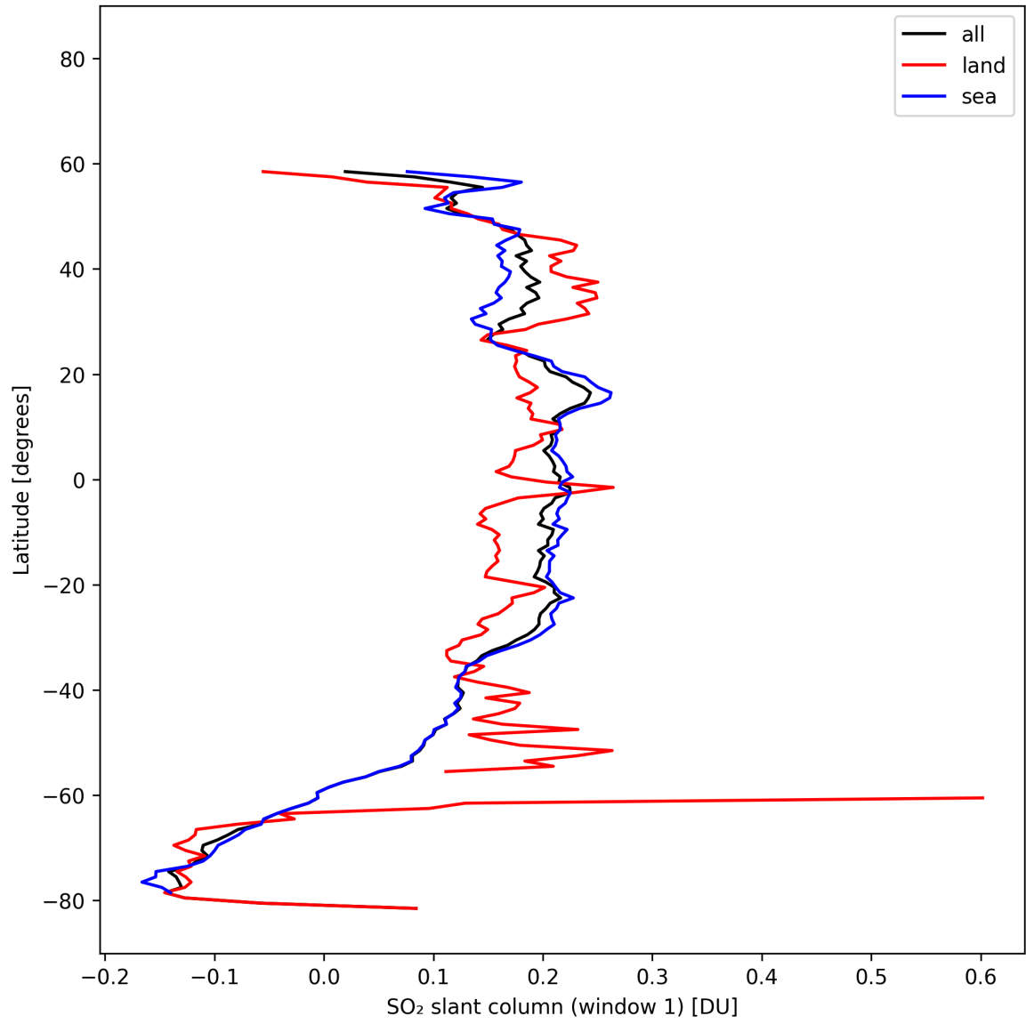
Figure 37: Zonal average of “SO 2 slant column (window 1)” for 2025-10-22 to 2025-10-23.
