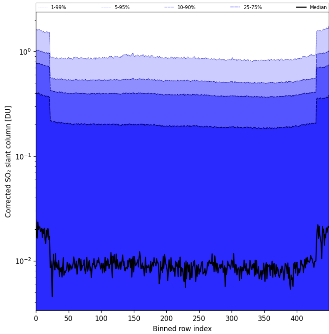
Figure 86: Along track statistics of "Corrected SO 2 slant column" for 2025-10-22 to 2025-10-23
