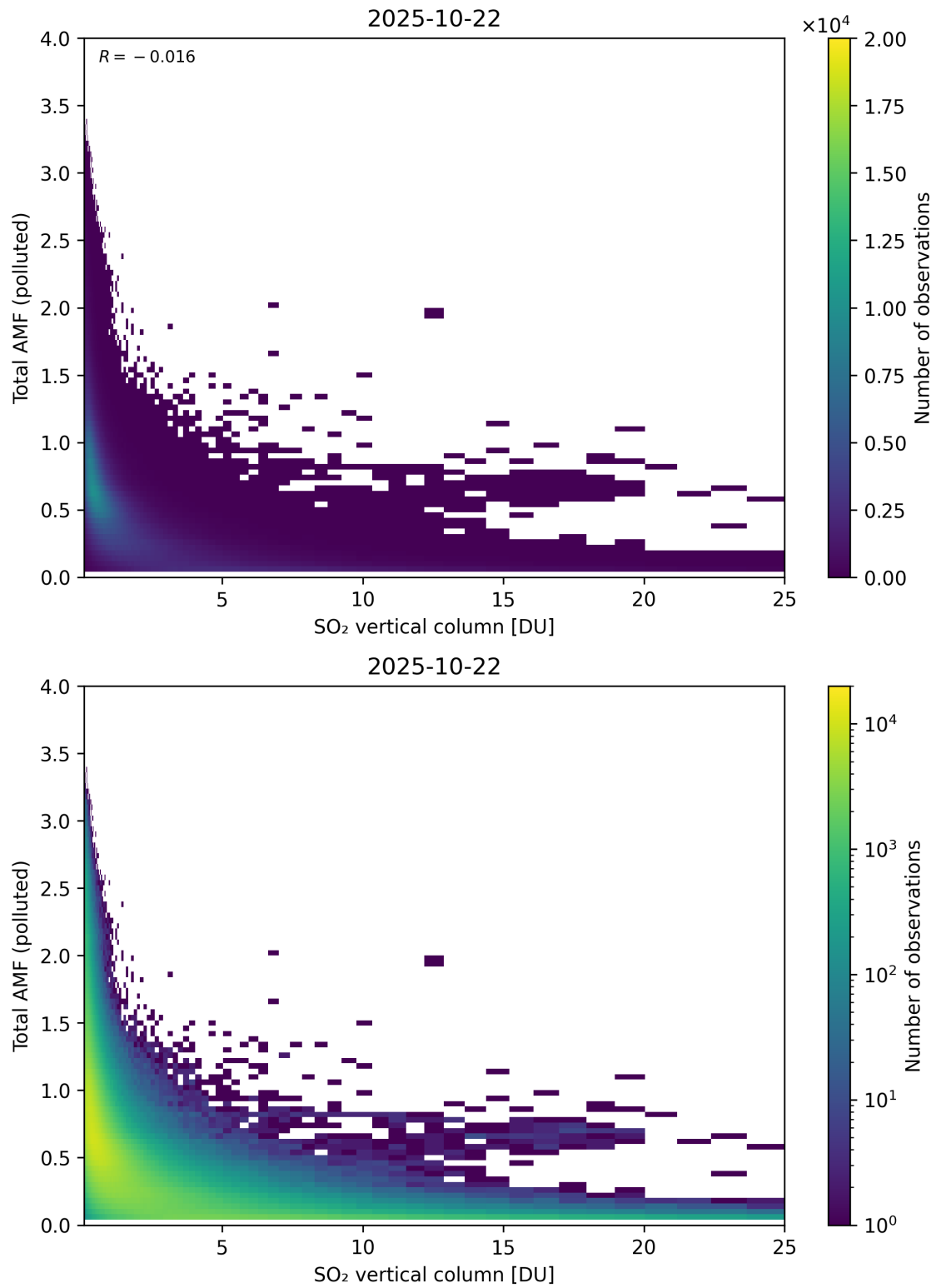
Figure 359: Scatter density plot of “SO 2 vertical column” against “Total AMF (polluted)” for 2025-10-22 to 2025-10-23.
