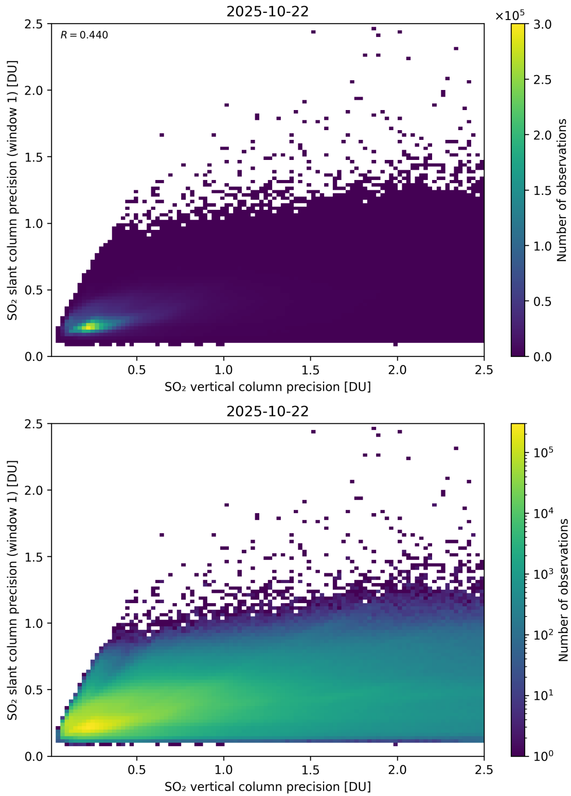
Figure 342: Scatter density plot of “SO 2 vertical column precision” against “SO 2 slant column precision (window 1)” for 2025-10-22 to 2025-10-23.
