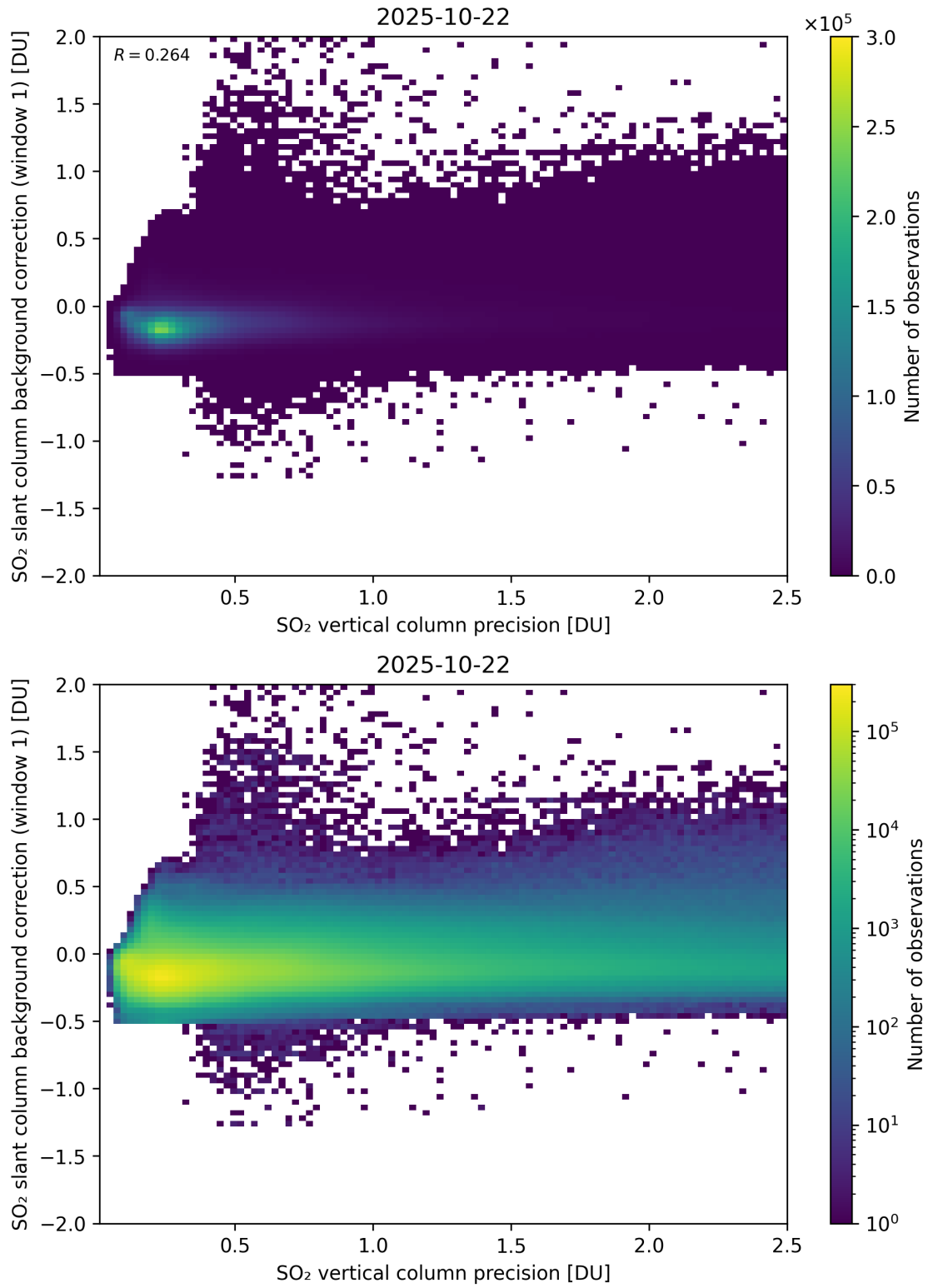
Figure 329: Scatter density plot of “SO 2 vertical column precision” against “SO 2 slant column background correction (window 1)” for 2025-10-22 to 2025-10-23.
