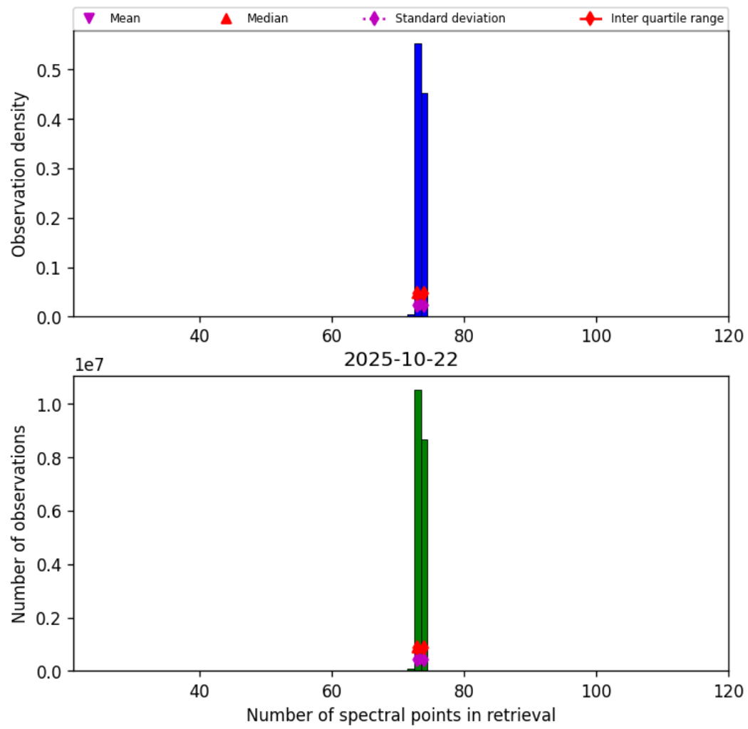
Figure 82: Histogram of “Number of spectral points in retrieval” for 2025-10-22 to 2025-10-23
