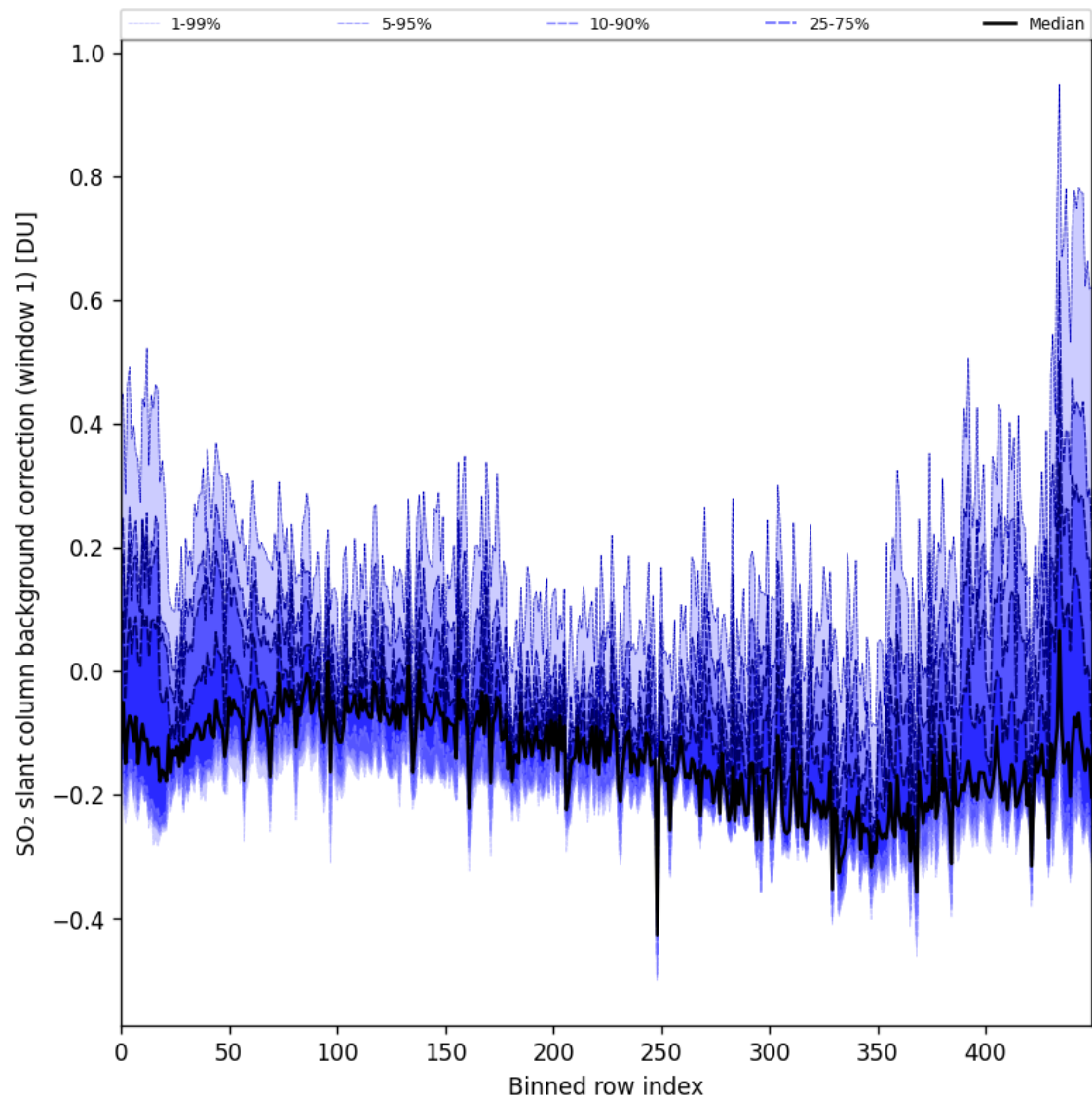
Figure 92: Along track statistics of “SO 2 slant column background correction (window 1)” for 2025-10-22 to 2025-10-23
