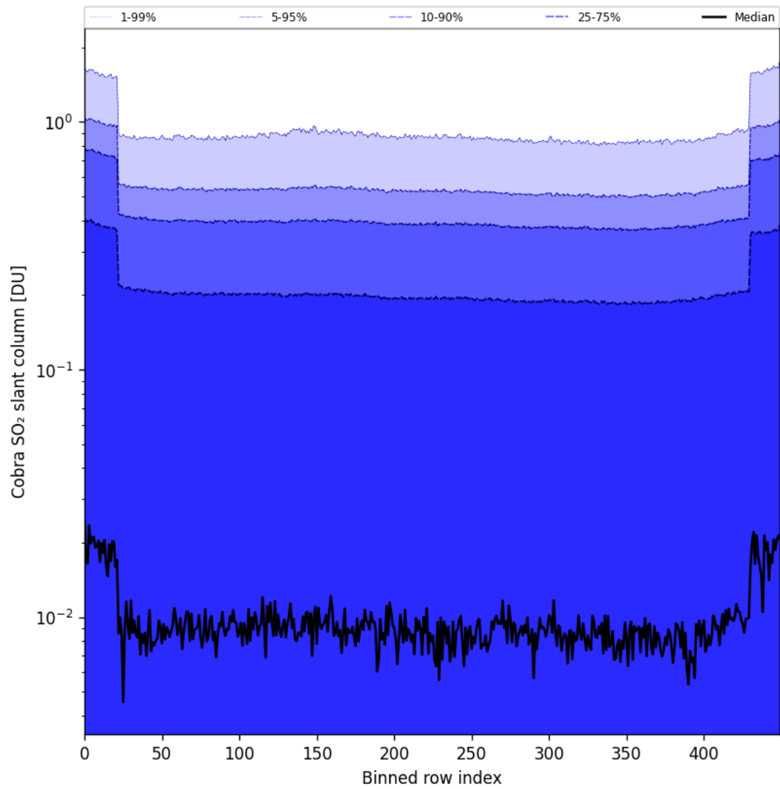
Figure 87: Along track statistics of “Cobra SO 2 slant column” for 2025-10-22 to 2025-10-23
