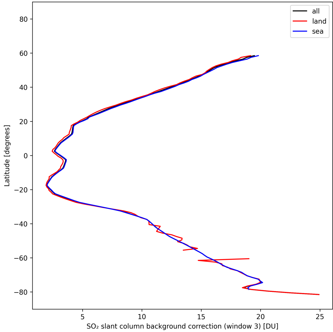
Figure 48: Zonal average of “SO 2 slant column background correction (window 3)” for 2025-10-22 to 2025-10-23.
