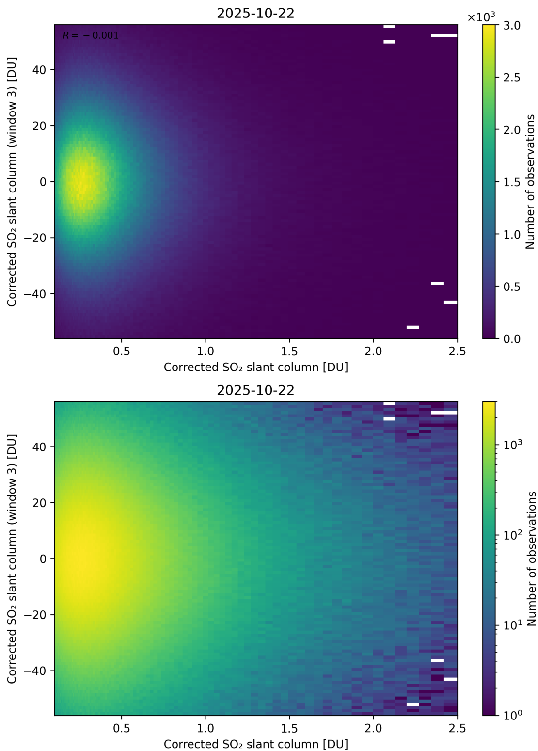
Figure 236: Scatter density plot of “Corrected SO 2 slant column” against “Corrected SO 2 slant column (window 3)” for 2025-10-22 to 2025-10-23.
