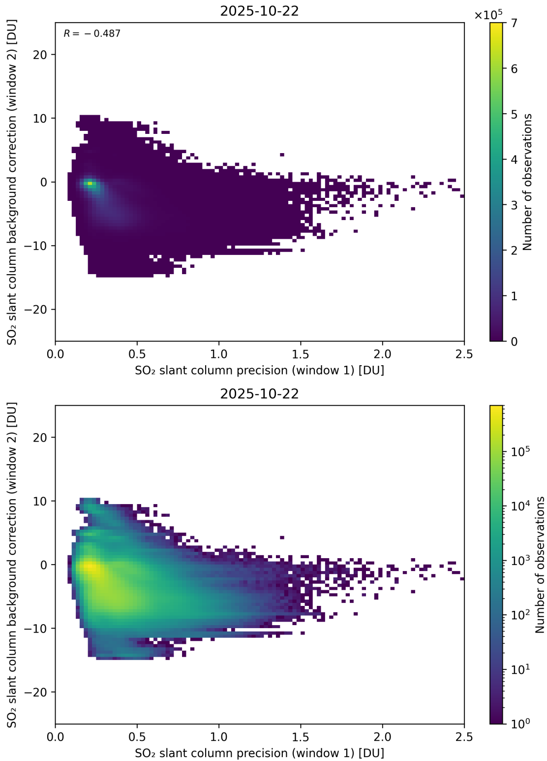
Figure 269: Scatter density plot of “SO 2 slant column precision (window 1)” against “SO 2 slant column background correction (window 2)” for 2025-10-22 to 2025-10-23.
