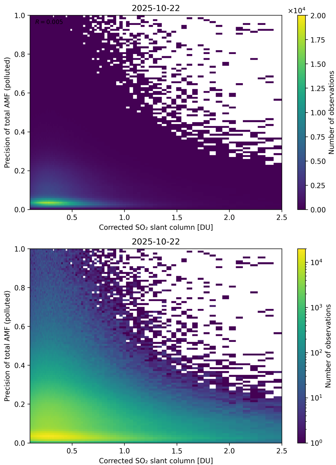
Figure 243: Scatter density plot of “Corrected SO 2 slant column” against “Precision of total AMF (polluted)” for 2025-10-22 to 2025-10-23.
