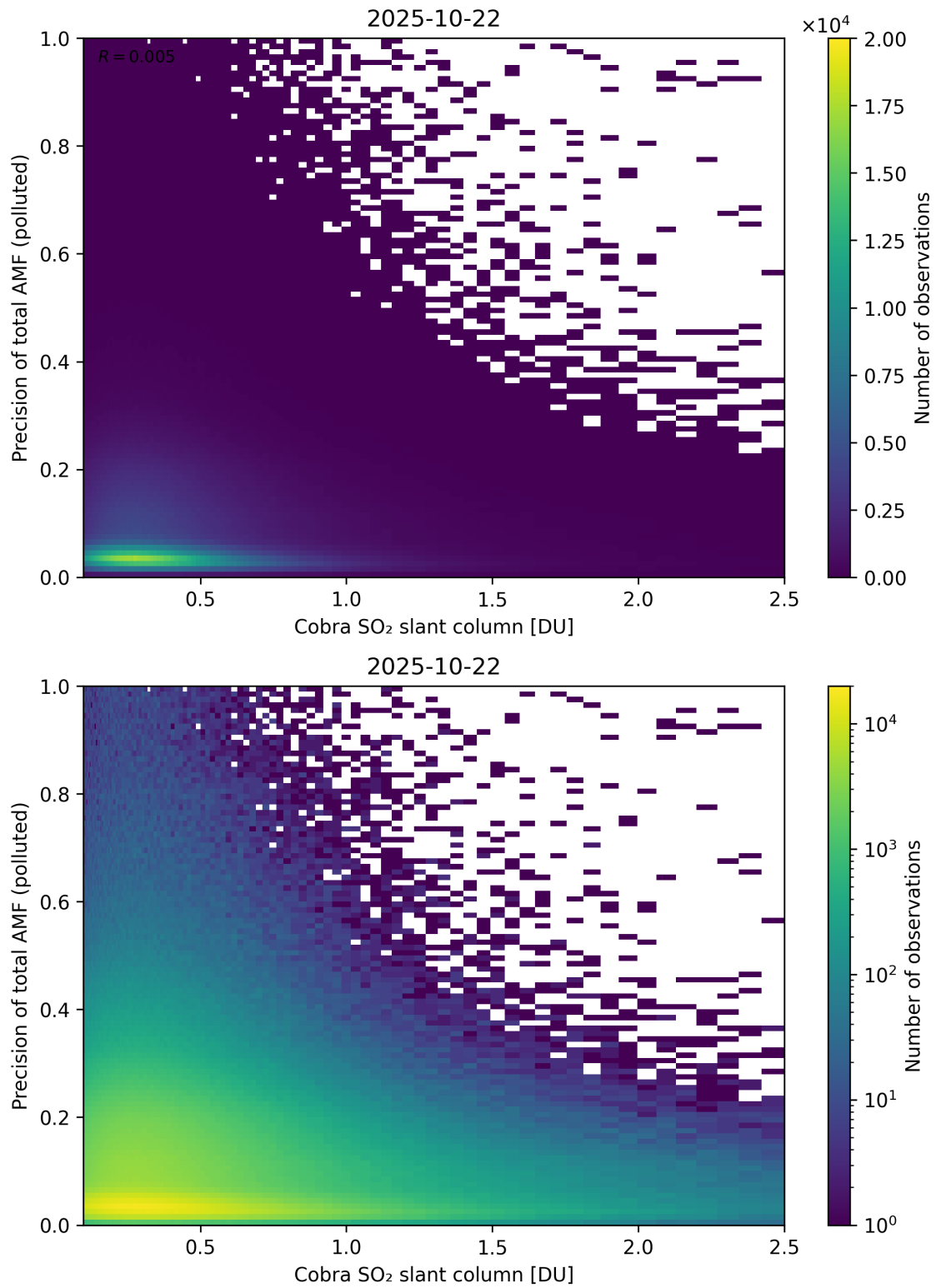
Figure 225: Scatter density plot of “Cobra SO 2 slant column” against “Precision of total AMF (polluted)” for 2025-10-22 to 2025-10-23.
