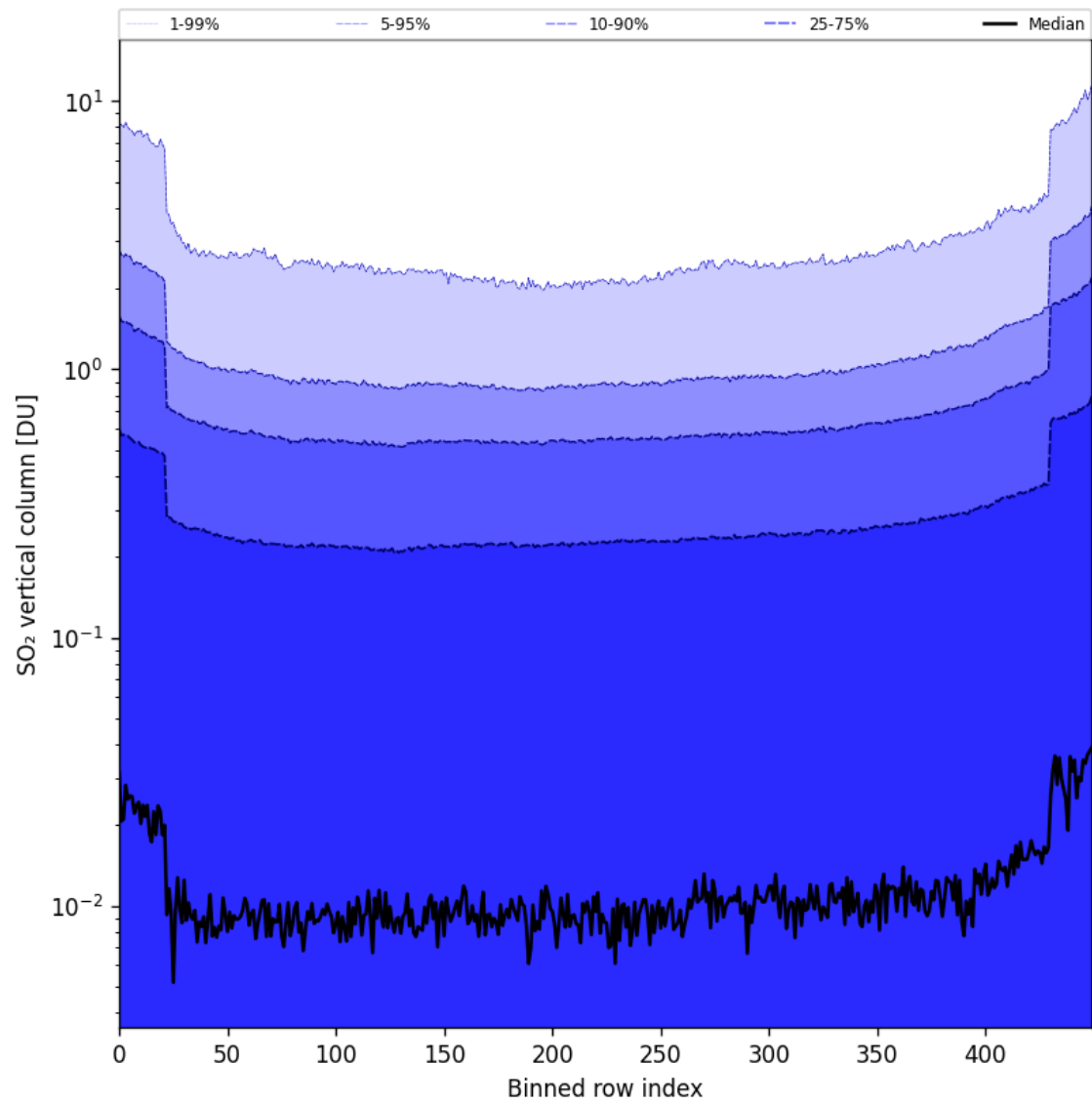
Figure 84: Along track statistics of “SO 2 vertical column” for 2025-10-22 to 2025-10-23
