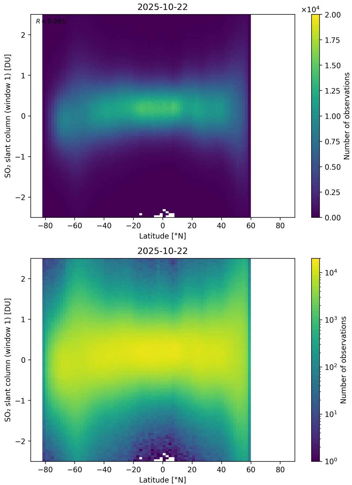
Figure 162: Scatter density plot of “Latitude” against “SO 2 slant column (window 1)” for 2025-10-22 to 2025-10-23.
