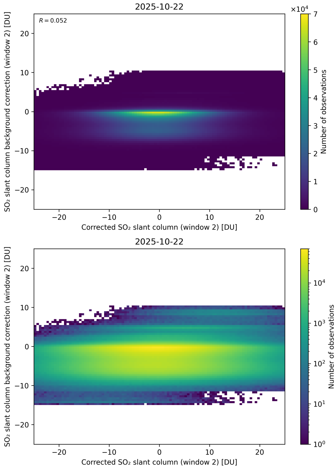
Figure 244: Scatter density plot of “Corrected SO 2 slant column (window 2)” against “SO 2 slant column background correction (window 2)” for 2025-10-22 to 2025-10-23.
