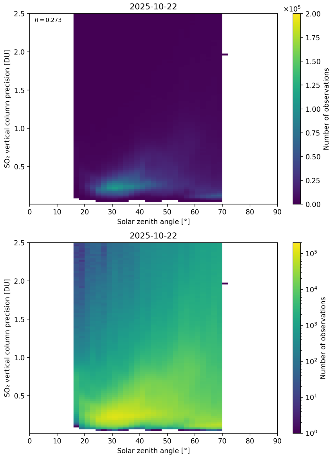
Figure 192: Scatter density plot of “Solar zenith angle” against “SO 2 vertical column precision” for 2025-10-22 to 2025-10-23.
