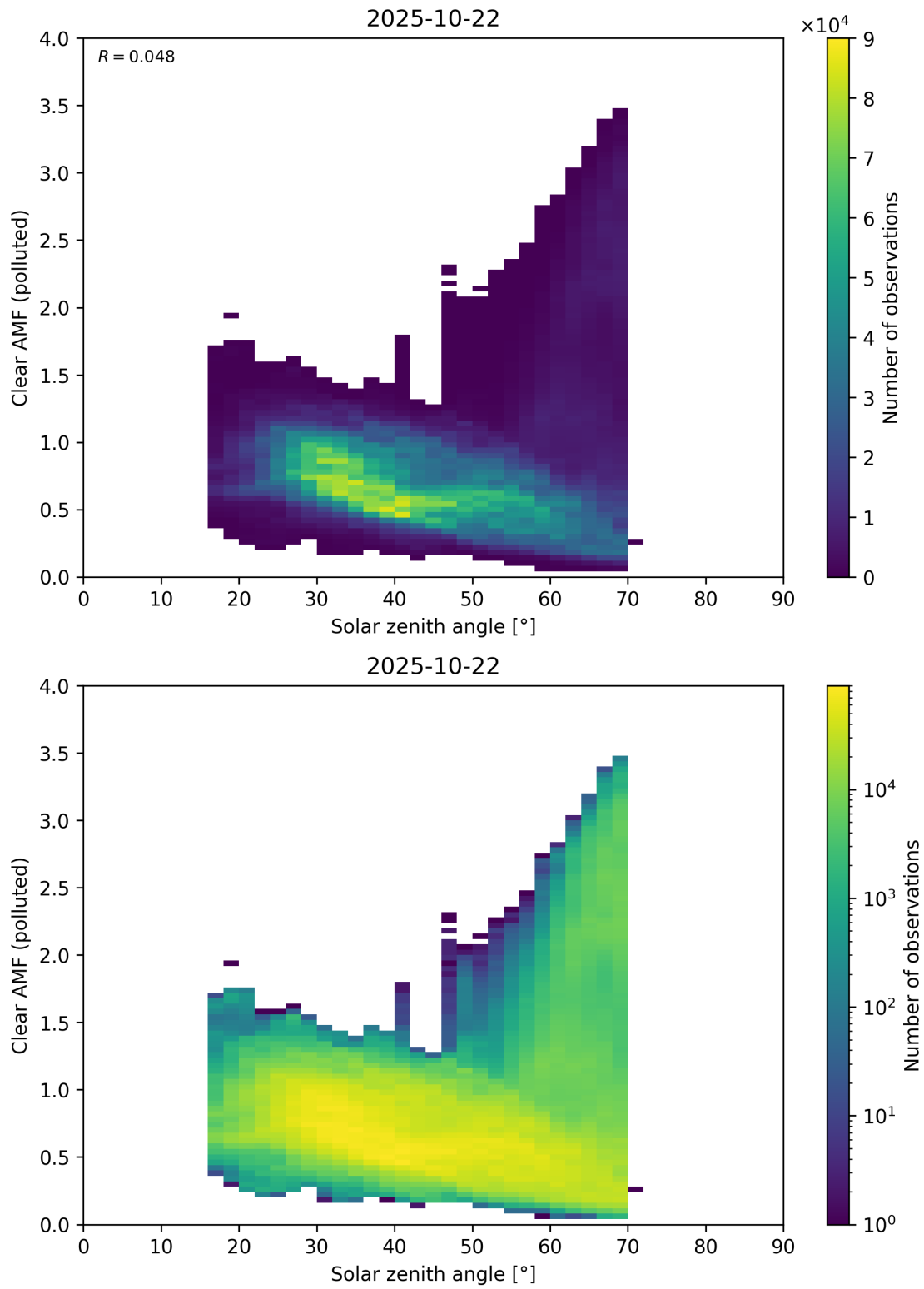
Figure 178: Scatter density plot of “Solar zenith angle” against “Clear AMF (polluted)” for 2025-10-22 to 2025-10-23.
