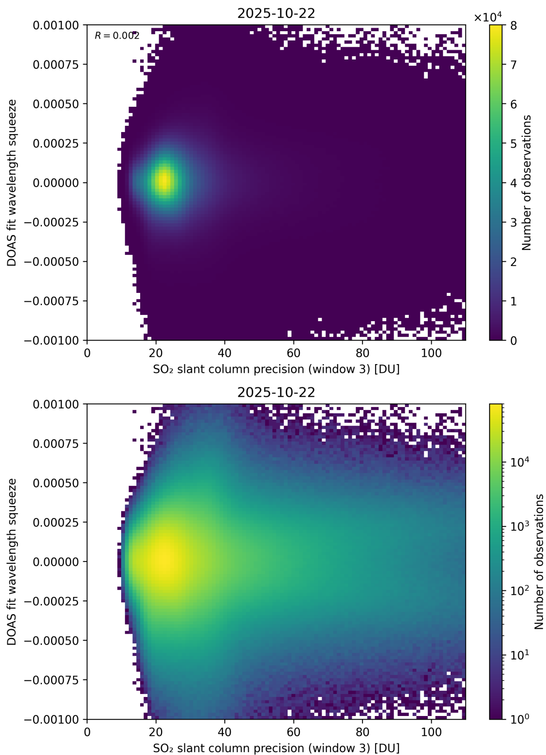
Figure 309: Scatter density plot of “SO 2 slant column precision (window 3)” against “DOAS fit wavelength squeeze” for 2025-10-22 to 2025-10-23.
