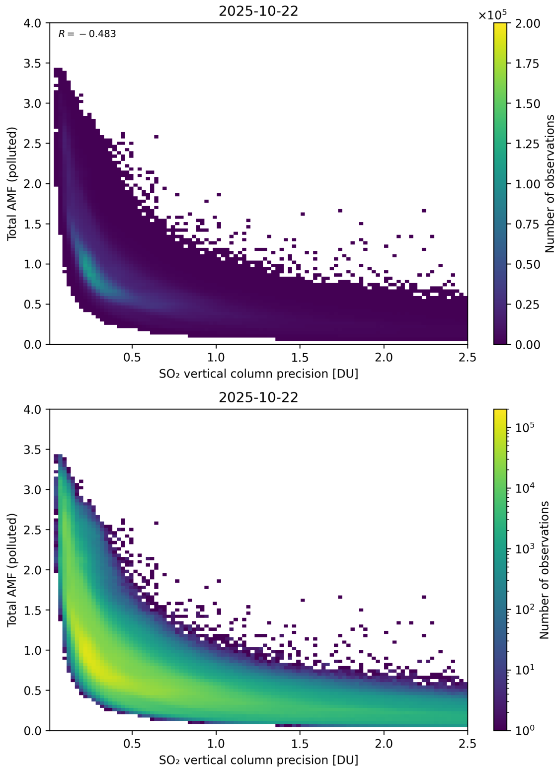
Figure 346: Scatter density plot of “SO 2 vertical column precision” against “Total AMF (polluted)” for 2025-10-22 to 2025-10-23.
