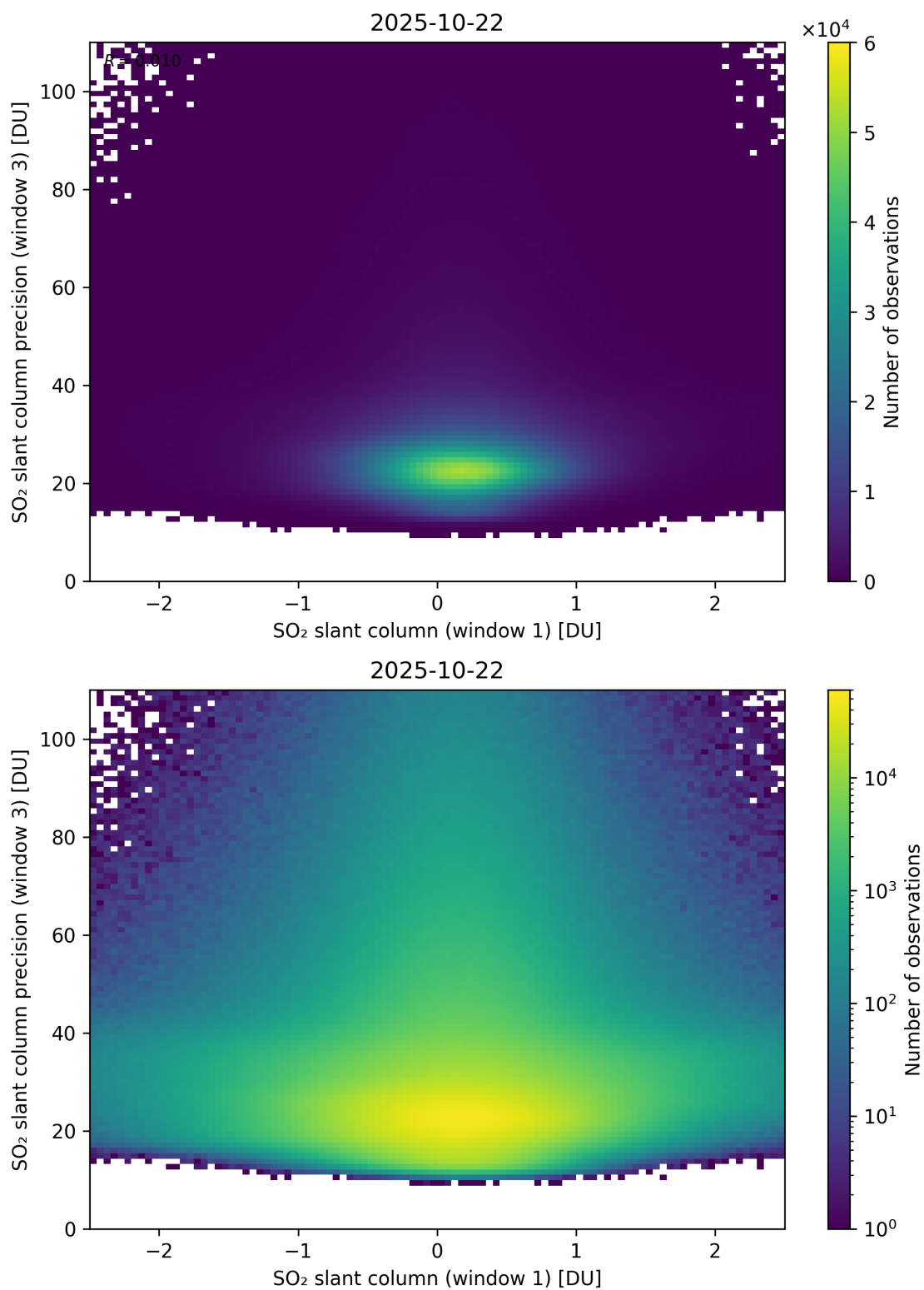
Figure 288: Scatter density plot of “SO 2 slant column (window 1)” against “SO 2 slant column precision (window 3)” for 2025-10-22 to 2025-10-23.
