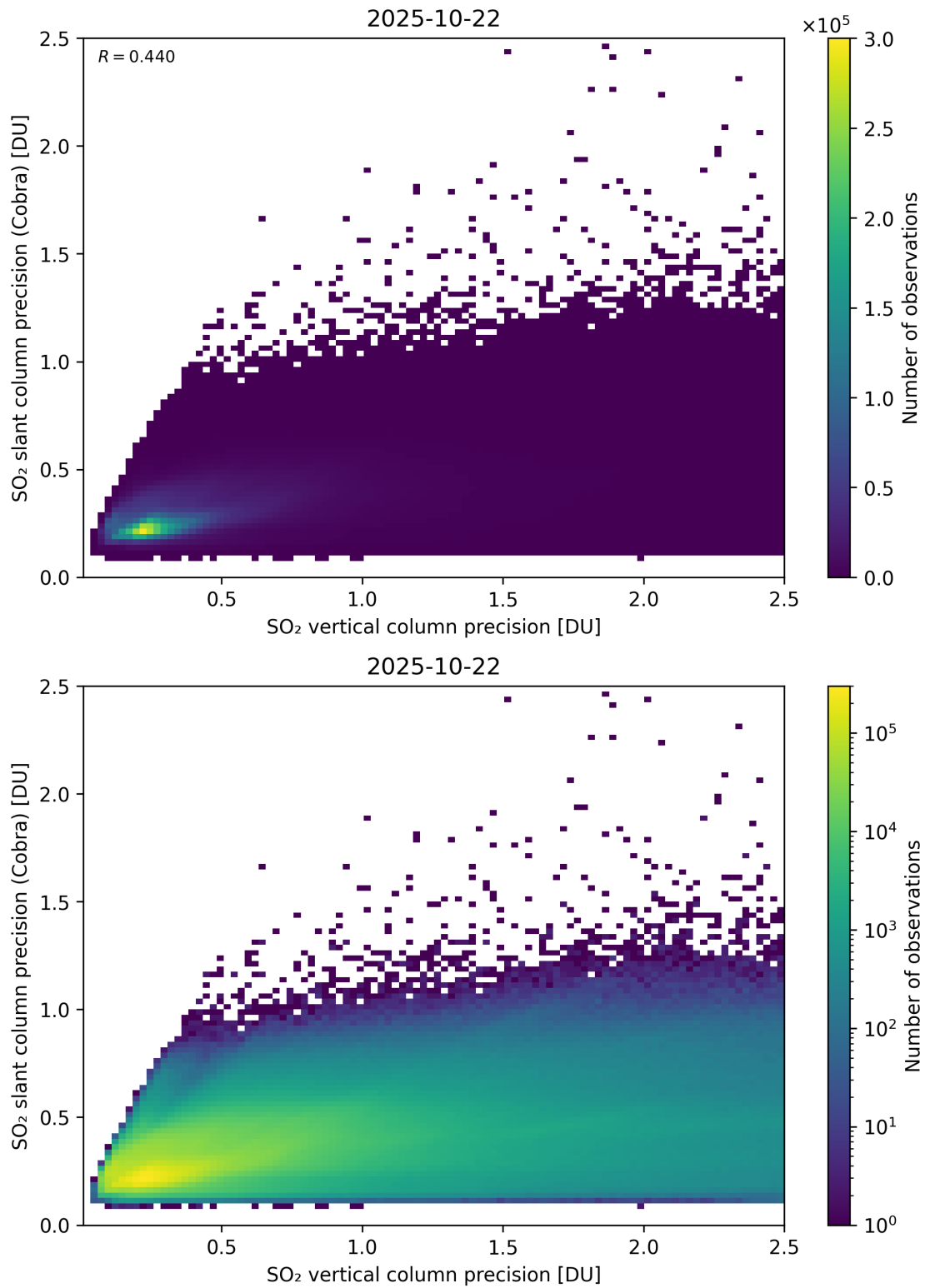
Figure 337: Scatter density plot of “SO 2 vertical column precision” against “SO 2 slant column precision (Cobra)” for 2025-10-22 to 2025-10-23.
