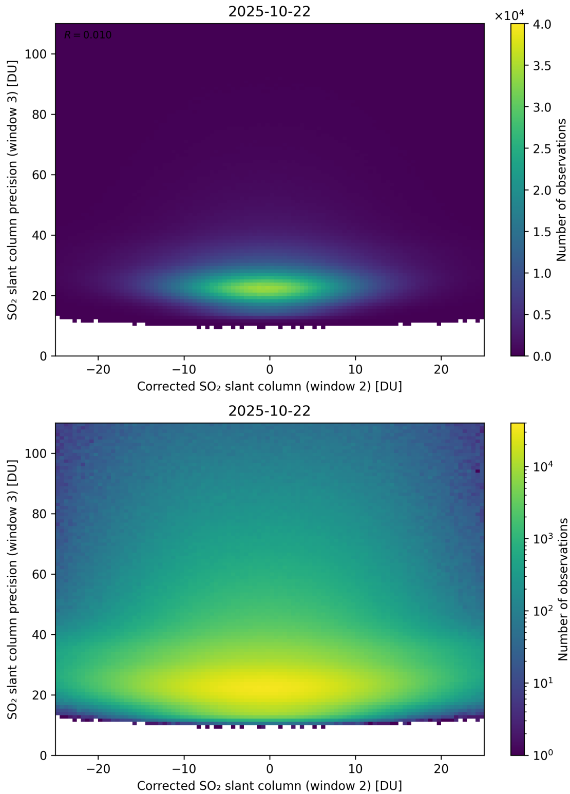
Figure 252: Scatter density plot of “Corrected SO 2 slant column (window 2)” against “SO 2 slant column precision (window 3)” for 2025-10-22 to 2025-10-23.
