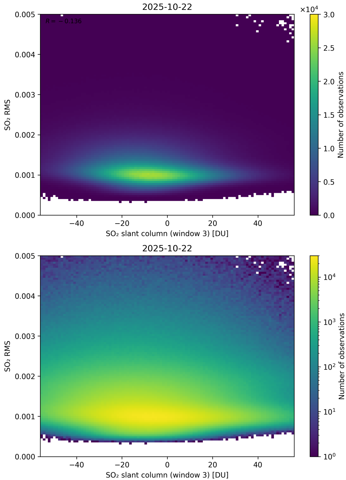
Figure 306: Scatter density plot of “SO 2 slant column (window 3)” against “SO 2 RMS” for 2025-10-22 to 2025-10-23.
