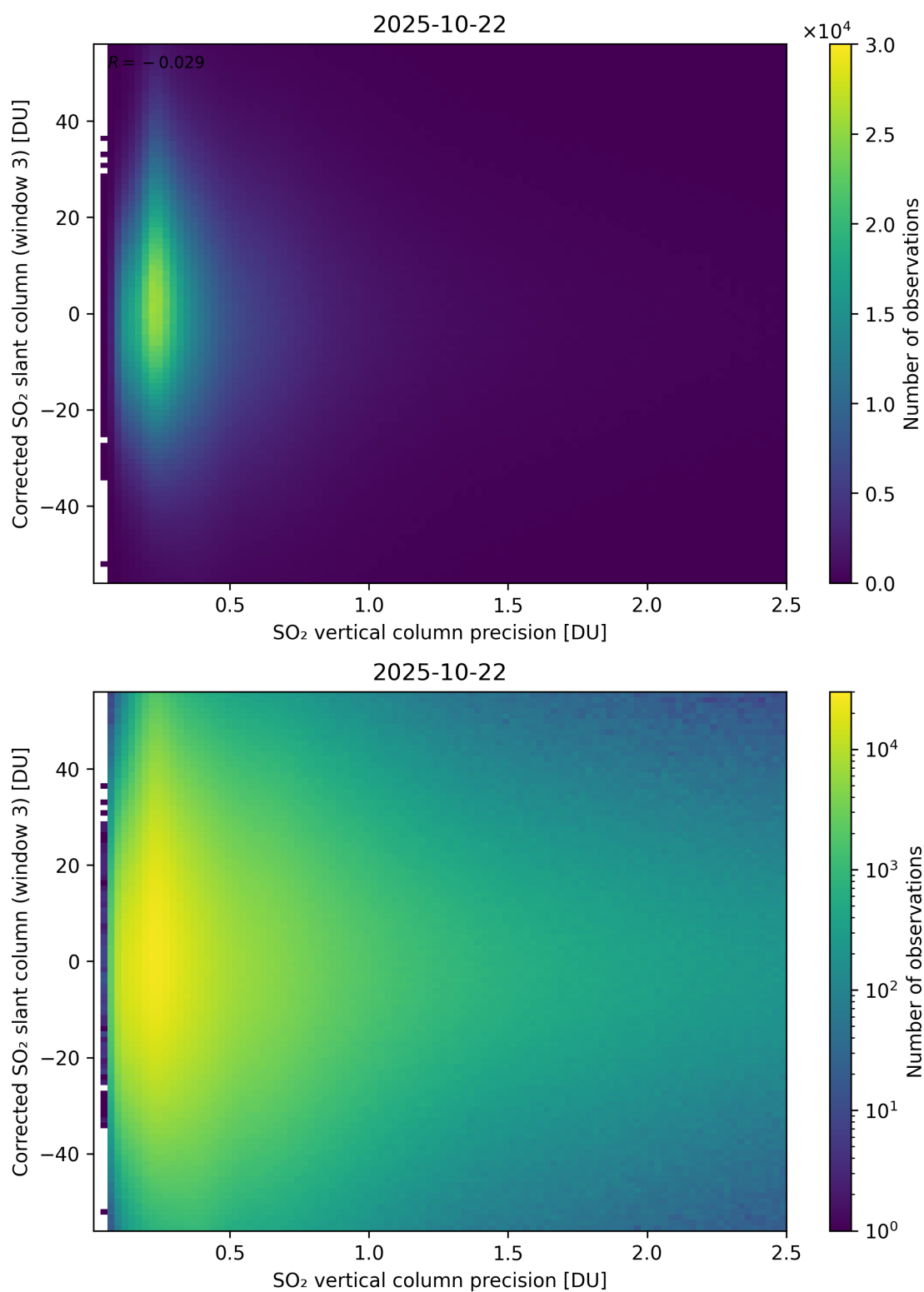
Figure 340: Scatter density plot of “SO 2 vertical column precision” against “Corrected SO 2 slant column (window 3)” for 2025-10-22 to 2025-10-23.
