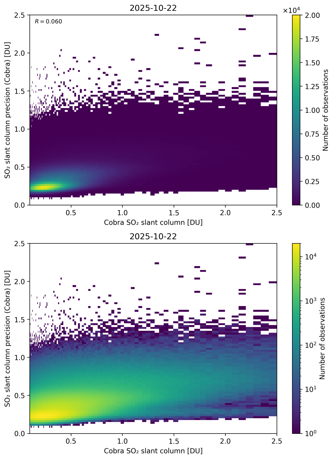
Figure 216: Scatter density plot of “Cobra SO 2 slant column” against “SO 2 slant column precision (Cobra)” for 2025-10-22 to 2025-10-23.
