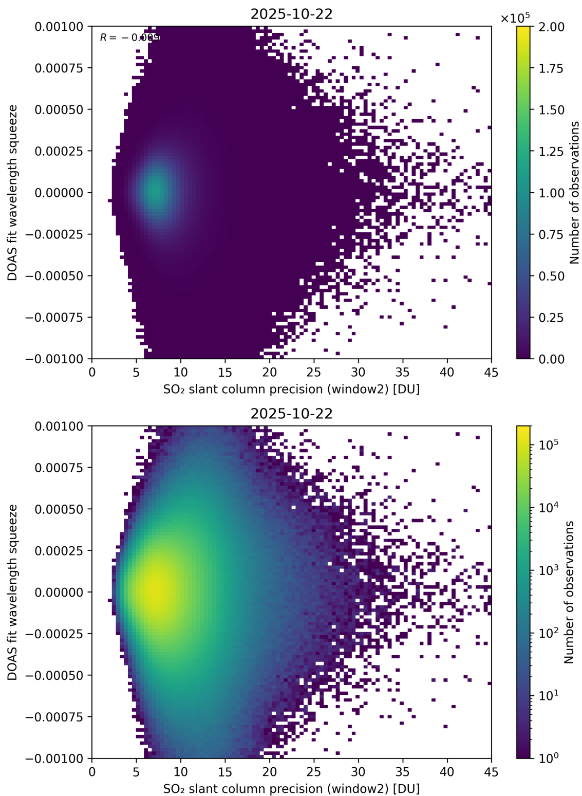
Figure 294: Scatter density plot of “SO 2 slant column precision (window2)” against “DOAS fit wavelength squeeze” for 2025-10-22 to 2025-10-23.
