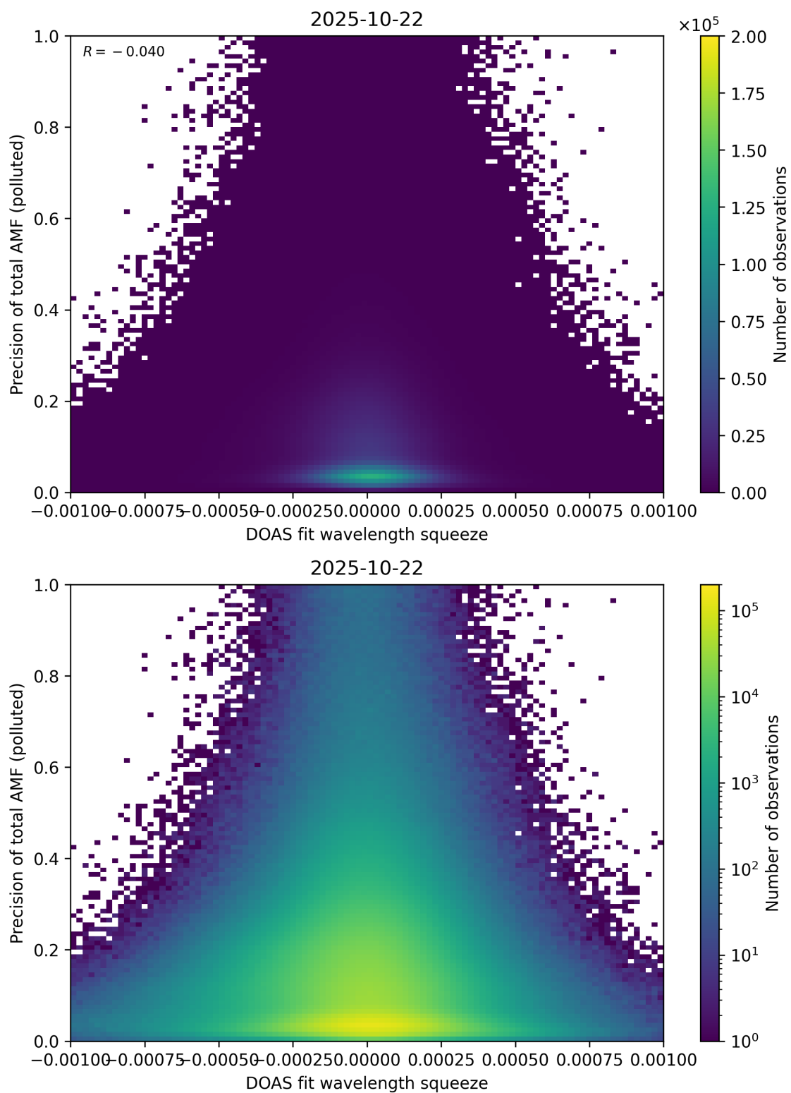
Figure 146: Scatter density plot of “DOAS fit wavelength squeeze” against “Precision of total AMF (polluted)” for 2025-10-22 to 2025-10-23.
