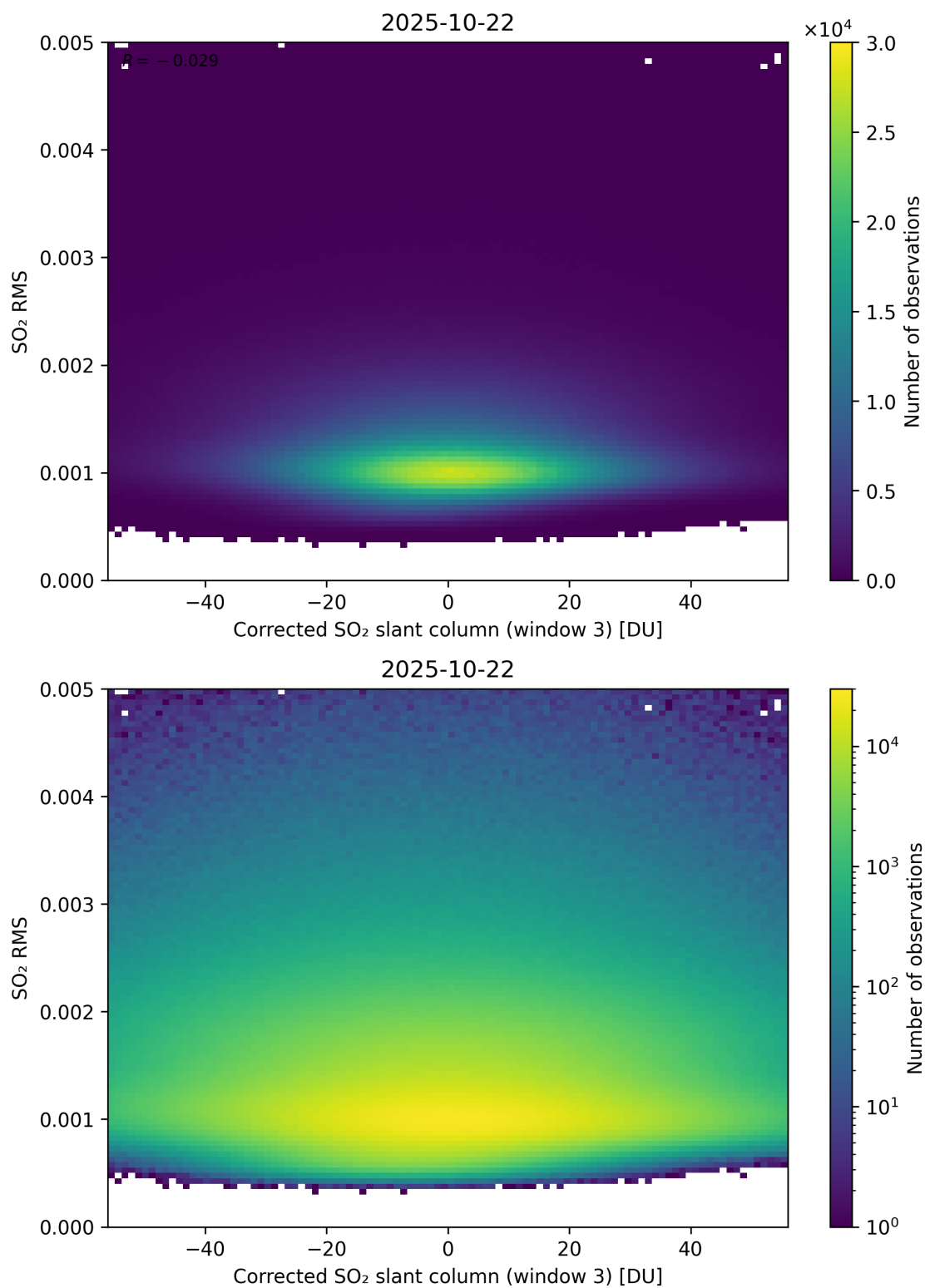
Figure 258: Scatter density plot of “Corrected SO 2 slant column (window 3)” against “SO 2 RMS” for 2025-10-22 to 2025-10-23.
