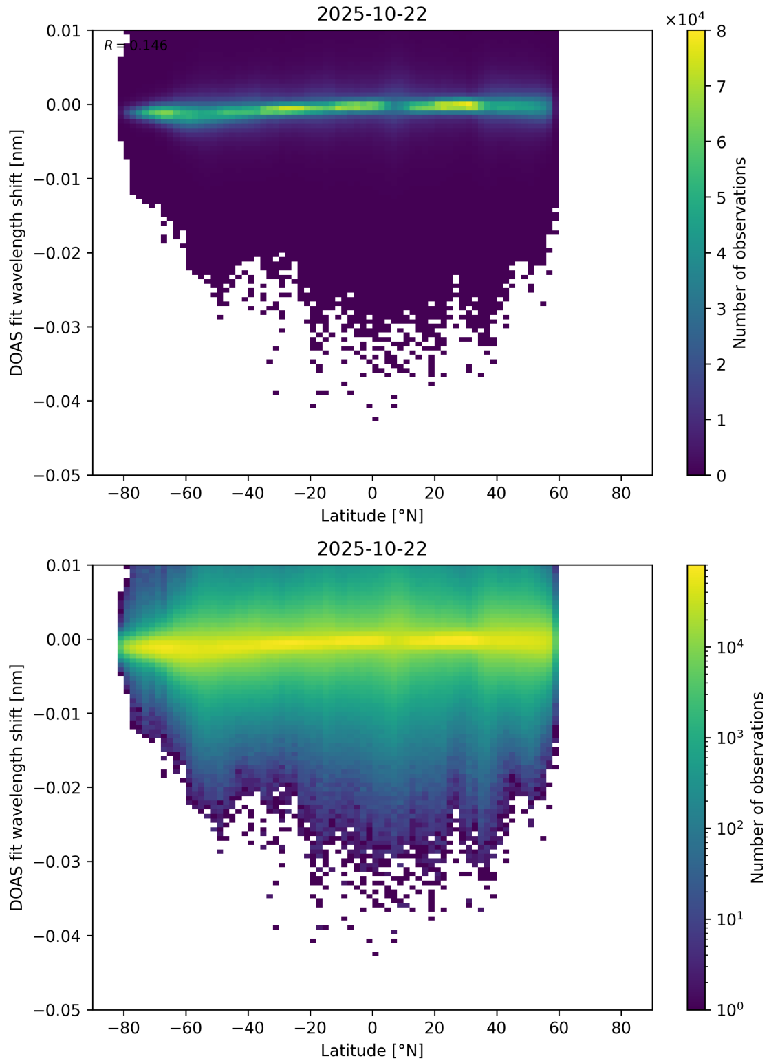
Figure 153: Scatter density plot of “Latitude” against “DOAS fit wavelength shift” for 2025-10-22 to 2025-10-23.
