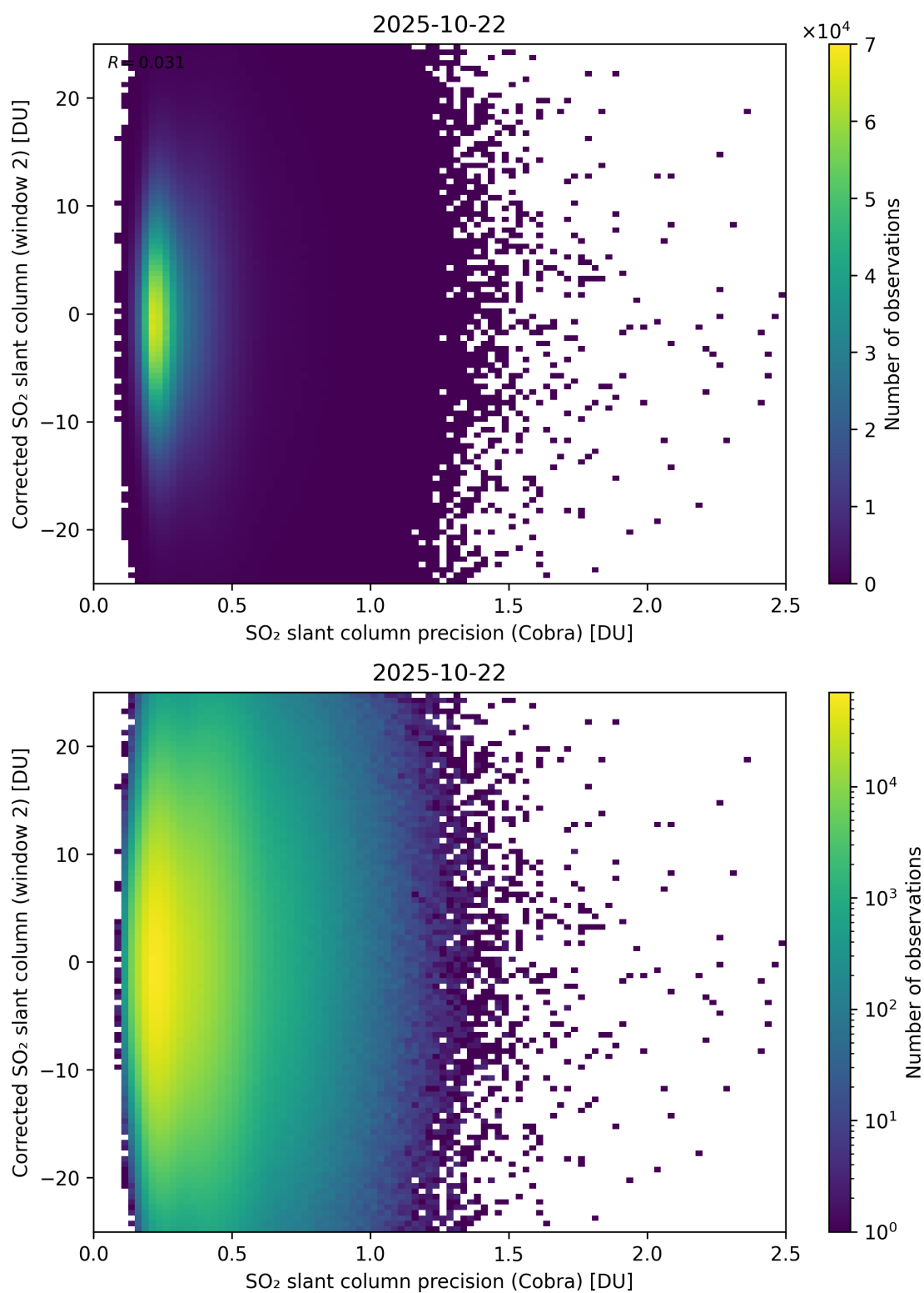
Figure 206: Scatter density plot of “SO 2 slant column precision (Cobra)” against “Corrected SO 2 slant column (window 2)” for 2025-10-22 to 2025-10-23.
