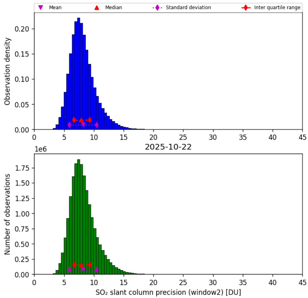
Figure 68: Histogram of “SO 2 slant column precision (window2)” for 2025-10-22 to 2025-10-23
