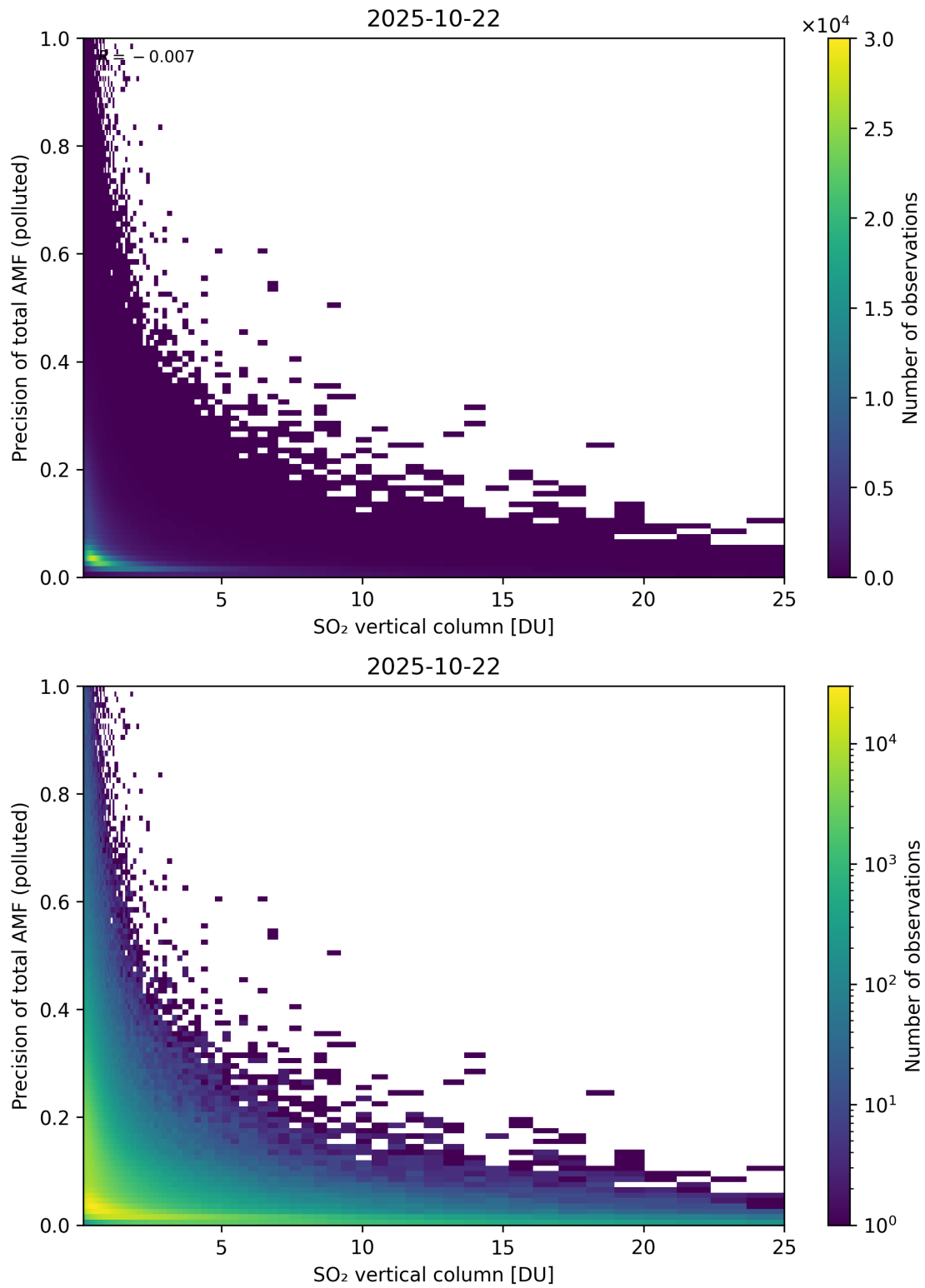
Figure 360: Scatter density plot of “SO 2 vertical column” against “Precision of total AMF (polluted)” for 2025-10-22 to 2025-10-23.
