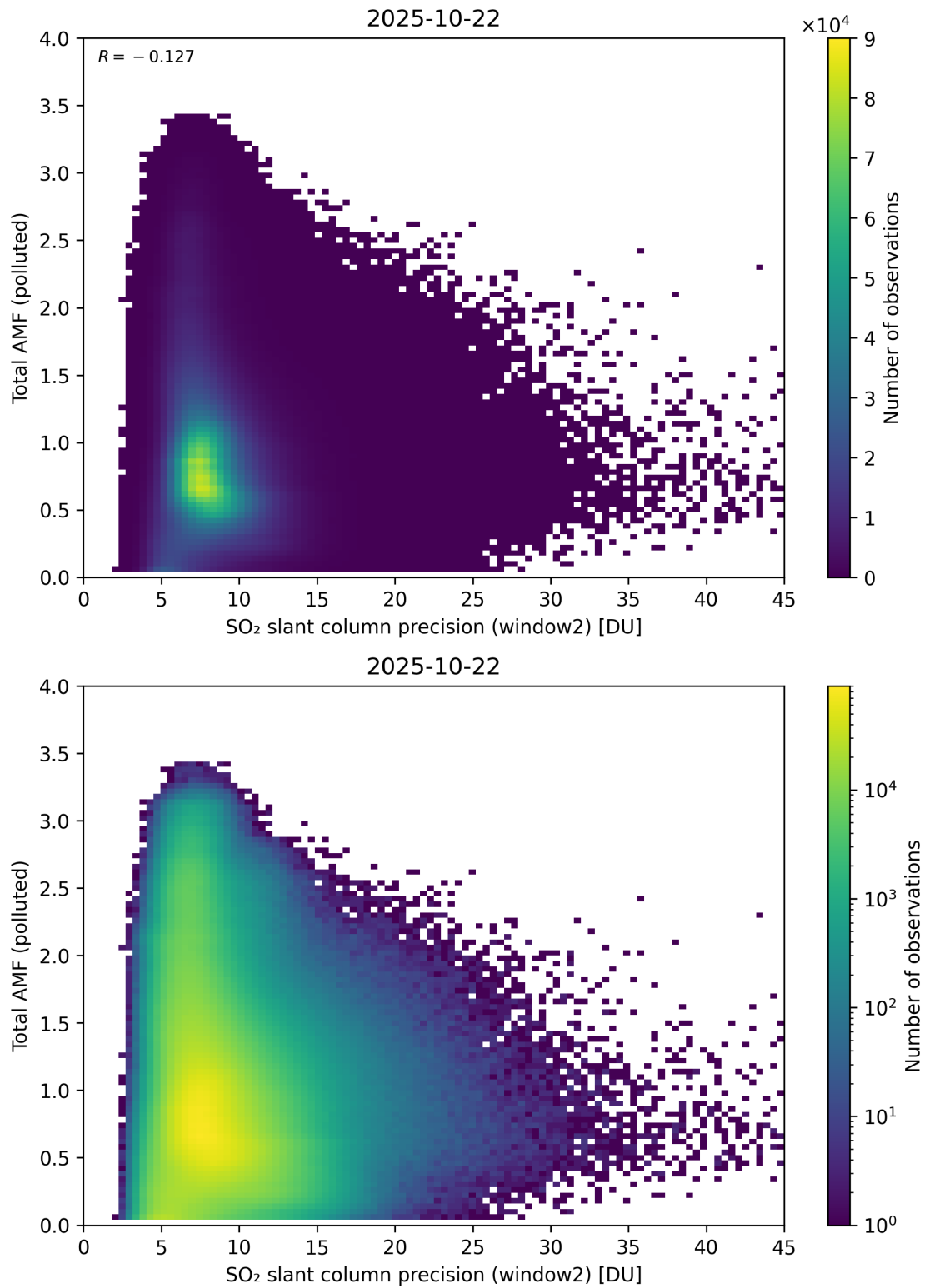
Figure 301: Scatter density plot of “SO 2 slant column precision (window2)” against “Total AMF (polluted)” for 2025-10-22 to 2025-10-23.
