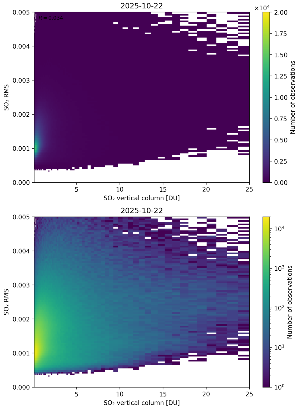
Figure 328: Scatter density plot of “SO 2 vertical column” against “SO 2 RMS” for 2025-10-22 to 2025-10-23.
