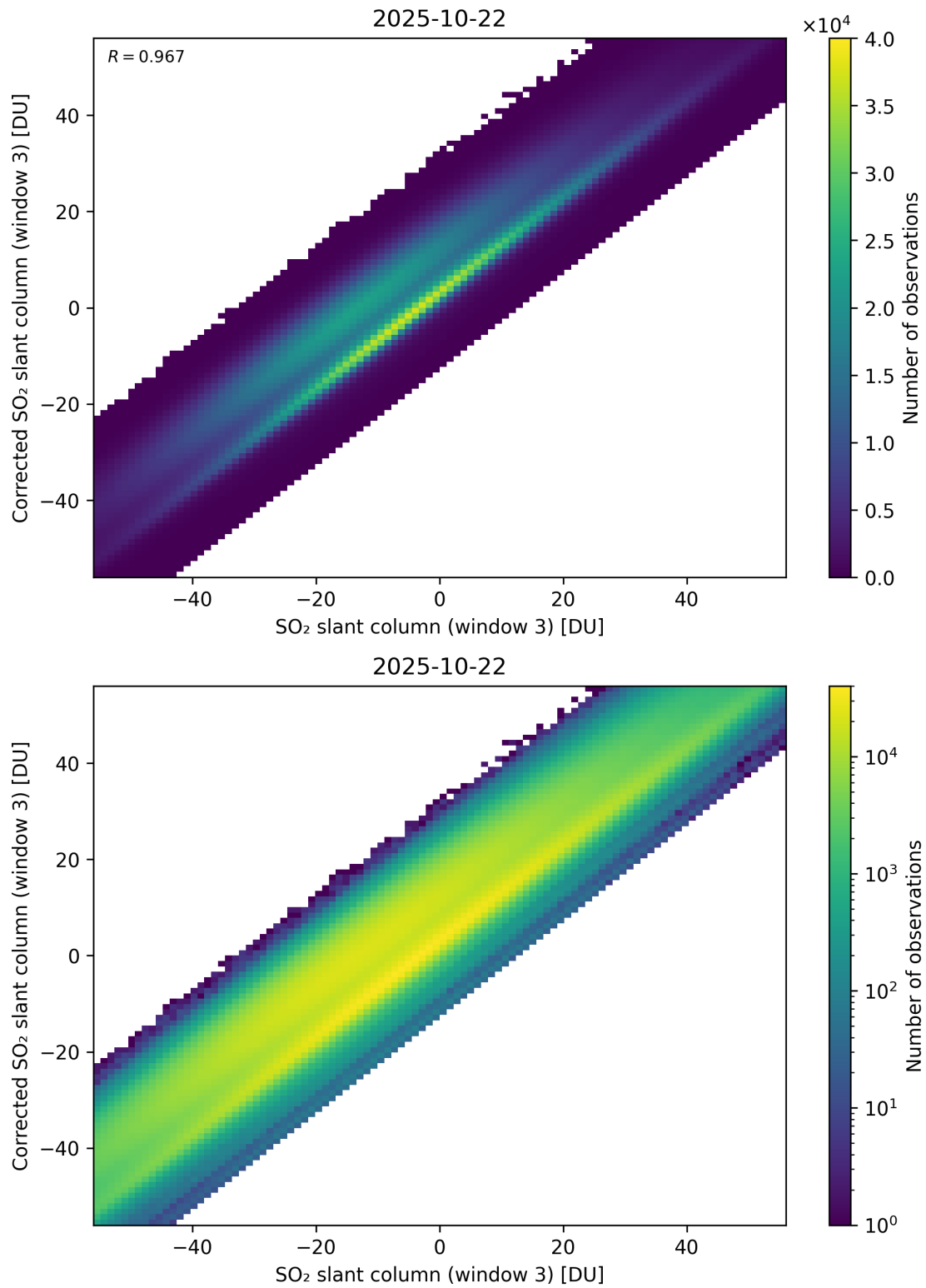
Figure 316: Scatter density plot of “SO 2 slant column (window 3)” against “Corrected SO 2 slant column (window 3)” for 2025-10-22 to 2025-10-23.
