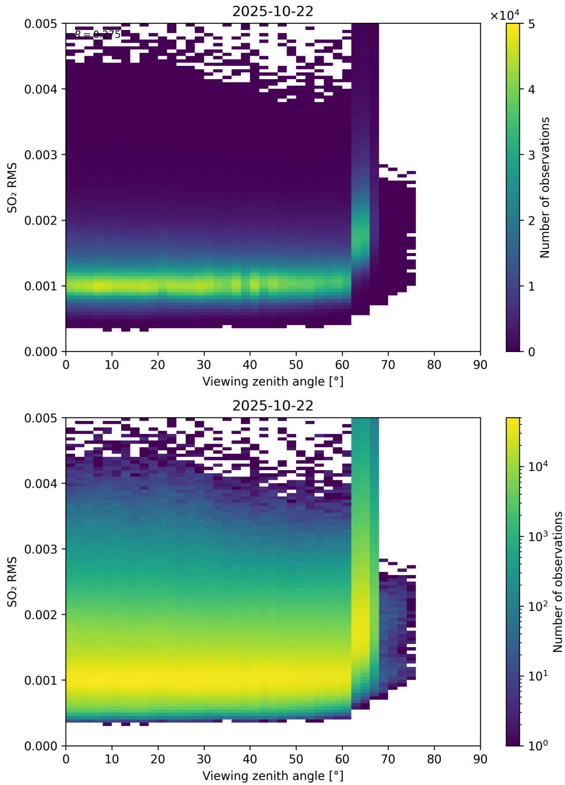
Figure 367: Scatter density plot of “Viewing zenith angle” against “SO 2 RMS” for 2025-10-22 to 2025-10-23.
