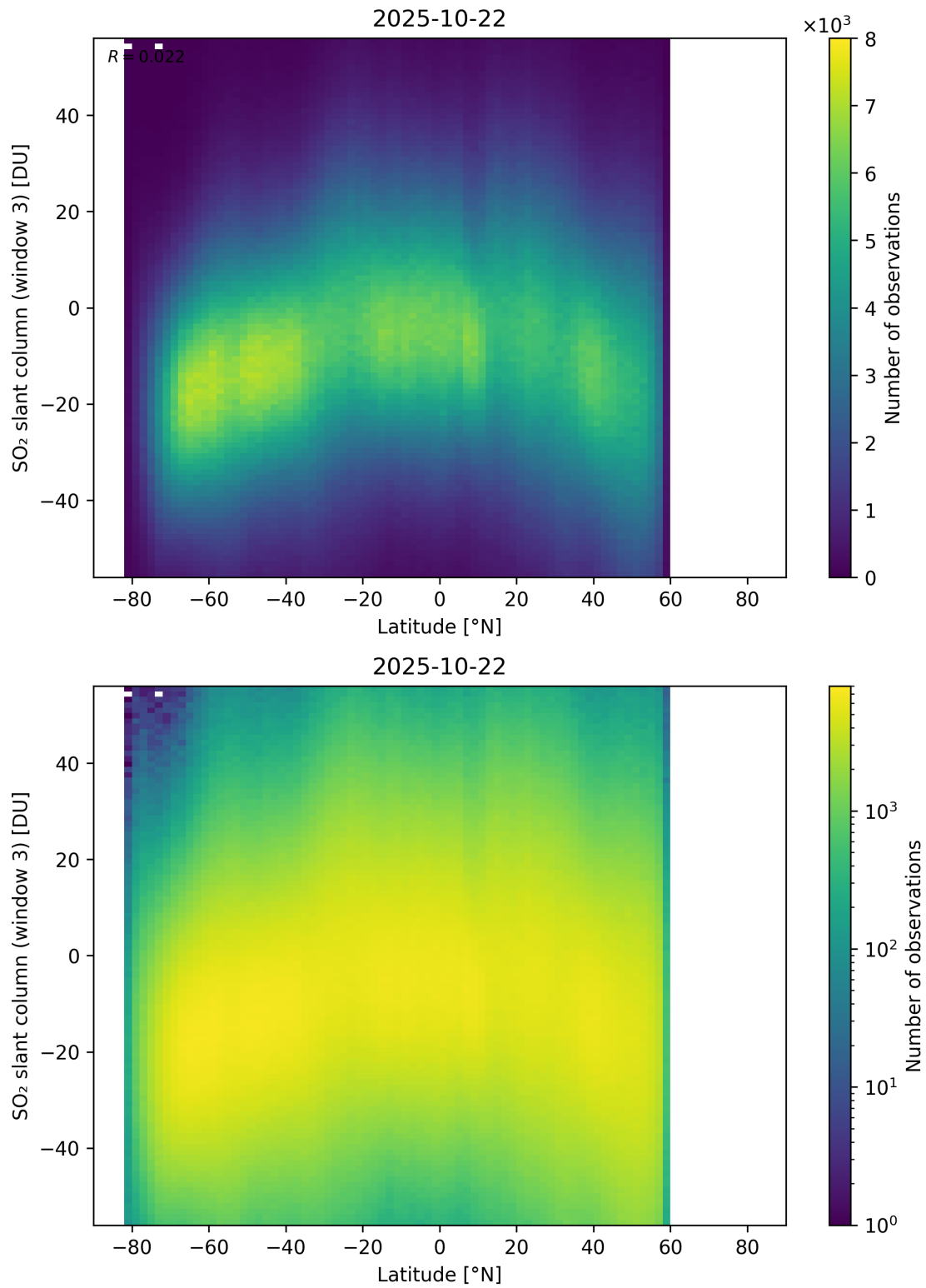
Figure 165: Scatter density plot of “Latitude” against “SO 2 slant column (window 3)” for 2025-10-22 to 2025-10-23.
