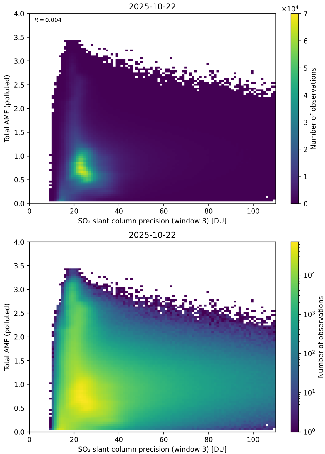
Figure 313: Scatter density plot of “SO 2 slant column precision (window 3)” against “Total AMF (polluted)” for 2025-10-22 to 2025-10-23.
