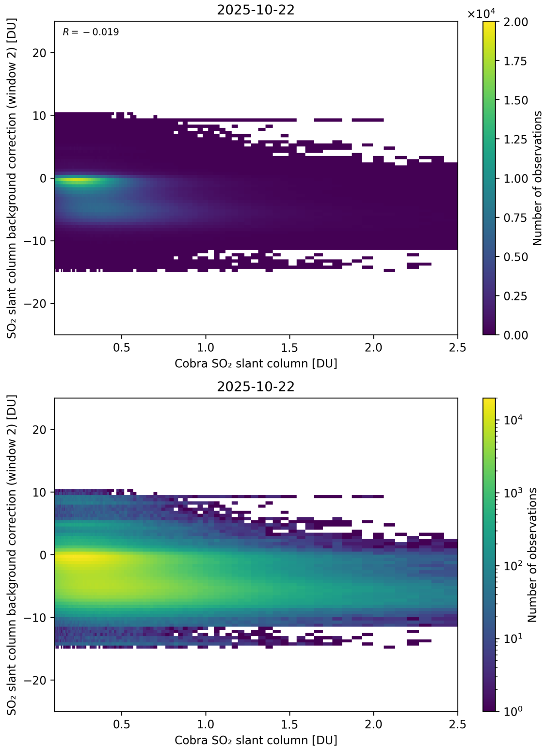
Figure 194: Scatter density plot of “Cobra SO 2 slant column” against “SO 2 slant column background correction (window 2)” for 2025-10-22 to 2025-10-23.
