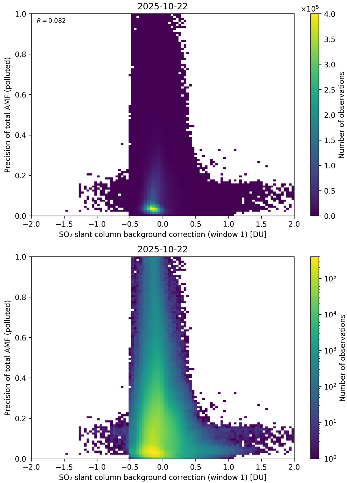
Figure 121: Scatter density plot of “SO 2 slant column background correction (window 1)” against “Precision of total AMF (polluted)” for 2025-10-22 to 2025-10-23.
