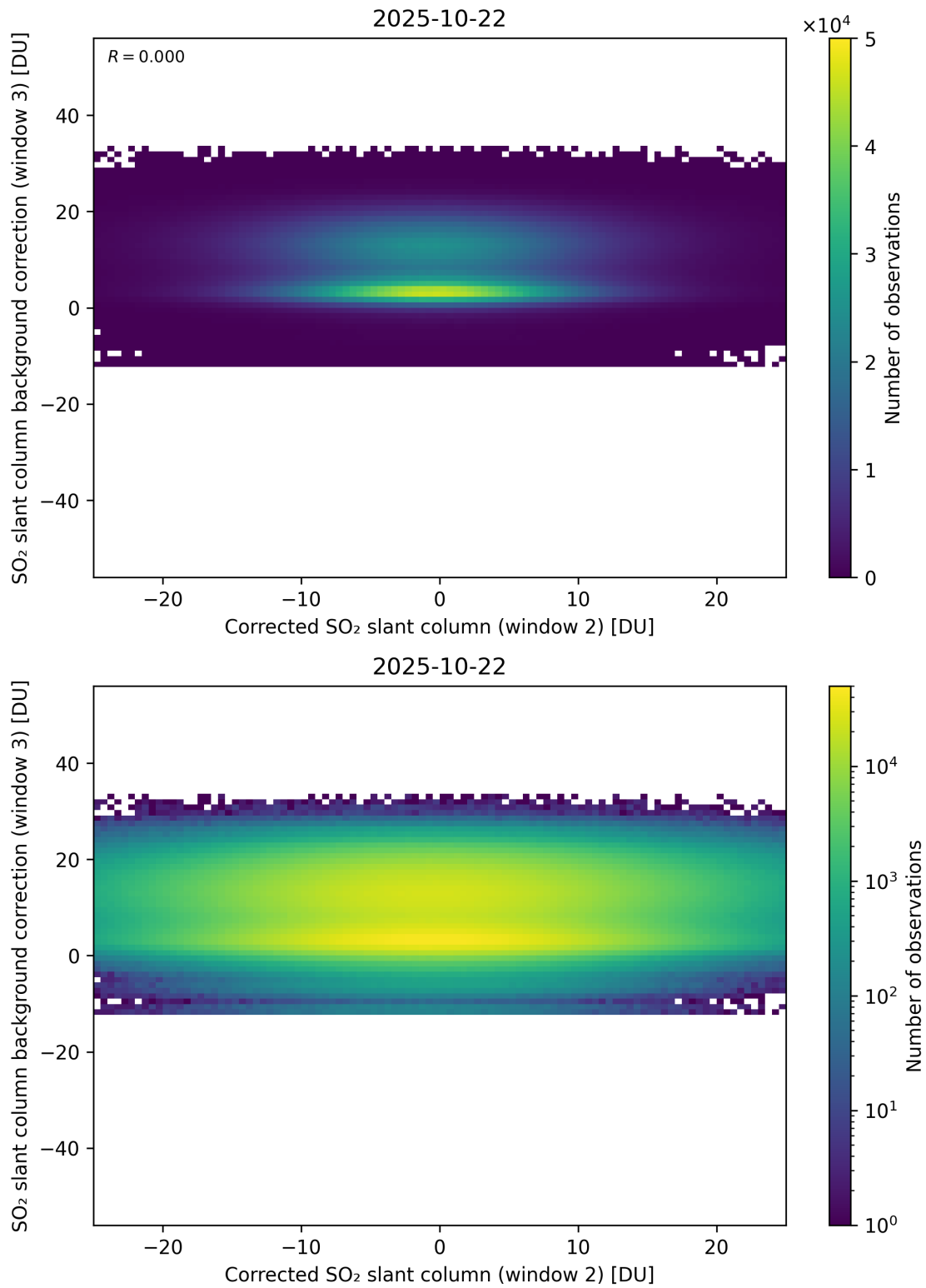
Figure 245: Scatter density plot of “Corrected SO 2 slant column (window 2)” against “SO 2 slant column background correction (window 3)” for 2025-10-22 to 2025-10-23.
