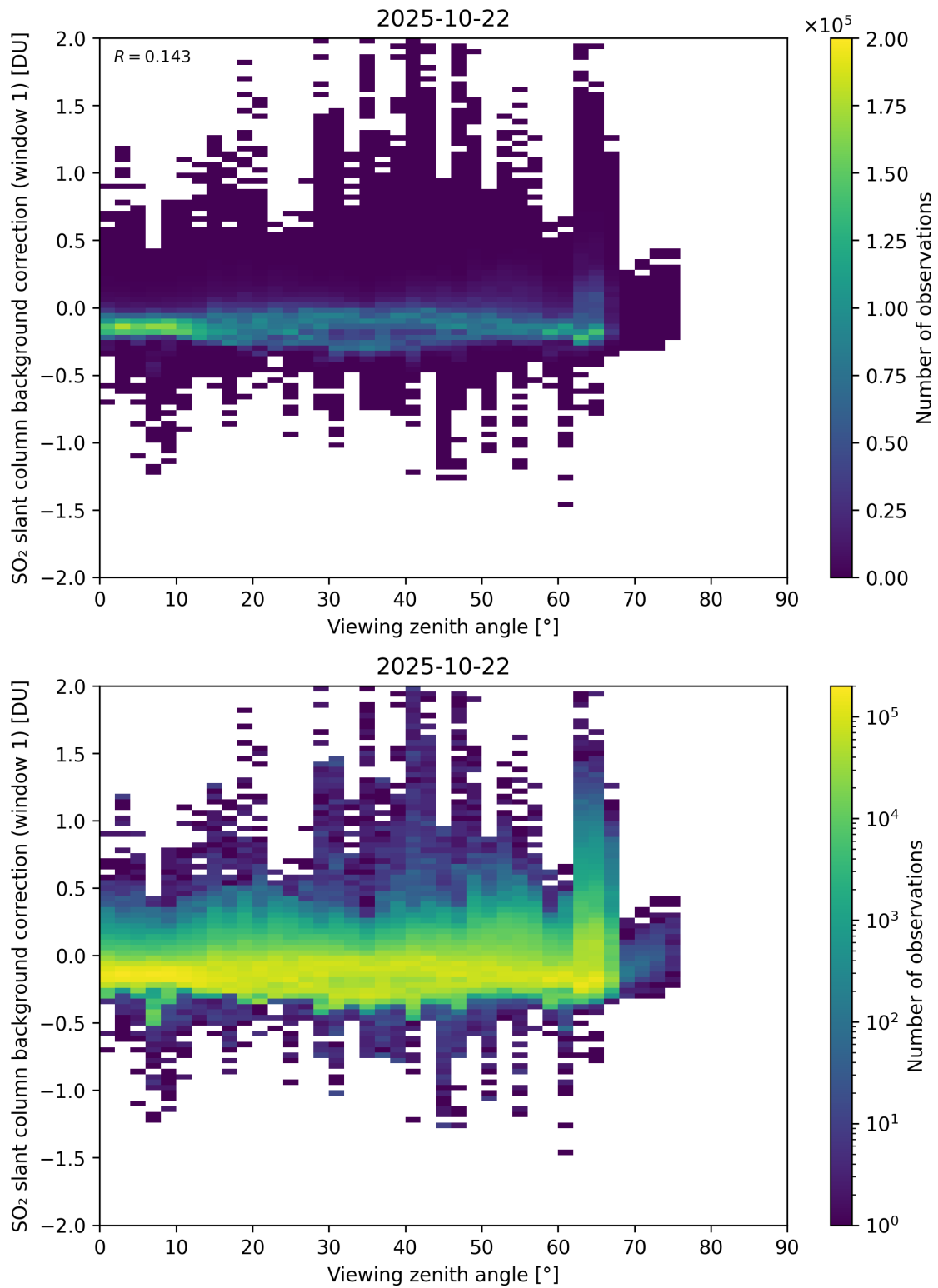
Figure 362: Scatter density plot of “Viewing zenith angle” against “SO 2 slant column background correction (window 1)” for 2025-10-22 to 2025-10-23.
