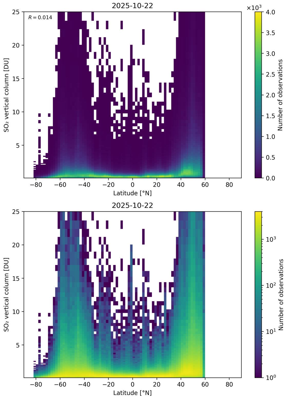
Figure 169: Scatter density plot of “Latitude” against “SO 2 vertical column” for 2025-10-22 to 2025-10-23.
