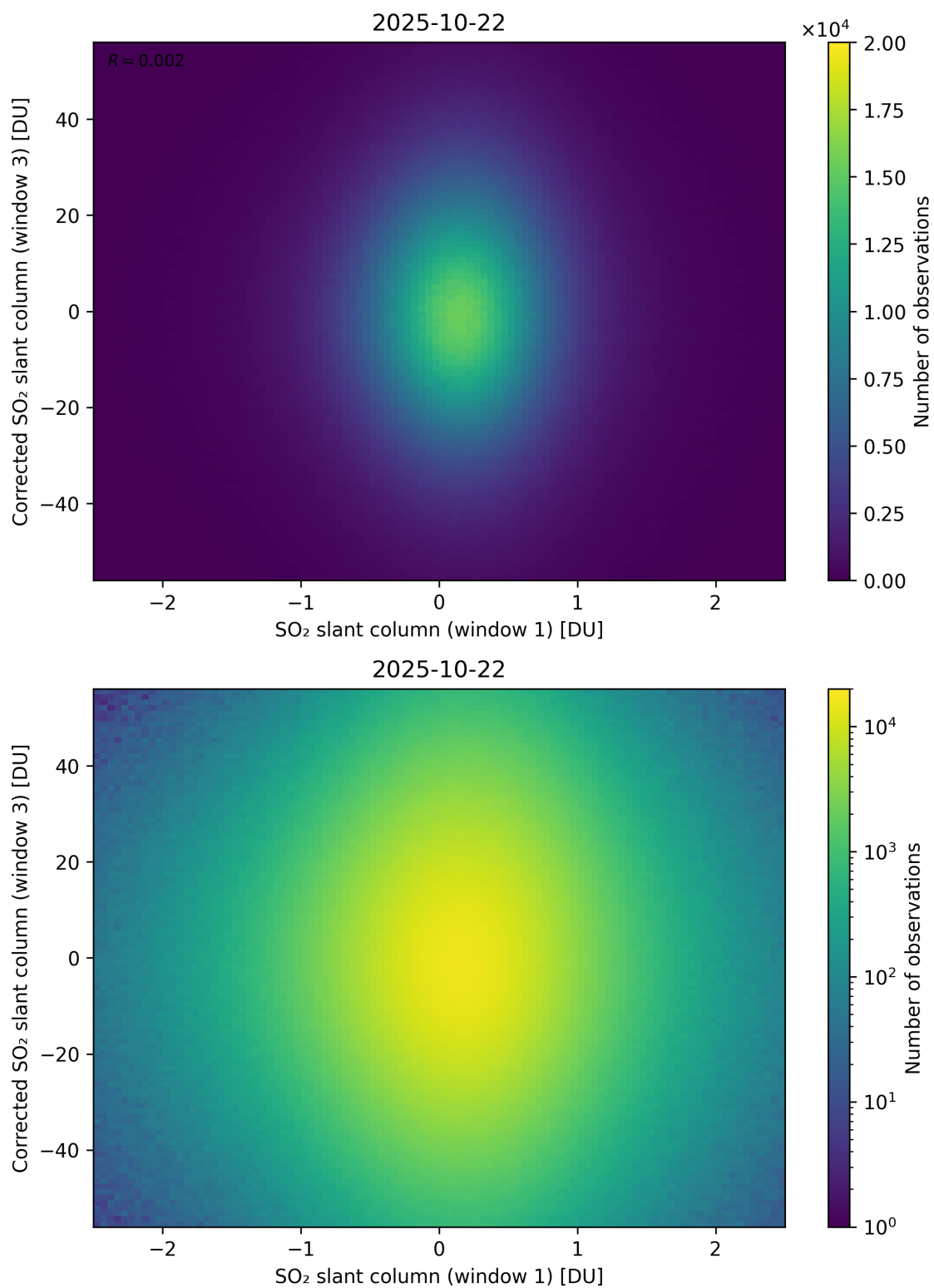
Figure 284: Scatter density plot of “SO 2 slant column (window 1)” against “Corrected SO 2 slant column (window 3)” for 2025-10-22 to 2025-10-23.
