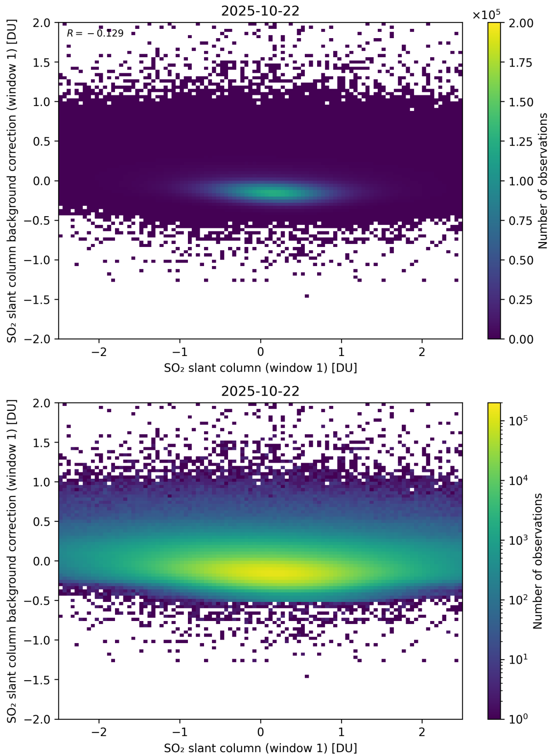
Figure 262: Scatter density plot of “SO 2 slant column (window 1)” against “SO 2 slant column background correction (window 1)” for 2025-10-22 to 2025-10-23.
