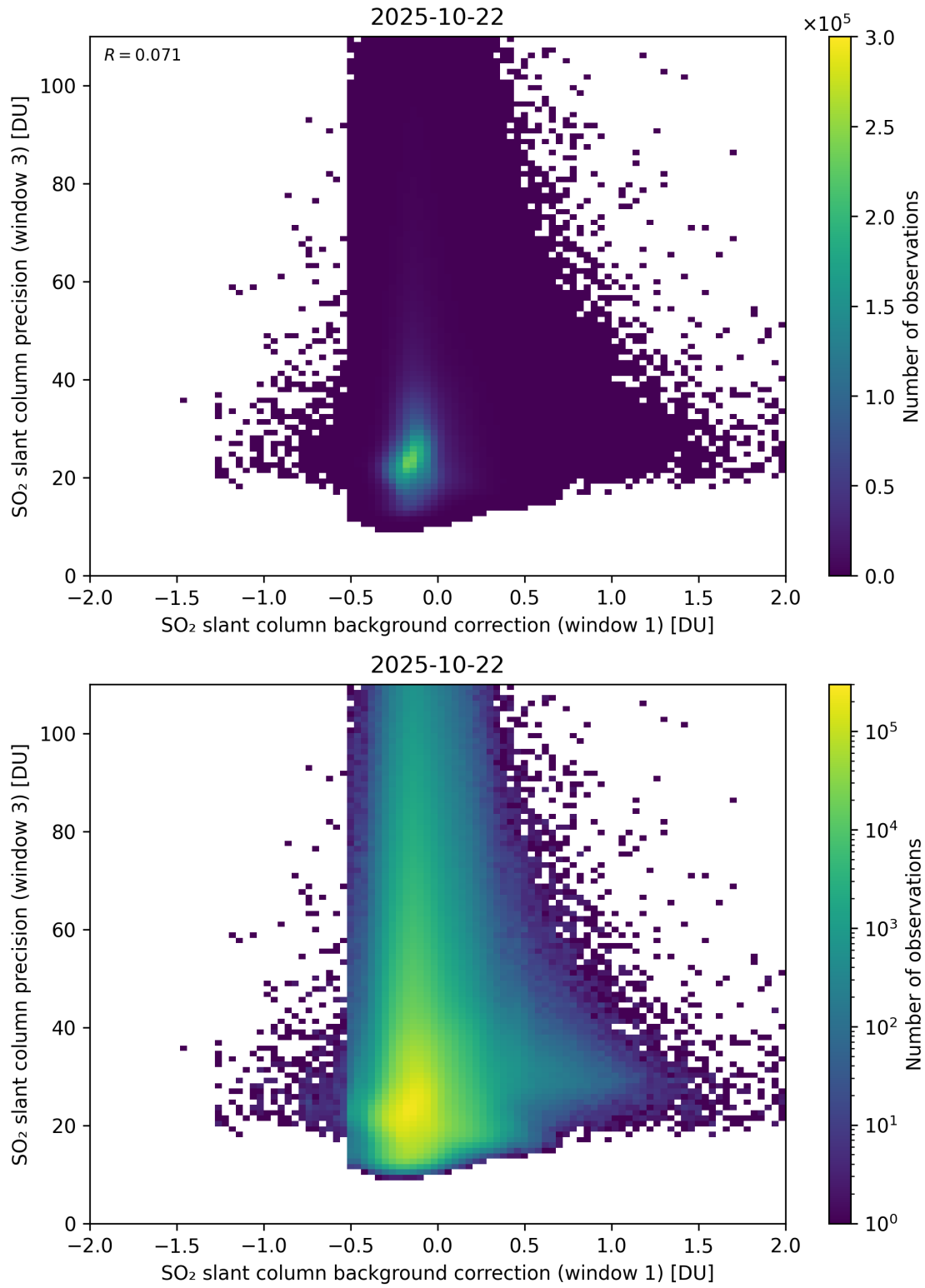
Figure 119: Scatter density plot of “SO 2 slant column background correction (window 1)” against “SO 2 slant column precision (window 3)” for 2025-10-22 to 2025-10-23.
