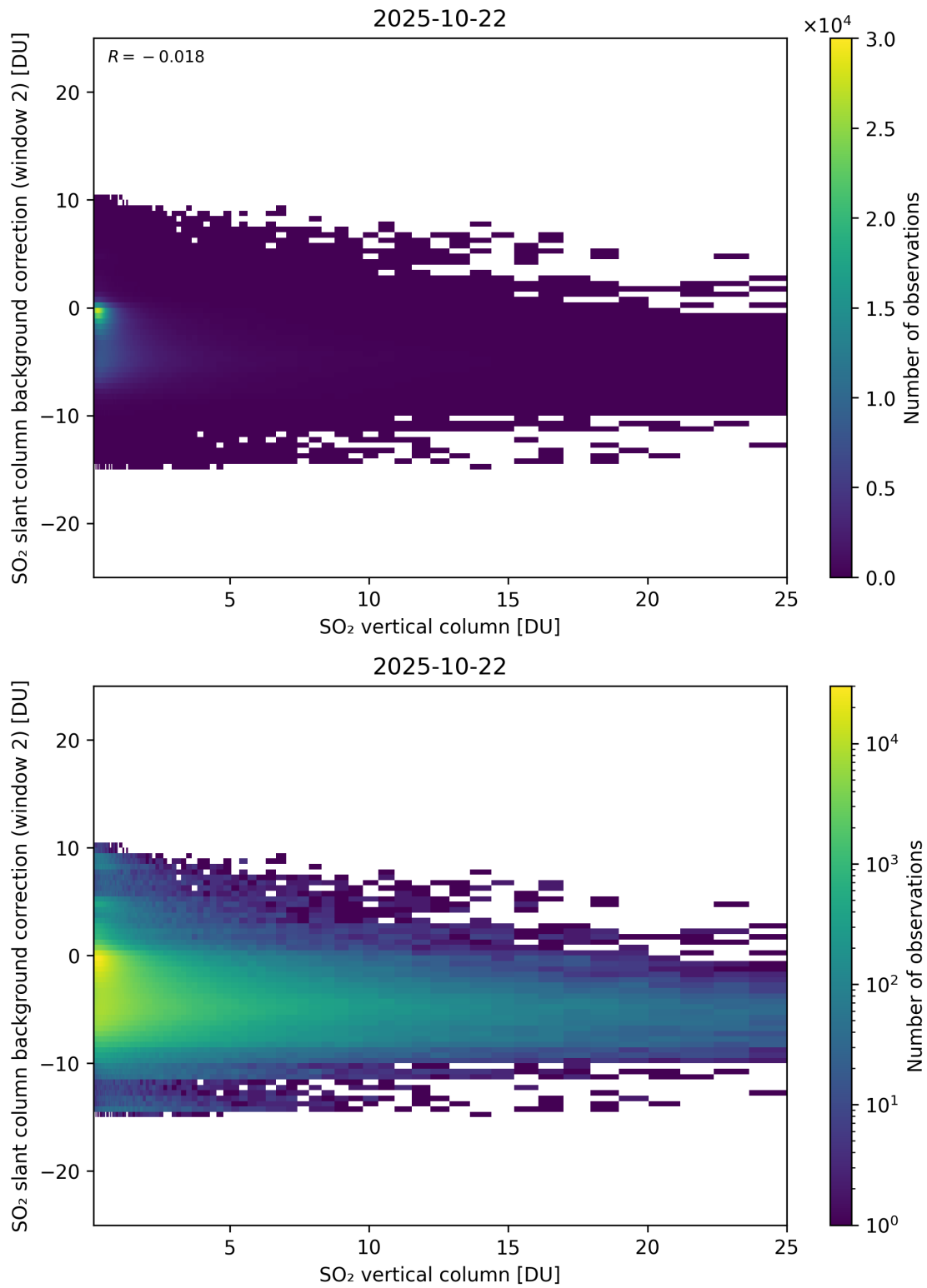
Figure 324: Scatter density plot of “SO 2 vertical column” against “SO 2 slant column background correction (window 2)” for 2025-10-22 to 2025-10-23.
