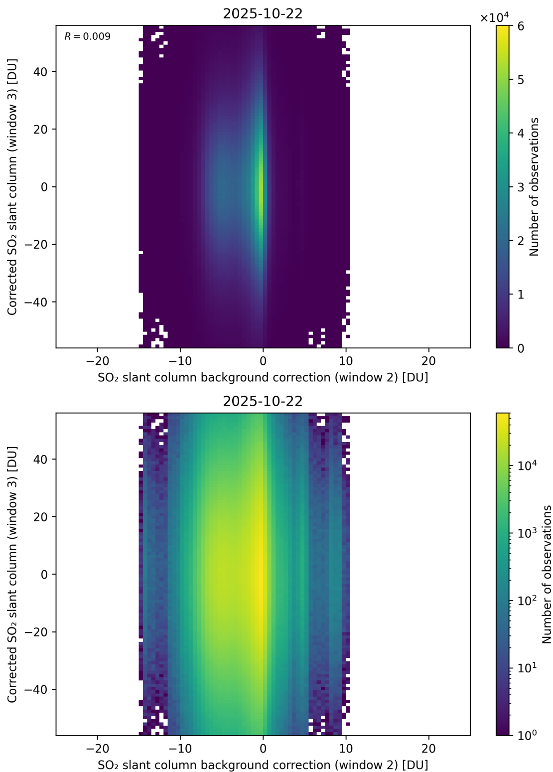
Figure 127: Scatter density plot of “SO 2 slant column background correction (window 2)” against “Corrected SO 2 slant column (window 3)” for 2025-10-22 to 2025-10-23.
