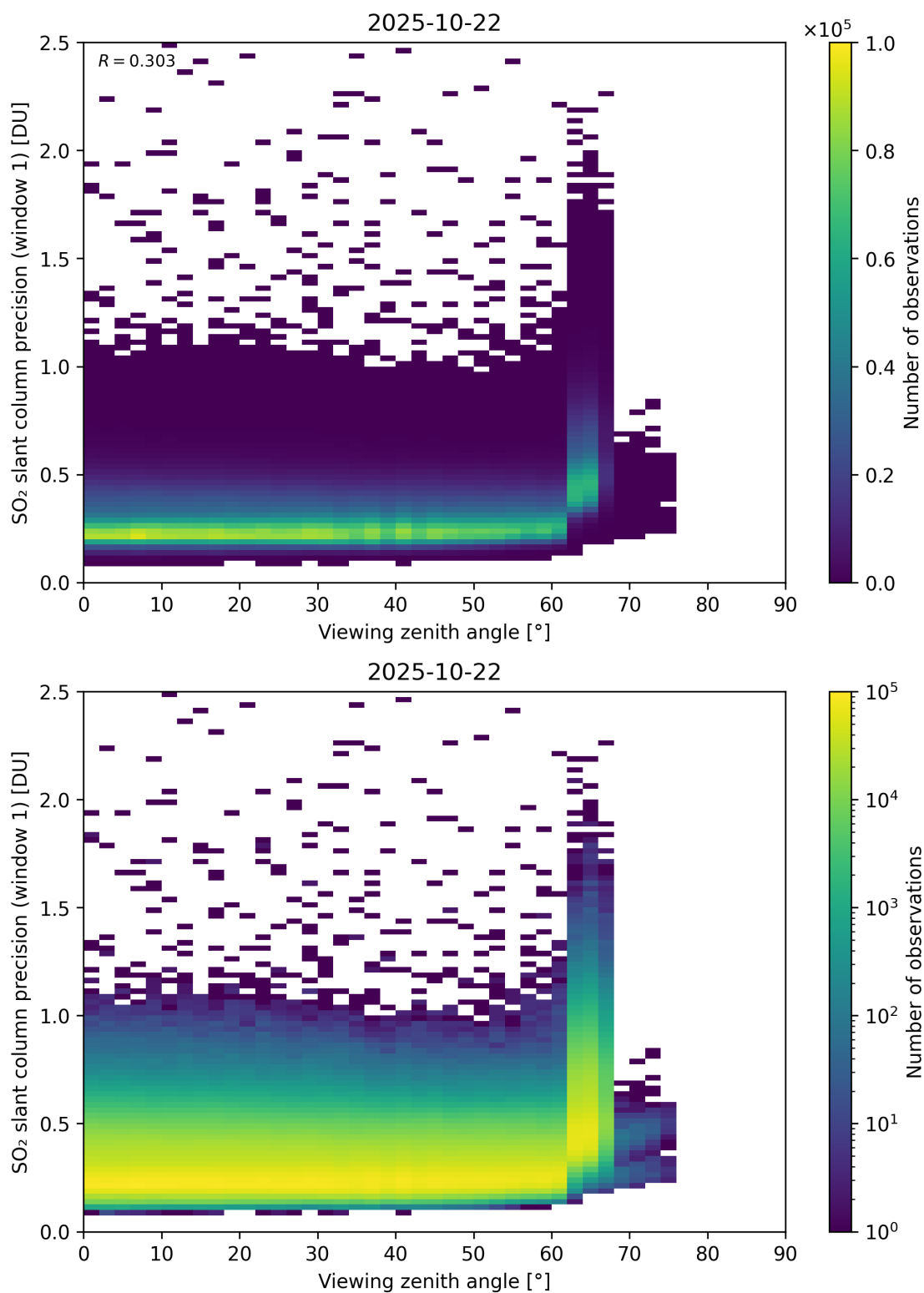
Figure 377: Scatter density plot of “Viewing zenith angle” against “SO 2 slant column precision (window 1)” for 2025-10-22 to 2025-10-23.
