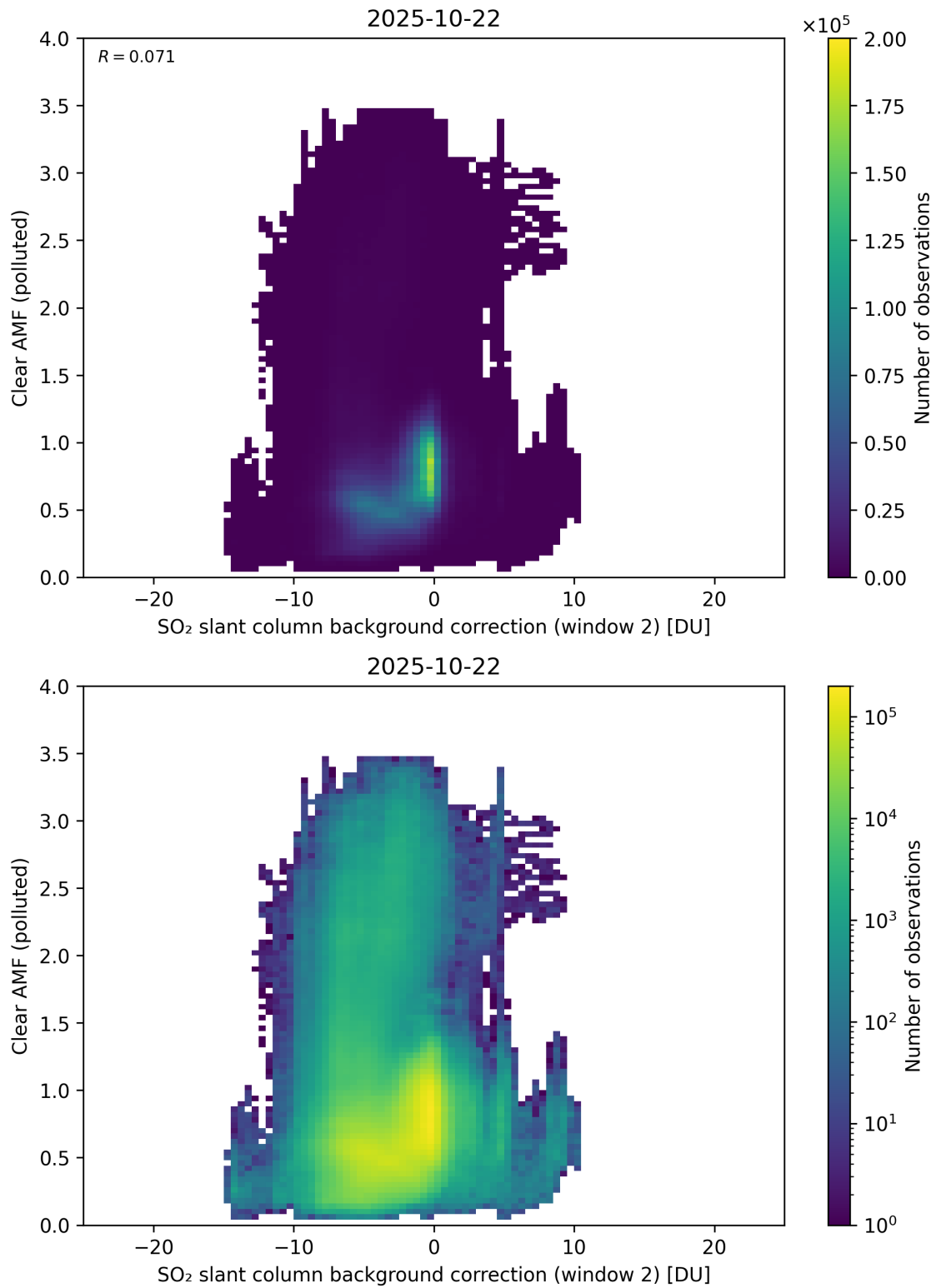
Figure 126: Scatter density plot of “SO 2 slant column background correction (window 2)” against “Clear AMF (polluted)” for 2025-10-22 to 2025-10-23.
