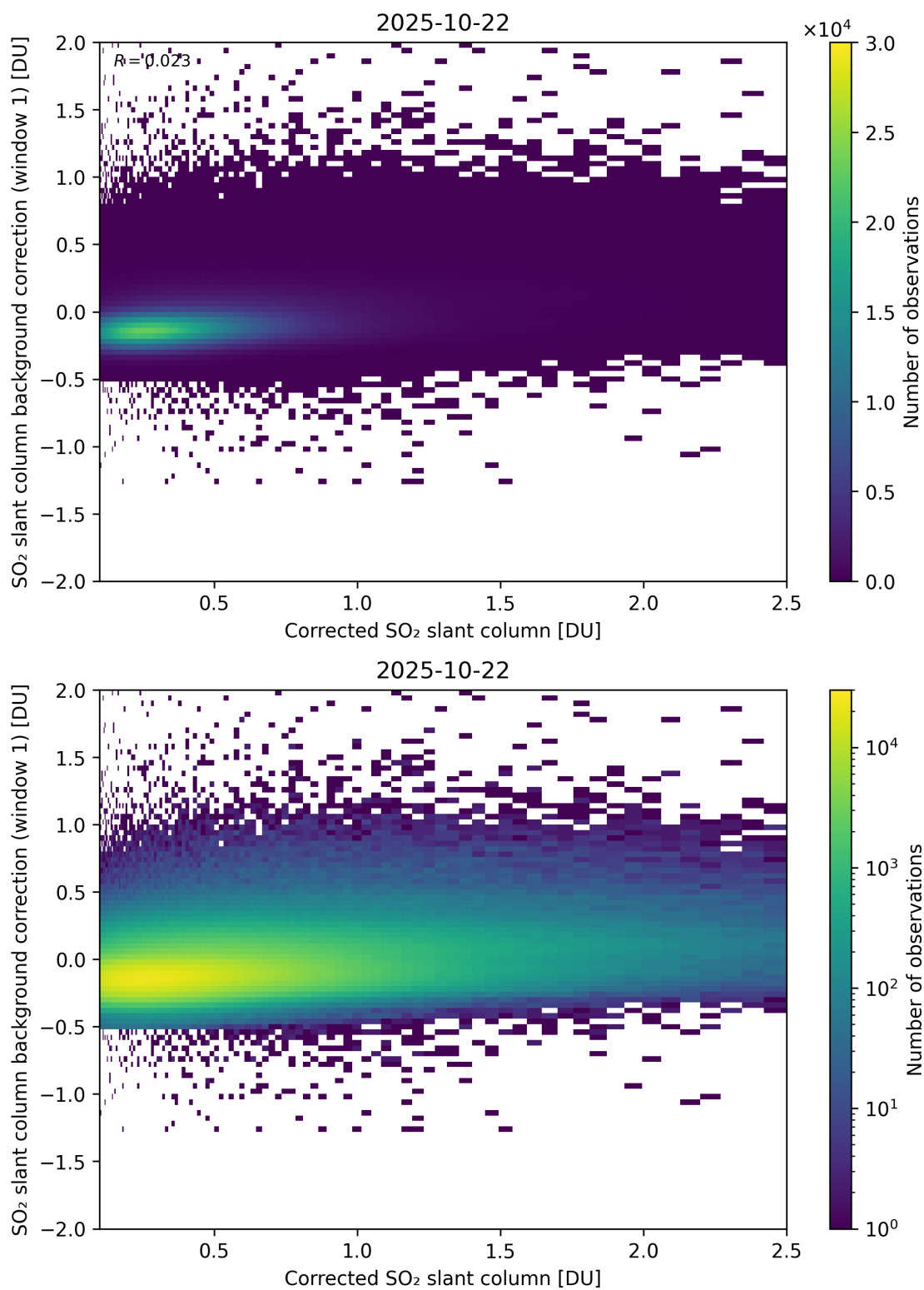
Figure 226: Scatter density plot of “Corrected SO 2 slant column” against “SO 2 slant column background correction (window 1)” for 2025-10-22 to 2025-10-23.
