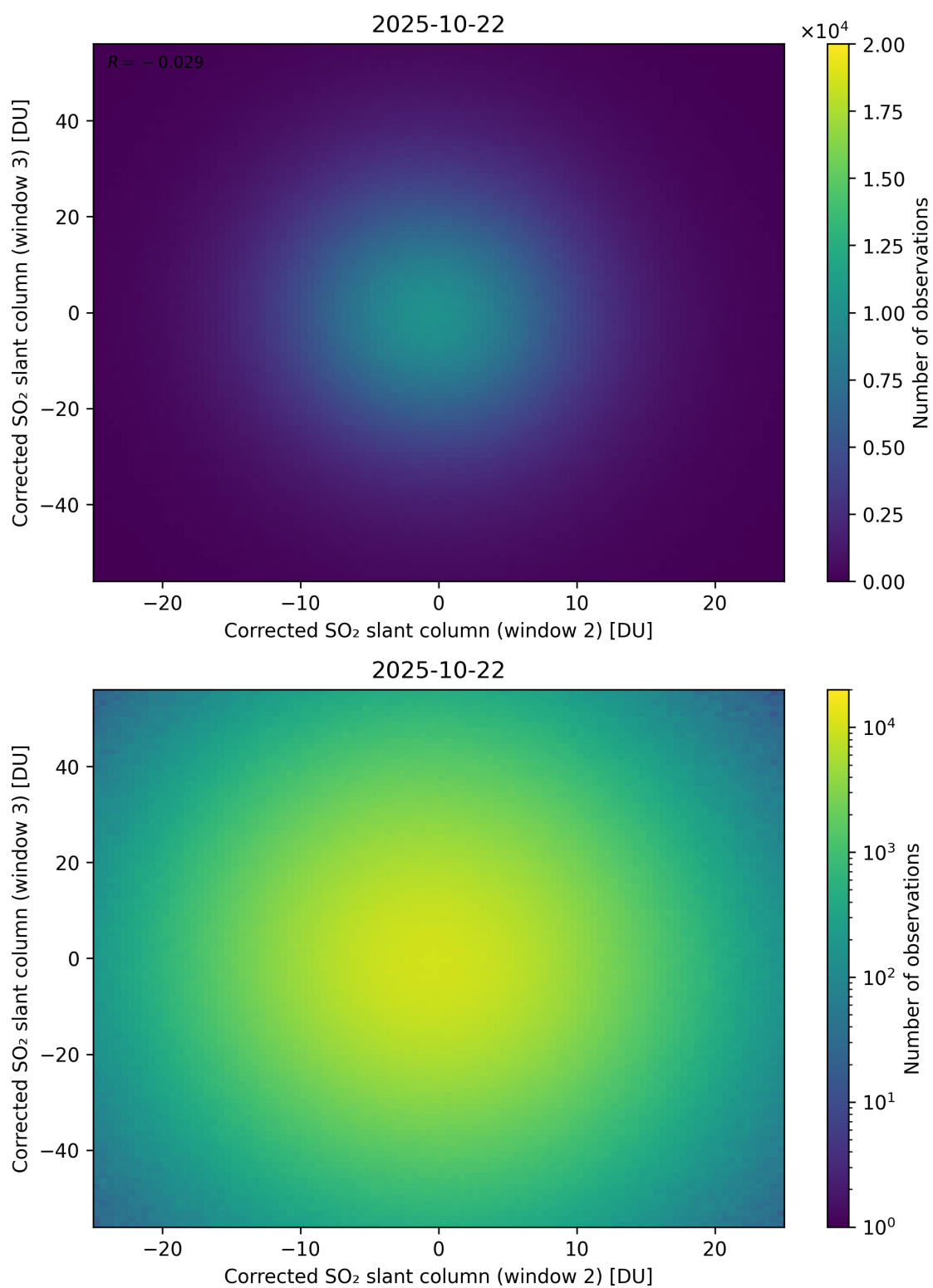
Figure 250: Scatter density plot of “Corrected SO 2 slant column (window 2)” against “Corrected SO 2 slant column (window 3)” for 2025-10-22 to 2025-10-23.
