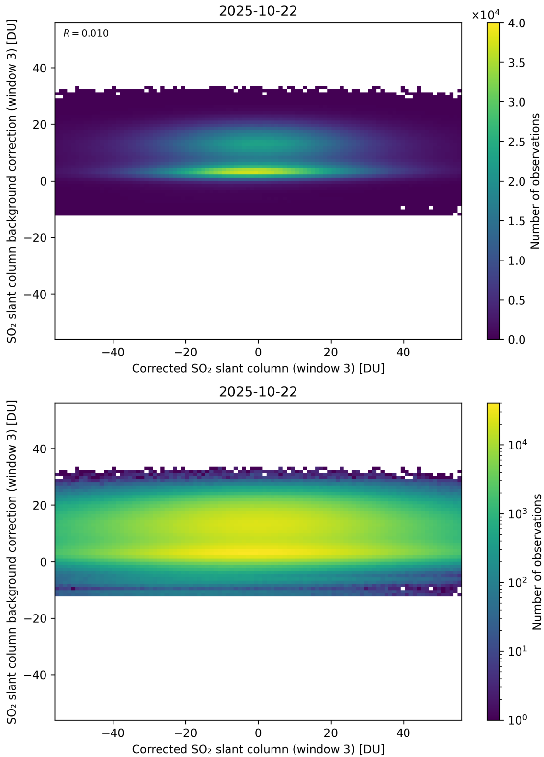
Figure 255: Scatter density plot of “Corrected SO 2 slant column (window 3)” against “SO 2 slant column background correction (window 3)” for 2025-10-22 to 2025-10-23.
