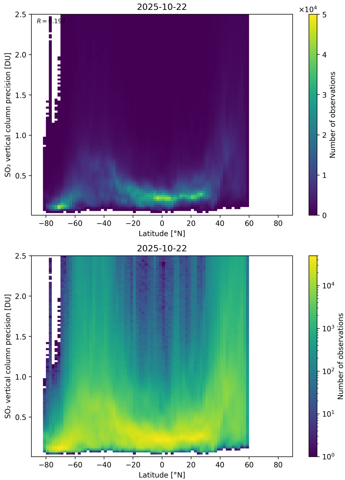
Figure 170: Scatter density plot of “Latitude” against “SO 2 vertical column precision” for 2025-10-22 to 2025-10-23.
