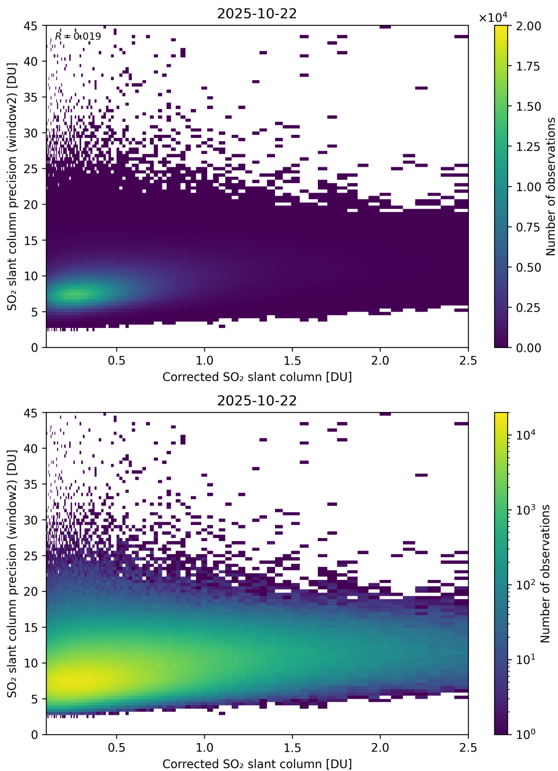
Figure 239: Scatter density plot of “Corrected SO 2 slant column” against “SO 2 slant column precision (window2)” for 2025-10-22 to 2025-10-23.
