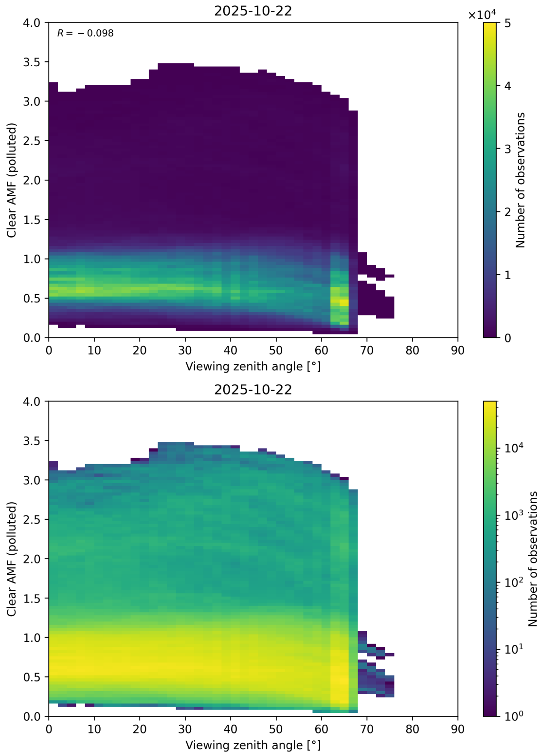
Figure 370: Scatter density plot of “Viewing zenith angle” against “Clear AMF (polluted)” for 2025-10-22 to 2025-10-23.
