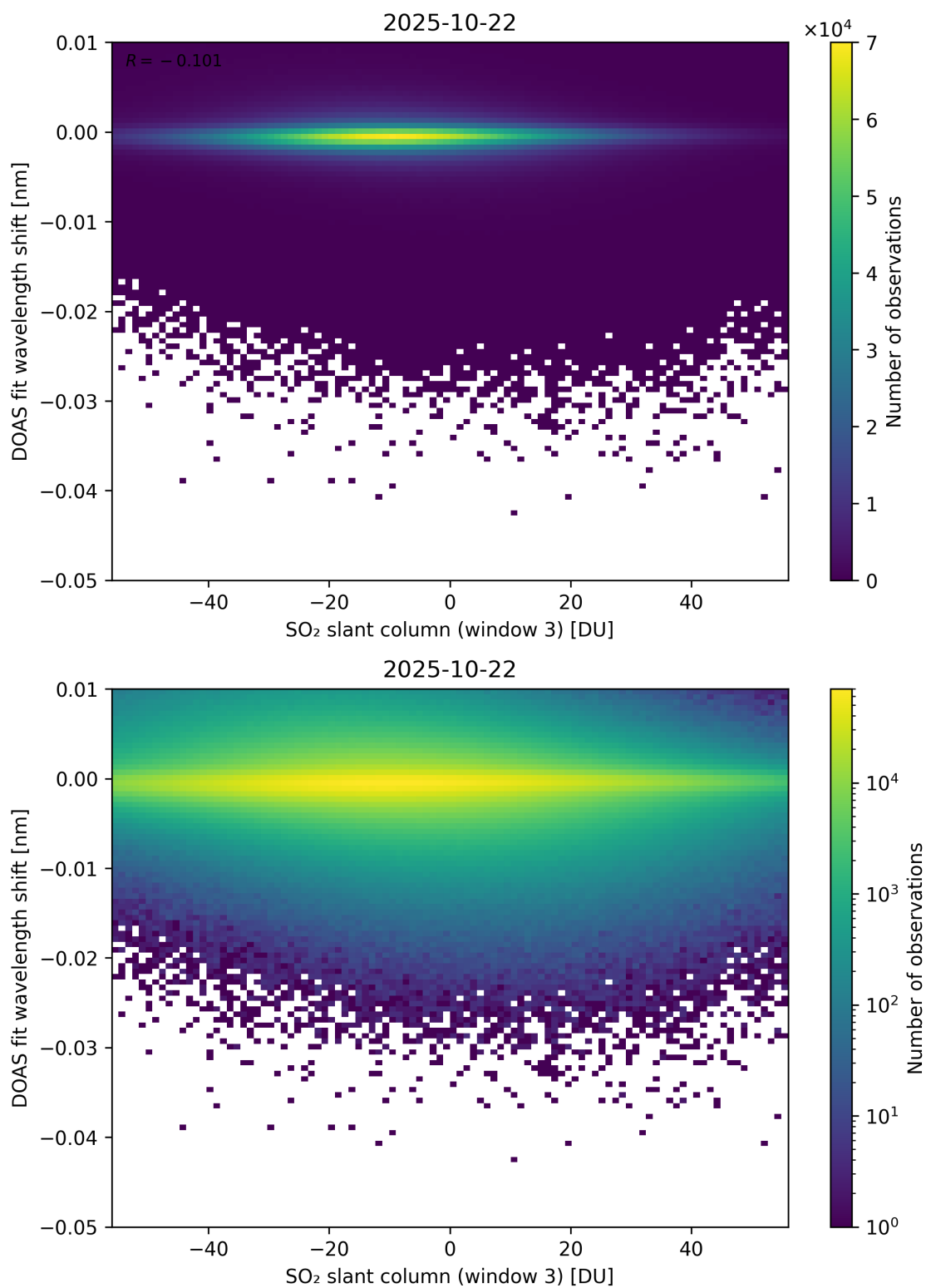
Figure 304: Scatter density plot of “SO 2 slant column (window 3)” against “DOAS fit wavelength shift” for 2025-10-22 to 2025-10-23.
