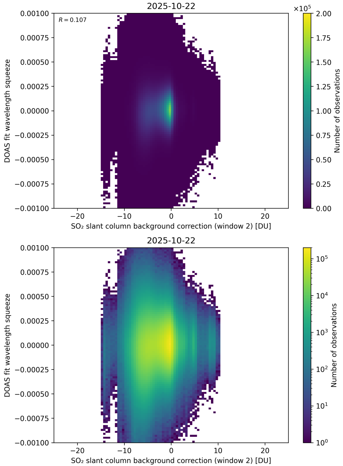
Figure 124: Scatter density plot of “SO 2 slant column background correction (window 2)” against “DOAS fit wavelength squeeze” for 2025-10-22 to 2025-10-23.
