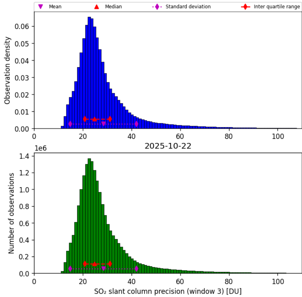
Figure 72: Histogram of “SO 2 slant column precision (window 3)” for 2025-10-22 to 2025-10-23
