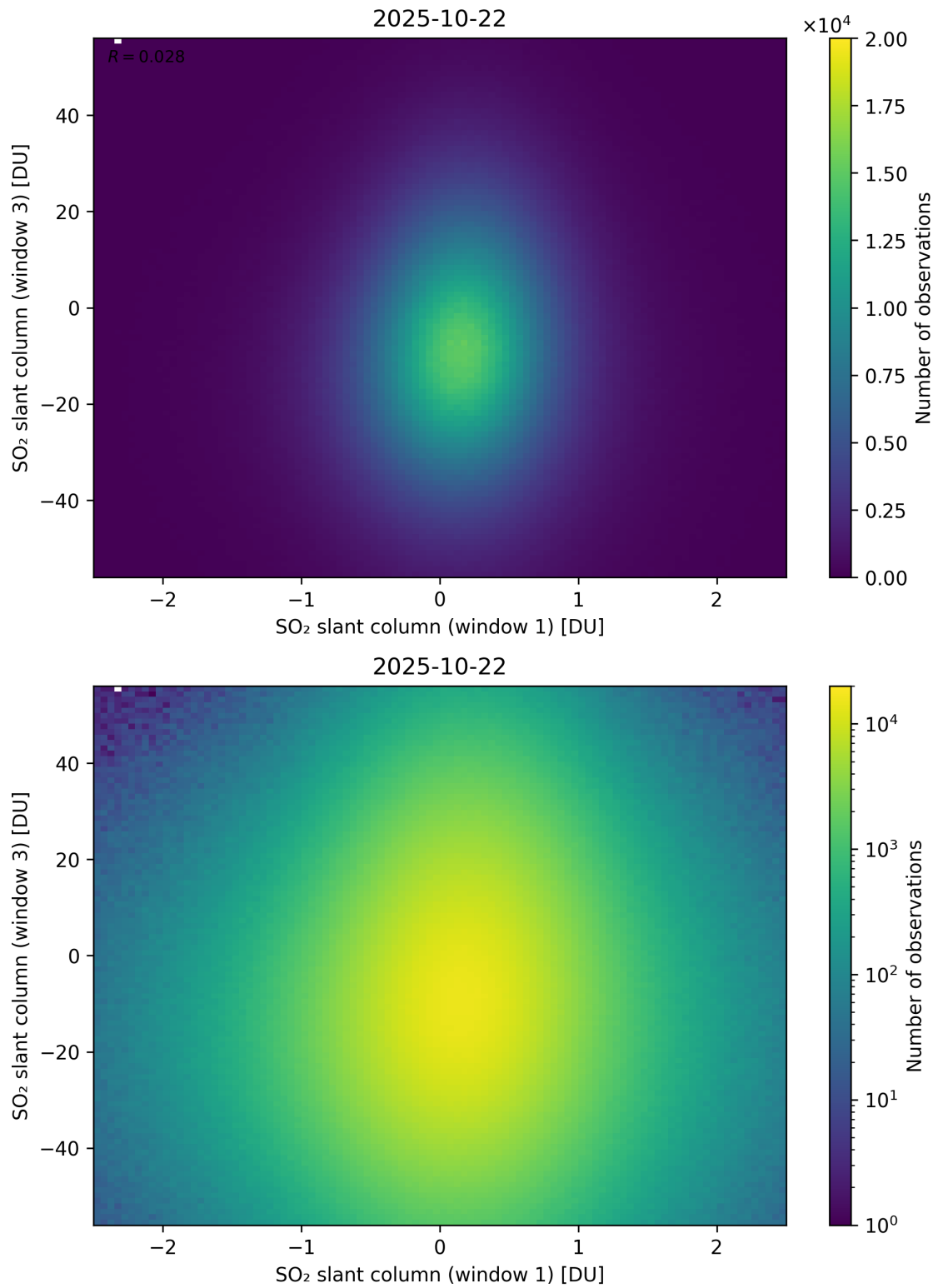
Figure 287: Scatter density plot of “SO 2 slant column (window 1)” against “SO 2 slant column (window 3)” for 2025-10-22 to 2025-10-23.
