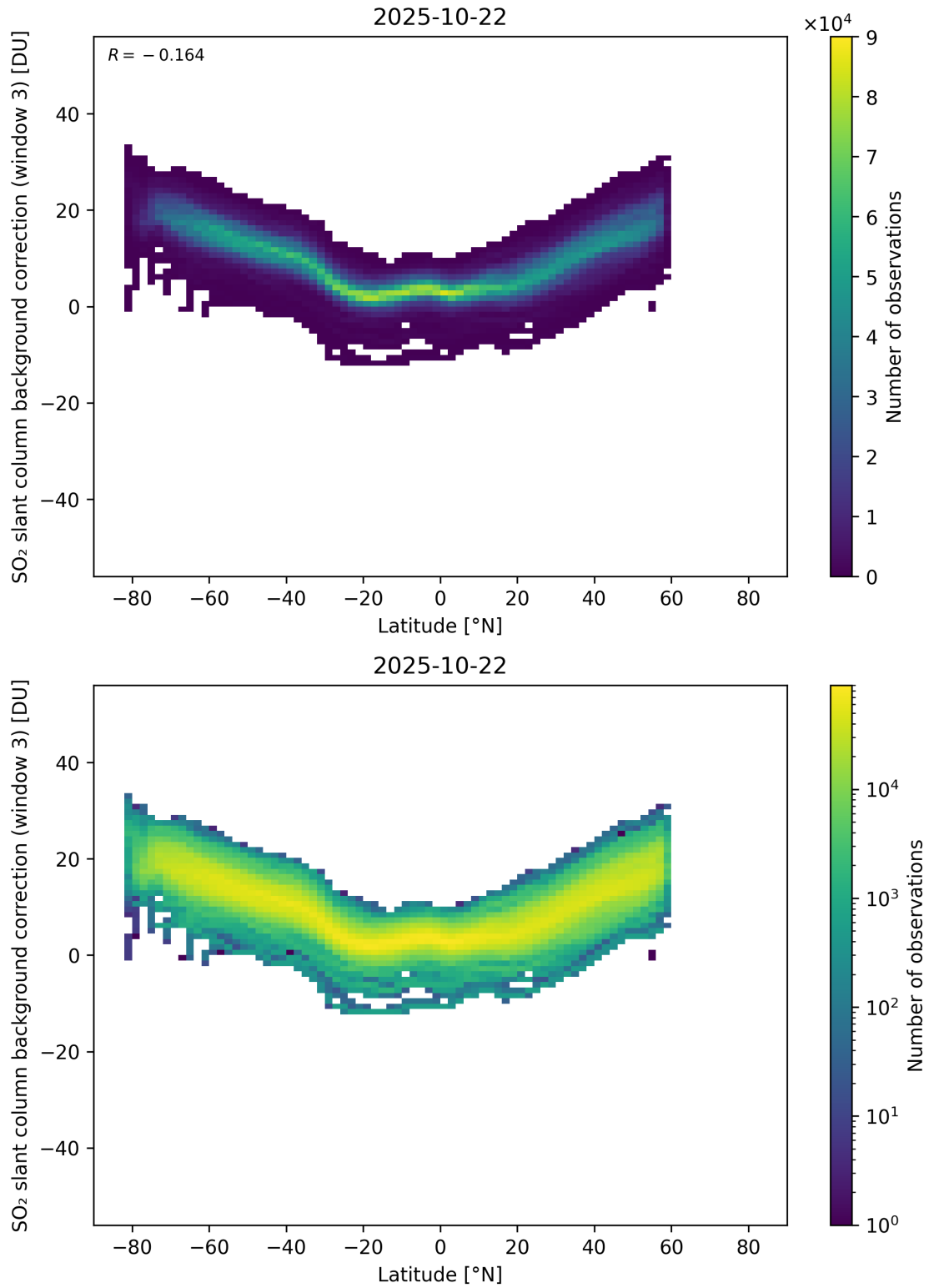
Figure 152: Scatter density plot of “Latitude” against “SO 2 slant column background correction (window 3)” for 2025-10-22 to 2025-10-23.
