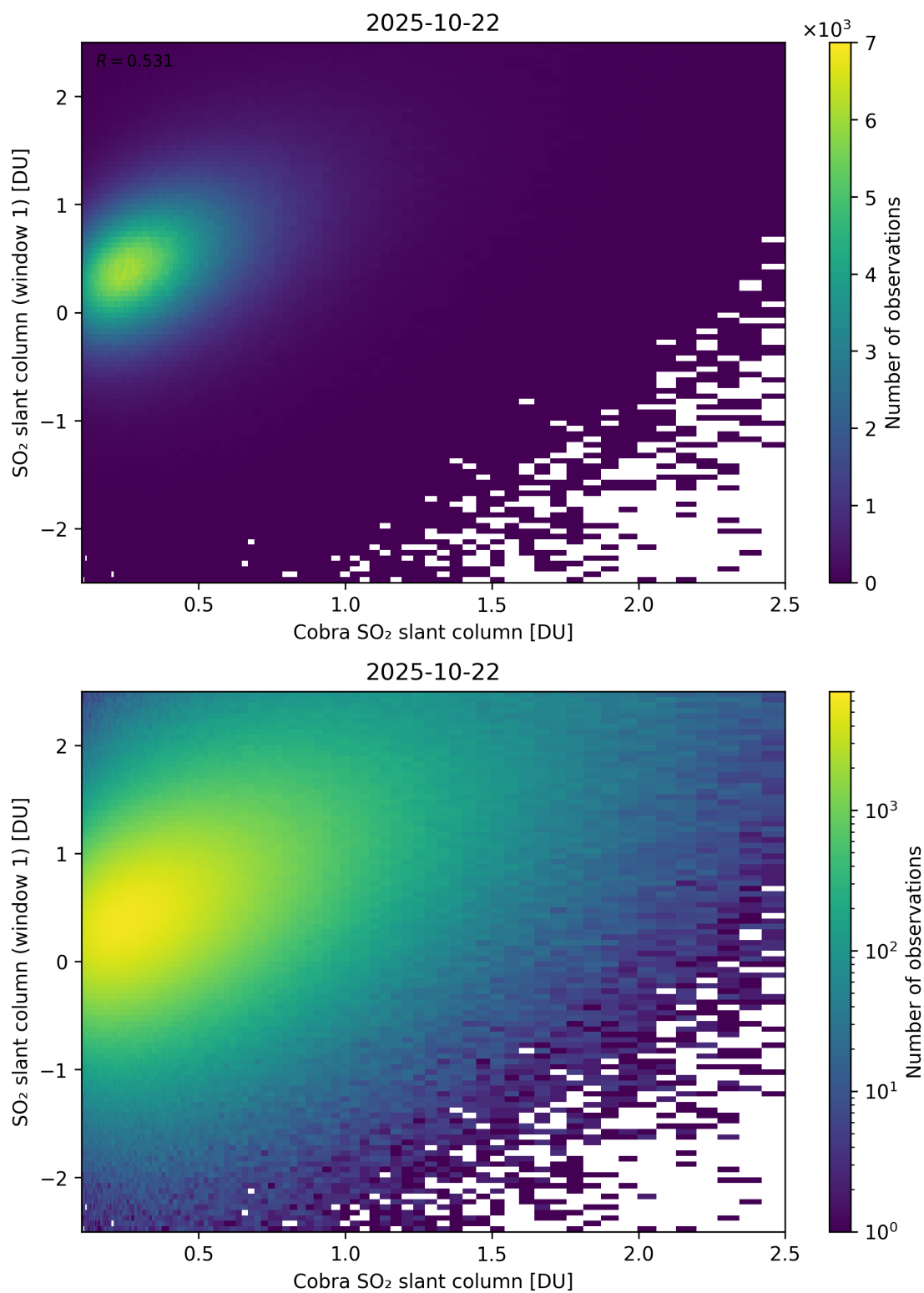
Figure 219: Scatter density plot of “Cobra SO 2 slant column” against “SO 2 slant column (window 1)” for 2025-10-22 to 2025-10-23.
