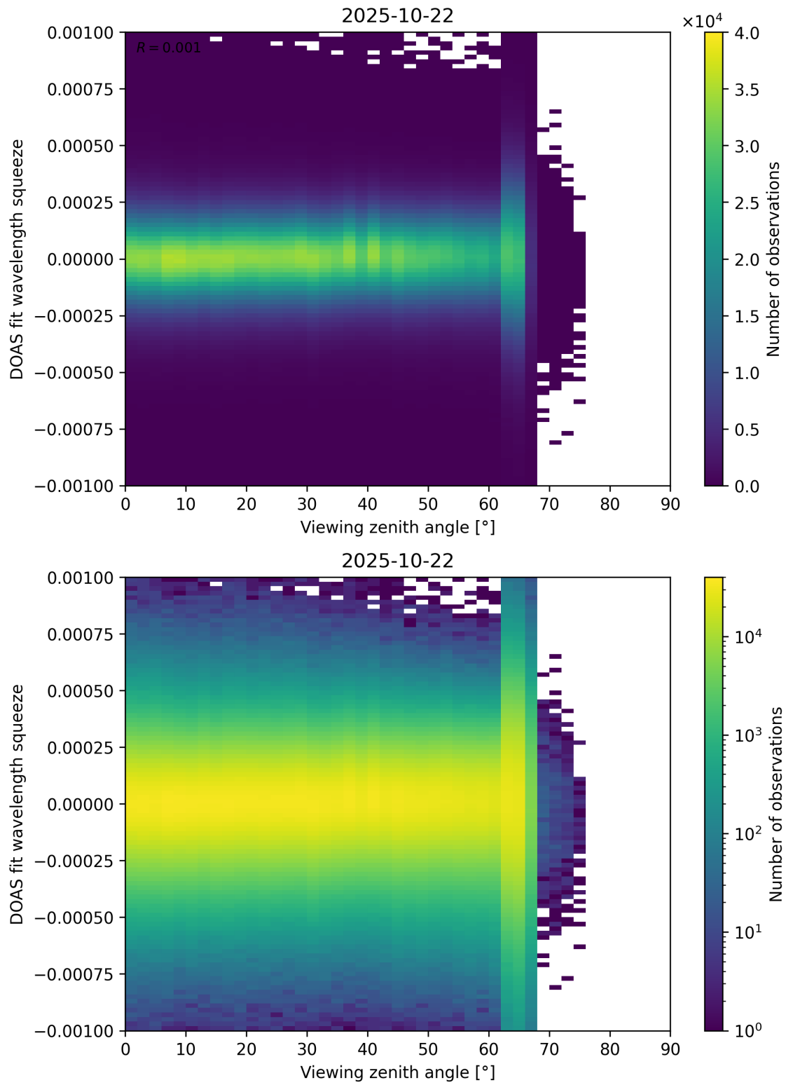
Figure 366: Scatter density plot of “Viewing zenith angle” against “DOAS fit wavelength squeeze” for 2025-10-22 to 2025-10-23.
