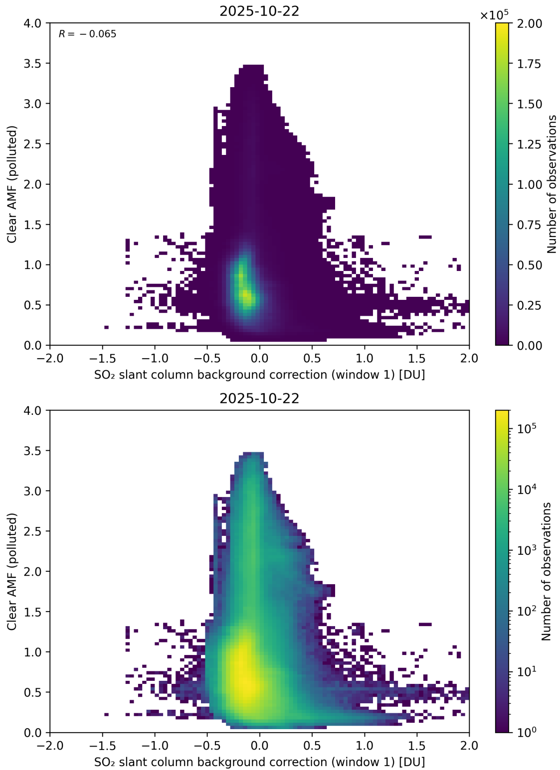
Figure 114: Scatter density plot of “SO 2 slant column background correction (window 1)” against “Clear AMF (polluted)” for 2025-10-22 to 2025-10-23.
