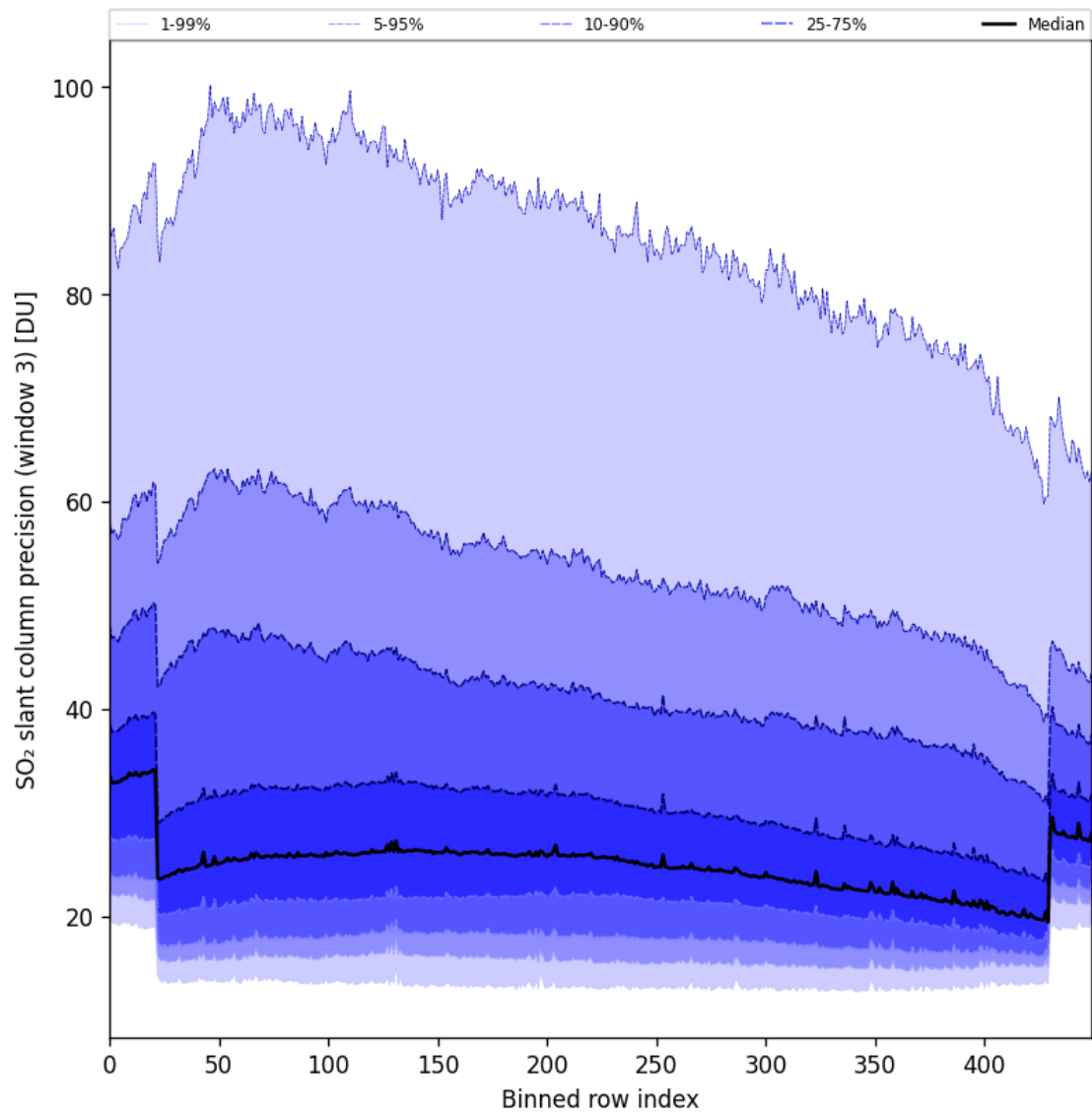
Figure 98: Along track statistics of “SO 2 slant column precision (window 3)” for 2025-10-22 to 2025-10-23
