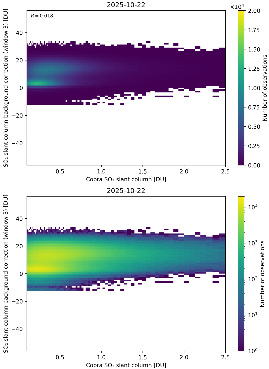
Figure 195: Scatter density plot of “Cobra SO 2 slant column” against “SO 2 slant column background correction (window 3)” for 2025-10-22 to 2025-10-23.
