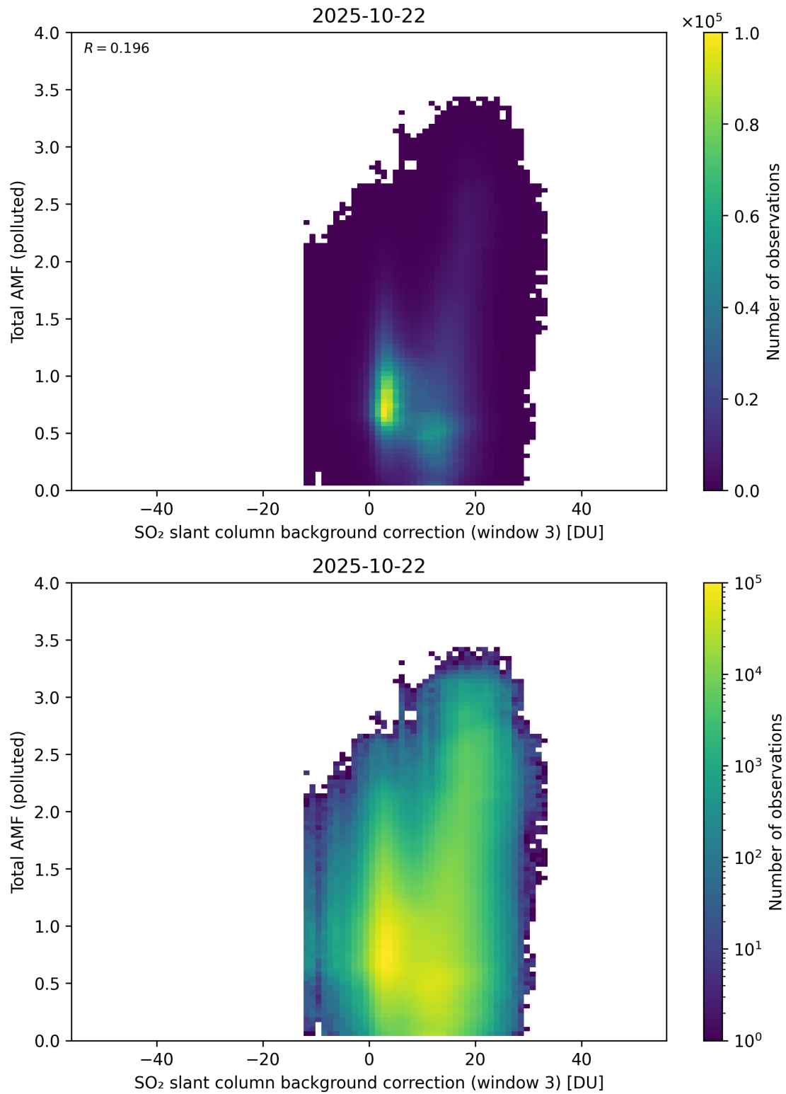
Figure 136: Scatter density plot of “SO 2 slant column background correction (window 3)” against “Total AMF (polluted)” for 2025-10-22 to 2025-10-23.
