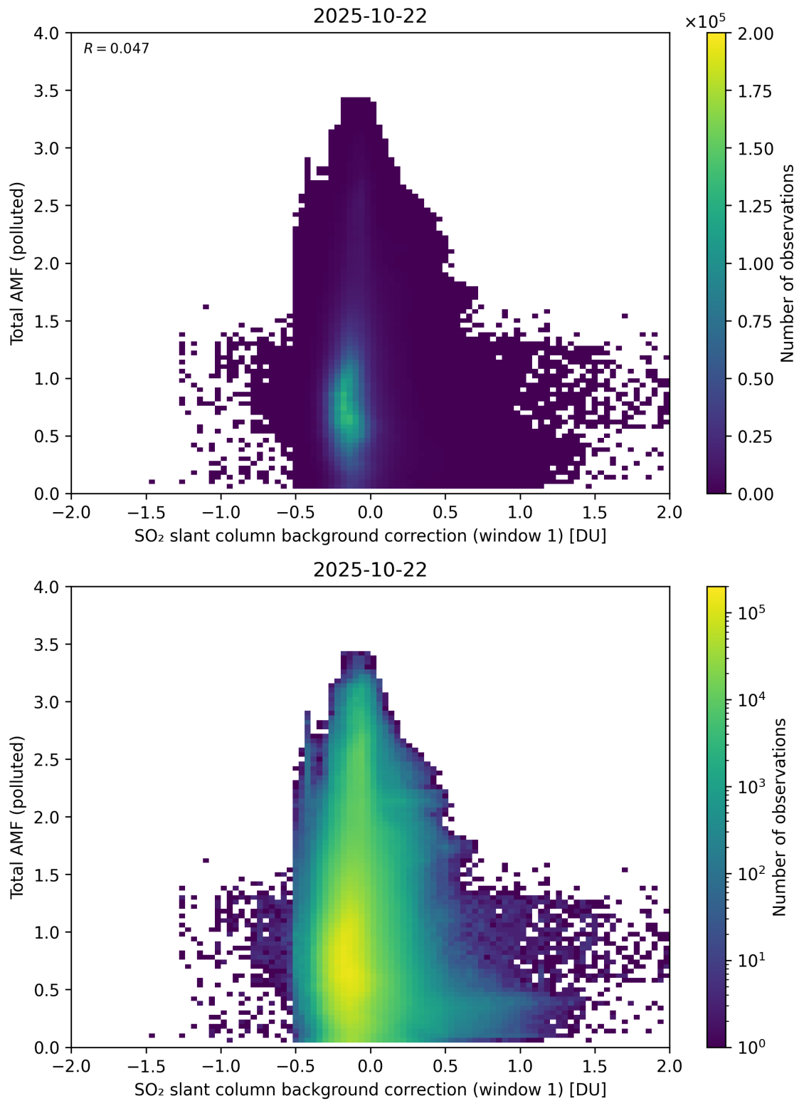
Figure 120: Scatter density plot of “SO 2 slant column background correction (window 1)” against “Total AMF (polluted)” for 2025-10-22 to 2025-10-23.
