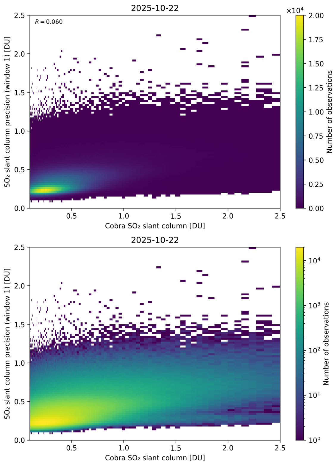
Figure 220: Scatter density plot of “Cobra SO 2 slant column” against “SO 2 slant column precision (window 1)” for 2025-10-22 to 2025-10-23.
