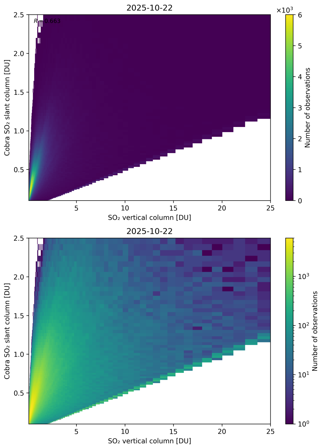
Figure 349: Scatter density plot of “SO 2 vertical column” against “Cobra SO 2 slant column” for 2025-10-22 to 2025-10-23.
