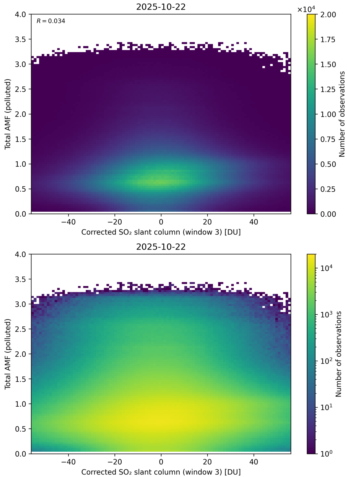
Figure 260: Scatter density plot of “Corrected SO 2 slant column (window 3)” against “Total AMF (polluted)” for 2025-10-22 to 2025-10-23.
