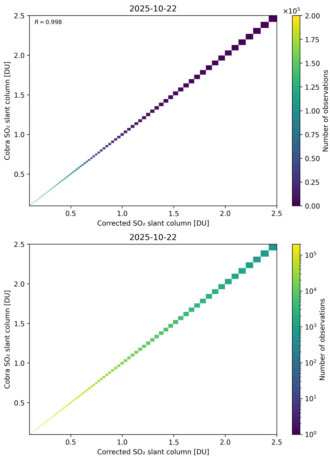
Figure 233: Scatter density plot of “Corrected SO 2 slant column” against “Cobra SO 2 slant column” for 2025-10-22 to 2025-10-23.
