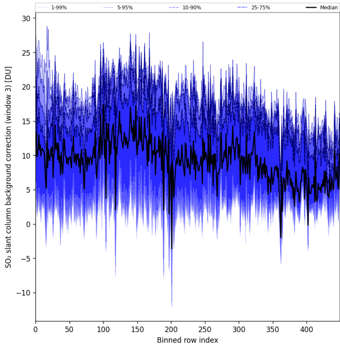
Figure 100: Along track statistics of “SO 2 slant column background correction (window 3)” for 2025-10-22 to 2025-10-23
