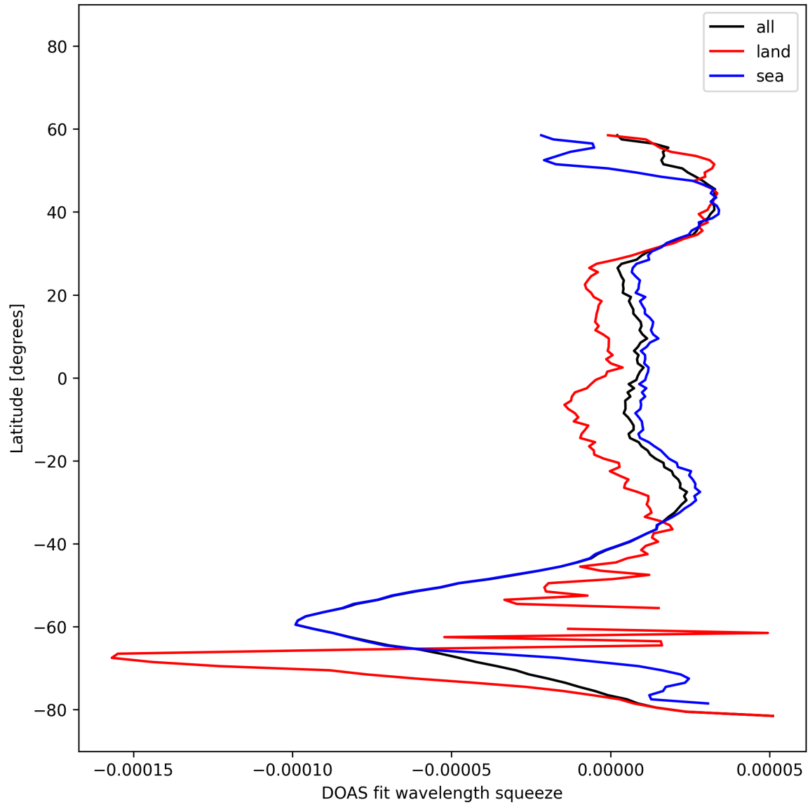
Figure 51: Zonal average of “DOAS fit wavelength squeeze” for 2025-10-22 to 2025-10-23.
