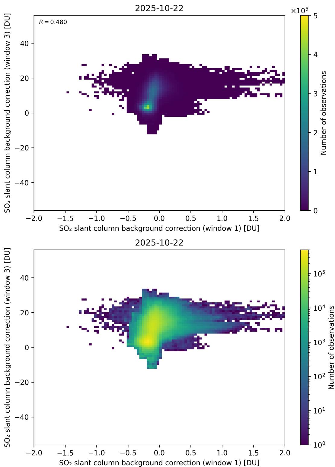
Figure 110: Scatter density plot of “SO 2 slant column background correction (window 1)” against “SO 2 slant column background correction (window 3)” for 2025-10-22 to 2025-10-23.
