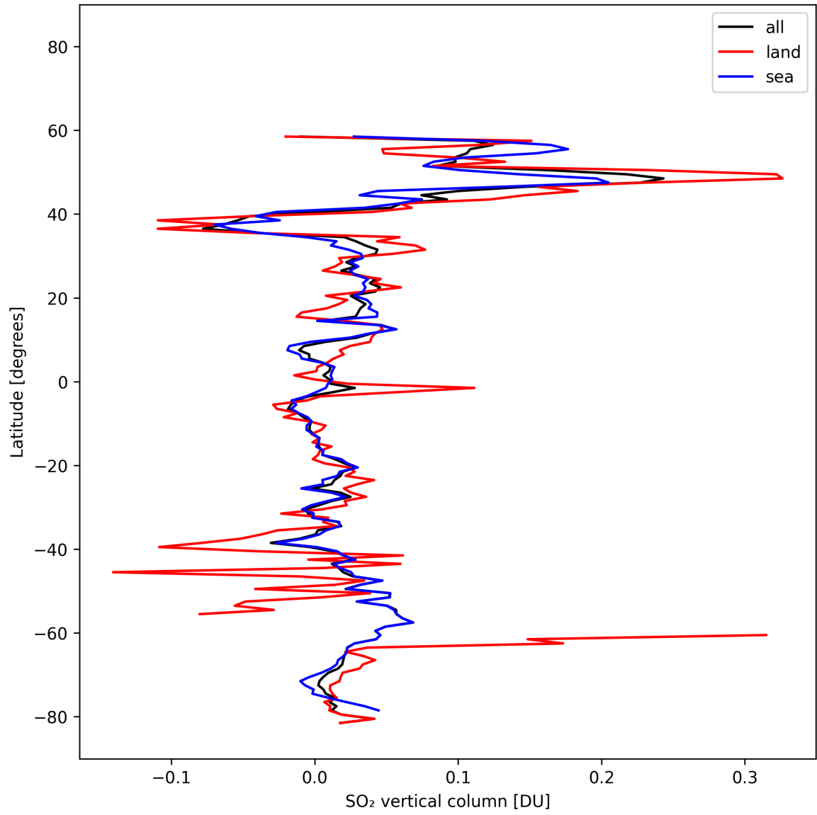
Figure 32: Zonal average of “SO 2 vertical column” for 2025-10-22 to 2025-10-23.
