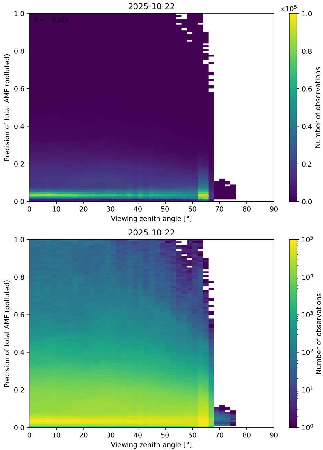
Figure 382: Scatter density plot of “Viewing zenith angle” against “Precision of total AMF (polluted)” for 2025-10-22 to 2025-10-23.
