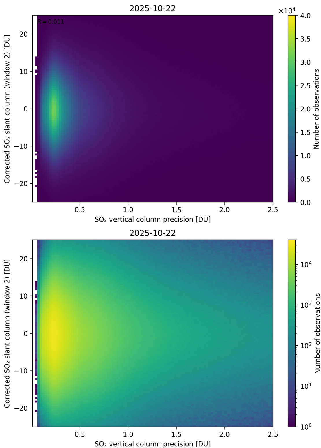
Figure 339: Scatter density plot of “SO 2 vertical column precision” against “Corrected SO 2 slant column (window 2)” for 2025-10-22 to 2025-10-23.
