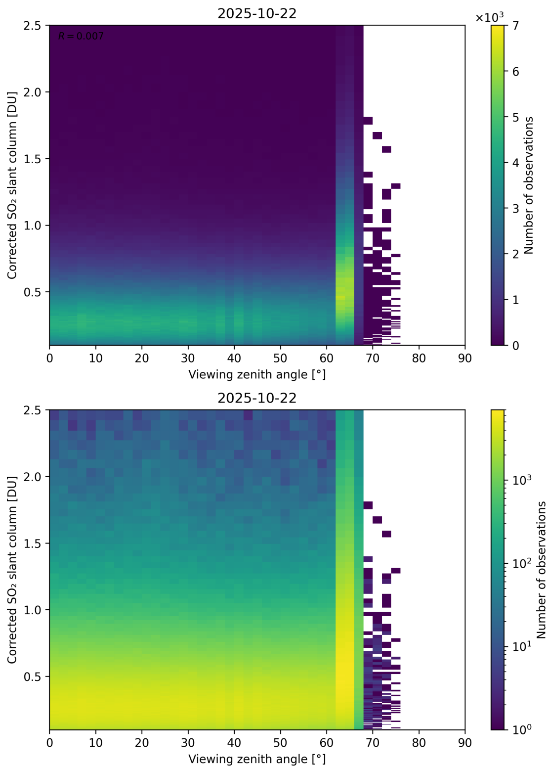
Figure 373: Scatter density plot of “Viewing zenith angle” against “Corrected SO 2 slant column” for 2025-10-22 to 2025-10-23.
