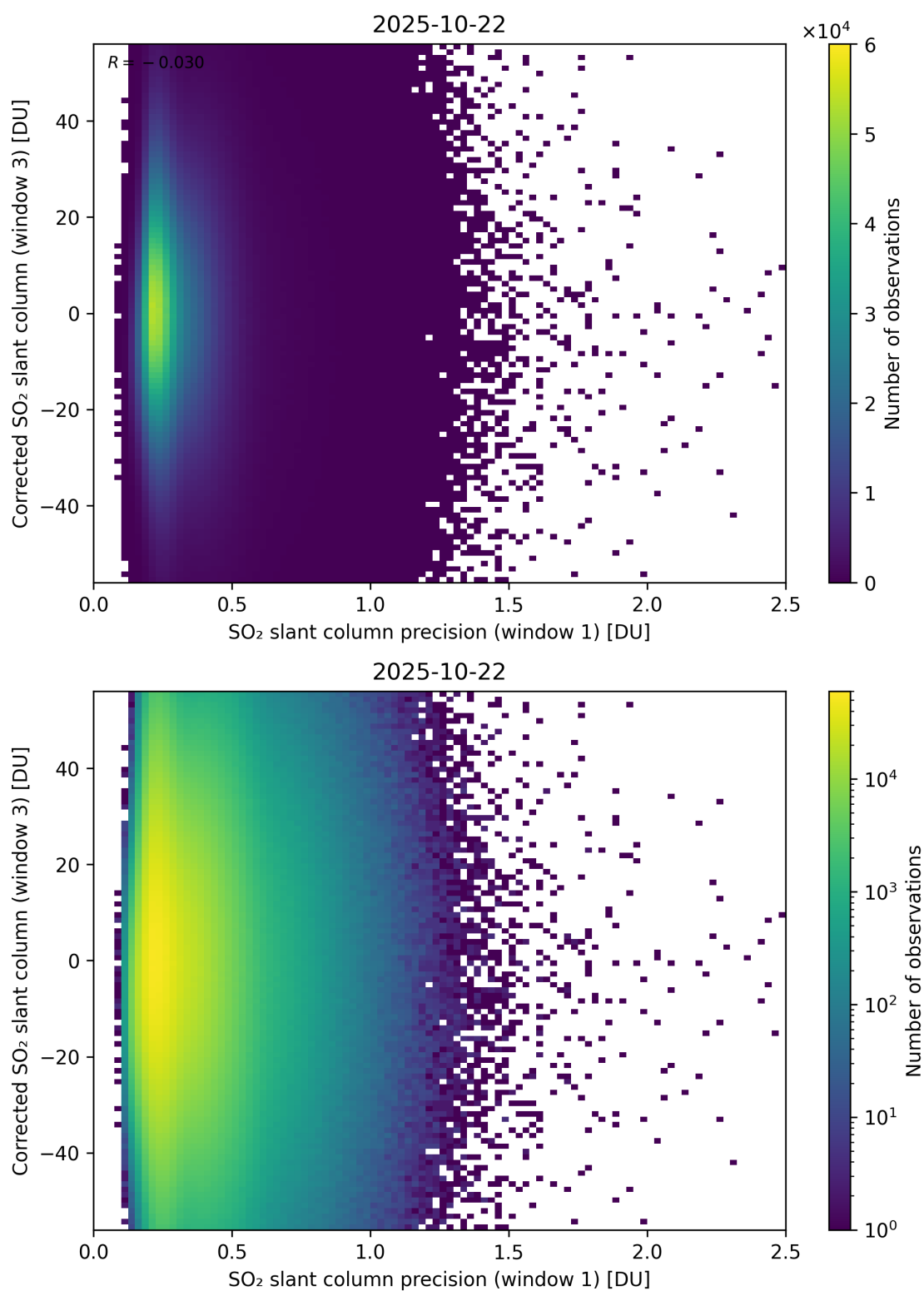
Figure 276: Scatter density plot of “SO 2 slant column precision (window 1)” against “Corrected SO 2 slant column (window 3)” for 2025-10-22 to 2025-10-23.
