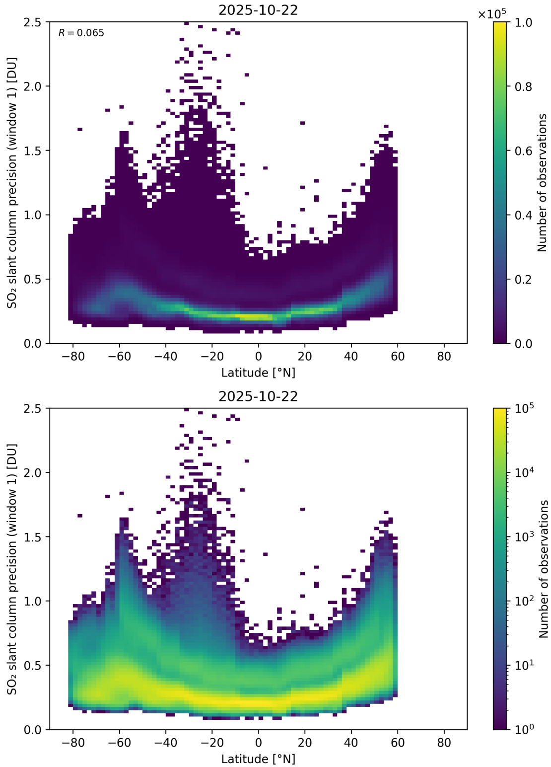
Figure 163: Scatter density plot of “Latitude” against “SO 2 slant column precision (window 1)” for 2025-10-22 to 2025-10-23.
