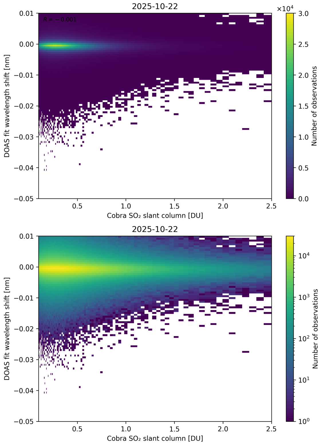
Figure 196: Scatter density plot of “Cobra SO 2 slant column” against “DOAS fit wavelength shift” for 2025-10-22 to 2025-10-23.
