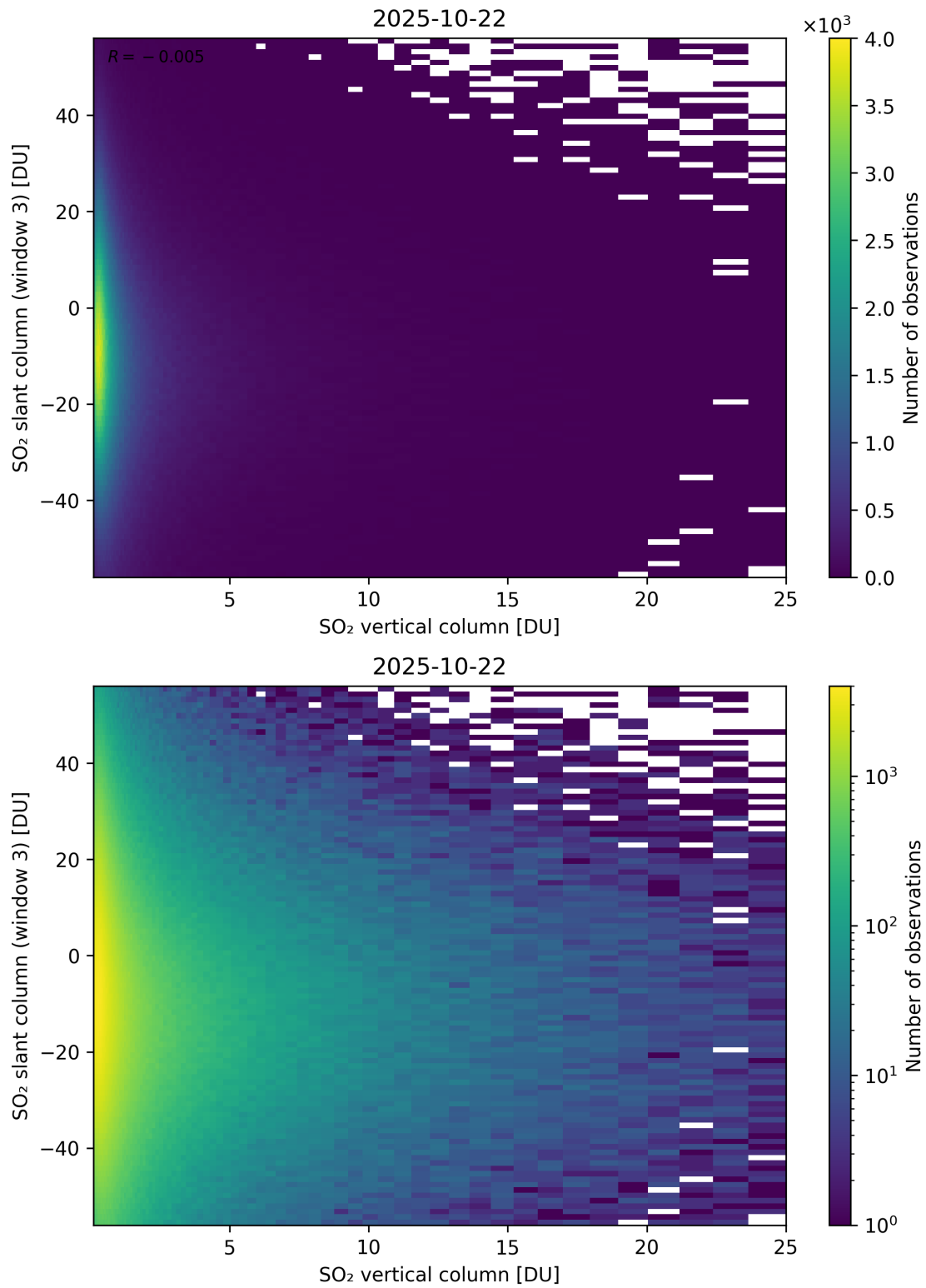
Figure 357: Scatter density plot of “SO 2 vertical column” against “SO 2 slant column (window 3)” for 2025-10-22 to 2025-10-23.
