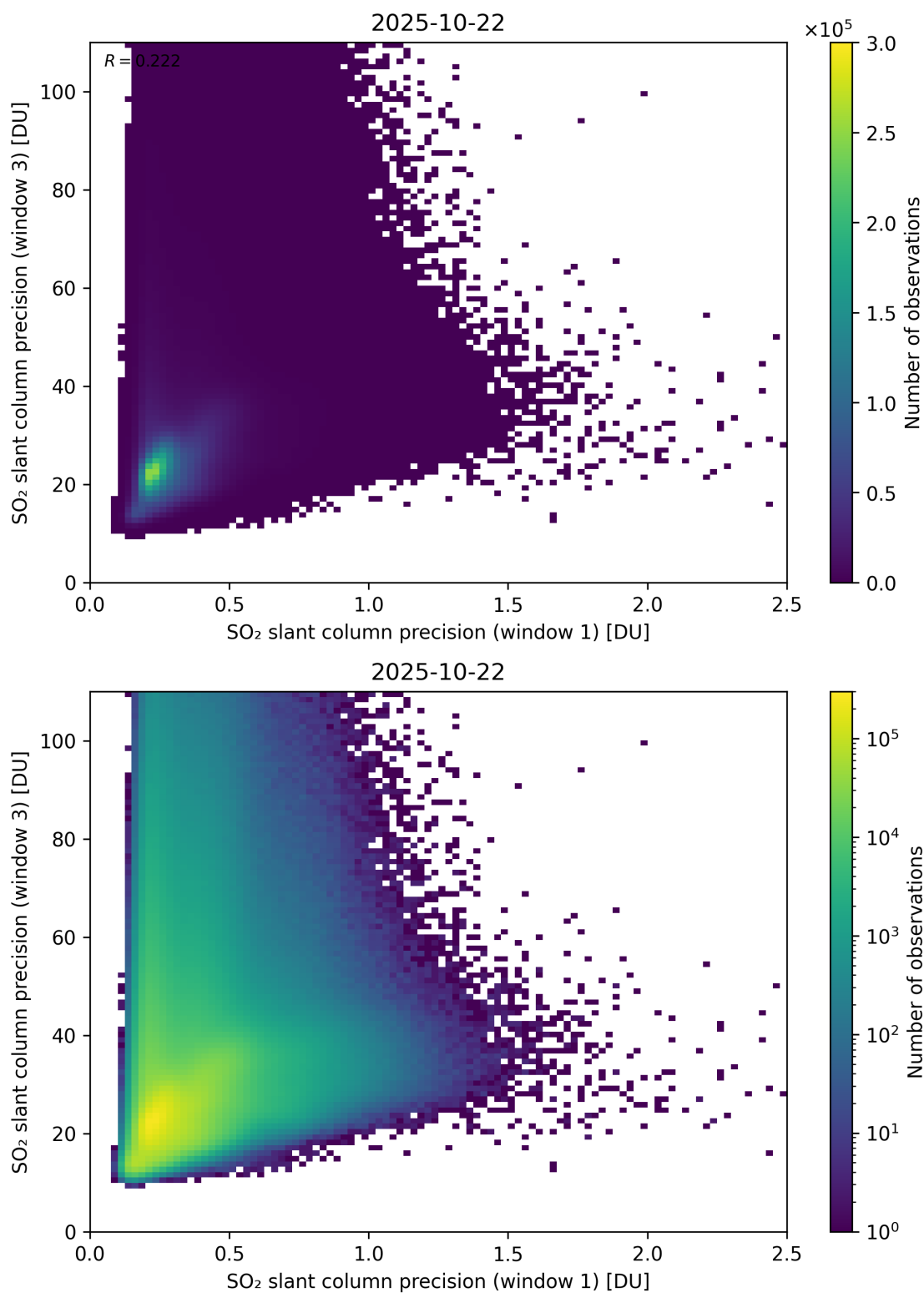
Figure 279: Scatter density plot of “SO 2 slant column precision (window 1)” against “SO 2 slant column precision (window 3)” for 2025-10-22 to 2025-10-23.
