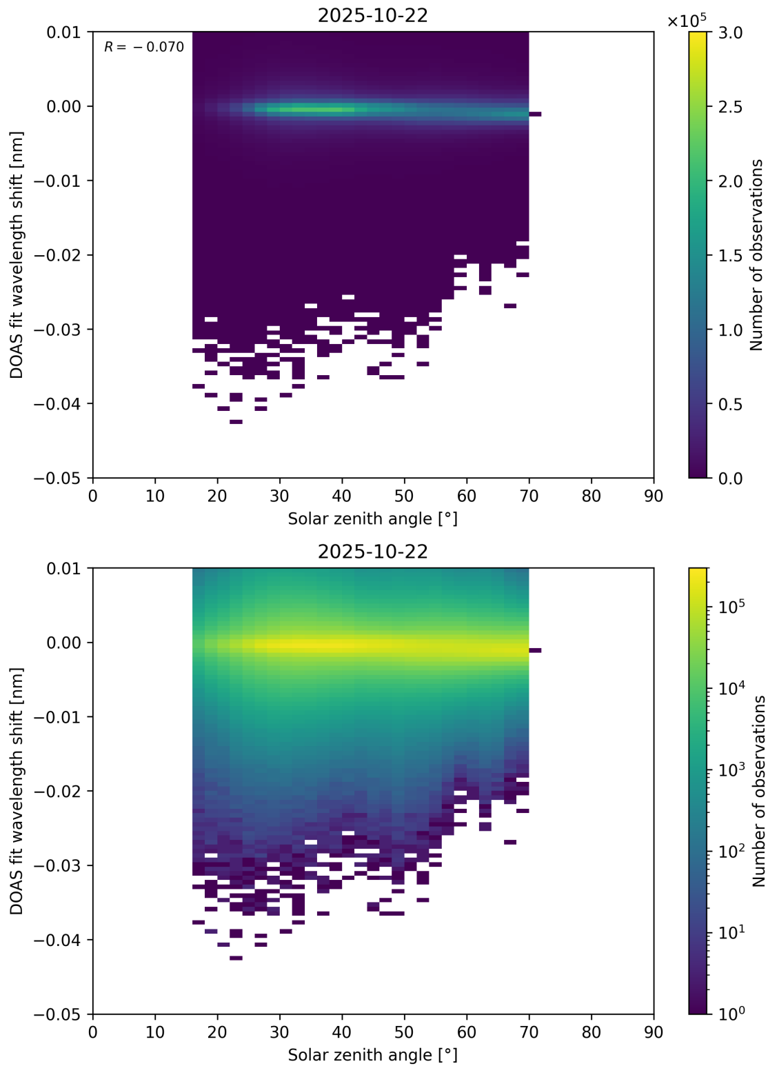
Figure 174: Scatter density plot of “Solar zenith angle” against “DOAS fit wavelength shift” for 2025-10-22 to 2025-10-23.
