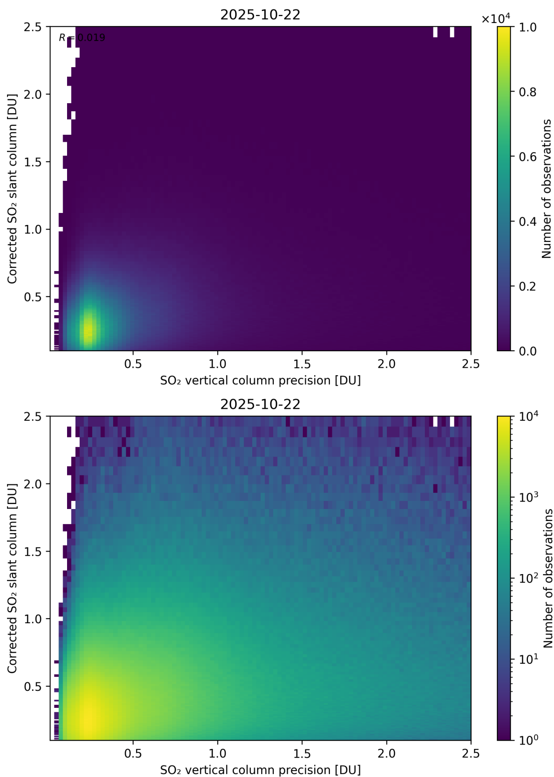
Figure 338: Scatter density plot of “SO 2 vertical column precision” against “Corrected SO 2 slant column” for 2025-10-22 to 2025-10-23.
