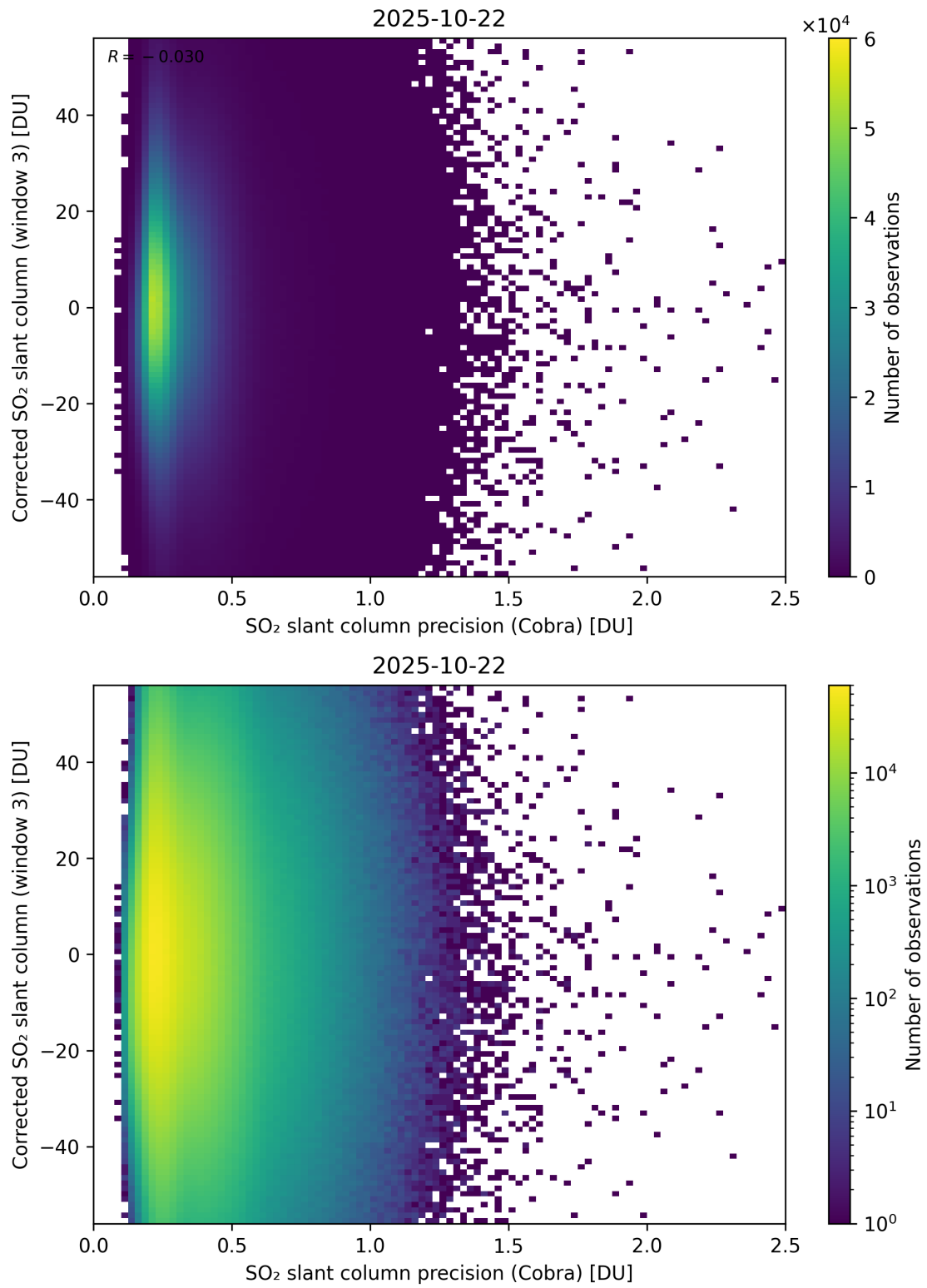
Figure 207: Scatter density plot of “SO 2 slant column precision (Cobra)” against “Corrected SO 2 slant column (window 3)” for 2025-10-22 to 2025-10-23.
