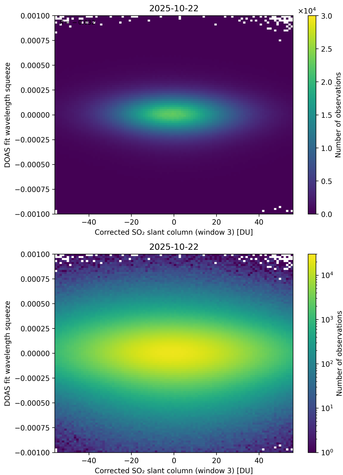
Figure 257: Scatter density plot of “Corrected SO 2 slant column (window 3)” against “DOAS fit wavelength squeeze” for 2025-10-22 to 2025-10-23.
