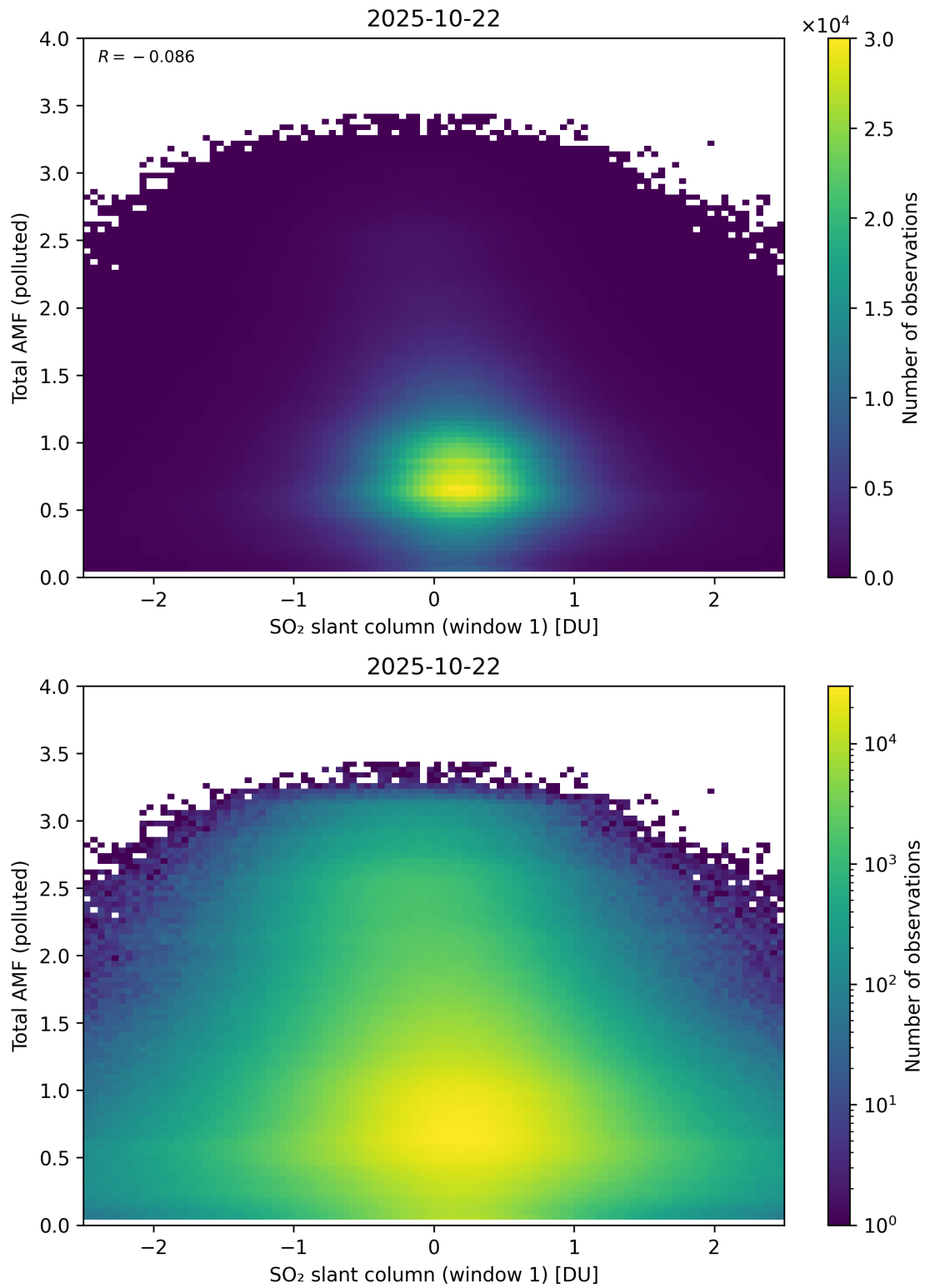
Figure 289: Scatter density plot of “SO 2 slant column (window 1)” against “Total AMF (polluted)” for 2025-10-22 to 2025-10-23.
