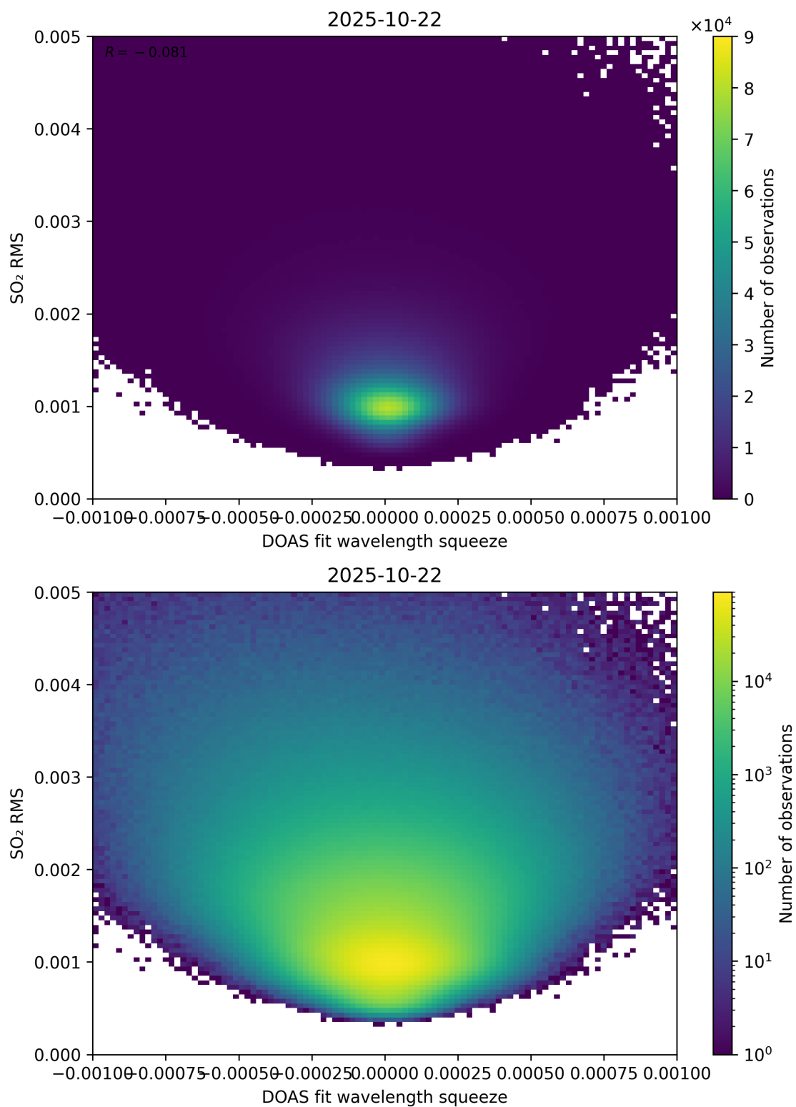
Figure 143: Scatter density plot of “DOAS fit wavelength squeeze” against “SO 2 RMS” for 2025-10-22 to 2025-10-23.
