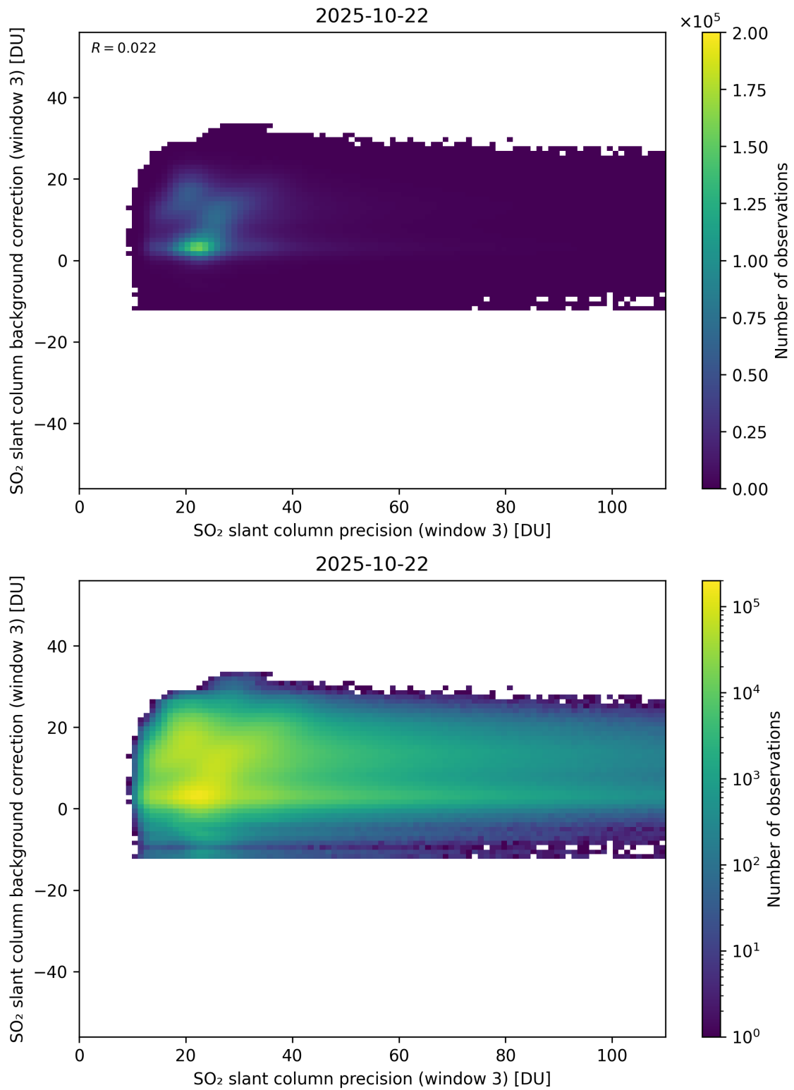
Figure 307: Scatter density plot of “SO 2 slant column precision (window 3)” against “SO 2 slant column background correction (window 3)” for 2025-10-22 to 2025-10-23.
