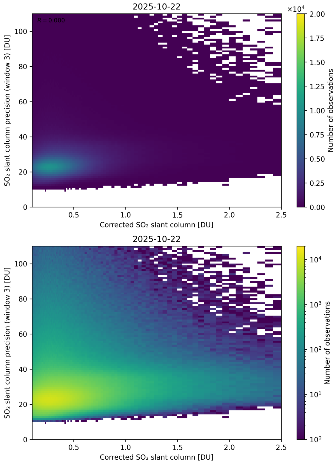
Figure 241: Scatter density plot of “Corrected SO 2 slant column” against “SO 2 slant column precision (window 3)” for 2025-10-22 to 2025-10-23.
