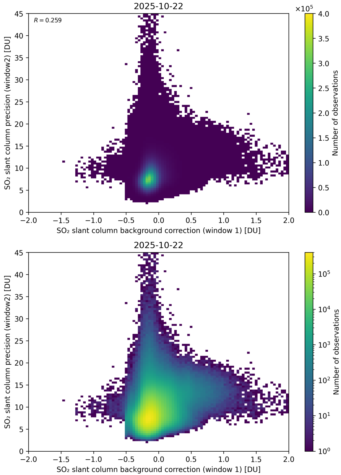
Figure 117: Scatter density plot of “SO 2 slant column background correction (window 1)” against “SO 2 slant column precision (window2)” for 2025-10-22 to 2025-10-23.
