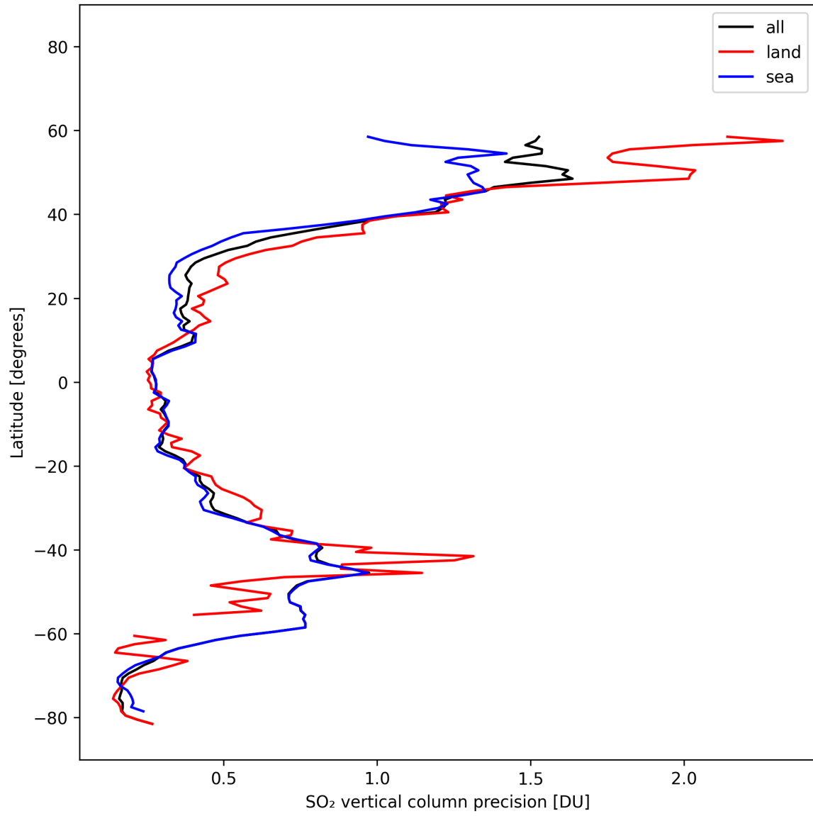
Figure 33: Zonal average of “SO 2 vertical column precision” for 2025-10-22 to 2025-10-23.
