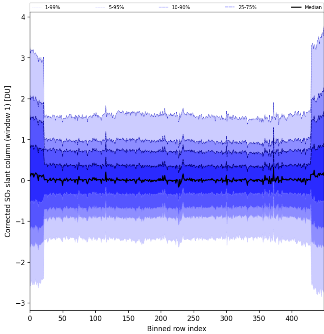
Figure 91: Along track statistics of “Corrected SO 2 slant column (window 1)” for 2025-10-22 to 2025-10-23
