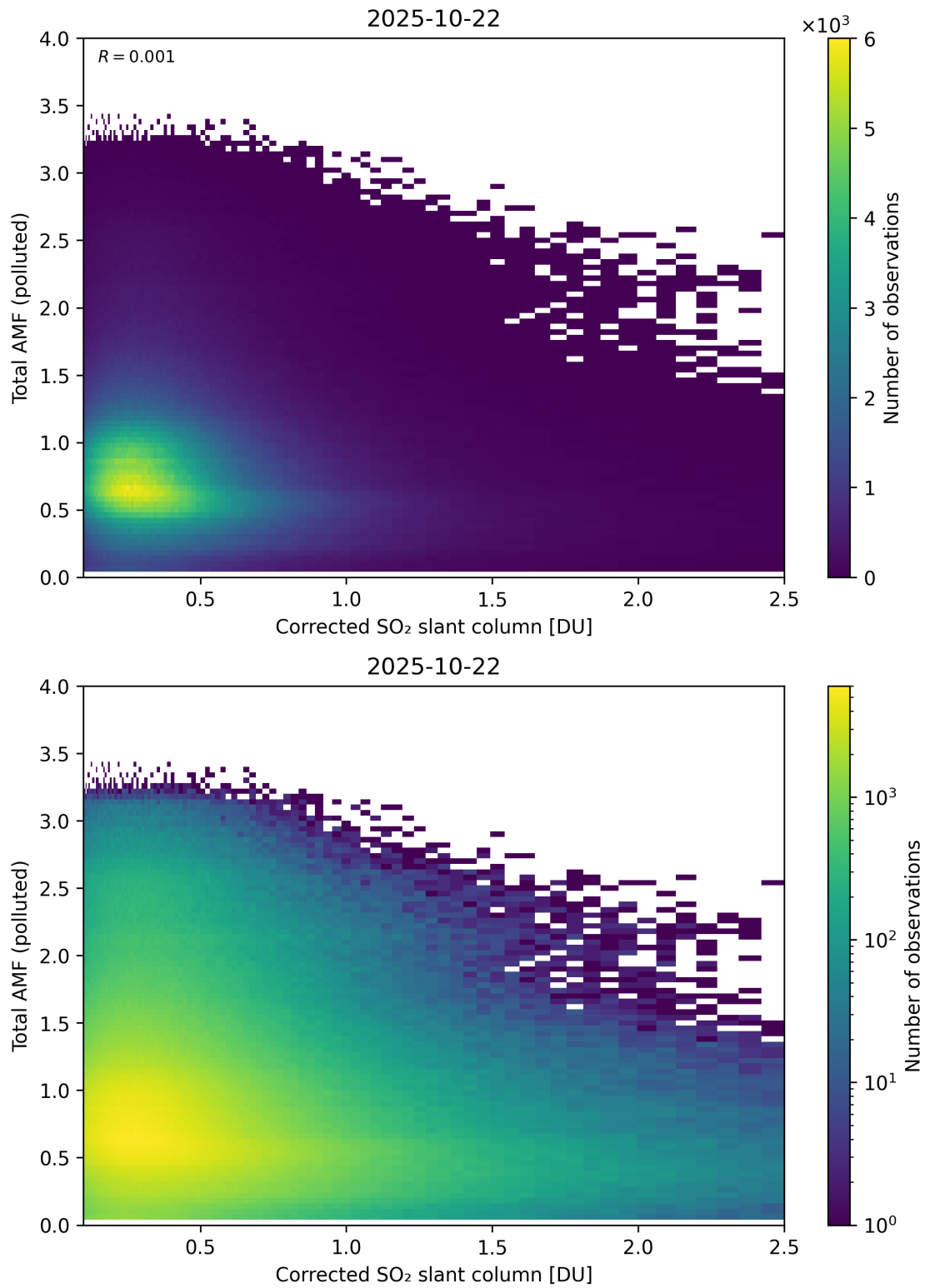
Figure 242: Scatter density plot of “Corrected SO 2 slant column” against “Total AMF (polluted)” for 2025-10-22 to 2025-10-23.
