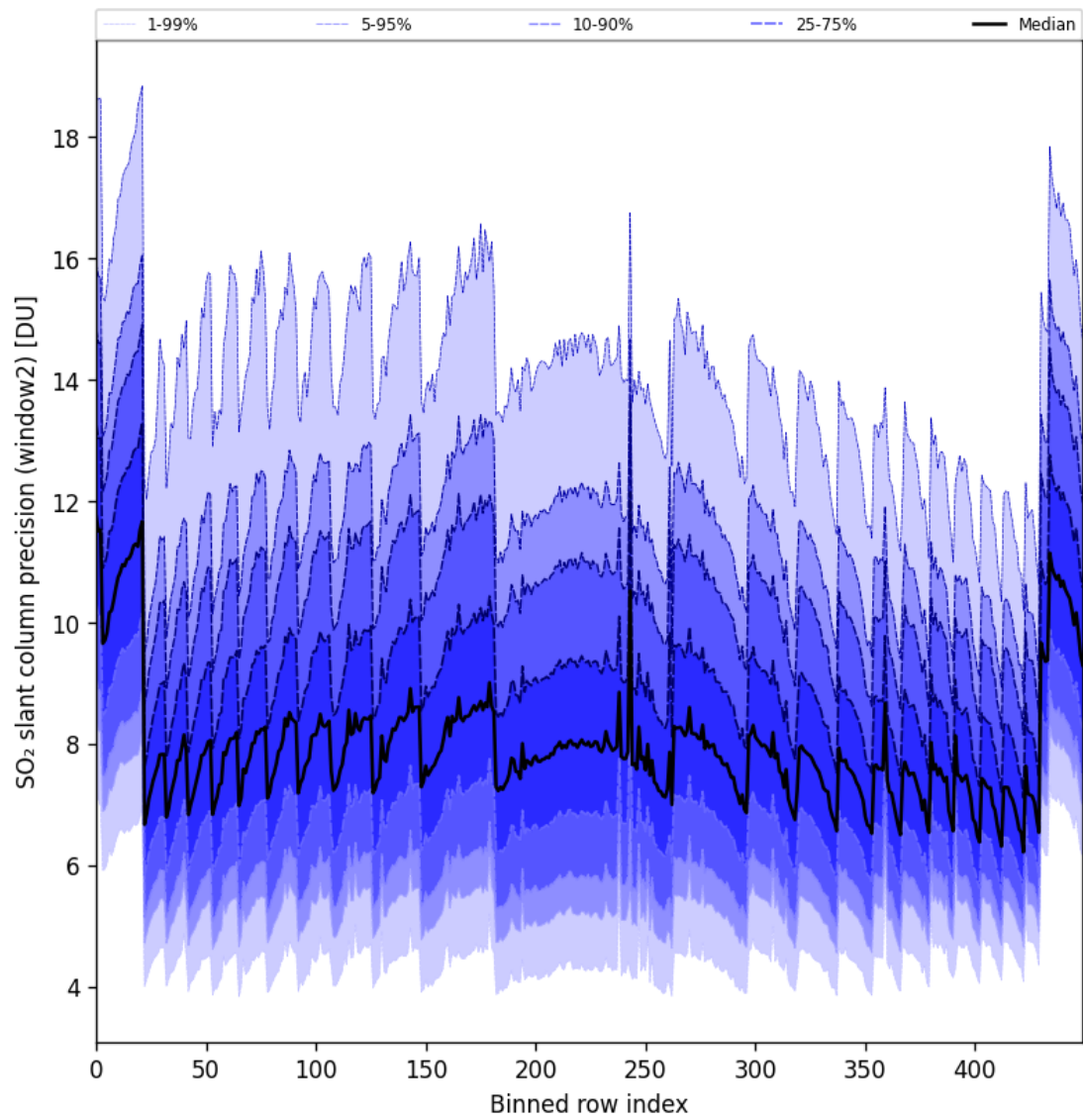
Figure 94: Along track statistics of “SO 2 slant column precision (window2)” for 2025-10-22 to 2025-10-23
