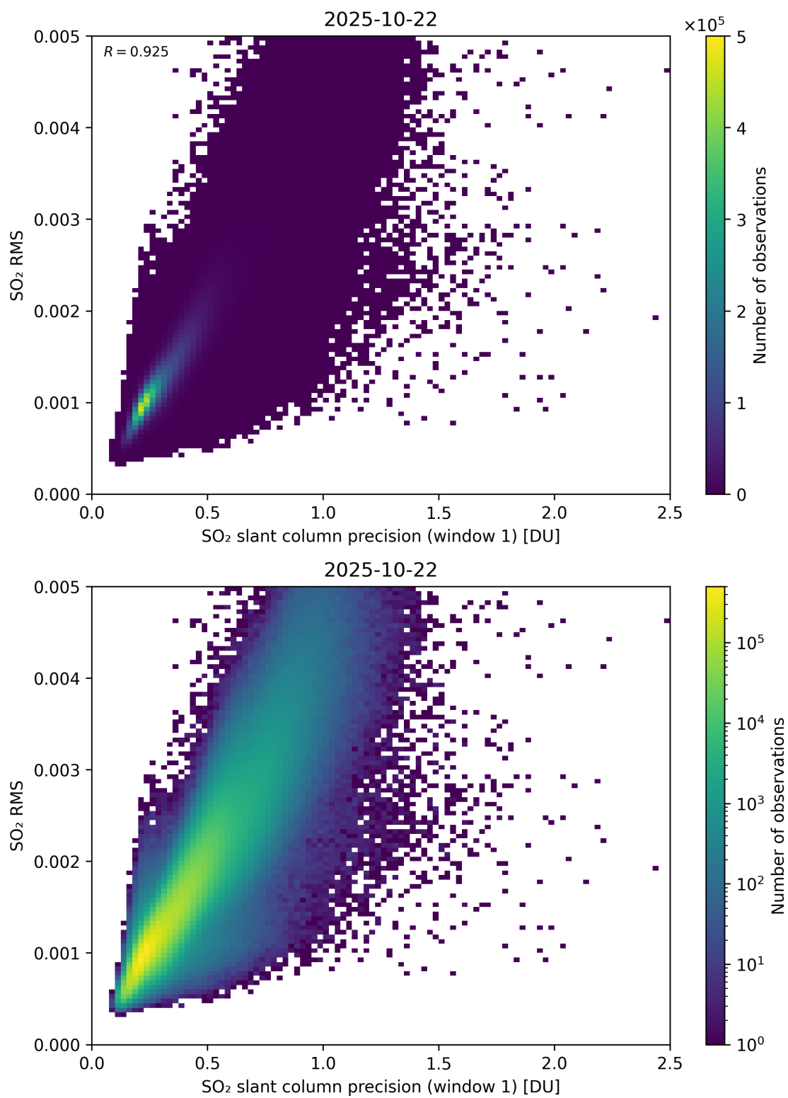
Figure 273: Scatter density plot of “SO 2 slant column precision (window 1)” against “SO 2 RMS” for 2025-10-22 to 2025-10-23.
