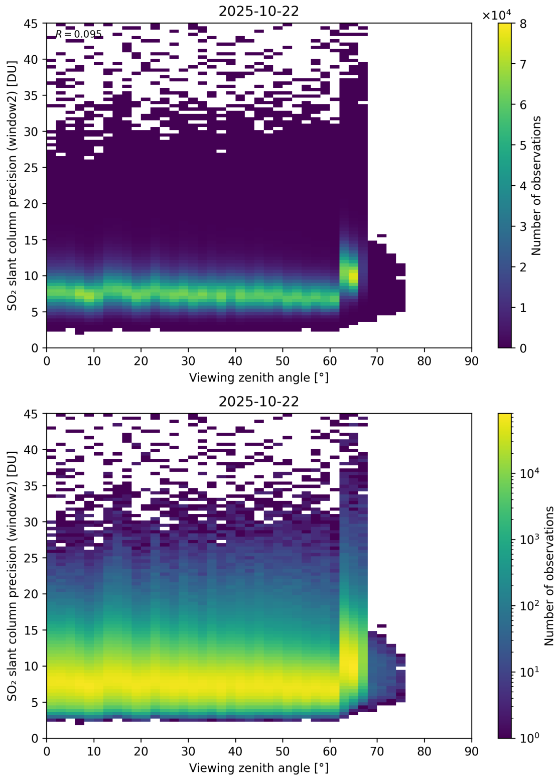
Figure 378: Scatter density plot of “Viewing zenith angle” against “SO 2 slant column precision (window2)” for 2025-10-22 to 2025-10-23.
