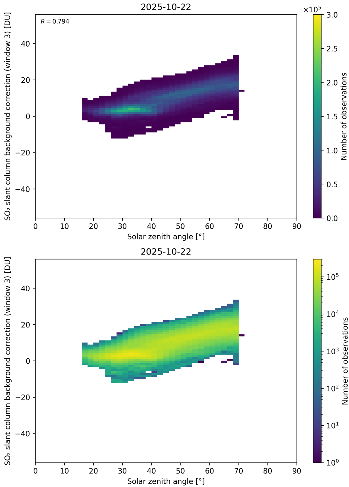
Figure 173: Scatter density plot of “Solar zenith angle” against “SO 2 slant column background correction (window 3)” for 2025-10-22 to 2025-10-23.
