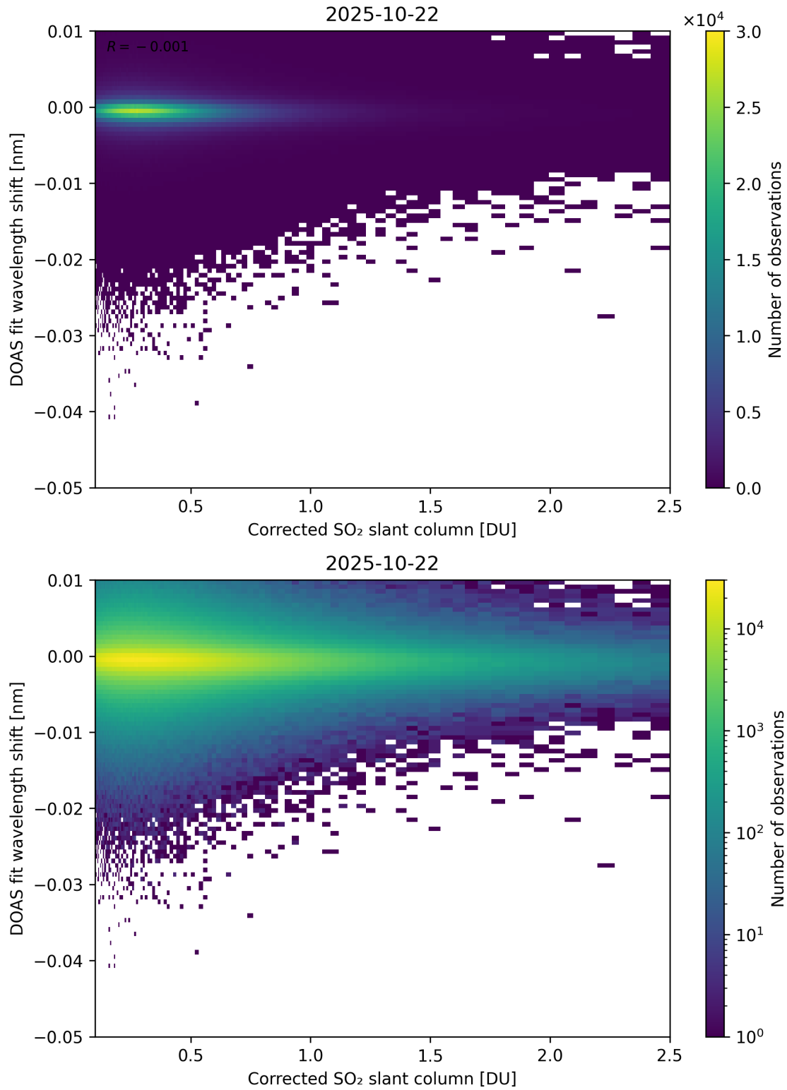
Figure 229: Scatter density plot of “Corrected SO 2 slant column” against “DOAS fit wavelength shift” for 2025-10-22 to 2025-10-23.
