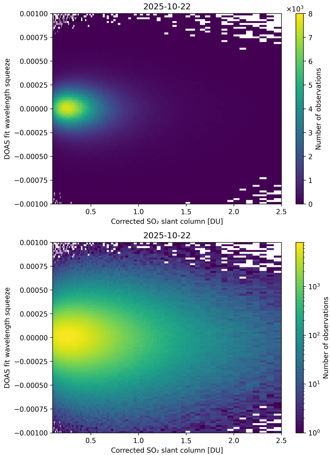
Figure 230: Scatter density plot of “Corrected SO 2 slant column” against “DOAS fit wavelength squeeze” for 2025-10-22 to 2025-10-23.
