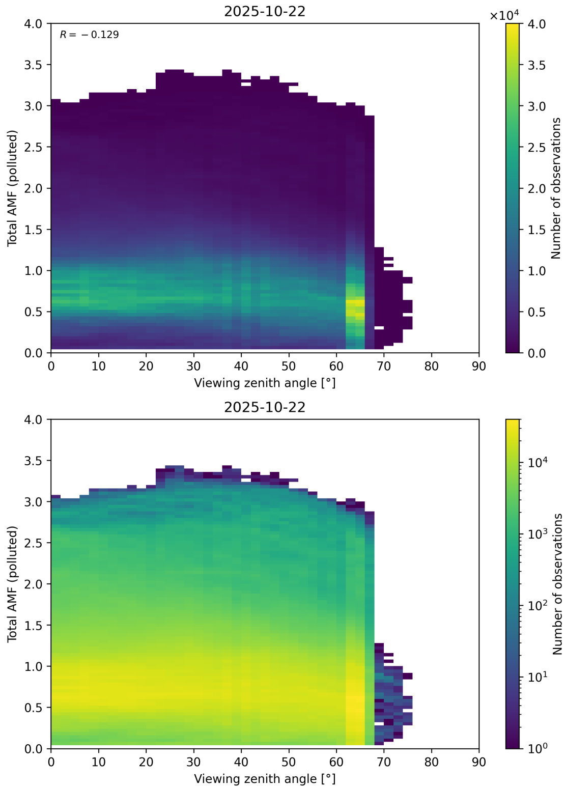
Figure 381: Scatter density plot of “Viewing zenith angle” against “Total AMF (polluted)” for 2025-10-22 to 2025-10-23.
