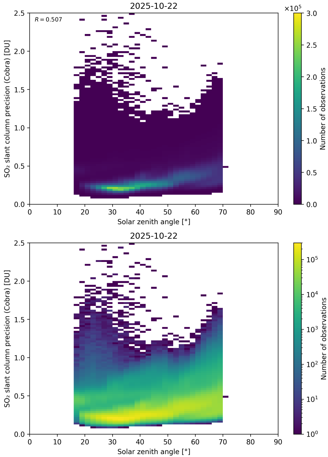
Figure 180: Scatter density plot of “Solar zenith angle” against “SO 2 slant column precision (Cobra)” for 2025-10-22 to 2025-10-23.
