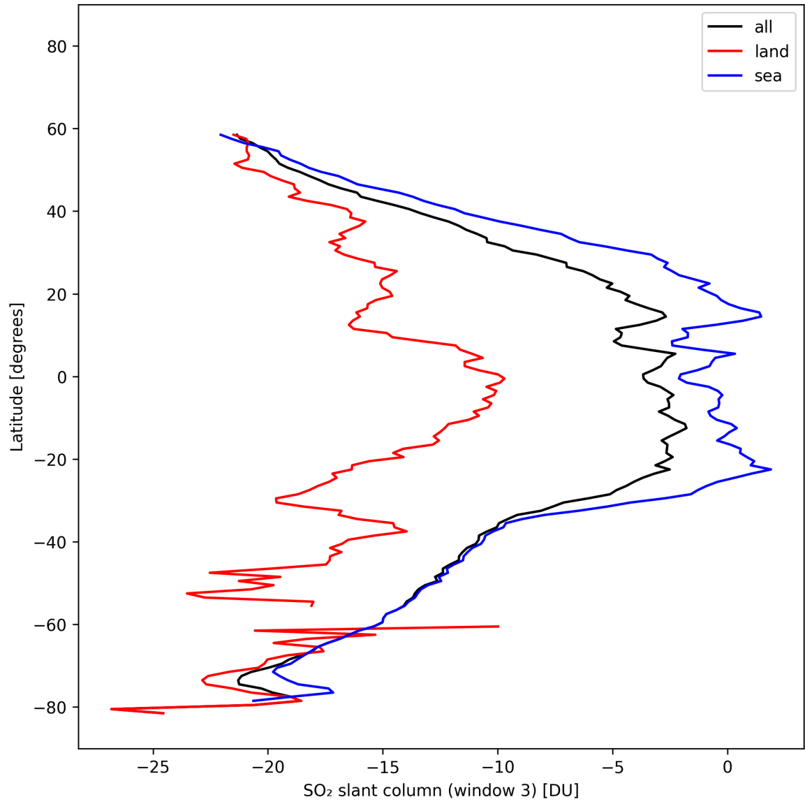
Figure 45: Zonal average of “SO 2 slant column (window 3)” for 2025-10-22 to 2025-10-23.
