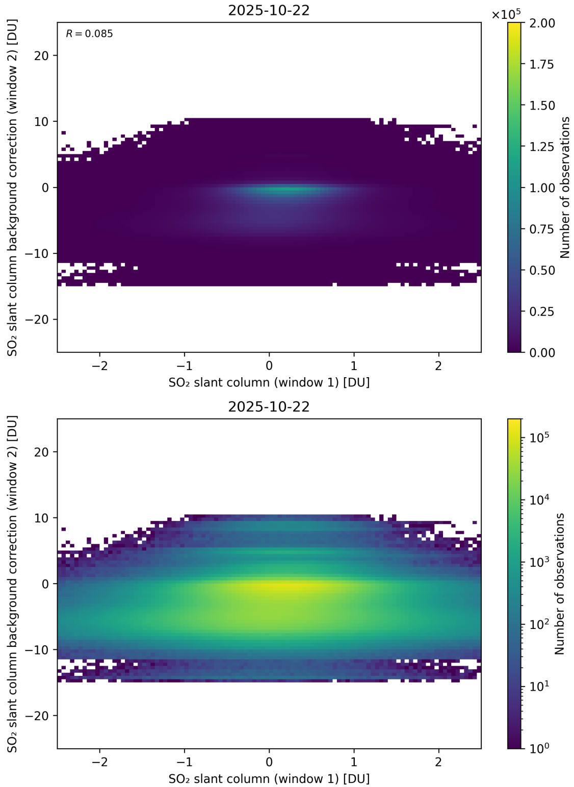
Figure 263: Scatter density plot of “SO 2 slant column (window 1)” against “SO 2 slant column background correction (window 2)” for 2025-10-22 to 2025-10-23.
