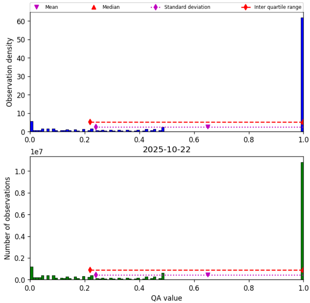
Figure 57: Histogram of “QA value” for 2025-10-22 to 2025-10-23
