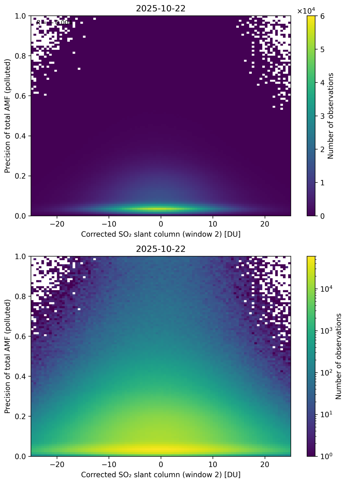
Figure 254: Scatter density plot of “Corrected SO 2 slant column (window 2)” against “Precision of total AMF (polluted)” for 2025-10-22 to 2025-10-23.
