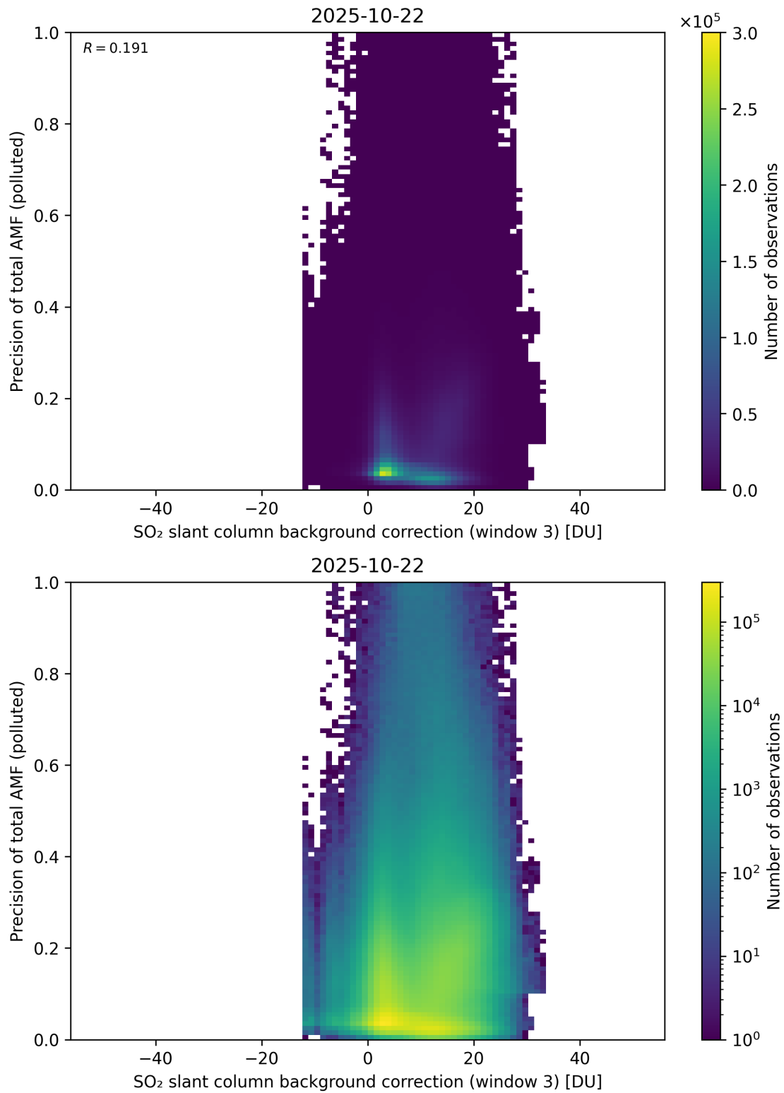
Figure 137: Scatter density plot of “SO 2 slant column background correction (window 3)” against “Precision of total AMF (polluted)” for 2025-10-22 to 2025-10-23.
