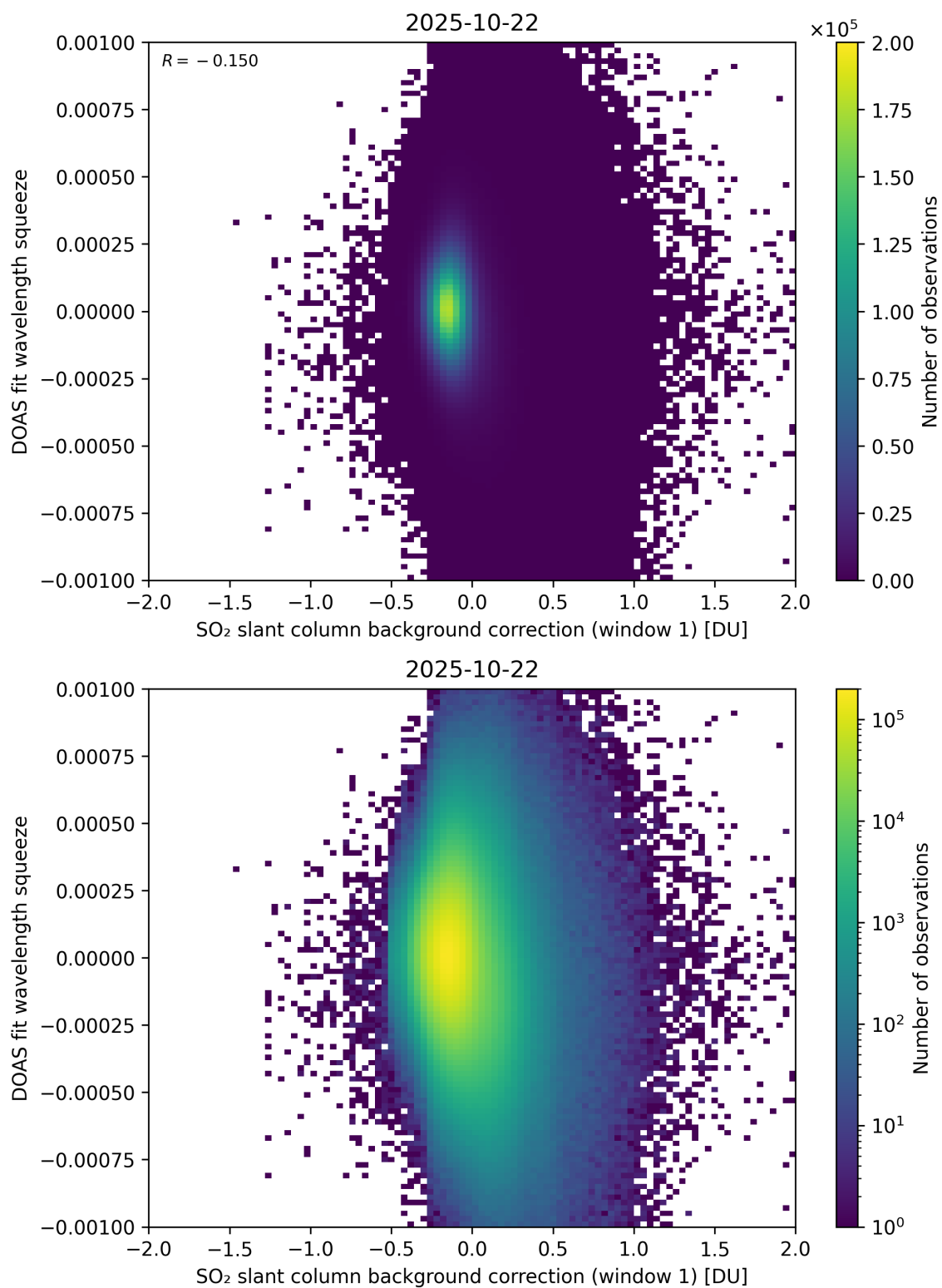
Figure 112: Scatter density plot of “SO 2 slant column background correction (window 1)” against “DOAS fit wavelength squeeze” for 2025-10-22 to 2025-10-23.
