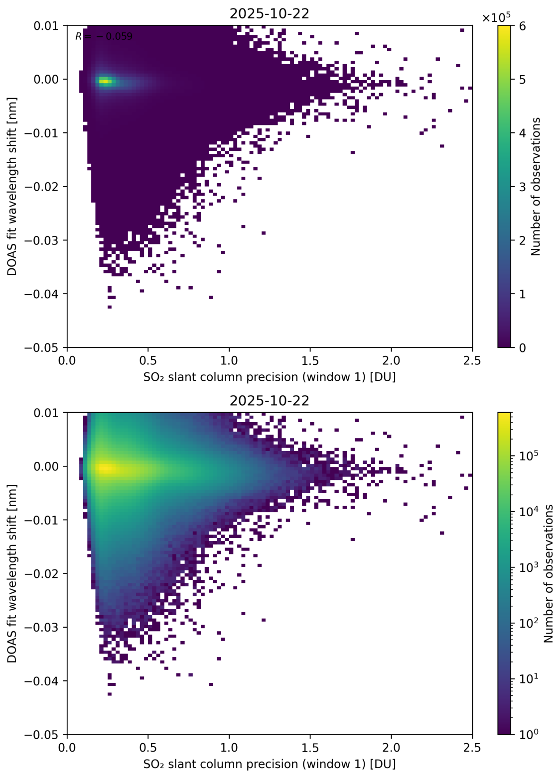
Figure 271: Scatter density plot of “SO 2 slant column precision (window 1)” against “DOAS fit wavelength shift” for 2025-10-22 to 2025-10-23.
