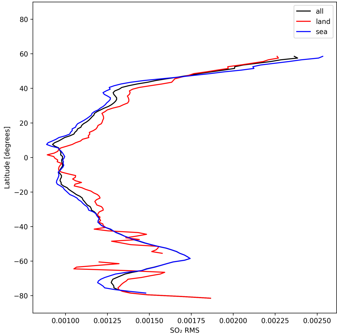
Figure 52: Zonal average of “SO 2 RMS” for 2025-10-22 to 2025-10-23.
