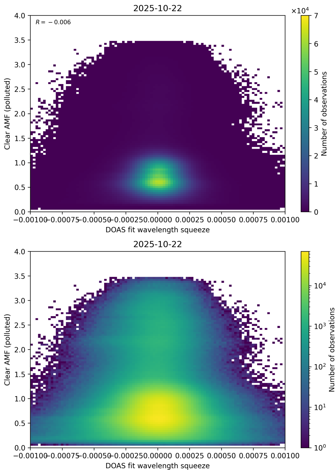
Figure 144: Scatter density plot of “DOAS fit wavelength squeeze” against “Clear AMF (polluted)” for 2025-10-22 to 2025-10-23.
