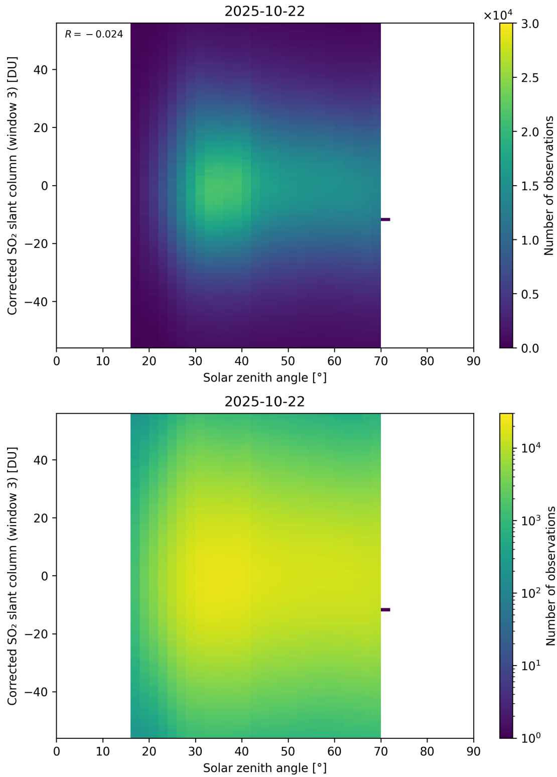
Figure 183: Scatter density plot of “Solar zenith angle” against “Corrected SO 2 slant column (window 3)” for 2025-10-22 to 2025-10-23.
