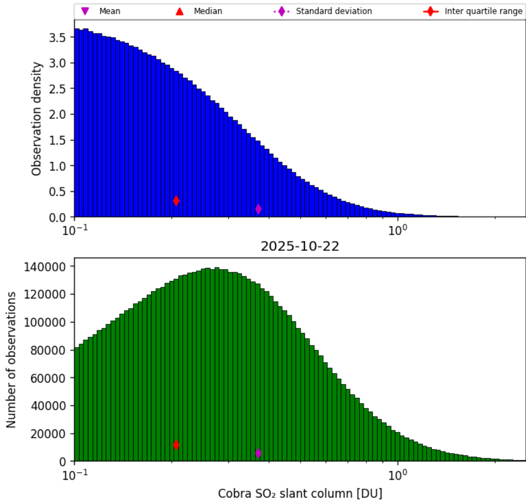
Figure 61: Histogram of “Cobra SO 2 slant column” for 2025-10-22 to 2025-10-23
