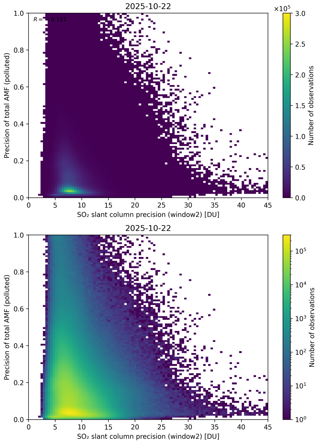
Figure 302: Scatter density plot of “SO 2 slant column precision (window2)” against “Precision of total AMF (polluted)” for 2025-10-22 to 2025-10-23.
