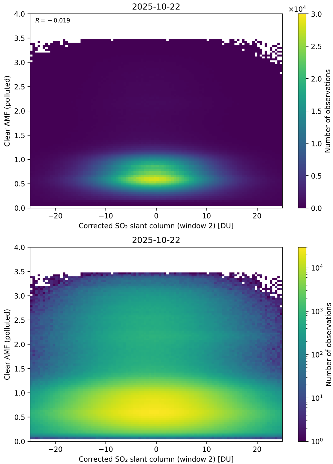
Figure 249: Scatter density plot of “Corrected SO 2 slant column (window 2)” against “Clear AMF (polluted)” for 2025-10-22 to 2025-10-23.
