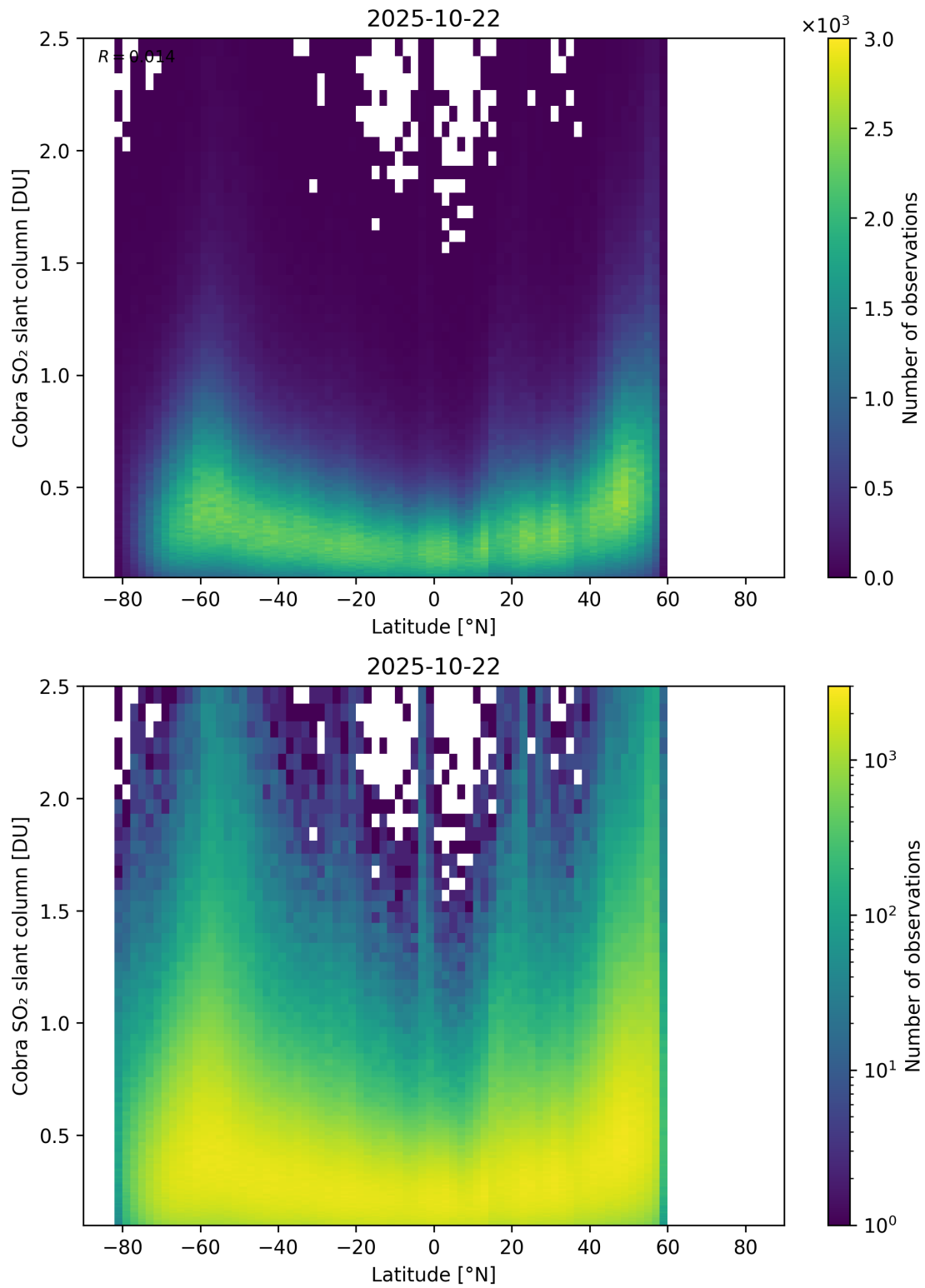
Figure 157: Scatter density plot of “Latitude” against “Cobra SO 2 slant column” for 2025-10-22 to 2025-10-23.
