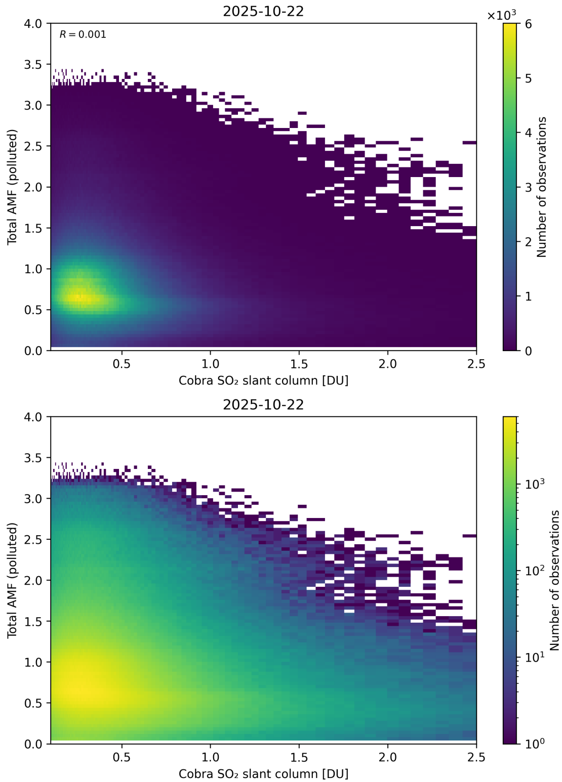
Figure 224: Scatter density plot of “Cobra SO 2 slant column” against “Total AMF (polluted)” for 2025-10-22 to 2025-10-23.
