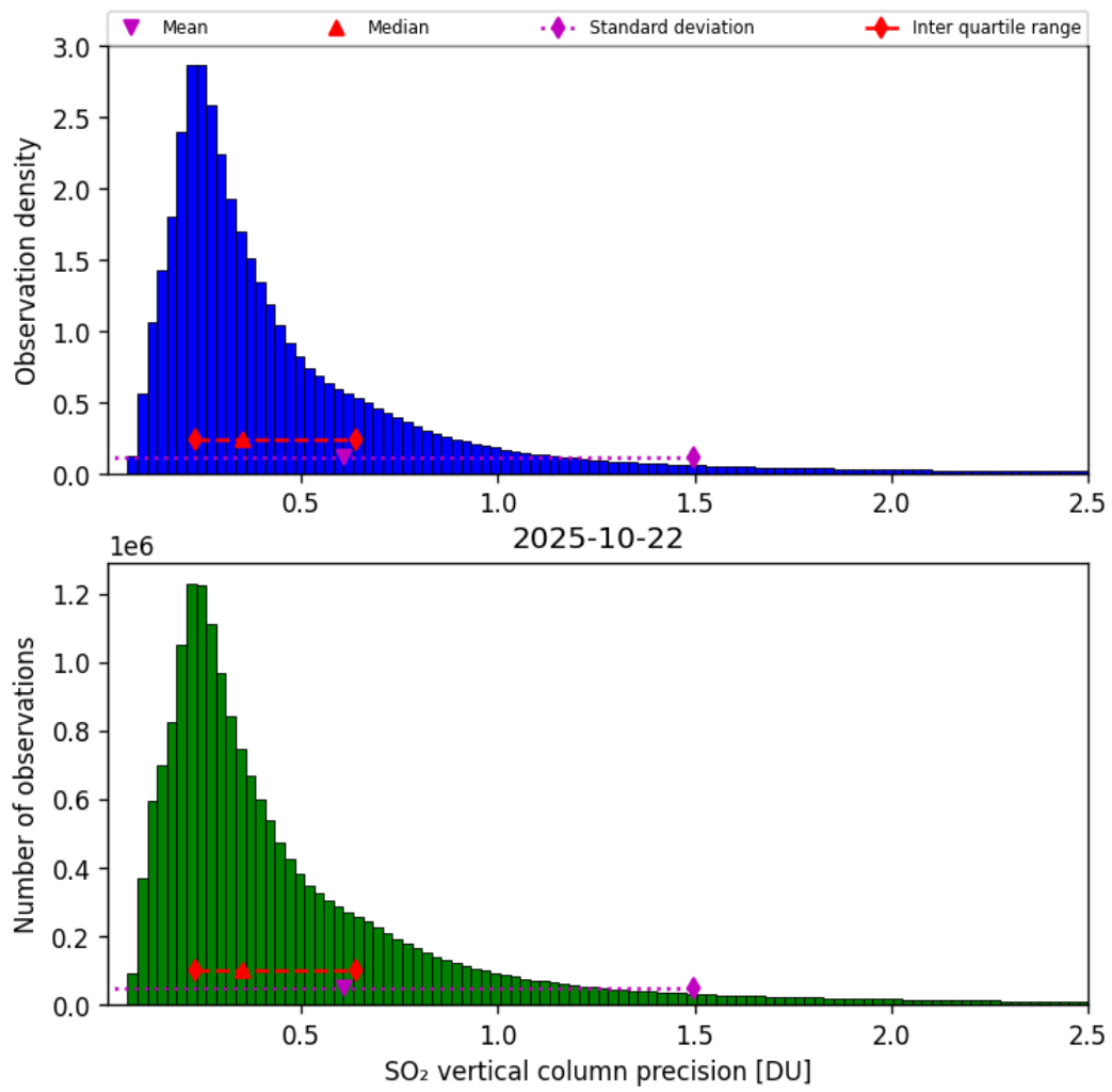
Figure 59: Histogram of “SO 2 vertical column precision” for 2025-10-22 to 2025-10-23
