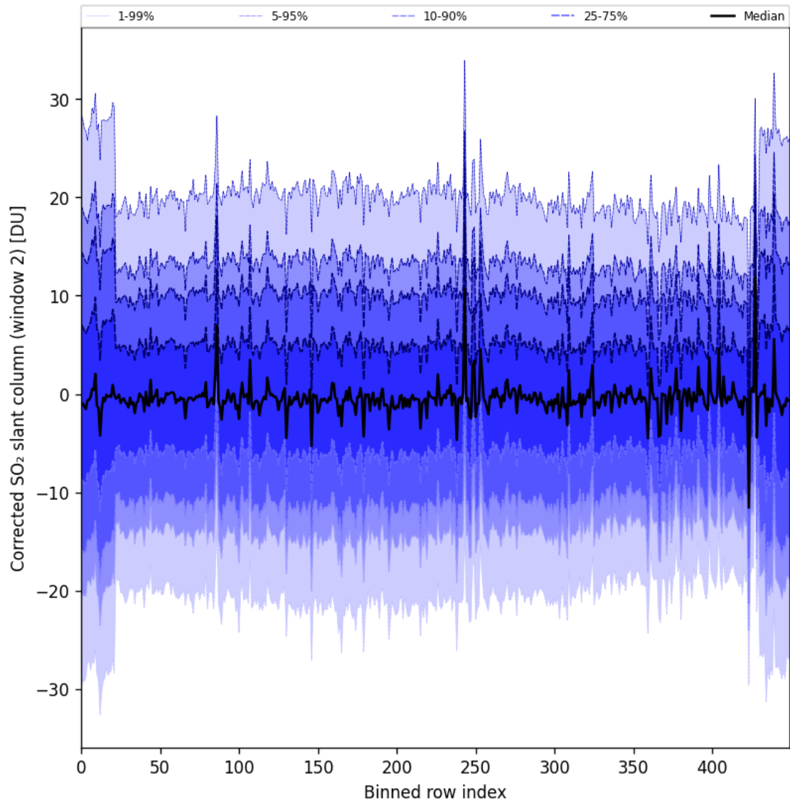
Figure 95: Along track statistics of “Corrected SO 2 slant column (window 2)” for 2025-10-22 to 2025-10-23
