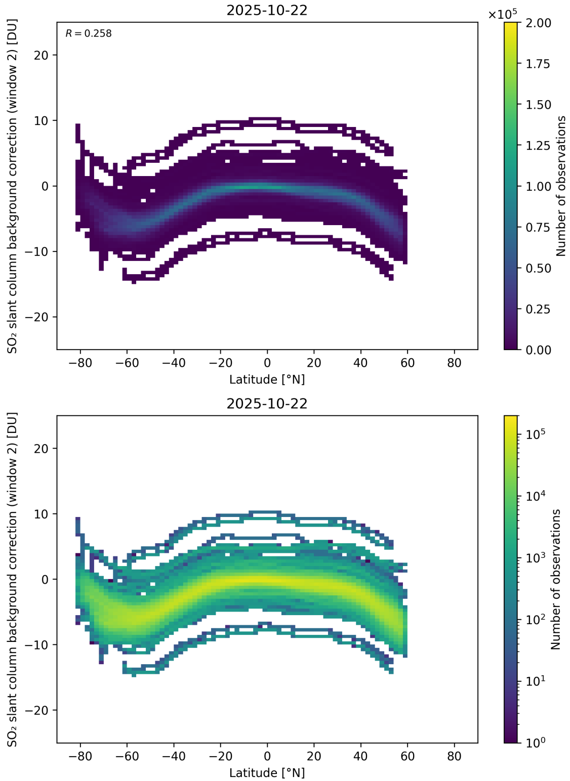
Figure 151: Scatter density plot of “Latitude” against “SO 2 slant column background correction (window 2)” for 2025-10-22 to 2025-10-23.
