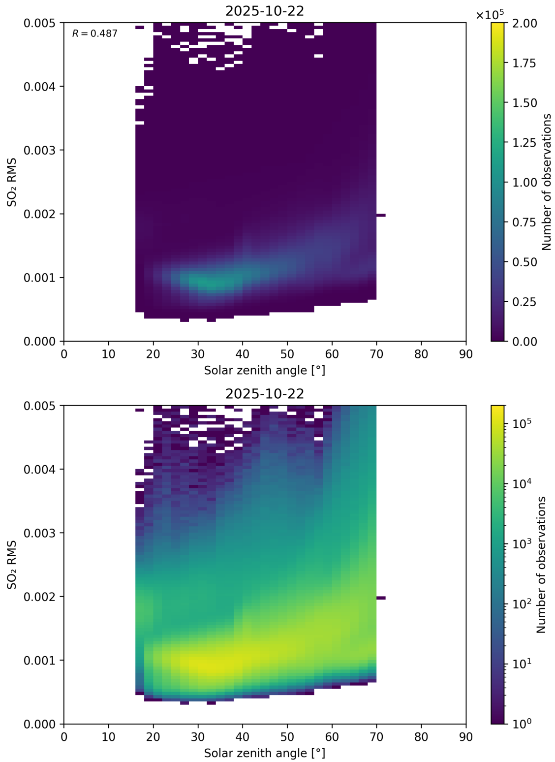
Figure 176: Scatter density plot of “Solar zenith angle” against “SO 2 RMS” for 2025-10-22 to 2025-10-23.
