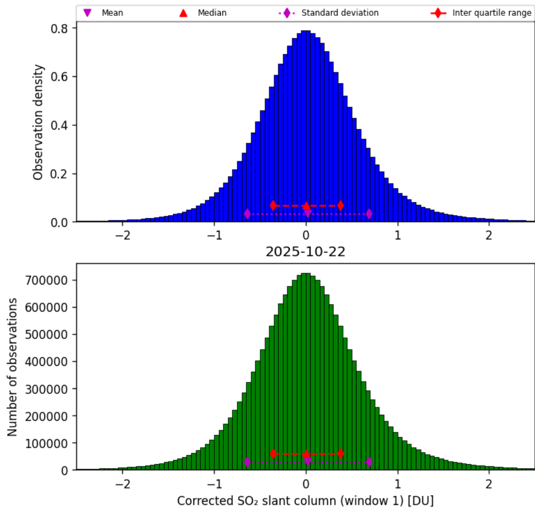
Figure 65: Histogram of “Corrected SO 2 slant column (window 1)” for 2025-10-22 to 2025-10-23
