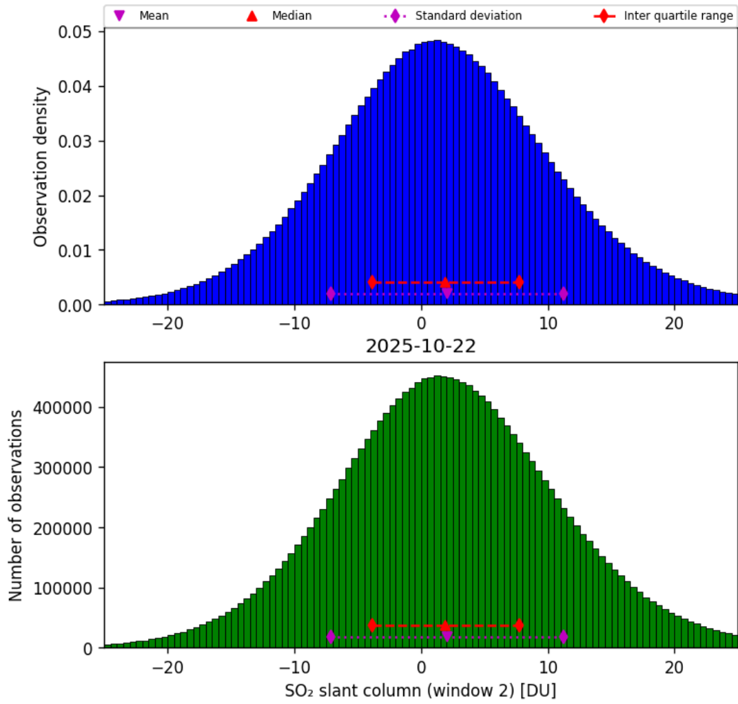
Figure 67: Histogram of “SO 2 slant column (window 2)” for 2025-10-22 to 2025-10-23
