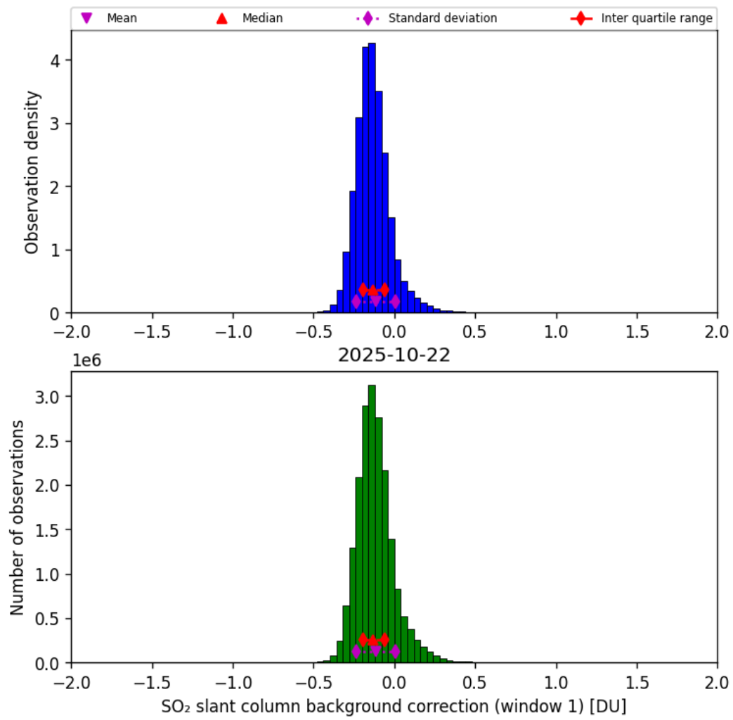
Figure 66: Histogram of “SO 2 slant column background correction (window 1)” for 2025-10-22 to 2025-10-23
