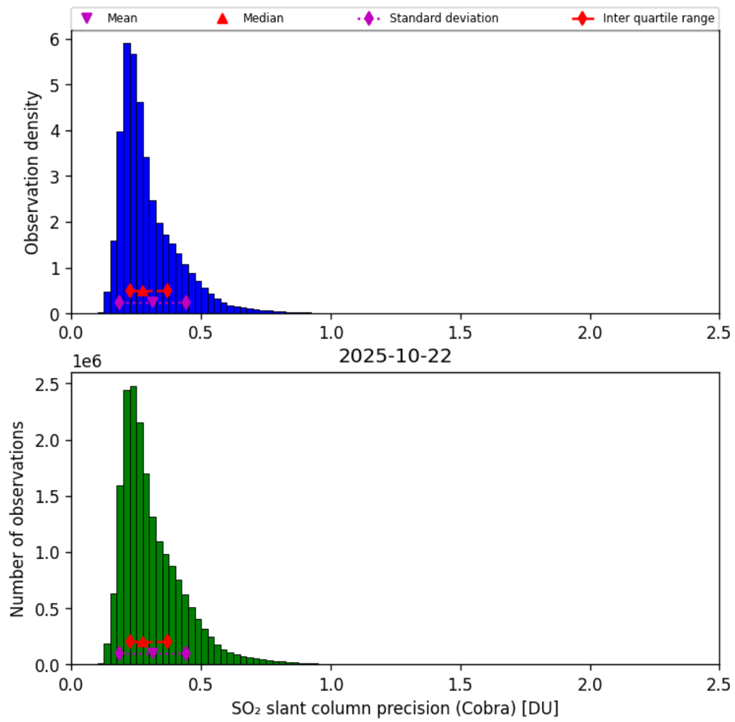
Figure 62: Histogram of “SO 2 slant column precision (Cobra)” for 2025-10-22 to 2025-10-23
