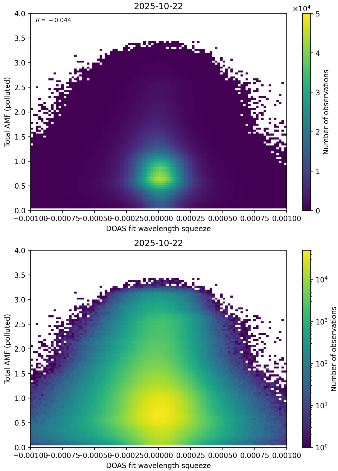
Figure 145: Scatter density plot of “DOAS fit wavelength squeeze” against “Total AMF (polluted)” for 2025-10-22 to 2025-10-23.
