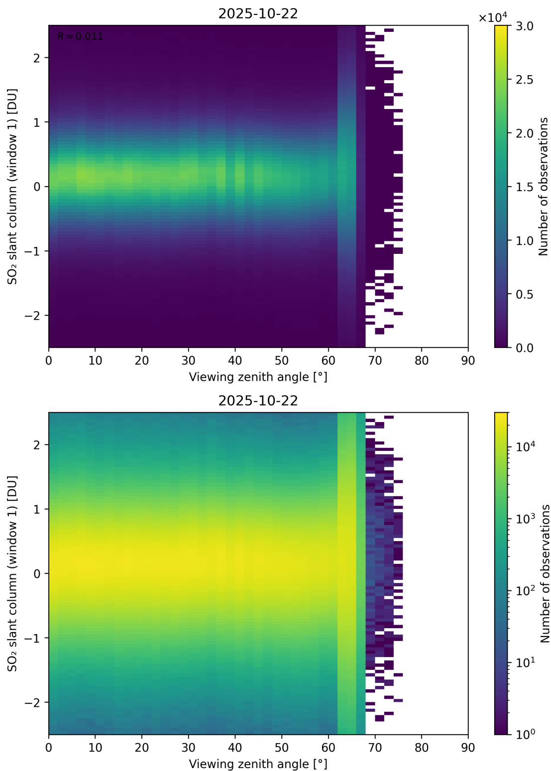
Figure 376: Scatter density plot of “Viewing zenith angle” against “SO 2 slant column (window 1)” for 2025-10-22 to 2025-10-23.
