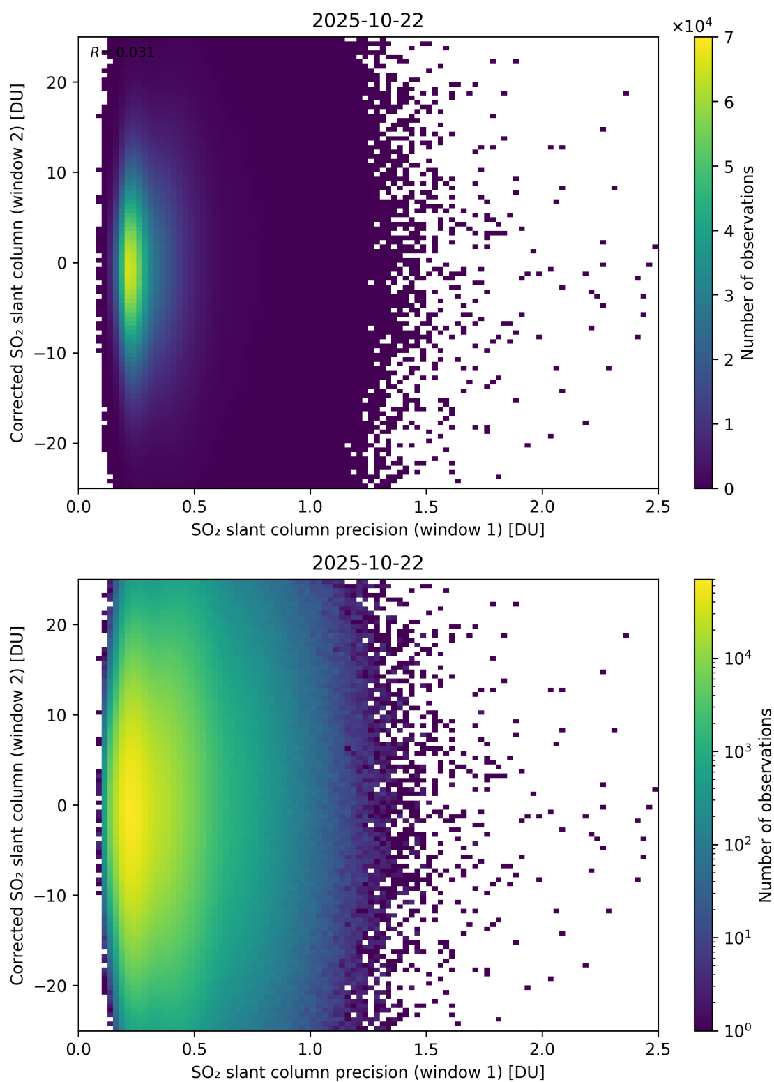
Figure 275: Scatter density plot of “SO 2 slant column precision (window 1)” against “Corrected SO 2 slant column (window 2)” for 2025-10-22 to 2025-10-23.
