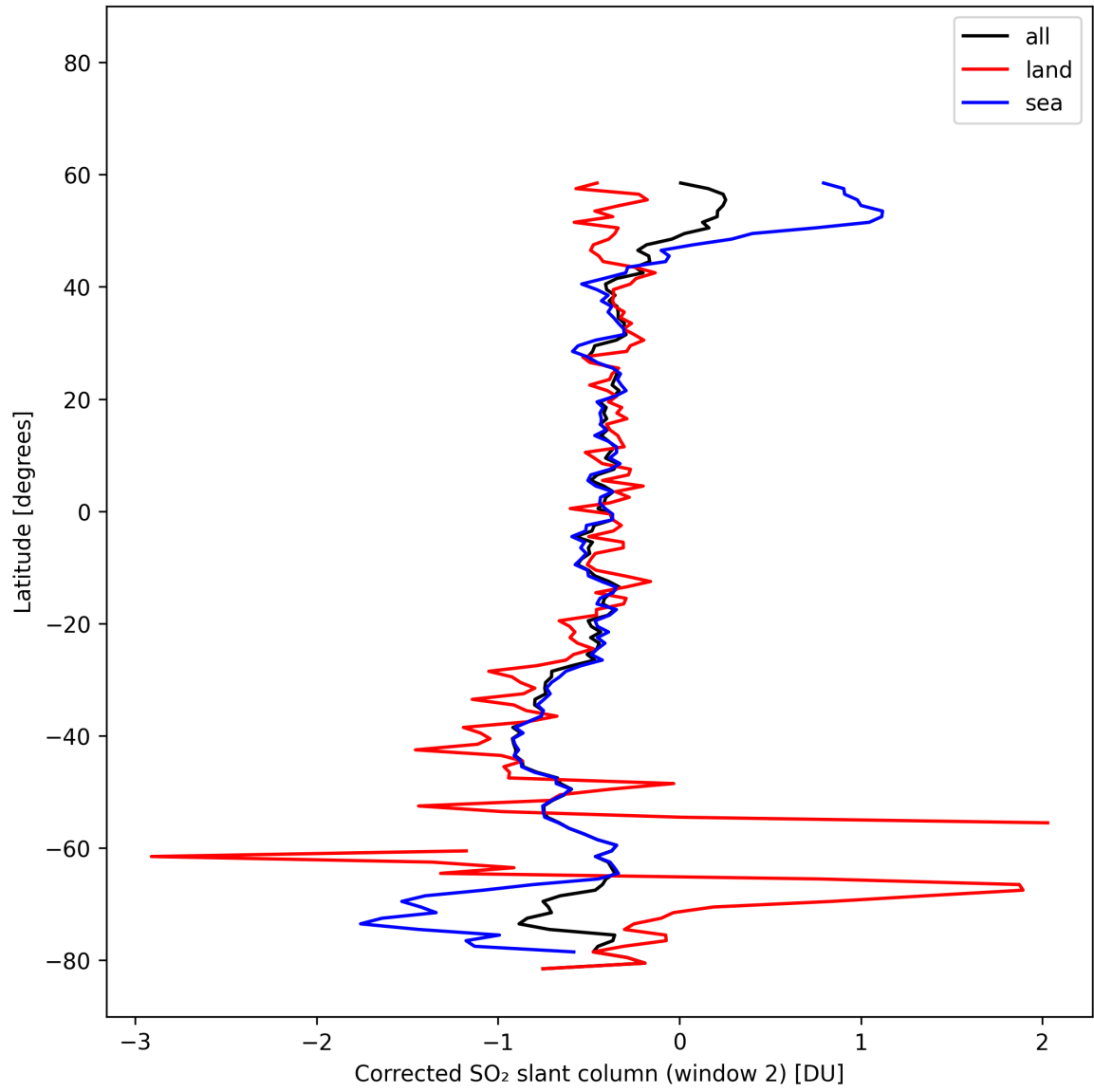
Figure 43: Zonal average of “Corrected SO 2 slant column (window 2)” for 2025-10-22 to 2025-10-23.
