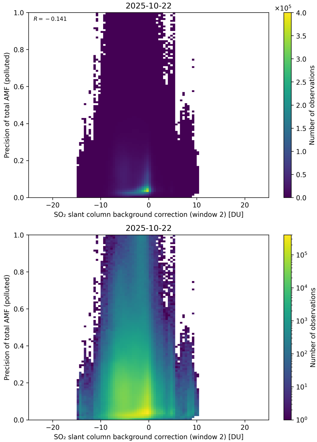
Figure 131: Scatter density plot of “SO 2 slant column background correction (window 2)” against “Precision of total AMF (polluted)” for 2025-10-22 to 2025-10-23.
