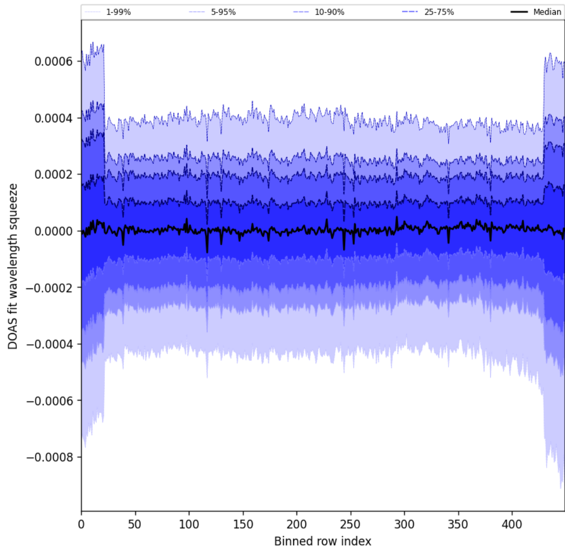
Figure 103: Along track statistics of “DOAS fit wavelength squeeze” for 2025-10-22 to 2025-10-23
