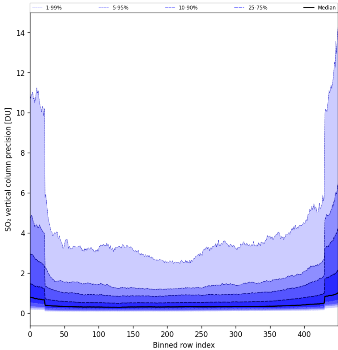
Figure 85: Along track statistics of “SO 2 vertical column precision” for 2025-10-22 to 2025-10-23
