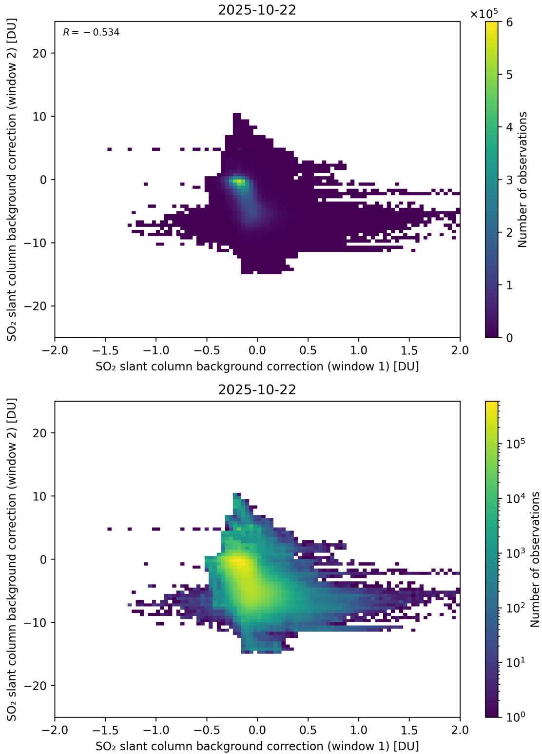
Figure 109: Scatter density plot of “SO 2 slant column background correction (window 1)” against “SO 2 slant column background correction (window 2)” for 2025-10-22 to 2025-10-23.
