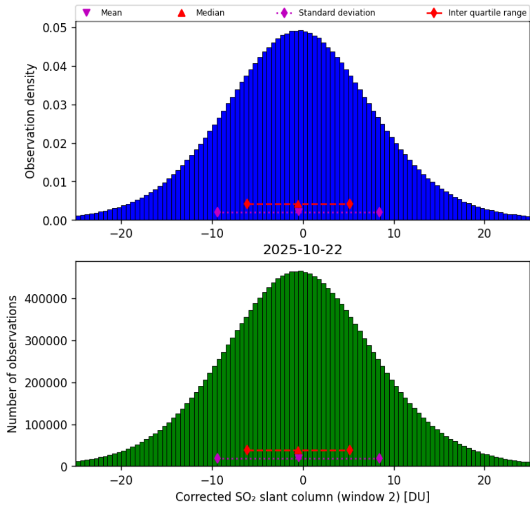
Figure 69: Histogram of “Corrected SO 2 slant column (window 2)” for 2025-10-22 to 2025-10-23
