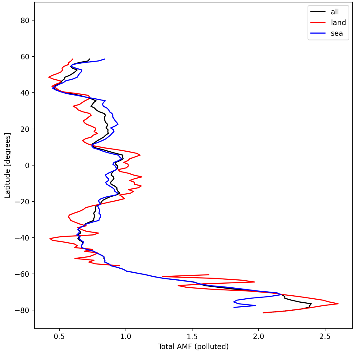
Figure 53: Zonal average of “Total AMF (polluted)” for 2025-10-22 to 2025-10-23.
