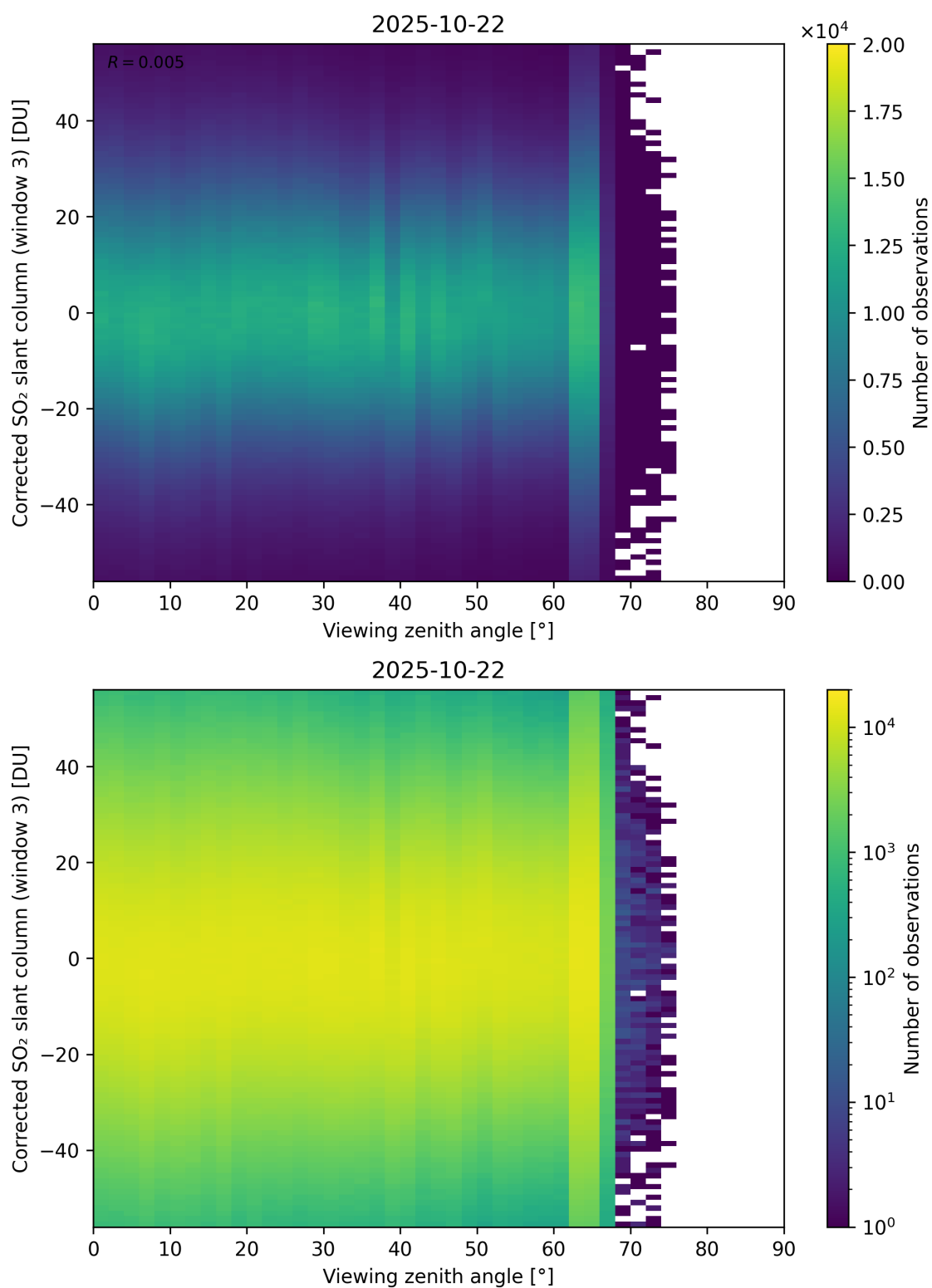
Figure 375: Scatter density plot of “Viewing zenith angle” against “Corrected SO 2 slant column (window 3)” for 2025-10-22 to 2025-10-23.
