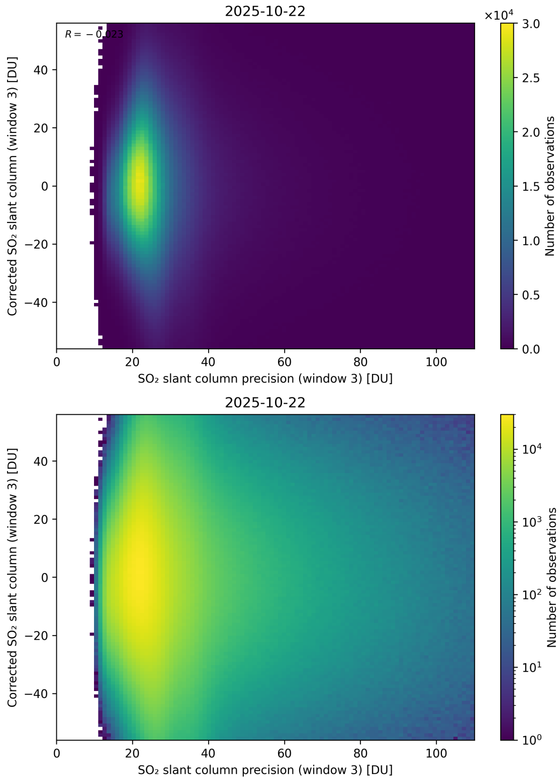
Figure 312: Scatter density plot of “SO 2 slant column precision (window 3)” against “Corrected SO 2 slant column (window 3)” for 2025-10-22 to 2025-10-23.
