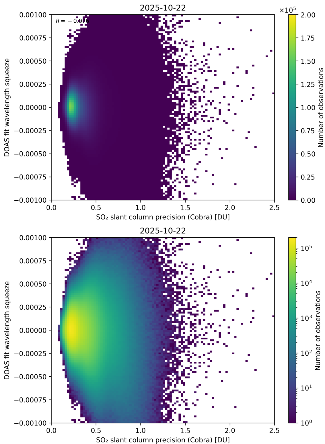
Figure 203: Scatter density plot of “SO 2 slant column precision (Cobra)” against “DOAS fit wavelength squeeze” for 2025-10-22 to 2025-10-23.
