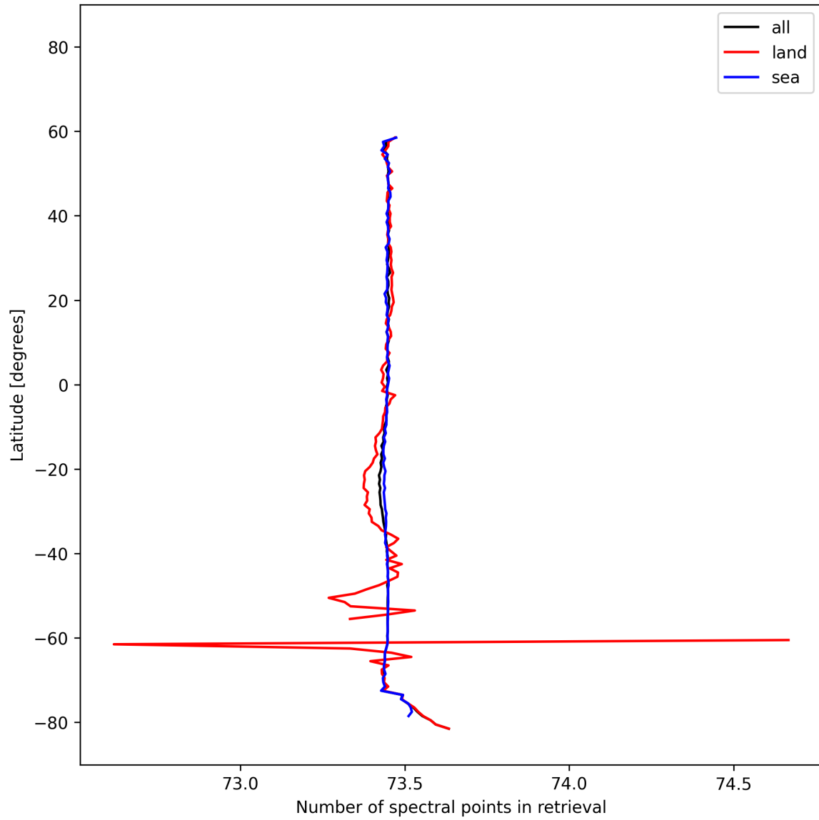
Figure 56: Zonal average of “Number of spectral points in retrieval” for 2025-10-22 to 2025-10-23.
