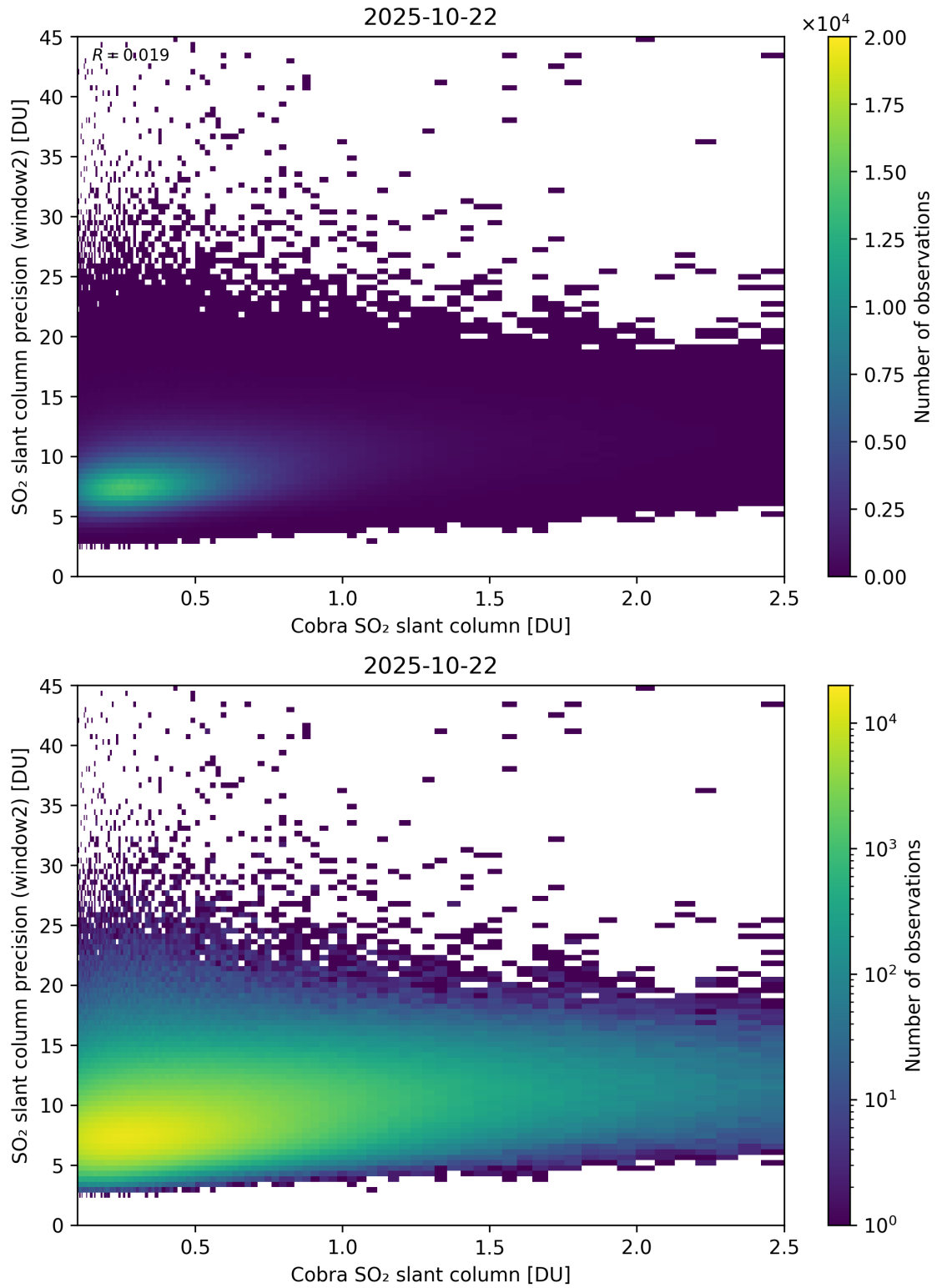
Figure 221: Scatter density plot of “Cobra SO 2 slant column” against “SO 2 slant column precision (window2)” for 2025-10-22 to 2025-10-23.
