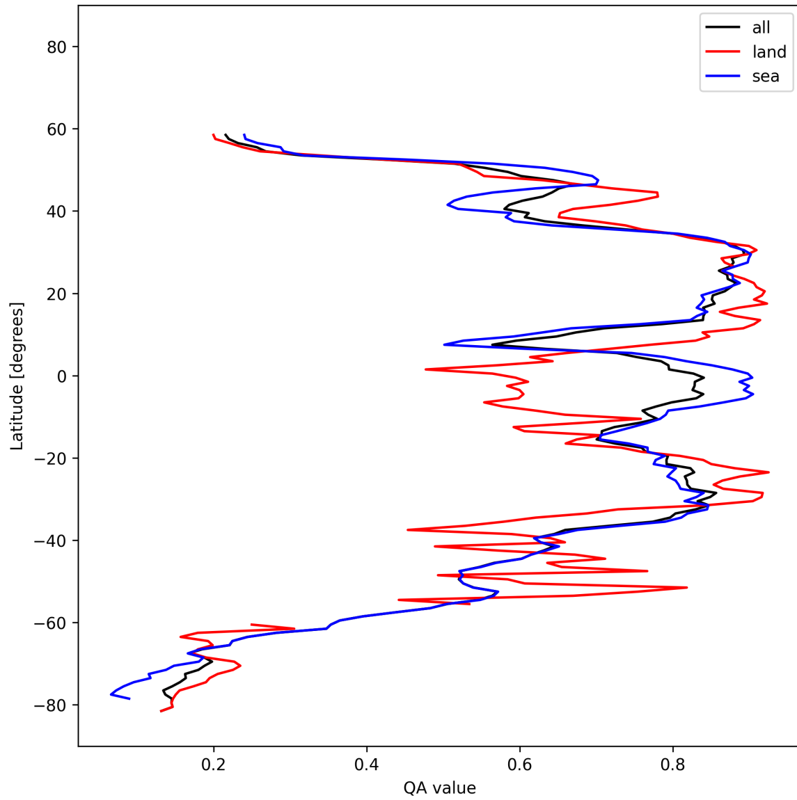
Figure 31: Zonal average of “QA value” for 2025-10-22 to 2025-10-23.
