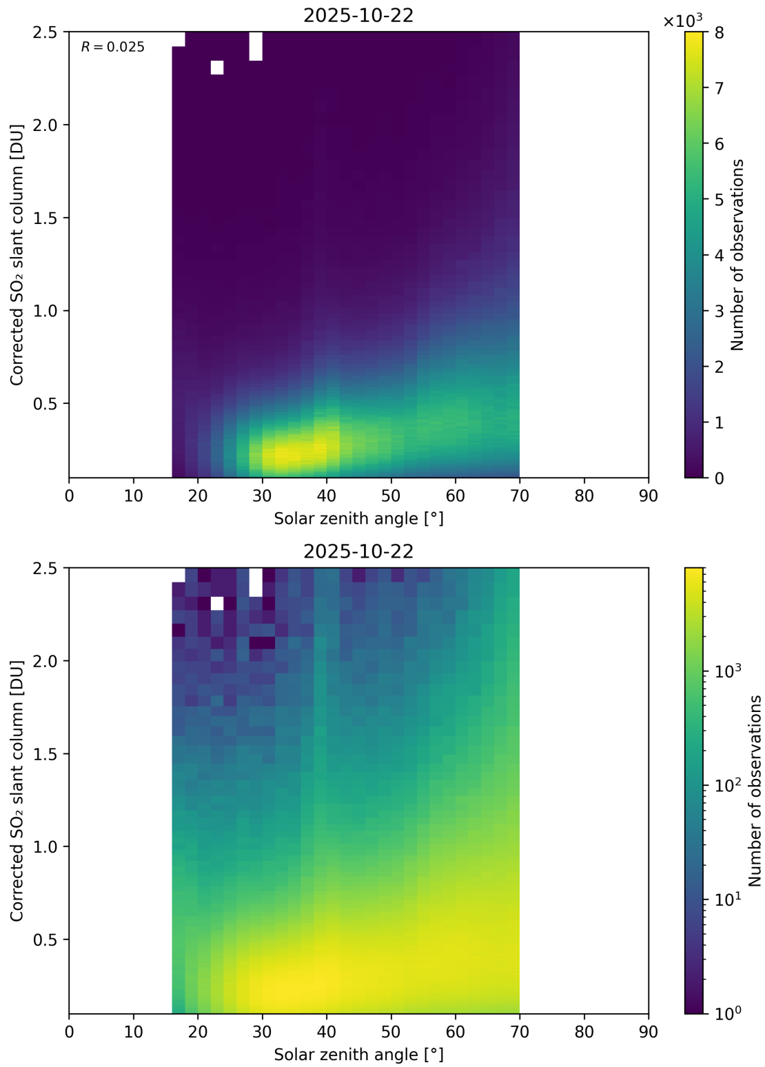
Figure 181: Scatter density plot of “Solar zenith angle” against “Corrected SO 2 slant column” for 2025-10-22 to 2025-10-23.
