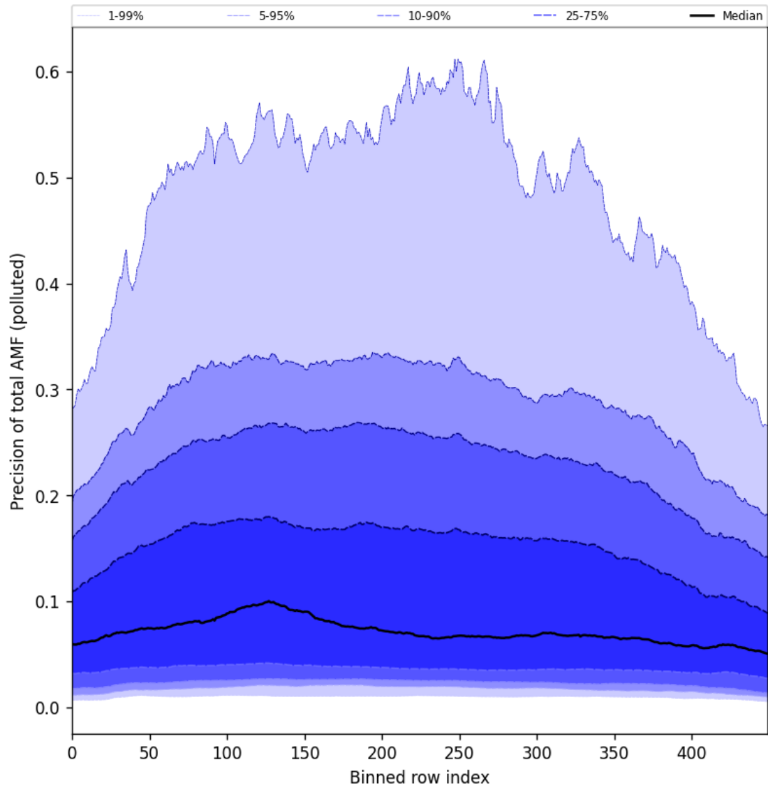
Figure 106: Along track statistics of “Precision of total AMF (polluted)” for 2025-10-22 to 2025-10-23
