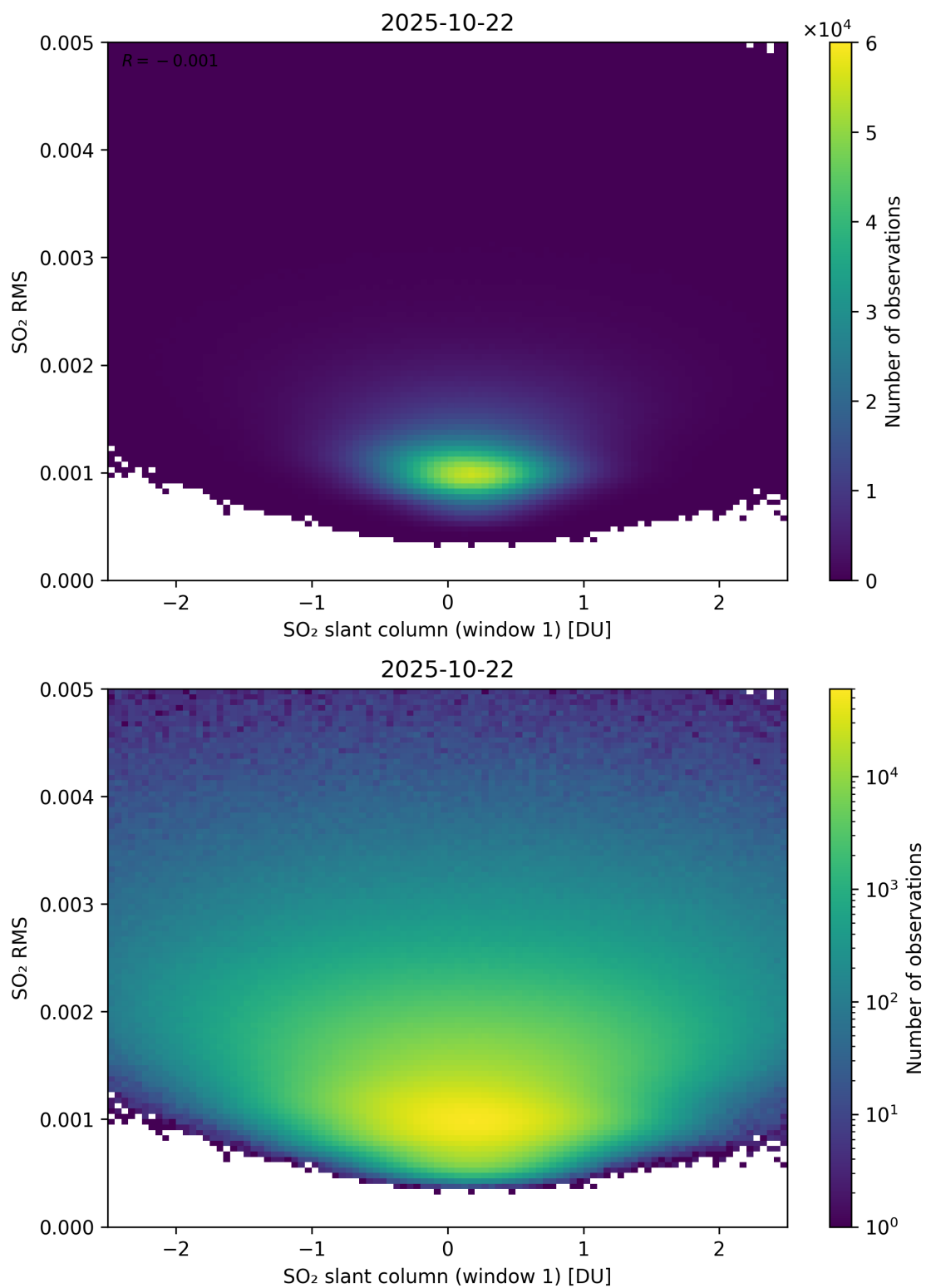
Figure 267: Scatter density plot of “SO 2 slant column (window 1)” against “SO 2 RMS” for 2025-10-22 to 2025-10-23.
