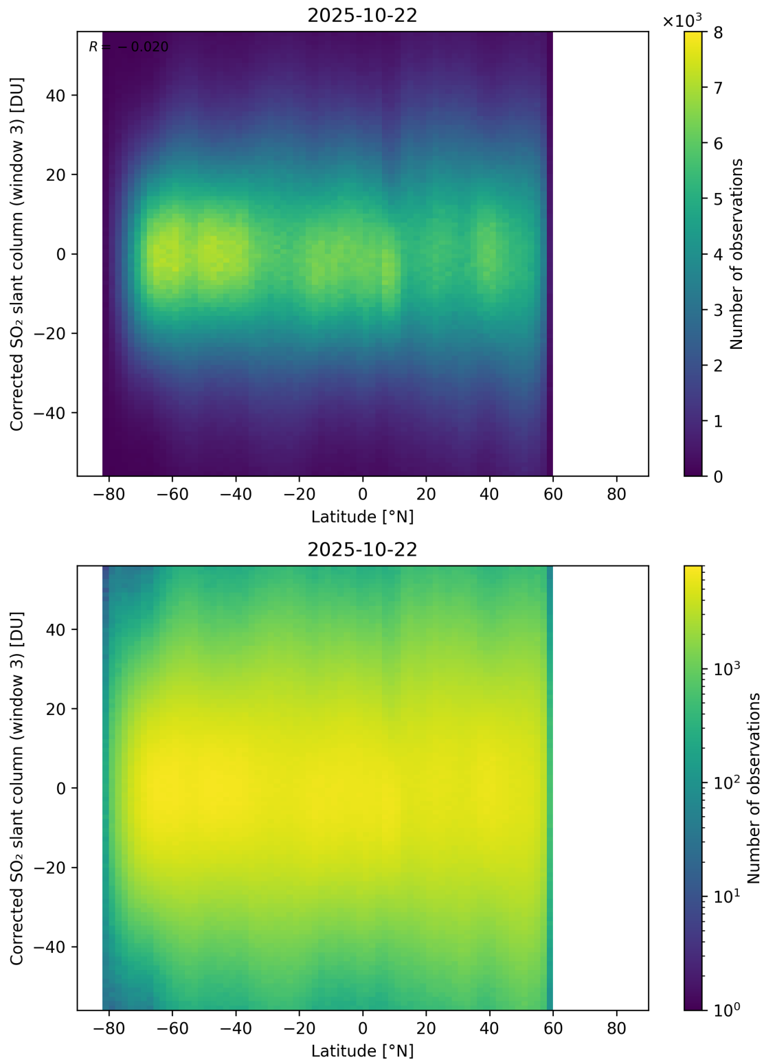
Figure 161: Scatter density plot of “Latitude” against “Corrected SO 2 slant column (window 3)” for 2025-10-22 to 2025-10-23.
