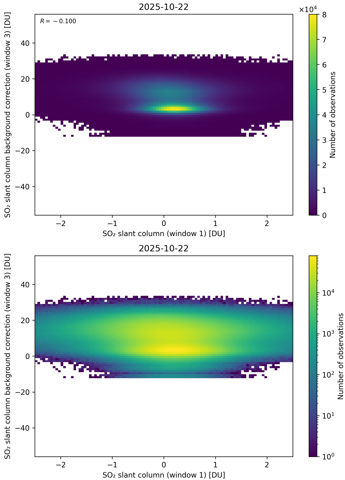
Figure 264: Scatter density plot of “SO 2 slant column (window 1)” against “SO 2 slant column background correction (window 3)” for 2025-10-22 to 2025-10-23.
