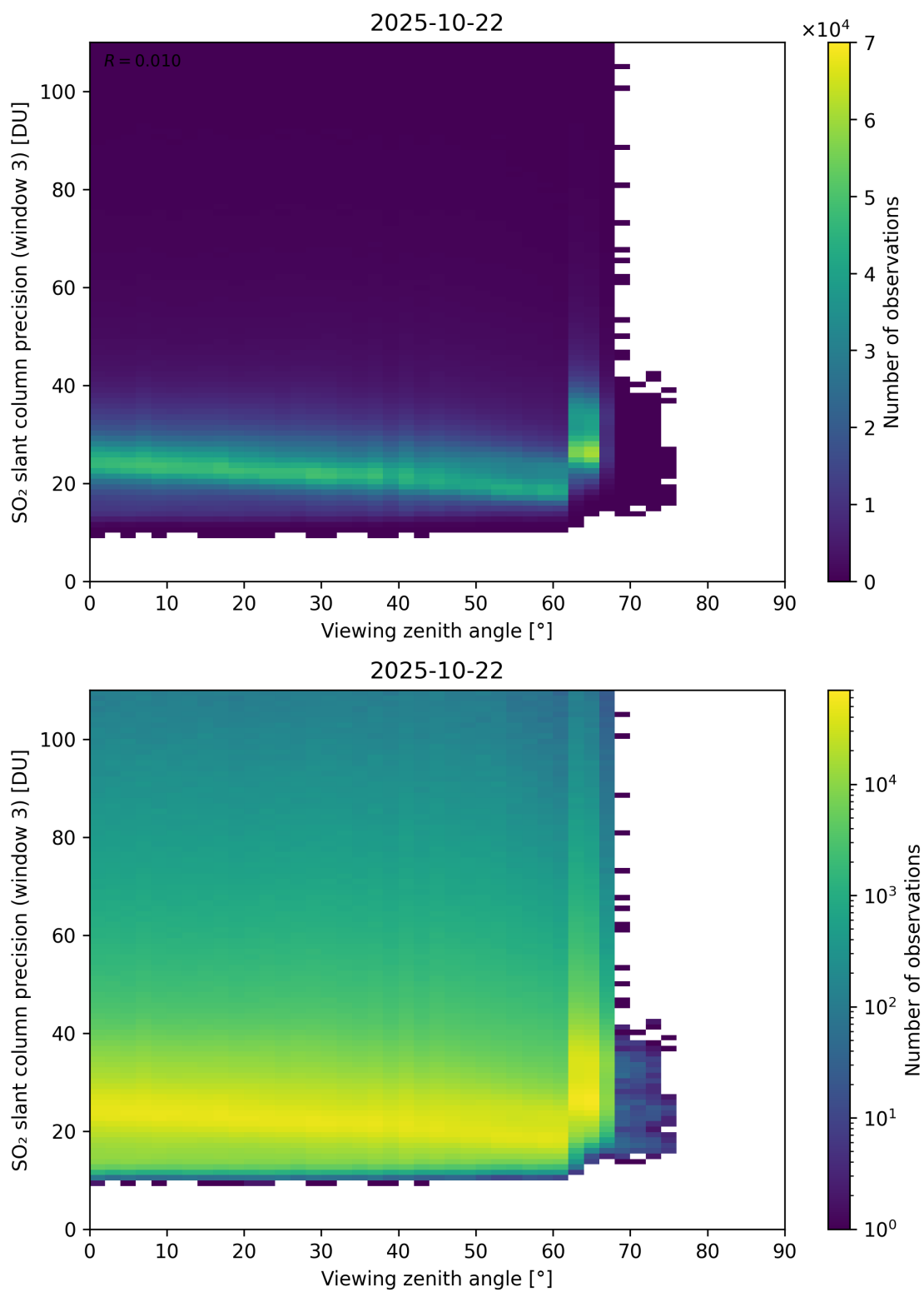
Figure 380: Scatter density plot of “Viewing zenith angle” against “SO 2 slant column precision (window 3)” for 2025-10-22 to 2025-10-23.
