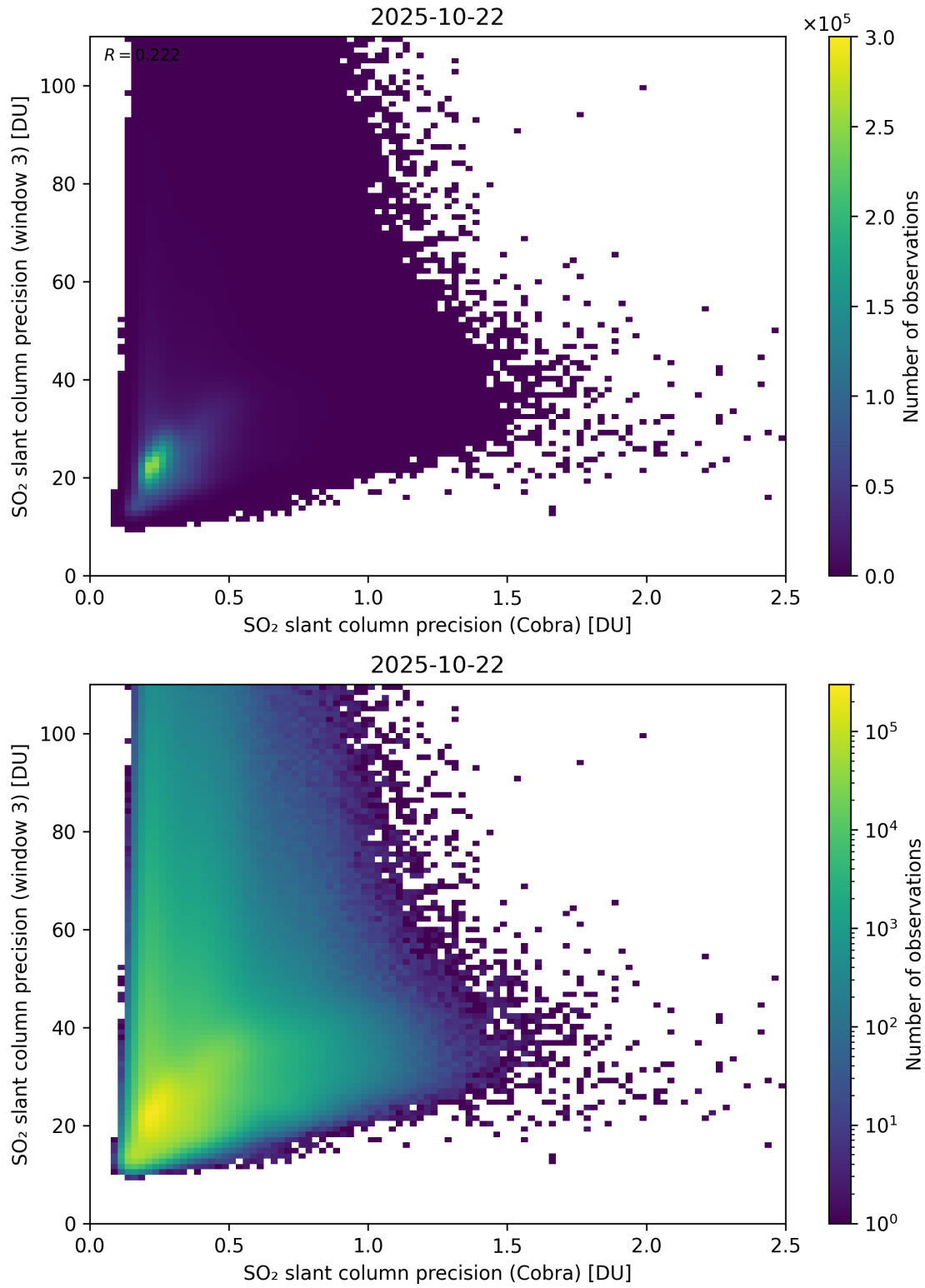
Figure 212: Scatter density plot of “SO 2 slant column precision (Cobra)” against “SO 2 slant column precision (window 3)” for 2025-10-22 to 2025-10-23.
