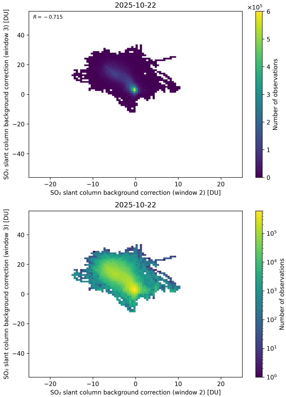
Figure 122: Scatter density plot of “SO 2 slant column background correction (window 2)” against “SO 2 slant column background correction (window 3)” for 2025-10-22 to 2025-10-23.
