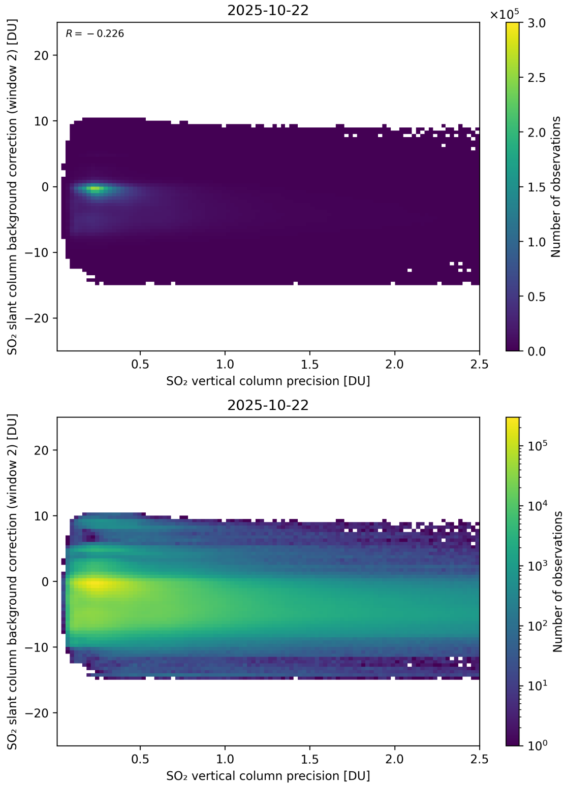
Figure 330: Scatter density plot of “SO 2 vertical column precision” against “SO 2 slant column background correction (window 2)” for 2025-10-22 to 2025-10-23.
