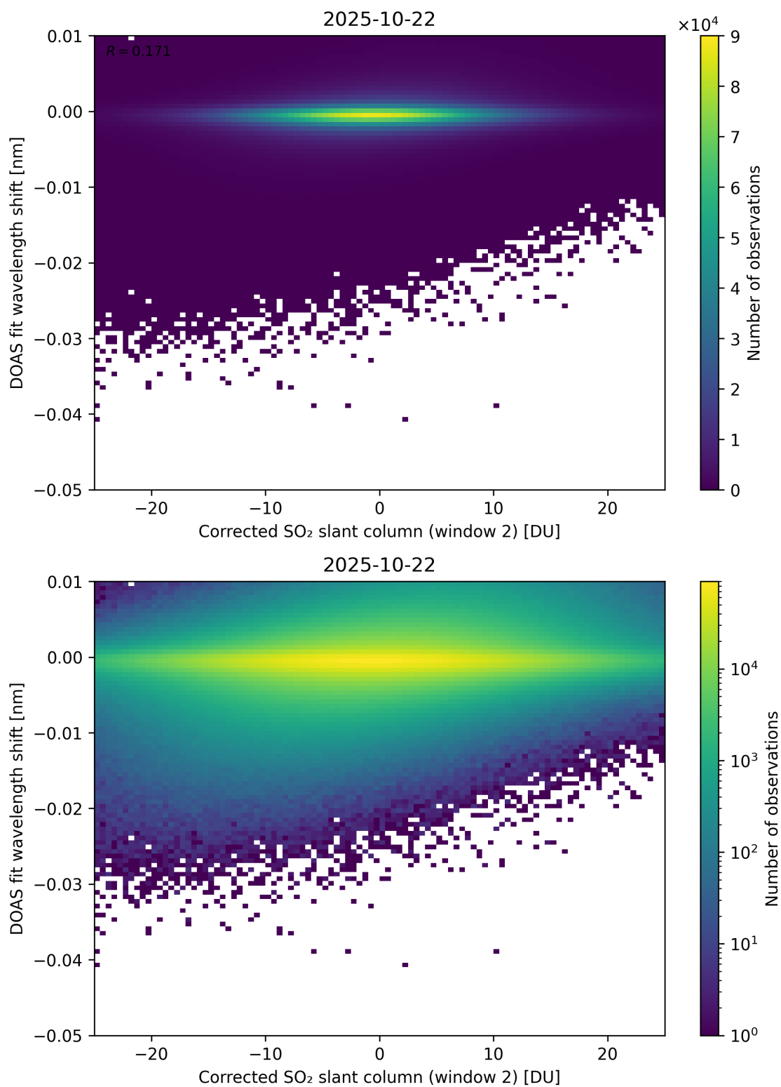
Figure 246: Scatter density plot of “Corrected SO 2 slant column (window 2)” against “DOAS fit wavelength shift” for 2025-10-22 to 2025-10-23.
