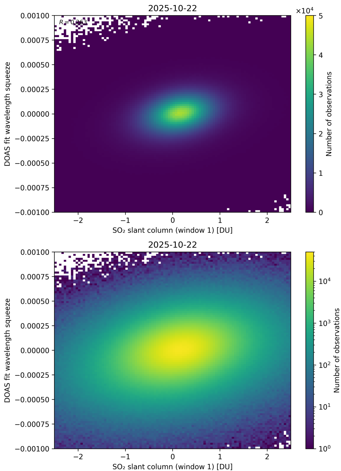
Figure 266: Scatter density plot of “SO 2 slant column (window 1)” against “DOAS fit wavelength squeeze” for 2025-10-22 to 2025-10-23.
