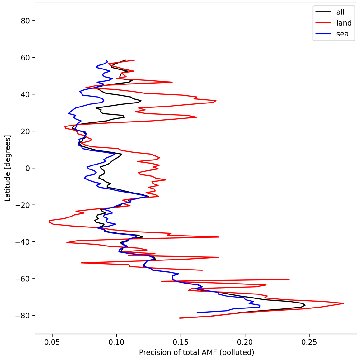
Figure 54: Zonal average of “Precision of total AMF (polluted)” for 2025-10-22 to 2025-10-23.
