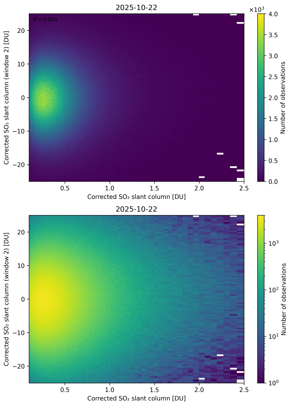
Figure 235: Scatter density plot of “Corrected SO 2 slant column” against “Corrected SO 2 slant column (window 2)” for 2025-10-22 to 2025-10-23.
