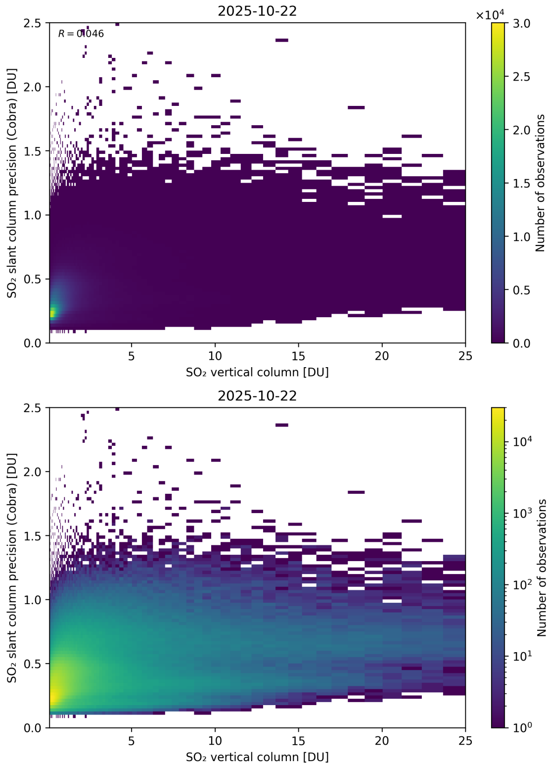
Figure 350: Scatter density plot of “SO 2 vertical column” against “SO 2 slant column precision (Cobra)” for 2025-10-22 to 2025-10-23.
