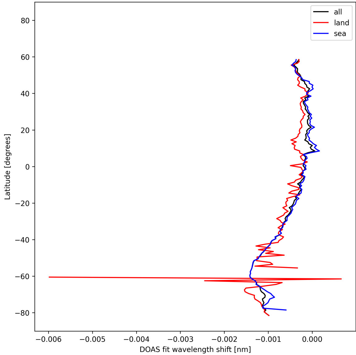
Figure 50: Zonal average of "DOAS fit wavelength shift" for 2025-10-22 to 2025-10-23.
