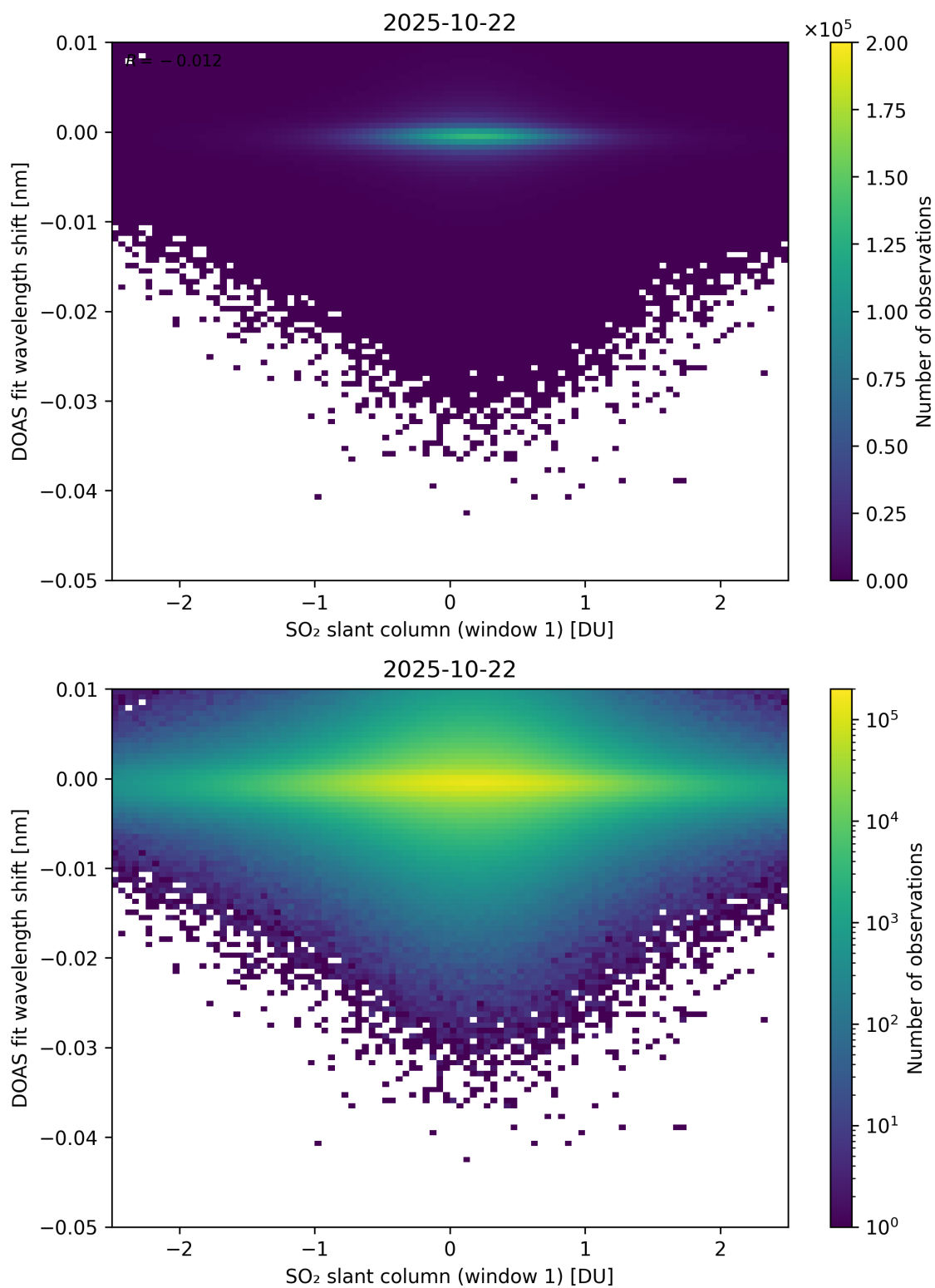
Figure 265: Scatter density plot of “SO 2 slant column (window 1)” against “DOAS fit wavelength shift” for 2025-10-22 to 2025-10-23.
