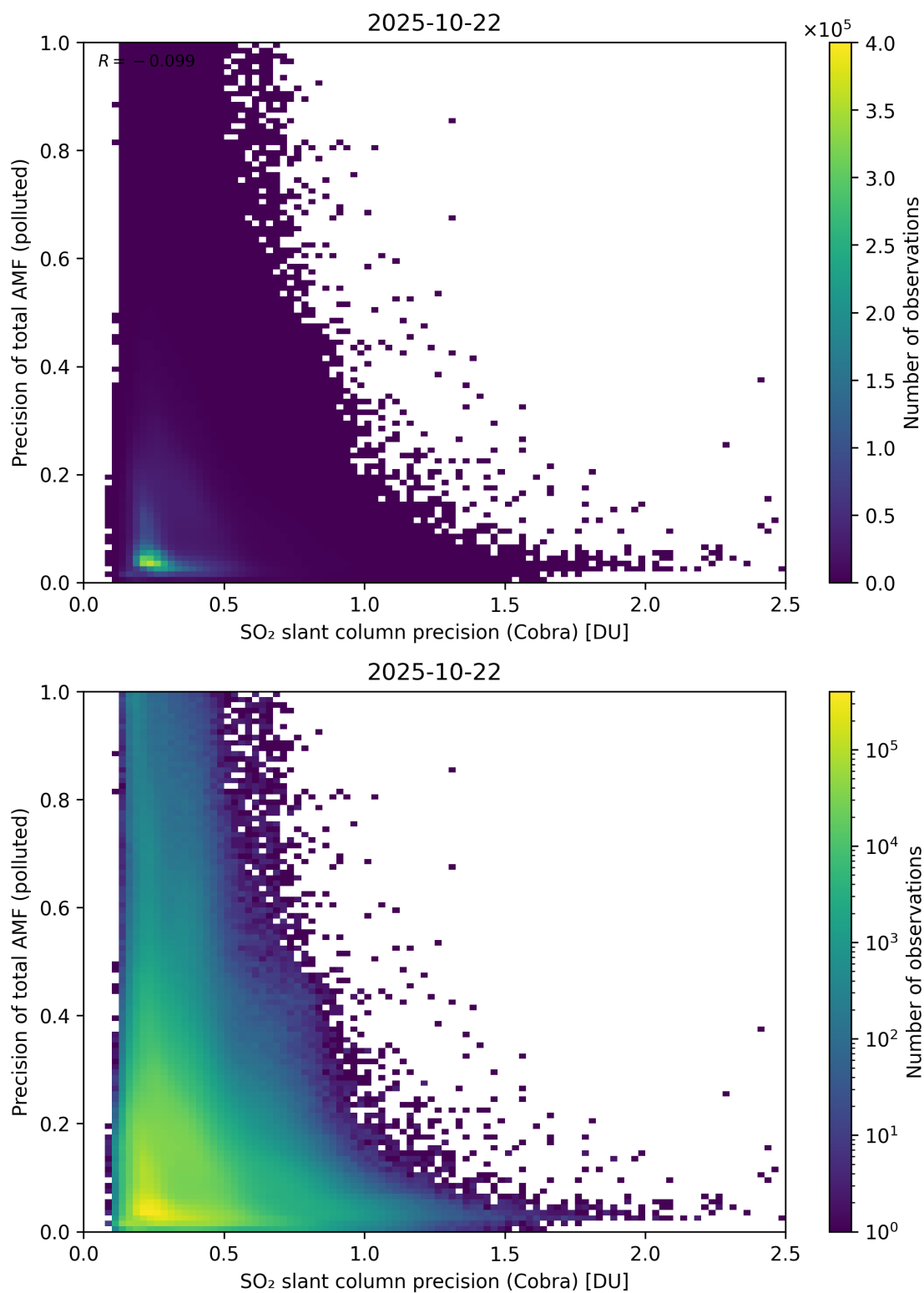
Figure 214: Scatter density plot of “SO 2 slant column precision (Cobra)” against “Precision of total AMF (polluted)” for 2025-10-22 to 2025-10-23.
