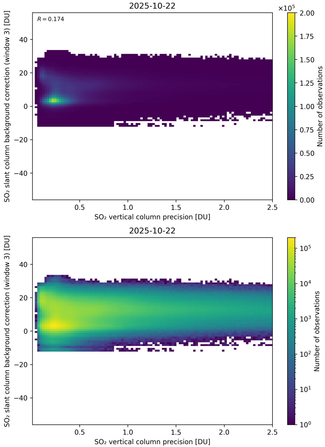
Figure 331: Scatter density plot of “SO 2 vertical column precision” against “SO 2 slant column background correction (window 3)” for 2025-10-22 to 2025-10-23.
