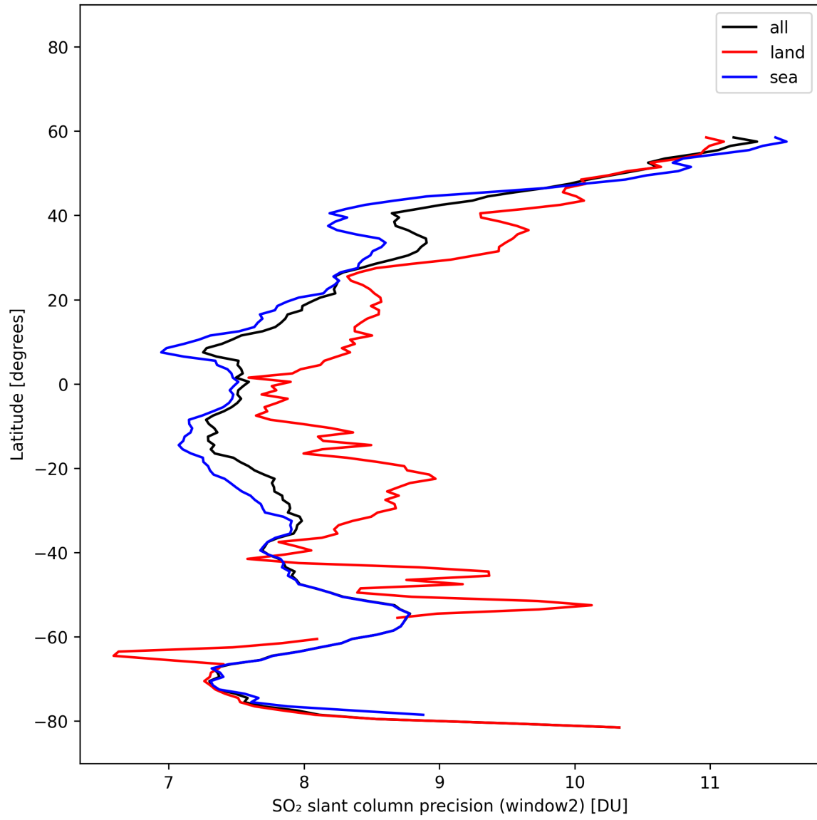
Figure 42: Zonal average of “SO 2 slant column precision (window2)” for 2025-10-22 to 2025-10-23.
