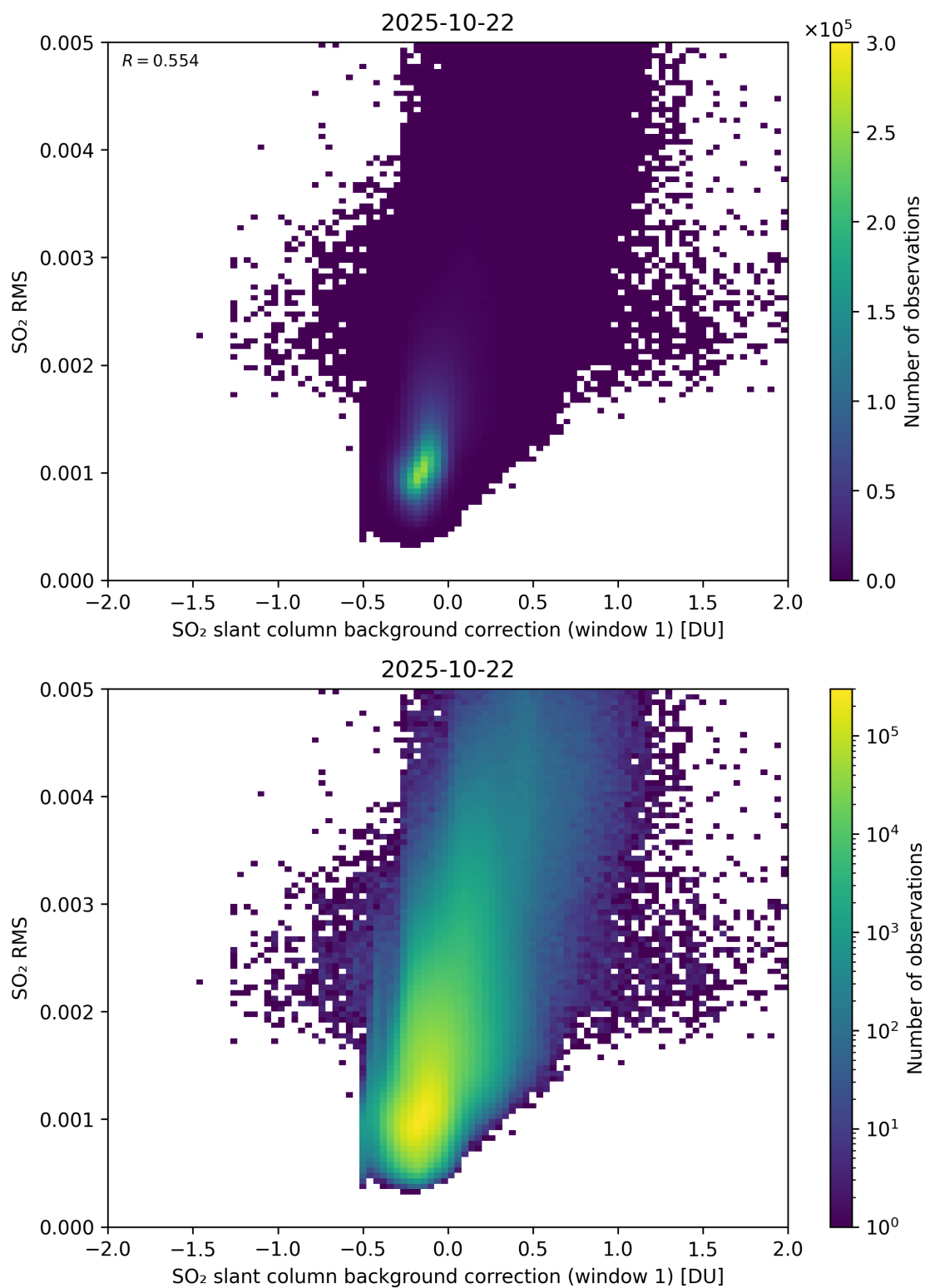
Figure 113: Scatter density plot of “SO 2 slant column background correction (window 1)” against “SO 2 RMS” for 2025-10-22 to 2025-10-23.
