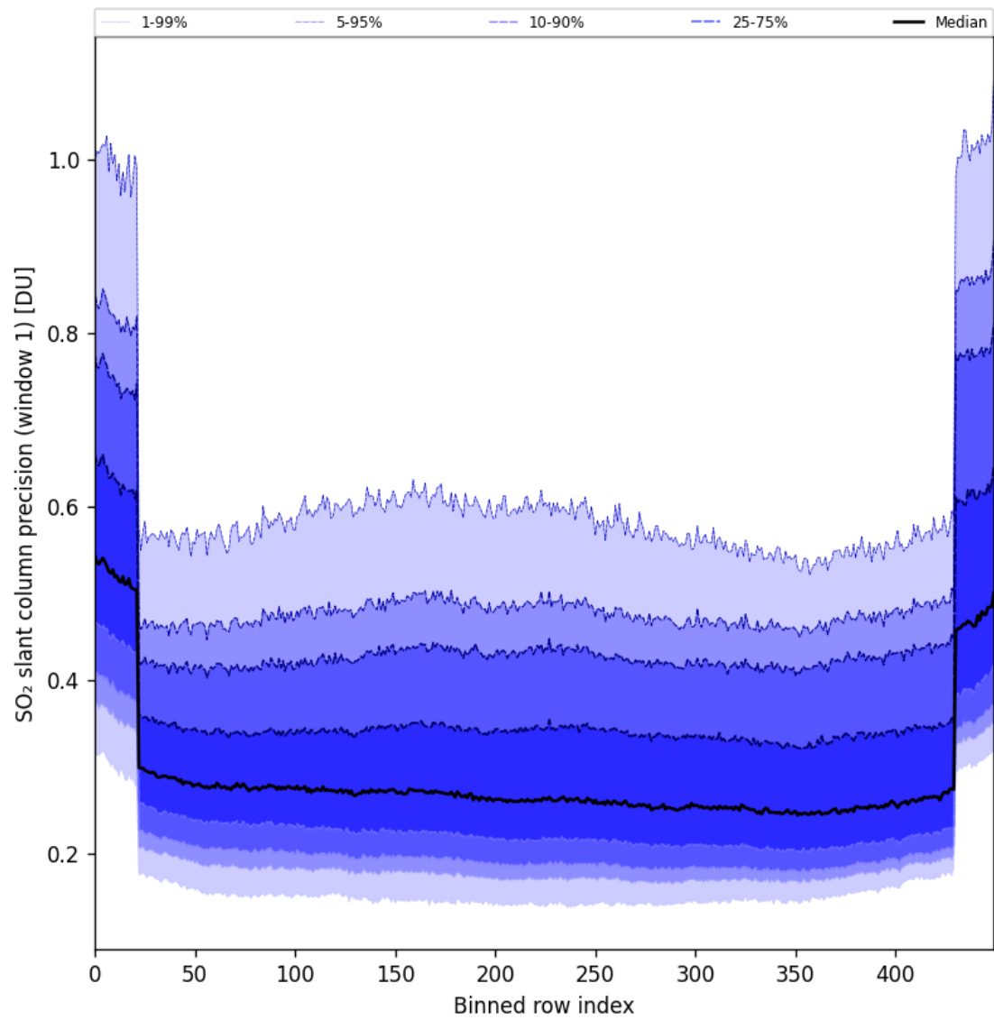
Figure 90: Along track statistics of “SO 2 slant column precision (window 1)” for 2025-10-22 to 2025-10-23
