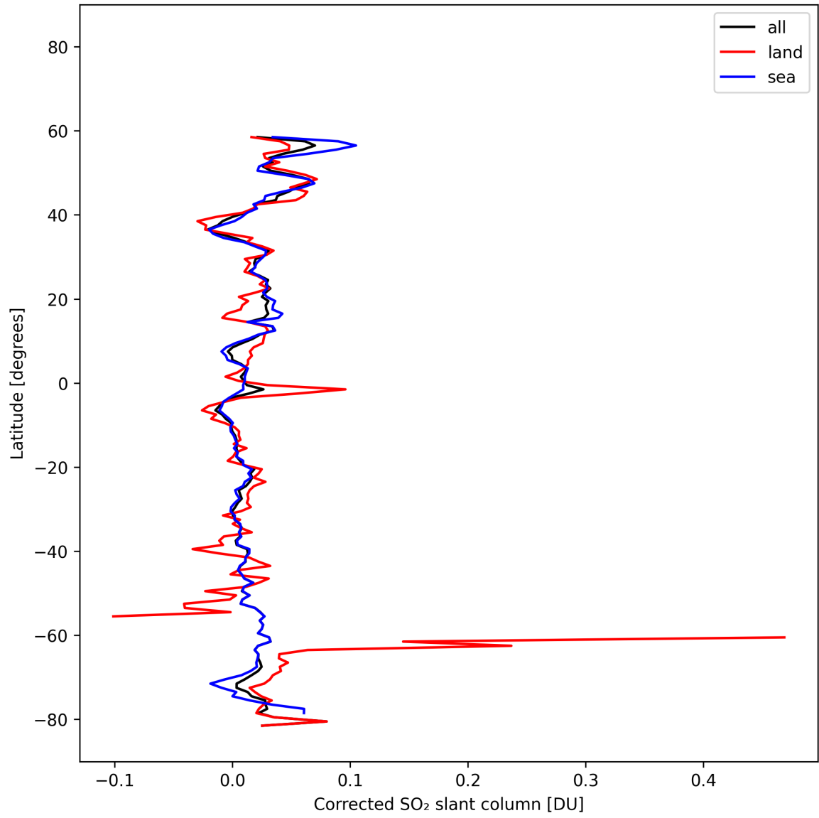
Figure 34: Zonal average of “Corrected SO 2 slant column” for 2025-10-22 to 2025-10-23.
