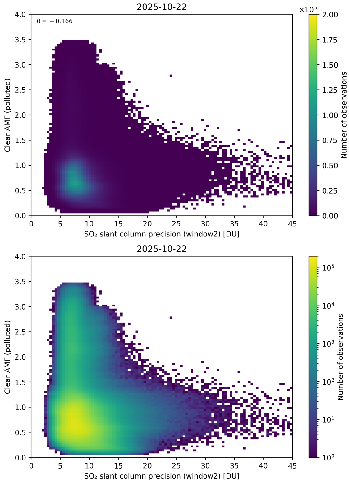
Figure 296: Scatter density plot of “SO 2 slant column precision (window2)” against “Clear AMF (polluted)” for 2025-10-22 to 2025-10-23.
