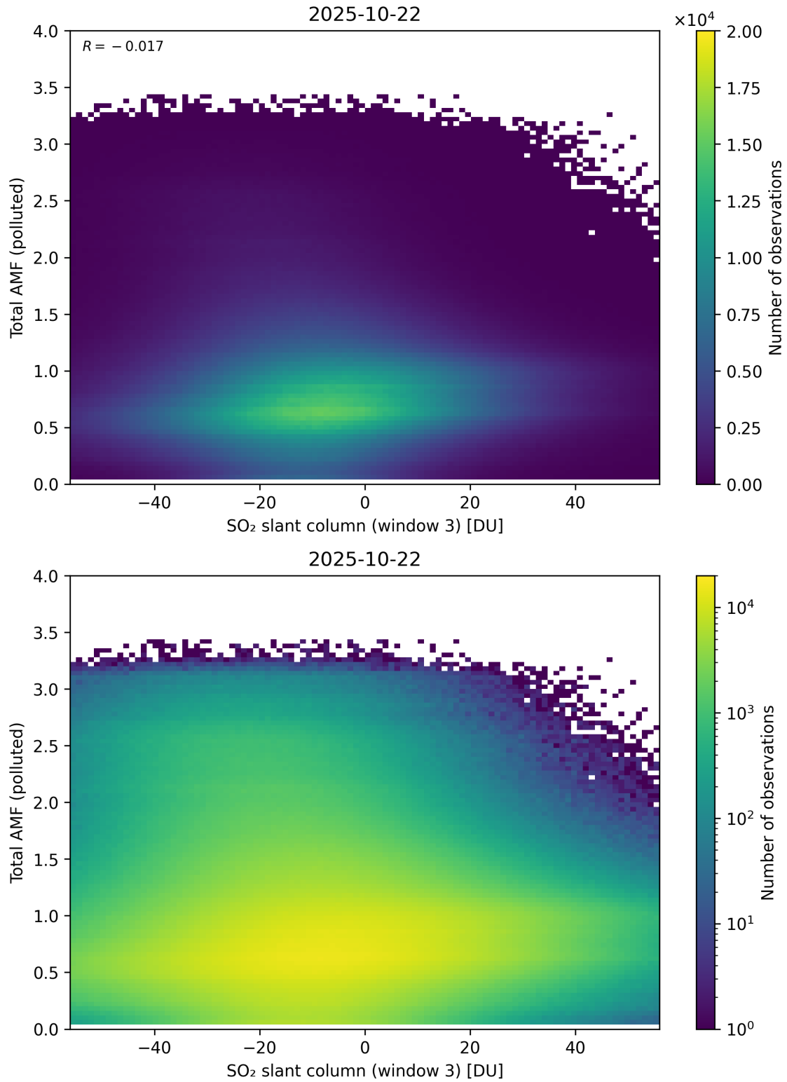
Figure 318: Scatter density plot of “SO 2 slant column (window 3)” against “Total AMF (polluted)” for 2025-10-22 to 2025-10-23.
