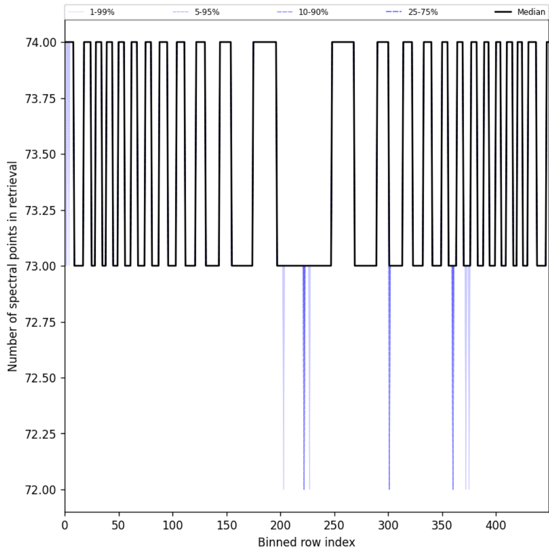
Figure 108: Along track statistics of “Number of spectral points in retrieval” for 2025-10-22 to 2025-10-23
