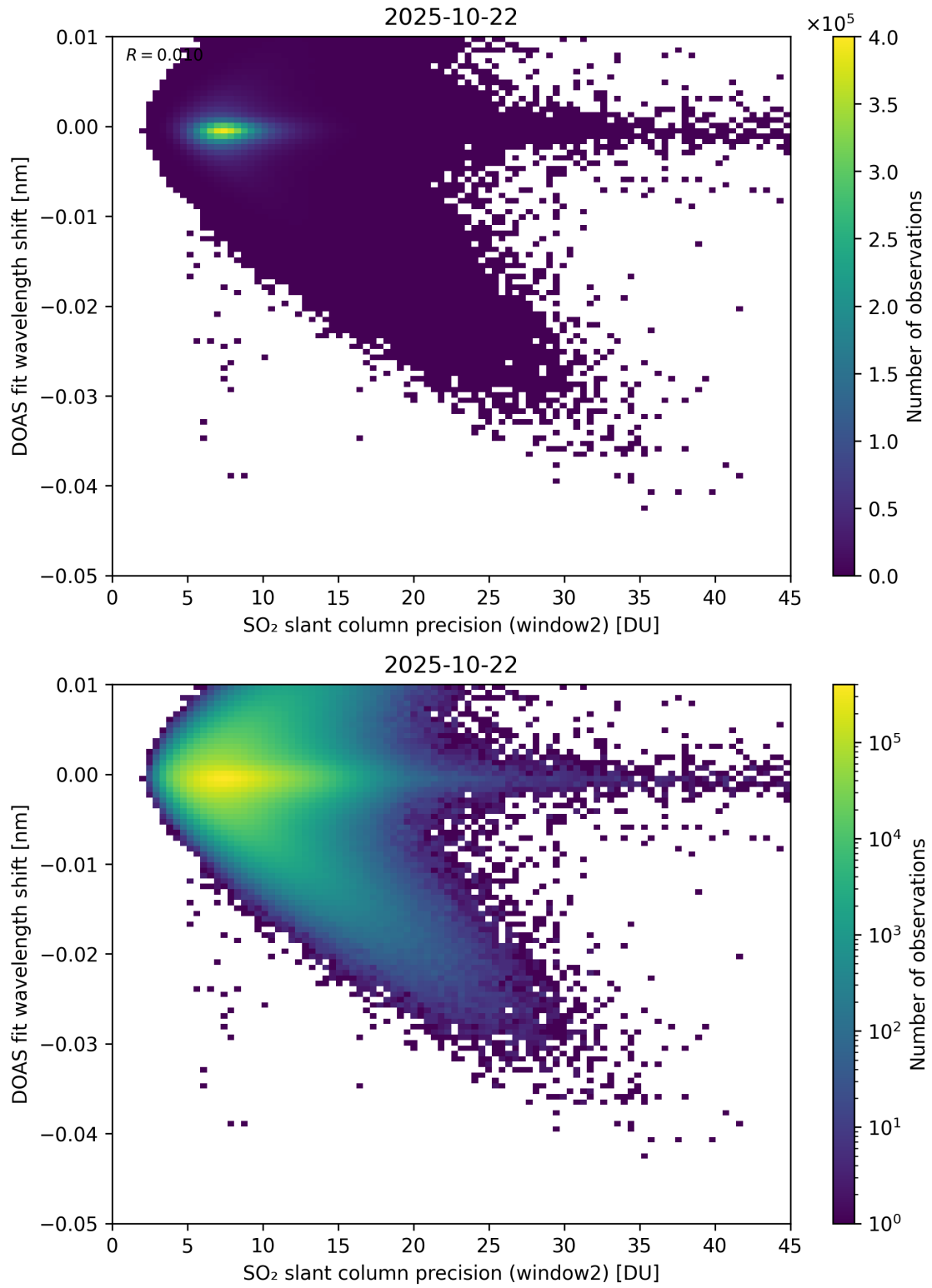
Figure 293: Scatter density plot of “SO 2 slant column precision (window2)” against “DOAS fit wavelength shift” for 2025-10-22 to 2025-10-23.
