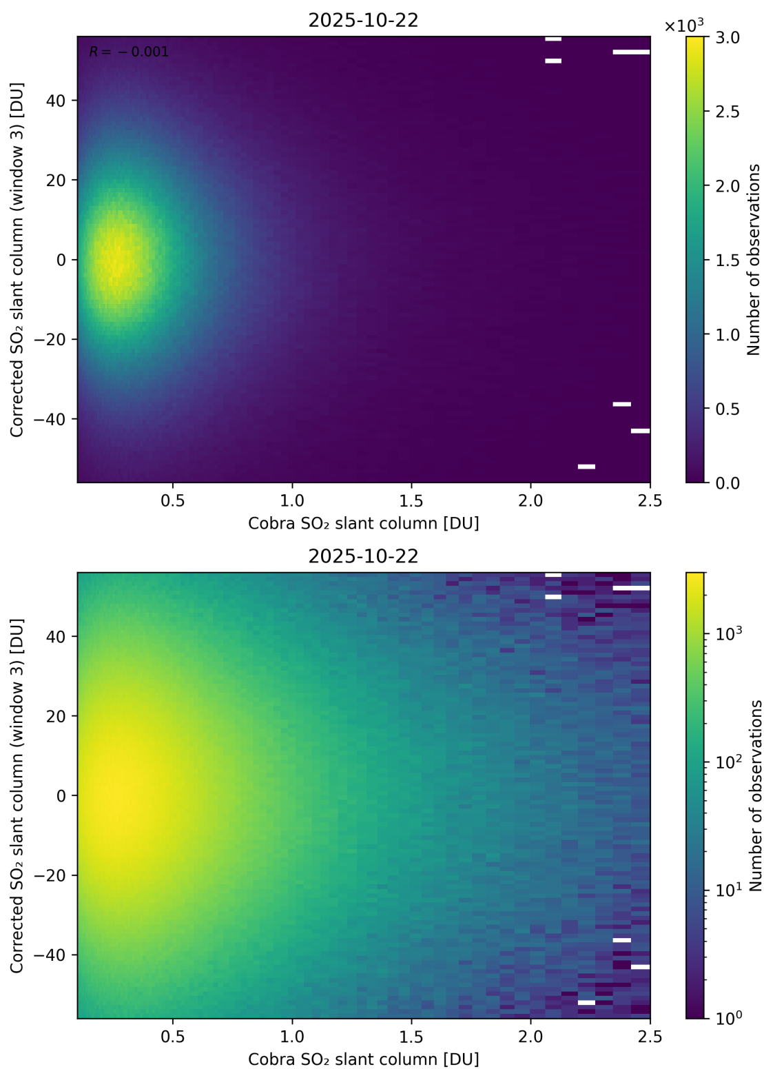
Figure 218: Scatter density plot of “Cobra SO 2 slant column” against “Corrected SO 2 slant column (window 3)” for 2025-10-22 to 2025-10-23.
