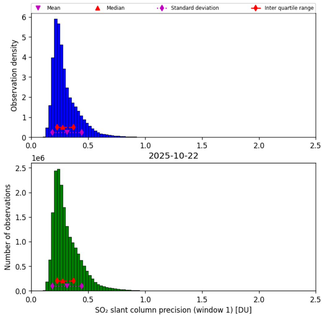
Figure 64: Histogram of “SO 2 slant column precision (window 1)” for 2025-10-22 to 2025-10-23
