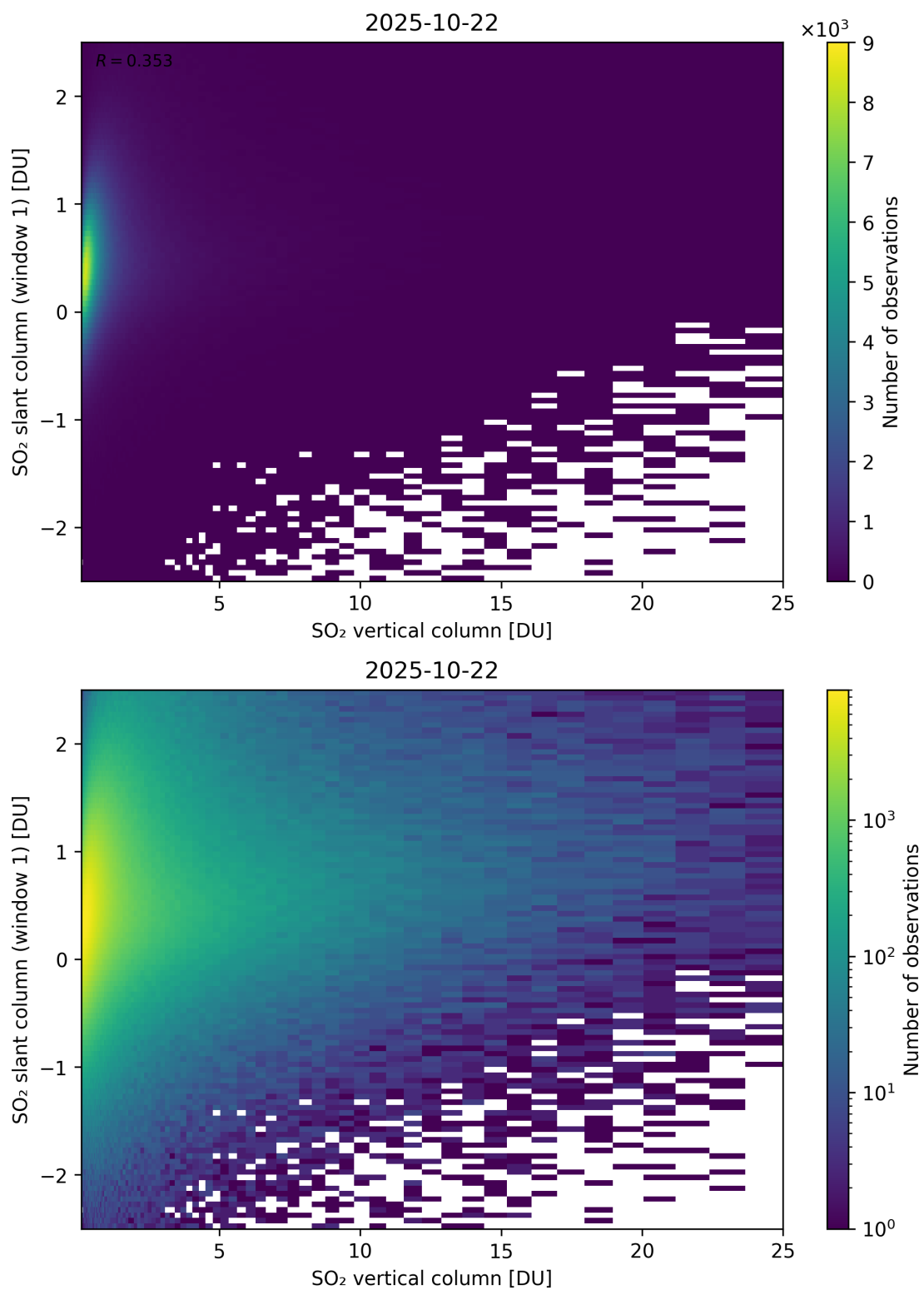
Figure 354: Scatter density plot of “SO 2 vertical column” against “SO 2 slant column (window 1)” for 2025-10-22 to 2025-10-23.
