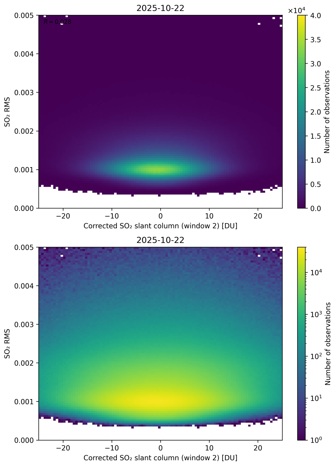
Figure 248: Scatter density plot of “Corrected SO 2 slant column (window 2)” against “SO 2 RMS” for 2025-10-22 to 2025-10-23.
