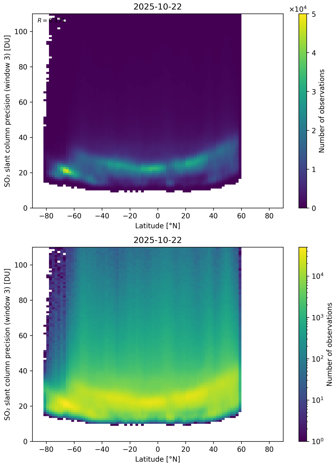
Figure 166: Scatter density plot of “Latitude” against “SO 2 slant column precision (window 3)” for 2025-10-22 to 2025-10-23.
