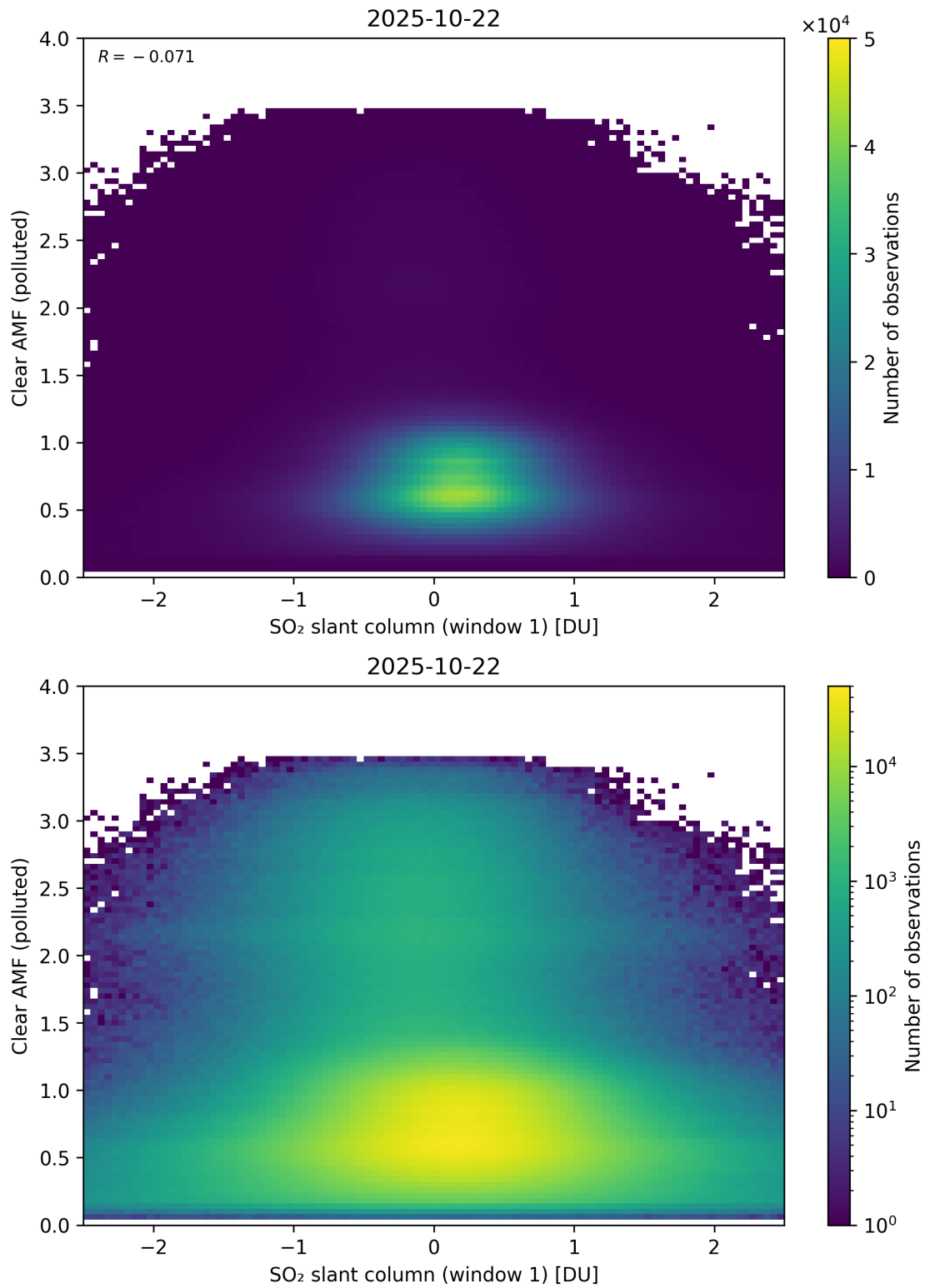
Figure 282: Scatter density plot of “SO 2 slant column (window 1)” against “Clear AMF (polluted)” for 2025-10-22 to 2025-10-23.
