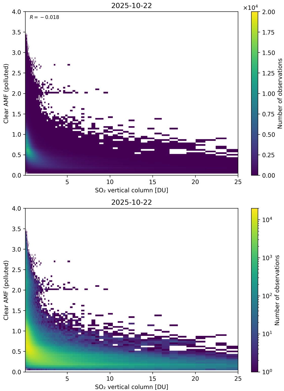
Figure 348: Scatter density plot of “SO 2 vertical column” against “Clear AMF (polluted)” for 2025-10-22 to 2025-10-23.
