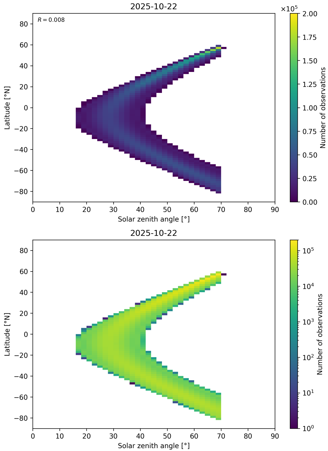
Figure 177: Scatter density plot of “Solar zenith angle” against “Latitude” for 2025-10-22 to 2025-10-23.
