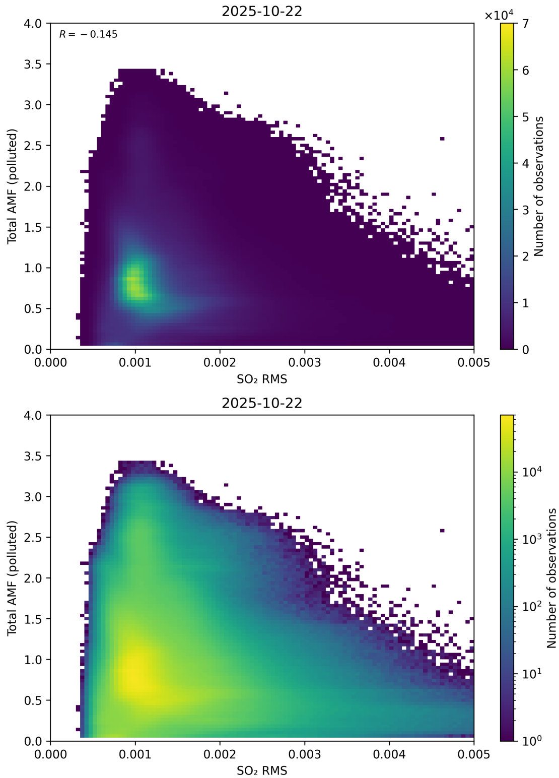
Figure 148: Scatter density plot of “SO 2 RMS” against “Total AMF (polluted)” for 2025-10-22 to 2025-10-23.
