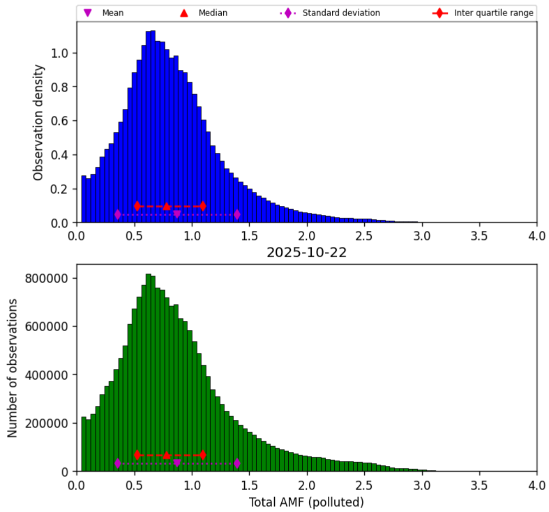
Figure 79: Histogram of “Total AMF (polluted)” for 2025-10-22 to 2025-10-23
