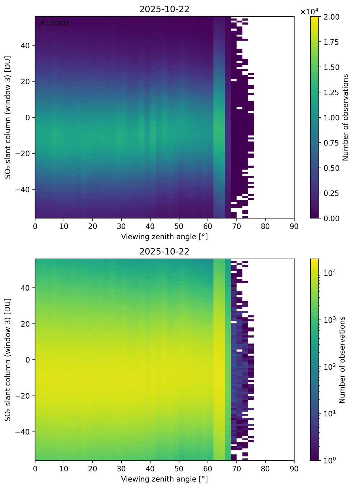
Figure 379: Scatter density plot of “Viewing zenith angle” against “SO 2 slant column (window 3)” for 2025-10-22 to 2025-10-23.
