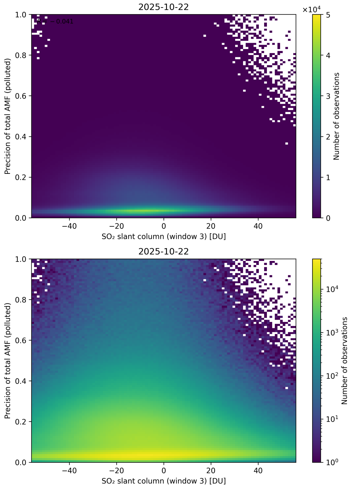
Figure 319: Scatter density plot of “SO 2 slant column (window 3)” against “Precision of total AMF (polluted)” for 2025-10-22 to 2025-10-23.
