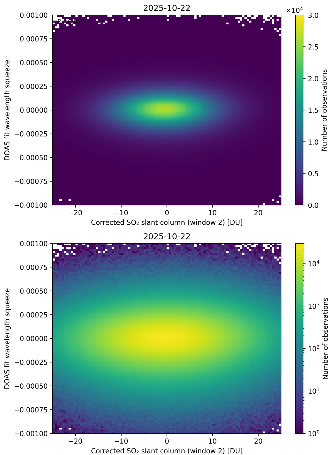
Figure 247: Scatter density plot of “Corrected SO 2 slant column (window 2)” against “DOAS fit wavelength squeeze” for 2025-10-22 to 2025-10-23.
