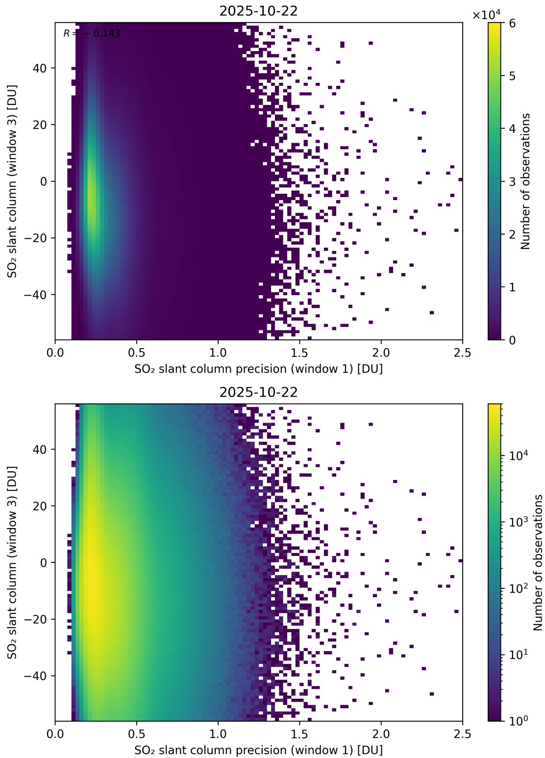
Figure 278: Scatter density plot of “SO 2 slant column precision (window 1)” against “SO 2 slant column (window 3)” for 2025-10-22 to 2025-10-23.
