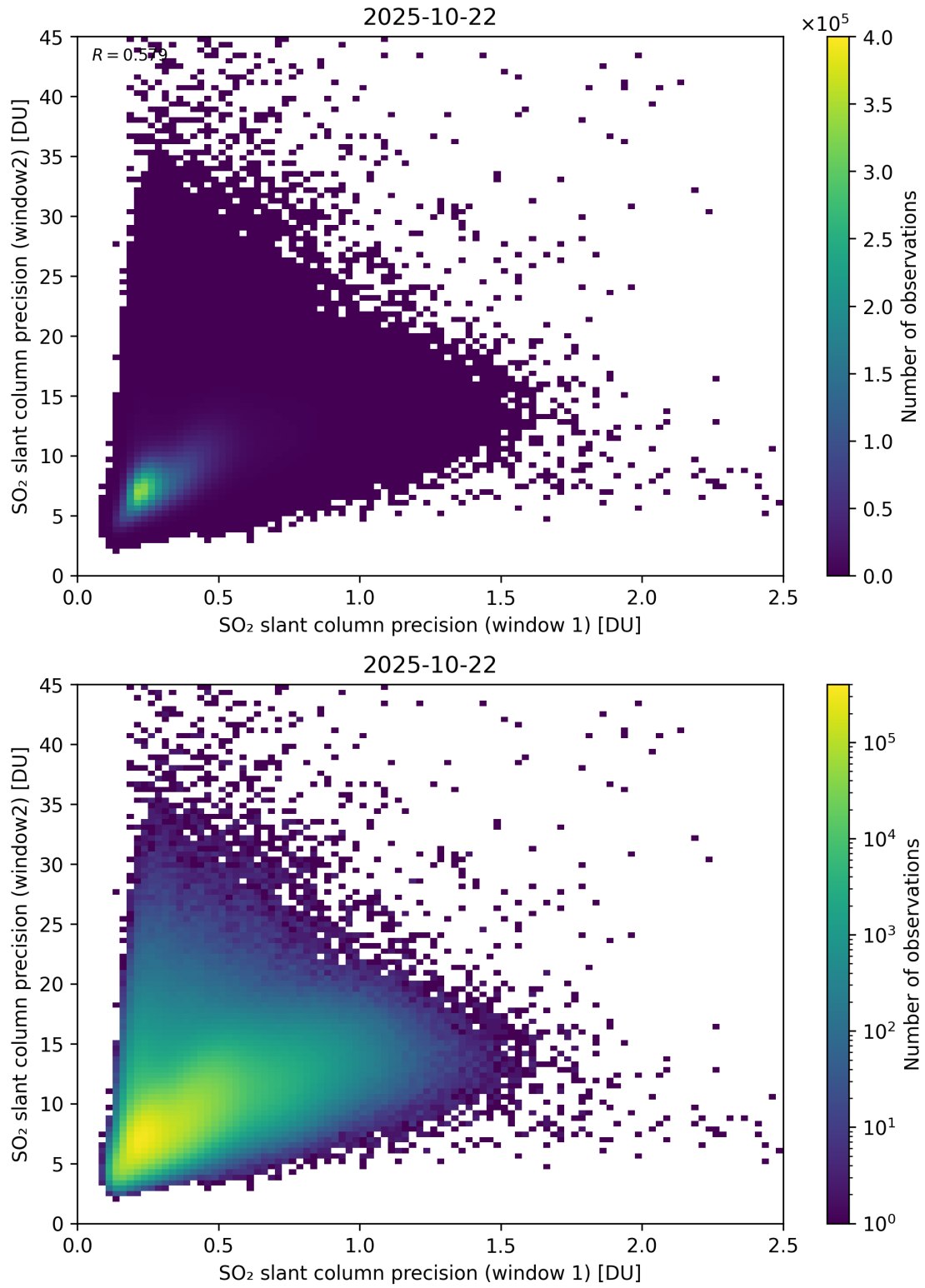
Figure 277: Scatter density plot of “SO 2 slant column precision (window 1)” against “SO 2 slant column precision (window2)” for 2025-10-22 to 2025-10-23.
