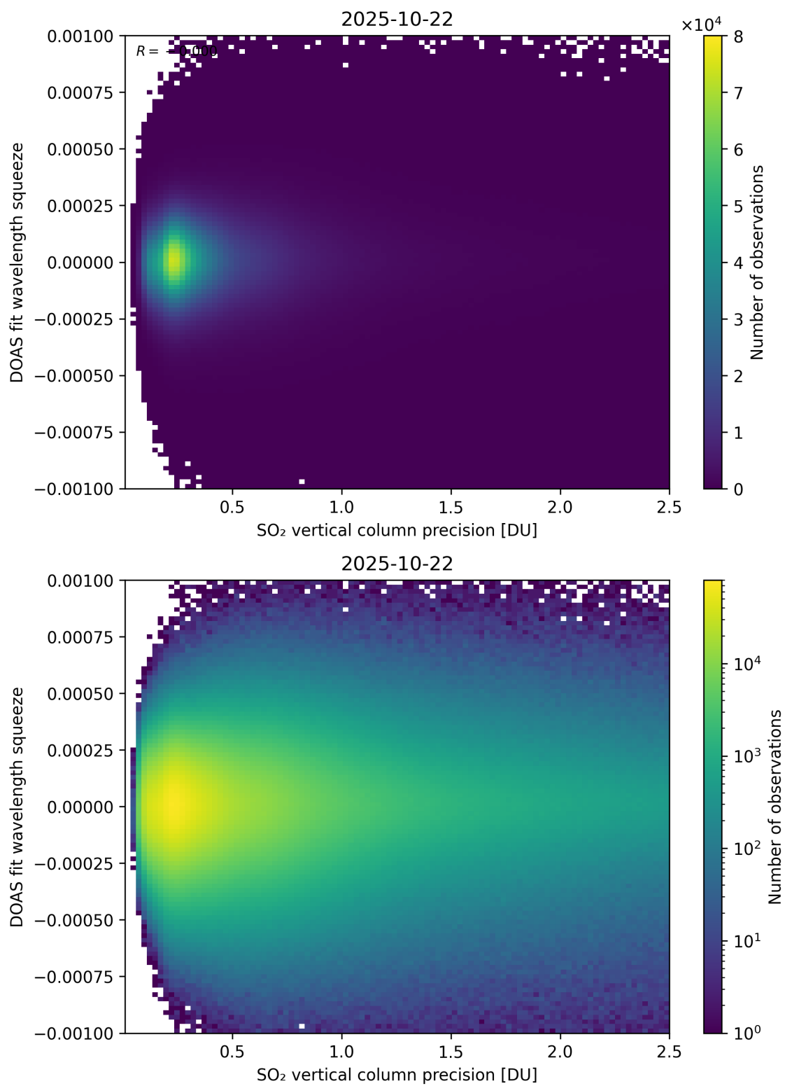
Figure 333: Scatter density plot of “SO 2 vertical column precision” against “DOAS fit wavelength squeeze” for 2025-10-22 to 2025-10-23.
