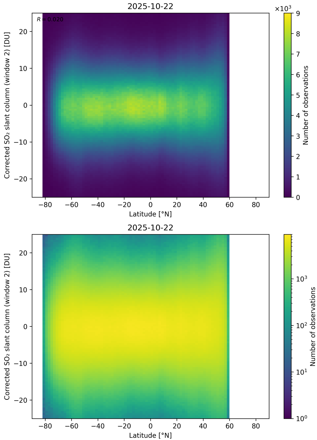
Figure 160: Scatter density plot of “Latitude” against “Corrected SO 2 slant column (window 2)” for 2025-10-22 to 2025-10-23.
