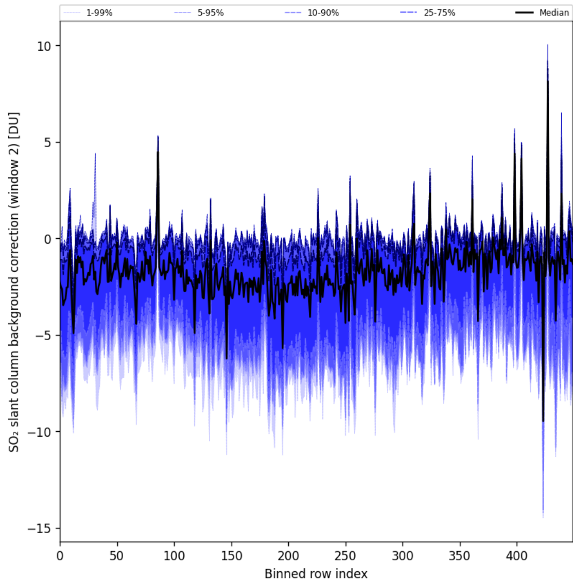
Figure 96: Along track statistics of “SO 2 slant column background correction (window 2)” for 2025-10-22 to 2025-10-23
