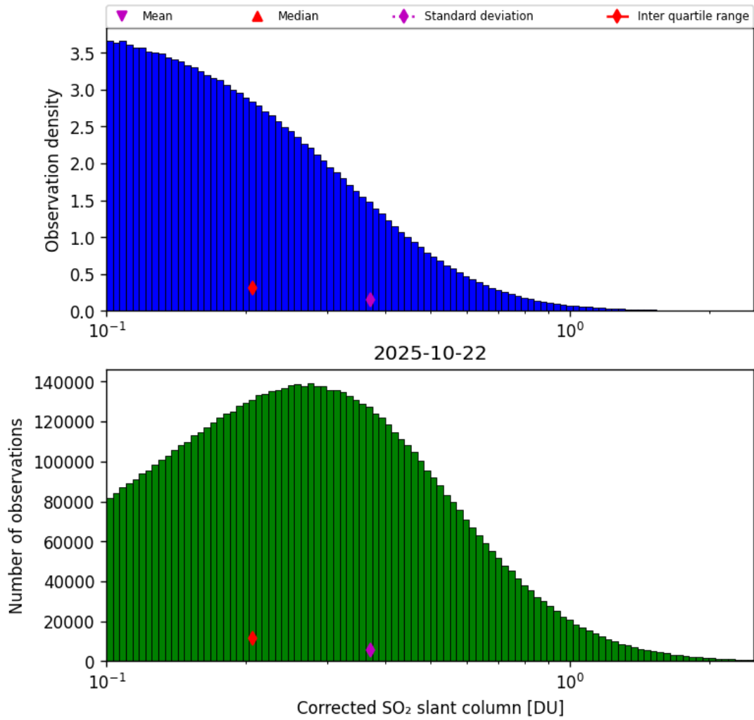
Figure 60: Histogram of "Corrected SO 2 slant column" for 2025-10-22 to 2025-10-23
