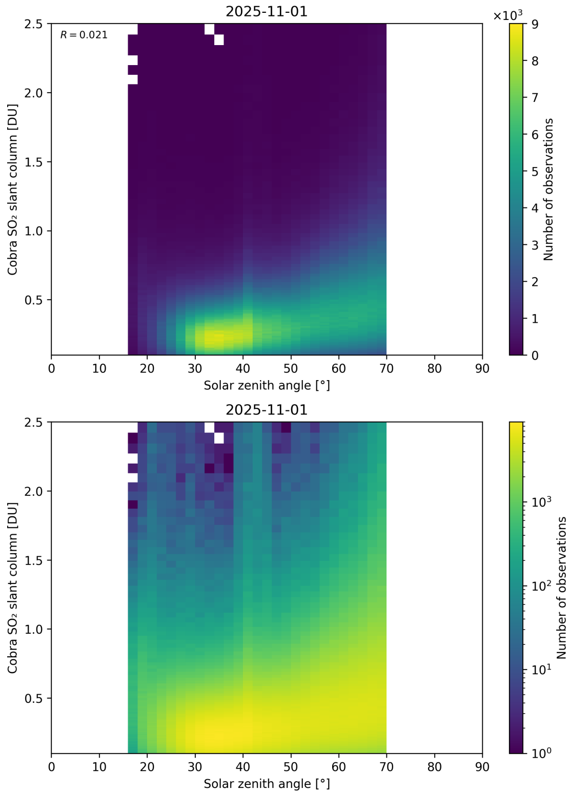
Figure 179: Scatter density plot of “Solar zenith angle” against “Cobra SO 2 slant column” for 2025-10-31 to 2025-11-02.
