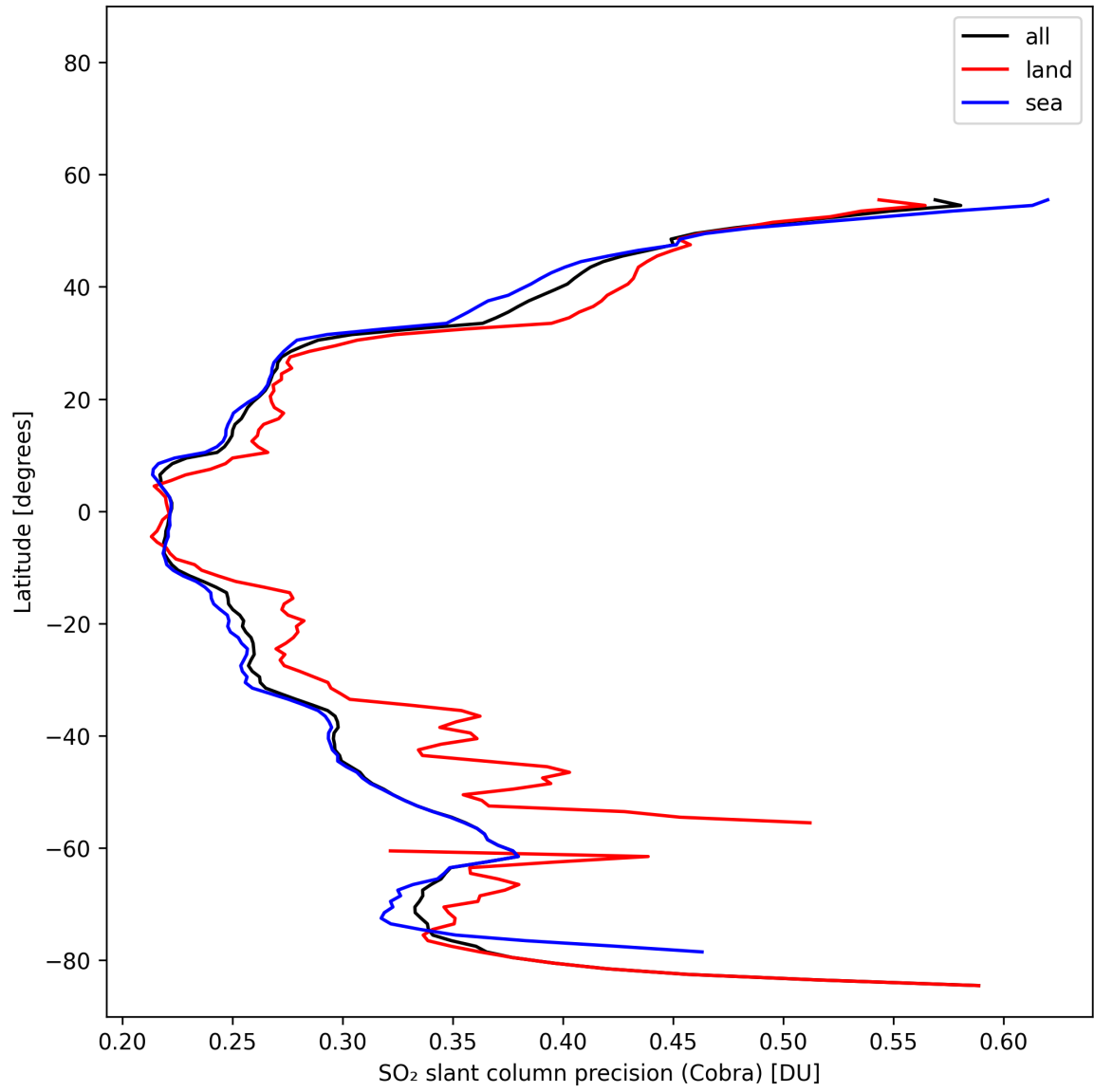
Figure 36: Zonal average of “SO 2 slant column precision (Cobra)” for 2025-10-31 to 2025-11-02.
