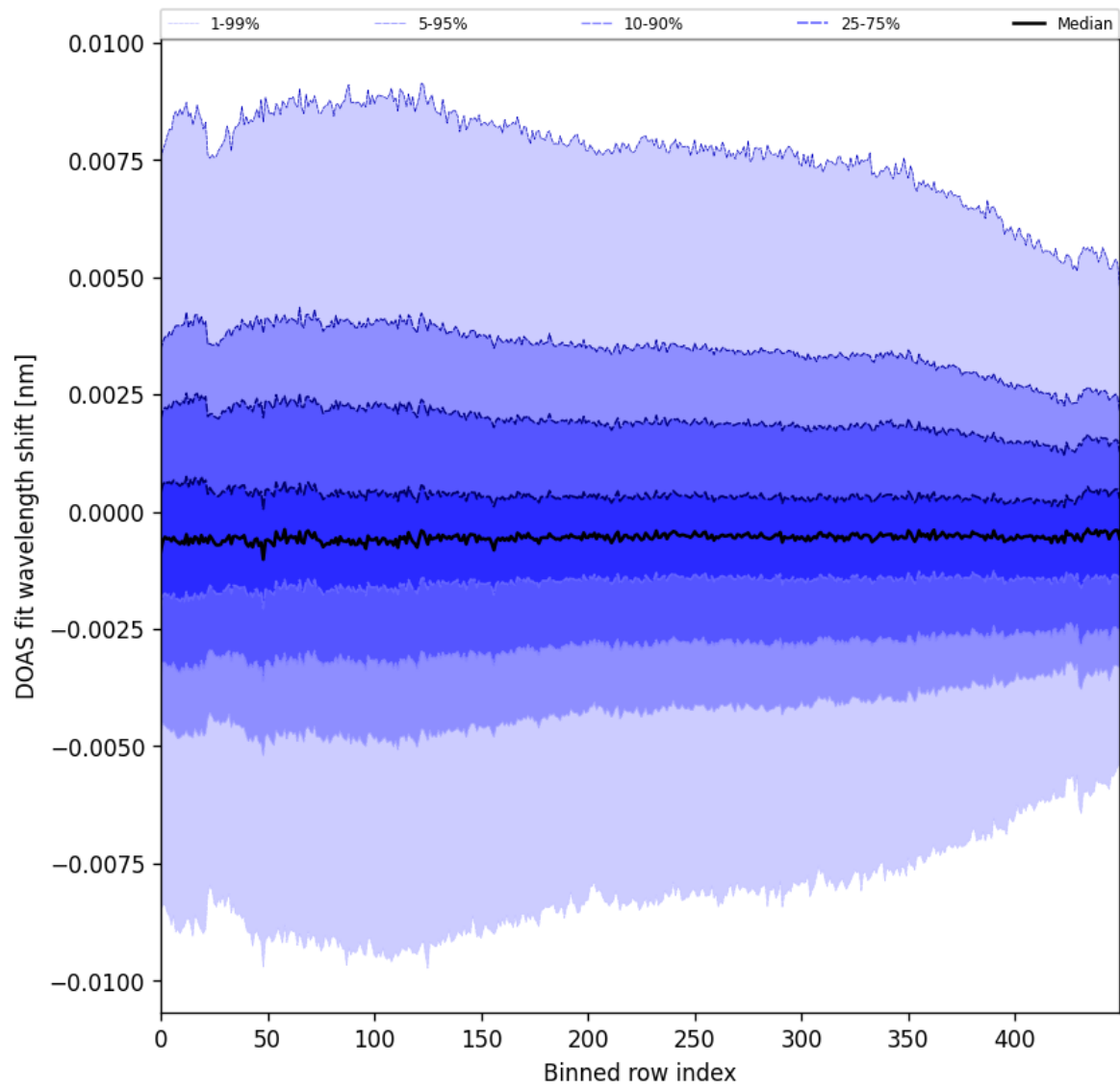
Figure 102: Along track statistics of “DOAS fit wavelength shift” for 2025-10-31 to 2025-11-02
