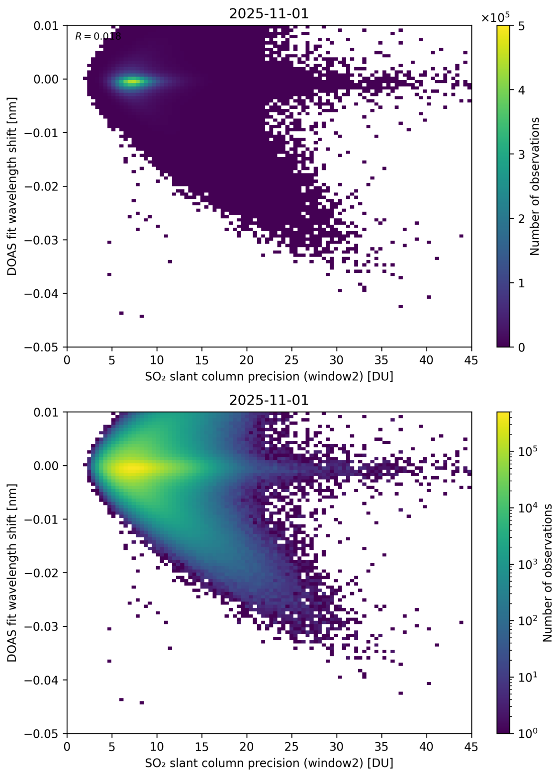
Figure 293: Scatter density plot of “SO 2 slant column precision (window2)” against “DOAS fit wavelength shift” for 2025-10-31 to 2025-11-02.
