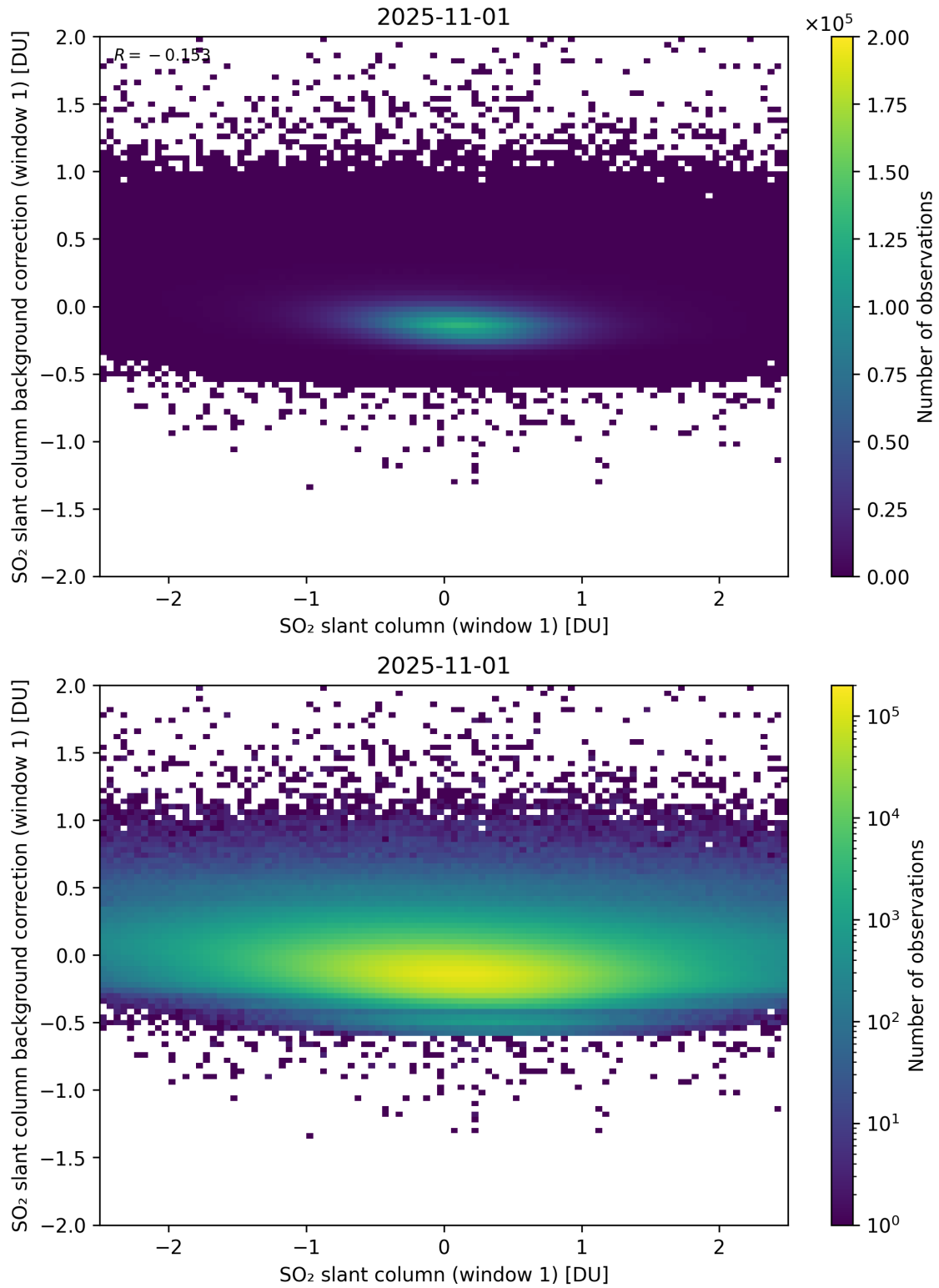
Figure 262: Scatter density plot of “SO 2 slant column (window 1)” against “SO 2 slant column background correction (window 1)” for 2025-10-31 to 2025-11-02.
