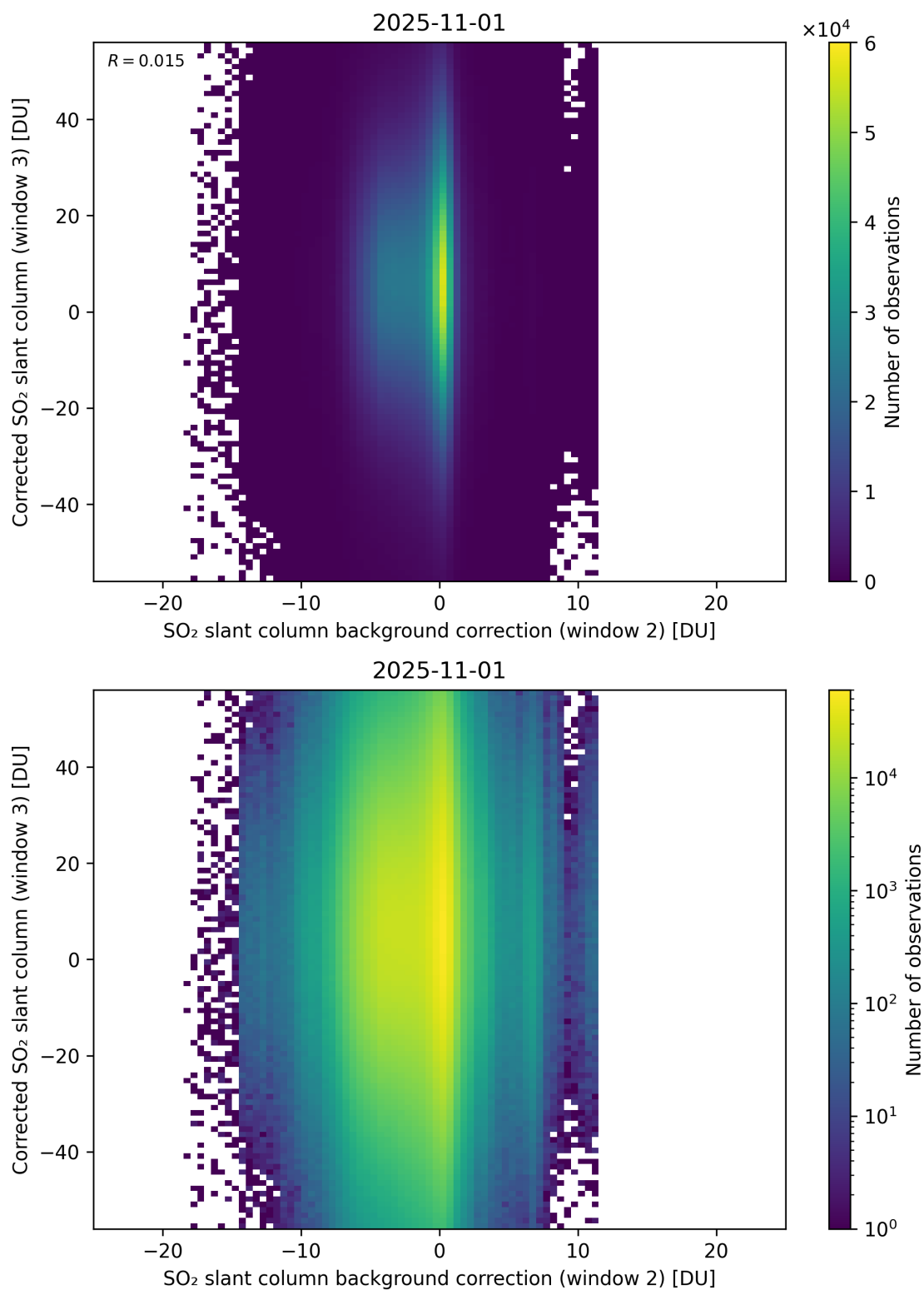
Figure 127: Scatter density plot of “SO 2 slant column background correction (window 2)” against “Corrected SO 2 slant column (window 3)” for 2025-10-31 to 2025-11-02.
