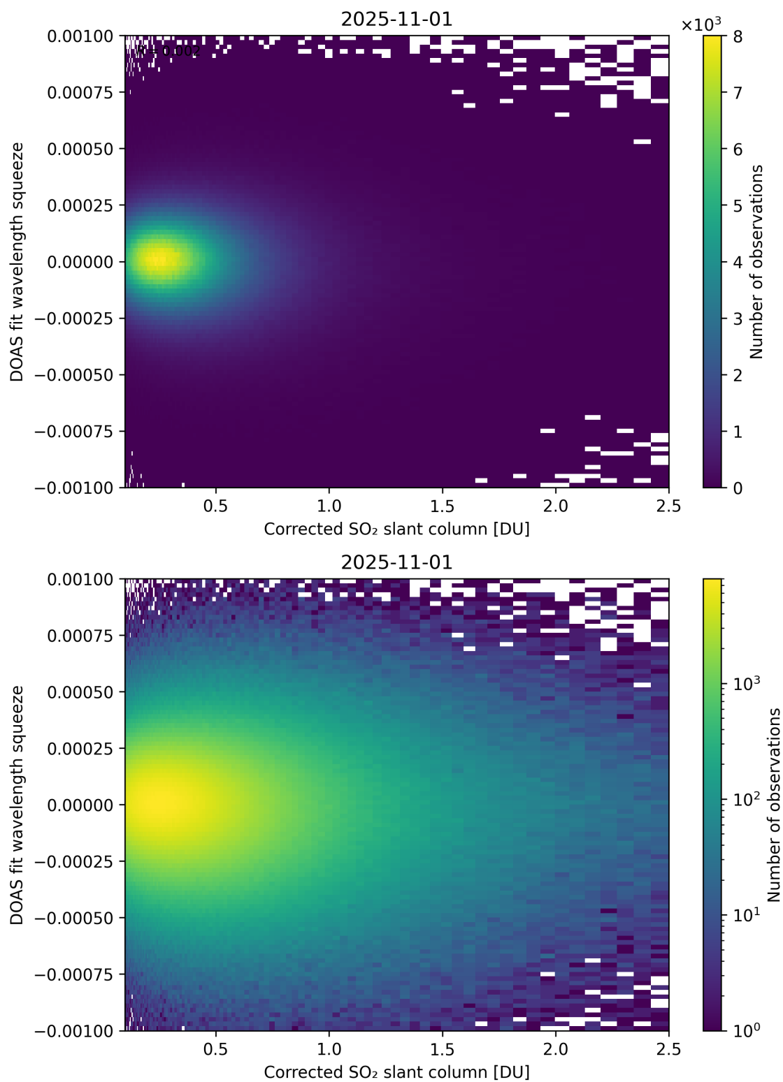
Figure 230: Scatter density plot of "Corrected SO 2 slant column" against "DOAS fit wavelength squeeze" for 2025-10-31 to 2025-11-02.
