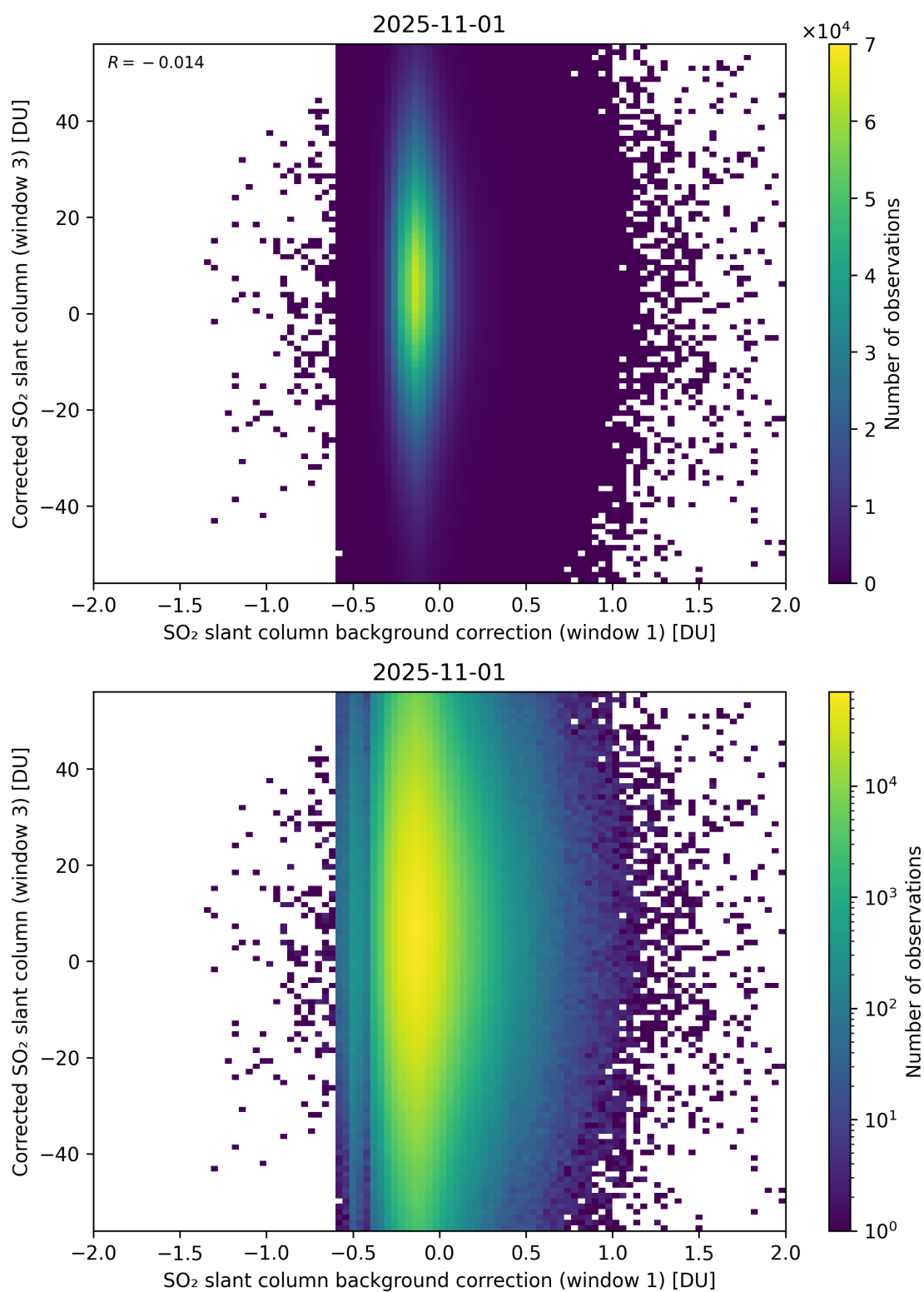
Figure 116: Scatter density plot of “SO 2 slant column background correction (window 1)” against “Corrected SO 2 slant column (window 3)” for 2025-10-31 to 2025-11-02.
