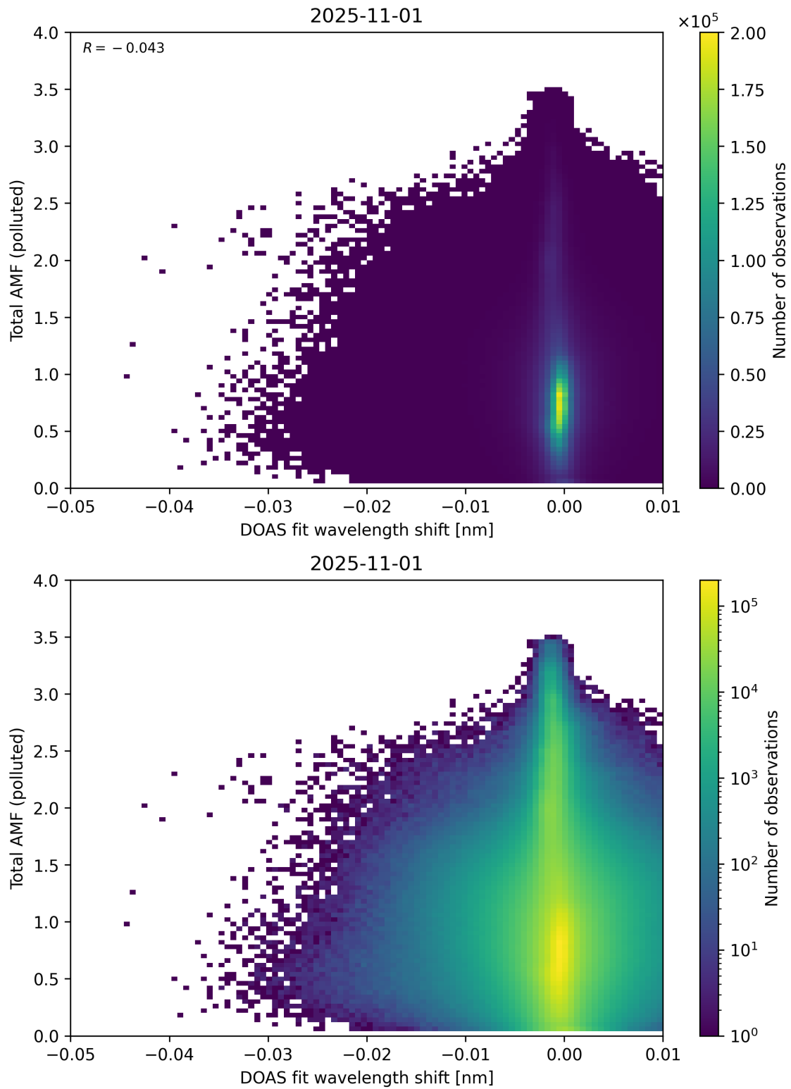
Figure 141: Scatter density plot of “DOAS fit wavelength shift” against “Total AMF (polluted)” for 2025-10-31 to 2025-11-02.
