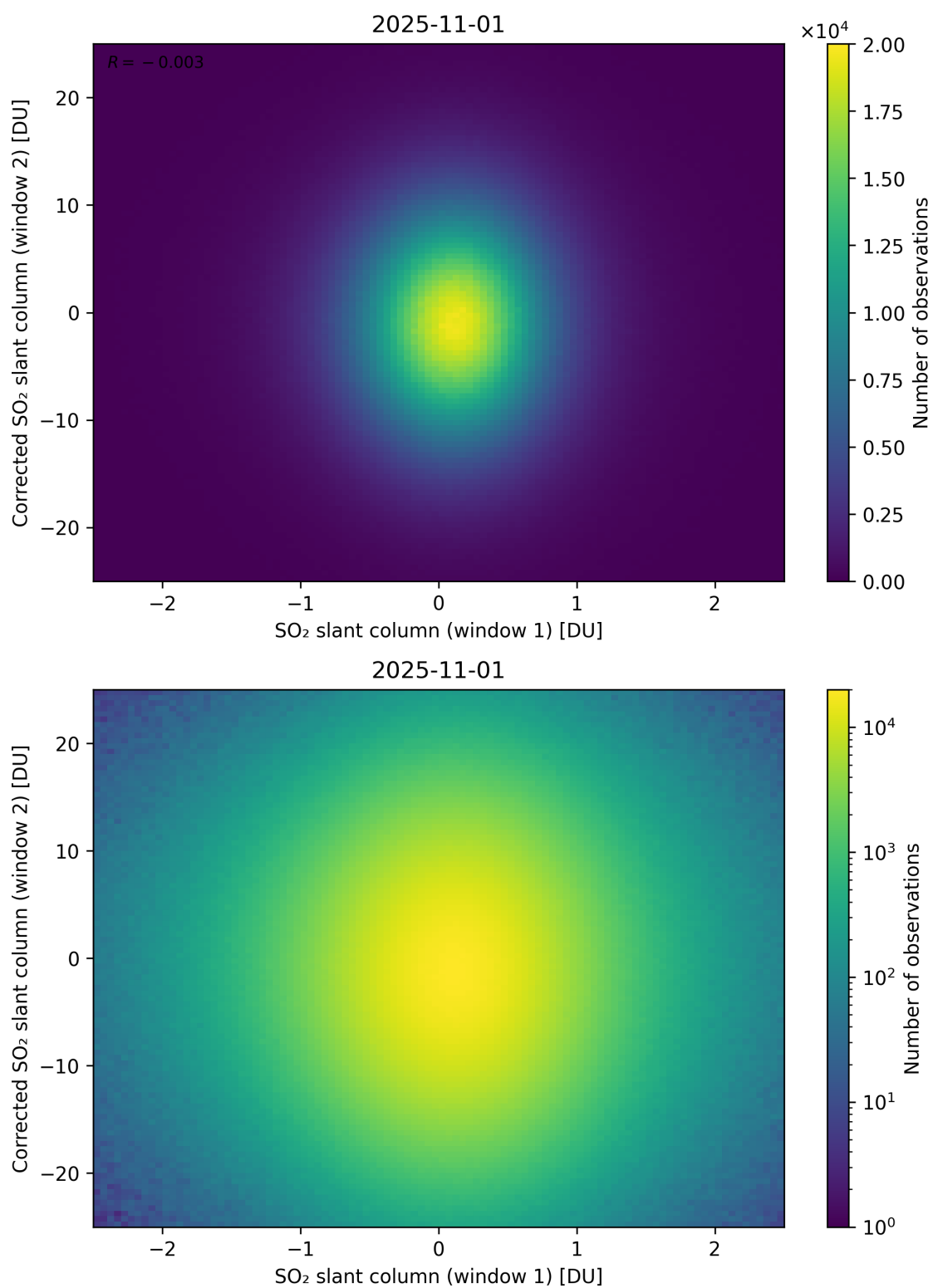
Figure 283: Scatter density plot of “SO 2 slant column (window 1)” against “Corrected SO 2 slant column (window 2)” for 2025-10-31 to 2025-11-02.
