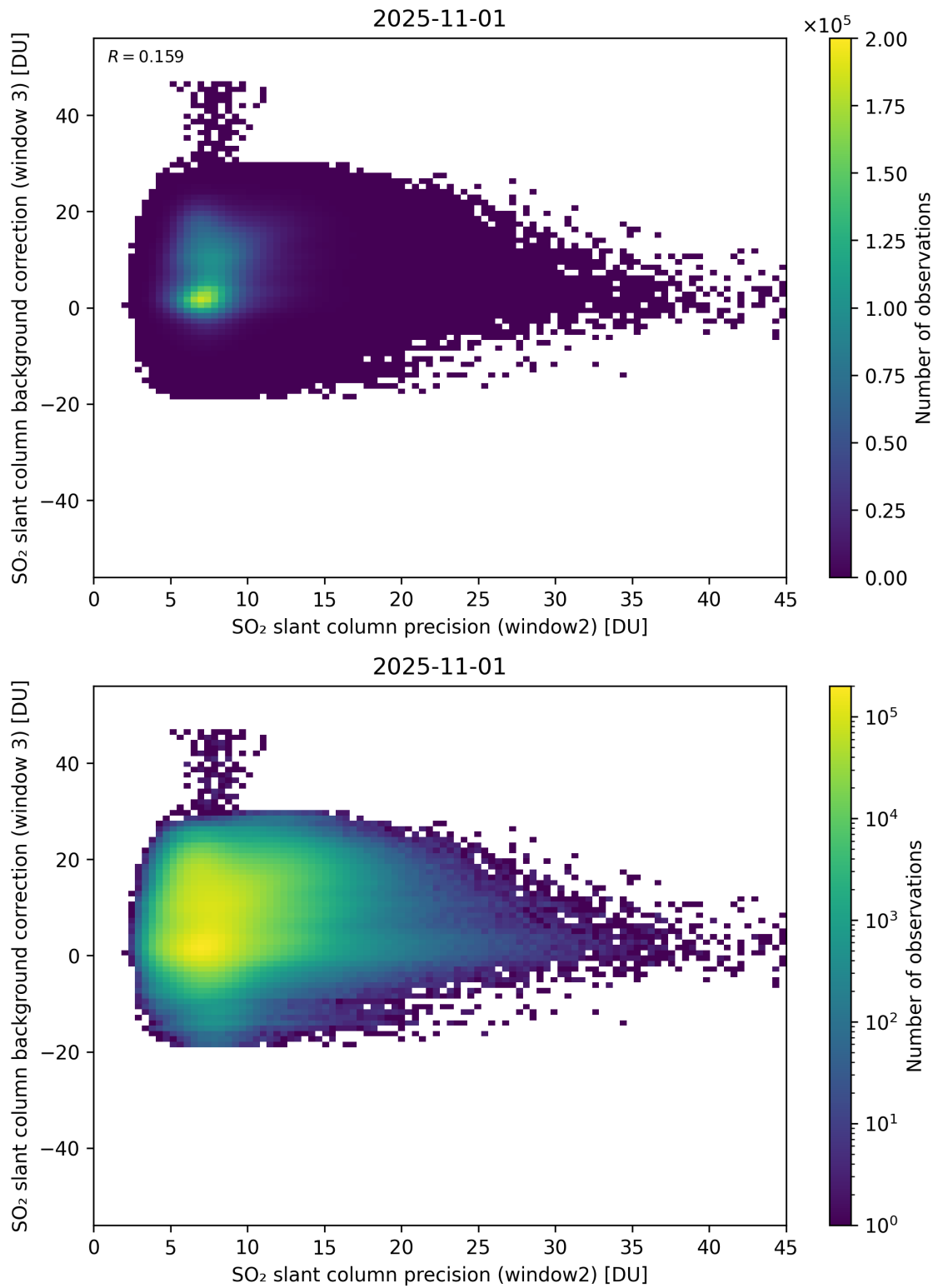
Figure 292: Scatter density plot of “SO 2 slant column precision (window2)” against “SO 2 slant column background correction (window 3)” for 2025-10-31 to 2025-11-02.
