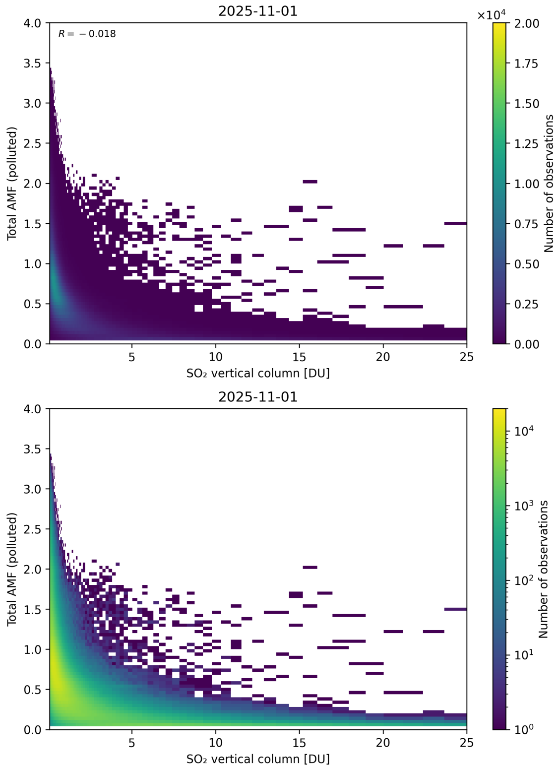
Figure 359: Scatter density plot of “SO 2 vertical column” against “Total AMF (polluted)” for 2025-10-31 to 2025-11-02.
