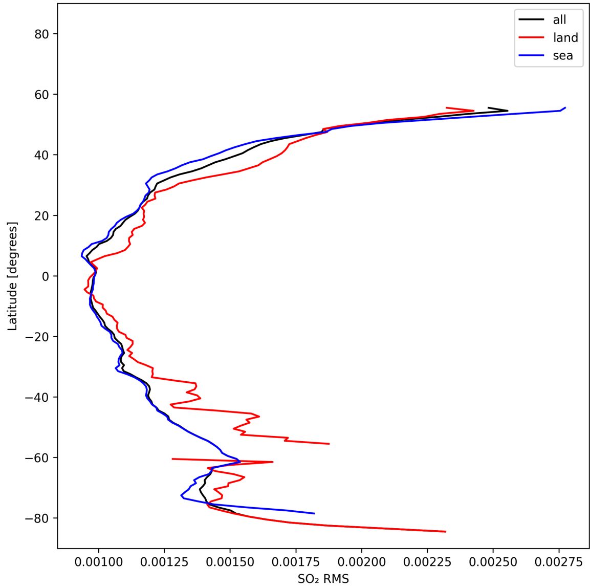
Figure 52: Zonal average of “SO 2 RMS” for 2025-10-31 to 2025-11-02.
