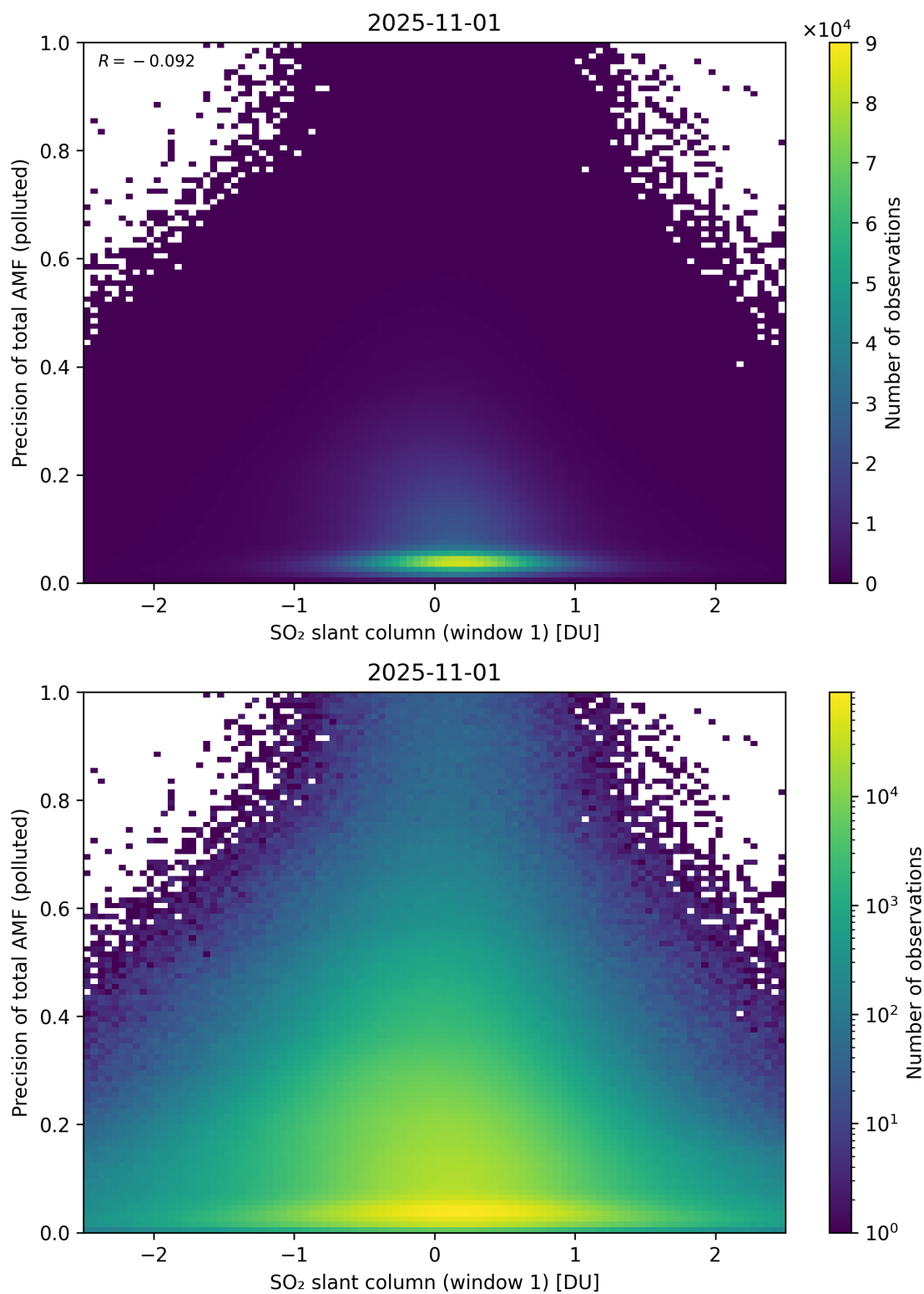
Figure 290: Scatter density plot of “SO 2 slant column (window 1)” against “Precision of total AMF (polluted)” for 2025-10-31 to 2025-11-02.
