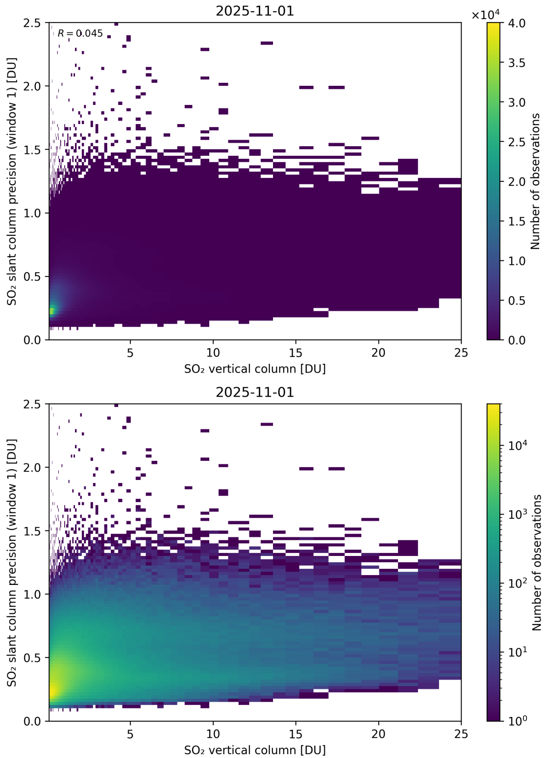
Figure 355: Scatter density plot of “SO 2 vertical column” against “SO 2 slant column precision (window 1)” for 2025-10-31 to 2025-11-02.
