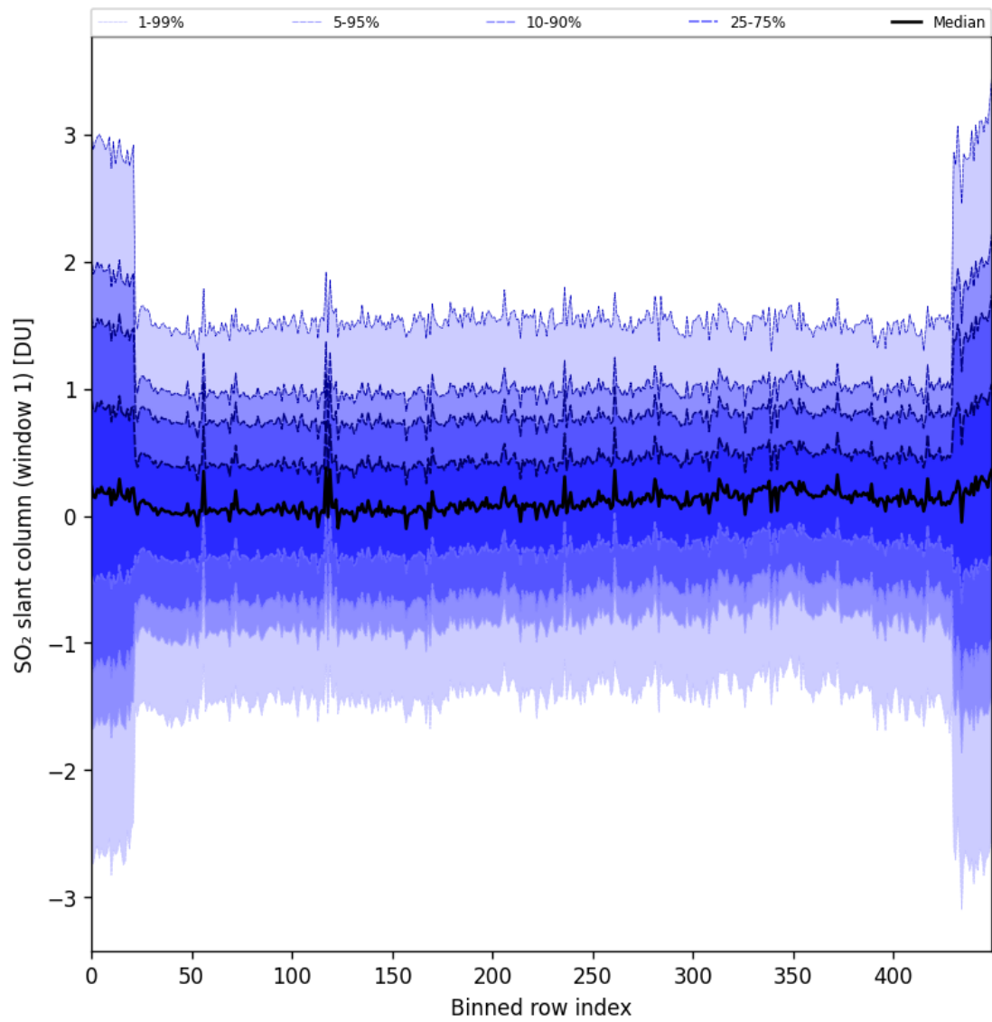
Figure 89: Along track statistics of “SO 2 slant column (window 1)” for 2025-10-31 to 2025-11-02
