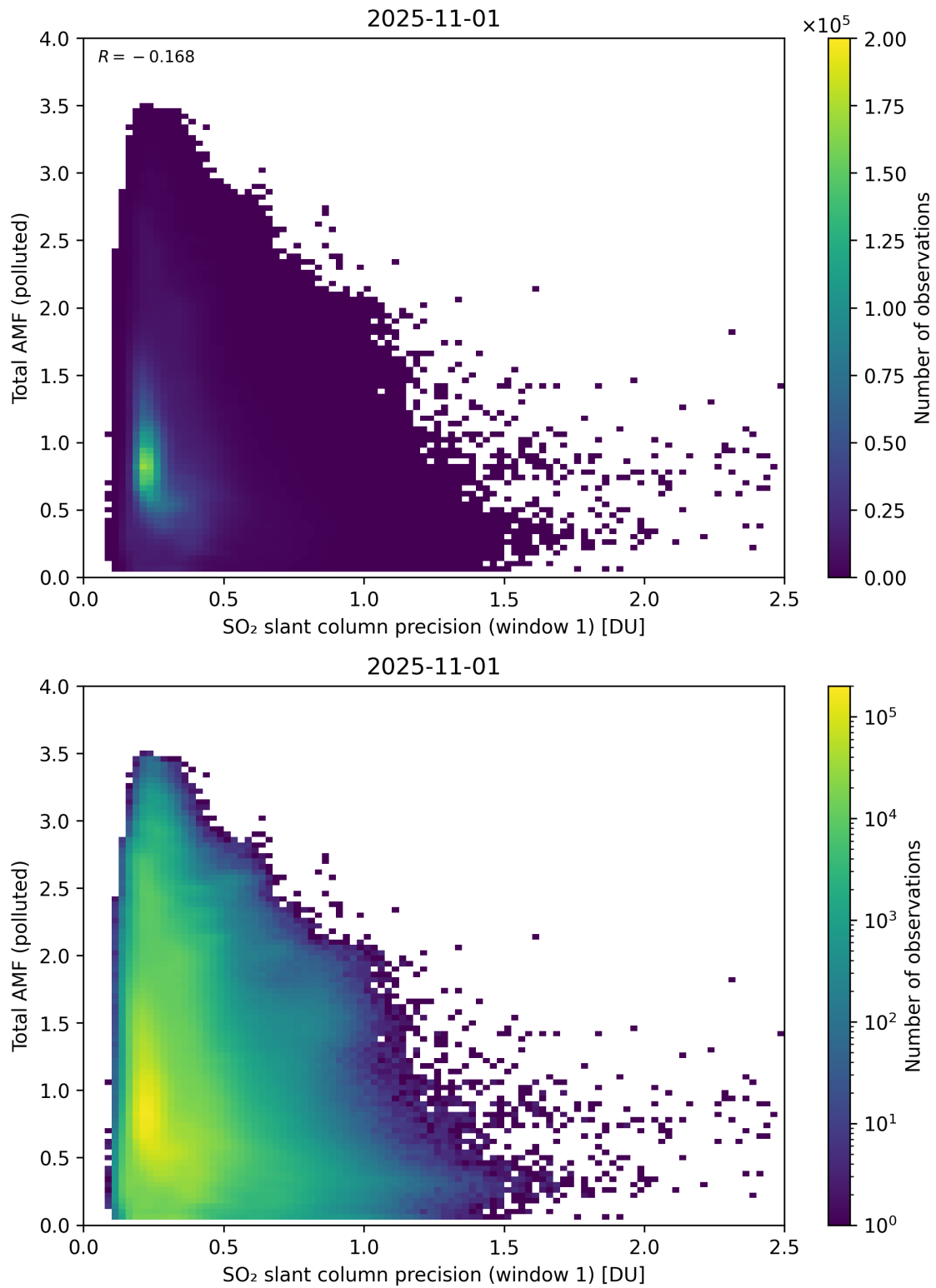
Figure 280: Scatter density plot of “SO 2 slant column precision (window 1)” against “Total AMF (polluted)” for 2025-10-31 to 2025-11-02.
