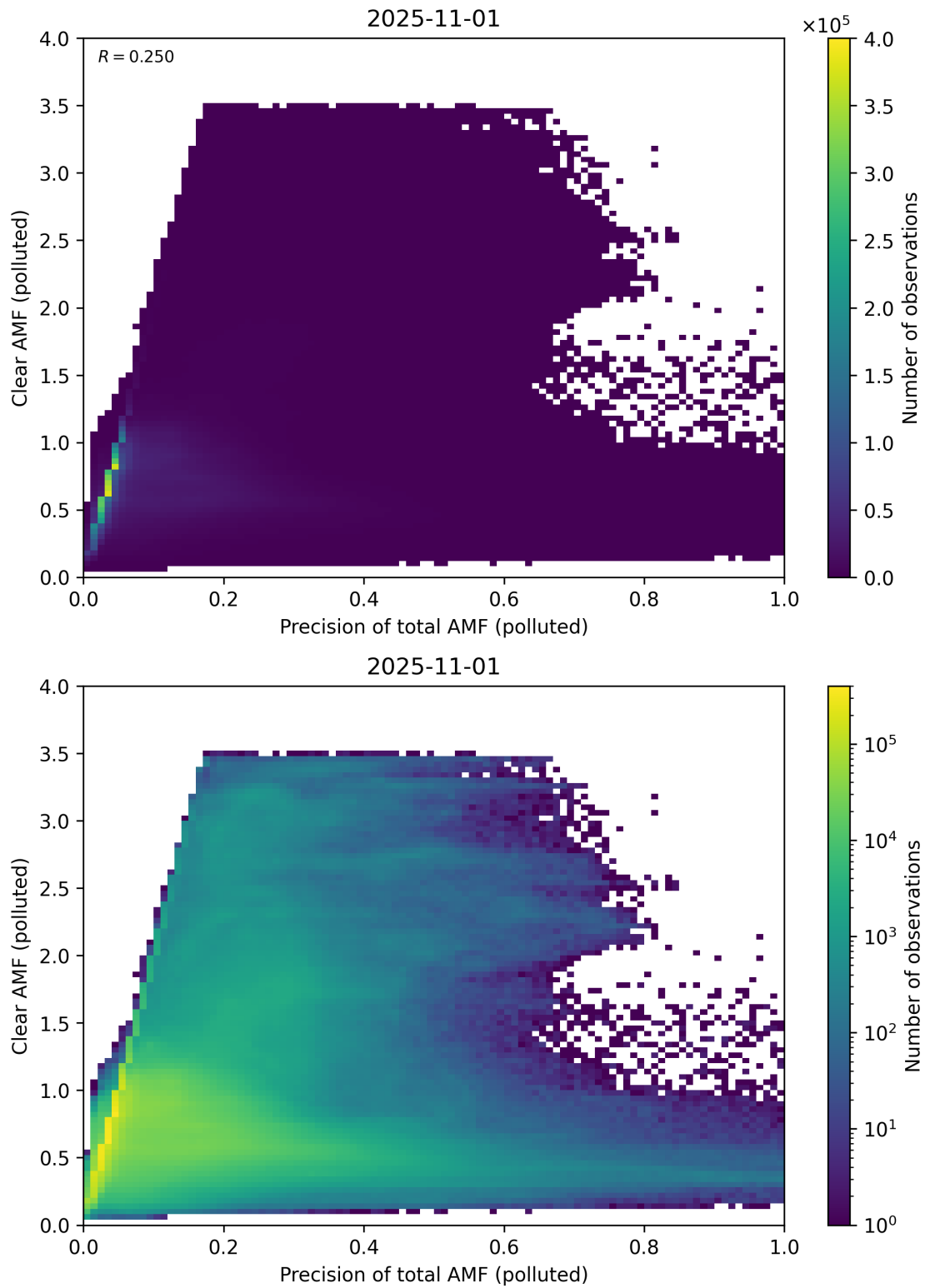
Figure 320: Scatter density plot of “Precision of total AMF (polluted)” against “Clear AMF (polluted)” for 2025-10-31 to 2025-11-02.
