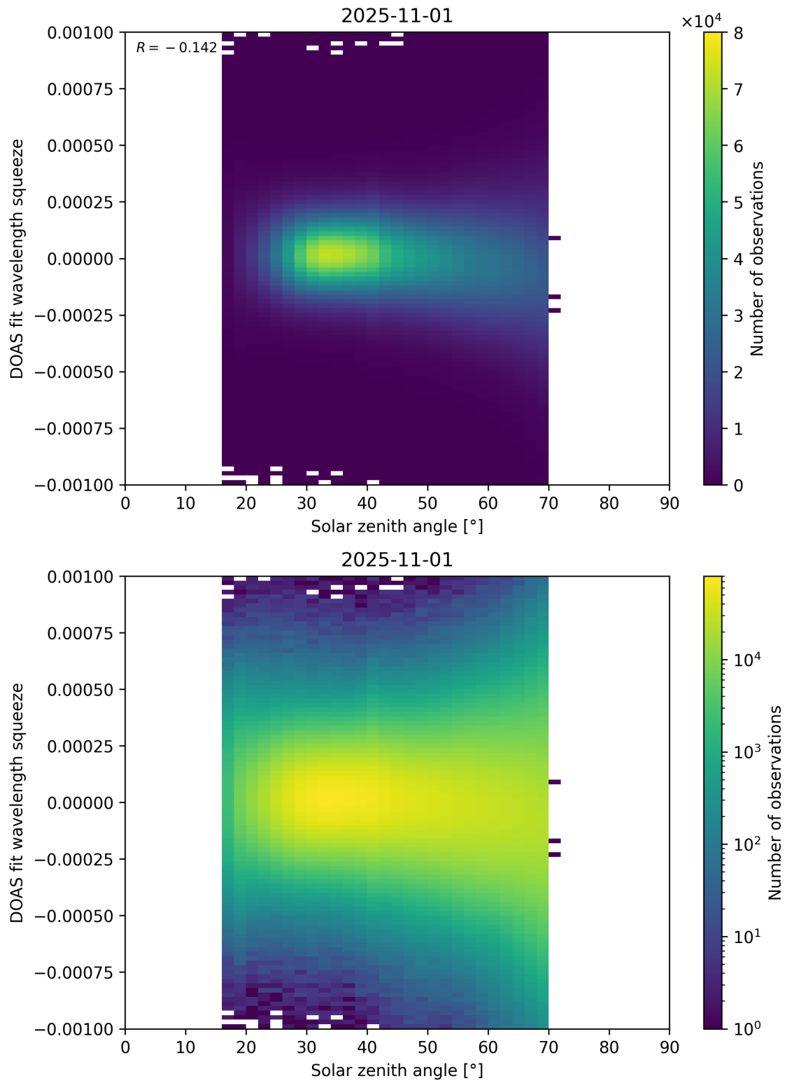
Figure 175: Scatter density plot of “Solar zenith angle” against “DOAS fit wavelength squeeze” for 2025-10-31 to 2025-11-02.
