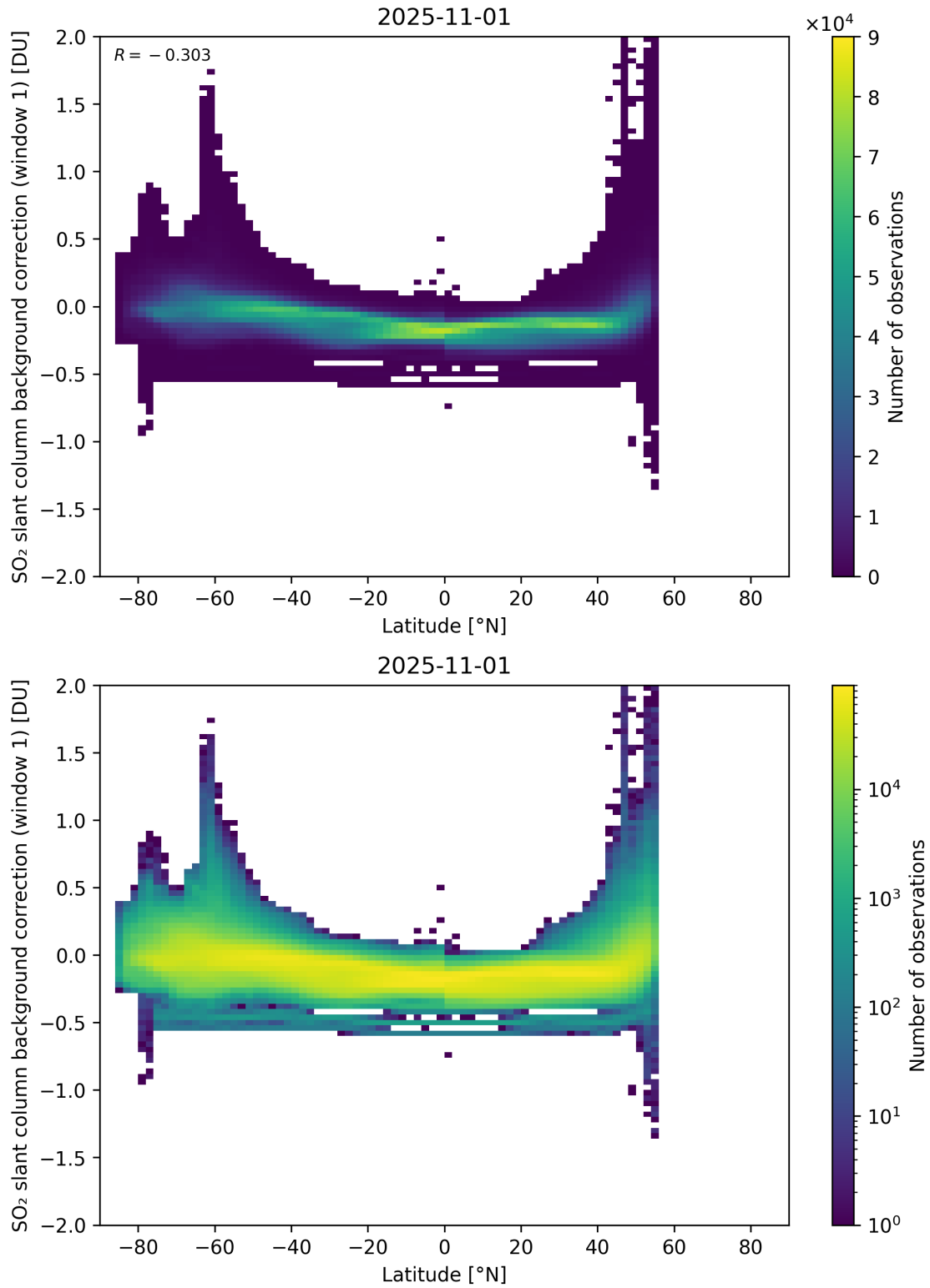
Figure 150: Scatter density plot of “Latitude” against “SO 2 slant column background correction (window 1)” for 2025-10-31 to 2025-11-02.
