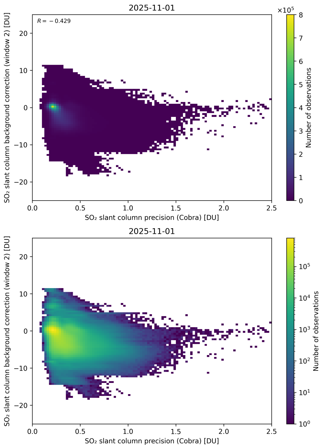
Figure 200: Scatter density plot of “SO 2 slant column precision (Cobra)” against “SO 2 slant column background correction (window 2)” for 2025-10-31 to 2025-11-02.
