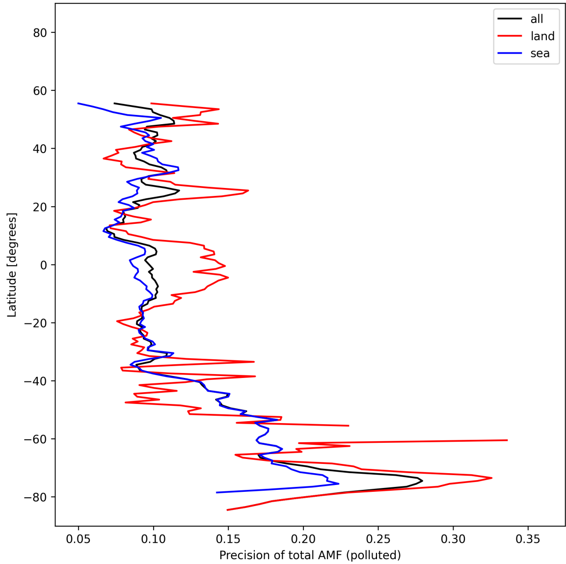
Figure 54: Zonal average of “Precision of total AMF (polluted)” for 2025-10-31 to 2025-11-02.
