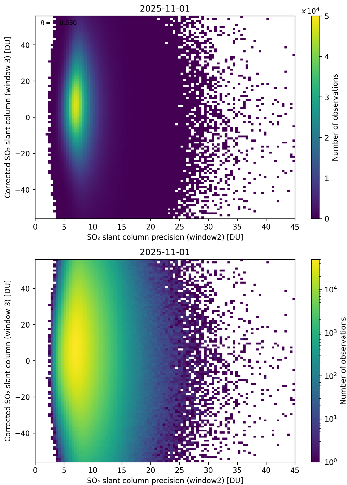
Figure 298: Scatter density plot of “SO 2 slant column precision (window2)” against “Corrected SO 2 slant column (window 3)” for 2025-10-31 to 2025-11-02.
