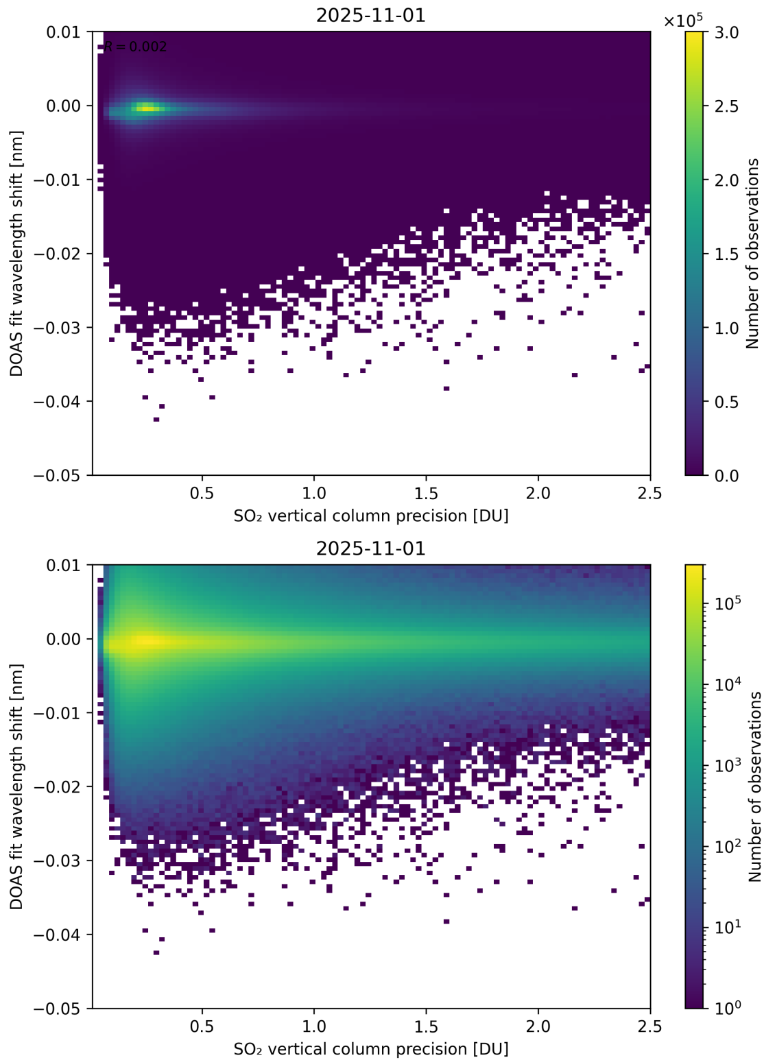
Figure 332: Scatter density plot of “SO 2 vertical column precision” against “DOAS fit wavelength shift” for 2025-10-31 to 2025-11-02.
