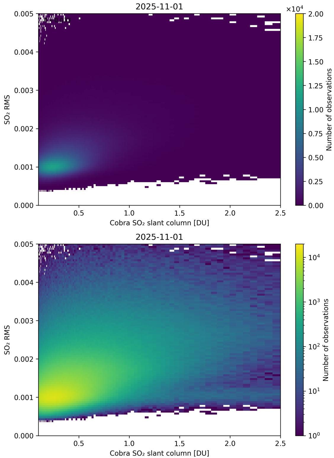
Figure 198: Scatter density plot of “Cobra SO 2 slant column” against “SO 2 RMS” for 2025-10-31 to 2025-11-02.
