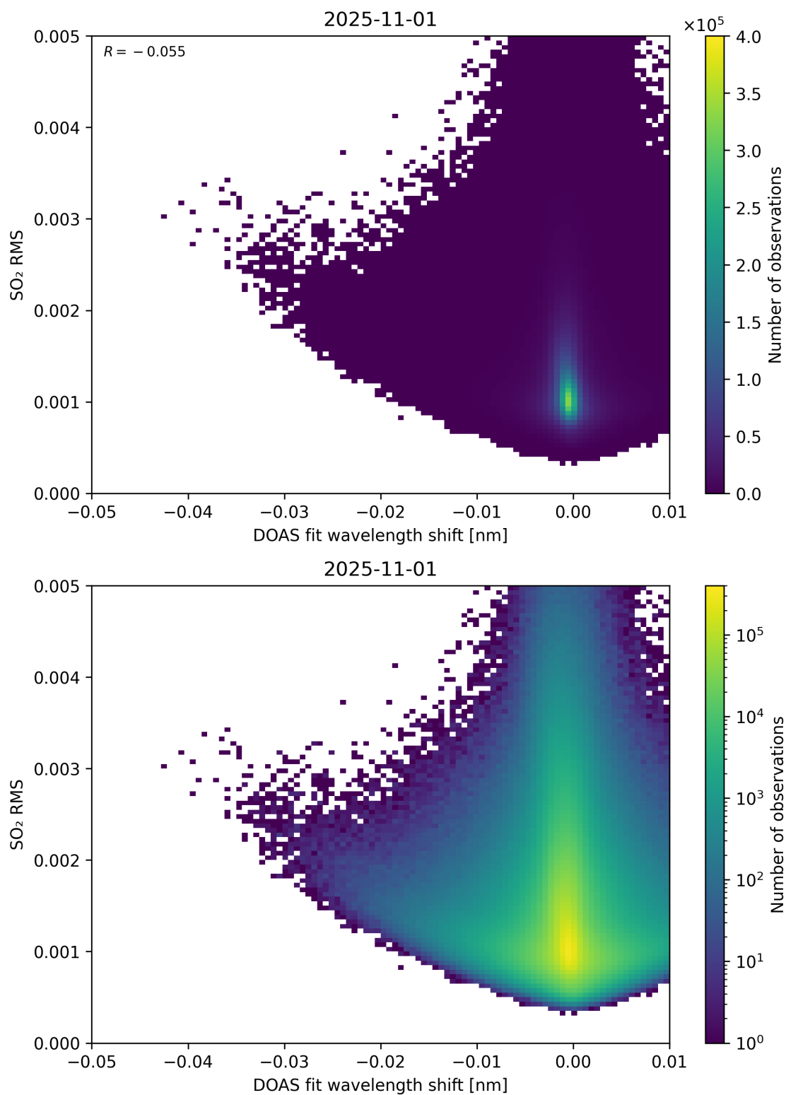
Figure 139: Scatter density plot of “DOAS fit wavelength shift” against “SO 2 RMS” for 2025-10-31 to 2025-11-02.
