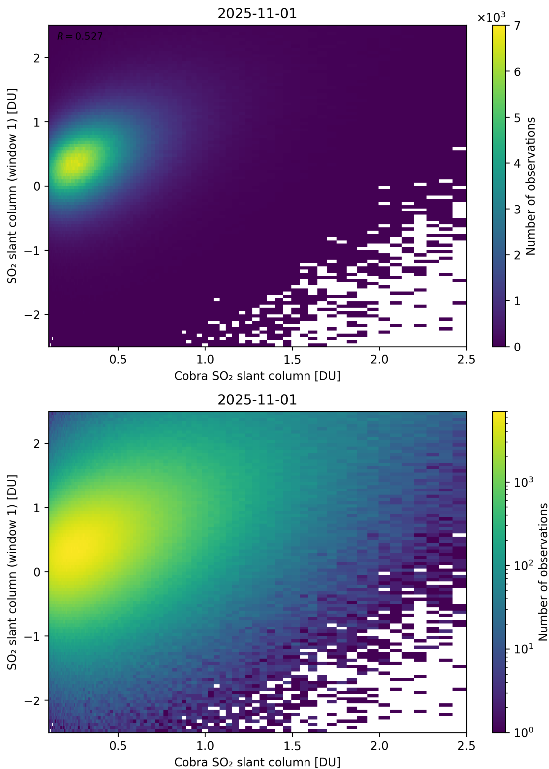
Figure 219: Scatter density plot of “Cobra SO 2 slant column” against “SO 2 slant column (window 1)” for 2025-10-31 to 2025-11-02.
