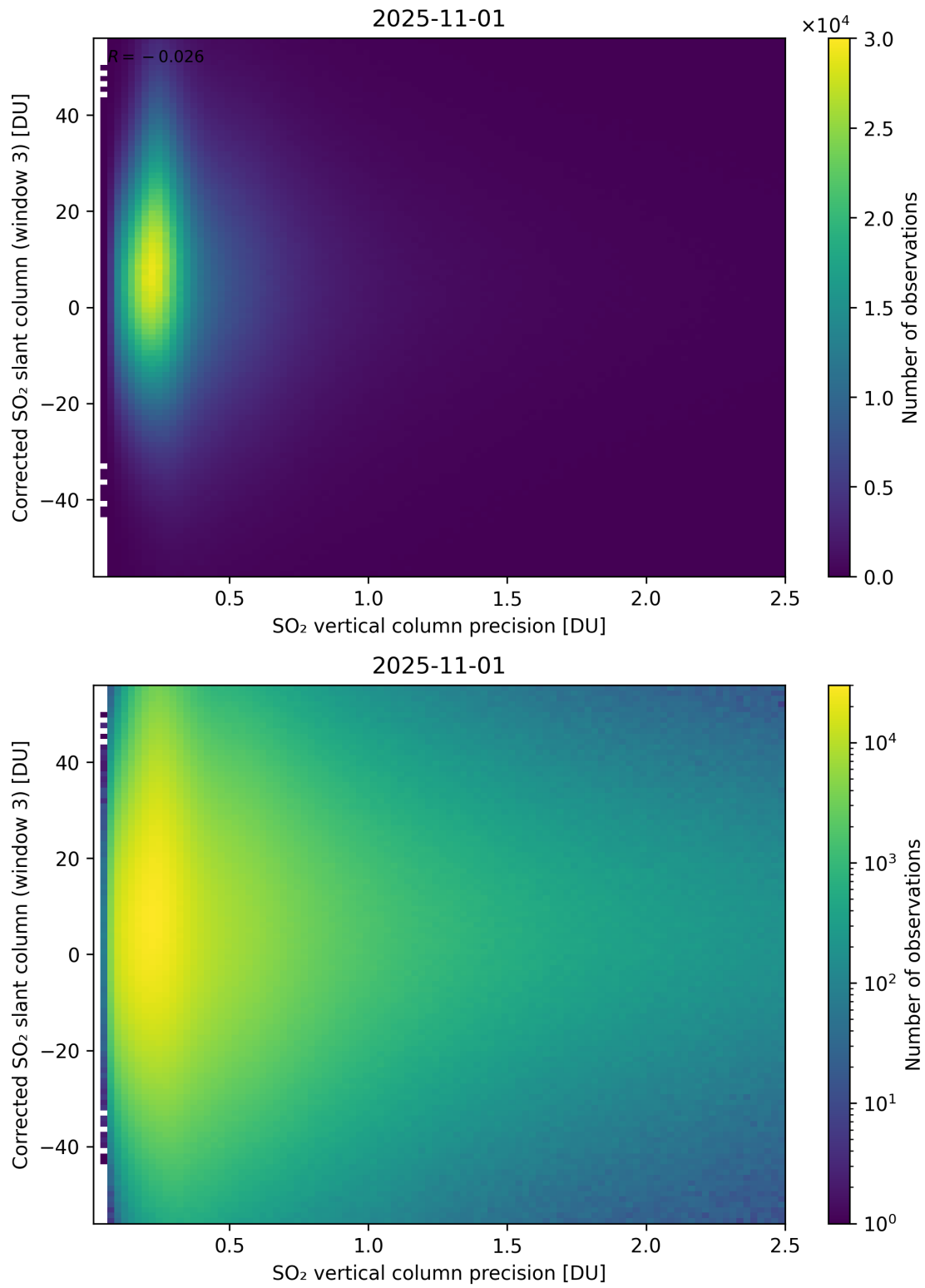
Figure 340: Scatter density plot of “SO 2 vertical column precision” against “Corrected SO 2 slant column (window 3)” for 2025-10-31 to 2025-11-02.
