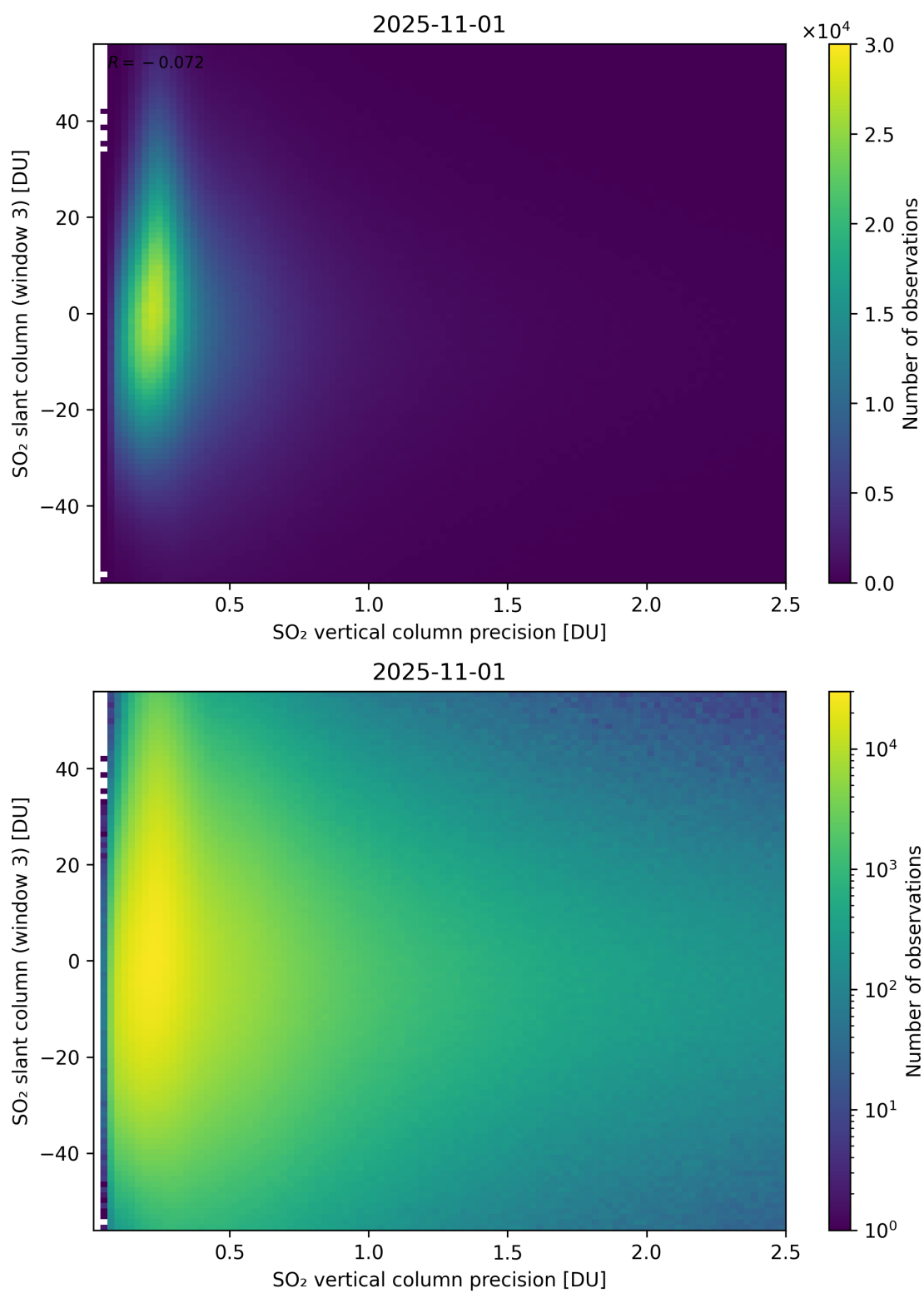
Figure 344: Scatter density plot of “SO 2 vertical column precision” against “SO 2 slant column (window 3)” for 2025-10-31 to 2025-11-02.
