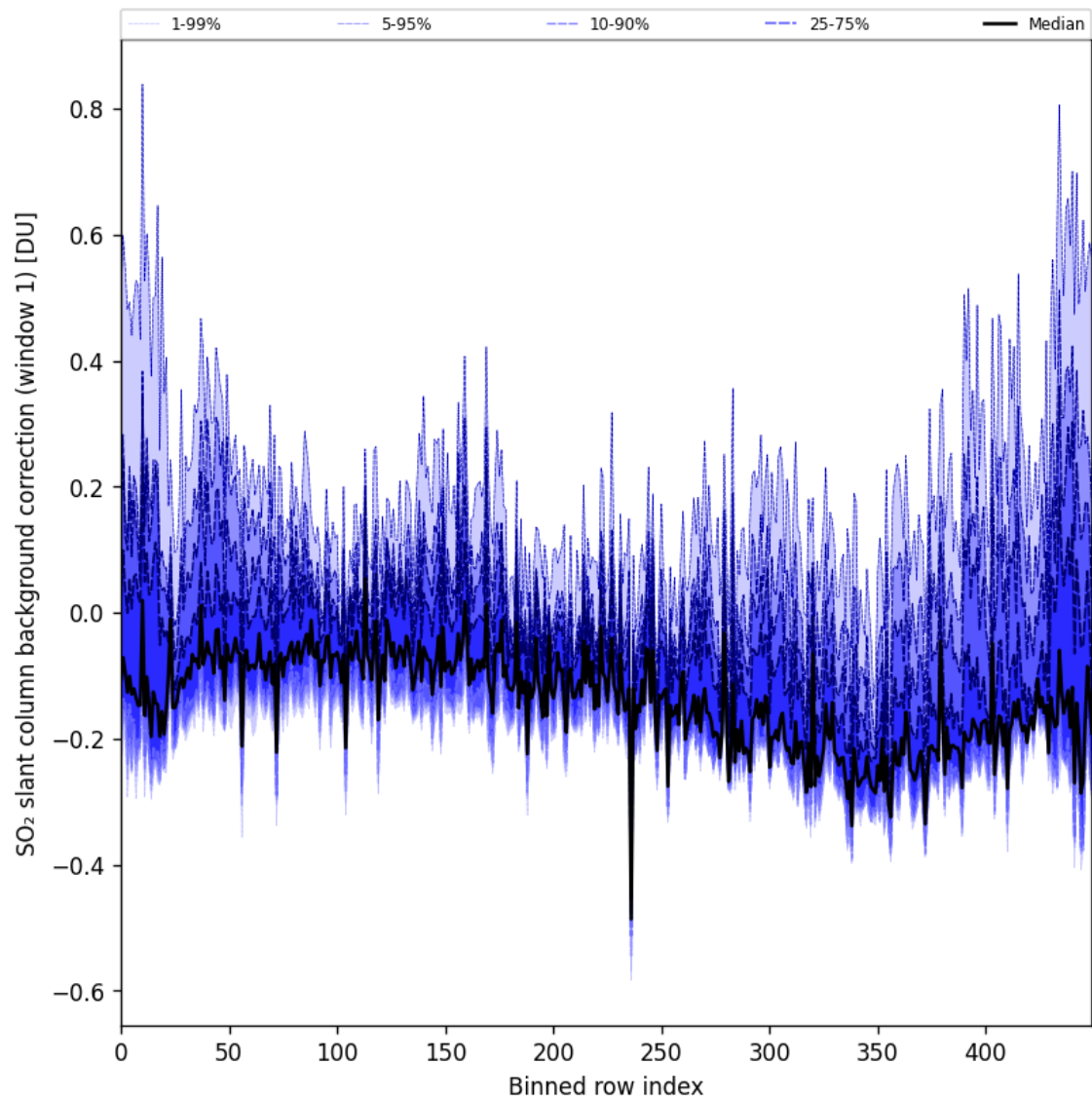
Figure 92: Along track statistics of “SO 2 slant column background correction (window 1)” for 2025-10-31 to 2025-11-02
