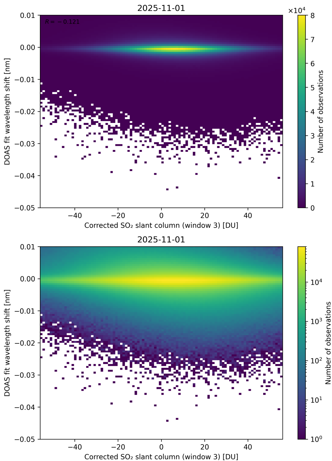
Figure 256: Scatter density plot of “Corrected SO 2 slant column (window 3)” against “DOAS fit wavelength shift” for 2025-10-31 to 2025-11-02.
