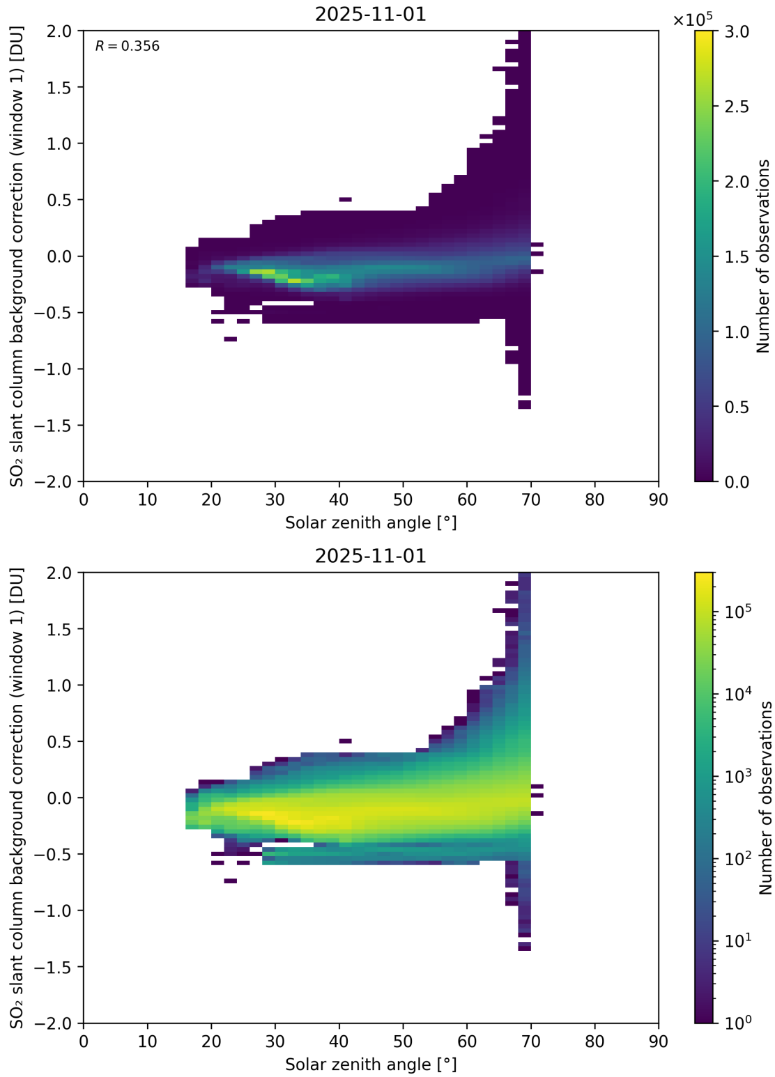
Figure 171: Scatter density plot of “Solar zenith angle” against “SO 2 slant column background correction (window 1)” for 2025-10-31 to 2025-11-02.
