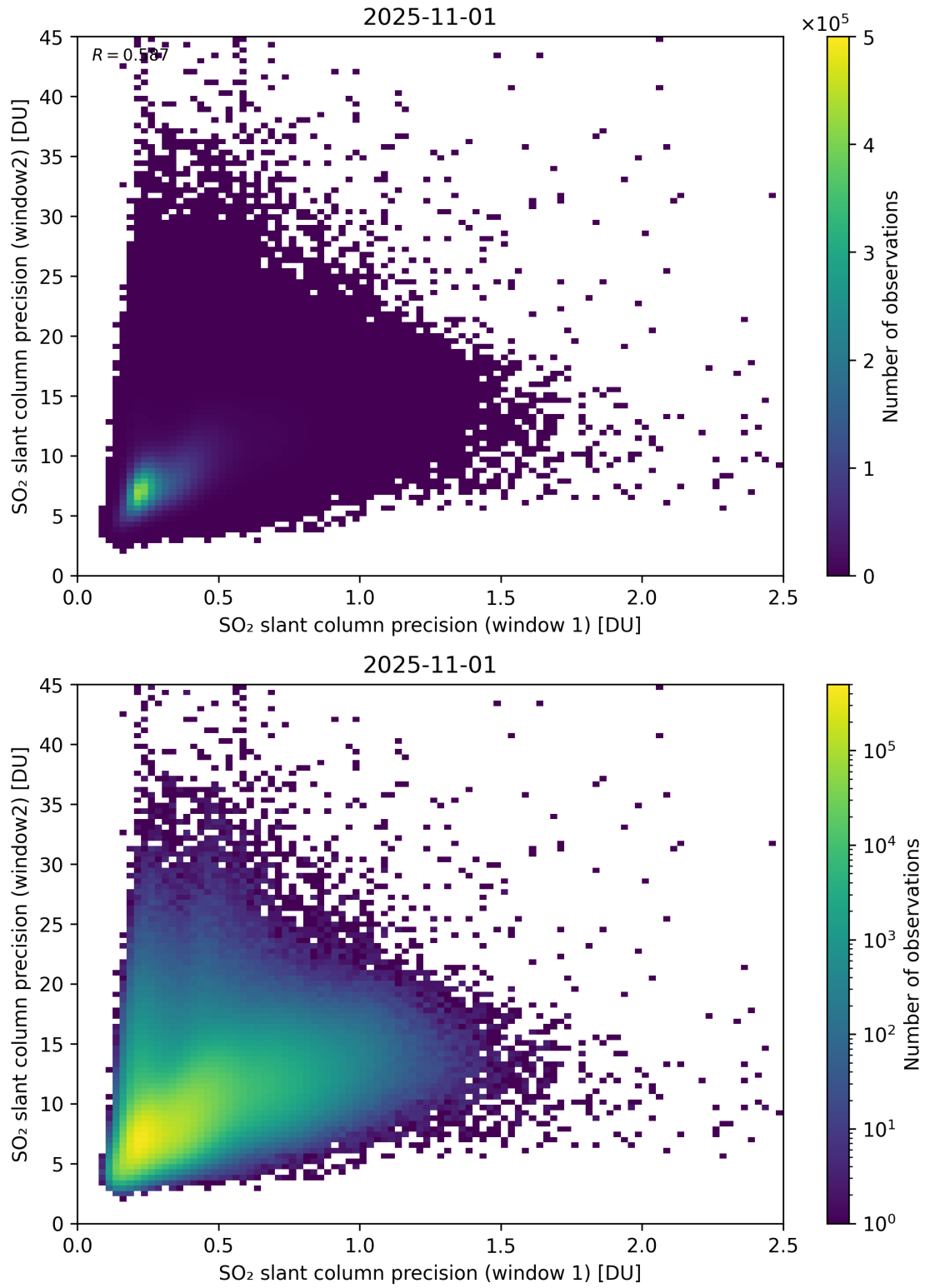
Figure 277: Scatter density plot of “SO 2 slant column precision (window 1)” against “SO 2 slant column precision (window2)” for 2025-10-31 to 2025-11-02.
