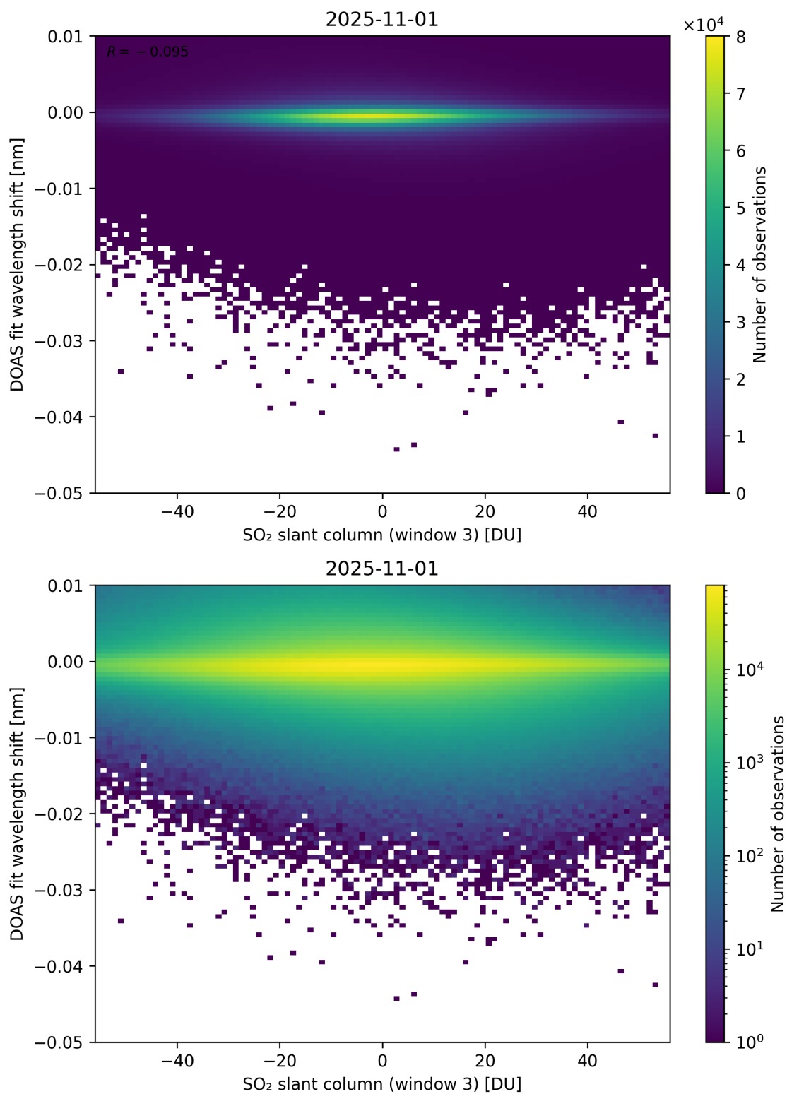
Figure 304: Scatter density plot of “SO 2 slant column (window 3)” against “DOAS fit wavelength shift” for 2025-10-31 to 2025-11-02.
