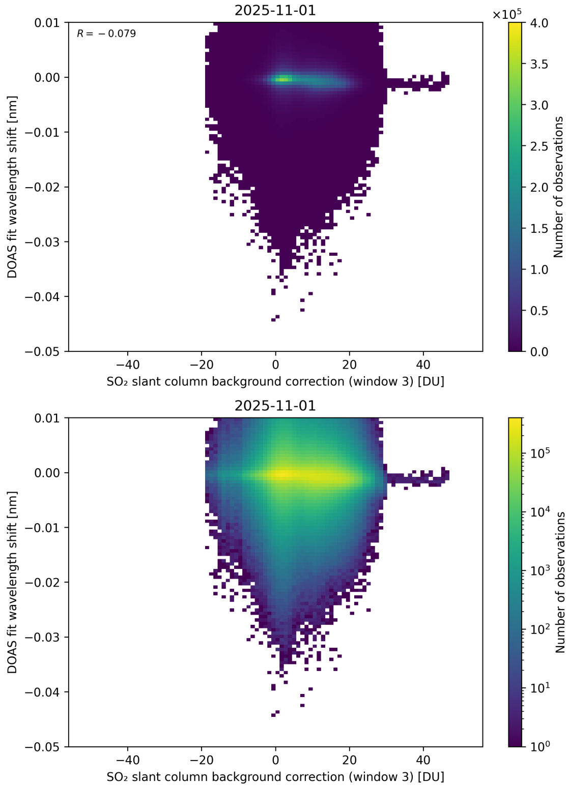
Figure 132: Scatter density plot of “SO 2 slant column background correction (window 3)” against “DOAS fit wavelength shift” for 2025-10-31 to 2025-11-02.
