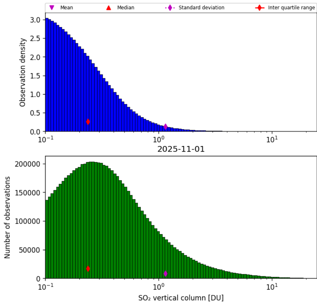
Figure 58: Histogram of “SO 2 vertical column” for 2025-10-31 to 2025-11-02
