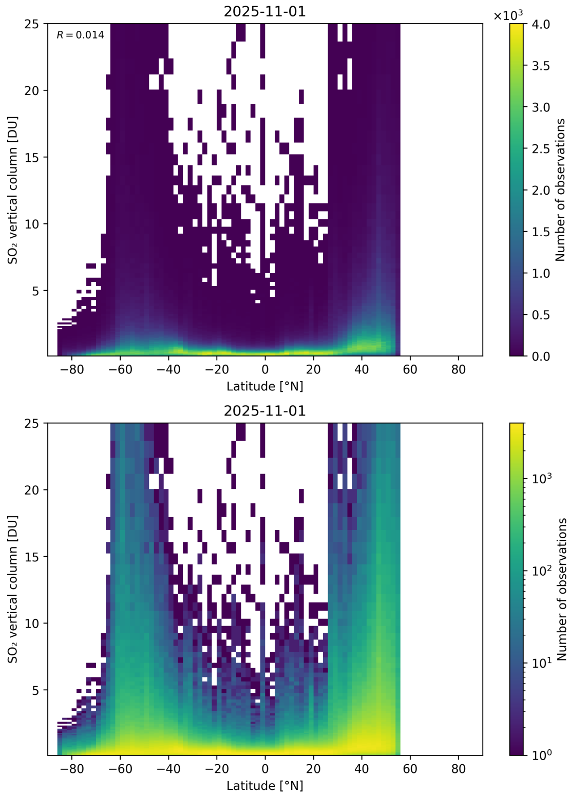
Figure 169: Scatter density plot of “Latitude” against “SO 2 vertical column” for 2025-10-31 to 2025-11-02.
