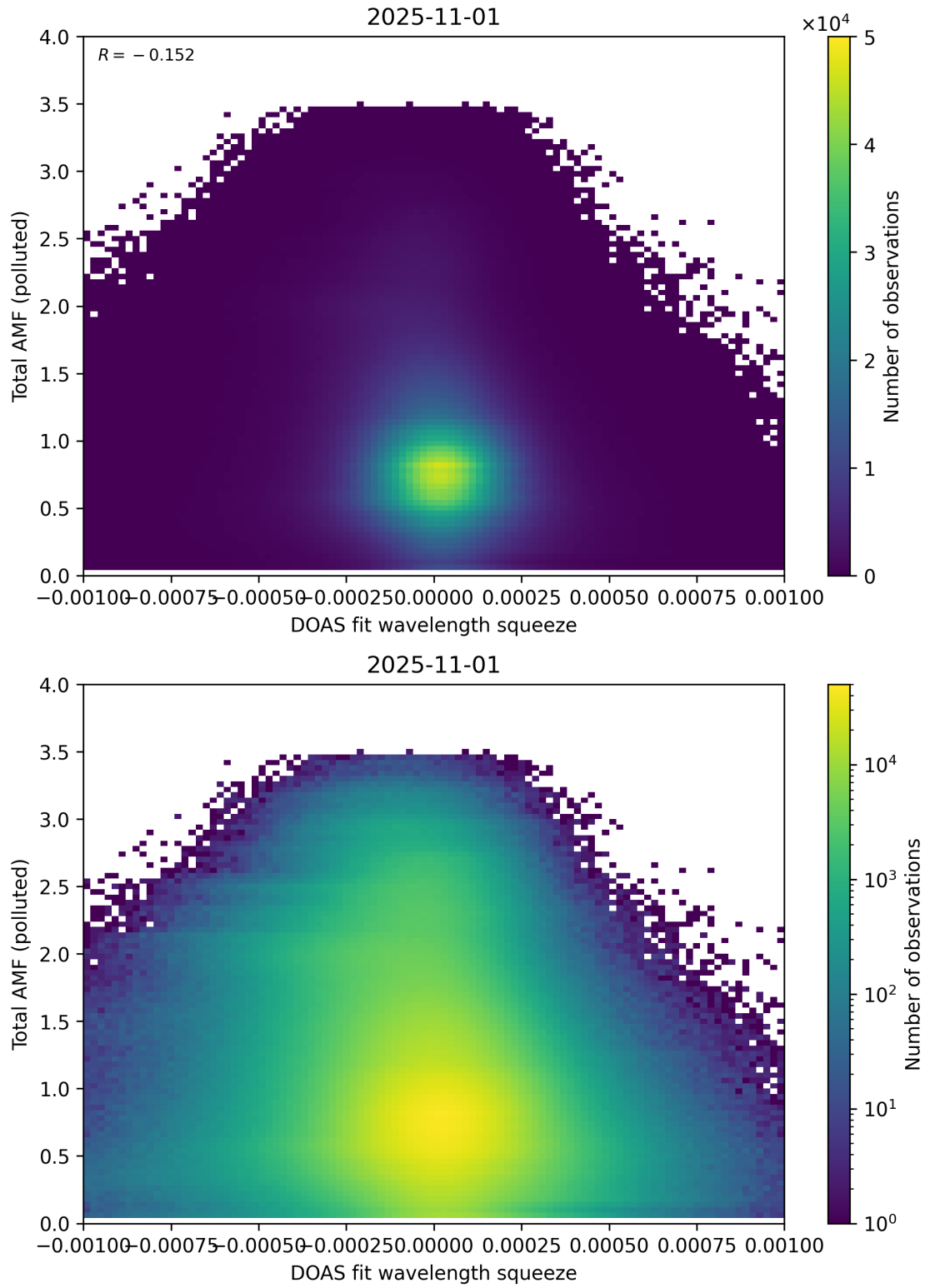
Figure 145: Scatter density plot of “DOAS fit wavelength squeeze” against “Total AMF (polluted)” for 2025-10-31 to 2025-11-02.
