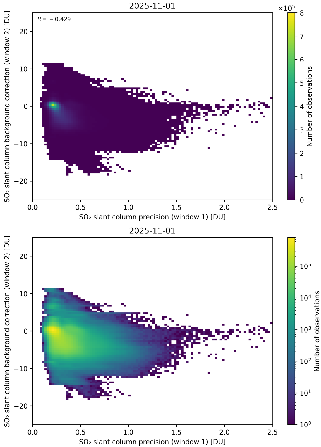
Figure 269: Scatter density plot of “SO 2 slant column precision (window 1)” against “SO 2 slant column background correction (window 2)” for 2025-10-31 to 2025-11-02.
