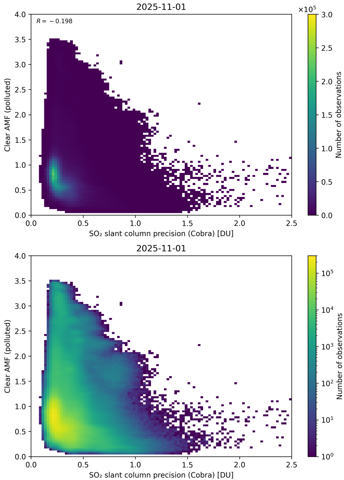
Figure 205: Scatter density plot of “SO 2 slant column precision (Cobra)” against “Clear AMF (polluted)” for 2025-10-31 to 2025-11-02.
