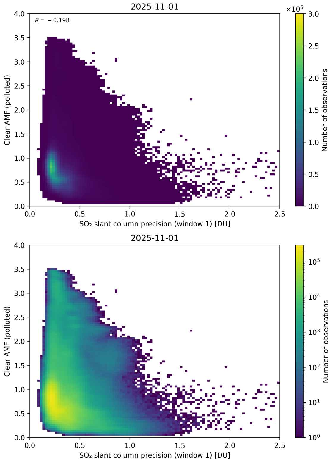
Figure 274: Scatter density plot of “SO 2 slant column precision (window 1)” against “Clear AMF (polluted)” for 2025-10-31 to 2025-11-02.
