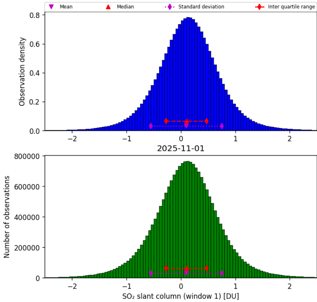
Figure 63: Histogram of “SO 2 slant column (window 1)” for 2025-10-31 to 2025-11-02
