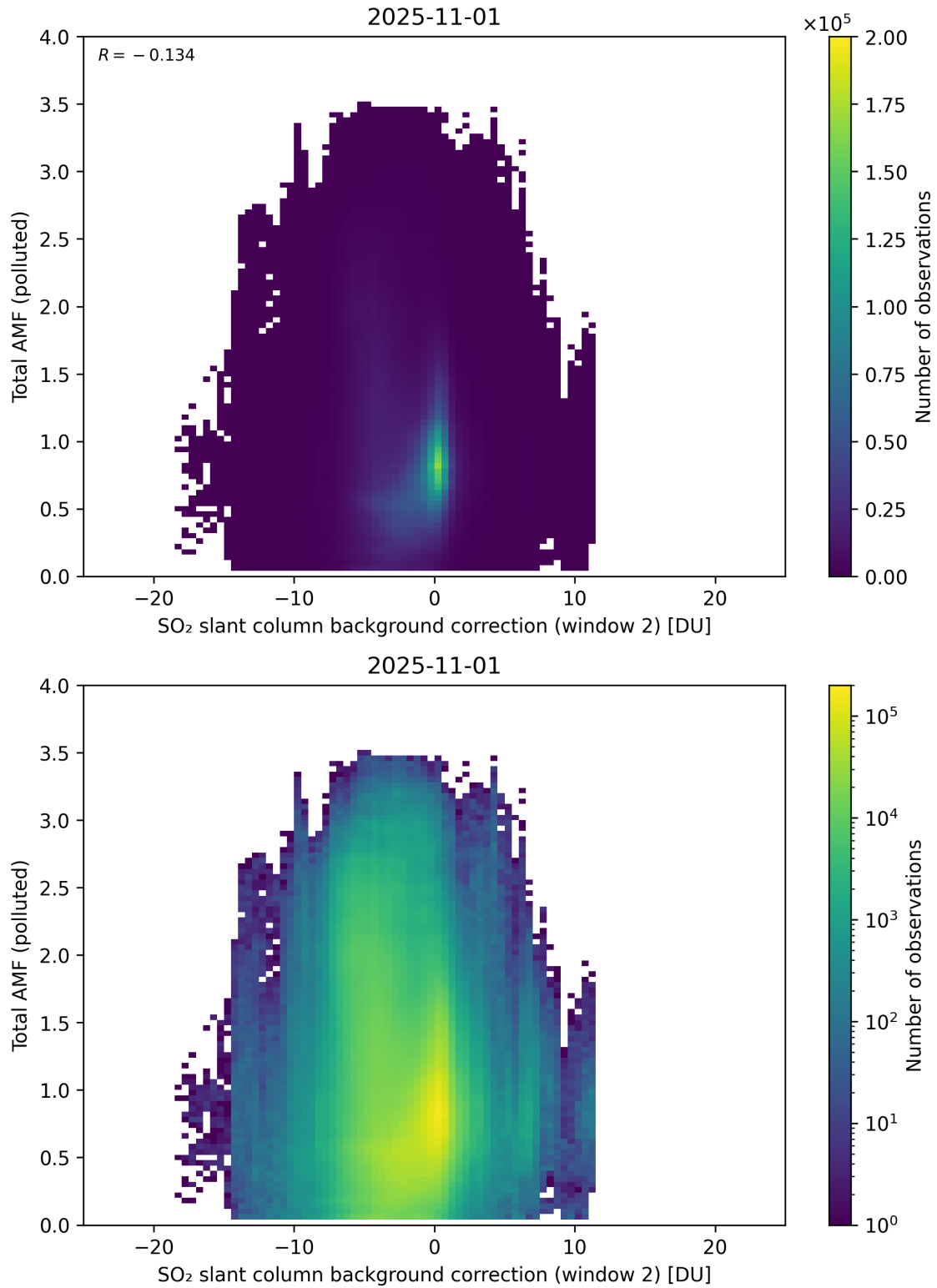
Figure 130: Scatter density plot of “SO 2 slant column background correction (window 2)” against “Total AMF (polluted)” for 2025-10-31 to 2025-11-02.
