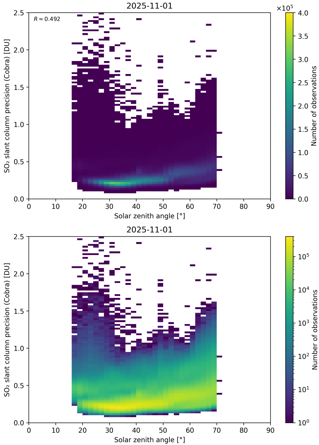
Figure 180: Scatter density plot of “Solar zenith angle” against “SO 2 slant column precision (Cobra)” for 2025-10-31 to 2025-11-02.
