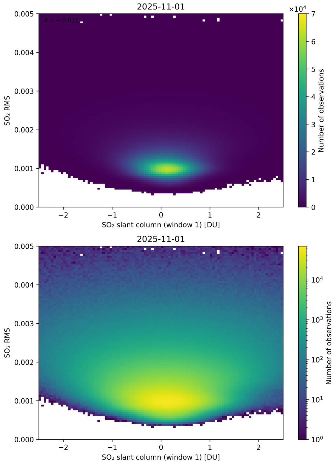
Figure 267: Scatter density plot of “SO 2 slant column (window 1)” against “SO 2 RMS” for 2025-10-31 to 2025-11-02.
