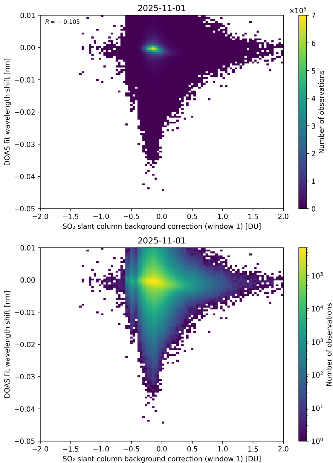
Figure 111: Scatter density plot of “SO 2 slant column background correction (window 1)” against “DOAS fit wavelength shift” for 2025-10-31 to 2025-11-02.
