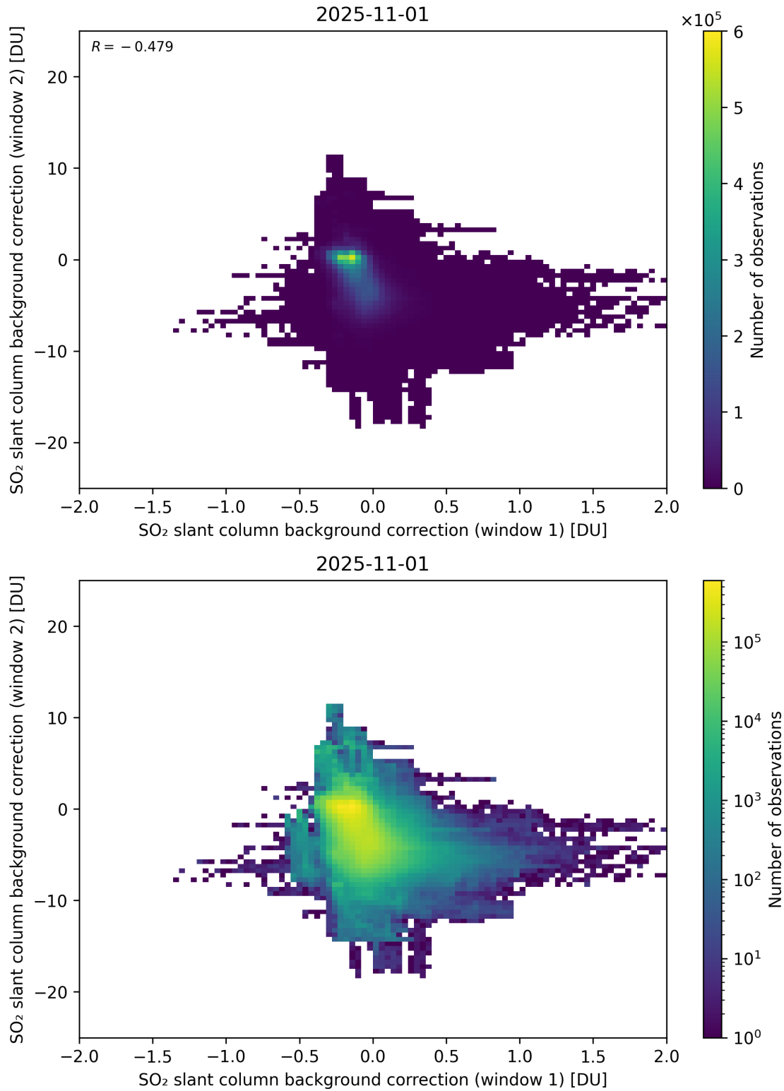
Figure 109: Scatter density plot of “SO 2 slant column background correction (window 1)” against “SO 2 slant column background correction (window 2)” for 2025-10-31 to 2025-11-02.
