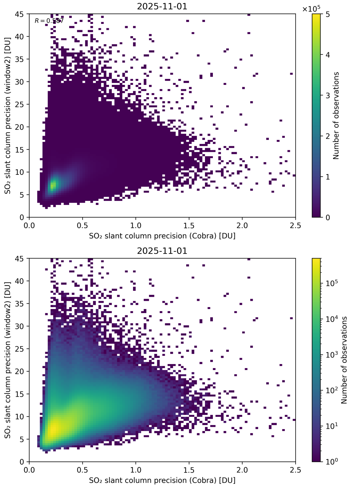
Figure 210: Scatter density plot of “SO 2 slant column precision (Cobra)” against “SO 2 slant column precision (window2)” for 2025-10-31 to 2025-11-02.
