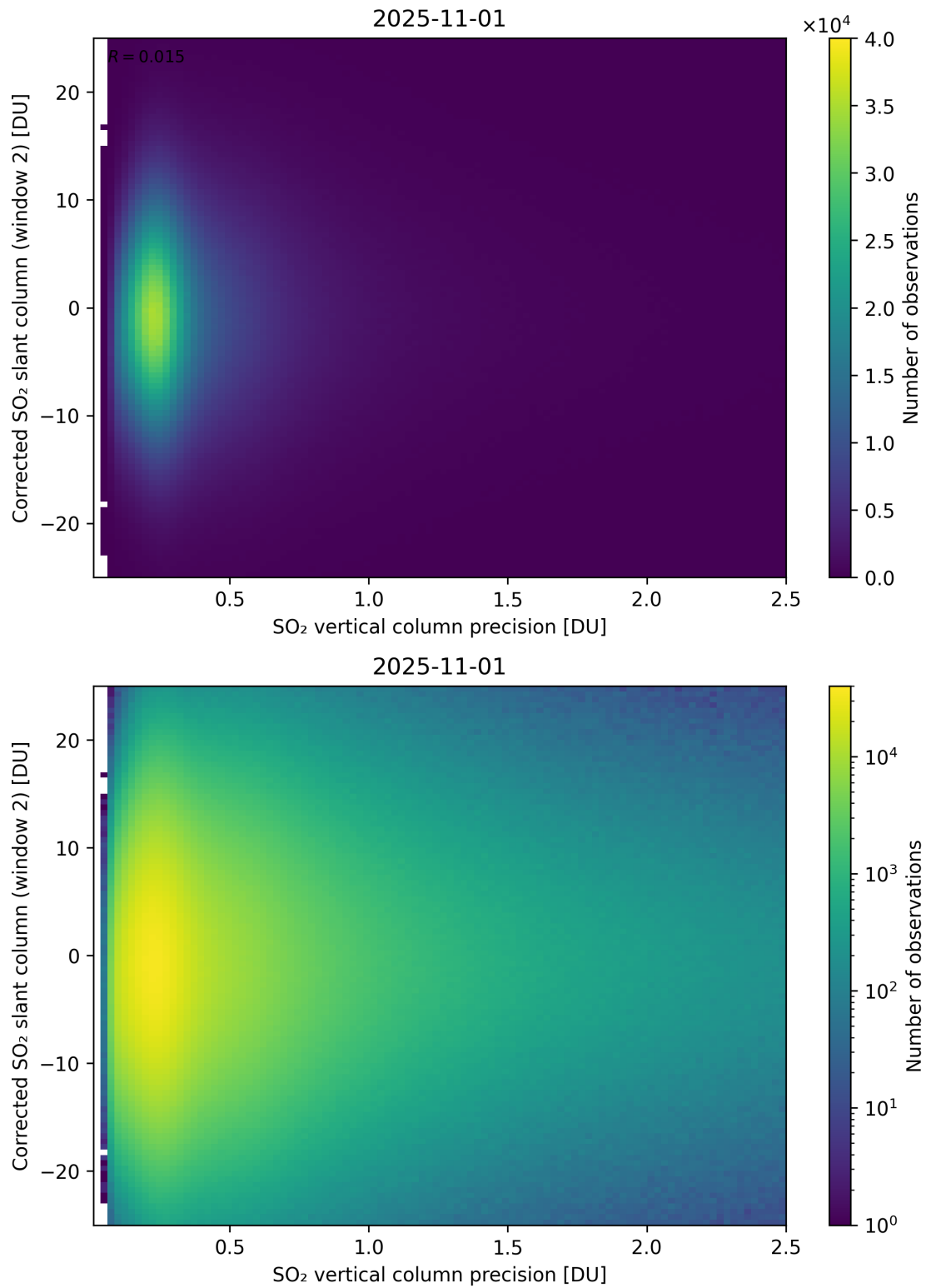
Figure 339: Scatter density plot of “SO 2 vertical column precision” against “Corrected SO 2 slant column (window 2)” for 2025-10-31 to 2025-11-02.
