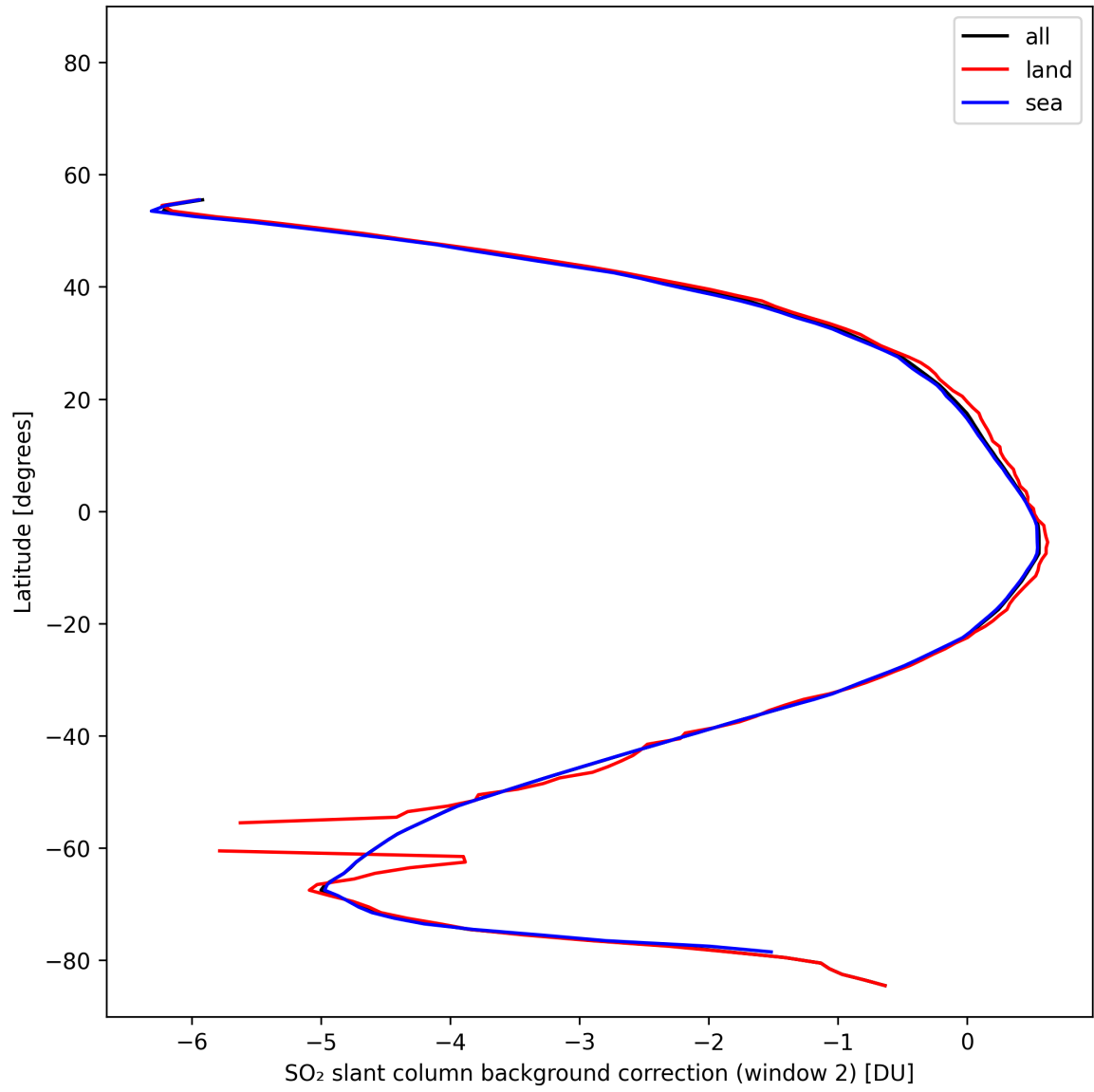
Figure 44: Zonal average of “SO 2 slant column background correction (window 2)” for 2025-10-31 to 2025-11-02.
