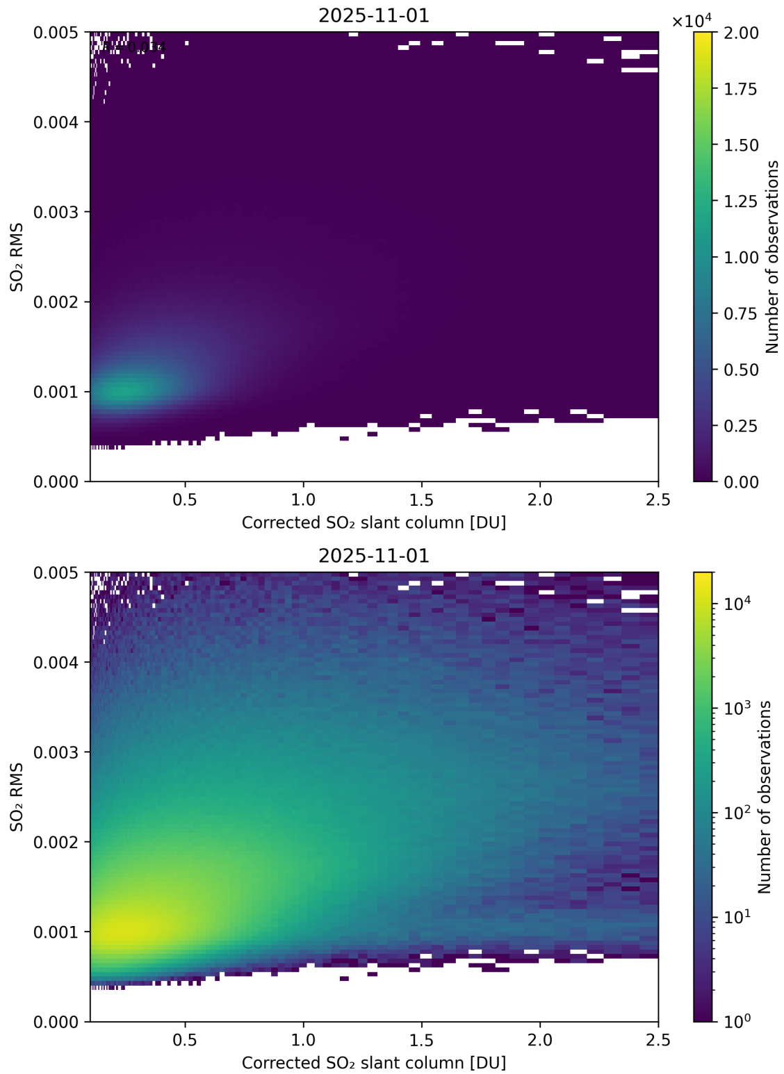
Figure 231: Scatter density plot of “Corrected SO 2 slant column” against “SO 2 RMS” for 2025-10-31 to 2025-11-02.
