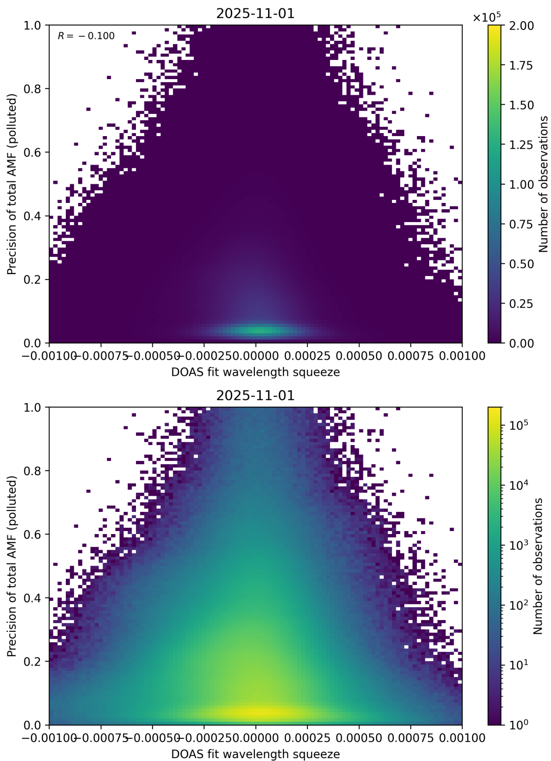
Figure 146: Scatter density plot of “DOAS fit wavelength squeeze” against “Precision of total AMF (polluted)” for 2025-10-31 to 2025-11-02.
