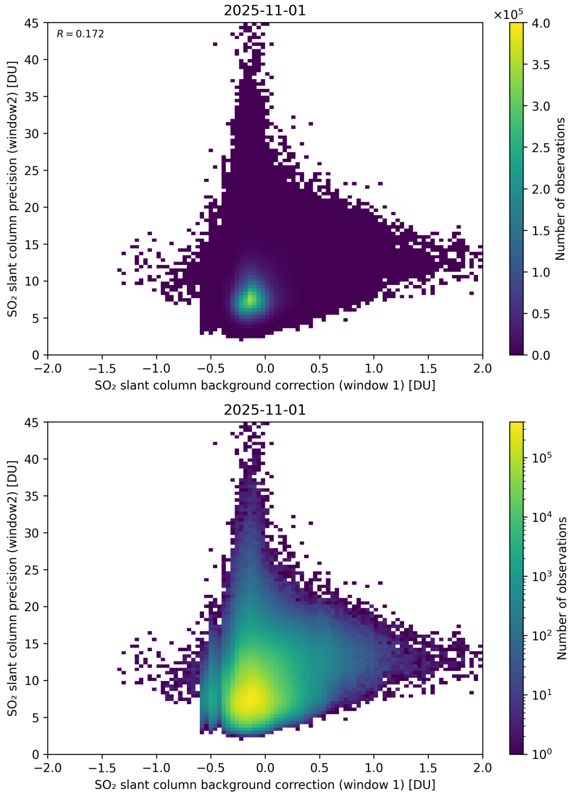
Figure 117: Scatter density plot of “SO 2 slant column background correction (window 1)” against “SO 2 slant column precision (window2)” for 2025-10-31 to 2025-11-02.
