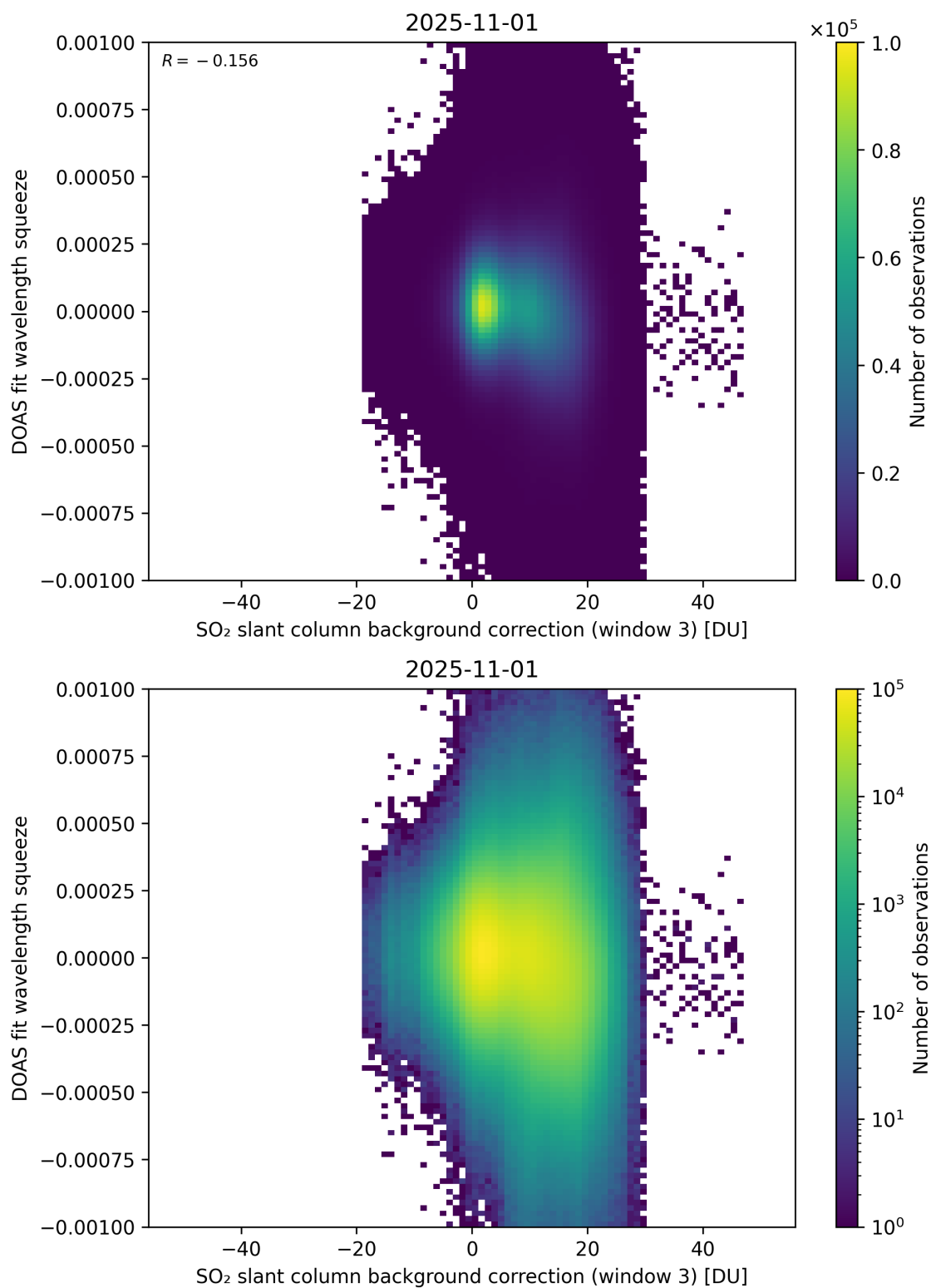
Figure 133: Scatter density plot of “SO 2 slant column background correction (window 3)” against “DOAS fit wavelength squeeze” for 2025-10-31 to 2025-11-02.
