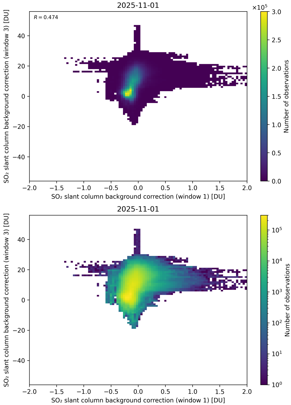
Figure 110: Scatter density plot of “SO 2 slant column background correction (window 1)” against “SO 2 slant column background correction (window 3)” for 2025-10-31 to 2025-11-02.
