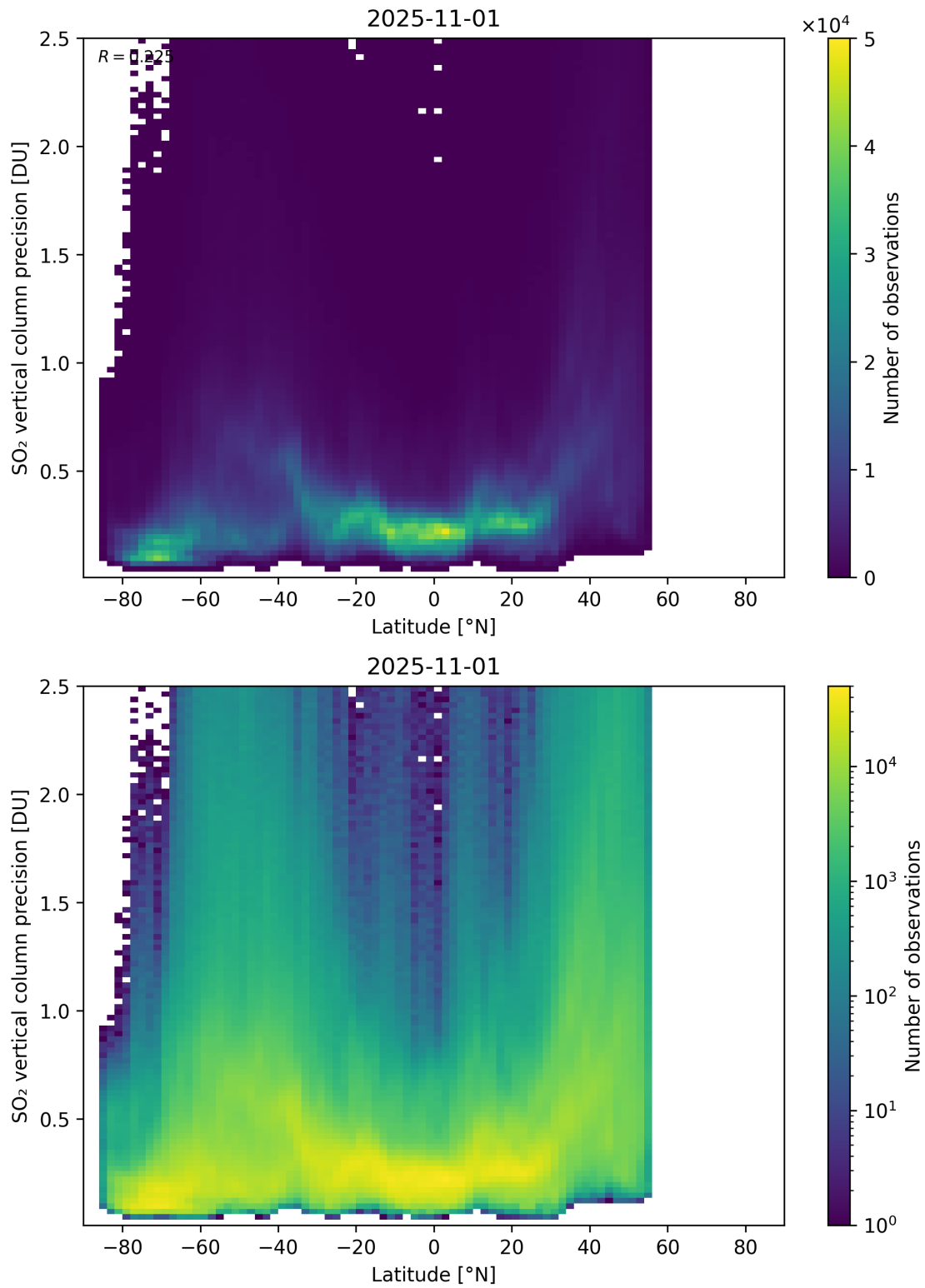
Figure 170: Scatter density plot of “Latitude” against “SO 2 vertical column precision” for 2025-10-31 to 2025-11-02.
