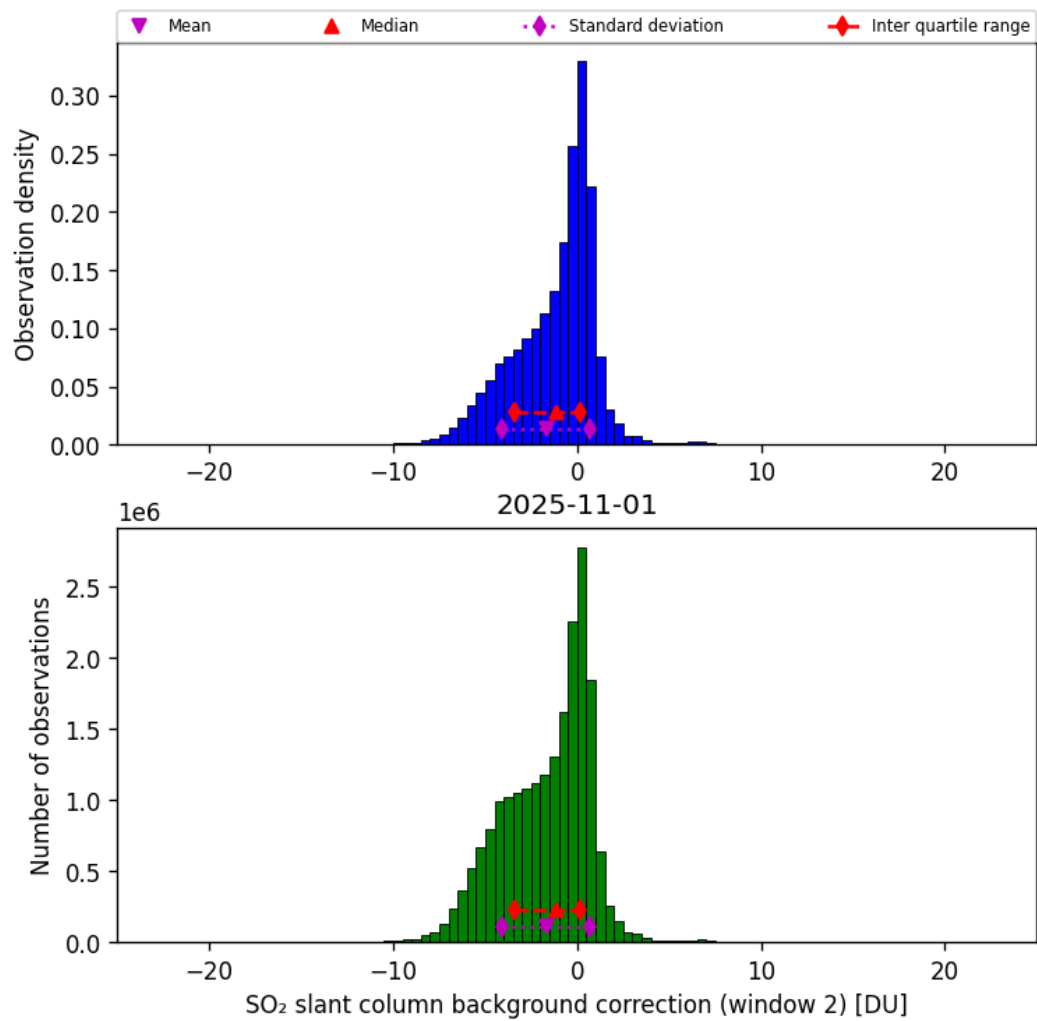
Figure 70: Histogram of “SO 2 slant column background correction (window 2)” for 2025-10-31 to 2025-11-02
