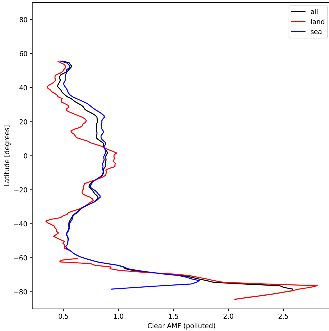
Figure 55: Zonal average of “Clear AMF (polluted)” for 2025-10-31 to 2025-11-02.
