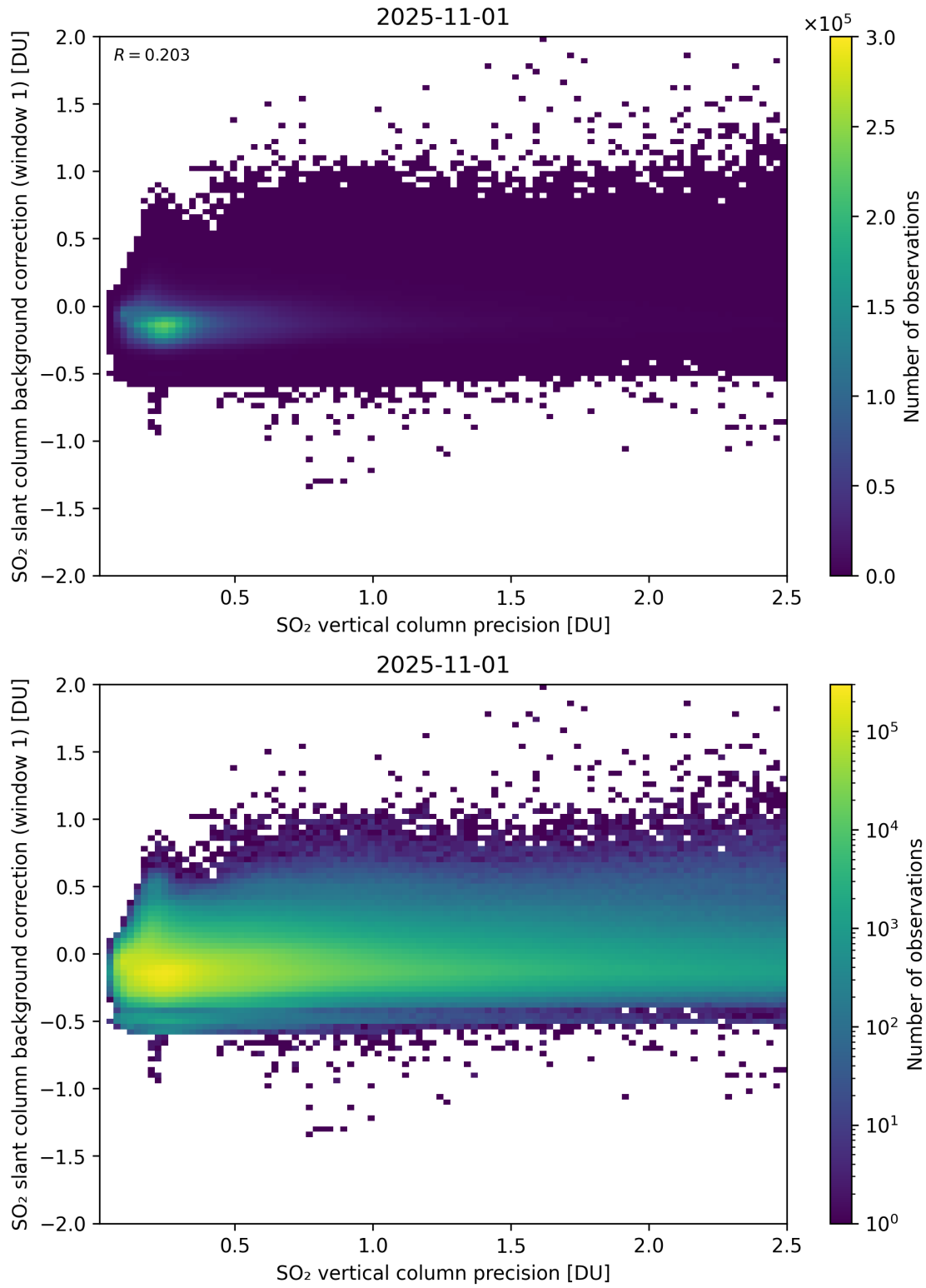
Figure 329: Scatter density plot of “SO 2 vertical column precision” against “SO 2 slant column background correction (window 1)” for 2025-10-31 to 2025-11-02.
