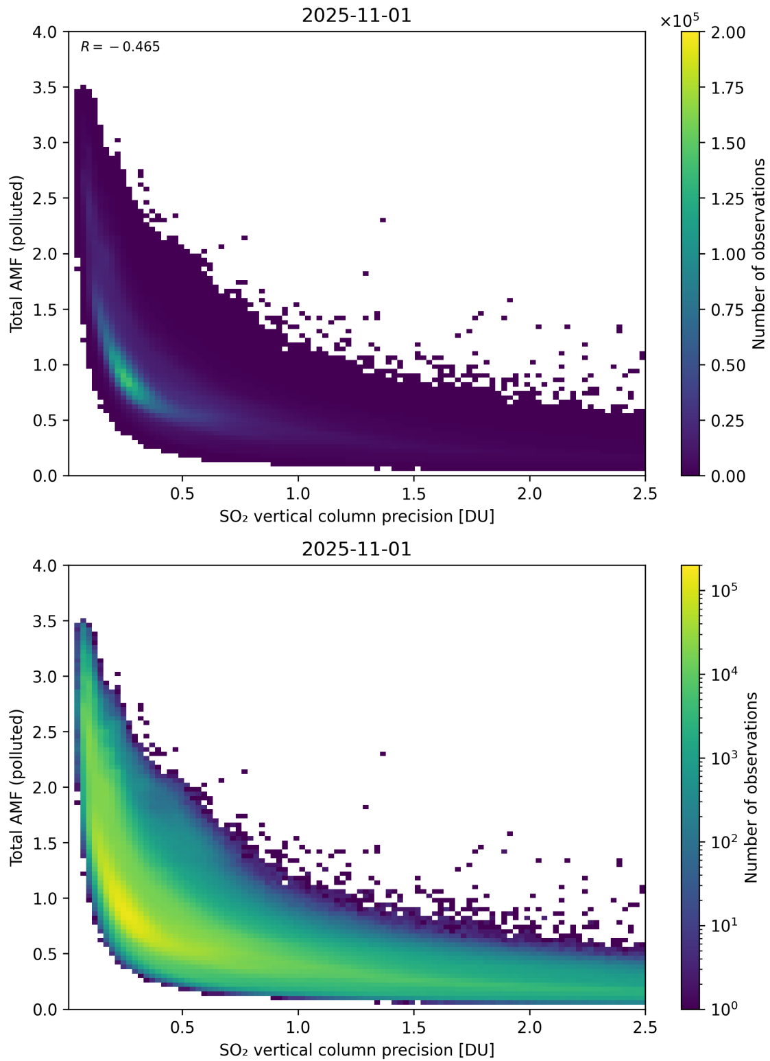
Figure 346: Scatter density plot of “SO 2 vertical column precision” against “Total AMF (polluted)” for 2025-10-31 to 2025-11-02.
