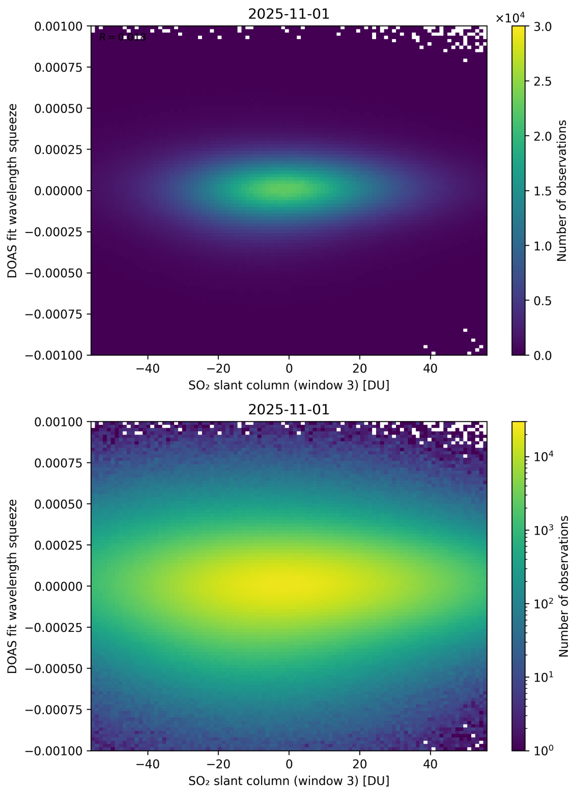
Figure 305: Scatter density plot of “SO 2 slant column (window 3)” against “DOAS fit wavelength squeeze” for 2025-10-31 to 2025-11-02.
