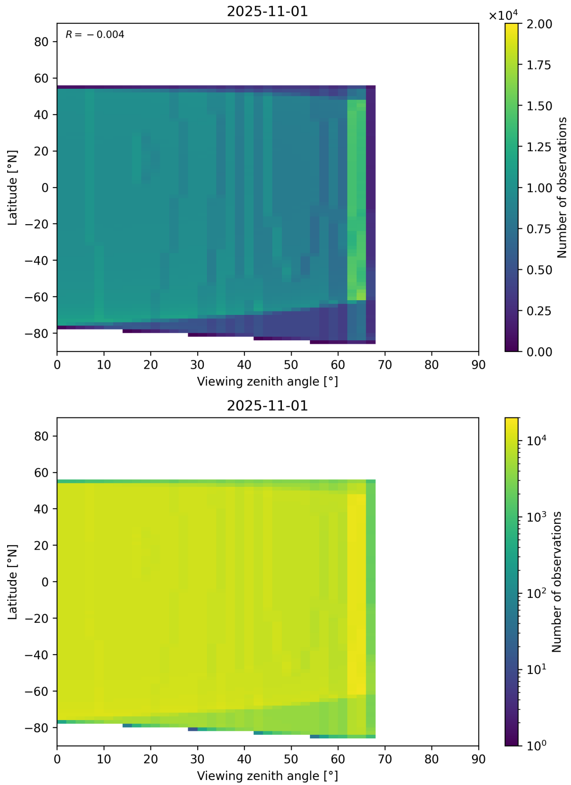
Figure 368: Scatter density plot of “Viewing zenith angle” against “Latitude” for 2025-10-31 to 2025-11-02.
