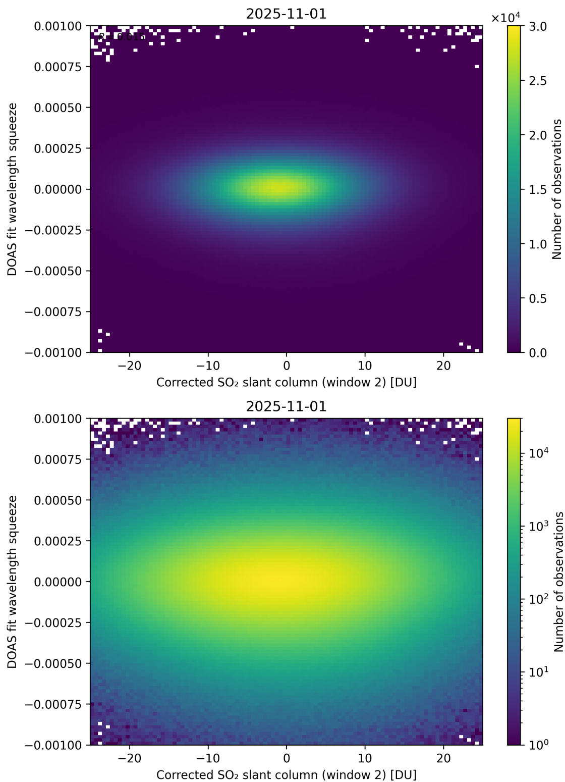
Figure 247: Scatter density plot of “Corrected SO 2 slant column (window 2)” against “DOAS fit wavelength squeeze” for 2025-10-31 to 2025-11-02.
