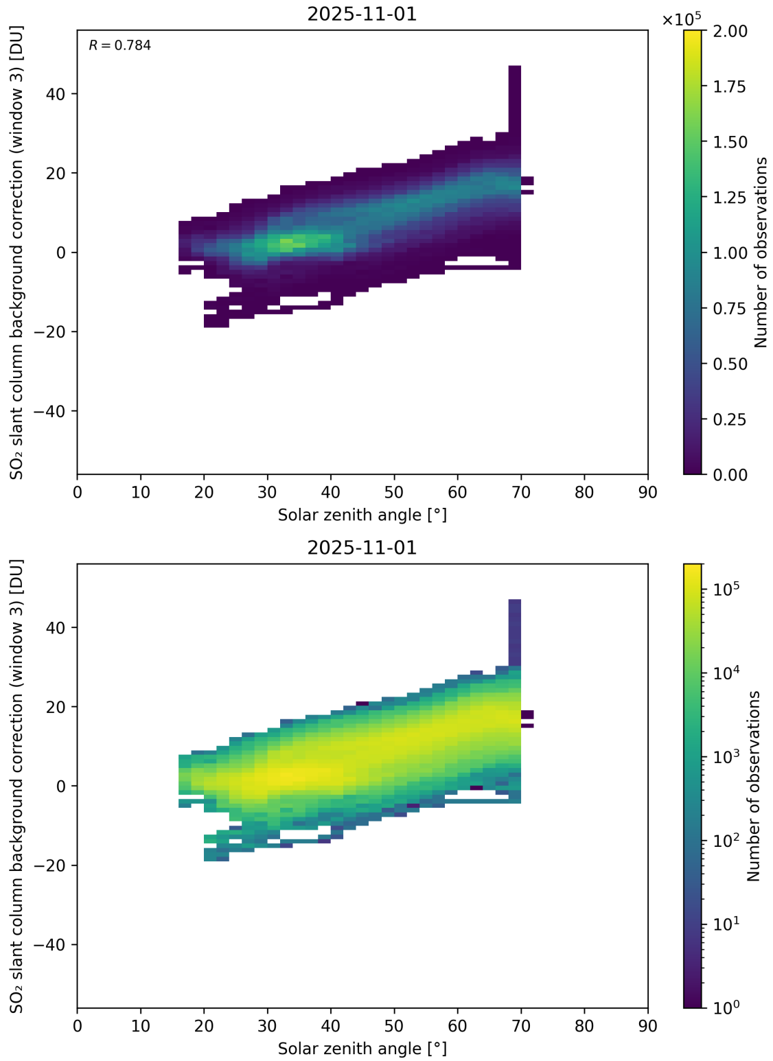
Figure 173: Scatter density plot of “Solar zenith angle” against “SO 2 slant column background correction (window 3)” for 2025-10-31 to 2025-11-02.
