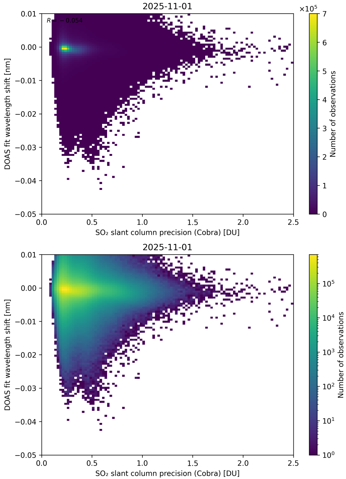
Figure 202: Scatter density plot of “SO 2 slant column precision (Cobra)” against “DOAS fit wavelength shift” for 2025-10-31 to 2025-11-02.
