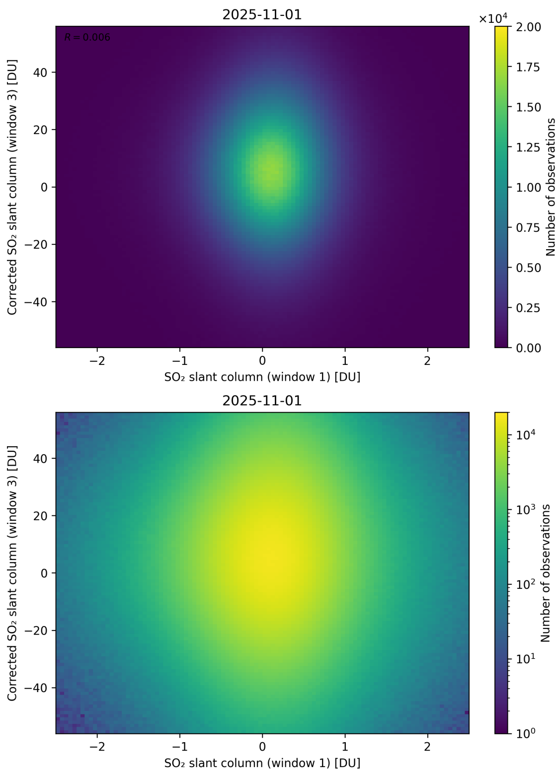
Figure 284: Scatter density plot of “SO 2 slant column (window 1)” against “Corrected SO 2 slant column (window 3)” for 2025-10-31 to 2025-11-02.
