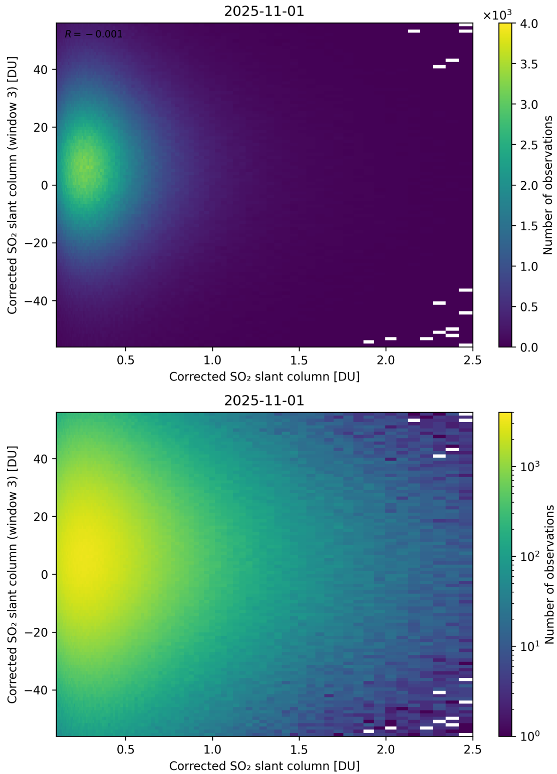
Figure 236: Scatter density plot of “Corrected SO 2 slant column” against “Corrected SO 2 slant column (window 3)” for 2025-10-31 to 2025-11-02.
