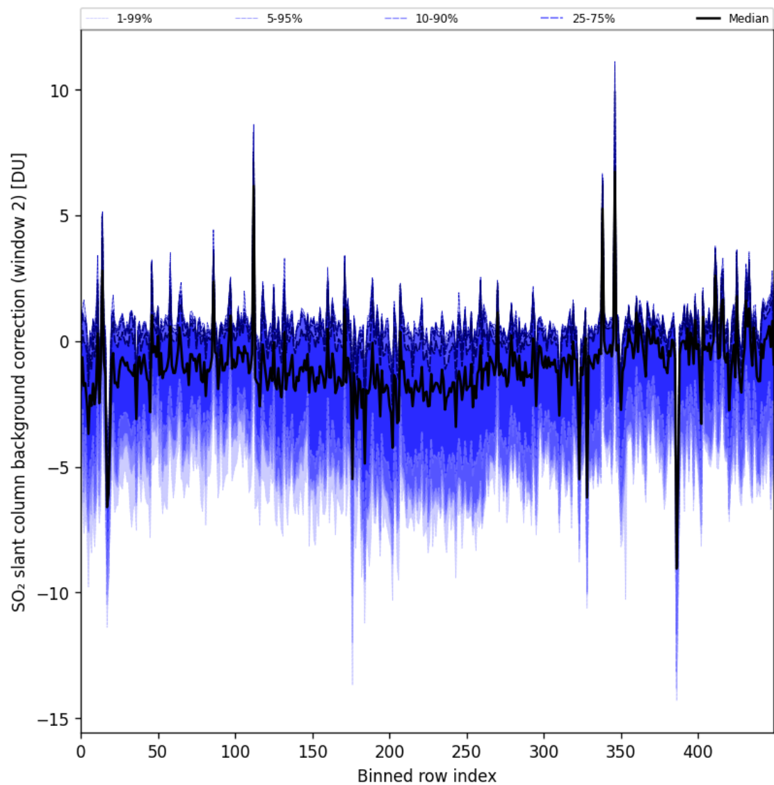
Figure 96: Along track statistics of “SO 2 slant column background correction (window 2)” for 2025-10-31 to 2025-11-02
