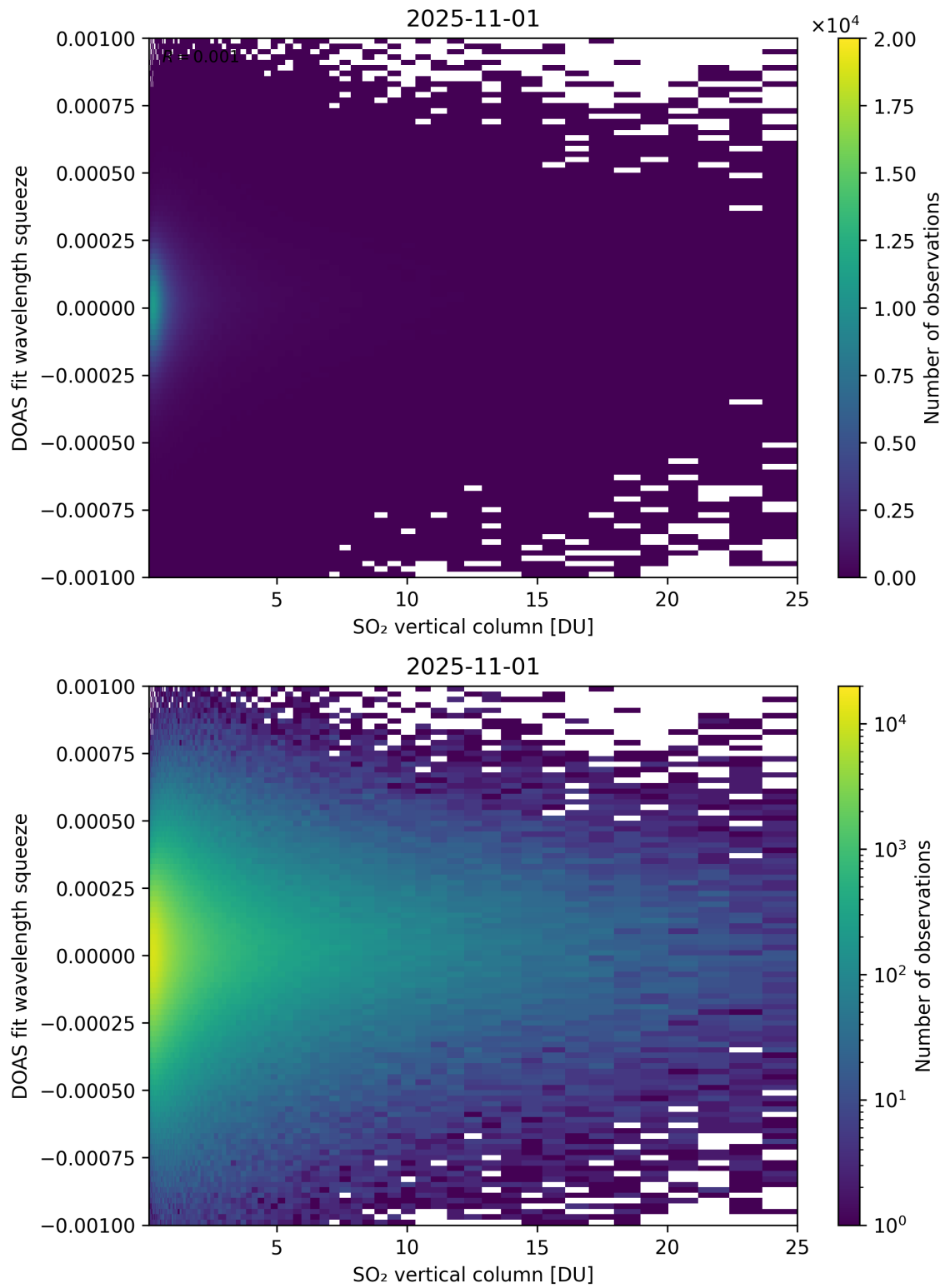
Figure 327: Scatter density plot of “SO 2 vertical column” against “DOAS fit wavelength squeeze” for 2025-10-31 to 2025-11-02.
