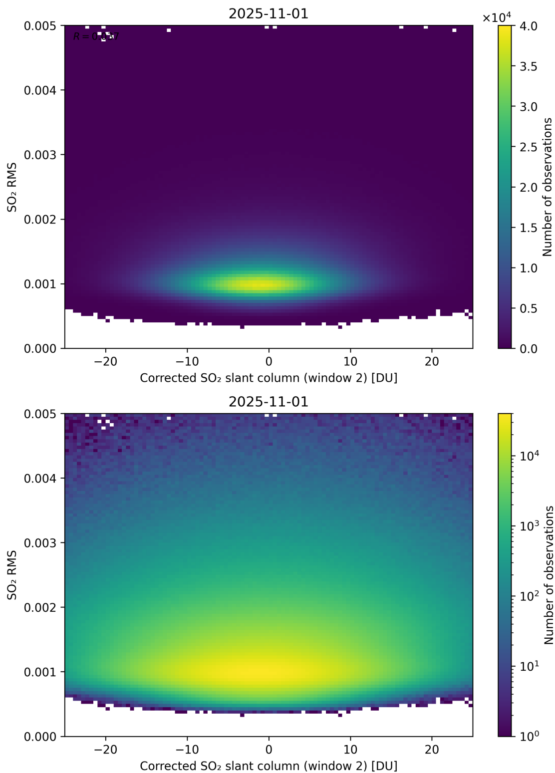
Figure 248: Scatter density plot of “Corrected SO 2 slant column (window 2)” against “SO 2 RMS” for 2025-10-31 to 2025-11-02.
