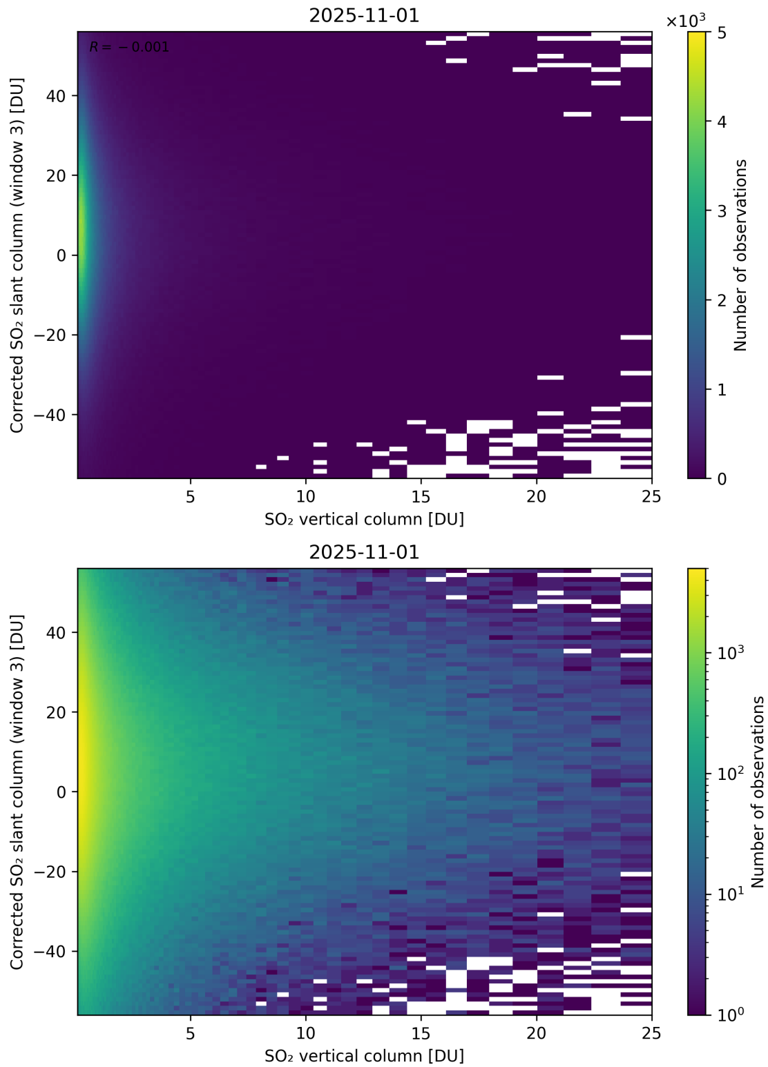
Figure 353: Scatter density plot of “SO 2 vertical column” against “Corrected SO 2 slant column (window 3)” for 2025-10-31 to 2025-11-02.
