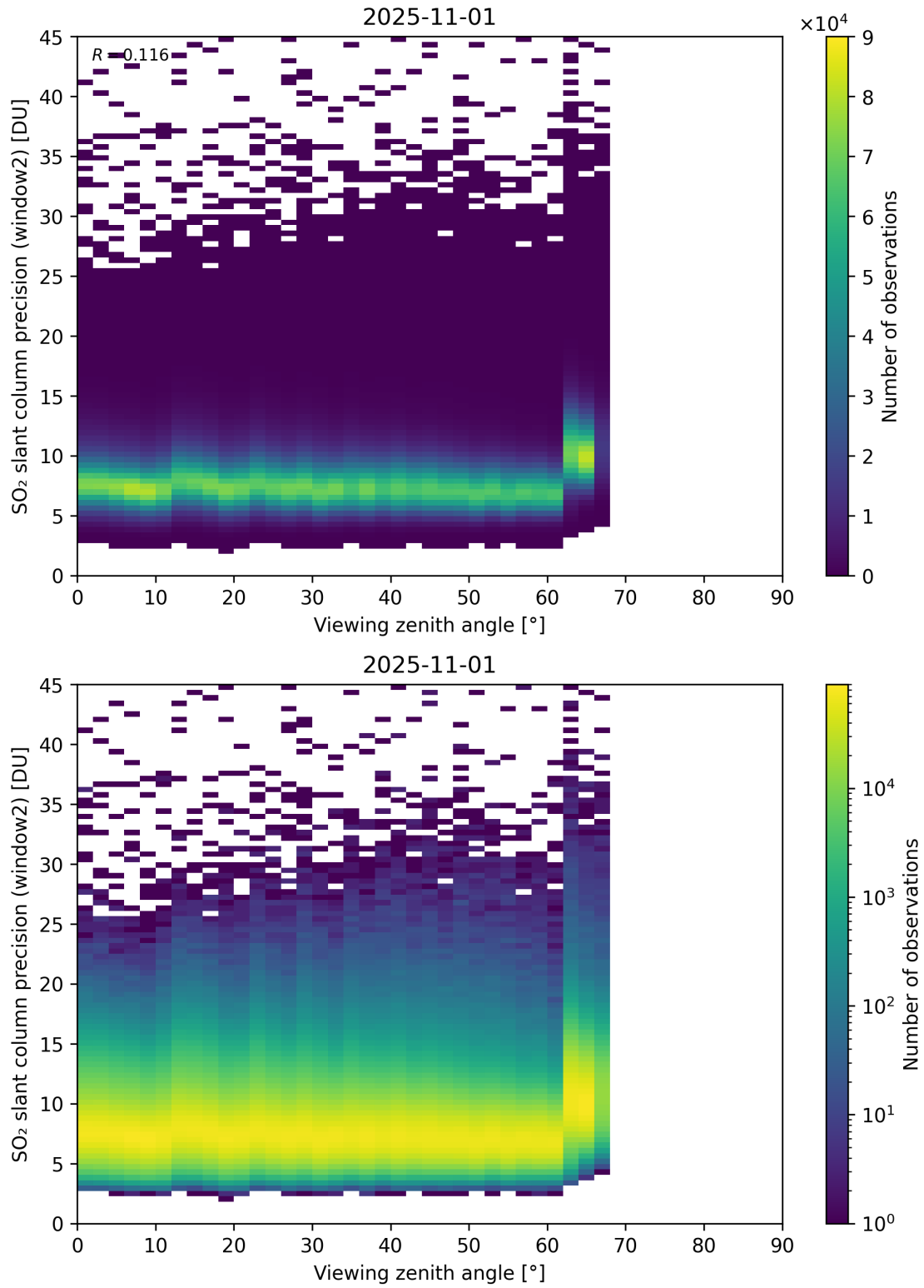
Figure 378: Scatter density plot of “Viewing zenith angle” against “SO 2 slant column precision (window2)” for 2025-10-31 to 2025-11-02.
