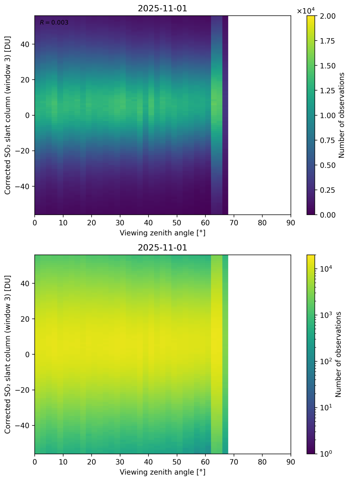
Figure 375: Scatter density plot of “Viewing zenith angle” against “Corrected SO 2 slant column (window 3)” for 2025-10-31 to 2025-11-02.
