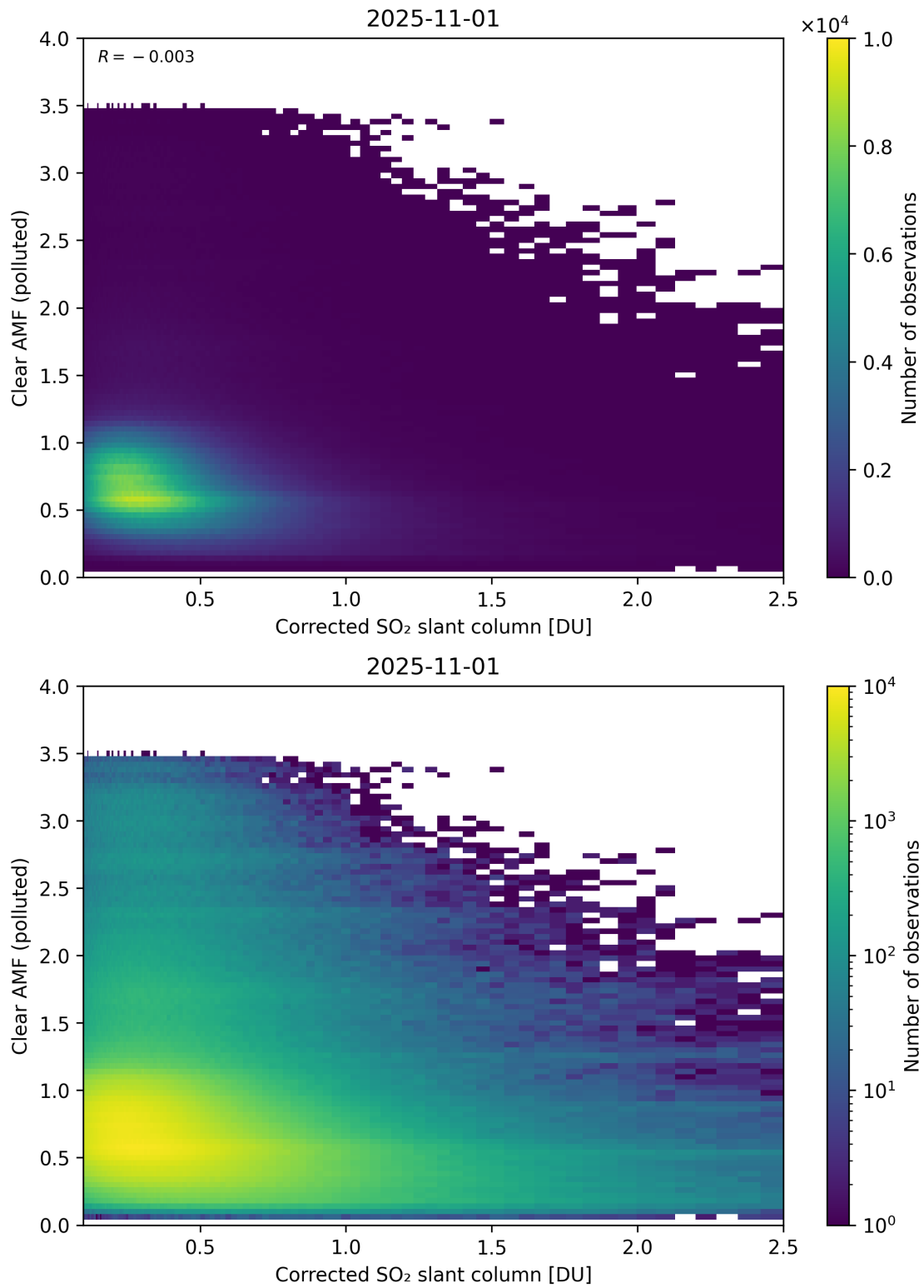
Figure 232: Scatter density plot of “Corrected SO 2 slant column” against “Clear AMF (polluted)” for 2025-10-31 to 2025-11-02.
