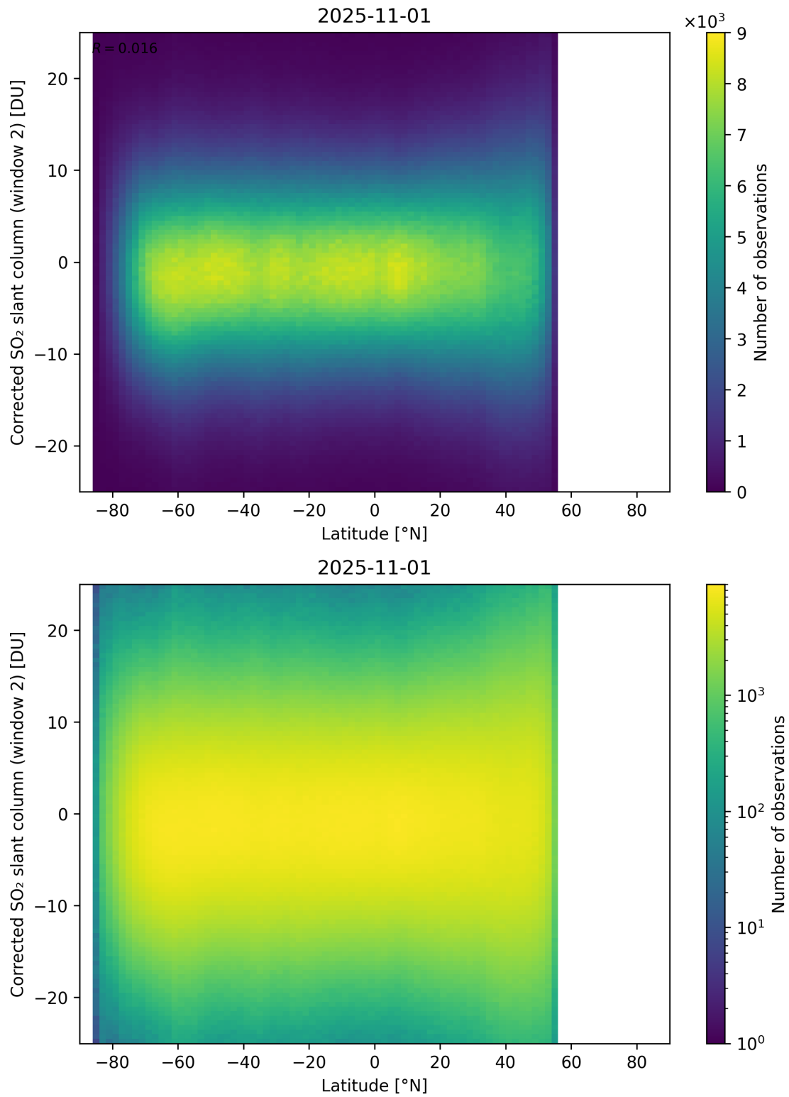
Figure 160: Scatter density plot of “Latitude” against “Corrected SO 2 slant column (window 2)” for 2025-10-31 to 2025-11-02.
