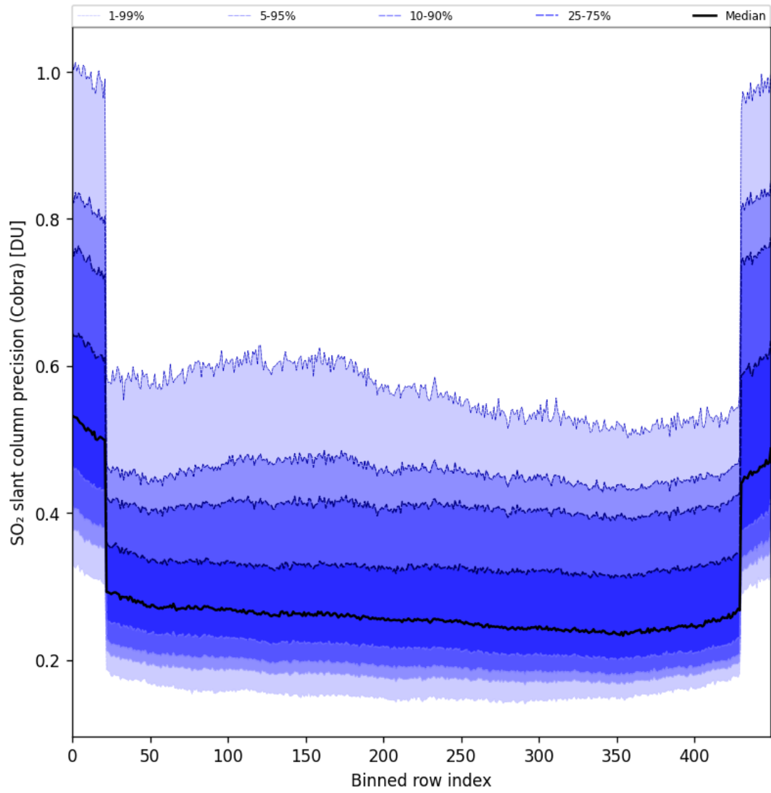
Figure 88: Along track statistics of “SO 2 slant column precision (Cobra)” for 2025-10-31 to 2025-11-02
