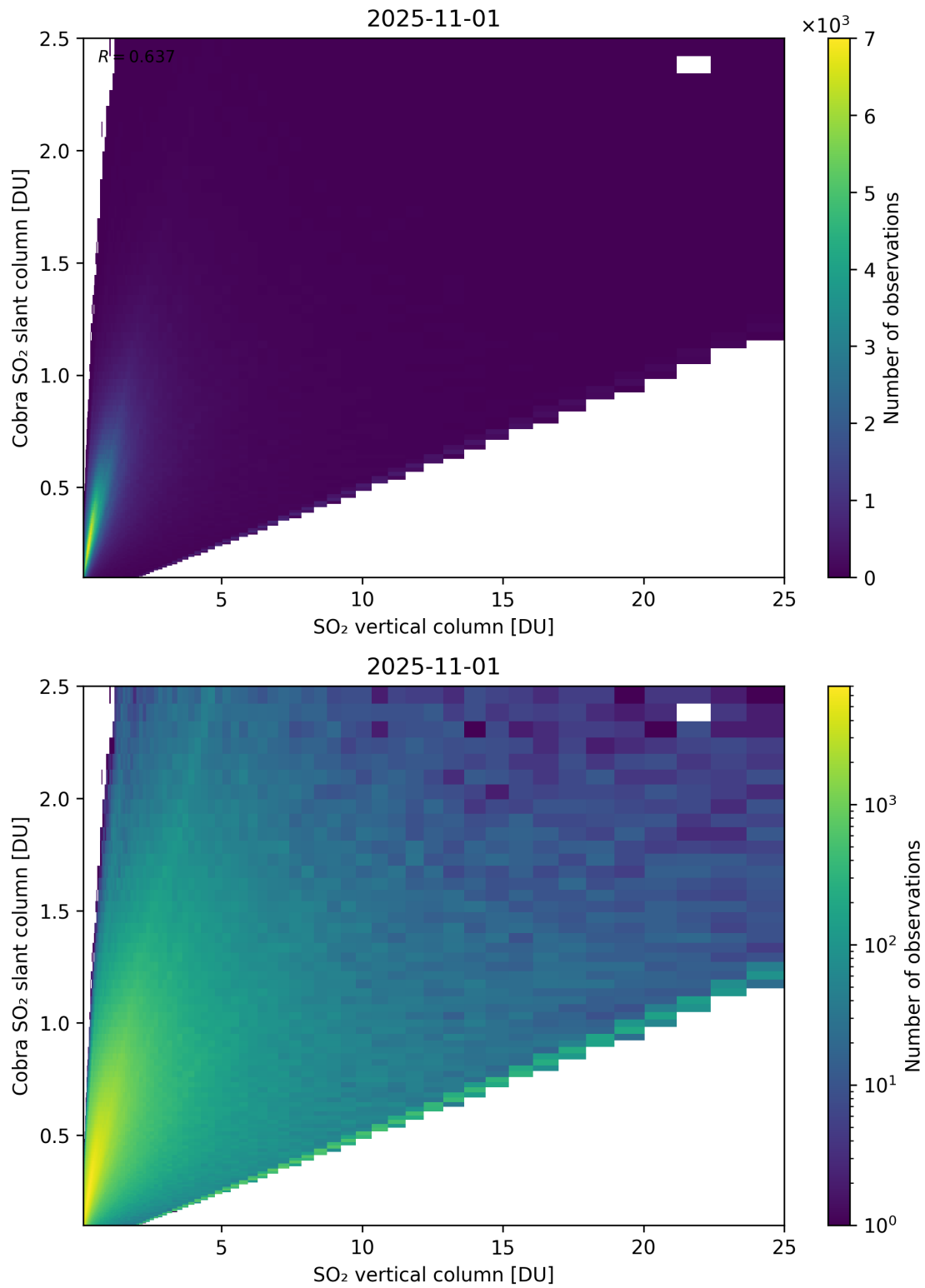
Figure 349: Scatter density plot of “SO 2 vertical column” against “Cobra SO 2 slant column” for 2025-10-31 to 2025-11-02.
