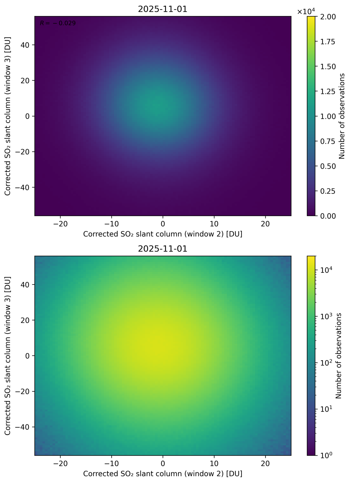
Figure 250: Scatter density plot of “Corrected SO 2 slant column (window 2)” against “Corrected SO 2 slant column (window 3)” for 2025-10-31 to 2025-11-02.
