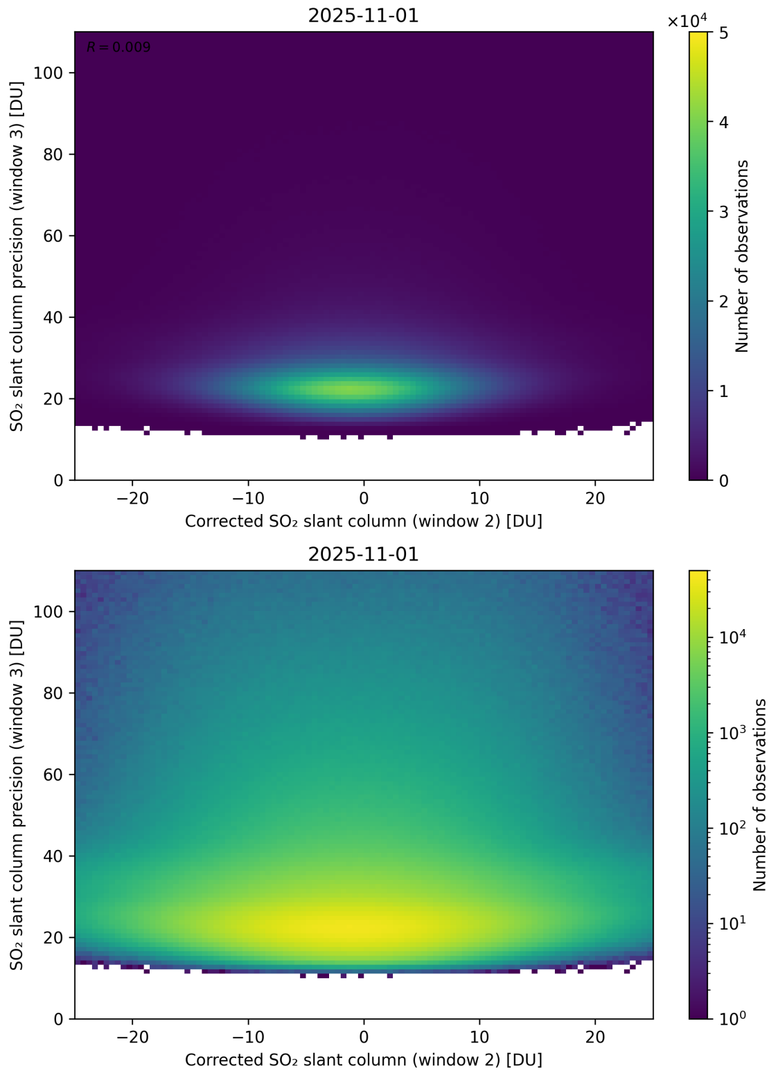
Figure 252: Scatter density plot of “Corrected SO 2 slant column (window 2)” against “SO 2 slant column precision (window 3)” for 2025-10-31 to 2025-11-02.
