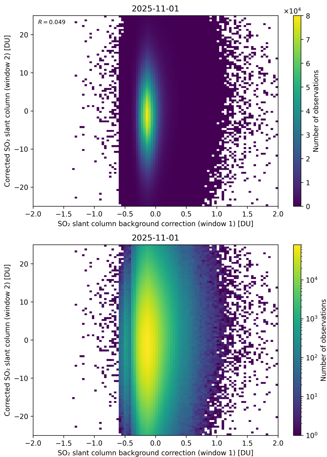
Figure 115: Scatter density plot of “SO 2 slant column background correction (window 1)” against “Corrected SO 2 slant column (window 2)” for 2025-10-31 to 2025-11-02.
