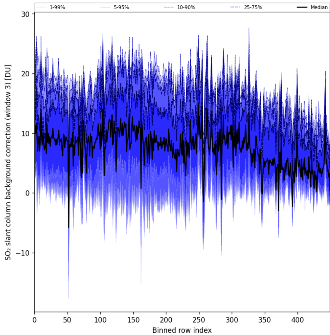
Figure 100: Along track statistics of “SO 2 slant column background correction (window 3)” for 2025-10-31 to 2025-11-02
