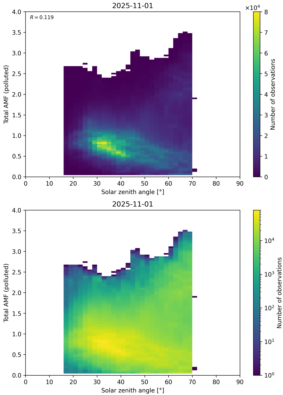
Figure 189: Scatter density plot of “Solar zenith angle” against “Total AMF (polluted)” for 2025-10-31 to 2025-11-02.
