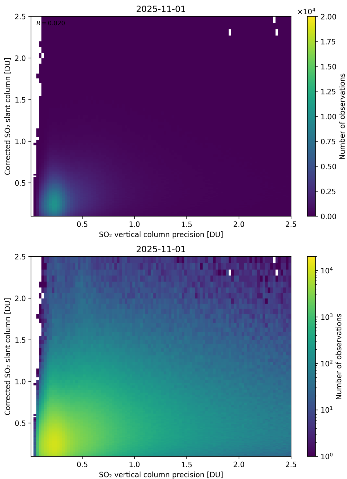
Figure 338: Scatter density plot of “SO 2 vertical column precision” against “Corrected SO 2 slant column” for 2025-10-31 to 2025-11-02.
