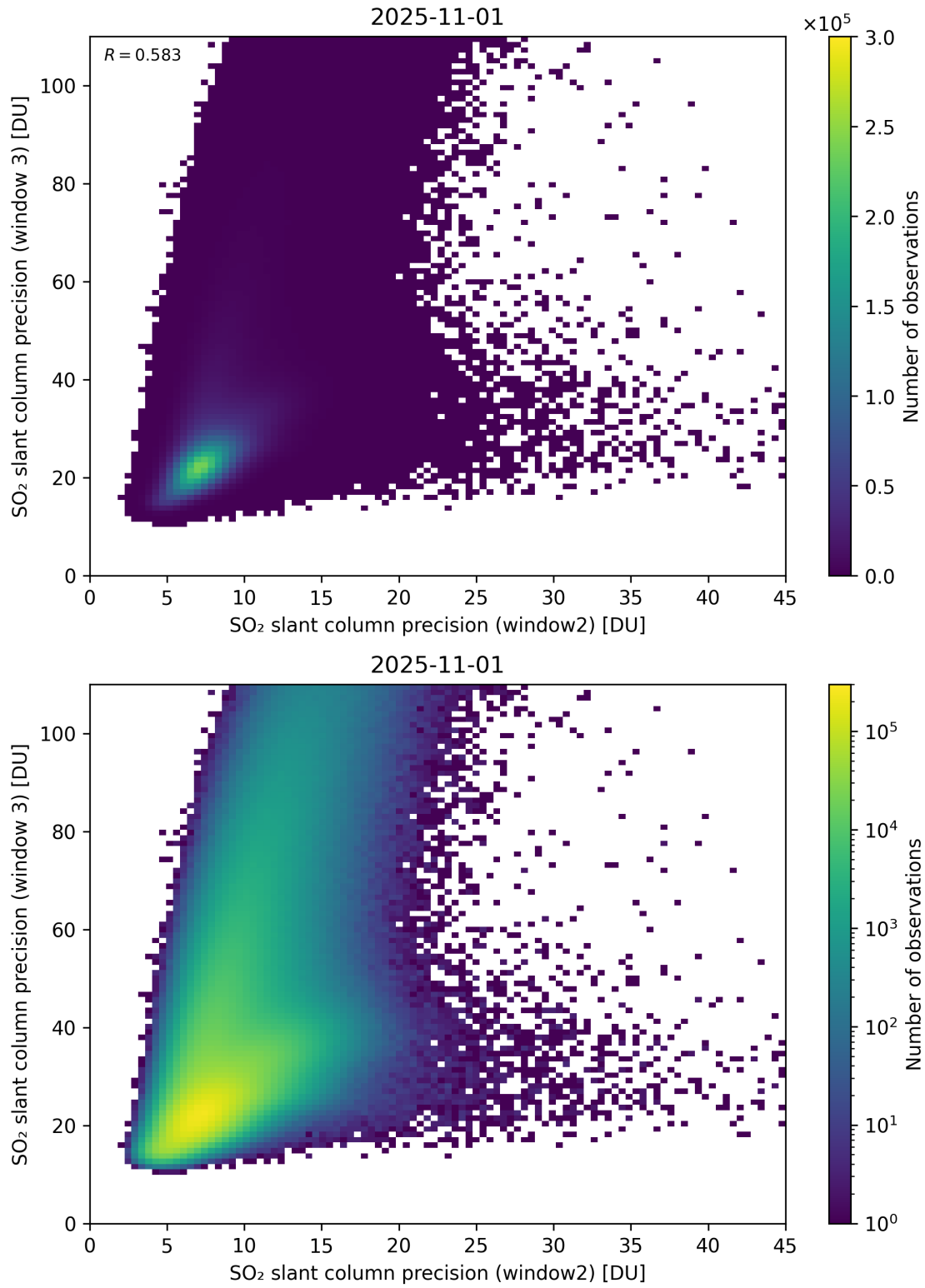
Figure 300: Scatter density plot of “SO 2 slant column precision (window2)” against “SO 2 slant column precision (window 3)” for 2025-10-31 to 2025-11-02.
