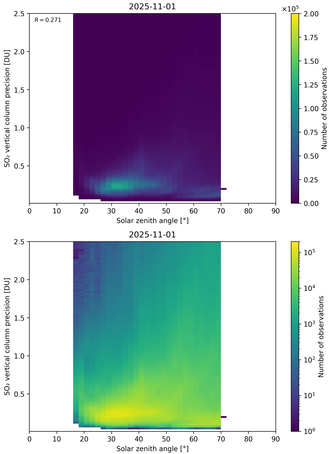
Figure 192: Scatter density plot of “Solar zenith angle” against “SO 2 vertical column precision” for 2025-10-31 to 2025-11-02.
