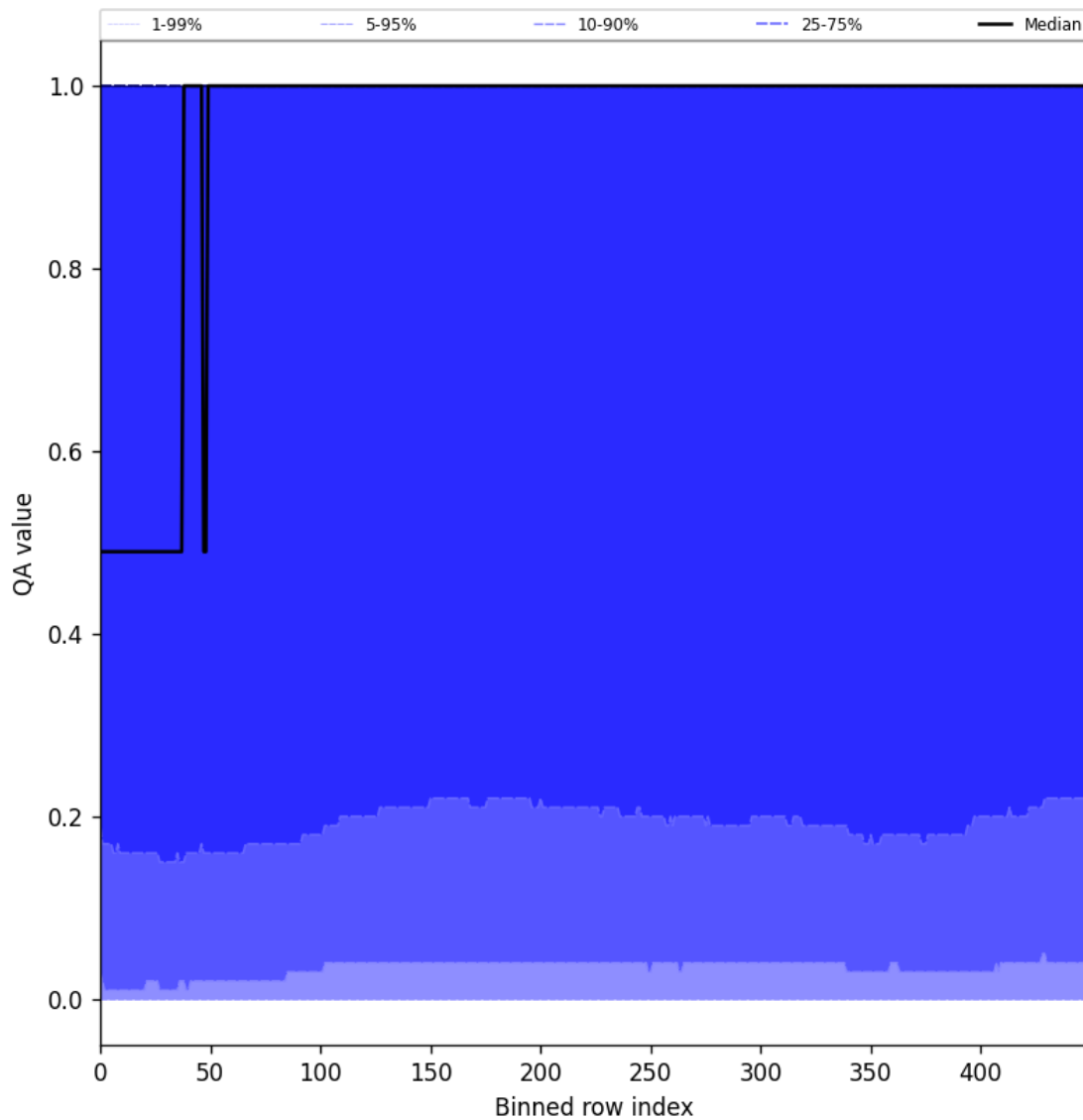
Figure 83: Along track statistics of “QA value” for 2025-10-31 to 2025-11-02
