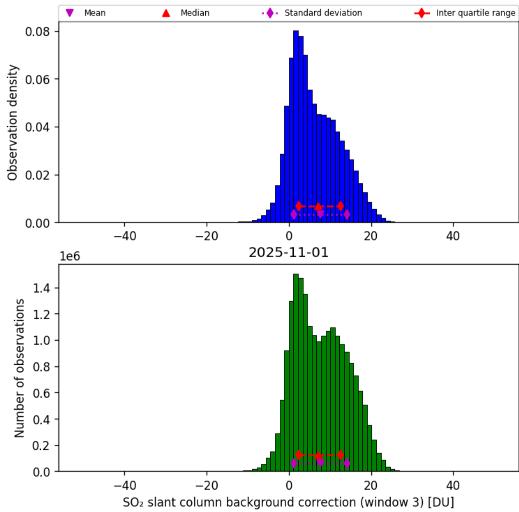
Figure 74: Histogram of “SO 2 slant column background correction (window 3)” for 2025-10-31 to 2025-11-02
