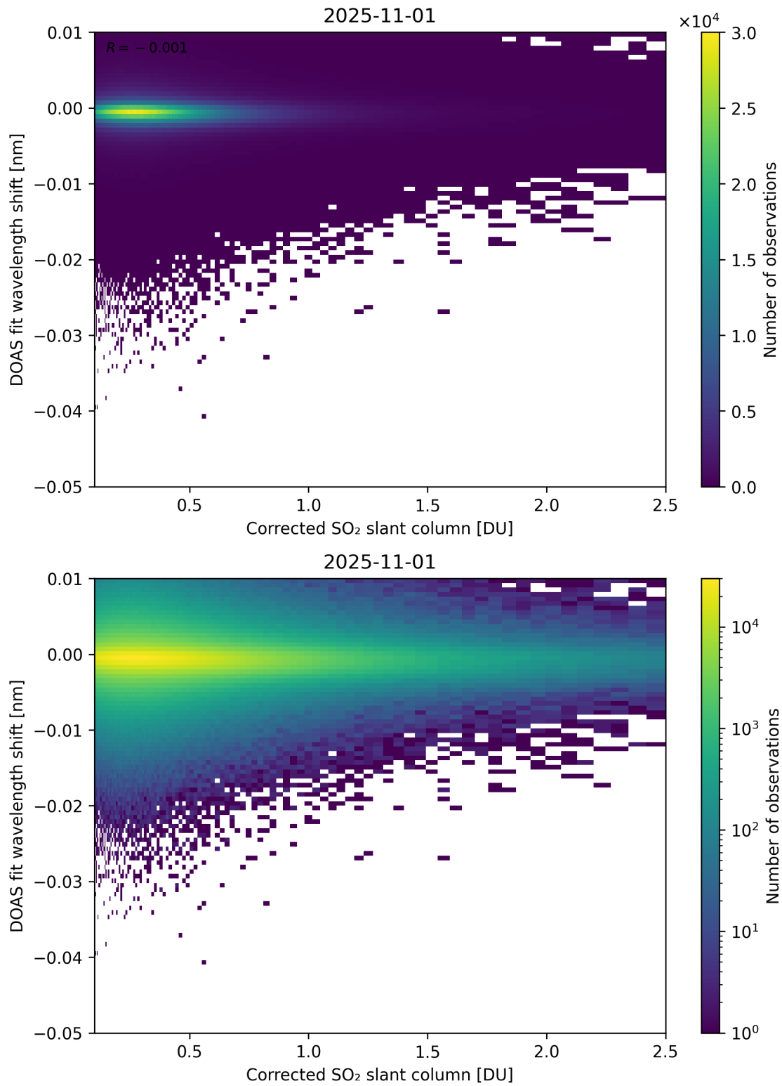
Figure 229: Scatter density plot of “Corrected SO 2 slant column” against “DOAS fit wavelength shift” for 2025-10-31 to 2025-11-02.
