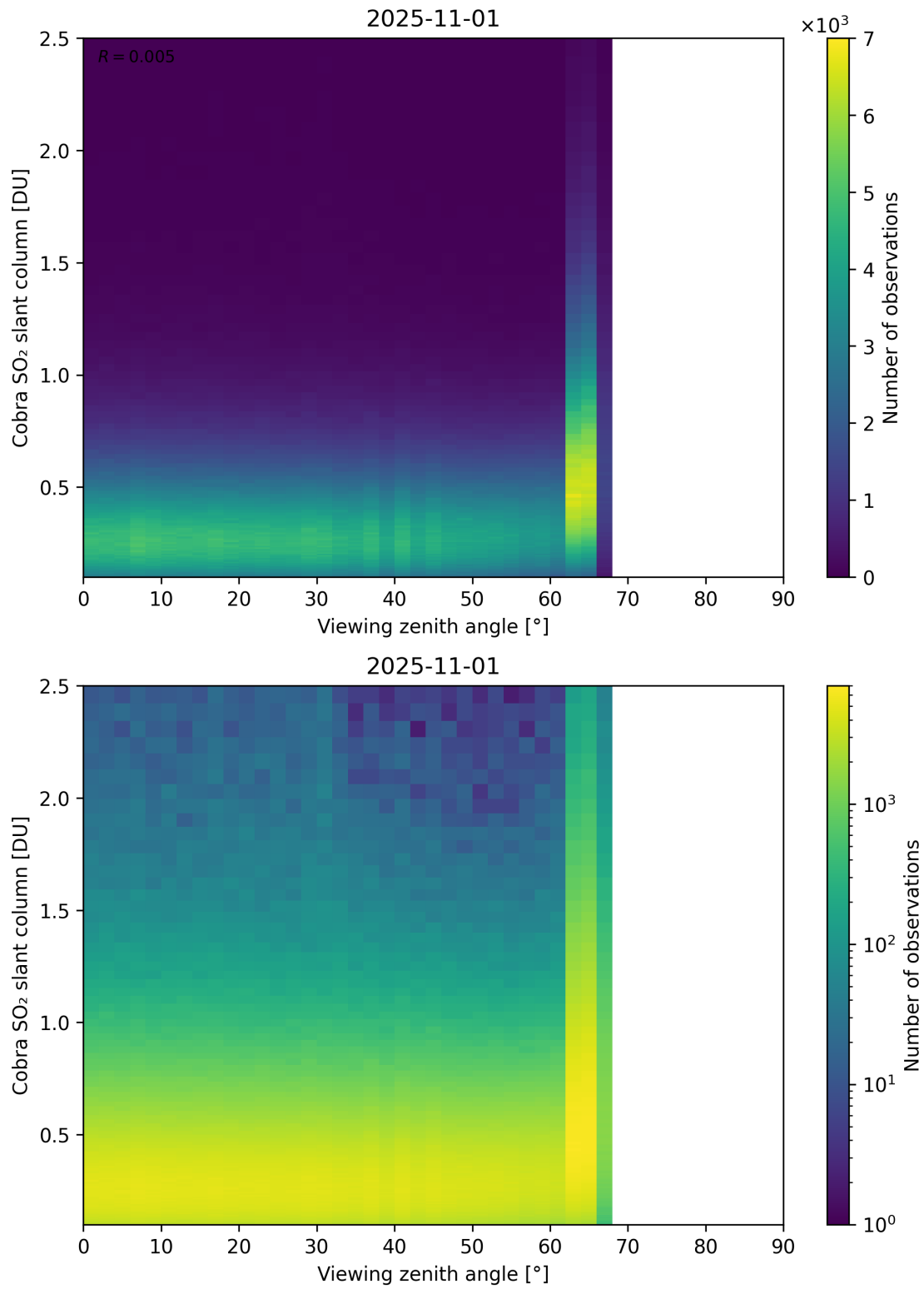
Figure 371: Scatter density plot of “Viewing zenith angle” against “Cobra SO 2 slant column” for 2025-10-31 to 2025-11-02.
