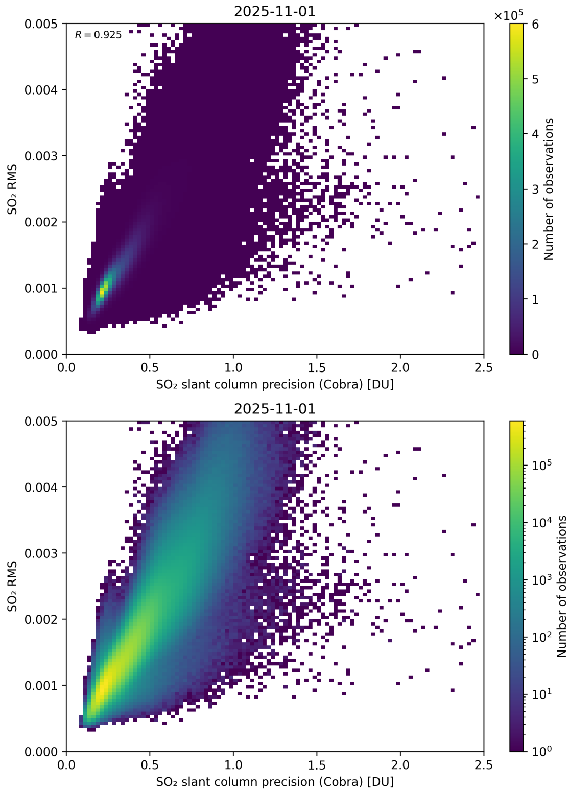
Figure 204: Scatter density plot of “SO 2 slant column precision (Cobra)” against “SO 2 RMS” for 2025-10-31 to 2025-11-02.
