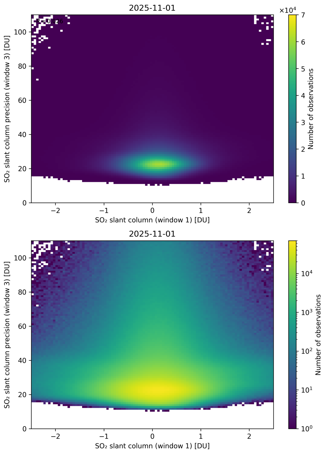
Figure 288: Scatter density plot of “SO 2 slant column (window 1)” against “SO 2 slant column precision (window 3)” for 2025-10-31 to 2025-11-02.
