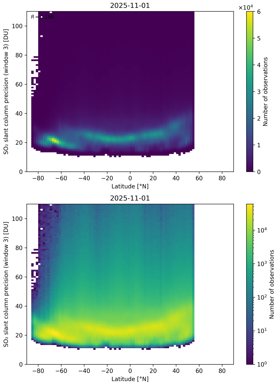
Figure 166: Scatter density plot of “Latitude” against “SO 2 slant column precision (window 3)” for 2025-10-31 to 2025-11-02.
