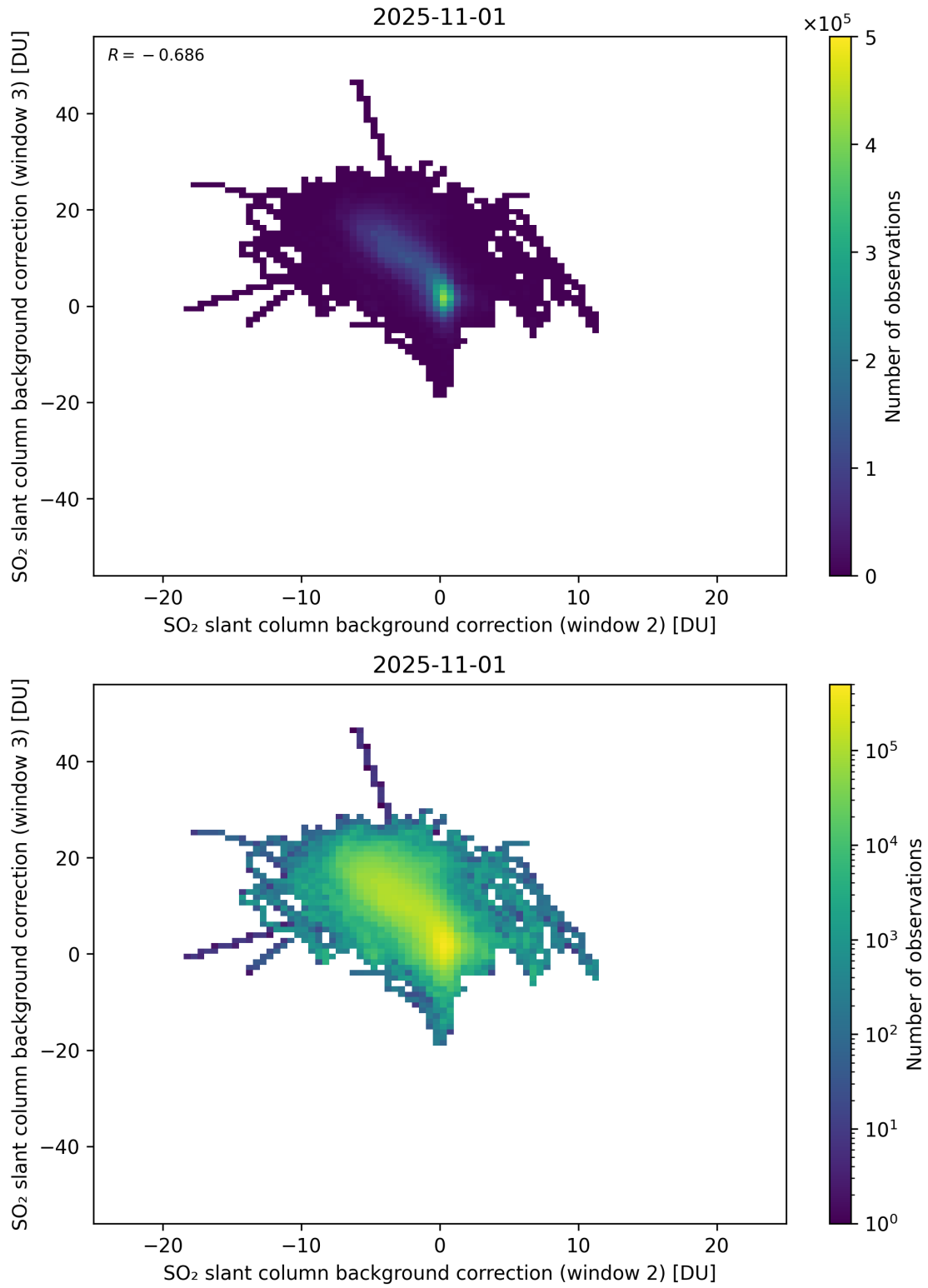
Figure 122: Scatter density plot of “SO 2 slant column background correction (window 2)” against “SO 2 slant column background correction (window 3)” for 2025-10-31 to 2025-11-02.
