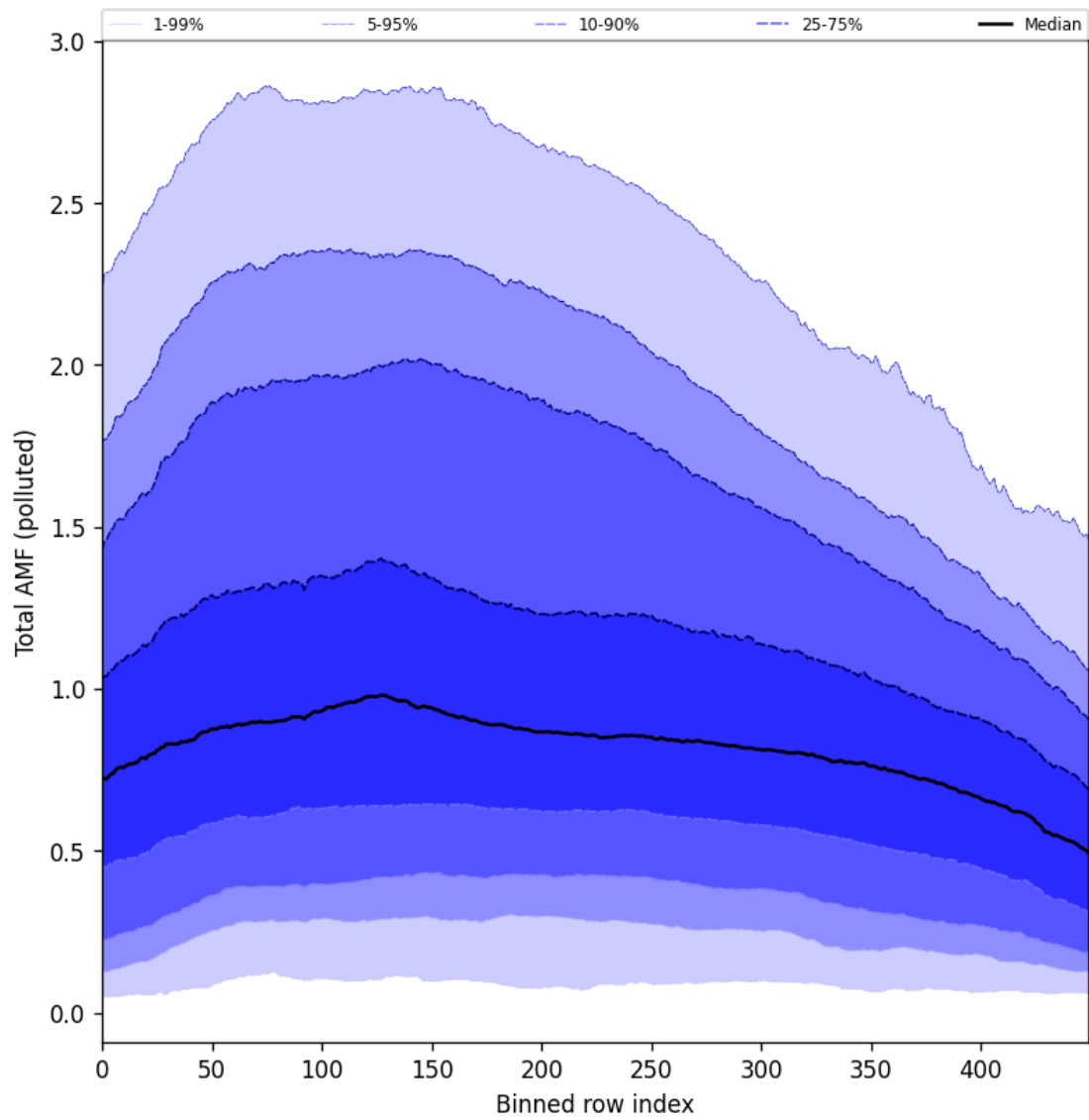
Figure 105: Along track statistics of “Total AMF (polluted)” for 2025-10-31 to 2025-11-02
