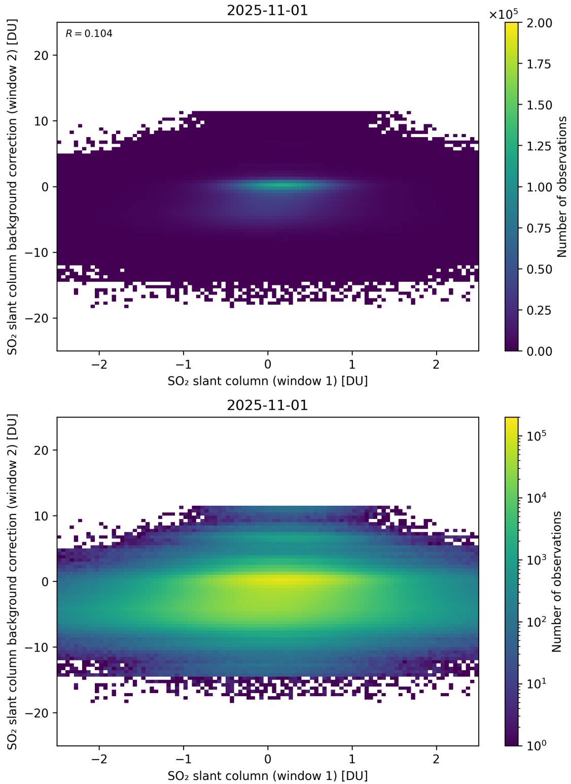
Figure 263: Scatter density plot of “SO 2 slant column (window 1)” against “SO 2 slant column background correction (window 2)” for 2025-10-31 to 2025-11-02.
