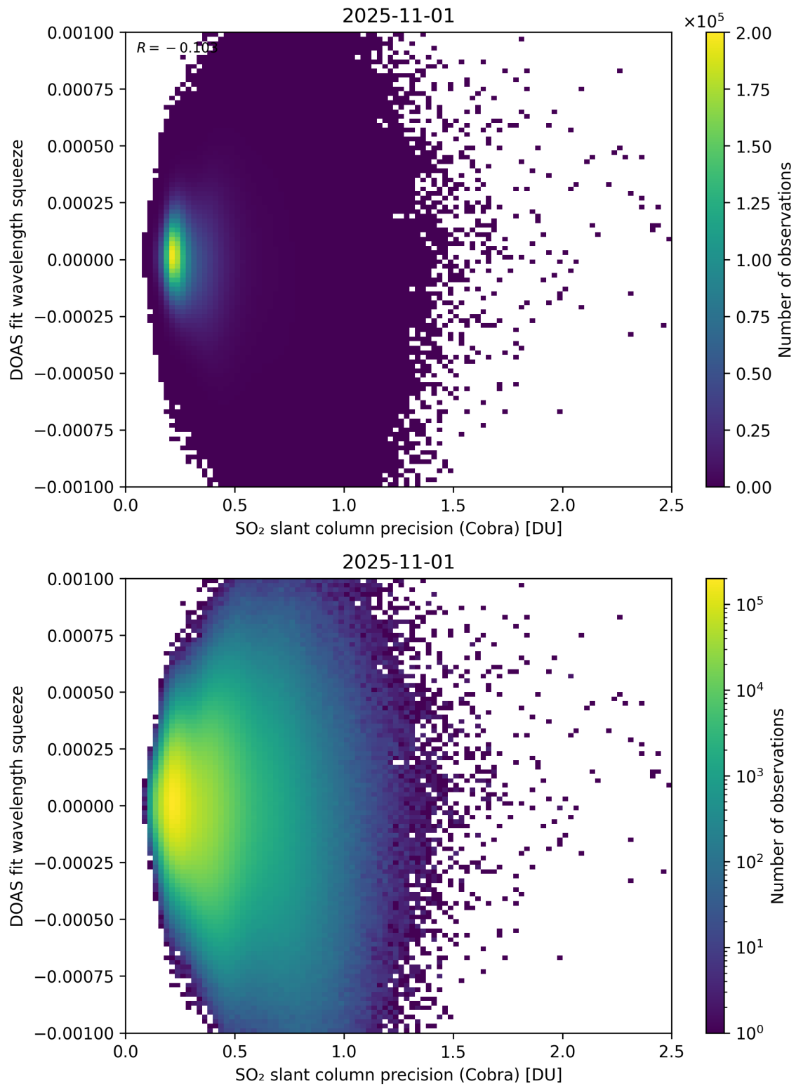
Figure 203: Scatter density plot of “SO 2 slant column precision (Cobra)” against “DOAS fit wavelength squeeze” for 2025-10-31 to 2025-11-02.
