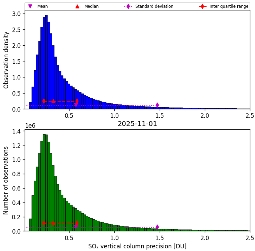
Figure 59: Histogram of “SO 2 vertical column precision” for 2025-10-31 to 2025-11-02
