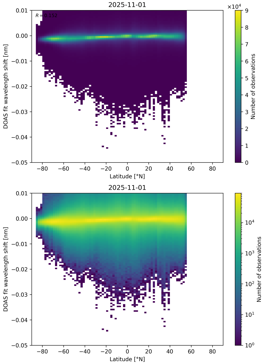
Figure 153: Scatter density plot of “Latitude” against “DOAS fit wavelength shift” for 2025-10-31 to 2025-11-02.
