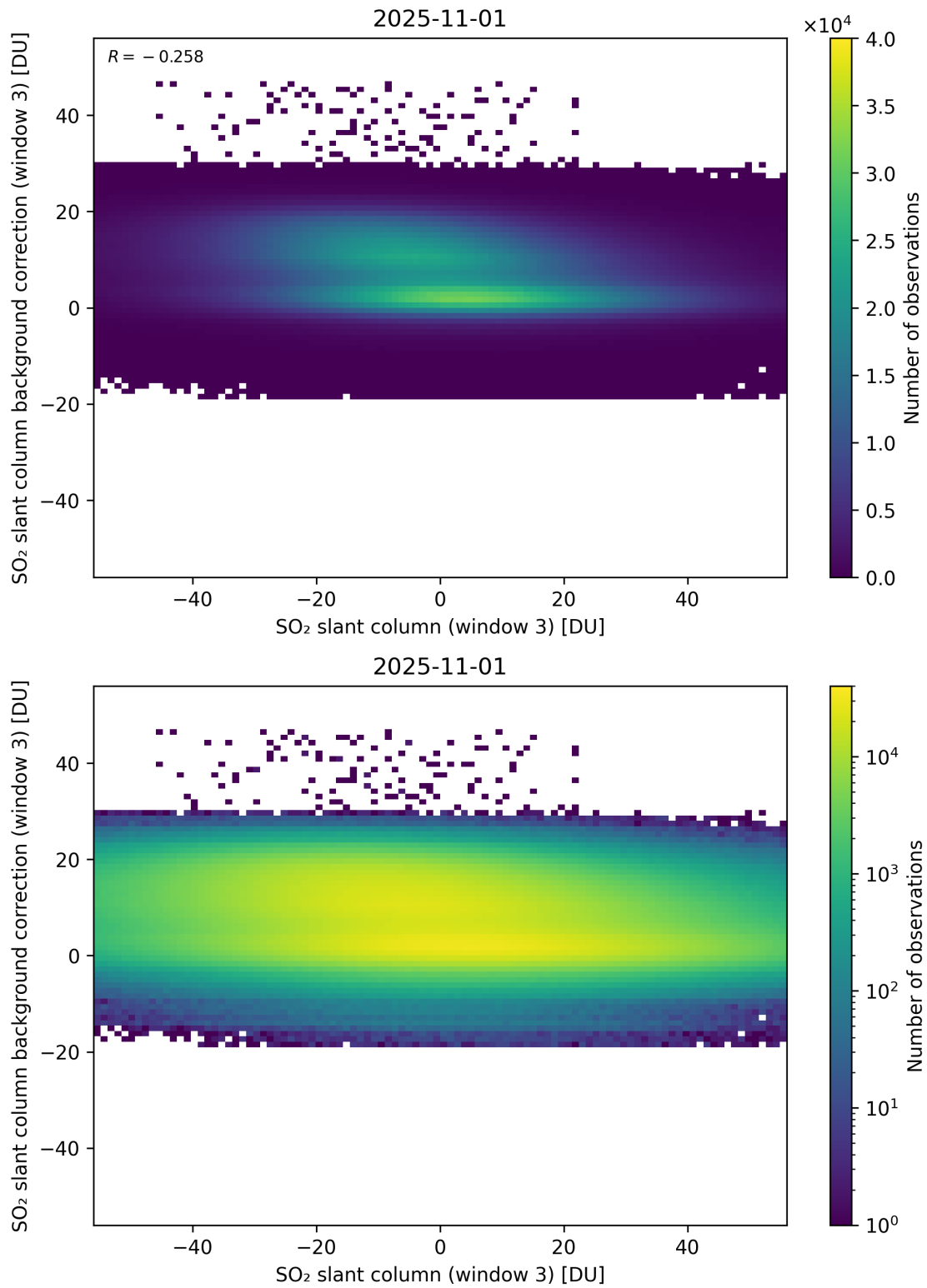
Figure 303: Scatter density plot of “SO 2 slant column (window 3)” against “SO 2 slant column background correction (window 3)” for 2025-10-31 to 2025-11-02.
