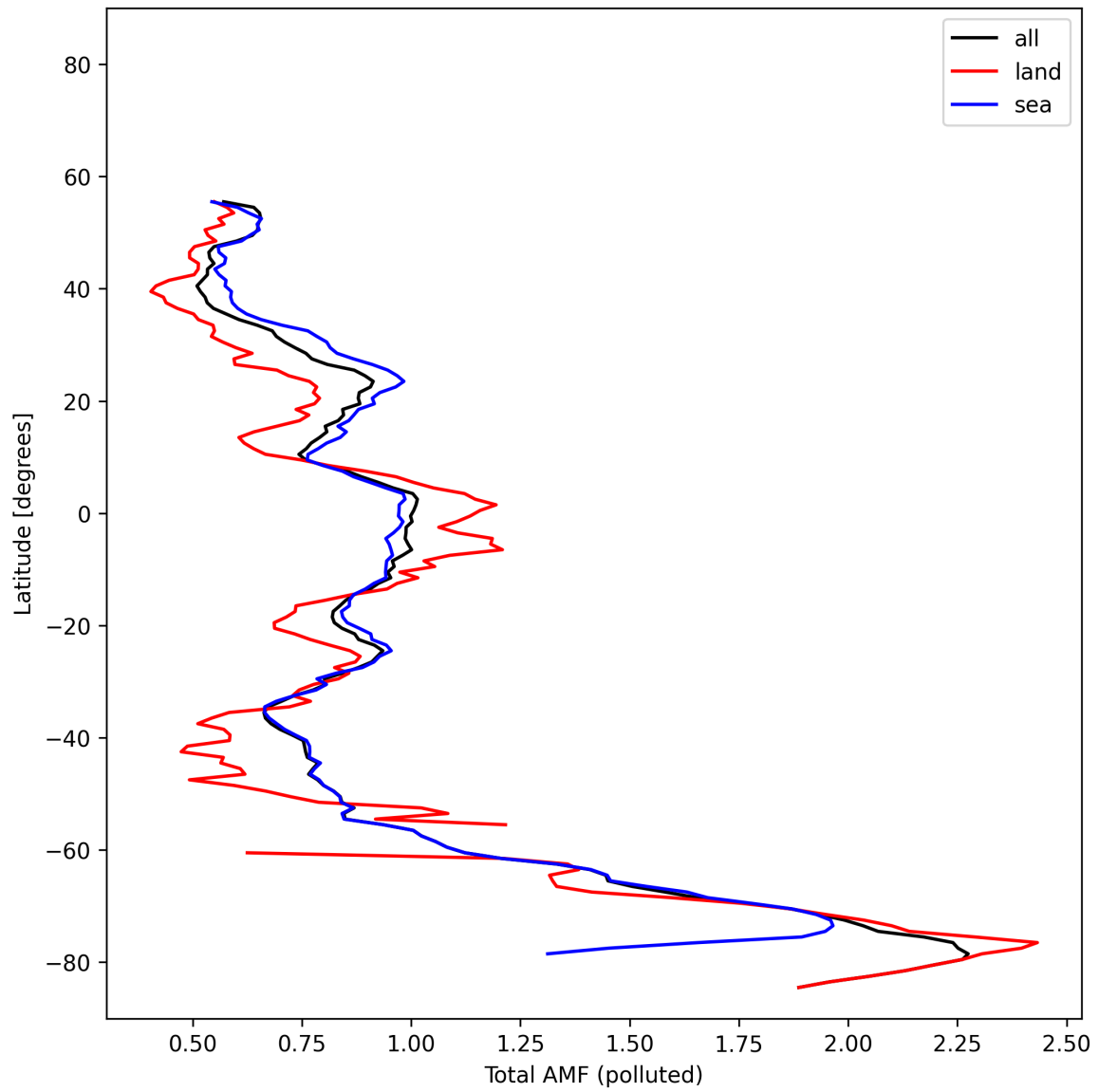
Figure 53: Zonal average of “Total AMF (polluted)” for 2025-10-31 to 2025-11-02.
