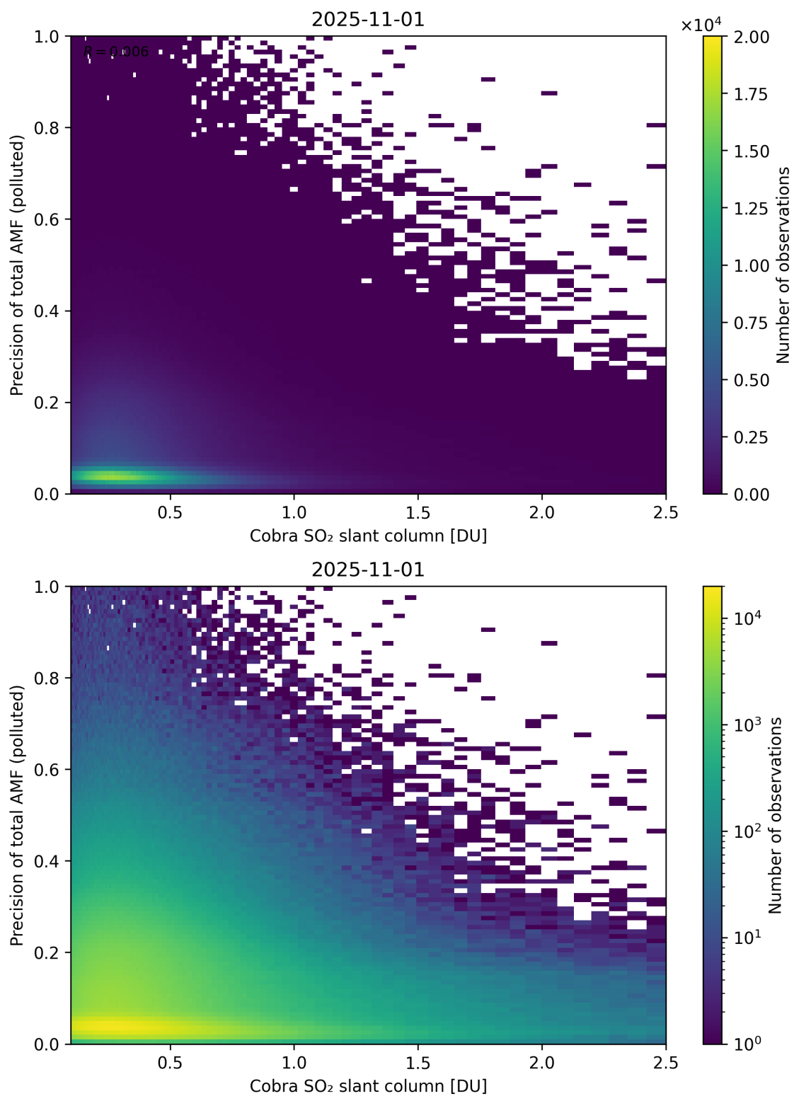
Figure 225: Scatter density plot of “Cobra SO 2 slant column” against “Precision of total AMF (polluted)” for 2025-10-31 to 2025-11-02.
