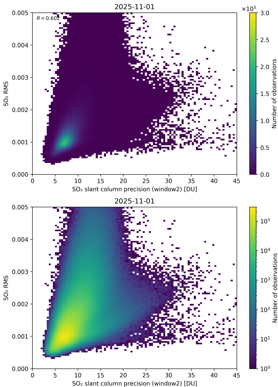
Figure 295: Scatter density plot of “SO 2 slant column precision (window2)” against “SO 2 RMS” for 2025-10-31 to 2025-11-02.
