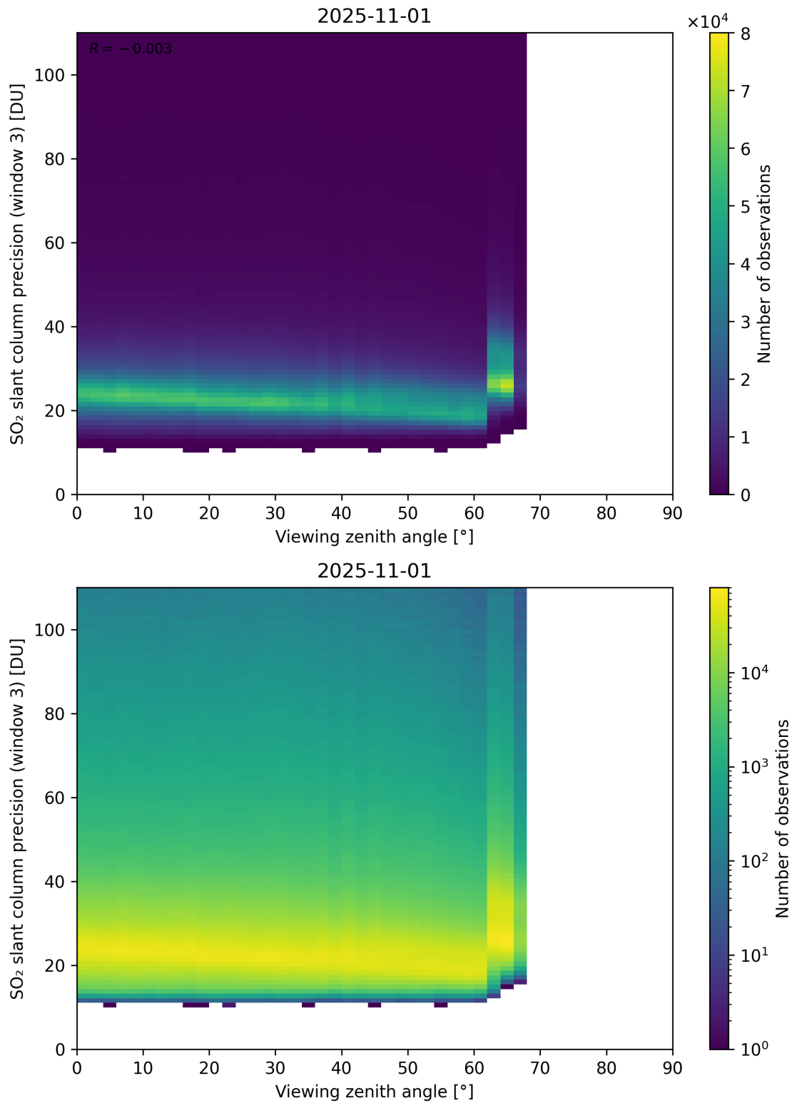
Figure 380: Scatter density plot of “Viewing zenith angle” against “SO 2 slant column precision (window 3)” for 2025-10-31 to 2025-11-02.
