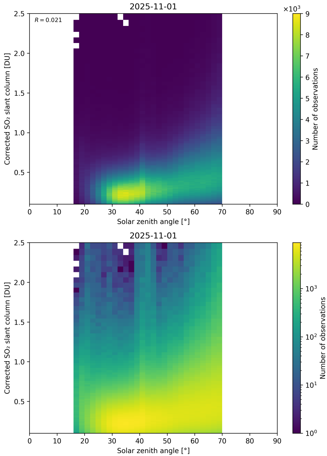
Figure 181: Scatter density plot of “Solar zenith angle” against “Corrected SO 2 slant column” for 2025-10-31 to 2025-11-02.
