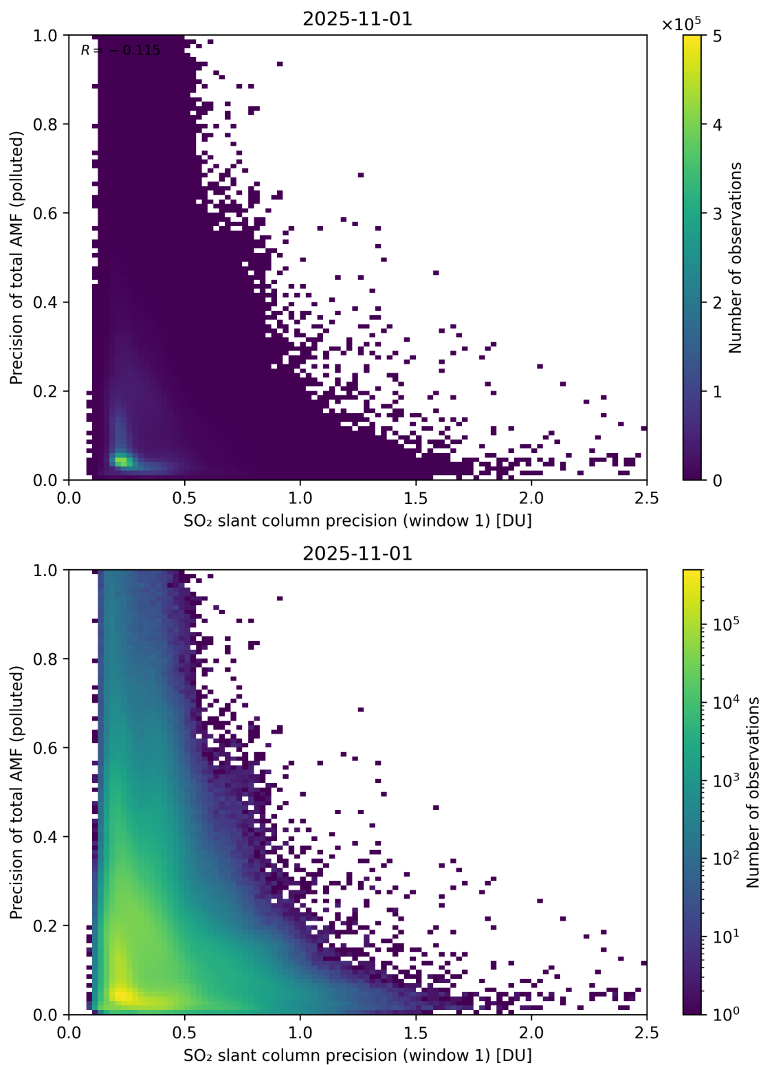
Figure 281: Scatter density plot of “SO 2 slant column precision (window 1)” against “Precision of total AMF (polluted)” for 2025-10-31 to 2025-11-02.
