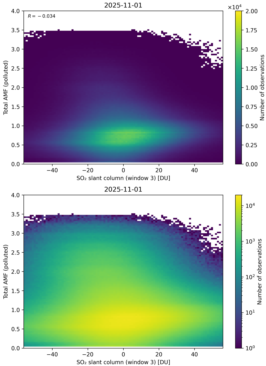
Figure 318: Scatter density plot of “SO 2 slant column (window 3)” against “Total AMF (polluted)” for 2025-10-31 to 2025-11-02.
