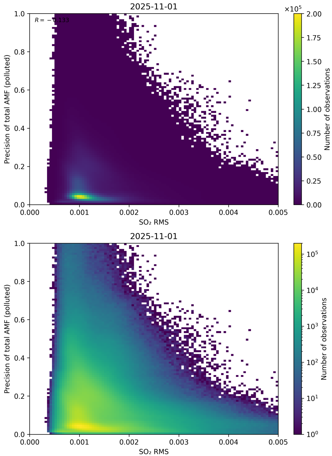
Figure 149: Scatter density plot of “SO 2 RMS” against “Precision of total AMF (polluted)” for 2025-10-31 to 2025-11-02.
