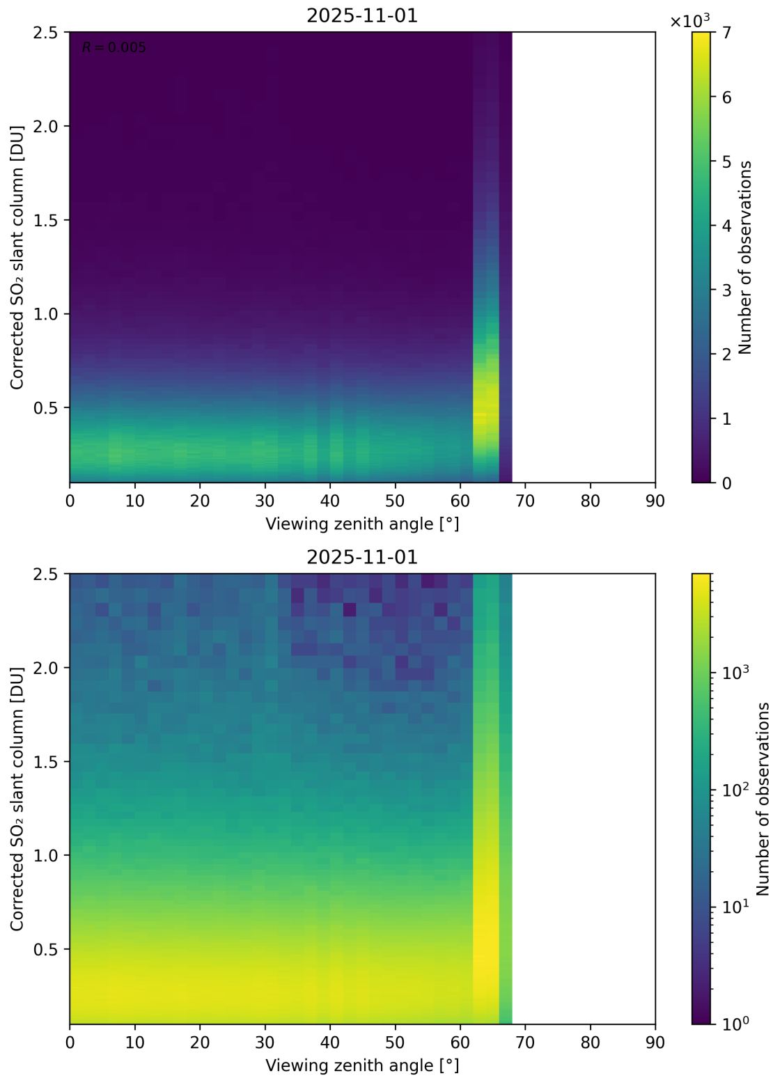
Figure 373: Scatter density plot of “Viewing zenith angle” against “Corrected SO 2 slant column” for 2025-10-31 to 2025-11-02.
