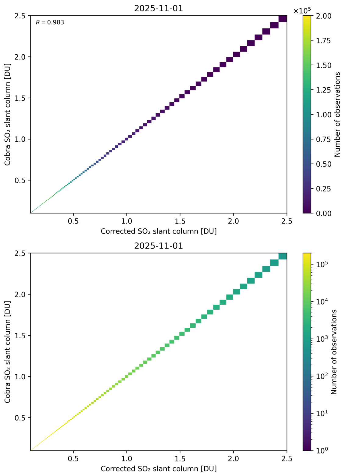
Figure 233: Scatter density plot of “Corrected SO 2 slant column” against “Cobra SO 2 slant column” for 2025-10-31 to 2025-11-02.
