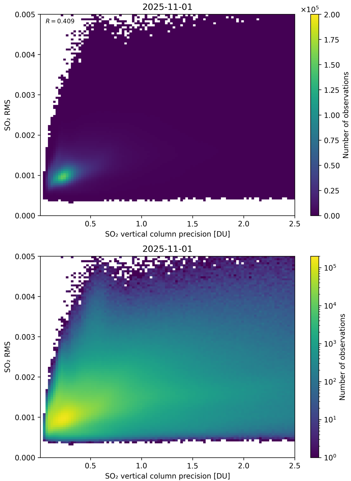
Figure 334: Scatter density plot of “SO 2 vertical column precision” against “SO 2 RMS” for 2025-10-31 to 2025-11-02.
