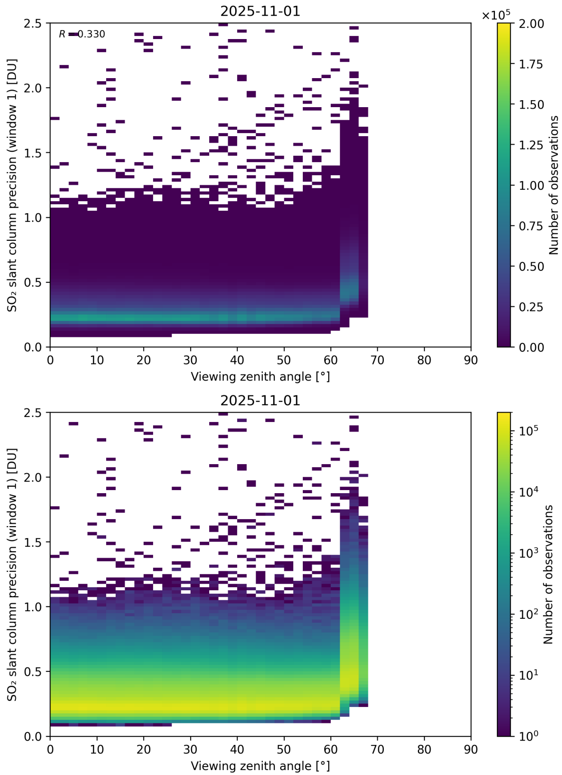
Figure 377: Scatter density plot of “Viewing zenith angle” against “SO 2 slant column precision (window 1)” for 2025-10-31 to 2025-11-02.
