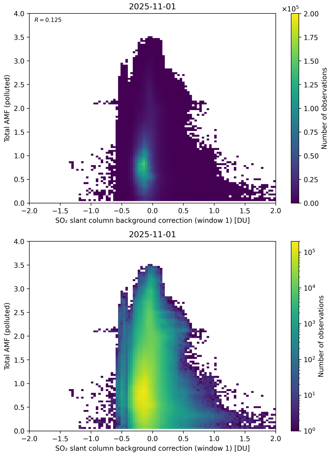
Figure 120: Scatter density plot of “SO 2 slant column background correction (window 1)” against “Total AMF (polluted)” for 2025-10-31 to 2025-11-02.
