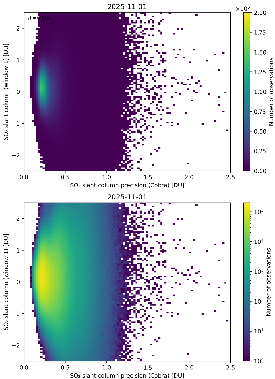
Figure 208: Scatter density plot of “SO 2 slant column precision (Cobra)” against “SO 2 slant column (window 1)” for 2025-10-31 to 2025-11-02.
