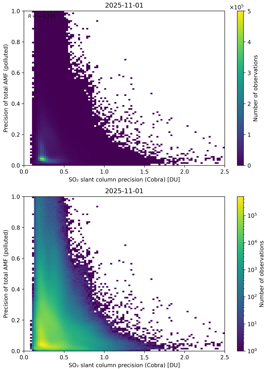
Figure 214: Scatter density plot of “SO 2 slant column precision (Cobra)” against “Precision of total AMF (polluted)” for 2025-10-31 to 2025-11-02.
