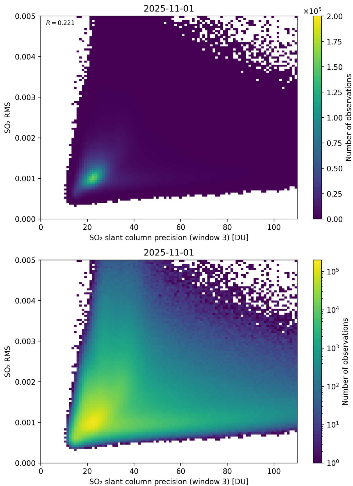
Figure 310: Scatter density plot of “SO 2 slant column precision (window 3)” against “SO 2 RMS” for 2025-10-31 to 2025-11-02.
