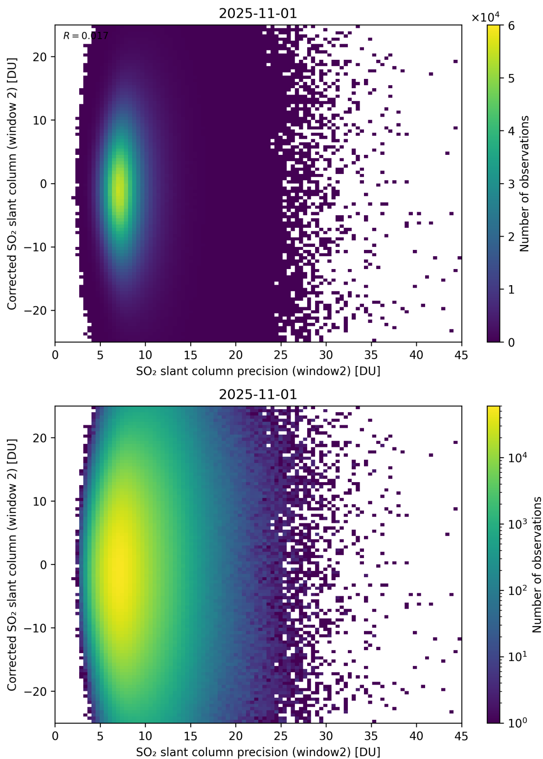
Figure 297: Scatter density plot of “SO 2 slant column precision (window2)” against “Corrected SO 2 slant column (window 2)” for 2025-10-31 to 2025-11-02.
