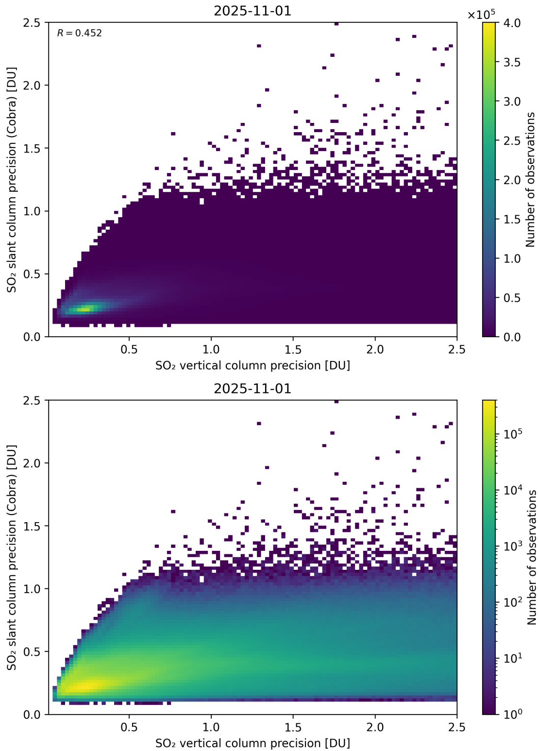
Figure 337: Scatter density plot of “SO 2 vertical column precision” against “SO 2 slant column precision (Cobra)” for 2025-10-31 to 2025-11-02.
