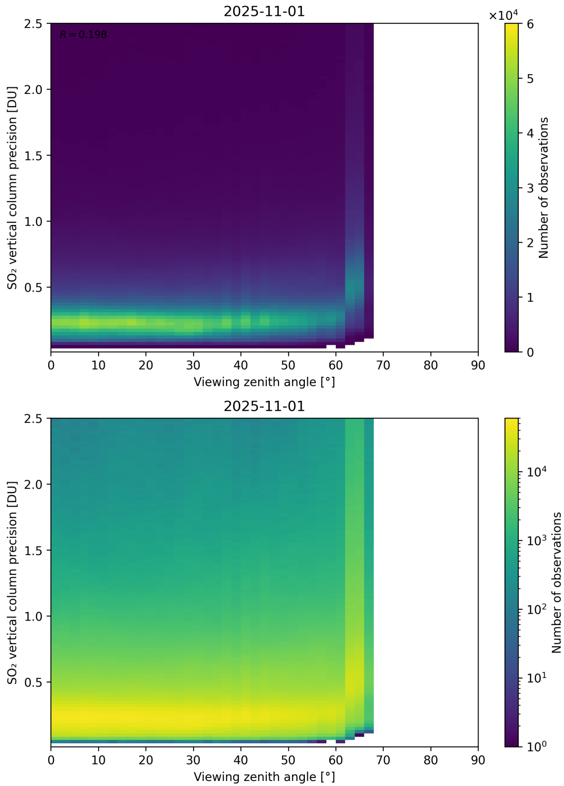
Figure 384: Scatter density plot of “Viewing zenith angle” against “SO 2 vertical column precision” for 2025-10-31 to 2025-11-02.
