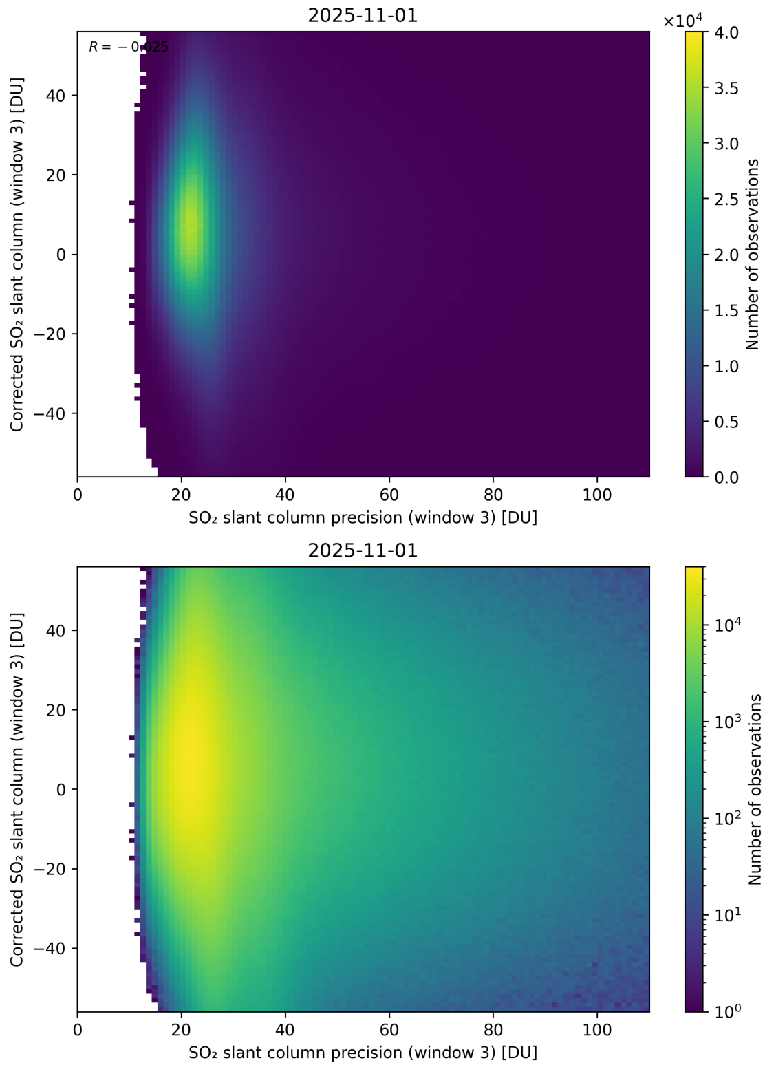
Figure 312: Scatter density plot of “SO 2 slant column precision (window 3)” against “Corrected SO 2 slant column (window 3)” for 2025-10-31 to 2025-11-02.
