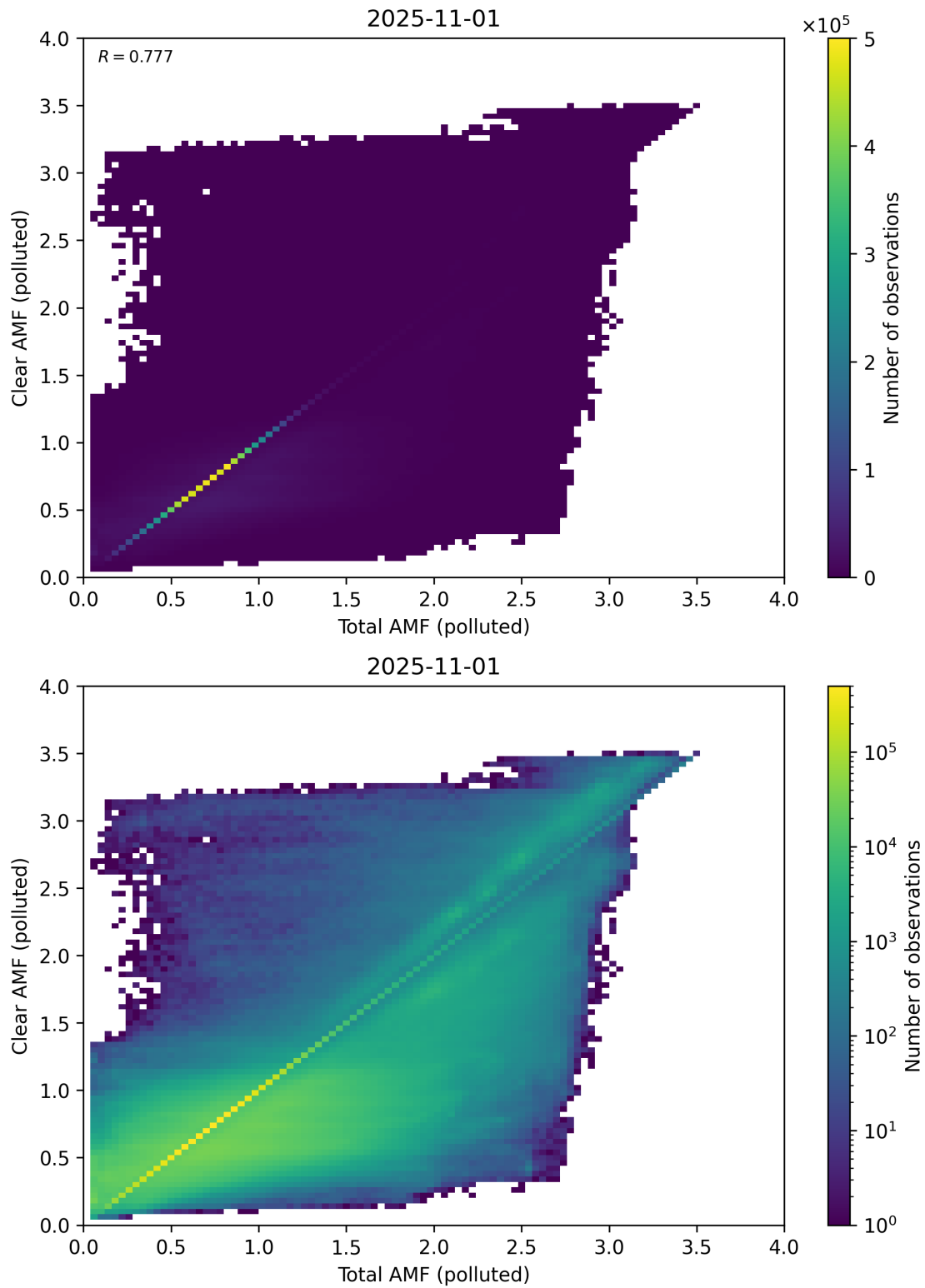
Figure 321: Scatter density plot of “Total AMF (polluted)” against “Clear AMF (polluted)” for 2025-10-31 to 2025-11-02.
