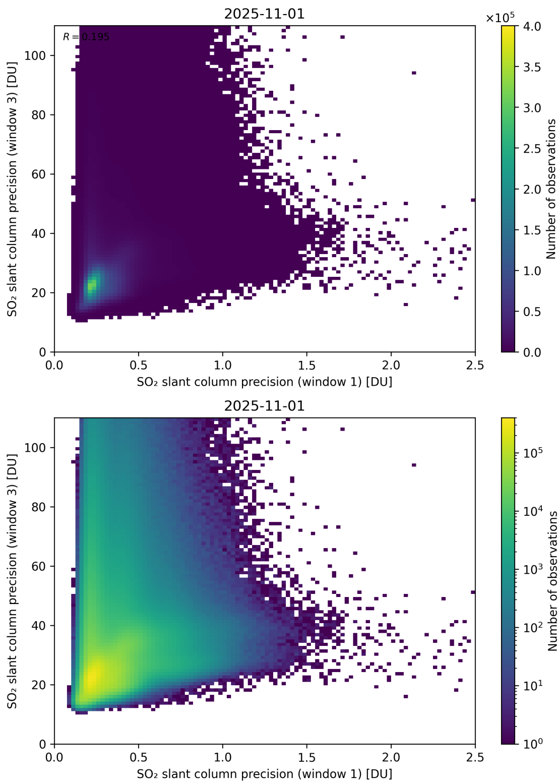
Figure 279: Scatter density plot of “SO 2 slant column precision (window 1)” against “SO 2 slant column precision (window 3)” for 2025-10-31 to 2025-11-02.
