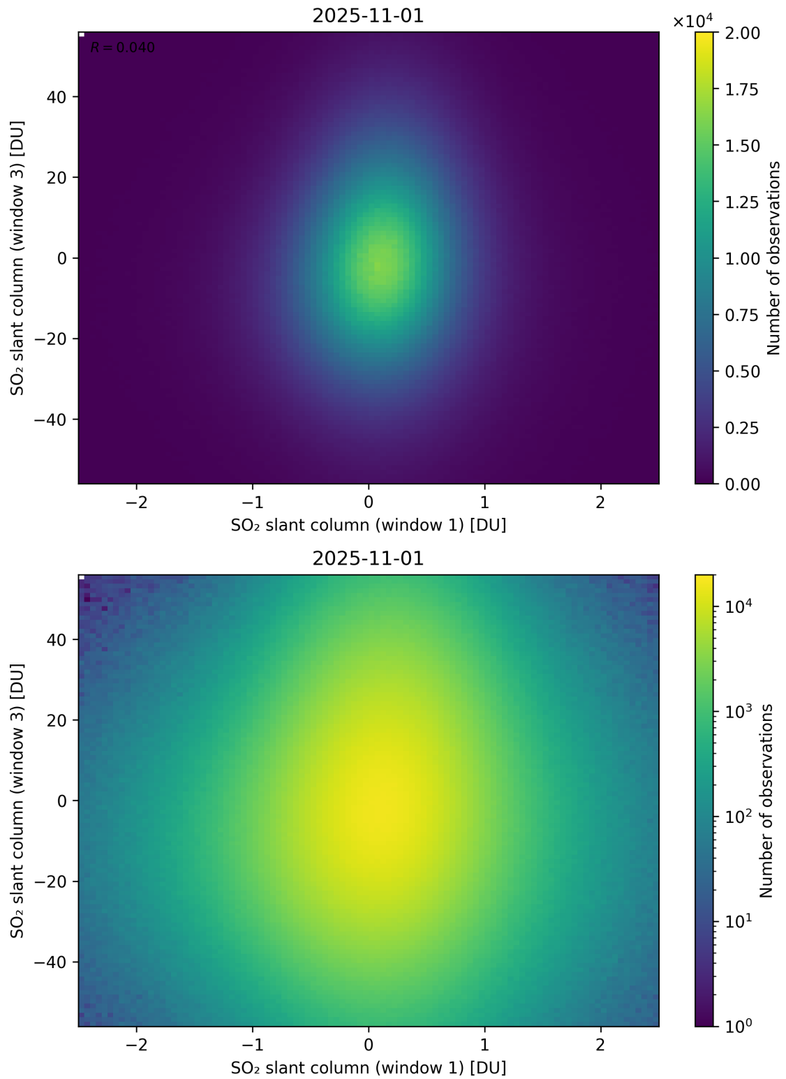
Figure 287: Scatter density plot of “SO 2 slant column (window 1)” against “SO 2 slant column (window 3)” for 2025-10-31 to 2025-11-02.
