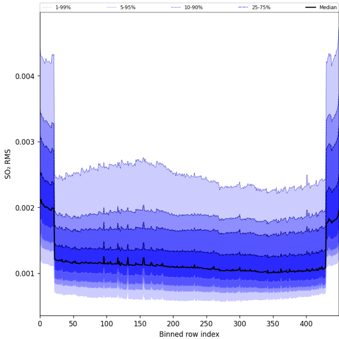
Figure 104: Along track statistics of “SO 2 RMS” for 2025-10-31 to 2025-11-02
