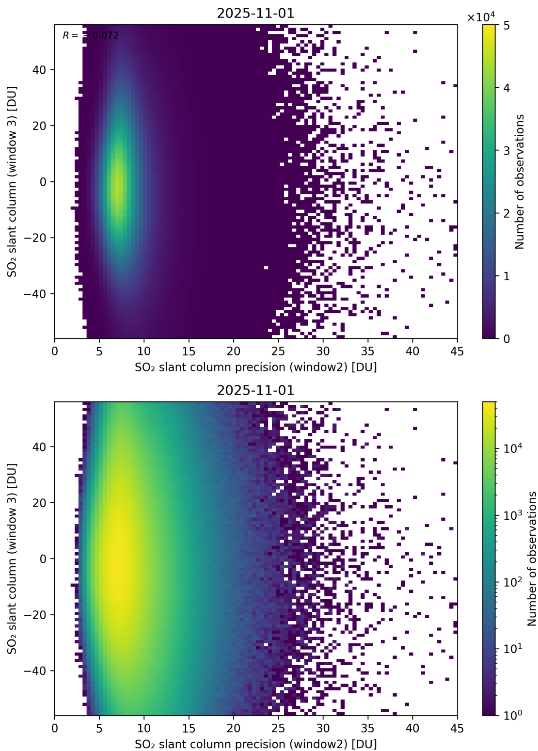
Figure 299: Scatter density plot of “SO 2 slant column precision (window2)” against “SO 2 slant column (window 3)” for 2025-10-31 to 2025-11-02.
