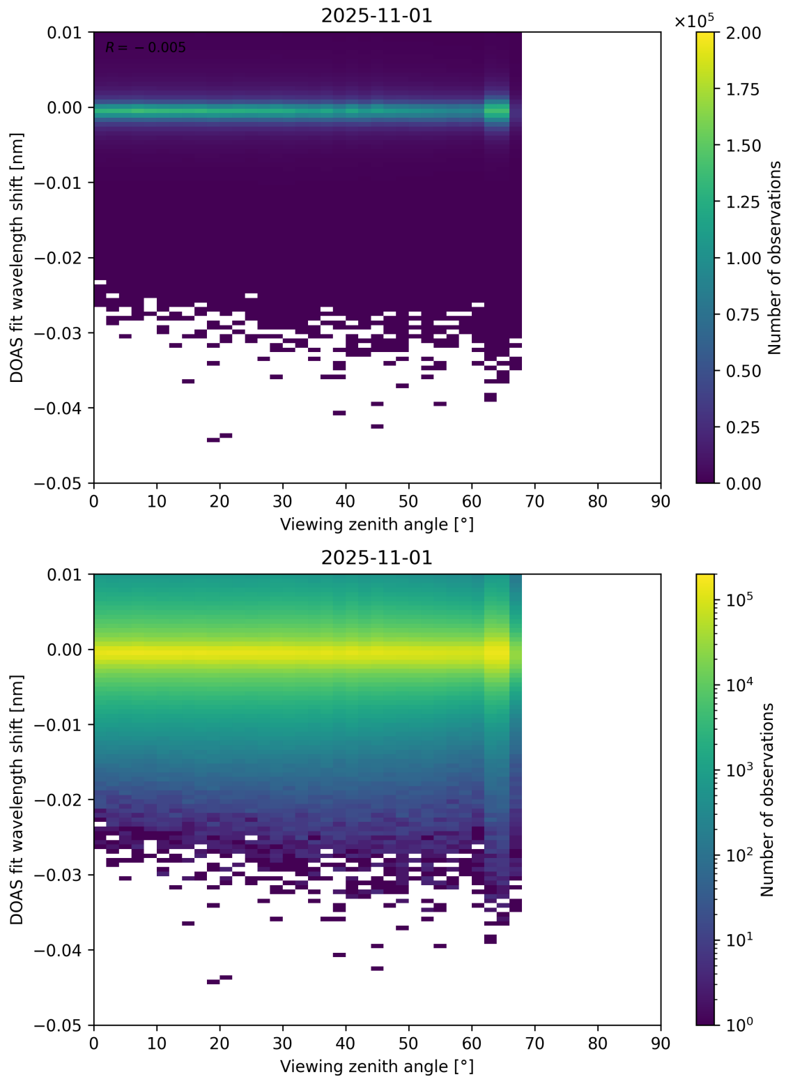
Figure 365: Scatter density plot of “Viewing zenith angle” against “DOAS fit wavelength shift” for 2025-10-31 to 2025-11-02.
