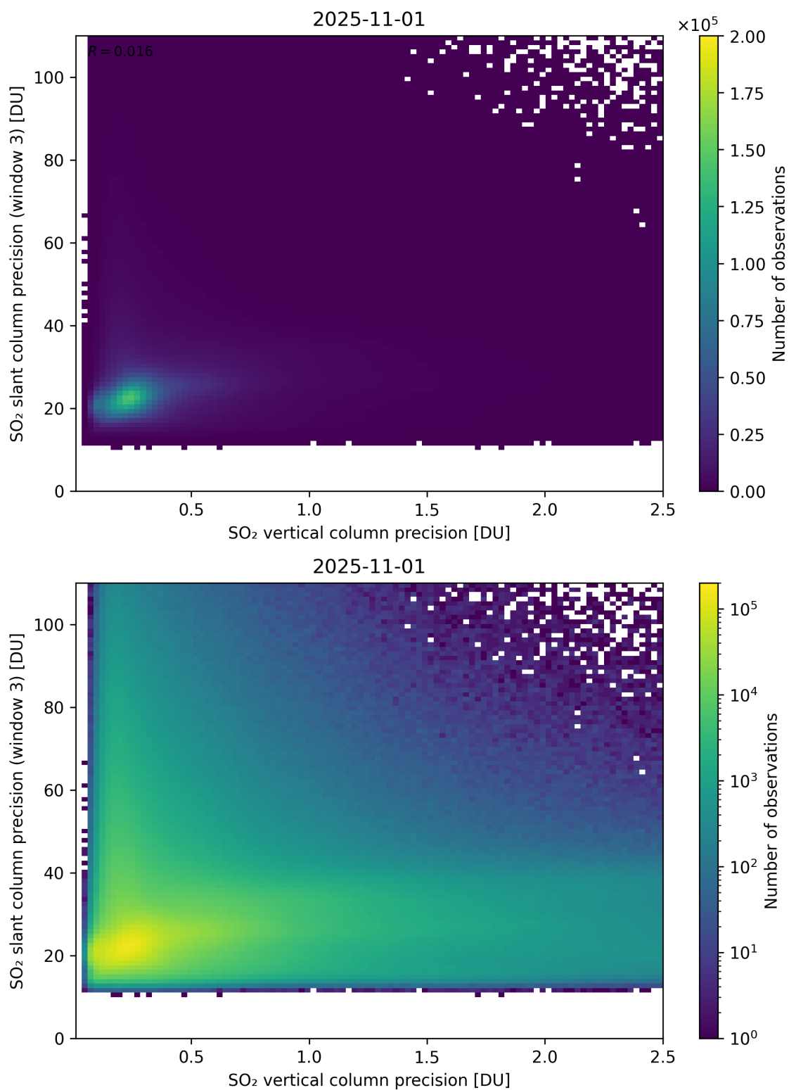
Figure 345: Scatter density plot of “SO 2 vertical column precision” against “SO 2 slant column precision (window 3)” for 2025-10-31 to 2025-11-02.
