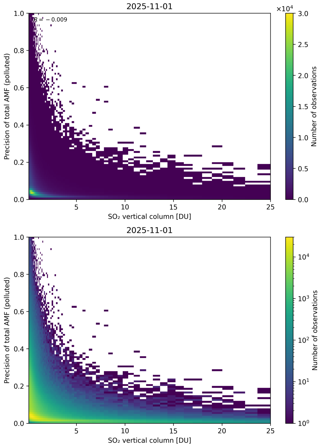
Figure 360: Scatter density plot of “SO 2 vertical column” against “Precision of total AMF (polluted)” for 2025-10-31 to 2025-11-02.
