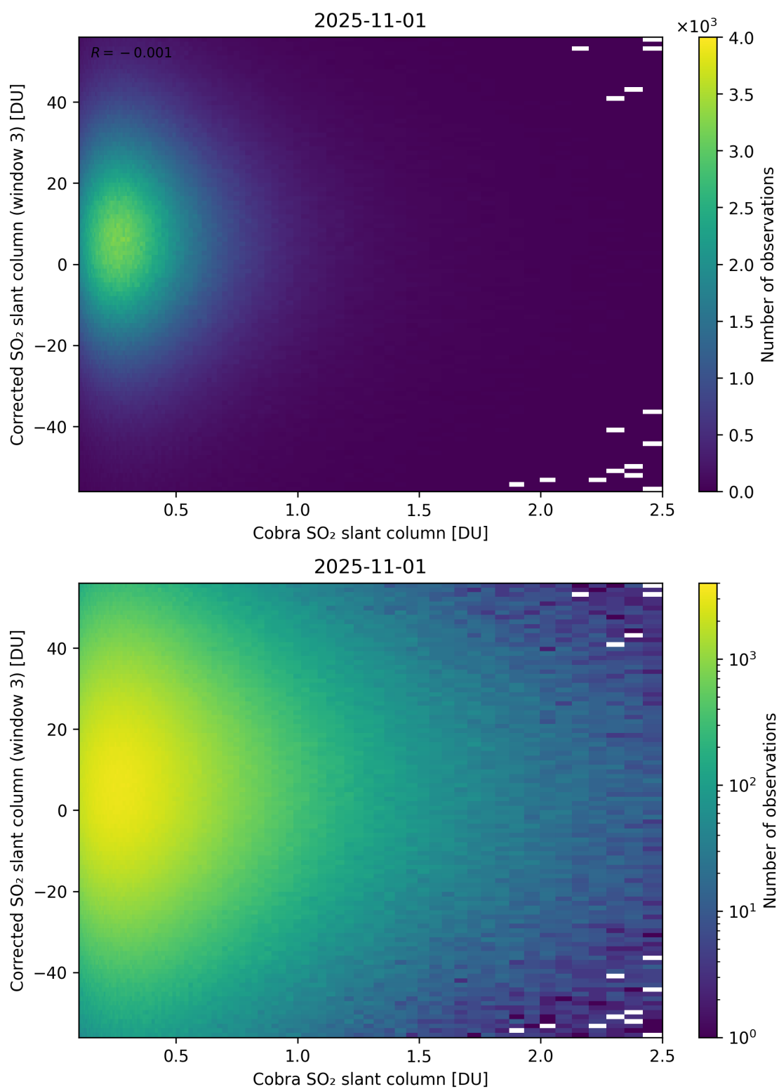
Figure 218: Scatter density plot of “Cobra SO 2 slant column” against “Corrected SO 2 slant column (window 3)” for 2025-10-31 to 2025-11-02.
