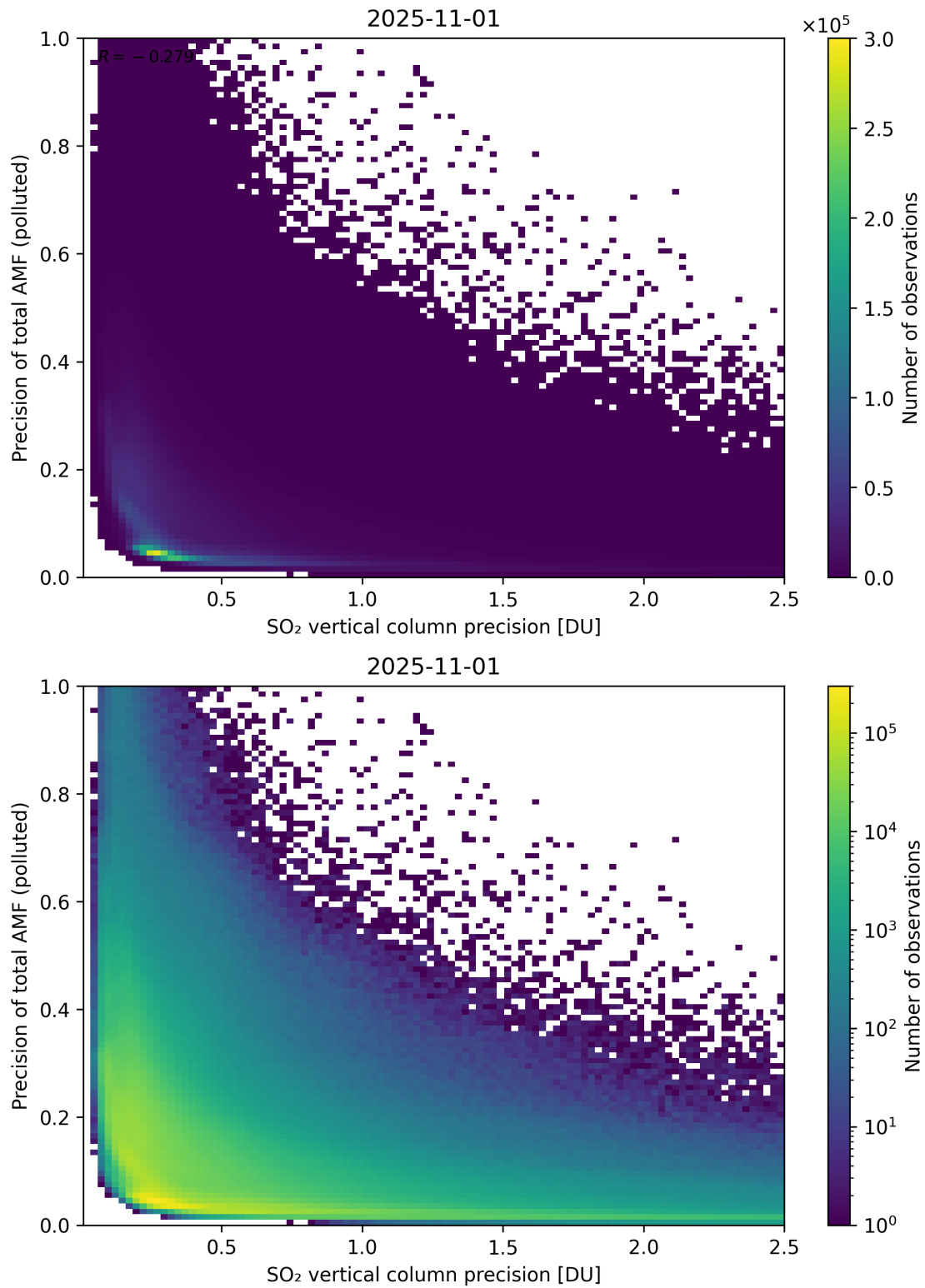
Figure 347: Scatter density plot of “SO 2 vertical column precision” against “Precision of total AMF (polluted)” for 2025-10-31 to 2025-11-02.
