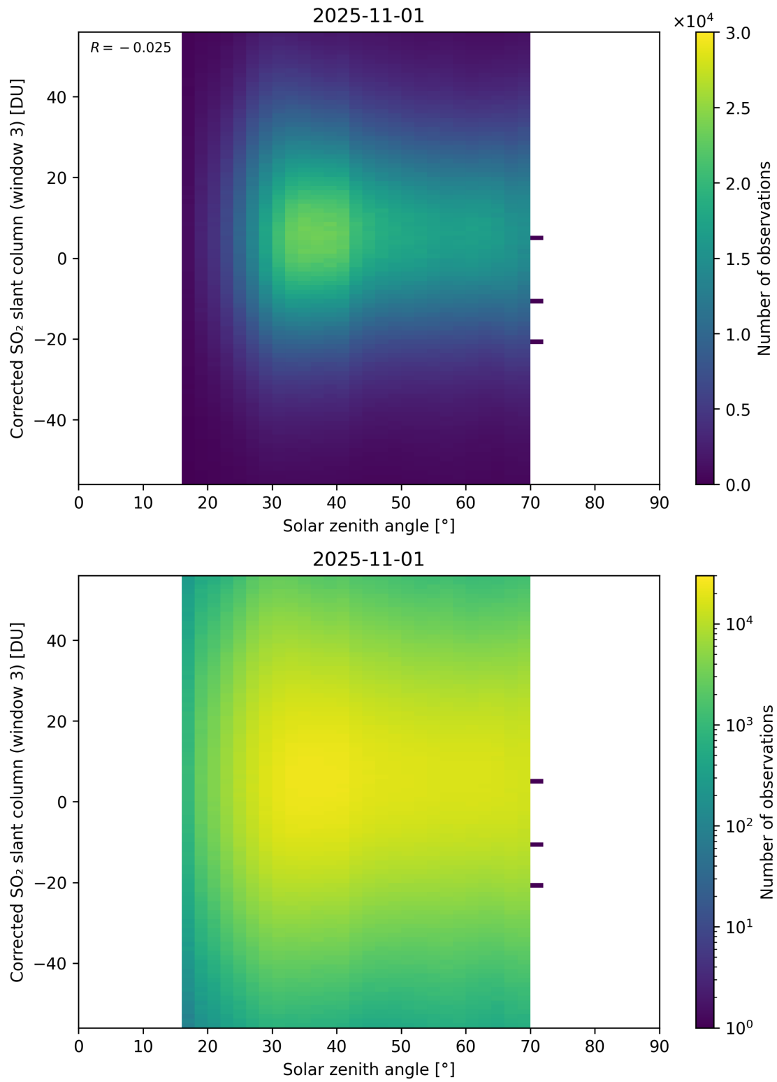
Figure 183: Scatter density plot of “Solar zenith angle” against “Corrected SO 2 slant column (window 3)” for 2025-10-31 to 2025-11-02.
