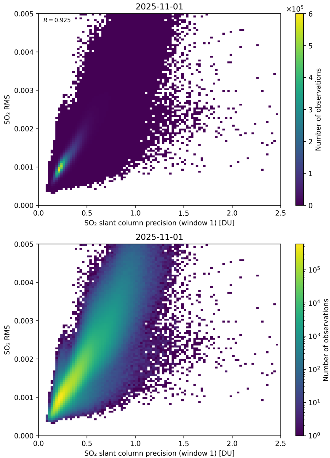
Figure 273: Scatter density plot of “SO 2 slant column precision (window 1)” against “SO 2 RMS” for 2025-10-31 to 2025-11-02.
