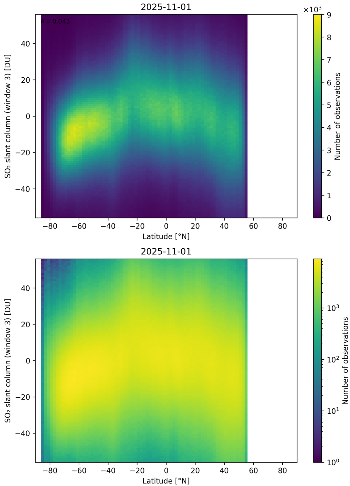
Figure 165: Scatter density plot of “Latitude” against “SO 2 slant column (window 3)” for 2025-10-31 to 2025-11-02.
