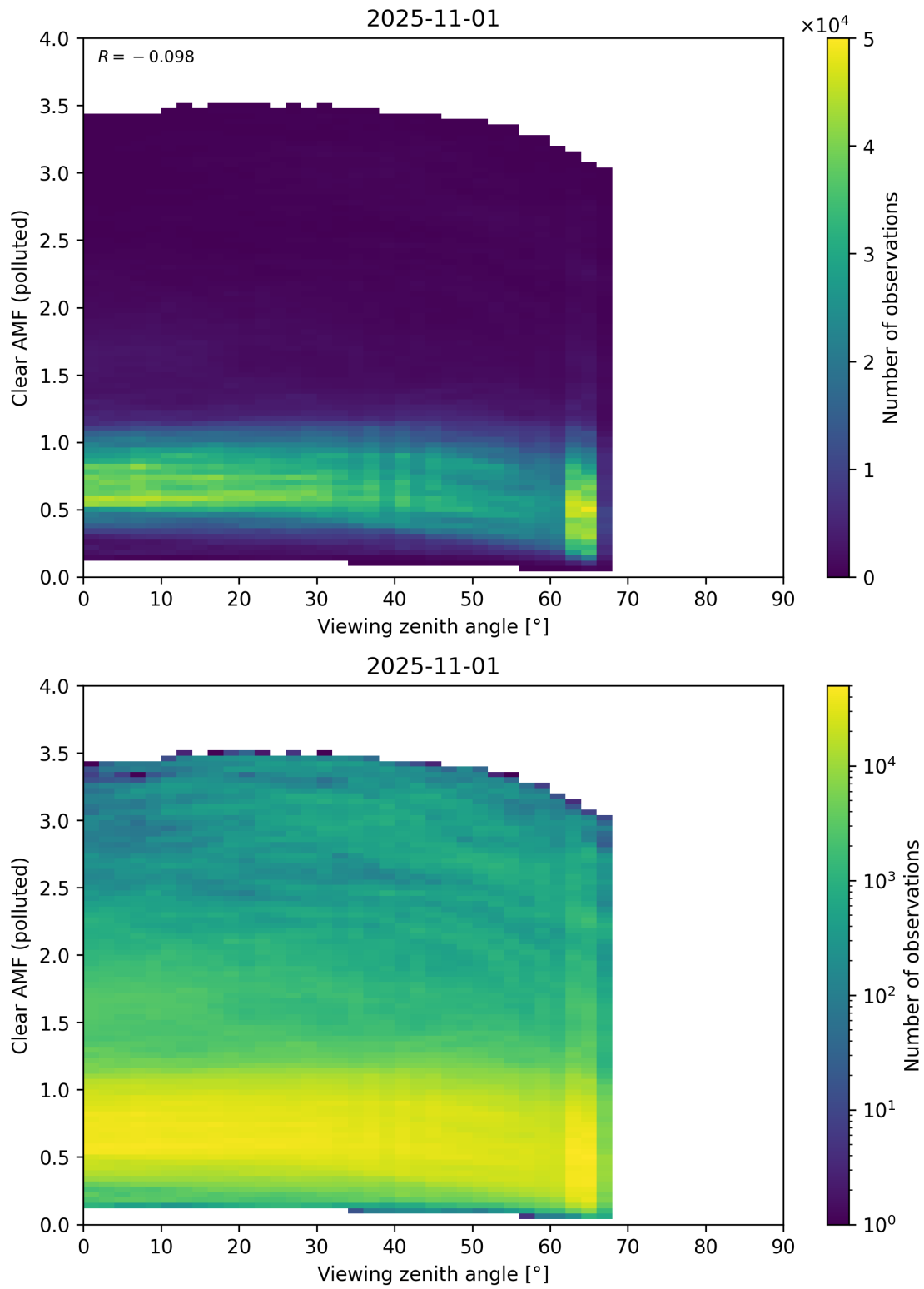
Figure 370: Scatter density plot of “Viewing zenith angle” against “Clear AMF (polluted)” for 2025-10-31 to 2025-11-02.
