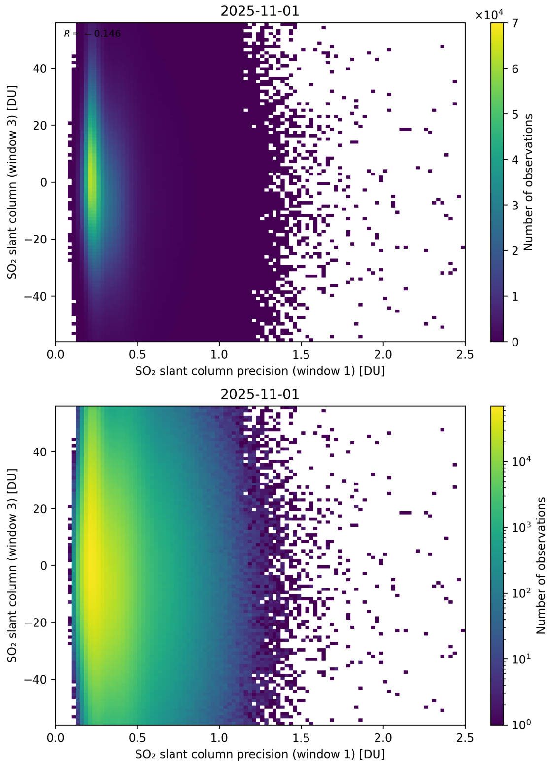
Figure 278: Scatter density plot of “SO 2 slant column precision (window 1)” against “SO 2 slant column (window 3)” for 2025-10-31 to 2025-11-02.
