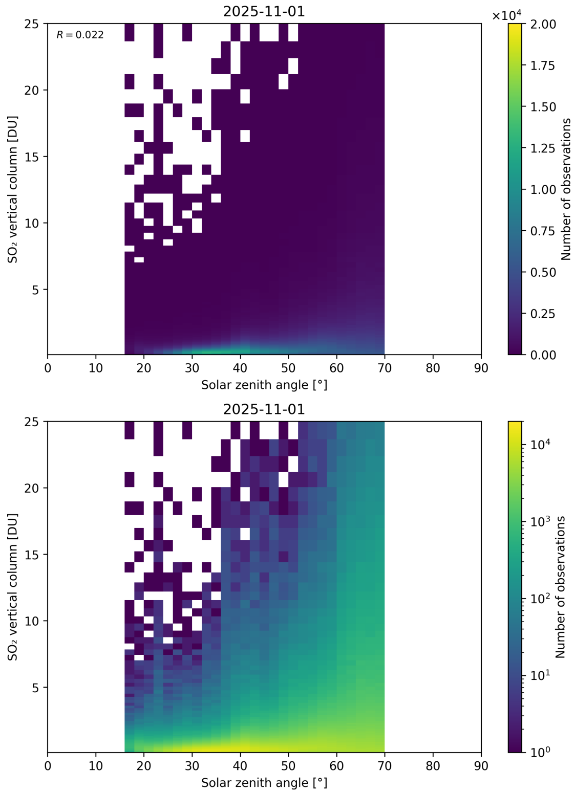
Figure 191: Scatter density plot of “Solar zenith angle” against “SO 2 vertical column” for 2025-10-31 to 2025-11-02.
