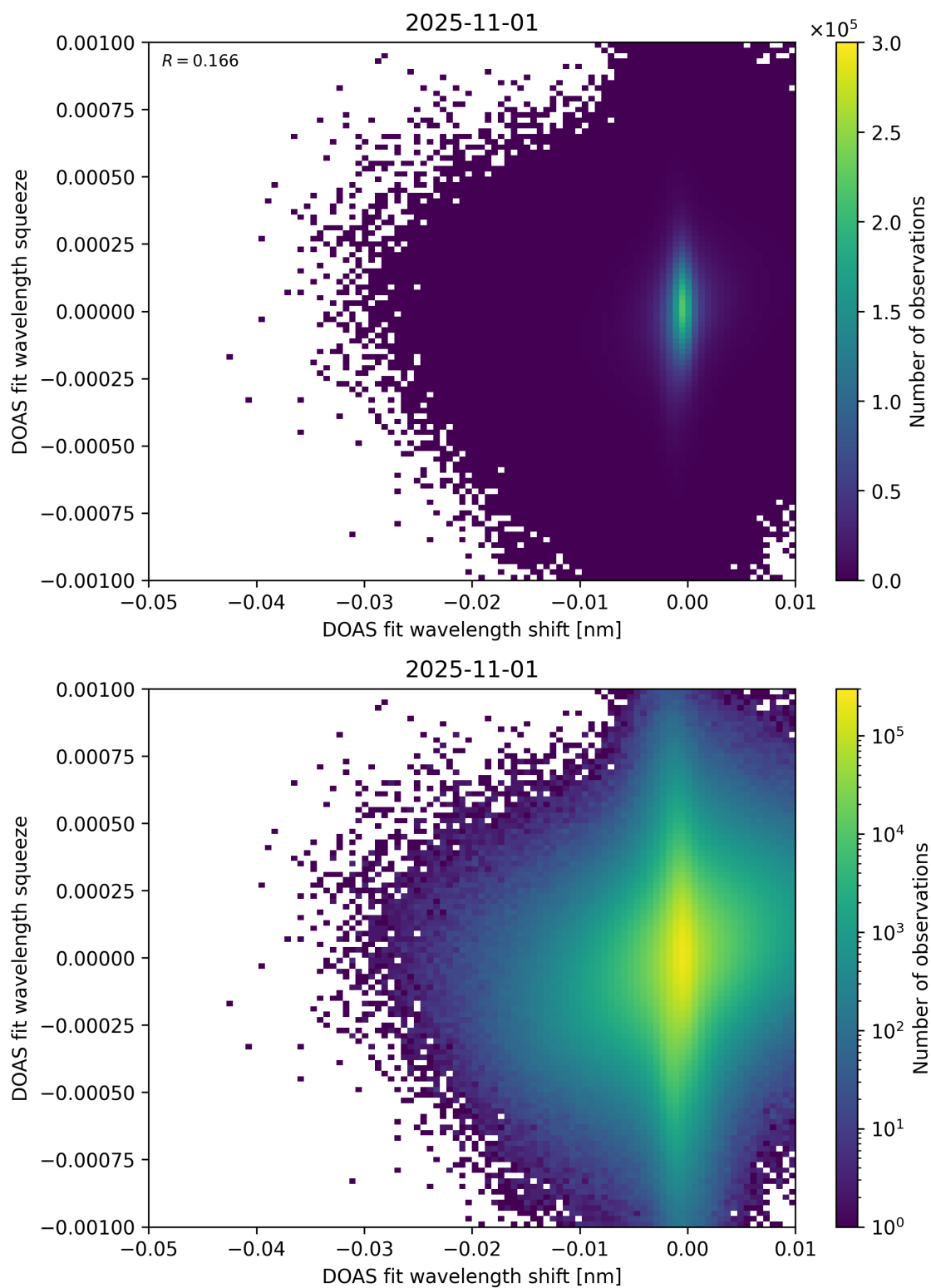
Figure 138: Scatter density plot of “DOAS fit wavelength shift” against “DOAS fit wavelength squeeze” for 2025-10-31 to 2025-11-02.
