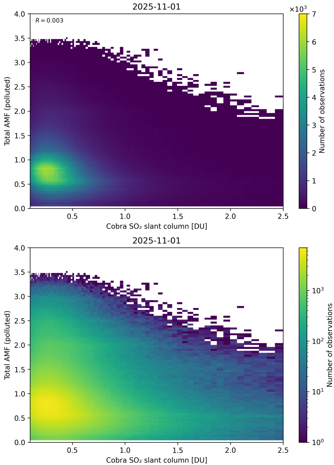
Figure 224: Scatter density plot of “Cobra SO 2 slant column” against “Total AMF (polluted)” for 2025-10-31 to 2025-11-02.
