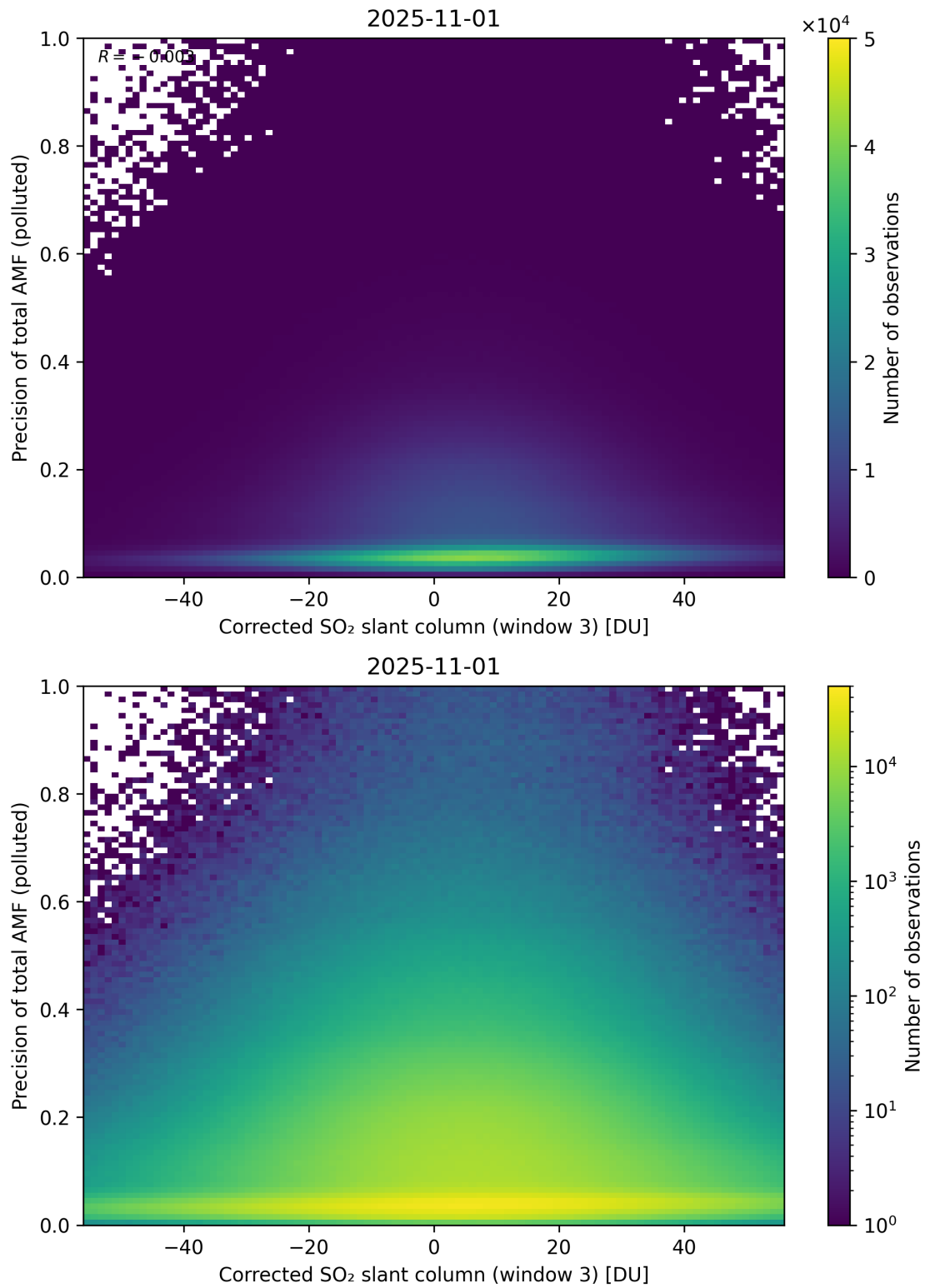
Figure 261: Scatter density plot of “Corrected SO 2 slant column (window 3)” against “Precision of total AMF (polluted)” for 2025-10-31 to 2025-11-02.
