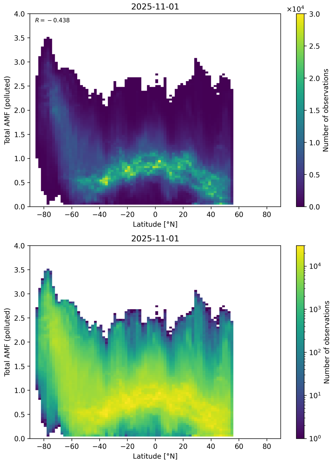
Figure 167: Scatter density plot of “Latitude” against “Total AMF (polluted)” for 2025-10-31 to 2025-11-02.
