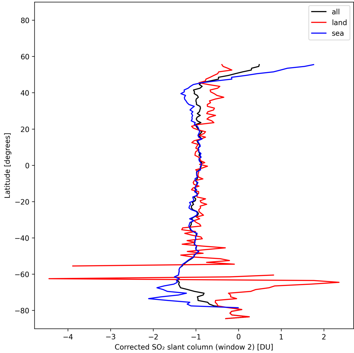
Figure 43: Zonal average of “Corrected SO 2 slant column (window 2)” for 2025-10-31 to 2025-11-02.
