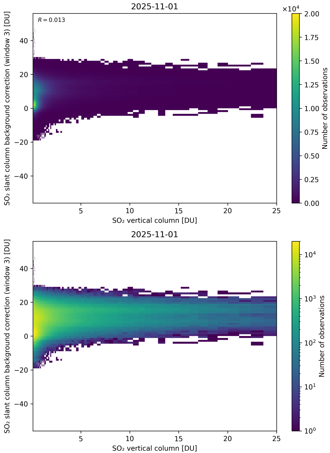
Figure 325: Scatter density plot of “SO 2 vertical column” against “SO 2 slant column background correction (window 3)” for 2025-10-31 to 2025-11-02.
