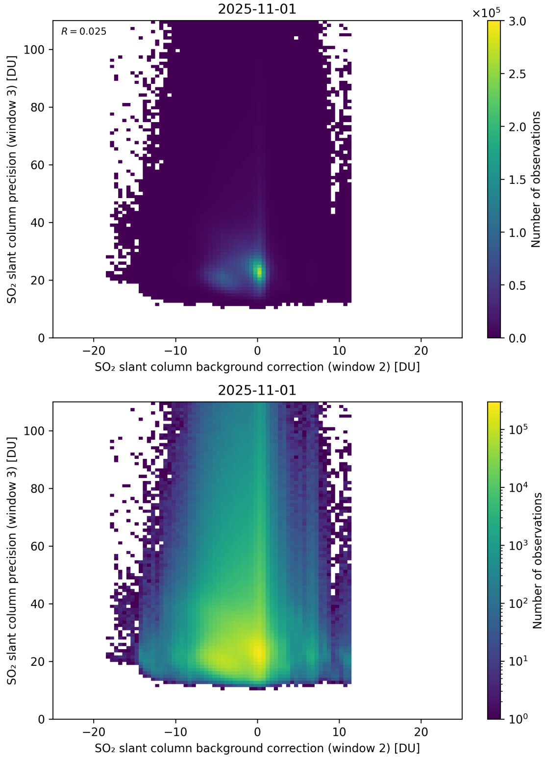
Figure 129: Scatter density plot of “SO 2 slant column background correction (window 2)” against “SO 2 slant column precision (window 3)” for 2025-10-31 to 2025-11-02.
