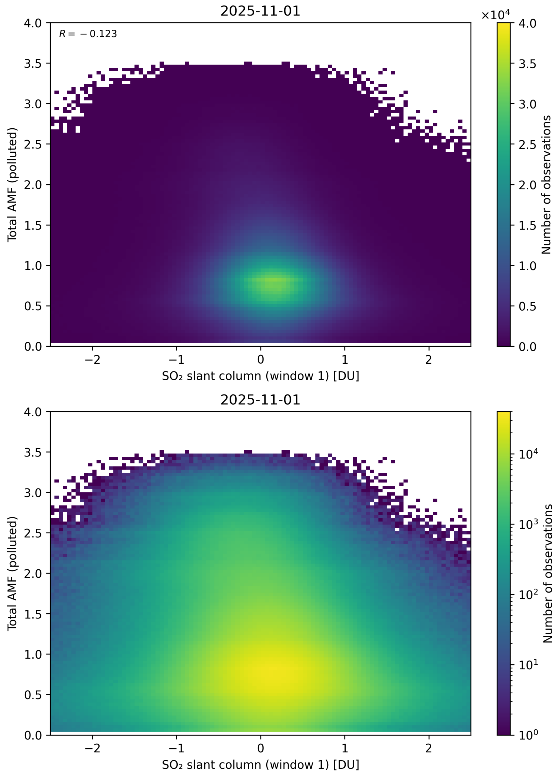
Figure 289: Scatter density plot of “SO 2 slant column (window 1)” against “Total AMF (polluted)” for 2025-10-31 to 2025-11-02.
