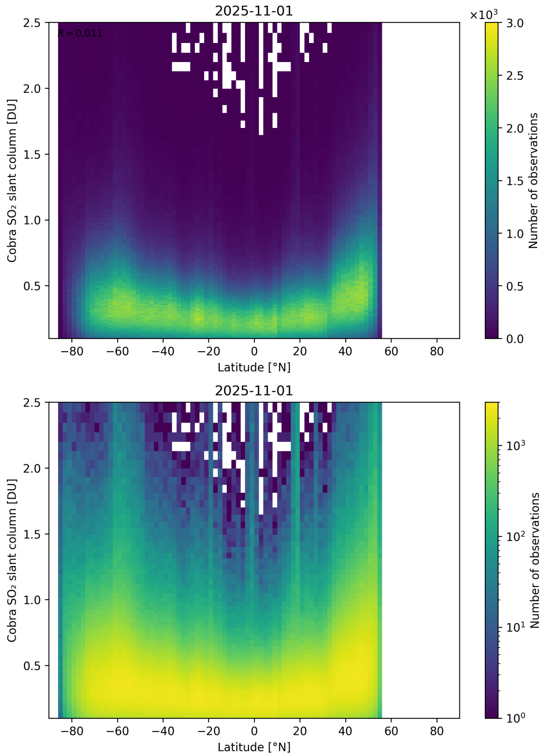
Figure 157: Scatter density plot of “Latitude” against “Cobra SO 2 slant column” for 2025-10-31 to 2025-11-02.
