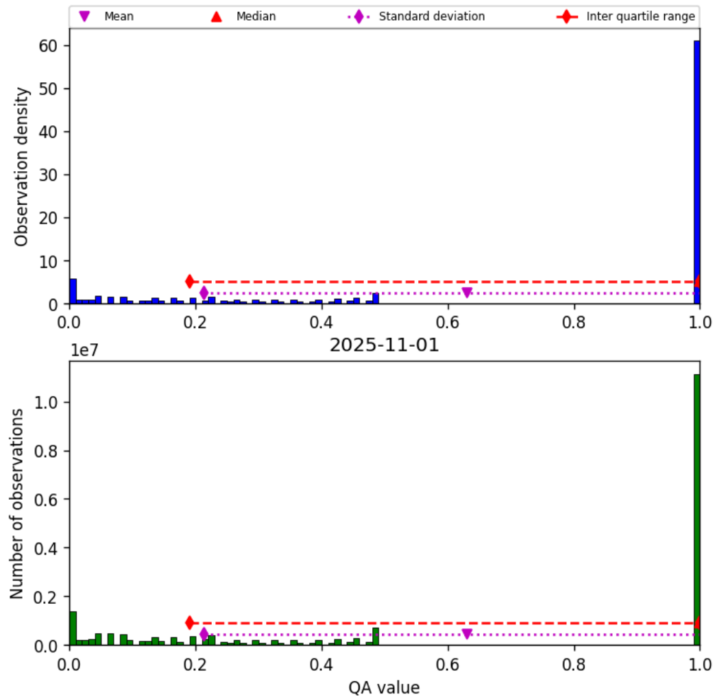
Figure 57: Histogram of “QA value” for 2025-10-31 to 2025-11-02
