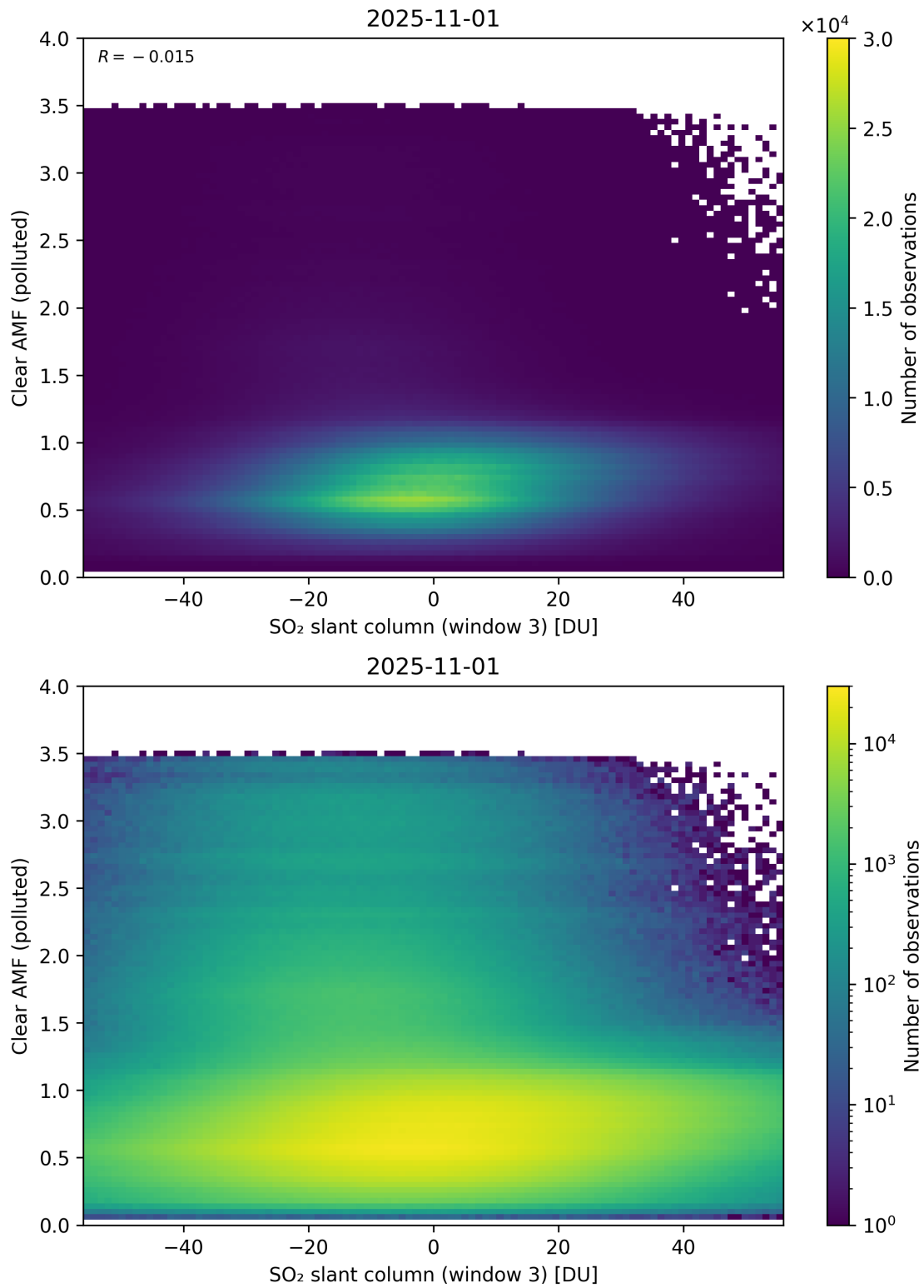
Figure 315: Scatter density plot of “SO 2 slant column (window 3)” against “Clear AMF (polluted)” for 2025-10-31 to 2025-11-02.
