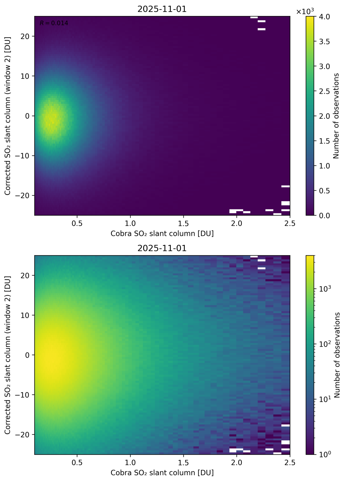
Figure 217: Scatter density plot of “Cobra SO 2 slant column” against “Corrected SO 2 slant column (window 2)” for 2025-10-31 to 2025-11-02.
