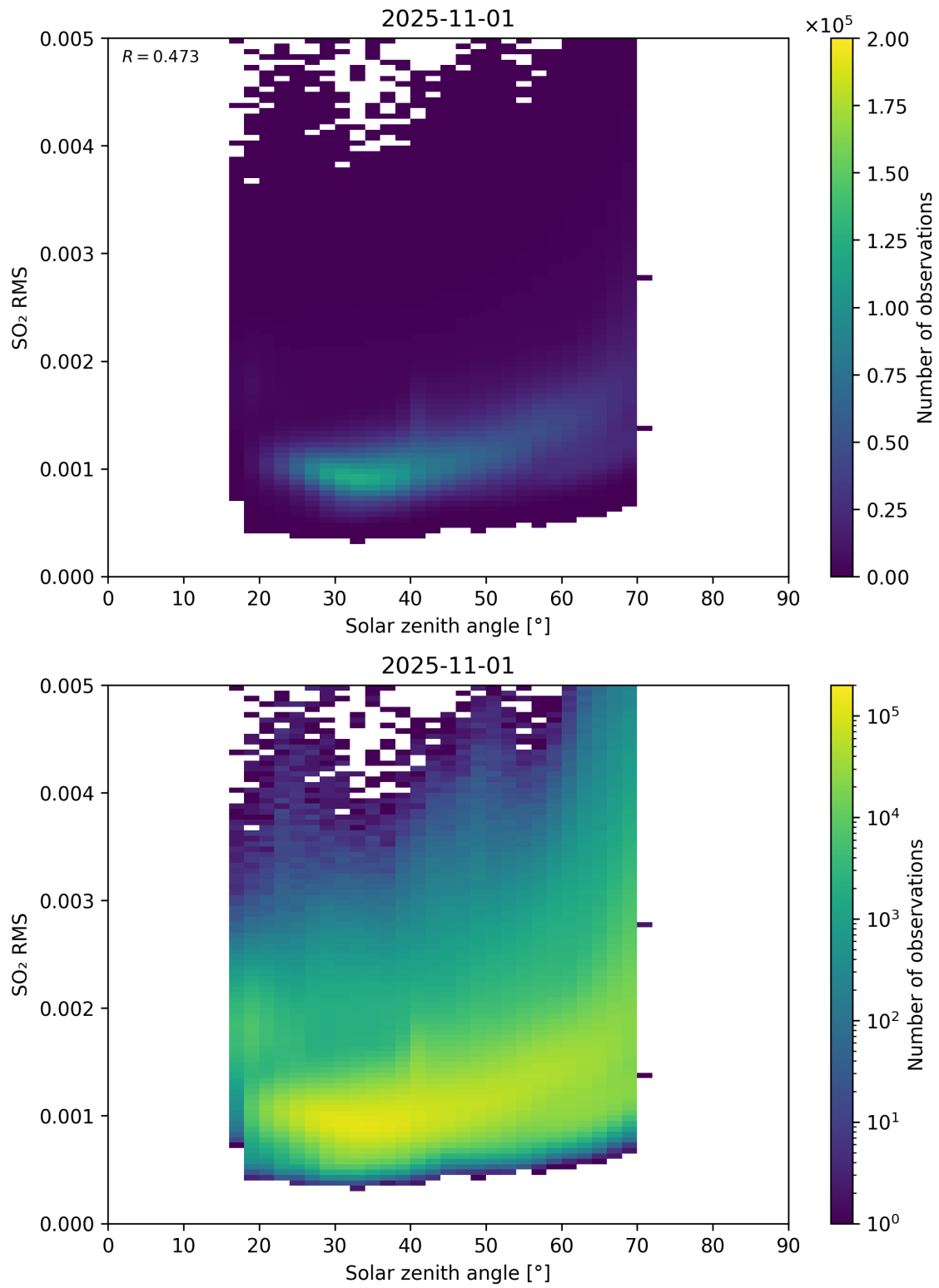
Figure 176: Scatter density plot of “Solar zenith angle” against “SO 2 RMS” for 2025-10-31 to 2025-11-02.
