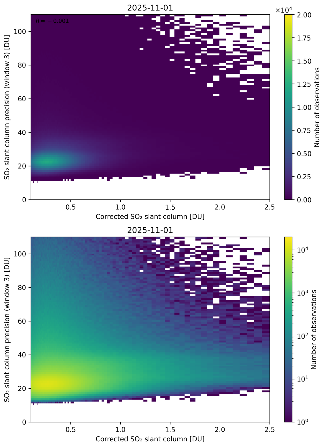
Figure 241: Scatter density plot of “Corrected SO 2 slant column” against “SO 2 slant column precision (window 3)” for 2025-10-31 to 2025-11-02.
