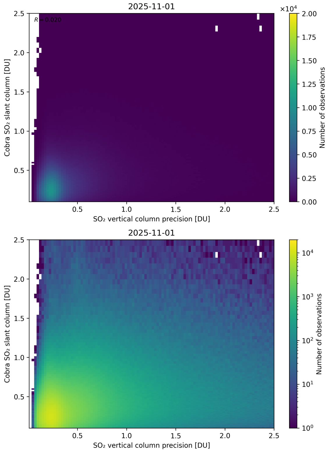
Figure 336: Scatter density plot of “SO 2 vertical column precision” against “Cobra SO 2 slant column” for 2025-10-31 to 2025-11-02.
