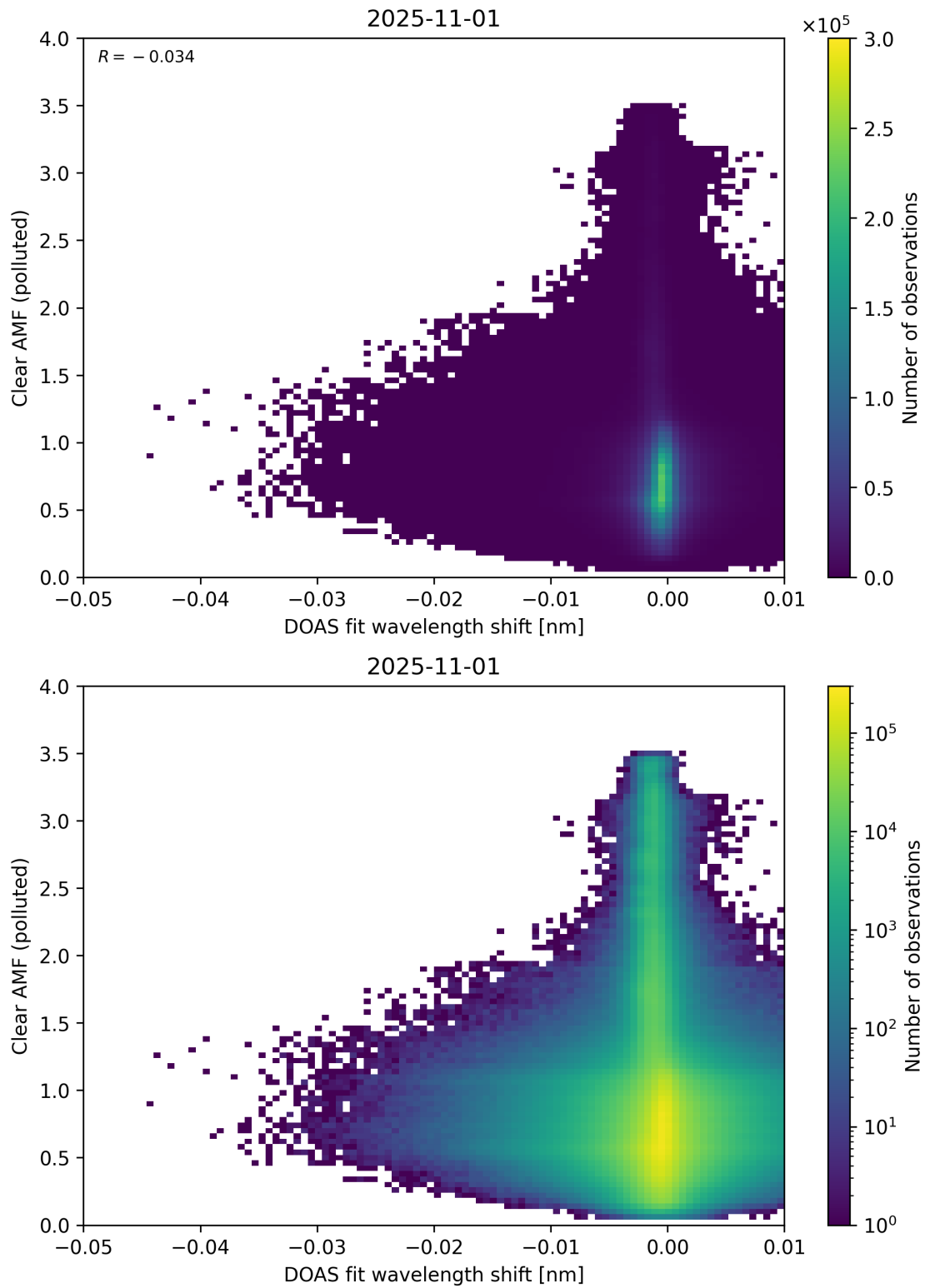
Figure 140: Scatter density plot of “DOAS fit wavelength shift” against “Clear AMF (polluted)” for 2025-10-31 to 2025-11-02.
