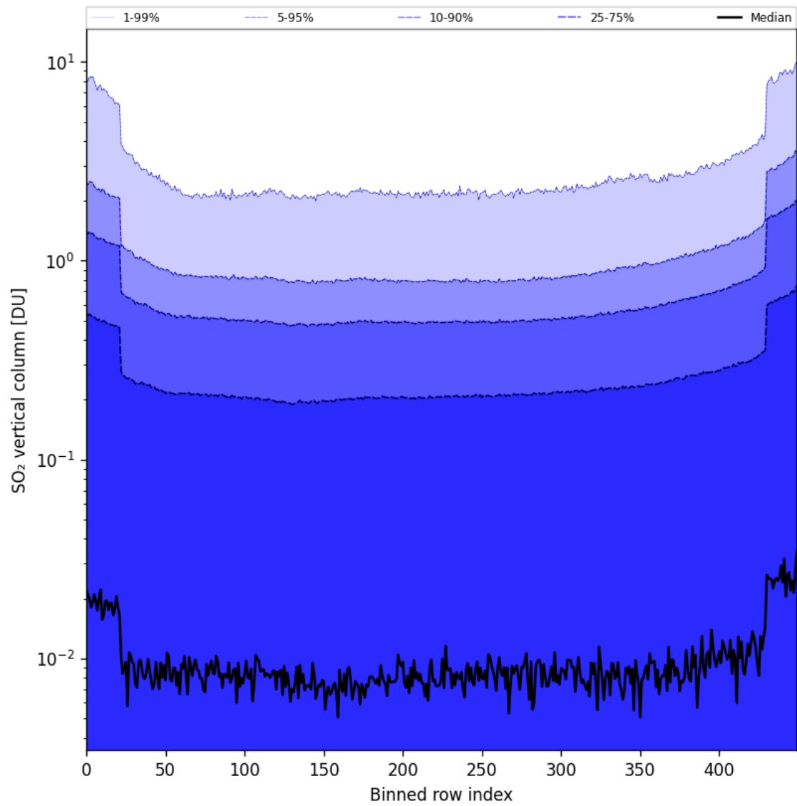
Figure 84: Along track statistics of “SO 2 vertical column” for 2025-10-31 to 2025-11-02
