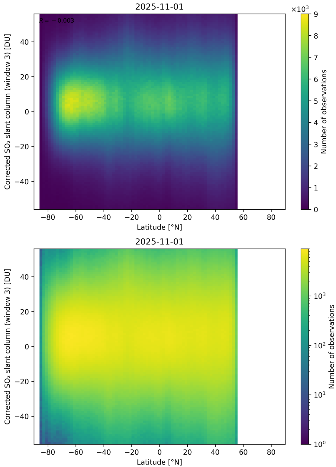
Figure 161: Scatter density plot of “Latitude” against “Corrected SO 2 slant column (window 3)” for 2025-10-31 to 2025-11-02.
