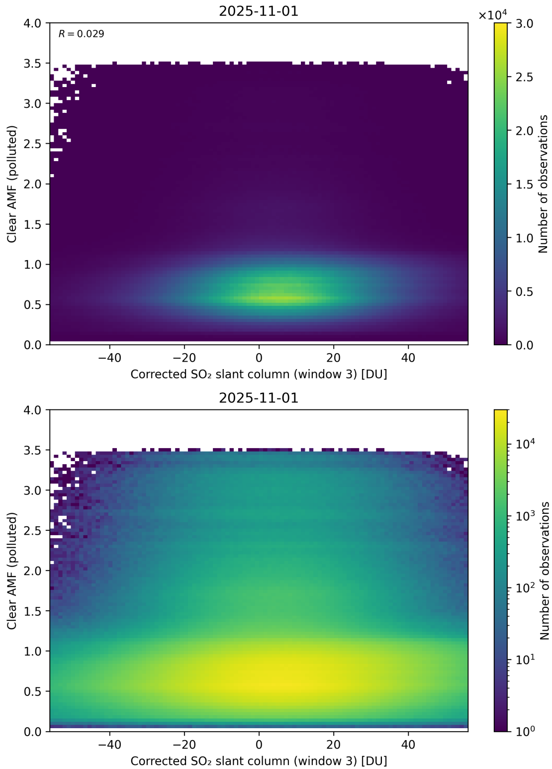
Figure 259: Scatter density plot of “Corrected SO 2 slant column (window 3)” against “Clear AMF (polluted)” for 2025-10-31 to 2025-11-02.
