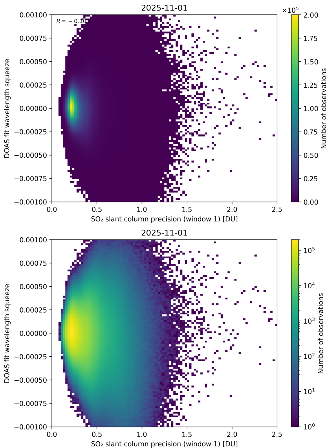
Figure 272: Scatter density plot of “SO 2 slant column precision (window 1)” against “DOAS fit wavelength squeeze” for 2025-10-31 to 2025-11-02.
