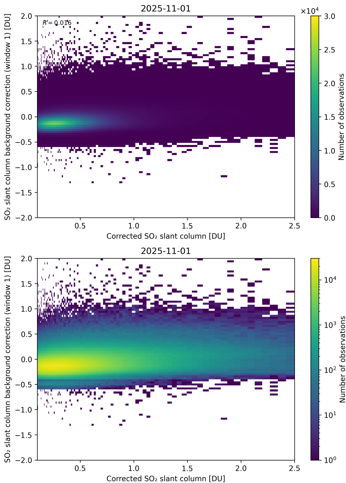
Figure 226: Scatter density plot of “Corrected SO 2 slant column” against “SO 2 slant column background correction (window 1)” for 2025-10-31 to 2025-11-02.
