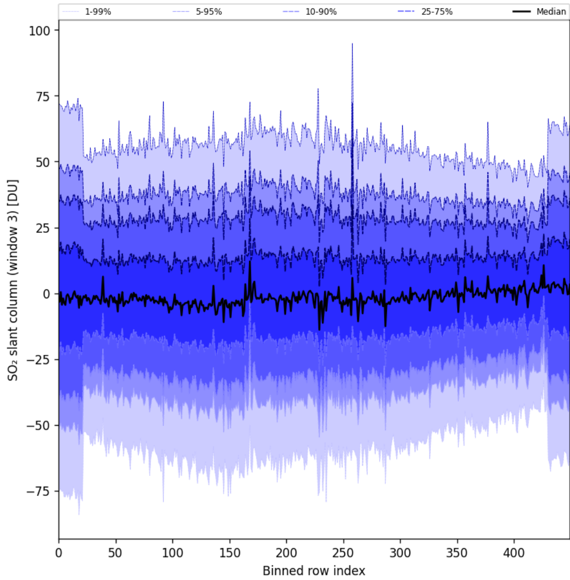
Figure 97: Along track statistics of “SO 2 slant column (window 3)” for 2025-10-31 to 2025-11-02
