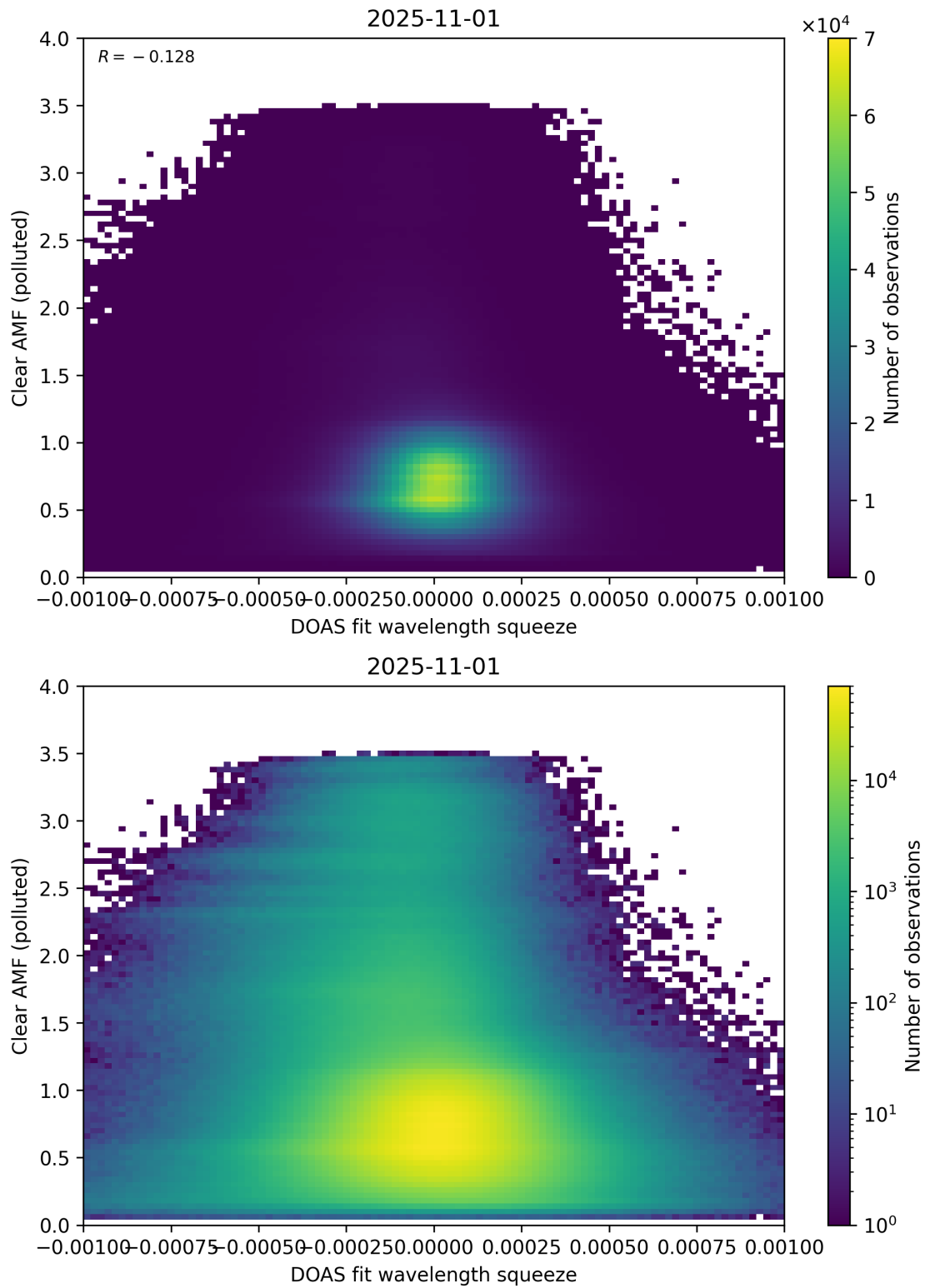
Figure 144: Scatter density plot of “DOAS fit wavelength squeeze” against “Clear AMF (polluted)” for 2025-10-31 to 2025-11-02.
