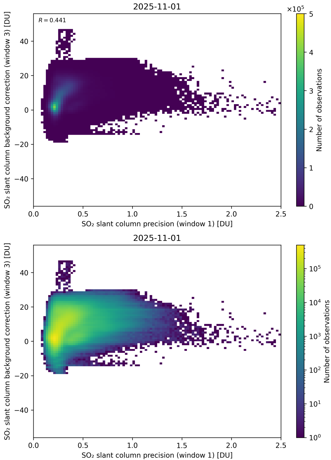
Figure 270: Scatter density plot of “SO 2 slant column precision (window 1)” against “SO 2 slant column background correction (window 3)” for 2025-10-31 to 2025-11-02.
