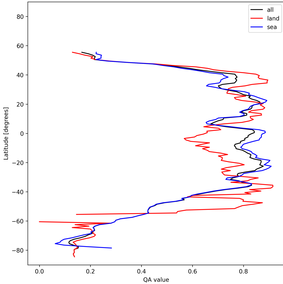
Figure 31: Zonal average of “QA value” for 2025-10-31 to 2025-11-02.
