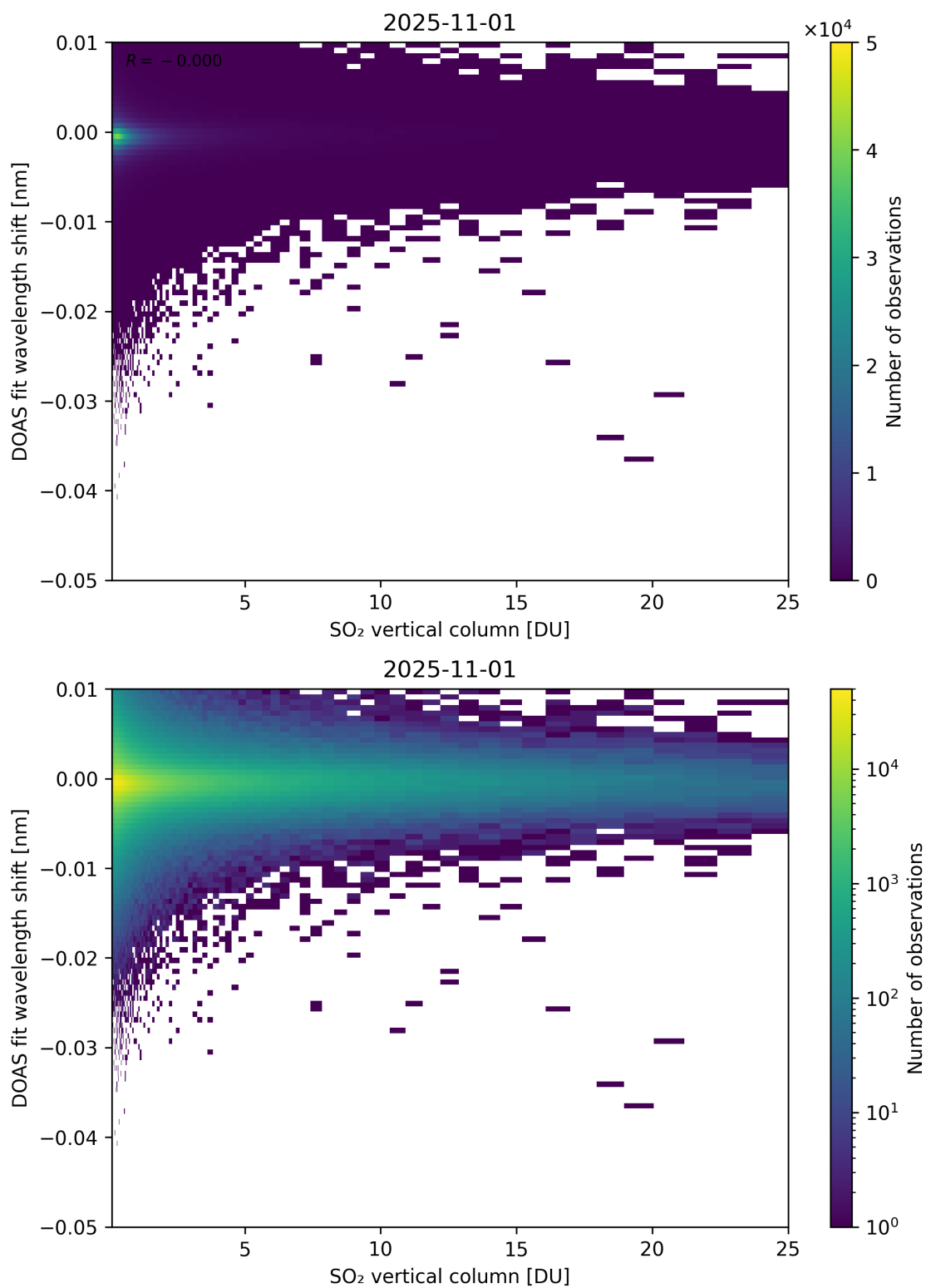
Figure 326: Scatter density plot of “SO 2 vertical column” against “DOAS fit wavelength shift” for 2025-10-31 to 2025-11-02.
