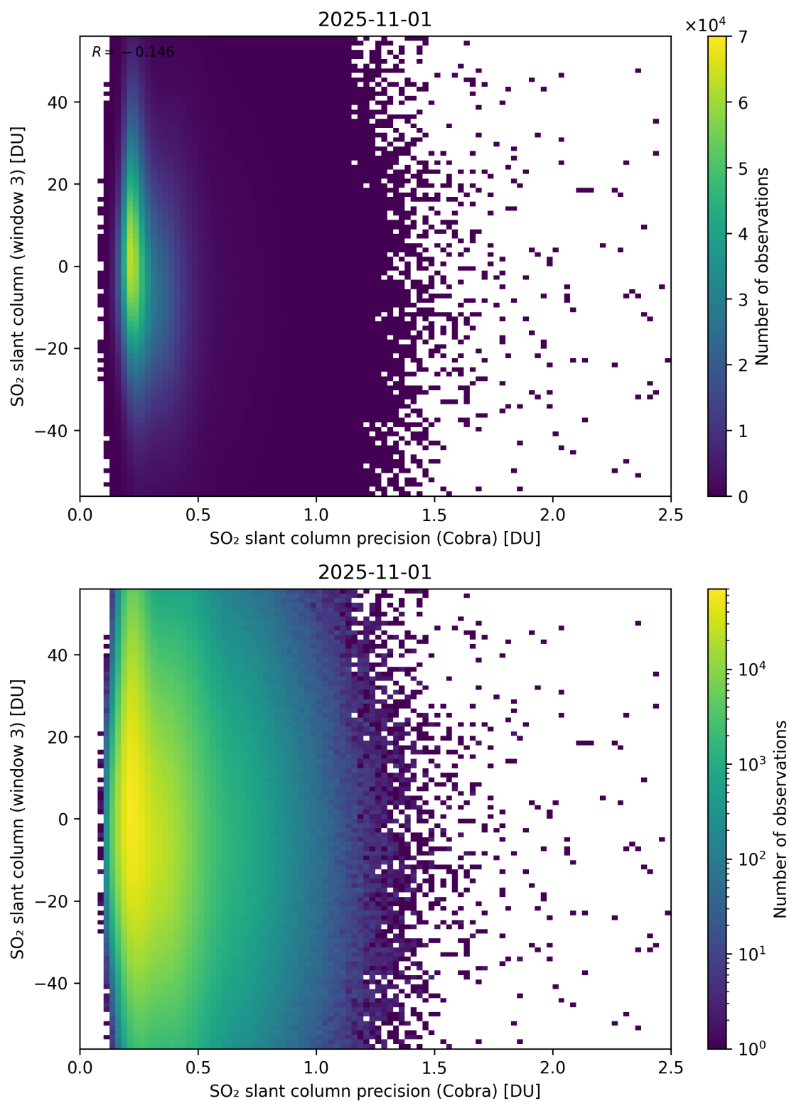
Figure 211: Scatter density plot of “SO 2 slant column precision (Cobra)” against “SO 2 slant column (window 3)” for 2025-10-31 to 2025-11-02.
