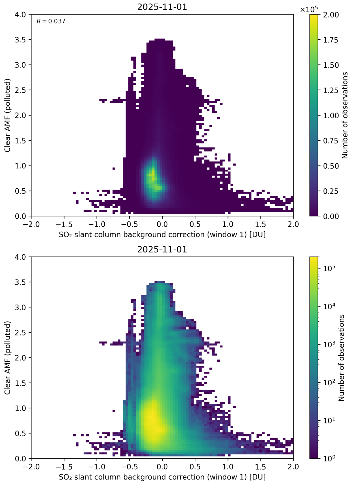
Figure 114: Scatter density plot of “SO 2 slant column background correction (window 1)” against “Clear AMF (polluted)” for 2025-10-31 to 2025-11-02.
