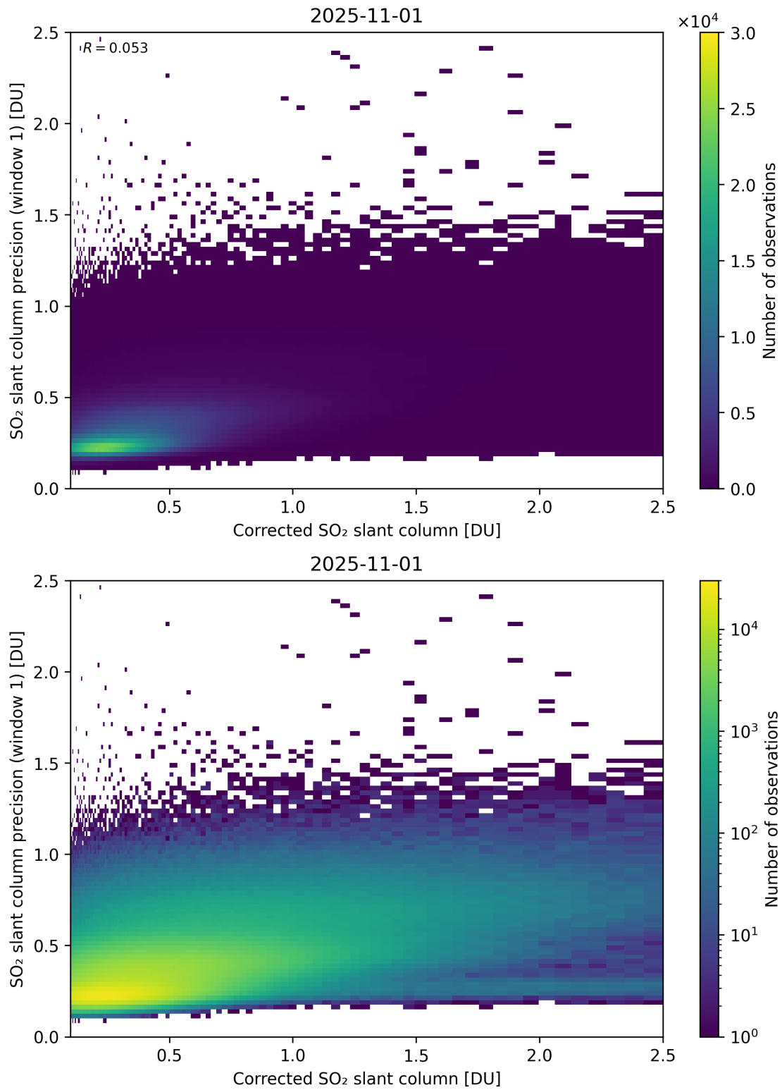
Figure 238: Scatter density plot of “Corrected SO 2 slant column” against “SO 2 slant column precision (window 1)” for 2025-10-31 to 2025-11-02.
