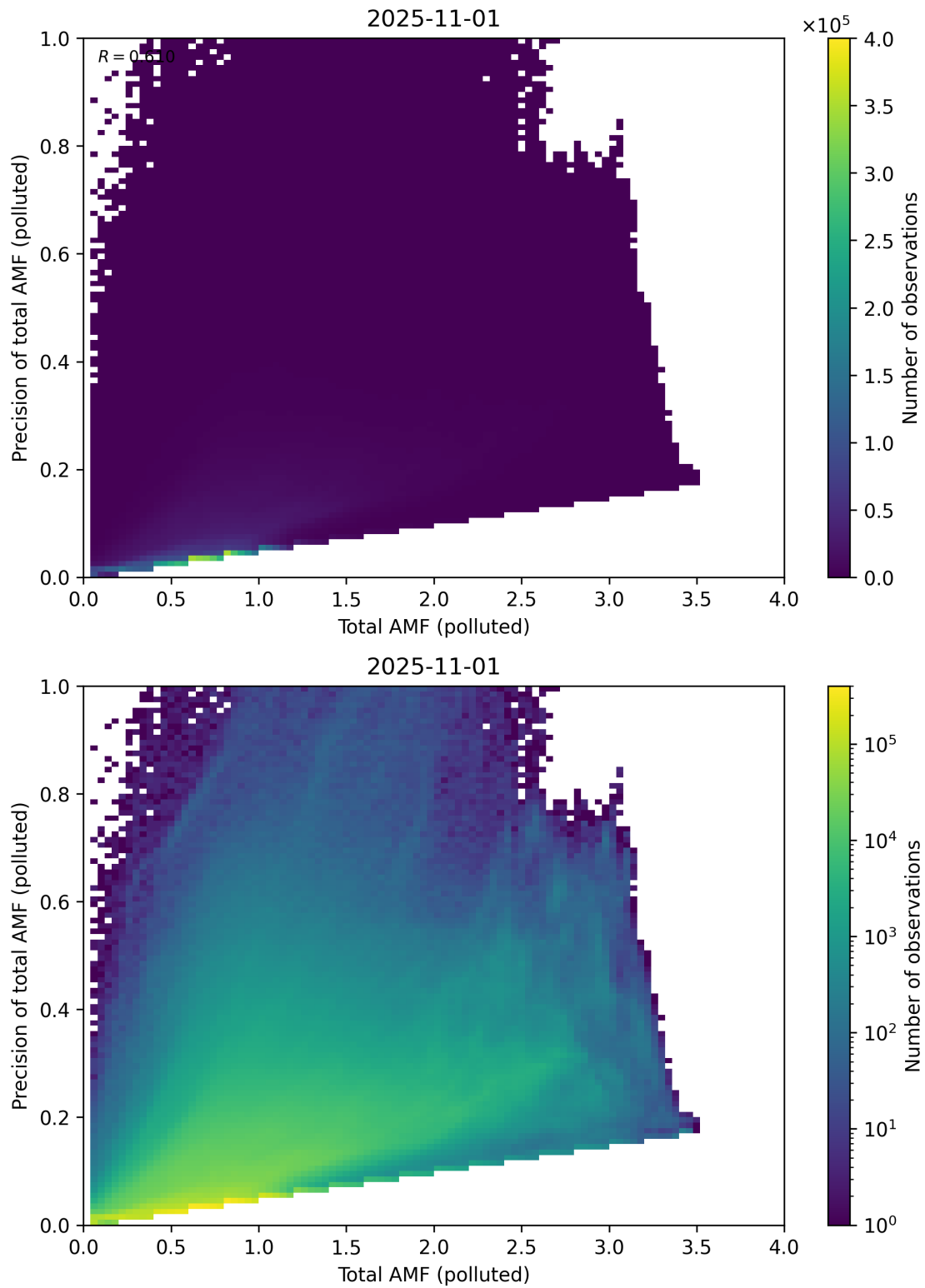
Figure 322: Scatter density plot of “Total AMF (polluted)” against “Precision of total AMF (polluted)” for 2025-10-31 to 2025-11-02.
