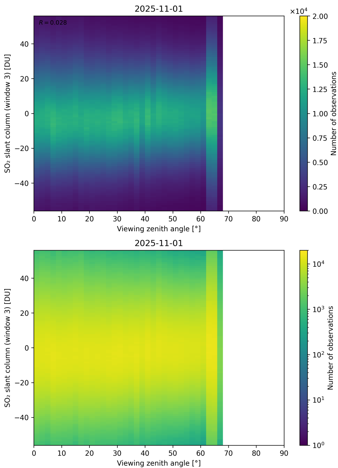
Figure 379: Scatter density plot of “Viewing zenith angle” against “SO 2 slant column (window 3)” for 2025-10-31 to 2025-11-02.
