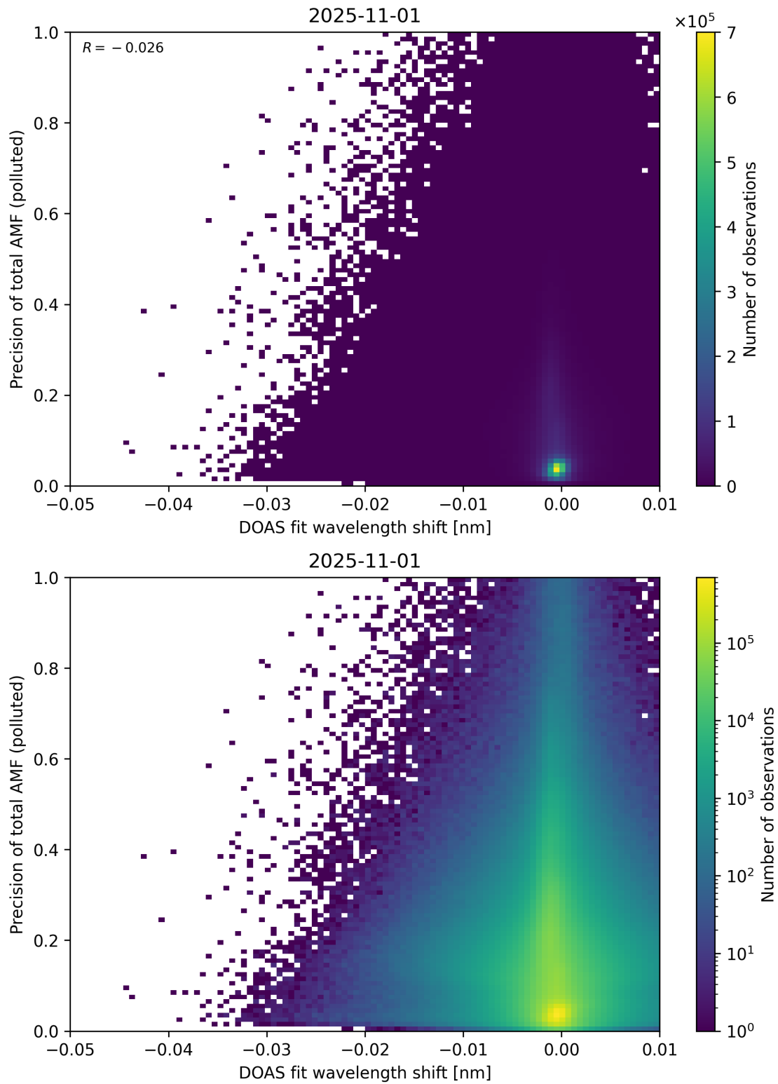
Figure 142: Scatter density plot of “DOAS fit wavelength shift” against “Precision of total AMF (polluted)” for 2025-10-31 to 2025-11-02.
