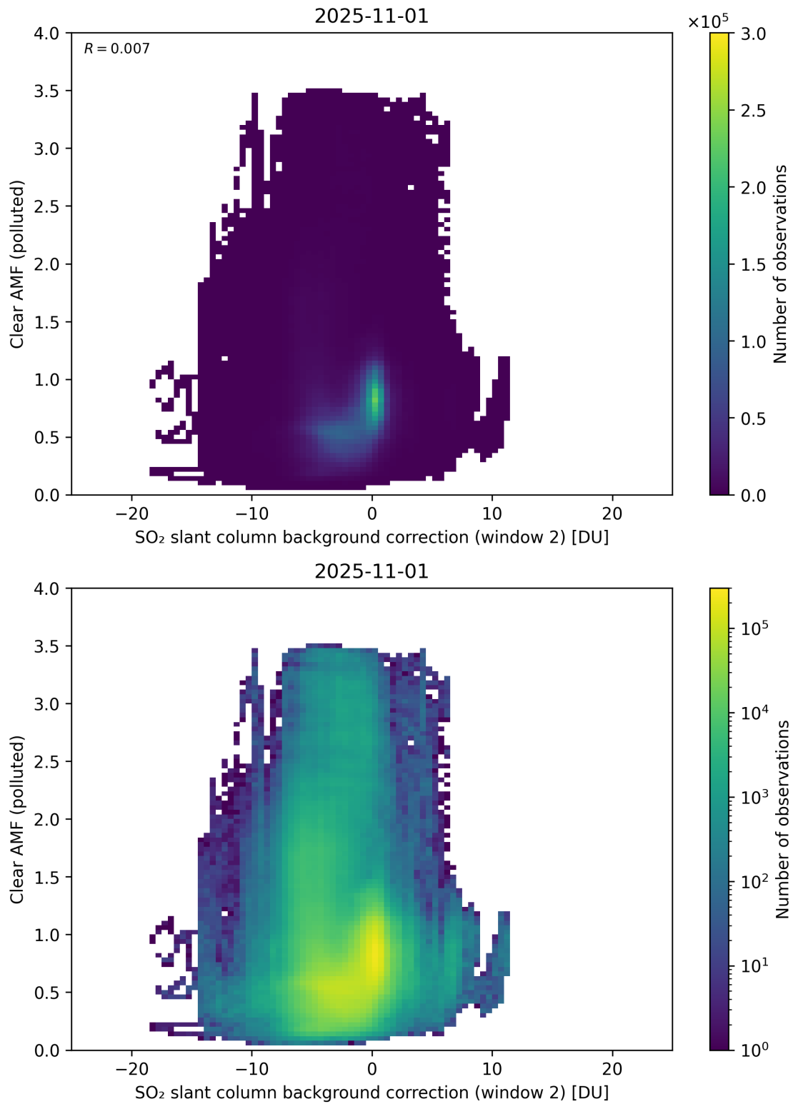
Figure 126: Scatter density plot of “SO 2 slant column background correction (window 2)” against “Clear AMF (polluted)” for 2025-10-31 to 2025-11-02.
