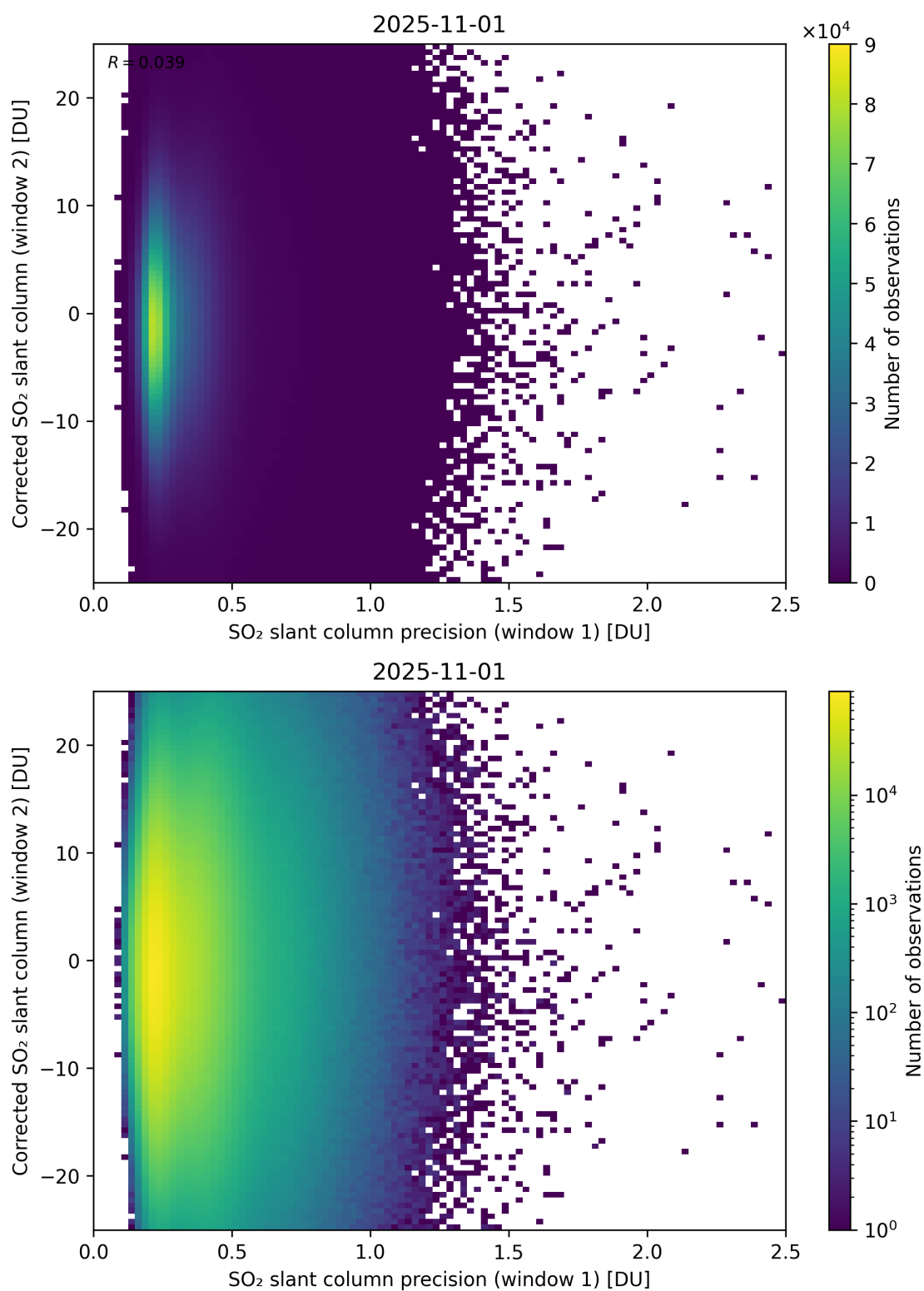
Figure 275: Scatter density plot of “SO 2 slant column precision (window 1)” against “Corrected SO 2 slant column (window 2)” for 2025-10-31 to 2025-11-02.
