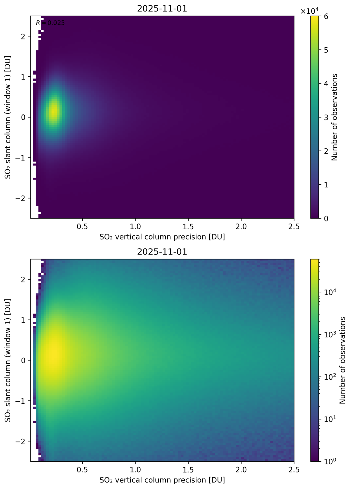
Figure 341: Scatter density plot of “SO 2 vertical column precision” against “SO 2 slant column (window 1)” for 2025-10-31 to 2025-11-02.
