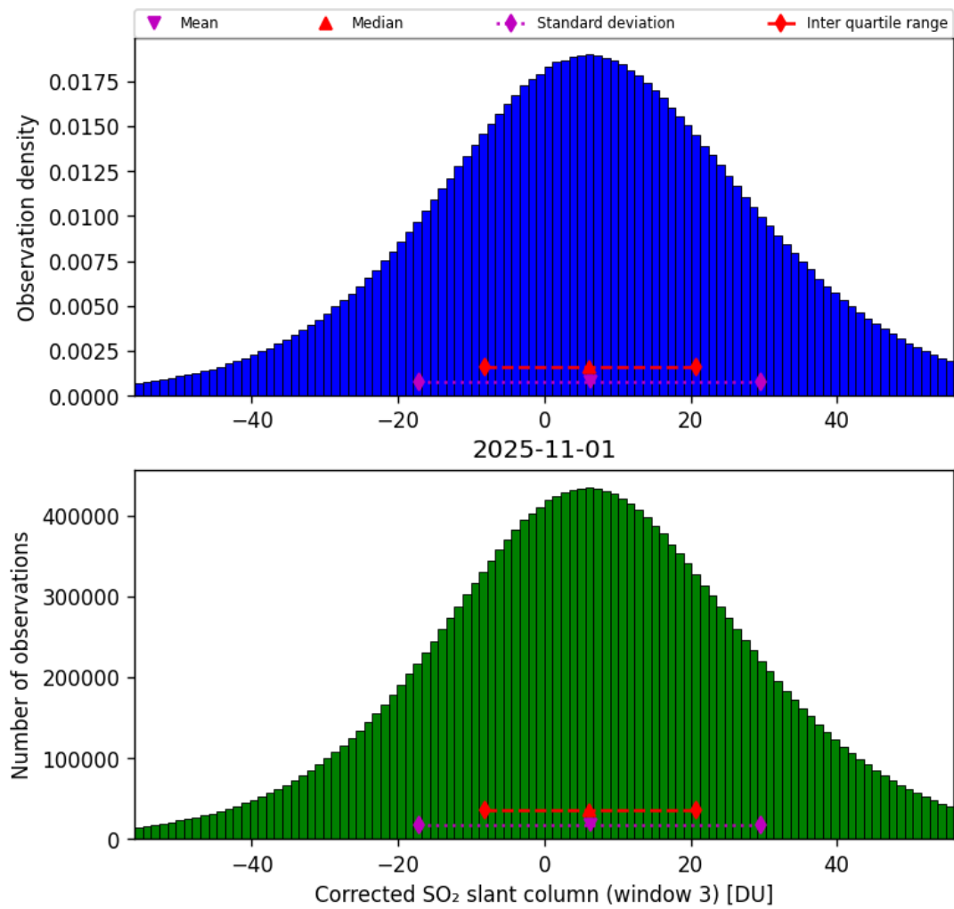
Figure 73: Histogram of “Corrected SO 2 slant column (window 3)” for 2025-10-31 to 2025-11-02
