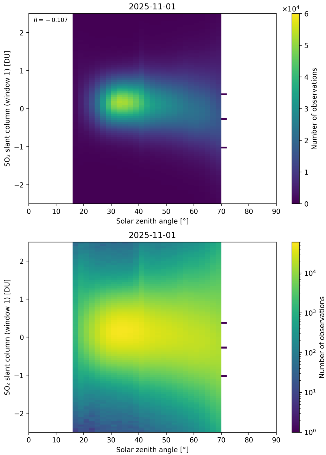
Figure 184: Scatter density plot of “Solar zenith angle” against “SO 2 slant column (window 1)” for 2025-10-31 to 2025-11-02.
