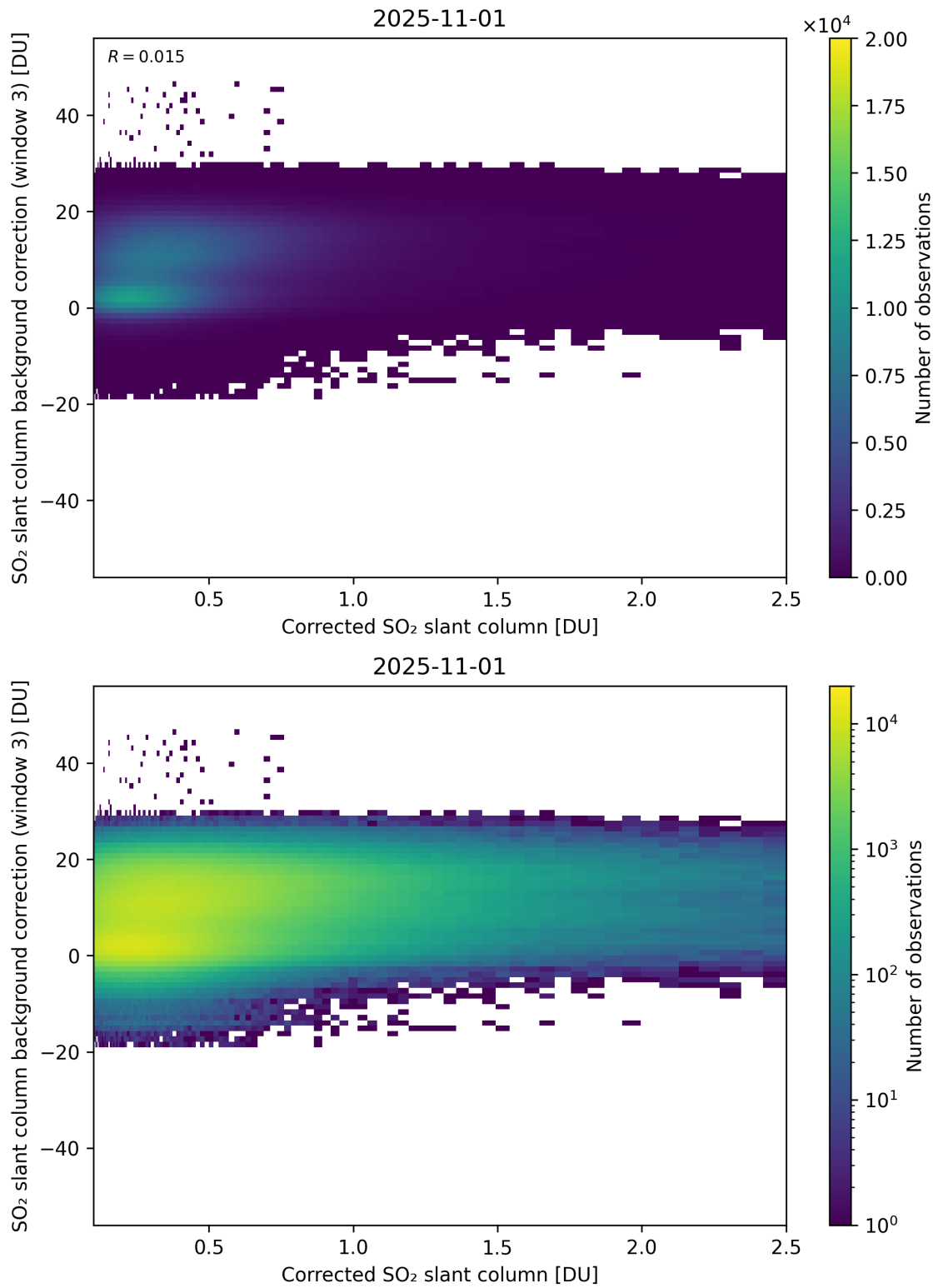
Figure 228: Scatter density plot of “Corrected SO 2 slant column” against “SO 2 slant column background correction (window 3)” for 2025-10-31 to 2025-11-02.
