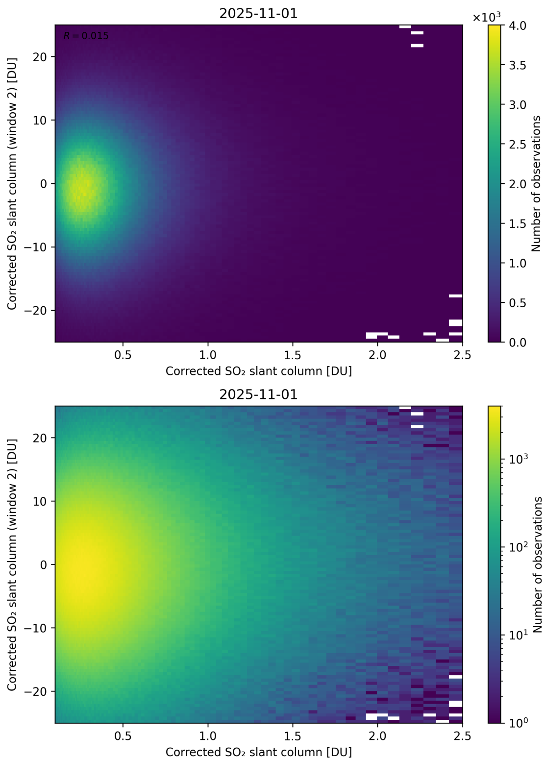
Figure 235: Scatter density plot of “Corrected SO 2 slant column” against “Corrected SO 2 slant column (window 2)” for 2025-10-31 to 2025-11-02.
