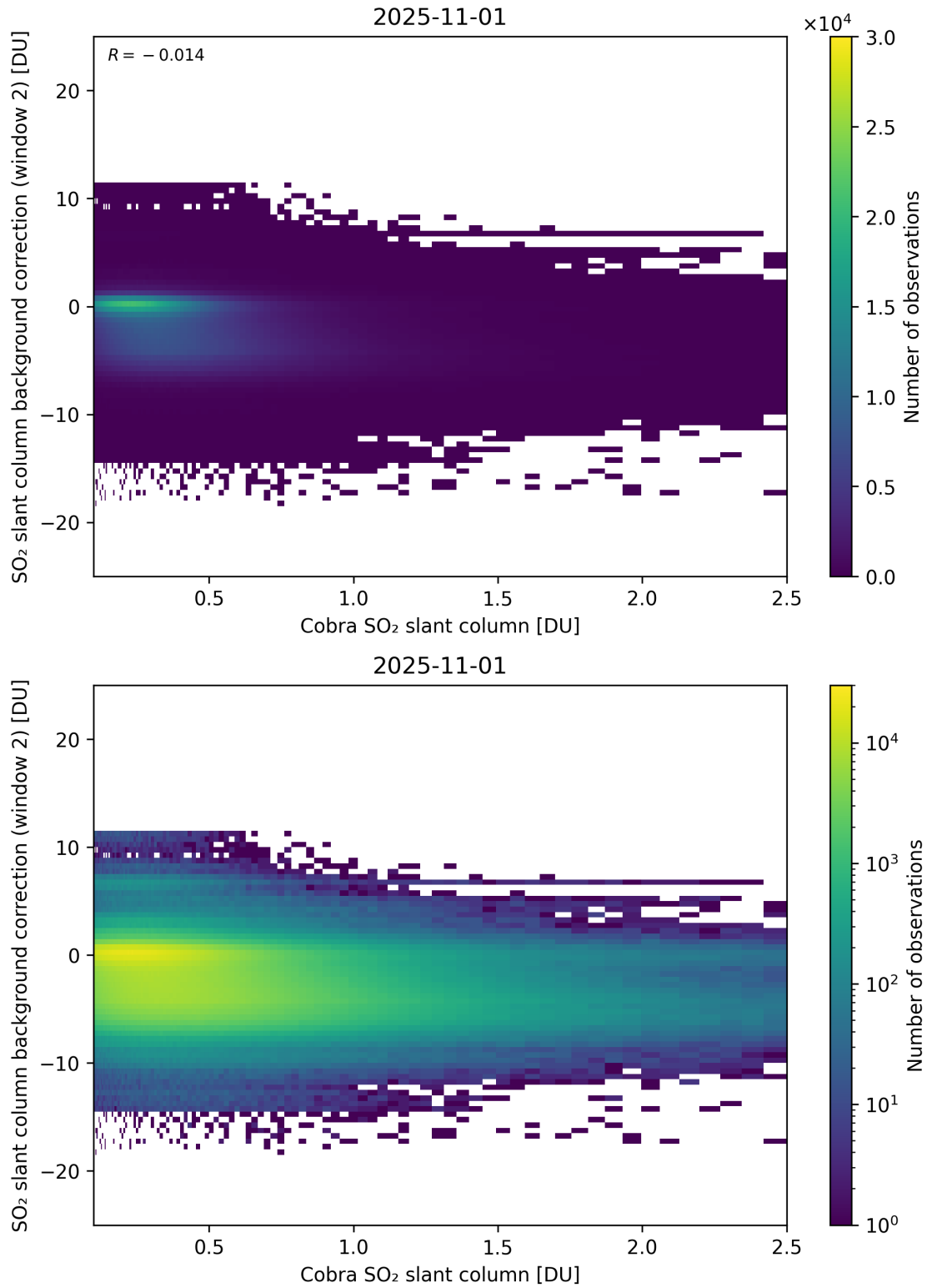
Figure 194: Scatter density plot of “Cobra SO 2 slant column” against “SO 2 slant column background correction (window 2)” for 2025-10-31 to 2025-11-02.
