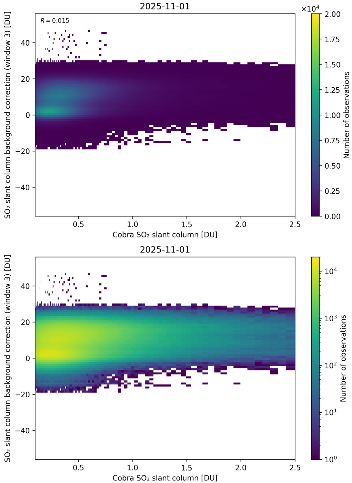
Figure 195: Scatter density plot of “Cobra SO 2 slant column” against “SO 2 slant column background correction (window 3)” for 2025-10-31 to 2025-11-02.
