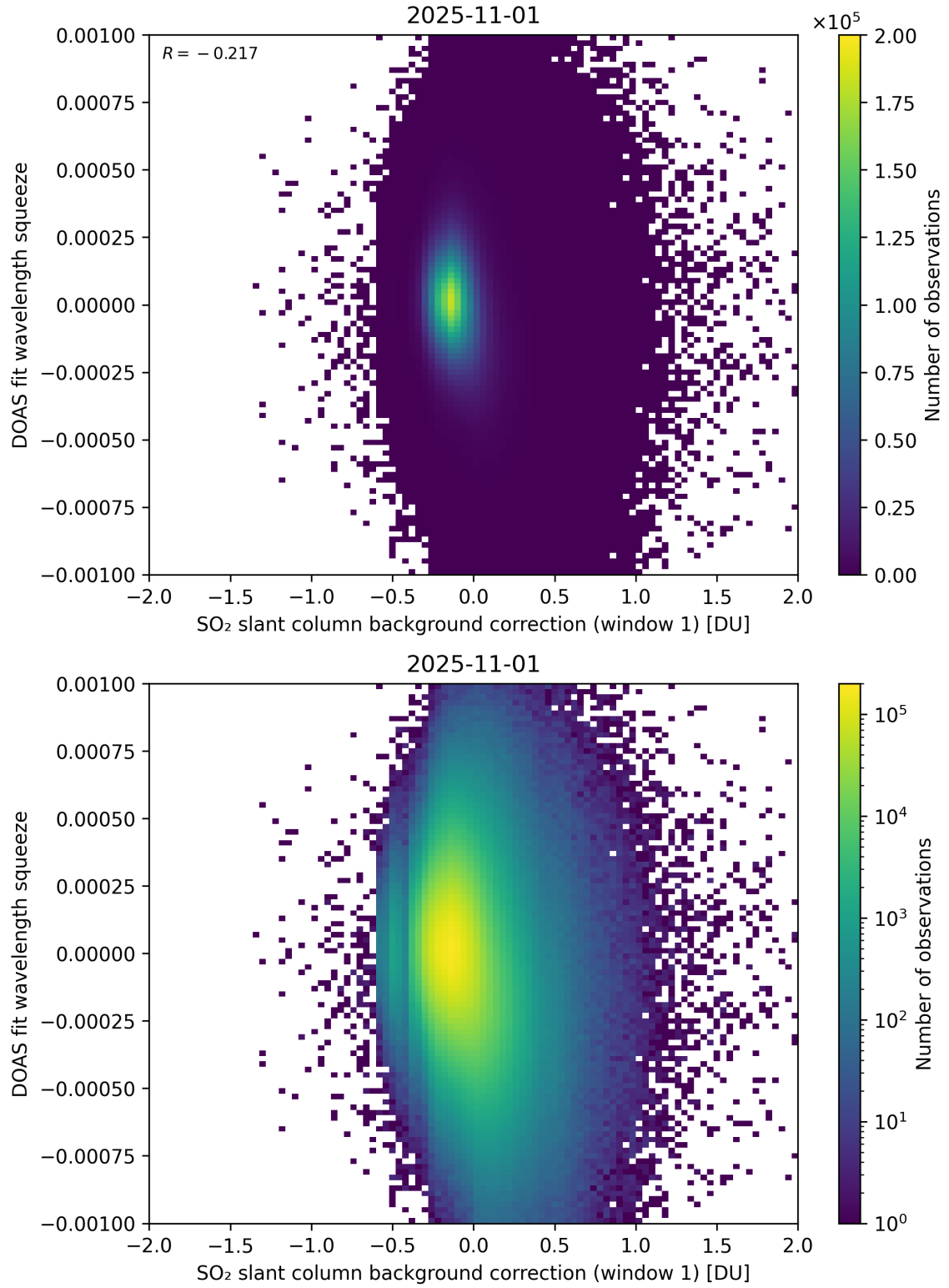
Figure 112: Scatter density plot of “SO 2 slant column background correction (window 1)” against “DOAS fit wavelength squeeze” for 2025-10-31 to 2025-11-02.
