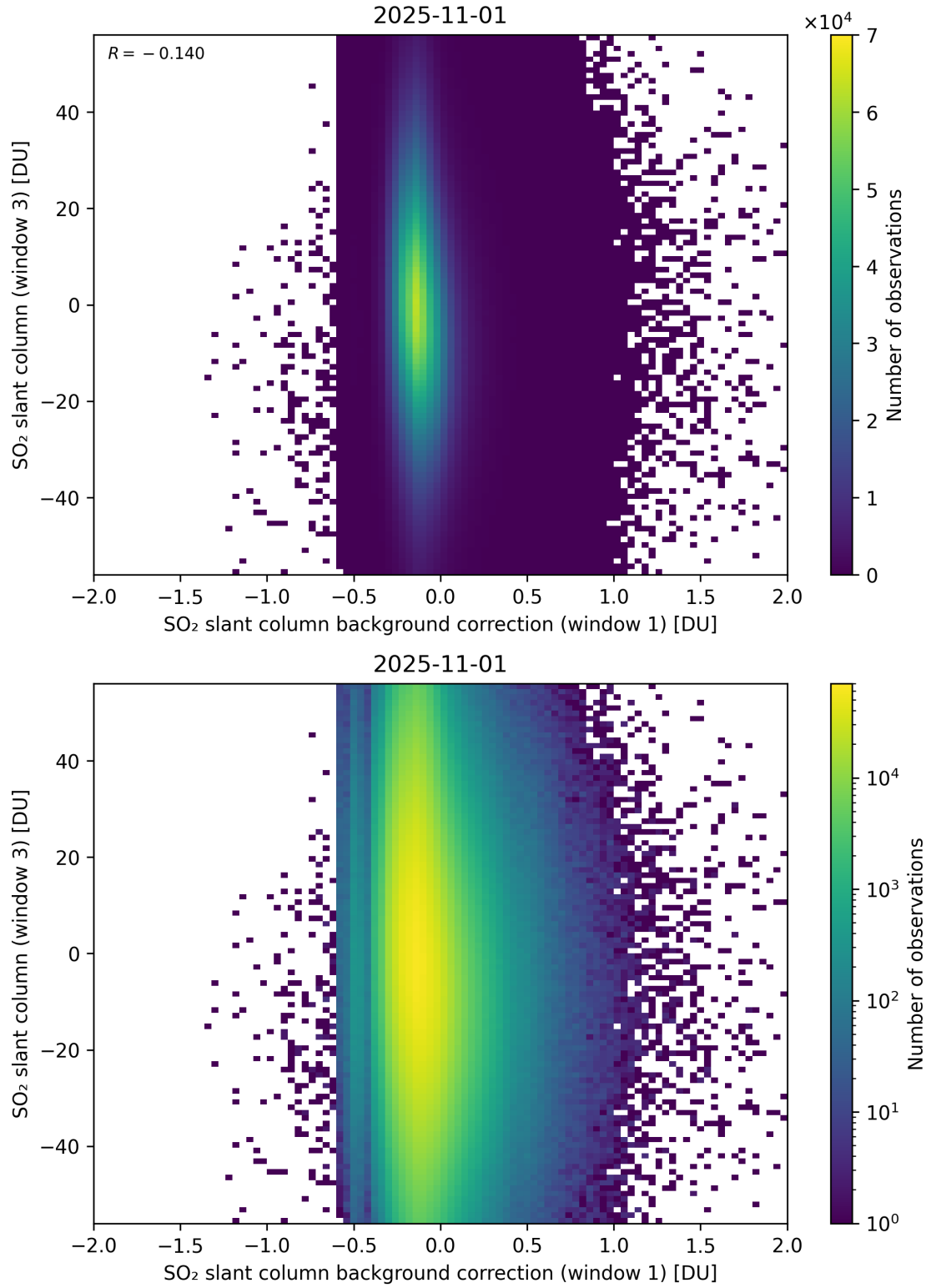
Figure 118: Scatter density plot of “SO 2 slant column background correction (window 1)” against “SO 2 slant column (window 3)” for 2025-10-31 to 2025-11-02.
