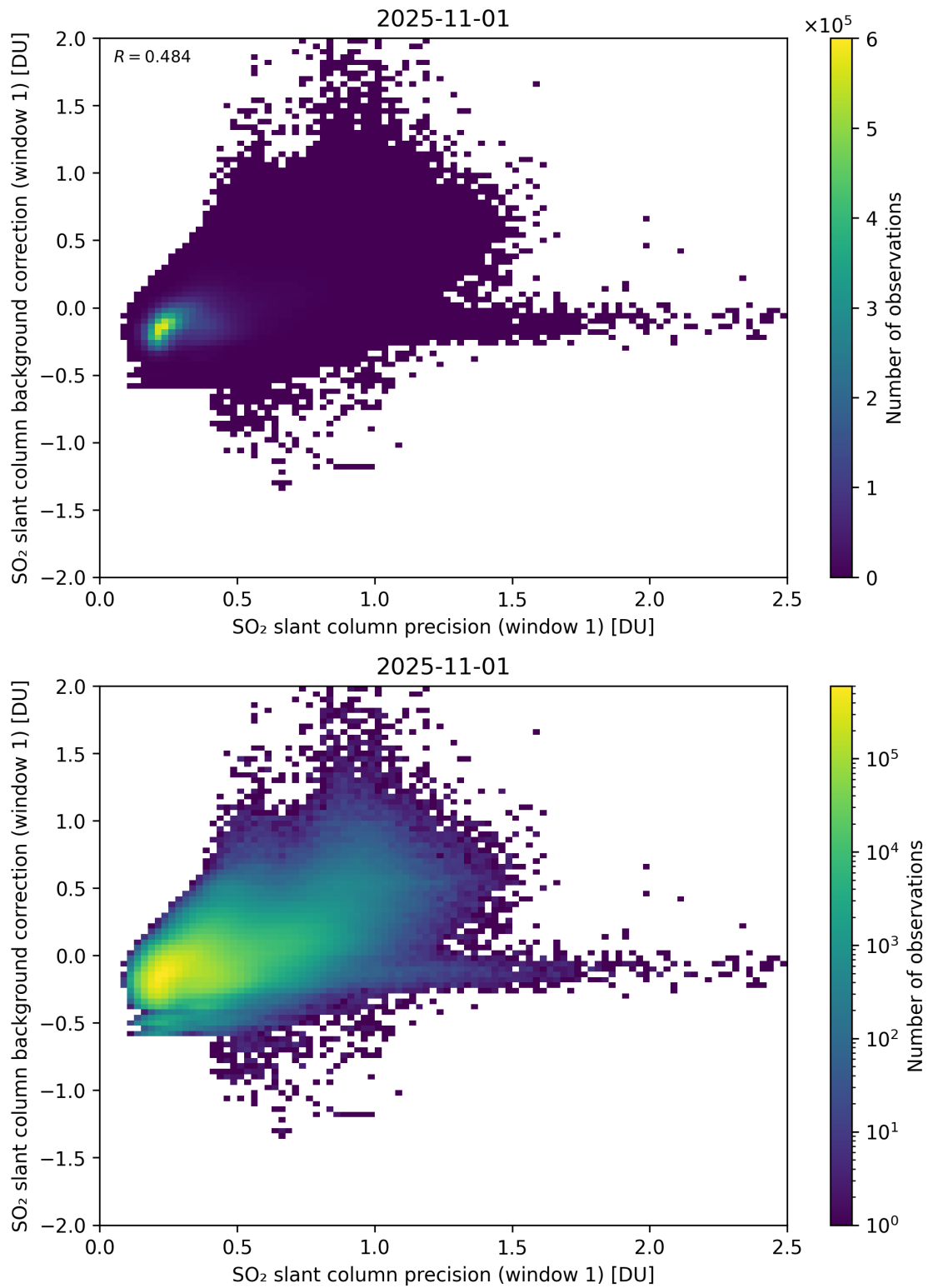
Figure 268: Scatter density plot of “SO 2 slant column precision (window 1)” against “SO 2 slant column background correction (window 1)” for 2025-10-31 to 2025-11-02.
