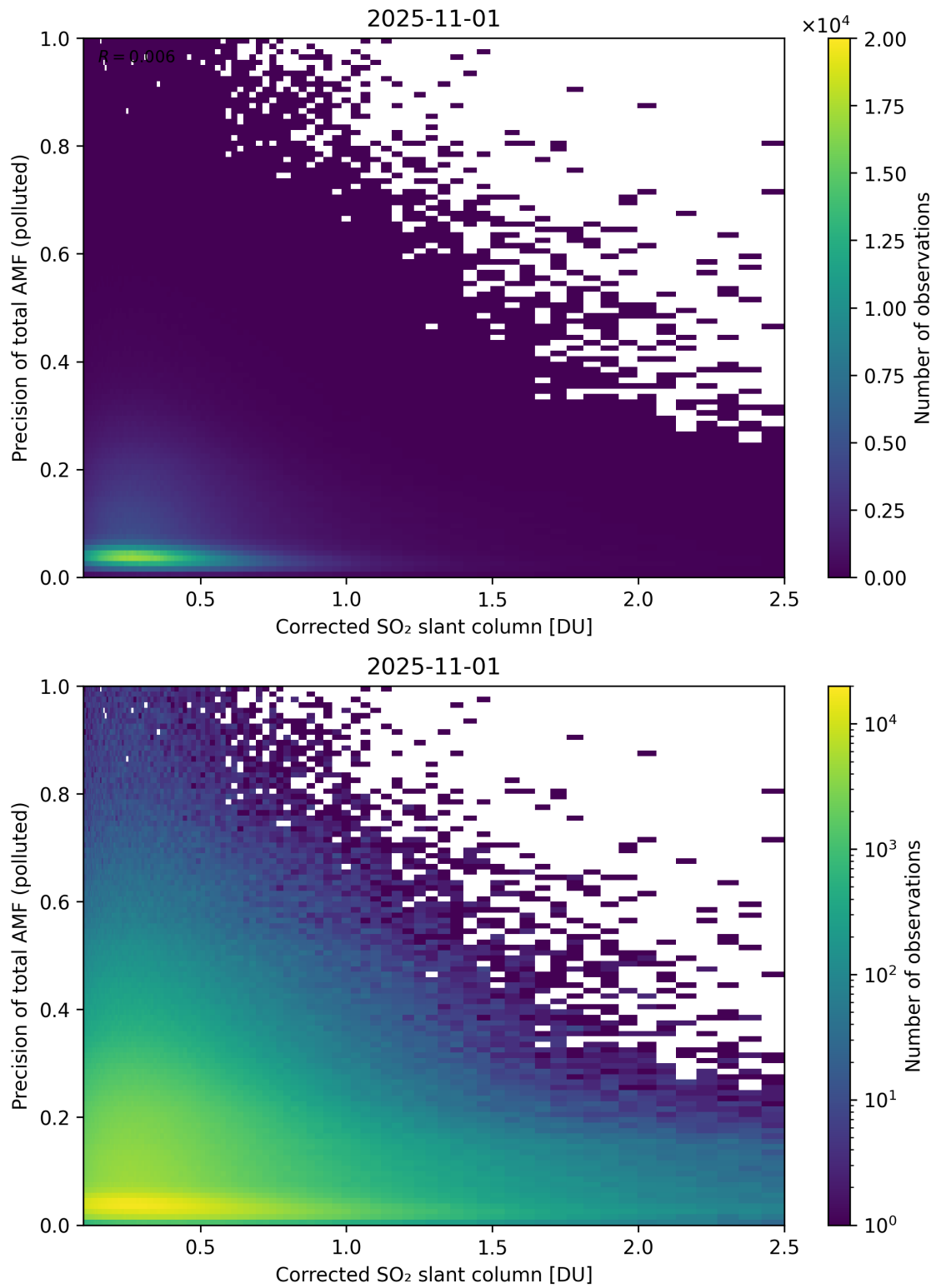
Figure 243: Scatter density plot of “Corrected SO 2 slant column” against “Precision of total AMF (polluted)” for 2025-10-31 to 2025-11-02.
