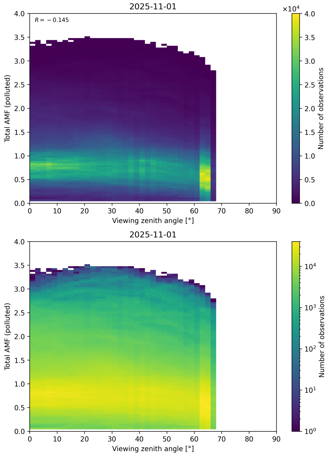
Figure 381: Scatter density plot of “Viewing zenith angle” against “Total AMF (polluted)” for 2025-10-31 to 2025-11-02.
