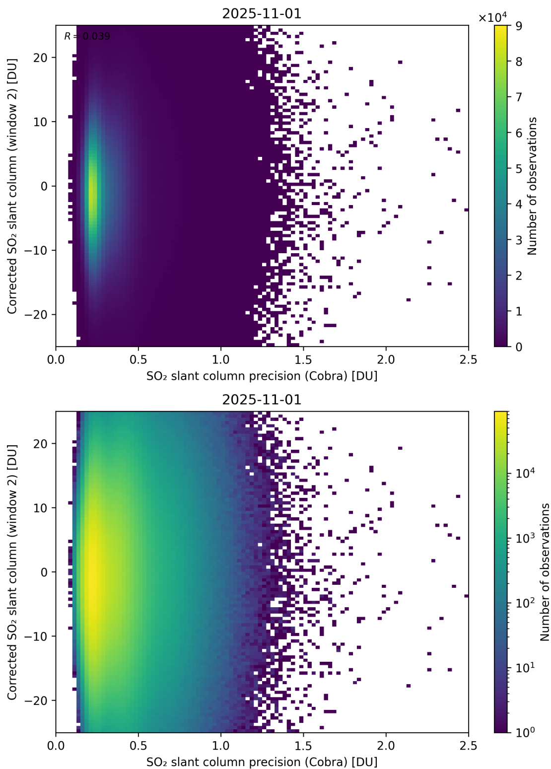
Figure 206: Scatter density plot of “SO 2 slant column precision (Cobra)” against “Corrected SO 2 slant column (window 2)” for 2025-10-31 to 2025-11-02.
