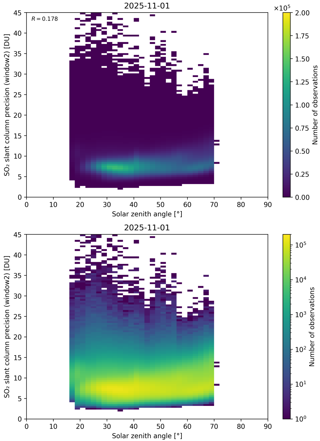
Figure 186: Scatter density plot of “Solar zenith angle” against “SO 2 slant column precision (window2)” for 2025-10-31 to 2025-11-02.
