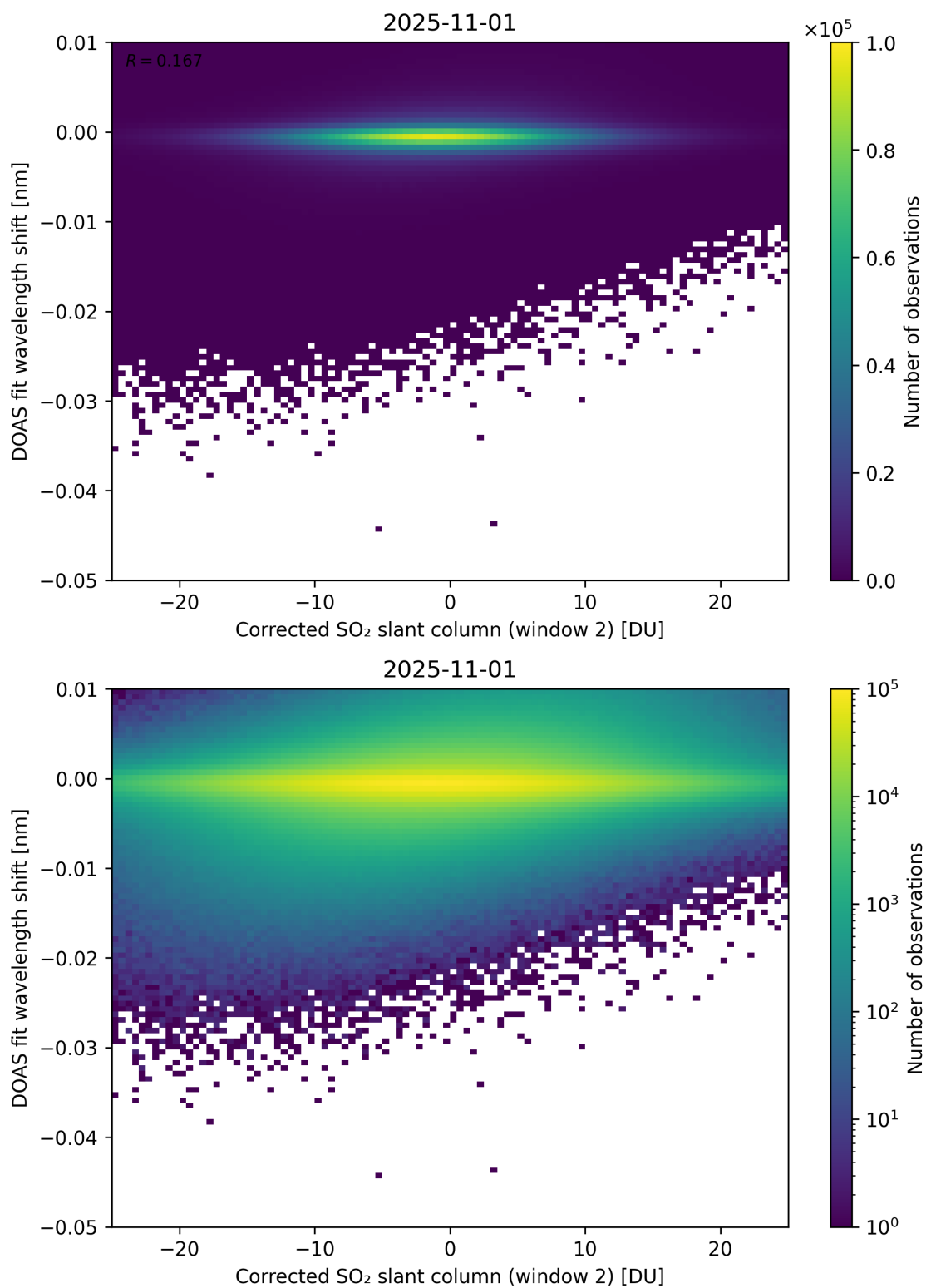
Figure 246: Scatter density plot of “Corrected SO 2 slant column (window 2)” against “DOAS fit wavelength shift” for 2025-10-31 to 2025-11-02.
