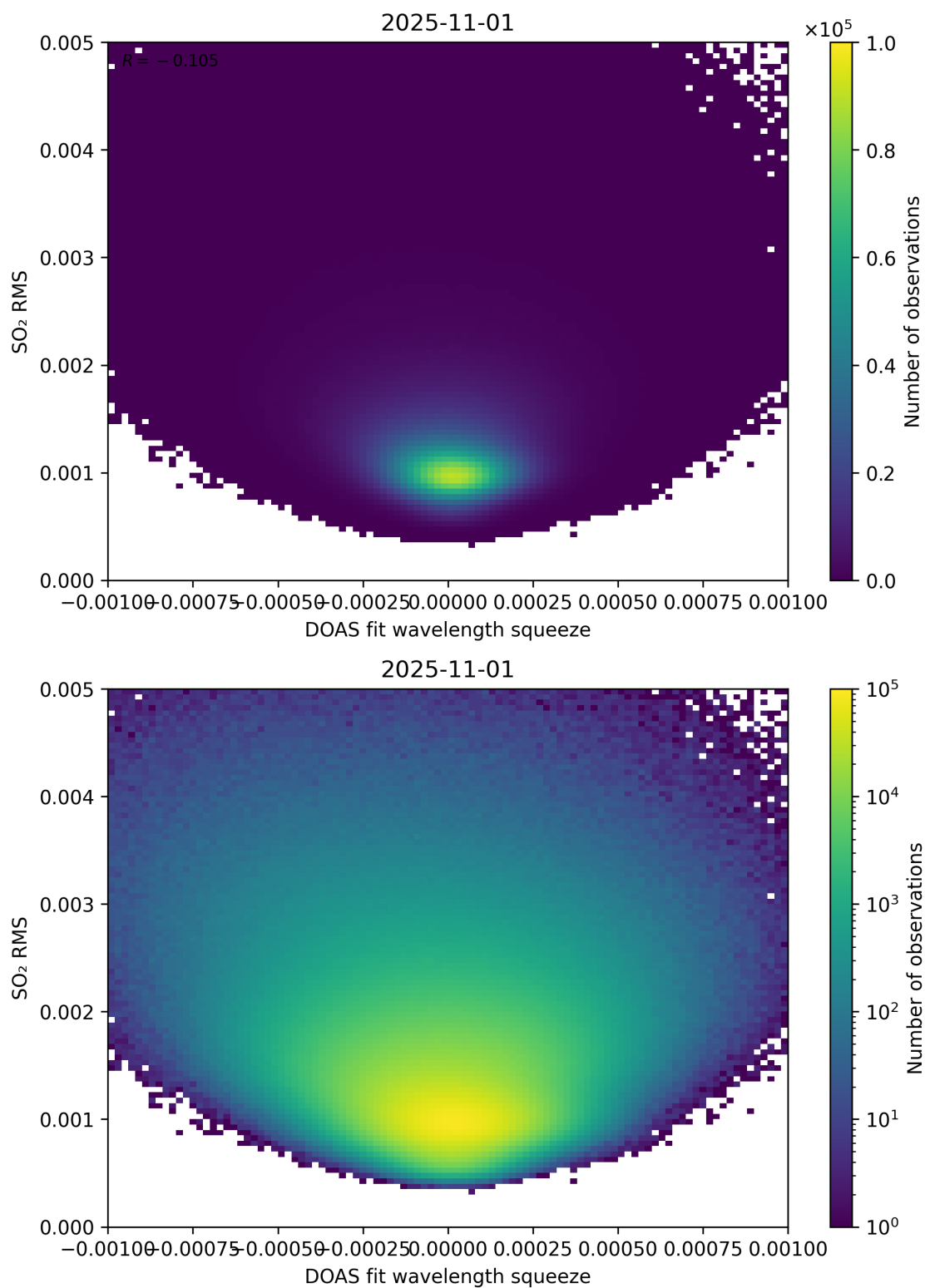
Figure 143: Scatter density plot of “DOAS fit wavelength squeeze” against “SO 2 RMS” for 2025-10-31 to 2025-11-02.
