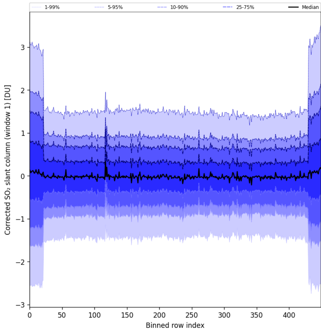
Figure 91: Along track statistics of “Corrected SO 2 slant column (window 1)” for 2025-10-31 to 2025-11-02
