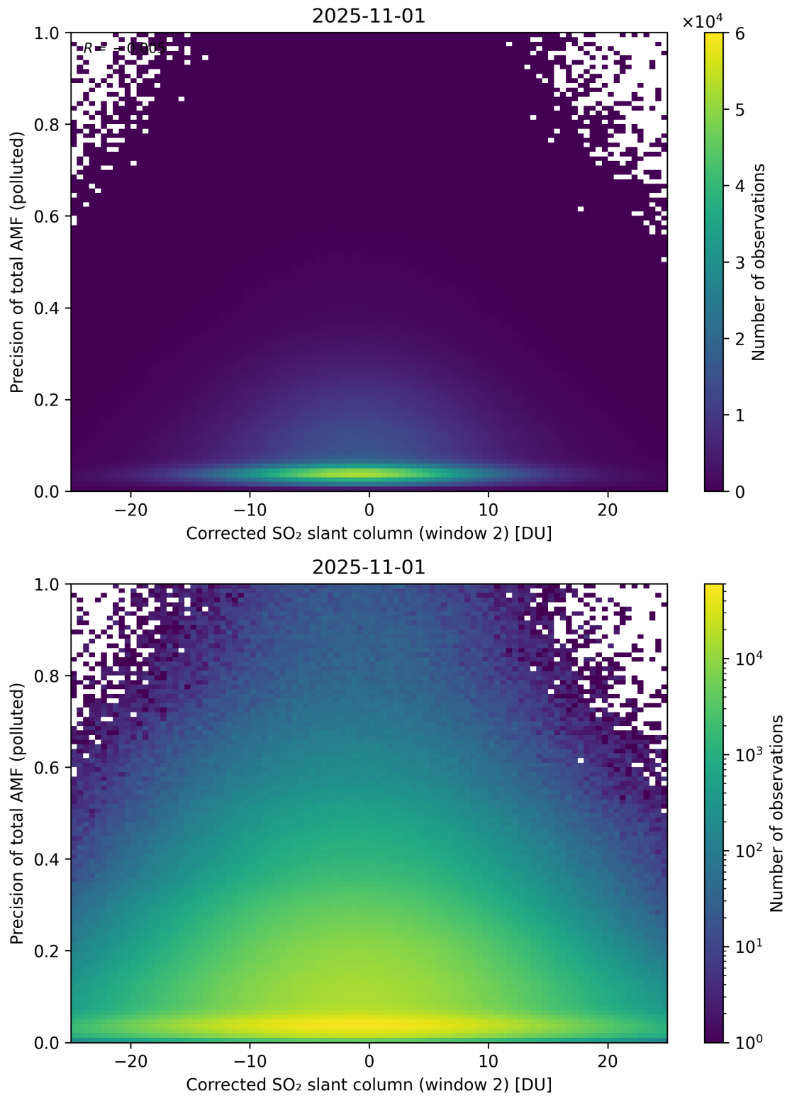
Figure 254: Scatter density plot of “Corrected SO 2 slant column (window 2)” against “Precision of total AMF (polluted)” for 2025-10-31 to 2025-11-02.
