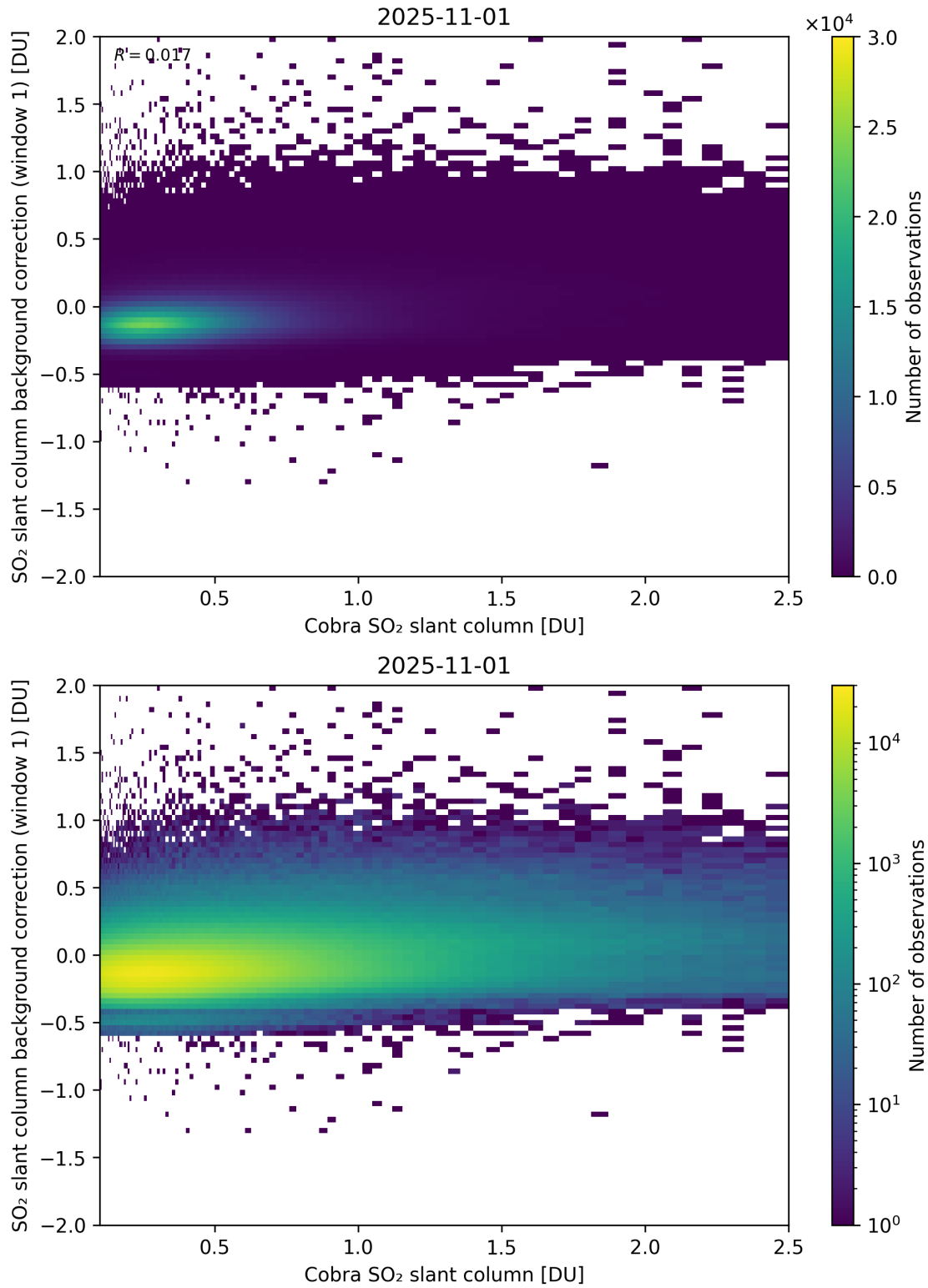
Figure 193: Scatter density plot of “Cobra SO 2 slant column” against “SO 2 slant column background correction (window 1)” for 2025-10-31 to 2025-11-02.
