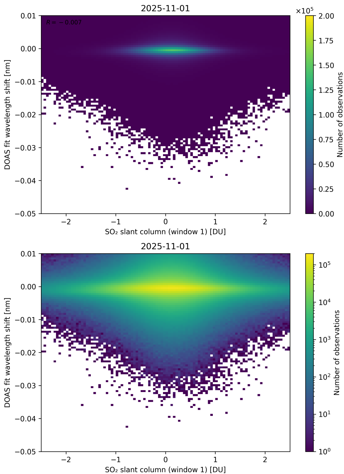
Figure 265: Scatter density plot of “SO 2 slant column (window 1)” against “DOAS fit wavelength shift” for 2025-10-31 to 2025-11-02.
