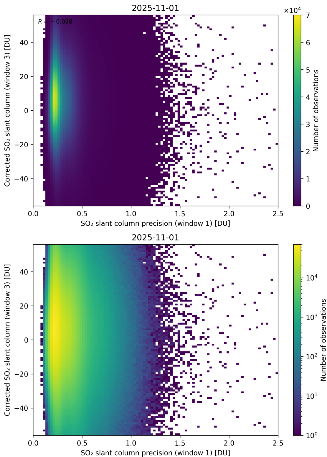
Figure 276: Scatter density plot of “SO 2 slant column precision (window 1)” against “Corrected SO 2 slant column (window 3)” for 2025-10-31 to 2025-11-02.
