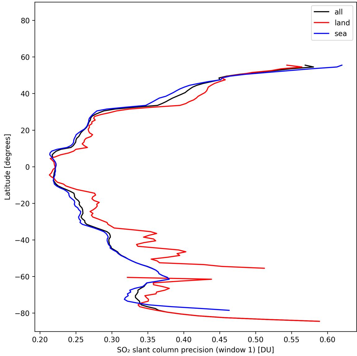
Figure 38: Zonal average of “SO 2 slant column precision (window 1)” for 2025-10-31 to 2025-11-02.
