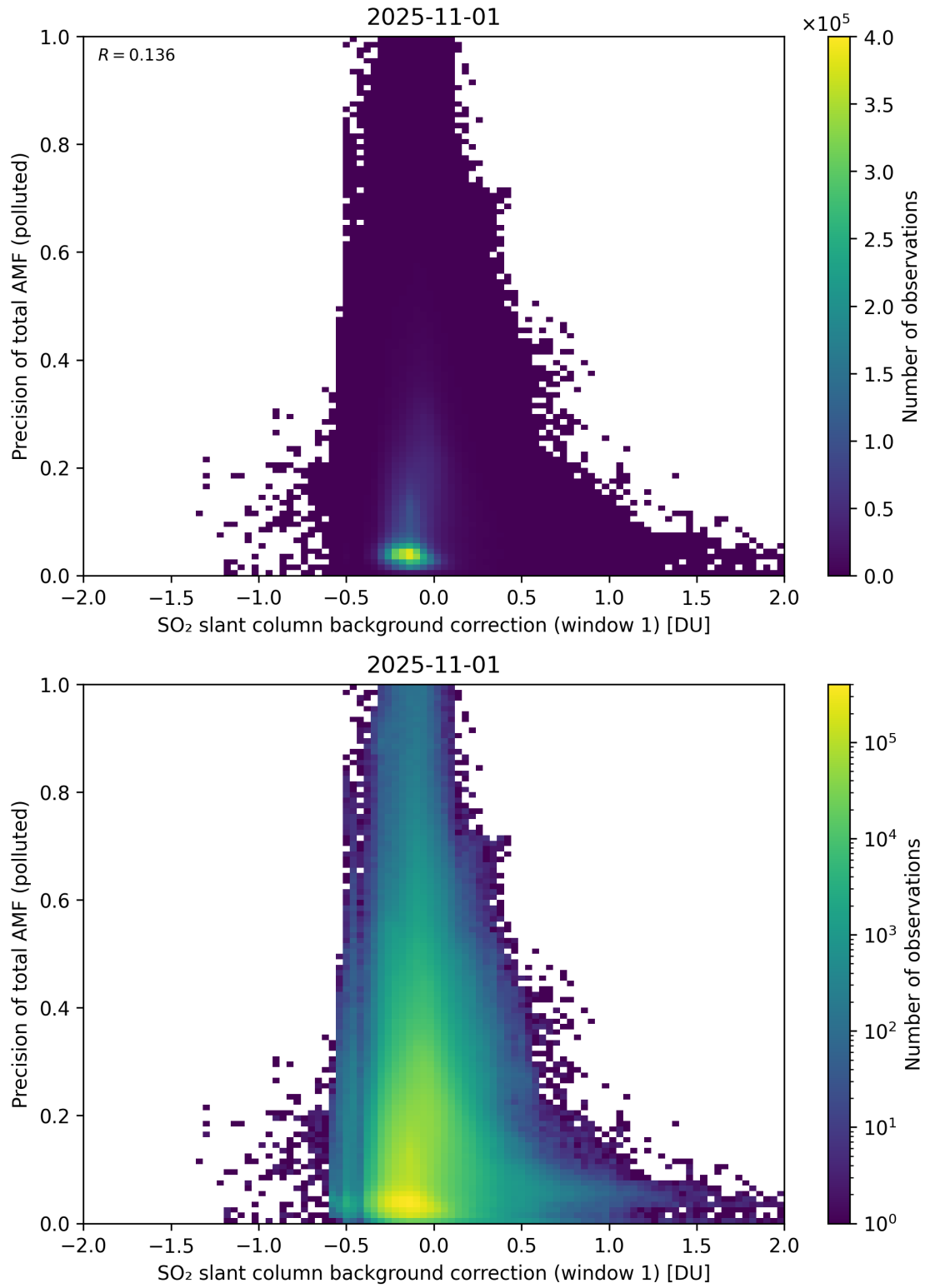
Figure 121: Scatter density plot of “SO 2 slant column background correction (window 1)” against “Precision of total AMF (polluted)” for 2025-10-31 to 2025-11-02.
