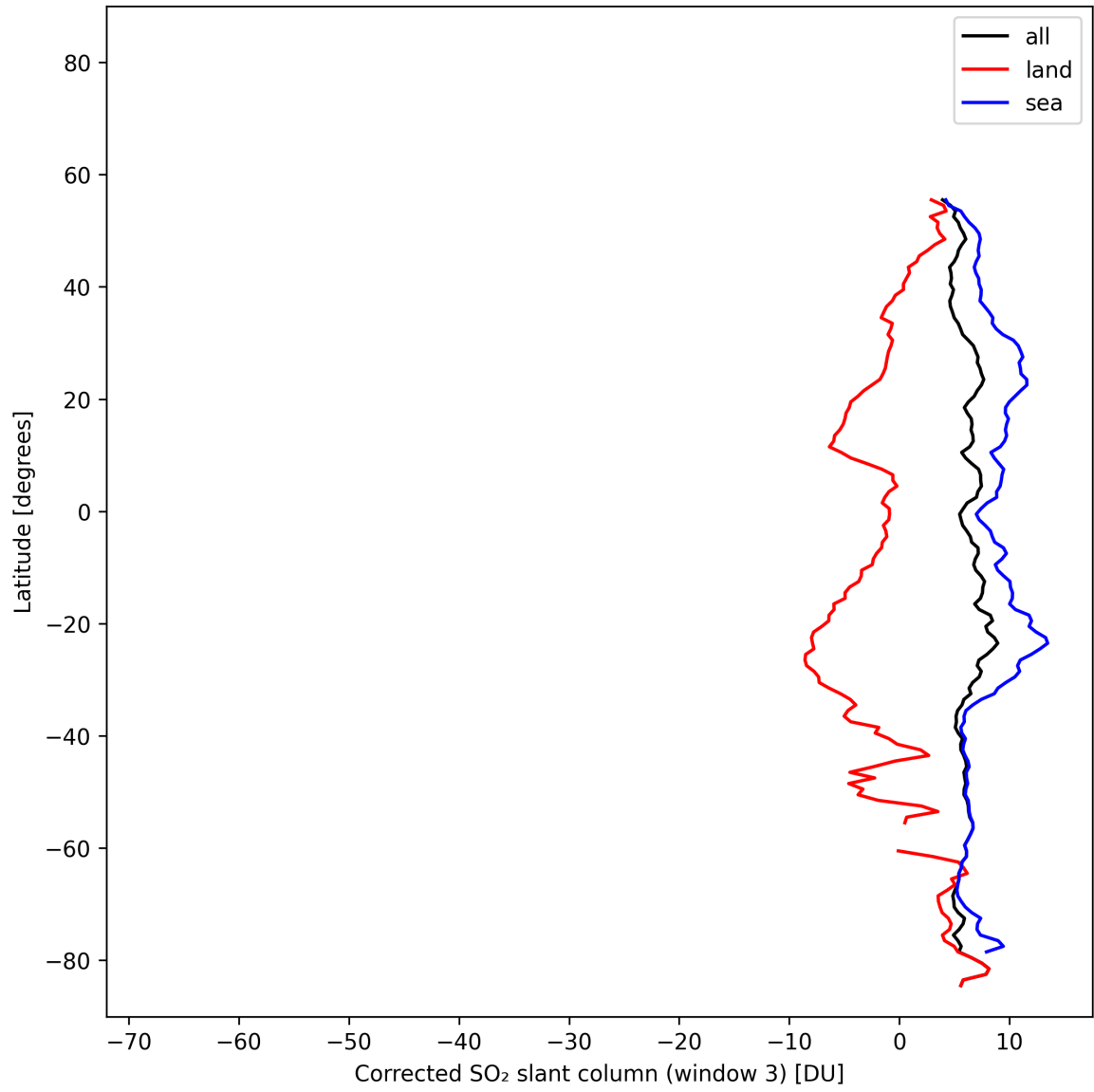
Figure 47: Zonal average of “Corrected SO 2 slant column (window 3)” for 2025-10-31 to 2025-11-02.
