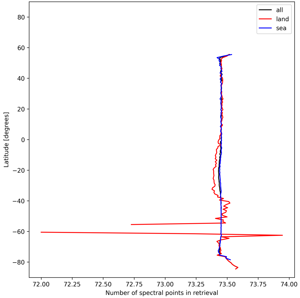
Figure 56: Zonal average of “Number of spectral points in retrieval” for 2025-10-31 to 2025-11-02.
