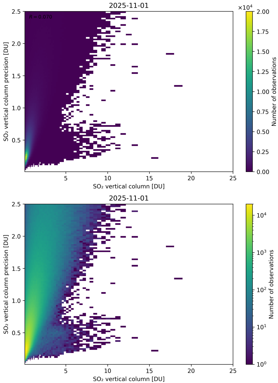
Figure 361: Scatter density plot of “SO 2 vertical column” against “SO 2 vertical column precision” for 2025-10-31 to 2025-11-02.
