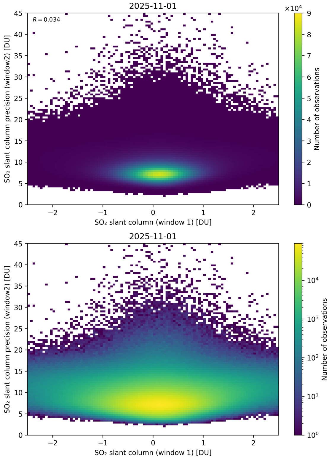
Figure 286: Scatter density plot of “SO 2 slant column (window 1)” against “SO 2 slant column precision (window2)” for 2025-10-31 to 2025-11-02.
