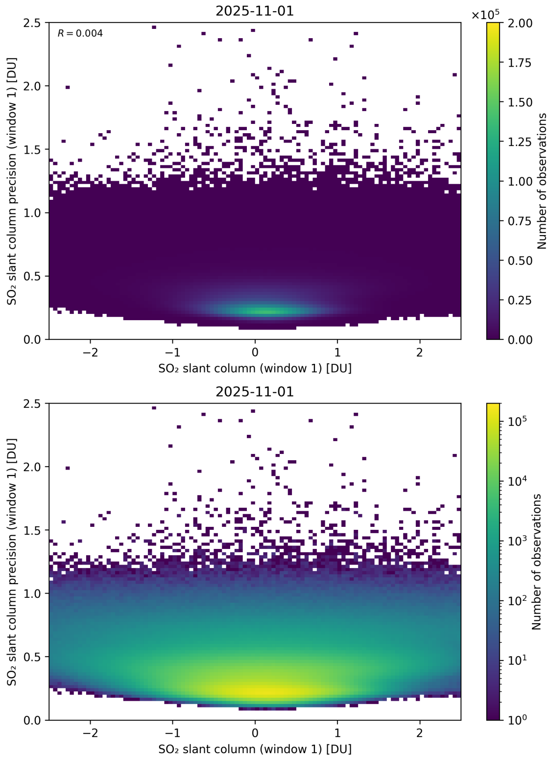
Figure 285: Scatter density plot of “SO 2 slant column (window 1)” against “SO 2 slant column precision (window 1)” for 2025-10-31 to 2025-11-02.
