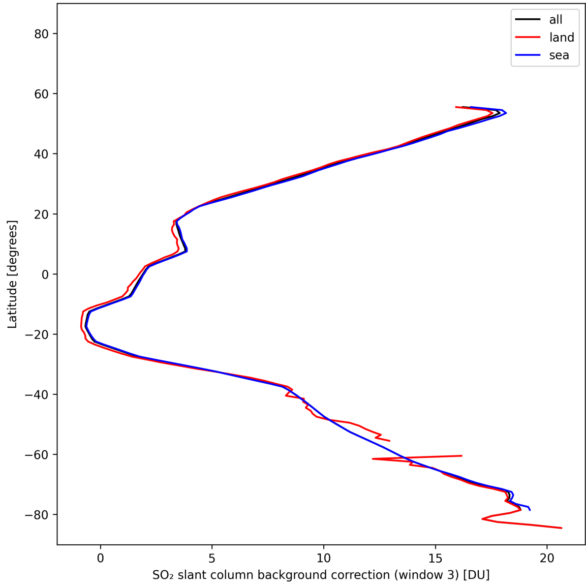
Figure 48: Zonal average of “SO 2 slant column background correction (window 3)” for 2025-10-31 to 2025-11-02.
