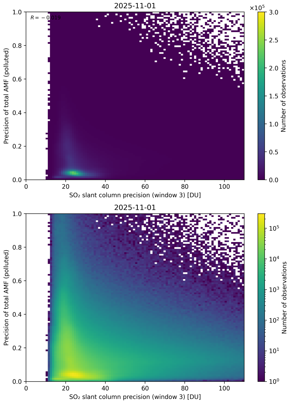
Figure 314: Scatter density plot of “SO 2 slant column precision (window 3)” against “Precision of total AMF (polluted)” for 2025-10-31 to 2025-11-02.
