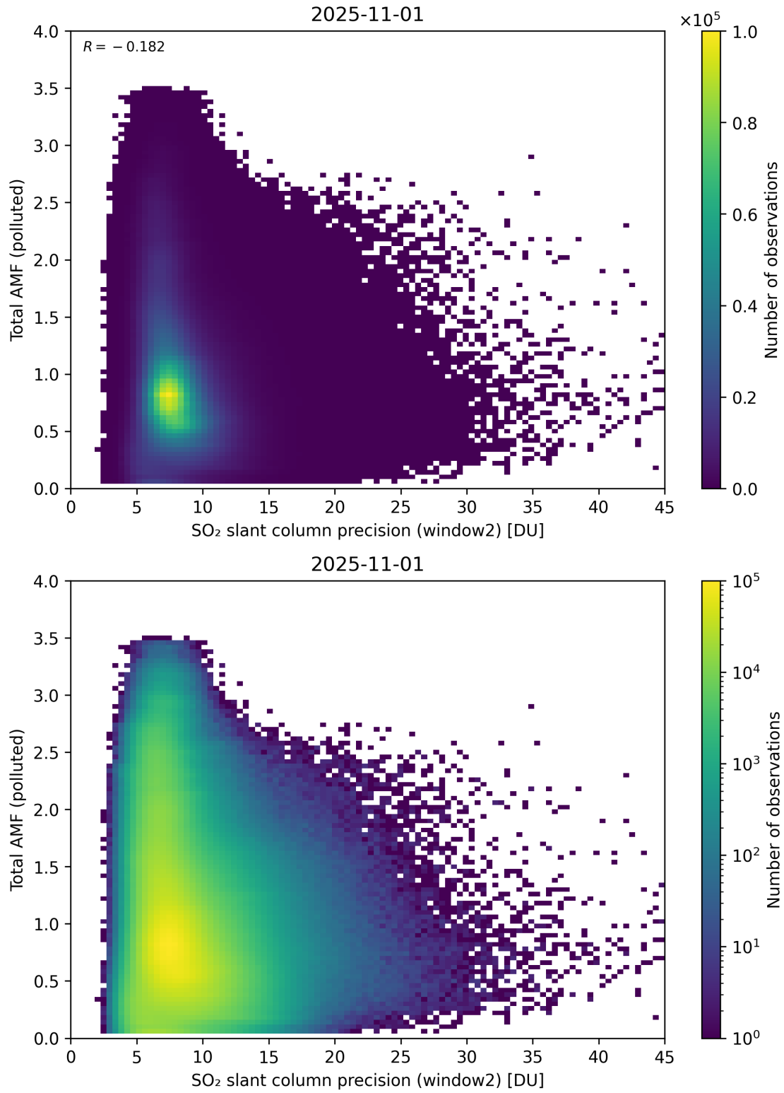
Figure 301: Scatter density plot of “SO 2 slant column precision (window2)” against “Total AMF (polluted)” for 2025-10-31 to 2025-11-02.
