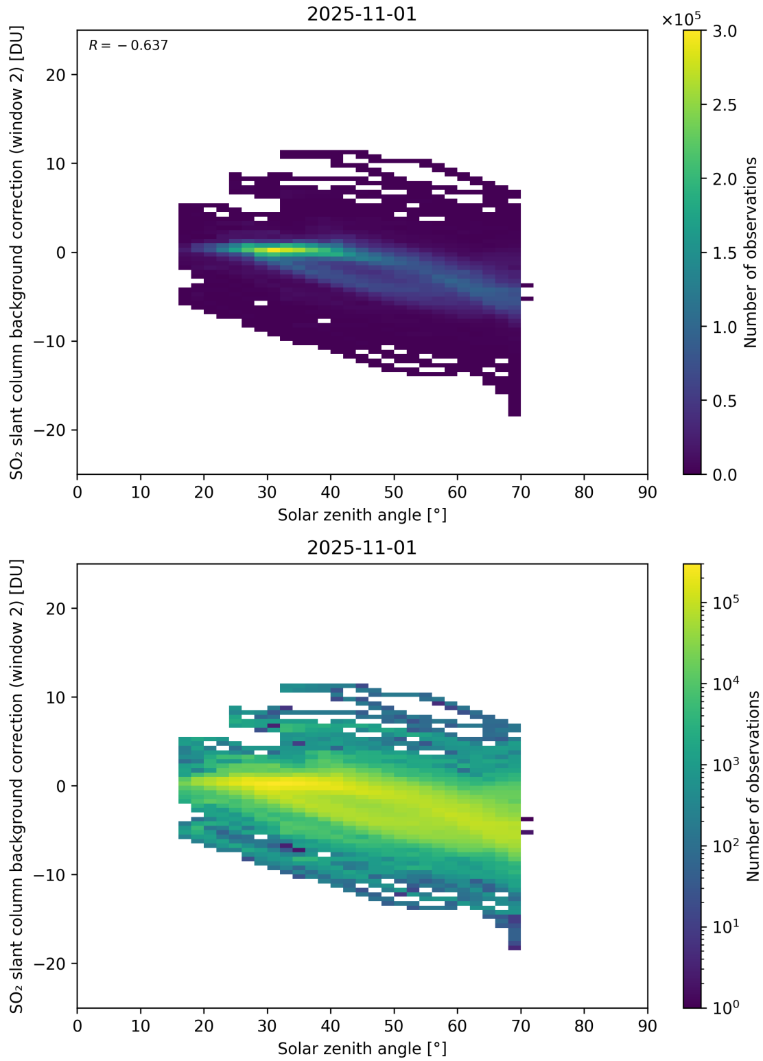
Figure 172: Scatter density plot of “Solar zenith angle” against “SO 2 slant column background correction (window 2)” for 2025-10-31 to 2025-11-02.
