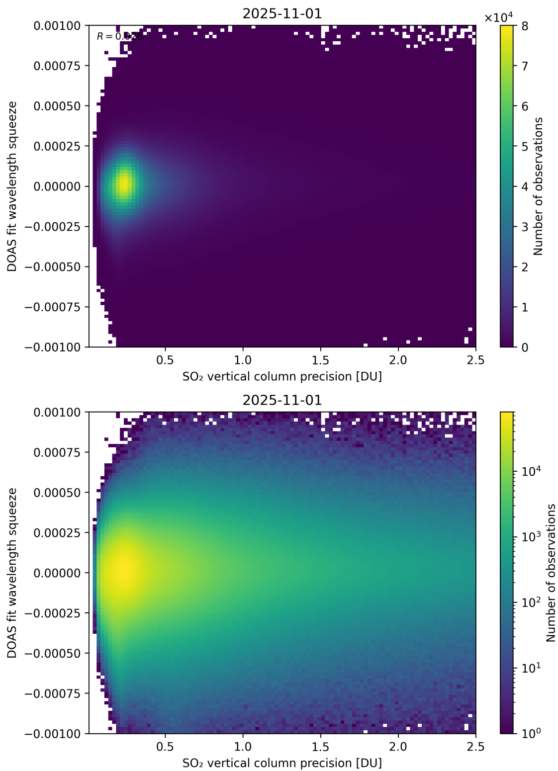
Figure 333: Scatter density plot of “SO 2 vertical column precision” against “DOAS fit wavelength squeeze” for 2025-10-31 to 2025-11-02.
