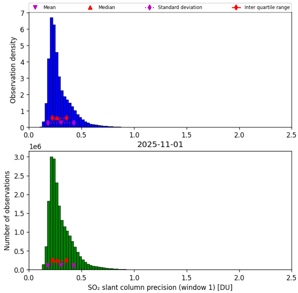
Figure 64: Histogram of “SO 2 slant column precision (window 1)” for 2025-10-31 to 2025-11-02
