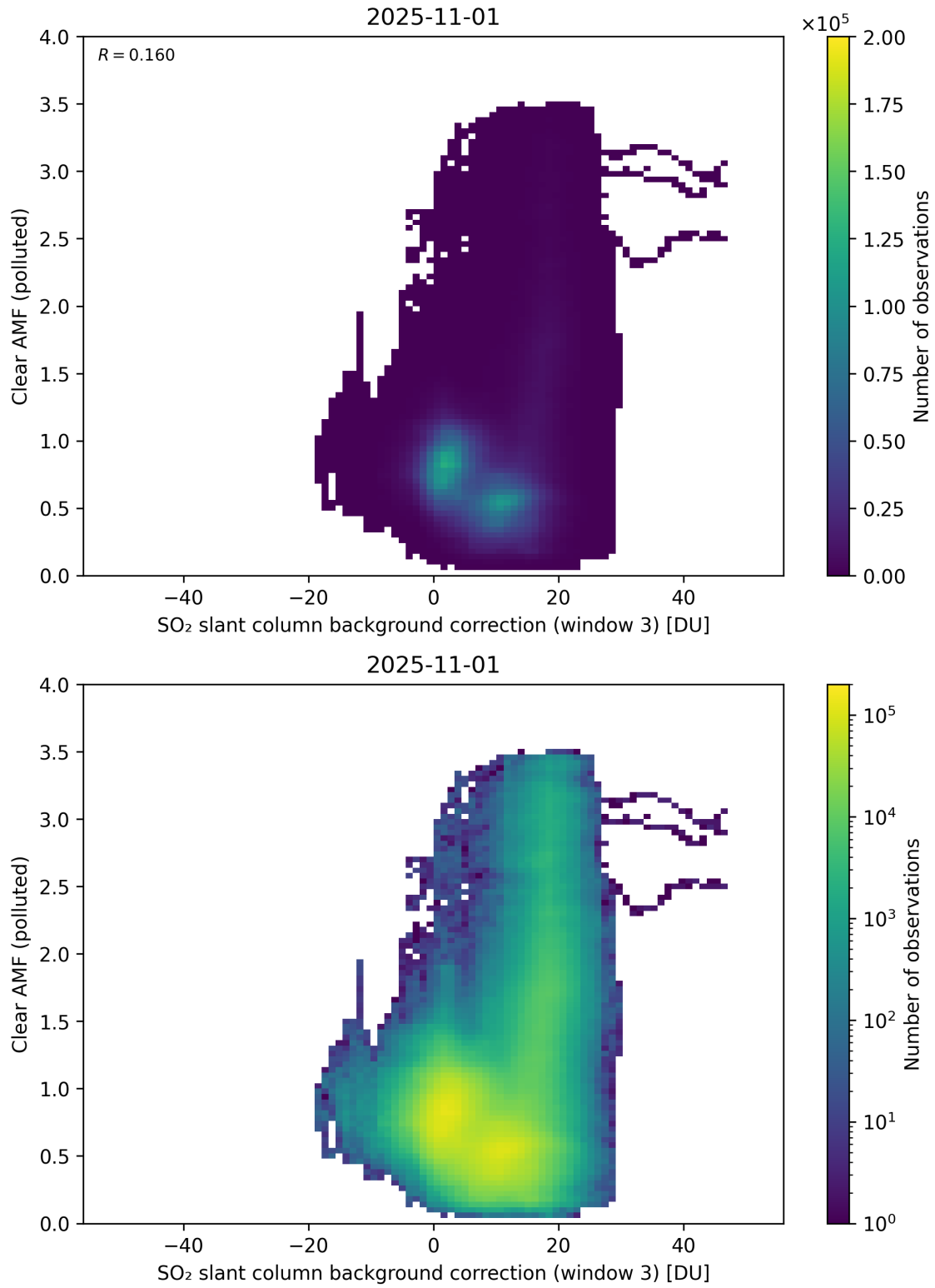
Figure 135: Scatter density plot of “SO 2 slant column background correction (window 3)” against “Clear AMF (polluted)” for 2025-10-31 to 2025-11-02.
