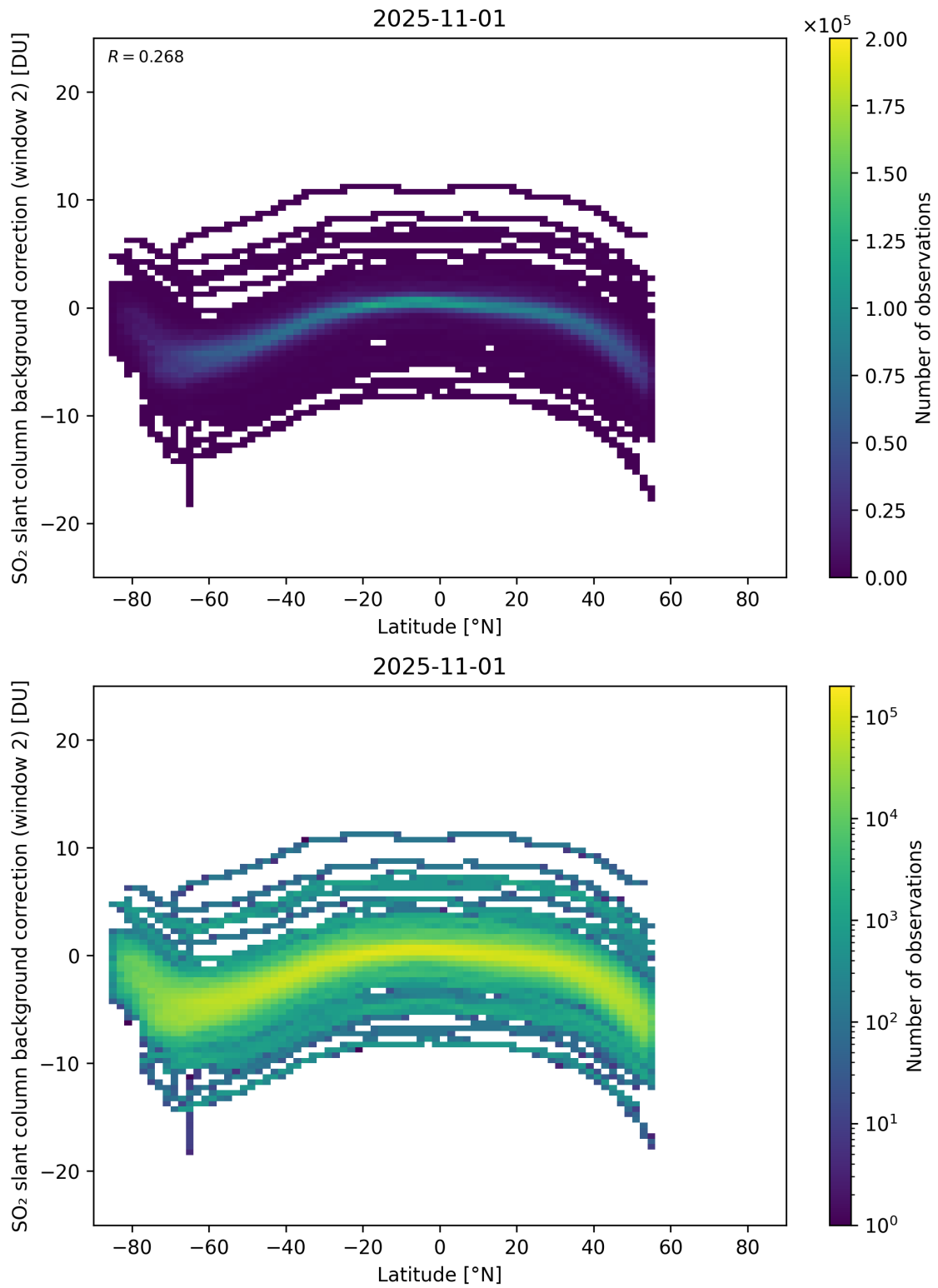
Figure 151: Scatter density plot of “Latitude” against “SO 2 slant column background correction (window 2)” for 2025-10-31 to 2025-11-02.
