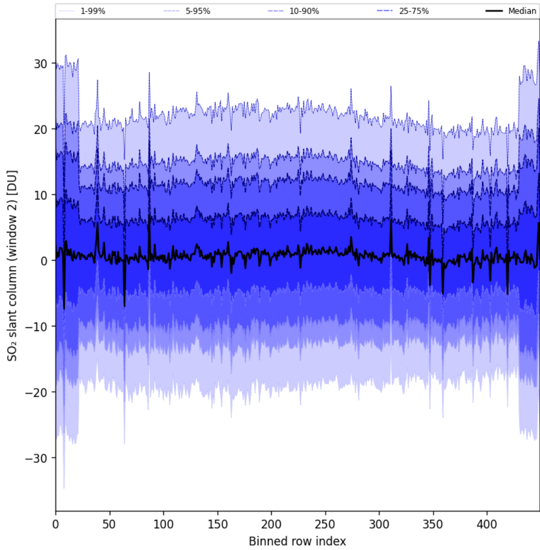
Figure 93: Along track statistics of “SO 2 slant column (window 2)” for 2025-10-31 to 2025-11-02
