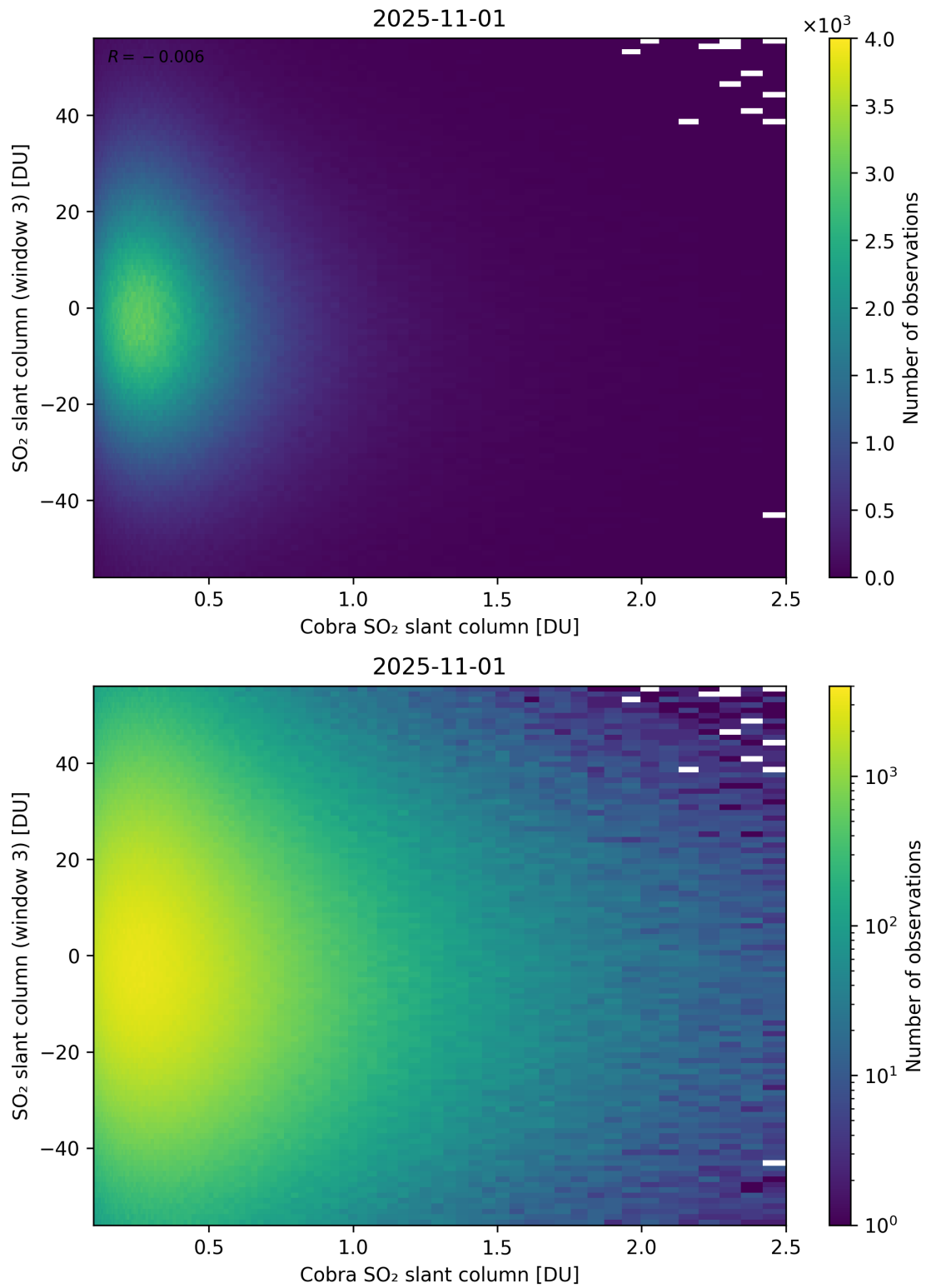
Figure 222: Scatter density plot of “Cobra SO 2 slant column” against “SO 2 slant column (window 3)” for 2025-10-31 to 2025-11-02.
