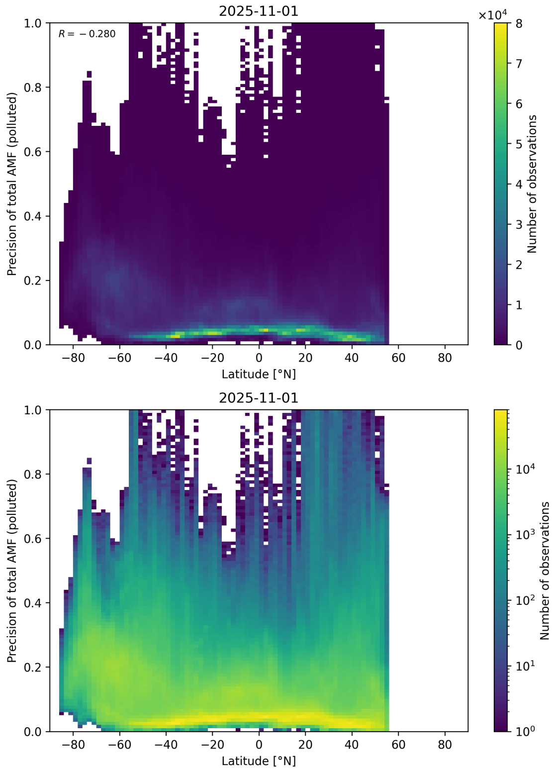
Figure 168: Scatter density plot of “Latitude” against “Precision of total AMF (polluted)” for 2025-10-31 to 2025-11-02.
