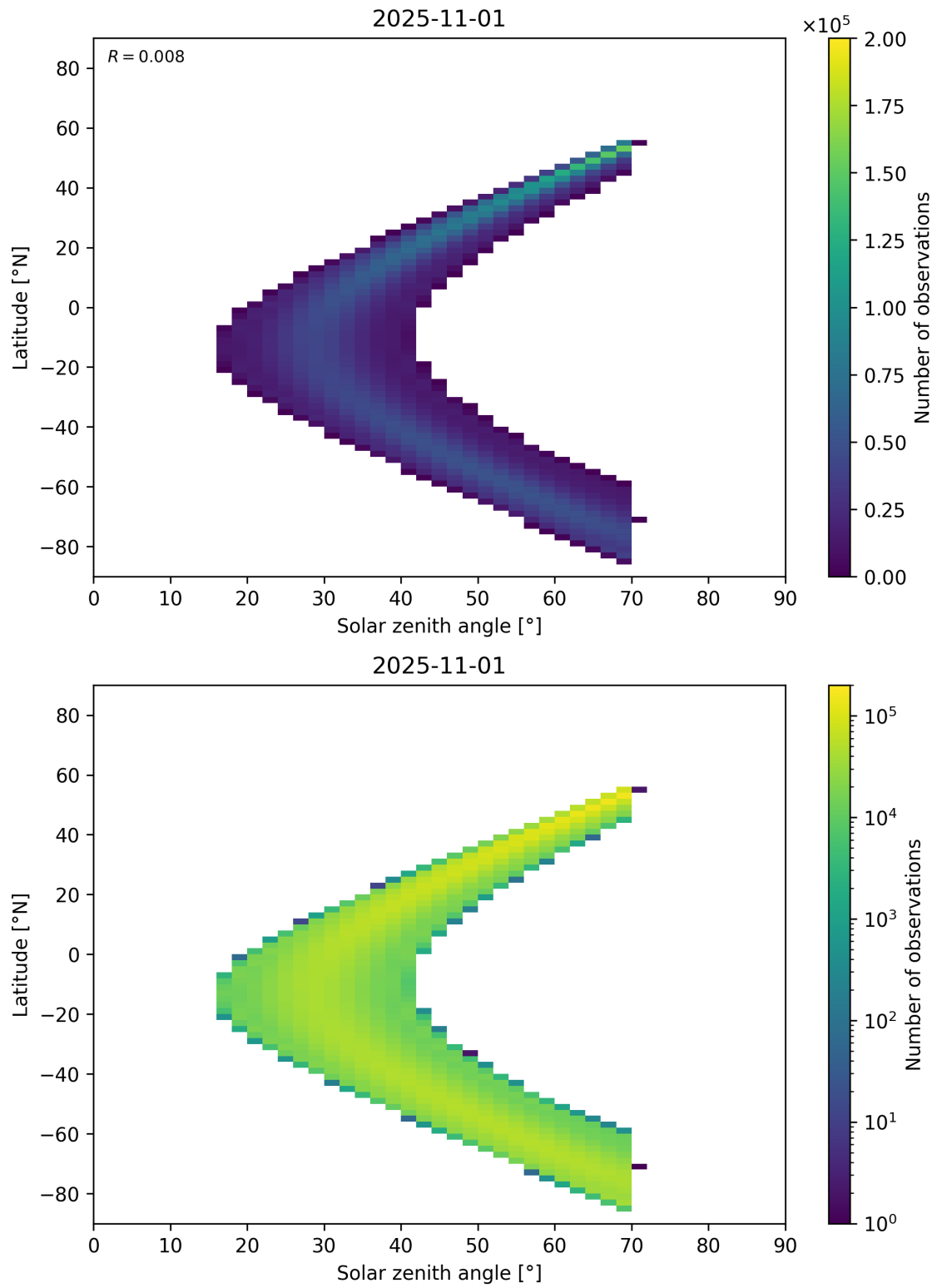
Figure 177: Scatter density plot of “Solar zenith angle” against “Latitude” for 2025-10-31 to 2025-11-02.
