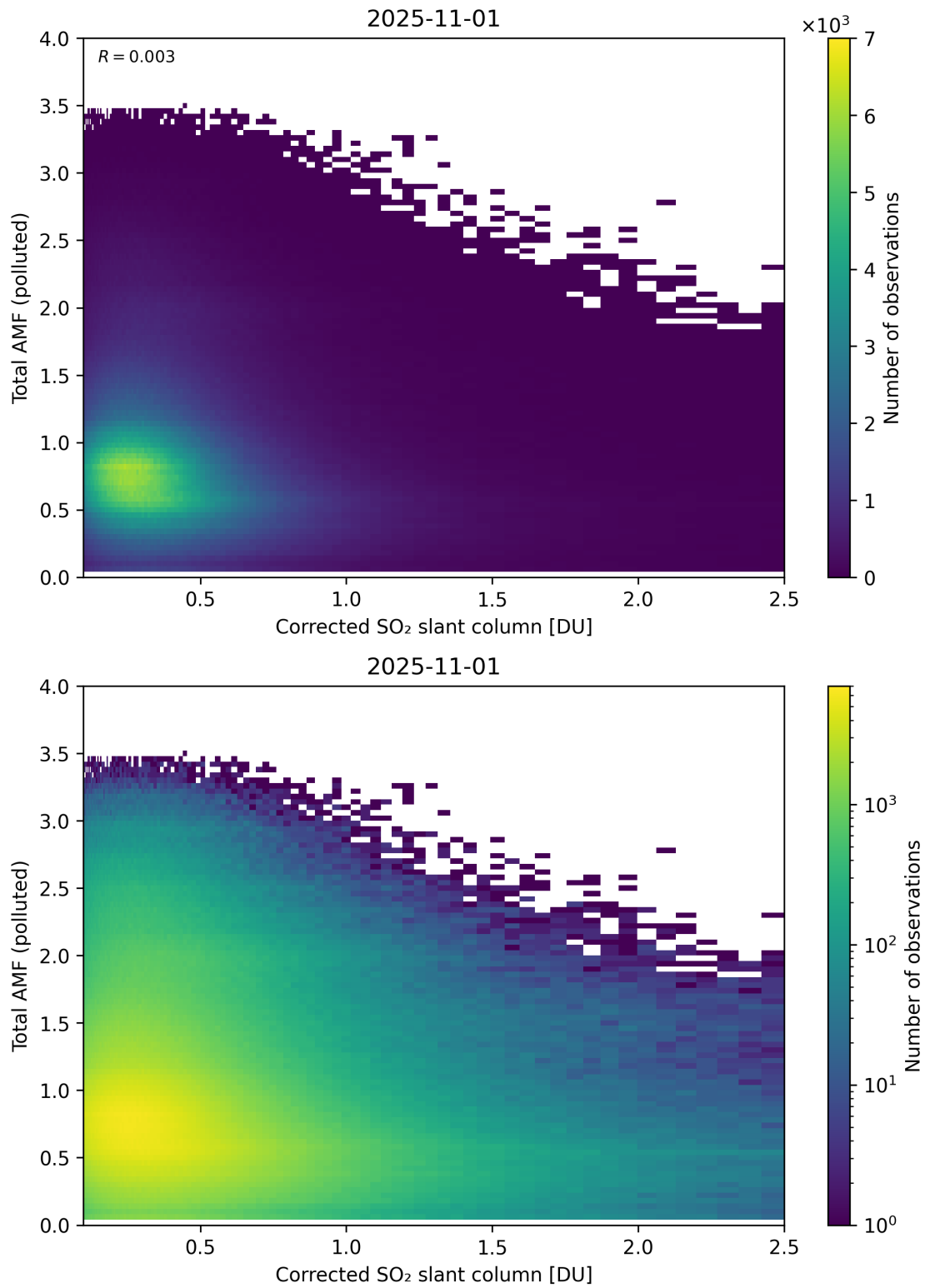
Figure 242: Scatter density plot of “Corrected SO 2 slant column” against “Total AMF (polluted)” for 2025-10-31 to 2025-11-02.
