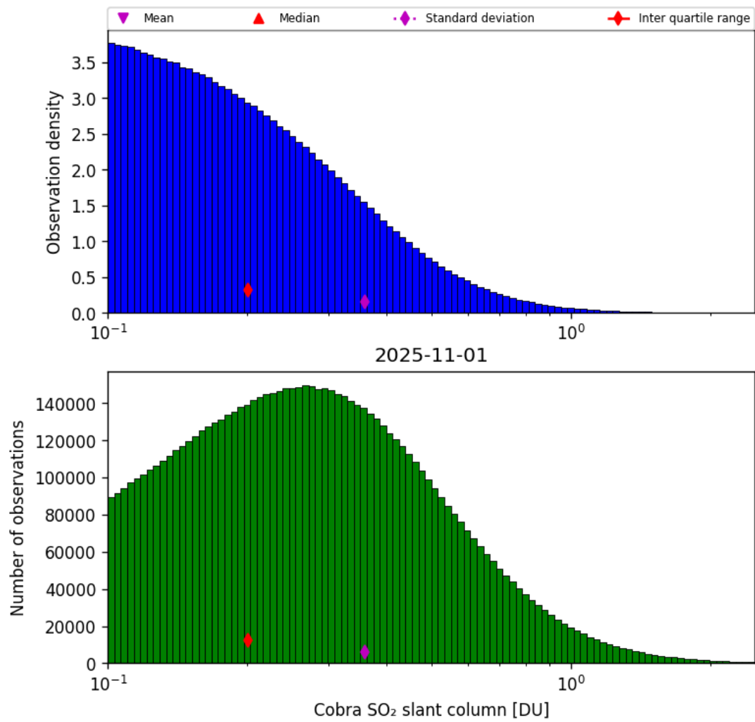
Figure 61: Histogram of “Cobra SO 2 slant column” for 2025-10-31 to 2025-11-02
