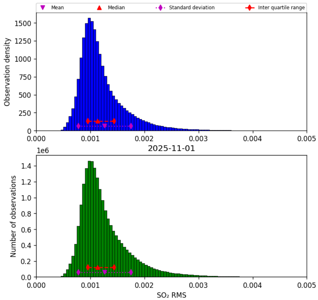
Figure 78: Histogram of “SO 2 RMS” for 2025-10-31 to 2025-11-02
