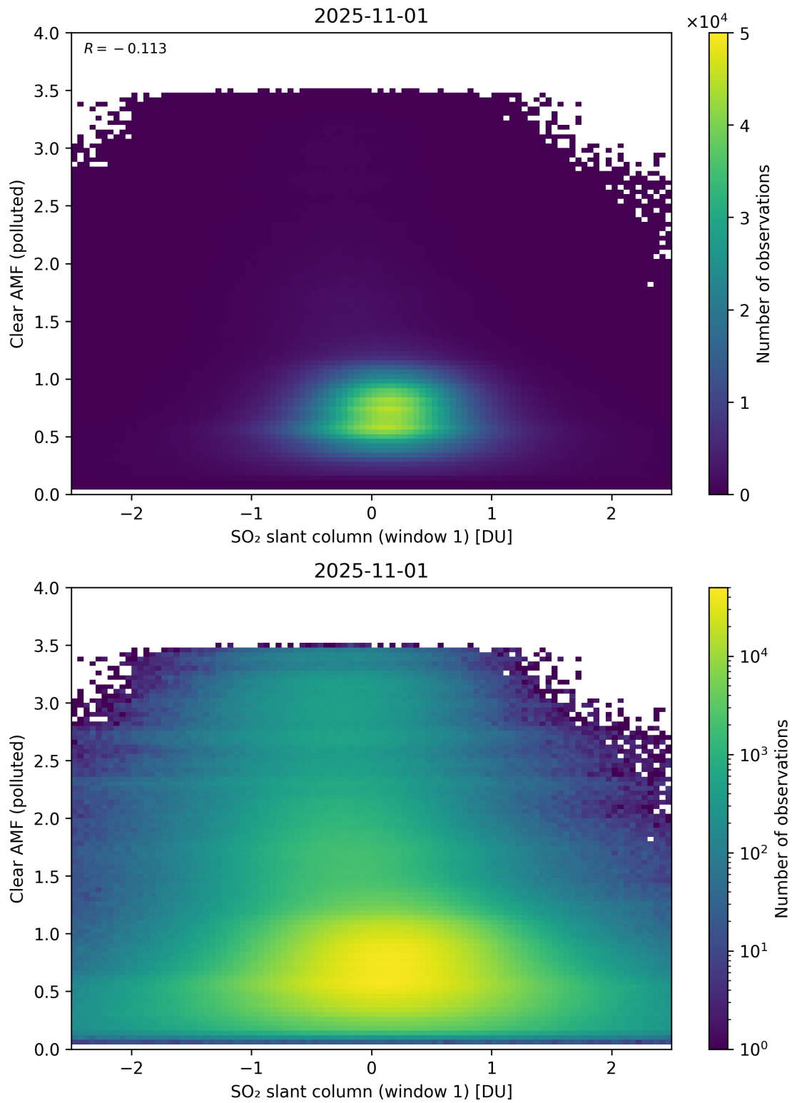
Figure 282: Scatter density plot of “SO 2 slant column (window 1)” against “Clear AMF (polluted)” for 2025-10-31 to 2025-11-02.
