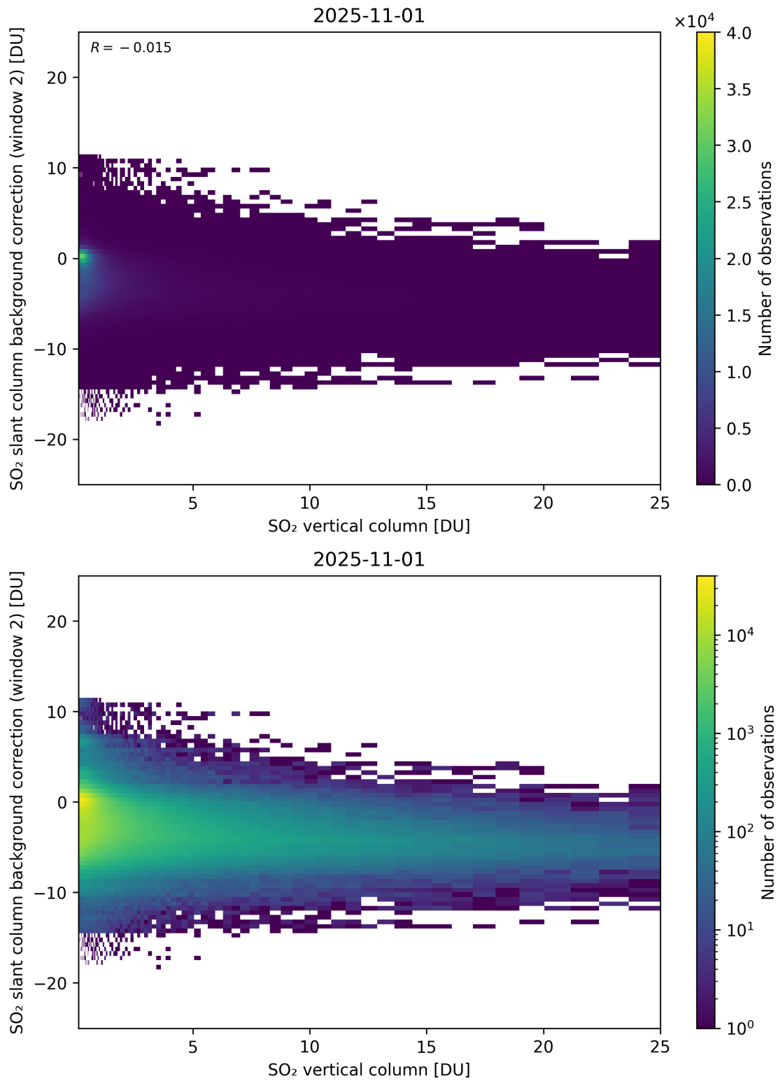
Figure 324: Scatter density plot of “SO 2 vertical column” against “SO 2 slant column background correction (window 2)” for 2025-10-31 to 2025-11-02.
