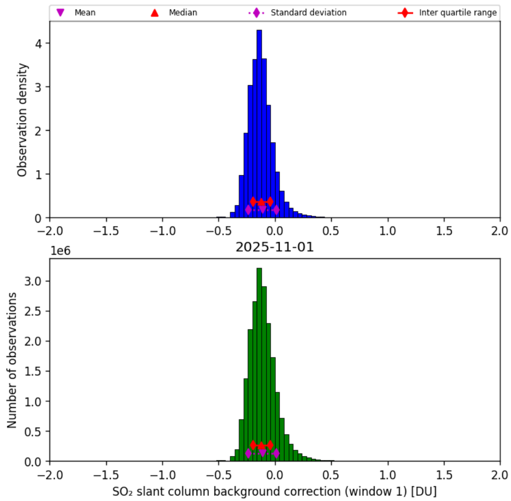
Figure 66: Histogram of “SO 2 slant column background correction (window 1)” for 2025-10-31 to 2025-11-02
