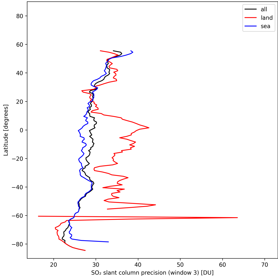
Figure 46: Zonal average of “SO 2 slant column precision (window 3)” for 2025-10-31 to 2025-11-02.
