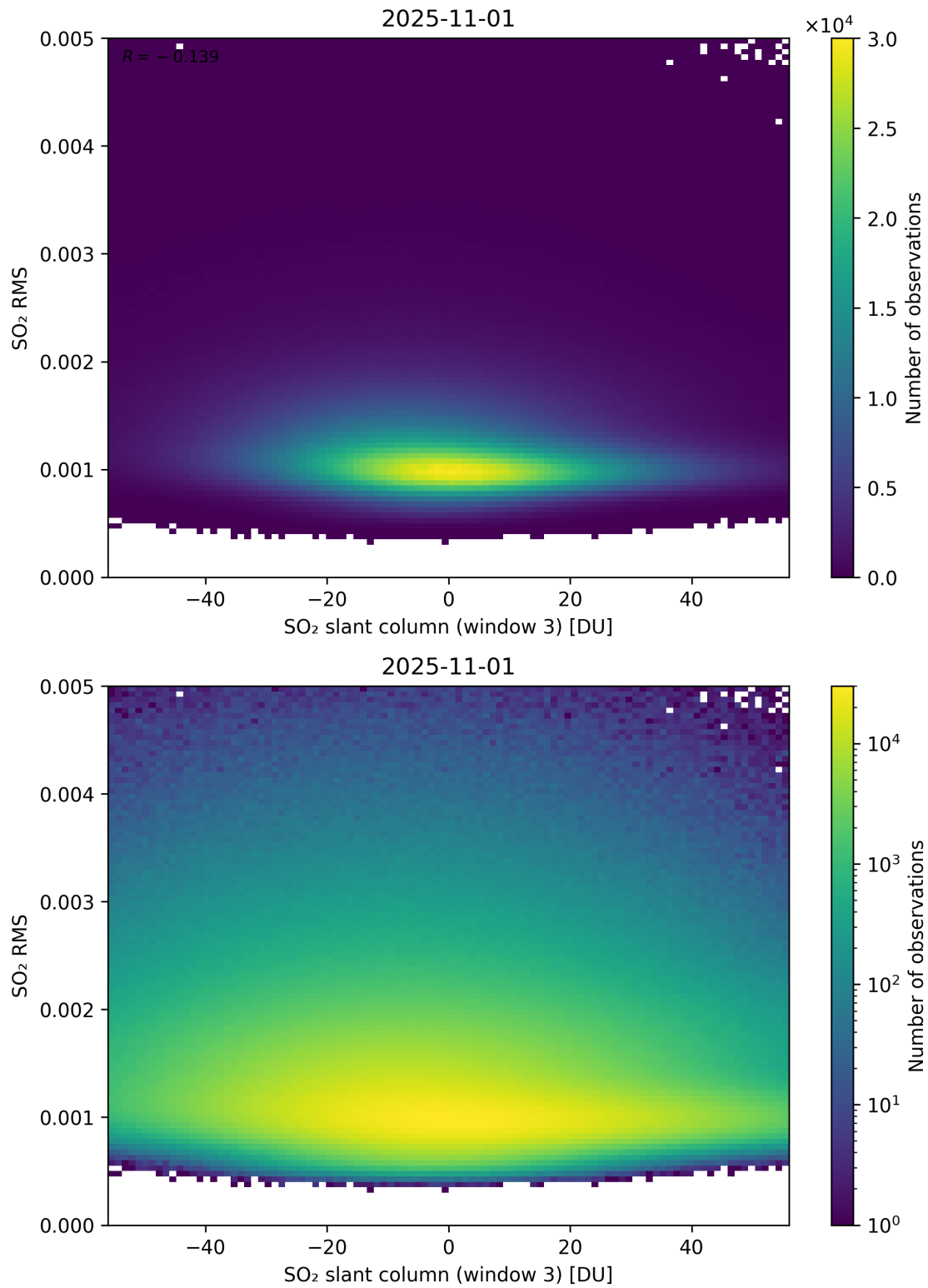
Figure 306: Scatter density plot of “SO 2 slant column (window 3)” against “SO 2 RMS” for 2025-10-31 to 2025-11-02.
