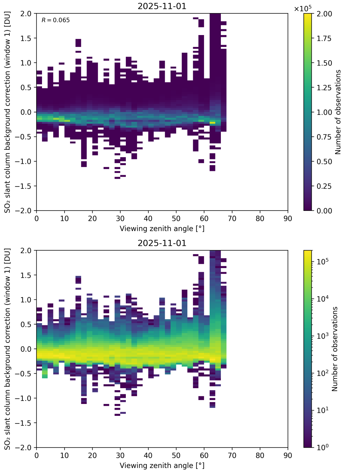
Figure 362: Scatter density plot of “Viewing zenith angle” against “SO 2 slant column background correction (window 1)” for 2025-10-31 to 2025-11-02.
