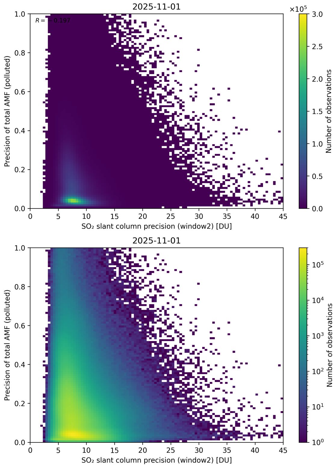
Figure 302: Scatter density plot of “SO 2 slant column precision (window2)” against “Precision of total AMF (polluted)” for 2025-10-31 to 2025-11-02.
