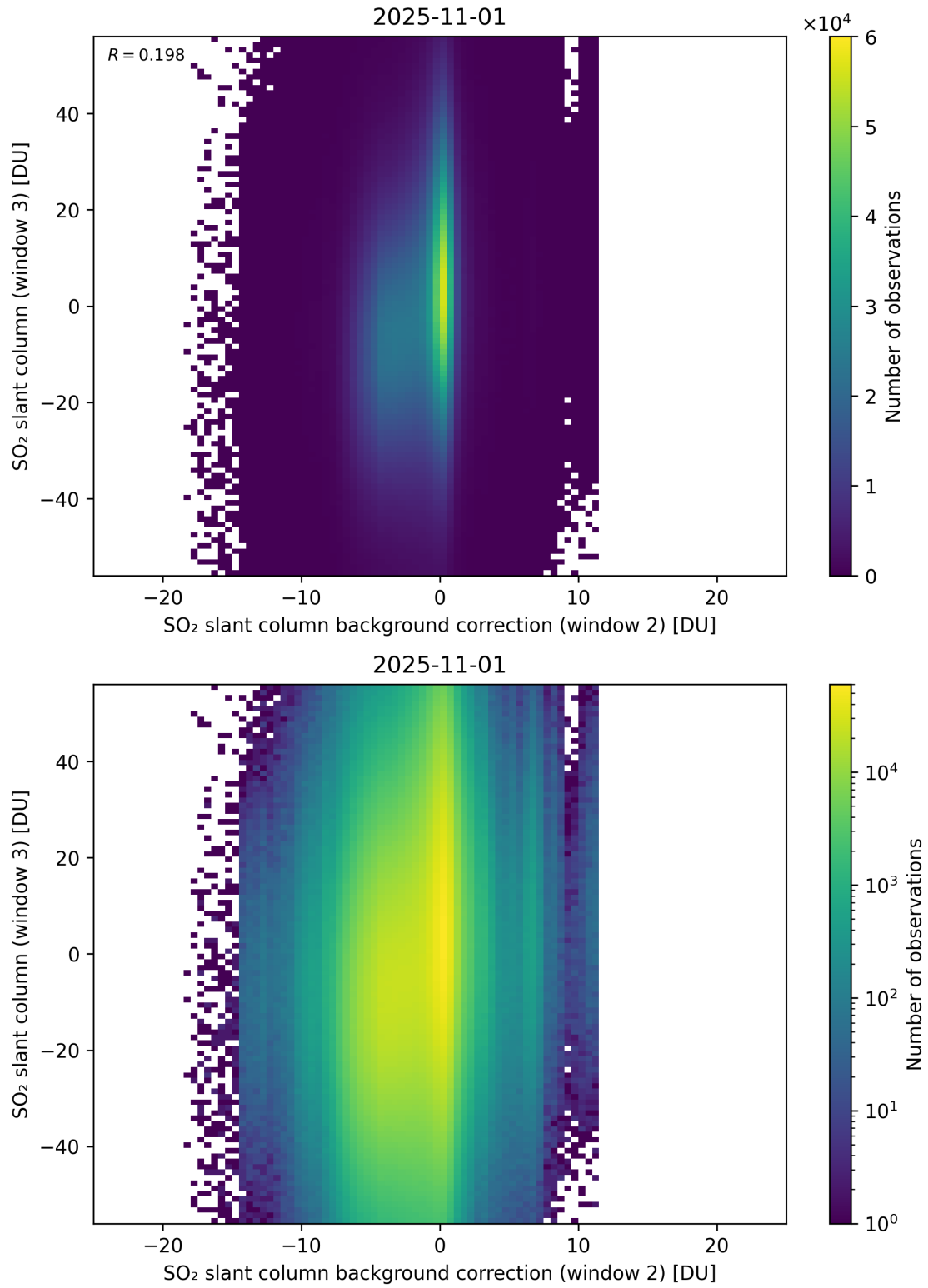
Figure 128: Scatter density plot of “SO 2 slant column background correction (window 2)” against “SO 2 slant column (window 3)” for 2025-10-31 to 2025-11-02.
