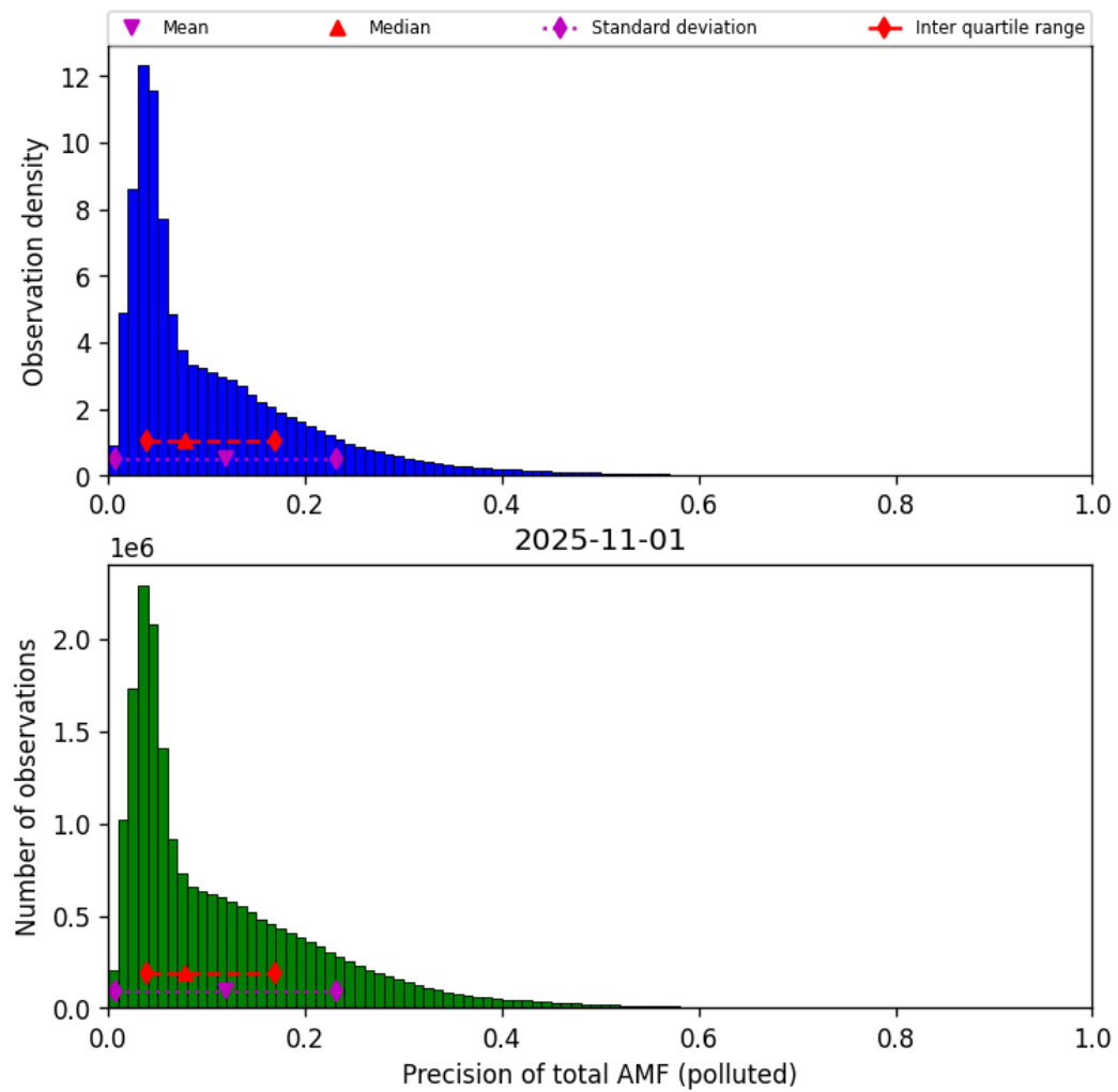
Figure 80: Histogram of “Precision of total AMF (polluted)” for 2025-10-31 to 2025-11-02
