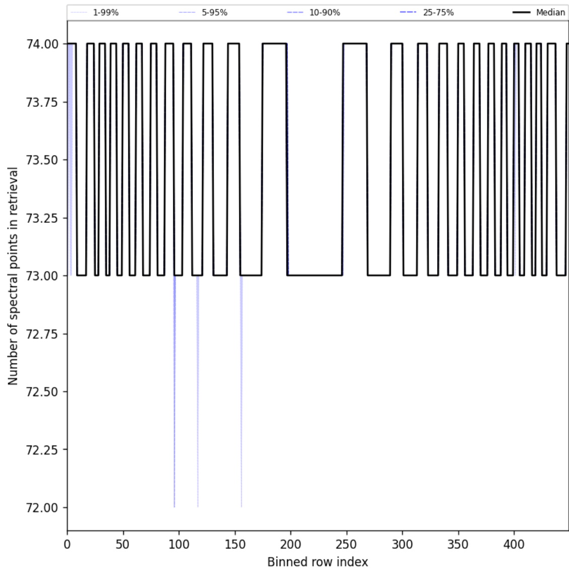
Figure 108: Along track statistics of “Number of spectral points in retrieval” for 2025-10-31 to 2025-11-02
