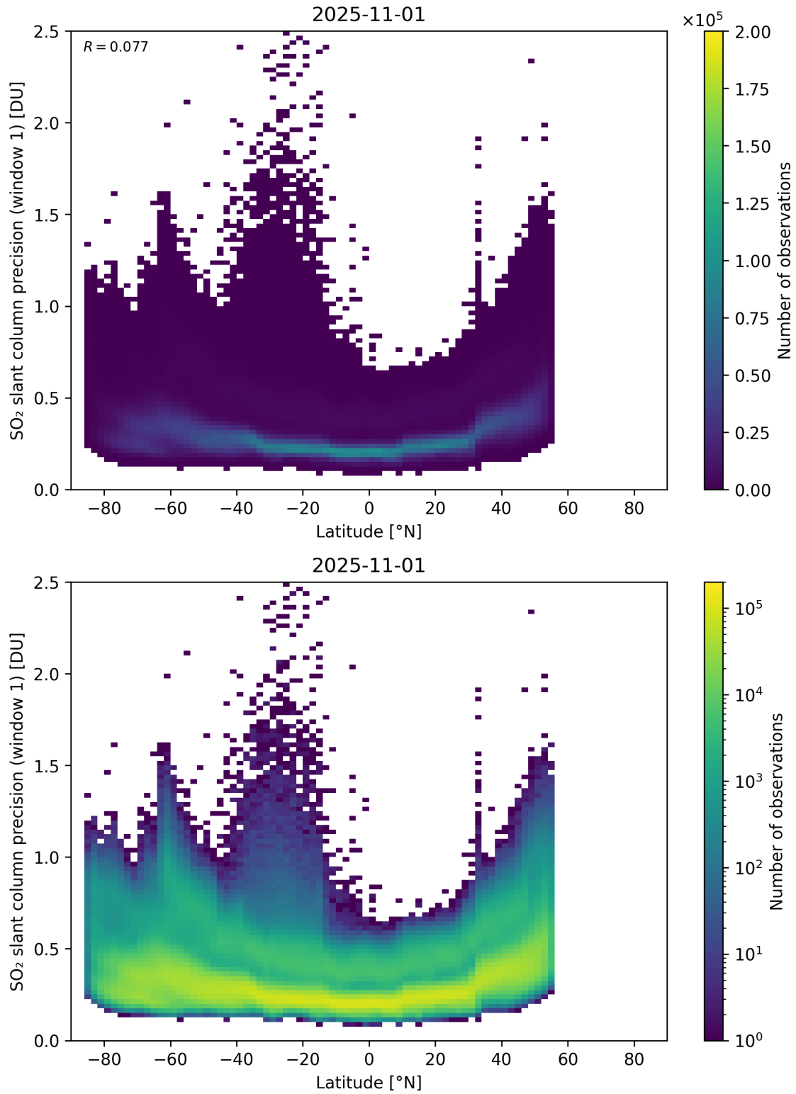
Figure 163: Scatter density plot of “Latitude” against “SO 2 slant column precision (window 1)” for 2025-10-31 to 2025-11-02.
