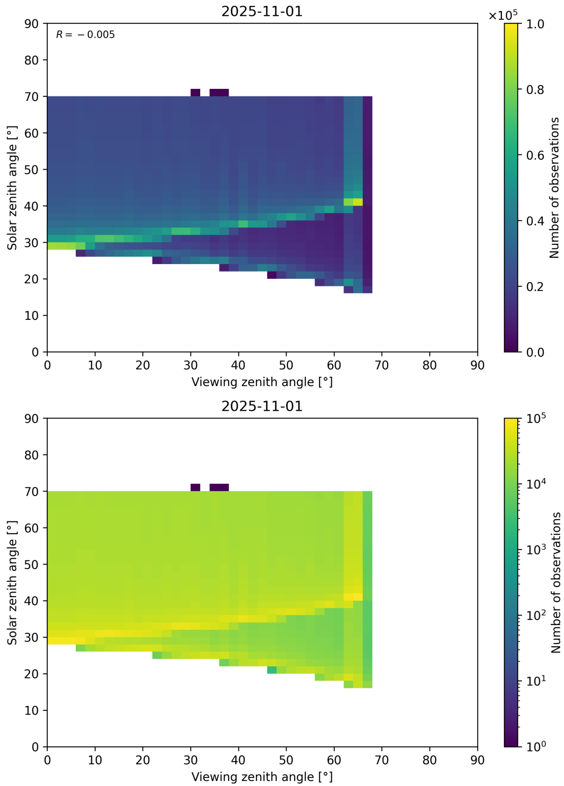
Figure 369: Scatter density plot of “Viewing zenith angle” against “Solar zenith angle” for 2025-10-31 to 2025-11-02.
