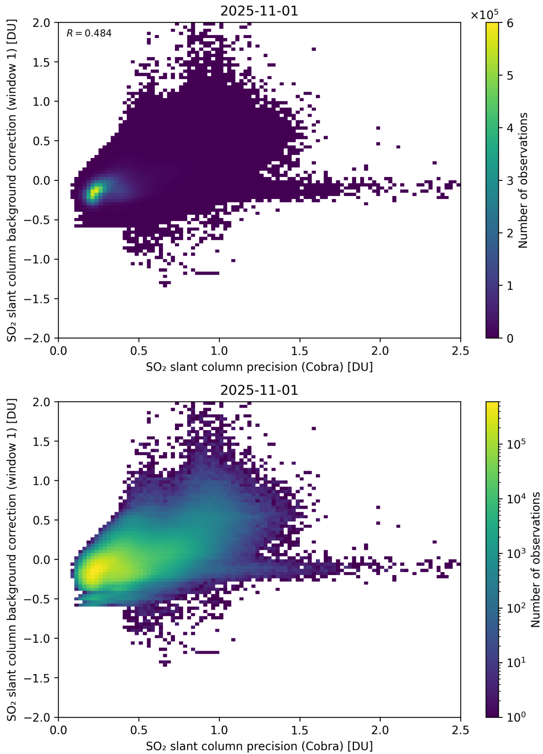
Figure 199: Scatter density plot of “SO 2 slant column precision (Cobra)” against “SO 2 slant column background correction (window 1)” for 2025-10-31 to 2025-11-02.
