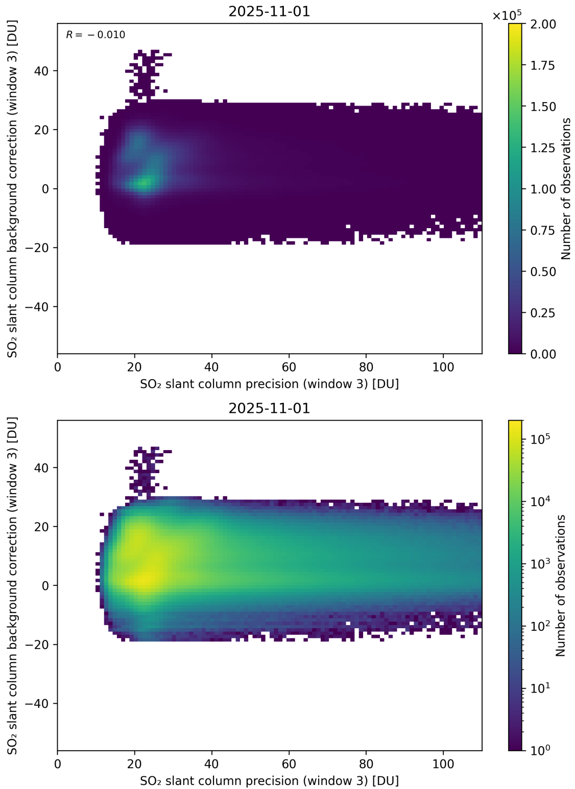
Figure 307: Scatter density plot of “SO 2 slant column precision (window 3)” against “SO 2 slant column background correction (window 3)” for 2025-10-31 to 2025-11-02.
