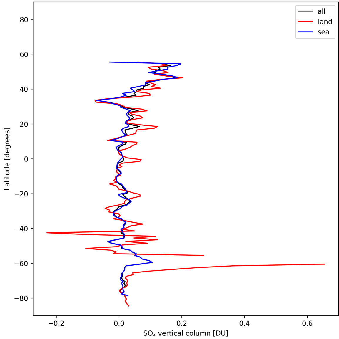
Figure 32: Zonal average of “SO 2 vertical column” for 2025-10-31 to 2025-11-02.
