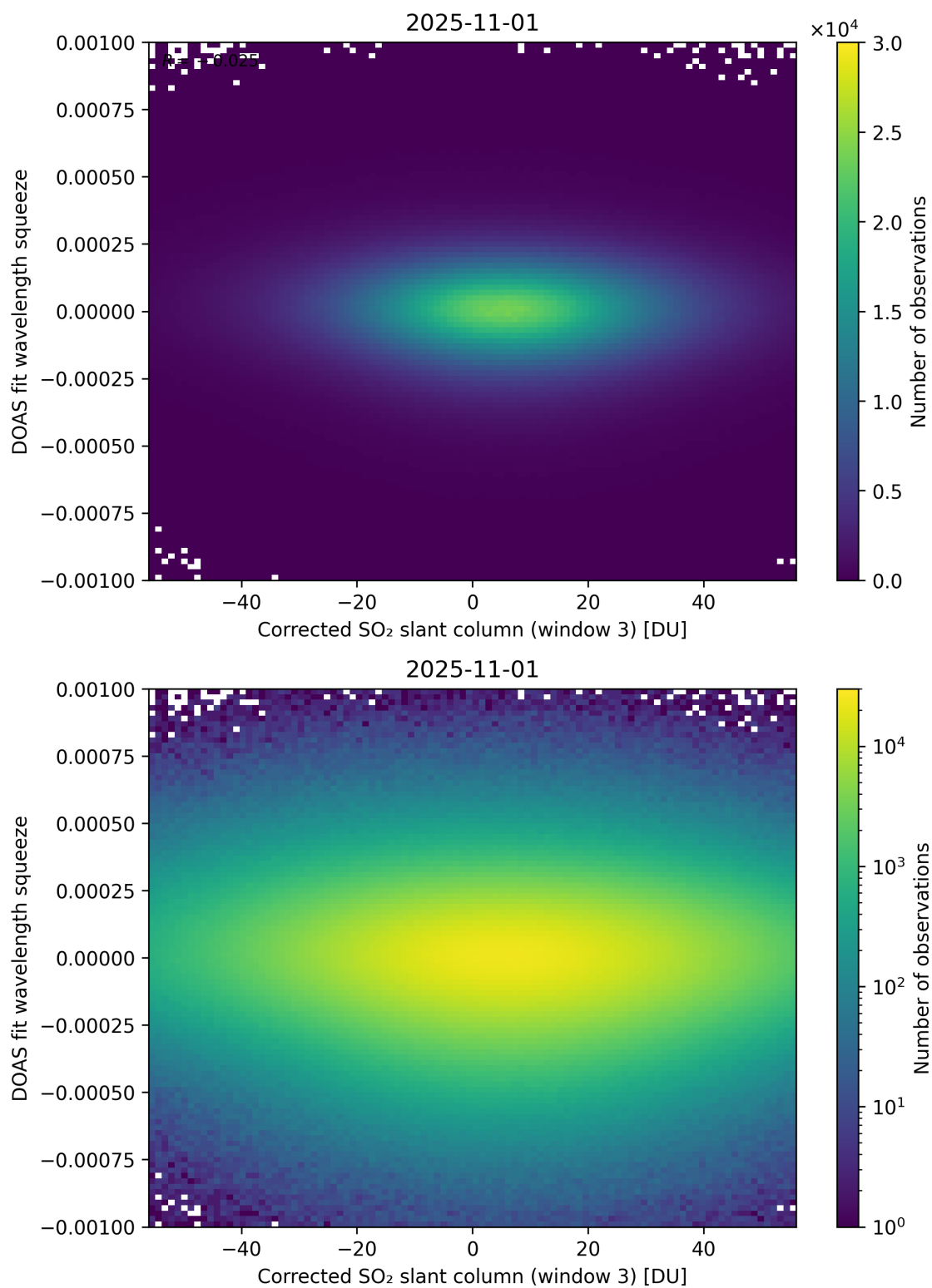
Figure 257: Scatter density plot of “Corrected SO 2 slant column (window 3)” against “DOAS fit wavelength squeeze” for 2025-10-31 to 2025-11-02.
