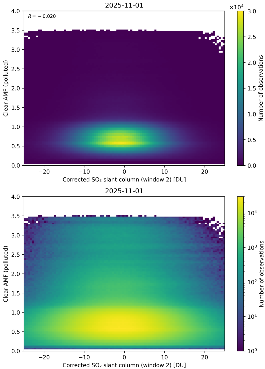
Figure 249: Scatter density plot of “Corrected SO 2 slant column (window 2)” against “Clear AMF (polluted)” for 2025-10-31 to 2025-11-02.
