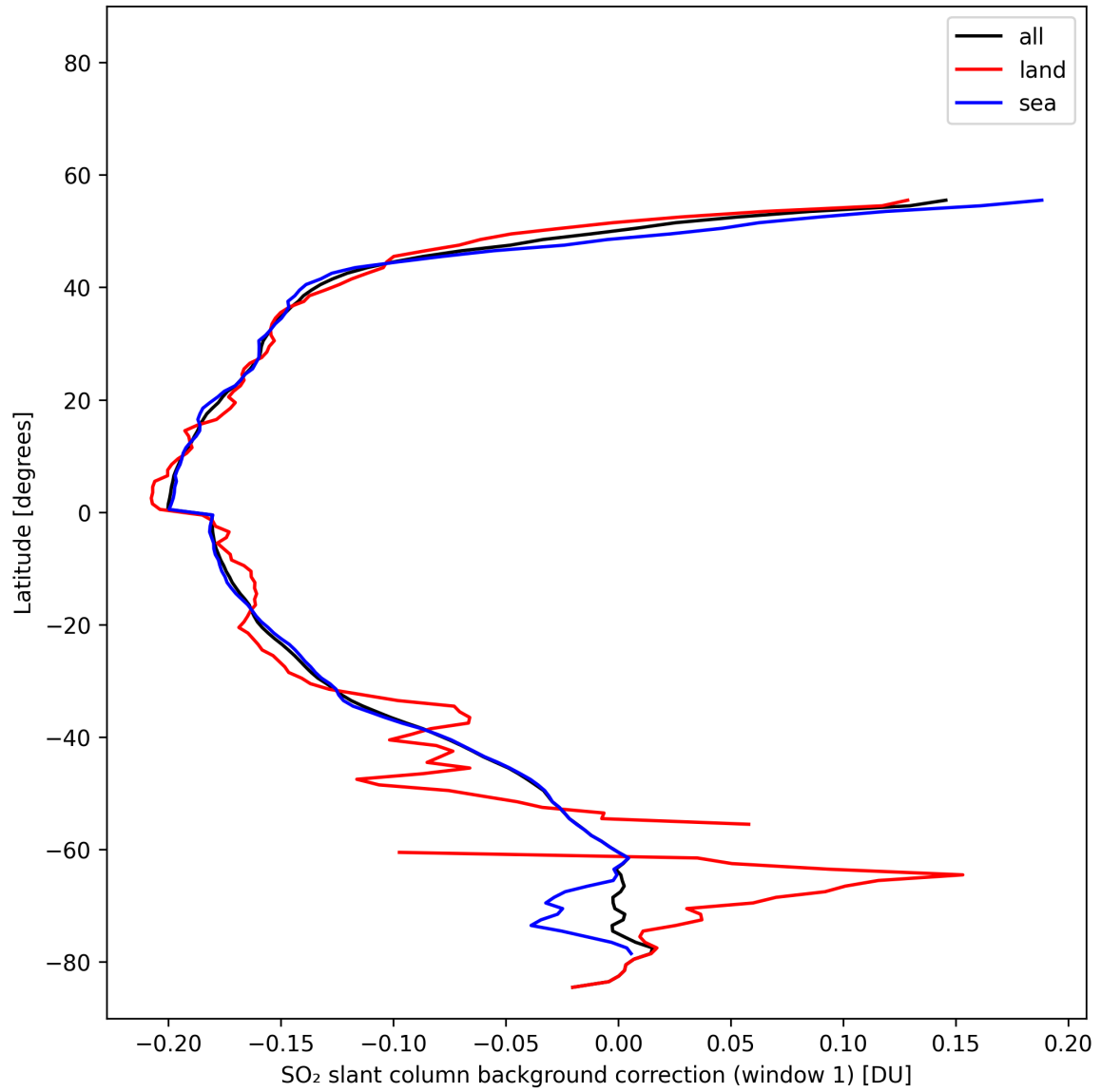
Figure 40: Zonal average of “SO 2 slant column background correction (window 1)” for 2025-10-31 to 2025-11-02.
