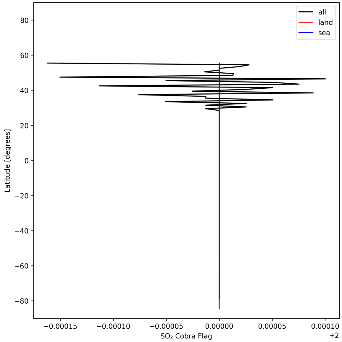
Figure 49: Zonal average of "SO 2 Cobra Flag" for 2025-10-31 to 2025-11-02.
