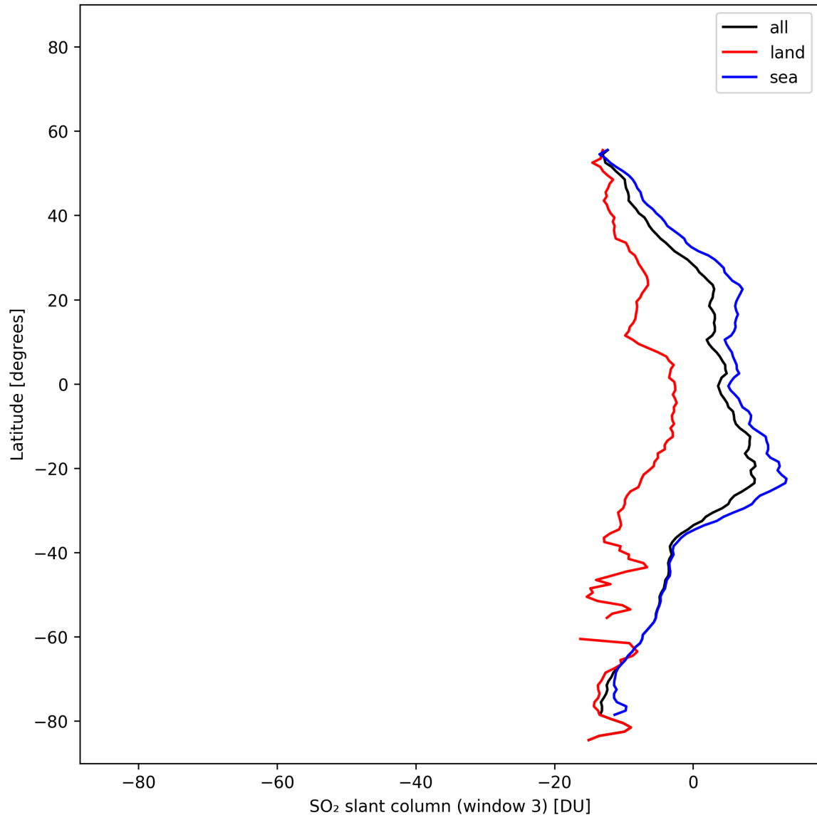
Figure 45: Zonal average of “SO 2 slant column (window 3)” for 2025-10-31 to 2025-11-02.
