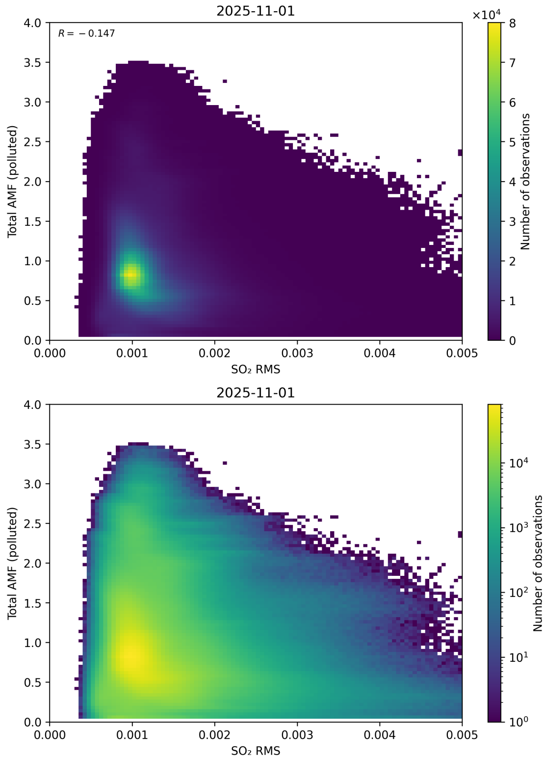
Figure 148: Scatter density plot of “SO 2 RMS” against “Total AMF (polluted)” for 2025-10-31 to 2025-11-02.
