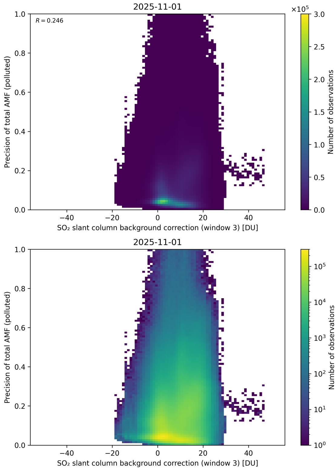
Figure 137: Scatter density plot of “SO 2 slant column background correction (window 3)” against “Precision of total AMF (polluted)” for 2025-10-31 to 2025-11-02.
