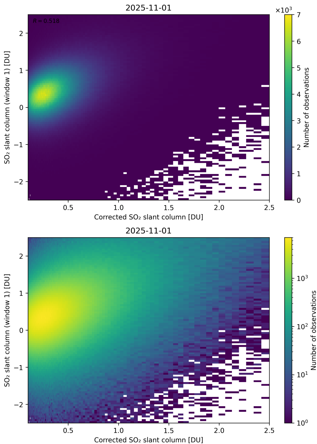
Figure 237: Scatter density plot of “Corrected SO 2 slant column” against “SO 2 slant column (window 1)” for 2025-10-31 to 2025-11-02.
