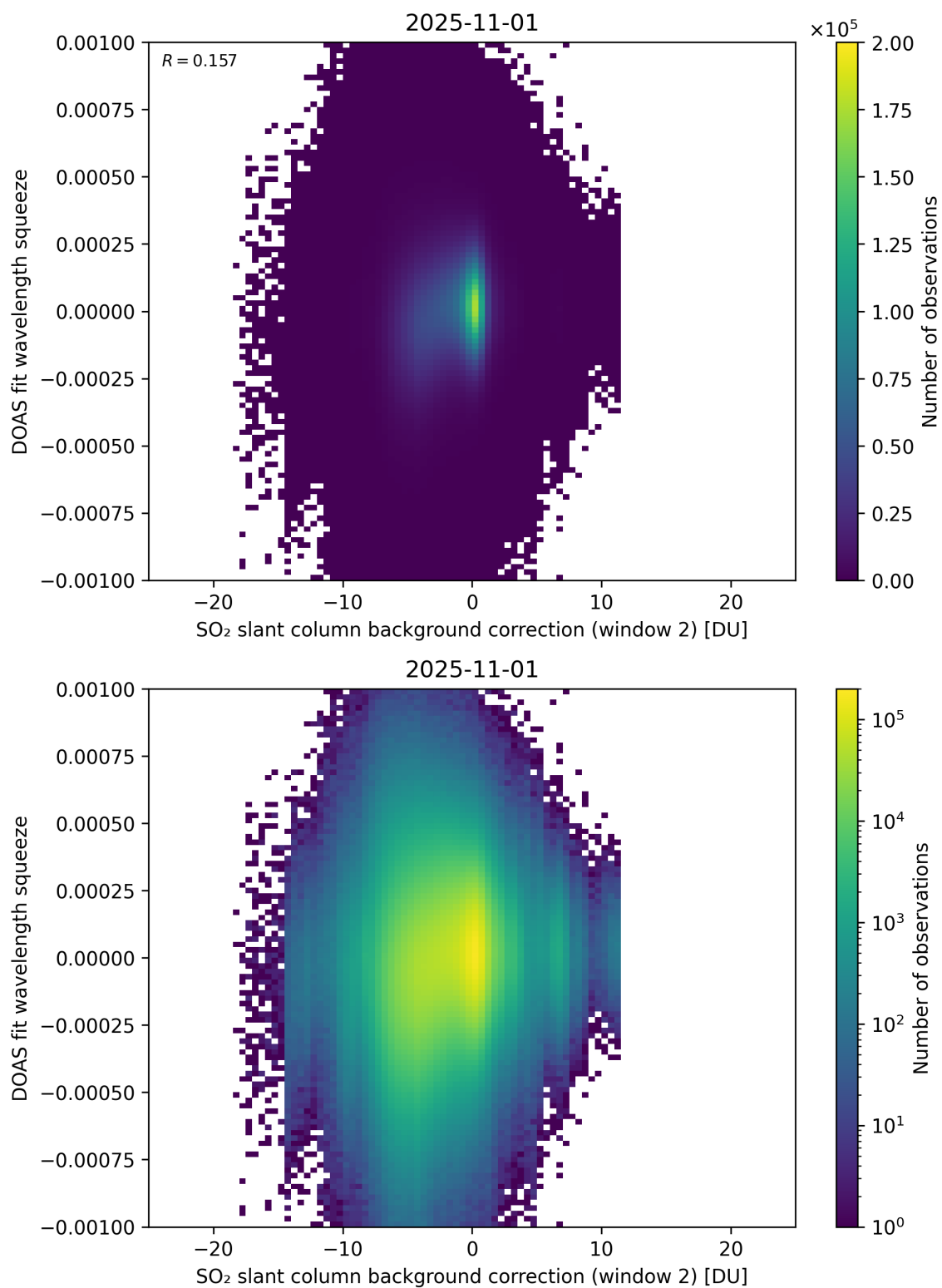
Figure 124: Scatter density plot of “SO 2 slant column background correction (window 2)” against “DOAS fit wavelength squeeze” for 2025-10-31 to 2025-11-02.
