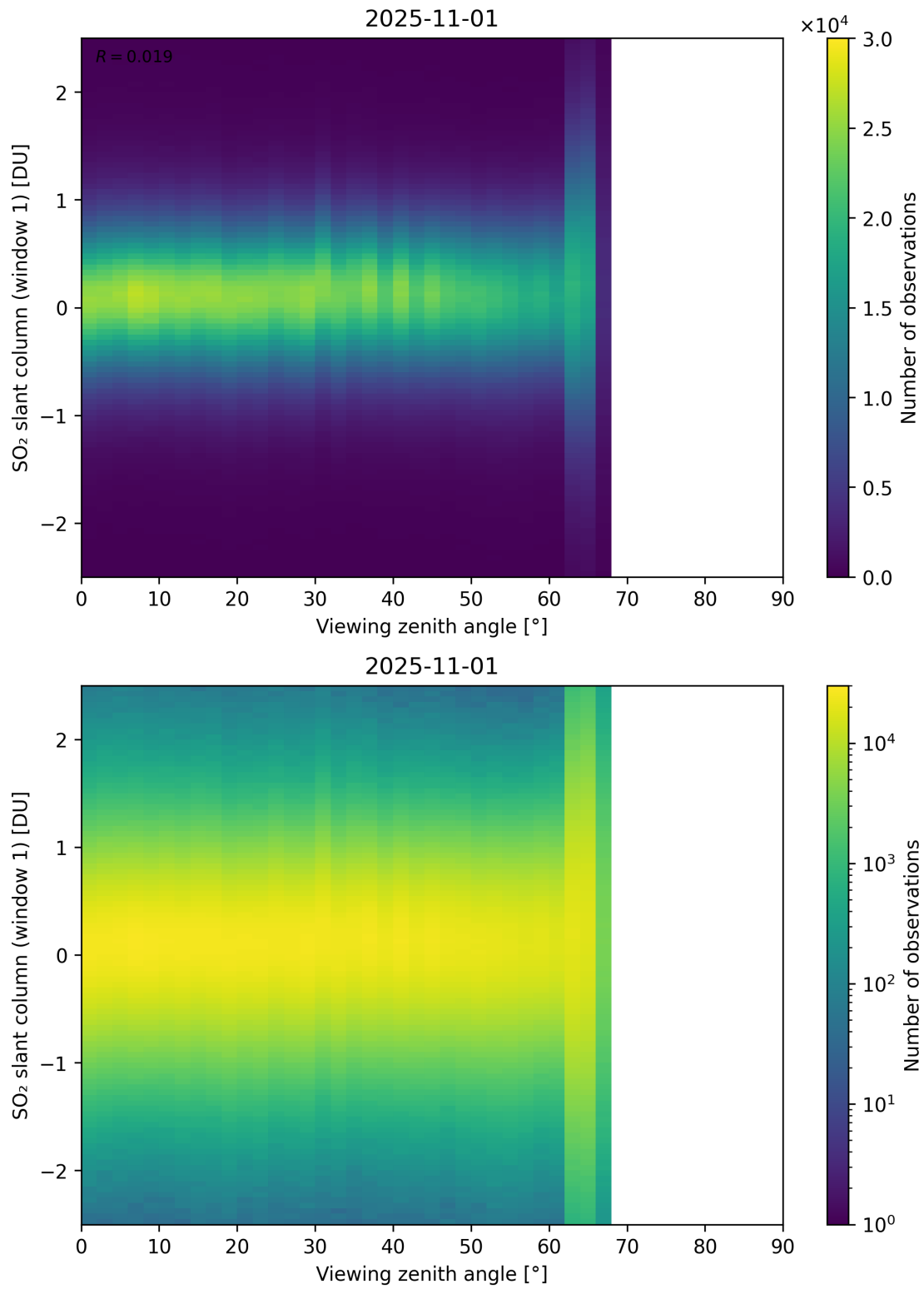
Figure 376: Scatter density plot of “Viewing zenith angle” against “SO 2 slant column (window 1)” for 2025-10-31 to 2025-11-02.
