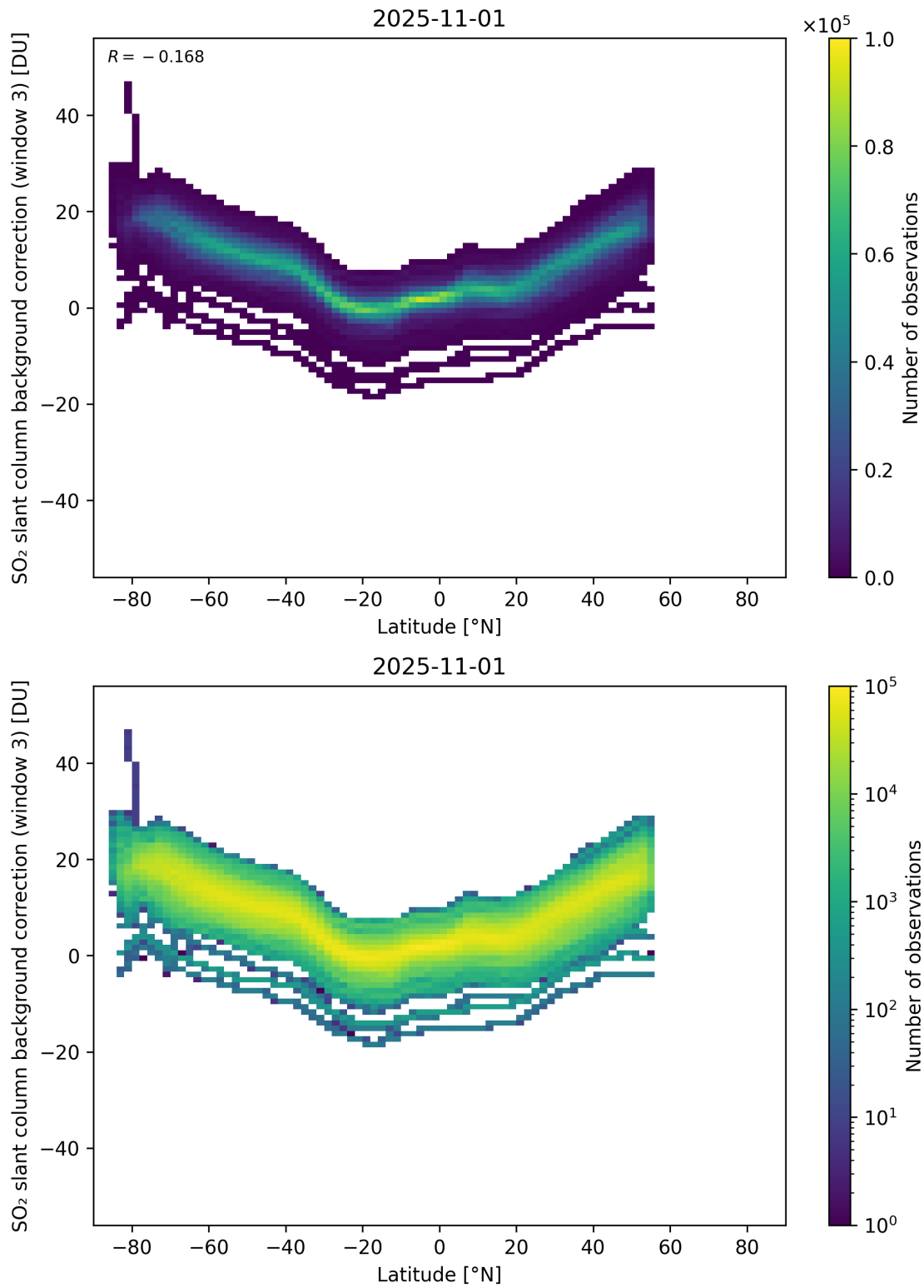
Figure 152: Scatter density plot of “Latitude” against “SO 2 slant column background correction (window 3)” for 2025-10-31 to 2025-11-02.
