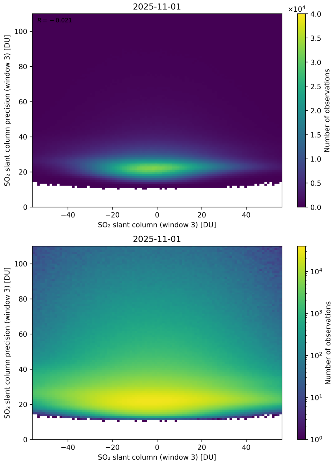
Figure 317: Scatter density plot of “SO 2 slant column (window 3)” against “SO 2 slant column precision (window 3)” for 2025-10-31 to 2025-11-02.
