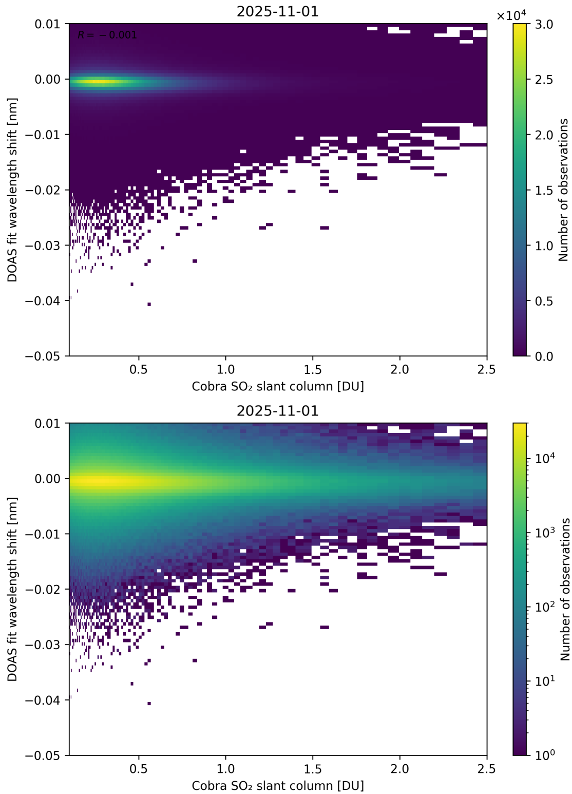
Figure 196: Scatter density plot of “Cobra SO 2 slant column” against “DOAS fit wavelength shift” for 2025-10-31 to 2025-11-02.
