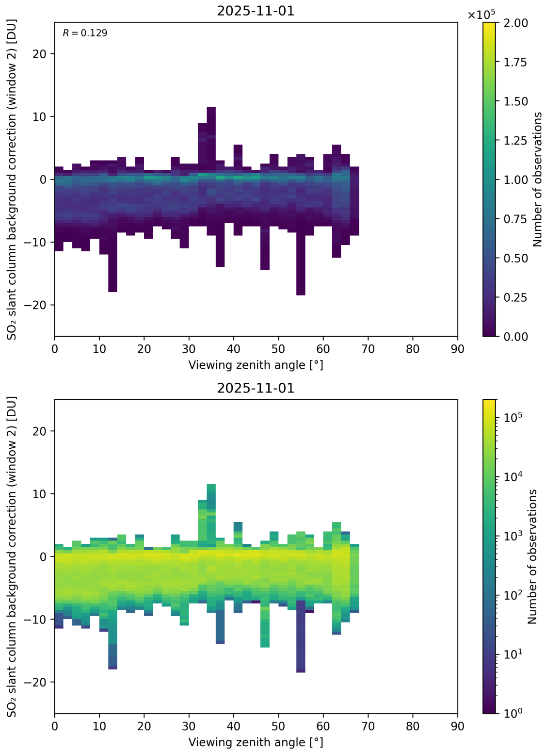
Figure 363: Scatter density plot of “Viewing zenith angle” against “SO 2 slant column background correction (window 2)” for 2025-10-31 to 2025-11-02.
