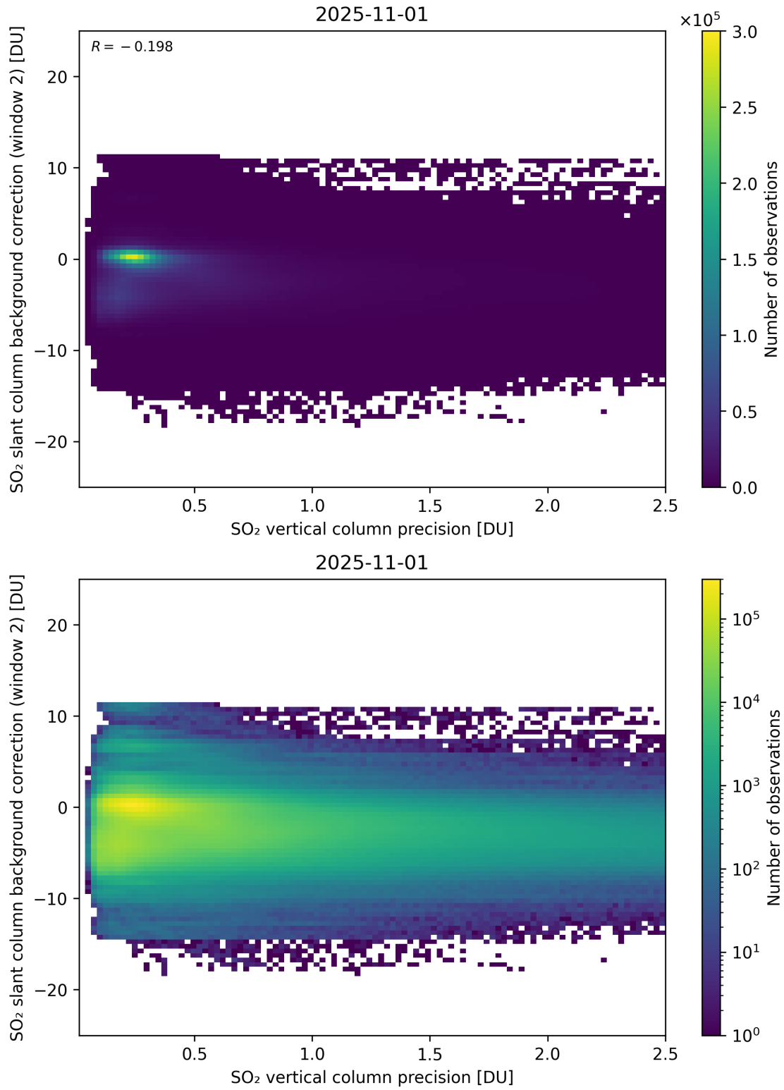
Figure 330: Scatter density plot of “SO 2 vertical column precision” against “SO 2 slant column background correction (window 2)” for 2025-10-31 to 2025-11-02.
