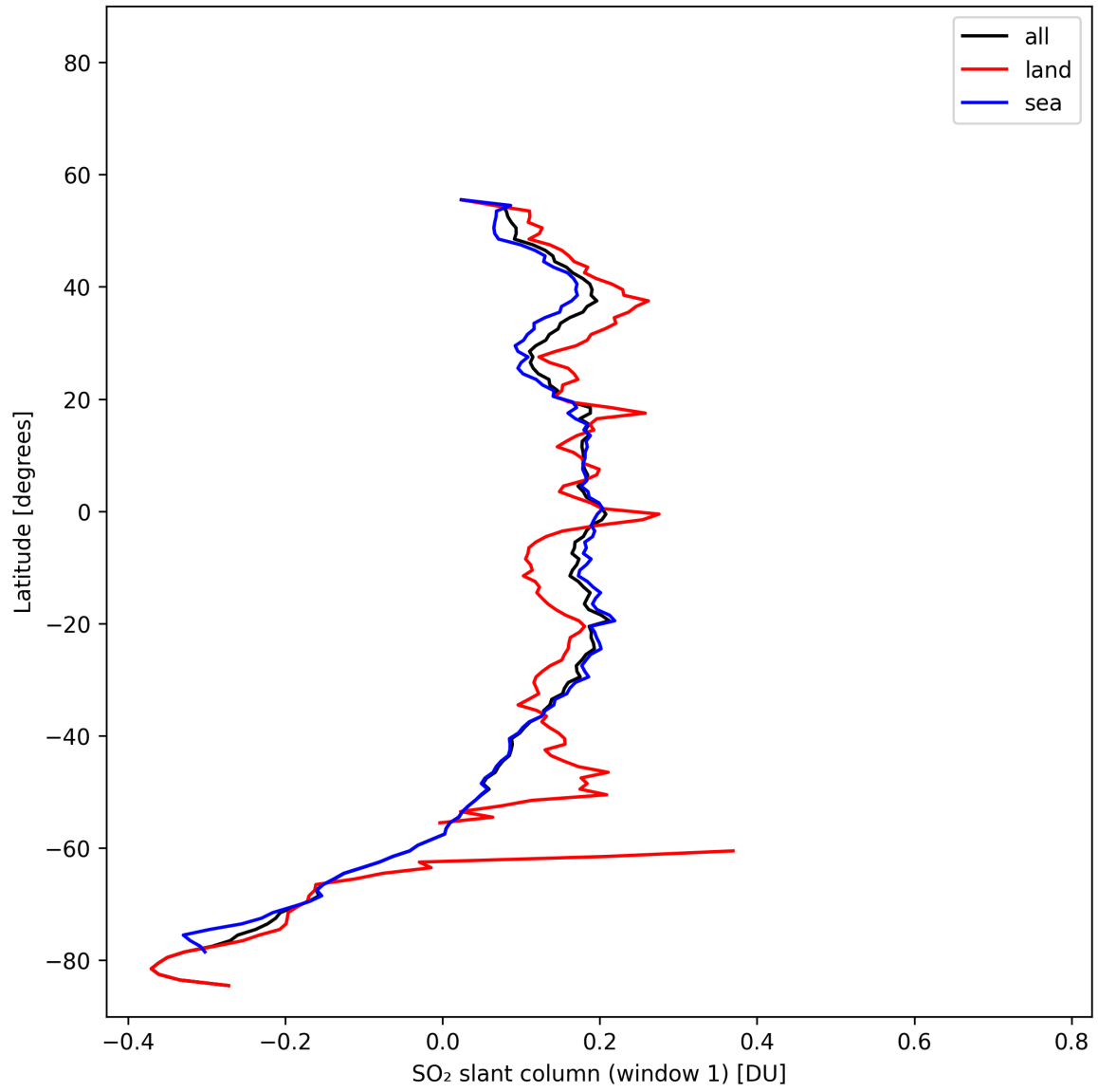
Figure 37: Zonal average of “SO 2 slant column (window 1)” for 2025-10-31 to 2025-11-02.
