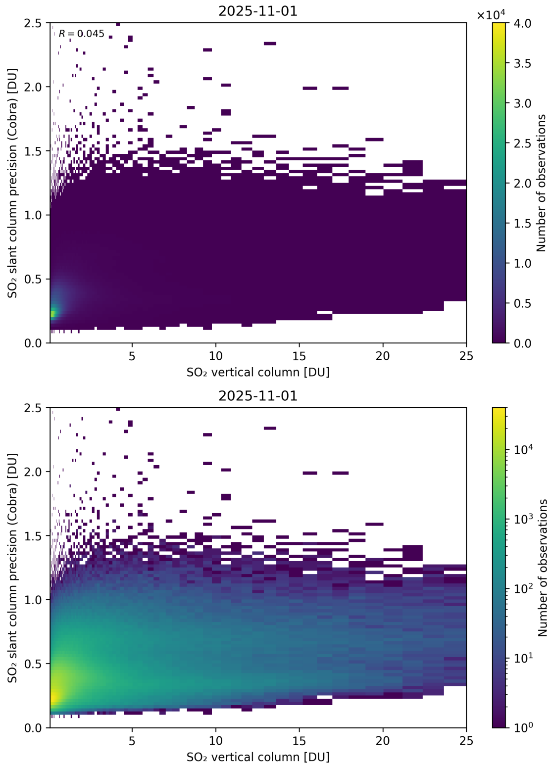
Figure 350: Scatter density plot of “SO 2 vertical column” against “SO 2 slant column precision (Cobra)” for 2025-10-31 to 2025-11-02.
