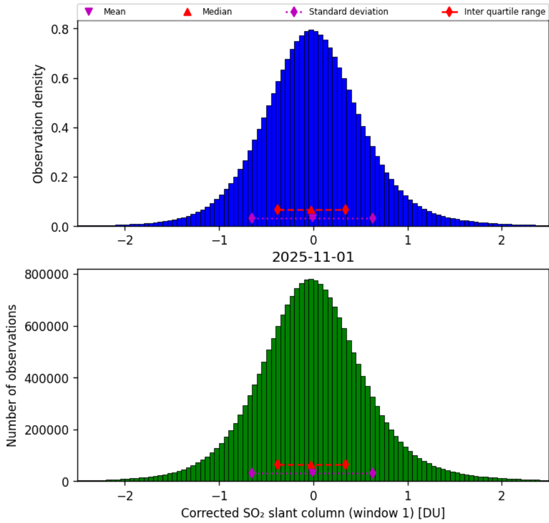
Figure 65: Histogram of “Corrected SO 2 slant column (window 1)” for 2025-10-31 to 2025-11-02
