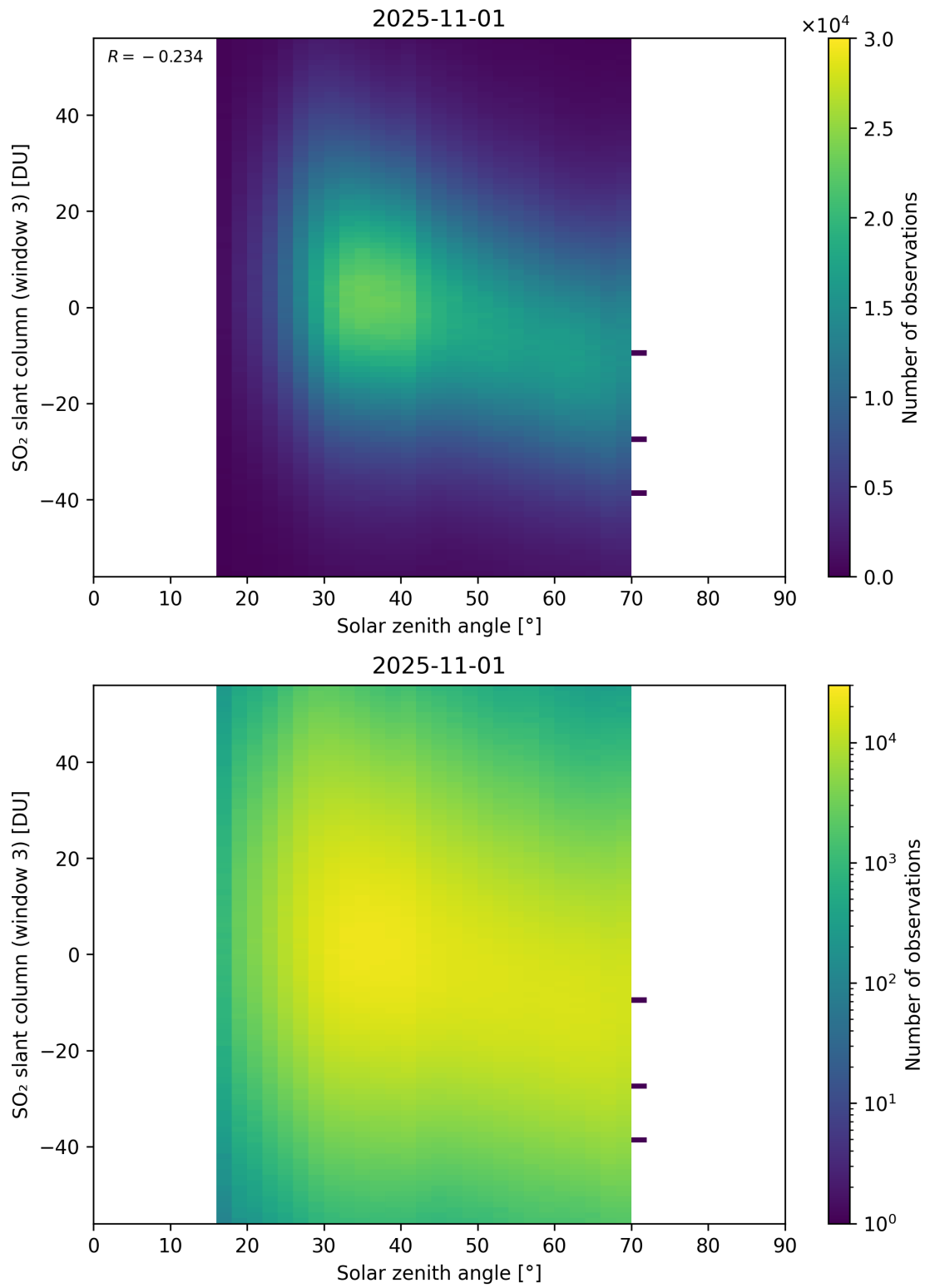
Figure 187: Scatter density plot of “Solar zenith angle” against “SO 2 slant column (window 3)” for 2025-10-31 to 2025-11-02.
