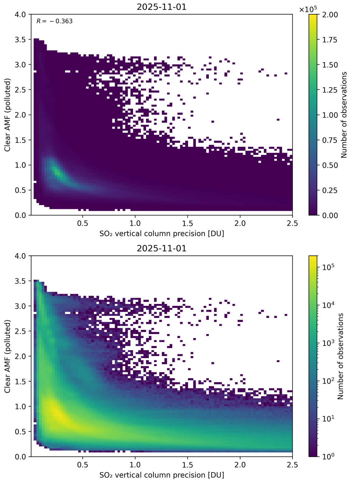
Figure 335: Scatter density plot of “SO 2 vertical column precision” against “Clear AMF (polluted)” for 2025-10-31 to 2025-11-02.
