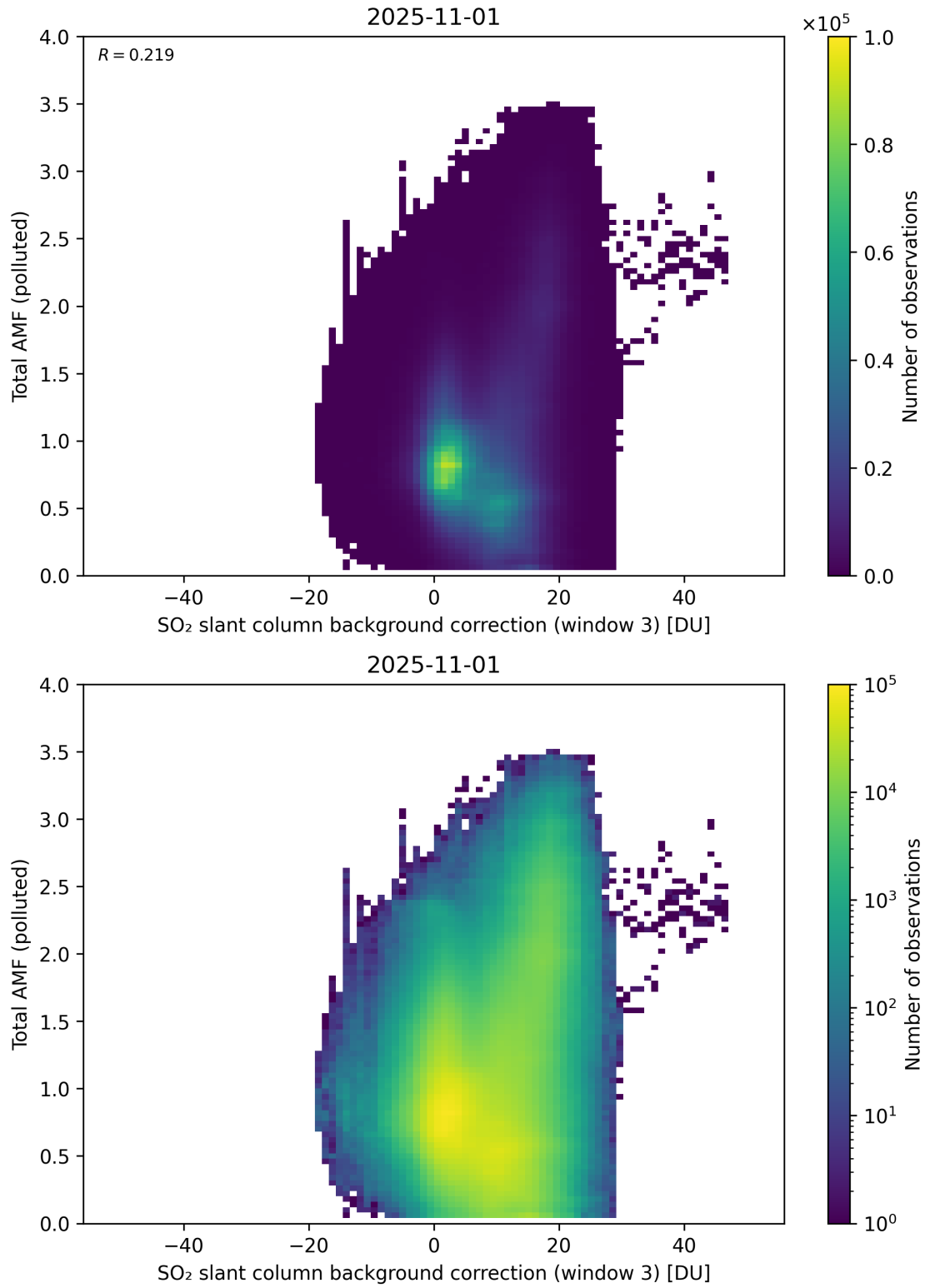
Figure 136: Scatter density plot of “SO 2 slant column background correction (window 3)” against “Total AMF (polluted)” for 2025-10-31 to 2025-11-02.
