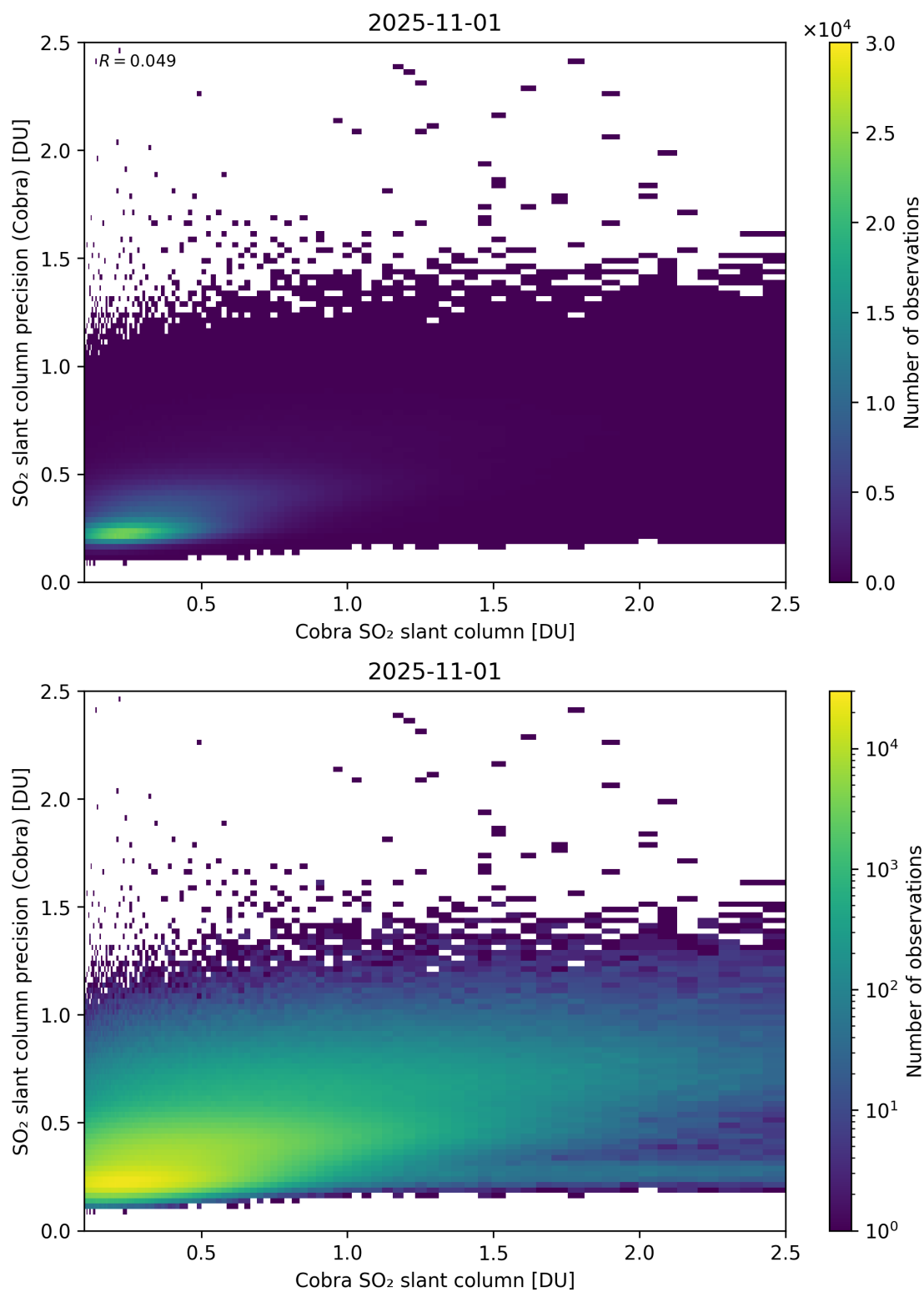
Figure 216: Scatter density plot of “Cobra SO 2 slant column” against “SO 2 slant column precision (Cobra)” for 2025-10-31 to 2025-11-02.
