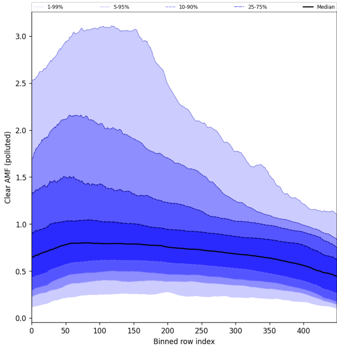
Figure 107: Along track statistics of “Clear AMF (polluted)” for 2025-10-31 to 2025-11-02
