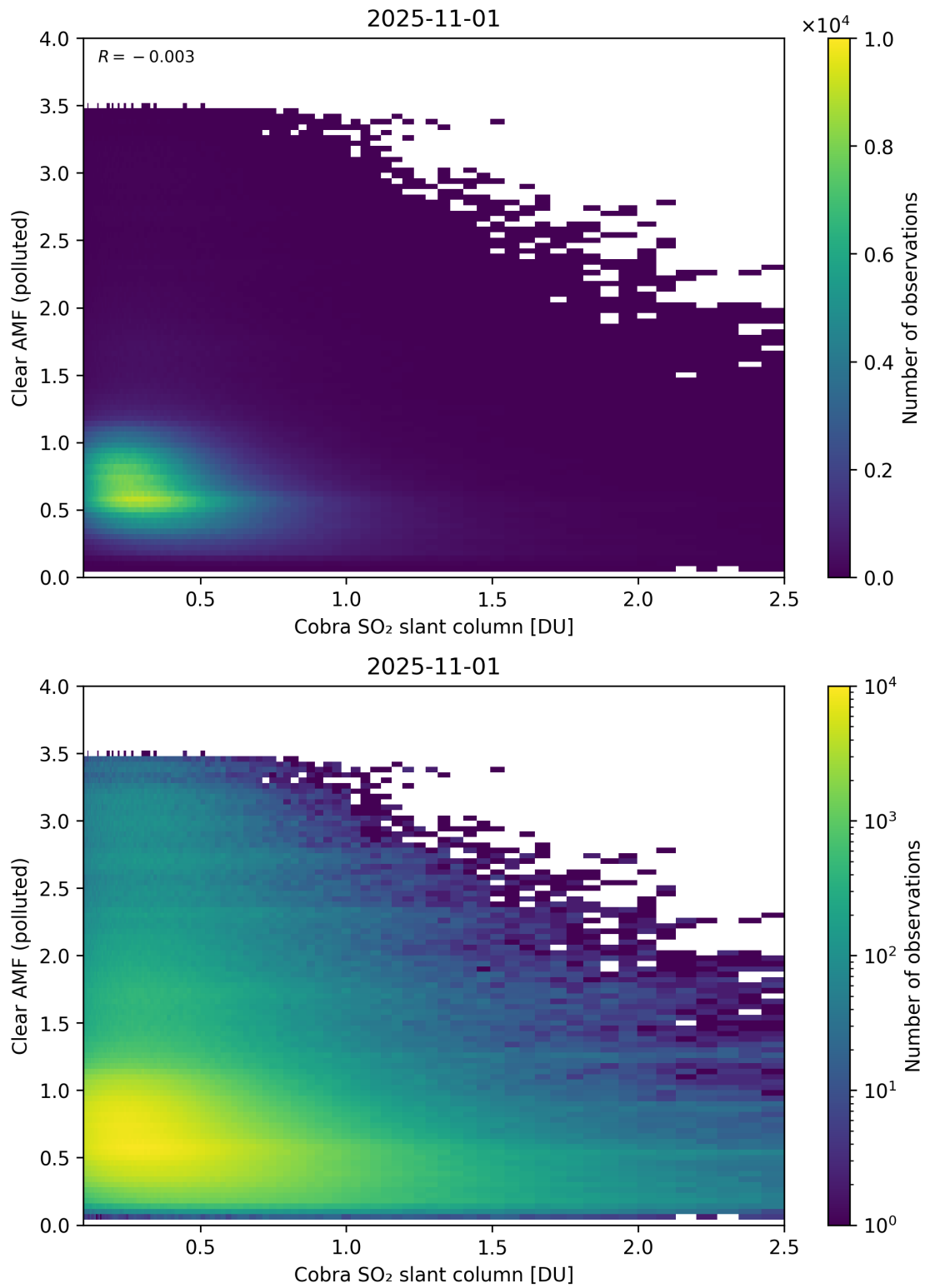
Figure 215: Scatter density plot of “Cobra SO 2 slant column” against “Clear AMF (polluted)” for 2025-10-31 to 2025-11-02.
