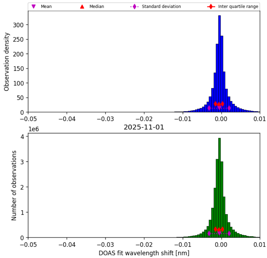
Figure 76: Histogram of “DOAS fit wavelength shift” for 2025-10-31 to 2025-11-02
