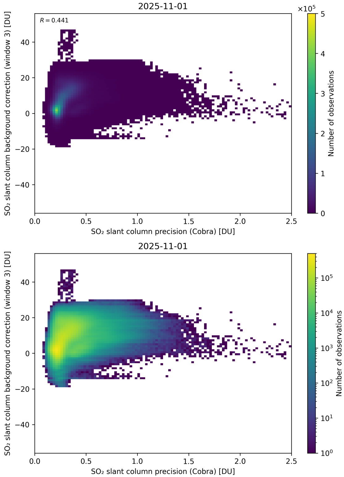
Figure 201: Scatter density plot of “SO 2 slant column precision (Cobra)” against “SO 2 slant column background correction (window 3)” for 2025-10-31 to 2025-11-02.
