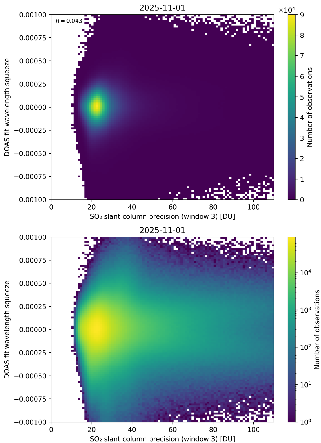
Figure 309: Scatter density plot of “SO 2 slant column precision (window 3)” against “DOAS fit wavelength squeeze” for 2025-10-31 to 2025-11-02.
