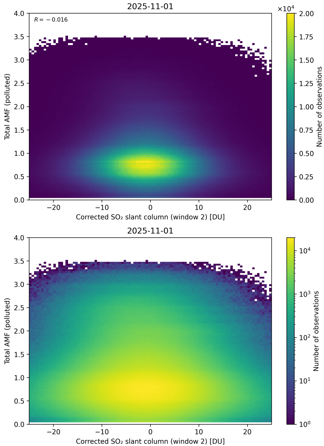
Figure 253: Scatter density plot of “Corrected SO 2 slant column (window 2)” against “Total AMF (polluted)” for 2025-10-31 to 2025-11-02.
