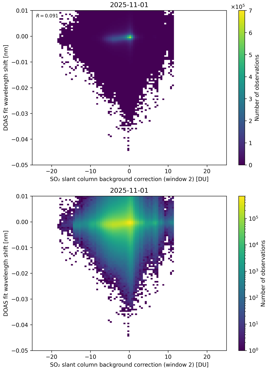
Figure 123: Scatter density plot of “SO 2 slant column background correction (window 2)” against “DOAS fit wavelength shift” for 2025-10-31 to 2025-11-02.
