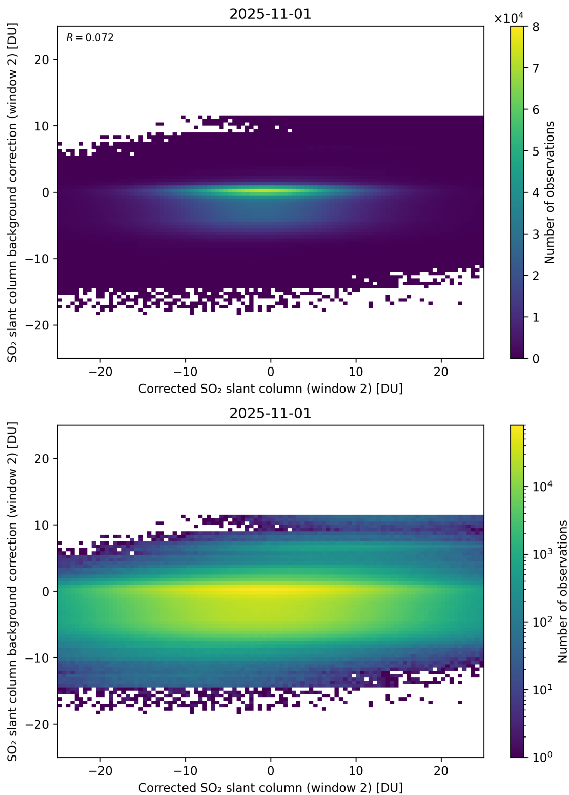
Figure 244: Scatter density plot of “Corrected SO 2 slant column (window 2)” against “SO 2 slant column background correction (window 2)” for 2025-10-31 to 2025-11-02.
