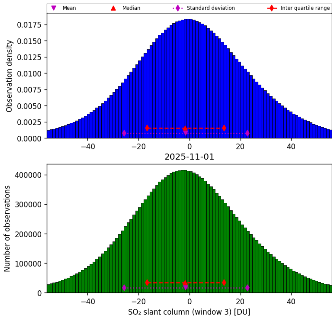
Figure 71: Histogram of “SO 2 slant column (window 3)” for 2025-10-31 to 2025-11-02
