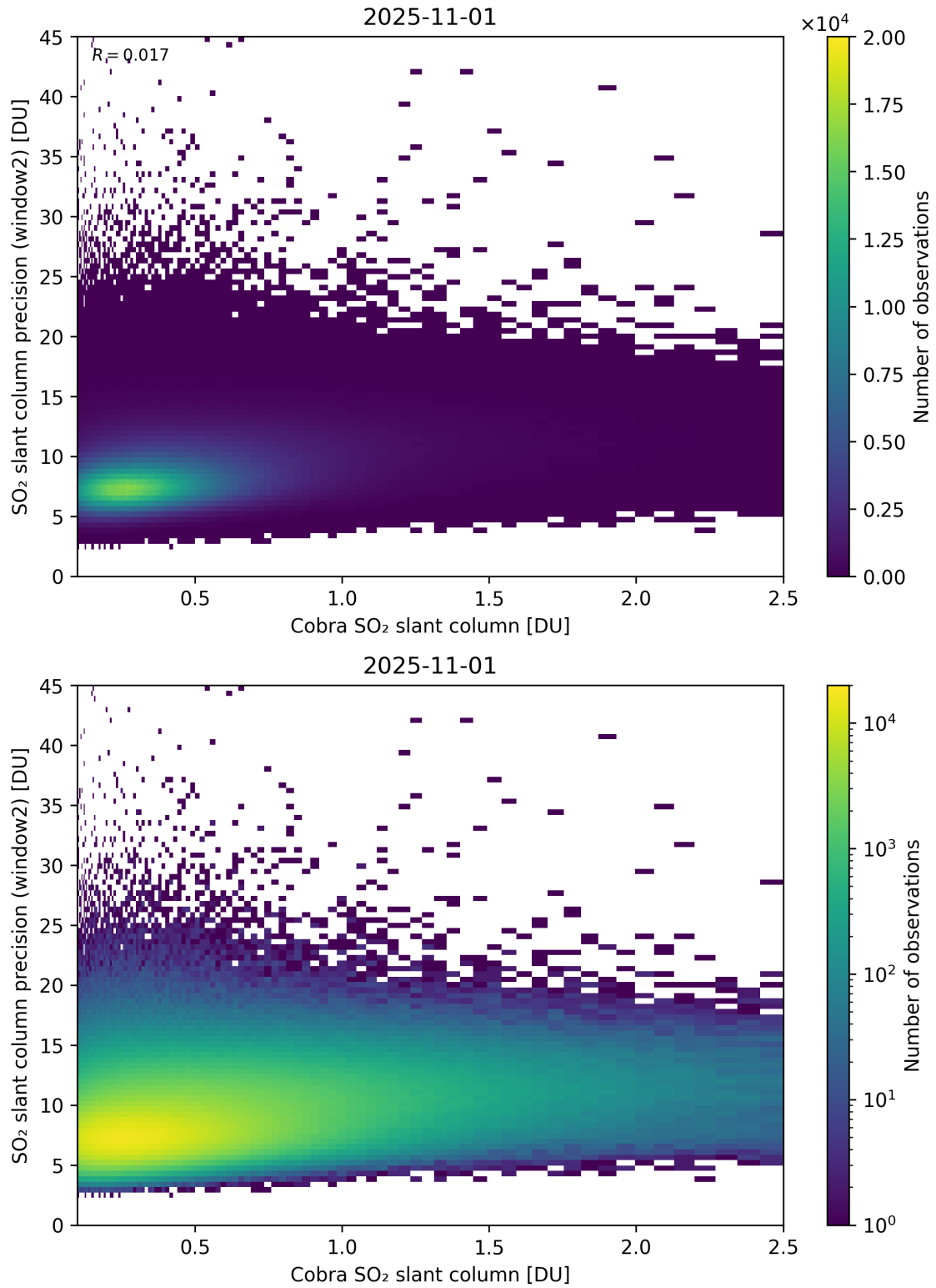
Figure 221: Scatter density plot of “Cobra SO 2 slant column” against “SO 2 slant column precision (window2)” for 2025-10-31 to 2025-11-02.
