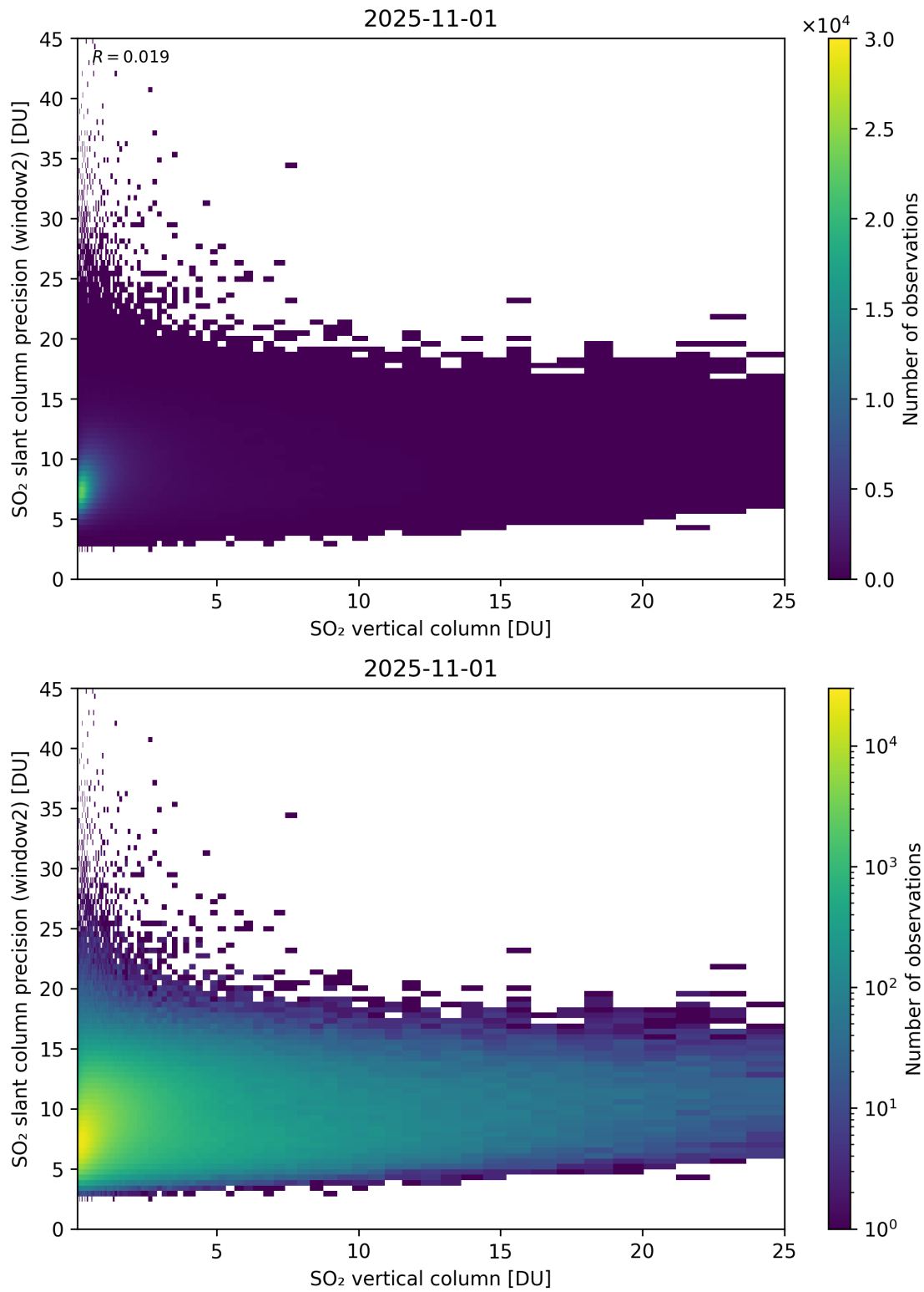
Figure 356: Scatter density plot of “SO 2 vertical column” against “SO 2 slant column precision (window2)” for 2025-10-31 to 2025-11-02.
