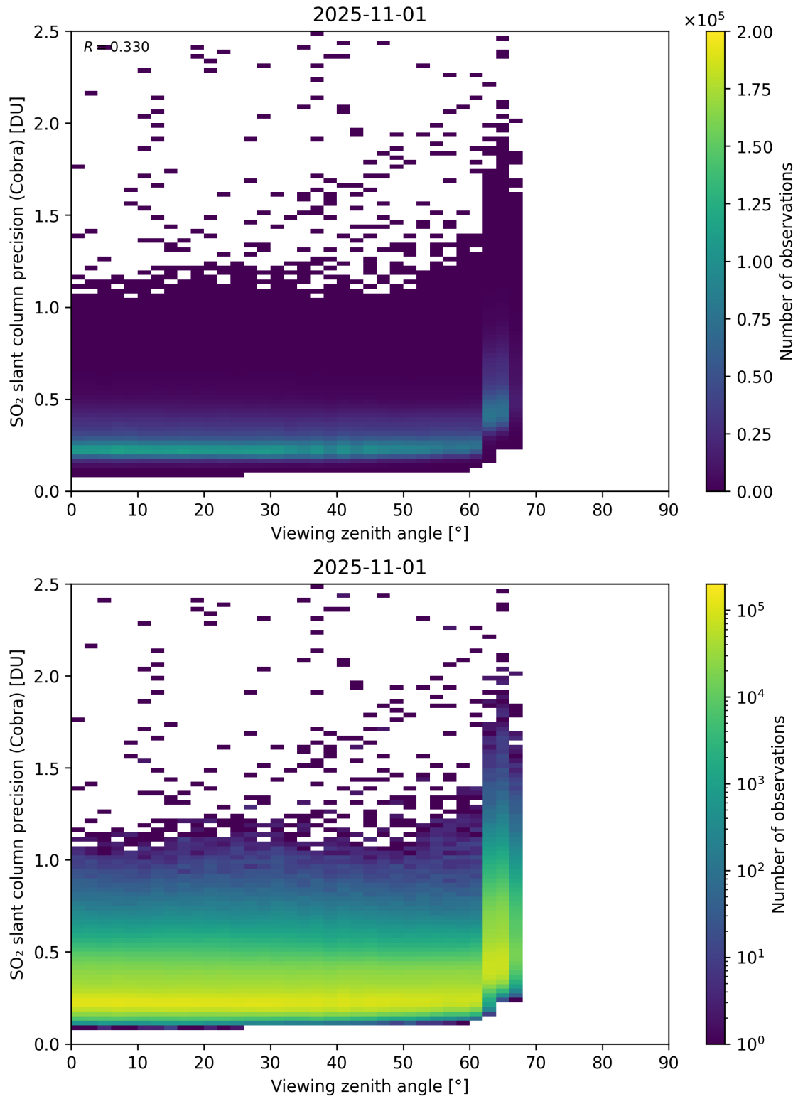
Figure 372: Scatter density plot of “Viewing zenith angle” against “SO 2 slant column precision (Cobra)” for 2025-10-31 to 2025-11-02.
