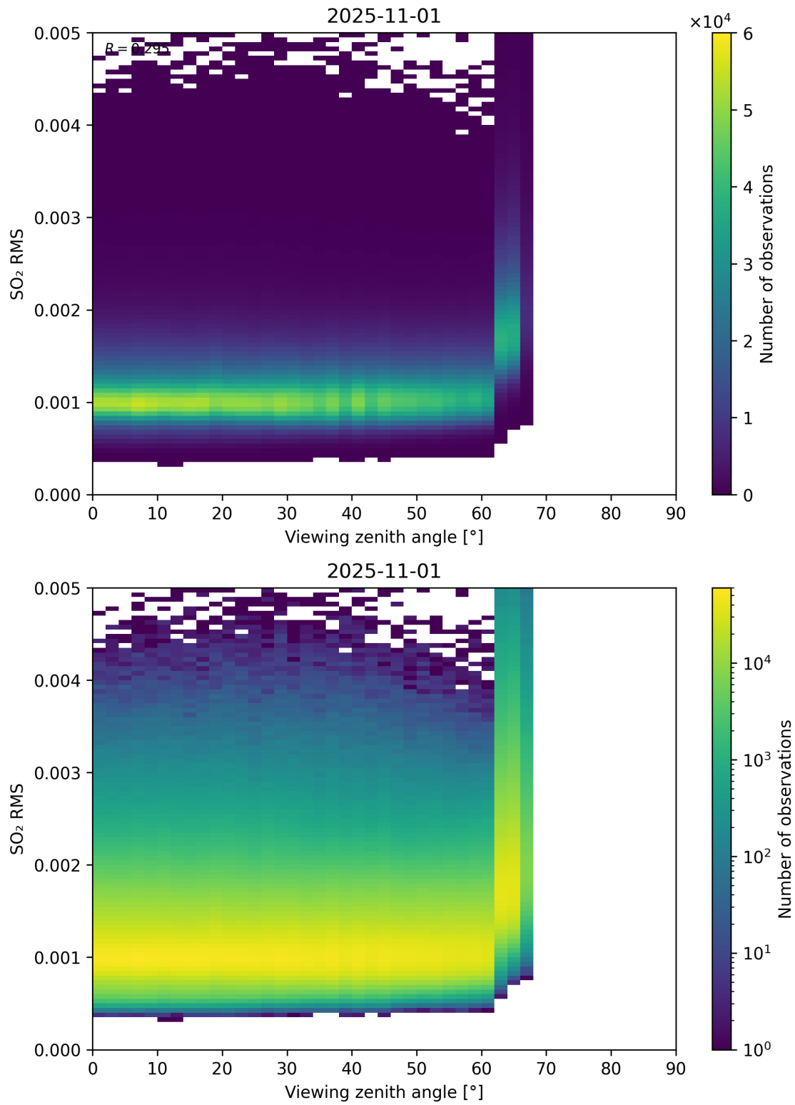
Figure 367: Scatter density plot of “Viewing zenith angle” against “SO 2 RMS” for 2025-10-31 to 2025-11-02.
