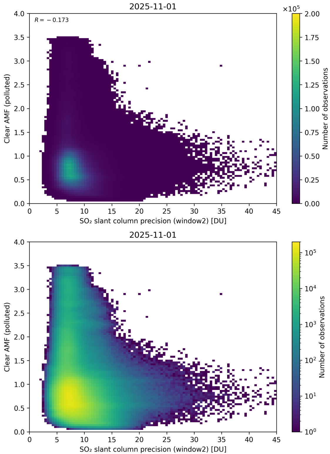
Figure 296: Scatter density plot of “SO 2 slant column precision (window2)” against “Clear AMF (polluted)” for 2025-10-31 to 2025-11-02.
