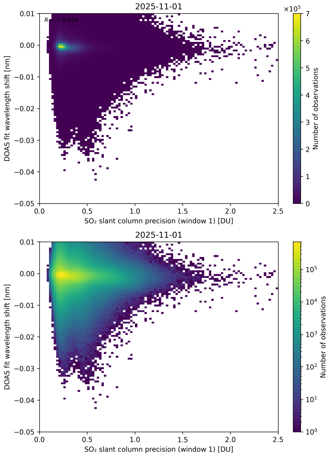
Figure 271: Scatter density plot of “SO 2 slant column precision (window 1)” against “DOAS fit wavelength shift” for 2025-10-31 to 2025-11-02.
