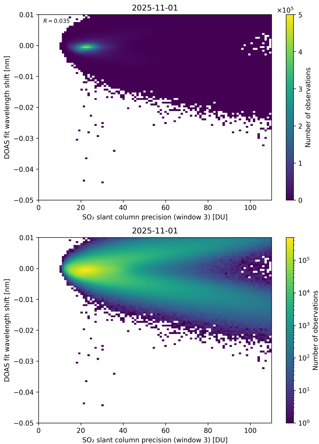
Figure 308: Scatter density plot of “SO 2 slant column precision (window 3)” against “DOAS fit wavelength shift” for 2025-10-31 to 2025-11-02.
