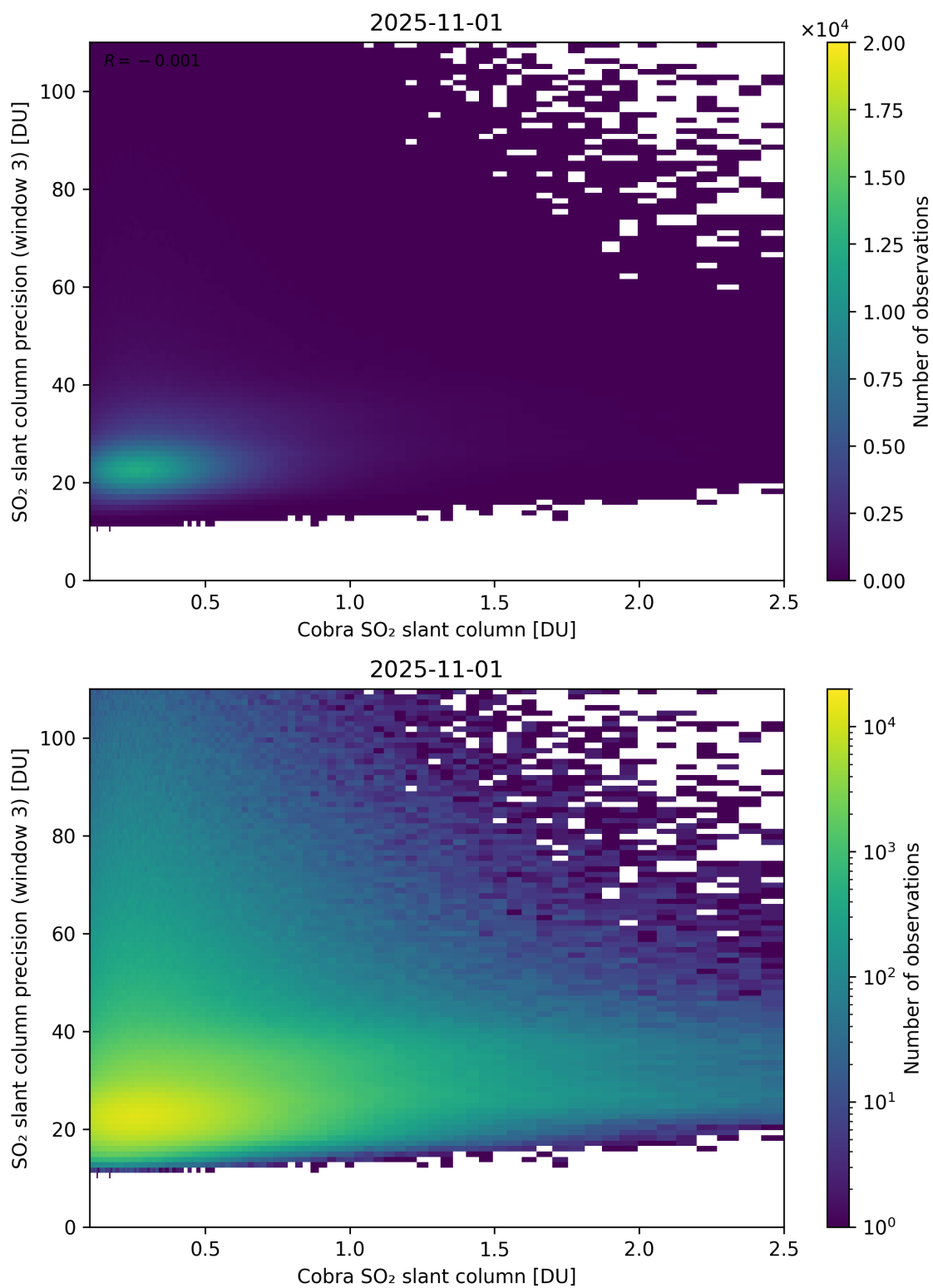
Figure 223: Scatter density plot of “Cobra SO 2 slant column” against “SO 2 slant column precision (window 3)” for 2025-10-31 to 2025-11-02.
