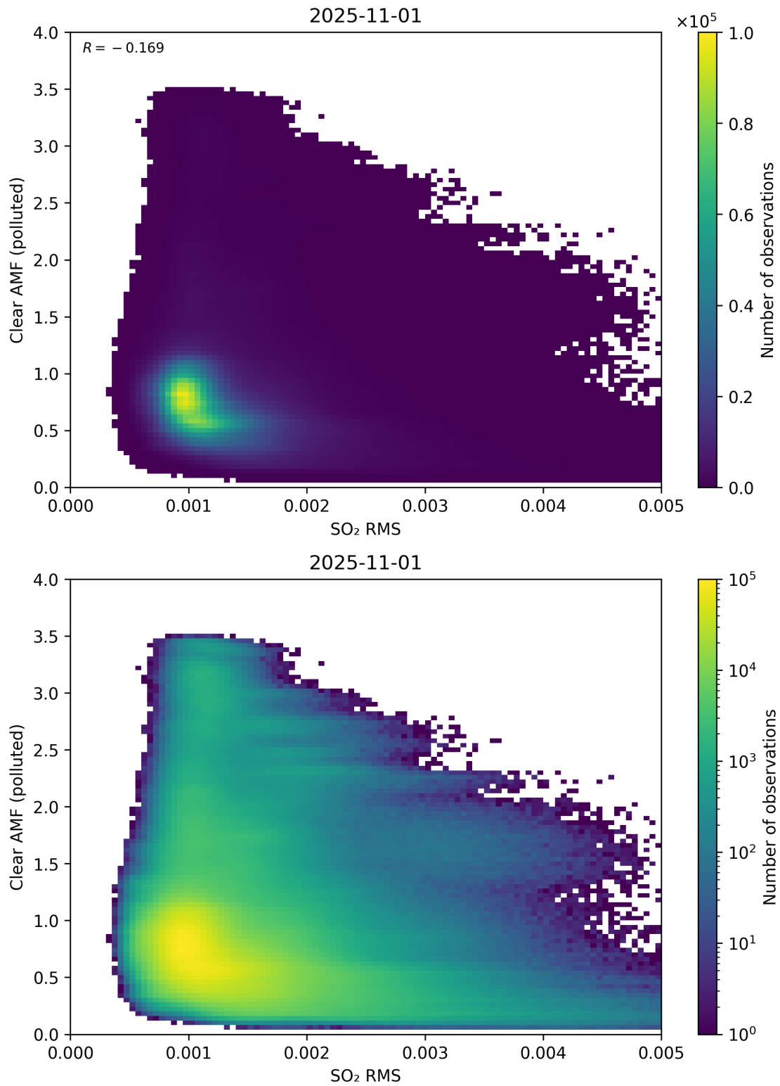
Figure 147: Scatter density plot of “SO 2 RMS” against “Clear AMF (polluted)” for 2025-10-31 to 2025-11-02.
