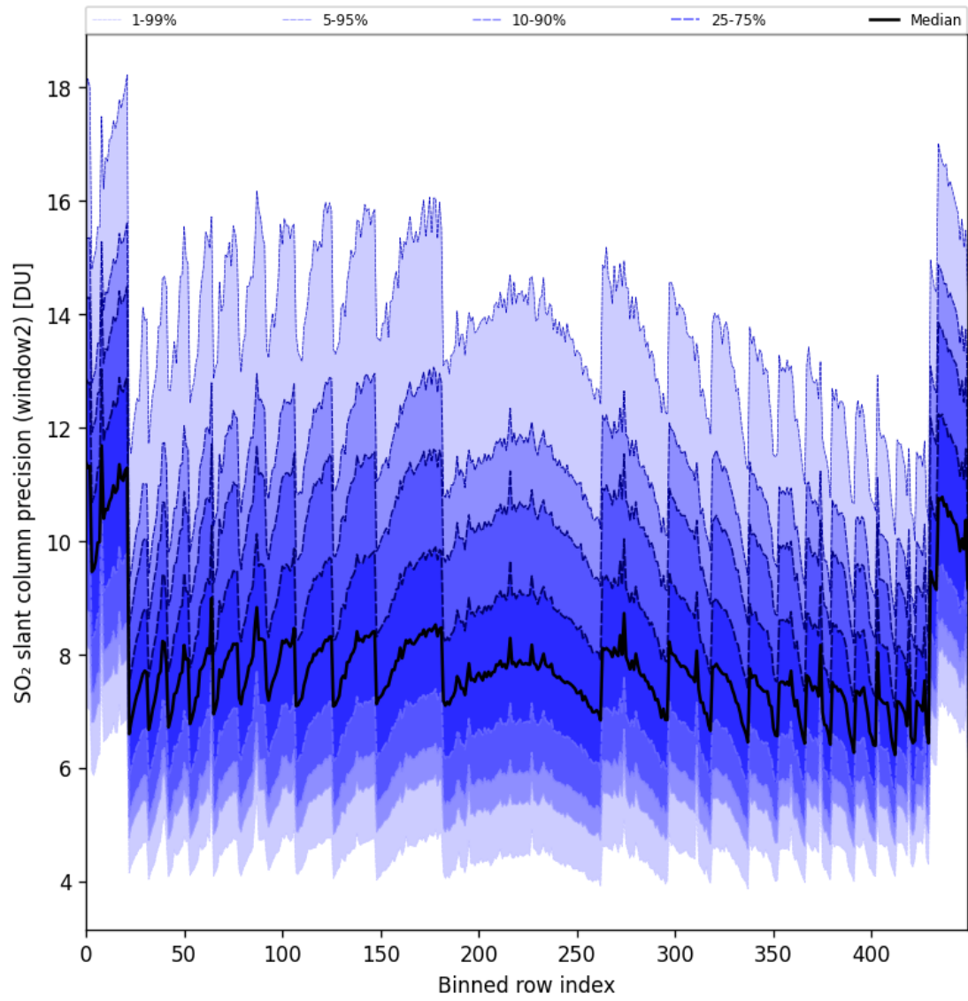
Figure 94: Along track statistics of “SO 2 slant column precision (window2)” for 2025-10-31 to 2025-11-02
