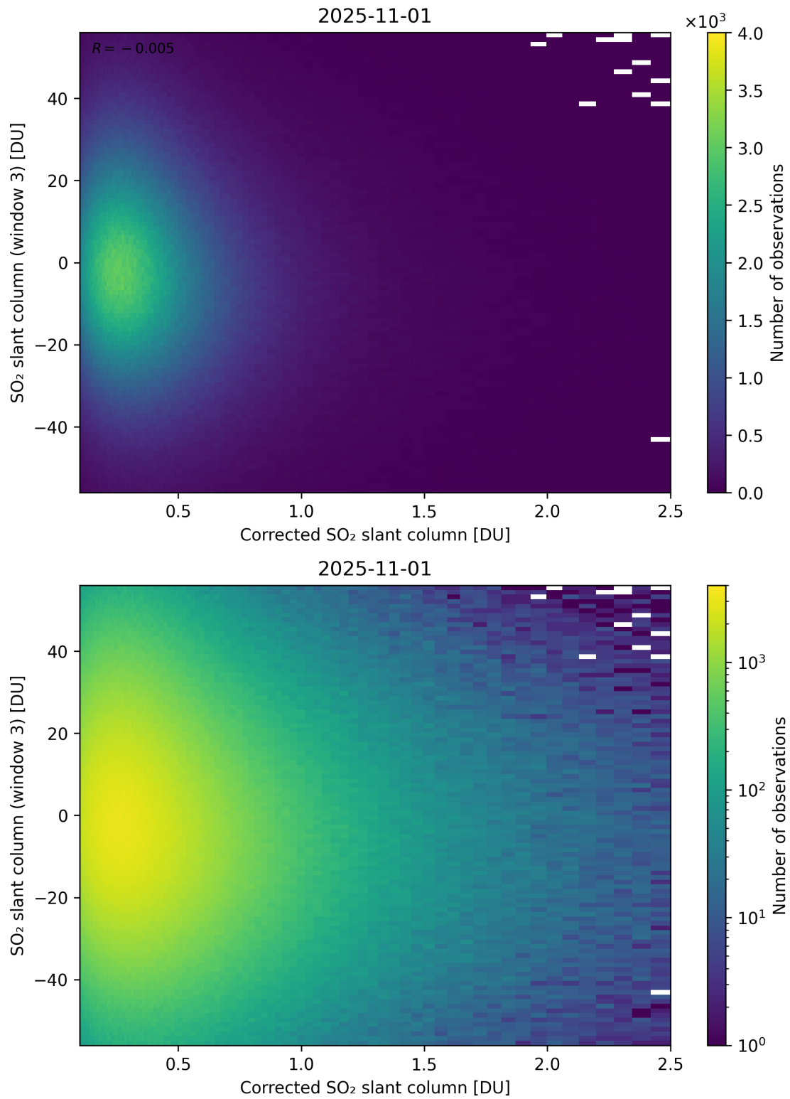
Figure 240: Scatter density plot of “Corrected SO 2 slant column” against “SO 2 slant column (window 3)” for 2025-10-31 to 2025-11-02.
