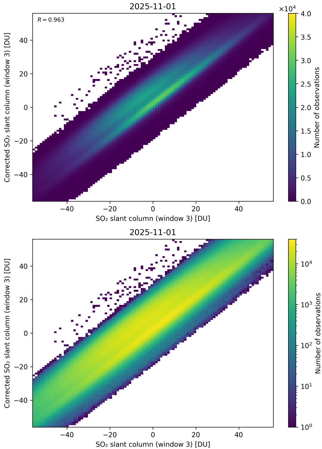
Figure 316: Scatter density plot of “SO 2 slant column (window 3)” against “Corrected SO 2 slant column (window 3)” for 2025-10-31 to 2025-11-02.
