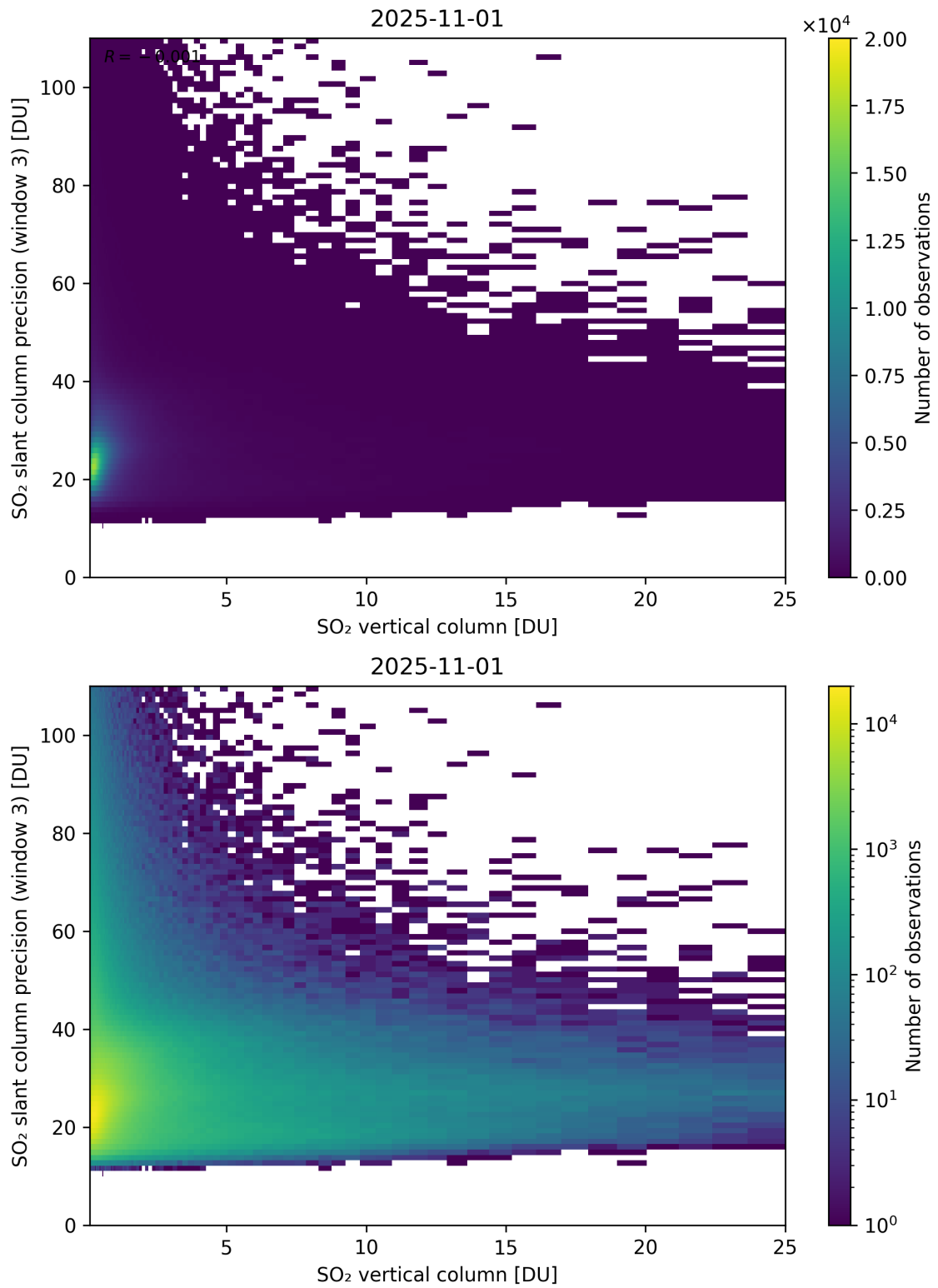
Figure 358: Scatter density plot of “SO 2 vertical column” against “SO 2 slant column precision (window 3)” for 2025-10-31 to 2025-11-02.
