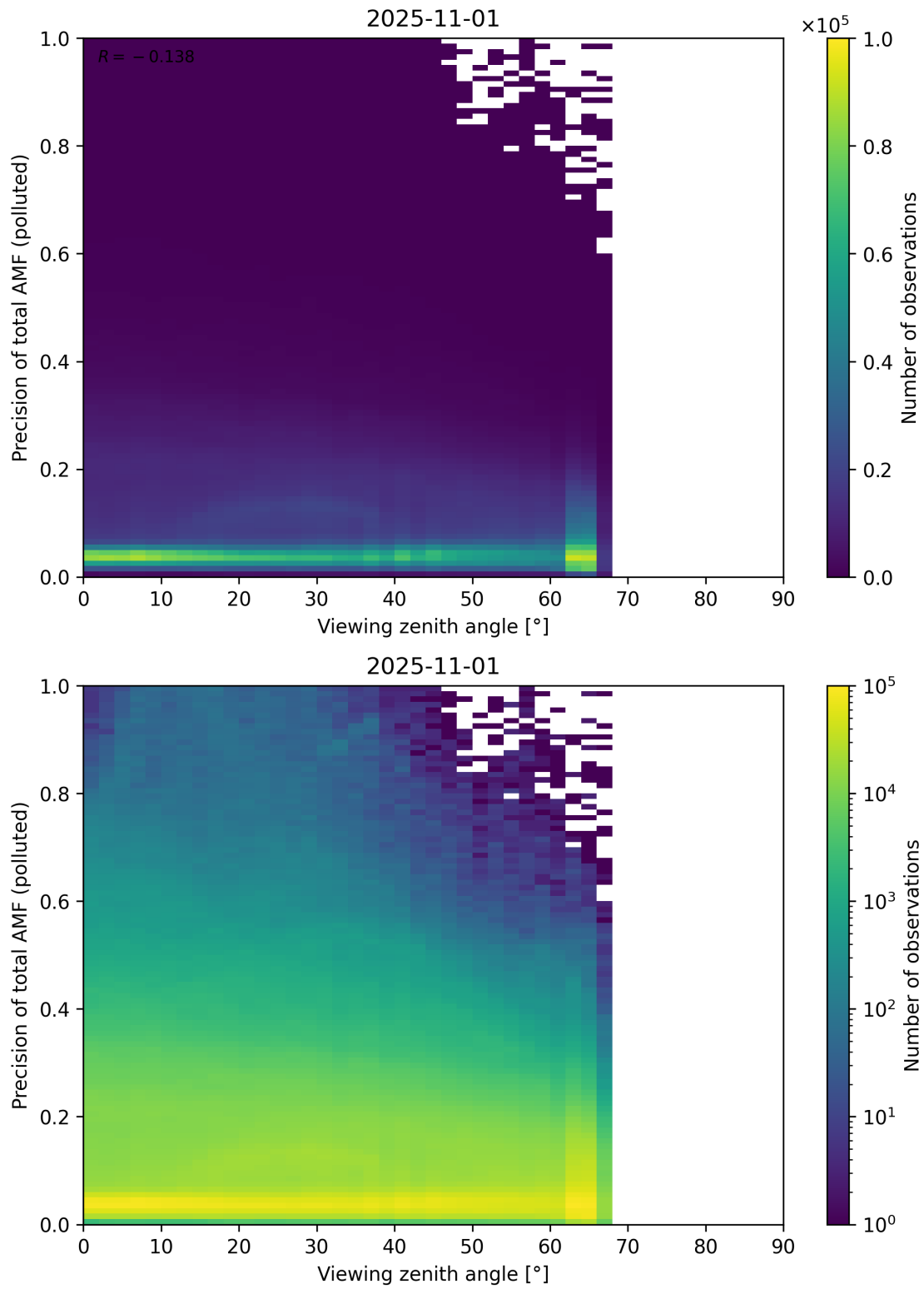
Figure 382: Scatter density plot of “Viewing zenith angle” against “Precision of total AMF (polluted)” for 2025-10-31 to 2025-11-02.
