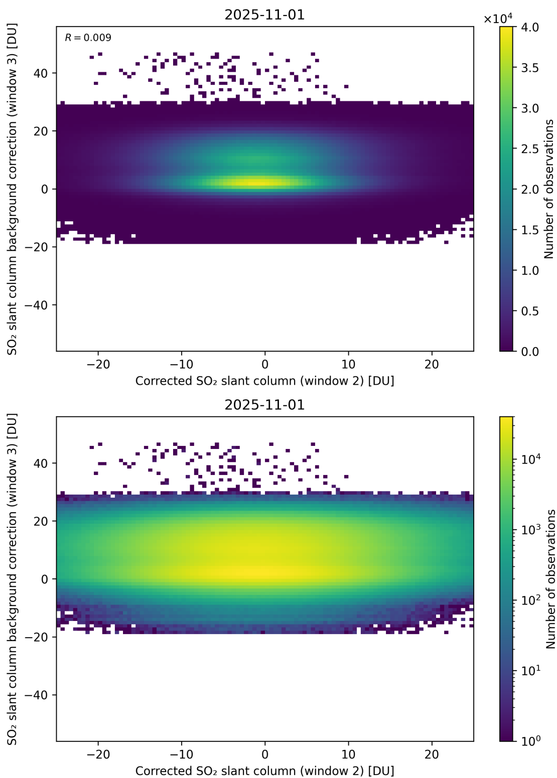
Figure 245: Scatter density plot of “Corrected SO 2 slant column (window 2)” against “SO 2 slant column background correction (window 3)” for 2025-10-31 to 2025-11-02.
