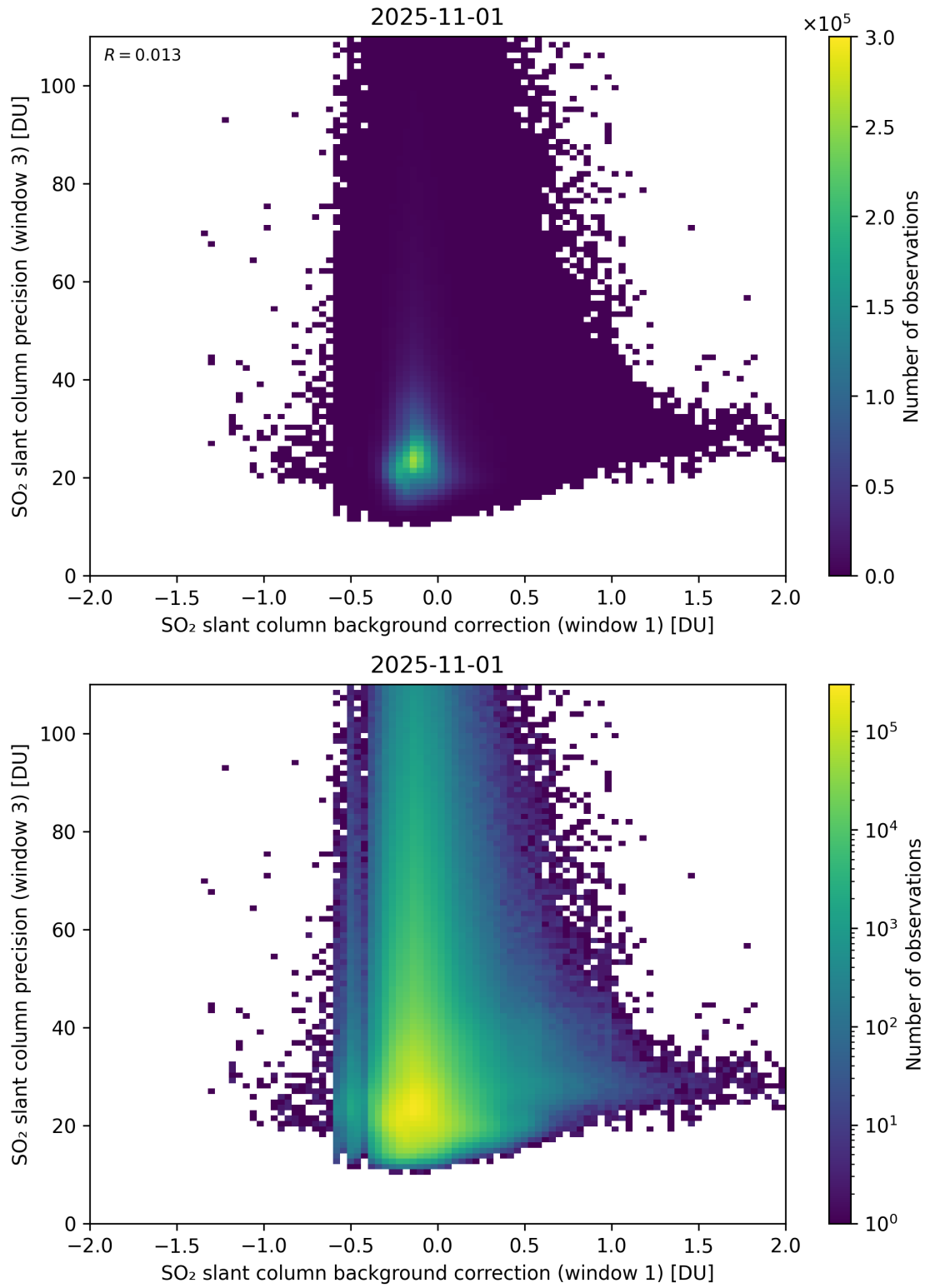
Figure 119: Scatter density plot of “SO 2 slant column background correction (window 1)” against “SO 2 slant column precision (window 3)” for 2025-10-31 to 2025-11-02.
