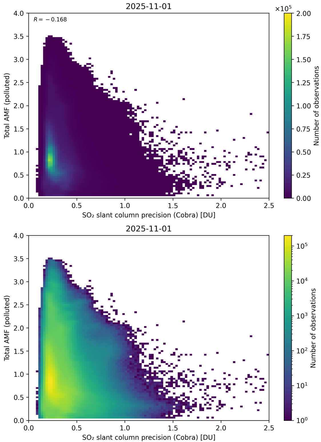
Figure 213: Scatter density plot of “SO 2 slant column precision (Cobra)” against “Total AMF (polluted)” for 2025-10-31 to 2025-11-02.
