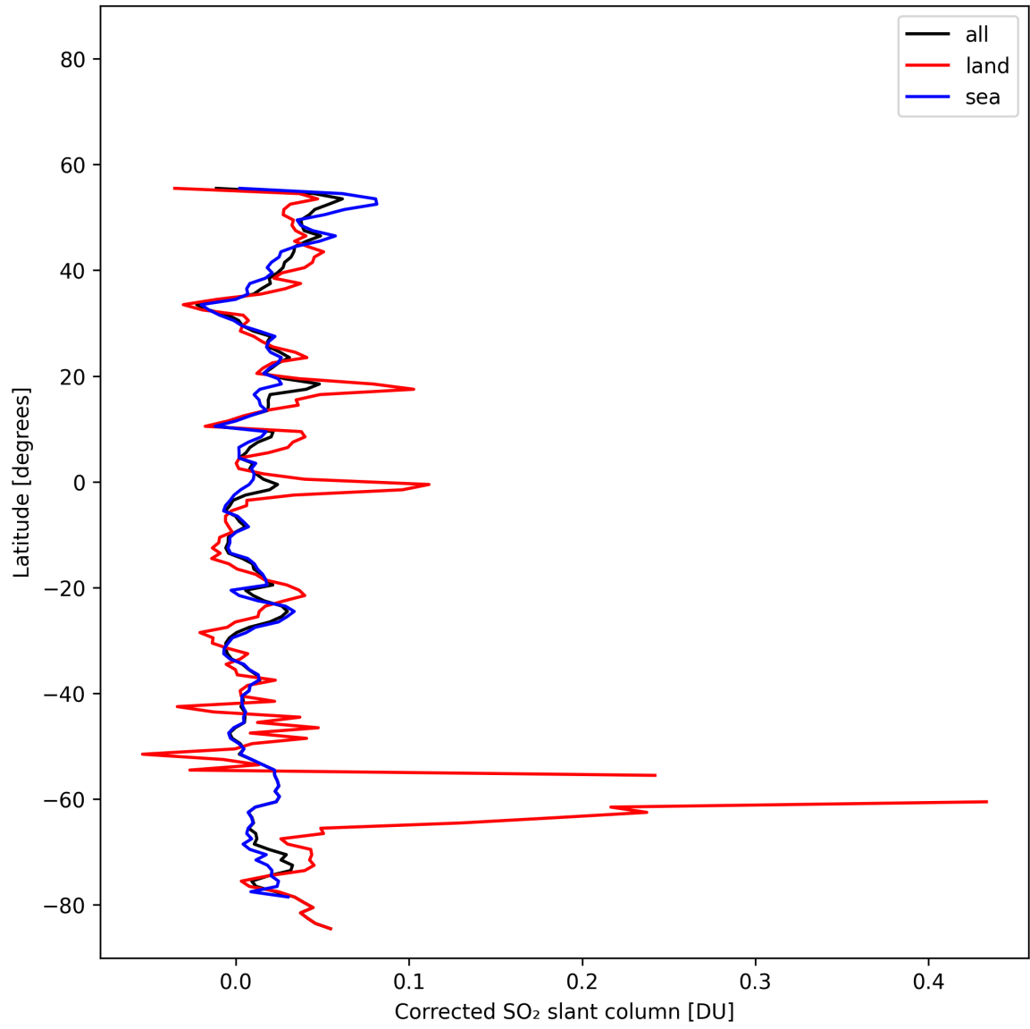
Figure 34: Zonal average of “Corrected SO 2 slant column” for 2025-10-31 to 2025-11-02.
