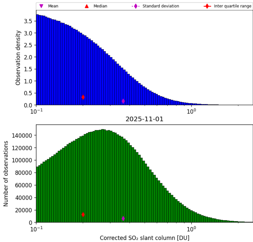
Figure 60: Histogram of "Corrected SO 2 slant column" for 2025-10-31 to 2025-11-02
