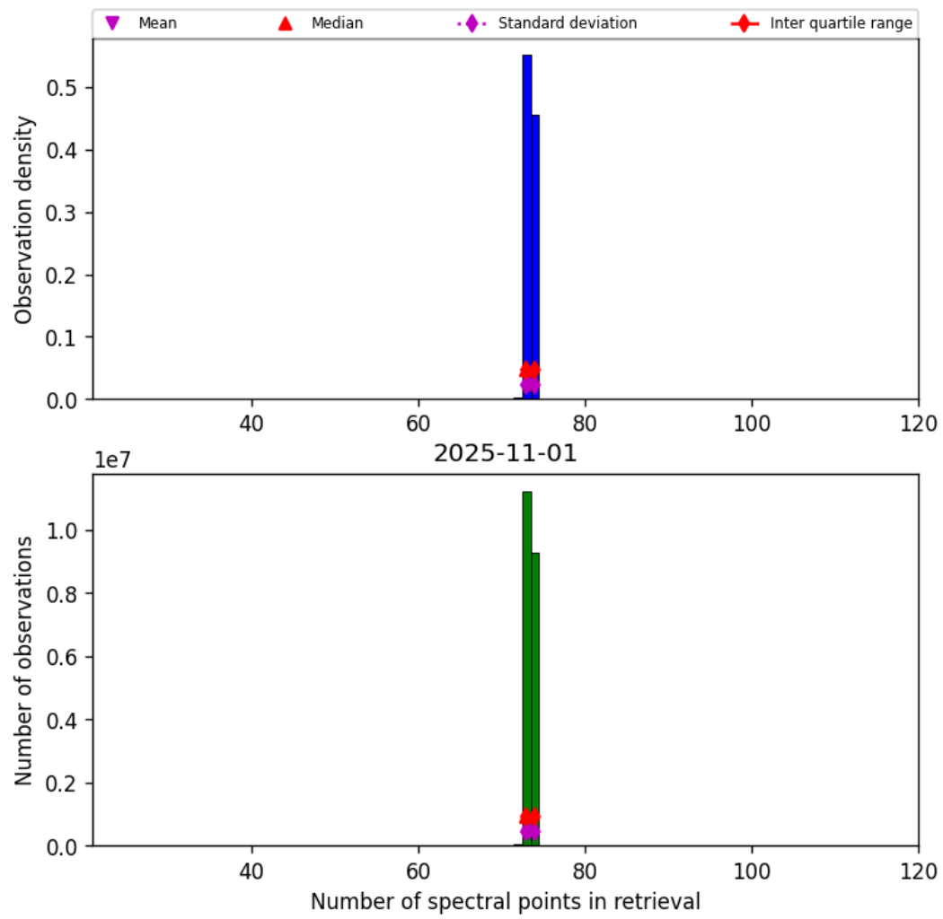
Figure 82: Histogram of “Number of spectral points in retrieval” for 2025-10-31 to 2025-11-02
