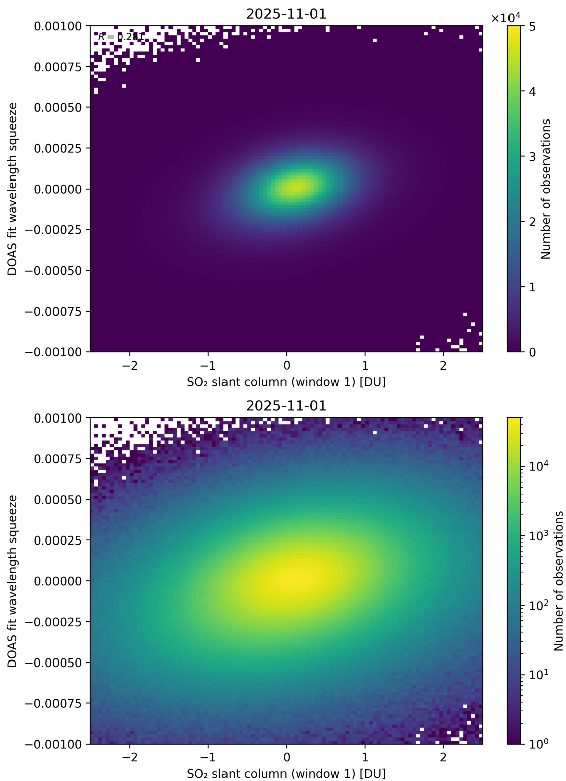
Figure 266: Scatter density plot of “SO 2 slant column (window 1)” against “DOAS fit wavelength squeeze” for 2025-10-31 to 2025-11-02.
