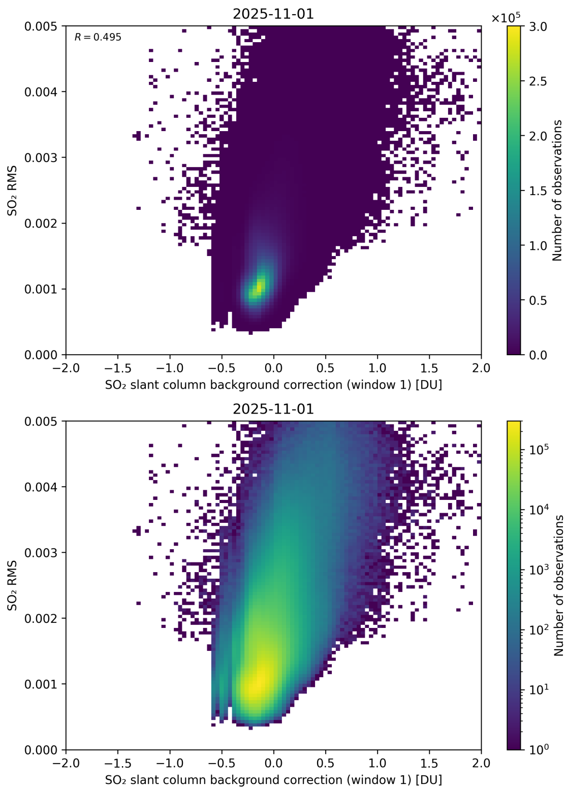
Figure 113: Scatter density plot of “SO 2 slant column background correction (window 1)” against “SO 2 RMS” for 2025-10-31 to 2025-11-02.
