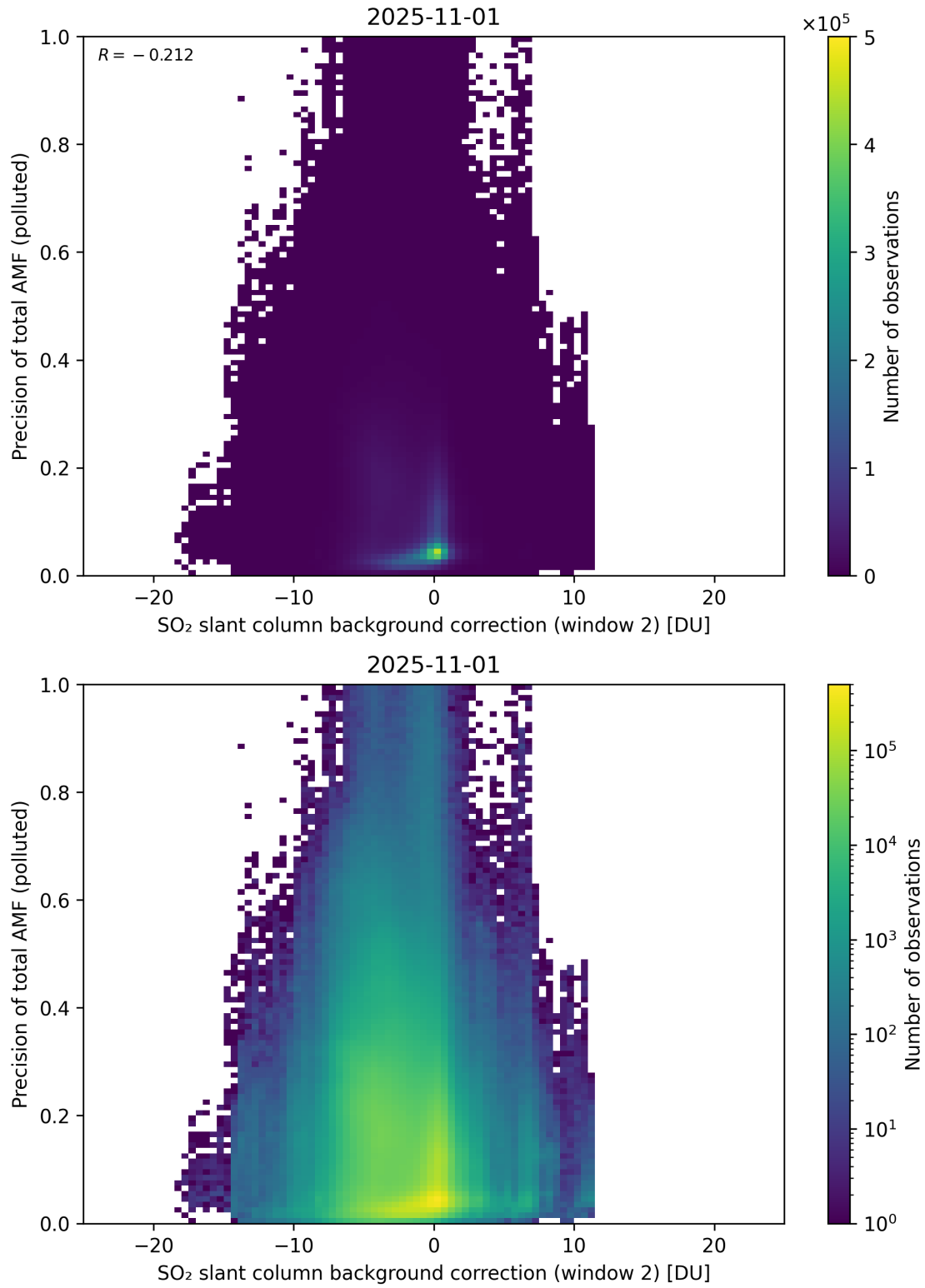
Figure 131: Scatter density plot of “SO 2 slant column background correction (window 2)” against “Precision of total AMF (polluted)” for 2025-10-31 to 2025-11-02.
