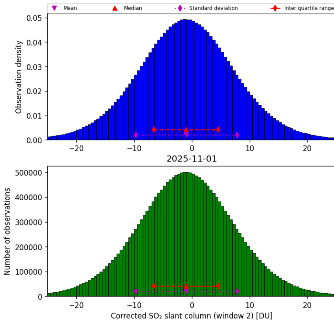
Figure 69: Histogram of “Corrected SO 2 slant column (window 2)” for 2025-10-31 to 2025-11-02
