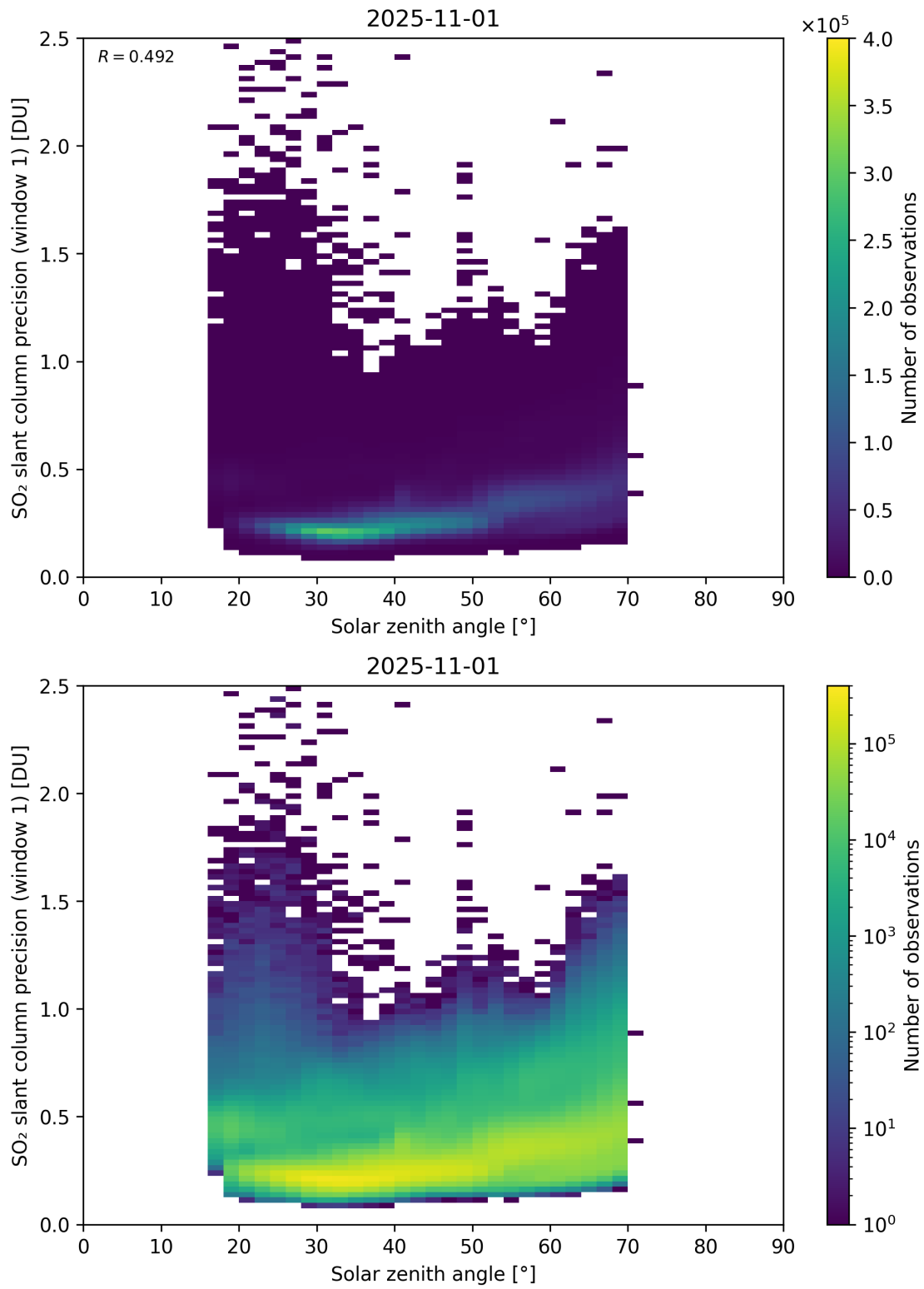
Figure 185: Scatter density plot of “Solar zenith angle” against “SO 2 slant column precision (window 1)” for 2025-10-31 to 2025-11-02.
