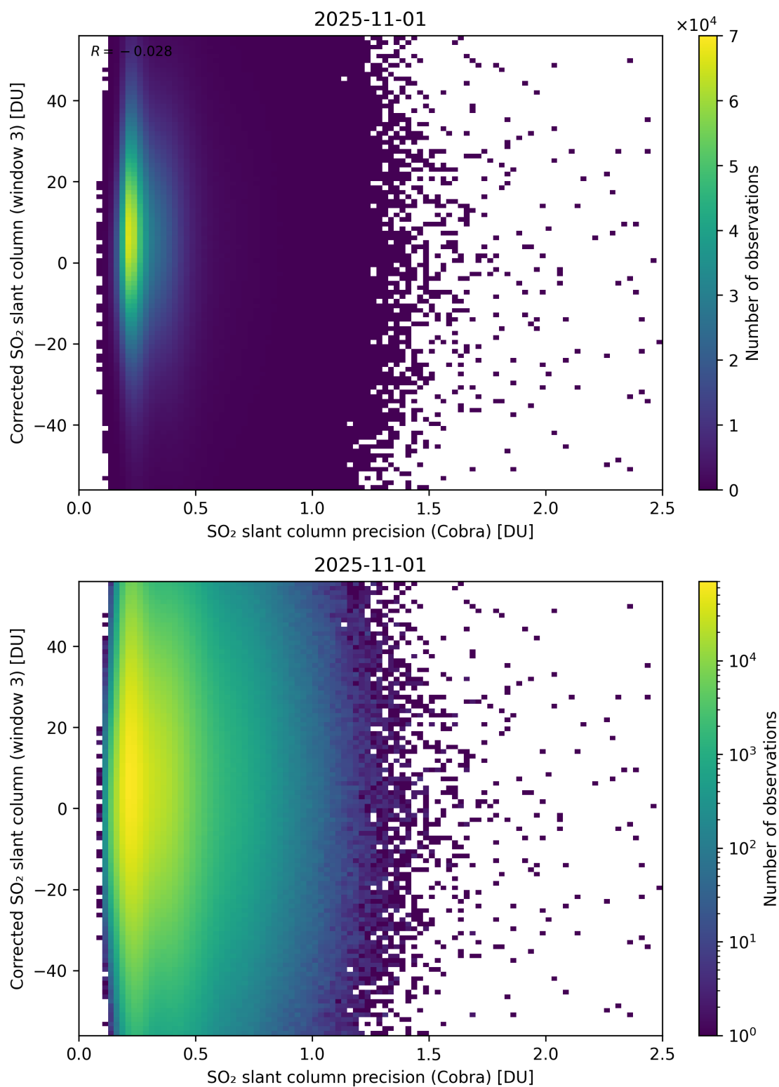
Figure 207: Scatter density plot of “SO 2 slant column precision (Cobra)” against “Corrected SO 2 slant column (window 3)” for 2025-10-31 to 2025-11-02.
