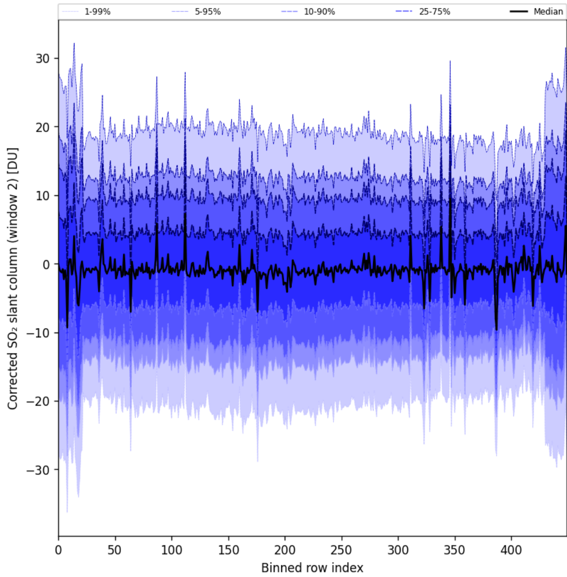
Figure 95: Along track statistics of “Corrected SO 2 slant column (window 2)” for 2025-10-31 to 2025-11-02
