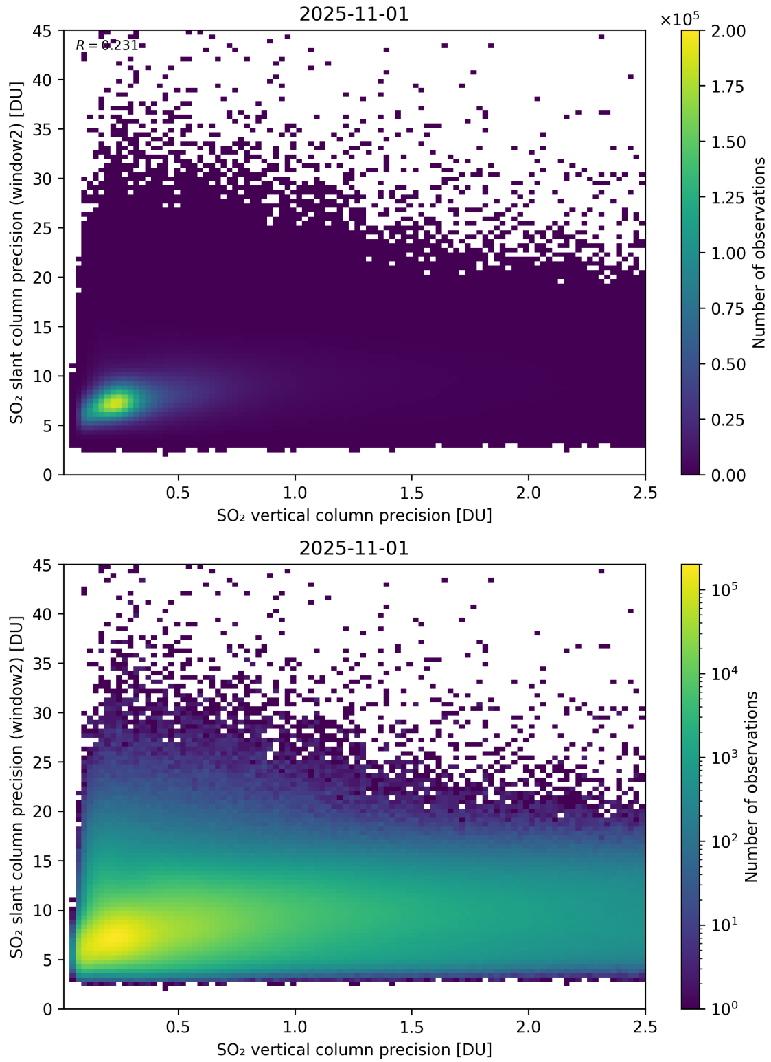
Figure 343: Scatter density plot of “SO 2 vertical column precision” against “SO 2 slant column precision (window2)” for 2025-10-31 to 2025-11-02.
