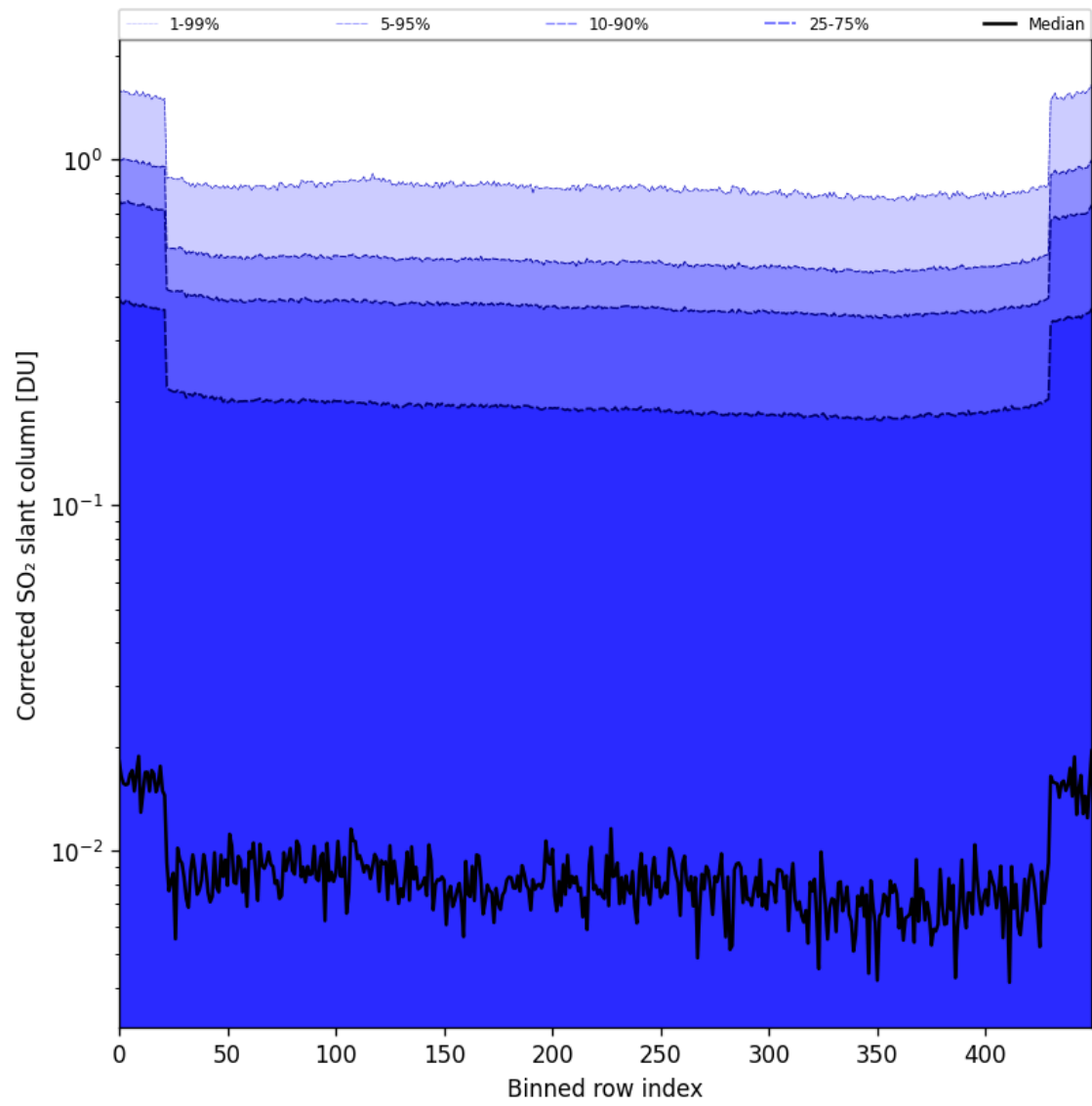
Figure 86: Along track statistics of “Corrected SO 2 slant column” for 2025-10-31 to 2025-11-02
