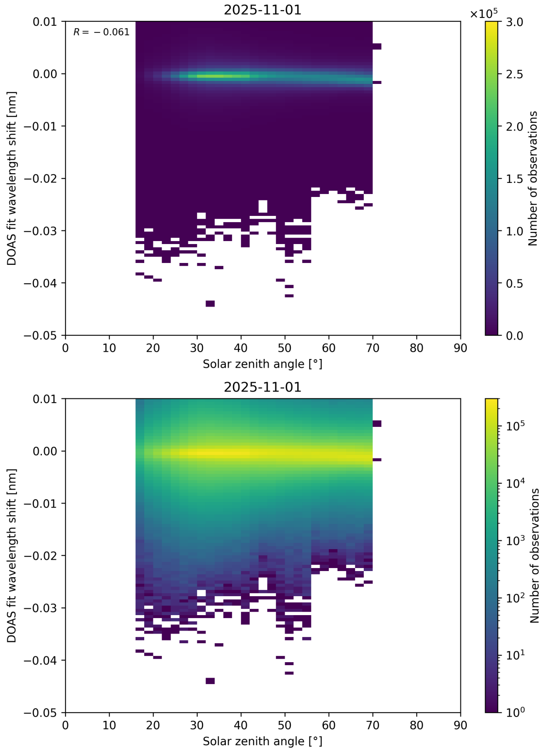
Figure 174: Scatter density plot of “Solar zenith angle” against “DOAS fit wavelength shift” for 2025-10-31 to 2025-11-02.
