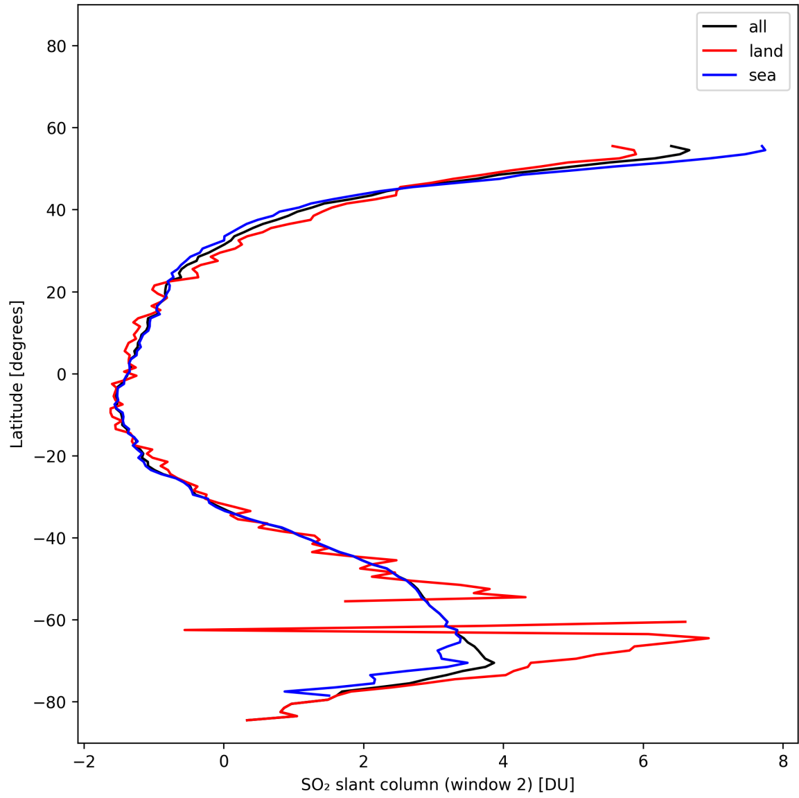
Figure 41: Zonal average of “SO 2 slant column (window 2)” for 2025-10-31 to 2025-11-02.
