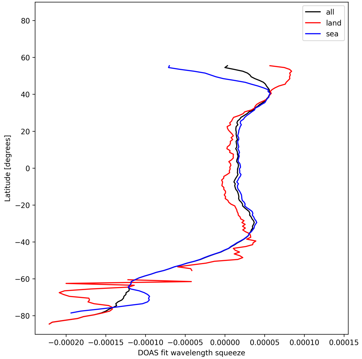
Figure 51: Zonal average of “DOAS fit wavelength squeeze” for 2025-10-31 to 2025-11-02.
