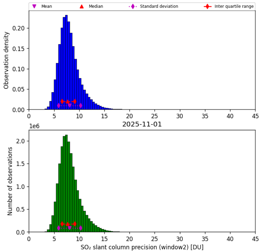
Figure 68: Histogram of “SO 2 slant column precision (window2)” for 2025-10-31 to 2025-11-02
