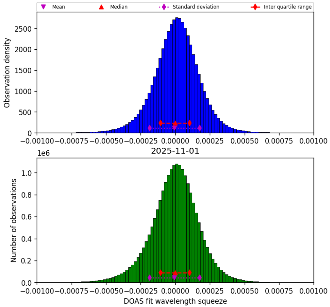
Figure 77: Histogram of “DOAS fit wavelength squeeze” for 2025-10-31 to 2025-11-02
