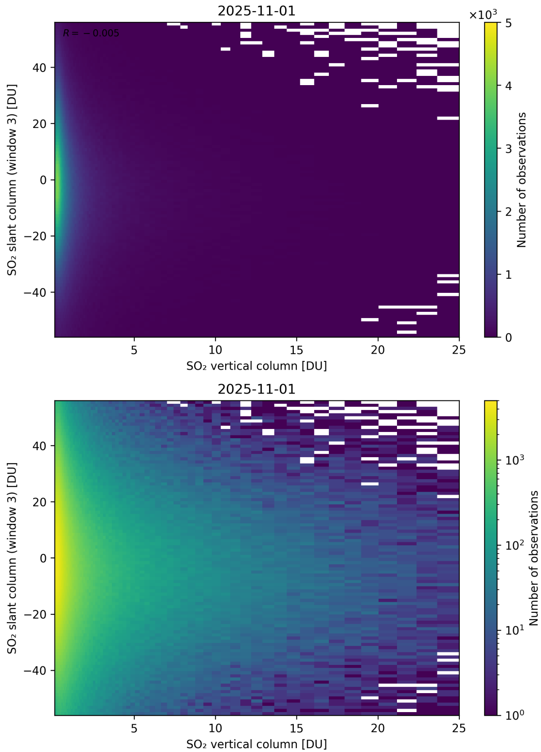
Figure 357: Scatter density plot of “SO 2 vertical column” against “SO 2 slant column (window 3)” for 2025-10-31 to 2025-11-02.
