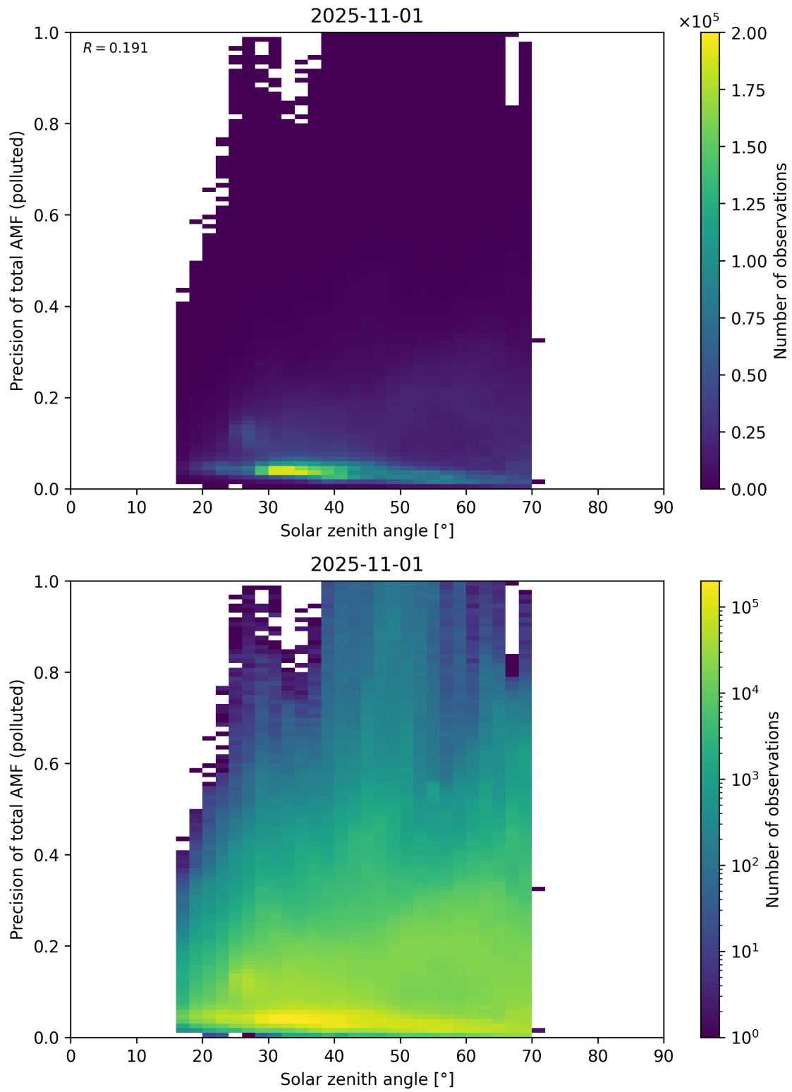
Figure 190: Scatter density plot of “Solar zenith angle” against “Precision of total AMF (polluted)” for 2025-10-31 to 2025-11-02.
