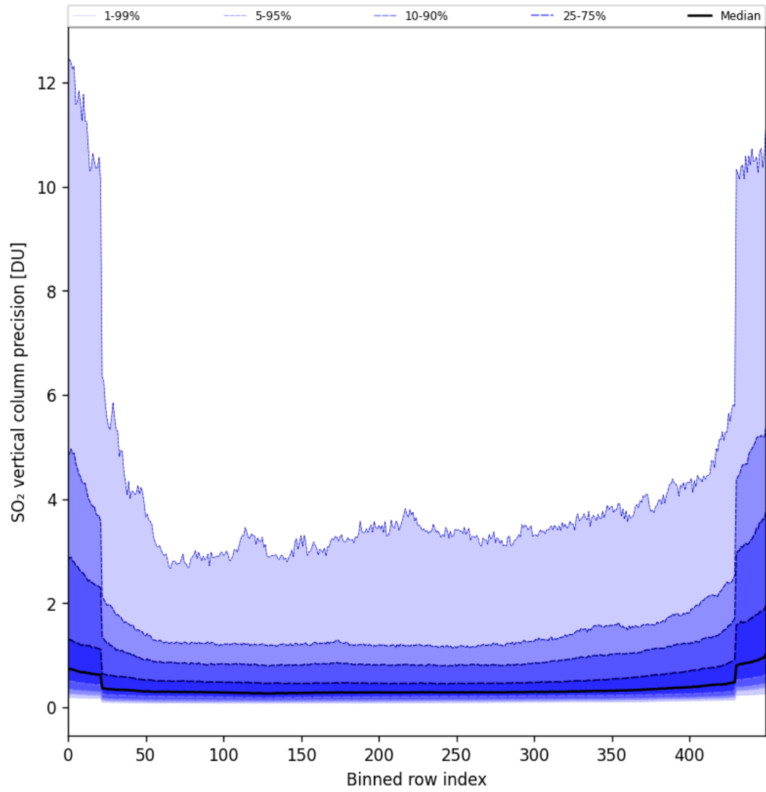
Figure 85: Along track statistics of “SO 2 vertical column precision” for 2025-10-31 to 2025-11-02
