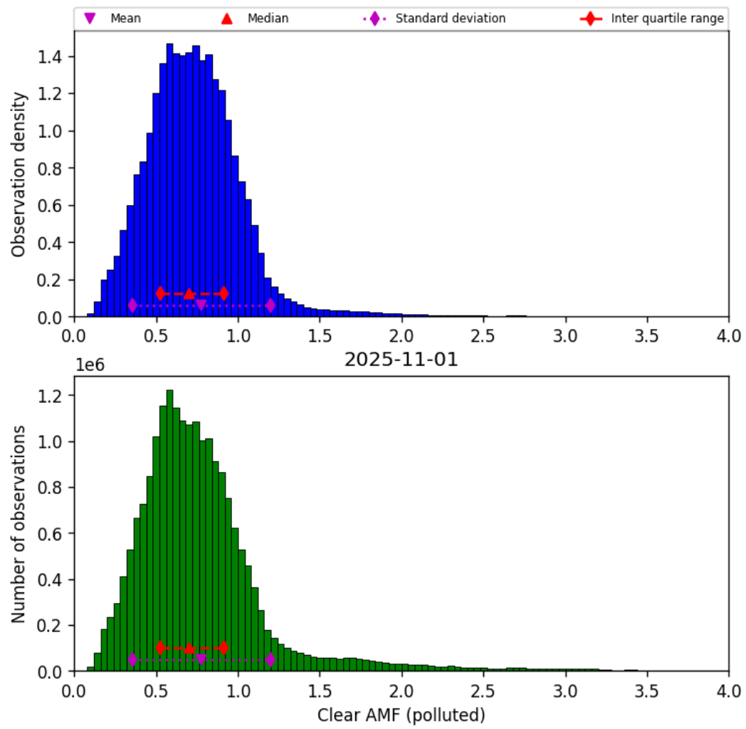
Figure 81: Histogram of “Clear AMF (polluted)” for 2025-10-31 to 2025-11-02
