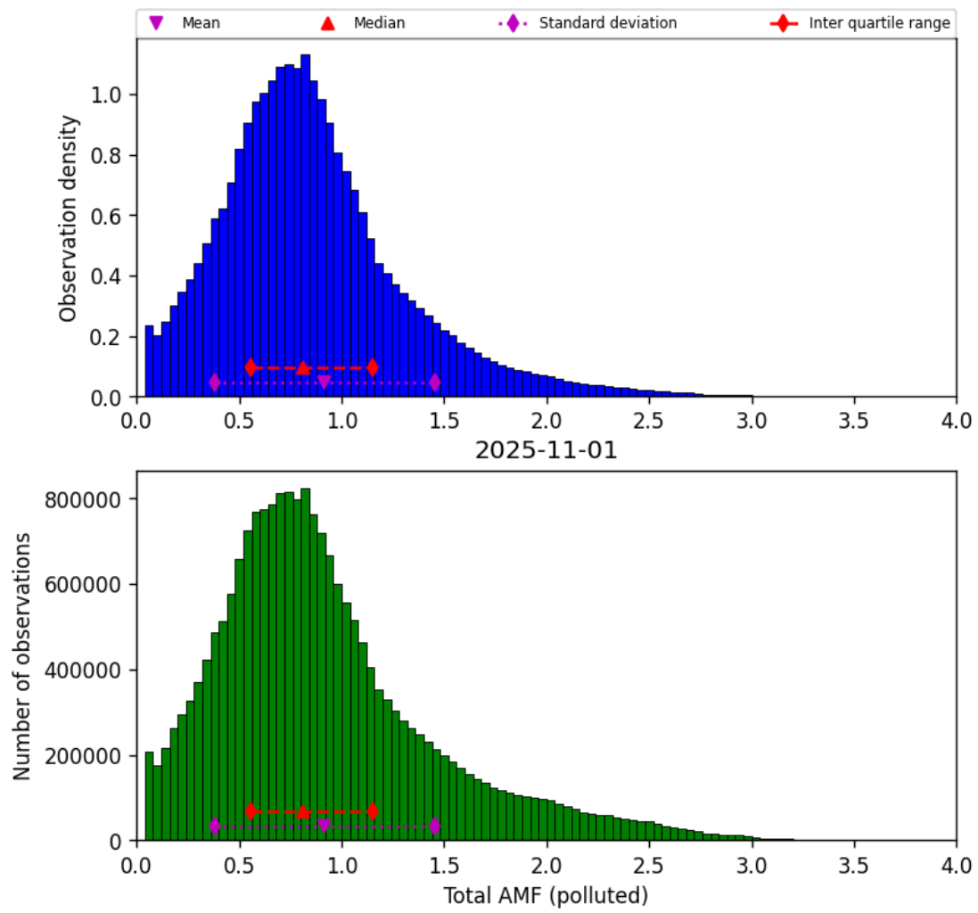
Figure 79: Histogram of “Total AMF (polluted)” for 2025-10-31 to 2025-11-02
