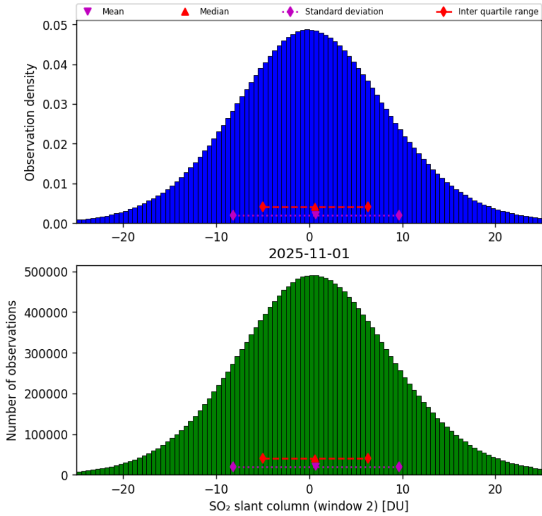
Figure 67: Histogram of “SO 2 slant column (window 2)” for 2025-10-31 to 2025-11-02
