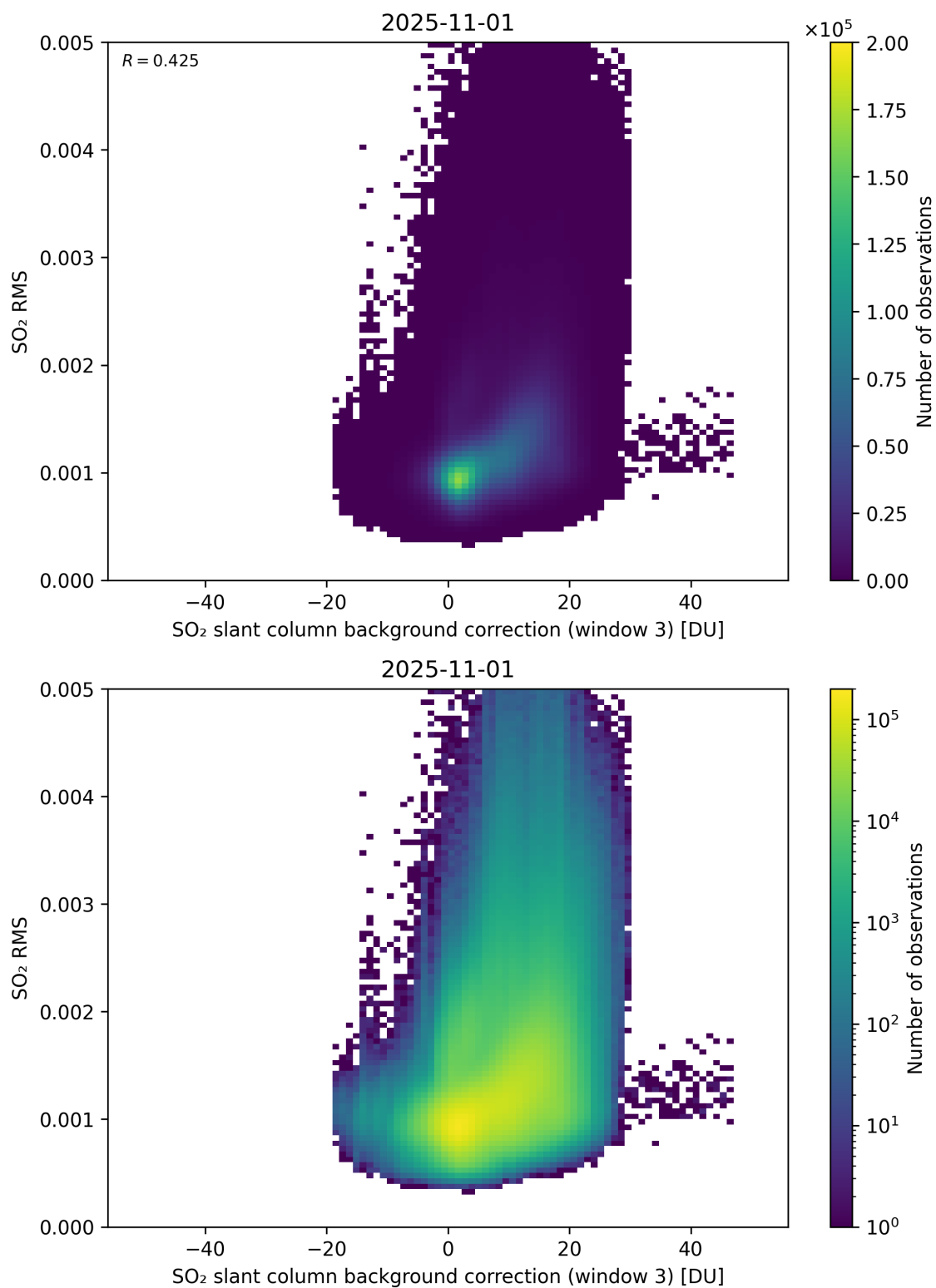
Figure 134: Scatter density plot of “SO 2 slant column background correction (window 3)” against “SO 2 RMS” for 2025-10-31 to 2025-11-02.
