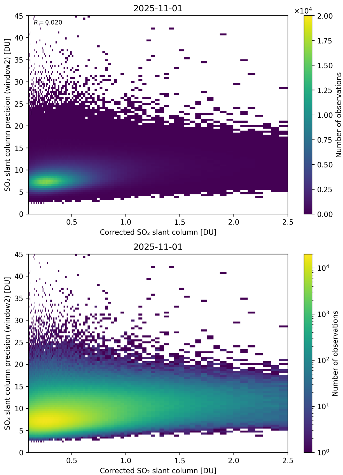
Figure 239: Scatter density plot of “Corrected SO 2 slant column” against “SO 2 slant column precision (window2)” for 2025-10-31 to 2025-11-02.
