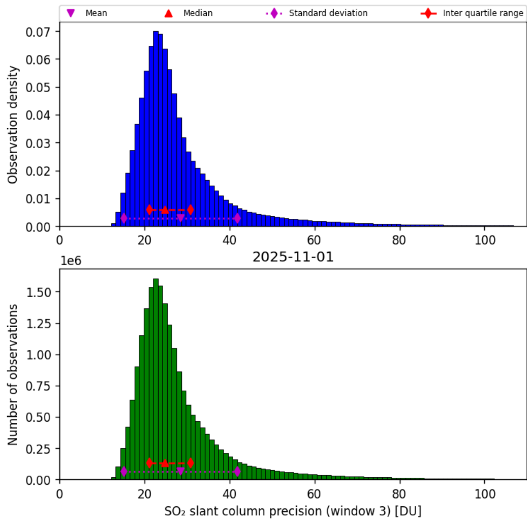
Figure 72: Histogram of “SO 2 slant column precision (window 3)” for 2025-10-31 to 2025-11-02
