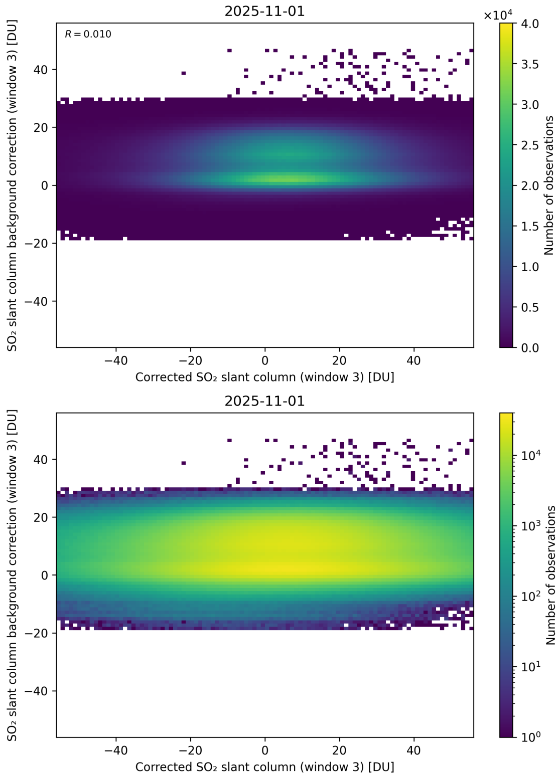
Figure 255: Scatter density plot of “Corrected SO 2 slant column (window 3)” against “SO 2 slant column background correction (window 3)” for 2025-10-31 to 2025-11-02.
