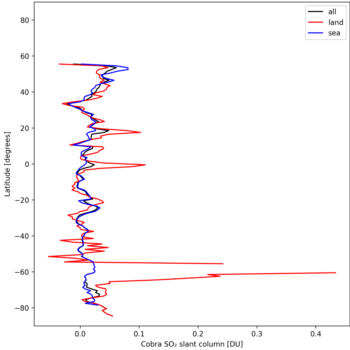
Figure 35: Zonal average of “Cobra SO 2 slant column” for 2025-10-31 to 2025-11-02.
