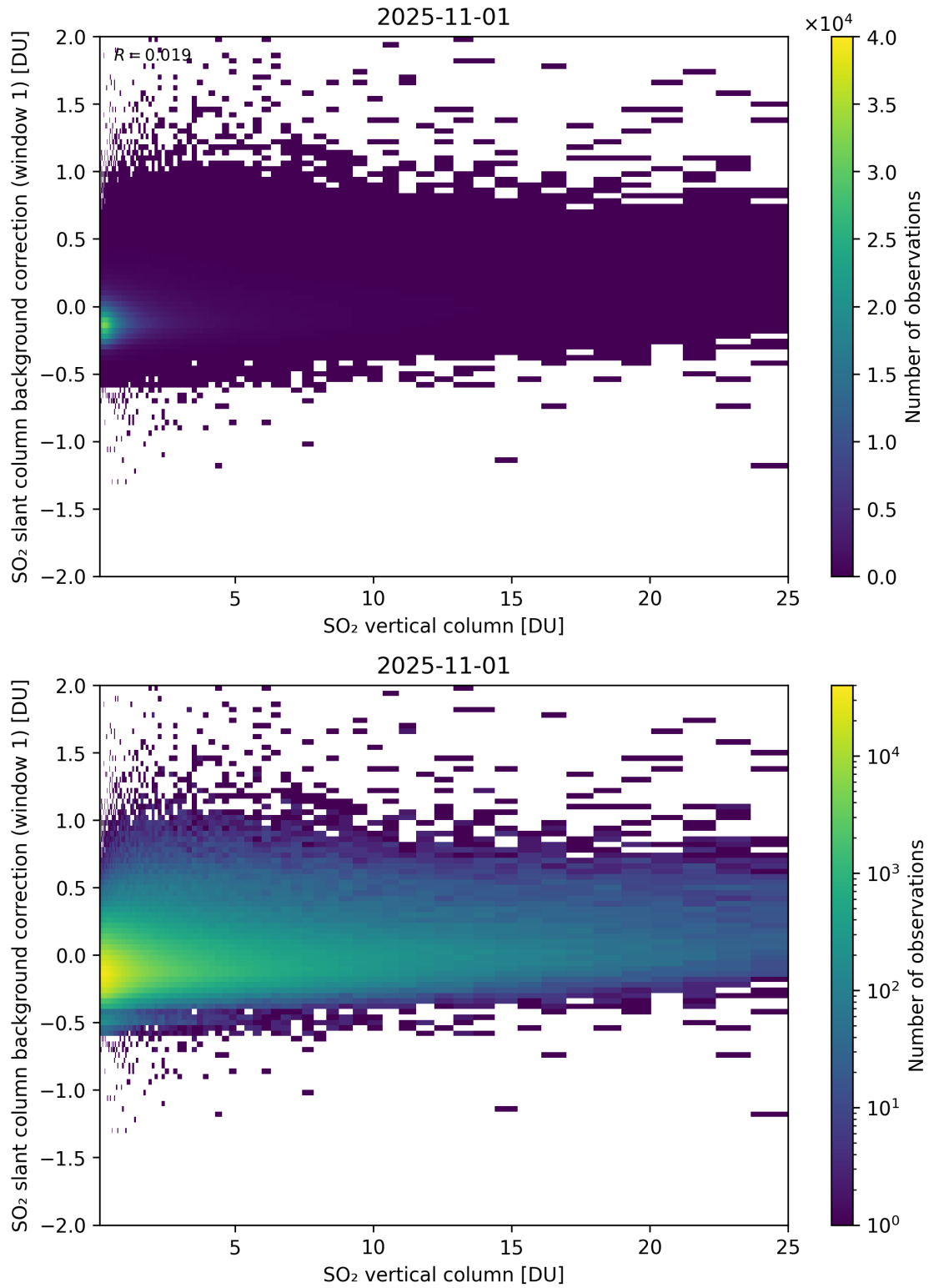
Figure 323: Scatter density plot of “SO 2 vertical column” against “SO 2 slant column background correction (window 1)” for 2025-10-31 to 2025-11-02.
