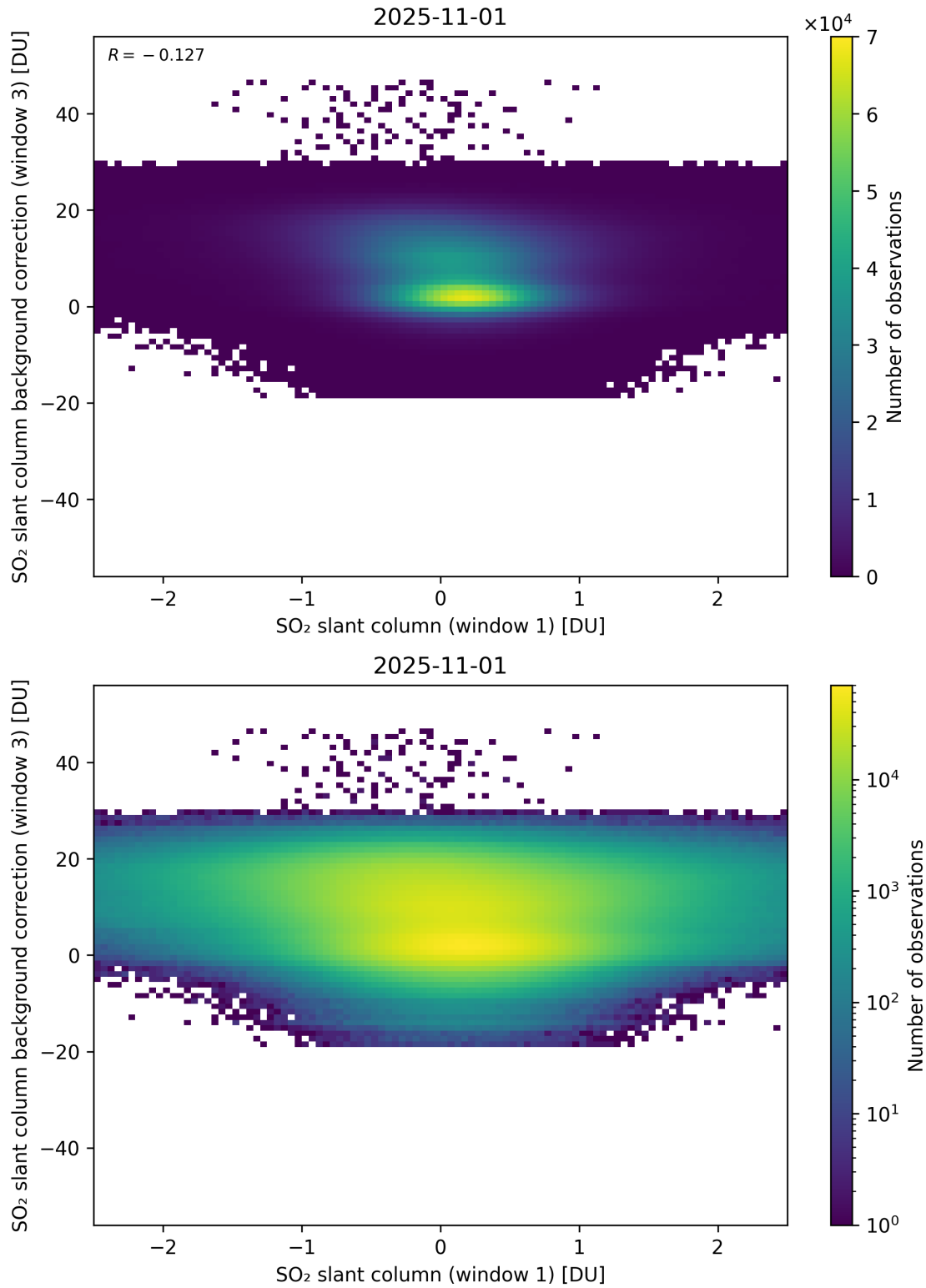
Figure 264: Scatter density plot of “SO 2 slant column (window 1)” against “SO 2 slant column background correction (window 3)” for 2025-10-31 to 2025-11-02.
