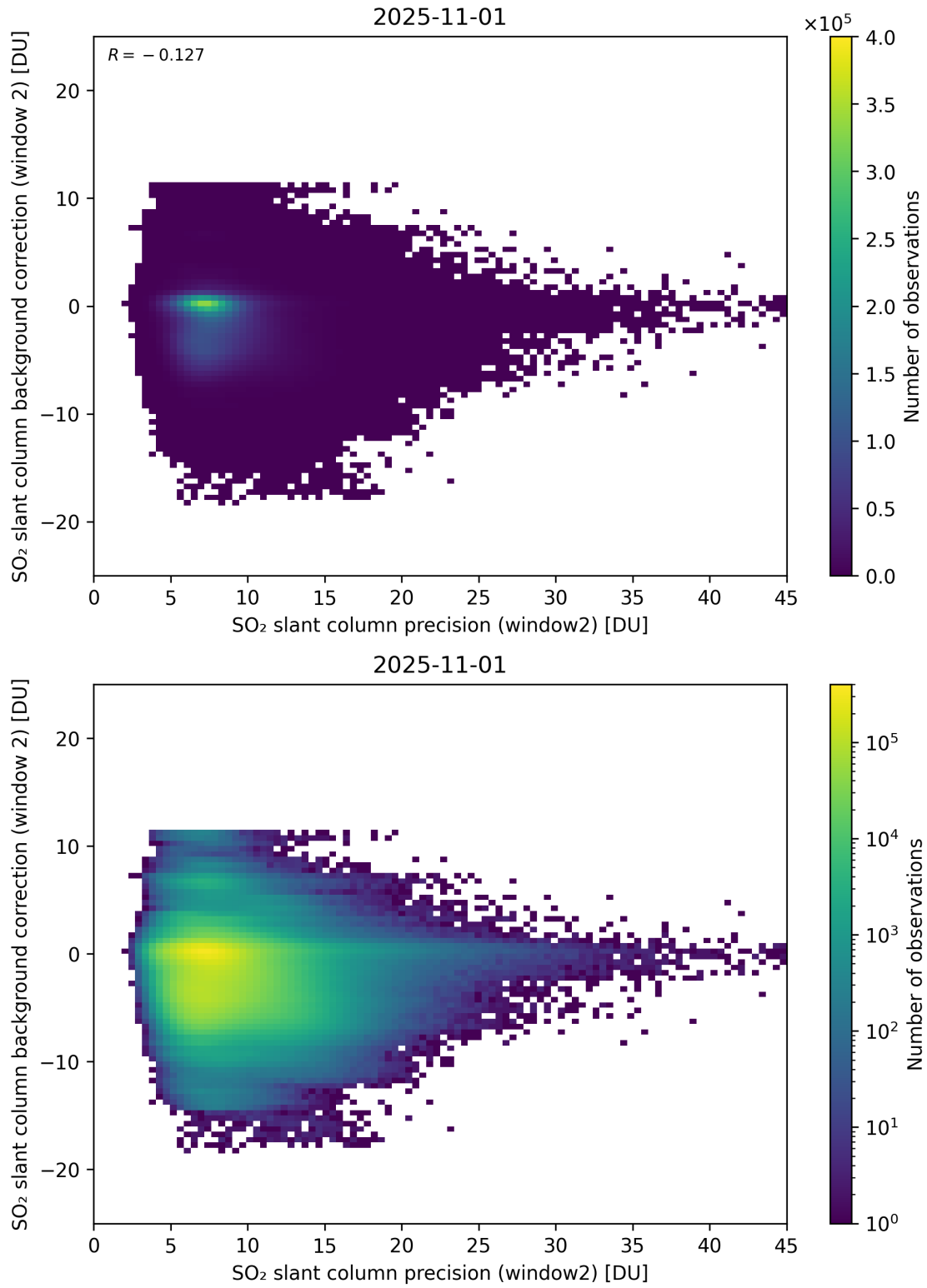
Figure 291: Scatter density plot of “SO 2 slant column precision (window2)” against “SO 2 slant column background correction (window 2)” for 2025-10-31 to 2025-11-02.
