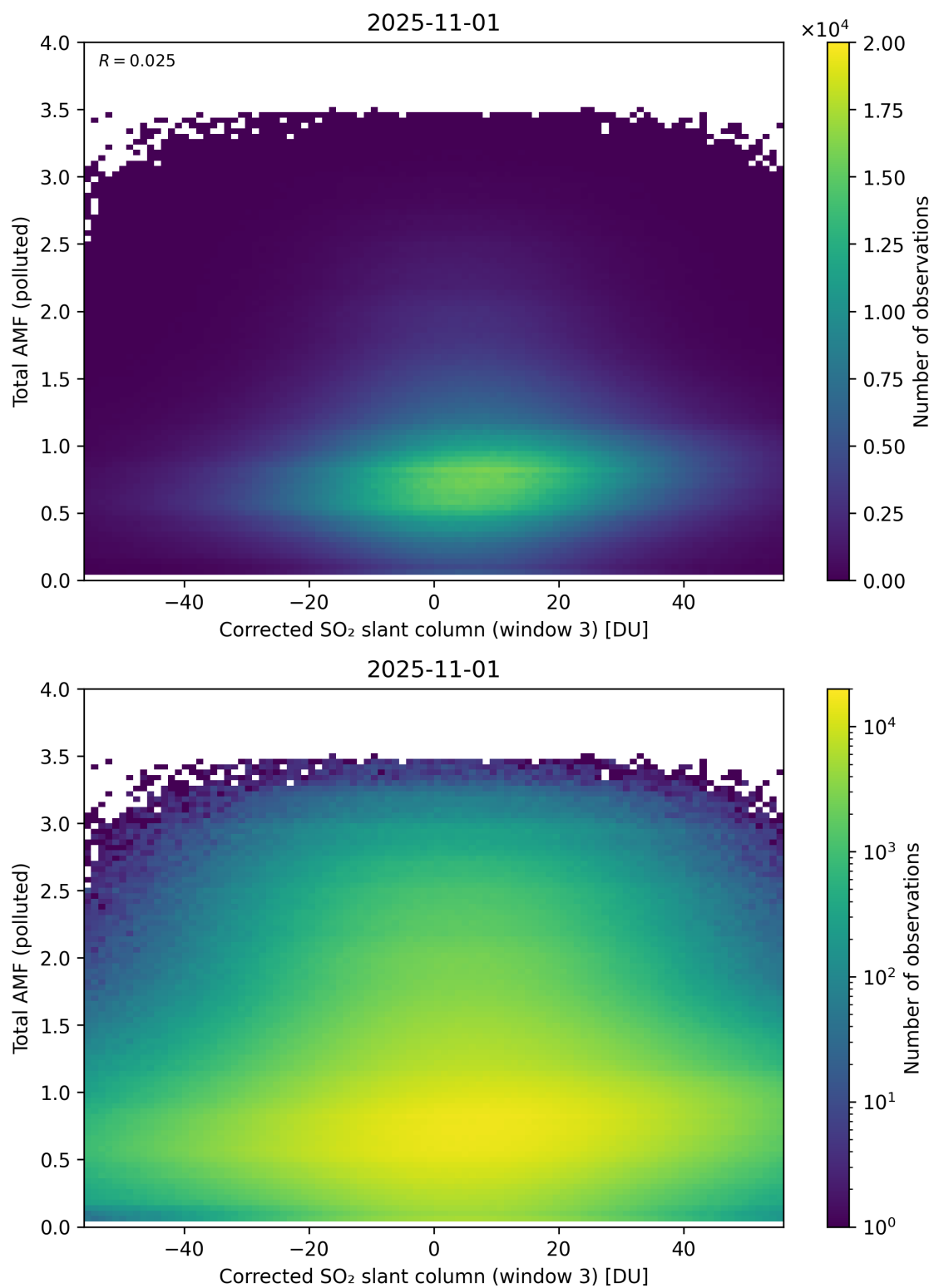
Figure 260: Scatter density plot of “Corrected SO 2 slant column (window 3)” against “Total AMF (polluted)” for 2025-10-31 to 2025-11-02.
