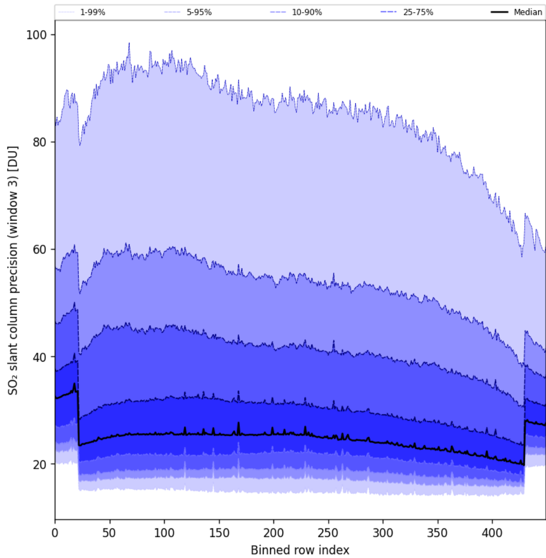
Figure 98: Along track statistics of “SO 2 slant column precision (window 3)” for 2025-10-31 to 2025-11-02
