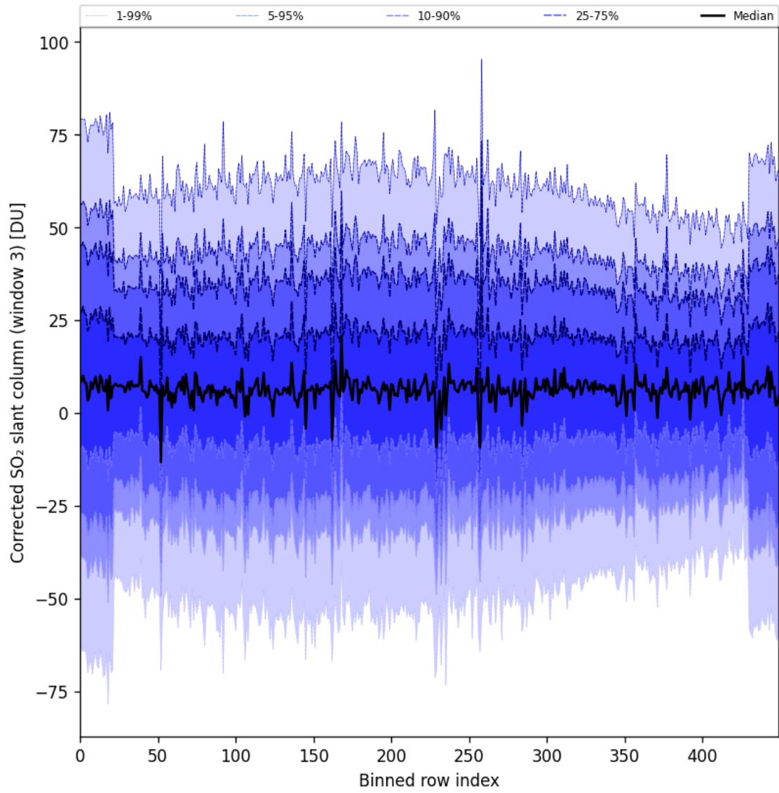
Figure 99: Along track statistics of “Corrected SO 2 slant column (window 3)” for 2025-10-31 to 2025-11-02
