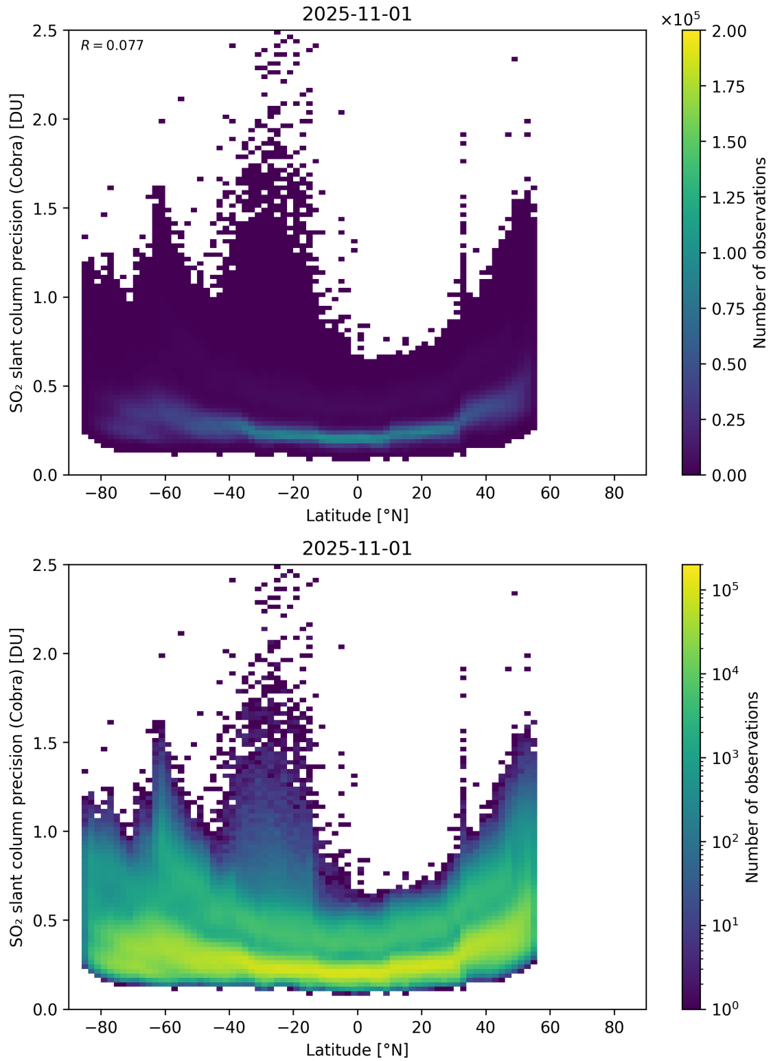
Figure 158: Scatter density plot of “Latitude” against “SO 2 slant column precision (Cobra)” for 2025-10-31 to 2025-11-02.
