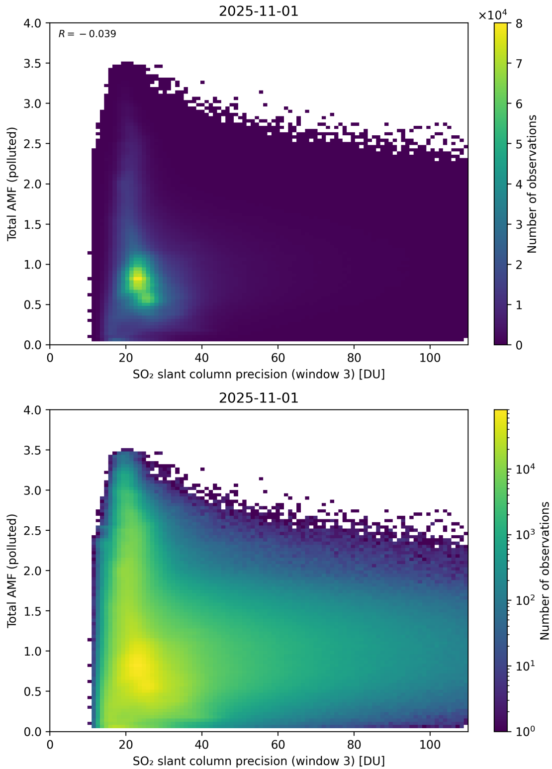
Figure 313: Scatter density plot of “SO 2 slant column precision (window 3)” against “Total AMF (polluted)” for 2025-10-31 to 2025-11-02.
