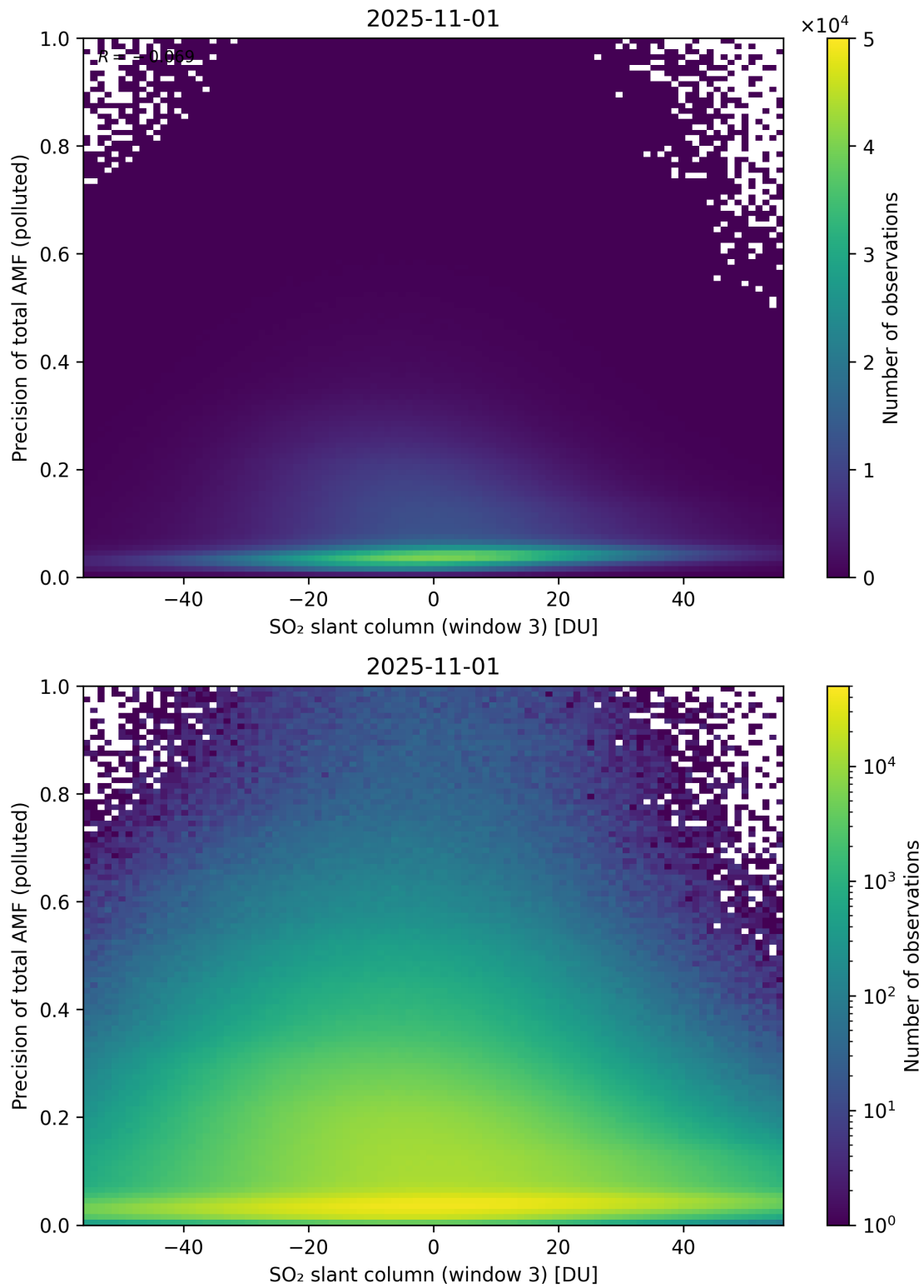
Figure 319: Scatter density plot of “SO 2 slant column (window 3)” against “Precision of total AMF (polluted)” for 2025-10-31 to 2025-11-02.
