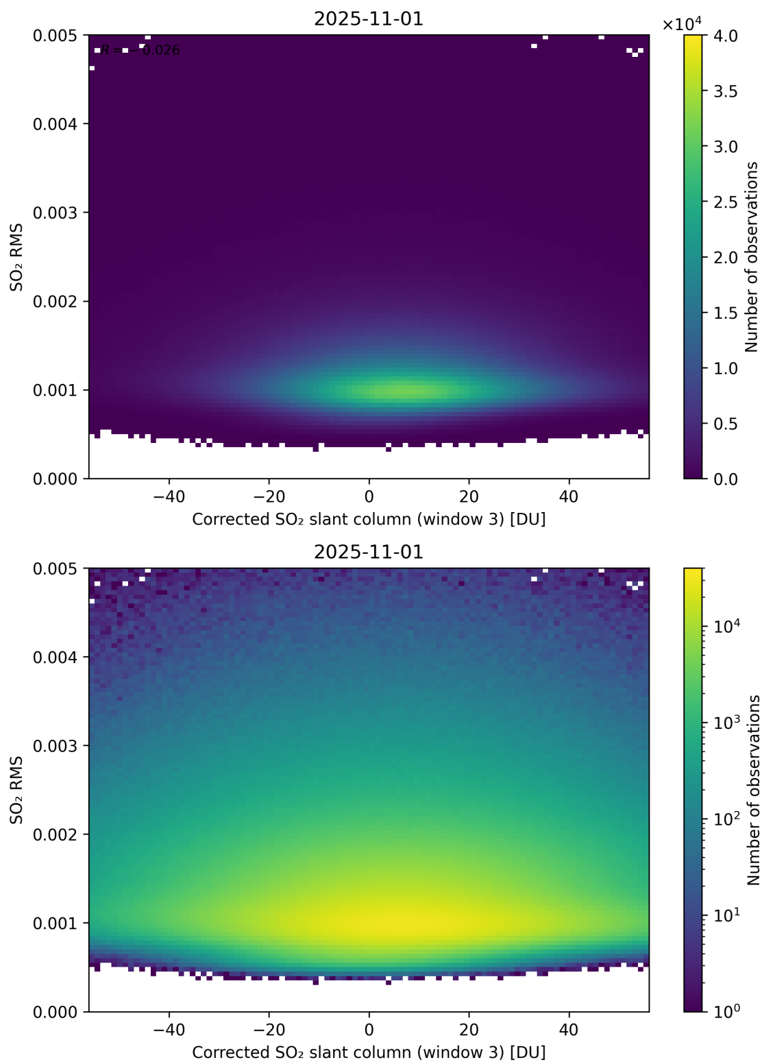
Figure 258: Scatter density plot of “Corrected SO 2 slant column (window 3)” against “SO 2 RMS” for 2025-10-31 to 2025-11-02.
