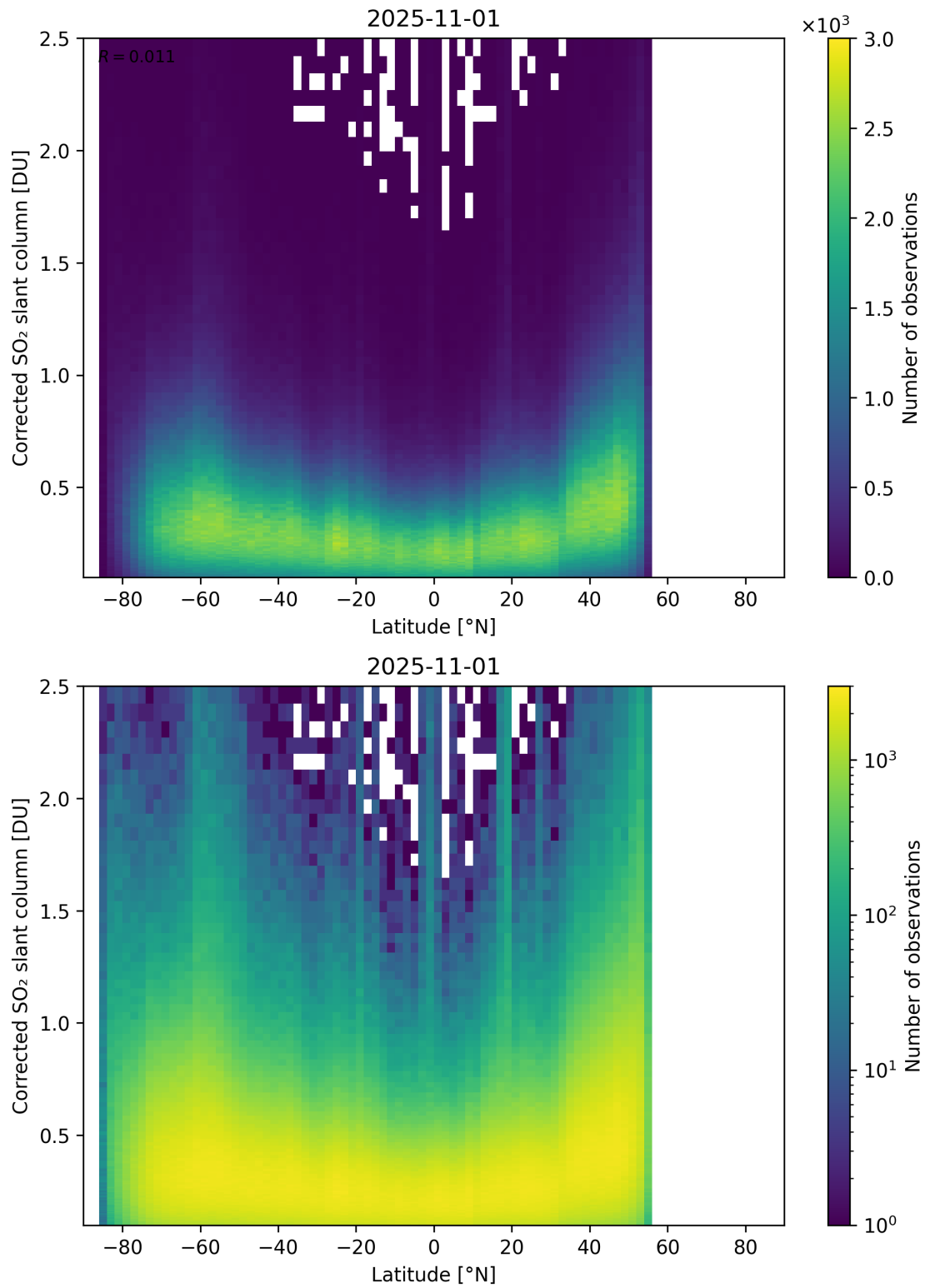
Figure 159: Scatter density plot of “Latitude” against “Corrected SO 2 slant column” for 2025-10-31 to 2025-11-02.
