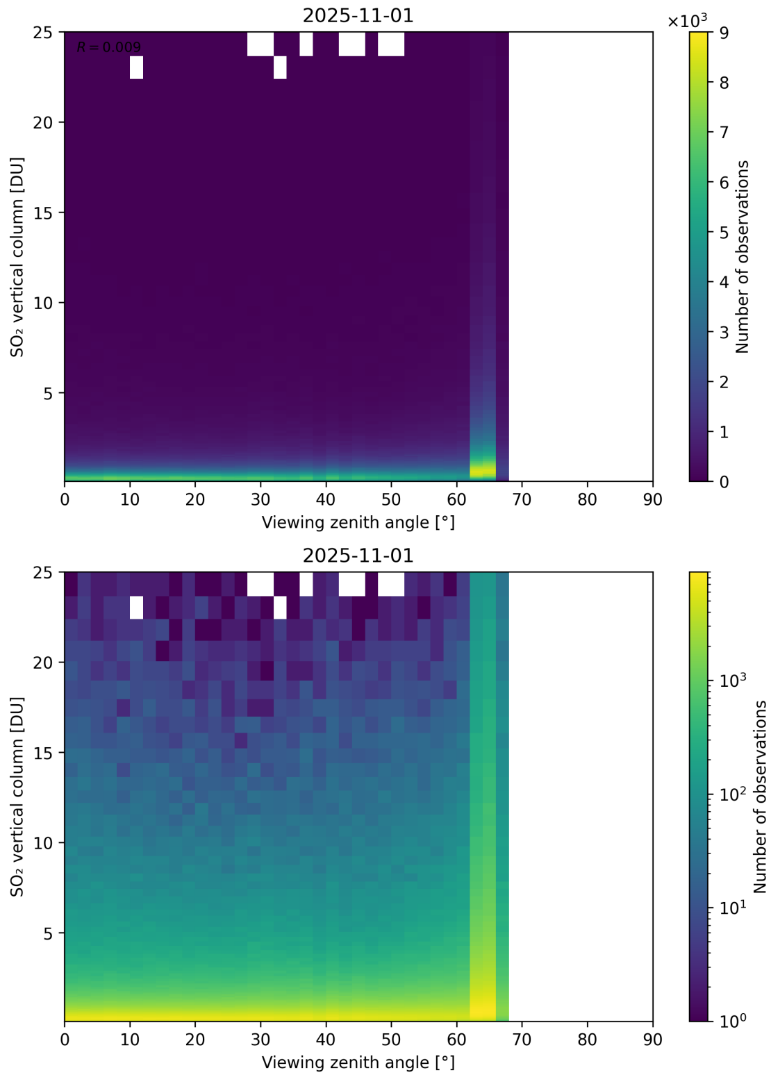
Figure 383: Scatter density plot of “Viewing zenith angle” against “SO 2 vertical column” for 2025-10-31 to 2025-11-02.
