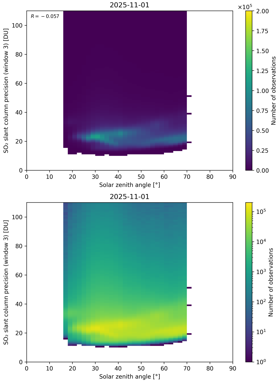
Figure 188: Scatter density plot of “Solar zenith angle” against “SO 2 slant column precision (window 3)” for 2025-10-31 to 2025-11-02.
