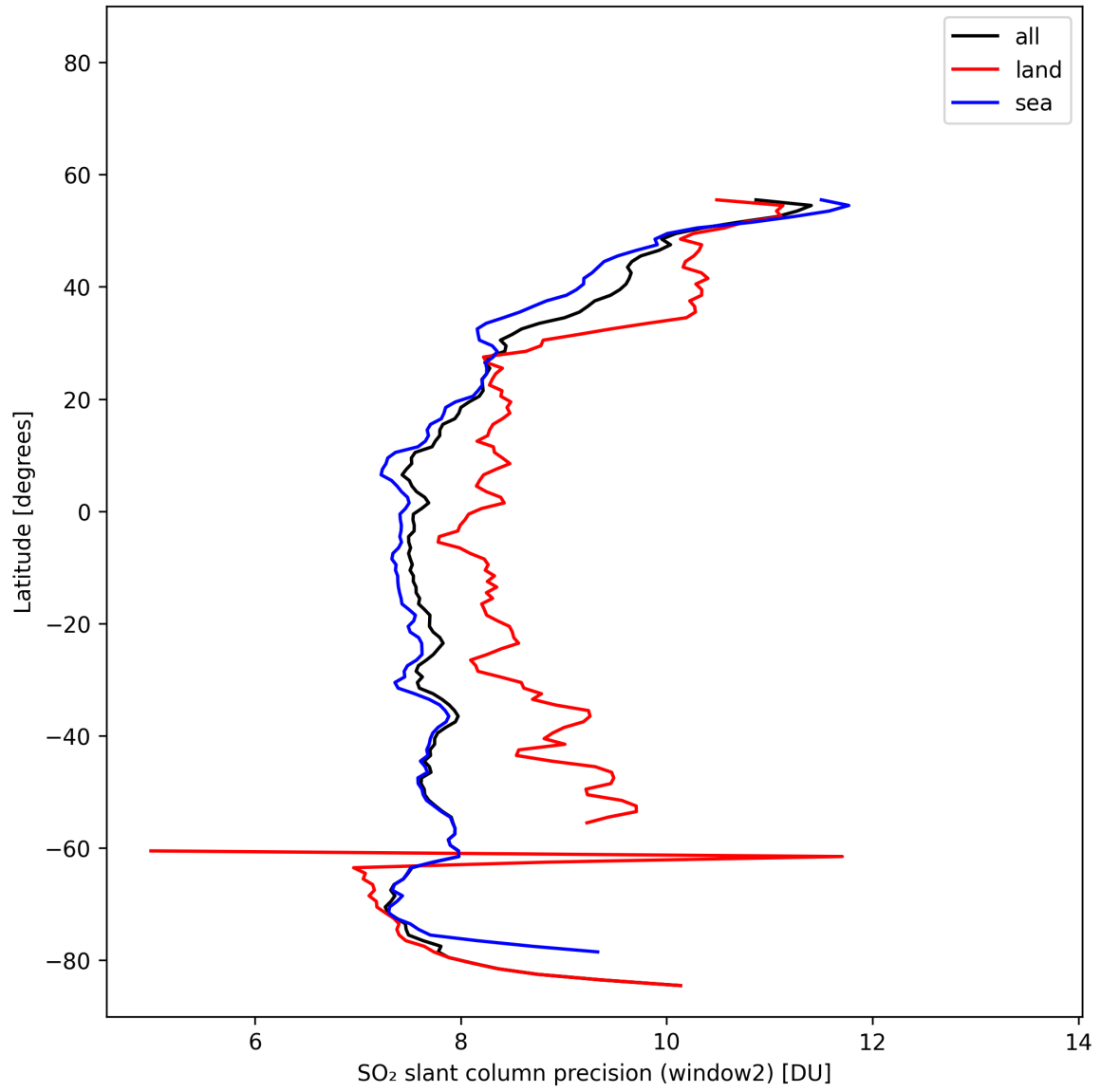
Figure 42: Zonal average of “SO 2 slant column precision (window2)” for 2025-10-31 to 2025-11-02.
