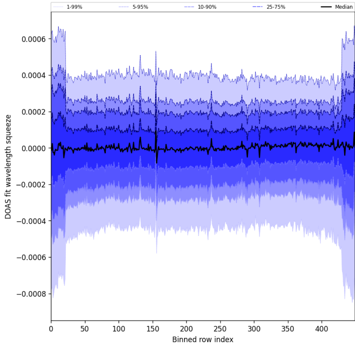
Figure 103: Along track statistics of “DOAS fit wavelength squeeze” for 2025-10-31 to 2025-11-02
