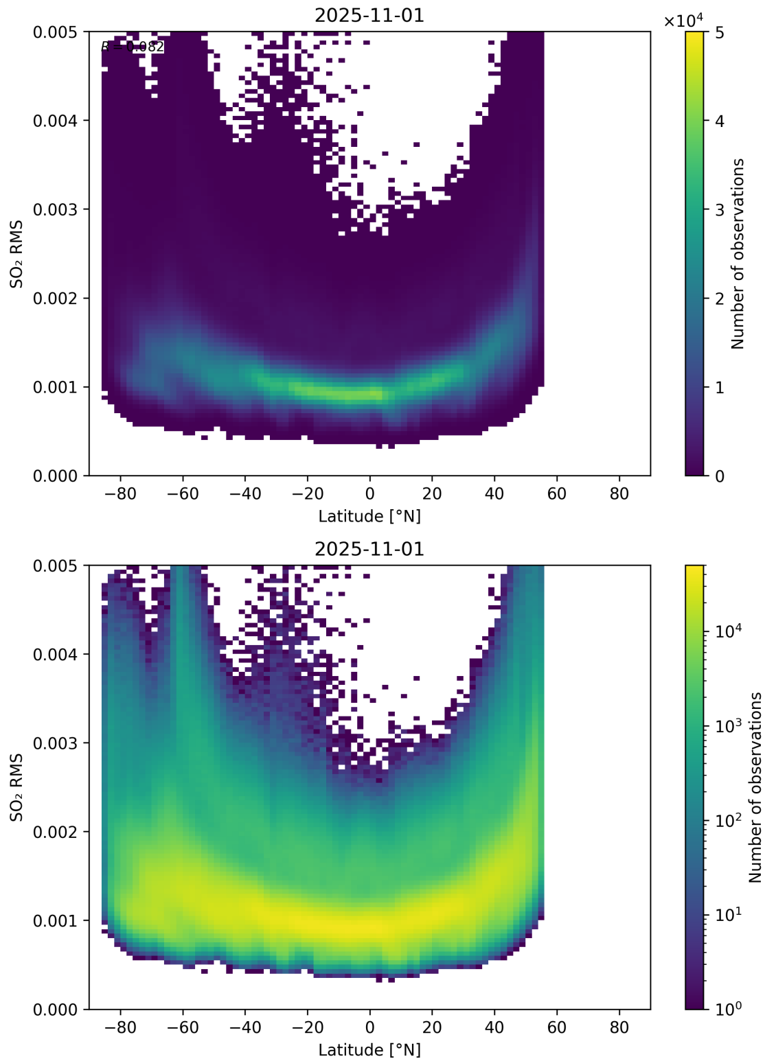
Figure 155: Scatter density plot of “Latitude” against “SO 2 RMS” for 2025-10-31 to 2025-11-02.
