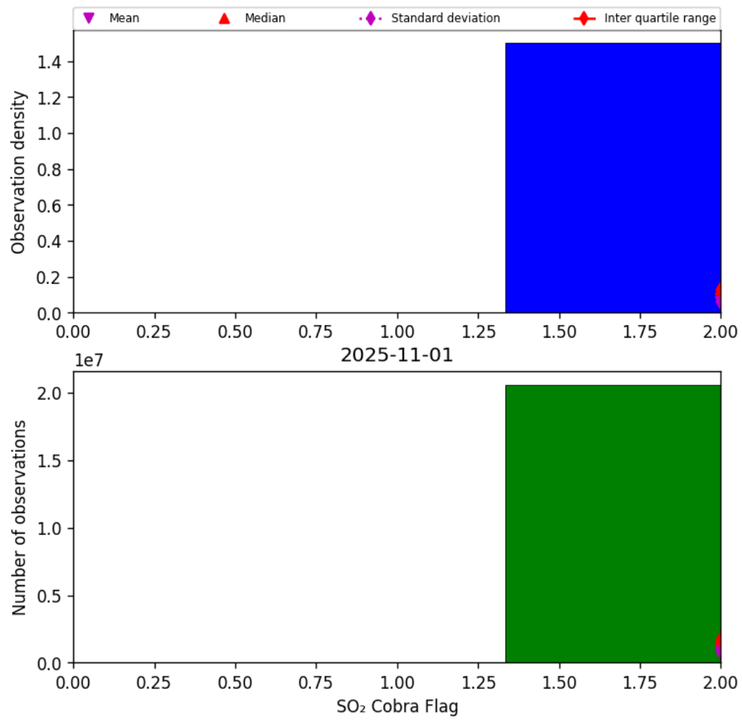
Figure 75: Histogram of “SO 2 Cobra Flag” for 2025-10-31 to 2025-11-02
