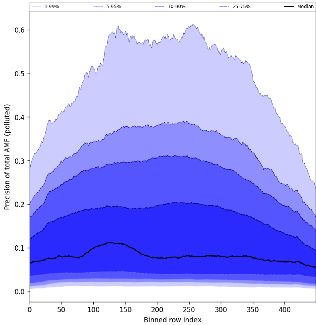
Figure 106: Along track statistics of “Precision of total AMF (polluted)” for 2025-10-31 to 2025-11-02
