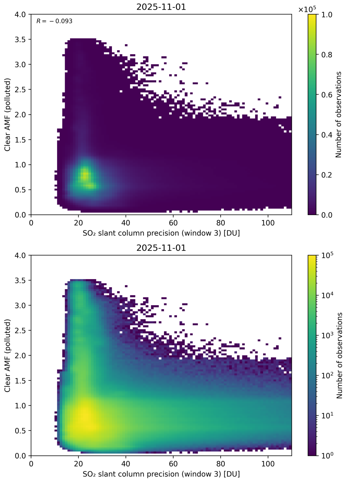
Figure 311: Scatter density plot of “SO 2 slant column precision (window 3)” against “Clear AMF (polluted)” for 2025-10-31 to 2025-11-02.
