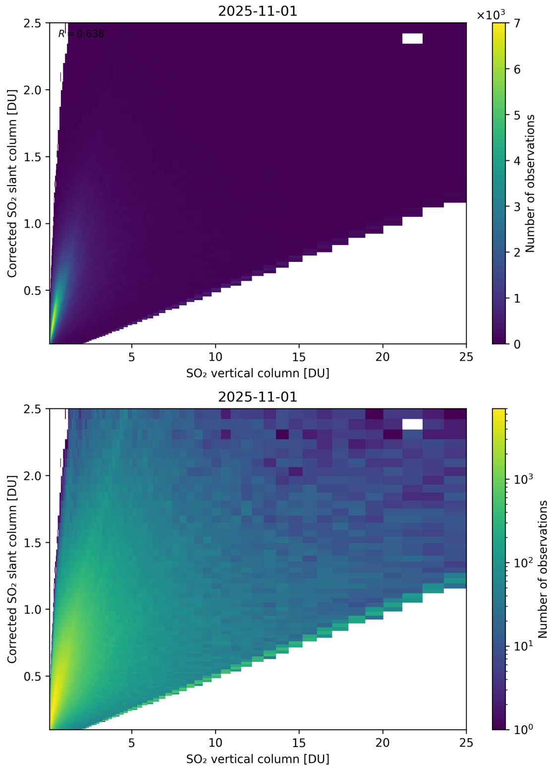
Figure 351: Scatter density plot of “SO 2 vertical column” against “Corrected SO 2 slant column” for 2025-10-31 to 2025-11-02.
