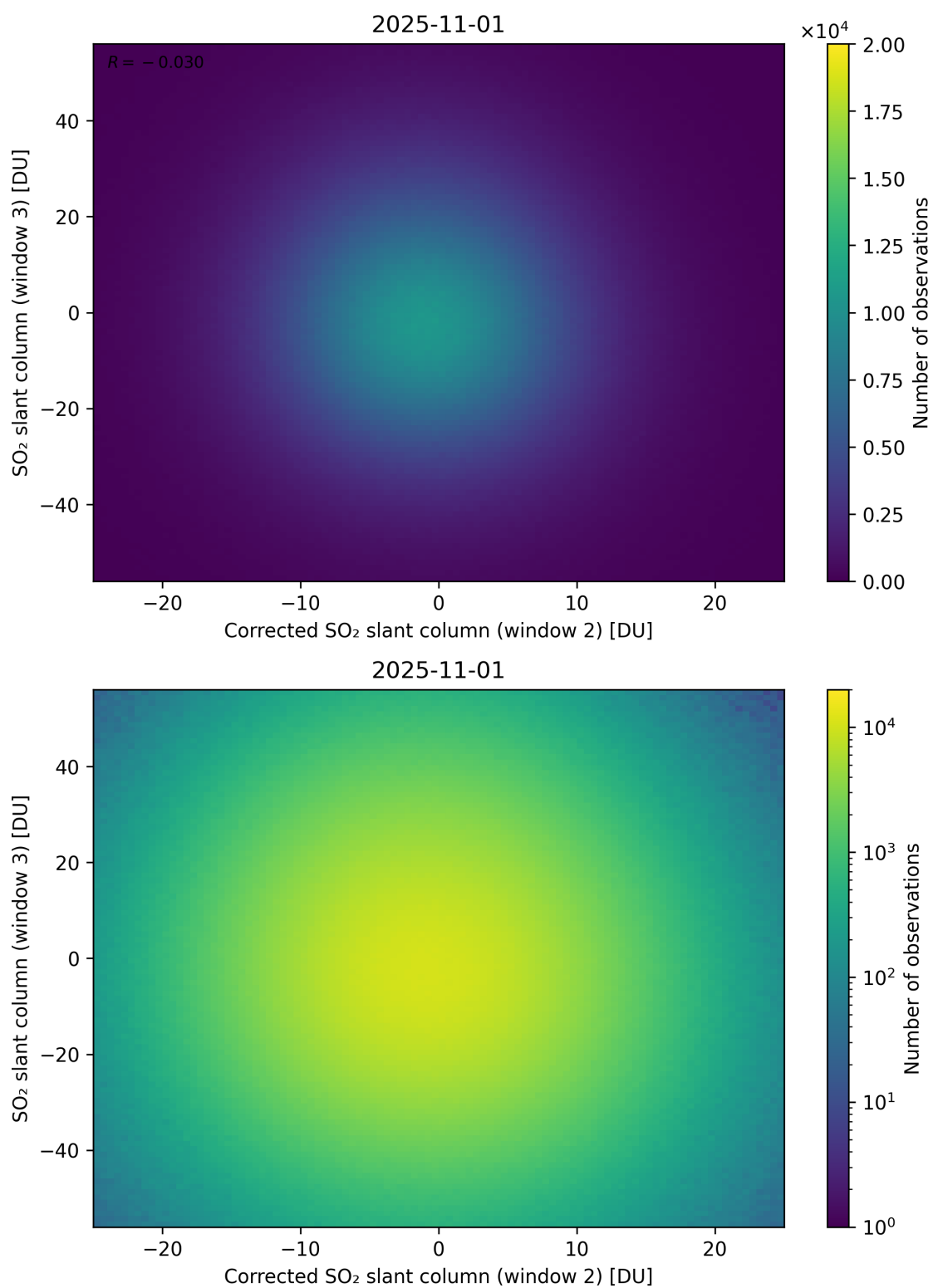
Figure 251: Scatter density plot of “Corrected SO 2 slant column (window 2)” against “SO 2 slant column (window 3)” for 2025-10-31 to 2025-11-02.
