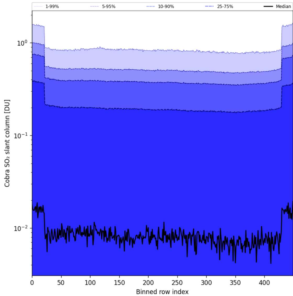
Figure 87: Along track statistics of “Cobra SO 2 slant column” for 2025-10-31 to 2025-11-02
