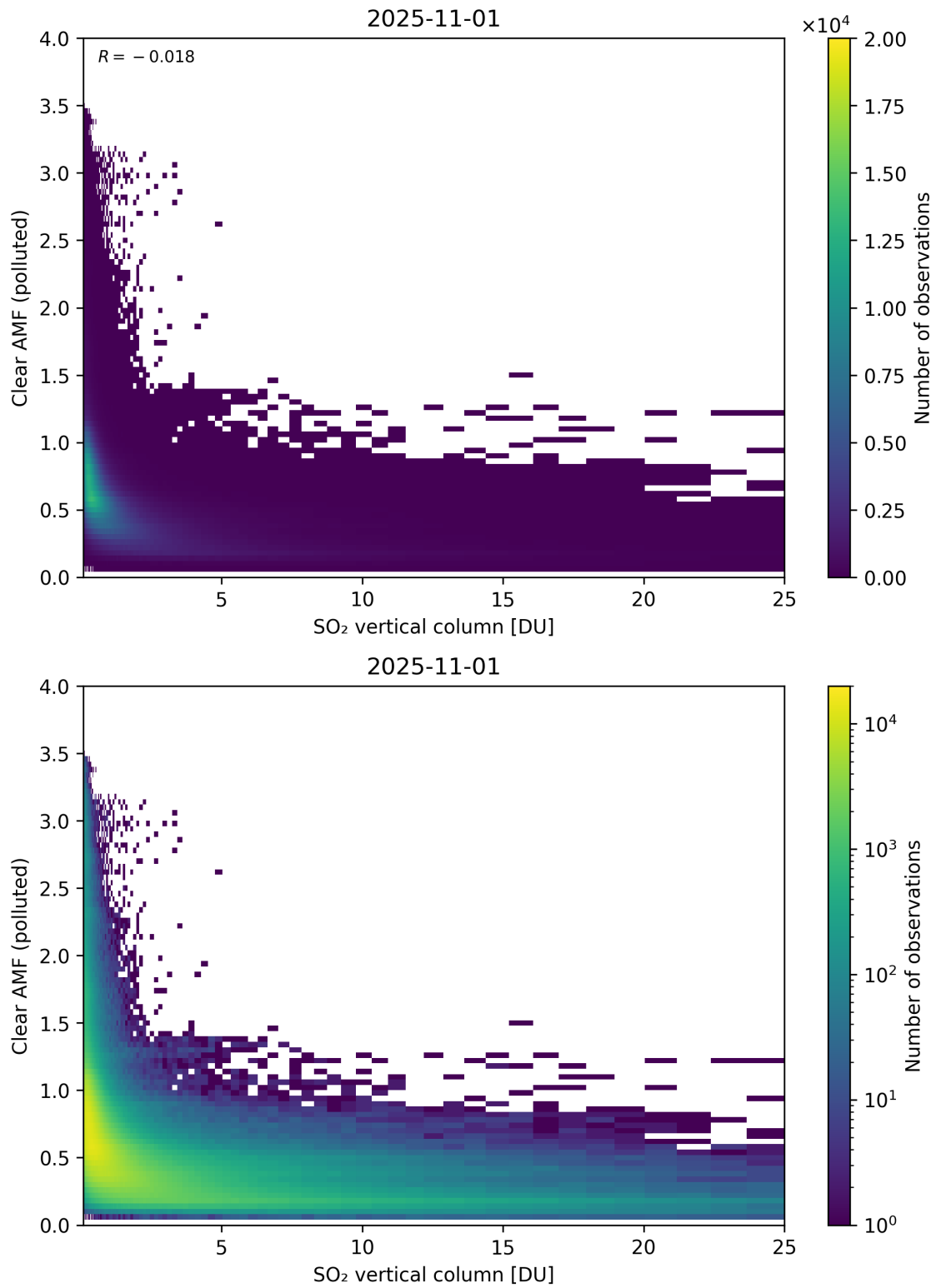
Figure 348: Scatter density plot of “SO 2 vertical column” against “Clear AMF (polluted)” for 2025-10-31 to 2025-11-02.
