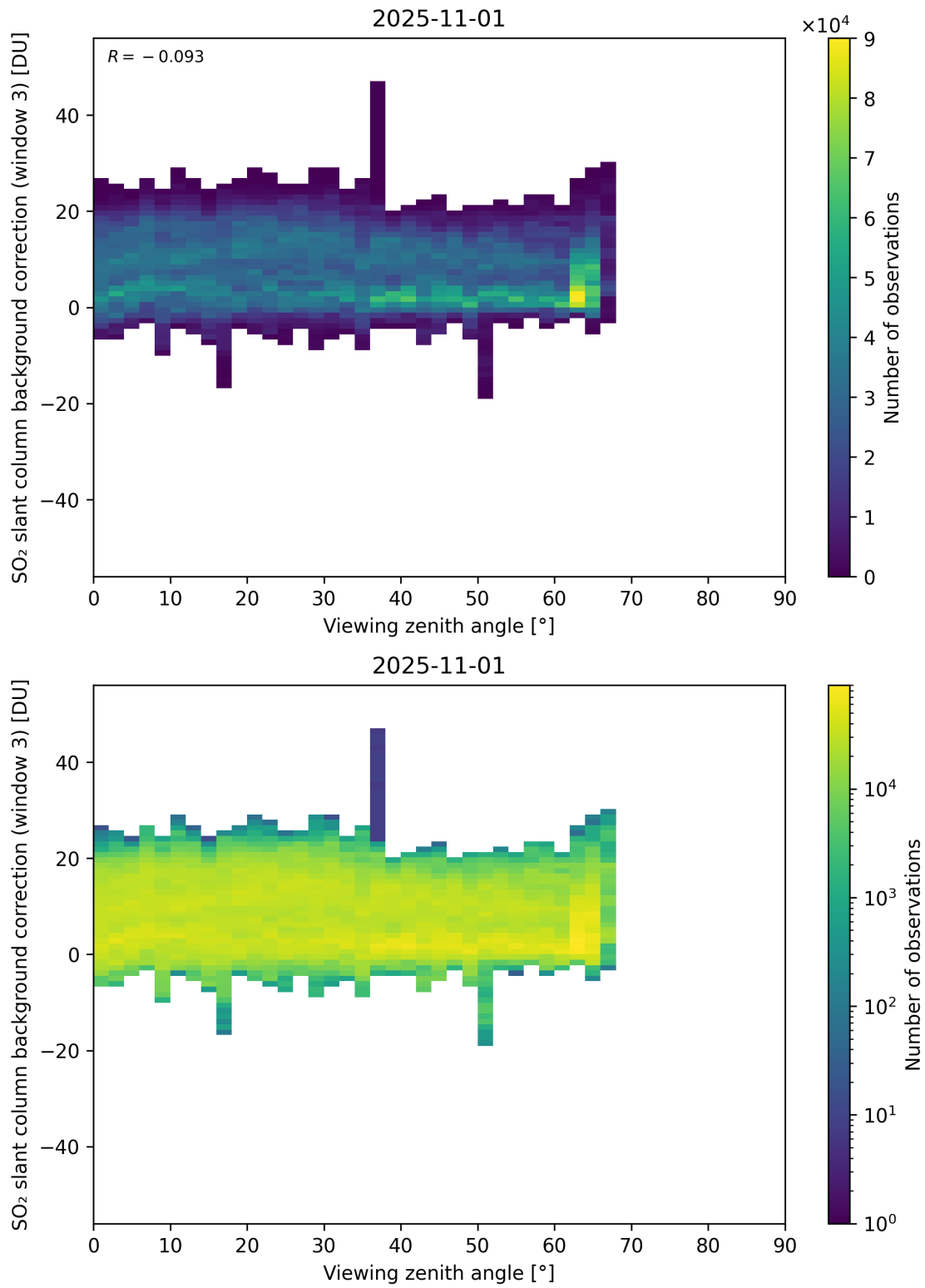
Figure 364: Scatter density plot of “Viewing zenith angle” against “SO 2 slant column background correction (window 3)” for 2025-10-31 to 2025-11-02.
