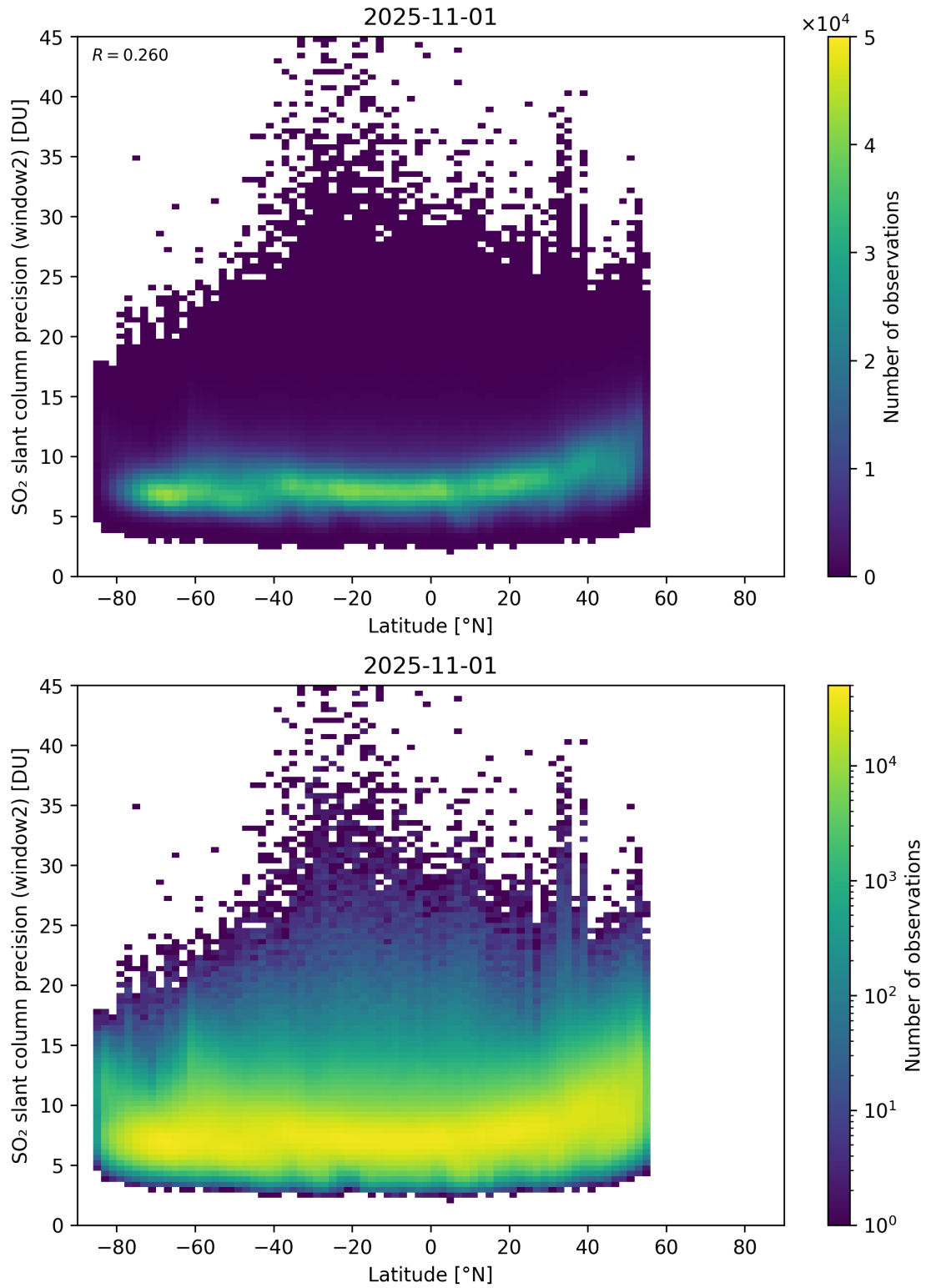
Figure 164: Scatter density plot of “Latitude” against “SO 2 slant column precision (window2)” for 2025-10-31 to 2025-11-02.
