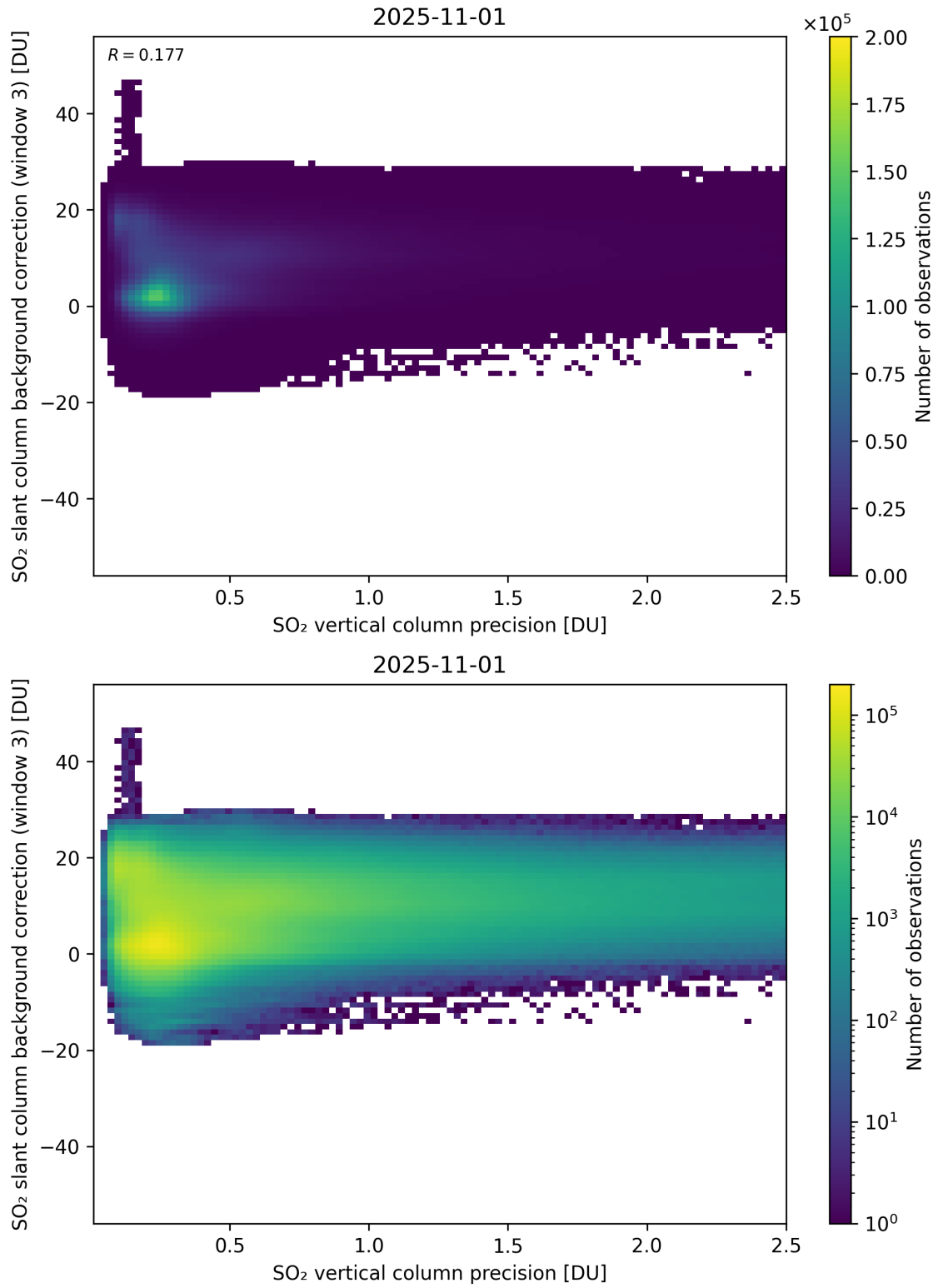
Figure 331: Scatter density plot of “SO 2 vertical column precision” against “SO 2 slant column background correction (window 3)” for 2025-10-31 to 2025-11-02.
