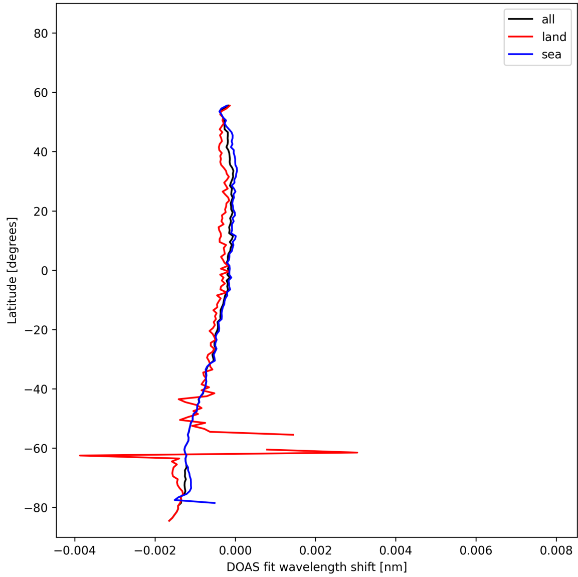
Figure 50: Zonal average of “DOAS fit wavelength shift” for 2025-10-31 to 2025-11-02.
