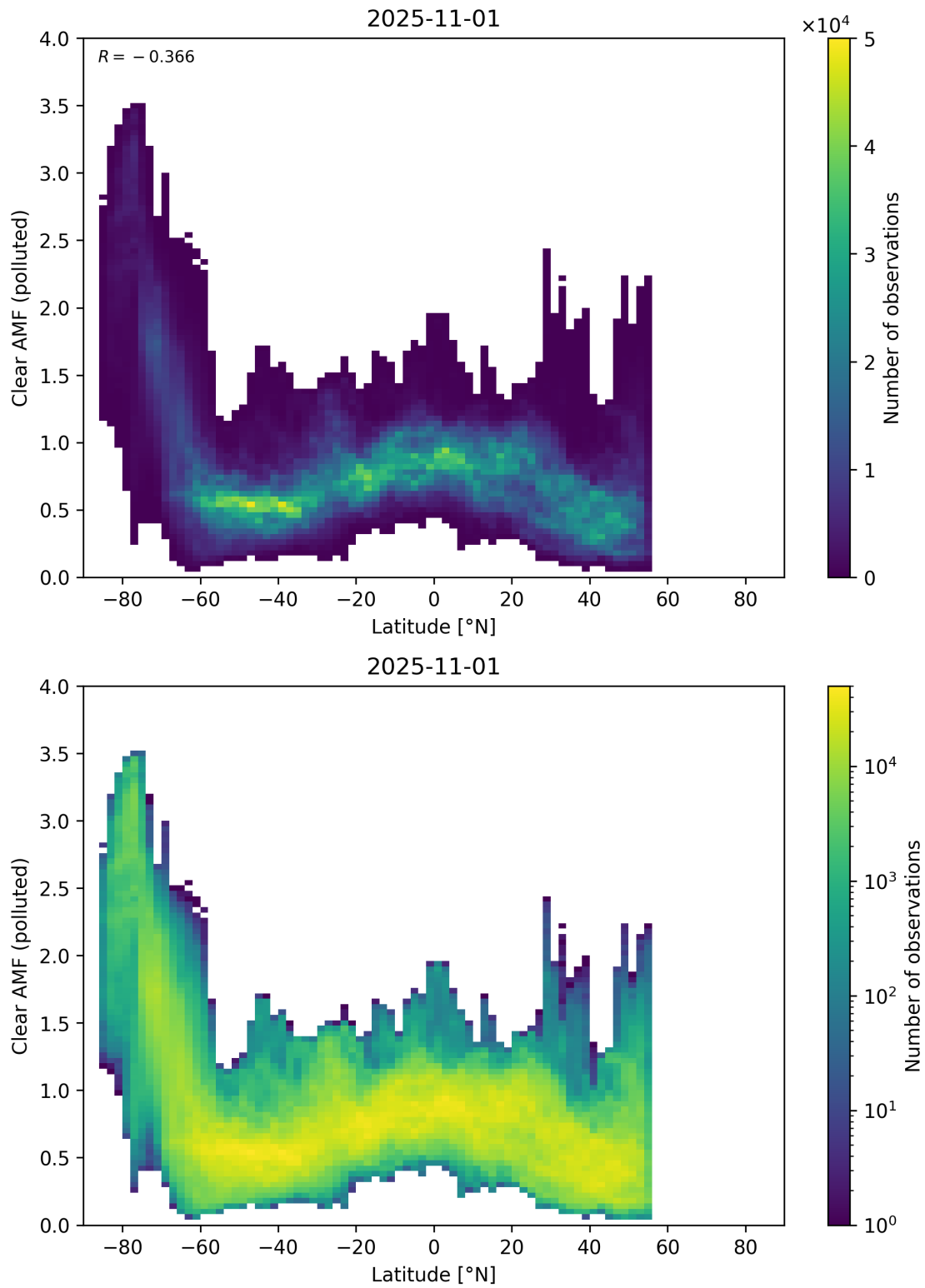
Figure 156: Scatter density plot of “Latitude” against “Clear AMF (polluted)” for 2025-10-31 to 2025-11-02.
