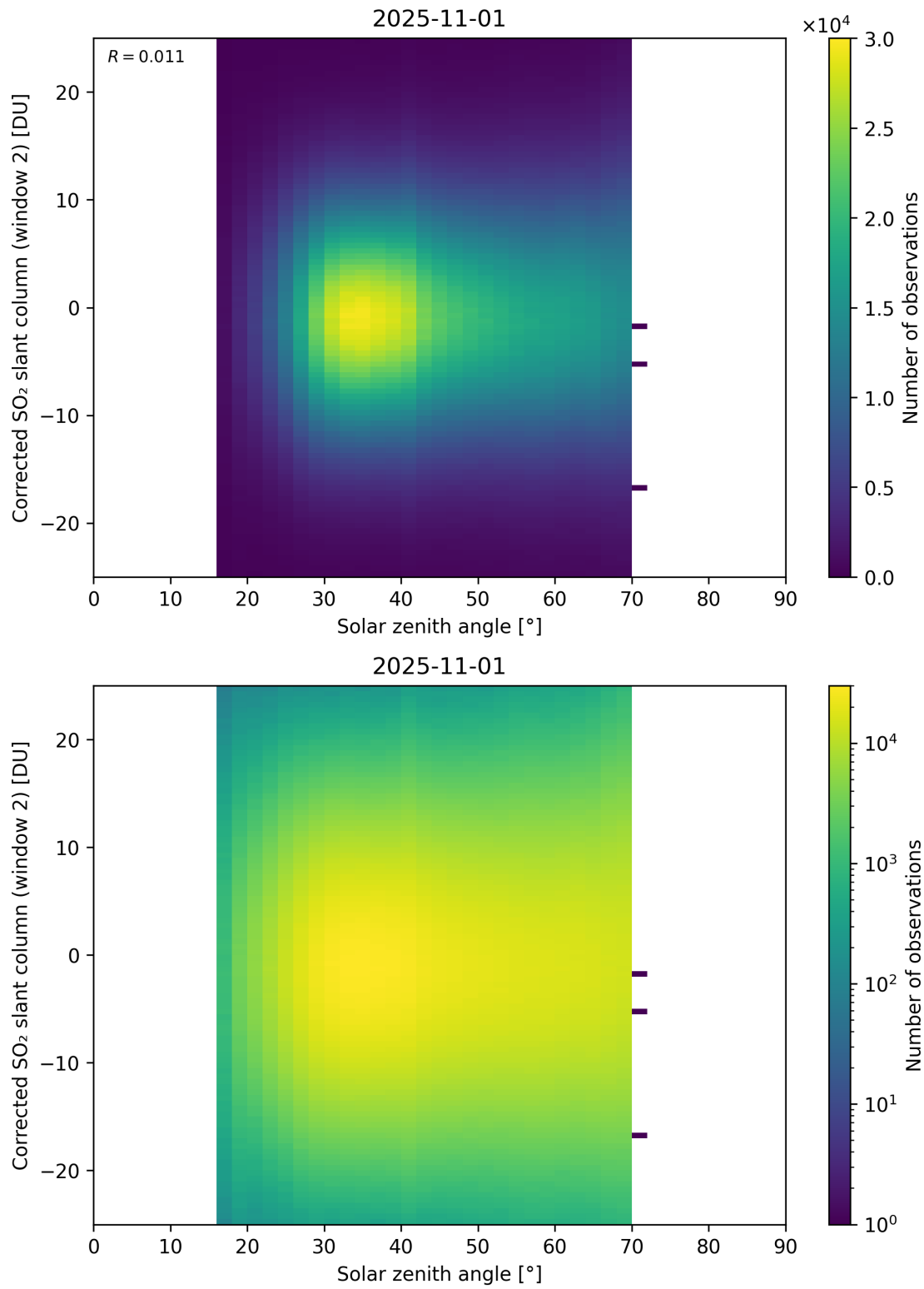
Figure 182: Scatter density plot of “Solar zenith angle” against “Corrected SO 2 slant column (window 2)” for 2025-10-31 to 2025-11-02.
