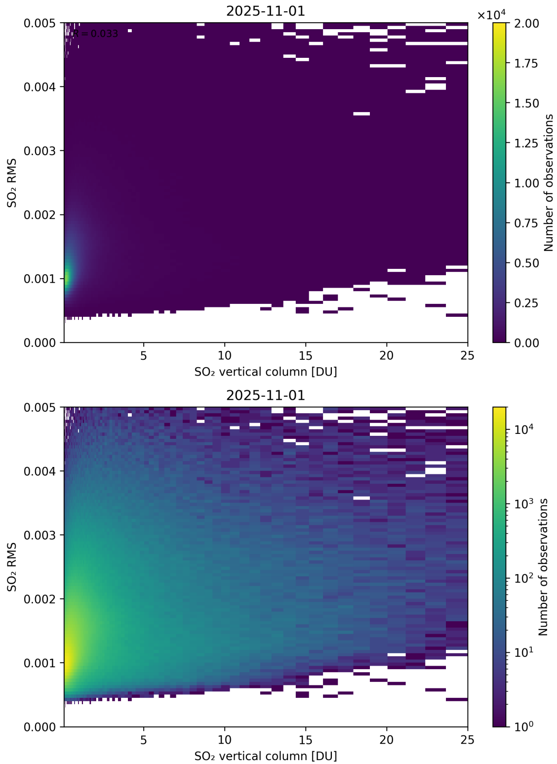
Figure 328: Scatter density plot of “SO 2 vertical column” against “SO 2 RMS” for 2025-10-31 to 2025-11-02.
