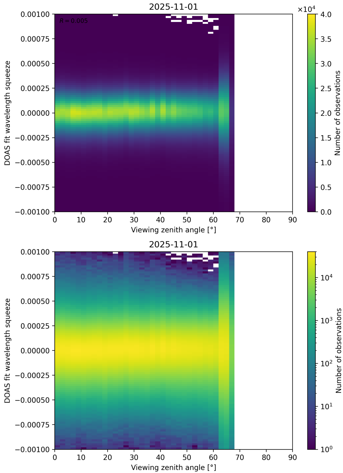
Figure 366: Scatter density plot of “Viewing zenith angle” against “DOAS fit wavelength squeeze” for 2025-10-31 to 2025-11-02.
