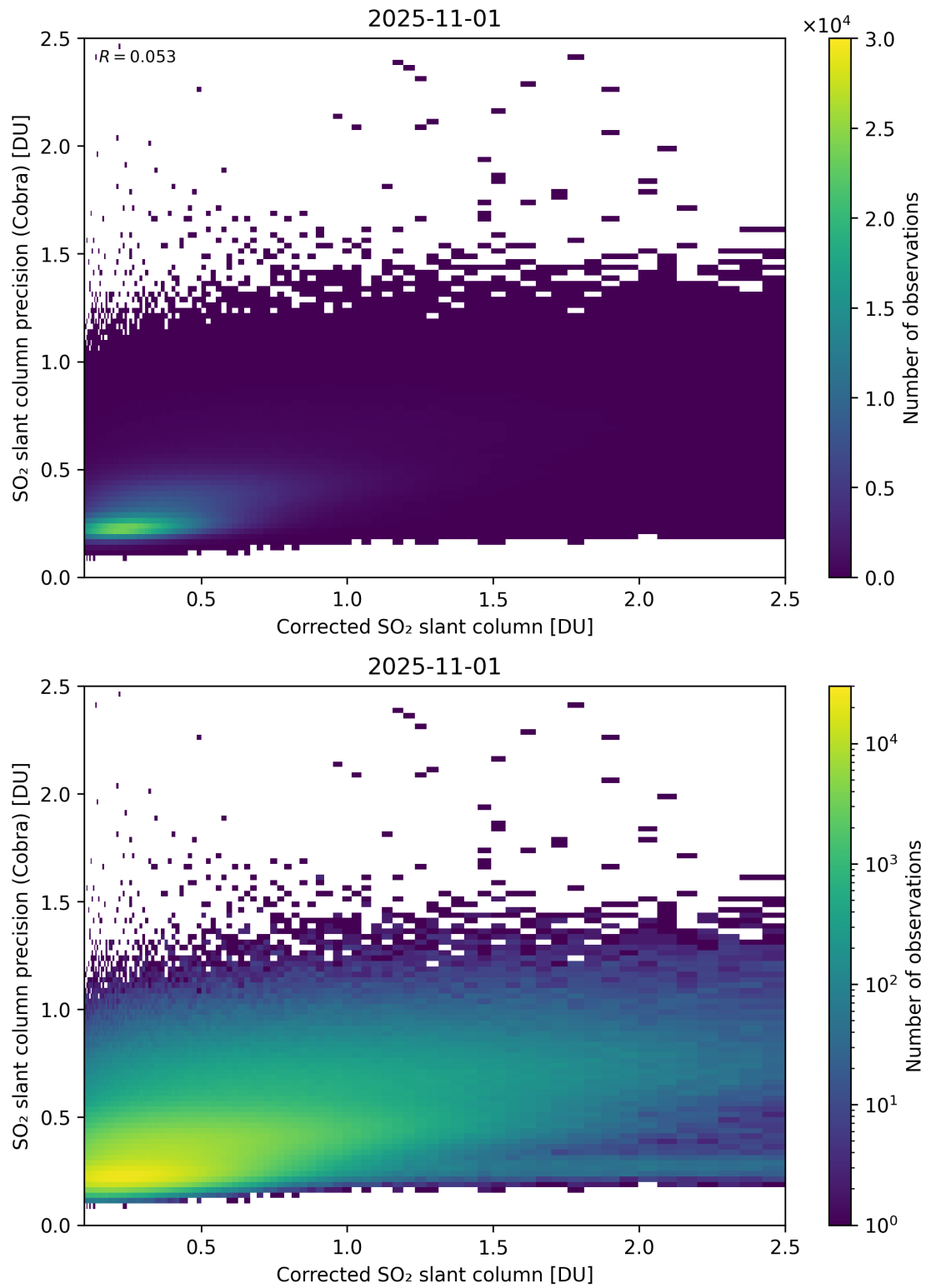
Figure 234: Scatter density plot of “Corrected SO 2 slant column” against “SO 2 slant column precision (Cobra)” for 2025-10-31 to 2025-11-02.
