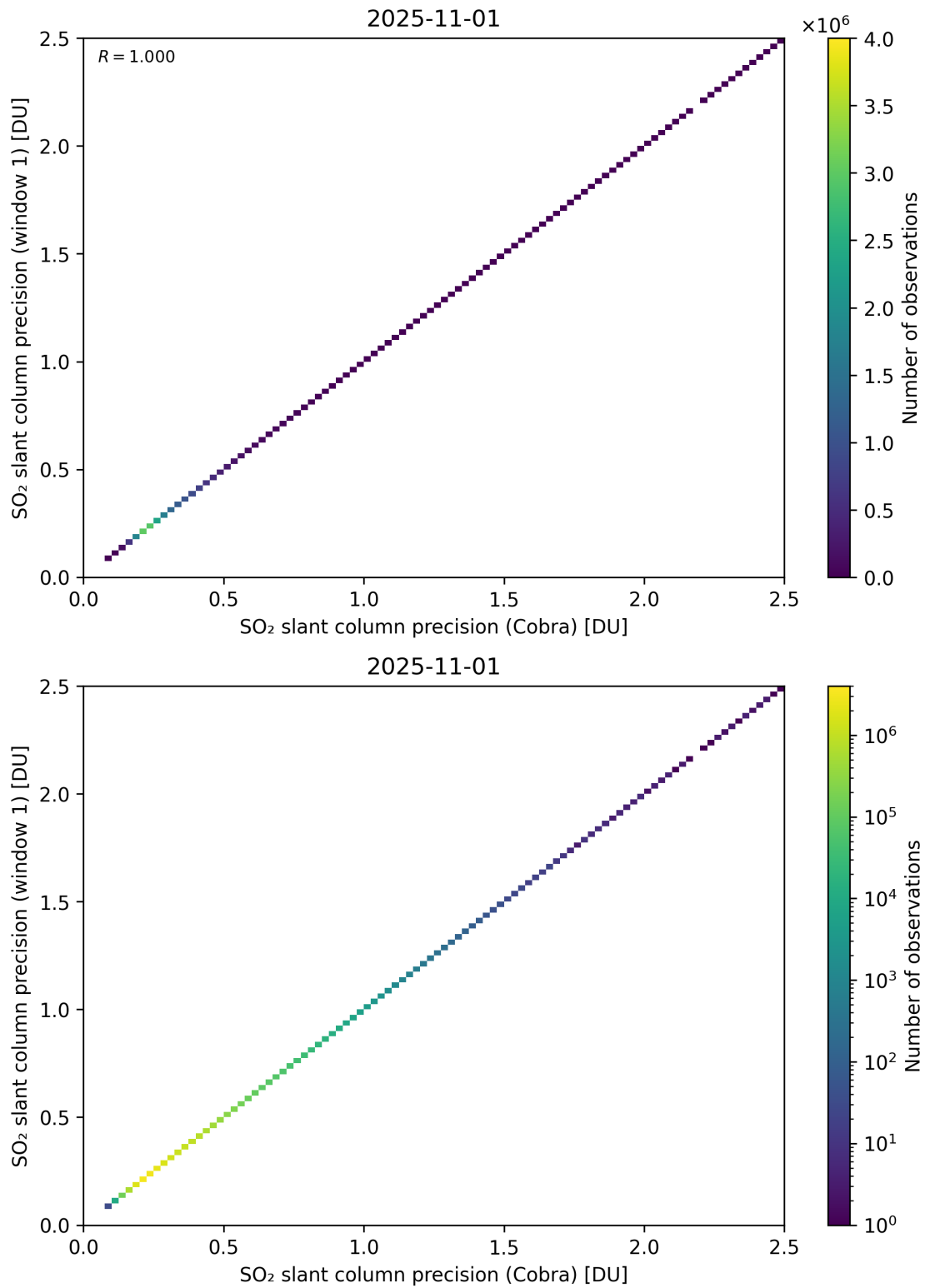
Figure 209: Scatter density plot of “SO 2 slant column precision (Cobra)” against “SO 2 slant column precision (window 1)” for 2025-10-31 to 2025-11-02.
