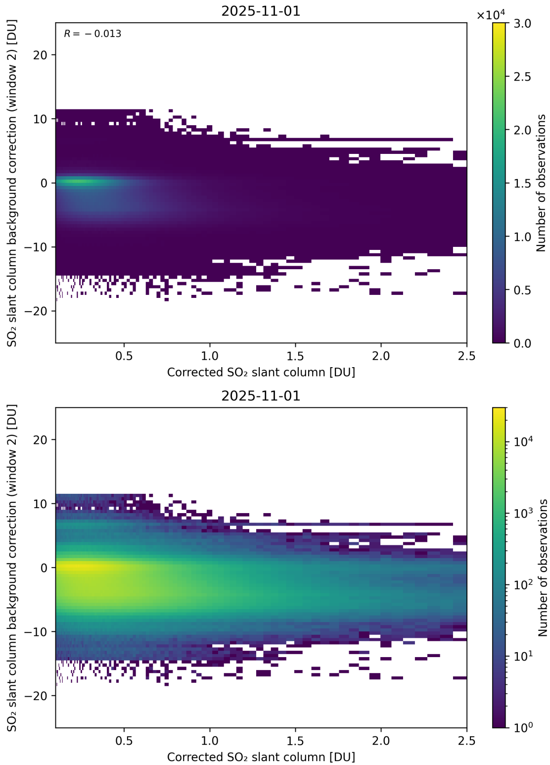
Figure 227: Scatter density plot of “Corrected SO 2 slant column” against “SO 2 slant column background correction (window 2)” for 2025-10-31 to 2025-11-02.
