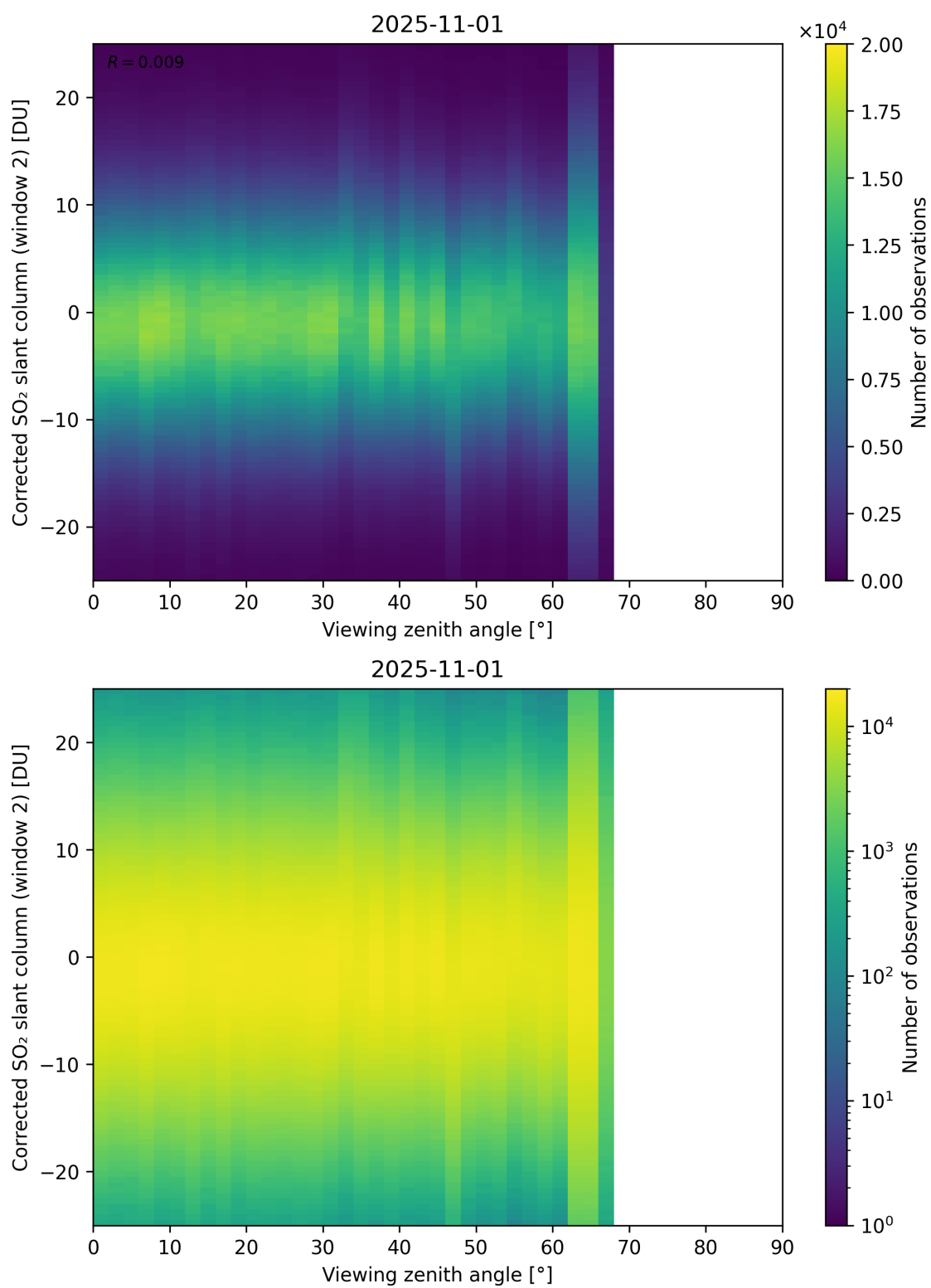
Figure 374: Scatter density plot of “Viewing zenith angle” against “Corrected SO 2 slant column (window 2)” for 2025-10-31 to 2025-11-02.
