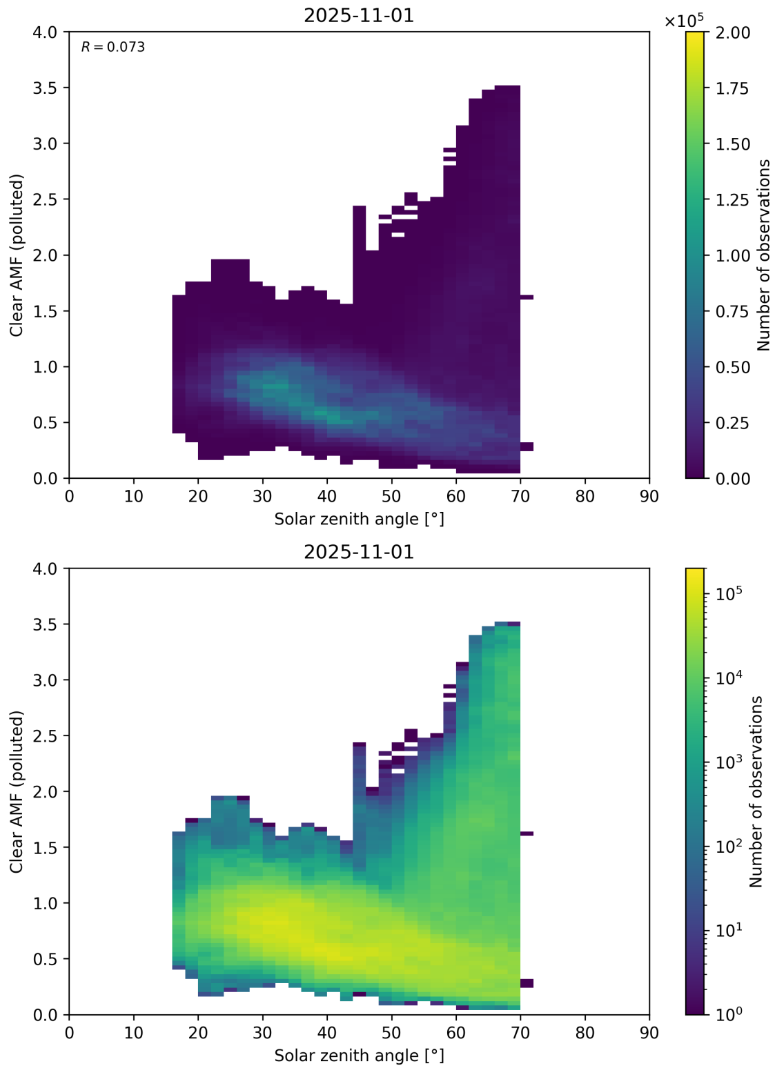
Figure 178: Scatter density plot of “Solar zenith angle” against “Clear AMF (polluted)” for 2025-10-31 to 2025-11-02.
