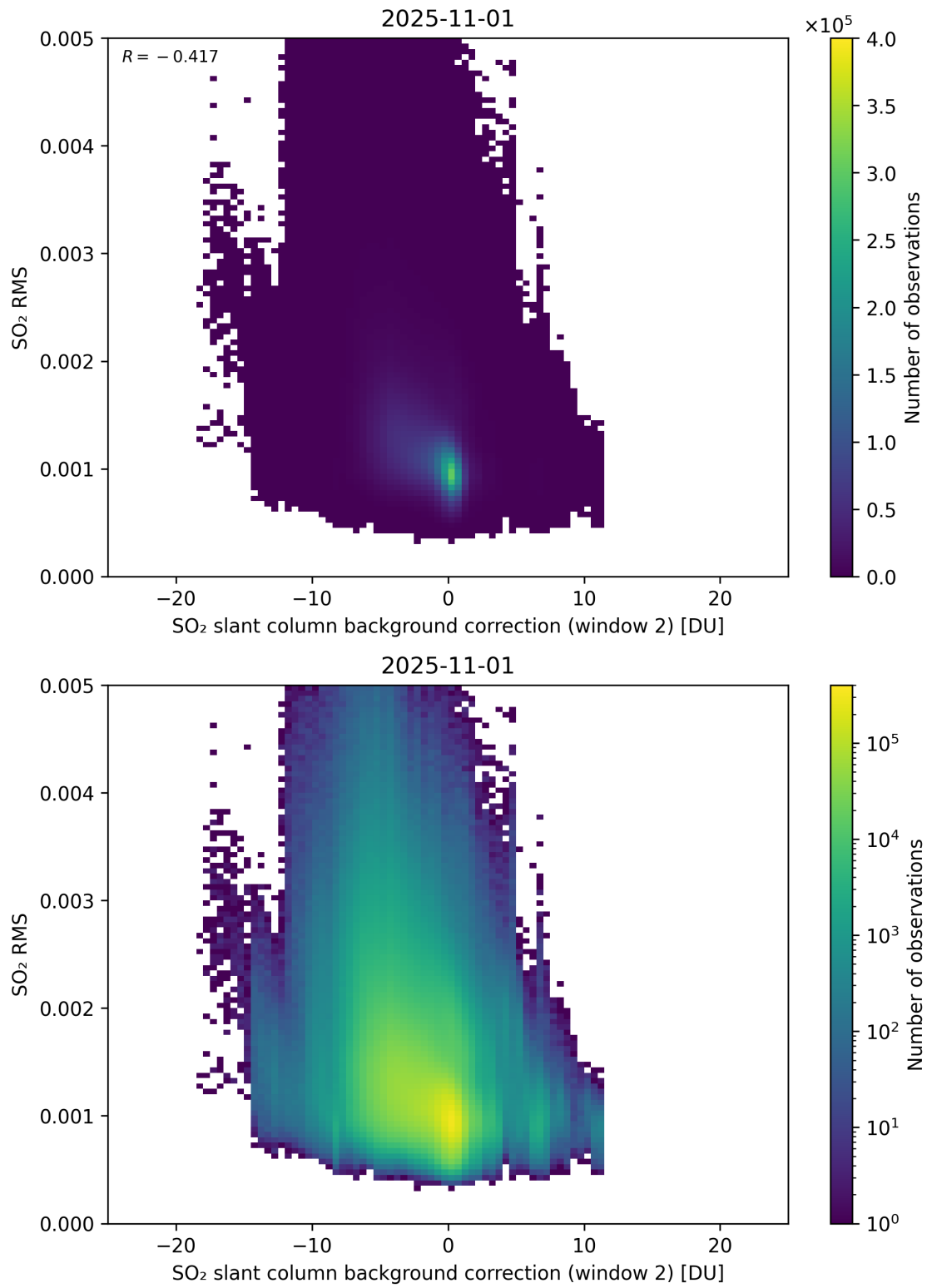
Figure 125: Scatter density plot of “SO 2 slant column background correction (window 2)” against “SO 2 RMS” for 2025-10-31 to 2025-11-02.
