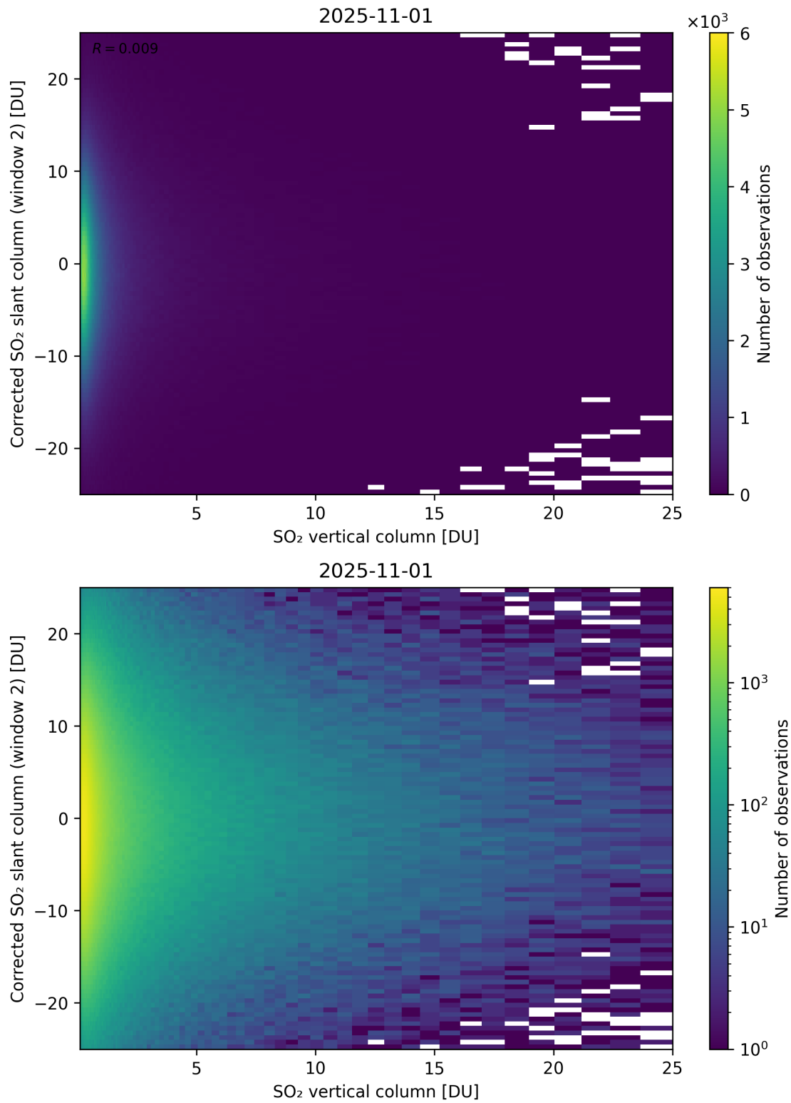
Figure 352: Scatter density plot of “SO 2 vertical column” against “Corrected SO 2 slant column (window 2)” for 2025-10-31 to 2025-11-02.
