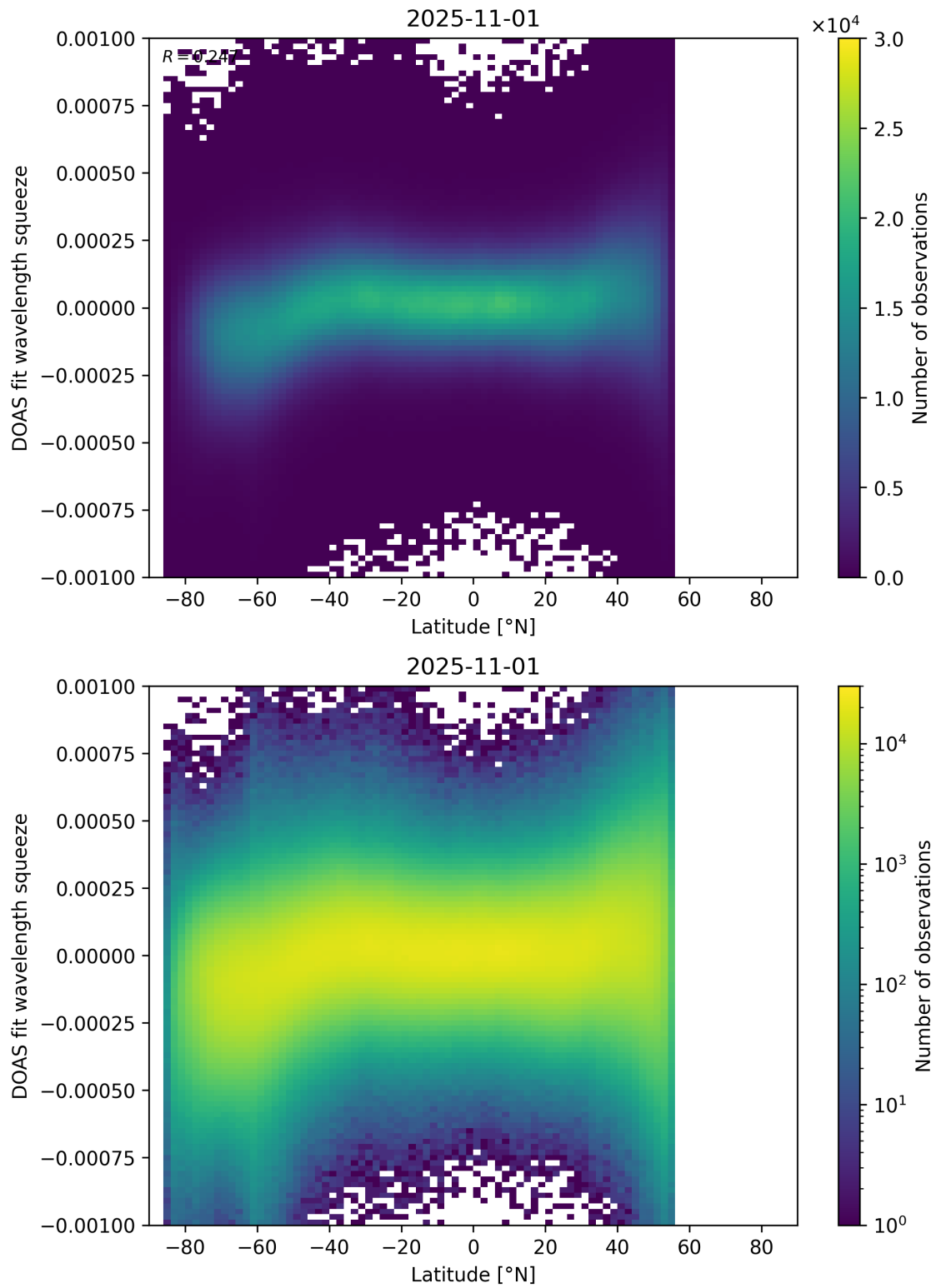
Figure 154: Scatter density plot of “Latitude” against “DOAS fit wavelength squeeze” for 2025-10-31 to 2025-11-02.
