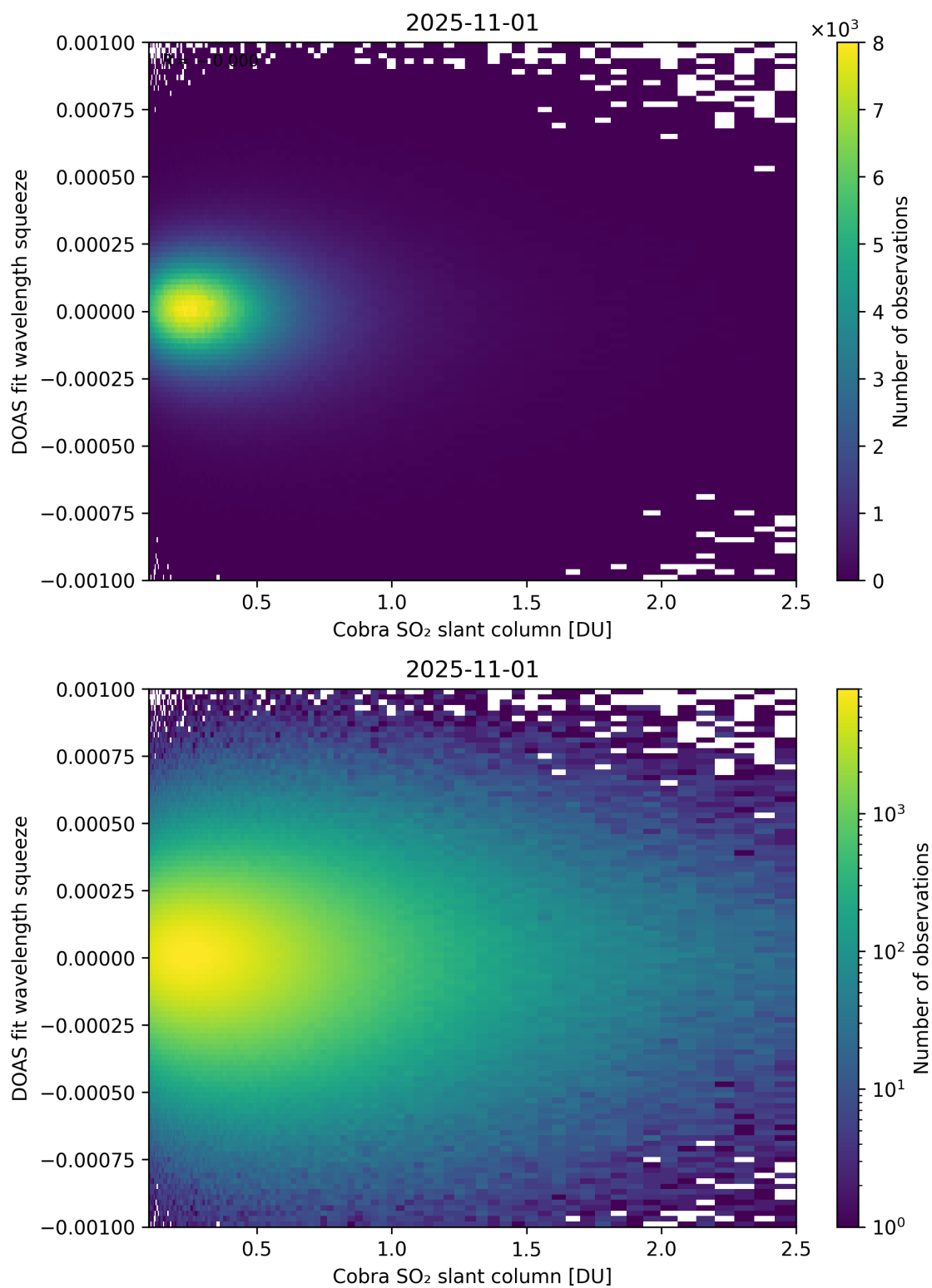
Figure 197: Scatter density plot of “Cobra SO 2 slant column” against “DOAS fit wavelength squeeze” for 2025-10-31 to 2025-11-02.
