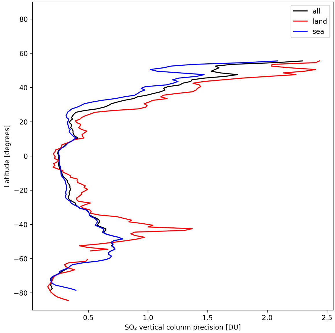
Figure 33: Zonal average of “SO 2 vertical column precision” for 2025-10-31 to 2025-11-02.
