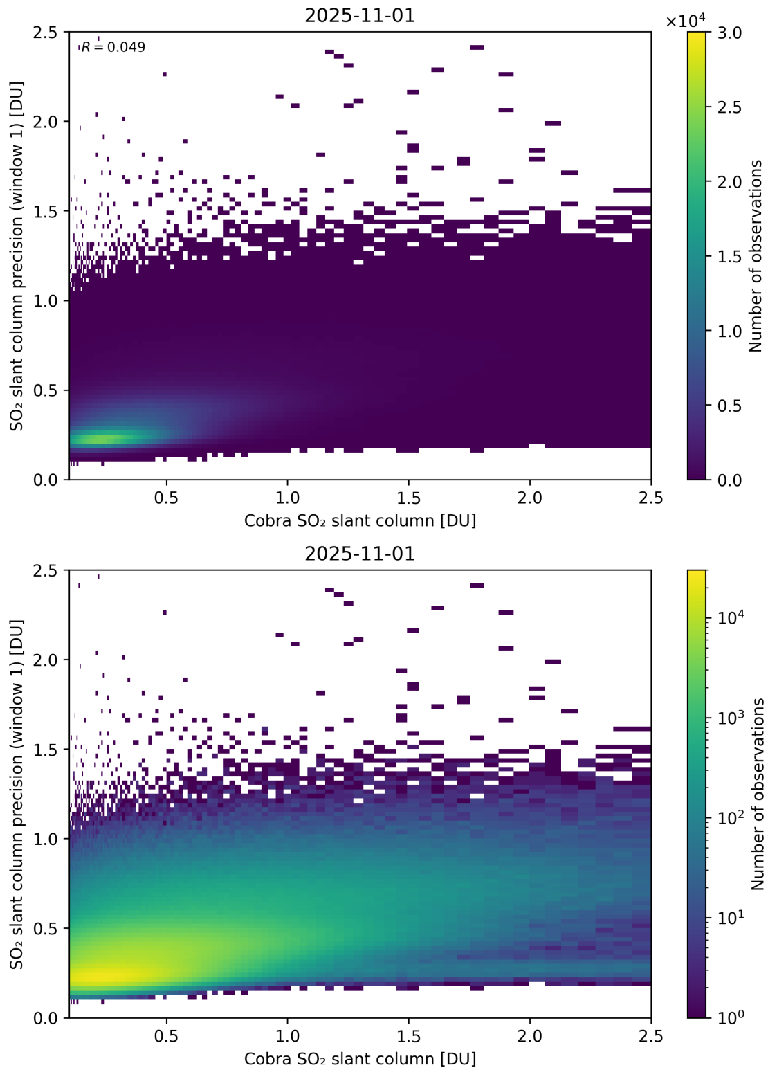
Figure 220: Scatter density plot of “Cobra SO 2 slant column” against “SO 2 slant column precision (window 1)” for 2025-10-31 to 2025-11-02.
