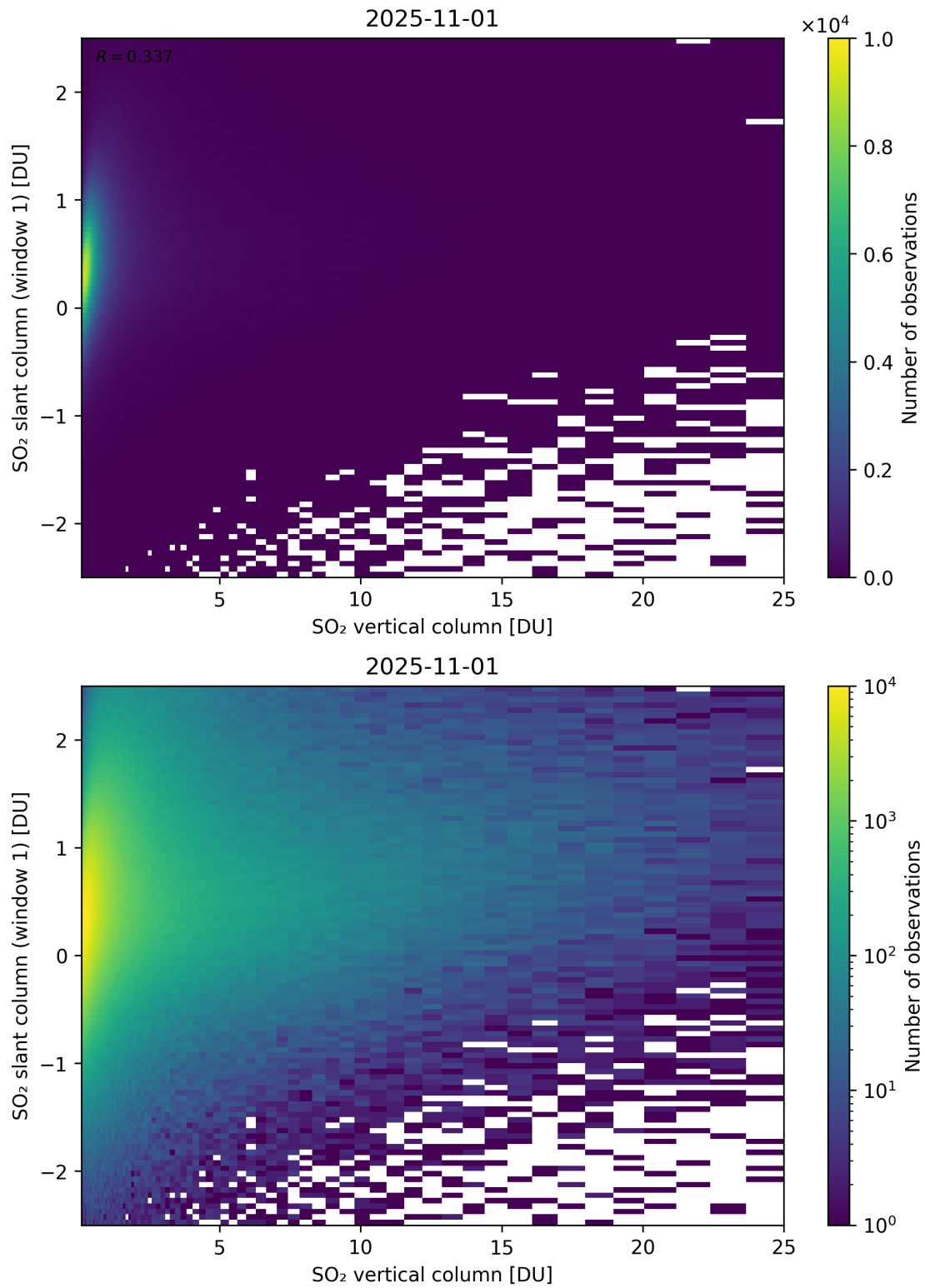
Figure 354: Scatter density plot of “SO 2 vertical column” against “SO 2 slant column (window 1)” for 2025-10-31 to 2025-11-02.
