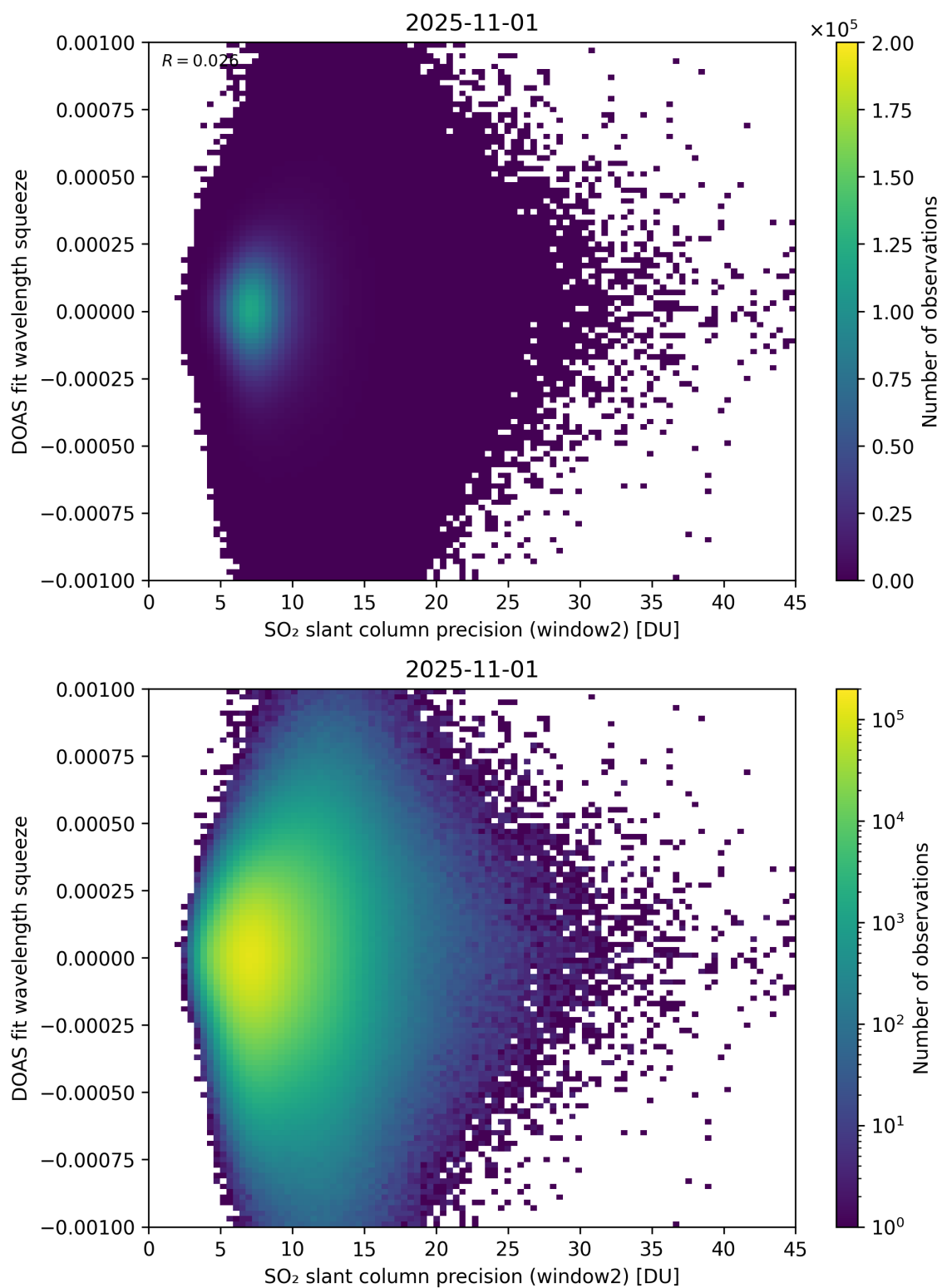
Figure 294: Scatter density plot of “SO 2 slant column precision (window2)” against “DOAS fit wavelength squeeze” for 2025-10-31 to 2025-11-02.
