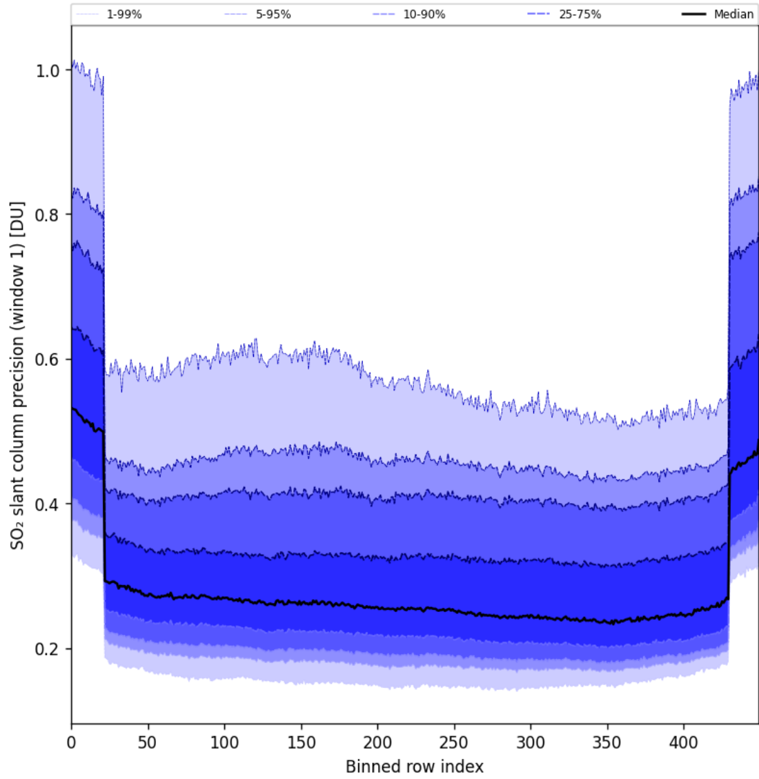
Figure 90: Along track statistics of “SO 2 slant column precision (window 1)” for 2025-10-31 to 2025-11-02
