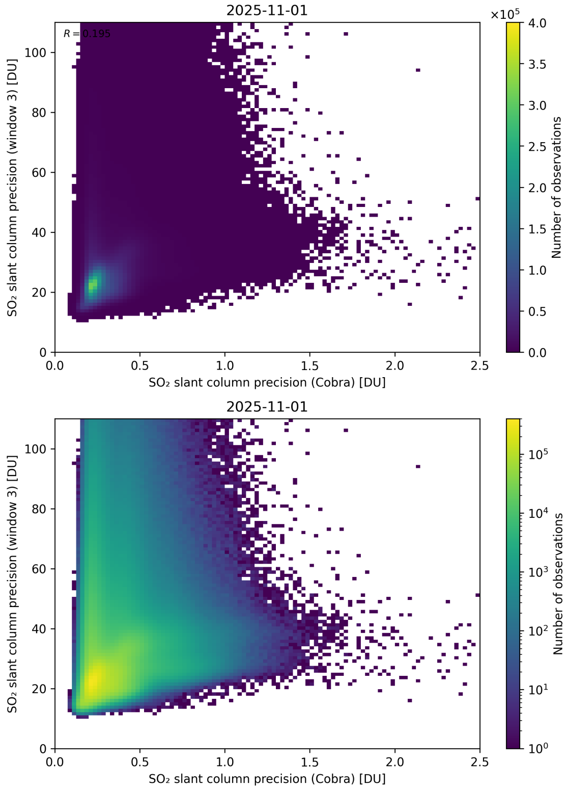
Figure 212: Scatter density plot of “SO 2 slant column precision (Cobra)” against “SO 2 slant column precision (window 3)” for 2025-10-31 to 2025-11-02.
