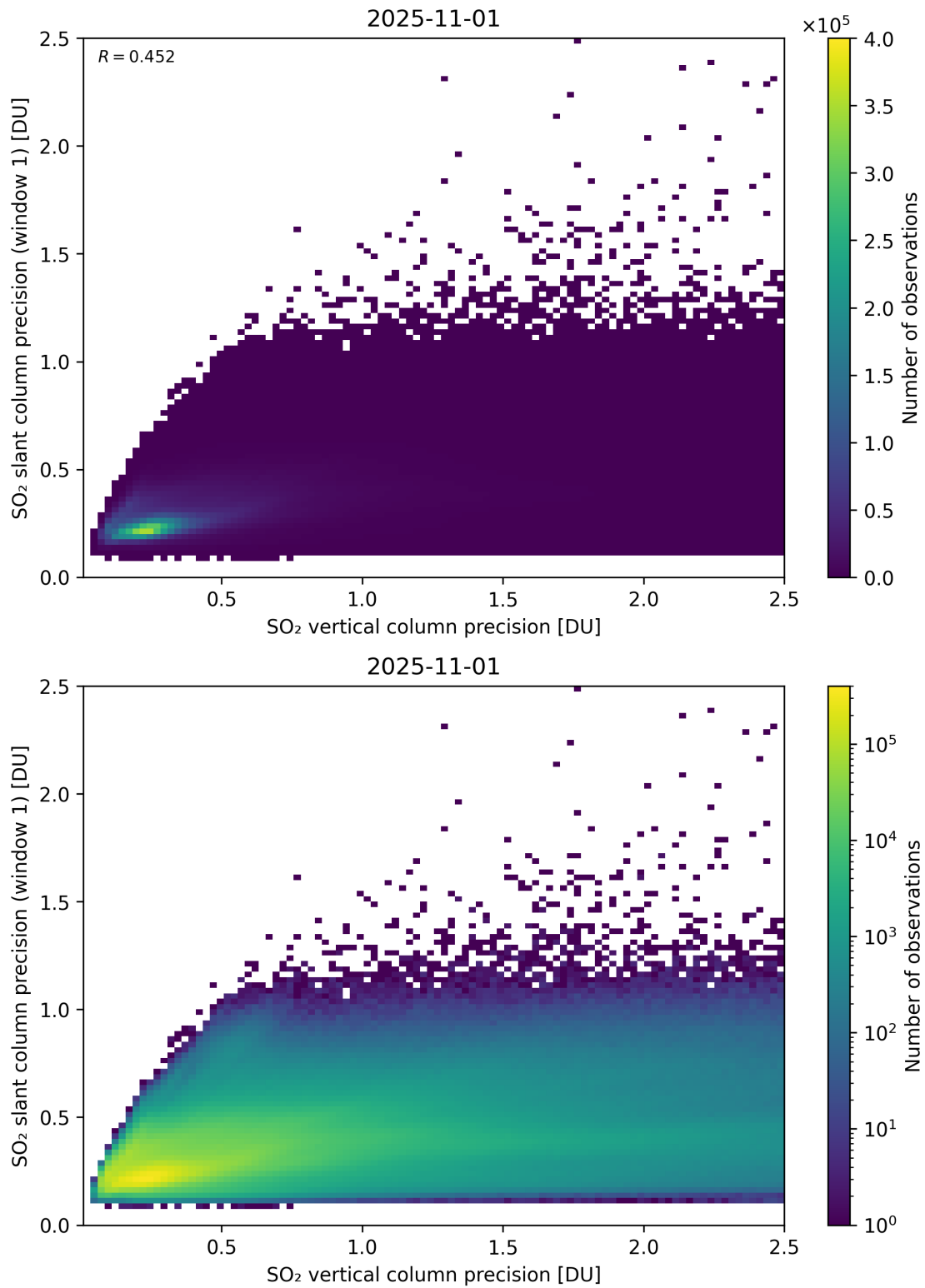
Figure 342: Scatter density plot of “SO 2 vertical column precision” against “SO 2 slant column precision (window 1)” for 2025-10-31 to 2025-11-02.
