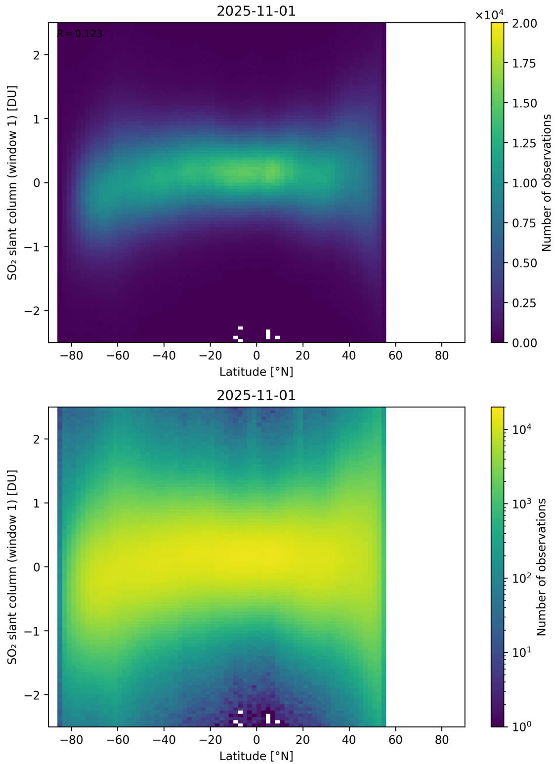
Figure 162: Scatter density plot of “Latitude” against “SO 2 slant column (window 1)” for 2025-10-31 to 2025-11-02.
