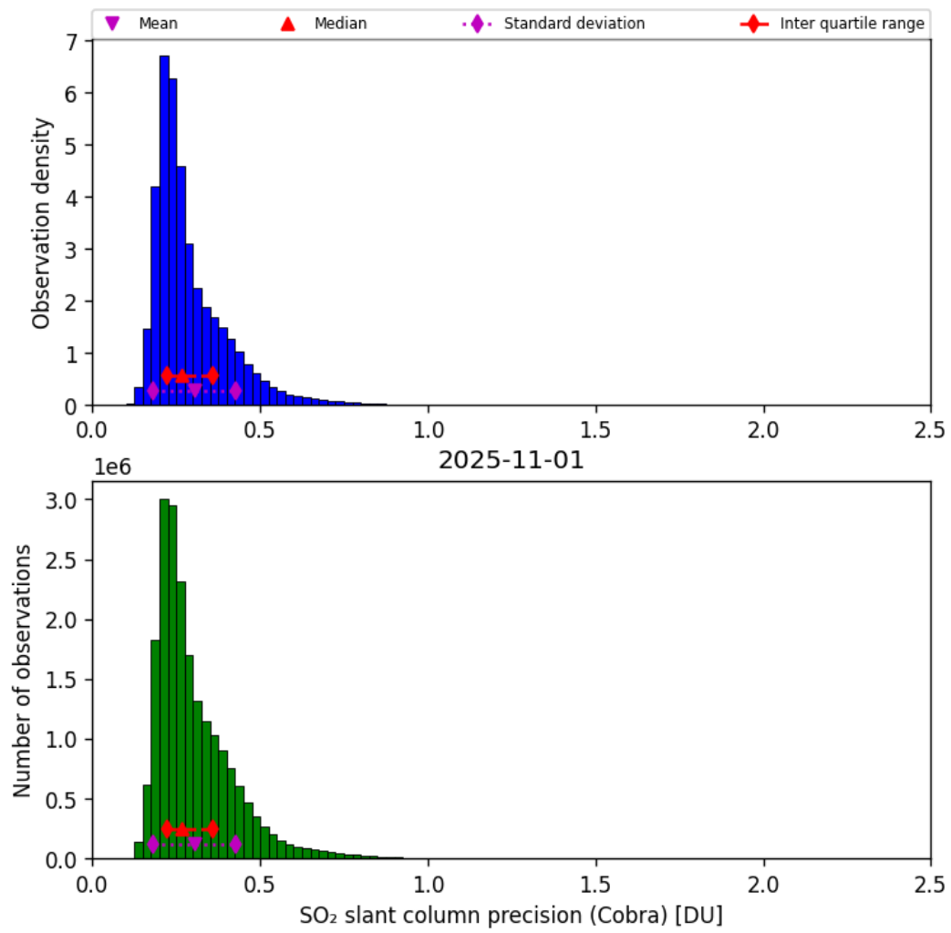
Figure 62: Histogram of “SO 2 slant column precision (Cobra)” for 2025-10-31 to 2025-11-02
