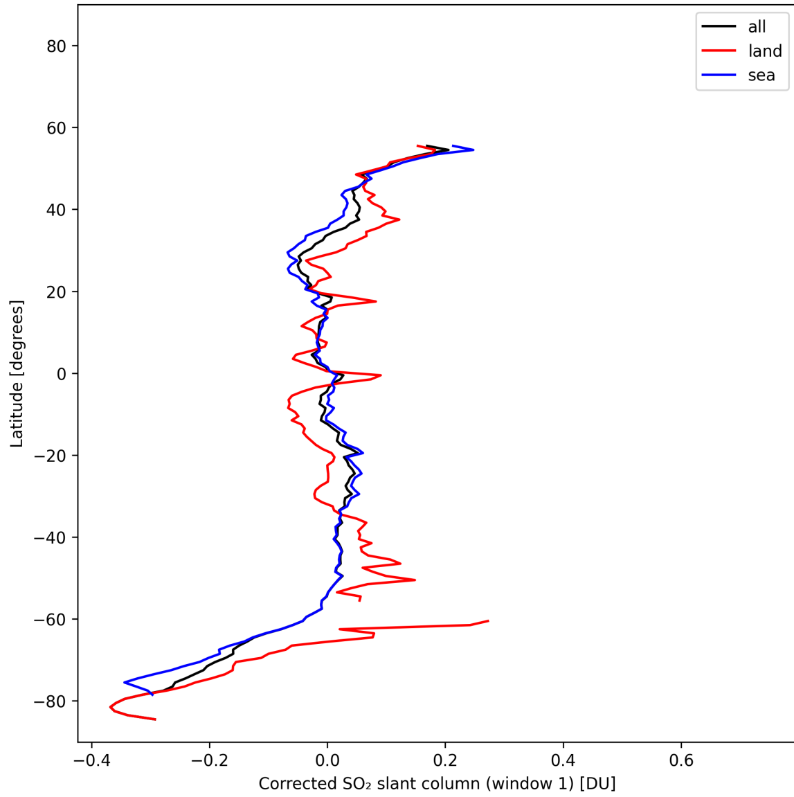
Figure 39: Zonal average of “Corrected SO 2 slant column (window 1)” for 2025-10-31 to 2025-11-02.
