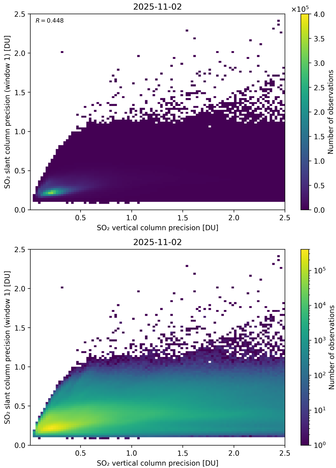
Figure 342: Scatter density plot of “SO 2 vertical column precision” against “SO 2 slant column precision (window 1)” for 2025-11-02 to 2025-11-03.
