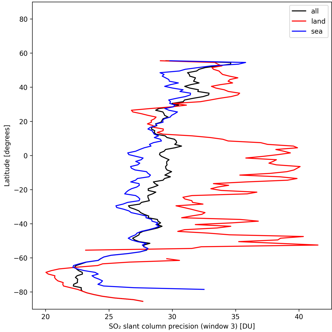
Figure 46: Zonal average of “SO 2 slant column precision (window 3)” for 2025-11-02 to 2025-11-03.
