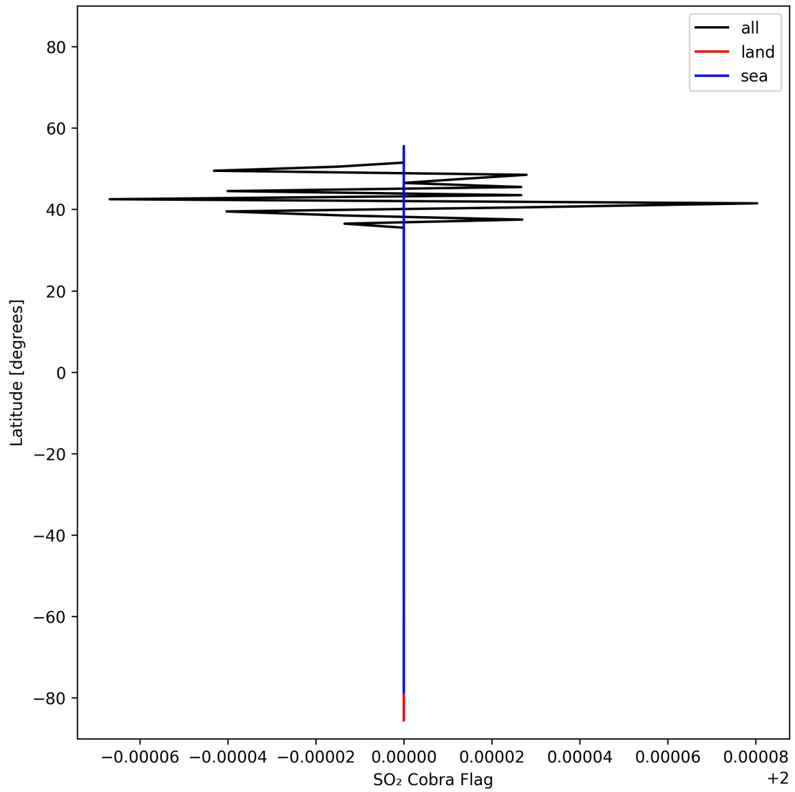
Figure 49: Zonal average of “SO 2 Cobra Flag” for 2025-11-02 to 2025-11-03.
