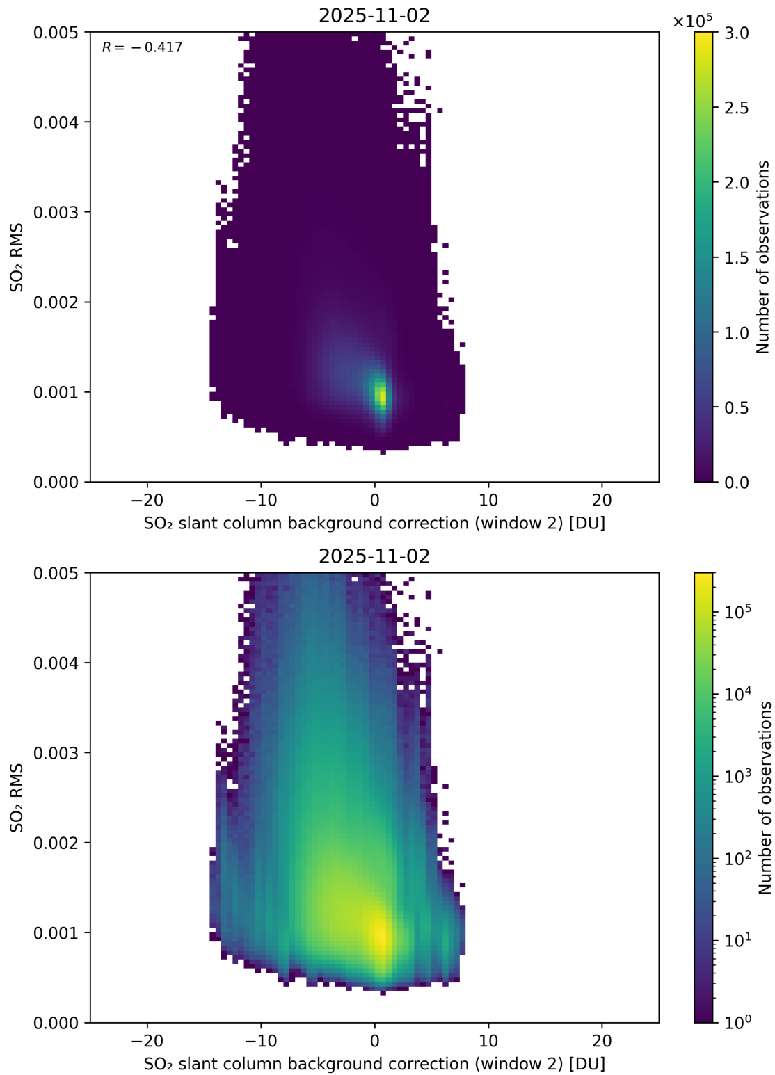
Figure 125: Scatter density plot of “SO 2 slant column background correction (window 2)” against “SO 2 RMS” for 2025-11-02 to 2025-11-03.
