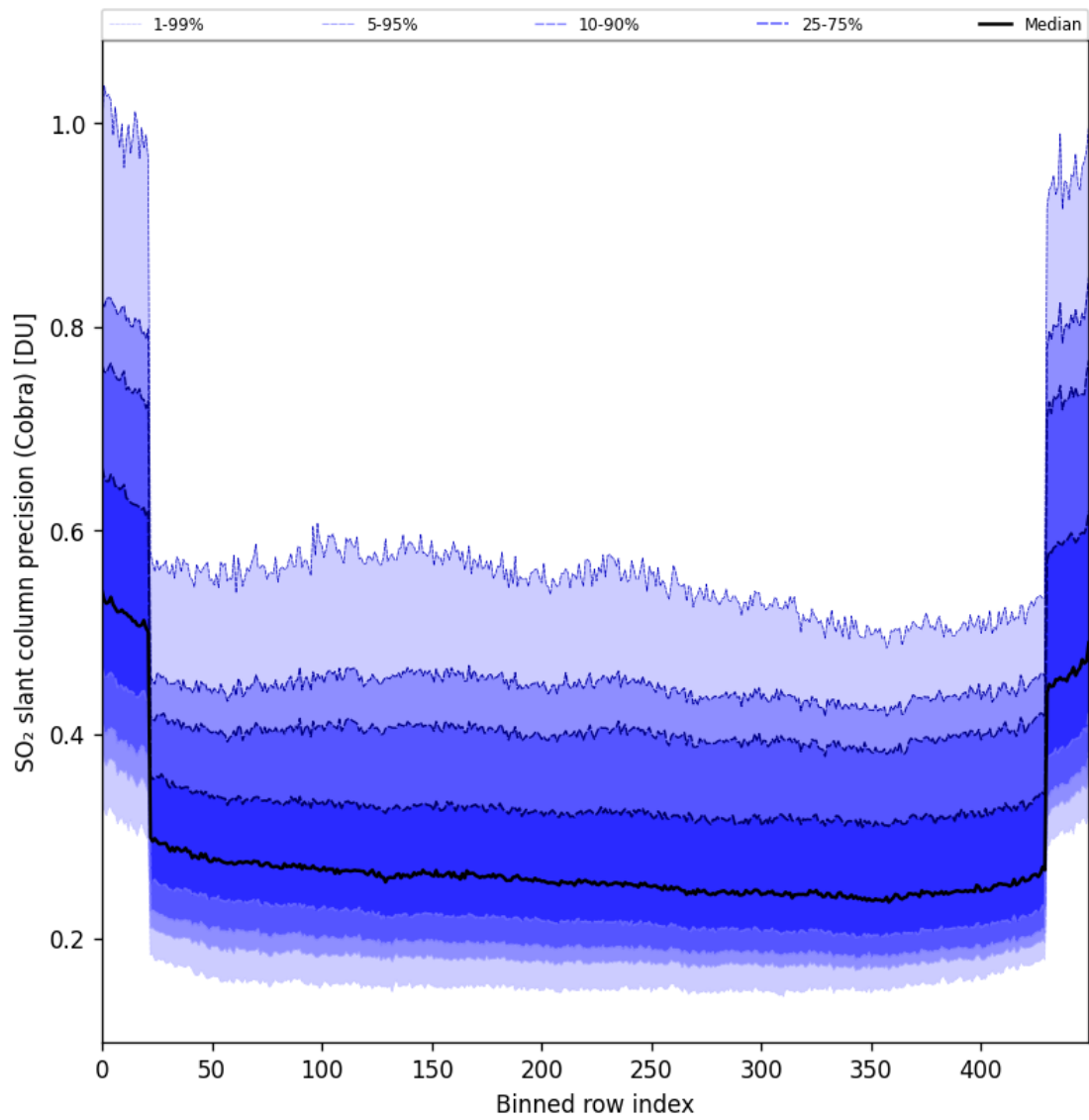
Figure 88: Along track statistics of “SO 2 slant column precision (Cobra)” for 2025-11-02 to 2025-11-03
