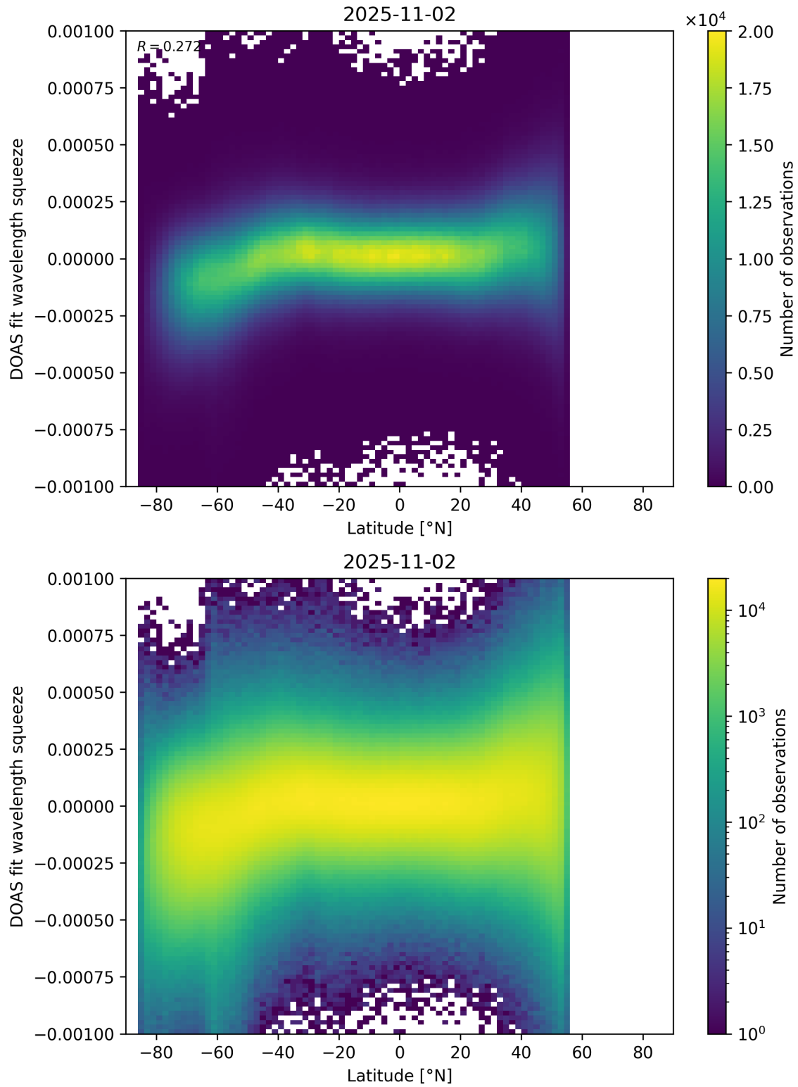
Figure 154: Scatter density plot of “Latitude” against “DOAS fit wavelength squeeze” for 2025-11-02 to 2025-11-03.
