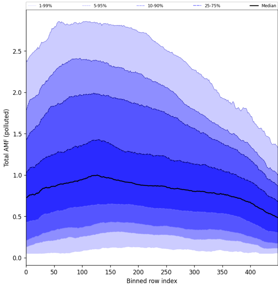
Figure 105: Along track statistics of “Total AMF (polluted)” for 2025-11-02 to 2025-11-03
