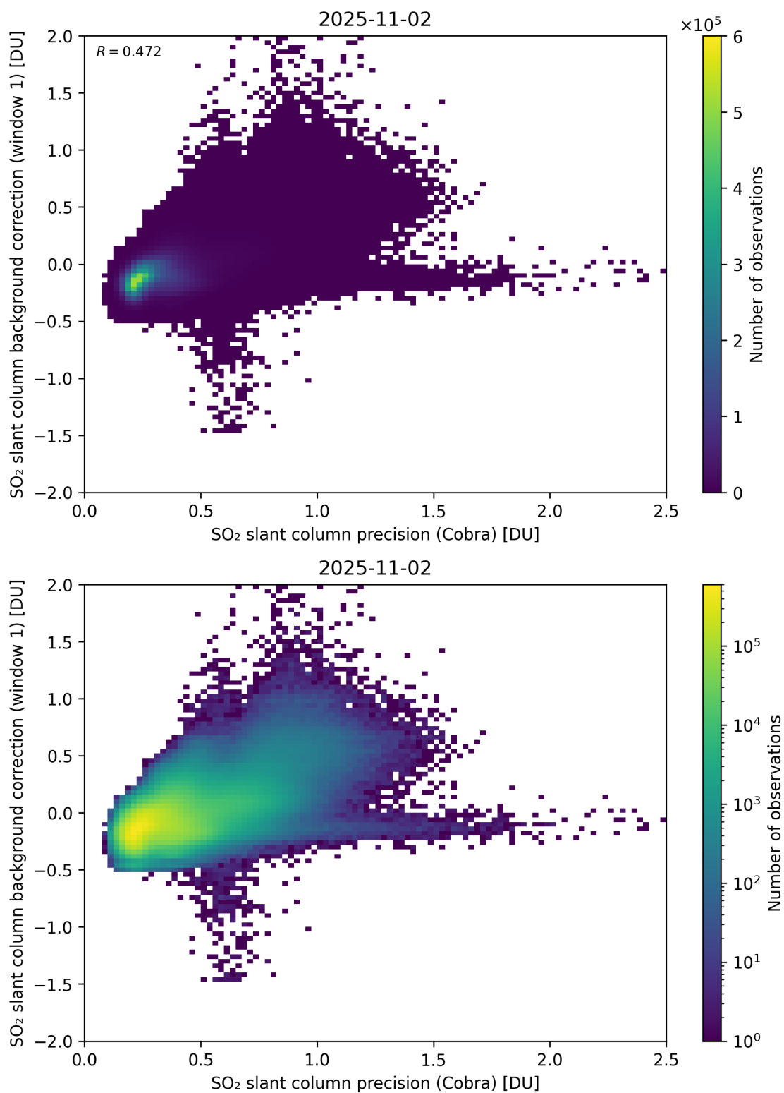
Figure 199: Scatter density plot of “SO 2 slant column precision (Cobra)” against “SO 2 slant column background correction (window 1)” for 2025-11-02 to 2025-11-03.
