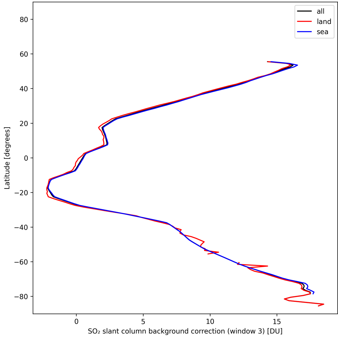
Figure 48: Zonal average of “SO 2 slant column background correction (window 3)” for 2025-11-02 to 2025-11-03.
