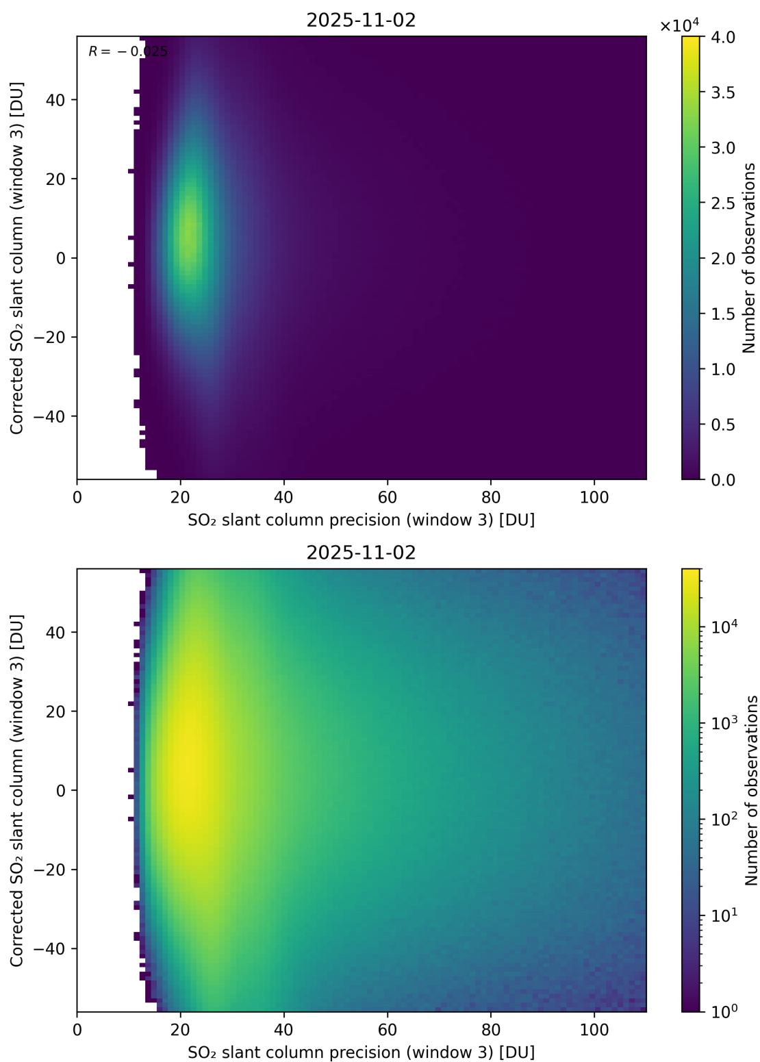
Figure 312: Scatter density plot of “SO 2 slant column precision (window 3)” against “Corrected SO 2 slant column (window 3)” for 2025-11-02 to 2025-11-03.
