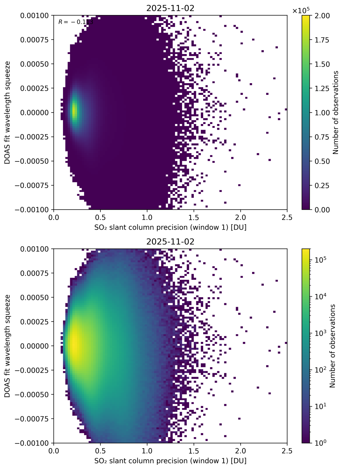
Figure 272: Scatter density plot of “SO 2 slant column precision (window 1)” against “DOAS fit wavelength squeeze” for 2025-11-02 to 2025-11-03.
