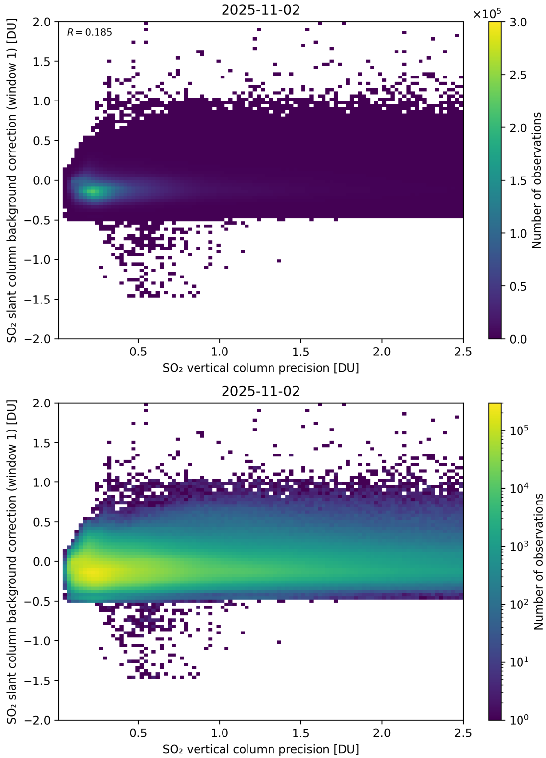
Figure 329: Scatter density plot of “SO 2 vertical column precision” against “SO 2 slant column background correction (window 1)” for 2025-11-02 to 2025-11-03.
