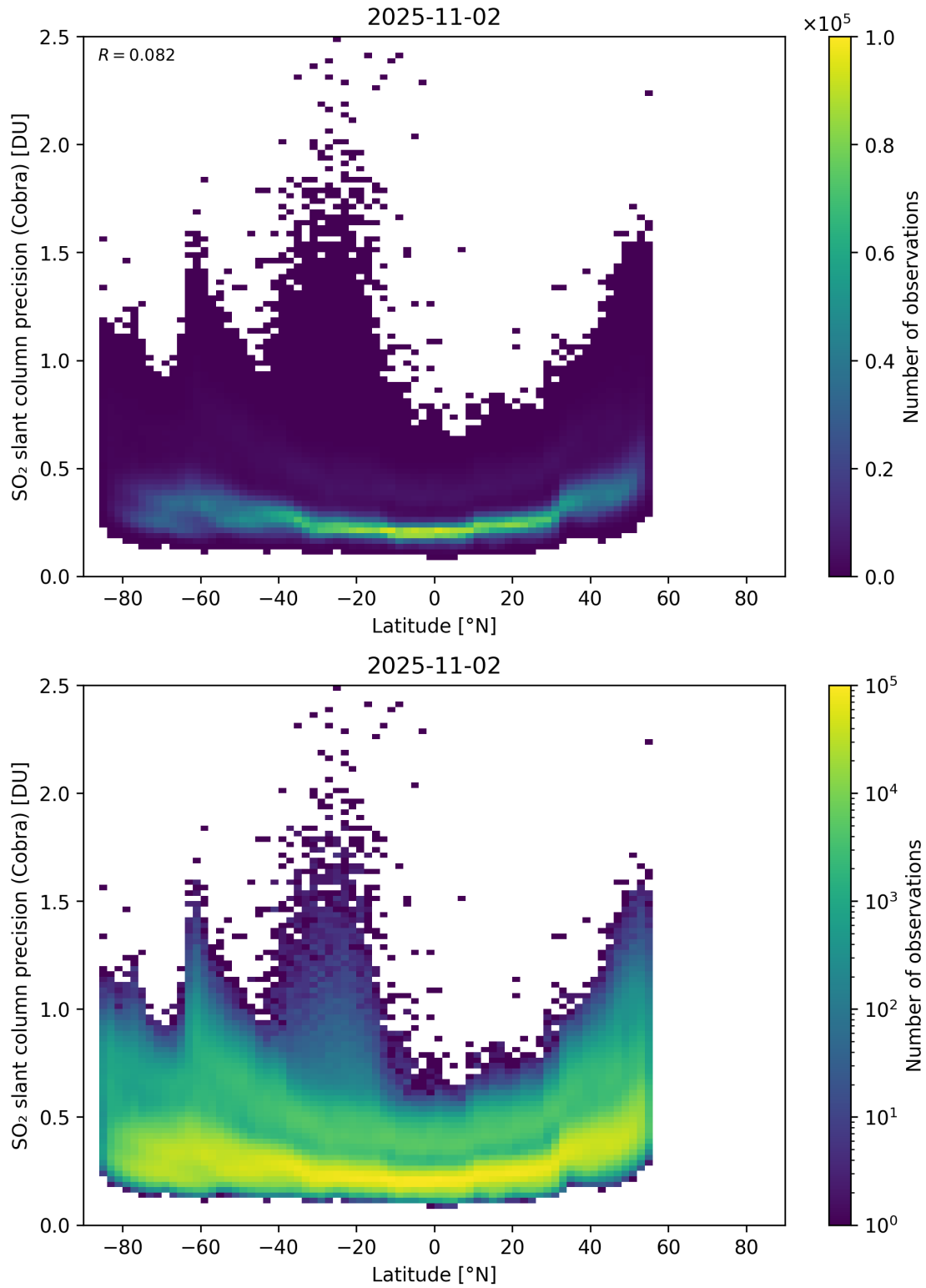
Figure 158: Scatter density plot of “Latitude” against “SO 2 slant column precision (Cobra)” for 2025-11-02 to 2025-11-03.
