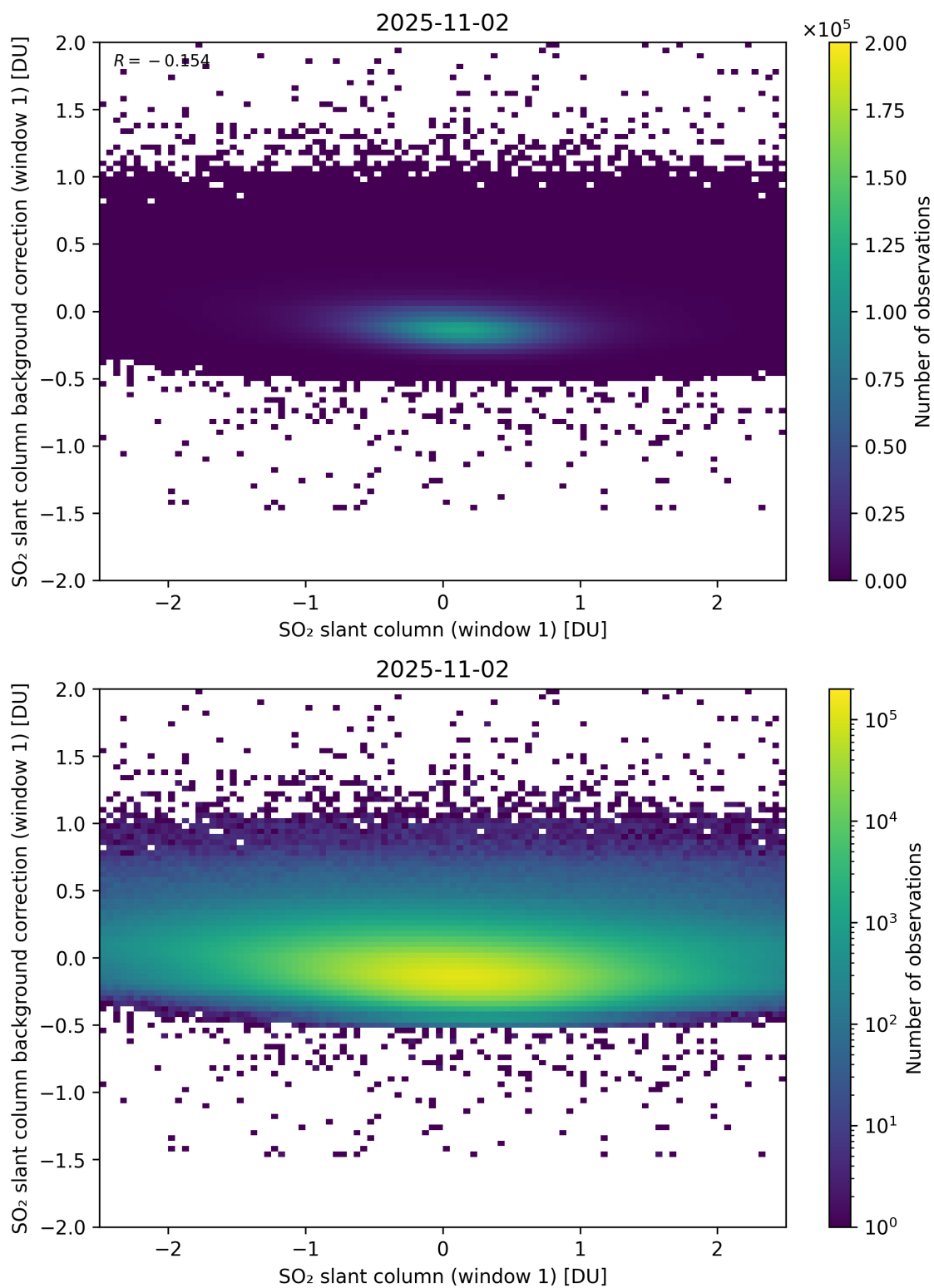
Figure 262: Scatter density plot of “SO 2 slant column (window 1)” against “SO 2 slant column background correction (window 1)” for 2025-11-02 to 2025-11-03.
