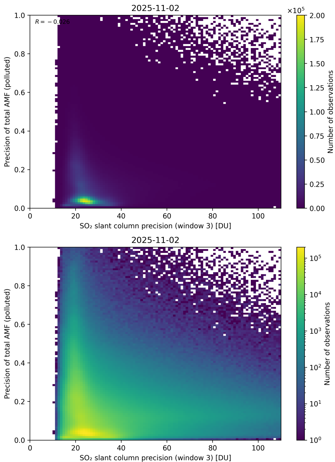
Figure 314: Scatter density plot of “SO 2 slant column precision (window 3)” against “Precision of total AMF (polluted)” for 2025-11-02 to 2025-11-03.
