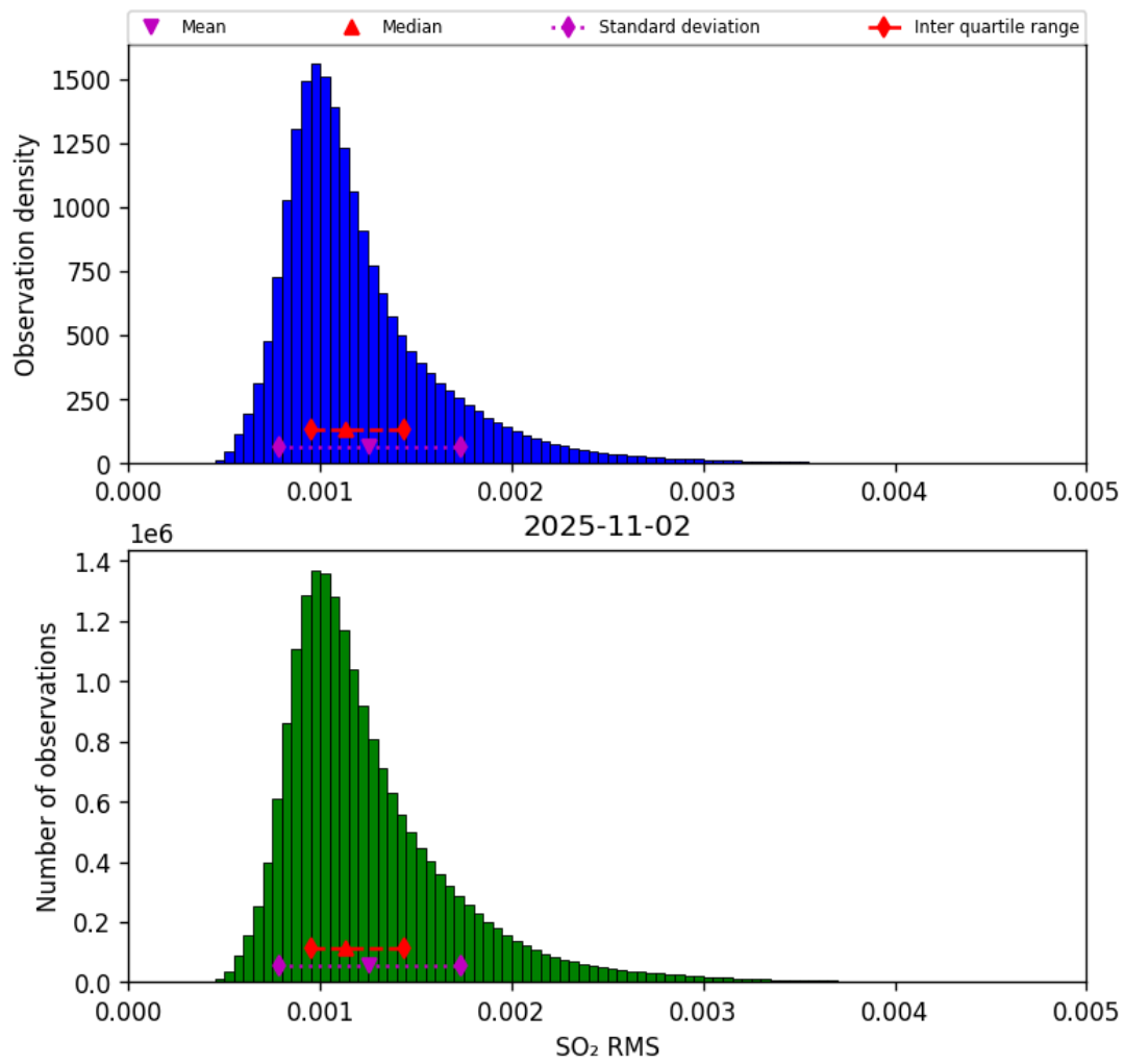
Figure 78: Histogram of “SO 2 RMS” for 2025-11-02 to 2025-11-03
