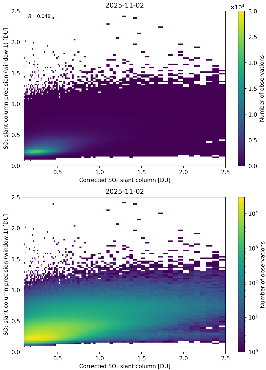
Figure 238: Scatter density plot of “Corrected SO 2 slant column” against “SO 2 slant column precision (window 1)” for 2025-11-02 to 2025-11-03.
