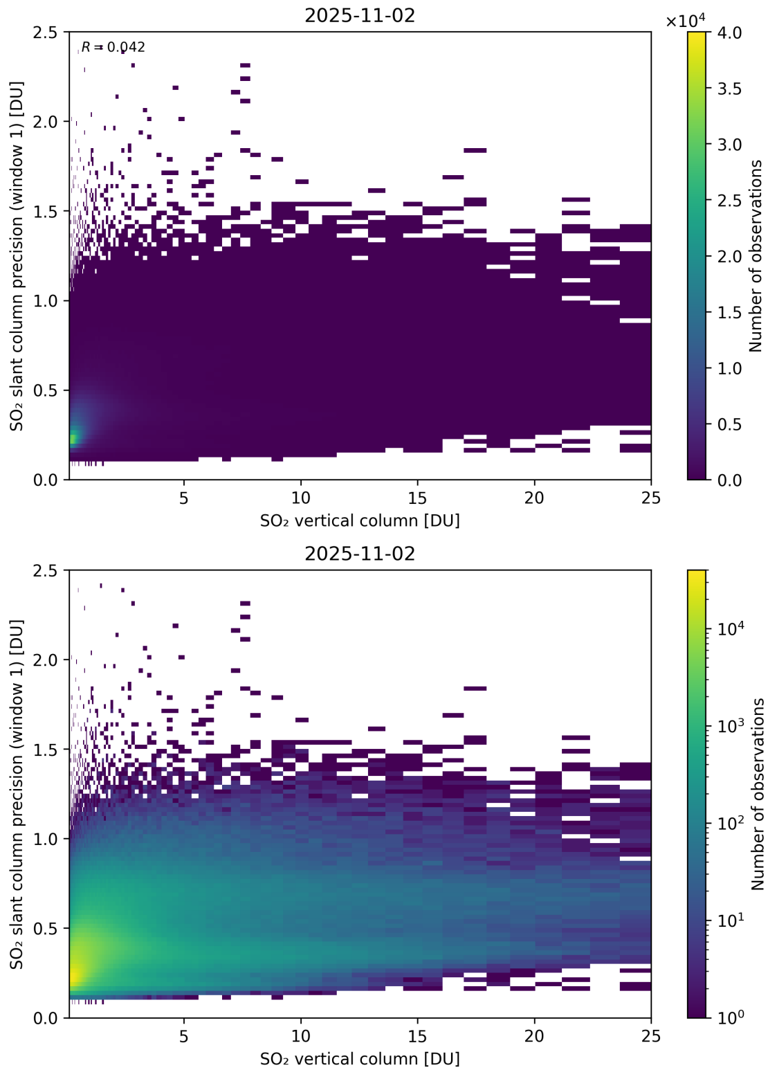
Figure 355: Scatter density plot of “SO 2 vertical column” against “SO 2 slant column precision (window 1)” for 2025-11-02 to 2025-11-03.
