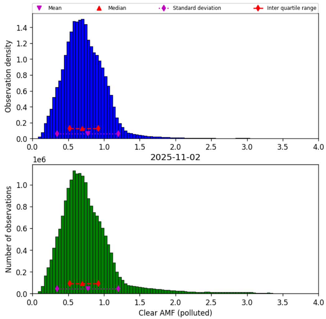
Figure 81: Histogram of “Clear AMF (polluted)” for 2025-11-02 to 2025-11-03
