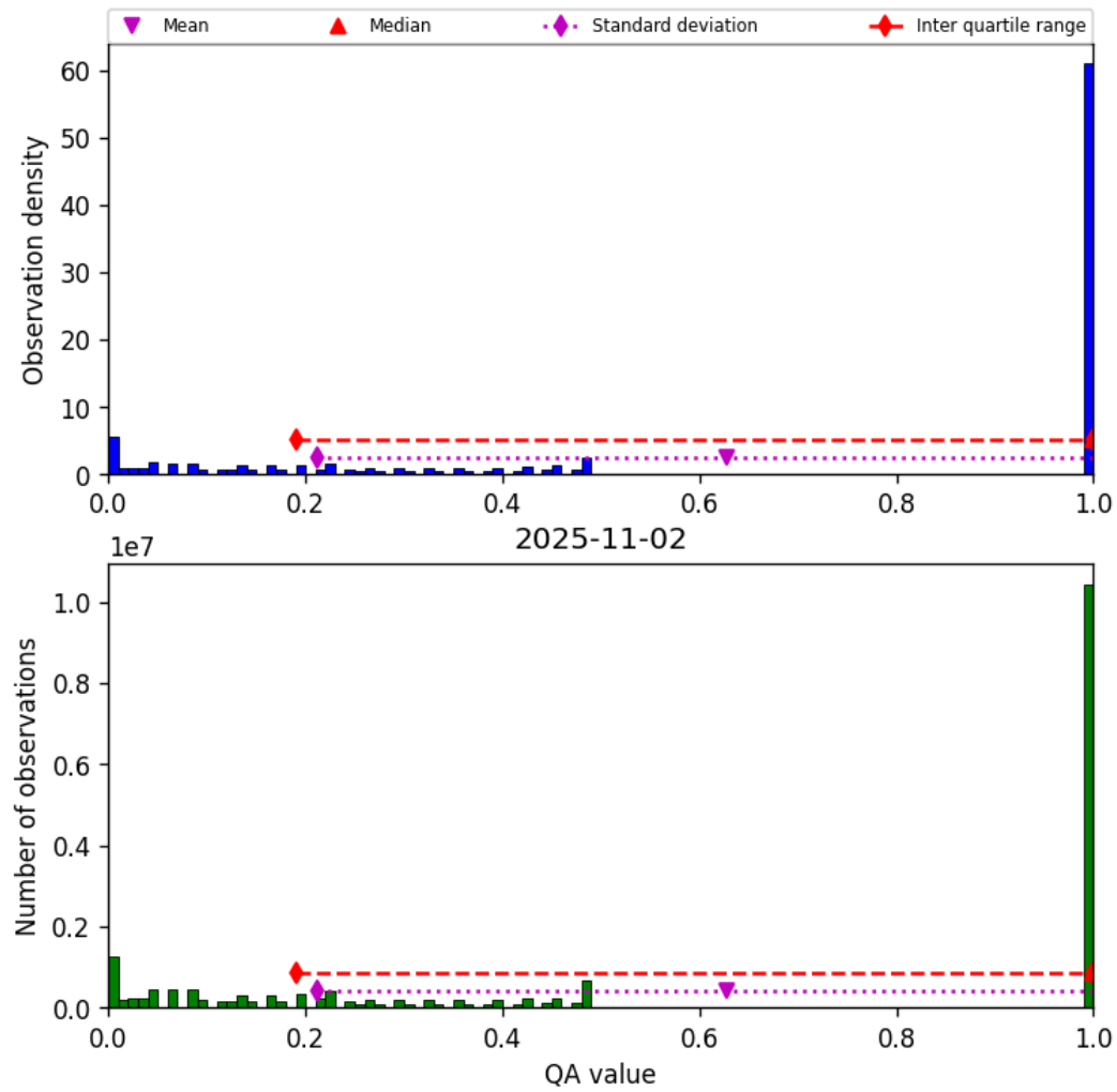
Figure 57: Histogram of “QA value” for 2025-11-02 to 2025-11-03
