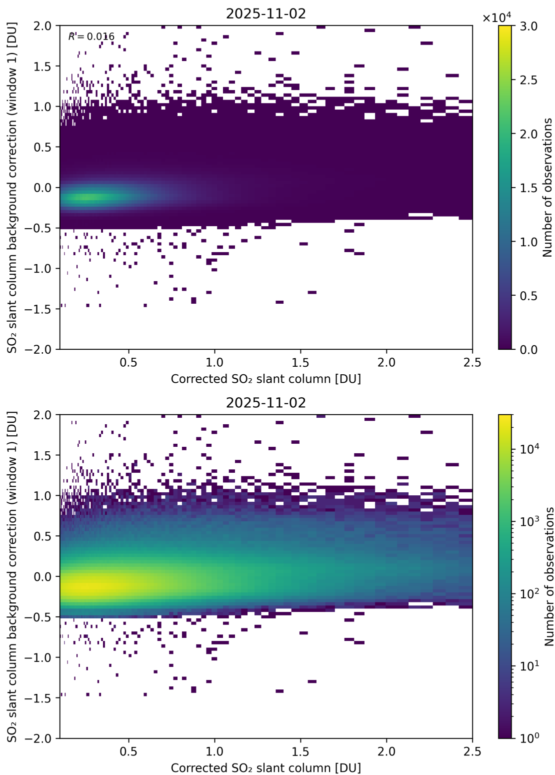
Figure 226: Scatter density plot of “Corrected SO 2 slant column” against “SO 2 slant column background correction (window 1)” for 2025-11-02 to 2025-11-03.
