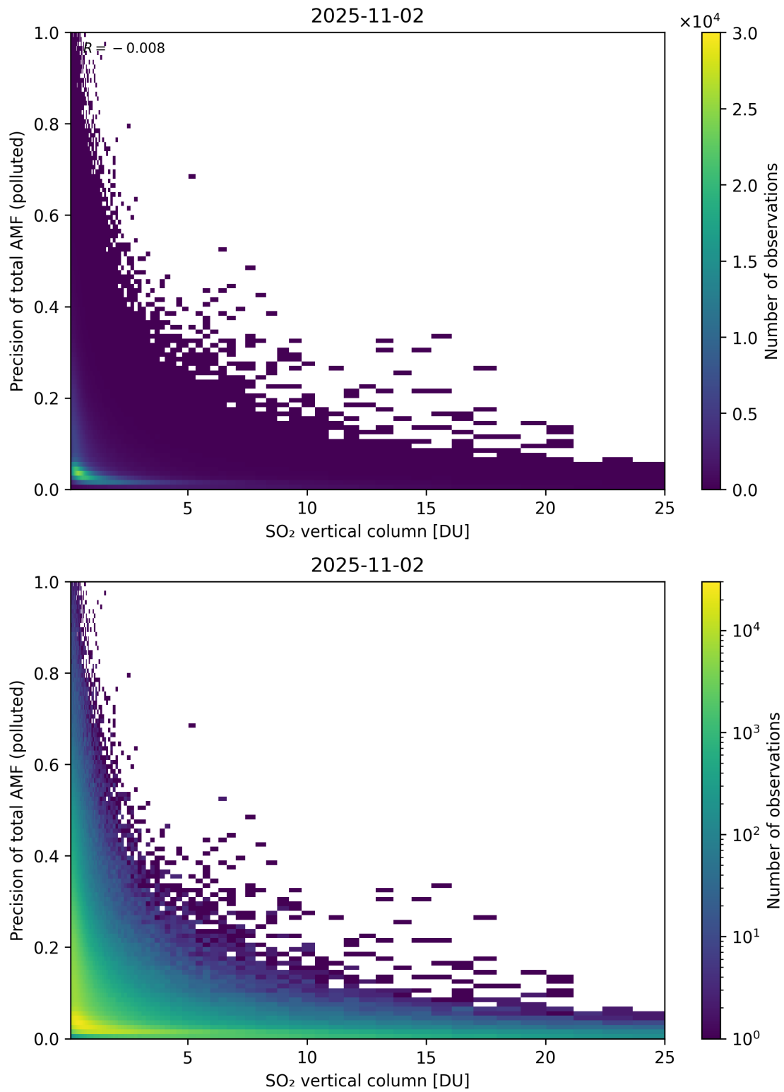
Figure 360: Scatter density plot of “SO 2 vertical column” against “Precision of total AMF (polluted)” for 2025-11-02 to 2025-11-03.
