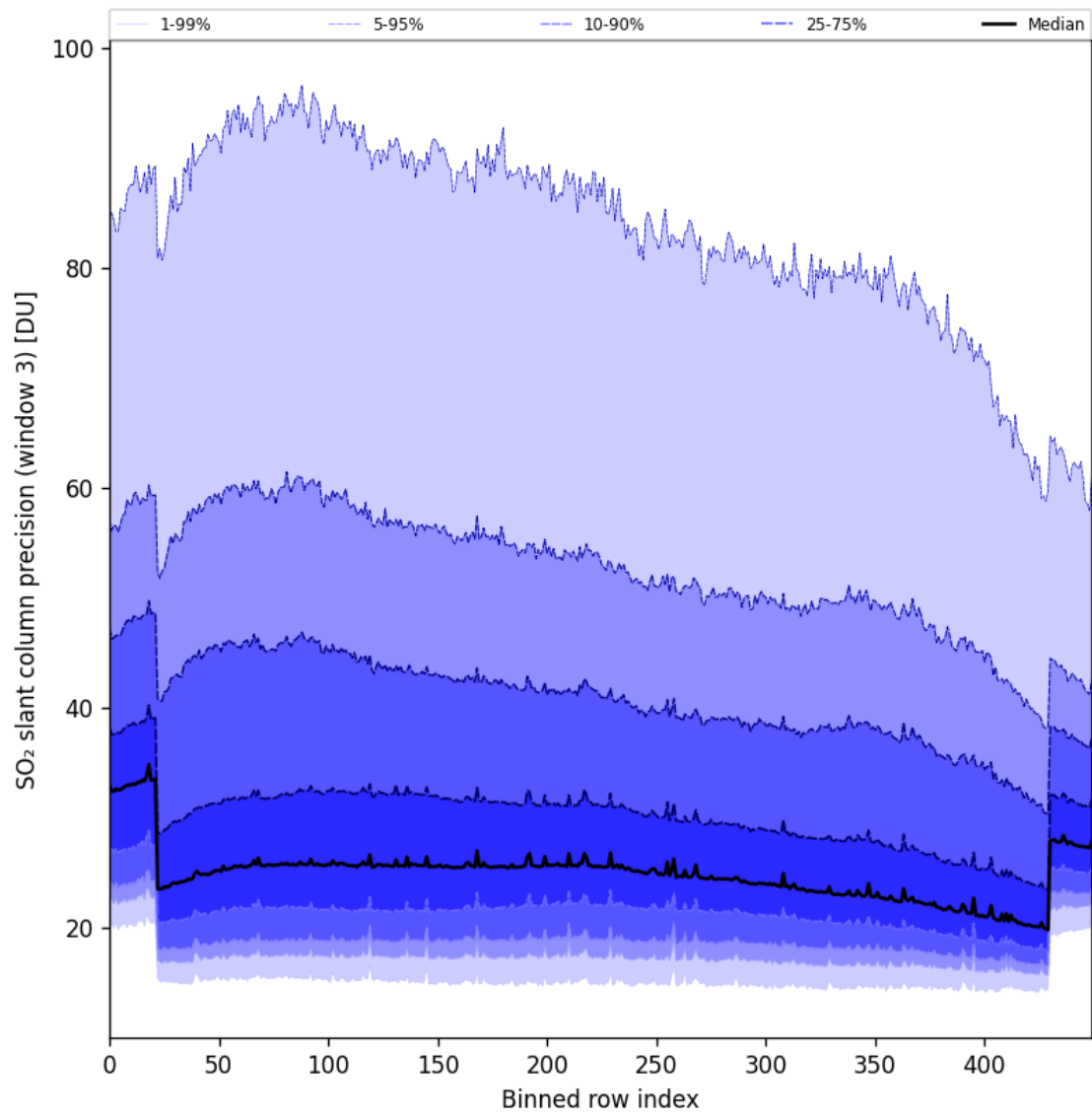
Figure 98: Along track statistics of “SO 2 slant column precision (window 3)” for 2025-11-02 to 2025-11-03
