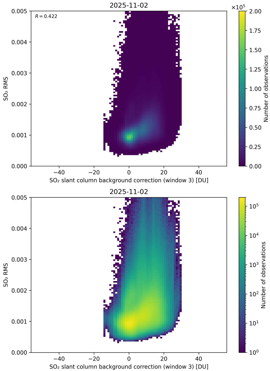
Figure 134: Scatter density plot of “SO 2 slant column background correction (window 3)” against “SO 2 RMS” for 2025-11-02 to 2025-11-03.
