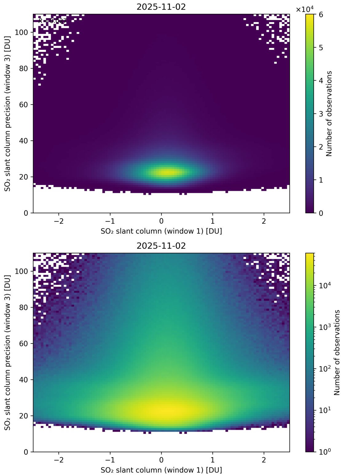
Figure 288: Scatter density plot of “SO 2 slant column (window 1)” against “SO 2 slant column precision (window 3)” for 2025-11-02 to 2025-11-03.
