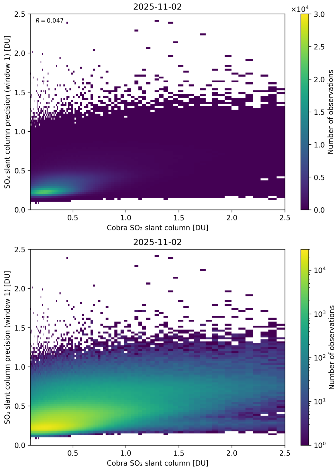
Figure 220: Scatter density plot of “Cobra SO 2 slant column” against “SO 2 slant column precision (window 1)” for 2025-11-02 to 2025-11-03.
