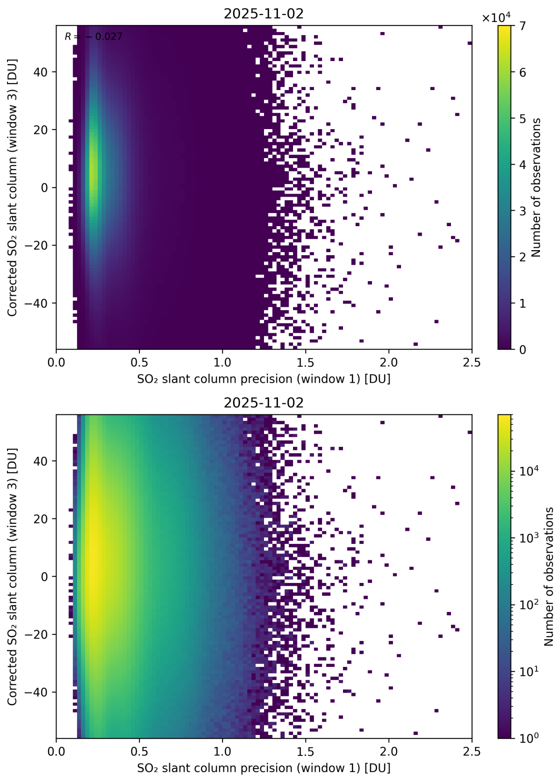
Figure 276: Scatter density plot of “SO 2 slant column precision (window 1)” against “Corrected SO 2 slant column (window 3)” for 2025-11-02 to 2025-11-03.
