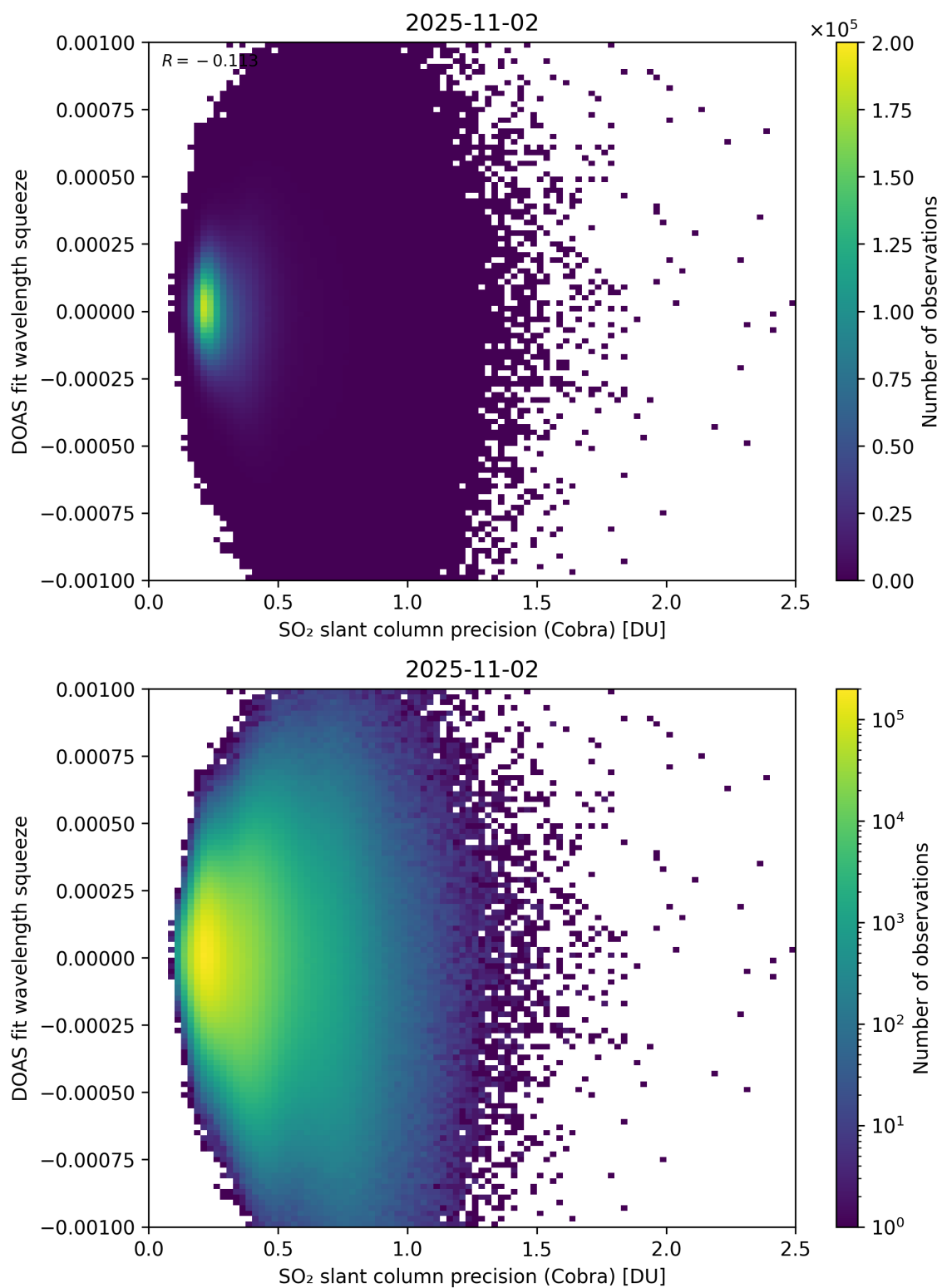
Figure 203: Scatter density plot of “SO 2 slant column precision (Cobra)” against “DOAS fit wavelength squeeze” for 2025-11-02 to 2025-11-03.
