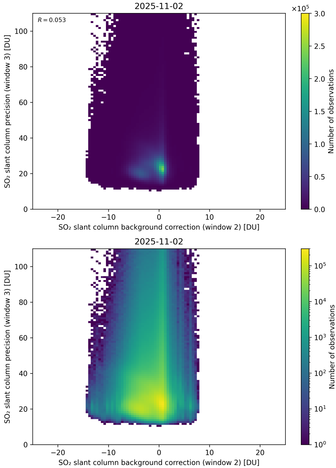
Figure 129: Scatter density plot of “SO 2 slant column background correction (window 2)” against “SO 2 slant column precision (window 3)” for 2025-11-02 to 2025-11-03.
