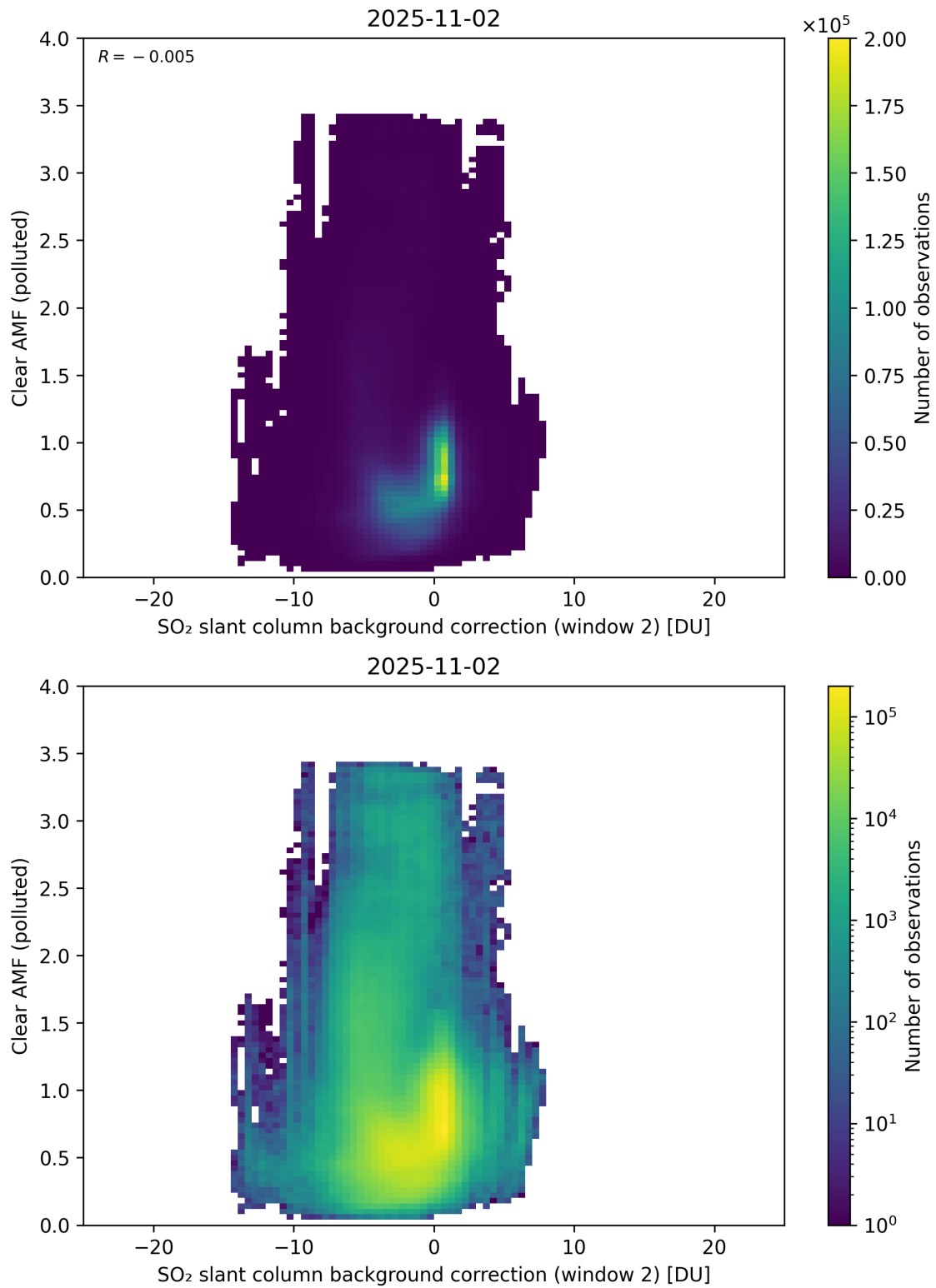
Figure 126: Scatter density plot of “SO 2 slant column background correction (window 2)” against “Clear AMF (polluted)” for 2025-11-02 to 2025-11-03.
