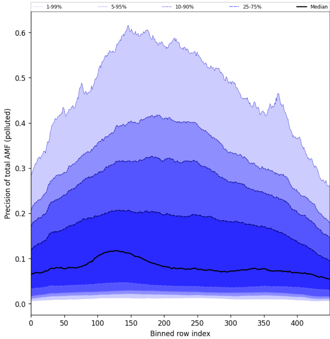
Figure 106: Along track statistics of “Precision of total AMF (polluted)” for 2025-11-02 to 2025-11-03
