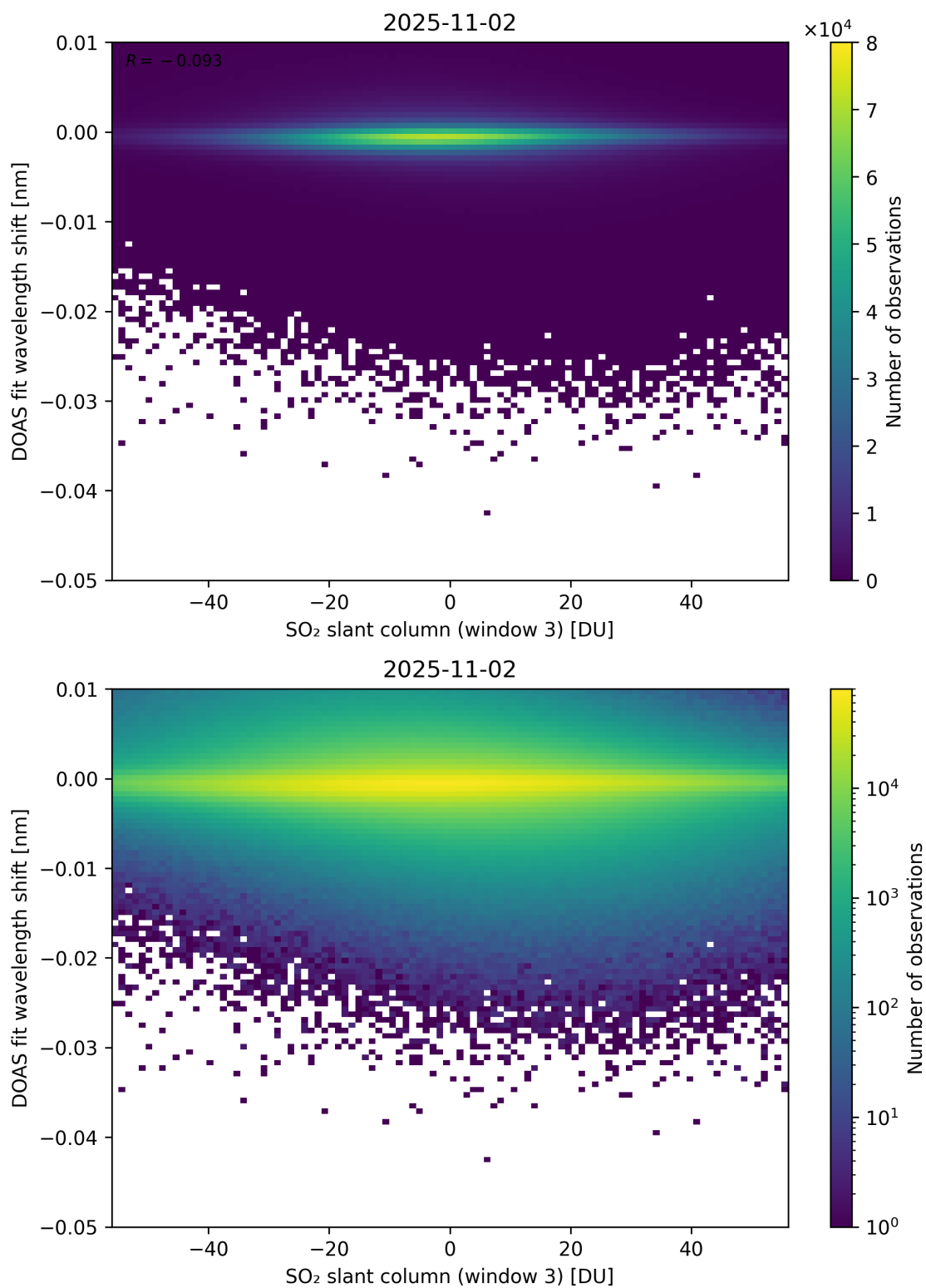
Figure 304: Scatter density plot of “SO 2 slant column (window 3)” against “DOAS fit wavelength shift” for 2025-11-02 to 2025-11-03.
