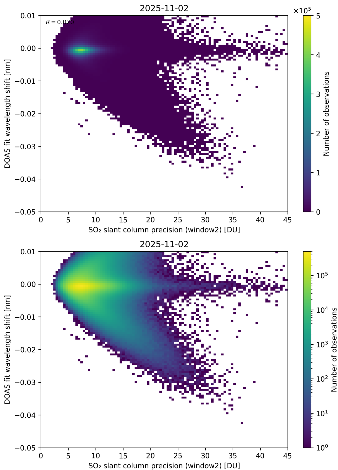
Figure 293: Scatter density plot of “SO 2 slant column precision (window2)” against “DOAS fit wavelength shift” for 2025-11-02 to 2025-11-03.
