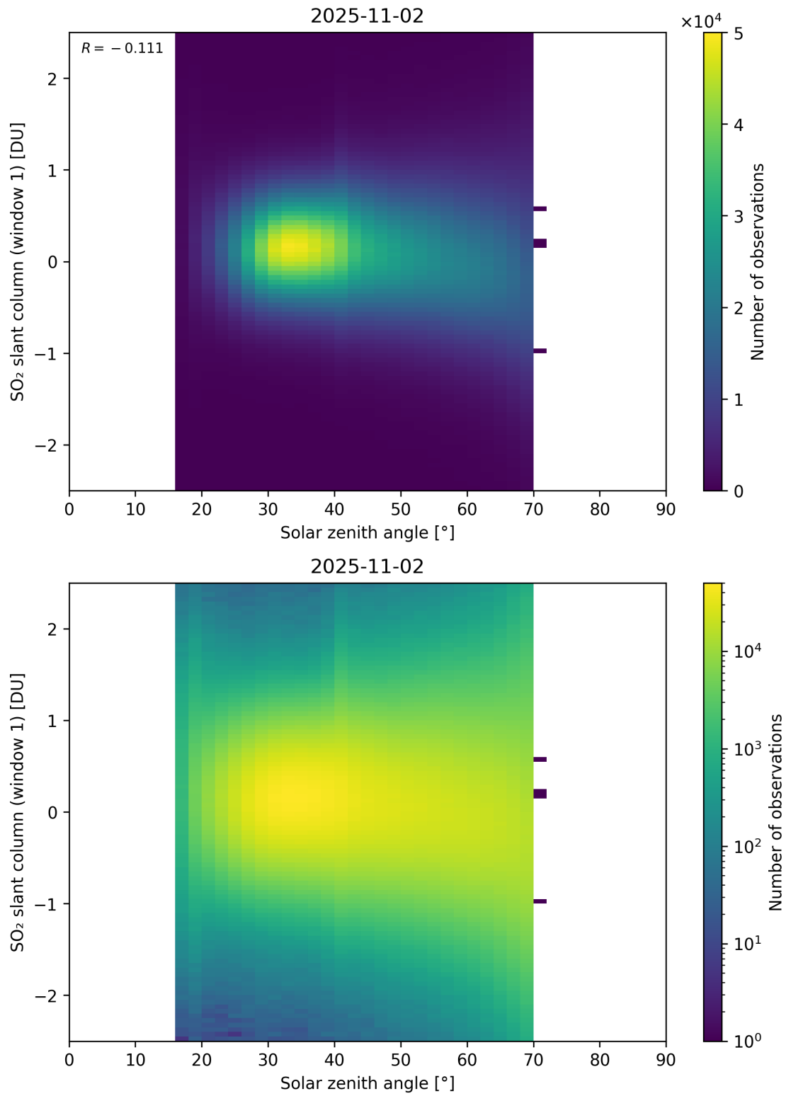
Figure 184: Scatter density plot of “Solar zenith angle” against “SO 2 slant column (window 1)” for 2025-11-02 to 2025-11-03.
