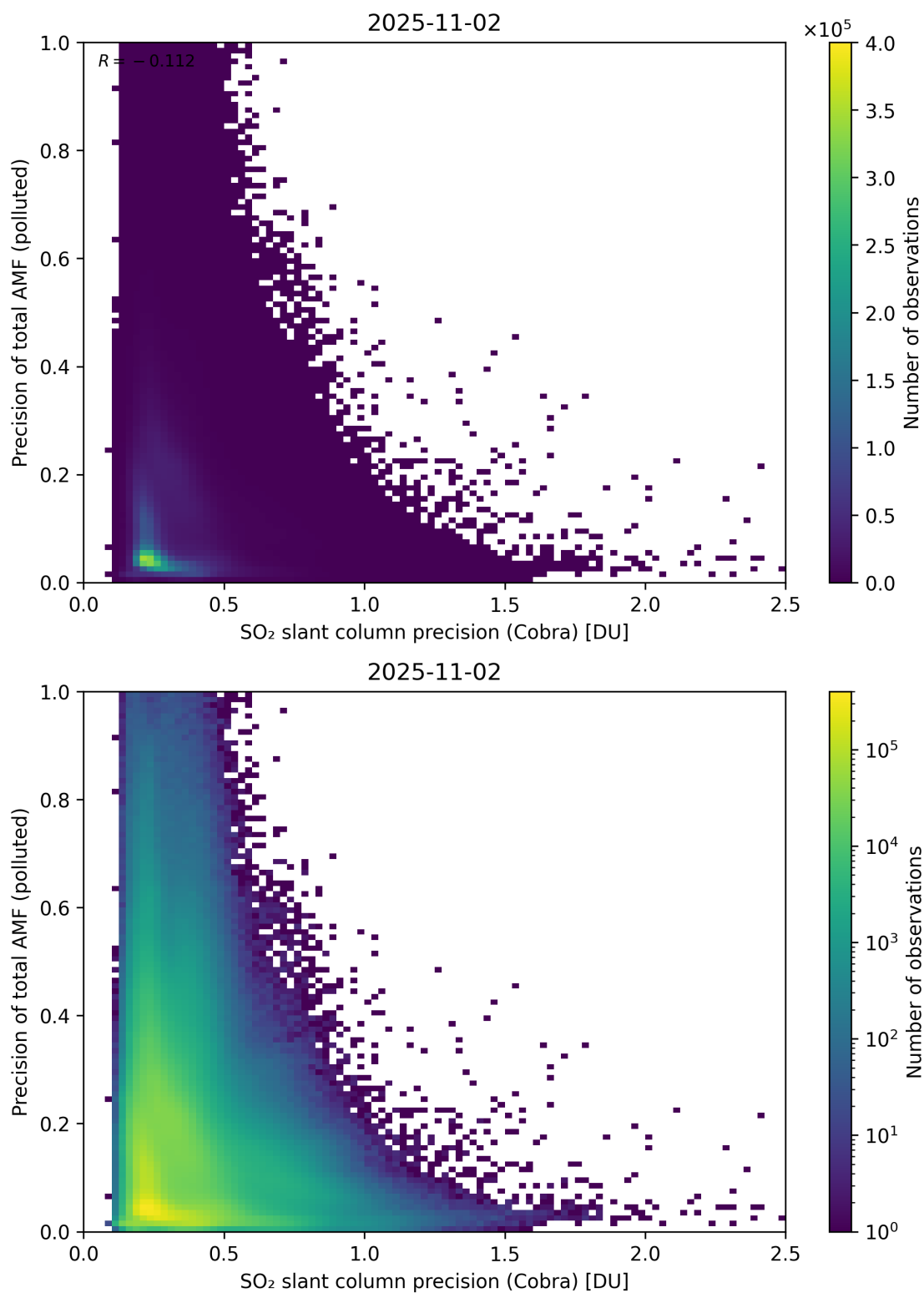
Figure 214: Scatter density plot of “SO 2 slant column precision (Cobra)” against “Precision of total AMF (polluted)” for 2025-11-02 to 2025-11-03.
