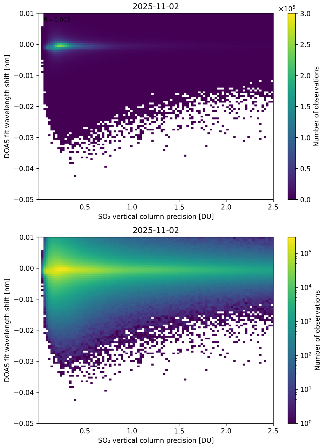
Figure 332: Scatter density plot of “SO 2 vertical column precision” against “DOAS fit wavelength shift” for 2025-11-02 to 2025-11-03.
