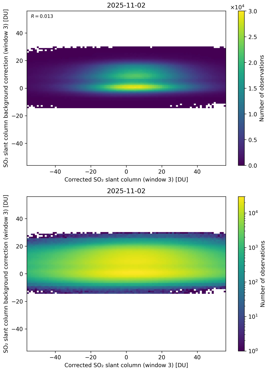
Figure 255: Scatter density plot of “Corrected SO 2 slant column (window 3)” against “SO 2 slant column background correction (window 3)” for 2025-11-02 to 2025-11-03.
