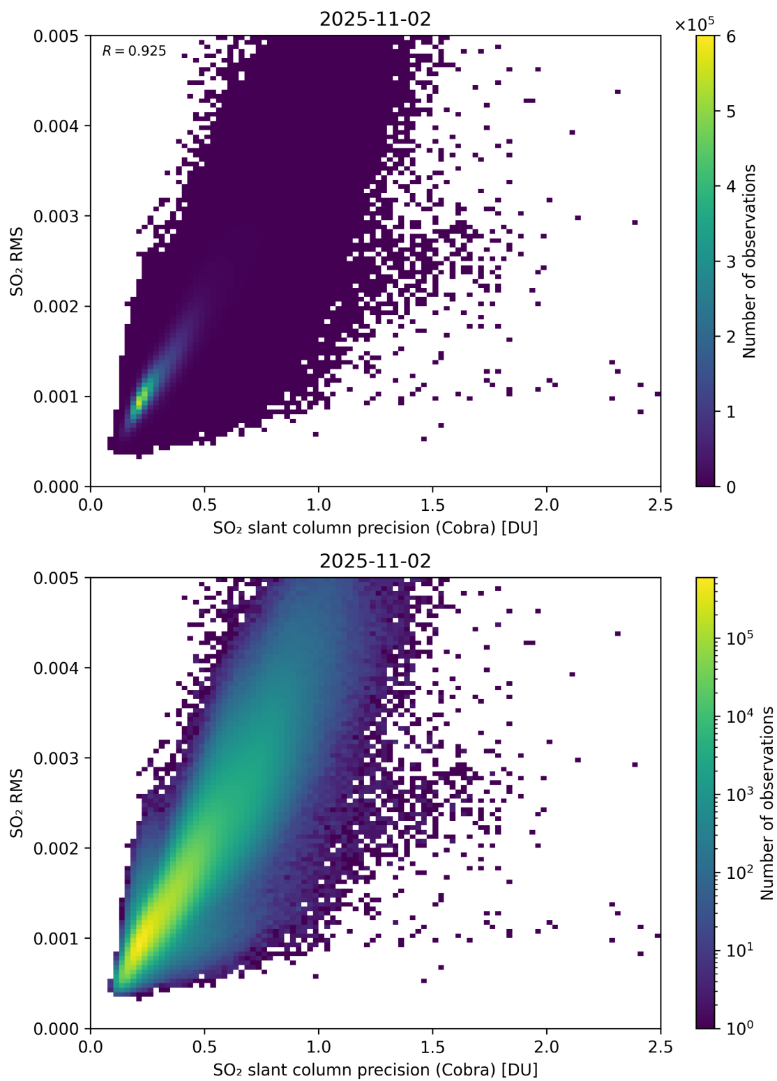
Figure 204: Scatter density plot of “SO 2 slant column precision (Cobra)” against “SO 2 RMS” for 2025-11-02 to 2025-11-03.
