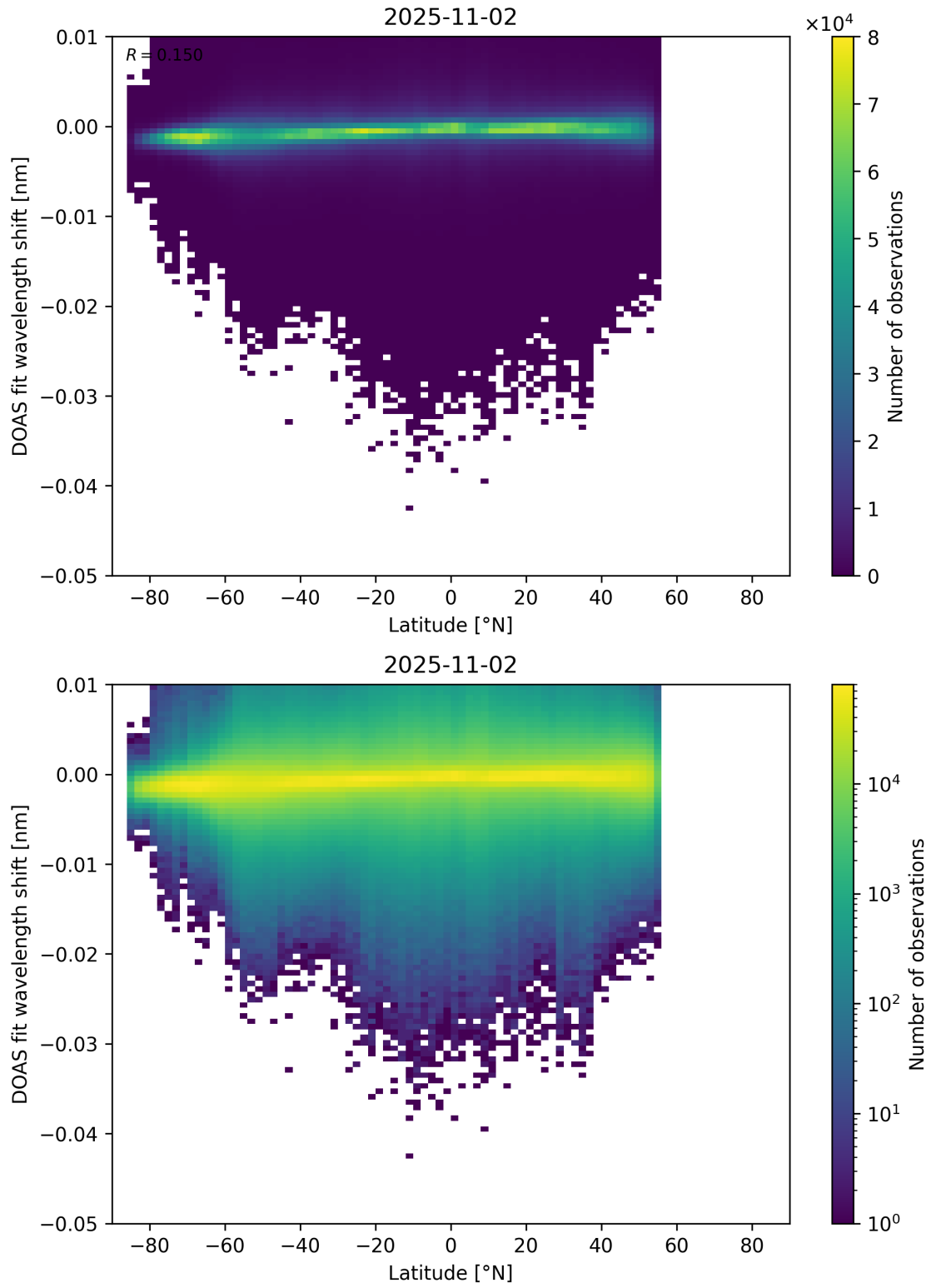
Figure 153: Scatter density plot of “Latitude” against “DOAS fit wavelength shift” for 2025-11-02 to 2025-11-03.
