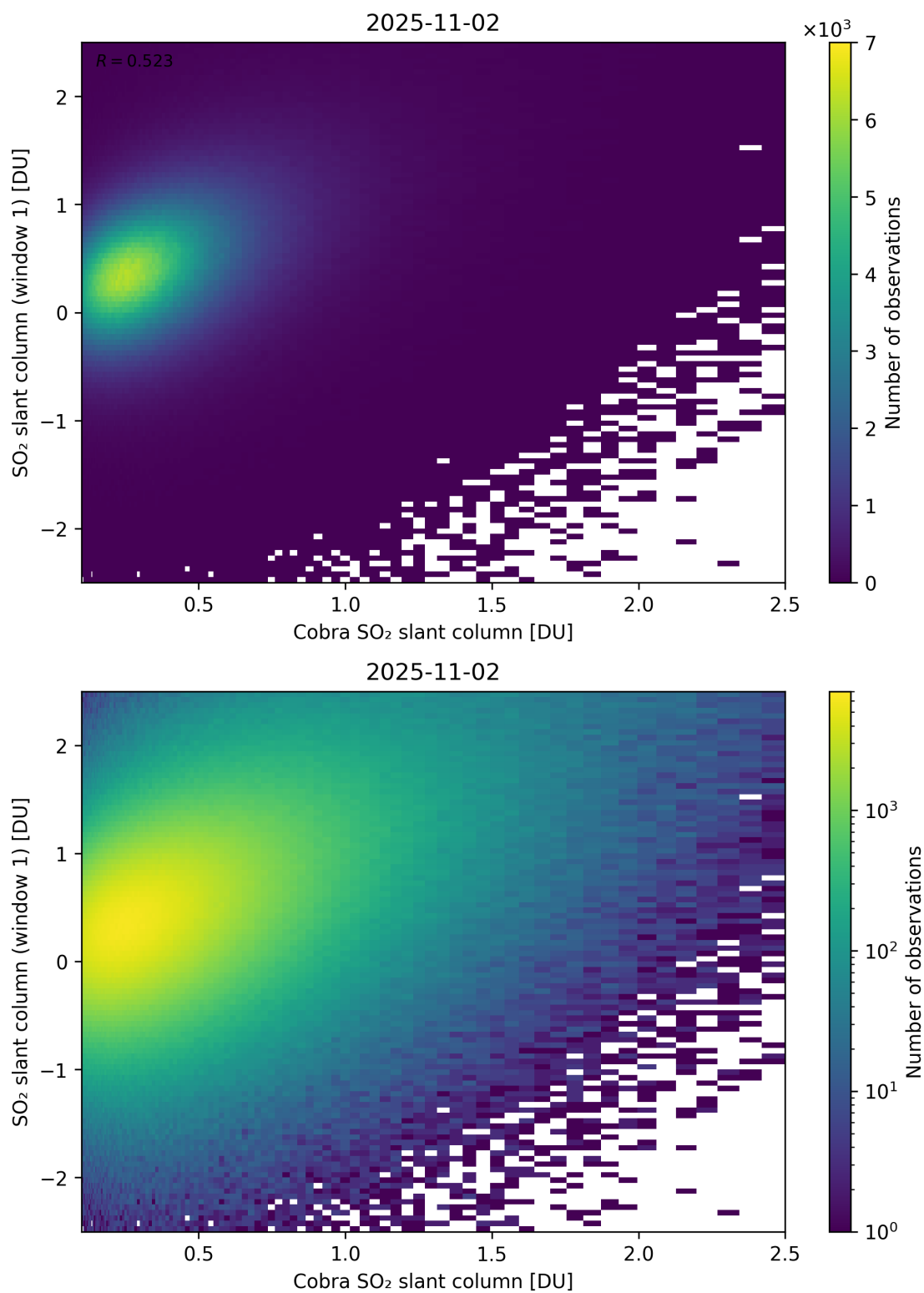
Figure 219: Scatter density plot of “Cobra SO 2 slant column” against “SO 2 slant column (window 1)” for 2025-11-02 to 2025-11-03.
