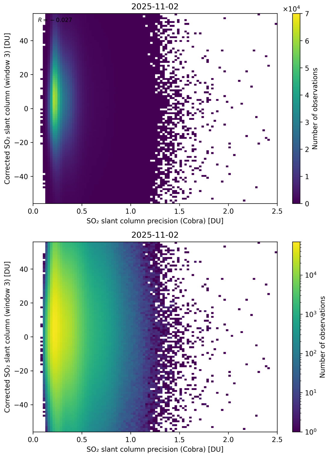
Figure 207: Scatter density plot of “SO 2 slant column precision (Cobra)” against “Corrected SO 2 slant column (window 3)” for 2025-11-02 to 2025-11-03.
