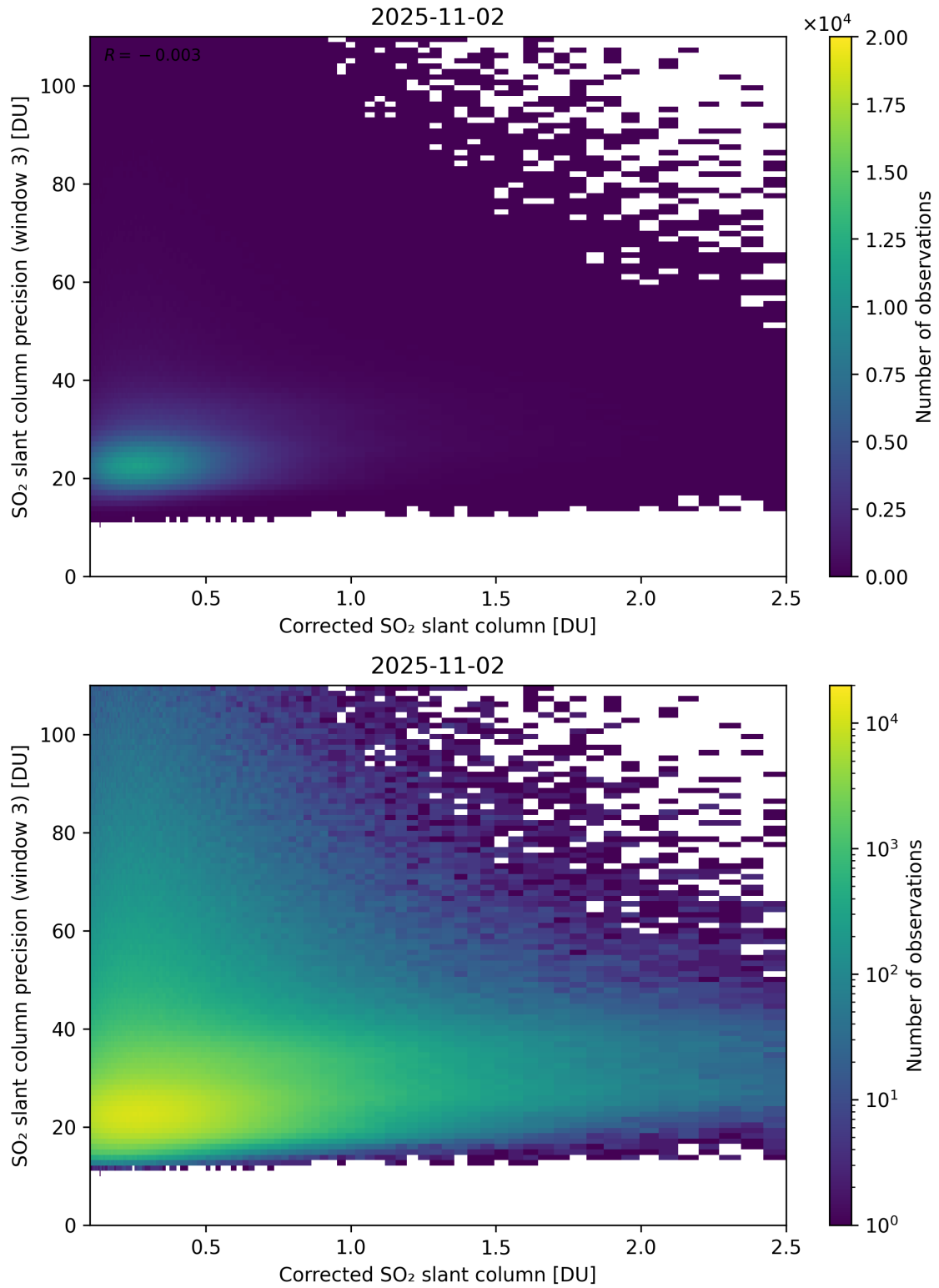
Figure 241: Scatter density plot of “Corrected SO 2 slant column” against “SO 2 slant column precision (window 3)” for 2025-11-02 to 2025-11-03.
