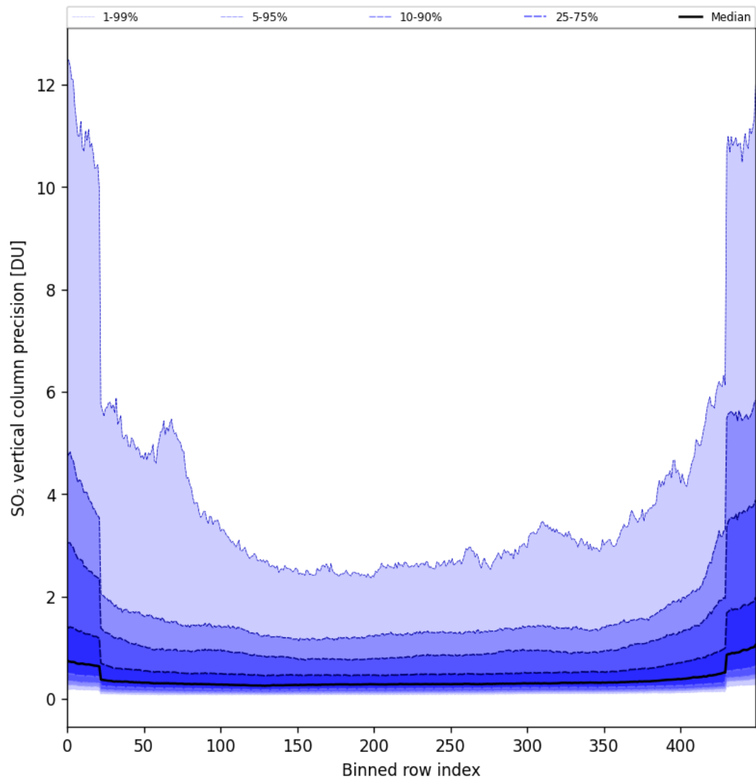
Figure 85: Along track statistics of “SO 2 vertical column precision” for 2025-11-02 to 2025-11-03
