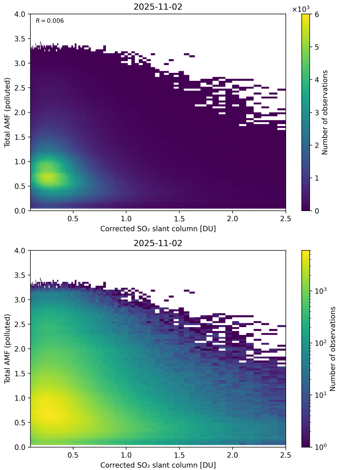
Figure 242: Scatter density plot of “Corrected SO 2 slant column” against “Total AMF (polluted)” for 2025-11-02 to 2025-11-03.
