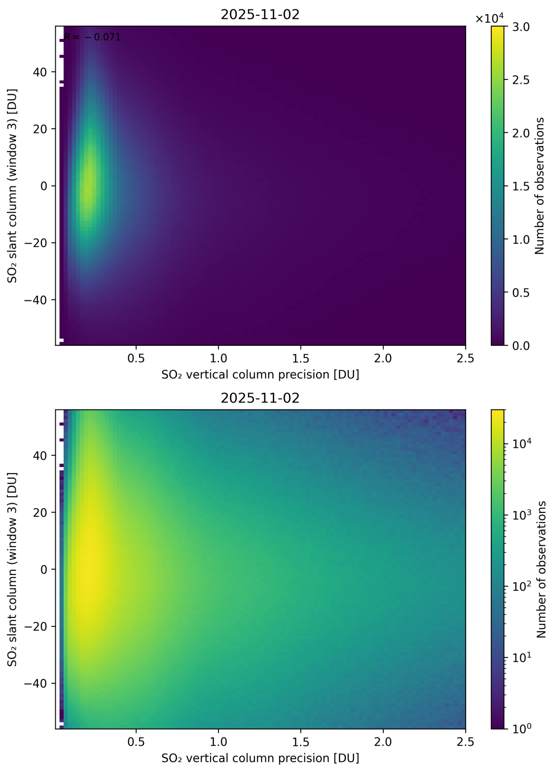
Figure 344: Scatter density plot of “SO 2 vertical column precision” against “SO 2 slant column (window 3)” for 2025-11-02 to 2025-11-03.
