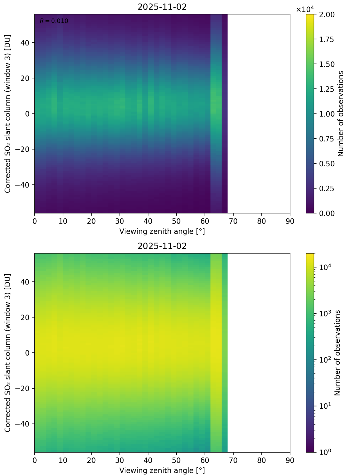
Figure 375: Scatter density plot of “Viewing zenith angle” against “Corrected SO 2 slant column (window 3)” for 2025-11-02 to 2025-11-03.
