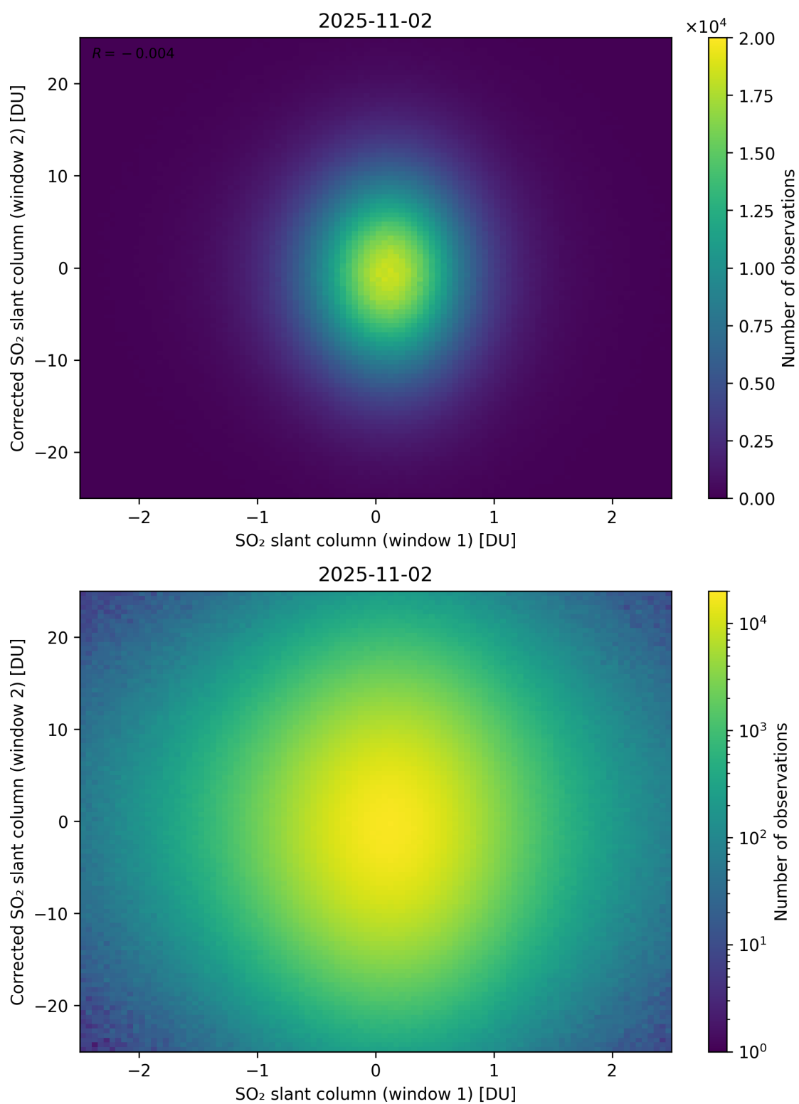
Figure 283: Scatter density plot of “SO 2 slant column (window 1)” against “Corrected SO 2 slant column (window 2)” for 2025-11-02 to 2025-11-03.
