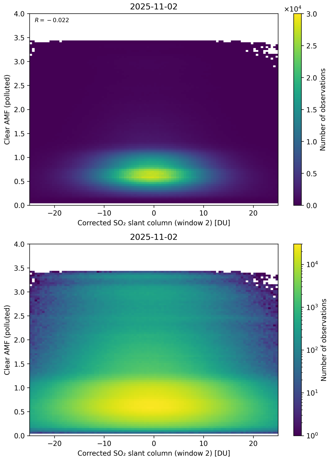
Figure 249: Scatter density plot of “Corrected SO 2 slant column (window 2)” against “Clear AMF (polluted)” for 2025-11-02 to 2025-11-03.
