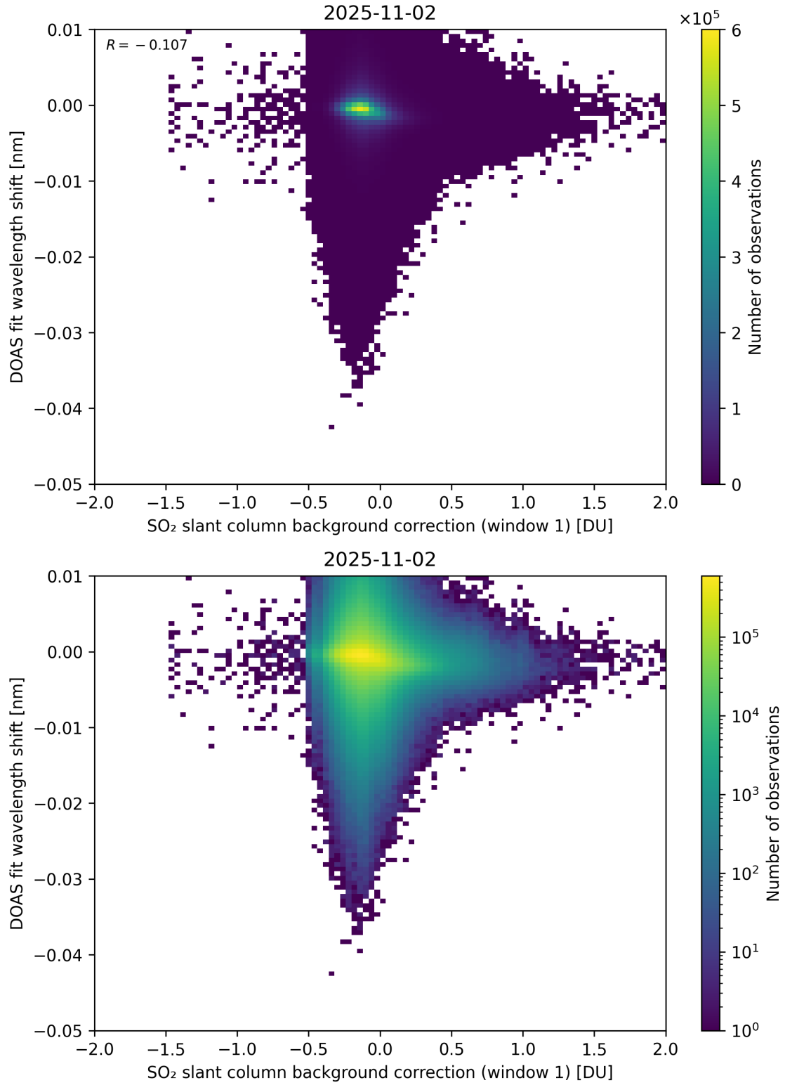
Figure 111: Scatter density plot of “SO 2 slant column background correction (window 1)” against “DOAS fit wavelength shift” for 2025-11-02 to 2025-11-03.
