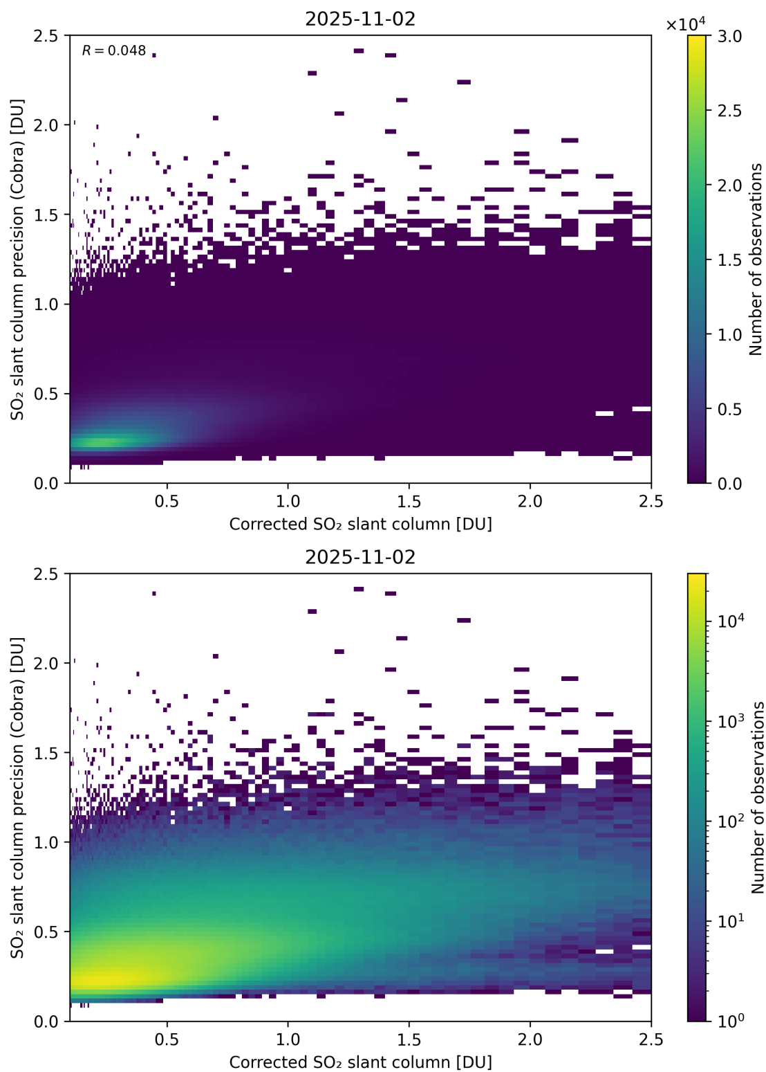
Figure 234: Scatter density plot of “Corrected SO 2 slant column” against “SO 2 slant column precision (Cobra)” for 2025-11-02 to 2025-11-03.
