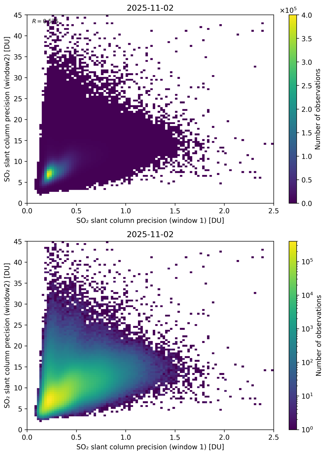
Figure 277: Scatter density plot of “SO 2 slant column precision (window 1)” against “SO 2 slant column precision (window2)” for 2025-11-02 to 2025-11-03.
