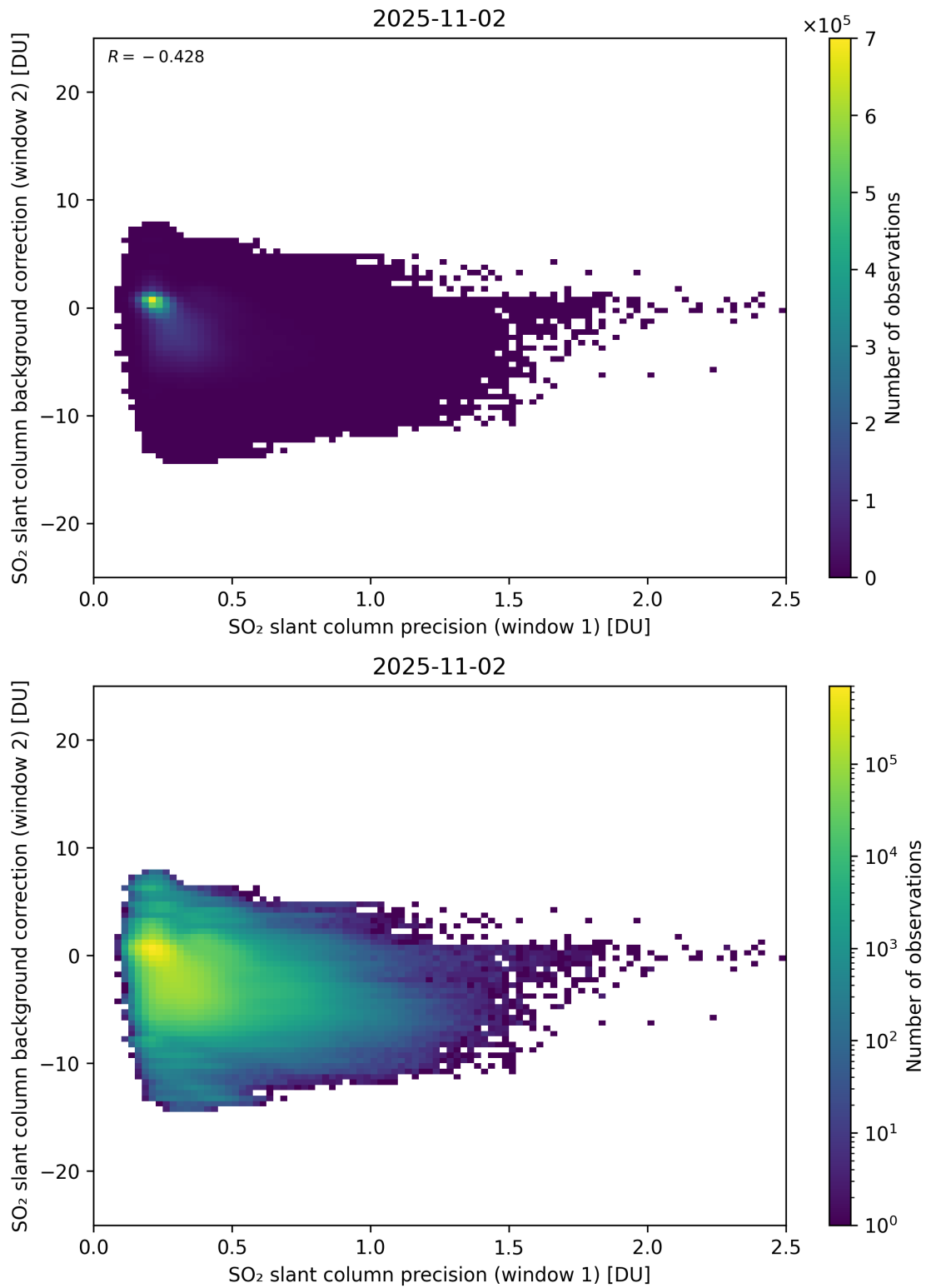
Figure 269: Scatter density plot of “SO 2 slant column precision (window 1)” against “SO 2 slant column background correction (window 2)” for 2025-11-02 to 2025-11-03.
