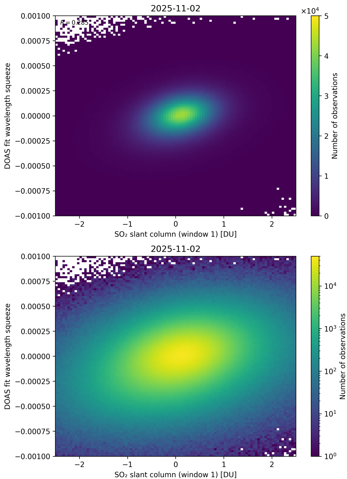
Figure 266: Scatter density plot of “SO 2 slant column (window 1)” against “DOAS fit wavelength squeeze” for 2025-11-02 to 2025-11-03.
