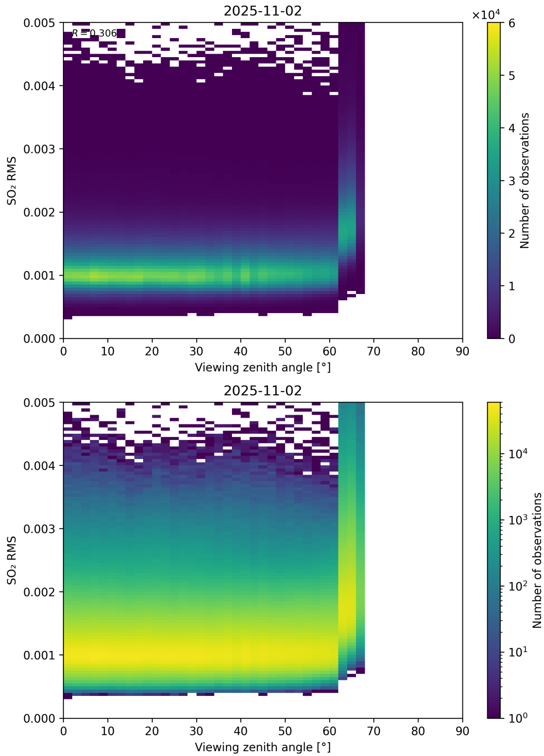
Figure 367: Scatter density plot of “Viewing zenith angle” against “SO 2 RMS” for 2025-11-02 to 2025-11-03.
