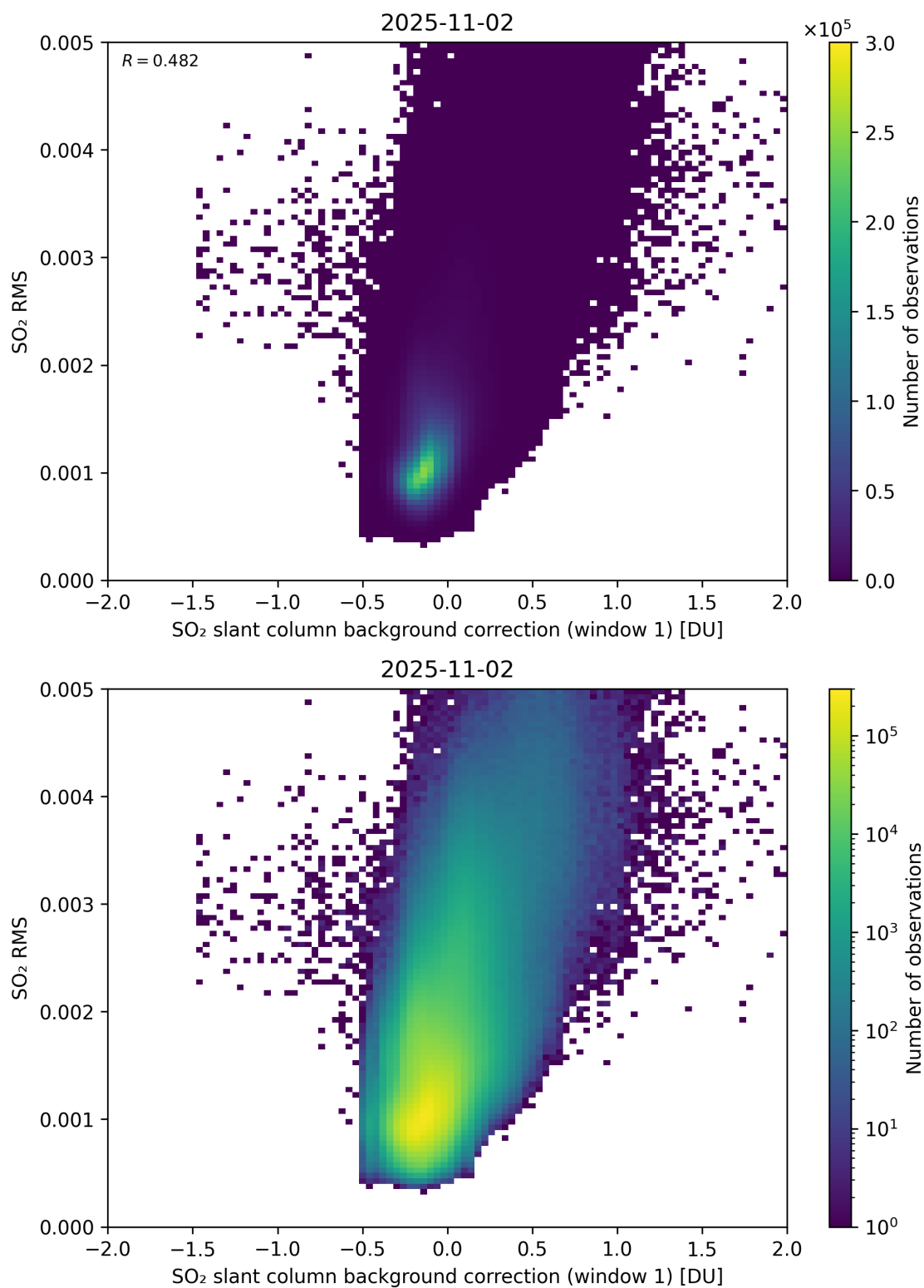
Figure 113: Scatter density plot of “SO 2 slant column background correction (window 1)” against “SO 2 RMS” for 2025-11-02 to 2025-11-03.
