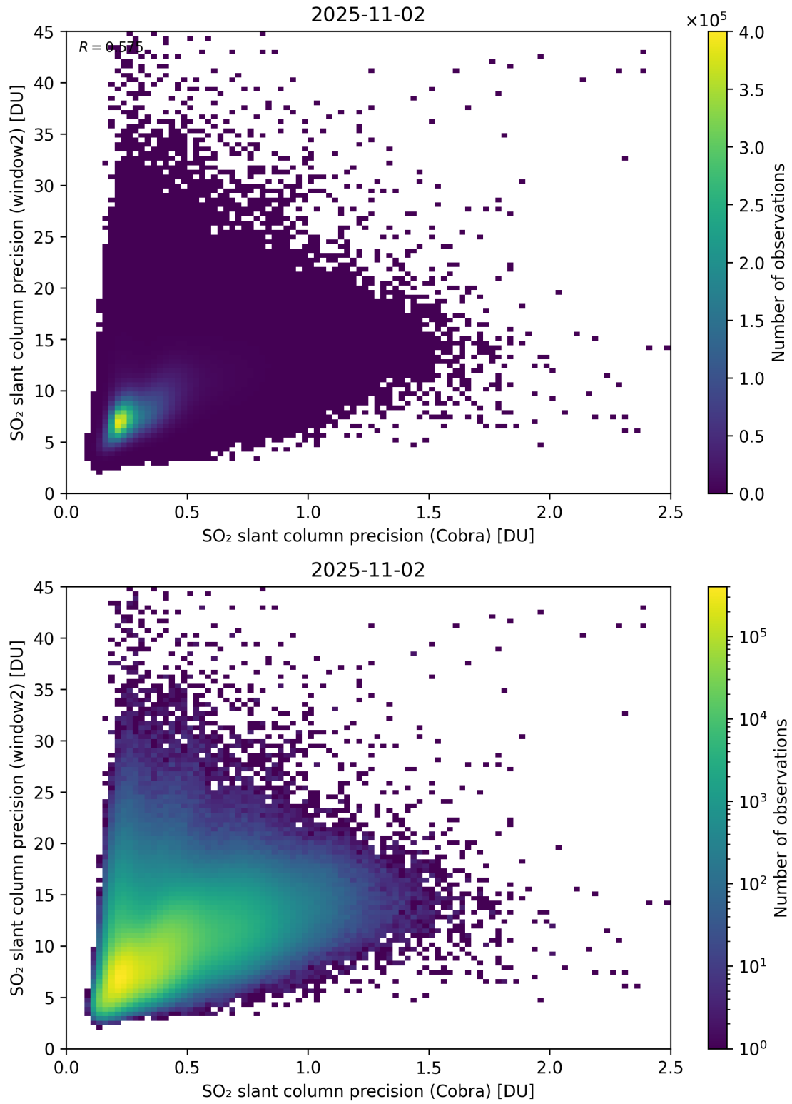
Figure 210: Scatter density plot of “SO 2 slant column precision (Cobra)” against “SO 2 slant column precision (window2)” for 2025-11-02 to 2025-11-03.
