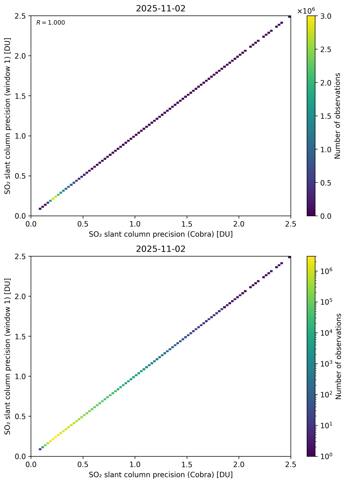
Figure 209: Scatter density plot of “SO 2 slant column precision (Cobra)” against “SO 2 slant column precision (window 1)” for 2025-11-02 to 2025-11-03.
