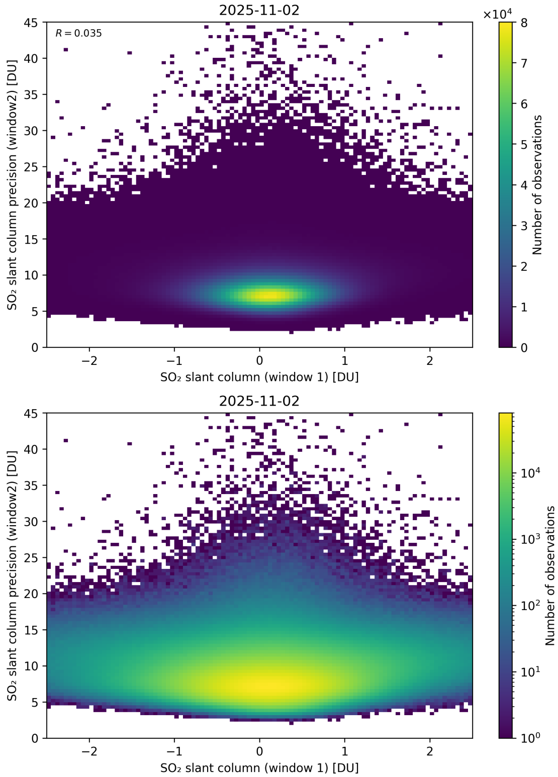
Figure 286: Scatter density plot of “SO 2 slant column (window 1)” against “SO 2 slant column precision (window2)” for 2025-11-02 to 2025-11-03.
