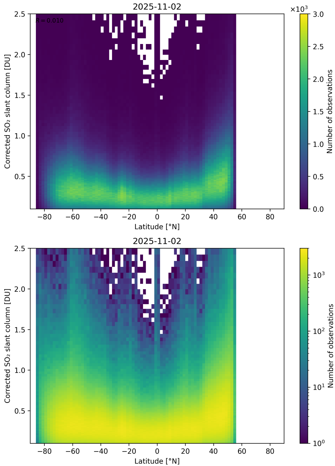
Figure 159: Scatter density plot of “Latitude” against “Corrected SO 2 slant column” for 2025-11-02 to 2025-11-03.
