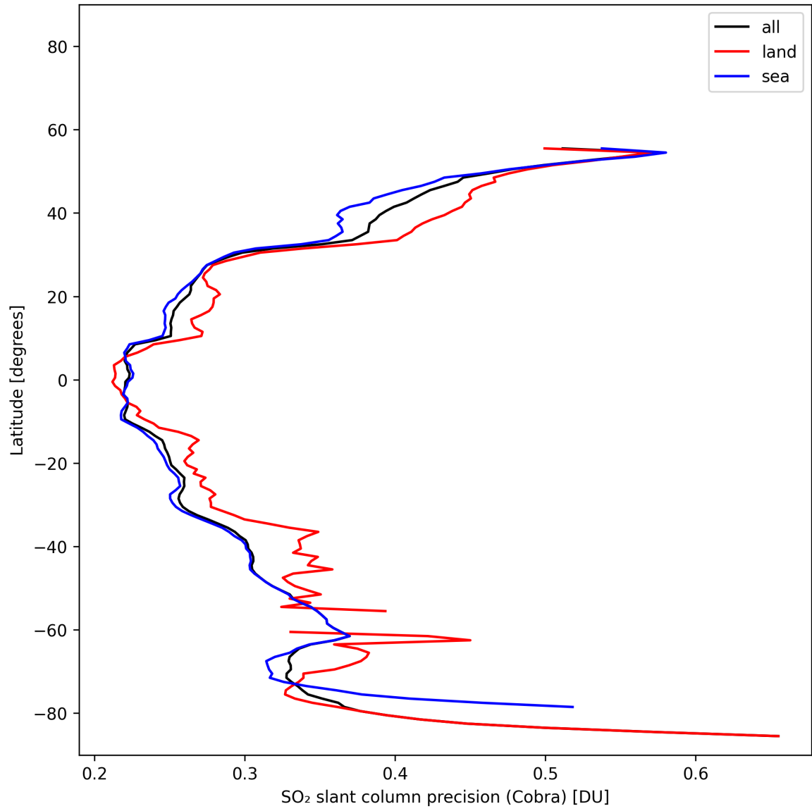
Figure 36: Zonal average of “SO 2 slant column precision (Cobra)” for 2025-11-02 to 2025-11-03.
