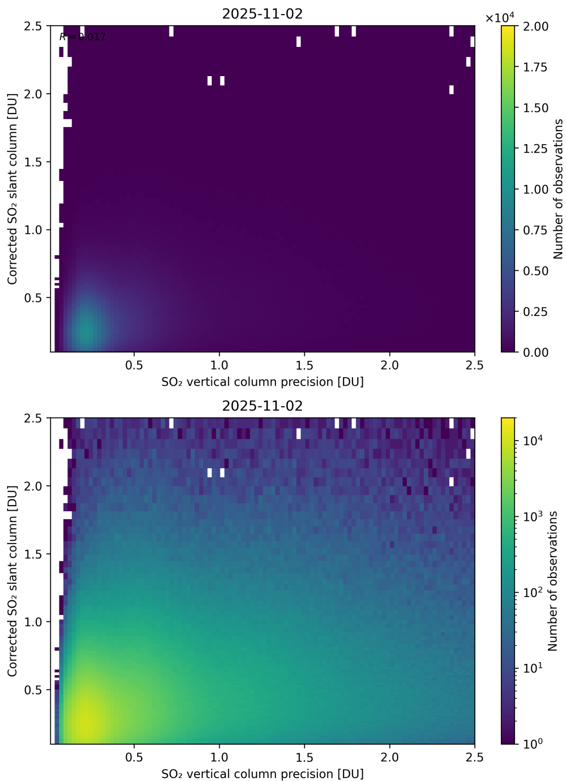
Figure 338: Scatter density plot of “SO 2 vertical column precision” against “Corrected SO 2 slant column” for 2025-11-02 to 2025-11-03.
