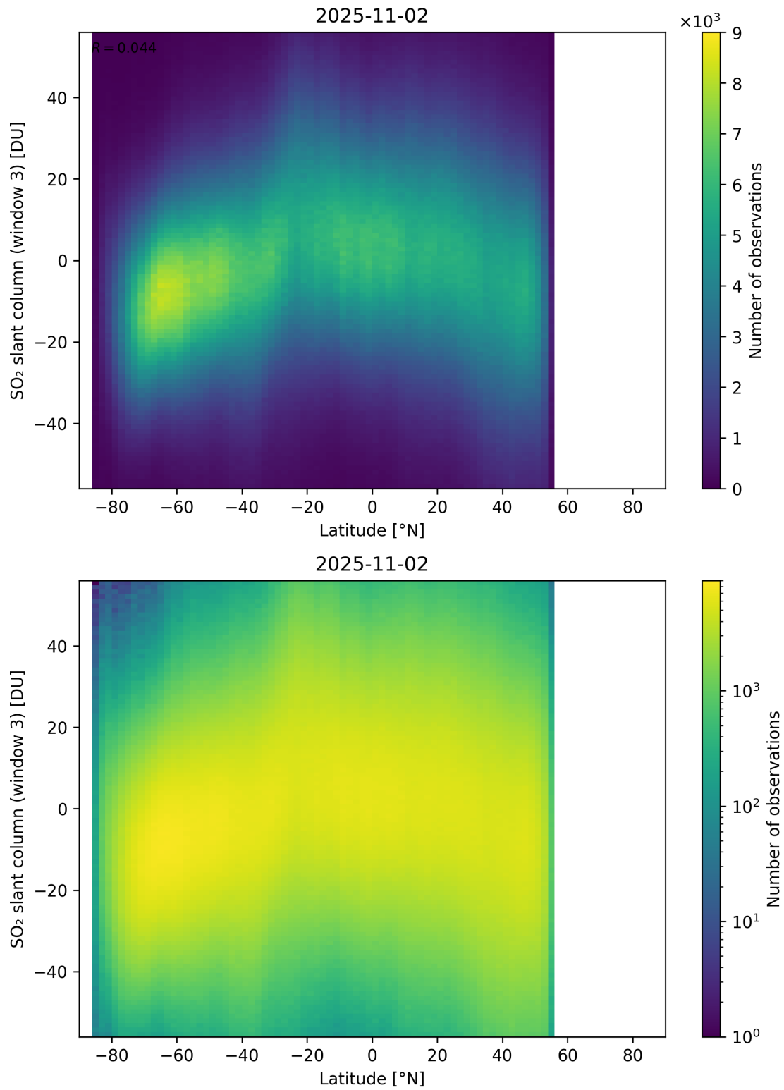
Figure 165: Scatter density plot of “Latitude” against “SO 2 slant column (window 3)” for 2025-11-02 to 2025-11-03.
