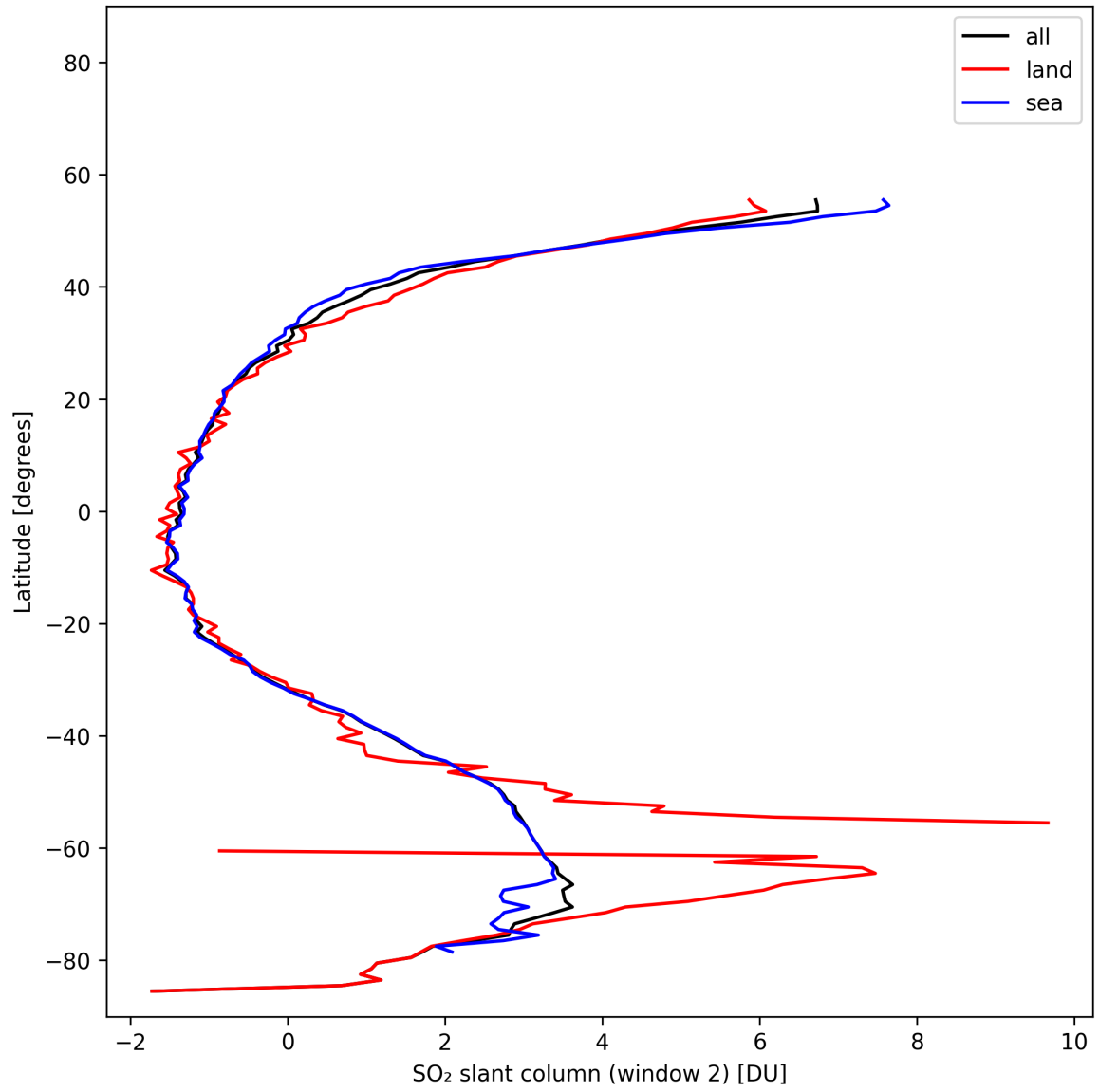
Figure 41: Zonal average of “SO 2 slant column (window 2)” for 2025-11-02 to 2025-11-03.
