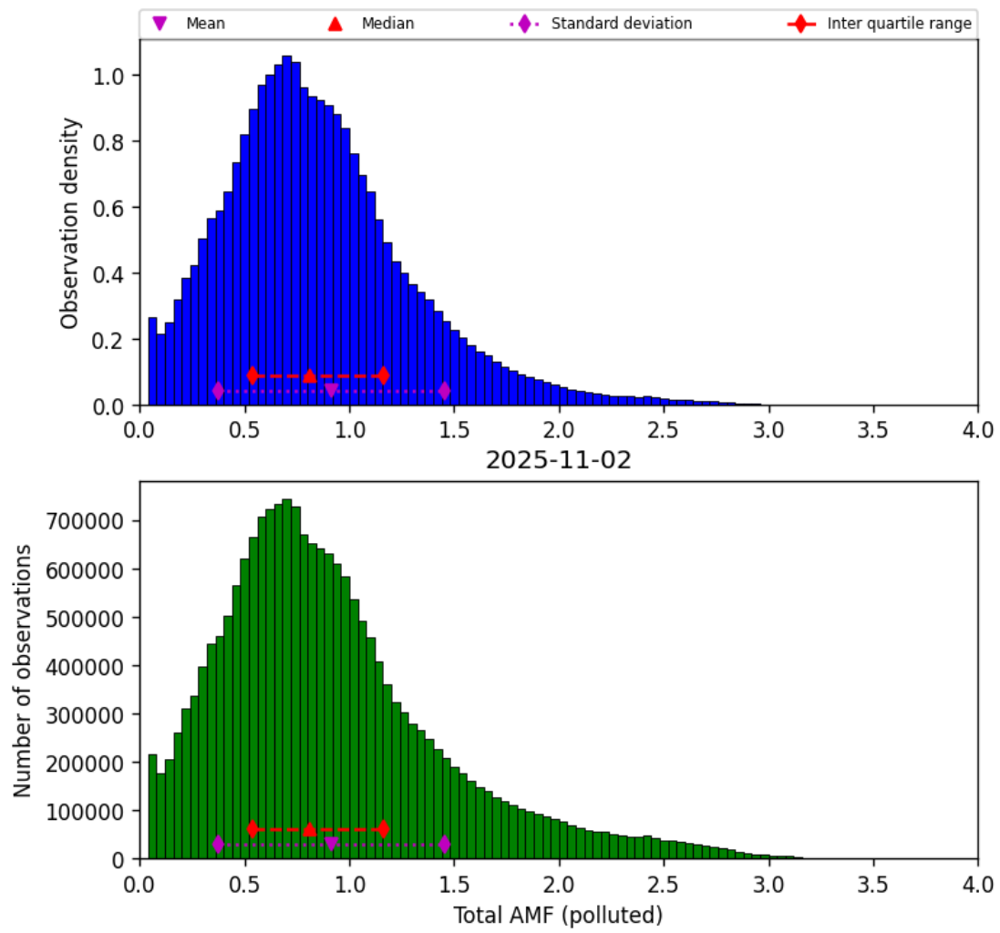
Figure 79: Histogram of “Total AMF (polluted)” for 2025-11-02 to 2025-11-03
