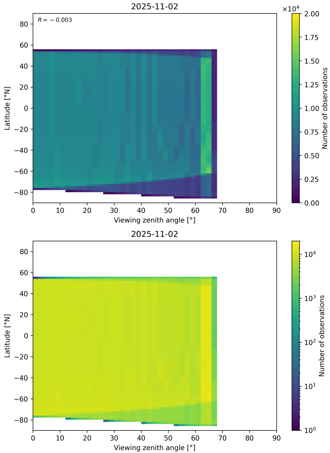
Figure 368: Scatter density plot of “Viewing zenith angle” against “Latitude” for 2025-11-02 to 2025-11-03.
