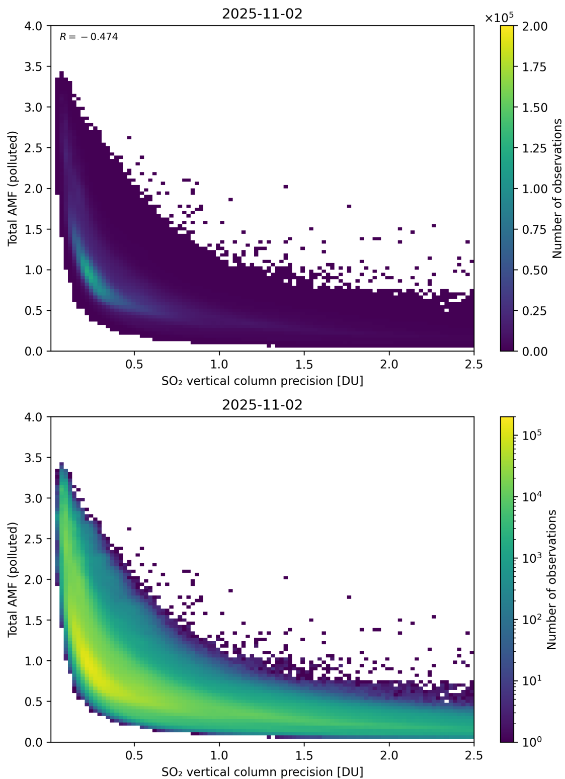
Figure 346: Scatter density plot of “SO 2 vertical column precision” against “Total AMF (polluted)” for 2025-11-02 to 2025-11-03.
