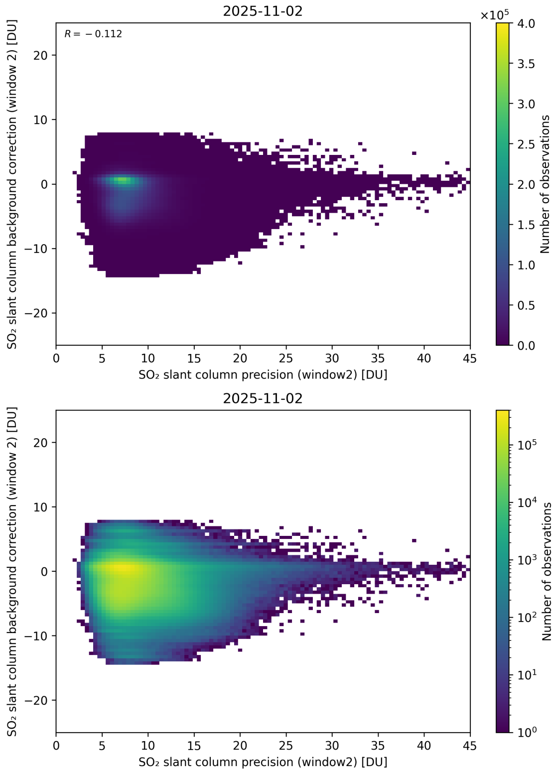
Figure 291: Scatter density plot of “SO 2 slant column precision (window2)” against “SO 2 slant column background correction (window 2)” for 2025-11-02 to 2025-11-03.
