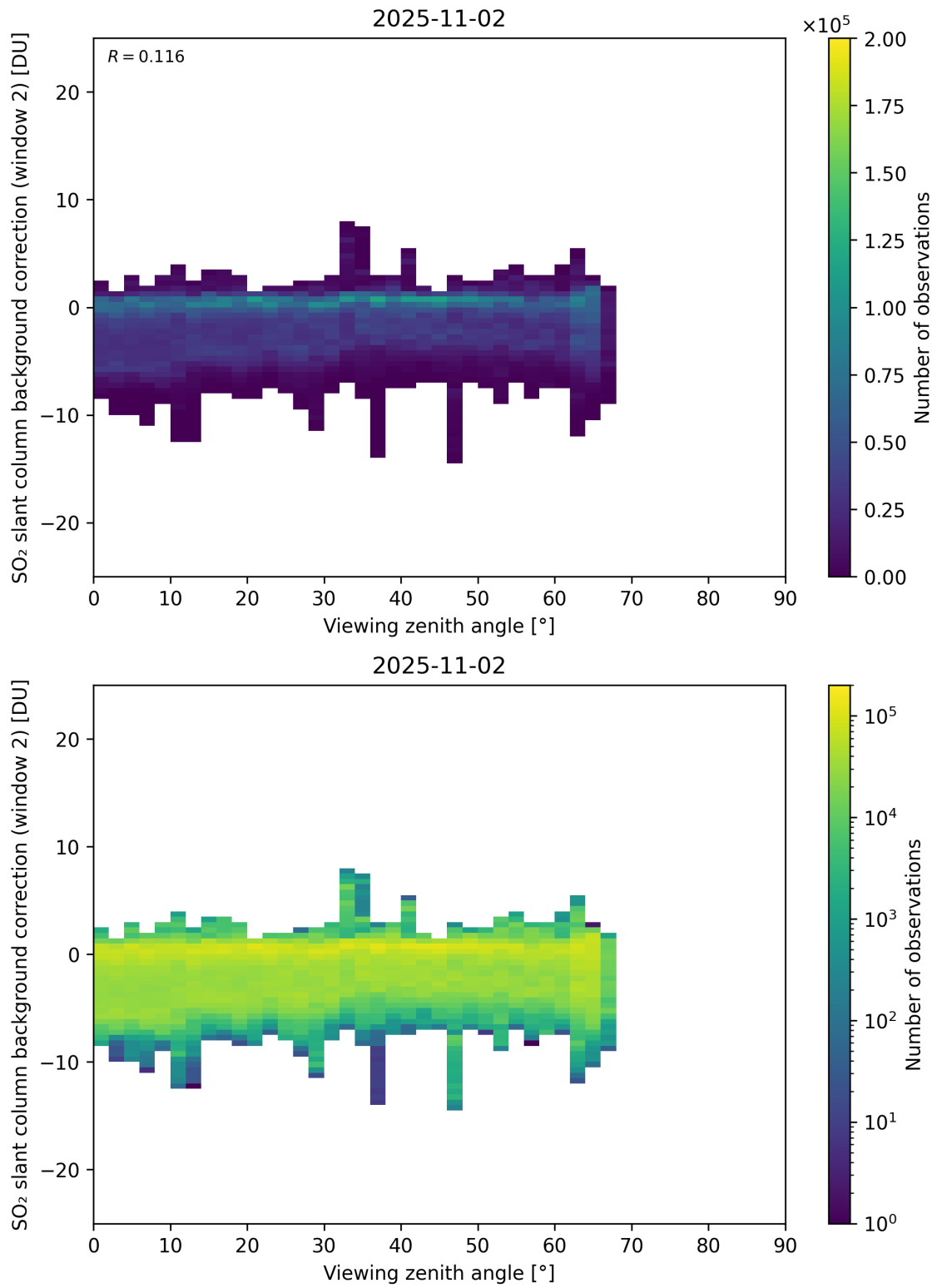
Figure 363: Scatter density plot of “Viewing zenith angle” against “SO 2 slant column background correction (window 2)” for 2025-11-02 to 2025-11-03.
