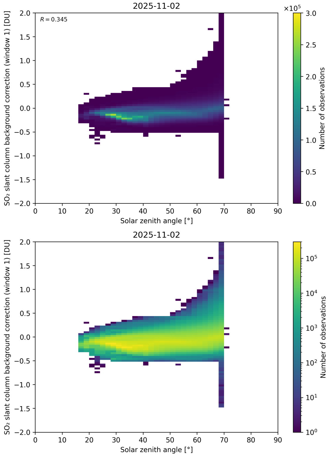
Figure 171: Scatter density plot of “Solar zenith angle” against “SO 2 slant column background correction (window 1)” for 2025-11-02 to 2025-11-03.
