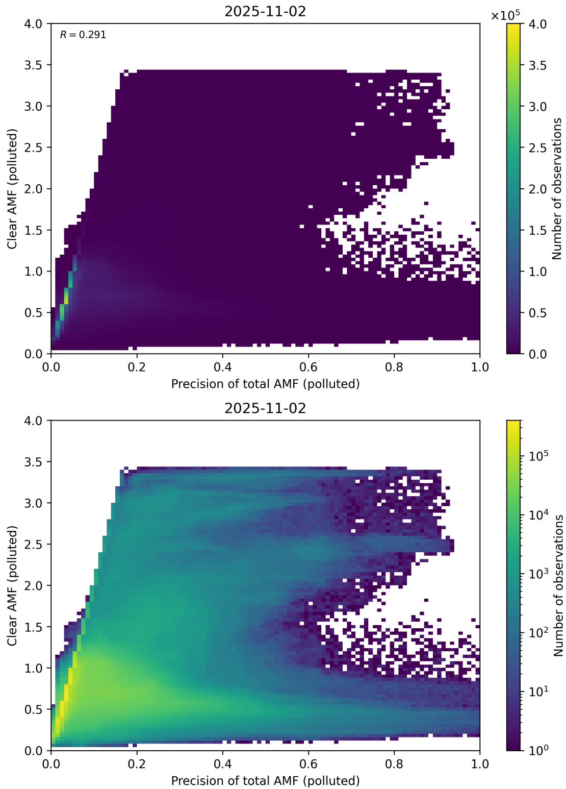
Figure 320: Scatter density plot of “Precision of total AMF (polluted)” against “Clear AMF (polluted)” for 2025-11-02 to 2025-11-03.
