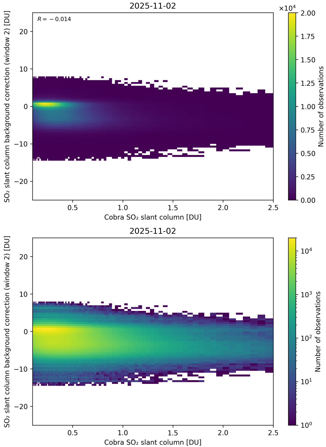
Figure 194: Scatter density plot of “Cobra SO 2 slant column” against “SO 2 slant column background correction (window 2)” for 2025-11-02 to 2025-11-03.
