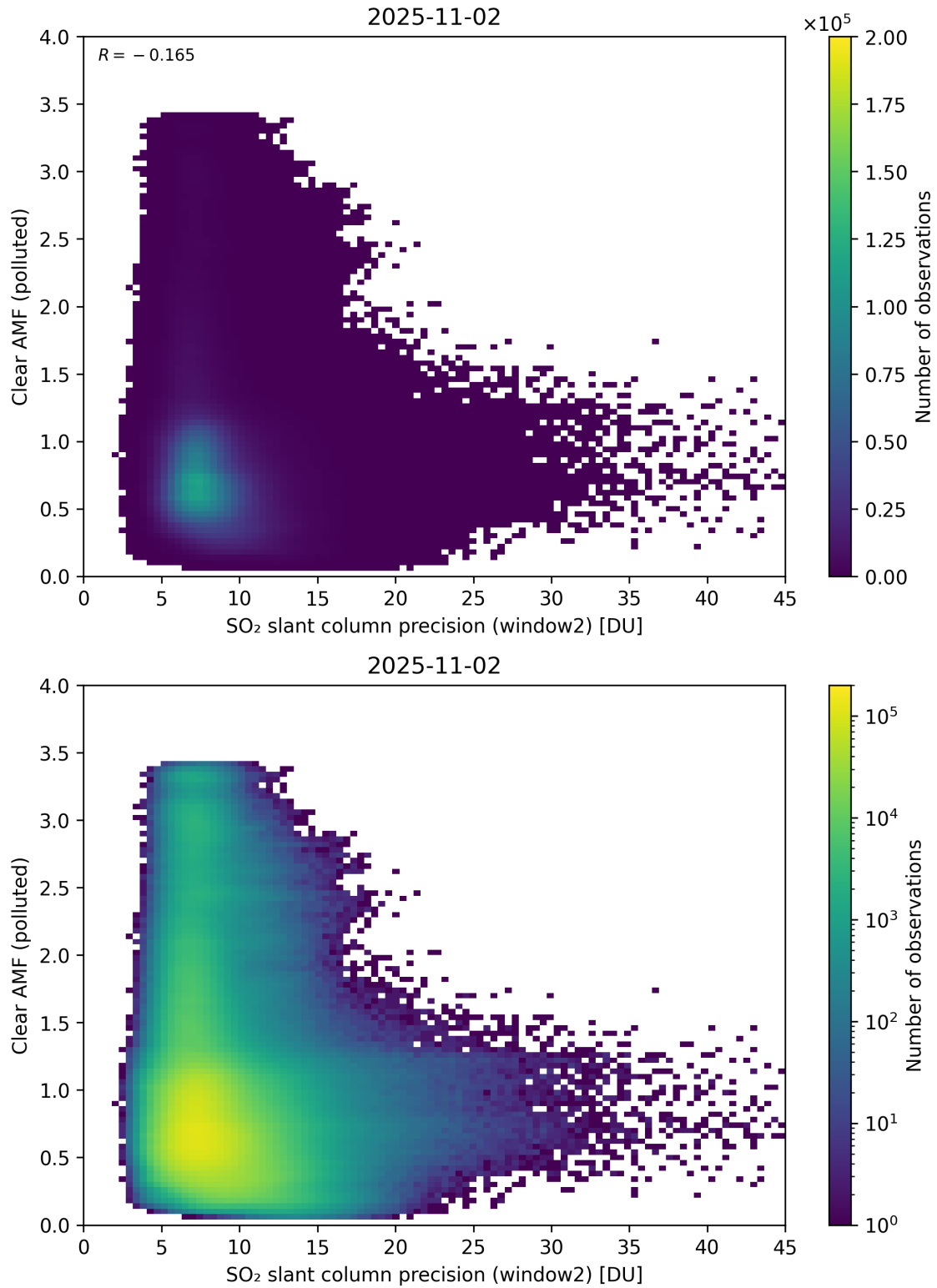
Figure 296: Scatter density plot of “SO 2 slant column precision (window2)” against “Clear AMF (polluted)” for 2025-11-02 to 2025-11-03.
