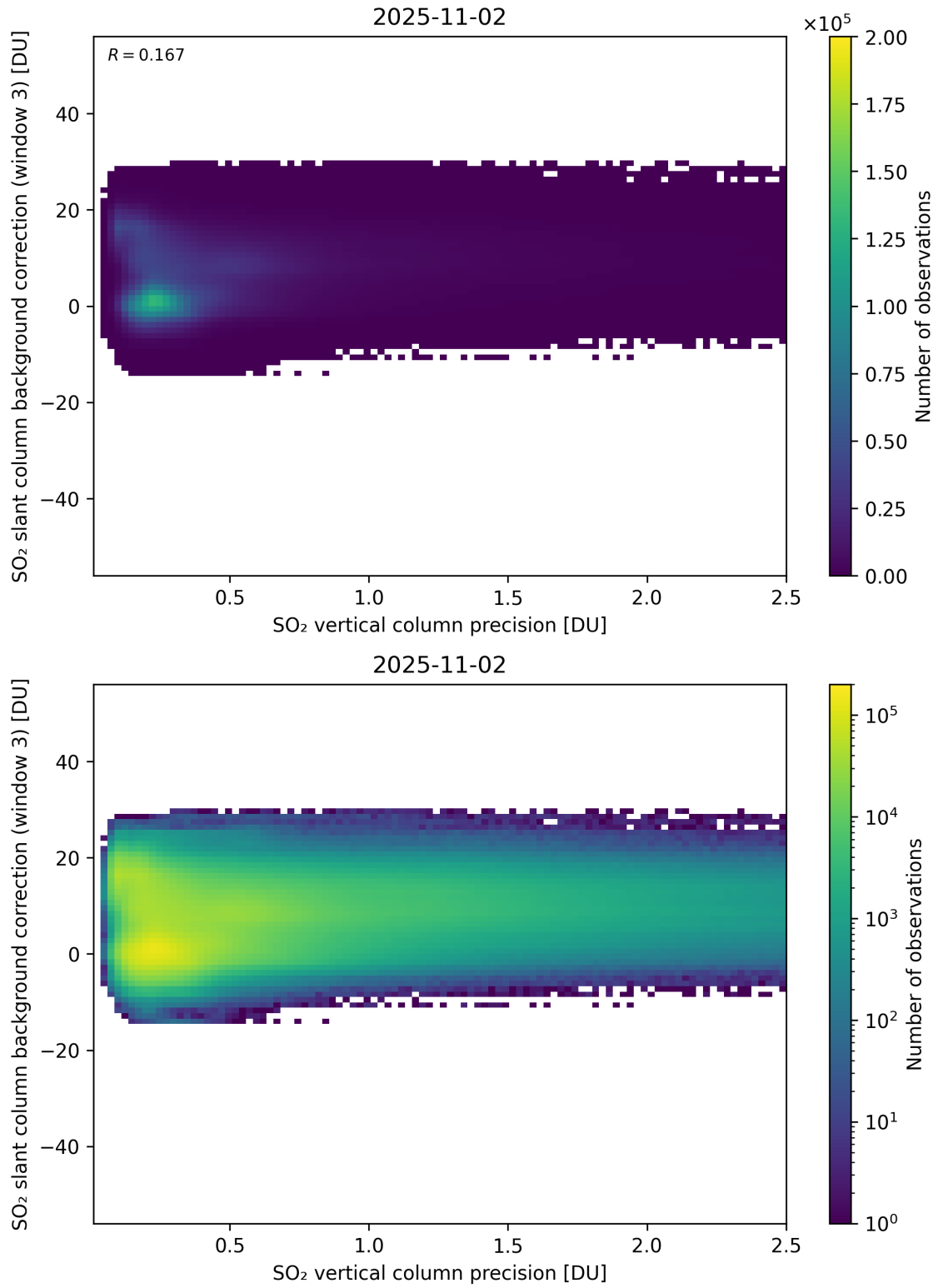
Figure 331: Scatter density plot of “SO 2 vertical column precision” against “SO 2 slant column background correction (window 3)” for 2025-11-02 to 2025-11-03.
