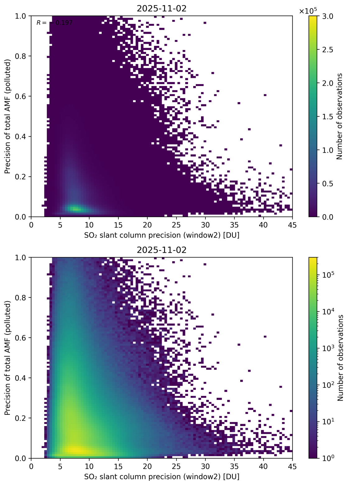
Figure 302: Scatter density plot of “SO 2 slant column precision (window2)” against “Precision of total AMF (polluted)” for 2025-11-02 to 2025-11-03.
