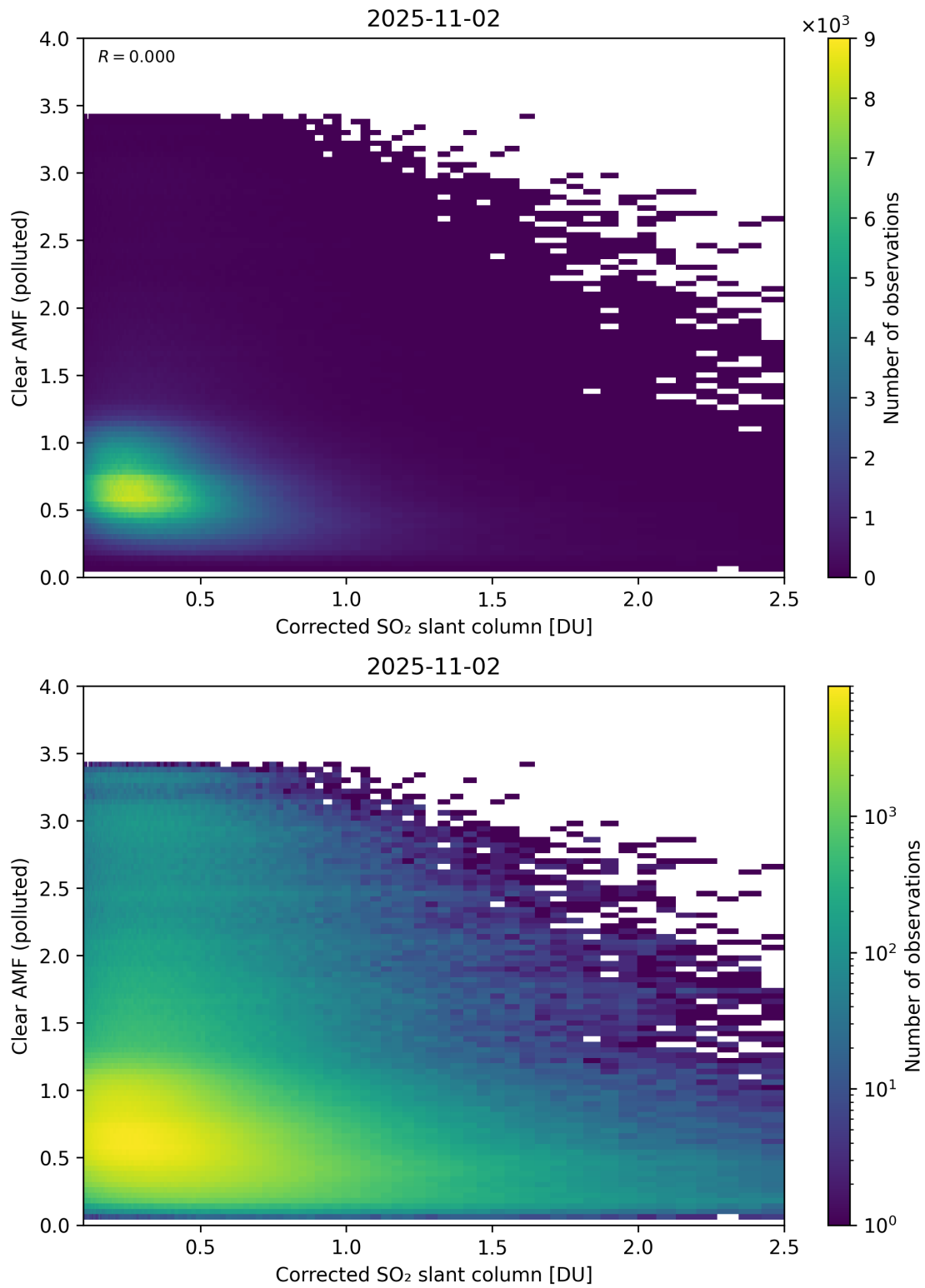
Figure 232: Scatter density plot of “Corrected SO 2 slant column” against “Clear AMF (polluted)” for 2025-11-02 to 2025-11-03.
