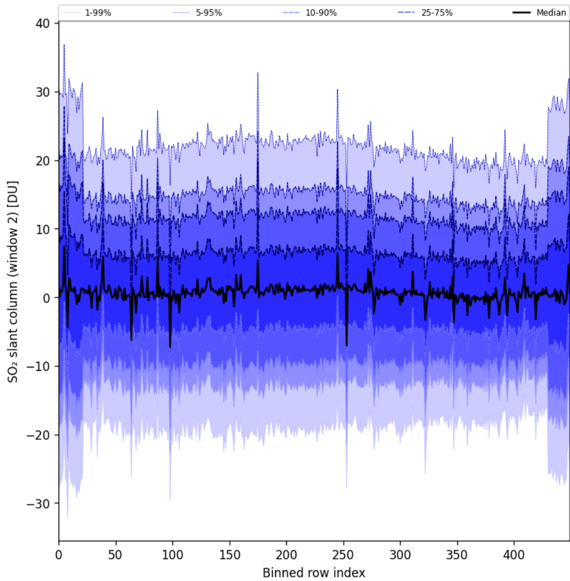
Figure 93: Along track statistics of “SO 2 slant column (window 2)” for 2025-11-02 to 2025-11-03
