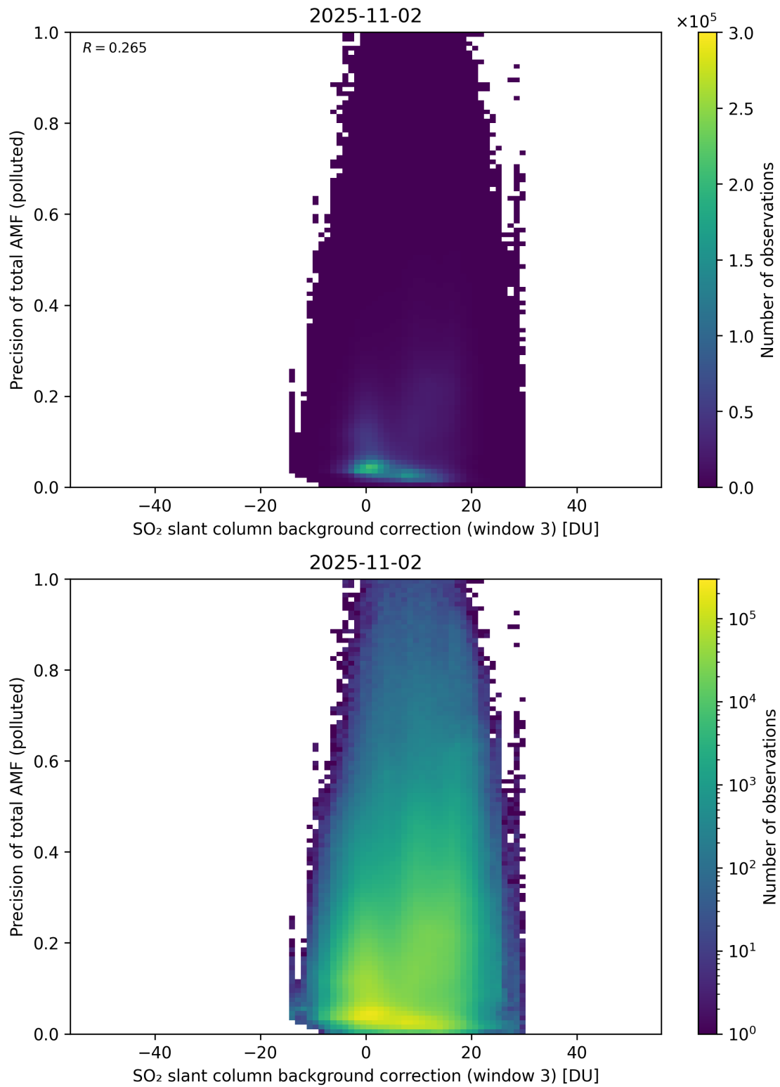
Figure 137: Scatter density plot of “SO 2 slant column background correction (window 3)” against “Precision of total AMF (polluted)” for 2025-11-02 to 2025-11-03.
