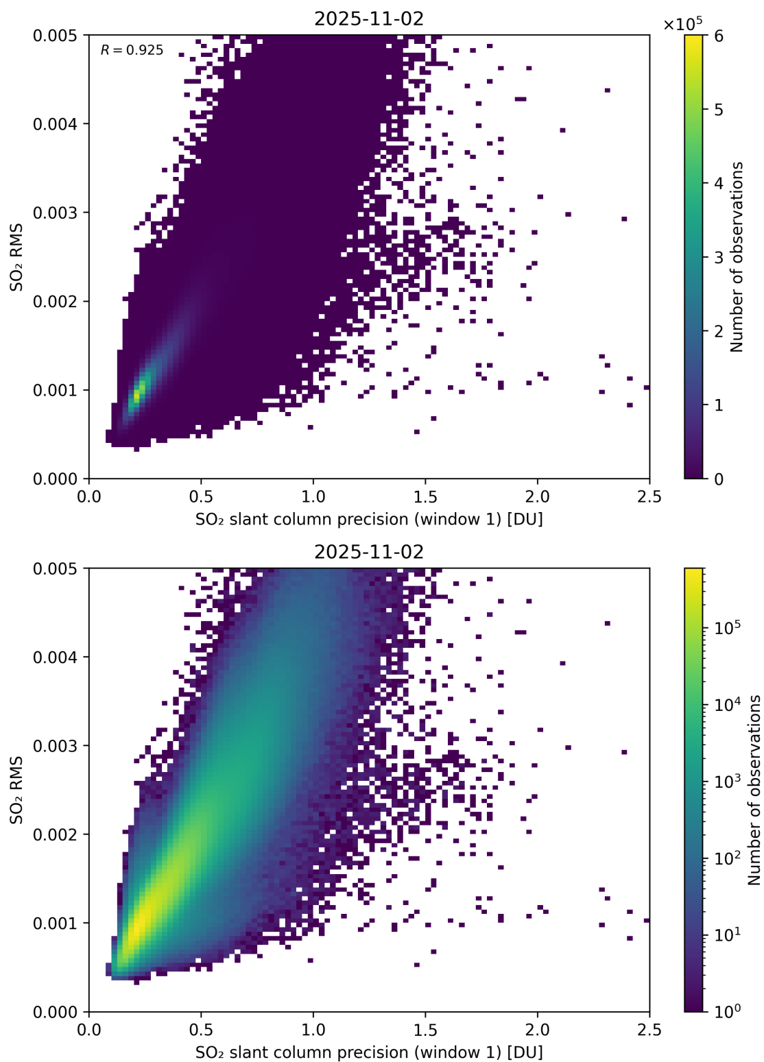
Figure 273: Scatter density plot of “SO 2 slant column precision (window 1)” against “SO 2 RMS” for 2025-11-02 to 2025-11-03.
