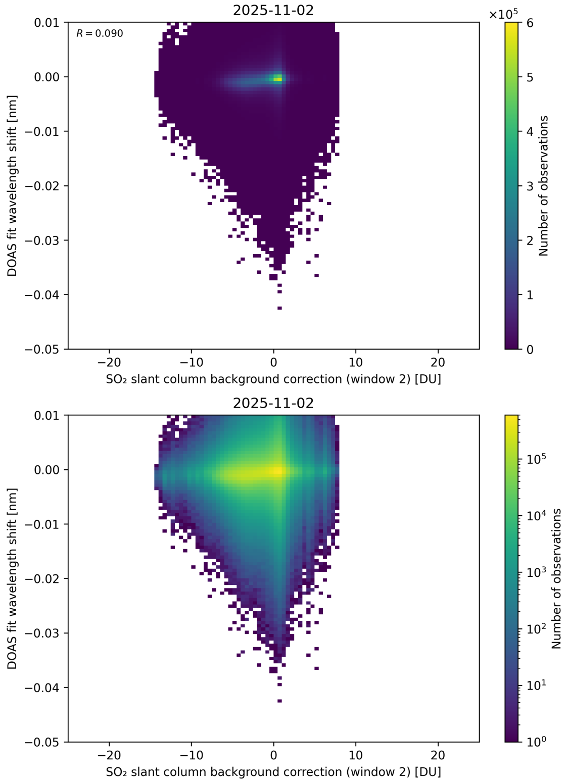
Figure 123: Scatter density plot of “SO 2 slant column background correction (window 2)” against “DOAS fit wavelength shift” for 2025-11-02 to 2025-11-03.
