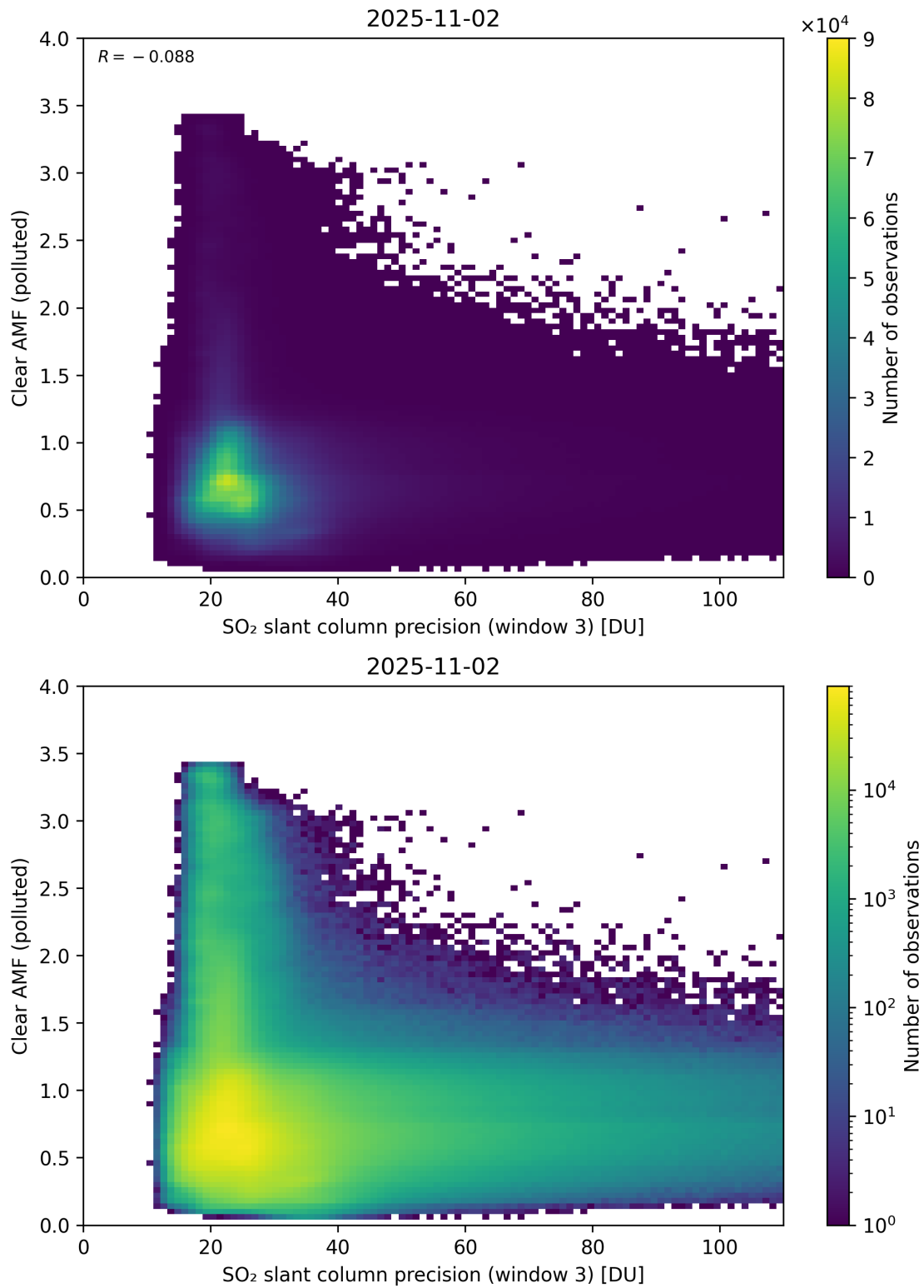
Figure 311: Scatter density plot of “SO 2 slant column precision (window 3)” against “Clear AMF (polluted)” for 2025-11-02 to 2025-11-03.
