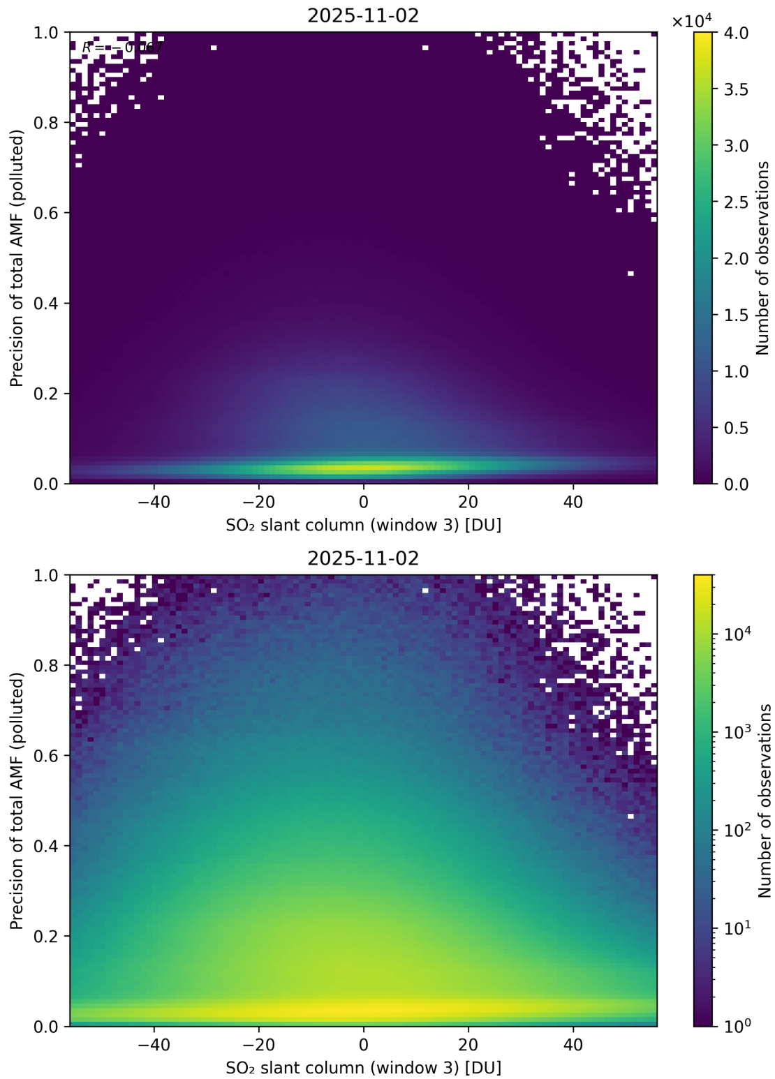
Figure 319: Scatter density plot of “SO 2 slant column (window 3)” against “Precision of total AMF (polluted)” for 2025-11-02 to 2025-11-03.
