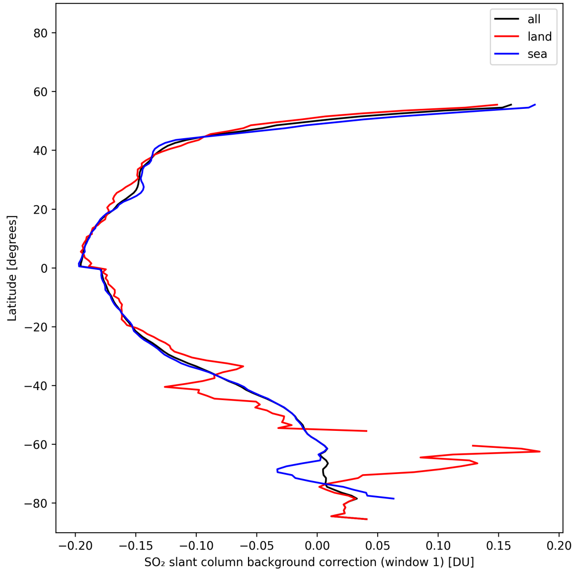
Figure 40: Zonal average of “SO 2 slant column background correction (window 1)” for 2025-11-02 to 2025-11-03.
