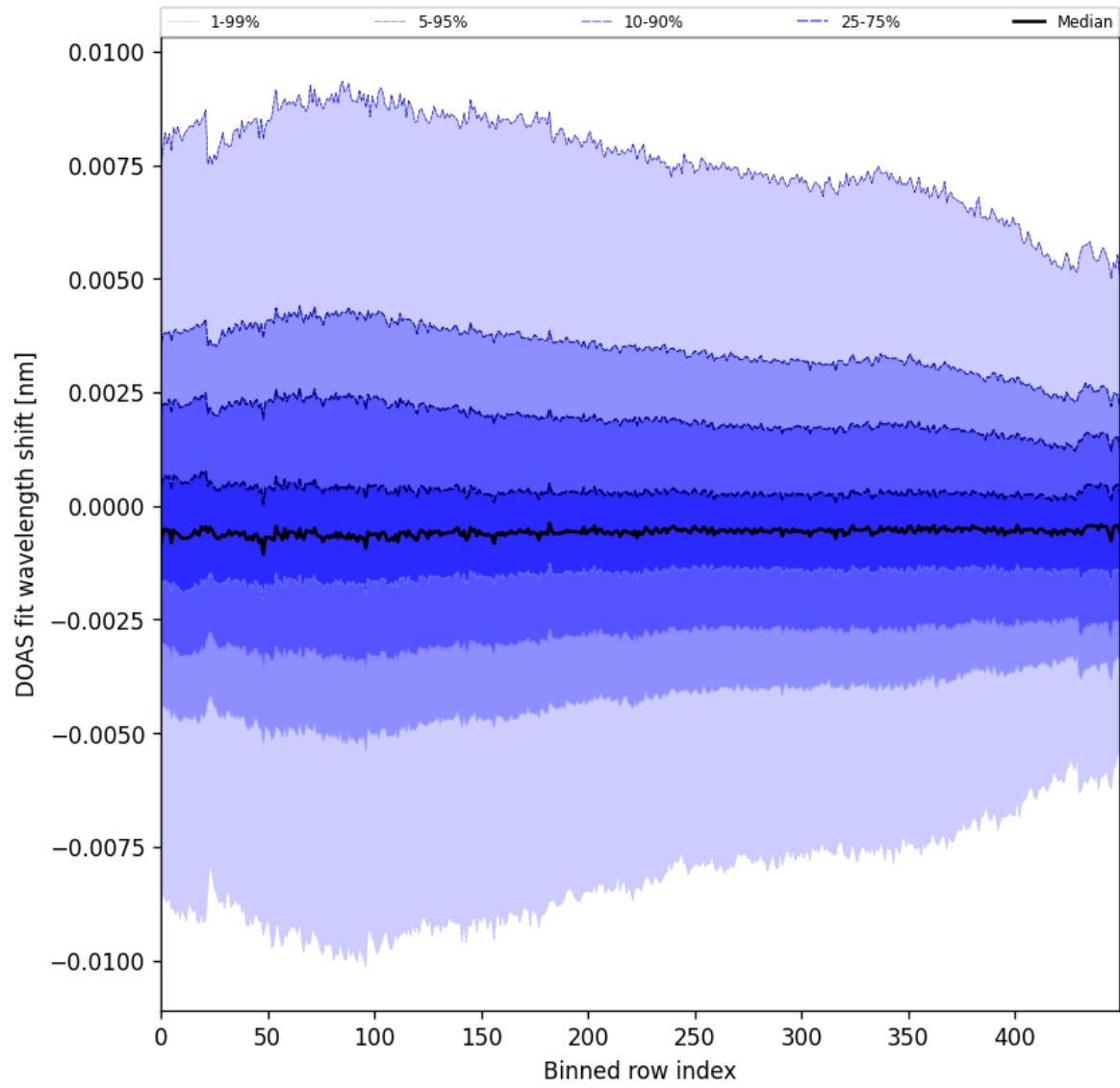
Figure 102: Along track statistics of “DOAS fit wavelength shift” for 2025-11-02 to 2025-11-03
