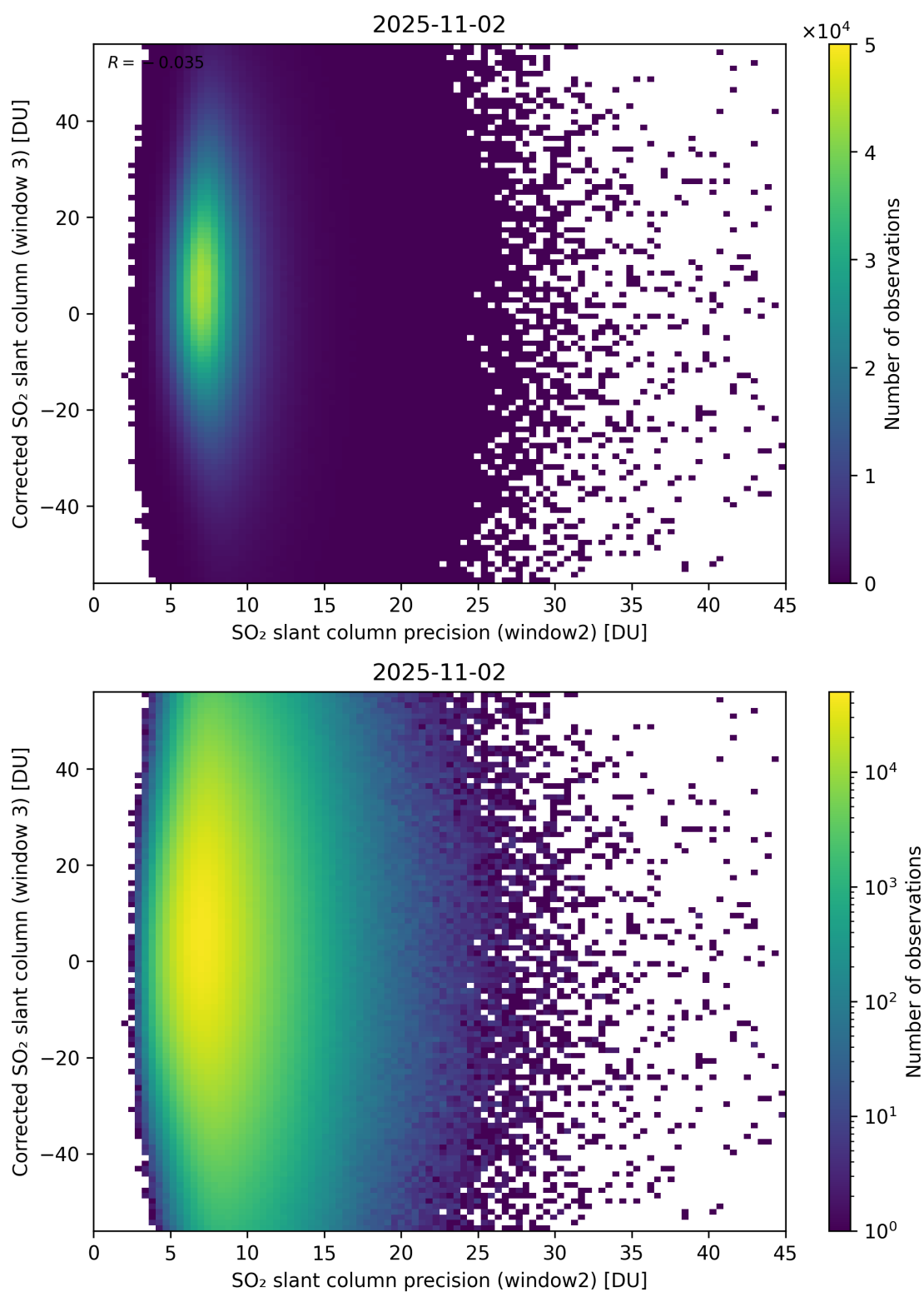
Figure 298: Scatter density plot of “SO 2 slant column precision (window2)” against “Corrected SO 2 slant column (window 3)” for 2025-11-02 to 2025-11-03.
