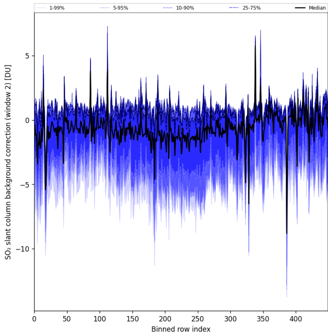
Figure 96: Along track statistics of “SO 2 slant column background correction (window 2)” for 2025-11-02 to 2025-11-03
