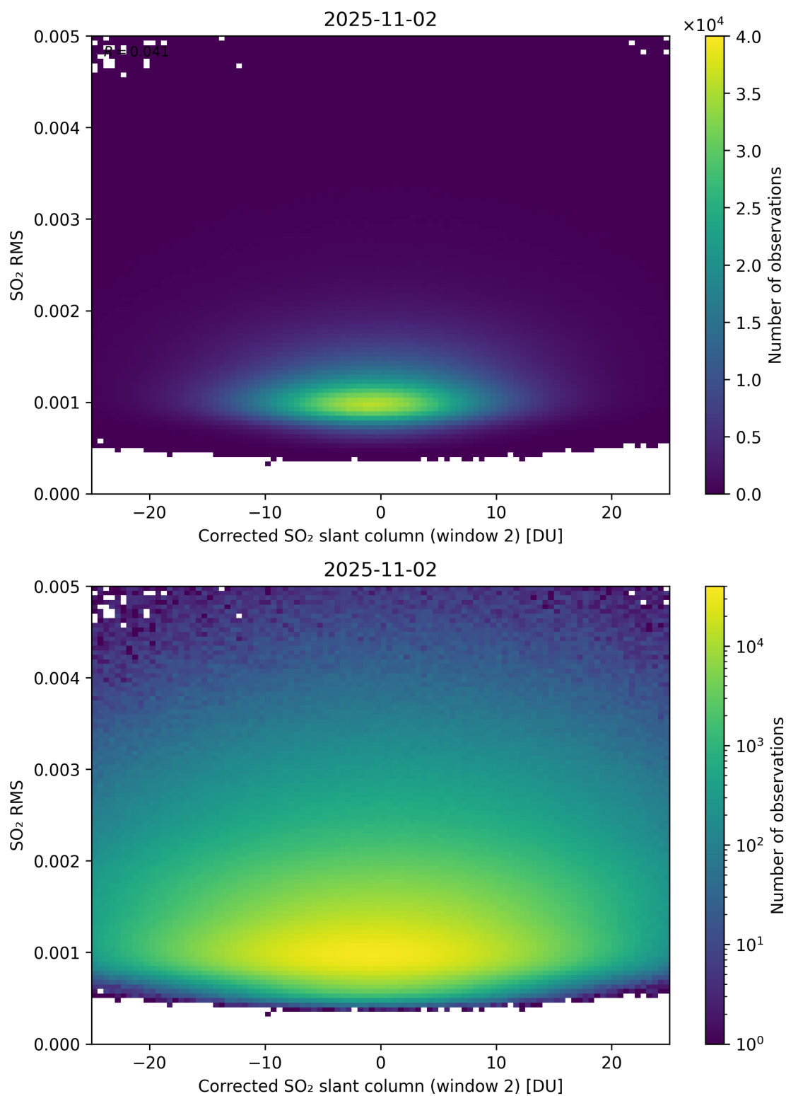
Figure 248: Scatter density plot of “Corrected SO 2 slant column (window 2)” against “SO 2 RMS” for 2025-11-02 to 2025-11-03.
