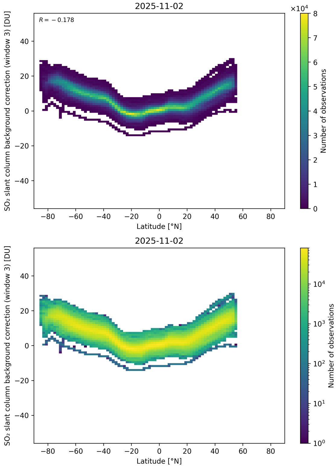
Figure 152: Scatter density plot of “Latitude” against “SO 2 slant column background correction (window 3)” for 2025-11-02 to 2025-11-03.
