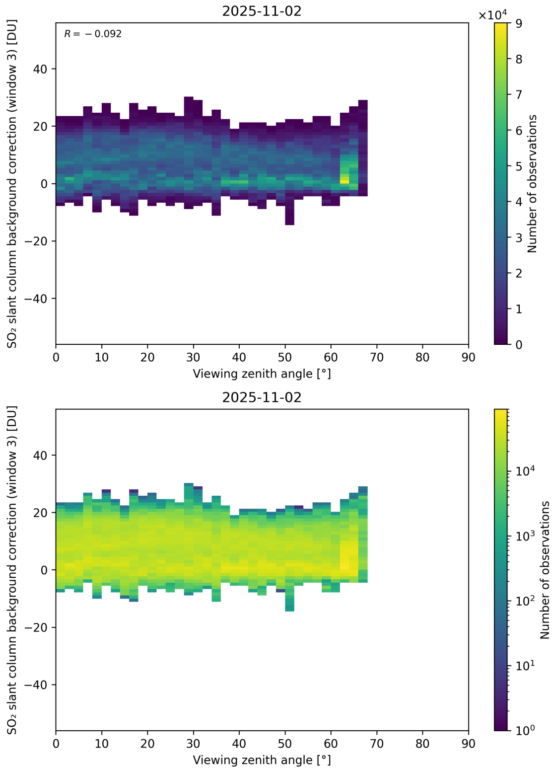
Figure 364: Scatter density plot of “Viewing zenith angle” against “SO 2 slant column background correction (window 3)” for 2025-11-02 to 2025-11-03.
