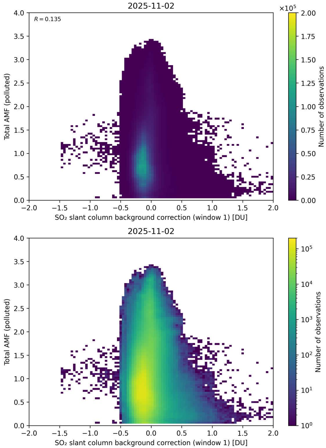
Figure 120: Scatter density plot of “SO 2 slant column background correction (window 1)” against “Total AMF (polluted)” for 2025-11-02 to 2025-11-03.
