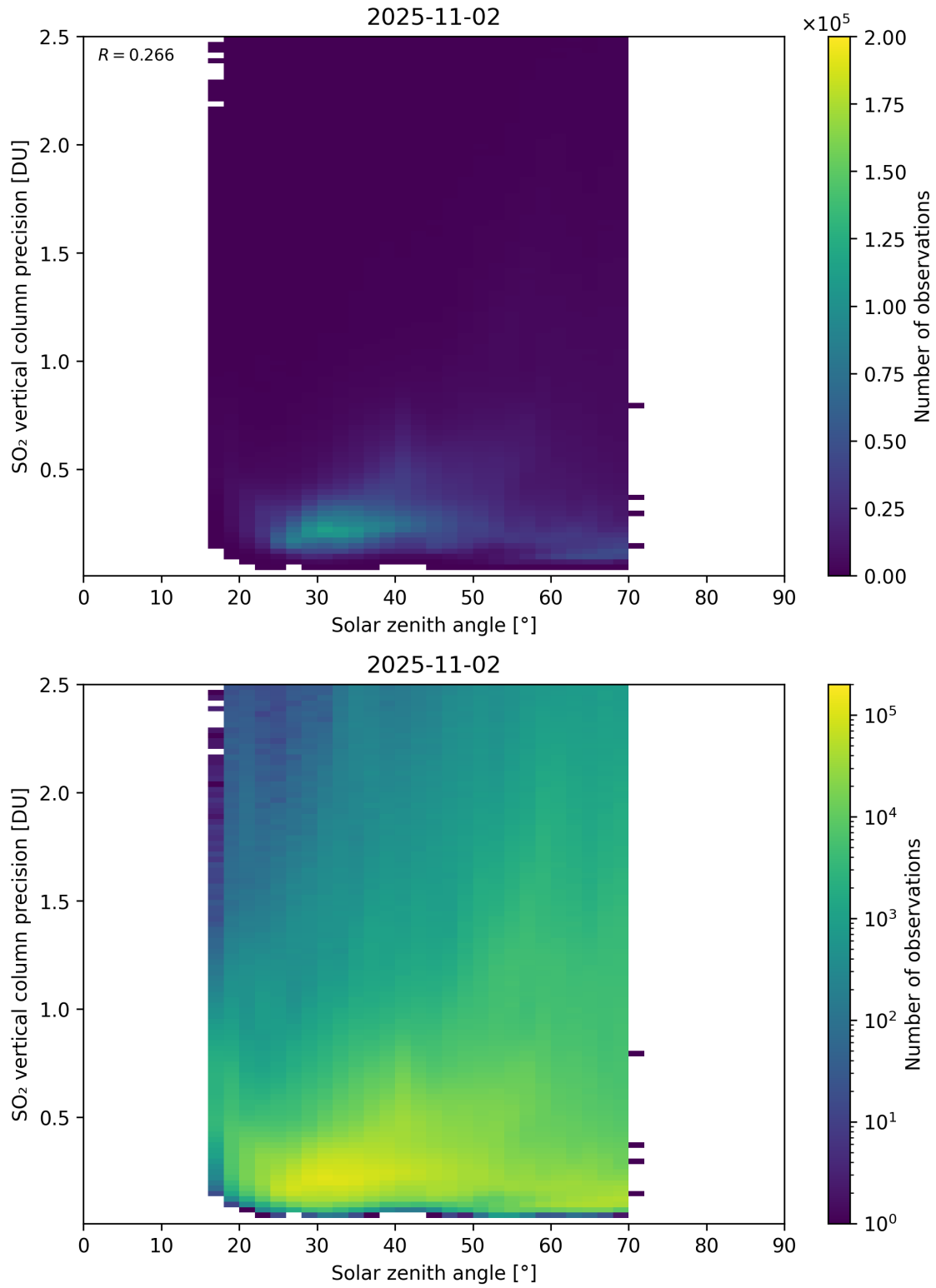
Figure 192: Scatter density plot of “Solar zenith angle” against “SO 2 vertical column precision” for 2025-11-02 to 2025-11-03.
