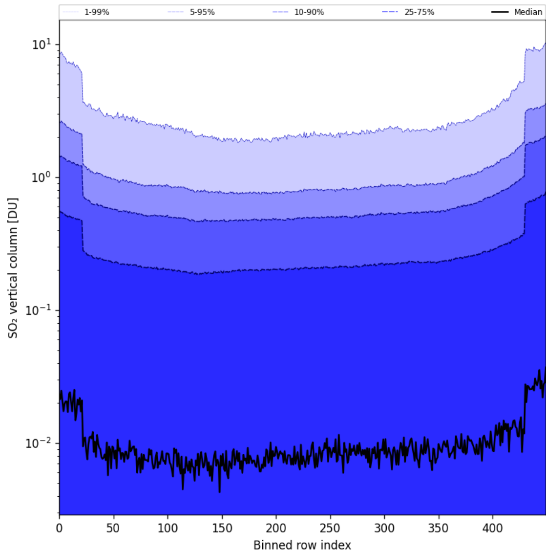
Figure 84: Along track statistics of “SO 2 vertical column” for 2025-11-02 to 2025-11-03
