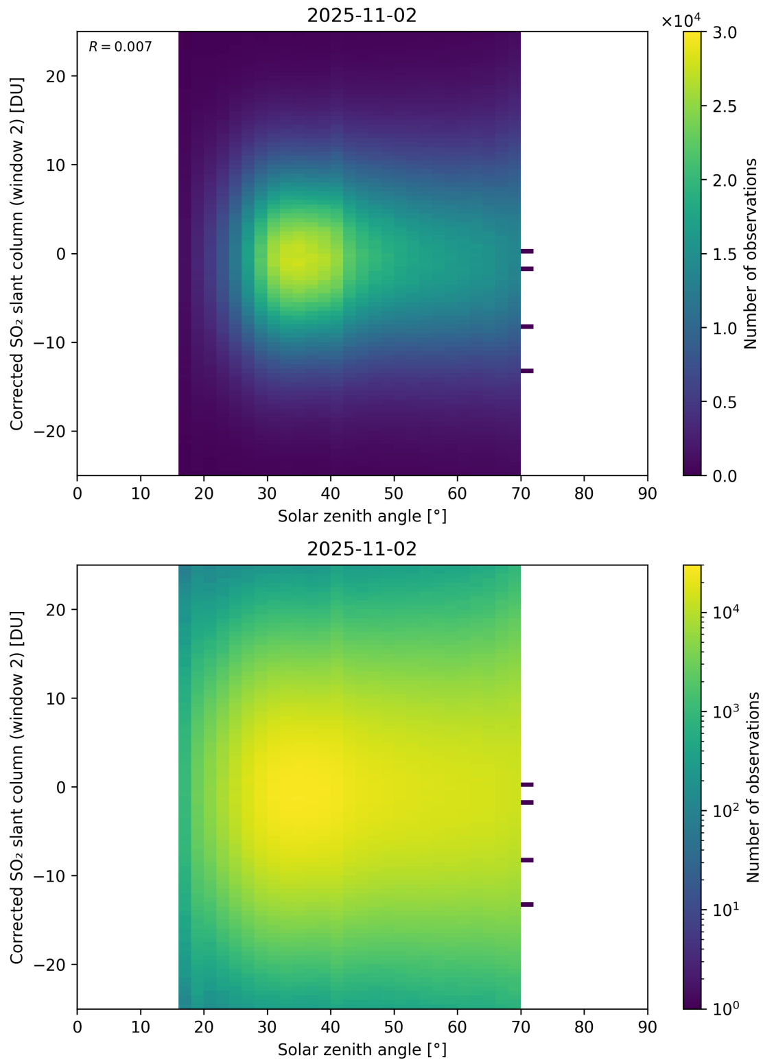
Figure 182: Scatter density plot of “Solar zenith angle” against “Corrected SO 2 slant column (window 2)” for 2025-11-02 to 2025-11-03.
