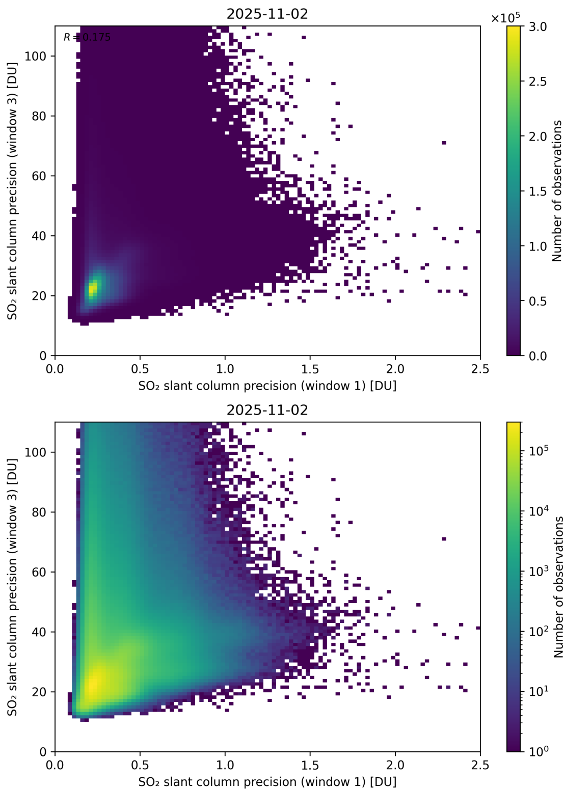
Figure 279: Scatter density plot of “SO 2 slant column precision (window 1)” against “SO 2 slant column precision (window 3)” for 2025-11-02 to 2025-11-03.
