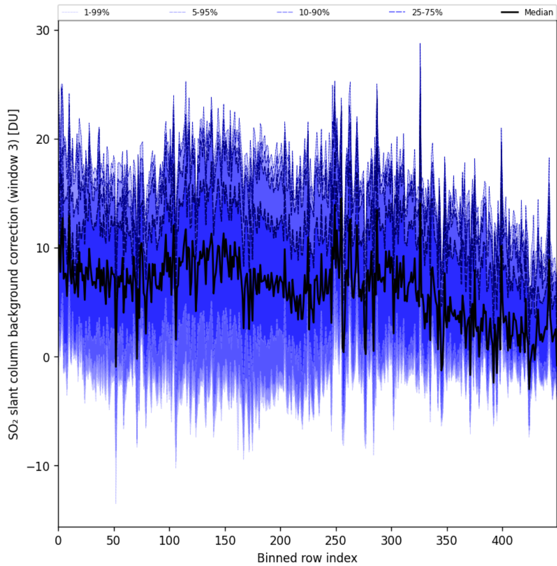
Figure 100: Along track statistics of “SO 2 slant column background correction (window 3)” for 2025-11-02 to 2025-11-03
