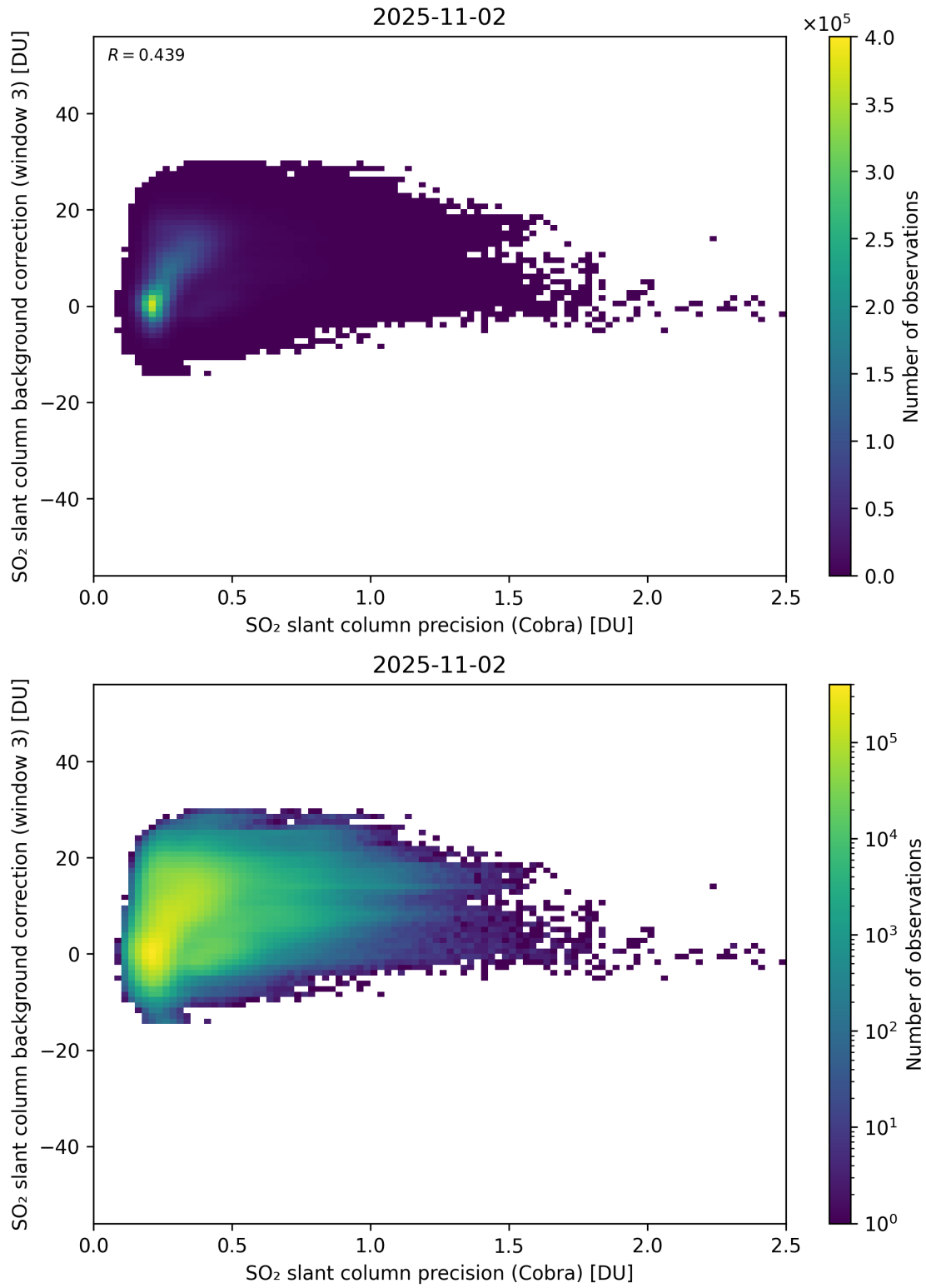
Figure 201: Scatter density plot of “SO 2 slant column precision (Cobra)” against “SO 2 slant column background correction (window 3)” for 2025-11-02 to 2025-11-03.
