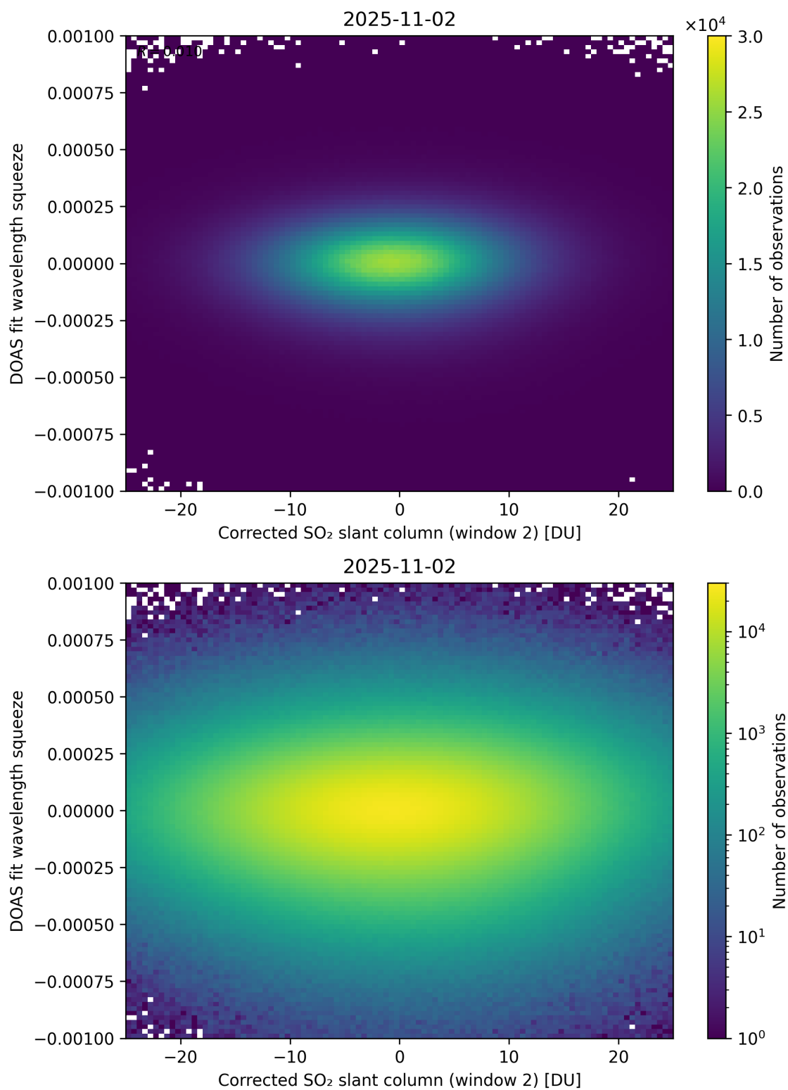
Figure 247: Scatter density plot of “Corrected SO 2 slant column (window 2)” against “DOAS fit wavelength squeeze” for 2025-11-02 to 2025-11-03.
