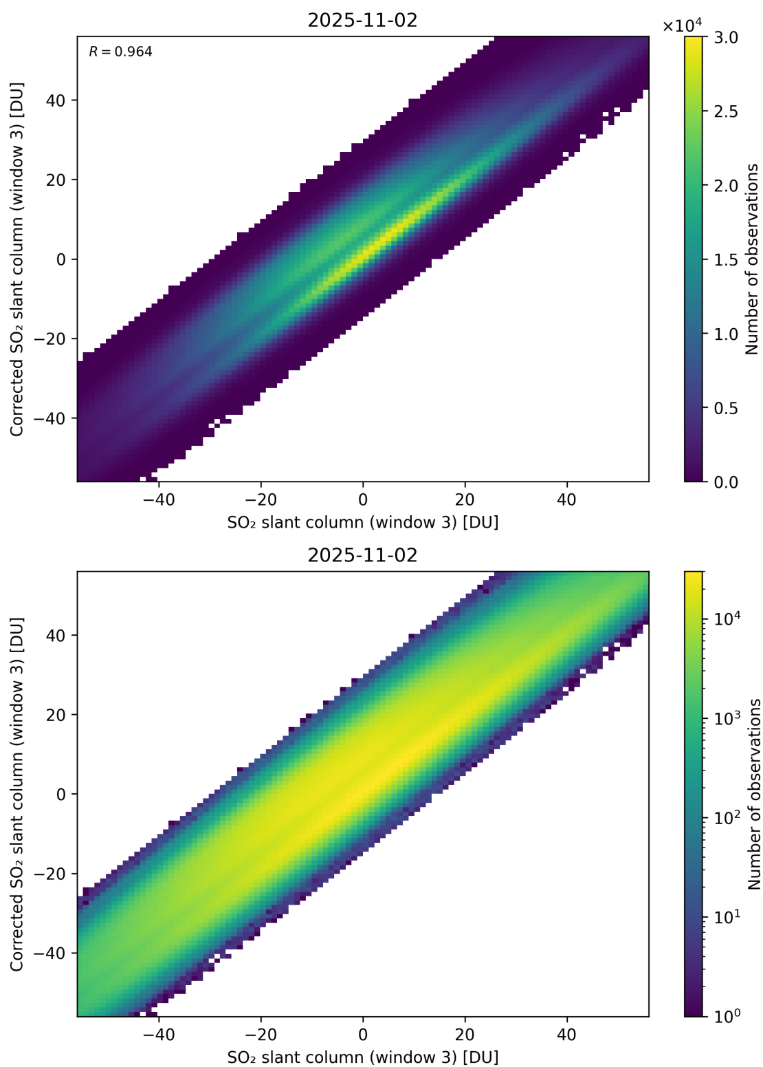
Figure 316: Scatter density plot of “SO 2 slant column (window 3)” against “Corrected SO 2 slant column (window 3)” for 2025-11-02 to 2025-11-03.
