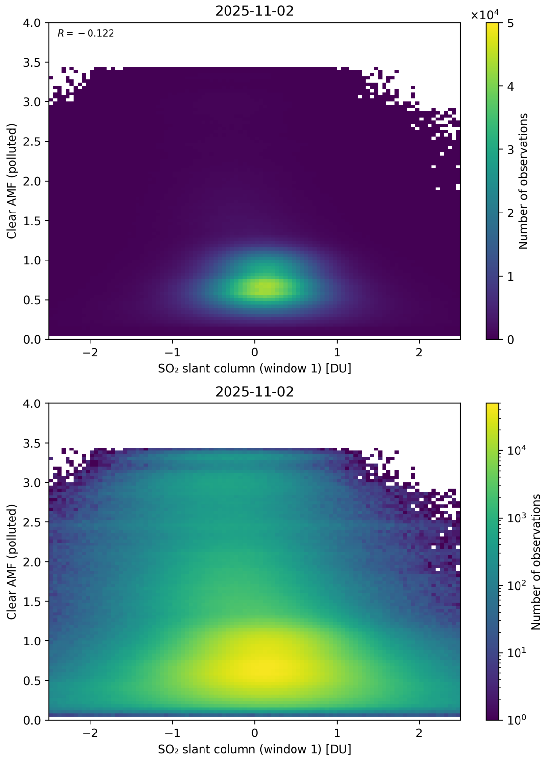
Figure 282: Scatter density plot of “SO 2 slant column (window 1)” against “Clear AMF (polluted)” for 2025-11-02 to 2025-11-03.
