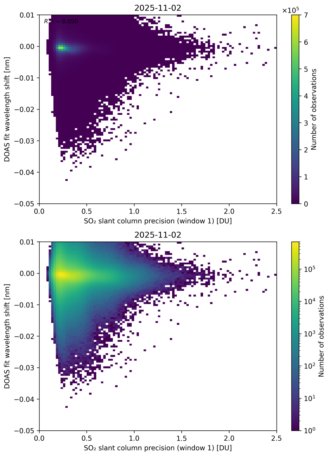
Figure 271: Scatter density plot of “SO 2 slant column precision (window 1)” against “DOAS fit wavelength shift” for 2025-11-02 to 2025-11-03.
