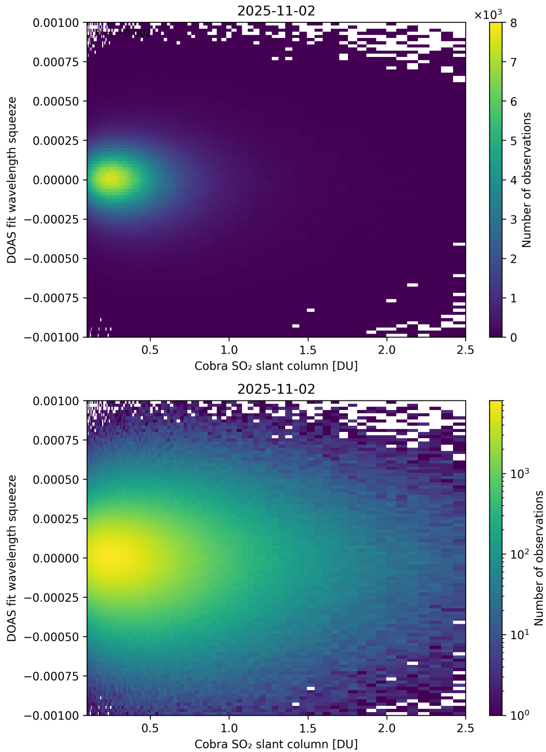
Figure 197: Scatter density plot of “Cobra SO 2 slant column” against “DOAS fit wavelength squeeze” for 2025-11-02 to 2025-11-03.
