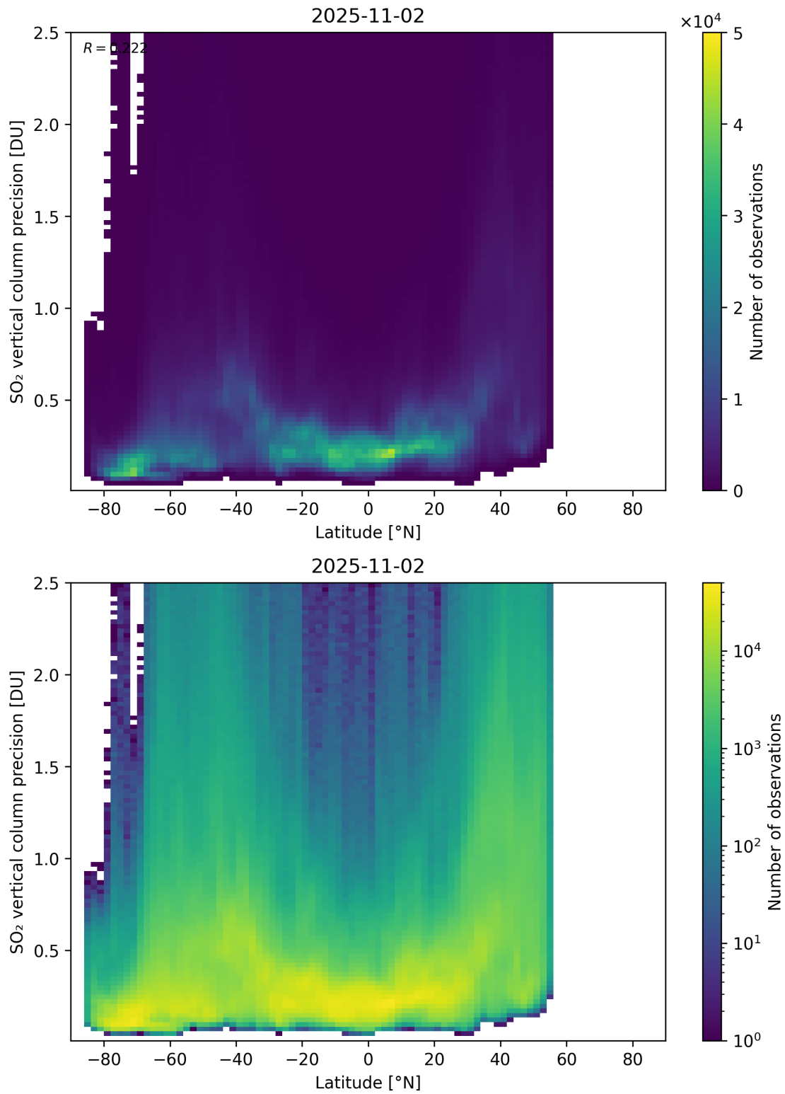
Figure 170: Scatter density plot of “Latitude” against “SO 2 vertical column precision” for 2025-11-02 to 2025-11-03.
