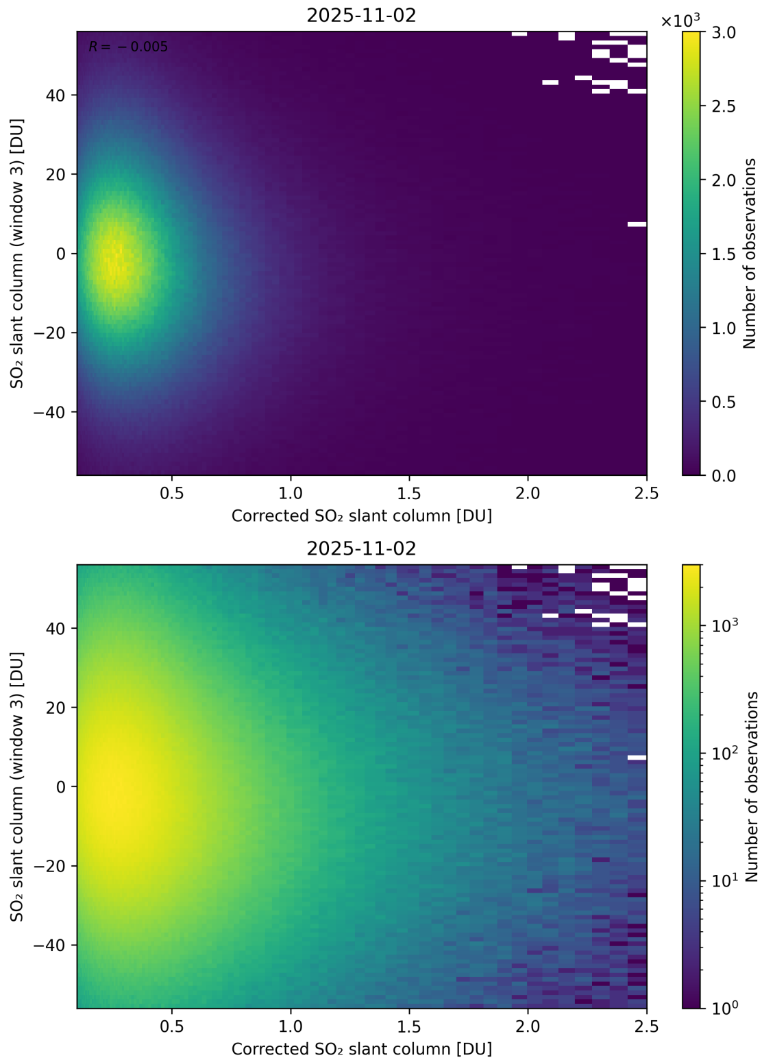
Figure 240: Scatter density plot of “Corrected SO 2 slant column” against “SO 2 slant column (window 3)” for 2025-11-02 to 2025-11-03.
