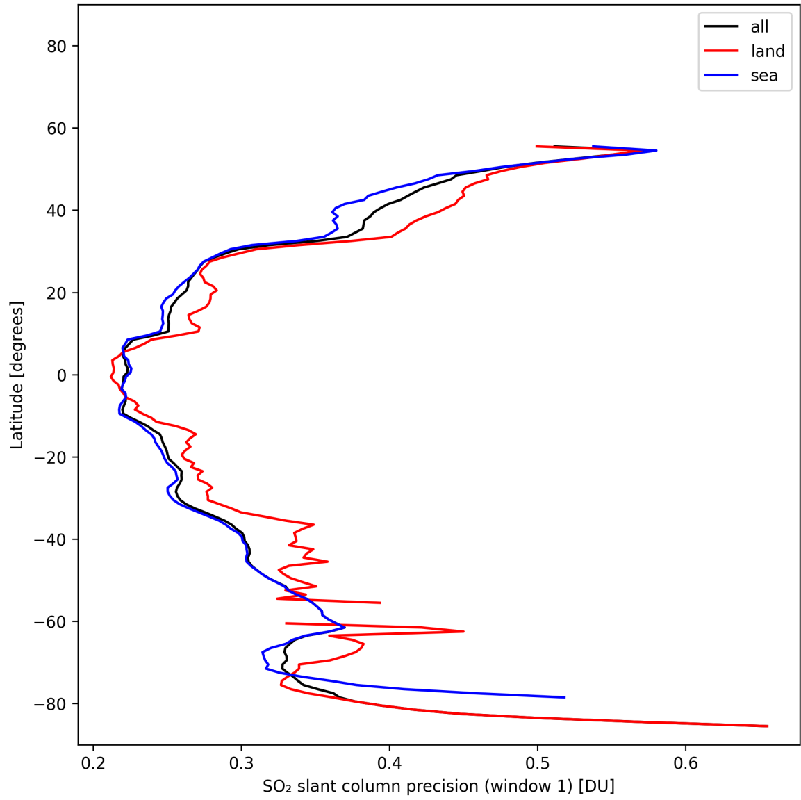
Figure 38: Zonal average of “SO 2 slant column precision (window 1)” for 2025-11-02 to 2025-11-03.
