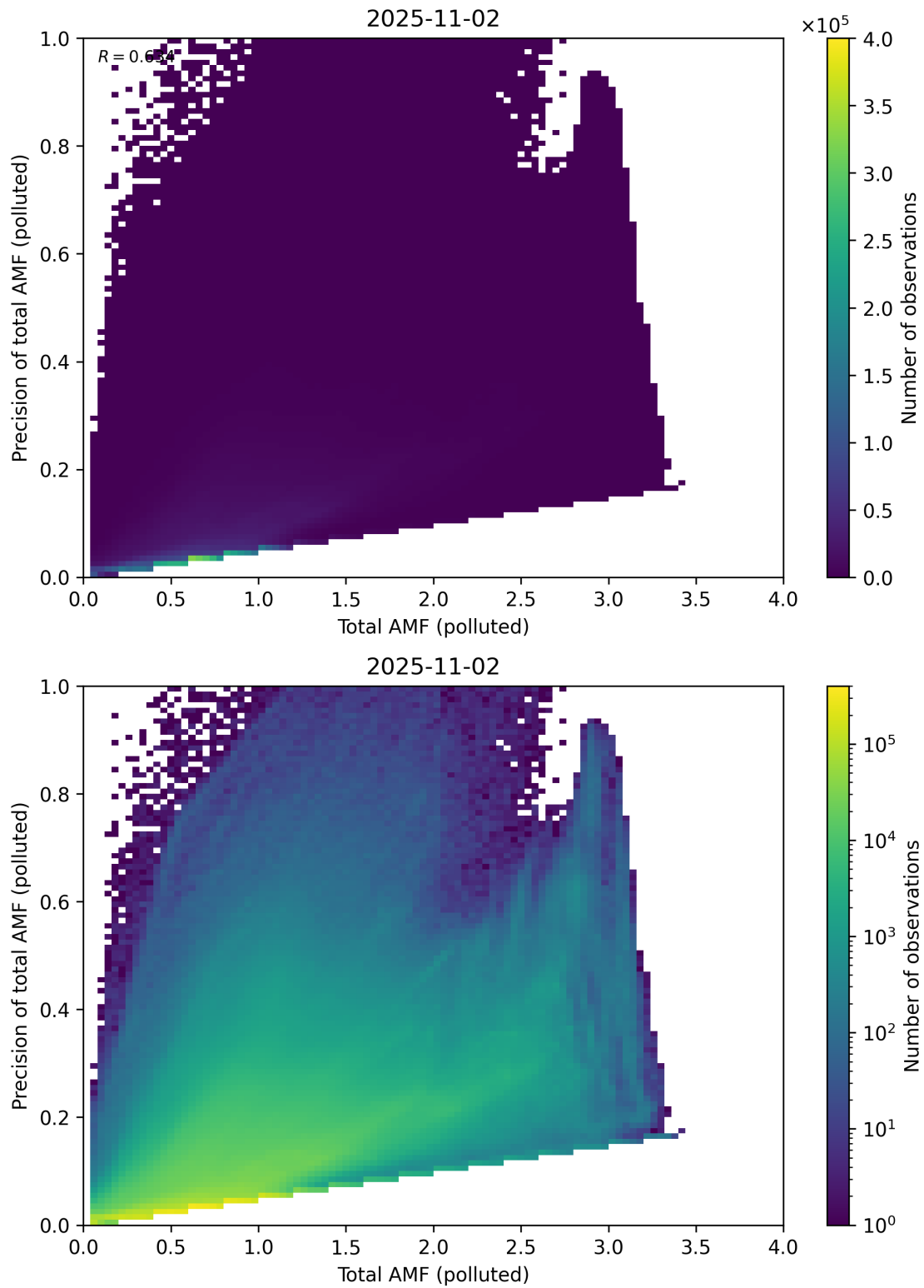
Figure 322: Scatter density plot of “Total AMF (polluted)” against “Precision of total AMF (polluted)” for 2025-11-02 to 2025-11-03.
