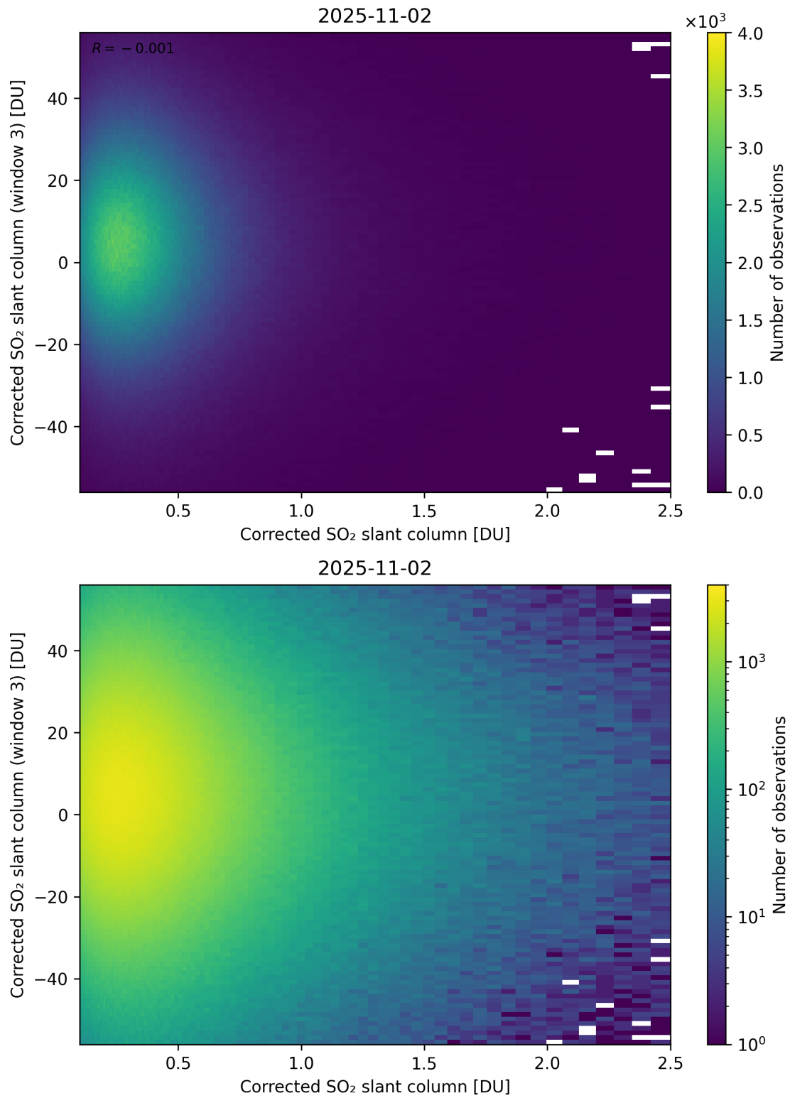
Figure 236: Scatter density plot of “Corrected SO 2 slant column” against “Corrected SO 2 slant column (window 3)” for 2025-11-02 to 2025-11-03.
