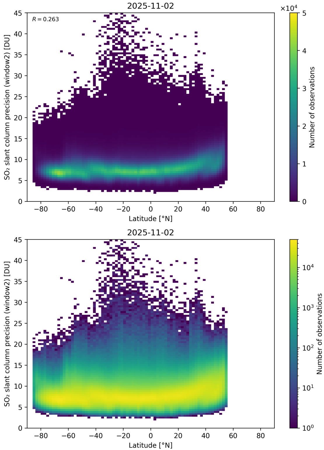
Figure 164: Scatter density plot of “Latitude” against “SO 2 slant column precision (window2)” for 2025-11-02 to 2025-11-03.
