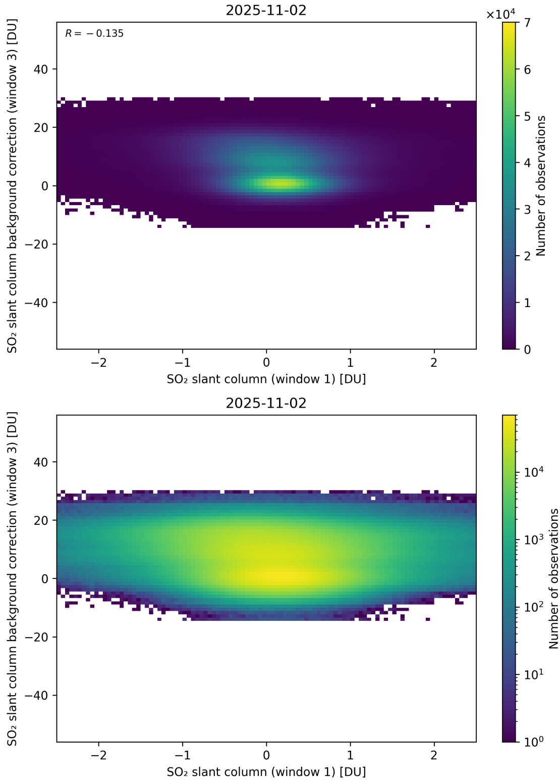
Figure 264: Scatter density plot of “SO 2 slant column (window 1)” against “SO 2 slant column background correction (window 3)” for 2025-11-02 to 2025-11-03.
