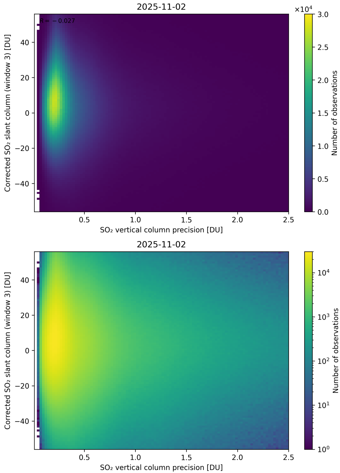
Figure 340: Scatter density plot of “SO 2 vertical column precision” against “Corrected SO 2 slant column (window 3)” for 2025-11-02 to 2025-11-03.
