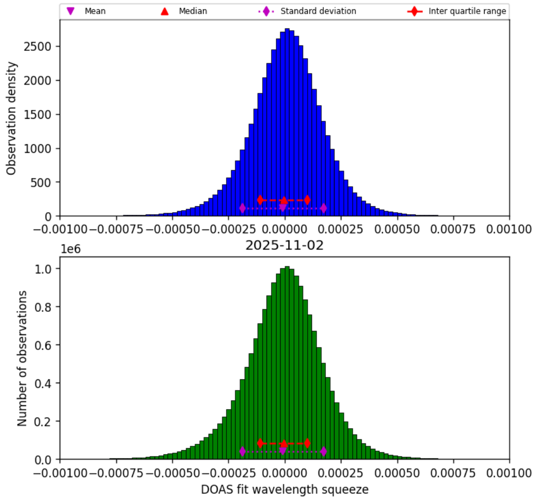
Figure 77: Histogram of “DOAS fit wavelength squeeze” for 2025-11-02 to 2025-11-03
