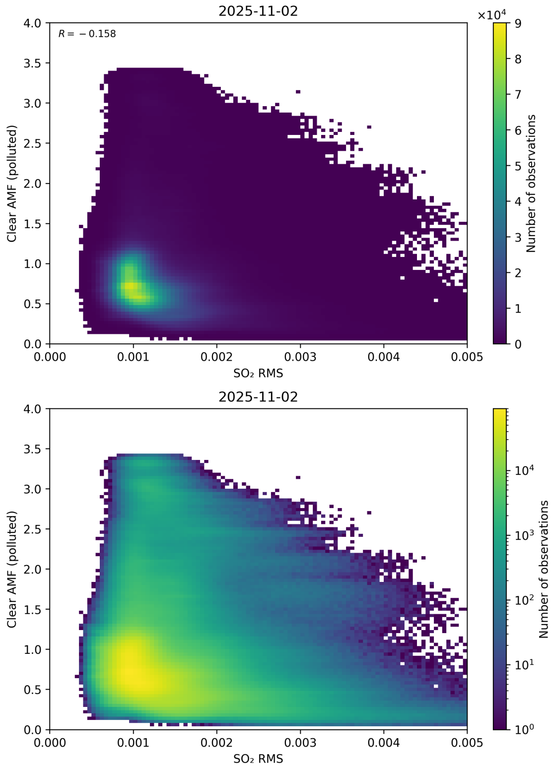
Figure 147: Scatter density plot of “SO 2 RMS” against “Clear AMF (polluted)” for 2025-11-02 to 2025-11-03.
