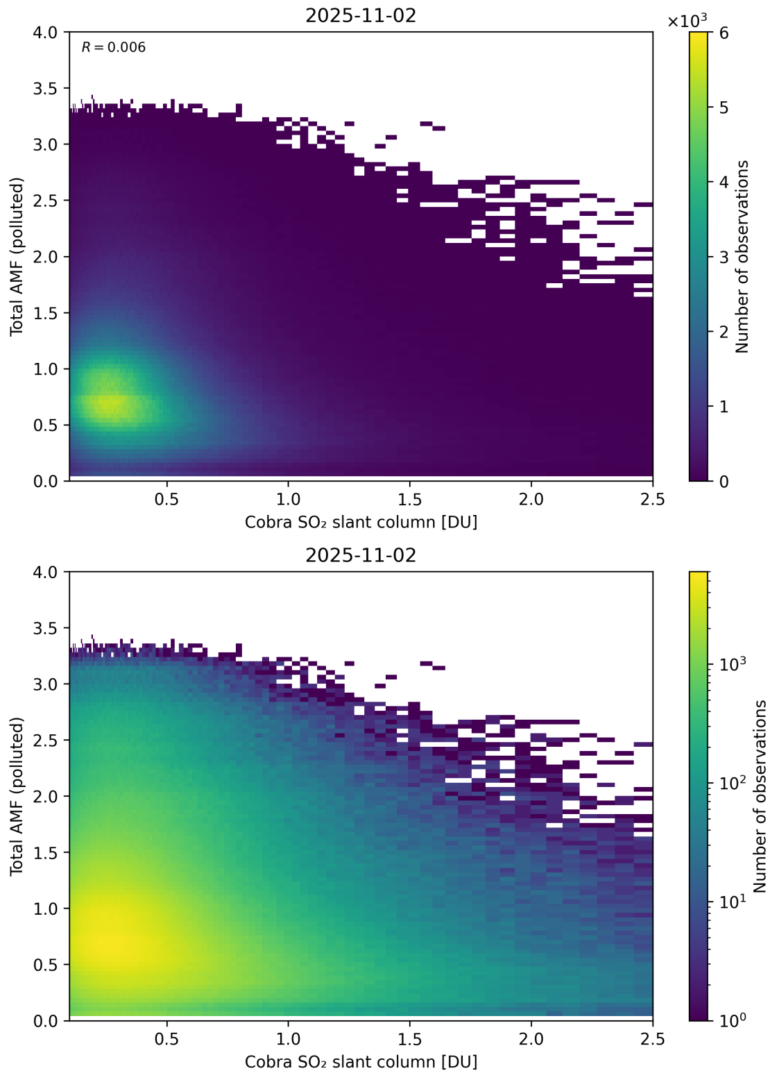
Figure 224: Scatter density plot of “Cobra SO 2 slant column” against “Total AMF (polluted)” for 2025-11-02 to 2025-11-03.
