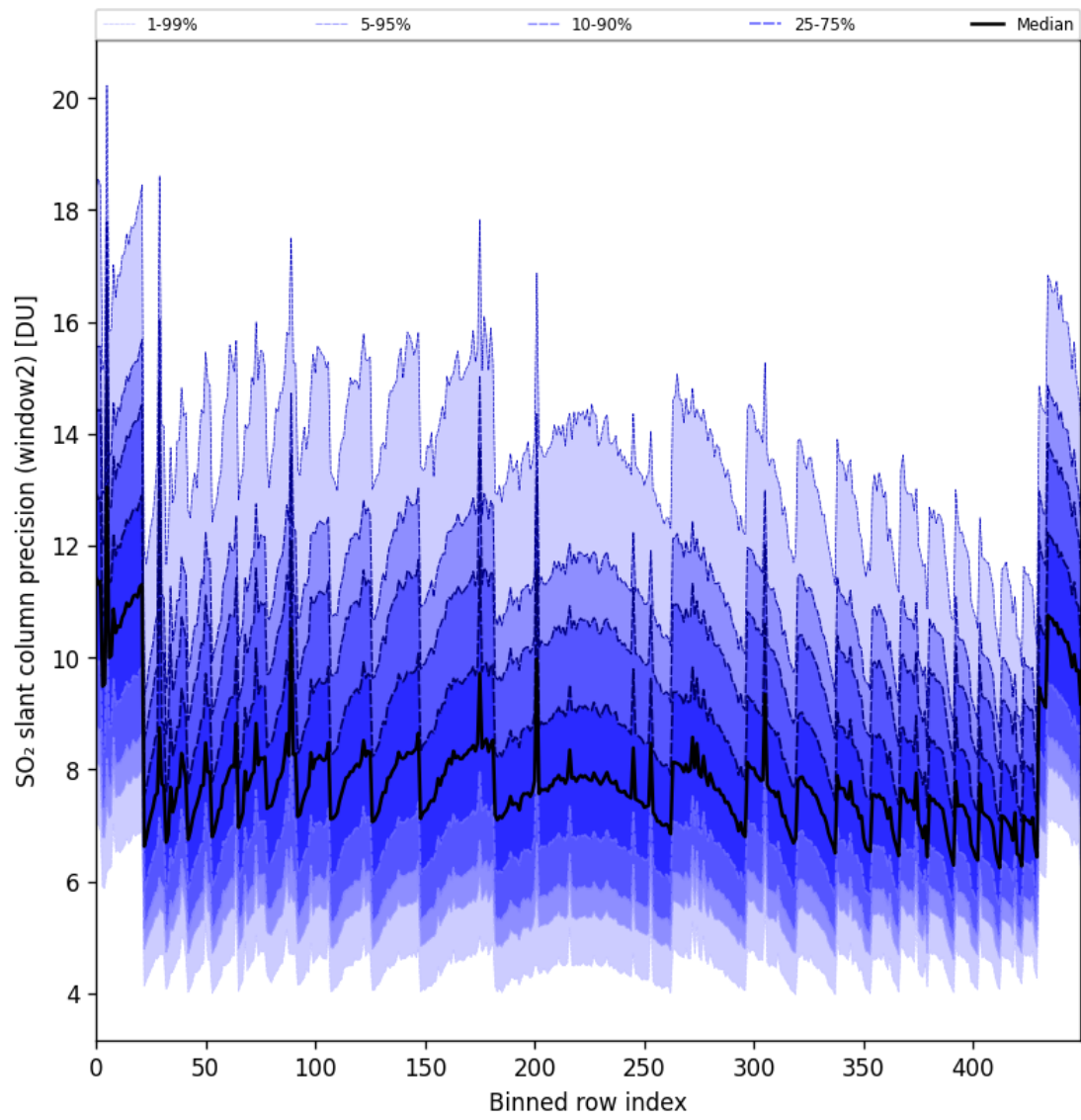
Figure 94: Along track statistics of “SO 2 slant column precision (window2)” for 2025-11-02 to 2025-11-03
