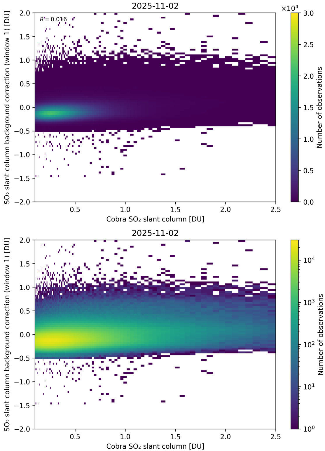
Figure 193: Scatter density plot of “Cobra SO 2 slant column” against “SO 2 slant column background correction (window 1)” for 2025-11-02 to 2025-11-03.
