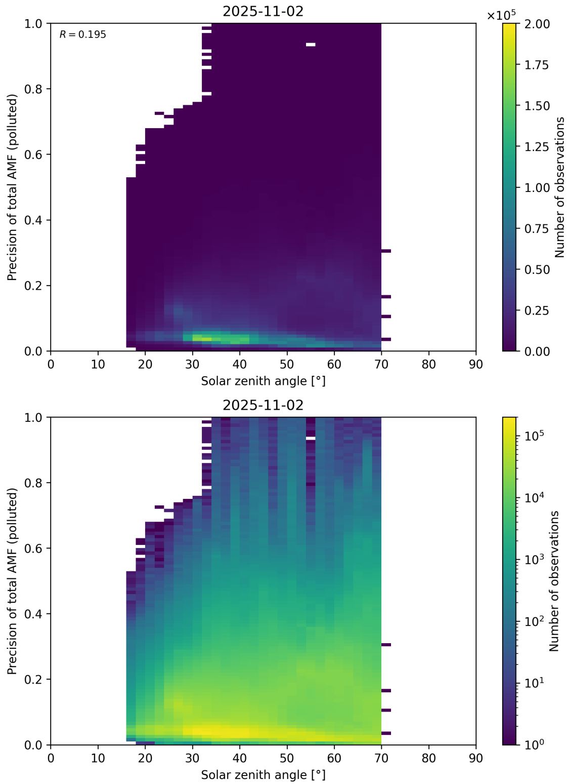
Figure 190: Scatter density plot of “Solar zenith angle” against “Precision of total AMF (polluted)” for 2025-11-02 to 2025-11-03.
