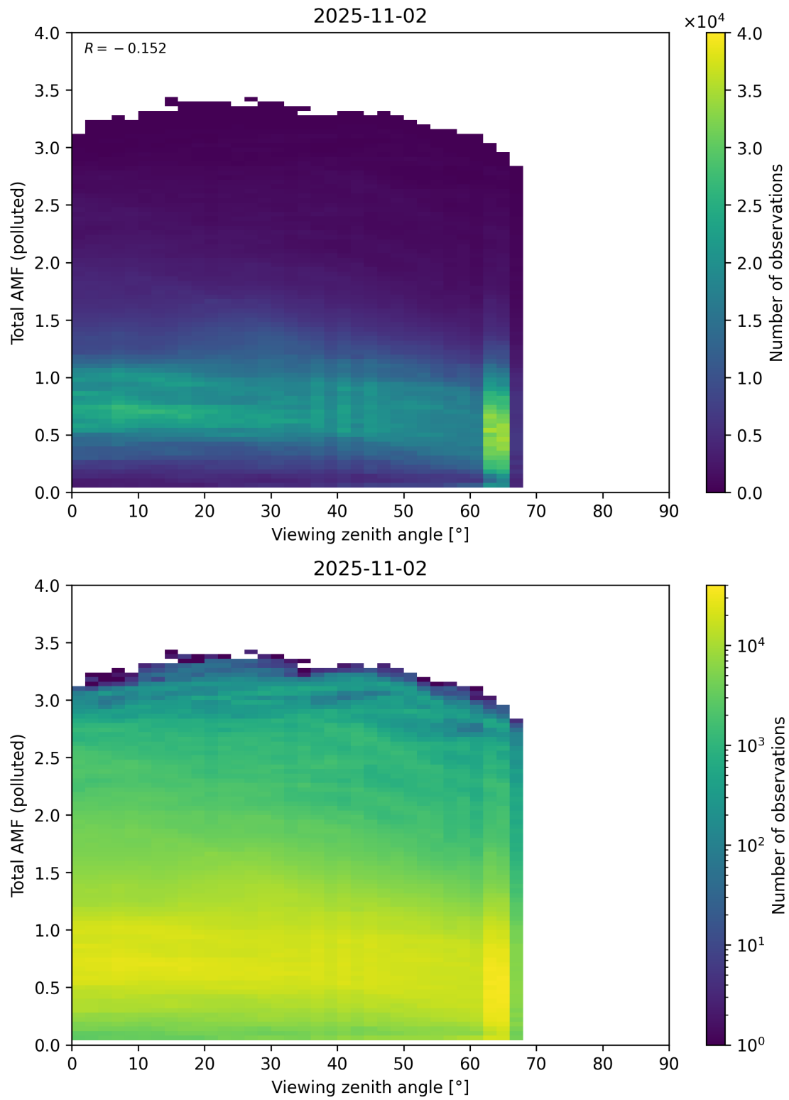
Figure 381: Scatter density plot of “Viewing zenith angle” against “Total AMF (polluted)” for 2025-11-02 to 2025-11-03.
