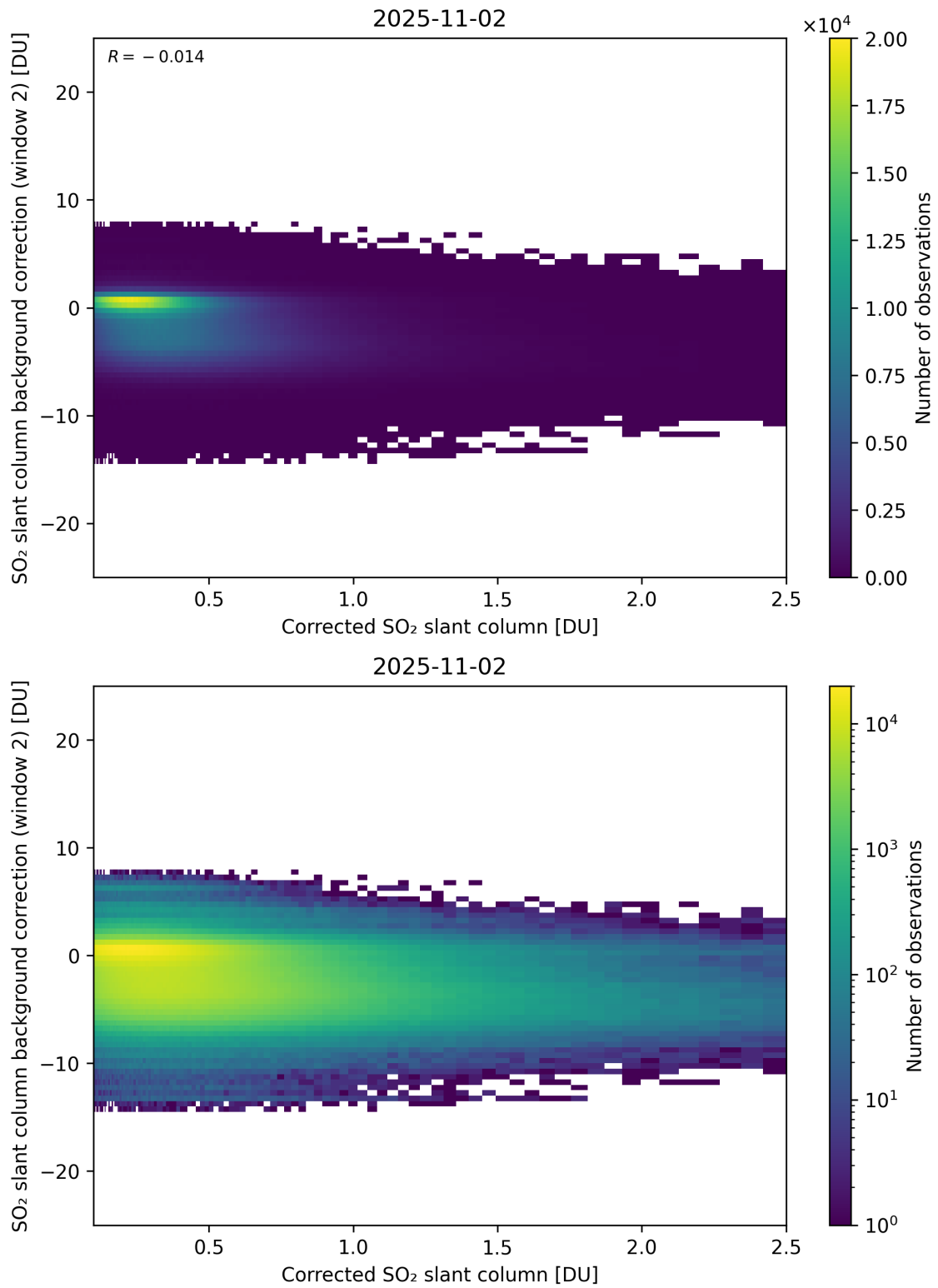
Figure 227: Scatter density plot of “Corrected SO 2 slant column” against “SO 2 slant column background correction (window 2)” for 2025-11-02 to 2025-11-03.
