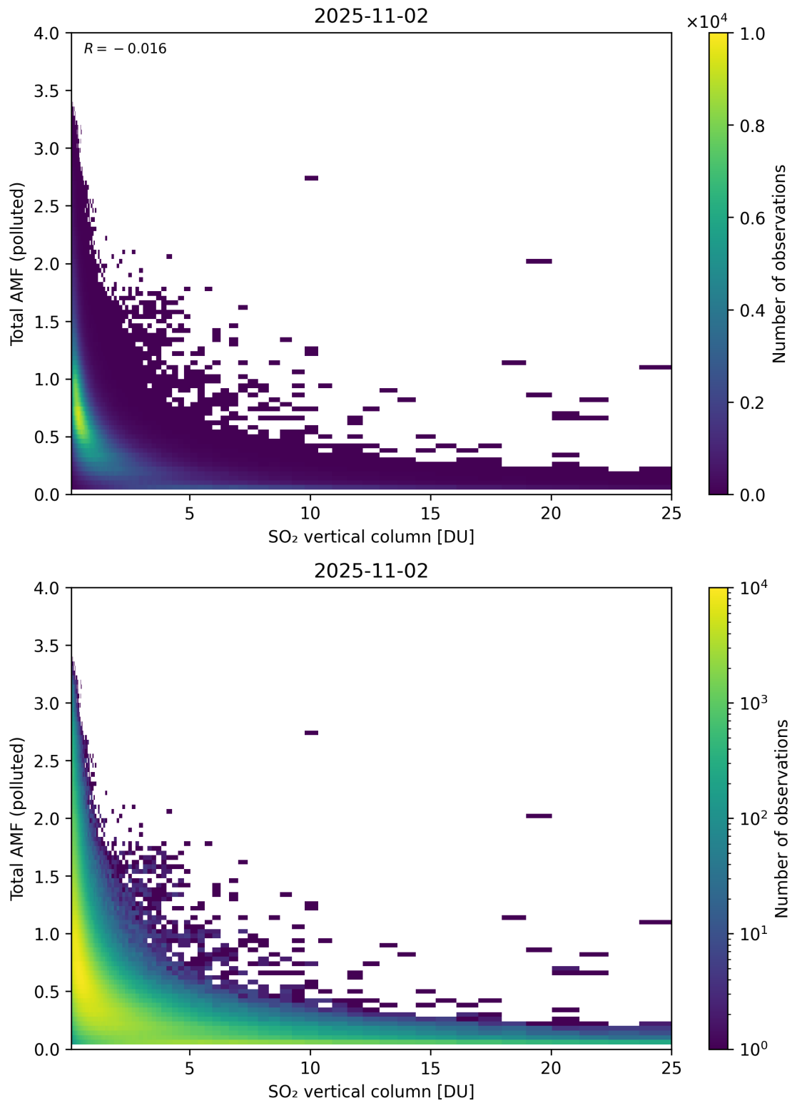
Figure 359: Scatter density plot of “SO 2 vertical column” against “Total AMF (polluted)” for 2025-11-02 to 2025-11-03.
