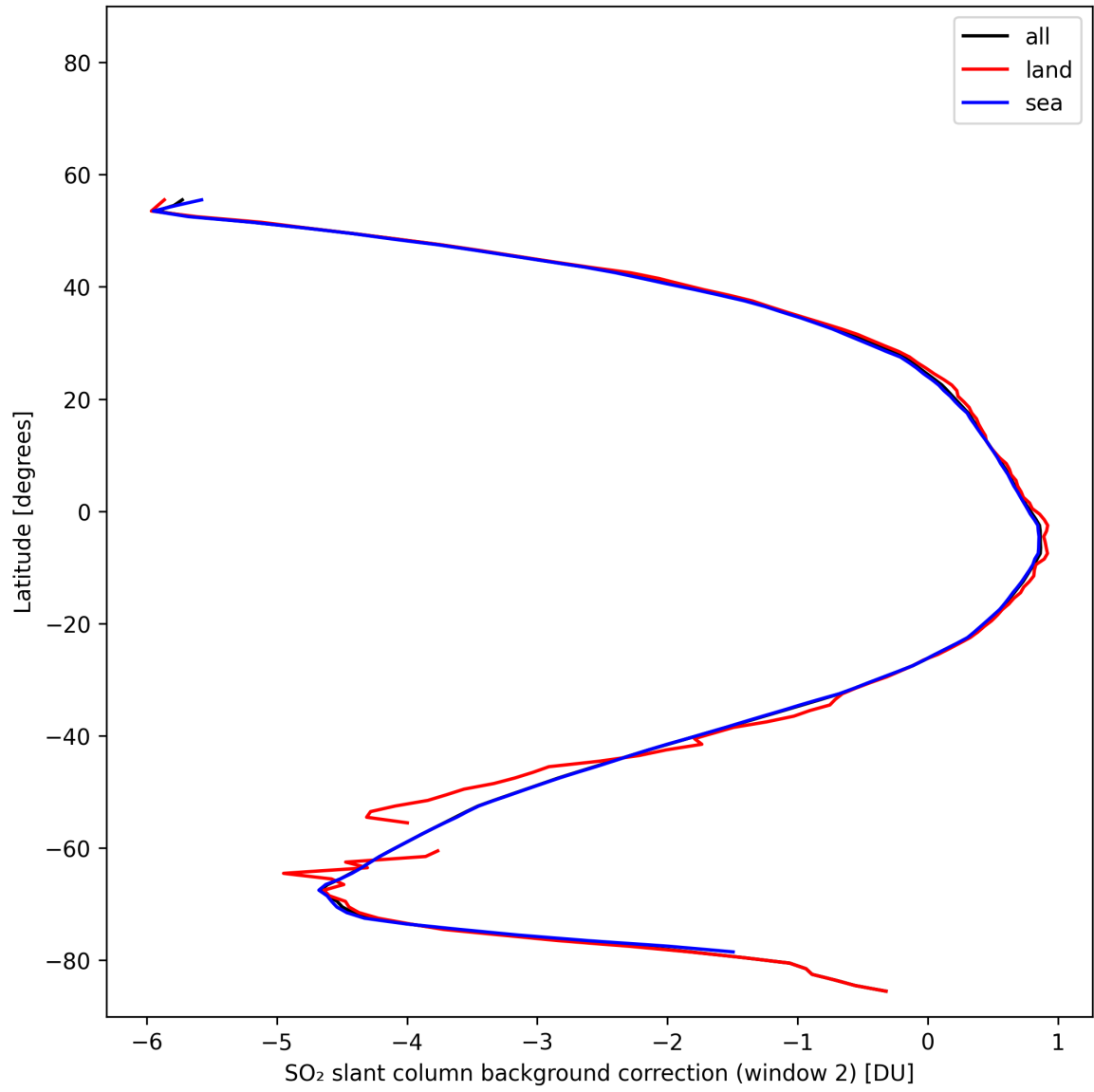
Figure 44: Zonal average of “SO 2 slant column background correction (window 2)” for 2025-11-02 to 2025-11-03.
