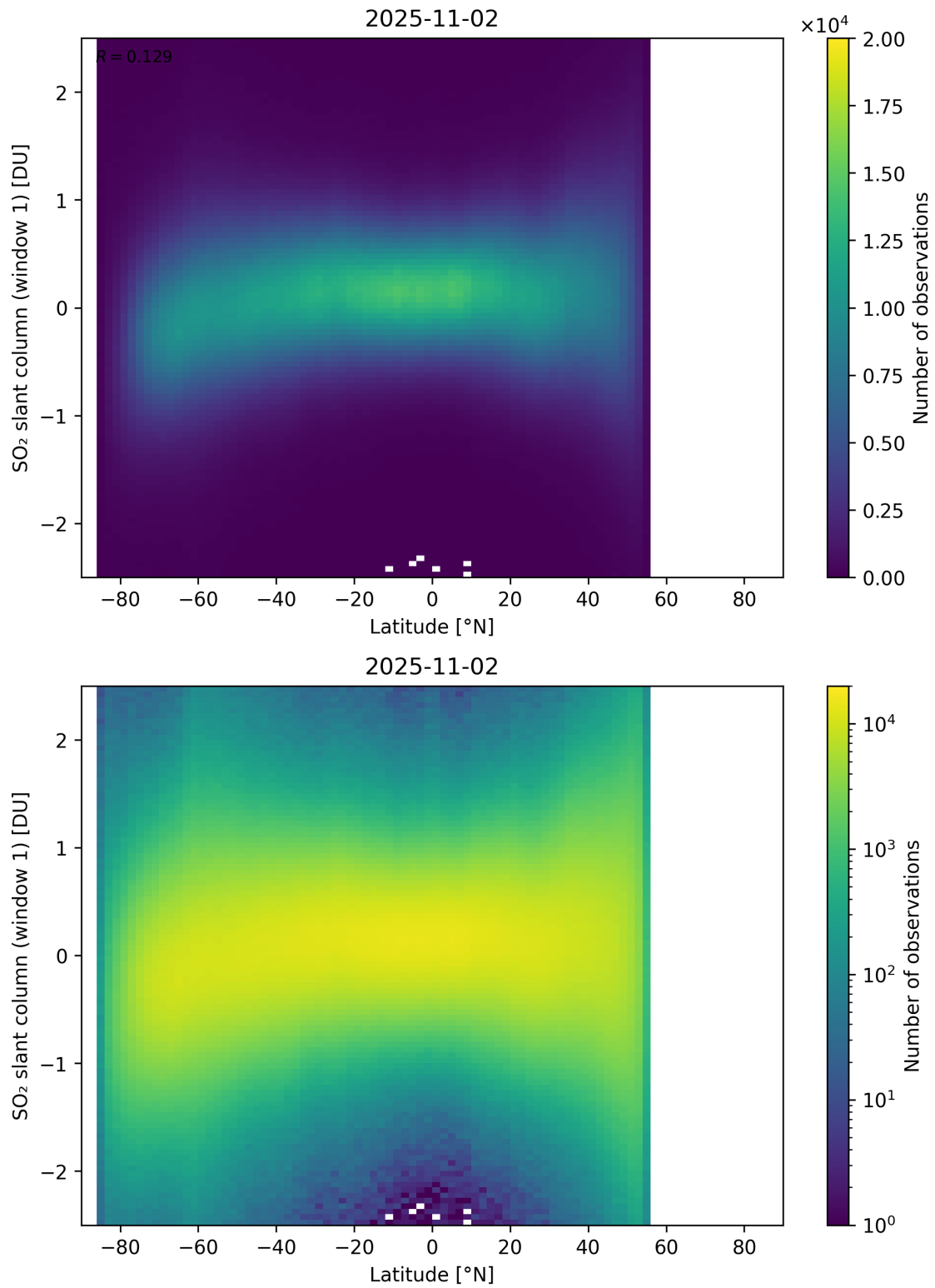
Figure 162: Scatter density plot of “Latitude” against “SO 2 slant column (window 1)” for 2025-11-02 to 2025-11-03.
