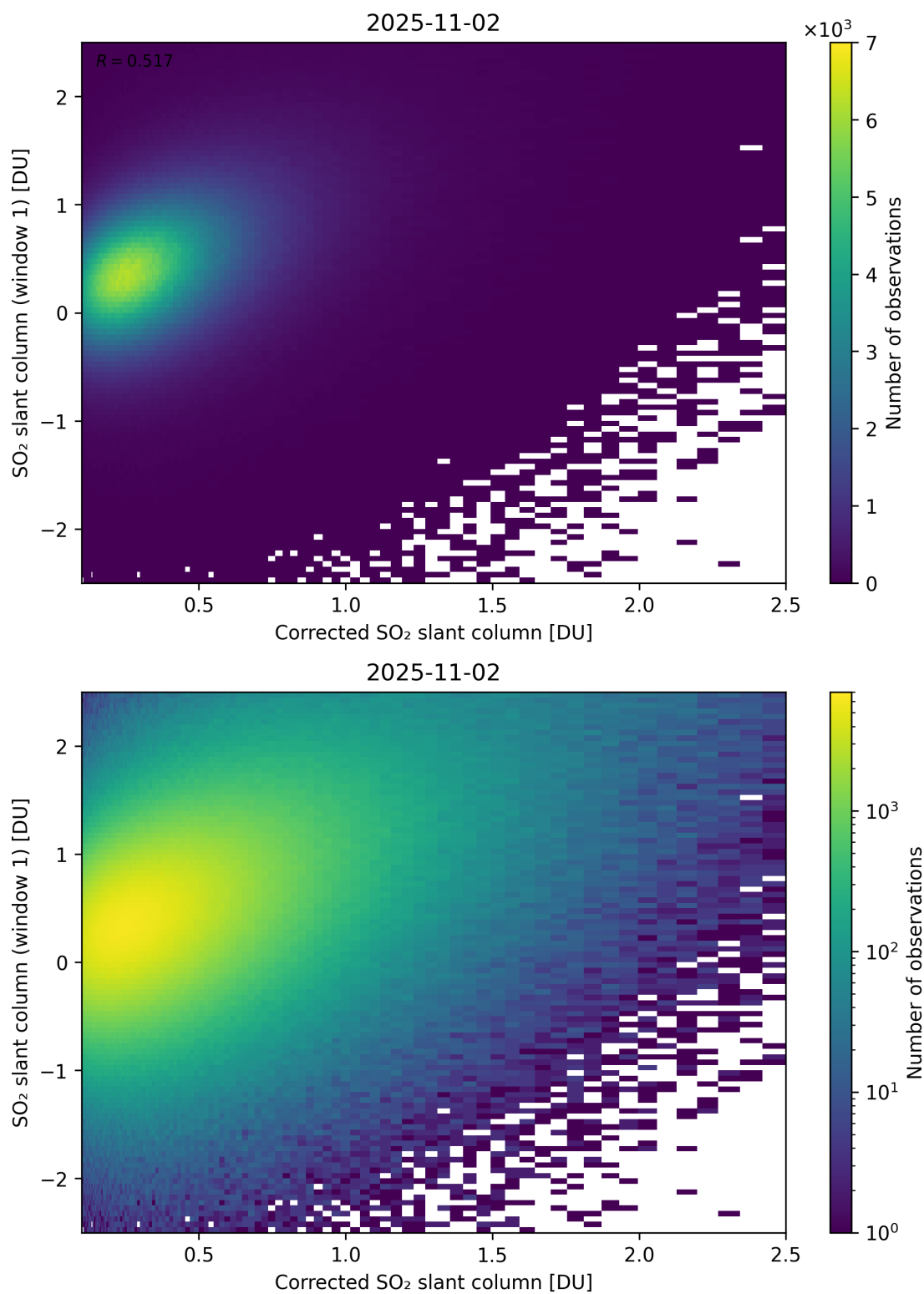
Figure 237: Scatter density plot of “Corrected SO 2 slant column” against “SO 2 slant column (window 1)” for 2025-11-02 to 2025-11-03.
