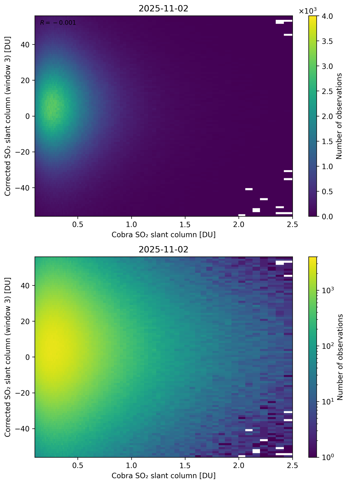
Figure 218: Scatter density plot of “Cobra SO 2 slant column” against “Corrected SO 2 slant column (window 3)” for 2025-11-02 to 2025-11-03.
