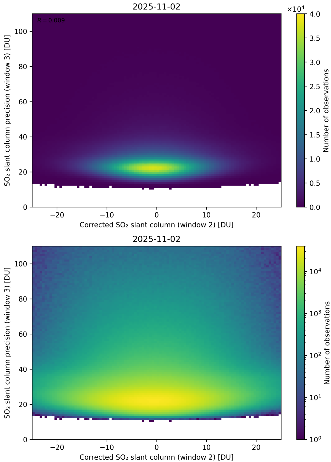
Figure 252: Scatter density plot of “Corrected SO 2 slant column (window 2)” against “SO 2 slant column precision (window 3)” for 2025-11-02 to 2025-11-03.
