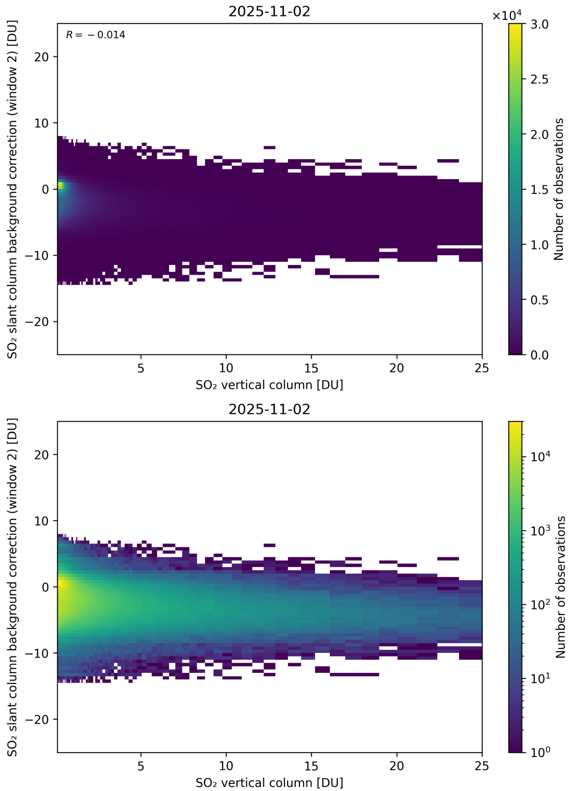
Figure 324: Scatter density plot of “SO 2 vertical column” against “SO 2 slant column background correction (window 2)” for 2025-11-02 to 2025-11-03.
