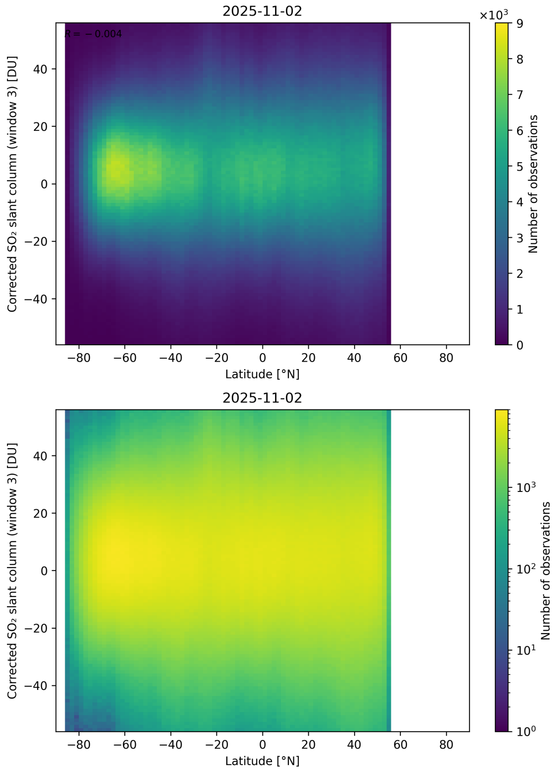
Figure 161: Scatter density plot of “Latitude” against “Corrected SO 2 slant column (window 3)” for 2025-11-02 to 2025-11-03.
