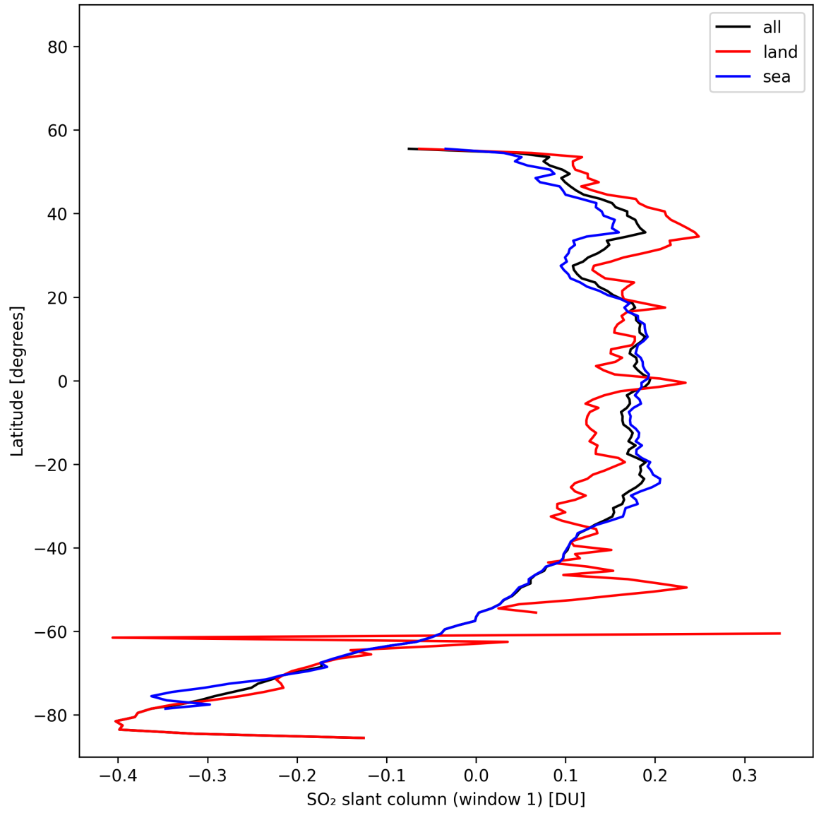
Figure 37: Zonal average of “SO 2 slant column (window 1)” for 2025-11-02 to 2025-11-03.
