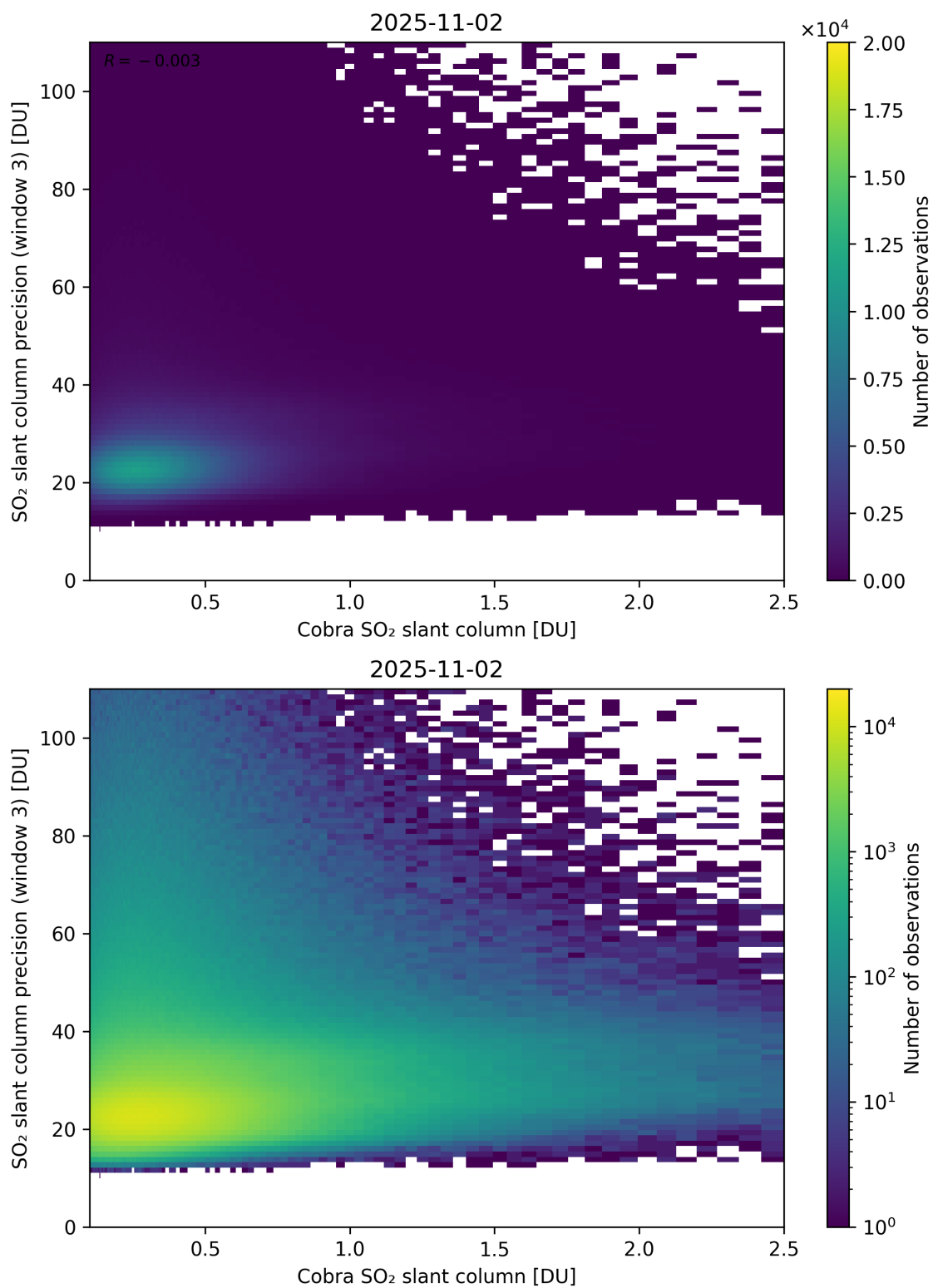
Figure 223: Scatter density plot of “Cobra SO 2 slant column” against “SO 2 slant column precision (window 3)” for 2025-11-02 to 2025-11-03.
