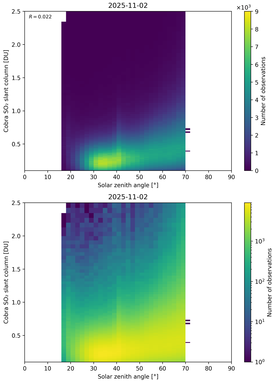
Figure 179: Scatter density plot of “Solar zenith angle” against “Cobra SO 2 slant column” for 2025-11-02 to 2025-11-03.
