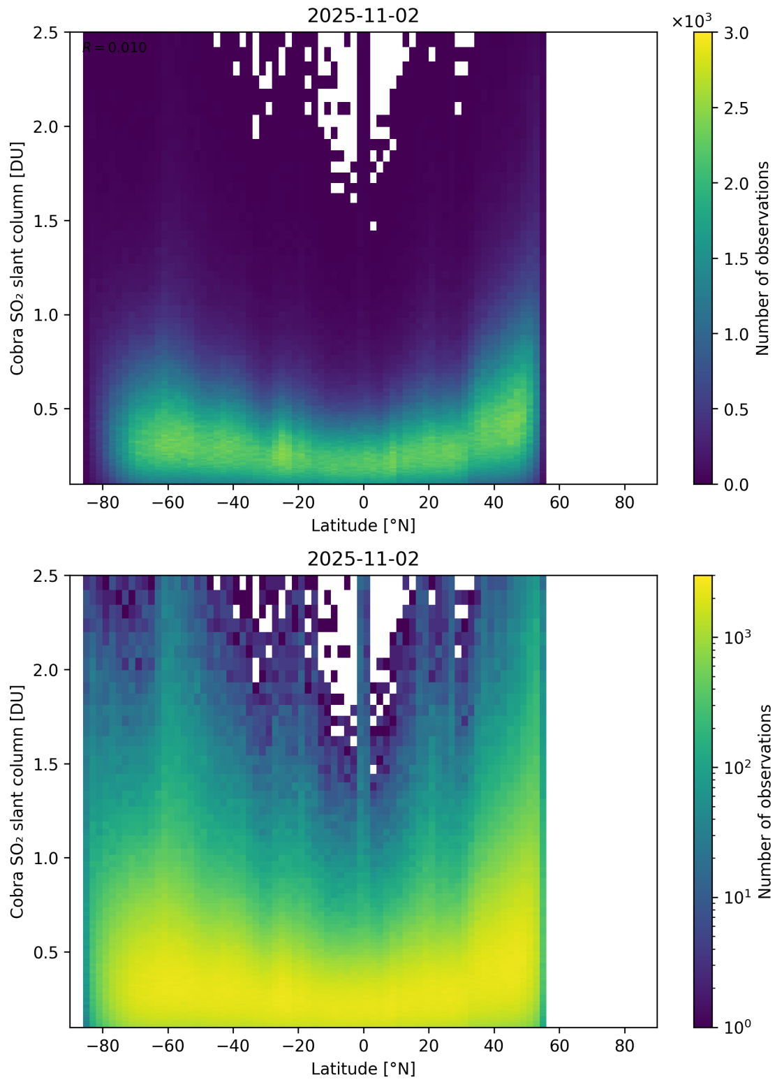
Figure 157: Scatter density plot of “Latitude” against “Cobra SO 2 slant column” for 2025-11-02 to 2025-11-03.
