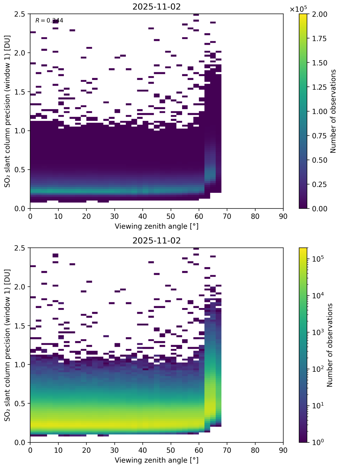
Figure 377: Scatter density plot of “Viewing zenith angle” against “SO 2 slant column precision (window 1)” for 2025-11-02 to 2025-11-03.
