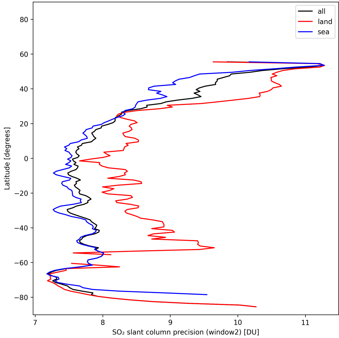
Figure 42: Zonal average of “SO 2 slant column precision (window2)” for 2025-11-02 to 2025-11-03.
