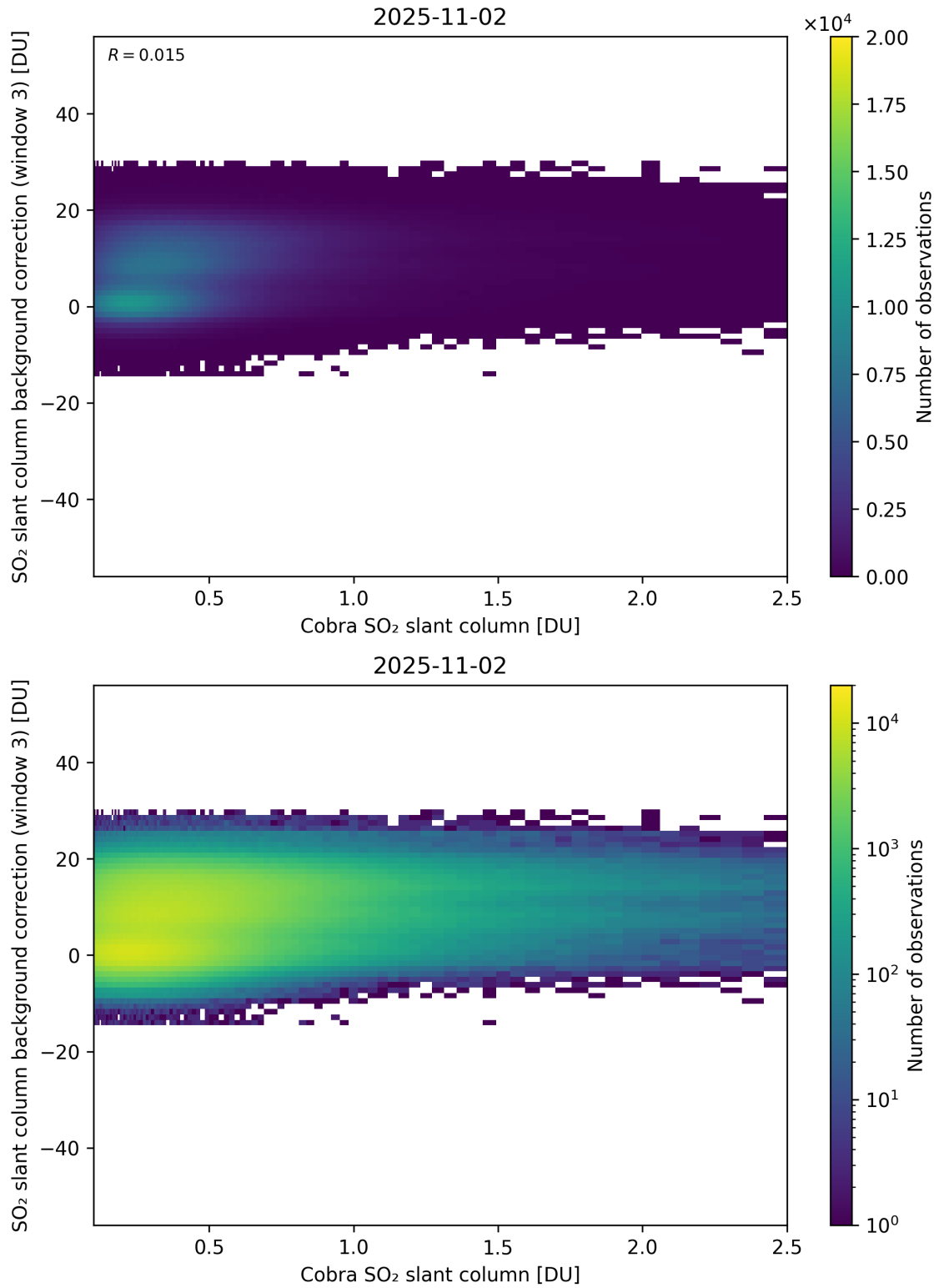
Figure 195: Scatter density plot of “Cobra SO 2 slant column” against “SO 2 slant column background correction (window 3)” for 2025-11-02 to 2025-11-03.
