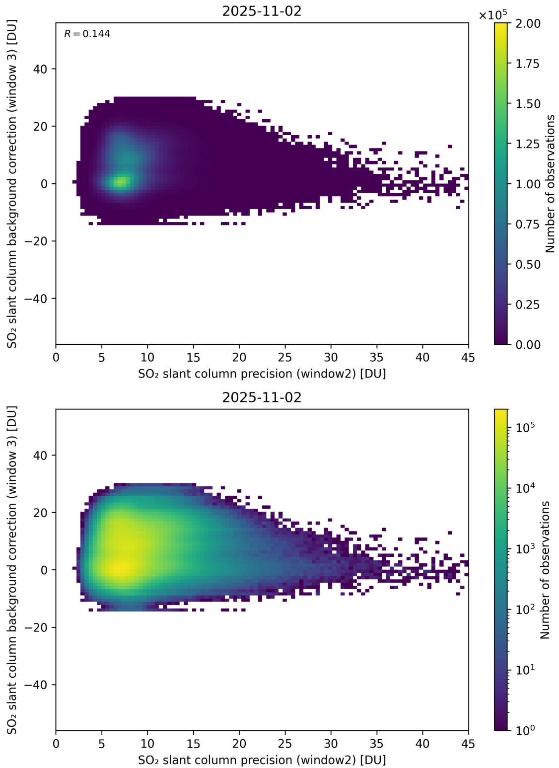
Figure 292: Scatter density plot of “SO 2 slant column precision (window2)” against “SO 2 slant column background correction (window 3)” for 2025-11-02 to 2025-11-03.
