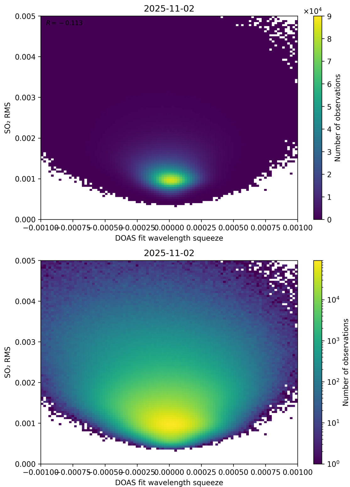
Figure 143: Scatter density plot of “DOAS fit wavelength squeeze” against “SO 2 RMS” for 2025-11-02 to 2025-11-03.
