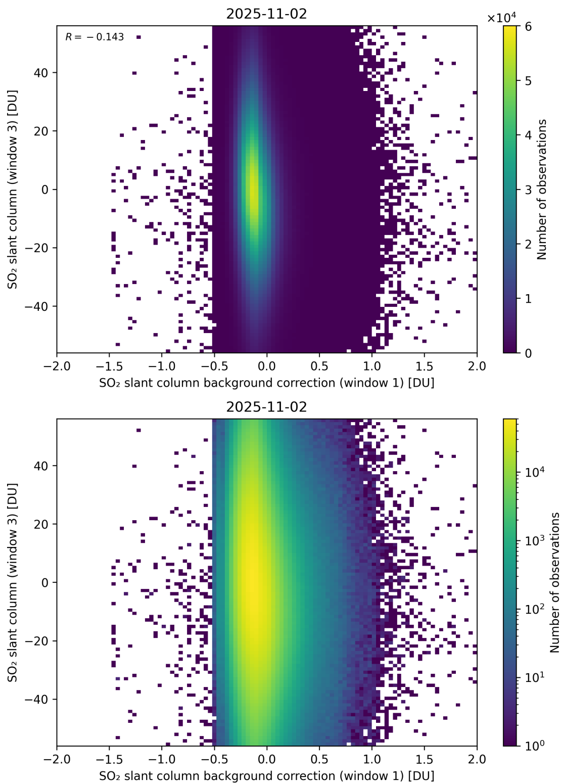
Figure 118: Scatter density plot of “SO 2 slant column background correction (window 1)” against “SO 2 slant column (window 3)” for 2025-11-02 to 2025-11-03.
