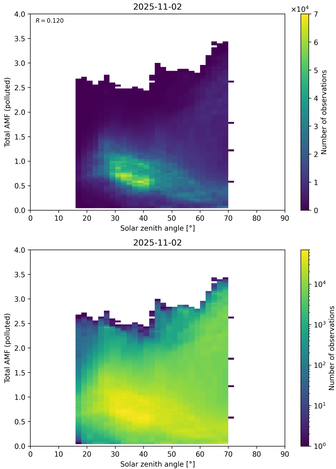
Figure 189: Scatter density plot of “Solar zenith angle” against “Total AMF (polluted)” for 2025-11-02 to 2025-11-03.
