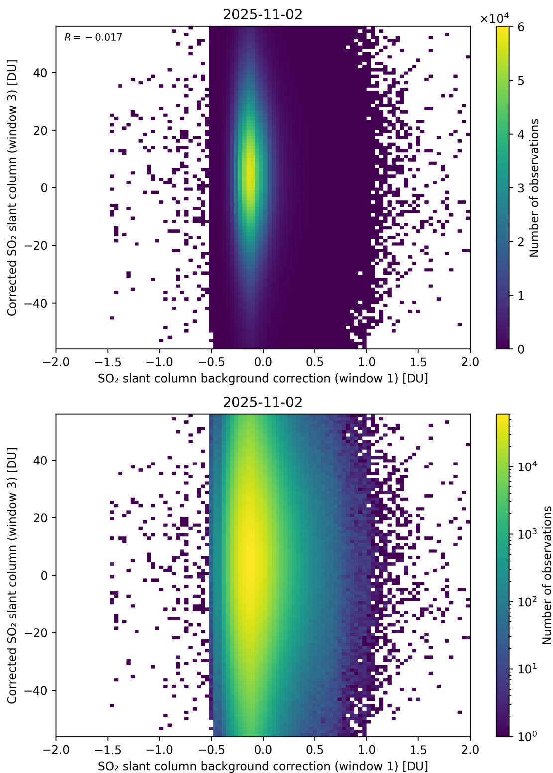
Figure 116: Scatter density plot of “SO 2 slant column background correction (window 1)” against “Corrected SO 2 slant column (window 3)” for 2025-11-02 to 2025-11-03.
