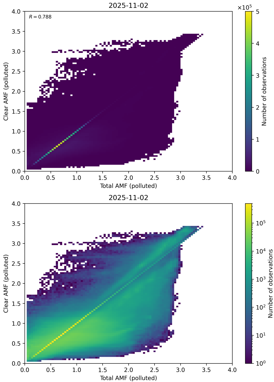
Figure 321: Scatter density plot of “Total AMF (polluted)” against “Clear AMF (polluted)” for 2025-11-02 to 2025-11-03.
