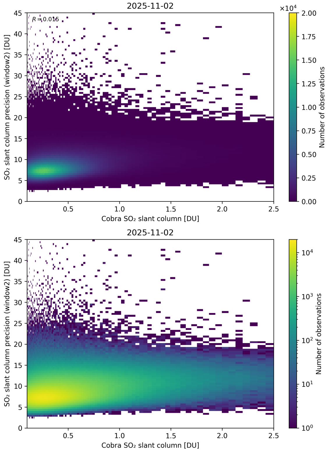
Figure 221: Scatter density plot of “Cobra SO 2 slant column” against “SO 2 slant column precision (window2)” for 2025-11-02 to 2025-11-03.
