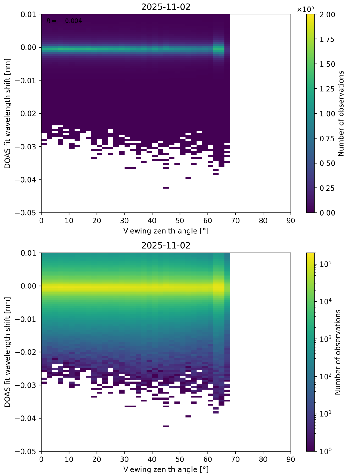
Figure 365: Scatter density plot of “Viewing zenith angle” against “DOAS fit wavelength shift” for 2025-11-02 to 2025-11-03.
