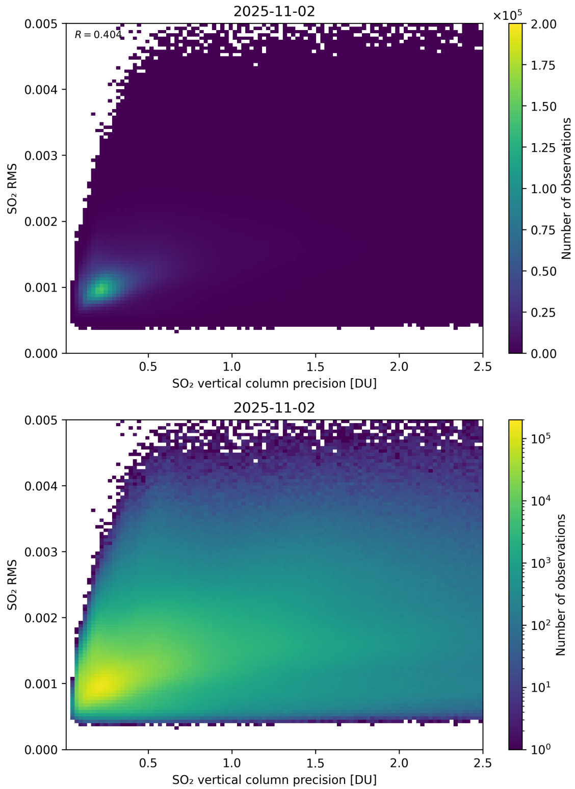
Figure 334: Scatter density plot of “SO 2 vertical column precision” against “SO 2 RMS” for 2025-11-02 to 2025-11-03.
