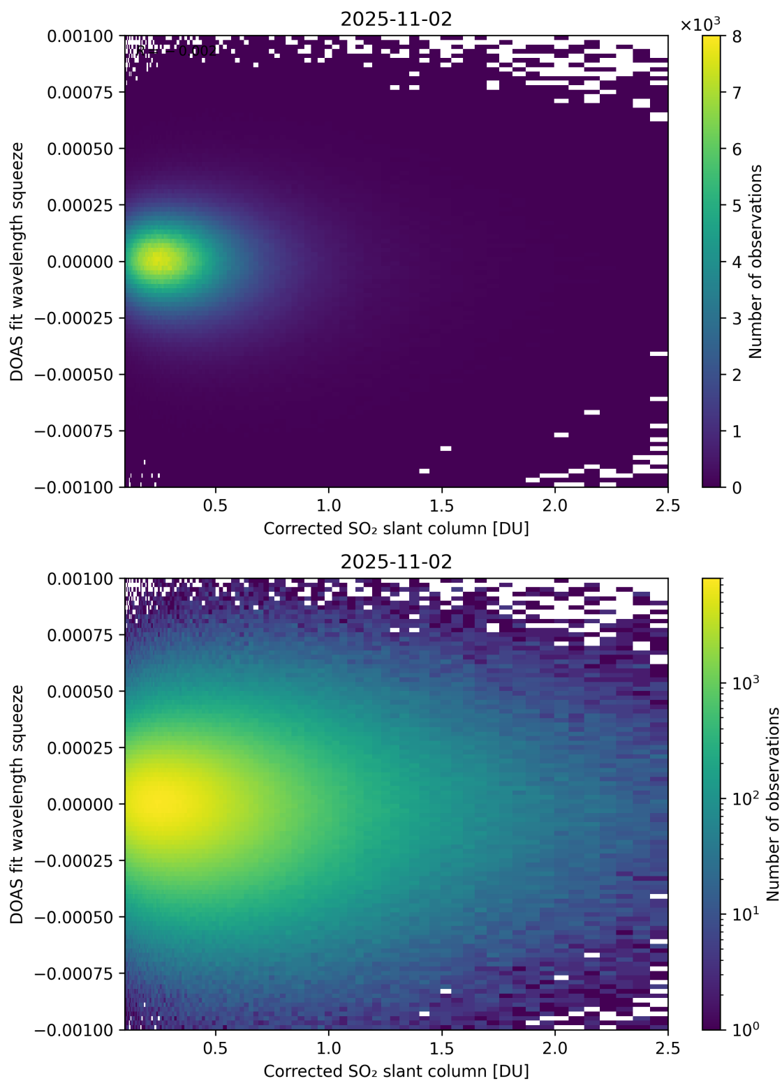
Figure 230: Scatter density plot of “Corrected SO 2 slant column” against “DOAS fit wavelength squeeze” for 2025-11-02 to 2025-11-03.
