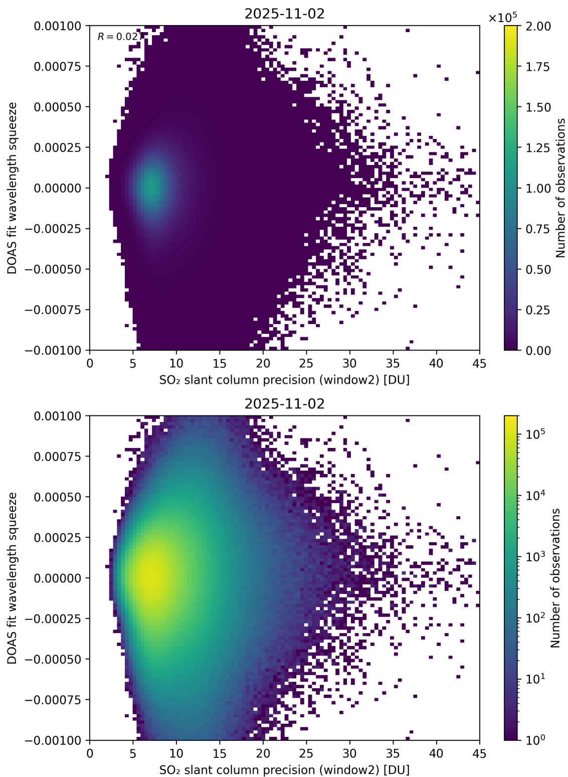
Figure 294: Scatter density plot of “SO 2 slant column precision (window2)” against “DOAS fit wavelength squeeze” for 2025-11-02 to 2025-11-03.
