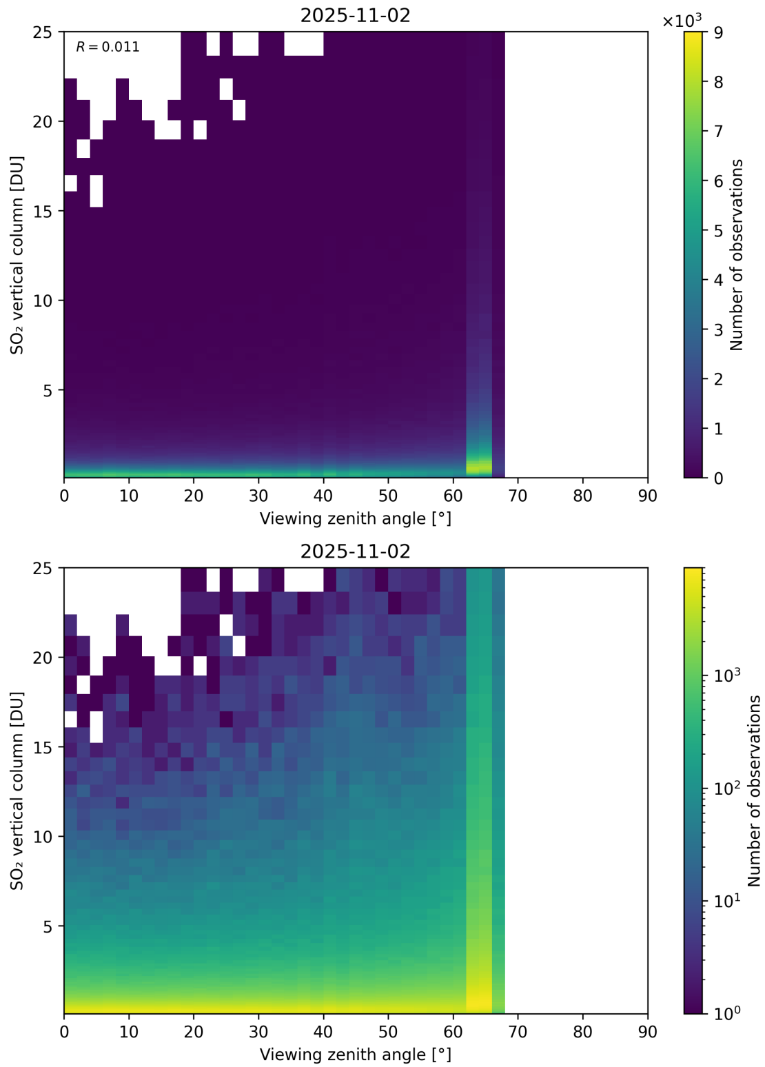
Figure 383: Scatter density plot of “Viewing zenith angle” against “SO 2 vertical column” for 2025-11-02 to 2025-11-03.
