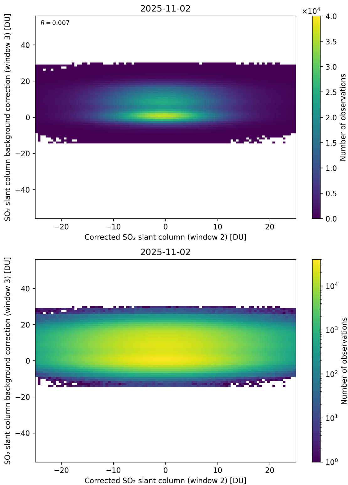
Figure 245: Scatter density plot of “Corrected SO 2 slant column (window 2)” against “SO 2 slant column background correction (window 3)” for 2025-11-02 to 2025-11-03.
