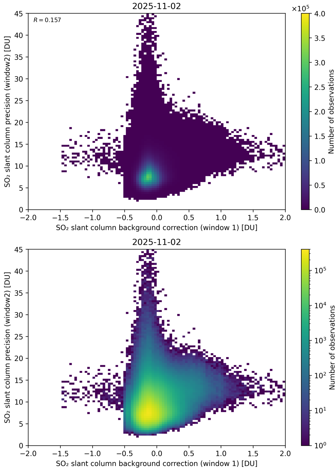
Figure 117: Scatter density plot of “SO 2 slant column background correction (window 1)” against “SO 2 slant column precision (window2)” for 2025-11-02 to 2025-11-03.
