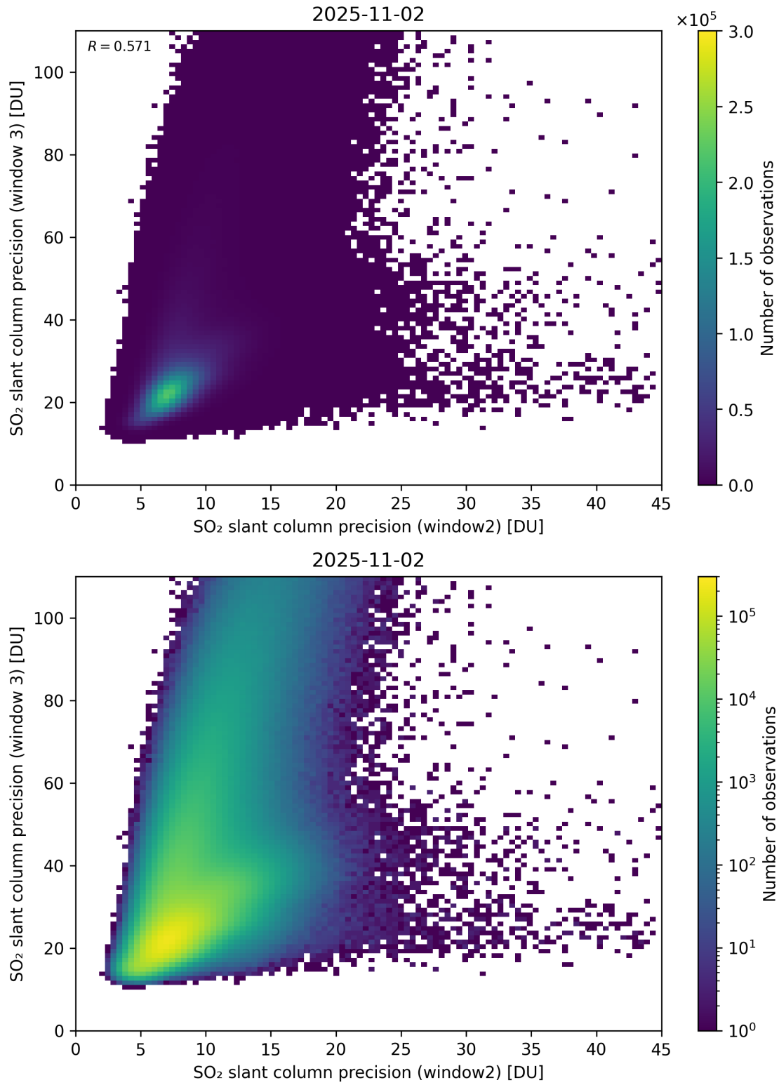
Figure 300: Scatter density plot of “SO 2 slant column precision (window2)” against “SO 2 slant column precision (window 3)” for 2025-11-02 to 2025-11-03.
