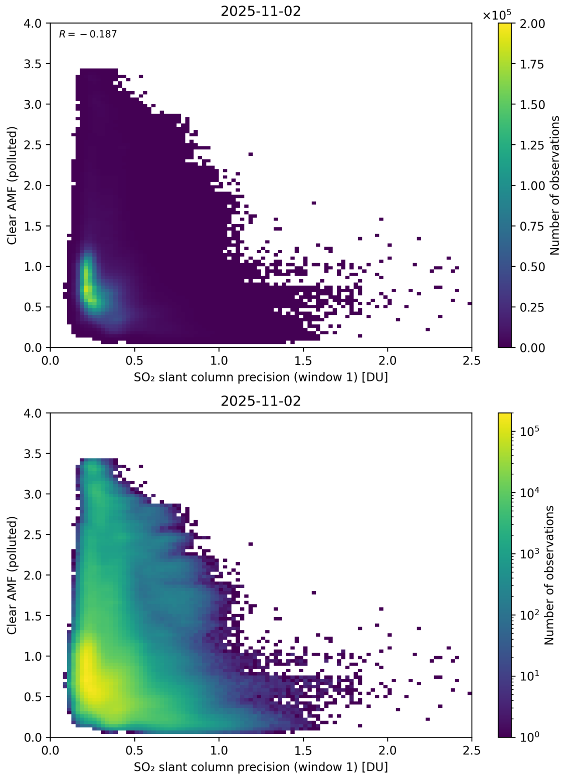
Figure 274: Scatter density plot of “SO 2 slant column precision (window 1)” against “Clear AMF (polluted)” for 2025-11-02 to 2025-11-03.
