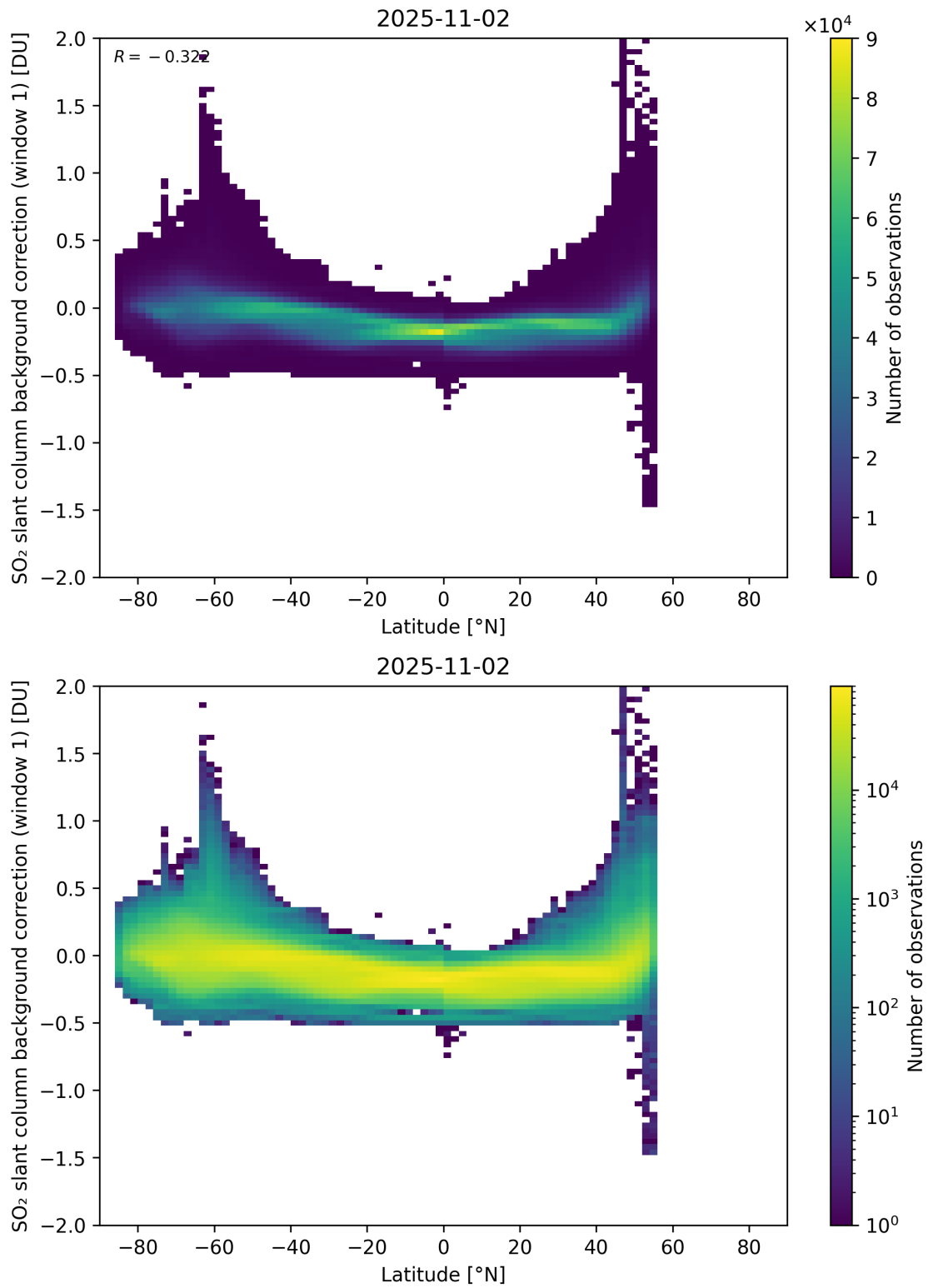
Figure 150: Scatter density plot of “Latitude” against “SO 2 slant column background correction (window 1)” for 2025-11-02 to 2025-11-03.
