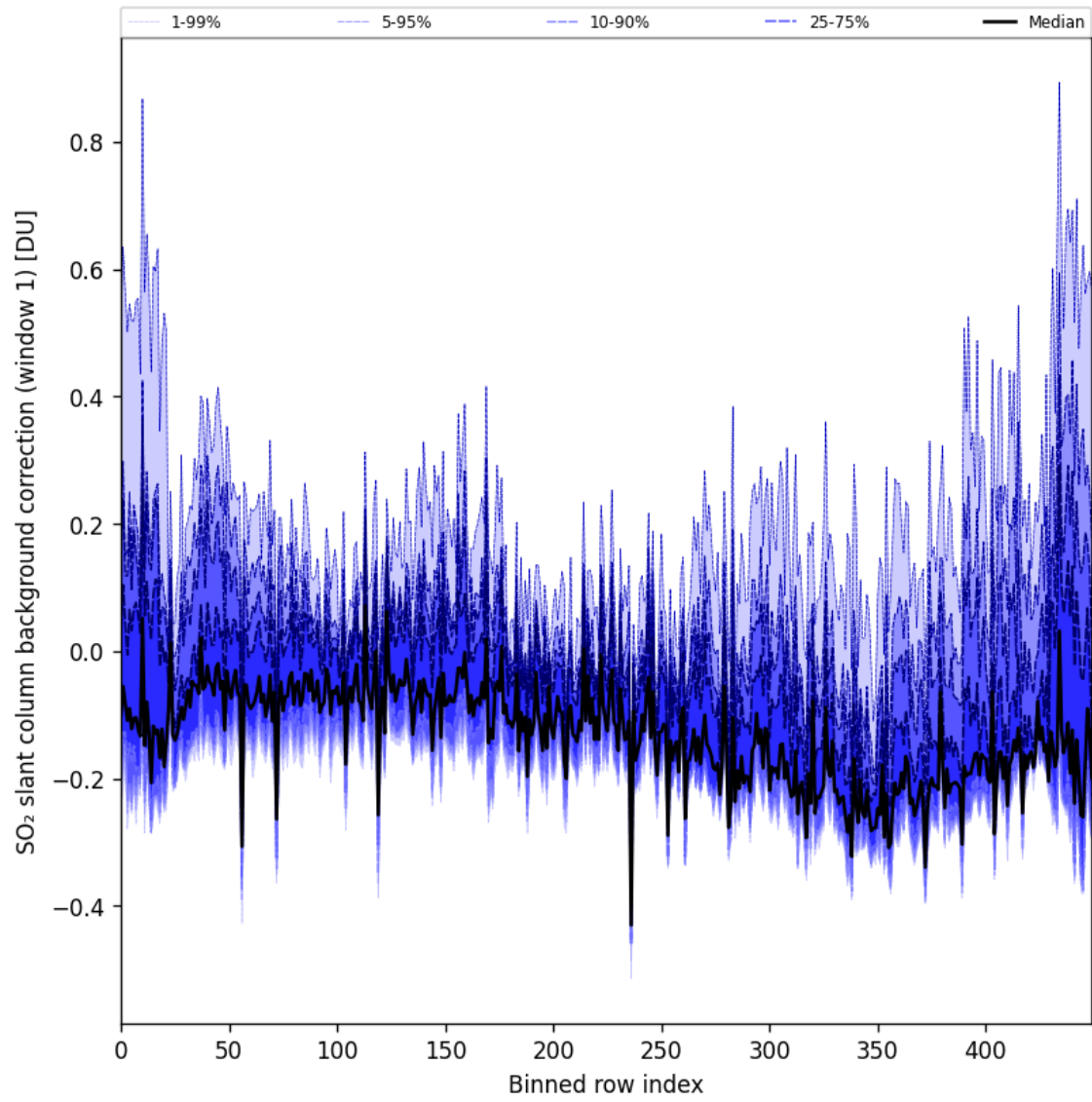
Figure 92: Along track statistics of “SO 2 slant column background correction (window 1)” for 2025-11-02 to 2025-11-03
