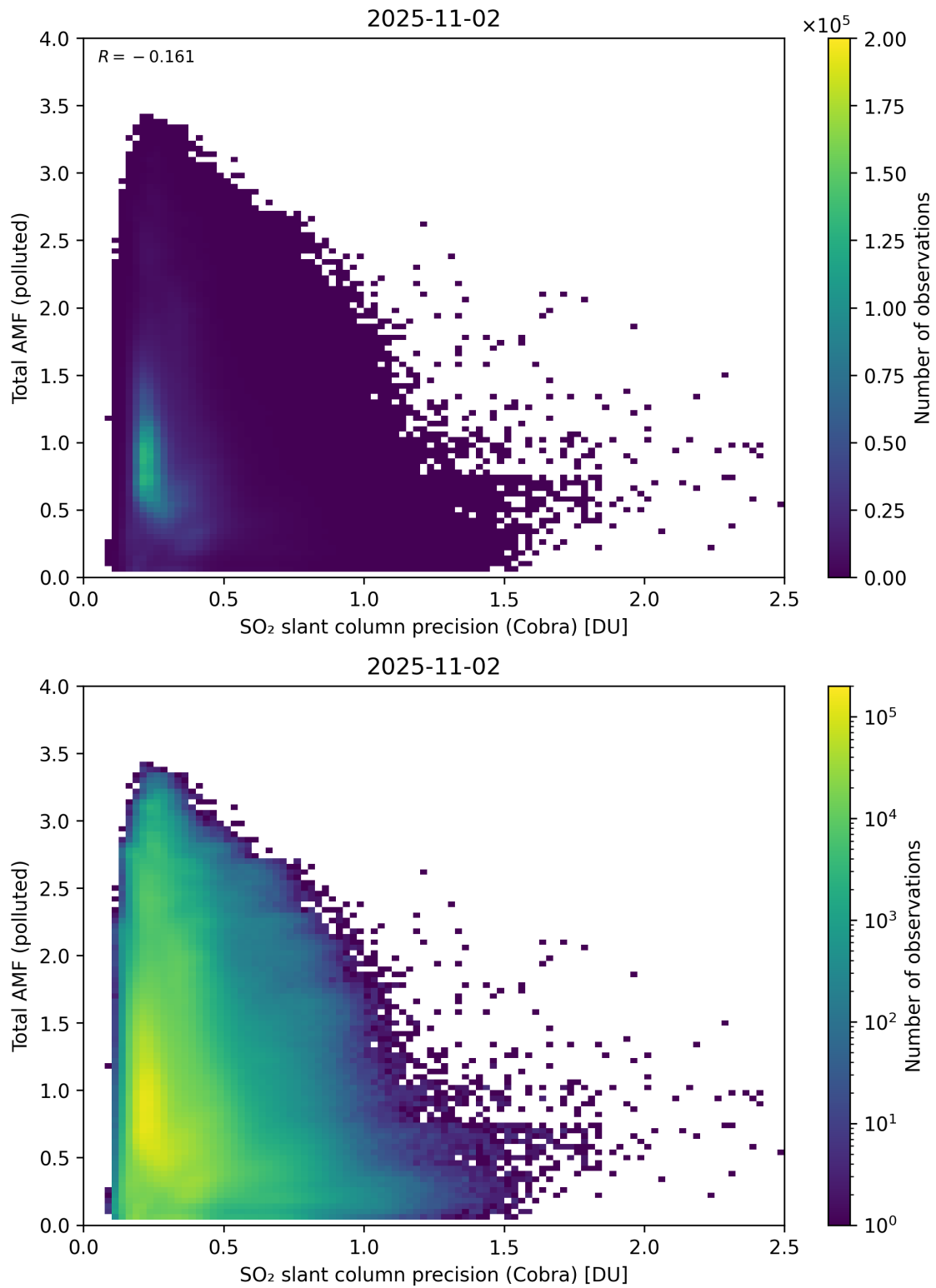
Figure 213: Scatter density plot of “SO 2 slant column precision (Cobra)” against “Total AMF (polluted)” for 2025-11-02 to 2025-11-03.
