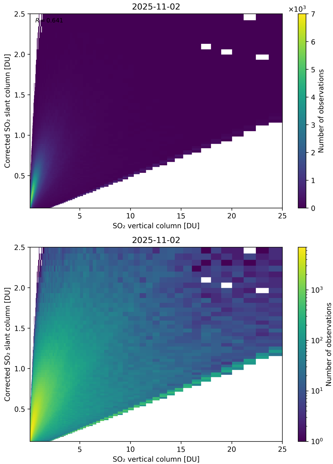
Figure 351: Scatter density plot of “SO 2 vertical column” against “Corrected SO 2 slant column” for 2025-11-02 to 2025-11-03.
