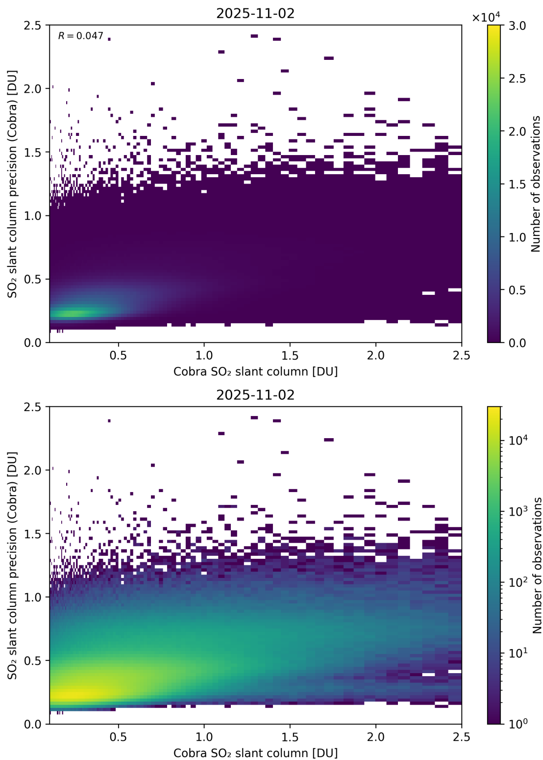
Figure 216: Scatter density plot of “Cobra SO 2 slant column” against “SO 2 slant column precision (Cobra)” for 2025-11-02 to 2025-11-03.
