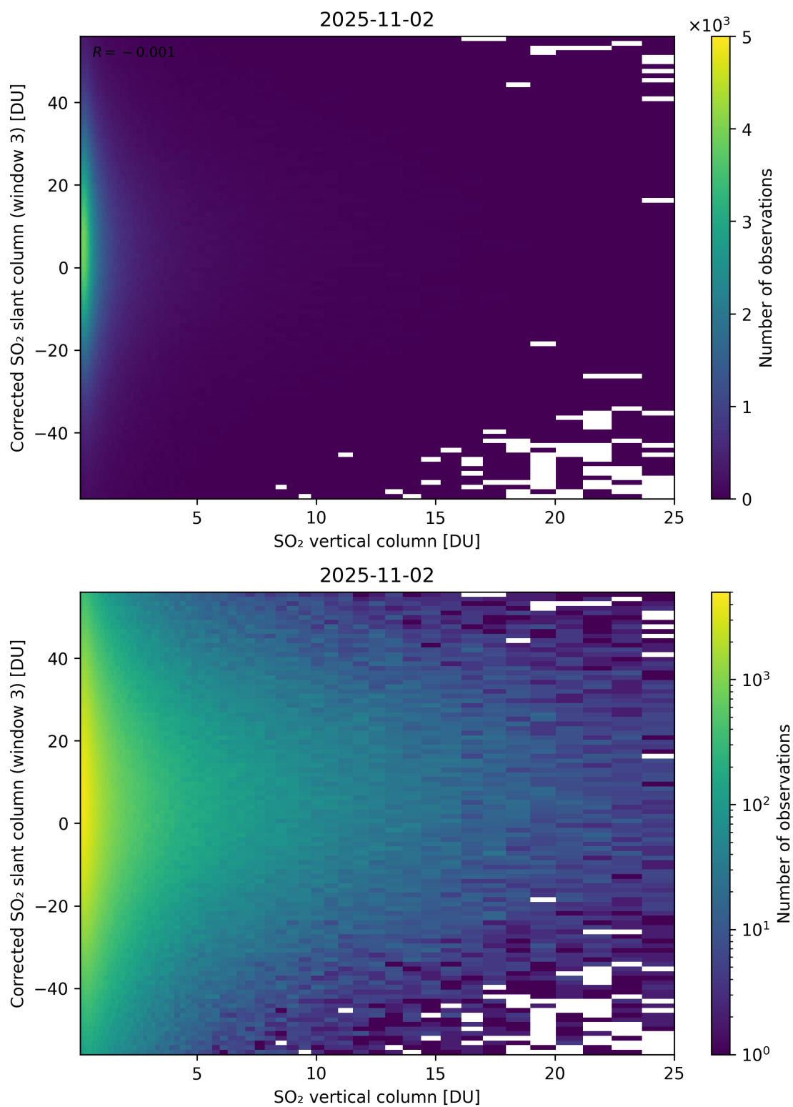
Figure 353: Scatter density plot of “SO 2 vertical column” against “Corrected SO 2 slant column (window 3)” for 2025-11-02 to 2025-11-03.
