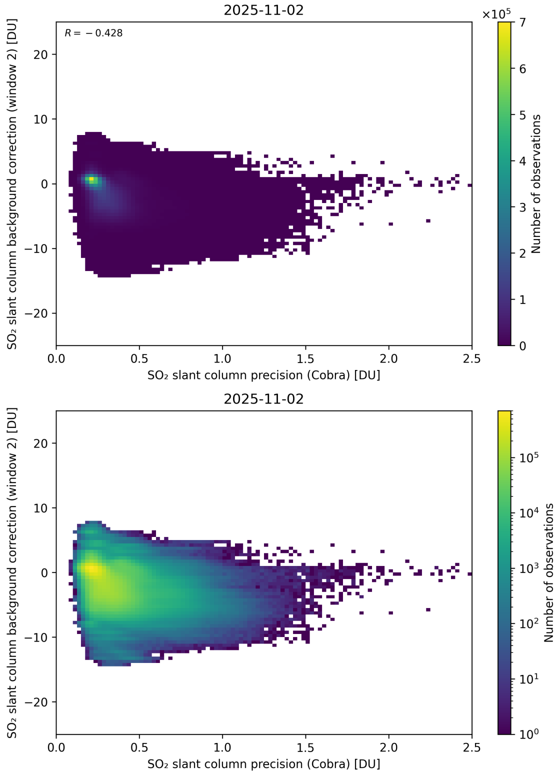
Figure 200: Scatter density plot of “SO 2 slant column precision (Cobra)” against “SO 2 slant column background correction (window 2)” for 2025-11-02 to 2025-11-03.
