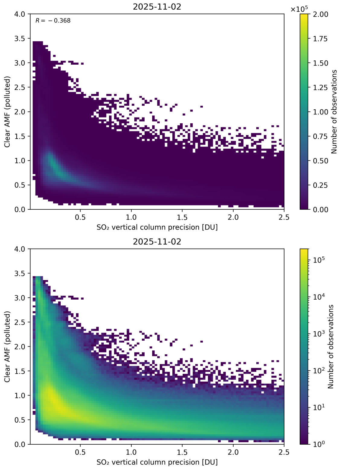
Figure 335: Scatter density plot of “SO 2 vertical column precision” against “Clear AMF (polluted)” for 2025-11-02 to 2025-11-03.
