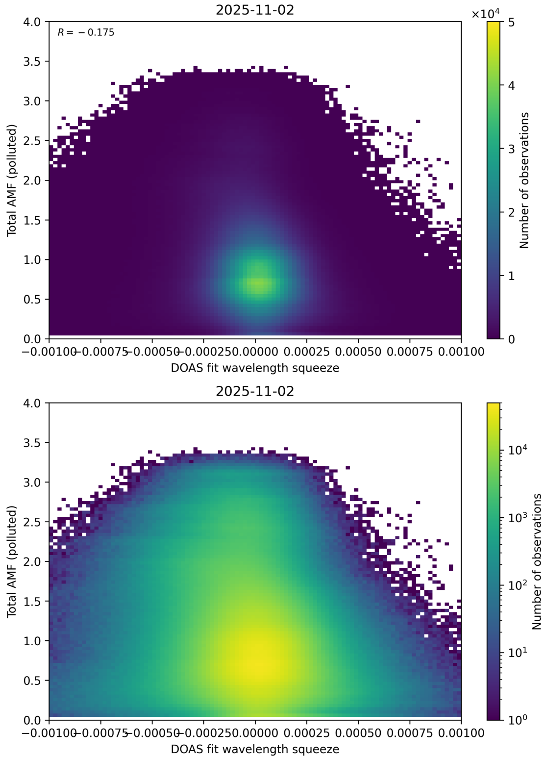
Figure 145: Scatter density plot of “DOAS fit wavelength squeeze” against “Total AMF (polluted)” for 2025-11-02 to 2025-11-03.
