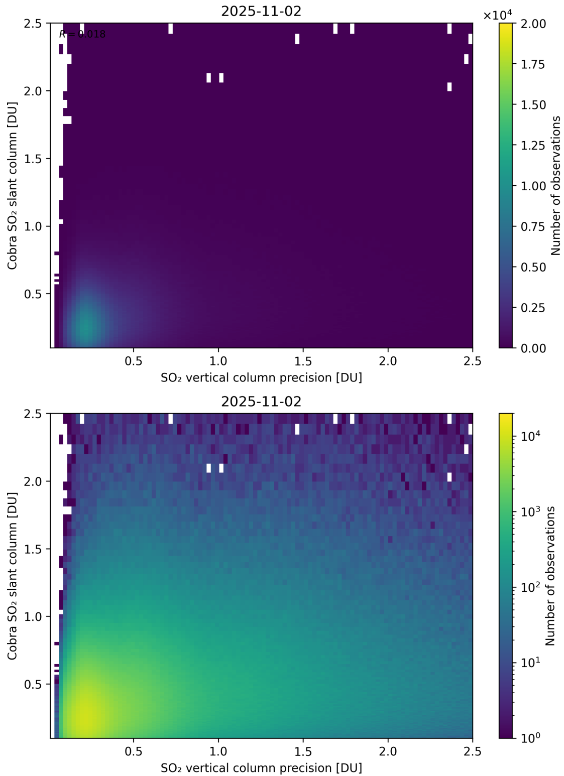
Figure 336: Scatter density plot of “SO 2 vertical column precision” against “Cobra SO 2 slant column” for 2025-11-02 to 2025-11-03.
