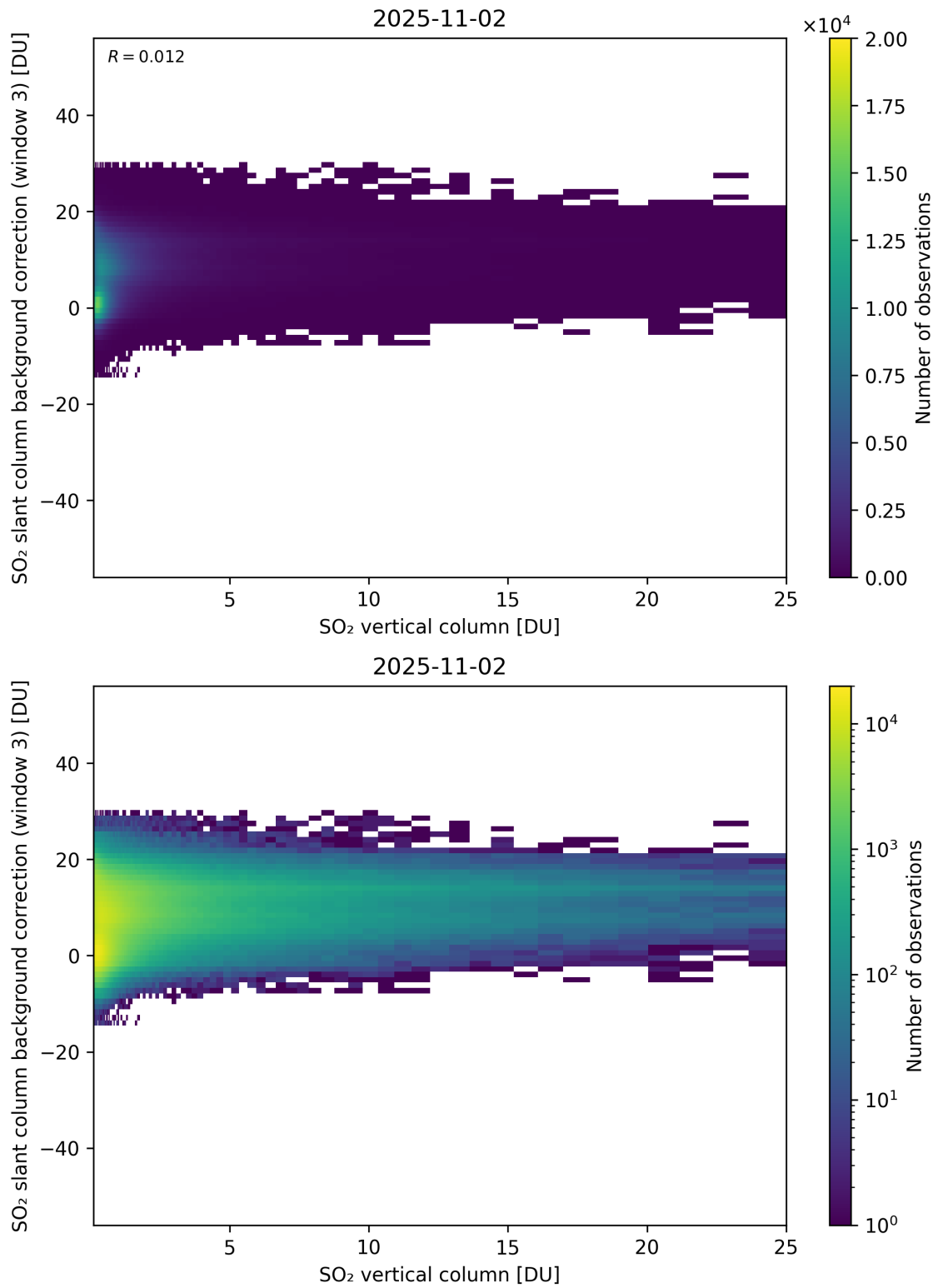
Figure 325: Scatter density plot of “SO 2 vertical column” against “SO 2 slant column background correction (window 3)” for 2025-11-02 to 2025-11-03.
