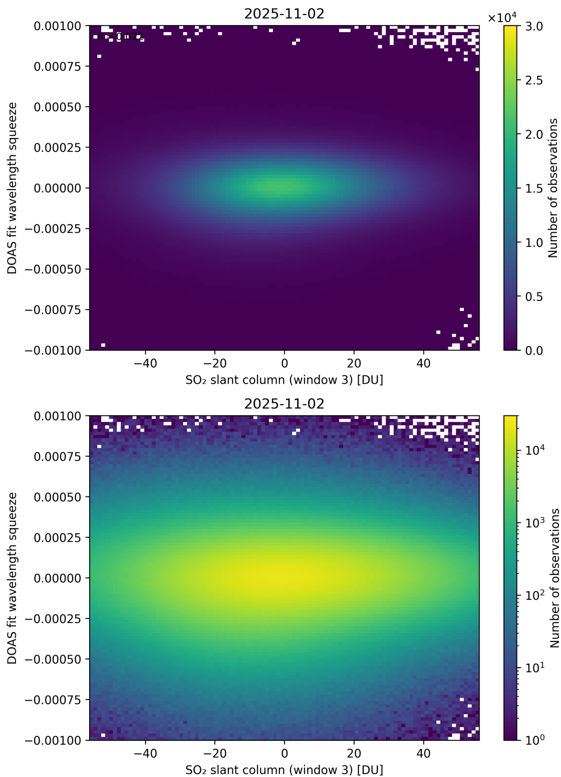
Figure 305: Scatter density plot of “SO 2 slant column (window 3)” against “DOAS fit wavelength squeeze” for 2025-11-02 to 2025-11-03.
