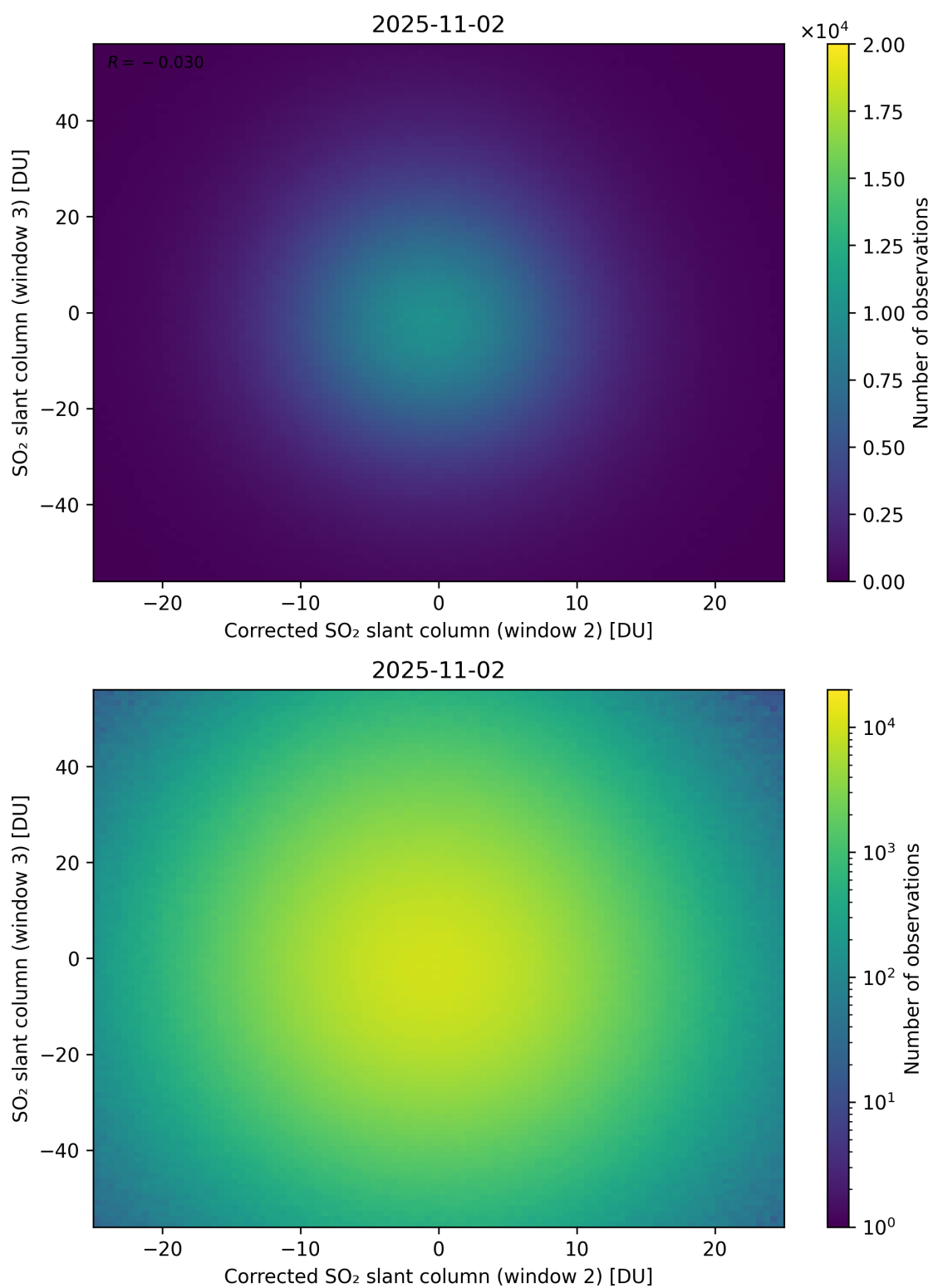
Figure 251: Scatter density plot of “Corrected SO 2 slant column (window 2)” against “SO 2 slant column (window 3)” for 2025-11-02 to 2025-11-03.
