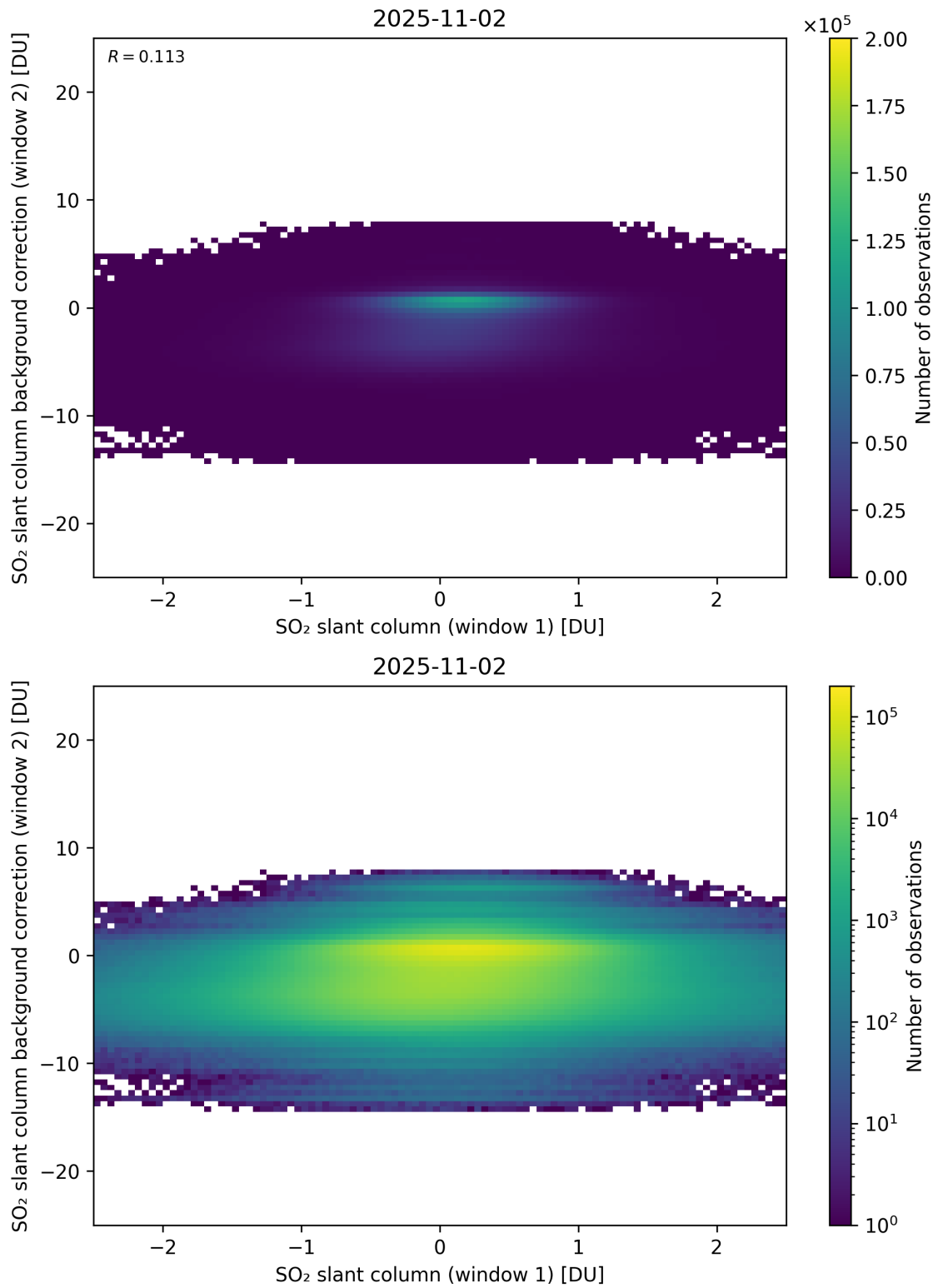
Figure 263: Scatter density plot of “SO 2 slant column (window 1)” against “SO 2 slant column background correction (window 2)” for 2025-11-02 to 2025-11-03.
