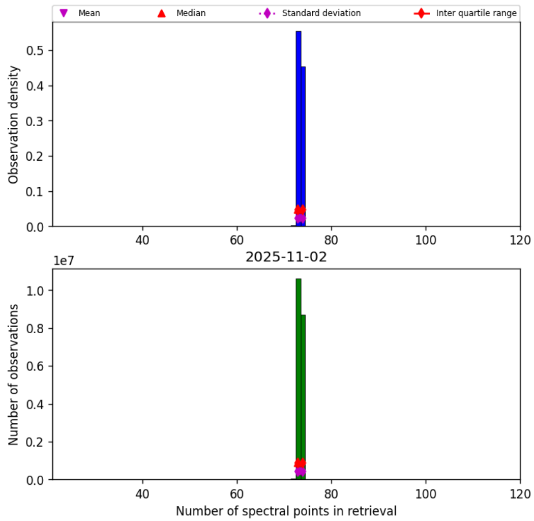
Figure 82: Histogram of “Number of spectral points in retrieval” for 2025-11-02 to 2025-11-03
