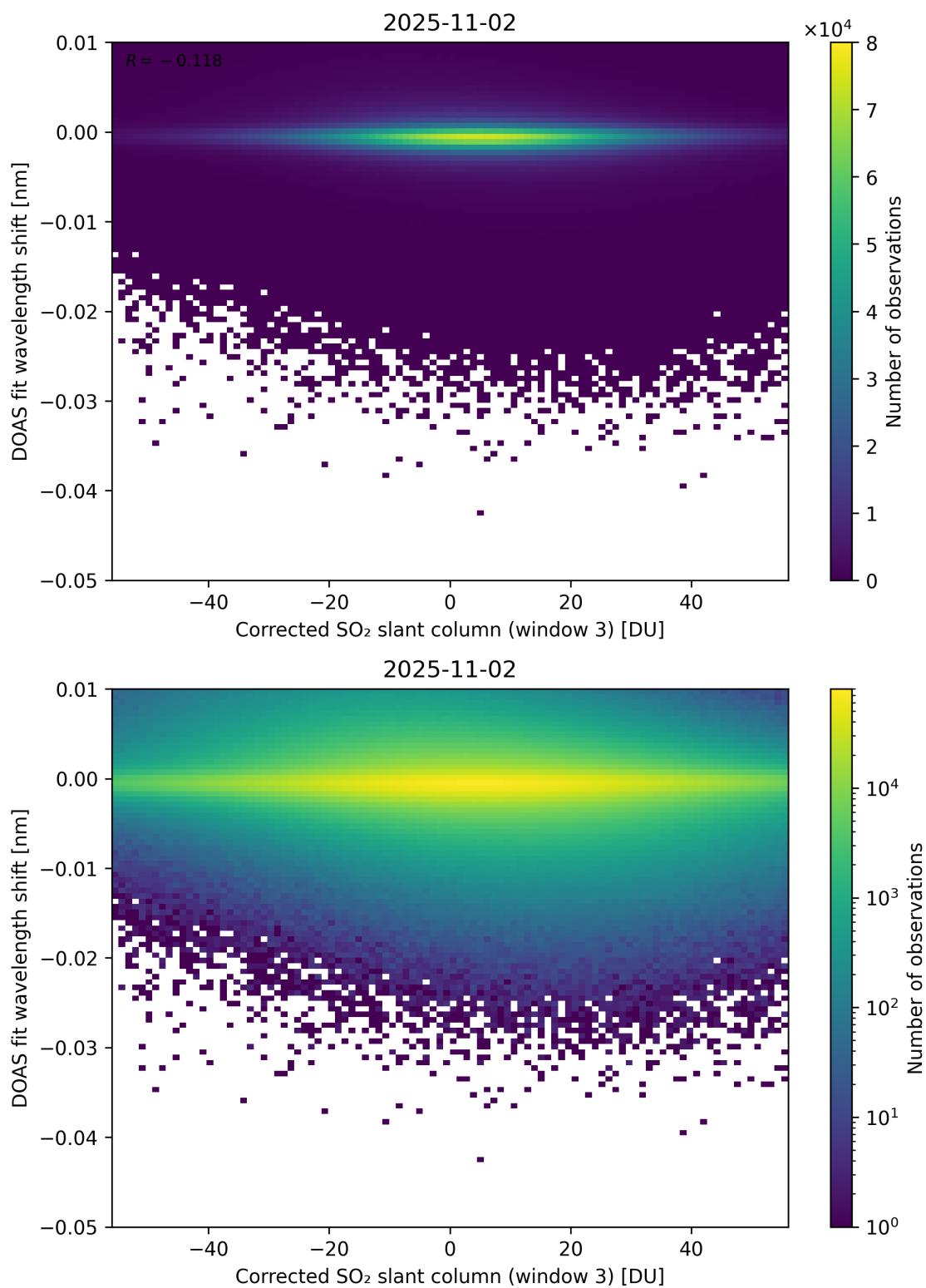
Figure 256: Scatter density plot of “Corrected SO 2 slant column (window 3)” against “DOAS fit wavelength shift” for 2025-11-02 to 2025-11-03.
