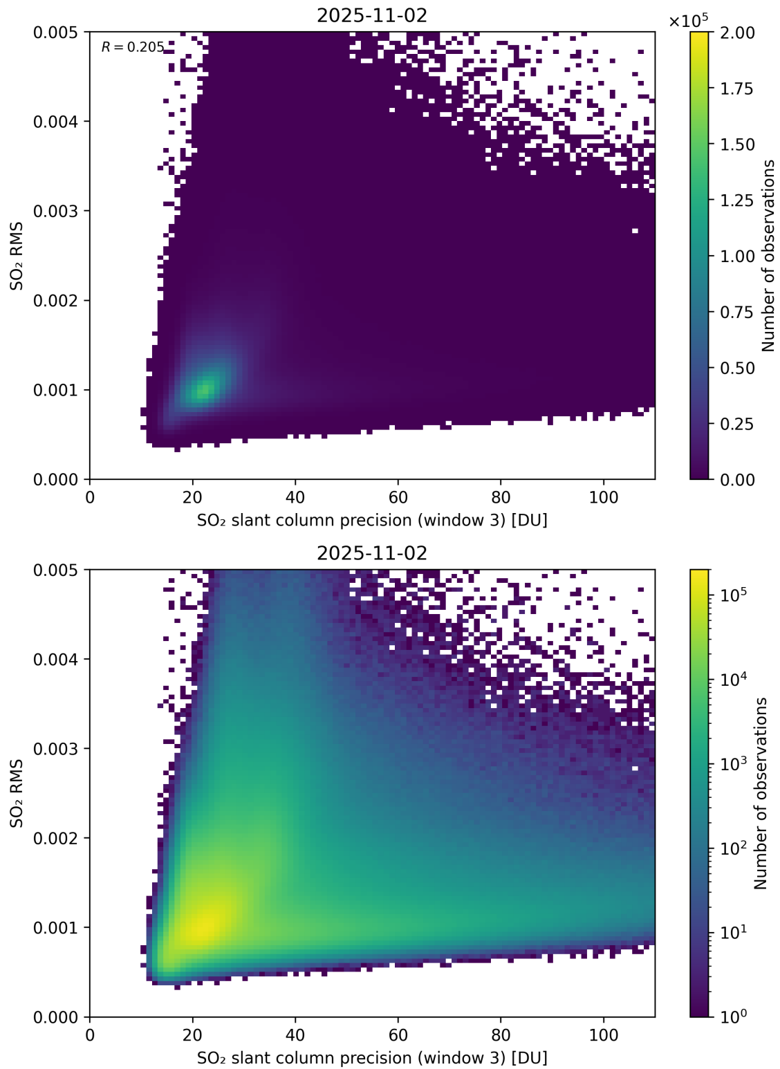
Figure 310: Scatter density plot of “SO 2 slant column precision (window 3)” against “SO 2 RMS” for 2025-11-02 to 2025-11-03.
