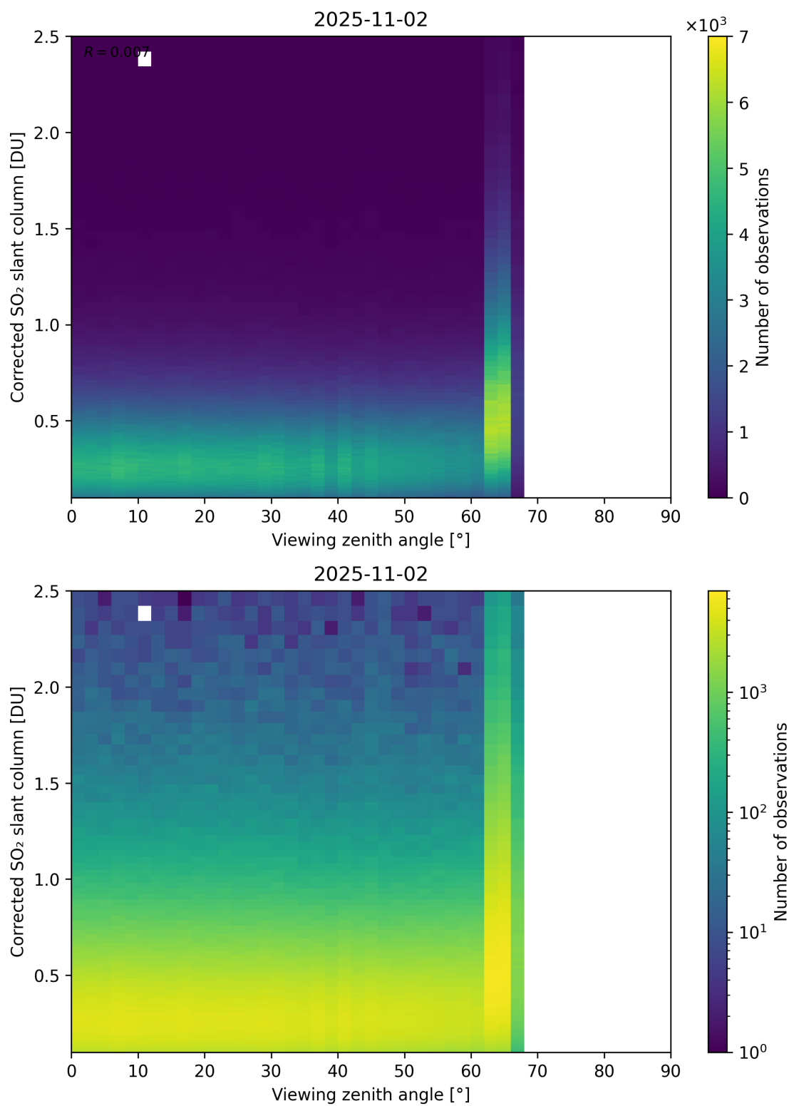
Figure 373: Scatter density plot of “Viewing zenith angle” against “Corrected SO 2 slant column” for 2025-11-02 to 2025-11-03.
