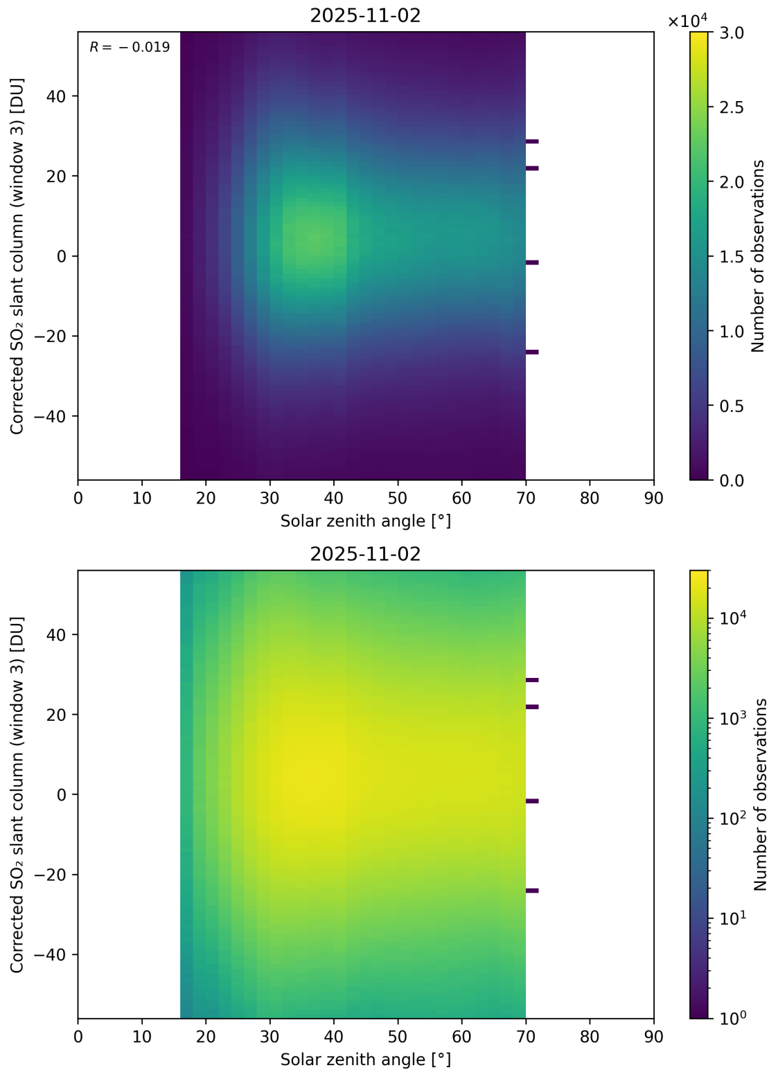
Figure 183: Scatter density plot of “Solar zenith angle” against “Corrected SO 2 slant column (window 3)” for 2025-11-02 to 2025-11-03.
