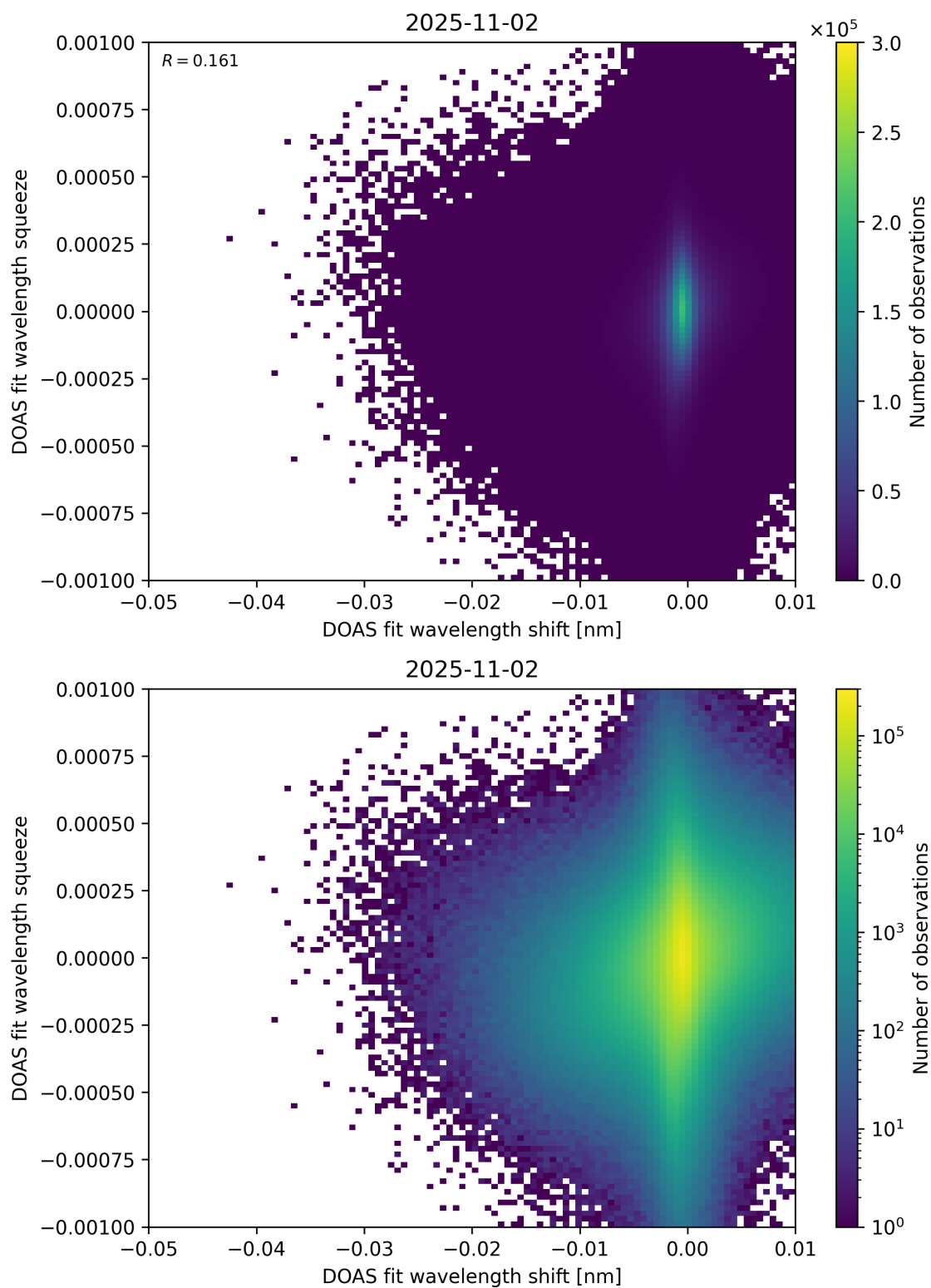
Figure 138: Scatter density plot of “DOAS fit wavelength shift” against “DOAS fit wavelength squeeze” for 2025-11-02 to 2025-11-03.
