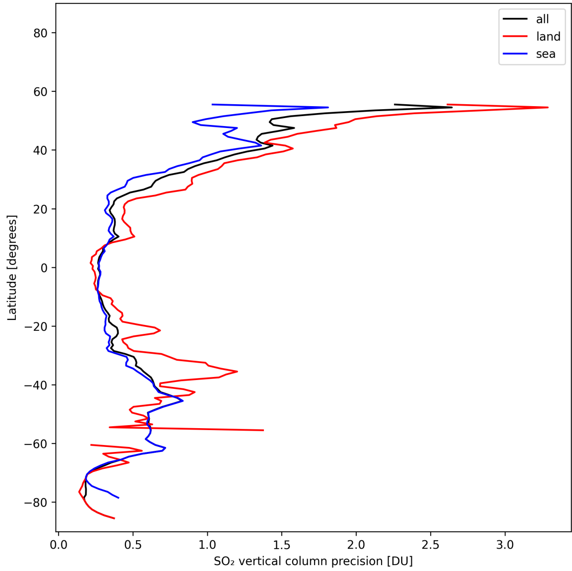
Figure 33: Zonal average of “SO 2 vertical column precision” for 2025-11-02 to 2025-11-03.
