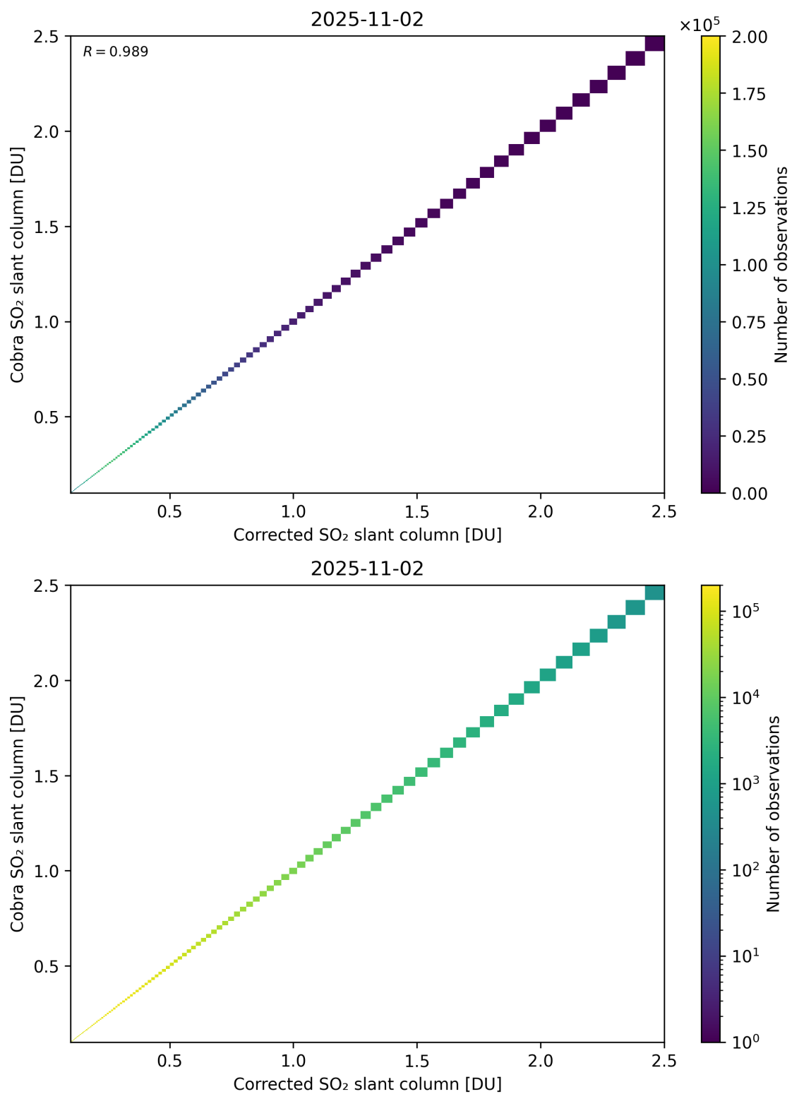
Figure 233: Scatter density plot of “Corrected SO 2 slant column” against “Cobra SO 2 slant column” for 2025-11-02 to 2025-11-03.
