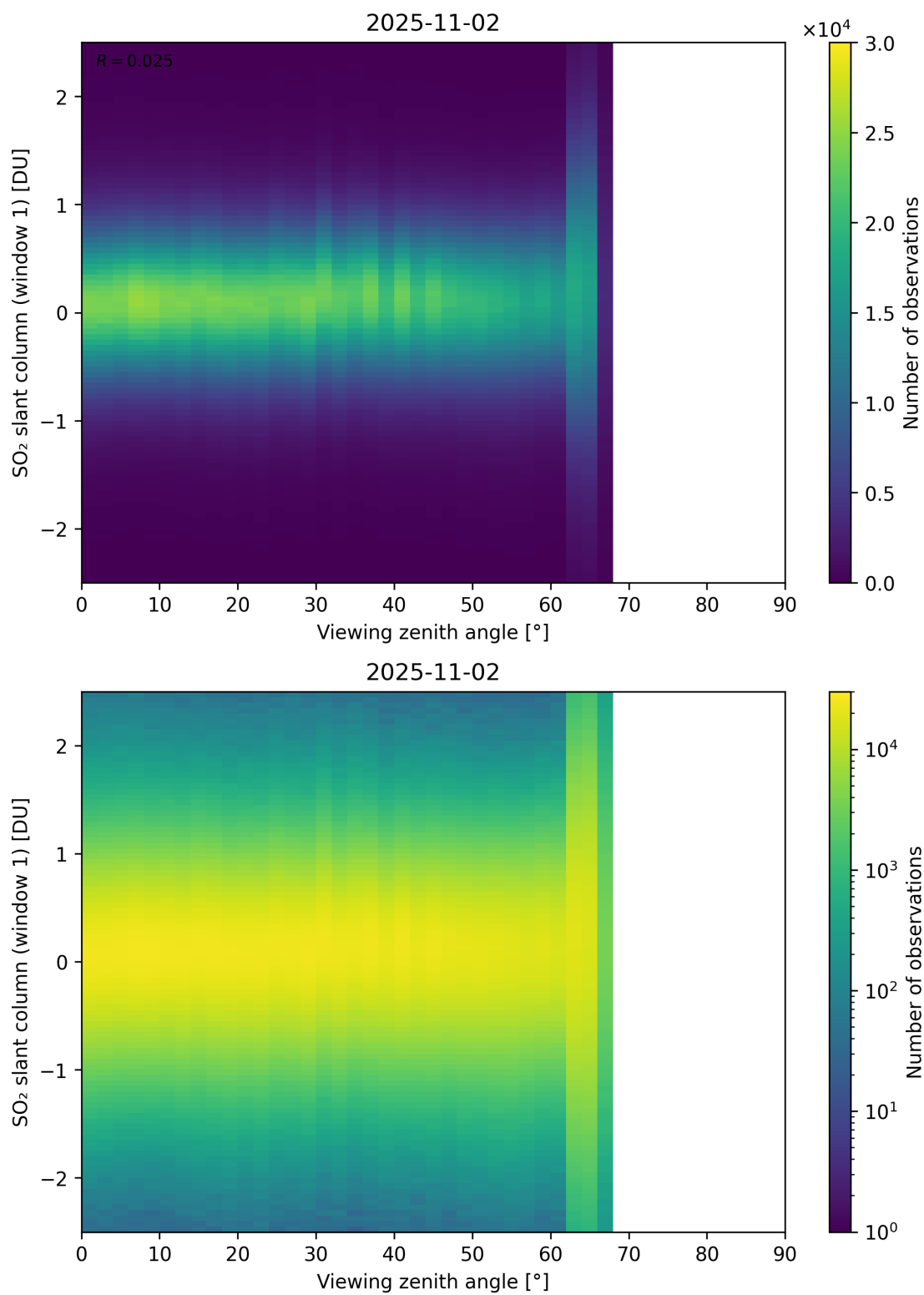
Figure 376: Scatter density plot of “Viewing zenith angle” against “SO 2 slant column (window 1)” for 2025-11-02 to 2025-11-03.
