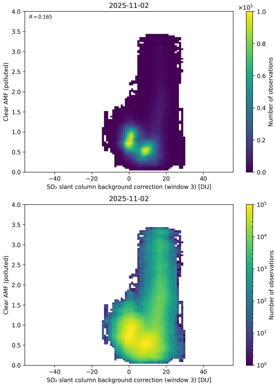
Figure 135: Scatter density plot of “SO 2 slant column background correction (window 3)” against “Clear AMF (polluted)” for 2025-11-02 to 2025-11-03.
