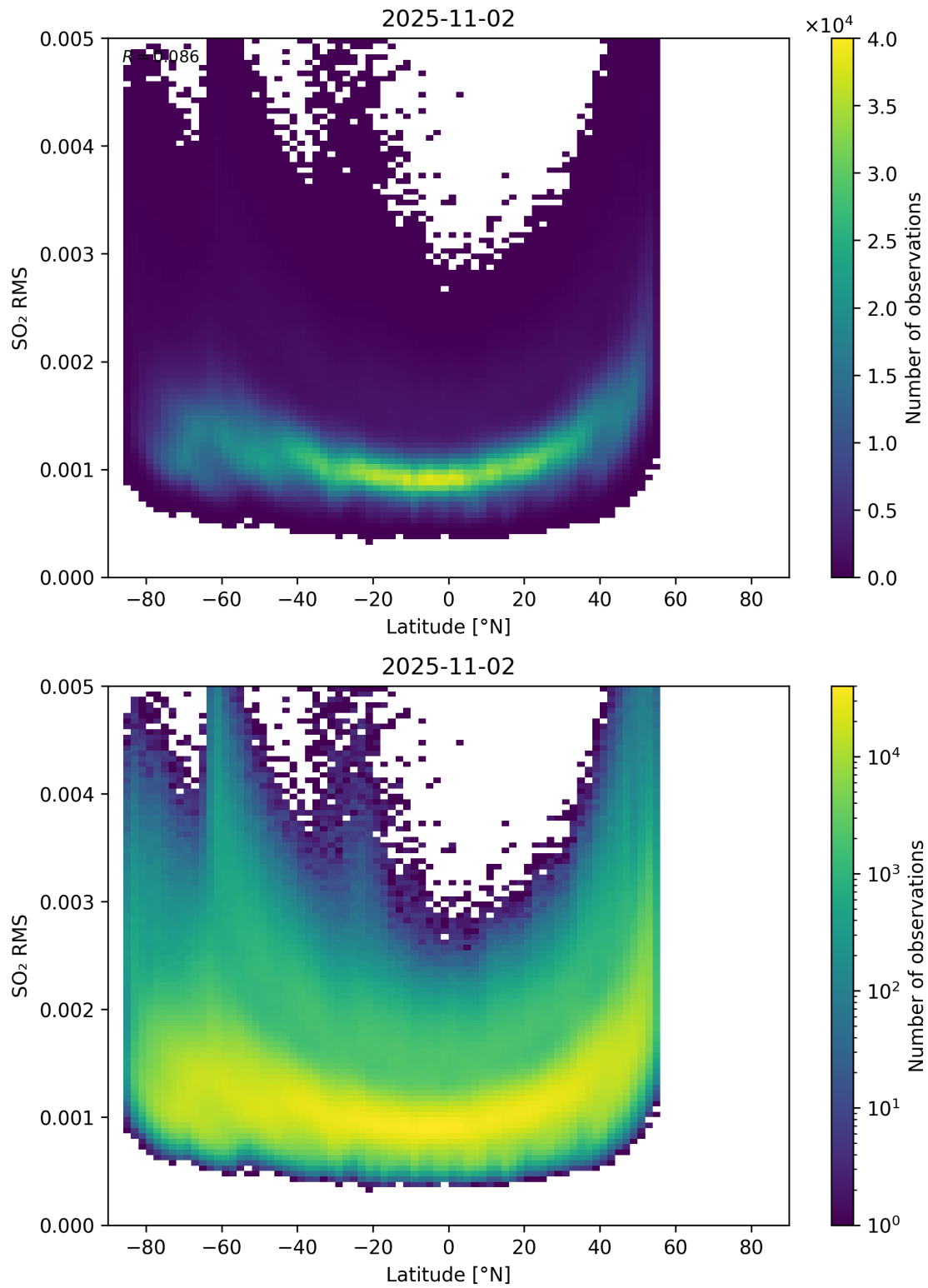
Figure 155: Scatter density plot of “Latitude” against “SO 2 RMS” for 2025-11-02 to 2025-11-03.
