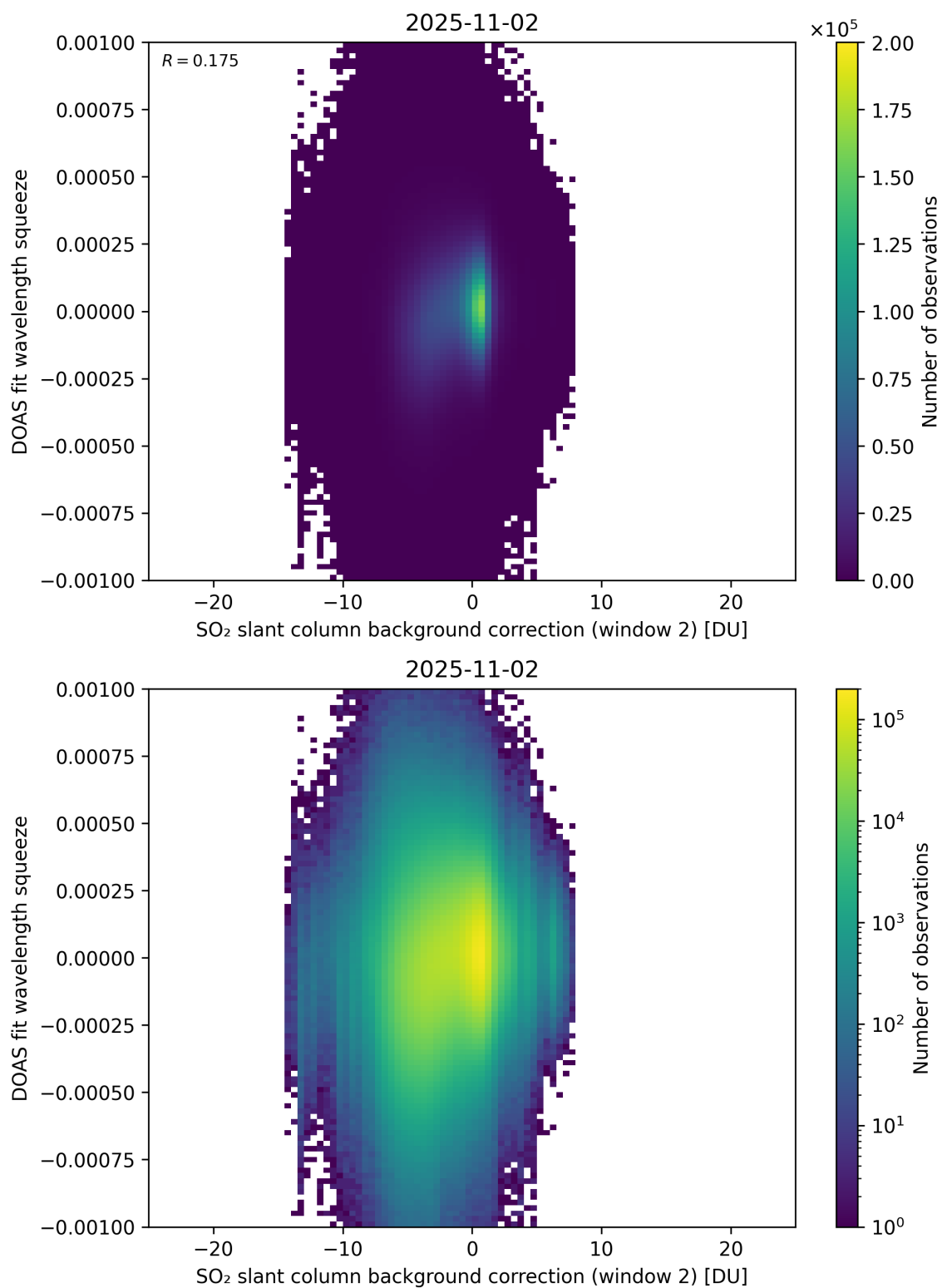
Figure 124: Scatter density plot of “SO 2 slant column background correction (window 2)” against “DOAS fit wavelength squeeze” for 2025-11-02 to 2025-11-03.
