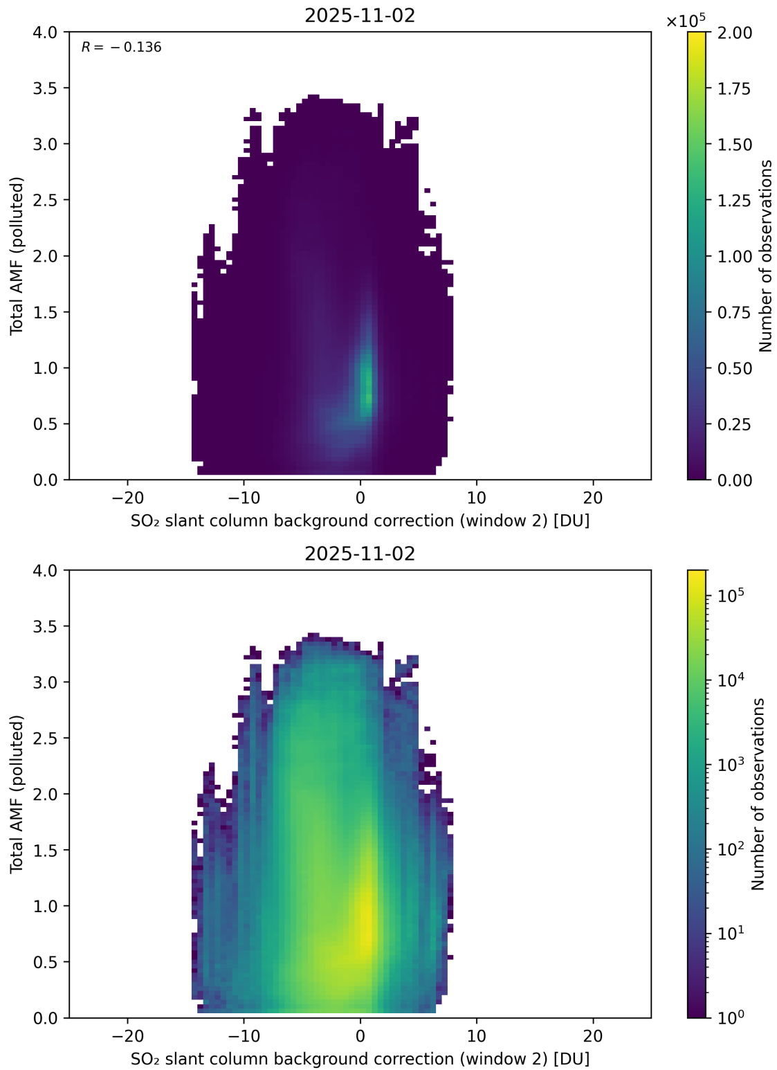
Figure 130: Scatter density plot of “SO 2 slant column background correction (window 2)” against “Total AMF (polluted)” for 2025-11-02 to 2025-11-03.
