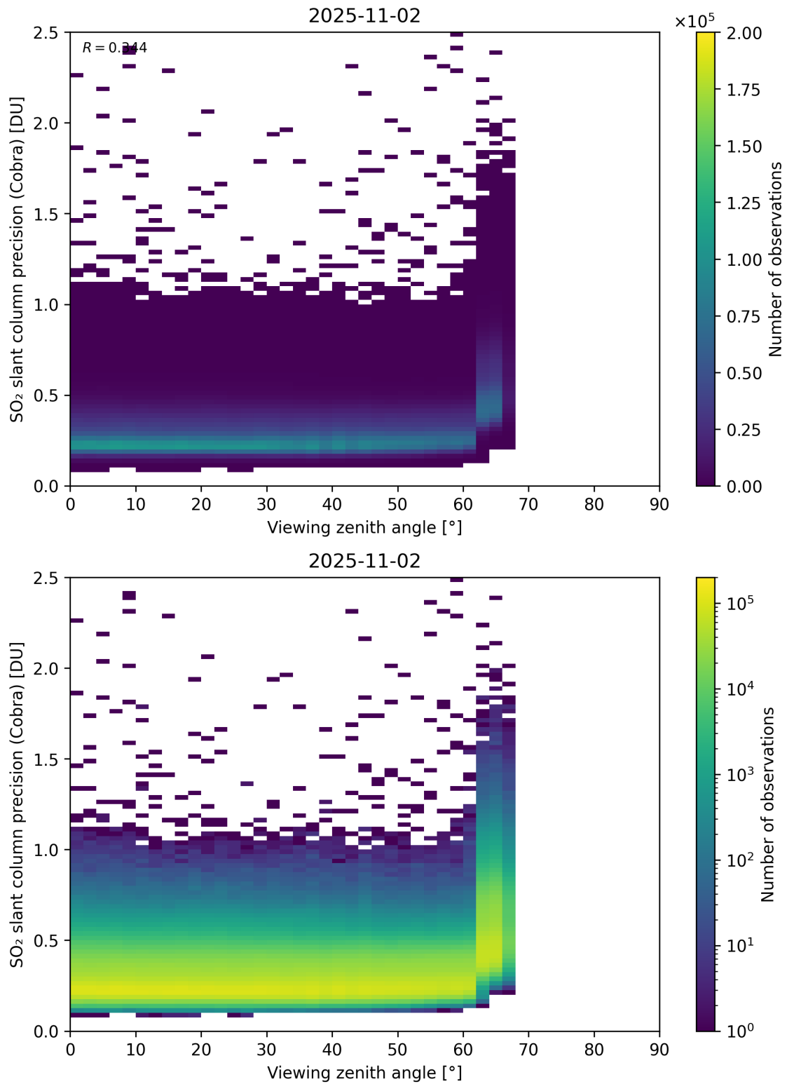
Figure 372: Scatter density plot of “Viewing zenith angle” against “SO 2 slant column precision (Cobra)” for 2025-11-02 to 2025-11-03.
