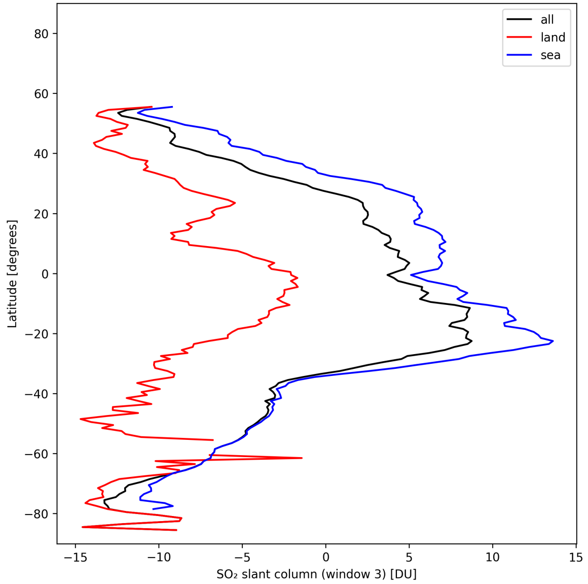
Figure 45: Zonal average of “SO 2 slant column (window 3)” for 2025-11-02 to 2025-11-03.
