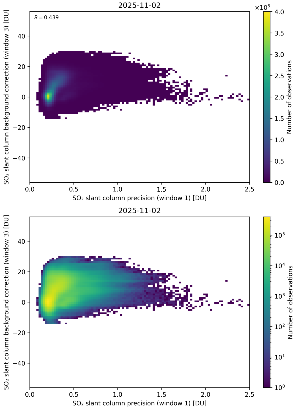
Figure 270: Scatter density plot of “SO 2 slant column precision (window 1)” against “SO 2 slant column background correction (window 3)” for 2025-11-02 to 2025-11-03.
