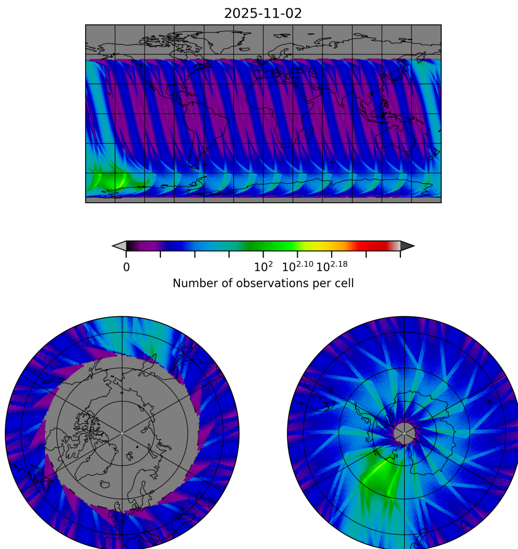
Figure 30: Map of the number of observations for 2025-11-02 to 2025-11-03
