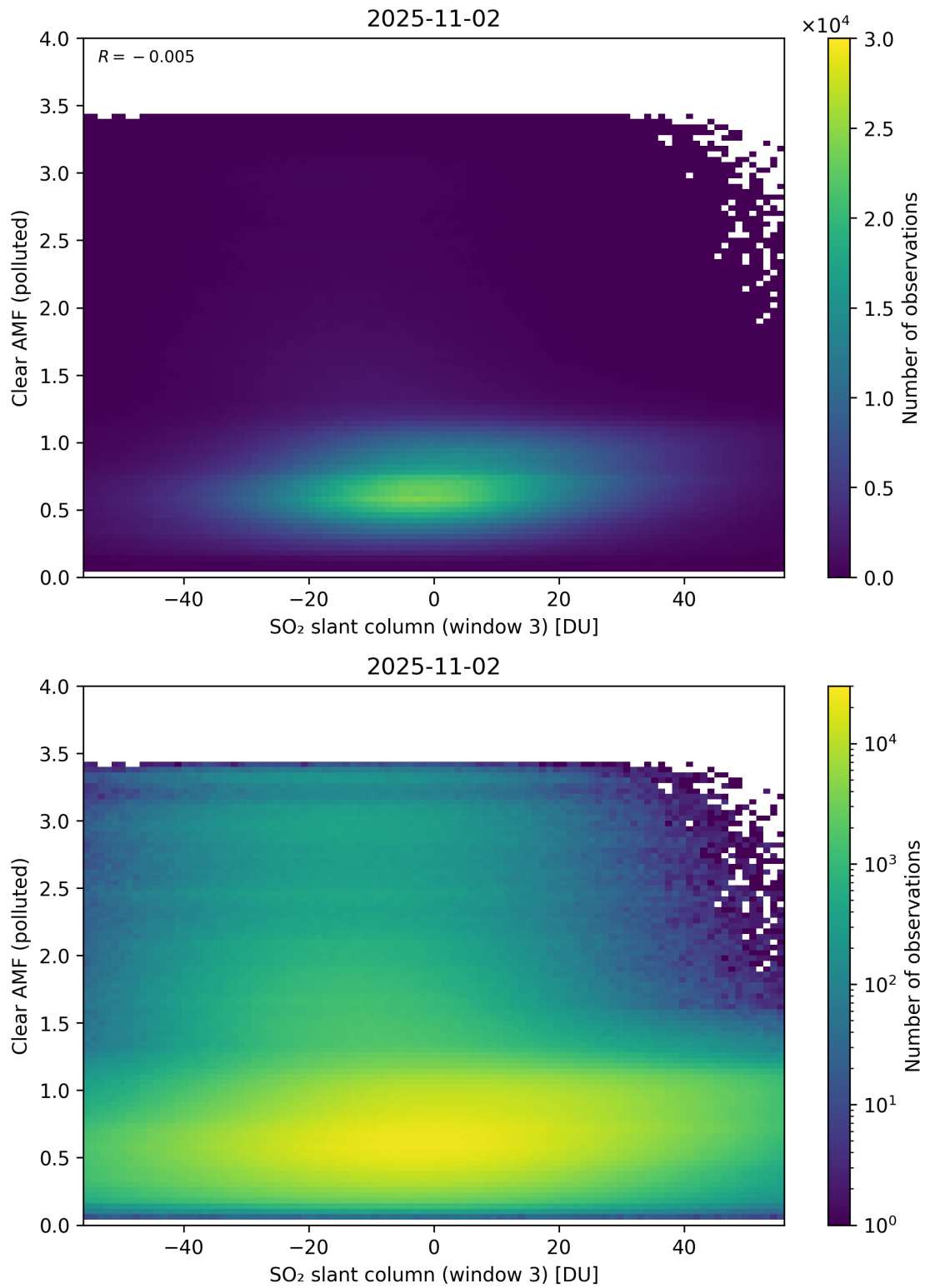
Figure 315: Scatter density plot of “SO 2 slant column (window 3)” against “Clear AMF (polluted)” for 2025-11-02 to 2025-11-03.
