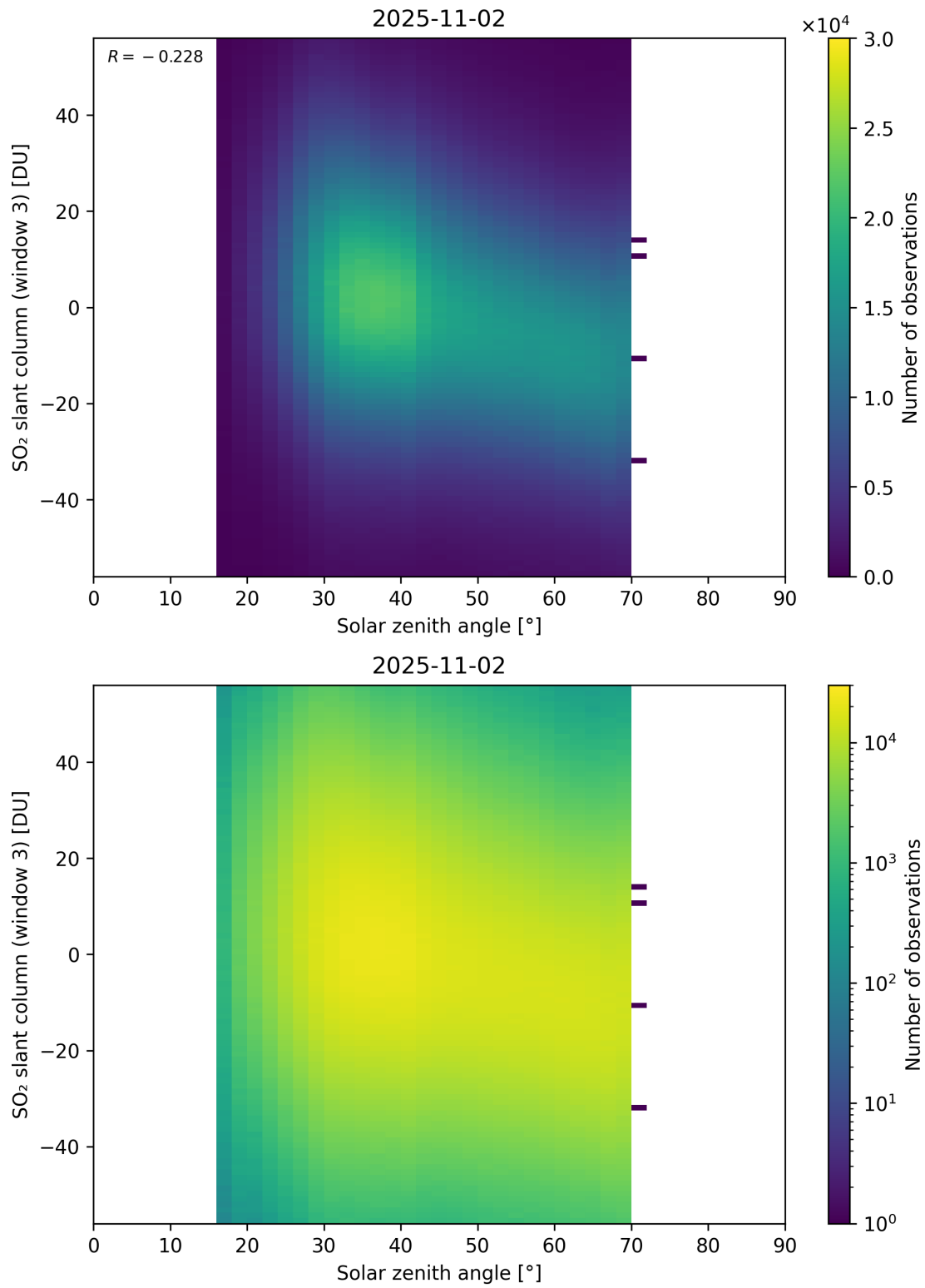
Figure 187: Scatter density plot of “Solar zenith angle” against “SO 2 slant column (window 3)” for 2025-11-02 to 2025-11-03.
