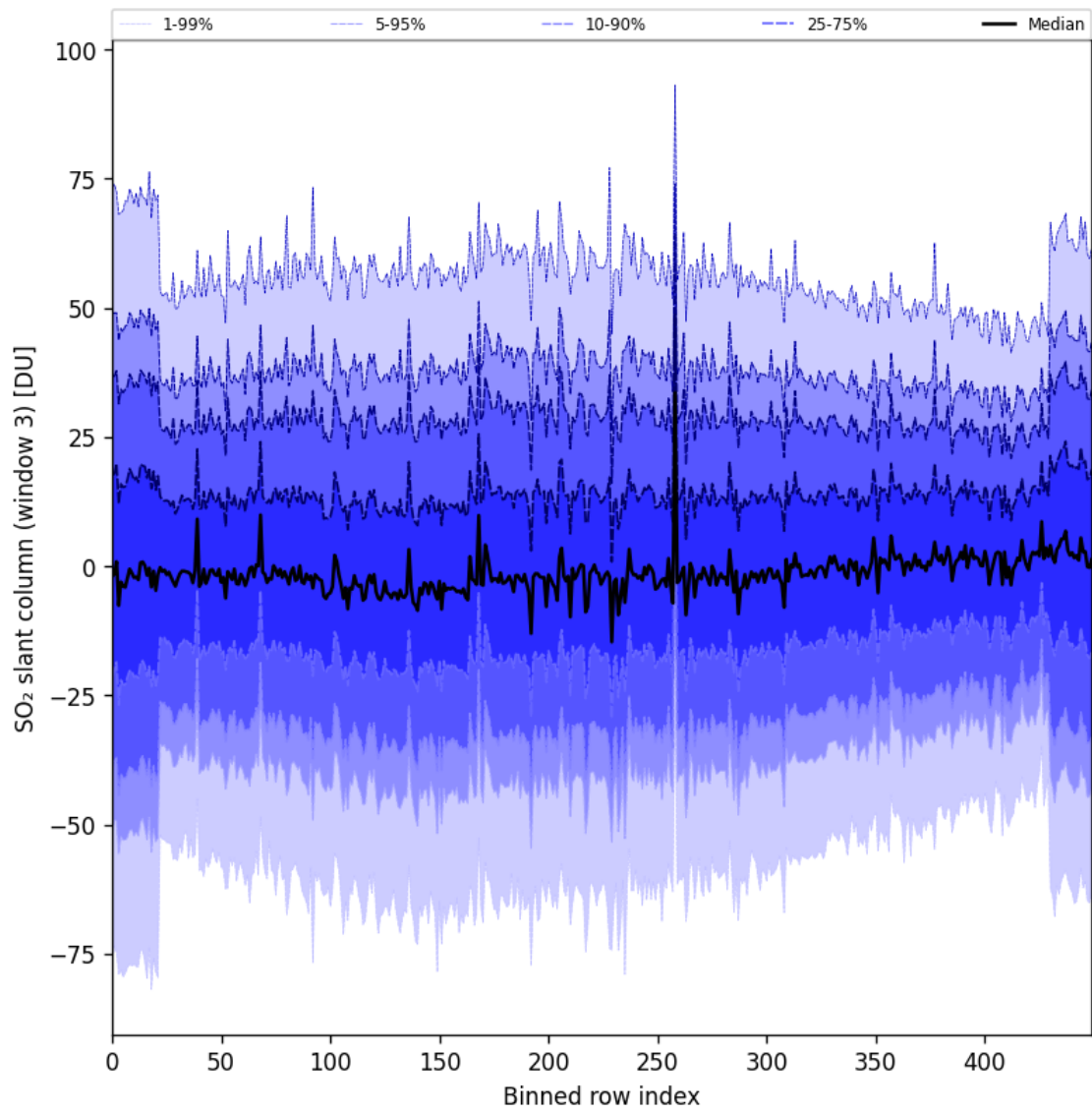
Figure 97: Along track statistics of “SO 2 slant column (window 3)” for 2025-11-02 to 2025-11-03
