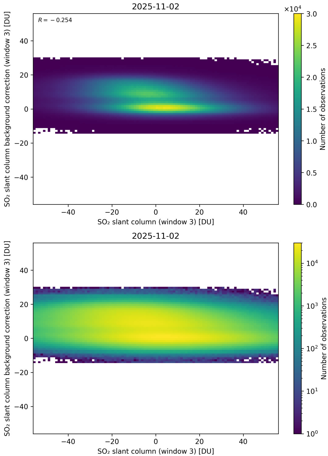
Figure 303: Scatter density plot of “SO 2 slant column (window 3)” against “SO 2 slant column background correction (window 3)” for 2025-11-02 to 2025-11-03.
