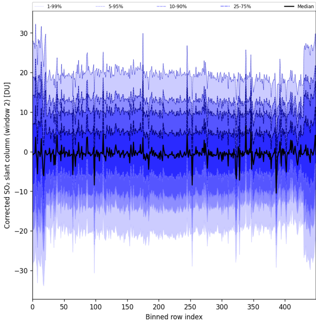
Figure 95: Along track statistics of “Corrected SO 2 slant column (window 2)” for 2025-11-02 to 2025-11-03
