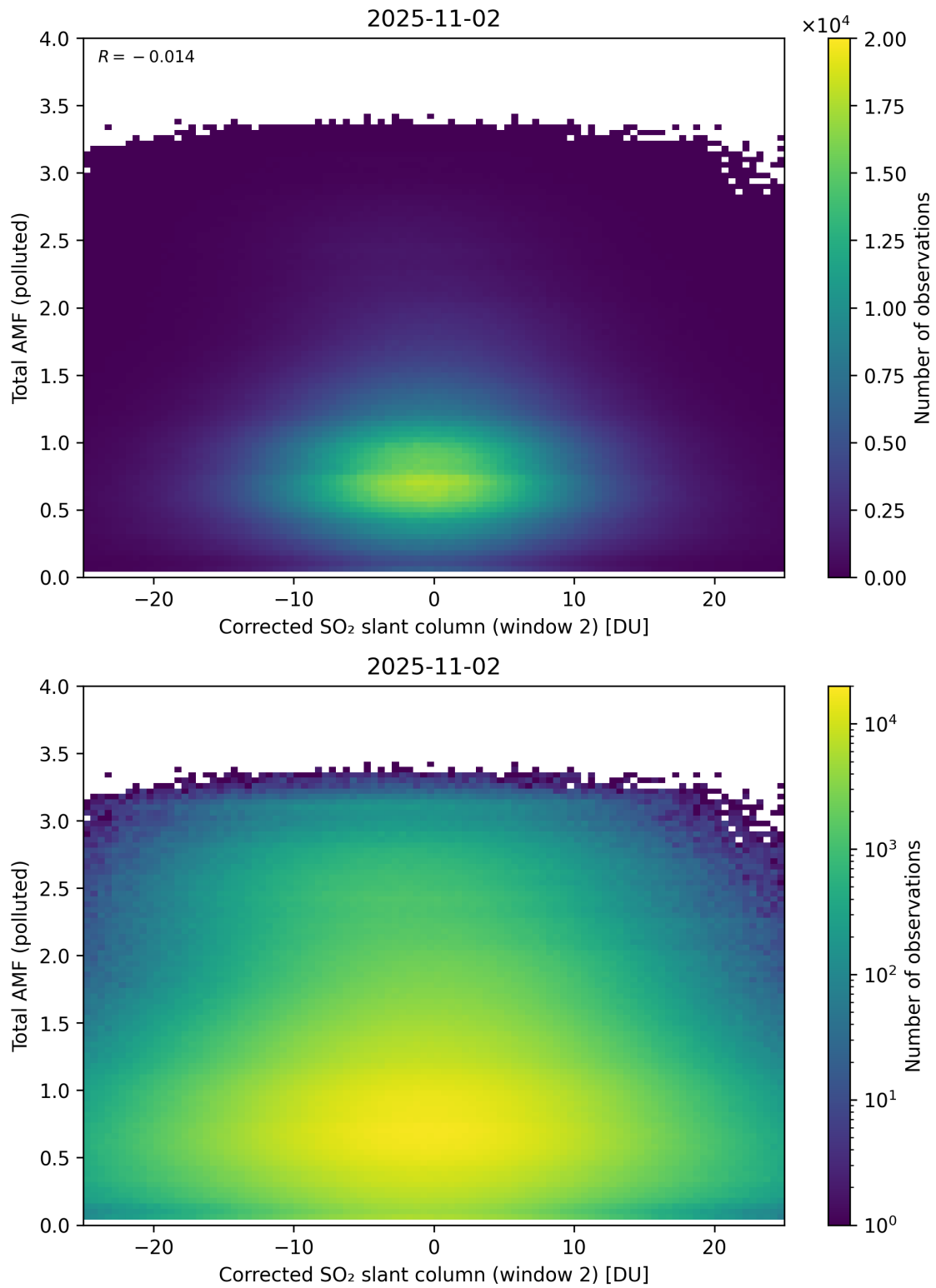
Figure 253: Scatter density plot of “Corrected SO 2 slant column (window 2)” against “Total AMF (polluted)” for 2025-11-02 to 2025-11-03.
