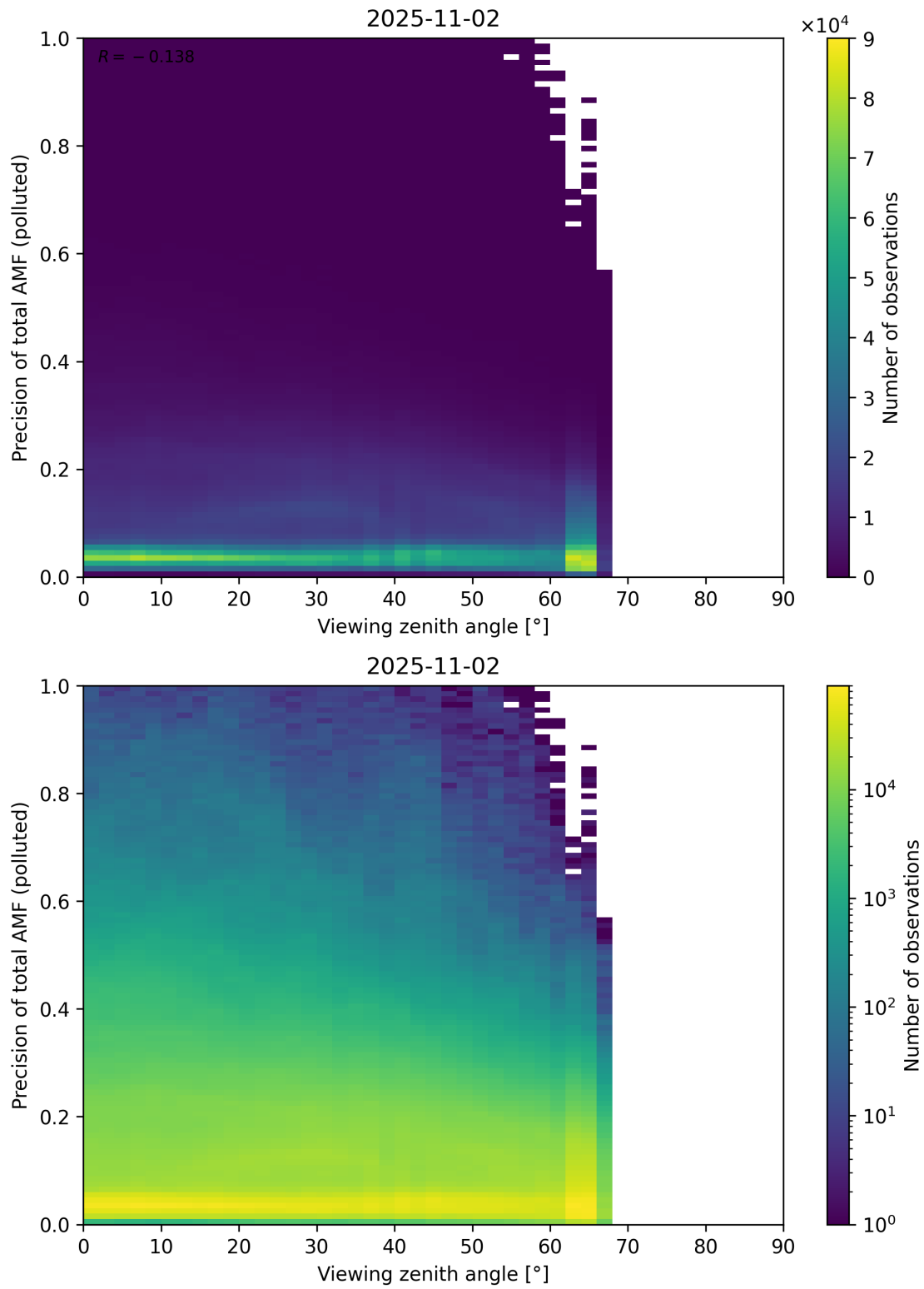
Figure 382: Scatter density plot of “Viewing zenith angle” against “Precision of total AMF (polluted)” for 2025-11-02 to 2025-11-03.
