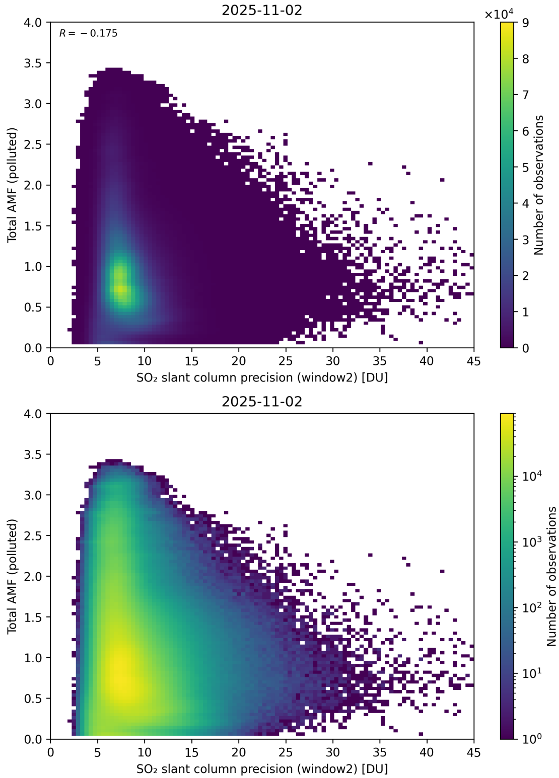
Figure 301: Scatter density plot of “SO 2 slant column precision (window2)” against “Total AMF (polluted)” for 2025-11-02 to 2025-11-03.
