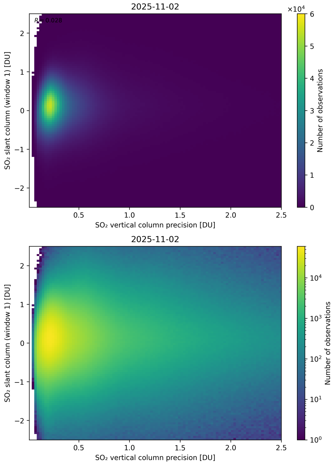
Figure 341: Scatter density plot of “SO 2 vertical column precision” against “SO 2 slant column (window 1)” for 2025-11-02 to 2025-11-03.
