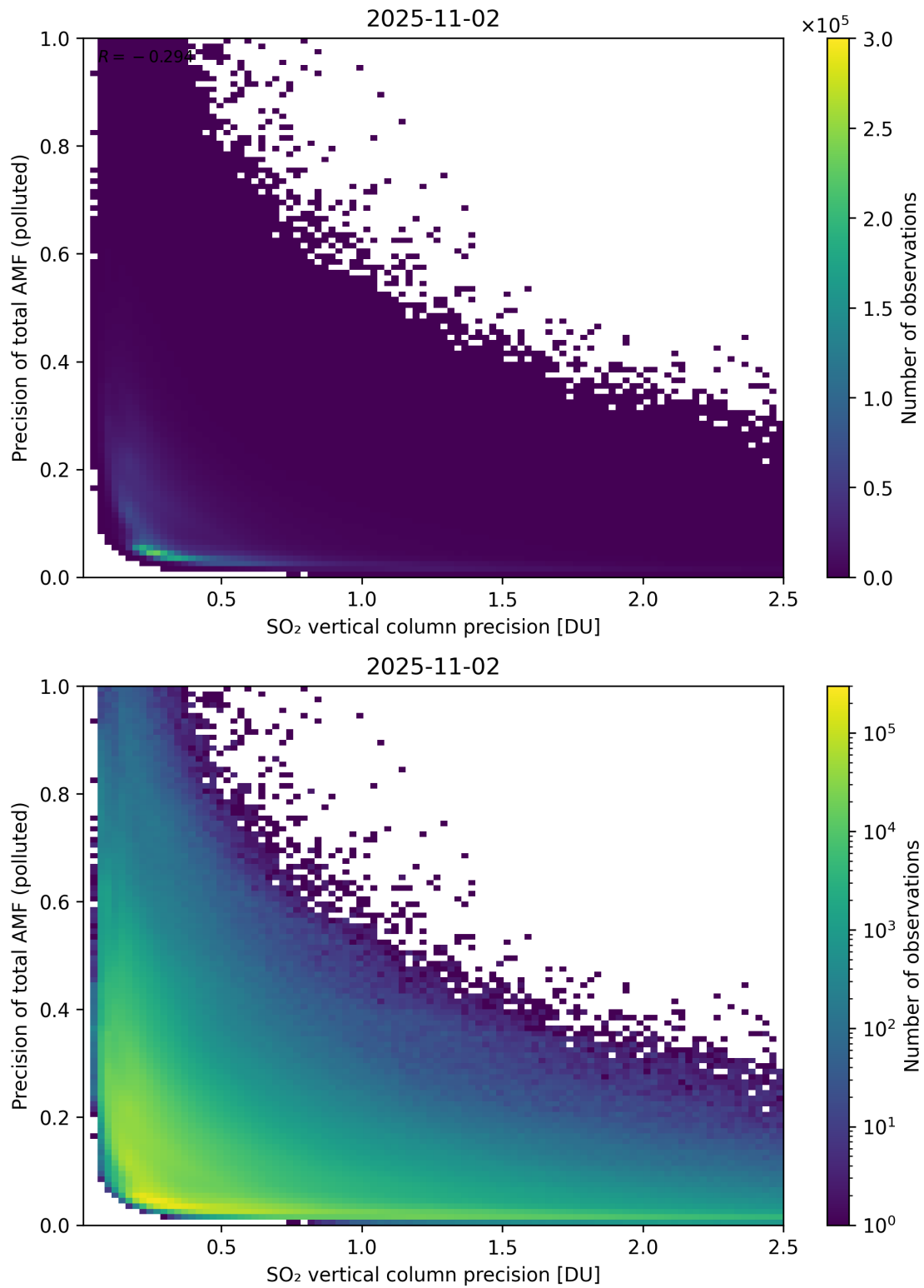
Figure 347: Scatter density plot of “SO 2 vertical column precision” against “Precision of total AMF (polluted)” for 2025-11-02 to 2025-11-03.
