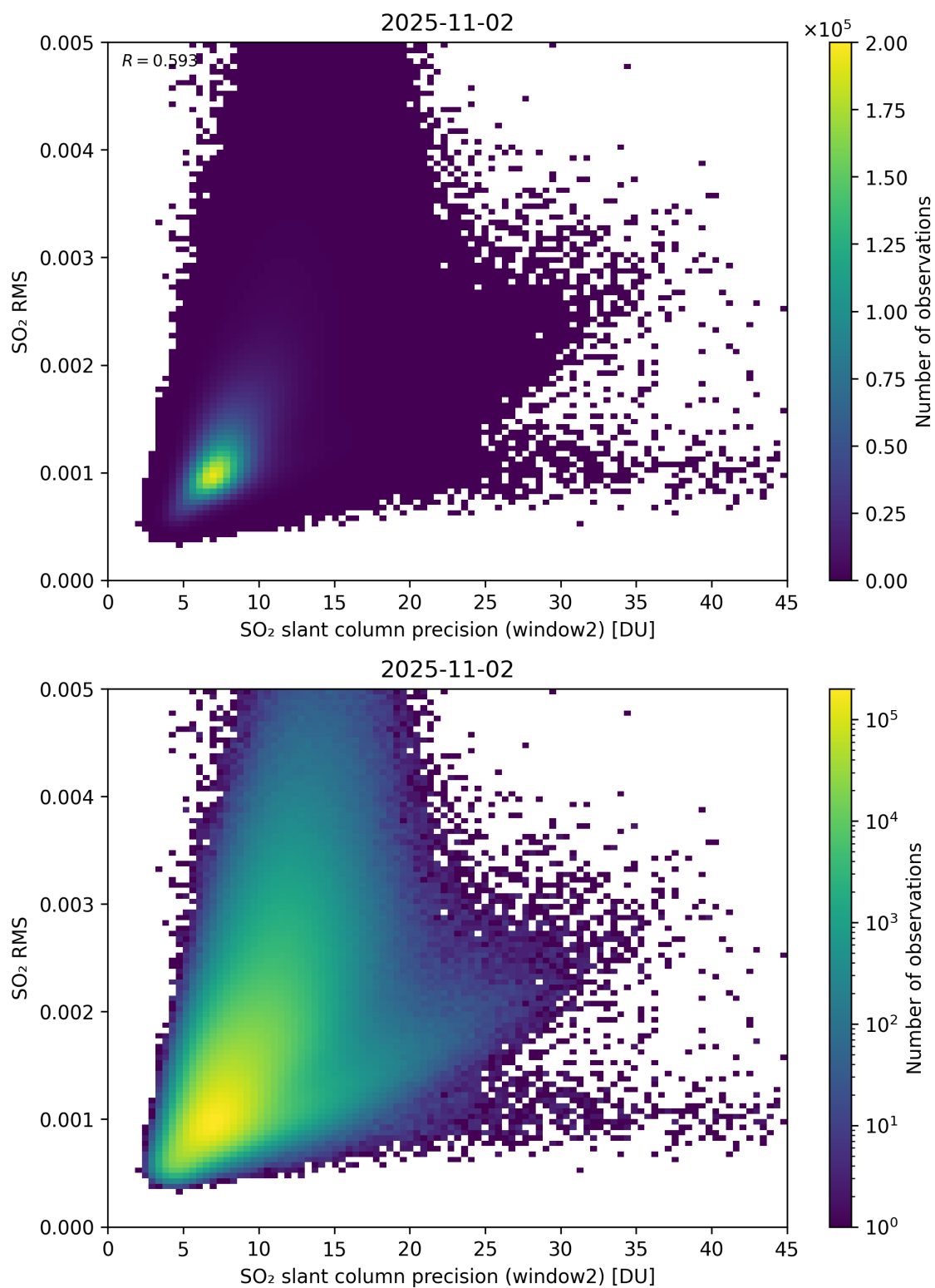
Figure 295: Scatter density plot of “SO 2 slant column precision (window2)” against “SO 2 RMS” for 2025-11-02 to 2025-11-03.
