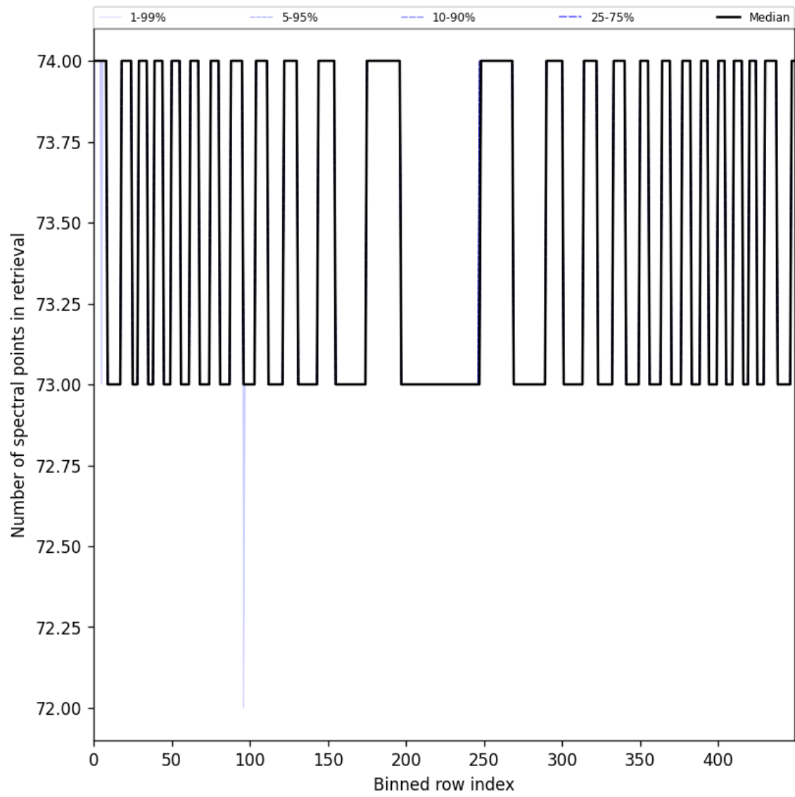
Figure 108: Along track statistics of “Number of spectral points in retrieval” for 2025-11-02 to 2025-11-03
