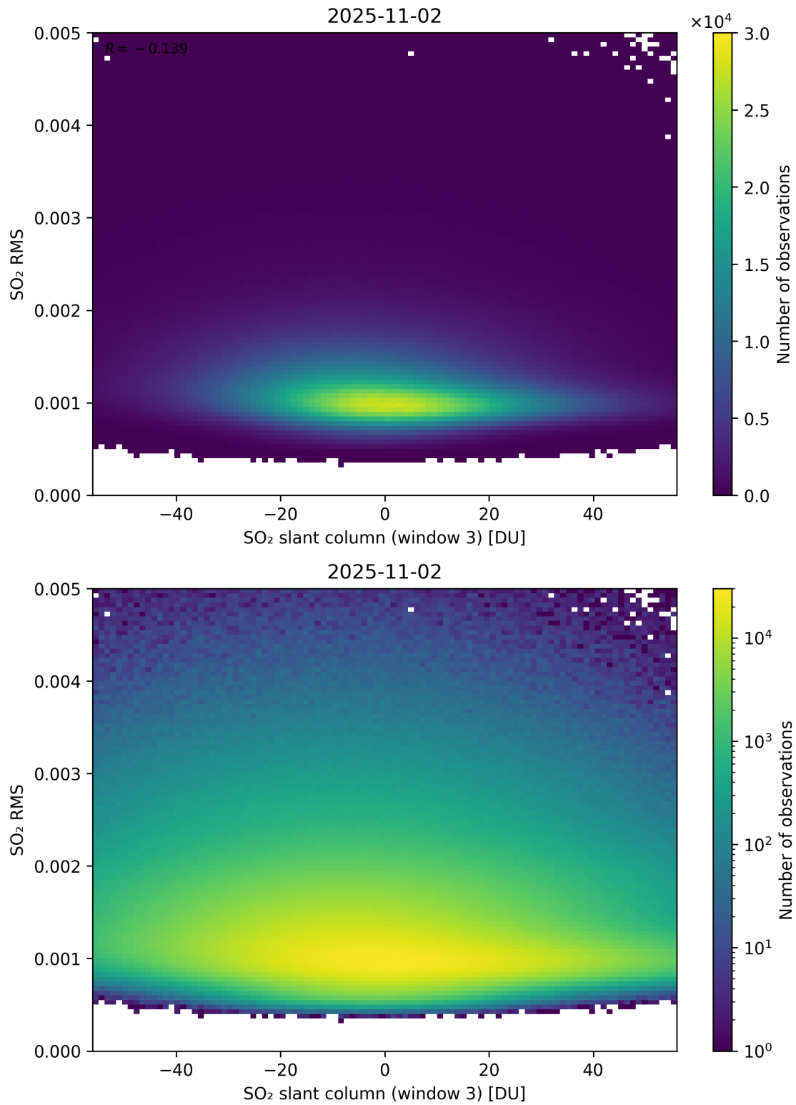
Figure 306: Scatter density plot of “SO 2 slant column (window 3)” against “SO 2 RMS” for 2025-11-02 to 2025-11-03.
