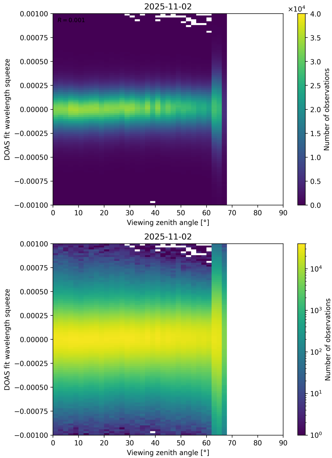
Figure 366: Scatter density plot of “Viewing zenith angle” against “DOAS fit wavelength squeeze” for 2025-11-02 to 2025-11-03.
