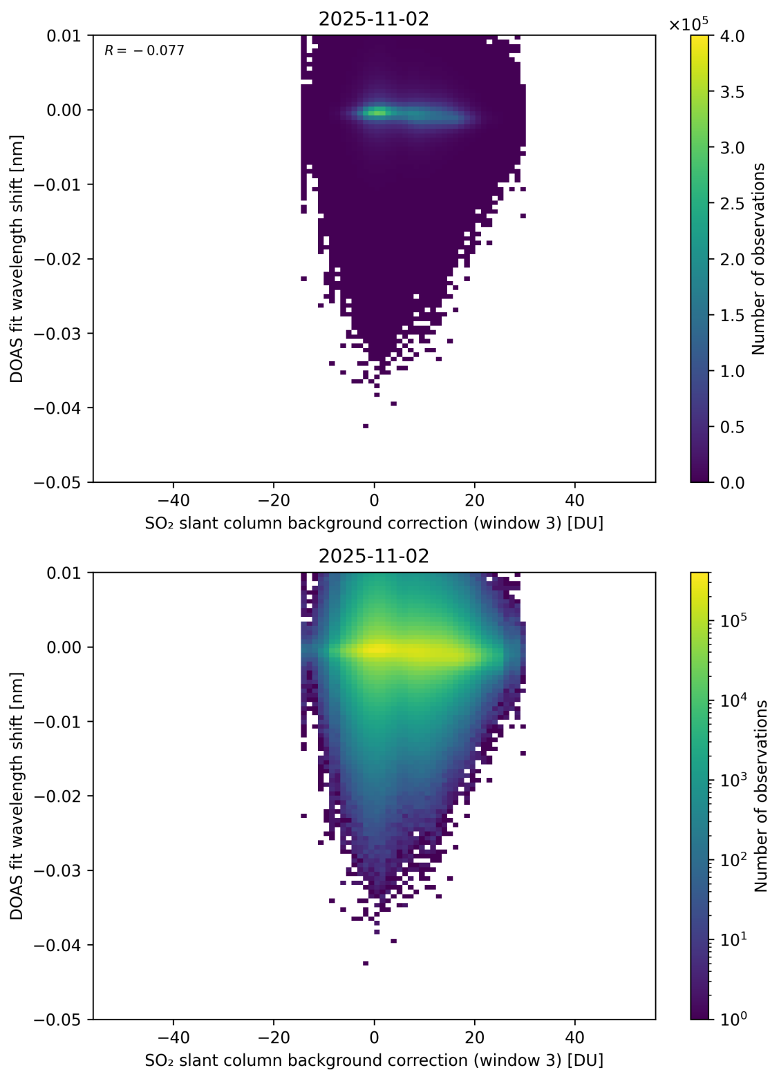
Figure 132: Scatter density plot of “SO 2 slant column background correction (window 3)” against “DOAS fit wavelength shift” for 2025-11-02 to 2025-11-03.
