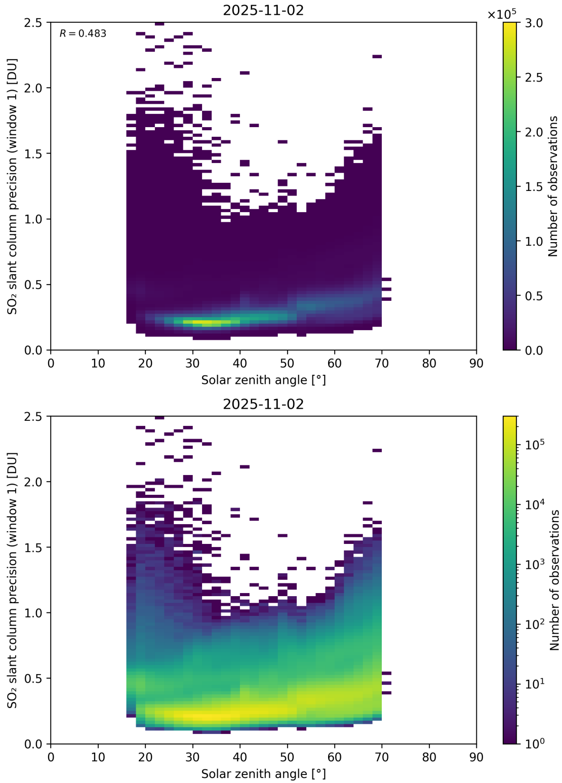
Figure 185: Scatter density plot of “Solar zenith angle” against “SO 2 slant column precision (window 1)” for 2025-11-02 to 2025-11-03.
