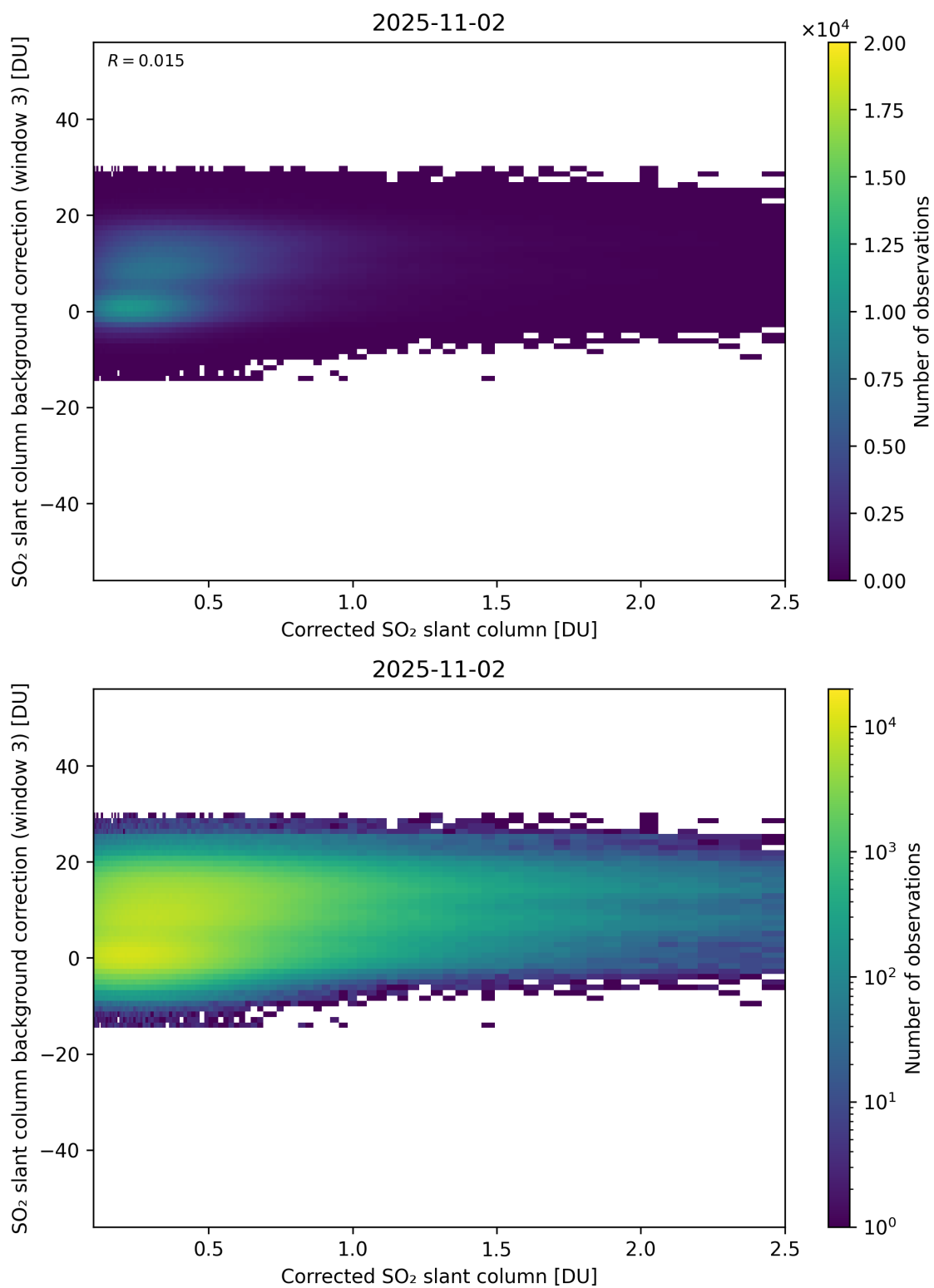
Figure 228: Scatter density plot of “Corrected SO 2 slant column” against “SO 2 slant column background correction (window 3)” for 2025-11-02 to 2025-11-03.
