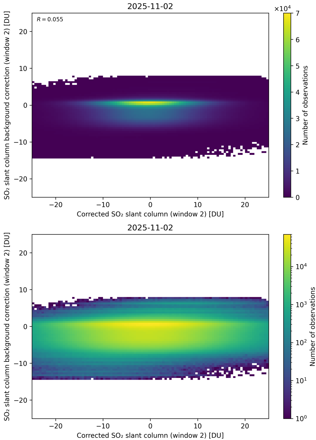
Figure 244: Scatter density plot of “Corrected SO 2 slant column (window 2)” against “SO 2 slant column background correction (window 2)” for 2025-11-02 to 2025-11-03.
