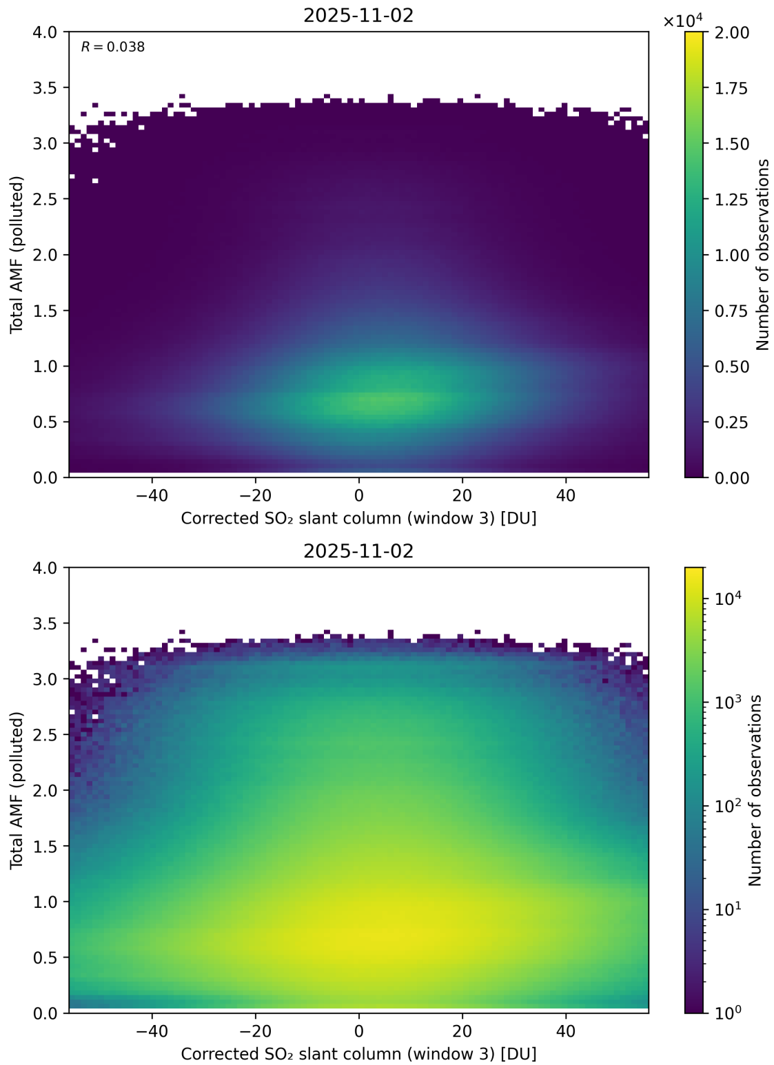
Figure 260: Scatter density plot of “Corrected SO 2 slant column (window 3)” against “Total AMF (polluted)” for 2025-11-02 to 2025-11-03.
