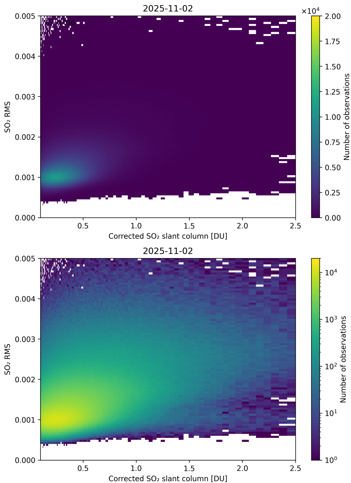
Figure 231: Scatter density plot of “Corrected SO 2 slant column” against “SO 2 RMS” for 2025-11-02 to 2025-11-03.
