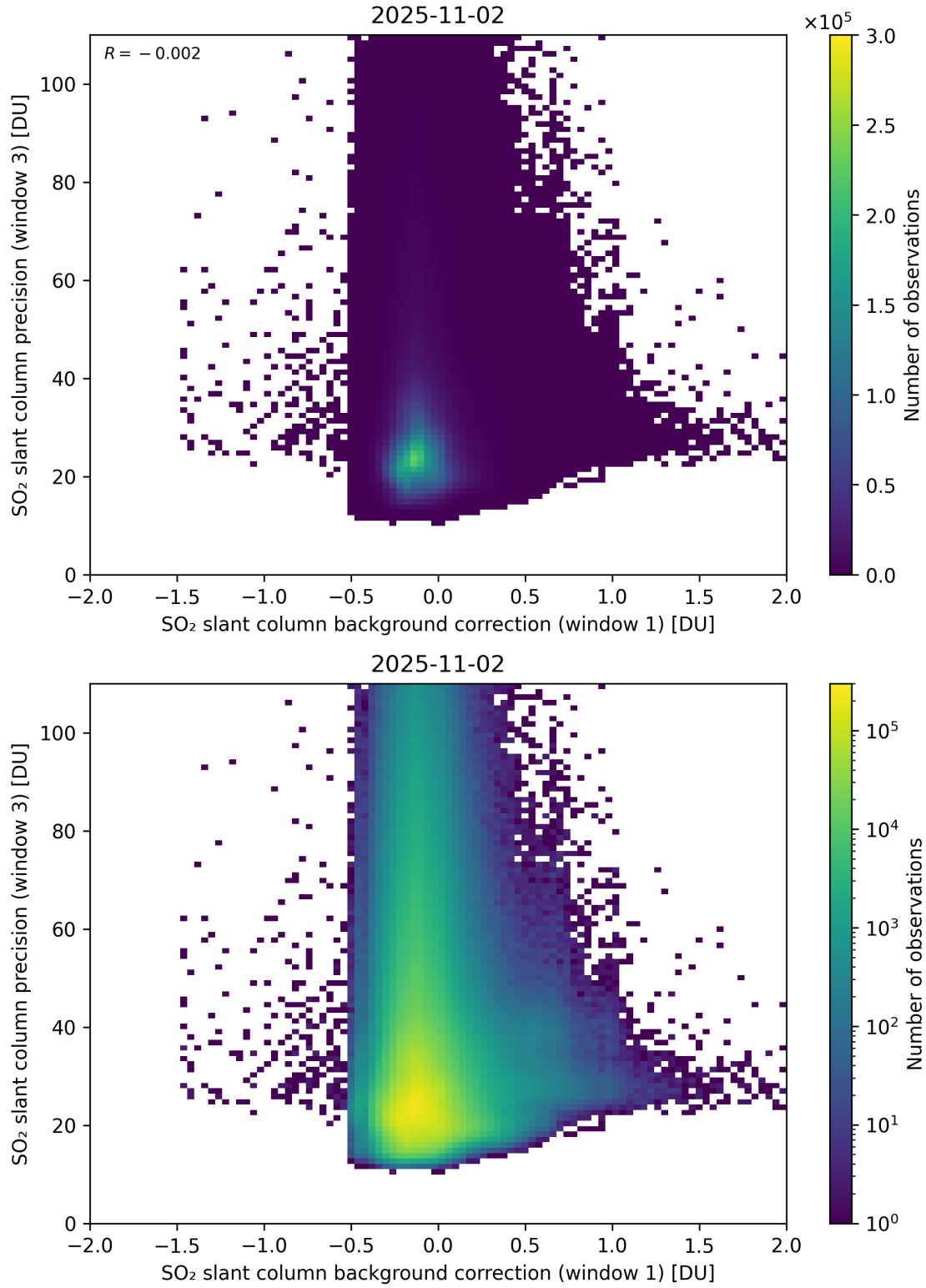
Figure 119: Scatter density plot of “SO 2 slant column background correction (window 1)” against “SO 2 slant column precision (window 3)” for 2025-11-02 to 2025-11-03.
