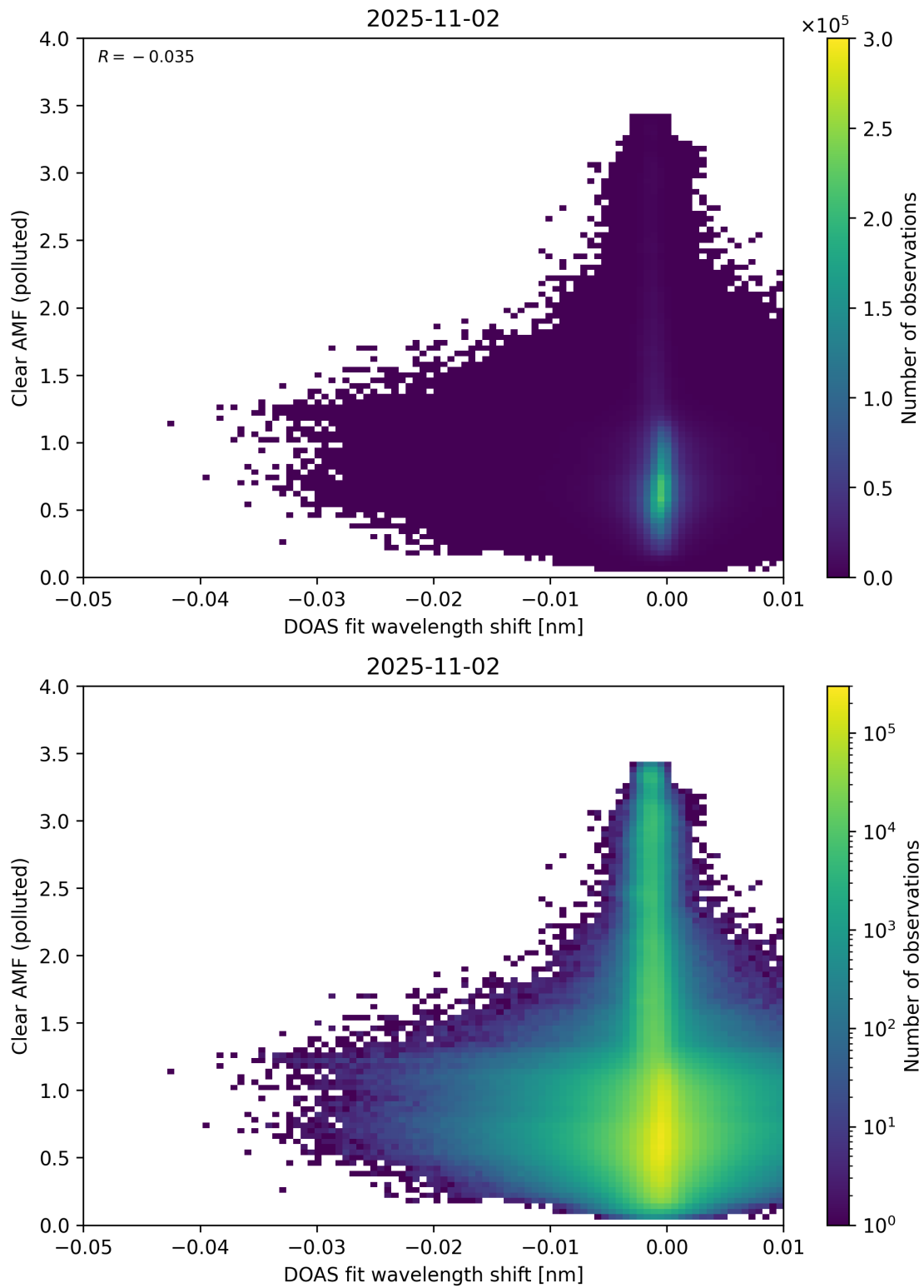
Figure 140: Scatter density plot of “DOAS fit wavelength shift” against “Clear AMF (polluted)” for 2025-11-02 to 2025-11-03.
