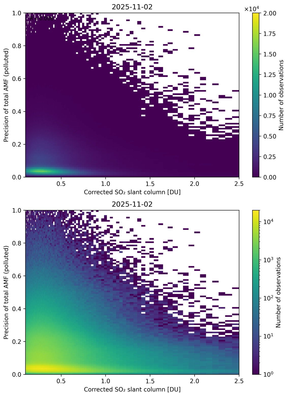
Figure 243: Scatter density plot of “Corrected SO 2 slant column” against “Precision of total AMF (polluted)” for 2025-11-02 to 2025-11-03.
