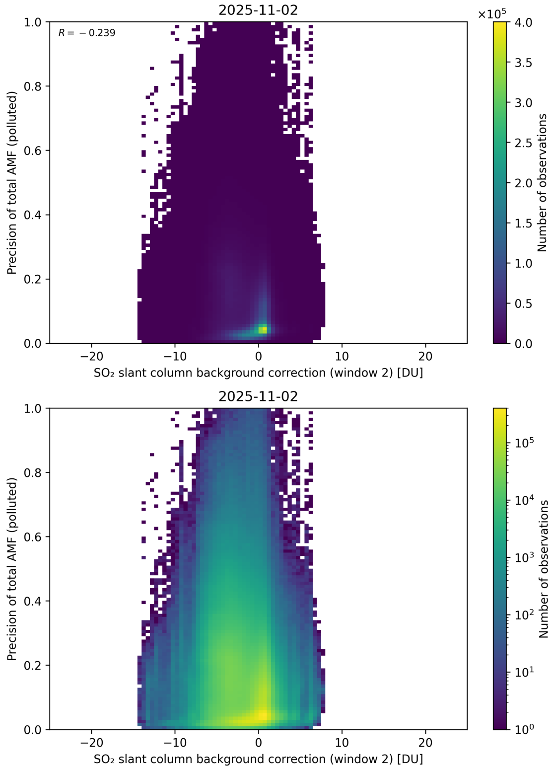
Figure 131: Scatter density plot of “SO 2 slant column background correction (window 2)” against “Precision of total AMF (polluted)” for 2025-11-02 to 2025-11-03.
