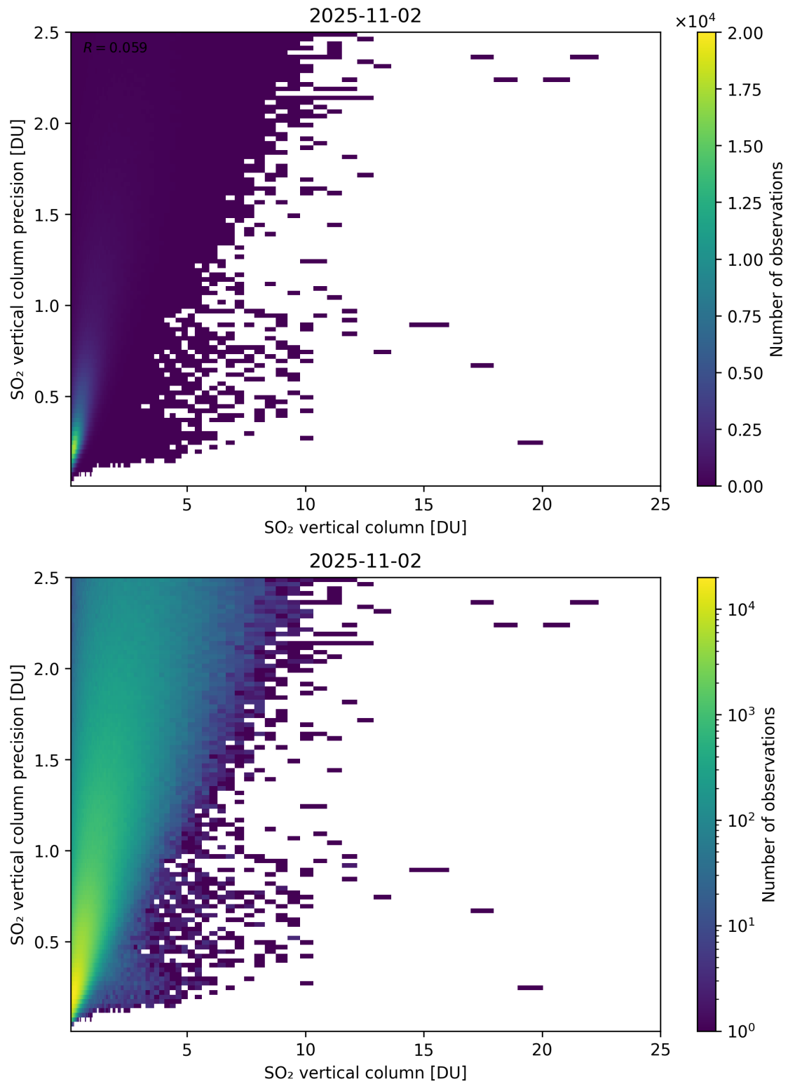
Figure 361: Scatter density plot of “SO 2 vertical column” against “SO 2 vertical column precision” for 2025-11-02 to 2025-11-03.
