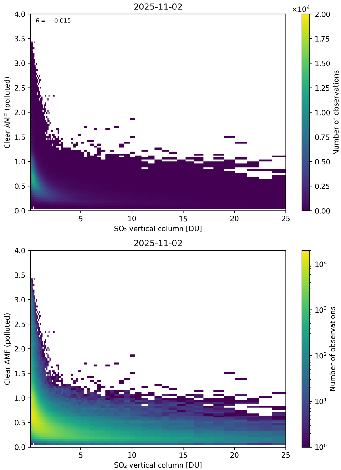
Figure 348: Scatter density plot of “SO 2 vertical column” against “Clear AMF (polluted)” for 2025-11-02 to 2025-11-03.
