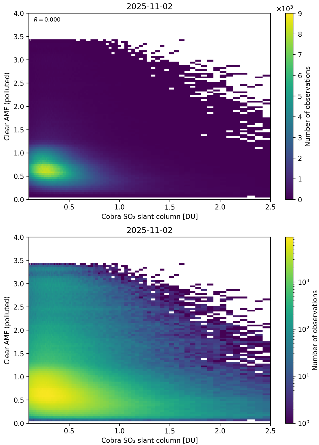
Figure 215: Scatter density plot of “Cobra SO 2 slant column” against “Clear AMF (polluted)” for 2025-11-02 to 2025-11-03.
