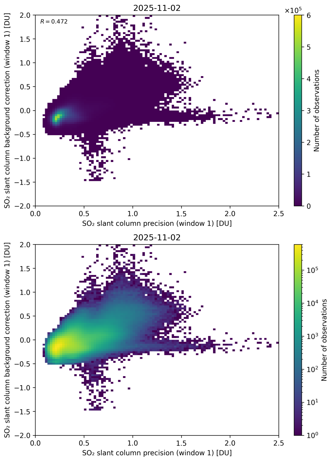
Figure 268: Scatter density plot of “SO 2 slant column precision (window 1)” against “SO 2 slant column background correction (window 1)” for 2025-11-02 to 2025-11-03.
