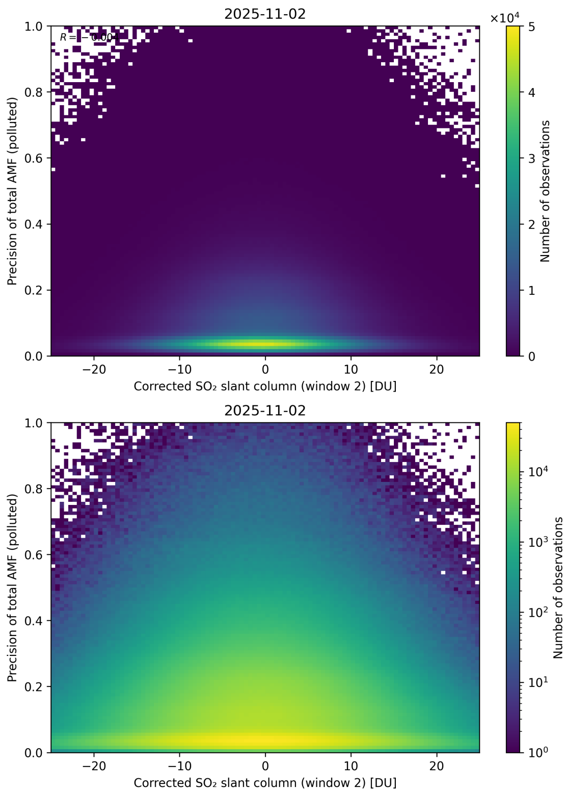
Figure 254: Scatter density plot of “Corrected SO 2 slant column (window 2)” against “Precision of total AMF (polluted)” for 2025-11-02 to 2025-11-03.
