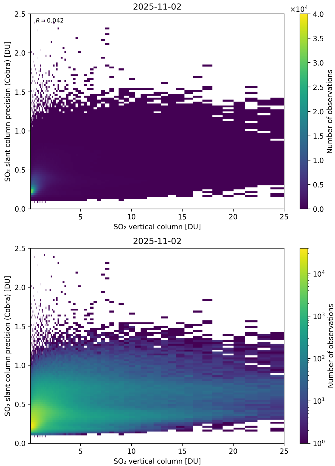
Figure 350: Scatter density plot of “SO 2 vertical column” against “SO 2 slant column precision (Cobra)” for 2025-11-02 to 2025-11-03.
