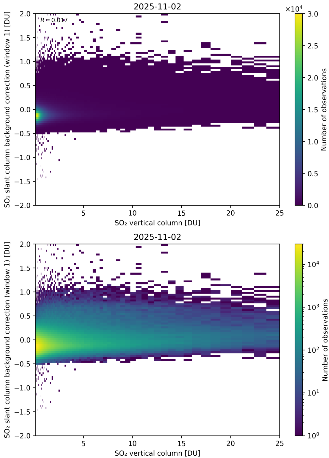
Figure 323: Scatter density plot of “SO 2 vertical column” against “SO 2 slant column background correction (window 1)” for 2025-11-02 to 2025-11-03.
