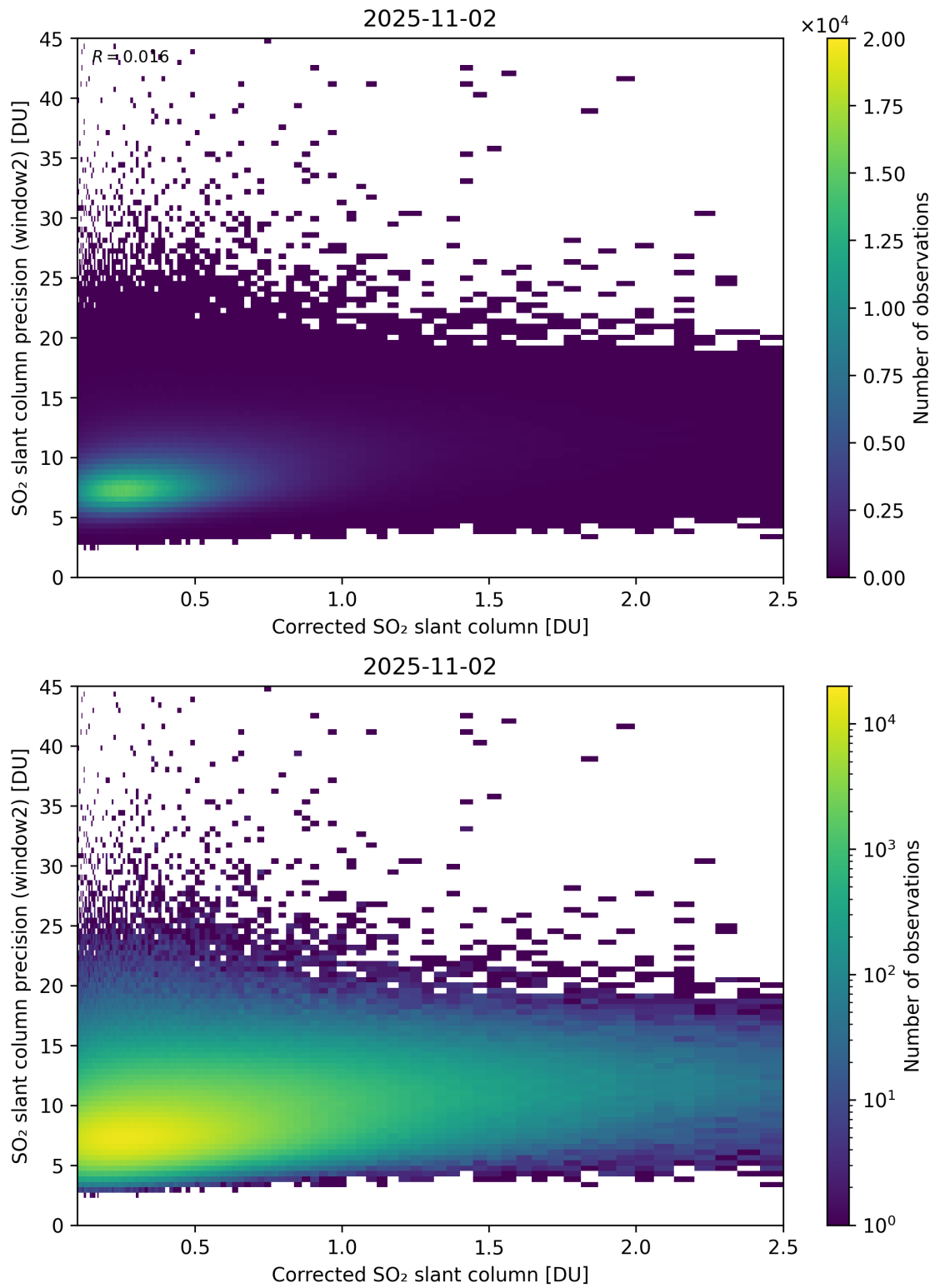
Figure 239: Scatter density plot of “Corrected SO 2 slant column” against “SO 2 slant column precision (window2)” for 2025-11-02 to 2025-11-03.
