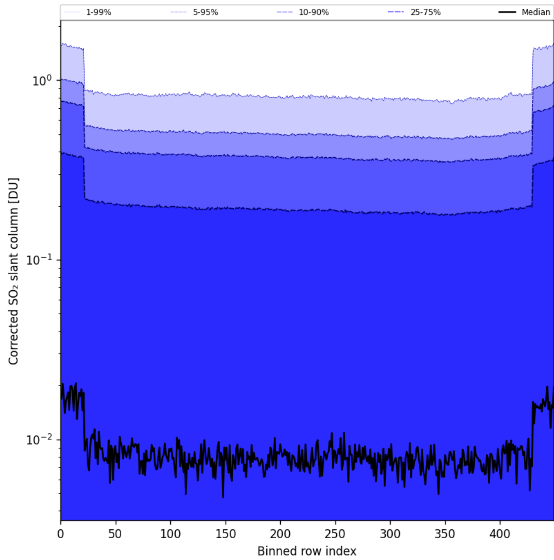
Figure 86: Along track statistics of "Corrected SO 2 slant column" for 2025-11-02 to 2025-11-03
