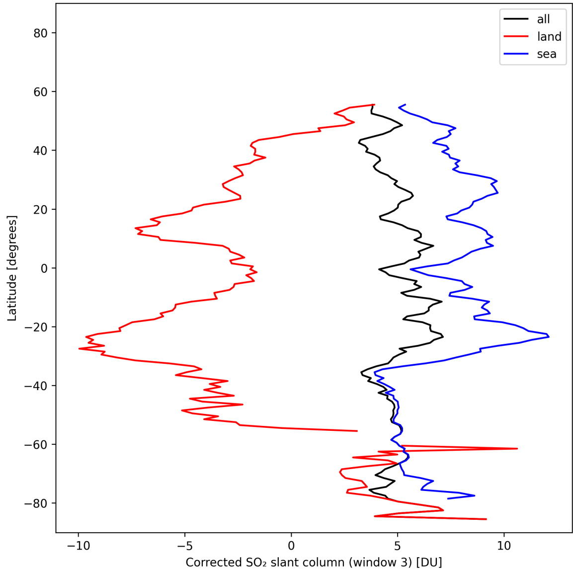
Figure 47: Zonal average of “Corrected SO 2 slant column (window 3)” for 2025-11-02 to 2025-11-03.
