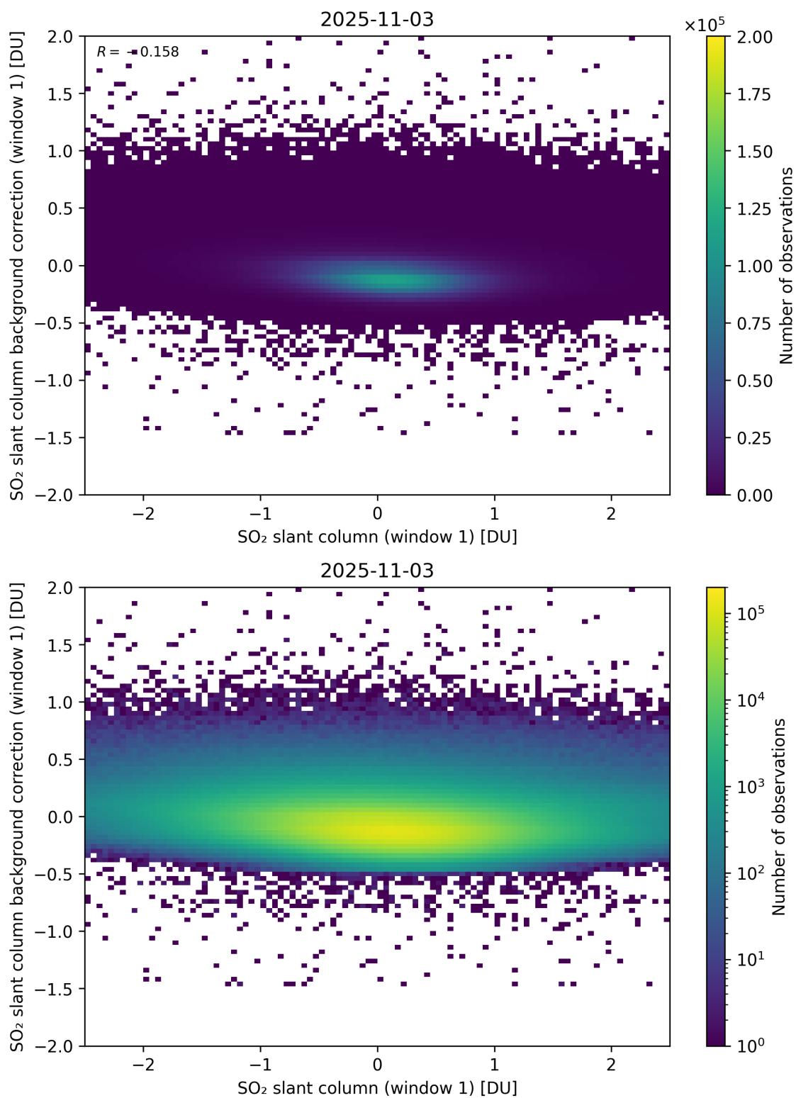
Figure 262: Scatter density plot of “SO 2 slant column (window 1)” against “SO 2 slant column background correction (window 1)” for 2025-11-02 to 2025-11-04.
