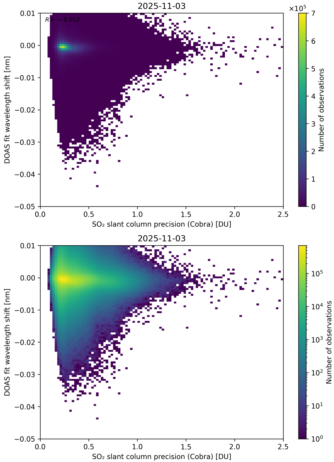
Figure 202: Scatter density plot of “SO 2 slant column precision (Cobra)” against “DOAS fit wavelength shift” for 2025-11-02 to 2025-11-04.
