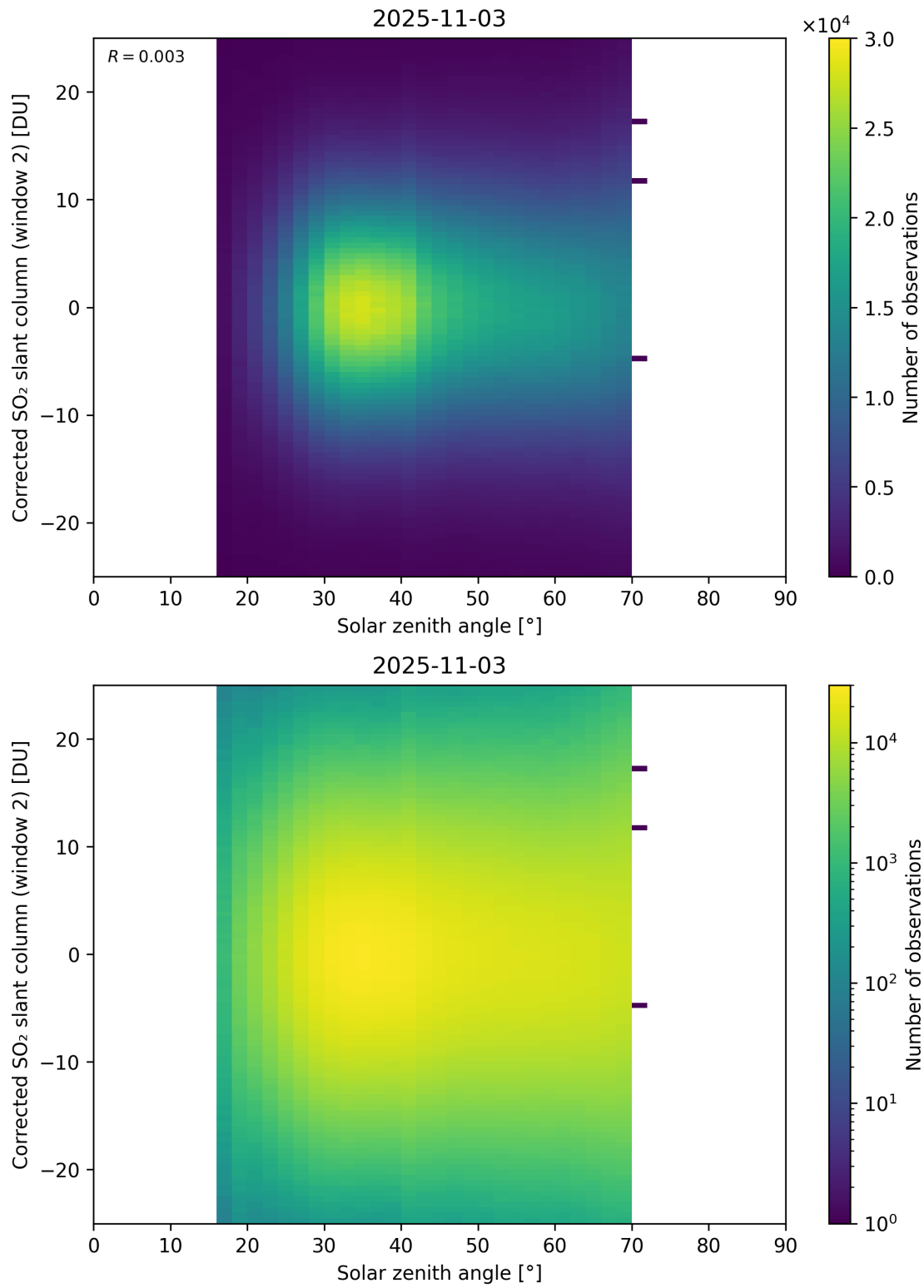
Figure 182: Scatter density plot of “Solar zenith angle” against “Corrected SO 2 slant column (window 2)” for 2025-11-02 to 2025-11-04.
