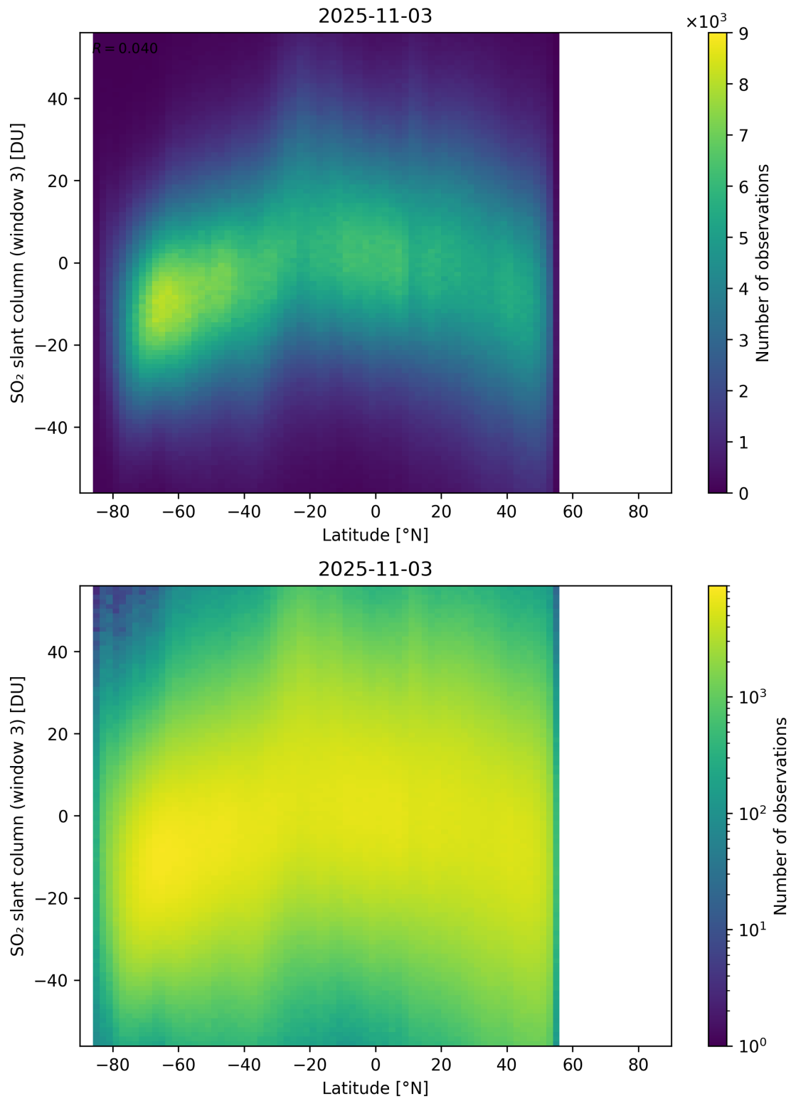
Figure 165: Scatter density plot of “Latitude” against “SO 2 slant column (window 3)” for 2025-11-02 to 2025-11-04.
