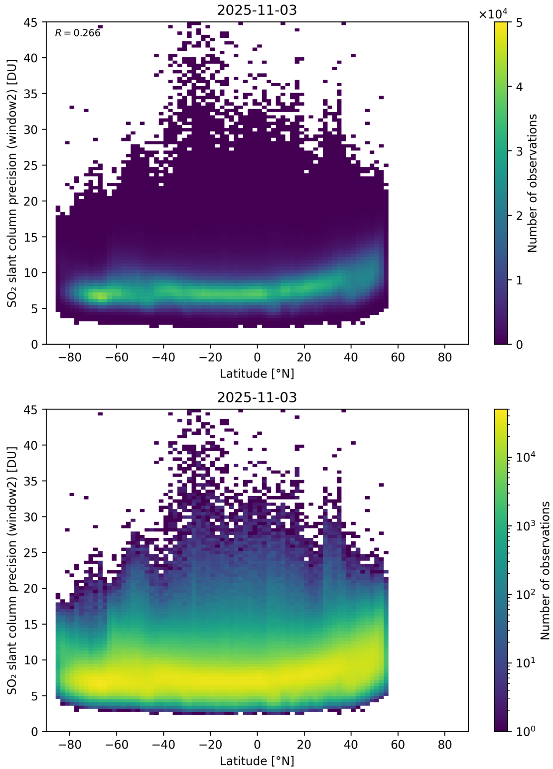
Figure 164: Scatter density plot of “Latitude” against “SO 2 slant column precision (window2)” for 2025-11-02 to 2025-11-04.
