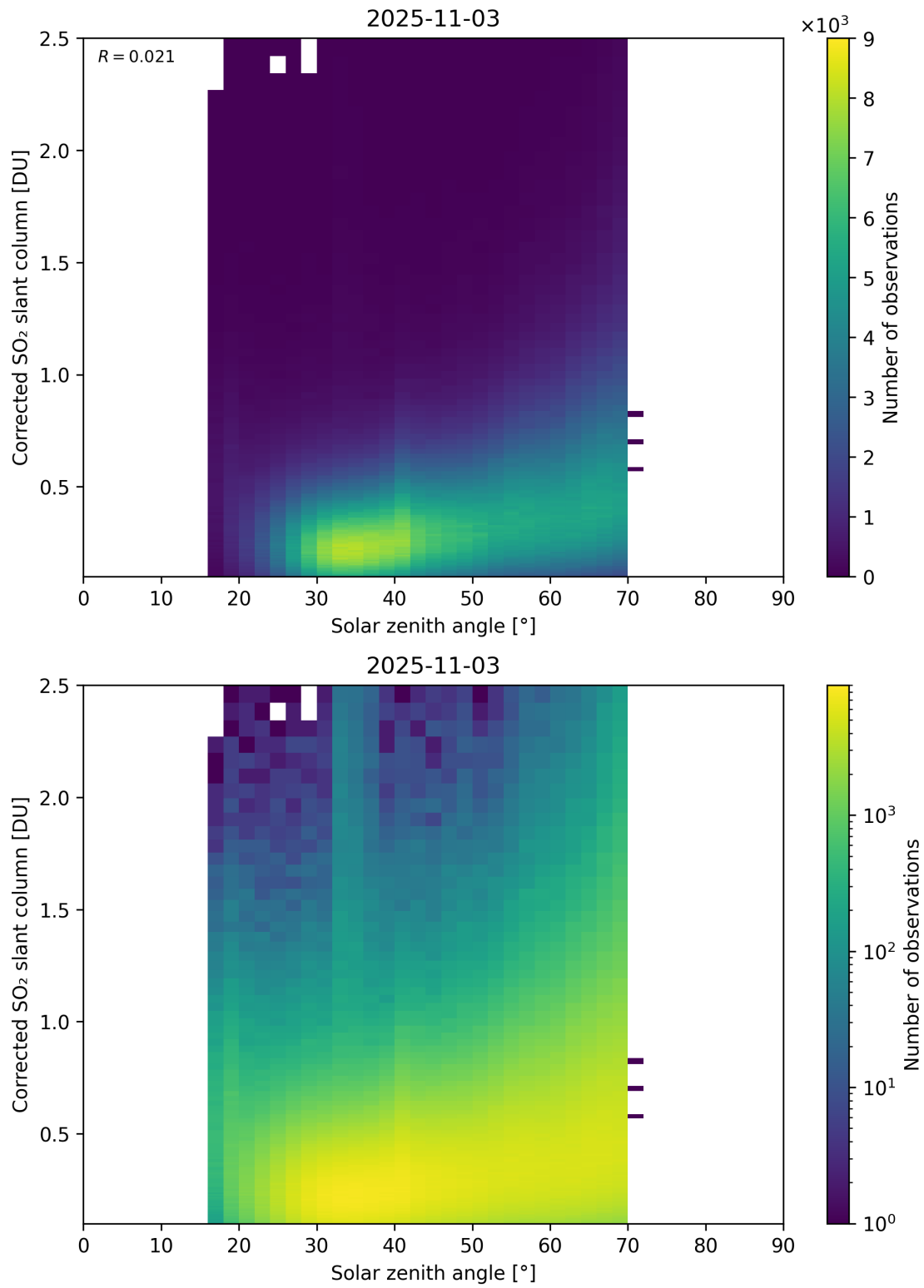
Figure 181: Scatter density plot of “Solar zenith angle” against “Corrected SO 2 slant column” for 2025-11-02 to 2025-11-04.
