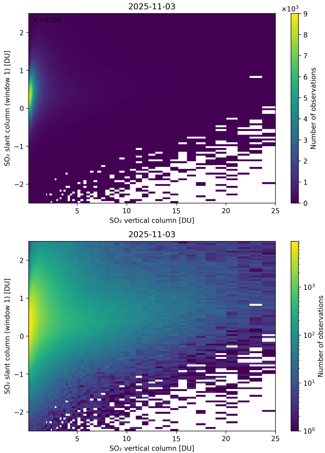
Figure 354: Scatter density plot of “SO 2 vertical column” against “SO 2 slant column (window 1)” for 2025-11-02 to 2025-11-04.
