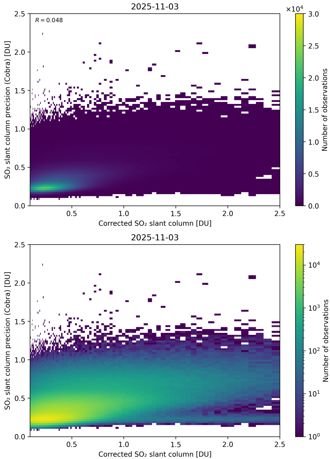
Figure 234: Scatter density plot of “Corrected SO 2 slant column” against “SO 2 slant column precision (Cobra)” for 2025-11-02 to 2025-11-04.
