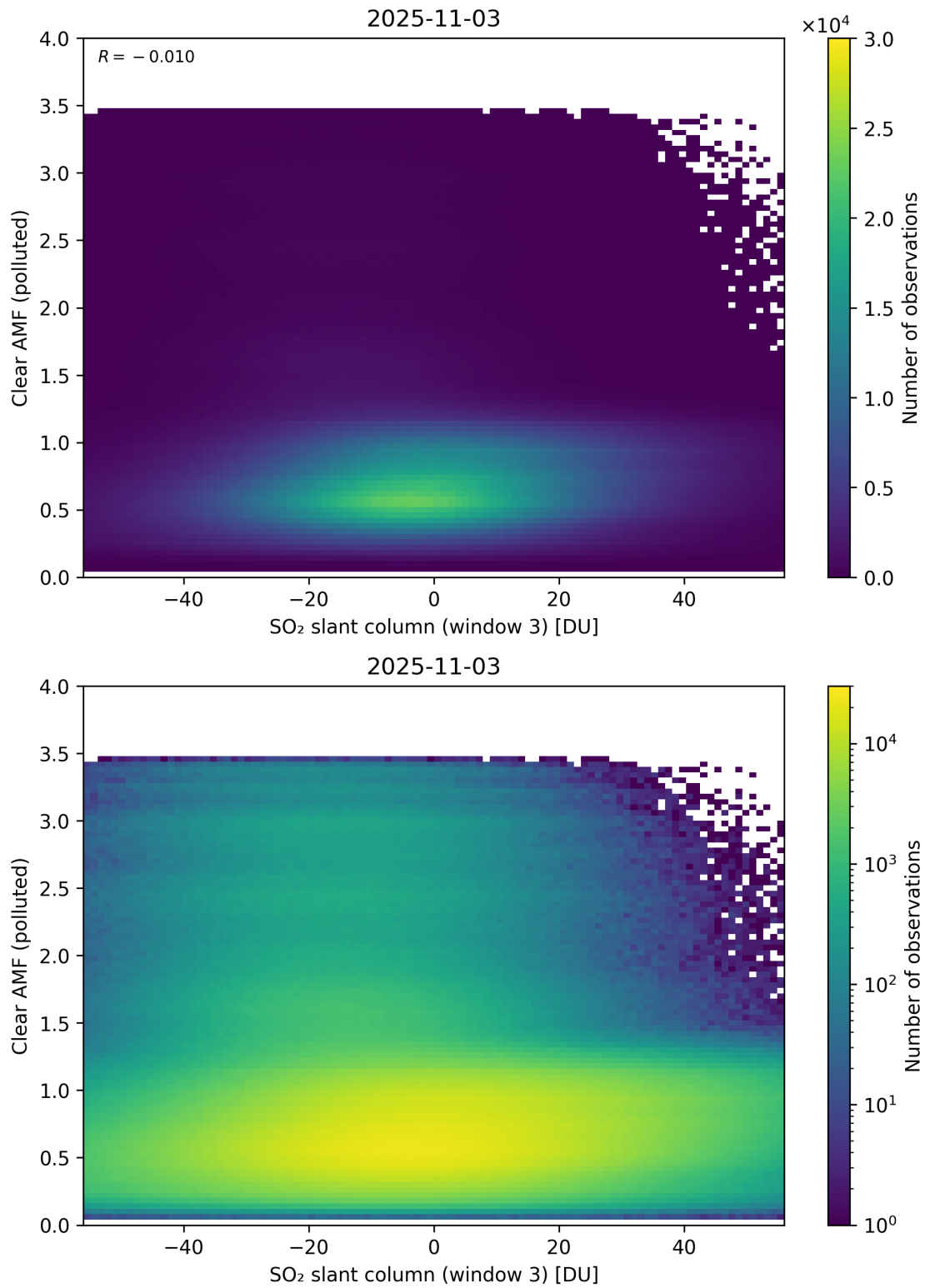
Figure 315: Scatter density plot of “SO 2 slant column (window 3)” against “Clear AMF (polluted)” for 2025-11-02 to 2025-11-04.
