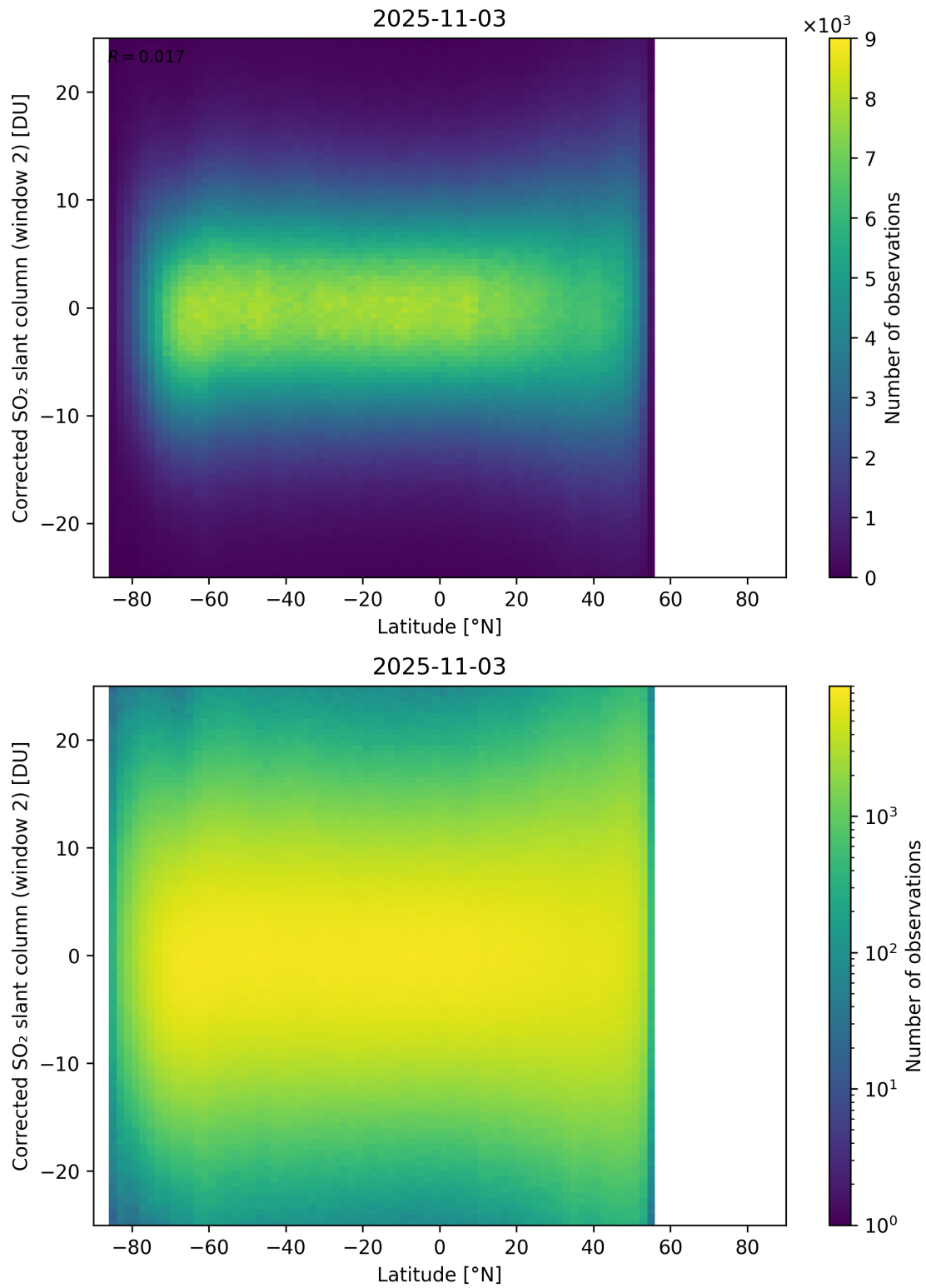
Figure 160: Scatter density plot of “Latitude” against “Corrected SO 2 slant column (window 2)” for 2025-11-02 to 2025-11-04.
