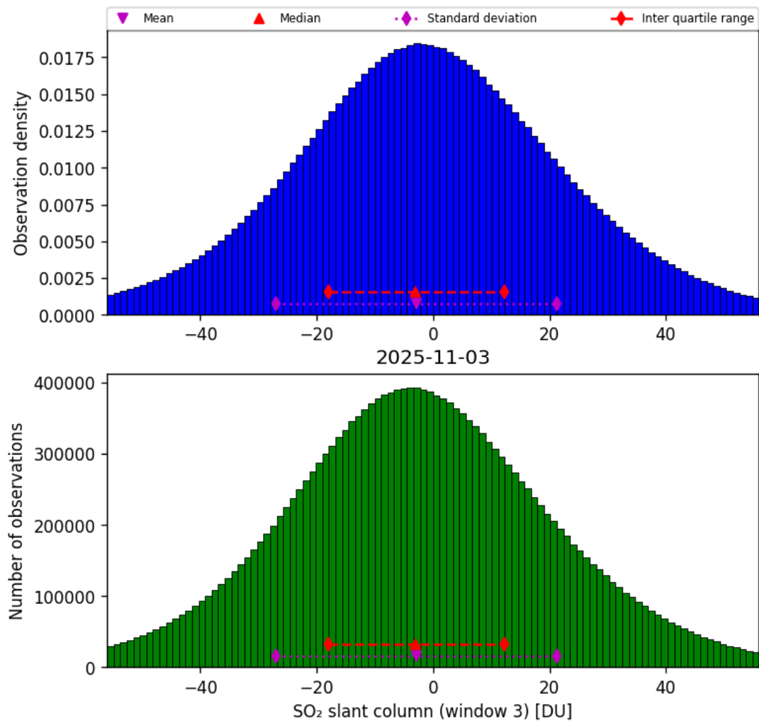
Figure 71: Histogram of “SO 2 slant column (window 3)” for 2025-11-02 to 2025-11-04
