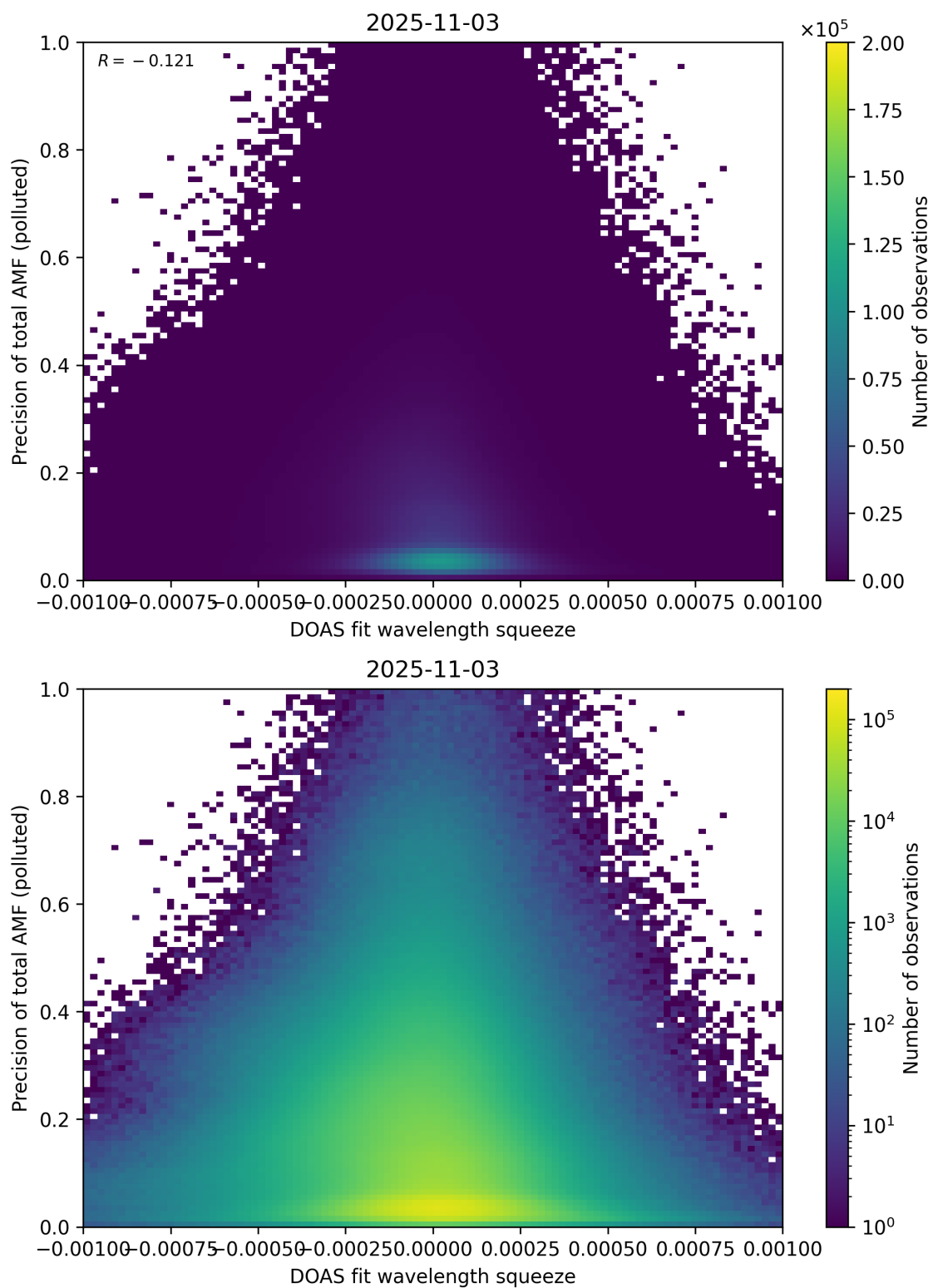
Figure 146: Scatter density plot of “DOAS fit wavelength squeeze” against “Precision of total AMF (polluted)” for 2025-11-02 to 2025-11-04.
