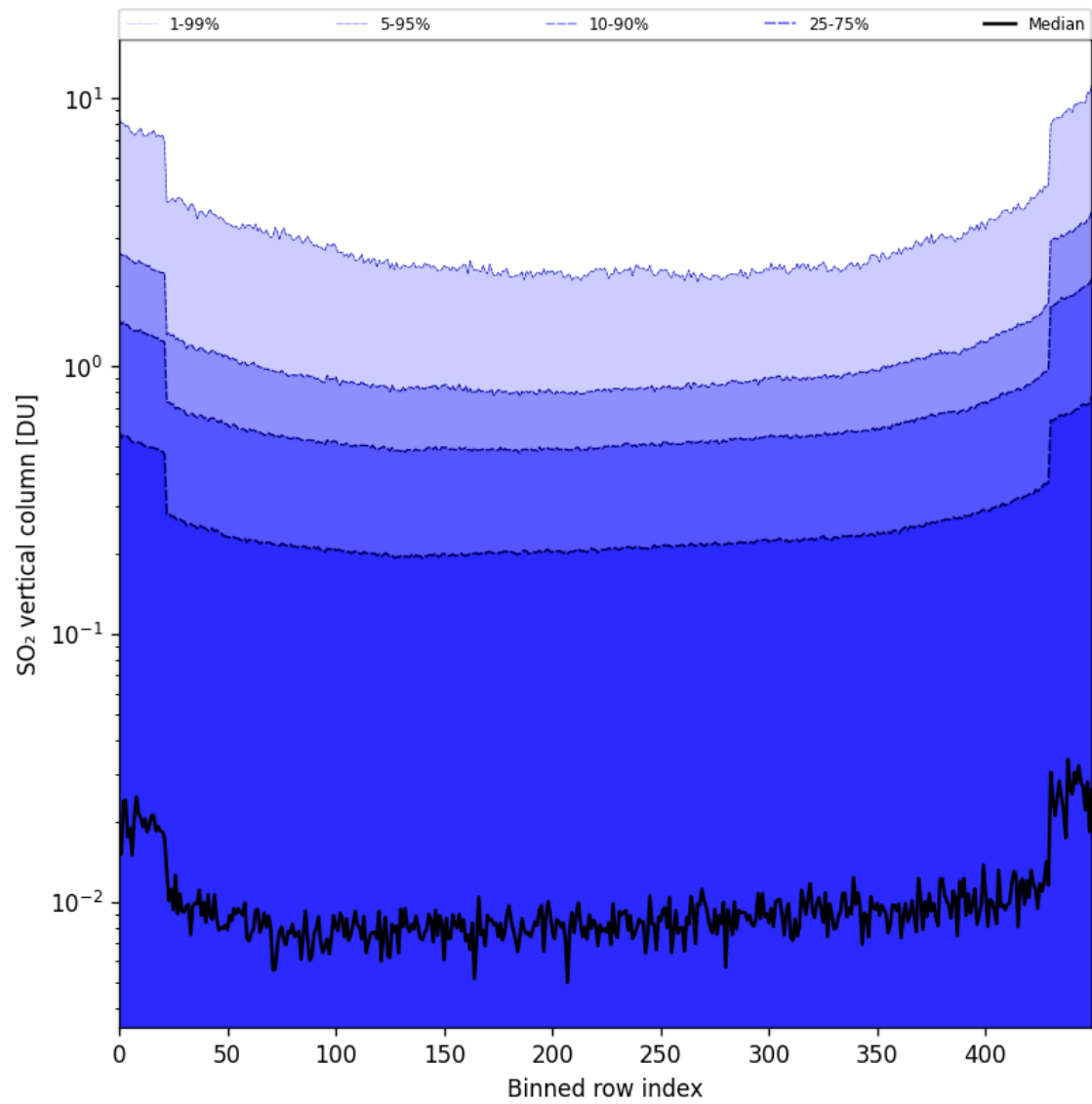
Figure 84: Along track statistics of “SO 2 vertical column” for 2025-11-02 to 2025-11-04
