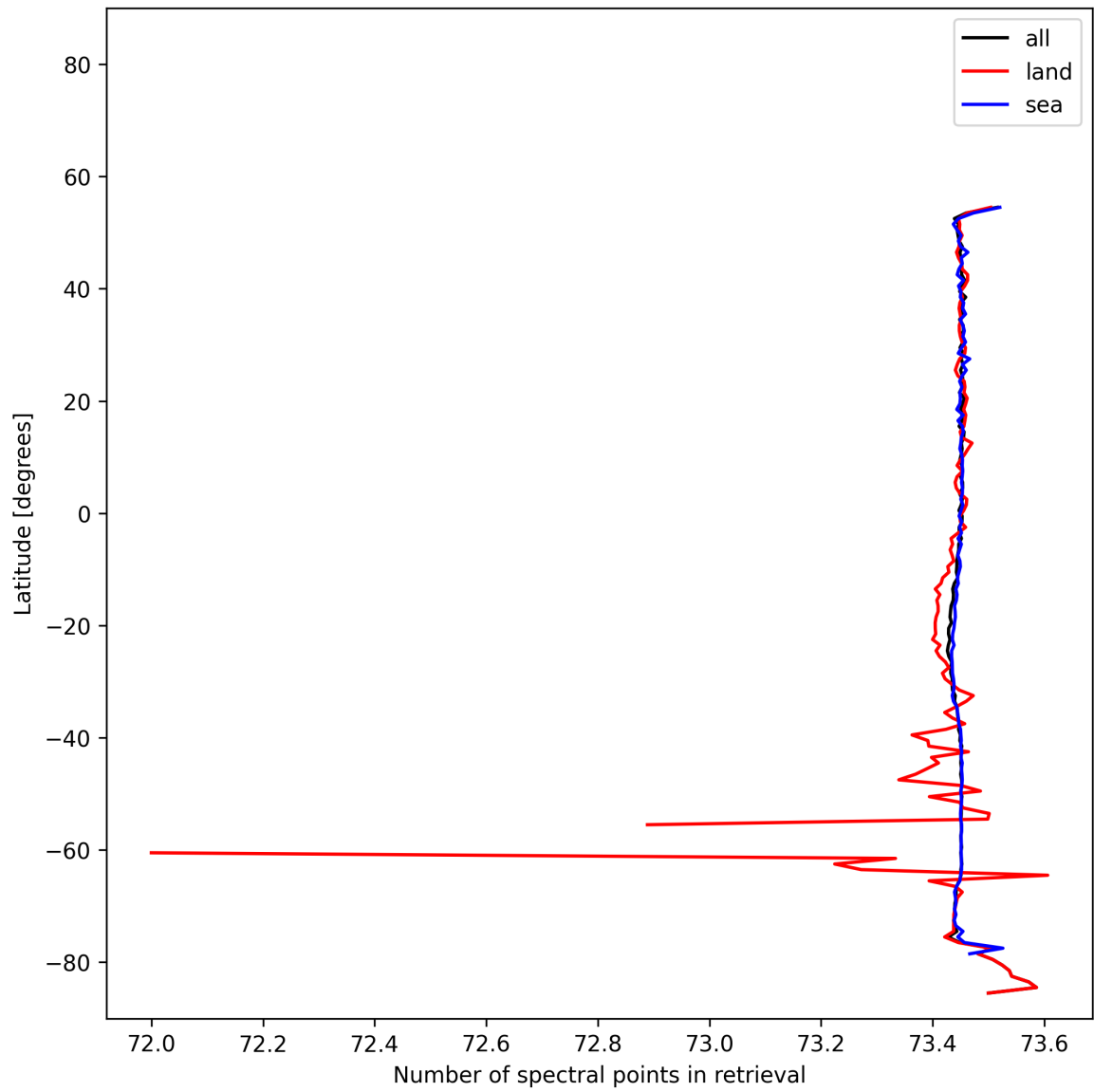
Figure 56: Zonal average of “Number of spectral points in retrieval” for 2025-11-02 to 2025-11-04.
