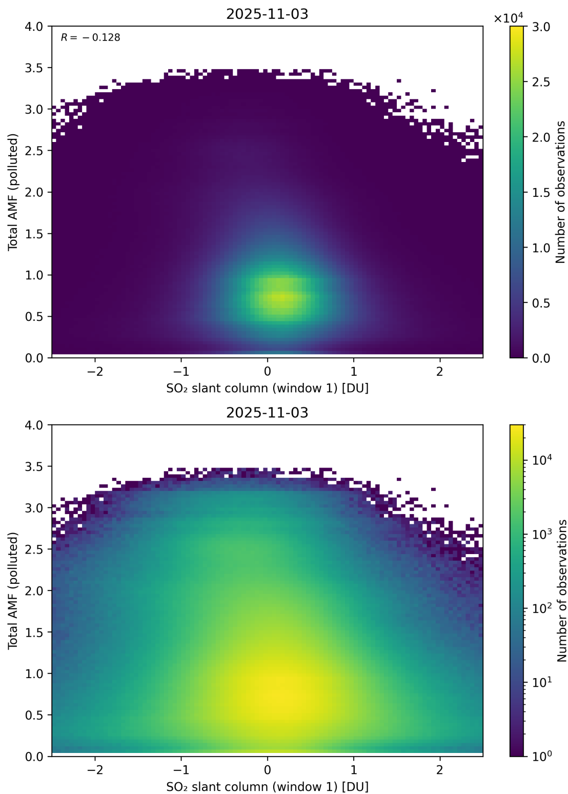
Figure 289: Scatter density plot of “SO 2 slant column (window 1)” against “Total AMF (polluted)” for 2025-11-02 to 2025-11-04.
