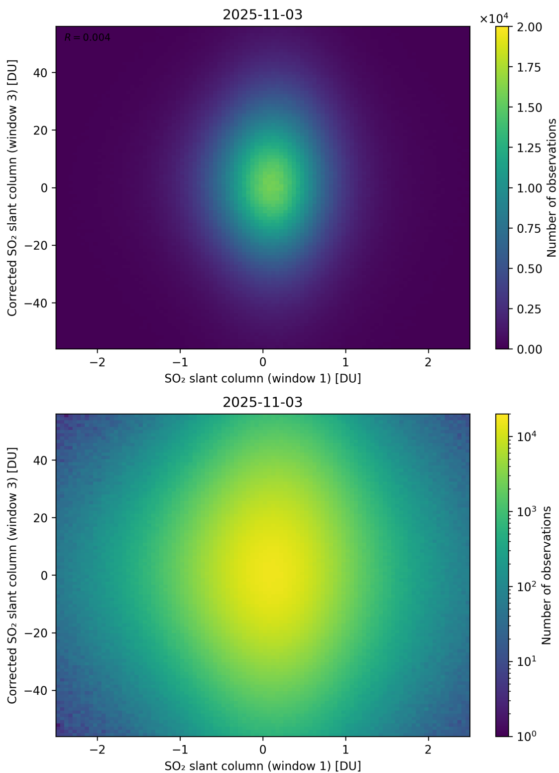
Figure 284: Scatter density plot of “SO 2 slant column (window 1)” against “Corrected SO 2 slant column (window 3)” for 2025-11-02 to 2025-11-04.
