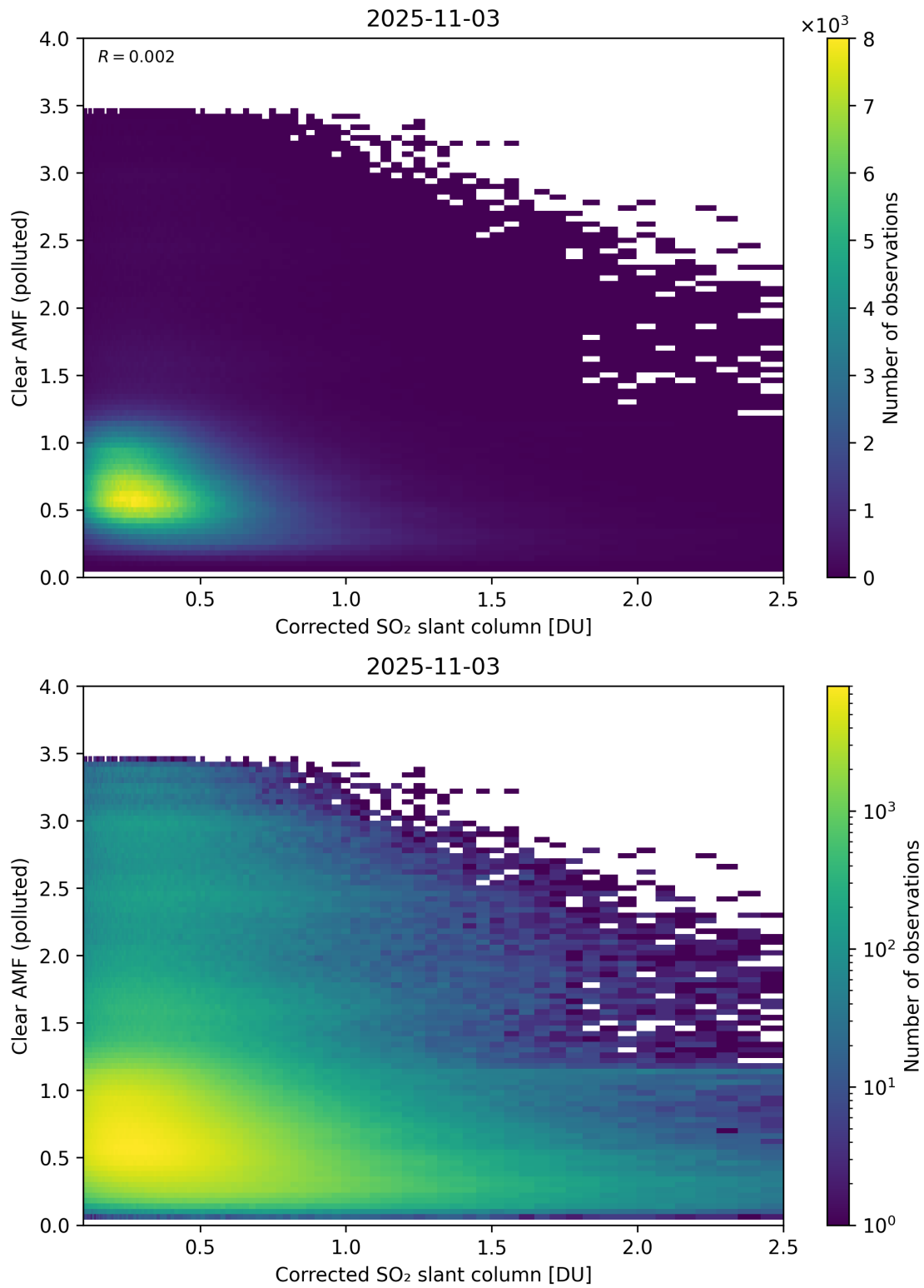
Figure 232: Scatter density plot of “Corrected SO 2 slant column” against “Clear AMF (polluted)” for 2025-11-02 to 2025-11-04.
