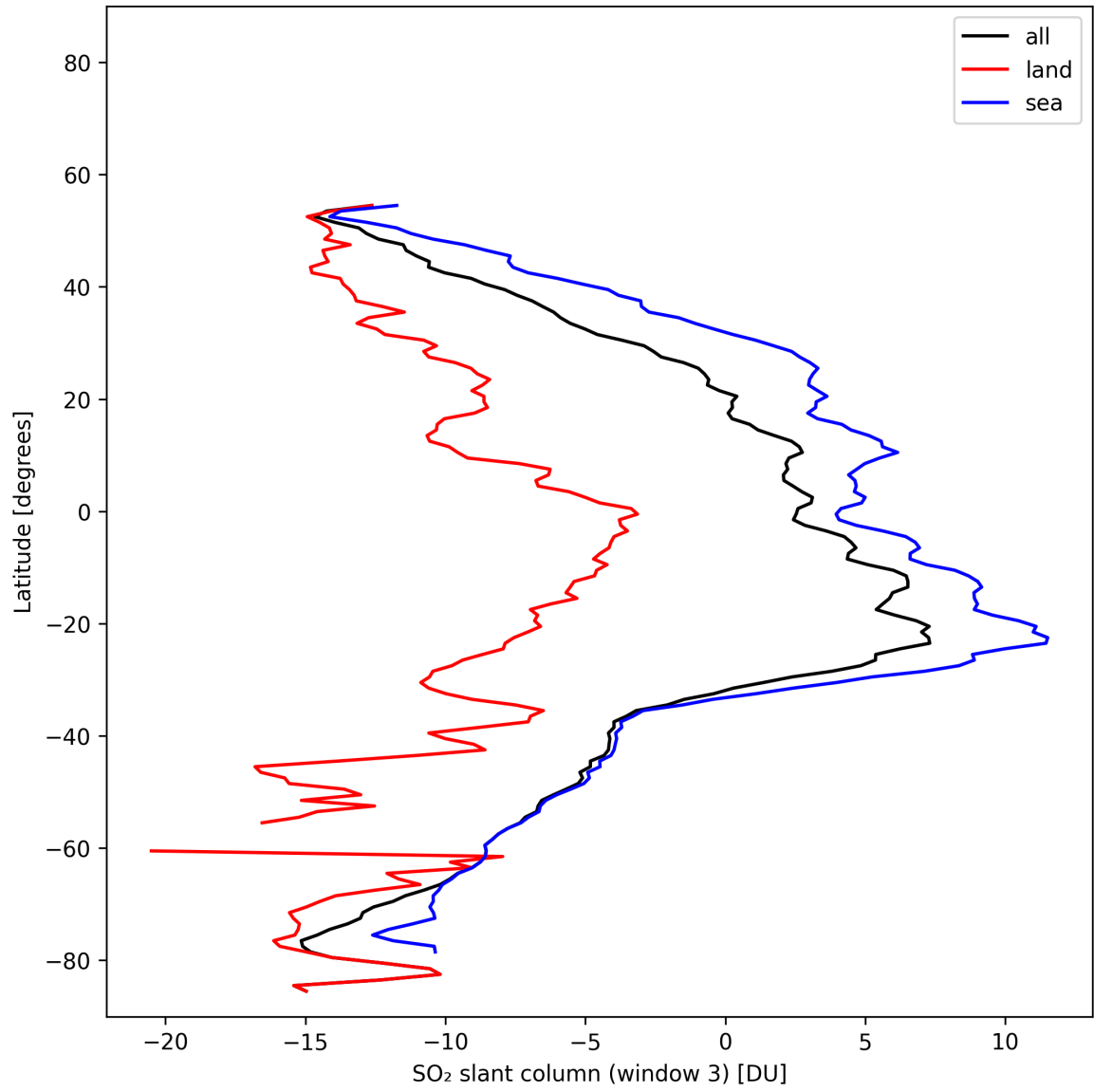
Figure 45: Zonal average of “SO 2 slant column (window 3)” for 2025-11-02 to 2025-11-04.
