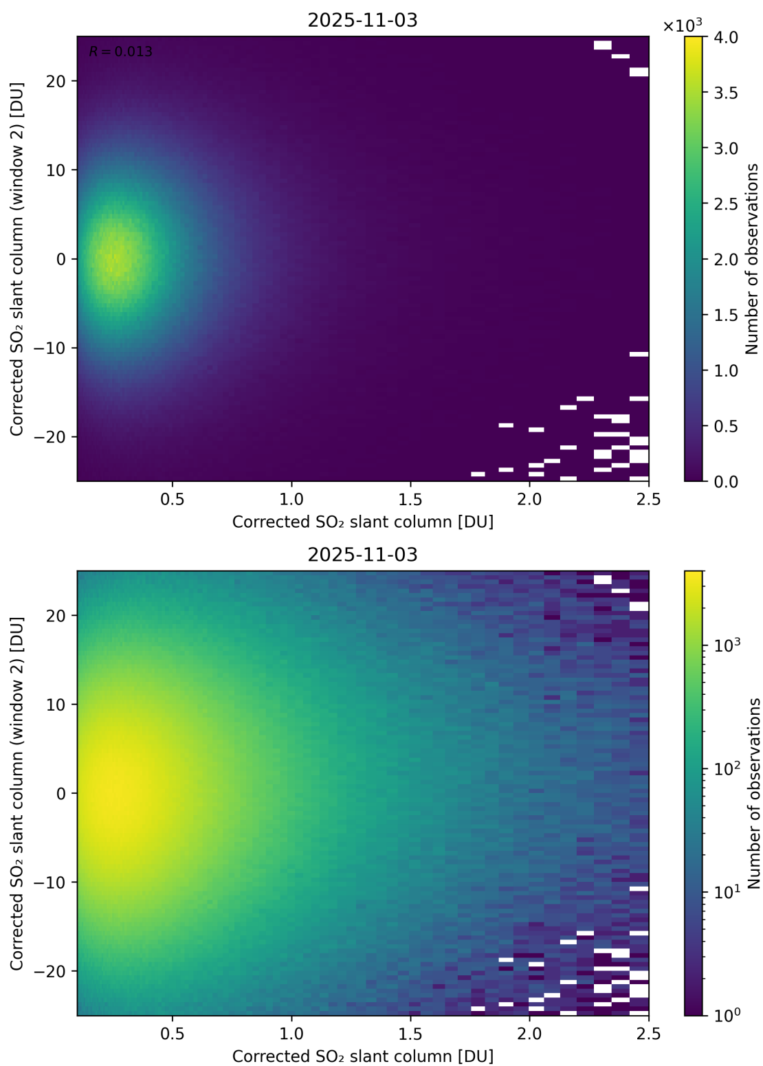
Figure 235: Scatter density plot of “Corrected SO 2 slant column” against “Corrected SO 2 slant column (window 2)” for 2025-11-02 to 2025-11-04.
