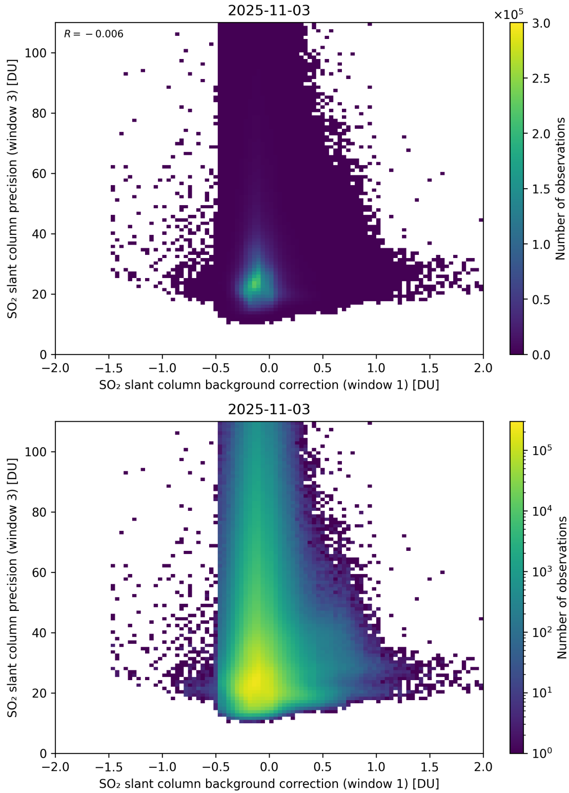
Figure 119: Scatter density plot of “SO 2 slant column background correction (window 1)” against “SO 2 slant column precision (window 3)” for 2025-11-02 to 2025-11-04.
