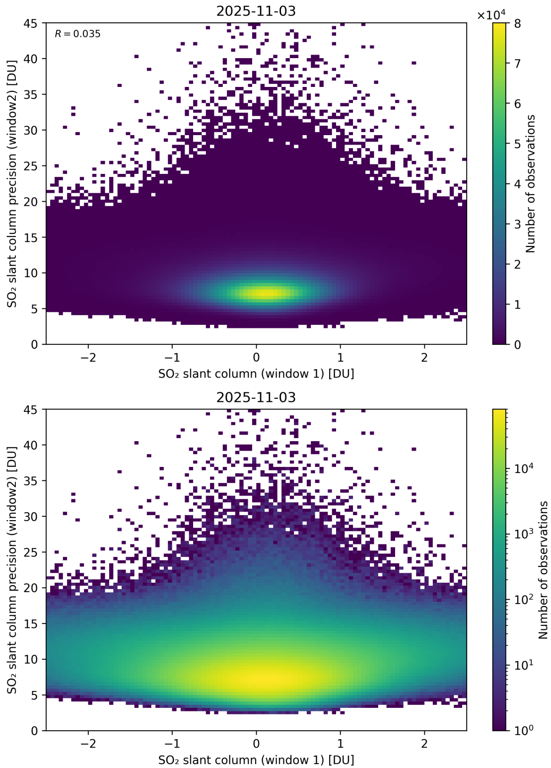
Figure 286: Scatter density plot of “SO 2 slant column (window 1)” against “SO 2 slant column precision (window2)” for 2025-11-02 to 2025-11-04.
