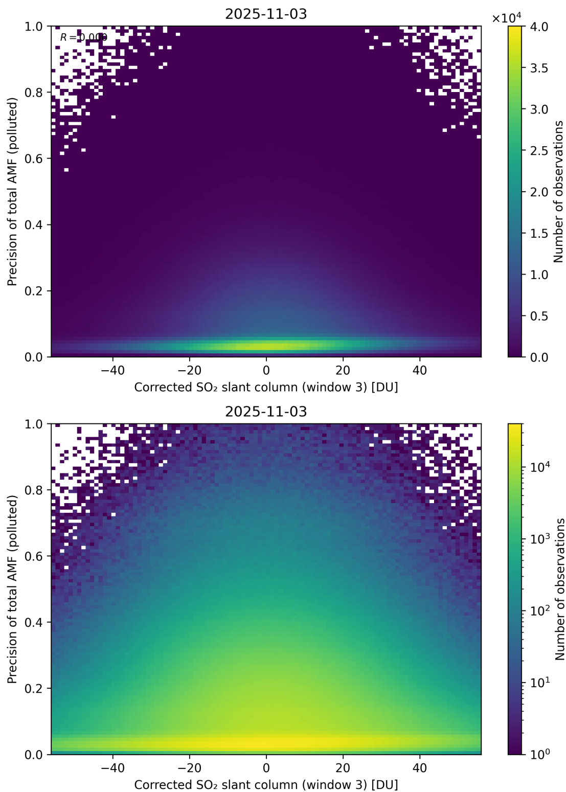
Figure 261: Scatter density plot of “Corrected SO 2 slant column (window 3)” against “Precision of total AMF (polluted)” for 2025-11-02 to 2025-11-04.
