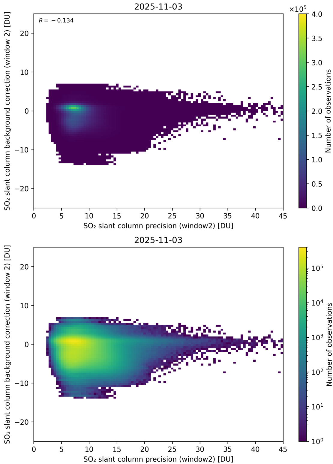
Figure 291: Scatter density plot of “SO 2 slant column precision (window2)” against “SO 2 slant column background correction (window 2)” for 2025-11-02 to 2025-11-04.
