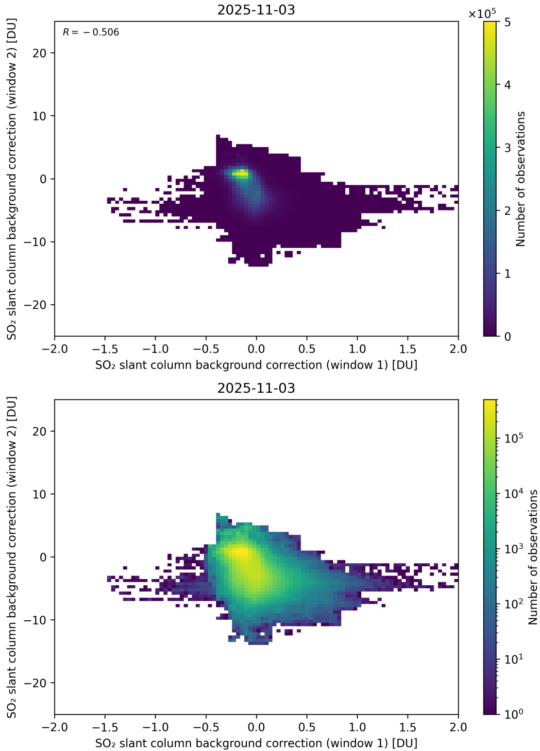
Figure 109: Scatter density plot of “SO 2 slant column background correction (window 1)” against “SO 2 slant column background correction (window 2)” for 2025-11-02 to 2025-11-04.
