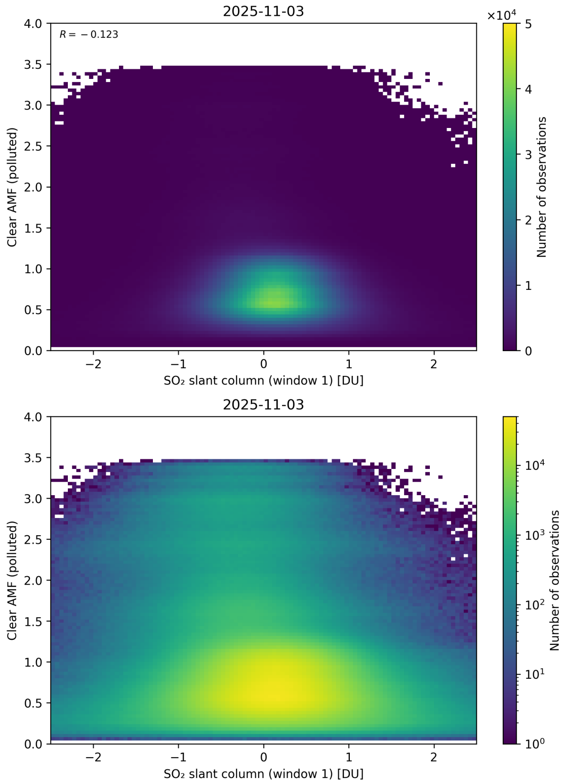
Figure 282: Scatter density plot of “SO 2 slant column (window 1)” against “Clear AMF (polluted)” for 2025-11-02 to 2025-11-04.
