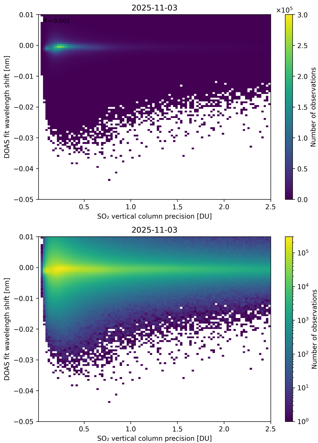
Figure 332: Scatter density plot of “SO 2 vertical column precision” against “DOAS fit wavelength shift” for 2025-11-02 to 2025-11-04.
