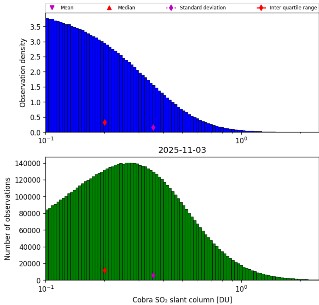
Figure 61: Histogram of “Cobra SO 2 slant column” for 2025-11-02 to 2025-11-04
