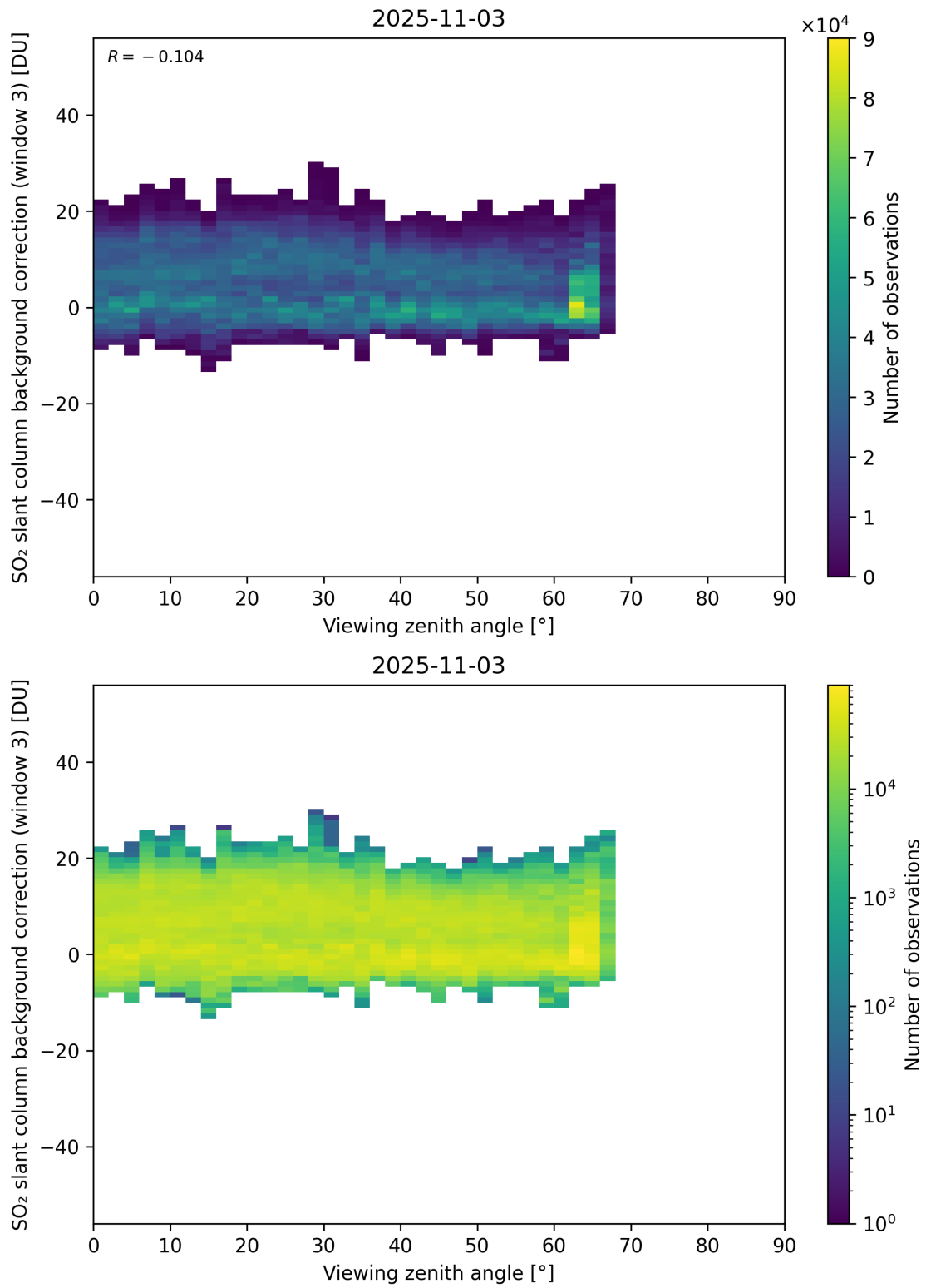
Figure 364: Scatter density plot of “Viewing zenith angle” against “SO 2 slant column background correction (window 3)” for 2025-11-02 to 2025-11-04.
