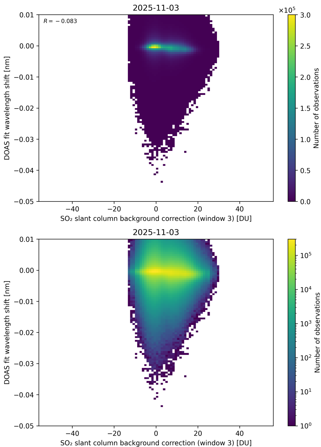
Figure 132: Scatter density plot of “SO 2 slant column background correction (window 3)” against “DOAS fit wavelength shift” for 2025-11-02 to 2025-11-04.
