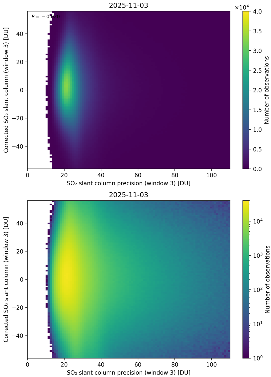
Figure 312: Scatter density plot of “SO 2 slant column precision (window 3)” against “Corrected SO 2 slant column (window 3)” for 2025-11-02 to 2025-11-04.
