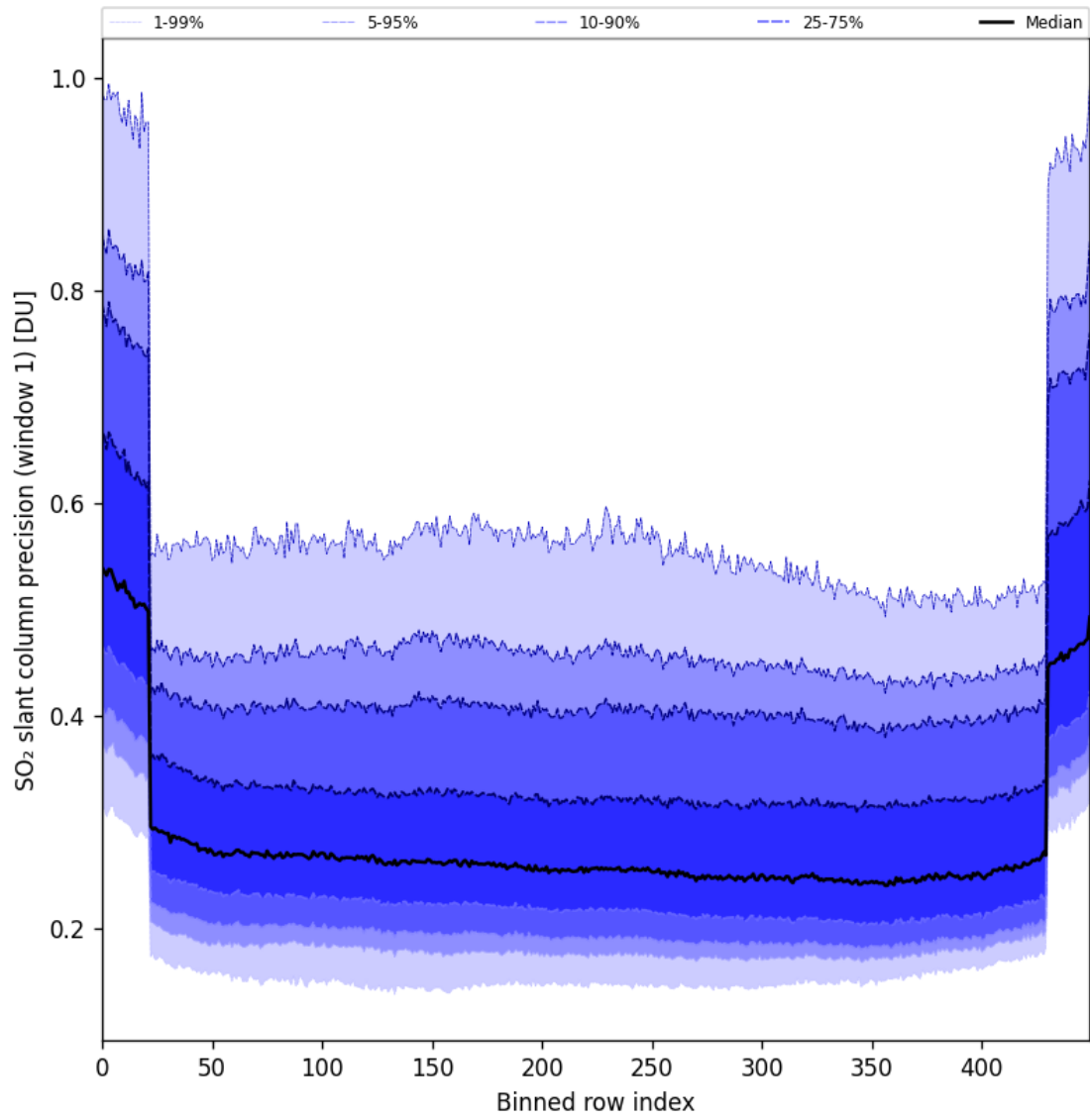
Figure 90: Along track statistics of “SO 2 slant column precision (window 1)” for 2025-11-02 to 2025-11-04
