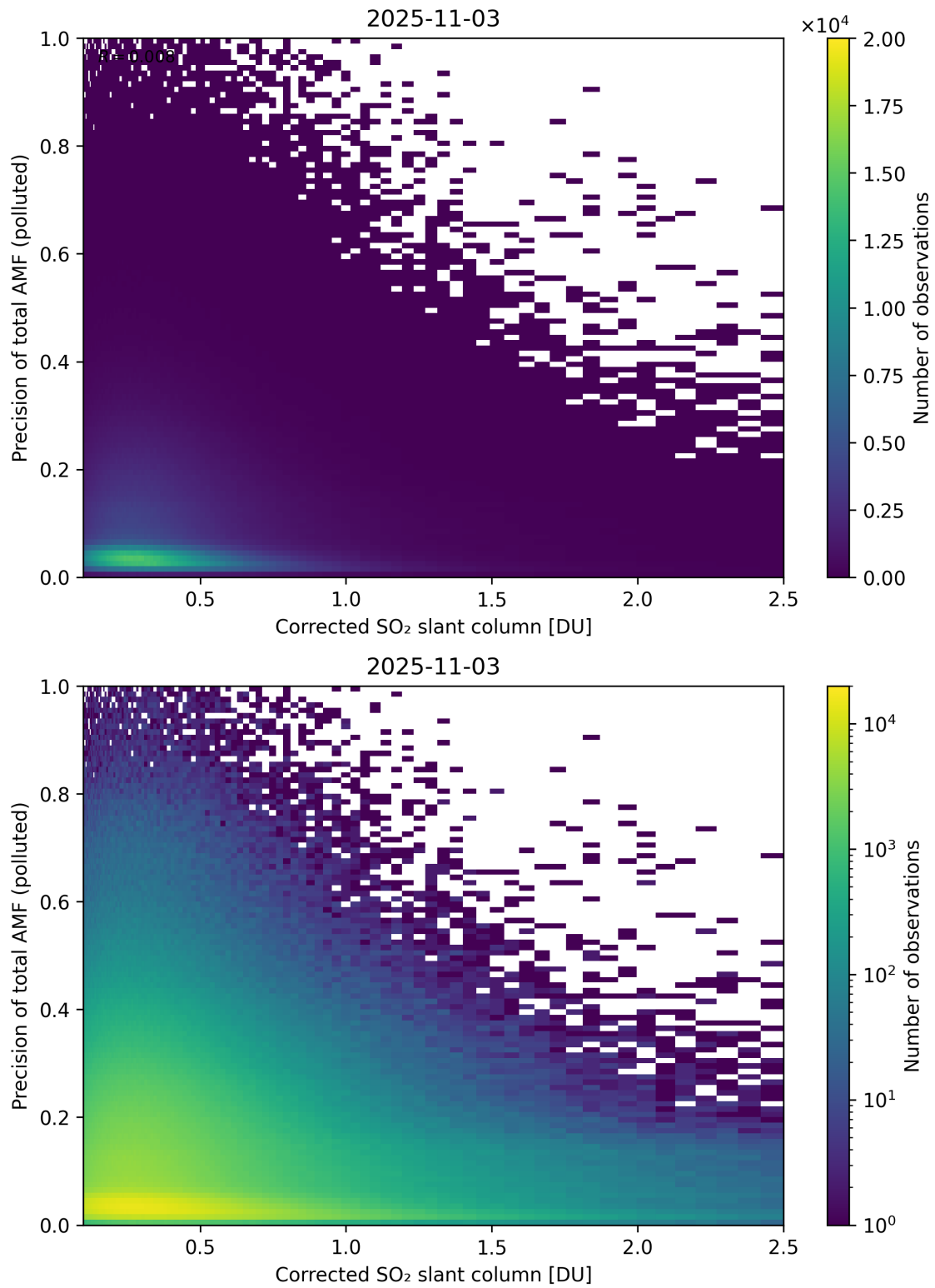
Figure 243: Scatter density plot of “Corrected SO 2 slant column” against “Precision of total AMF (polluted)” for 2025-11-02 to 2025-11-04.
