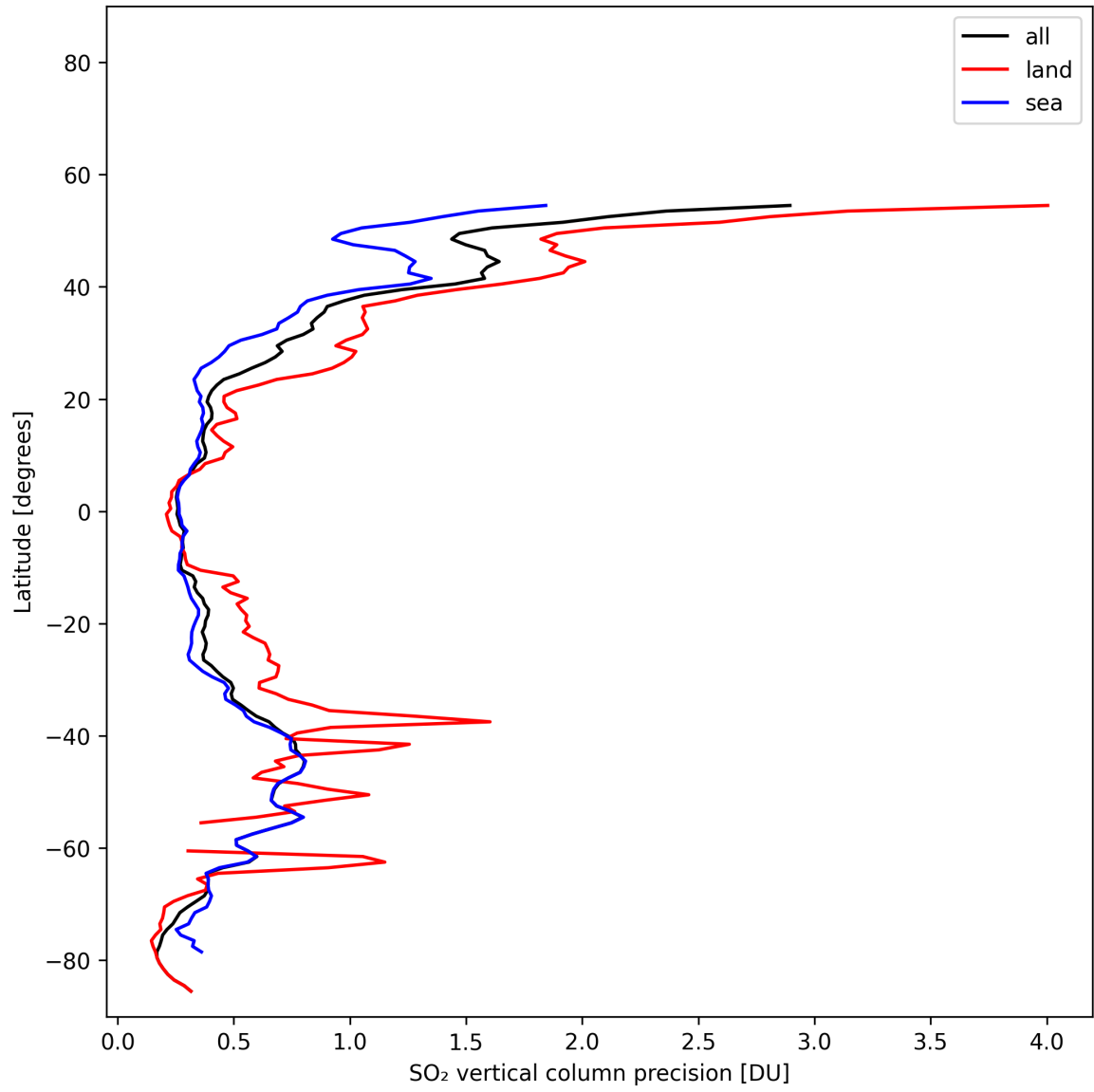
Figure 33: Zonal average of “SO 2 vertical column precision” for 2025-11-02 to 2025-11-04.
