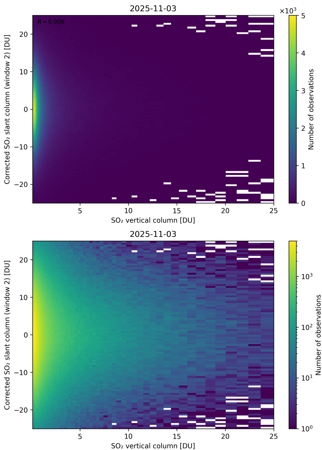
Figure 352: Scatter density plot of “SO 2 vertical column” against “Corrected SO 2 slant column (window 2)” for 2025-11-02 to 2025-11-04.
