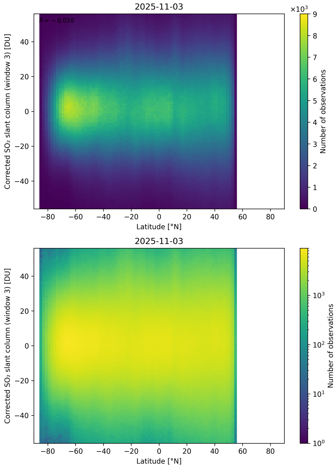
Figure 161: Scatter density plot of “Latitude” against “Corrected SO 2 slant column (window 3)” for 2025-11-02 to 2025-11-04.
