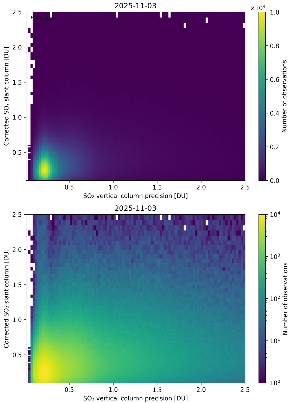
Figure 338: Scatter density plot of “SO 2 vertical column precision” against “Corrected SO 2 slant column” for 2025-11-02 to 2025-11-04.
