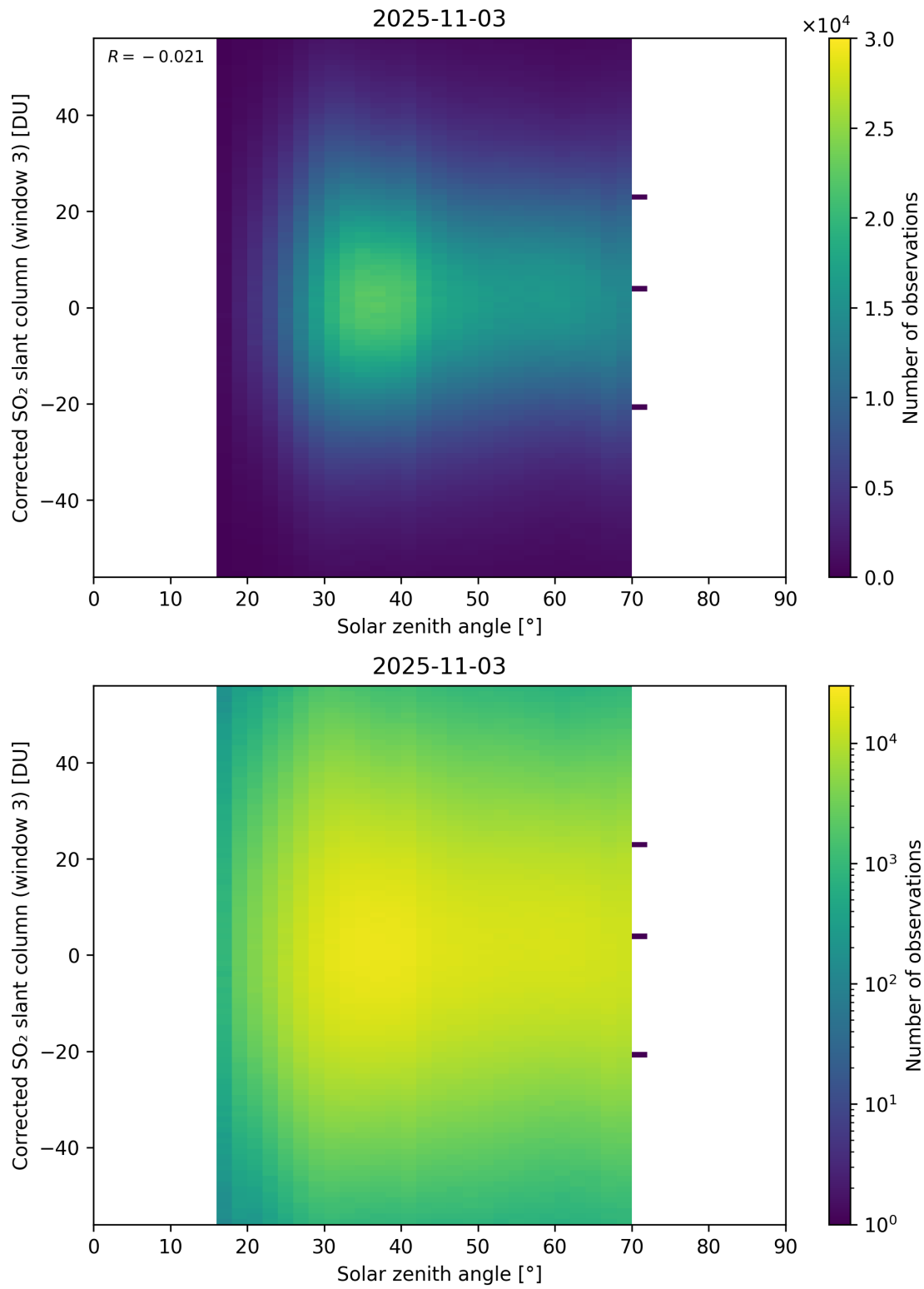
Figure 183: Scatter density plot of “Solar zenith angle” against “Corrected SO 2 slant column (window 3)” for 2025-11-02 to 2025-11-04.
