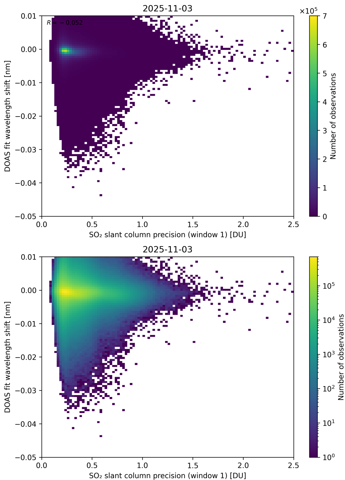
Figure 271: Scatter density plot of “SO 2 slant column precision (window 1)” against “DOAS fit wavelength shift” for 2025-11-02 to 2025-11-04.
