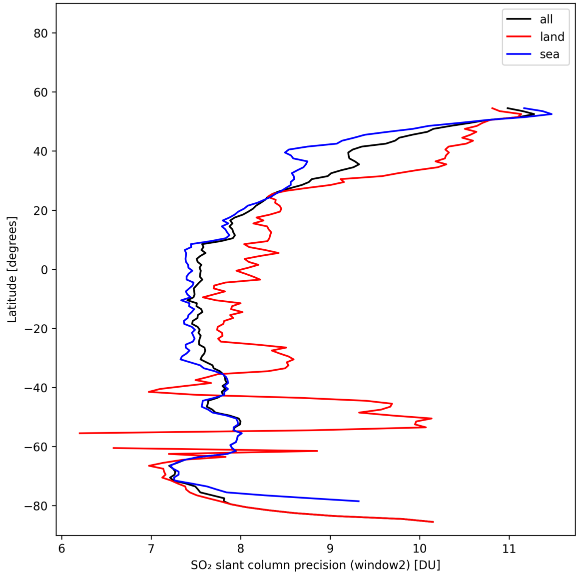
Figure 42: Zonal average of “SO 2 slant column precision (window2)” for 2025-11-02 to 2025-11-04.
