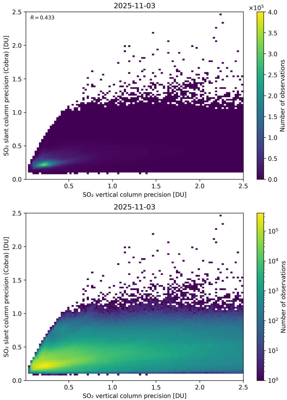
Figure 337: Scatter density plot of “SO 2 vertical column precision” against “SO 2 slant column precision (Cobra)” for 2025-11-02 to 2025-11-04.
