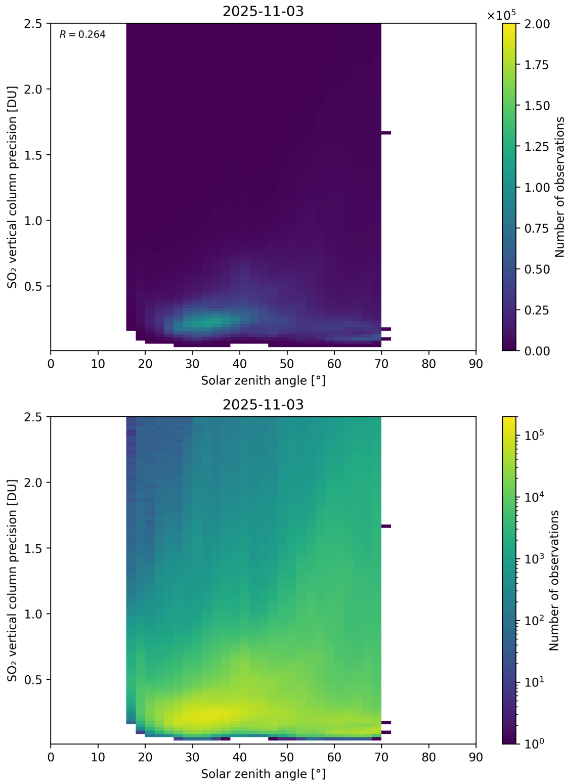
Figure 192: Scatter density plot of “Solar zenith angle” against “SO 2 vertical column precision” for 2025-11-02 to 2025-11-04.
