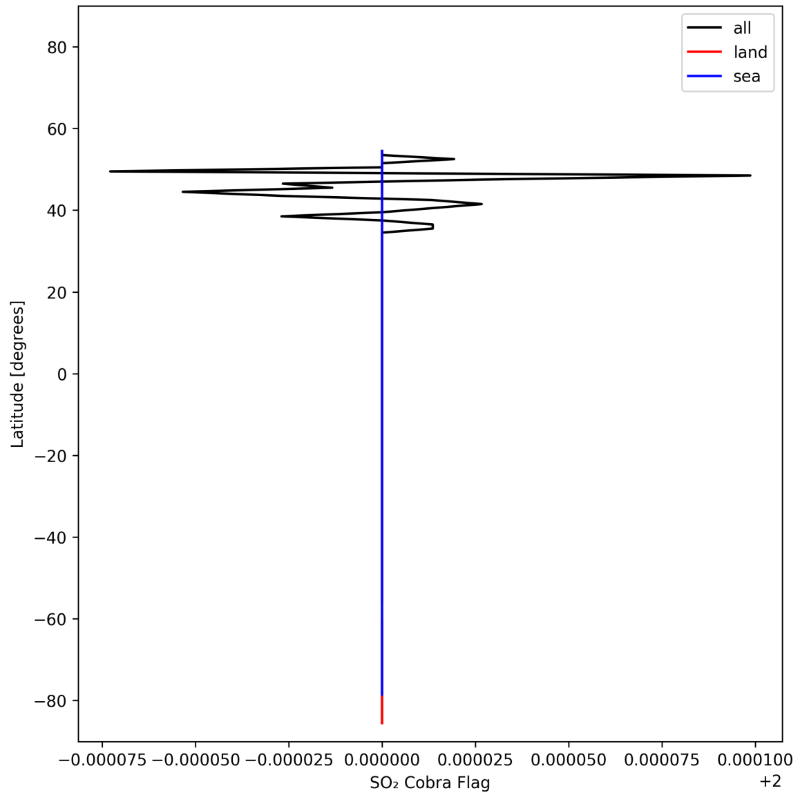
Figure 49: Zonal average of “SO 2 Cobra Flag” for 2025-11-02 to 2025-11-04.
