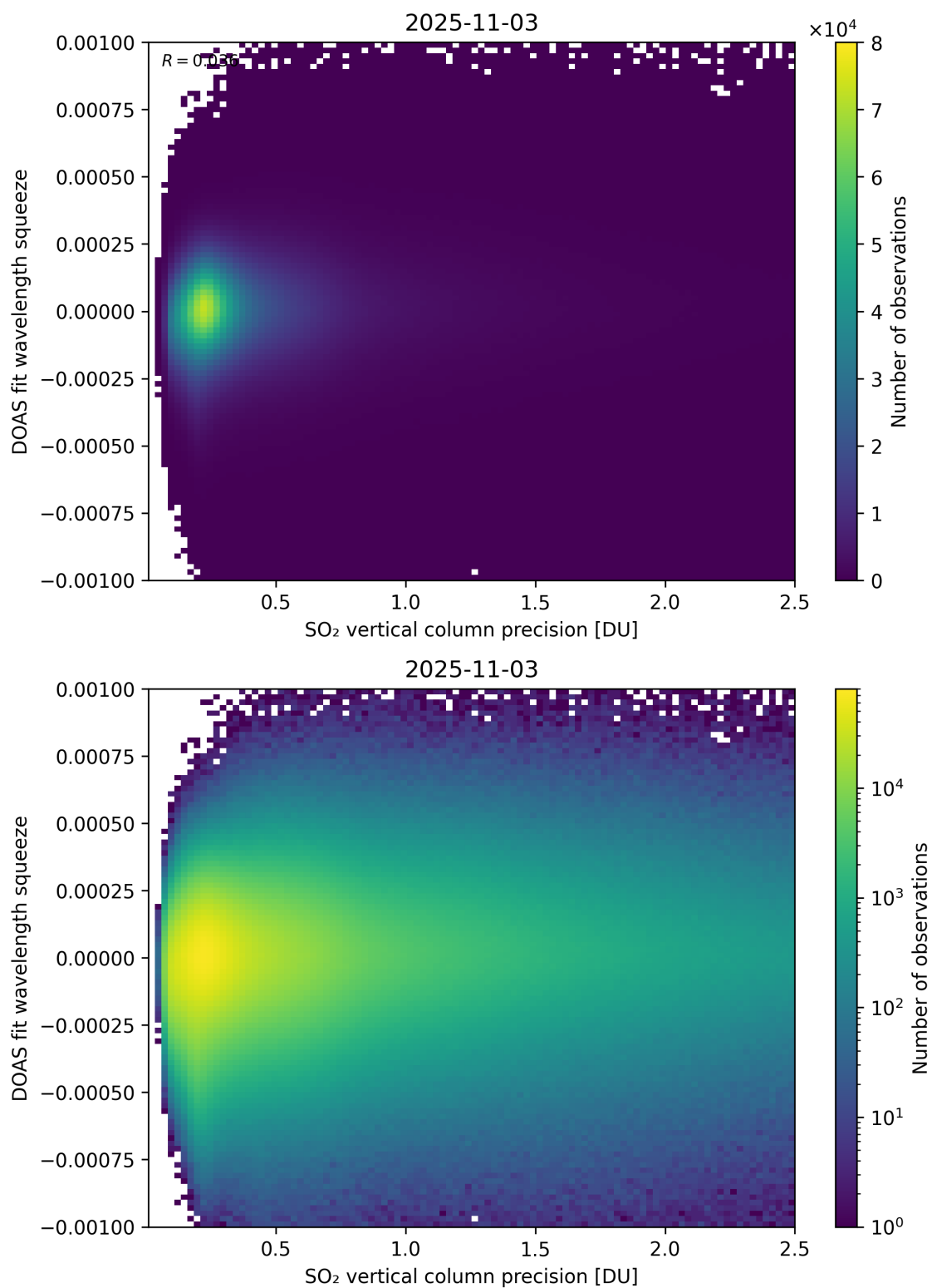
Figure 333: Scatter density plot of “SO 2 vertical column precision” against “DOAS fit wavelength squeeze” for 2025-11-02 to 2025-11-04.
