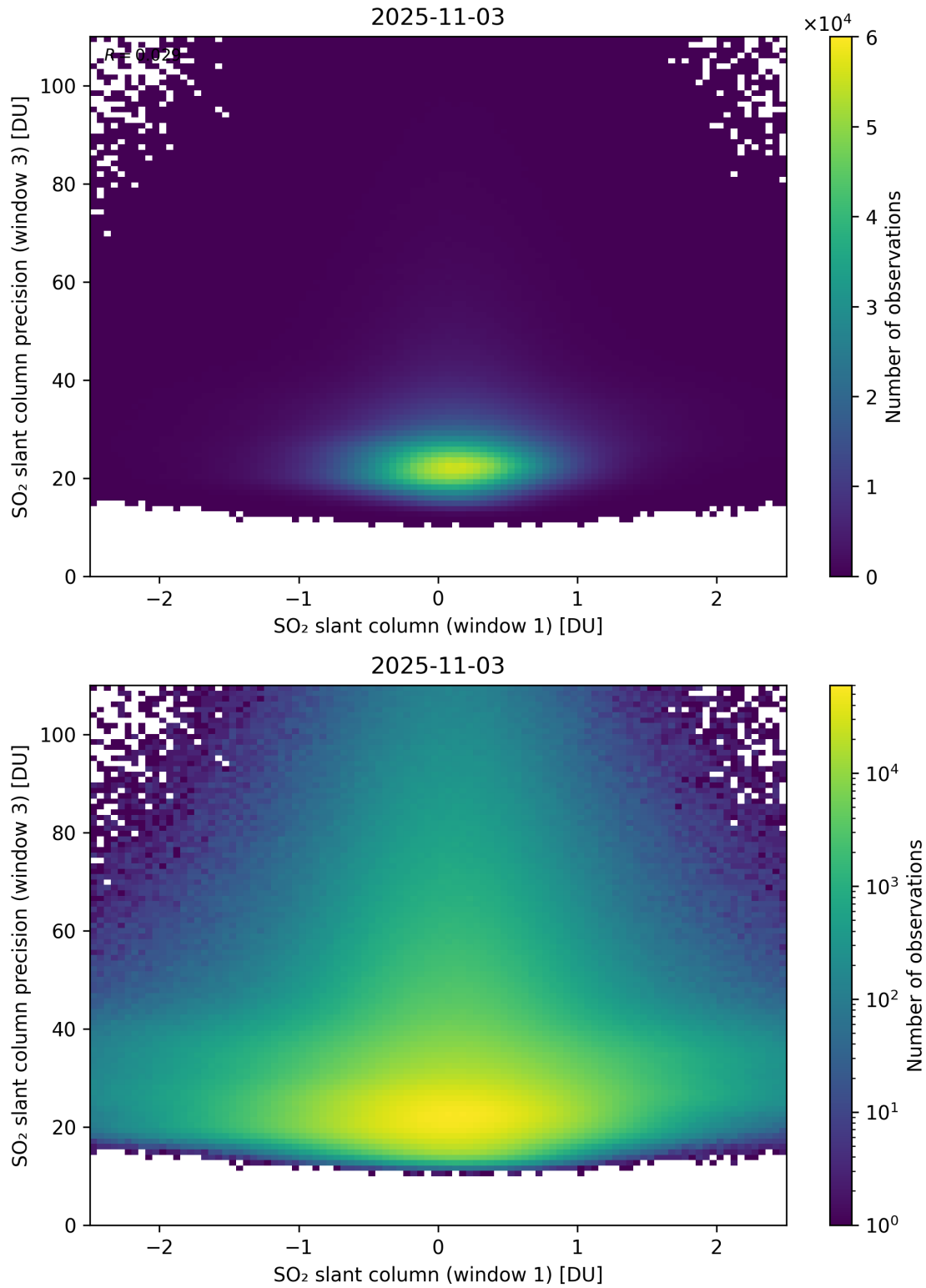
Figure 288: Scatter density plot of “SO 2 slant column (window 1)” against “SO 2 slant column precision (window 3)” for 2025-11-02 to 2025-11-04.
