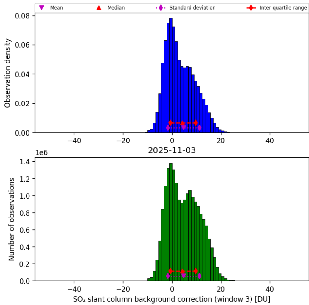
Figure 74: Histogram of “SO 2 slant column background correction (window 3)” for 2025-11-02 to 2025-11-04
