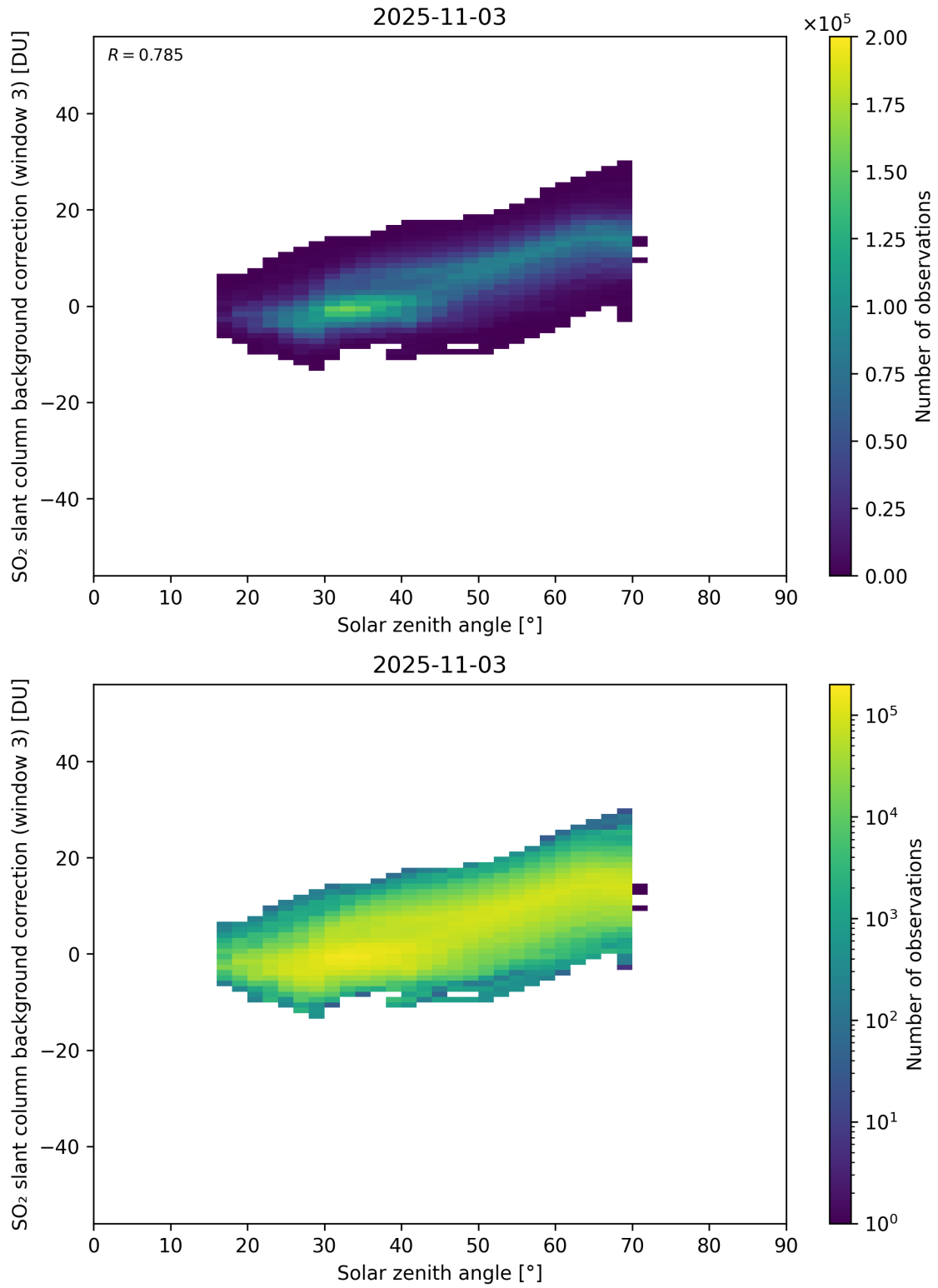
Figure 173: Scatter density plot of “Solar zenith angle” against “SO 2 slant column background correction (window 3)” for 2025-11-02 to 2025-11-04.
