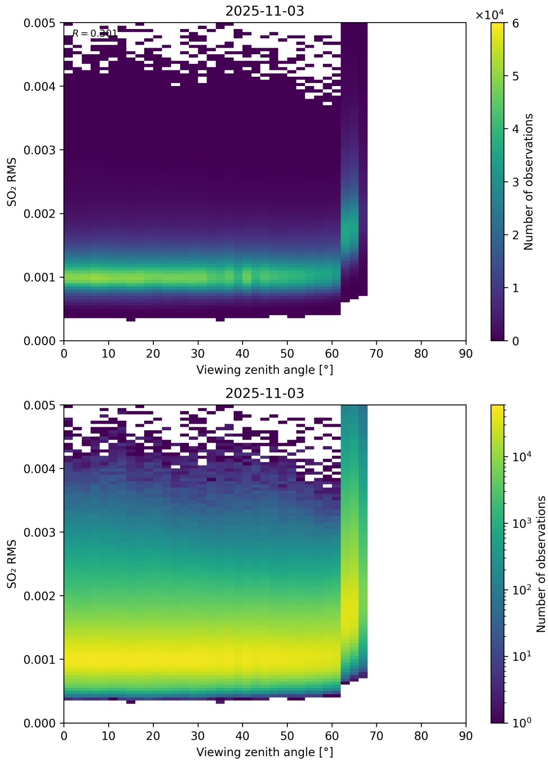
Figure 367: Scatter density plot of “Viewing zenith angle” against “SO 2 RMS” for 2025-11-02 to 2025-11-04.
