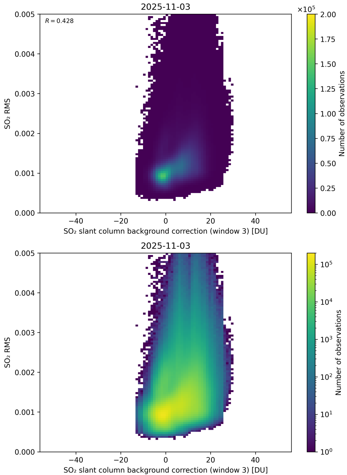
Figure 134: Scatter density plot of “SO 2 slant column background correction (window 3)” against “SO 2 RMS” for 2025-11-02 to 2025-11-04.
