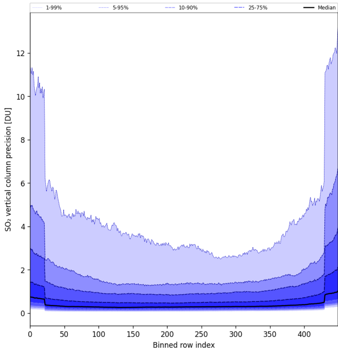
Figure 85: Along track statistics of “SO 2 vertical column precision” for 2025-11-02 to 2025-11-04
