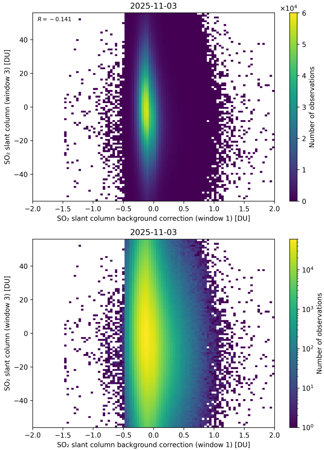
Figure 118: Scatter density plot of “SO 2 slant column background correction (window 1)” against “SO 2 slant column (window 3)” for 2025-11-02 to 2025-11-04.
