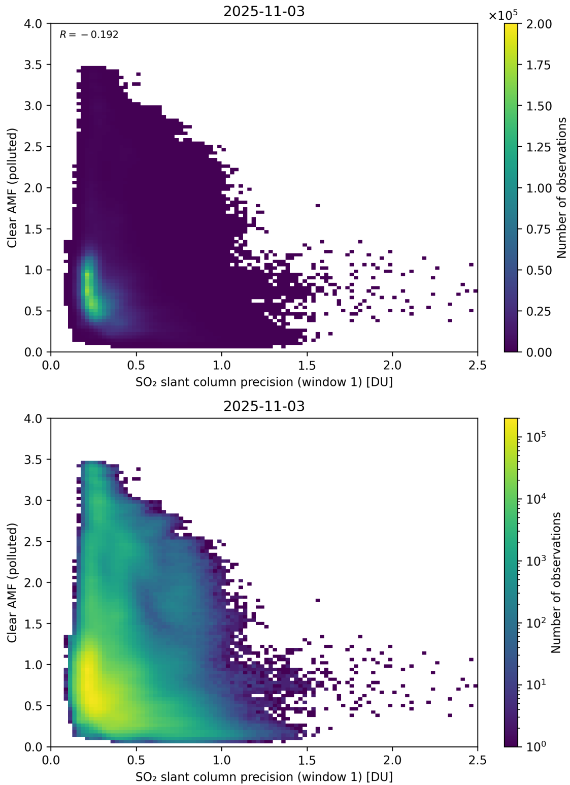
Figure 274: Scatter density plot of “SO 2 slant column precision (window 1)” against “Clear AMF (polluted)” for 2025-11-02 to 2025-11-04.
