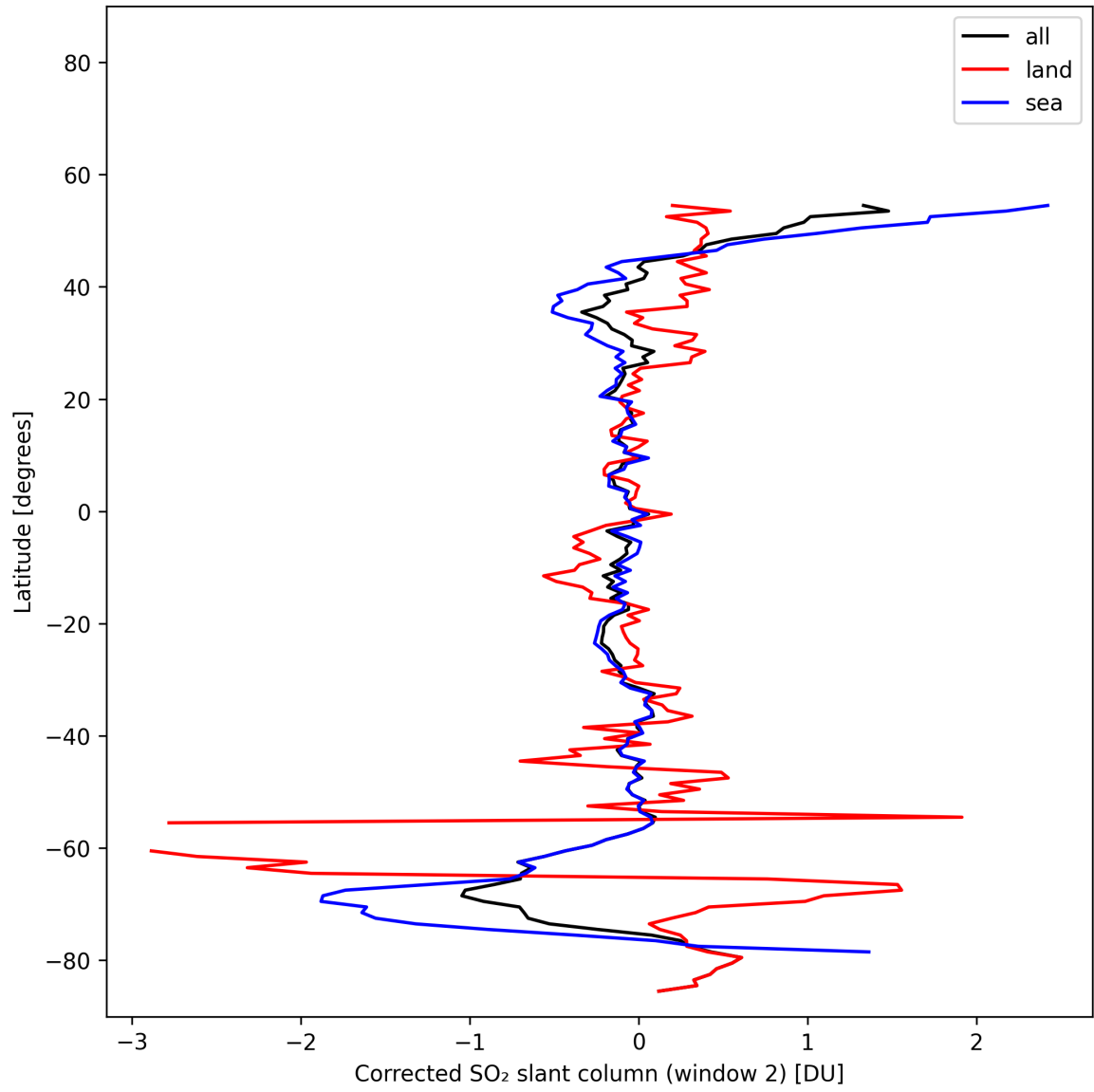
Figure 43: Zonal average of “Corrected SO 2 slant column (window 2)” for 2025-11-02 to 2025-11-04.
