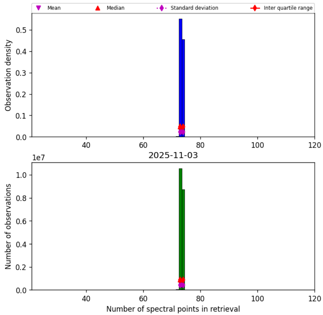
Figure 82: Histogram of “Number of spectral points in retrieval” for 2025-11-02 to 2025-11-04
