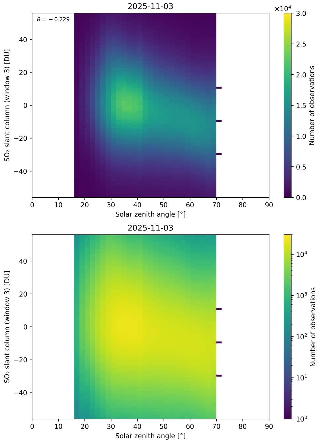
Figure 187: Scatter density plot of “Solar zenith angle” against “SO 2 slant column (window 3)” for 2025-11-02 to 2025-11-04.
