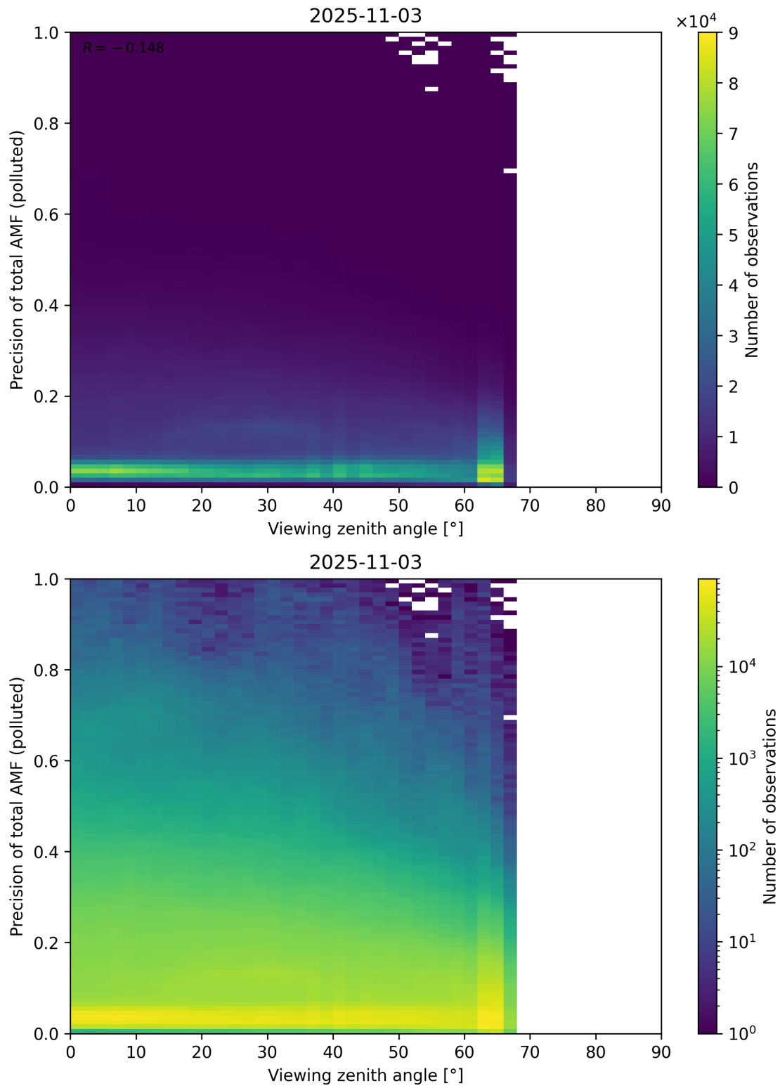
Figure 382: Scatter density plot of “Viewing zenith angle” against “Precision of total AMF (polluted)” for 2025-11-02 to 2025-11-04.
