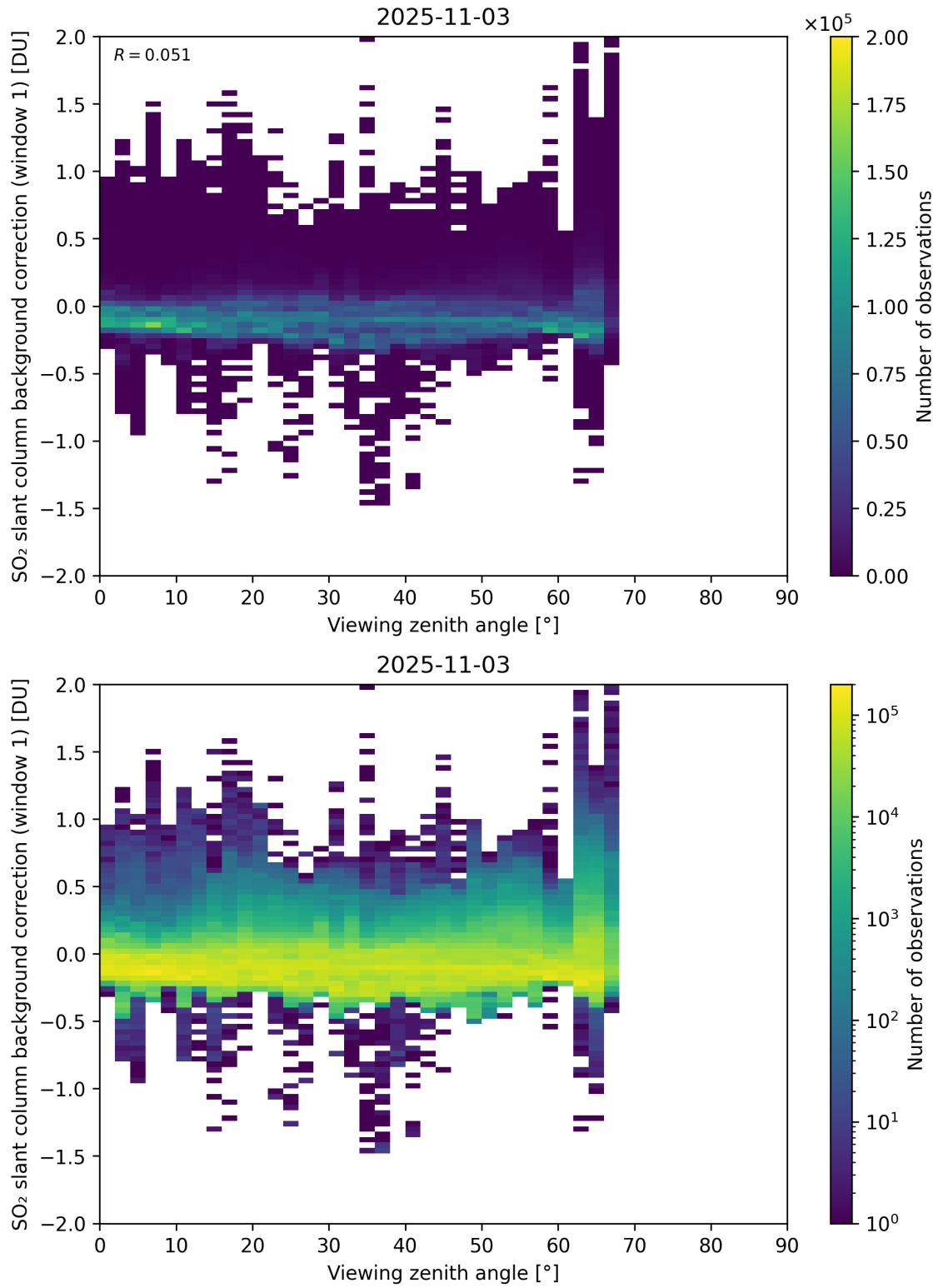
Figure 362: Scatter density plot of “Viewing zenith angle” against “SO 2 slant column background correction (window 1)” for 2025-11-02 to 2025-11-04.
