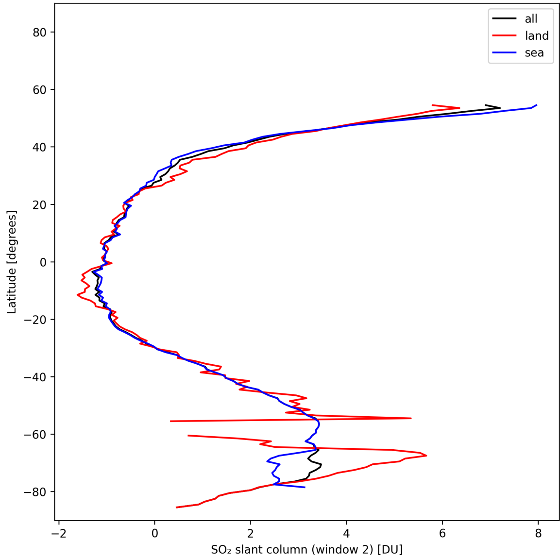
Figure 41: Zonal average of “SO 2 slant column (window 2)” for 2025-11-02 to 2025-11-04.
