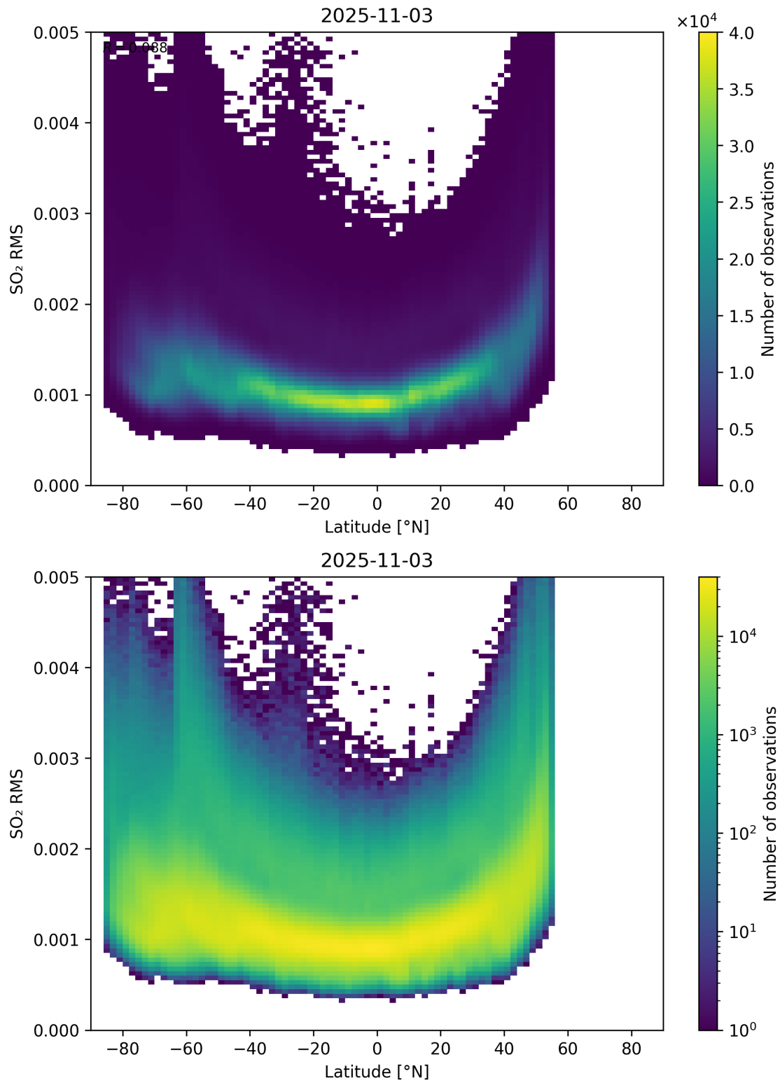
Figure 155: Scatter density plot of “Latitude” against “SO 2 RMS” for 2025-11-02 to 2025-11-04.
