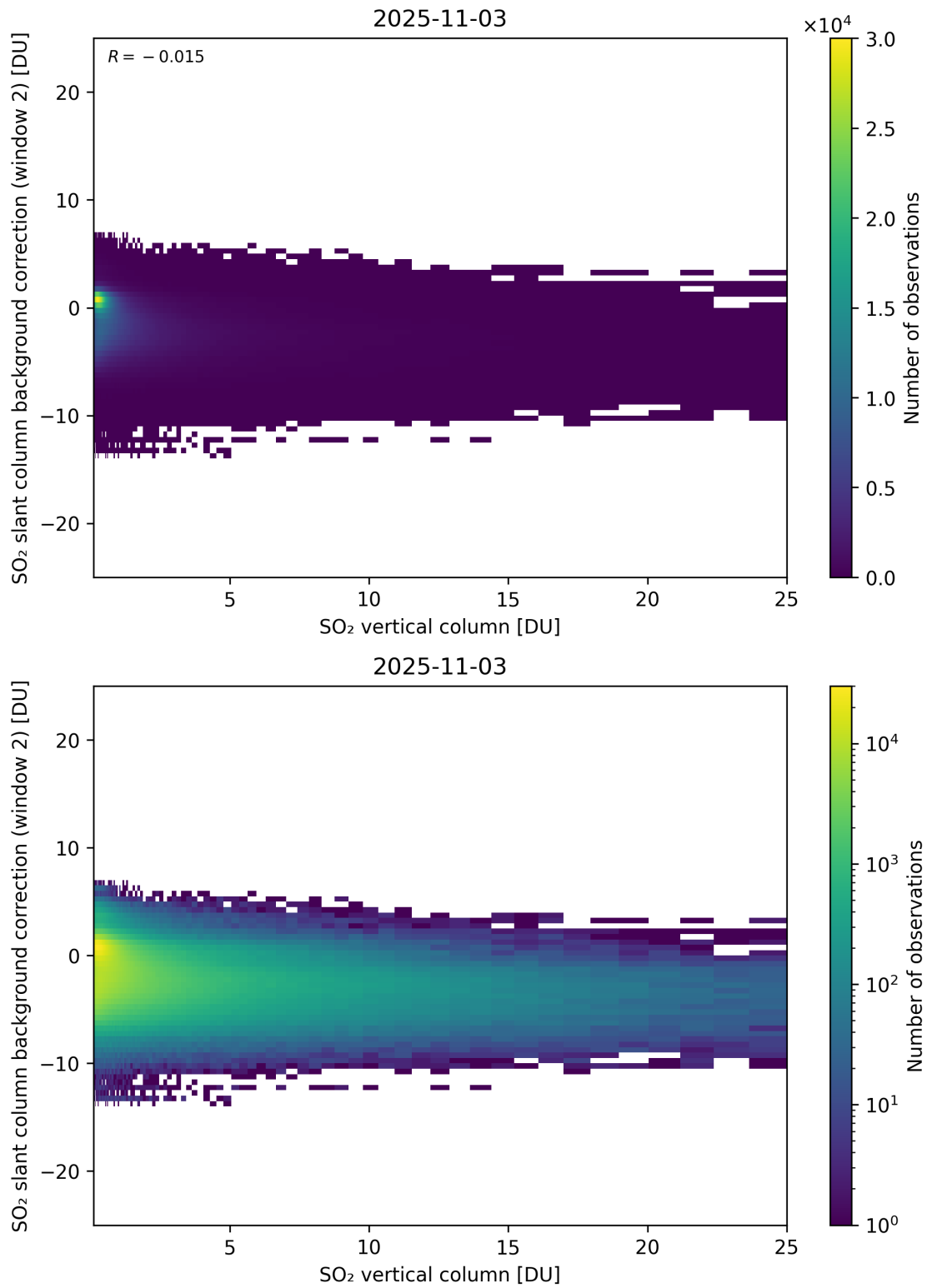
Figure 324: Scatter density plot of “SO 2 vertical column” against “SO 2 slant column background correction (window 2)” for 2025-11-02 to 2025-11-04.
