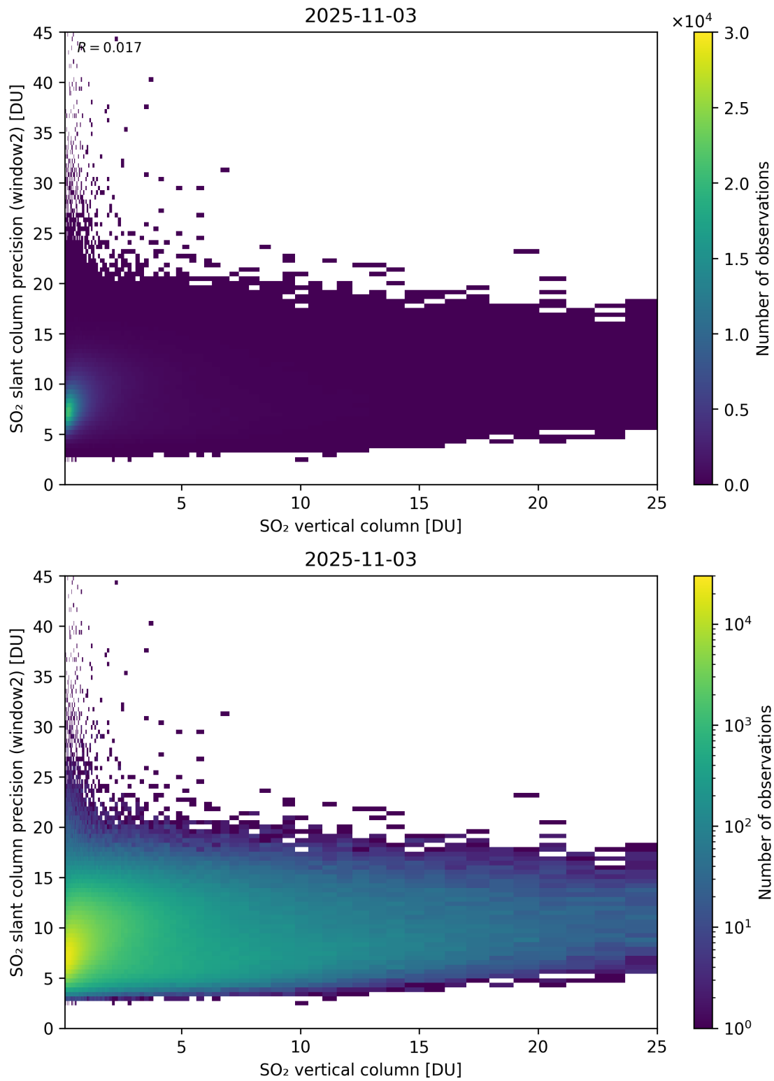
Figure 356: Scatter density plot of “SO 2 vertical column” against “SO 2 slant column precision (window2)” for 2025-11-02 to 2025-11-04.
