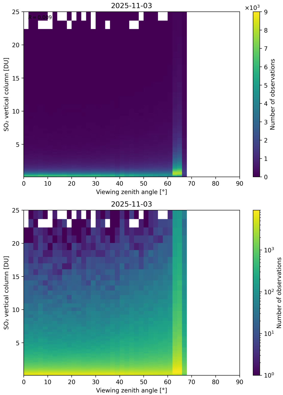
Figure 383: Scatter density plot of “Viewing zenith angle” against “SO 2 vertical column” for 2025-11-02 to 2025-11-04.
