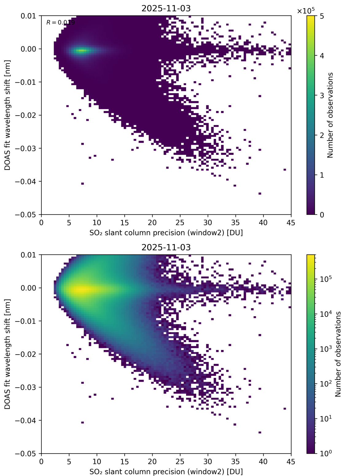
Figure 293: Scatter density plot of “SO 2 slant column precision (window2)” against “DOAS fit wavelength shift” for 2025-11-02 to 2025-11-04.
