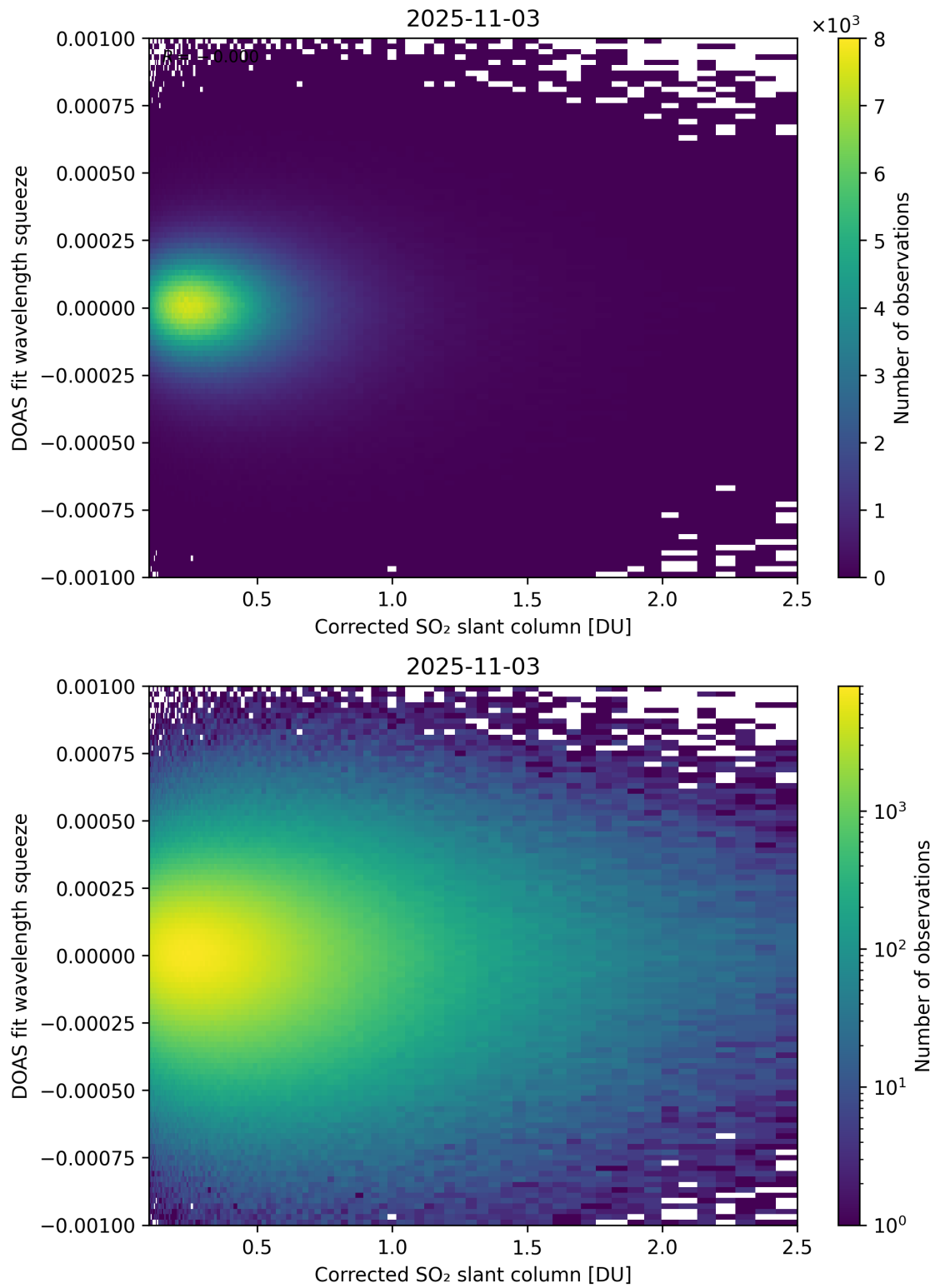
Figure 230: Scatter density plot of “Corrected SO 2 slant column” against “DOAS fit wavelength squeeze” for 2025-11-02 to 2025-11-04.
