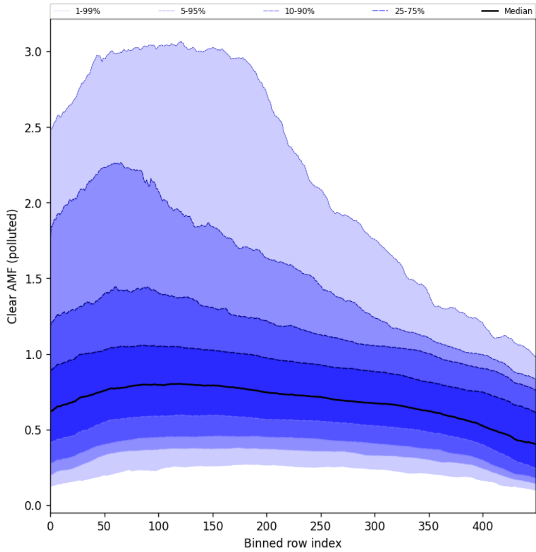
Figure 107: Along track statistics of “Clear AMF (polluted)” for 2025-11-02 to 2025-11-04
