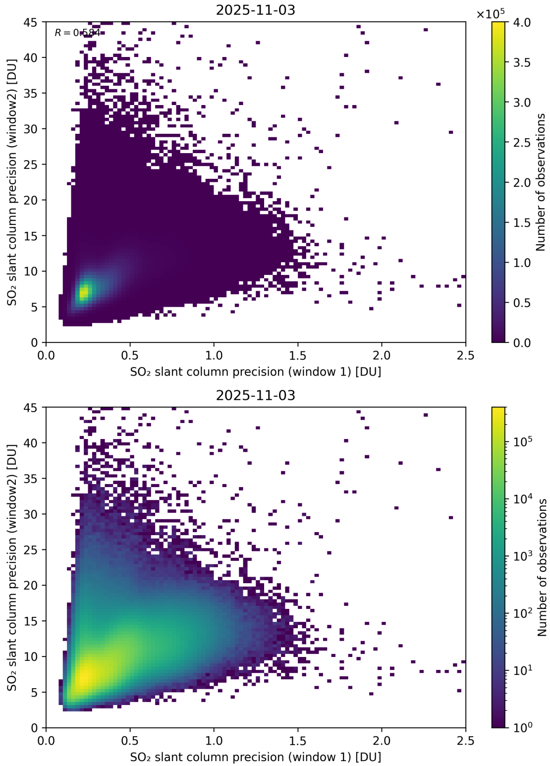
Figure 277: Scatter density plot of “SO 2 slant column precision (window 1)” against “SO 2 slant column precision (window2)” for 2025-11-02 to 2025-11-04.
