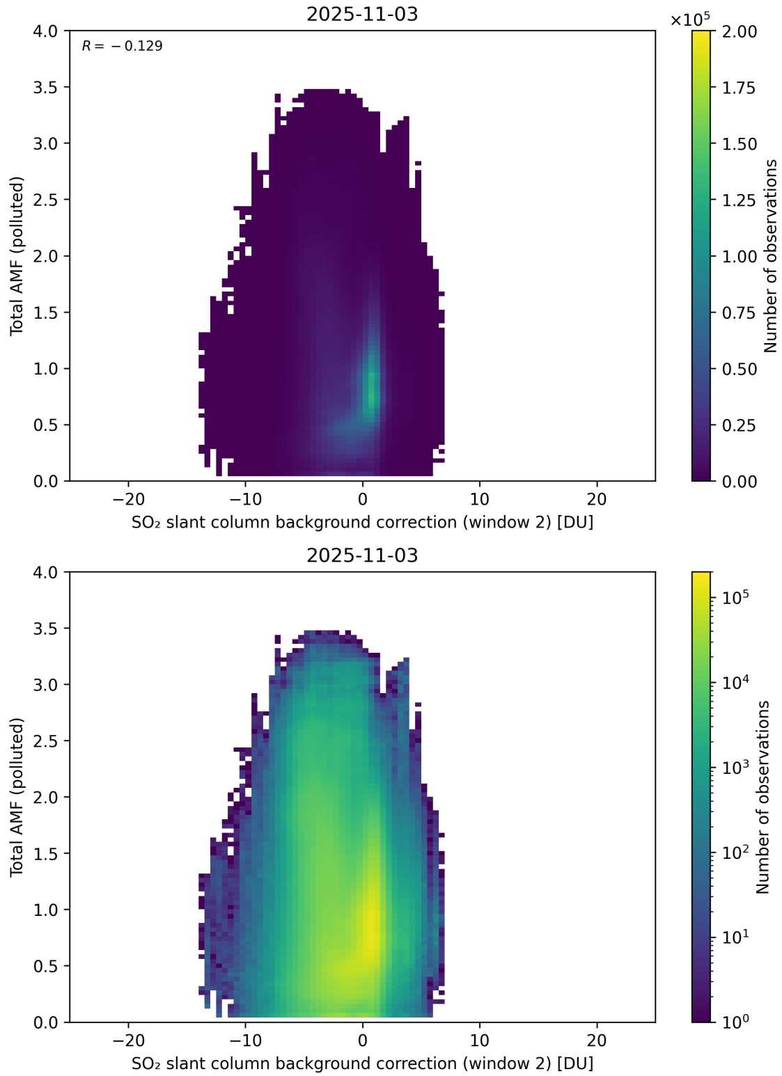
Figure 130: Scatter density plot of “SO 2 slant column background correction (window 2)” against “Total AMF (polluted)” for 2025-11-02 to 2025-11-04.
