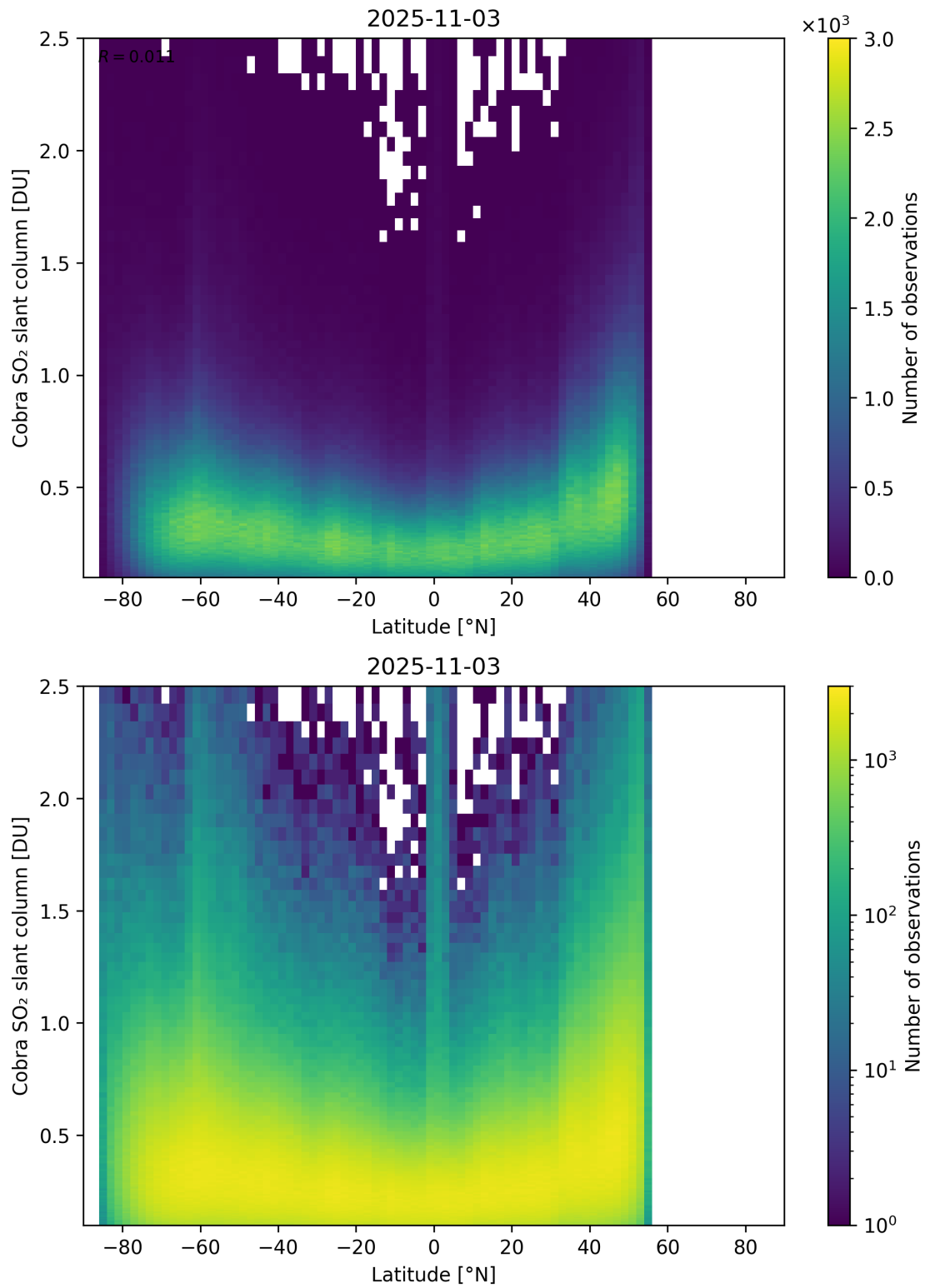
Figure 157: Scatter density plot of “Latitude” against “Cobra SO 2 slant column” for 2025-11-02 to 2025-11-04.
