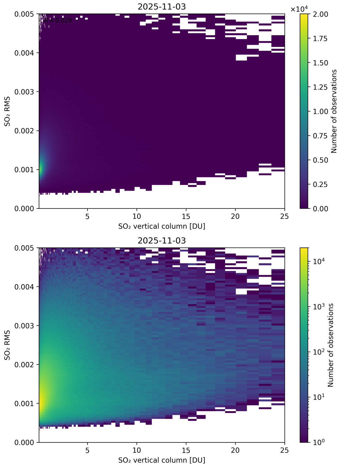
Figure 328: Scatter density plot of “SO 2 vertical column” against “SO 2 RMS” for 2025-11-02 to 2025-11-04.
