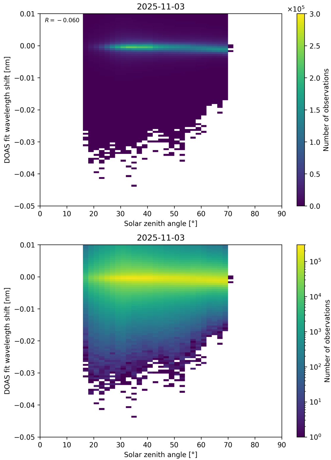
Figure 174: Scatter density plot of “Solar zenith angle” against “DOAS fit wavelength shift” for 2025-11-02 to 2025-11-04.
