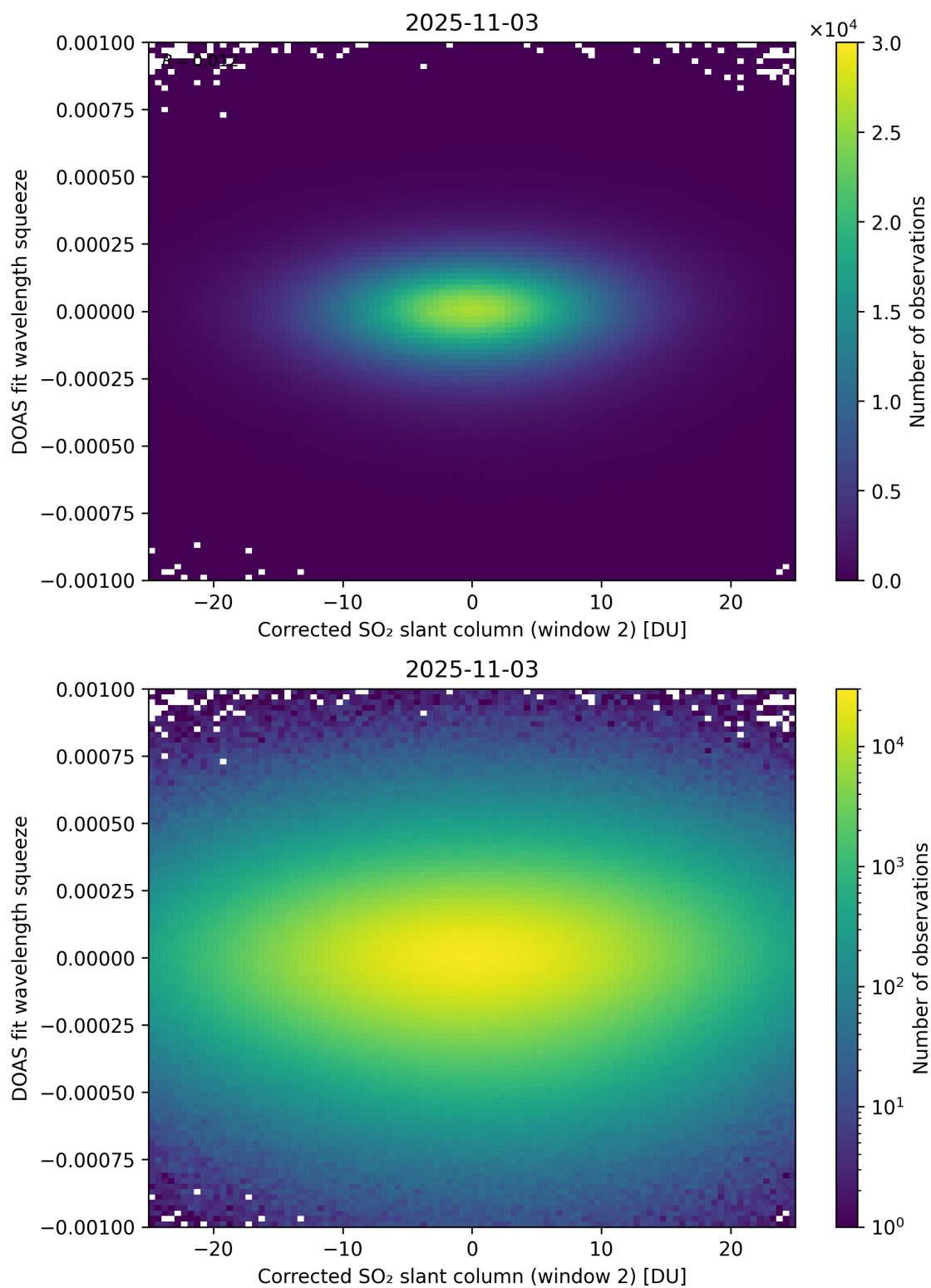
Figure 247: Scatter density plot of “Corrected SO 2 slant column (window 2)” against “DOAS fit wavelength squeeze” for 2025-11-02 to 2025-11-04.
