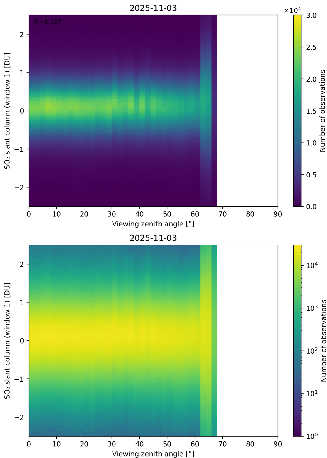
Figure 376: Scatter density plot of “Viewing zenith angle” against “SO 2 slant column (window 1)” for 2025-11-02 to 2025-11-04.
