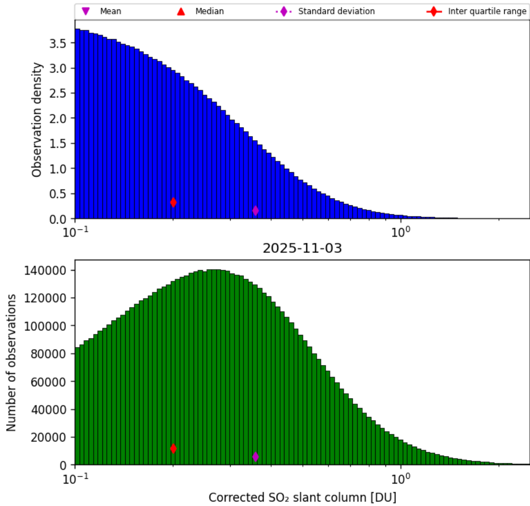
Figure 60: Histogram of “Corrected SO 2 slant column” for 2025-11-02 to 2025-11-04
