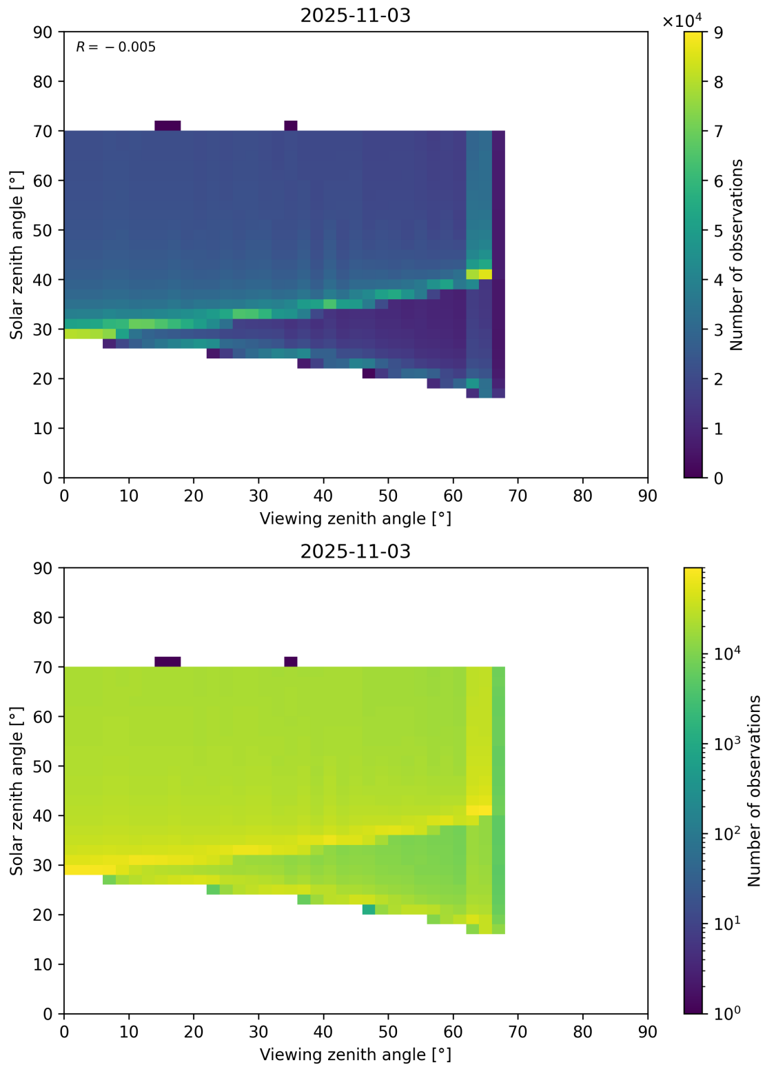
Figure 369: Scatter density plot of “Viewing zenith angle” against “Solar zenith angle” for 2025-11-02 to 2025-11-04.
