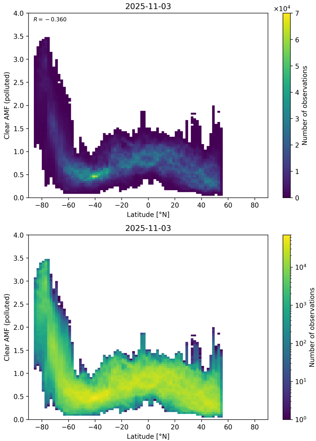
Figure 156: Scatter density plot of “Latitude” against “Clear AMF (polluted)” for 2025-11-02 to 2025-11-04.
