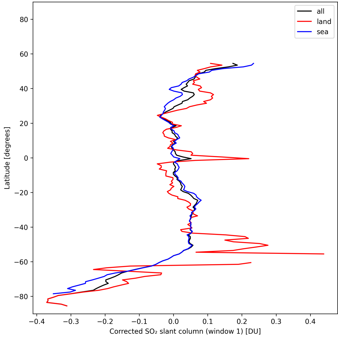
Figure 39: Zonal average of “Corrected SO 2 slant column (window 1)” for 2025-11-02 to 2025-11-04.
