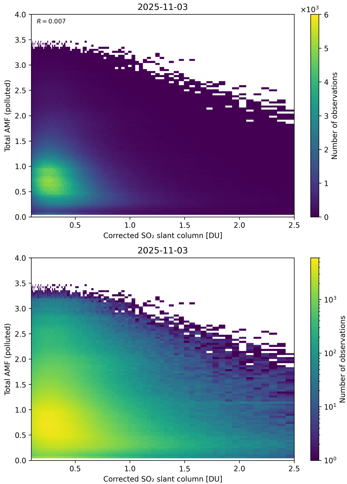
Figure 242: Scatter density plot of “Corrected SO 2 slant column” against “Total AMF (polluted)” for 2025-11-02 to 2025-11-04.
