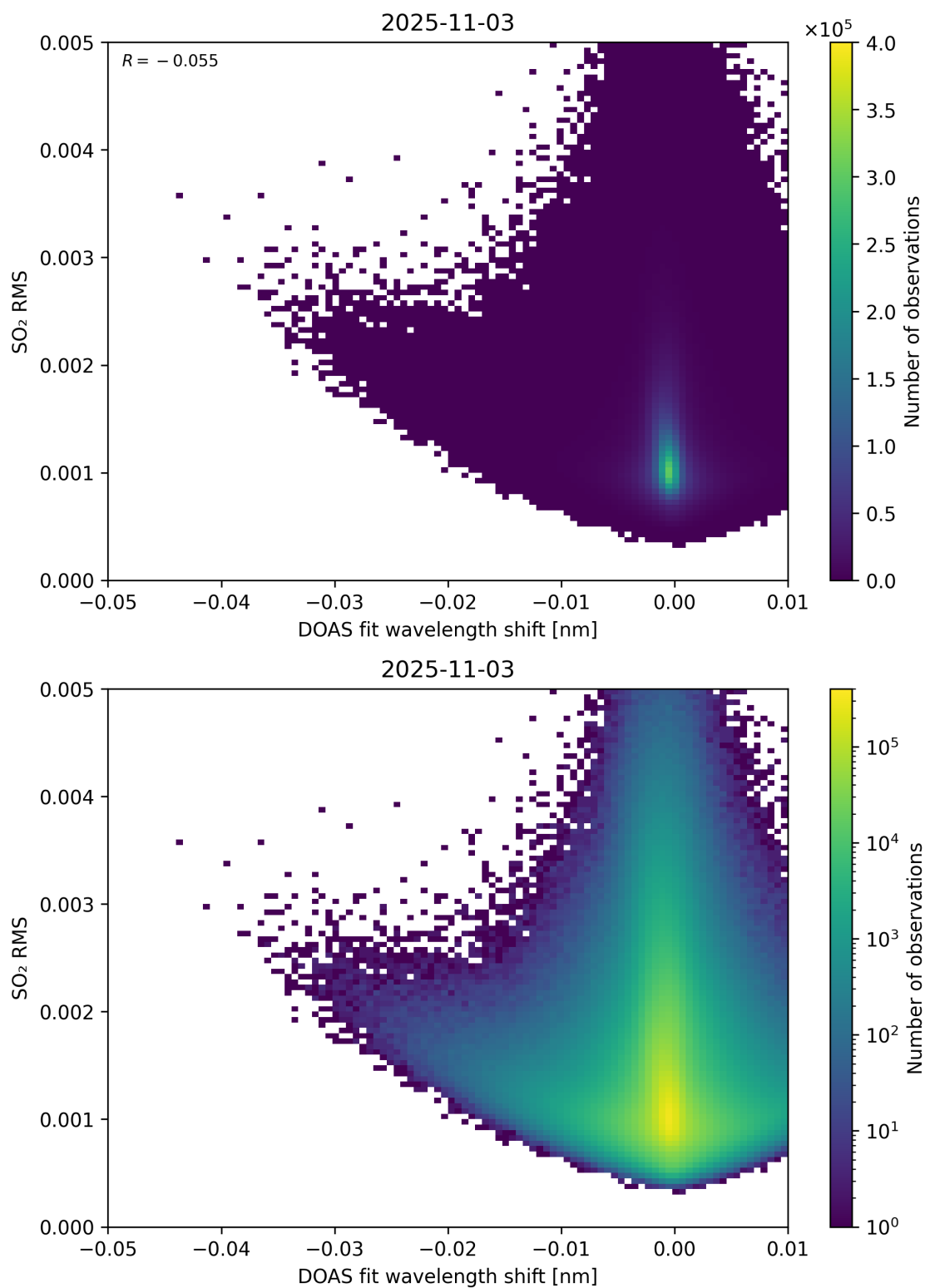
Figure 139: Scatter density plot of “DOAS fit wavelength shift” against “SO 2 RMS” for 2025-11-02 to 2025-11-04.
