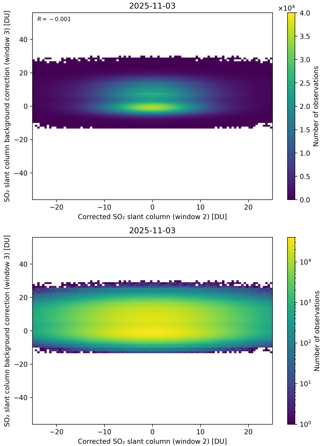
Figure 245: Scatter density plot of “Corrected SO 2 slant column (window 2)” against “SO 2 slant column background correction (window 3)” for 2025-11-02 to 2025-11-04.
