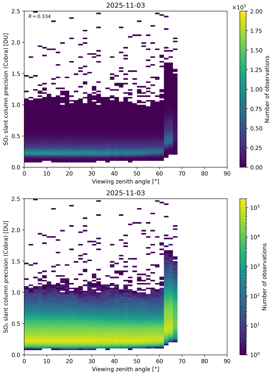
Figure 372: Scatter density plot of “Viewing zenith angle” against “SO 2 slant column precision (Cobra)” for 2025-11-02 to 2025-11-04.
