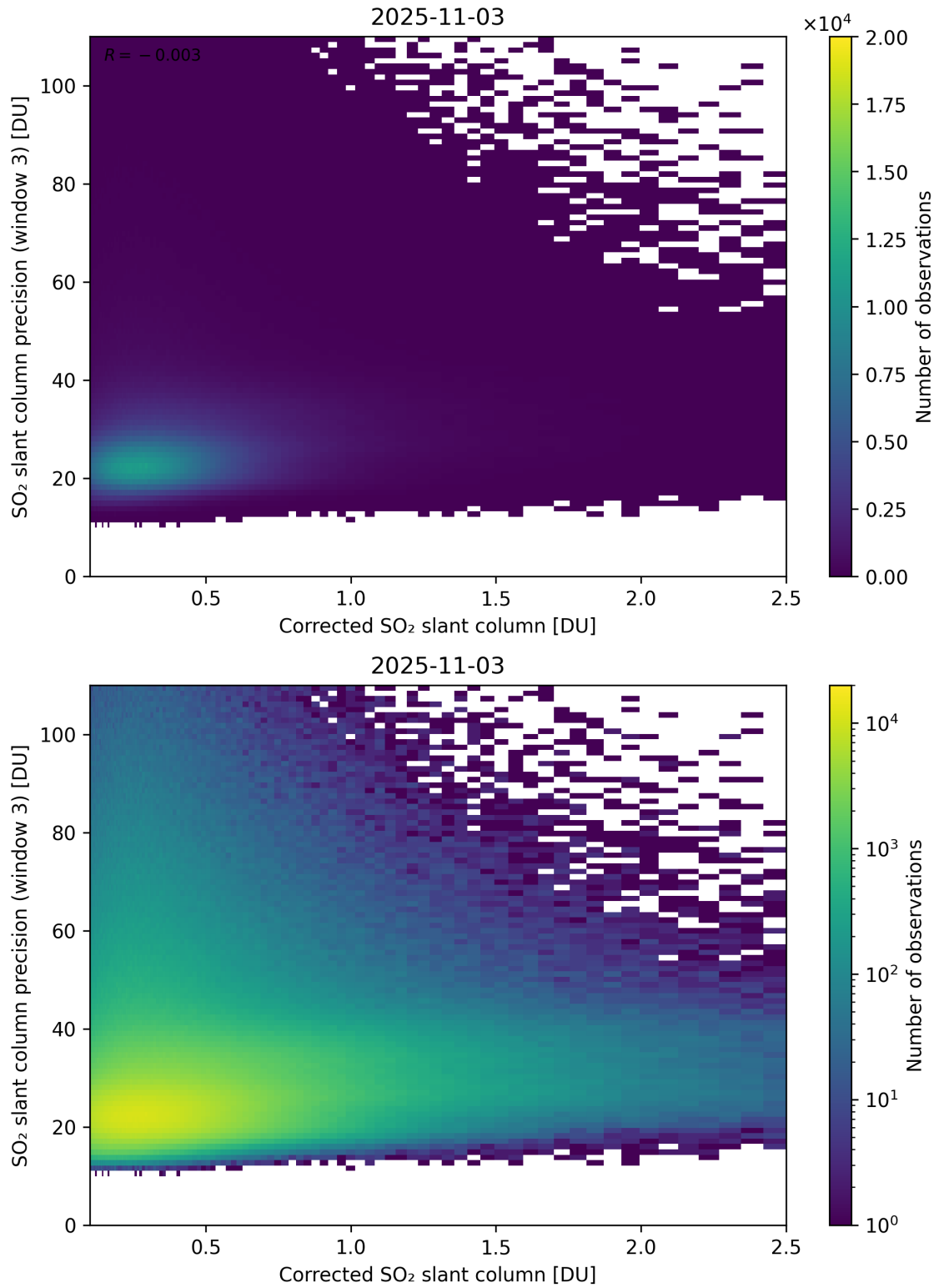
Figure 241: Scatter density plot of “Corrected SO 2 slant column” against “SO 2 slant column precision (window 3)” for 2025-11-02 to 2025-11-04.
