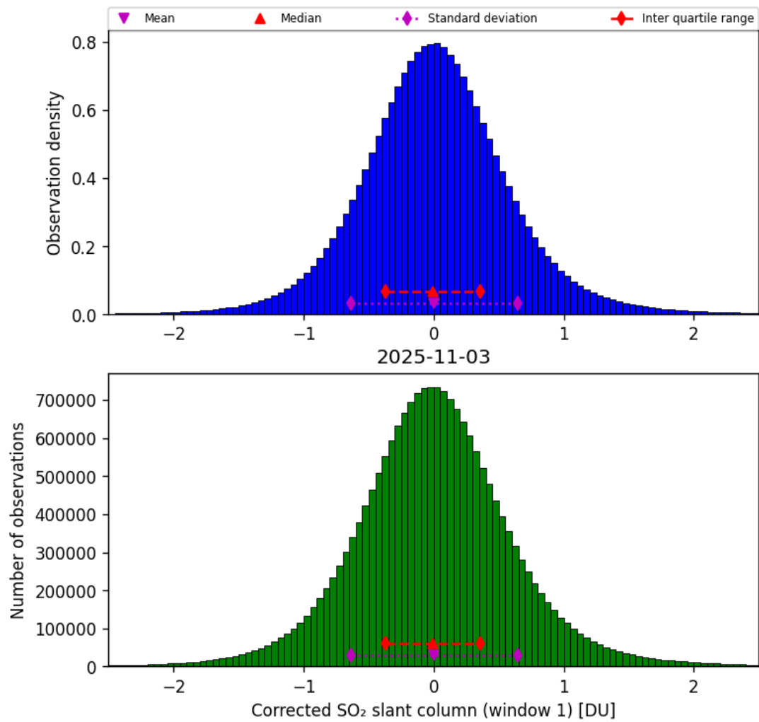
Figure 65: Histogram of “Corrected SO 2 slant column (window 1)” for 2025-11-02 to 2025-11-04
