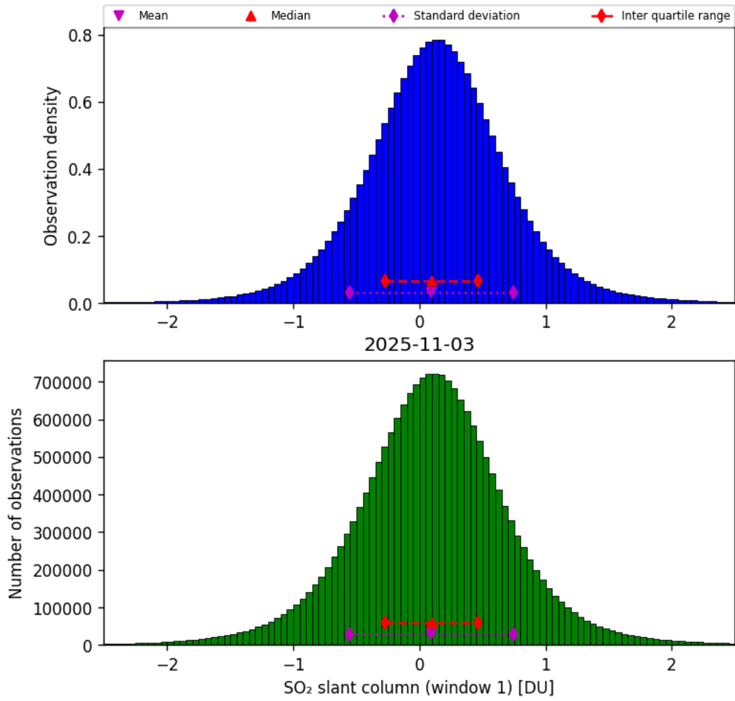
Figure 63: Histogram of “SO 2 slant column (window 1)” for 2025-11-02 to 2025-11-04
