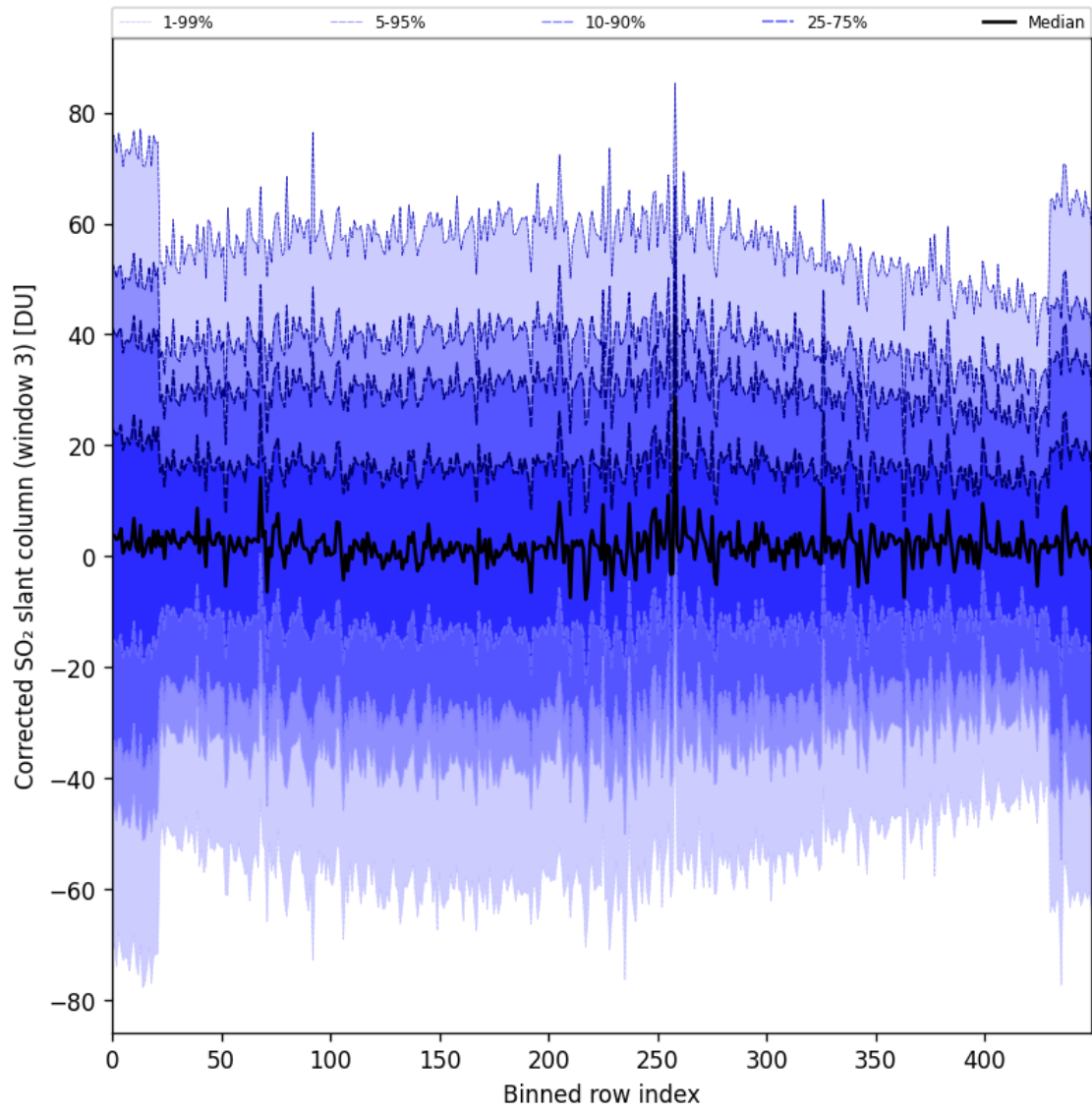
Figure 99: Along track statistics of “Corrected SO 2 slant column (window 3)” for 2025-11-02 to 2025-11-04
