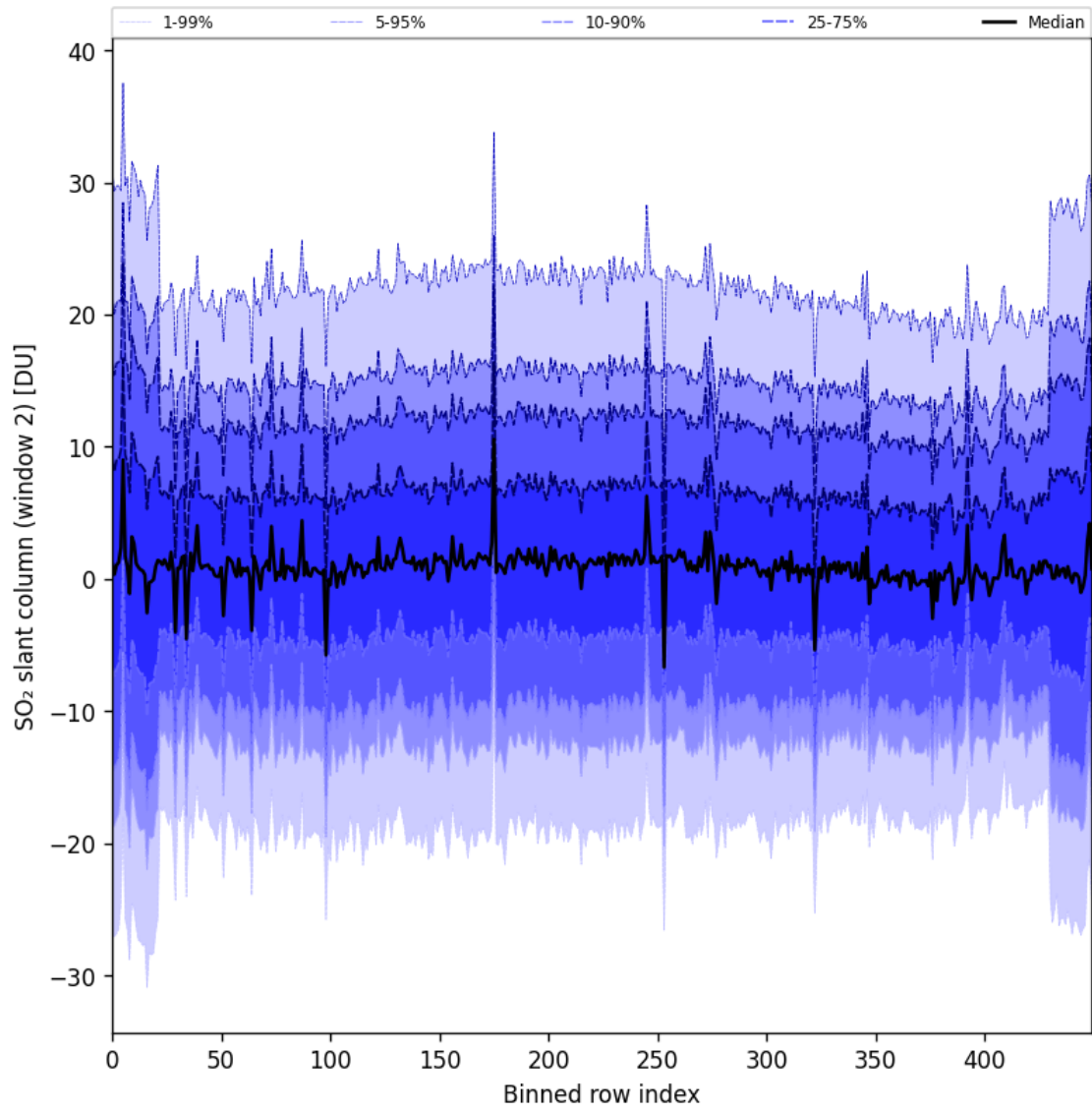
Figure 93: Along track statistics of “SO 2 slant column (window 2)” for 2025-11-02 to 2025-11-04
