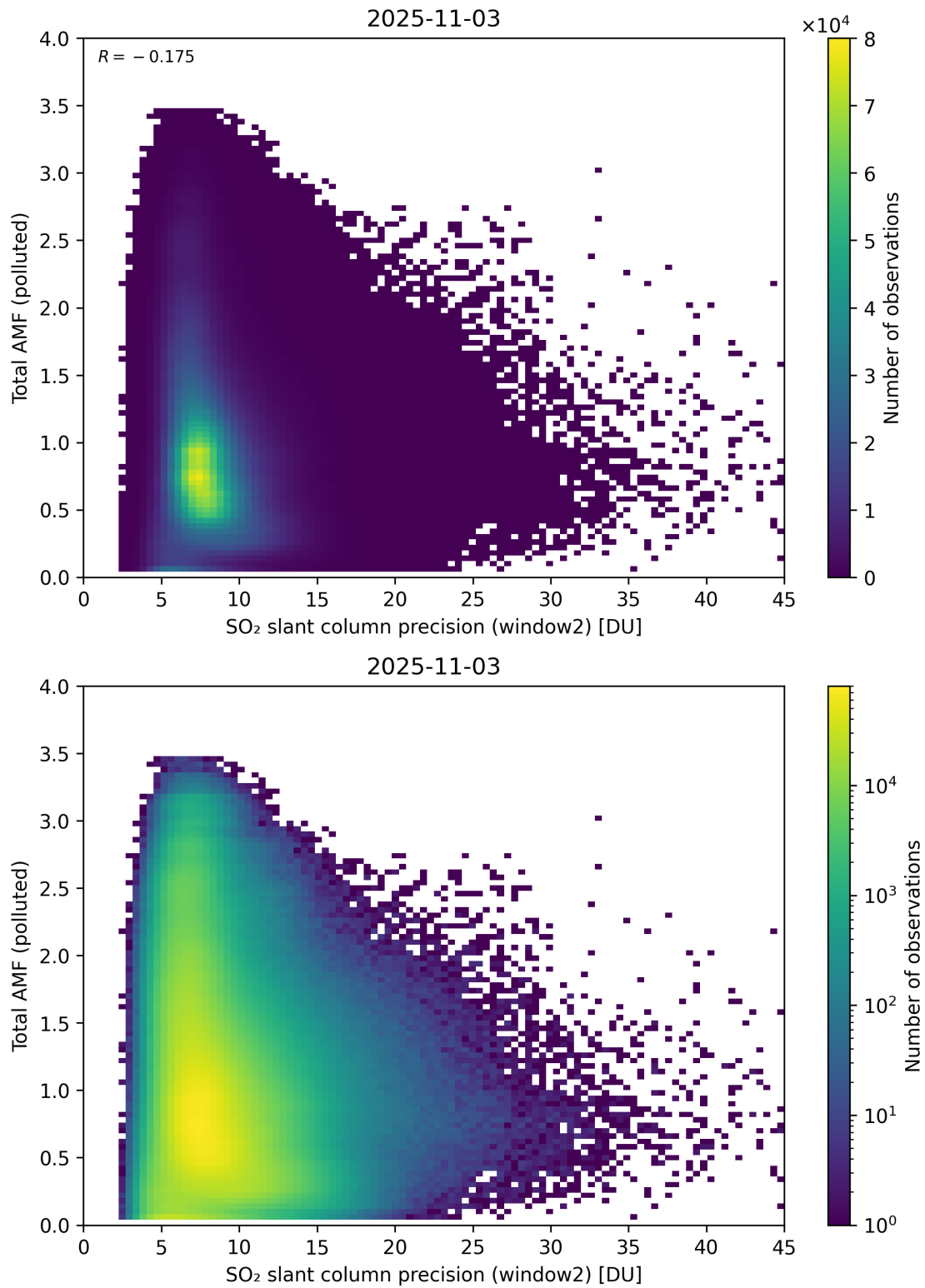
Figure 301: Scatter density plot of “SO 2 slant column precision (window2)” against “Total AMF (polluted)” for 2025-11-02 to 2025-11-04.
