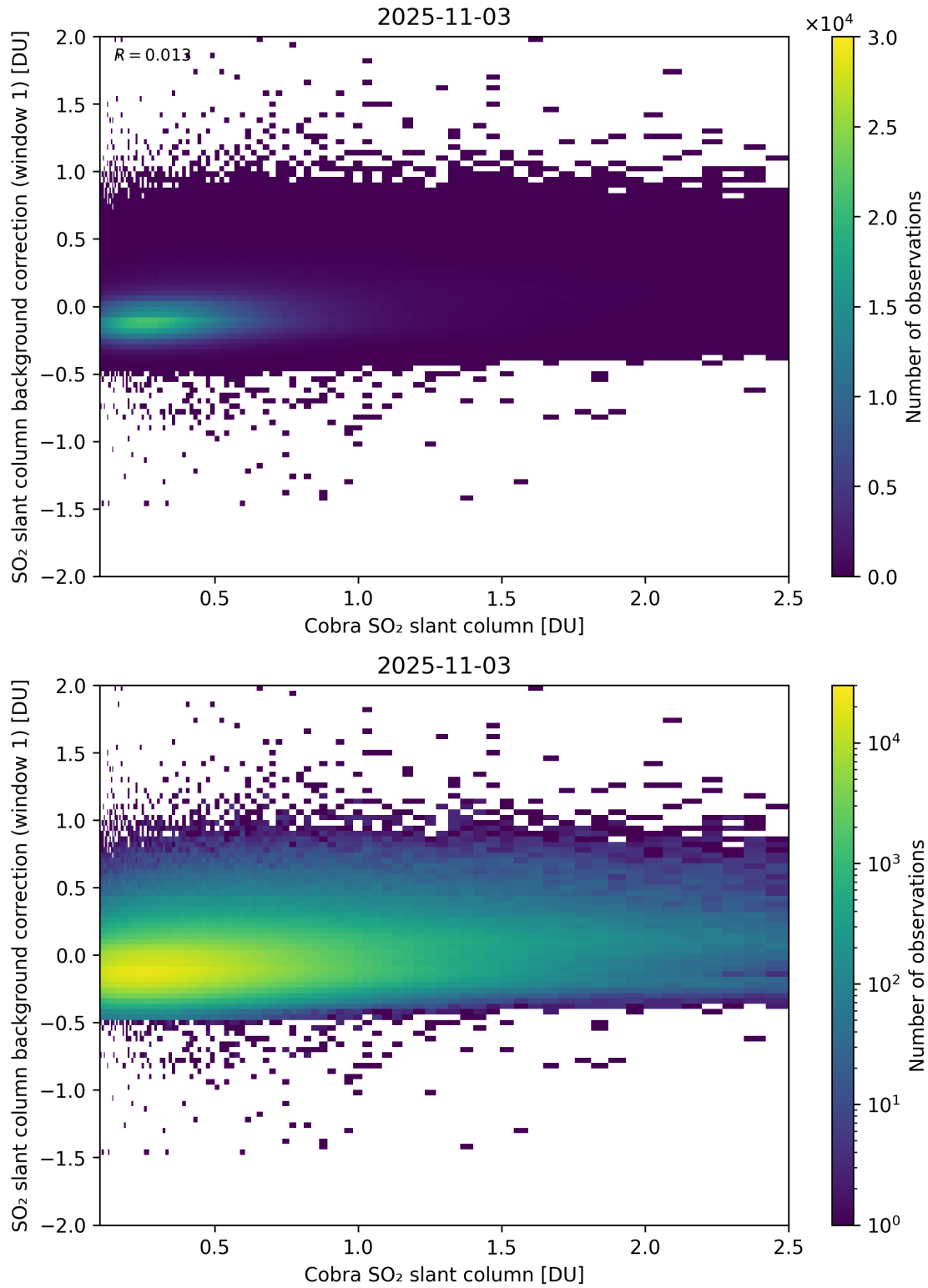
Figure 193: Scatter density plot of “Cobra SO 2 slant column” against “SO 2 slant column background correction (window 1)” for 2025-11-02 to 2025-11-04.
