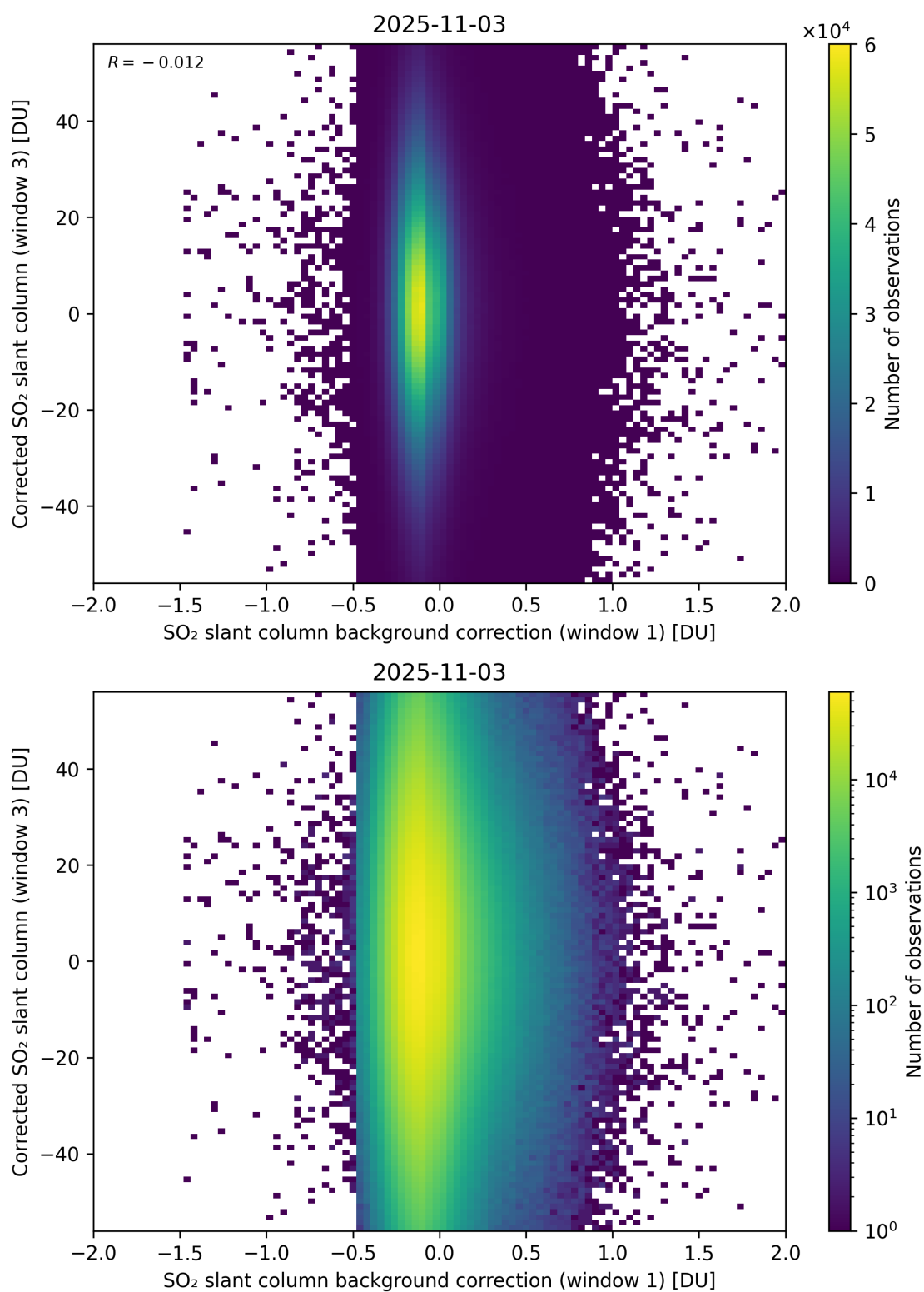
Figure 116: Scatter density plot of “SO 2 slant column background correction (window 1)” against “Corrected SO 2 slant column (window 3)” for 2025-11-02 to 2025-11-04.
