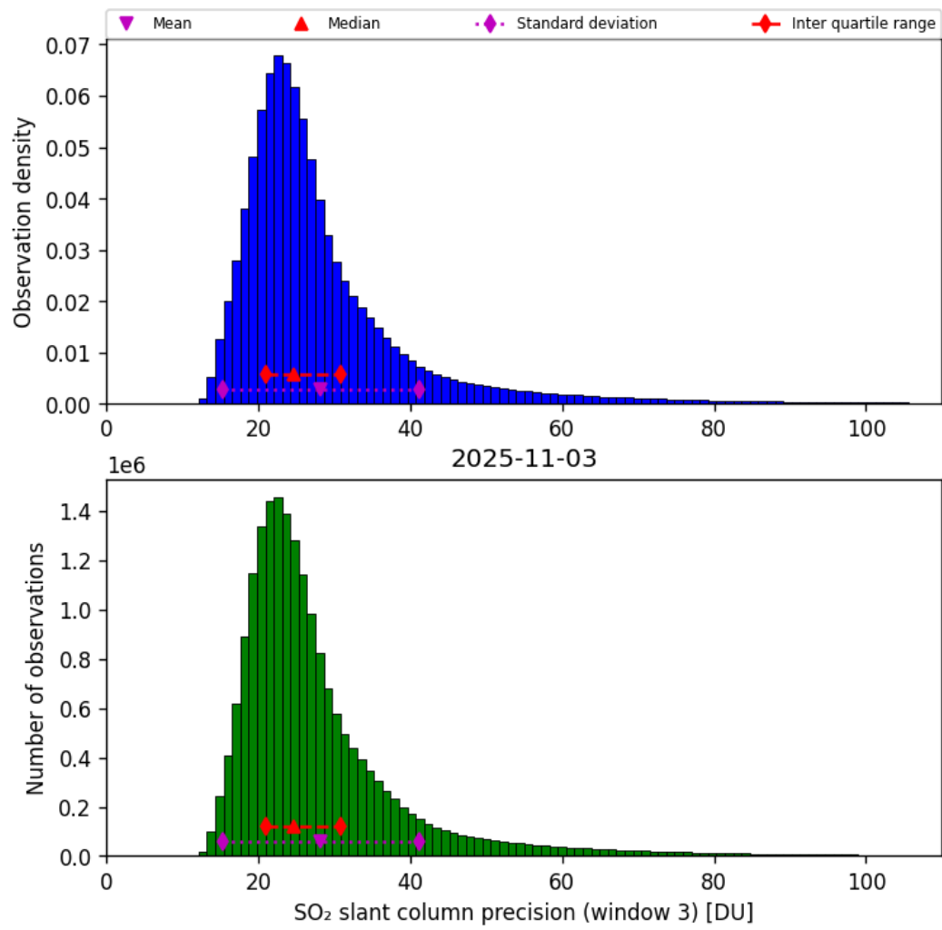
Figure 72: Histogram of “SO 2 slant column precision (window 3)” for 2025-11-02 to 2025-11-04
