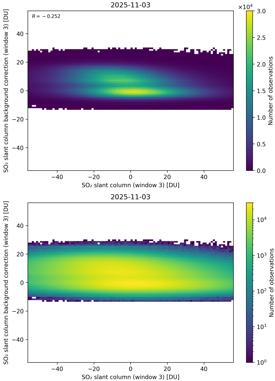
Figure 303: Scatter density plot of “SO 2 slant column (window 3)” against “SO 2 slant column background correction (window 3)” for 2025-11-02 to 2025-11-04.
