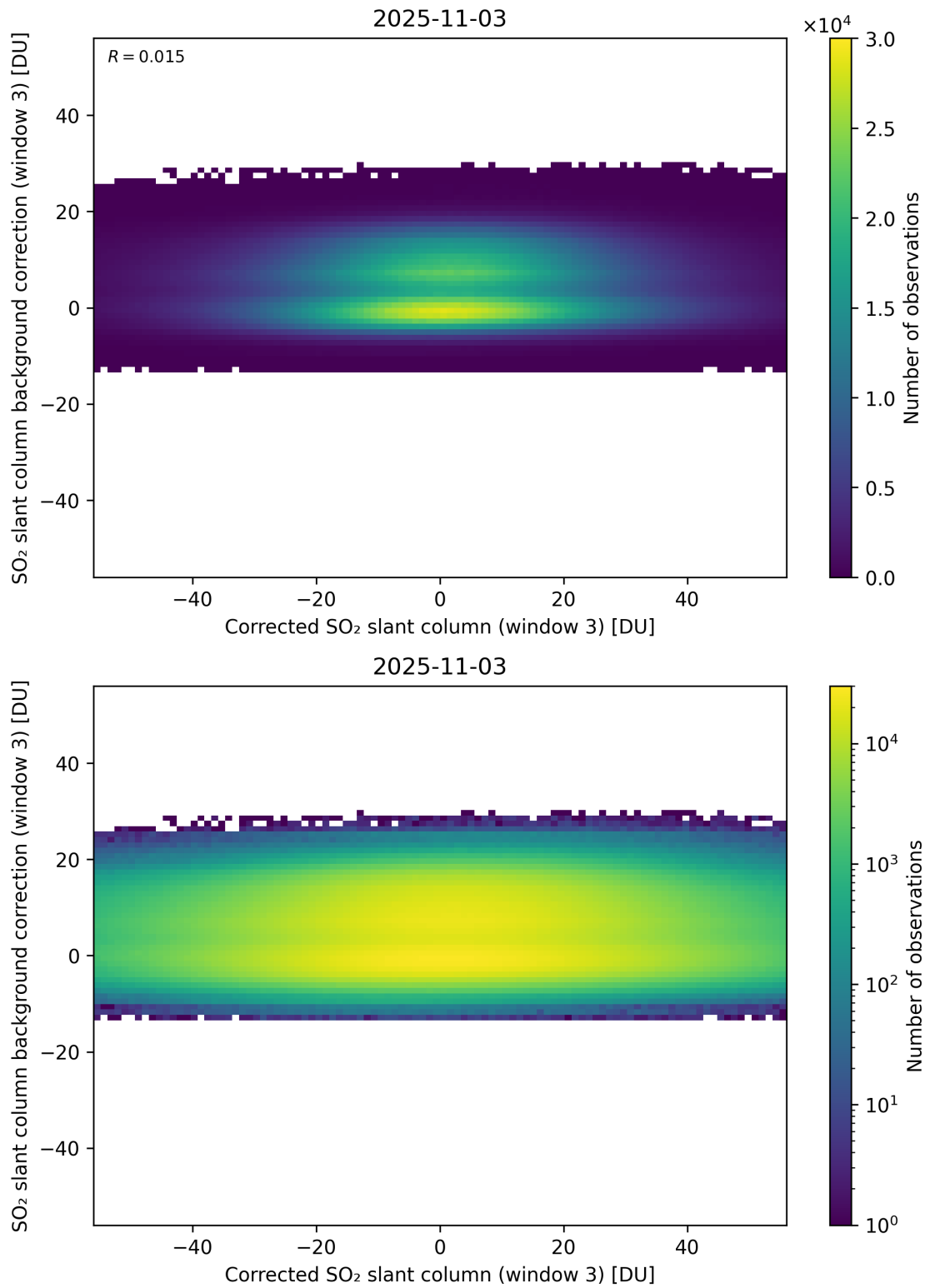
Figure 255: Scatter density plot of “Corrected SO 2 slant column (window 3)” against “SO 2 slant column background correction (window 3)” for 2025-11-02 to 2025-11-04.
