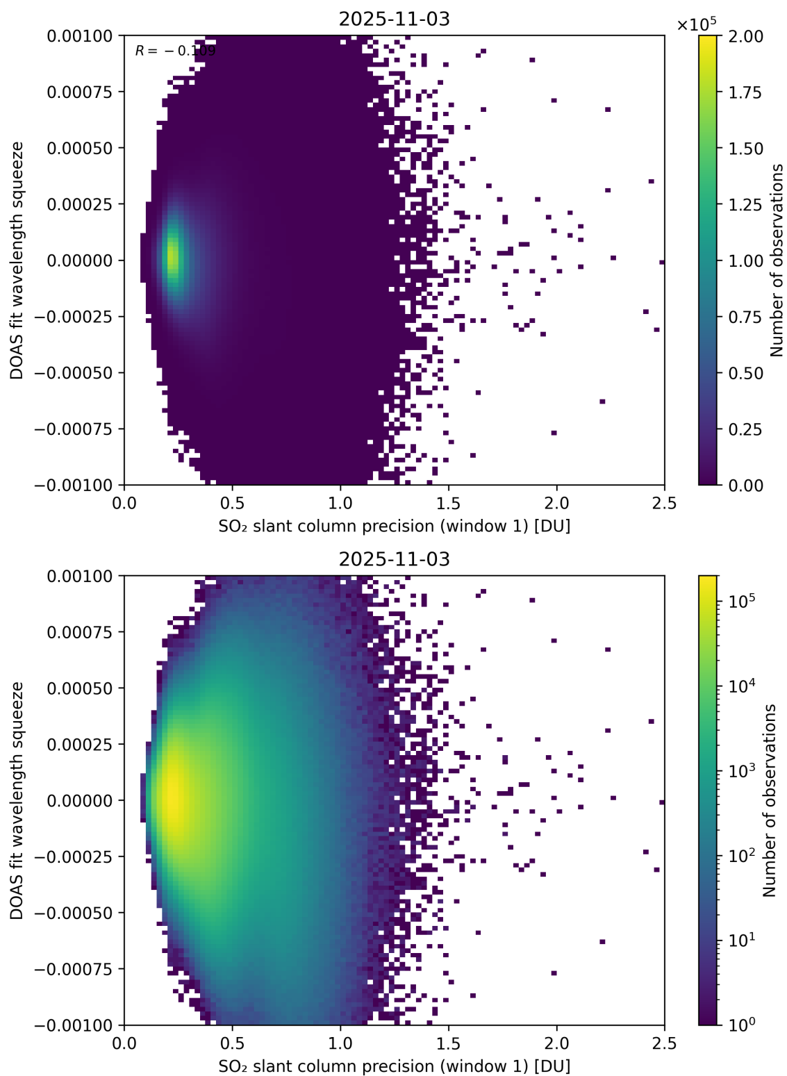
Figure 272: Scatter density plot of “SO 2 slant column precision (window 1)” against “DOAS fit wavelength squeeze” for 2025-11-02 to 2025-11-04.
