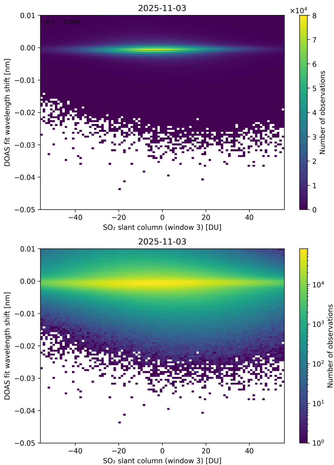
Figure 304: Scatter density plot of “SO 2 slant column (window 3)” against “DOAS fit wavelength shift” for 2025-11-02 to 2025-11-04.
