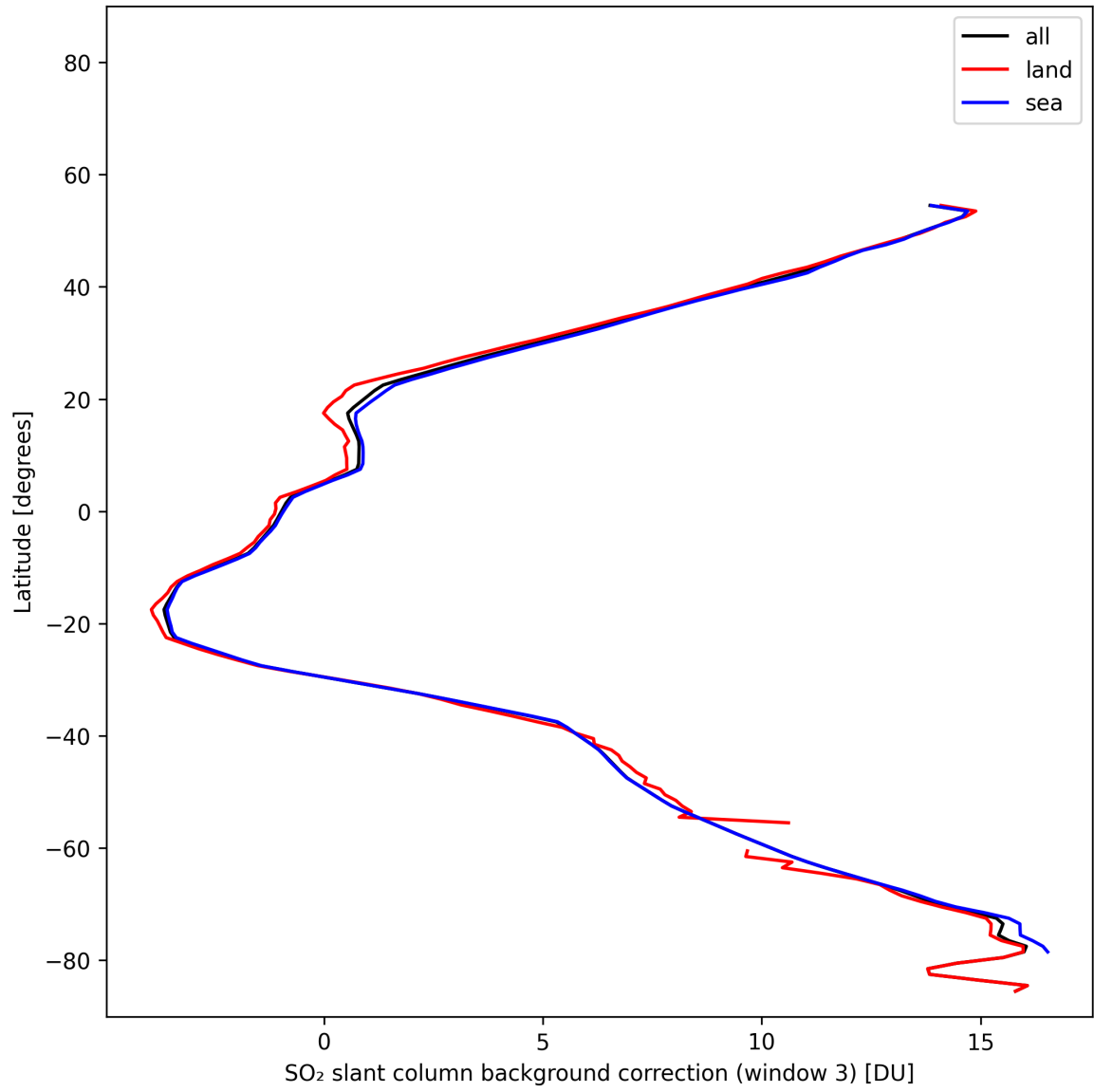
Figure 48: Zonal average of “SO 2 slant column background correction (window 3)” for 2025-11-02 to 2025-11-04.
