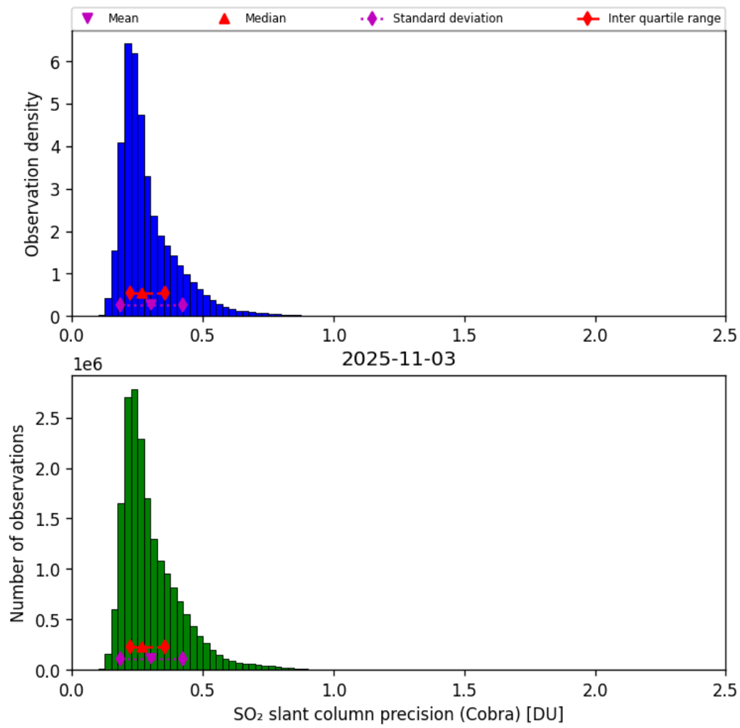
Figure 62: Histogram of “SO 2 slant column precision (Cobra)” for 2025-11-02 to 2025-11-04
