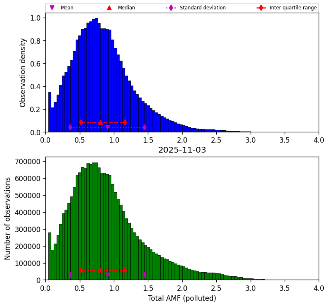
Figure 79: Histogram of “Total AMF (polluted)” for 2025-11-02 to 2025-11-04
