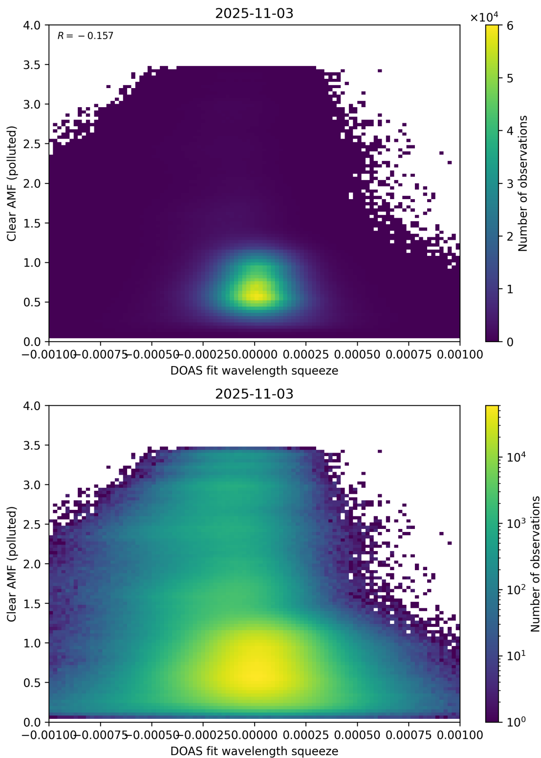
Figure 144: Scatter density plot of “DOAS fit wavelength squeeze” against “Clear AMF (polluted)” for 2025-11-02 to 2025-11-04.
