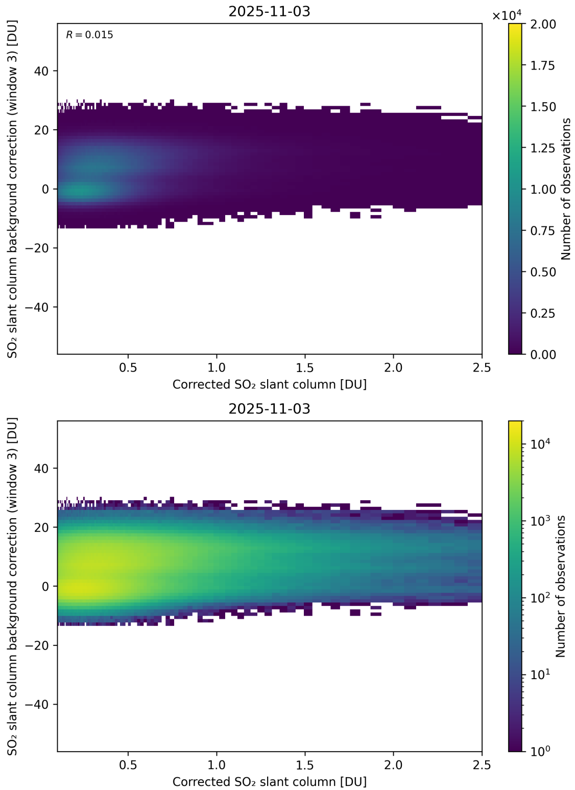
Figure 228: Scatter density plot of “Corrected SO 2 slant column” against “SO 2 slant column background correction (window 3)” for 2025-11-02 to 2025-11-04.
