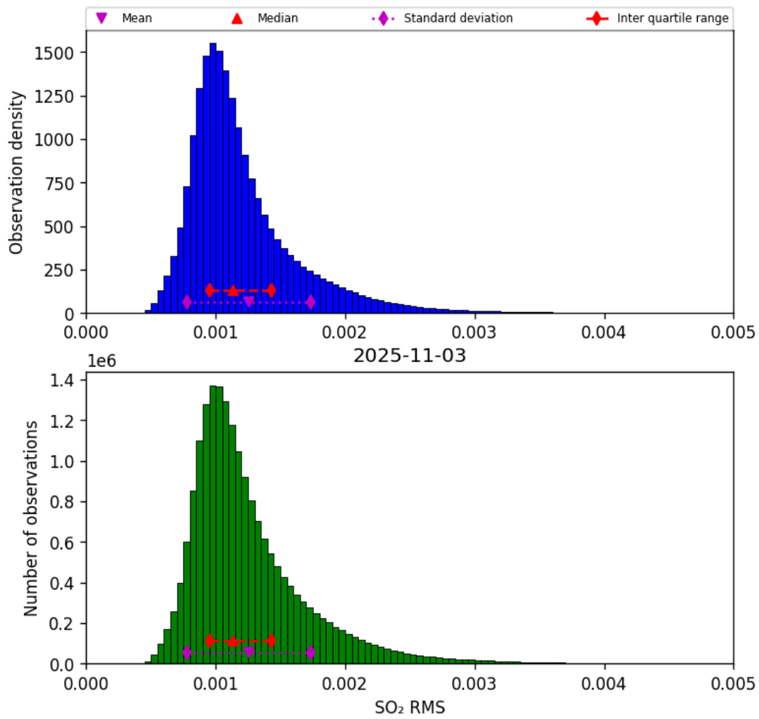
Figure 78: Histogram of “SO 2 RMS” for 2025-11-02 to 2025-11-04
