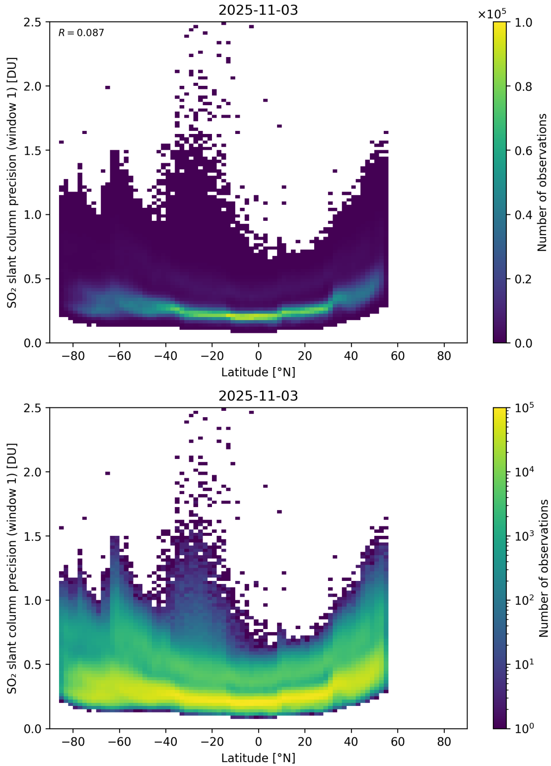
Figure 163: Scatter density plot of “Latitude” against “SO 2 slant column precision (window 1)” for 2025-11-02 to 2025-11-04.
