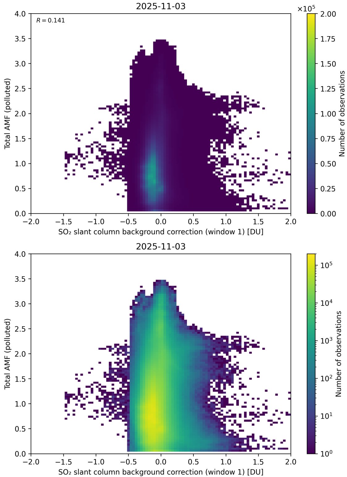
Figure 120: Scatter density plot of “SO 2 slant column background correction (window 1)” against “Total AMF (polluted)” for 2025-11-02 to 2025-11-04.
