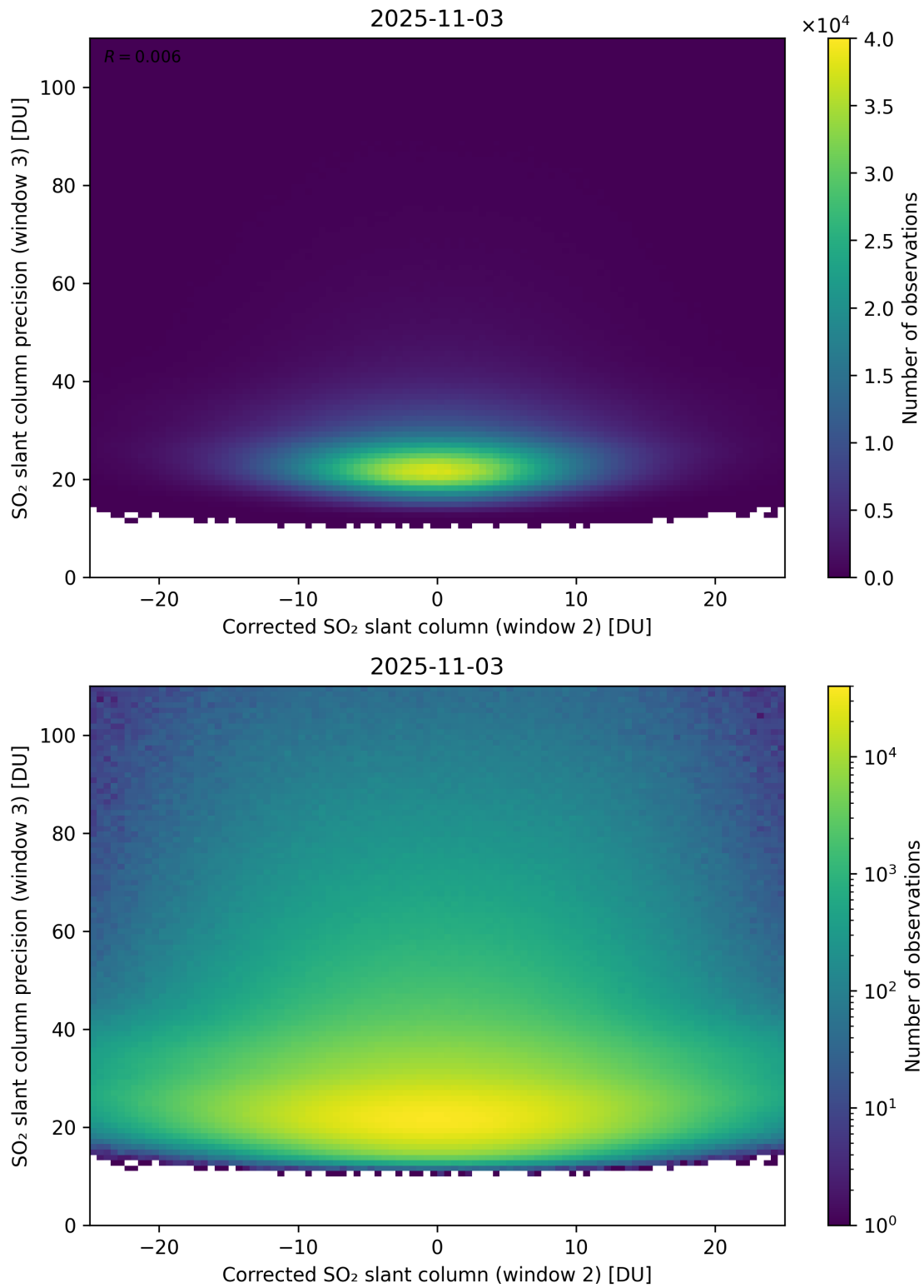
Figure 252: Scatter density plot of “Corrected SO 2 slant column (window 2)” against “SO 2 slant column precision (window 3)” for 2025-11-02 to 2025-11-04.
