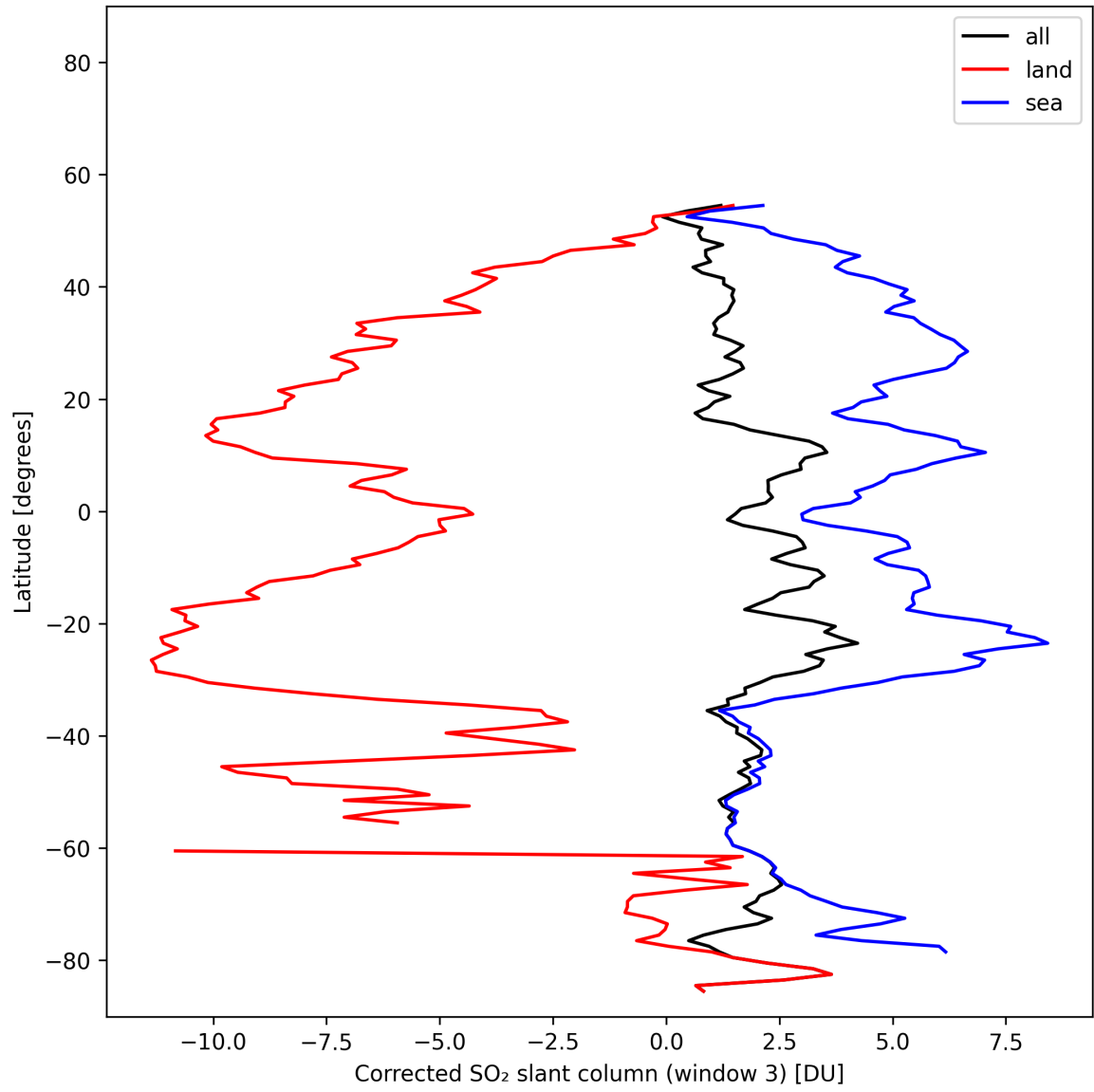
Figure 47: Zonal average of “Corrected SO 2 slant column (window 3)” for 2025-11-02 to 2025-11-04.
