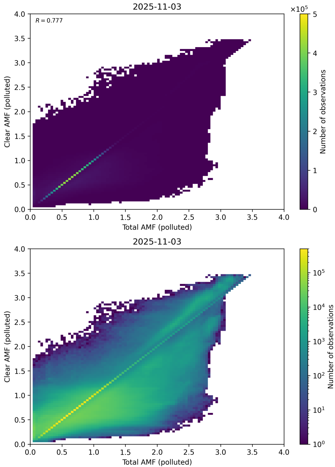
Figure 321: Scatter density plot of “Total AMF (polluted)” against “Clear AMF (polluted)” for 2025-11-02 to 2025-11-04.
