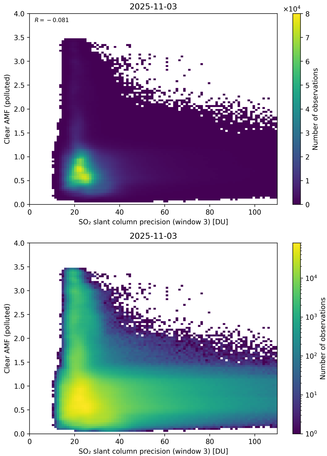
Figure 311: Scatter density plot of “SO 2 slant column precision (window 3)” against “Clear AMF (polluted)” for 2025-11-02 to 2025-11-04.
