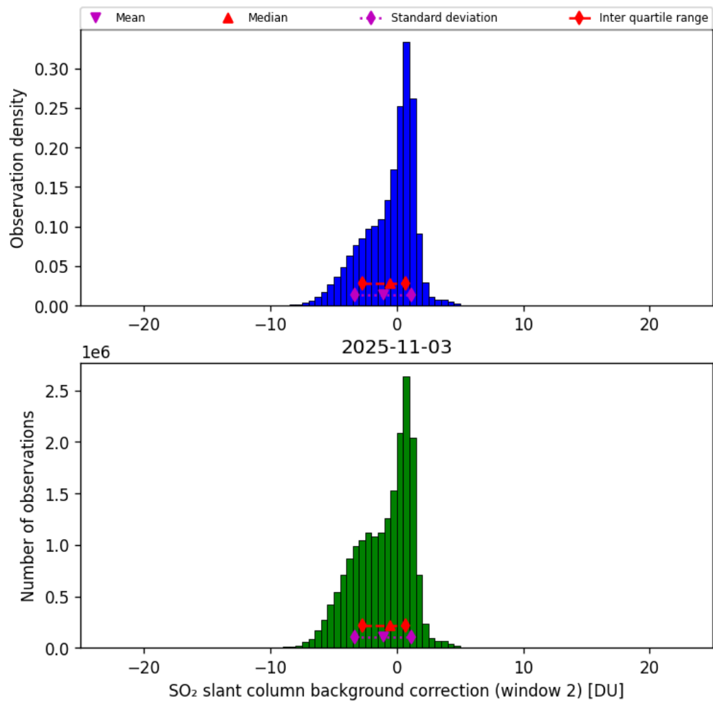
Figure 70: Histogram of “SO 2 slant column background correction (window 2)” for 2025-11-02 to 2025-11-04
