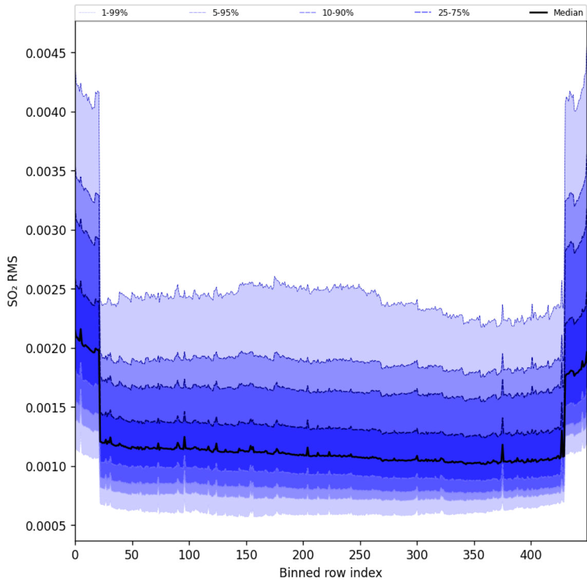
Figure 104: Along track statistics of “SO 2 RMS” for 2025-11-02 to 2025-11-04
