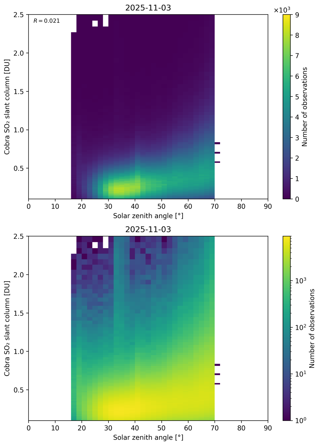
Figure 179: Scatter density plot of “Solar zenith angle” against “Cobra SO 2 slant column” for 2025-11-02 to 2025-11-04.
