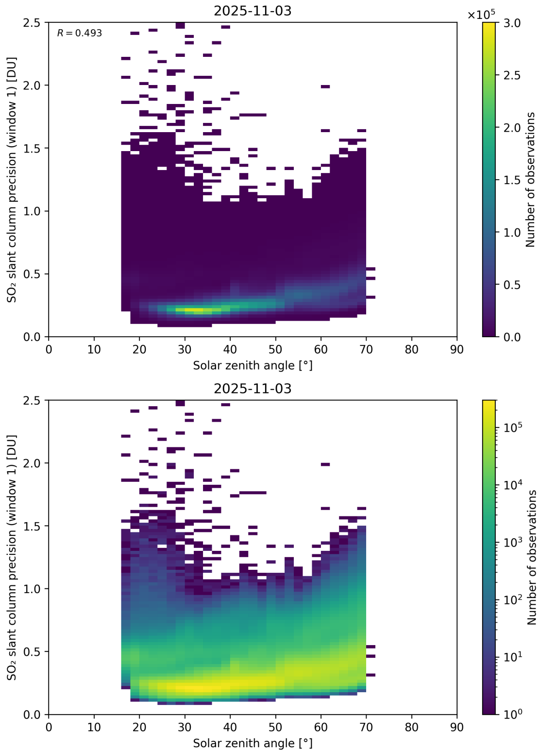
Figure 185: Scatter density plot of “Solar zenith angle” against “SO 2 slant column precision (window 1)” for 2025-11-02 to 2025-11-04.
