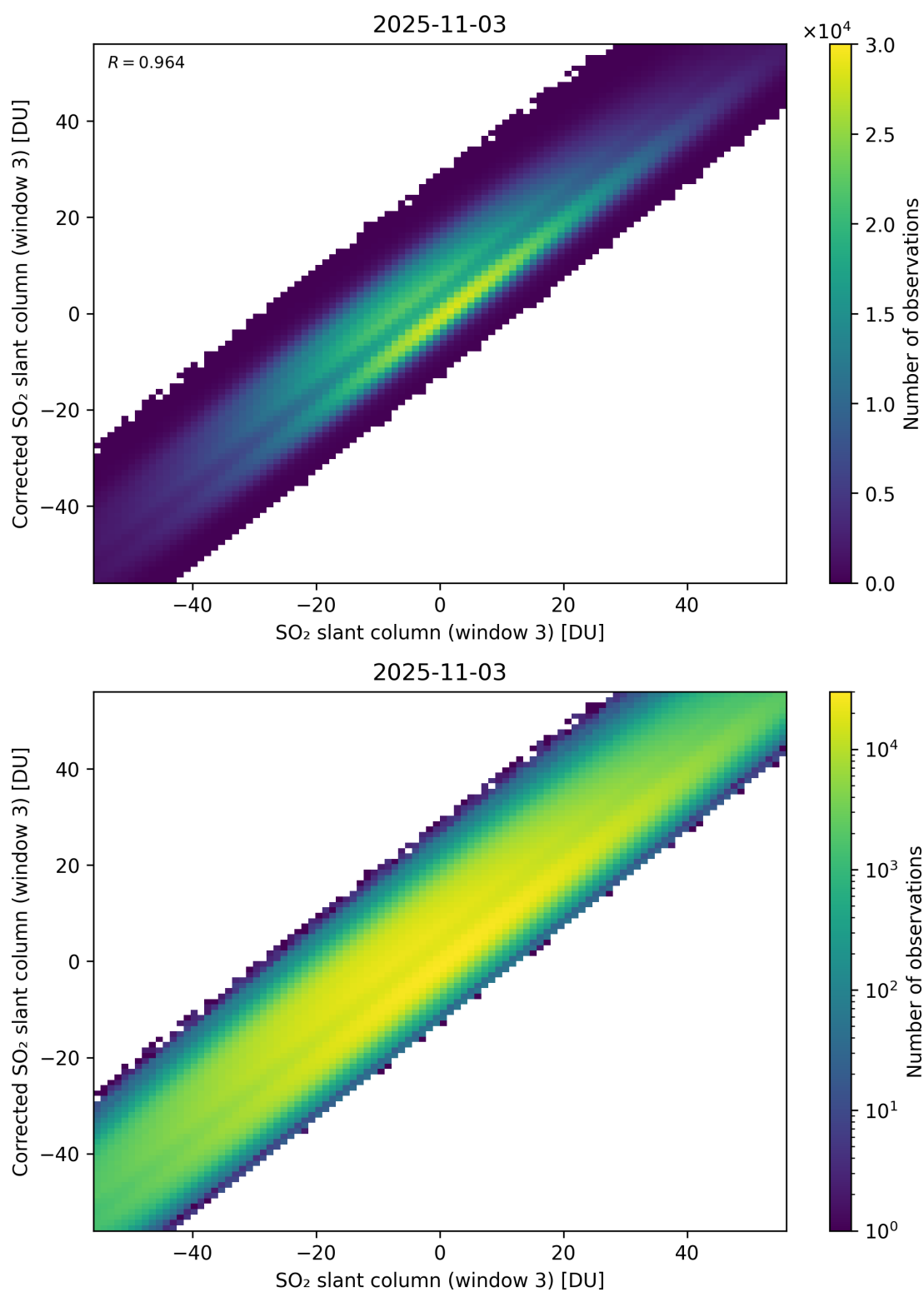
Figure 316: Scatter density plot of “SO 2 slant column (window 3)” against “Corrected SO 2 slant column (window 3)” for 2025-11-02 to 2025-11-04.
