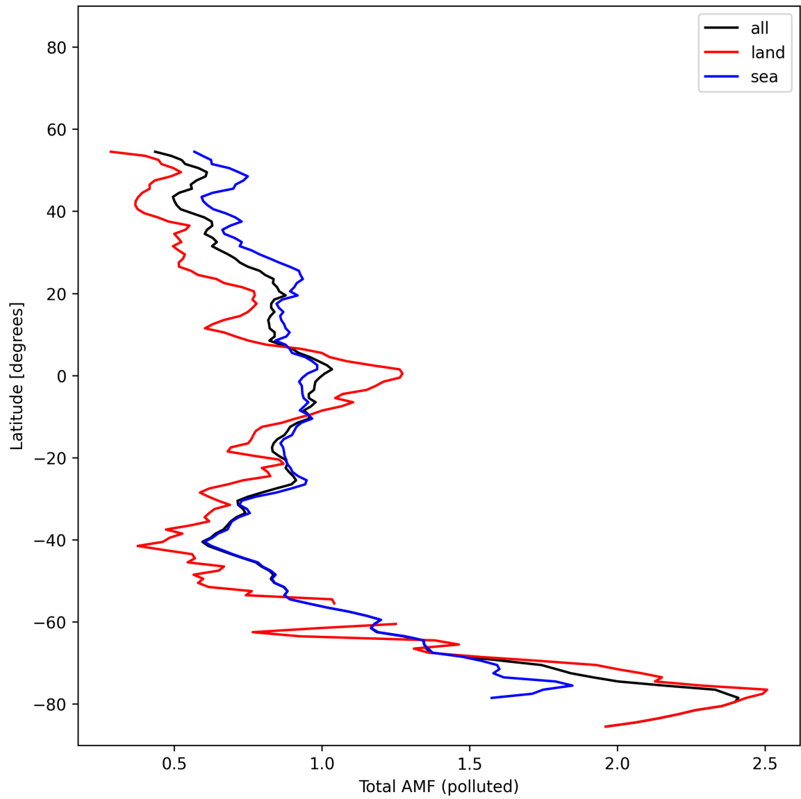
Figure 53: Zonal average of “Total AMF (polluted)” for 2025-11-02 to 2025-11-04.
