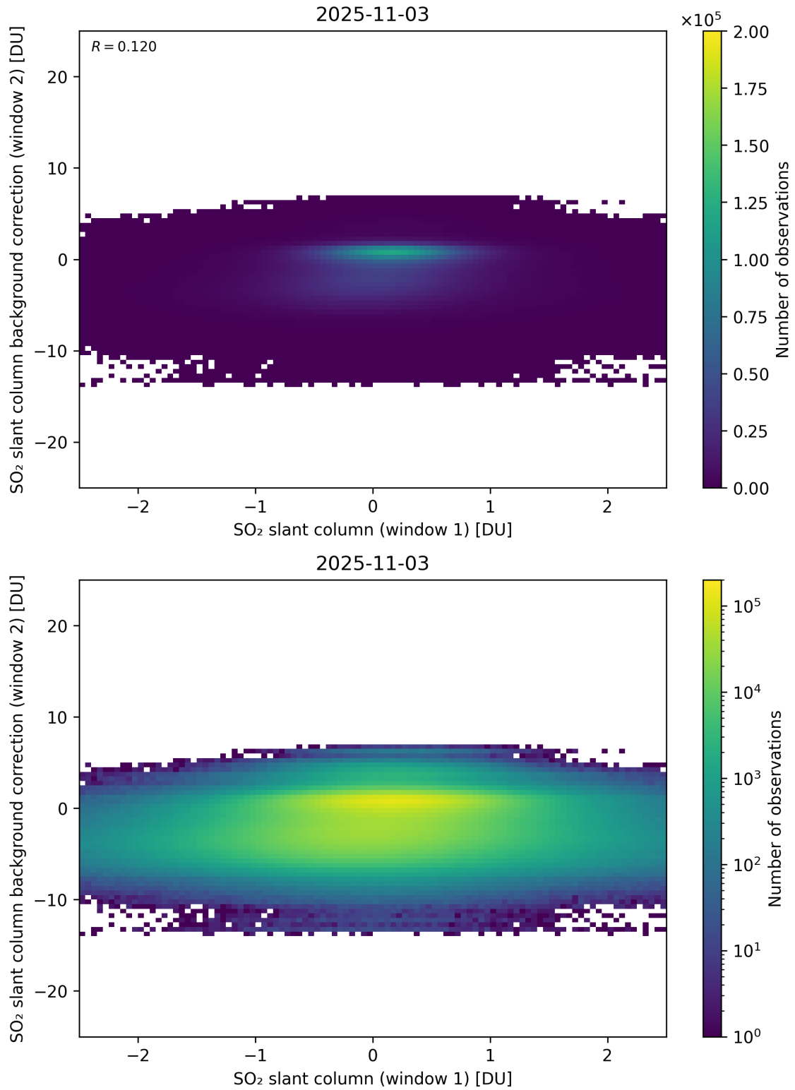
Figure 263: Scatter density plot of “SO 2 slant column (window 1)” against “SO 2 slant column background correction (window 2)” for 2025-11-02 to 2025-11-04.
