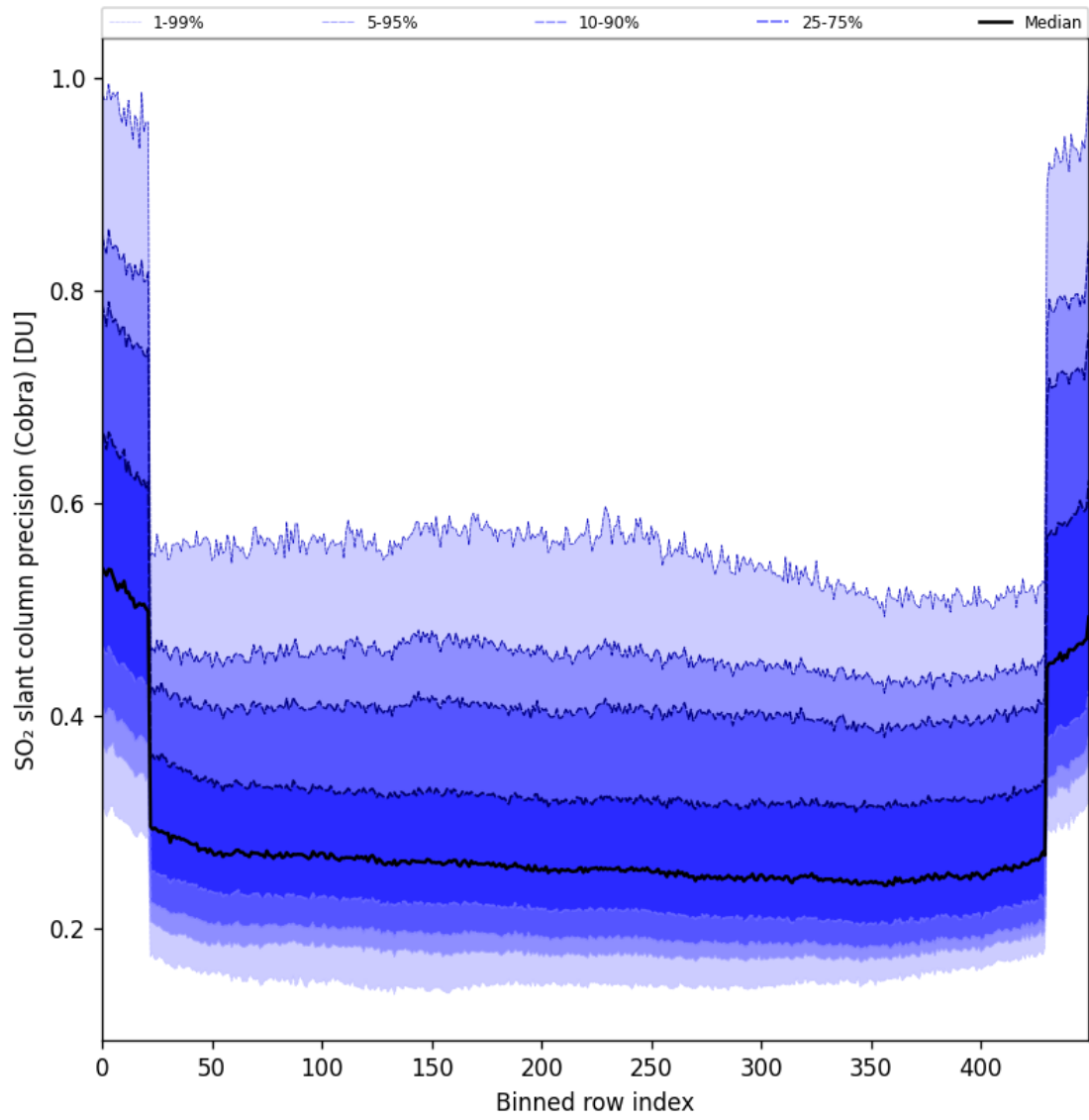
Figure 88: Along track statistics of “SO 2 slant column precision (Cobra)” for 2025-11-02 to 2025-11-04
