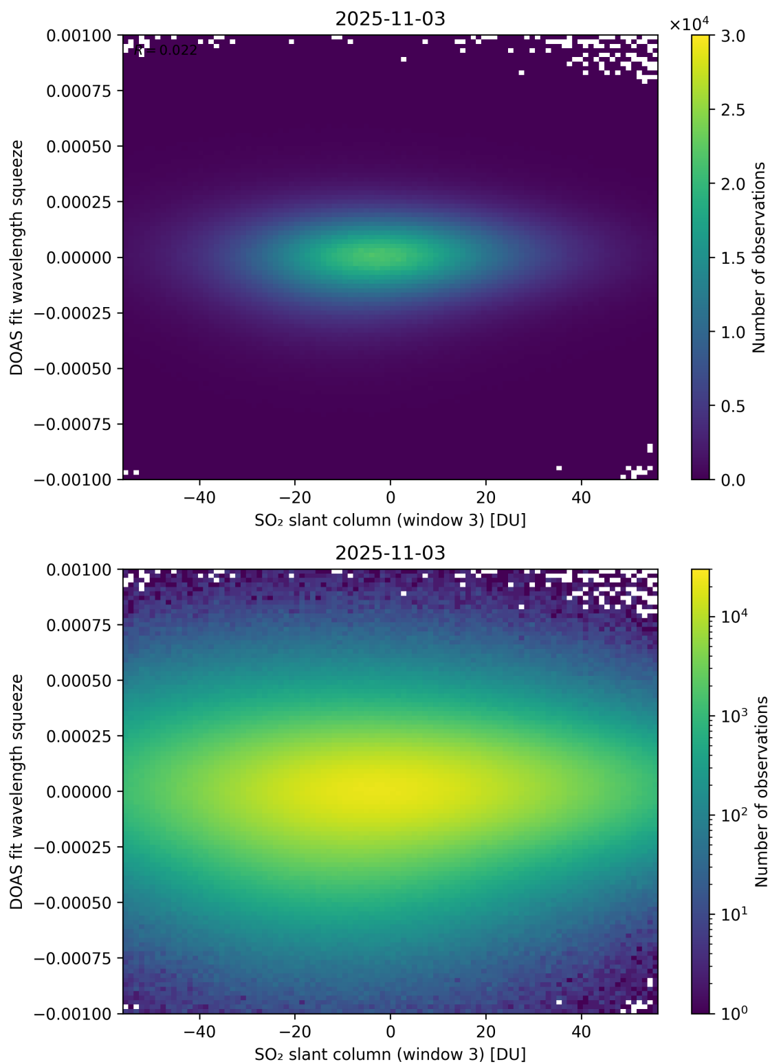
Figure 305: Scatter density plot of “SO 2 slant column (window 3)” against “DOAS fit wavelength squeeze” for 2025-11-02 to 2025-11-04.
