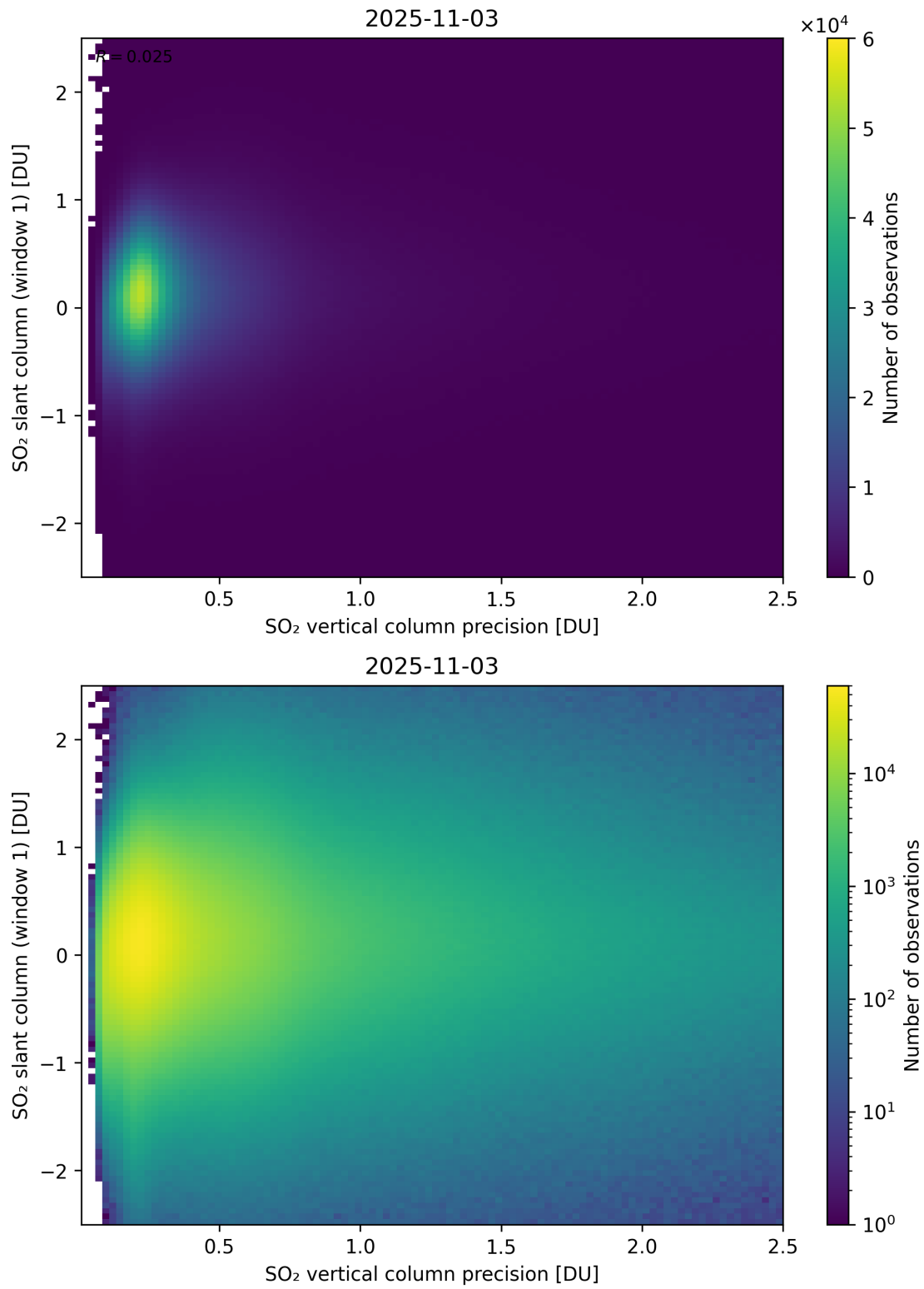
Figure 341: Scatter density plot of “SO 2 vertical column precision” against “SO 2 slant column (window 1)” for 2025-11-02 to 2025-11-04.
