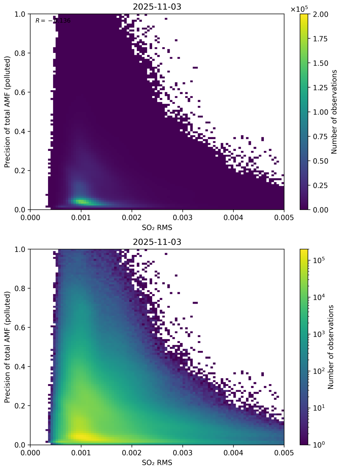
Figure 149: Scatter density plot of “SO 2 RMS” against “Precision of total AMF (polluted)” for 2025-11-02 to 2025-11-04.
