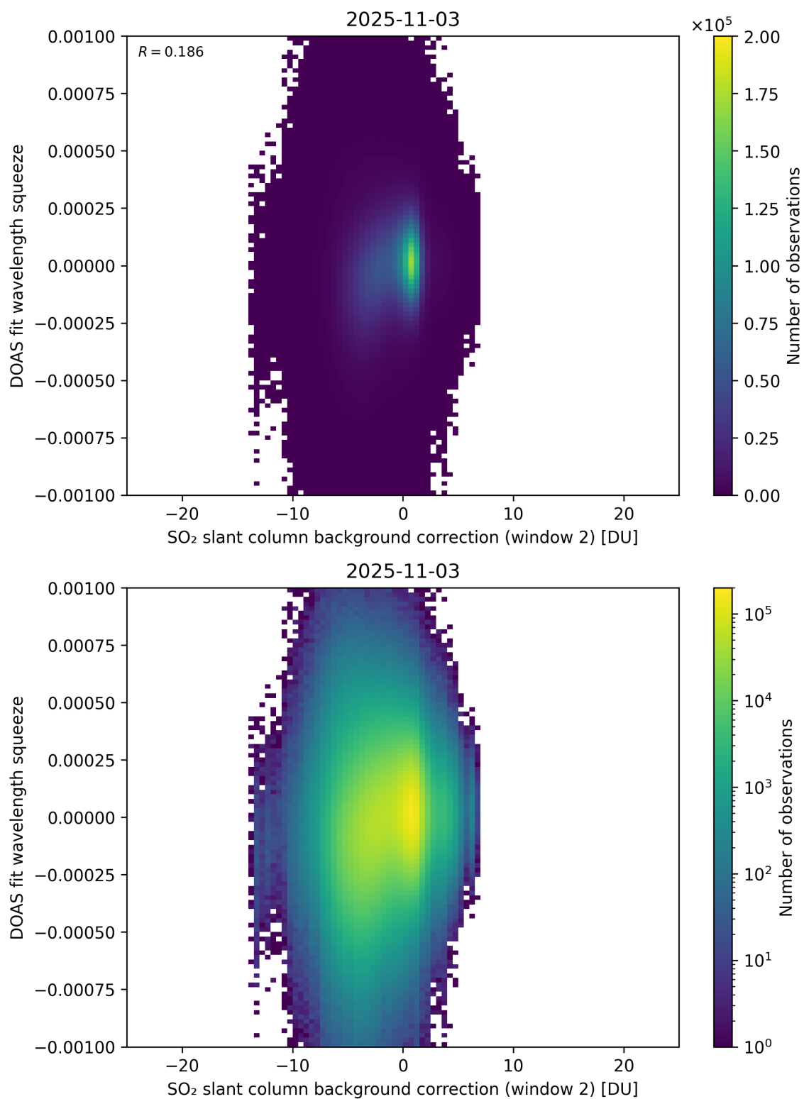
Figure 124: Scatter density plot of “SO 2 slant column background correction (window 2)” against “DOAS fit wavelength squeeze” for 2025-11-02 to 2025-11-04.
