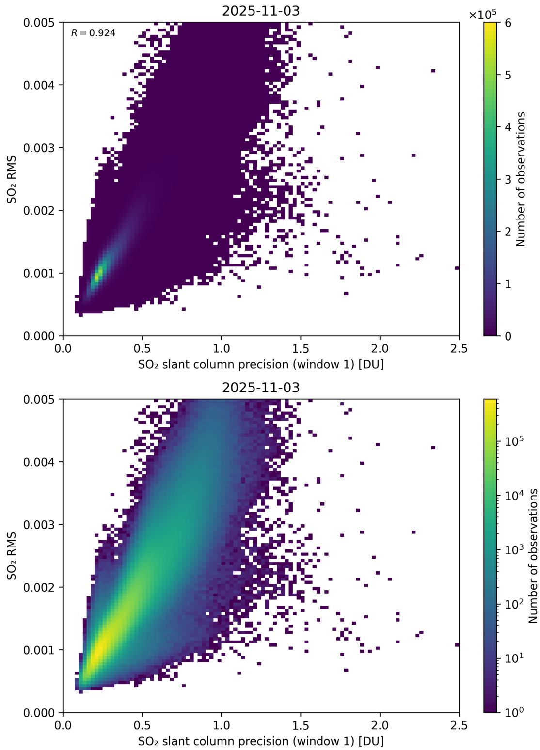
Figure 273: Scatter density plot of “SO 2 slant column precision (window 1)” against “SO 2 RMS” for 2025-11-02 to 2025-11-04.
