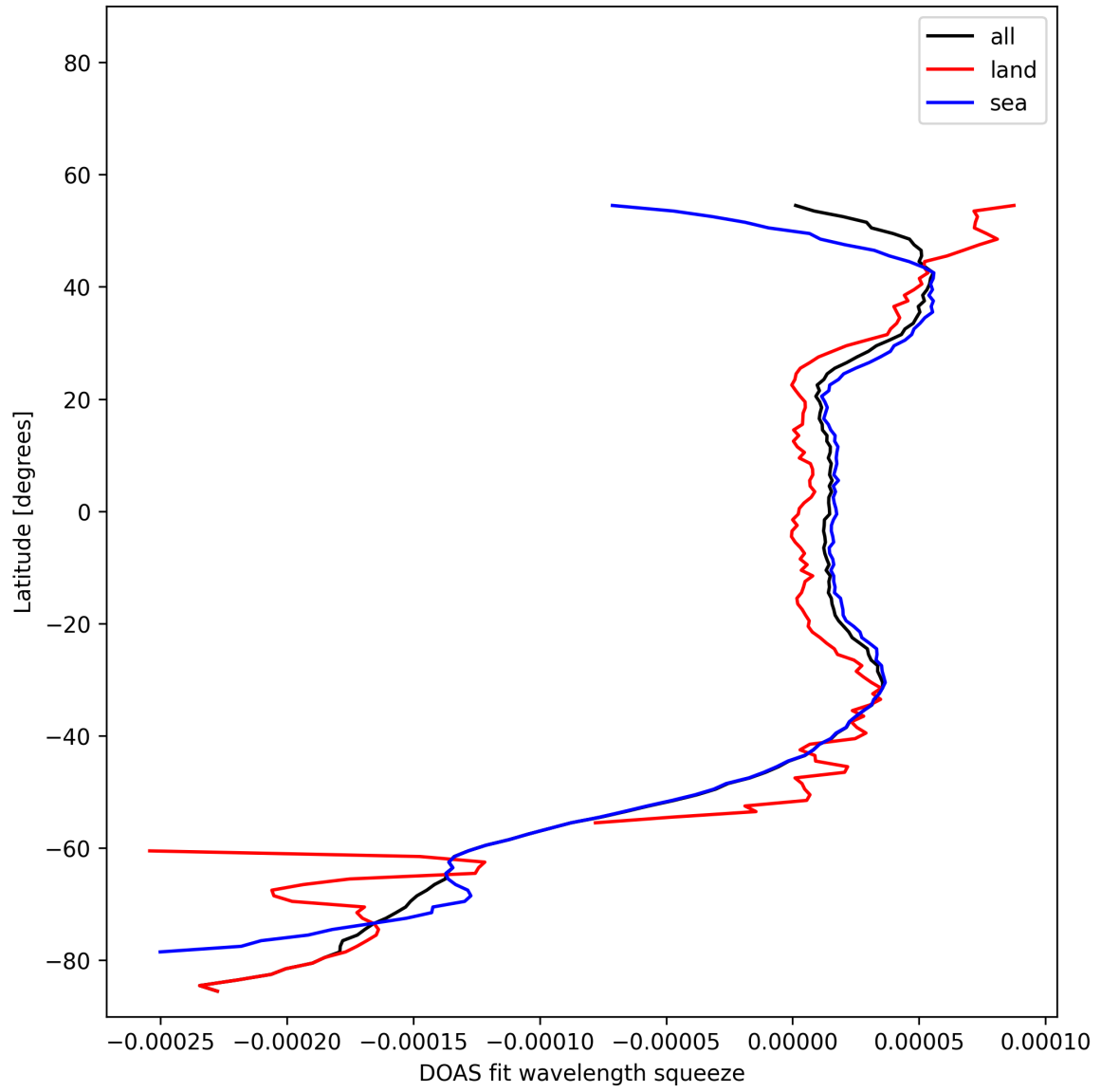
Figure 51: Zonal average of “DOAS fit wavelength squeeze” for 2025-11-02 to 2025-11-04.
