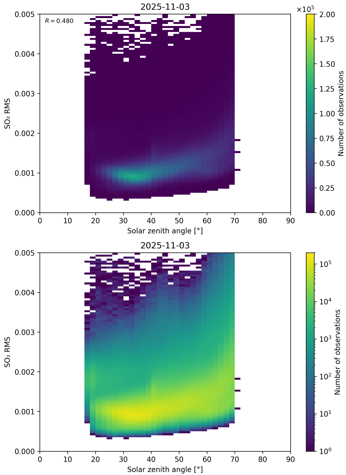
Figure 176: Scatter density plot of “Solar zenith angle” against “SO 2 RMS” for 2025-11-02 to 2025-11-04.
