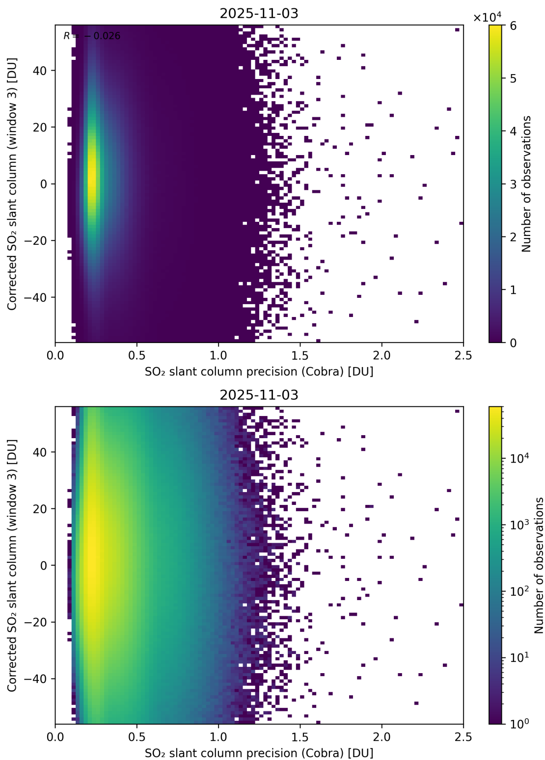
Figure 207: Scatter density plot of “SO 2 slant column precision (Cobra)” against “Corrected SO 2 slant column (window 3)” for 2025-11-02 to 2025-11-04.
