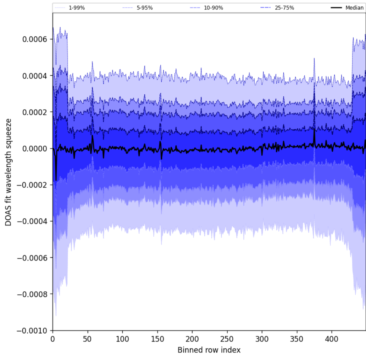
Figure 103: Along track statistics of “DOAS fit wavelength squeeze” for 2025-11-02 to 2025-11-04
