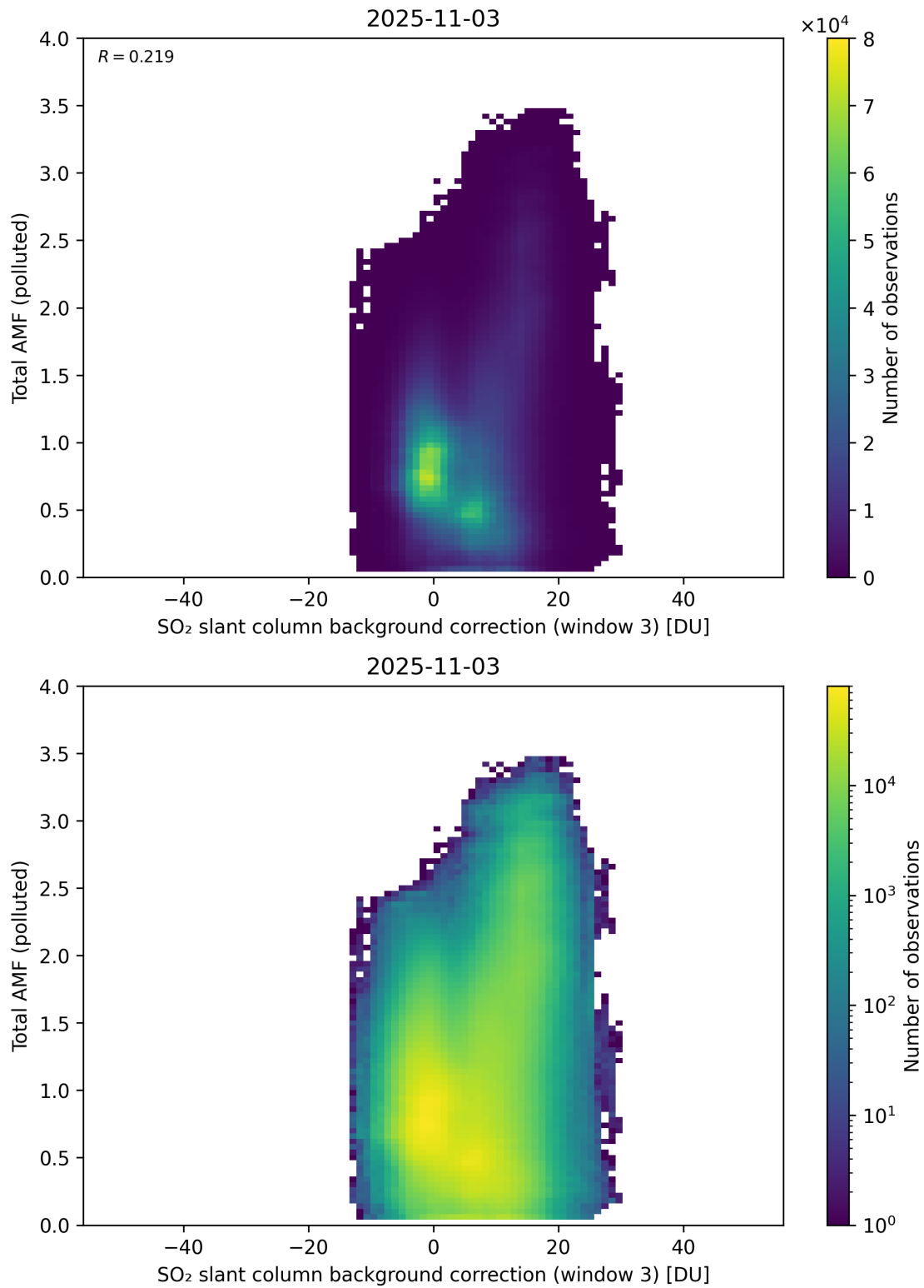
Figure 136: Scatter density plot of “SO 2 slant column background correction (window 3)” against “Total AMF (polluted)” for 2025-11-02 to 2025-11-04.
