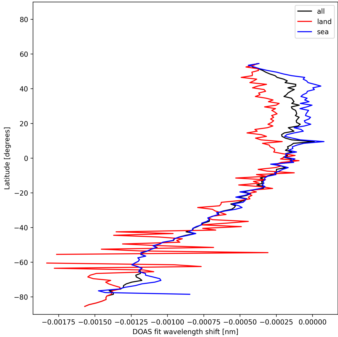
Figure 50: Zonal average of “DOAS fit wavelength shift” for 2025-11-02 to 2025-11-04.
