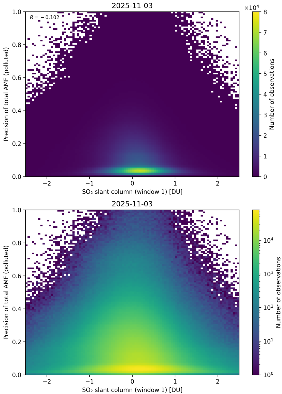
Figure 290: Scatter density plot of “SO 2 slant column (window 1)” against “Precision of total AMF (polluted)” for 2025-11-02 to 2025-11-04.
