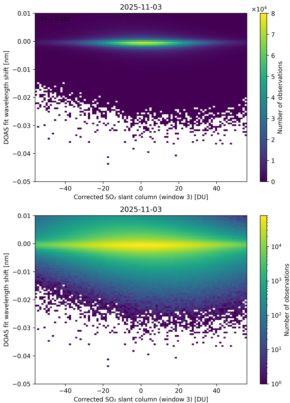
Figure 256: Scatter density plot of “Corrected SO 2 slant column (window 3)” against “DOAS fit wavelength shift” for 2025-11-02 to 2025-11-04.
