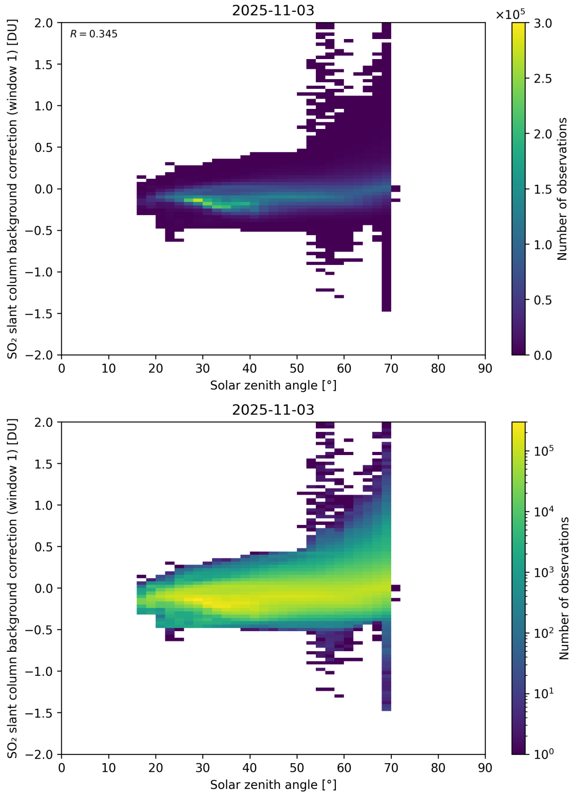
Figure 171: Scatter density plot of “Solar zenith angle” against “SO 2 slant column background correction (window 1)” for 2025-11-02 to 2025-11-04.
