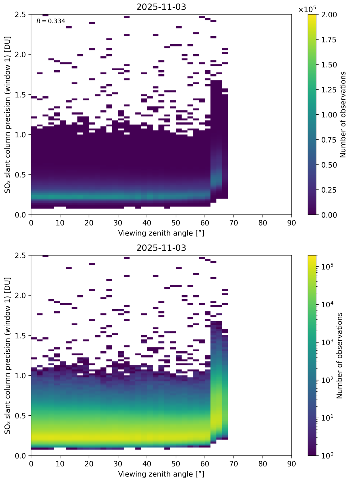
Figure 377: Scatter density plot of “Viewing zenith angle” against “SO 2 slant column precision (window 1)” for 2025-11-02 to 2025-11-04.
