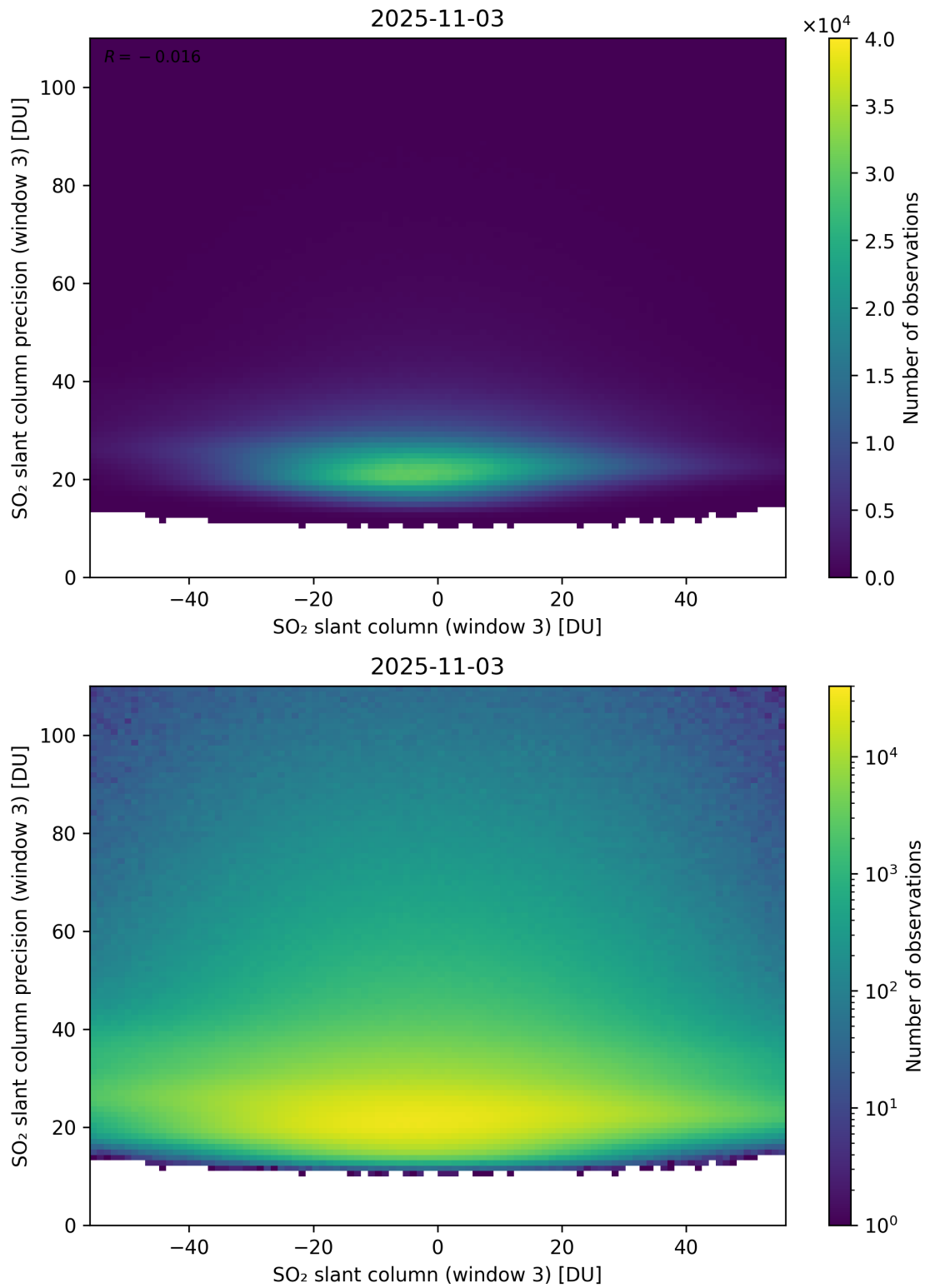
Figure 317: Scatter density plot of “SO 2 slant column (window 3)” against “SO 2 slant column precision (window 3)” for 2025-11-02 to 2025-11-04.
