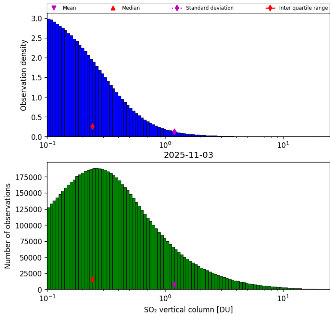
Figure 58: Histogram of “SO 2 vertical column” for 2025-11-02 to 2025-11-04
