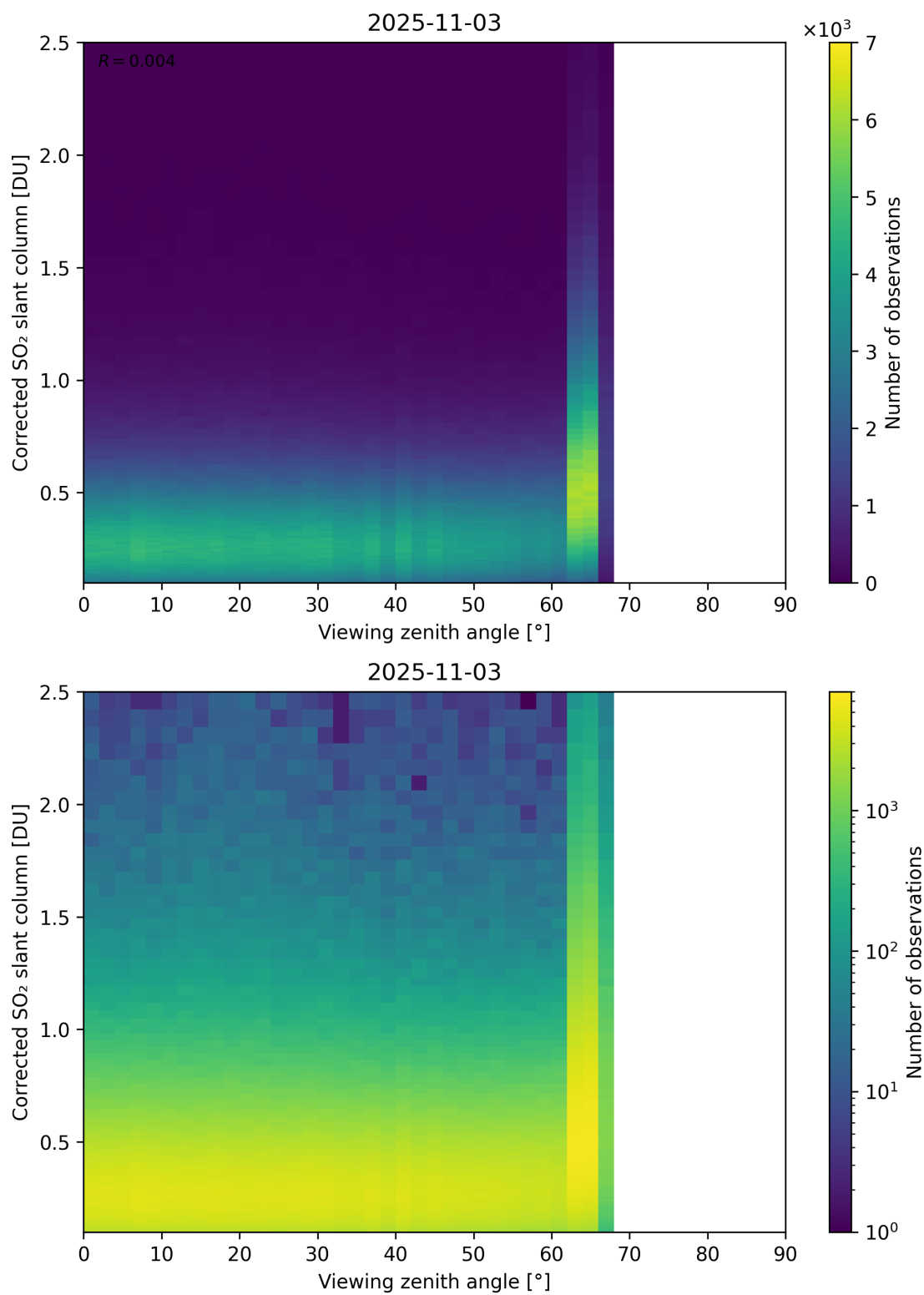
Figure 373: Scatter density plot of “Viewing zenith angle” against “Corrected SO 2 slant column” for 2025-11-02 to 2025-11-04.
