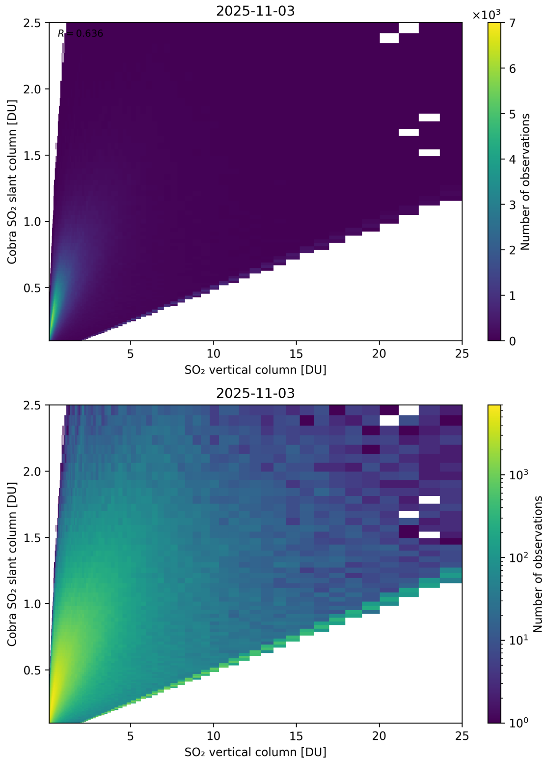
Figure 349: Scatter density plot of “SO 2 vertical column” against “Cobra SO 2 slant column” for 2025-11-02 to 2025-11-04.
