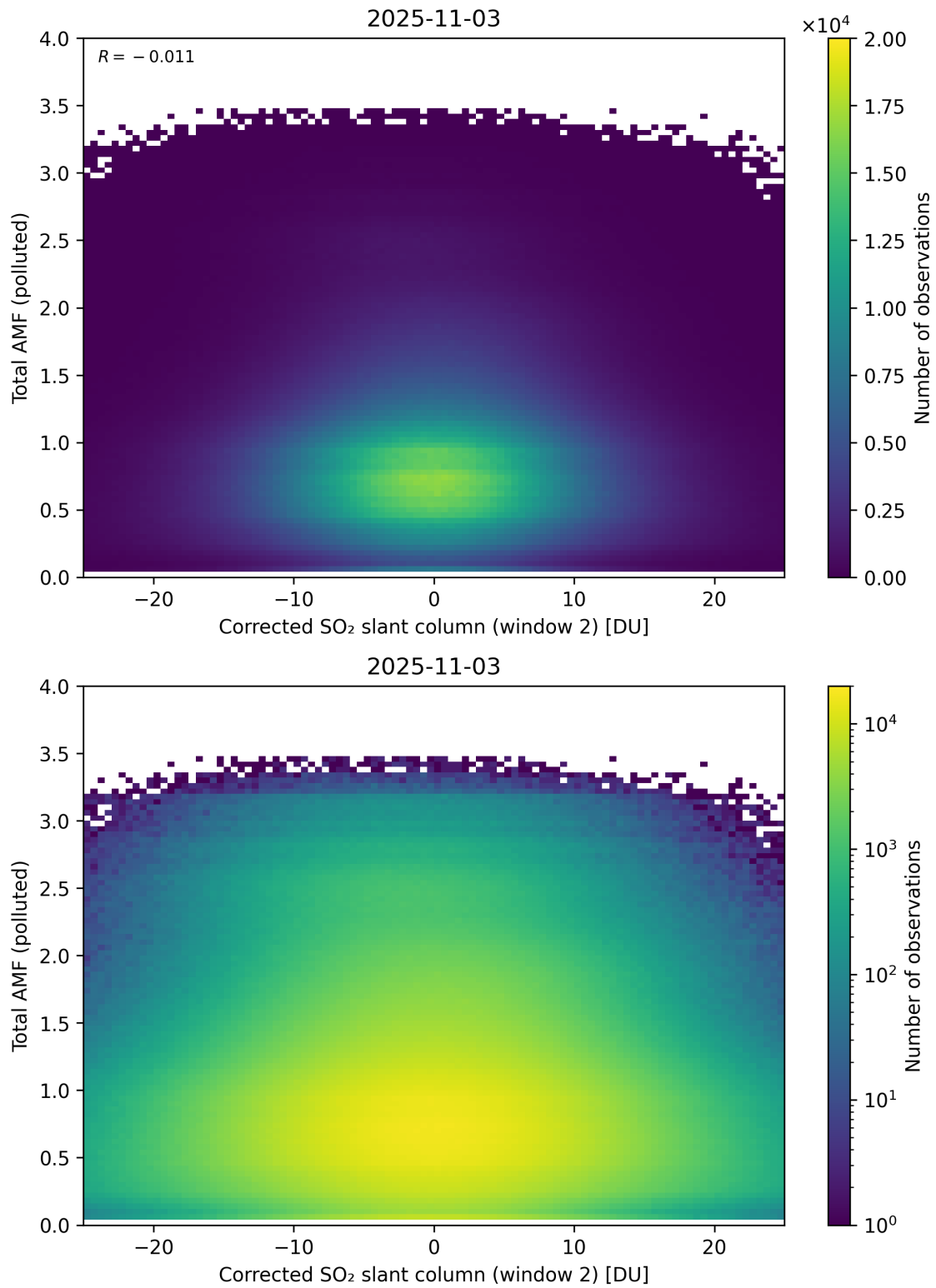
Figure 253: Scatter density plot of “Corrected SO 2 slant column (window 2)” against “Total AMF (polluted)” for 2025-11-02 to 2025-11-04.
