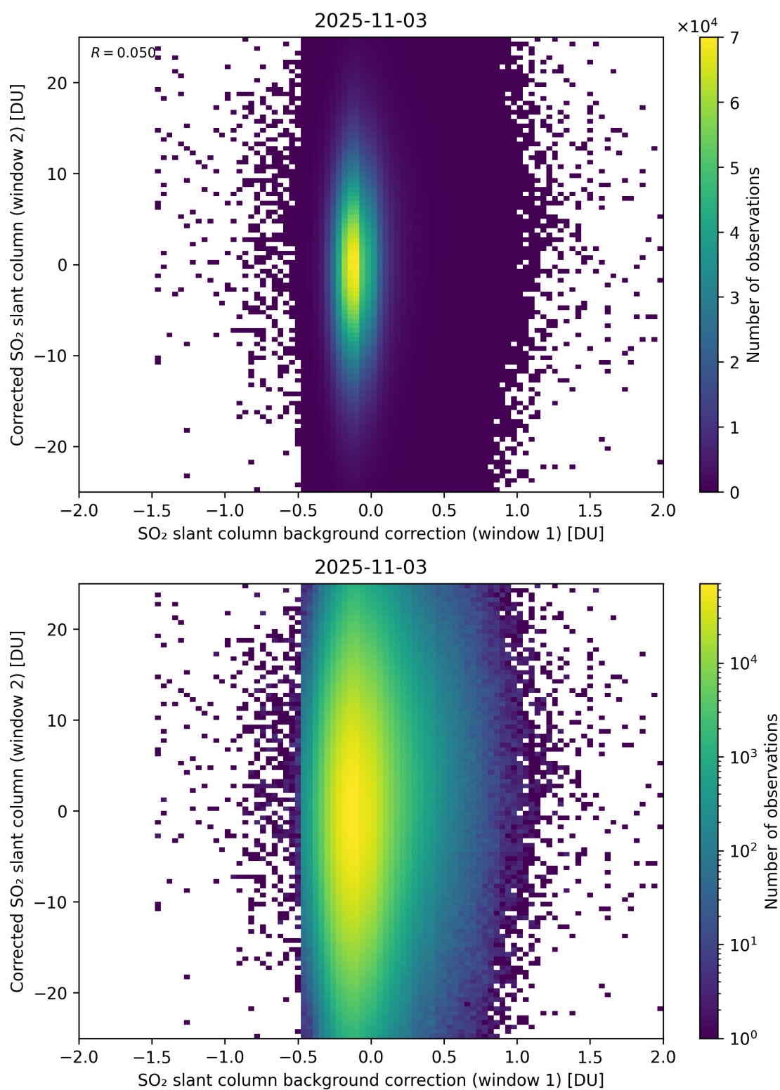
Figure 115: Scatter density plot of “SO 2 slant column background correction (window 1)” against “Corrected SO 2 slant column (window 2)” for 2025-11-02 to 2025-11-04.
