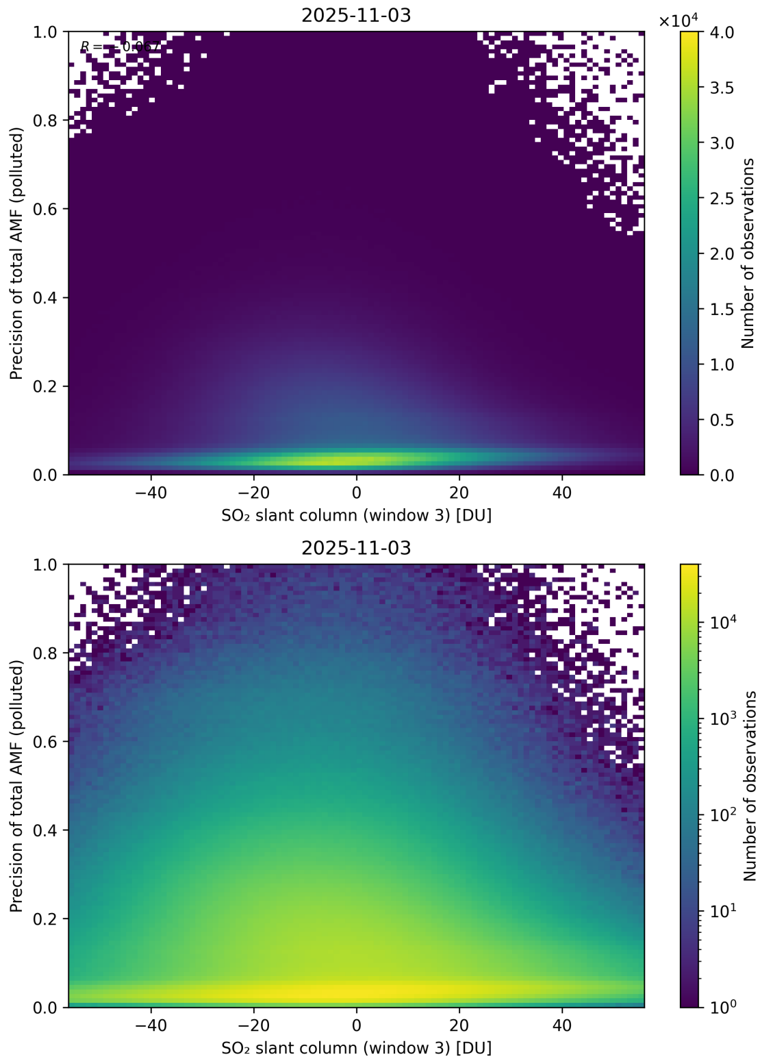
Figure 319: Scatter density plot of “SO 2 slant column (window 3)” against “Precision of total AMF (polluted)” for 2025-11-02 to 2025-11-04.
