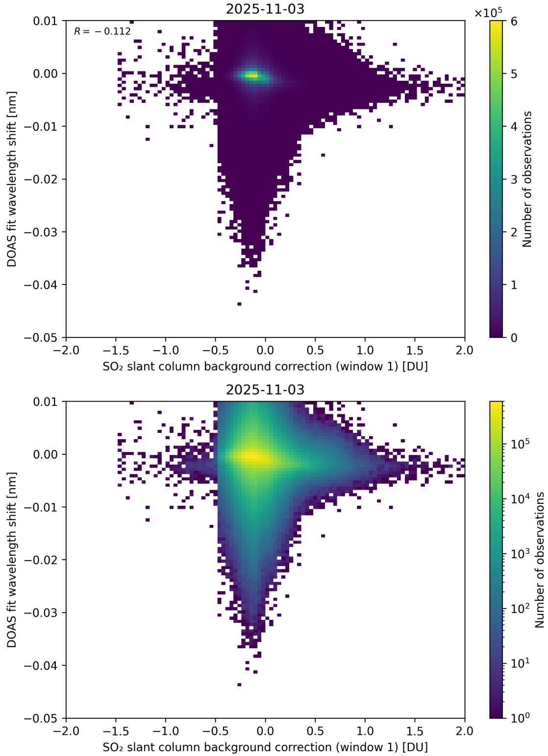
Figure 111: Scatter density plot of “SO 2 slant column background correction (window 1)” against “DOAS fit wavelength shift” for 2025-11-02 to 2025-11-04.
