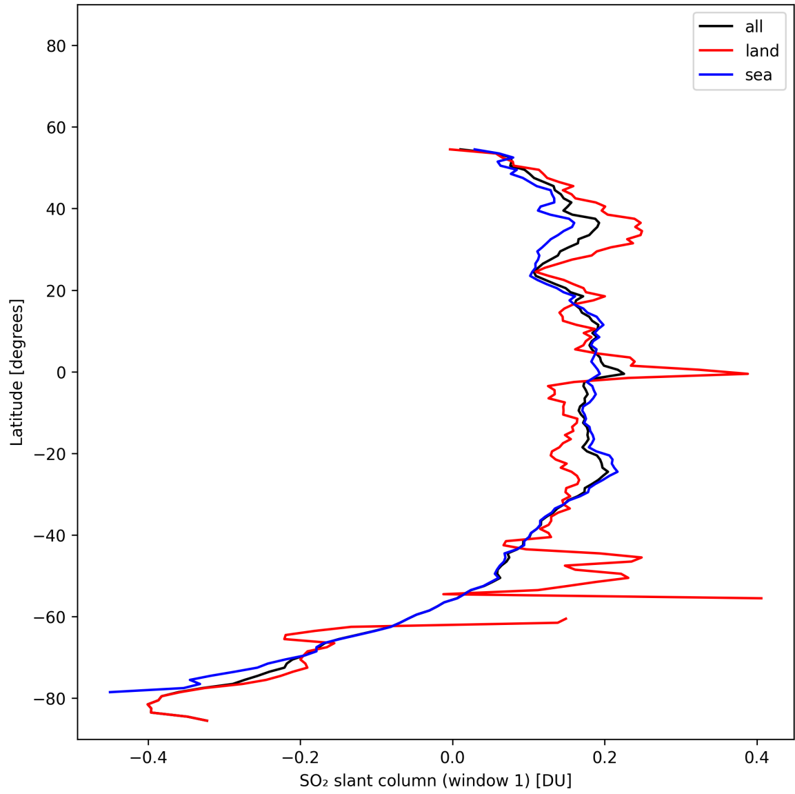
Figure 37: Zonal average of “SO 2 slant column (window 1)” for 2025-11-02 to 2025-11-04.
