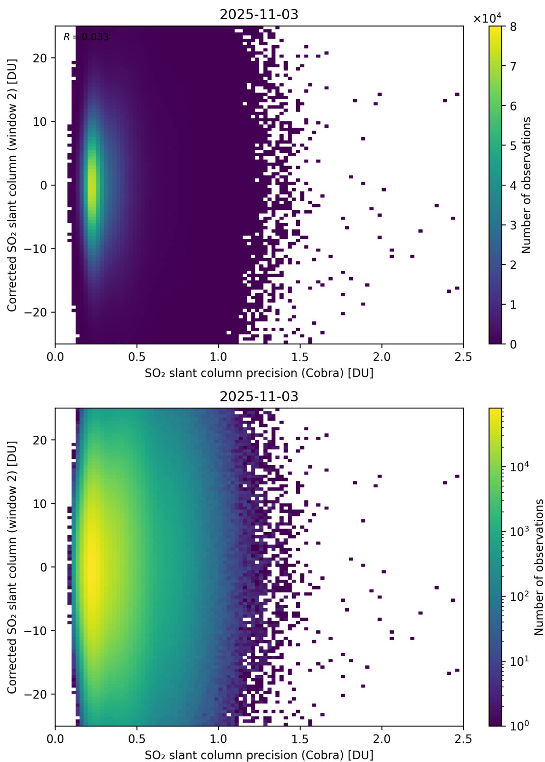
Figure 206: Scatter density plot of “SO 2 slant column precision (Cobra)” against “Corrected SO 2 slant column (window 2)” for 2025-11-02 to 2025-11-04.
