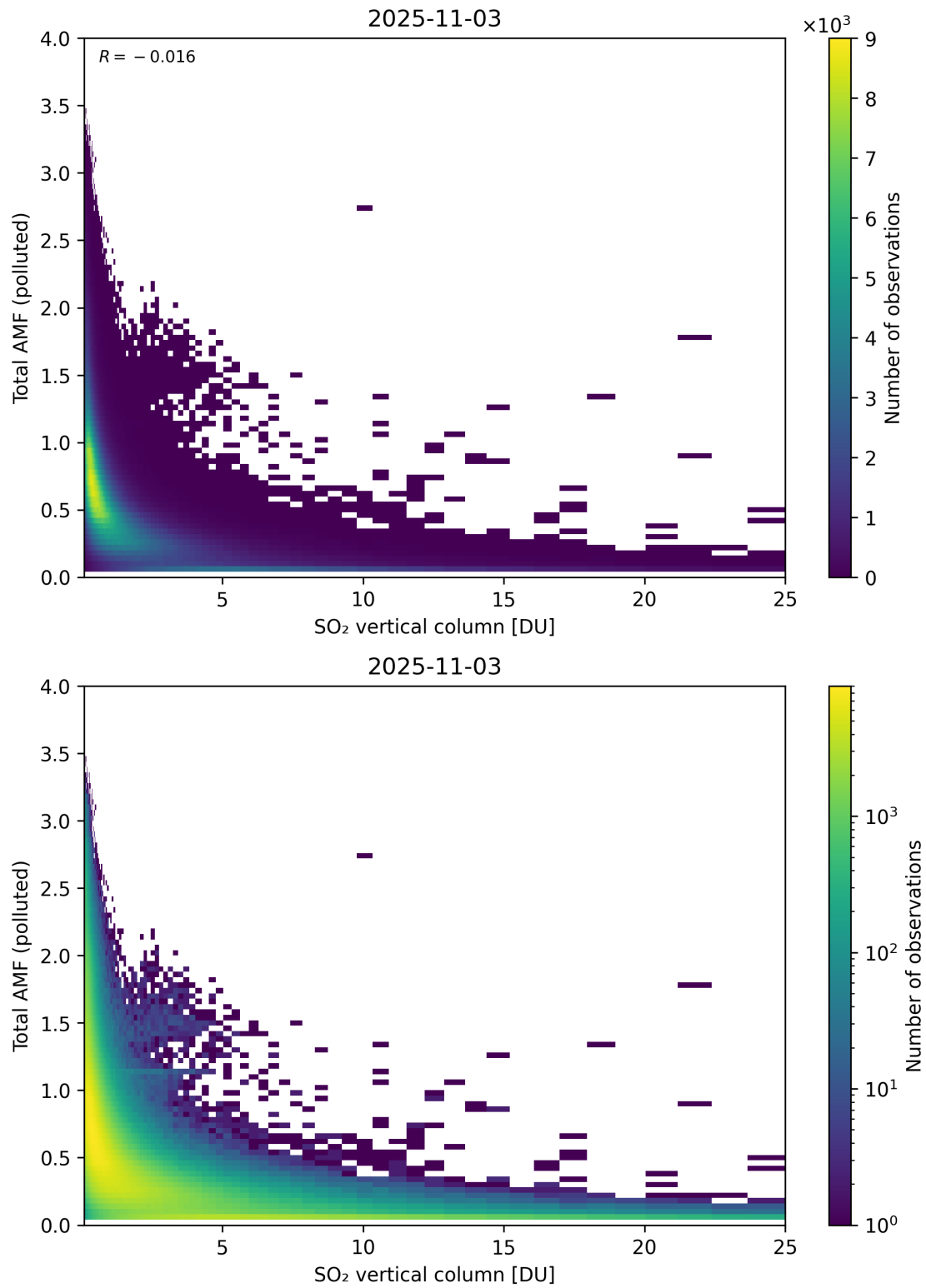
Figure 359: Scatter density plot of “SO 2 vertical column” against “Total AMF (polluted)” for 2025-11-02 to 2025-11-04.
