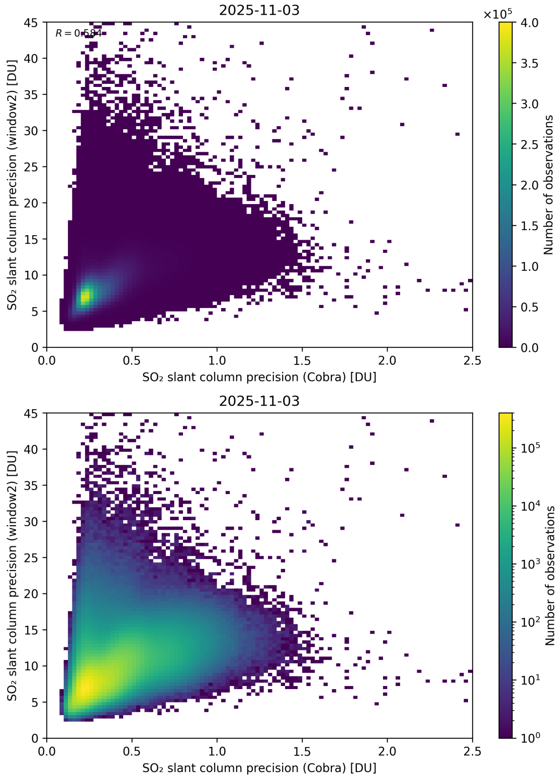
Figure 210: Scatter density plot of “SO 2 slant column precision (Cobra)” against “SO 2 slant column precision (window2)” for 2025-11-02 to 2025-11-04.
