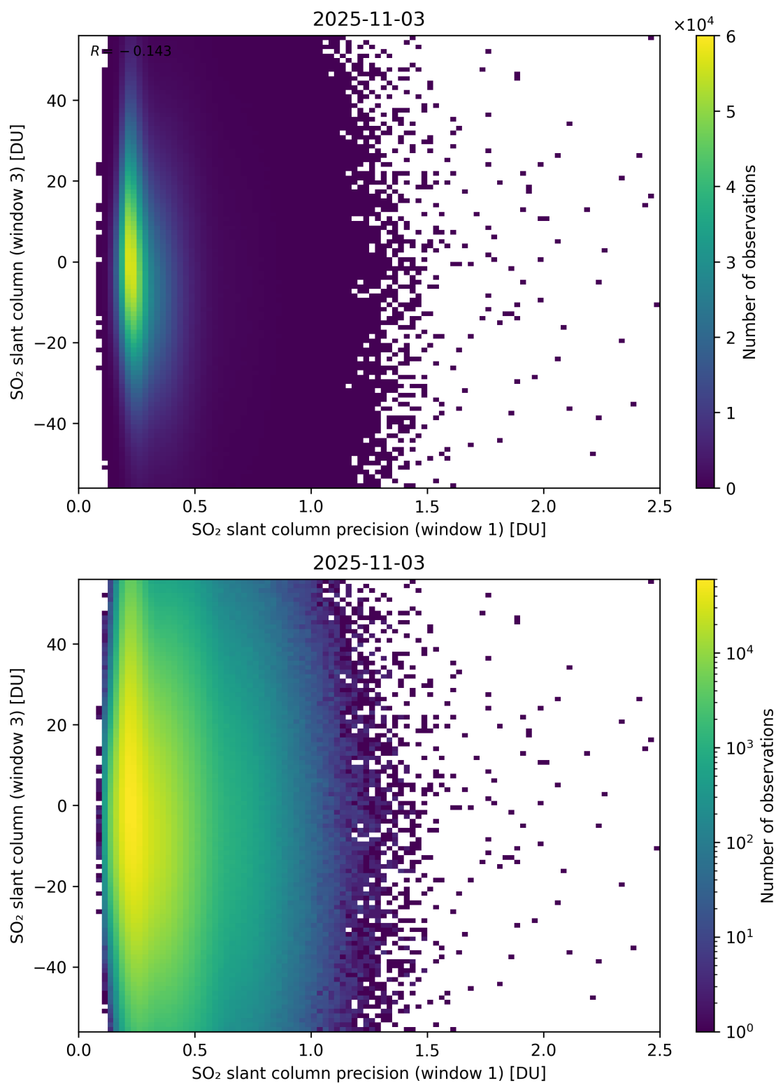
Figure 278: Scatter density plot of “SO 2 slant column precision (window 1)” against “SO 2 slant column (window 3)” for 2025-11-02 to 2025-11-04.
