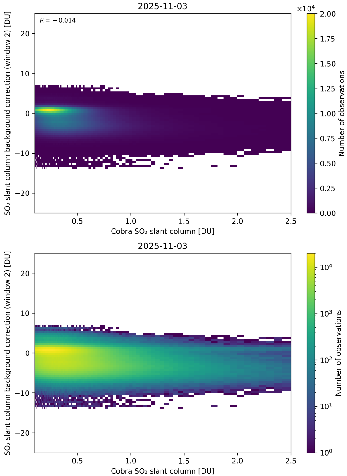
Figure 194: Scatter density plot of “Cobra SO 2 slant column” against “SO 2 slant column background correction (window 2)” for 2025-11-02 to 2025-11-04.
