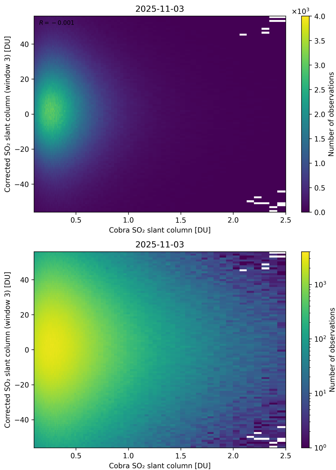
Figure 218: Scatter density plot of “Cobra SO 2 slant column” against “Corrected SO 2 slant column (window 3)” for 2025-11-02 to 2025-11-04.
