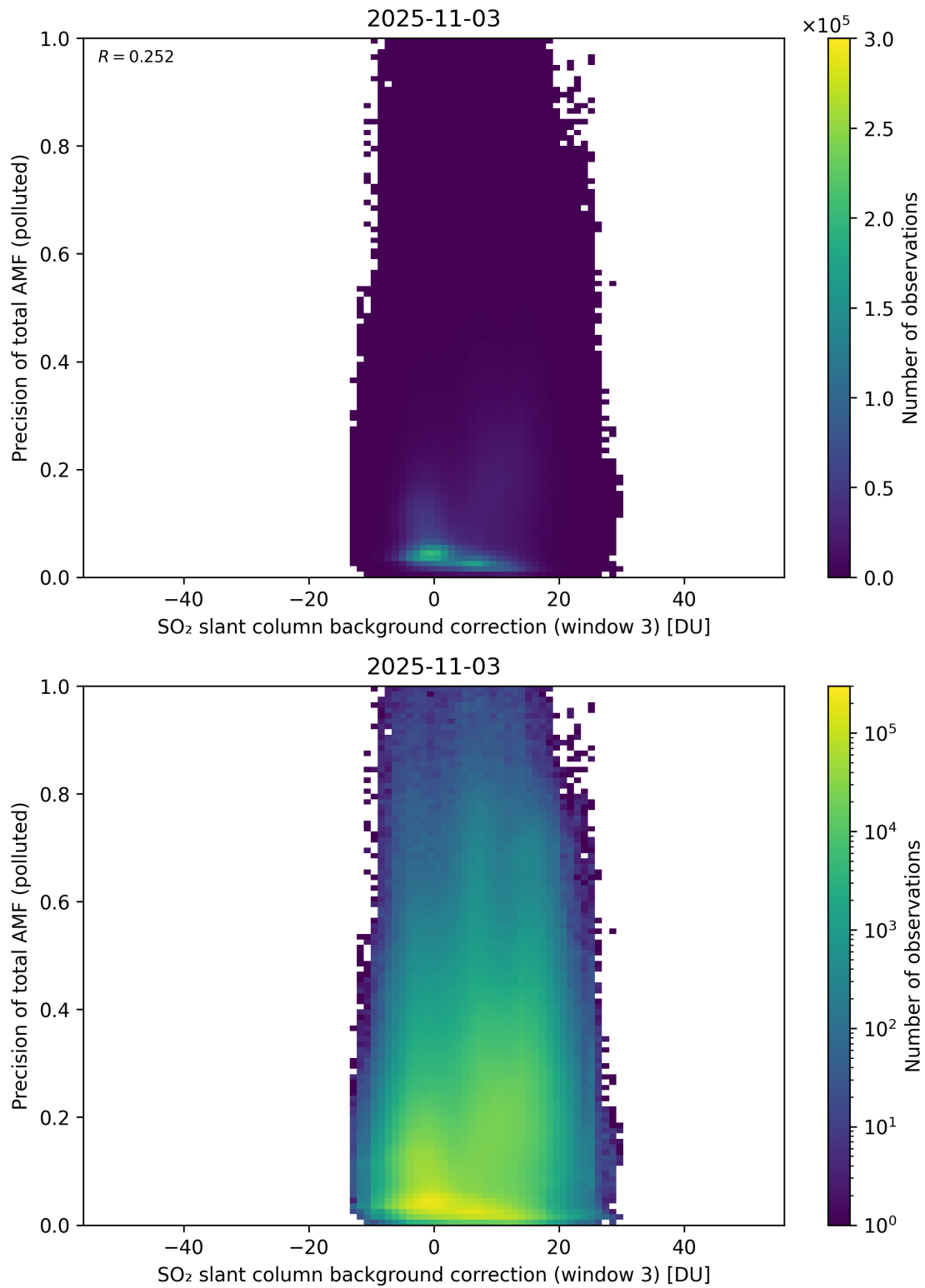
Figure 137: Scatter density plot of “SO 2 slant column background correction (window 3)” against “Precision of total AMF (polluted)” for 2025-11-02 to 2025-11-04.
