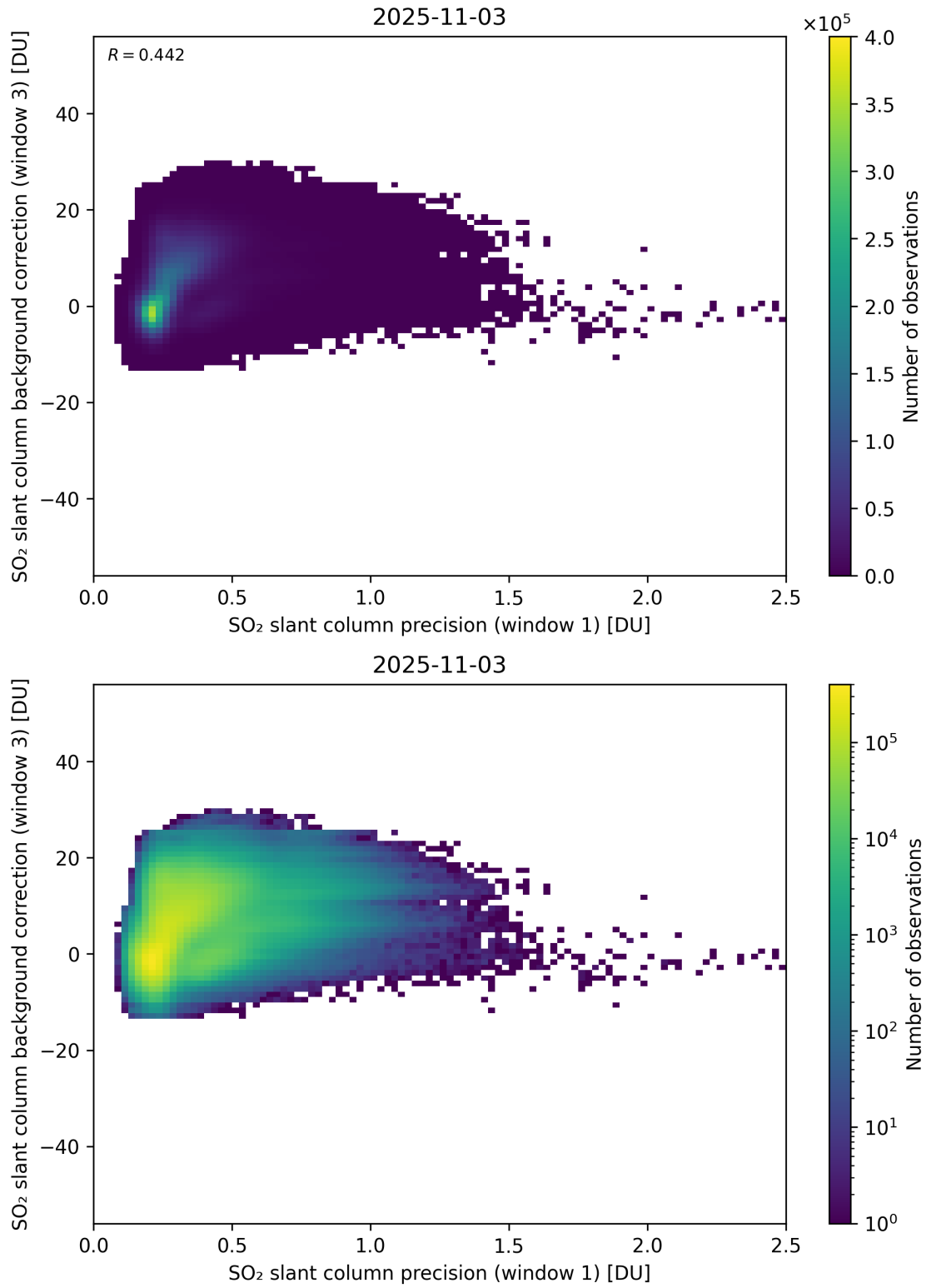
Figure 270: Scatter density plot of “SO 2 slant column precision (window 1)” against “SO 2 slant column background correction (window 3)” for 2025-11-02 to 2025-11-04.
