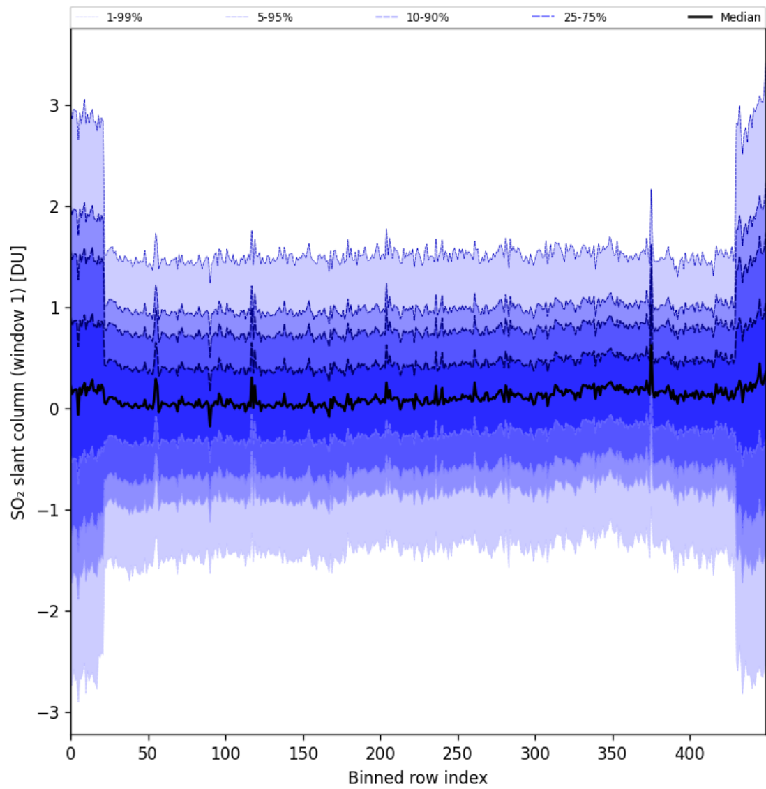
Figure 89: Along track statistics of “SO 2 slant column (window 1)” for 2025-11-02 to 2025-11-04
