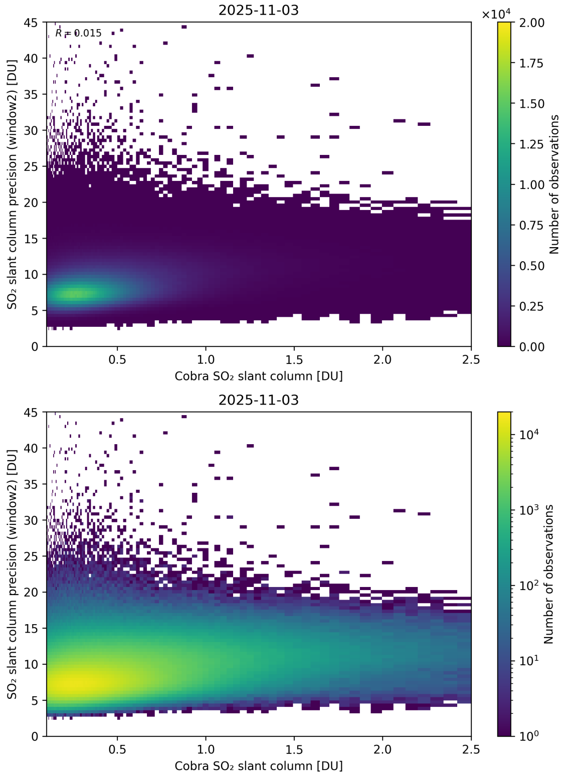
Figure 221: Scatter density plot of “Cobra SO 2 slant column” against “SO 2 slant column precision (window2)” for 2025-11-02 to 2025-11-04.
