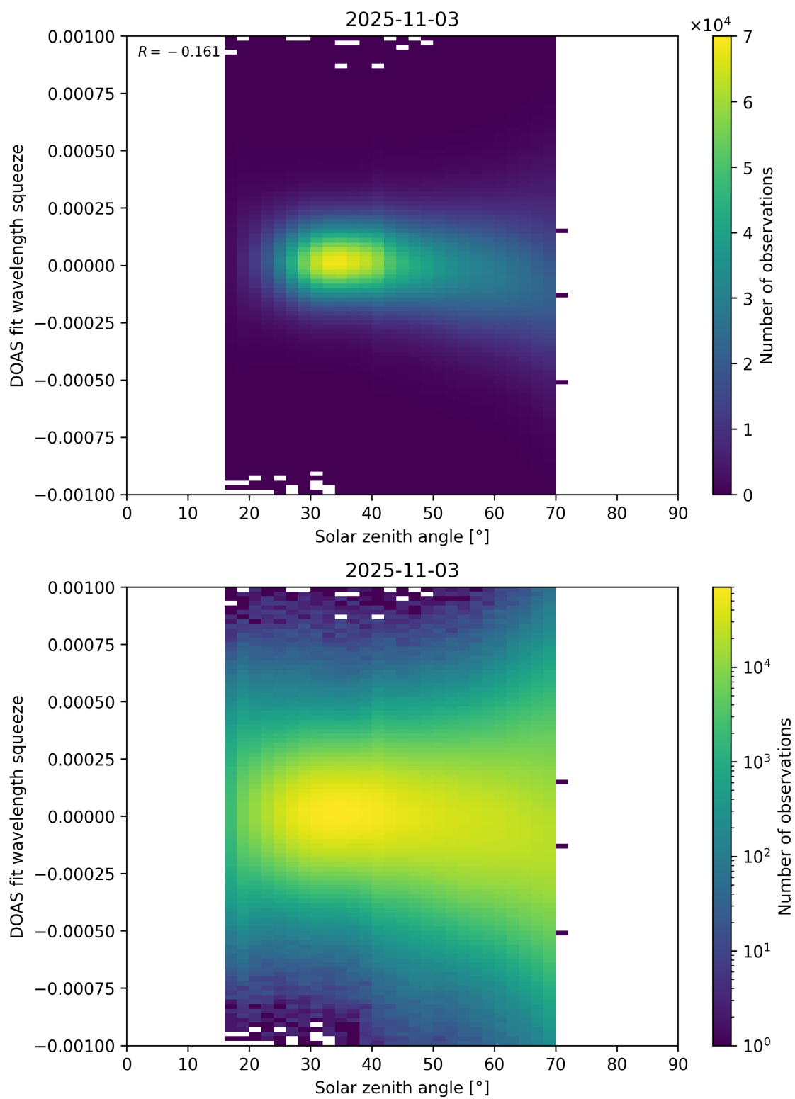
Figure 175: Scatter density plot of “Solar zenith angle” against “DOAS fit wavelength squeeze” for 2025-11-02 to 2025-11-04.
