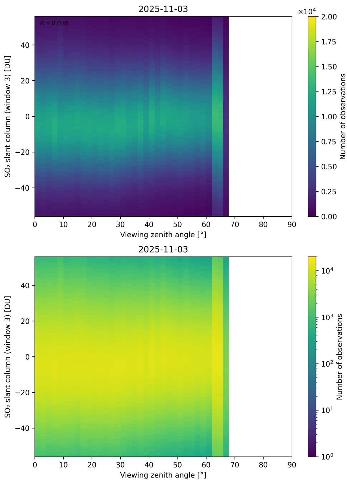
Figure 379: Scatter density plot of “Viewing zenith angle” against “SO 2 slant column (window 3)” for 2025-11-02 to 2025-11-04.
