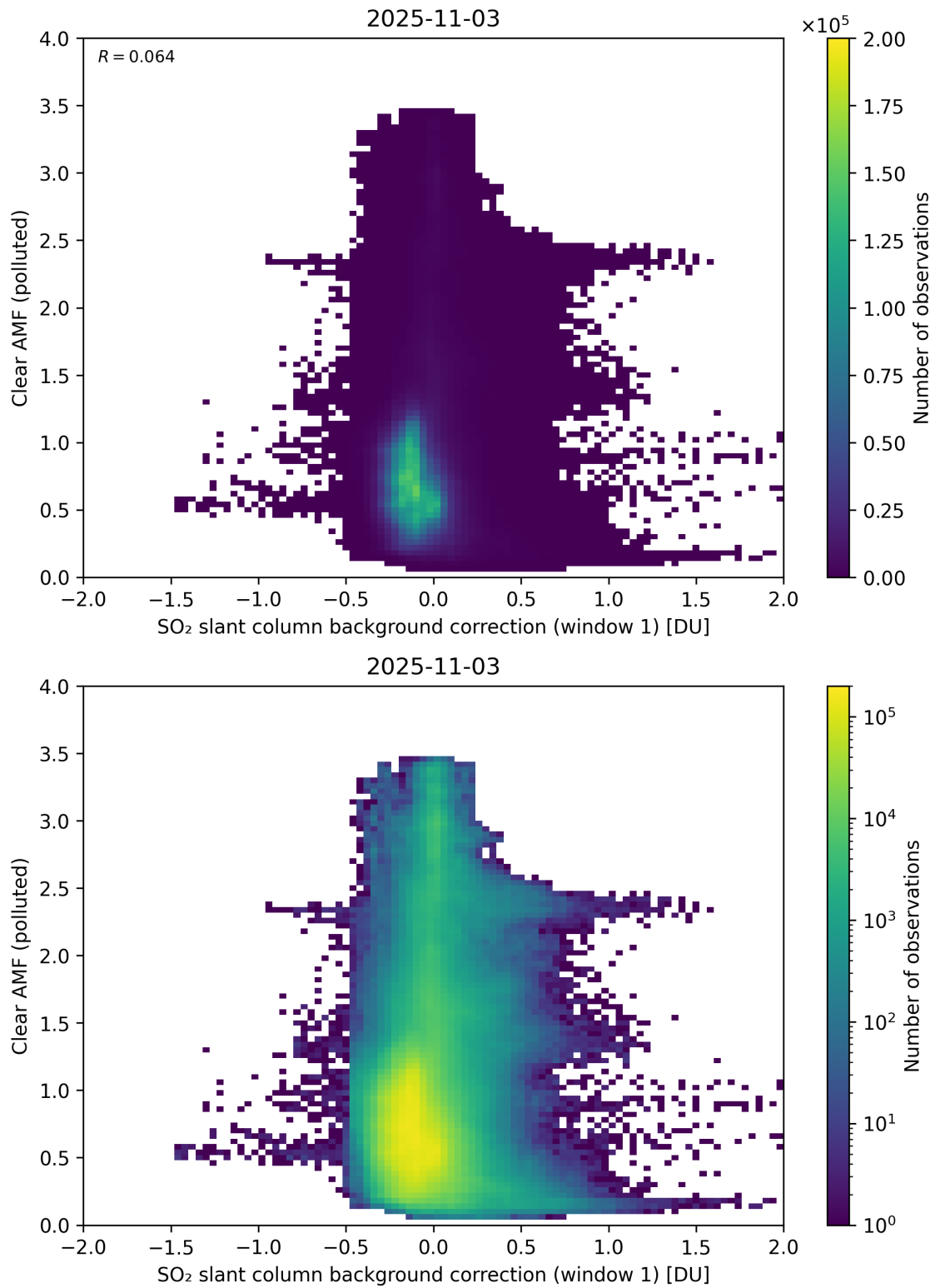
Figure 114: Scatter density plot of “SO 2 slant column background correction (window 1)” against “Clear AMF (polluted)” for 2025-11-02 to 2025-11-04.
