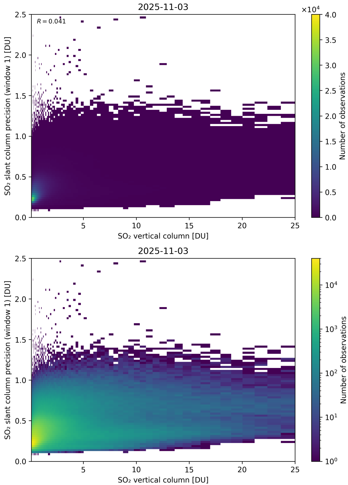
Figure 355: Scatter density plot of “SO 2 vertical column” against “SO 2 slant column precision (window 1)” for 2025-11-02 to 2025-11-04.
