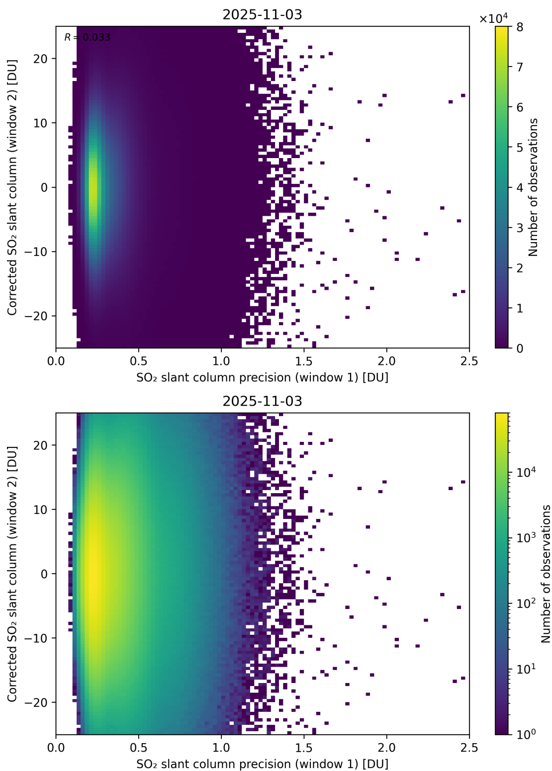
Figure 275: Scatter density plot of “SO 2 slant column precision (window 1)” against “Corrected SO 2 slant column (window 2)” for 2025-11-02 to 2025-11-04.
