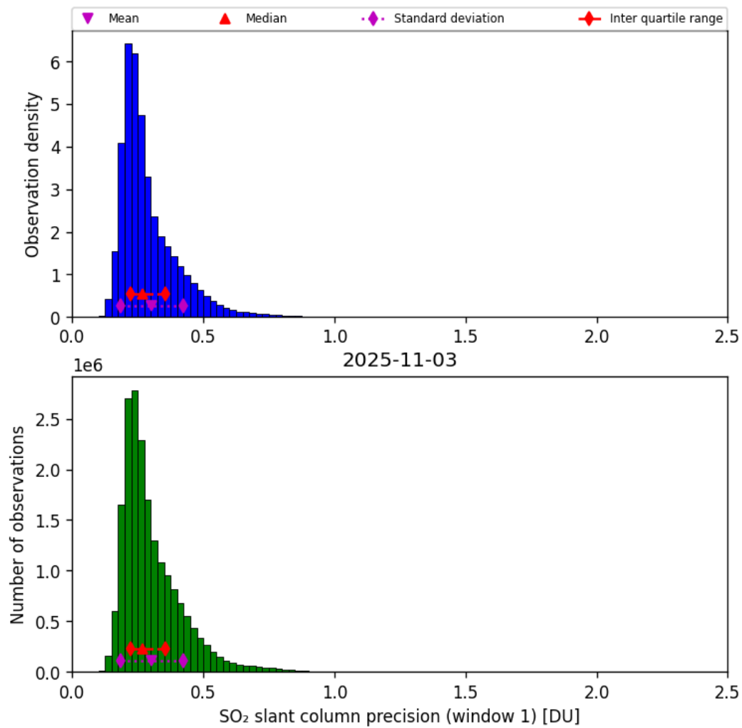
Figure 64: Histogram of “SO 2 slant column precision (window 1)” for 2025-11-02 to 2025-11-04
