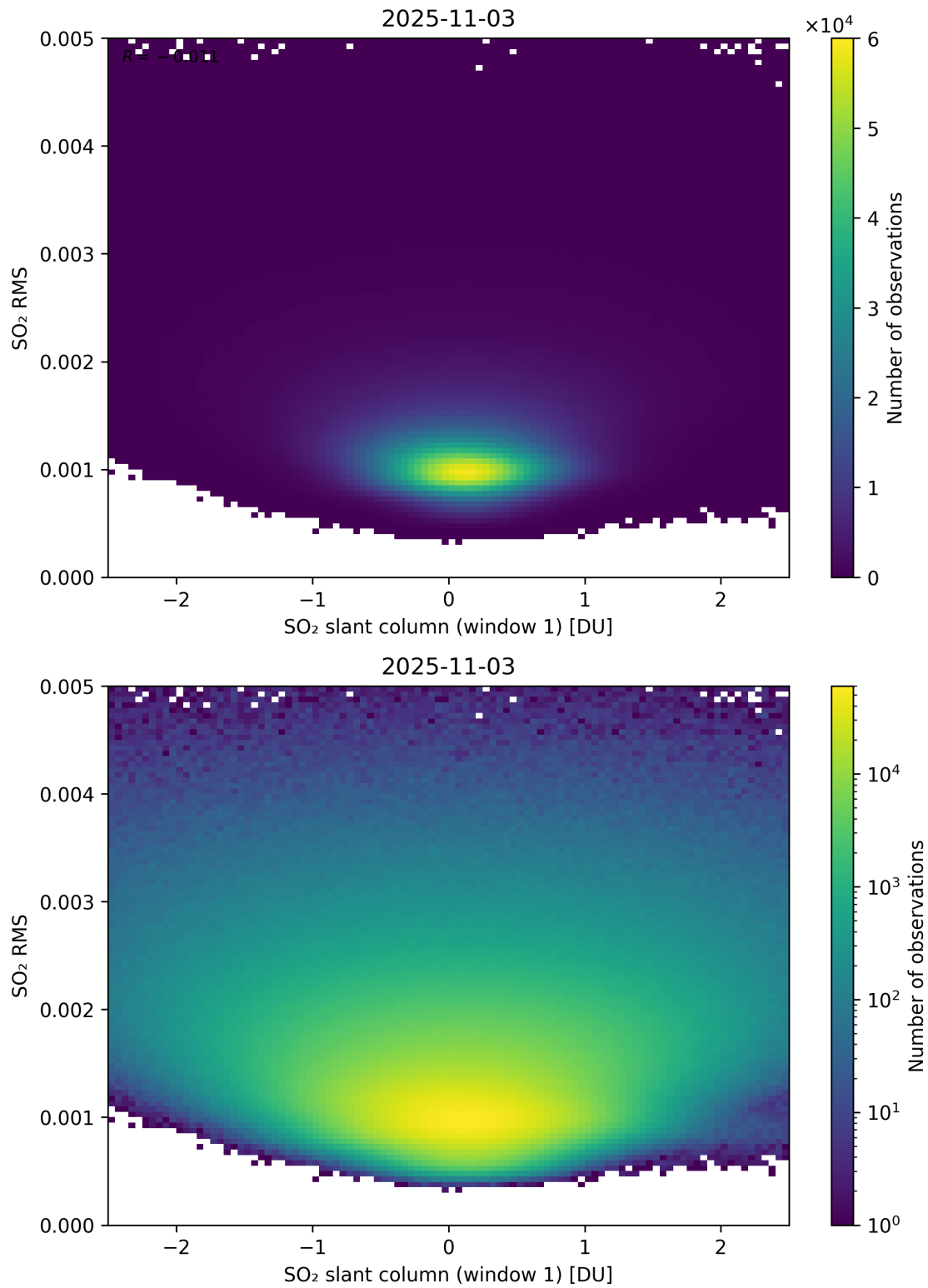
Figure 267: Scatter density plot of “SO 2 slant column (window 1)” against “SO 2 RMS” for 2025-11-02 to 2025-11-04.
