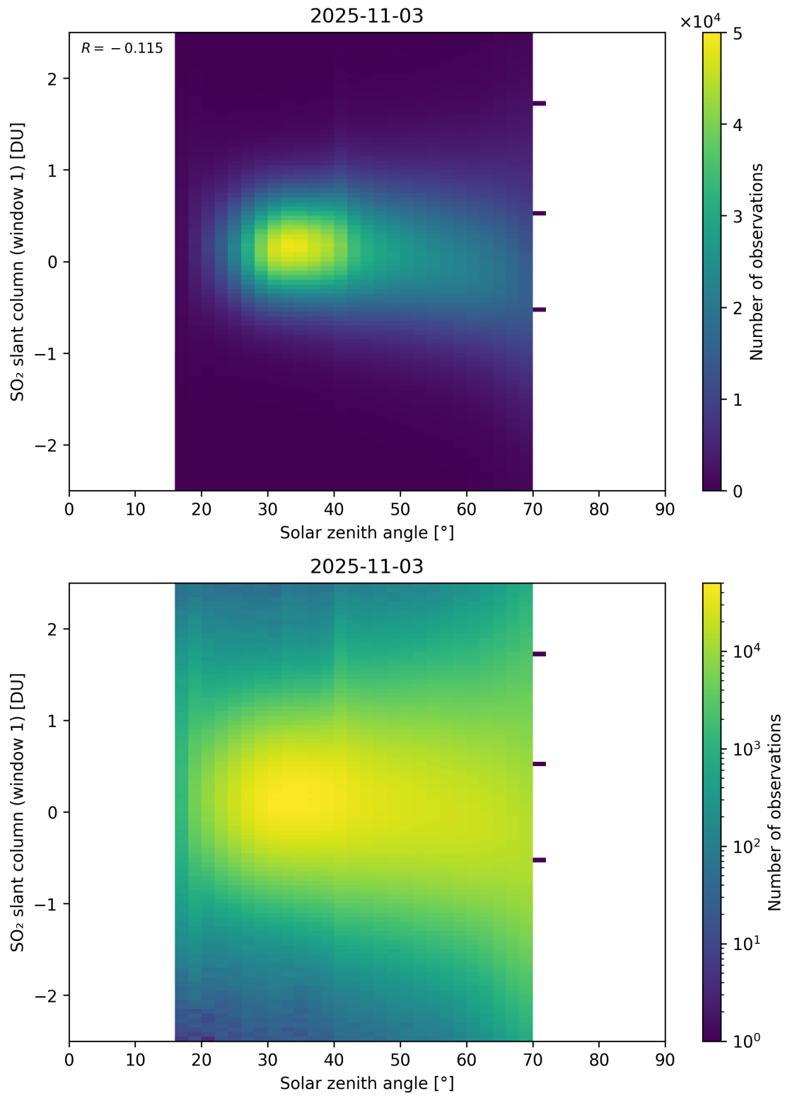
Figure 184: Scatter density plot of “Solar zenith angle” against “SO 2 slant column (window 1)” for 2025-11-02 to 2025-11-04.
