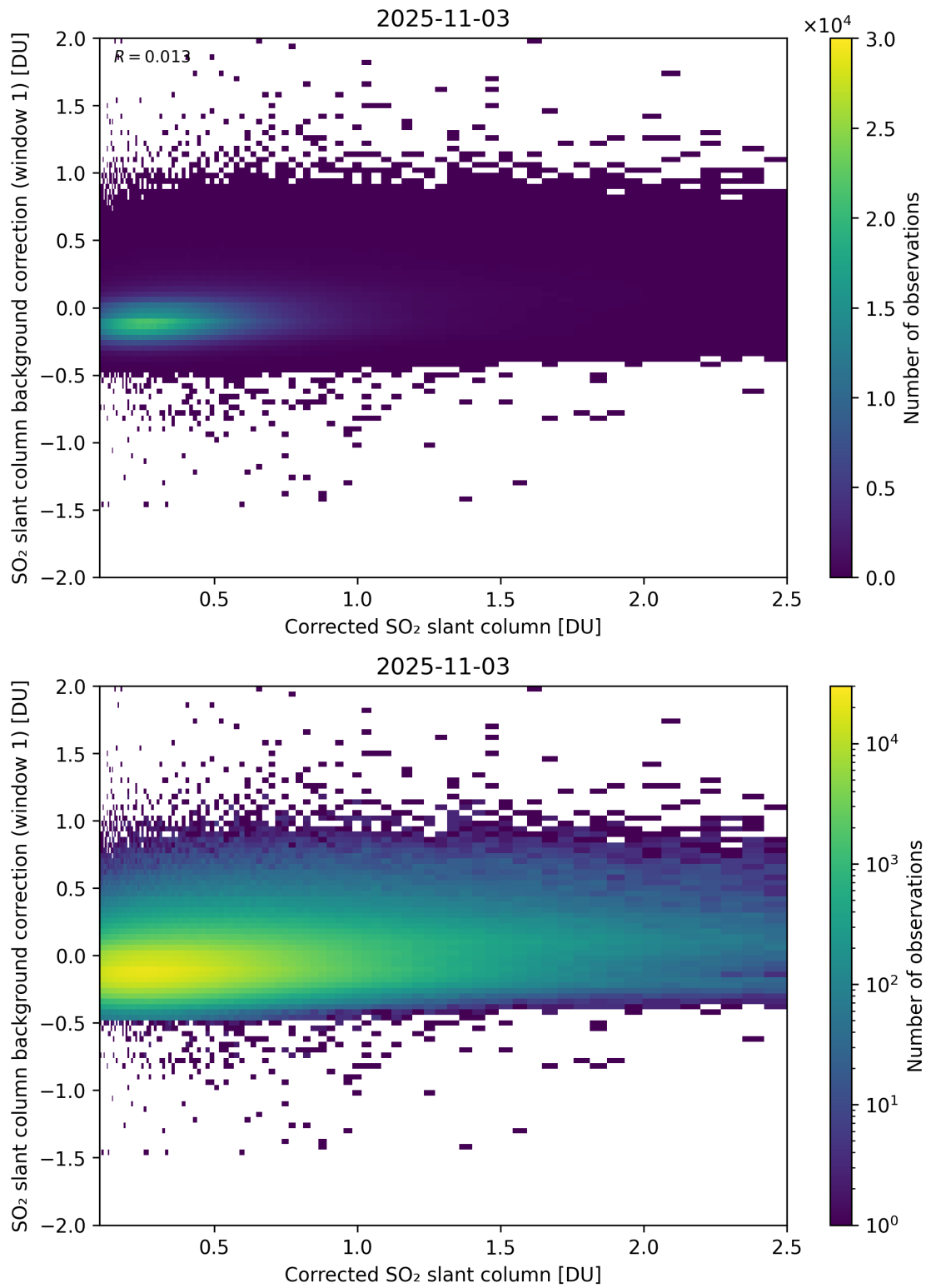
Figure 226: Scatter density plot of “Corrected SO 2 slant column” against “SO 2 slant column background correction (window 1)” for 2025-11-02 to 2025-11-04.
