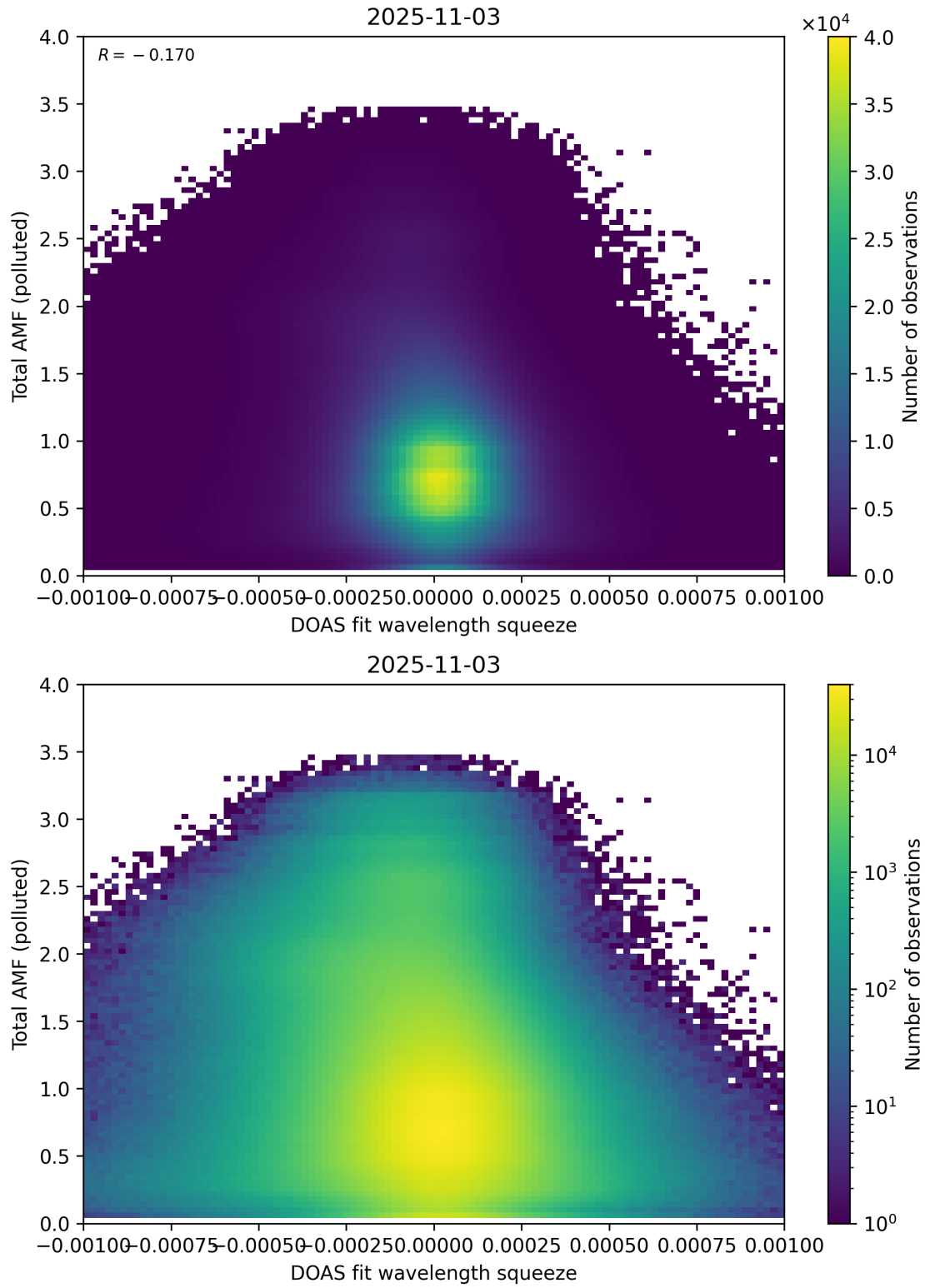
Figure 145: Scatter density plot of “DOAS fit wavelength squeeze” against “Total AMF (polluted)” for 2025-11-02 to 2025-11-04.
