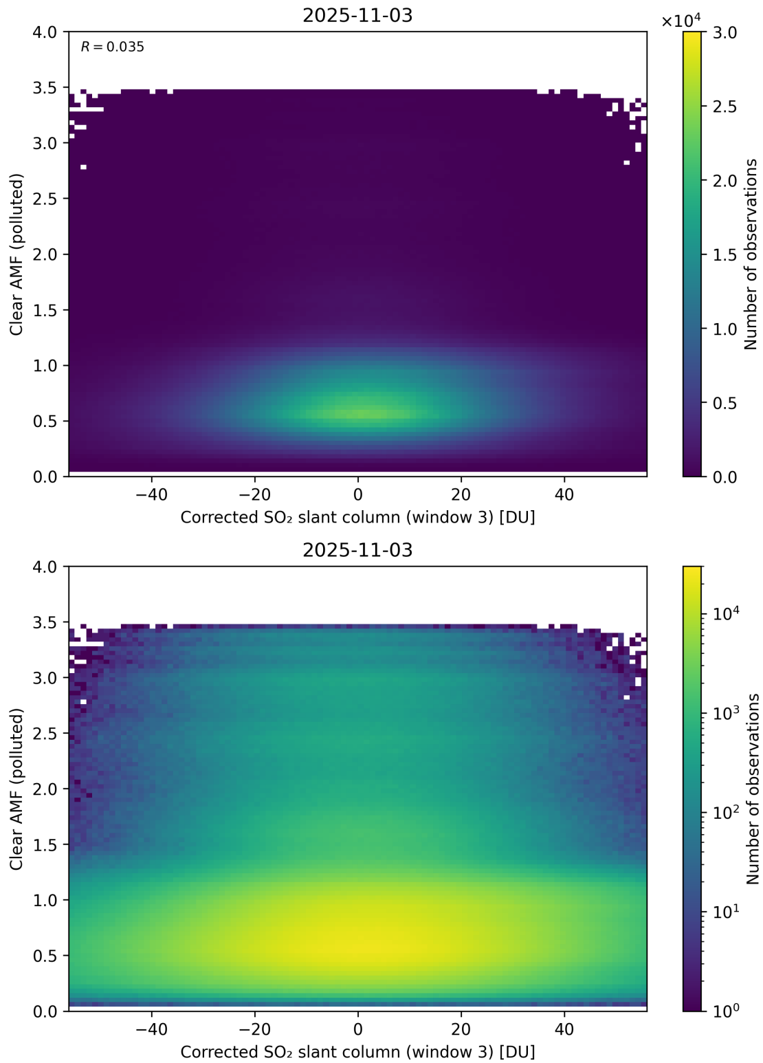
Figure 259: Scatter density plot of “Corrected SO 2 slant column (window 3)” against “Clear AMF (polluted)” for 2025-11-02 to 2025-11-04.
