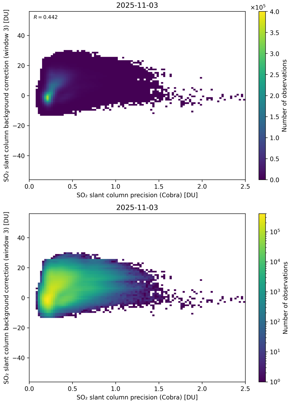
Figure 201: Scatter density plot of “SO 2 slant column precision (Cobra)” against “SO 2 slant column background correction (window 3)” for 2025-11-02 to 2025-11-04.
