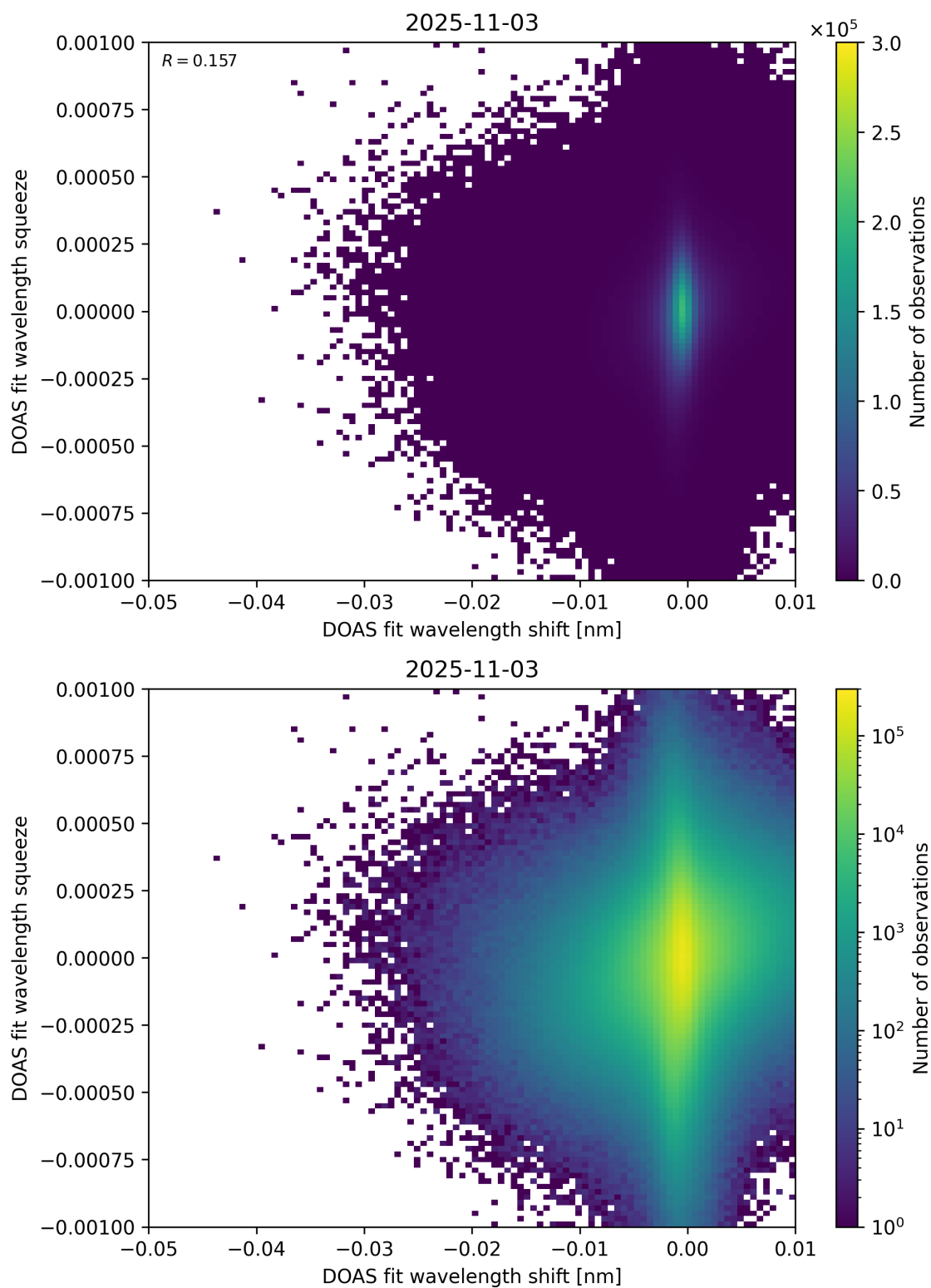
Figure 138: Scatter density plot of “DOAS fit wavelength shift” against “DOAS fit wavelength squeeze” for 2025-11-02 to 2025-11-04.
