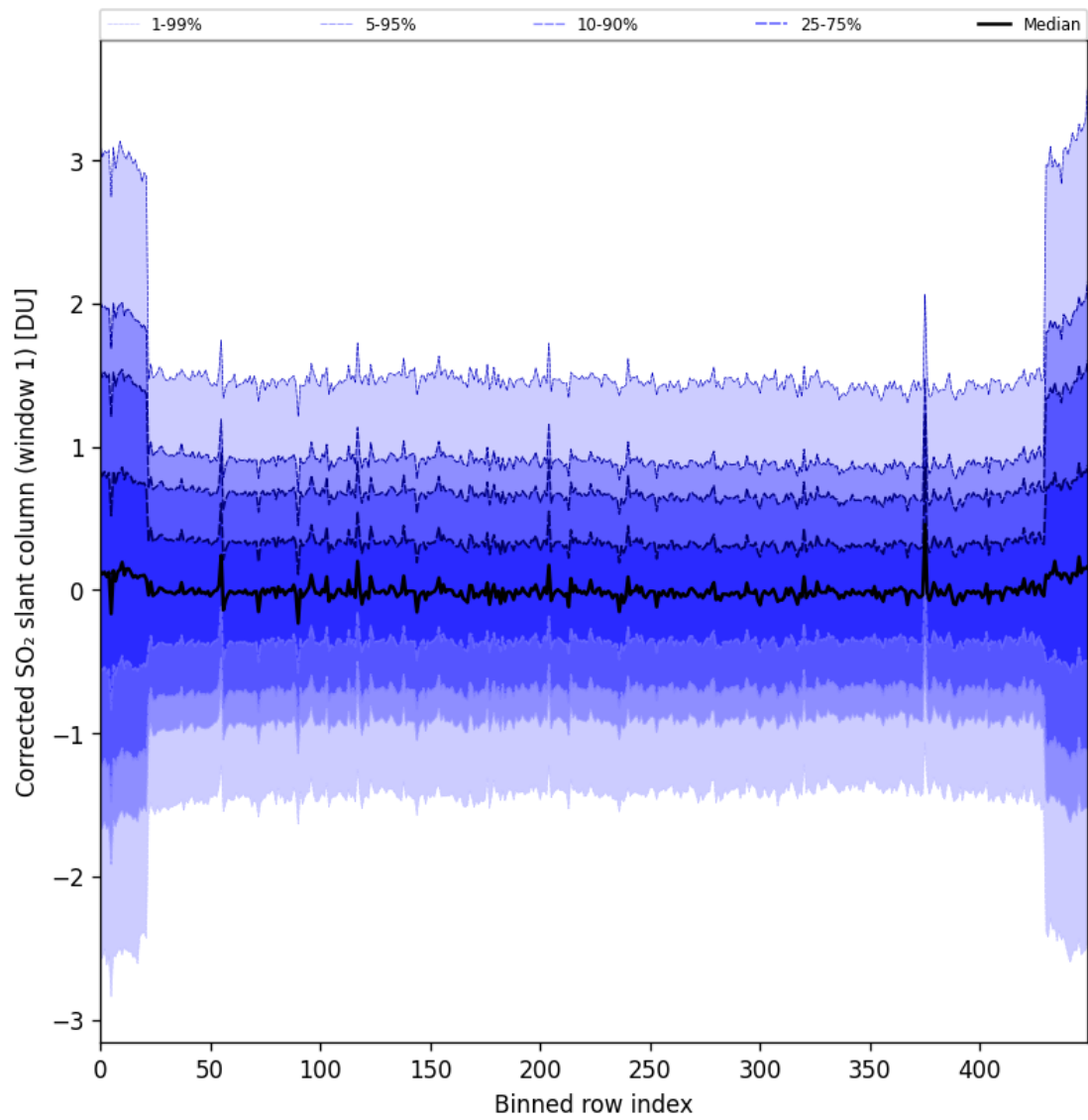
Figure 91: Along track statistics of “Corrected SO 2 slant column (window 1)” for 2025-11-02 to 2025-11-04
