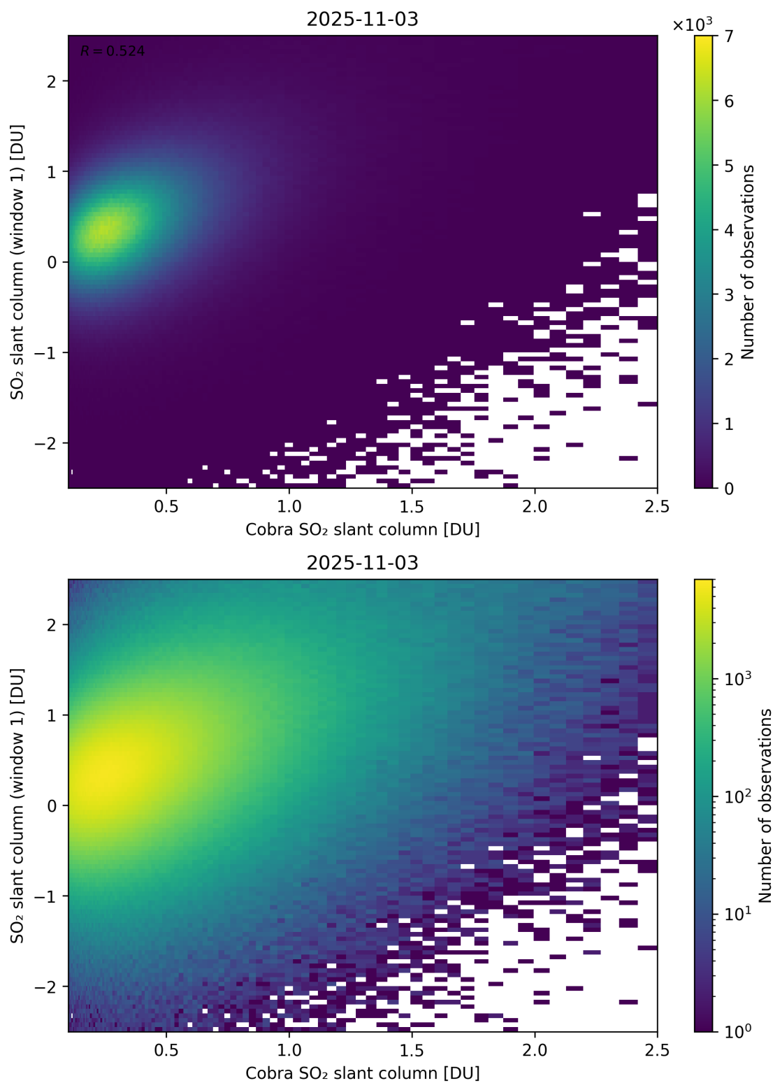
Figure 219: Scatter density plot of “Cobra SO 2 slant column” against “SO 2 slant column (window 1)” for 2025-11-02 to 2025-11-04.
