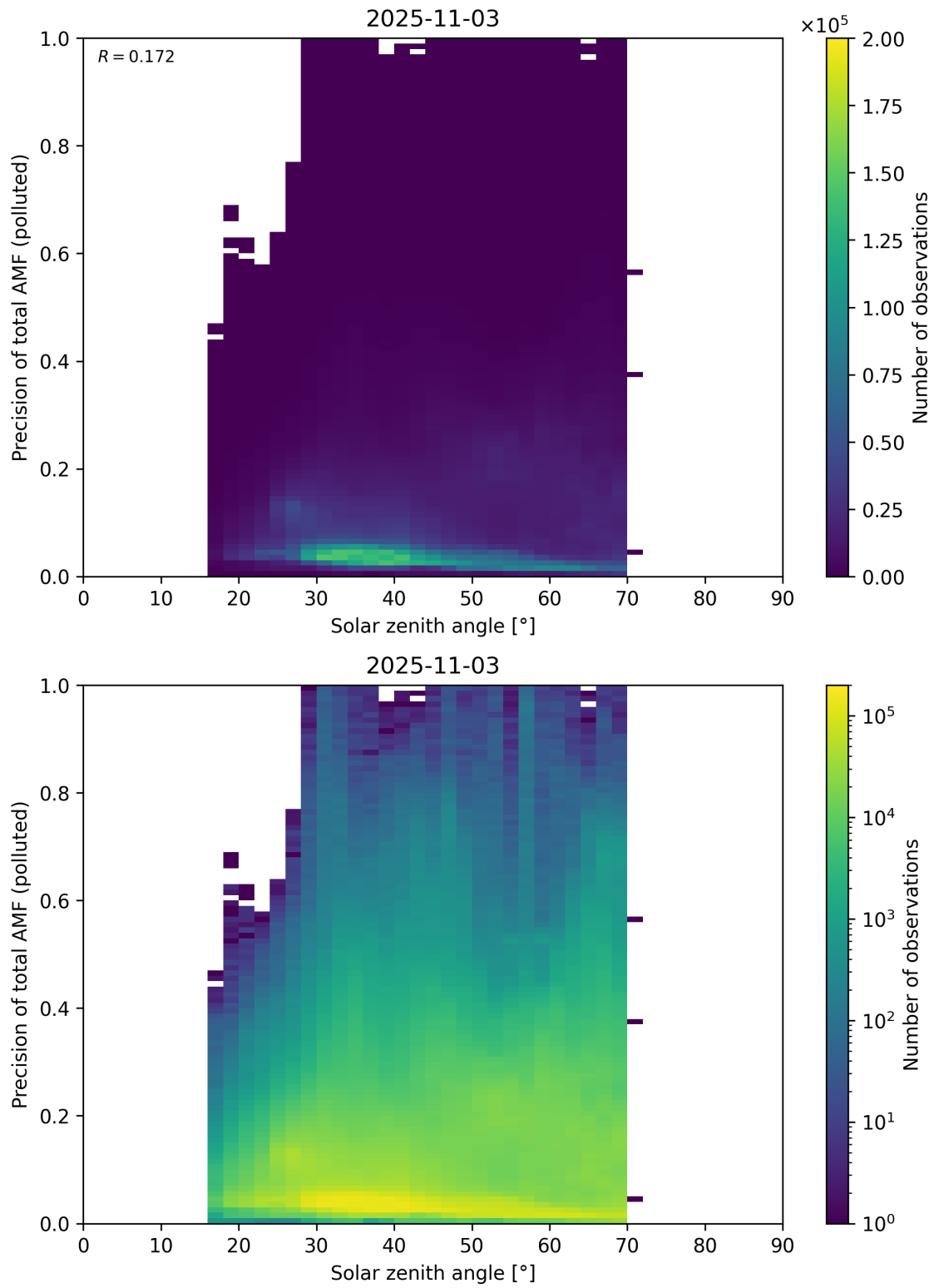
Figure 190: Scatter density plot of “Solar zenith angle” against “Precision of total AMF (polluted)” for 2025-11-02 to 2025-11-04.
