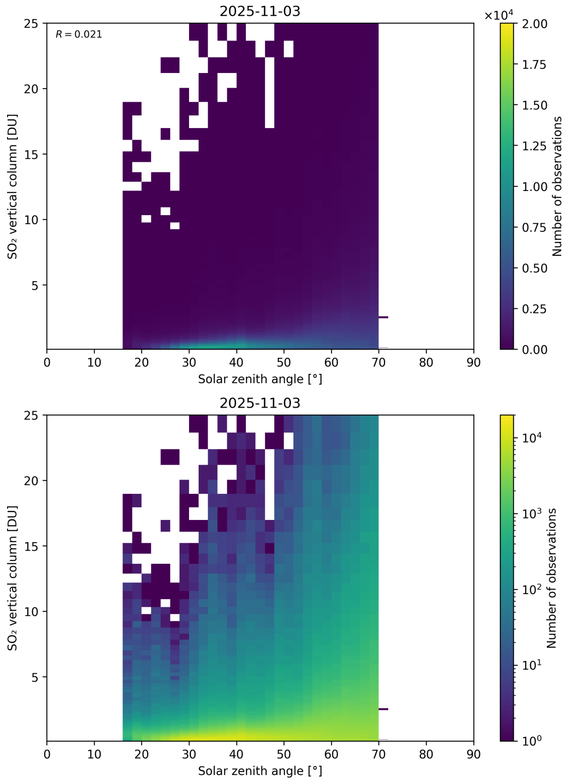
Figure 191: Scatter density plot of “Solar zenith angle” against “SO 2 vertical column” for 2025-11-02 to 2025-11-04.
