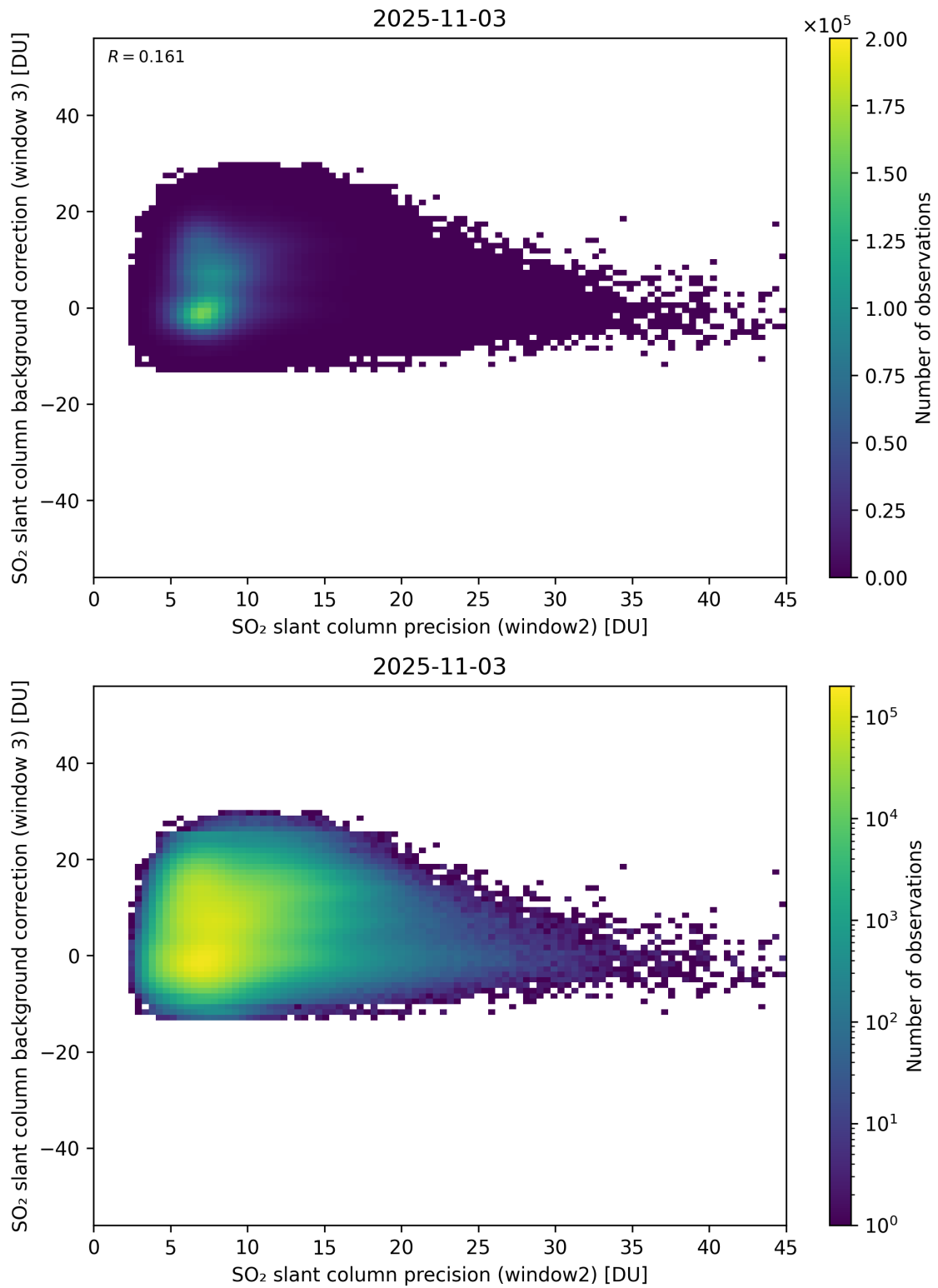
Figure 292: Scatter density plot of “SO 2 slant column precision (window2)” against “SO 2 slant column background correction (window 3)” for 2025-11-02 to 2025-11-04.
