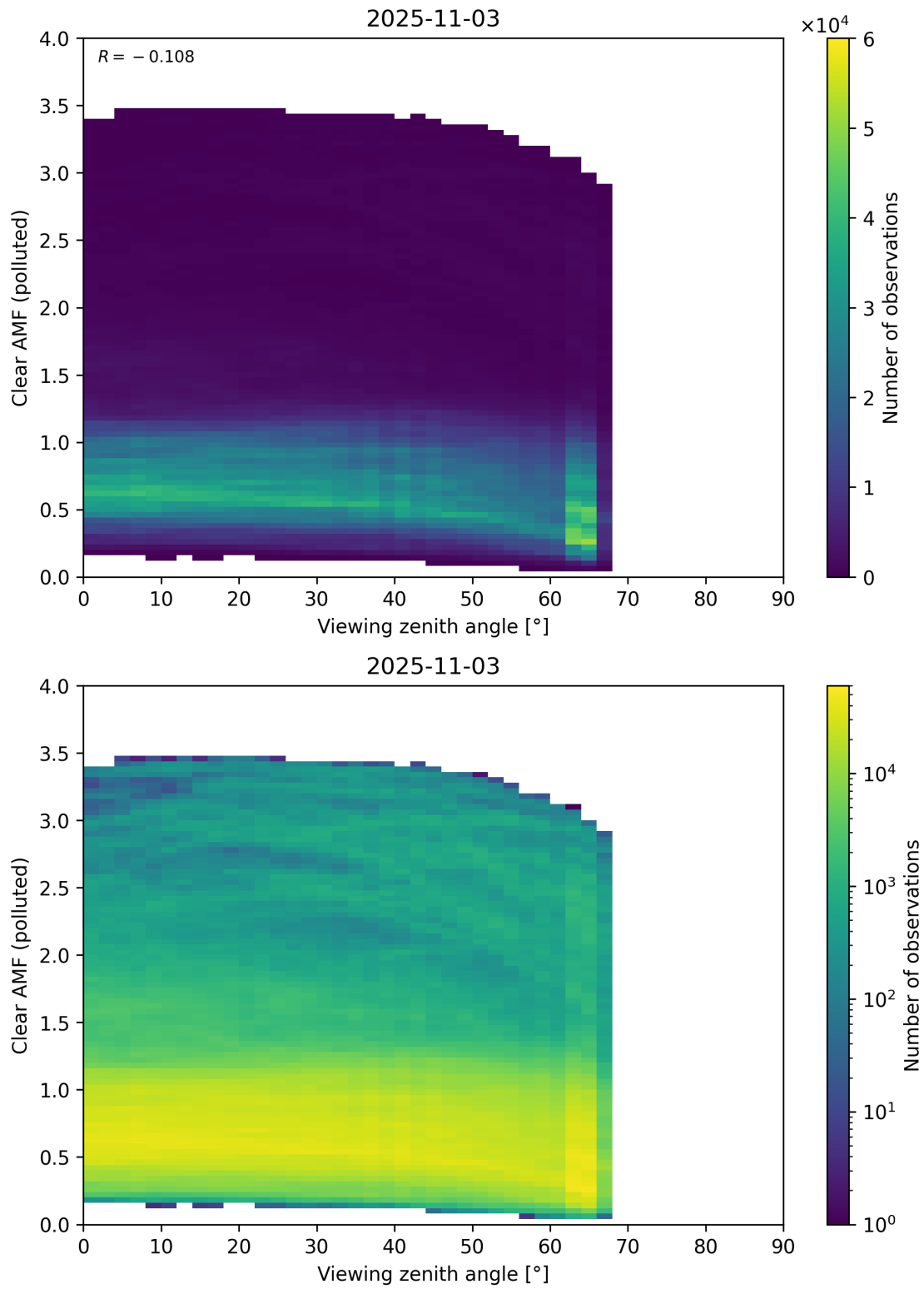
Figure 370: Scatter density plot of “Viewing zenith angle” against “Clear AMF (polluted)” for 2025-11-02 to 2025-11-04.
