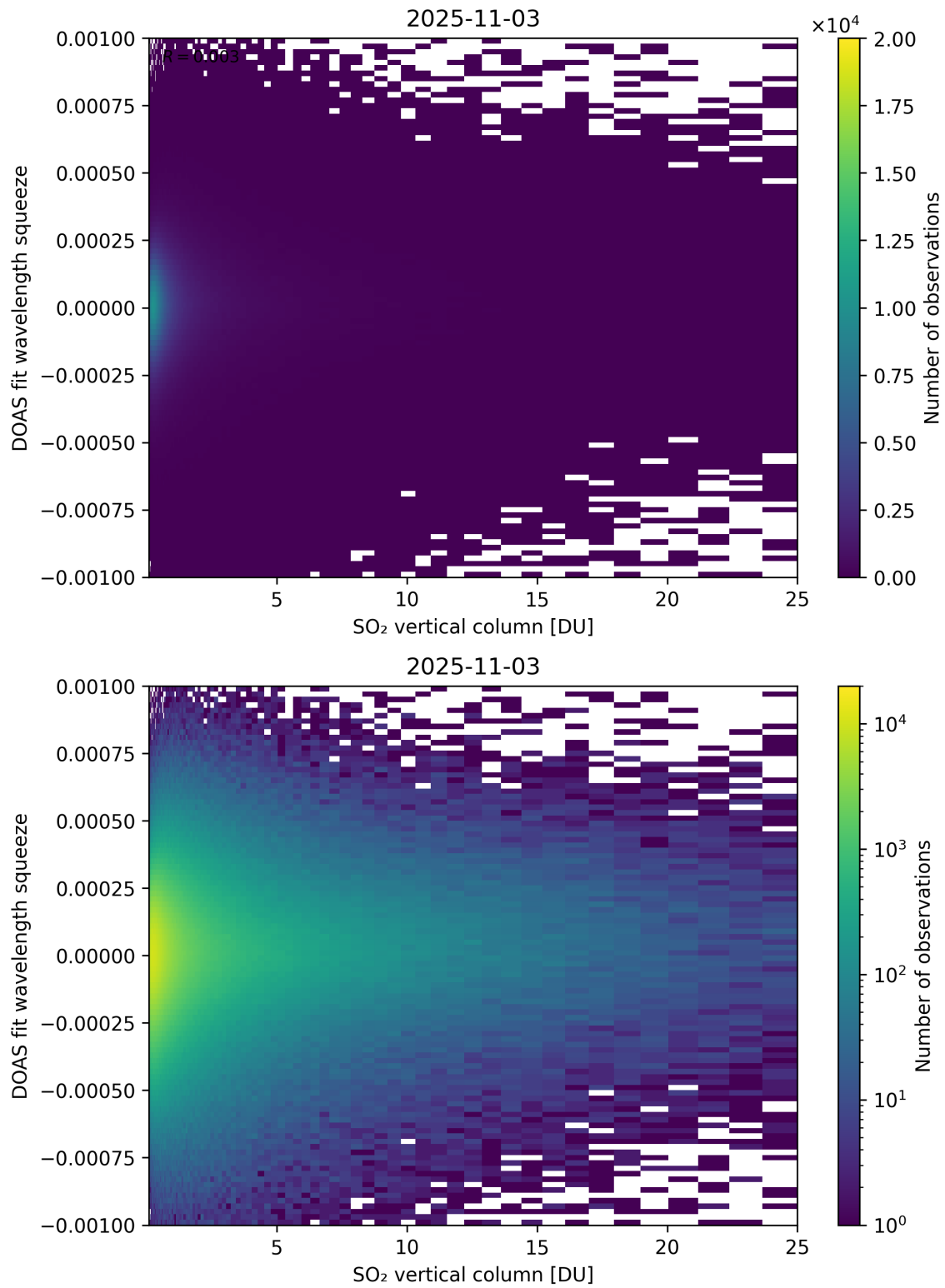
Figure 327: Scatter density plot of “SO 2 vertical column” against “DOAS fit wavelength squeeze” for 2025-11-02 to 2025-11-04.
