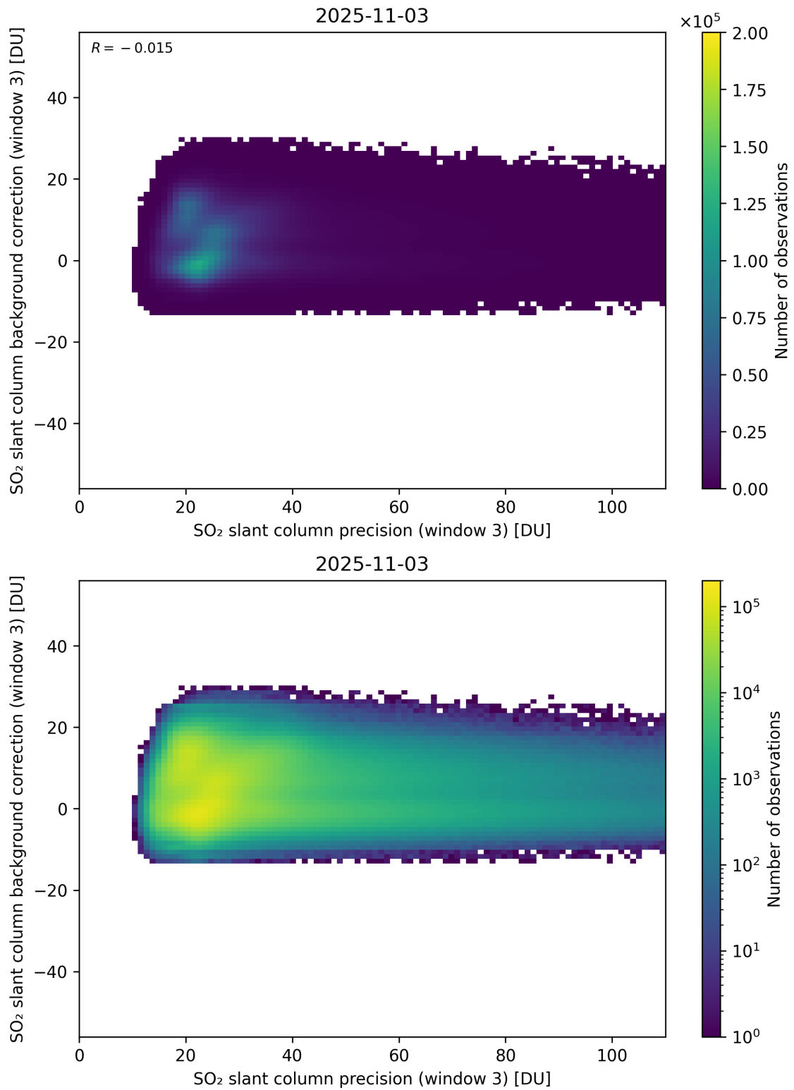
Figure 307: Scatter density plot of “SO 2 slant column precision (window 3)” against “SO 2 slant column background correction (window 3)” for 2025-11-02 to 2025-11-04.
