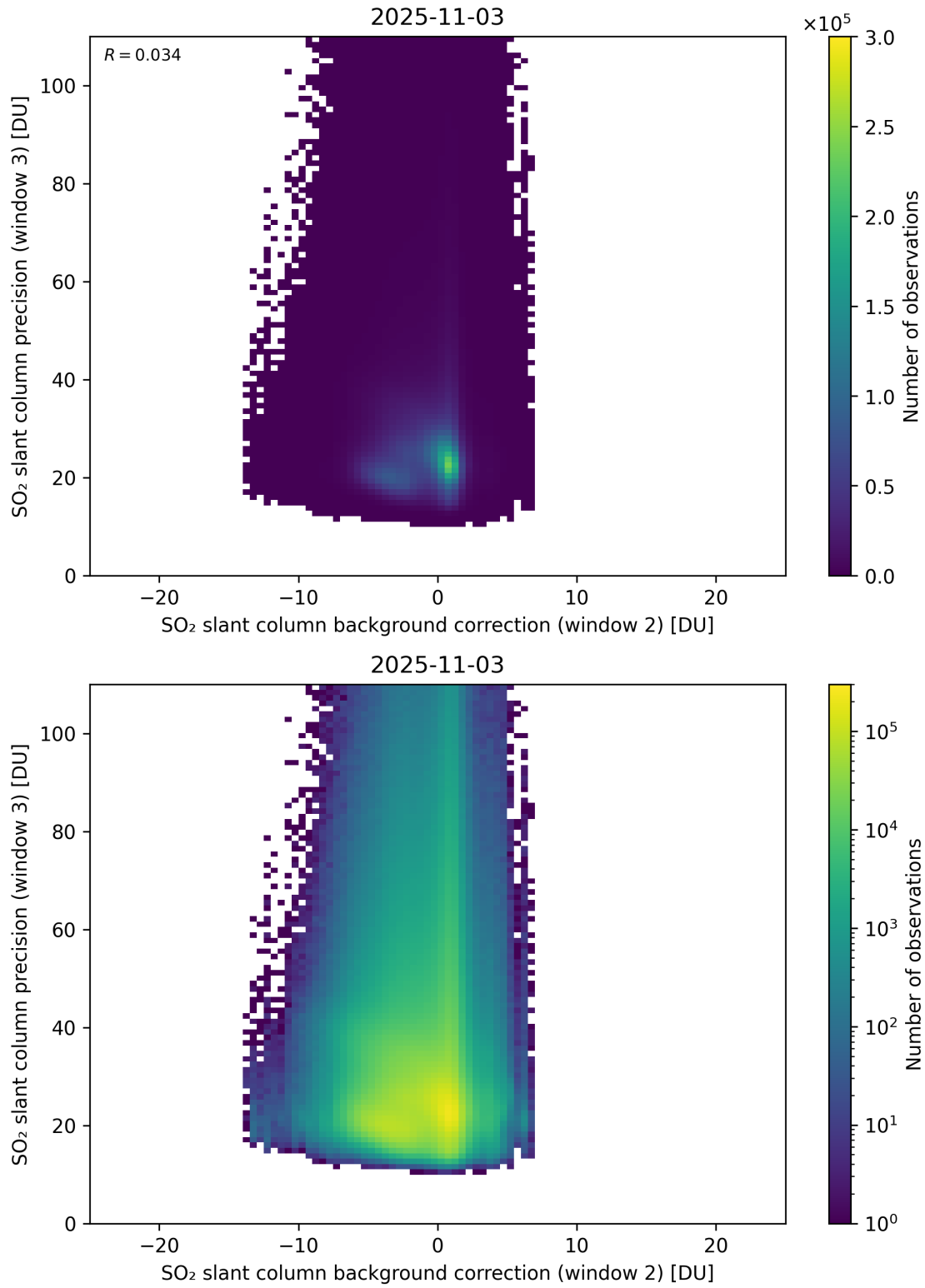
Figure 129: Scatter density plot of “SO 2 slant column background correction (window 2)” against “SO 2 slant column precision (window 3)” for 2025-11-02 to 2025-11-04.
