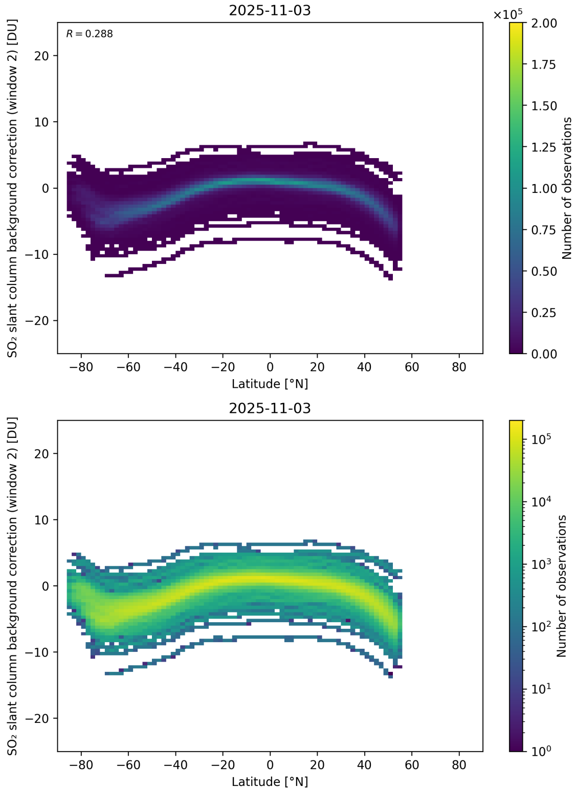
Figure 151: Scatter density plot of “Latitude” against “SO 2 slant column background correction (window 2)” for 2025-11-02 to 2025-11-04.
