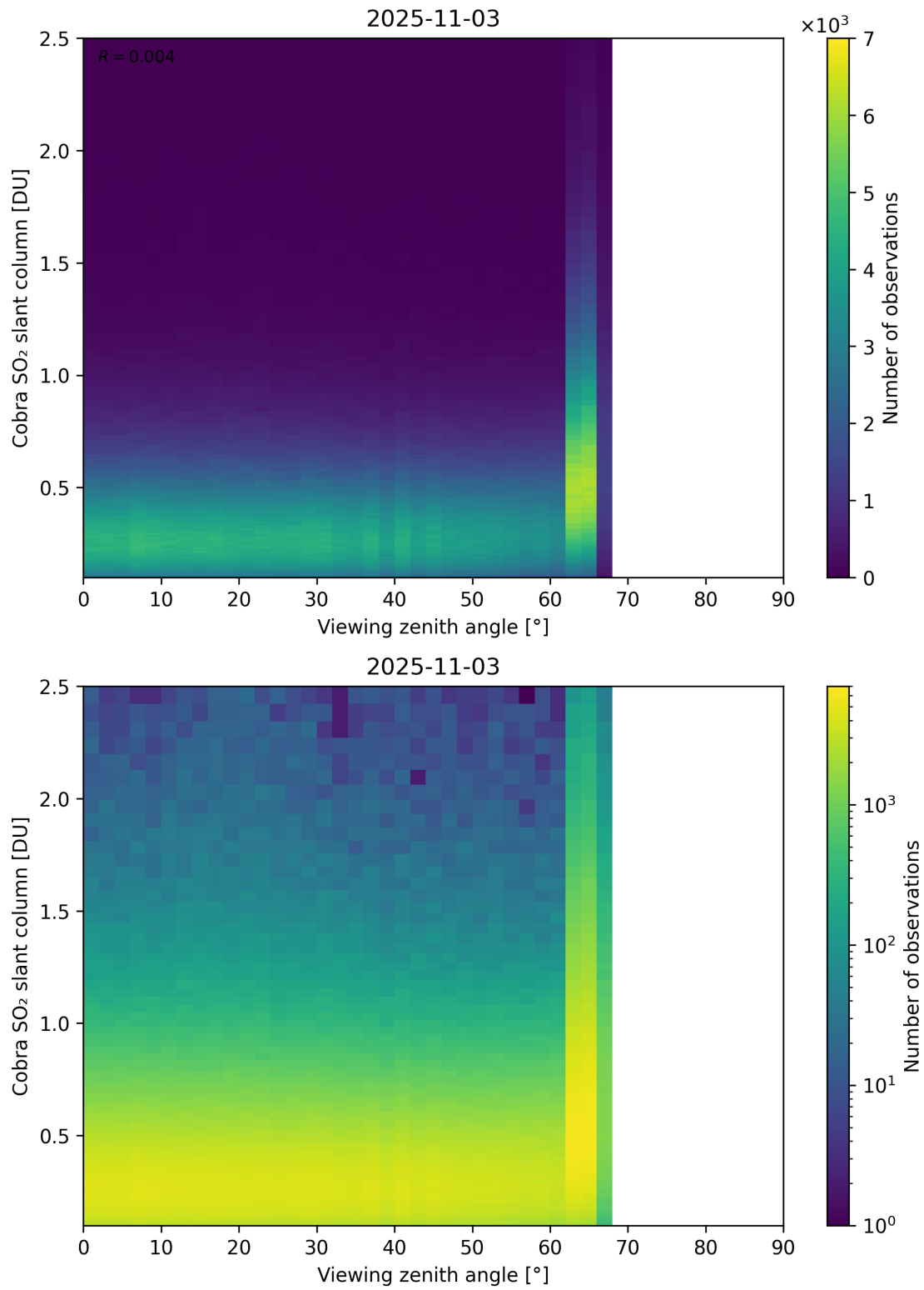
Figure 371: Scatter density plot of “Viewing zenith angle” against “Cobra SO 2 slant column” for 2025-11-02 to 2025-11-04.
