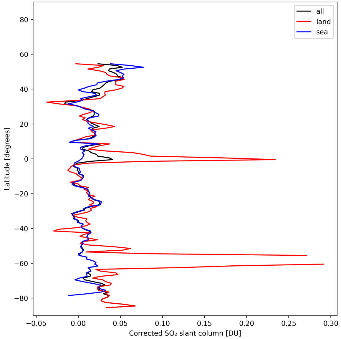
Figure 34: Zonal average of “Corrected SO 2 slant column” for 2025-11-02 to 2025-11-04.
