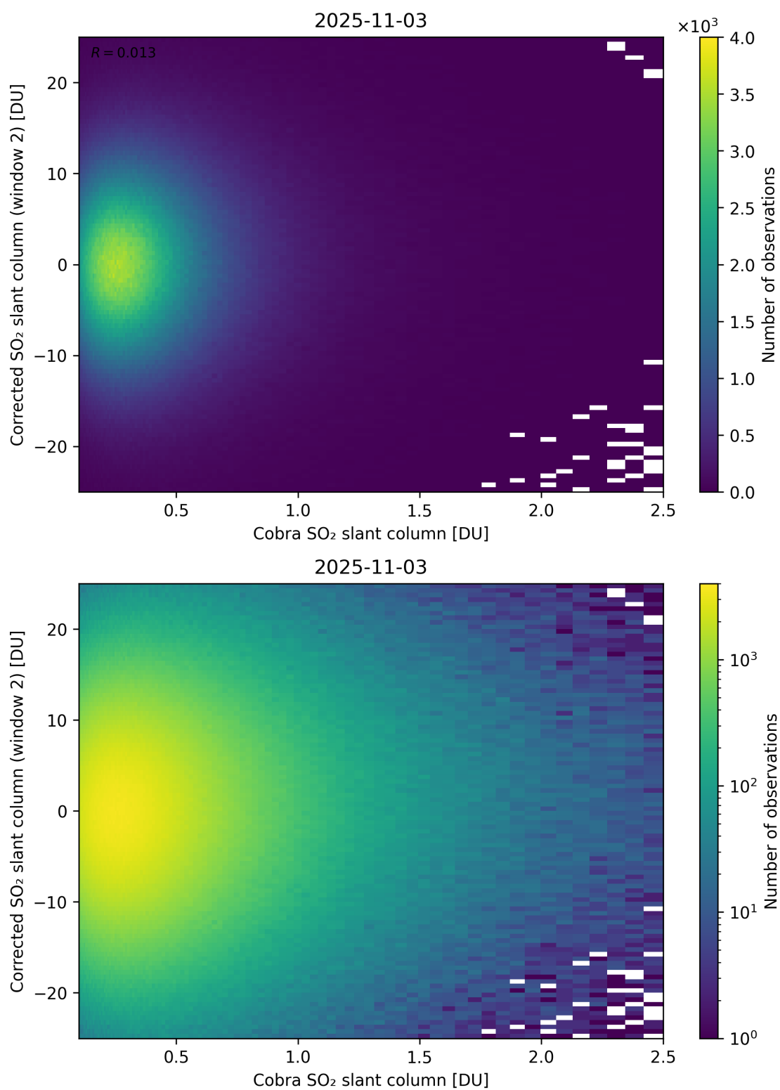
Figure 217: Scatter density plot of “Cobra SO 2 slant column” against “Corrected SO 2 slant column (window 2)” for 2025-11-02 to 2025-11-04.
