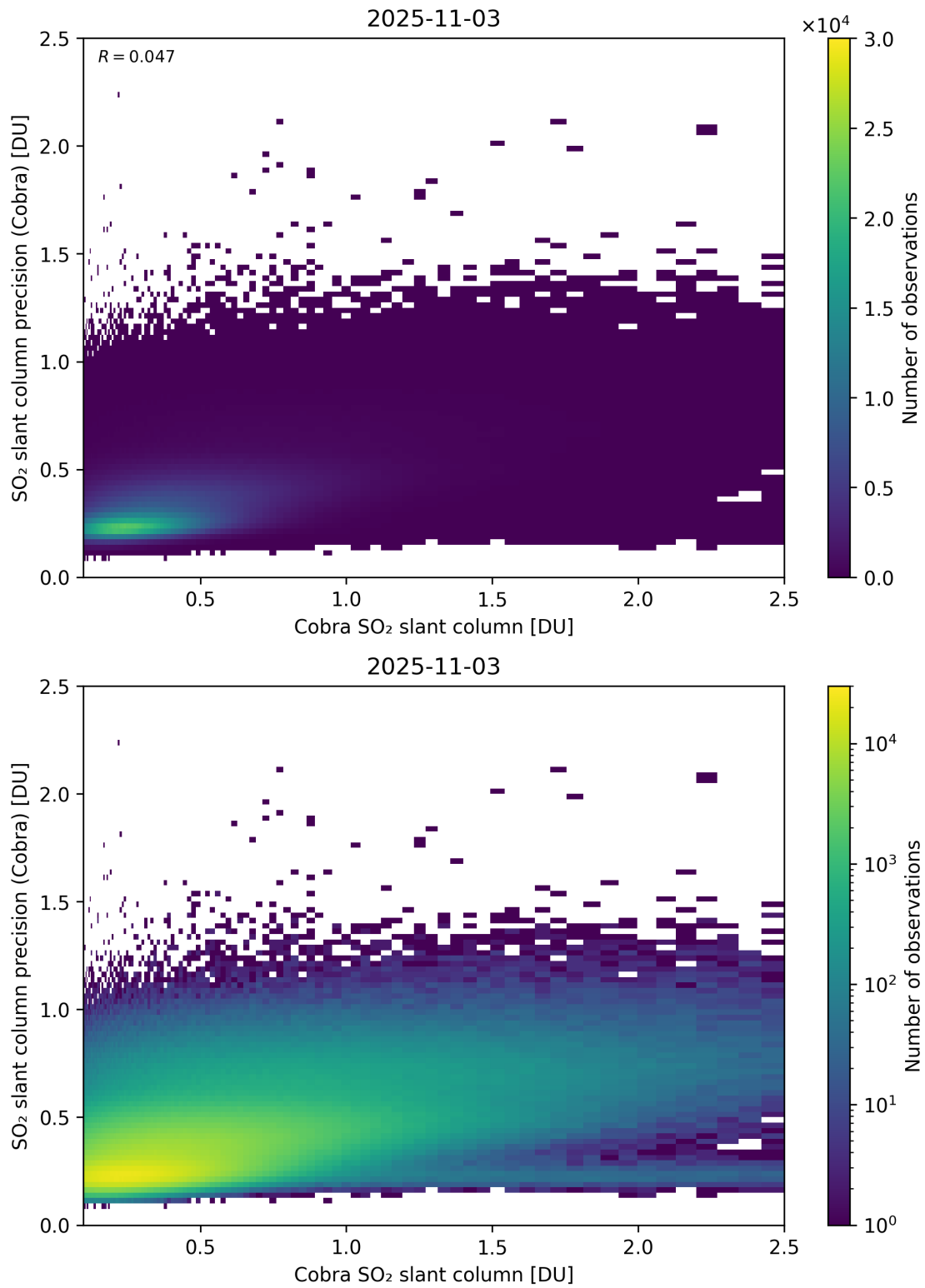
Figure 216: Scatter density plot of “Cobra SO 2 slant column” against “SO 2 slant column precision (Cobra)” for 2025-11-02 to 2025-11-04.
