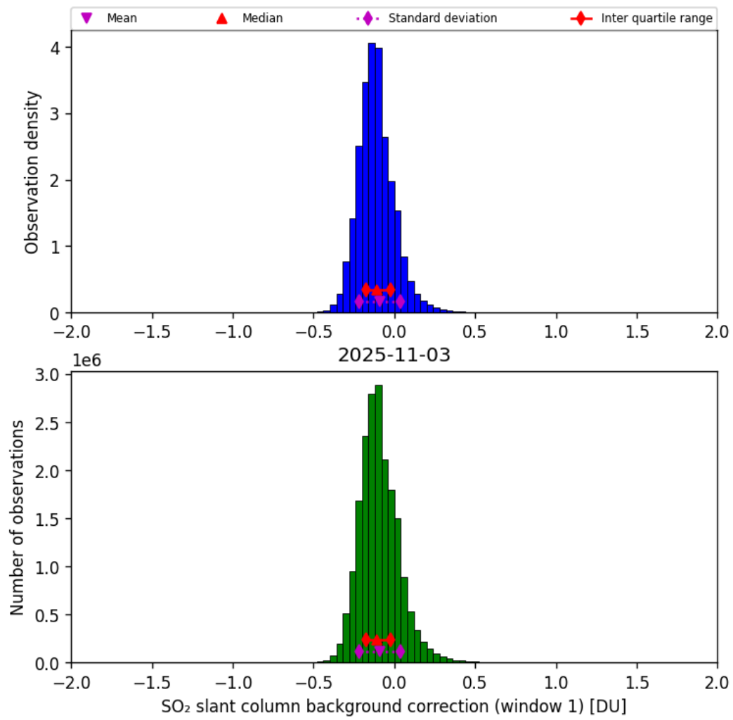
Figure 66: Histogram of “SO 2 slant column background correction (window 1)” for 2025-11-02 to 2025-11-04
