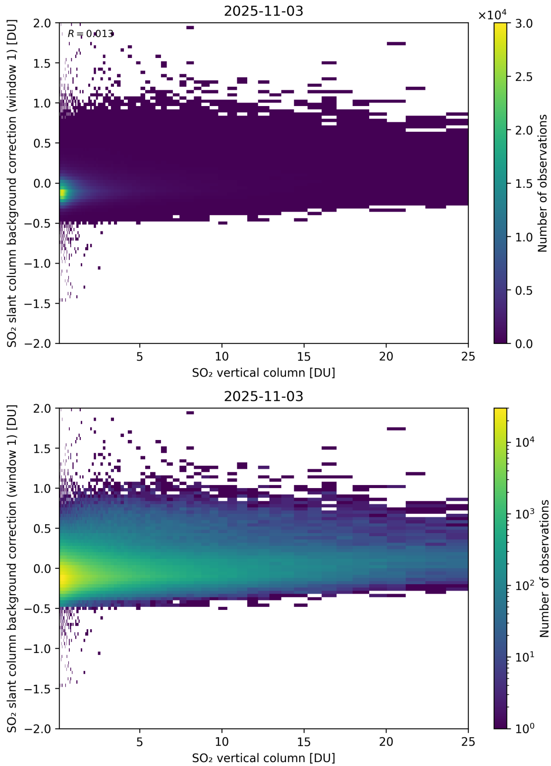
Figure 323: Scatter density plot of “SO 2 vertical column” against “SO 2 slant column background correction (window 1)” for 2025-11-02 to 2025-11-04.
