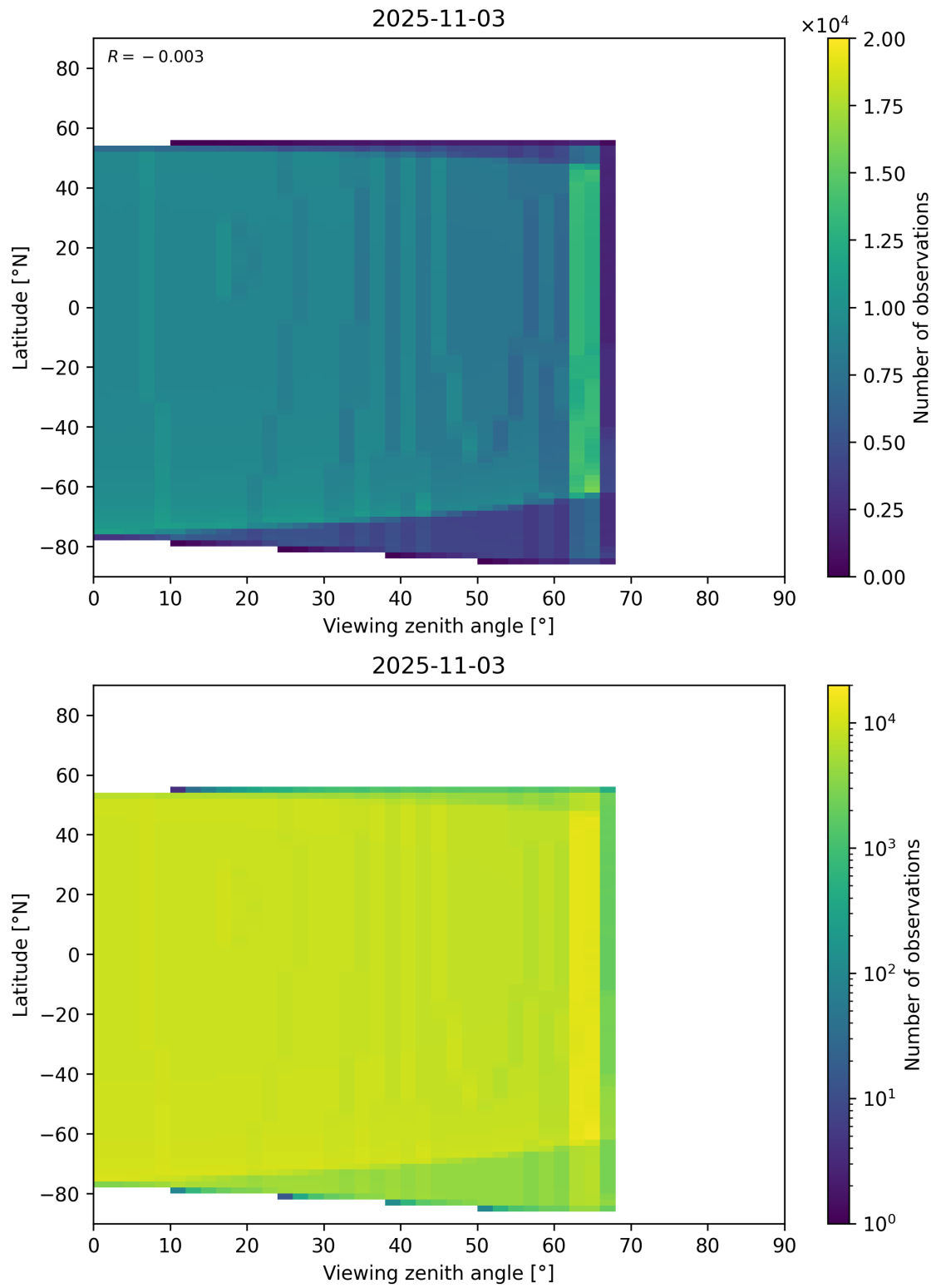
Figure 368: Scatter density plot of “Viewing zenith angle” against “Latitude” for 2025-11-02 to 2025-11-04.
