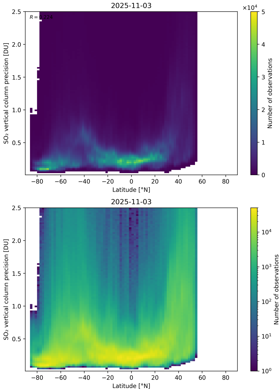
Figure 170: Scatter density plot of “Latitude” against “SO 2 vertical column precision” for 2025-11-02 to 2025-11-04.
