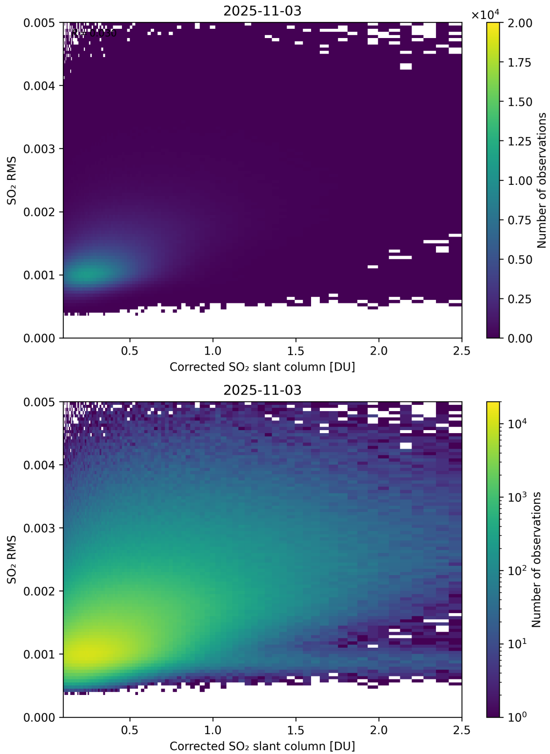
Figure 231: Scatter density plot of “Corrected SO 2 slant column” against “SO 2 RMS” for 2025-11-02 to 2025-11-04.
