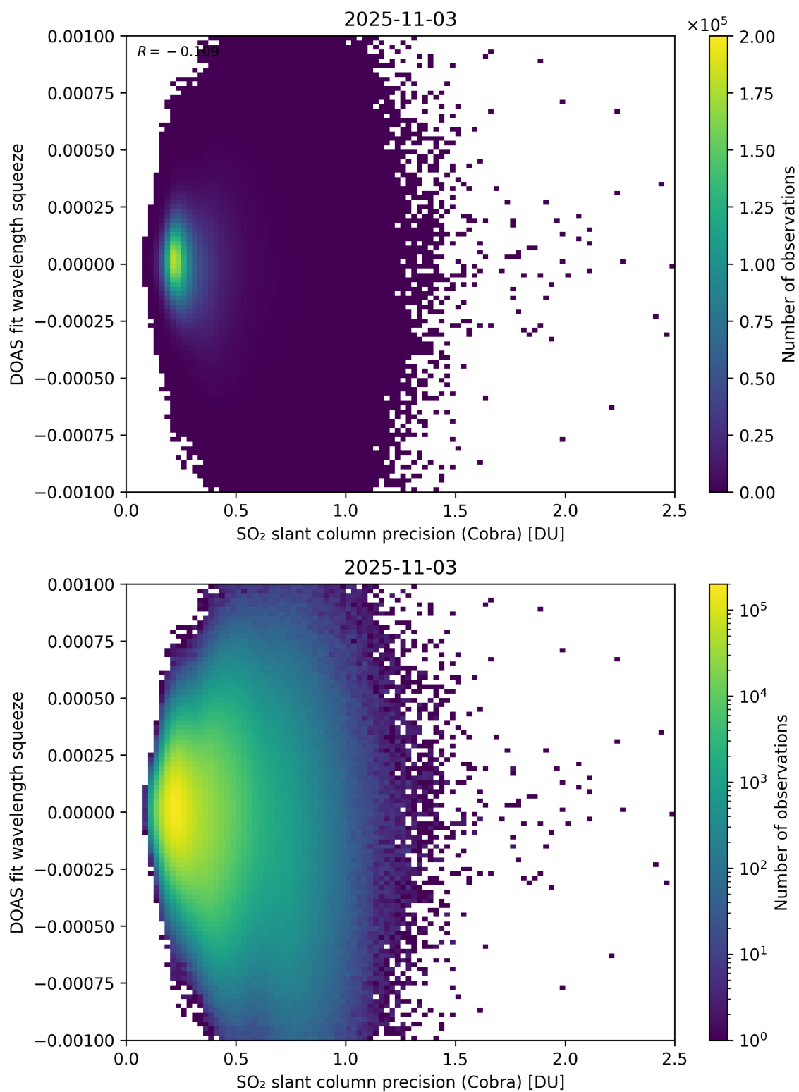
Figure 203: Scatter density plot of “SO 2 slant column precision (Cobra)” against “DOAS fit wavelength squeeze” for 2025-11-02 to 2025-11-04.
