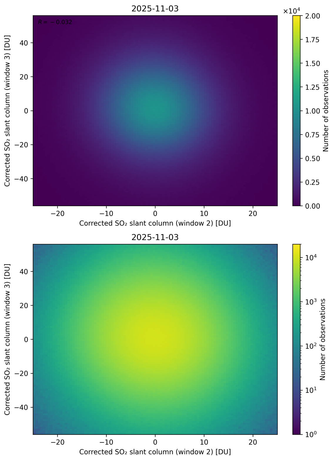
Figure 250: Scatter density plot of “Corrected SO 2 slant column (window 2)” against “Corrected SO 2 slant column (window 3)” for 2025-11-02 to 2025-11-04.
