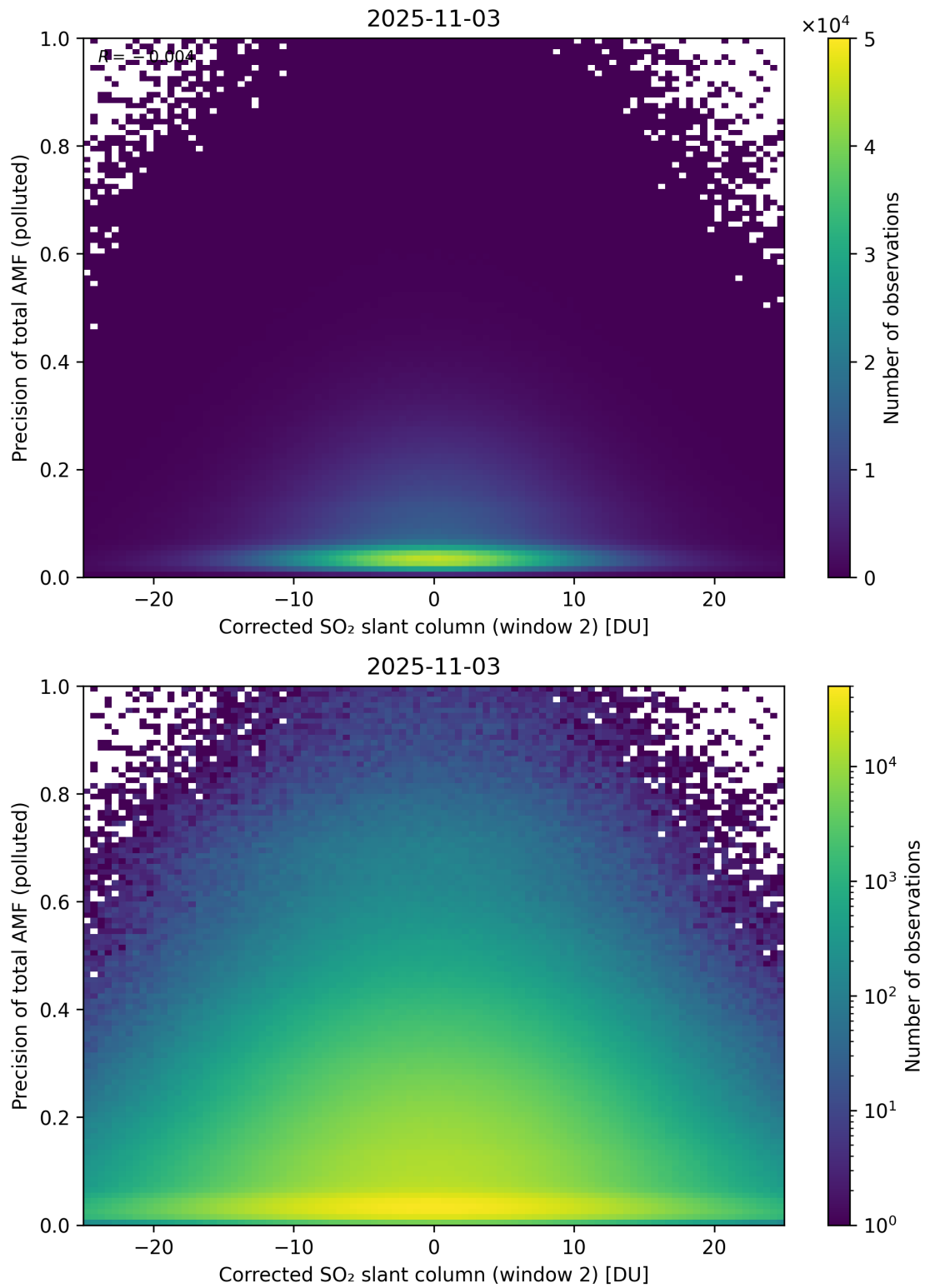
Figure 254: Scatter density plot of “Corrected SO 2 slant column (window 2)” against “Precision of total AMF (polluted)” for 2025-11-02 to 2025-11-04.
