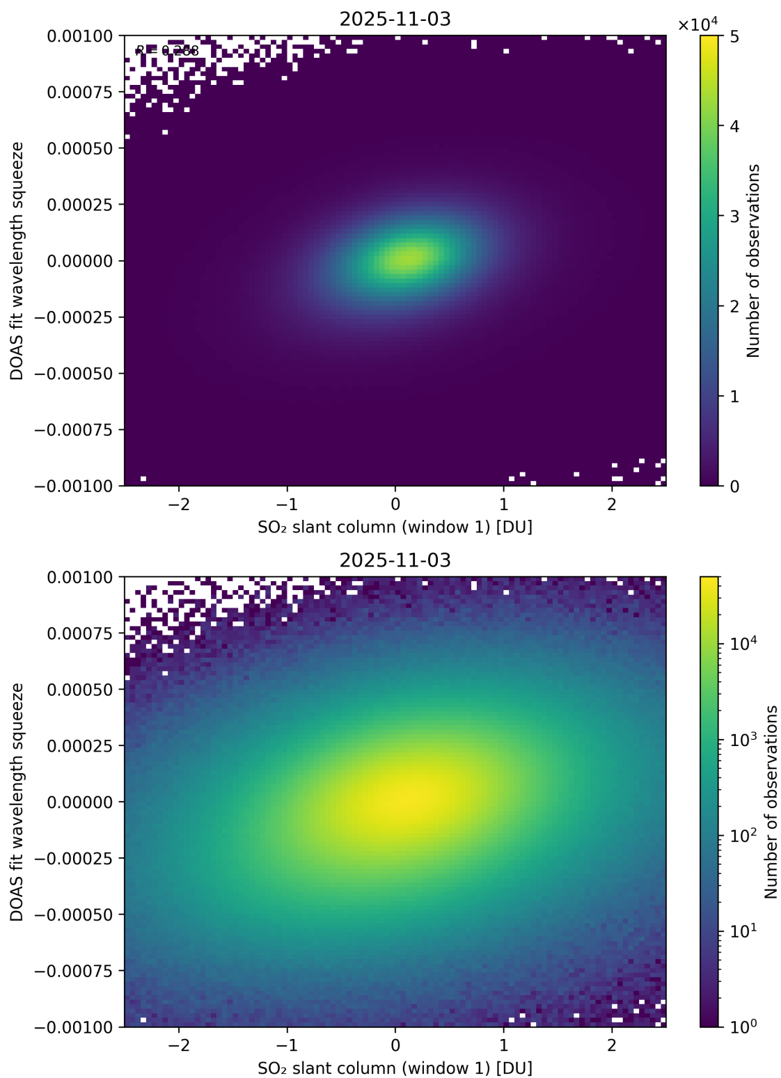
Figure 266: Scatter density plot of “SO 2 slant column (window 1)” against “DOAS fit wavelength squeeze” for 2025-11-02 to 2025-11-04.
