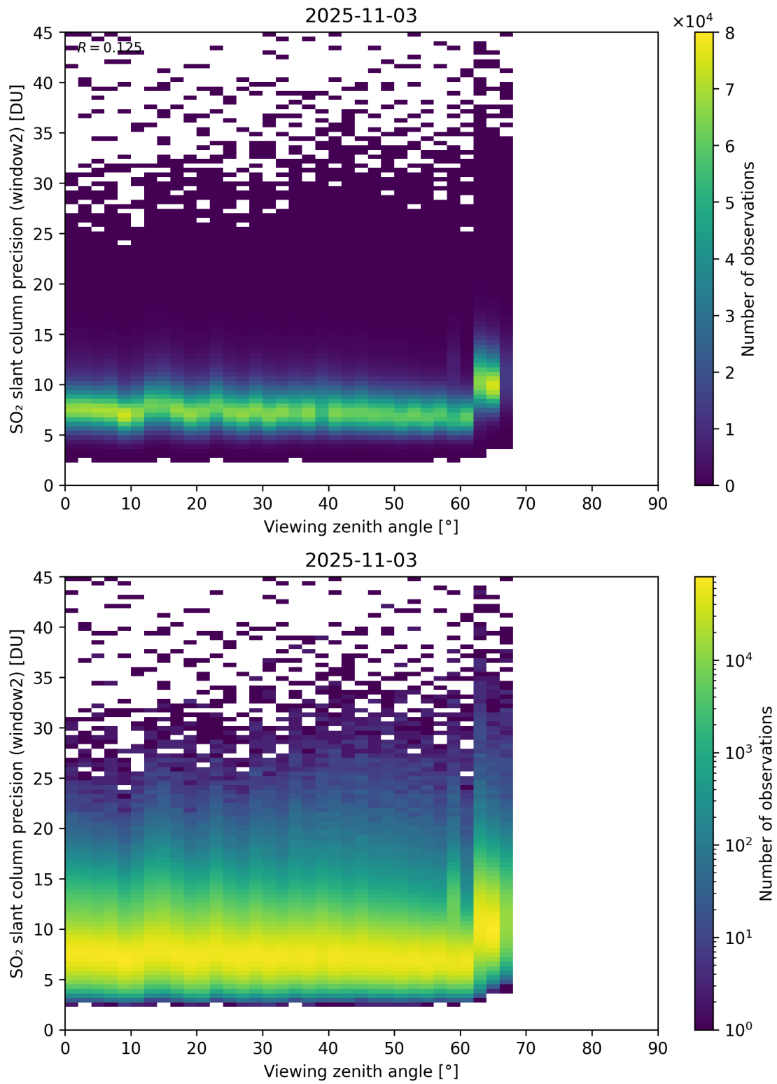
Figure 378: Scatter density plot of “Viewing zenith angle” against “SO 2 slant column precision (window2)” for 2025-11-02 to 2025-11-04.
