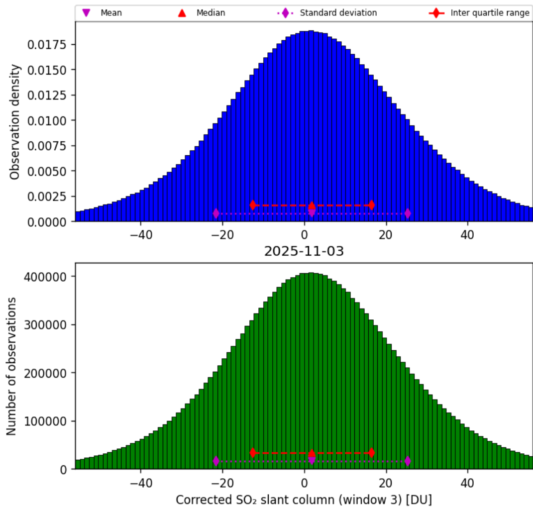
Figure 73: Histogram of “Corrected SO 2 slant column (window 3)” for 2025-11-02 to 2025-11-04
