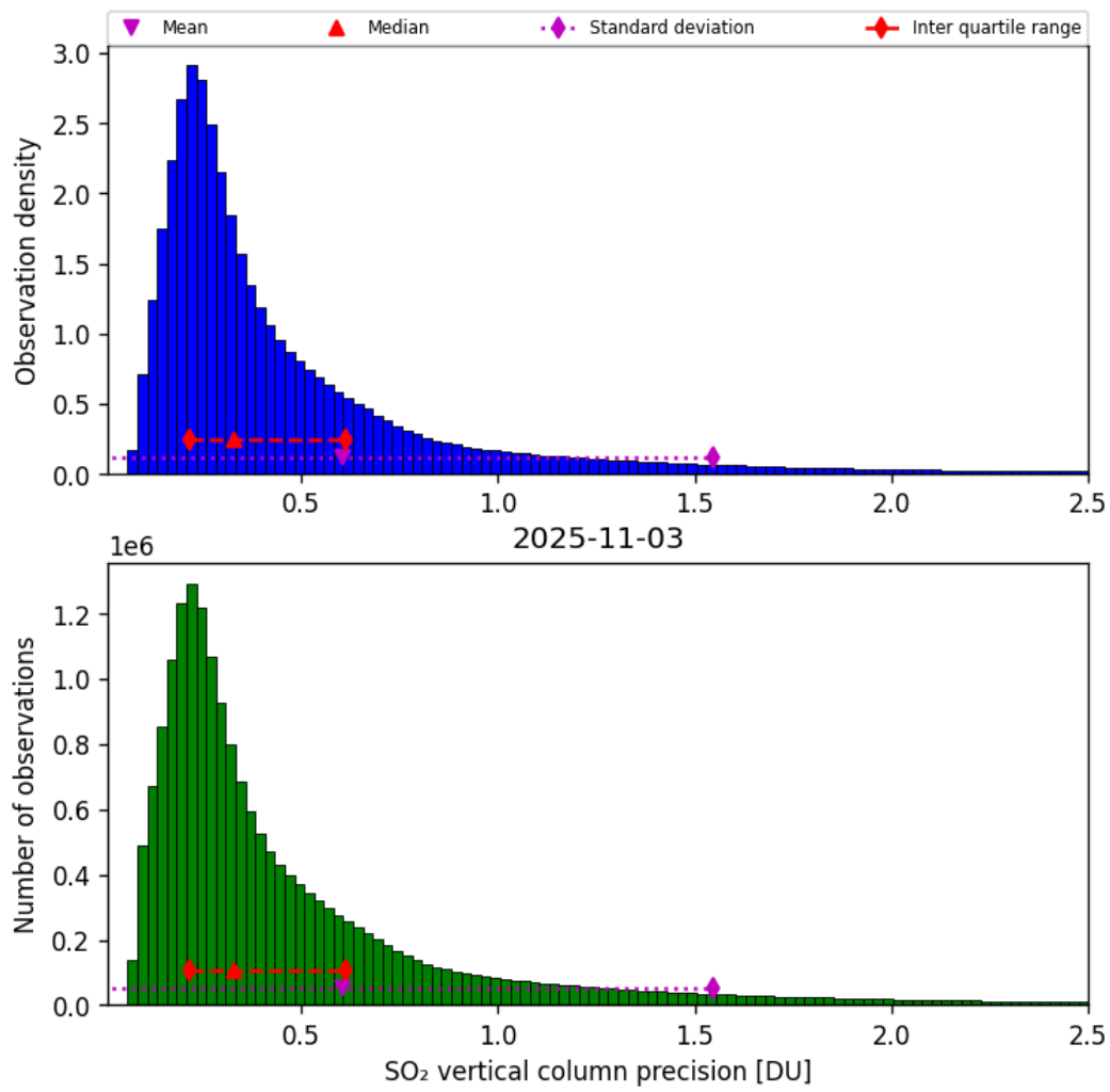
Figure 59: Histogram of “SO 2 vertical column precision” for 2025-11-02 to 2025-11-04
