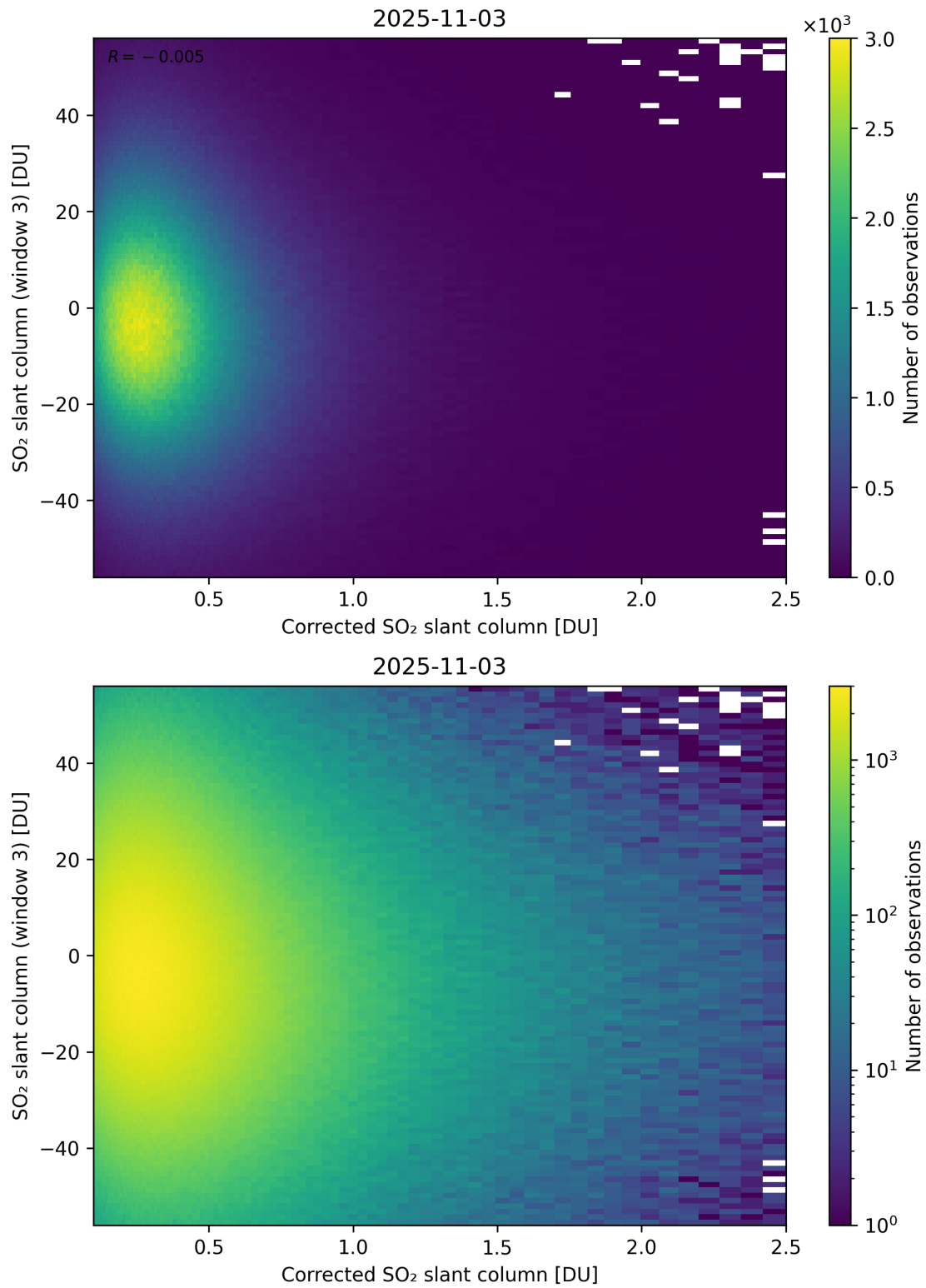
Figure 240: Scatter density plot of “Corrected SO 2 slant column” against “SO 2 slant column (window 3)” for 2025-11-02 to 2025-11-04.
