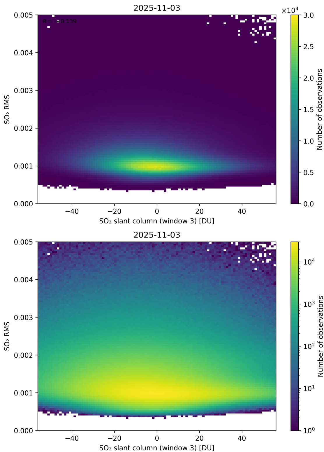
Figure 306: Scatter density plot of “SO 2 slant column (window 3)” against “SO 2 RMS” for 2025-11-02 to 2025-11-04.
