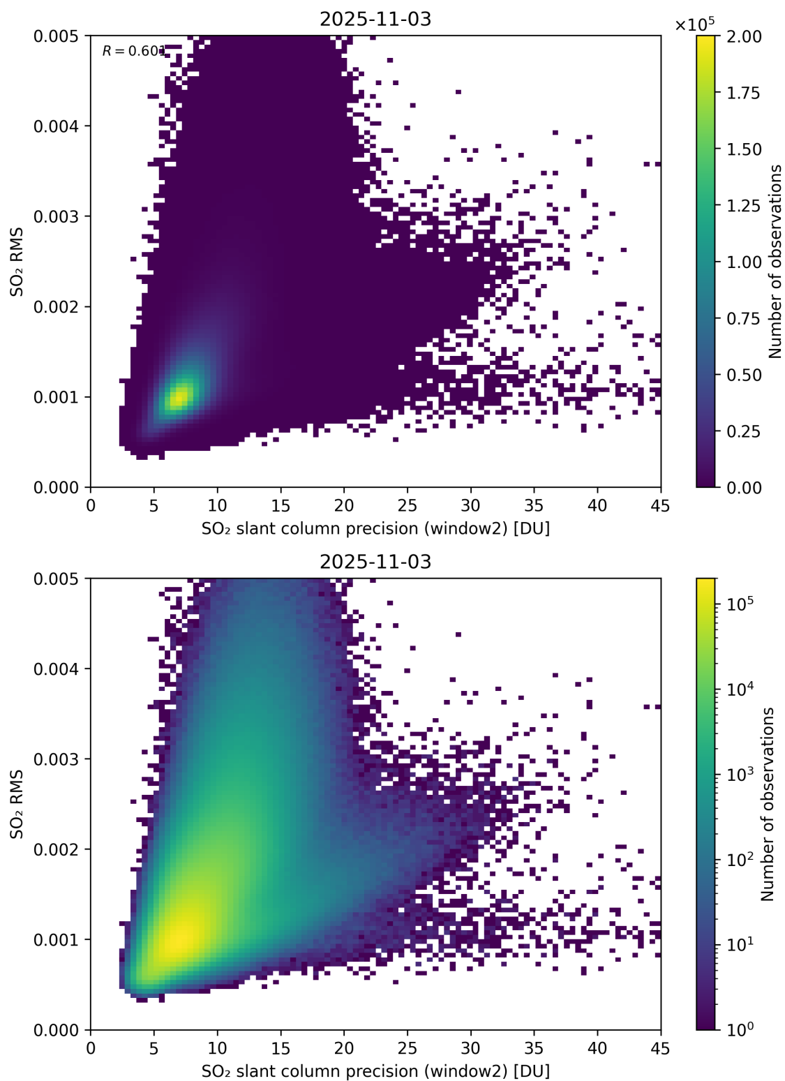
Figure 295: Scatter density plot of “SO 2 slant column precision (window2)” against “SO 2 RMS” for 2025-11-02 to 2025-11-04.
