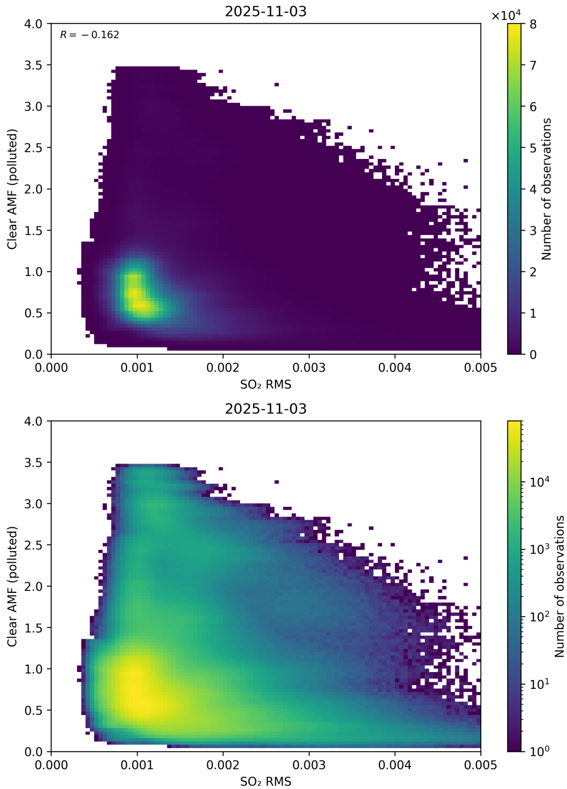
Figure 147: Scatter density plot of “SO 2 RMS” against “Clear AMF (polluted)” for 2025-11-02 to 2025-11-04.
