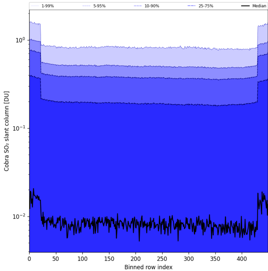
Figure 87: Along track statistics of “Cobra SO 2 slant column” for 2025-11-02 to 2025-11-04
