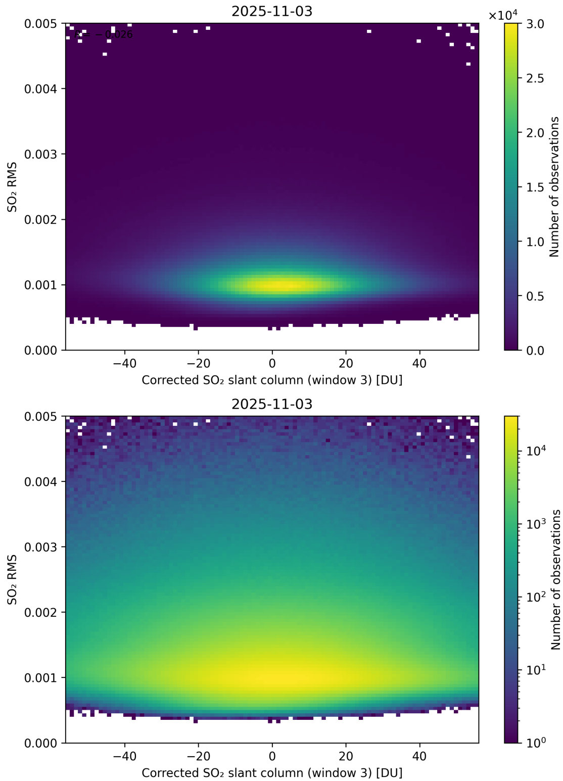
Figure 258: Scatter density plot of “Corrected SO 2 slant column (window 3)” against “SO 2 RMS” for 2025-11-02 to 2025-11-04.
