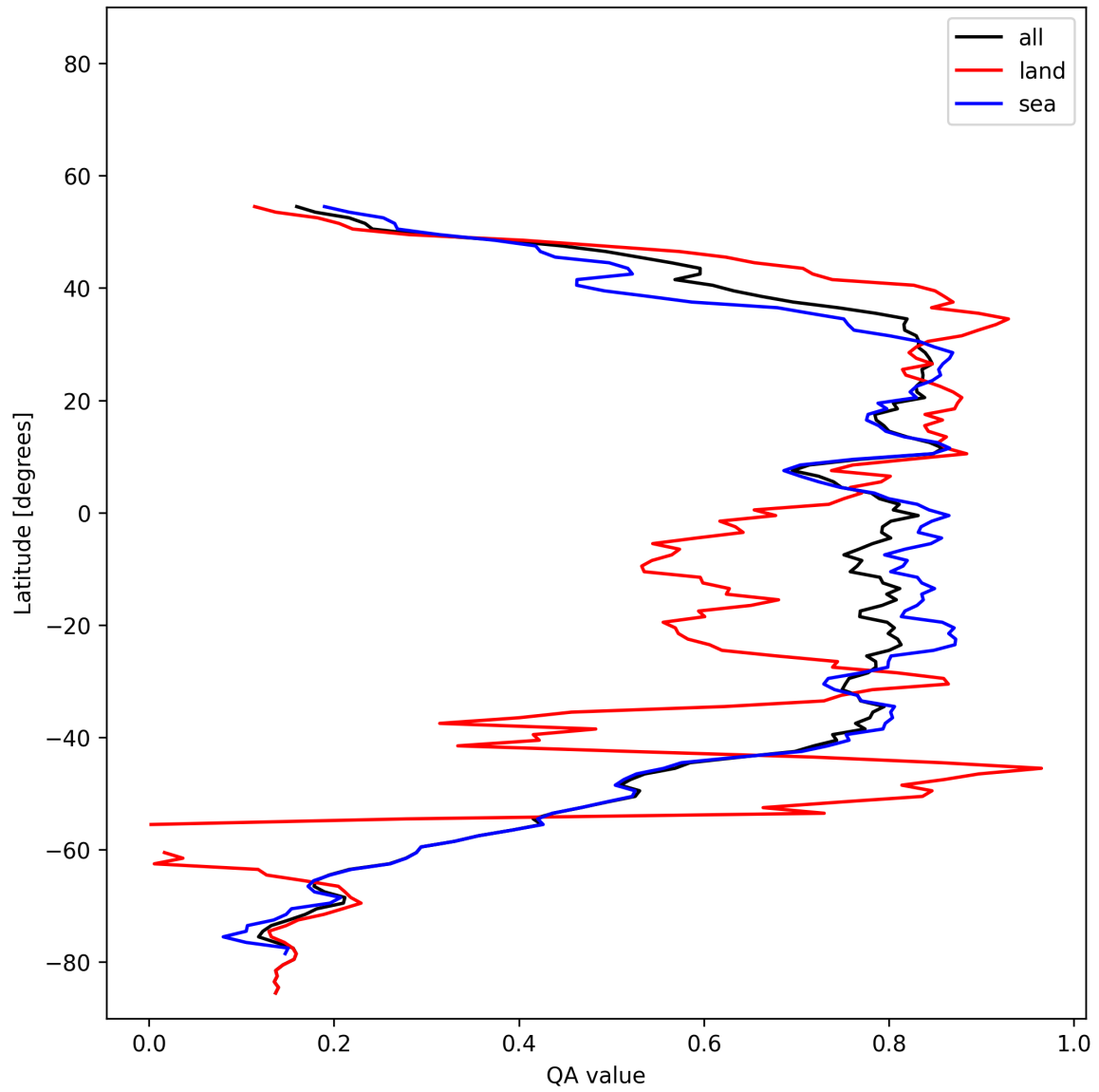
Figure 31: Zonal average of “QA value” for 2025-11-02 to 2025-11-04.
