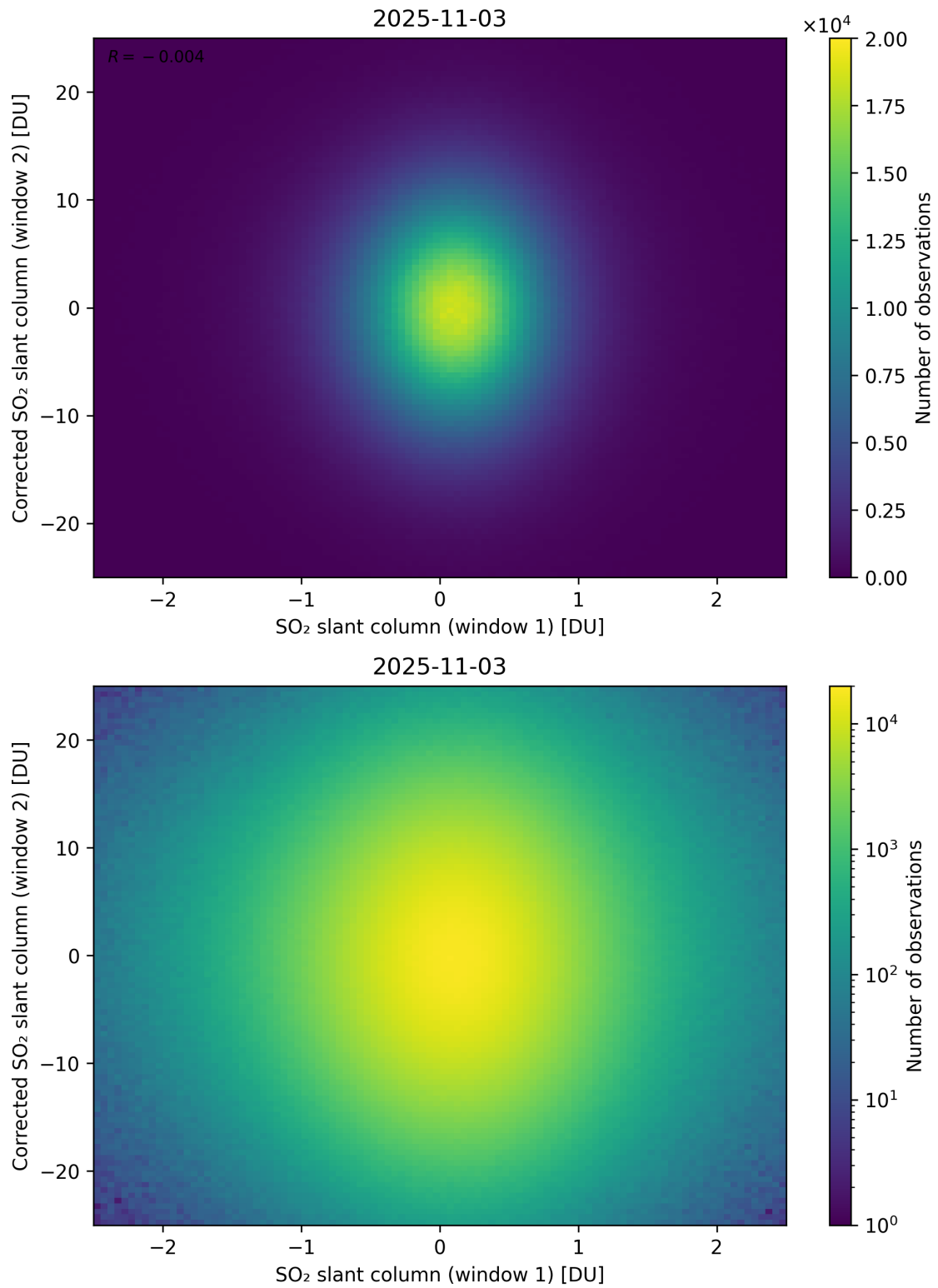
Figure 283: Scatter density plot of “SO 2 slant column (window 1)” against “Corrected SO 2 slant column (window 2)” for 2025-11-02 to 2025-11-04.
