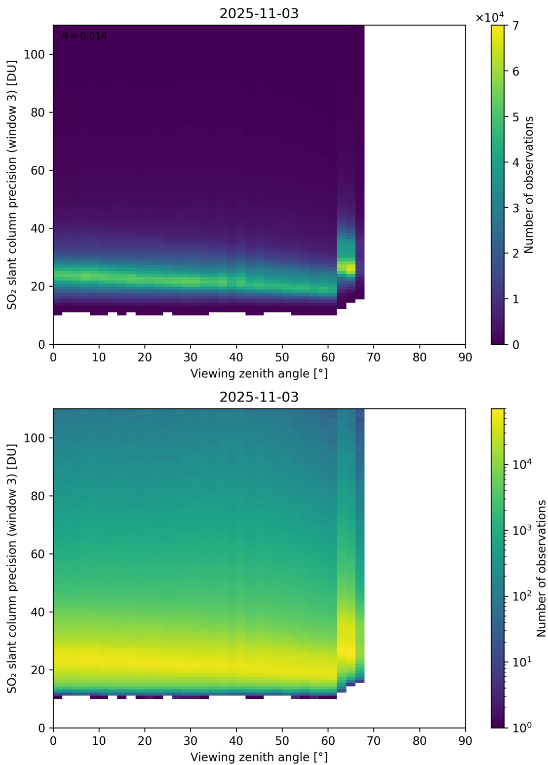
Figure 380: Scatter density plot of “Viewing zenith angle” against “SO 2 slant column precision (window 3)” for 2025-11-02 to 2025-11-04.
