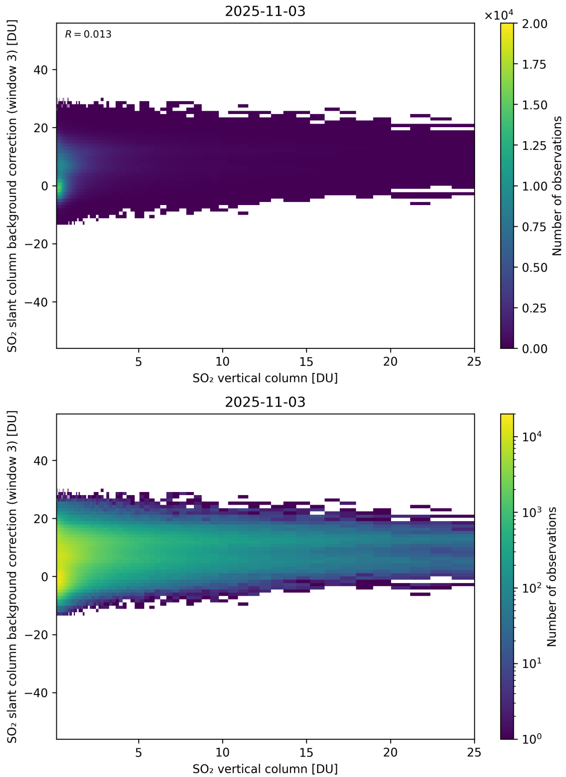
Figure 325: Scatter density plot of “SO 2 vertical column” against “SO 2 slant column background correction (window 3)” for 2025-11-02 to 2025-11-04.
