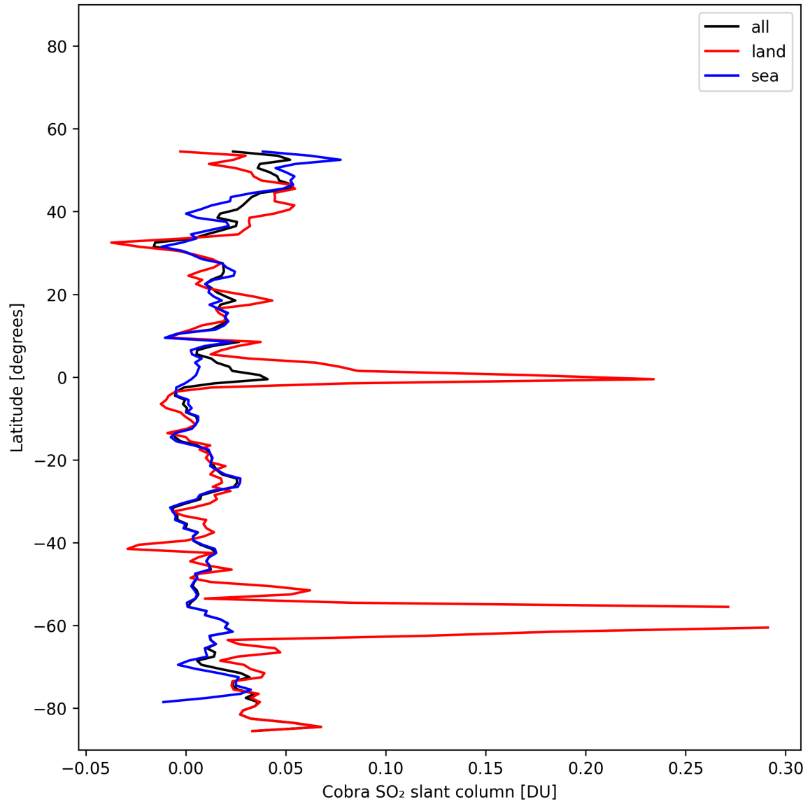
Figure 35: Zonal average of “Cobra SO 2 slant column” for 2025-11-02 to 2025-11-04.
