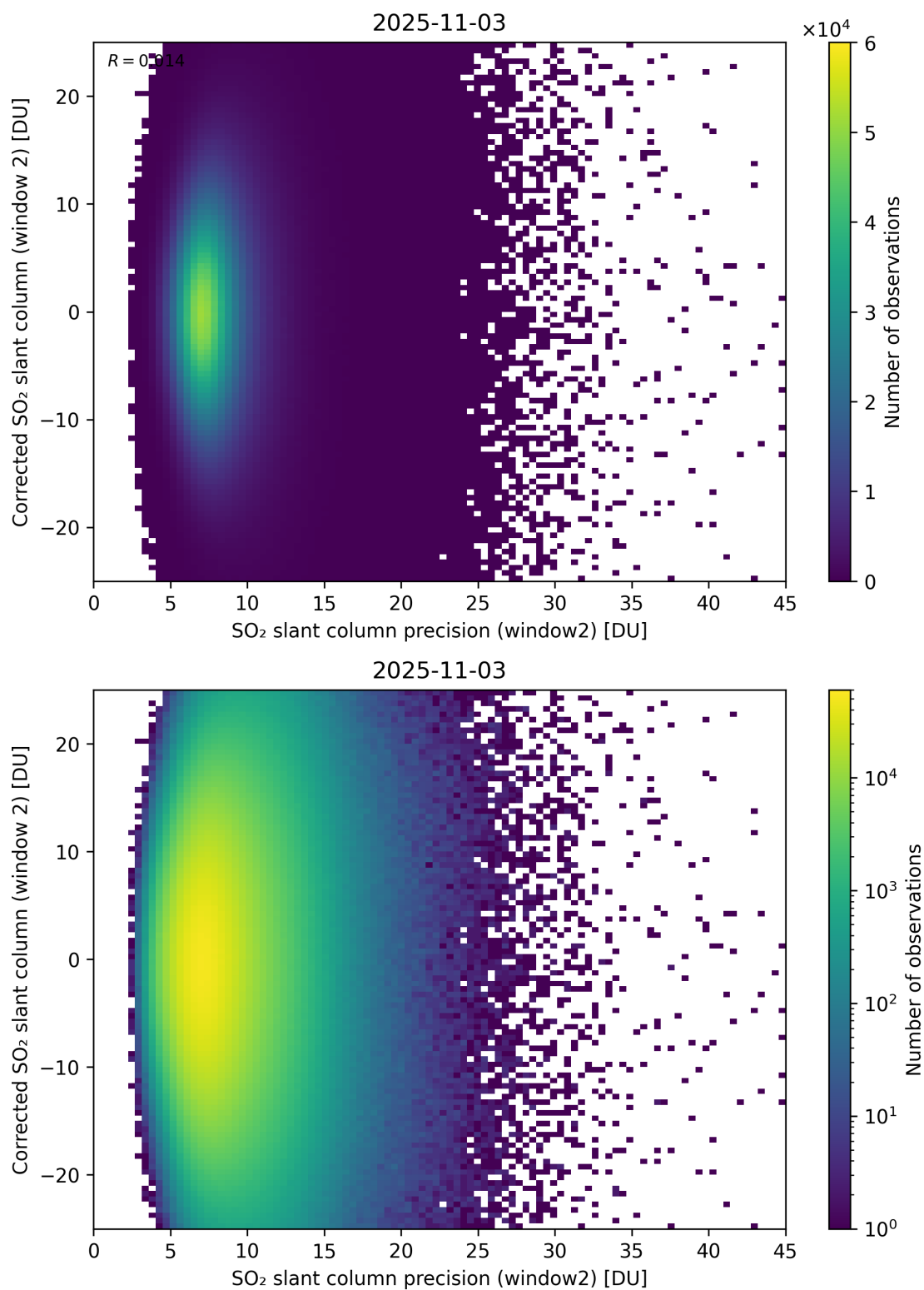
Figure 297: Scatter density plot of “SO 2 slant column precision (window2)” against “Corrected SO 2 slant column (window 2)” for 2025-11-02 to 2025-11-04.
