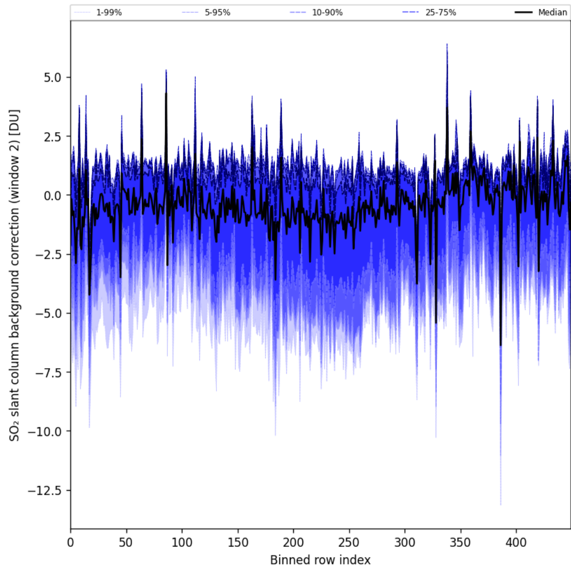
Figure 96: Along track statistics of “SO 2 slant column background correction (window 2)” for 2025-11-02 to 2025-11-04
