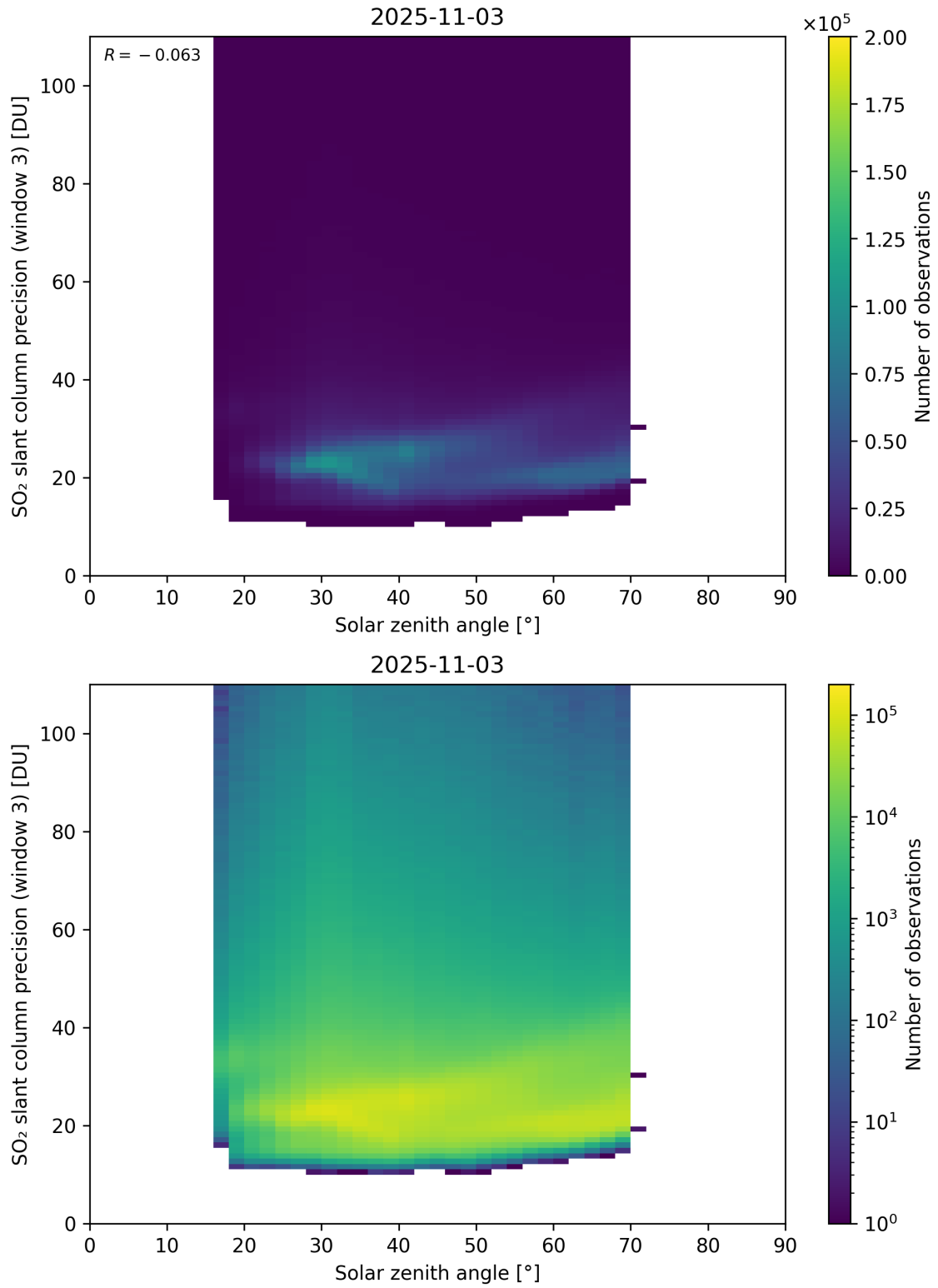
Figure 188: Scatter density plot of “Solar zenith angle” against “SO 2 slant column precision (window 3)” for 2025-11-02 to 2025-11-04.
