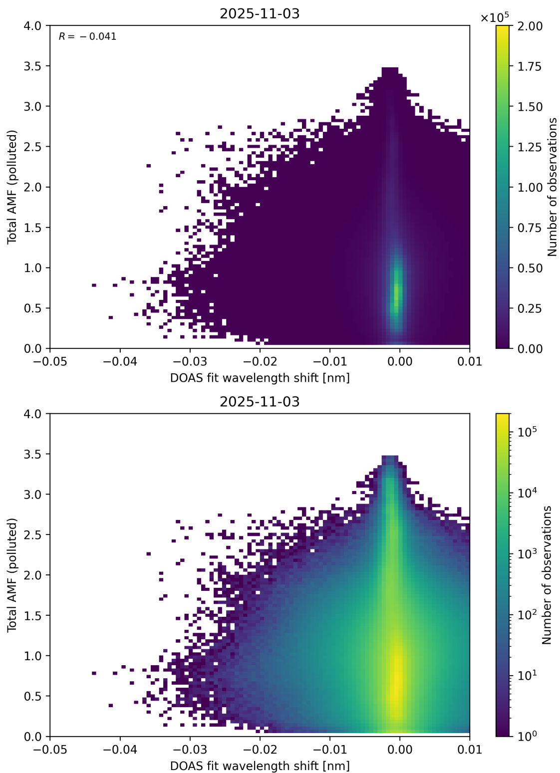
Figure 141: Scatter density plot of “DOAS fit wavelength shift” against “Total AMF (polluted)” for 2025-11-02 to 2025-11-04.
