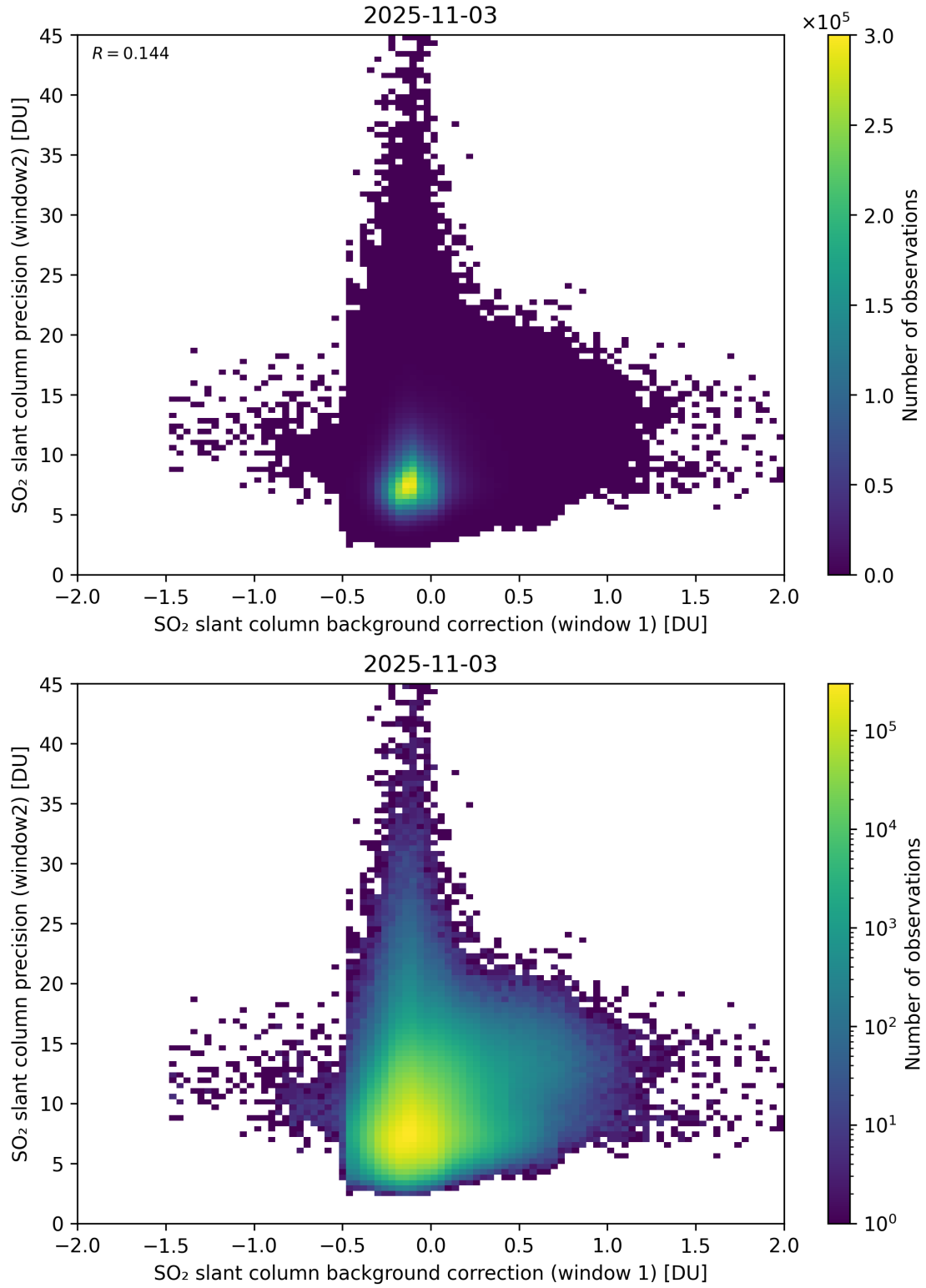
Figure 117: Scatter density plot of “SO 2 slant column background correction (window 1)” against “SO 2 slant column precision (window2)” for 2025-11-02 to 2025-11-04.
