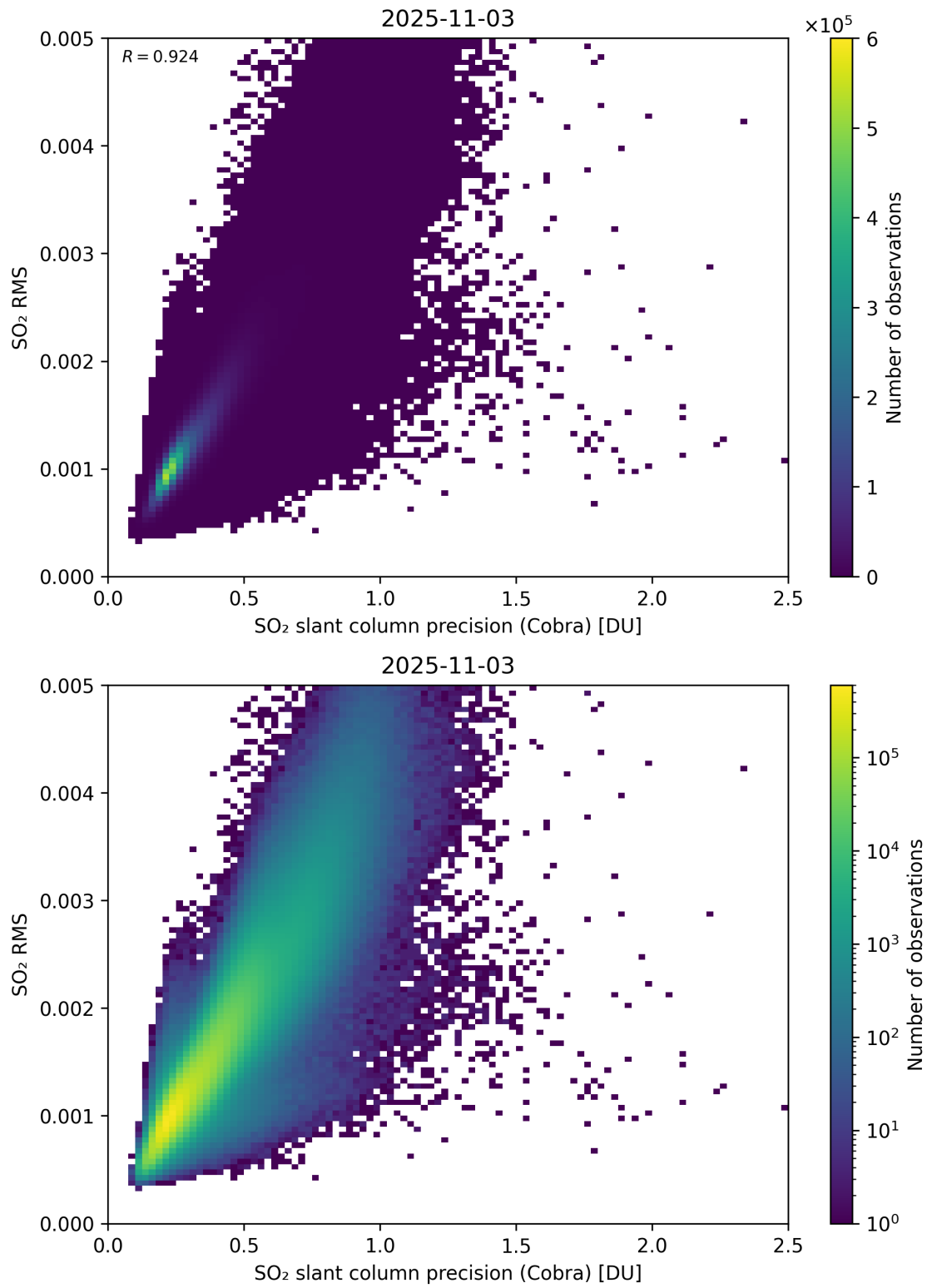
Figure 204: Scatter density plot of “SO 2 slant column precision (Cobra)” against “SO 2 RMS” for 2025-11-02 to 2025-11-04.
