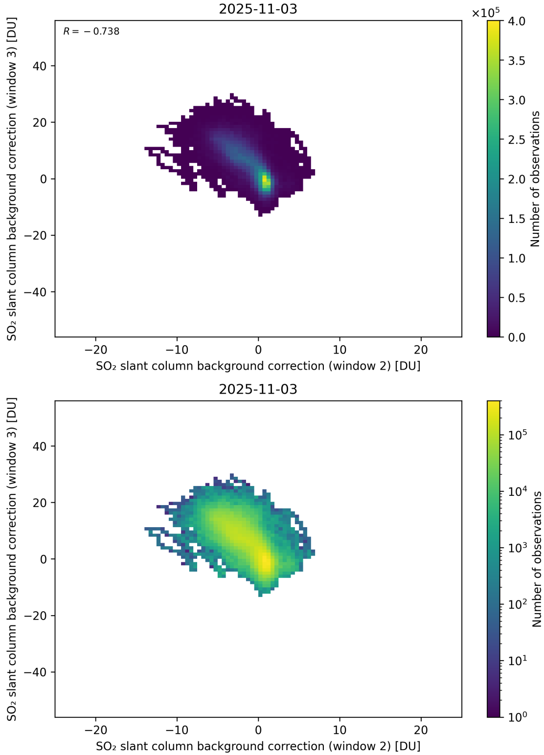
Figure 122: Scatter density plot of “SO 2 slant column background correction (window 2)” against “SO 2 slant column background correction (window 3)” for 2025-11-02 to 2025-11-04.
