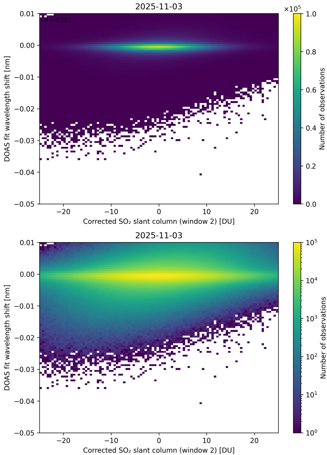
Figure 246: Scatter density plot of “Corrected SO 2 slant column (window 2)” against “DOAS fit wavelength shift” for 2025-11-02 to 2025-11-04.
