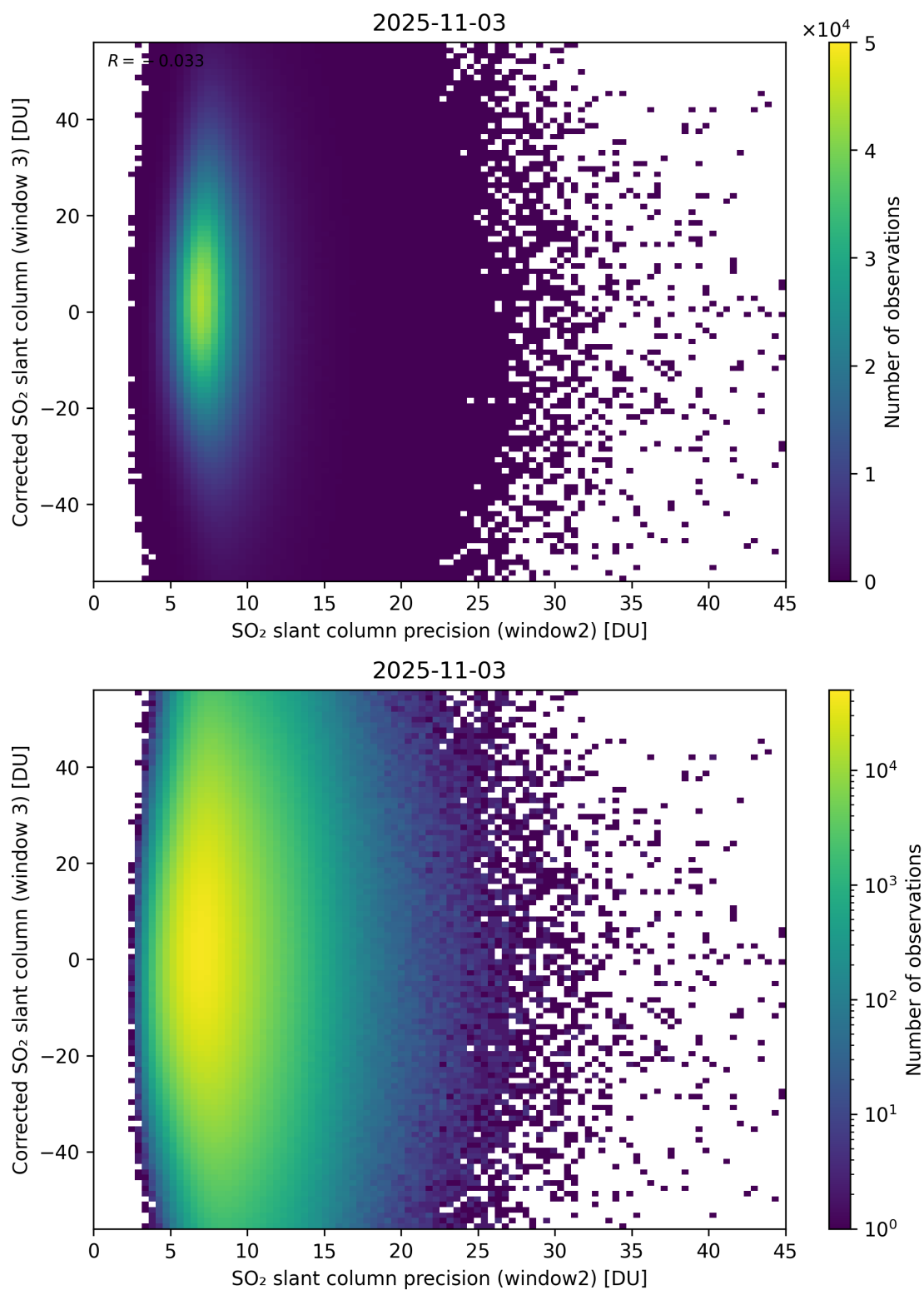
Figure 298: Scatter density plot of “SO 2 slant column precision (window2)” against “Corrected SO 2 slant column (window 3)” for 2025-11-02 to 2025-11-04.
