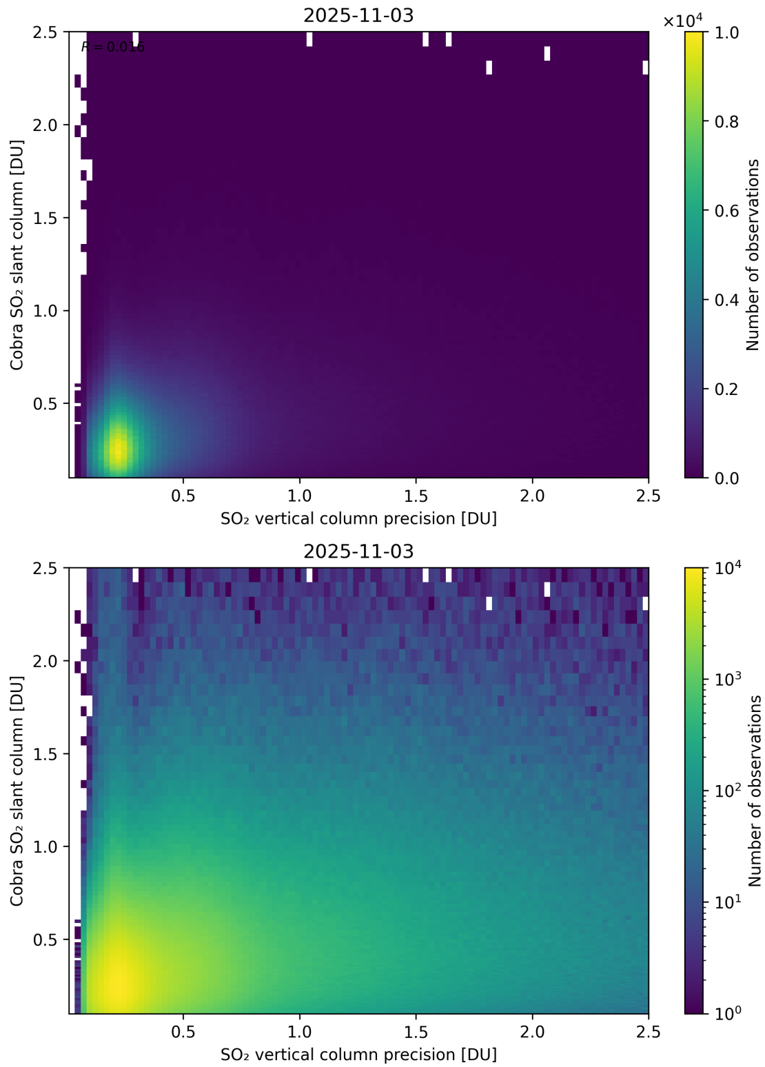
Figure 336: Scatter density plot of “SO 2 vertical column precision” against “Cobra SO 2 slant column” for 2025-11-02 to 2025-11-04.
