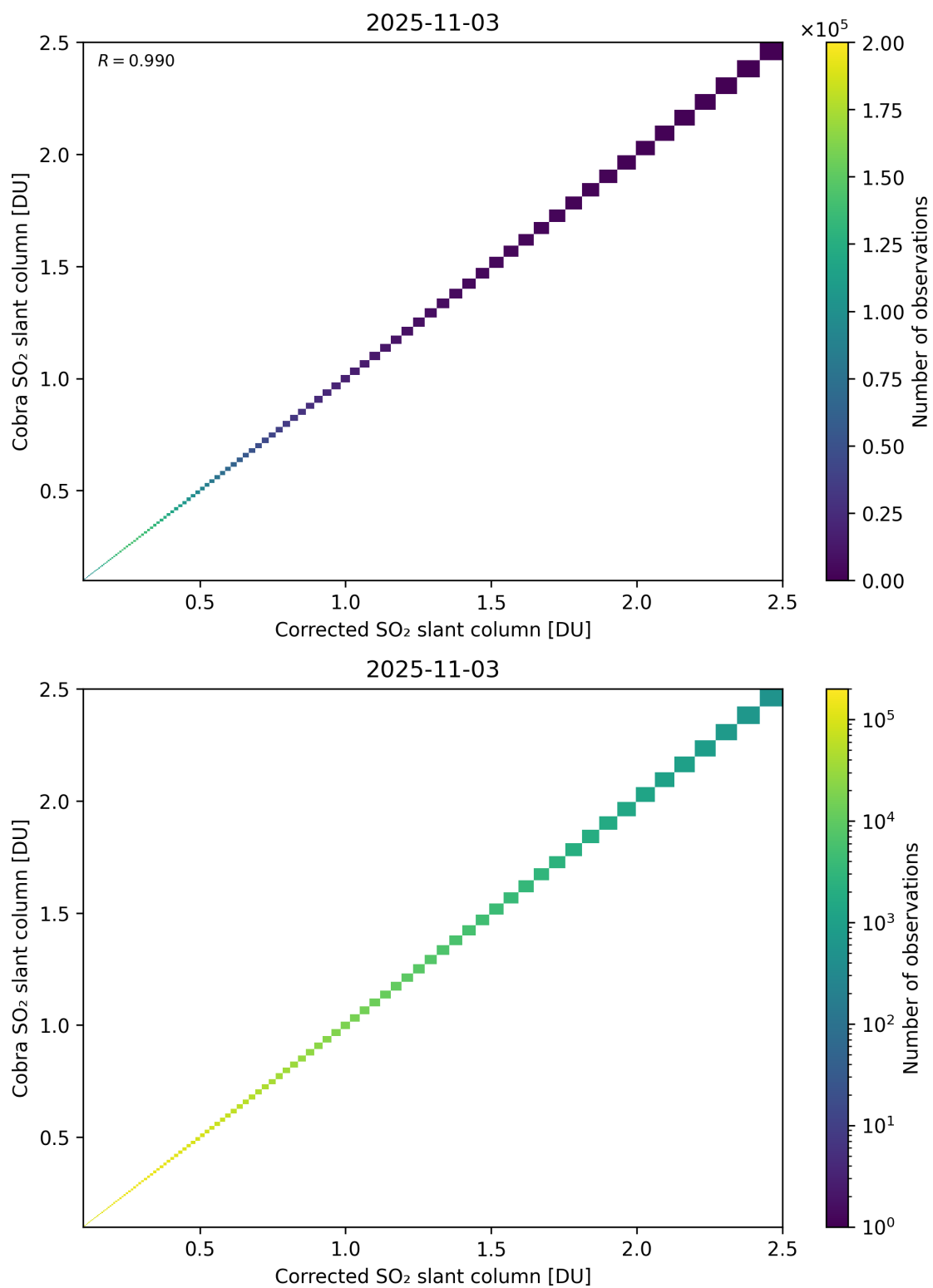
Figure 233: Scatter density plot of “Corrected SO 2 slant column” against “Cobra SO 2 slant column” for 2025-11-02 to 2025-11-04.
