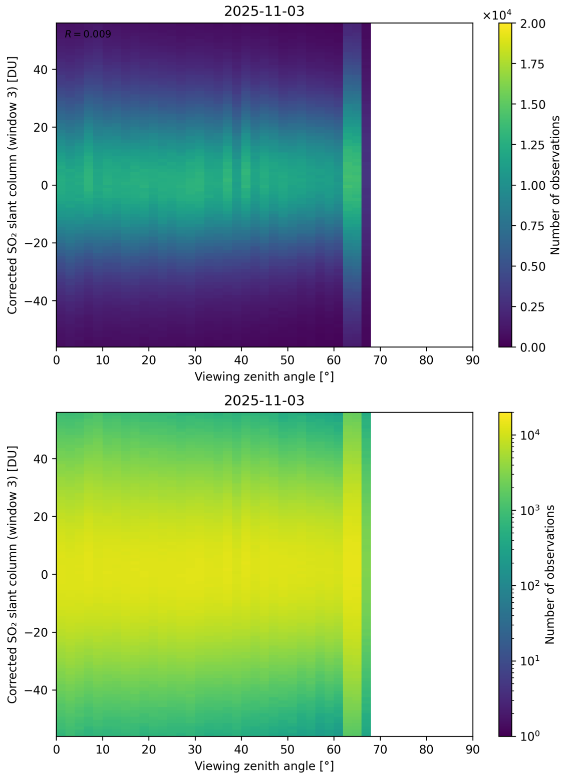
Figure 375: Scatter density plot of “Viewing zenith angle” against “Corrected SO 2 slant column (window 3)” for 2025-11-02 to 2025-11-04.
