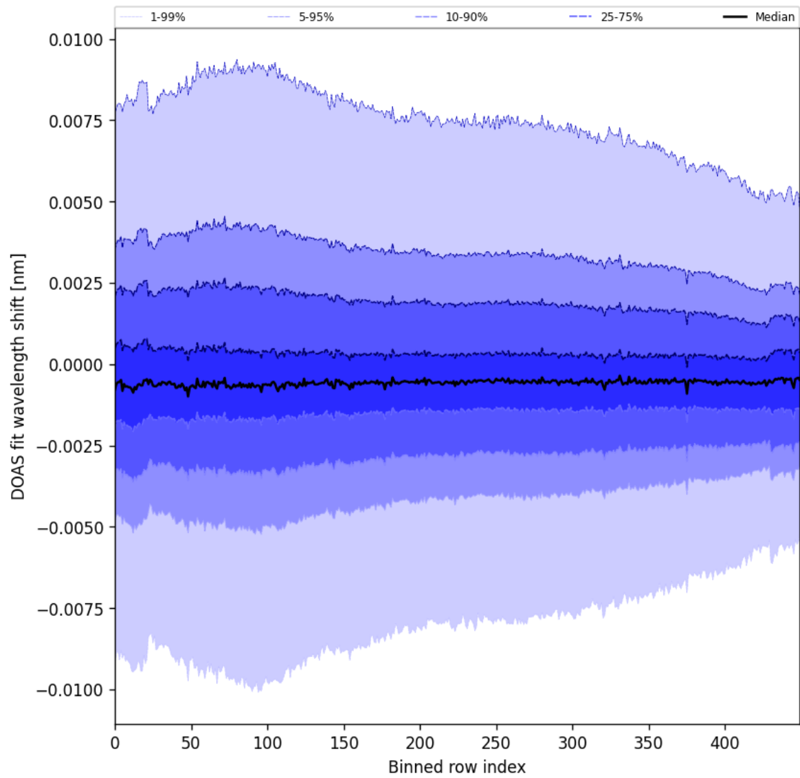
Figure 102: Along track statistics of “DOAS fit wavelength shift” for 2025-11-02 to 2025-11-04
