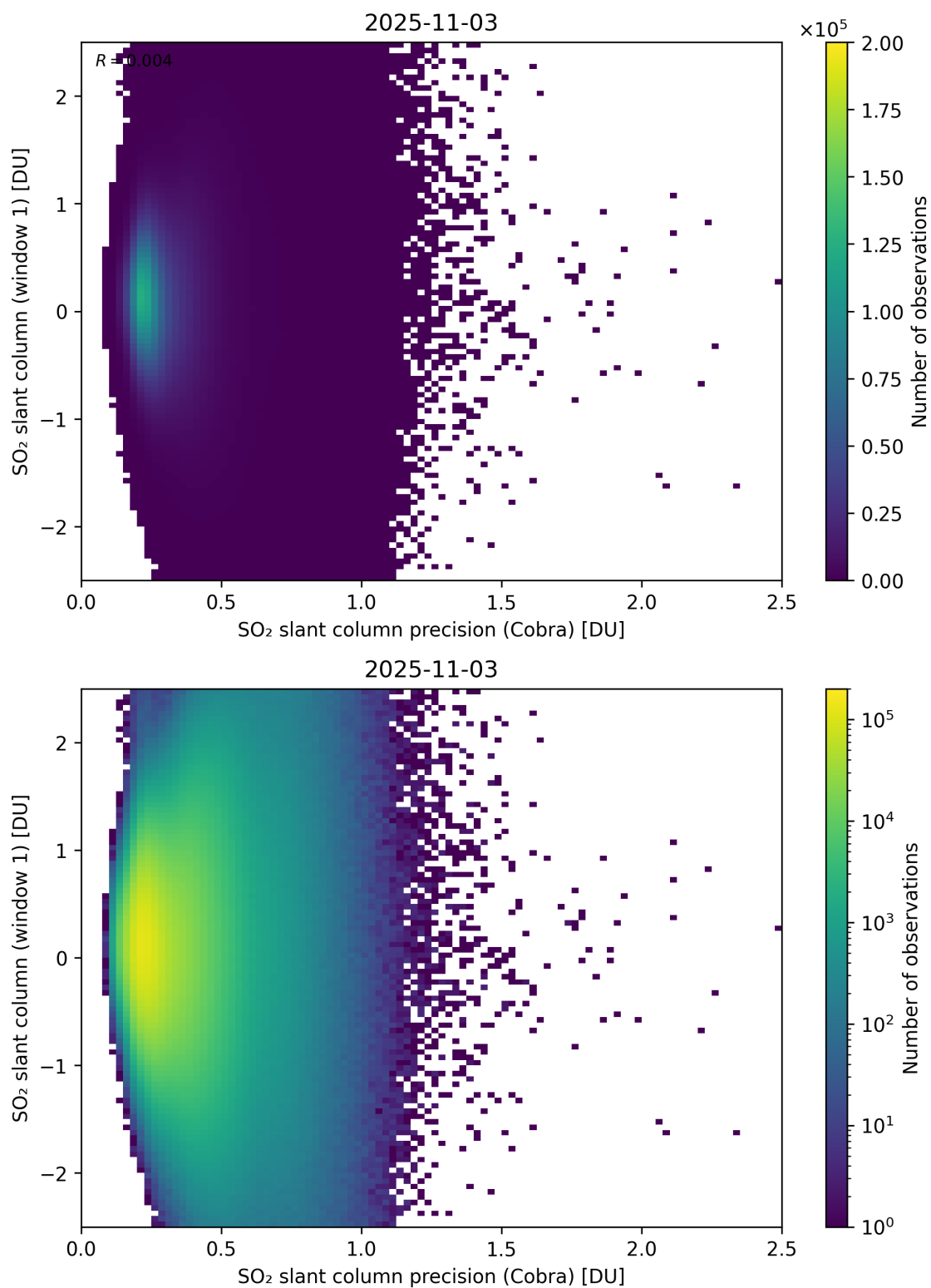
Figure 208: Scatter density plot of “SO 2 slant column precision (Cobra)” against “SO 2 slant column (window 1)” for 2025-11-02 to 2025-11-04.
