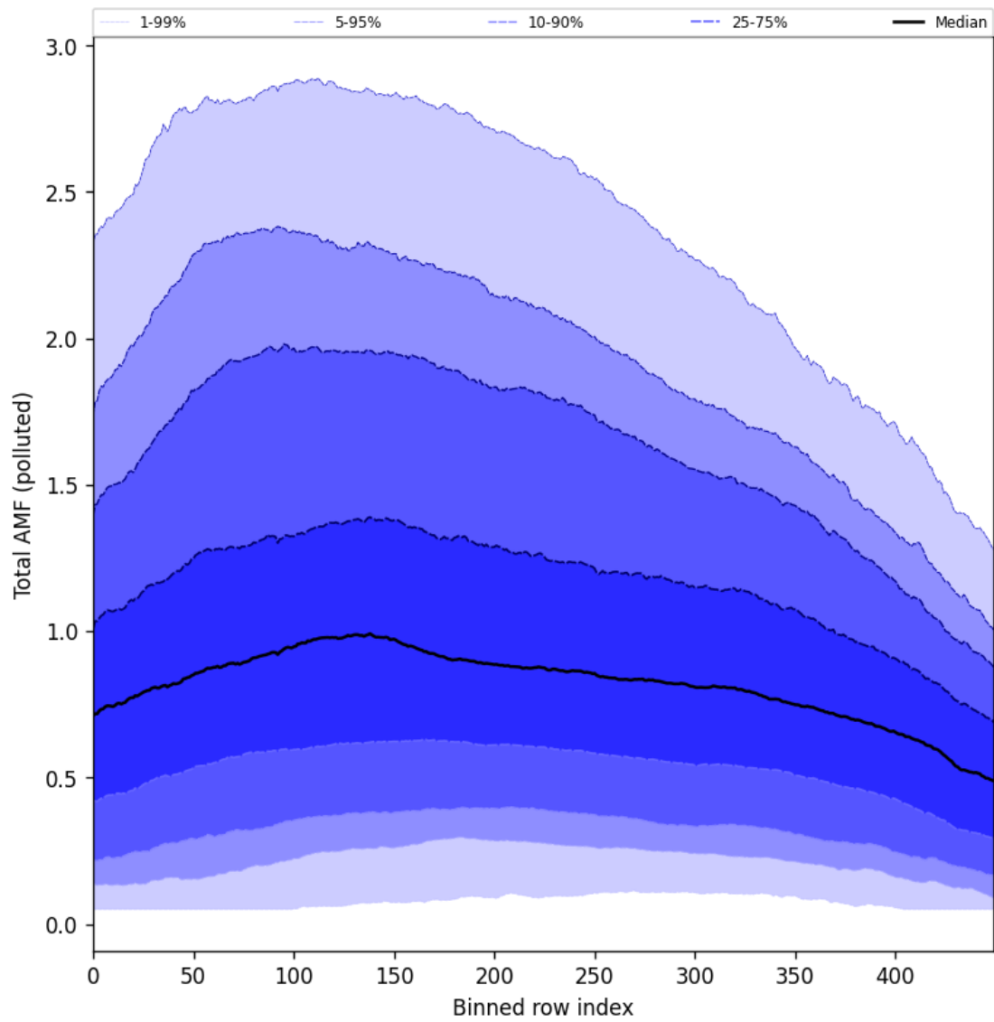
Figure 105: Along track statistics of “Total AMF (polluted)” for 2025-11-02 to 2025-11-04
