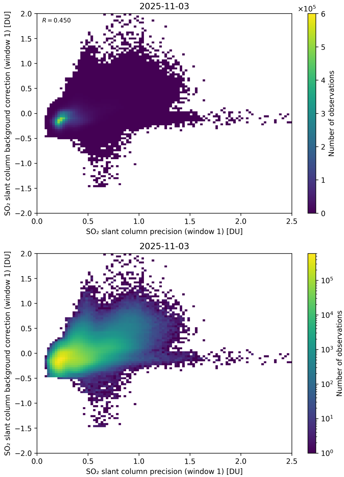
Figure 268: Scatter density plot of “SO 2 slant column precision (window 1)” against “SO 2 slant column background correction (window 1)” for 2025-11-02 to 2025-11-04.
