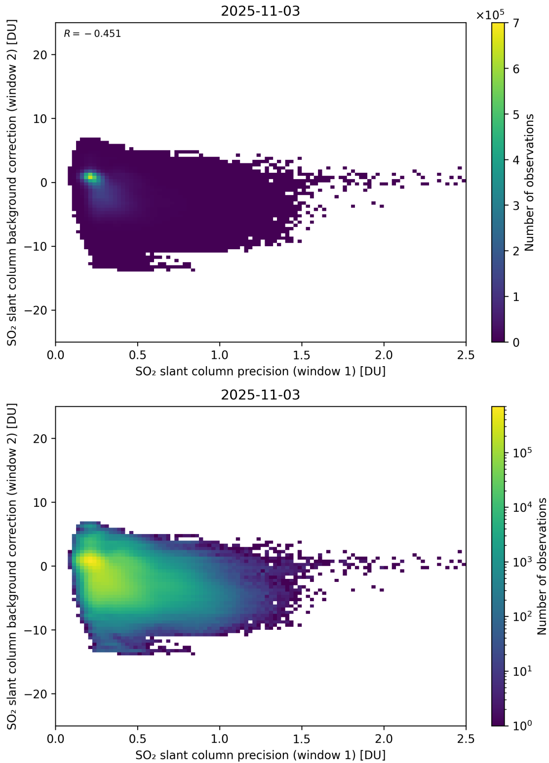
Figure 269: Scatter density plot of “SO 2 slant column precision (window 1)” against “SO 2 slant column background correction (window 2)” for 2025-11-02 to 2025-11-04.
