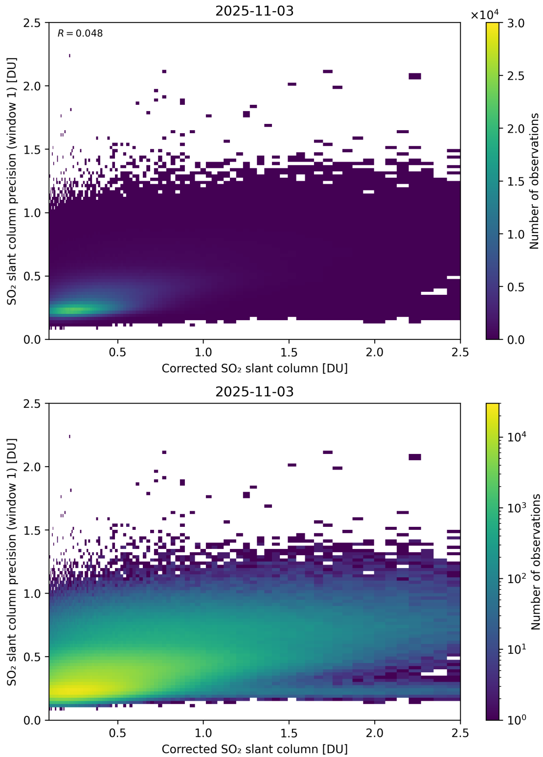
Figure 238: Scatter density plot of “Corrected SO 2 slant column” against “SO 2 slant column precision (window 1)” for 2025-11-02 to 2025-11-04.
