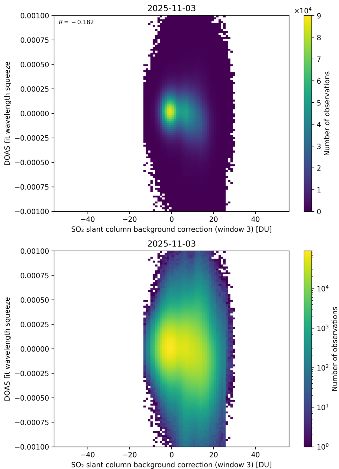
Figure 133: Scatter density plot of “SO 2 slant column background correction (window 3)” against “DOAS fit wavelength squeeze” for 2025-11-02 to 2025-11-04.
