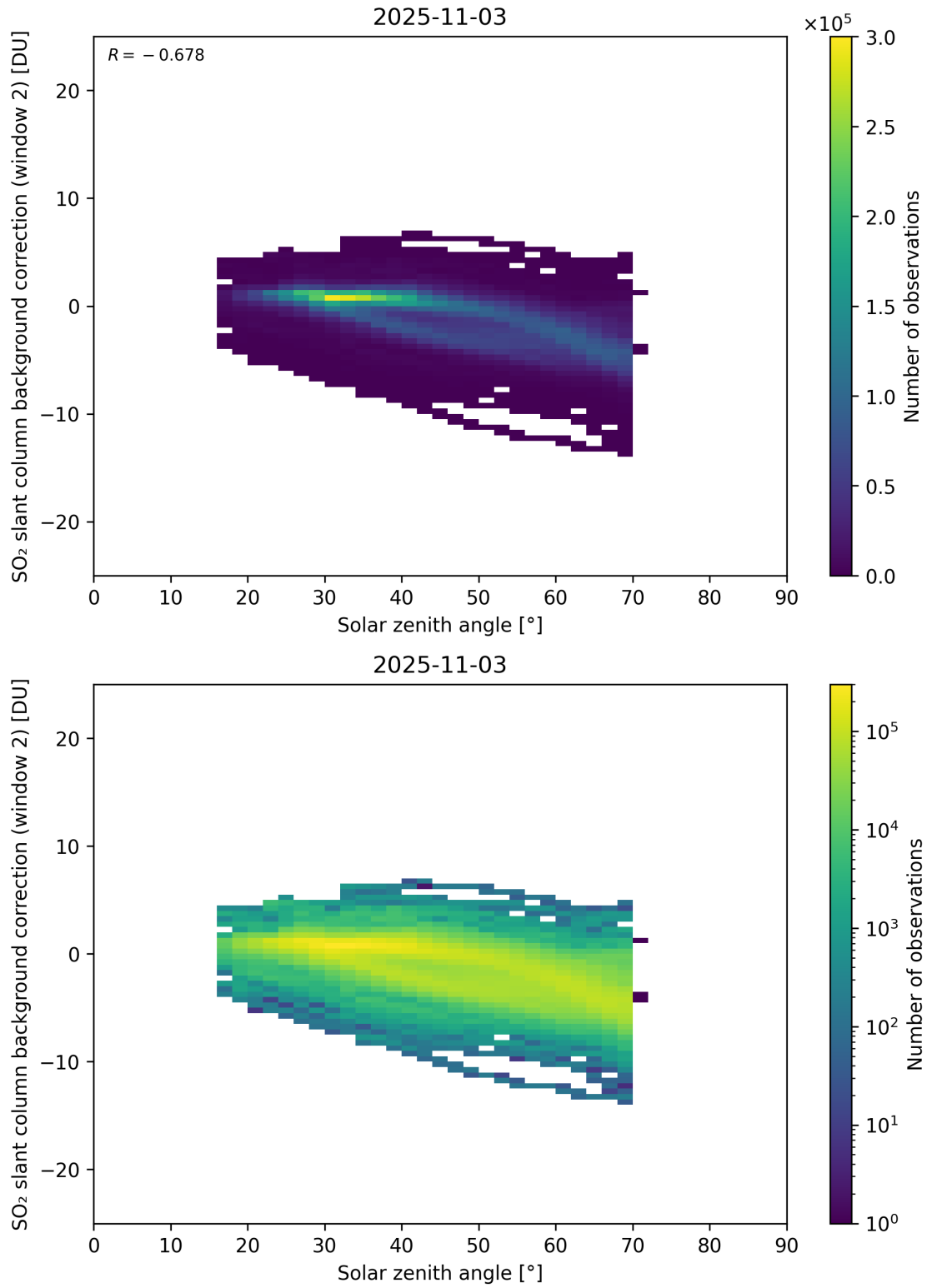
Figure 172: Scatter density plot of “Solar zenith angle” against “SO 2 slant column background correction (window 2)” for 2025-11-02 to 2025-11-04.
