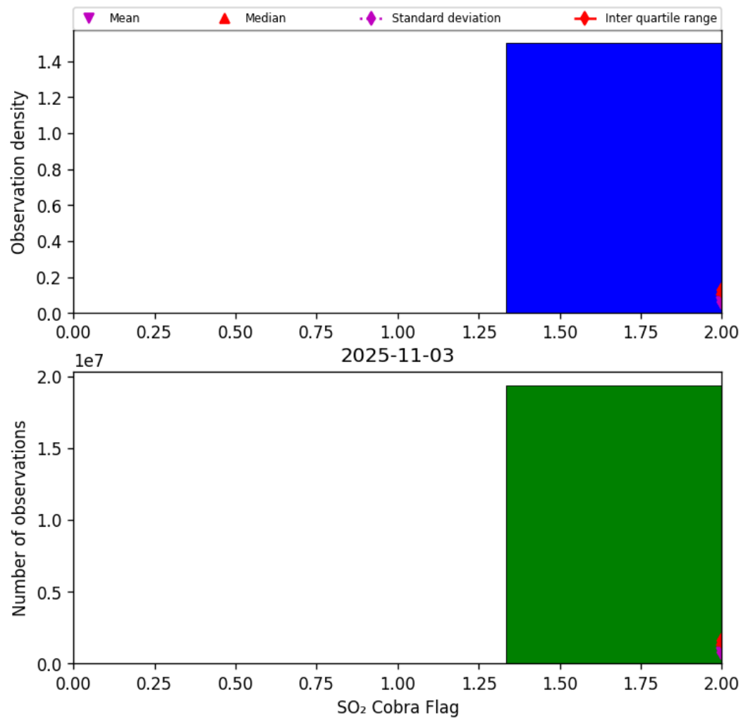
Figure 75: Histogram of “SO 2 Cobra Flag” for 2025-11-02 to 2025-11-04
