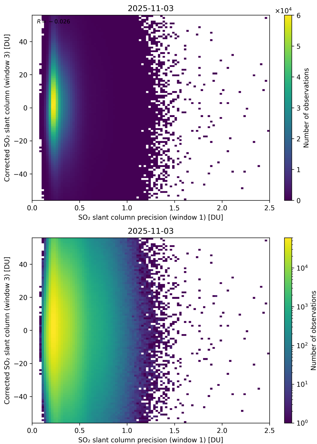
Figure 276: Scatter density plot of “SO 2 slant column precision (window 1)” against “Corrected SO 2 slant column (window 3)” for 2025-11-02 to 2025-11-04.
