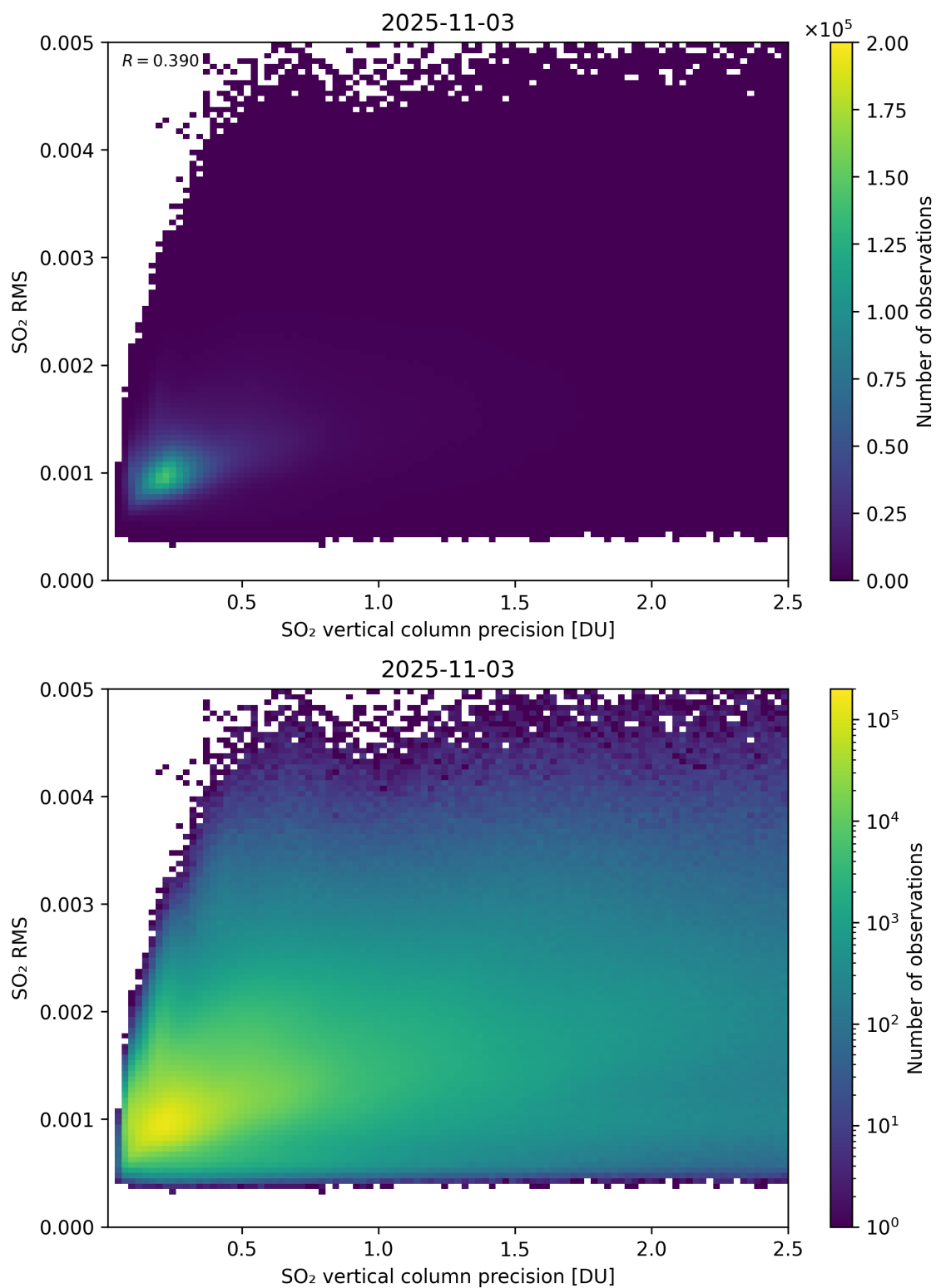
Figure 334: Scatter density plot of “SO 2 vertical column precision” against “SO 2 RMS” for 2025-11-02 to 2025-11-04.
