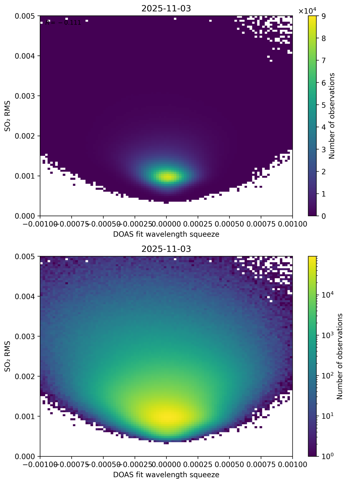
Figure 143: Scatter density plot of “DOAS fit wavelength squeeze” against “SO 2 RMS” for 2025-11-02 to 2025-11-04.
