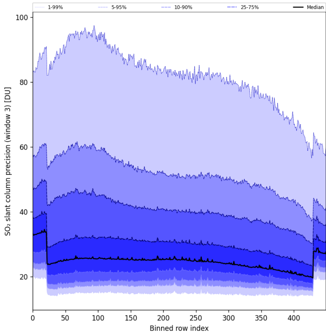
Figure 98: Along track statistics of “SO 2 slant column precision (window 3)” for 2025-11-02 to 2025-11-04
