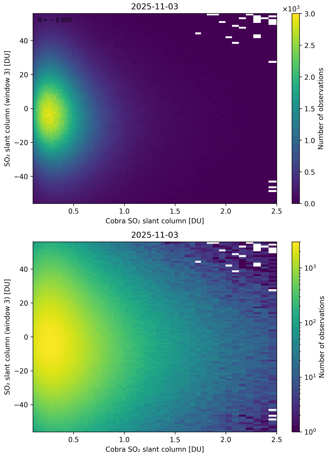
Figure 222: Scatter density plot of “Cobra SO 2 slant column” against “SO 2 slant column (window 3)” for 2025-11-02 to 2025-11-04.
