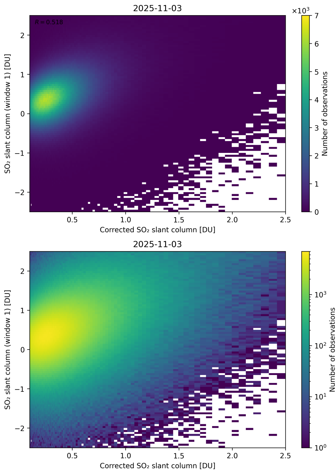
Figure 237: Scatter density plot of “Corrected SO 2 slant column” against “SO 2 slant column (window 1)” for 2025-11-02 to 2025-11-04.
