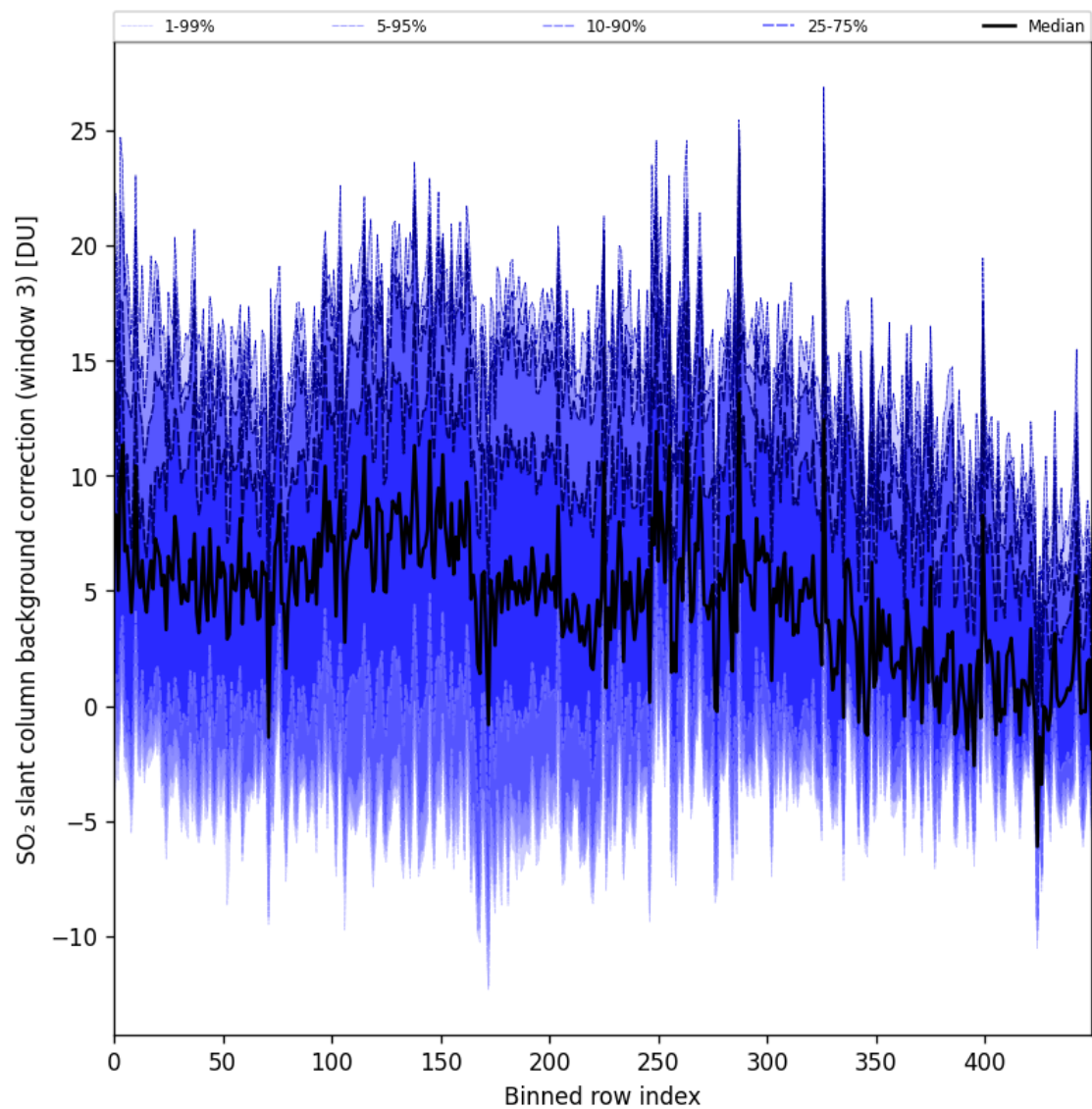
Figure 100: Along track statistics of “SO 2 slant column background correction (window 3)” for 2025-11-02 to 2025-11-04
