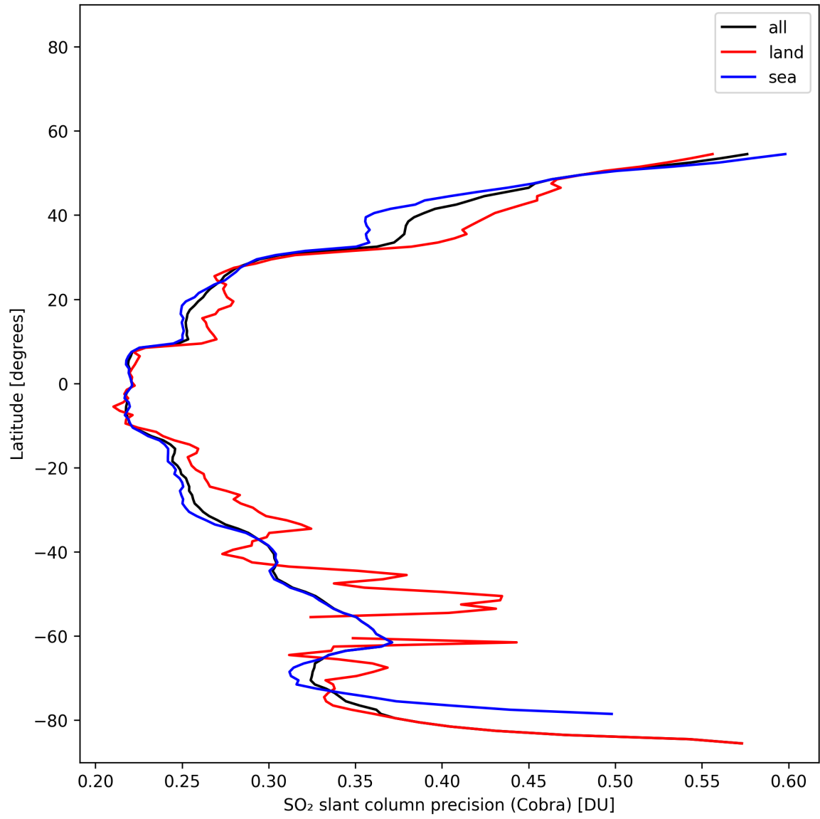
Figure 36: Zonal average of “SO 2 slant column precision (Cobra)” for 2025-11-02 to 2025-11-04.
