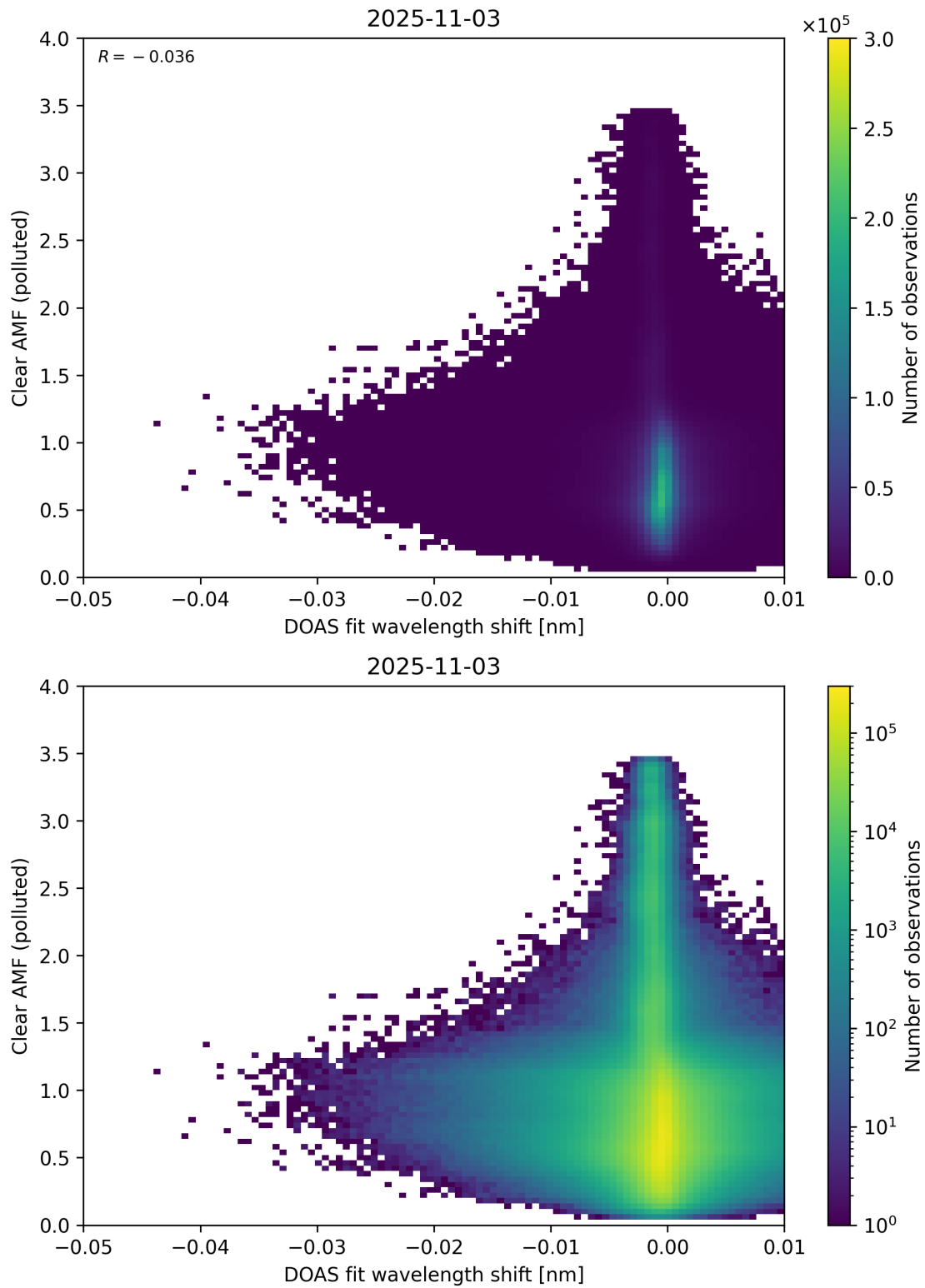
Figure 140: Scatter density plot of “DOAS fit wavelength shift” against “Clear AMF (polluted)” for 2025-11-02 to 2025-11-04.
