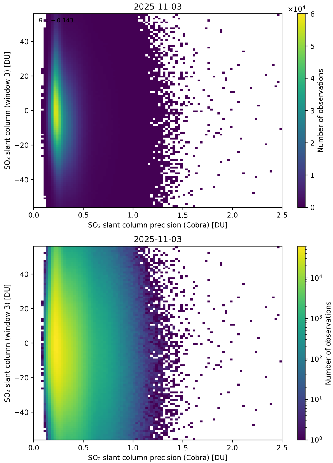
Figure 211: Scatter density plot of “SO 2 slant column precision (Cobra)” against “SO 2 slant column (window 3)” for 2025-11-02 to 2025-11-04.
