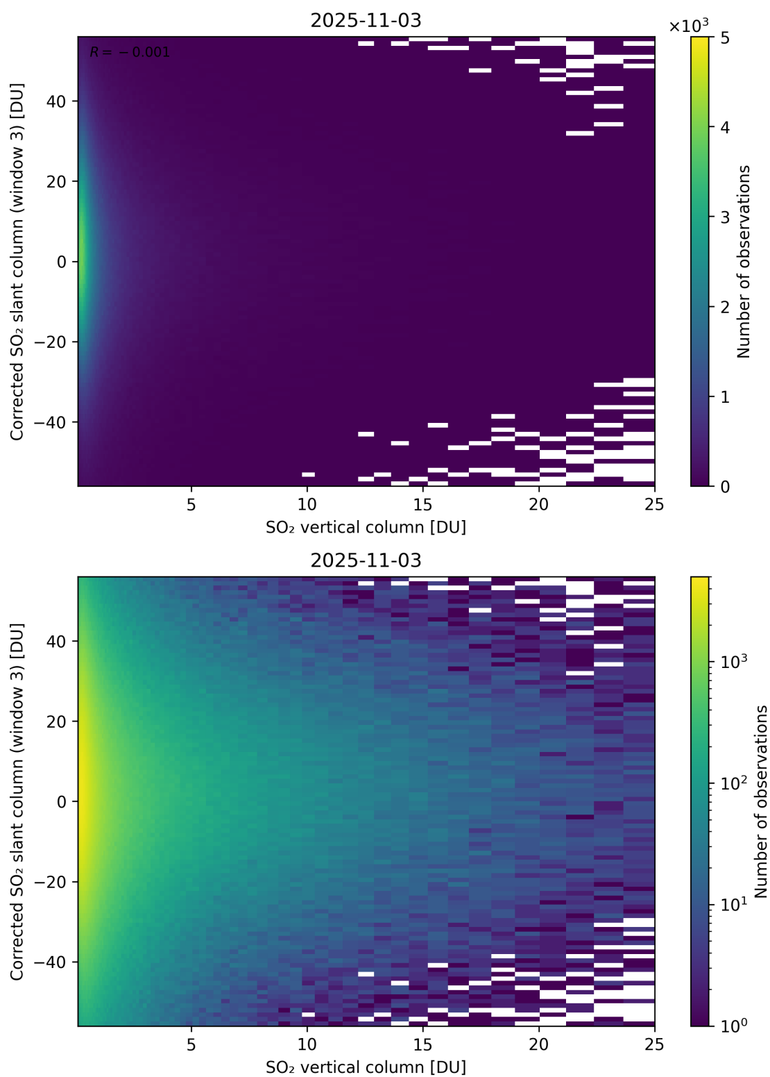
Figure 353: Scatter density plot of “SO 2 vertical column” against “Corrected SO 2 slant column (window 3)” for 2025-11-02 to 2025-11-04.
