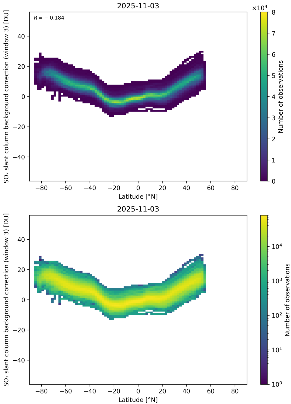
Figure 152: Scatter density plot of “Latitude” against “SO 2 slant column background correction (window 3)” for 2025-11-02 to 2025-11-04.
