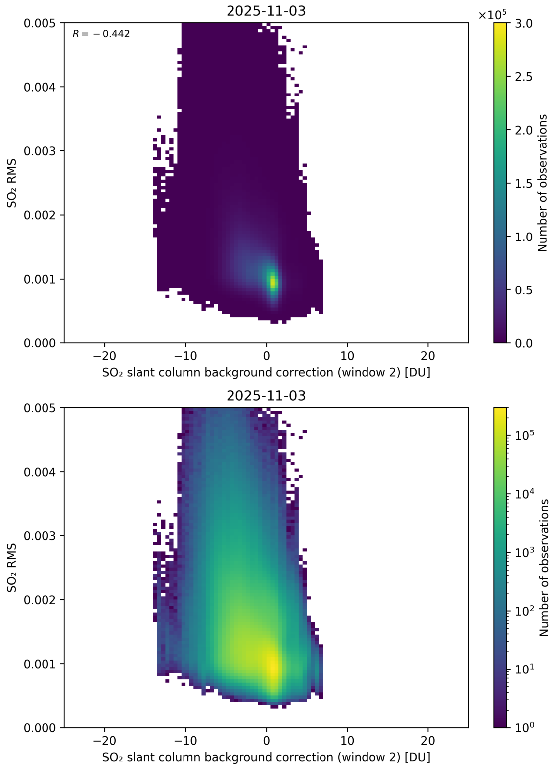
Figure 125: Scatter density plot of “SO 2 slant column background correction (window 2)” against “SO 2 RMS” for 2025-11-02 to 2025-11-04.
