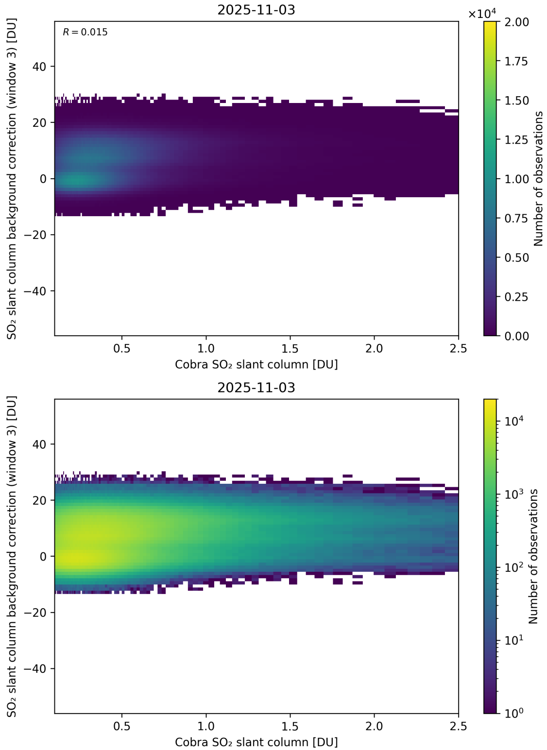
Figure 195: Scatter density plot of “Cobra SO 2 slant column” against “SO 2 slant column background correction (window 3)” for 2025-11-02 to 2025-11-04.
