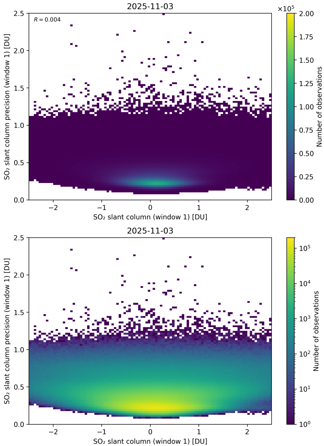
Figure 285: Scatter density plot of “SO 2 slant column (window 1)” against “SO 2 slant column precision (window 1)” for 2025-11-02 to 2025-11-04.
