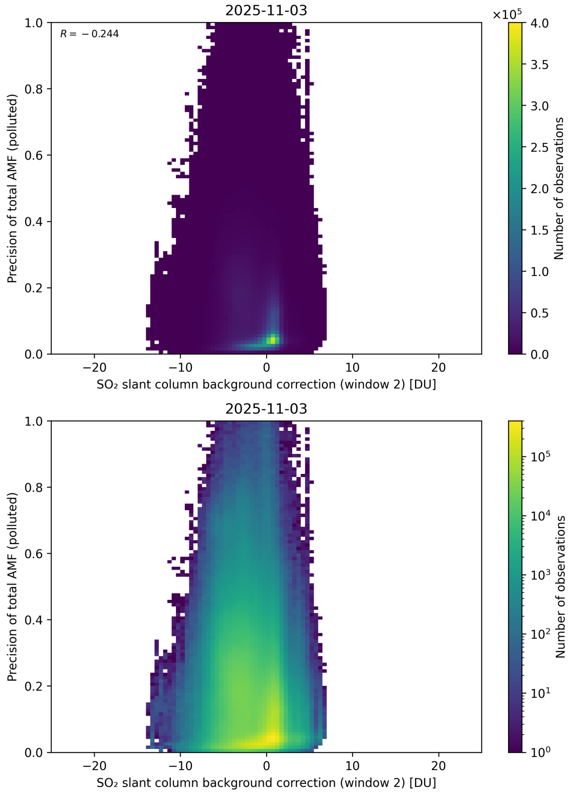
Figure 131: Scatter density plot of “SO 2 slant column background correction (window 2)” against “Precision of total AMF (polluted)” for 2025-11-02 to 2025-11-04.
