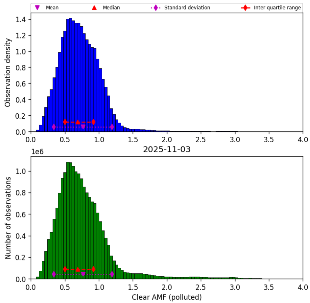
Figure 81: Histogram of “Clear AMF (polluted)” for 2025-11-02 to 2025-11-04
