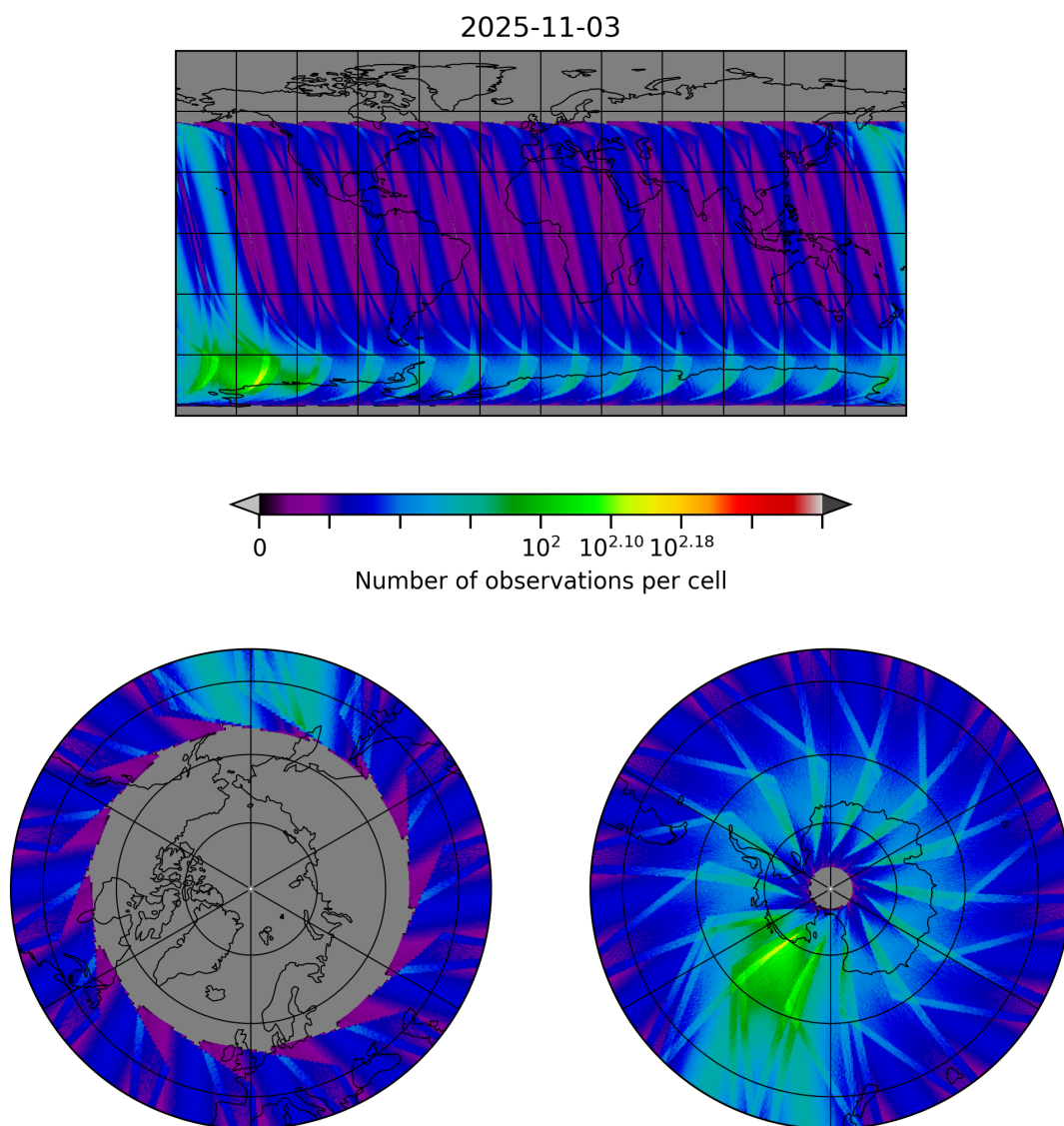
Figure 30: Map of the number of observations for 2025-11-02 to 2025-11-04
