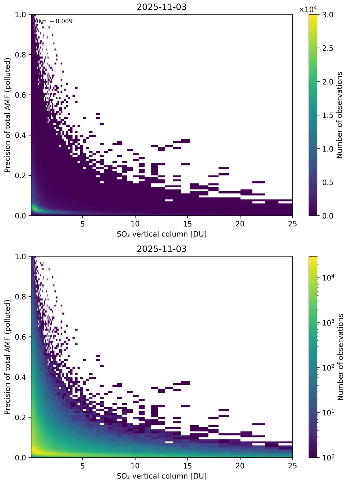
Figure 360: Scatter density plot of “SO 2 vertical column” against “Precision of total AMF (polluted)” for 2025-11-02 to 2025-11-04.
