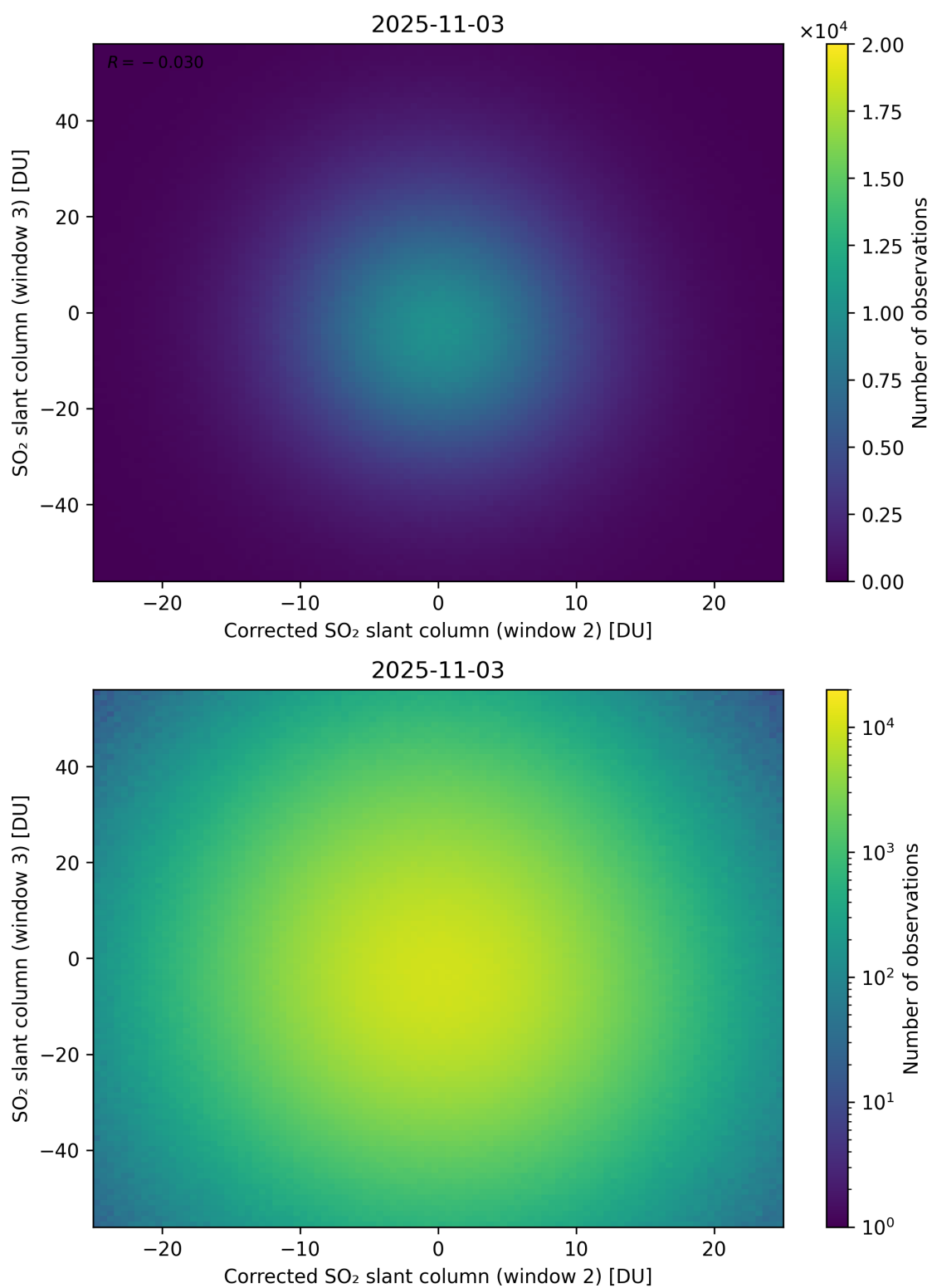
Figure 251: Scatter density plot of “Corrected SO 2 slant column (window 2)” against “SO 2 slant column (window 3)” for 2025-11-02 to 2025-11-04.
