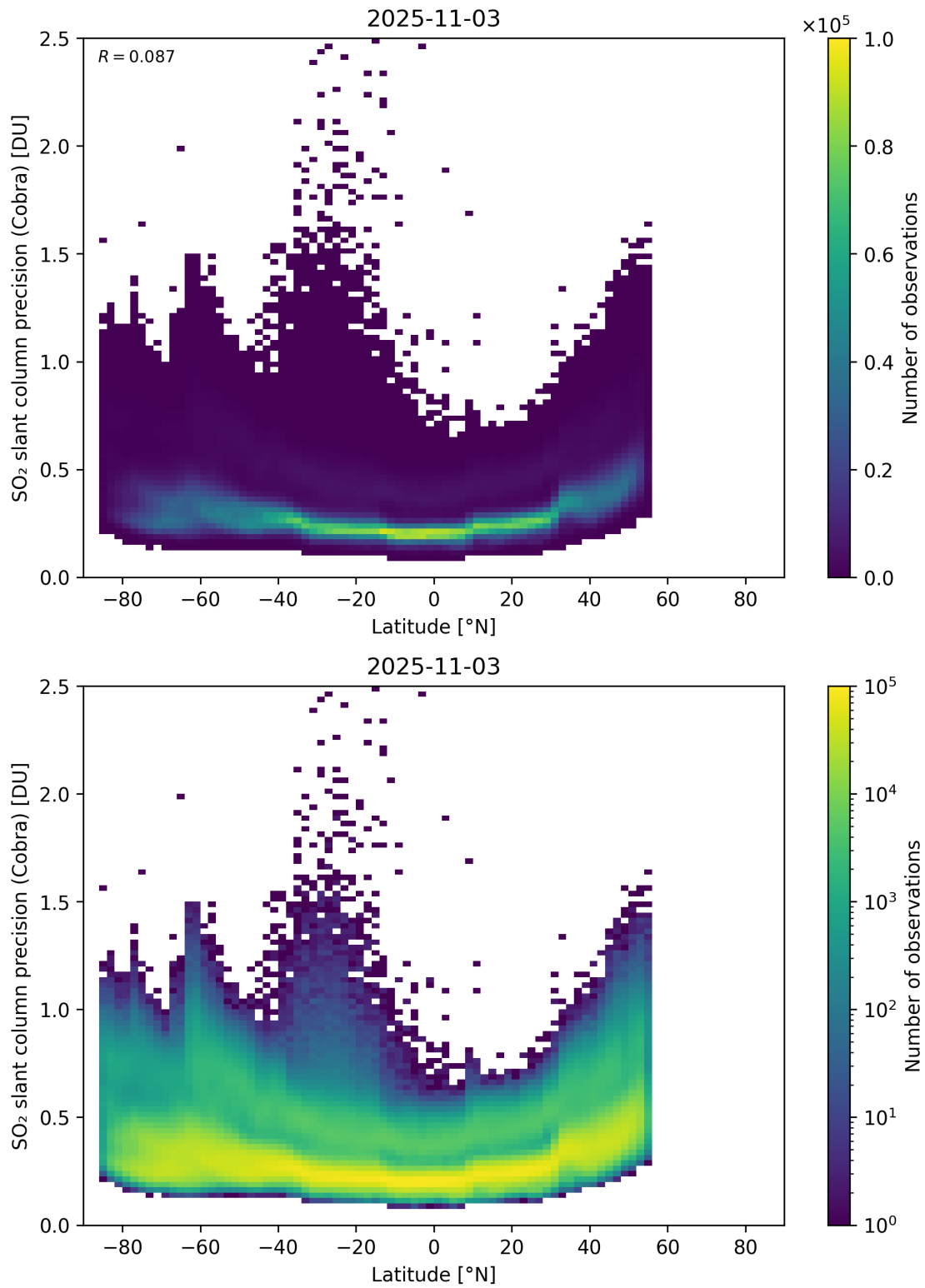
Figure 158: Scatter density plot of “Latitude” against “SO 2 slant column precision (Cobra)” for 2025-11-02 to 2025-11-04.
