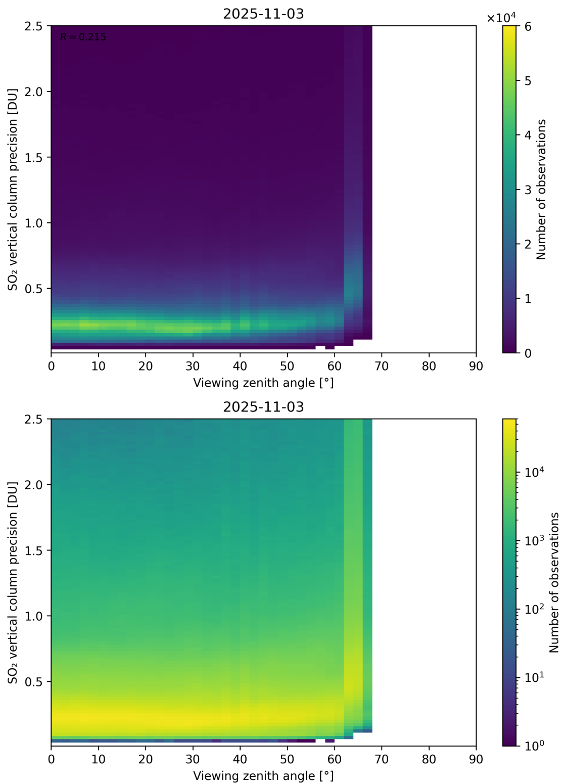
Figure 384: Scatter density plot of “Viewing zenith angle” against “SO 2 vertical column precision” for 2025-11-02 to 2025-11-04.
