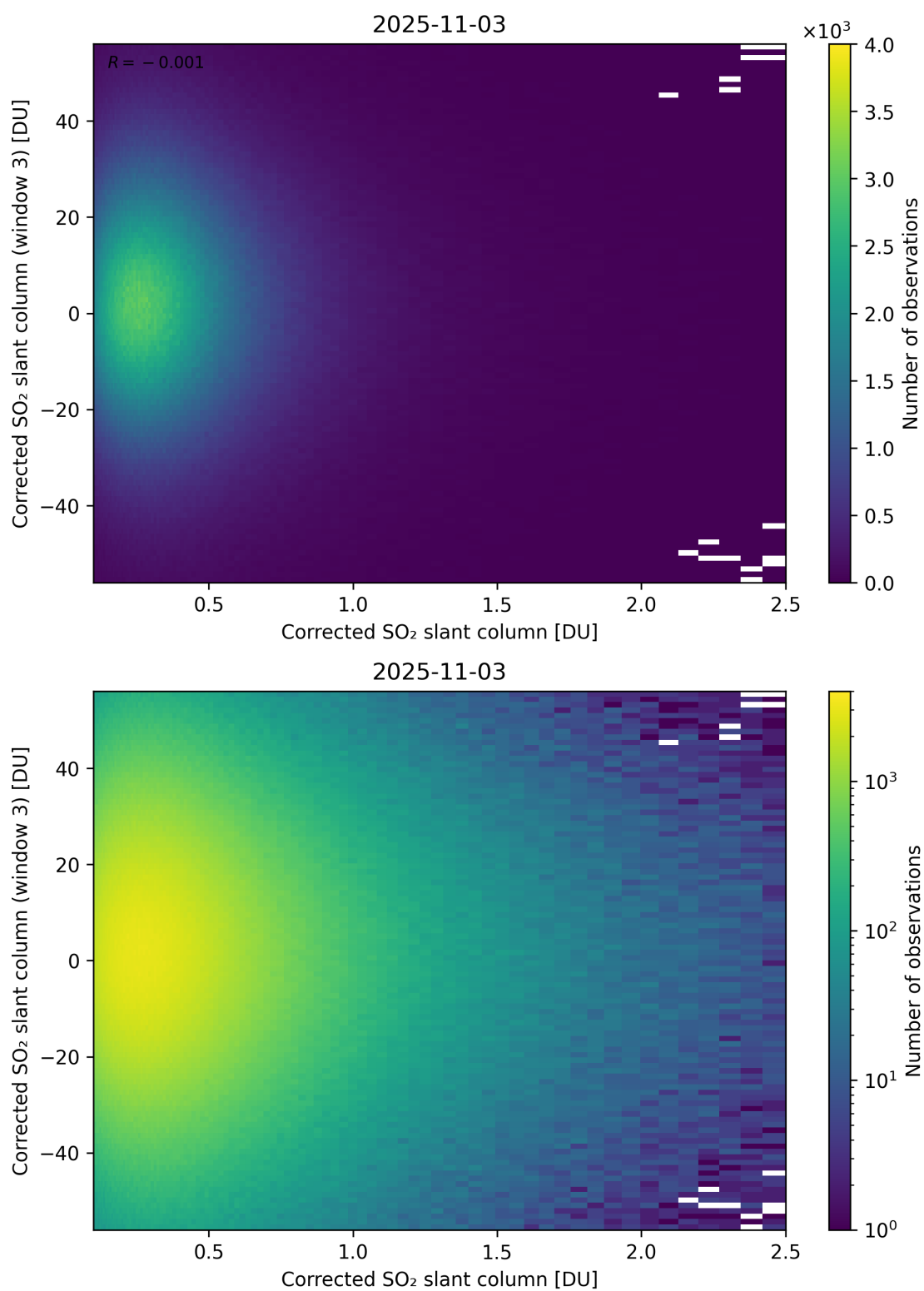
Figure 236: Scatter density plot of “Corrected SO 2 slant column” against “Corrected SO 2 slant column (window 3)” for 2025-11-02 to 2025-11-04.
