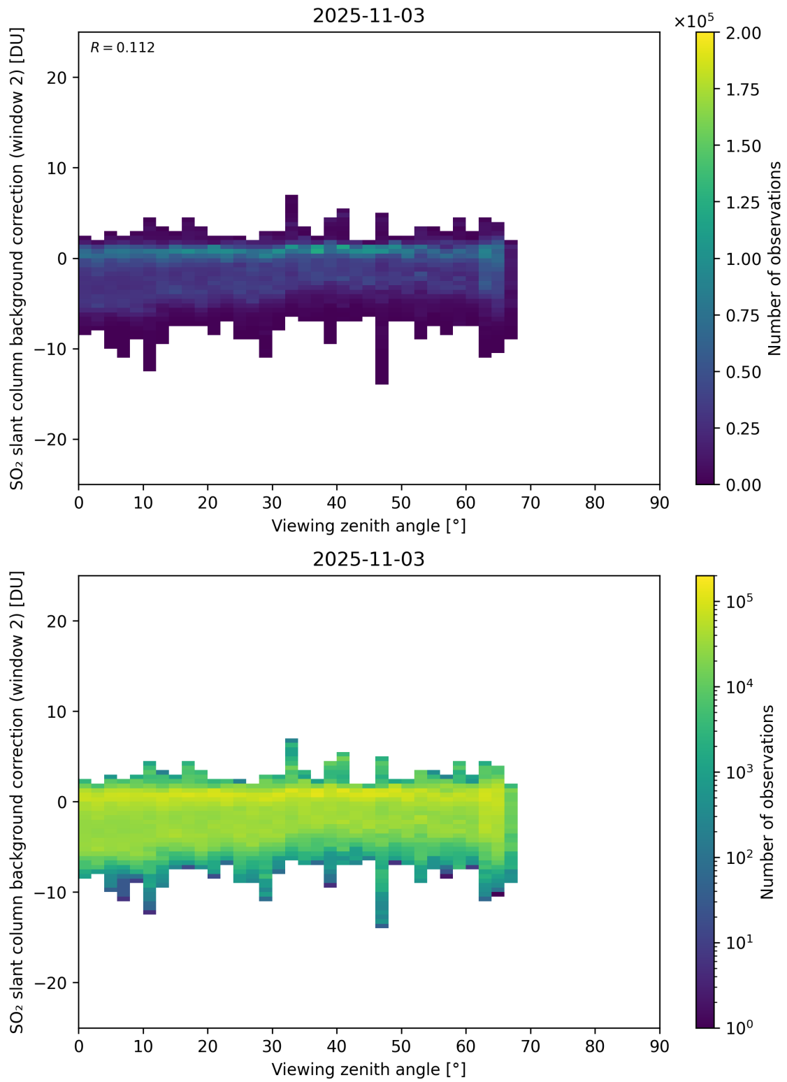
Figure 363: Scatter density plot of “Viewing zenith angle” against “SO 2 slant column background correction (window 2)” for 2025-11-02 to 2025-11-04.
