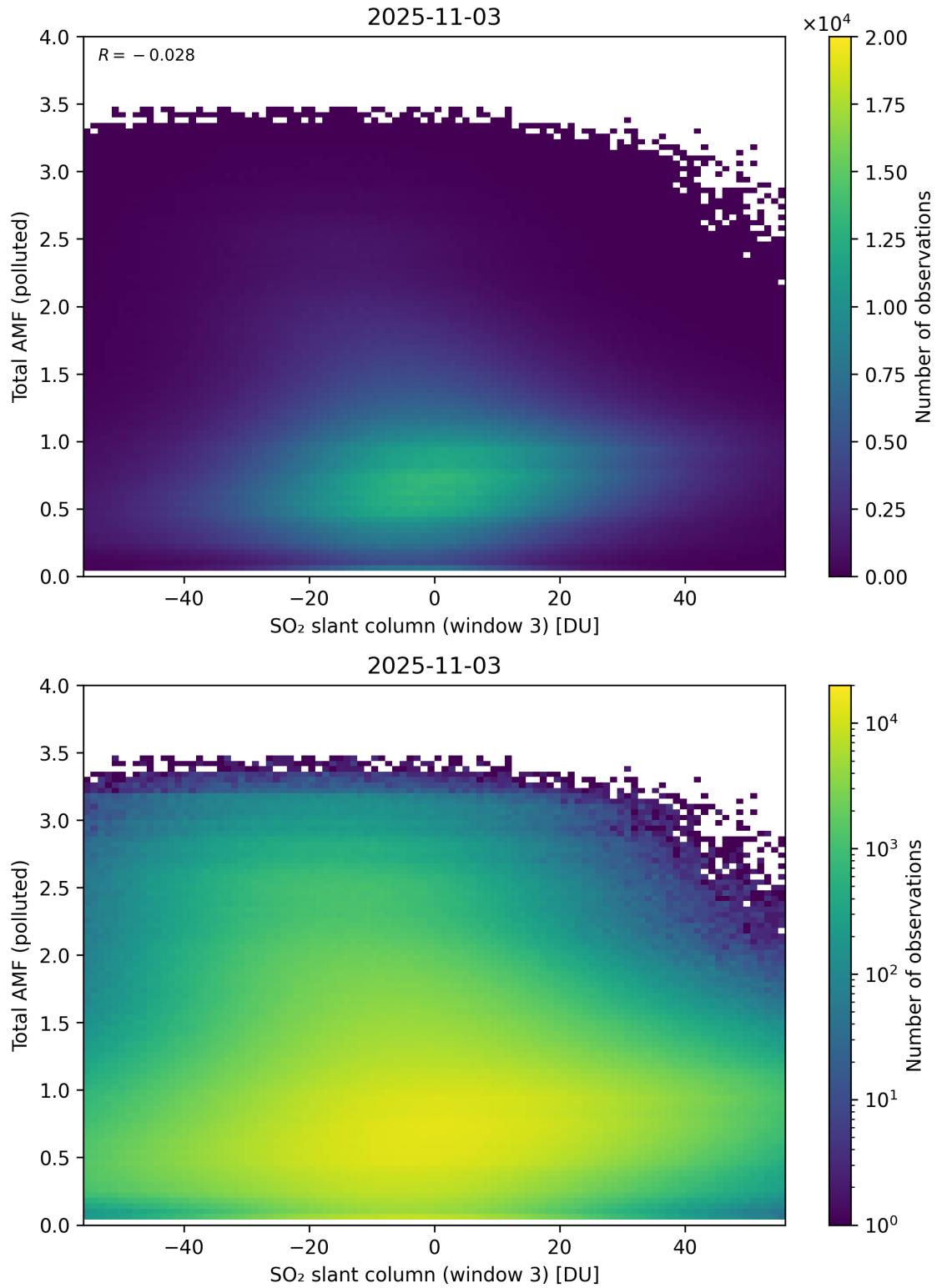
Figure 318: Scatter density plot of “SO 2 slant column (window 3)” against “Total AMF (polluted)” for 2025-11-02 to 2025-11-04.
