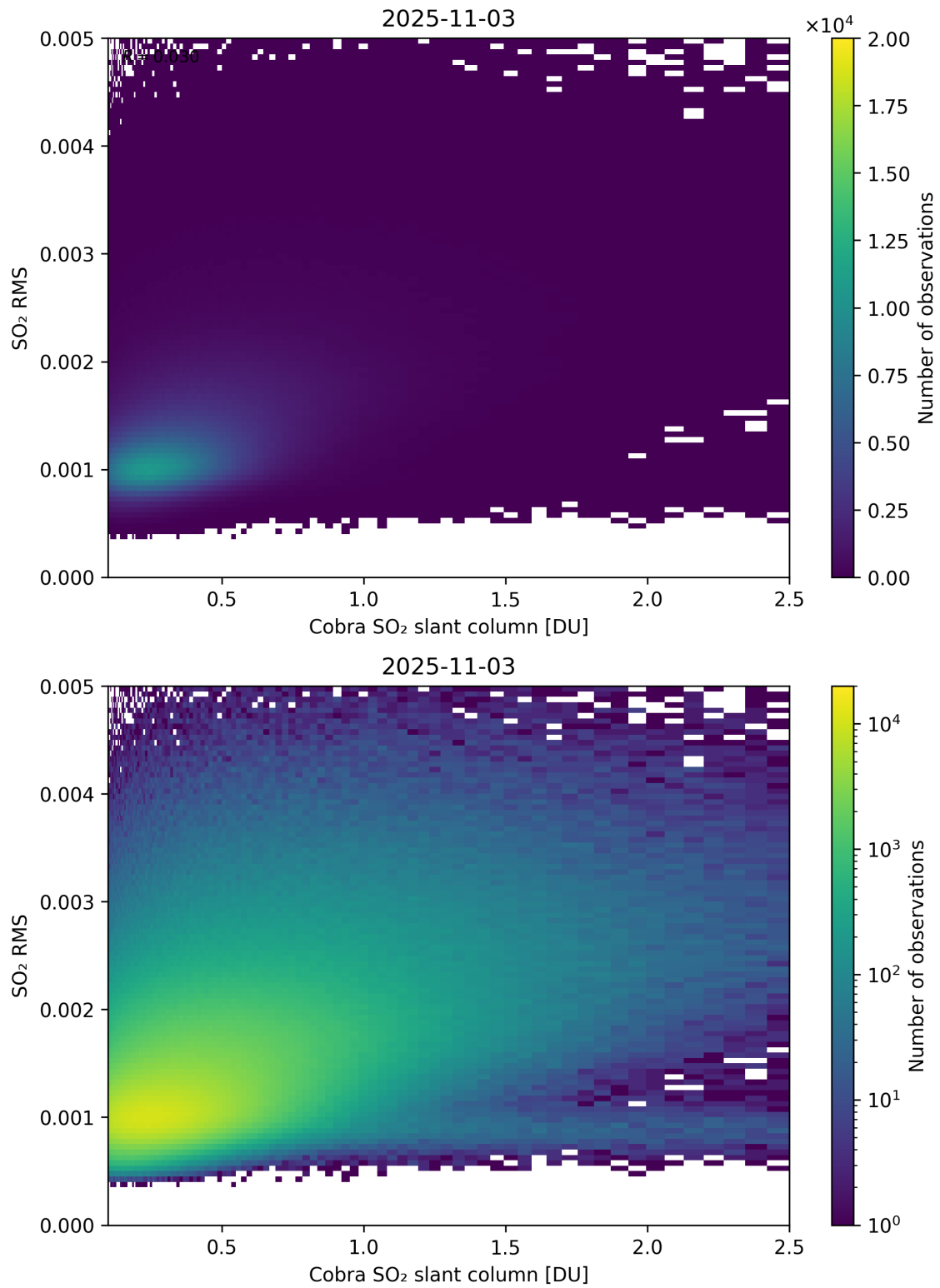
Figure 198: Scatter density plot of “Cobra SO 2 slant column” against “SO 2 RMS” for 2025-11-02 to 2025-11-04.
