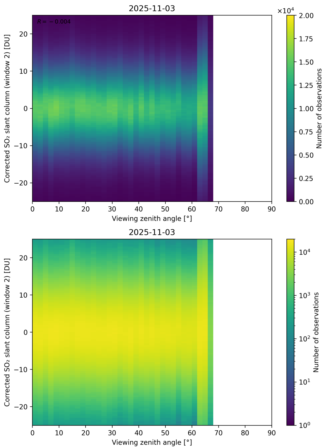
Figure 374: Scatter density plot of “Viewing zenith angle” against “Corrected SO 2 slant column (window 2)” for 2025-11-02 to 2025-11-04.
