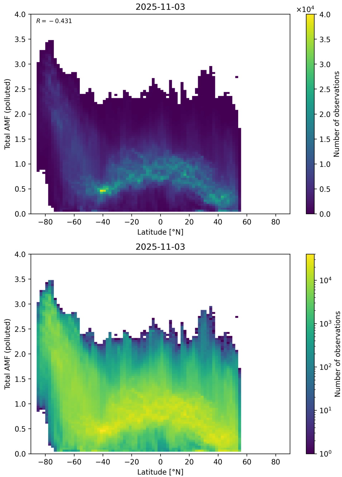
Figure 167: Scatter density plot of “Latitude” against “Total AMF (polluted)” for 2025-11-02 to 2025-11-04.
