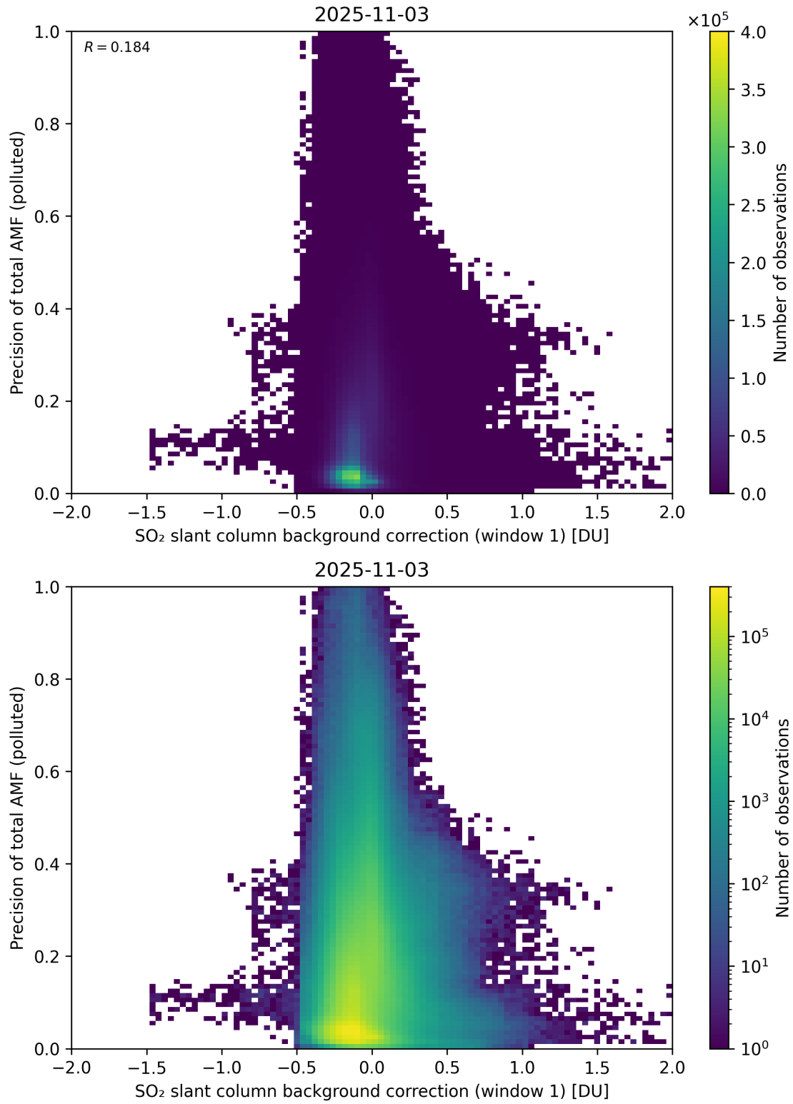
Figure 121: Scatter density plot of “SO 2 slant column background correction (window 1)” against “Precision of total AMF (polluted)” for 2025-11-02 to 2025-11-04.
