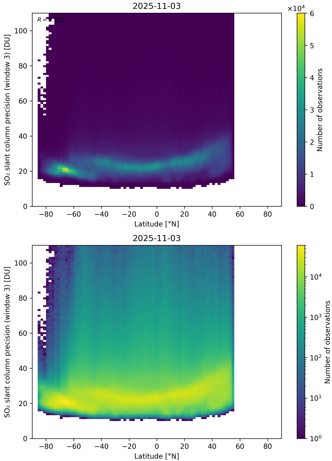
Figure 166: Scatter density plot of “Latitude” against “SO 2 slant column precision (window 3)” for 2025-11-02 to 2025-11-04.
