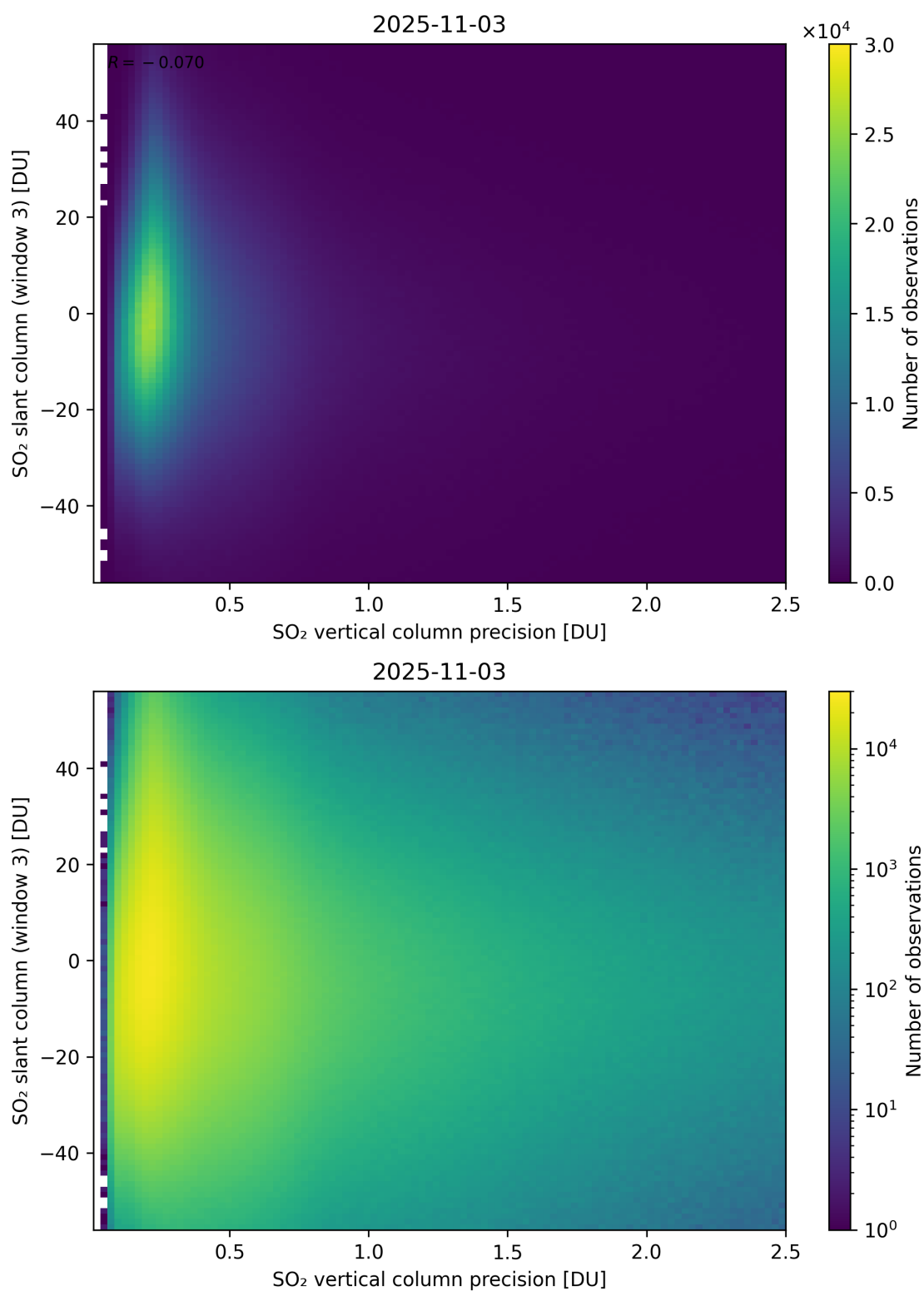
Figure 344: Scatter density plot of “SO 2 vertical column precision” against “SO 2 slant column (window 3)” for 2025-11-02 to 2025-11-04.
