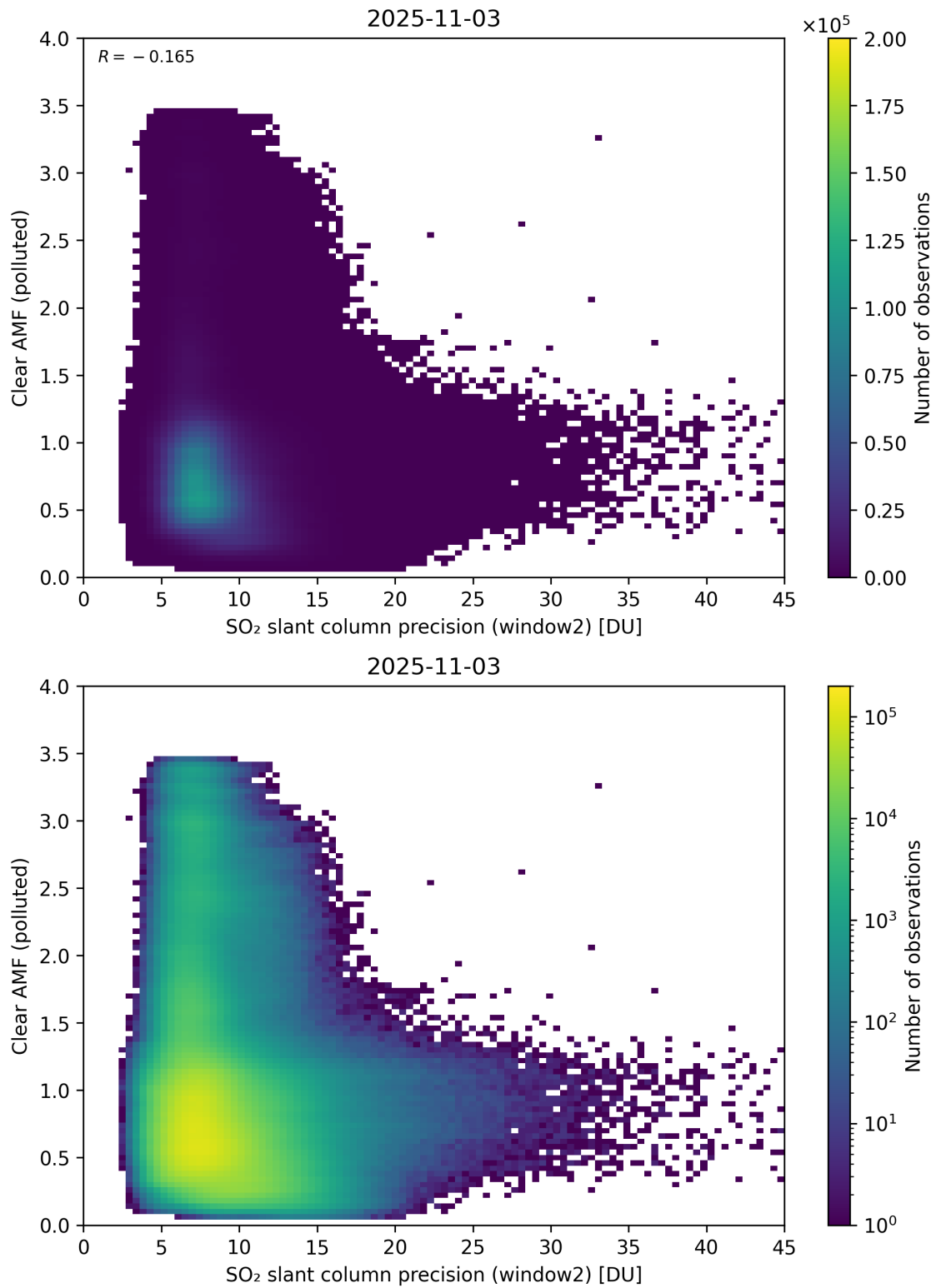
Figure 296: Scatter density plot of “SO 2 slant column precision (window2)” against “Clear AMF (polluted)” for 2025-11-02 to 2025-11-04.
