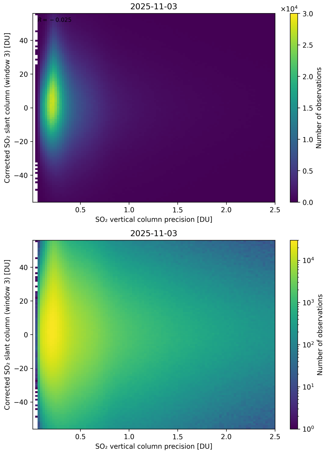
Figure 340: Scatter density plot of “SO 2 vertical column precision” against “Corrected SO 2 slant column (window 3)” for 2025-11-02 to 2025-11-04.
