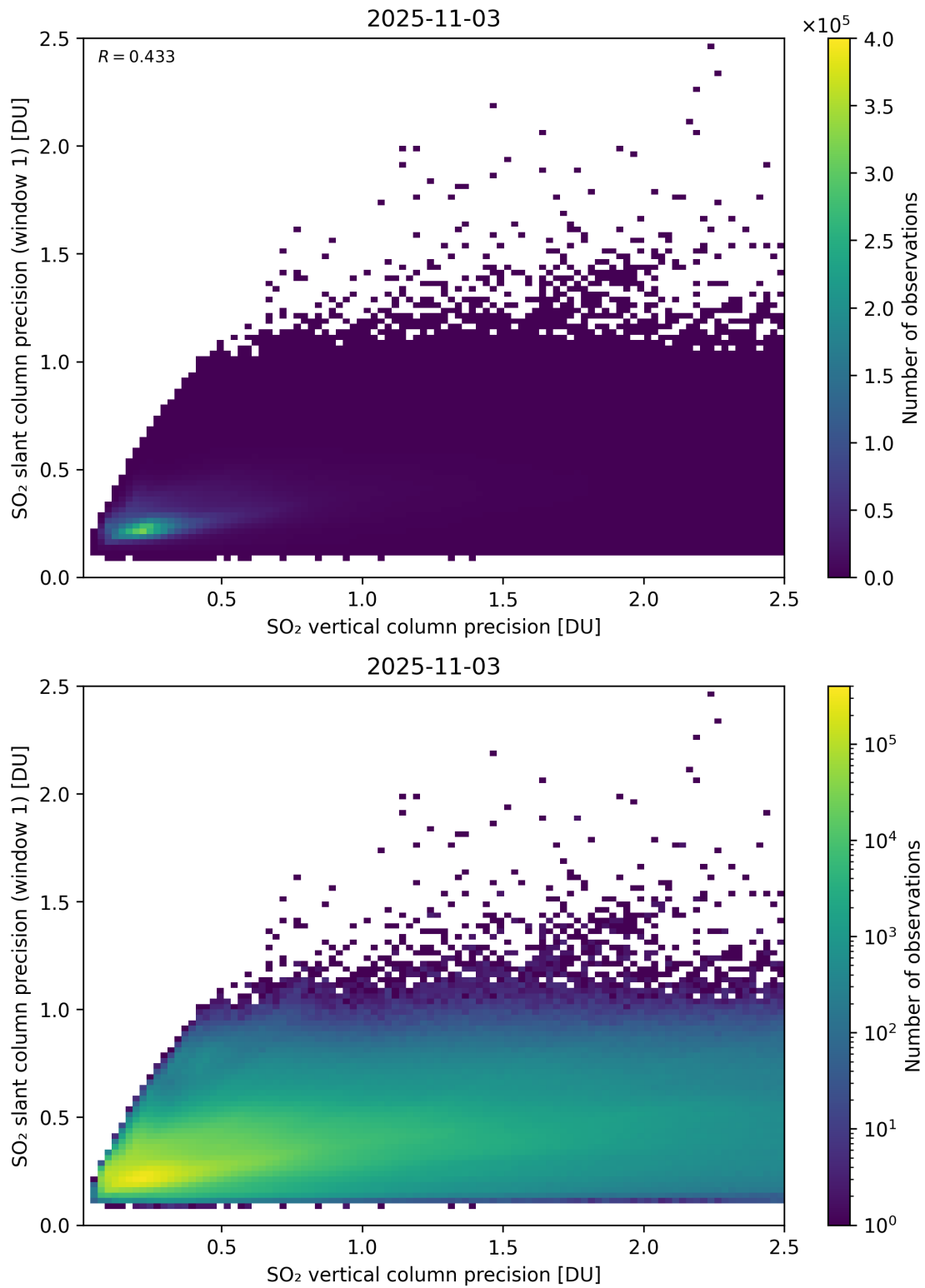
Figure 342: Scatter density plot of “SO 2 vertical column precision” against “SO 2 slant column precision (window 1)” for 2025-11-02 to 2025-11-04.
