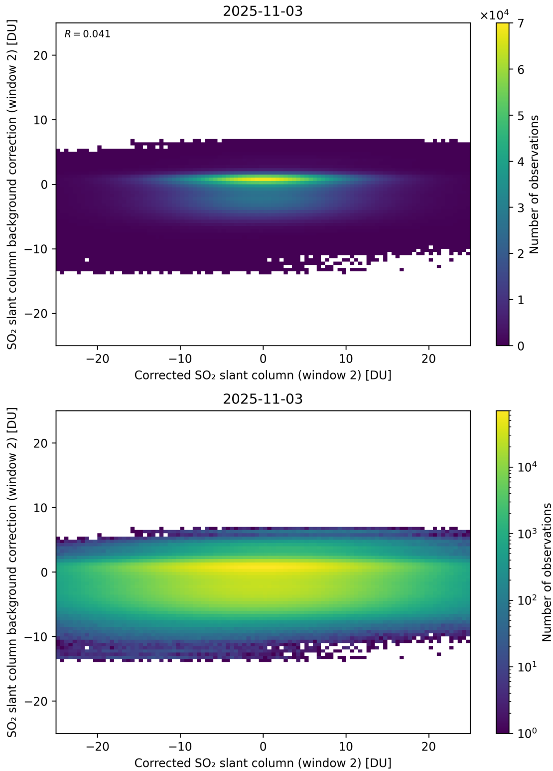
Figure 244: Scatter density plot of “Corrected SO 2 slant column (window 2)” against “SO 2 slant column background correction (window 2)” for 2025-11-02 to 2025-11-04.
