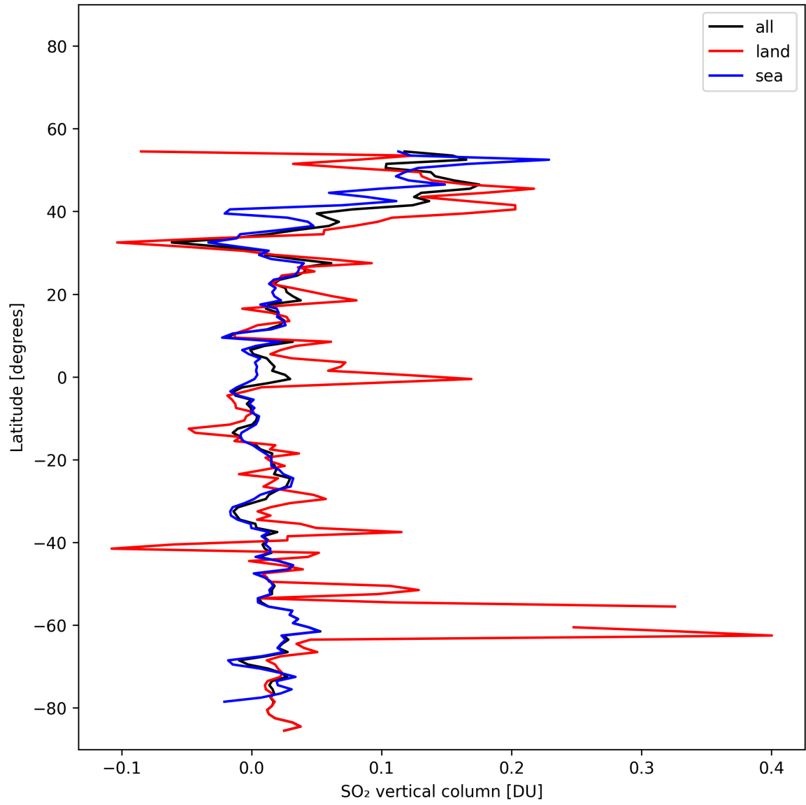
Figure 32: Zonal average of “SO 2 vertical column” for 2025-11-02 to 2025-11-04.
