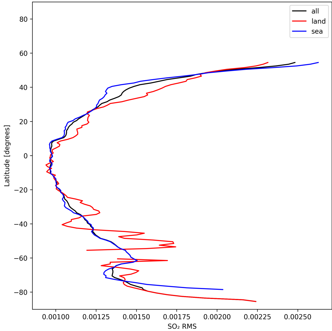
Figure 52: Zonal average of “SO 2 RMS” for 2025-11-02 to 2025-11-04.
