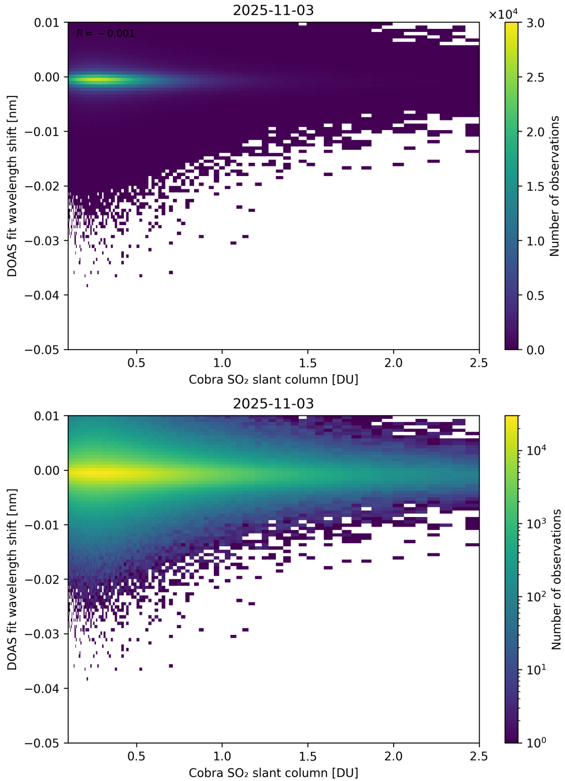
Figure 196: Scatter density plot of “Cobra SO 2 slant column” against “DOAS fit wavelength shift” for 2025-11-02 to 2025-11-04.
