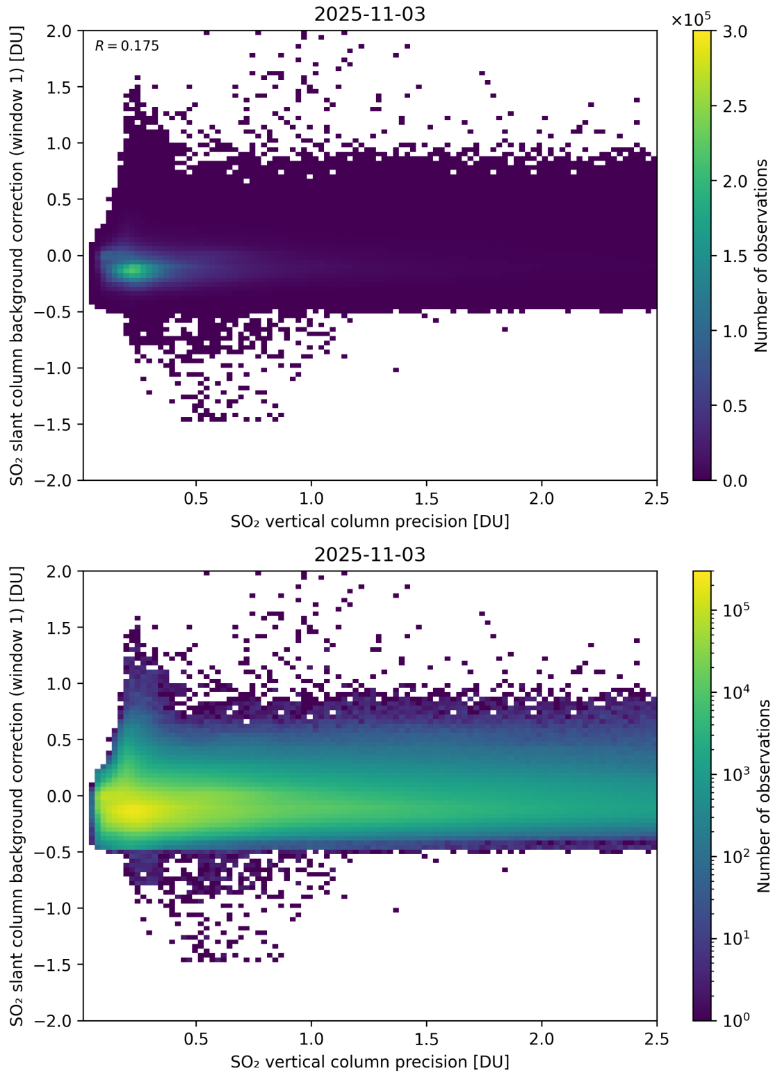
Figure 329: Scatter density plot of “SO 2 vertical column precision” against “SO 2 slant column background correction (window 1)” for 2025-11-02 to 2025-11-04.
