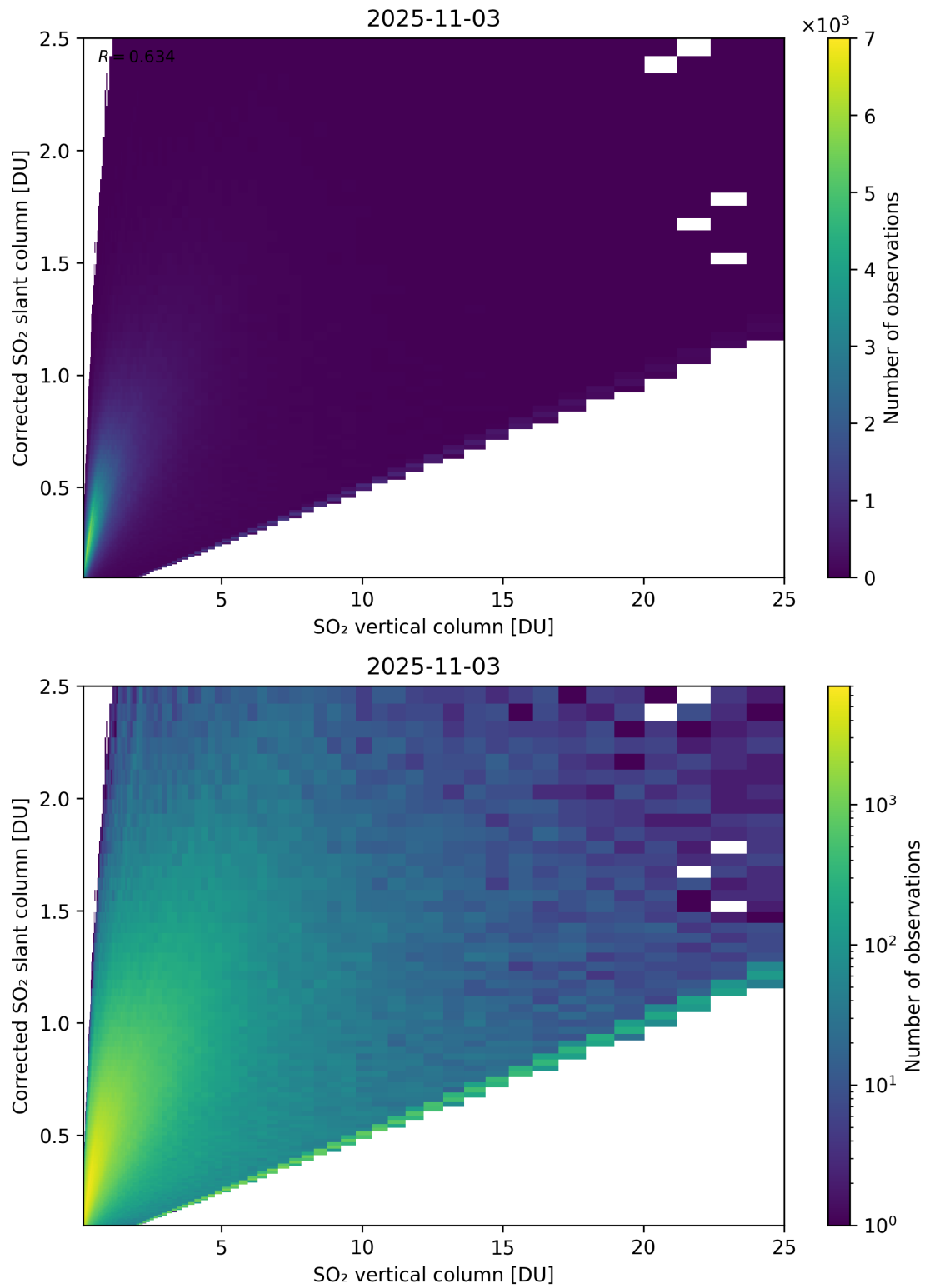
Figure 351: Scatter density plot of “SO 2 vertical column” against “Corrected SO 2 slant column” for 2025-11-02 to 2025-11-04.
