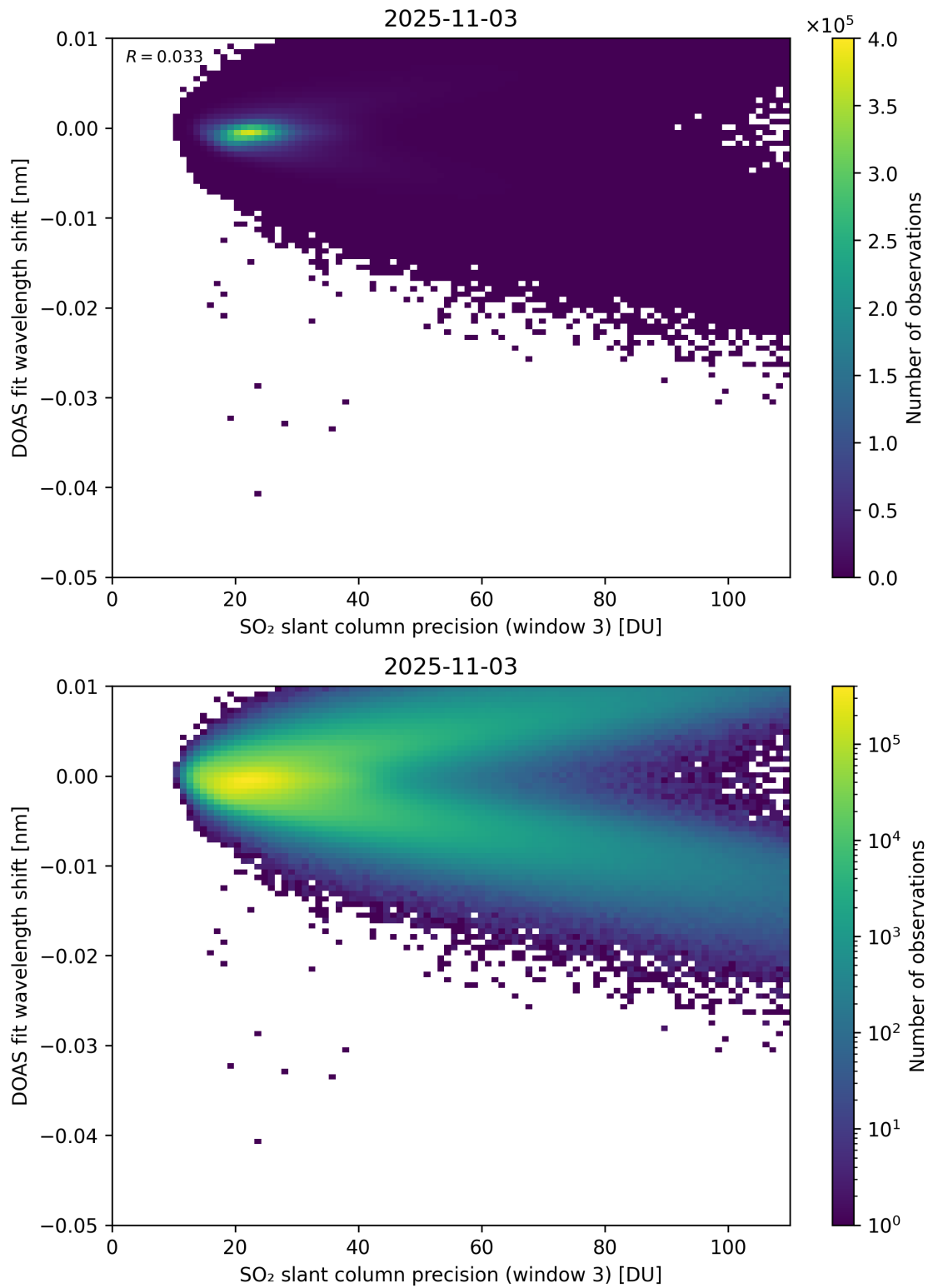
Figure 308: Scatter density plot of “SO 2 slant column precision (window 3)” against “DOAS fit wavelength shift” for 2025-11-02 to 2025-11-04.
