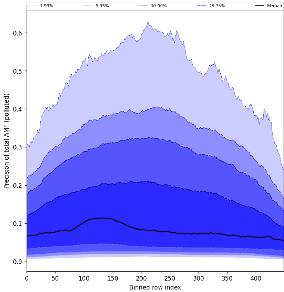
Figure 106: Along track statistics of “Precision of total AMF (polluted)” for 2025-11-02 to 2025-11-04
