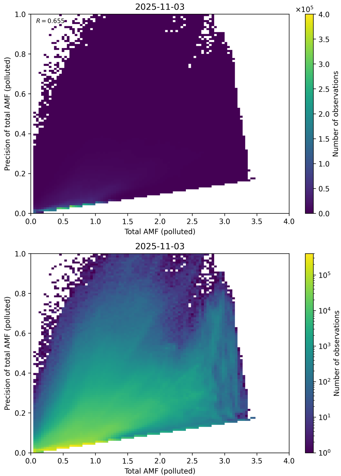
Figure 322: Scatter density plot of “Total AMF (polluted)” against “Precision of total AMF (polluted)” for 2025-11-02 to 2025-11-04.
