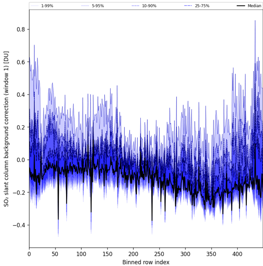
Figure 92: Along track statistics of “SO 2 slant column background correction (window 1)” for 2025-11-02 to 2025-11-04
