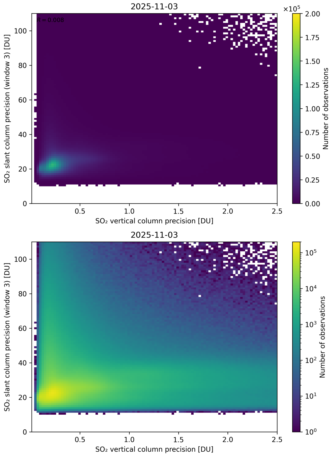
Figure 345: Scatter density plot of “SO 2 vertical column precision” against “SO 2 slant column precision (window 3)” for 2025-11-02 to 2025-11-04.
