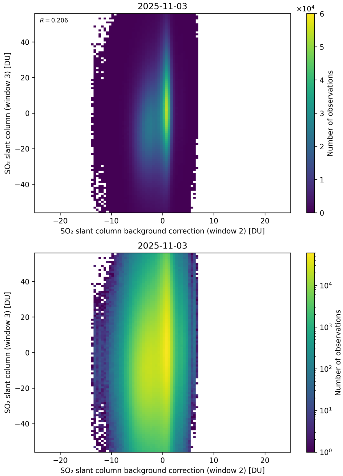
Figure 128: Scatter density plot of “SO 2 slant column background correction (window 2)” against “SO 2 slant column (window 3)” for 2025-11-02 to 2025-11-04.
