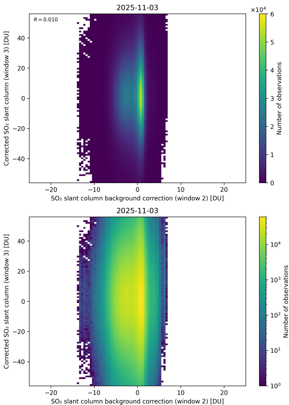
Figure 127: Scatter density plot of “SO 2 slant column background correction (window 2)” against “Corrected SO 2 slant column (window 3)” for 2025-11-02 to 2025-11-04.
