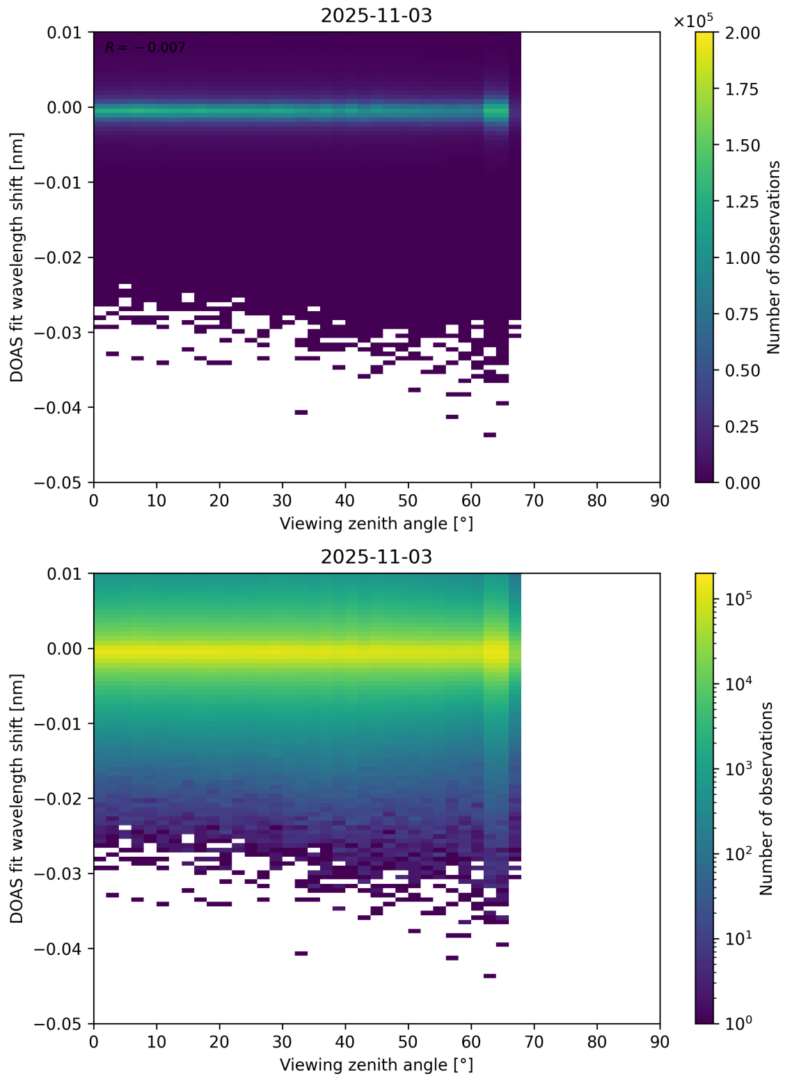
Figure 365: Scatter density plot of “Viewing zenith angle” against “DOAS fit wavelength shift” for 2025-11-02 to 2025-11-04.
