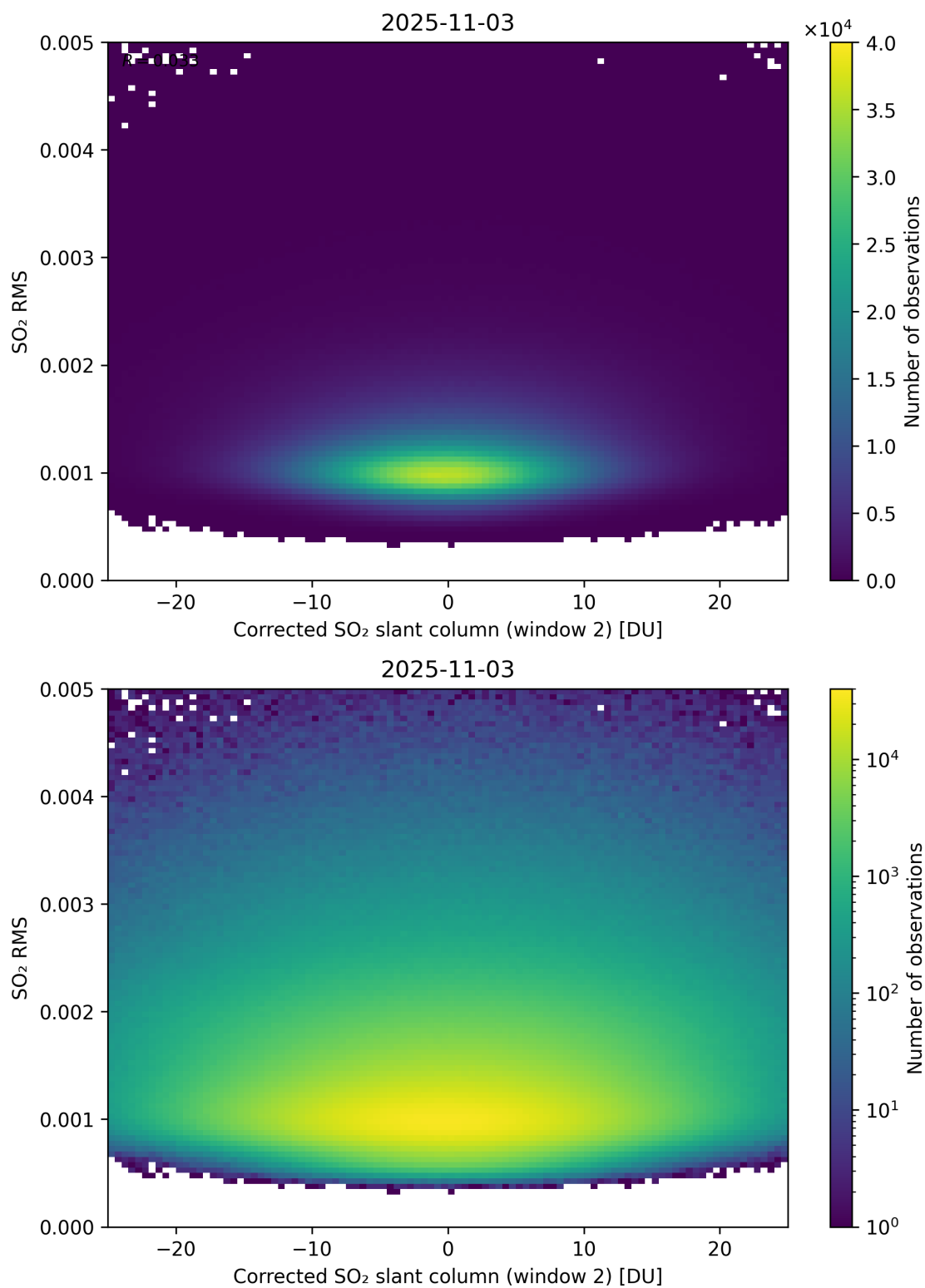
Figure 248: Scatter density plot of “Corrected SO 2 slant column (window 2)” against “SO 2 RMS” for 2025-11-02 to 2025-11-04.
