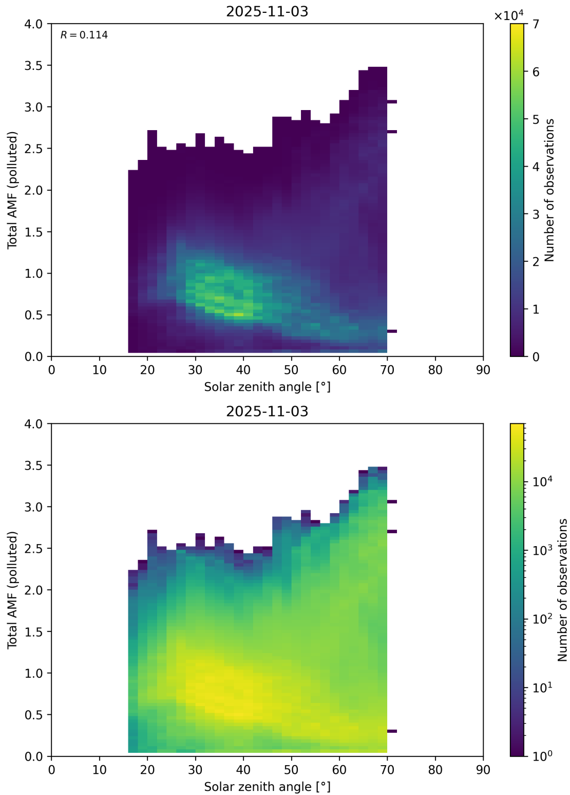
Figure 189: Scatter density plot of “Solar zenith angle” against “Total AMF (polluted)” for 2025-11-02 to 2025-11-04.
