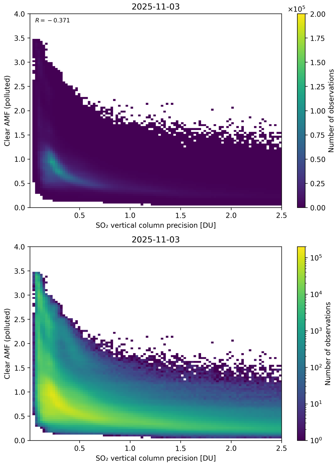
Figure 335: Scatter density plot of “SO 2 vertical column precision” against “Clear AMF (polluted)” for 2025-11-02 to 2025-11-04.
