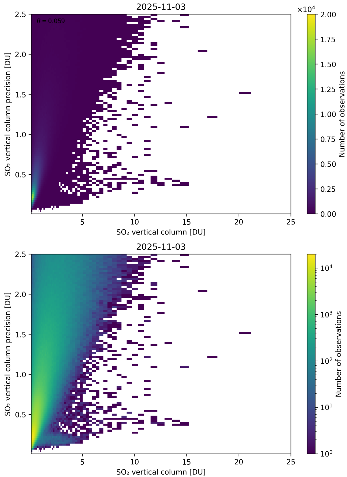
Figure 361: Scatter density plot of “SO 2 vertical column” against “SO 2 vertical column precision” for 2025-11-02 to 2025-11-04.
