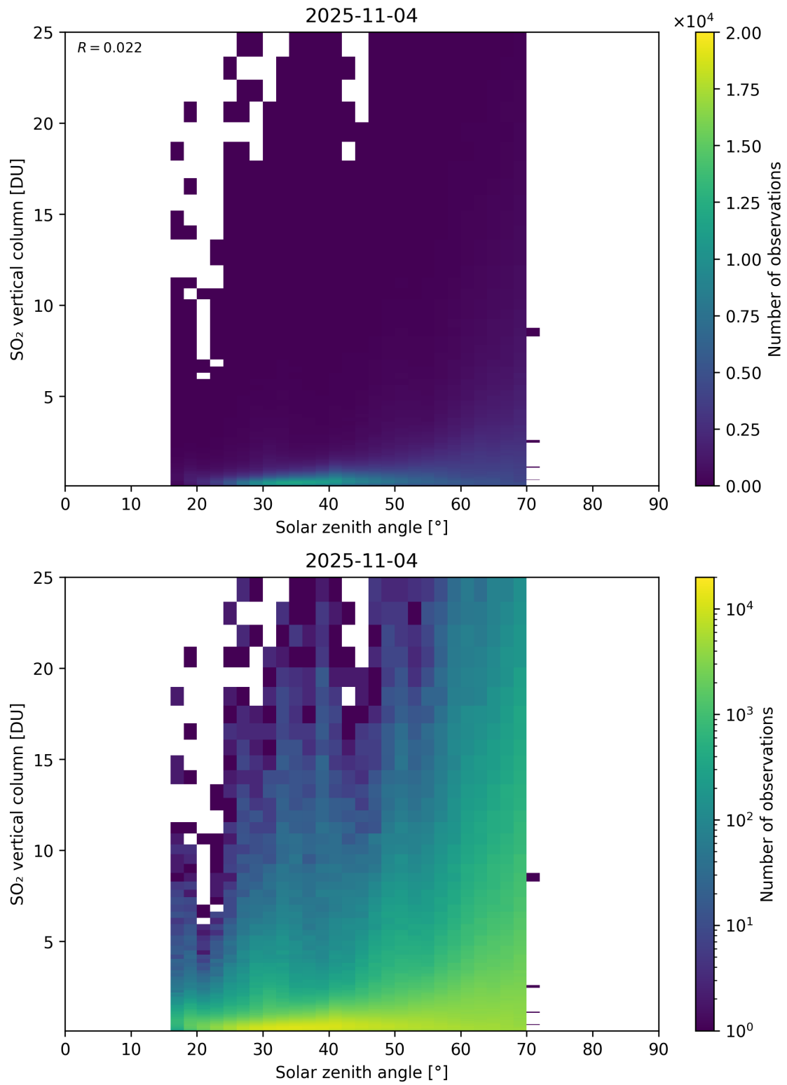
Figure 191: Scatter density plot of “Solar zenith angle” against “SO 2 vertical column” for 2025-11-03 to 2025-11-05.
