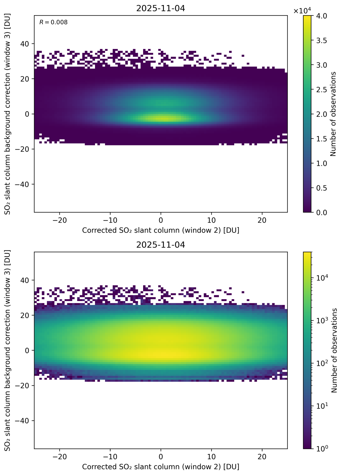
Figure 245: Scatter density plot of “Corrected SO 2 slant column (window 2)” against “SO 2 slant column background correction (window 3)” for 2025-11-03 to 2025-11-05.
