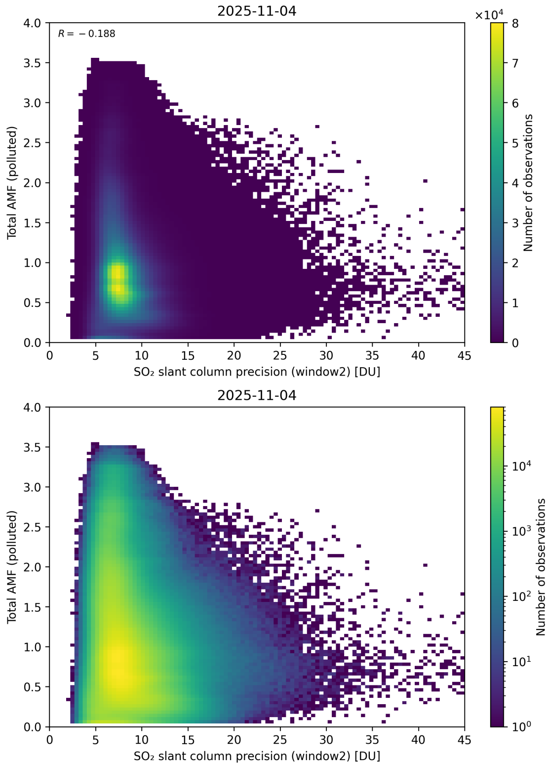
Figure 301: Scatter density plot of “SO 2 slant column precision (window2)” against “Total AMF (polluted)” for 2025-11-03 to 2025-11-05.
