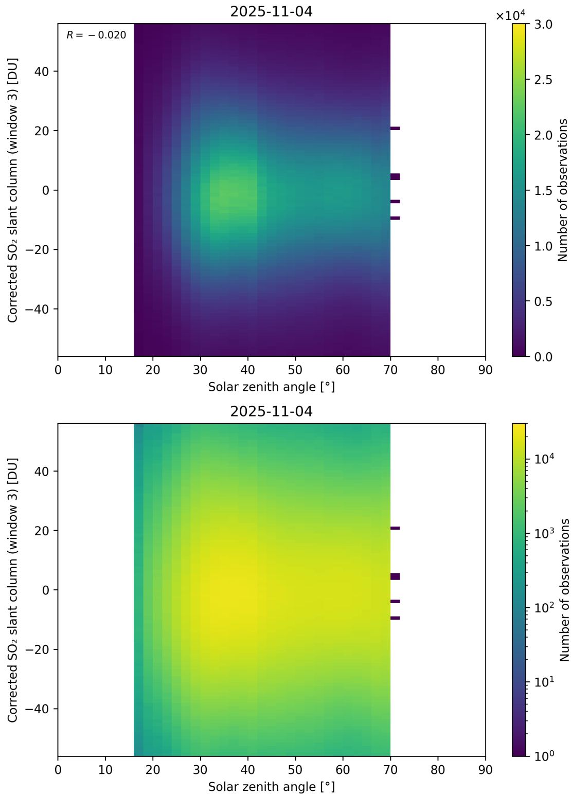
Figure 183: Scatter density plot of “Solar zenith angle” against “Corrected SO 2 slant column (window 3)” for 2025-11-03 to 2025-11-05.
