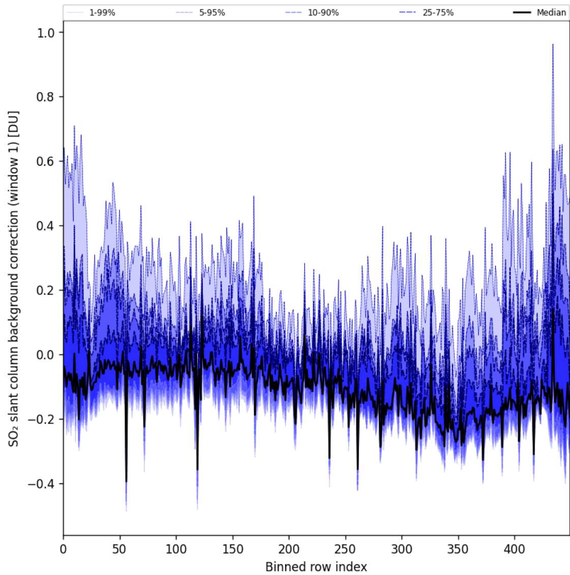
Figure 92: Along track statistics of “SO 2 slant column background correction (window 1)” for 2025-11-03 to 2025-11-05
