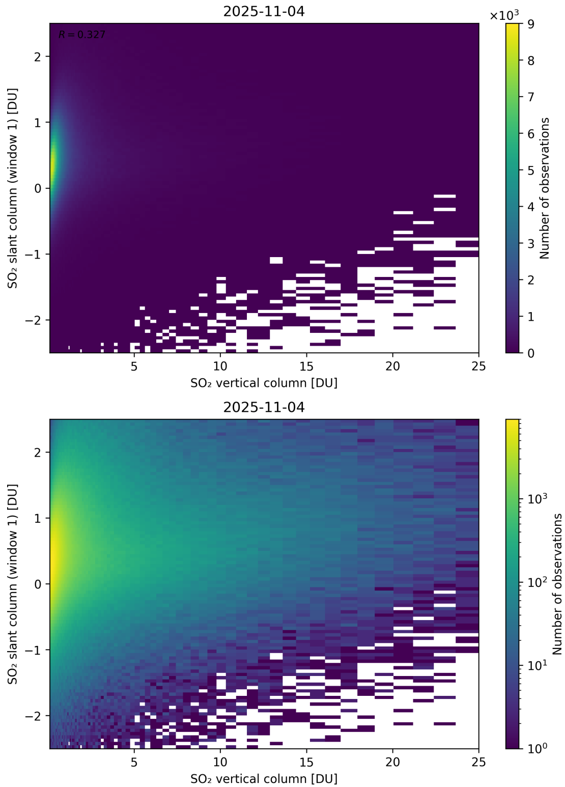
Figure 354: Scatter density plot of “SO 2 vertical column” against “SO 2 slant column (window 1)” for 2025-11-03 to 2025-11-05.
