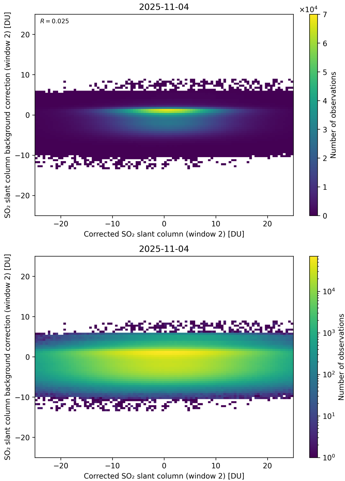
Figure 244: Scatter density plot of “Corrected SO 2 slant column (window 2)” against “SO 2 slant column background correction (window 2)” for 2025-11-03 to 2025-11-05.
