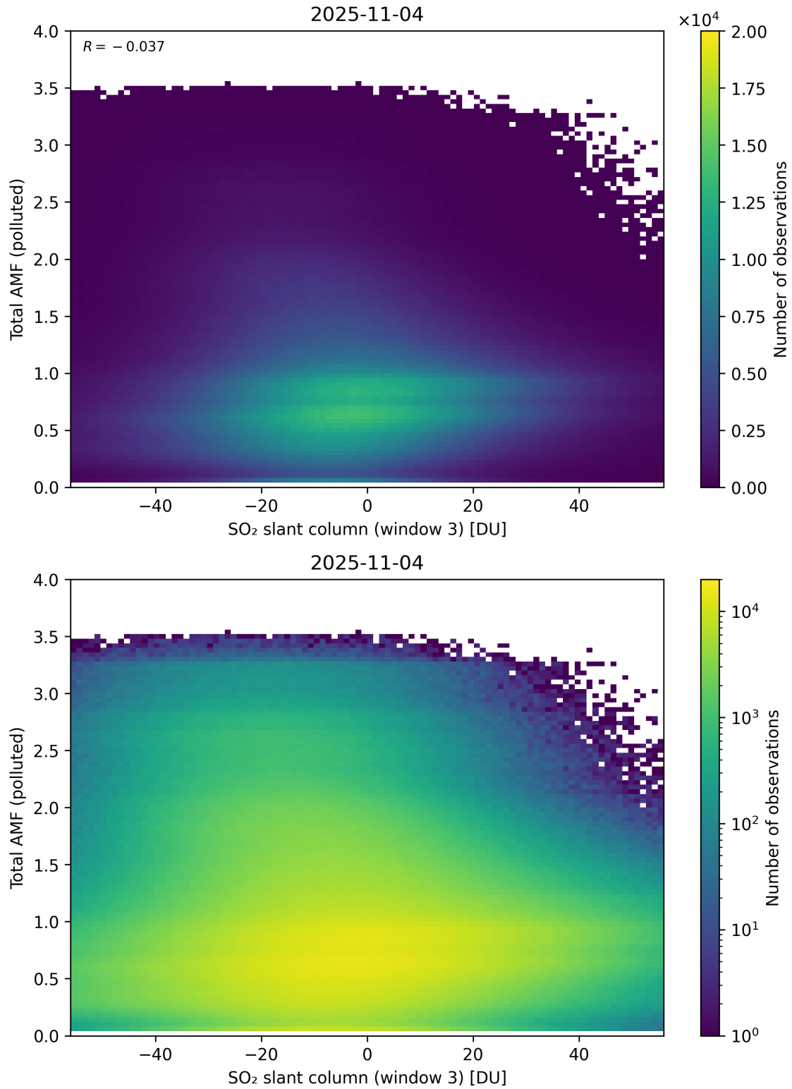
Figure 318: Scatter density plot of “SO 2 slant column (window 3)” against “Total AMF (polluted)” for 2025-11-03 to 2025-11-05.
