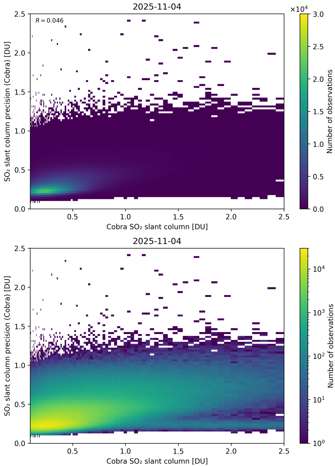
Figure 216: Scatter density plot of “Cobra SO 2 slant column” against “SO 2 slant column precision (Cobra)” for 2025-11-03 to 2025-11-05.
