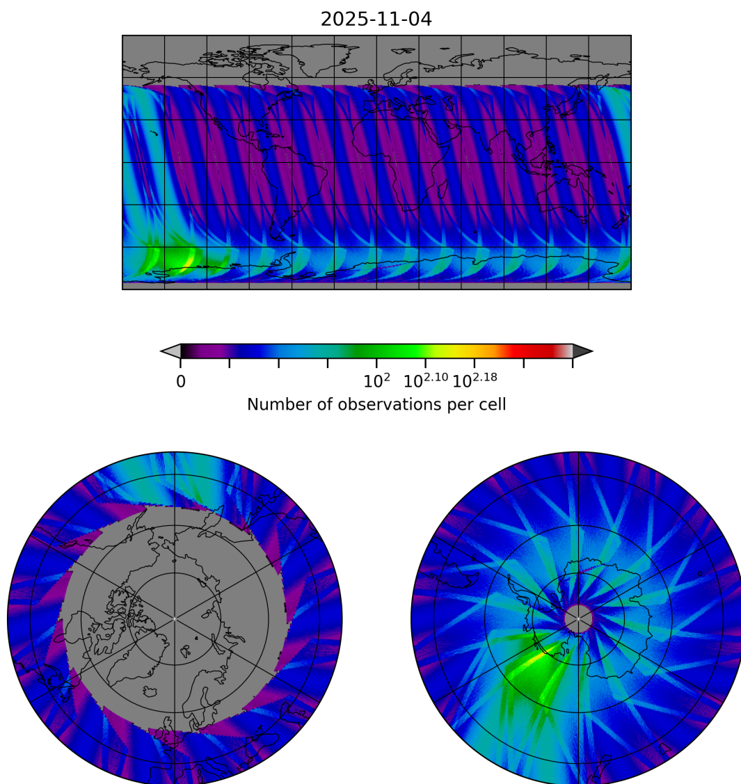
Figure 30: Map of the number of observations for 2025-11-03 to 2025-11-05
