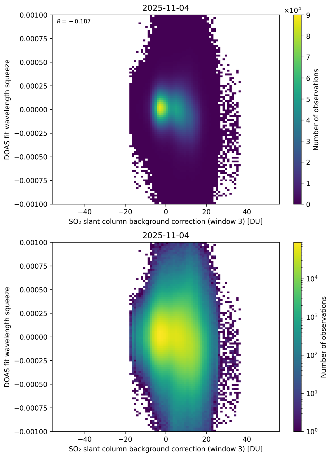
Figure 133: Scatter density plot of “SO 2 slant column background correction (window 3)” against “DOAS fit wavelength squeeze” for 2025-11-03 to 2025-11-05.
