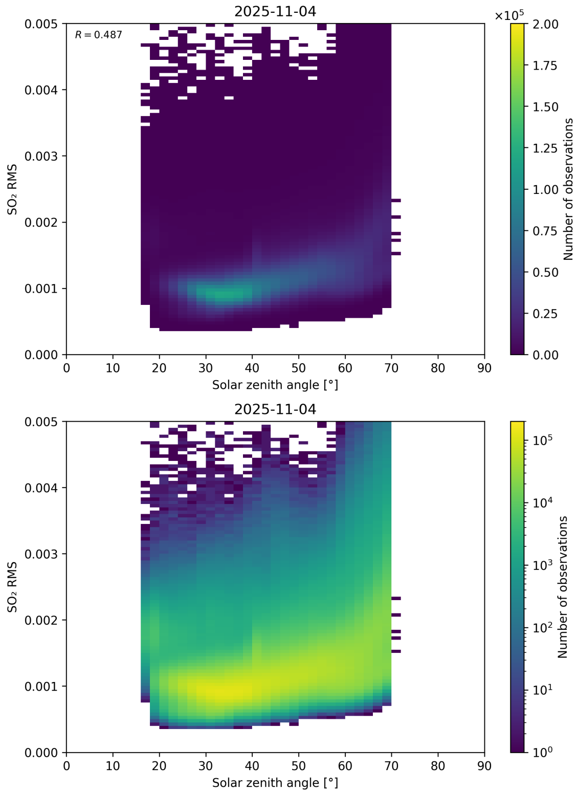
Figure 176: Scatter density plot of “Solar zenith angle” against “SO 2 RMS” for 2025-11-03 to 2025-11-05.
