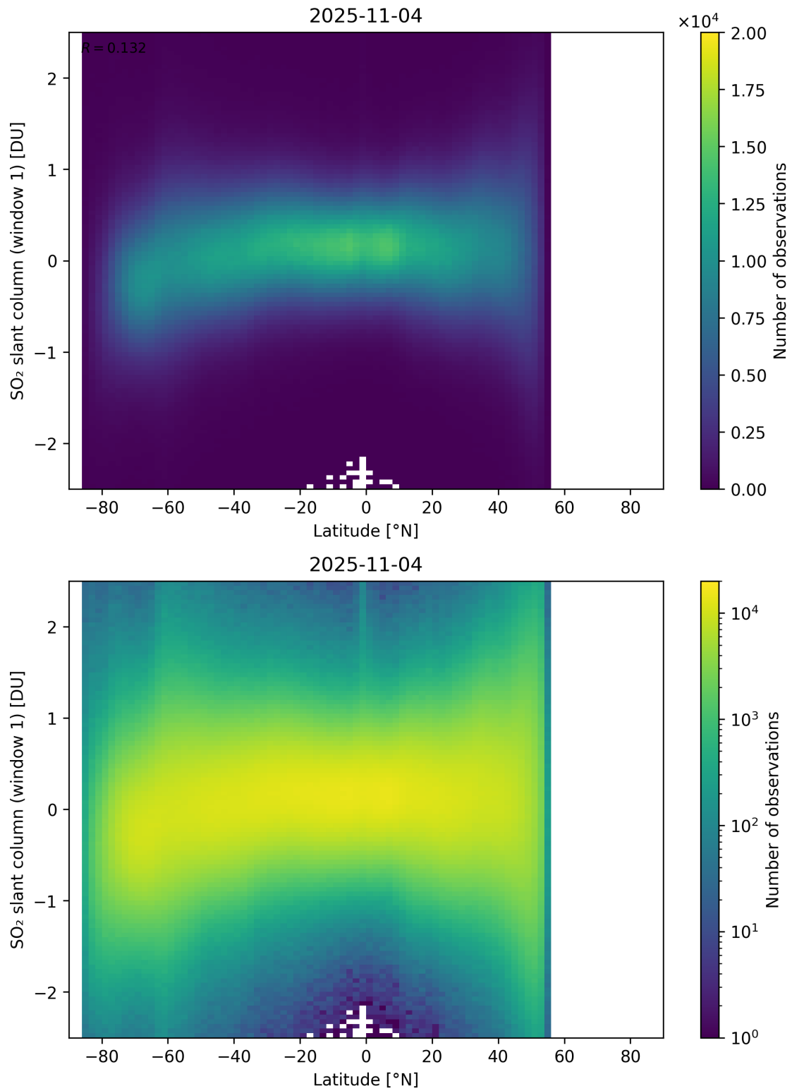
Figure 162: Scatter density plot of “Latitude” against “SO 2 slant column (window 1)” for 2025-11-03 to 2025-11-05.
