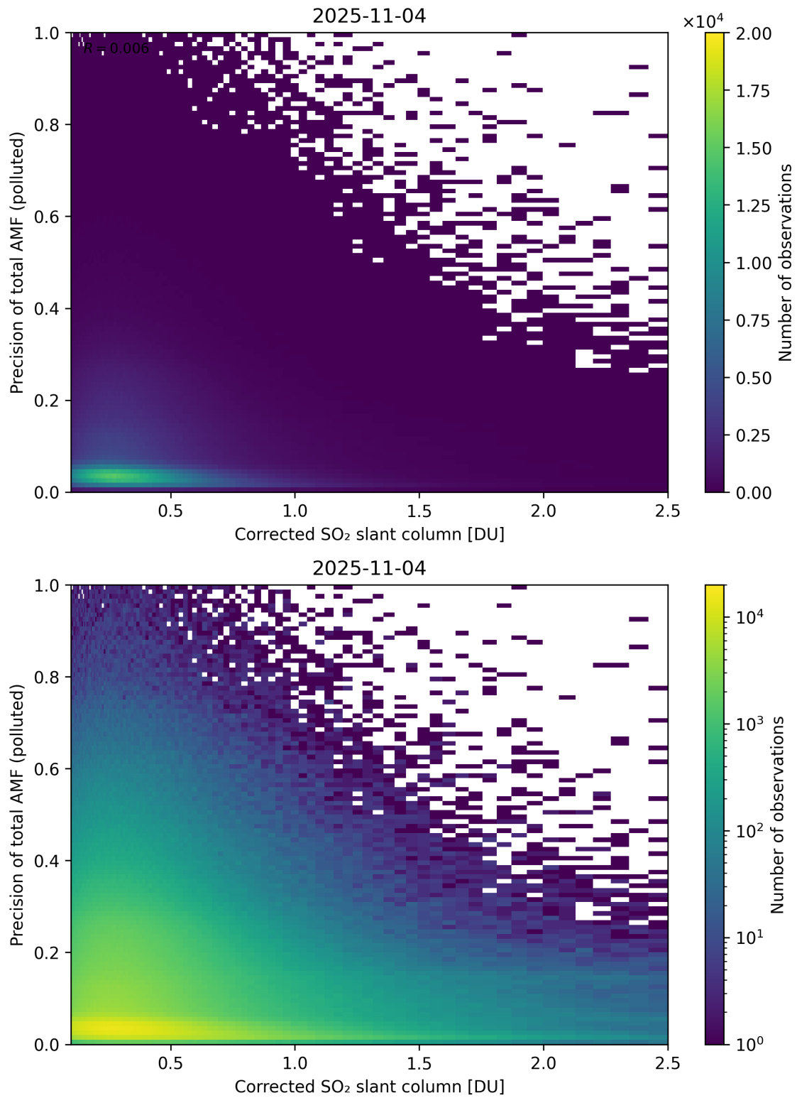
Figure 243: Scatter density plot of “Corrected SO 2 slant column” against “Precision of total AMF (polluted)” for 2025-11-03 to 2025-11-05.
