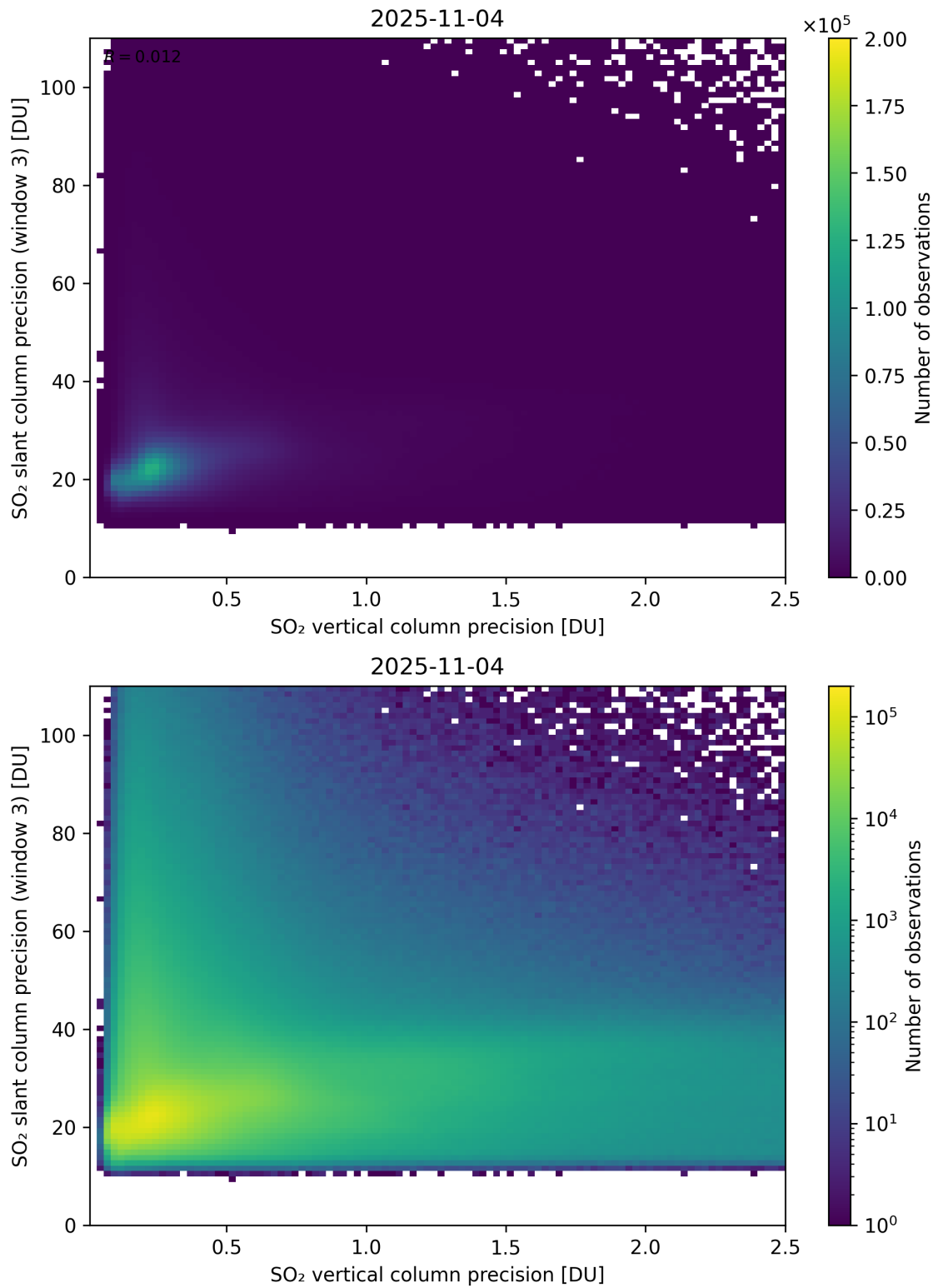
Figure 345: Scatter density plot of “SO 2 vertical column precision” against “SO 2 slant column precision (window 3)” for 2025-11-03 to 2025-11-05.
