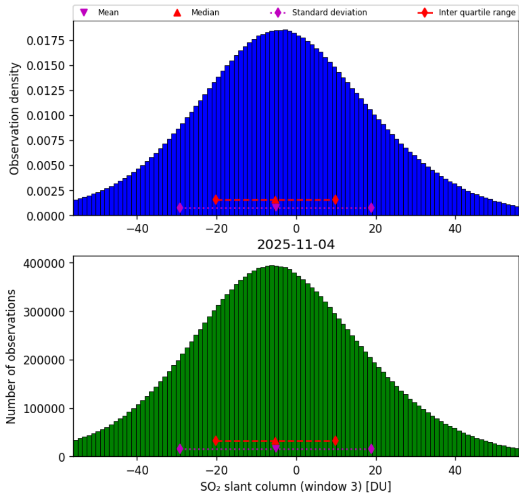
Figure 71: Histogram of “SO 2 slant column (window 3)” for 2025-11-03 to 2025-11-05
