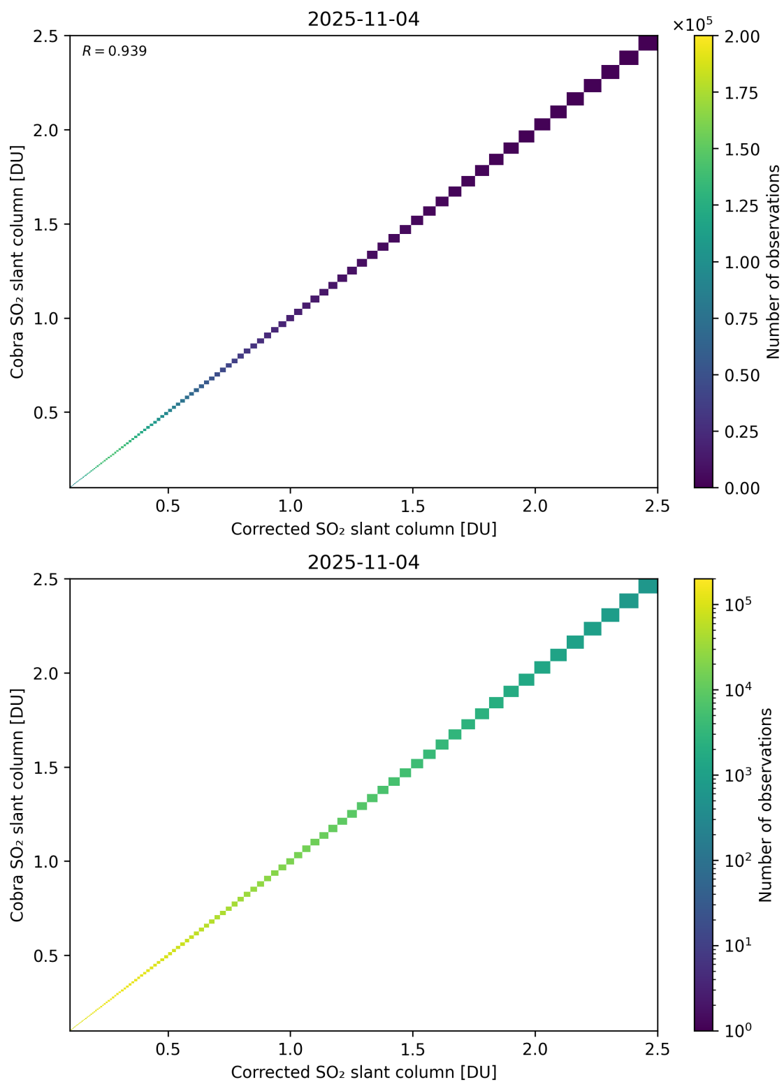
Figure 233: Scatter density plot of “Corrected SO 2 slant column” against “Cobra SO 2 slant column” for 2025-11-03 to 2025-11-05.
