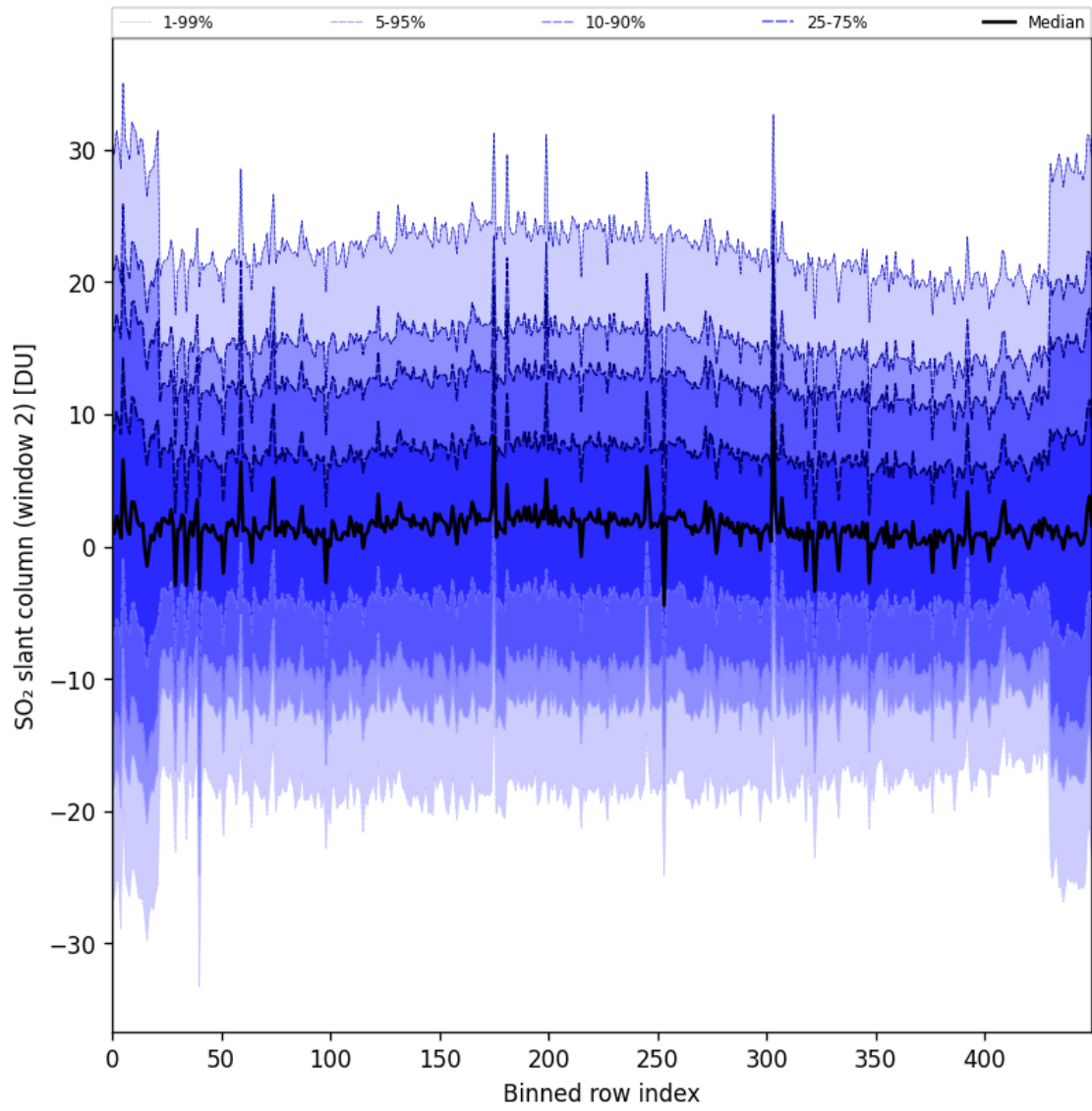
Figure 93: Along track statistics of “SO 2 slant column (window 2)” for 2025-11-03 to 2025-11-05
