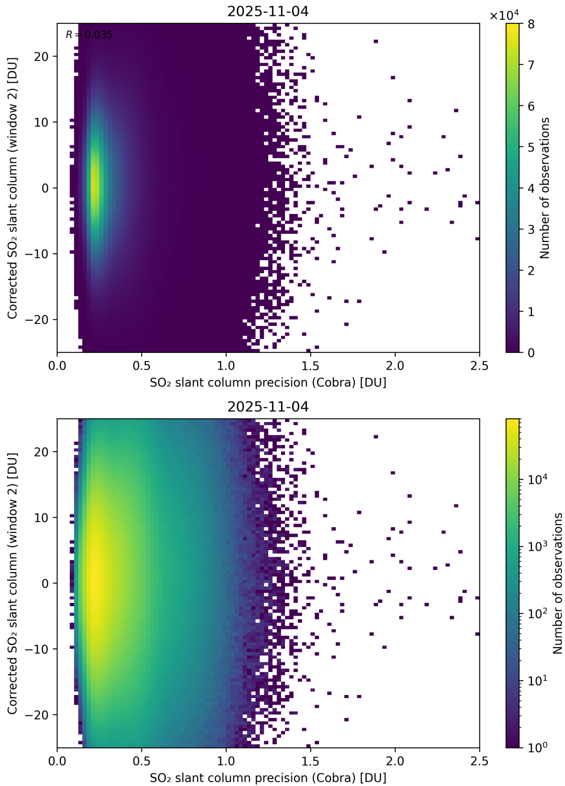
Figure 206: Scatter density plot of “SO 2 slant column precision (Cobra)” against “Corrected SO 2 slant column (window 2)” for 2025-11-03 to 2025-11-05.
