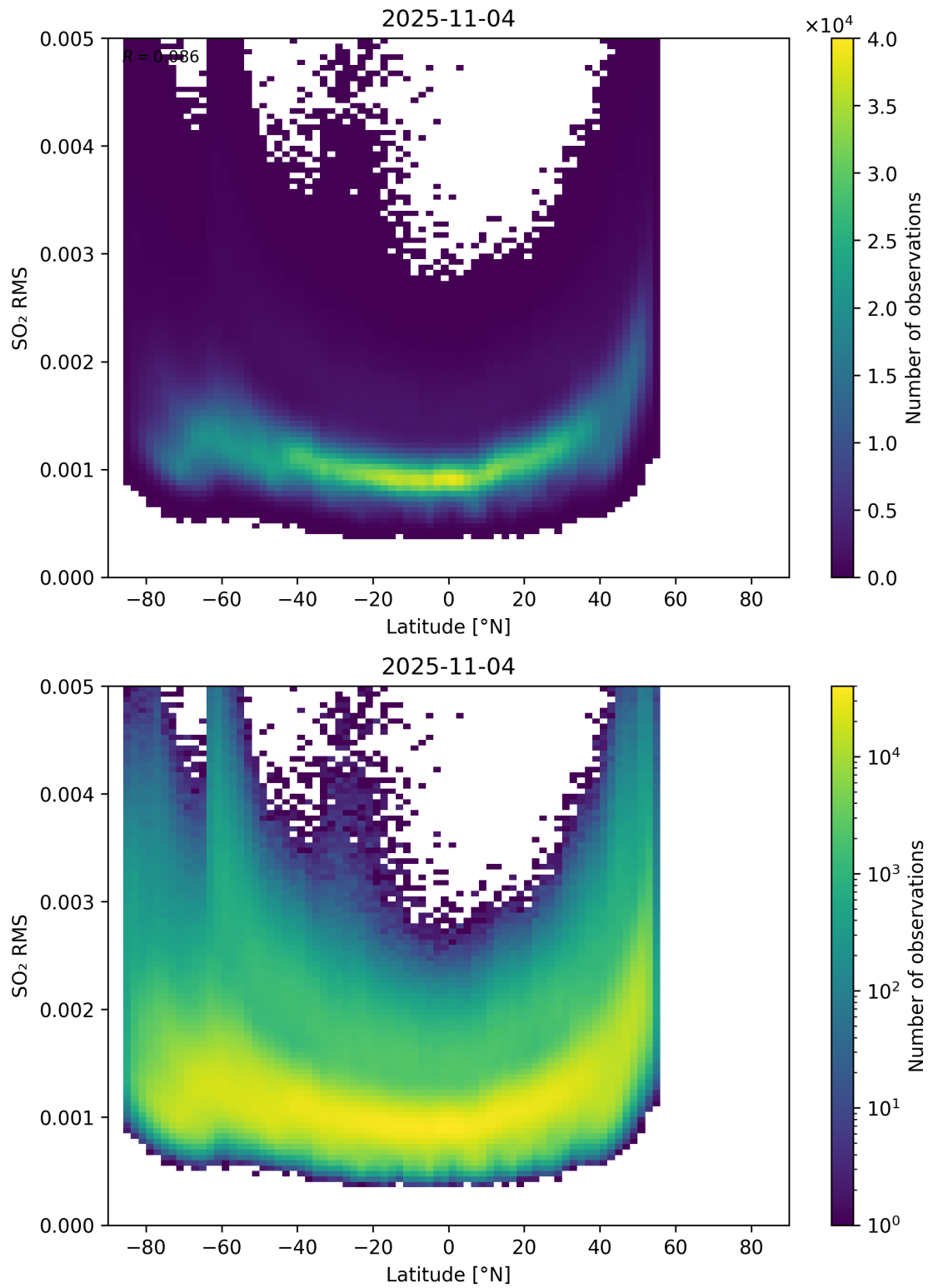
Figure 155: Scatter density plot of “Latitude” against “SO 2 RMS” for 2025-11-03 to 2025-11-05.
