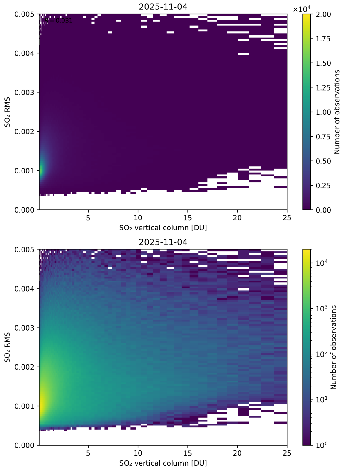
Figure 328: Scatter density plot of “SO 2 vertical column” against “SO 2 RMS” for 2025-11-03 to 2025-11-05.
