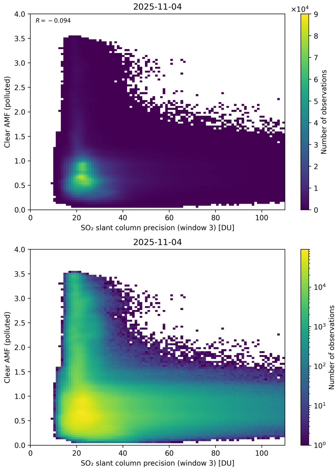
Figure 311: Scatter density plot of “SO 2 slant column precision (window 3)” against “Clear AMF (polluted)” for 2025-11-03 to 2025-11-05.
