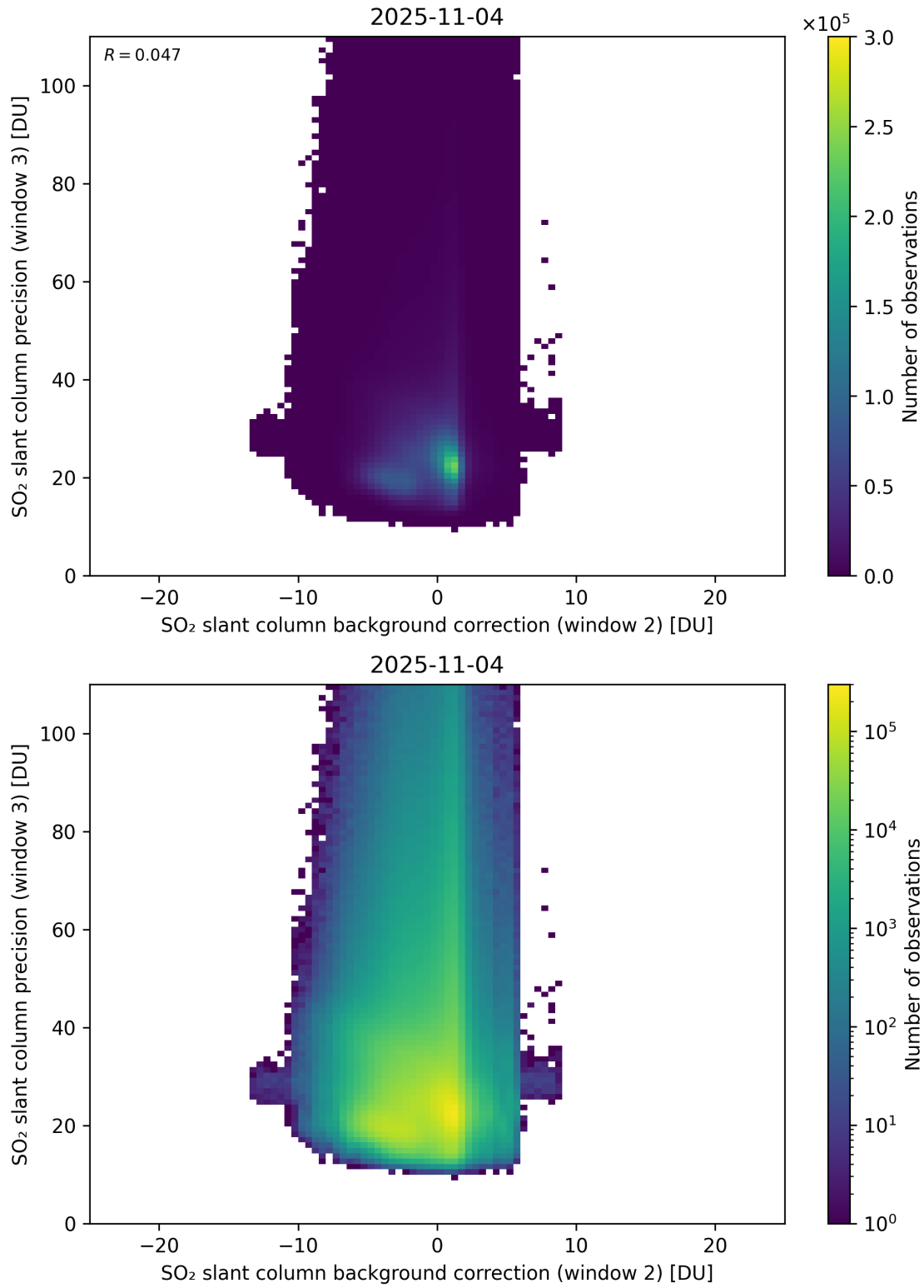
Figure 129: Scatter density plot of “SO 2 slant column background correction (window 2)” against “SO 2 slant column precision (window 3)” for 2025-11-03 to 2025-11-05.
