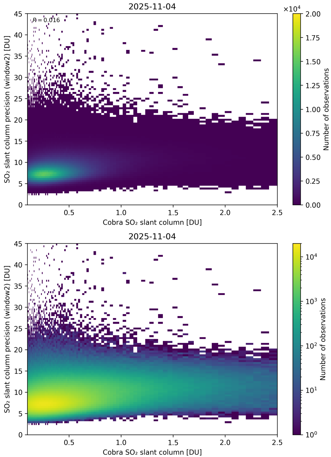
Figure 221: Scatter density plot of “Cobra SO 2 slant column” against “SO 2 slant column precision (window2)” for 2025-11-03 to 2025-11-05.
