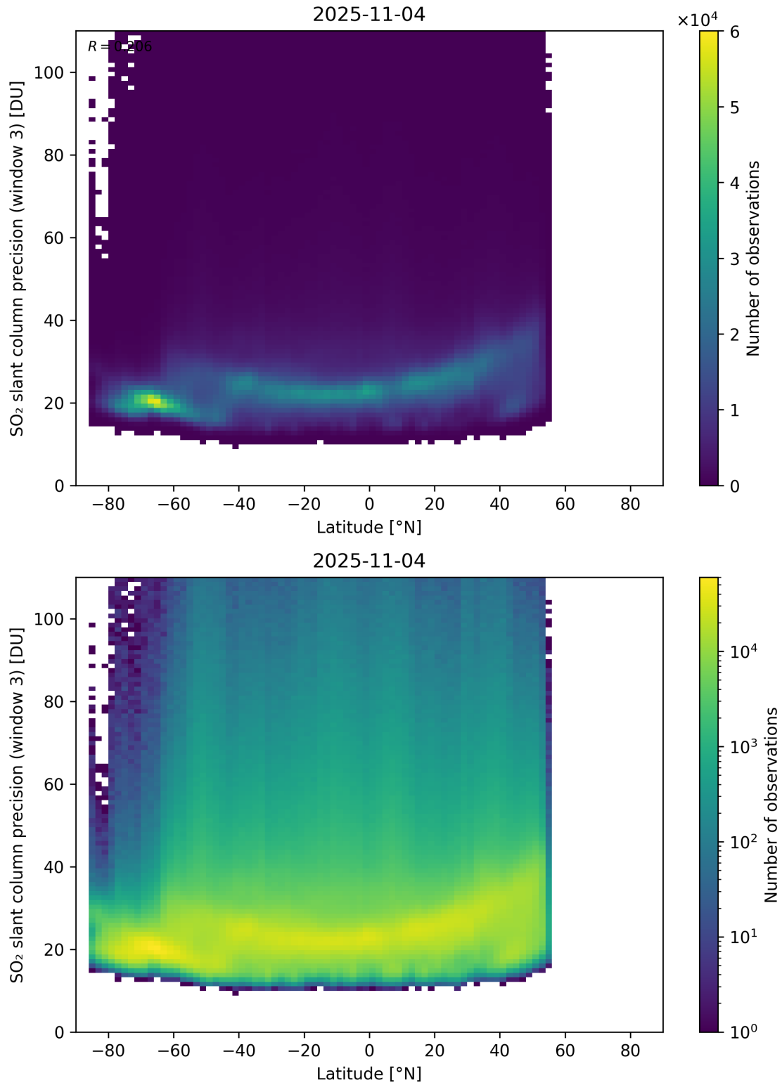
Figure 166: Scatter density plot of “Latitude” against “SO 2 slant column precision (window 3)” for 2025-11-03 to 2025-11-05.
