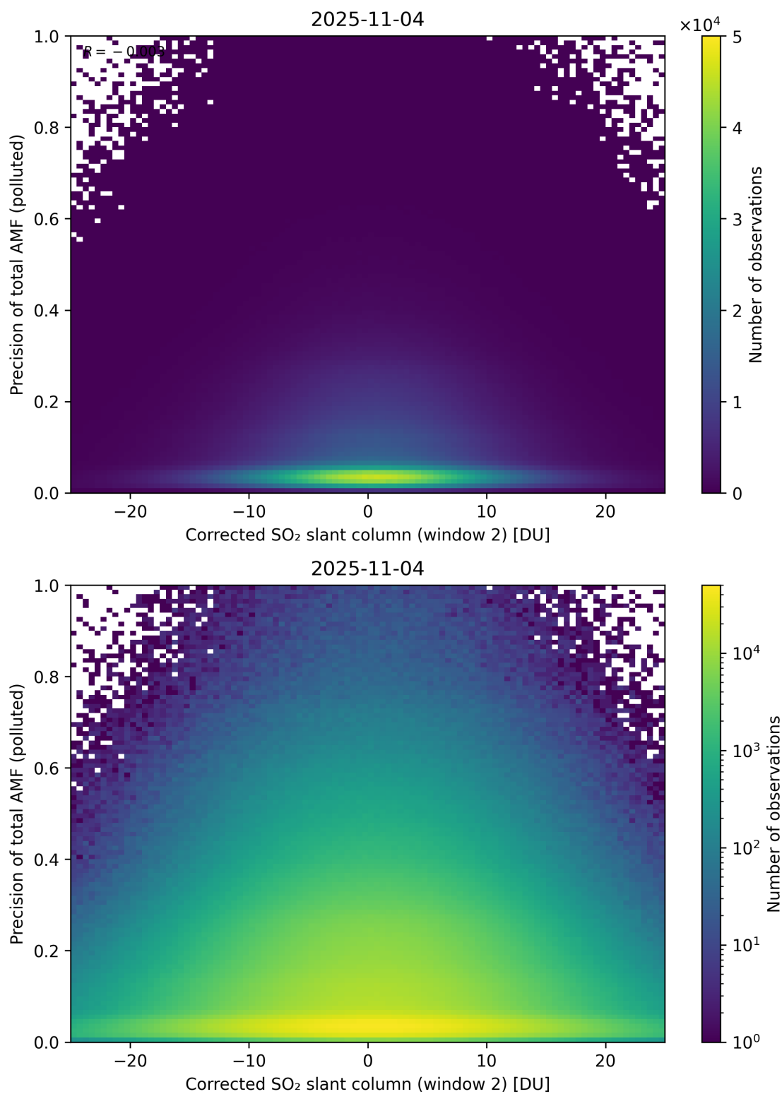
Figure 254: Scatter density plot of “Corrected SO 2 slant column (window 2)” against “Precision of total AMF (polluted)” for 2025-11-03 to 2025-11-05.
