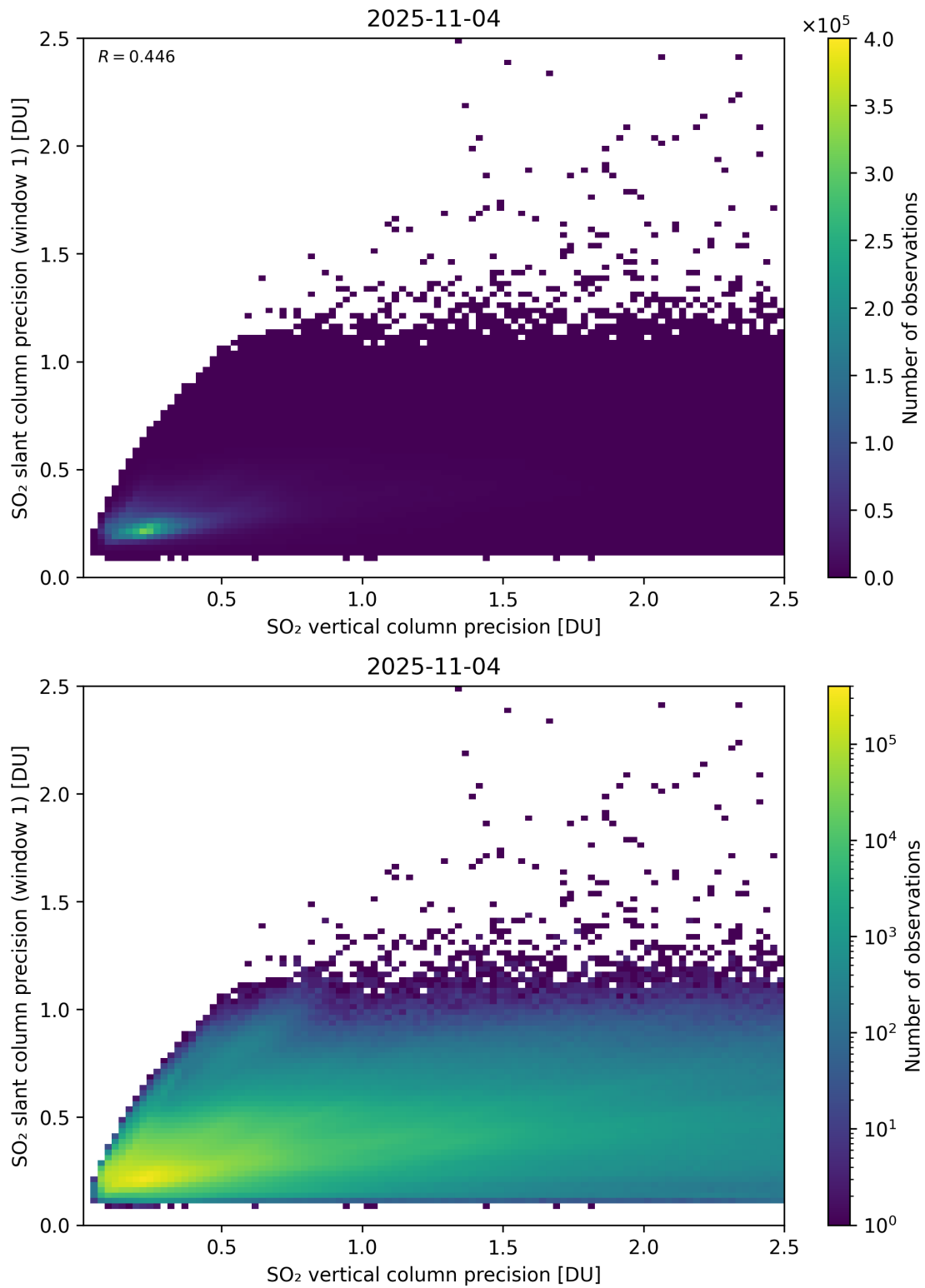
Figure 342: Scatter density plot of “SO 2 vertical column precision” against “SO 2 slant column precision (window 1)” for 2025-11-03 to 2025-11-05.
