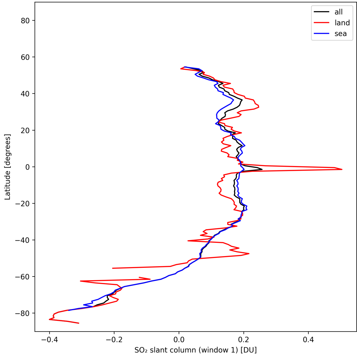
Figure 37: Zonal average of “SO 2 slant column (window 1)” for 2025-11-03 to 2025-11-05.
