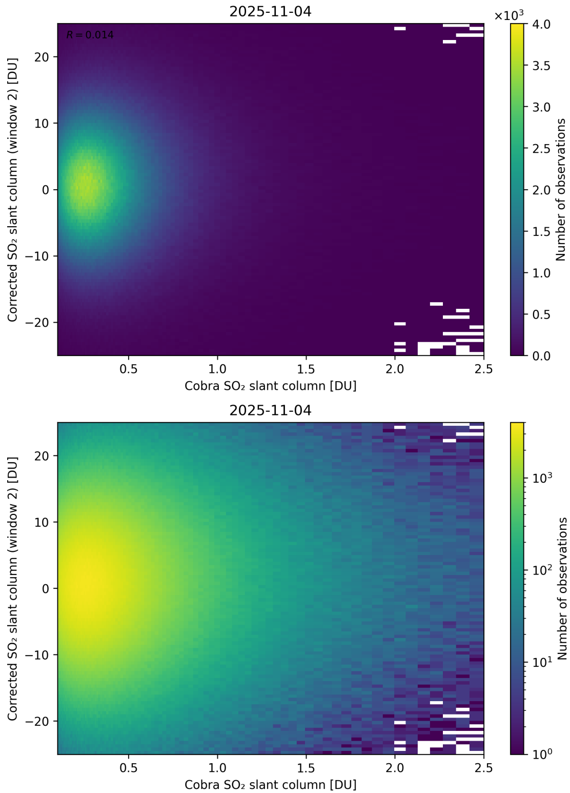
Figure 217: Scatter density plot of “Cobra SO 2 slant column” against “Corrected SO 2 slant column (window 2)” for 2025-11-03 to 2025-11-05.
