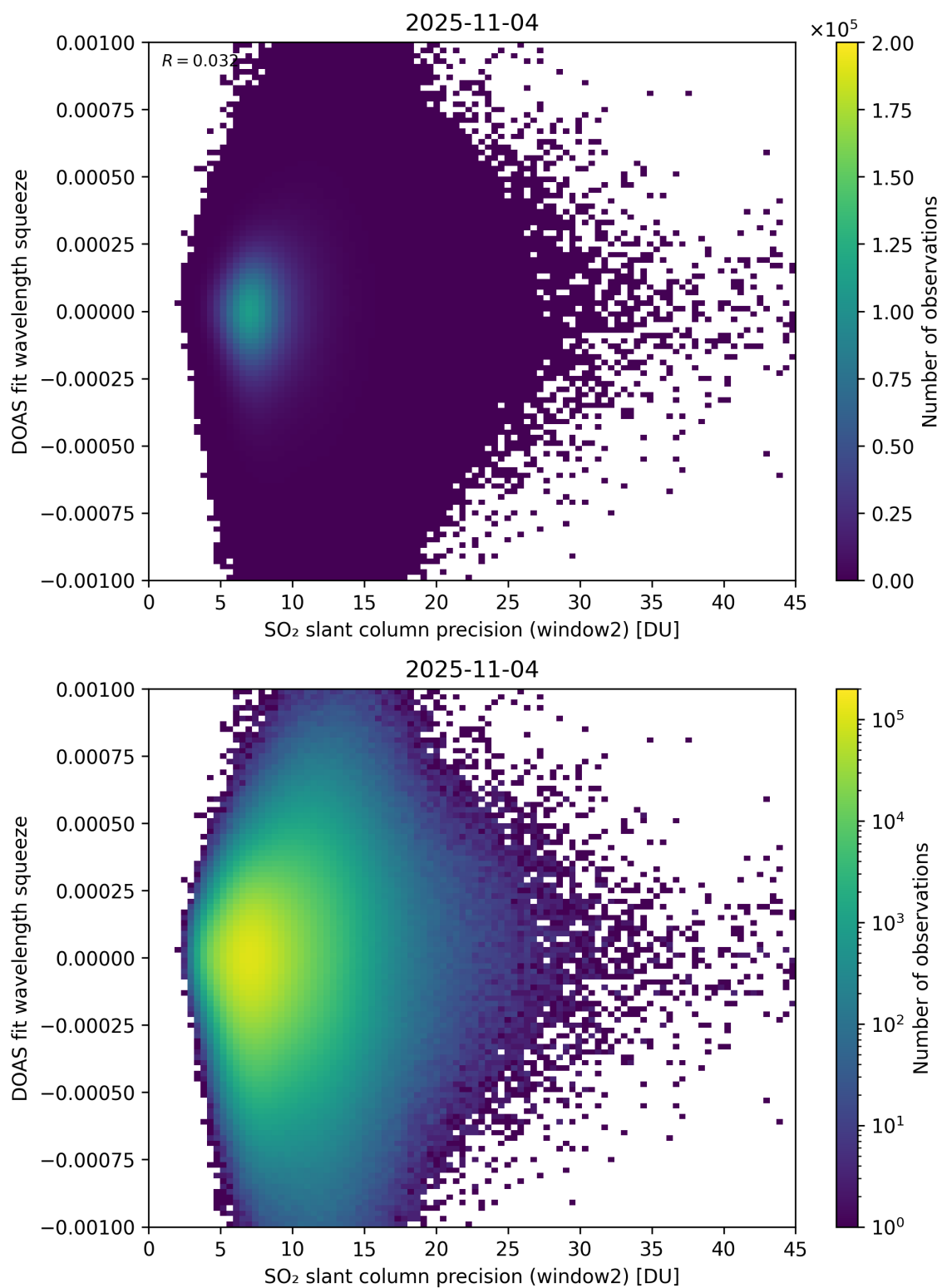
Figure 294: Scatter density plot of “SO 2 slant column precision (window2)” against “DOAS fit wavelength squeeze” for 2025-11-03 to 2025-11-05.
