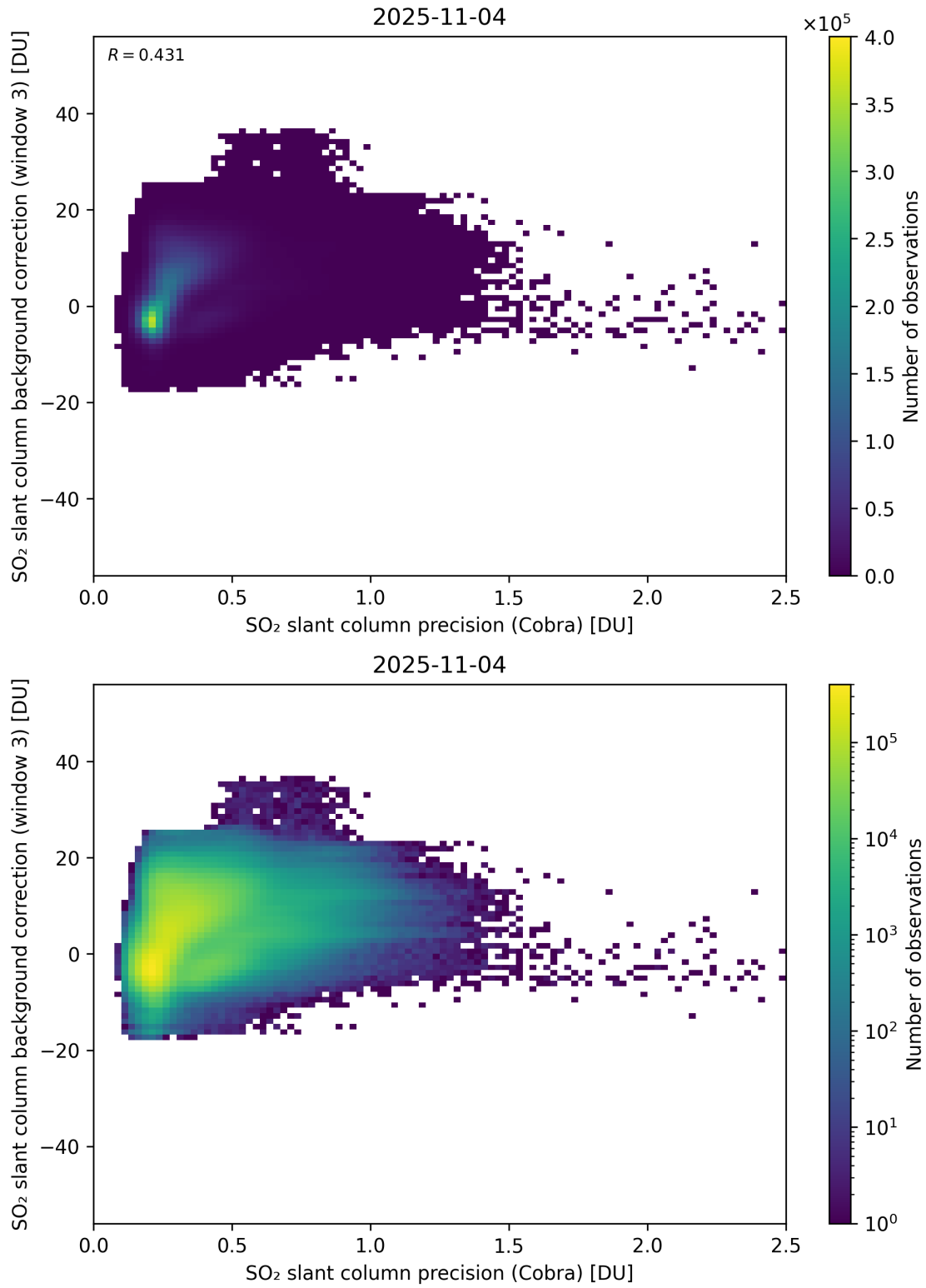
Figure 201: Scatter density plot of “SO 2 slant column precision (Cobra)” against “SO 2 slant column background correction (window 3)” for 2025-11-03 to 2025-11-05.
