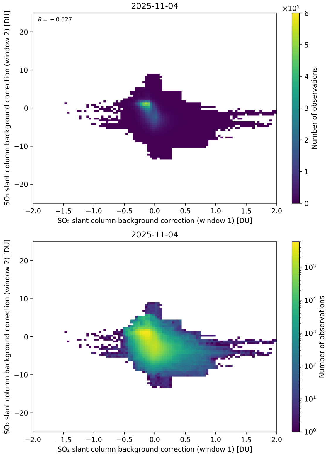
Figure 109: Scatter density plot of “SO 2 slant column background correction (window 1)” against “SO 2 slant column background correction (window 2)” for 2025-11-03 to 2025-11-05.
