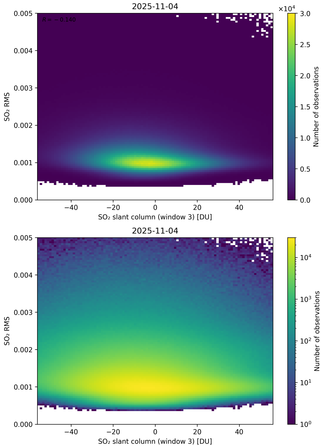
Figure 306: Scatter density plot of “SO 2 slant column (window 3)” against “SO 2 RMS” for 2025-11-03 to 2025-11-05.
