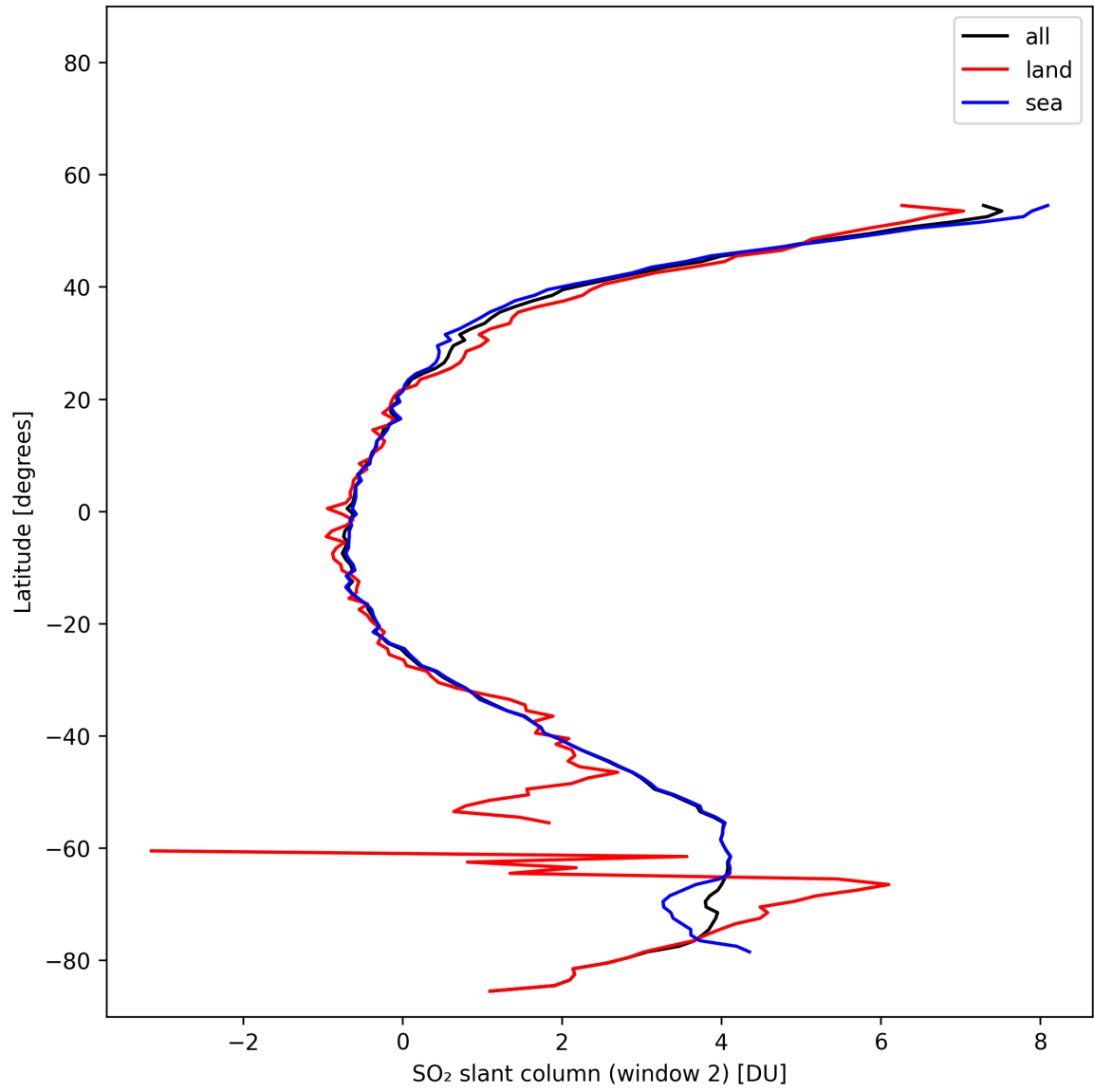
Figure 41: Zonal average of “SO 2 slant column (window 2)” for 2025-11-03 to 2025-11-05.
