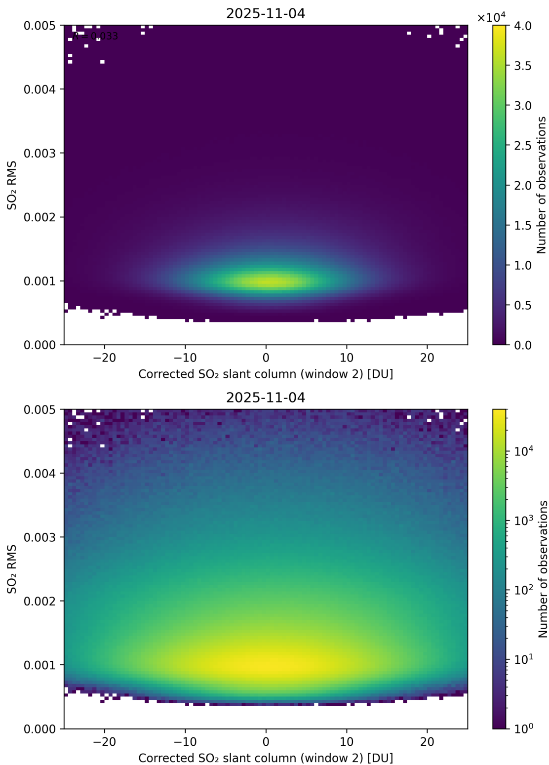
Figure 248: Scatter density plot of “Corrected SO 2 slant column (window 2)” against “SO 2 RMS” for 2025-11-03 to 2025-11-05.
