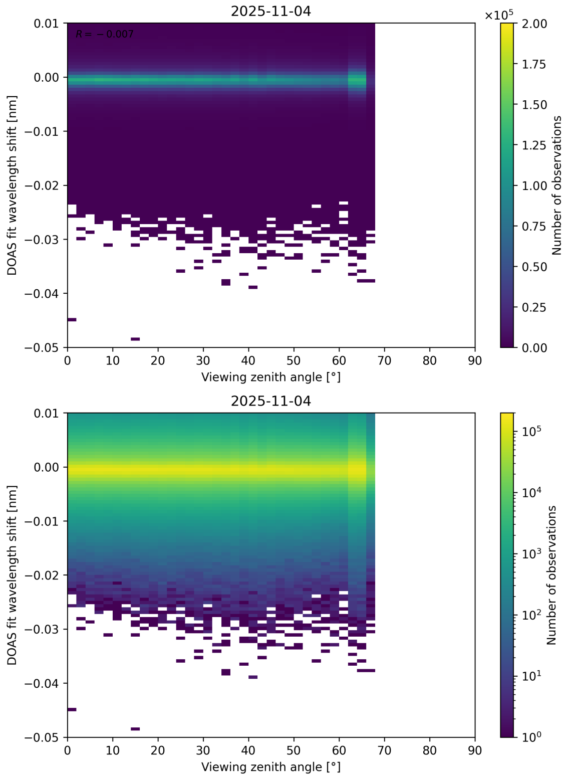
Figure 365: Scatter density plot of “Viewing zenith angle” against “DOAS fit wavelength shift” for 2025-11-03 to 2025-11-05.
