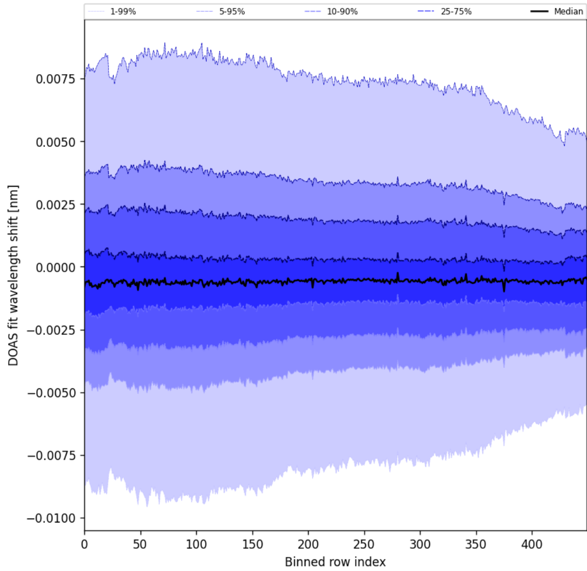
Figure 102: Along track statistics of “DOAS fit wavelength shift” for 2025-11-03 to 2025-11-05
