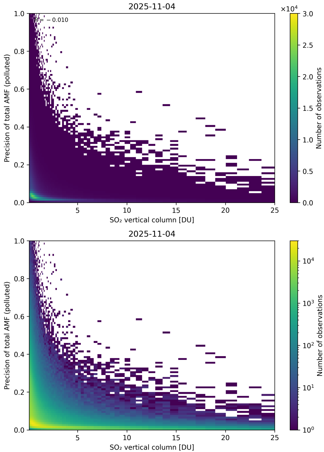
Figure 360: Scatter density plot of “SO 2 vertical column” against “Precision of total AMF (polluted)” for 2025-11-03 to 2025-11-05.
