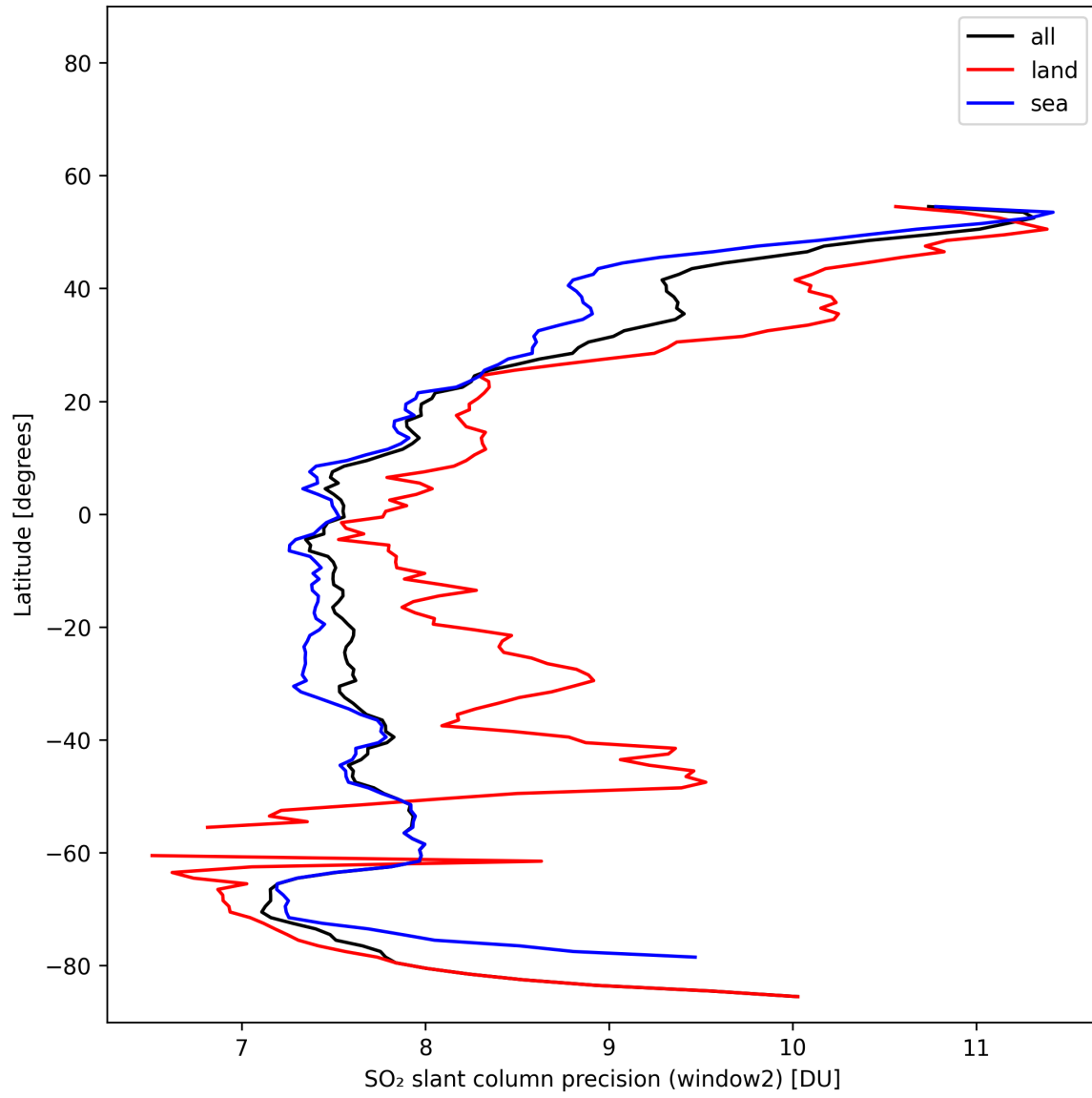
Figure 42: Zonal average of “SO 2 slant column precision (window2)” for 2025-11-03 to 2025-11-05.
