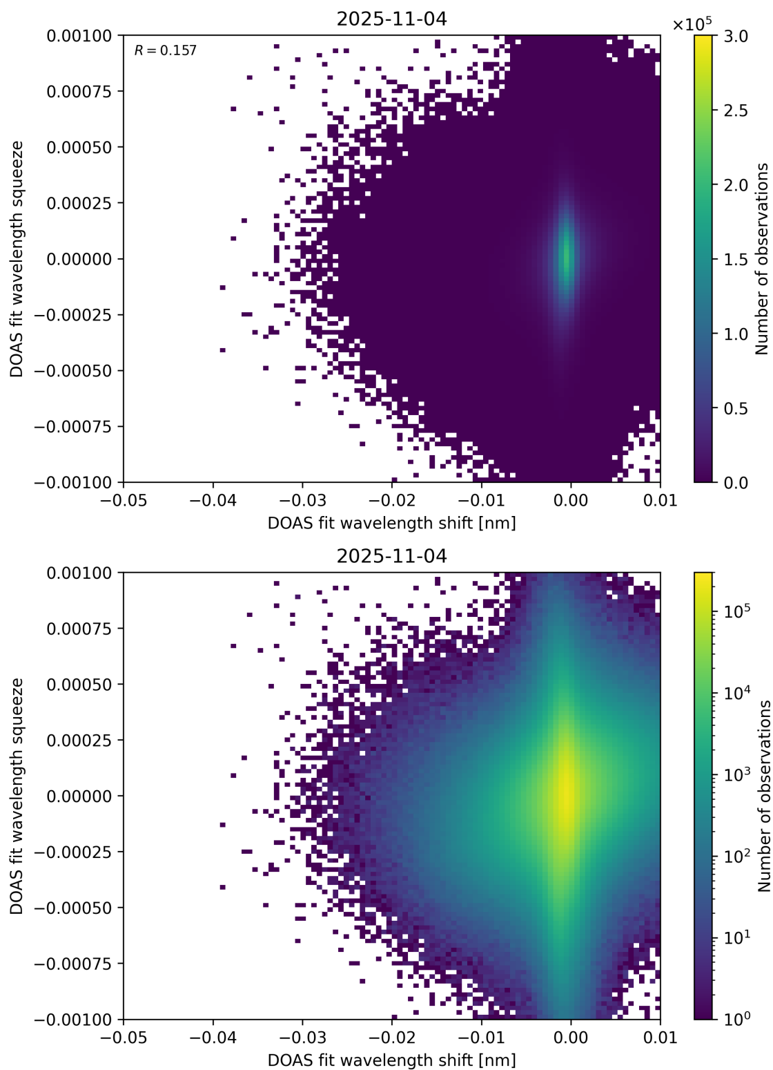
Figure 138: Scatter density plot of “DOAS fit wavelength shift” against “DOAS fit wavelength squeeze” for 2025-11-03 to 2025-11-05.
