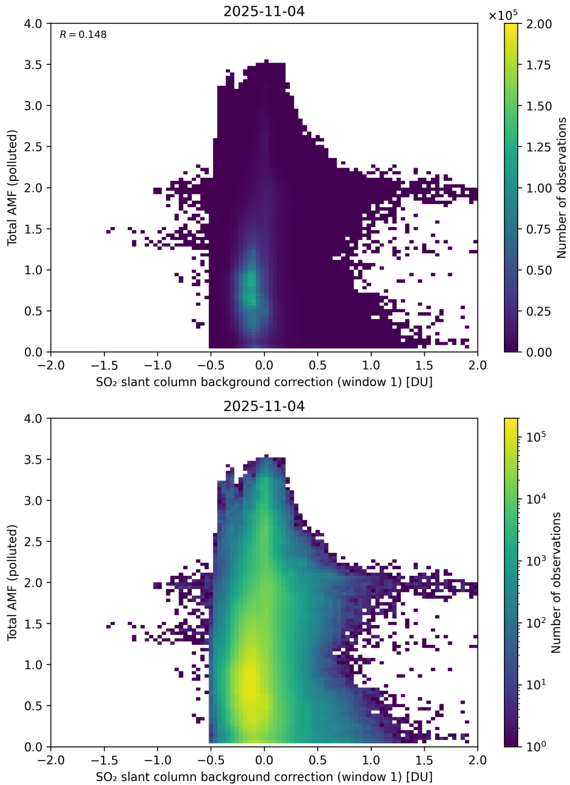
Figure 120: Scatter density plot of “SO 2 slant column background correction (window 1)” against “Total AMF (polluted)” for 2025-11-03 to 2025-11-05.
