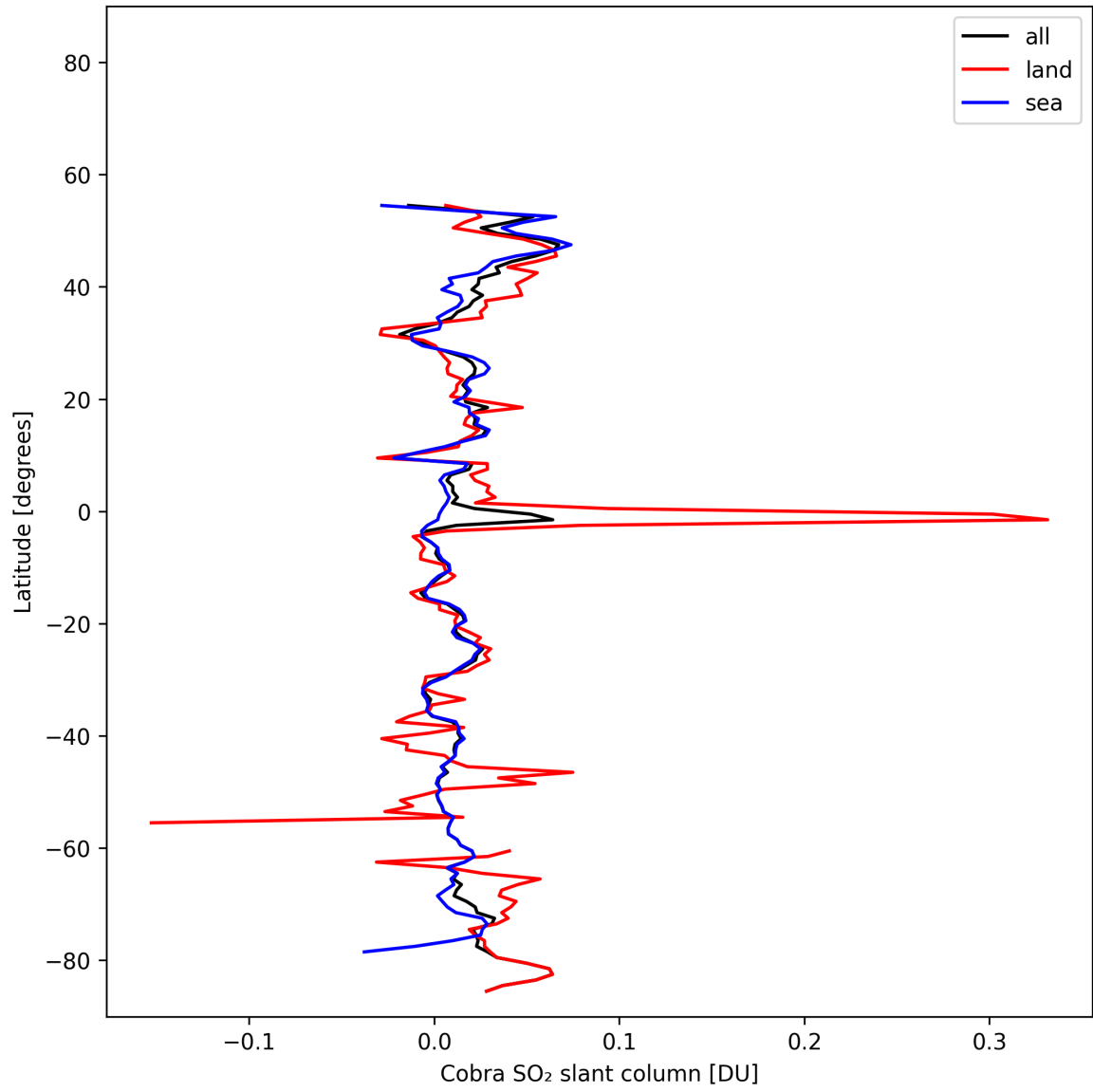
Figure 35: Zonal average of “Cobra SO 2 slant column” for 2025-11-03 to 2025-11-05.
