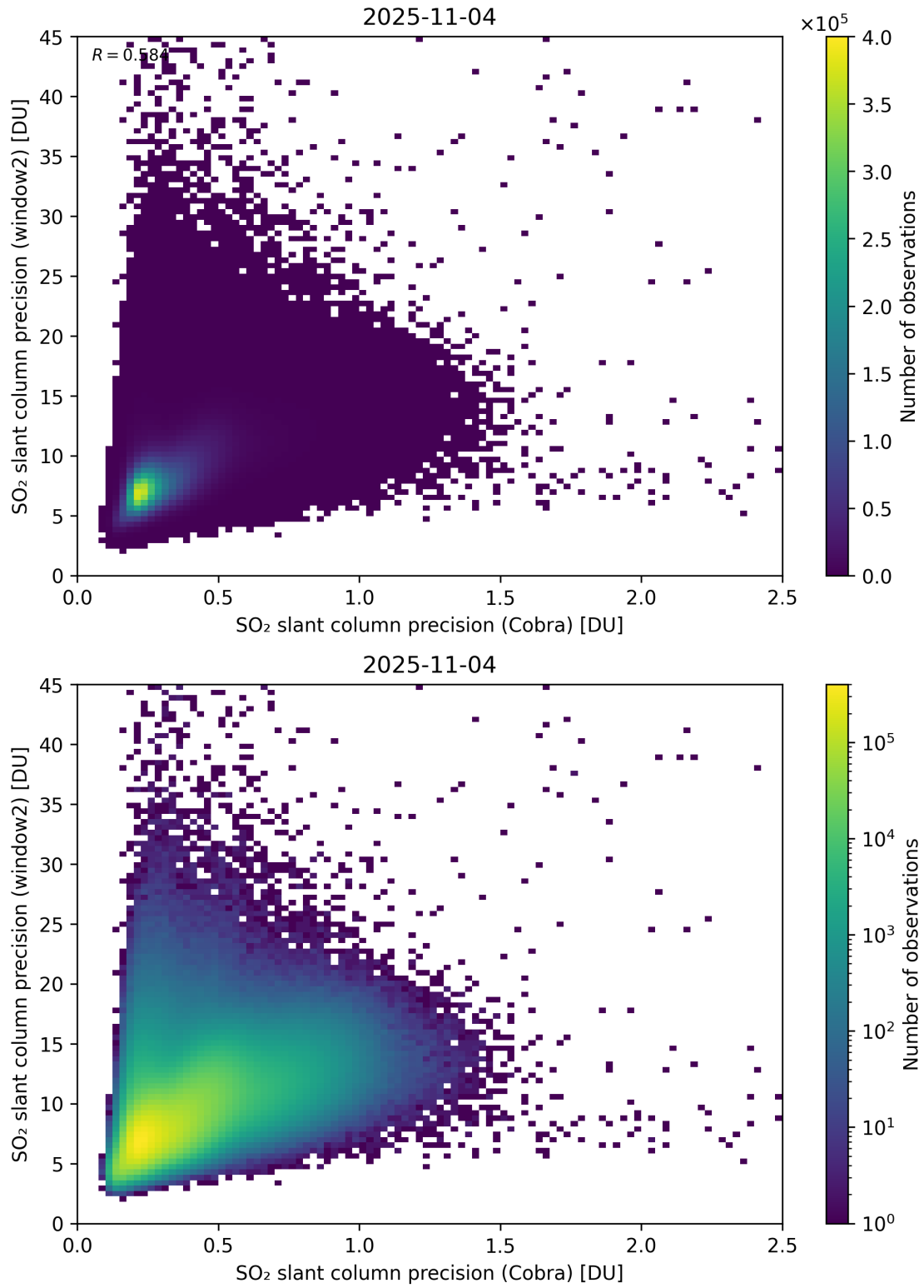
Figure 210: Scatter density plot of “SO 2 slant column precision (Cobra)” against “SO 2 slant column precision (window2)” for 2025-11-03 to 2025-11-05.
