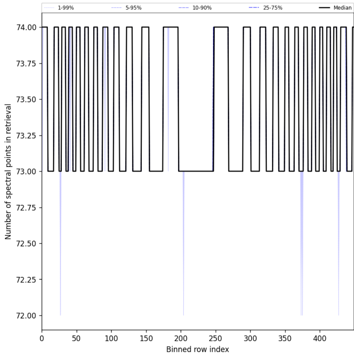
Figure 108: Along track statistics of “Number of spectral points in retrieval” for 2025-11-03 to 2025-11-05
