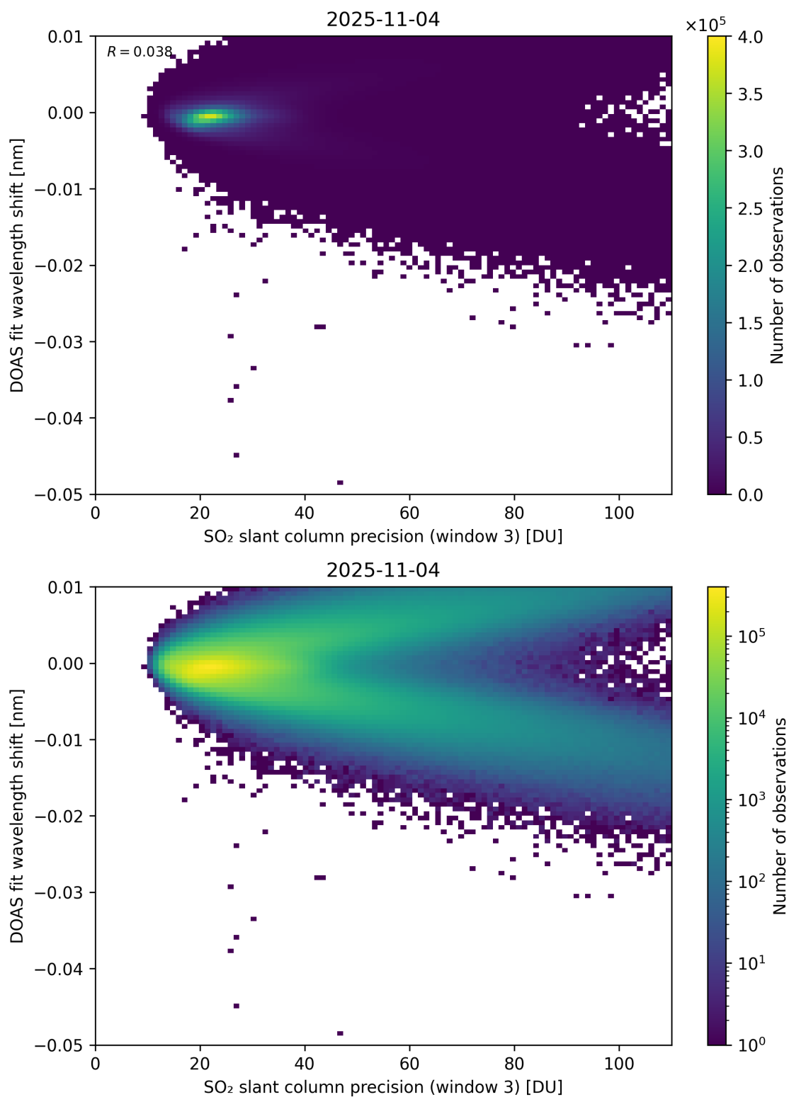
Figure 308: Scatter density plot of “SO 2 slant column precision (window 3)” against “DOAS fit wavelength shift” for 2025-11-03 to 2025-11-05.
