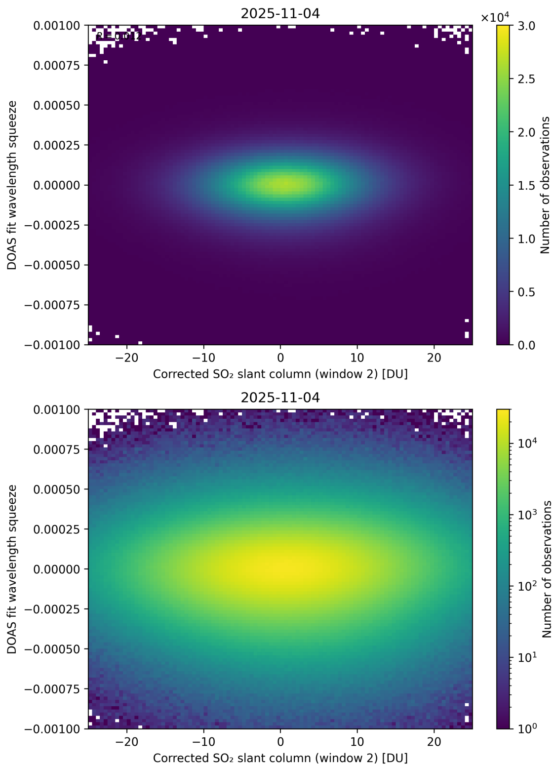
Figure 247: Scatter density plot of “Corrected SO 2 slant column (window 2)” against “DOAS fit wavelength squeeze” for 2025-11-03 to 2025-11-05.
