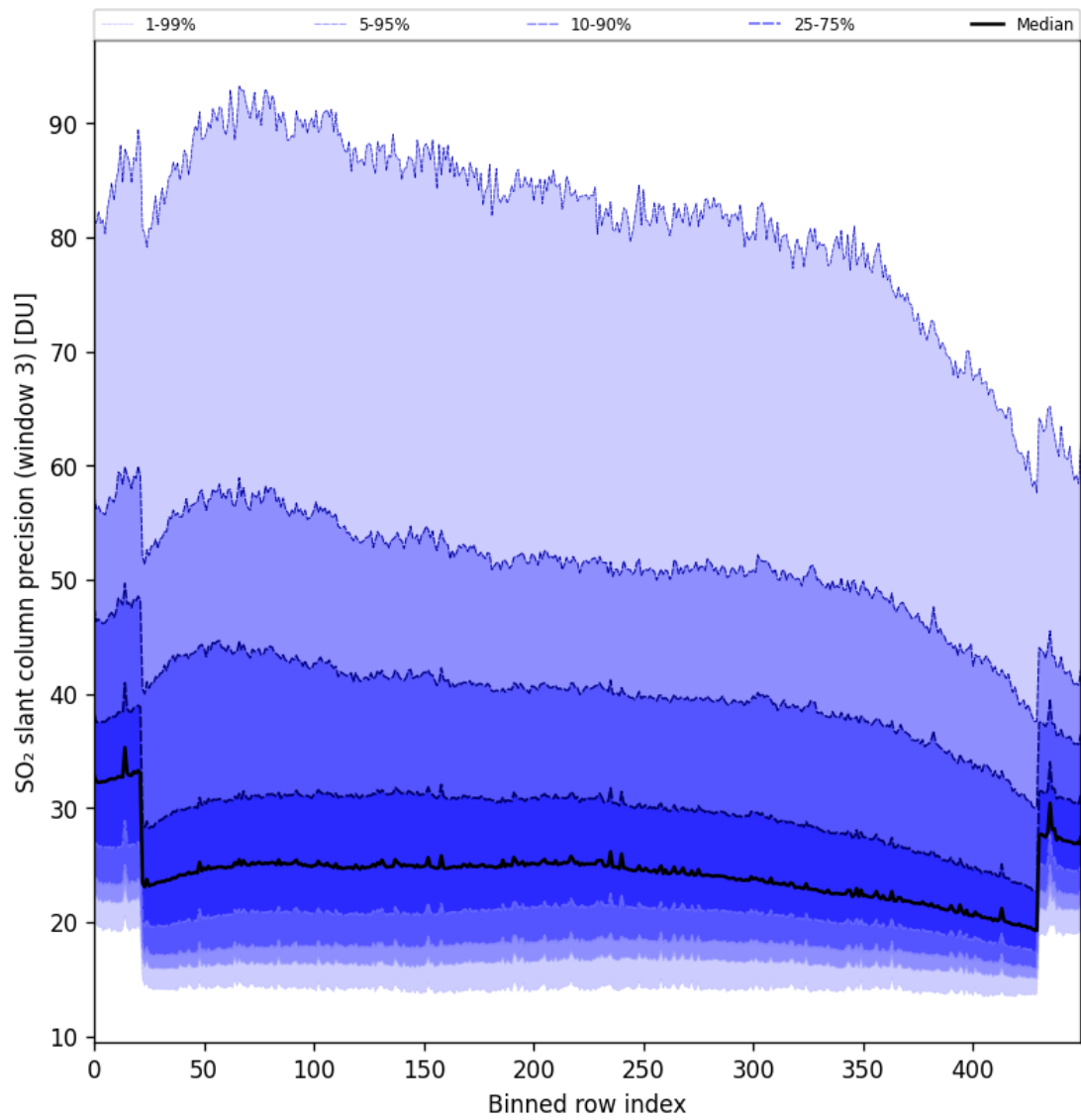
Figure 98: Along track statistics of “SO 2 slant column precision (window 3)” for 2025-11-03 to 2025-11-05
