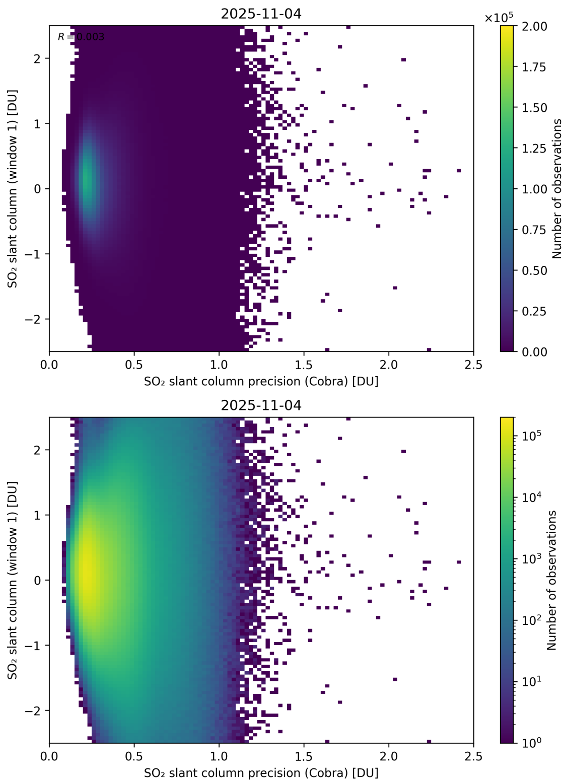
Figure 208: Scatter density plot of “SO 2 slant column precision (Cobra)” against “SO 2 slant column (window 1)” for 2025-11-03 to 2025-11-05.
