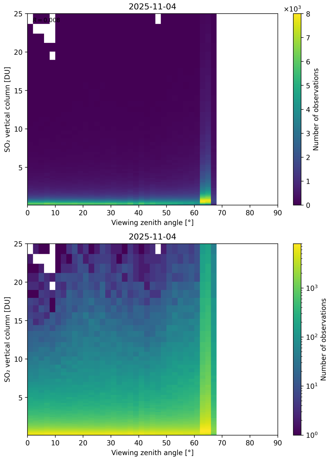
Figure 383: Scatter density plot of “Viewing zenith angle” against “SO 2 vertical column” for 2025-11-03 to 2025-11-05.
