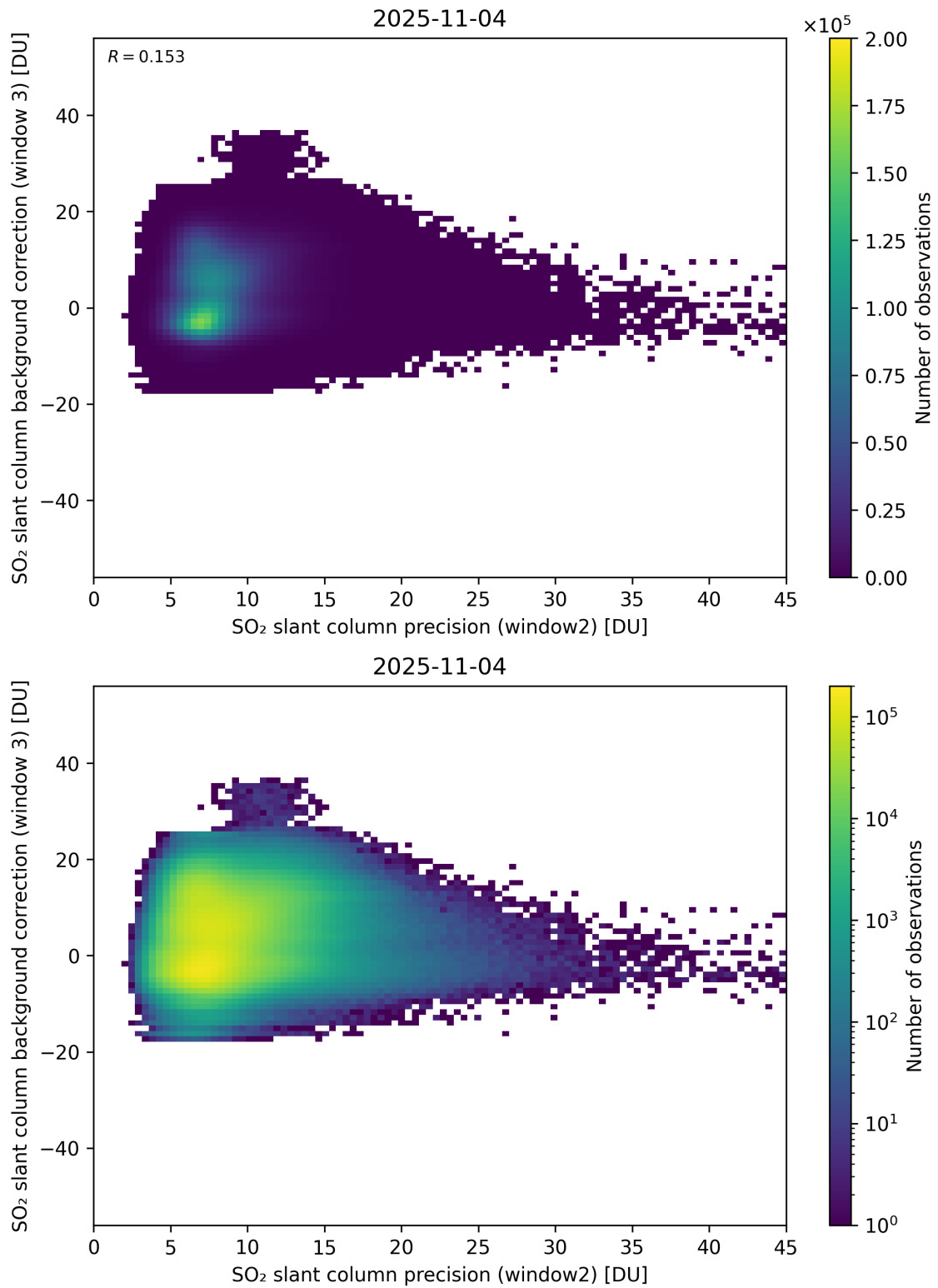
Figure 292: Scatter density plot of “SO 2 slant column precision (window2)” against “SO 2 slant column background correction (window 3)” for 2025-11-03 to 2025-11-05.
