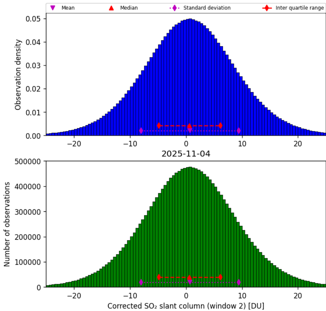
Figure 69: Histogram of “Corrected SO 2 slant column (window 2)” for 2025-11-03 to 2025-11-05
