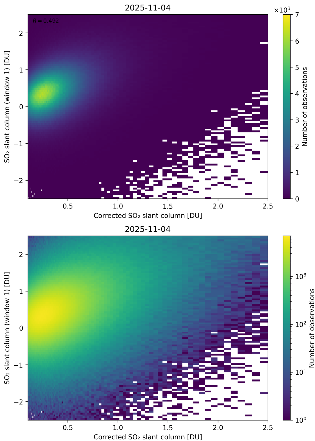
Figure 237: Scatter density plot of “Corrected SO 2 slant column” against “SO 2 slant column (window 1)” for 2025-11-03 to 2025-11-05.
