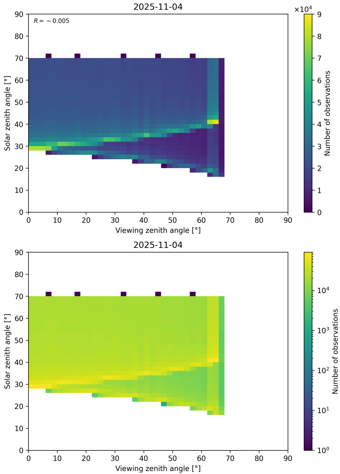
Figure 369: Scatter density plot of “Viewing zenith angle” against “Solar zenith angle” for 2025-11-03 to 2025-11-05.
