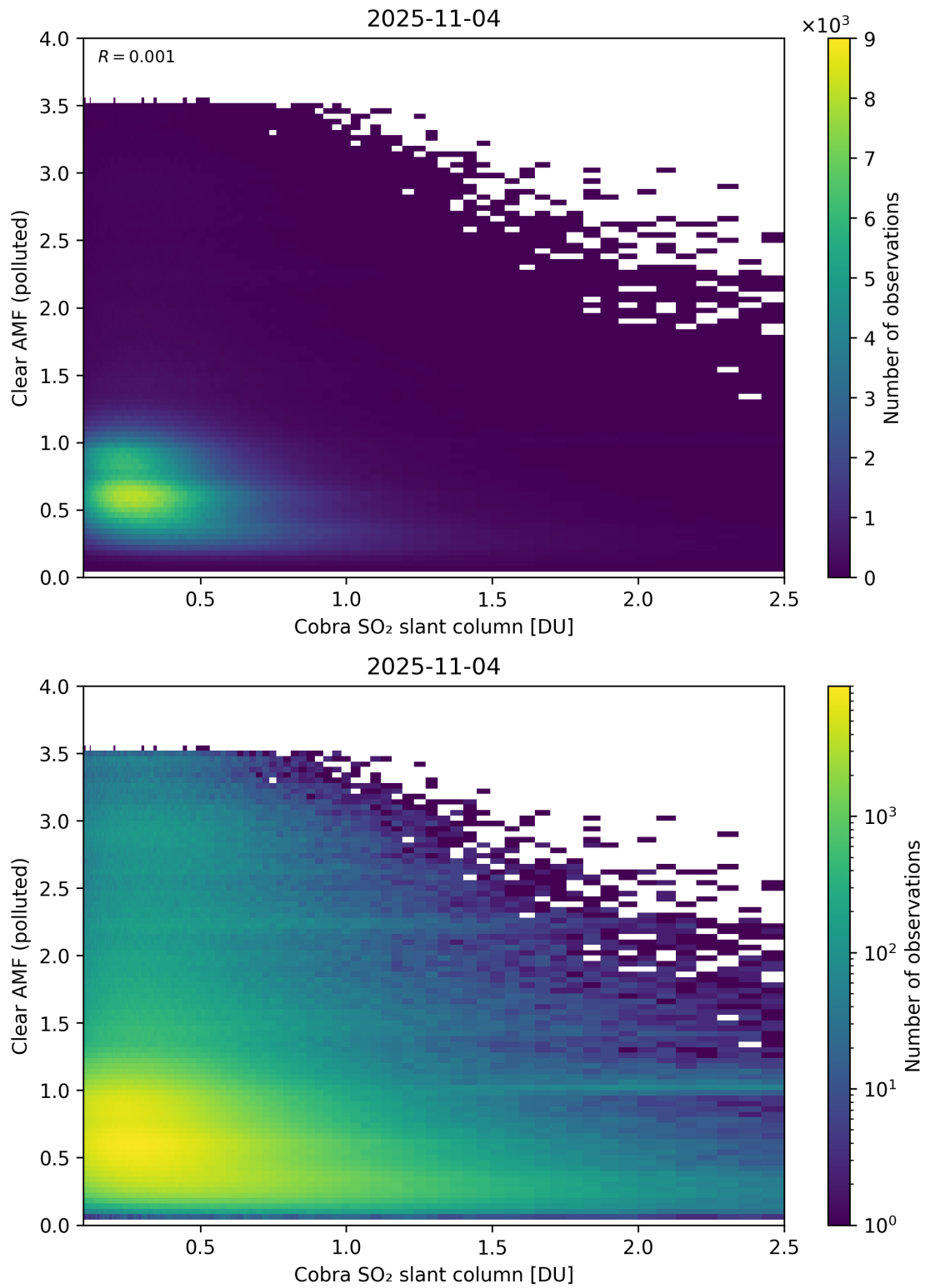
Figure 215: Scatter density plot of “Cobra SO 2 slant column” against “Clear AMF (polluted)” for 2025-11-03 to 2025-11-05.
