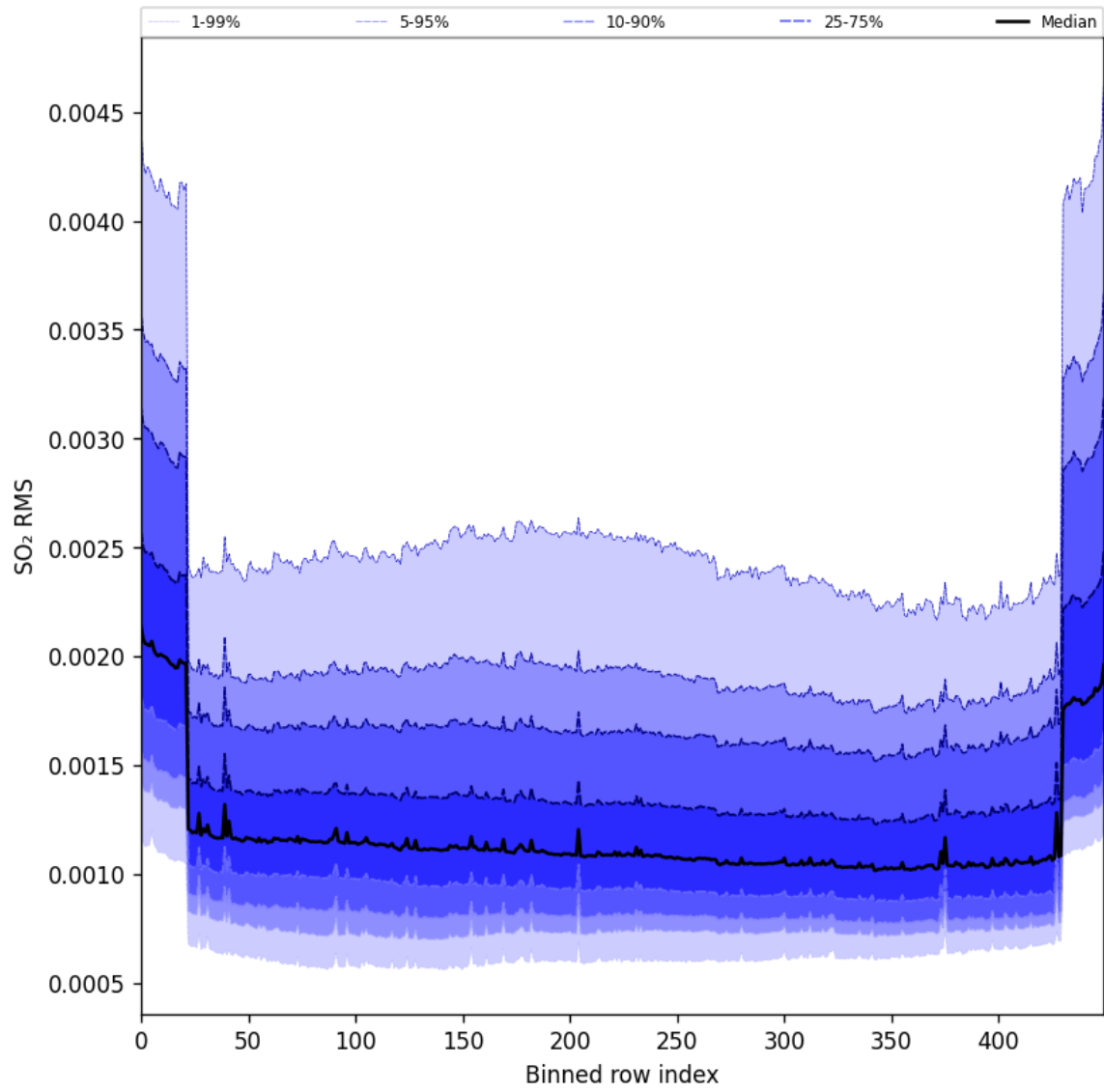
Figure 104: Along track statistics of “SO 2 RMS” for 2025-11-03 to 2025-11-05
