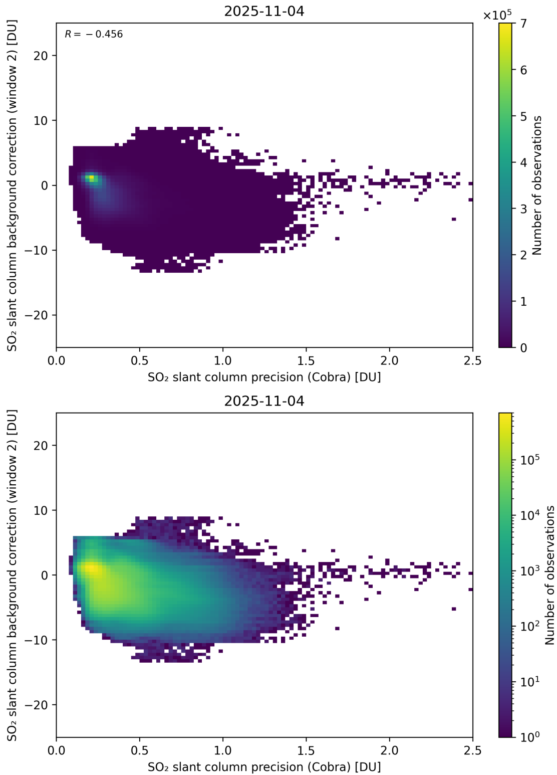
Figure 200: Scatter density plot of “SO 2 slant column precision (Cobra)” against “SO 2 slant column background correction (window 2)” for 2025-11-03 to 2025-11-05.
