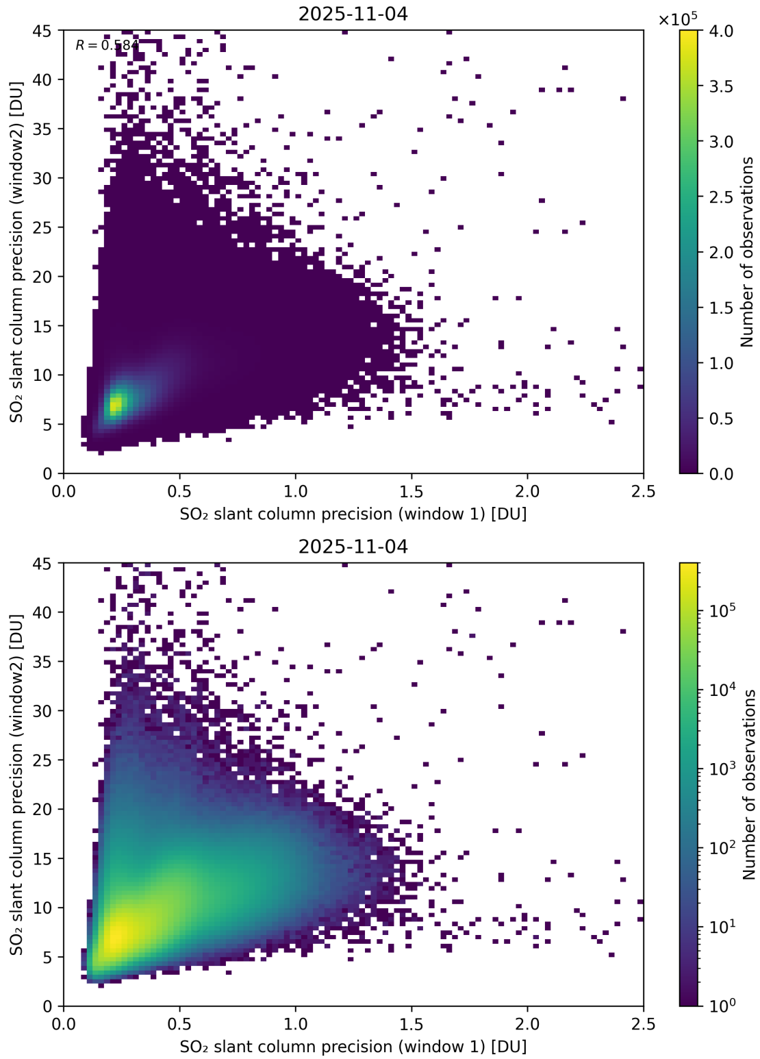
Figure 277: Scatter density plot of “SO 2 slant column precision (window 1)” against “SO 2 slant column precision (window2)” for 2025-11-03 to 2025-11-05.
