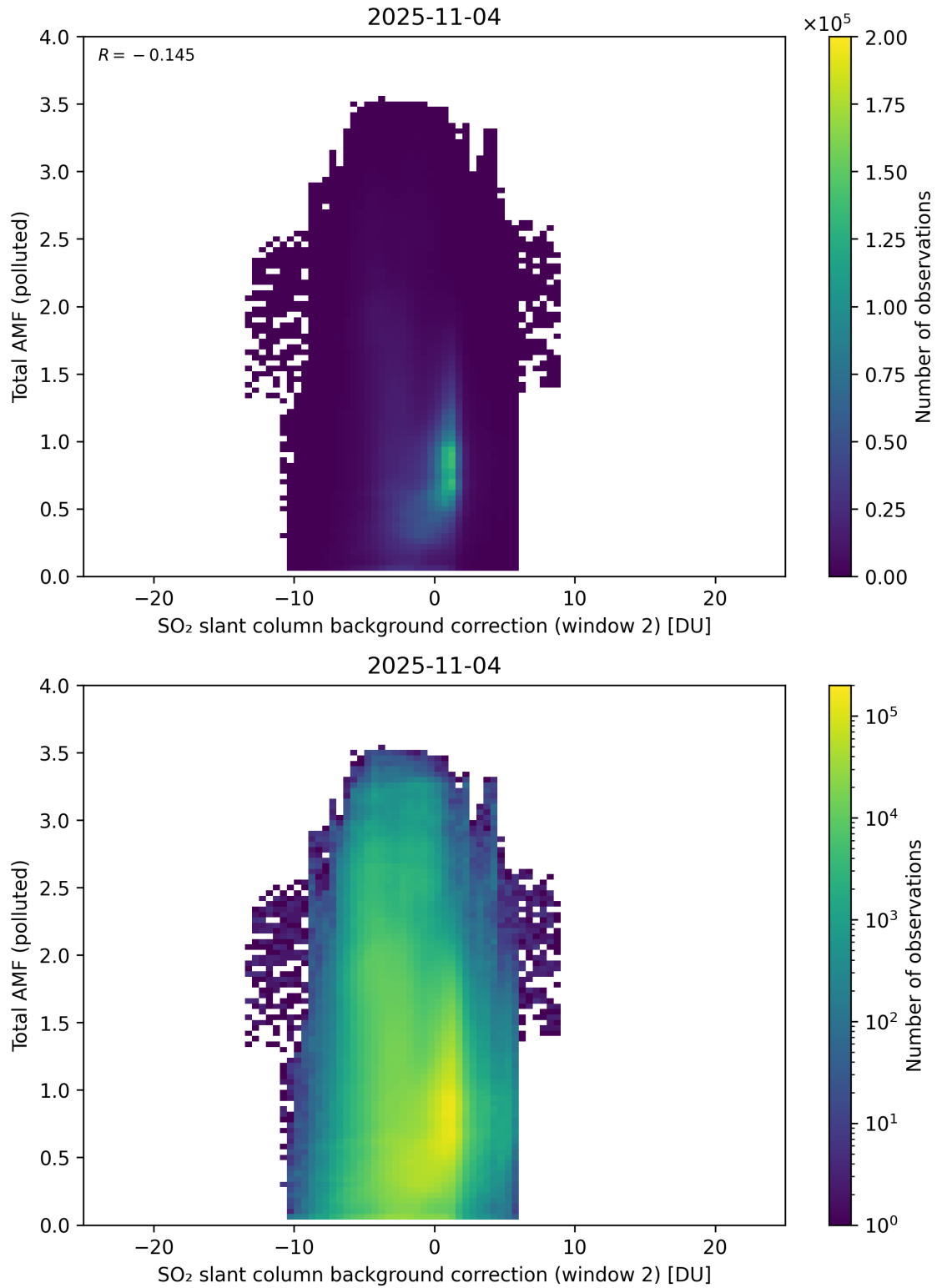
Figure 130: Scatter density plot of “SO 2 slant column background correction (window 2)” against “Total AMF (polluted)” for 2025-11-03 to 2025-11-05.
