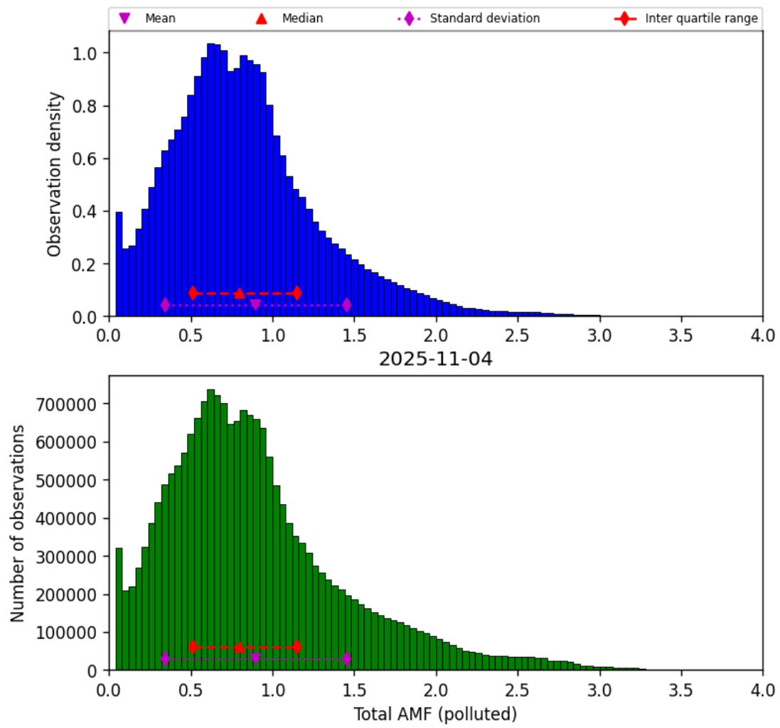
Figure 79: Histogram of “Total AMF (polluted)” for 2025-11-03 to 2025-11-05
