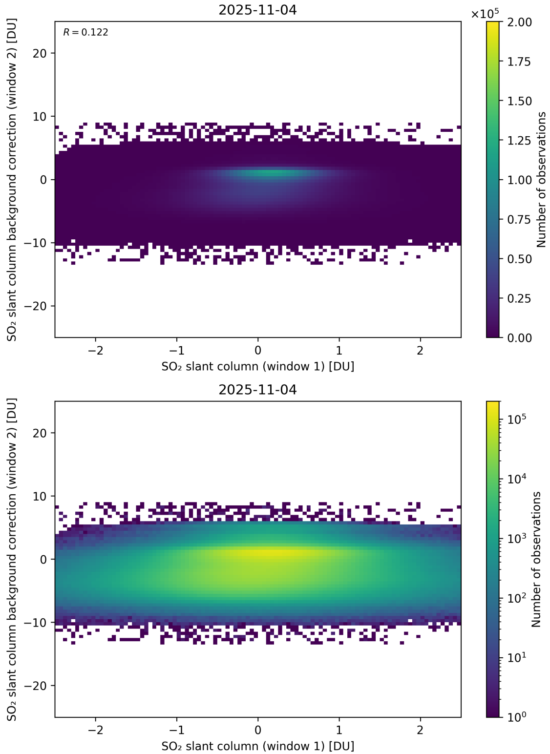
Figure 263: Scatter density plot of “SO 2 slant column (window 1)” against “SO 2 slant column background correction (window 2)” for 2025-11-03 to 2025-11-05.
