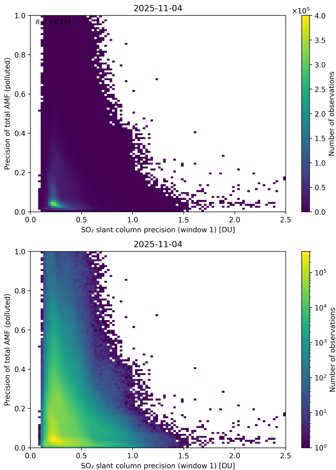
Figure 281: Scatter density plot of “SO 2 slant column precision (window 1)” against “Precision of total AMF (polluted)” for 2025-11-03 to 2025-11-05.
