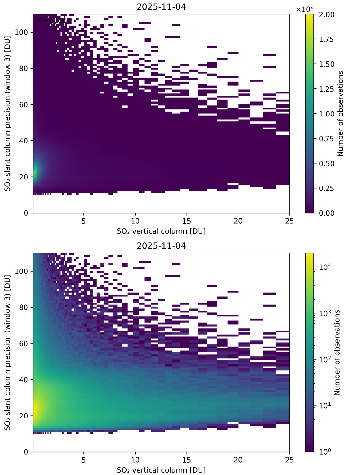
Figure 358: Scatter density plot of “SO 2 vertical column” against “SO 2 slant column precision (window 3)” for 2025-11-03 to 2025-11-05.
