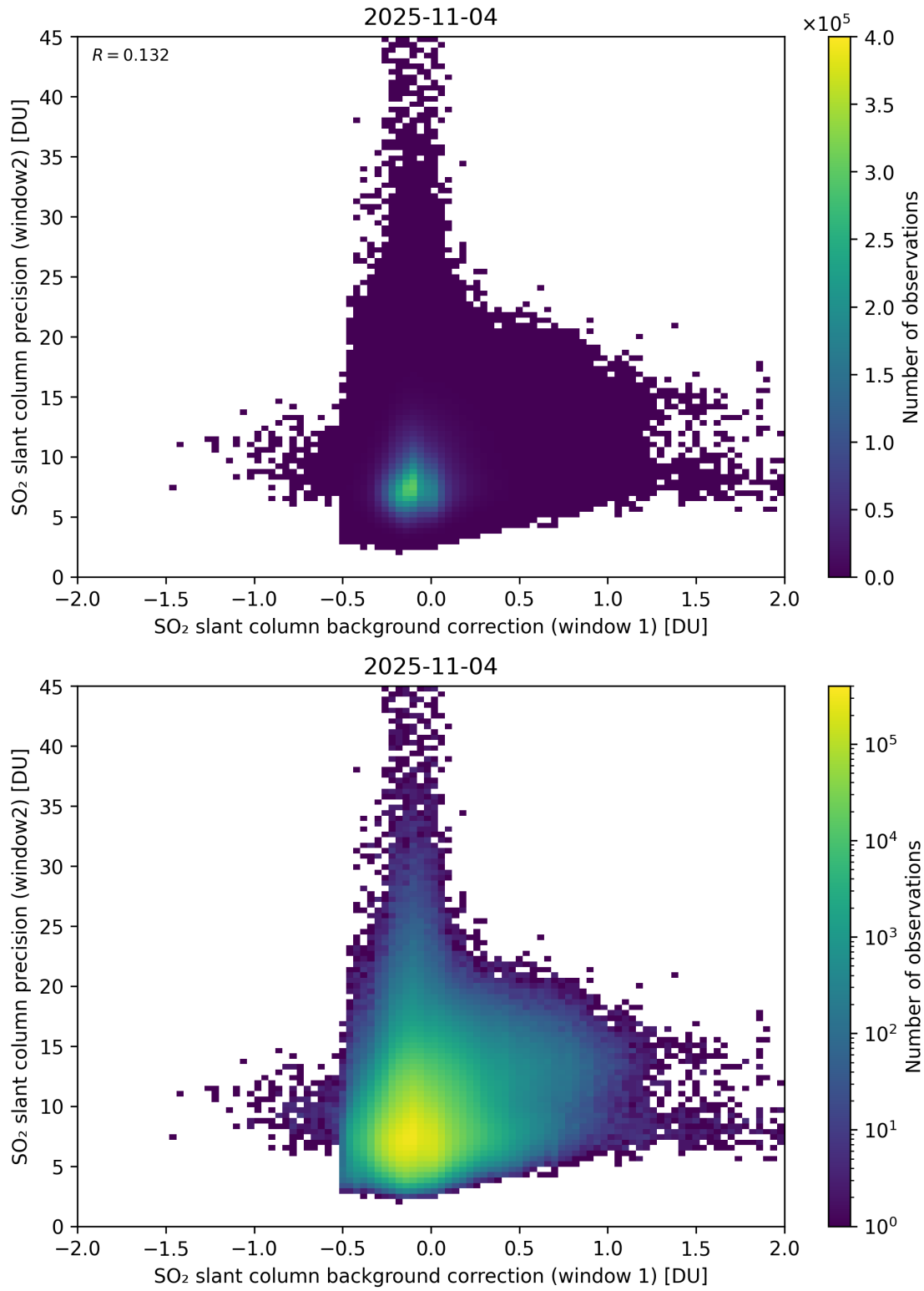
Figure 117: Scatter density plot of “SO 2 slant column background correction (window 1)” against “SO 2 slant column precision (window2)” for 2025-11-03 to 2025-11-05.
