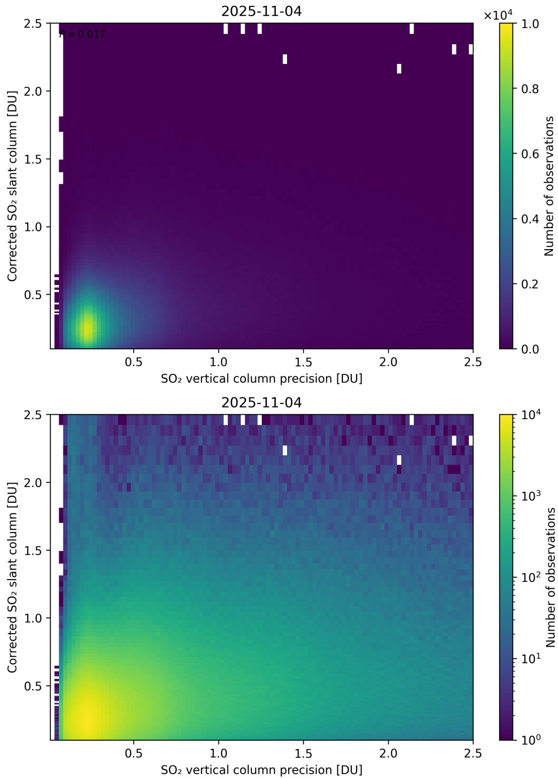
Figure 338: Scatter density plot of “SO 2 vertical column precision” against “Corrected SO 2 slant column” for 2025-11-03 to 2025-11-05.
