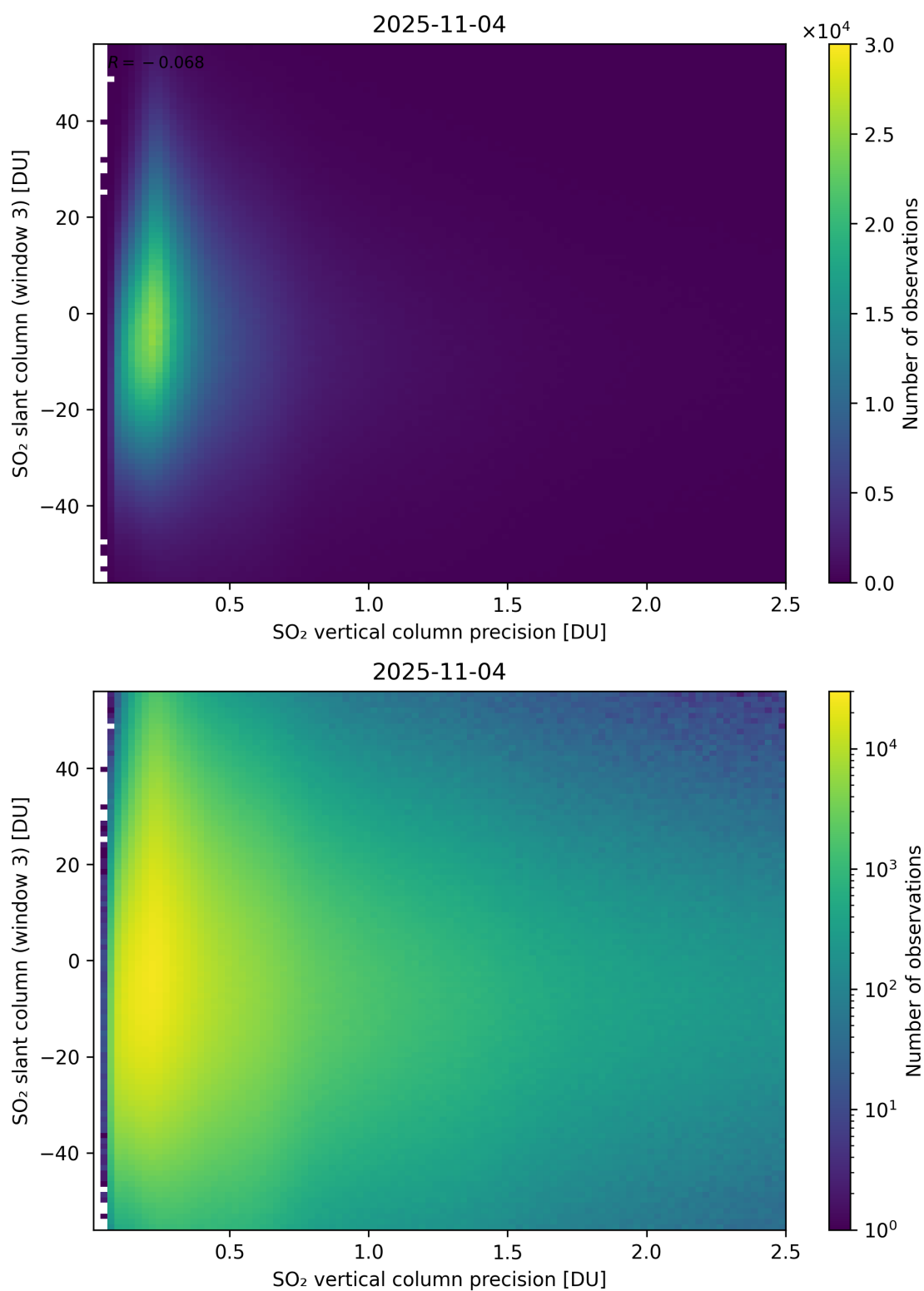
Figure 344: Scatter density plot of “SO 2 vertical column precision” against “SO 2 slant column (window 3)” for 2025-11-03 to 2025-11-05.
