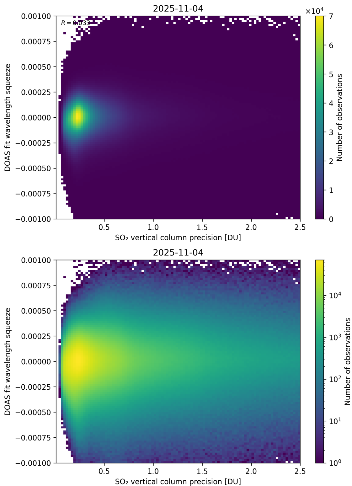
Figure 333: Scatter density plot of “SO 2 vertical column precision” against “DOAS fit wavelength squeeze” for 2025-11-03 to 2025-11-05.
