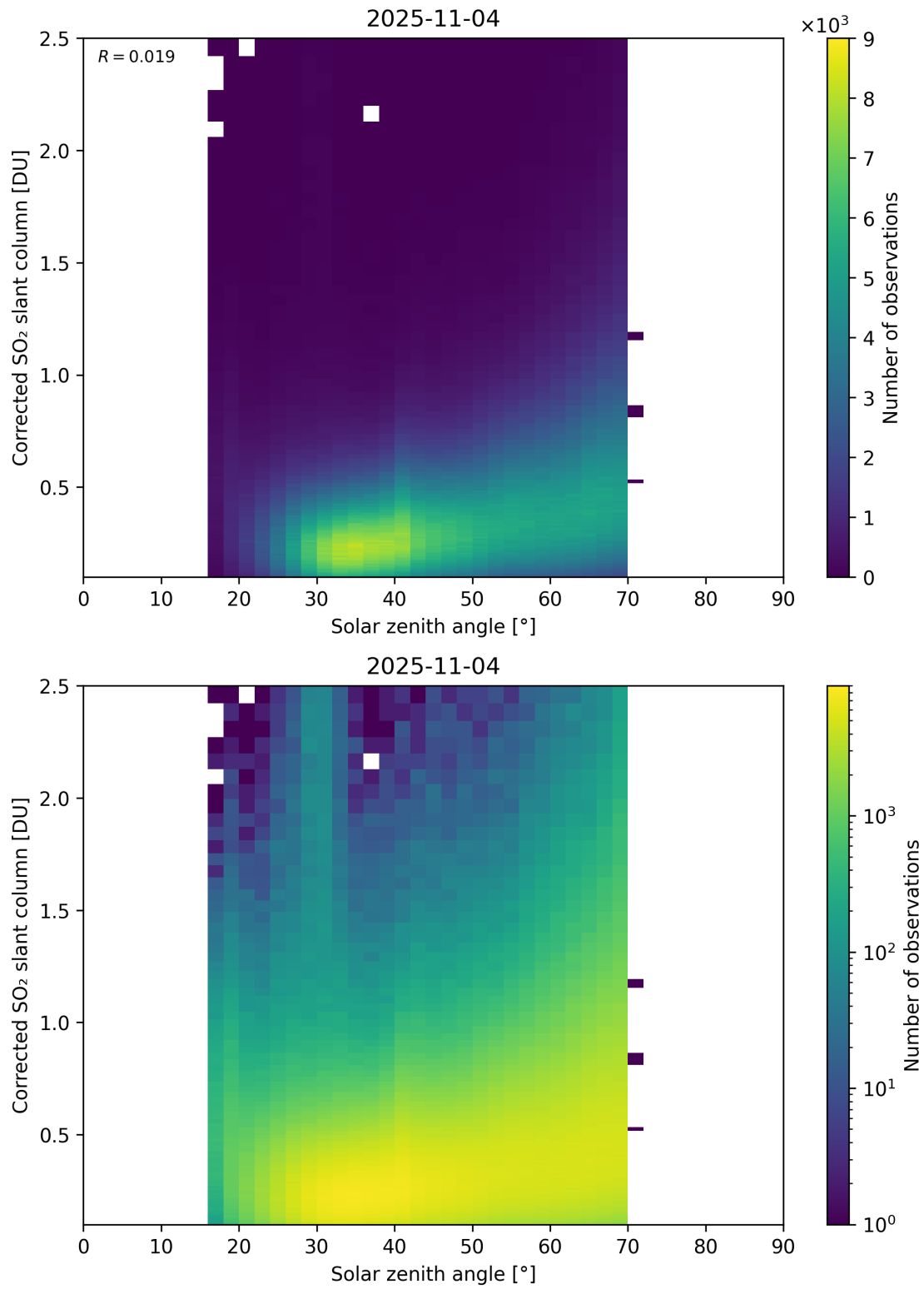
Figure 181: Scatter density plot of “Solar zenith angle” against “Corrected SO 2 slant column” for 2025-11-03 to 2025-11-05.
