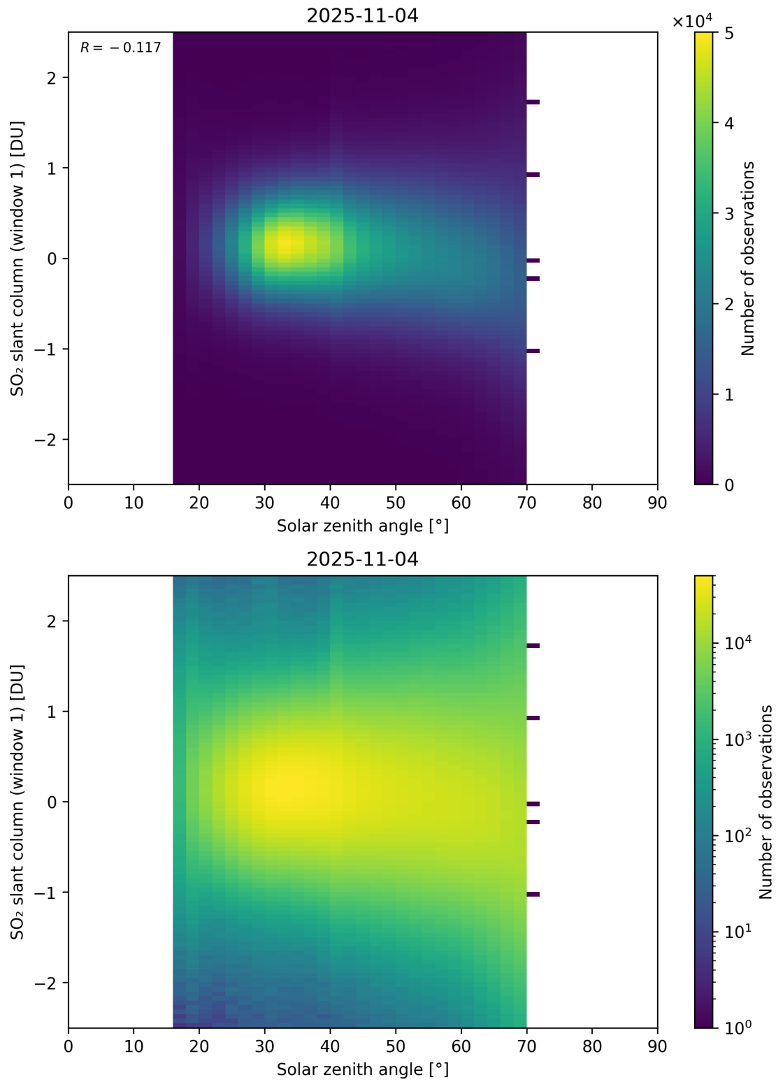
Figure 184: Scatter density plot of “Solar zenith angle” against “SO 2 slant column (window 1)” for 2025-11-03 to 2025-11-05.
