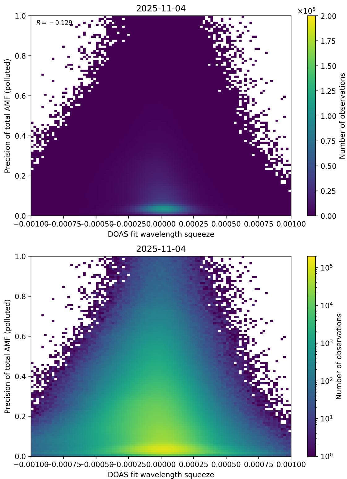
Figure 146: Scatter density plot of “DOAS fit wavelength squeeze” against “Precision of total AMF (polluted)” for 2025-11-03 to 2025-11-05.
