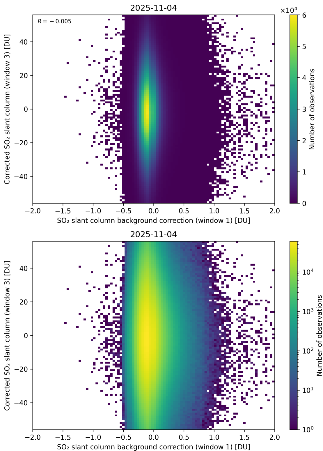
Figure 116: Scatter density plot of “SO 2 slant column background correction (window 1)” against “Corrected SO 2 slant column (window 3)” for 2025-11-03 to 2025-11-05.
