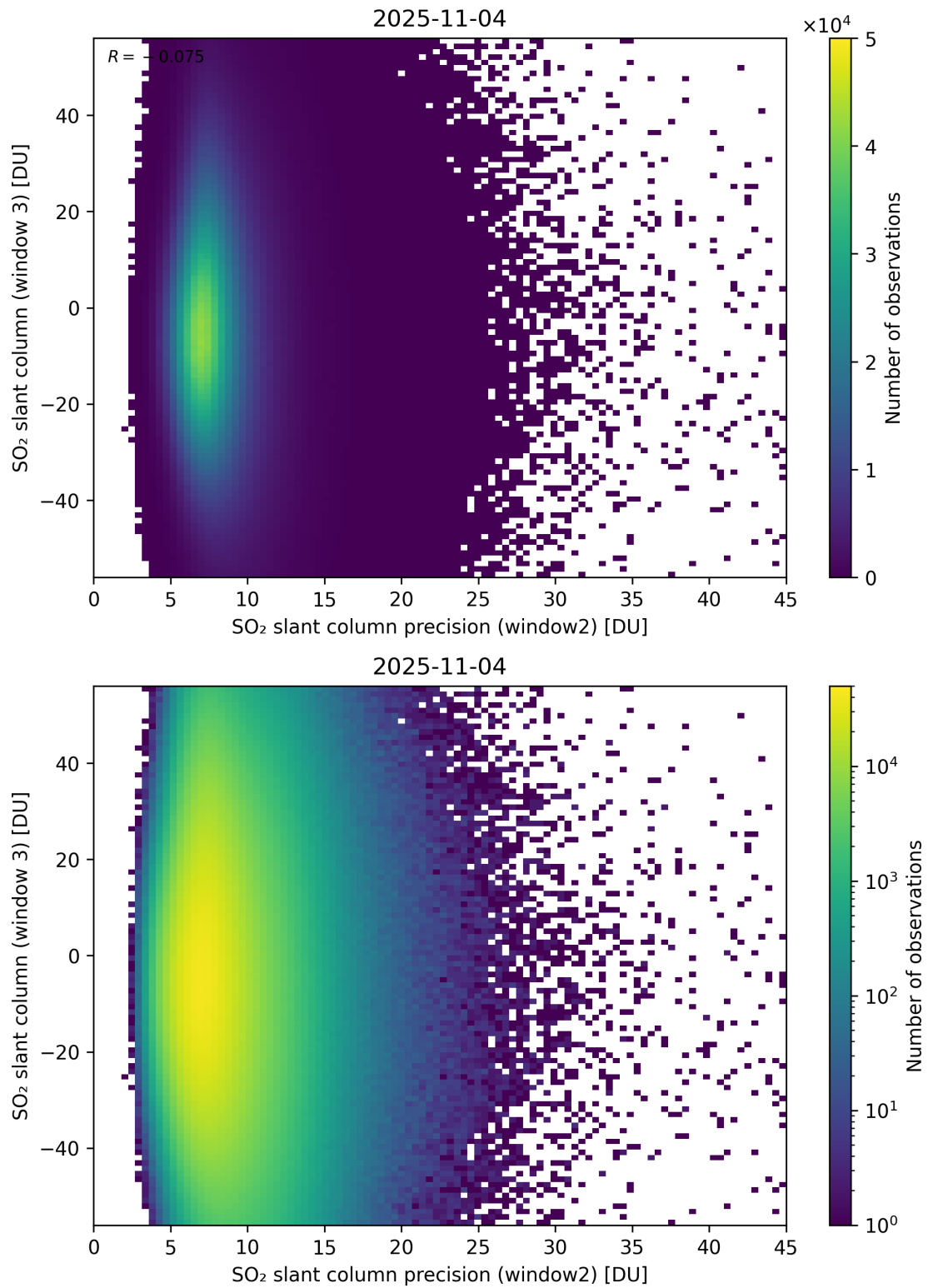
Figure 299: Scatter density plot of “SO 2 slant column precision (window2)” against “SO 2 slant column (window 3)” for 2025-11-03 to 2025-11-05.
