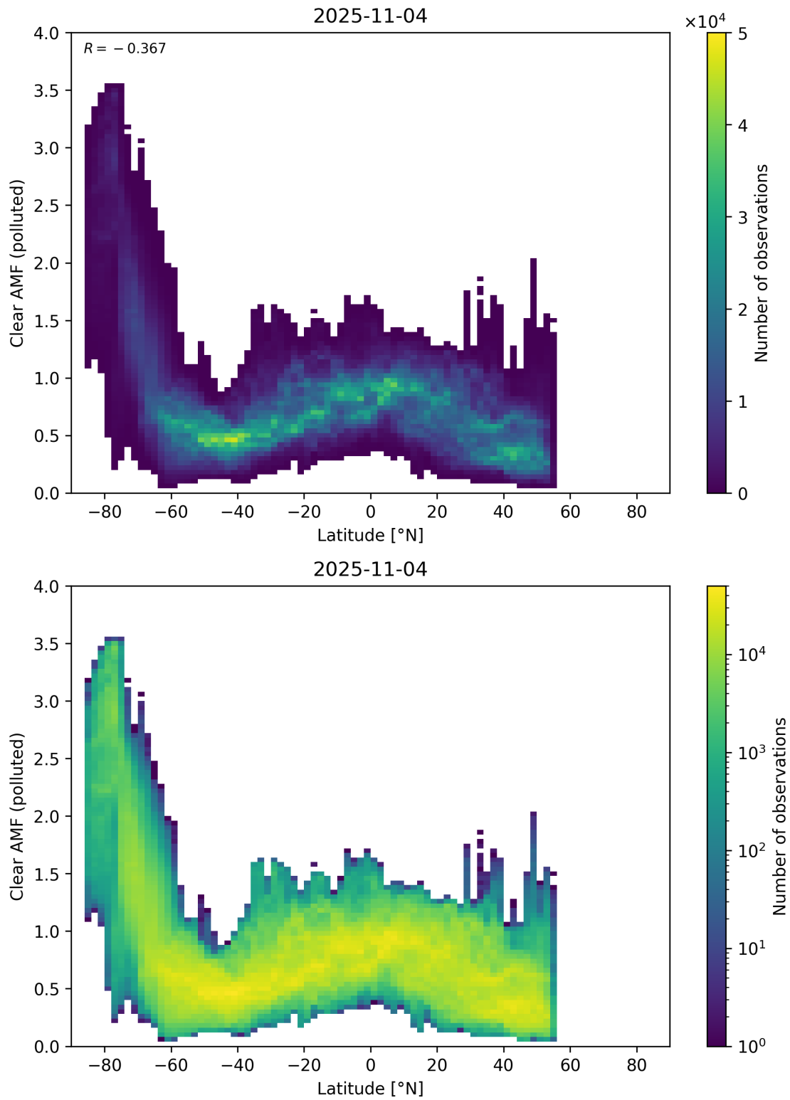
Figure 156: Scatter density plot of “Latitude” against “Clear AMF (polluted)” for 2025-11-03 to 2025-11-05.
