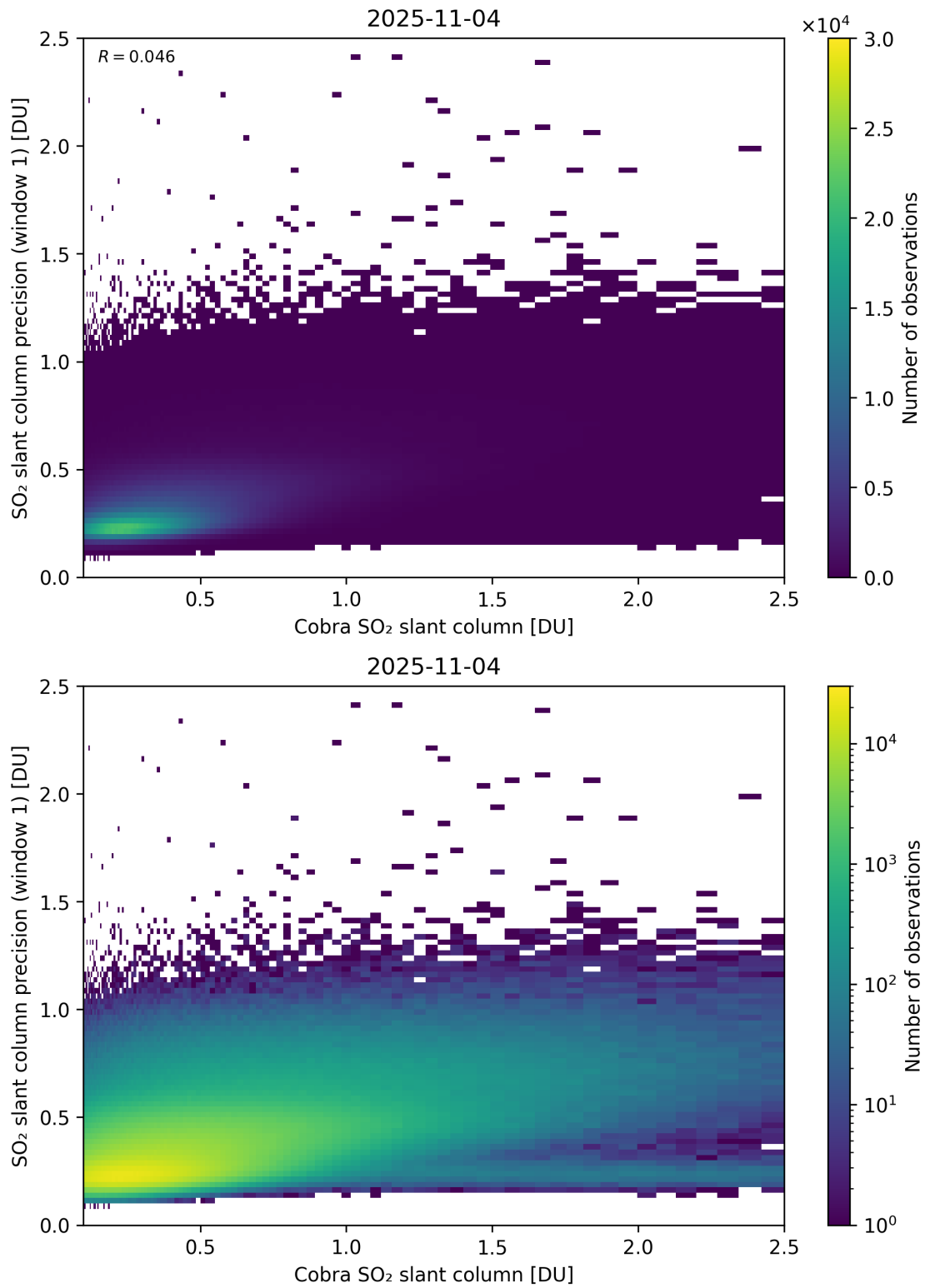
Figure 220: Scatter density plot of “Cobra SO 2 slant column” against “SO 2 slant column precision (window 1)” for 2025-11-03 to 2025-11-05.
