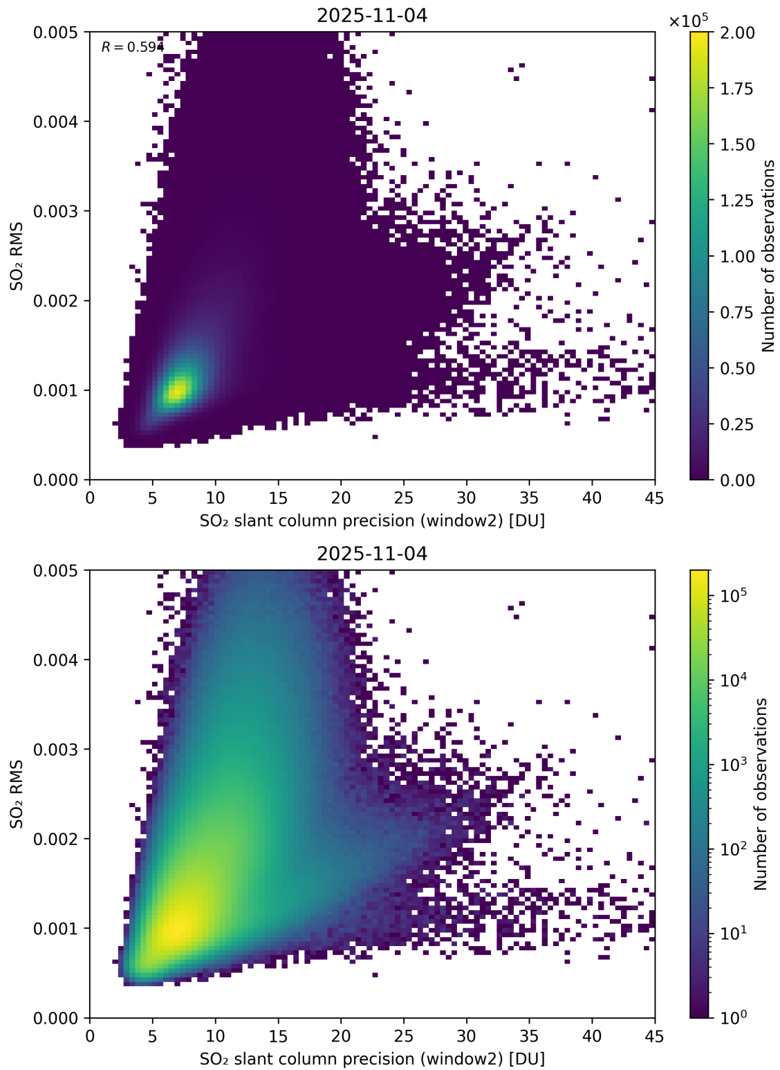
Figure 295: Scatter density plot of “SO 2 slant column precision (window2)” against “SO 2 RMS” for 2025-11-03 to 2025-11-05.
