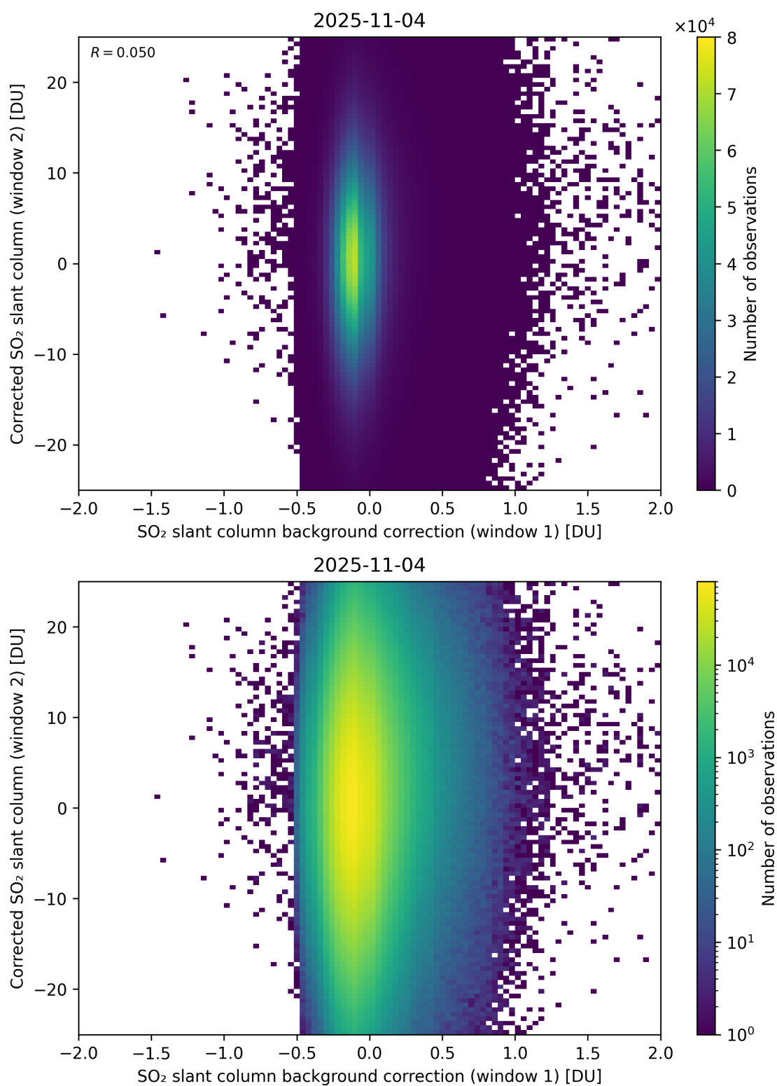
Figure 115: Scatter density plot of “SO 2 slant column background correction (window 1)” against “Corrected SO 2 slant column (window 2)” for 2025-11-03 to 2025-11-05.
