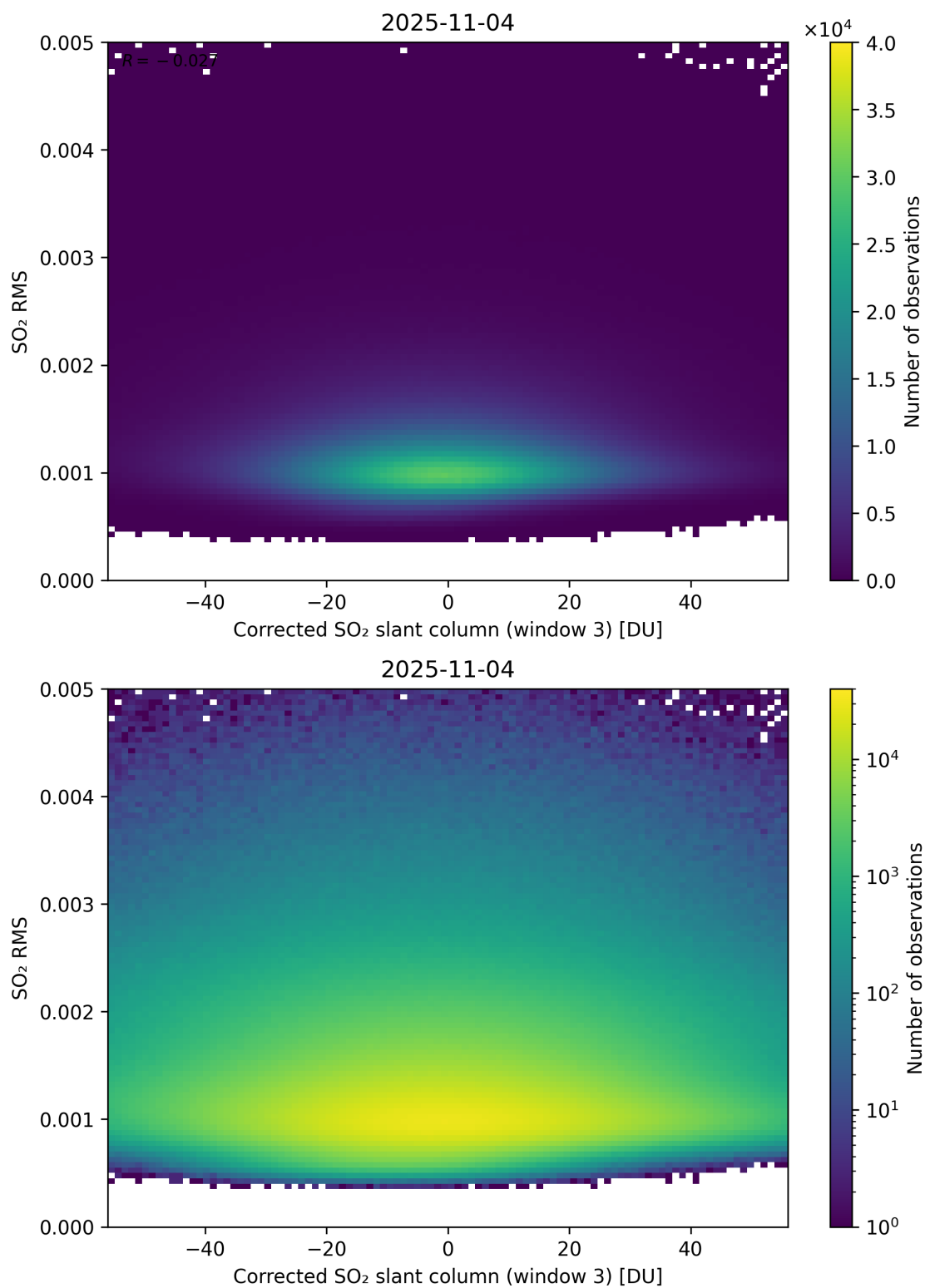
Figure 258: Scatter density plot of “Corrected SO 2 slant column (window 3)” against “SO 2 RMS” for 2025-11-03 to 2025-11-05.
