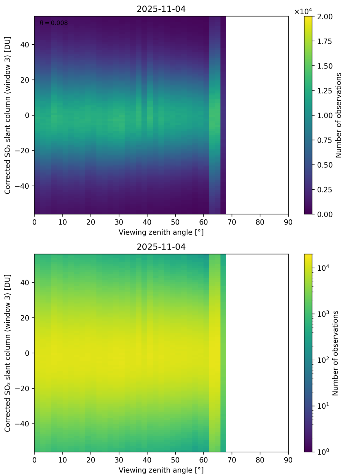
Figure 375: Scatter density plot of “Viewing zenith angle” against “Corrected SO 2 slant column (window 3)” for 2025-11-03 to 2025-11-05.
