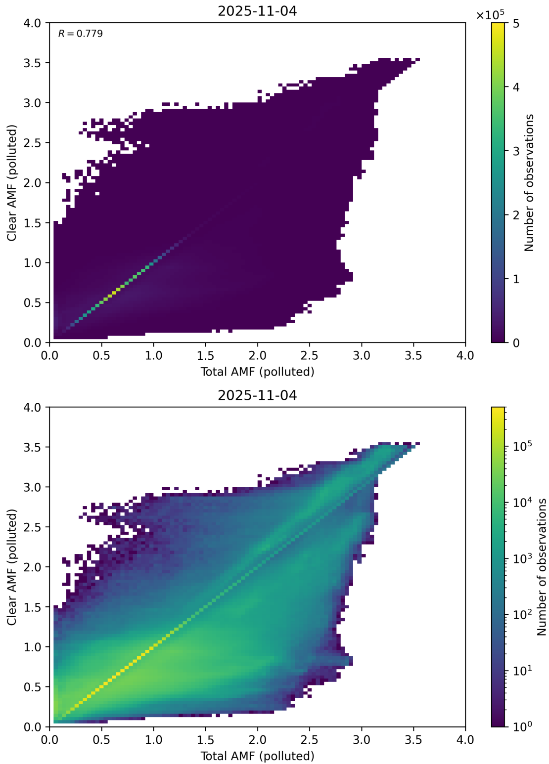
Figure 321: Scatter density plot of “Total AMF (polluted)” against “Clear AMF (polluted)” for 2025-11-03 to 2025-11-05.
