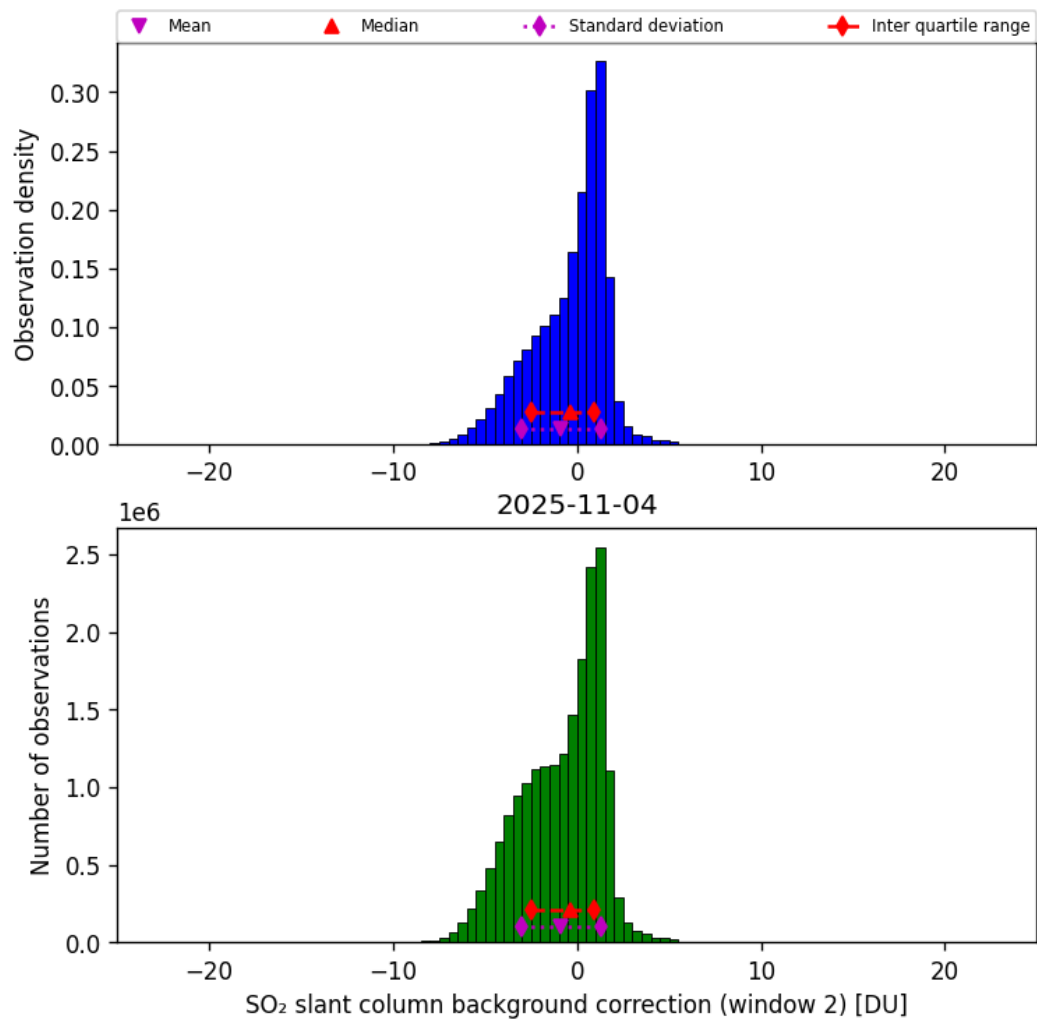
Figure 70: Histogram of “SO 2 slant column background correction (window 2)” for 2025-11-03 to 2025-11-05
