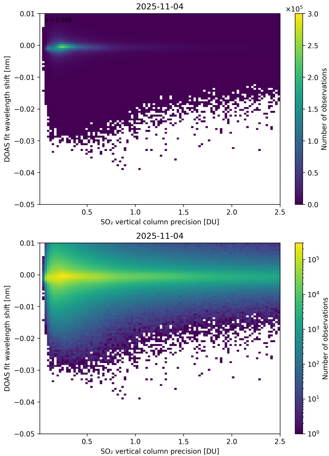
Figure 332: Scatter density plot of “SO 2 vertical column precision” against “DOAS fit wavelength shift” for 2025-11-03 to 2025-11-05.
