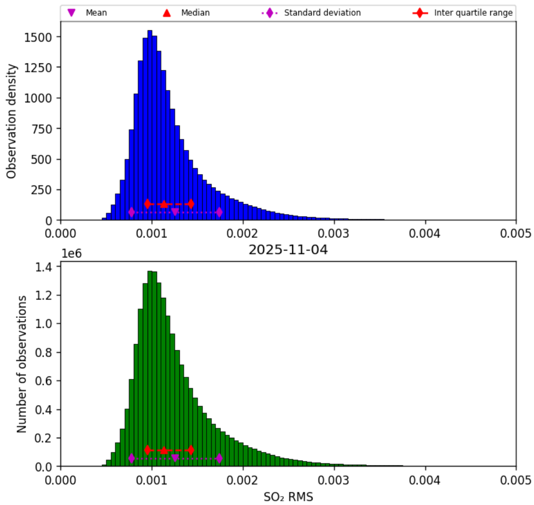
Figure 78: Histogram of “SO 2 RMS” for 2025-11-03 to 2025-11-05
