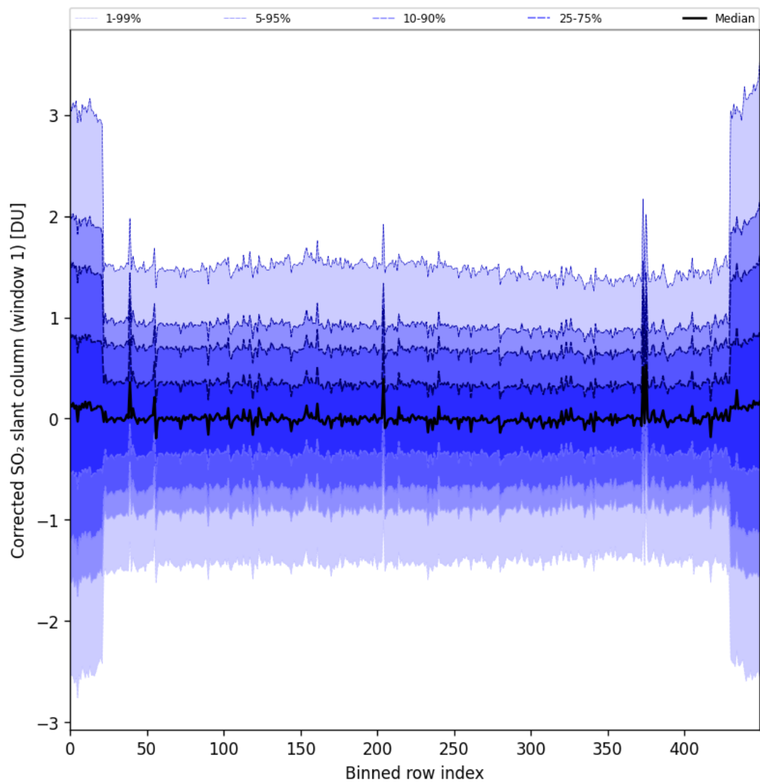
Figure 91: Along track statistics of “Corrected SO 2 slant column (window 1)” for 2025-11-03 to 2025-11-05
