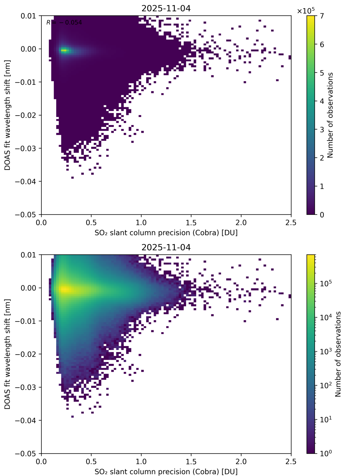
Figure 202: Scatter density plot of “SO 2 slant column precision (Cobra)” against “DOAS fit wavelength shift” for 2025-11-03 to 2025-11-05.
