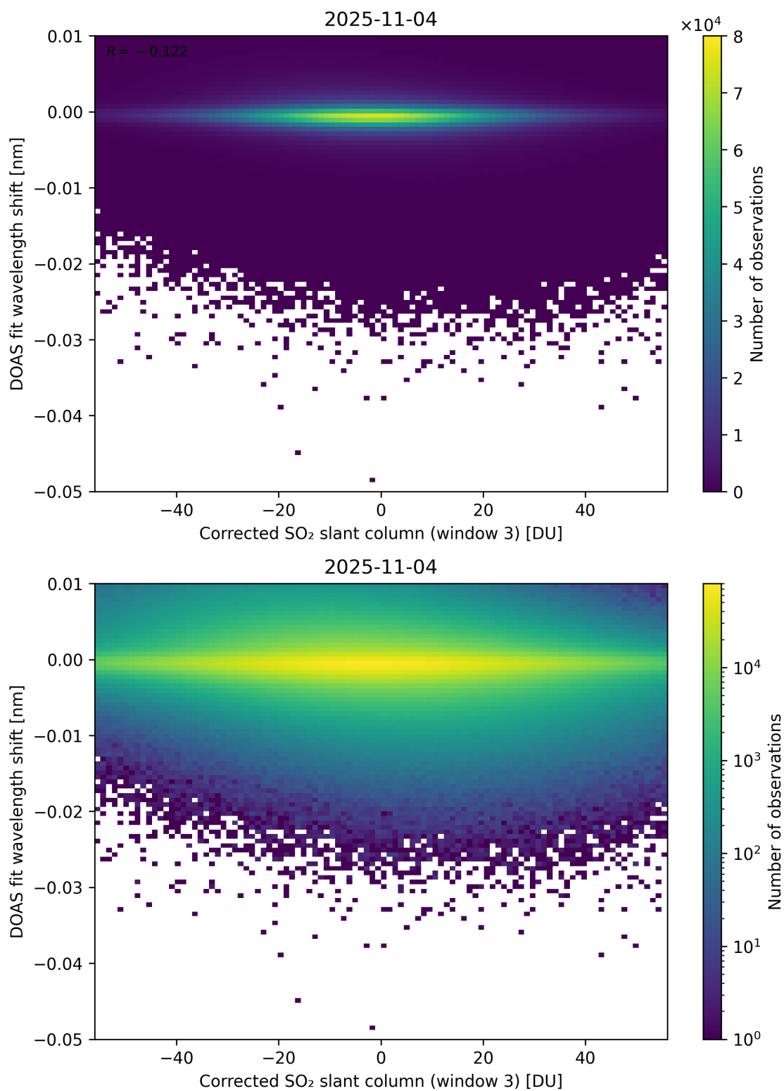
Figure 256: Scatter density plot of “Corrected SO 2 slant column (window 3)” against “DOAS fit wavelength shift” for 2025-11-03 to 2025-11-05.
