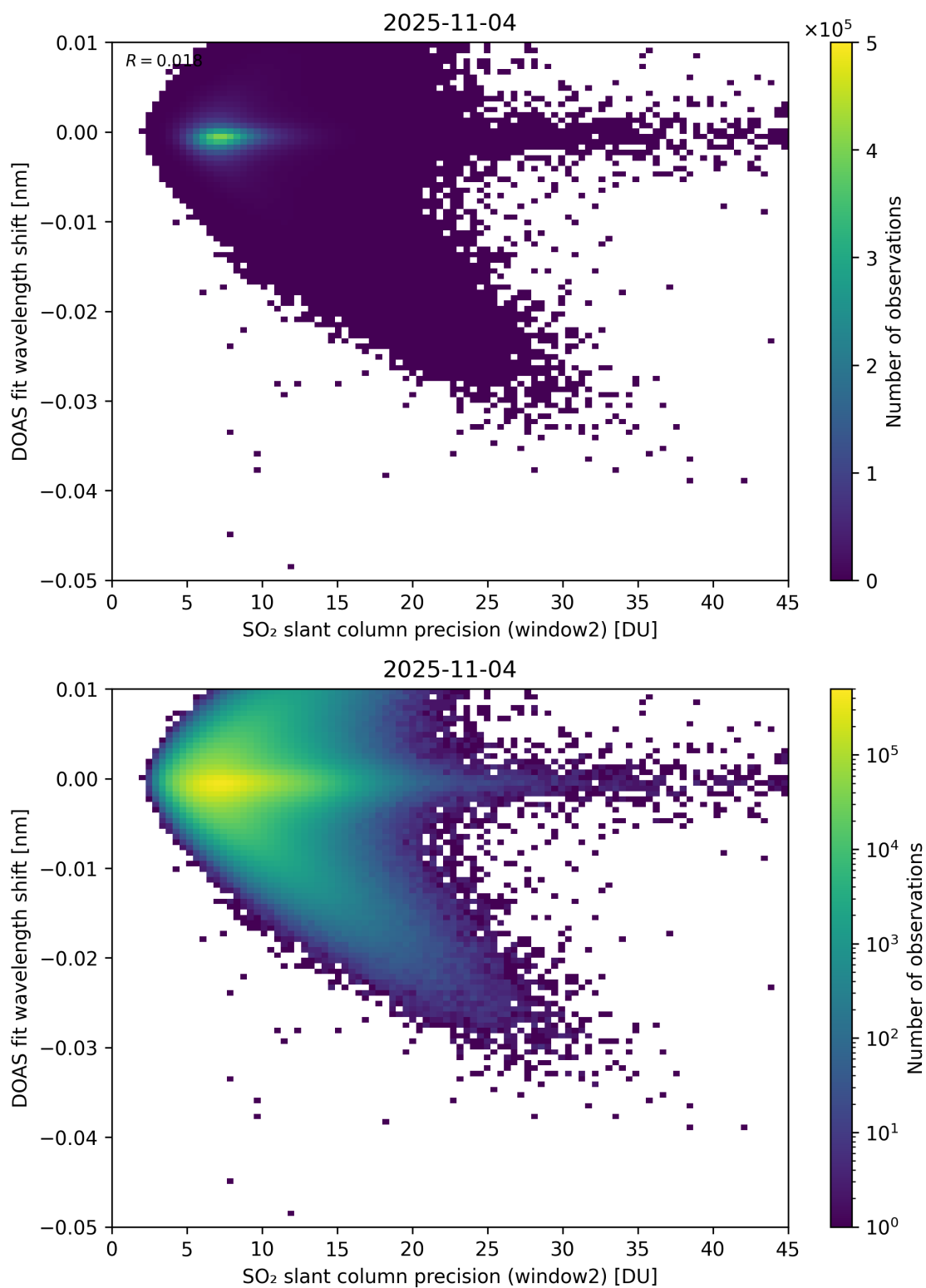
Figure 293: Scatter density plot of “SO 2 slant column precision (window2)” against “DOAS fit wavelength shift” for 2025-11-03 to 2025-11-05.
