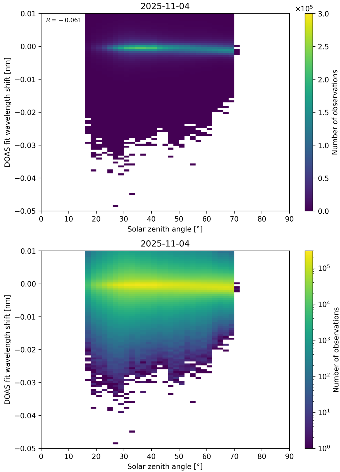
Figure 174: Scatter density plot of “Solar zenith angle” against “DOAS fit wavelength shift” for 2025-11-03 to 2025-11-05.
