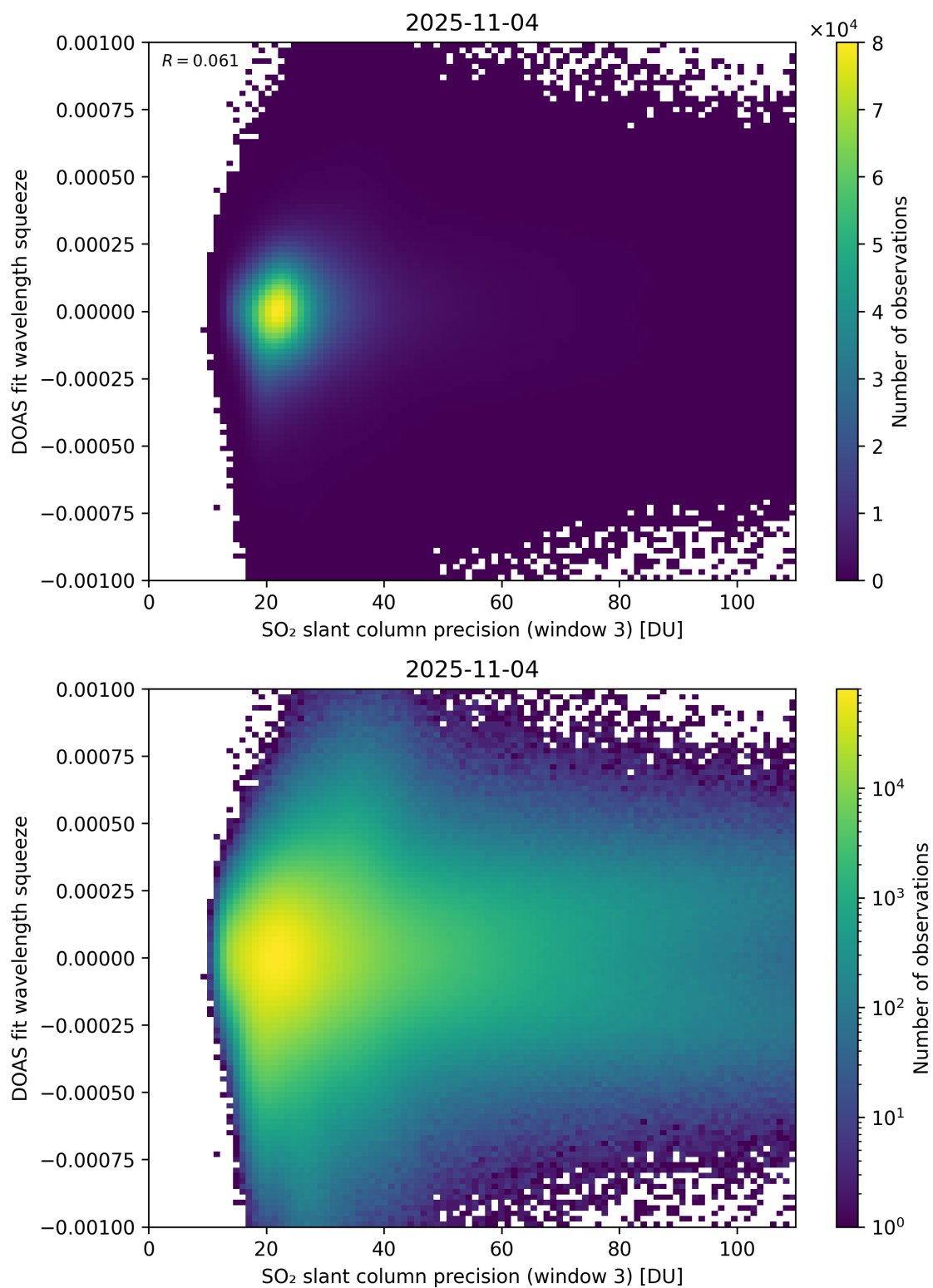
Figure 309: Scatter density plot of “SO 2 slant column precision (window 3)” against “DOAS fit wavelength squeeze” for 2025-11-03 to 2025-11-05.
