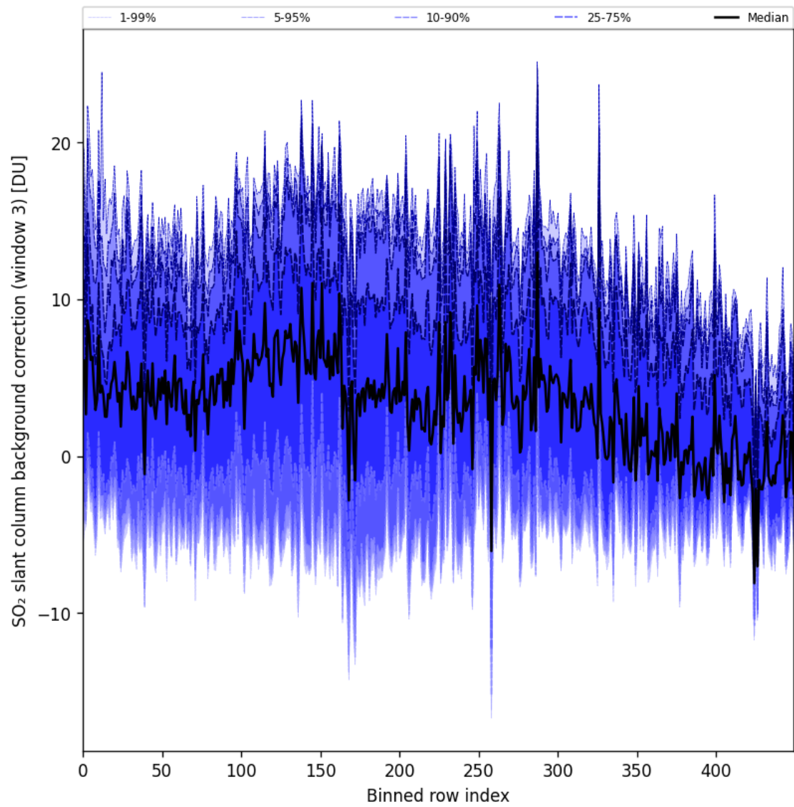
Figure 100: Along track statistics of “SO 2 slant column background correction (window 3)” for 2025-11-03 to 2025-11-05
