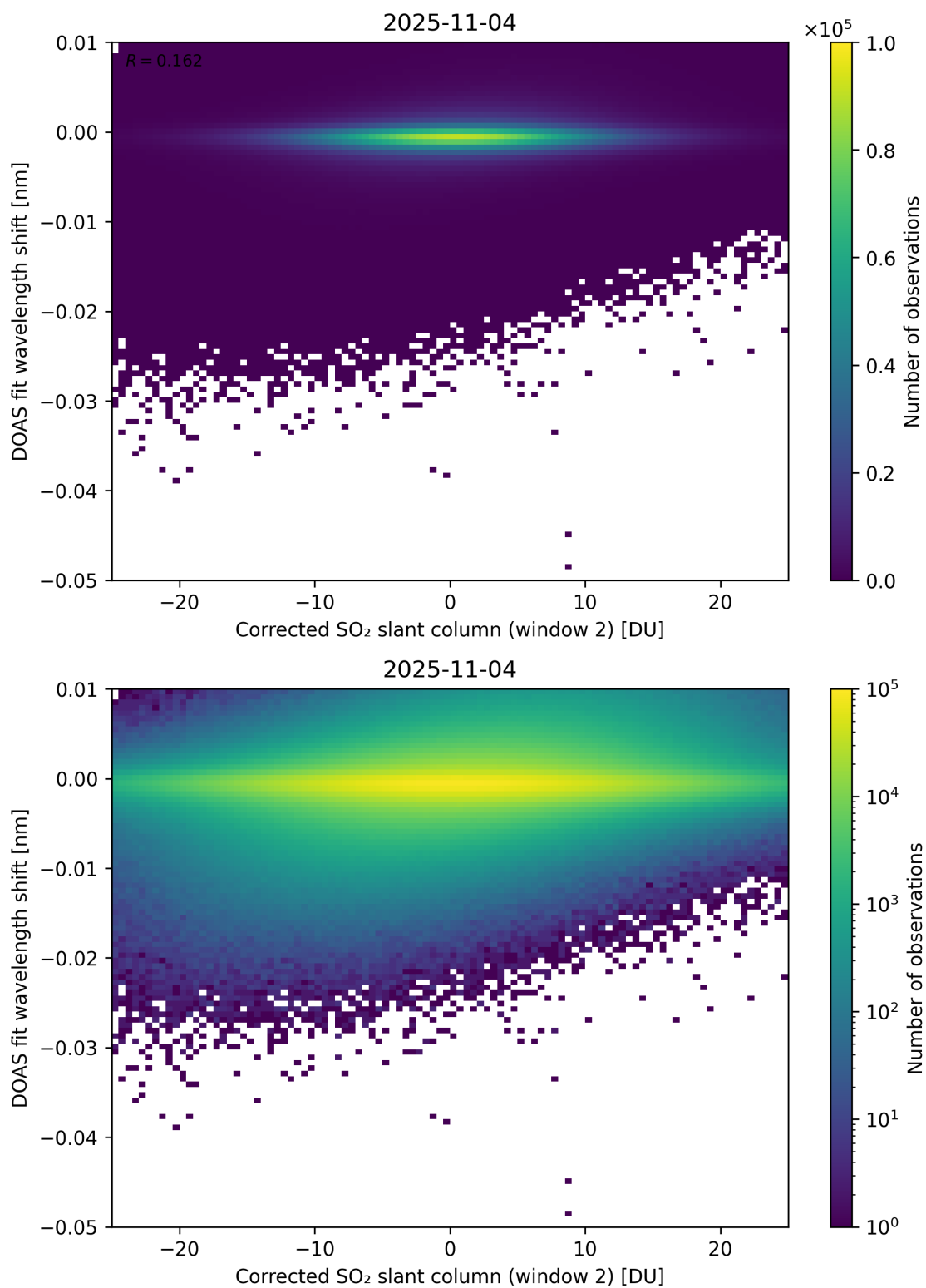
Figure 246: Scatter density plot of “Corrected SO 2 slant column (window 2)” against “DOAS fit wavelength shift” for 2025-11-03 to 2025-11-05.
