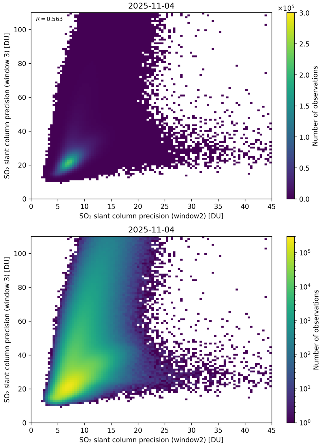
Figure 300: Scatter density plot of “SO 2 slant column precision (window2)” against “SO 2 slant column precision (window 3)” for 2025-11-03 to 2025-11-05.
