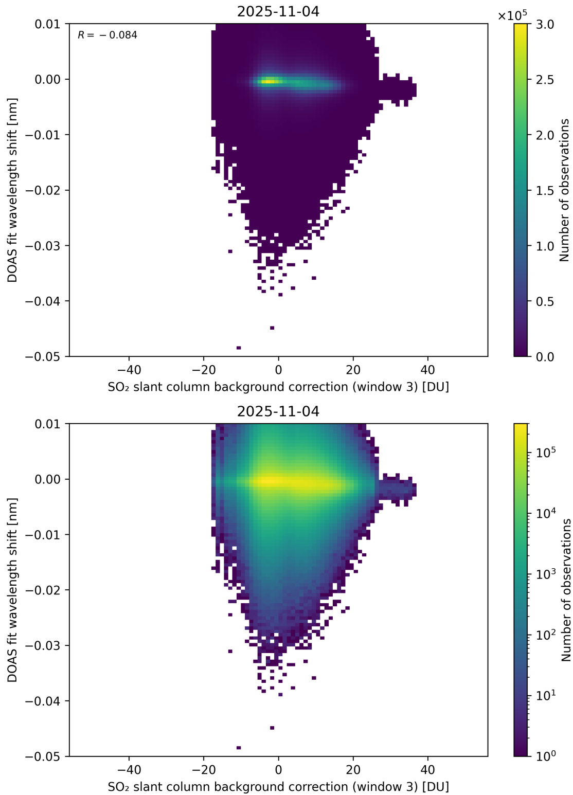
Figure 132: Scatter density plot of “SO 2 slant column background correction (window 3)” against “DOAS fit wavelength shift” for 2025-11-03 to 2025-11-05.
