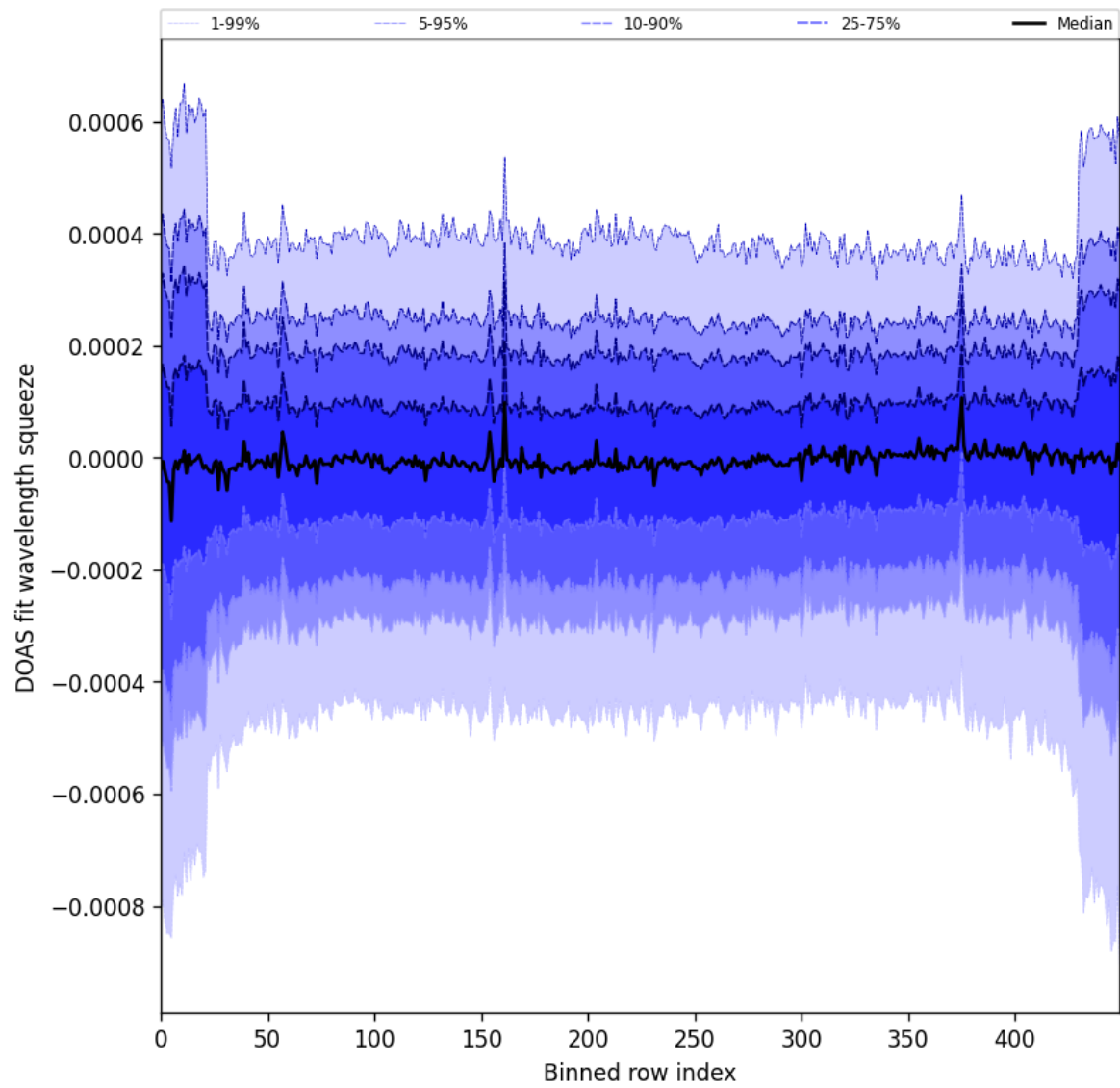
Figure 103: Along track statistics of “DOAS fit wavelength squeeze” for 2025-11-03 to 2025-11-05
