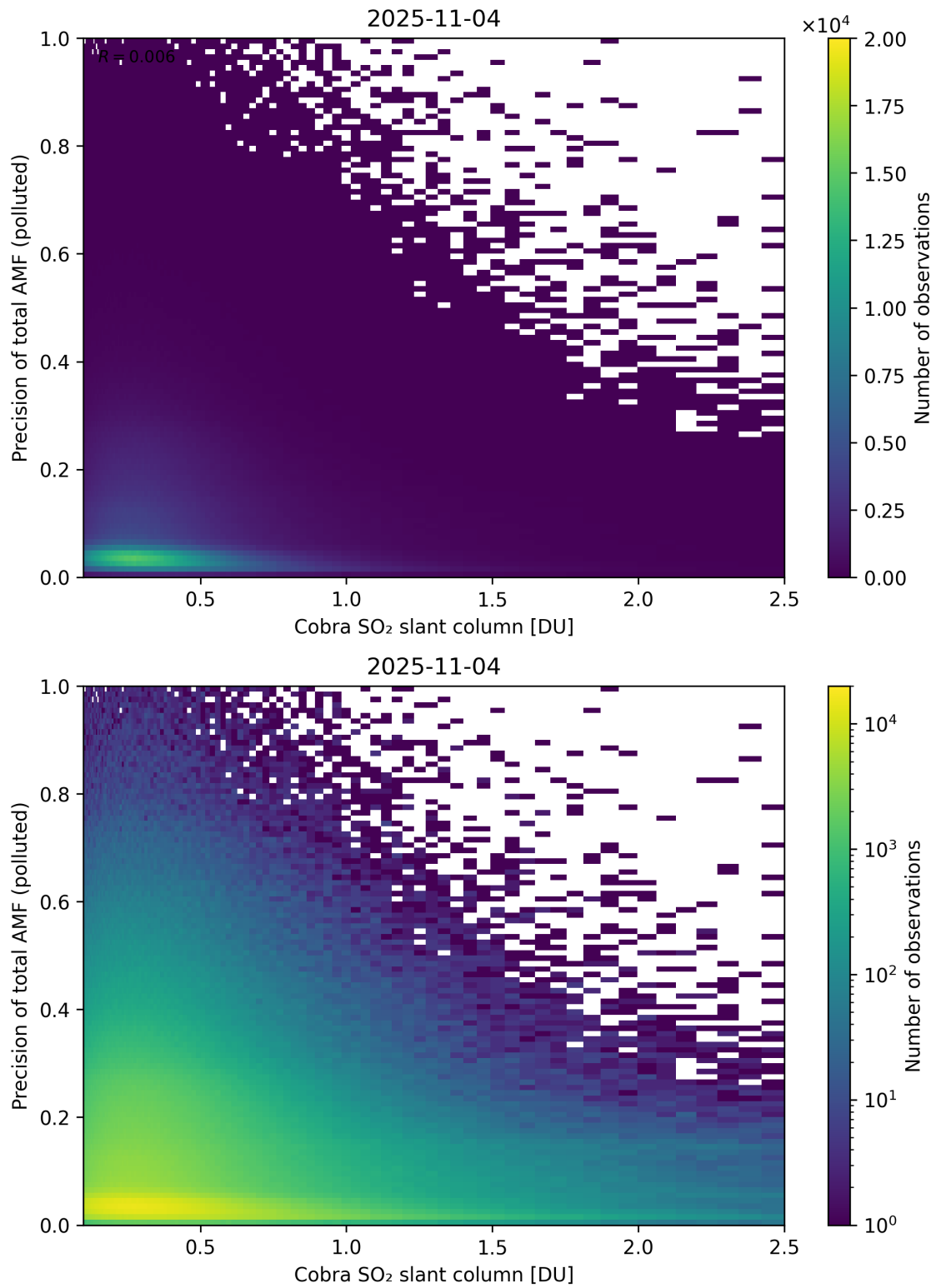
Figure 225: Scatter density plot of “Cobra SO 2 slant column” against “Precision of total AMF (polluted)” for 2025-11-03 to 2025-11-05.
