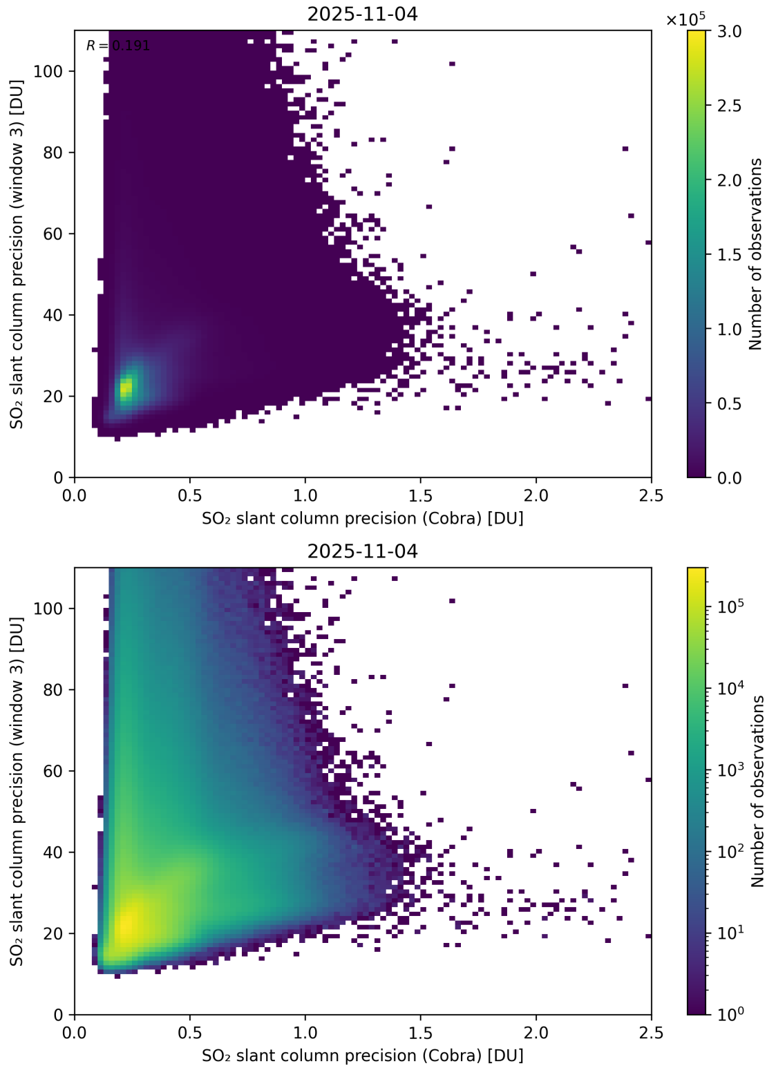
Figure 212: Scatter density plot of “SO 2 slant column precision (Cobra)” against “SO 2 slant column precision (window 3)” for 2025-11-03 to 2025-11-05.
