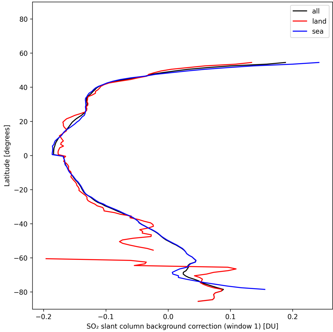
Figure 40: Zonal average of “SO 2 slant column background correction (window 1)” for 2025-11-03 to 2025-11-05.
