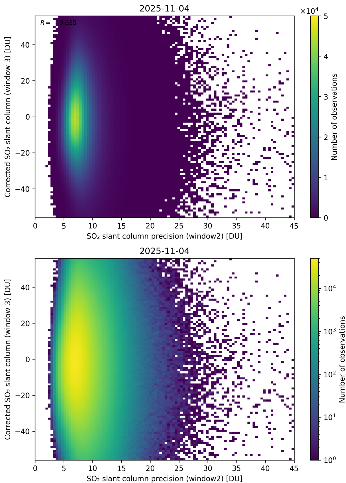
Figure 298: Scatter density plot of “SO 2 slant column precision (window2)” against “Corrected SO 2 slant column (window 3)” for 2025-11-03 to 2025-11-05.
