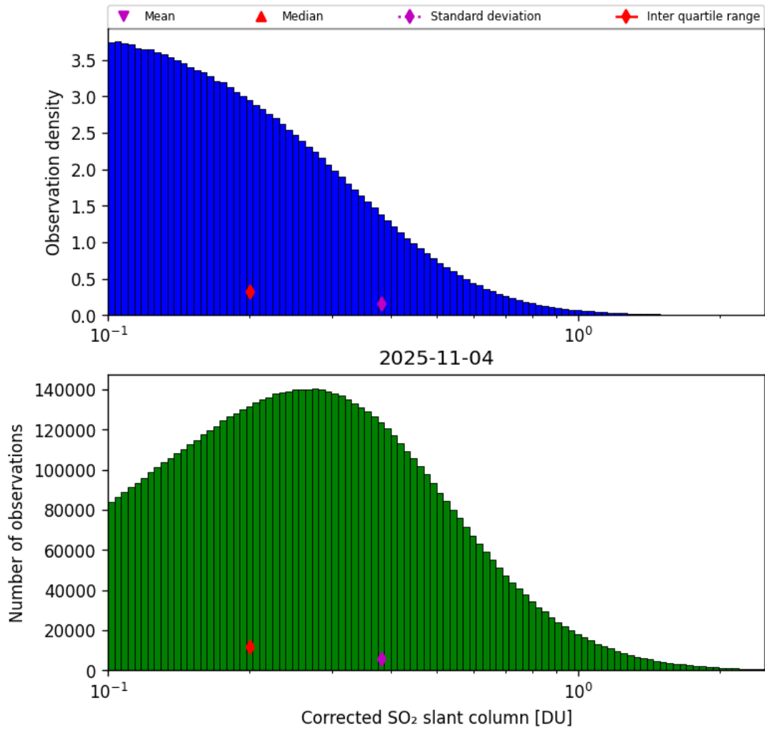
Figure 60: Histogram of “Corrected SO 2 slant column” for 2025-11-03 to 2025-11-05
