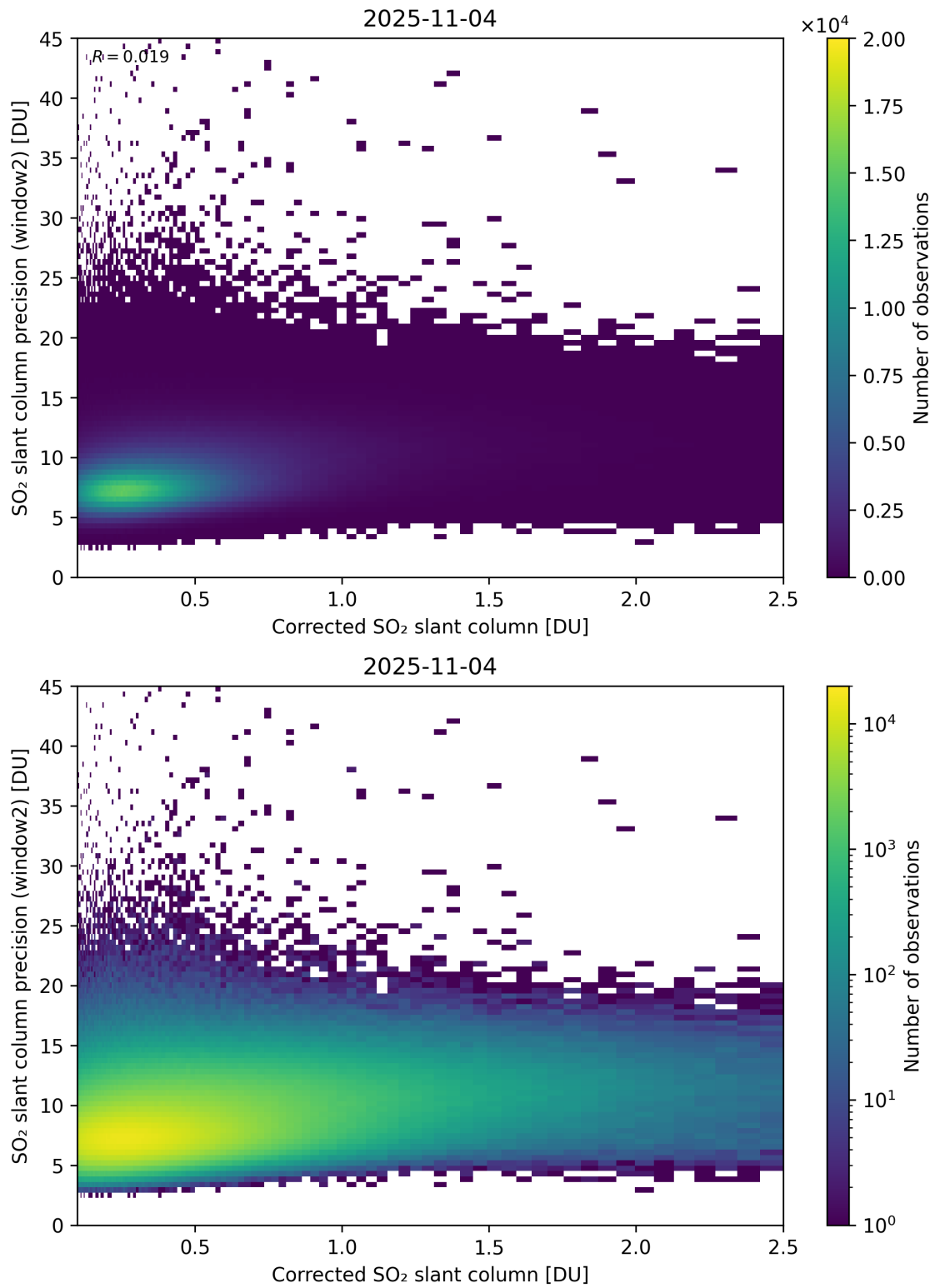
Figure 239: Scatter density plot of “Corrected SO 2 slant column” against “SO 2 slant column precision (window2)” for 2025-11-03 to 2025-11-05.
