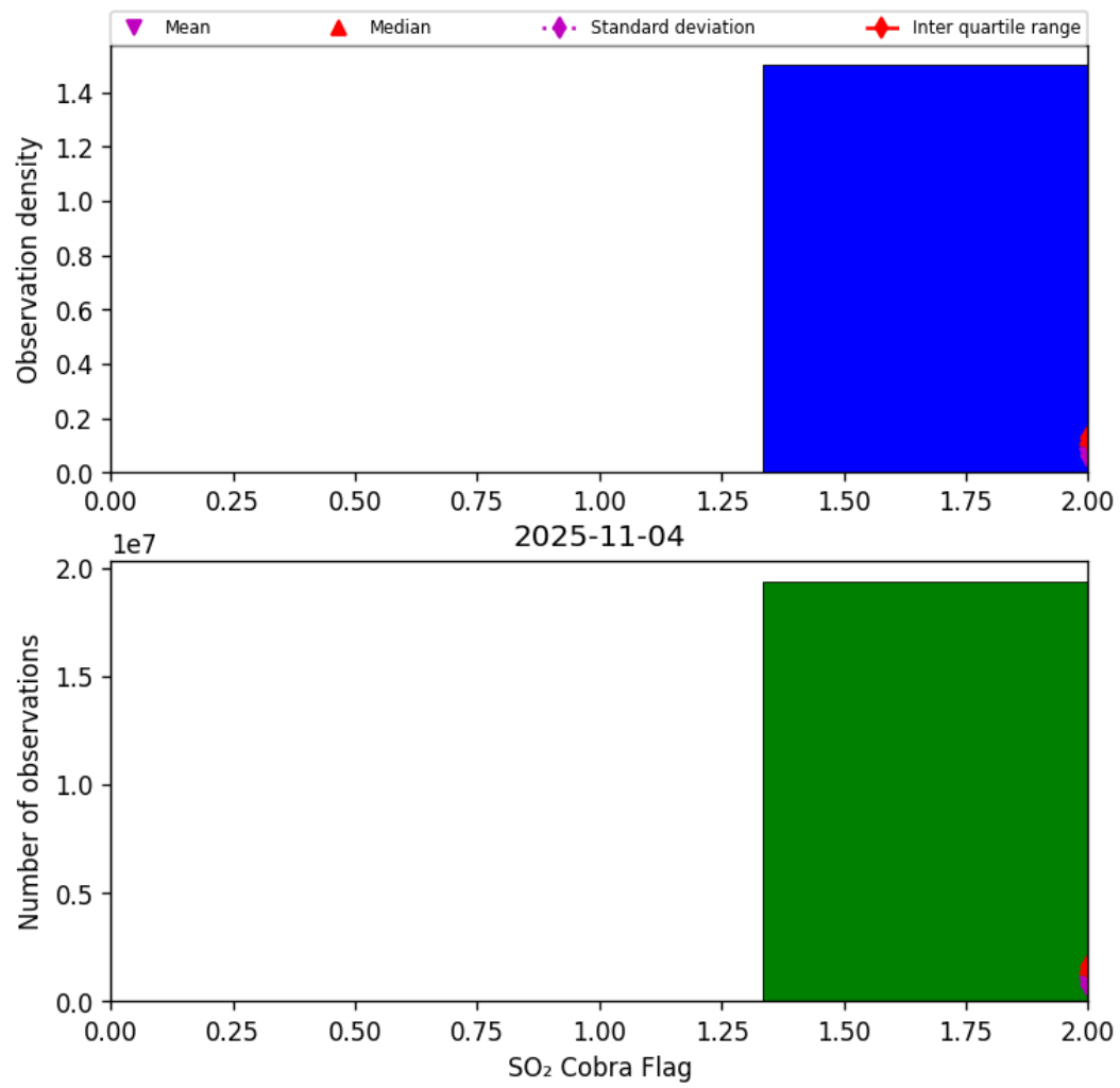
Figure 75: Histogram of “SO 2 Cobra Flag” for 2025-11-03 to 2025-11-05
