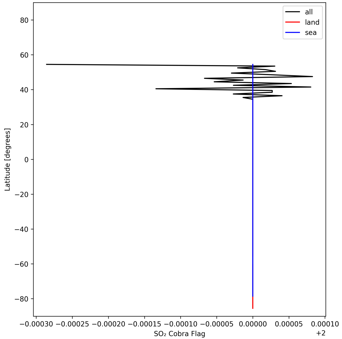
Figure 49: Zonal average of "SO 2 Cobra Flag" for 2025-11-03 to 2025-11-05.
