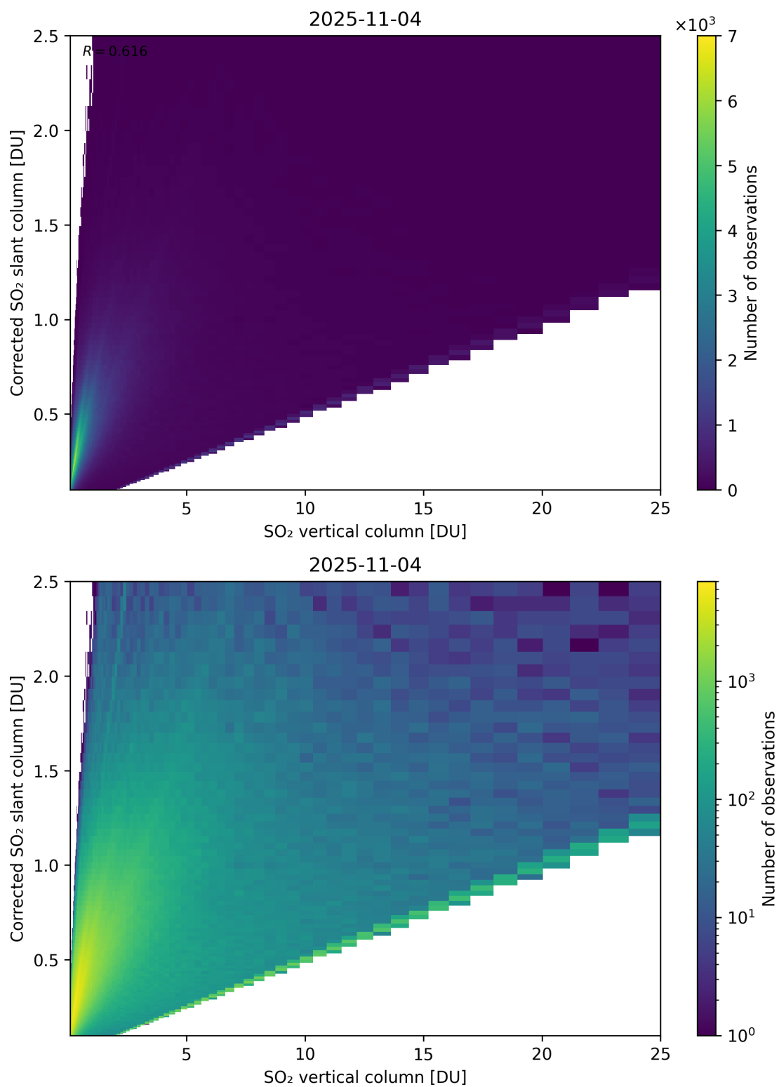
Figure 351: Scatter density plot of “SO 2 vertical column” against “Corrected SO 2 slant column” for 2025-11-03 to 2025-11-05.
