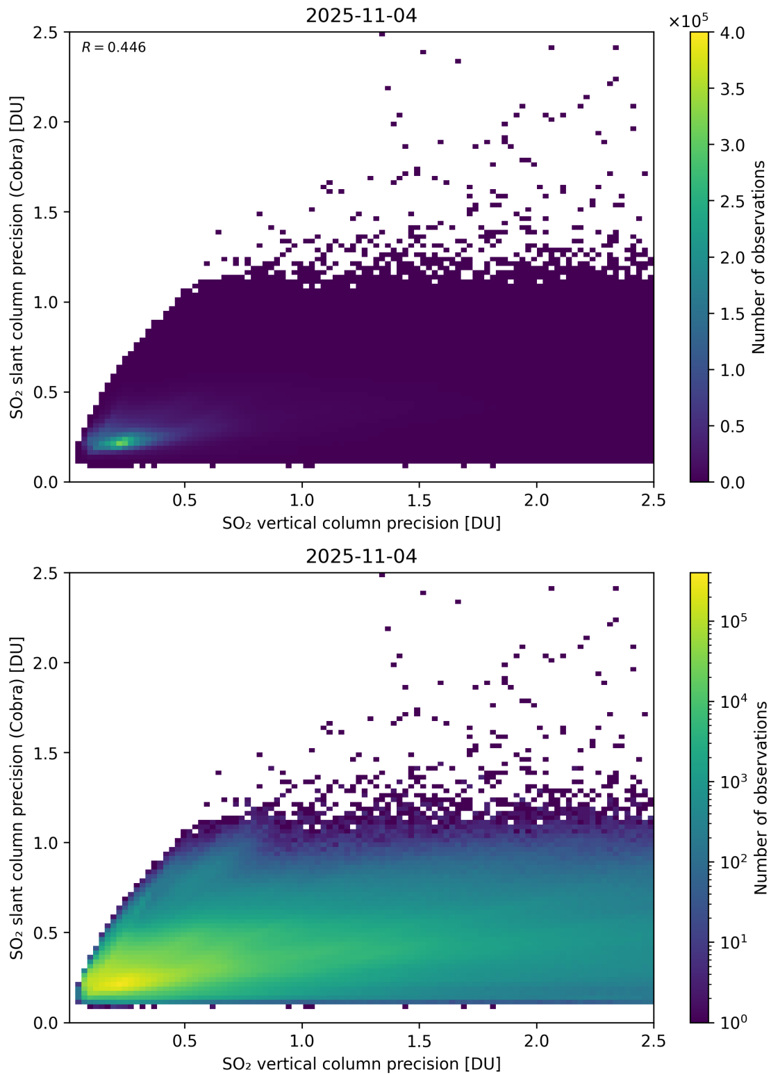
Figure 337: Scatter density plot of “SO 2 vertical column precision” against “SO 2 slant column precision (Cobra)” for 2025-11-03 to 2025-11-05.
