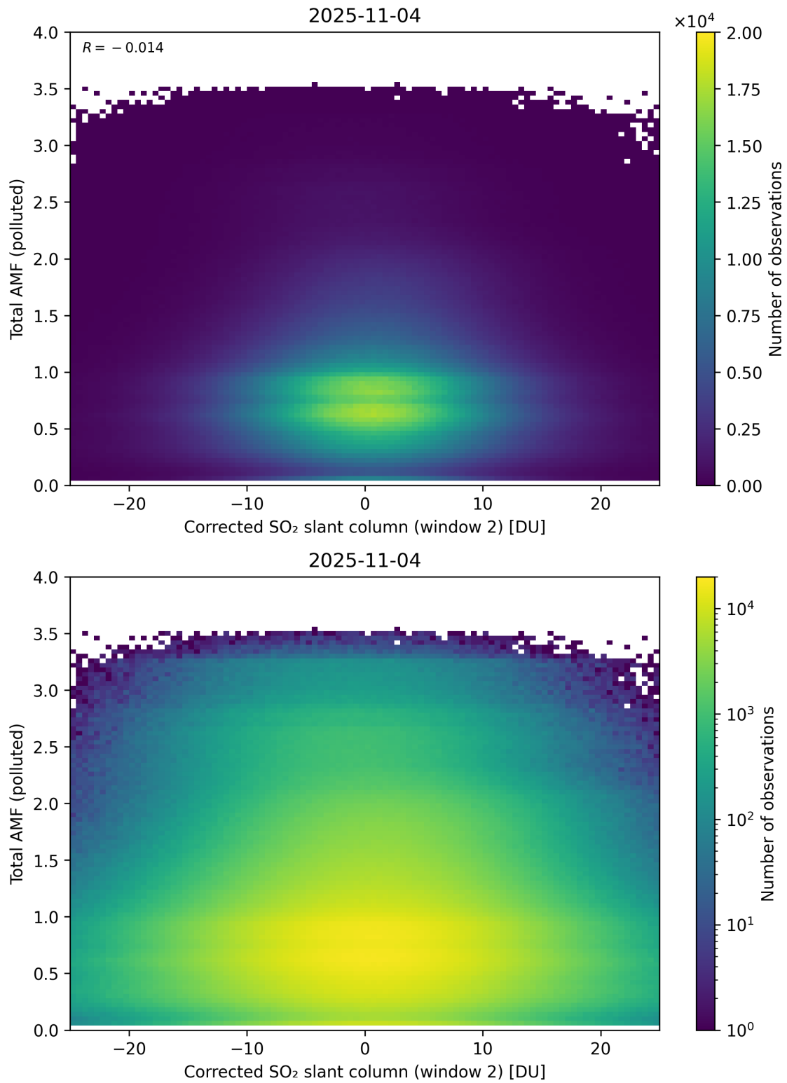
Figure 253: Scatter density plot of “Corrected SO 2 slant column (window 2)” against “Total AMF (polluted)” for 2025-11-03 to 2025-11-05.
