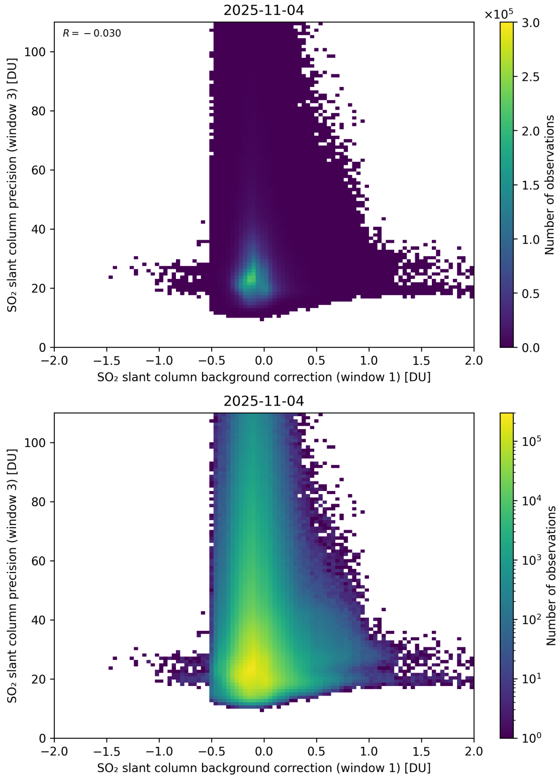
Figure 119: Scatter density plot of “SO 2 slant column background correction (window 1)” against “SO 2 slant column precision (window 3)” for 2025-11-03 to 2025-11-05.
