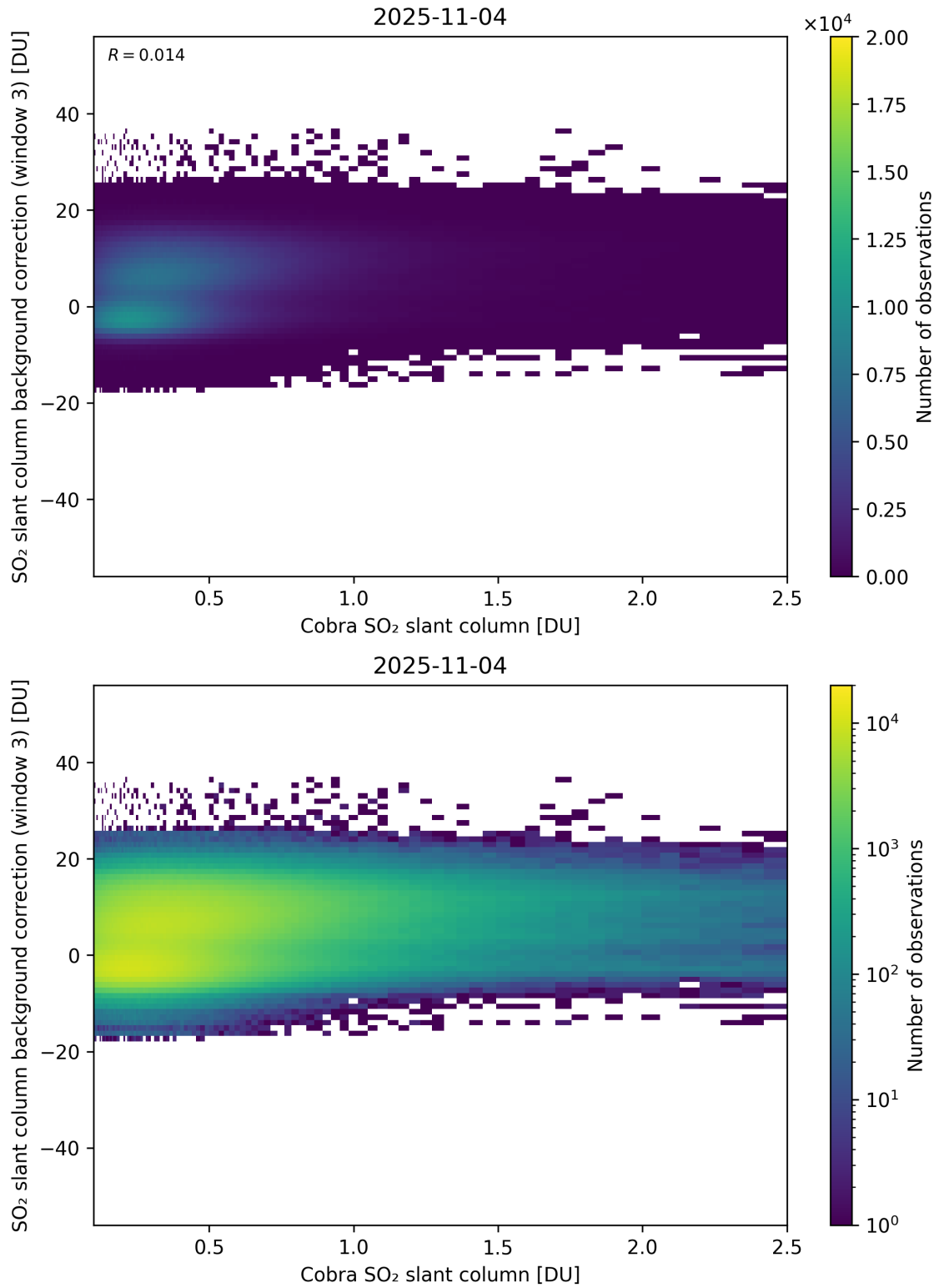
Figure 195: Scatter density plot of “Cobra SO 2 slant column” against “SO 2 slant column background correction (window 3)” for 2025-11-03 to 2025-11-05.
