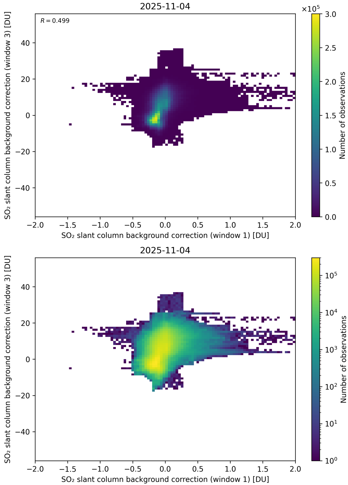
Figure 110: Scatter density plot of “SO 2 slant column background correction (window 1)” against “SO 2 slant column background correction (window 3)” for 2025-11-03 to 2025-11-05.
