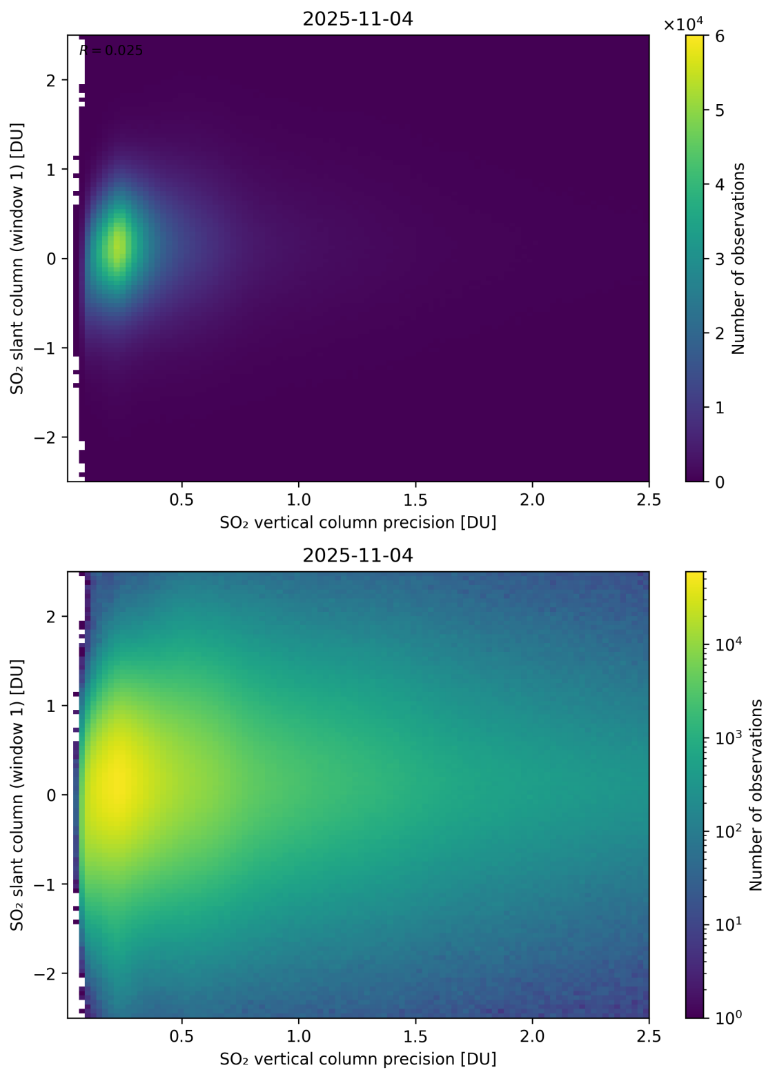
Figure 341: Scatter density plot of “SO 2 vertical column precision” against “SO 2 slant column (window 1)” for 2025-11-03 to 2025-11-05.
