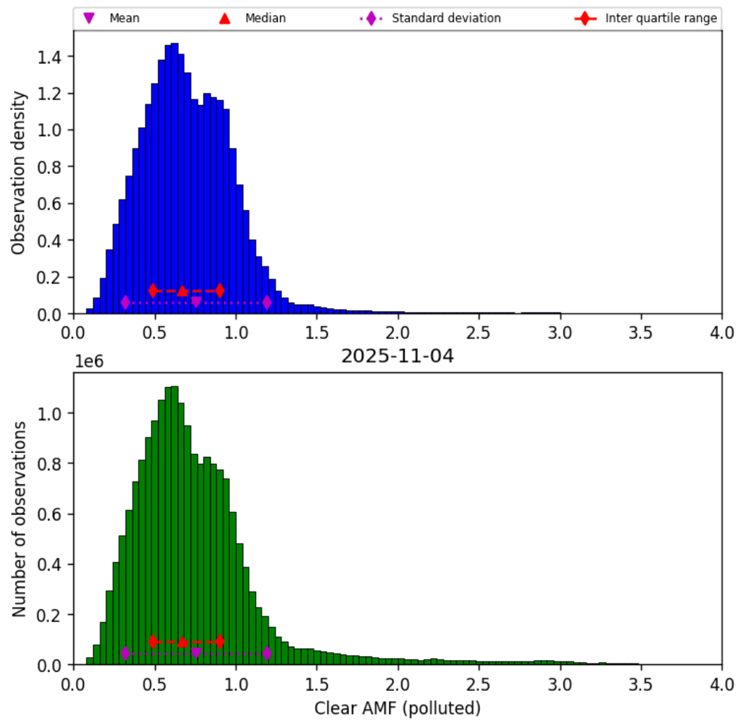
Figure 81: Histogram of “Clear AMF (polluted)” for 2025-11-03 to 2025-11-05
