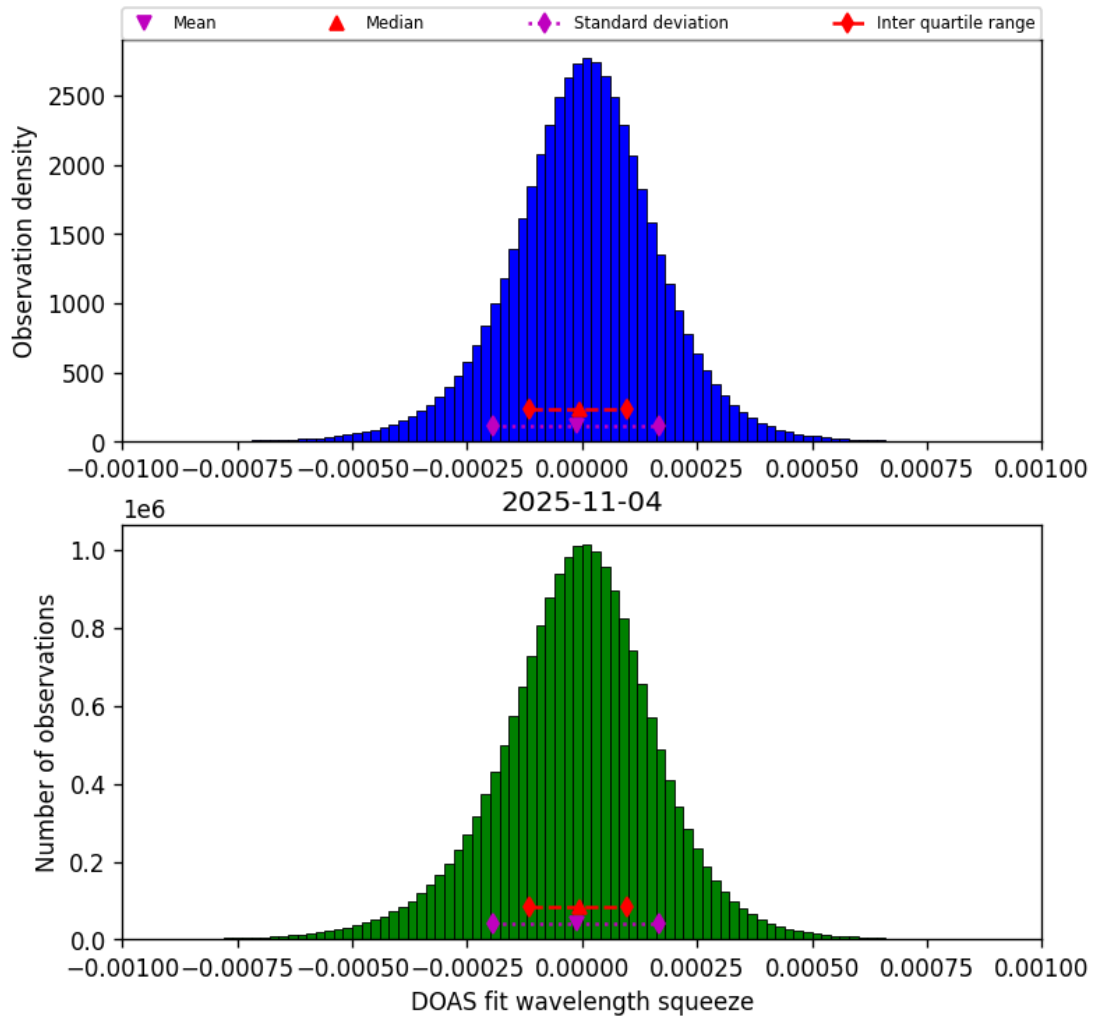
Figure 77: Histogram of “DOAS fit wavelength squeeze” for 2025-11-03 to 2025-11-05
