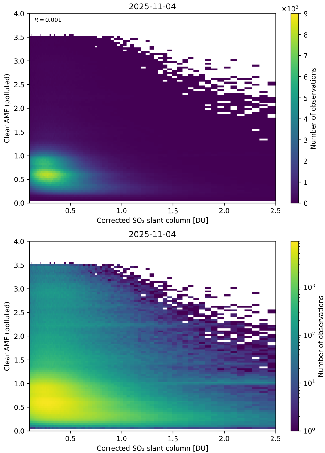
Figure 232: Scatter density plot of “Corrected SO 2 slant column” against “Clear AMF (polluted)” for 2025-11-03 to 2025-11-05.
