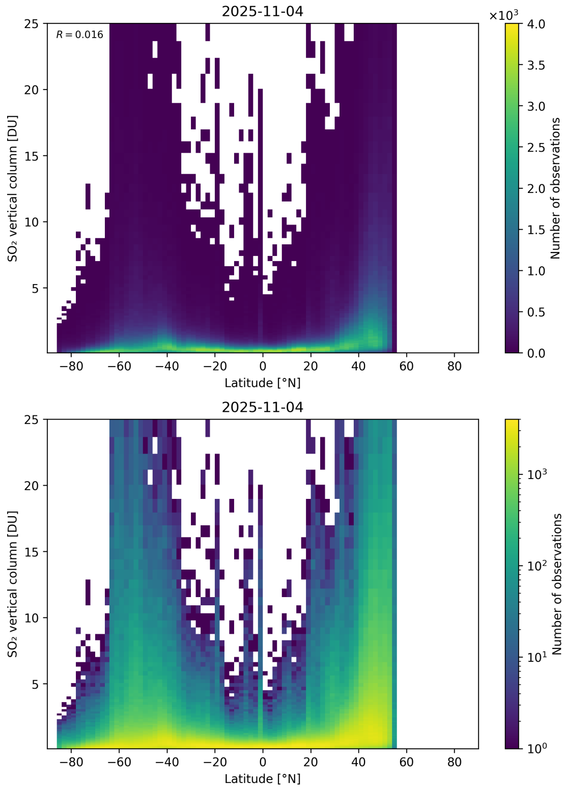
Figure 169: Scatter density plot of “Latitude” against “SO 2 vertical column” for 2025-11-03 to 2025-11-05.
