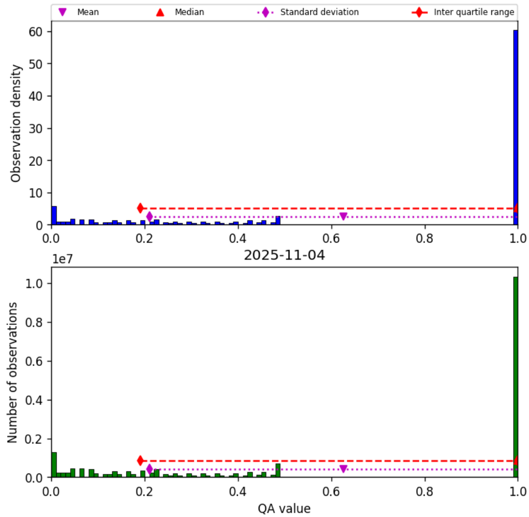
Figure 57: Histogram of “QA value” for 2025-11-03 to 2025-11-05
