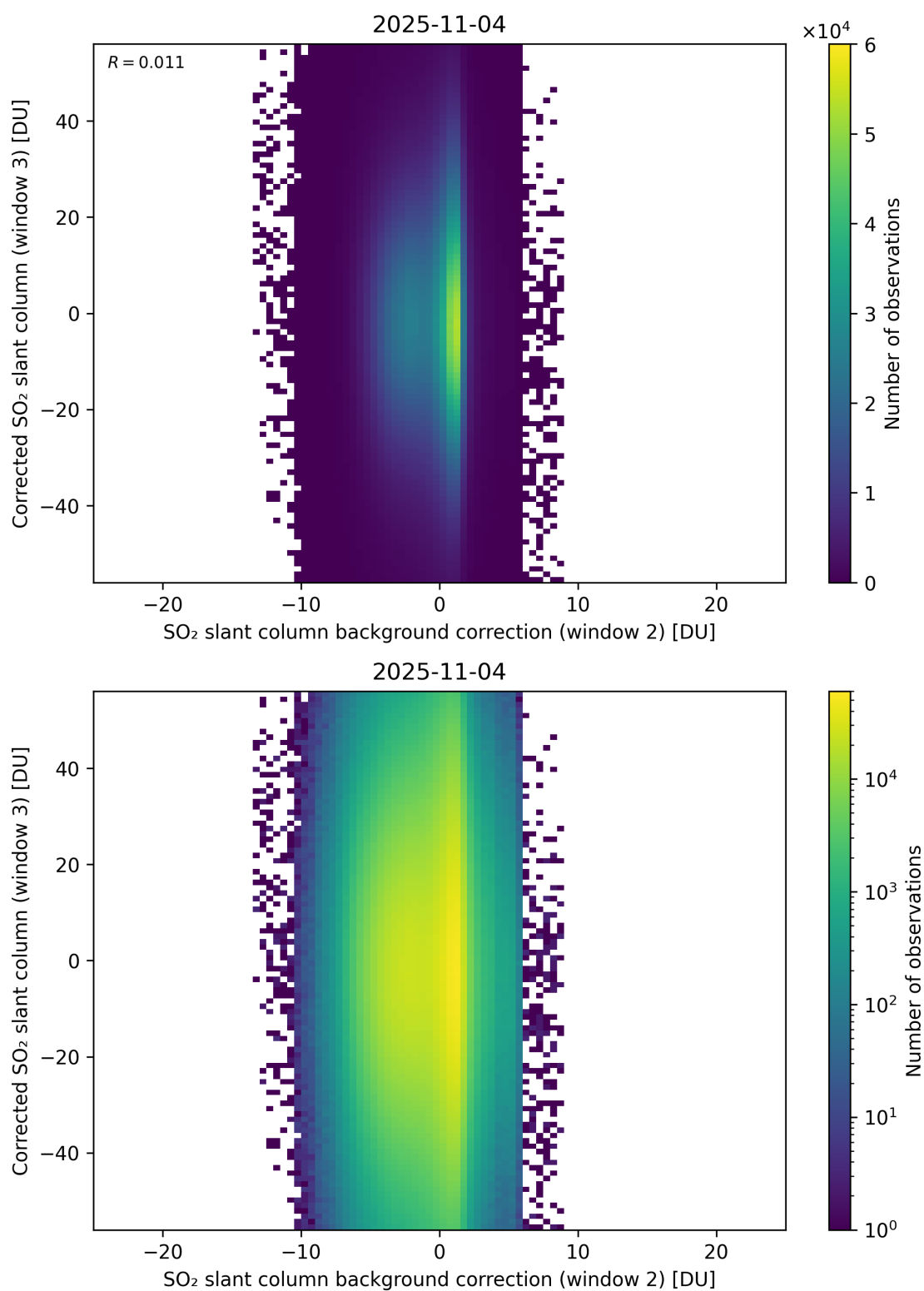
Figure 127: Scatter density plot of “SO 2 slant column background correction (window 2)” against “Corrected SO 2 slant column (window 3)” for 2025-11-03 to 2025-11-05.
