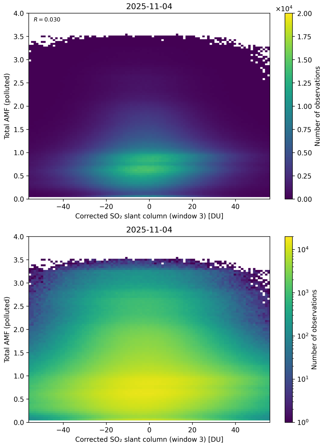
Figure 260: Scatter density plot of “Corrected SO 2 slant column (window 3)” against “Total AMF (polluted)” for 2025-11-03 to 2025-11-05.
