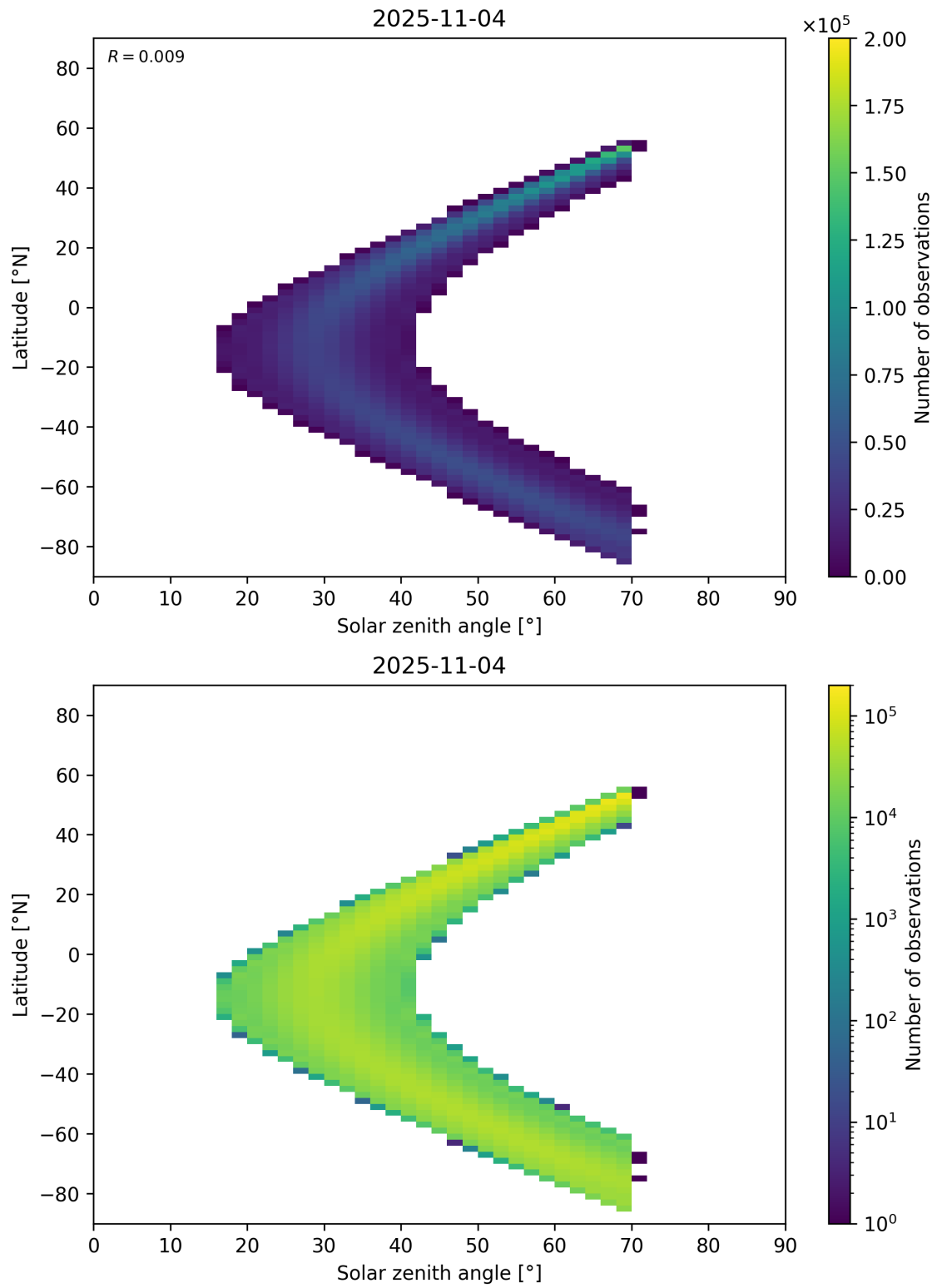
Figure 177: Scatter density plot of “Solar zenith angle” against “Latitude” for 2025-11-03 to 2025-11-05.
