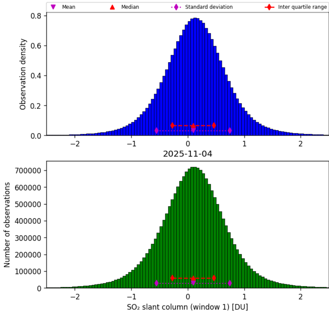
Figure 63: Histogram of “SO 2 slant column (window 1)” for 2025-11-03 to 2025-11-05
