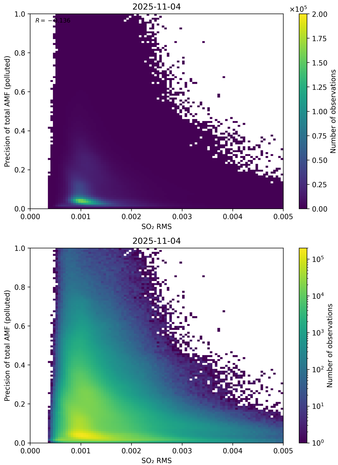
Figure 149: Scatter density plot of “SO 2 RMS” against “Precision of total AMF (polluted)” for 2025-11-03 to 2025-11-05.
