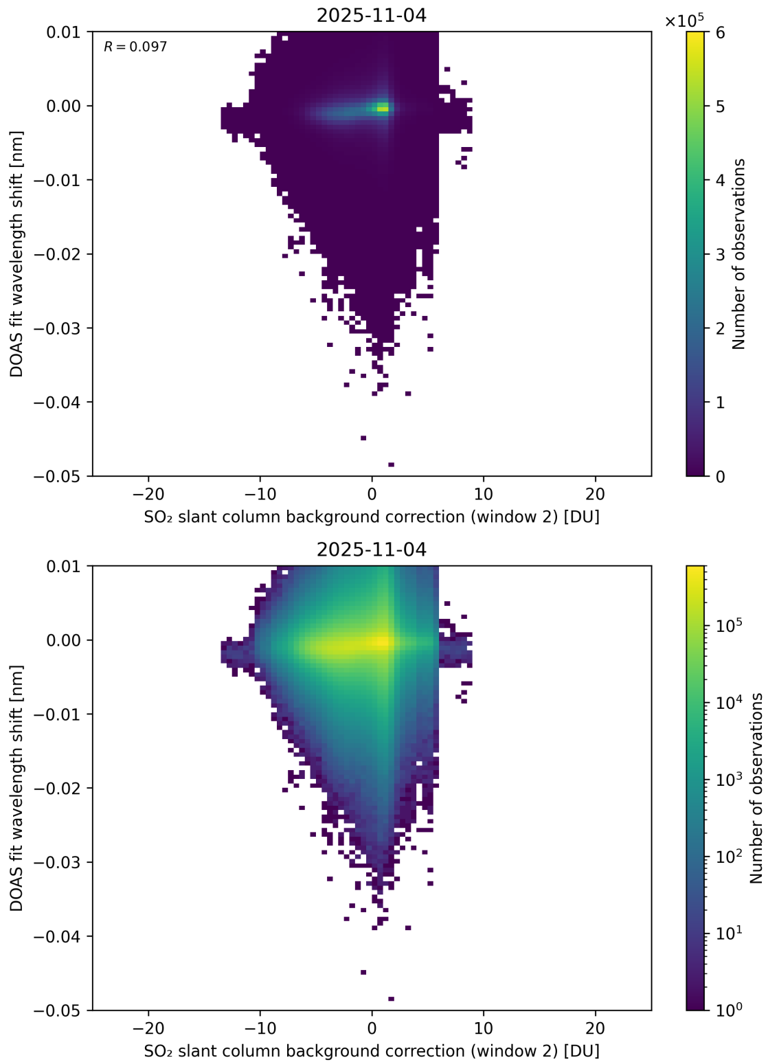
Figure 123: Scatter density plot of “SO 2 slant column background correction (window 2)” against “DOAS fit wavelength shift” for 2025-11-03 to 2025-11-05.
