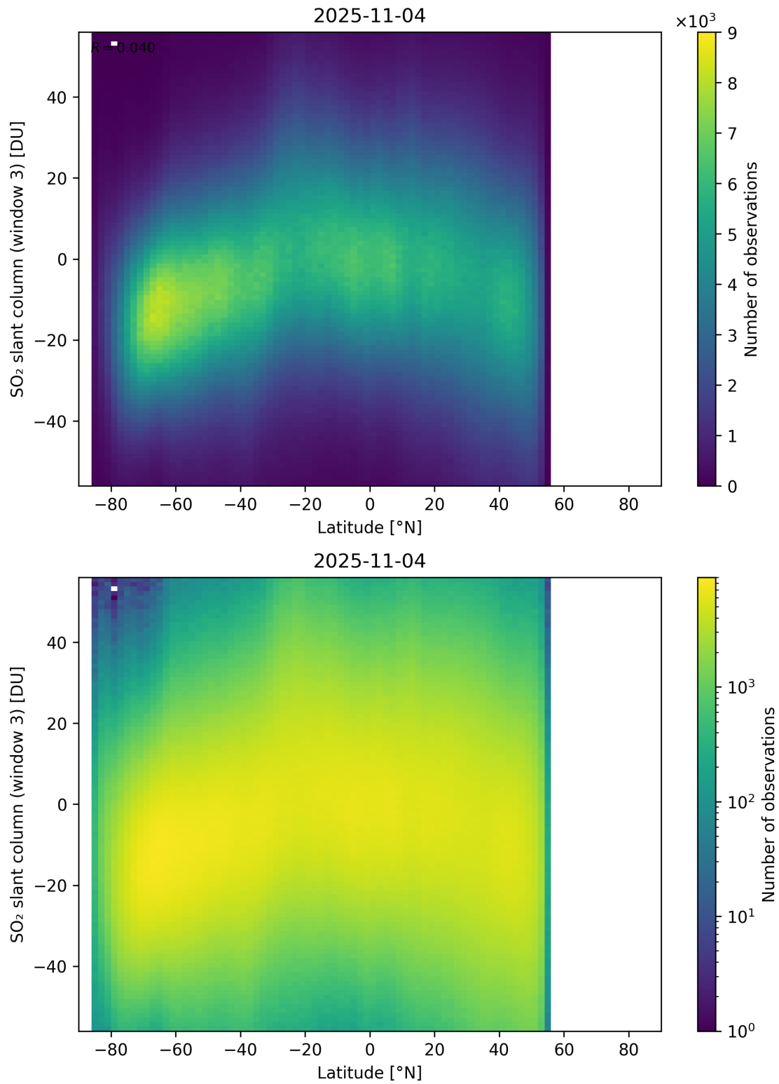
Figure 165: Scatter density plot of “Latitude” against “SO 2 slant column (window 3)” for 2025-11-03 to 2025-11-05.
