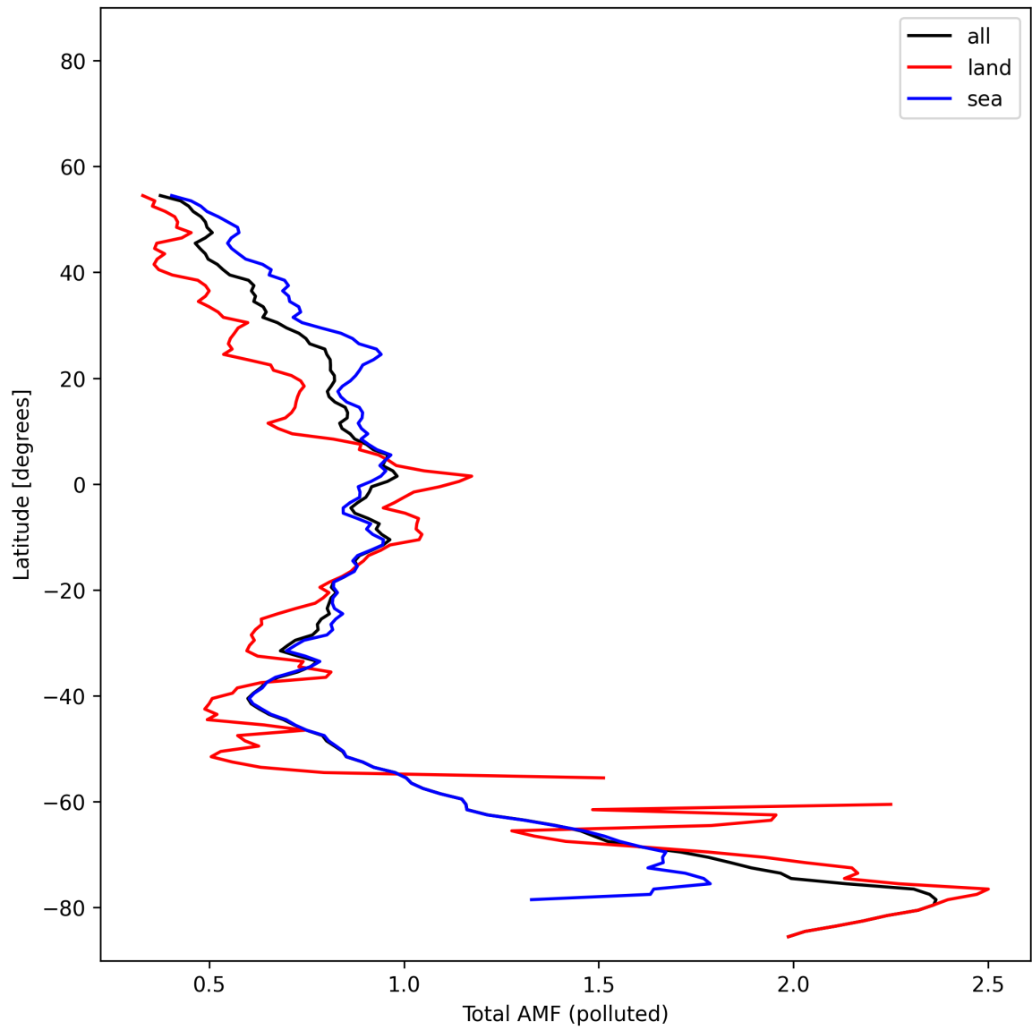
Figure 53: Zonal average of “Total AMF (polluted)” for 2025-11-03 to 2025-11-05.
