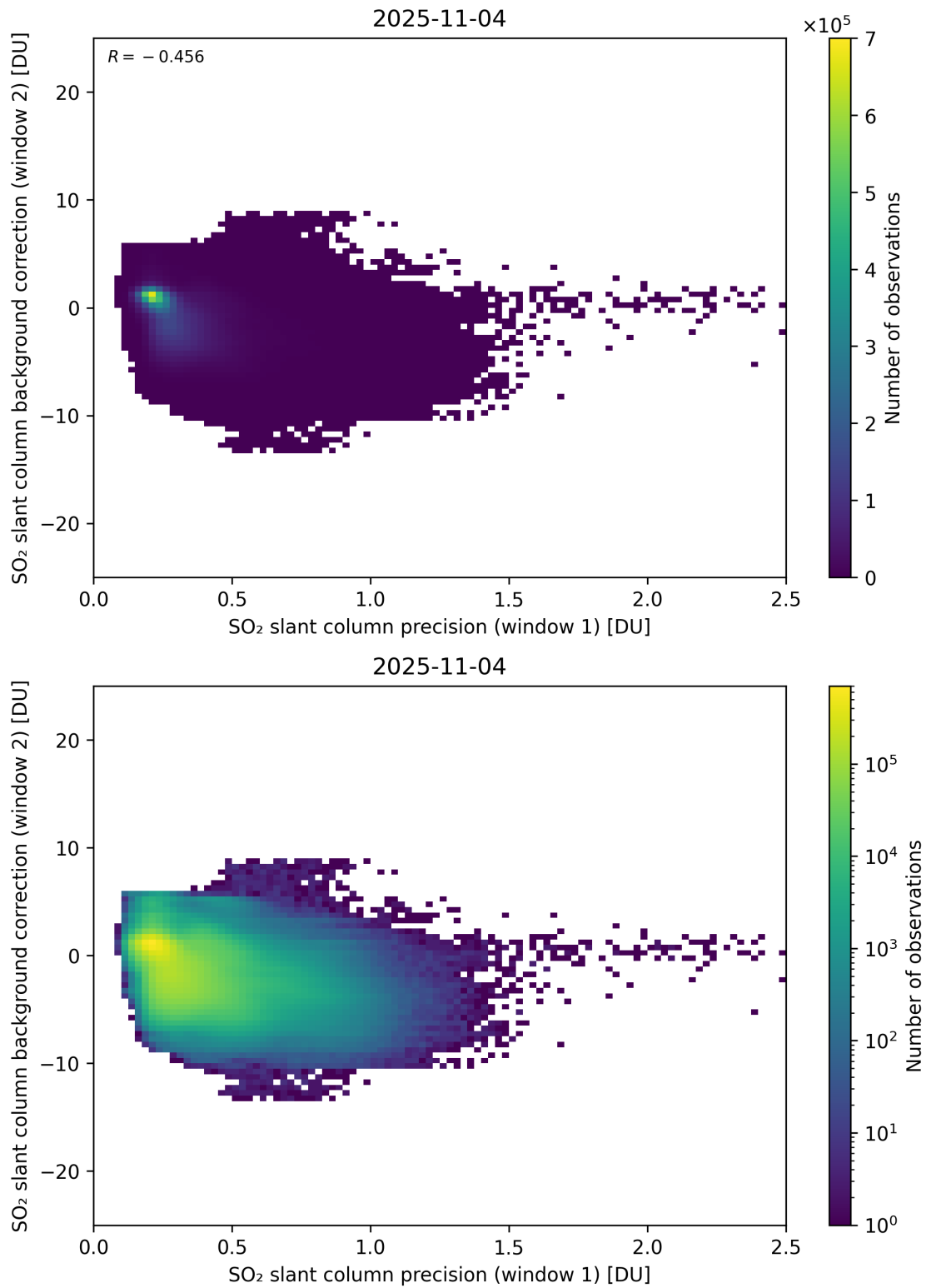
Figure 269: Scatter density plot of “SO 2 slant column precision (window 1)” against “SO 2 slant column background correction (window 2)” for 2025-11-03 to 2025-11-05.
