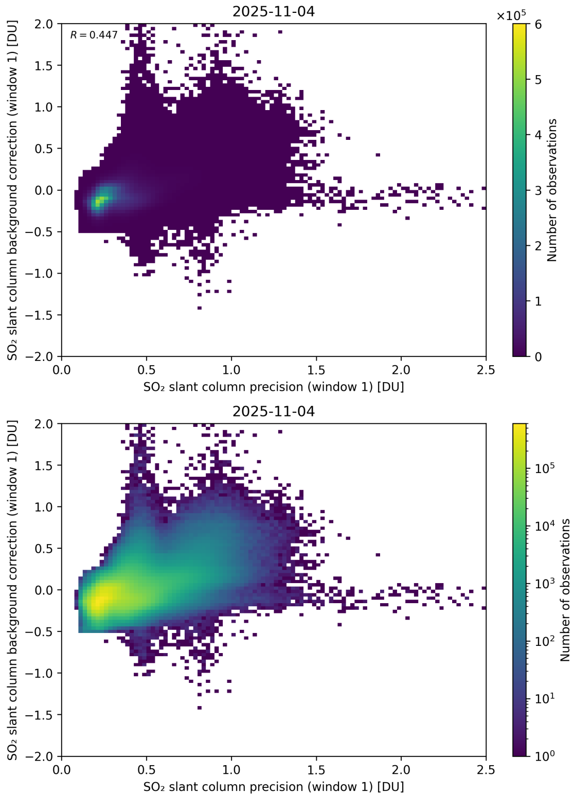
Figure 268: Scatter density plot of “SO 2 slant column precision (window 1)” against “SO 2 slant column background correction (window 1)” for 2025-11-03 to 2025-11-05.
