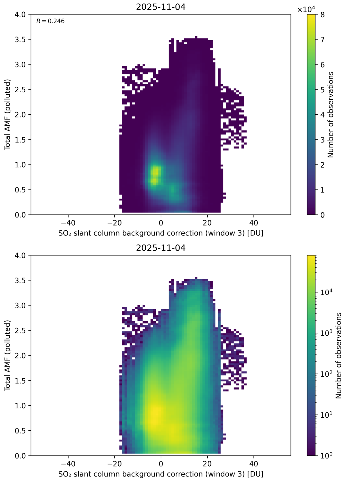
Figure 136: Scatter density plot of “SO 2 slant column background correction (window 3)” against “Total AMF (polluted)” for 2025-11-03 to 2025-11-05.
