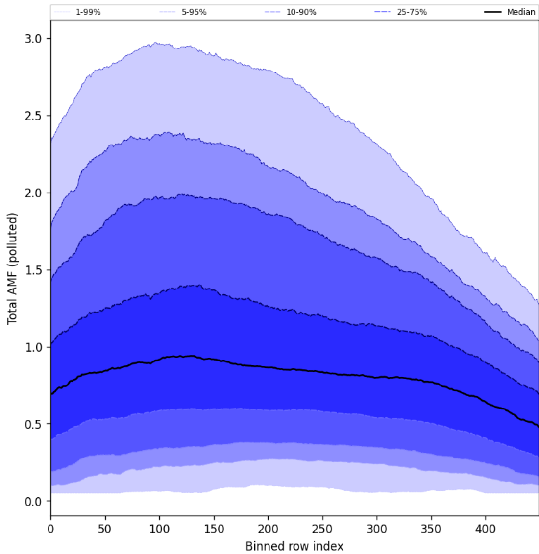
Figure 105: Along track statistics of “Total AMF (polluted)” for 2025-11-03 to 2025-11-05
