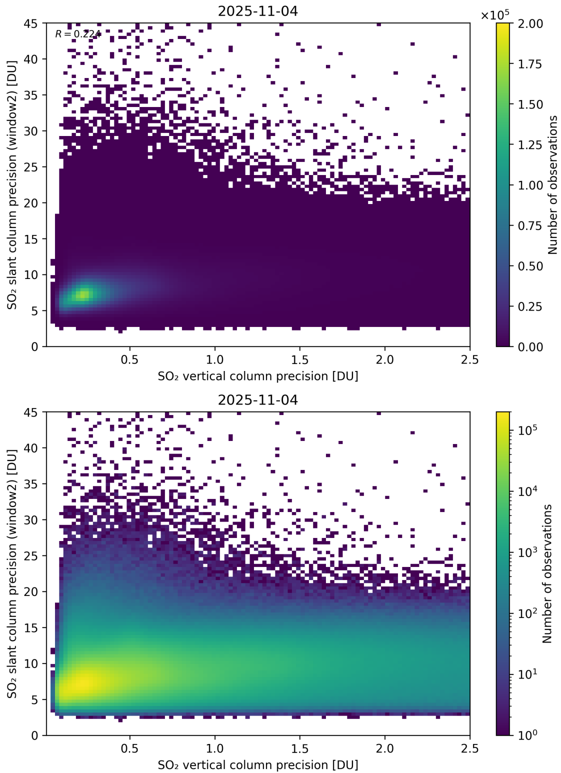
Figure 343: Scatter density plot of “SO 2 vertical column precision” against “SO 2 slant column precision (window2)” for 2025-11-03 to 2025-11-05.
