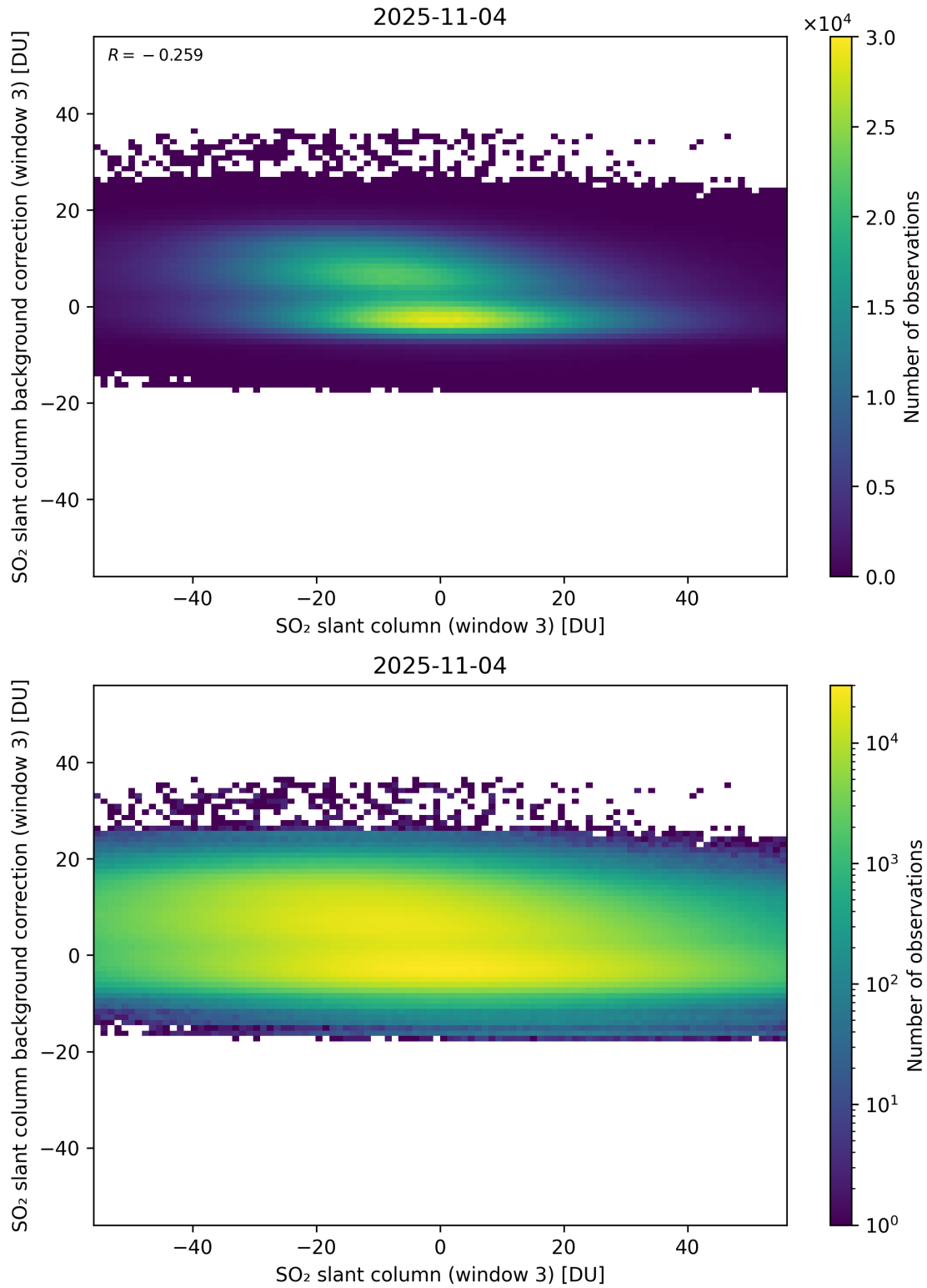
Figure 303: Scatter density plot of “SO 2 slant column (window 3)” against “SO 2 slant column background correction (window 3)” for 2025-11-03 to 2025-11-05.
