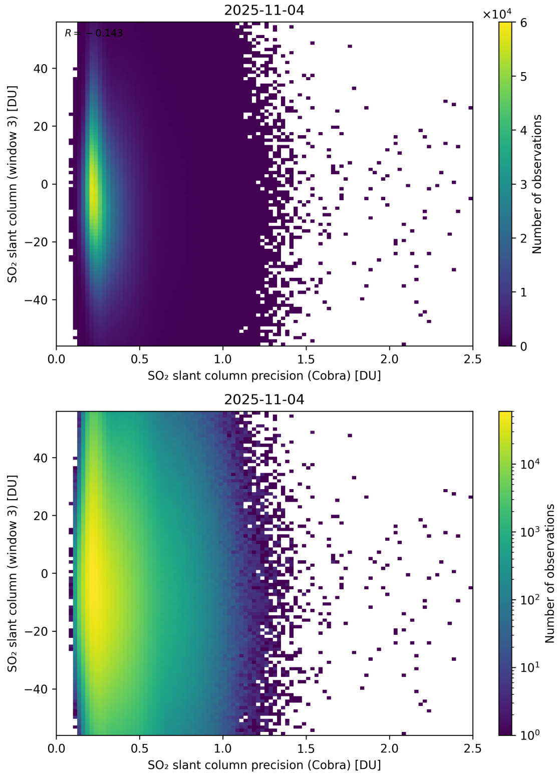
Figure 211: Scatter density plot of “SO 2 slant column precision (Cobra)” against “SO 2 slant column (window 3)” for 2025-11-03 to 2025-11-05.
