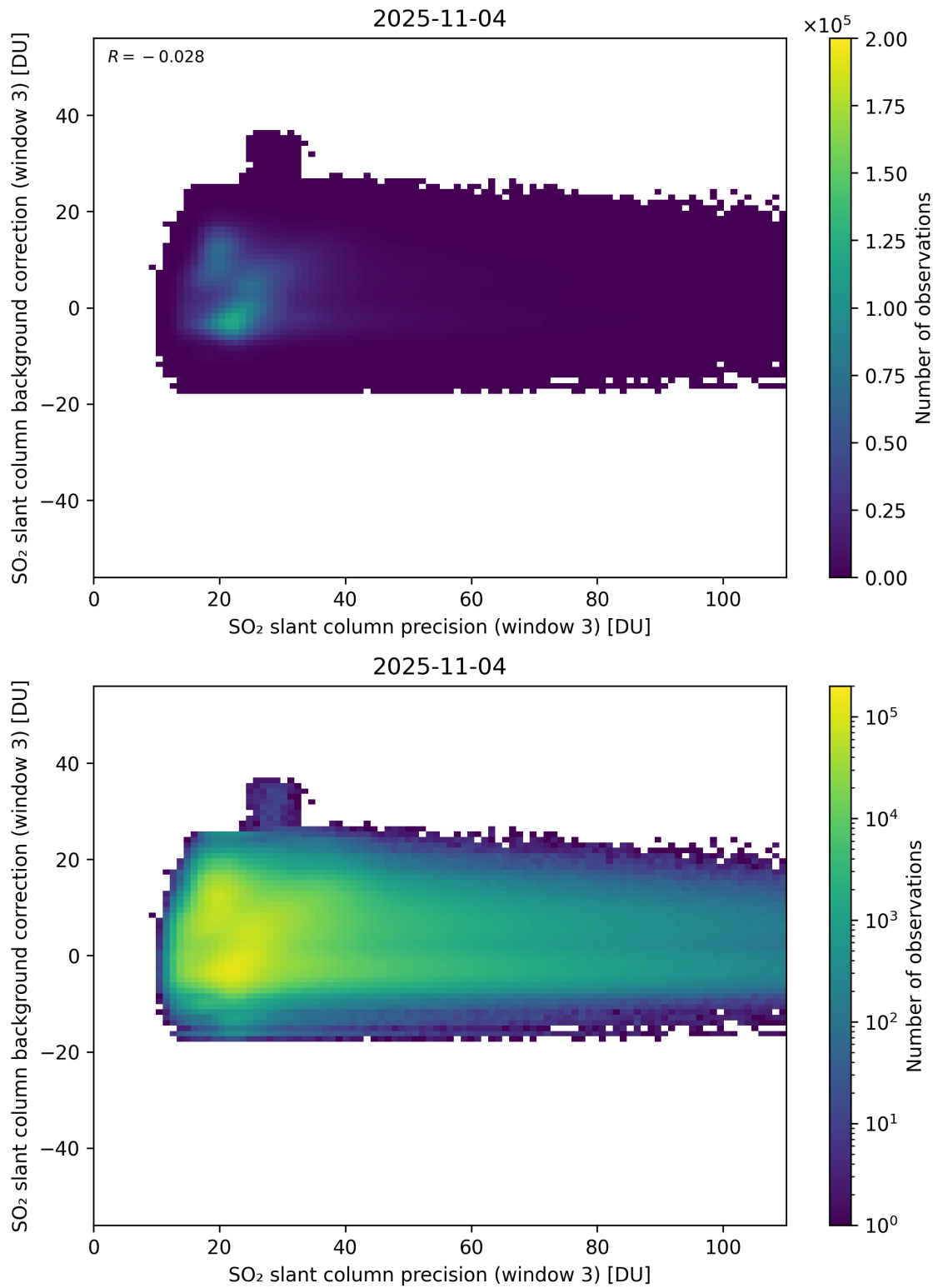
Figure 307: Scatter density plot of “SO 2 slant column precision (window 3)” against “SO 2 slant column background correction (window 3)” for 2025-11-03 to 2025-11-05.
