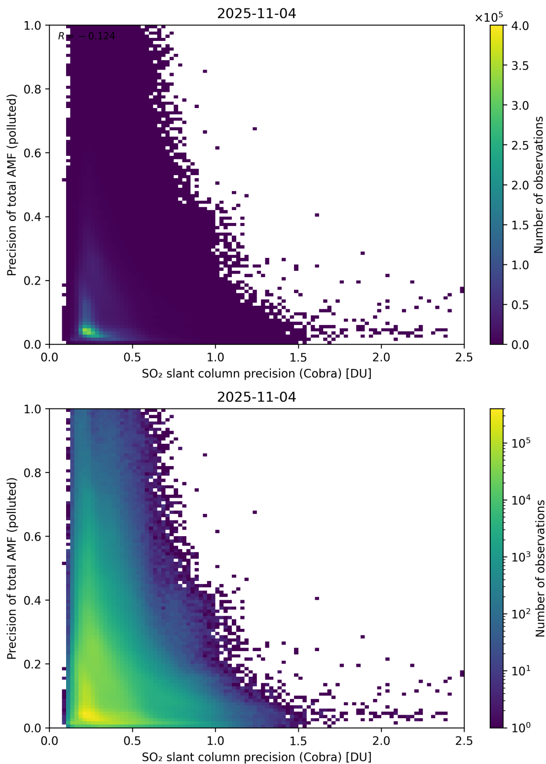
Figure 214: Scatter density plot of “SO 2 slant column precision (Cobra)” against “Precision of total AMF (polluted)” for 2025-11-03 to 2025-11-05.
