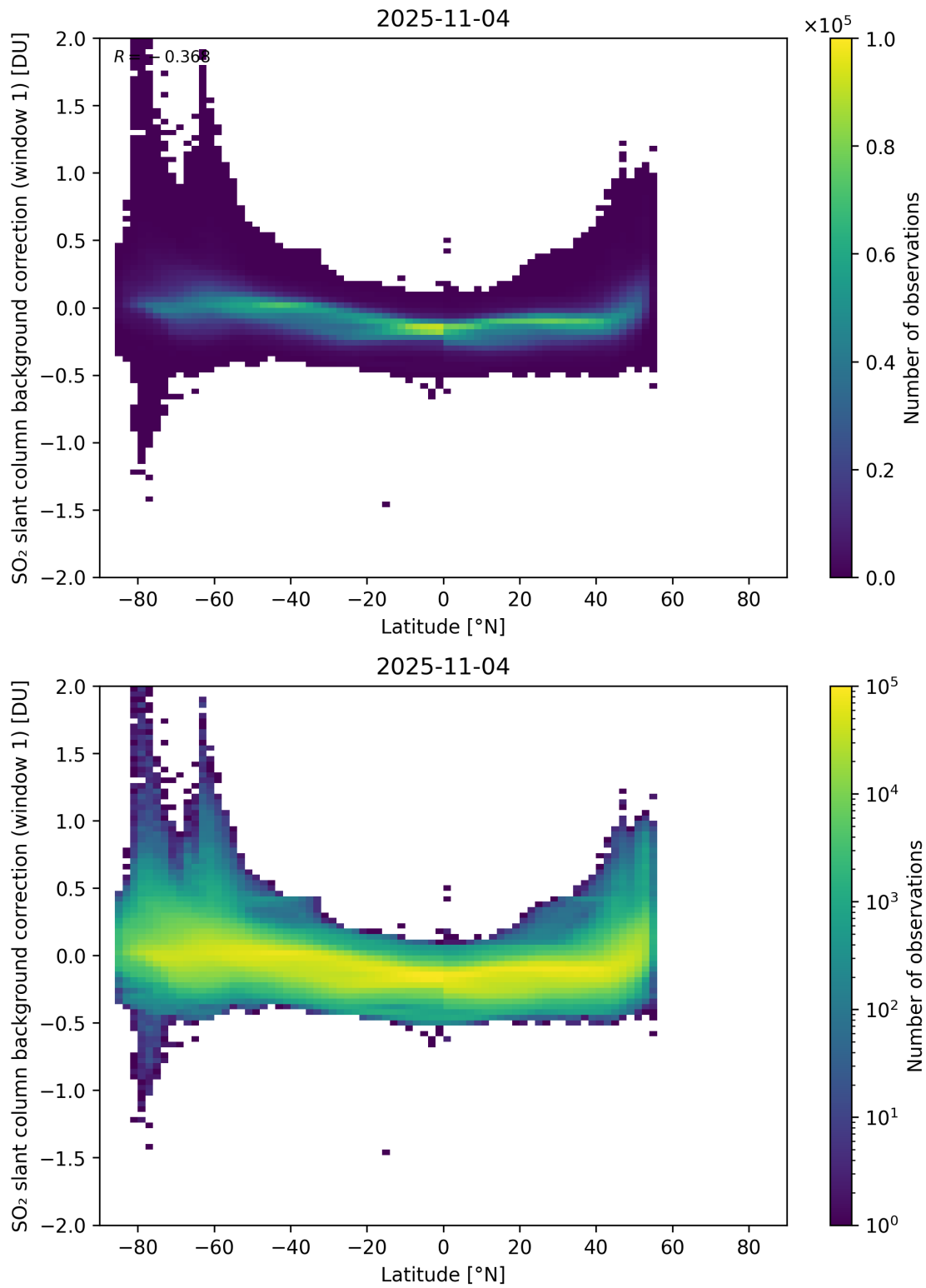
Figure 150: Scatter density plot of “Latitude” against “SO 2 slant column background correction (window 1)” for 2025-11-03 to 2025-11-05.
