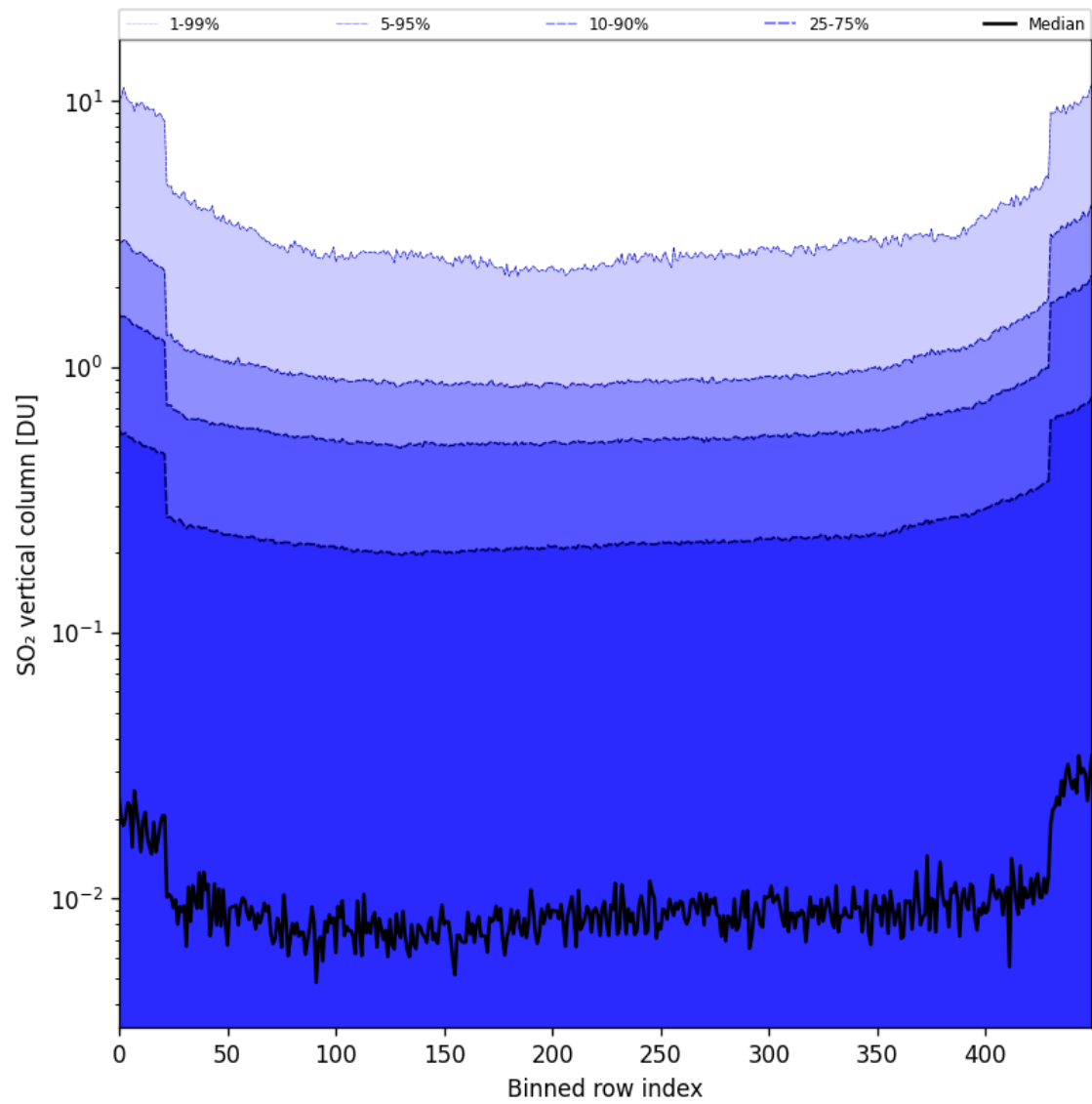
Figure 84: Along track statistics of “SO 2 vertical column” for 2025-11-03 to 2025-11-05
