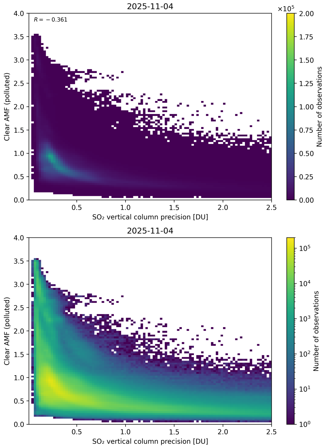
Figure 335: Scatter density plot of “SO 2 vertical column precision” against “Clear AMF (polluted)” for 2025-11-03 to 2025-11-05.
