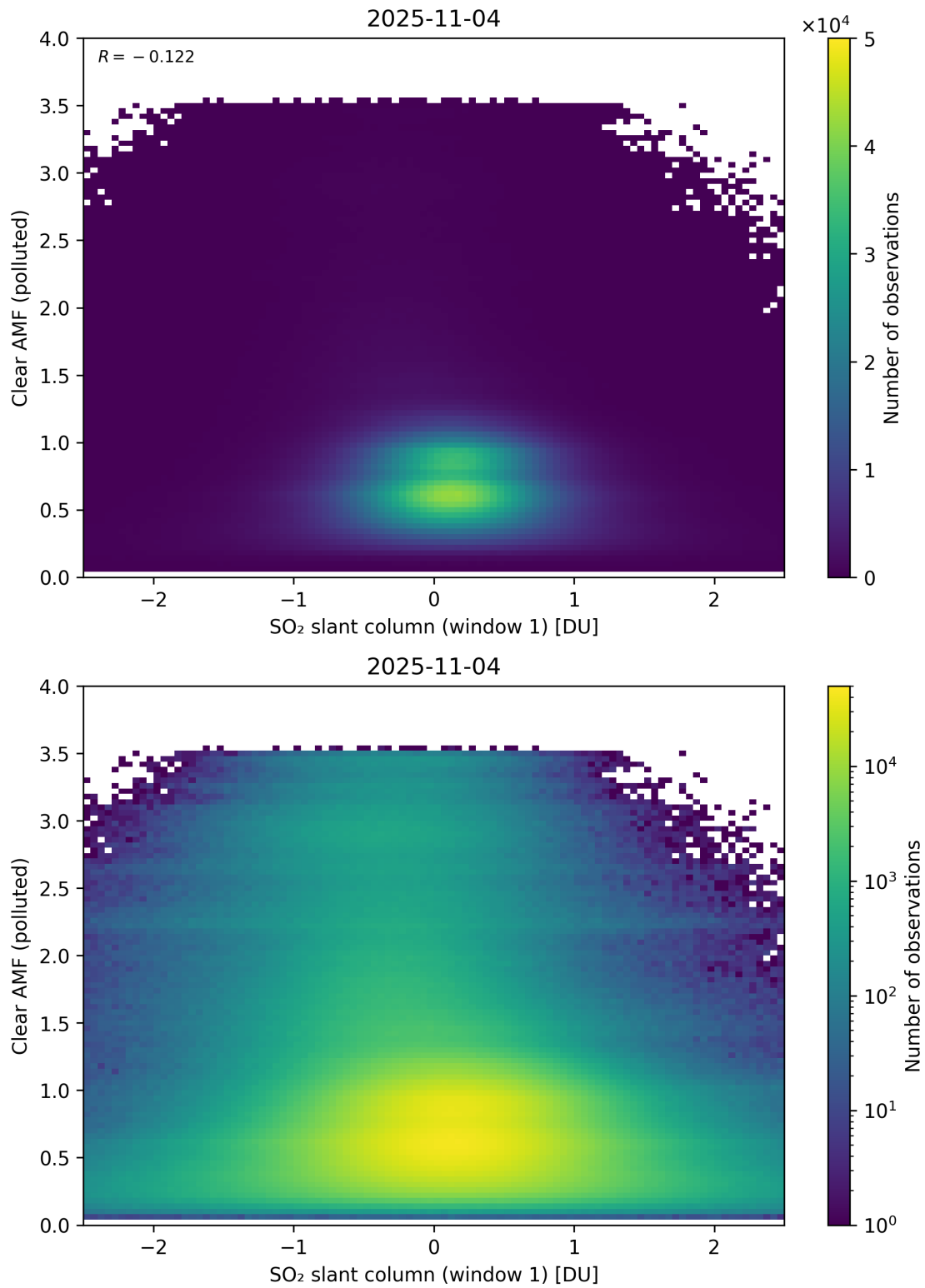
Figure 282: Scatter density plot of “SO 2 slant column (window 1)” against “Clear AMF (polluted)” for 2025-11-03 to 2025-11-05.
