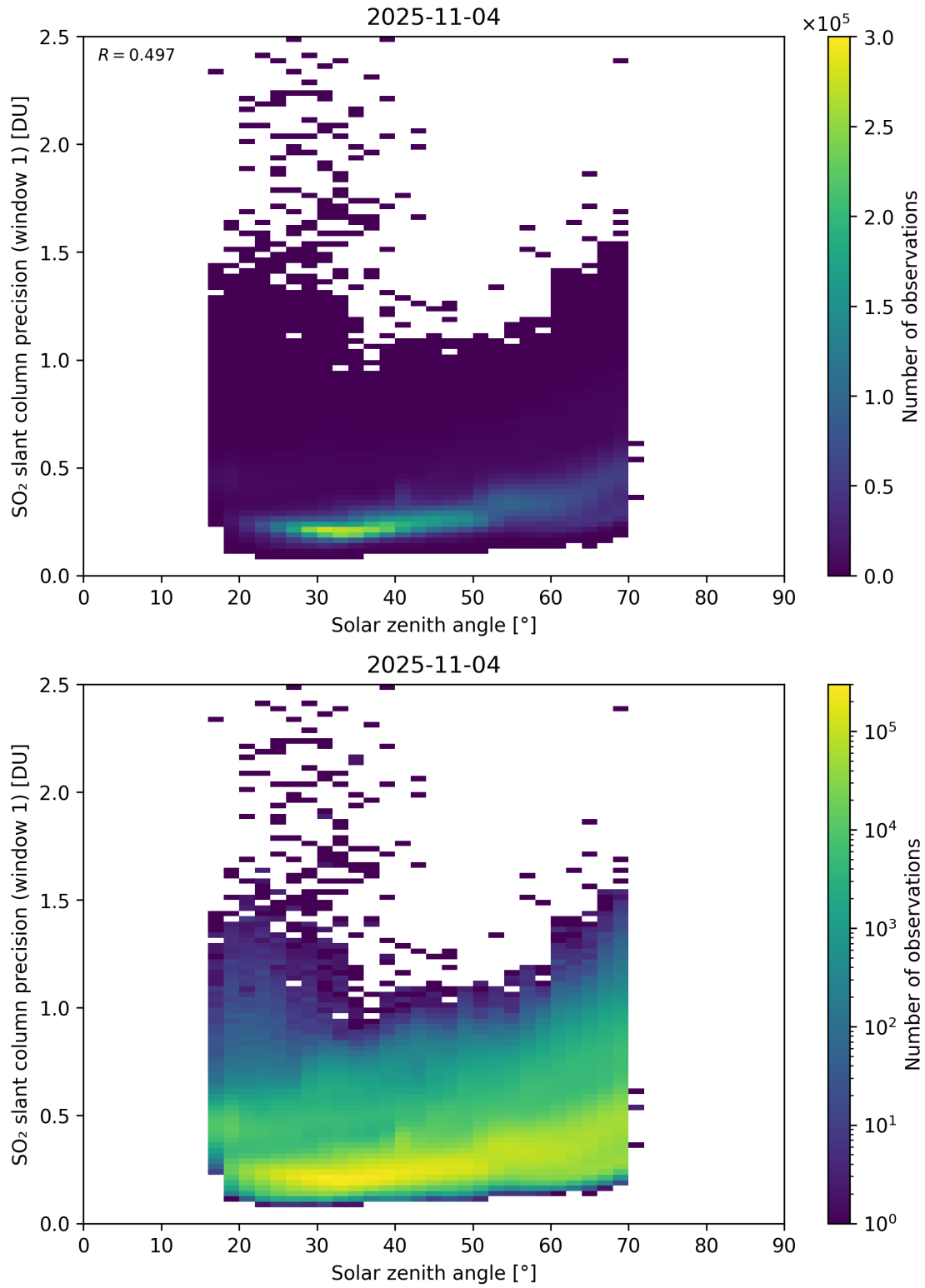
Figure 185: Scatter density plot of “Solar zenith angle” against “SO 2 slant column precision (window 1)” for 2025-11-03 to 2025-11-05.
