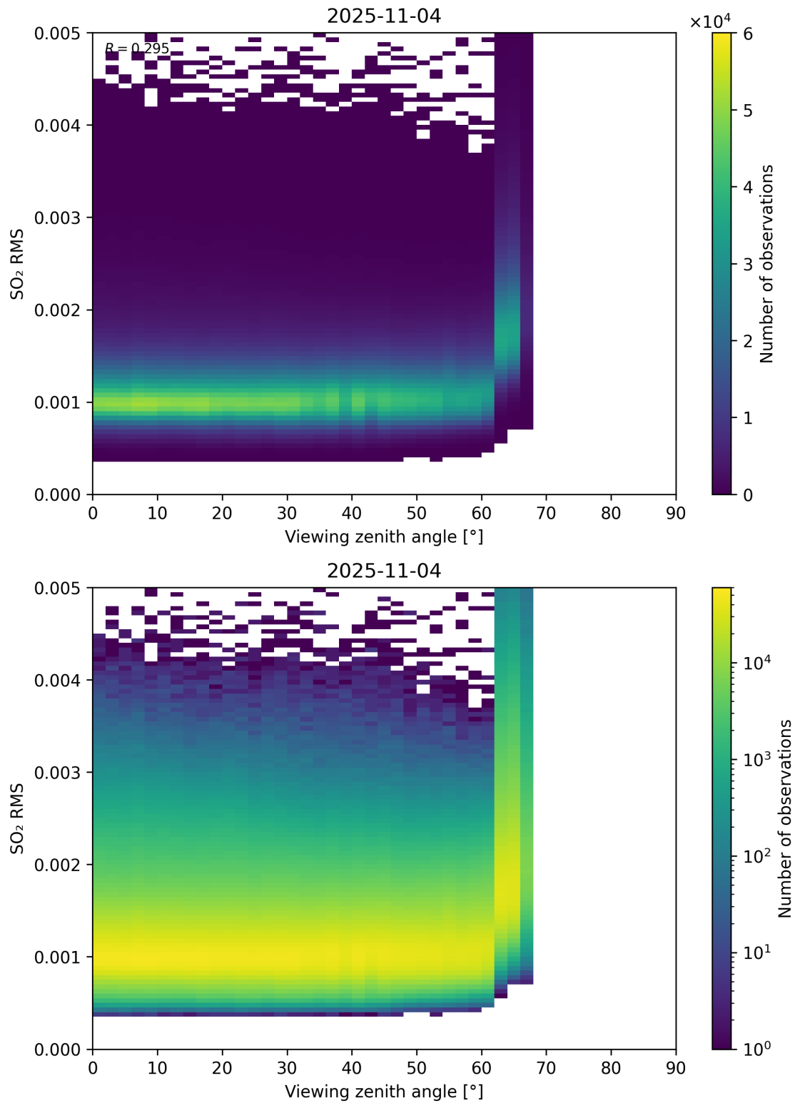
Figure 367: Scatter density plot of “Viewing zenith angle” against “SO 2 RMS” for 2025-11-03 to 2025-11-05.
