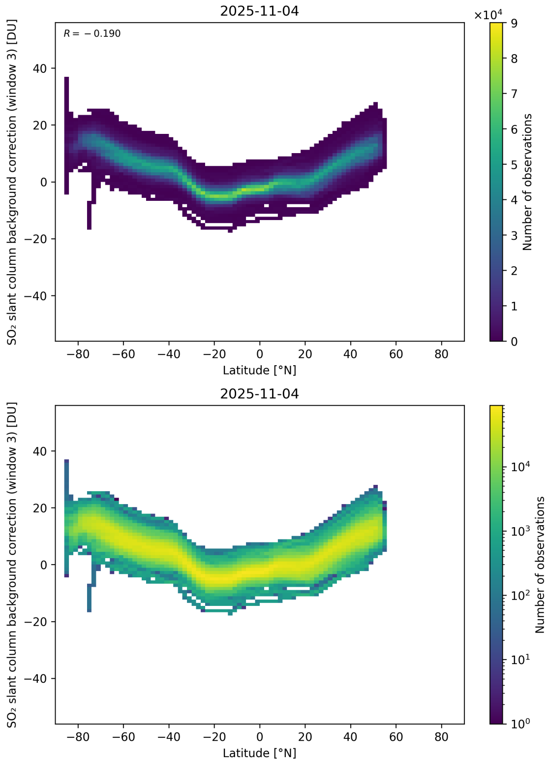
Figure 152: Scatter density plot of “Latitude” against “SO 2 slant column background correction (window 3)” for 2025-11-03 to 2025-11-05.
