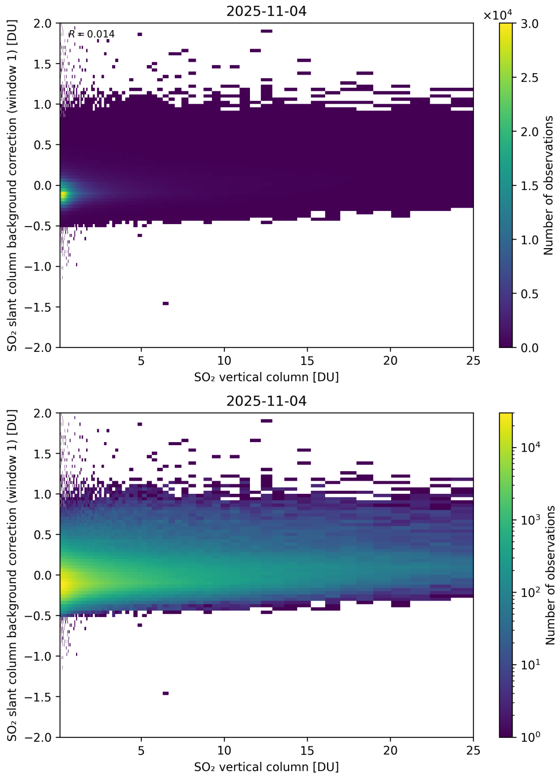
Figure 323: Scatter density plot of “SO 2 vertical column” against “SO 2 slant column background correction (window 1)” for 2025-11-03 to 2025-11-05.
