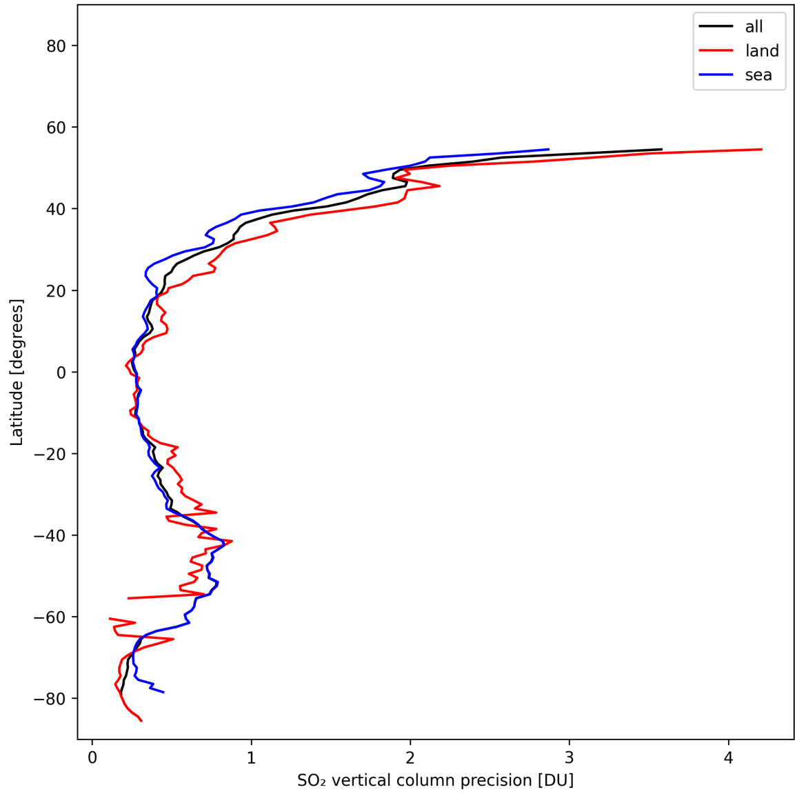
Figure 33: Zonal average of “SO 2 vertical column precision” for 2025-11-03 to 2025-11-05.
