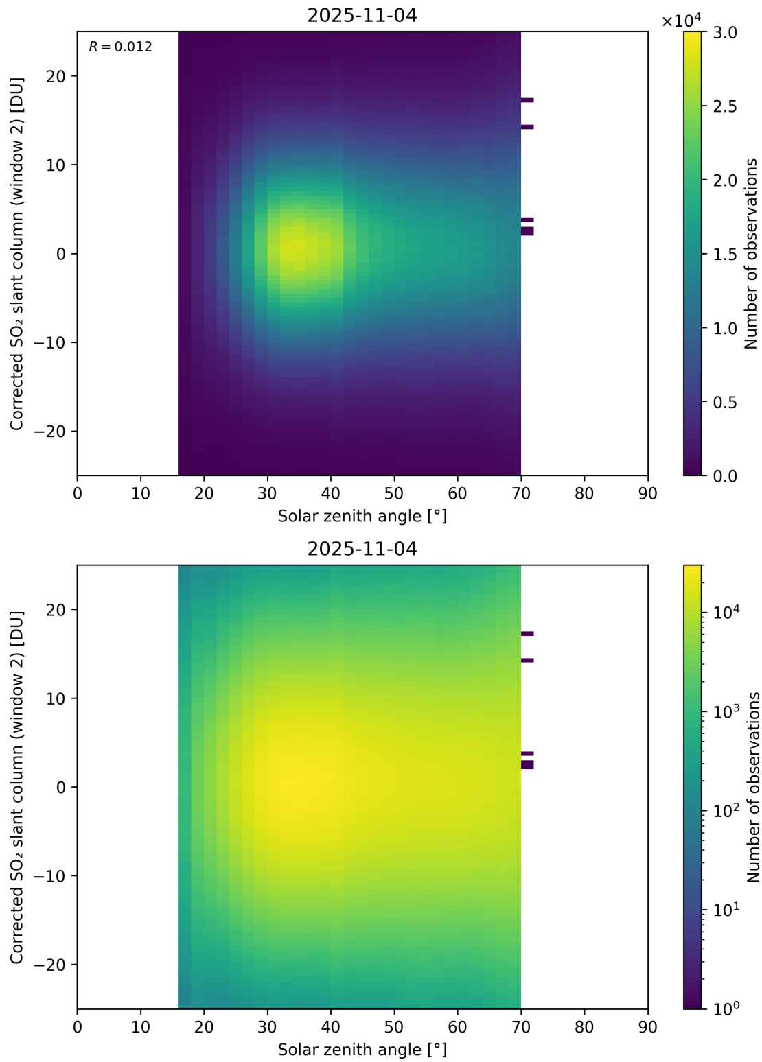
Figure 182: Scatter density plot of “Solar zenith angle” against “Corrected SO 2 slant column (window 2)” for 2025-11-03 to 2025-11-05.
