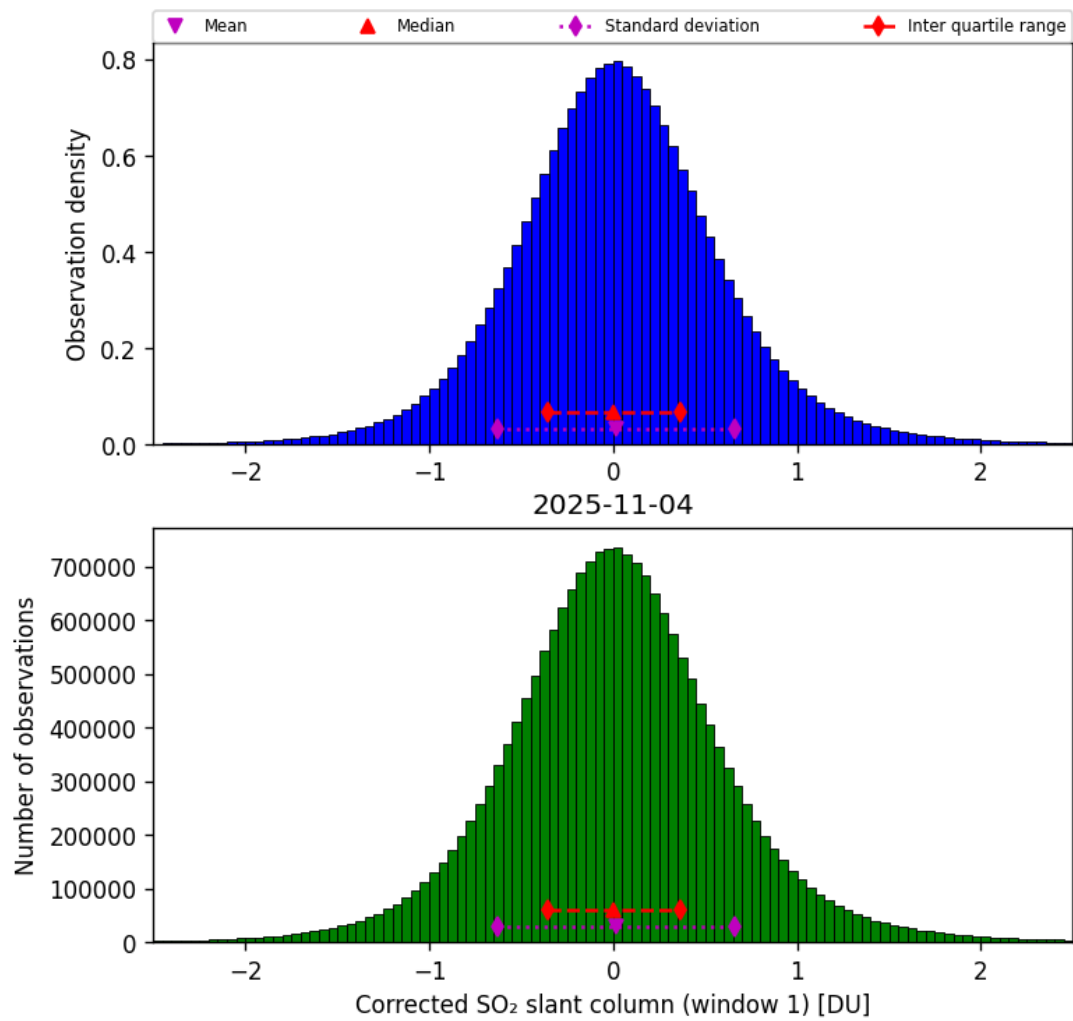
Figure 65: Histogram of “Corrected SO 2 slant column (window 1)” for 2025-11-03 to 2025-11-05
