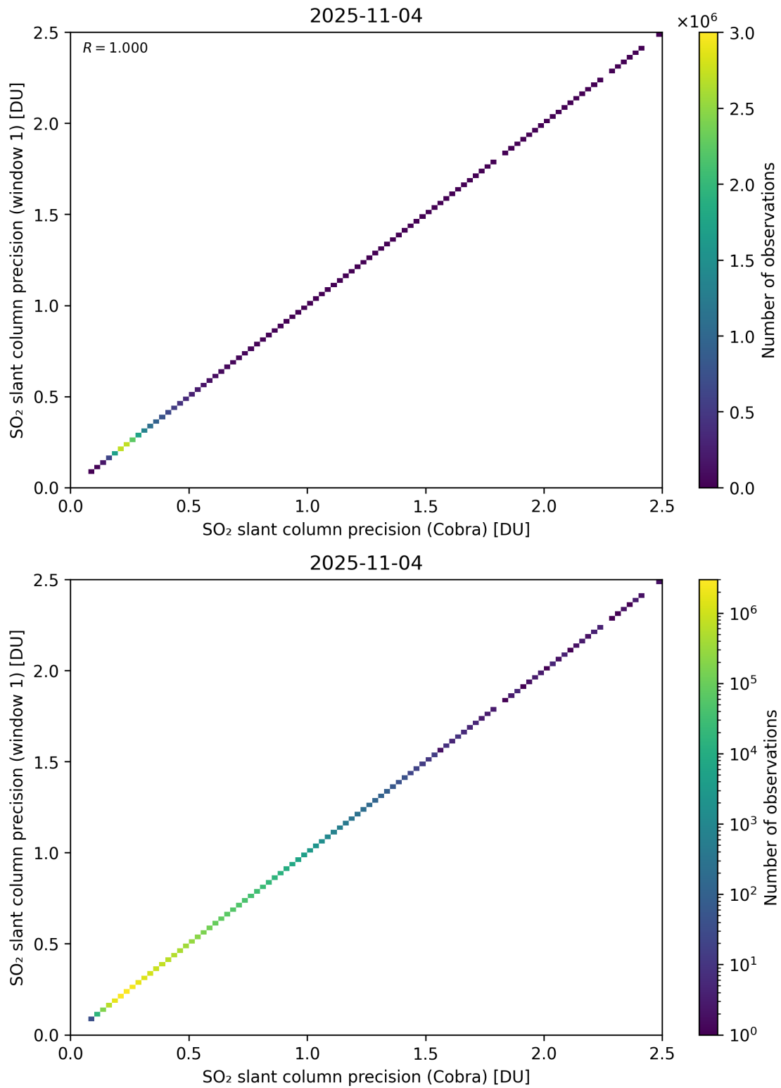
Figure 209: Scatter density plot of “SO 2 slant column precision (Cobra)” against “SO 2 slant column precision (window 1)” for 2025-11-03 to 2025-11-05.
