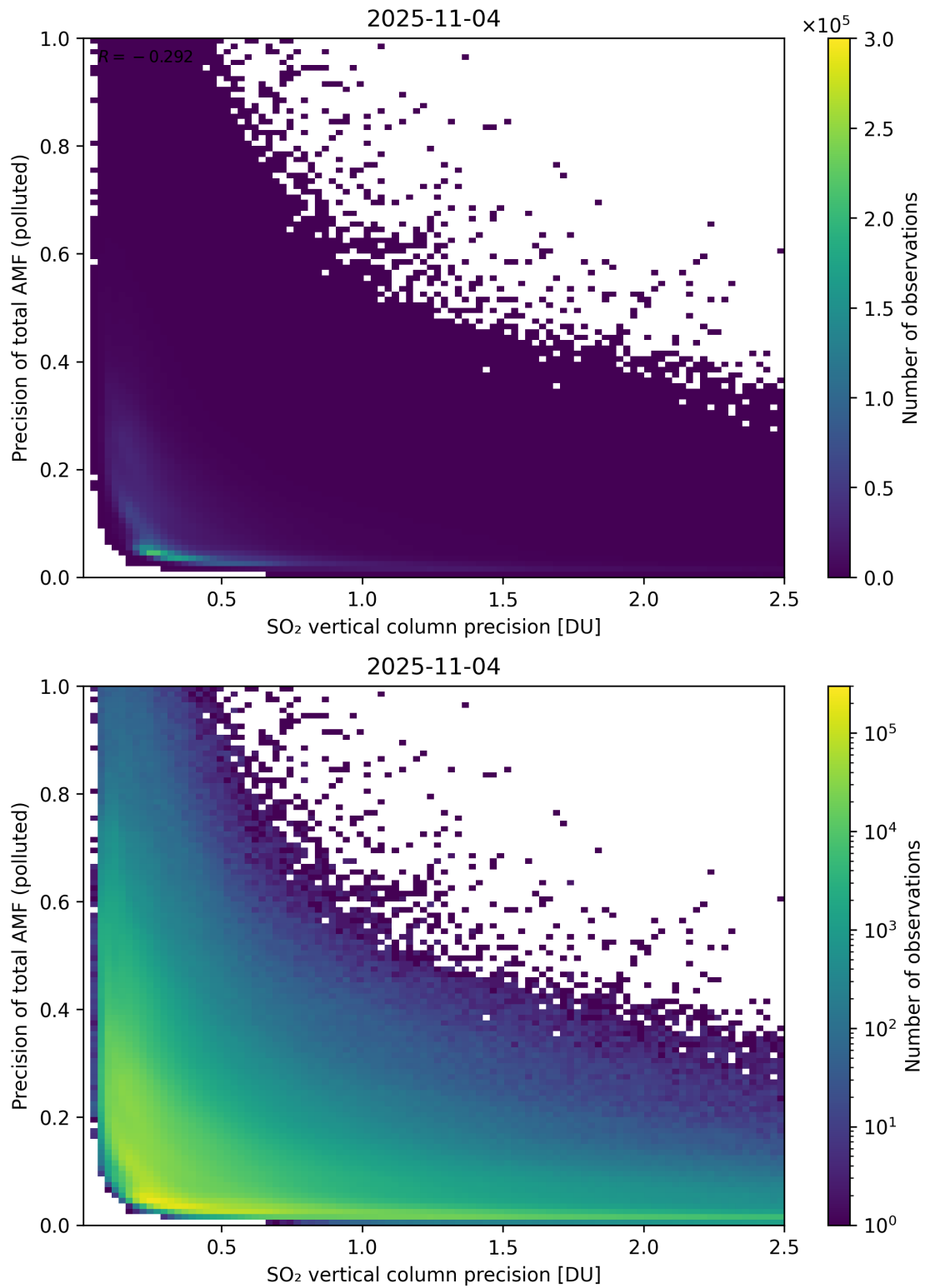
Figure 347: Scatter density plot of “SO 2 vertical column precision” against “Precision of total AMF (polluted)” for 2025-11-03 to 2025-11-05.
