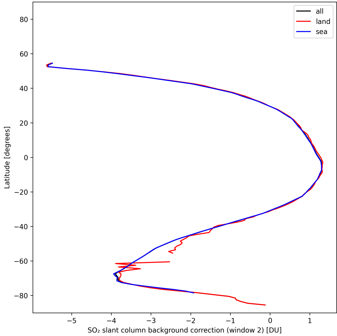
Figure 44: Zonal average of “SO 2 slant column background correction (window 2)” for 2025-11-03 to 2025-11-05.
