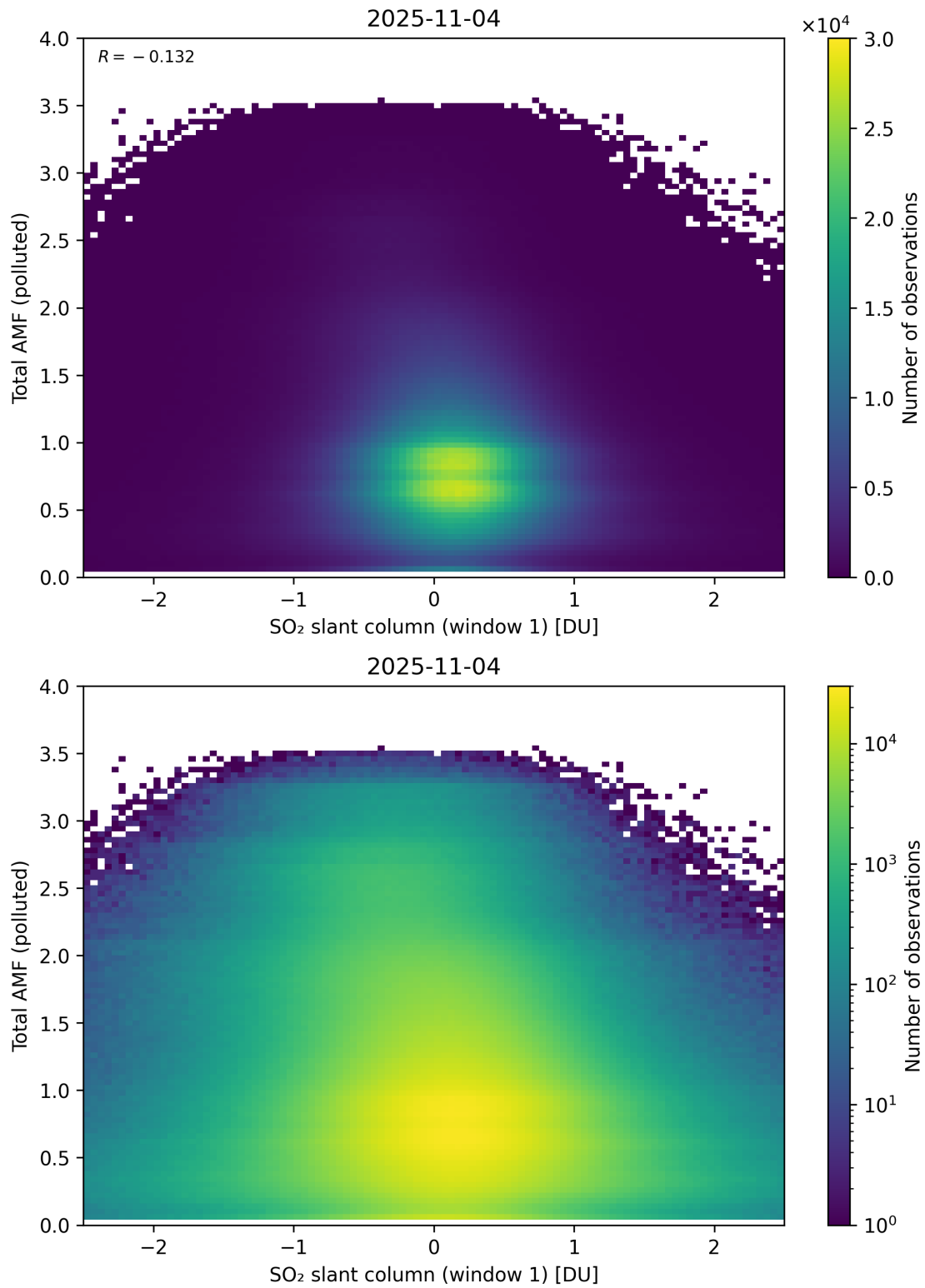
Figure 289: Scatter density plot of “SO 2 slant column (window 1)” against “Total AMF (polluted)” for 2025-11-03 to 2025-11-05.
