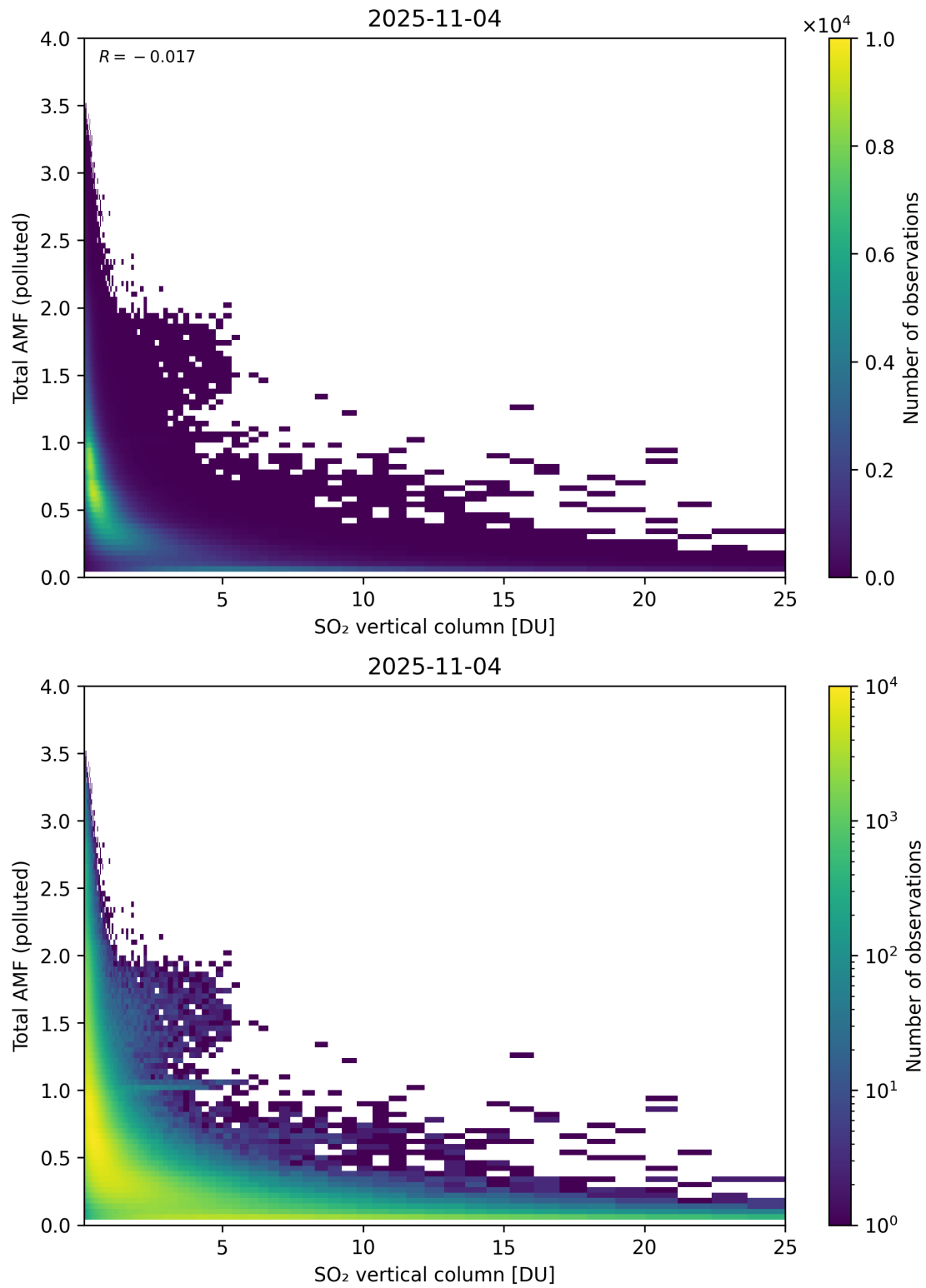
Figure 359: Scatter density plot of “SO 2 vertical column” against “Total AMF (polluted)” for 2025-11-03 to 2025-11-05.
