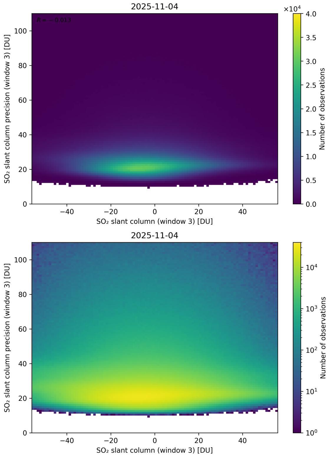
Figure 317: Scatter density plot of “SO 2 slant column (window 3)” against “SO 2 slant column precision (window 3)” for 2025-11-03 to 2025-11-05.
