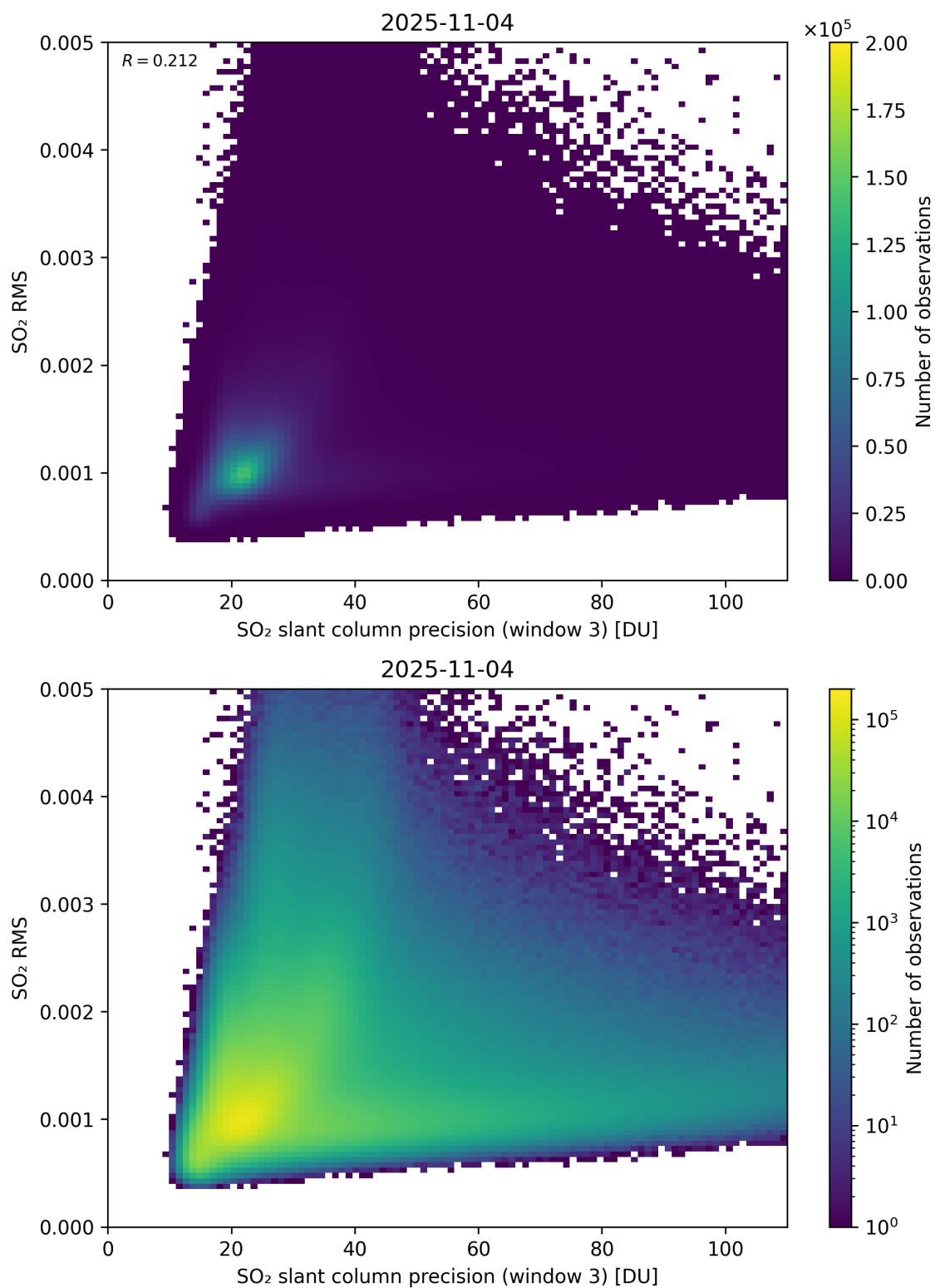
Figure 310: Scatter density plot of “SO 2 slant column precision (window 3)” against “SO 2 RMS” for 2025-11-03 to 2025-11-05.
