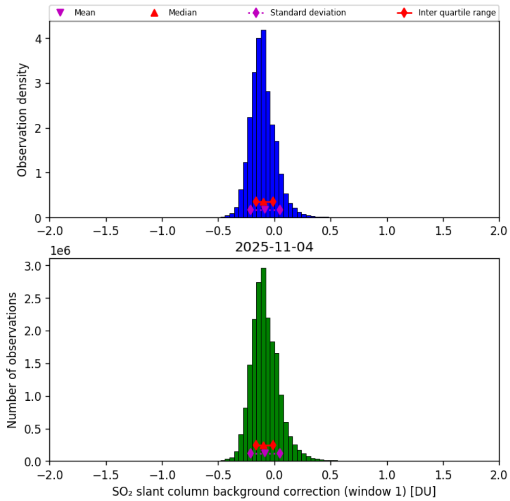
Figure 66: Histogram of “SO 2 slant column background correction (window 1)” for 2025-11-03 to 2025-11-05
