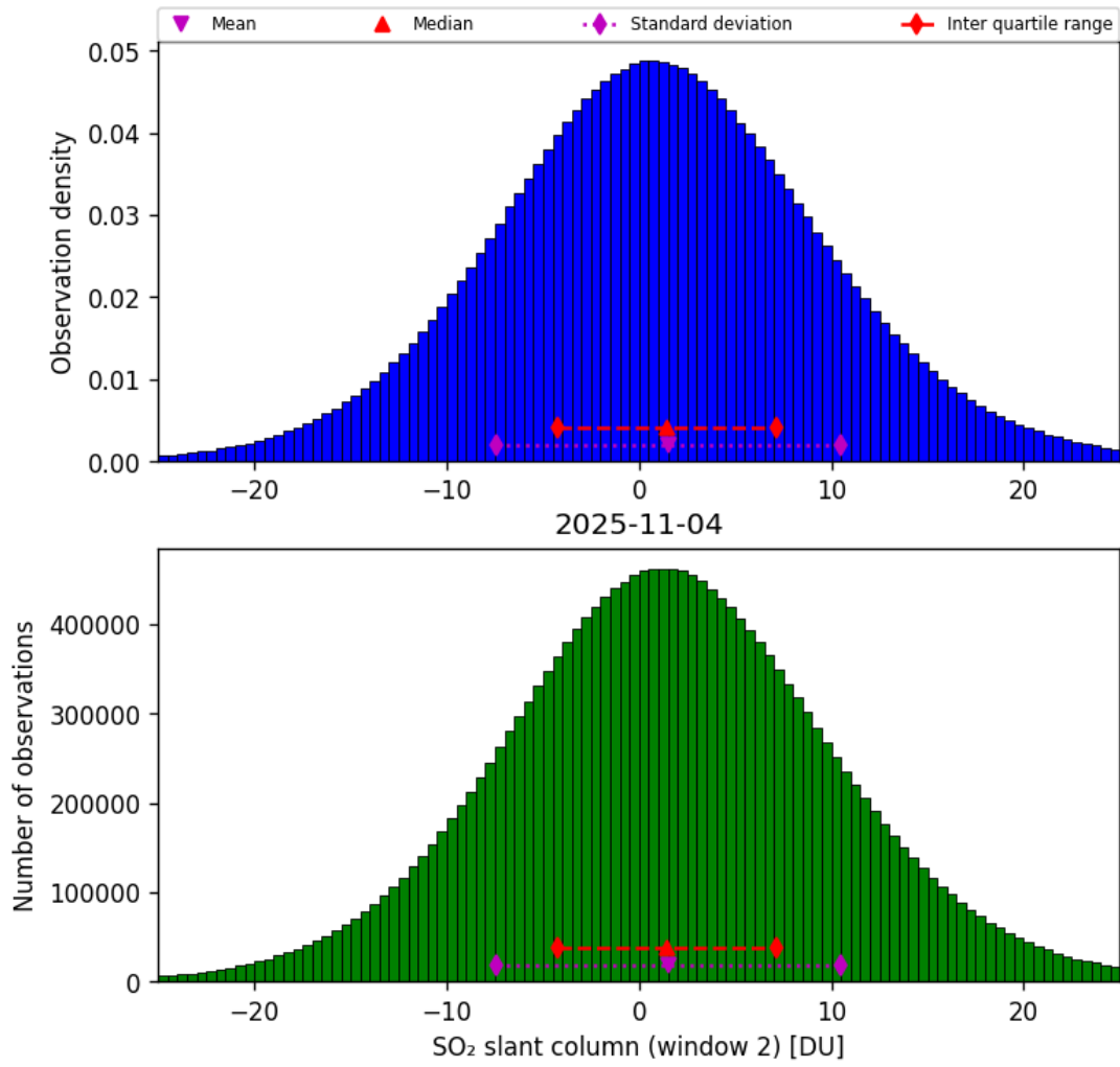
Figure 67: Histogram of “SO 2 slant column (window 2)” for 2025-11-03 to 2025-11-05
