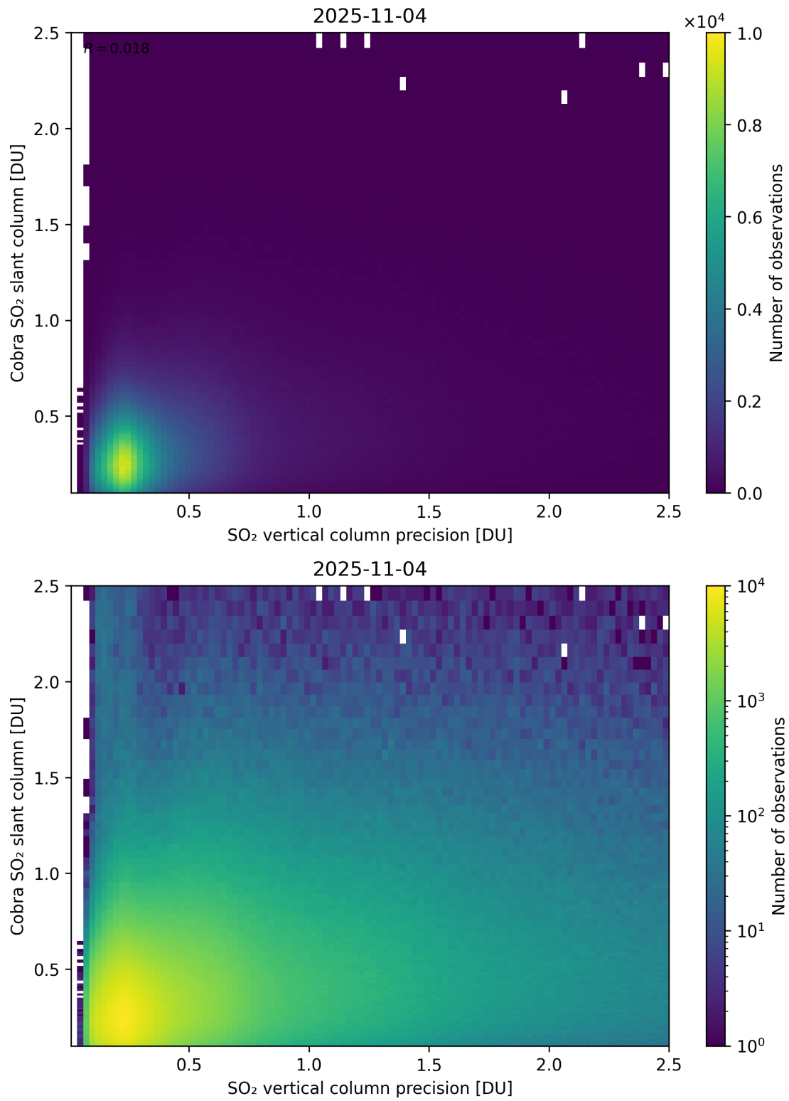
Figure 336: Scatter density plot of “SO 2 vertical column precision” against “Cobra SO 2 slant column” for 2025-11-03 to 2025-11-05.
