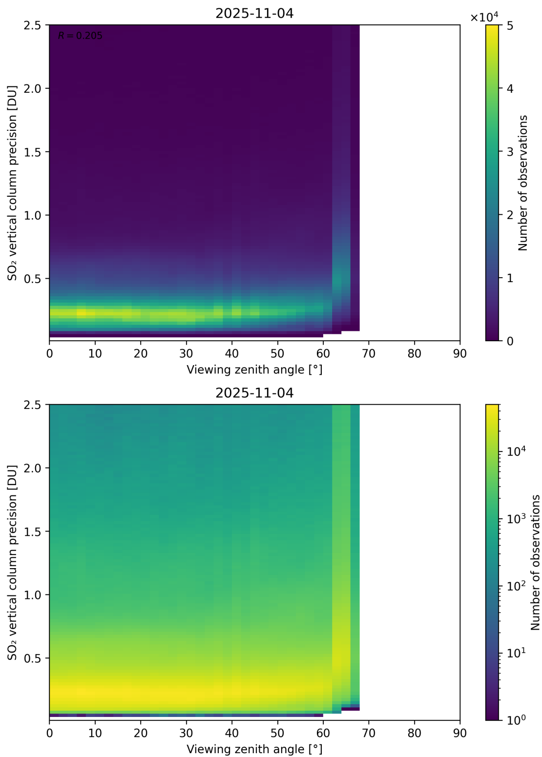
Figure 384: Scatter density plot of “Viewing zenith angle” against “SO 2 vertical column precision” for 2025-11-03 to 2025-11-05.
