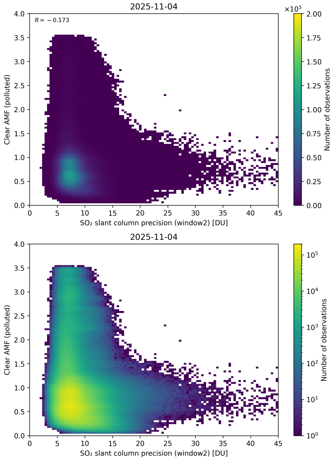
Figure 296: Scatter density plot of “SO 2 slant column precision (window2)” against “Clear AMF (polluted)” for 2025-11-03 to 2025-11-05.
