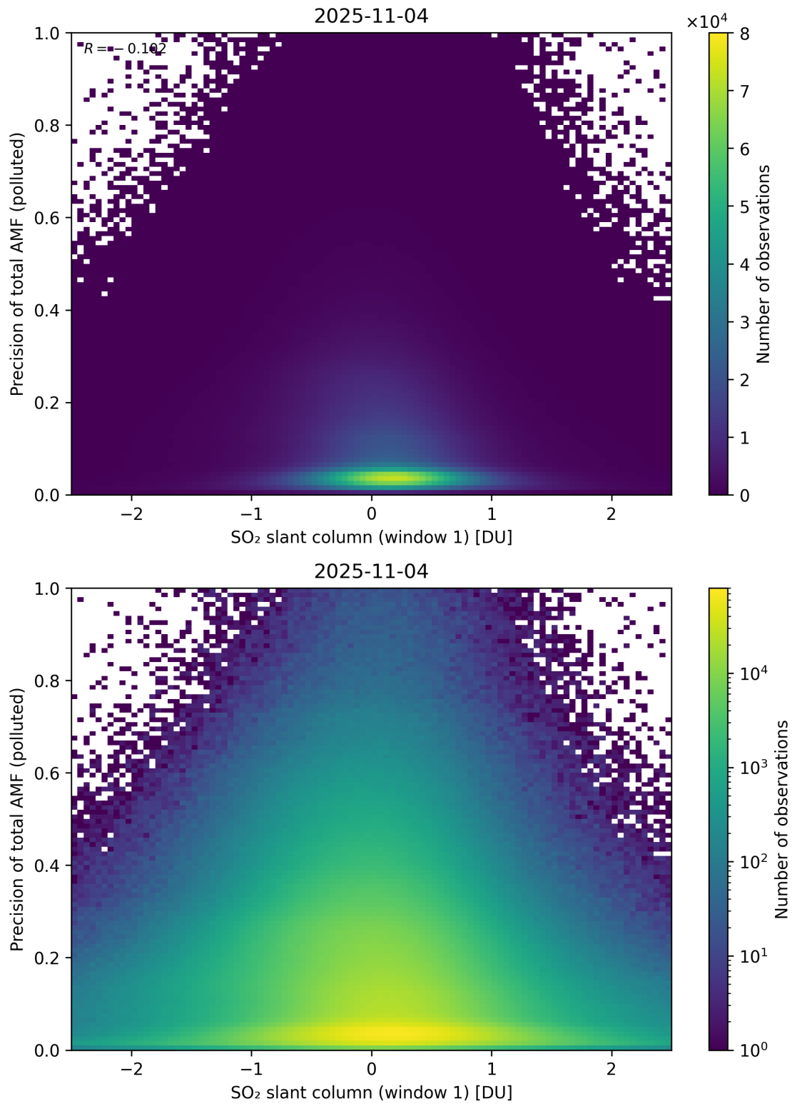
Figure 290: Scatter density plot of “SO 2 slant column (window 1)” against “Precision of total AMF (polluted)” for 2025-11-03 to 2025-11-05.
