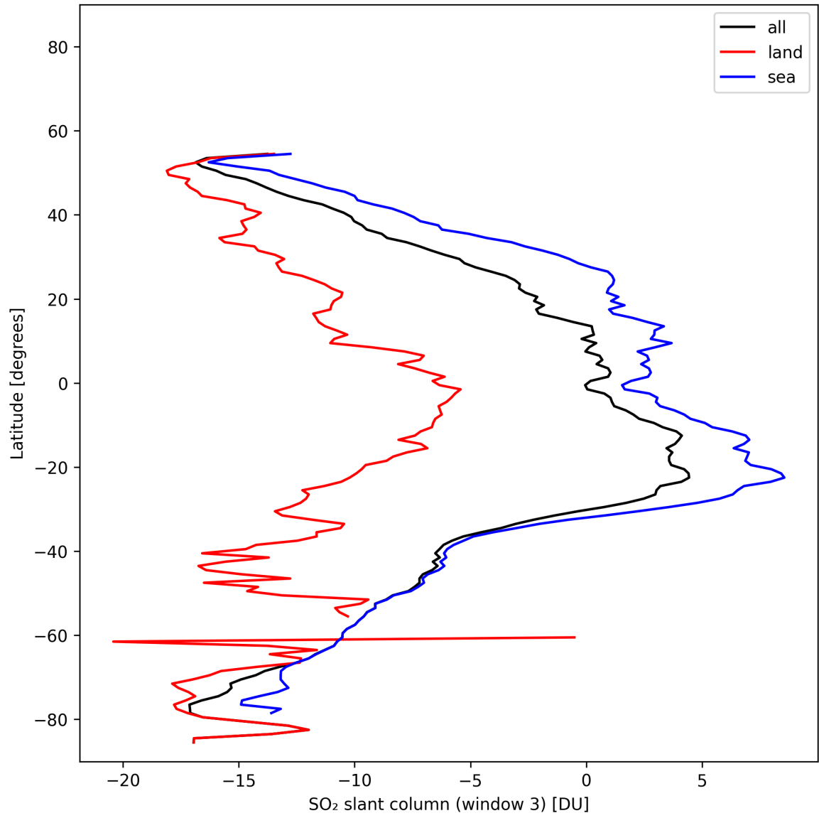
Figure 45: Zonal average of “SO 2 slant column (window 3)” for 2025-11-03 to 2025-11-05.
