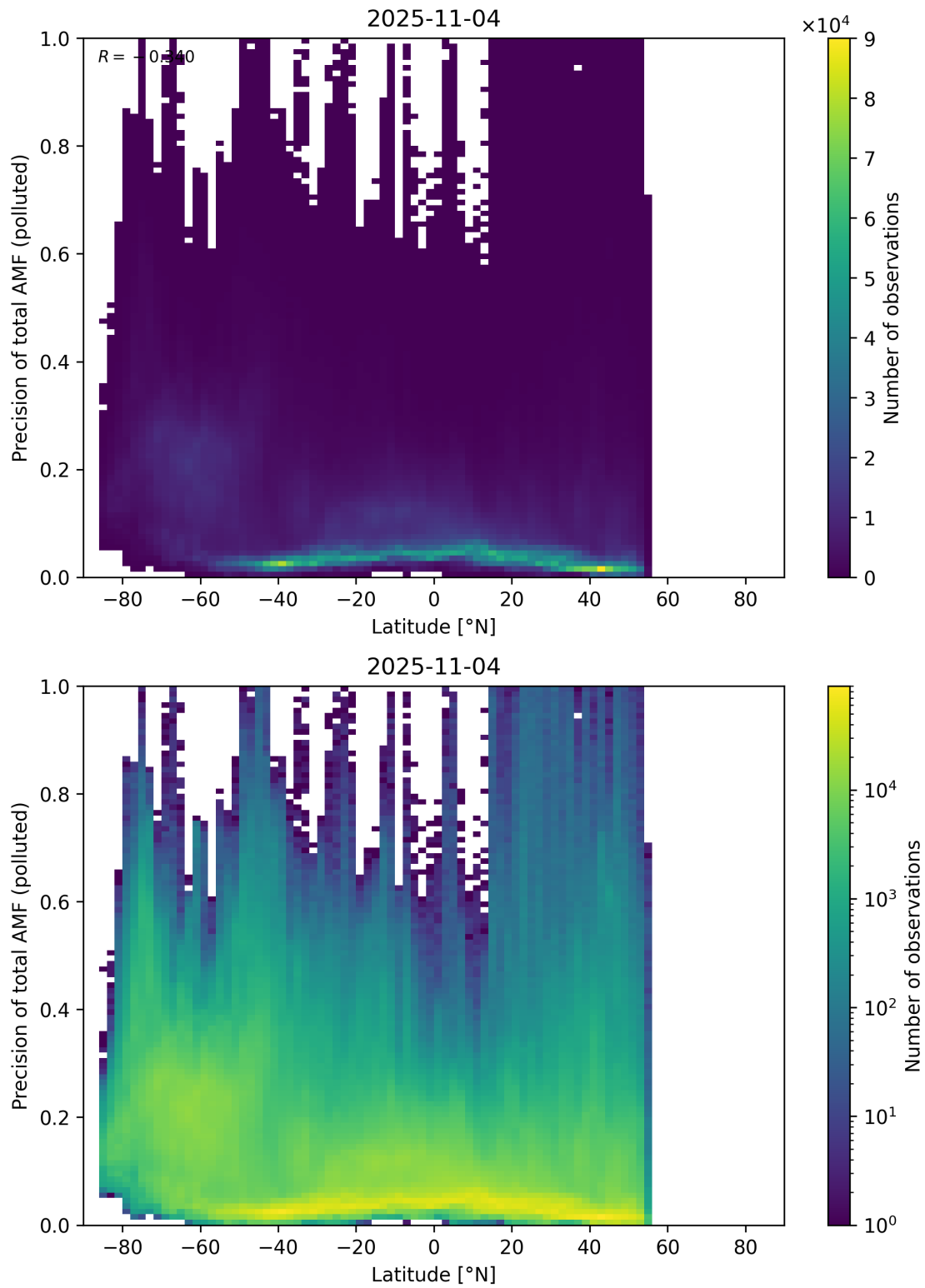
Figure 168: Scatter density plot of “Latitude” against “Precision of total AMF (polluted)” for 2025-11-03 to 2025-11-05.
