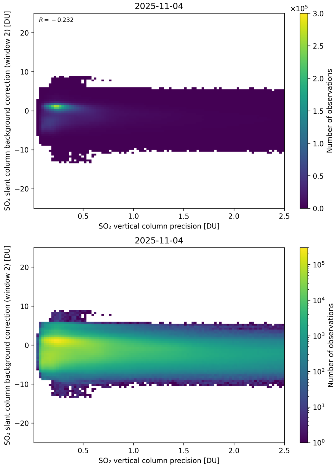
Figure 330: Scatter density plot of “SO 2 vertical column precision” against “SO 2 slant column background correction (window 2)” for 2025-11-03 to 2025-11-05.
