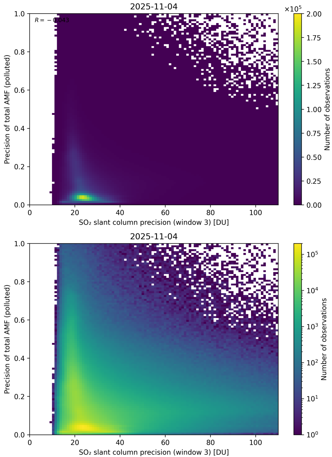
Figure 314: Scatter density plot of “SO 2 slant column precision (window 3)” against “Precision of total AMF (polluted)” for 2025-11-03 to 2025-11-05.
