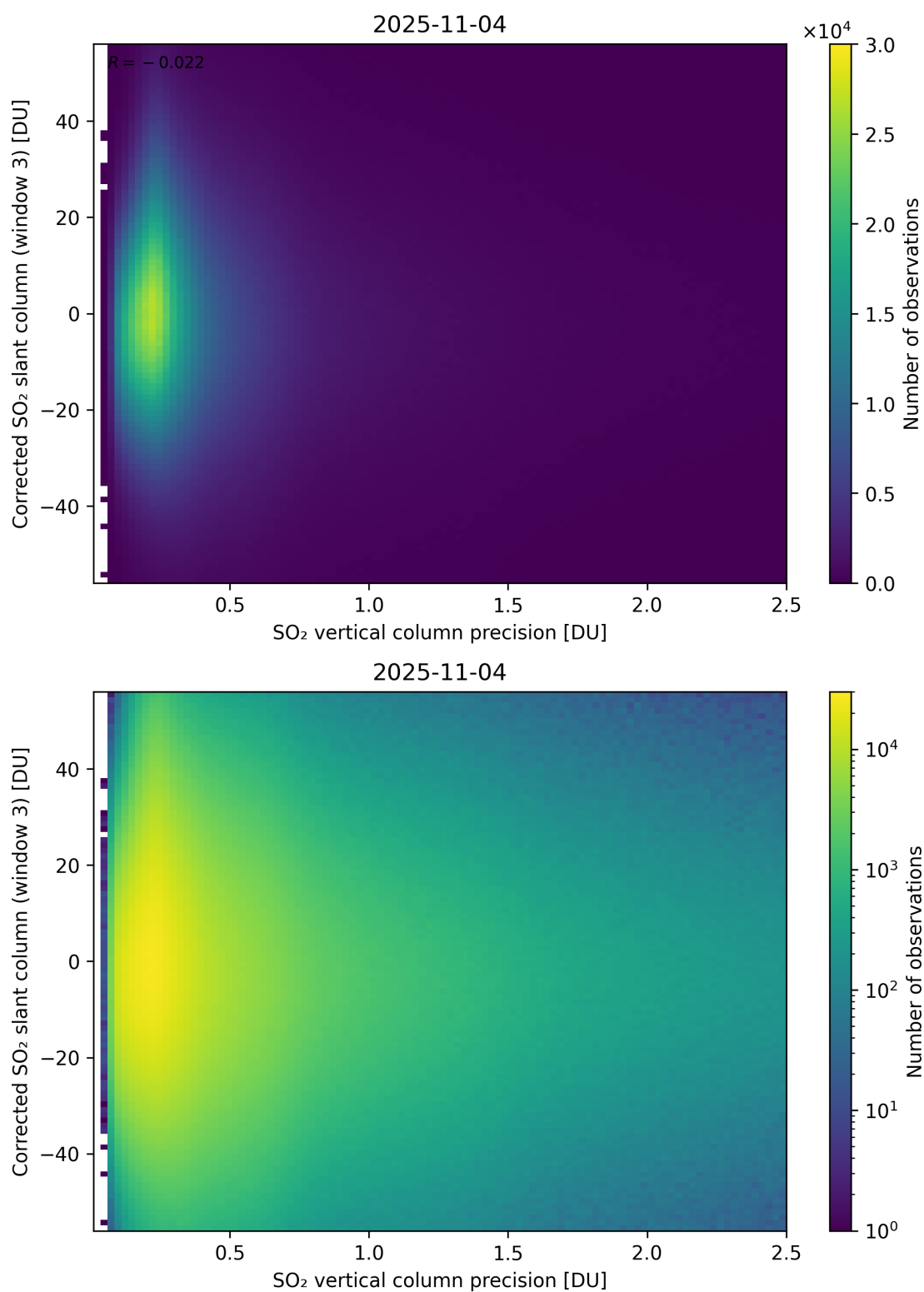
Figure 340: Scatter density plot of “SO 2 vertical column precision” against “Corrected SO 2 slant column (window 3)” for 2025-11-03 to 2025-11-05.
