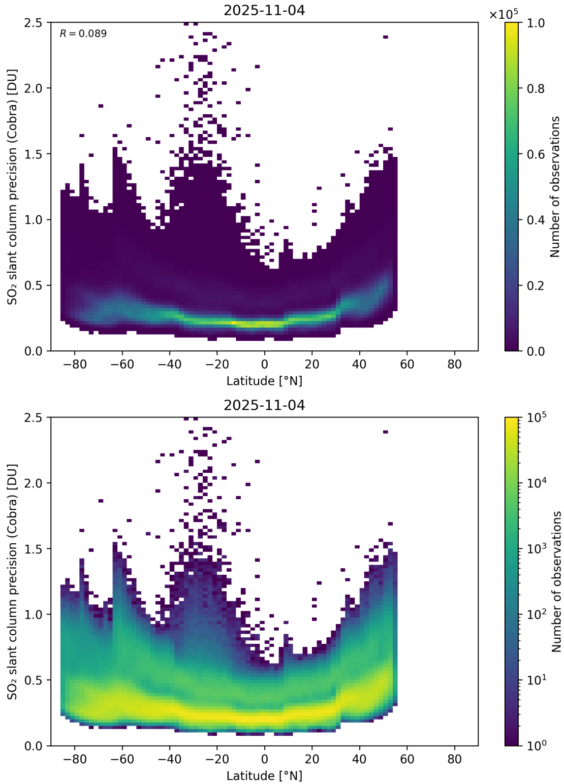
Figure 158: Scatter density plot of “Latitude” against “SO 2 slant column precision (Cobra)” for 2025-11-03 to 2025-11-05.
