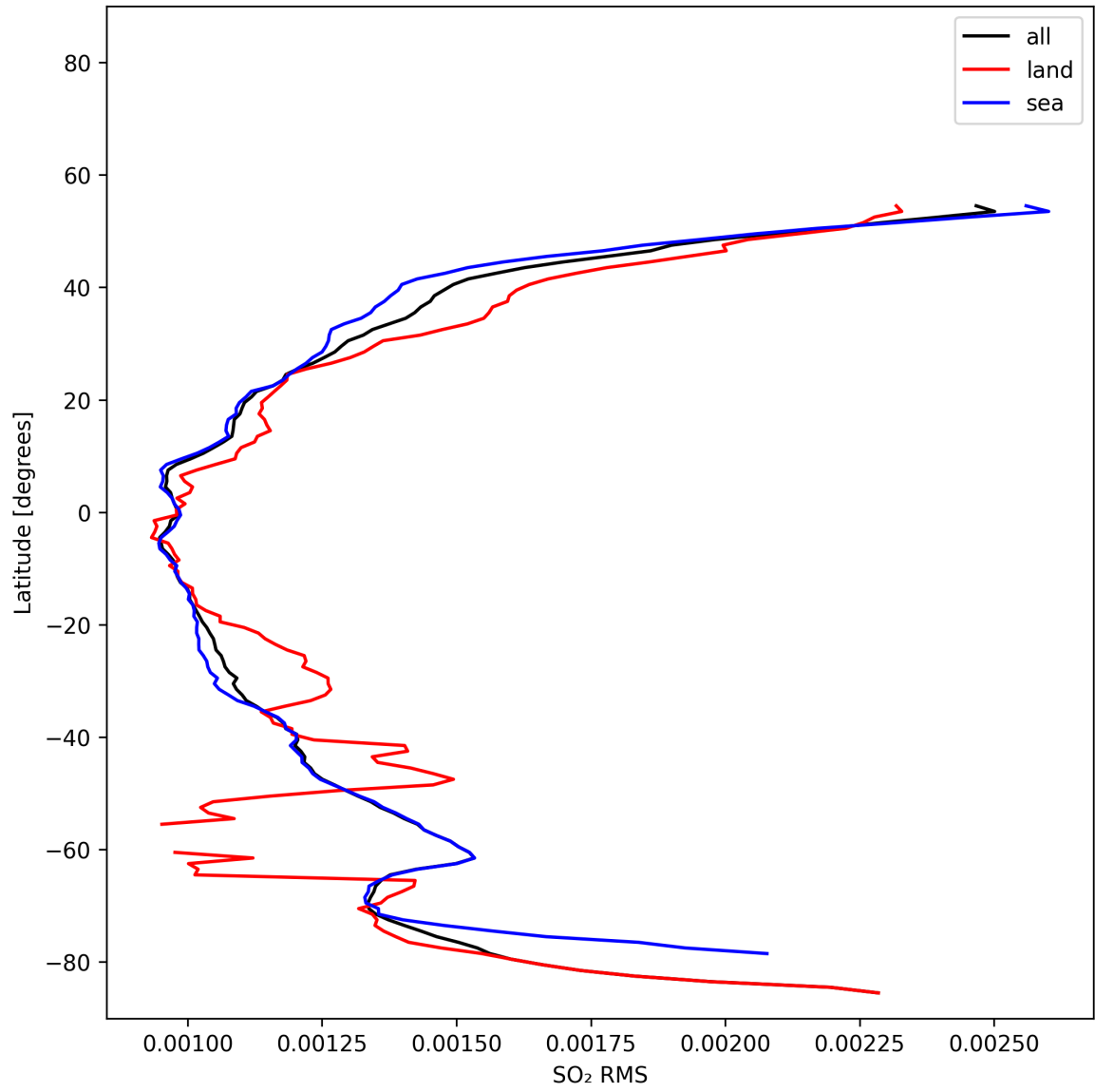
Figure 52: Zonal average of “SO 2 RMS” for 2025-11-03 to 2025-11-05.
