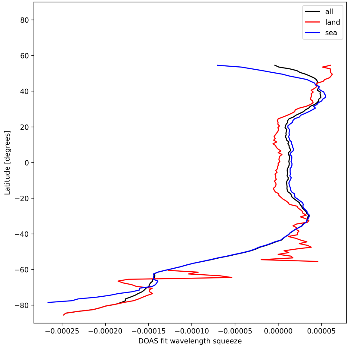
Figure 51: Zonal average of “DOAS fit wavelength squeeze” for 2025-11-03 to 2025-11-05.
