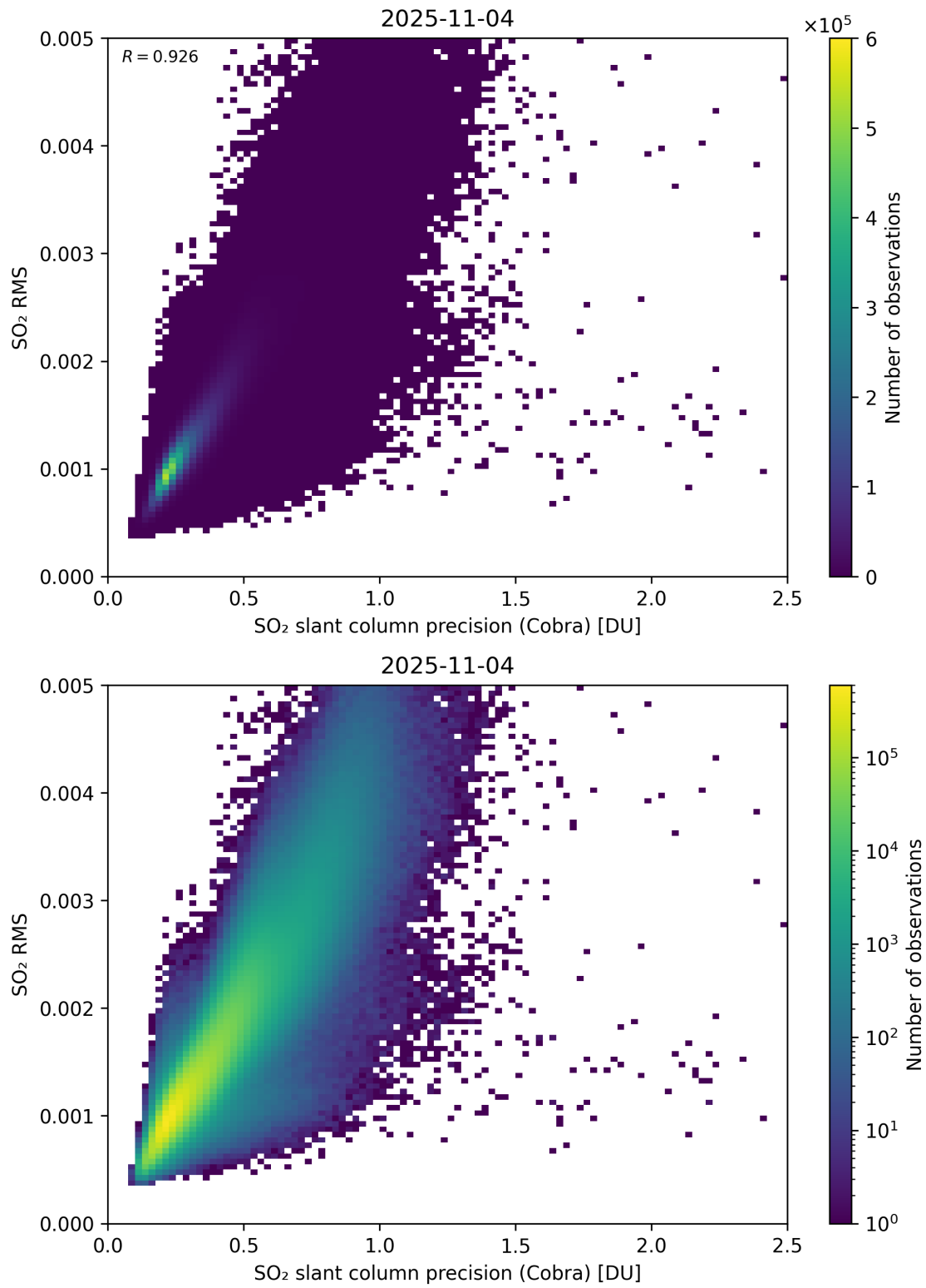
Figure 204: Scatter density plot of “SO 2 slant column precision (Cobra)” against “SO 2 RMS” for 2025-11-03 to 2025-11-05.
