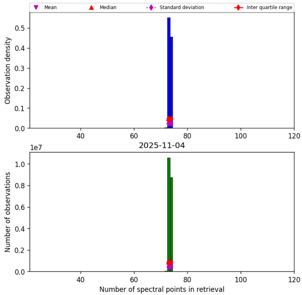
Figure 82: Histogram of “Number of spectral points in retrieval” for 2025-11-03 to 2025-11-05
