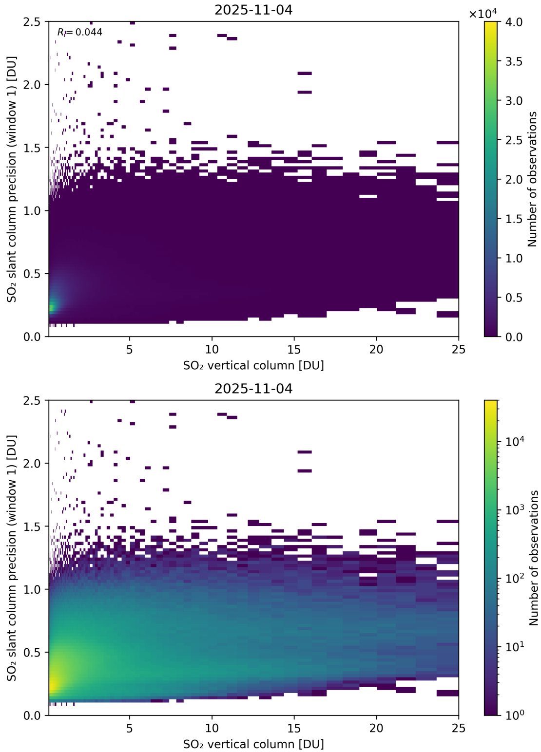
Figure 355: Scatter density plot of “SO 2 vertical column” against “SO 2 slant column precision (window 1)” for 2025-11-03 to 2025-11-05.
