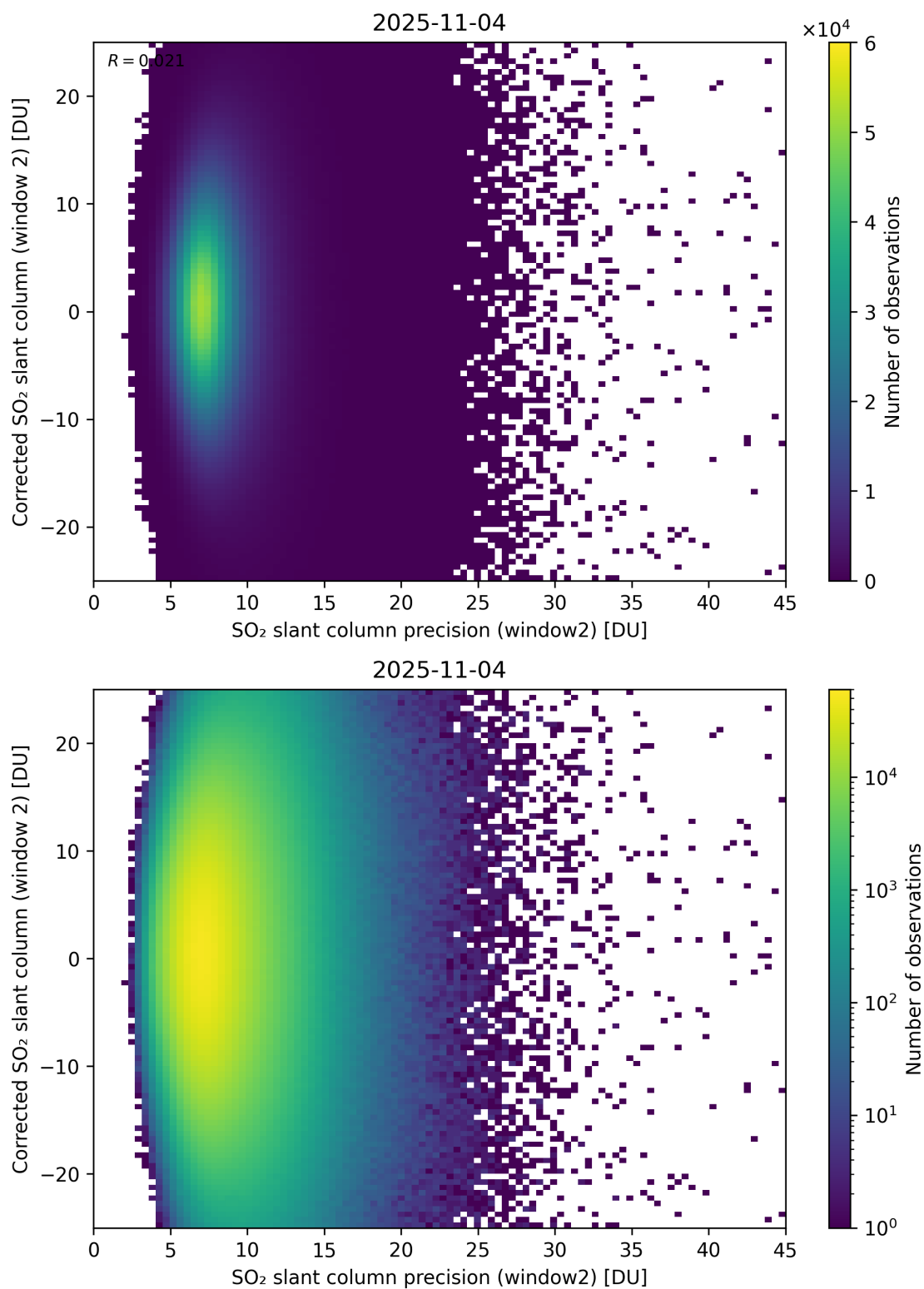
Figure 297: Scatter density plot of “SO 2 slant column precision (window2)” against “Corrected SO 2 slant column (window 2)” for 2025-11-03 to 2025-11-05.
