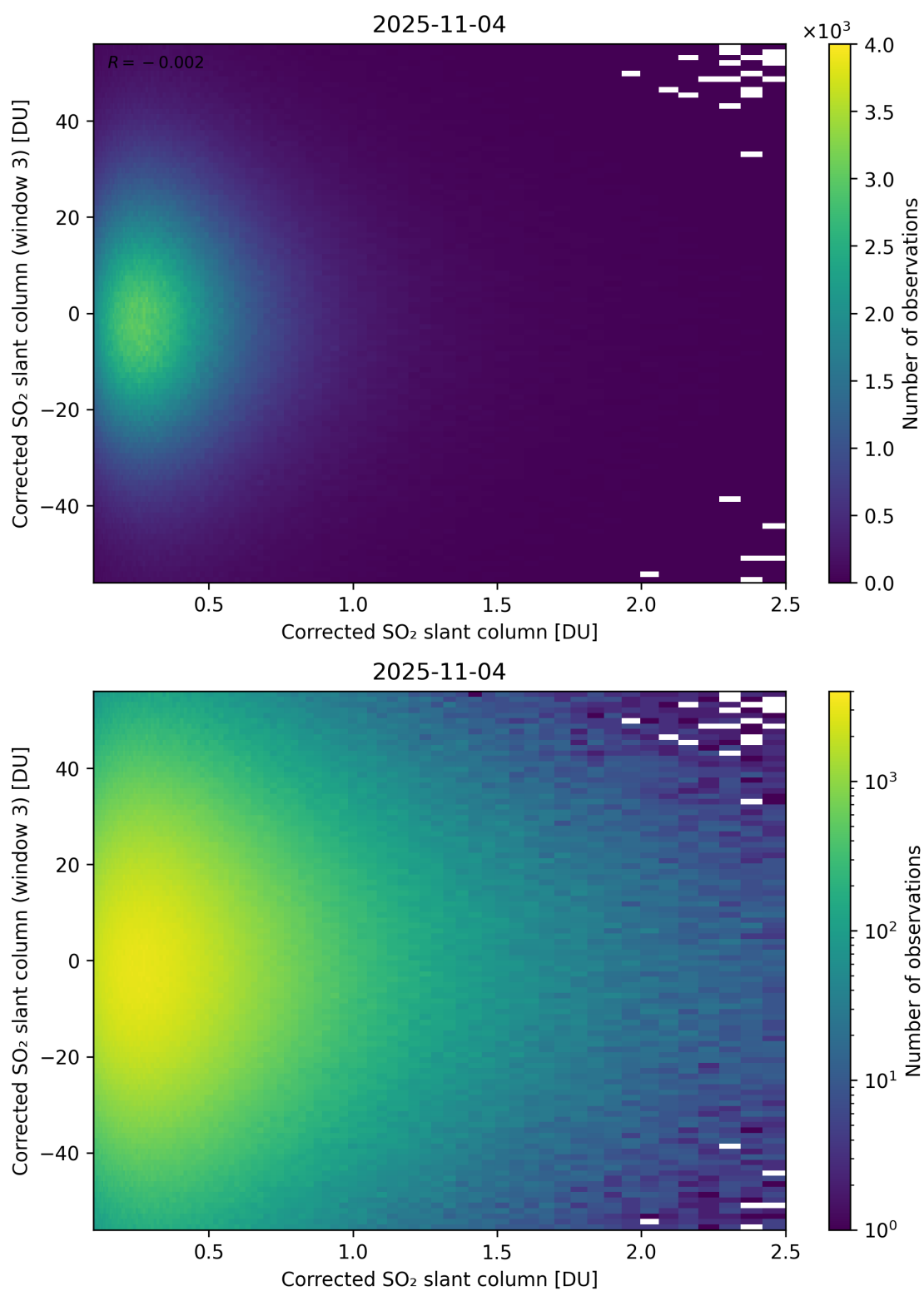
Figure 236: Scatter density plot of “Corrected SO 2 slant column” against “Corrected SO 2 slant column (window 3)” for 2025-11-03 to 2025-11-05.
