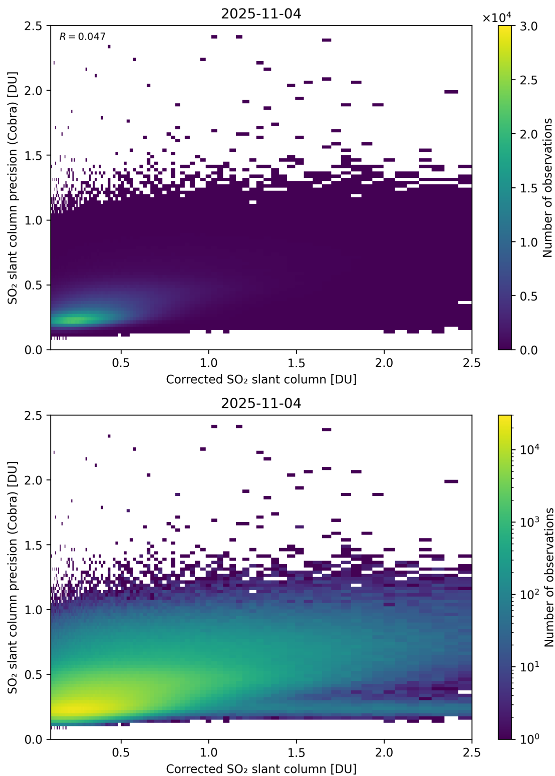
Figure 234: Scatter density plot of “Corrected SO 2 slant column” against “SO 2 slant column precision (Cobra)” for 2025-11-03 to 2025-11-05.
