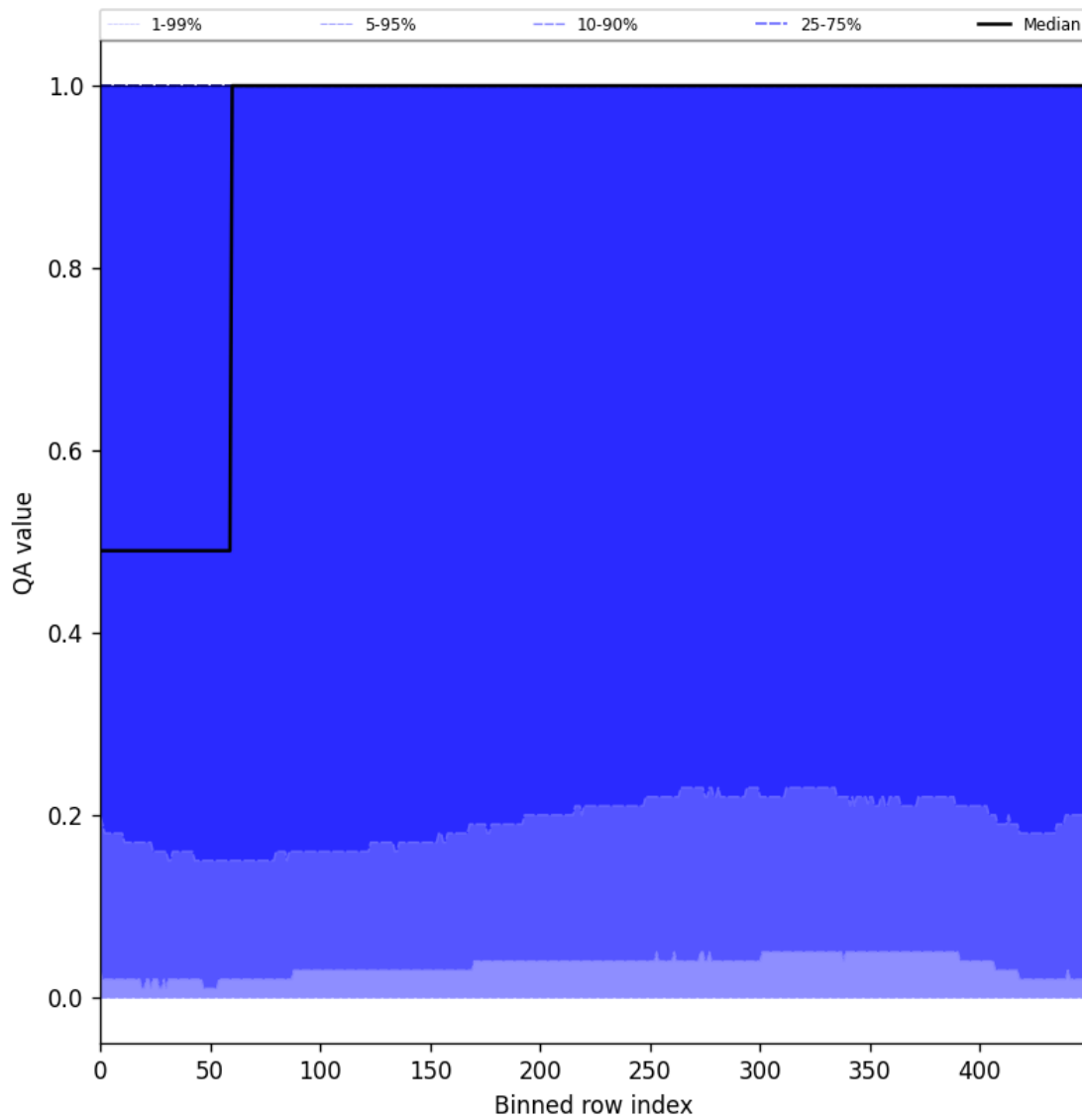
Figure 83: Along track statistics of “QA value” for 2025-11-03 to 2025-11-05
