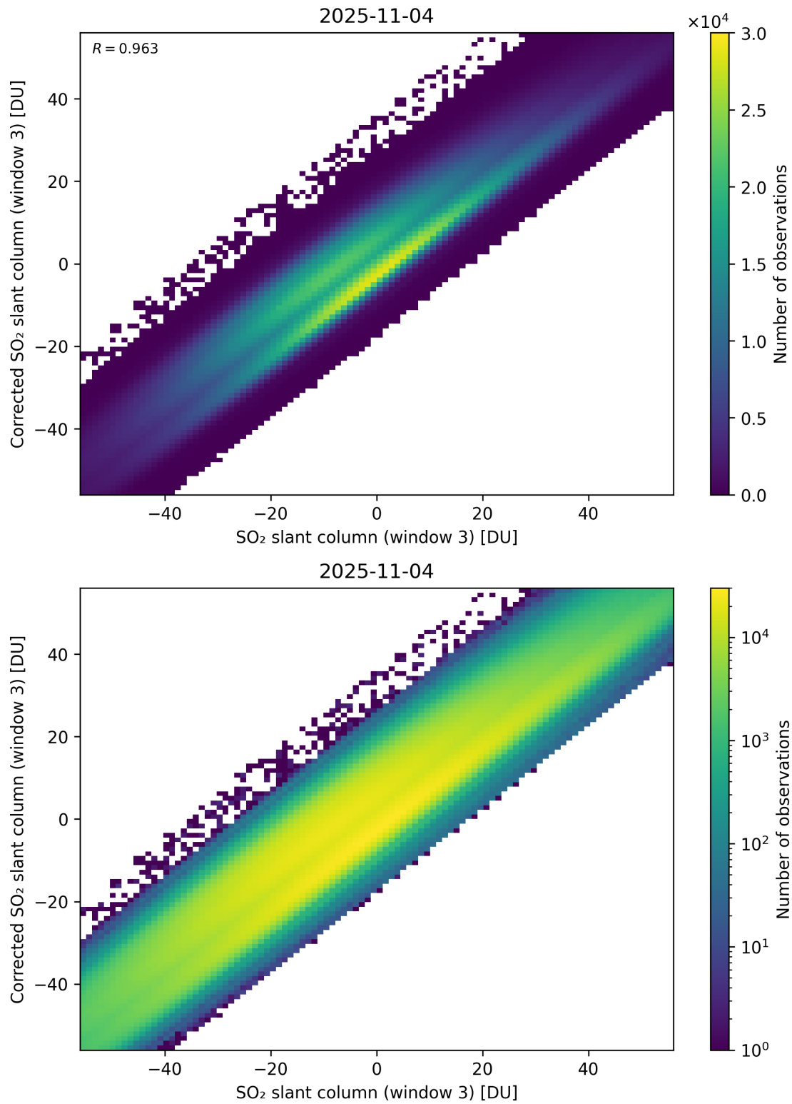
Figure 316: Scatter density plot of “SO 2 slant column (window 3)” against “Corrected SO 2 slant column (window 3)” for 2025-11-03 to 2025-11-05.
