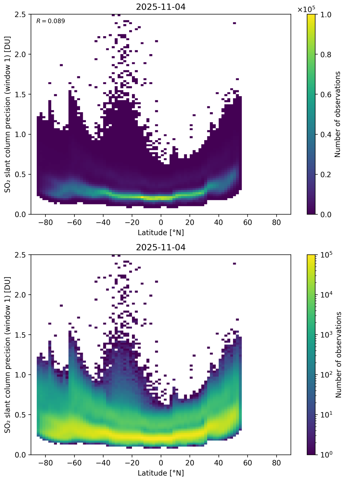
Figure 163: Scatter density plot of “Latitude” against “SO 2 slant column precision (window 1)” for 2025-11-03 to 2025-11-05.
