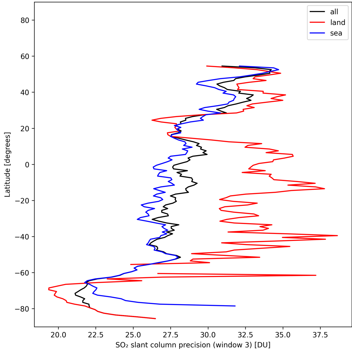
Figure 46: Zonal average of “SO 2 slant column precision (window 3)” for 2025-11-03 to 2025-11-05.
