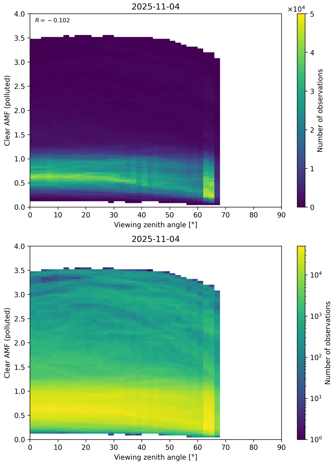
Figure 370: Scatter density plot of “Viewing zenith angle” against “Clear AMF (polluted)” for 2025-11-03 to 2025-11-05.
