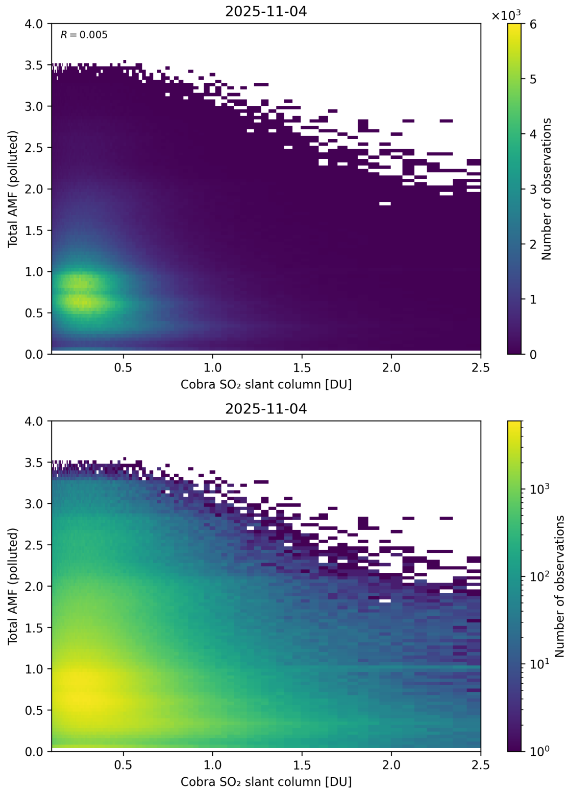
Figure 224: Scatter density plot of “Cobra SO 2 slant column” against “Total AMF (polluted)” for 2025-11-03 to 2025-11-05.
