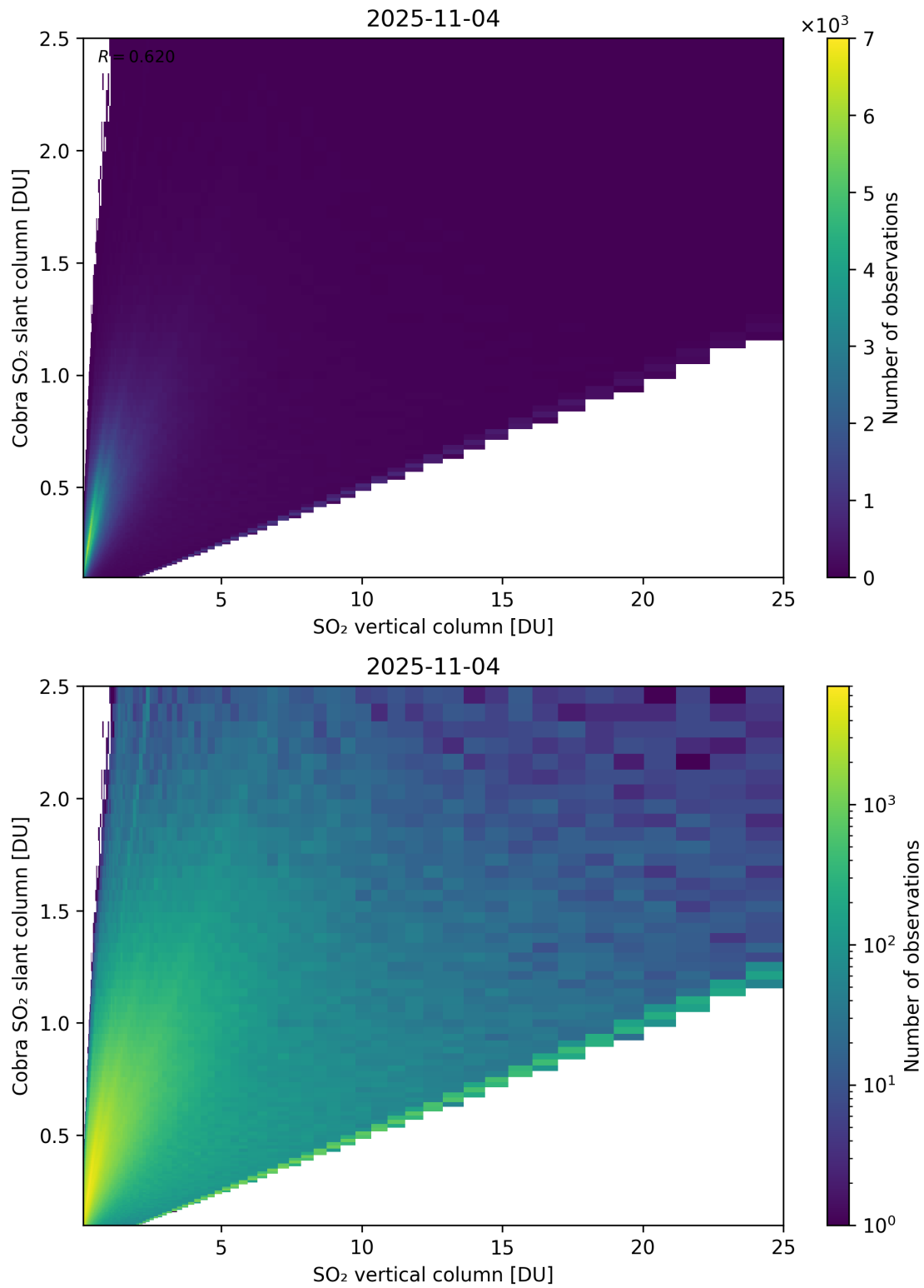
Figure 349: Scatter density plot of “SO 2 vertical column” against “Cobra SO 2 slant column” for 2025-11-03 to 2025-11-05.
