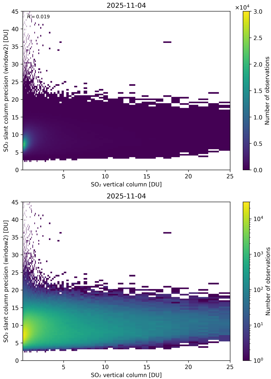
Figure 356: Scatter density plot of “SO 2 vertical column” against “SO 2 slant column precision (window2)” for 2025-11-03 to 2025-11-05.
