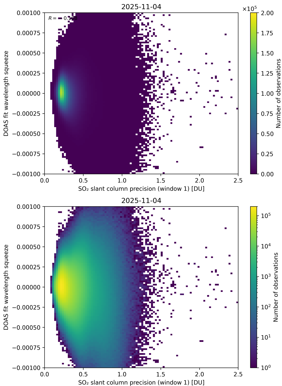
Figure 272: Scatter density plot of “SO 2 slant column precision (window 1)” against “DOAS fit wavelength squeeze” for 2025-11-03 to 2025-11-05.
