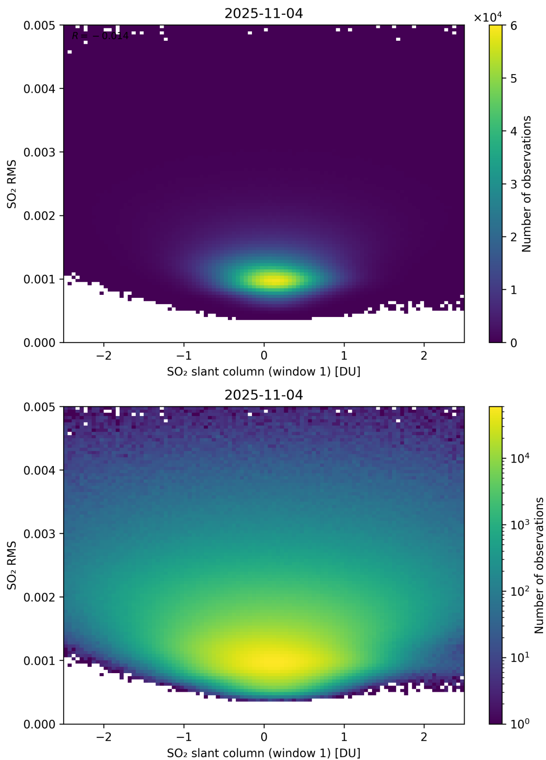
Figure 267: Scatter density plot of “SO 2 slant column (window 1)” against “SO 2 RMS” for 2025-11-03 to 2025-11-05.
