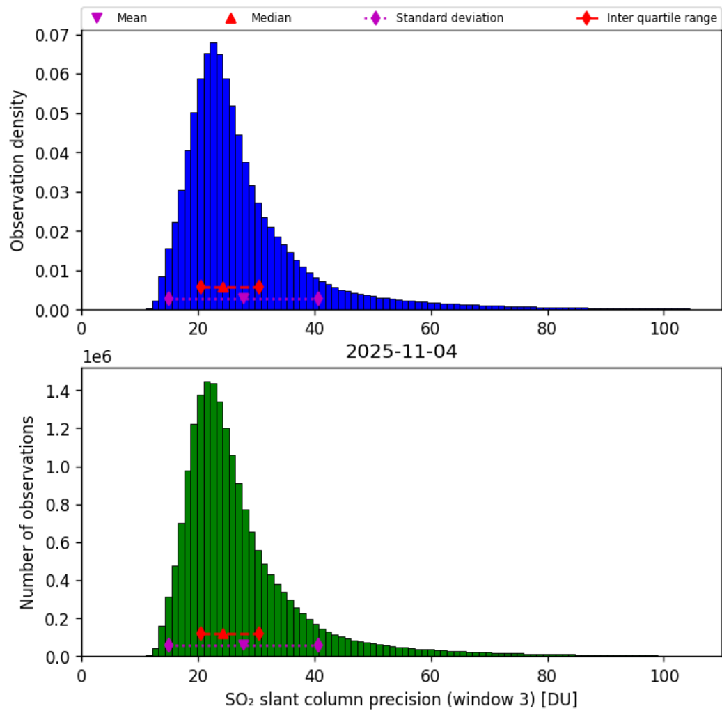
Figure 72: Histogram of “SO 2 slant column precision (window 3)” for 2025-11-03 to 2025-11-05
