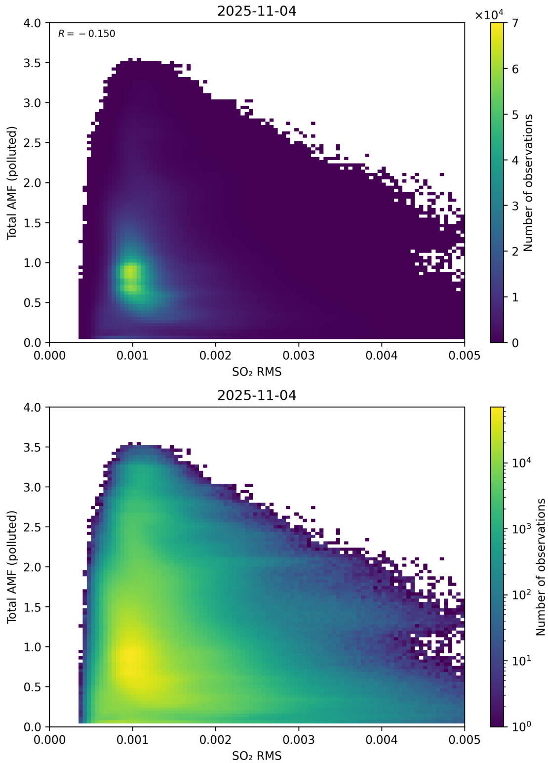
Figure 148: Scatter density plot of “SO 2 RMS” against “Total AMF (polluted)” for 2025-11-03 to 2025-11-05.
