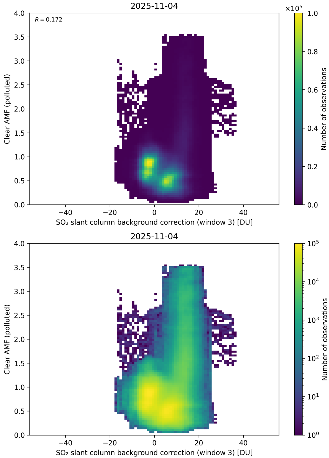
Figure 135: Scatter density plot of “SO 2 slant column background correction (window 3)” against “Clear AMF (polluted)” for 2025-11-03 to 2025-11-05.
