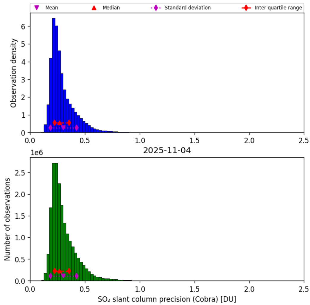
Figure 62: Histogram of “SO 2 slant column precision (Cobra)” for 2025-11-03 to 2025-11-05
