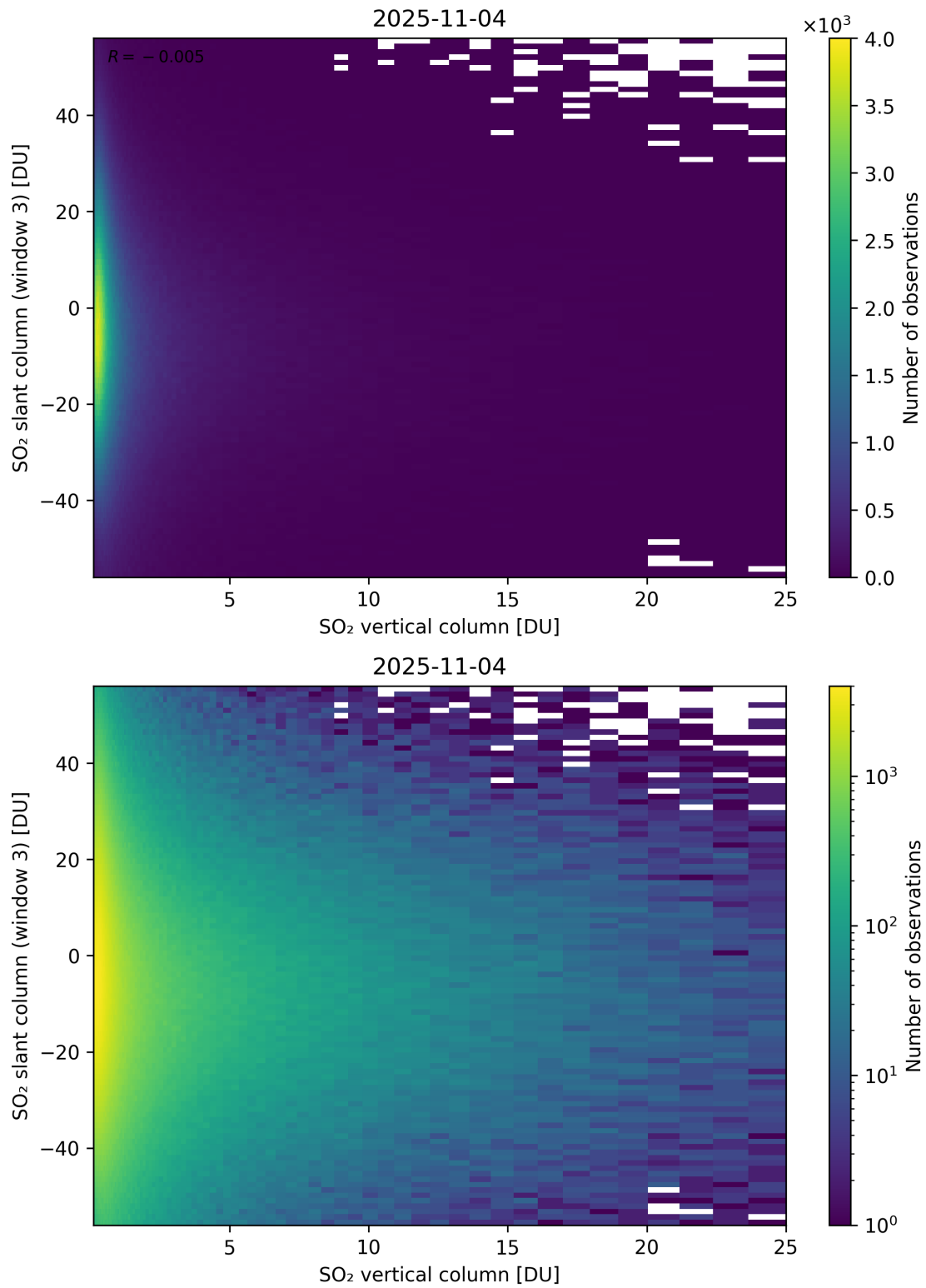
Figure 357: Scatter density plot of “SO 2 vertical column” against “SO 2 slant column (window 3)” for 2025-11-03 to 2025-11-05.
