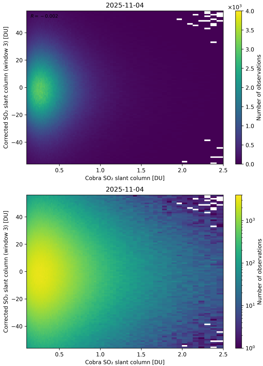
Figure 218: Scatter density plot of “Cobra SO 2 slant column” against “Corrected SO 2 slant column (window 3)” for 2025-11-03 to 2025-11-05.
