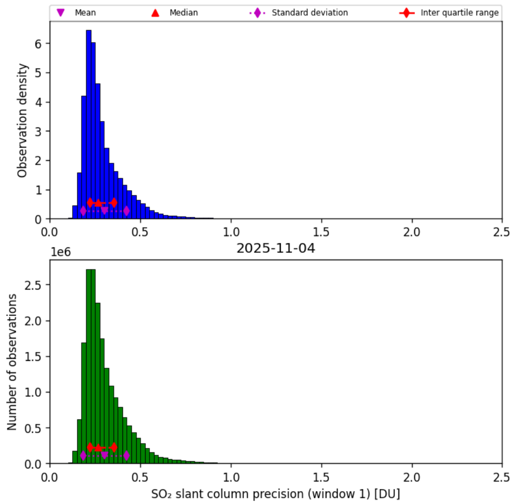
Figure 64: Histogram of “SO 2 slant column precision (window 1)” for 2025-11-03 to 2025-11-05
