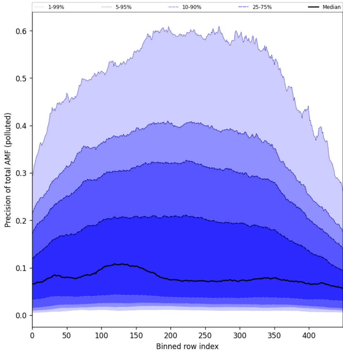
Figure 106: Along track statistics of “Precision of total AMF (polluted)” for 2025-11-03 to 2025-11-05
