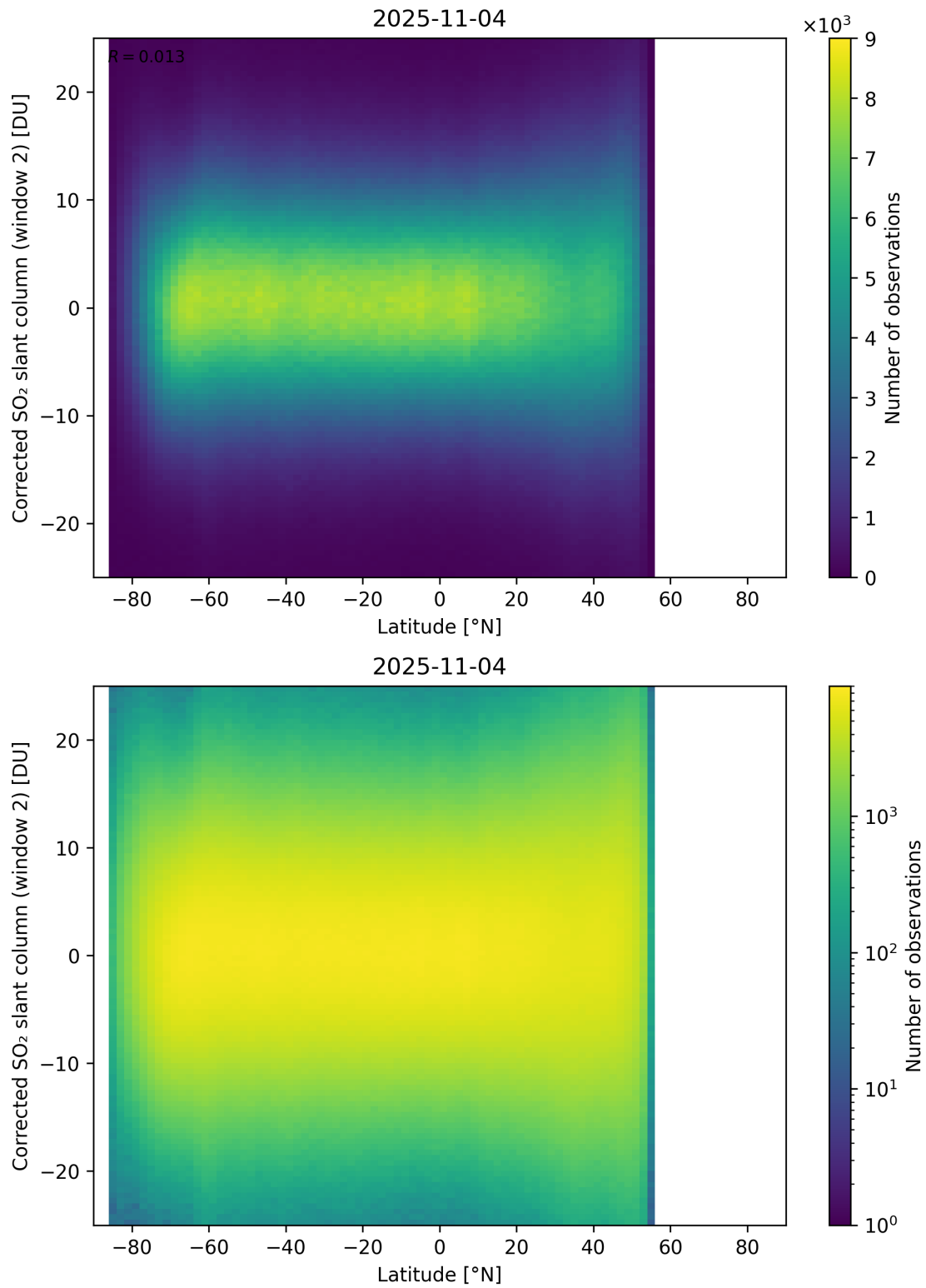
Figure 160: Scatter density plot of “Latitude” against “Corrected SO 2 slant column (window 2)” for 2025-11-03 to 2025-11-05.
