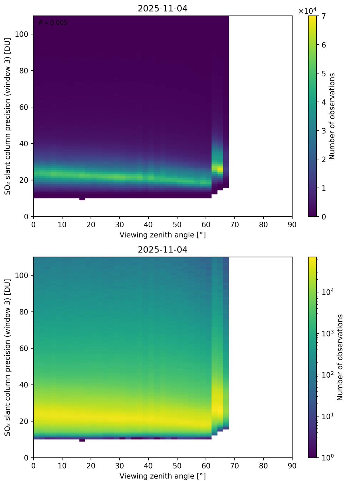
Figure 380: Scatter density plot of “Viewing zenith angle” against “SO 2 slant column precision (window 3)” for 2025-11-03 to 2025-11-05.
