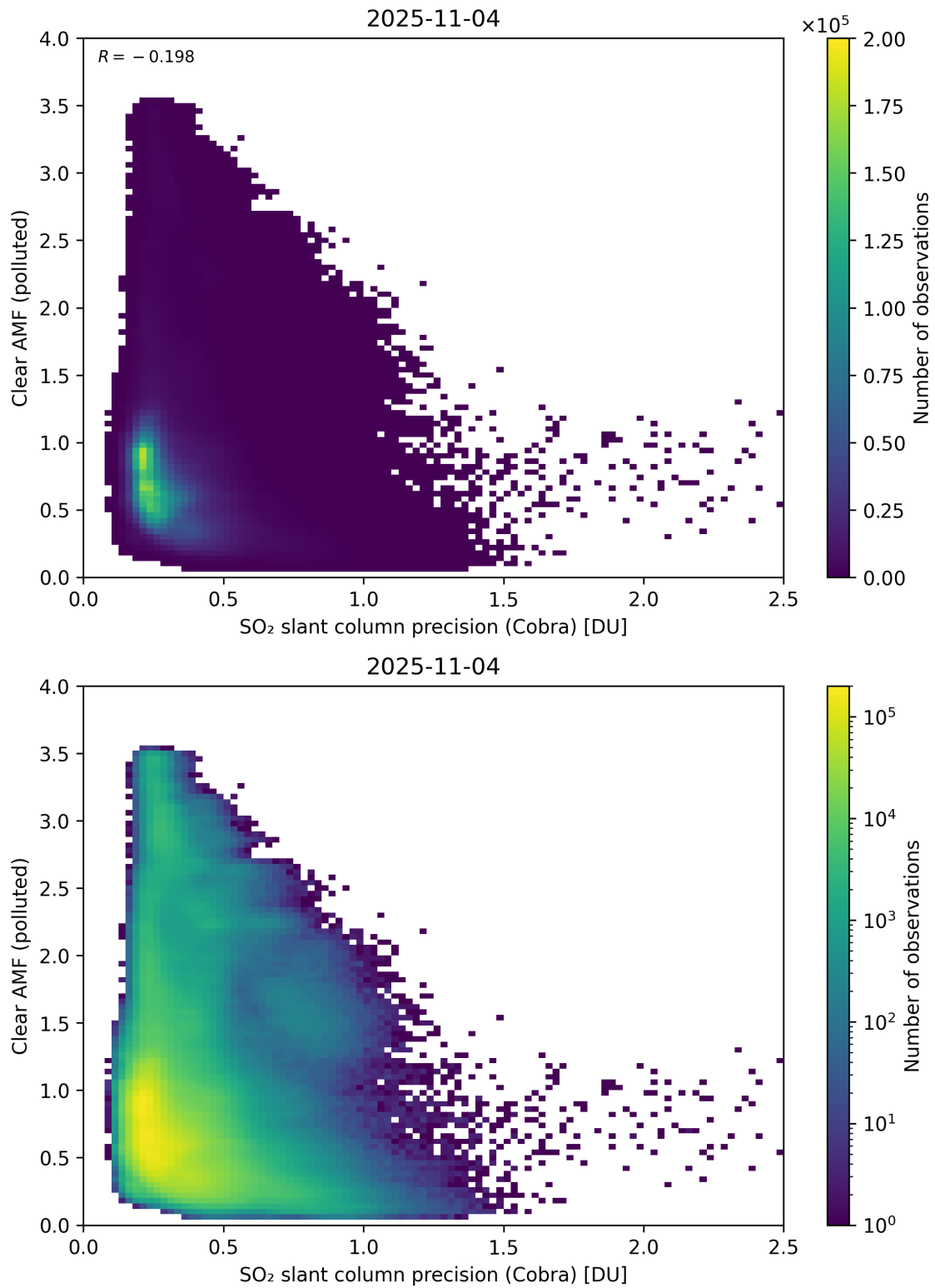
Figure 205: Scatter density plot of “SO 2 slant column precision (Cobra)” against “Clear AMF (polluted)” for 2025-11-03 to 2025-11-05.
