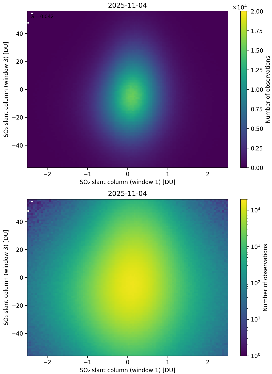
Figure 287: Scatter density plot of “SO 2 slant column (window 1)” against “SO 2 slant column (window 3)” for 2025-11-03 to 2025-11-05.
