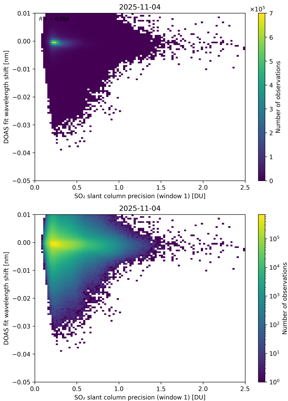
Figure 271: Scatter density plot of “SO 2 slant column precision (window 1)” against “DOAS fit wavelength shift” for 2025-11-03 to 2025-11-05.
