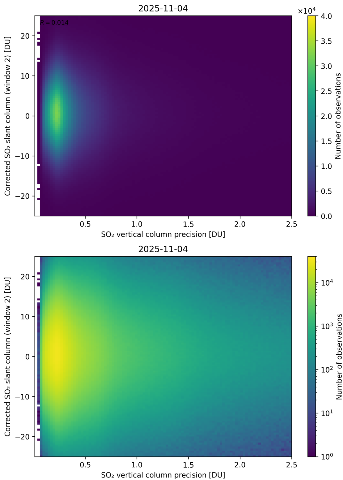
Figure 339: Scatter density plot of “SO 2 vertical column precision” against “Corrected SO 2 slant column (window 2)” for 2025-11-03 to 2025-11-05.
