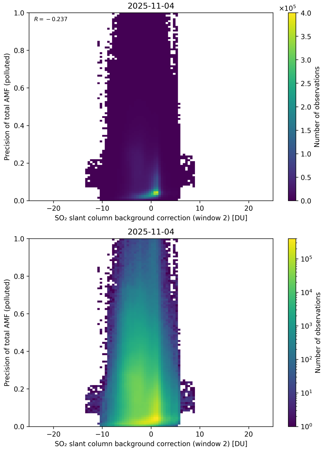
Figure 131: Scatter density plot of “SO 2 slant column background correction (window 2)” against “Precision of total AMF (polluted)” for 2025-11-03 to 2025-11-05.
