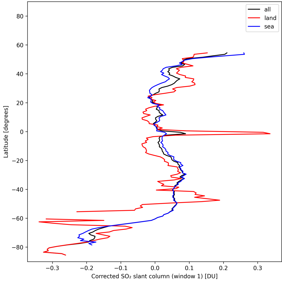
Figure 39: Zonal average of “Corrected SO 2 slant column (window 1)” for 2025-11-03 to 2025-11-05.
