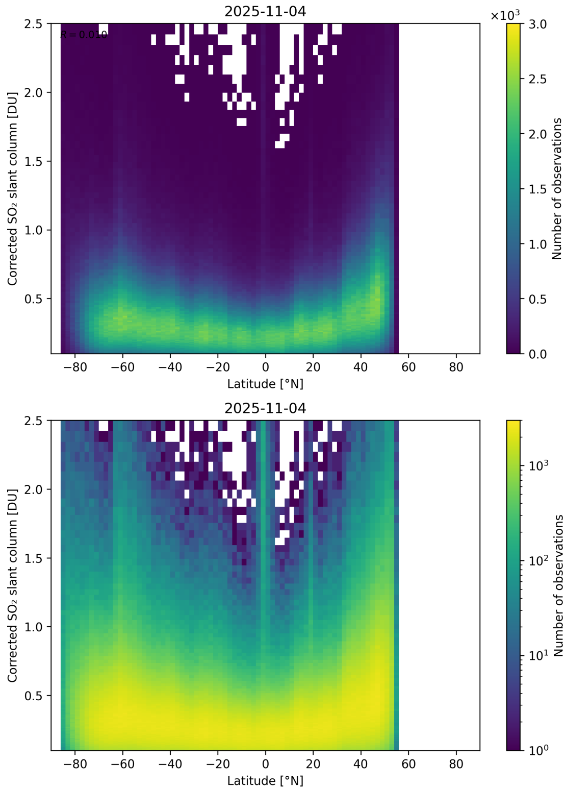
Figure 159: Scatter density plot of “Latitude” against “Corrected SO 2 slant column” for 2025-11-03 to 2025-11-05.
