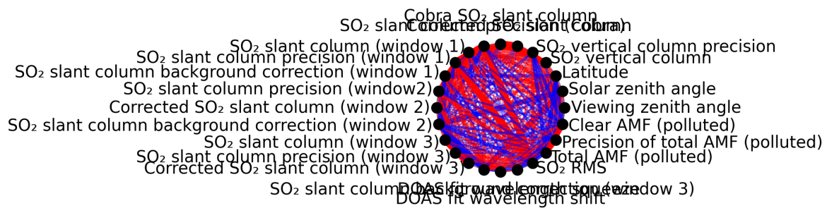
Figure 1: Map of correlation graph for 2025-11-03 to 2025-11-05.
