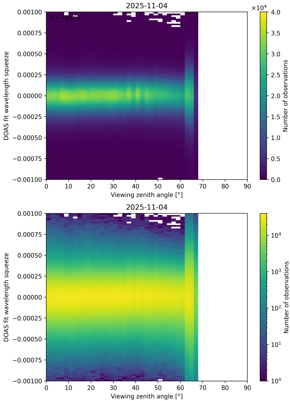
Figure 366: Scatter density plot of “Viewing zenith angle” against “DOAS fit wavelength squeeze” for 2025-11-03 to 2025-11-05.
