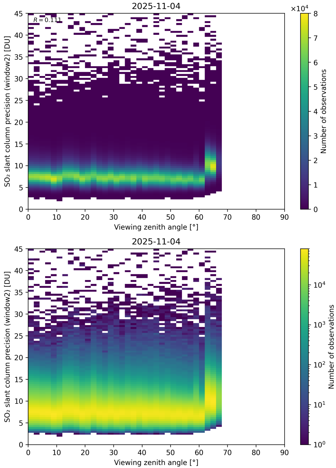
Figure 378: Scatter density plot of “Viewing zenith angle” against “SO 2 slant column precision (window2)” for 2025-11-03 to 2025-11-05.
