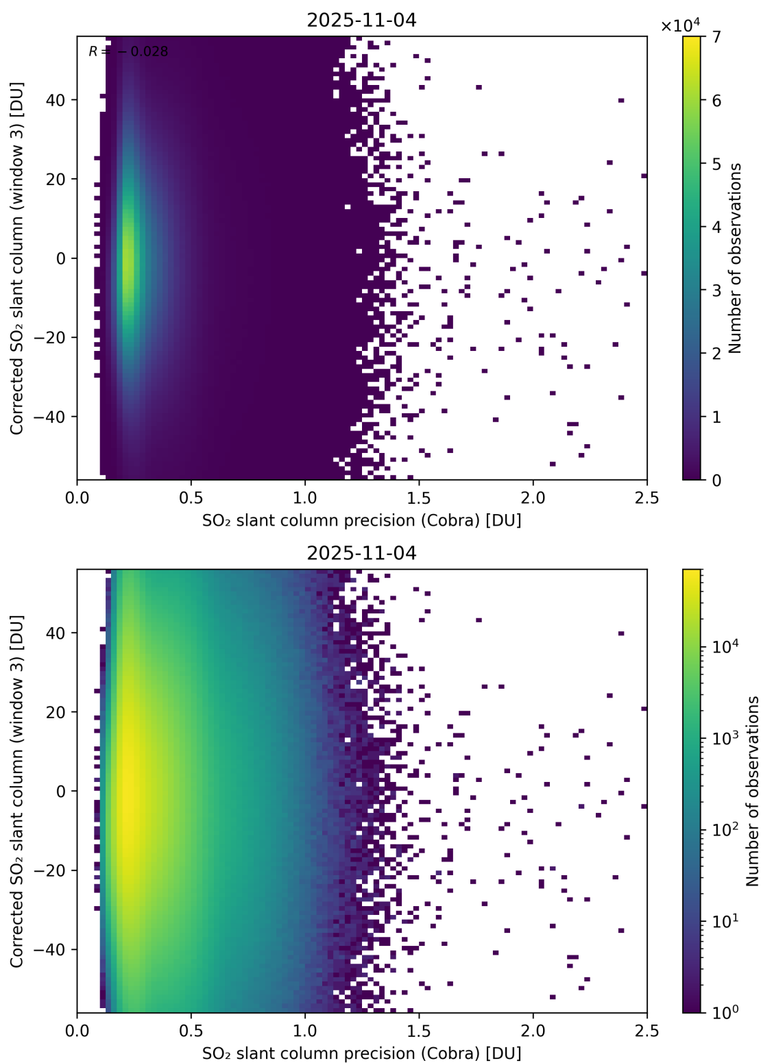
Figure 207: Scatter density plot of “SO 2 slant column precision (Cobra)” against “Corrected SO 2 slant column (window 3)” for 2025-11-03 to 2025-11-05.
