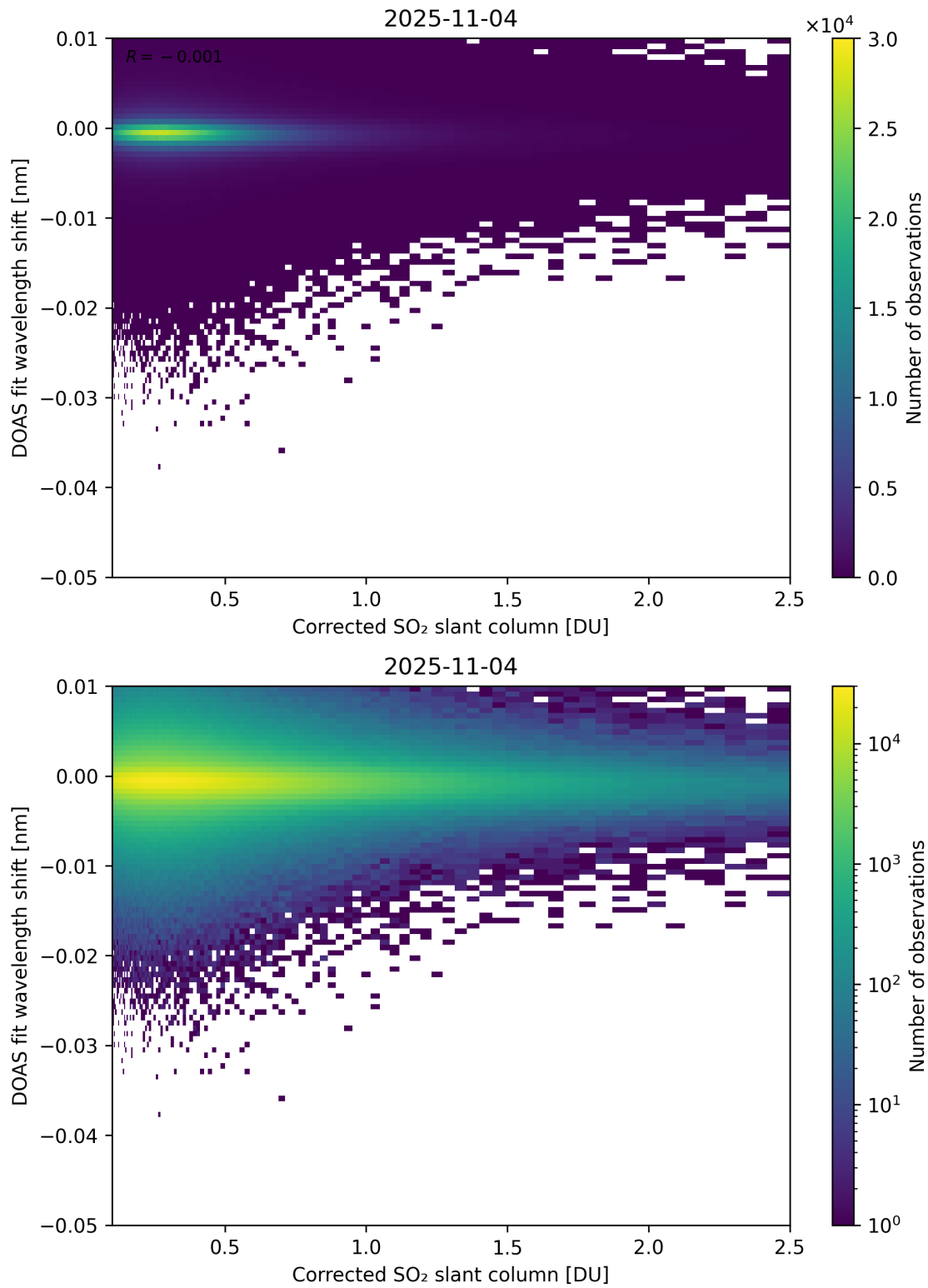
Figure 229: Scatter density plot of “Corrected SO 2 slant column” against “DOAS fit wavelength shift” for 2025-11-03 to 2025-11-05.
