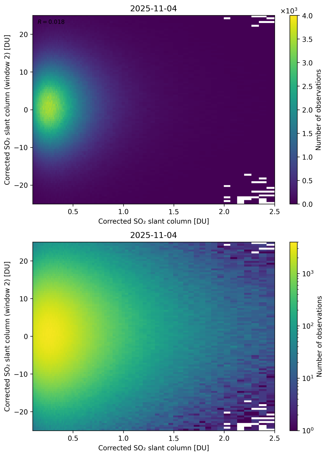
Figure 235: Scatter density plot of “Corrected SO 2 slant column” against “Corrected SO 2 slant column (window 2)” for 2025-11-03 to 2025-11-05.
