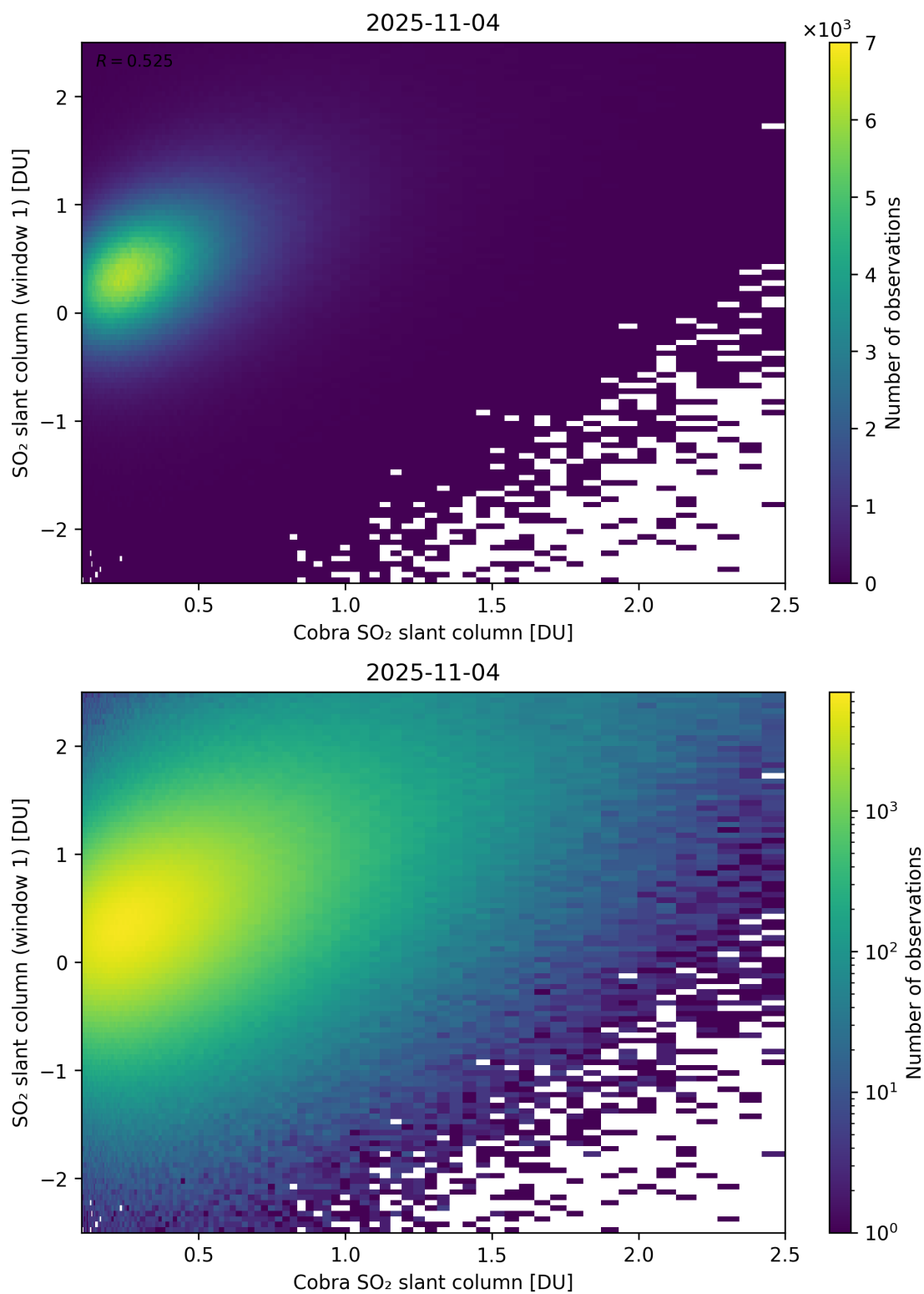
Figure 219: Scatter density plot of “Cobra SO 2 slant column” against “SO 2 slant column (window 1)” for 2025-11-03 to 2025-11-05.
