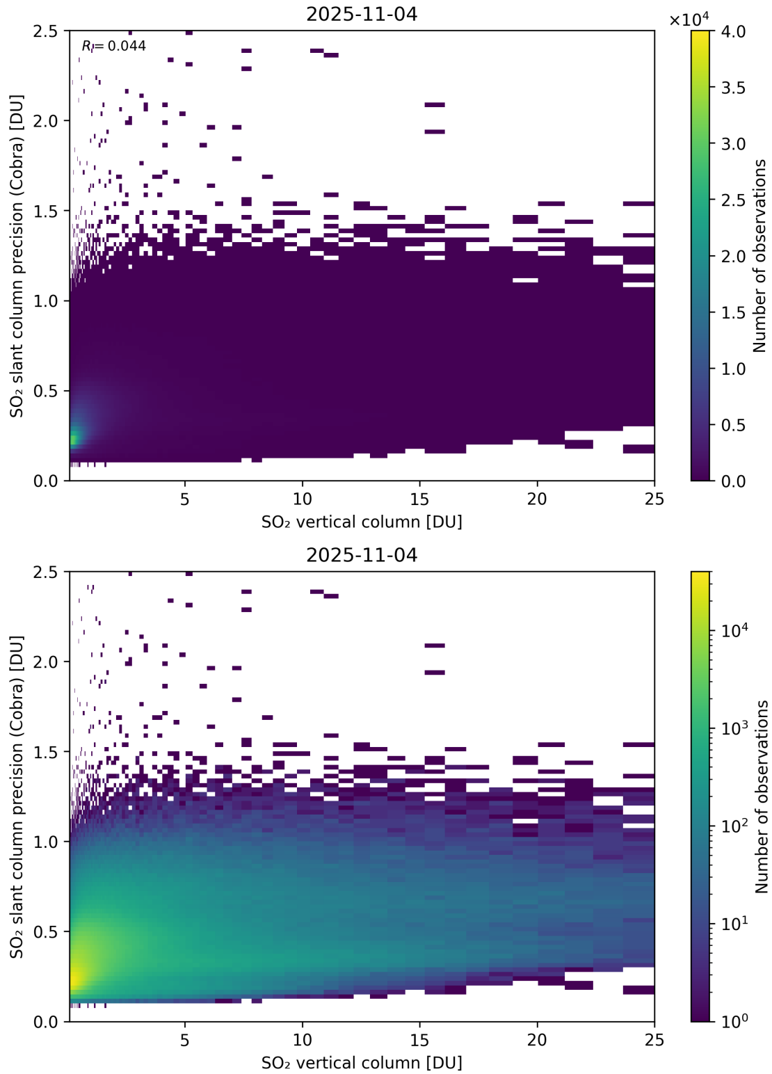
Figure 350: Scatter density plot of “SO 2 vertical column” against “SO 2 slant column precision (Cobra)” for 2025-11-03 to 2025-11-05.
