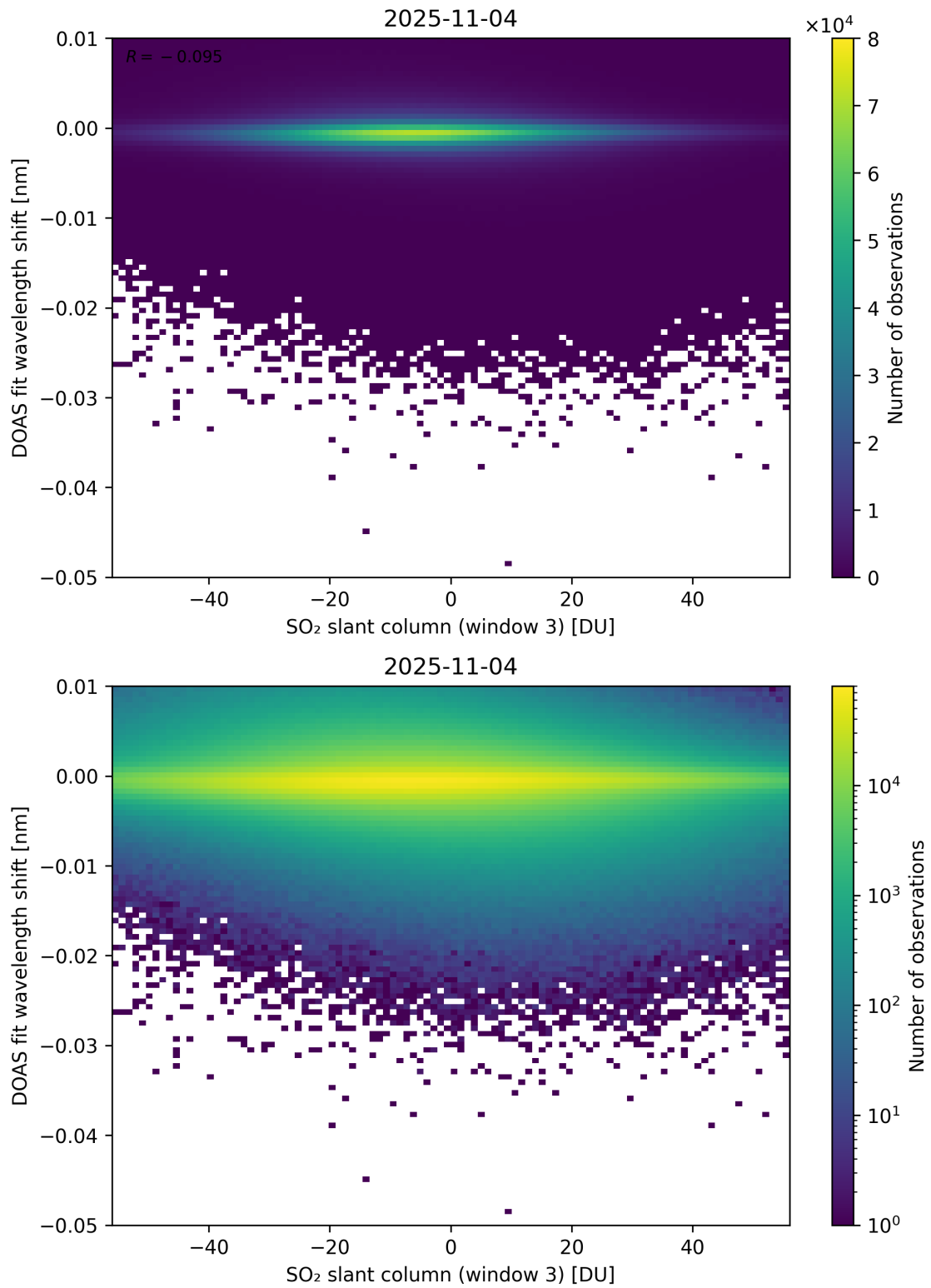
Figure 304: Scatter density plot of “SO 2 slant column (window 3)” against “DOAS fit wavelength shift” for 2025-11-03 to 2025-11-05.
