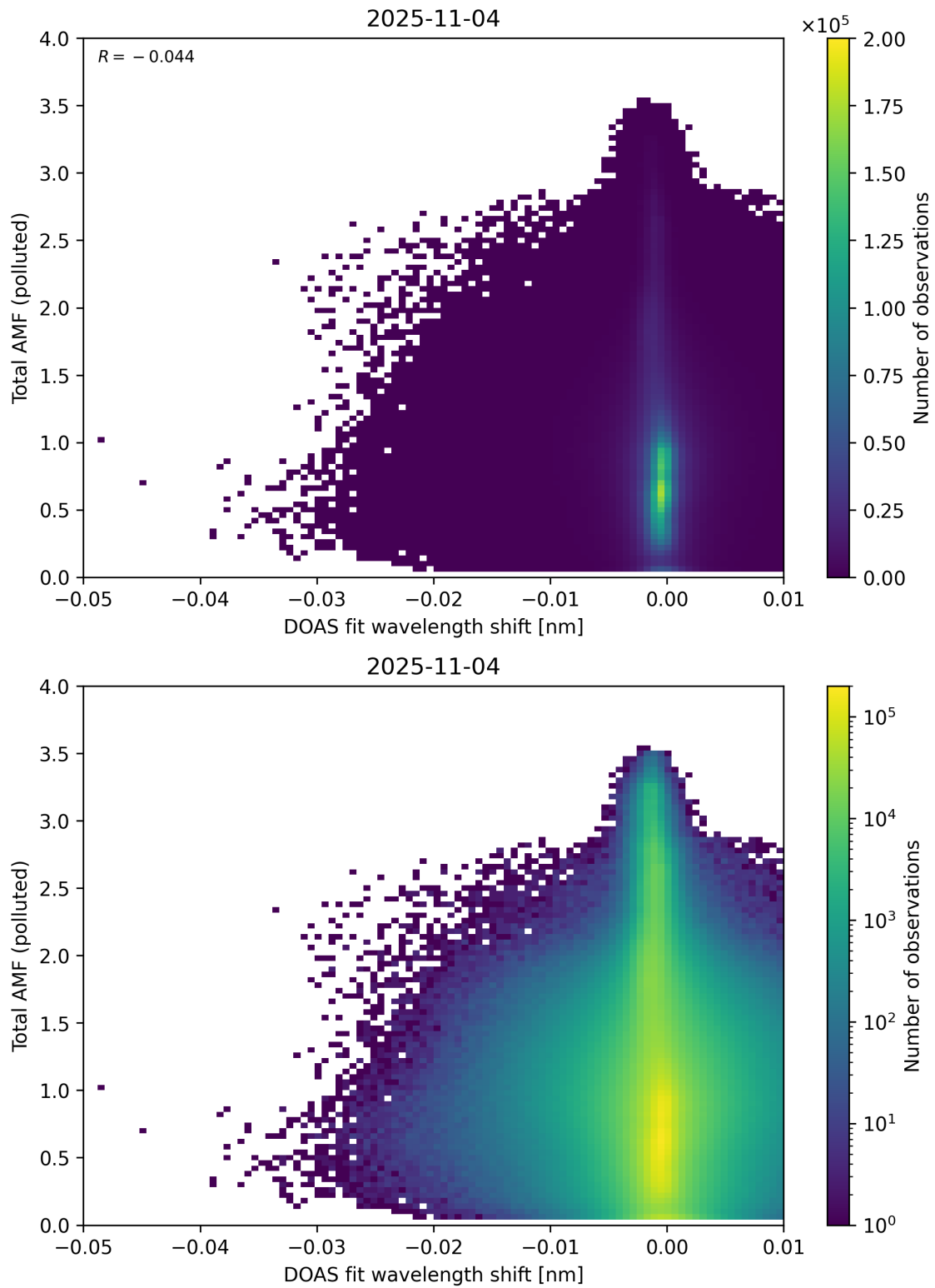
Figure 141: Scatter density plot of “DOAS fit wavelength shift” against “Total AMF (polluted)” for 2025-11-03 to 2025-11-05.
