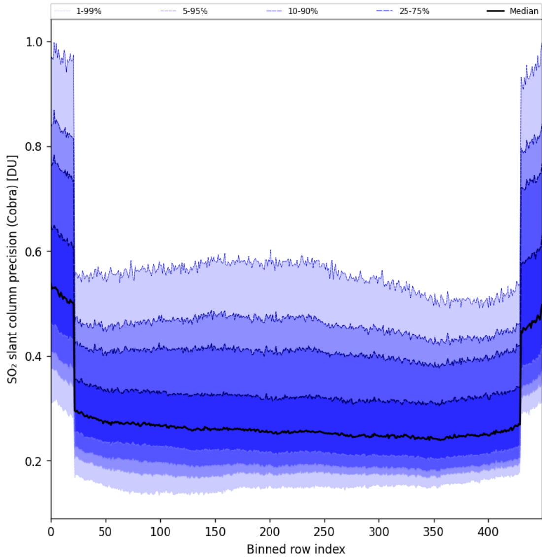
Figure 88: Along track statistics of “SO 2 slant column precision (Cobra)” for 2025-11-03 to 2025-11-05
