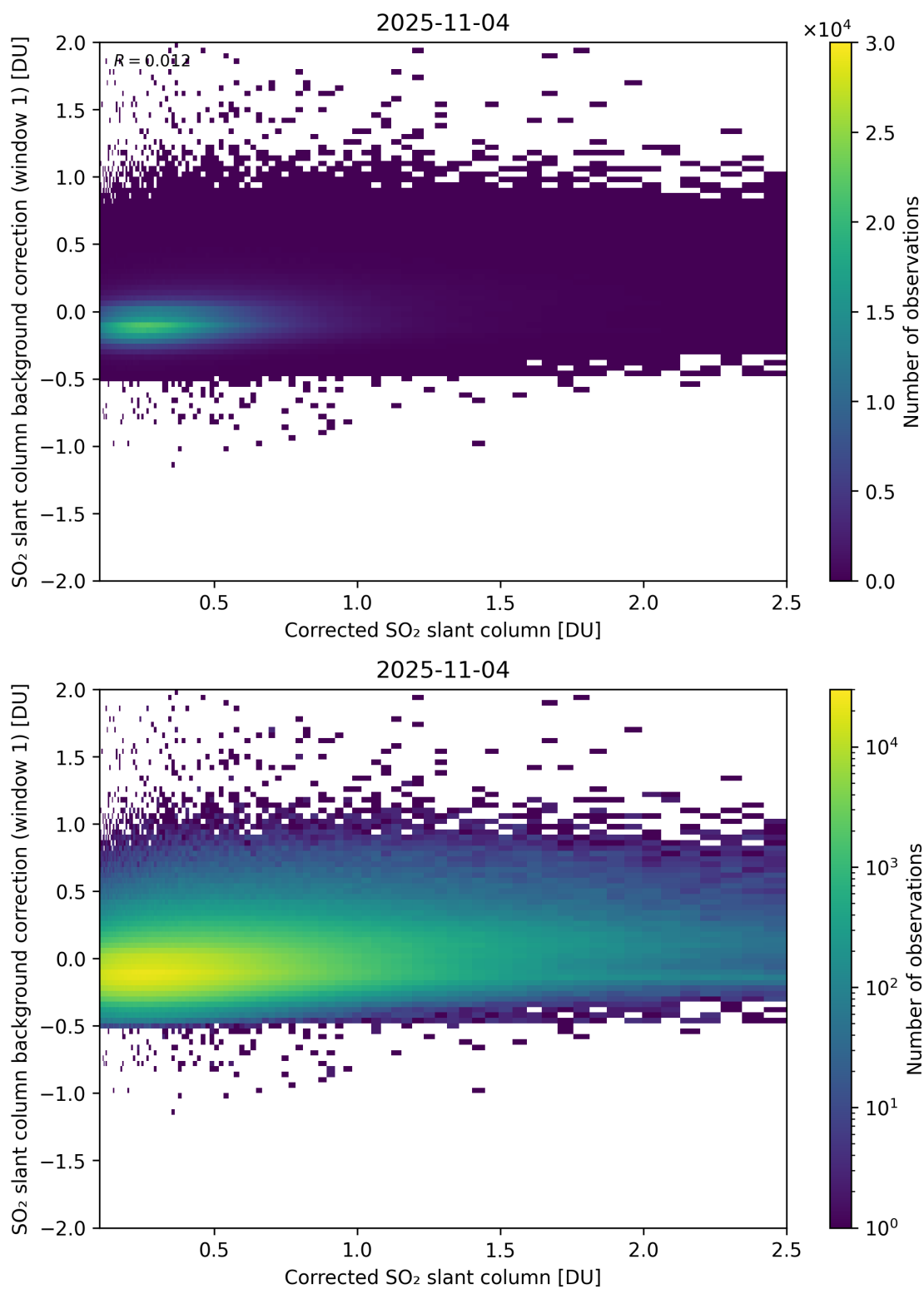
Figure 226: Scatter density plot of “Corrected SO 2 slant column” against “SO 2 slant column background correction (window 1)” for 2025-11-03 to 2025-11-05.
