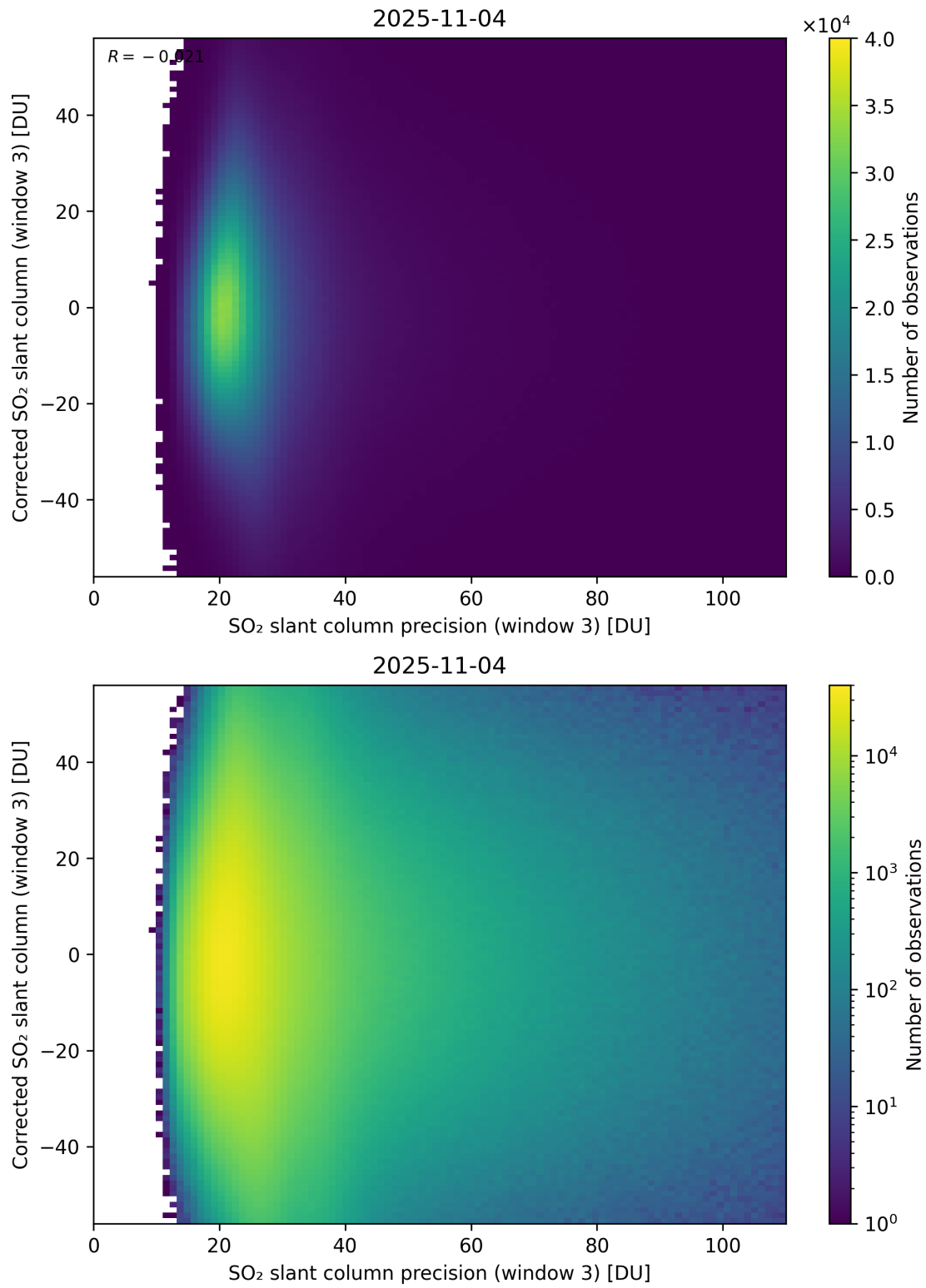
Figure 312: Scatter density plot of “SO 2 slant column precision (window 3)” against “Corrected SO 2 slant column (window 3)” for 2025-11-03 to 2025-11-05.
