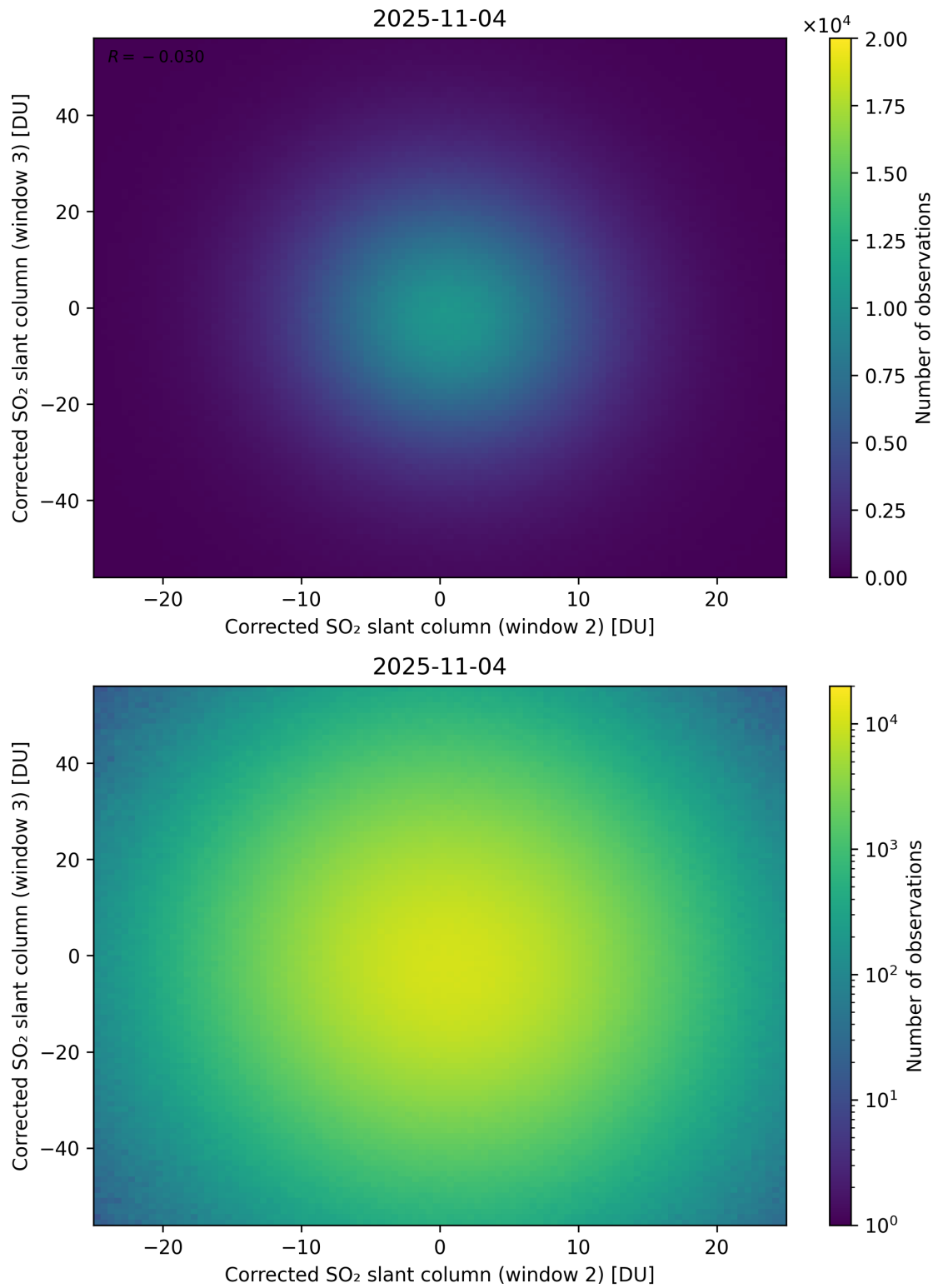
Figure 250: Scatter density plot of “Corrected SO 2 slant column (window 2)” against “Corrected SO 2 slant column (window 3)” for 2025-11-03 to 2025-11-05.
