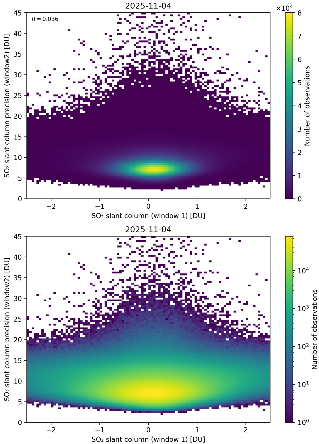
Figure 286: Scatter density plot of “SO 2 slant column (window 1)” against “SO 2 slant column precision (window2)” for 2025-11-03 to 2025-11-05.
