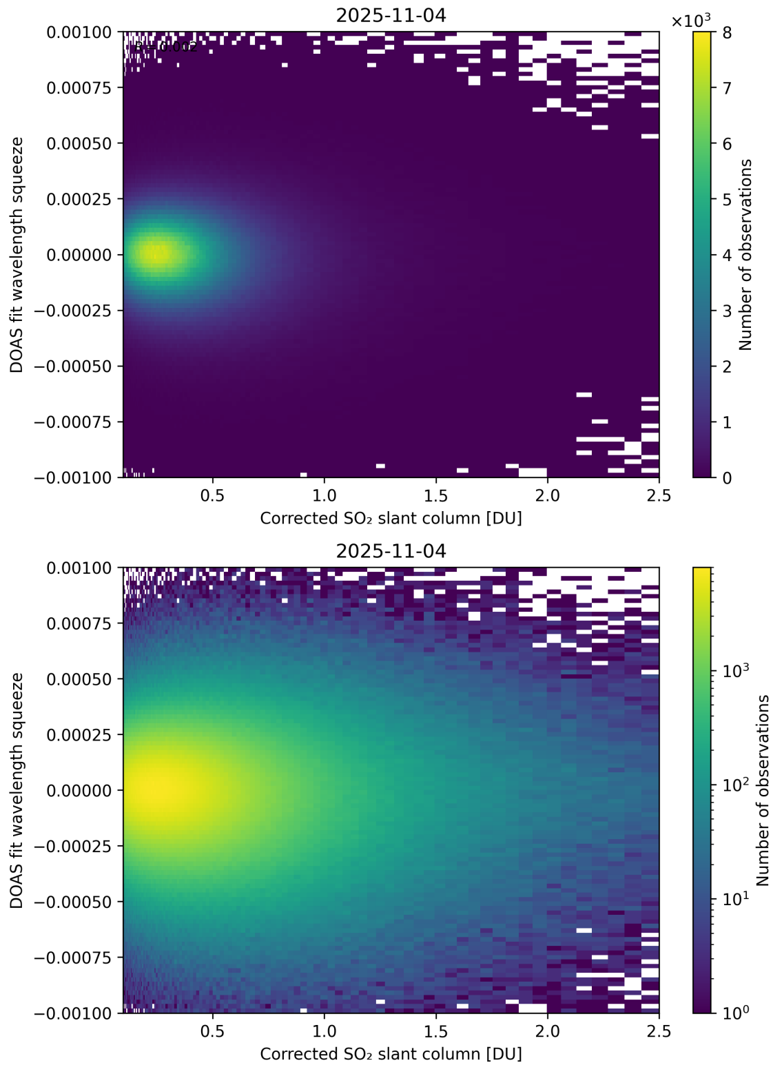
Figure 230: Scatter density plot of "Corrected SO 2 slant column" against "DOAS fit wavelength squeeze" for 2025-11-03 to 2025-11-05.
