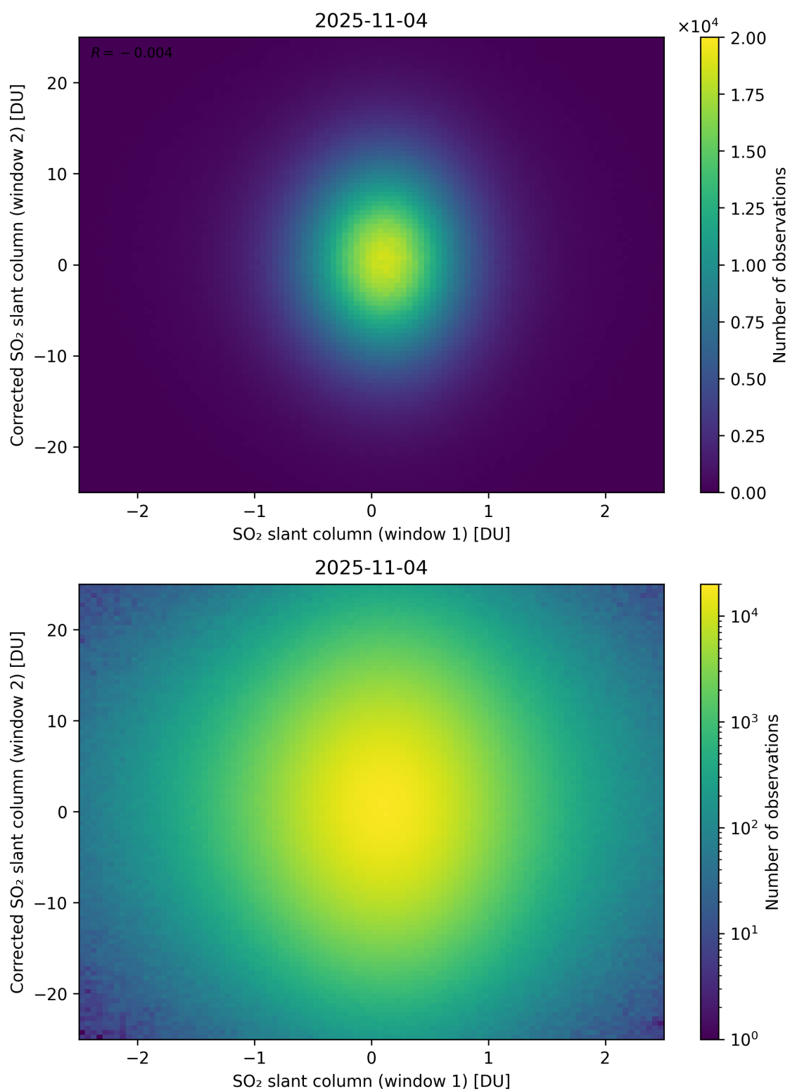
Figure 283: Scatter density plot of “SO 2 slant column (window 1)” against “Corrected SO 2 slant column (window 2)” for 2025-11-03 to 2025-11-05.
