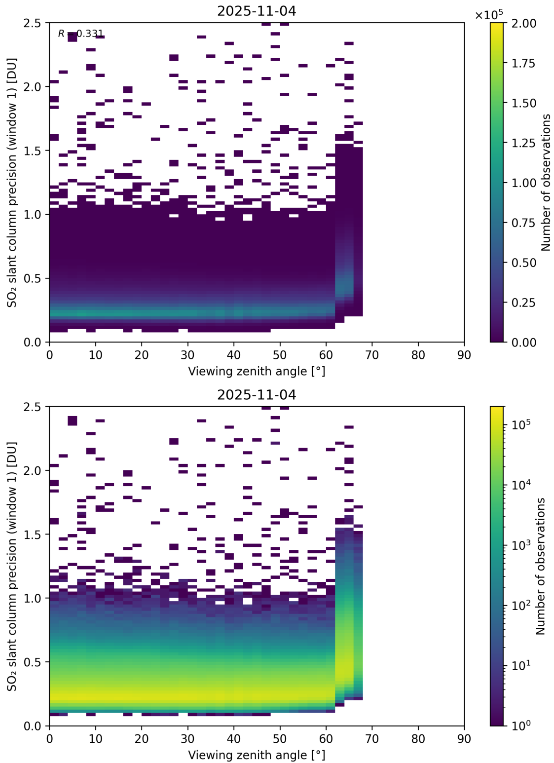
Figure 377: Scatter density plot of “Viewing zenith angle” against “SO 2 slant column precision (window 1)” for 2025-11-03 to 2025-11-05.
