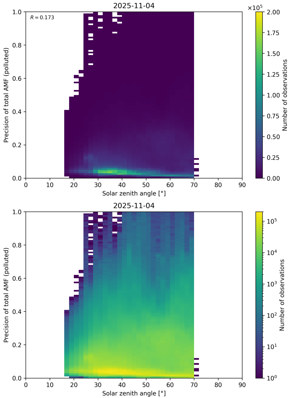
Figure 190: Scatter density plot of “Solar zenith angle” against “Precision of total AMF (polluted)” for 2025-11-03 to 2025-11-05.
