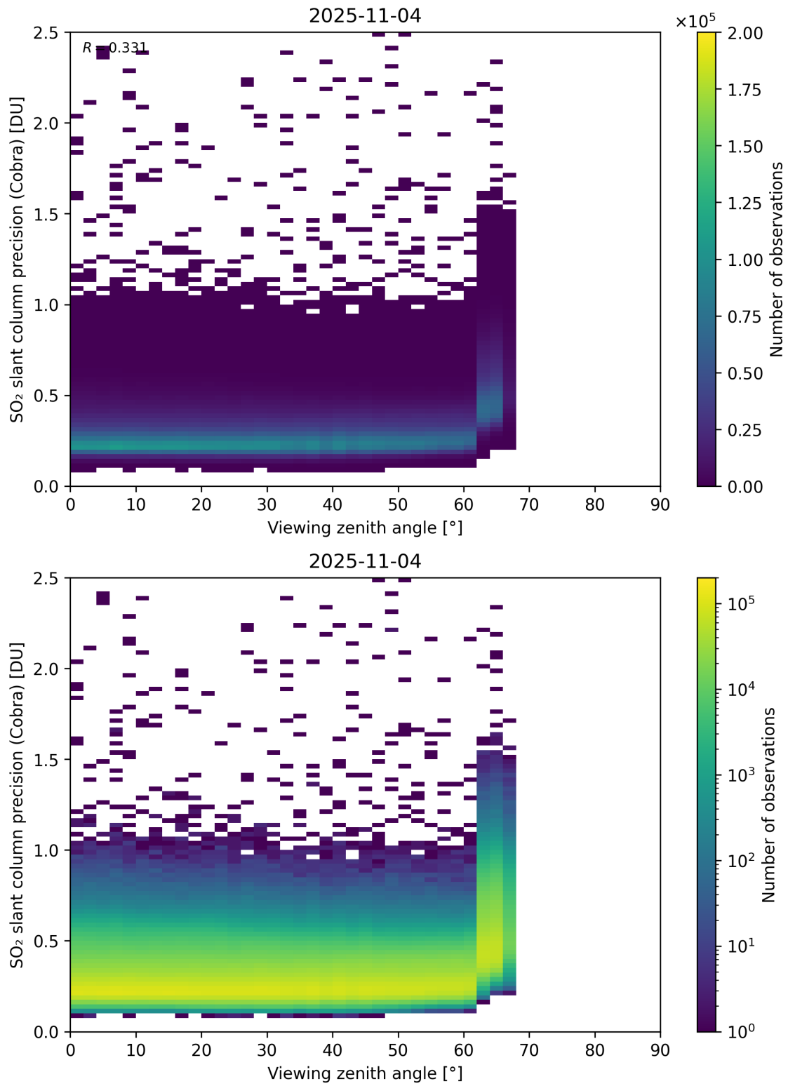
Figure 372: Scatter density plot of “Viewing zenith angle” against “SO 2 slant column precision (Cobra)” for 2025-11-03 to 2025-11-05.
