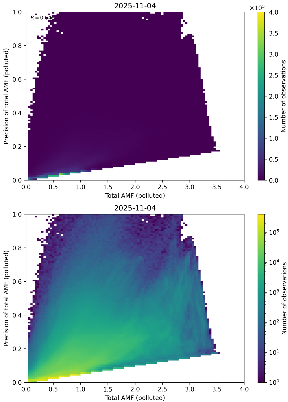
Figure 322: Scatter density plot of “Total AMF (polluted)” against “Precision of total AMF (polluted)” for 2025-11-03 to 2025-11-05.
