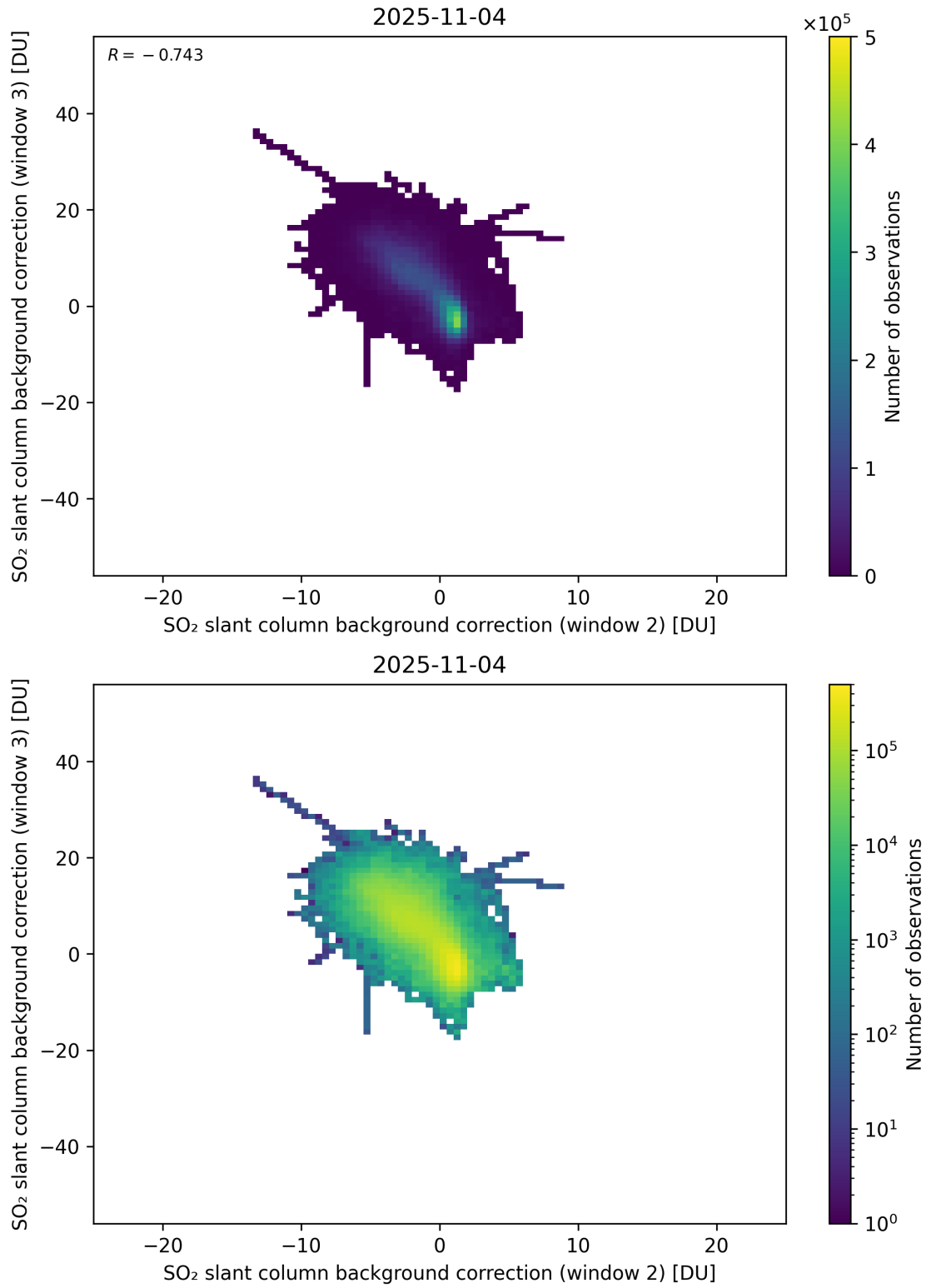
Figure 122: Scatter density plot of “SO 2 slant column background correction (window 2)” against “SO 2 slant column background correction (window 3)” for 2025-11-03 to 2025-11-05.
