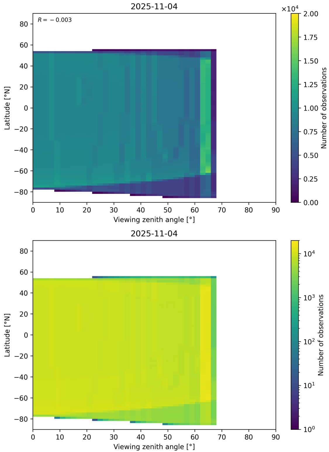
Figure 368: Scatter density plot of “Viewing zenith angle” against “Latitude” for 2025-11-03 to 2025-11-05.
