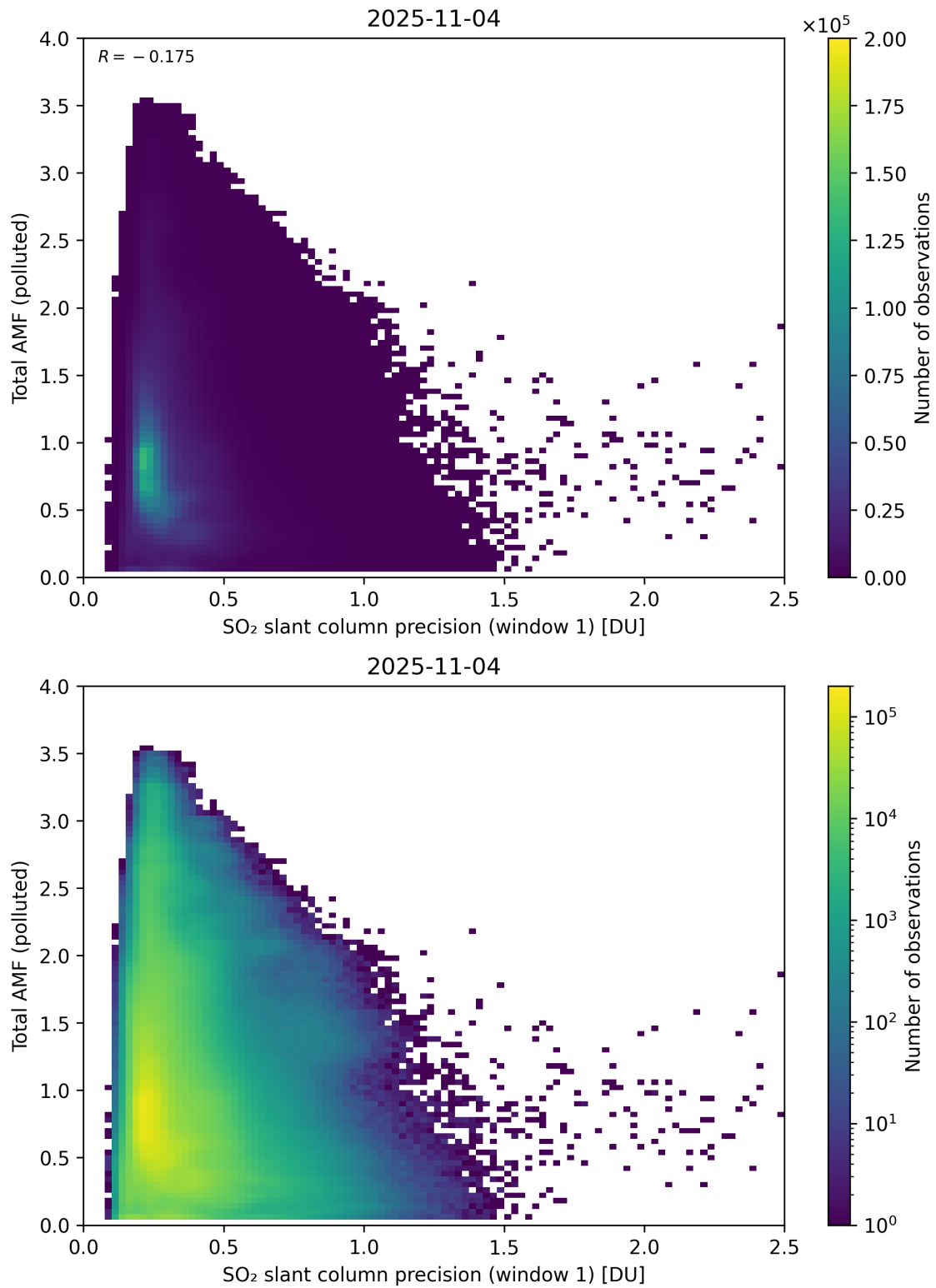
Figure 280: Scatter density plot of “SO 2 slant column precision (window 1)” against “Total AMF (polluted)” for 2025-11-03 to 2025-11-05.
