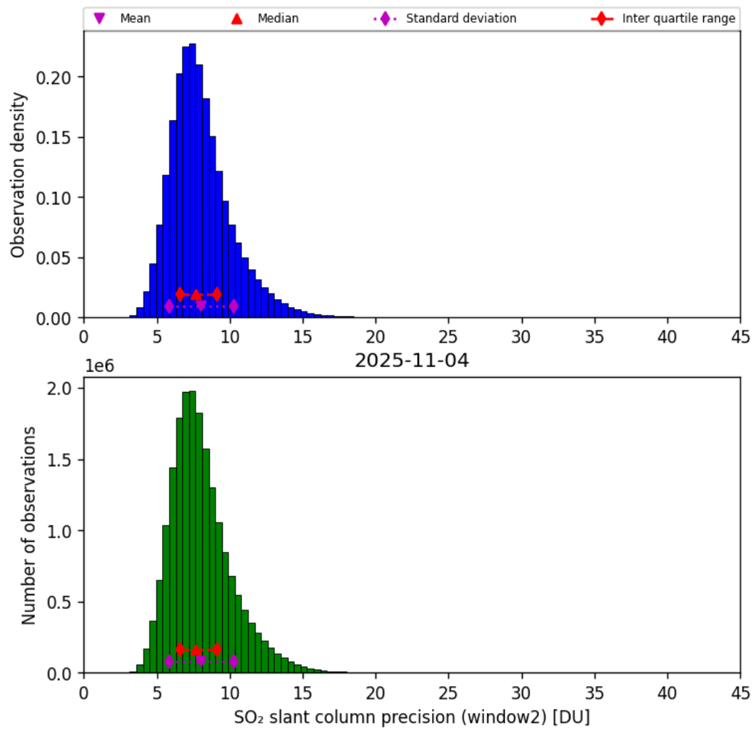
Figure 68: Histogram of “SO 2 slant column precision (window2)” for 2025-11-03 to 2025-11-05
