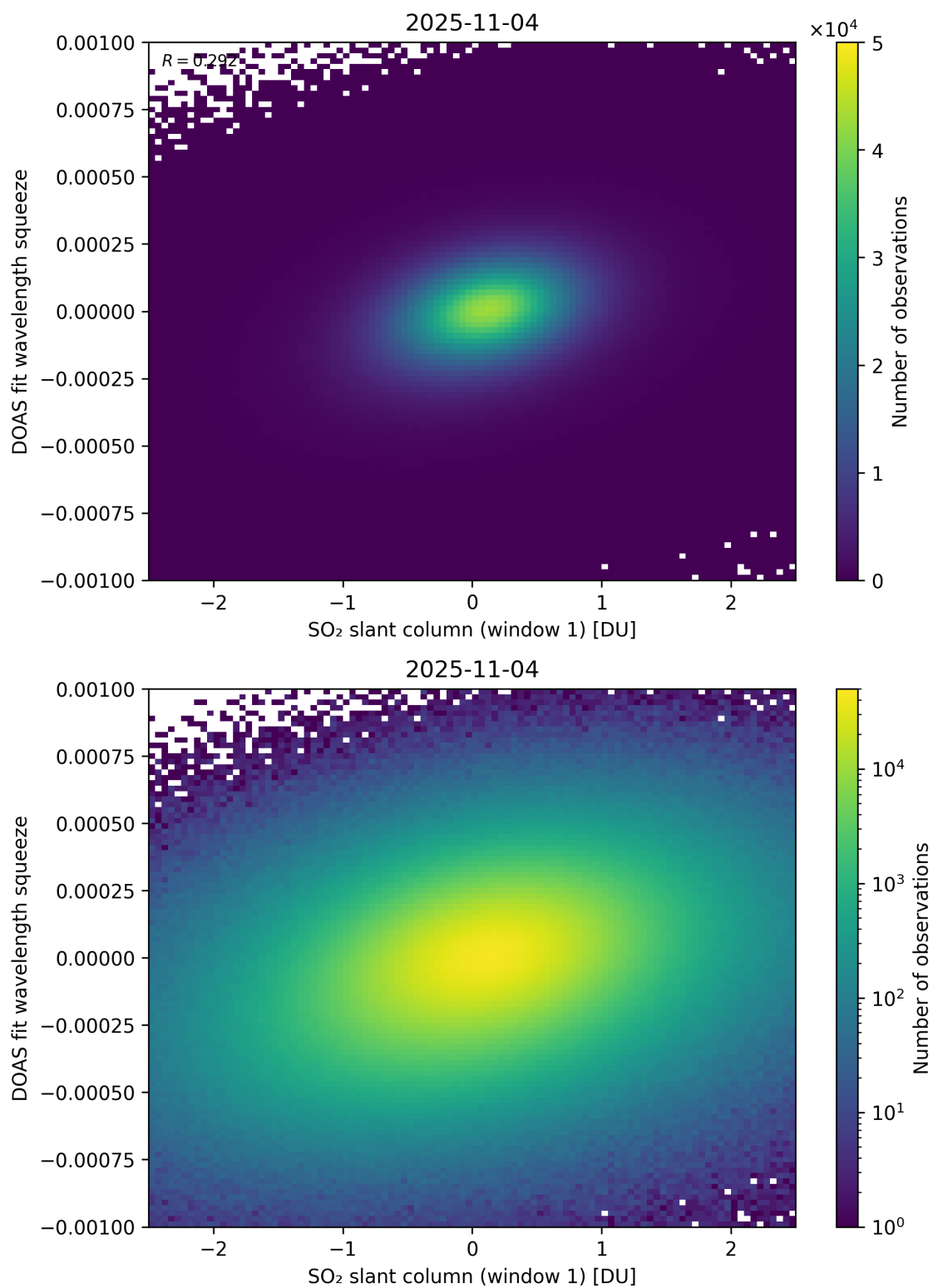
Figure 266: Scatter density plot of “SO 2 slant column (window 1)” against “DOAS fit wavelength squeeze” for 2025-11-03 to 2025-11-05.
