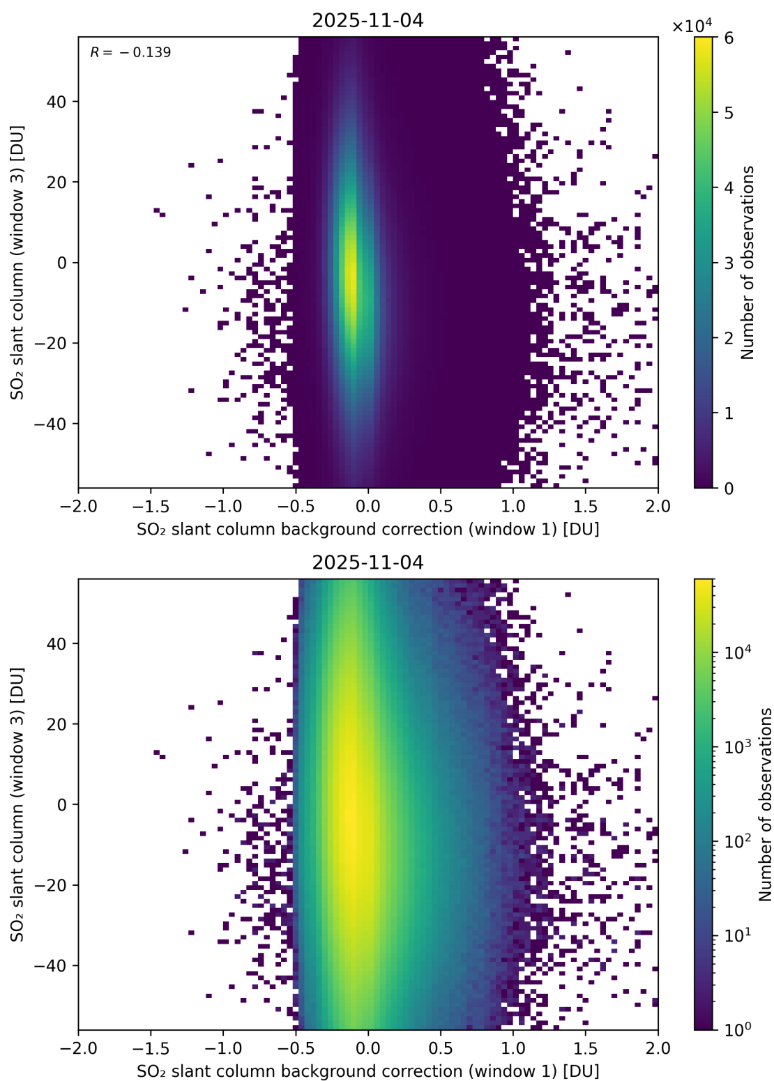
Figure 118: Scatter density plot of “SO 2 slant column background correction (window 1)” against “SO 2 slant column (window 3)” for 2025-11-03 to 2025-11-05.
