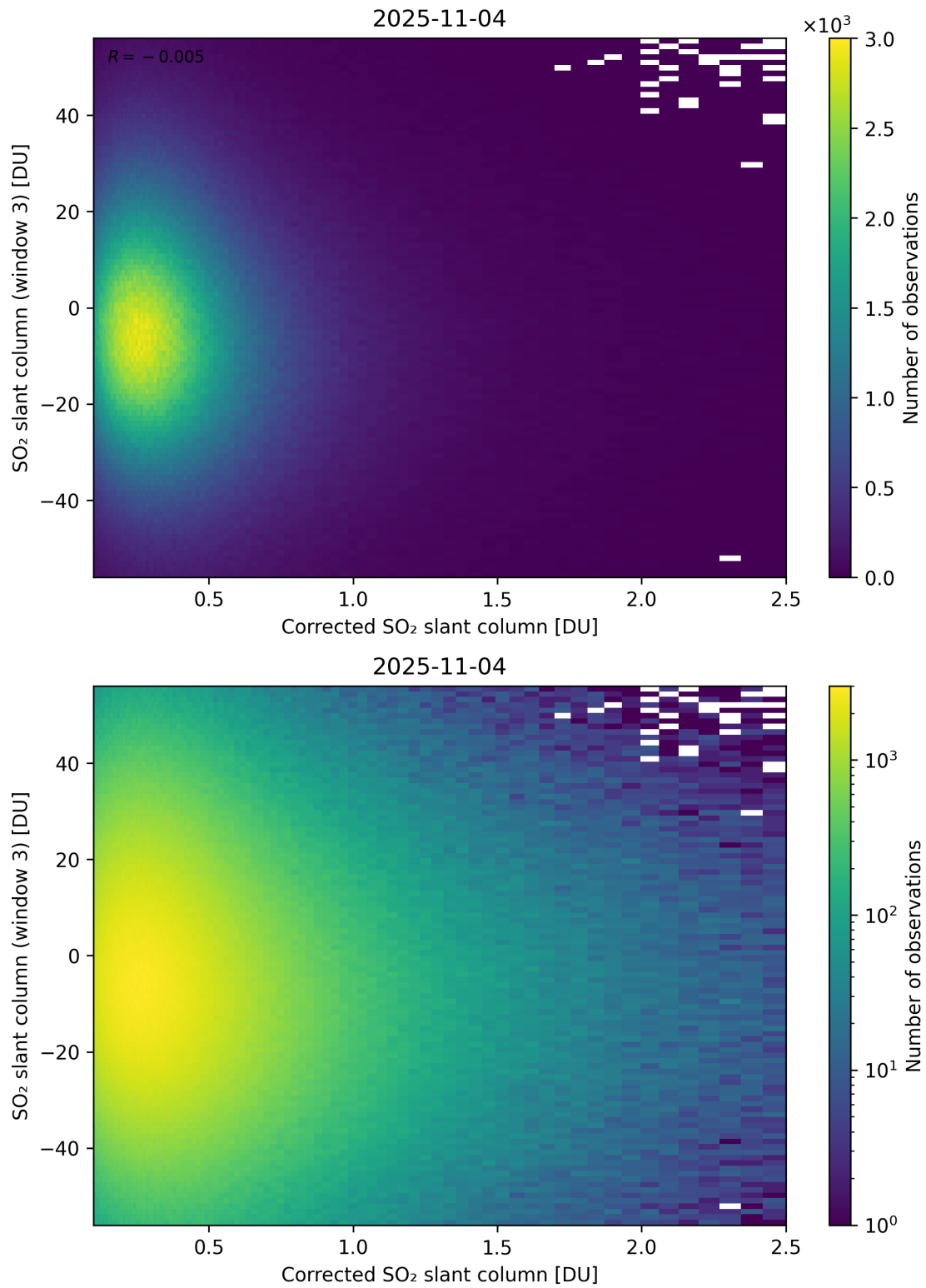
Figure 240: Scatter density plot of “Corrected SO 2 slant column” against “SO 2 slant column (window 3)” for 2025-11-03 to 2025-11-05.
