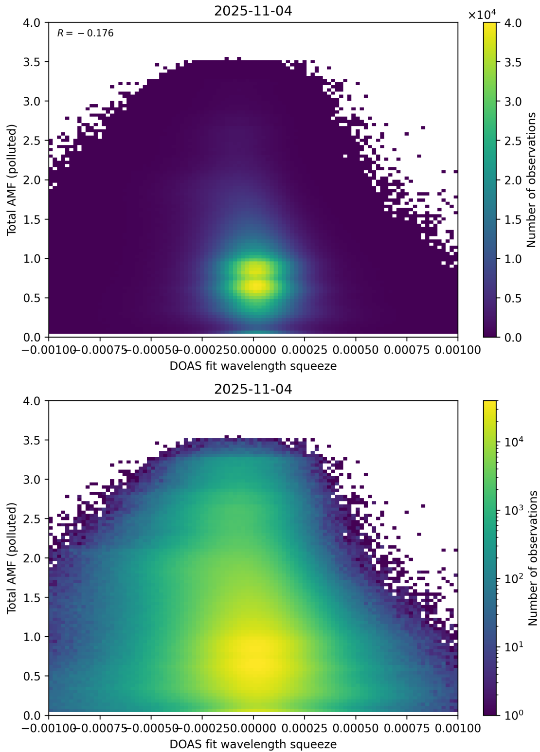
Figure 145: Scatter density plot of “DOAS fit wavelength squeeze” against “Total AMF (polluted)” for 2025-11-03 to 2025-11-05.
