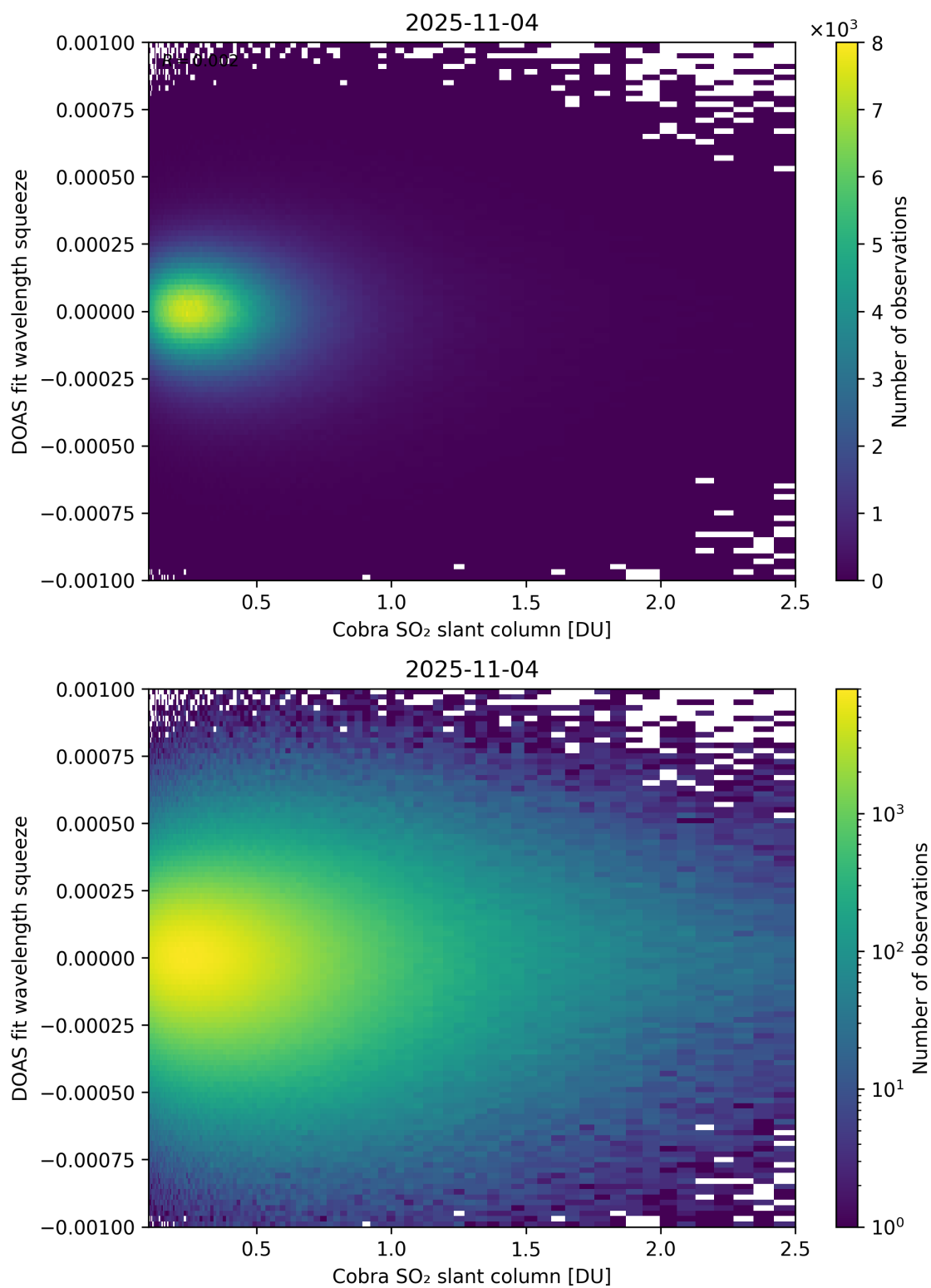
Figure 197: Scatter density plot of “Cobra SO 2 slant column” against “DOAS fit wavelength squeeze” for 2025-11-03 to 2025-11-05.
