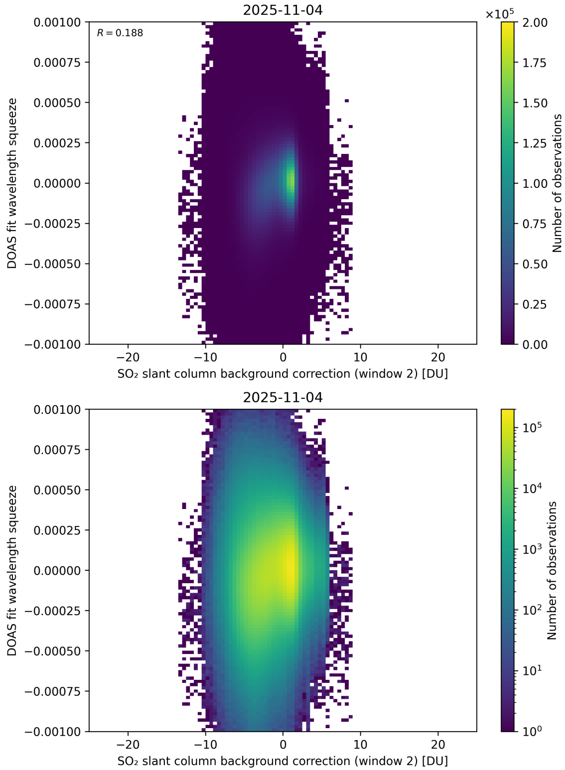
Figure 124: Scatter density plot of “SO 2 slant column background correction (window 2)” against “DOAS fit wavelength squeeze” for 2025-11-03 to 2025-11-05.
