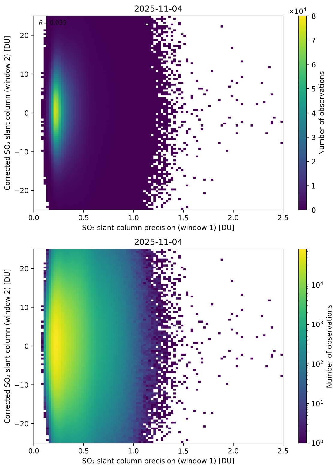
Figure 275: Scatter density plot of “SO 2 slant column precision (window 1)” against “Corrected SO 2 slant column (window 2)” for 2025-11-03 to 2025-11-05.
