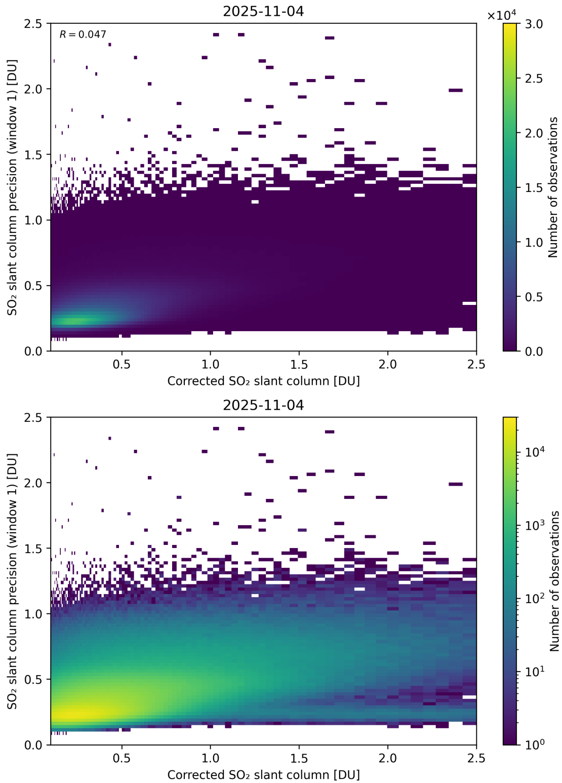
Figure 238: Scatter density plot of “Corrected SO 2 slant column” against “SO 2 slant column precision (window 1)” for 2025-11-03 to 2025-11-05.
