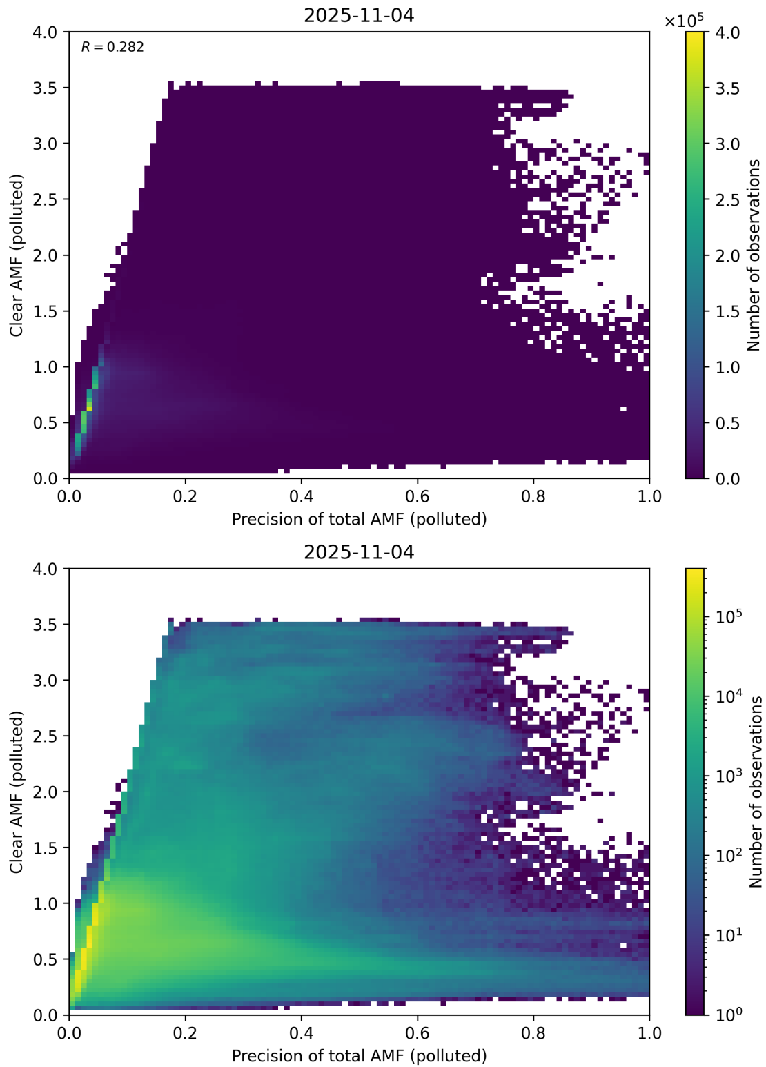
Figure 320: Scatter density plot of “Precision of total AMF (polluted)” against “Clear AMF (polluted)” for 2025-11-03 to 2025-11-05.
