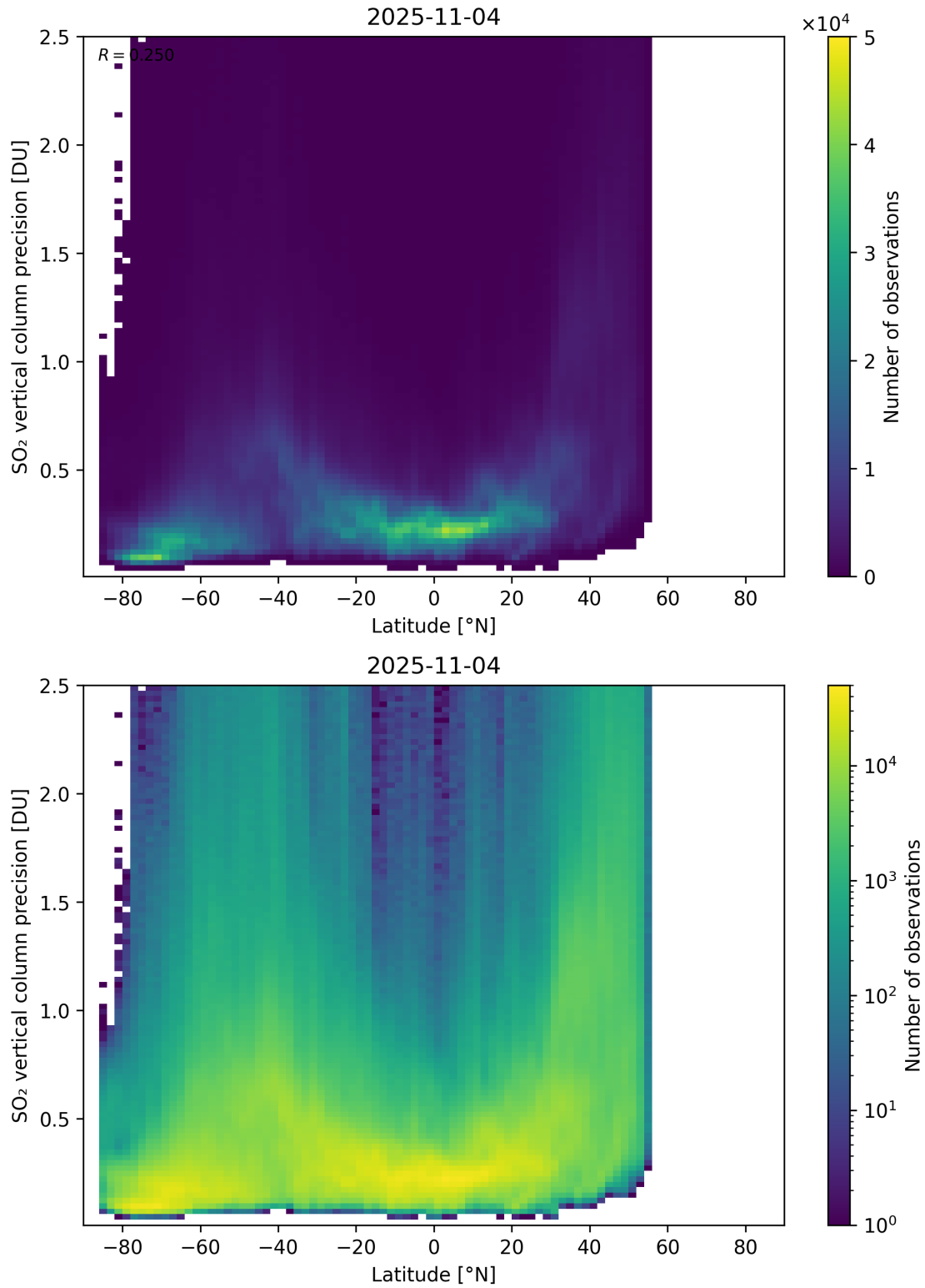
Figure 170: Scatter density plot of “Latitude” against “SO 2 vertical column precision” for 2025-11-03 to 2025-11-05.
