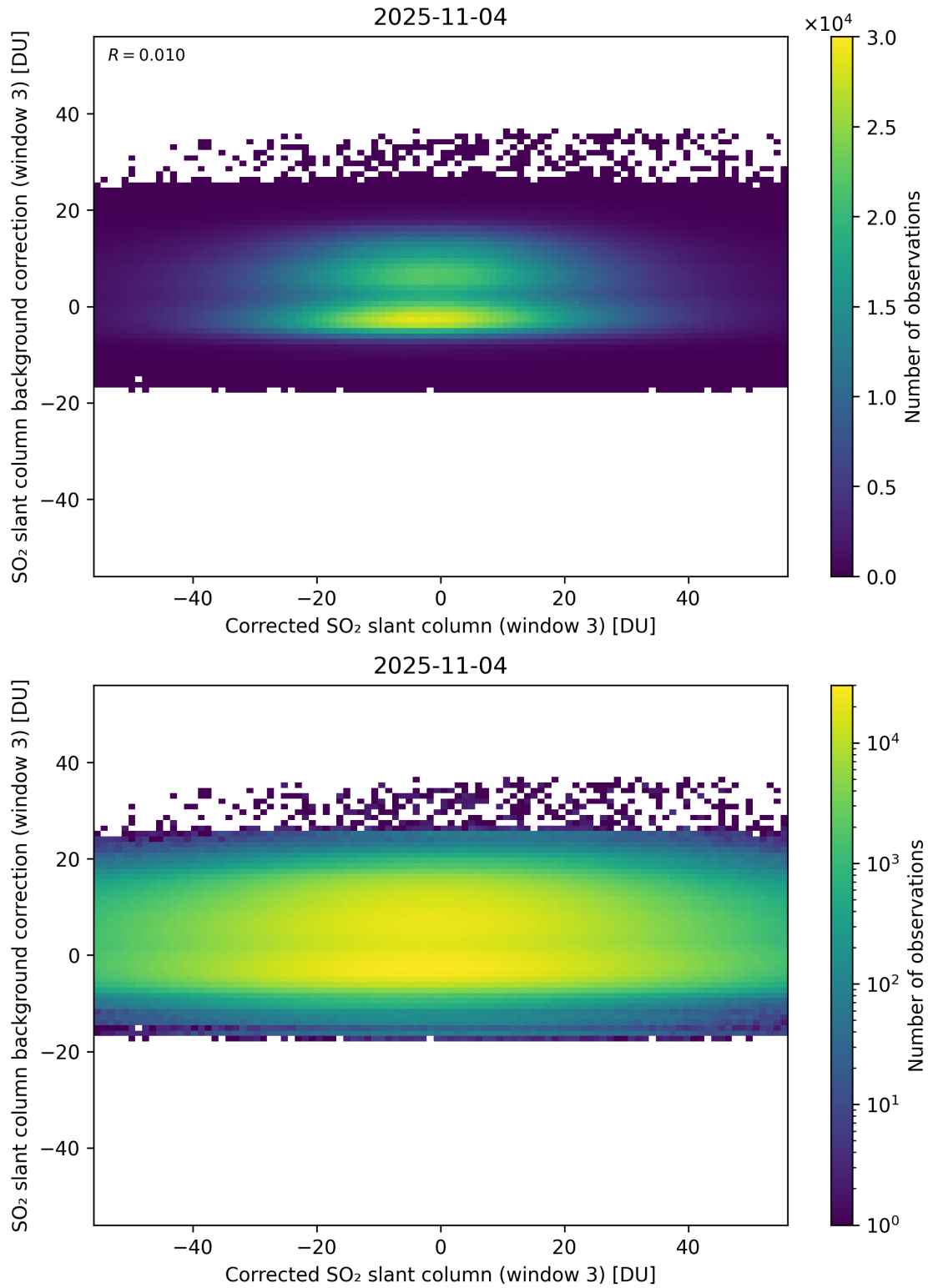
Figure 255: Scatter density plot of “Corrected SO 2 slant column (window 3)” against “SO 2 slant column background correction (window 3)” for 2025-11-03 to 2025-11-05.
