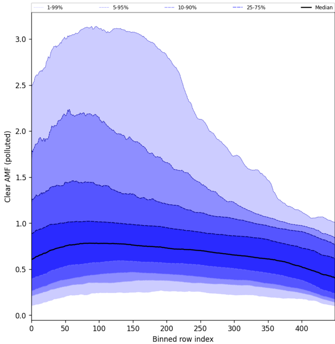
Figure 107: Along track statistics of “Clear AMF (polluted)” for 2025-11-03 to 2025-11-05
