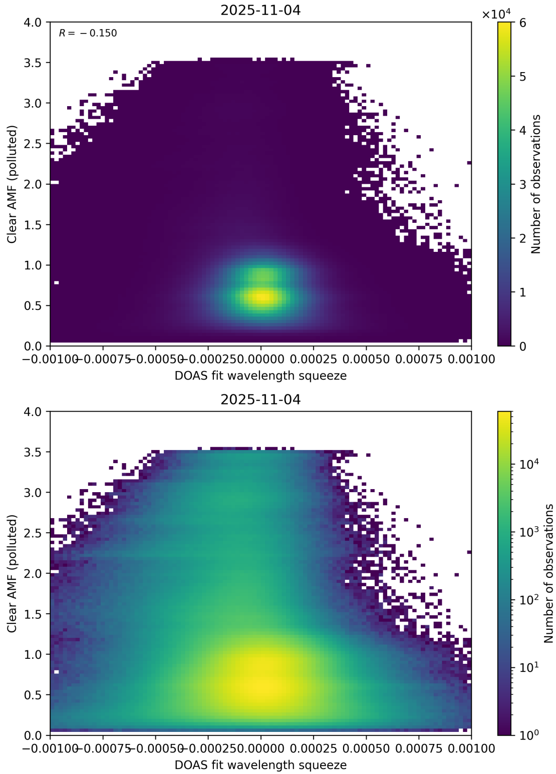
Figure 144: Scatter density plot of “DOAS fit wavelength squeeze” against “Clear AMF (polluted)” for 2025-11-03 to 2025-11-05.
