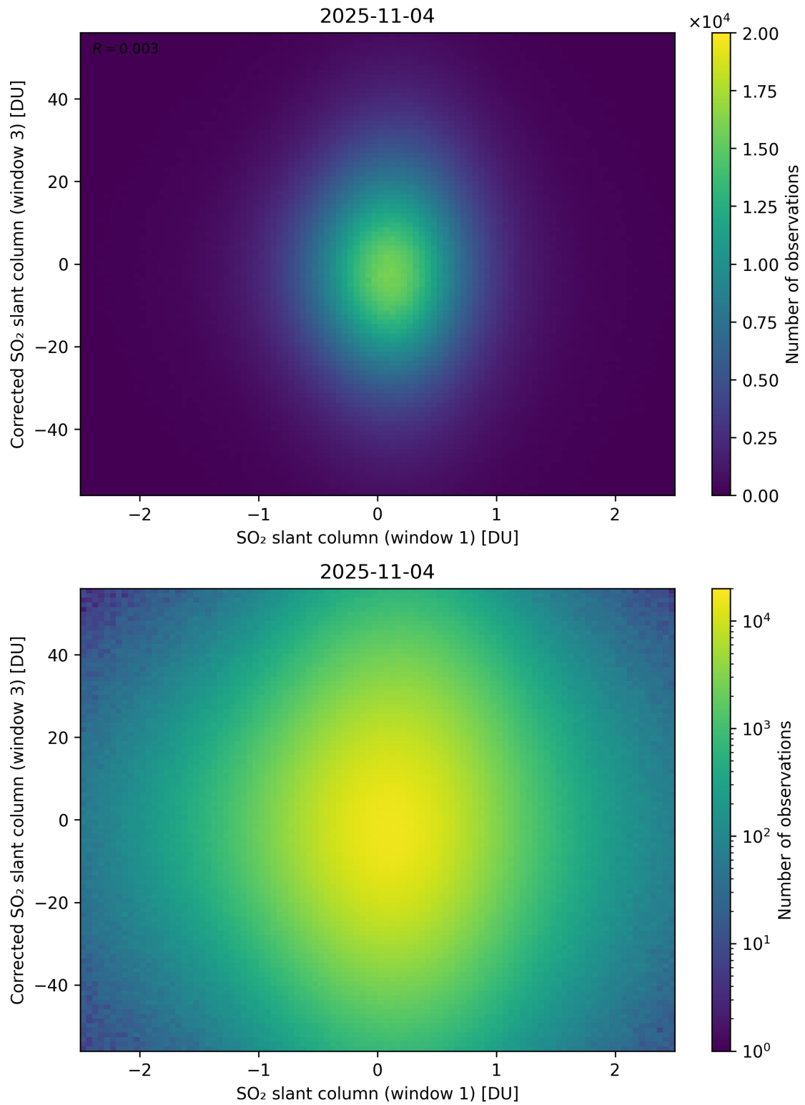
Figure 284: Scatter density plot of “SO 2 slant column (window 1)” against “Corrected SO 2 slant column (window 3)” for 2025-11-03 to 2025-11-05.
