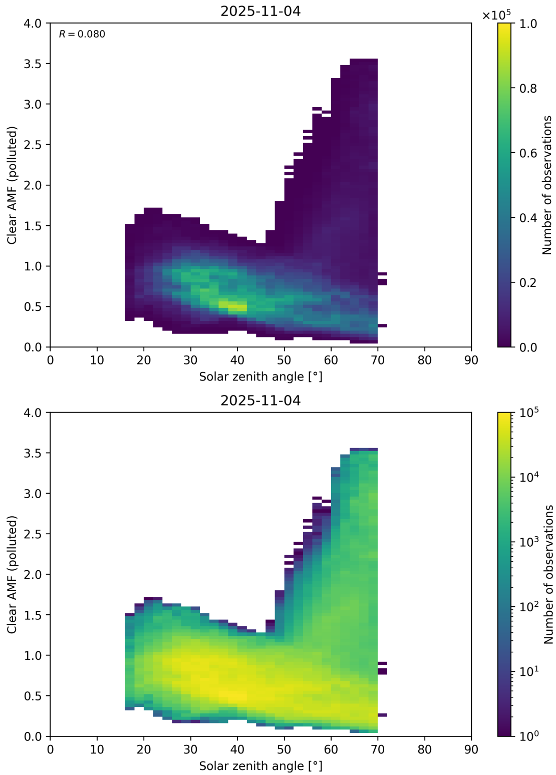
Figure 178: Scatter density plot of “Solar zenith angle” against “Clear AMF (polluted)” for 2025-11-03 to 2025-11-05.
