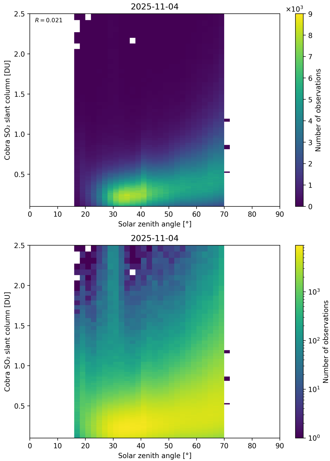
Figure 179: Scatter density plot of “Solar zenith angle” against “Cobra SO 2 slant column” for 2025-11-03 to 2025-11-05.
