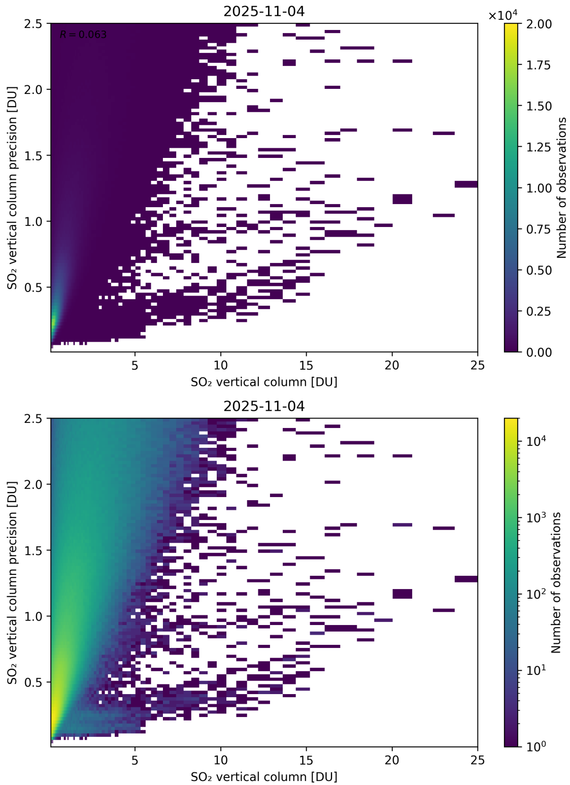
Figure 361: Scatter density plot of “SO 2 vertical column” against “SO 2 vertical column precision” for 2025-11-03 to 2025-11-05.
