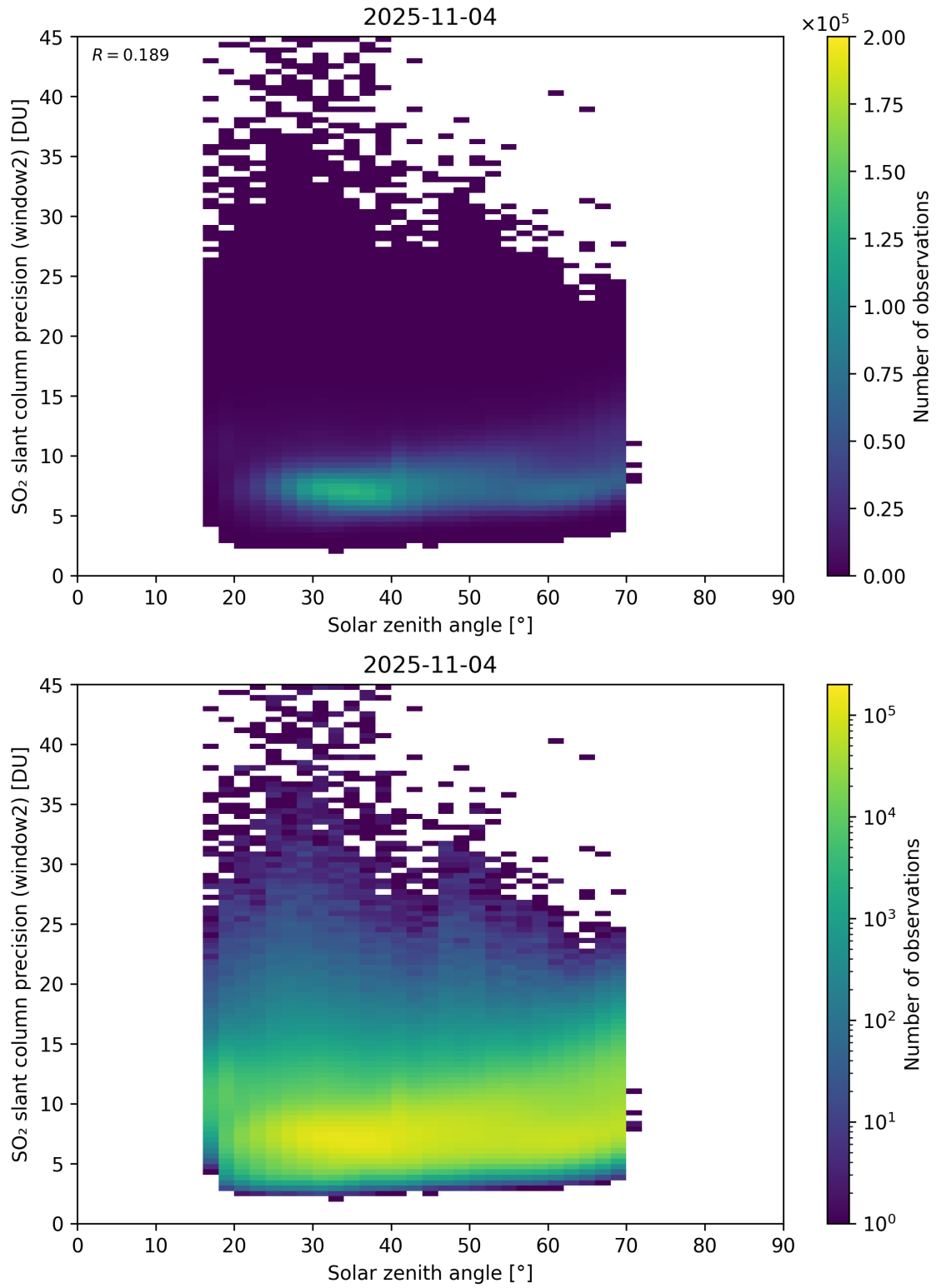
Figure 186: Scatter density plot of “Solar zenith angle” against “SO 2 slant column precision (window2)” for 2025-11-03 to 2025-11-05.
