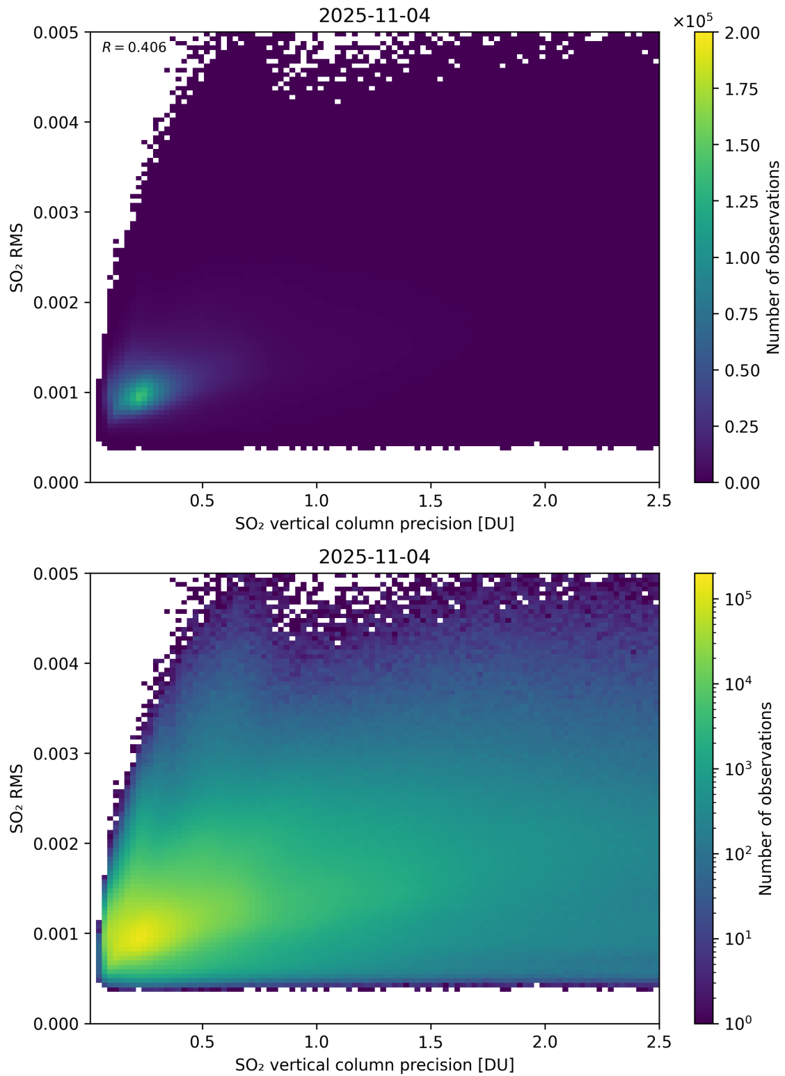
Figure 334: Scatter density plot of “SO 2 vertical column precision” against “SO 2 RMS” for 2025-11-03 to 2025-11-05.
