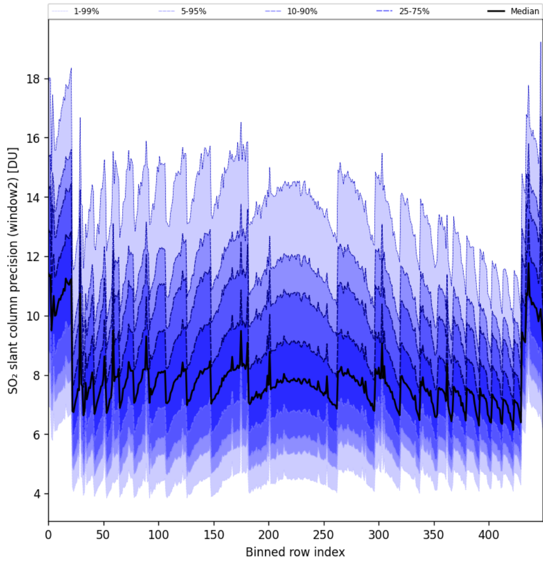
Figure 94: Along track statistics of “SO 2 slant column precision (window2)” for 2025-11-03 to 2025-11-05
