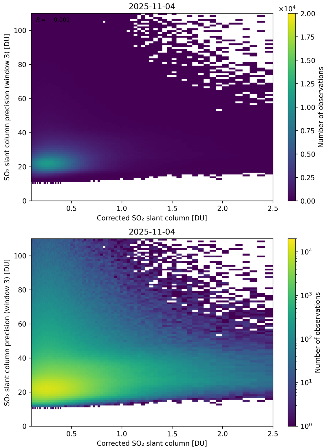
Figure 241: Scatter density plot of “Corrected SO 2 slant column” against “SO 2 slant column precision (window 3)” for 2025-11-03 to 2025-11-05.
