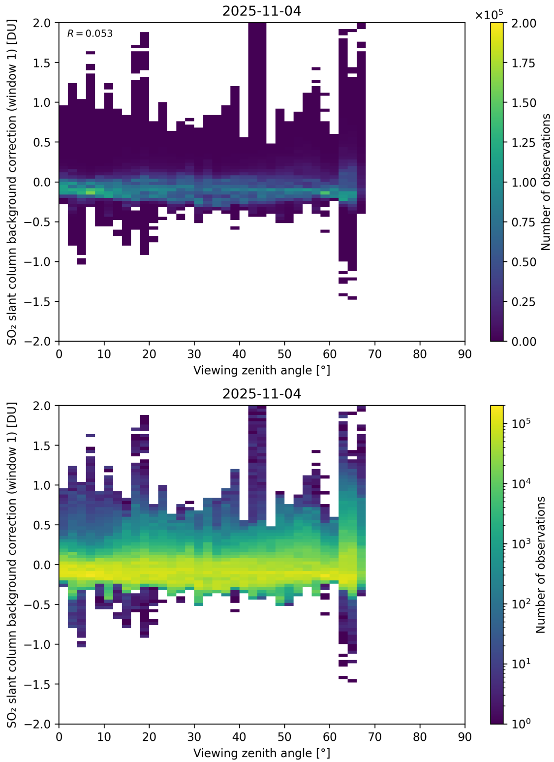
Figure 362: Scatter density plot of “Viewing zenith angle” against “SO 2 slant column background correction (window 1)” for 2025-11-03 to 2025-11-05.
