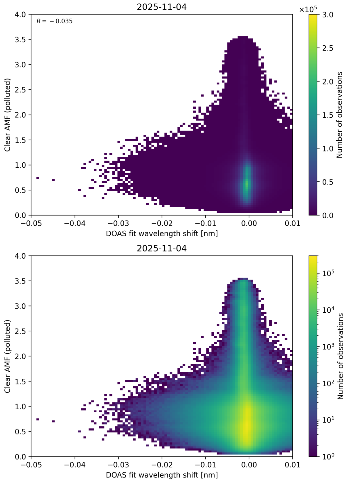
Figure 140: Scatter density plot of “DOAS fit wavelength shift” against “Clear AMF (polluted)” for 2025-11-03 to 2025-11-05.
