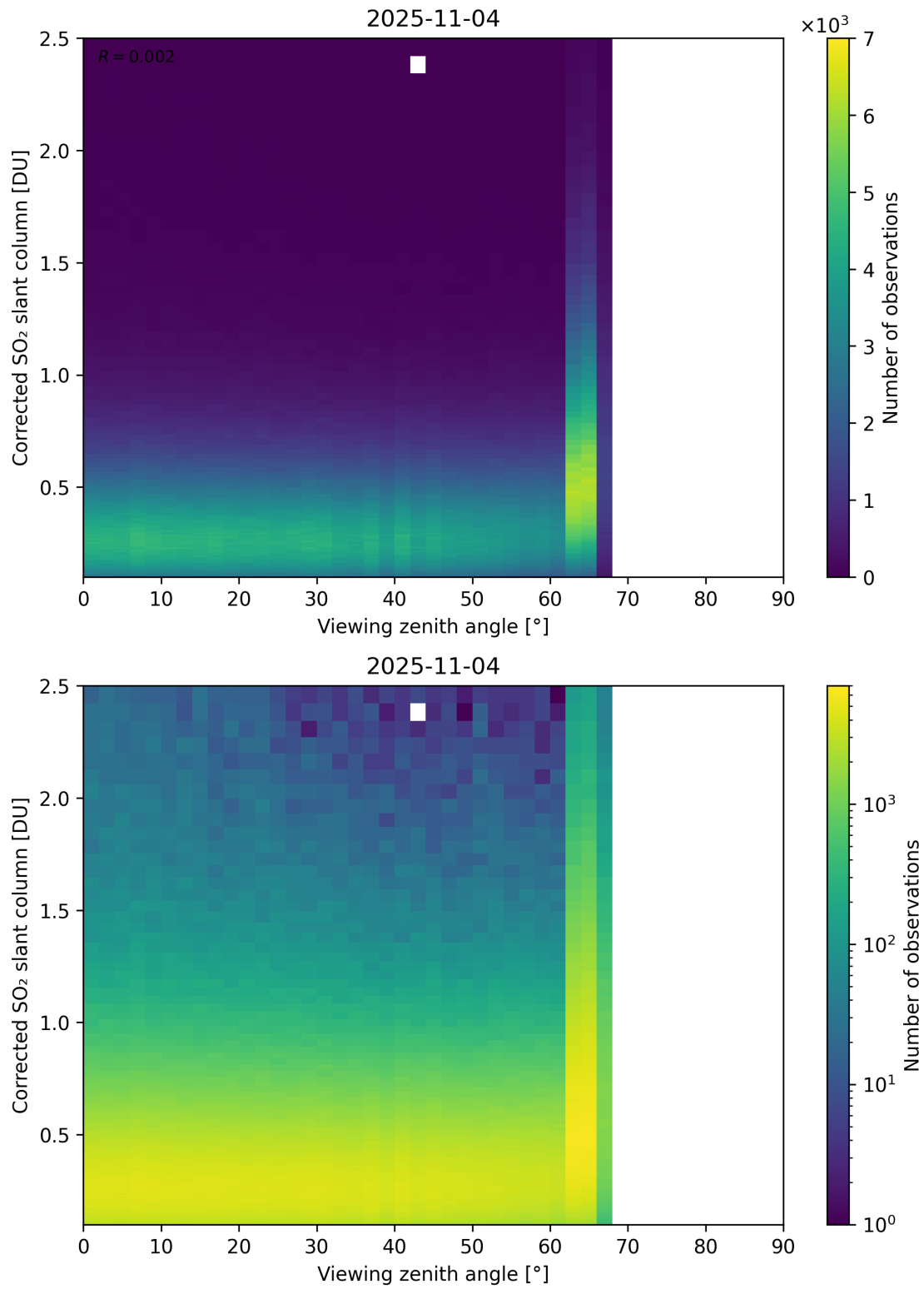
Figure 373: Scatter density plot of “Viewing zenith angle” against “Corrected SO 2 slant column” for 2025-11-03 to 2025-11-05.
