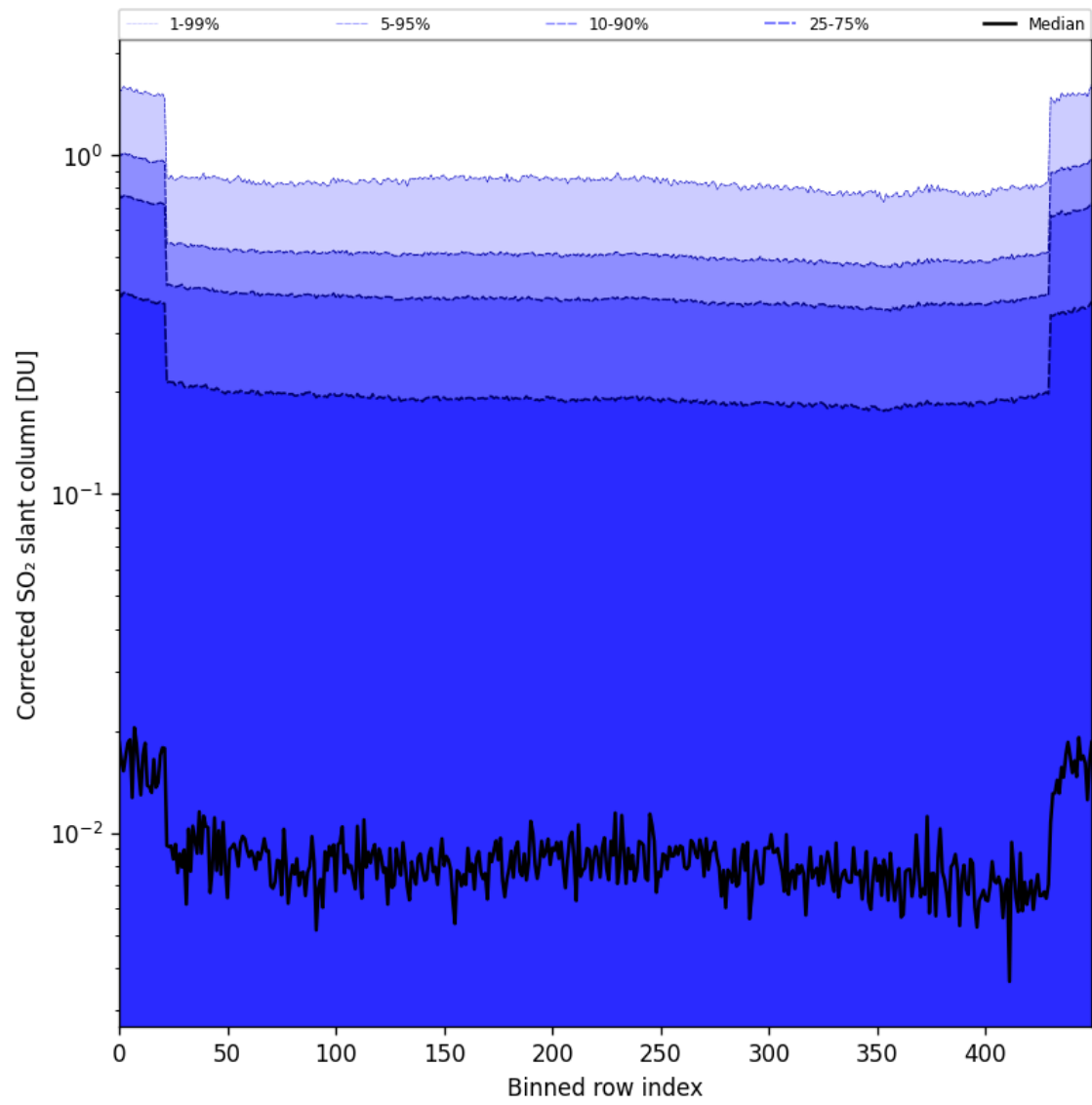
Figure 86: Along track statistics of “Corrected SO 2 slant column” for 2025-11-03 to 2025-11-05
