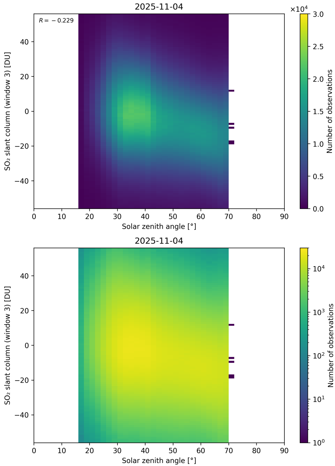
Figure 187: Scatter density plot of “Solar zenith angle” against “SO 2 slant column (window 3)” for 2025-11-03 to 2025-11-05.
