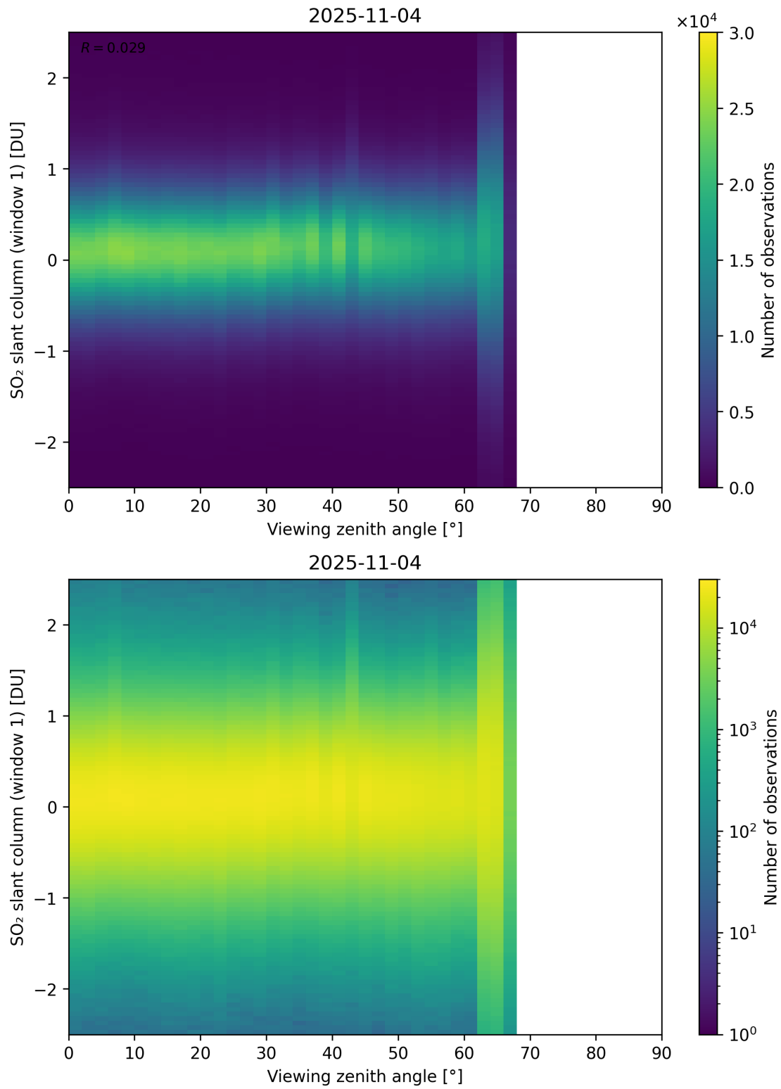
Figure 376: Scatter density plot of “Viewing zenith angle” against “SO 2 slant column (window 1)” for 2025-11-03 to 2025-11-05.
