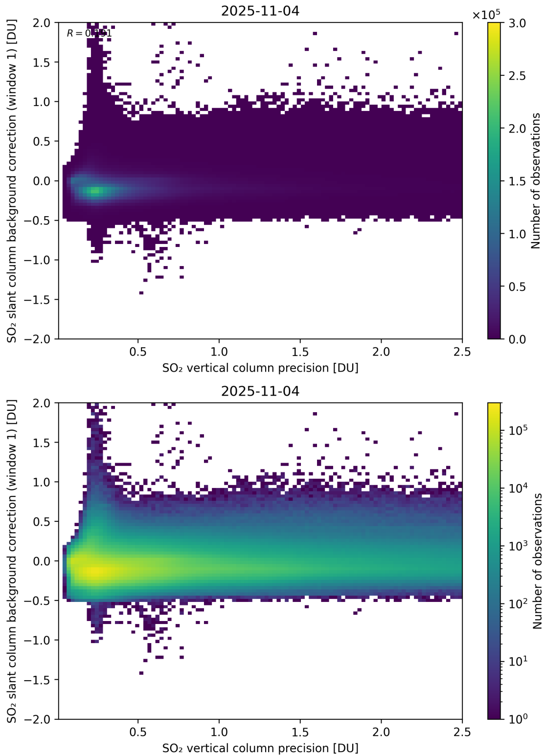
Figure 329: Scatter density plot of “SO 2 vertical column precision” against “SO 2 slant column background correction (window 1)” for 2025-11-03 to 2025-11-05.
