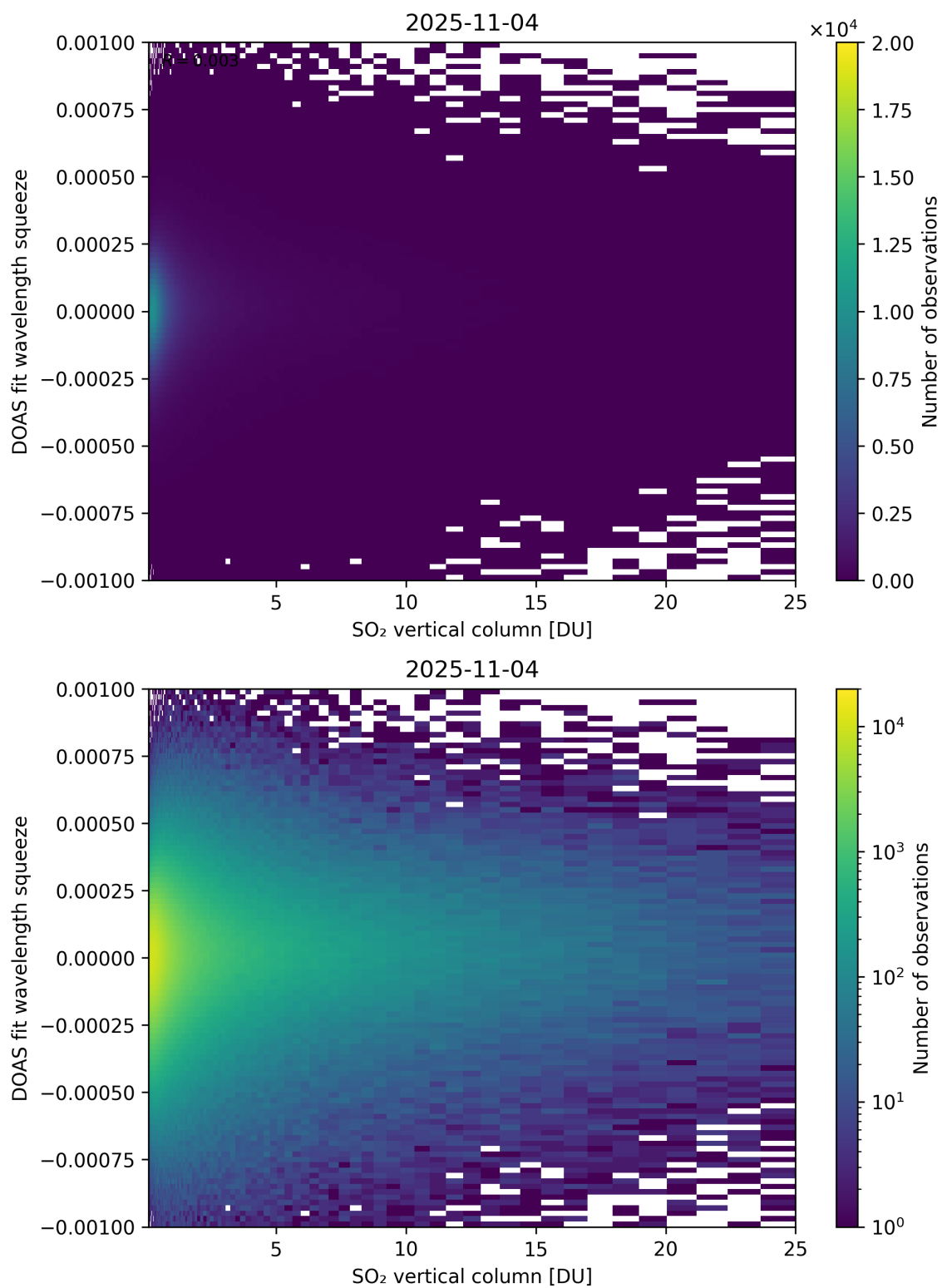
Figure 327: Scatter density plot of “SO 2 vertical column” against “DOAS fit wavelength squeeze” for 2025-11-03 to 2025-11-05.
