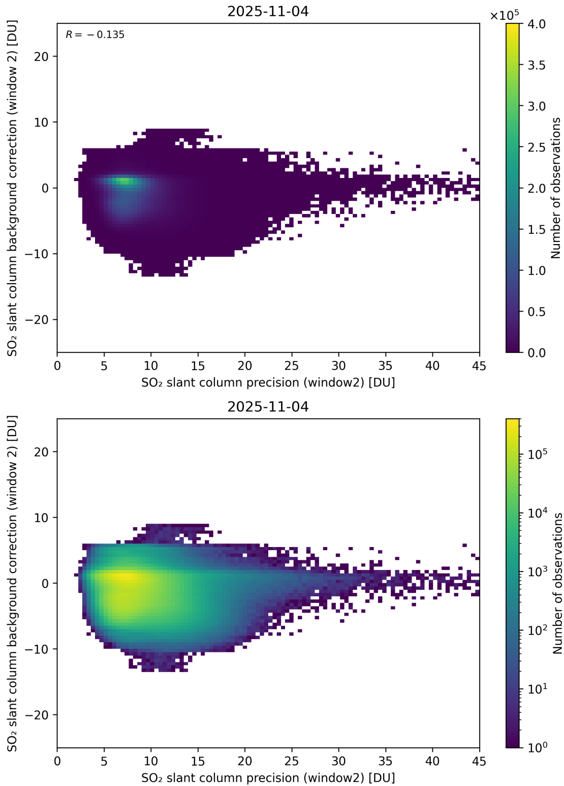
Figure 291: Scatter density plot of “SO 2 slant column precision (window2)” against “SO 2 slant column background correction (window 2)” for 2025-11-03 to 2025-11-05.
