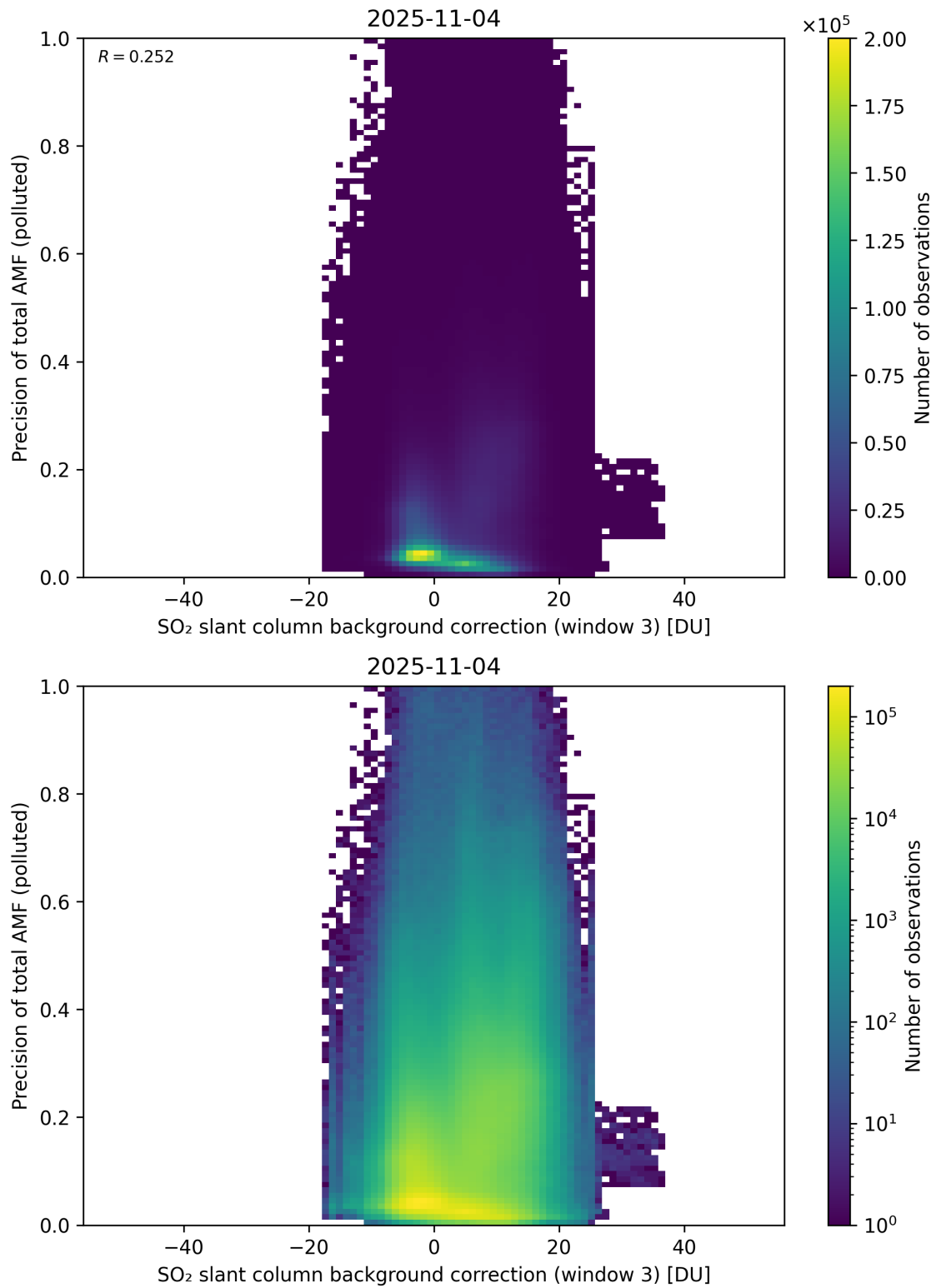
Figure 137: Scatter density plot of “SO 2 slant column background correction (window 3)” against “Precision of total AMF (polluted)” for 2025-11-03 to 2025-11-05.
