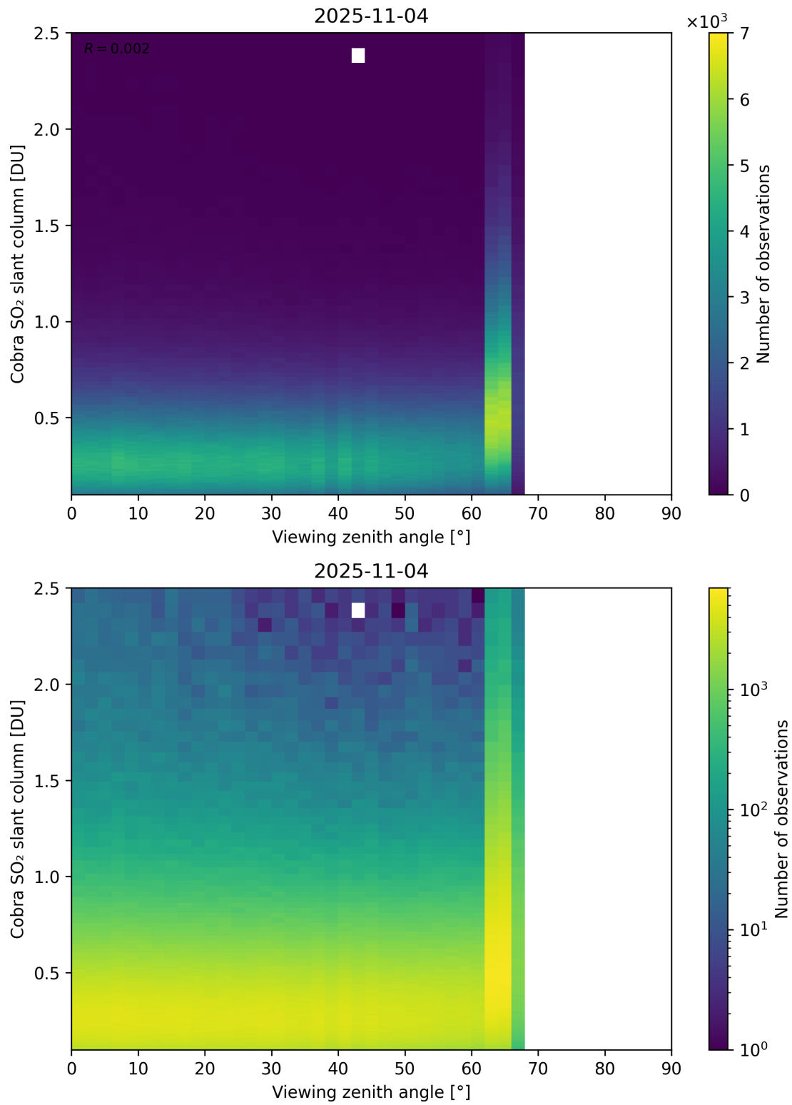
Figure 371: Scatter density plot of “Viewing zenith angle” against “Cobra SO 2 slant column” for 2025-11-03 to 2025-11-05.
