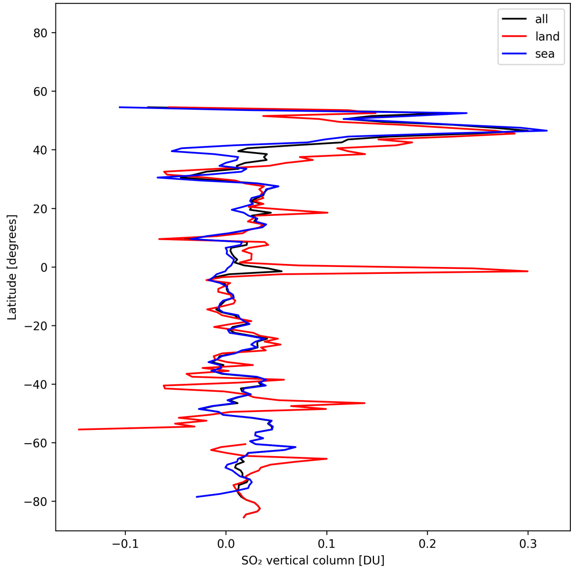
Figure 32: Zonal average of “SO 2 vertical column” for 2025-11-03 to 2025-11-05.
