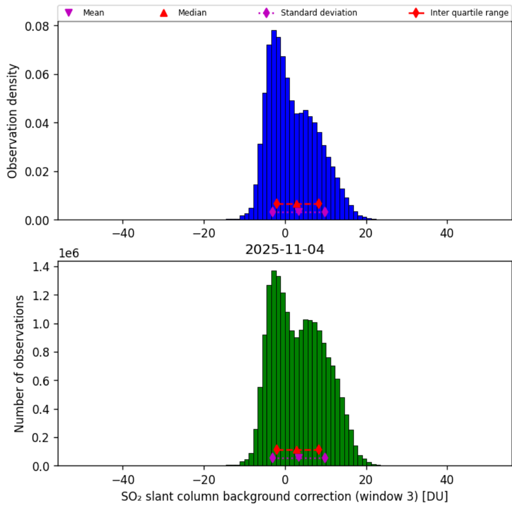
Figure 74: Histogram of “SO 2 slant column background correction (window 3)” for 2025-11-03 to 2025-11-05
