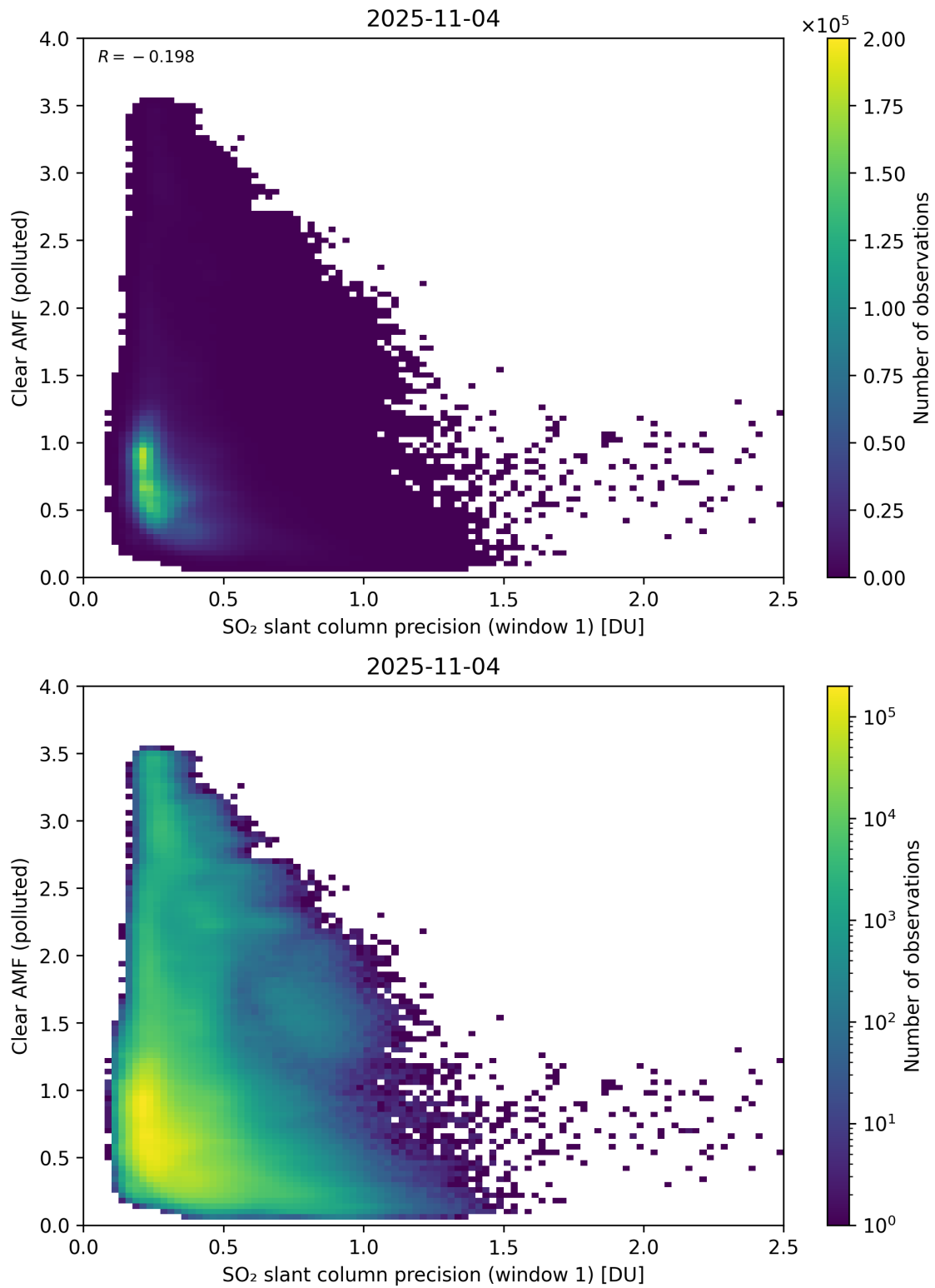
Figure 274: Scatter density plot of “SO 2 slant column precision (window 1)” against “Clear AMF (polluted)” for 2025-11-03 to 2025-11-05.
