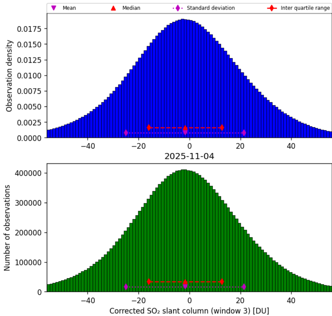
Figure 73: Histogram of “Corrected SO 2 slant column (window 3)” for 2025-11-03 to 2025-11-05
