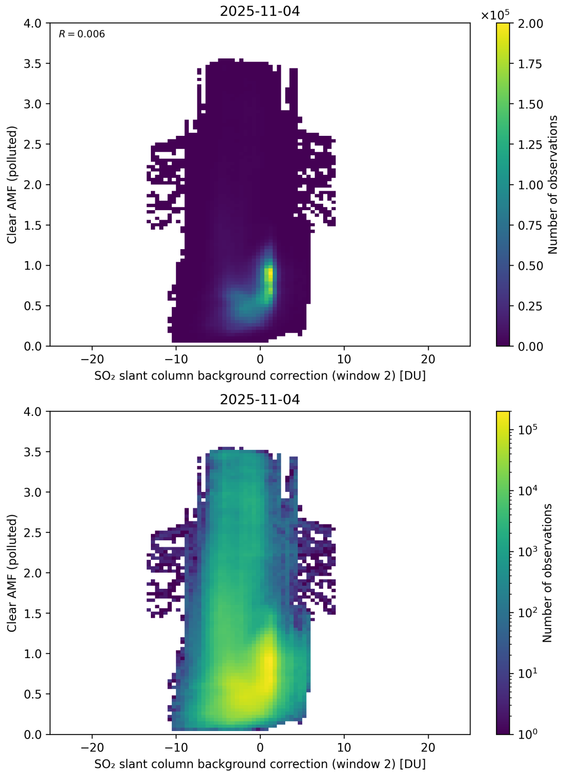
Figure 126: Scatter density plot of “SO 2 slant column background correction (window 2)” against “Clear AMF (polluted)” for 2025-11-03 to 2025-11-05.
