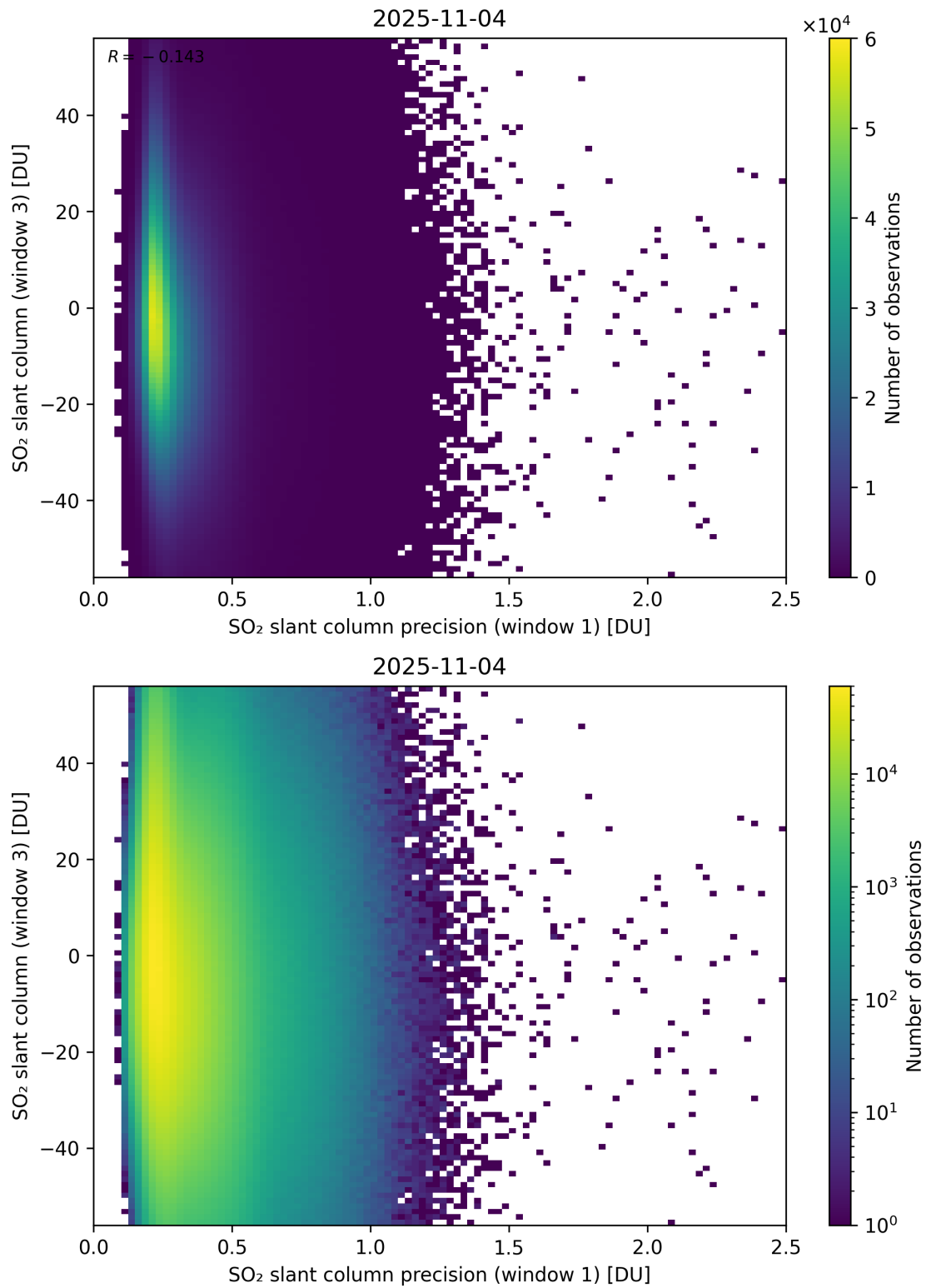
Figure 278: Scatter density plot of “SO 2 slant column precision (window 1)” against “SO 2 slant column (window 3)” for 2025-11-03 to 2025-11-05.
