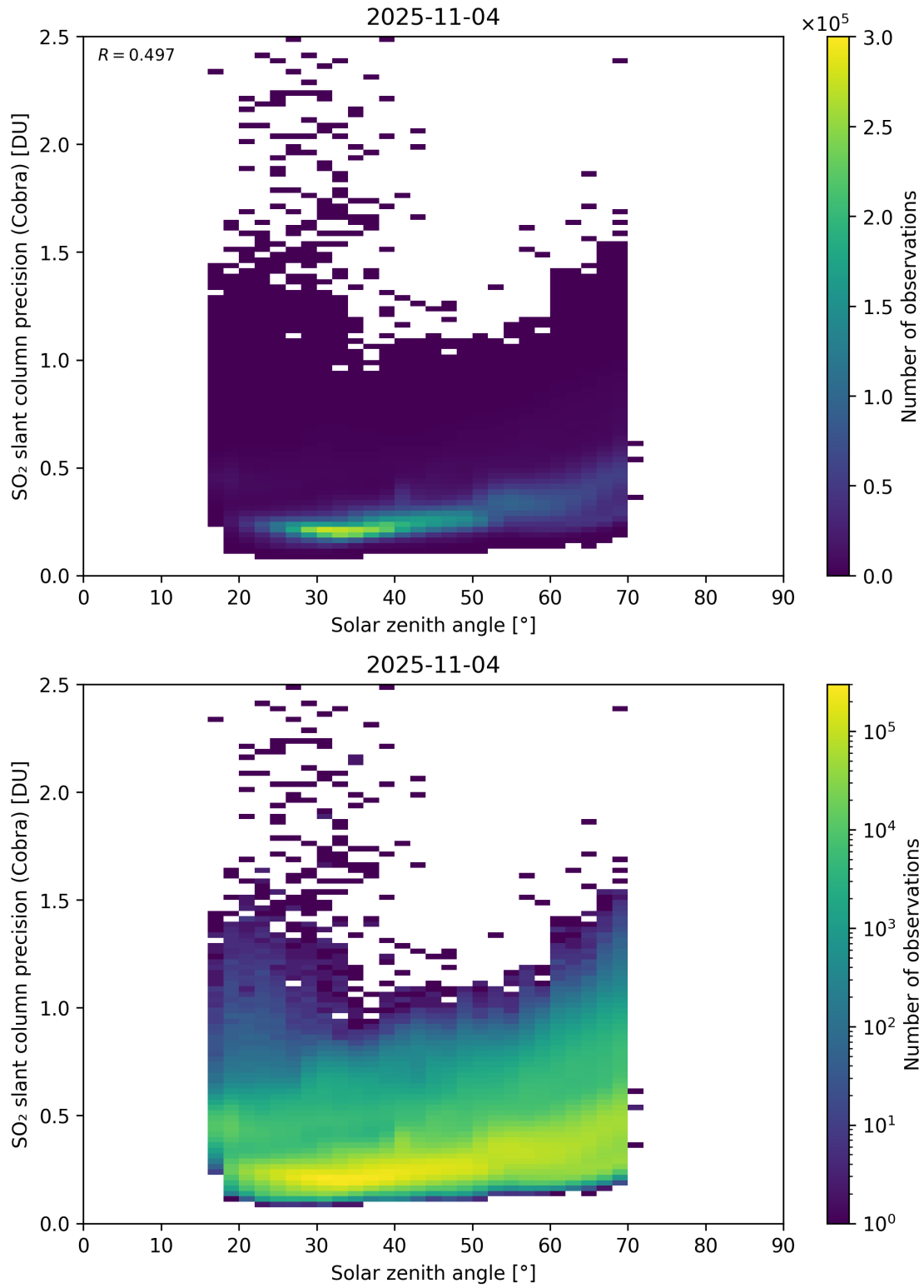
Figure 180: Scatter density plot of “Solar zenith angle” against “SO 2 slant column precision (Cobra)” for 2025-11-03 to 2025-11-05.
