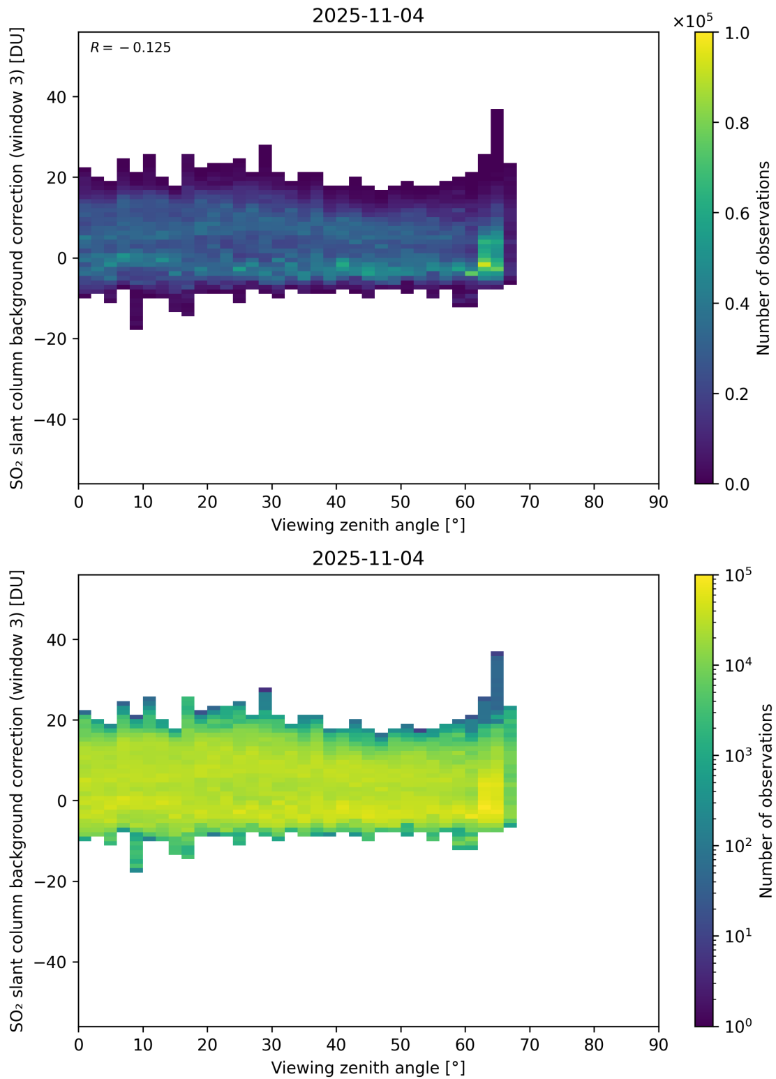
Figure 364: Scatter density plot of “Viewing zenith angle” against “SO 2 slant column background correction (window 3)” for 2025-11-03 to 2025-11-05.
