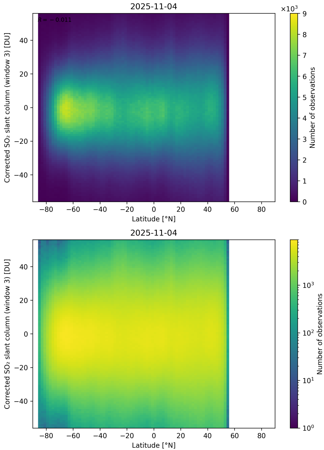
Figure 161: Scatter density plot of “Latitude” against “Corrected SO 2 slant column (window 3)” for 2025-11-03 to 2025-11-05.
