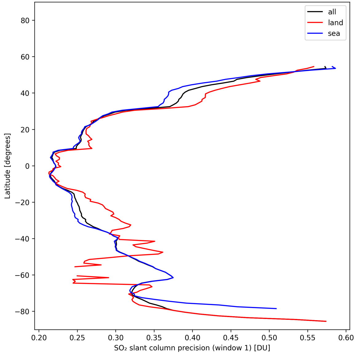
Figure 38: Zonal average of “SO 2 slant column precision (window 1)” for 2025-11-03 to 2025-11-05.
