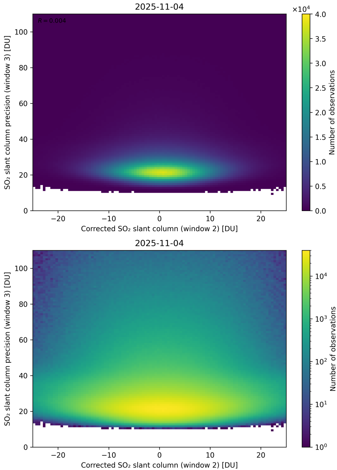
Figure 252: Scatter density plot of “Corrected SO 2 slant column (window 2)” against “SO 2 slant column precision (window 3)” for 2025-11-03 to 2025-11-05.
