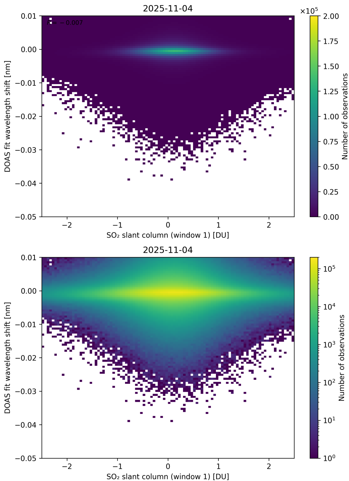
Figure 265: Scatter density plot of “SO 2 slant column (window 1)” against “DOAS fit wavelength shift” for 2025-11-03 to 2025-11-05.
