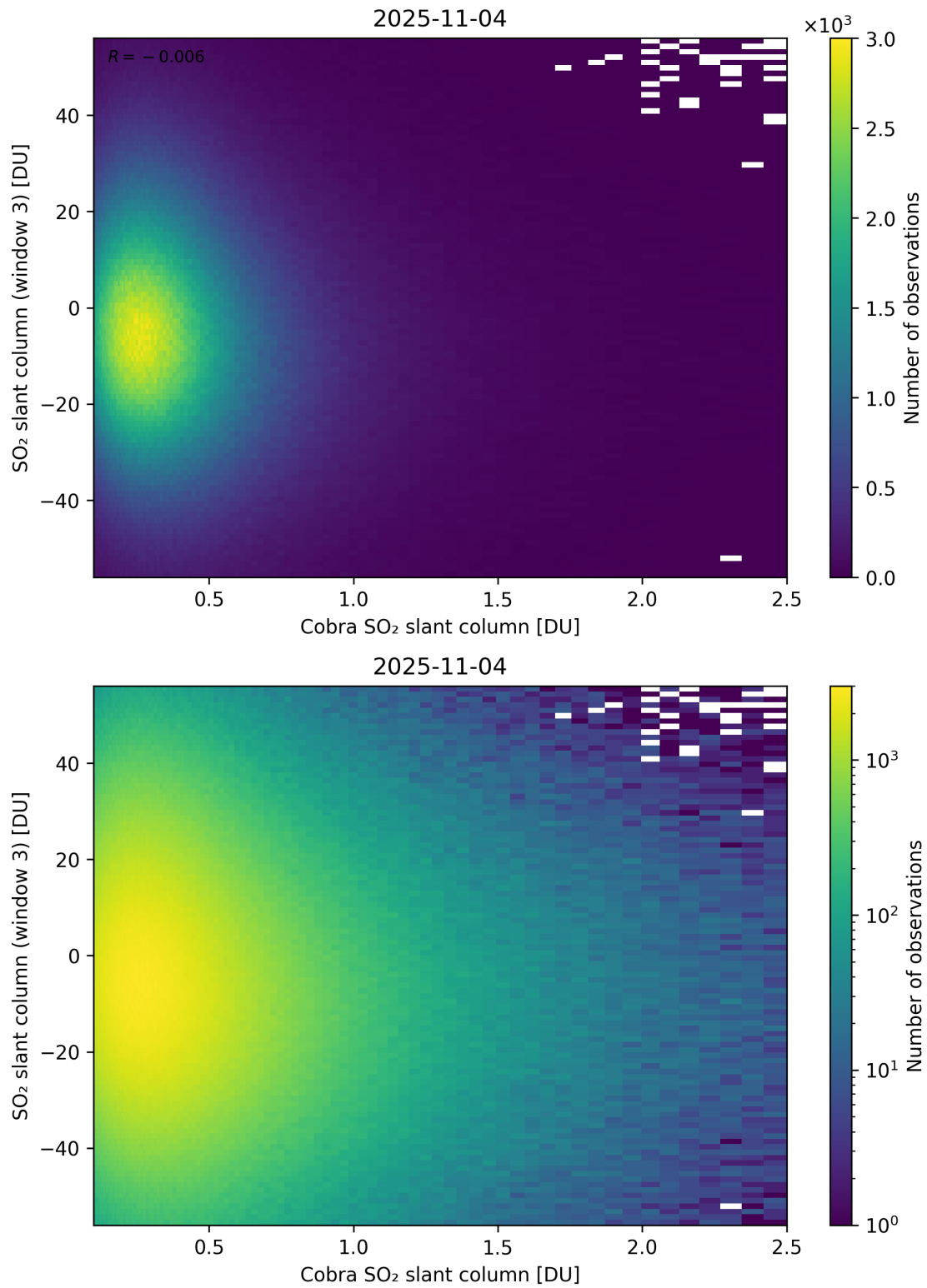
Figure 222: Scatter density plot of “Cobra SO 2 slant column” against “SO 2 slant column (window 3)” for 2025-11-03 to 2025-11-05.
