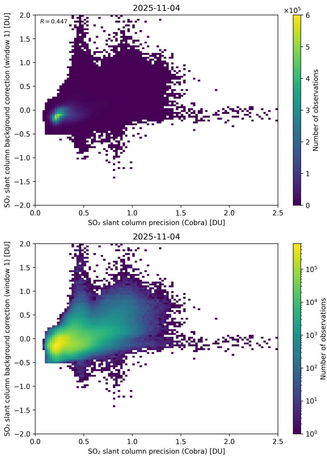
Figure 199: Scatter density plot of “SO 2 slant column precision (Cobra)” against “SO 2 slant column background correction (window 1)” for 2025-11-03 to 2025-11-05.
