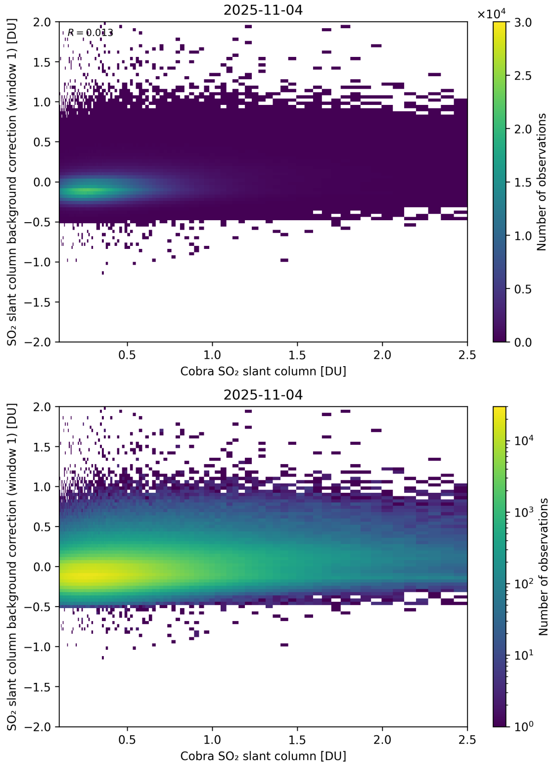
Figure 193: Scatter density plot of “Cobra SO 2 slant column” against “SO 2 slant column background correction (window 1)” for 2025-11-03 to 2025-11-05.
