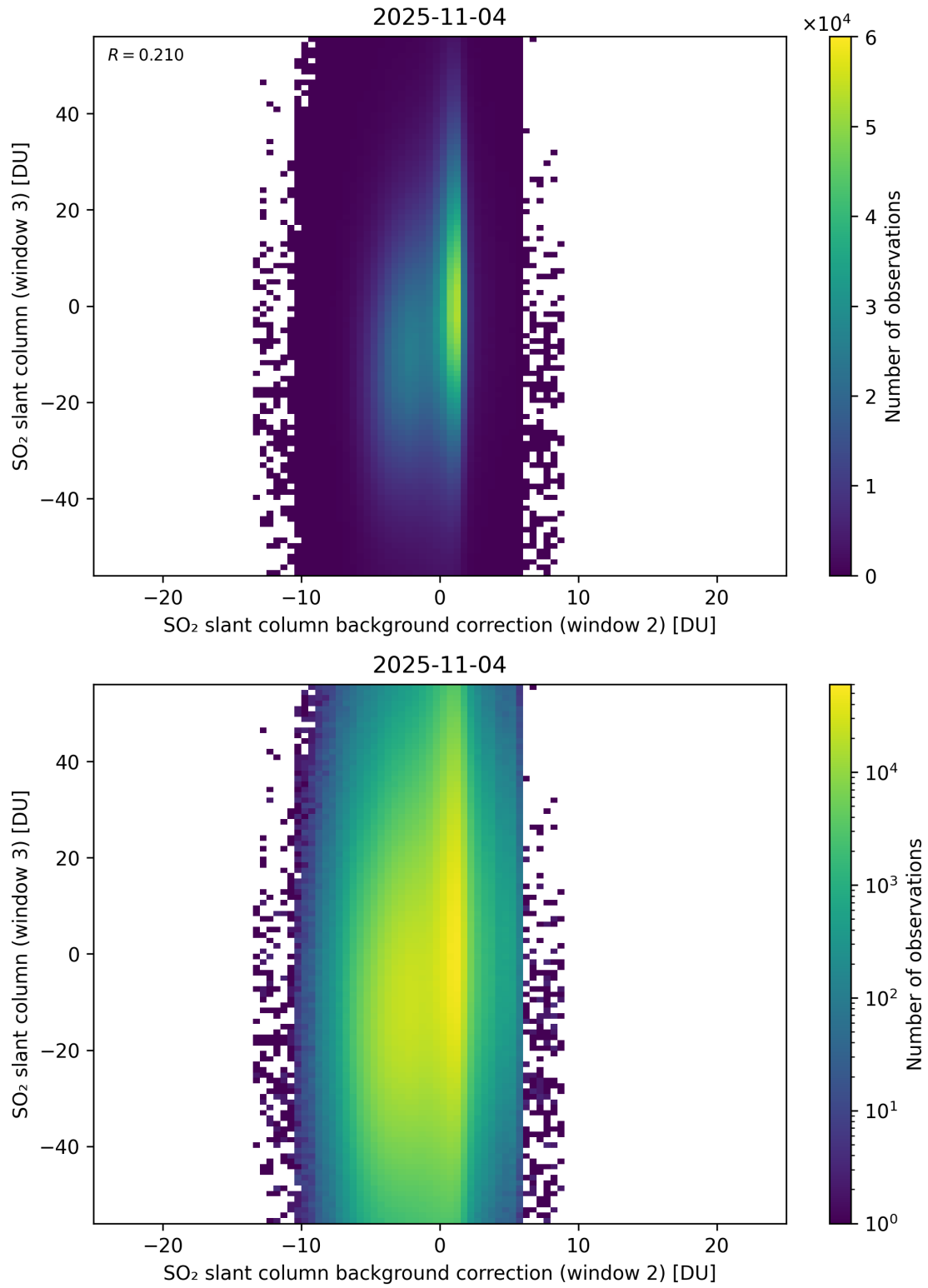
Figure 128: Scatter density plot of “SO 2 slant column background correction (window 2)” against “SO 2 slant column (window 3)” for 2025-11-03 to 2025-11-05.
