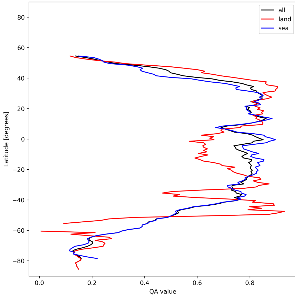
Figure 31: Zonal average of “QA value” for 2025-11-03 to 2025-11-05.
