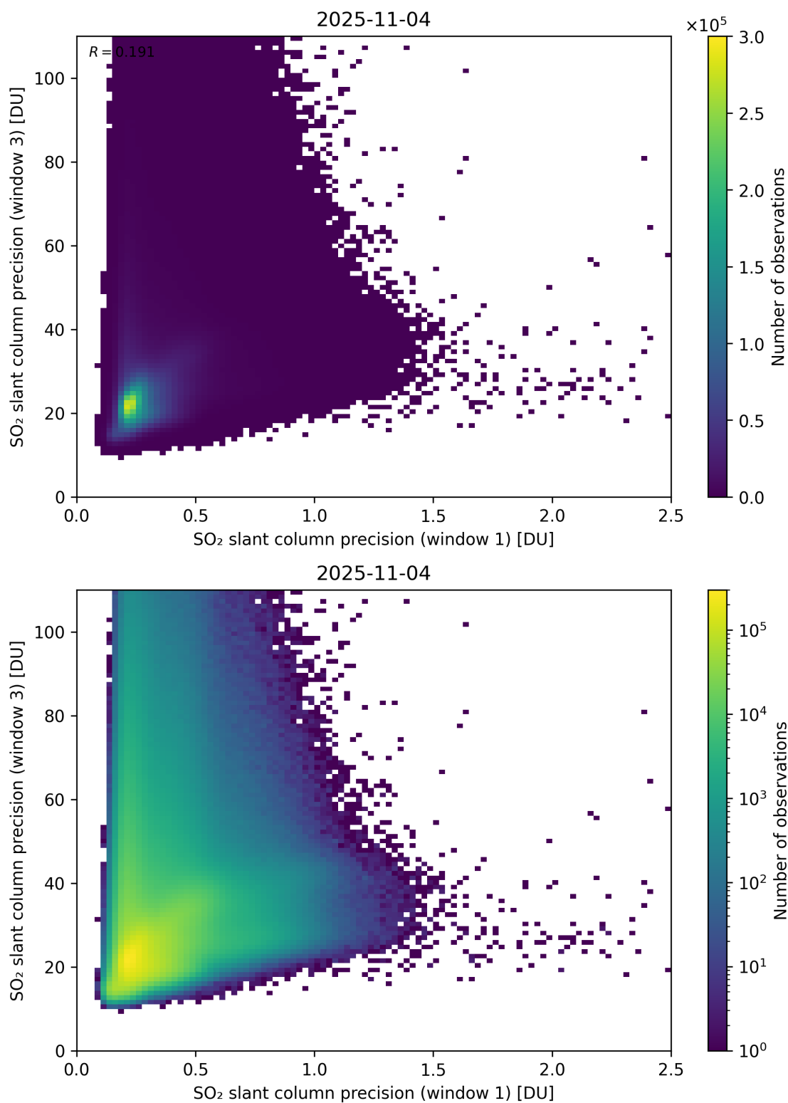
Figure 279: Scatter density plot of “SO 2 slant column precision (window 1)” against “SO 2 slant column precision (window 3)” for 2025-11-03 to 2025-11-05.
