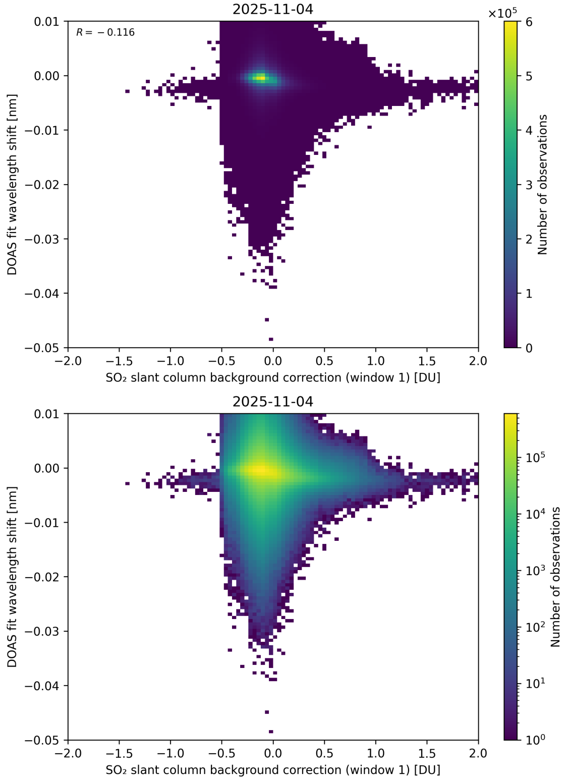
Figure 111: Scatter density plot of “SO 2 slant column background correction (window 1)” against “DOAS fit wavelength shift” for 2025-11-03 to 2025-11-05.
