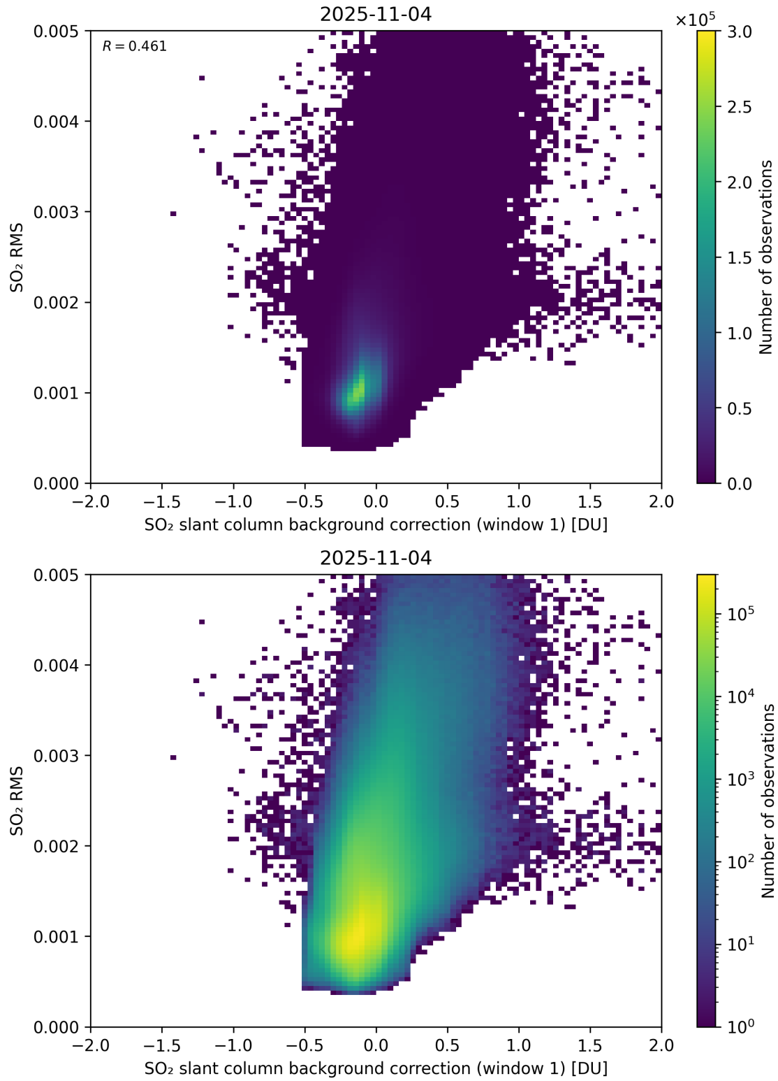
Figure 113: Scatter density plot of “SO 2 slant column background correction (window 1)” against “SO 2 RMS” for 2025-11-03 to 2025-11-05.
