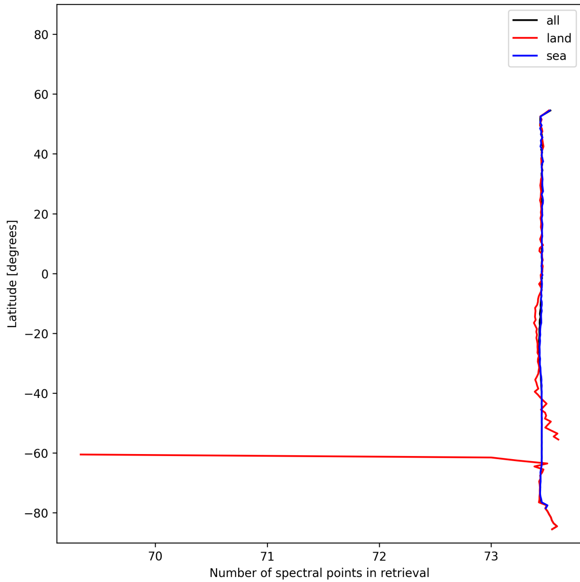
Figure 56: Zonal average of “Number of spectral points in retrieval” for 2025-11-03 to 2025-11-05.
