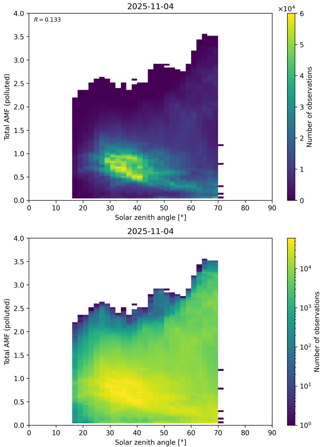
Figure 189: Scatter density plot of “Solar zenith angle” against “Total AMF (polluted)” for 2025-11-03 to 2025-11-05.
