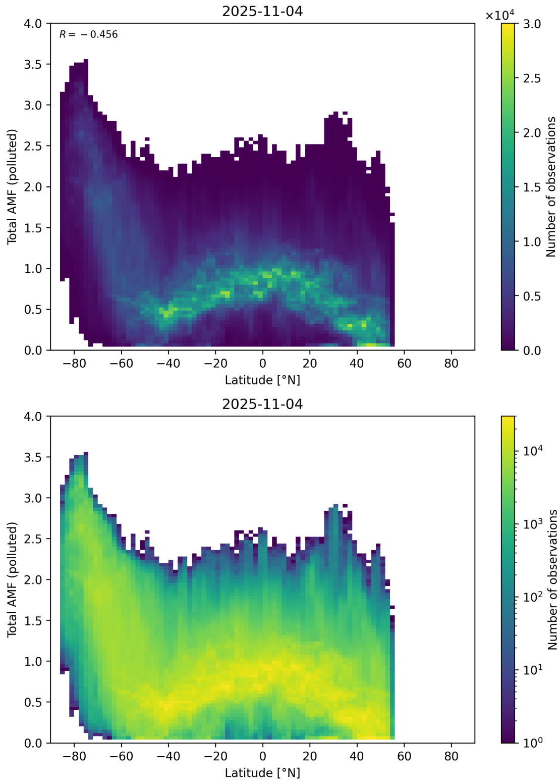
Figure 167: Scatter density plot of “Latitude” against “Total AMF (polluted)” for 2025-11-03 to 2025-11-05.
