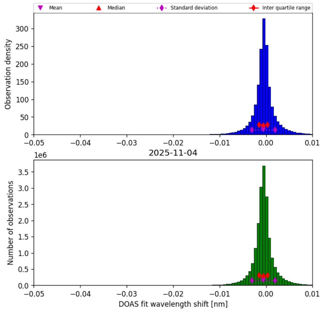
Figure 76: Histogram of “DOAS fit wavelength shift” for 2025-11-03 to 2025-11-05
