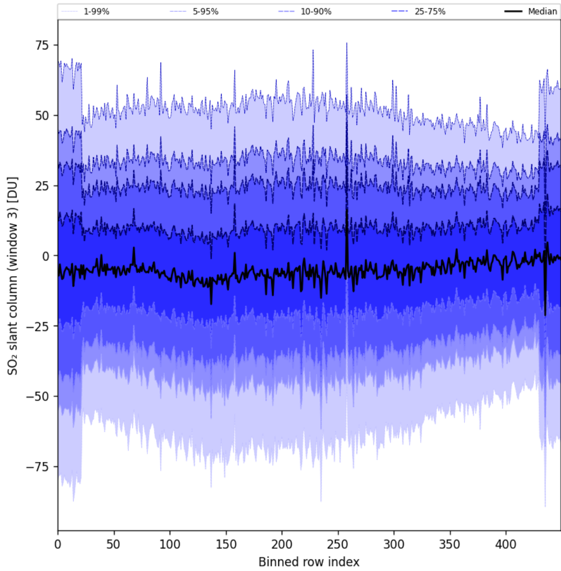
Figure 97: Along track statistics of “SO 2 slant column (window 3)” for 2025-11-03 to 2025-11-05
