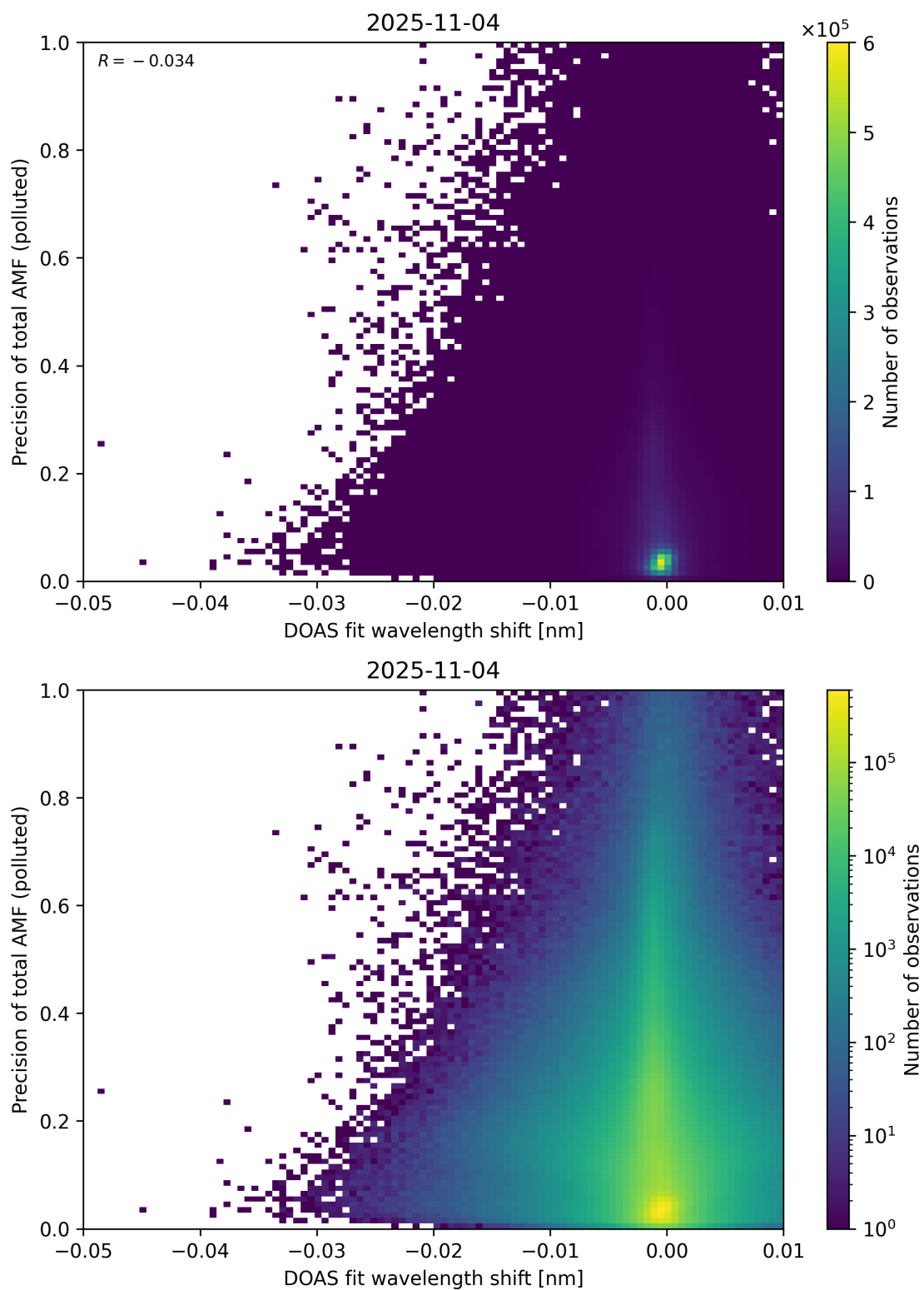
Figure 142: Scatter density plot of “DOAS fit wavelength shift” against “Precision of total AMF (polluted)” for 2025-11-03 to 2025-11-05.
