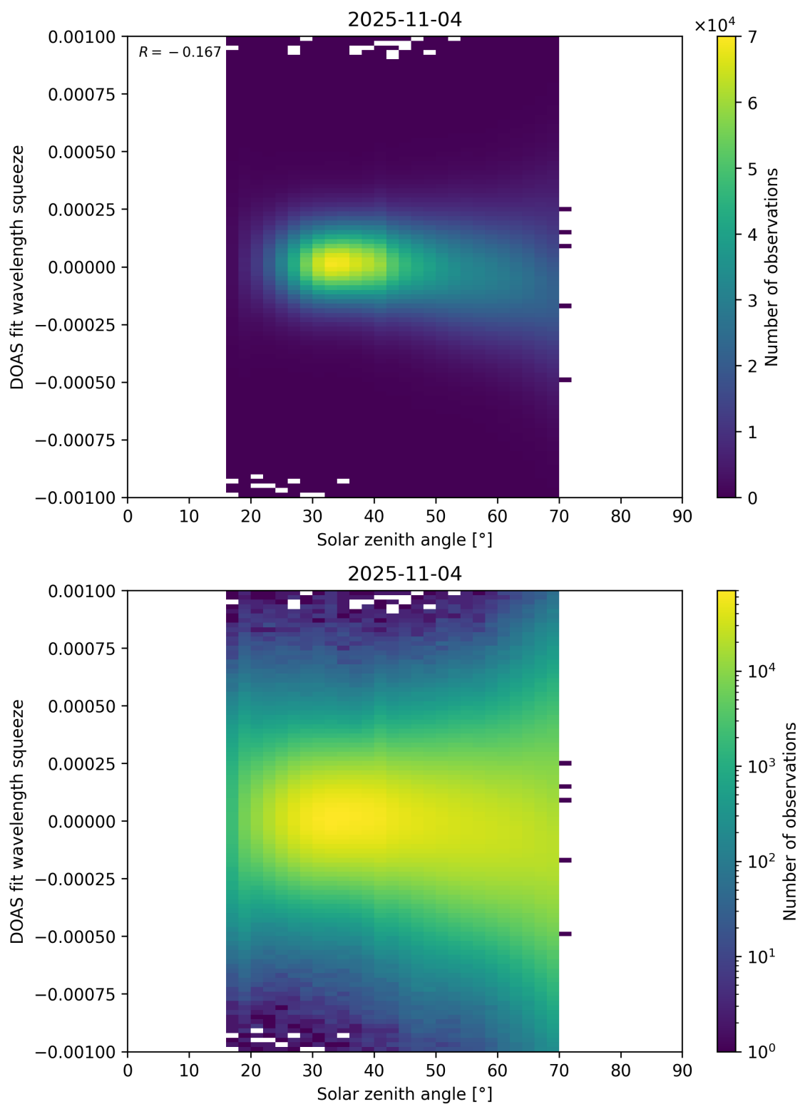
Figure 175: Scatter density plot of “Solar zenith angle” against “DOAS fit wavelength squeeze” for 2025-11-03 to 2025-11-05.
