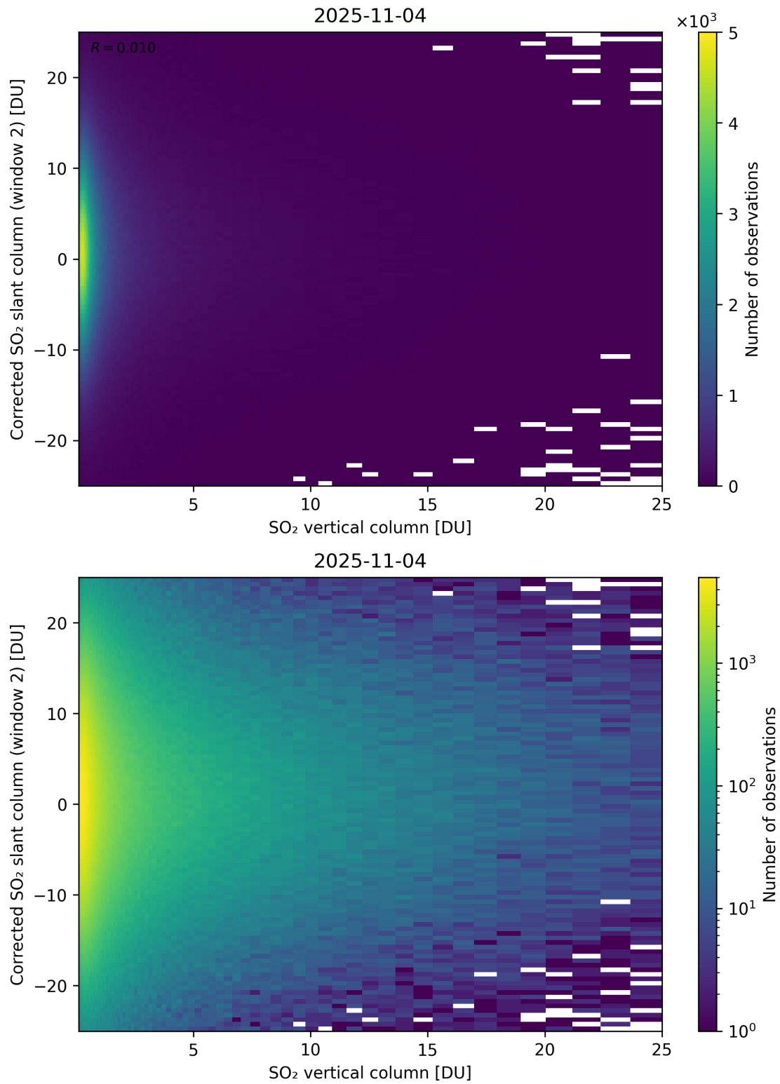
Figure 352: Scatter density plot of “SO 2 vertical column” against “Corrected SO 2 slant column (window 2)” for 2025-11-03 to 2025-11-05.
