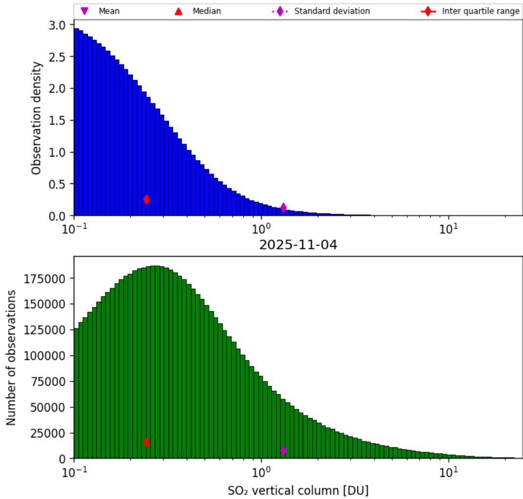
Figure 58: Histogram of “SO 2 vertical column” for 2025-11-03 to 2025-11-05
