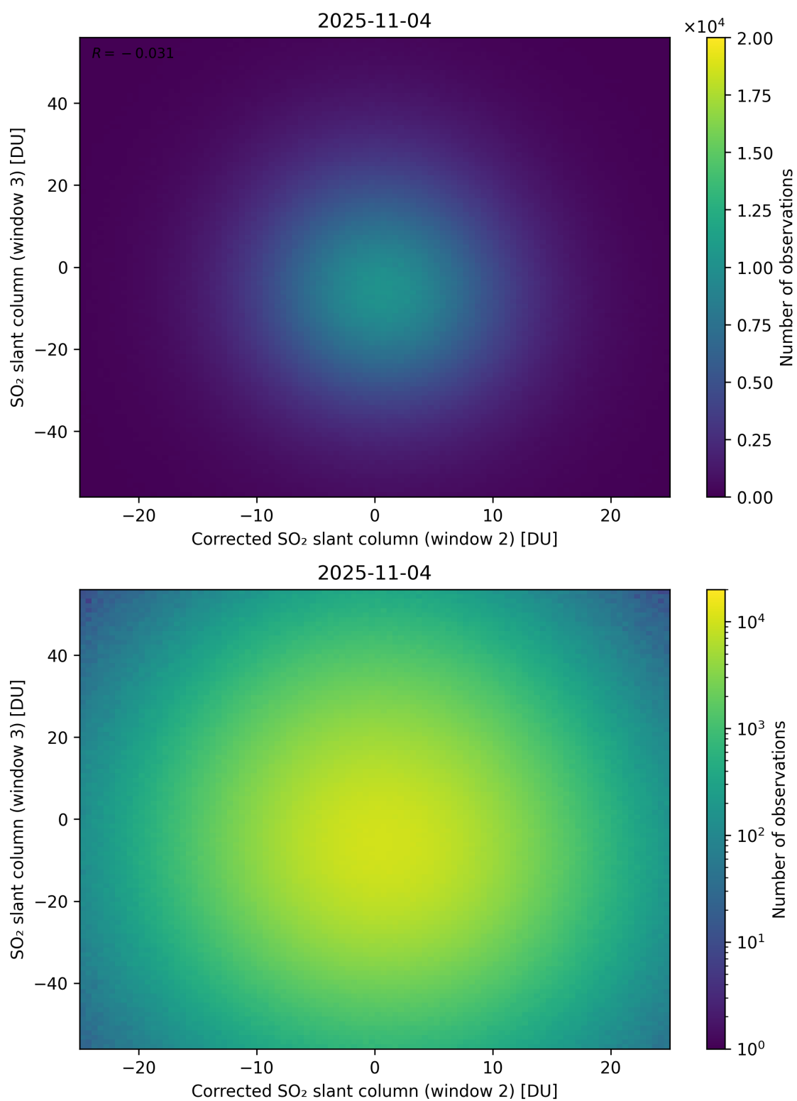
Figure 251: Scatter density plot of “Corrected SO 2 slant column (window 2)” against “SO 2 slant column (window 3)” for 2025-11-03 to 2025-11-05.
