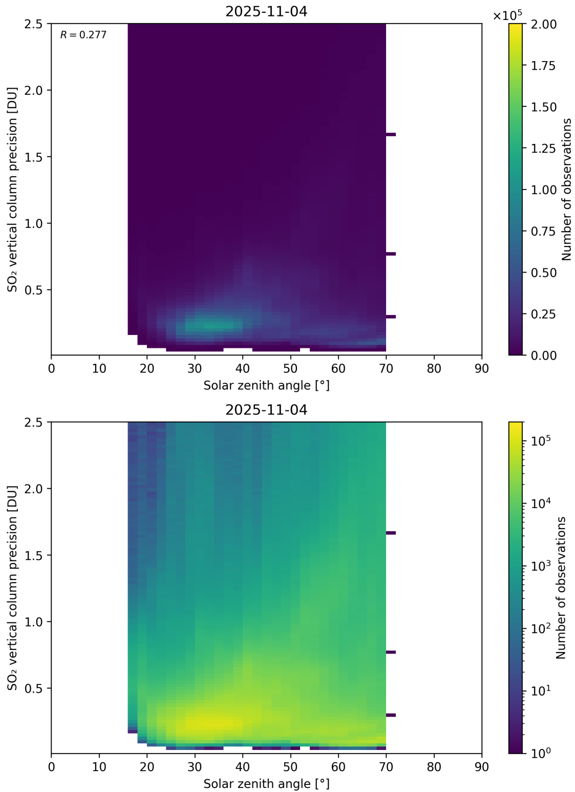
Figure 192: Scatter density plot of “Solar zenith angle” against “SO 2 vertical column precision” for 2025-11-03 to 2025-11-05.
