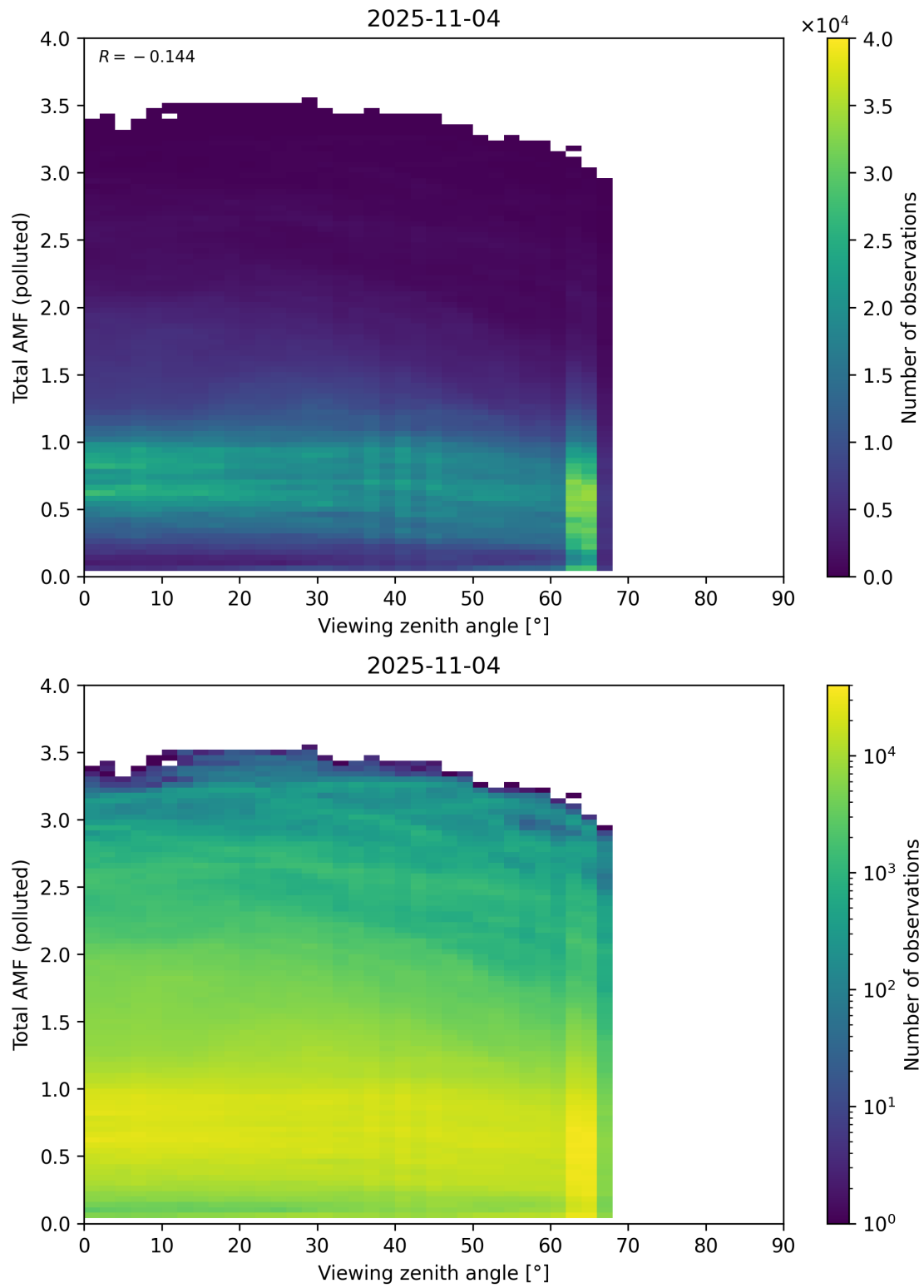
Figure 381: Scatter density plot of “Viewing zenith angle” against “Total AMF (polluted)” for 2025-11-03 to 2025-11-05.
