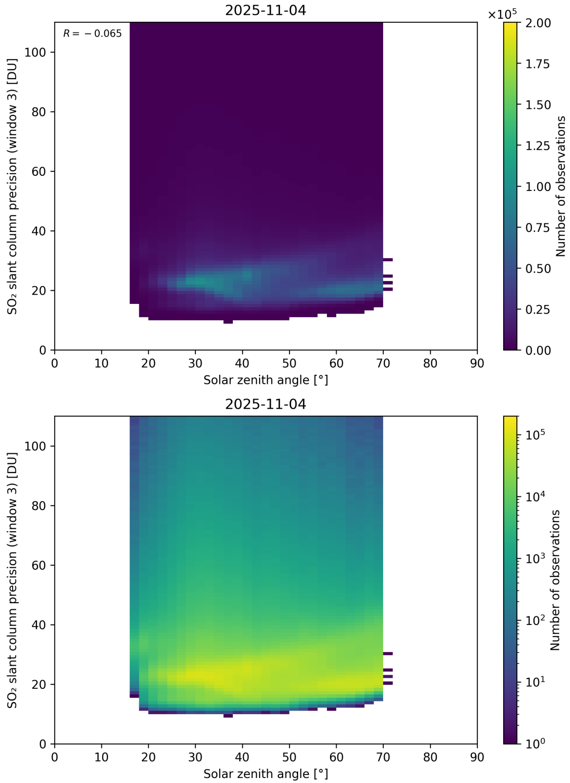
Figure 188: Scatter density plot of “Solar zenith angle” against “SO 2 slant column precision (window 3)” for 2025-11-03 to 2025-11-05.
