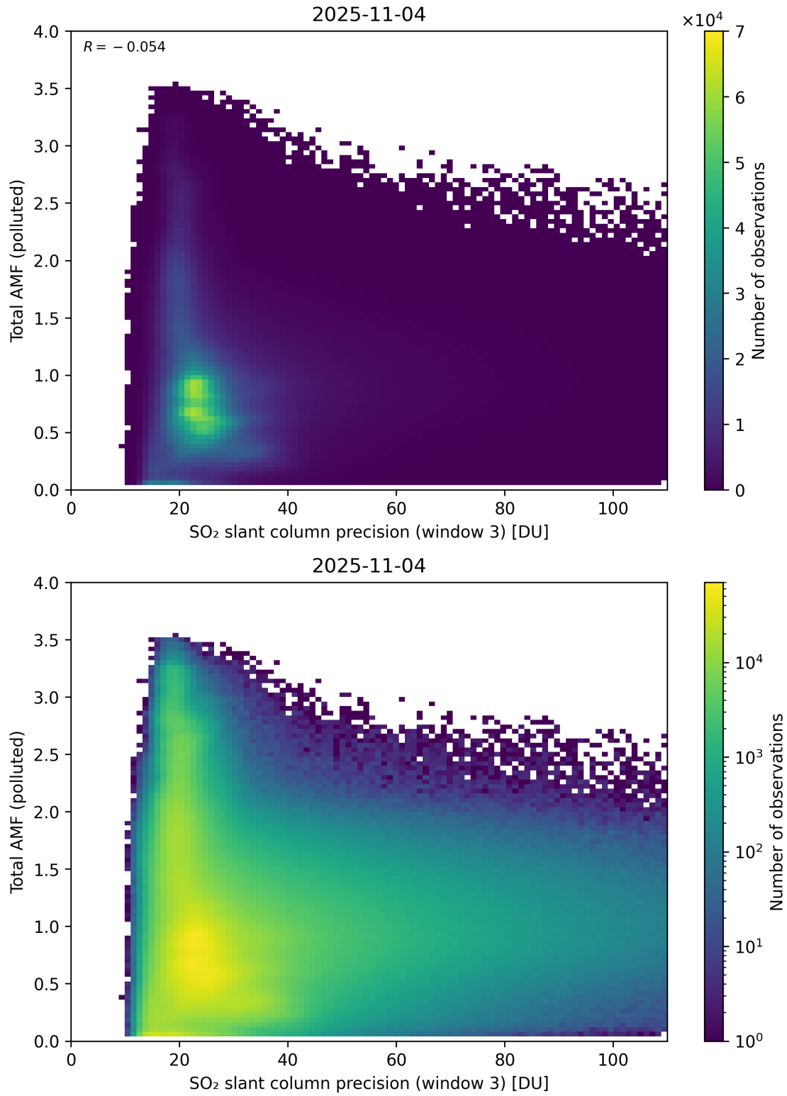
Figure 313: Scatter density plot of “SO 2 slant column precision (window 3)” against “Total AMF (polluted)” for 2025-11-03 to 2025-11-05.
