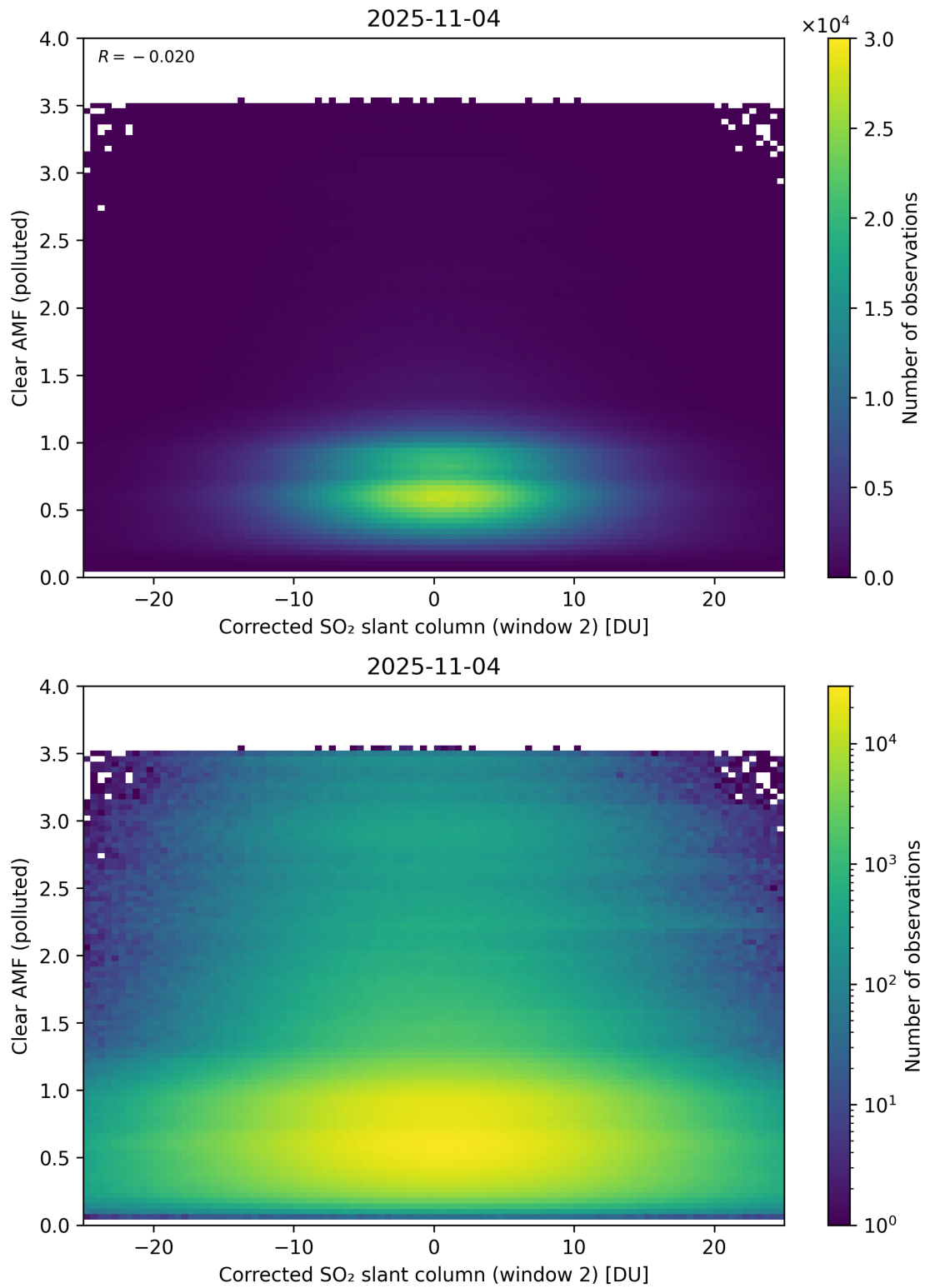
Figure 249: Scatter density plot of “Corrected SO 2 slant column (window 2)” against “Clear AMF (polluted)” for 2025-11-03 to 2025-11-05.
