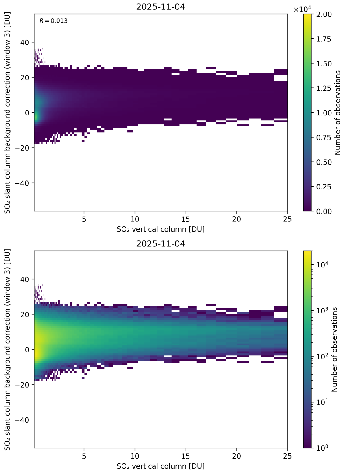
Figure 325: Scatter density plot of “SO 2 vertical column” against “SO 2 slant column background correction (window 3)” for 2025-11-03 to 2025-11-05.
