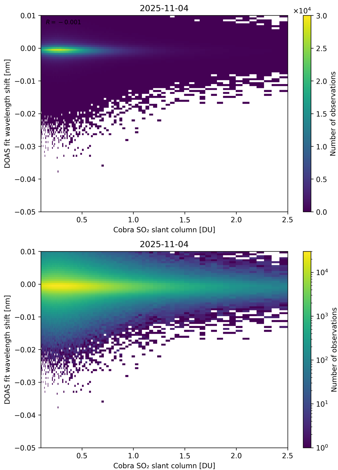
Figure 196: Scatter density plot of “Cobra SO 2 slant column” against “DOAS fit wavelength shift” for 2025-11-03 to 2025-11-05.
