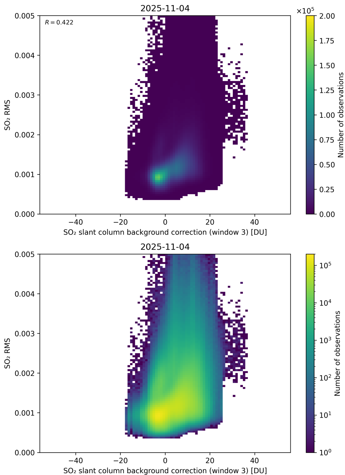
Figure 134: Scatter density plot of “SO 2 slant column background correction (window 3)” against “SO 2 RMS” for 2025-11-03 to 2025-11-05.
