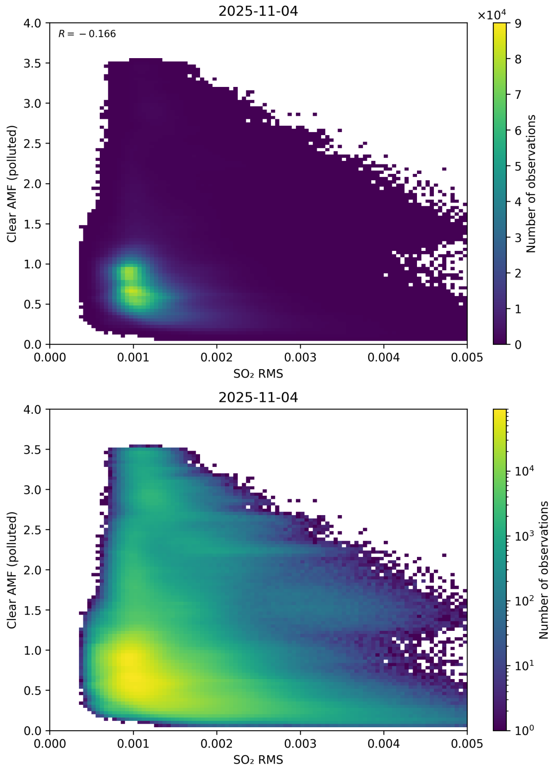
Figure 147: Scatter density plot of “SO 2 RMS” against “Clear AMF (polluted)” for 2025-11-03 to 2025-11-05.
