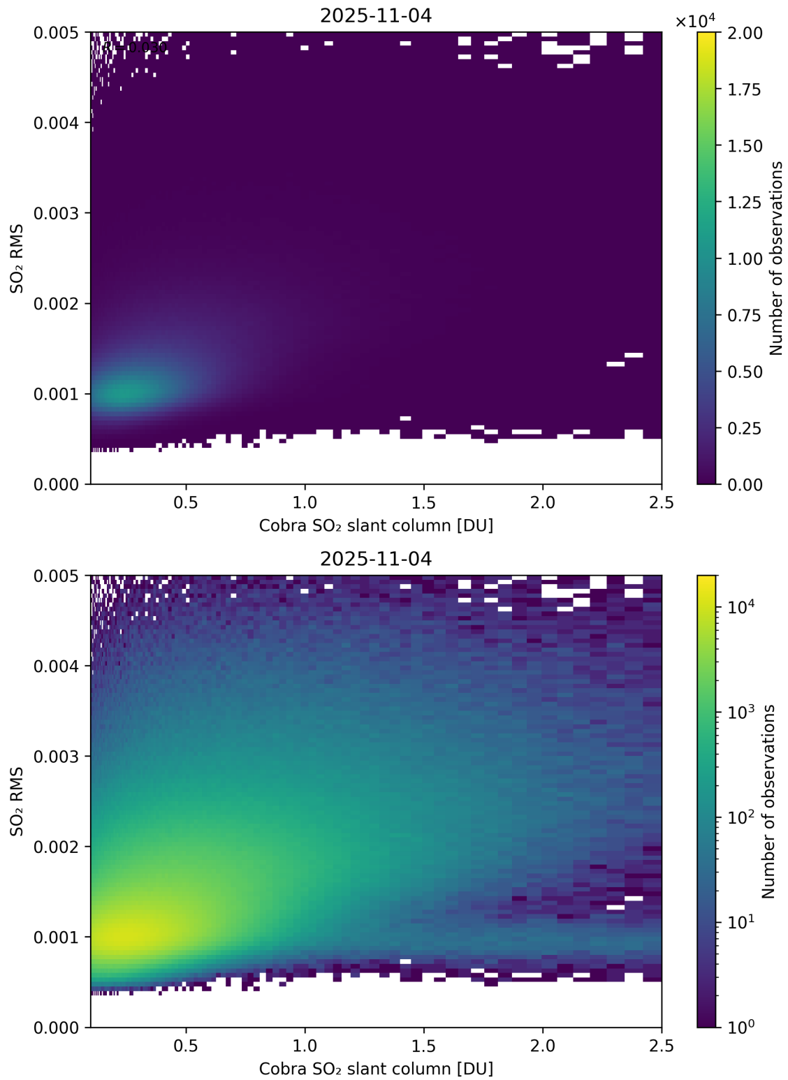
Figure 198: Scatter density plot of “Cobra SO 2 slant column” against “SO 2 RMS” for 2025-11-03 to 2025-11-05.
