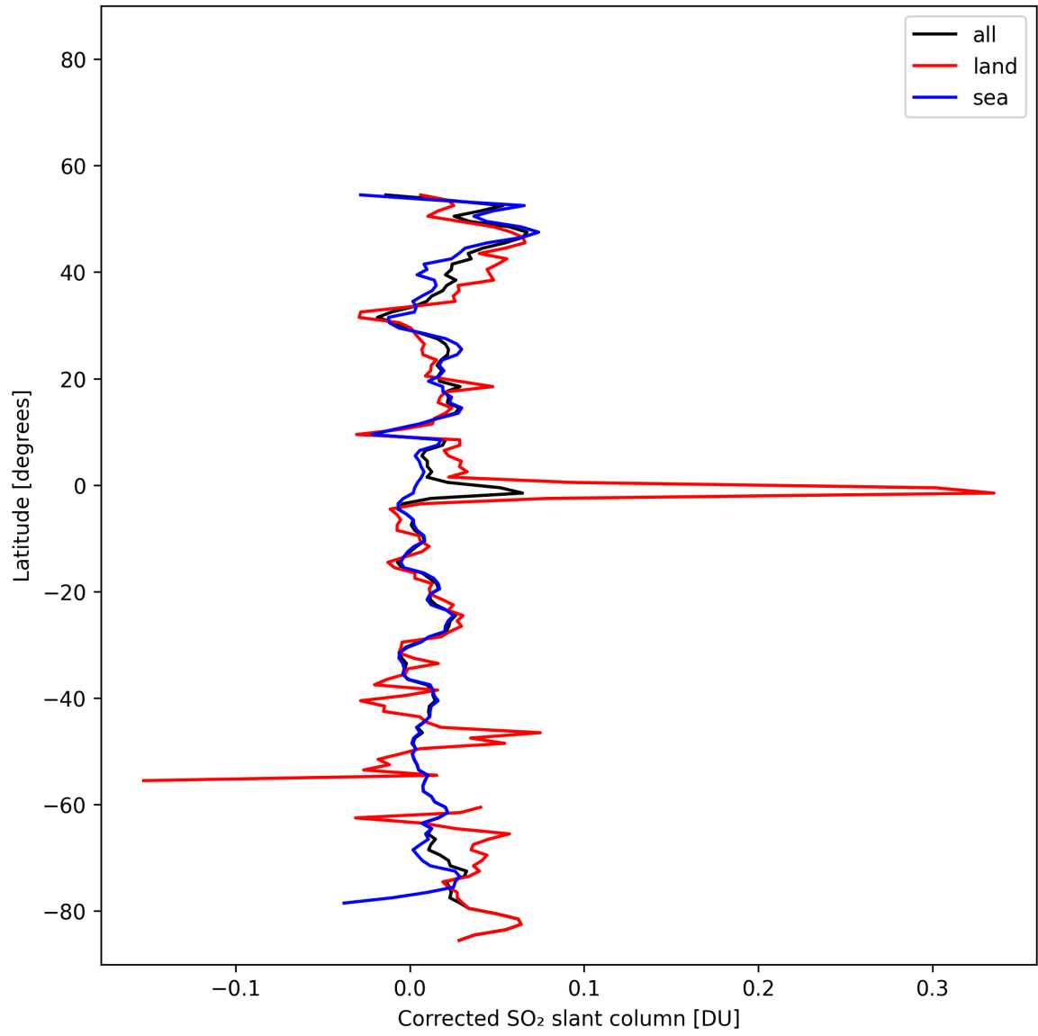
Figure 34: Zonal average of “Corrected SO 2 slant column” for 2025-11-03 to 2025-11-05.
