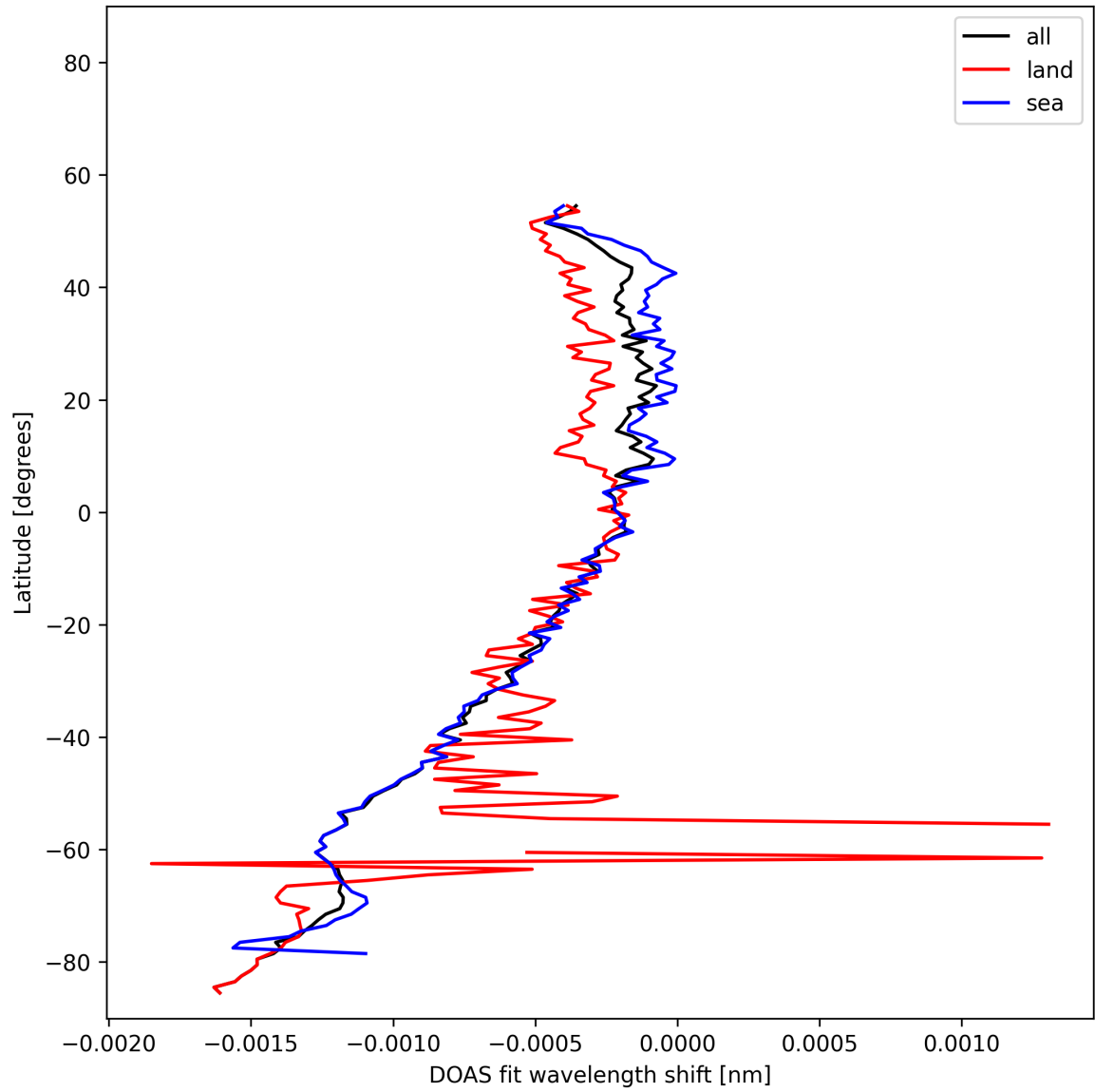
Figure 50: Zonal average of “DOAS fit wavelength shift” for 2025-11-03 to 2025-11-05.
