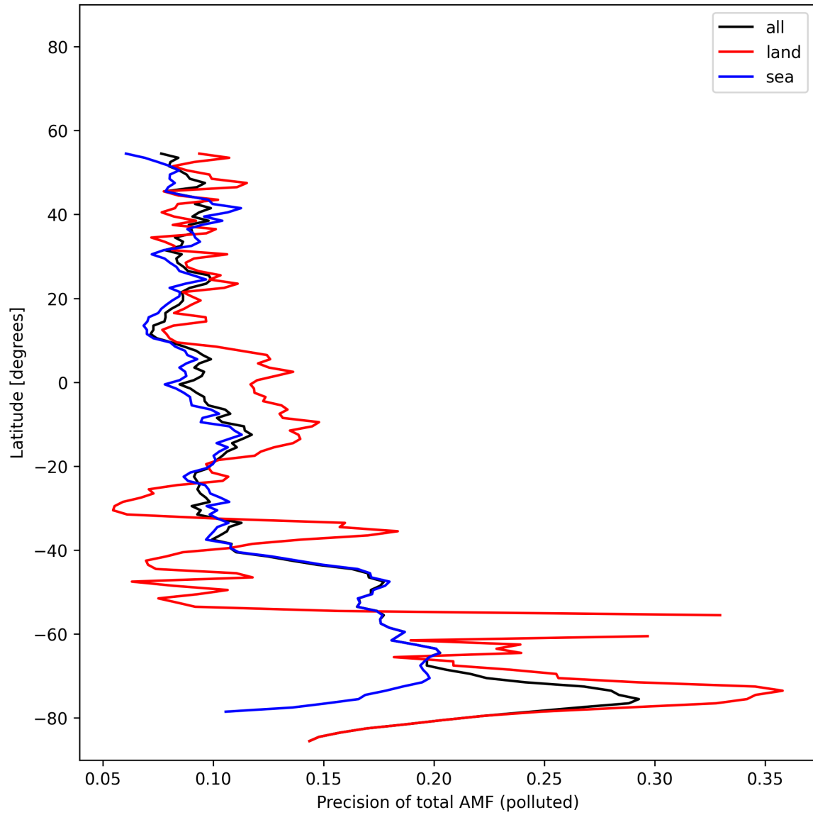
Figure 54: Zonal average of “Precision of total AMF (polluted)” for 2025-11-03 to 2025-11-05.
