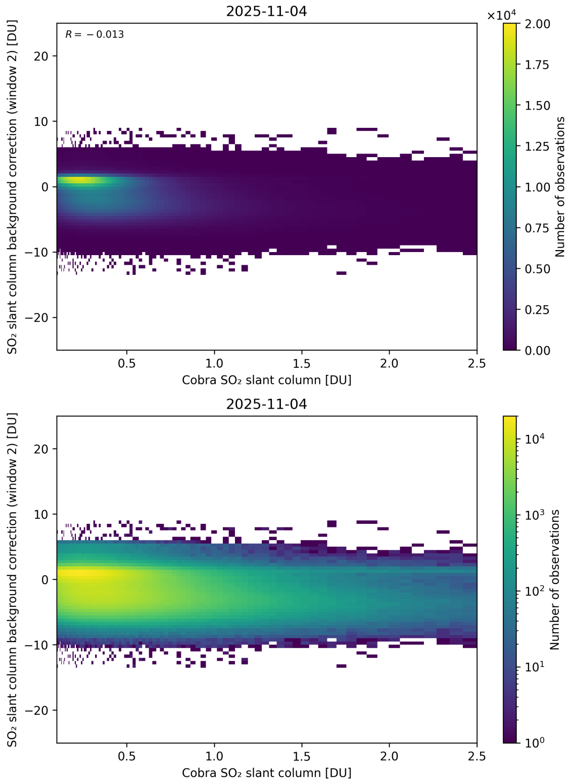
Figure 194: Scatter density plot of “Cobra SO 2 slant column” against “SO 2 slant column background correction (window 2)” for 2025-11-03 to 2025-11-05.
