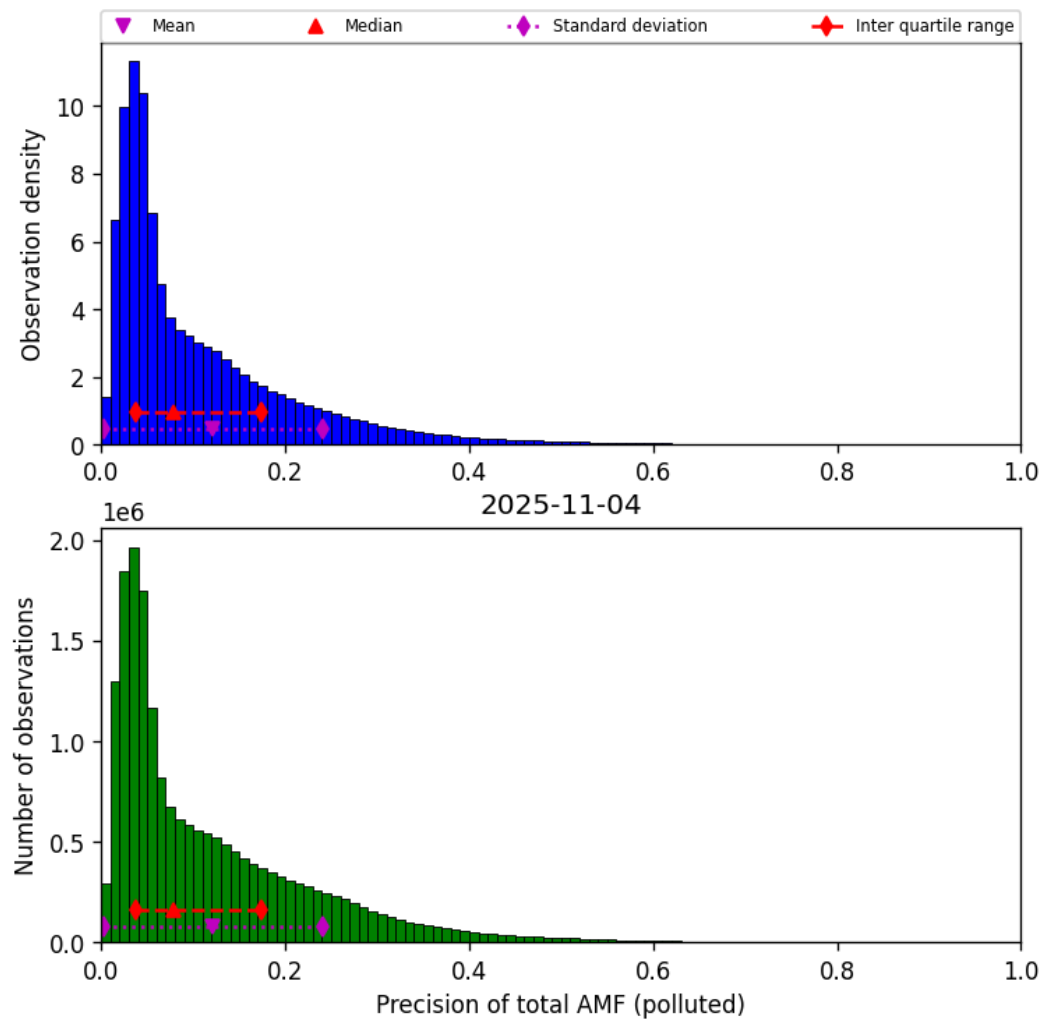
Figure 80: Histogram of “Precision of total AMF (polluted)” for 2025-11-03 to 2025-11-05
