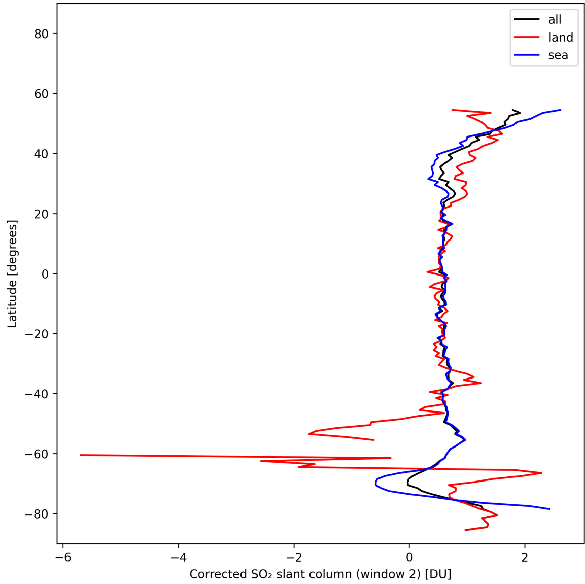
Figure 43: Zonal average of “Corrected SO 2 slant column (window 2)” for 2025-11-03 to 2025-11-05.
