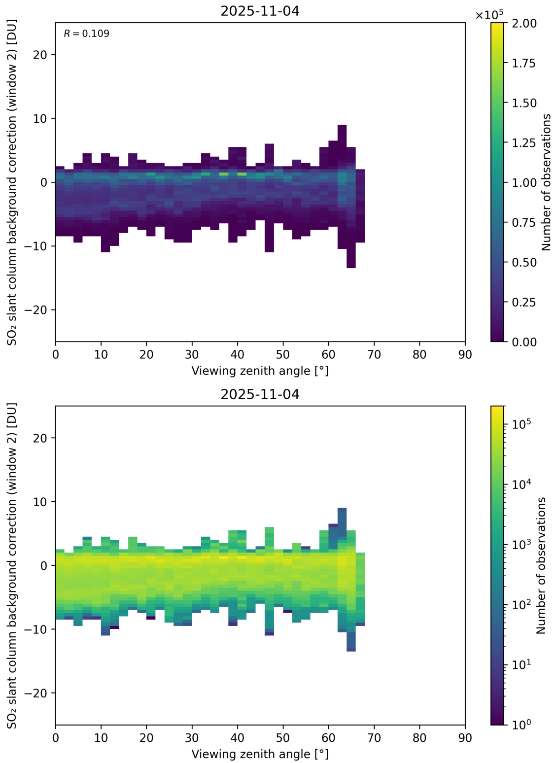
Figure 363: Scatter density plot of “Viewing zenith angle” against “SO 2 slant column background correction (window 2)” for 2025-11-03 to 2025-11-05.
