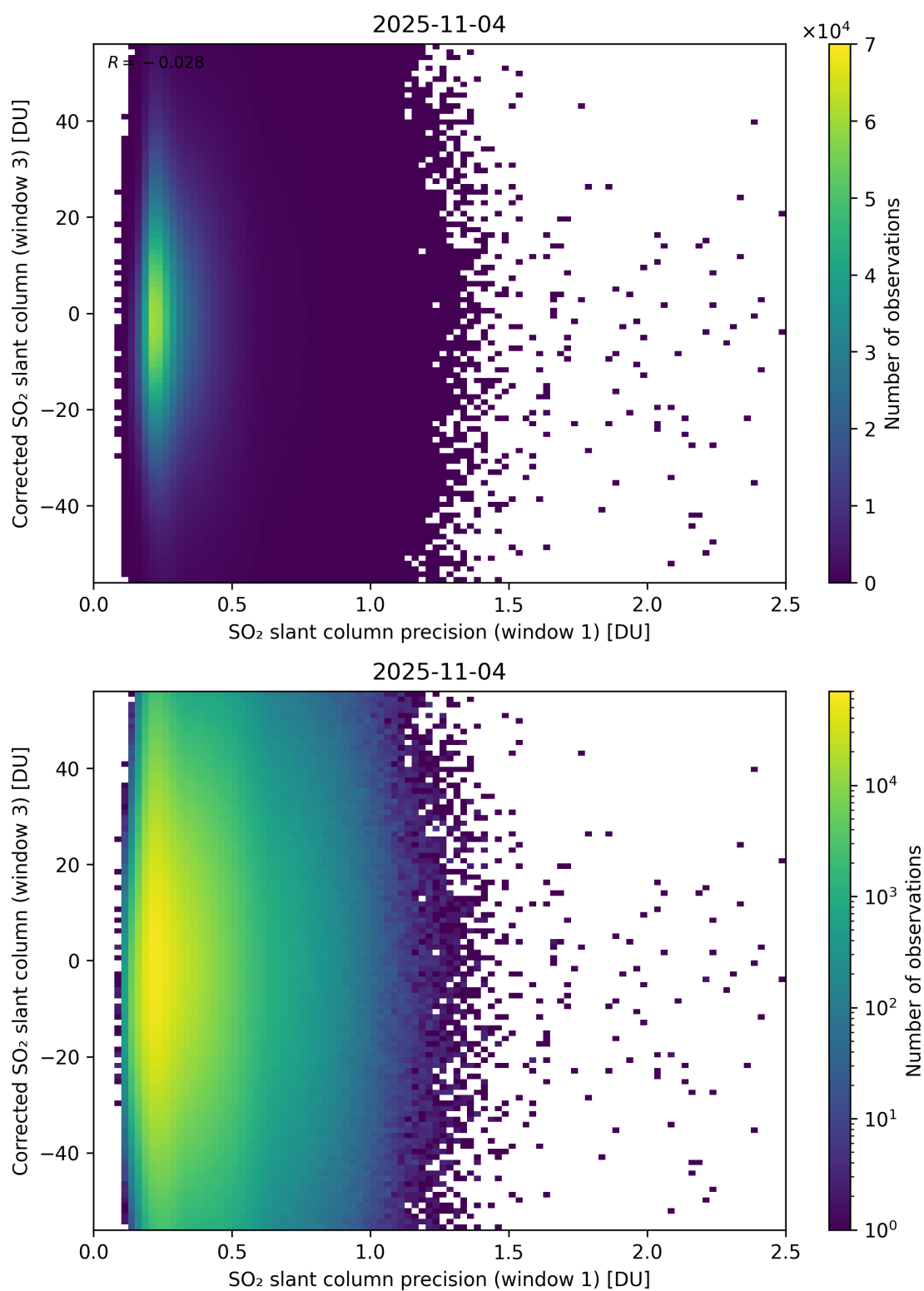
Figure 276: Scatter density plot of “SO 2 slant column precision (window 1)” against “Corrected SO 2 slant column (window 3)” for 2025-11-03 to 2025-11-05.
