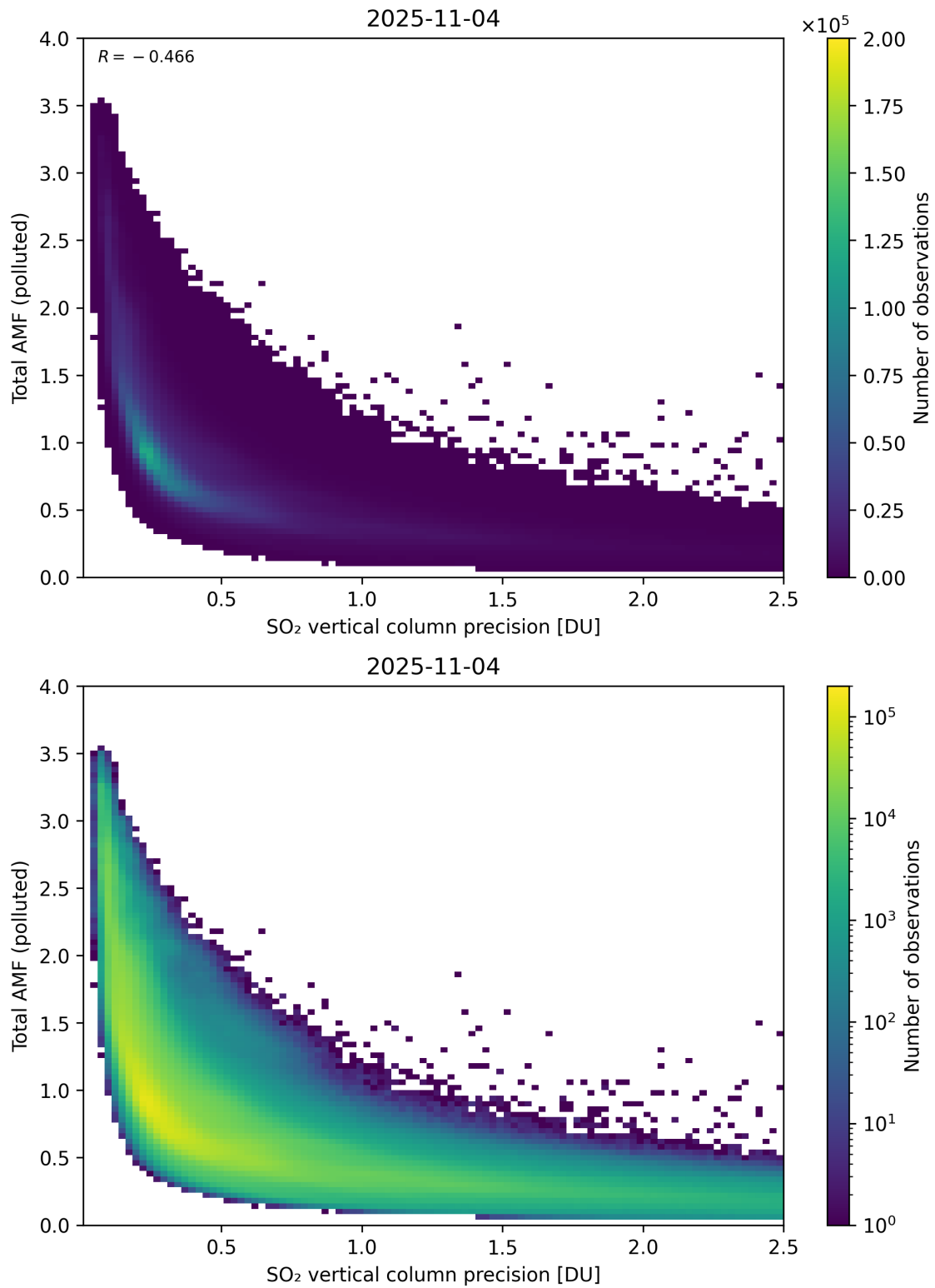
Figure 346: Scatter density plot of “SO 2 vertical column precision” against “Total AMF (polluted)” for 2025-11-03 to 2025-11-05.
