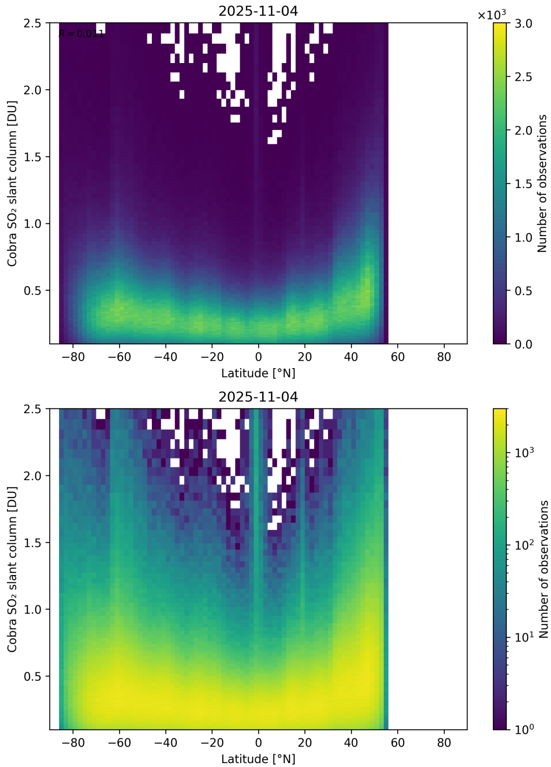
Figure 157: Scatter density plot of “Latitude” against “Cobra SO 2 slant column” for 2025-11-03 to 2025-11-05.
