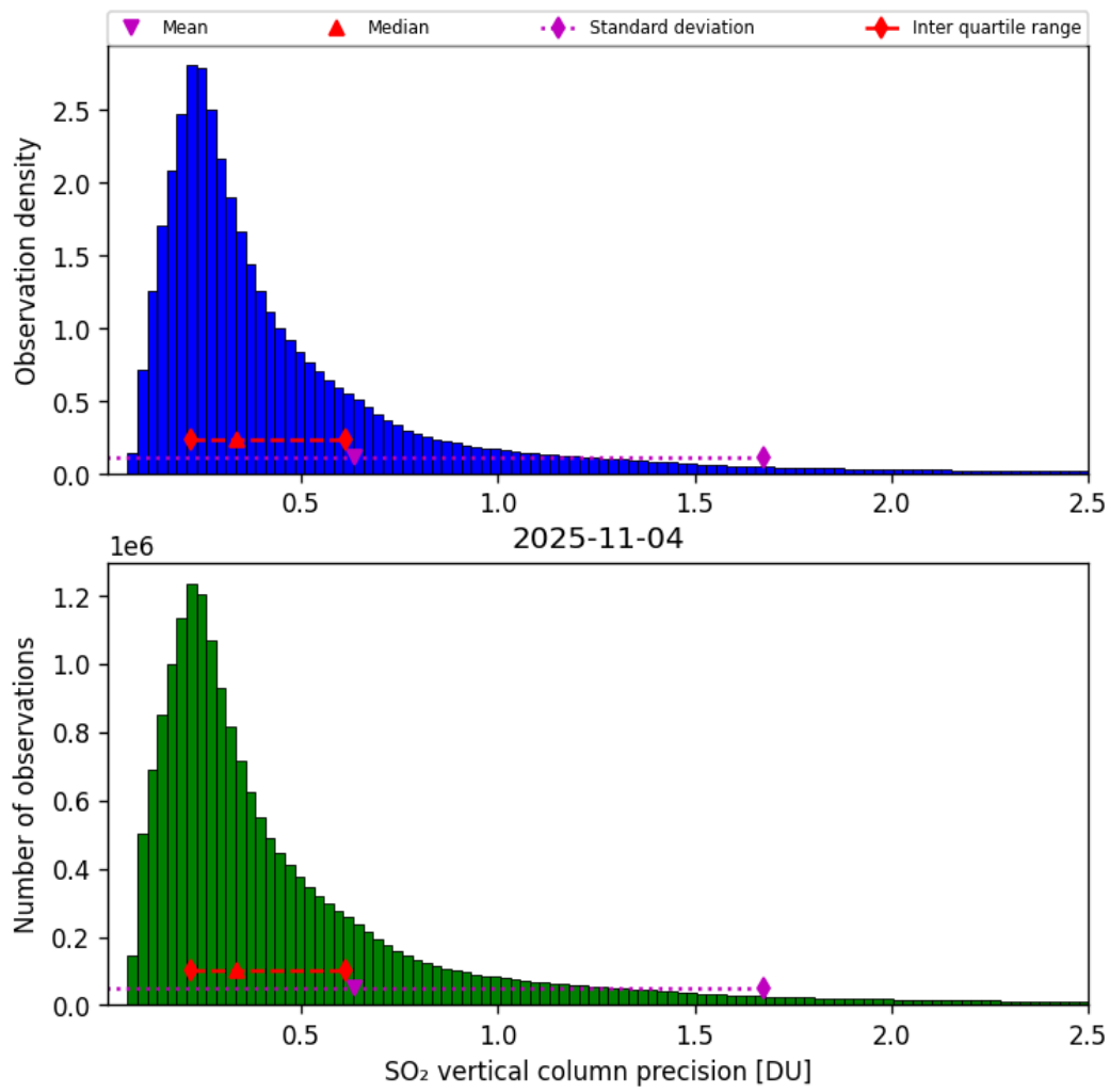
Figure 59: Histogram of “SO 2 vertical column precision” for 2025-11-03 to 2025-11-05
