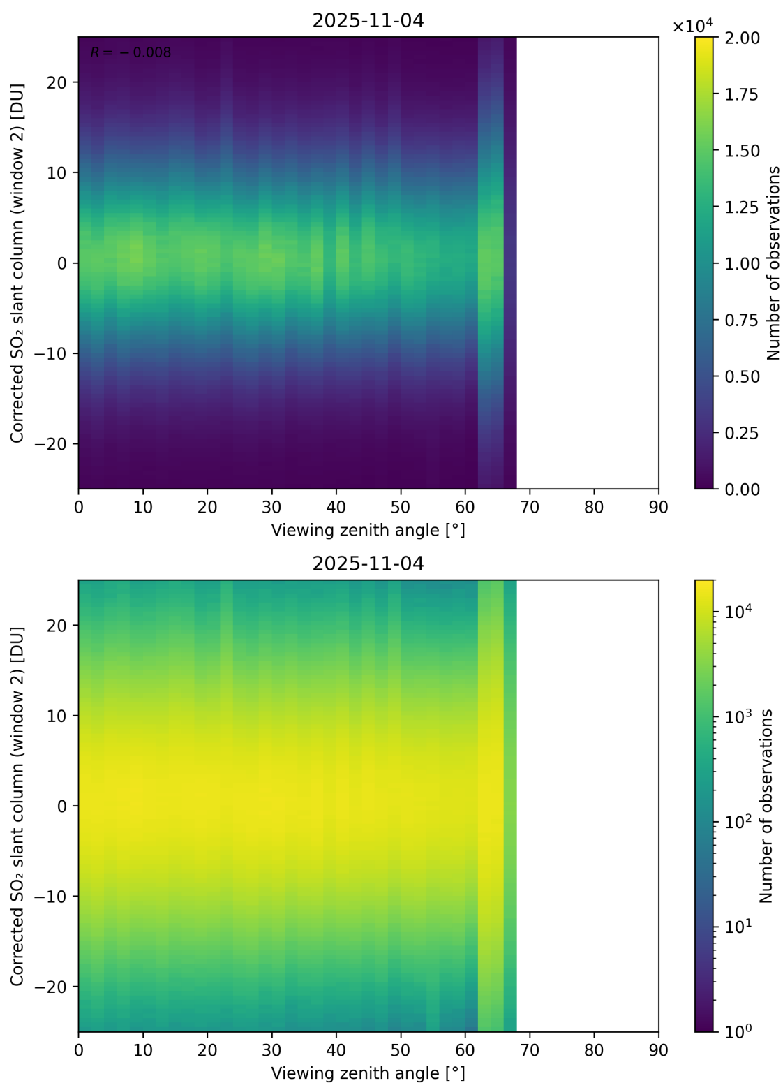
Figure 374: Scatter density plot of “Viewing zenith angle” against “Corrected SO 2 slant column (window 2)” for 2025-11-03 to 2025-11-05.
