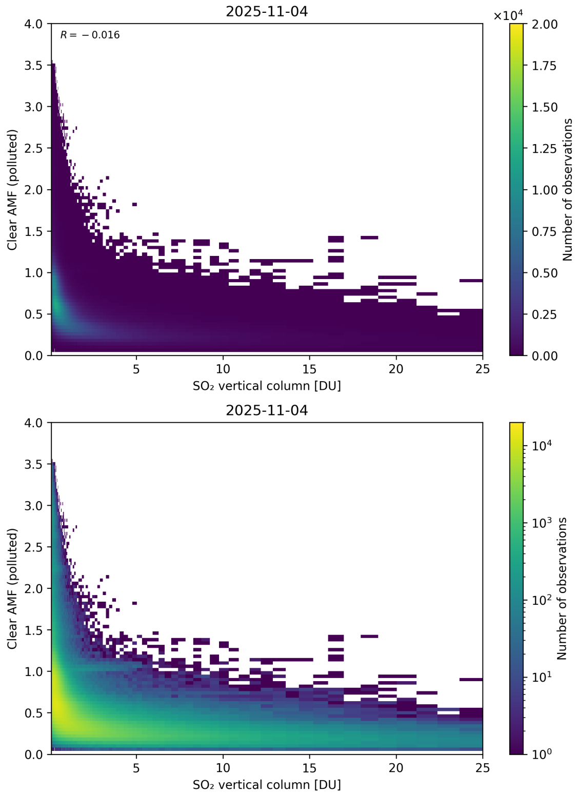
Figure 348: Scatter density plot of “SO 2 vertical column” against “Clear AMF (polluted)” for 2025-11-03 to 2025-11-05.
