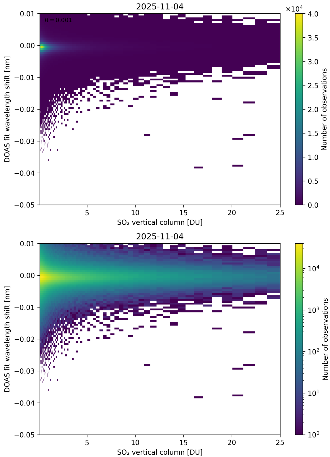
Figure 326: Scatter density plot of “SO 2 vertical column” against “DOAS fit wavelength shift” for 2025-11-03 to 2025-11-05.
