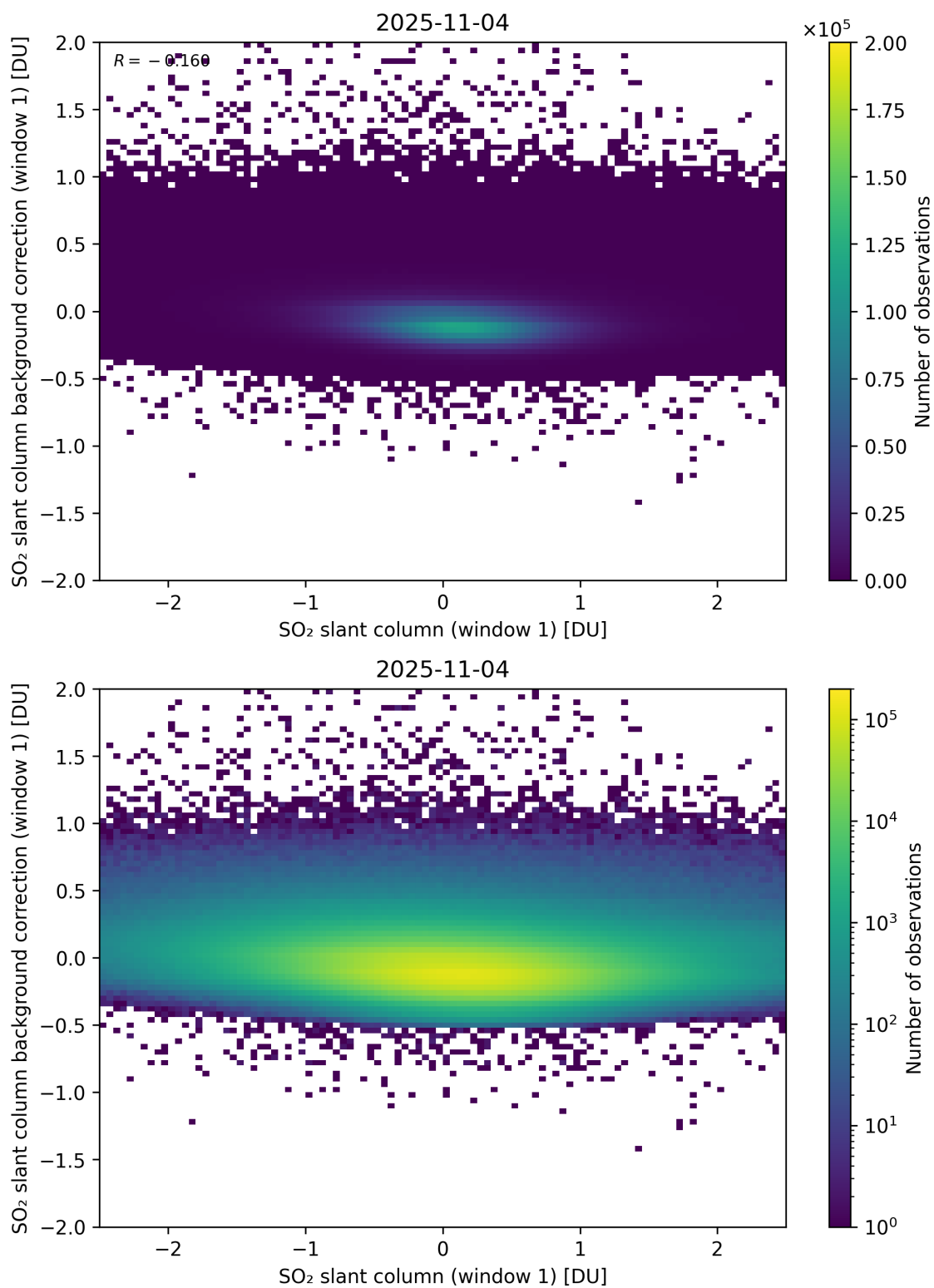
Figure 262: Scatter density plot of “SO 2 slant column (window 1)” against “SO 2 slant column background correction (window 1)” for 2025-11-03 to 2025-11-05.
