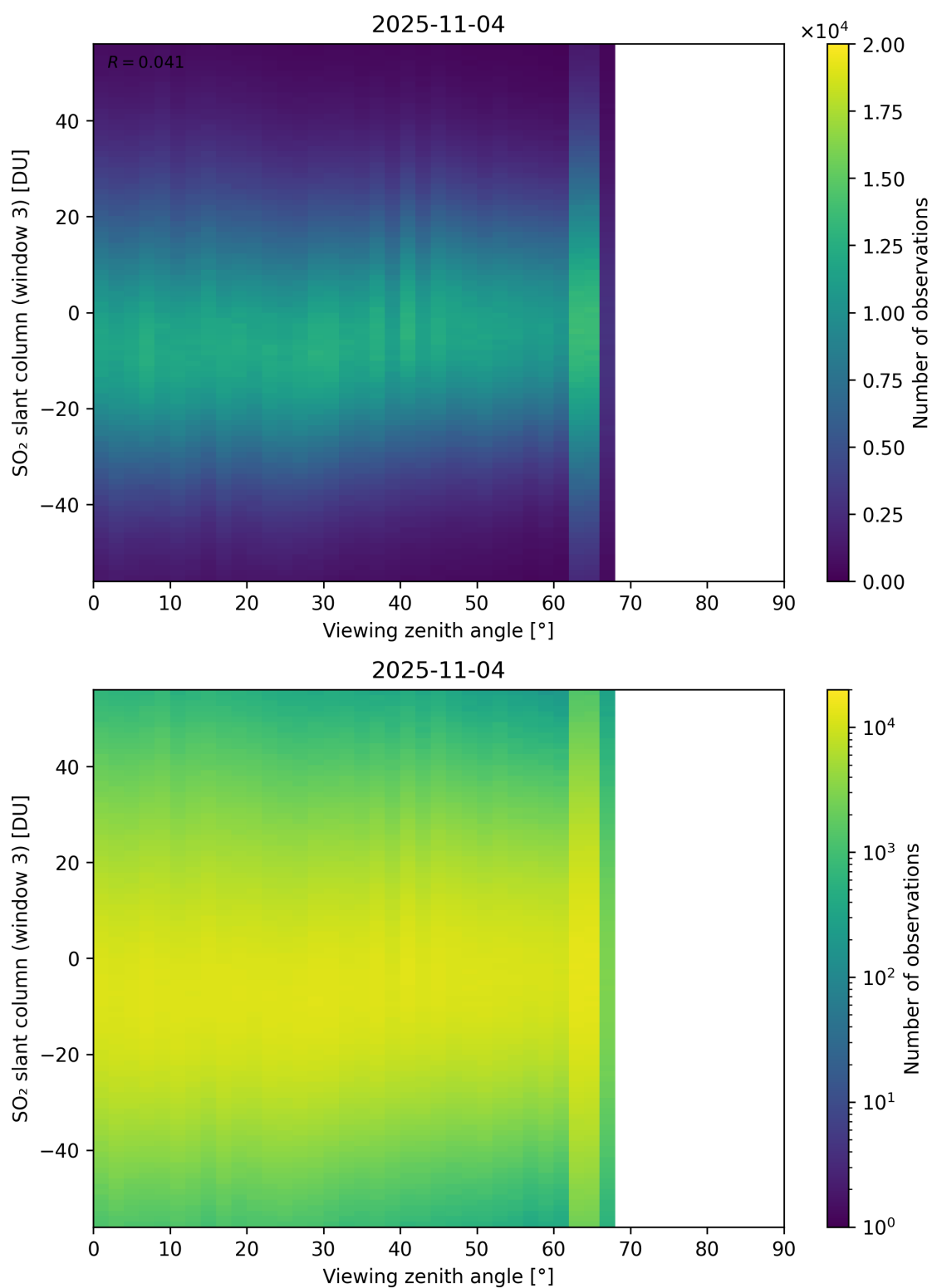
Figure 379: Scatter density plot of “Viewing zenith angle” against “SO 2 slant column (window 3)” for 2025-11-03 to 2025-11-05.
