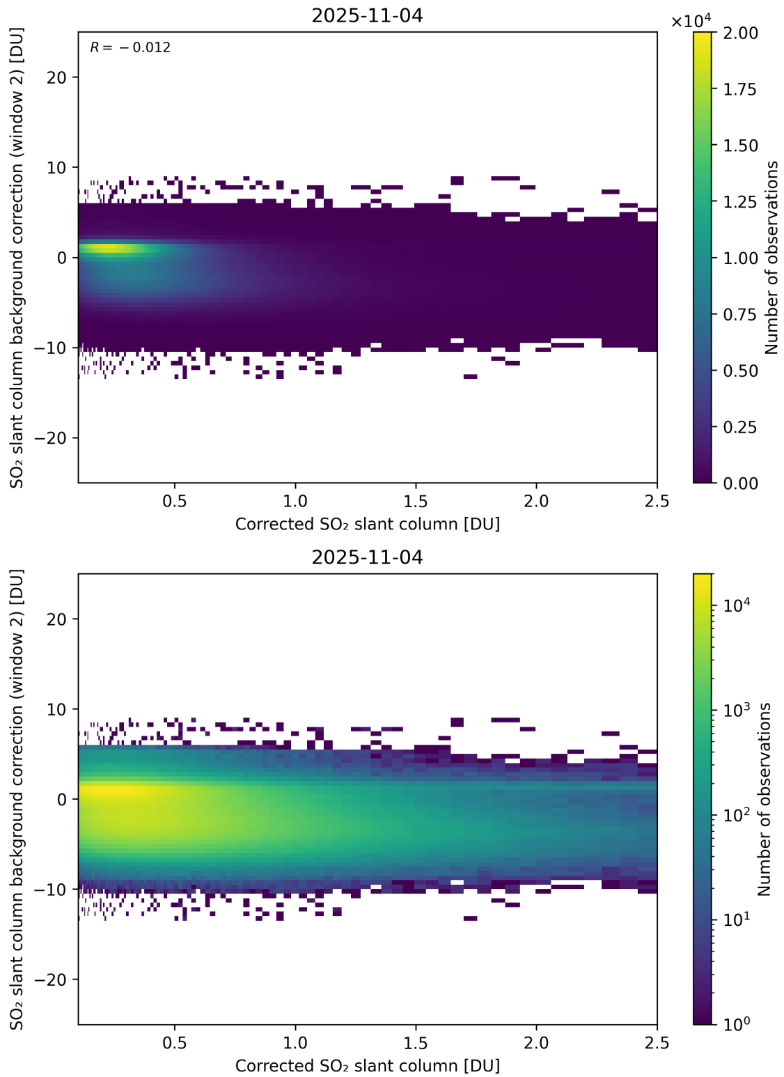
Figure 227: Scatter density plot of “Corrected SO 2 slant column” against “SO 2 slant column background correction (window 2)” for 2025-11-03 to 2025-11-05.
