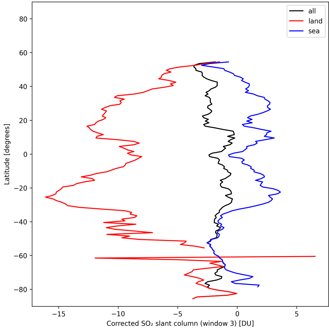
Figure 47: Zonal average of “Corrected SO 2 slant column (window 3)” for 2025-11-03 to 2025-11-05.
