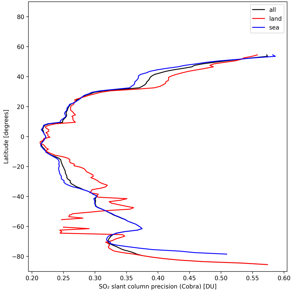
Figure 36: Zonal average of “SO 2 slant column precision (Cobra)” for 2025-11-03 to 2025-11-05.
