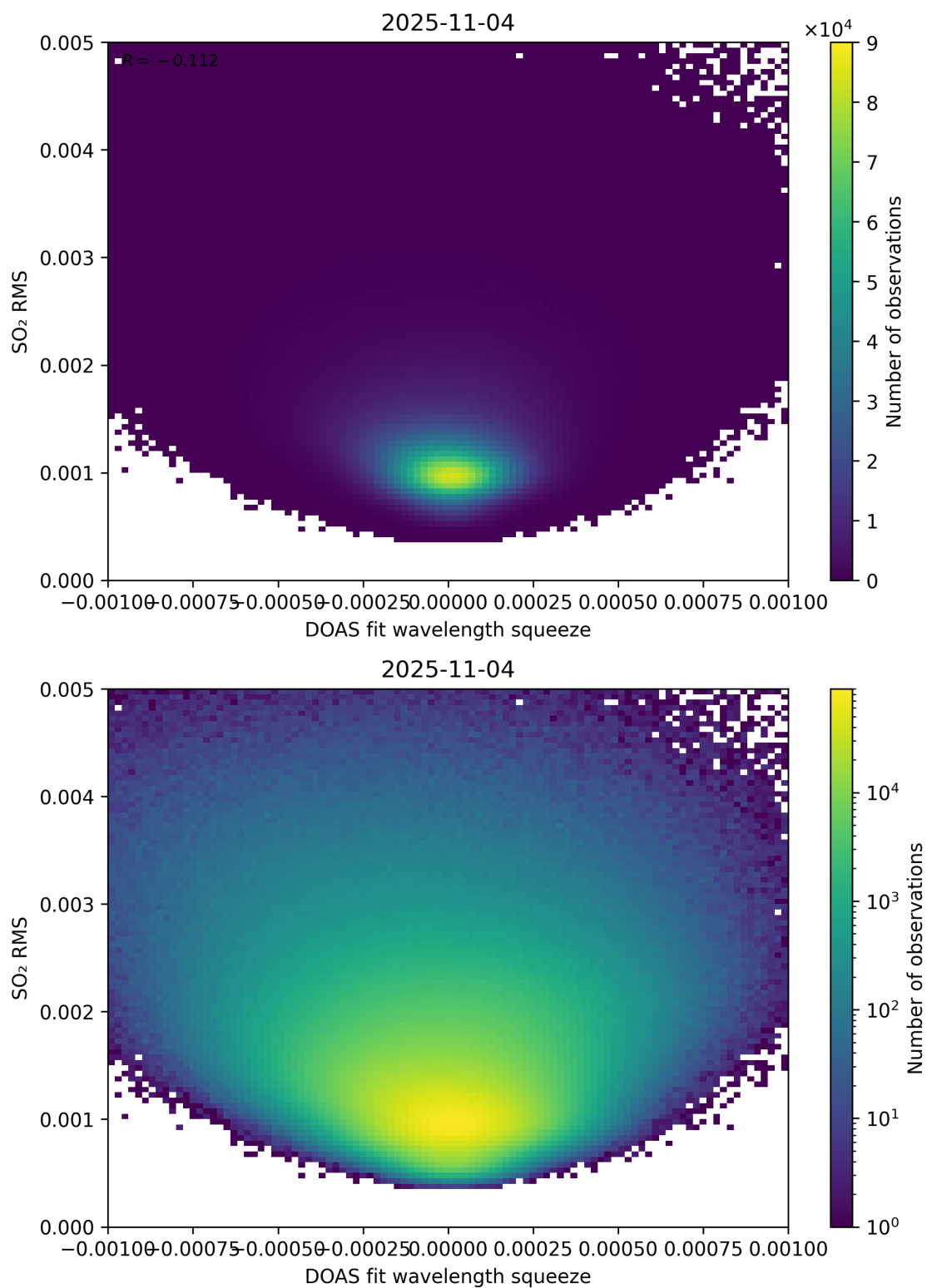
Figure 143: Scatter density plot of “DOAS fit wavelength squeeze” against “SO 2 RMS” for 2025-11-03 to 2025-11-05.
