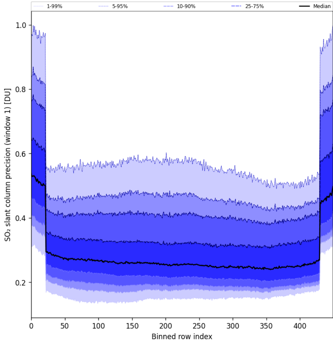
Figure 90: Along track statistics of “SO 2 slant column precision (window 1)” for 2025-11-03 to 2025-11-05
