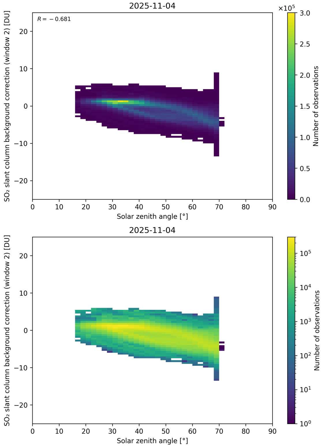
Figure 172: Scatter density plot of “Solar zenith angle” against “SO 2 slant column background correction (window 2)” for 2025-11-03 to 2025-11-05.
