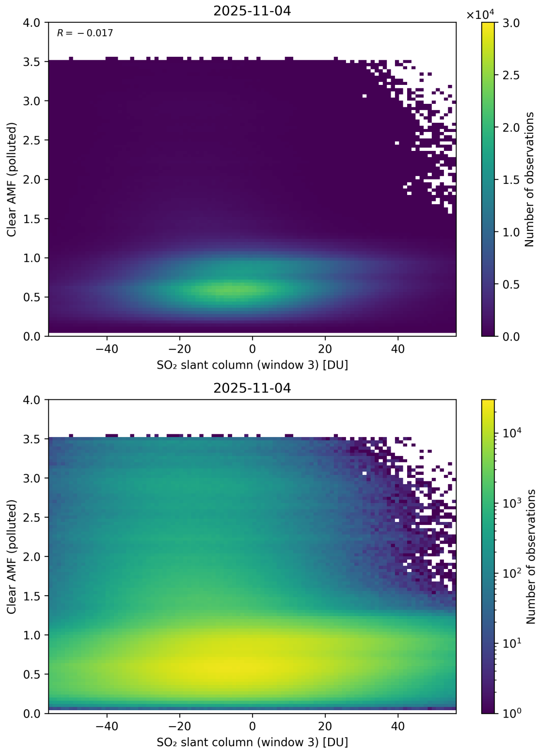
Figure 315: Scatter density plot of “SO 2 slant column (window 3)” against “Clear AMF (polluted)” for 2025-11-03 to 2025-11-05.
