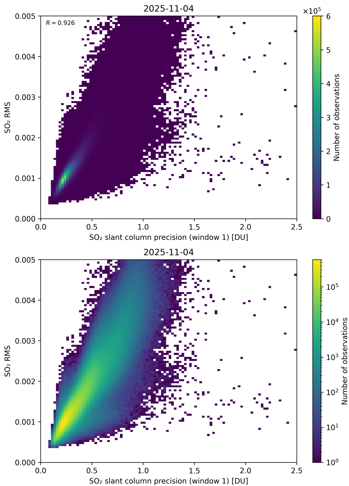
Figure 273: Scatter density plot of “SO 2 slant column precision (window 1)” against “SO 2 RMS” for 2025-11-03 to 2025-11-05.
