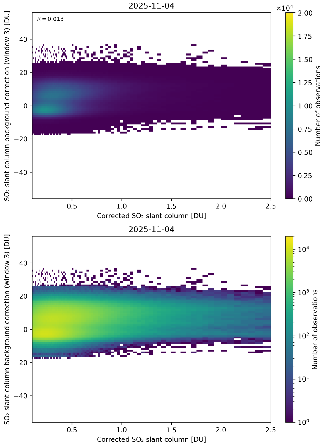
Figure 228: Scatter density plot of “Corrected SO 2 slant column” against “SO 2 slant column background correction (window 3)” for 2025-11-03 to 2025-11-05.
