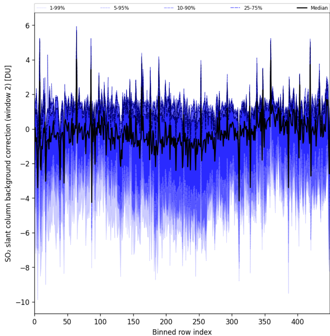
Figure 96: Along track statistics of “SO 2 slant column background correction (window 2)” for 2025-11-03 to 2025-11-05
