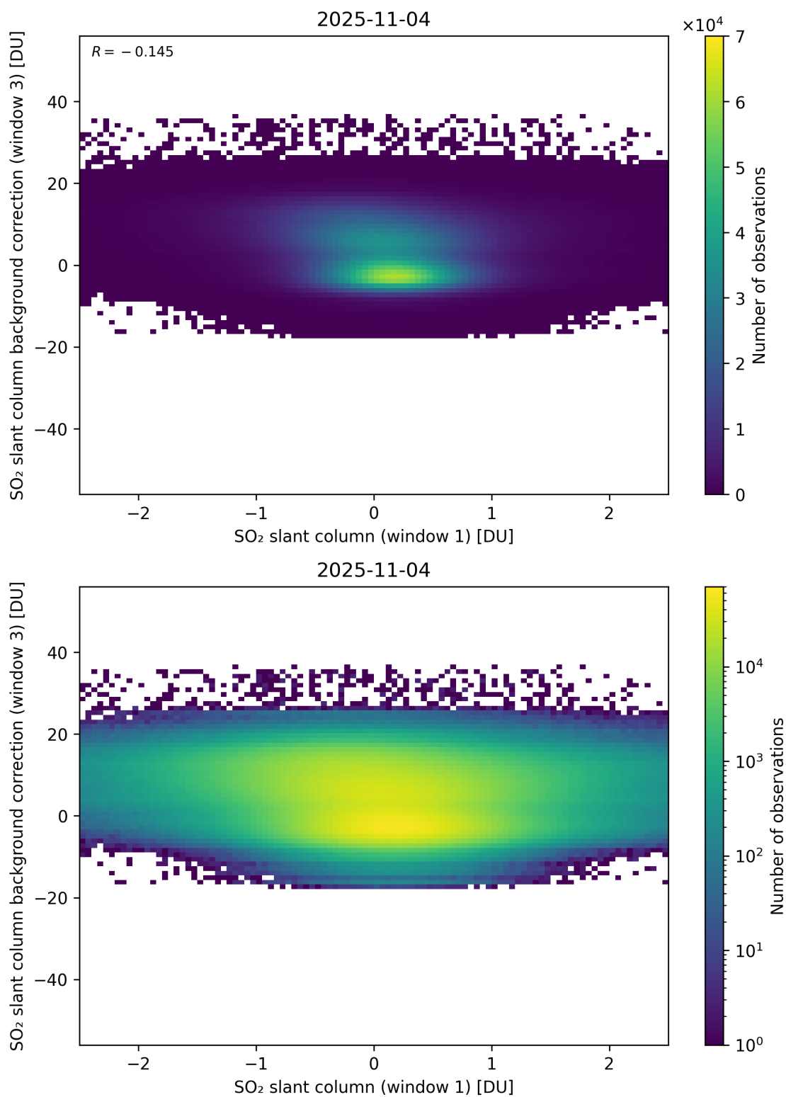
Figure 264: Scatter density plot of “SO 2 slant column (window 1)” against “SO 2 slant column background correction (window 3)” for 2025-11-03 to 2025-11-05.
