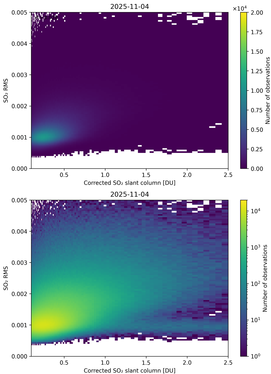
Figure 231: Scatter density plot of “Corrected SO 2 slant column” against “SO 2 RMS” for 2025-11-03 to 2025-11-05.
