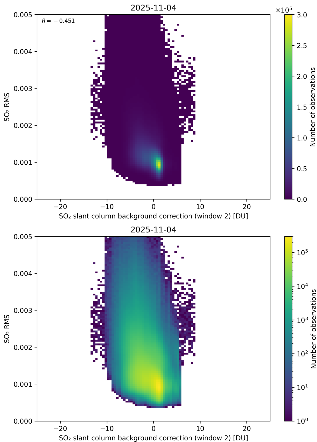
Figure 125: Scatter density plot of “SO 2 slant column background correction (window 2)” against “SO 2 RMS” for 2025-11-03 to 2025-11-05.
