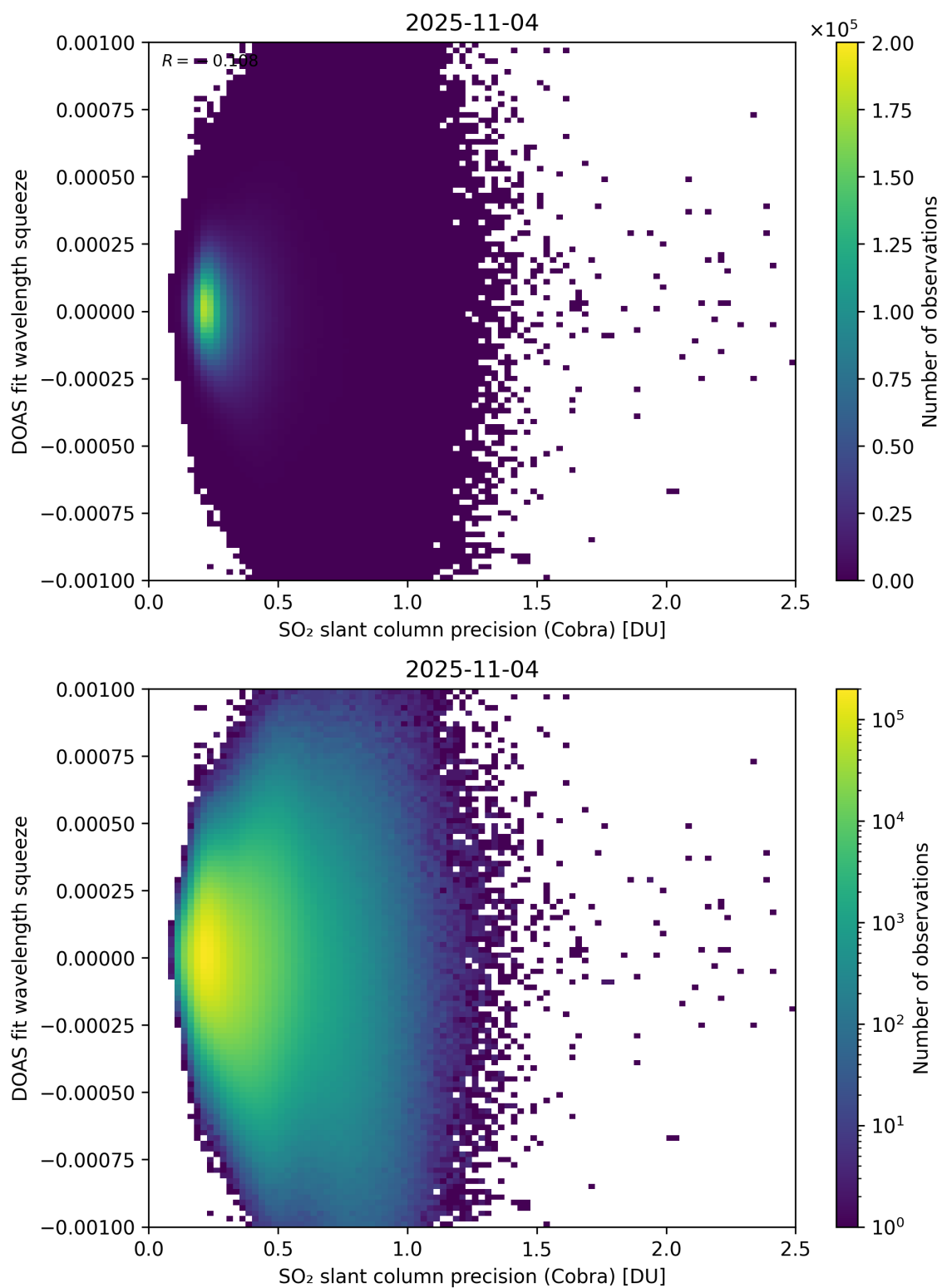
Figure 203: Scatter density plot of “SO 2 slant column precision (Cobra)” against “DOAS fit wavelength squeeze” for 2025-11-03 to 2025-11-05.
