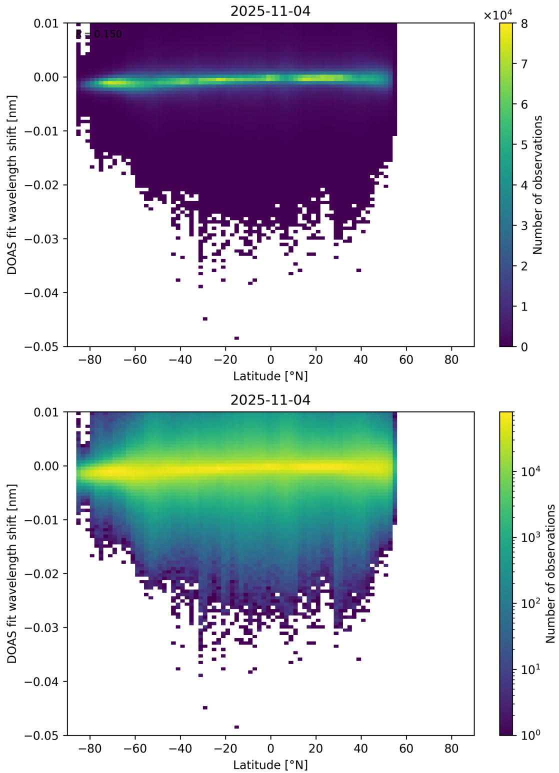
Figure 153: Scatter density plot of “Latitude” against “DOAS fit wavelength shift” for 2025-11-03 to 2025-11-05.
