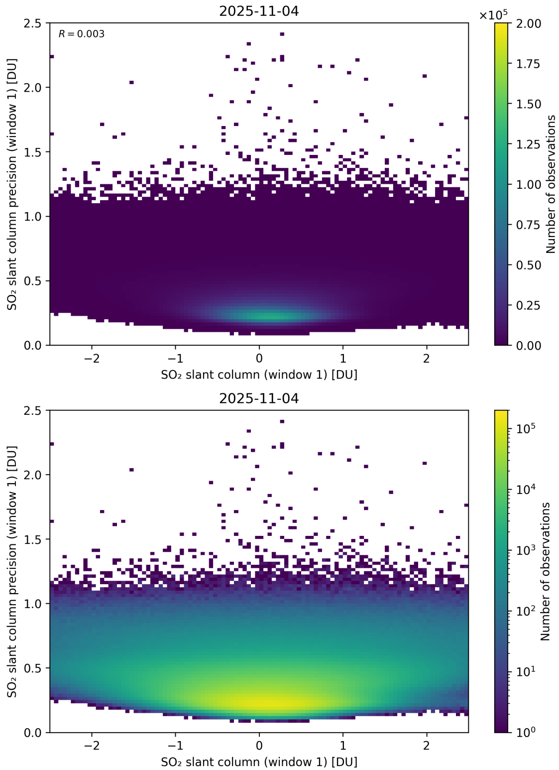
Figure 285: Scatter density plot of “SO 2 slant column (window 1)” against “SO 2 slant column precision (window 1)” for 2025-11-03 to 2025-11-05.
