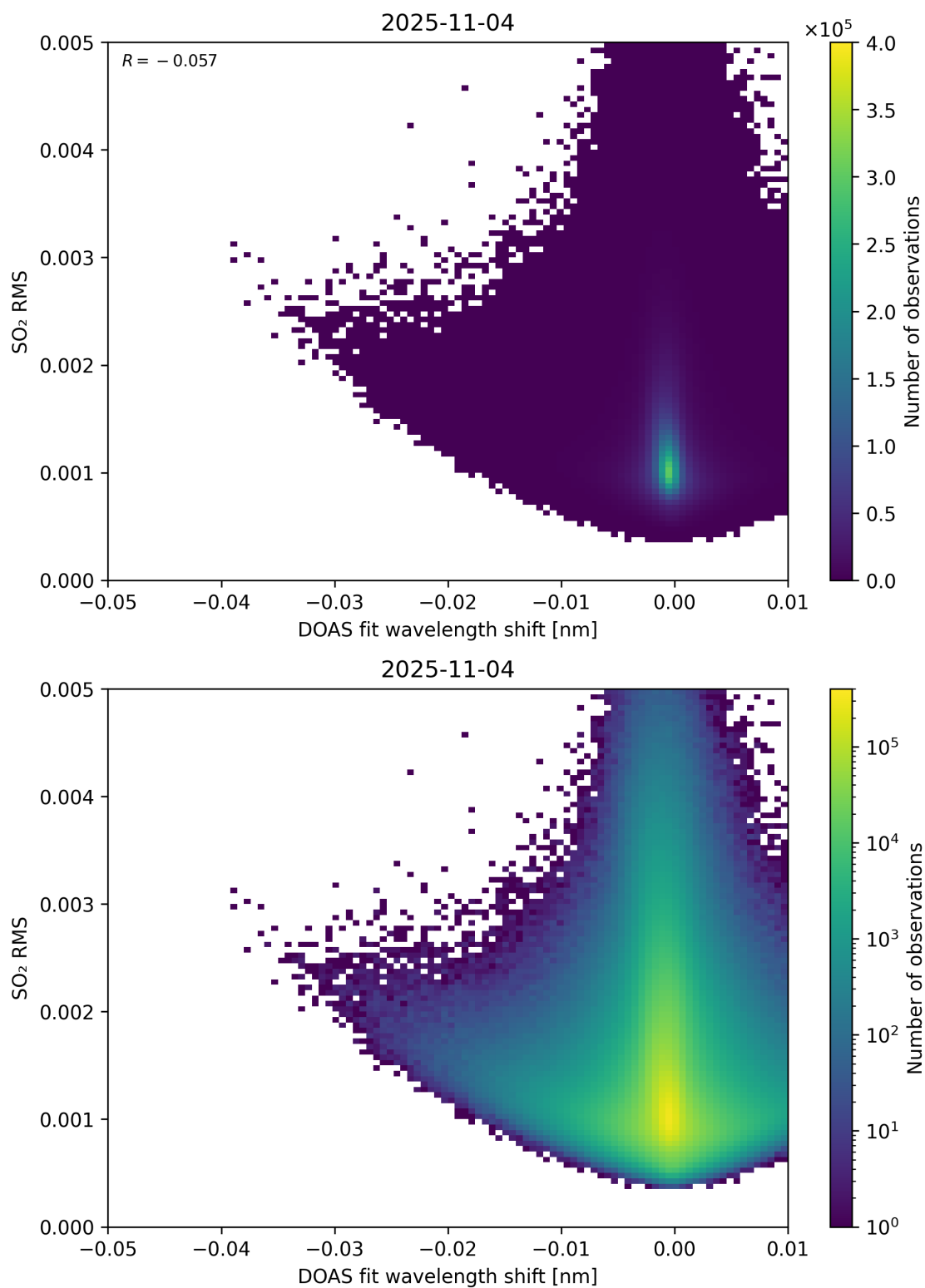
Figure 139: Scatter density plot of “DOAS fit wavelength shift” against “SO 2 RMS” for 2025-11-03 to 2025-11-05.
