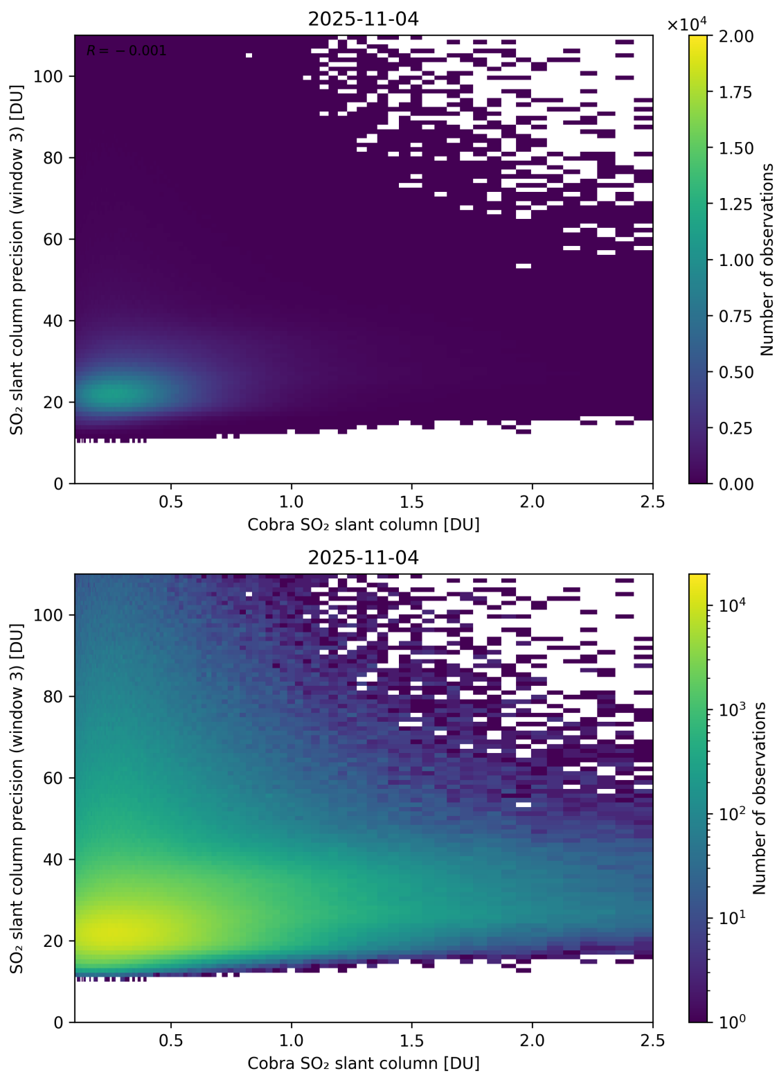
Figure 223: Scatter density plot of “Cobra SO 2 slant column” against “SO 2 slant column precision (window 3)” for 2025-11-03 to 2025-11-05.
