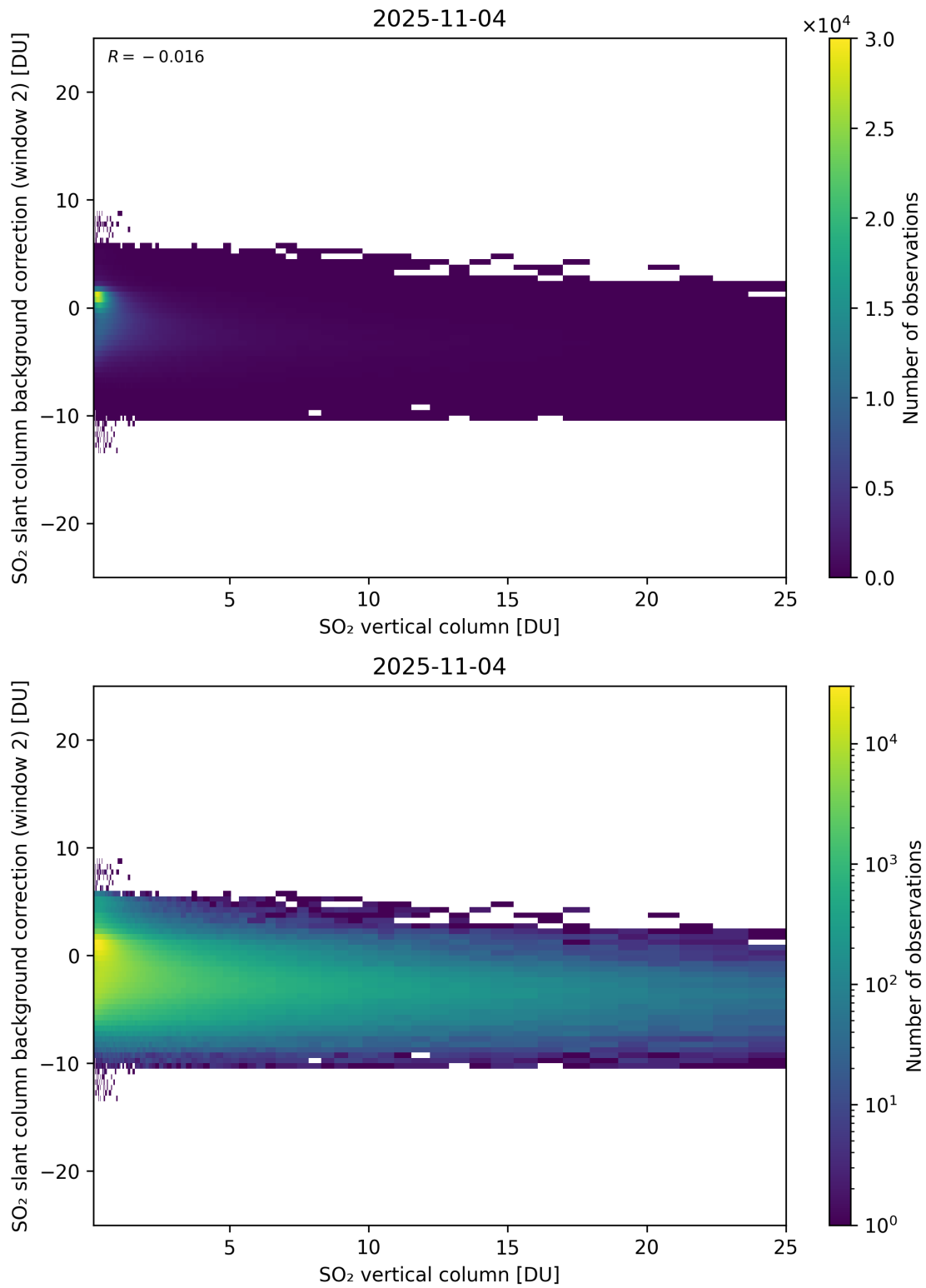
Figure 324: Scatter density plot of “SO 2 vertical column” against “SO 2 slant column background correction (window 2)” for 2025-11-03 to 2025-11-05.
