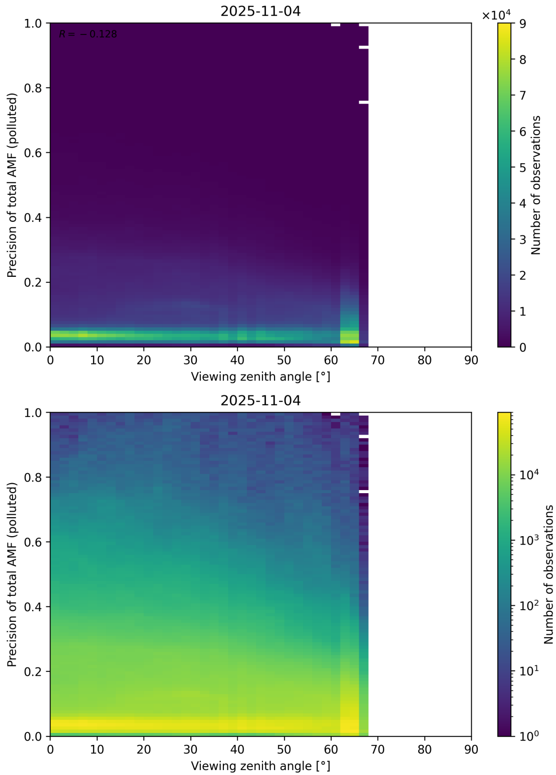
Figure 382: Scatter density plot of “Viewing zenith angle” against “Precision of total AMF (polluted)” for 2025-11-03 to 2025-11-05.
