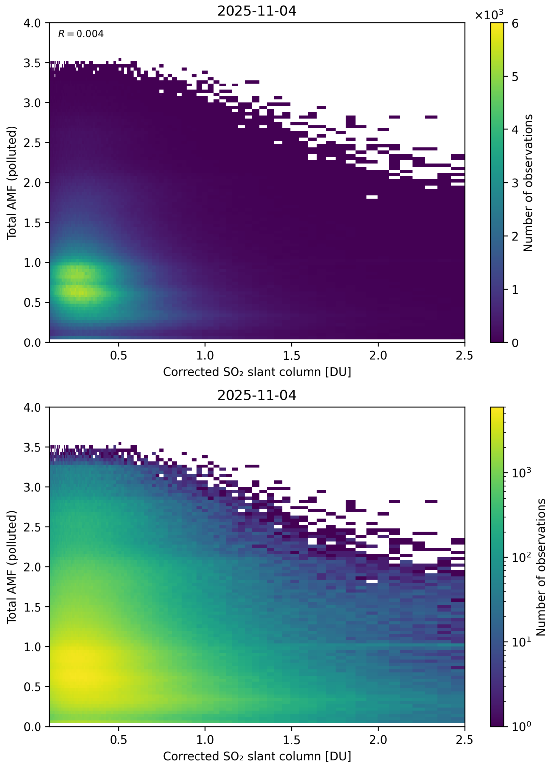
Figure 242: Scatter density plot of “Corrected SO 2 slant column” against “Total AMF (polluted)” for 2025-11-03 to 2025-11-05.
