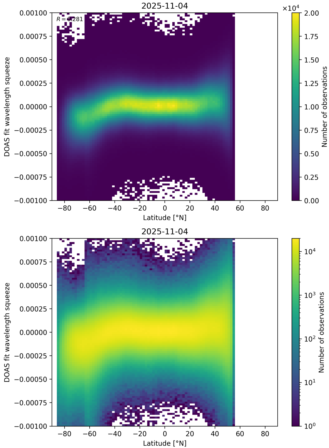
Figure 154: Scatter density plot of “Latitude” against “DOAS fit wavelength squeeze” for 2025-11-03 to 2025-11-05.
