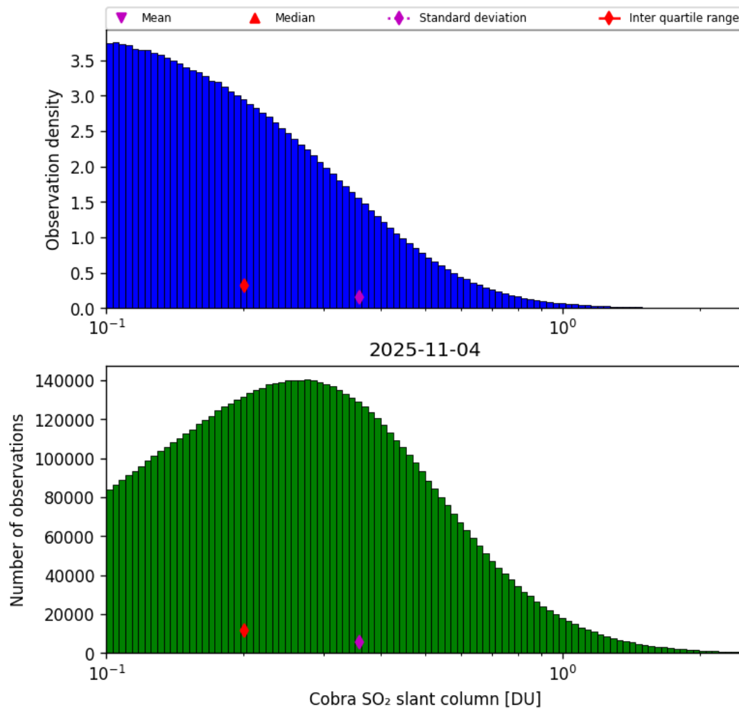
Figure 61: Histogram of “Cobra SO 2 slant column” for 2025-11-03 to 2025-11-05
