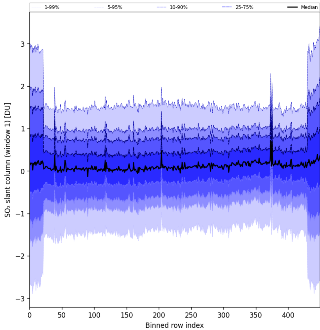
Figure 89: Along track statistics of “SO 2 slant column (window 1)” for 2025-11-03 to 2025-11-05
