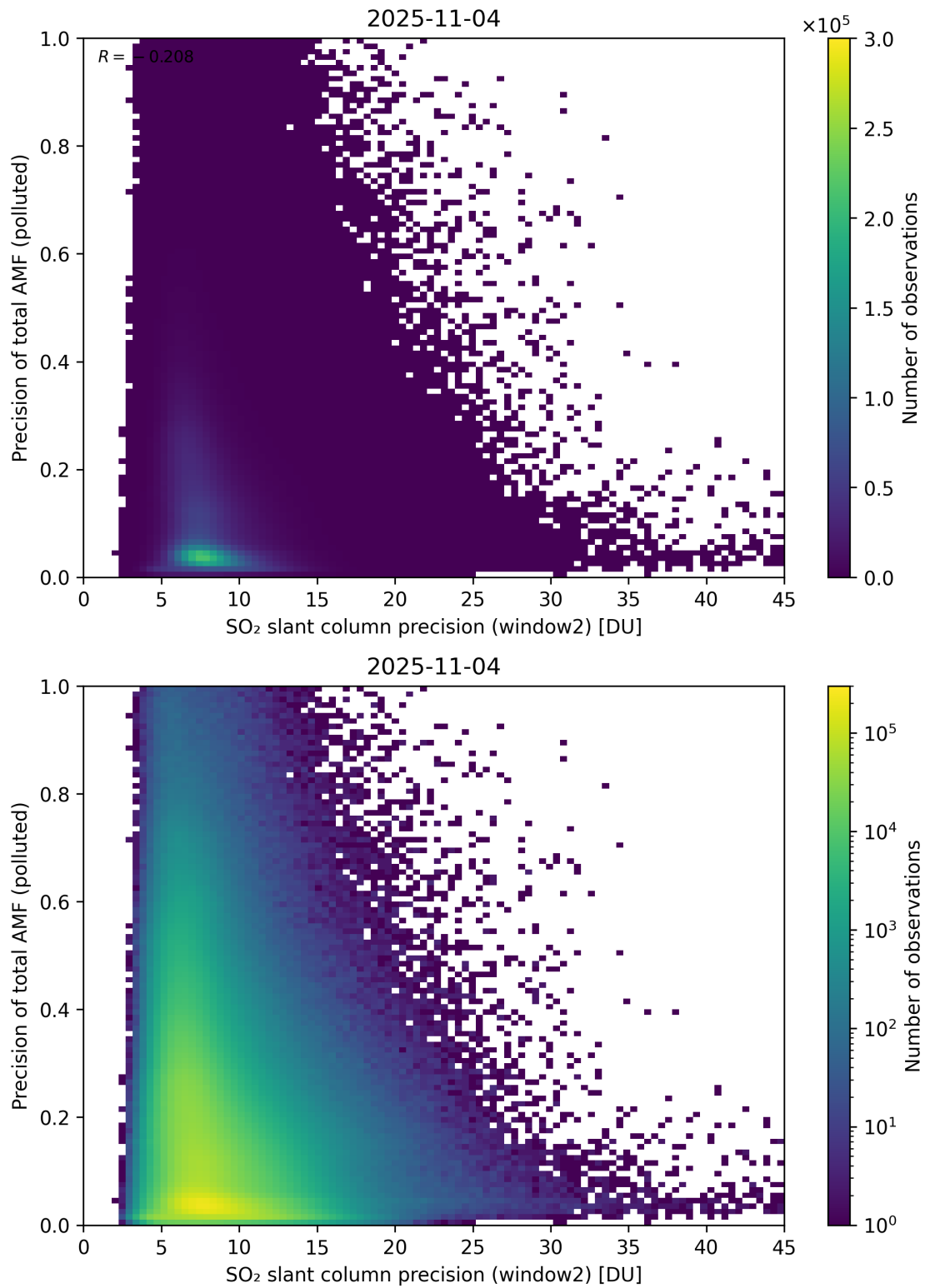
Figure 302: Scatter density plot of “SO 2 slant column precision (window2)” against “Precision of total AMF (polluted)” for 2025-11-03 to 2025-11-05.
