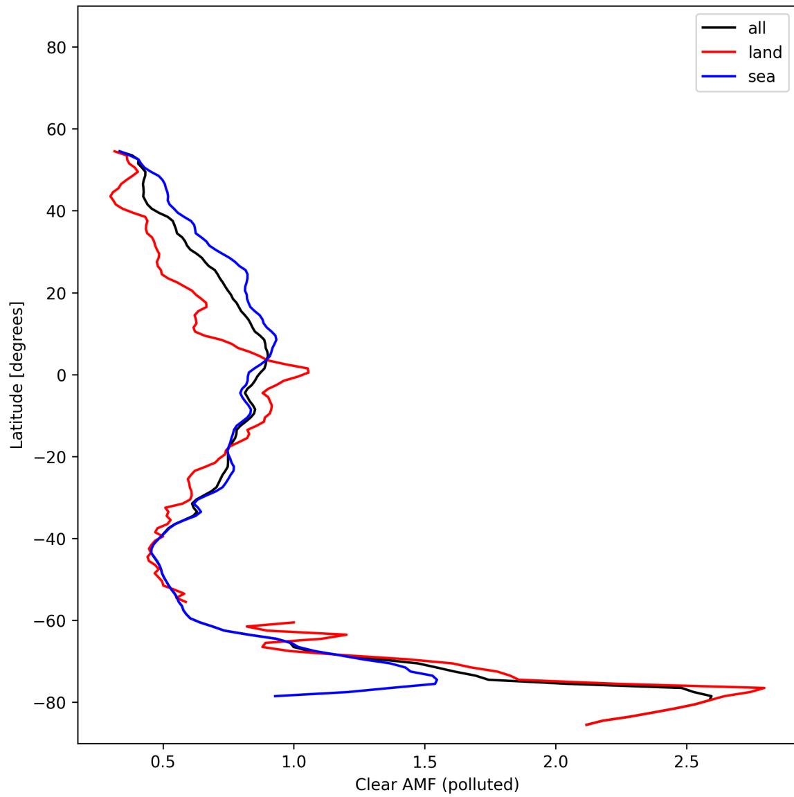
Figure 55: Zonal average of “Clear AMF (polluted)” for 2025-11-03 to 2025-11-05.
