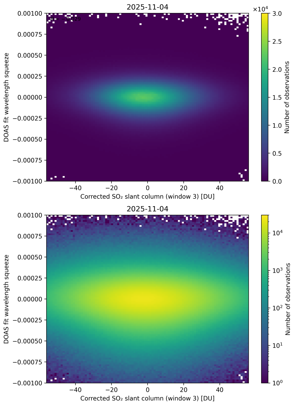
Figure 257: Scatter density plot of “Corrected SO 2 slant column (window 3)” against “DOAS fit wavelength squeeze” for 2025-11-03 to 2025-11-05.
