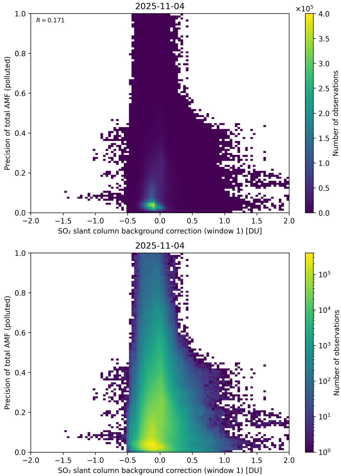
Figure 121: Scatter density plot of “SO 2 slant column background correction (window 1)” against “Precision of total AMF (polluted)” for 2025-11-03 to 2025-11-05.
