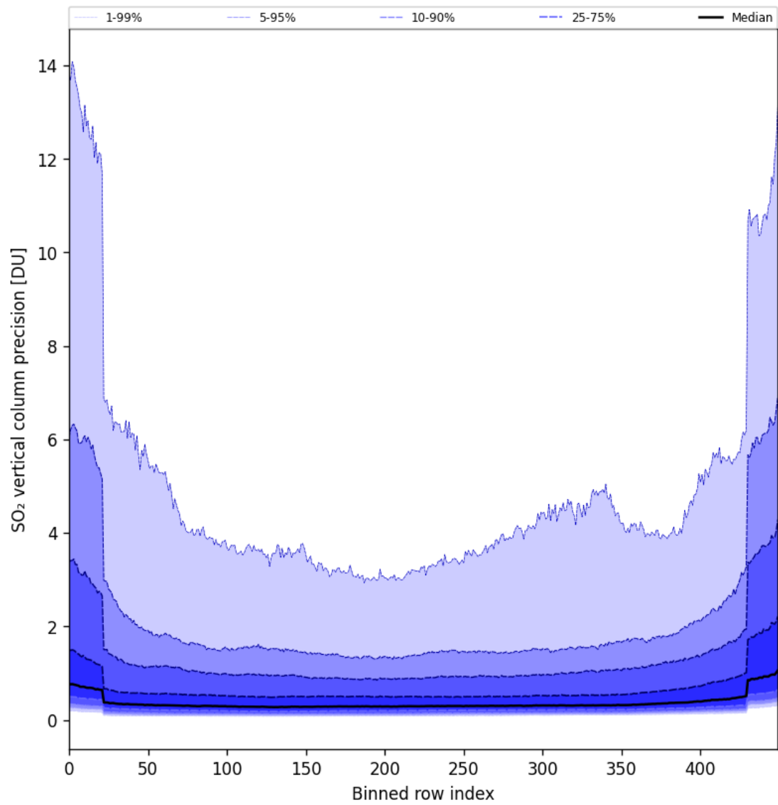
Figure 85: Along track statistics of “SO 2 vertical column precision” for 2025-11-03 to 2025-11-05
