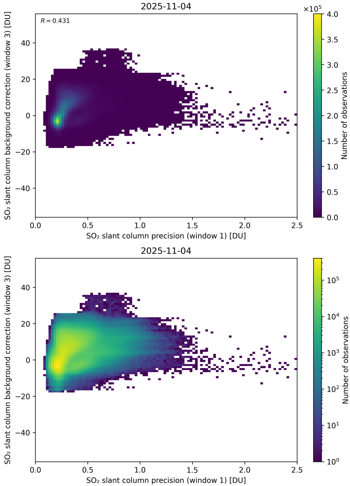
Figure 270: Scatter density plot of “SO 2 slant column precision (window 1)” against “SO 2 slant column background correction (window 3)” for 2025-11-03 to 2025-11-05.
