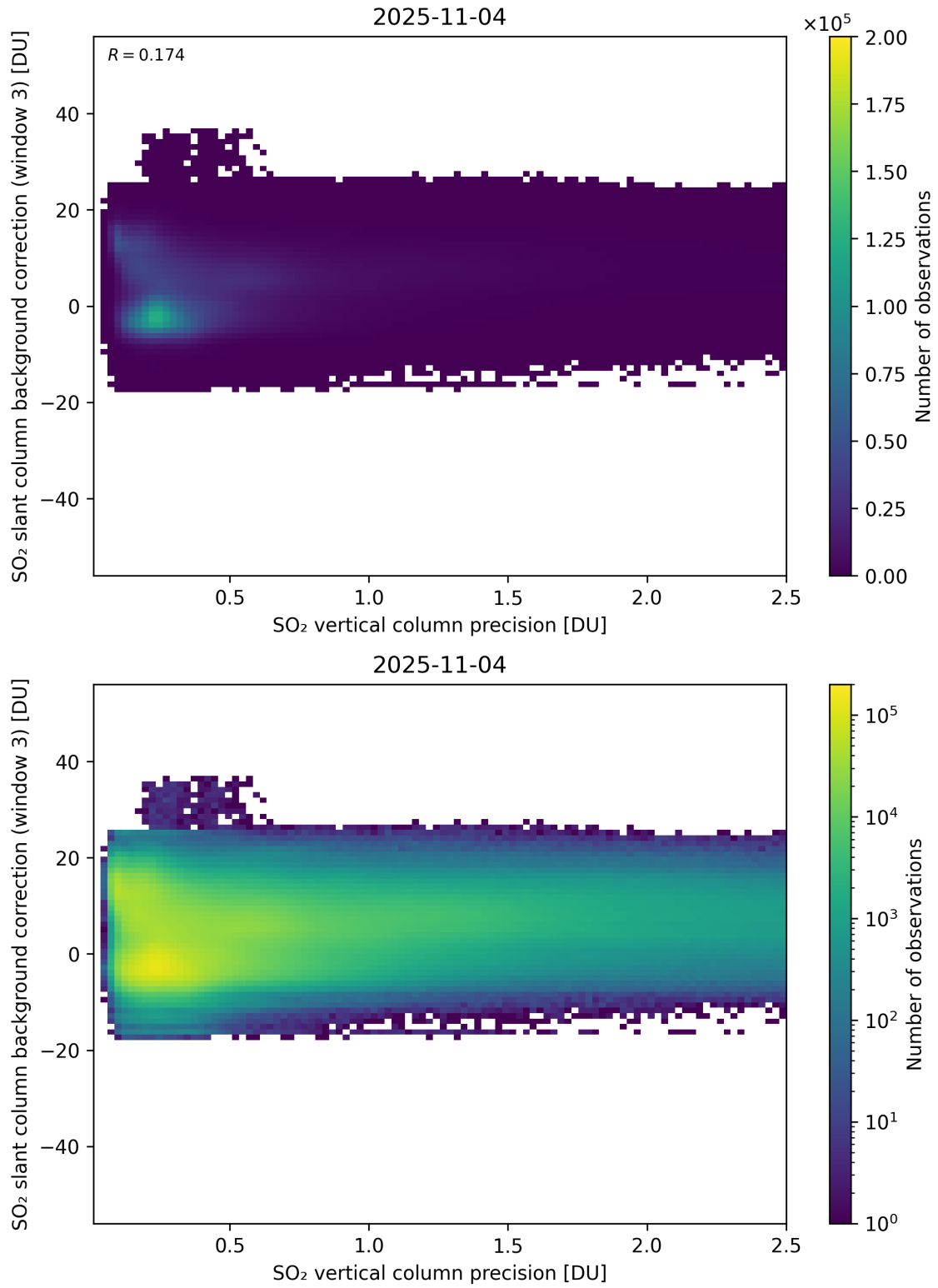
Figure 331: Scatter density plot of “SO 2 vertical column precision” against “SO 2 slant column background correction (window 3)” for 2025-11-03 to 2025-11-05.
