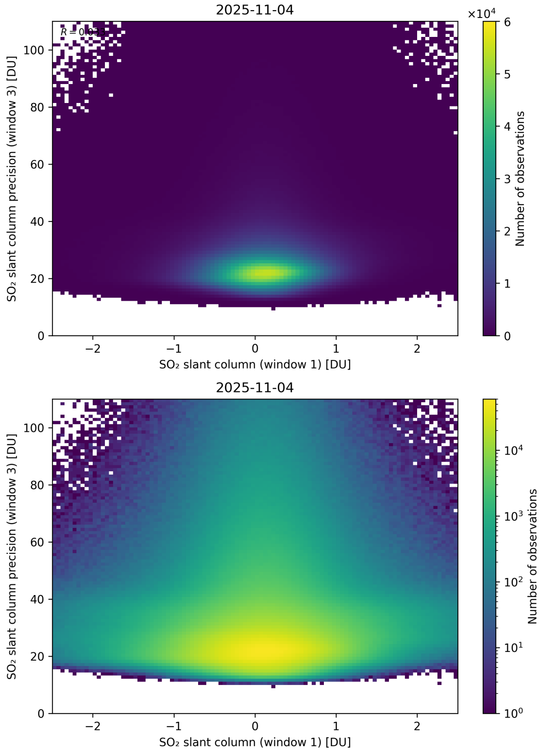
Figure 288: Scatter density plot of “SO 2 slant column (window 1)” against “SO 2 slant column precision (window 3)” for 2025-11-03 to 2025-11-05.
