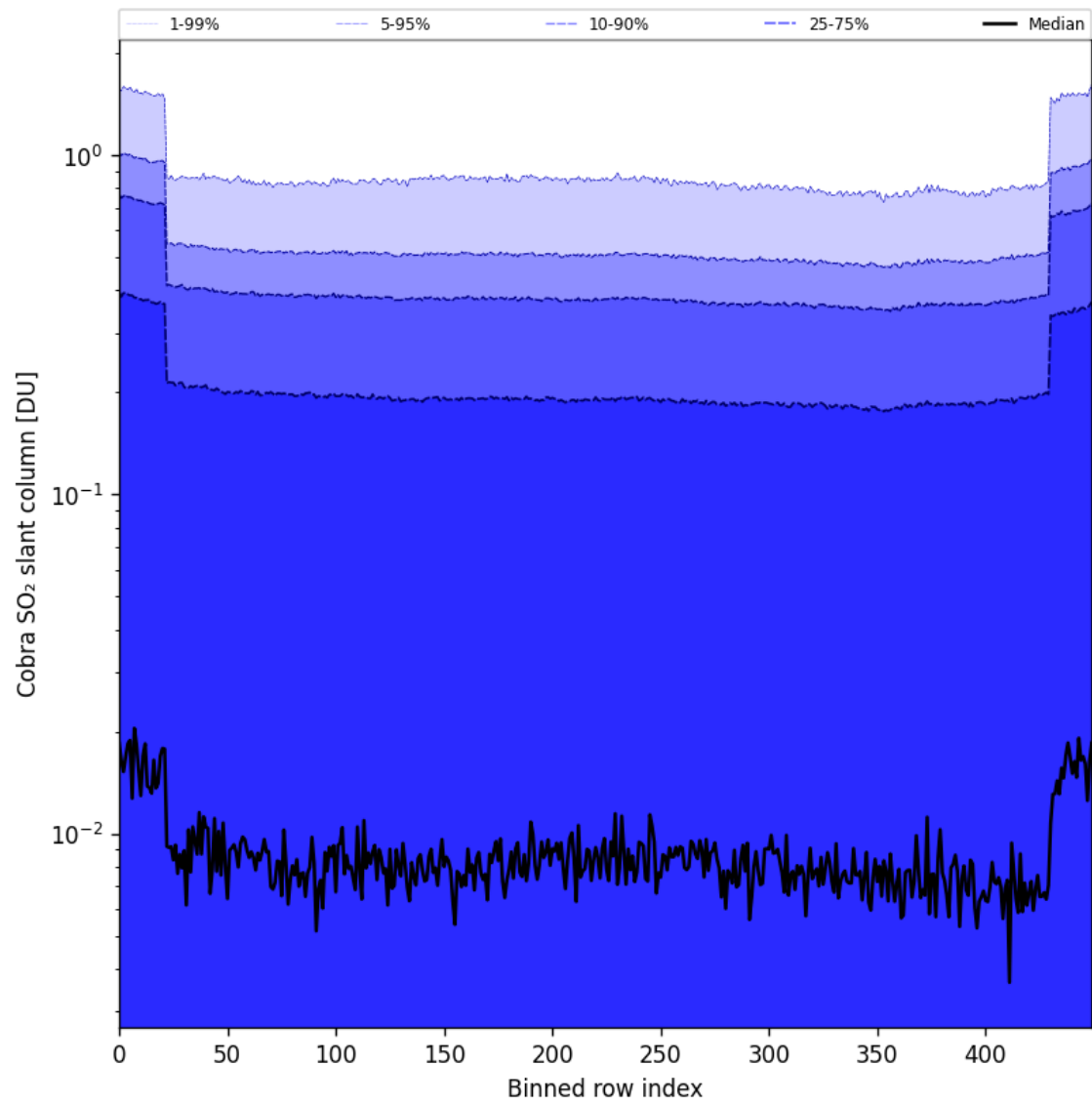
Figure 87: Along track statistics of “Cobra SO 2 slant column” for 2025-11-03 to 2025-11-05
