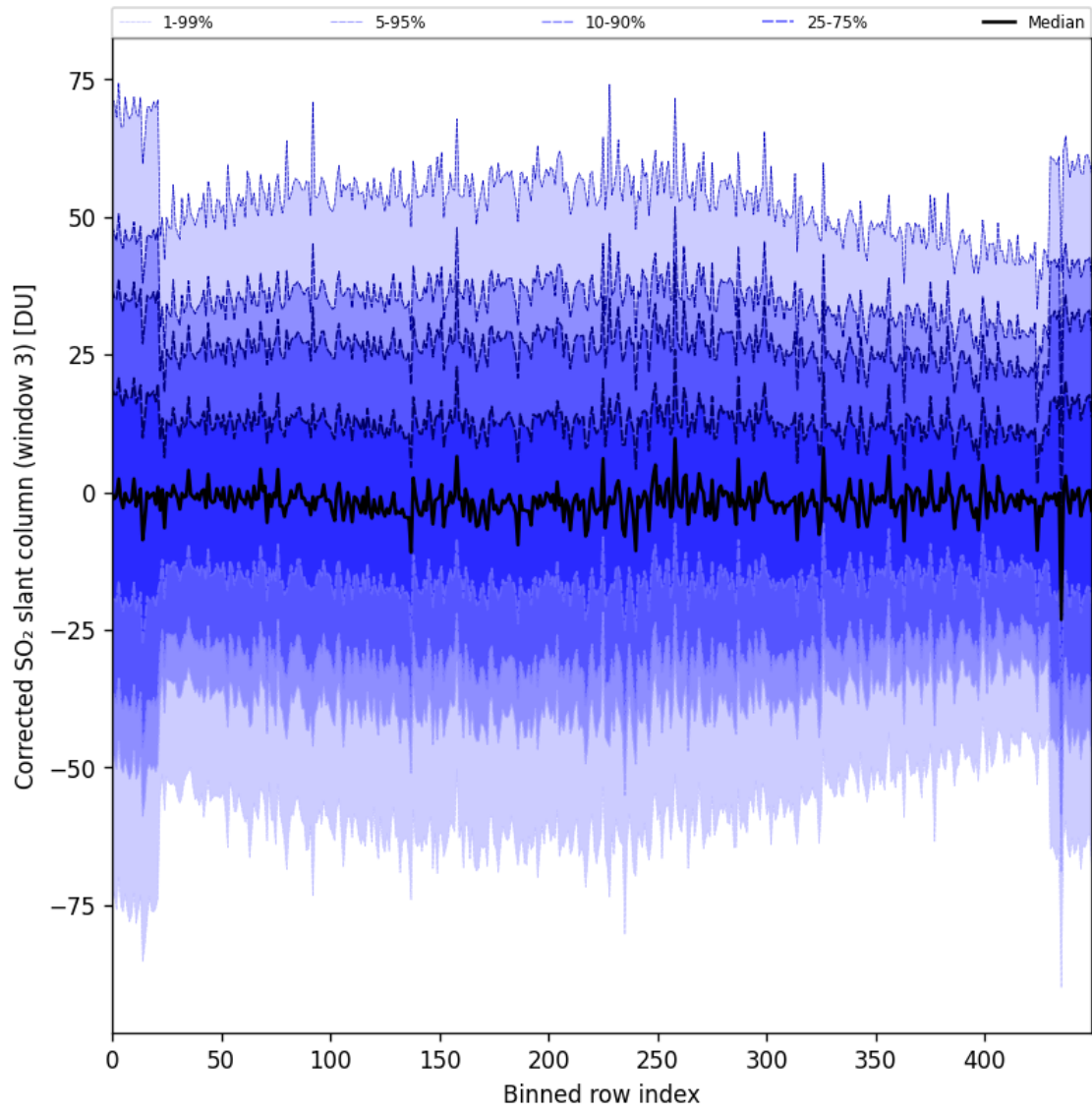
Figure 99: Along track statistics of “Corrected SO 2 slant column (window 3)” for 2025-11-03 to 2025-11-05
