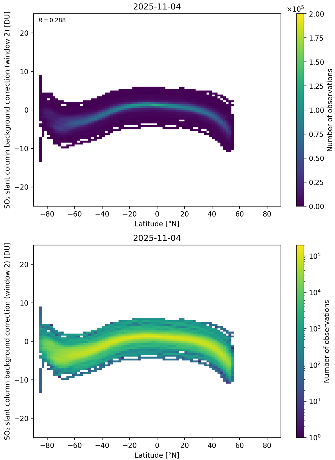
Figure 151: Scatter density plot of “Latitude” against “SO 2 slant column background correction (window 2)” for 2025-11-03 to 2025-11-05.
