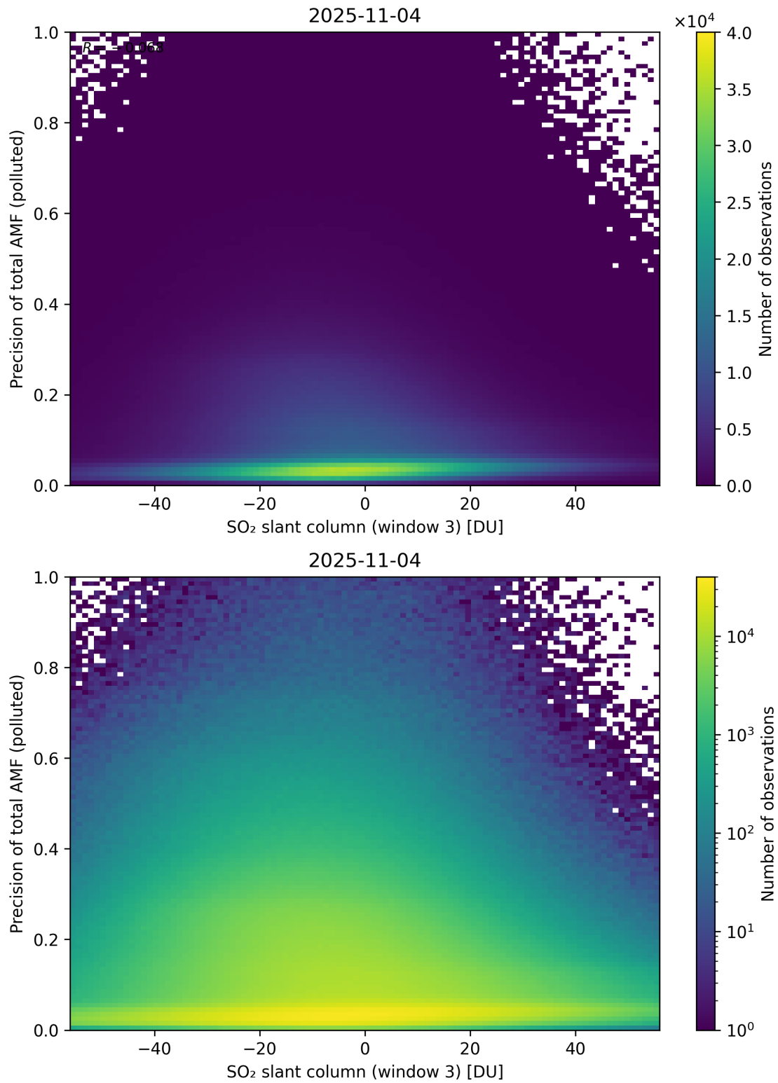
Figure 319: Scatter density plot of “SO 2 slant column (window 3)” against “Precision of total AMF (polluted)” for 2025-11-03 to 2025-11-05.
