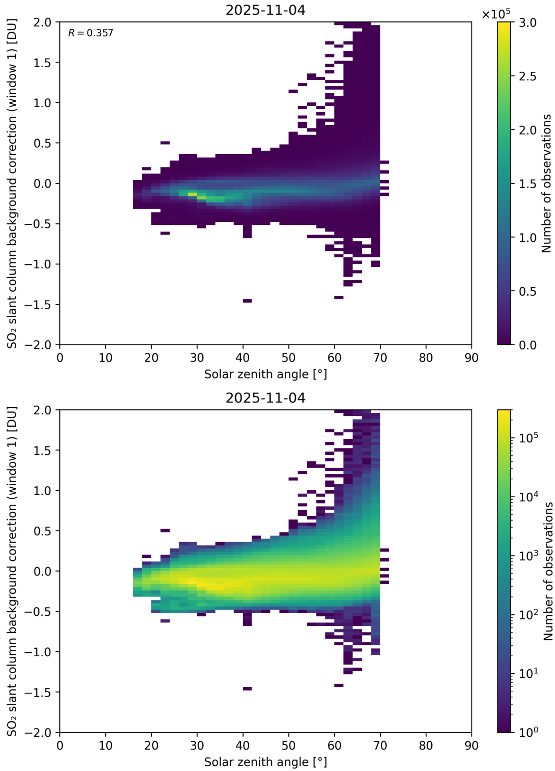
Figure 171: Scatter density plot of “Solar zenith angle” against “SO 2 slant column background correction (window 1)” for 2025-11-03 to 2025-11-05.
