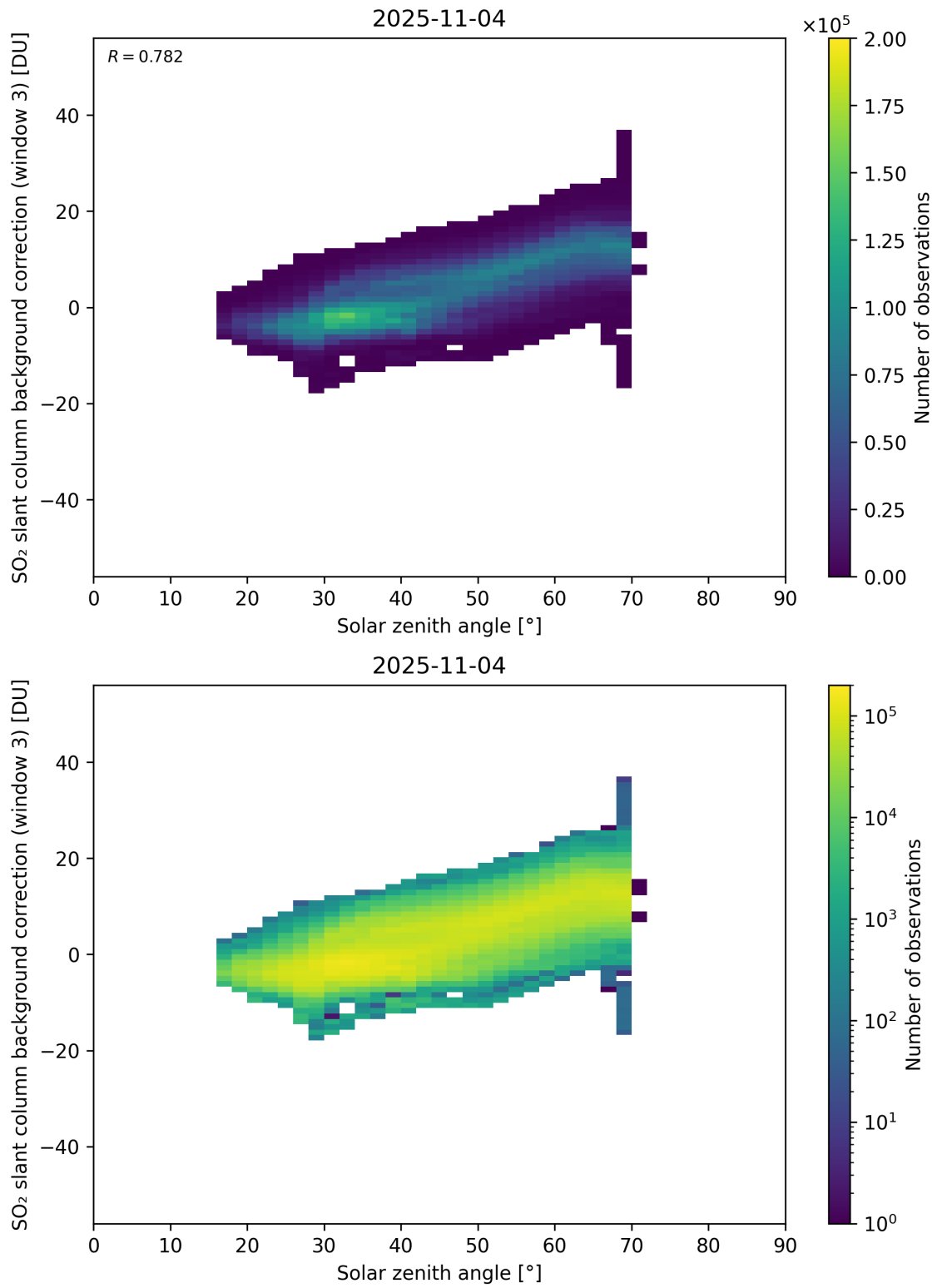
Figure 173: Scatter density plot of “Solar zenith angle” against “SO 2 slant column background correction (window 3)” for 2025-11-03 to 2025-11-05.
