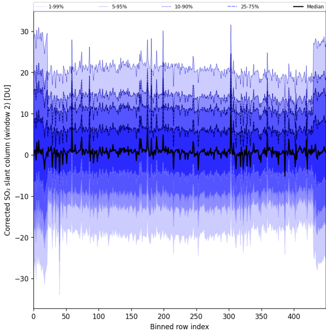
Figure 95: Along track statistics of “Corrected SO 2 slant column (window 2)” for 2025-11-03 to 2025-11-05
