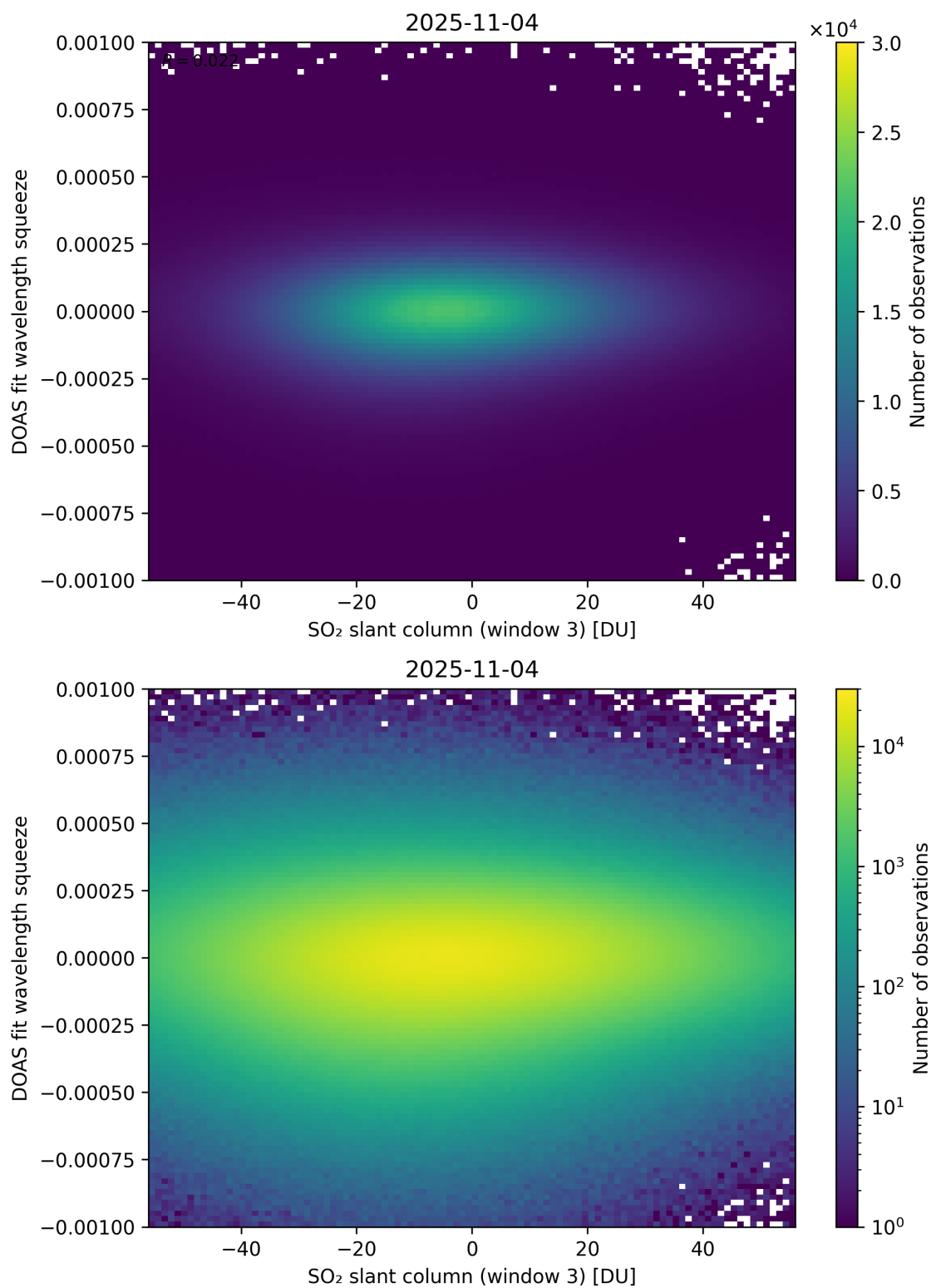
Figure 305: Scatter density plot of “SO 2 slant column (window 3)” against “DOAS fit wavelength squeeze” for 2025-11-03 to 2025-11-05.
