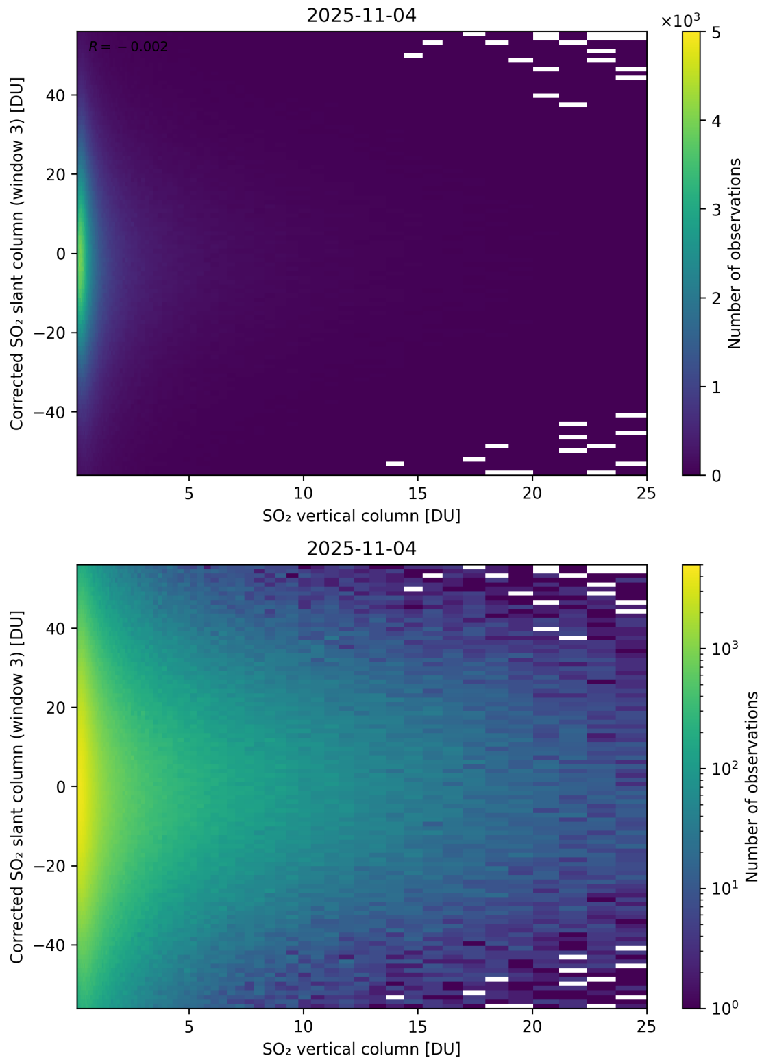
Figure 353: Scatter density plot of “SO 2 vertical column” against “Corrected SO 2 slant column (window 3)” for 2025-11-03 to 2025-11-05.
