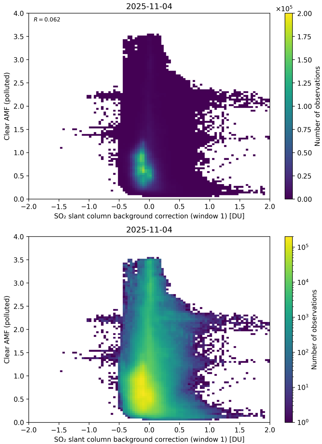
Figure 114: Scatter density plot of “SO 2 slant column background correction (window 1)” against “Clear AMF (polluted)” for 2025-11-03 to 2025-11-05.
