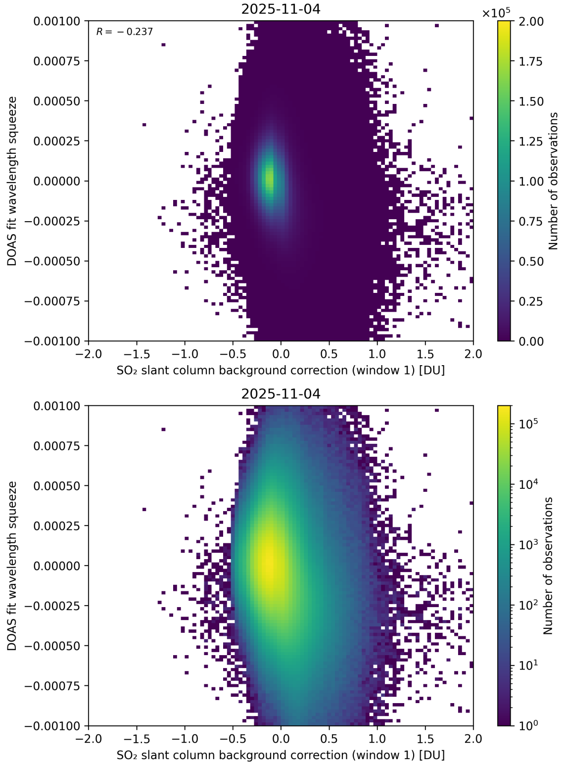
Figure 112: Scatter density plot of “SO 2 slant column background correction (window 1)” against “DOAS fit wavelength squeeze” for 2025-11-03 to 2025-11-05.
