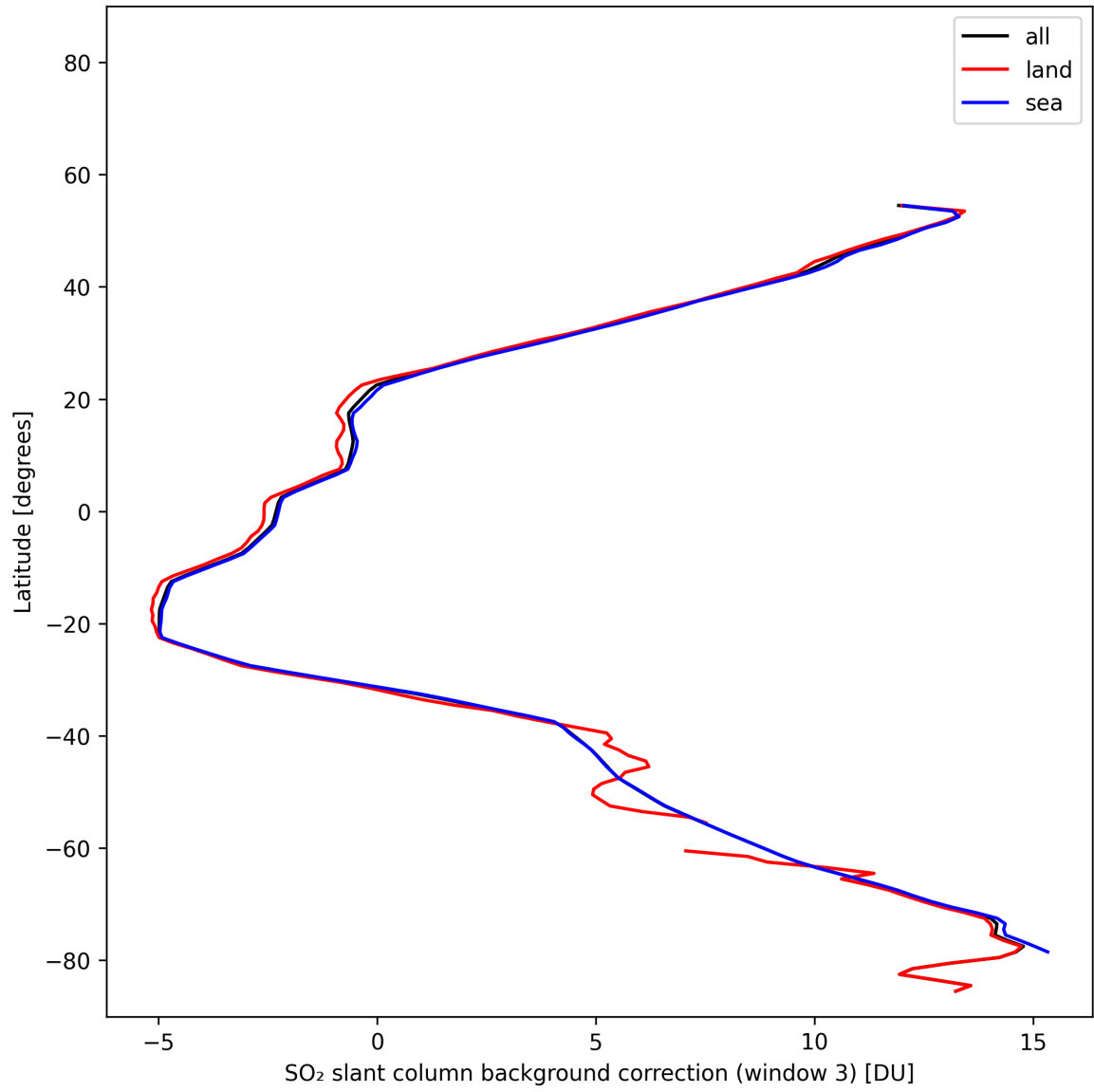
Figure 48: Zonal average of “SO 2 slant column background correction (window 3)” for 2025-11-03 to 2025-11-05.
