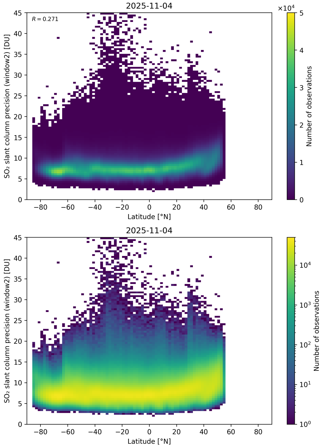
Figure 164: Scatter density plot of “Latitude” against “SO 2 slant column precision (window2)” for 2025-11-03 to 2025-11-05.
