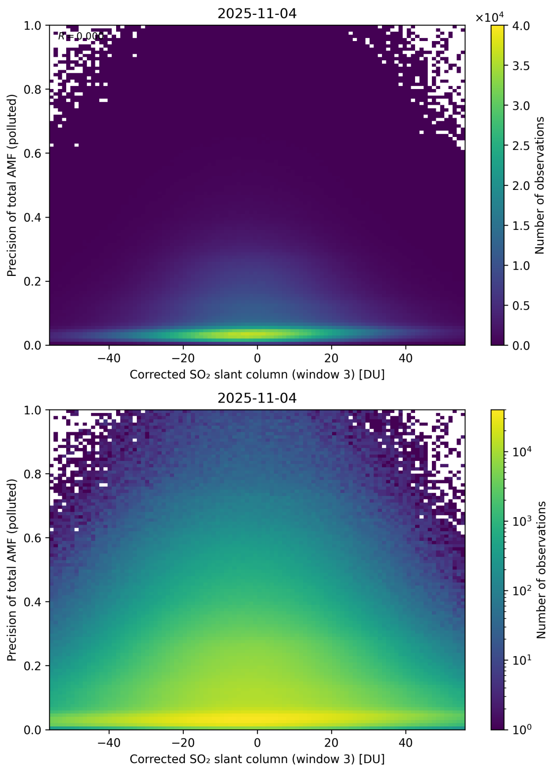
Figure 261: Scatter density plot of “Corrected SO 2 slant column (window 3)” against “Precision of total AMF (polluted)” for 2025-11-03 to 2025-11-05.
