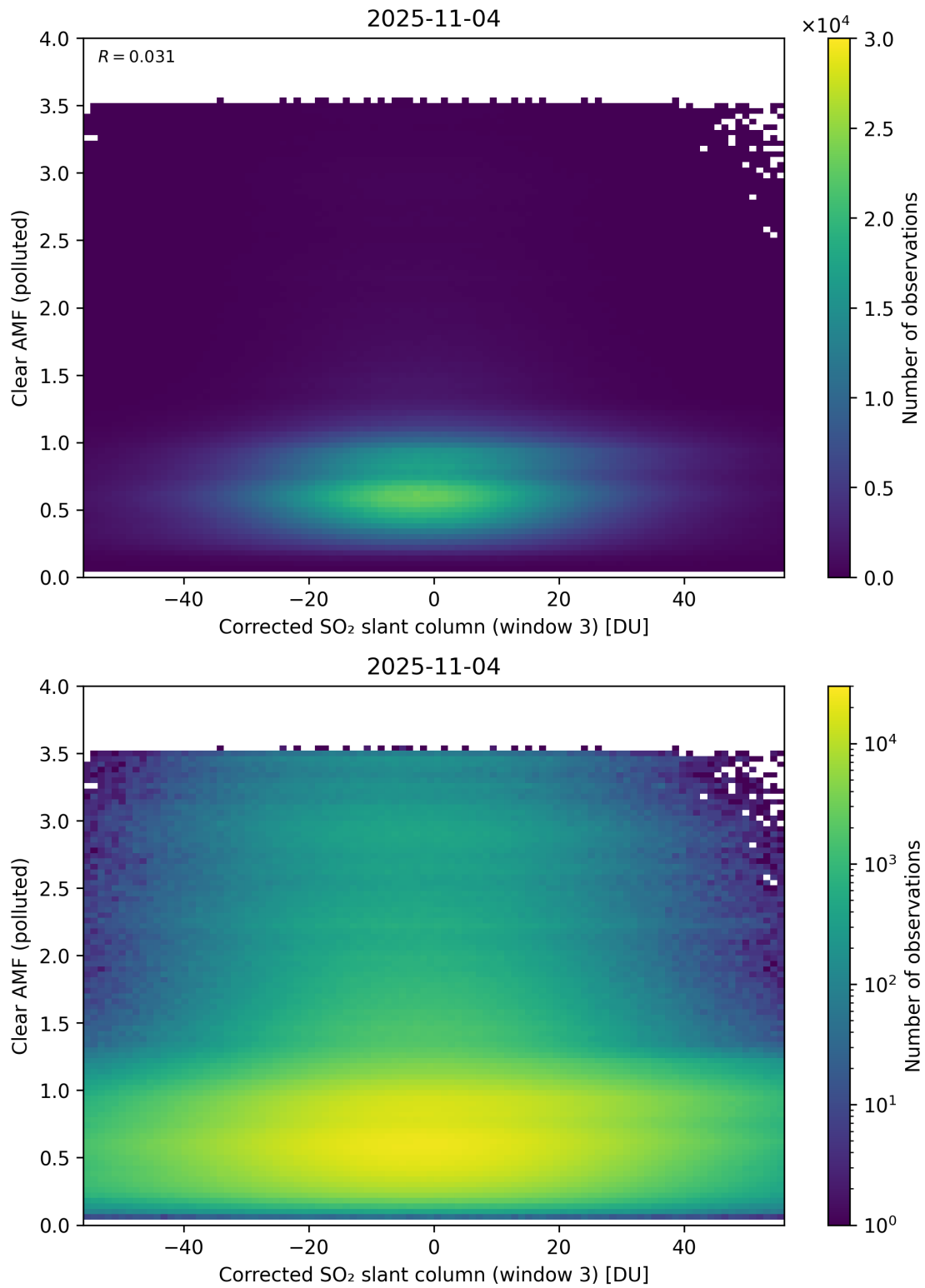
Figure 259: Scatter density plot of “Corrected SO 2 slant column (window 3)” against “Clear AMF (polluted)” for 2025-11-03 to 2025-11-05.
