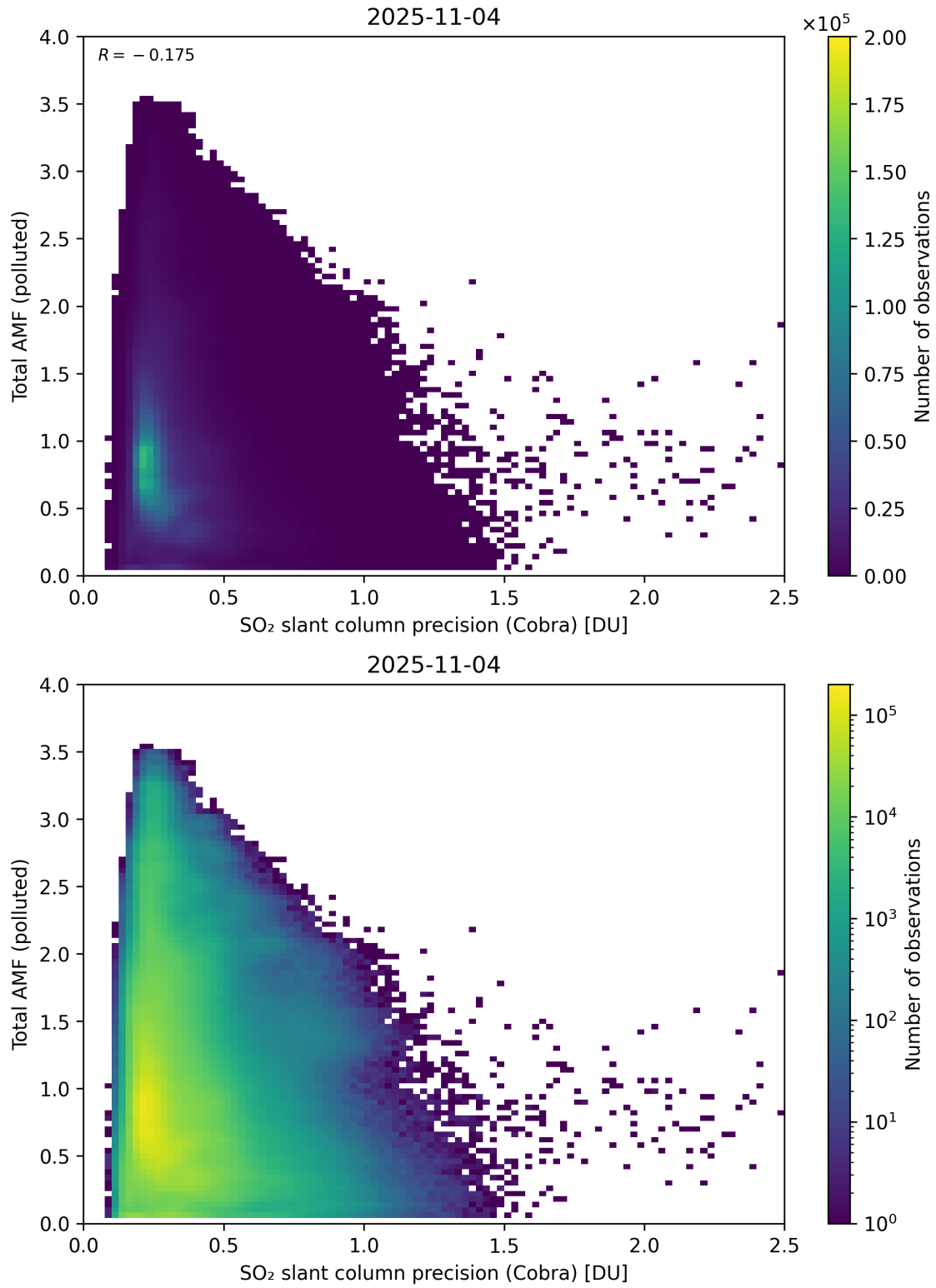
Figure 213: Scatter density plot of “SO 2 slant column precision (Cobra)” against “Total AMF (polluted)” for 2025-11-03 to 2025-11-05.
