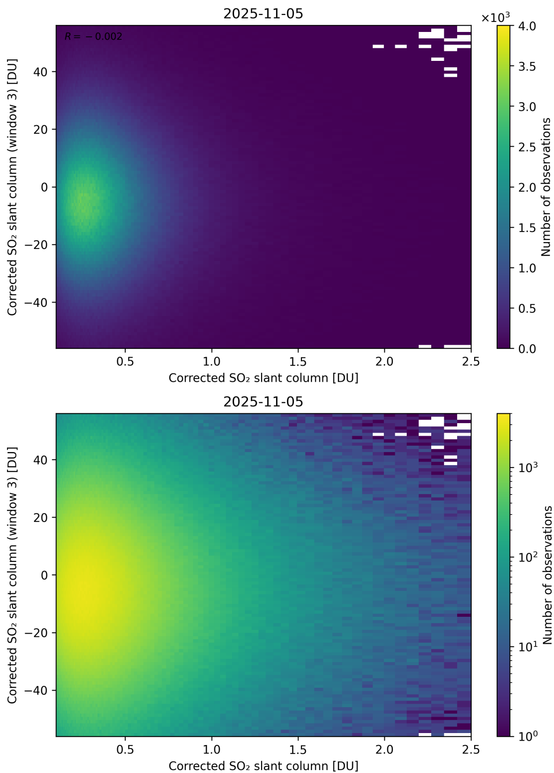
Figure 236: Scatter density plot of “Corrected SO 2 slant column” against “Corrected SO 2 slant column (window 3)” for 2025-11-04 to 2025-11-06.
