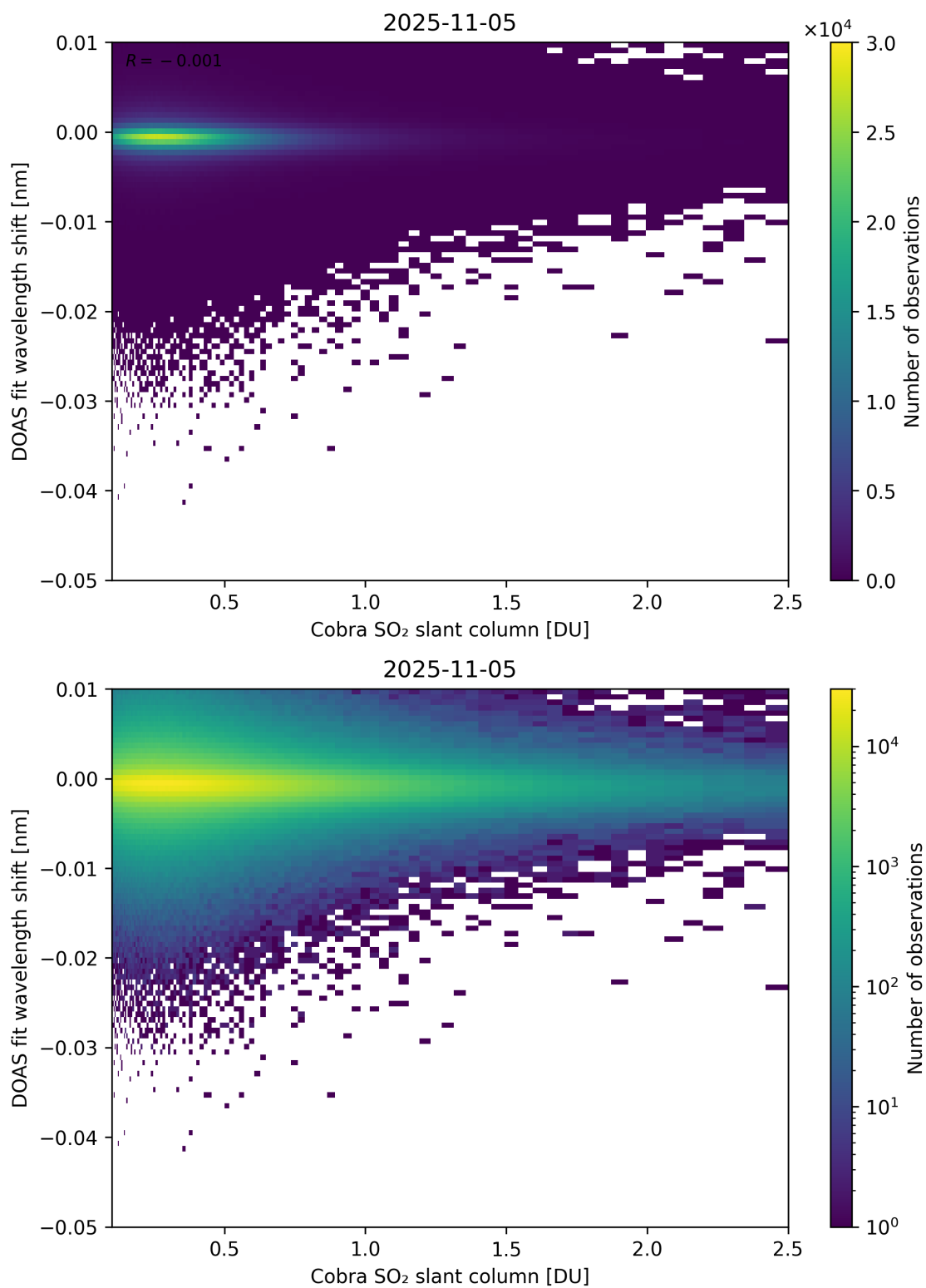
Figure 196: Scatter density plot of “Cobra SO 2 slant column” against “DOAS fit wavelength shift” for 2025-11-04 to 2025-11-06.
