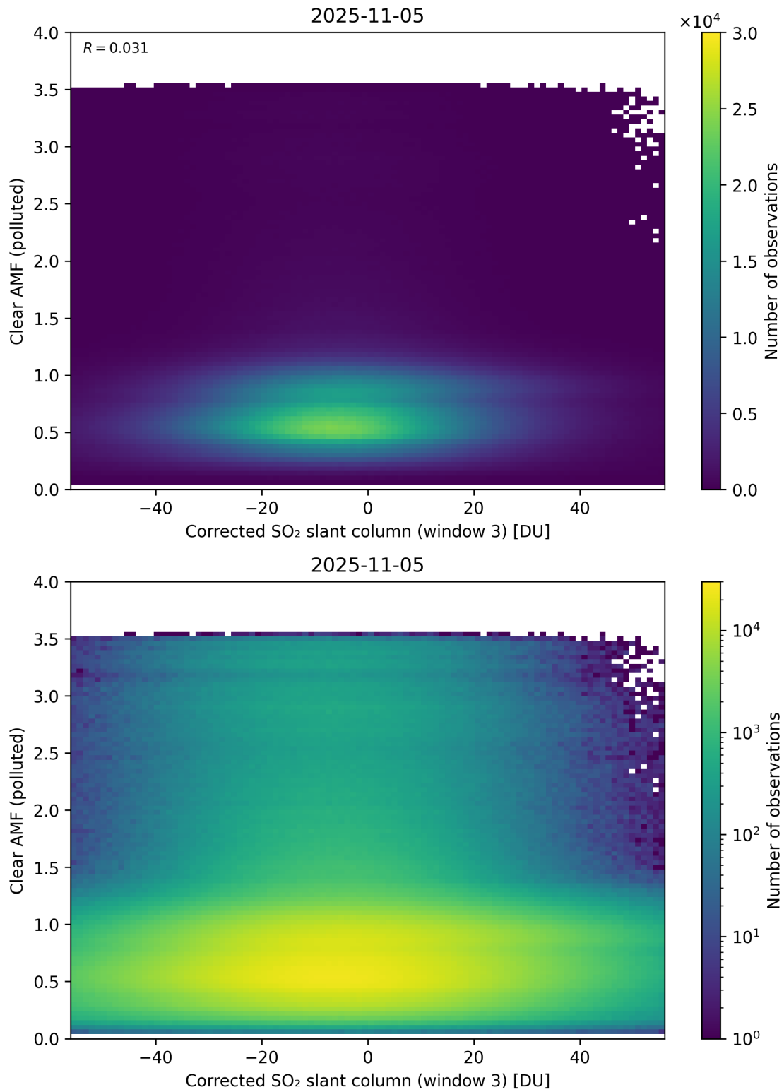
Figure 259: Scatter density plot of “Corrected SO 2 slant column (window 3)” against “Clear AMF (polluted)” for 2025-11-04 to 2025-11-06.
