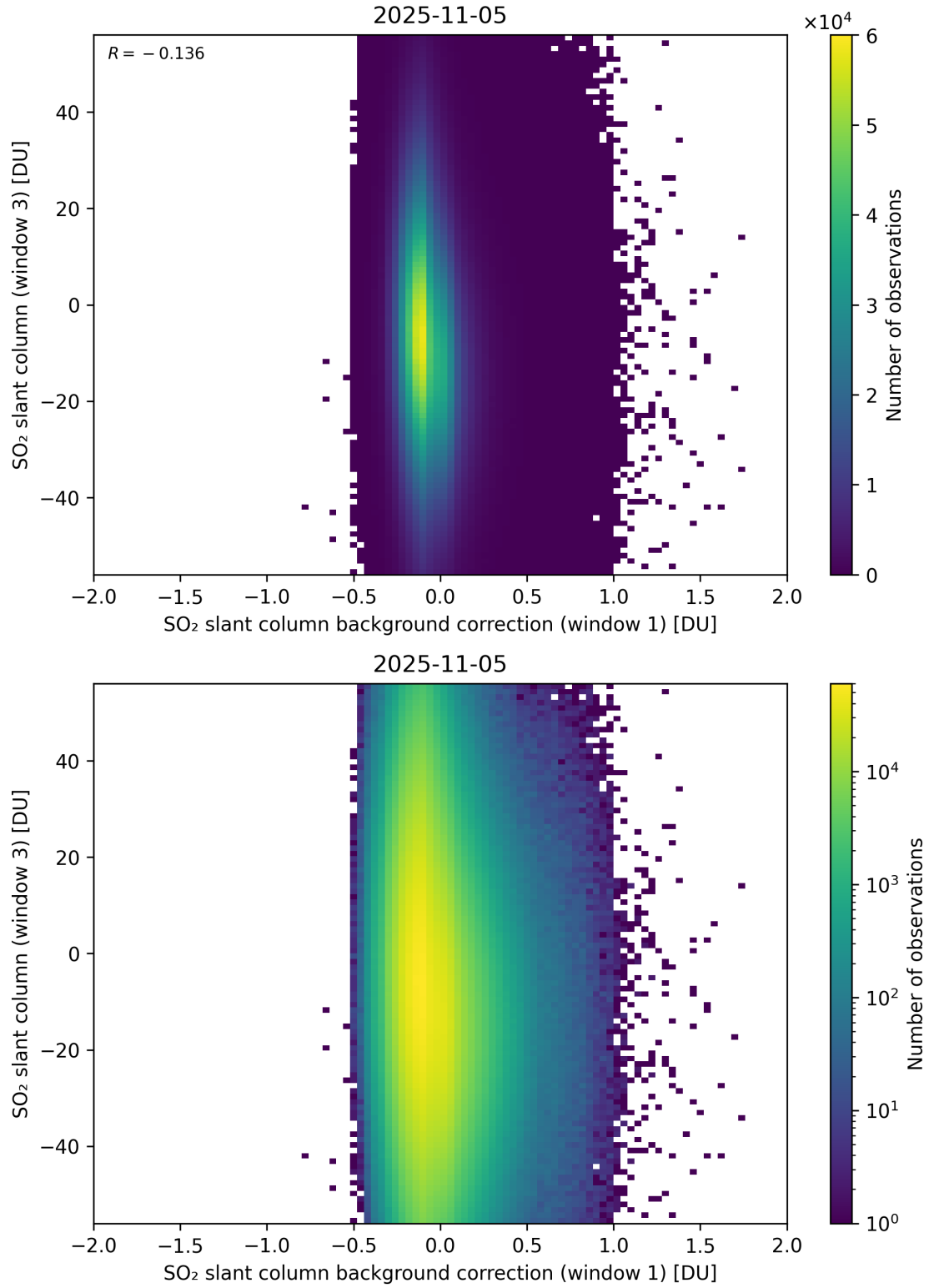
Figure 118: Scatter density plot of “SO 2 slant column background correction (window 1)” against “SO 2 slant column (window 3)” for 2025-11-04 to 2025-11-06.
