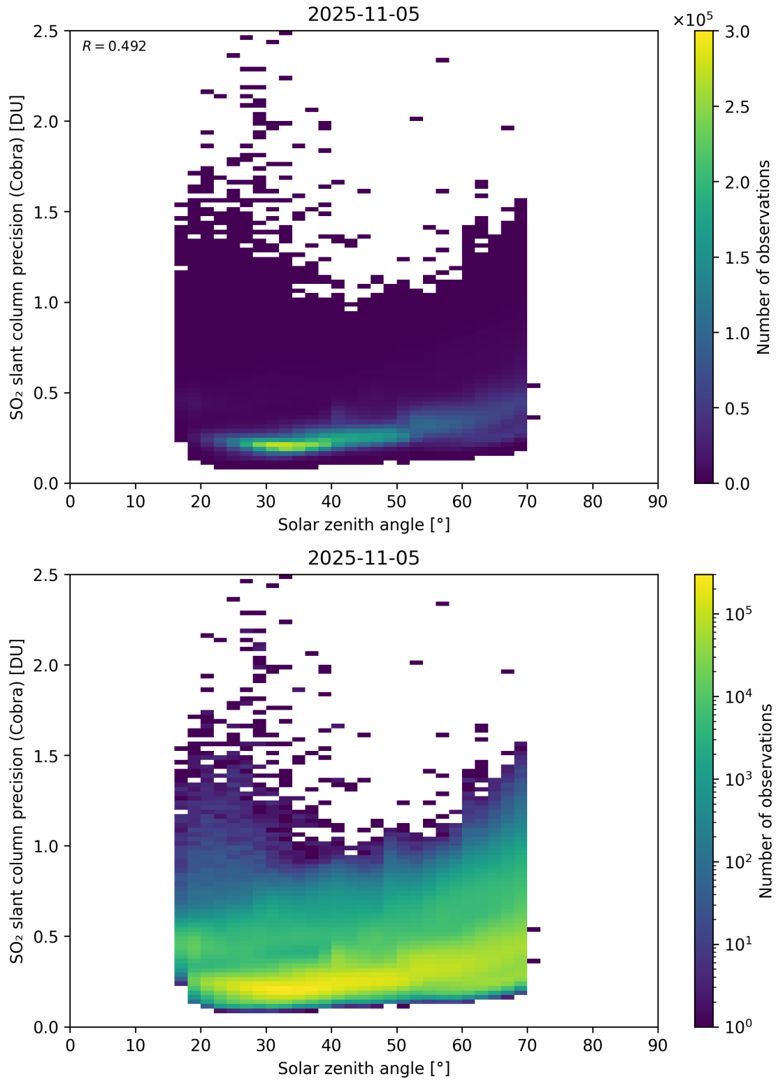
Figure 180: Scatter density plot of “Solar zenith angle” against “SO 2 slant column precision (Cobra)” for 2025-11-04 to 2025-11-06.
