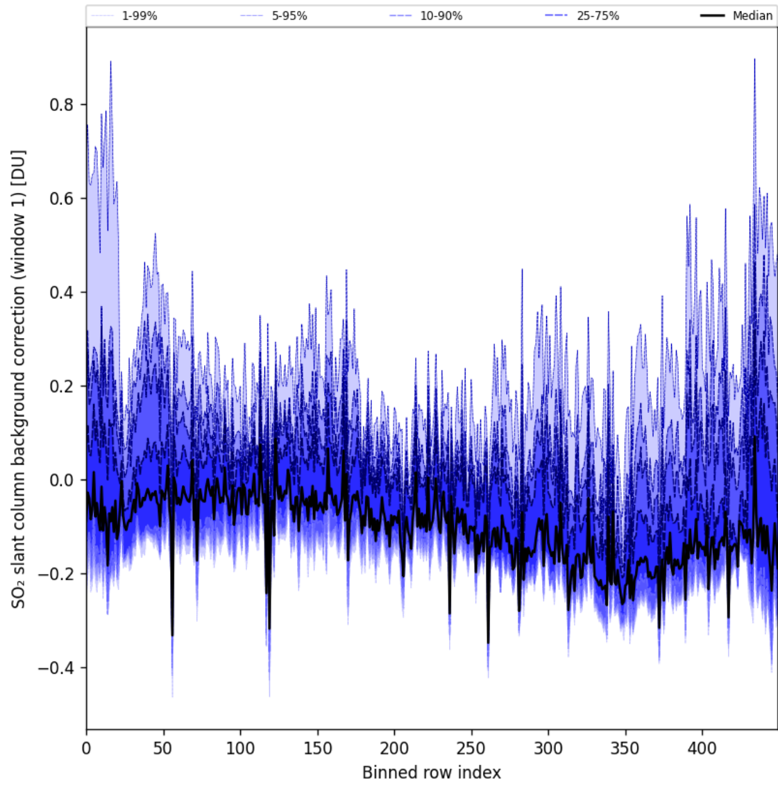
Figure 92: Along track statistics of “SO 2 slant column background correction (window 1)” for 2025-11-04 to 2025-11-06
