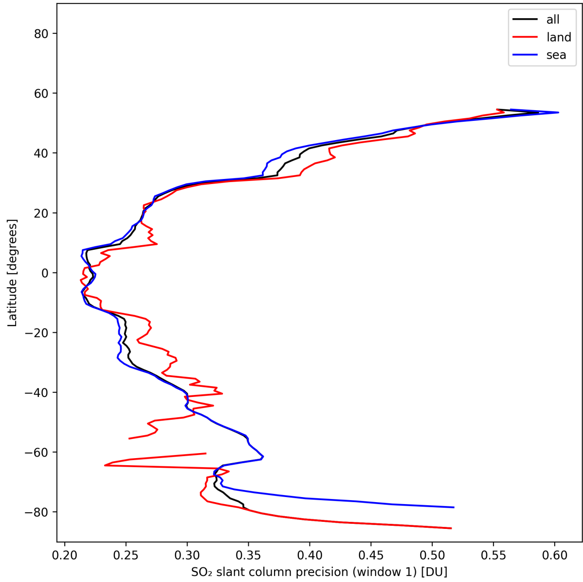
Figure 38: Zonal average of "SO 2 slant column precision (window 1)" for 2025-11-04 to 2025-11-06.
