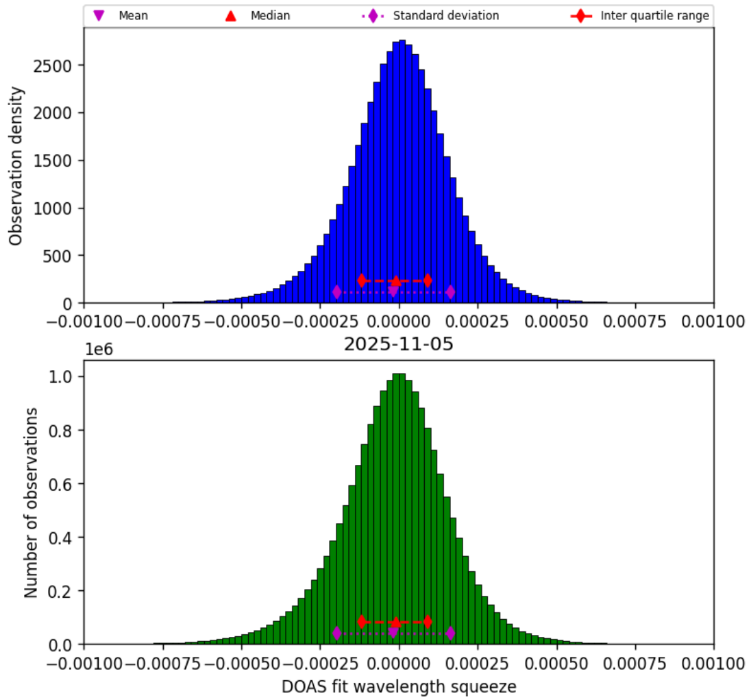
Figure 77: Histogram of “DOAS fit wavelength squeeze” for 2025-11-04 to 2025-11-06
