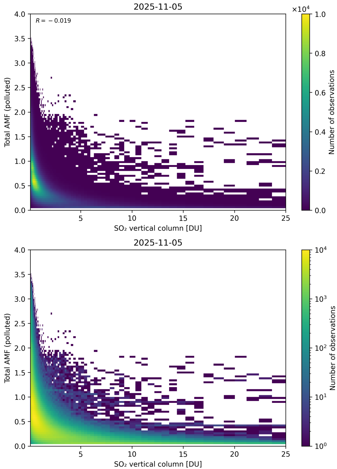
Figure 359: Scatter density plot of “SO 2 vertical column” against “Total AMF (polluted)” for 2025-11-04 to 2025-11-06.
