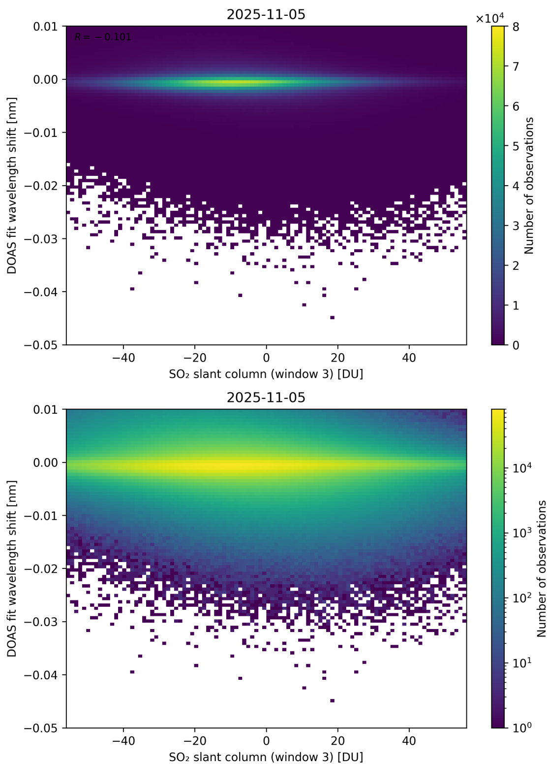
Figure 304: Scatter density plot of “SO 2 slant column (window 3)” against “DOAS fit wavelength shift” for 2025-11-04 to 2025-11-06.
