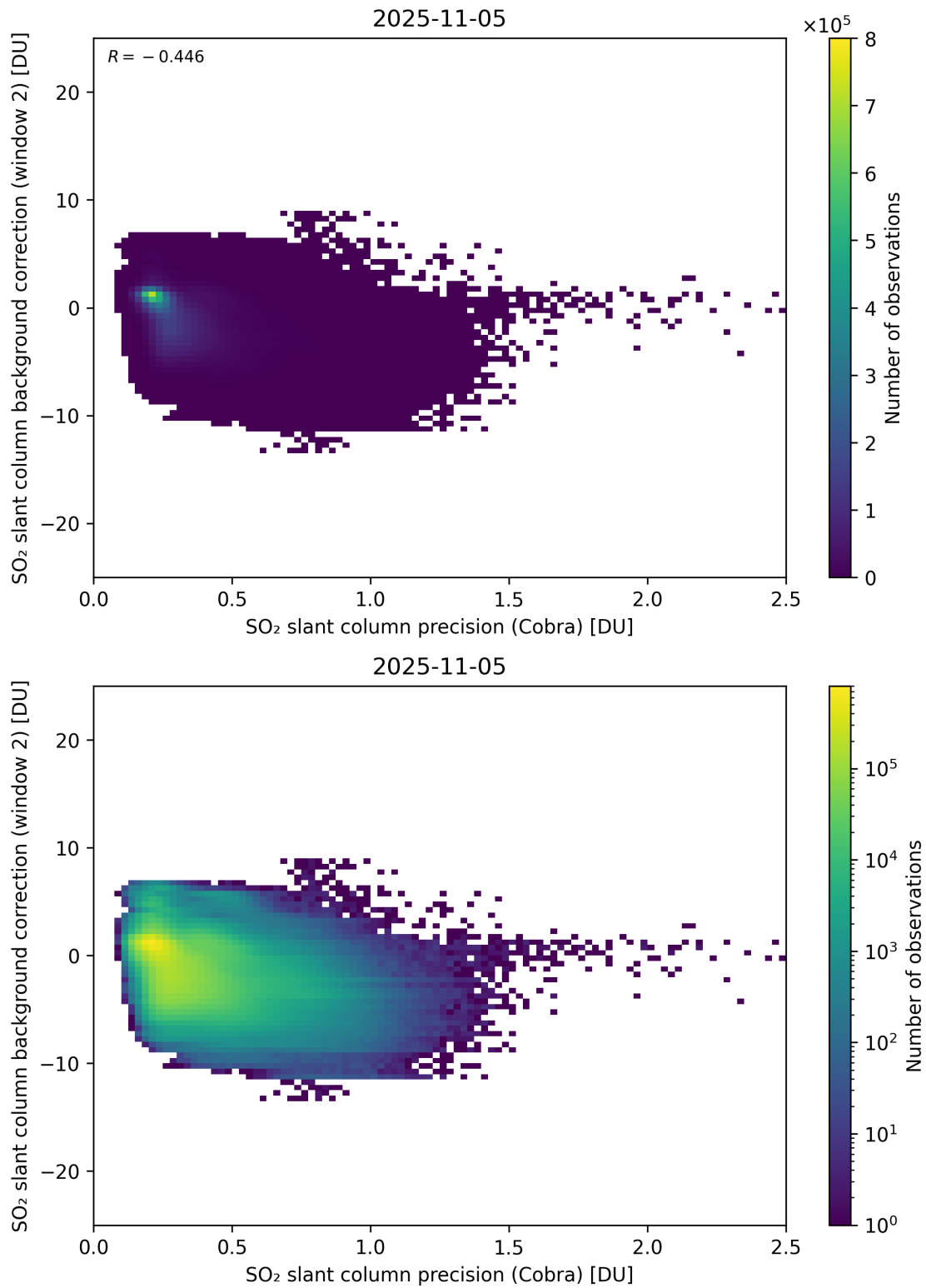
Figure 200: Scatter density plot of “SO 2 slant column precision (Cobra)” against “SO 2 slant column background correction (window 2)” for 2025-11-04 to 2025-11-06.
