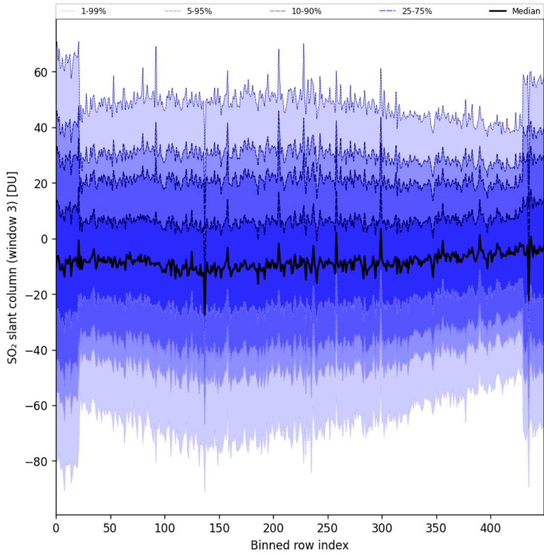
Figure 97: Along track statistics of “SO 2 slant column (window 3)” for 2025-11-04 to 2025-11-06
