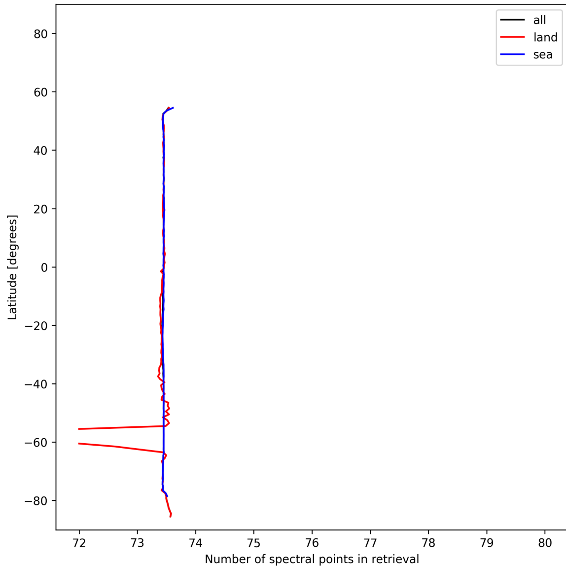
Figure 56: Zonal average of “Number of spectral points in retrieval” for 2025-11-04 to 2025-11-06.
