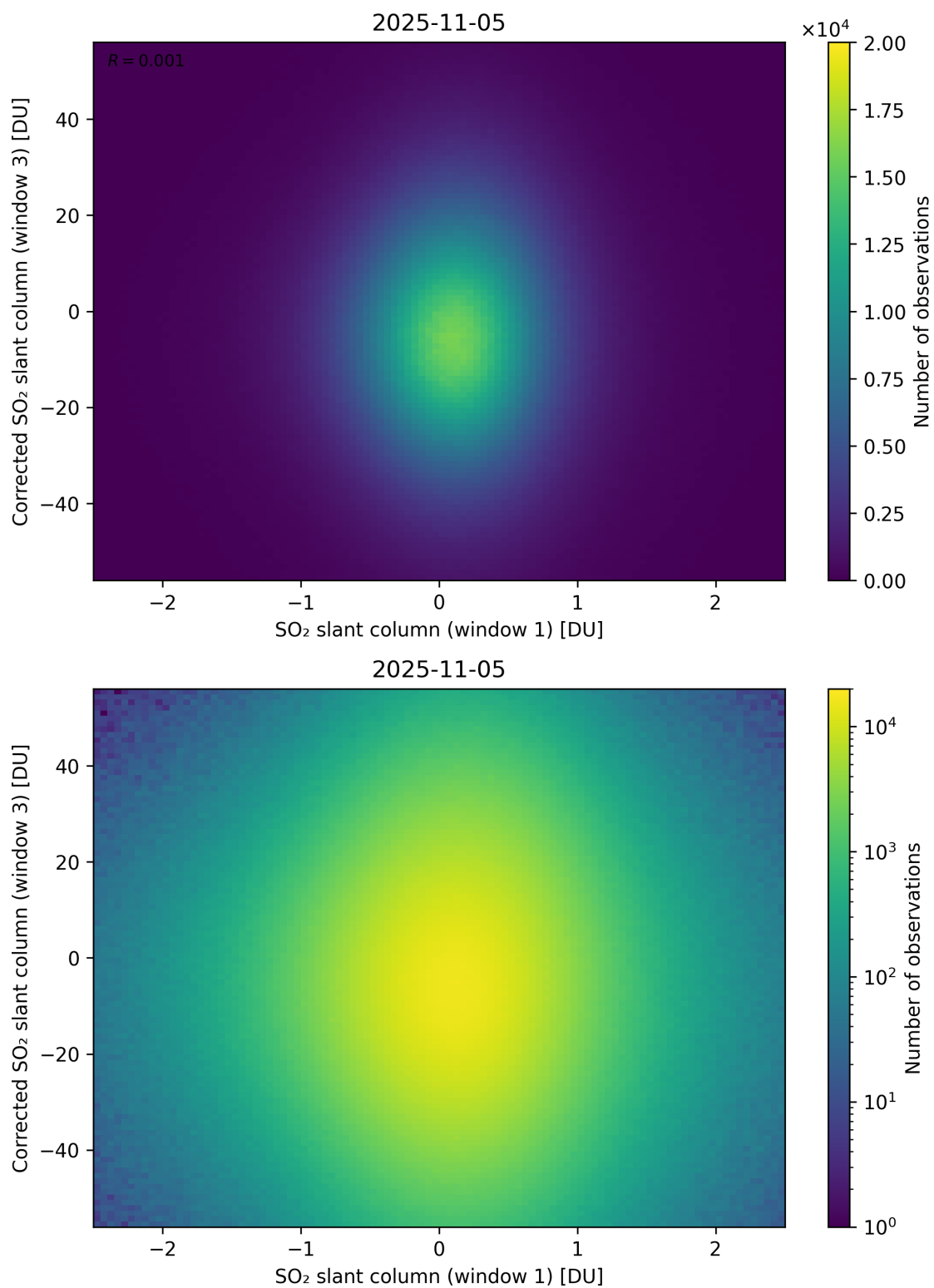
Figure 284: Scatter density plot of “SO 2 slant column (window 1)” against “Corrected SO 2 slant column (window 3)” for 2025-11-04 to 2025-11-06.
