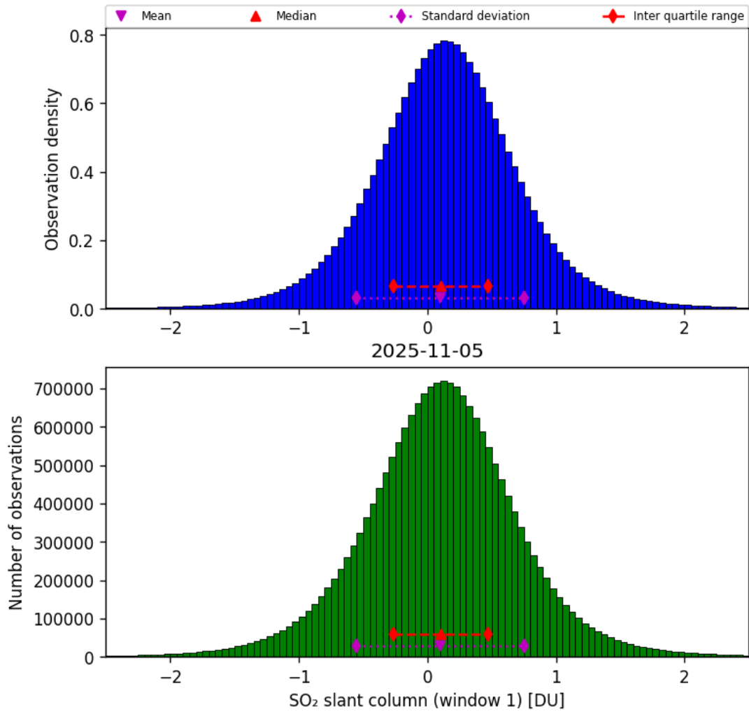
Figure 63: Histogram of “SO 2 slant column (window 1)” for 2025-11-04 to 2025-11-06
