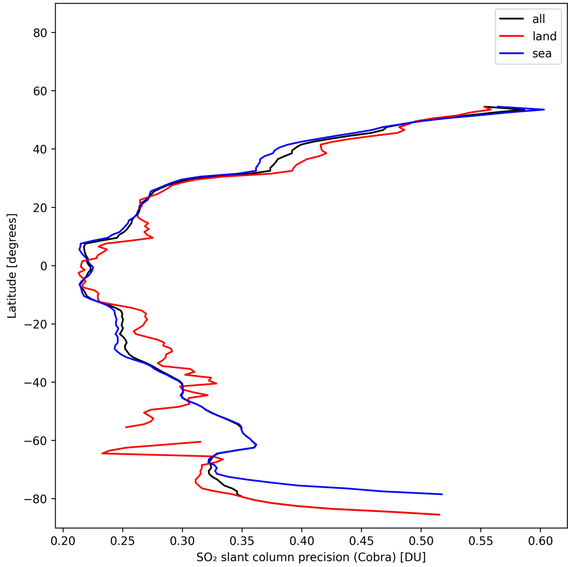
Figure 36: Zonal average of “SO 2 slant column precision (Cobra)” for 2025-11-04 to 2025-11-06.
