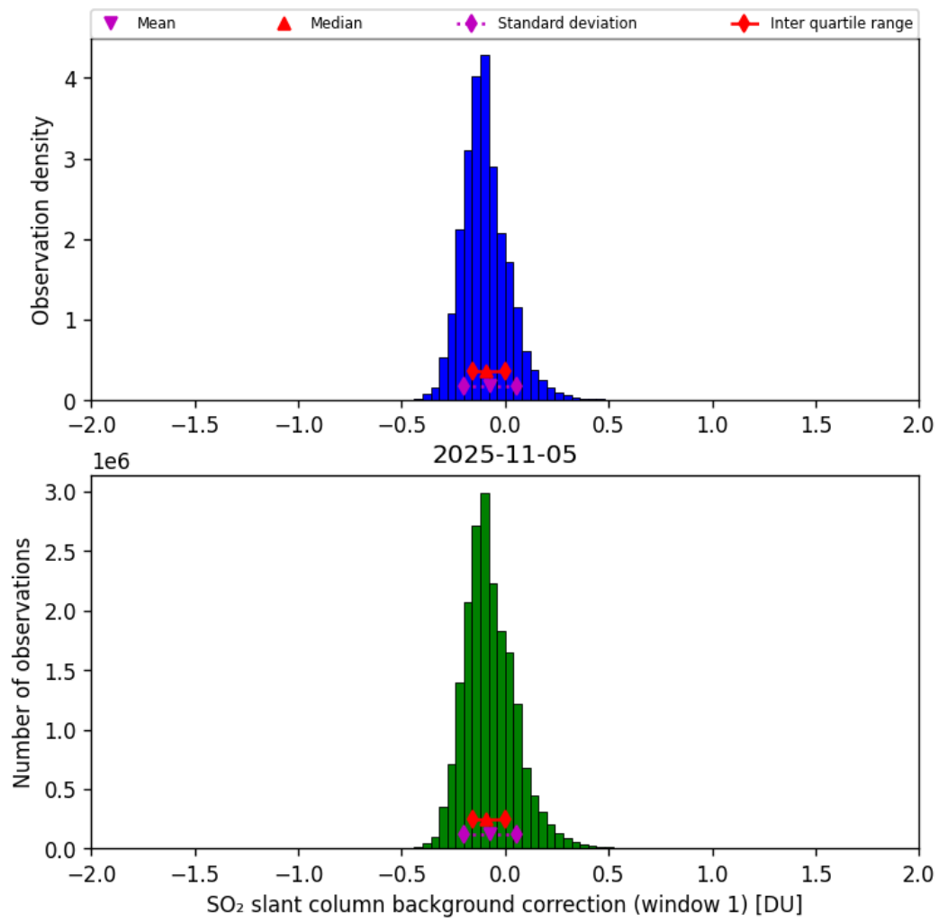
Figure 66: Histogram of “SO 2 slant column background correction (window 1)” for 2025-11-04 to 2025-11-06
