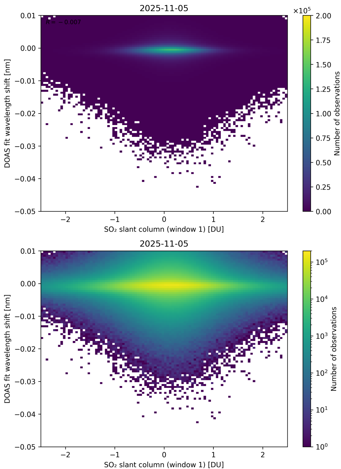
Figure 265: Scatter density plot of “SO 2 slant column (window 1)” against “DOAS fit wavelength shift” for 2025-11-04 to 2025-11-06.
