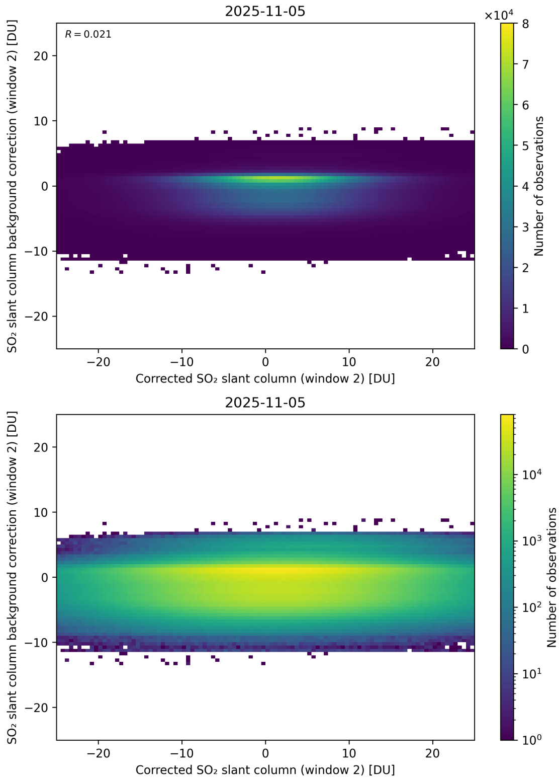
Figure 244: Scatter density plot of “Corrected SO 2 slant column (window 2)” against “SO 2 slant column background correction (window 2)” for 2025-11-04 to 2025-11-06.
