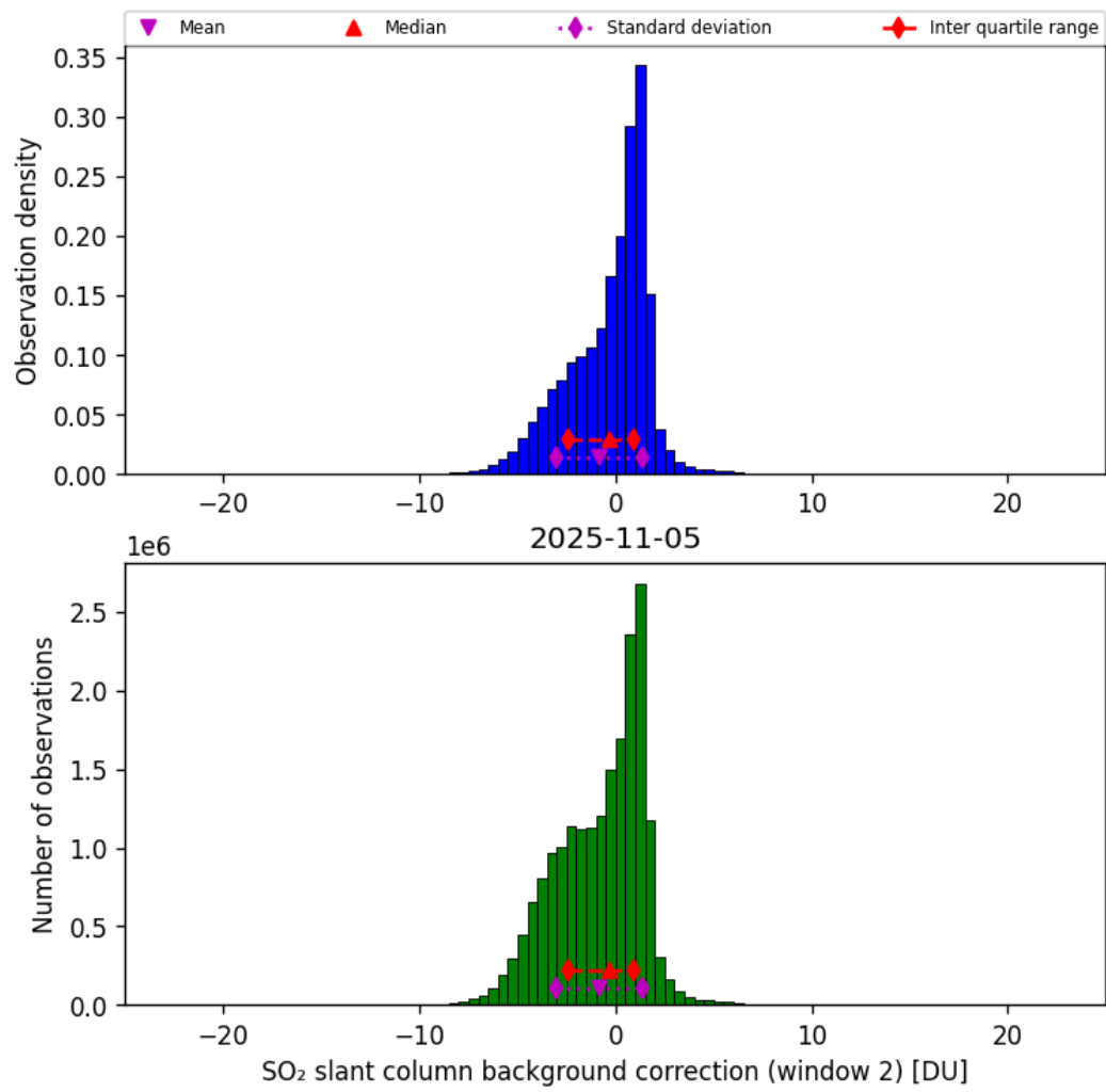
Figure 70: Histogram of “SO 2 slant column background correction (window 2)” for 2025-11-04 to 2025-11-06
