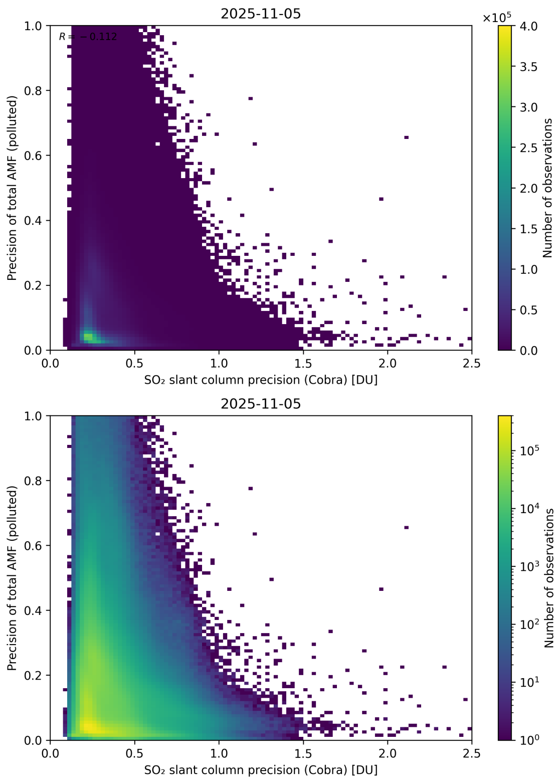
Figure 214: Scatter density plot of “SO 2 slant column precision (Cobra)” against “Precision of total AMF (polluted)” for 2025-11-04 to 2025-11-06.
