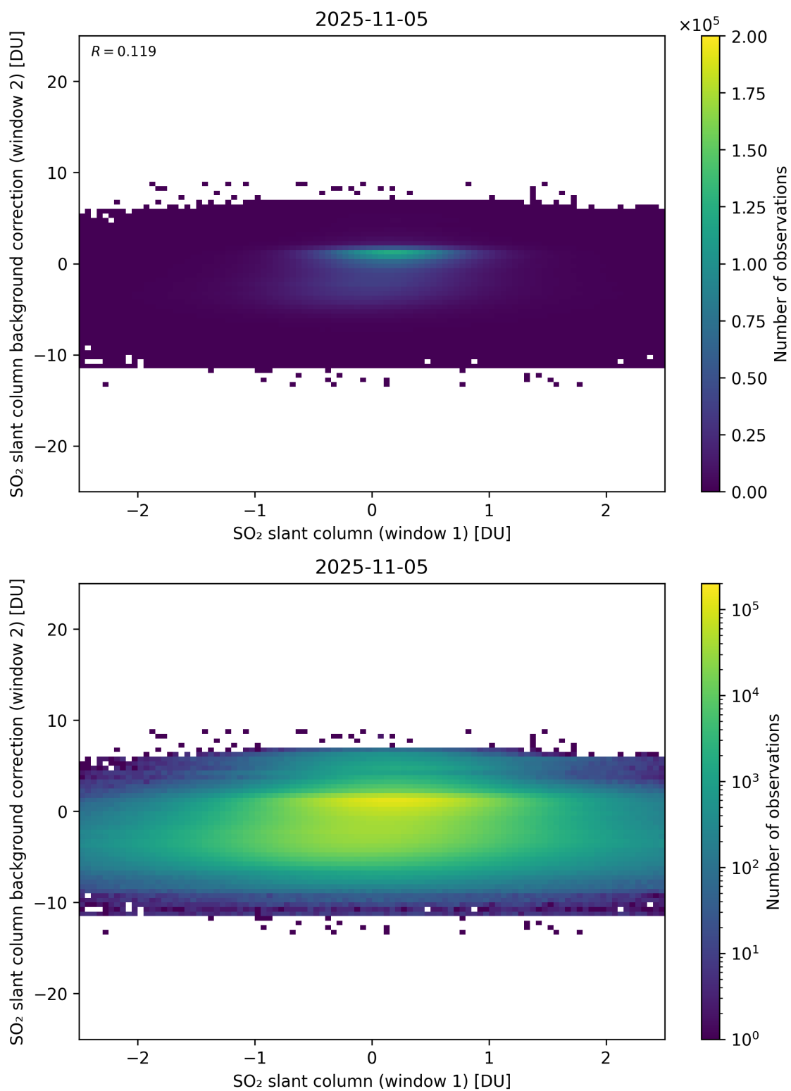
Figure 263: Scatter density plot of “SO 2 slant column (window 1)” against “SO 2 slant column background correction (window 2)” for 2025-11-04 to 2025-11-06.
