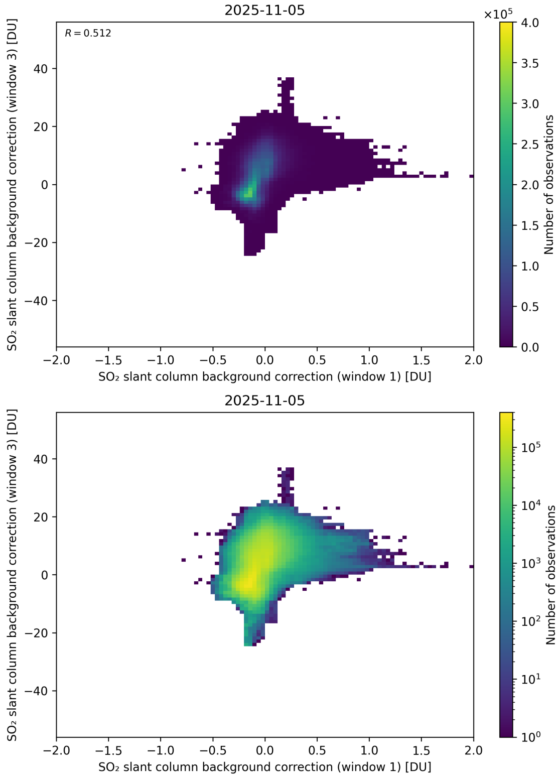
Figure 110: Scatter density plot of “SO 2 slant column background correction (window 1)” against “SO 2 slant column background correction (window 3)” for 2025-11-04 to 2025-11-06.
