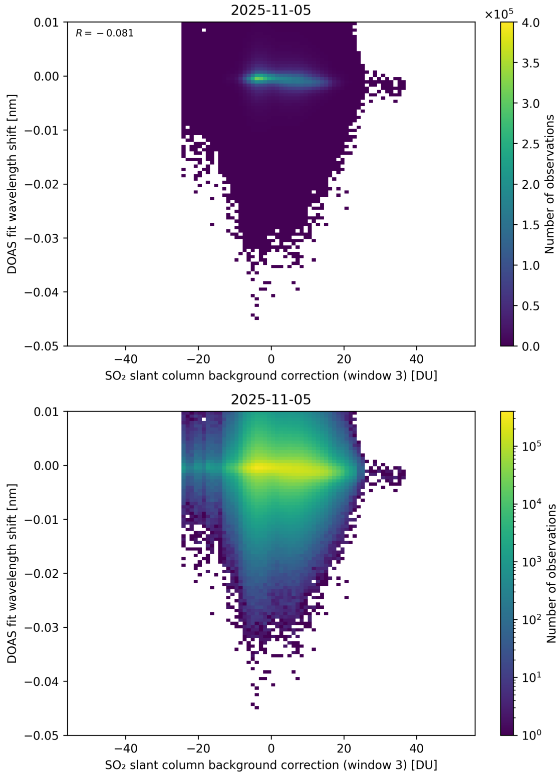
Figure 132: Scatter density plot of “SO 2 slant column background correction (window 3)” against “DOAS fit wavelength shift” for 2025-11-04 to 2025-11-06.
