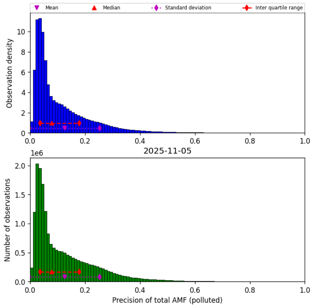
Figure 80: Histogram of “Precision of total AMF (polluted)” for 2025-11-04 to 2025-11-06
