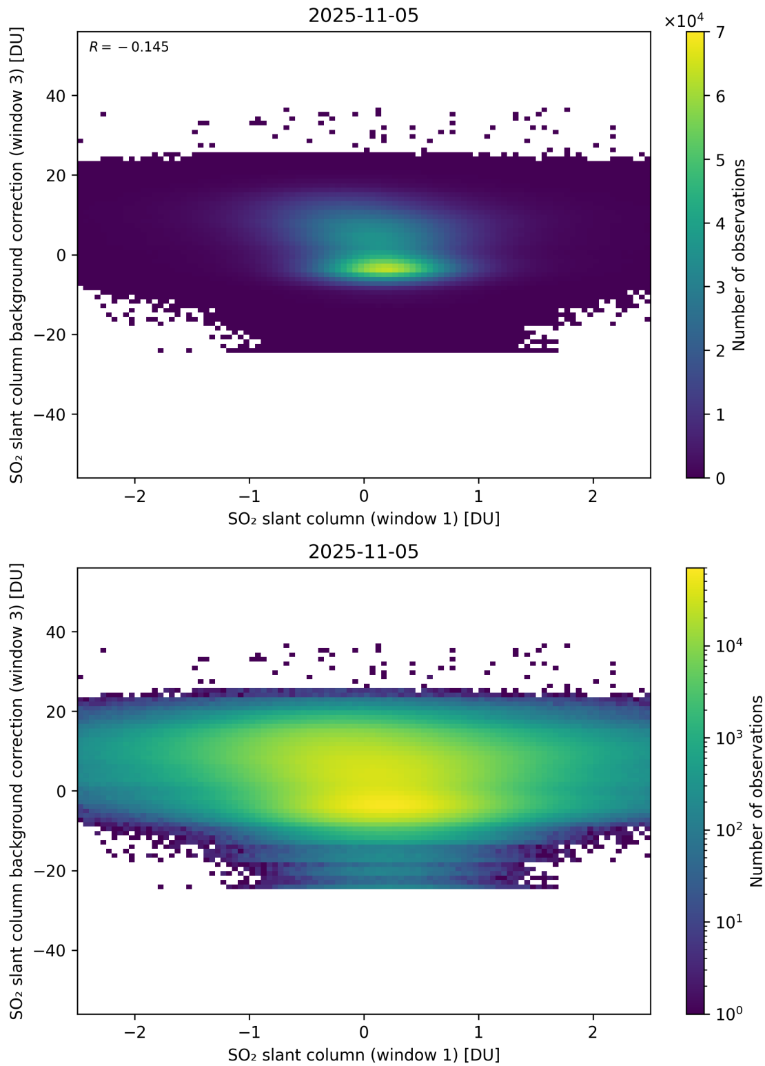
Figure 264: Scatter density plot of “SO 2 slant column (window 1)” against “SO 2 slant column background correction (window 3)” for 2025-11-04 to 2025-11-06.
