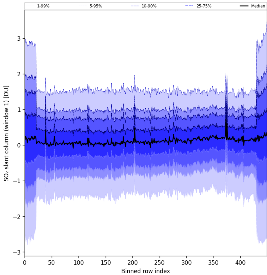
Figure 89: Along track statistics of “SO 2 slant column (window 1)” for 2025-11-04 to 2025-11-06
