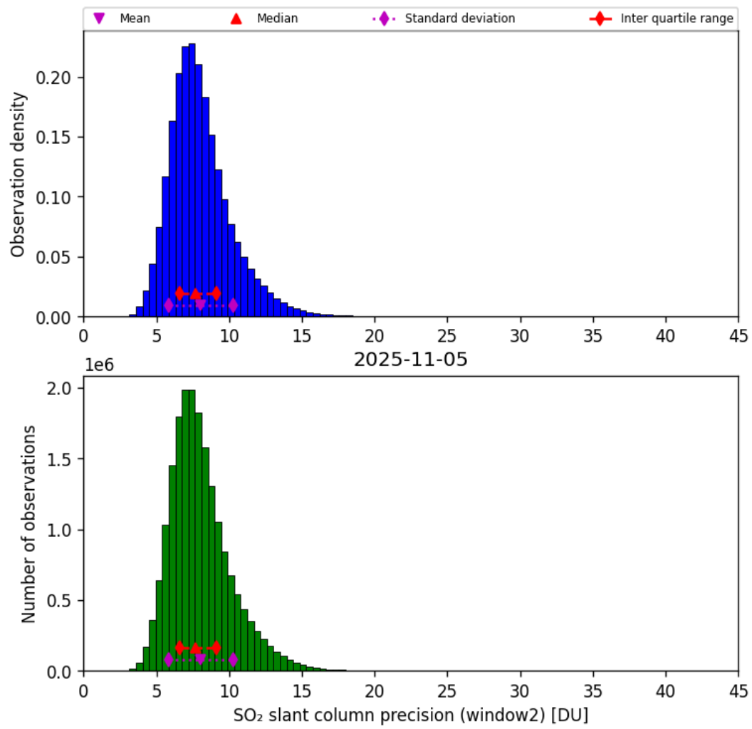
Figure 68: Histogram of “SO 2 slant column precision (window2)” for 2025-11-04 to 2025-11-06
