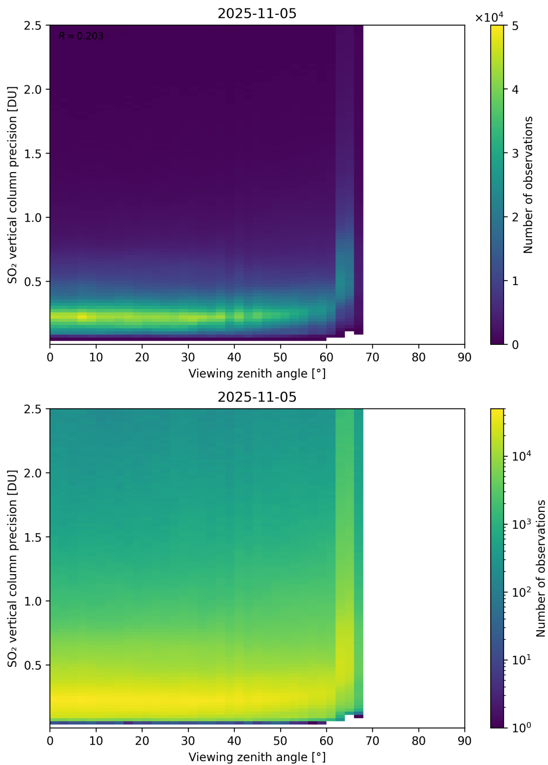
Figure 384: Scatter density plot of “Viewing zenith angle” against “SO 2 vertical column precision” for 2025-11-04 to 2025-11-06.
