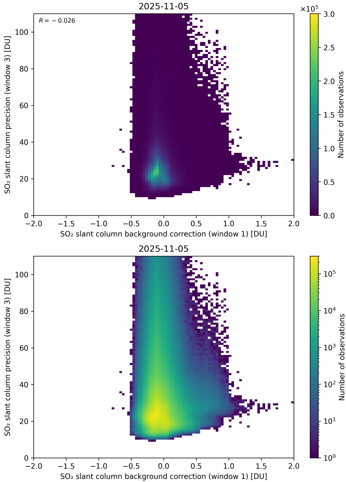
Figure 119: Scatter density plot of “SO 2 slant column background correction (window 1)” against “SO 2 slant column precision (window 3)” for 2025-11-04 to 2025-11-06.
