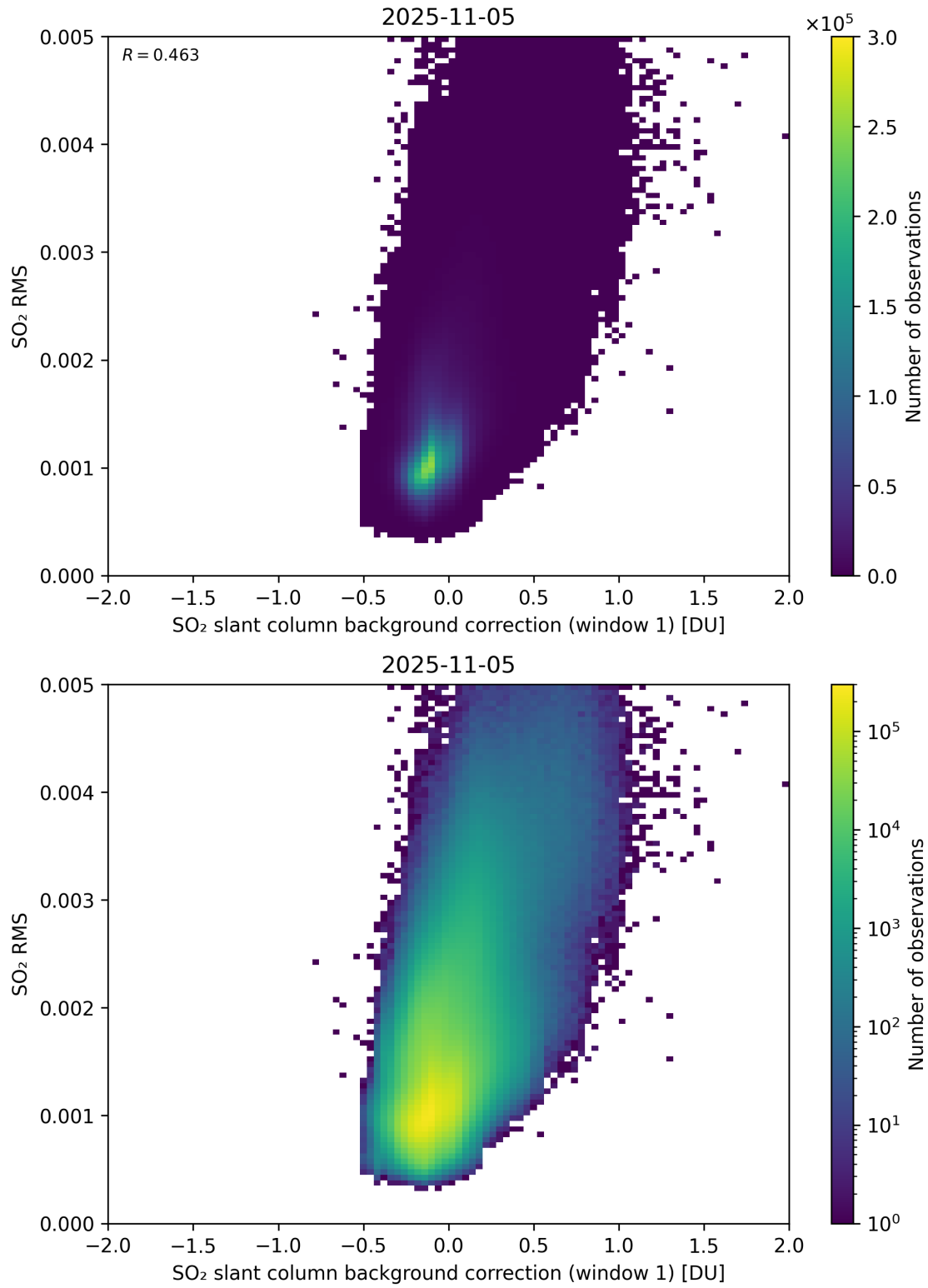
Figure 113: Scatter density plot of “SO 2 slant column background correction (window 1)” against “SO 2 RMS” for 2025-11-04 to 2025-11-06.
