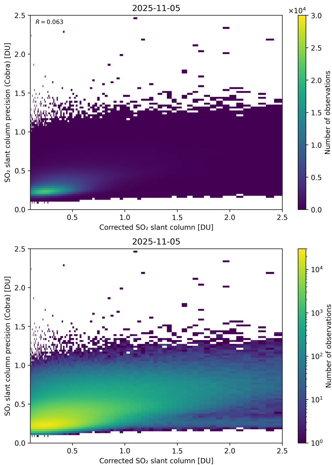
Figure 234: Scatter density plot of “Corrected SO 2 slant column” against “SO 2 slant column precision (Cobra)” for 2025-11-04 to 2025-11-06.
