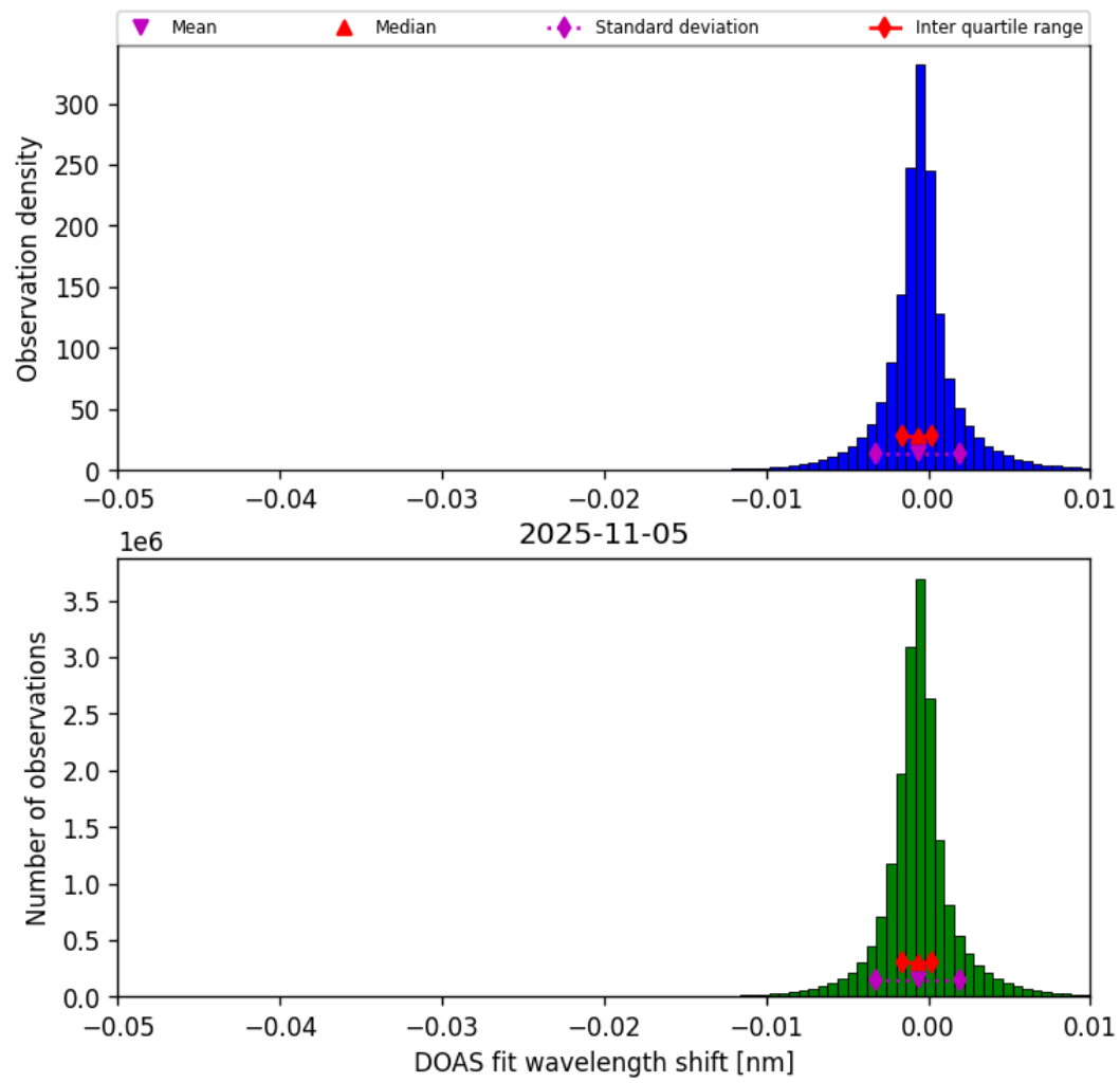
Figure 76: Histogram of “DOAS fit wavelength shift” for 2025-11-04 to 2025-11-06
