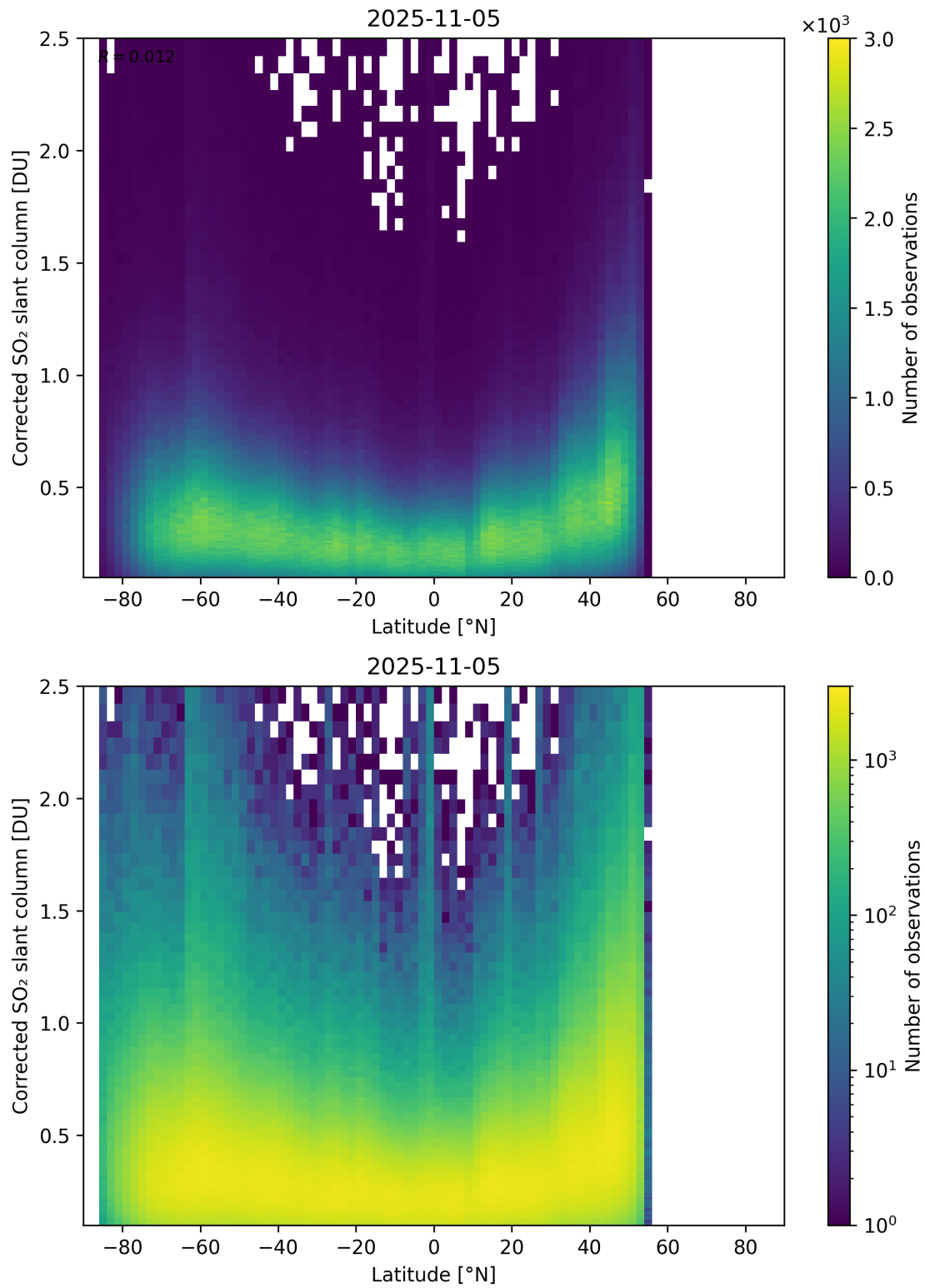
Figure 159: Scatter density plot of “Latitude” against “Corrected SO 2 slant column” for 2025-11-04 to 2025-11-06.
