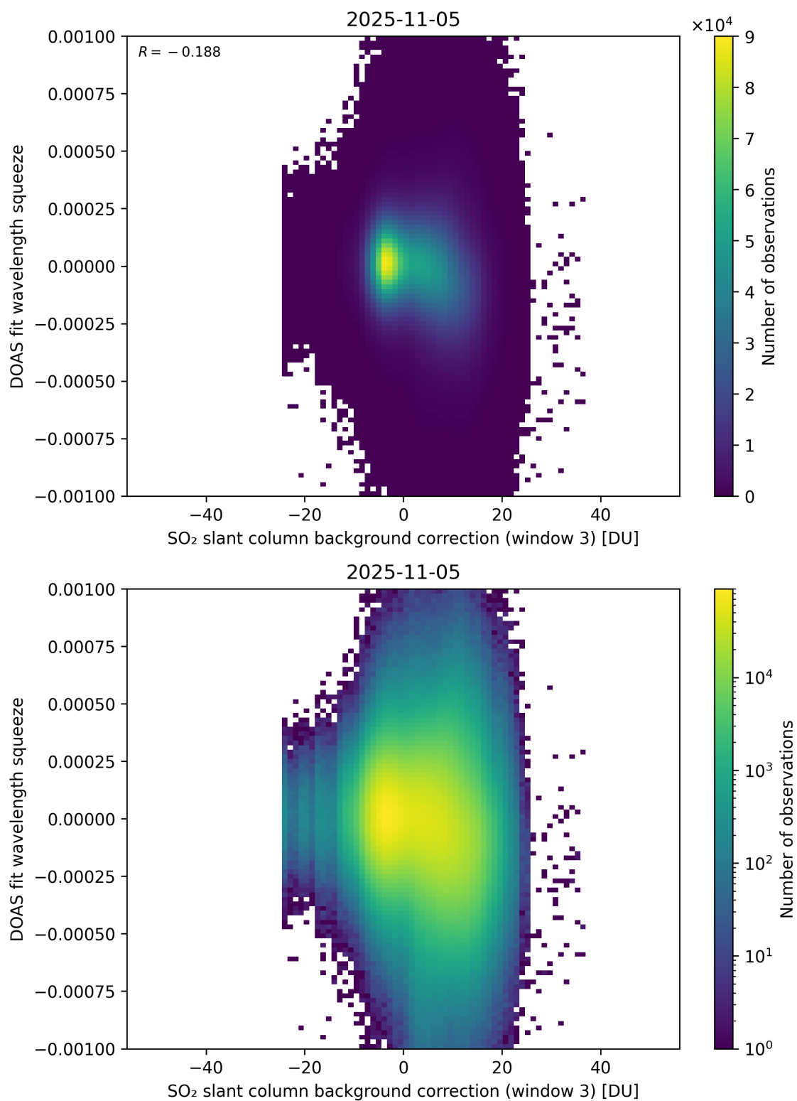
Figure 133: Scatter density plot of “SO 2 slant column background correction (window 3)” against “DOAS fit wavelength squeeze” for 2025-11-04 to 2025-11-06.
