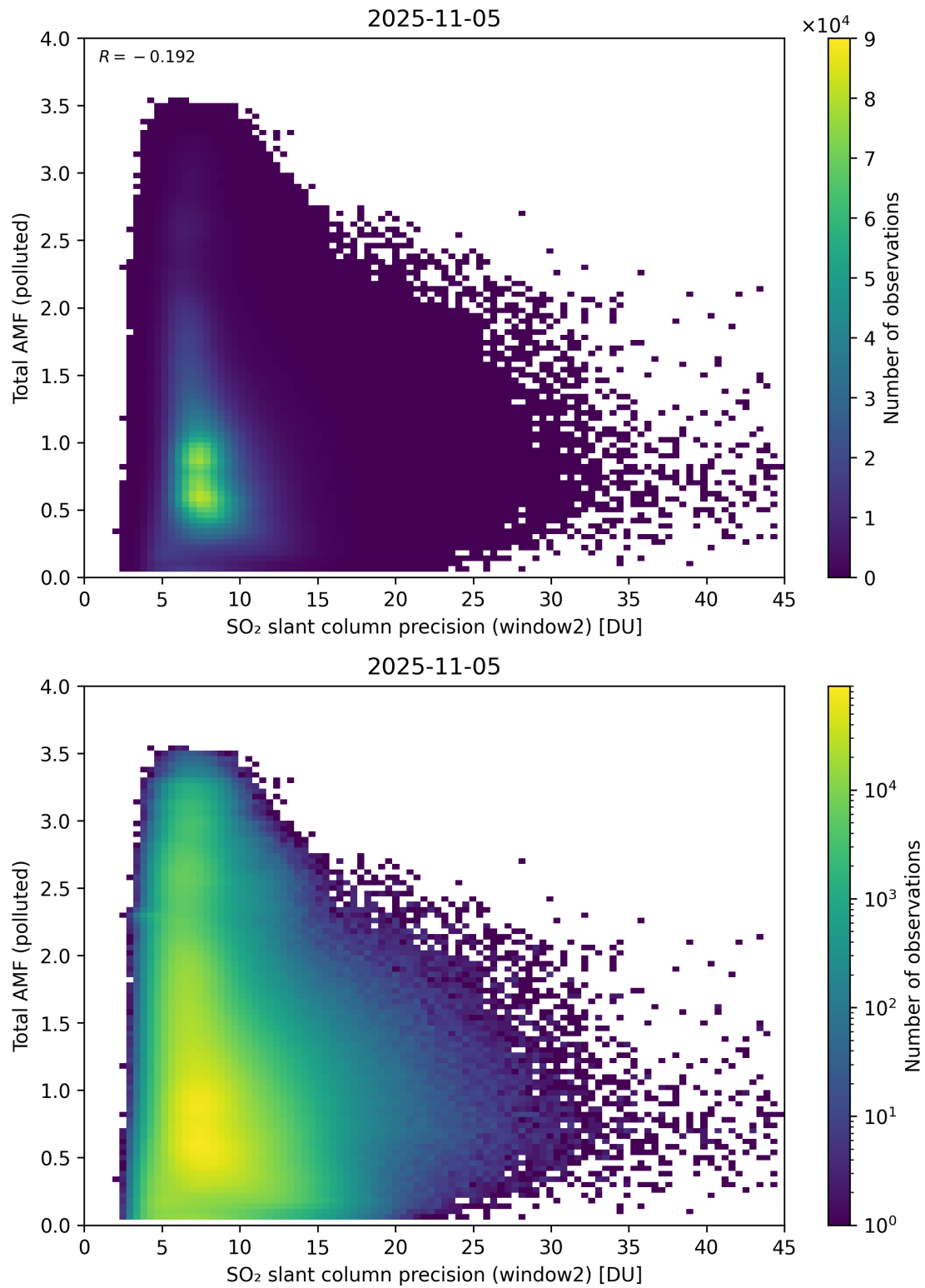
Figure 301: Scatter density plot of “SO 2 slant column precision (window2)” against “Total AMF (polluted)” for 2025-11-04 to 2025-11-06.
