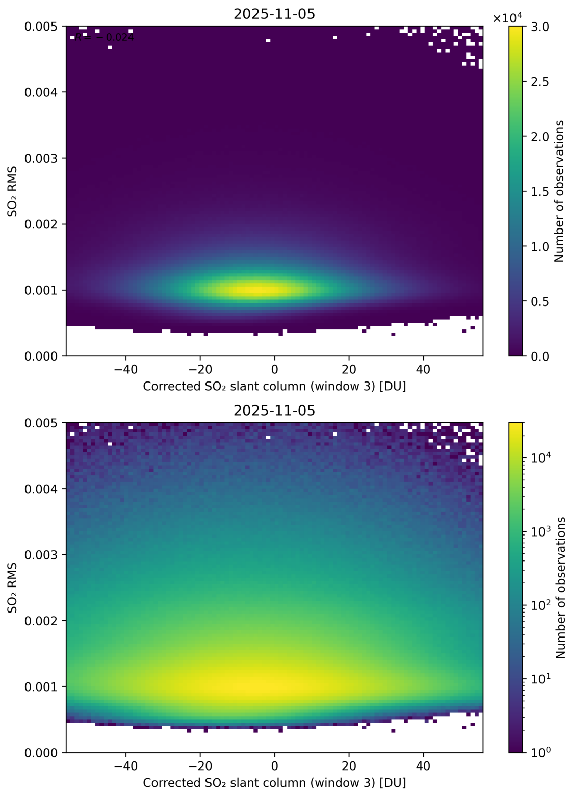
Figure 258: Scatter density plot of “Corrected SO 2 slant column (window 3)” against “SO 2 RMS” for 2025-11-04 to 2025-11-06.
