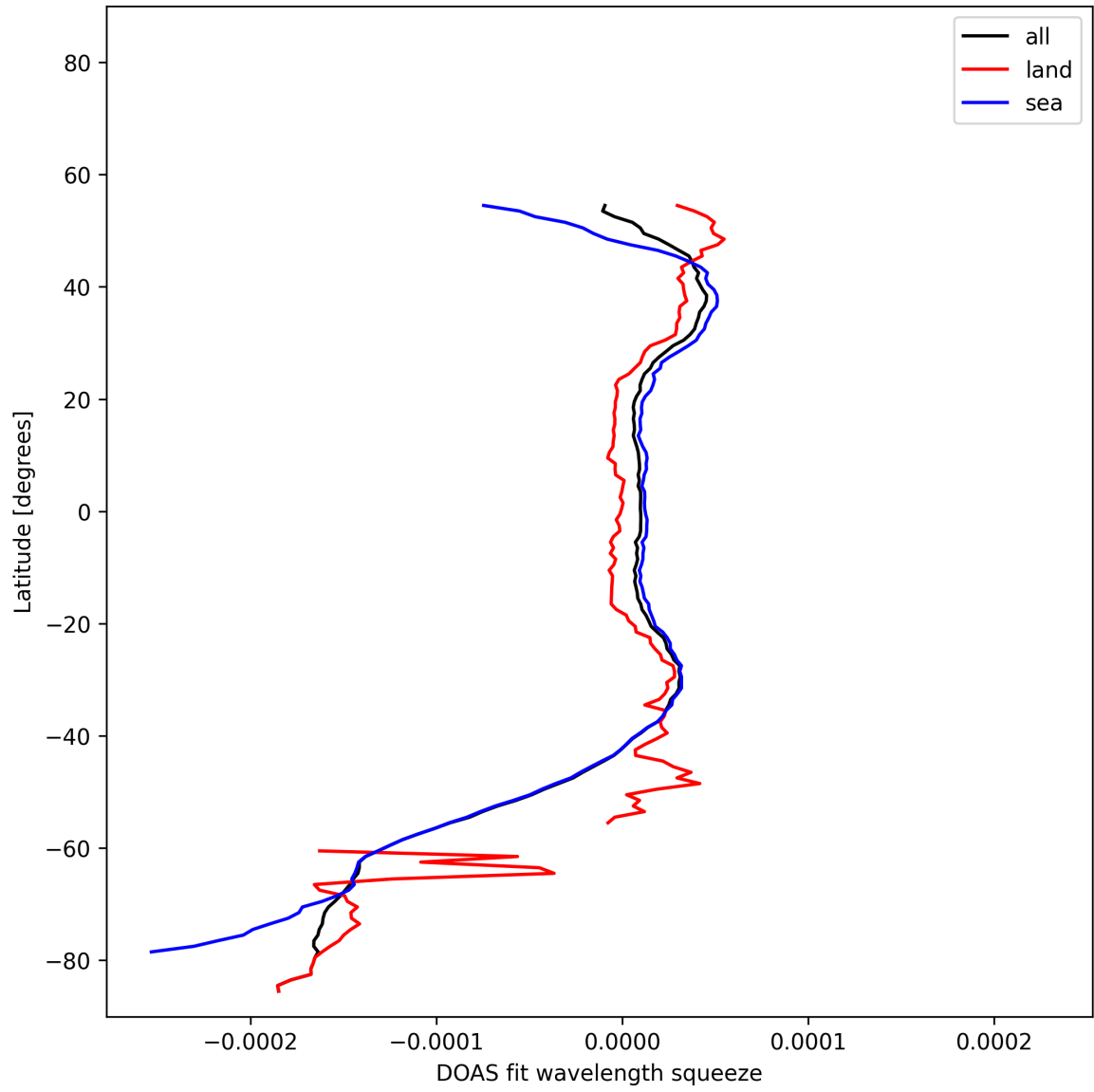
Figure 51: Zonal average of “DOAS fit wavelength squeeze” for 2025-11-04 to 2025-11-06.
