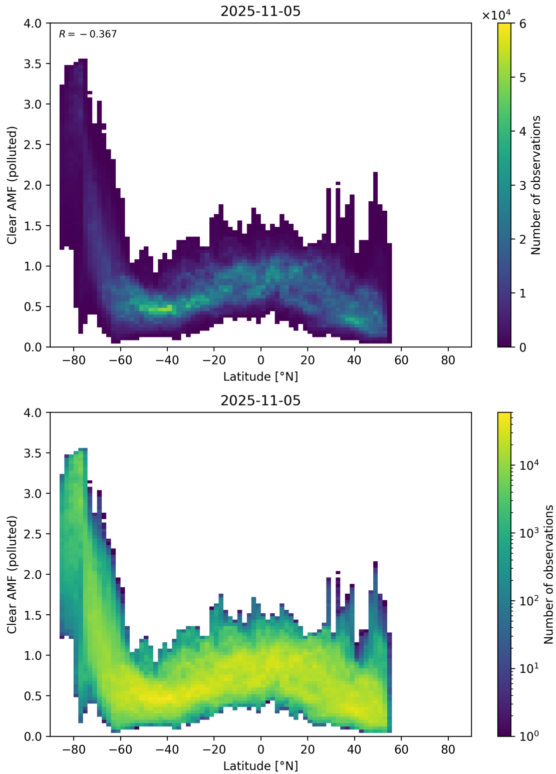
Figure 156: Scatter density plot of “Latitude” against “Clear AMF (polluted)” for 2025-11-04 to 2025-11-06.
