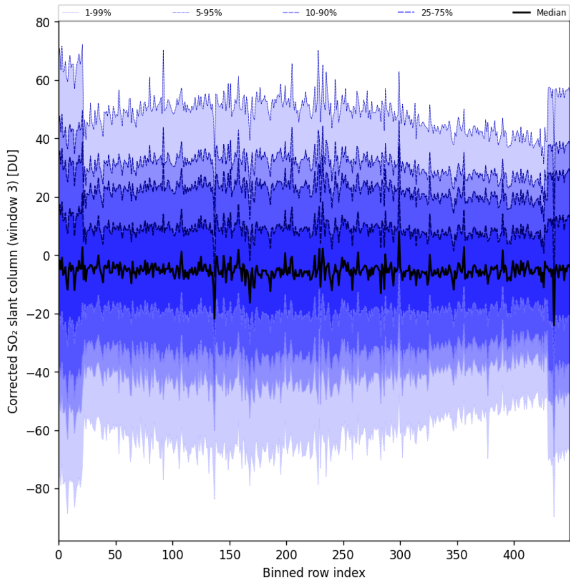
Figure 99: Along track statistics of “Corrected SO 2 slant column (window 3)” for 2025-11-04 to 2025-11-06
