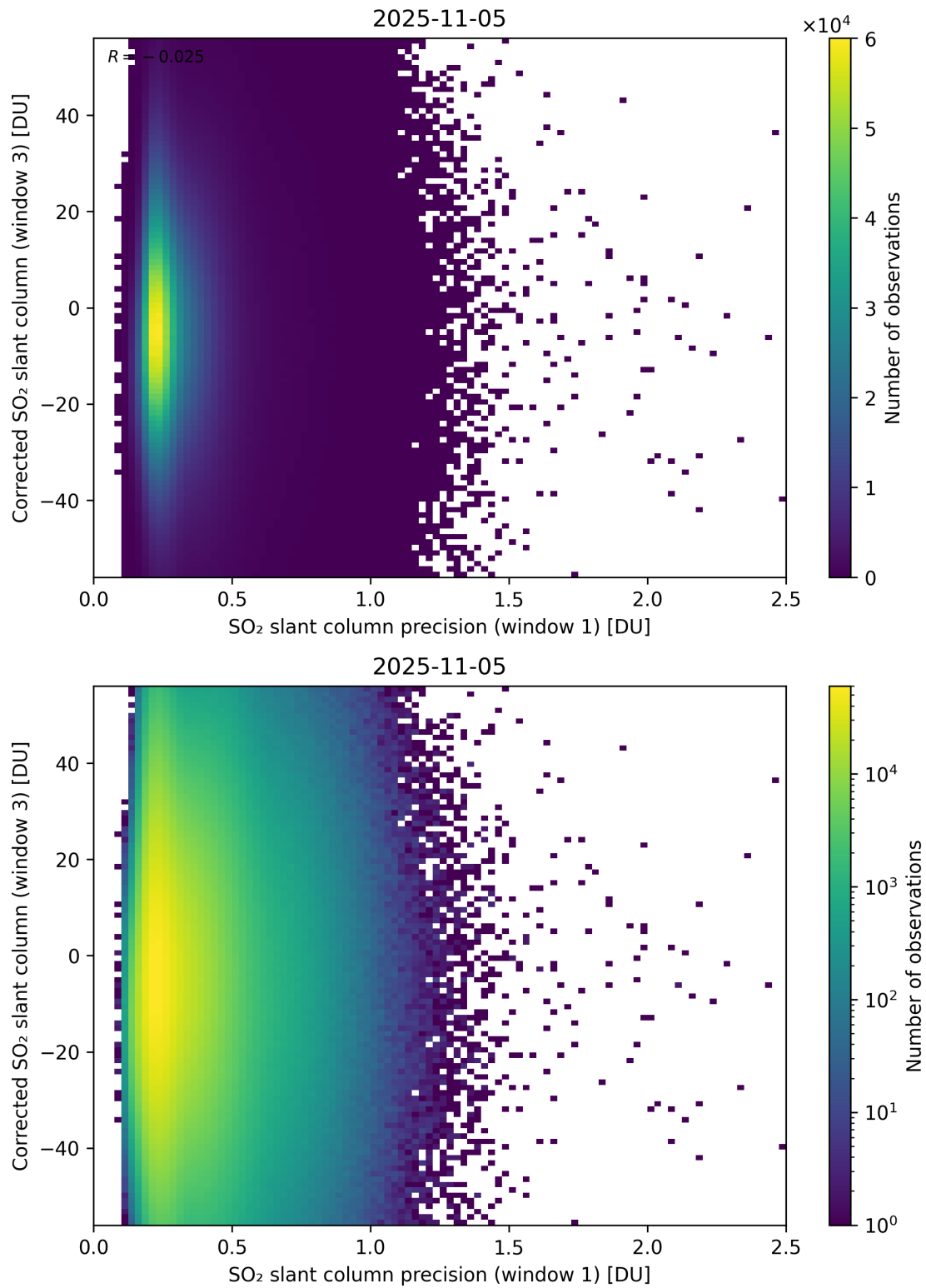
Figure 276: Scatter density plot of “SO 2 slant column precision (window 1)” against “Corrected SO 2 slant column (window 3)” for 2025-11-04 to 2025-11-06.
