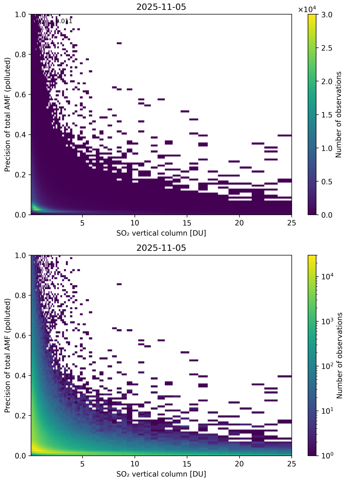
Figure 360: Scatter density plot of “SO 2 vertical column” against “Precision of total AMF (polluted)” for 2025-11-04 to 2025-11-06.
