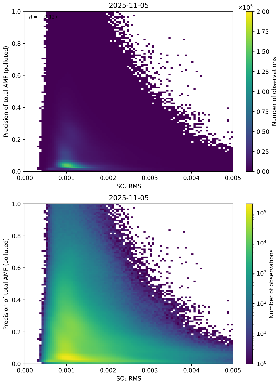
Figure 149: Scatter density plot of “SO 2 RMS” against “Precision of total AMF (polluted)” for 2025-11-04 to 2025-11-06.
