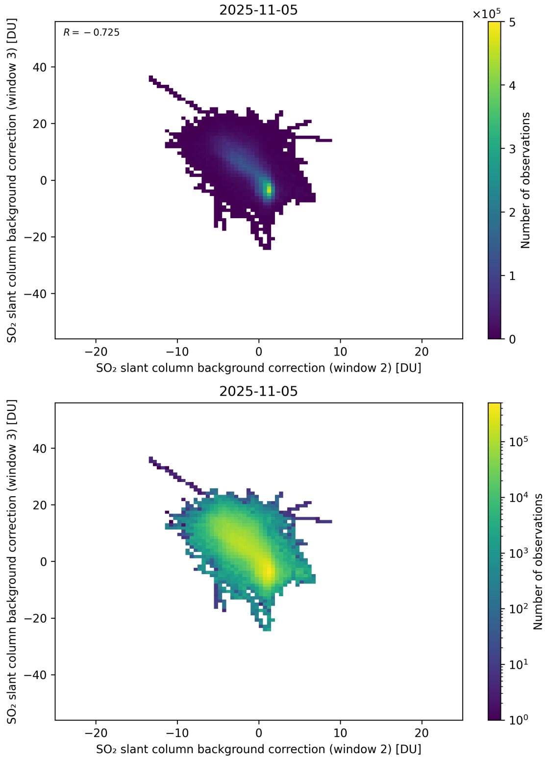
Figure 122: Scatter density plot of “SO 2 slant column background correction (window 2)” against “SO 2 slant column background correction (window 3)” for 2025-11-04 to 2025-11-06.
