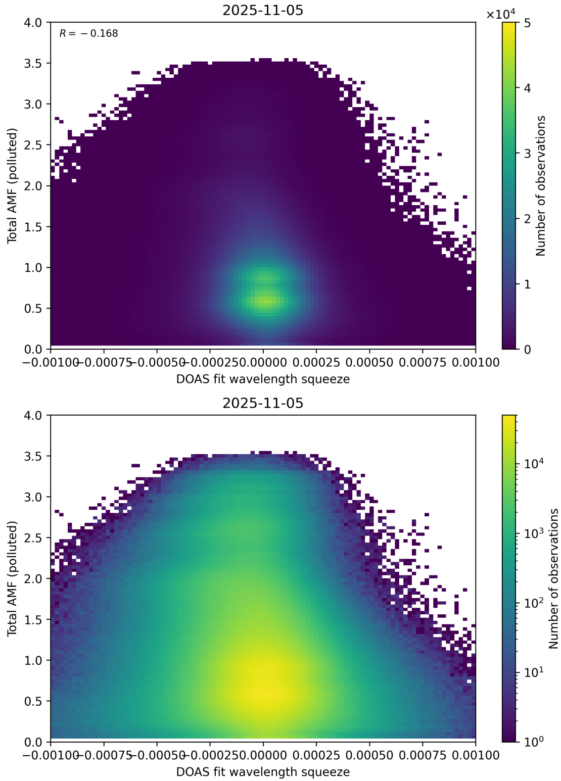
Figure 145: Scatter density plot of “DOAS fit wavelength squeeze” against “Total AMF (polluted)” for 2025-11-04 to 2025-11-06.
