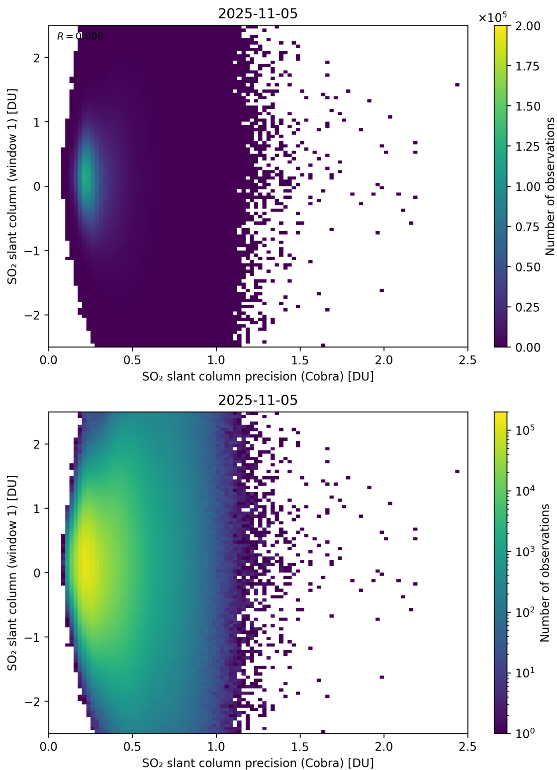
Figure 208: Scatter density plot of “SO 2 slant column precision (Cobra)” against “SO 2 slant column (window 1)” for 2025-11-04 to 2025-11-06.
