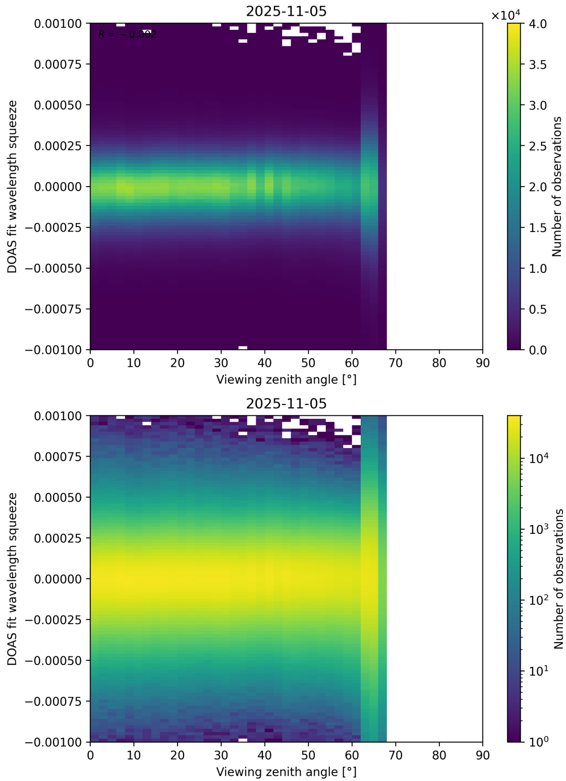
Figure 366: Scatter density plot of “Viewing zenith angle” against “DOAS fit wavelength squeeze” for 2025-11-04 to 2025-11-06.
