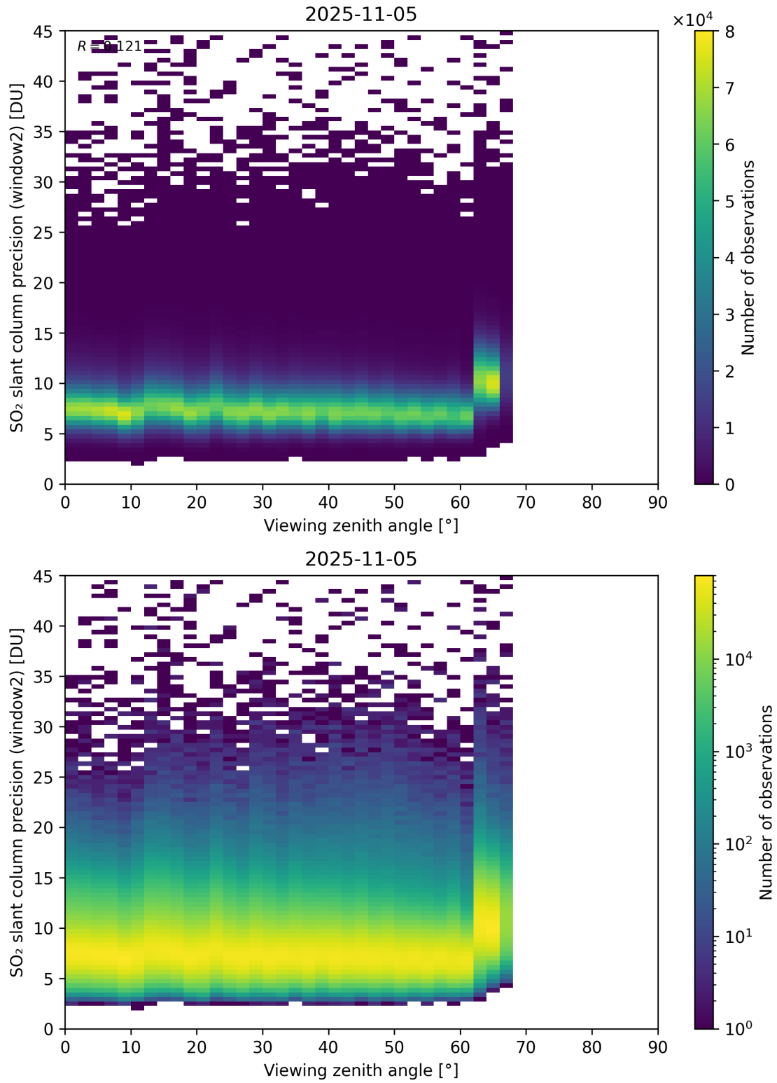
Figure 378: Scatter density plot of “Viewing zenith angle” against “SO 2 slant column precision (window2)” for 2025-11-04 to 2025-11-06.
