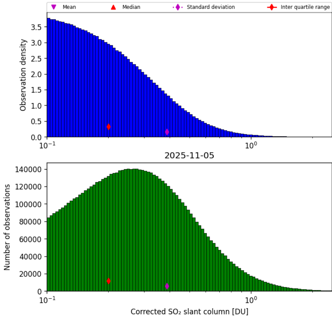
Figure 60: Histogram of “Corrected SO 2 slant column” for 2025-11-04 to 2025-11-06
