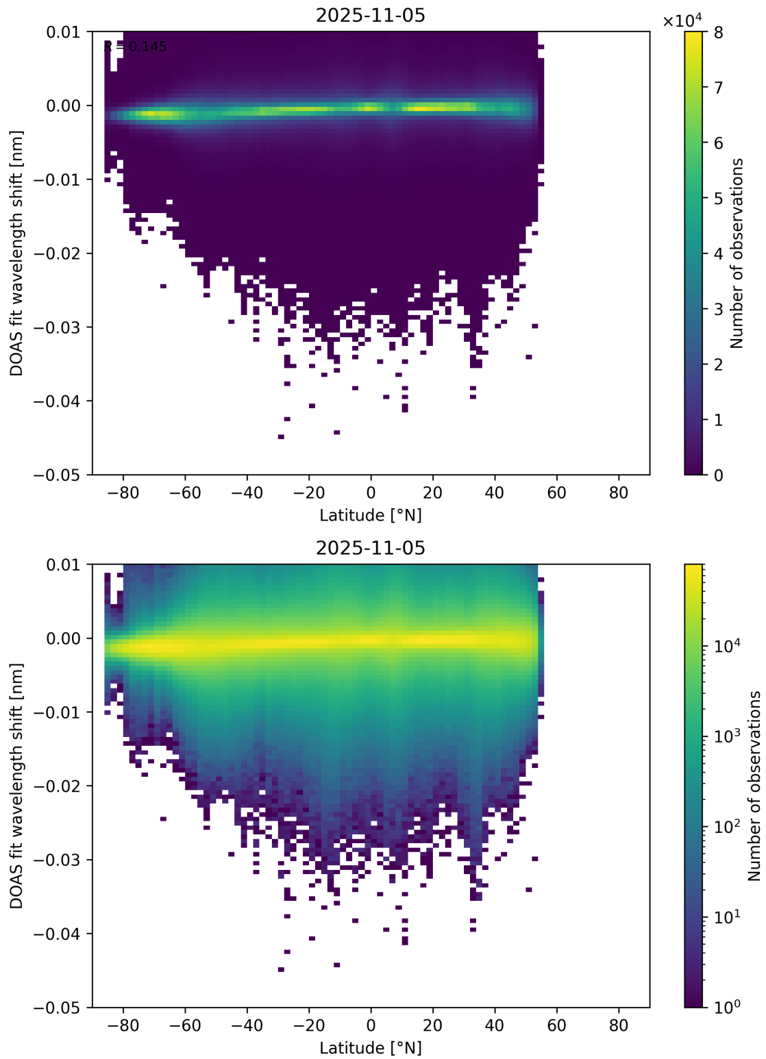
Figure 153: Scatter density plot of “Latitude” against “DOAS fit wavelength shift” for 2025-11-04 to 2025-11-06.
