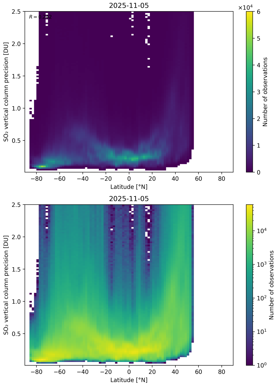
Figure 170: Scatter density plot of “Latitude” against “SO 2 vertical column precision” for 2025-11-04 to 2025-11-06.
