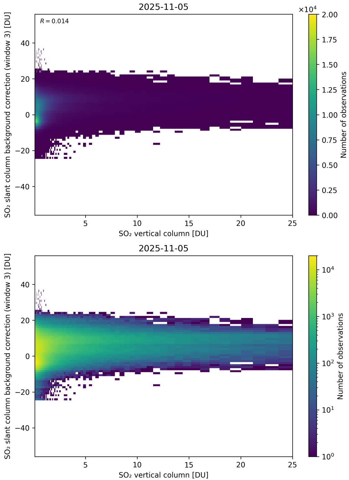
Figure 325: Scatter density plot of “SO 2 vertical column” against “SO 2 slant column background correction (window 3)” for 2025-11-04 to 2025-11-06.
