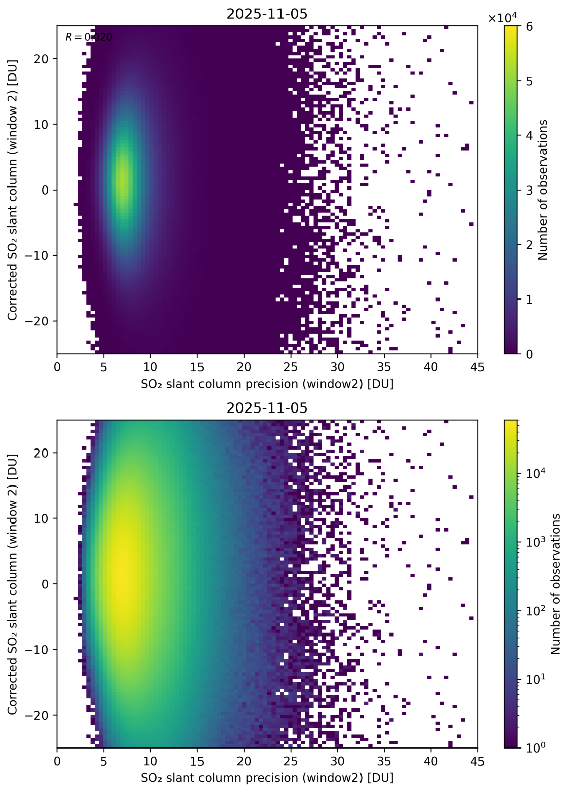
Figure 297: Scatter density plot of “SO 2 slant column precision (window2)” against “Corrected SO 2 slant column (window 2)” for 2025-11-04 to 2025-11-06.
