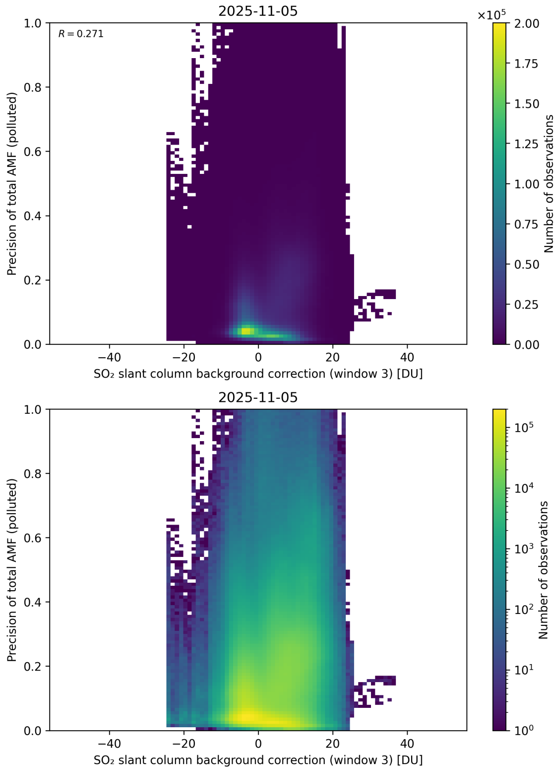
Figure 137: Scatter density plot of “SO 2 slant column background correction (window 3)” against “Precision of total AMF (polluted)” for 2025-11-04 to 2025-11-06.
