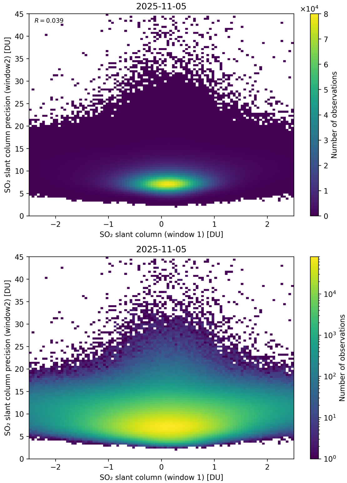
Figure 286: Scatter density plot of “SO 2 slant column (window 1)” against “SO 2 slant column precision (window2)” for 2025-11-04 to 2025-11-06.
