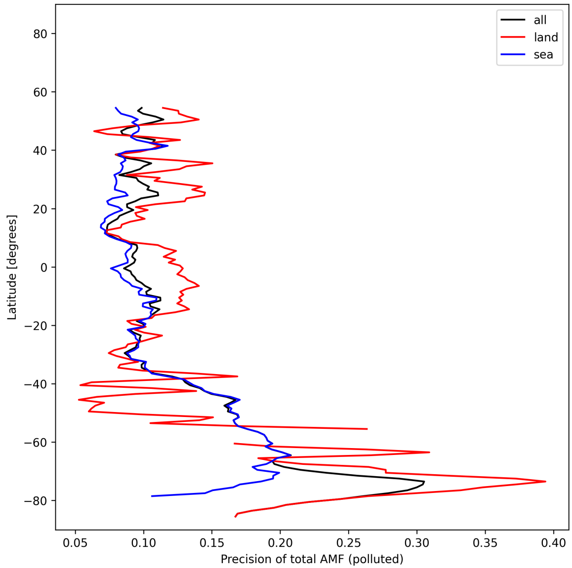
Figure 54: Zonal average of “Precision of total AMF (polluted)” for 2025-11-04 to 2025-11-06.
