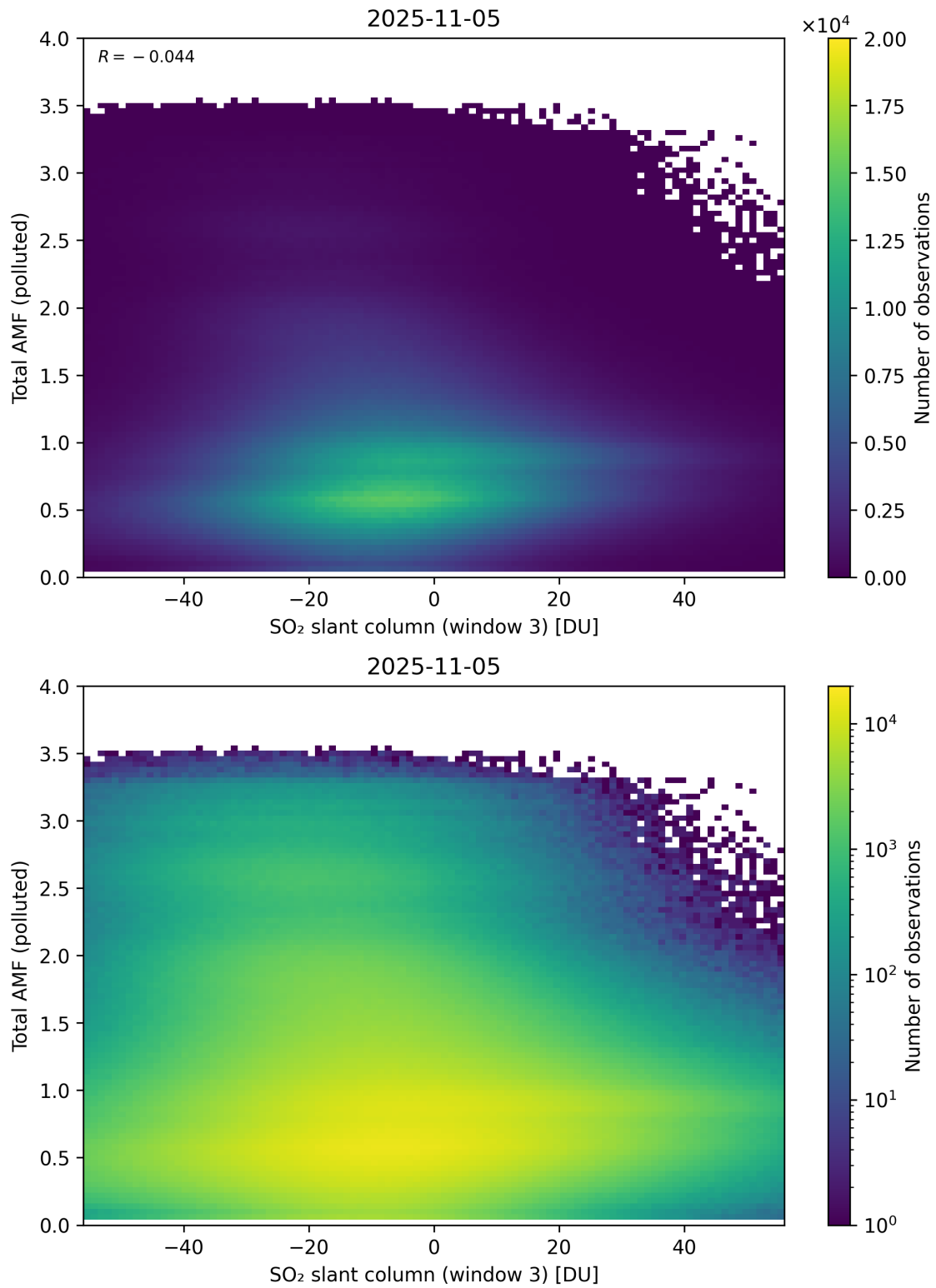
Figure 318: Scatter density plot of “SO 2 slant column (window 3)” against “Total AMF (polluted)” for 2025-11-04 to 2025-11-06.
