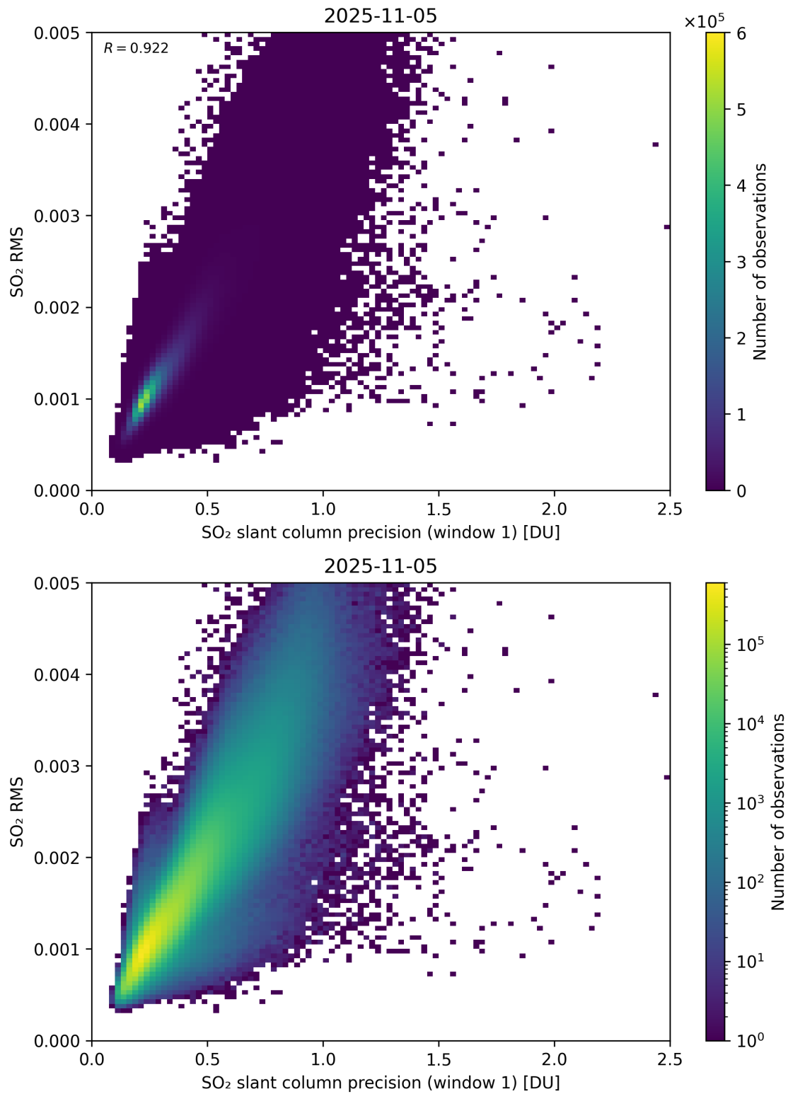
Figure 273: Scatter density plot of “SO 2 slant column precision (window 1)” against “SO 2 RMS” for 2025-11-04 to 2025-11-06.
