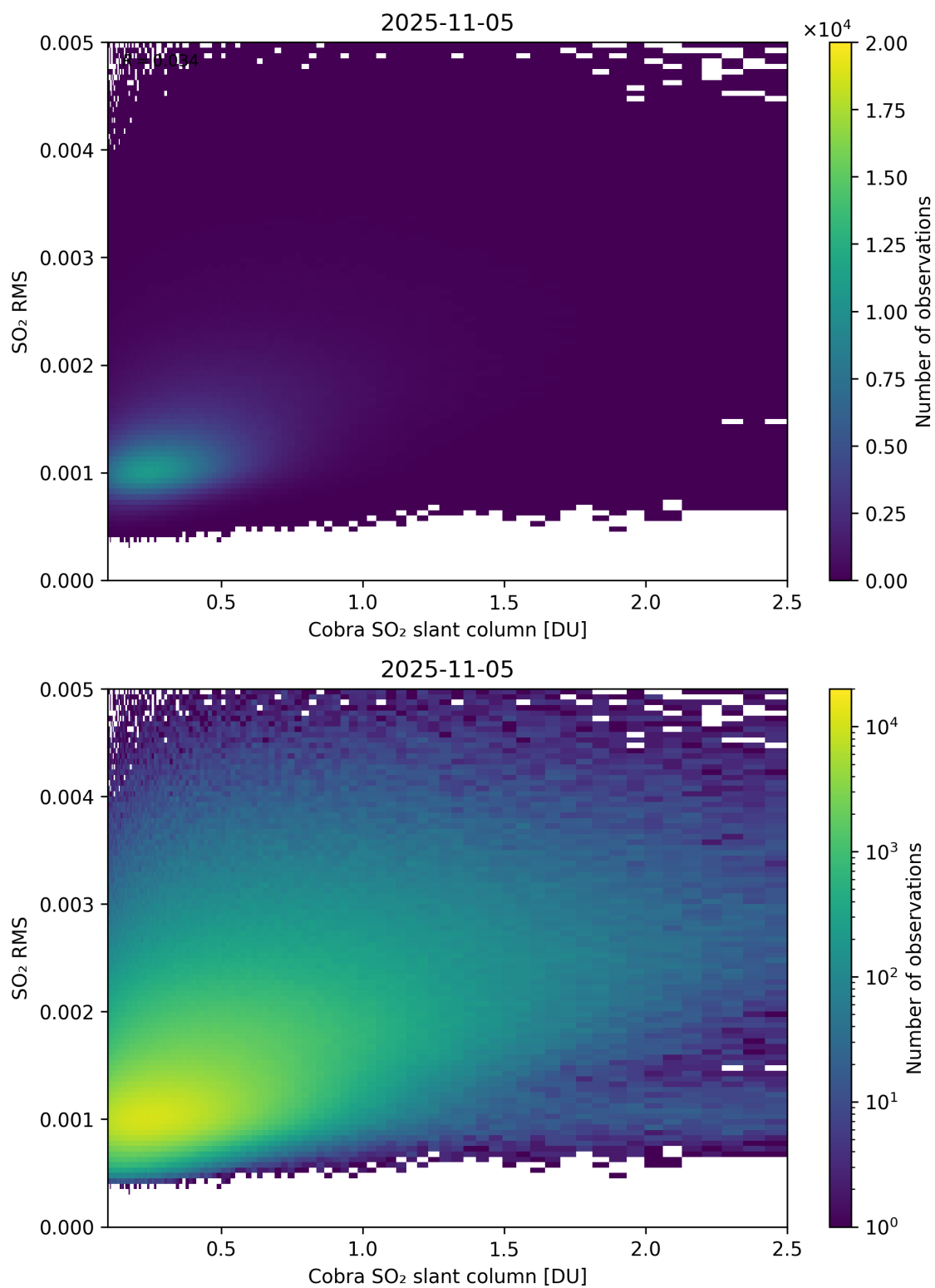
Figure 198: Scatter density plot of “Cobra SO 2 slant column” against “SO 2 RMS” for 2025-11-04 to 2025-11-06.
