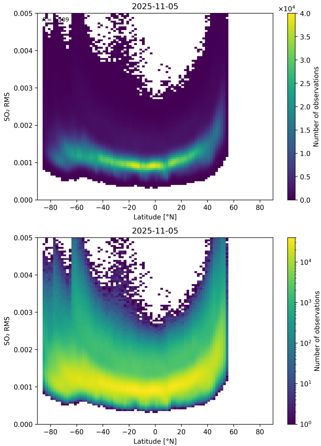
Figure 155: Scatter density plot of “Latitude” against “SO 2 RMS” for 2025-11-04 to 2025-11-06.
