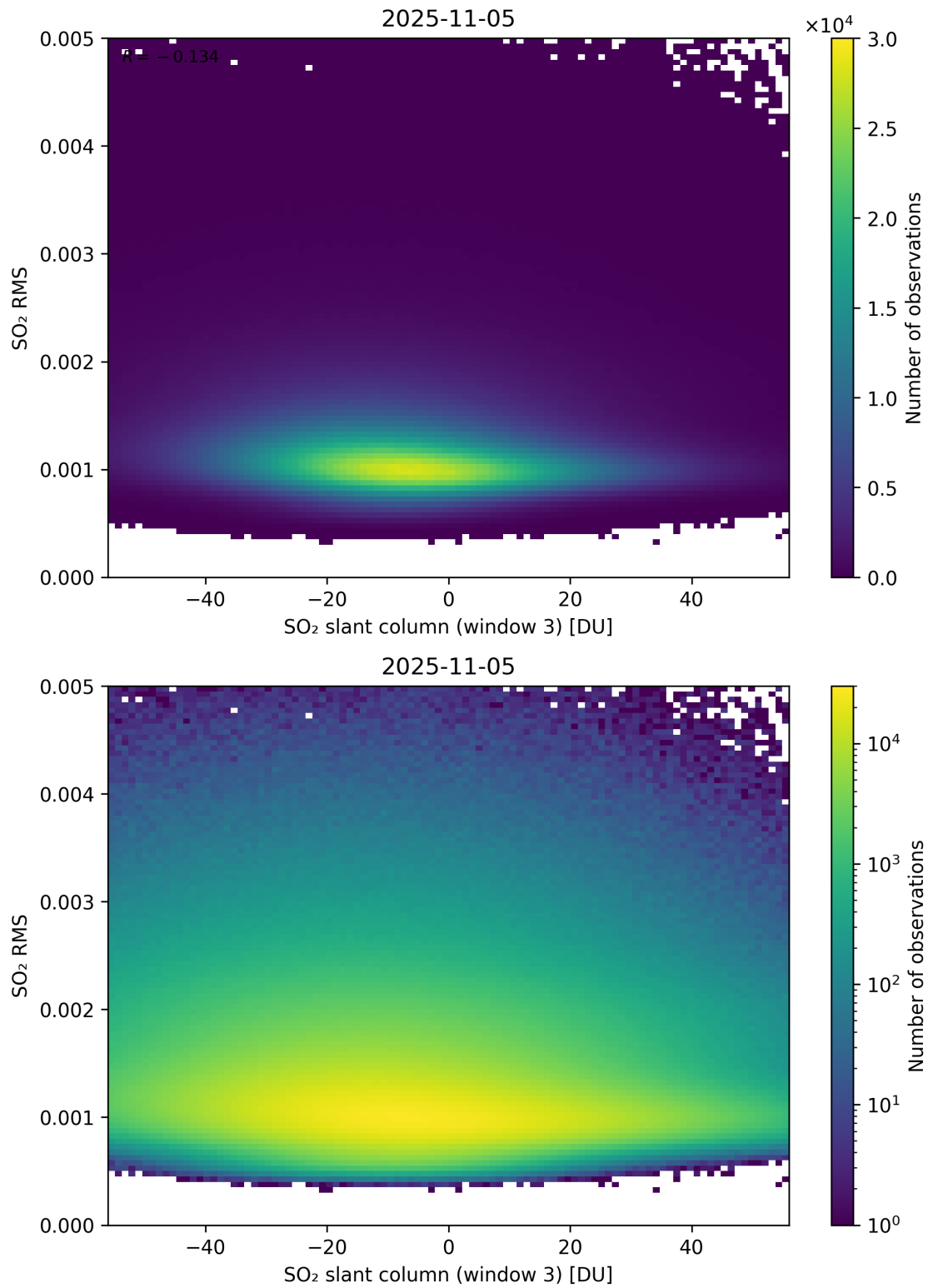
Figure 306: Scatter density plot of “SO 2 slant column (window 3)” against “SO 2 RMS” for 2025-11-04 to 2025-11-06.
