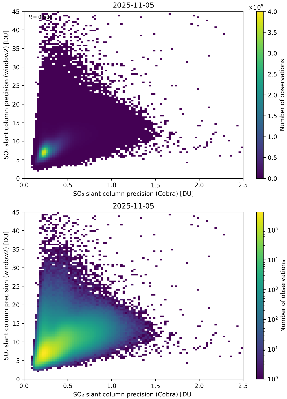
Figure 210: Scatter density plot of “SO 2 slant column precision (Cobra)” against “SO 2 slant column precision (window2)” for 2025-11-04 to 2025-11-06.
