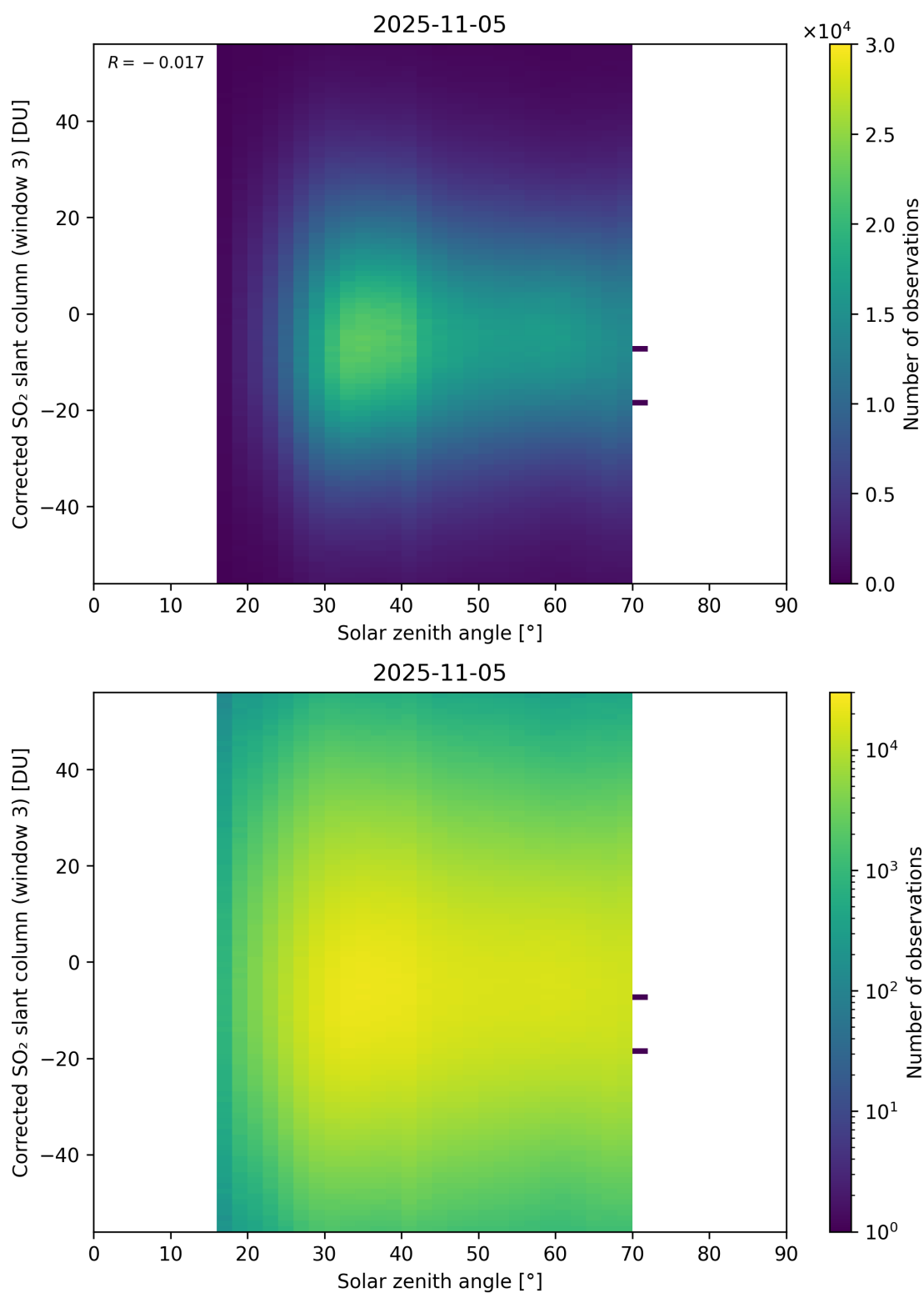
Figure 183: Scatter density plot of “Solar zenith angle” against “Corrected SO 2 slant column (window 3)” for 2025-11-04 to 2025-11-06.
