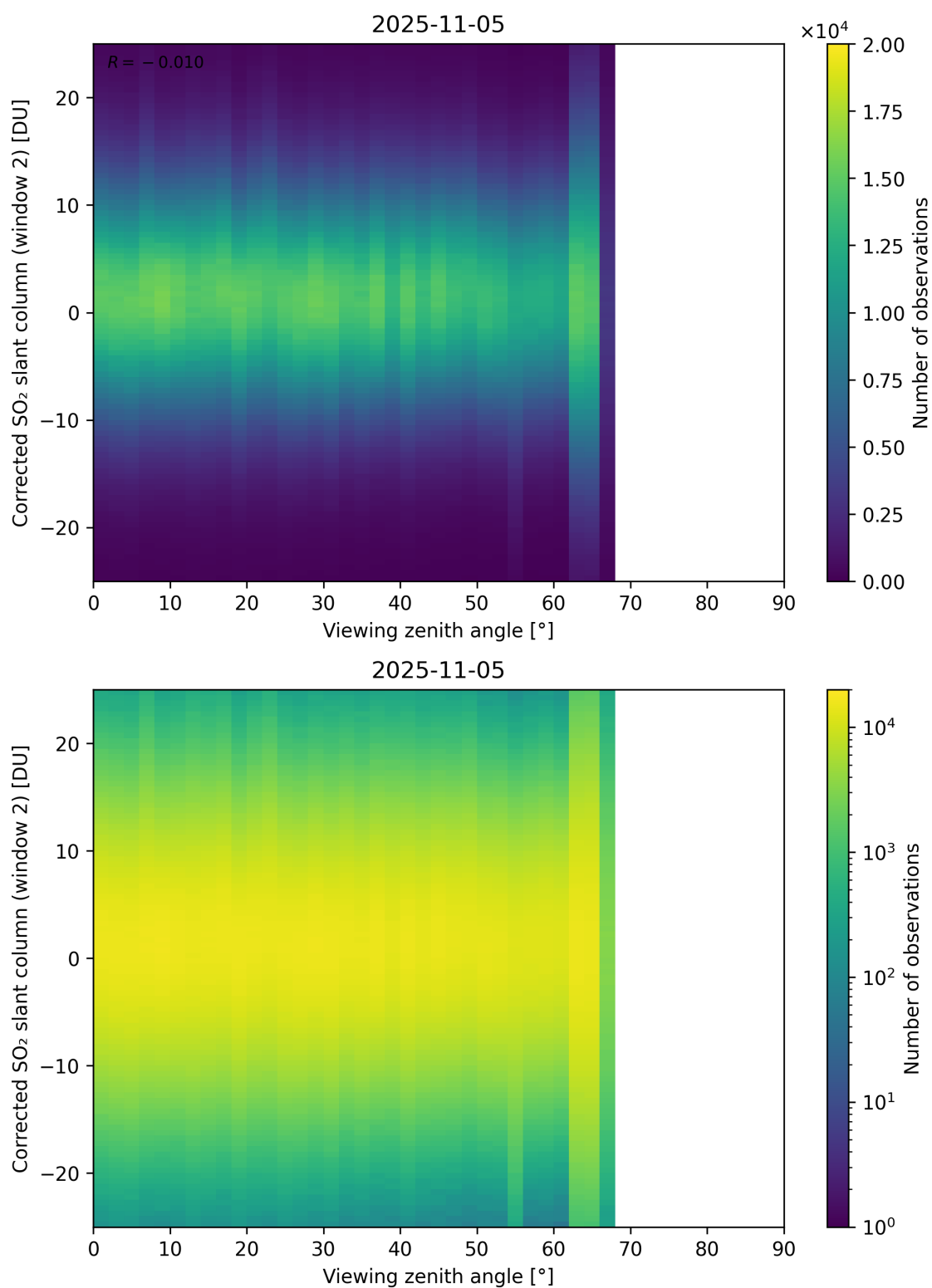
Figure 374: Scatter density plot of “Viewing zenith angle” against “Corrected SO 2 slant column (window 2)” for 2025-11-04 to 2025-11-06.
