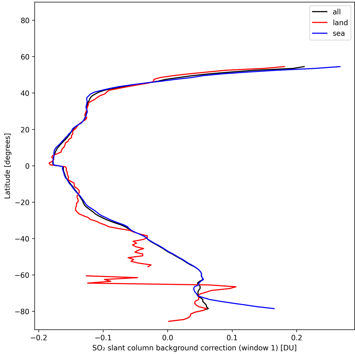
Figure 40: Zonal average of “SO 2 slant column background correction (window 1)” for 2025-11-04 to 2025-11-06.
