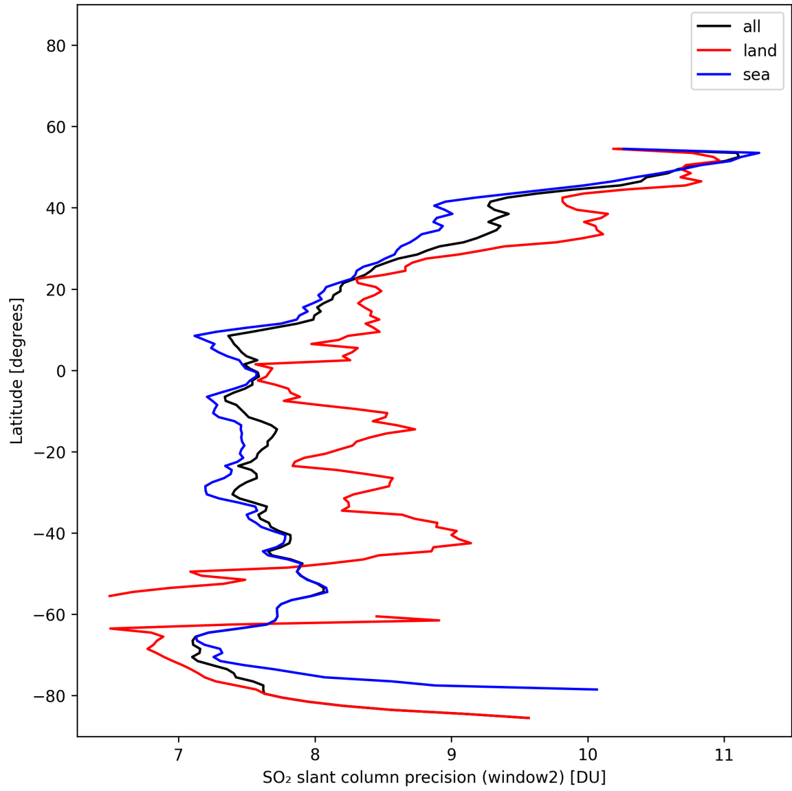
Figure 42: Zonal average of “SO 2 slant column precision (window2)” for 2025-11-04 to 2025-11-06.
