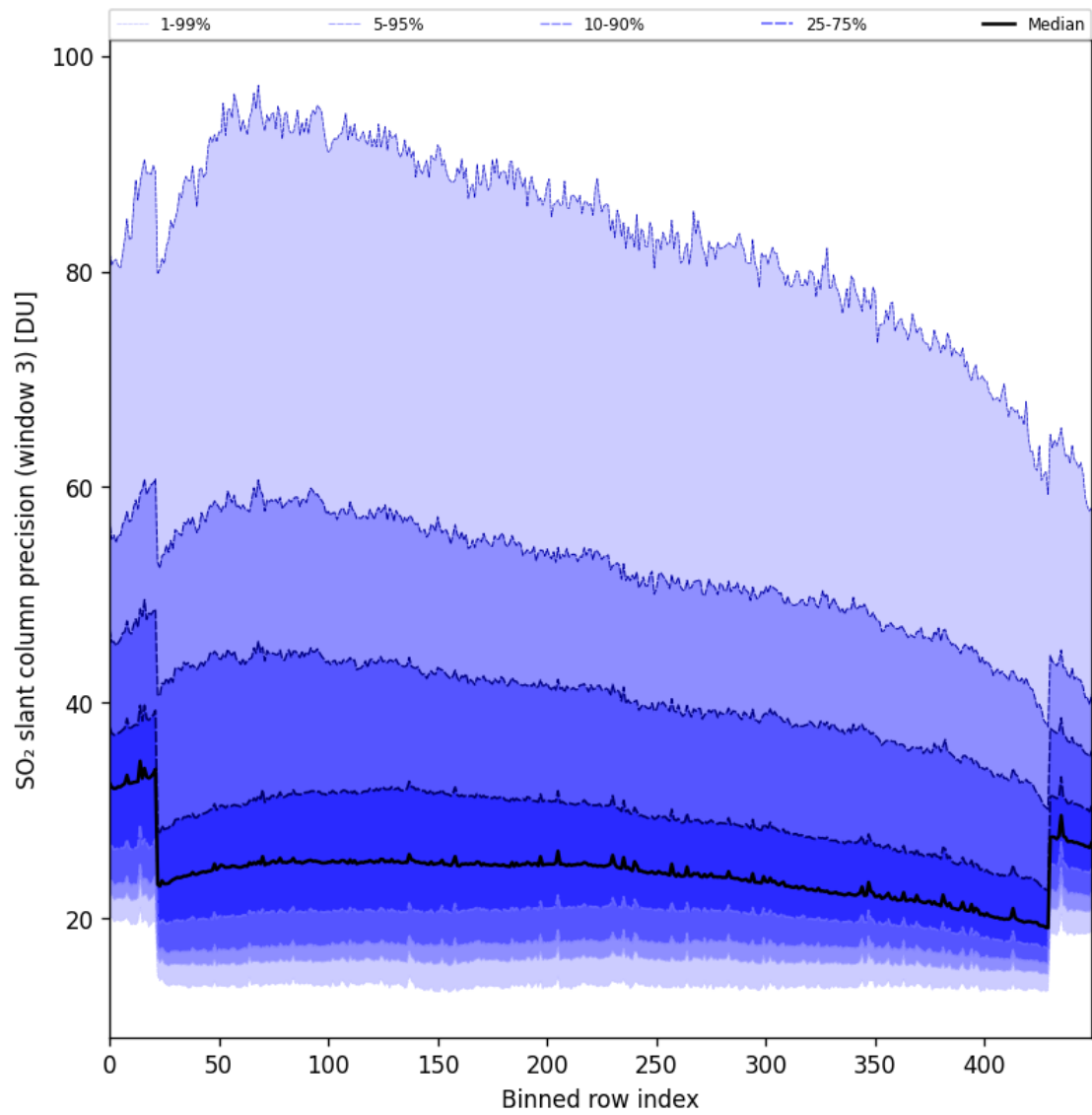
Figure 98: Along track statistics of “SO 2 slant column precision (window 3)” for 2025-11-04 to 2025-11-06
