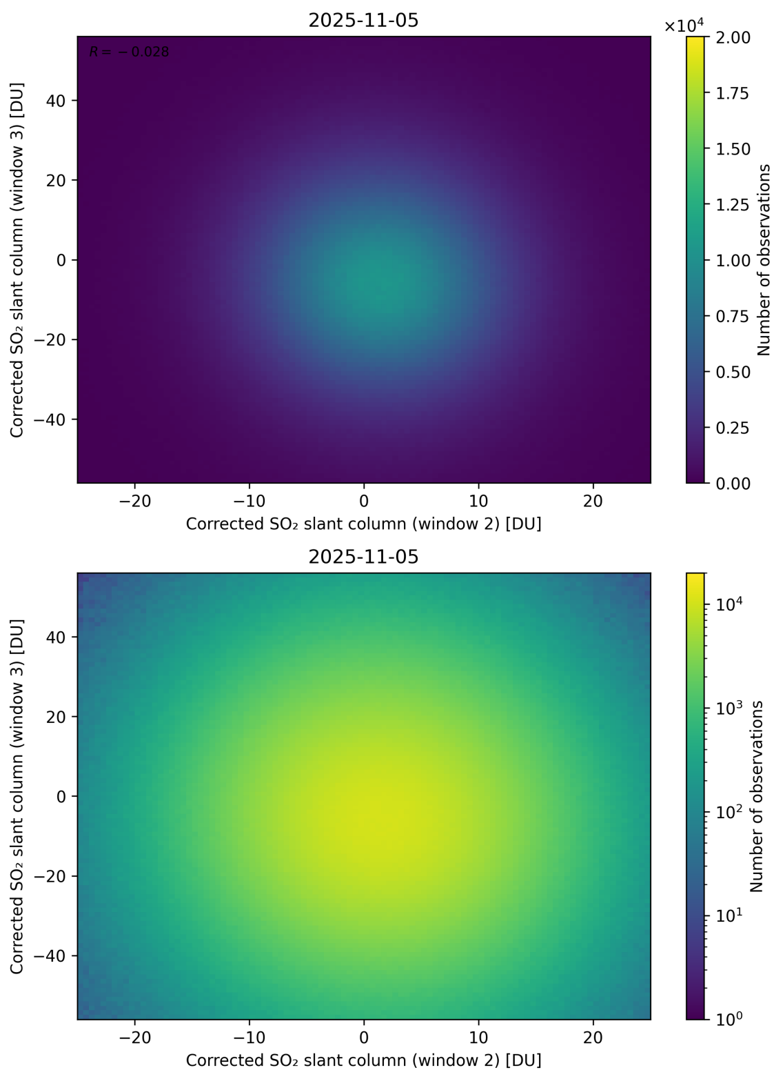
Figure 250: Scatter density plot of “Corrected SO 2 slant column (window 2)” against “Corrected SO 2 slant column (window 3)” for 2025-11-04 to 2025-11-06.
