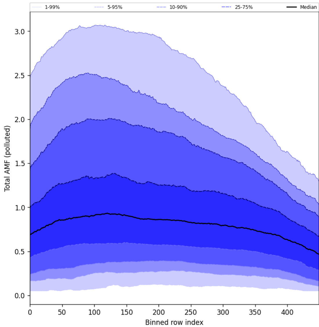
Figure 105: Along track statistics of “Total AMF (polluted)” for 2025-11-04 to 2025-11-06
