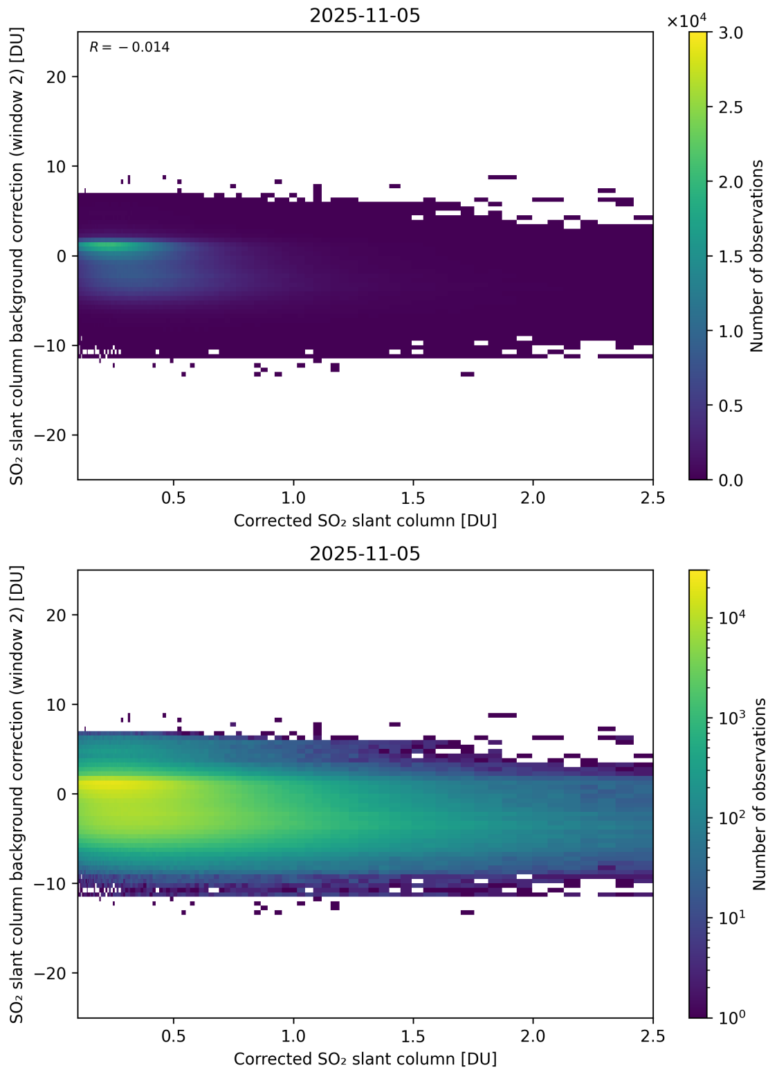
Figure 227: Scatter density plot of “Corrected SO 2 slant column” against “SO 2 slant column background correction (window 2)” for 2025-11-04 to 2025-11-06.
