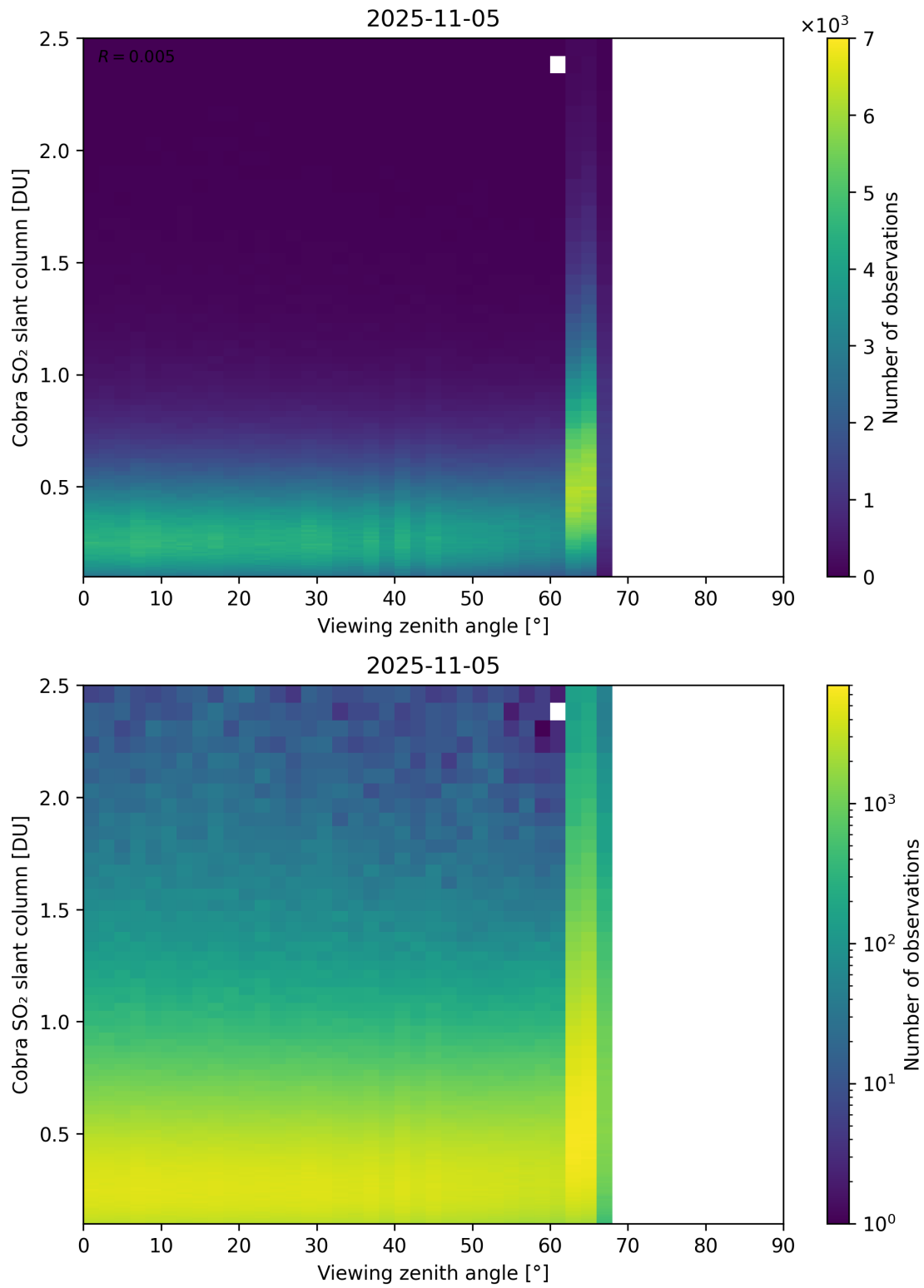
Figure 371: Scatter density plot of “Viewing zenith angle” against “Cobra SO 2 slant column” for 2025-11-04 to 2025-11-06.
