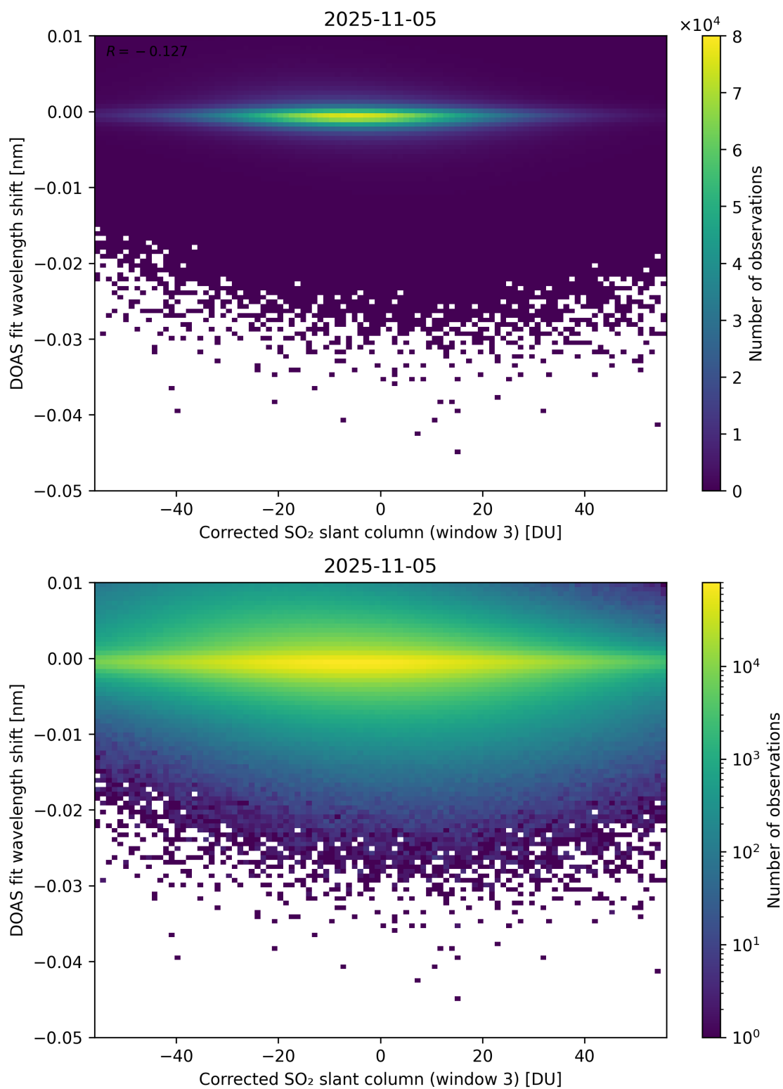
Figure 256: Scatter density plot of “Corrected SO 2 slant column (window 3)” against “DOAS fit wavelength shift” for 2025-11-04 to 2025-11-06.
