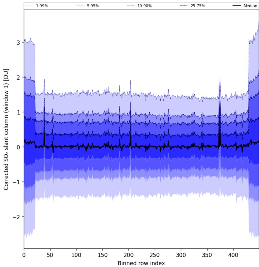
Figure 91: Along track statistics of “Corrected SO 2 slant column (window 1)” for 2025-11-04 to 2025-11-06
