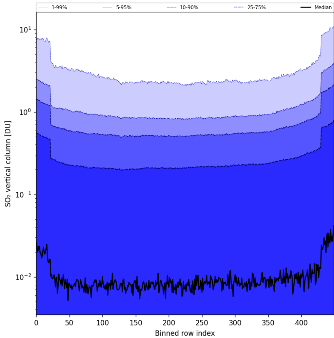
Figure 84: Along track statistics of “SO 2 vertical column” for 2025-11-04 to 2025-11-06
