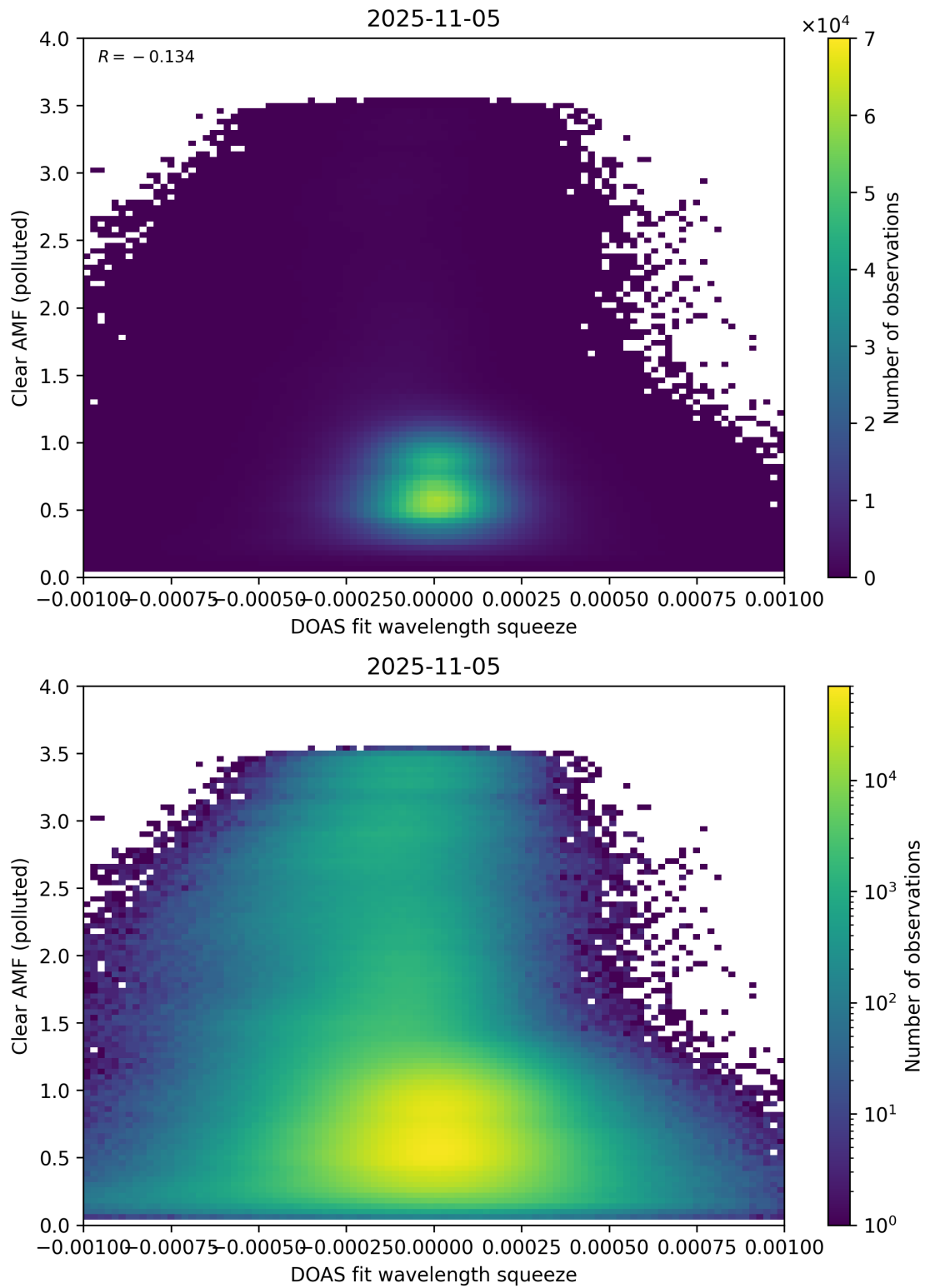
Figure 144: Scatter density plot of “DOAS fit wavelength squeeze” against “Clear AMF (polluted)” for 2025-11-04 to 2025-11-06.
