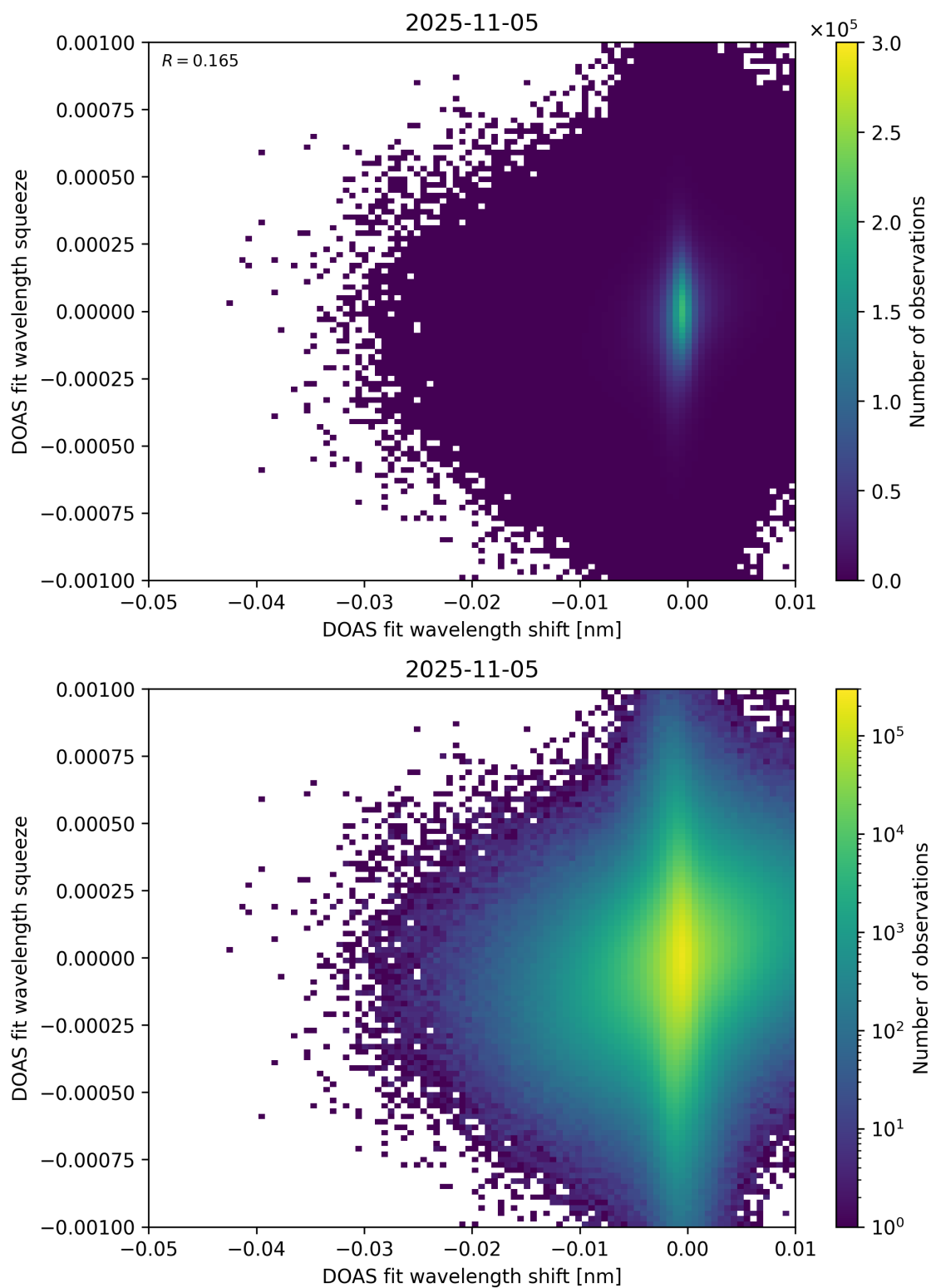
Figure 138: Scatter density plot of “DOAS fit wavelength shift” against “DOAS fit wavelength squeeze” for 2025-11-04 to 2025-11-06.
