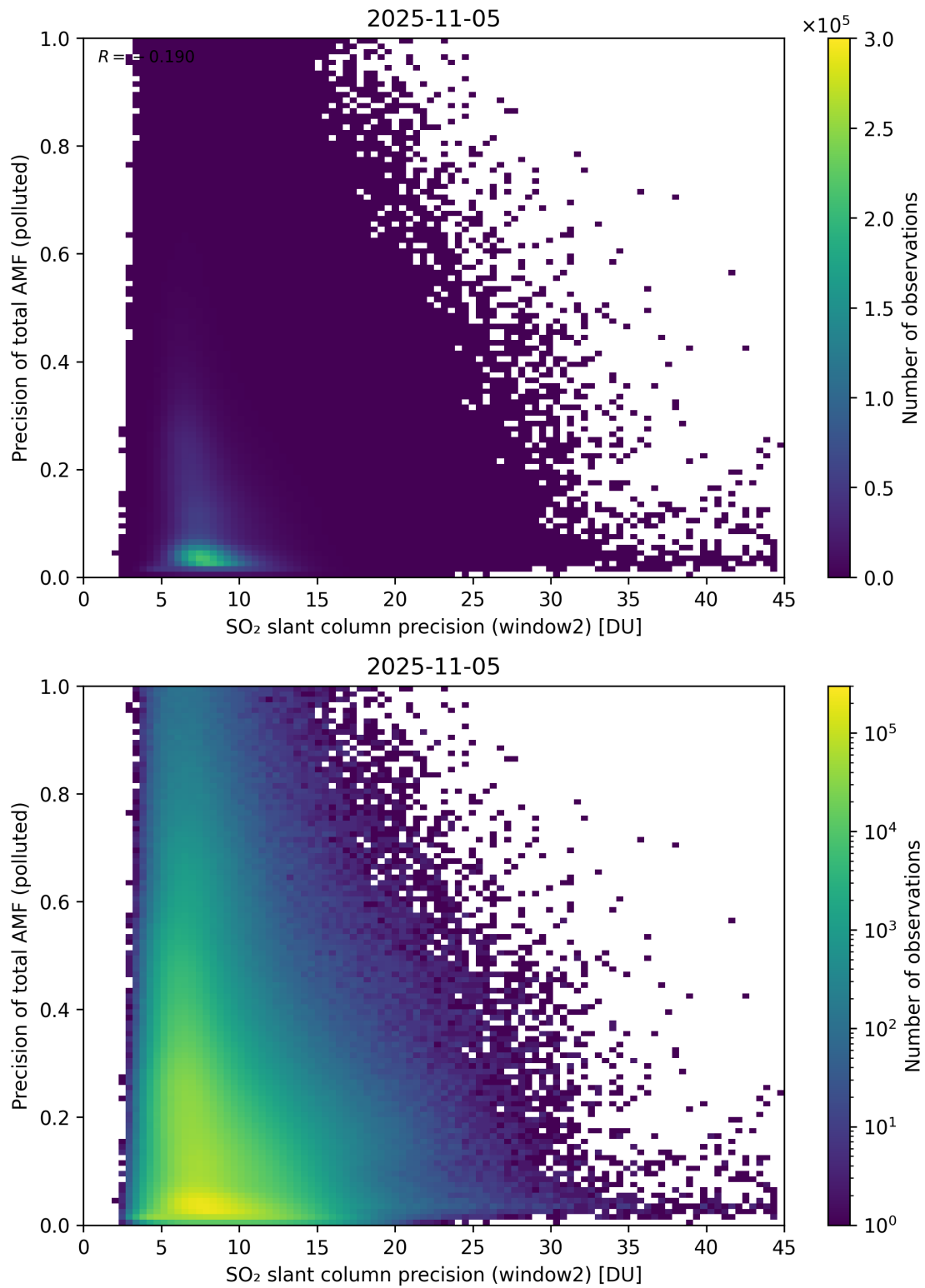
Figure 302: Scatter density plot of “SO 2 slant column precision (window2)” against “Precision of total AMF (polluted)” for 2025-11-04 to 2025-11-06.
