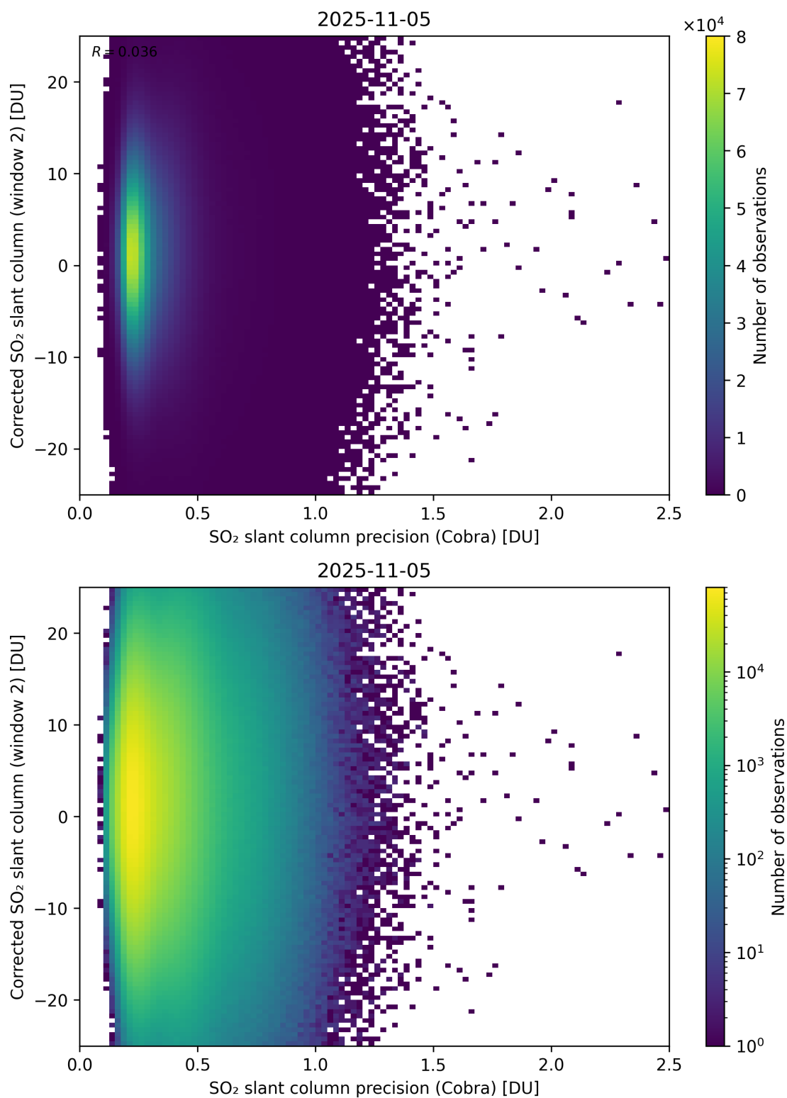
Figure 206: Scatter density plot of “SO 2 slant column precision (Cobra)” against “Corrected SO 2 slant column (window 2)” for 2025-11-04 to 2025-11-06.
