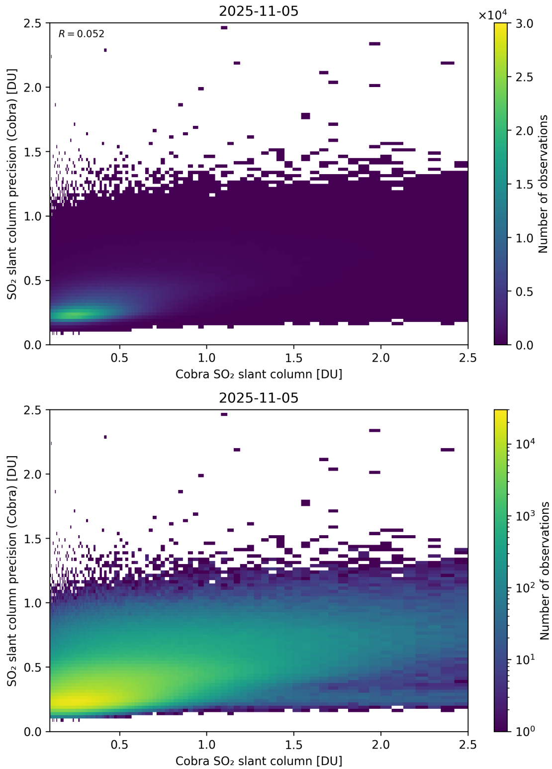
Figure 216: Scatter density plot of “Cobra SO 2 slant column” against “SO 2 slant column precision (Cobra)” for 2025-11-04 to 2025-11-06.
