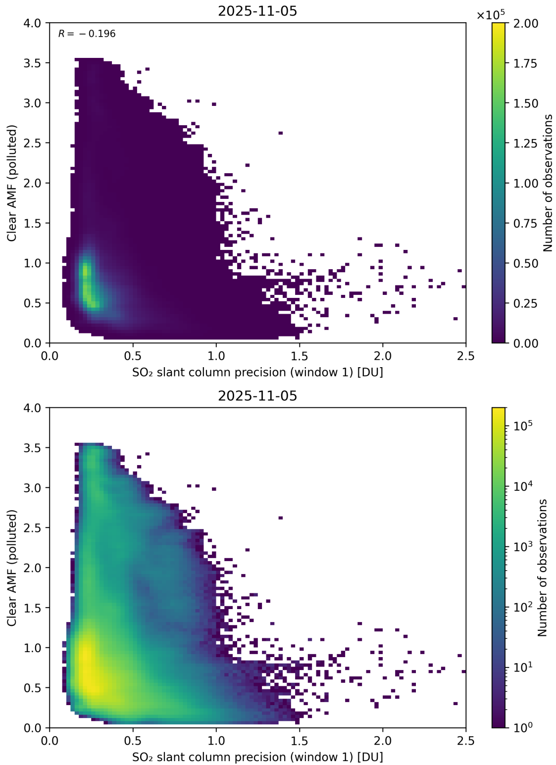
Figure 274: Scatter density plot of “SO 2 slant column precision (window 1)” against “Clear AMF (polluted)” for 2025-11-04 to 2025-11-06.
