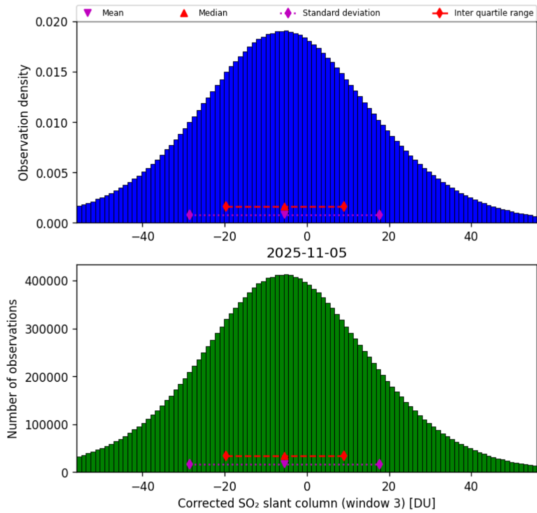
Figure 73: Histogram of “Corrected SO 2 slant column (window 3)” for 2025-11-04 to 2025-11-06
