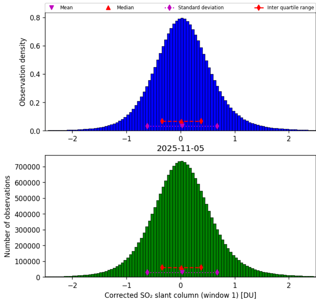
Figure 65: Histogram of “Corrected SO 2 slant column (window 1)” for 2025-11-04 to 2025-11-06
