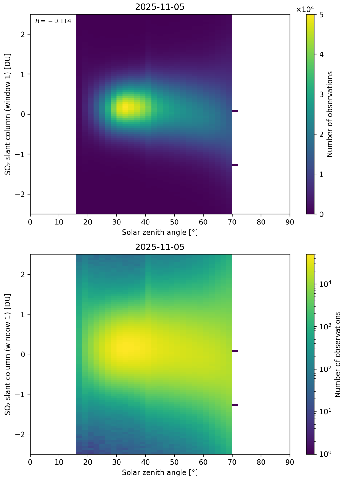
Figure 184: Scatter density plot of “Solar zenith angle” against “SO 2 slant column (window 1)” for 2025-11-04 to 2025-11-06.
