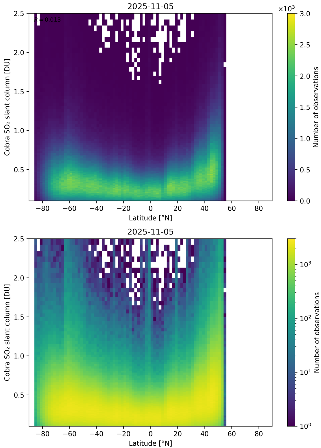
Figure 157: Scatter density plot of “Latitude” against “Cobra SO 2 slant column” for 2025-11-04 to 2025-11-06.
