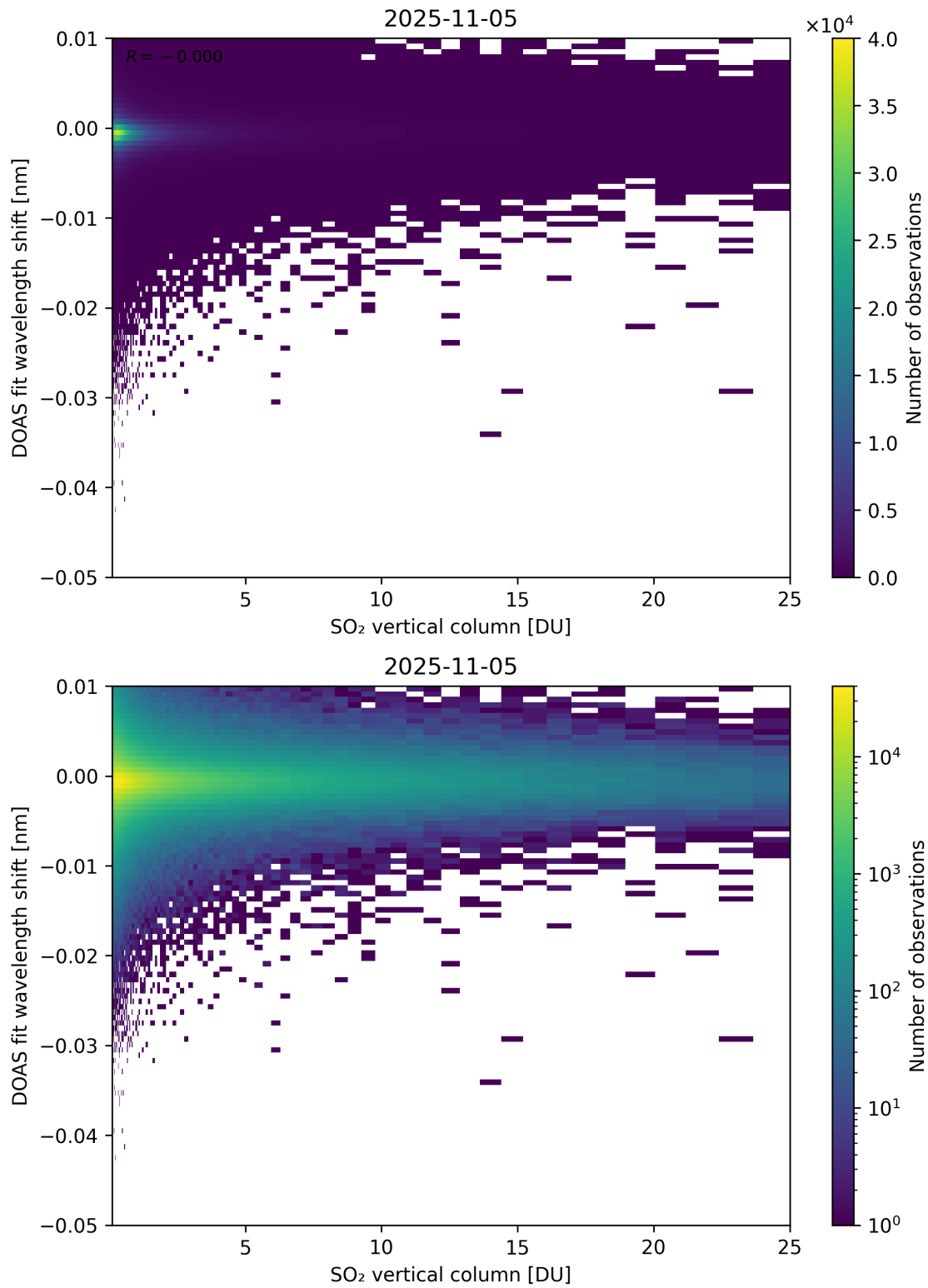
Figure 326: Scatter density plot of “SO 2 vertical column” against “DOAS fit wavelength shift” for 2025-11-04 to 2025-11-06.
