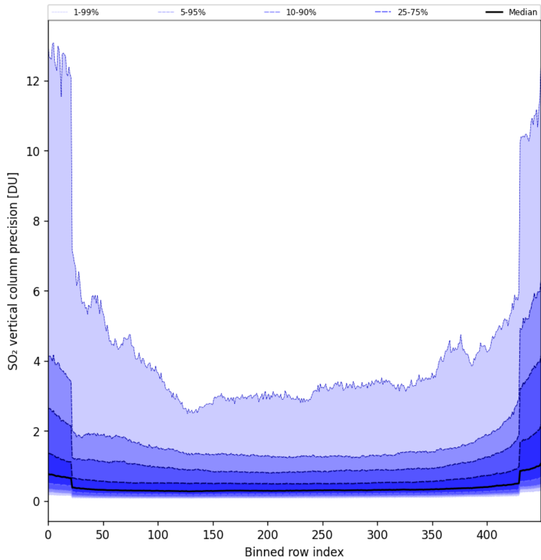
Figure 85: Along track statistics of “SO 2 vertical column precision” for 2025-11-04 to 2025-11-06
