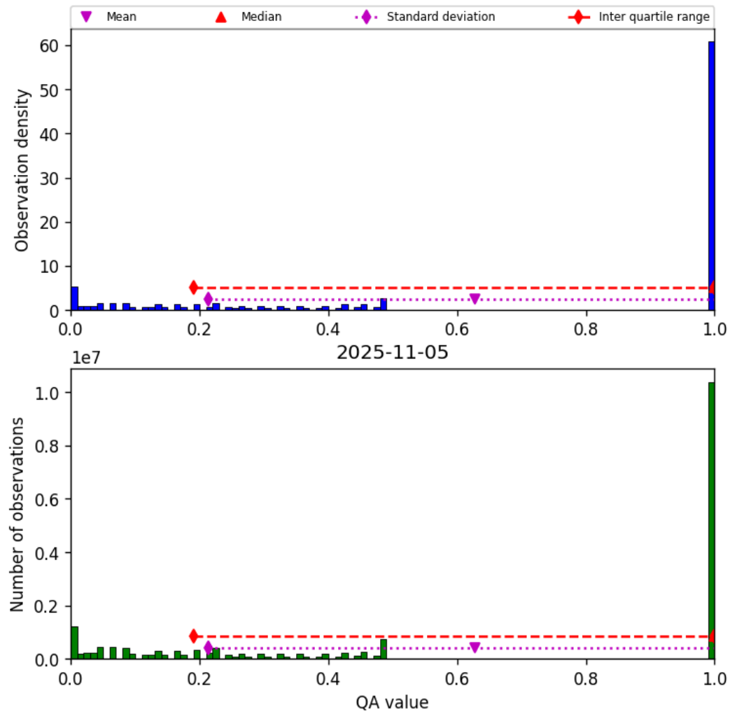
Figure 57: Histogram of “QA value” for 2025-11-04 to 2025-11-06
