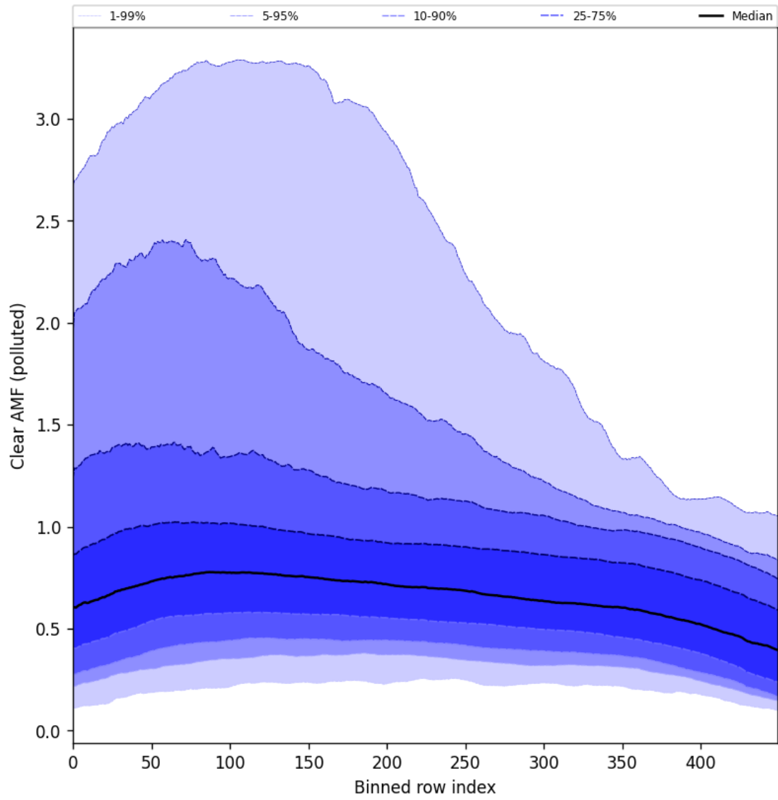
Figure 107: Along track statistics of “Clear AMF (polluted)” for 2025-11-04 to 2025-11-06
