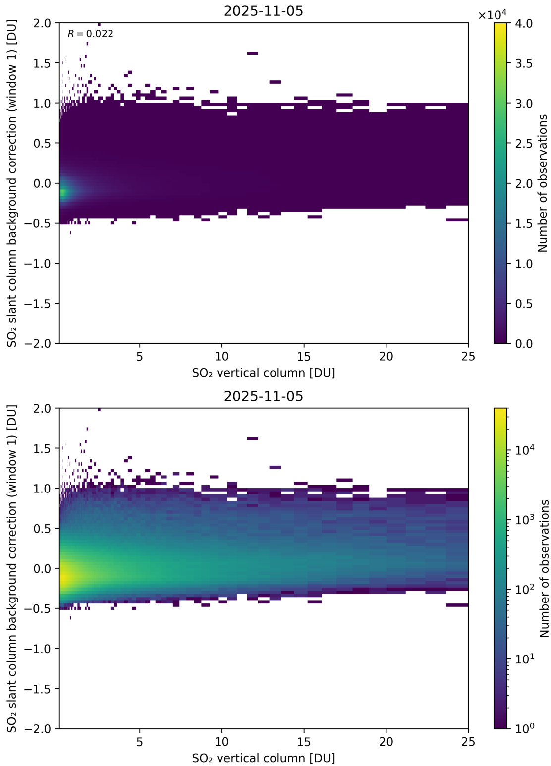
Figure 323: Scatter density plot of “SO 2 vertical column” against “SO 2 slant column background correction (window 1)” for 2025-11-04 to 2025-11-06.
