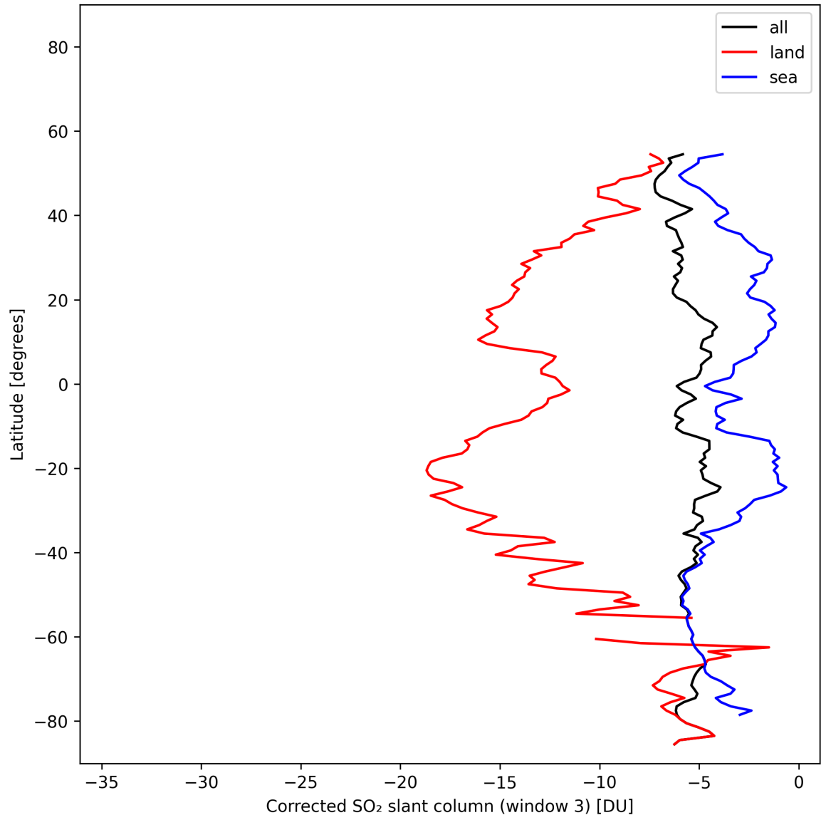
Figure 47: Zonal average of “Corrected SO 2 slant column (window 3)” for 2025-11-04 to 2025-11-06.
