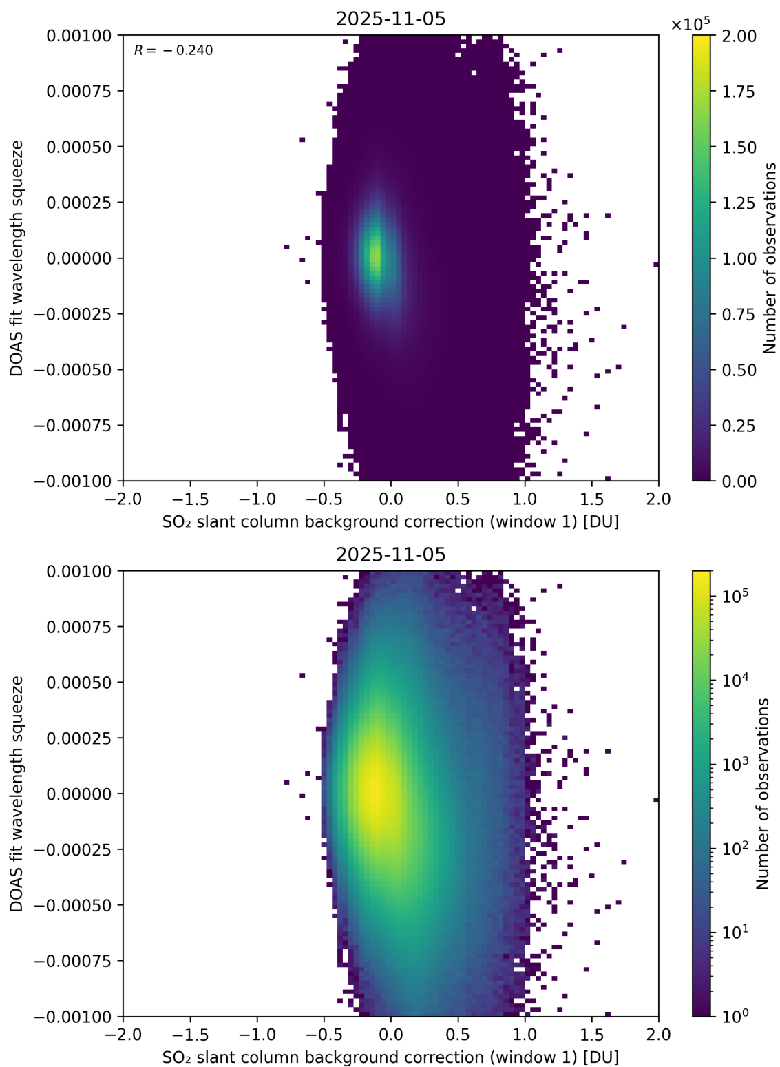
Figure 112: Scatter density plot of “SO 2 slant column background correction (window 1)” against “DOAS fit wavelength squeeze” for 2025-11-04 to 2025-11-06.
