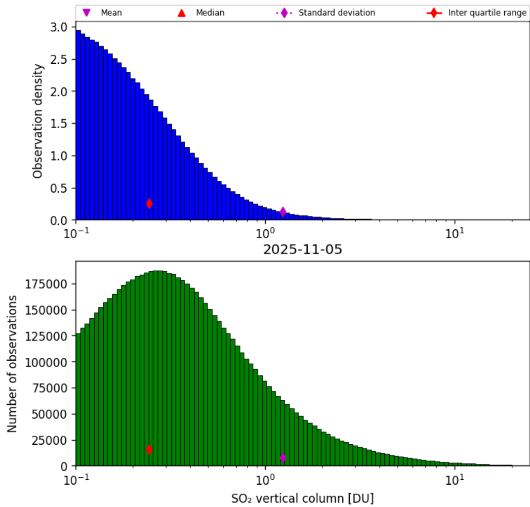
Figure 58: Histogram of “SO 2 vertical column” for 2025-11-04 to 2025-11-06
