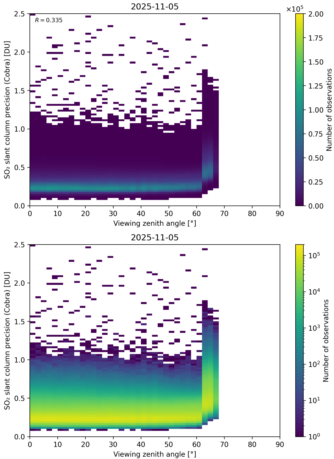
Figure 372: Scatter density plot of “Viewing zenith angle” against “SO 2 slant column precision (Cobra)” for 2025-11-04 to 2025-11-06.
