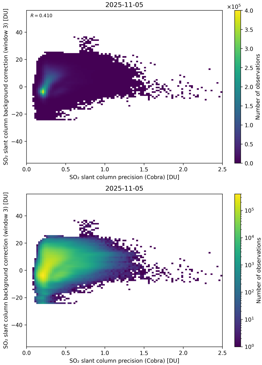
Figure 201: Scatter density plot of “SO 2 slant column precision (Cobra)” against “SO 2 slant column background correction (window 3)” for 2025-11-04 to 2025-11-06.
