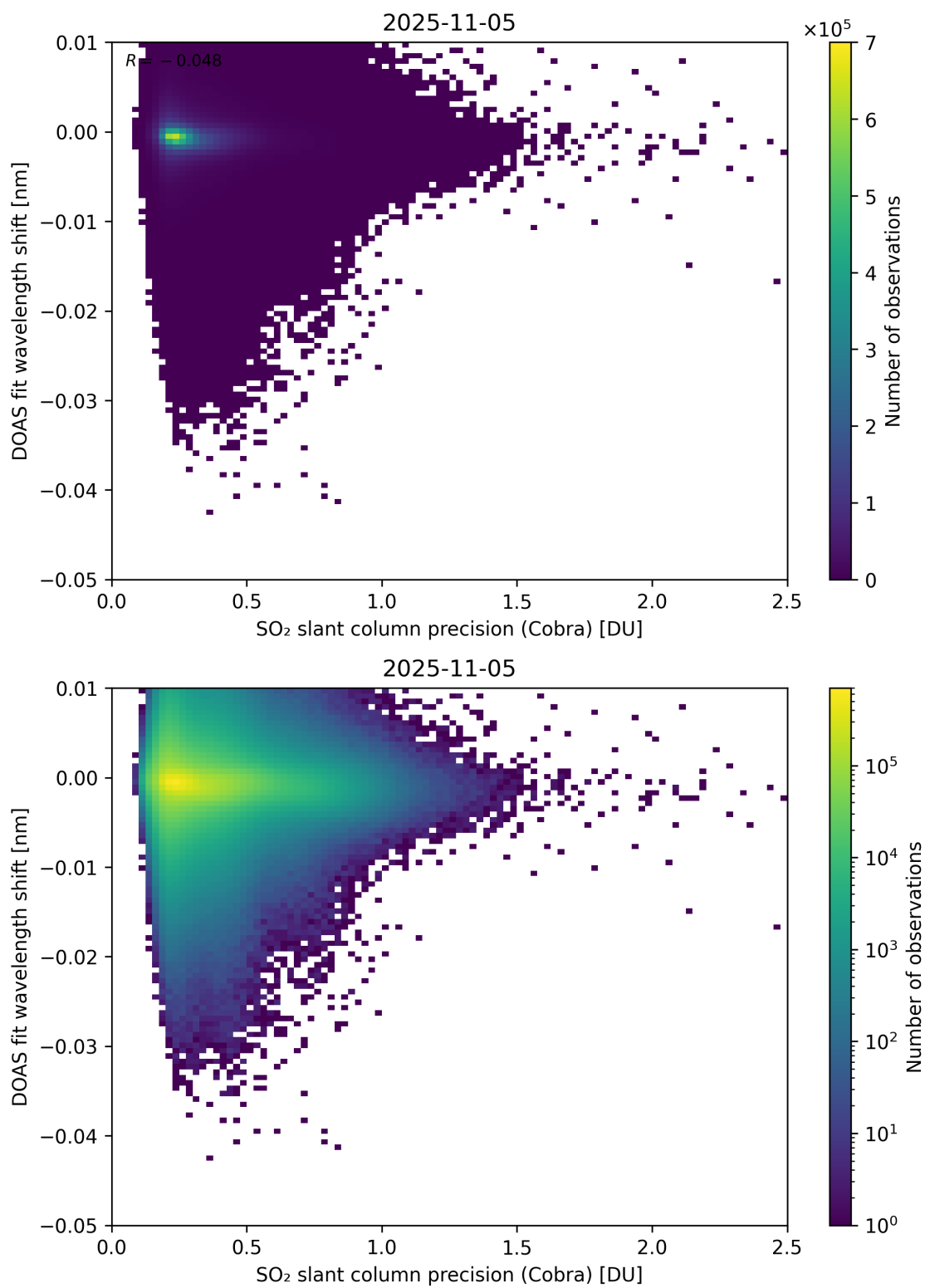
Figure 202: Scatter density plot of “SO 2 slant column precision (Cobra)” against “DOAS fit wavelength shift” for 2025-11-04 to 2025-11-06.
