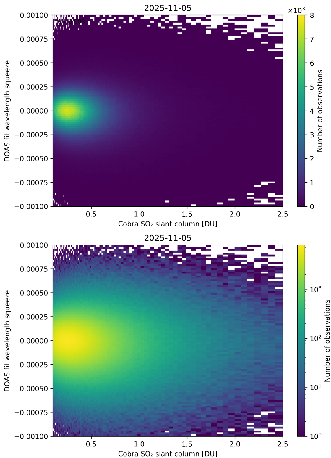
Figure 197: Scatter density plot of “Cobra SO 2 slant column” against “DOAS fit wavelength squeeze” for 2025-11-04 to 2025-11-06.
