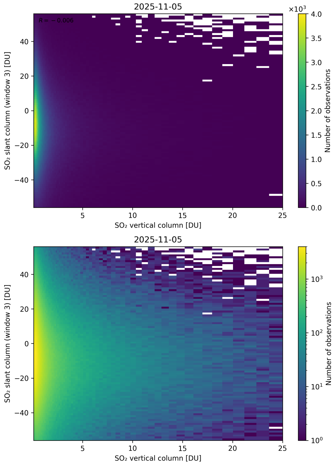
Figure 357: Scatter density plot of “SO 2 vertical column” against “SO 2 slant column (window 3)” for 2025-11-04 to 2025-11-06.
