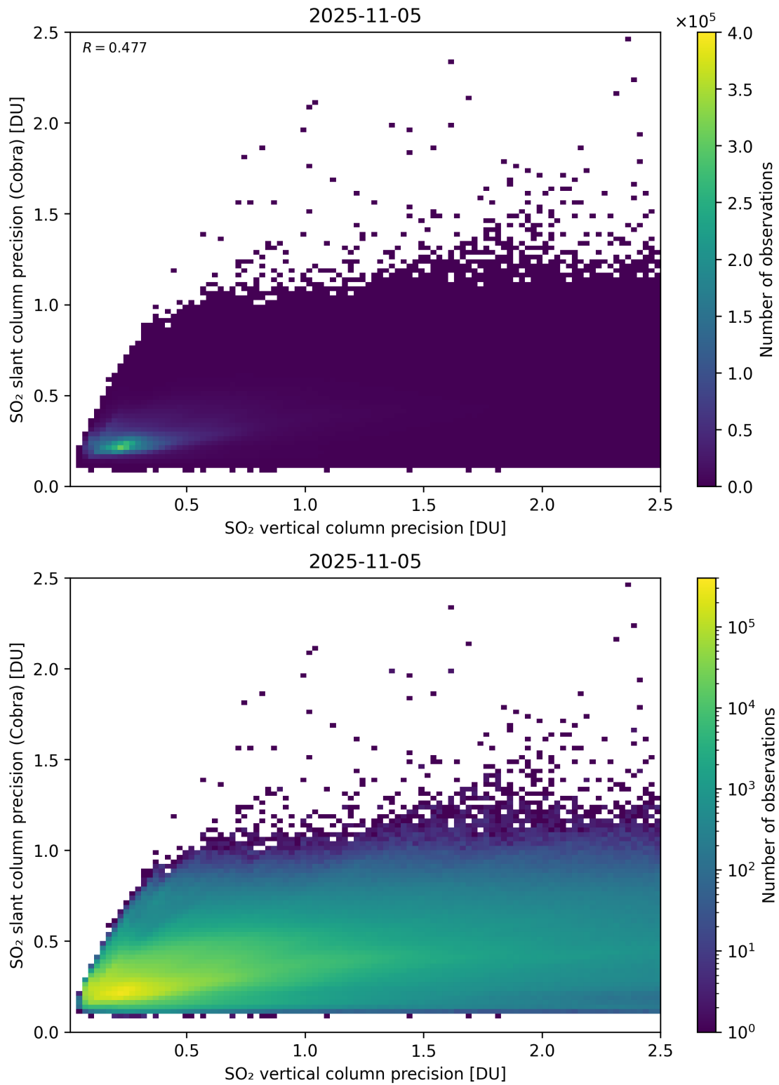
Figure 337: Scatter density plot of “SO 2 vertical column precision” against “SO 2 slant column precision (Cobra)” for 2025-11-04 to 2025-11-06.
