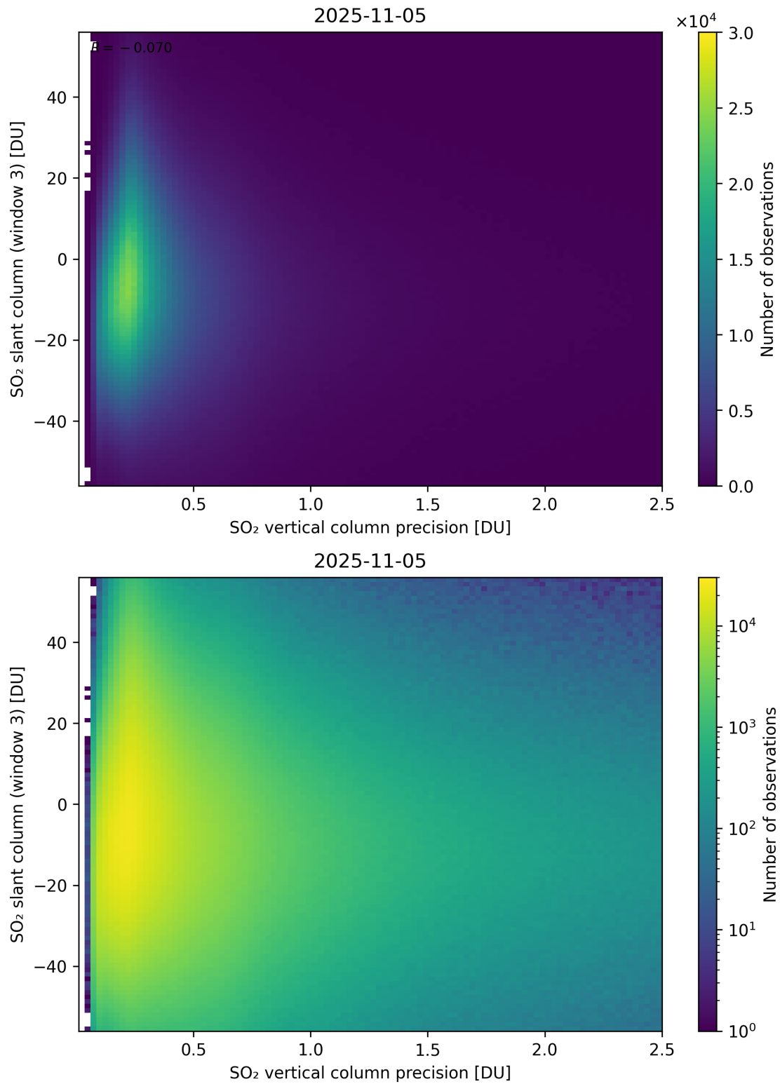
Figure 344: Scatter density plot of “SO 2 vertical column precision” against “SO 2 slant column (window 3)” for 2025-11-04 to 2025-11-06.
