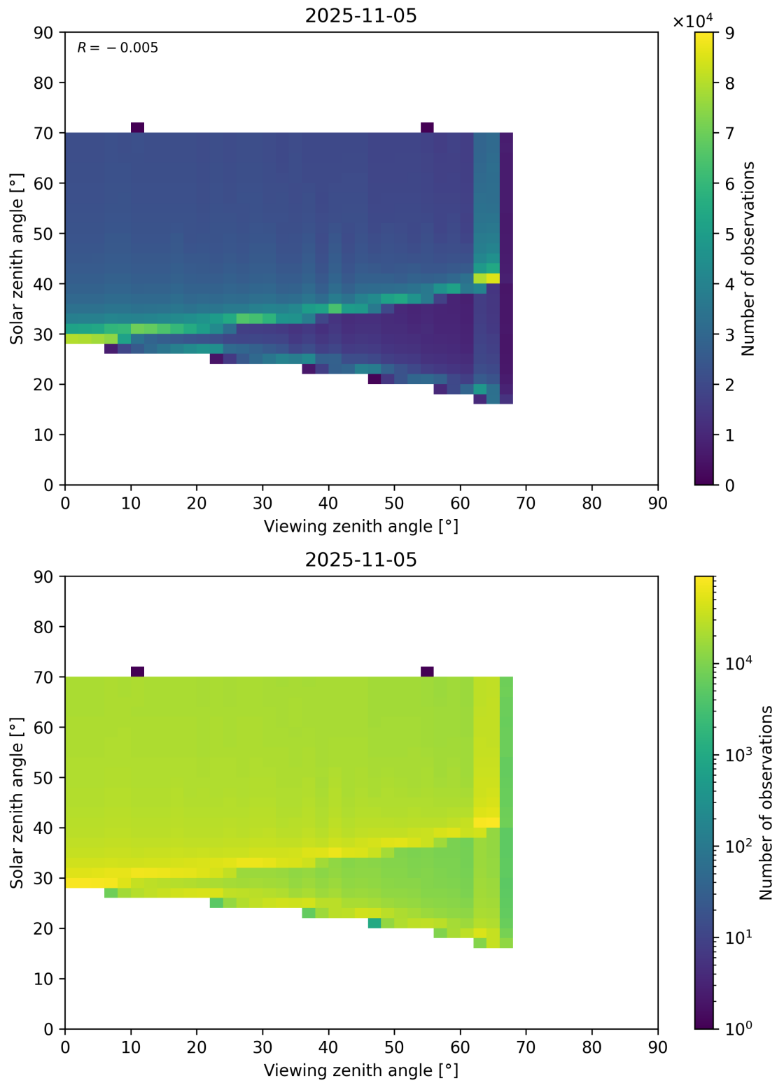
Figure 369: Scatter density plot of “Viewing zenith angle” against “Solar zenith angle” for 2025-11-04 to 2025-11-06.
