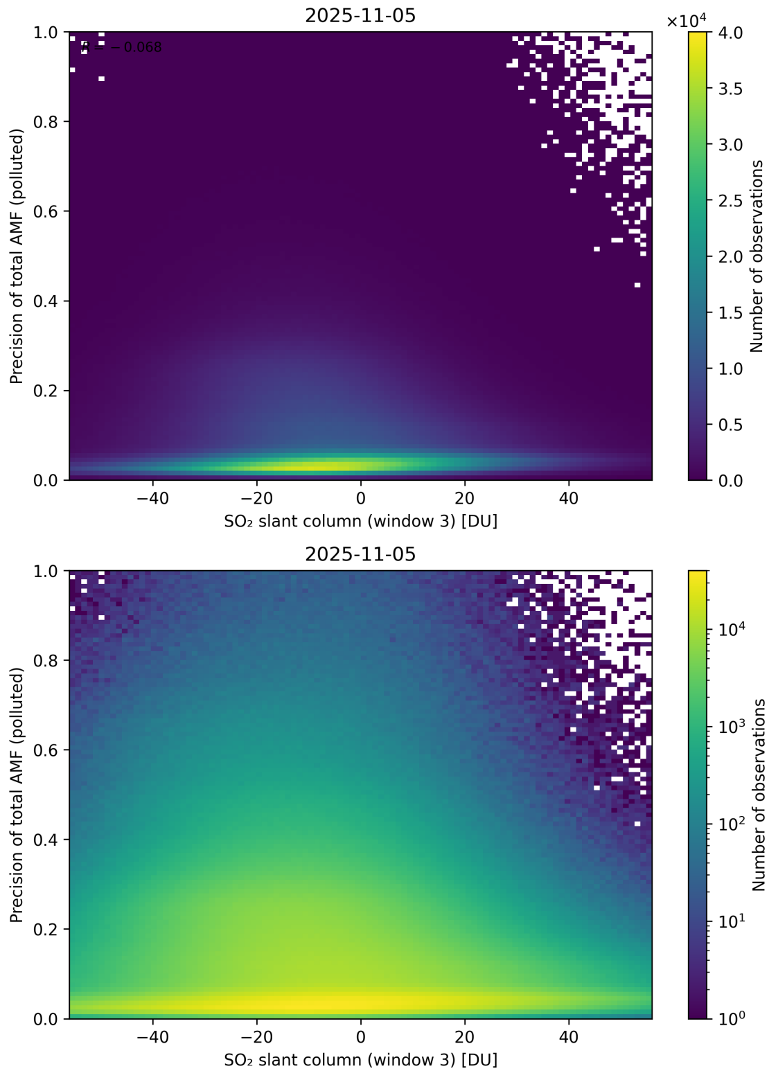
Figure 319: Scatter density plot of “SO 2 slant column (window 3)” against “Precision of total AMF (polluted)” for 2025-11-04 to 2025-11-06.
