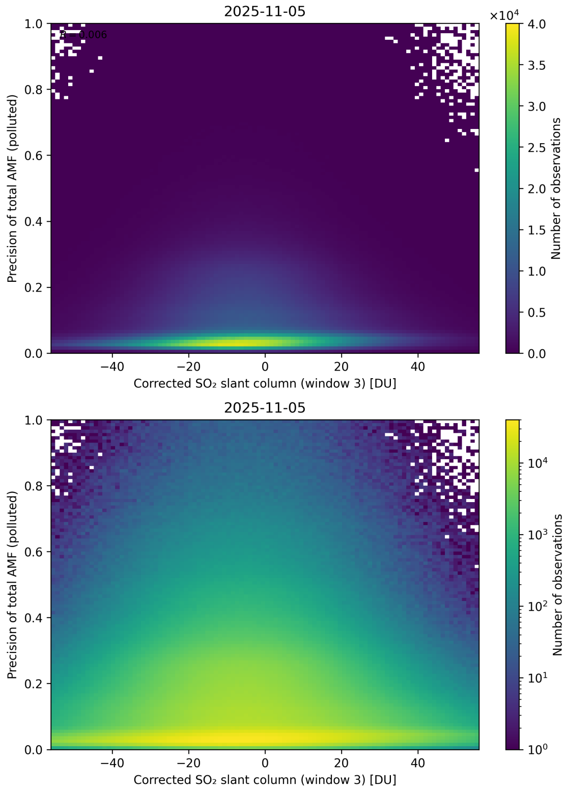
Figure 261: Scatter density plot of “Corrected SO 2 slant column (window 3)” against “Precision of total AMF (polluted)” for 2025-11-04 to 2025-11-06.
