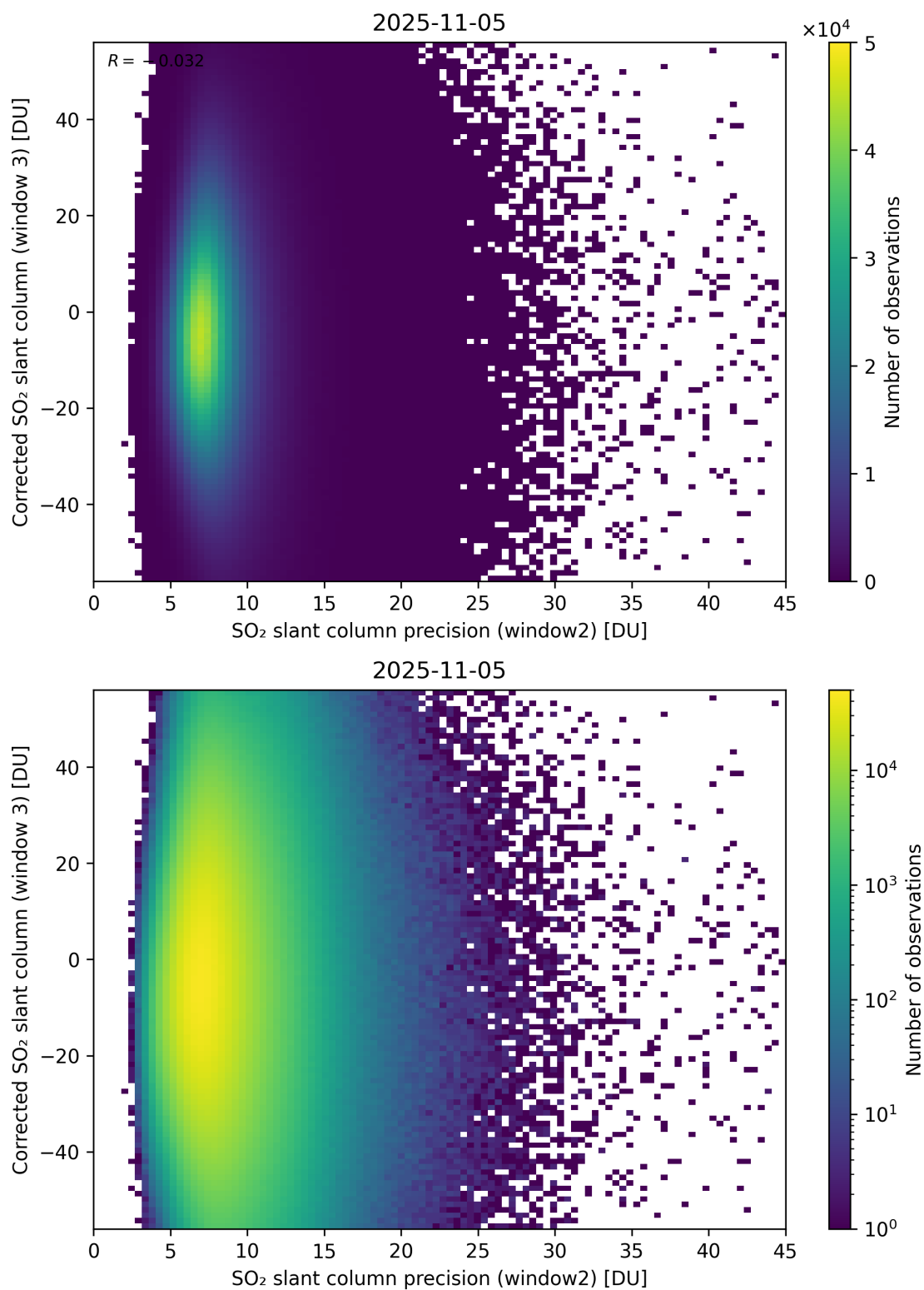
Figure 298: Scatter density plot of “SO 2 slant column precision (window2)” against “Corrected SO 2 slant column (window 3)” for 2025-11-04 to 2025-11-06.
