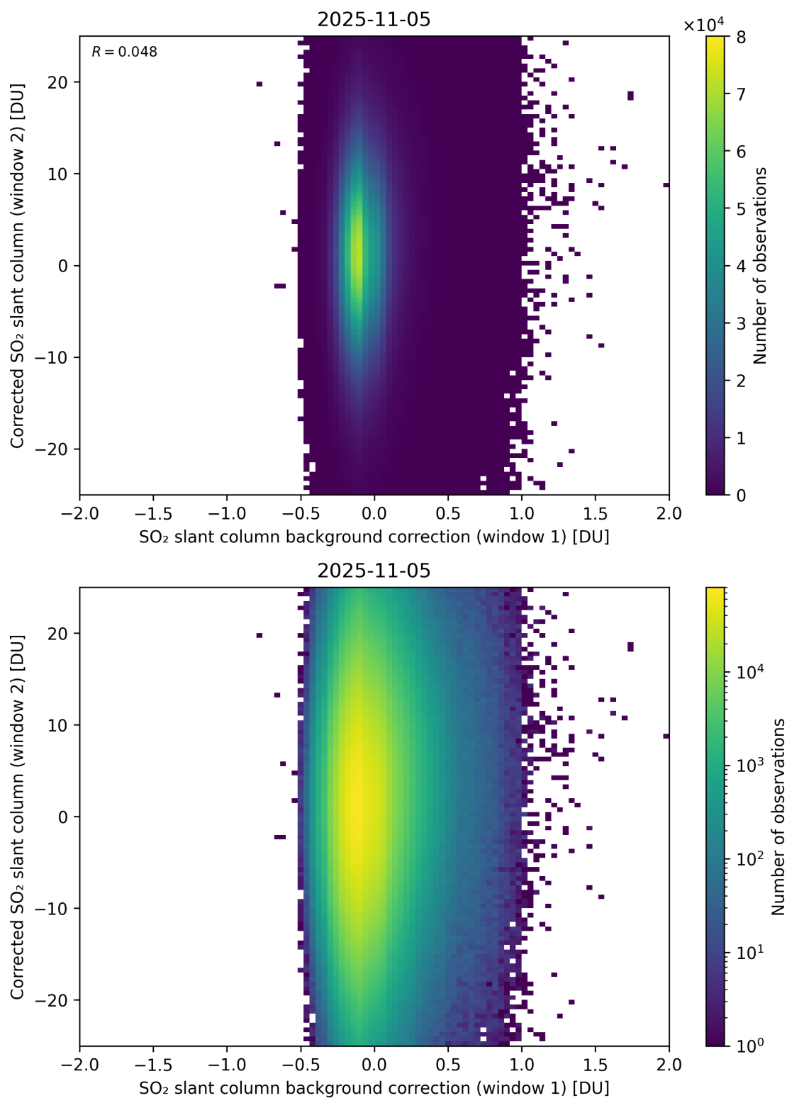
Figure 115: Scatter density plot of “SO 2 slant column background correction (window 1)” against “Corrected SO 2 slant column (window 2)” for 2025-11-04 to 2025-11-06.
