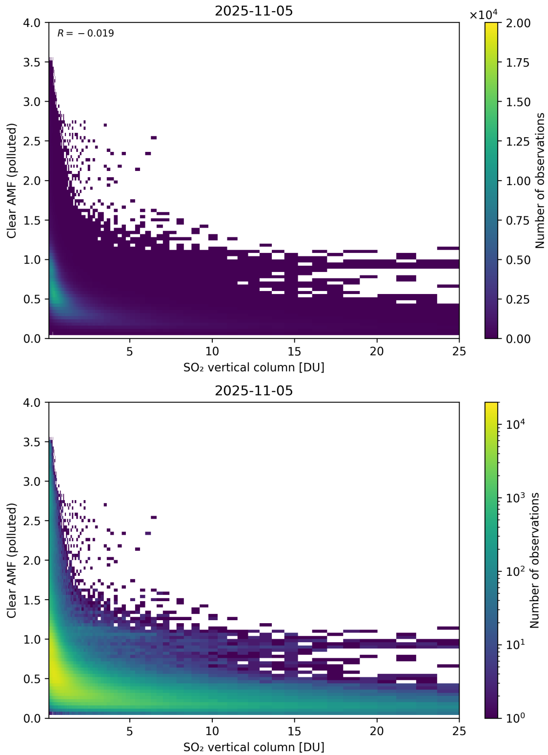
Figure 348: Scatter density plot of “SO 2 vertical column” against “Clear AMF (polluted)” for 2025-11-04 to 2025-11-06.
