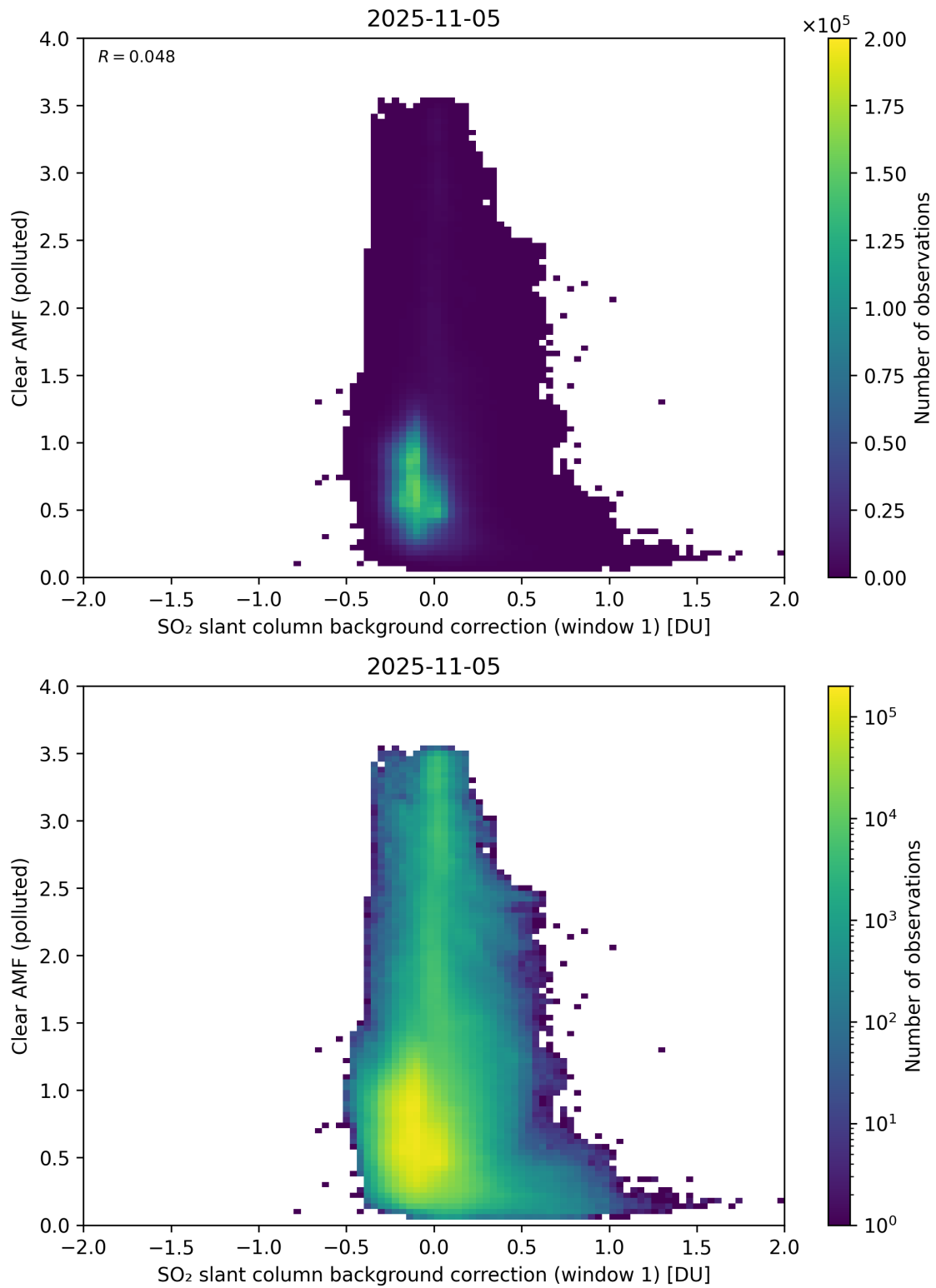
Figure 114: Scatter density plot of “SO 2 slant column background correction (window 1)” against “Clear AMF (polluted)” for 2025-11-04 to 2025-11-06.
