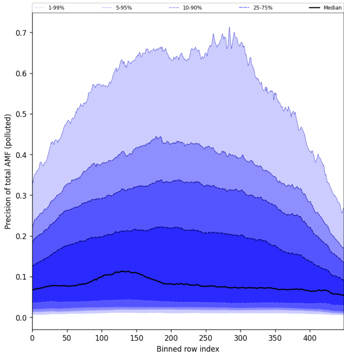
Figure 106: Along track statistics of “Precision of total AMF (polluted)” for 2025-11-04 to 2025-11-06
