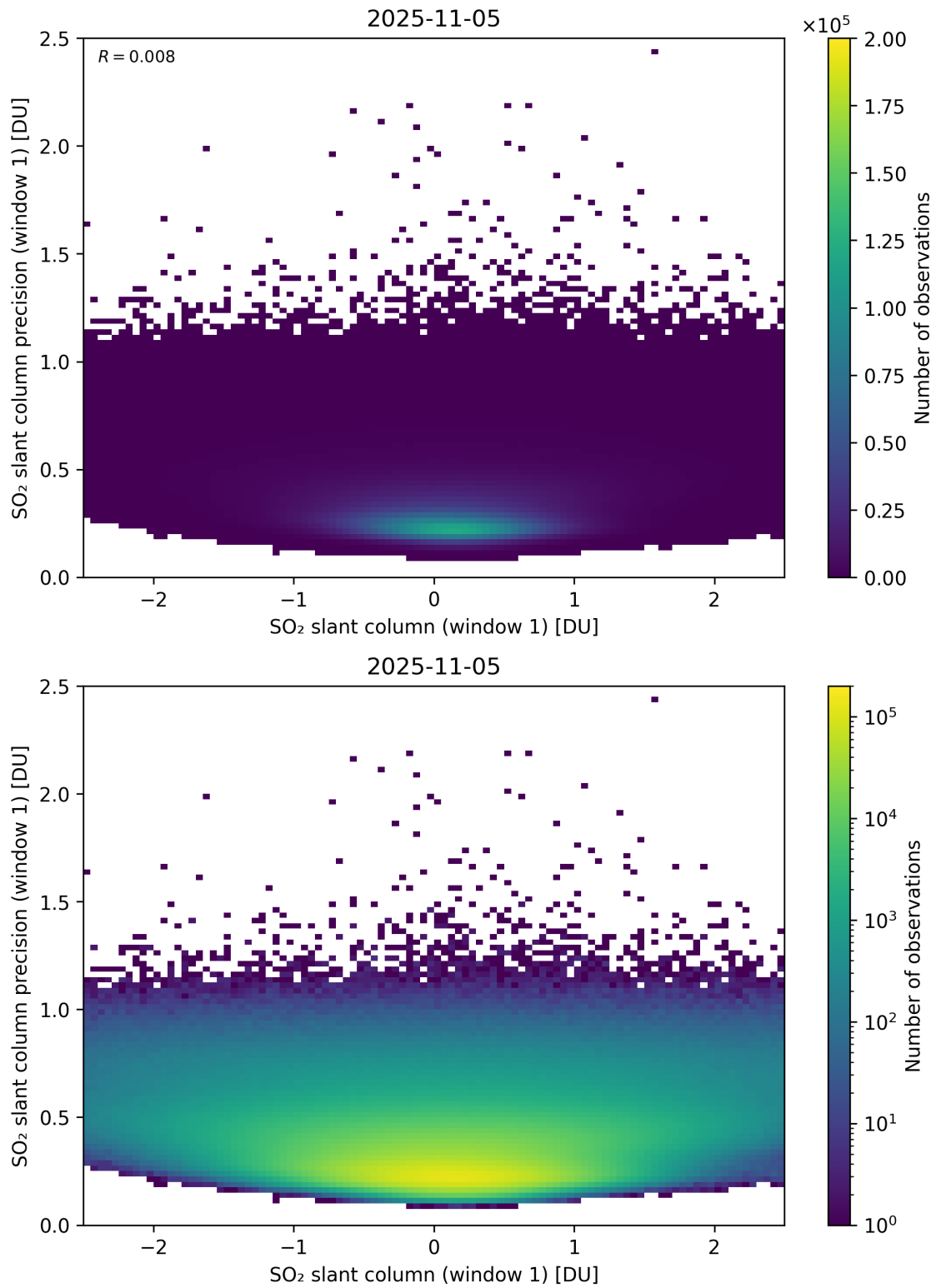
Figure 285: Scatter density plot of “SO 2 slant column (window 1)” against “SO 2 slant column precision (window 1)” for 2025-11-04 to 2025-11-06.
