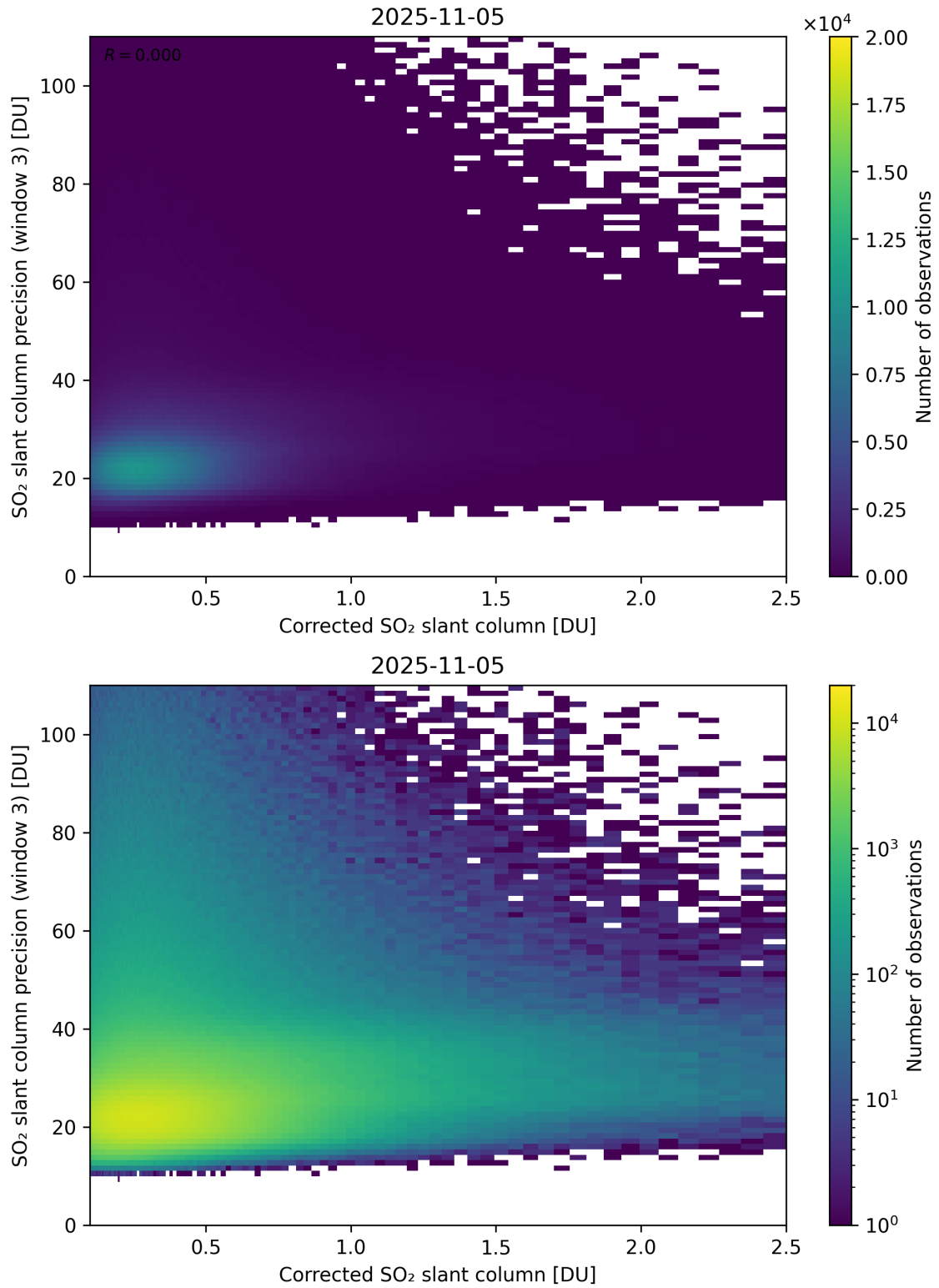
Figure 241: Scatter density plot of “Corrected SO 2 slant column” against “SO 2 slant column precision (window 3)” for 2025-11-04 to 2025-11-06.
