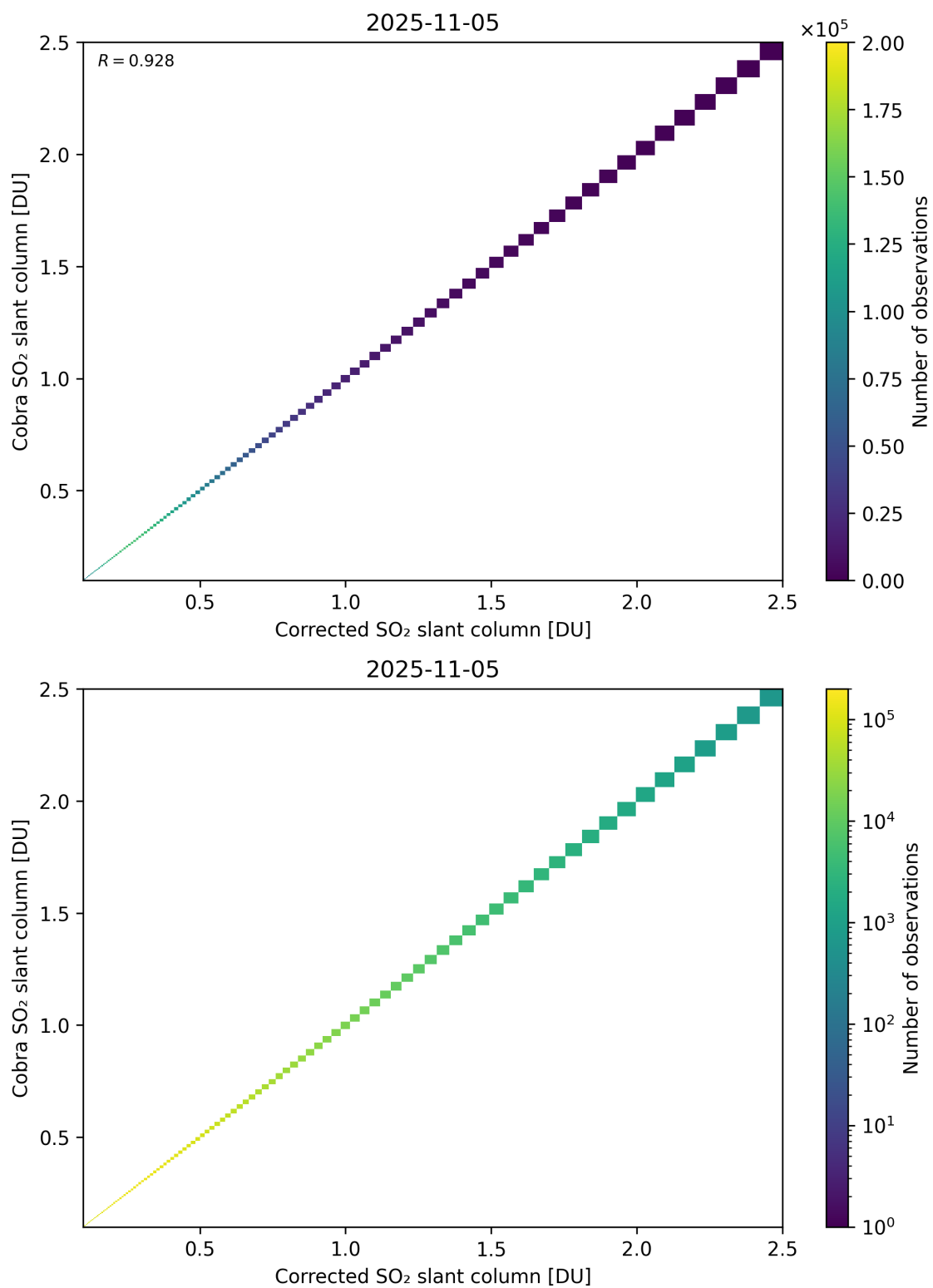
Figure 233: Scatter density plot of “Corrected SO 2 slant column” against “Cobra SO 2 slant column” for 2025-11-04 to 2025-11-06.
