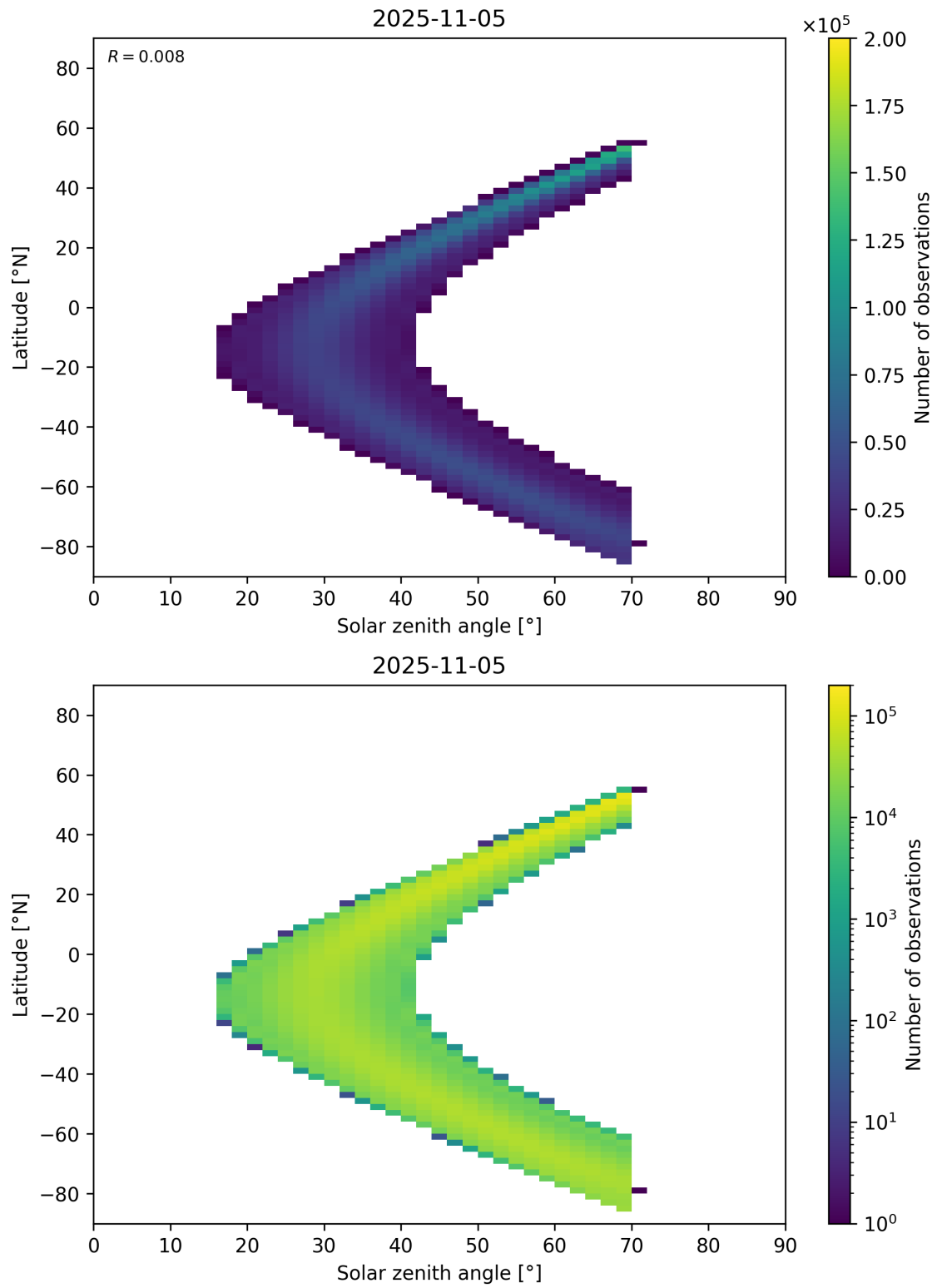
Figure 177: Scatter density plot of “Solar zenith angle” against “Latitude” for 2025-11-04 to 2025-11-06.
