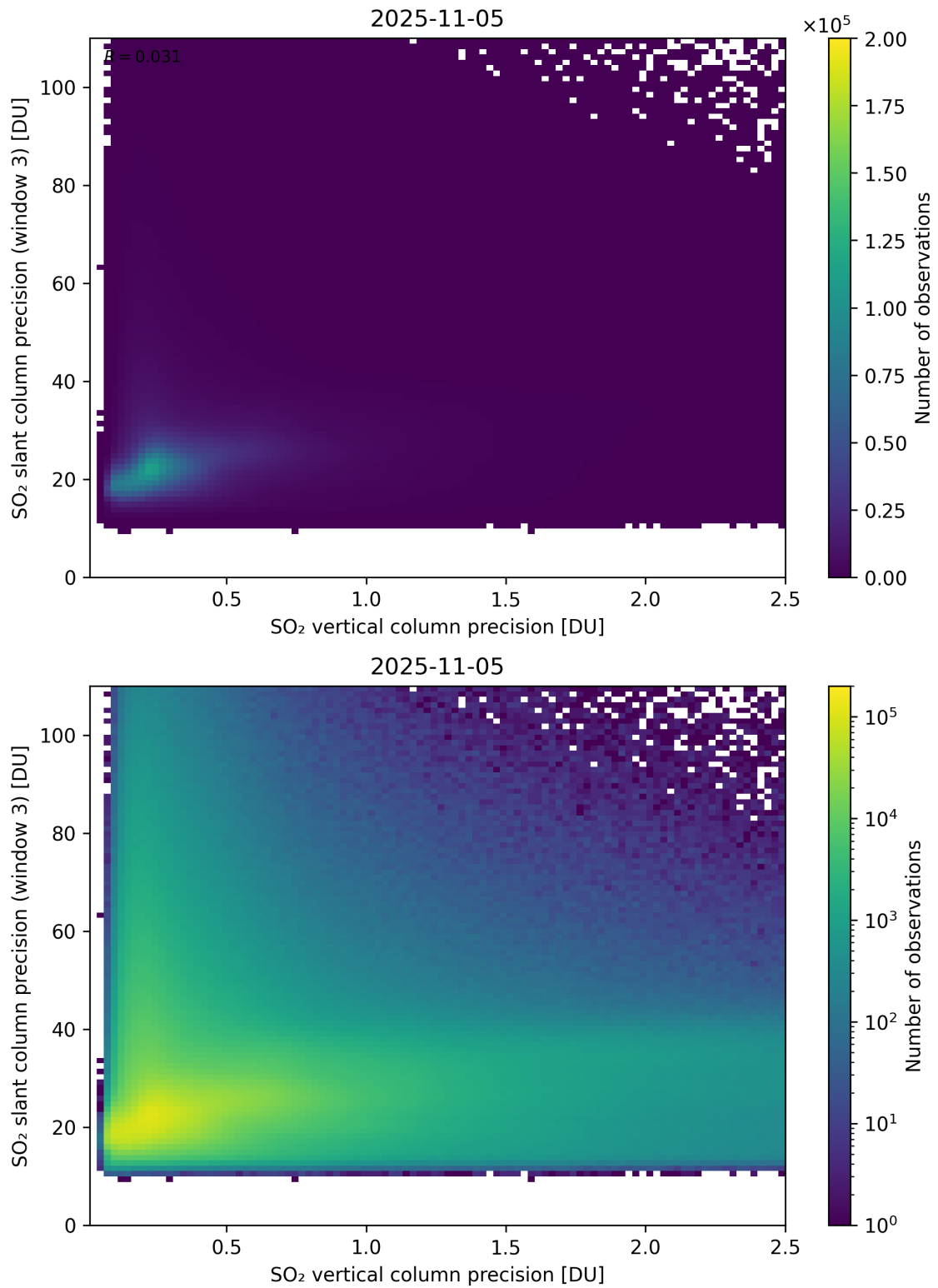
Figure 345: Scatter density plot of “SO 2 vertical column precision” against “SO 2 slant column precision (window 3)” for 2025-11-04 to 2025-11-06.
