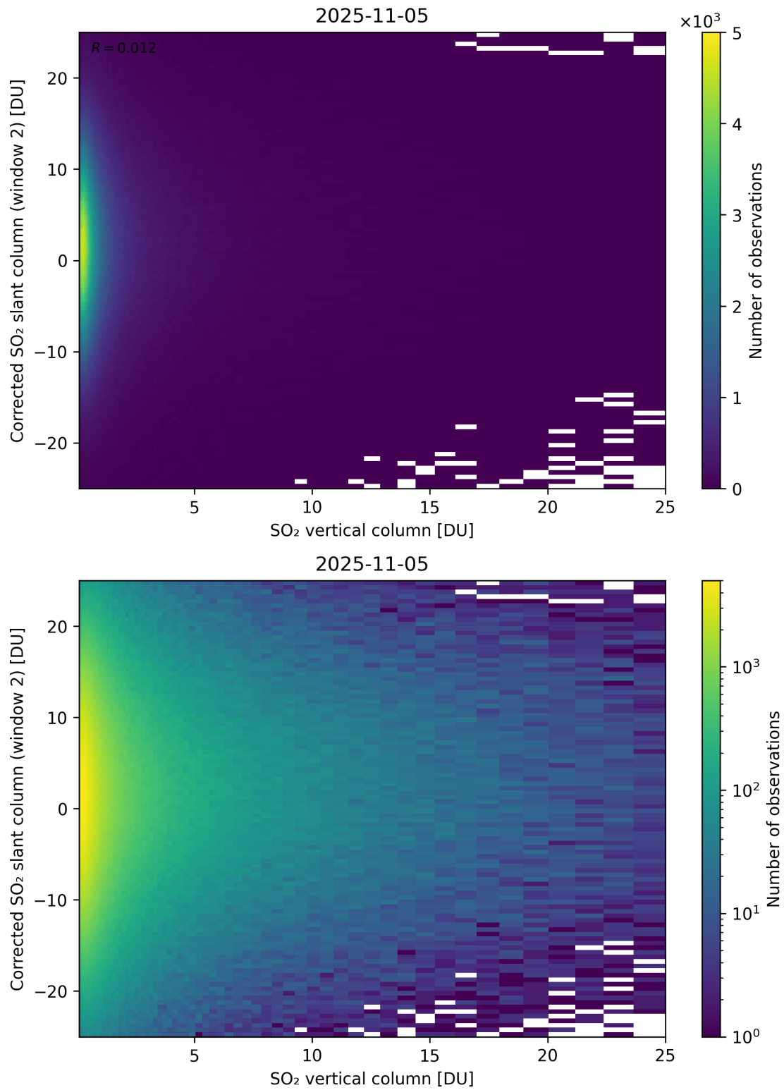
Figure 352: Scatter density plot of “SO 2 vertical column” against “Corrected SO 2 slant column (window 2)” for 2025-11-04 to 2025-11-06.
