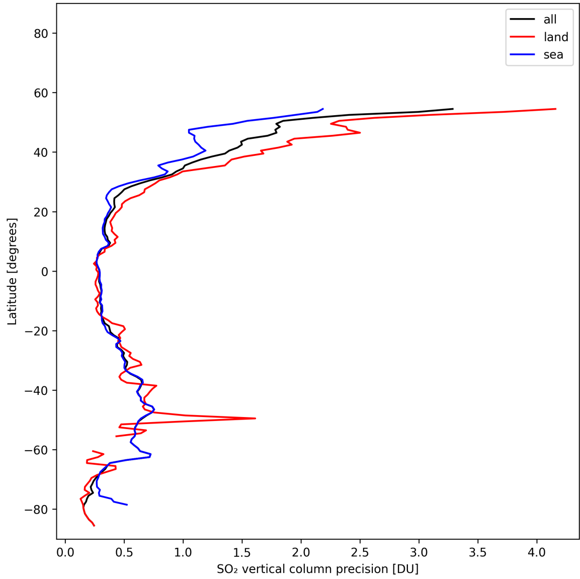
Figure 33: Zonal average of “SO 2 vertical column precision” for 2025-11-04 to 2025-11-06.
