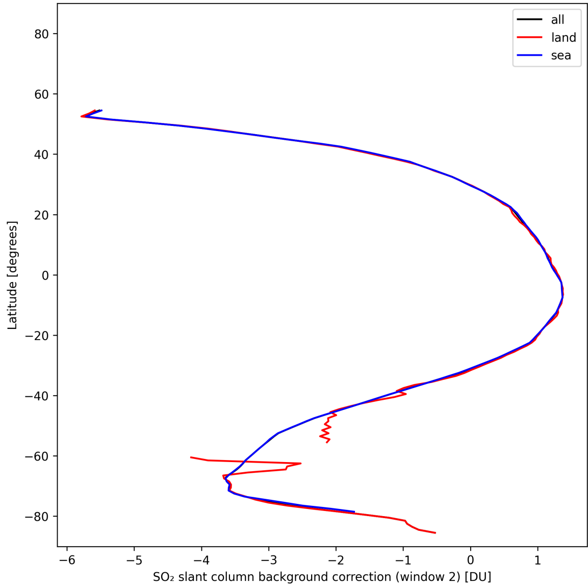
Figure 44: Zonal average of “SO 2 slant column background correction (window 2)” for 2025-11-04 to 2025-11-06.
