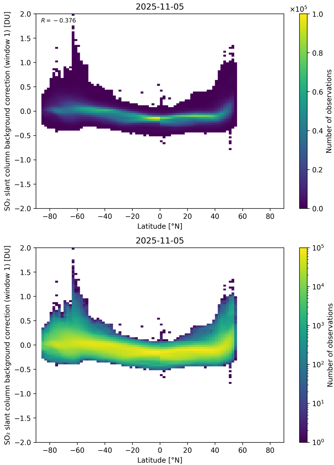
Figure 150: Scatter density plot of “Latitude” against “SO 2 slant column background correction (window 1)” for 2025-11-04 to 2025-11-06.
