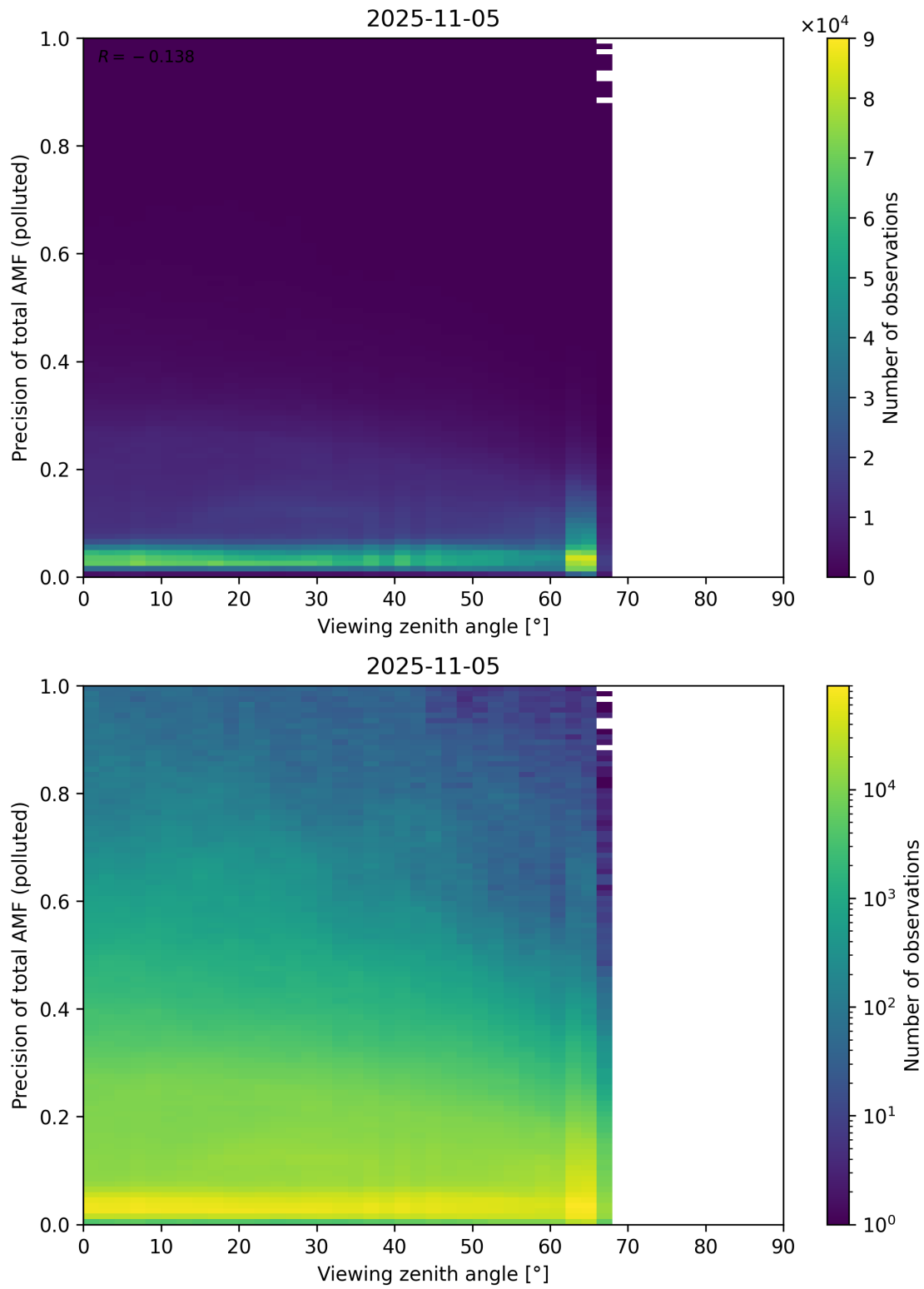
Figure 382: Scatter density plot of “Viewing zenith angle” against “Precision of total AMF (polluted)” for 2025-11-04 to 2025-11-06.
