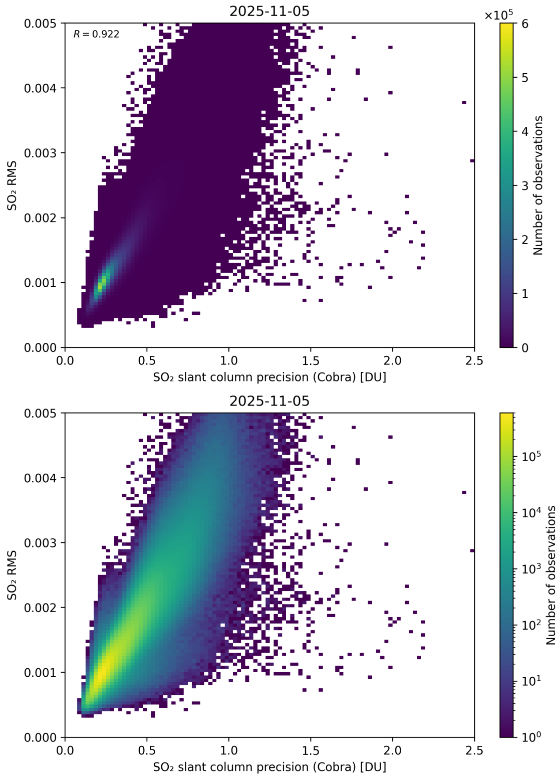
Figure 204: Scatter density plot of “SO 2 slant column precision (Cobra)” against “SO 2 RMS” for 2025-11-04 to 2025-11-06.
