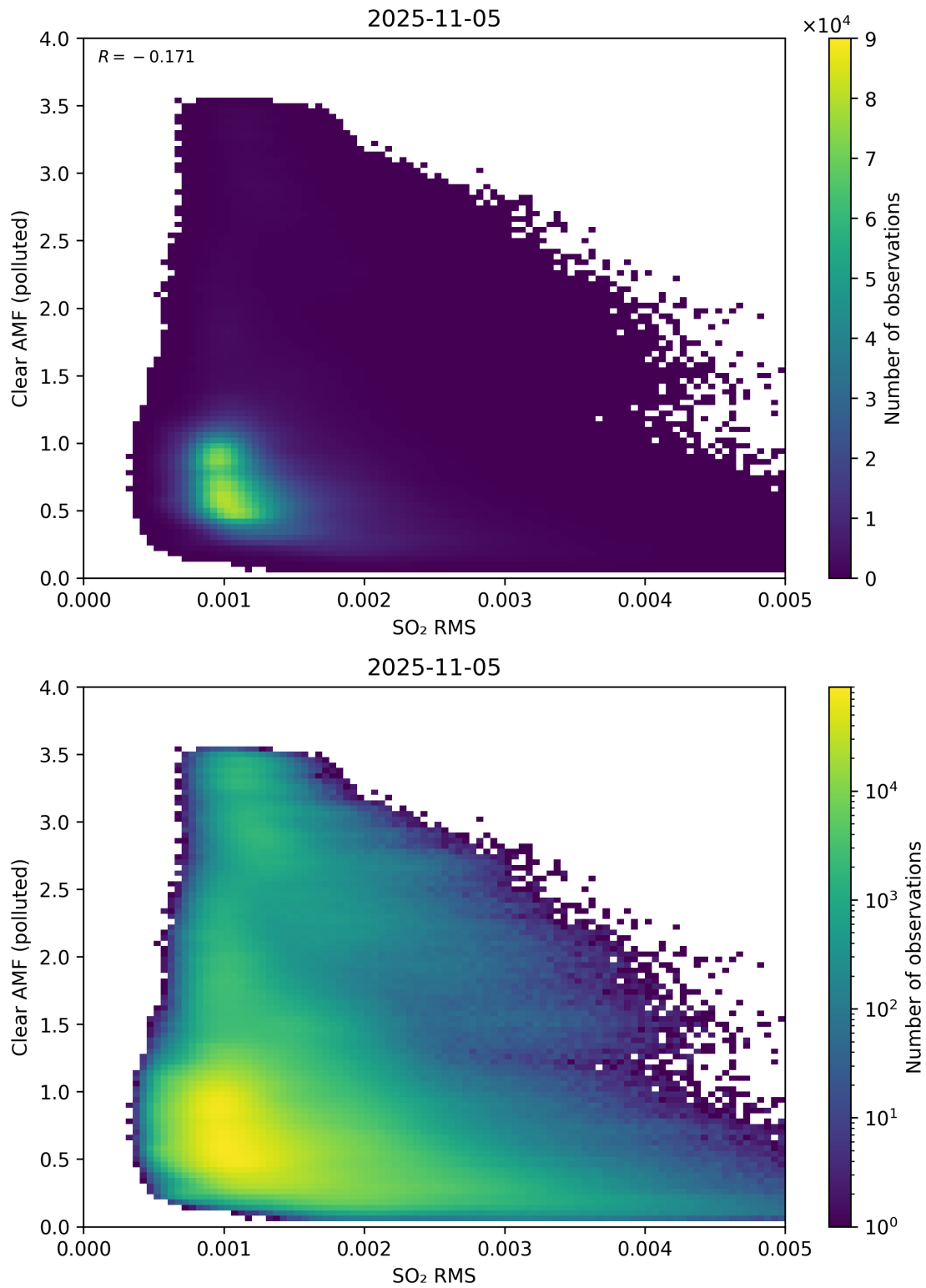
Figure 147: Scatter density plot of “SO 2 RMS” against “Clear AMF (polluted)” for 2025-11-04 to 2025-11-06.
