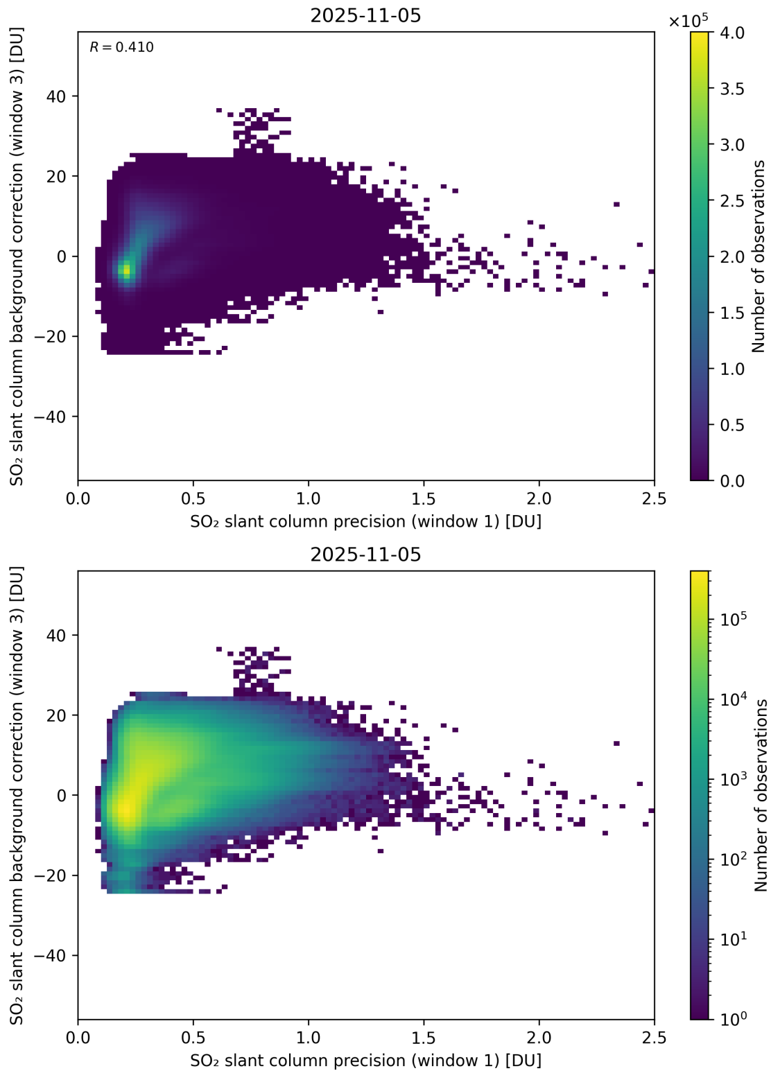
Figure 270: Scatter density plot of “SO 2 slant column precision (window 1)” against “SO 2 slant column background correction (window 3)” for 2025-11-04 to 2025-11-06.
