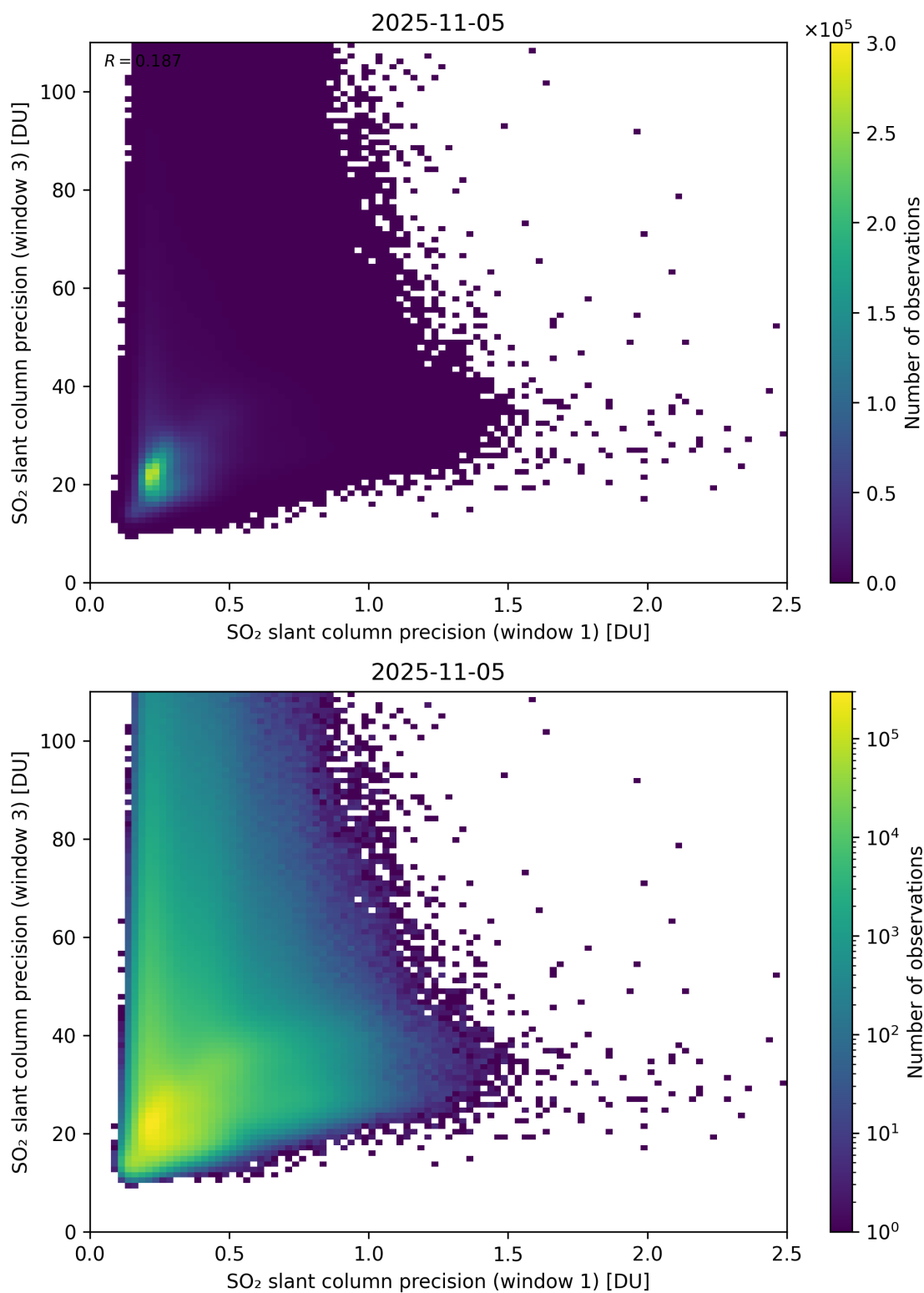
Figure 279: Scatter density plot of “SO 2 slant column precision (window 1)” against “SO 2 slant column precision (window 3)” for 2025-11-04 to 2025-11-06.
