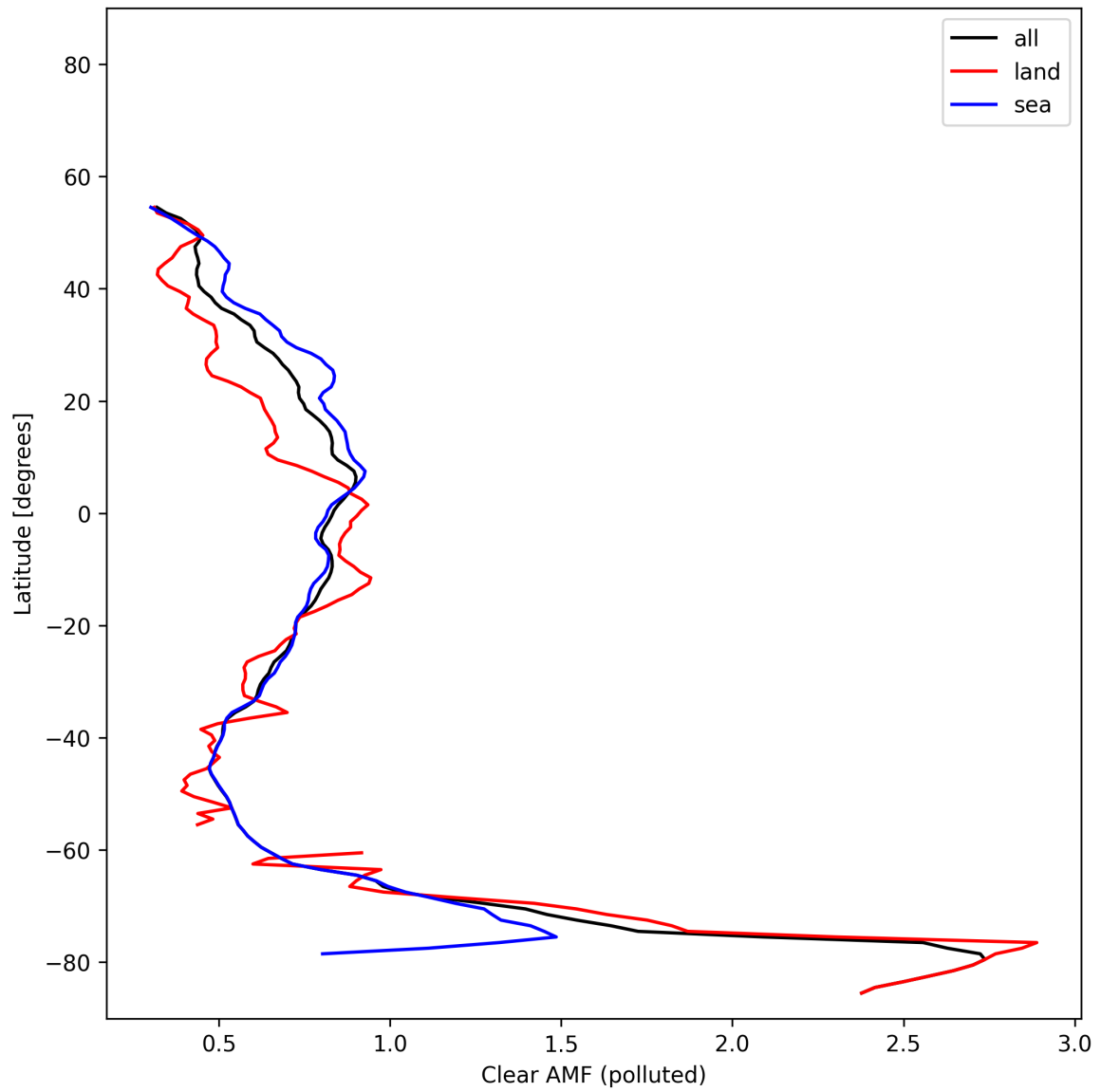
Figure 55: Zonal average of “Clear AMF (polluted)” for 2025-11-04 to 2025-11-06.
