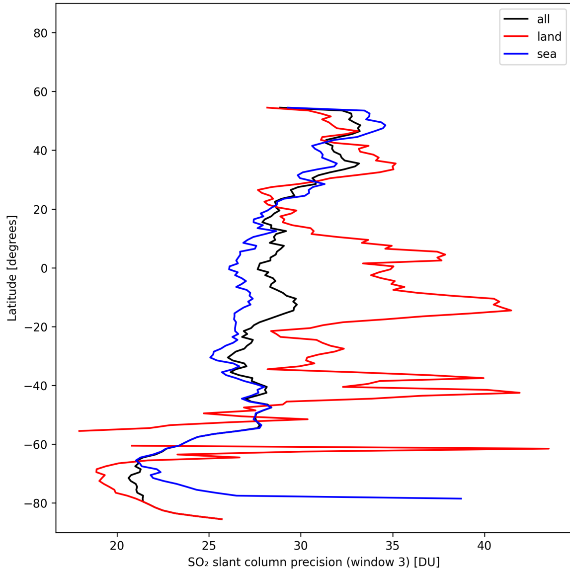
Figure 46: Zonal average of “SO 2 slant column precision (window 3)” for 2025-11-04 to 2025-11-06.
