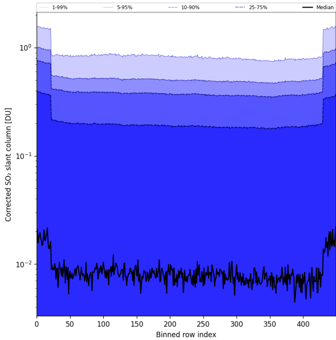
Figure 86: Along track statistics of "Corrected SO 2 slant column" for 2025-11-04 to 2025-11-06
