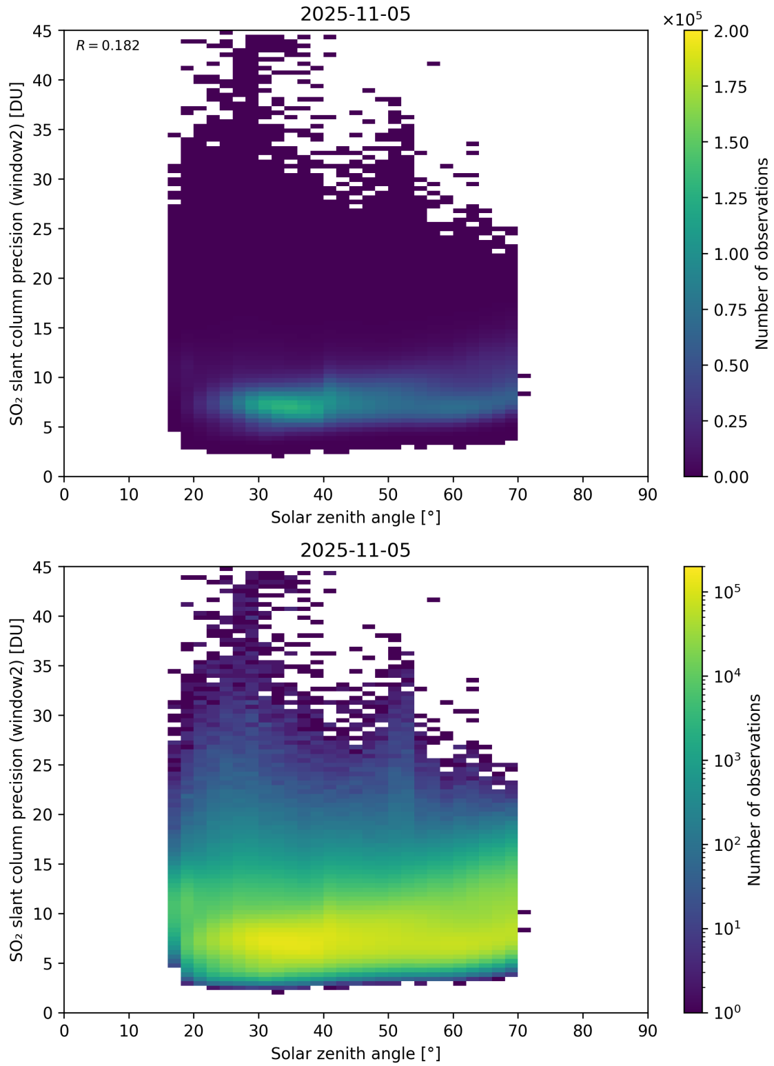
Figure 186: Scatter density plot of “Solar zenith angle” against “SO 2 slant column precision (window2)” for 2025-11-04 to 2025-11-06.
