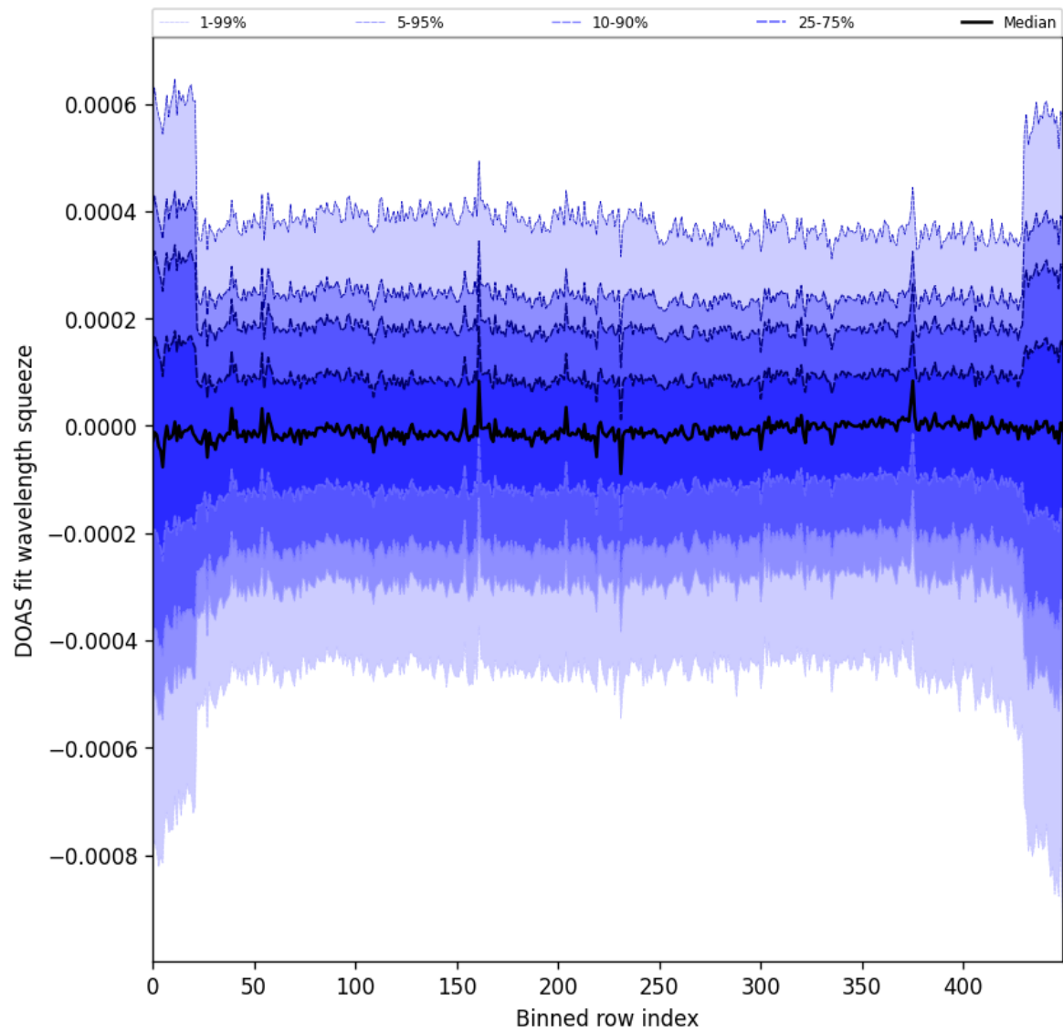
Figure 103: Along track statistics of “DOAS fit wavelength squeeze” for 2025-11-04 to 2025-11-06
