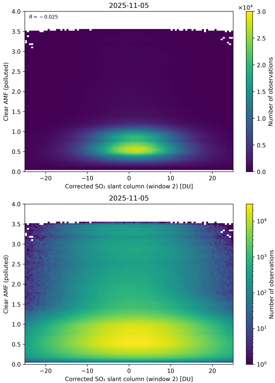
Figure 249: Scatter density plot of “Corrected SO 2 slant column (window 2)” against “Clear AMF (polluted)” for 2025-11-04 to 2025-11-06.
