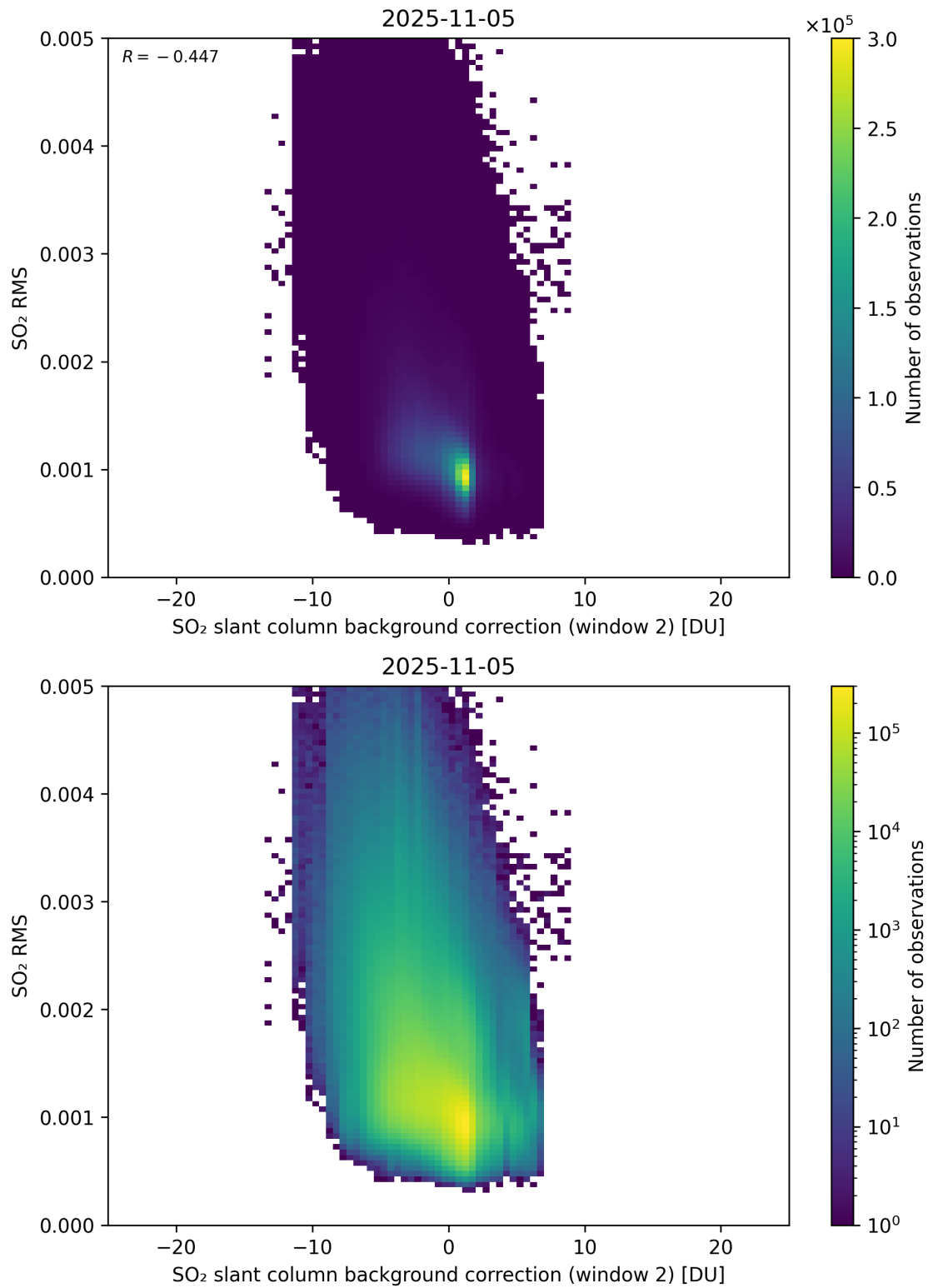
Figure 125: Scatter density plot of “SO 2 slant column background correction (window 2)” against “SO 2 RMS” for 2025-11-04 to 2025-11-06.
