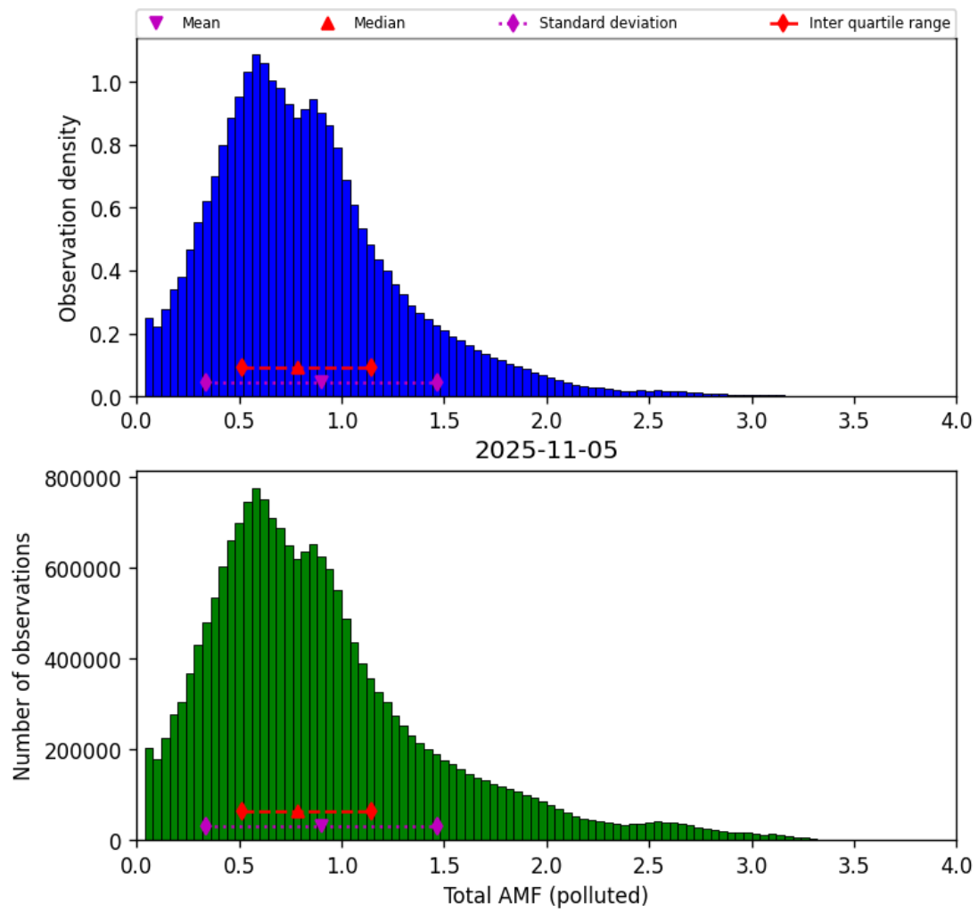
Figure 79: Histogram of “Total AMF (polluted)” for 2025-11-04 to 2025-11-06
