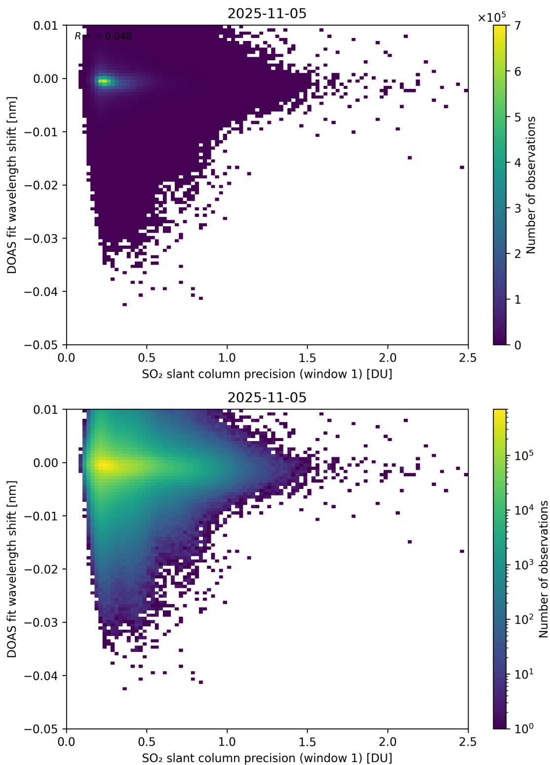
Figure 271: Scatter density plot of “SO 2 slant column precision (window 1)” against “DOAS fit wavelength shift” for 2025-11-04 to 2025-11-06.
