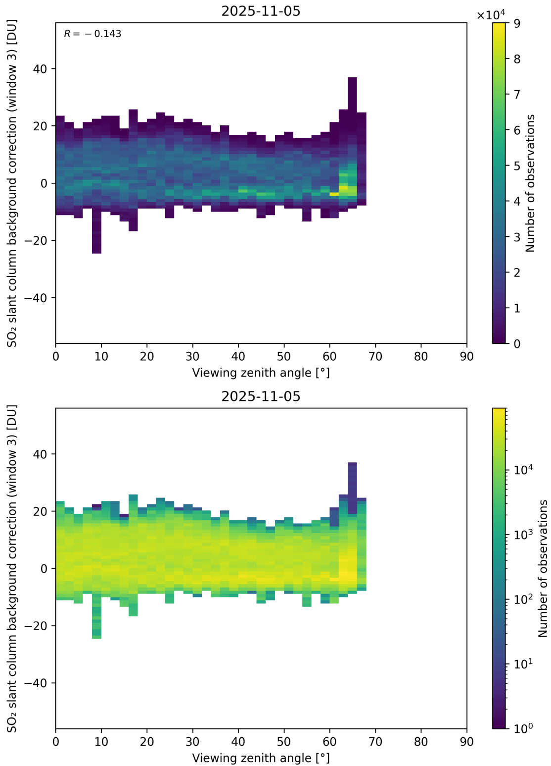
Figure 364: Scatter density plot of “Viewing zenith angle” against “SO 2 slant column background correction (window 3)” for 2025-11-04 to 2025-11-06.
