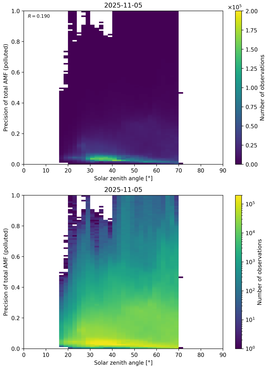
Figure 190: Scatter density plot of “Solar zenith angle” against “Precision of total AMF (polluted)” for 2025-11-04 to 2025-11-06.
