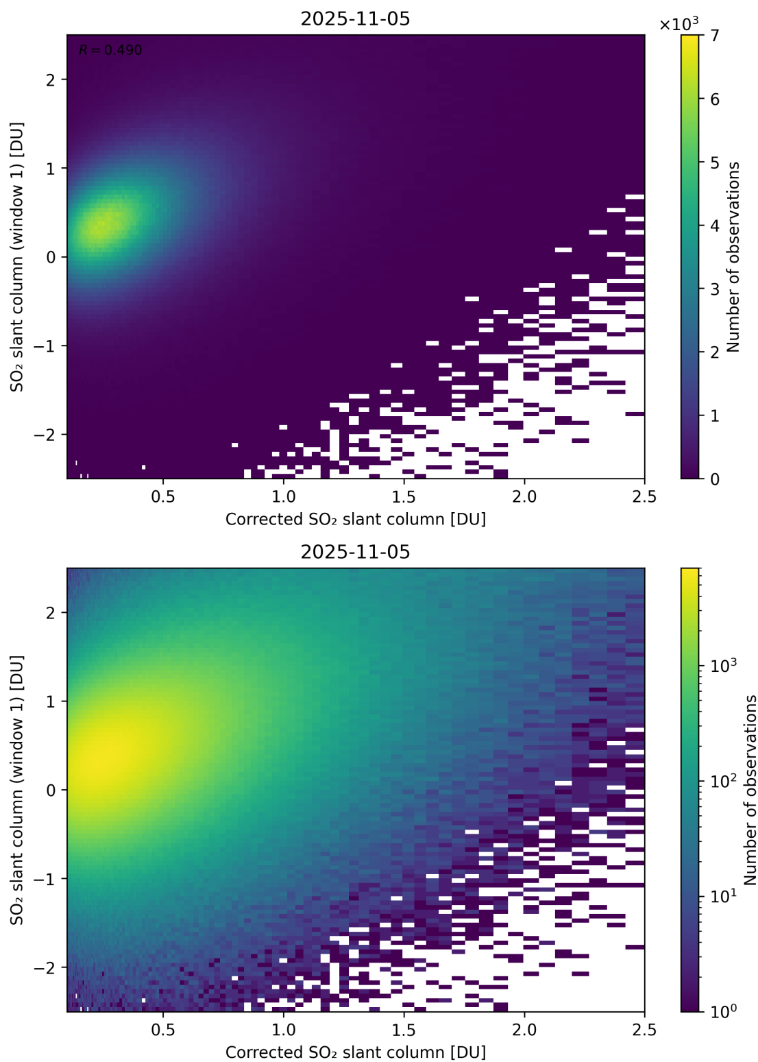
Figure 237: Scatter density plot of “Corrected SO 2 slant column” against “SO 2 slant column (window 1)” for 2025-11-04 to 2025-11-06.
