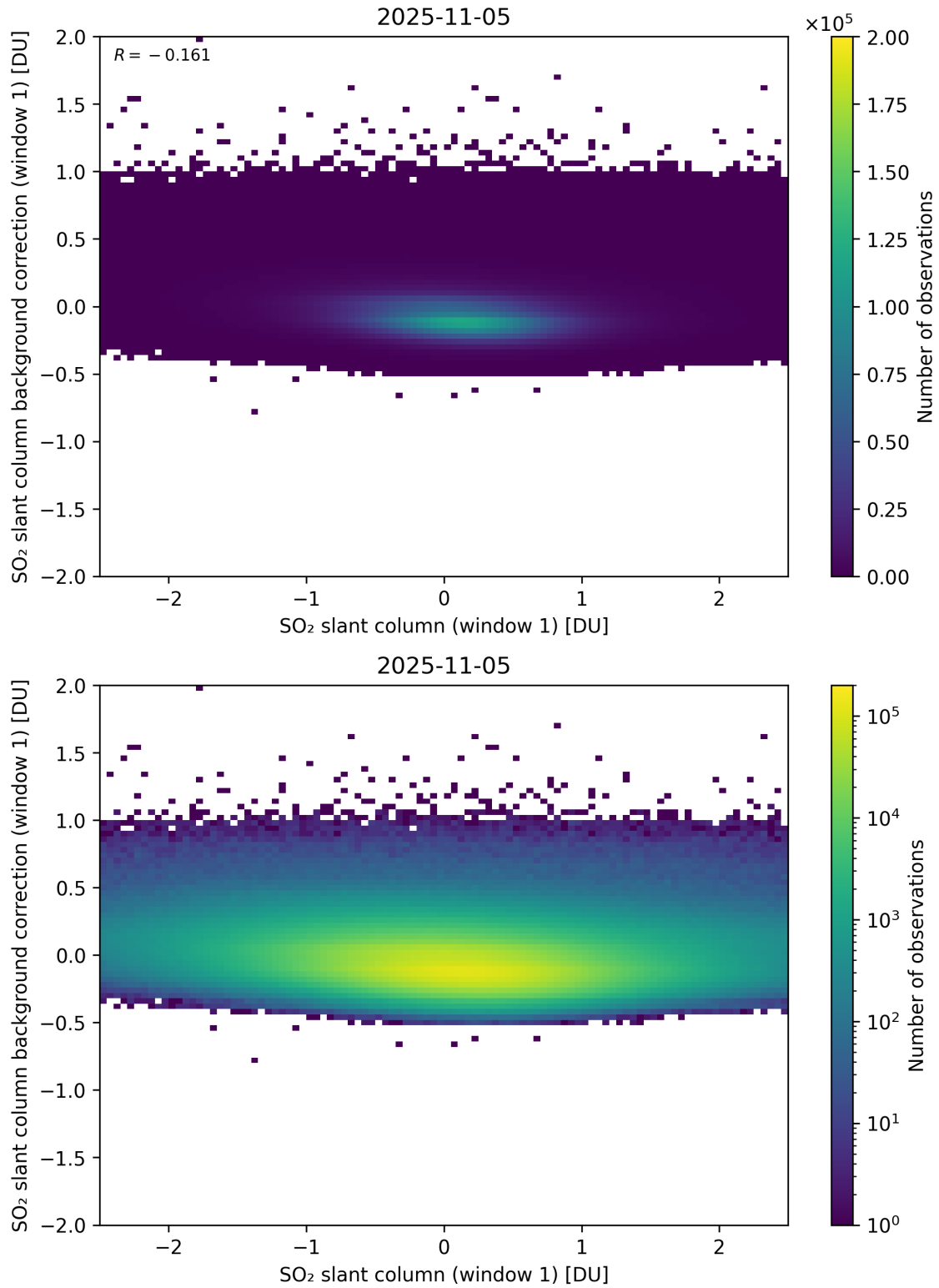
Figure 262: Scatter density plot of “SO 2 slant column (window 1)” against “SO 2 slant column background correction (window 1)” for 2025-11-04 to 2025-11-06.
