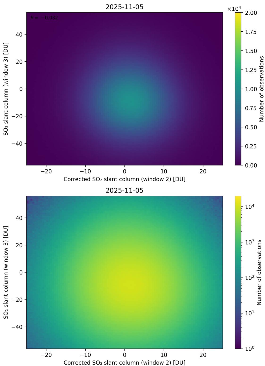
Figure 251: Scatter density plot of “Corrected SO 2 slant column (window 2)” against “SO 2 slant column (window 3)” for 2025-11-04 to 2025-11-06.
