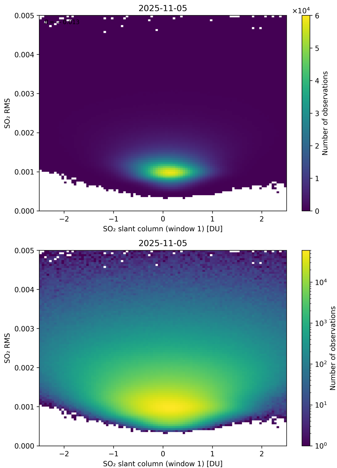
Figure 267: Scatter density plot of “SO 2 slant column (window 1)” against “SO 2 RMS” for 2025-11-04 to 2025-11-06.
