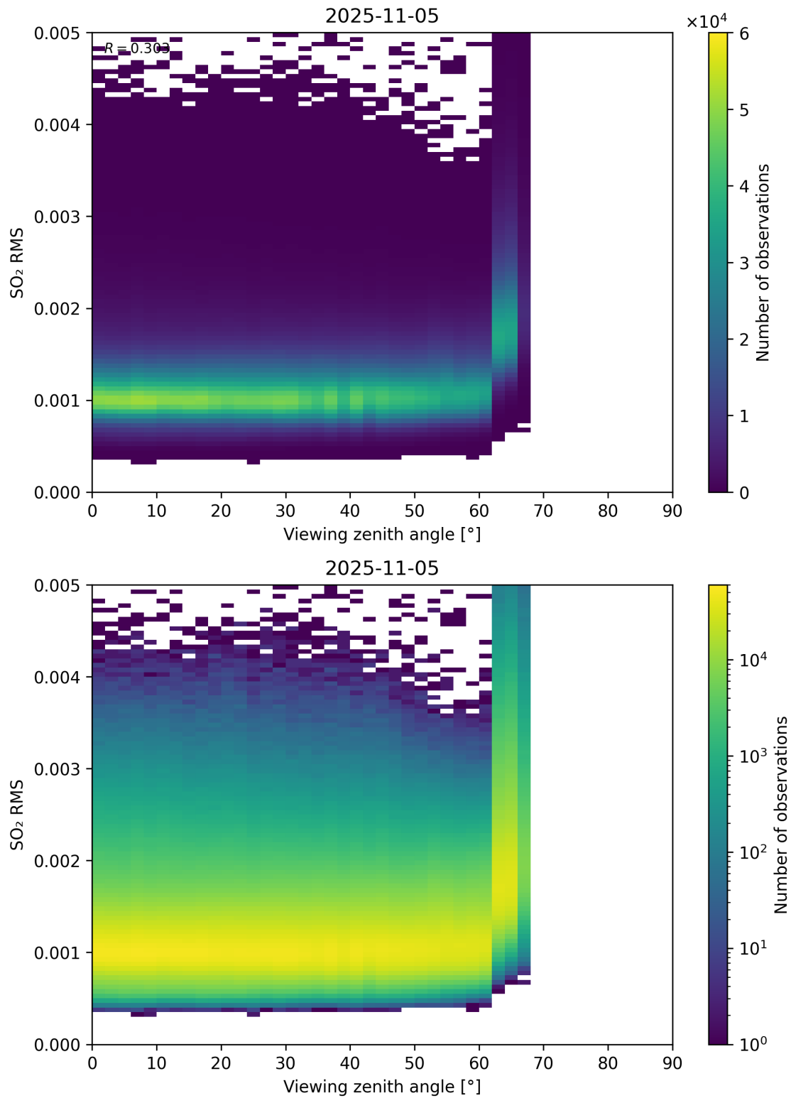
Figure 367: Scatter density plot of “Viewing zenith angle” against “SO 2 RMS” for 2025-11-04 to 2025-11-06.
