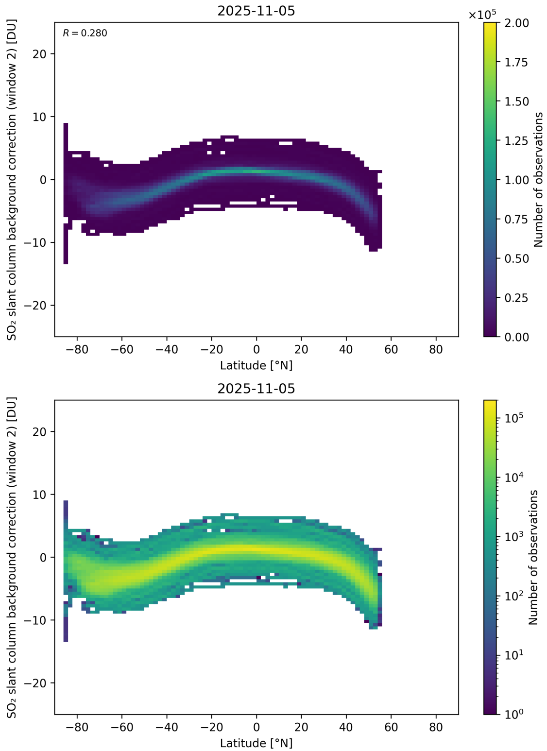
Figure 151: Scatter density plot of “Latitude” against “SO 2 slant column background correction (window 2)” for 2025-11-04 to 2025-11-06.
