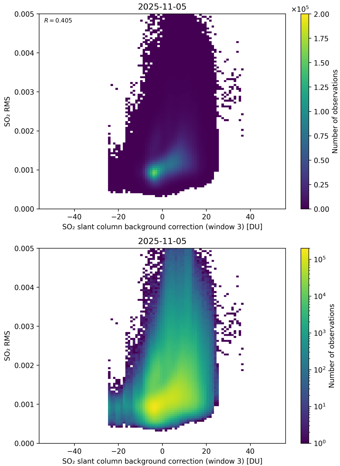
Figure 134: Scatter density plot of “SO 2 slant column background correction (window 3)” against “SO 2 RMS” for 2025-11-04 to 2025-11-06.
