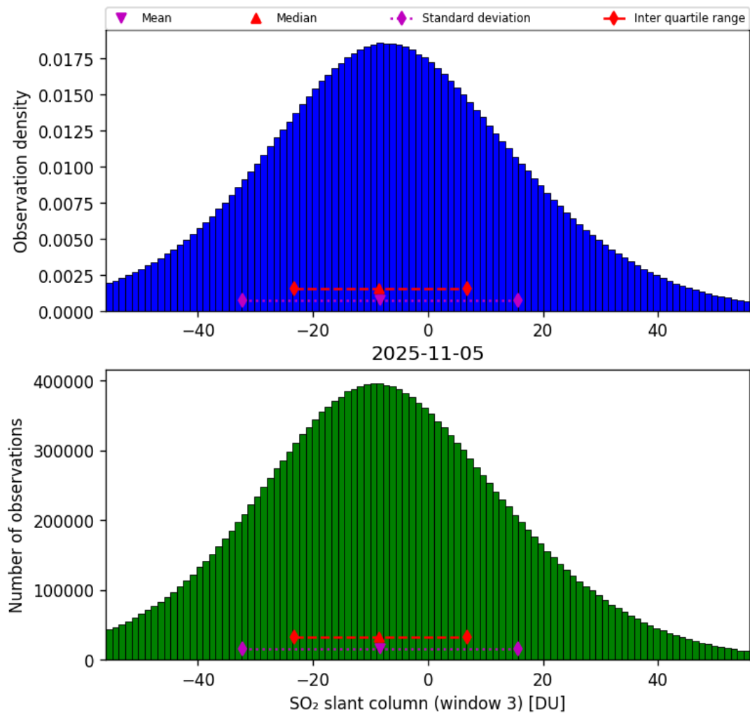
Figure 71: Histogram of “SO 2 slant column (window 3)” for 2025-11-04 to 2025-11-06
