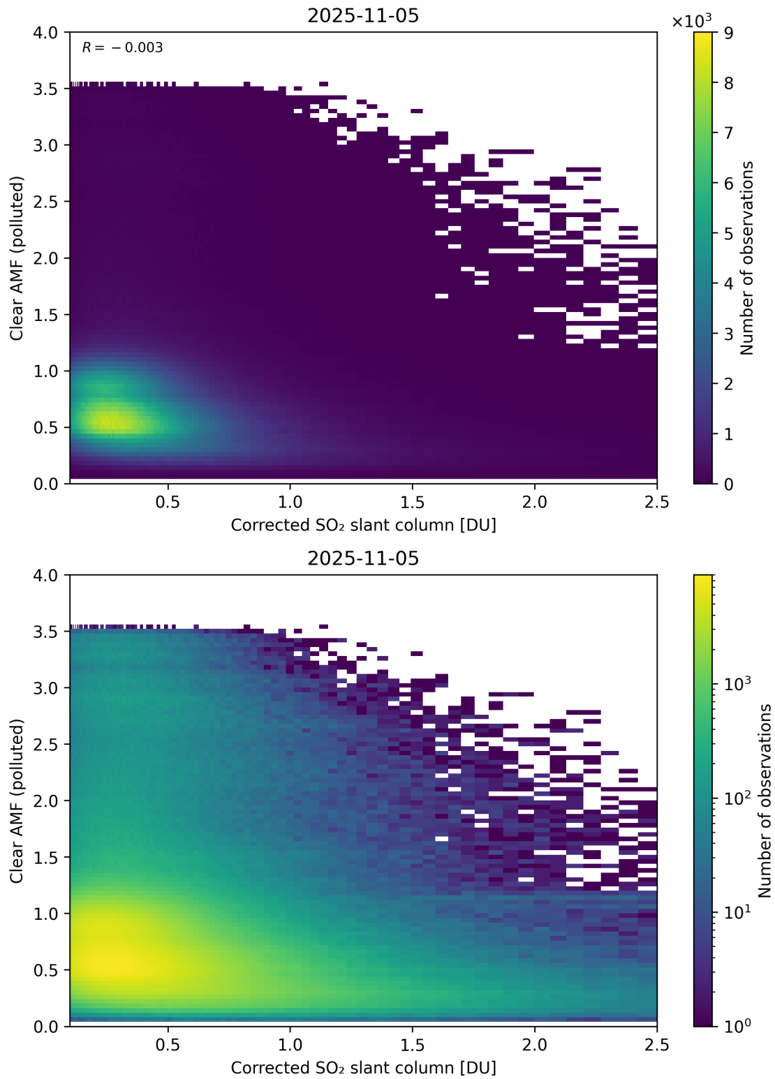
Figure 232: Scatter density plot of “Corrected SO 2 slant column” against “Clear AMF (polluted)” for 2025-11-04 to 2025-11-06.
