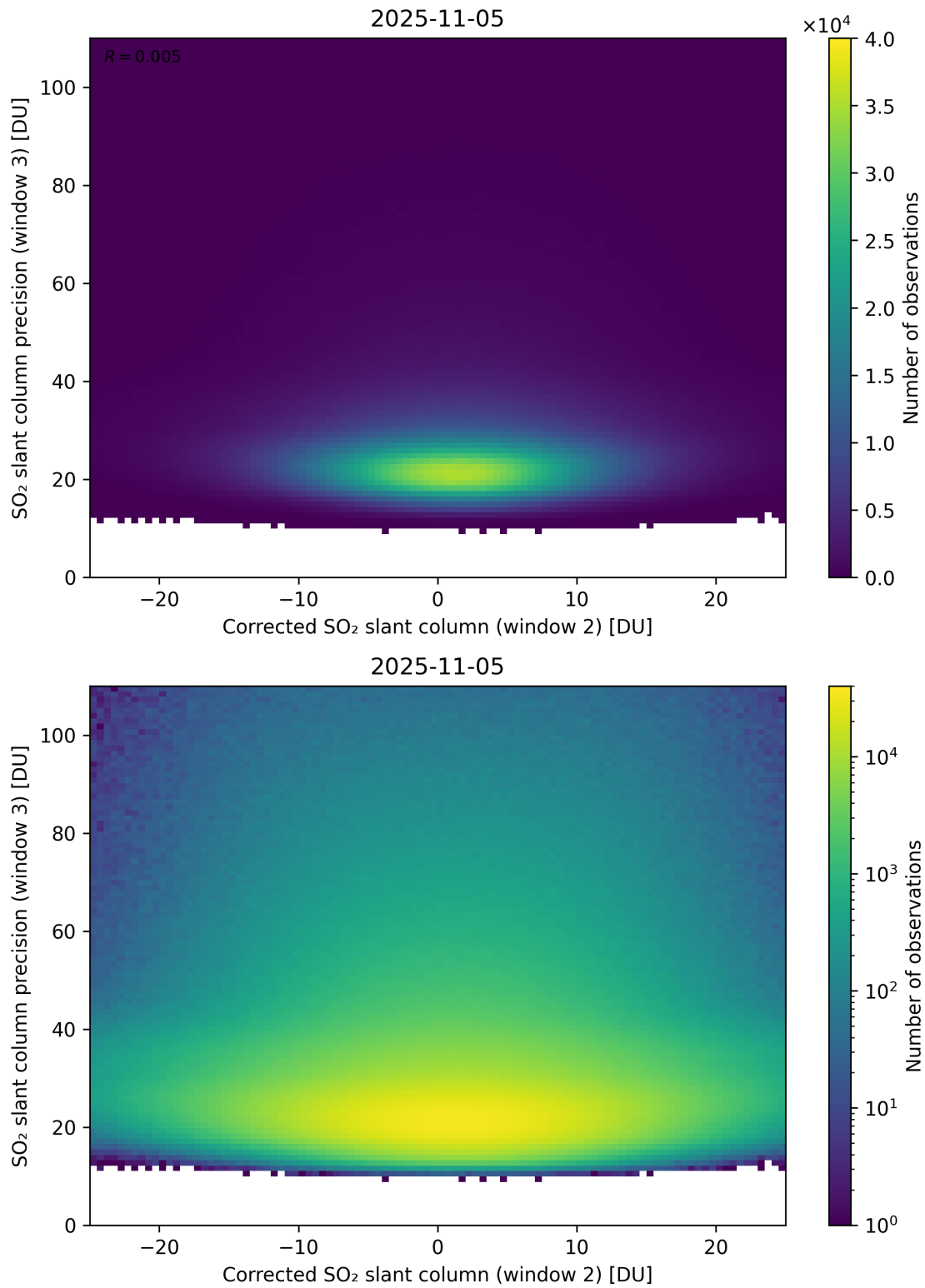
Figure 252: Scatter density plot of “Corrected SO 2 slant column (window 2)” against “SO 2 slant column precision (window 3)” for 2025-11-04 to 2025-11-06.
