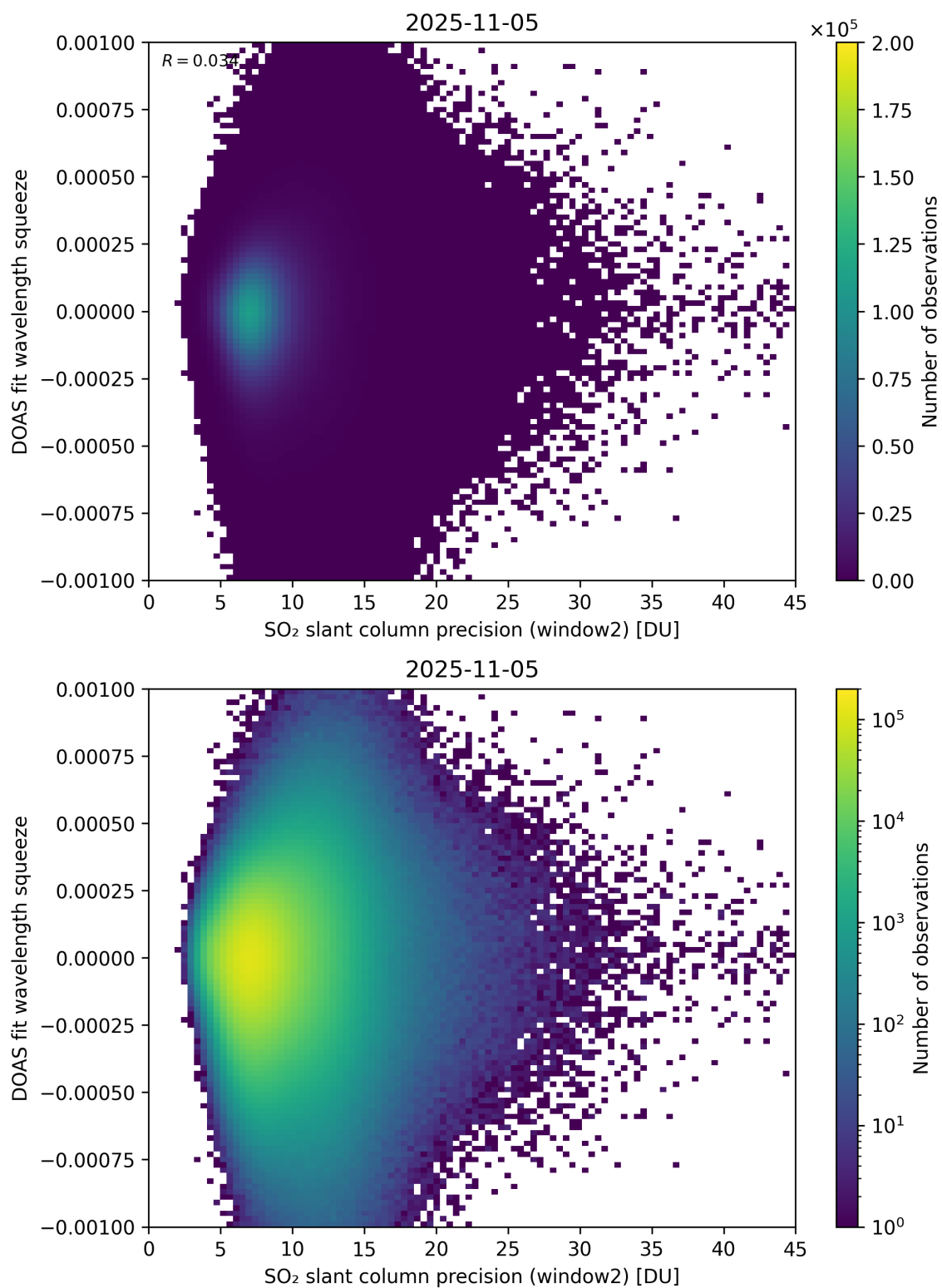
Figure 294: Scatter density plot of “SO 2 slant column precision (window2)” against “DOAS fit wavelength squeeze” for 2025-11-04 to 2025-11-06.
