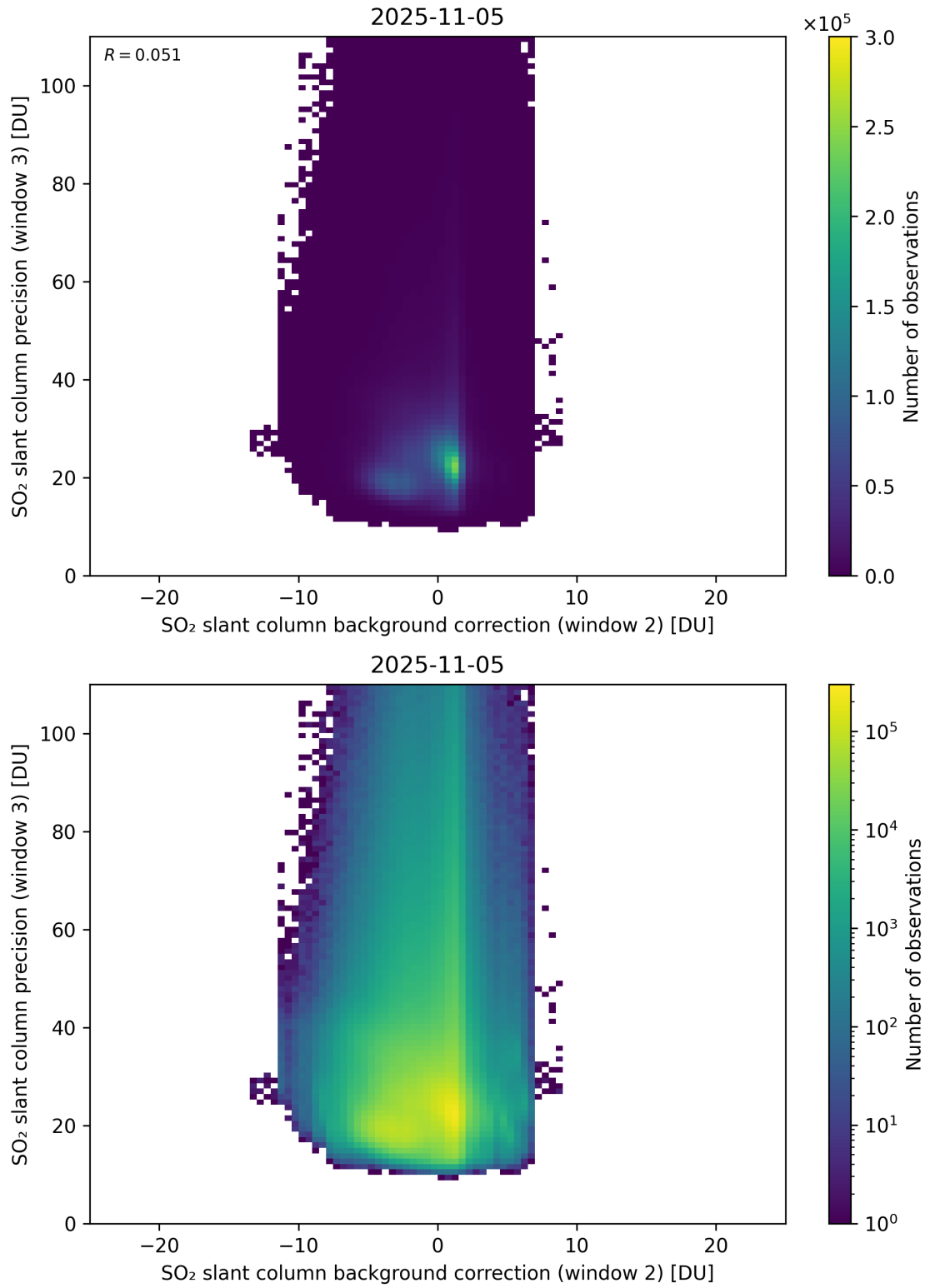
Figure 129: Scatter density plot of “SO 2 slant column background correction (window 2)” against “SO 2 slant column precision (window 3)” for 2025-11-04 to 2025-11-06.
