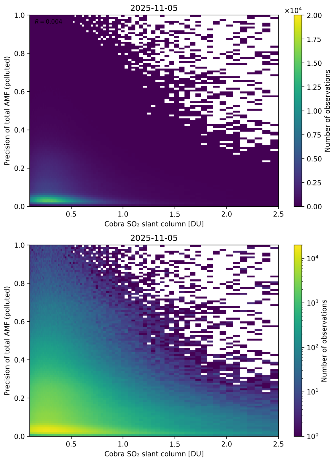
Figure 225: Scatter density plot of “Cobra SO 2 slant column” against “Precision of total AMF (polluted)” for 2025-11-04 to 2025-11-06.
