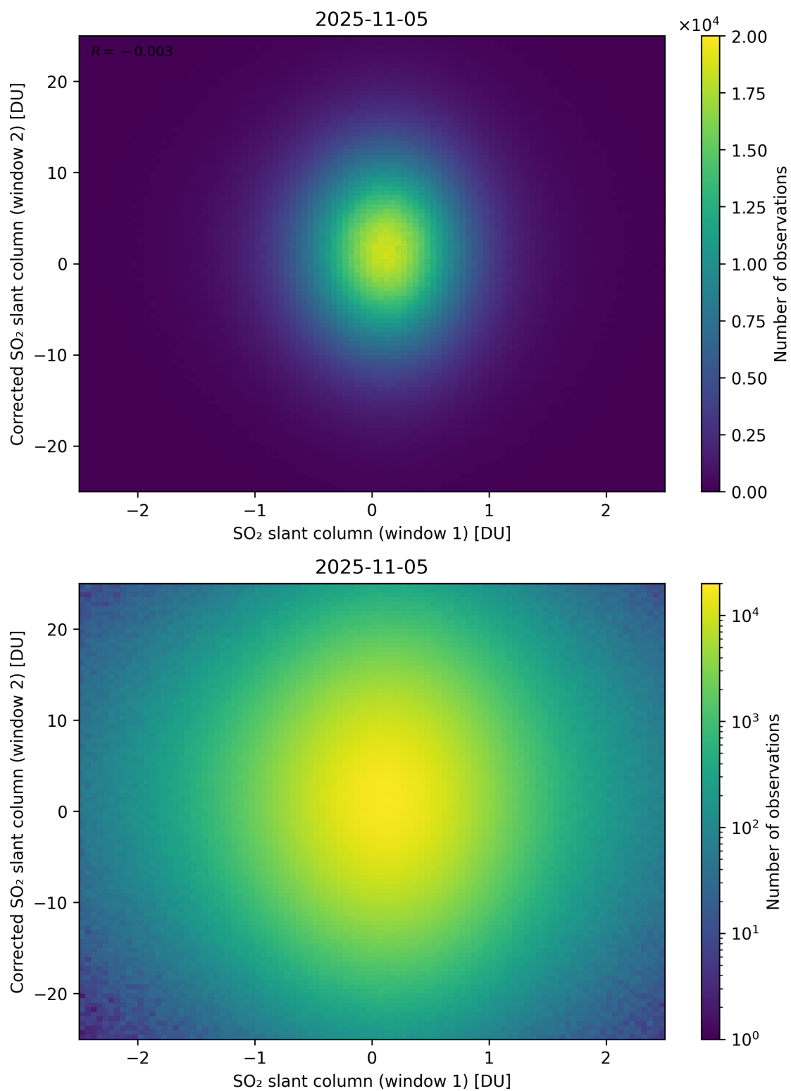
Figure 283: Scatter density plot of “SO 2 slant column (window 1)” against “Corrected SO 2 slant column (window 2)” for 2025-11-04 to 2025-11-06.
