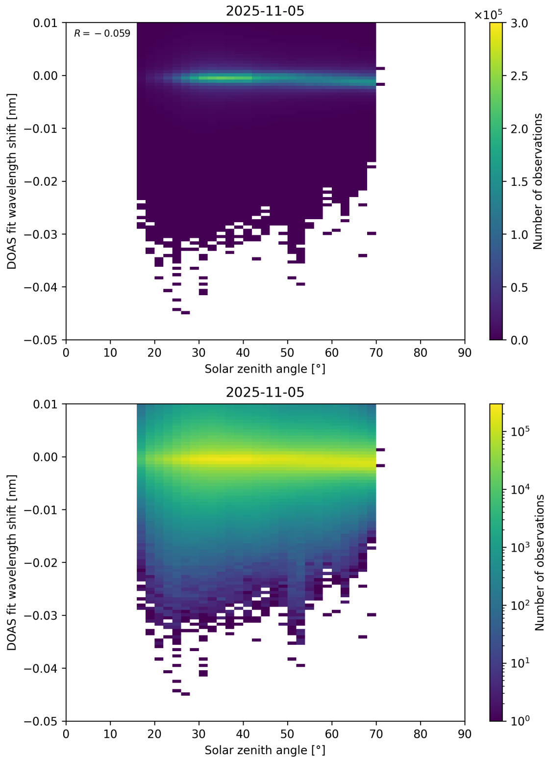
Figure 174: Scatter density plot of “Solar zenith angle” against “DOAS fit wavelength shift” for 2025-11-04 to 2025-11-06.
