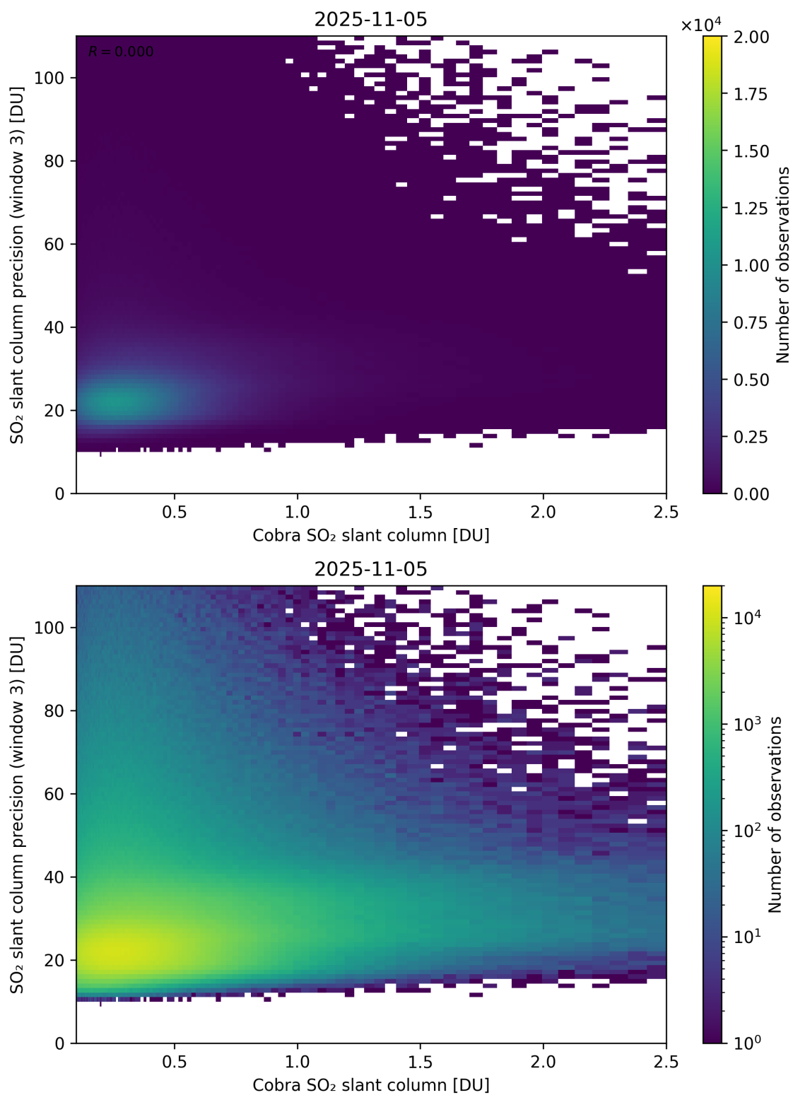
Figure 223: Scatter density plot of “Cobra SO 2 slant column” against “SO 2 slant column precision (window 3)” for 2025-11-04 to 2025-11-06.
