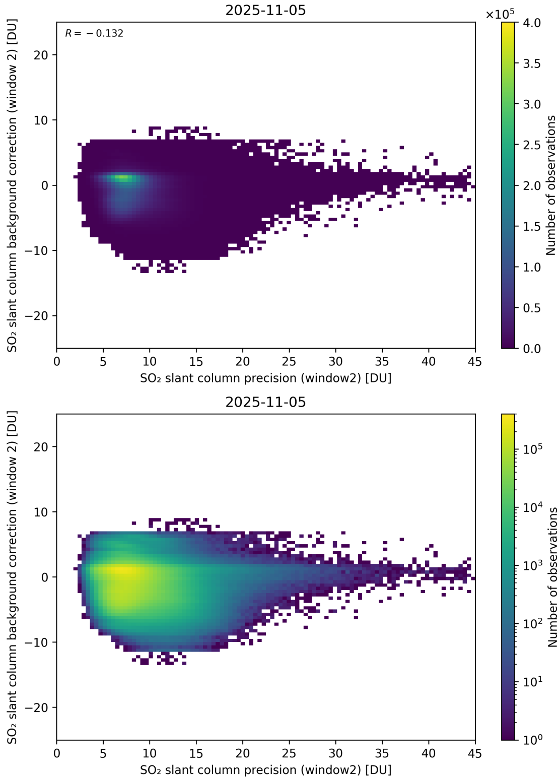
Figure 291: Scatter density plot of “SO 2 slant column precision (window2)” against “SO 2 slant column background correction (window 2)” for 2025-11-04 to 2025-11-06.
