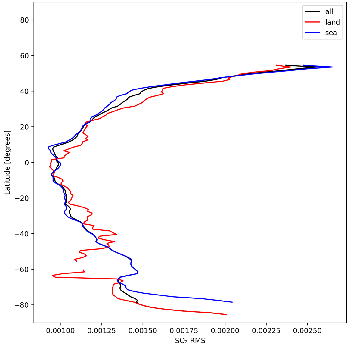
Figure 52: Zonal average of “SO 2 RMS” for 2025-11-04 to 2025-11-06.
