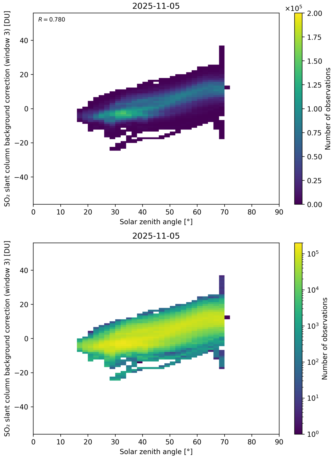
Figure 173: Scatter density plot of “Solar zenith angle” against “SO 2 slant column background correction (window 3)” for 2025-11-04 to 2025-11-06.
