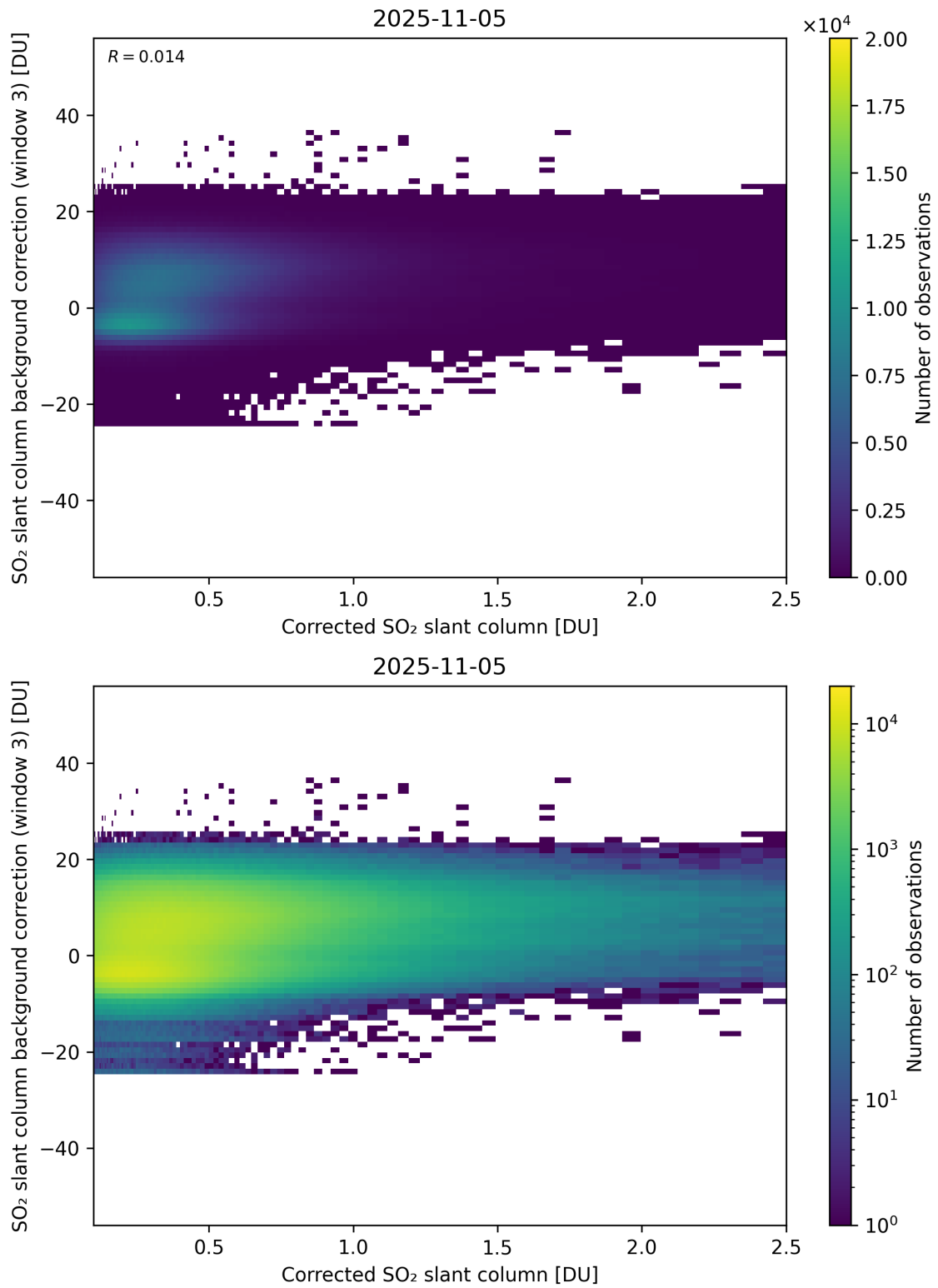
Figure 228: Scatter density plot of “Corrected SO 2 slant column” against “SO 2 slant column background correction (window 3)” for 2025-11-04 to 2025-11-06.
