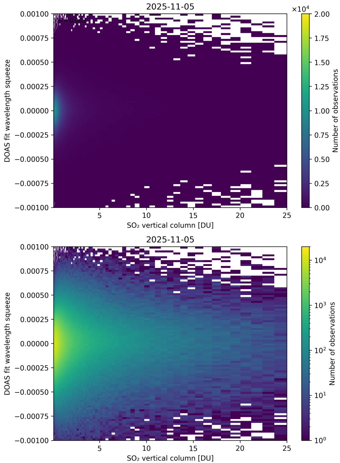
Figure 327: Scatter density plot of “SO 2 vertical column” against “DOAS fit wavelength squeeze” for 2025-11-04 to 2025-11-06.
