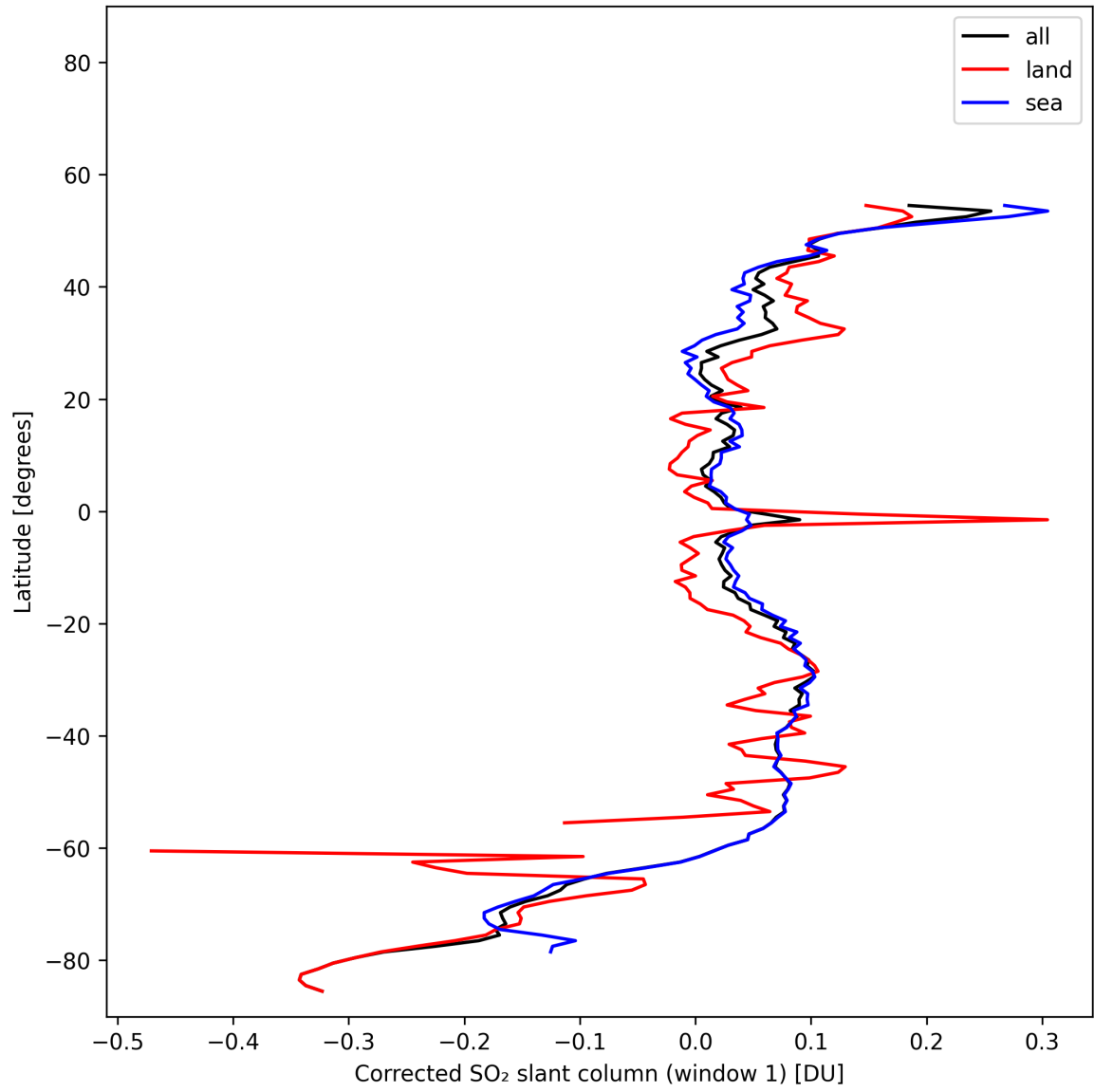
Figure 39: Zonal average of “Corrected SO 2 slant column (window 1)” for 2025-11-04 to 2025-11-06.
