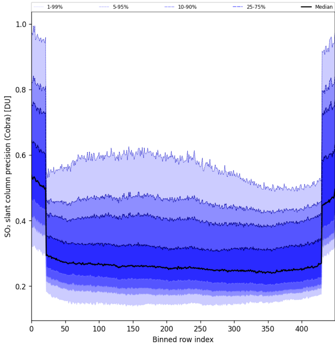
Figure 88: Along track statistics of “SO 2 slant column precision (Cobra)” for 2025-11-04 to 2025-11-06
