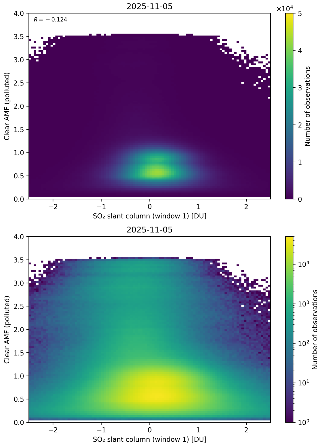
Figure 282: Scatter density plot of “SO 2 slant column (window 1)” against “Clear AMF (polluted)” for 2025-11-04 to 2025-11-06.
