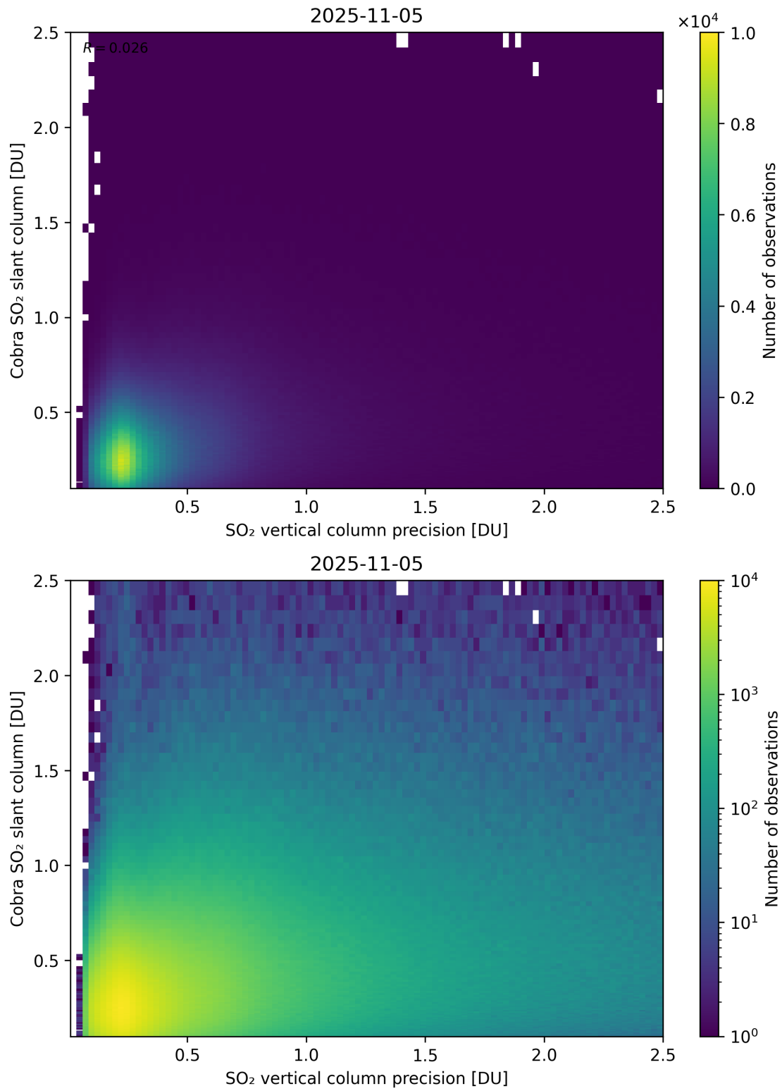
Figure 336: Scatter density plot of “SO 2 vertical column precision” against “Cobra SO 2 slant column” for 2025-11-04 to 2025-11-06.
