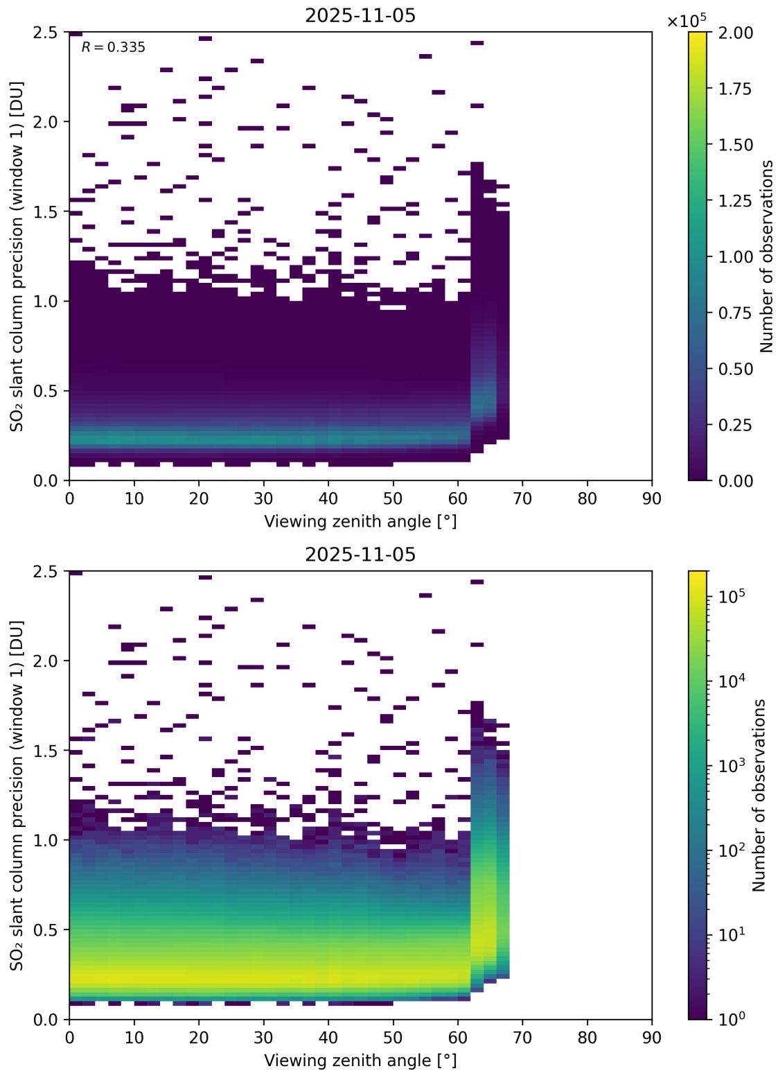
Figure 377: Scatter density plot of “Viewing zenith angle” against “SO 2 slant column precision (window 1)” for 2025-11-04 to 2025-11-06.
