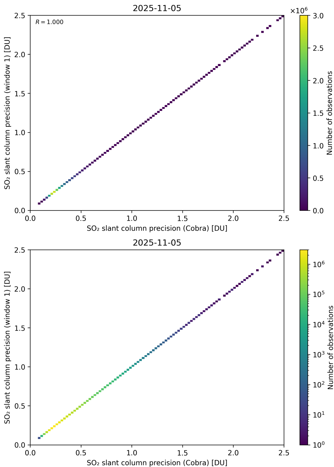
Figure 209: Scatter density plot of “SO 2 slant column precision (Cobra)” against “SO 2 slant column precision (window 1)” for 2025-11-04 to 2025-11-06.
