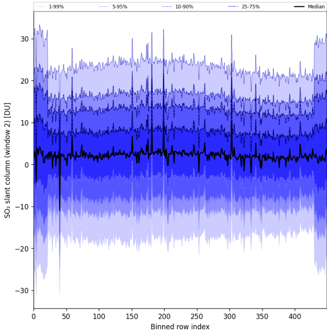
Figure 93: Along track statistics of “SO 2 slant column (window 2)” for 2025-11-04 to 2025-11-06
