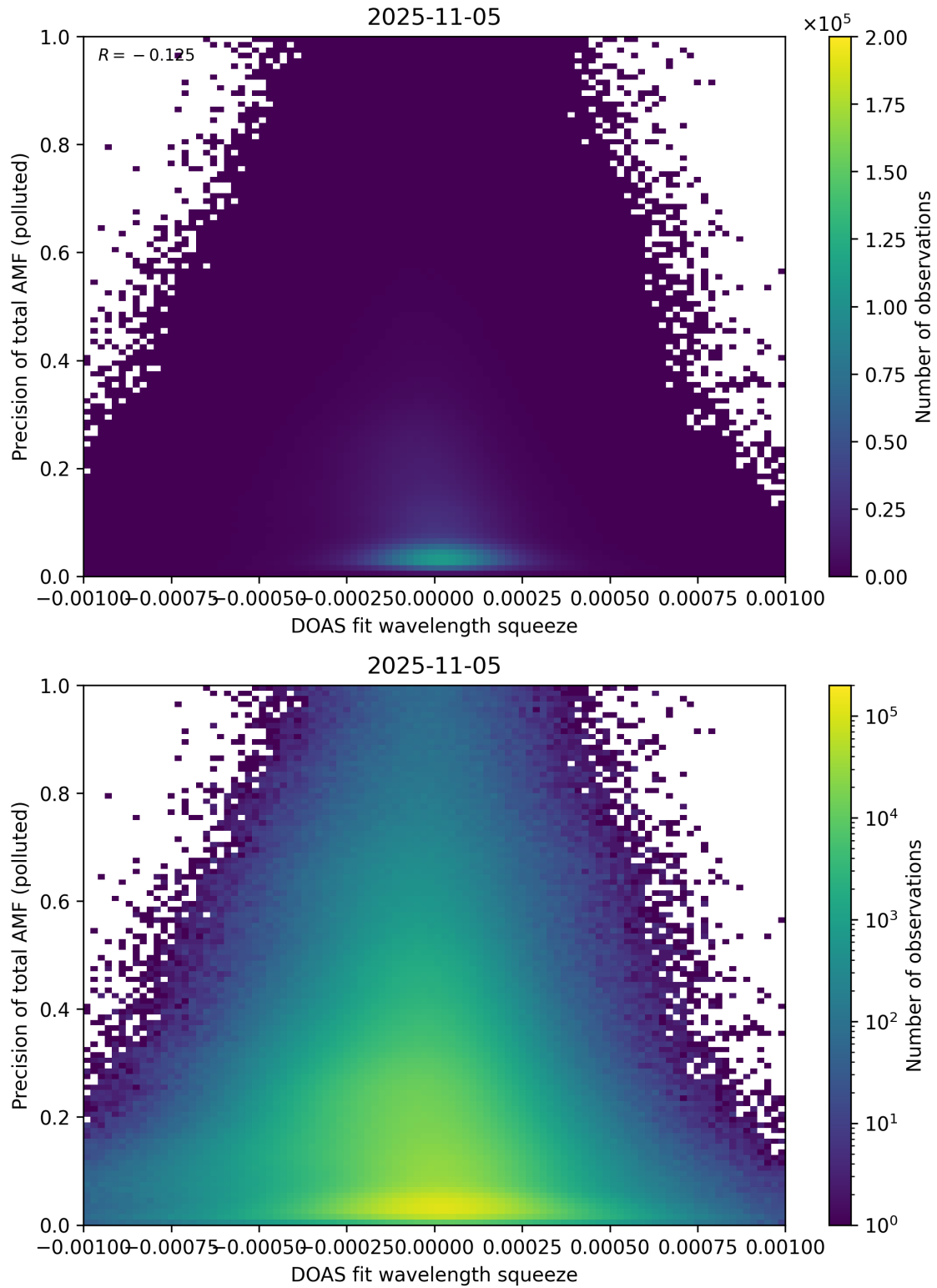
Figure 146: Scatter density plot of “DOAS fit wavelength squeeze” against “Precision of total AMF (polluted)” for 2025-11-04 to 2025-11-06.
