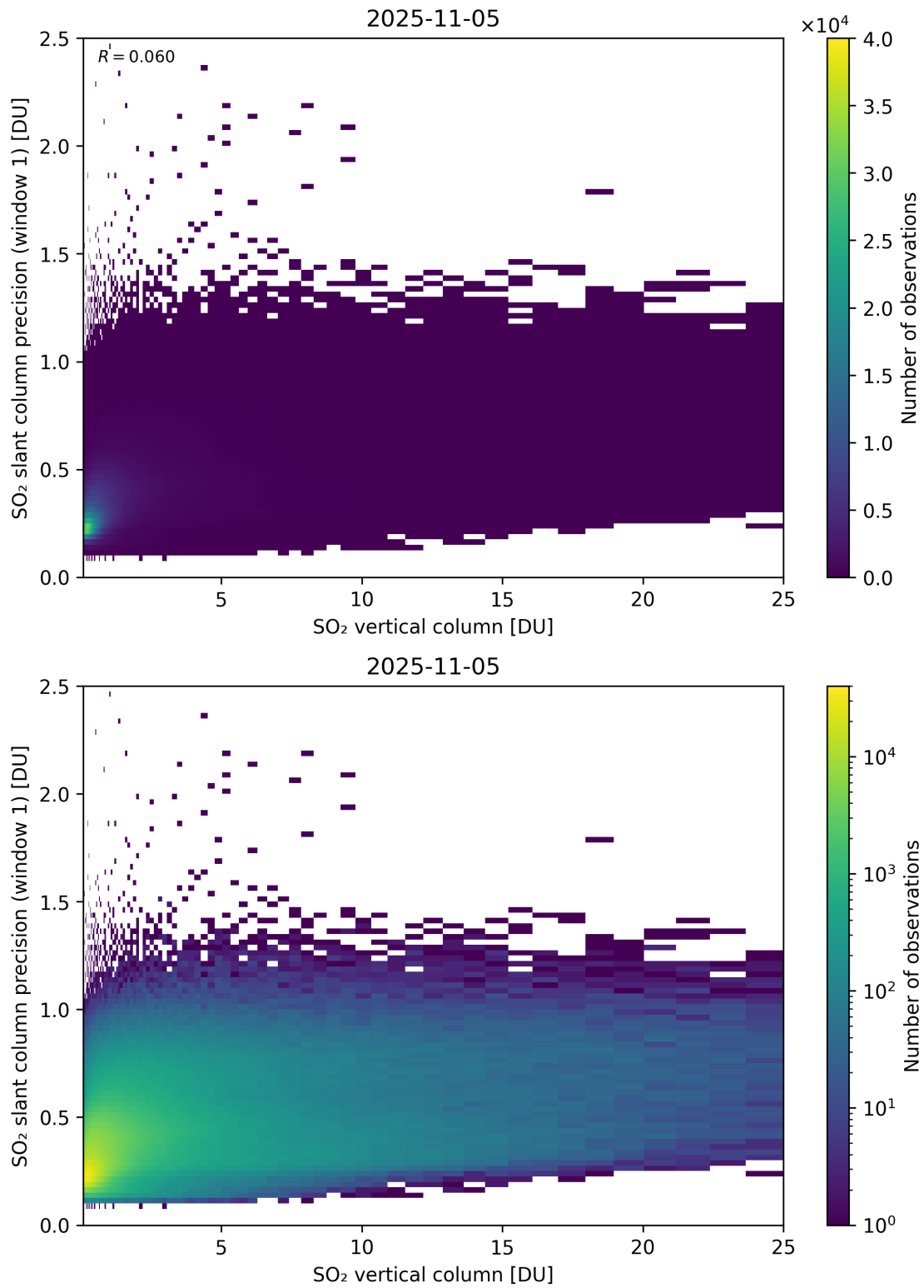
Figure 355: Scatter density plot of “SO 2 vertical column” against “SO 2 slant column precision (window 1)” for 2025-11-04 to 2025-11-06.
