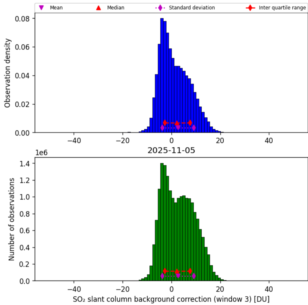
Figure 74: Histogram of “SO 2 slant column background correction (window 3)” for 2025-11-04 to 2025-11-06
