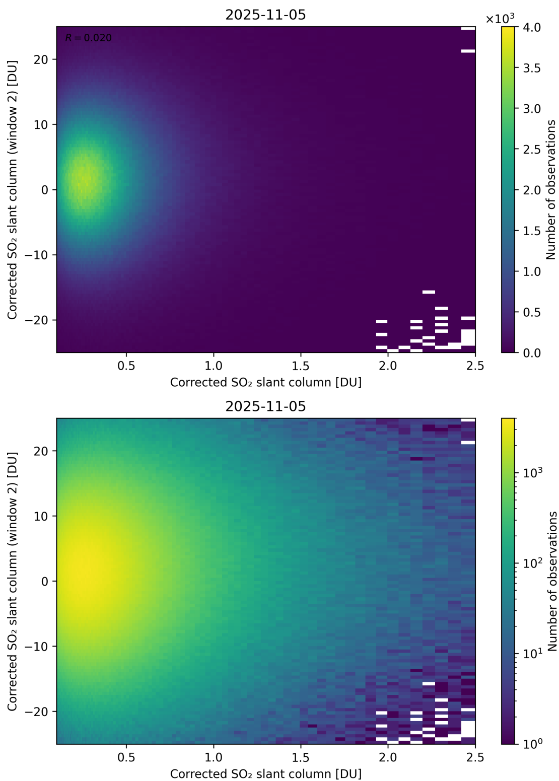
Figure 235: Scatter density plot of “Corrected SO 2 slant column” against “Corrected SO 2 slant column (window 2)” for 2025-11-04 to 2025-11-06.
