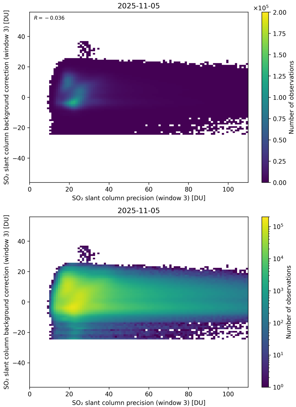
Figure 307: Scatter density plot of “SO 2 slant column precision (window 3)” against “SO 2 slant column background correction (window 3)” for 2025-11-04 to 2025-11-06.
