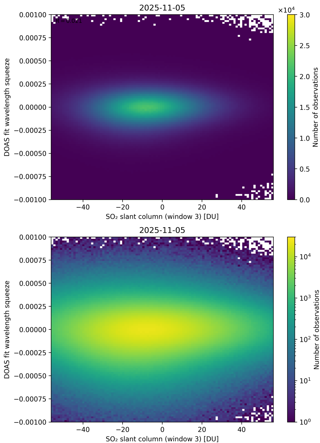
Figure 305: Scatter density plot of “SO 2 slant column (window 3)” against “DOAS fit wavelength squeeze” for 2025-11-04 to 2025-11-06.
