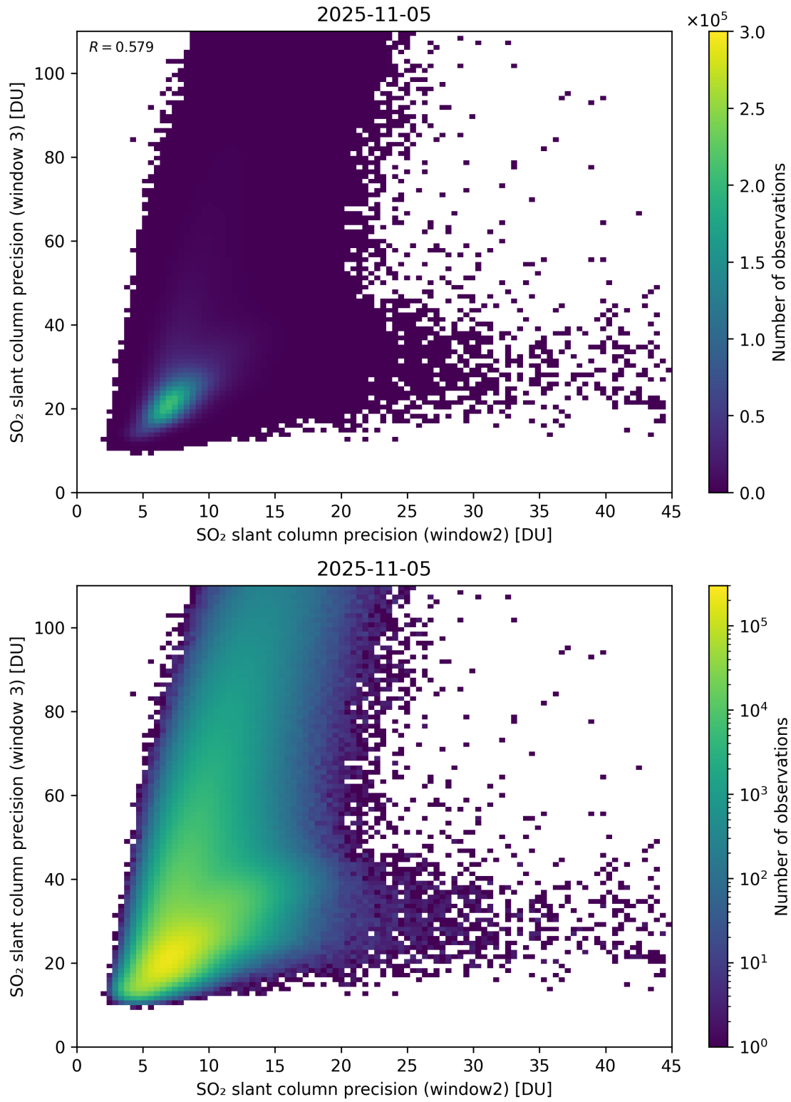
Figure 300: Scatter density plot of “SO 2 slant column precision (window2)” against “SO 2 slant column precision (window 3)” for 2025-11-04 to 2025-11-06.
