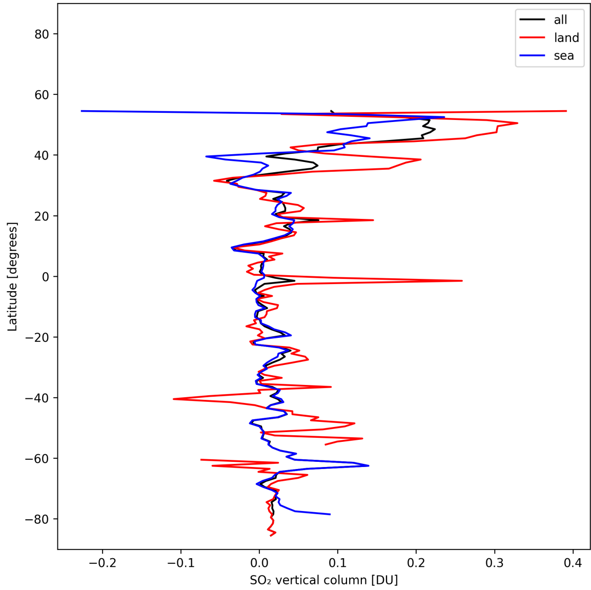
Figure 32: Zonal average of “SO 2 vertical column” for 2025-11-04 to 2025-11-06.
