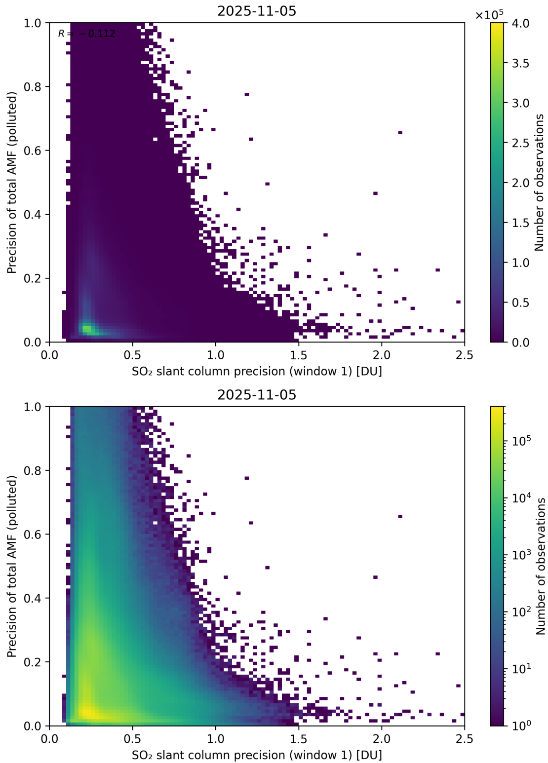
Figure 281: Scatter density plot of “SO 2 slant column precision (window 1)” against “Precision of total AMF (polluted)” for 2025-11-04 to 2025-11-06.
