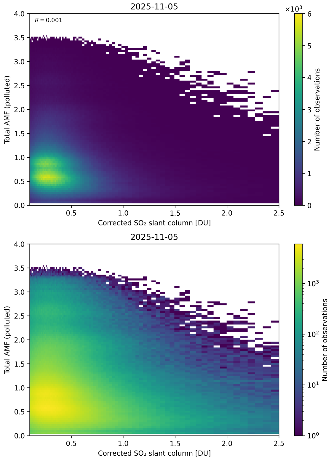
Figure 242: Scatter density plot of “Corrected SO 2 slant column” against “Total AMF (polluted)” for 2025-11-04 to 2025-11-06.
