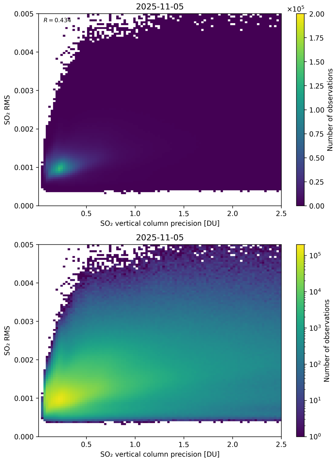
Figure 334: Scatter density plot of “SO 2 vertical column precision” against “SO 2 RMS” for 2025-11-04 to 2025-11-06.
