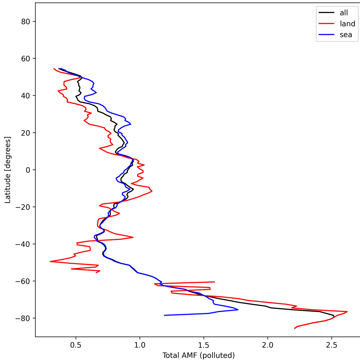
Figure 53: Zonal average of “Total AMF (polluted)” for 2025-11-04 to 2025-11-06.
