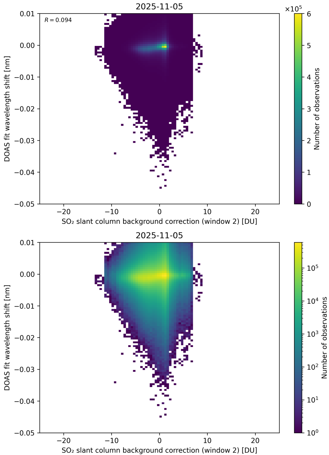
Figure 123: Scatter density plot of “SO 2 slant column background correction (window 2)” against “DOAS fit wavelength shift” for 2025-11-04 to 2025-11-06.
