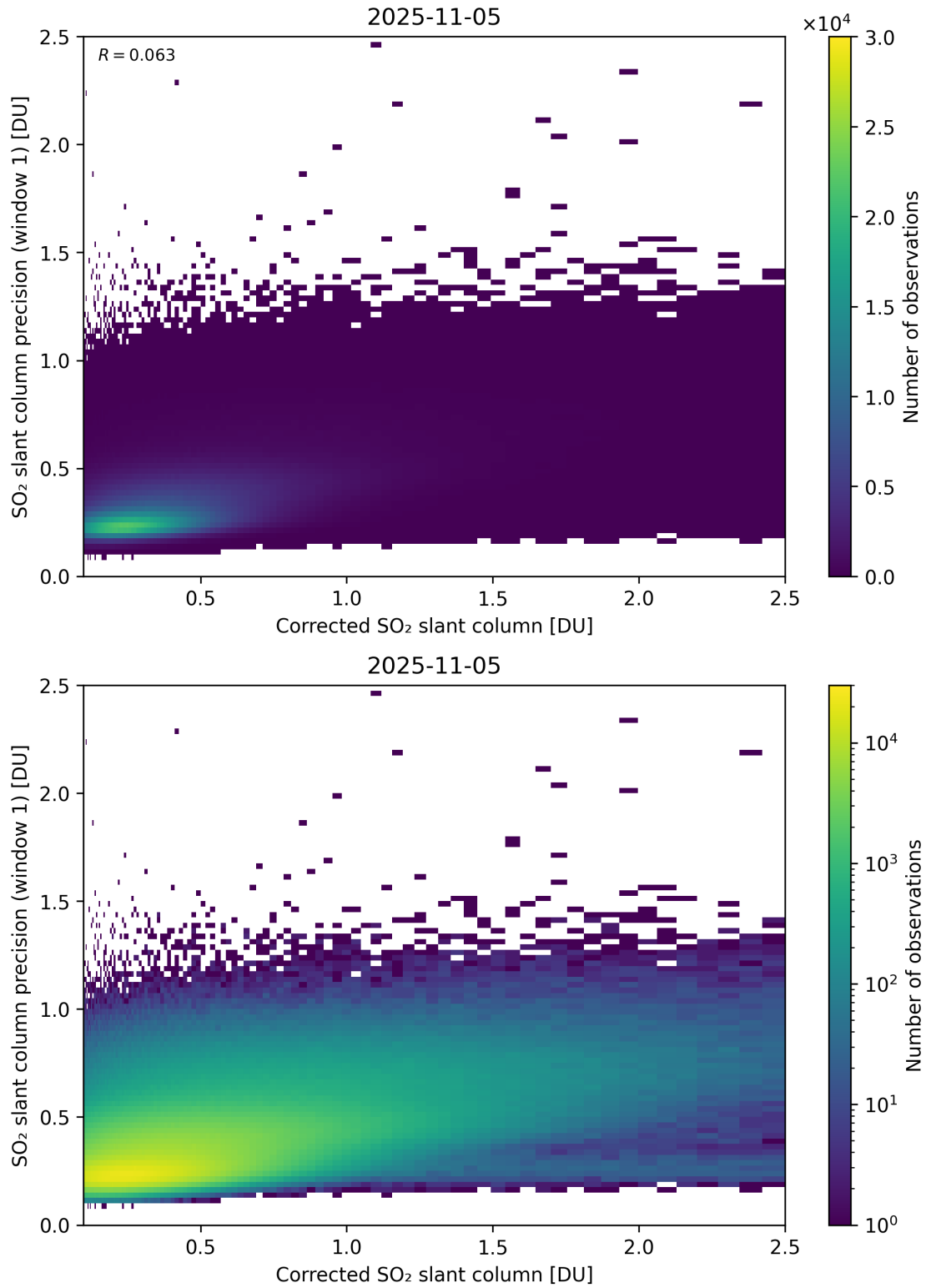
Figure 238: Scatter density plot of “Corrected SO 2 slant column” against “SO 2 slant column precision (window 1)” for 2025-11-04 to 2025-11-06.
