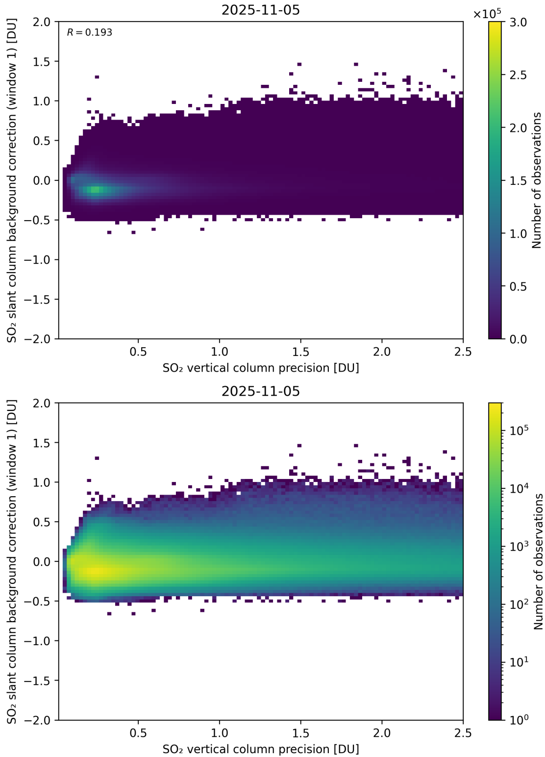
Figure 329: Scatter density plot of “SO 2 vertical column precision” against “SO 2 slant column background correction (window 1)” for 2025-11-04 to 2025-11-06.
