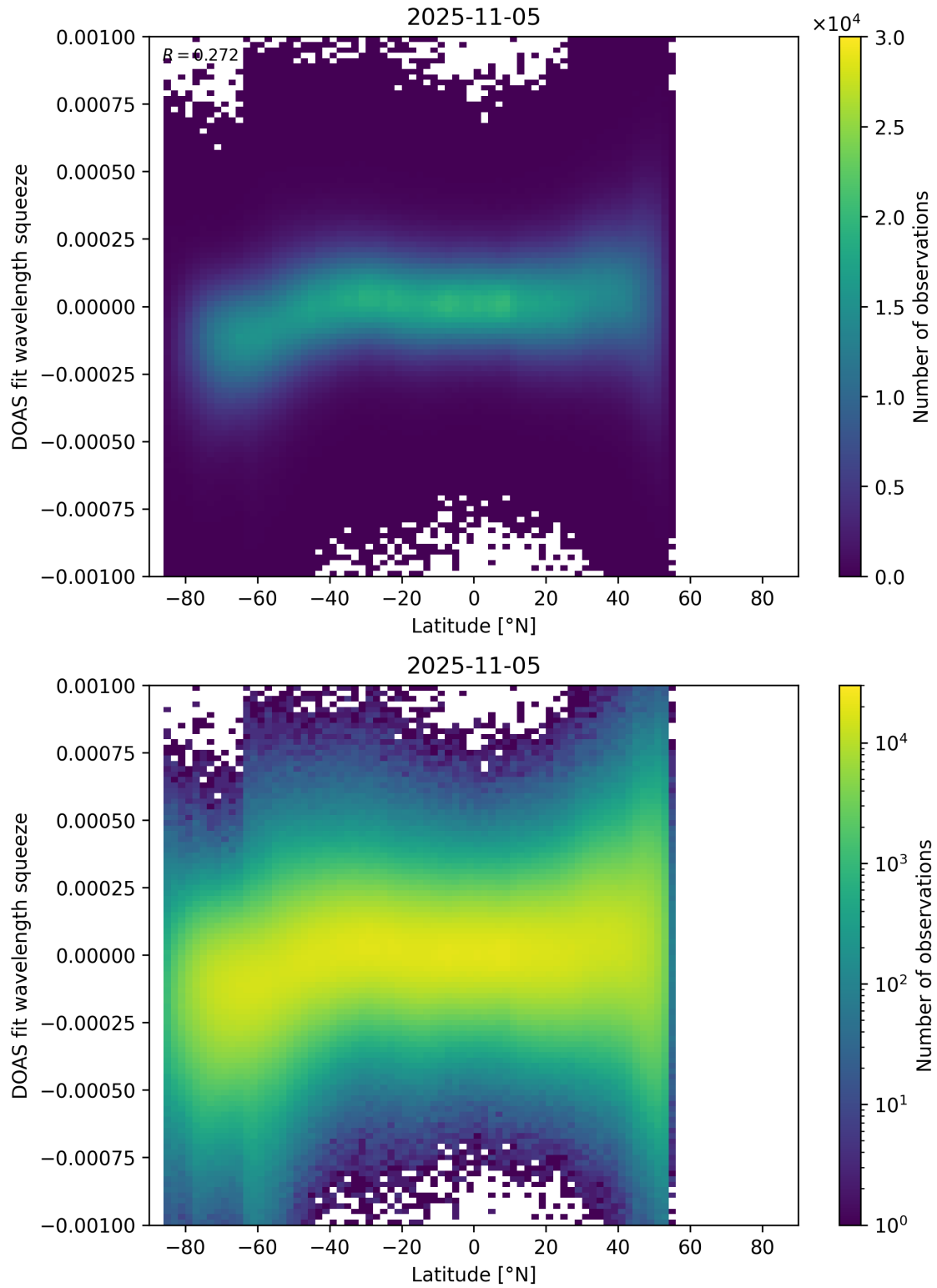
Figure 154: Scatter density plot of “Latitude” against “DOAS fit wavelength squeeze” for 2025-11-04 to 2025-11-06.
