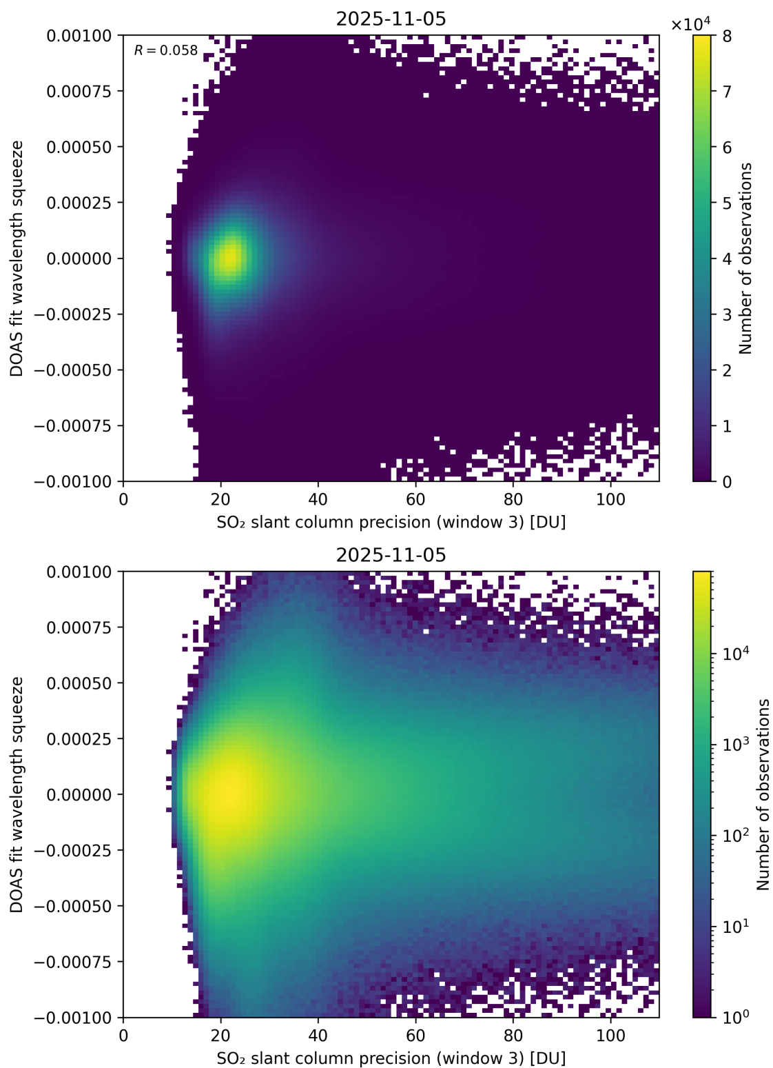
Figure 309: Scatter density plot of “SO 2 slant column precision (window 3)” against “DOAS fit wavelength squeeze” for 2025-11-04 to 2025-11-06.
