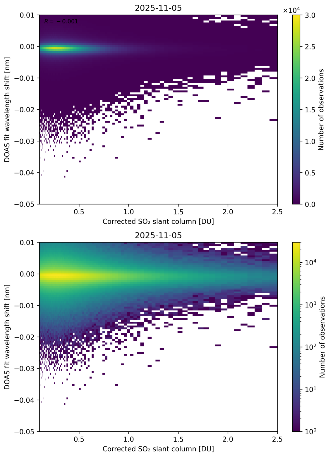
Figure 229: Scatter density plot of “Corrected SO 2 slant column” against “DOAS fit wavelength shift” for 2025-11-04 to 2025-11-06.
