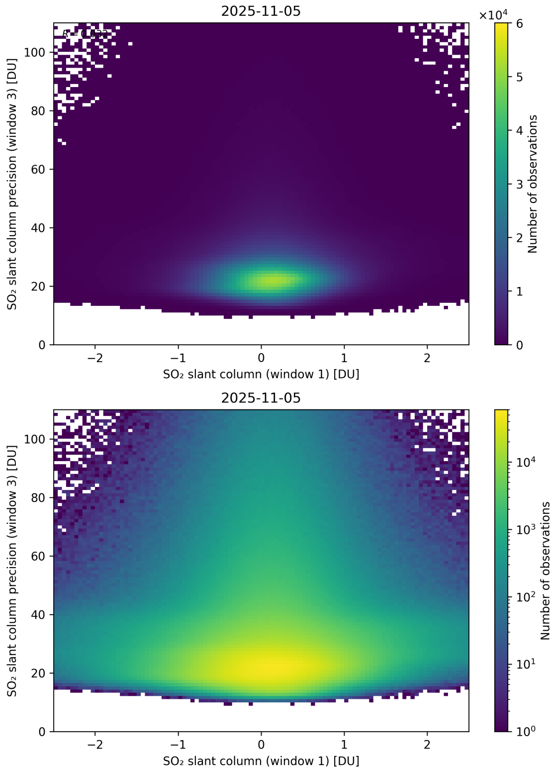
Figure 288: Scatter density plot of “SO 2 slant column (window 1)” against “SO 2 slant column precision (window 3)” for 2025-11-04 to 2025-11-06.
