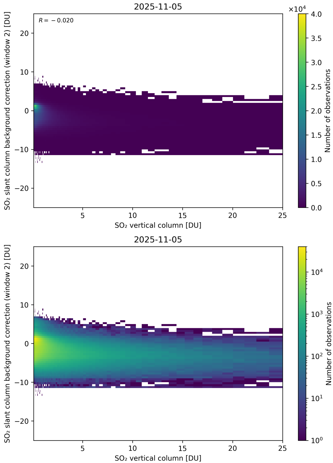
Figure 324: Scatter density plot of “SO 2 vertical column” against “SO 2 slant column background correction (window 2)” for 2025-11-04 to 2025-11-06.
