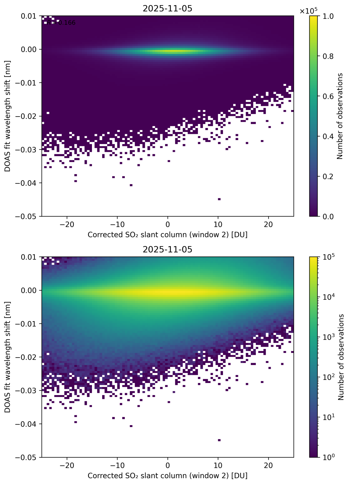
Figure 246: Scatter density plot of “Corrected SO 2 slant column (window 2)” against “DOAS fit wavelength shift” for 2025-11-04 to 2025-11-06.
