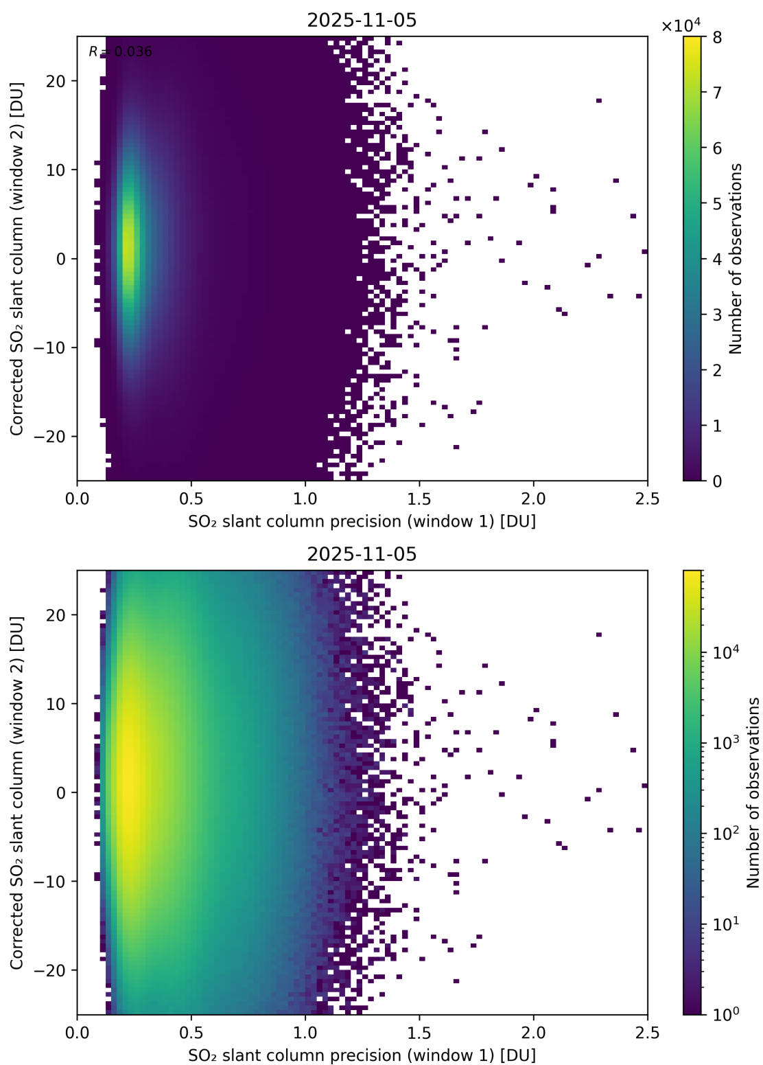
Figure 275: Scatter density plot of “SO 2 slant column precision (window 1)” against “Corrected SO 2 slant column (window 2)” for 2025-11-04 to 2025-11-06.
