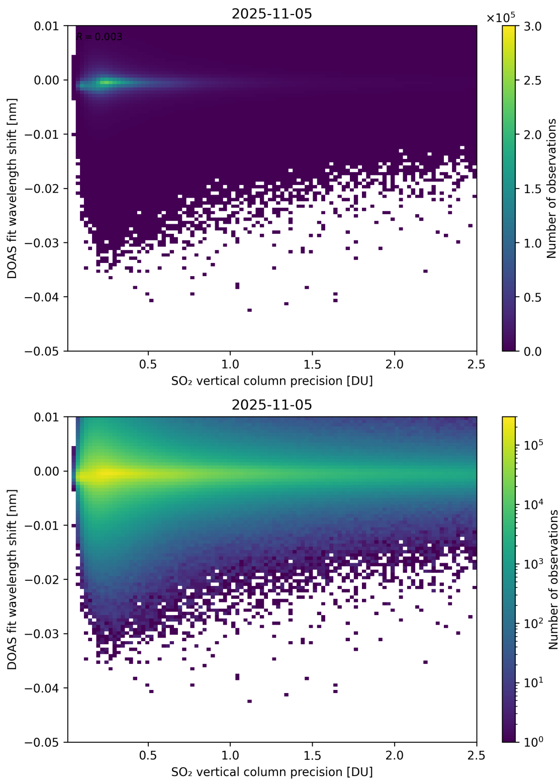
Figure 332: Scatter density plot of “SO 2 vertical column precision” against “DOAS fit wavelength shift” for 2025-11-04 to 2025-11-06.
