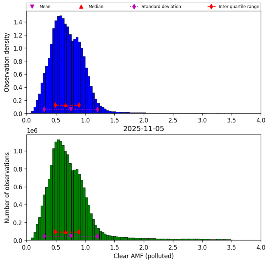
Figure 81: Histogram of “Clear AMF (polluted)” for 2025-11-04 to 2025-11-06
