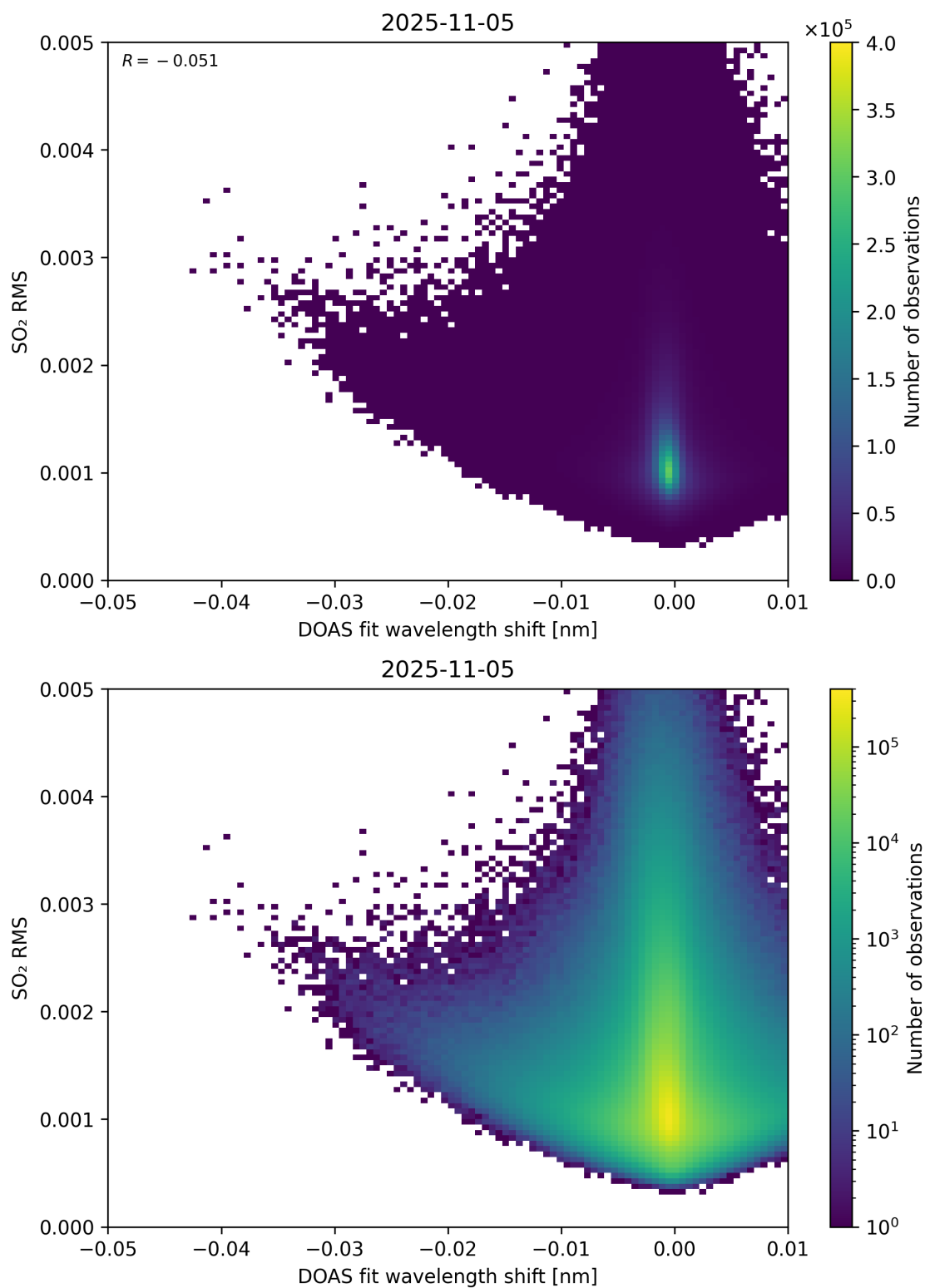
Figure 139: Scatter density plot of “DOAS fit wavelength shift” against “SO 2 RMS” for 2025-11-04 to 2025-11-06.
