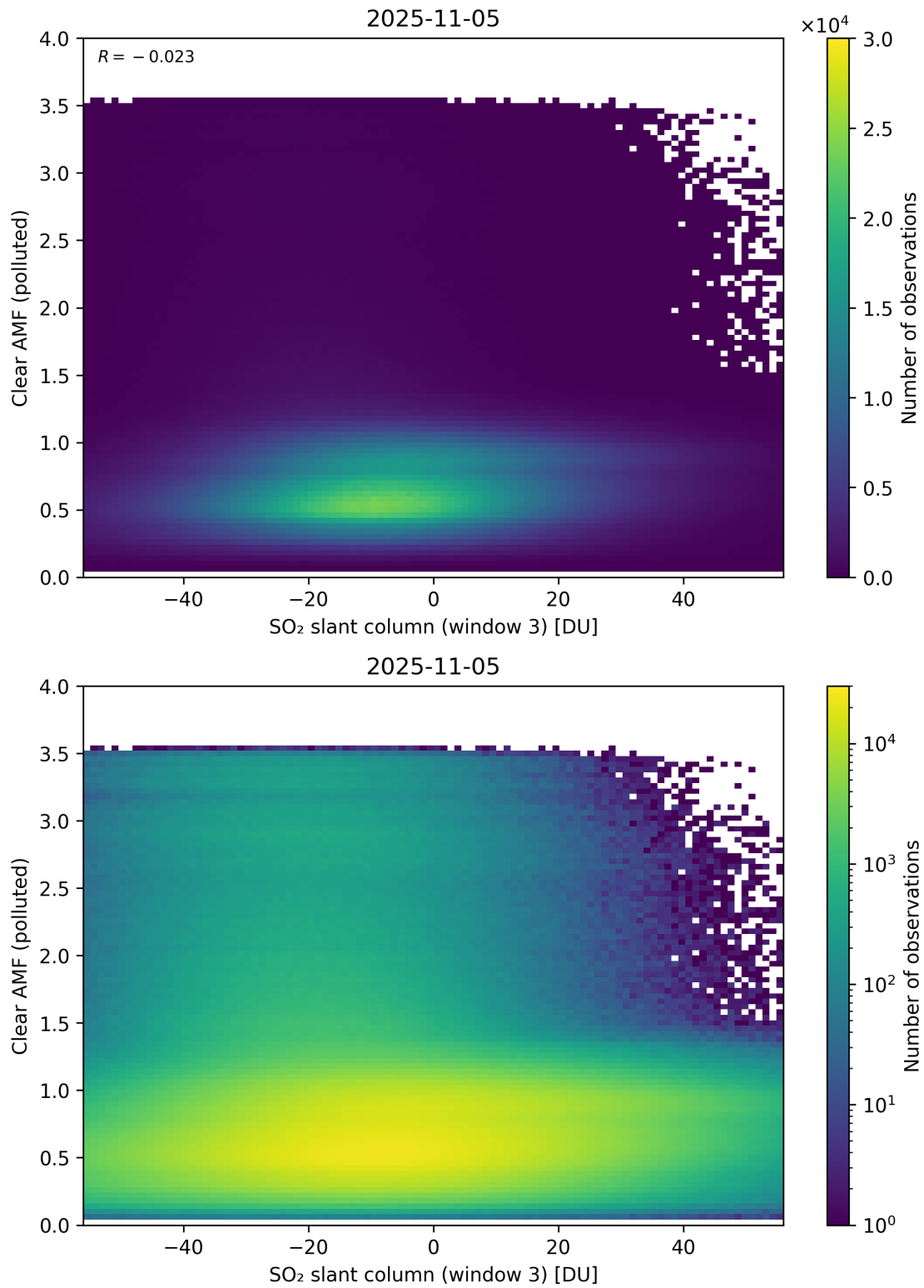
Figure 315: Scatter density plot of “SO 2 slant column (window 3)” against “Clear AMF (polluted)” for 2025-11-04 to 2025-11-06.
