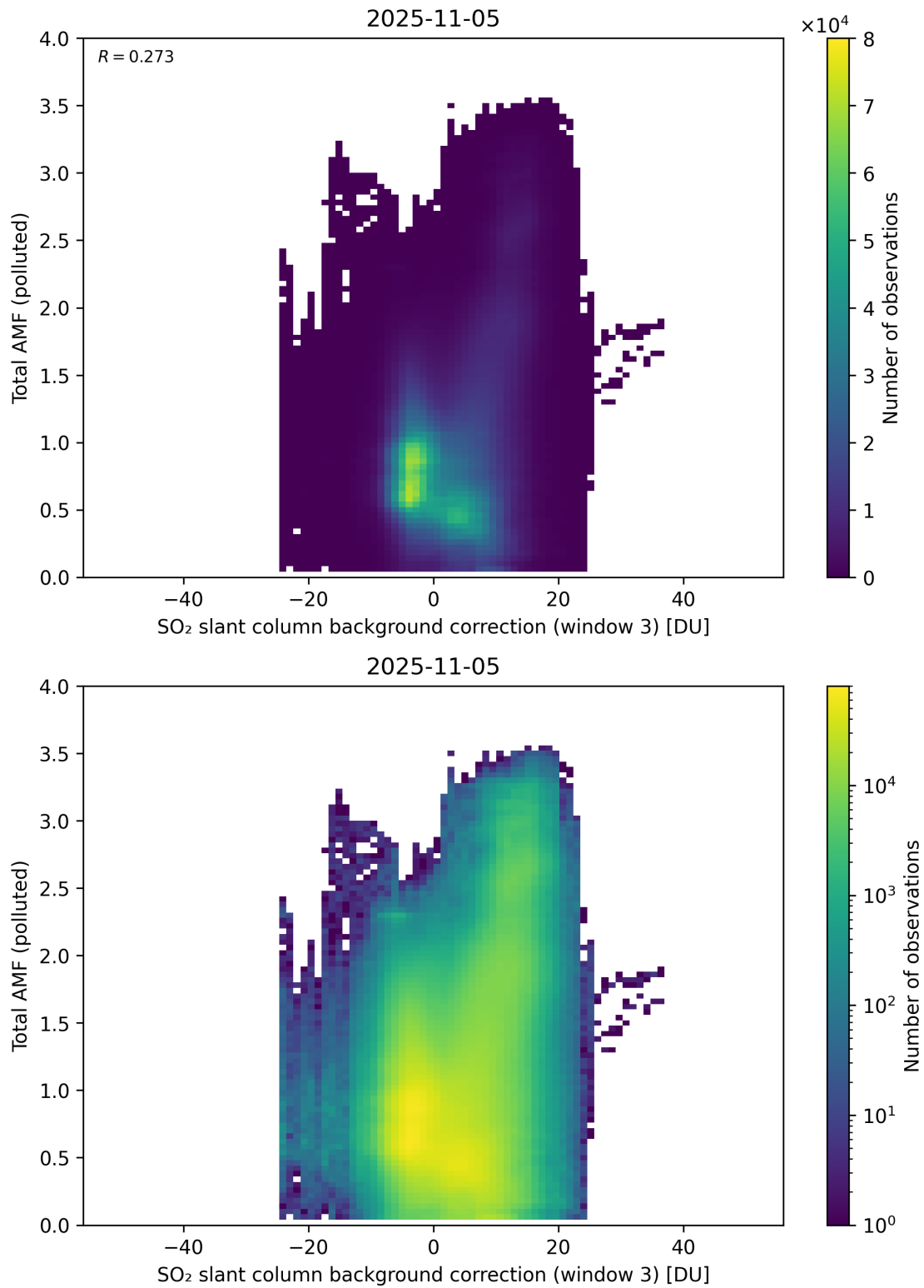
Figure 136: Scatter density plot of “SO 2 slant column background correction (window 3)” against “Total AMF (polluted)” for 2025-11-04 to 2025-11-06.
