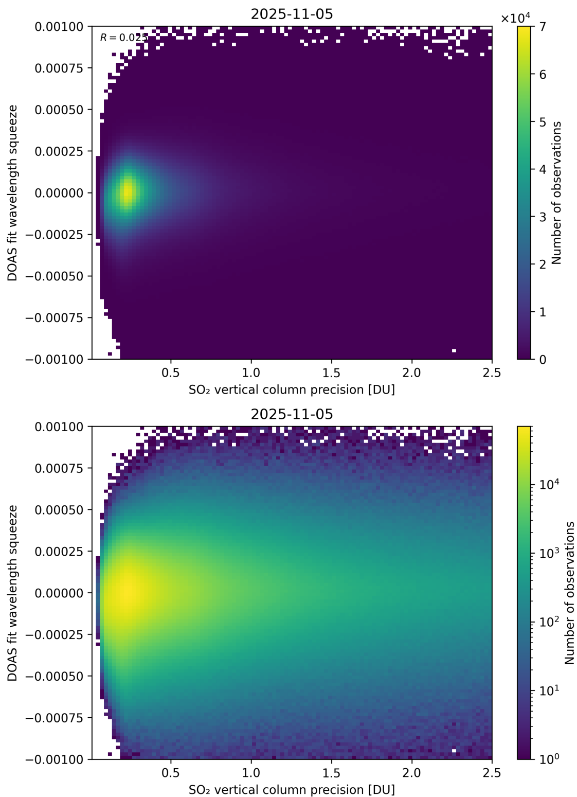
Figure 333: Scatter density plot of “SO 2 vertical column precision” against “DOAS fit wavelength squeeze” for 2025-11-04 to 2025-11-06.
