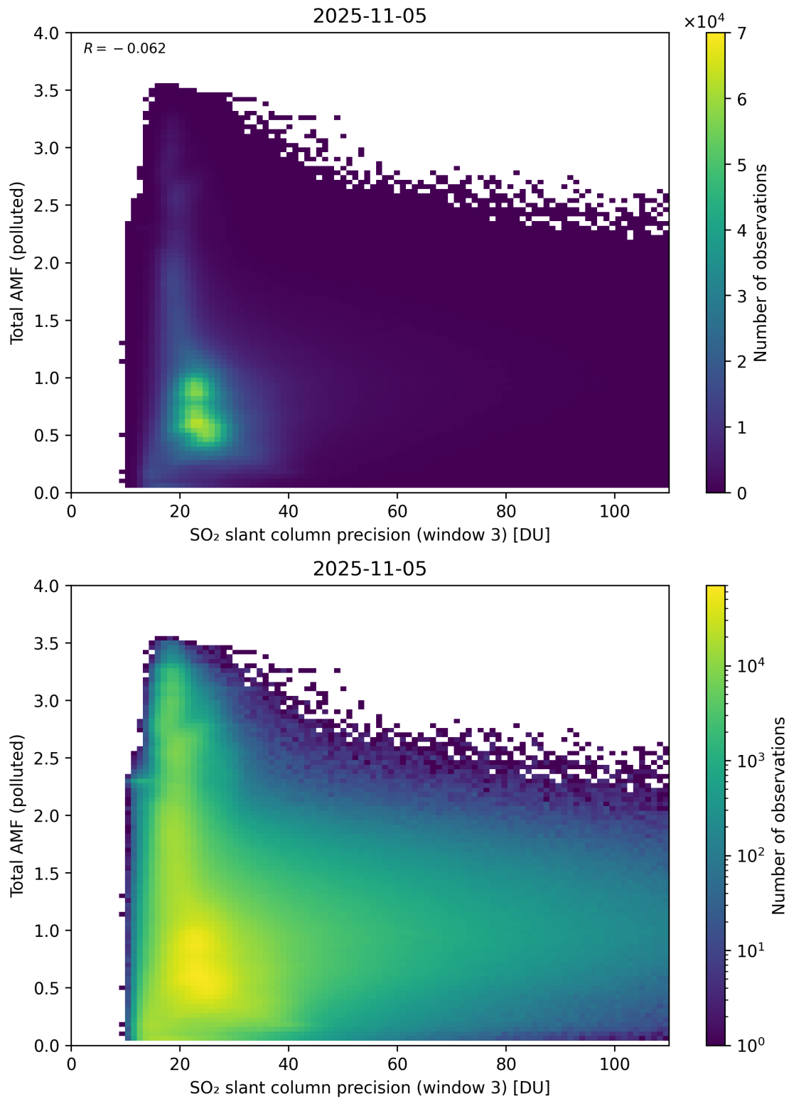
Figure 313: Scatter density plot of “SO 2 slant column precision (window 3)” against “Total AMF (polluted)” for 2025-11-04 to 2025-11-06.
