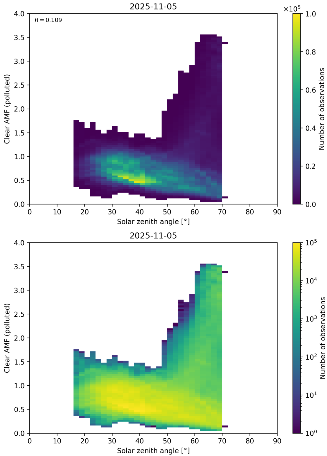
Figure 178: Scatter density plot of “Solar zenith angle” against “Clear AMF (polluted)” for 2025-11-04 to 2025-11-06.
