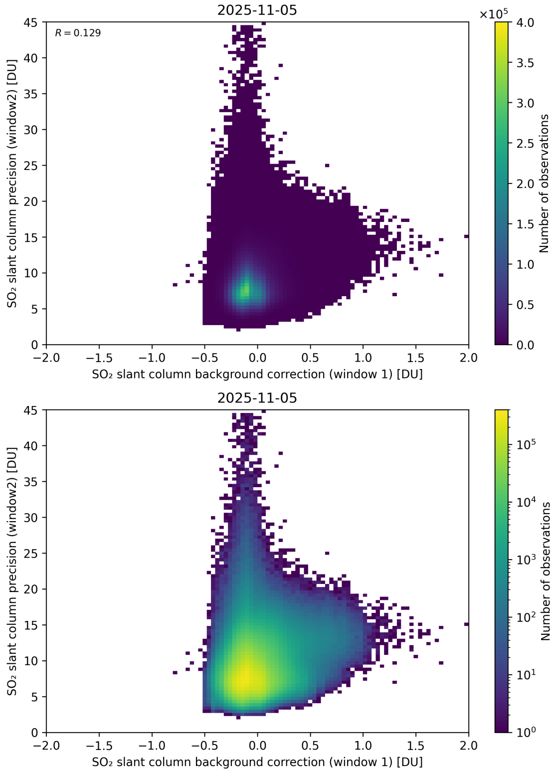
Figure 117: Scatter density plot of “SO 2 slant column background correction (window 1)” against “SO 2 slant column precision (window2)” for 2025-11-04 to 2025-11-06.
