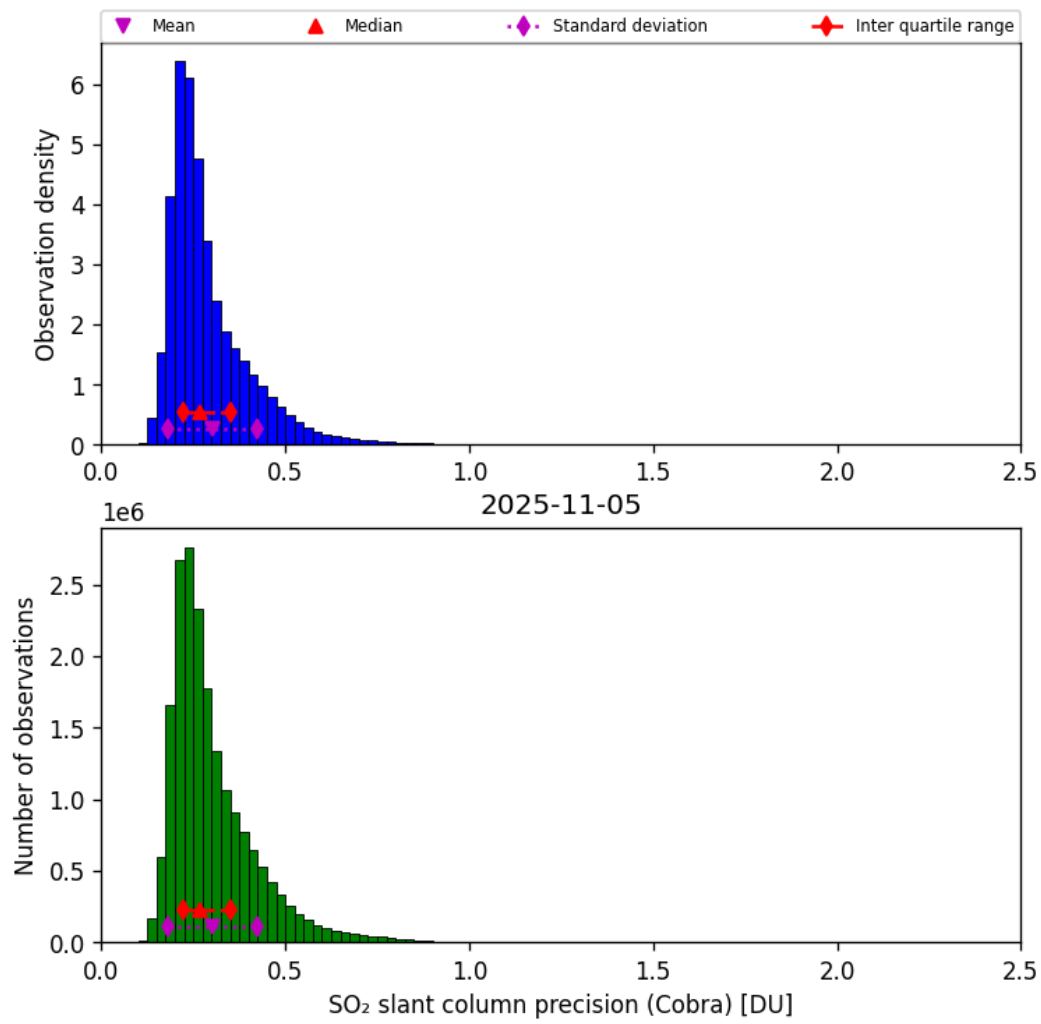
Figure 62: Histogram of “SO 2 slant column precision (Cobra)” for 2025-11-04 to 2025-11-06
