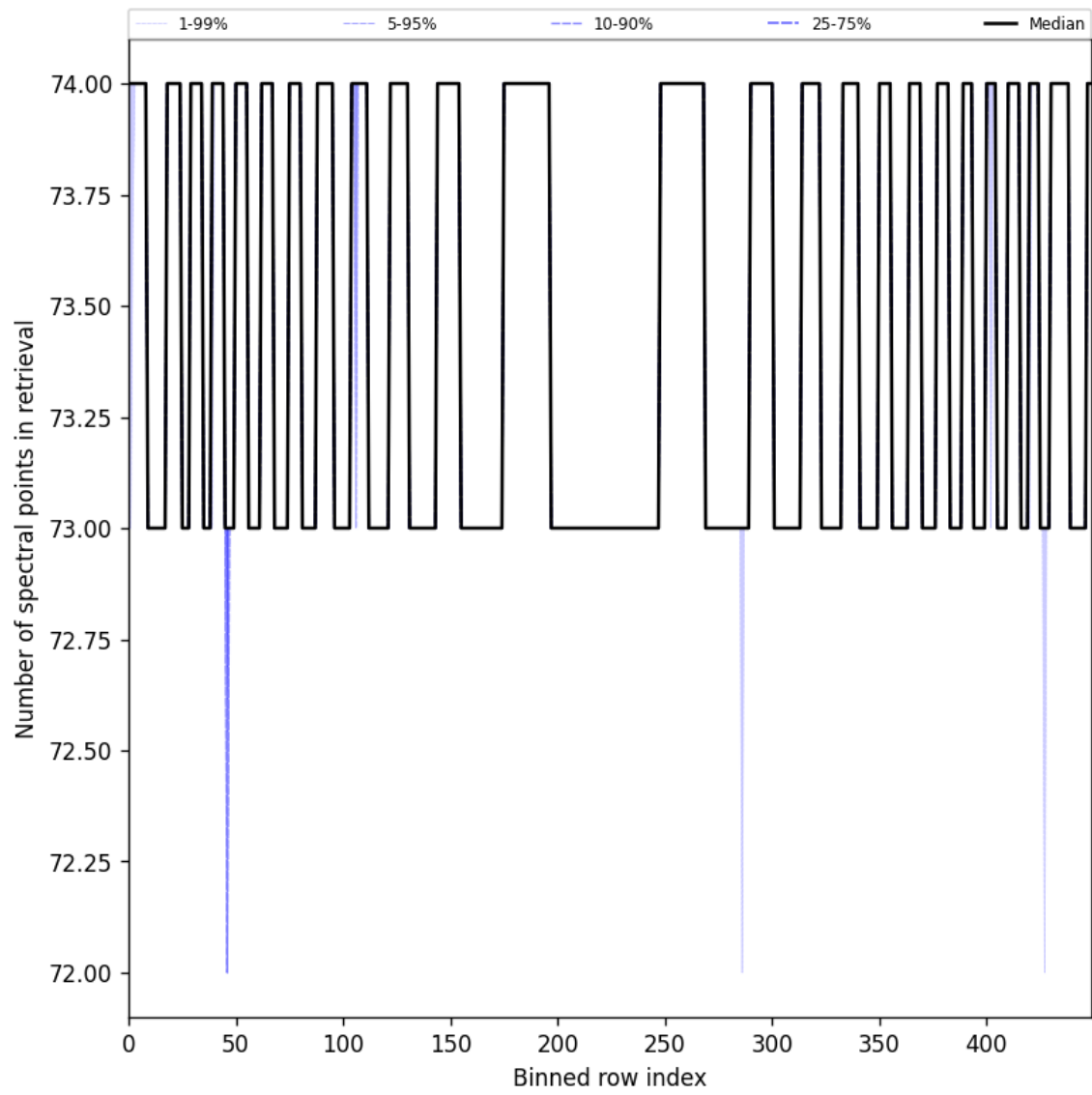
Figure 108: Along track statistics of “Number of spectral points in retrieval” for 2025-11-04 to 2025-11-06
