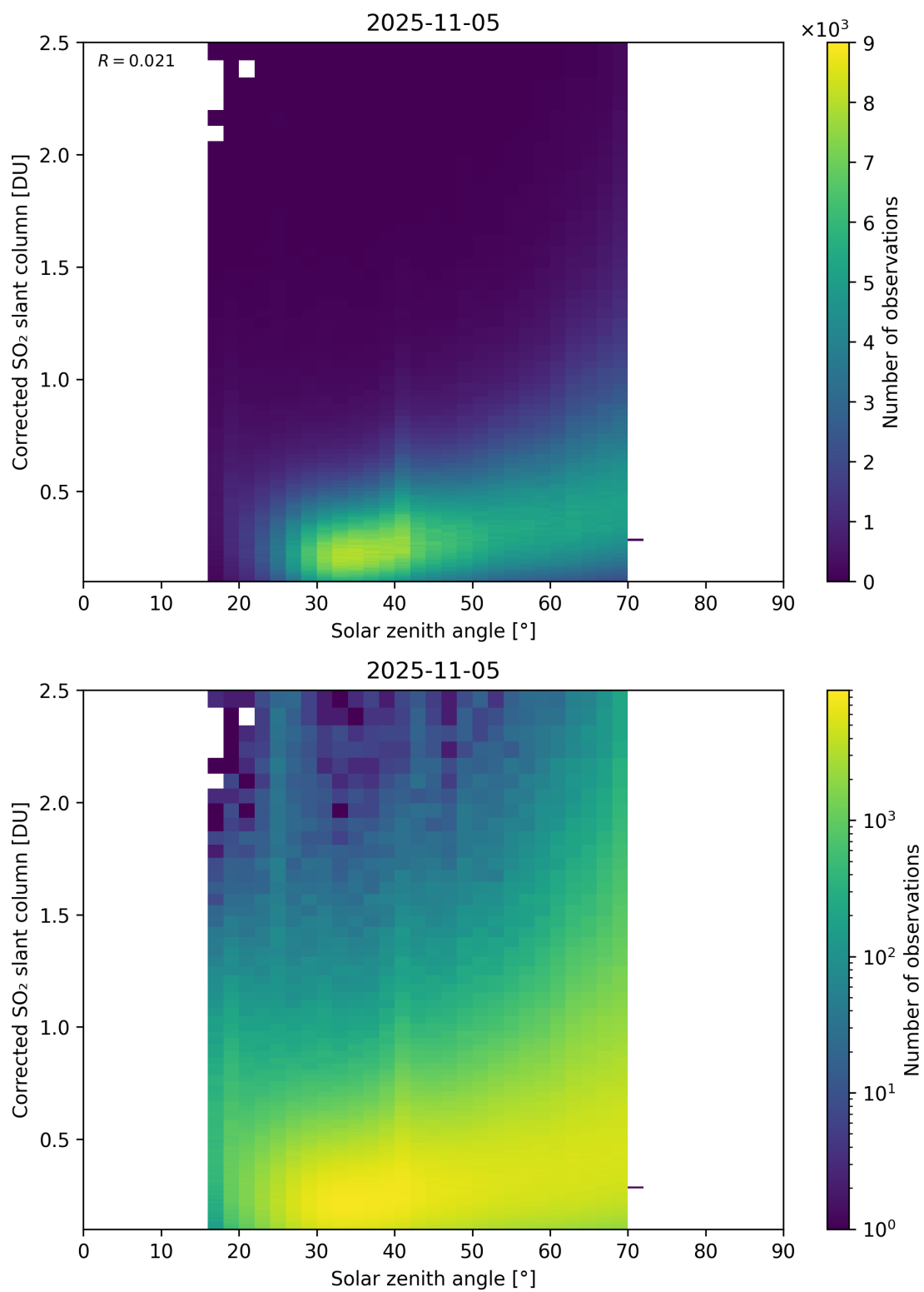
Figure 181: Scatter density plot of “Solar zenith angle” against “Corrected SO 2 slant column” for 2025-11-04 to 2025-11-06.
