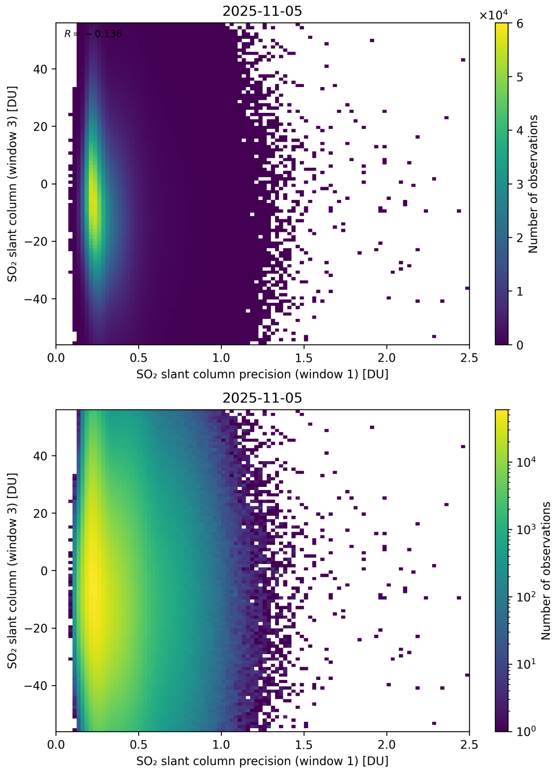
Figure 278: Scatter density plot of “SO 2 slant column precision (window 1)” against “SO 2 slant column (window 3)” for 2025-11-04 to 2025-11-06.
