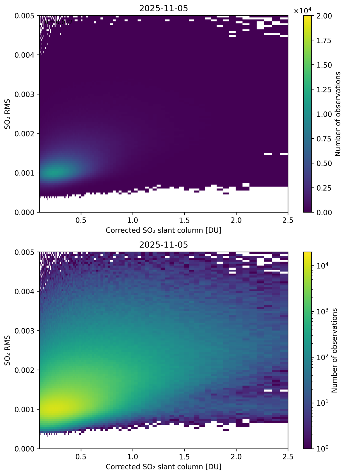
Figure 231: Scatter density plot of “Corrected SO 2 slant column” against “SO 2 RMS” for 2025-11-04 to 2025-11-06.
