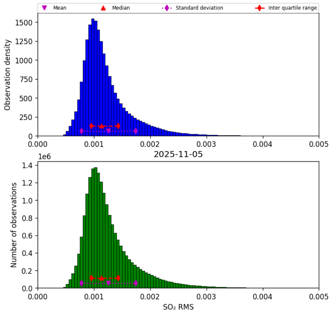
Figure 78: Histogram of “SO 2 RMS” for 2025-11-04 to 2025-11-06
