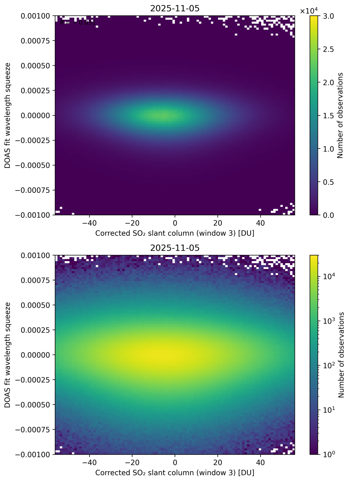
Figure 257: Scatter density plot of “Corrected SO 2 slant column (window 3)” against “DOAS fit wavelength squeeze” for 2025-11-04 to 2025-11-06.
