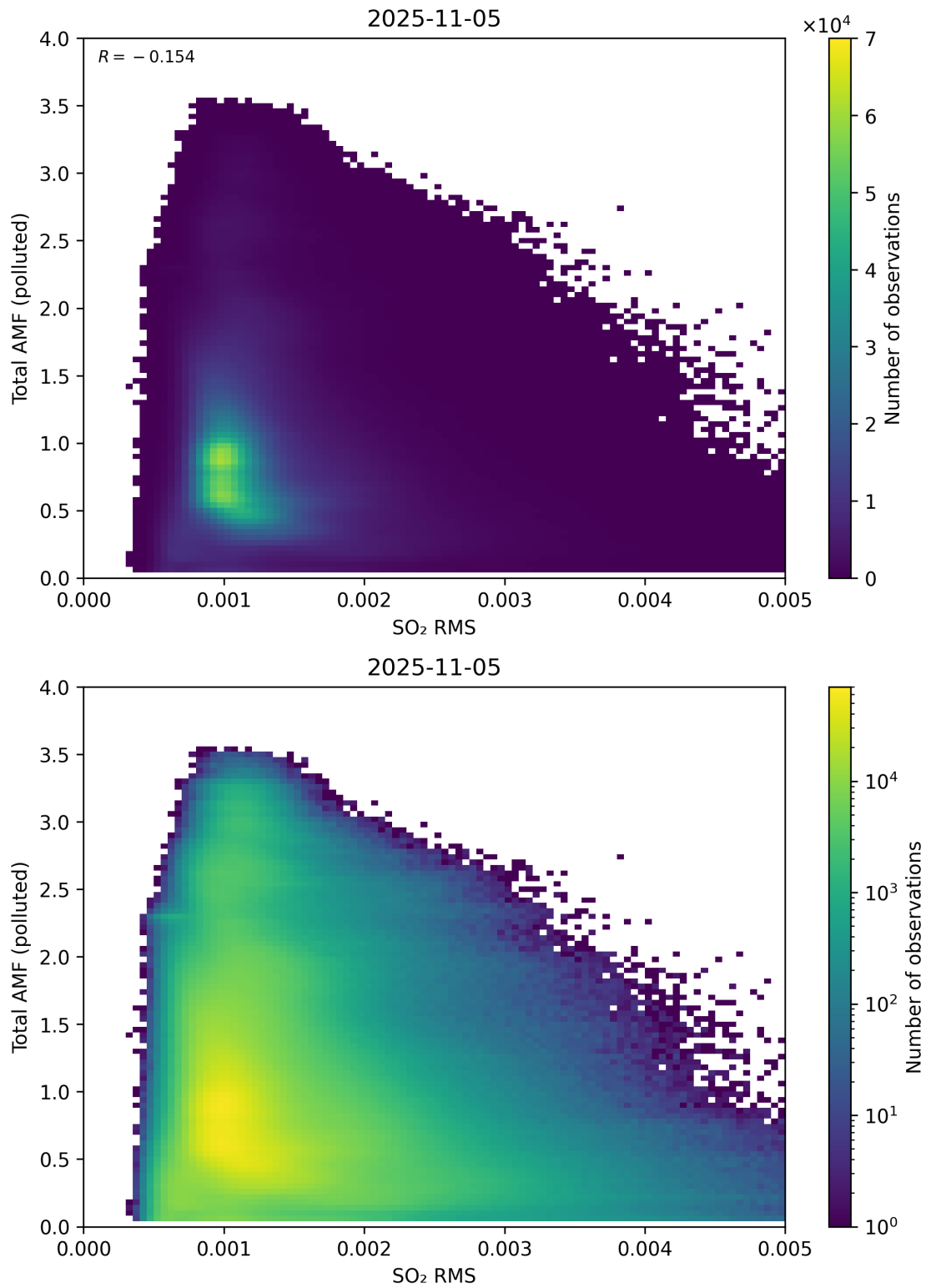
Figure 148: Scatter density plot of “SO 2 RMS” against “Total AMF (polluted)” for 2025-11-04 to 2025-11-06.
