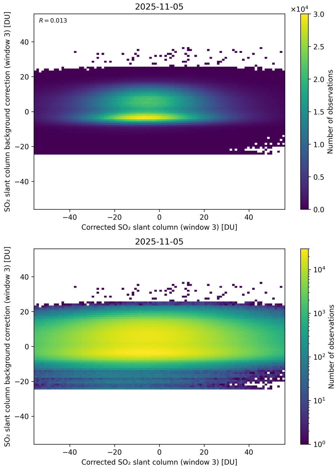
Figure 255: Scatter density plot of “Corrected SO 2 slant column (window 3)” against “SO 2 slant column background correction (window 3)” for 2025-11-04 to 2025-11-06.
