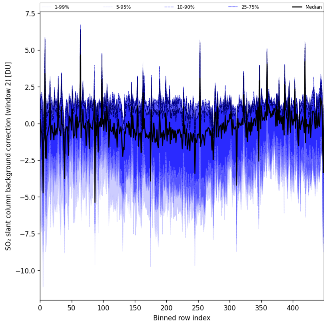
Figure 96: Along track statistics of “SO 2 slant column background correction (window 2)” for 2025-11-04 to 2025-11-06
