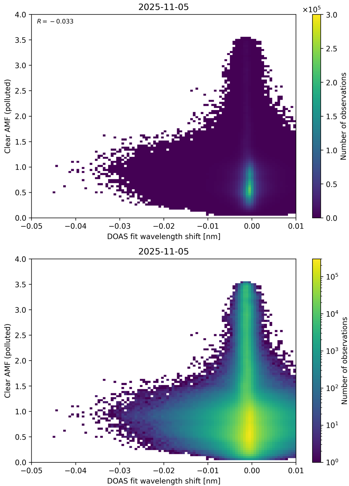
Figure 140: Scatter density plot of “DOAS fit wavelength shift” against “Clear AMF (polluted)” for 2025-11-04 to 2025-11-06.
