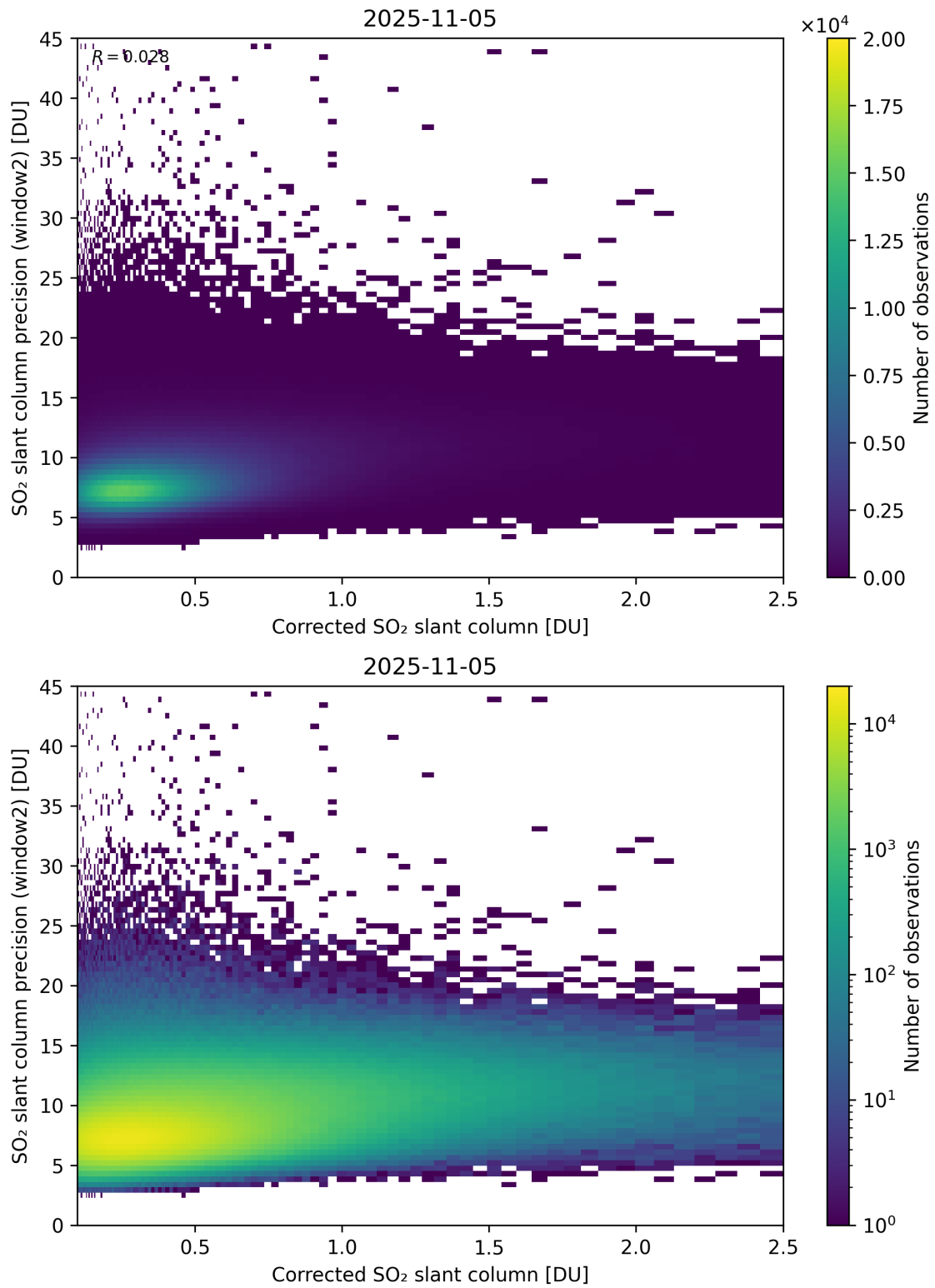
Figure 239: Scatter density plot of “Corrected SO 2 slant column” against “SO 2 slant column precision (window2)” for 2025-11-04 to 2025-11-06.
