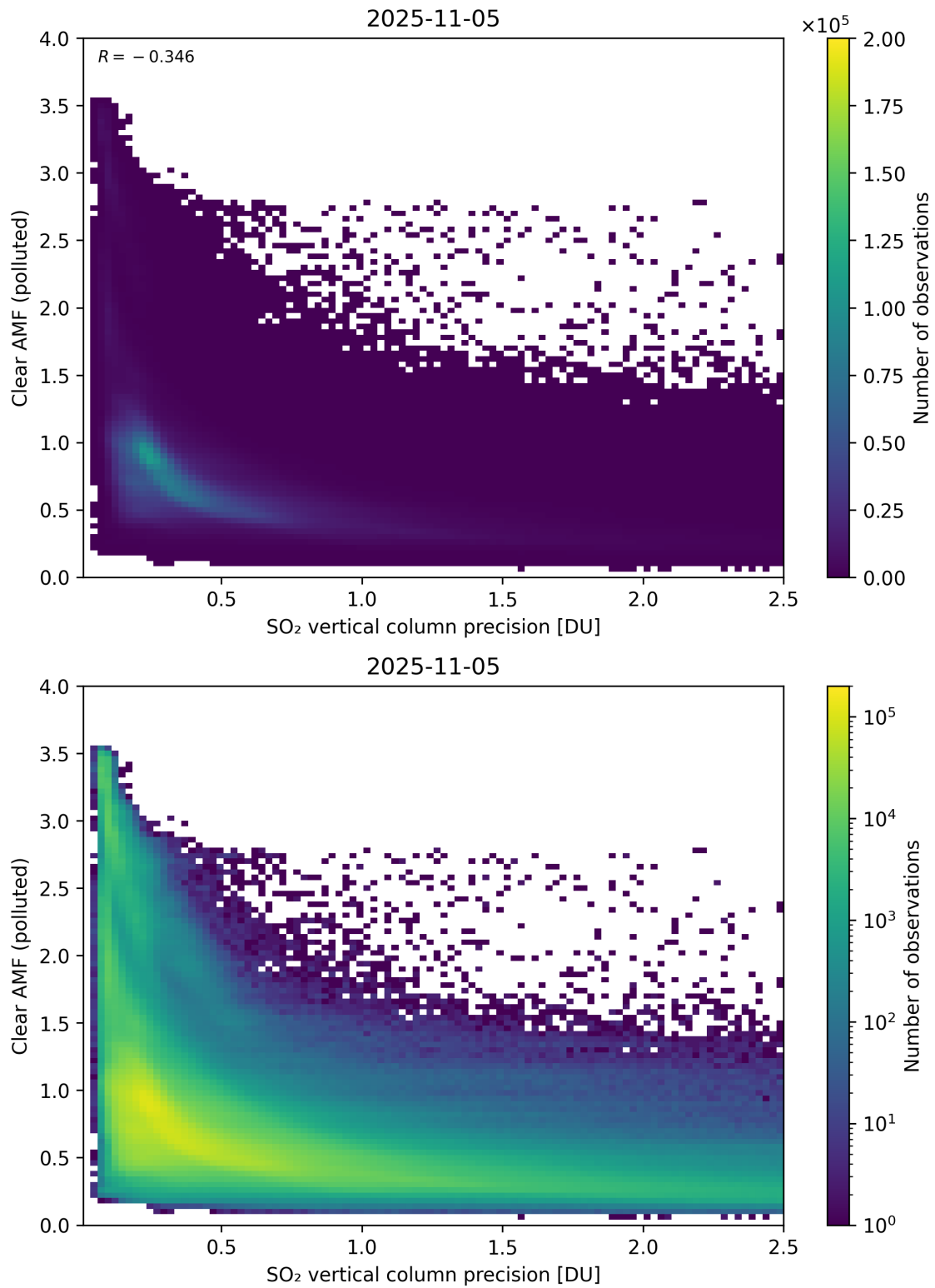
Figure 335: Scatter density plot of “SO 2 vertical column precision” against “Clear AMF (polluted)” for 2025-11-04 to 2025-11-06.
