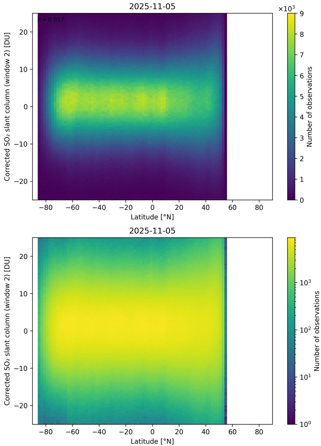
Figure 160: Scatter density plot of “Latitude” against “Corrected SO 2 slant column (window 2)” for 2025-11-04 to 2025-11-06.
