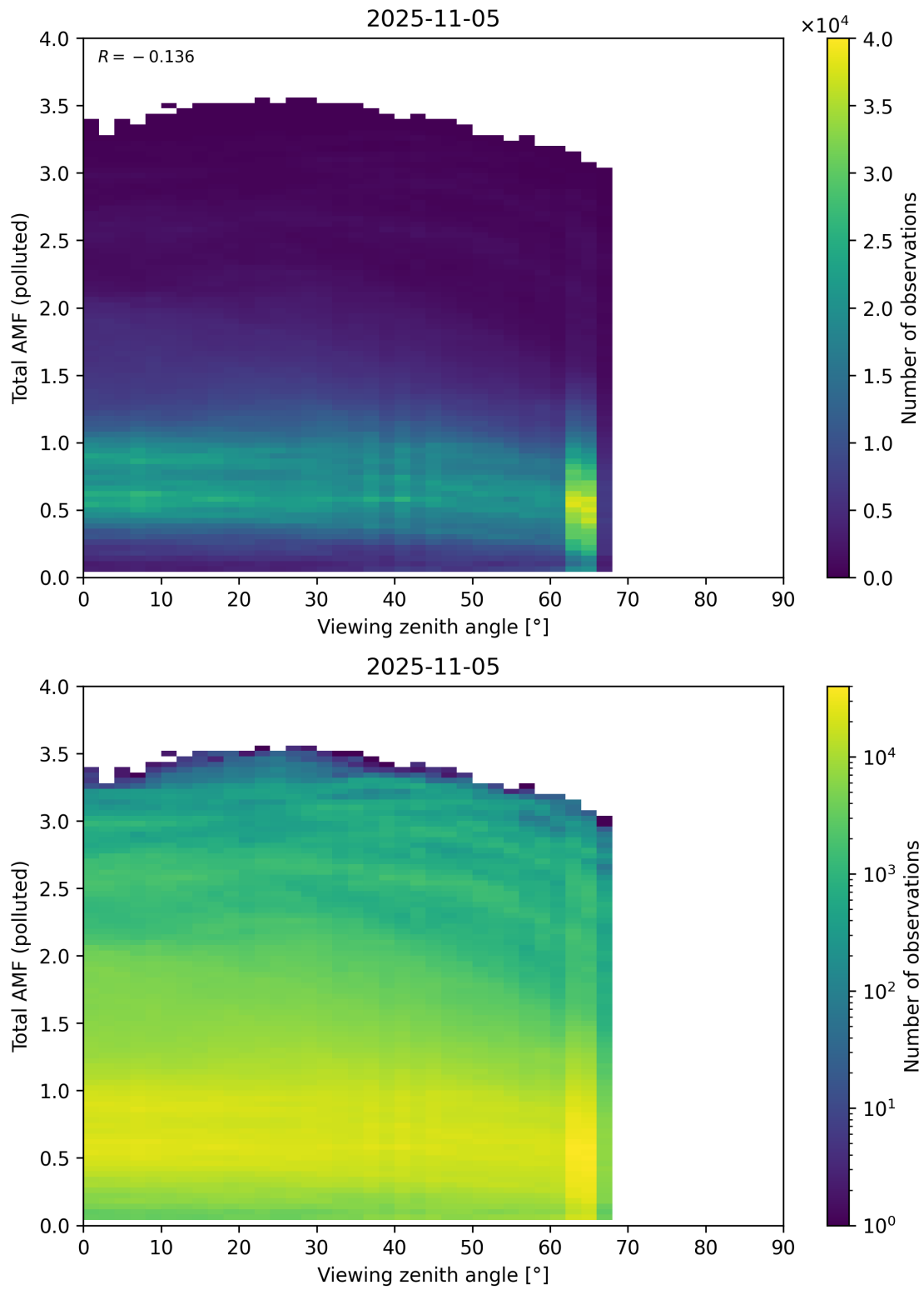
Figure 381: Scatter density plot of “Viewing zenith angle” against “Total AMF (polluted)” for 2025-11-04 to 2025-11-06.
