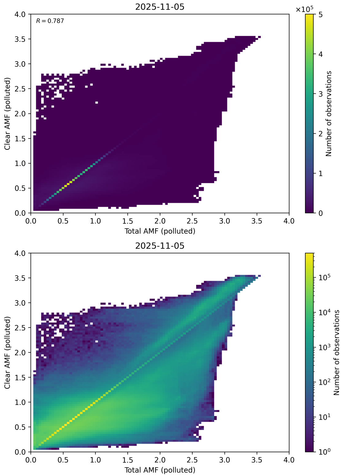
Figure 321: Scatter density plot of “Total AMF (polluted)” against “Clear AMF (polluted)” for 2025-11-04 to 2025-11-06.
