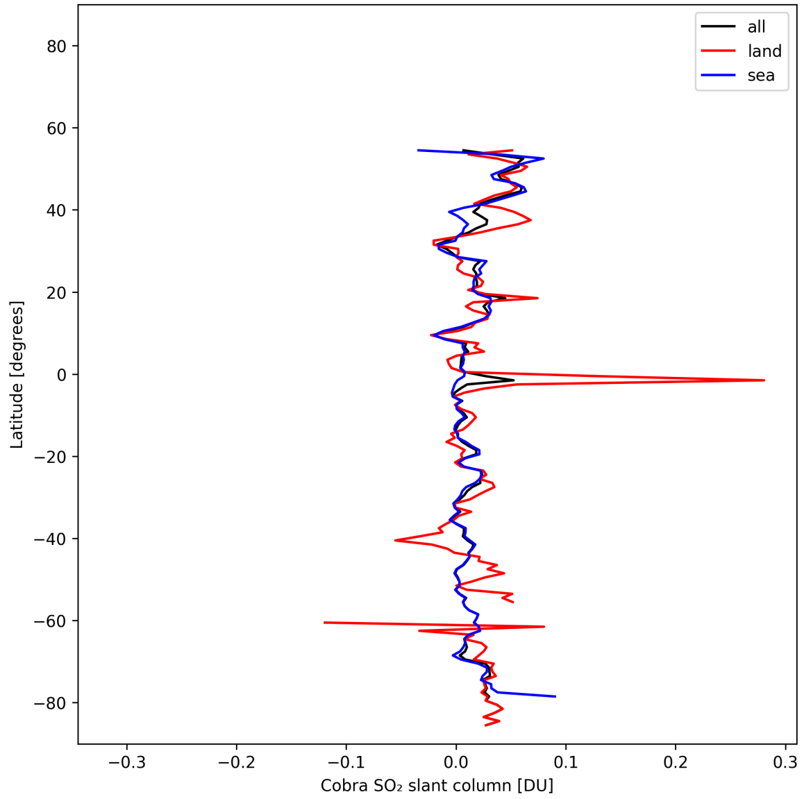
Figure 35: Zonal average of “Cobra SO 2 slant column” for 2025-11-04 to 2025-11-06.
