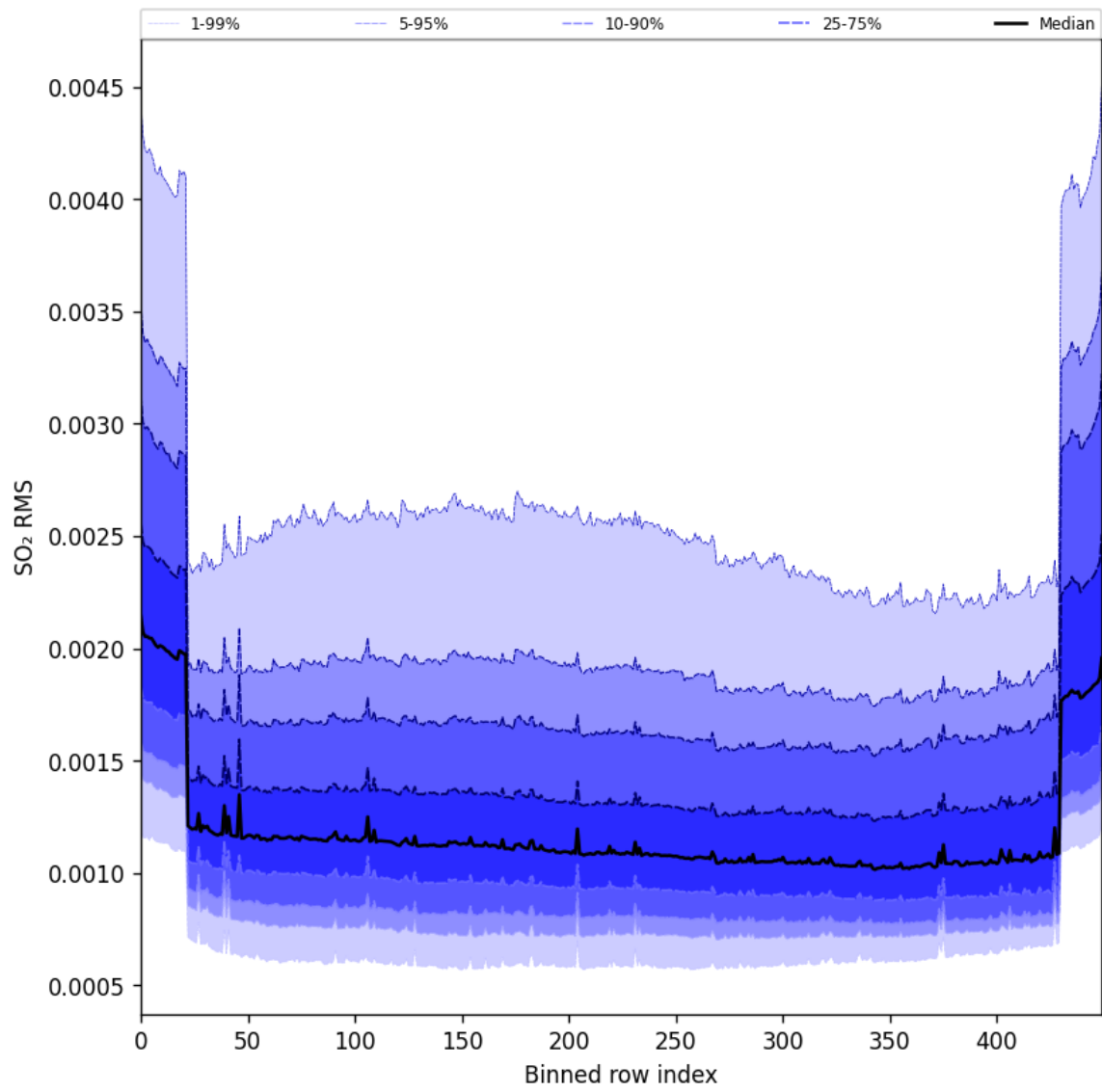
Figure 104: Along track statistics of “SO 2 RMS” for 2025-11-04 to 2025-11-06
