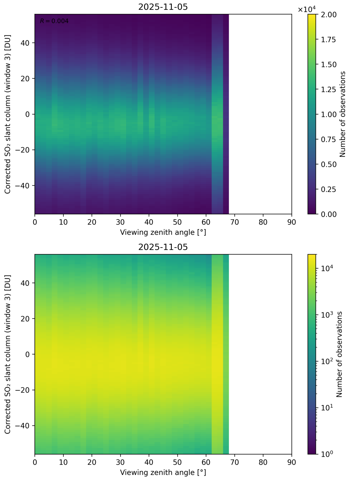
Figure 375: Scatter density plot of “Viewing zenith angle” against “Corrected SO 2 slant column (window 3)” for 2025-11-04 to 2025-11-06.
