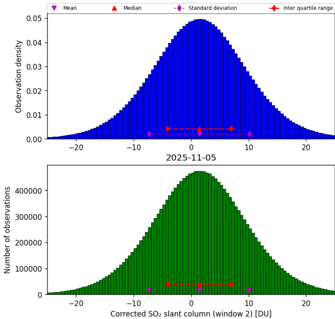
Figure 69: Histogram of “Corrected SO 2 slant column (window 2)” for 2025-11-04 to 2025-11-06
