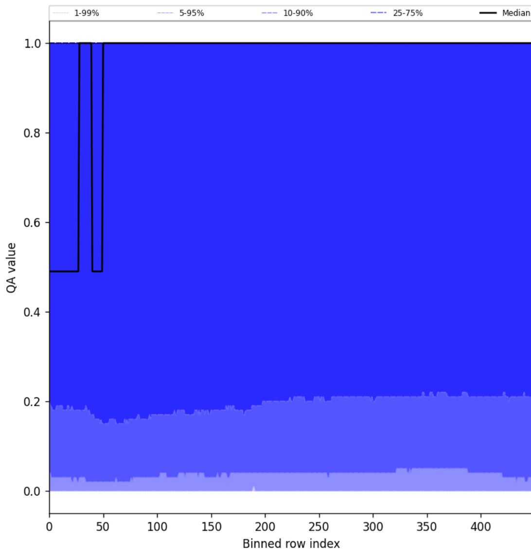
Figure 83: Along track statistics of “QA value” for 2025-11-04 to 2025-11-06
