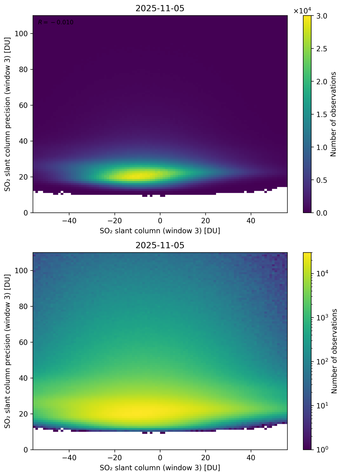
Figure 317: Scatter density plot of “SO 2 slant column (window 3)” against “SO 2 slant column precision (window 3)” for 2025-11-04 to 2025-11-06.
