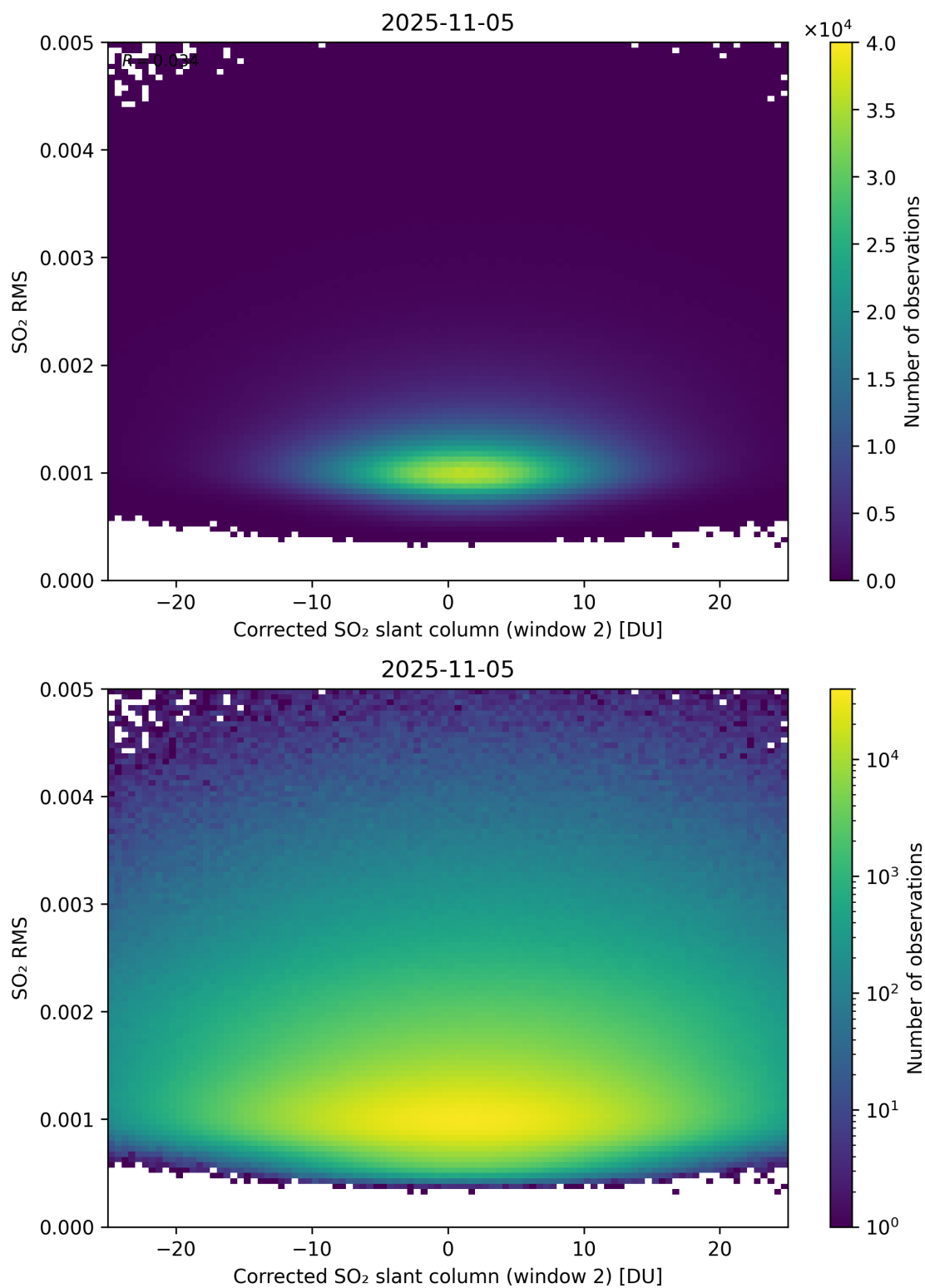
Figure 248: Scatter density plot of “Corrected SO 2 slant column (window 2)” against “SO 2 RMS” for 2025-11-04 to 2025-11-06.
