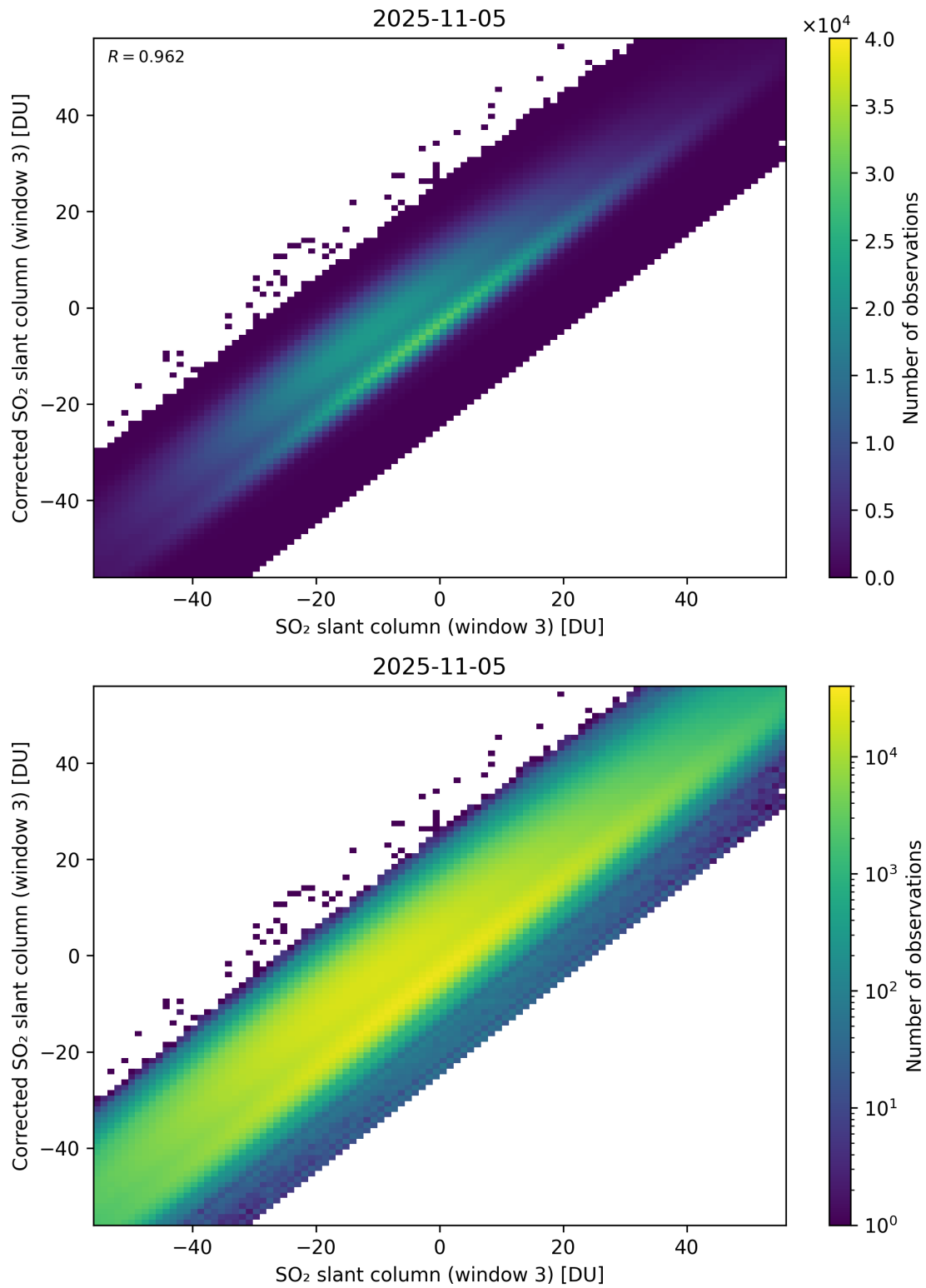
Figure 316: Scatter density plot of “SO 2 slant column (window 3)” against “Corrected SO 2 slant column (window 3)” for 2025-11-04 to 2025-11-06.
