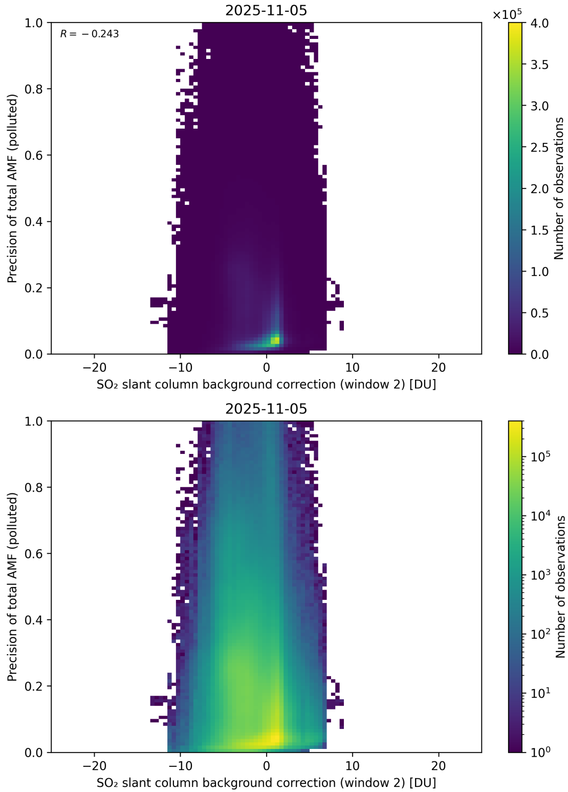
Figure 131: Scatter density plot of “SO 2 slant column background correction (window 2)” against “Precision of total AMF (polluted)” for 2025-11-04 to 2025-11-06.
