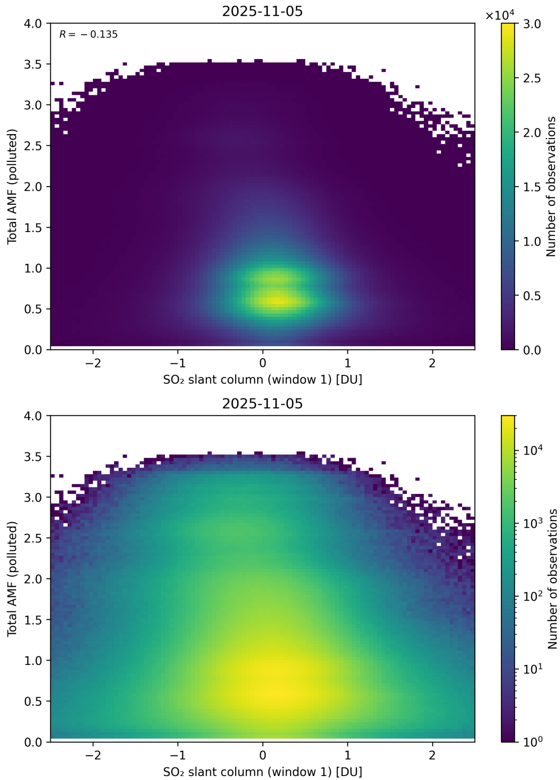
Figure 289: Scatter density plot of “SO 2 slant column (window 1)” against “Total AMF (polluted)” for 2025-11-04 to 2025-11-06.
