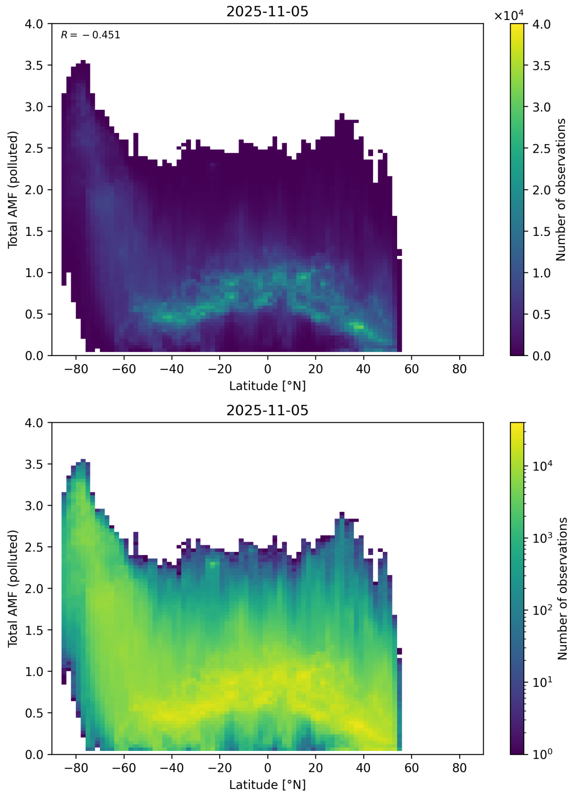
Figure 167: Scatter density plot of “Latitude” against “Total AMF (polluted)” for 2025-11-04 to 2025-11-06.
