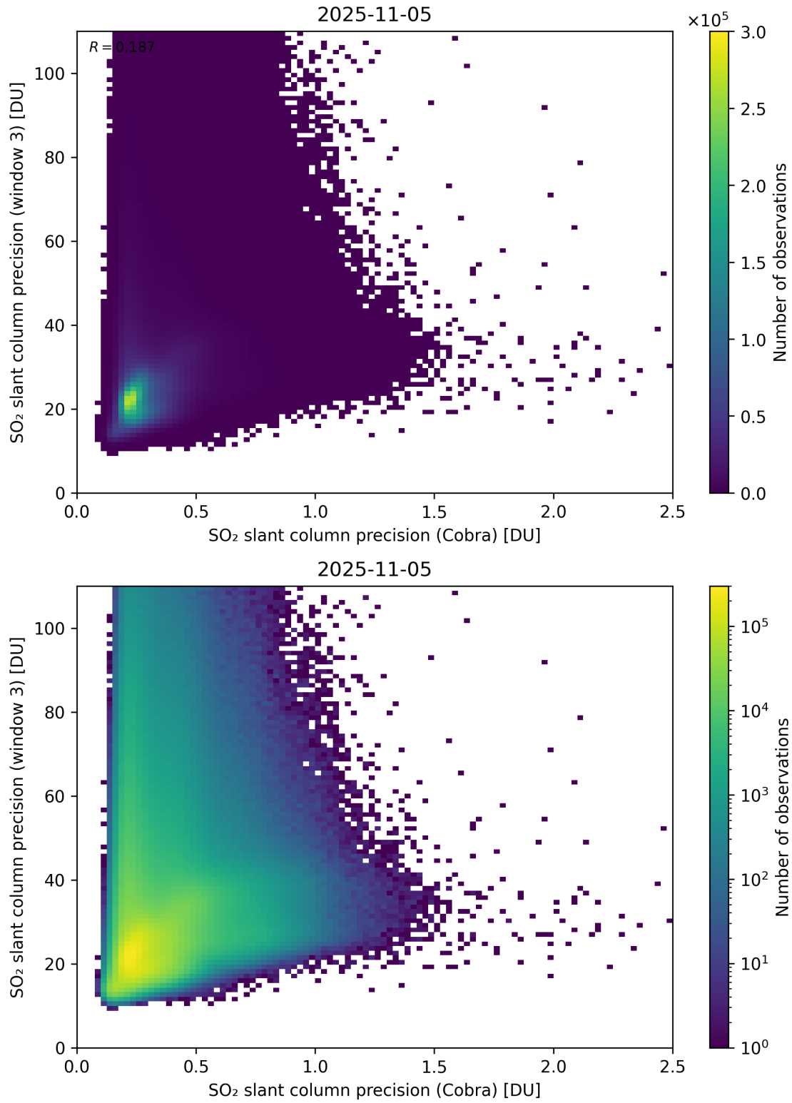
Figure 212: Scatter density plot of “SO 2 slant column precision (Cobra)” against “SO 2 slant column precision (window 3)” for 2025-11-04 to 2025-11-06.
