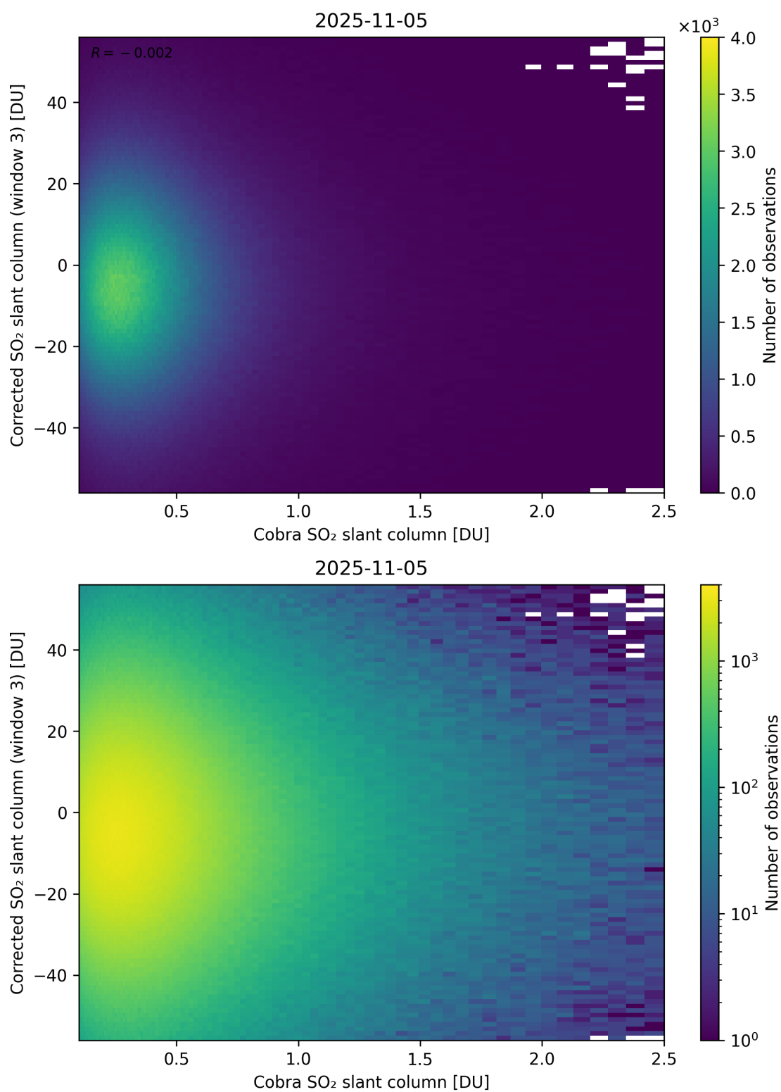
Figure 218: Scatter density plot of “Cobra SO 2 slant column” against “Corrected SO 2 slant column (window 3)” for 2025-11-04 to 2025-11-06.
