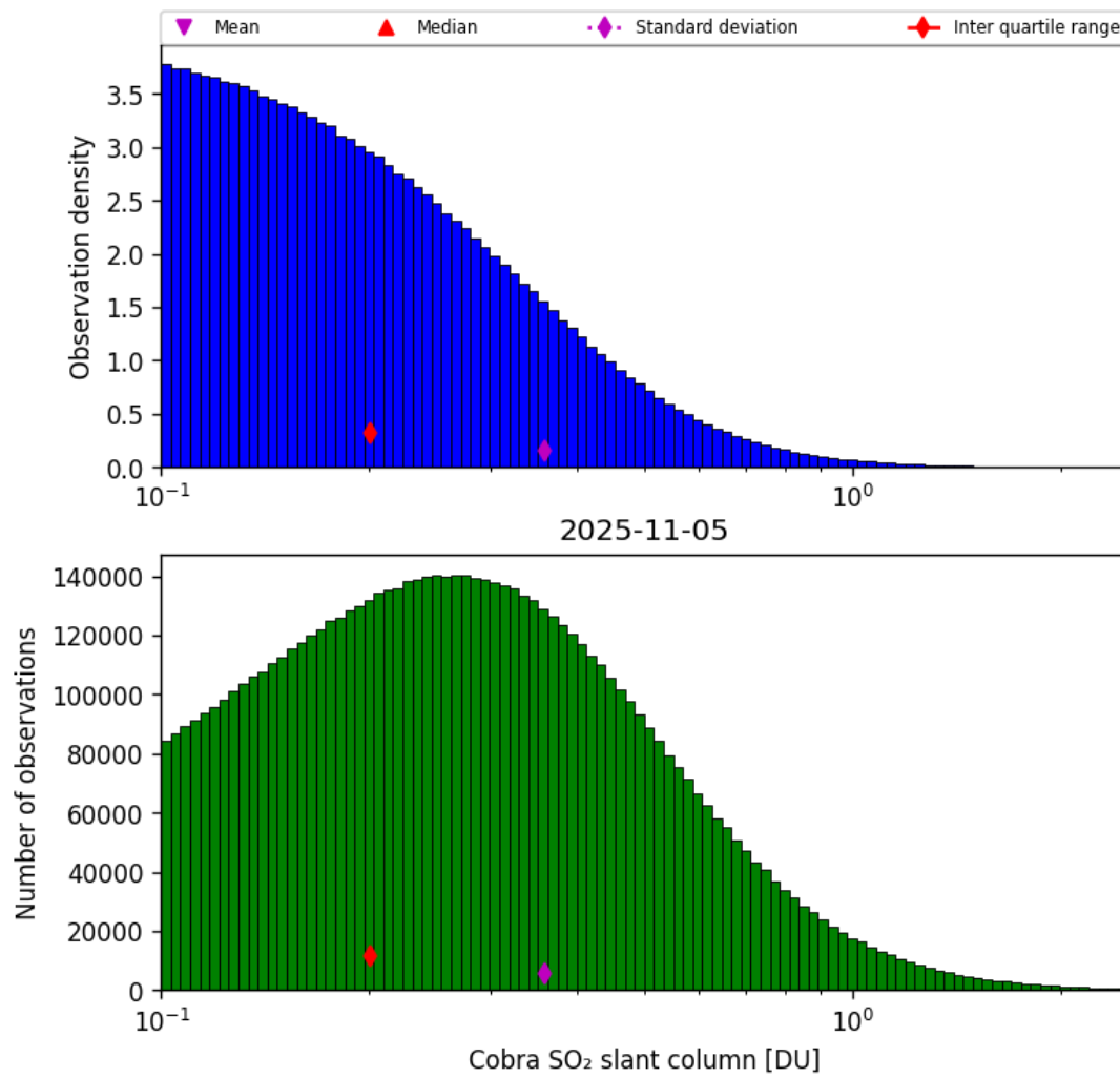
Figure 61: Histogram of “Cobra SO 2 slant column” for 2025-11-04 to 2025-11-06
