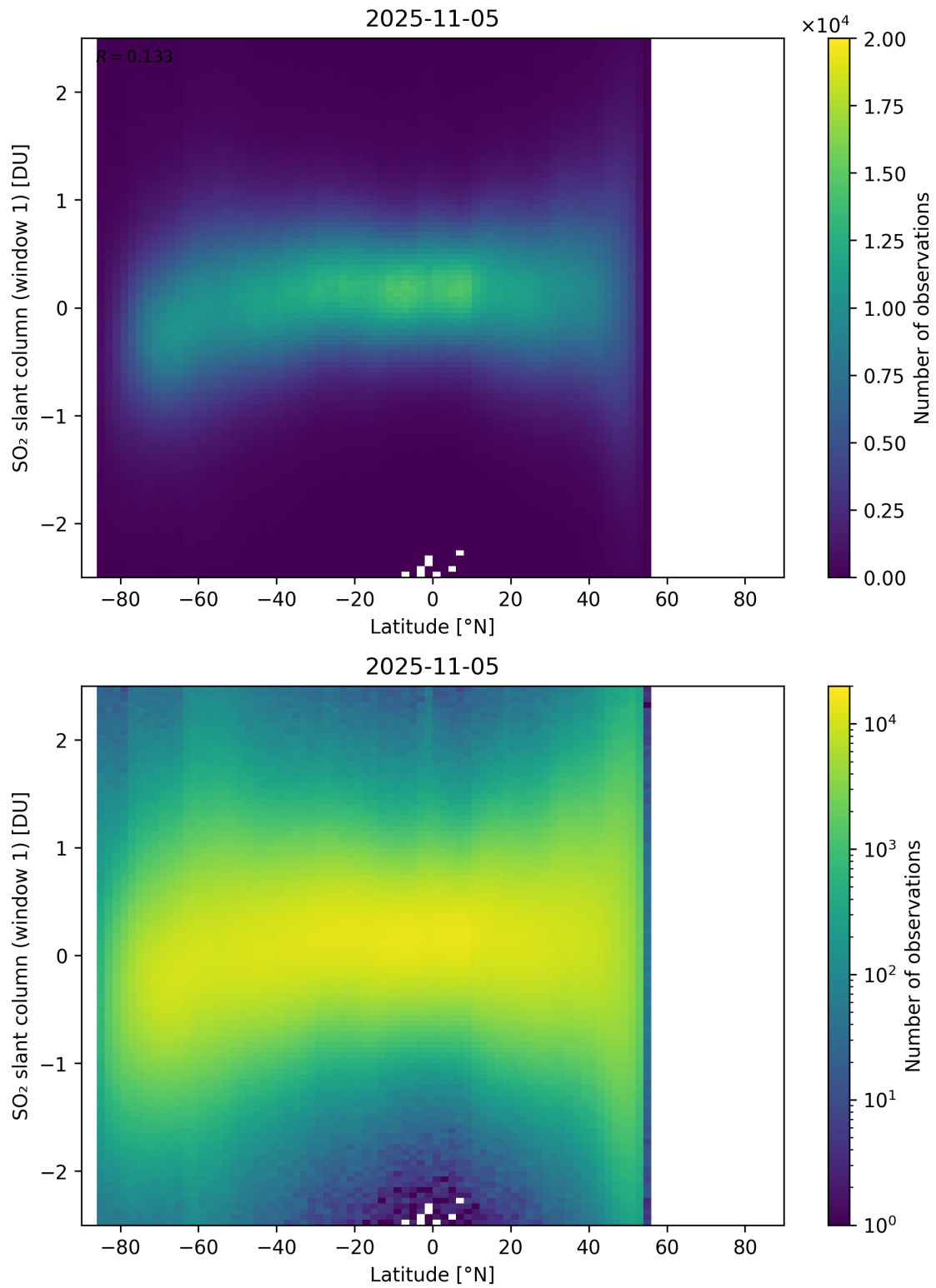
Figure 162: Scatter density plot of “Latitude” against “SO 2 slant column (window 1)” for 2025-11-04 to 2025-11-06.
