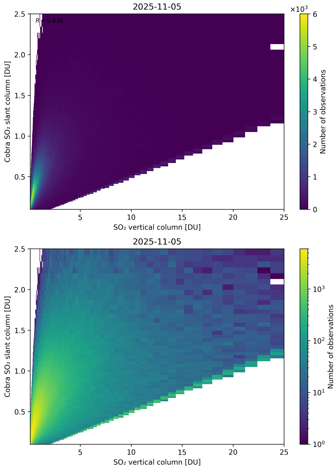
Figure 349: Scatter density plot of “SO 2 vertical column” against “Cobra SO 2 slant column” for 2025-11-04 to 2025-11-06.
