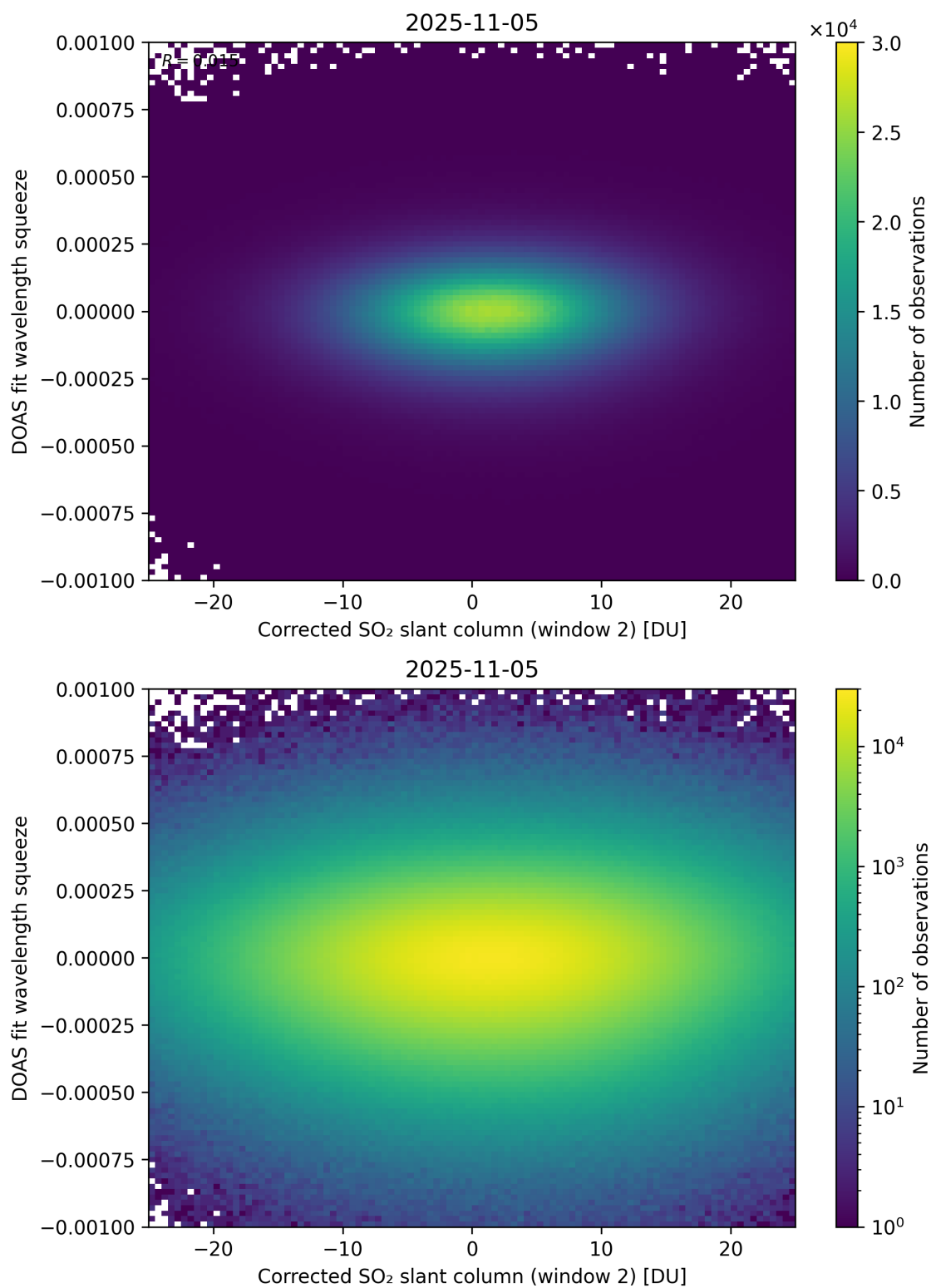
Figure 247: Scatter density plot of “Corrected SO 2 slant column (window 2)” against “DOAS fit wavelength squeeze” for 2025-11-04 to 2025-11-06.
