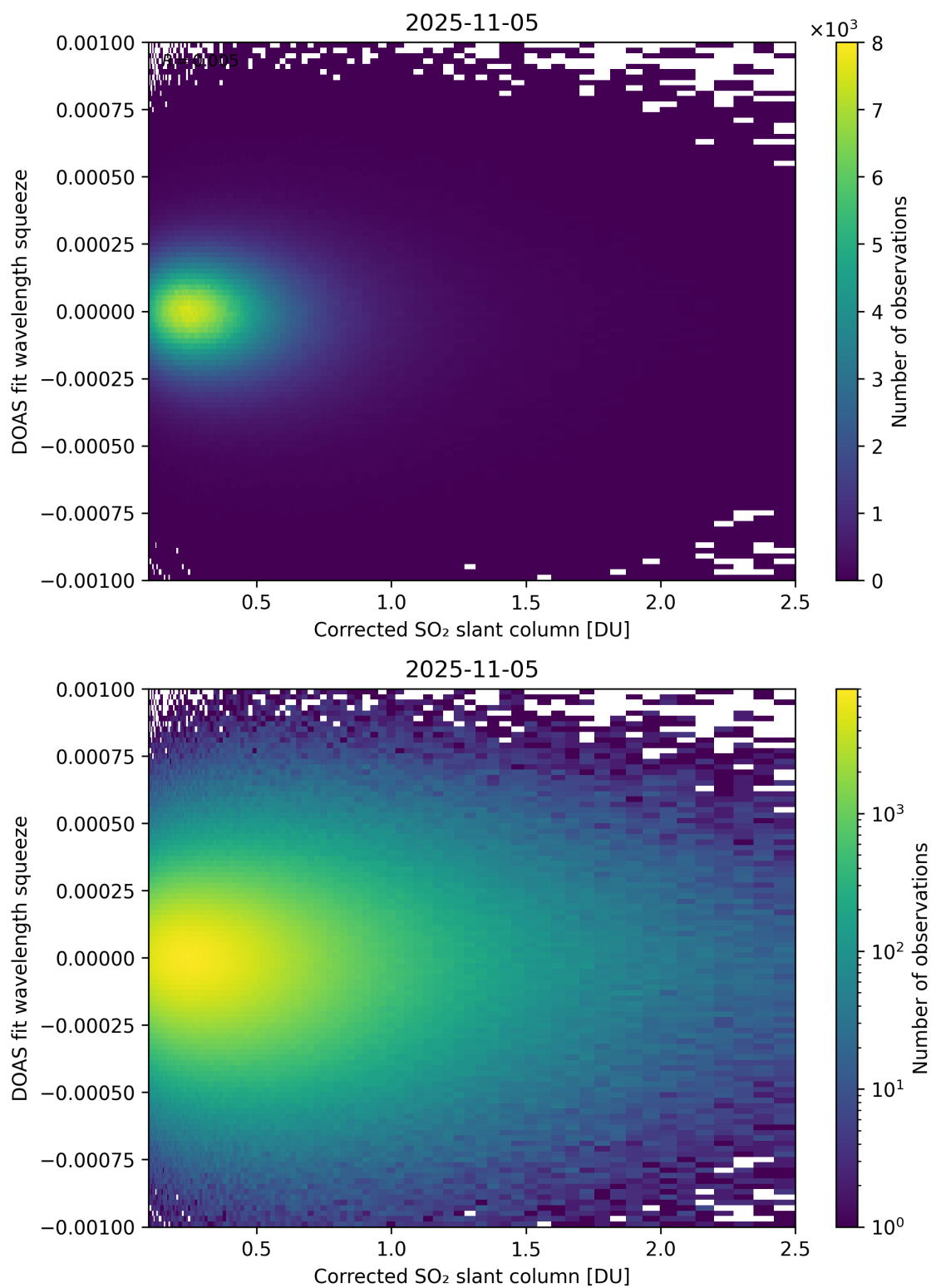
Figure 230: Scatter density plot of "Corrected SO 2 slant column" against "DOAS fit wavelength squeeze" for 2025-11-04 to 2025-11-06.
