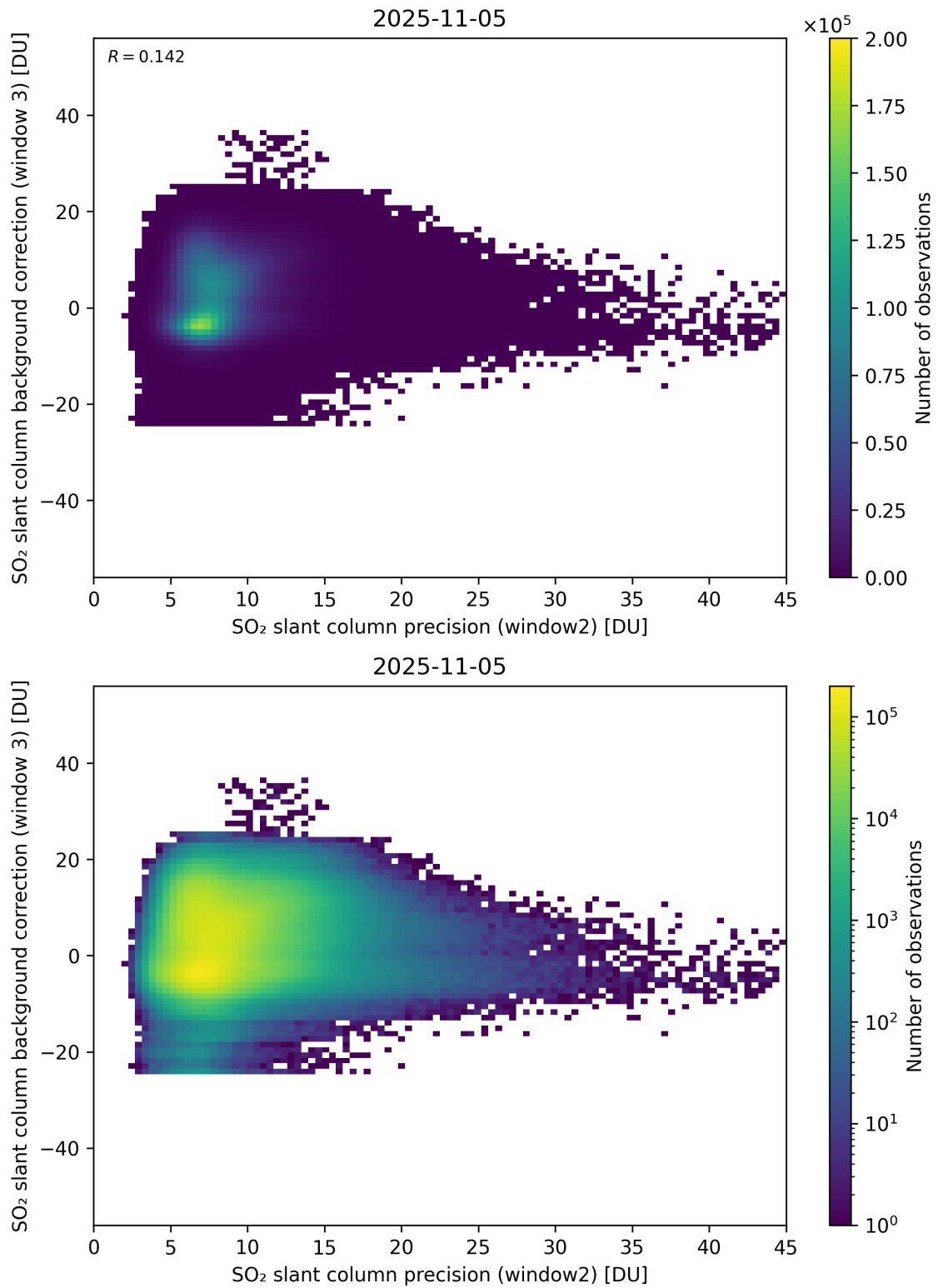
Figure 292: Scatter density plot of “SO 2 slant column precision (window2)” against “SO 2 slant column background correction (window 3)” for 2025-11-04 to 2025-11-06.
