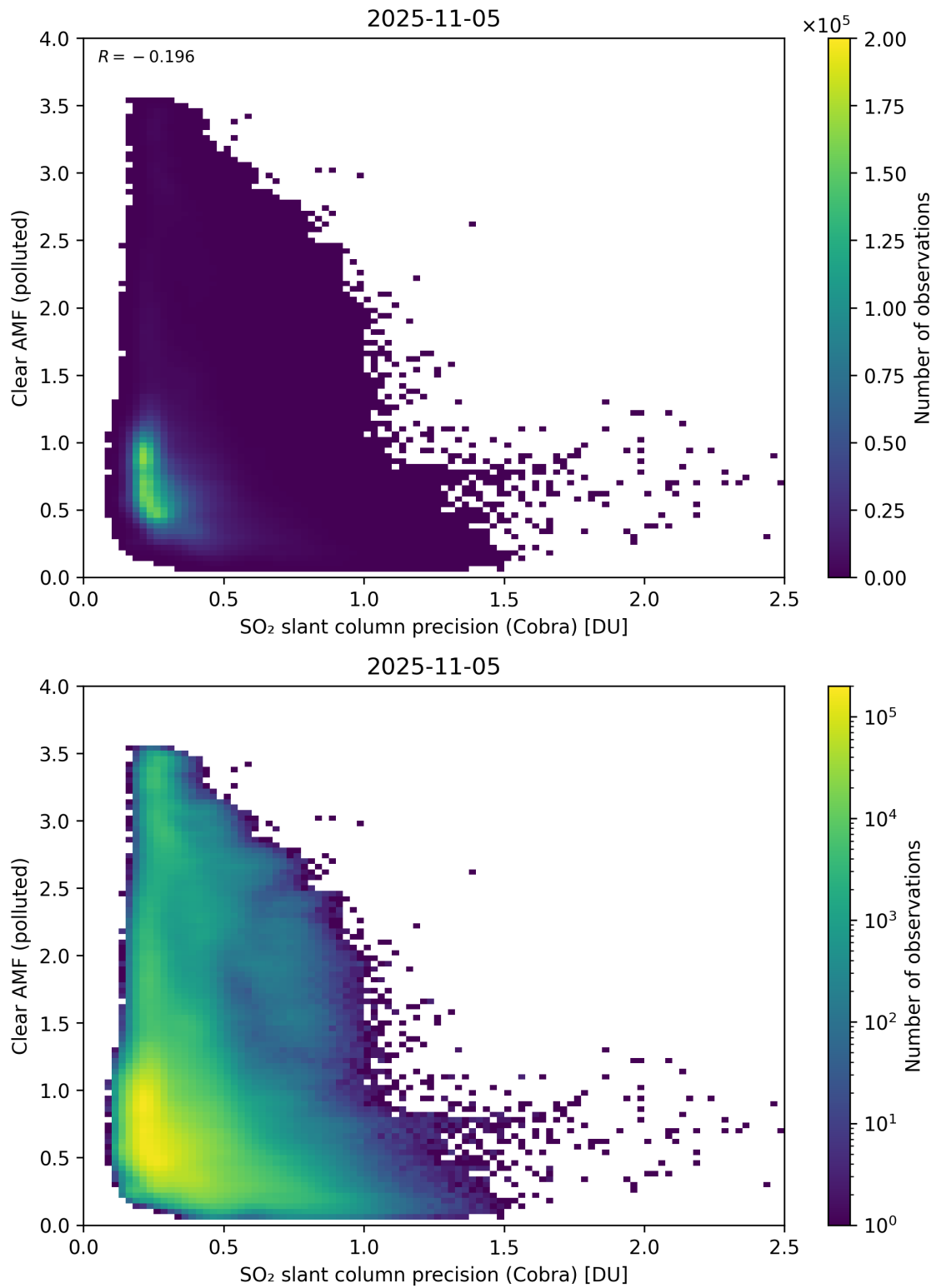
Figure 205: Scatter density plot of “SO 2 slant column precision (Cobra)” against “Clear AMF (polluted)” for 2025-11-04 to 2025-11-06.
