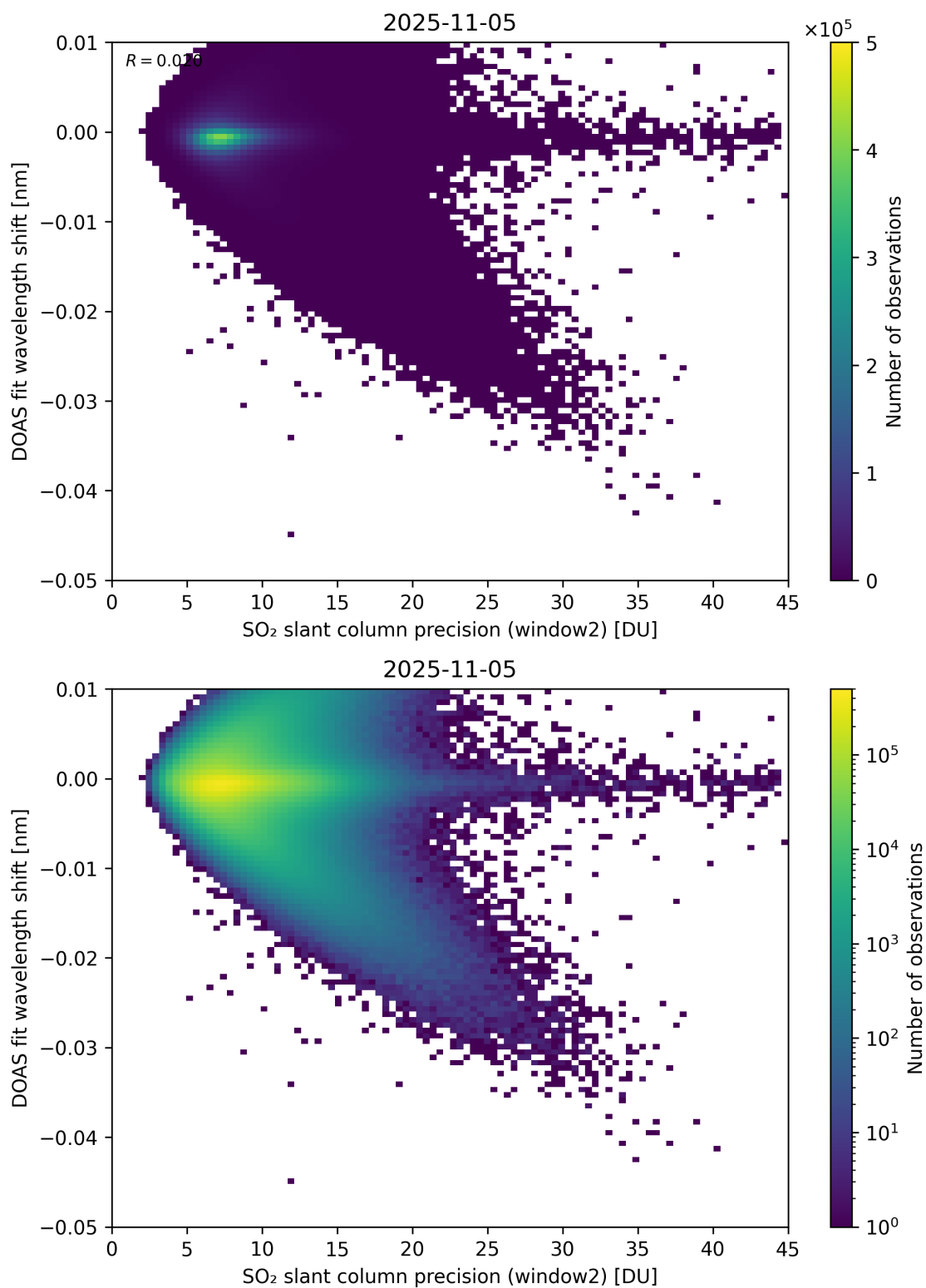
Figure 293: Scatter density plot of “SO 2 slant column precision (window2)” against “DOAS fit wavelength shift” for 2025-11-04 to 2025-11-06.
