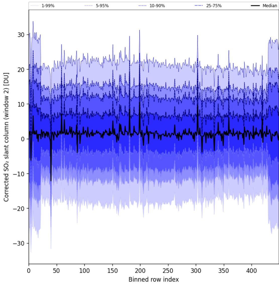
Figure 95: Along track statistics of “Corrected SO 2 slant column (window 2)” for 2025-11-04 to 2025-11-06
