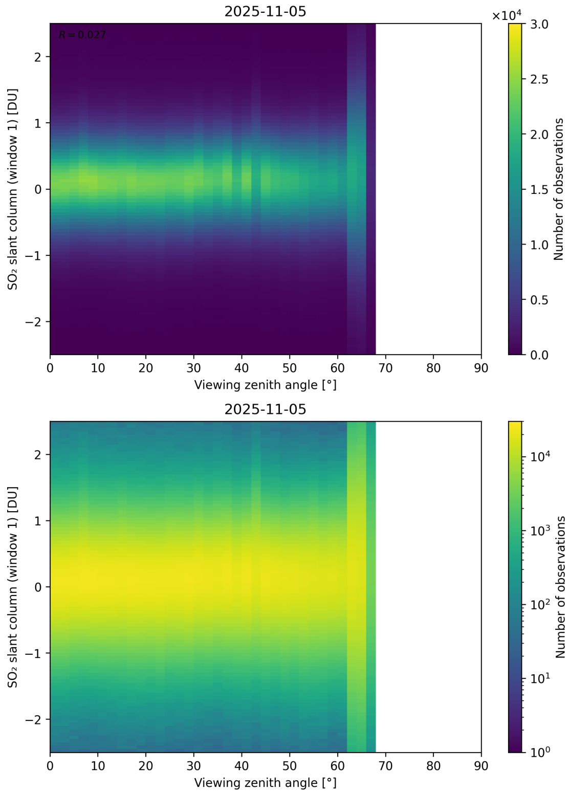
Figure 376: Scatter density plot of “Viewing zenith angle” against “SO 2 slant column (window 1)” for 2025-11-04 to 2025-11-06.
