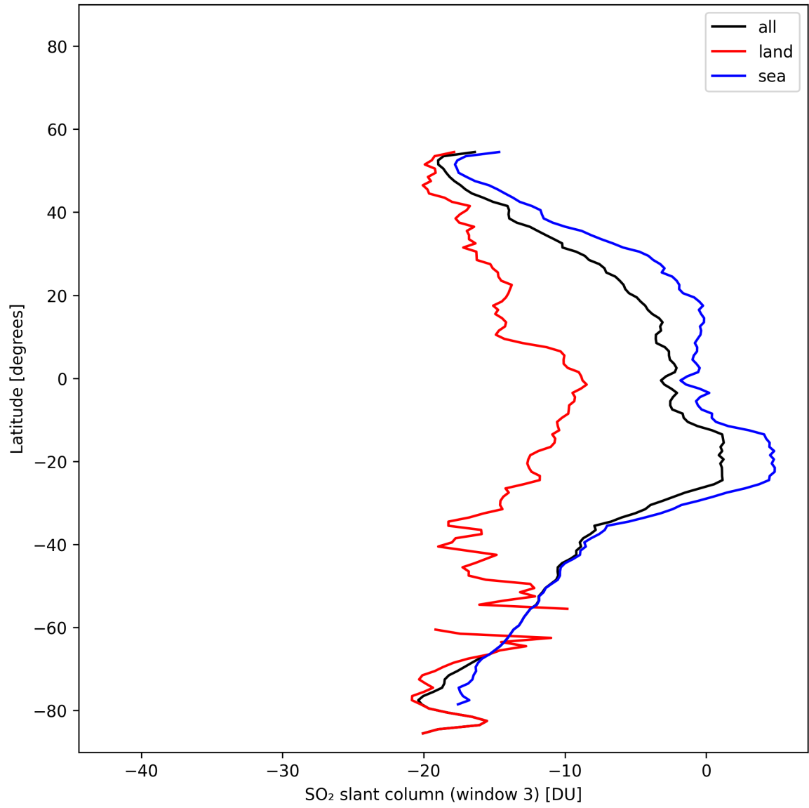
Figure 45: Zonal average of “SO 2 slant column (window 3)” for 2025-11-04 to 2025-11-06.
