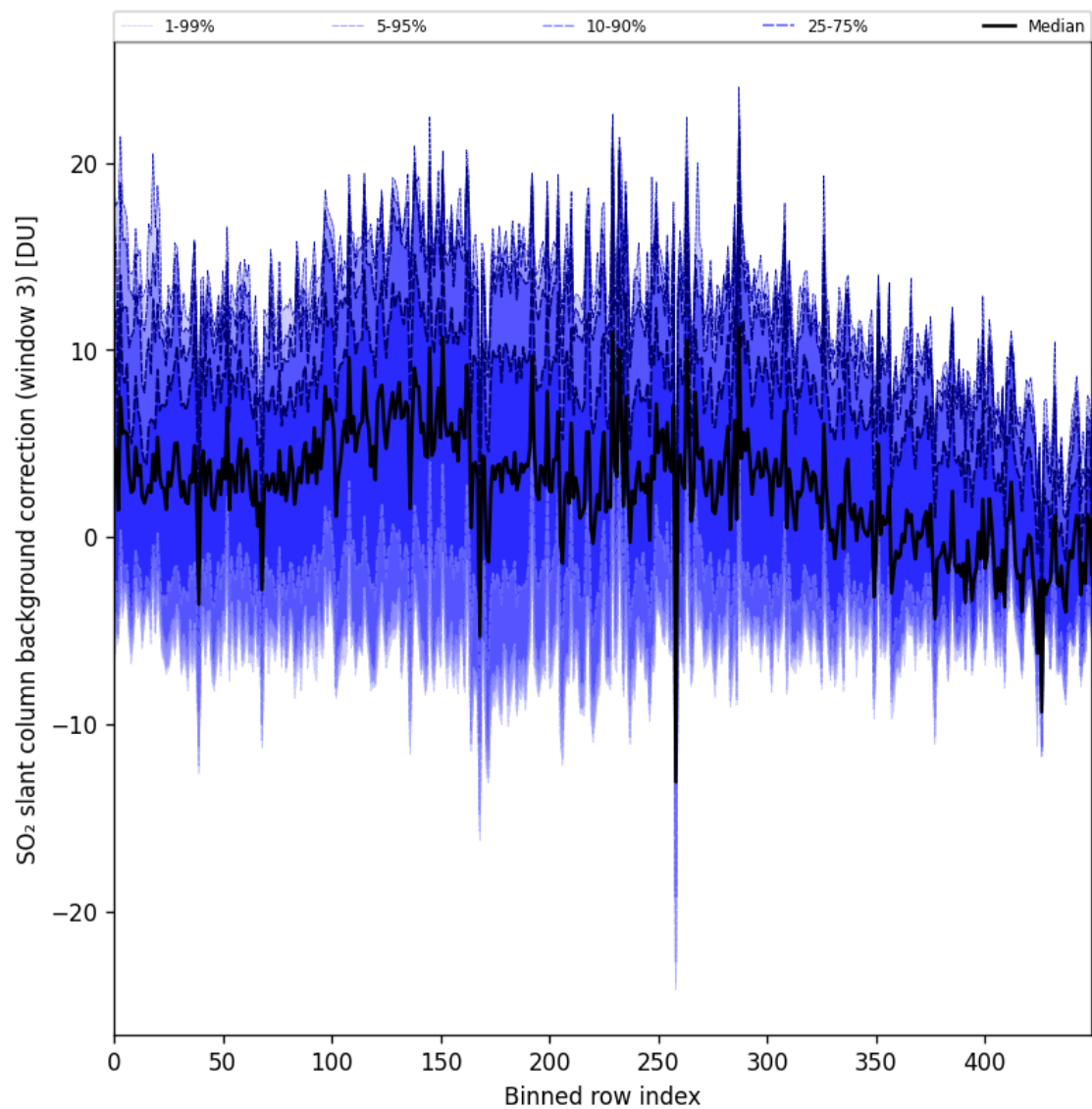
Figure 100: Along track statistics of “SO 2 slant column background correction (window 3)” for 2025-11-04 to 2025-11-06
