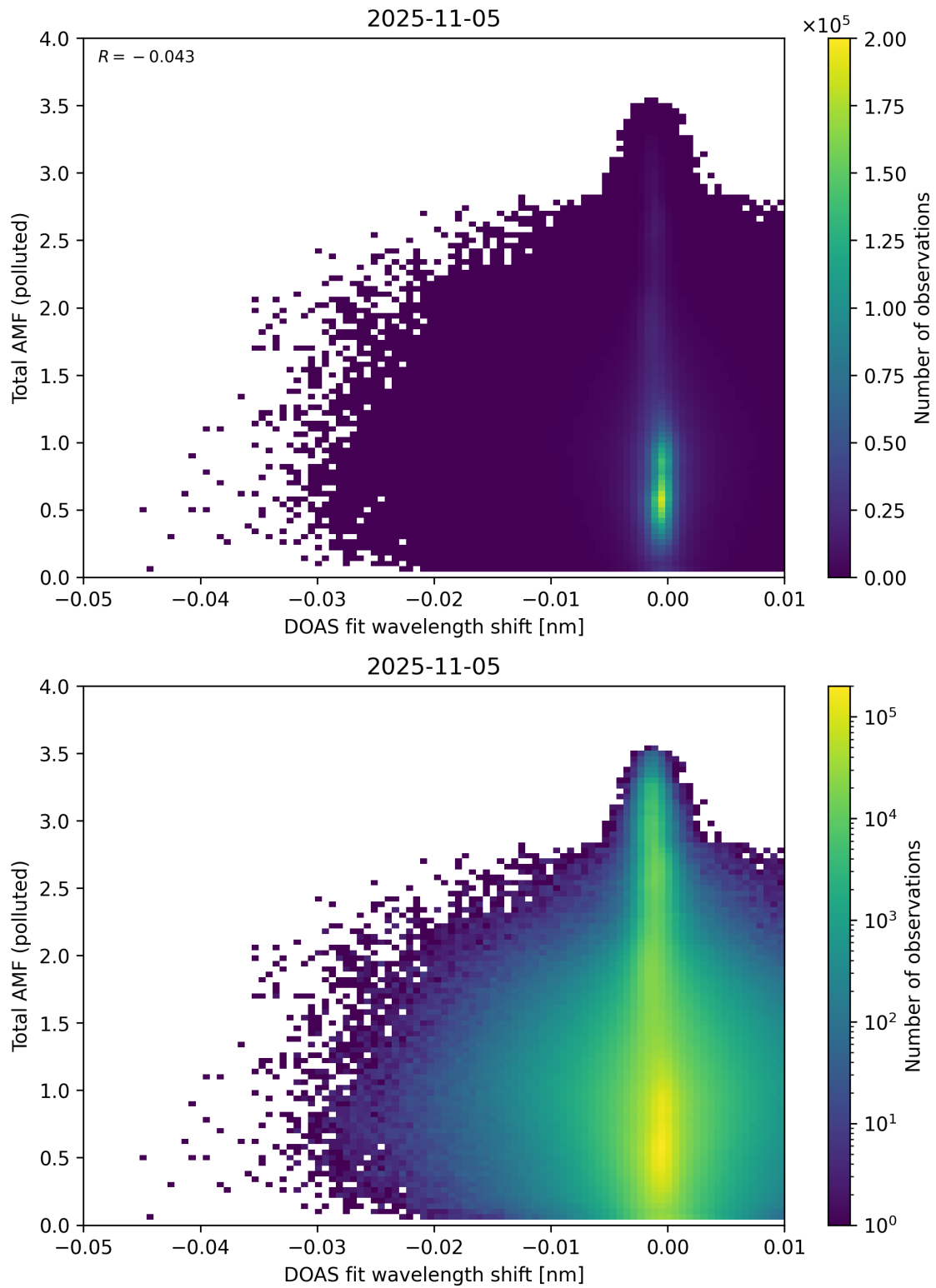
Figure 141: Scatter density plot of “DOAS fit wavelength shift” against “Total AMF (polluted)” for 2025-11-04 to 2025-11-06.
