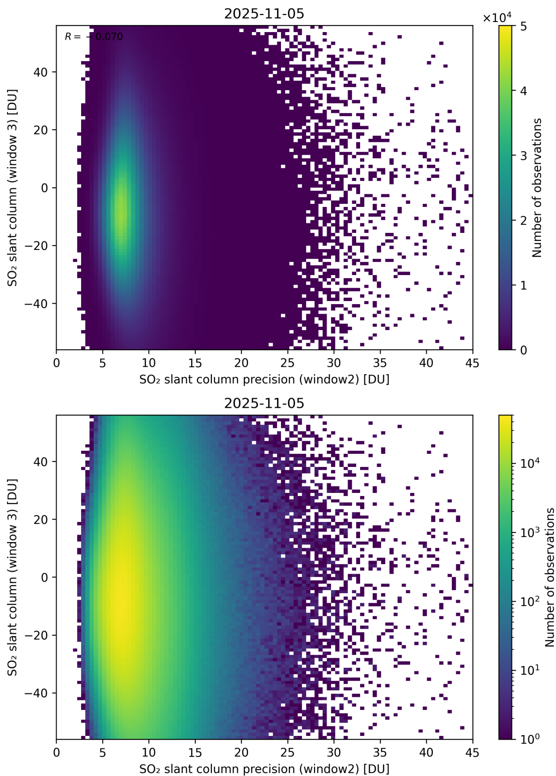
Figure 299: Scatter density plot of “SO 2 slant column precision (window2)” against “SO 2 slant column (window 3)” for 2025-11-04 to 2025-11-06.
