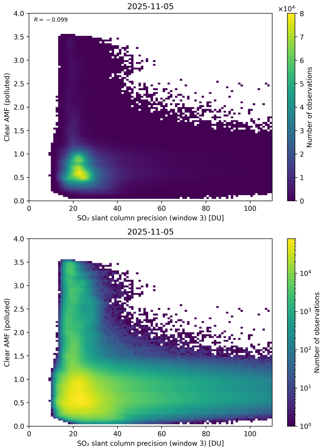
Figure 311: Scatter density plot of “SO 2 slant column precision (window 3)” against “Clear AMF (polluted)” for 2025-11-04 to 2025-11-06.
