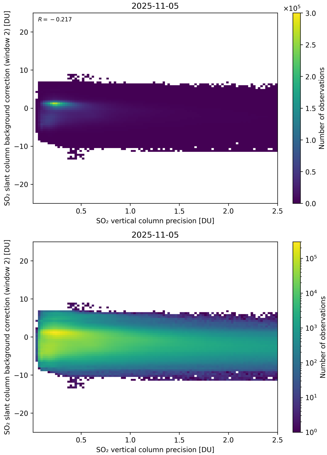
Figure 330: Scatter density plot of “SO 2 vertical column precision” against “SO 2 slant column background correction (window 2)” for 2025-11-04 to 2025-11-06.
