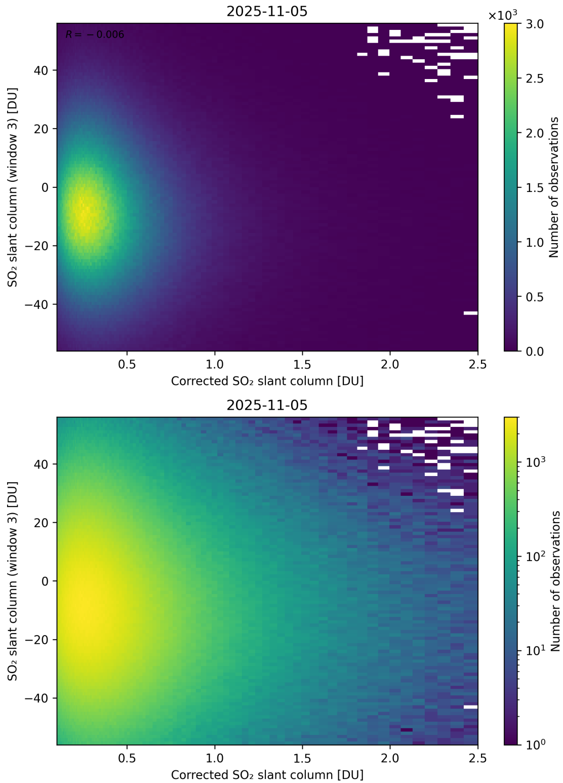
Figure 240: Scatter density plot of “Corrected SO 2 slant column” against “SO 2 slant column (window 3)” for 2025-11-04 to 2025-11-06.
