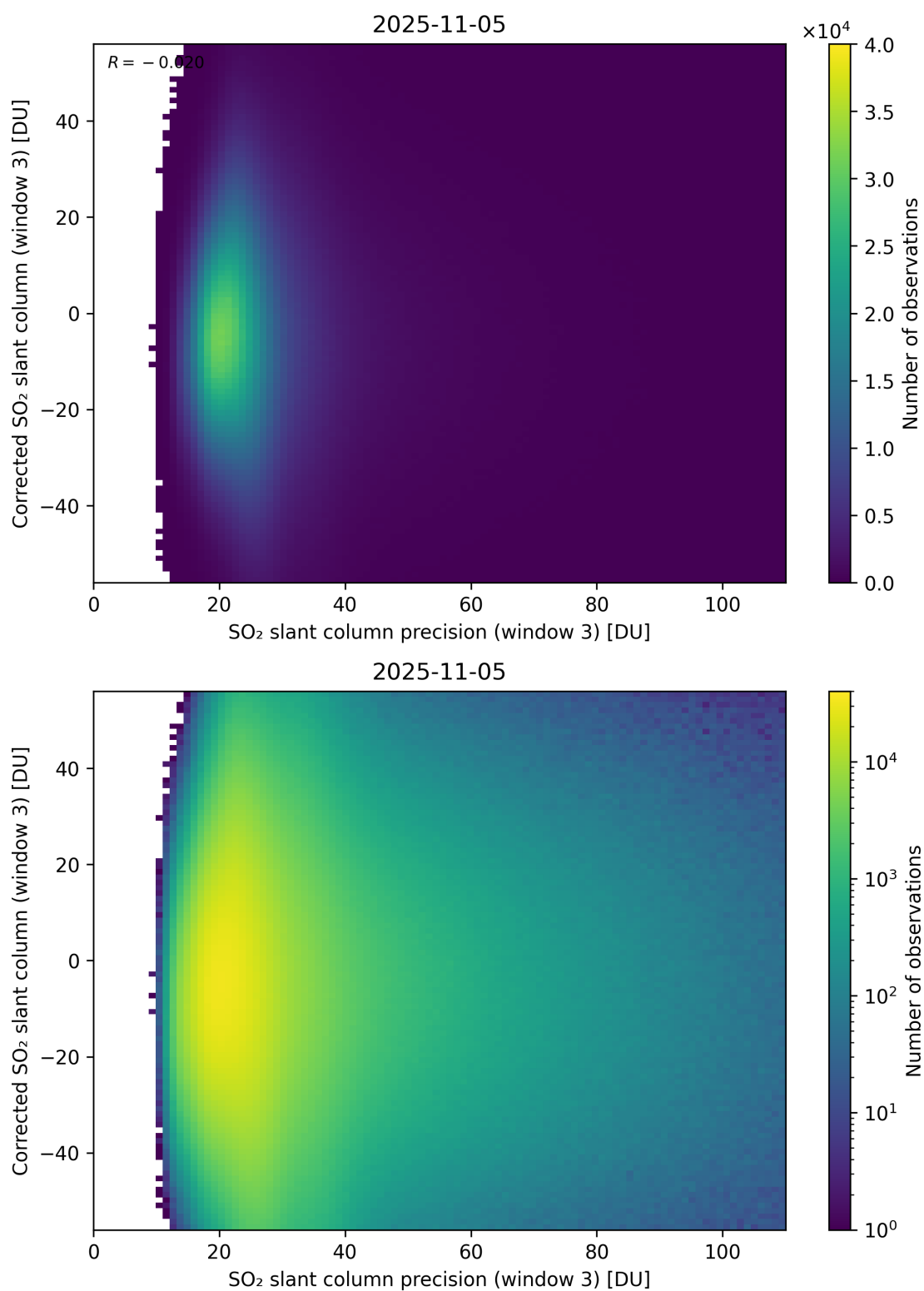
Figure 312: Scatter density plot of “SO 2 slant column precision (window 3)” against “Corrected SO 2 slant column (window 3)” for 2025-11-04 to 2025-11-06.
