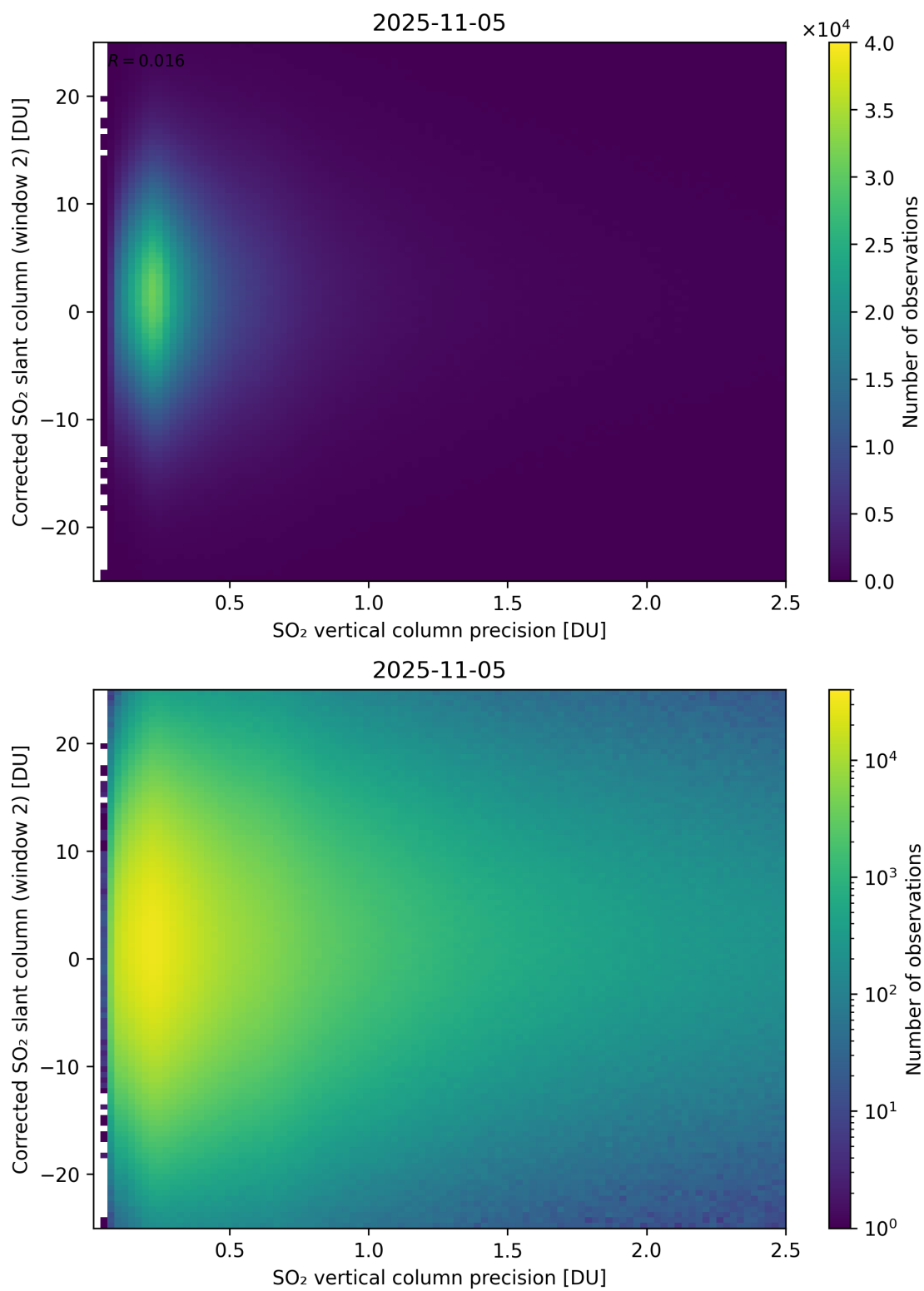
Figure 339: Scatter density plot of “SO 2 vertical column precision” against “Corrected SO 2 slant column (window 2)” for 2025-11-04 to 2025-11-06.
