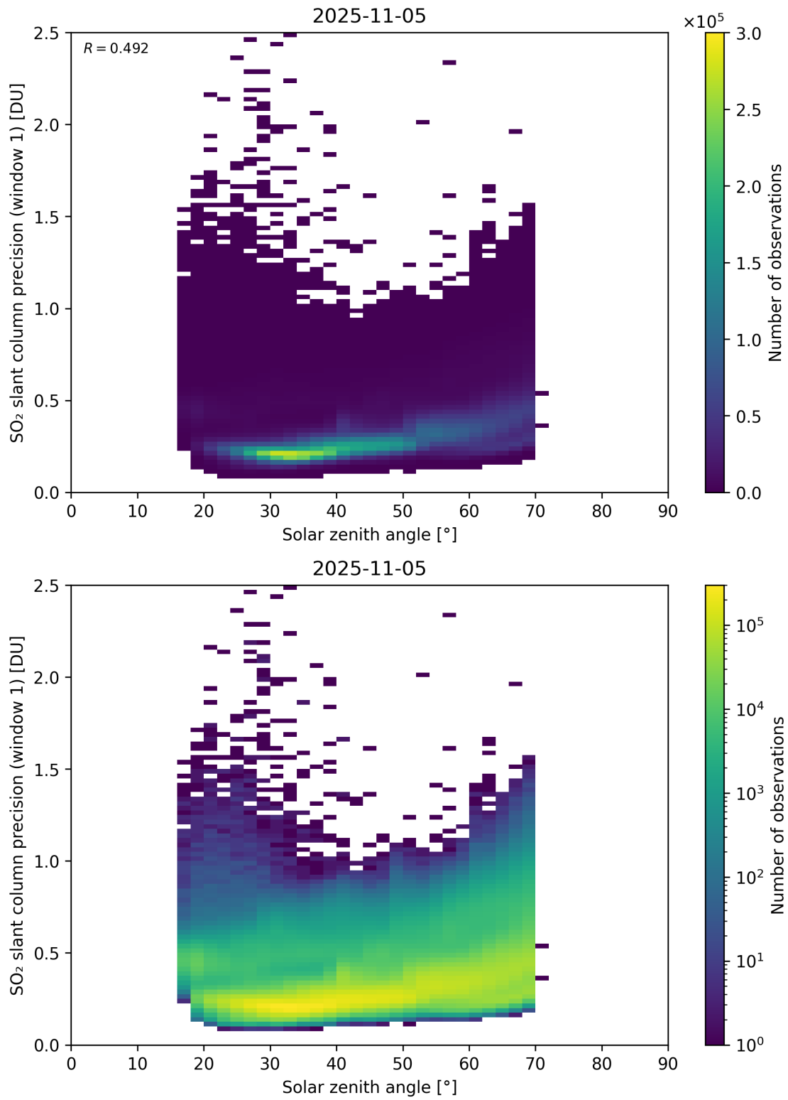
Figure 185: Scatter density plot of “Solar zenith angle” against “SO 2 slant column precision (window 1)” for 2025-11-04 to 2025-11-06.
