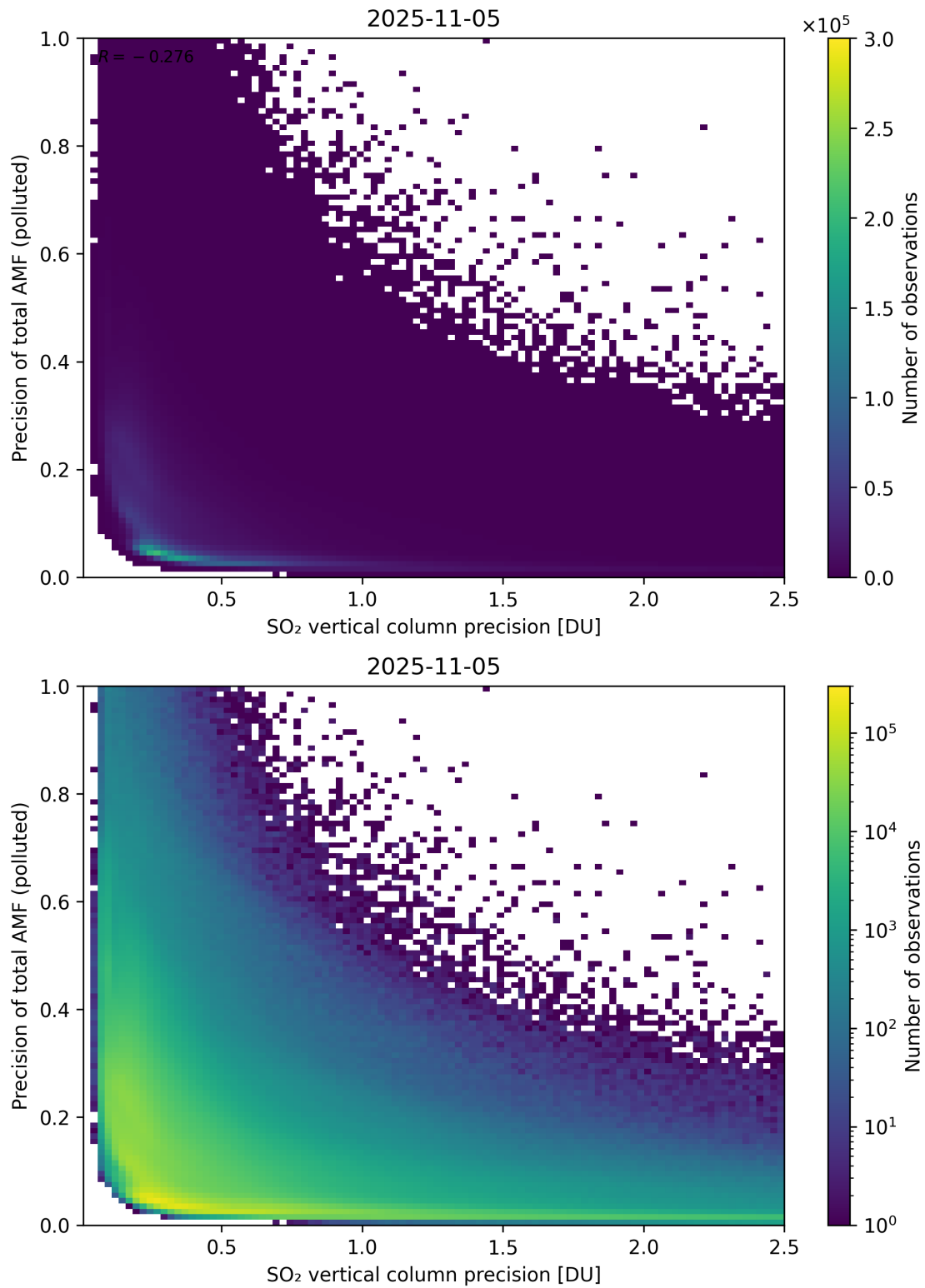
Figure 347: Scatter density plot of “SO 2 vertical column precision” against “Precision of total AMF (polluted)” for 2025-11-04 to 2025-11-06.
