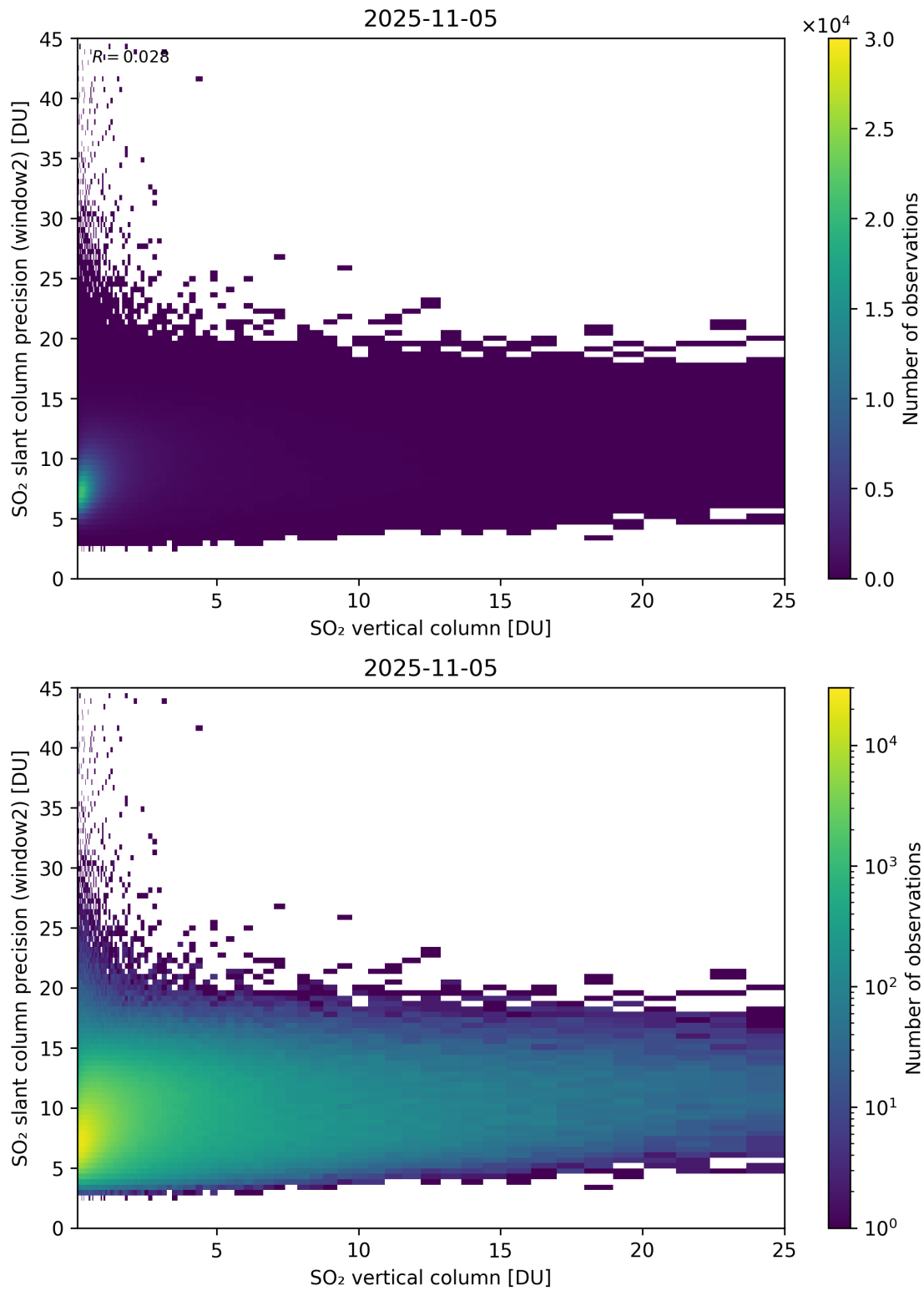
Figure 356: Scatter density plot of “SO 2 vertical column” against “SO 2 slant column precision (window2)” for 2025-11-04 to 2025-11-06.
