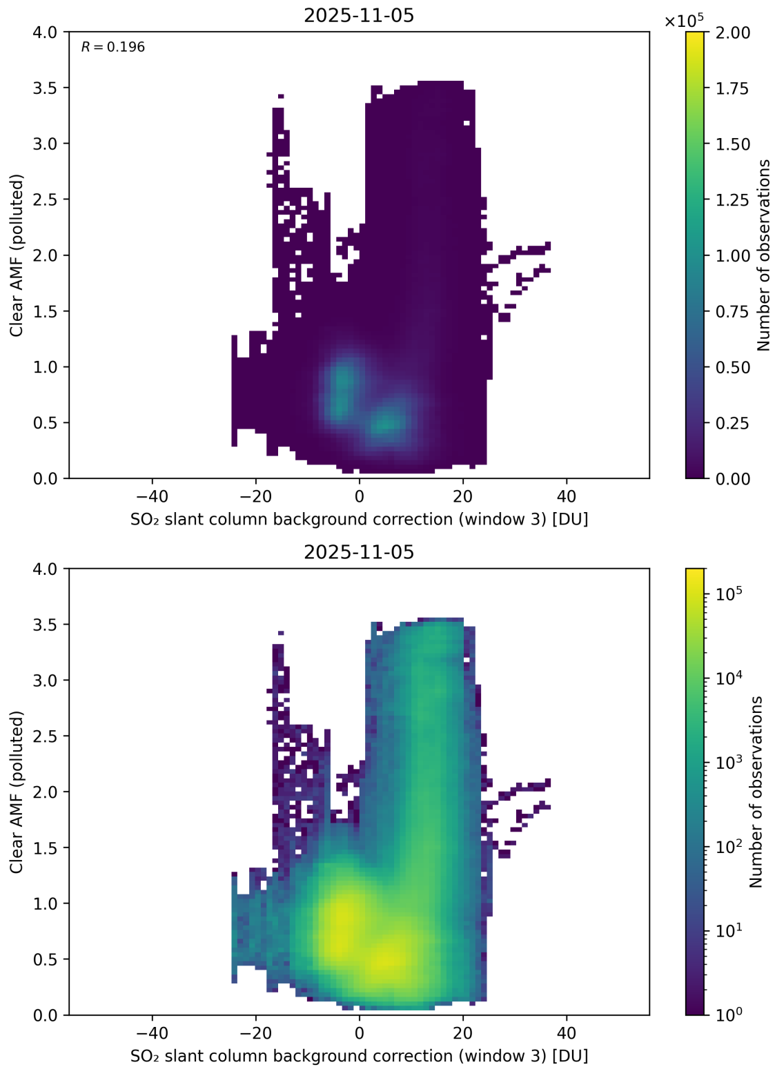
Figure 135: Scatter density plot of “SO 2 slant column background correction (window 3)” against “Clear AMF (polluted)” for 2025-11-04 to 2025-11-06.
