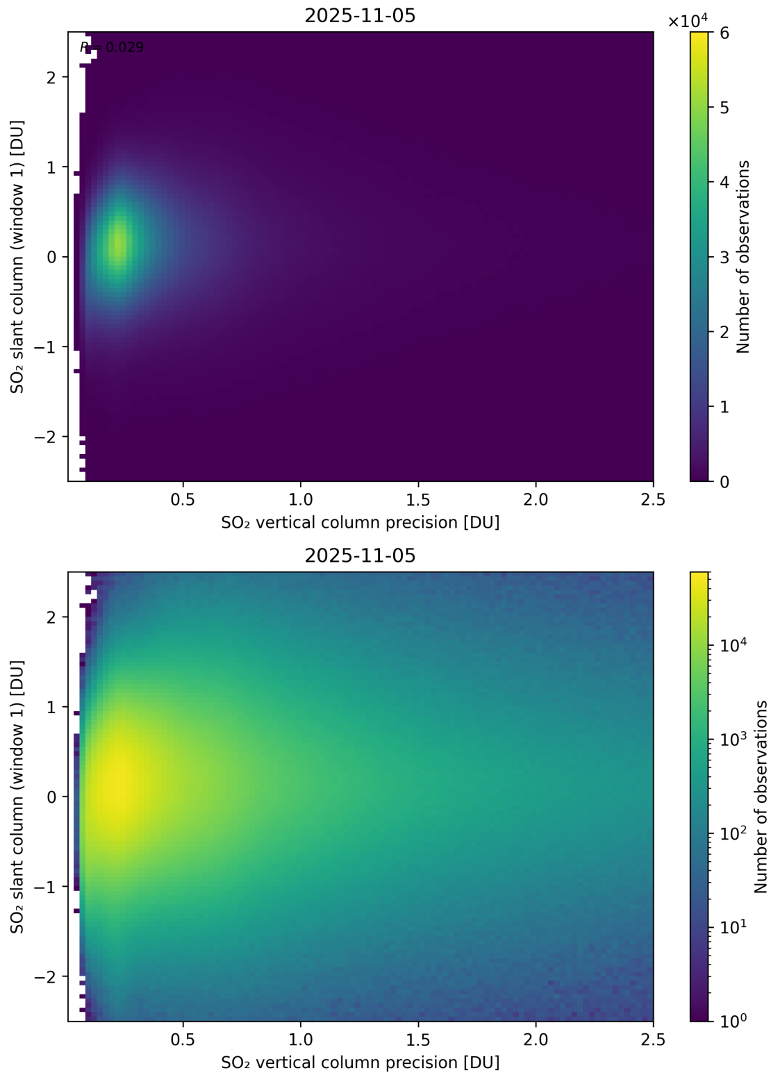
Figure 341: Scatter density plot of “SO 2 vertical column precision” against “SO 2 slant column (window 1)” for 2025-11-04 to 2025-11-06.
