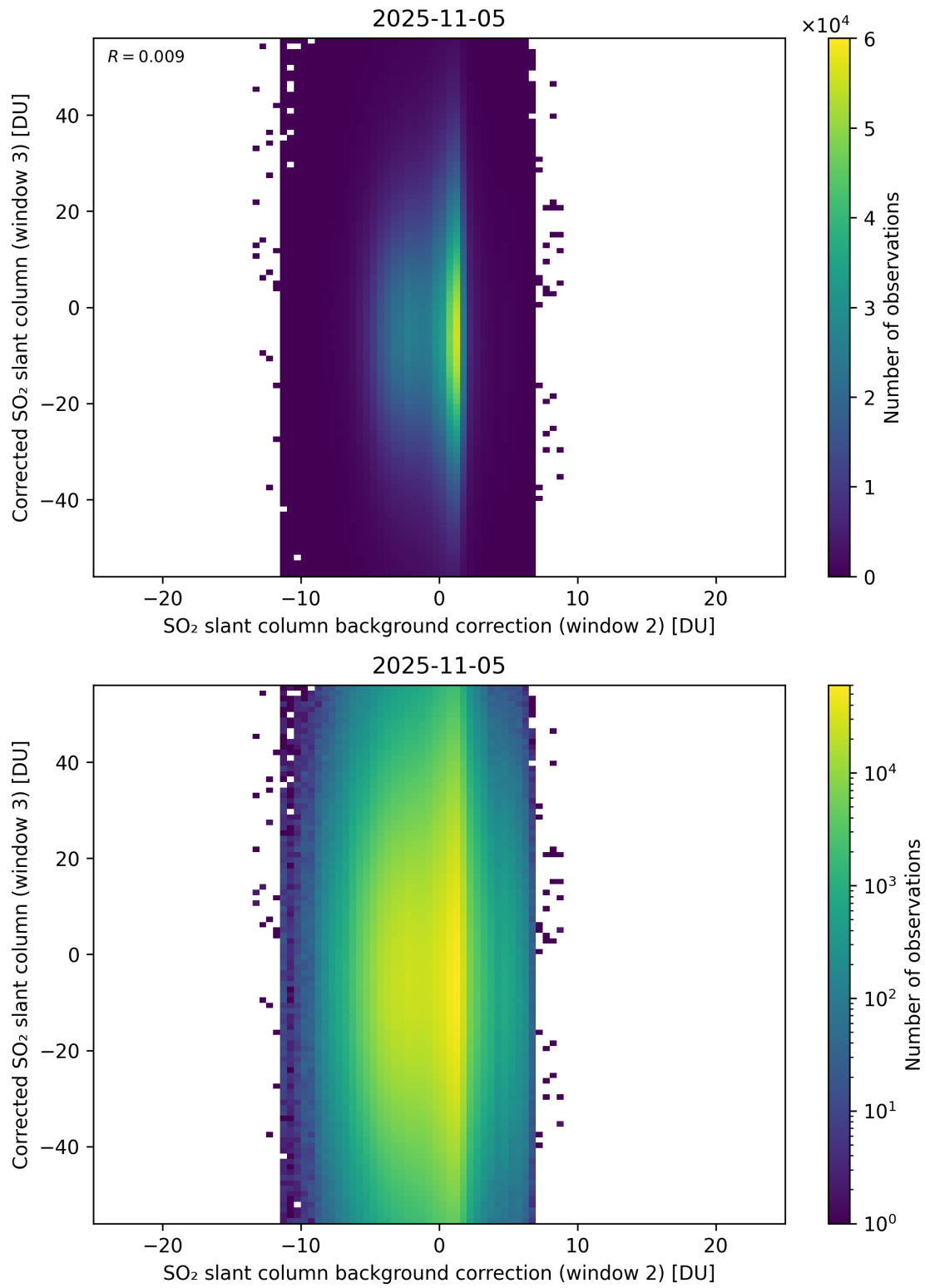
Figure 127: Scatter density plot of “SO 2 slant column background correction (window 2)” against “Corrected SO 2 slant column (window 3)” for 2025-11-04 to 2025-11-06.
