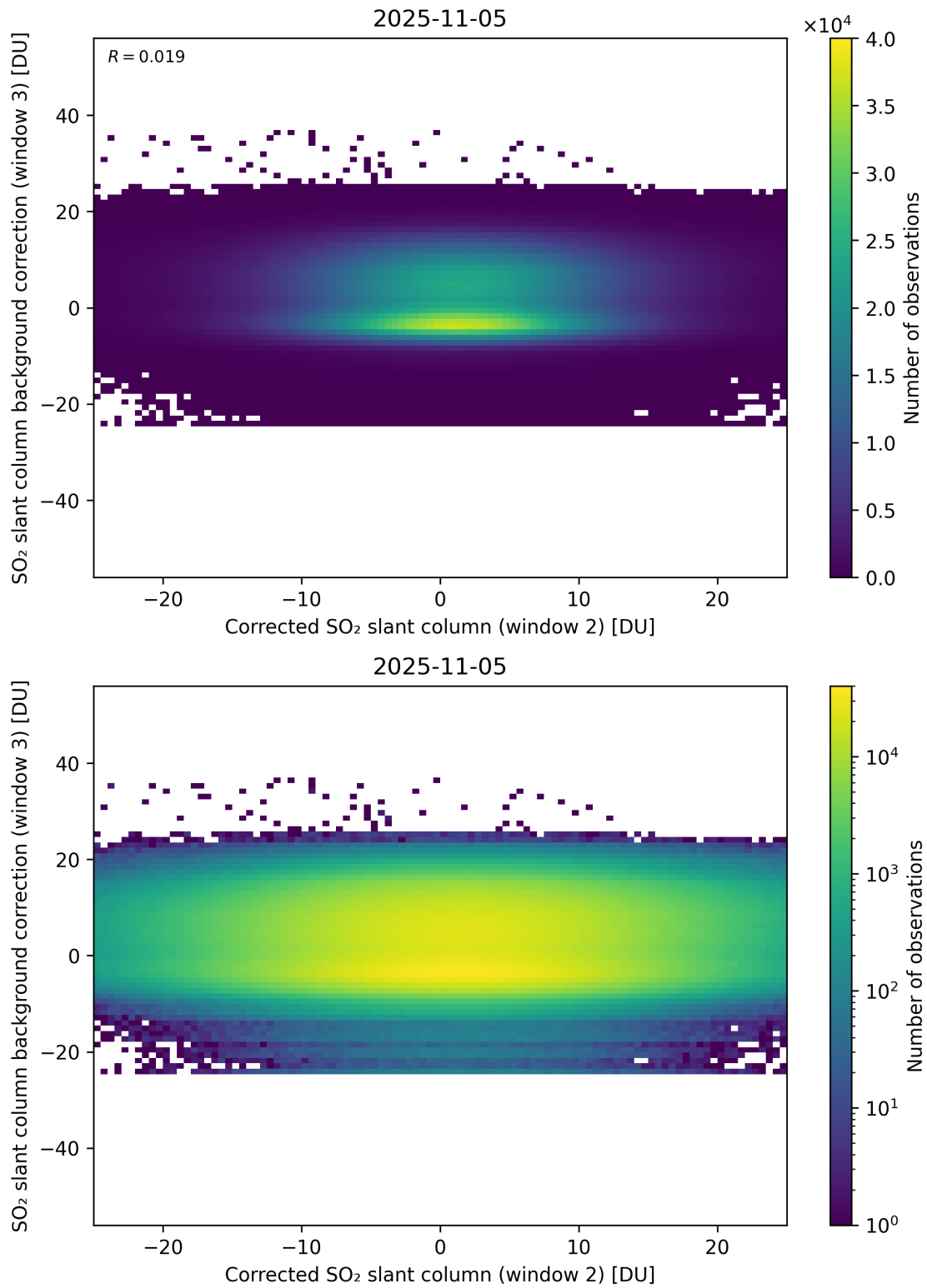
Figure 245: Scatter density plot of “Corrected SO 2 slant column (window 2)” against “SO 2 slant column background correction (window 3)” for 2025-11-04 to 2025-11-06.
