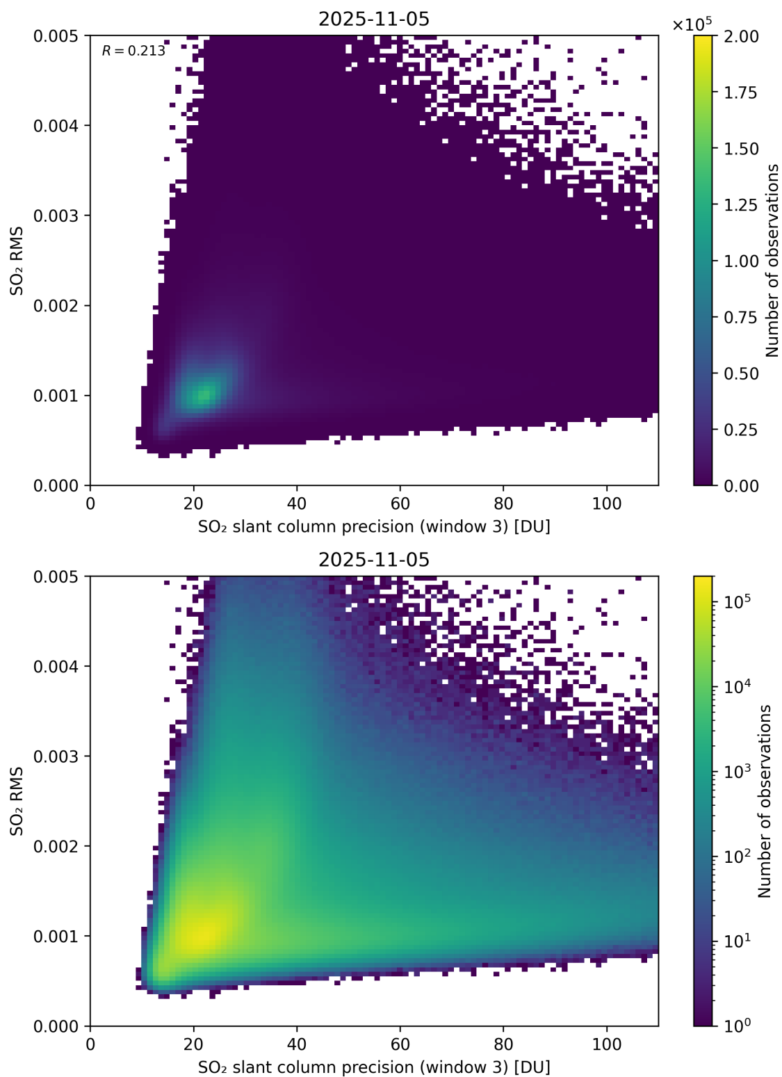
Figure 310: Scatter density plot of “SO 2 slant column precision (window 3)” against “SO 2 RMS” for 2025-11-04 to 2025-11-06.
