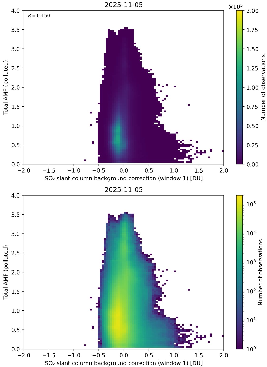
Figure 120: Scatter density plot of “SO 2 slant column background correction (window 1)” against “Total AMF (polluted)” for 2025-11-04 to 2025-11-06.
