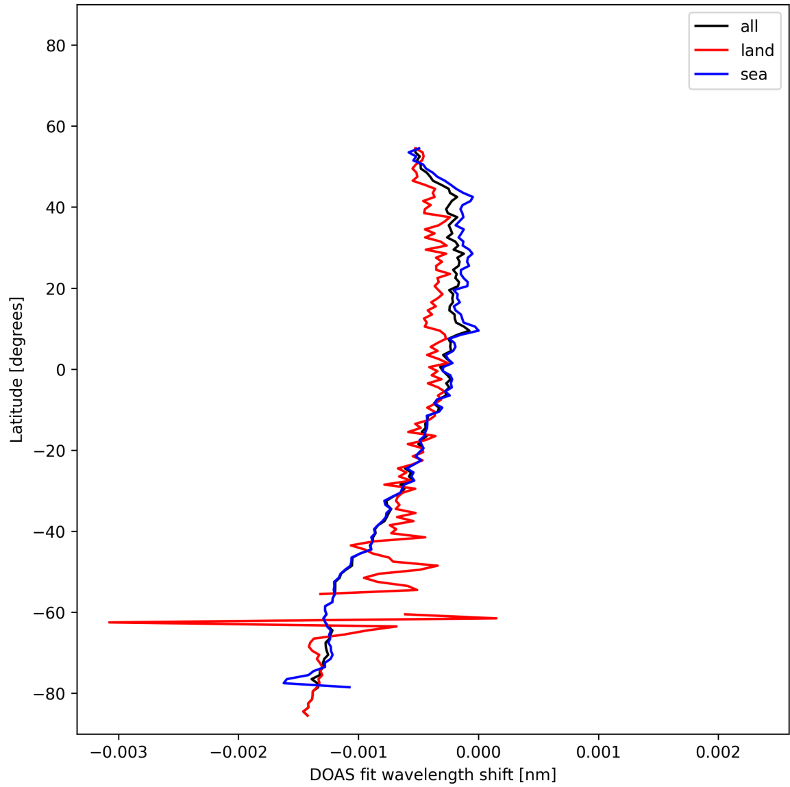
Figure 50: Zonal average of "DOAS fit wavelength shift" for 2025-11-04 to 2025-11-06.
