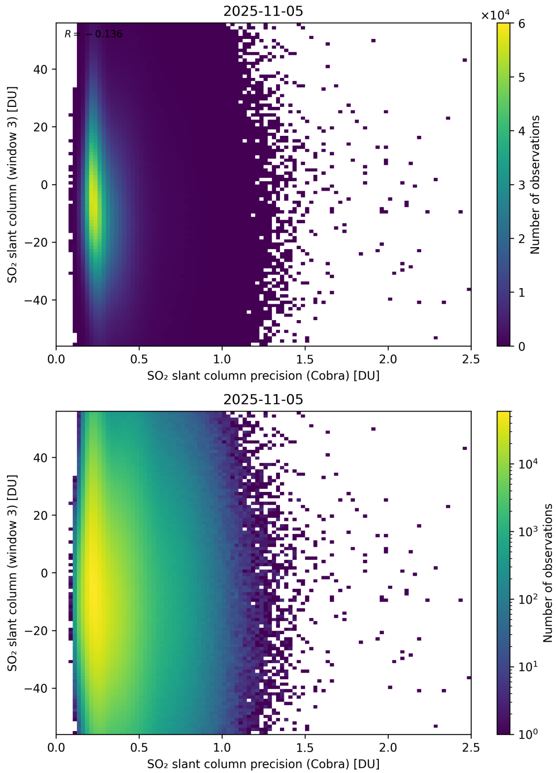
Figure 211: Scatter density plot of “SO 2 slant column precision (Cobra)” against “SO 2 slant column (window 3)” for 2025-11-04 to 2025-11-06.
