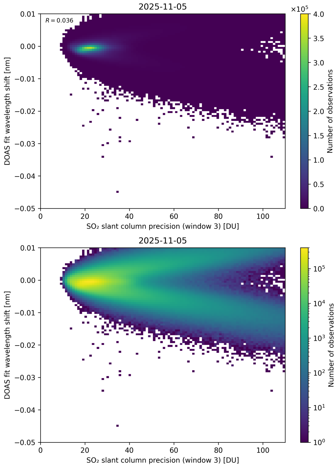
Figure 308: Scatter density plot of “SO 2 slant column precision (window 3)” against “DOAS fit wavelength shift” for 2025-11-04 to 2025-11-06.
