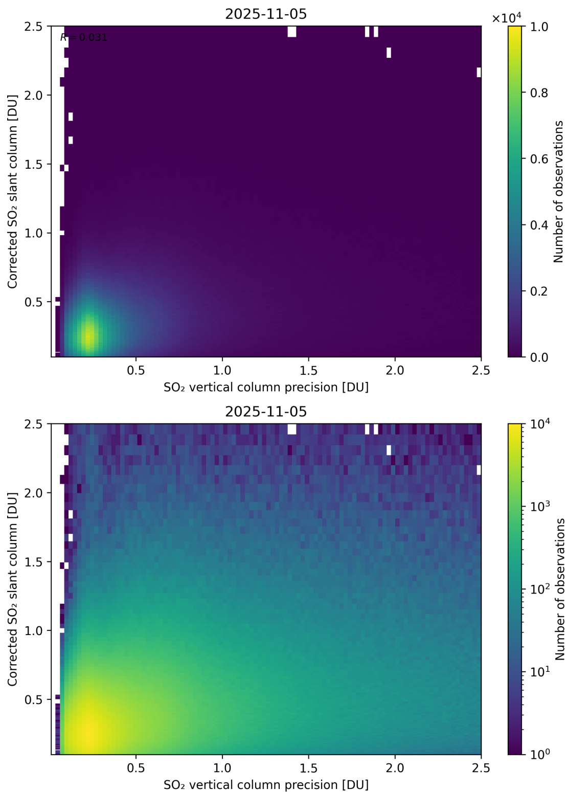
Figure 338: Scatter density plot of “SO 2 vertical column precision” against “Corrected SO 2 slant column” for 2025-11-04 to 2025-11-06.
