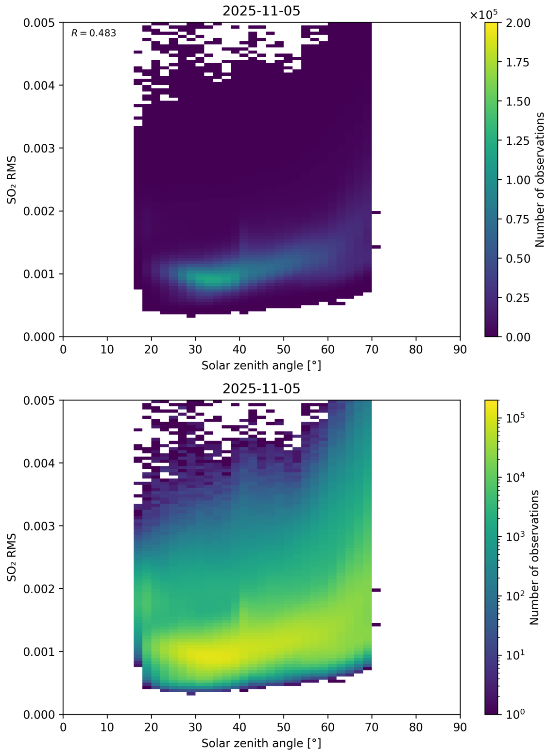
Figure 176: Scatter density plot of “Solar zenith angle” against “SO 2 RMS” for 2025-11-04 to 2025-11-06.
