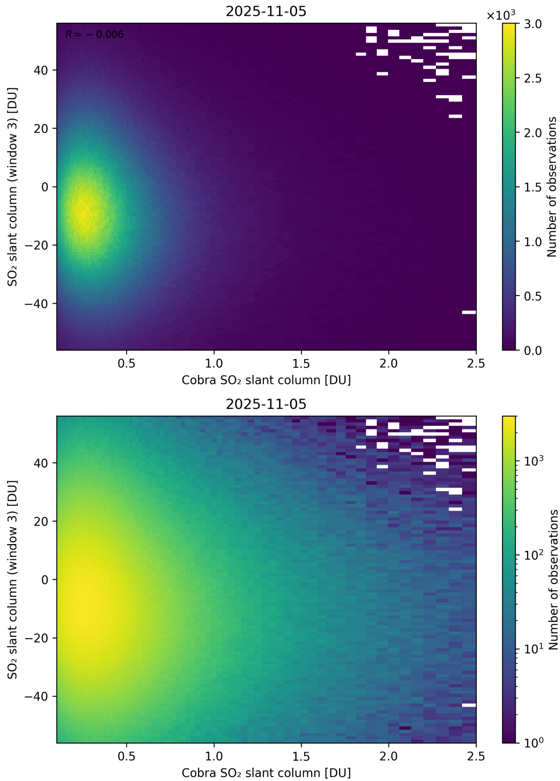
Figure 222: Scatter density plot of “Cobra SO 2 slant column” against “SO 2 slant column (window 3)” for 2025-11-04 to 2025-11-06.
