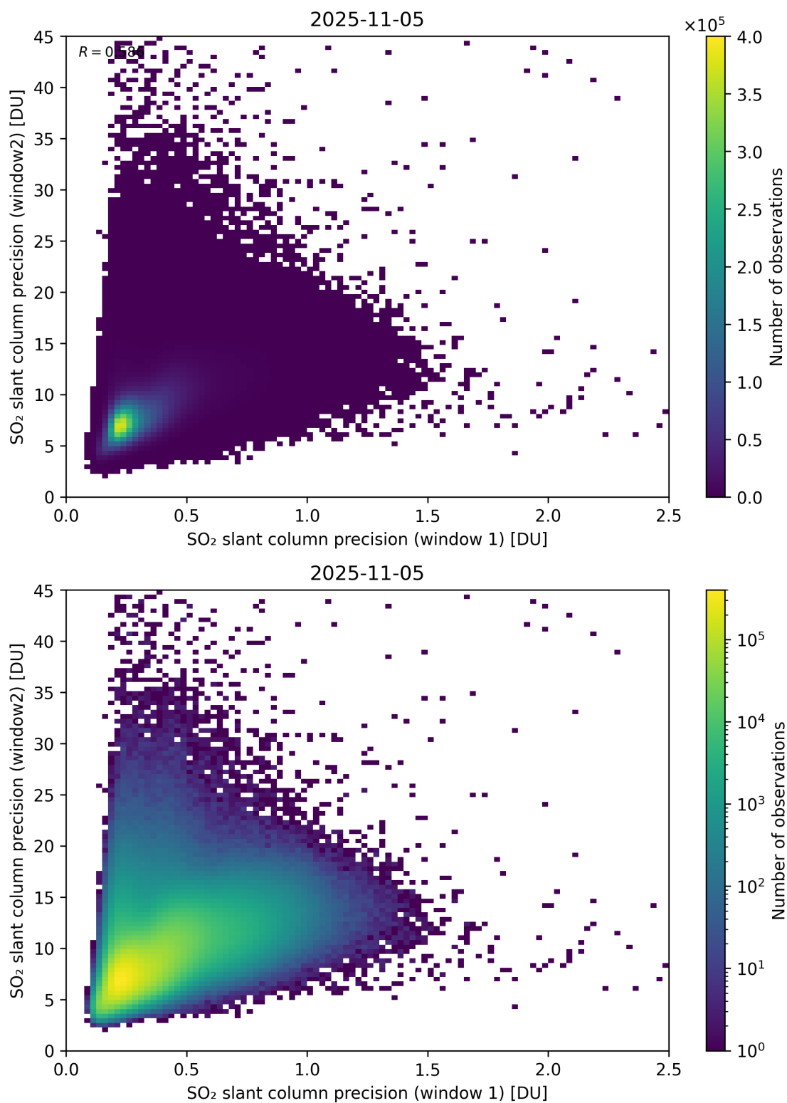
Figure 277: Scatter density plot of “SO 2 slant column precision (window 1)” against “SO 2 slant column precision (window2)” for 2025-11-04 to 2025-11-06.
