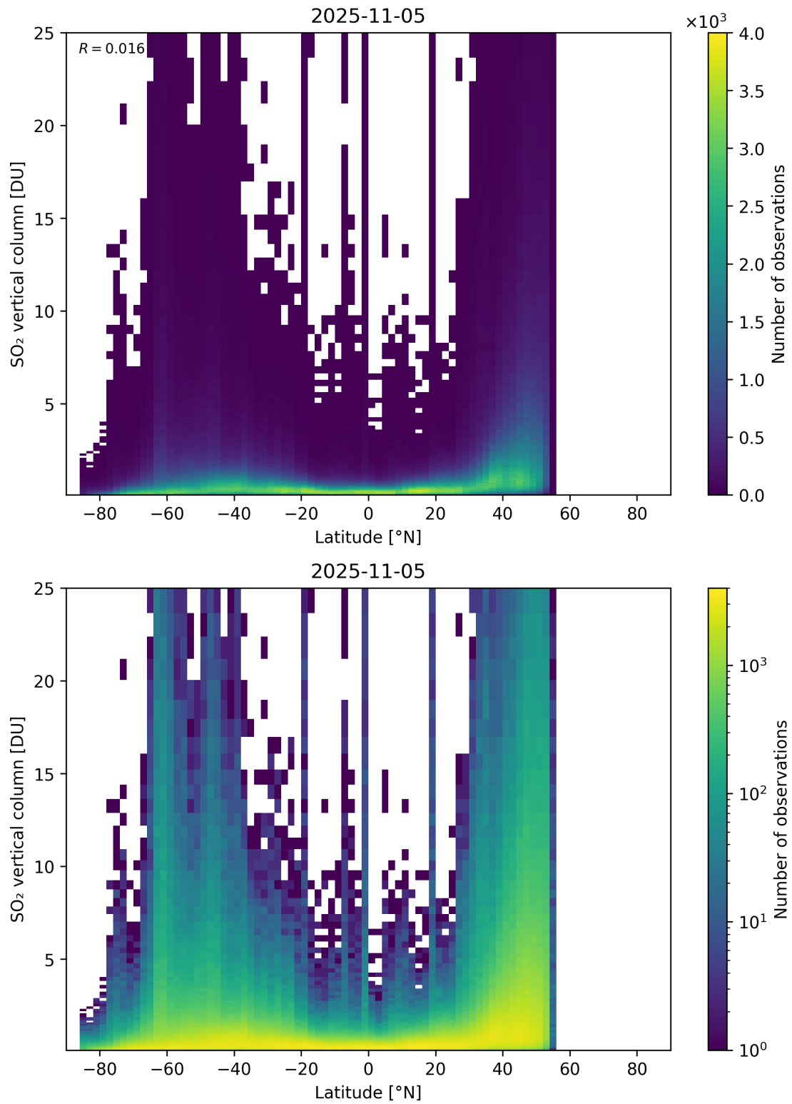
Figure 169: Scatter density plot of “Latitude” against “SO 2 vertical column” for 2025-11-04 to 2025-11-06.
