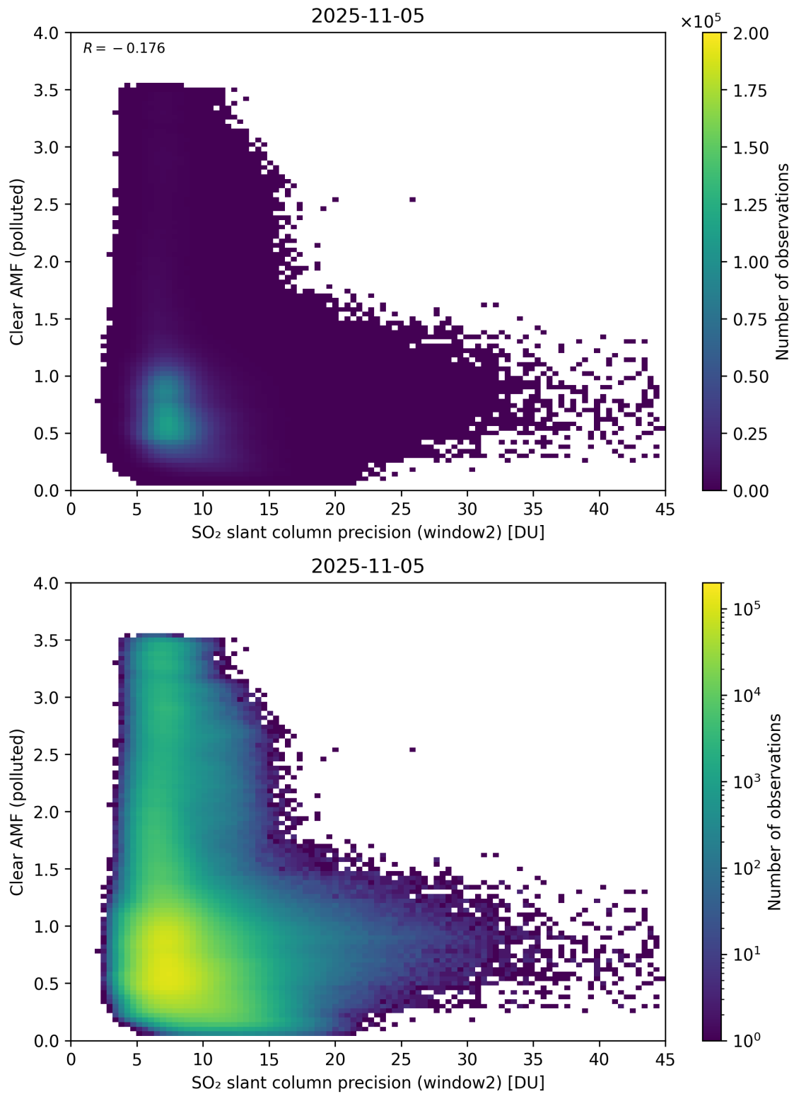
Figure 296: Scatter density plot of “SO 2 slant column precision (window2)” against “Clear AMF (polluted)” for 2025-11-04 to 2025-11-06.
