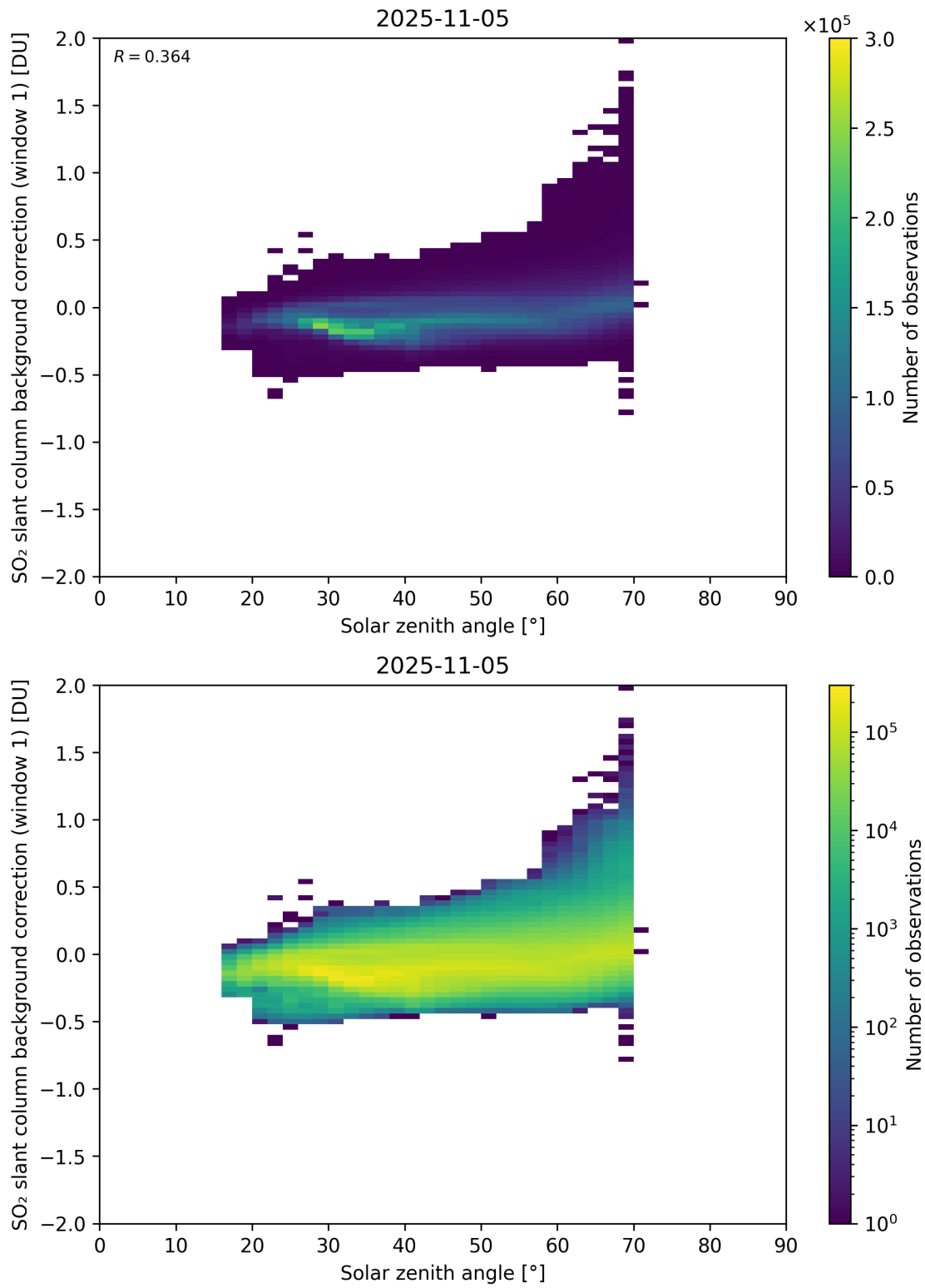
Figure 171: Scatter density plot of “Solar zenith angle” against “SO 2 slant column background correction (window 1)” for 2025-11-04 to 2025-11-06.
