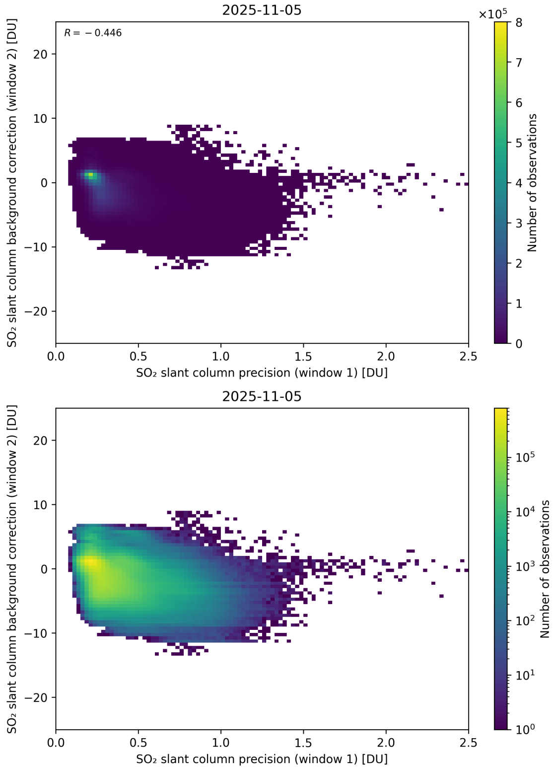
Figure 269: Scatter density plot of “SO 2 slant column precision (window 1)” against “SO 2 slant column background correction (window 2)” for 2025-11-04 to 2025-11-06.
