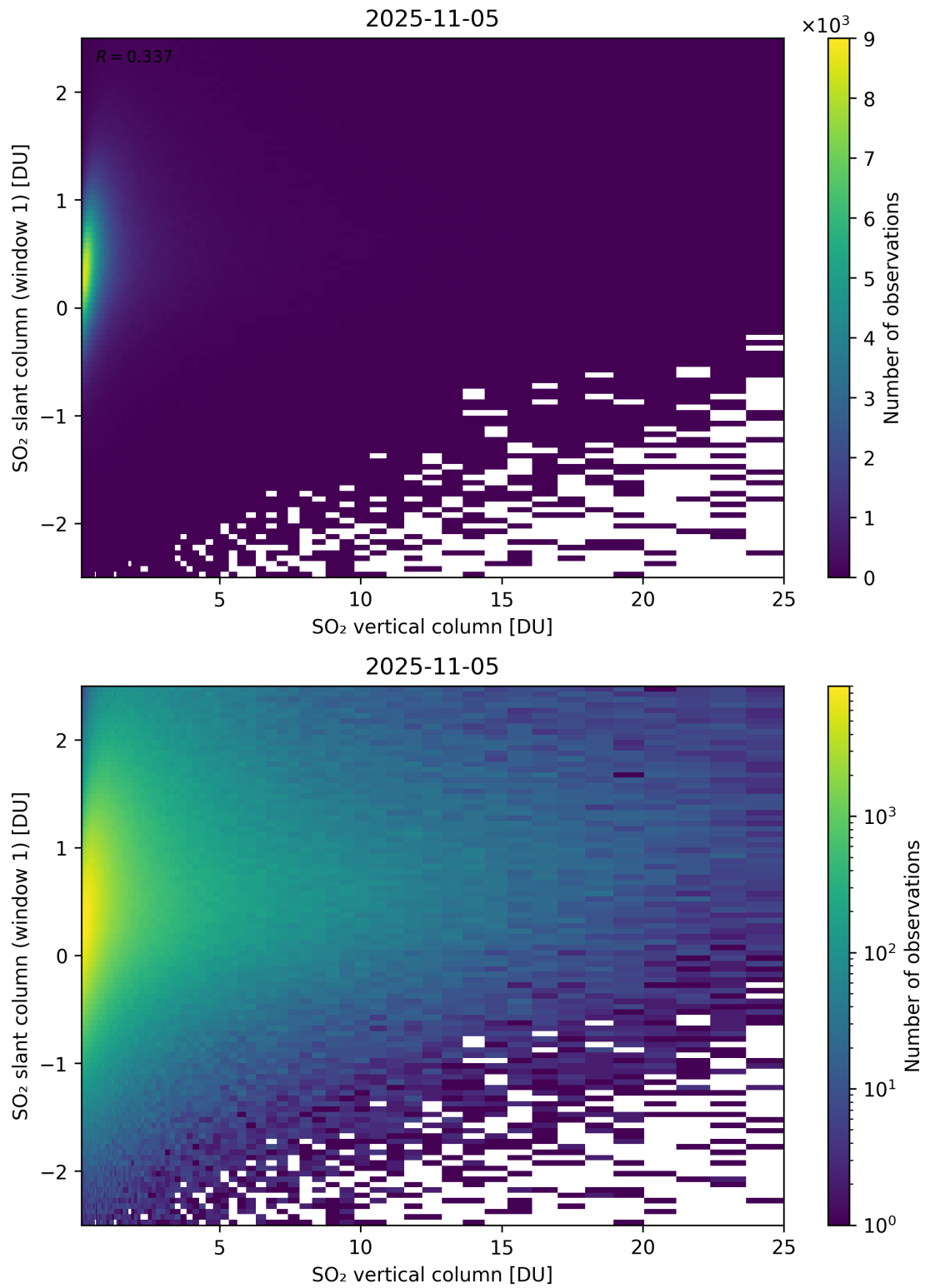
Figure 354: Scatter density plot of “SO 2 vertical column” against “SO 2 slant column (window 1)” for 2025-11-04 to 2025-11-06.
