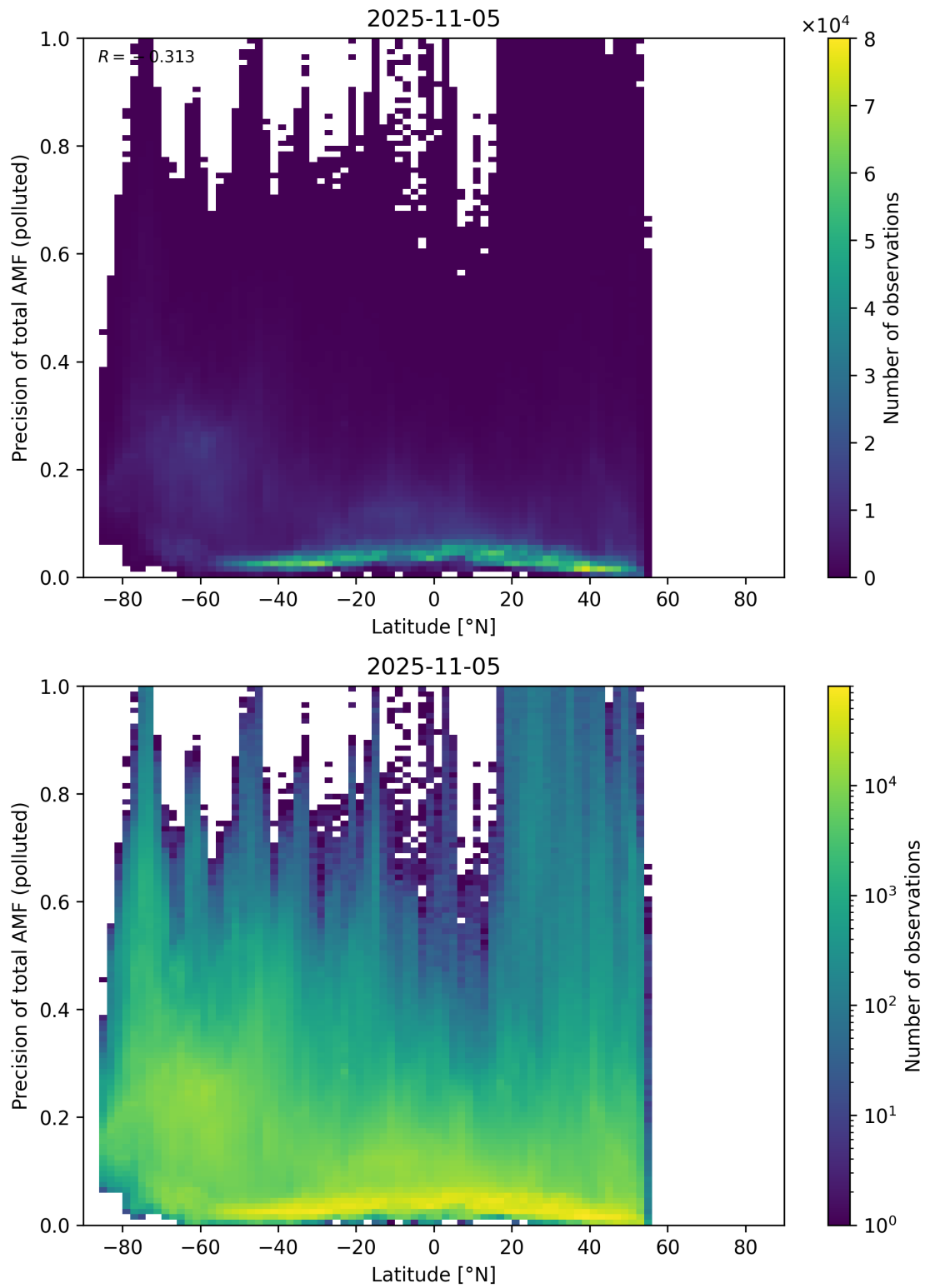
Figure 168: Scatter density plot of “Latitude” against “Precision of total AMF (polluted)” for 2025-11-04 to 2025-11-06.
