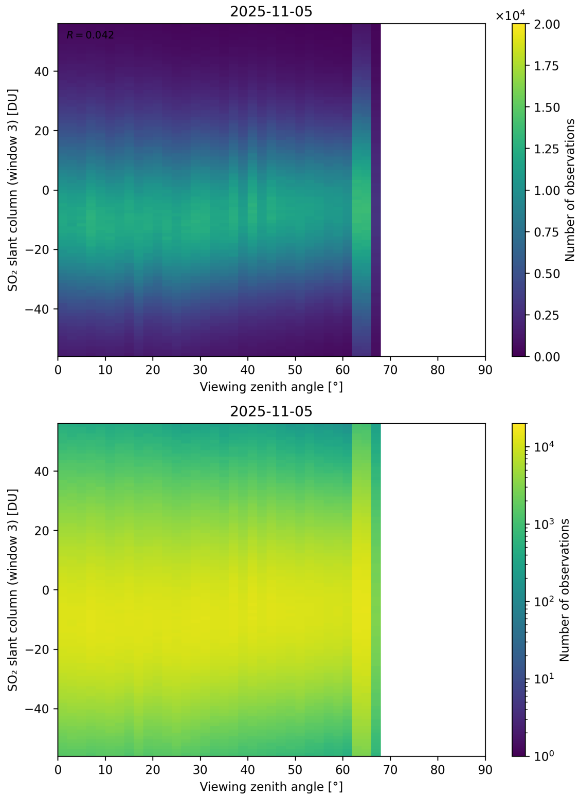
Figure 379: Scatter density plot of “Viewing zenith angle” against “SO 2 slant column (window 3)” for 2025-11-04 to 2025-11-06.
