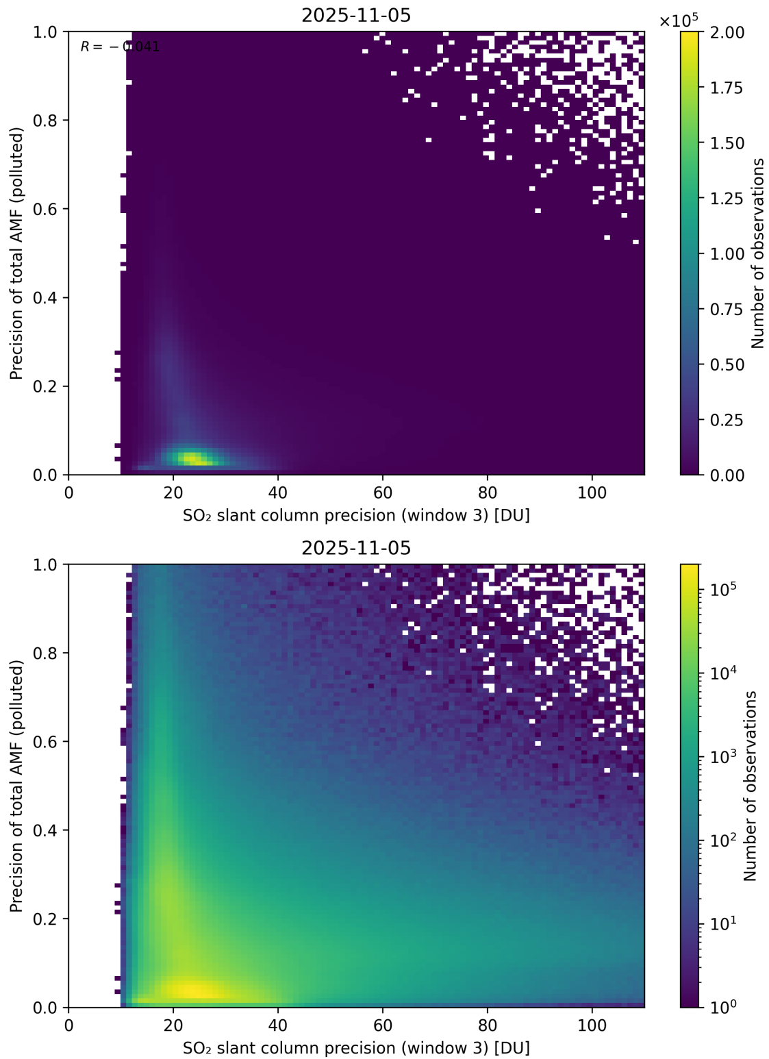
Figure 314: Scatter density plot of “SO 2 slant column precision (window 3)” against “Precision of total AMF (polluted)” for 2025-11-04 to 2025-11-06.
