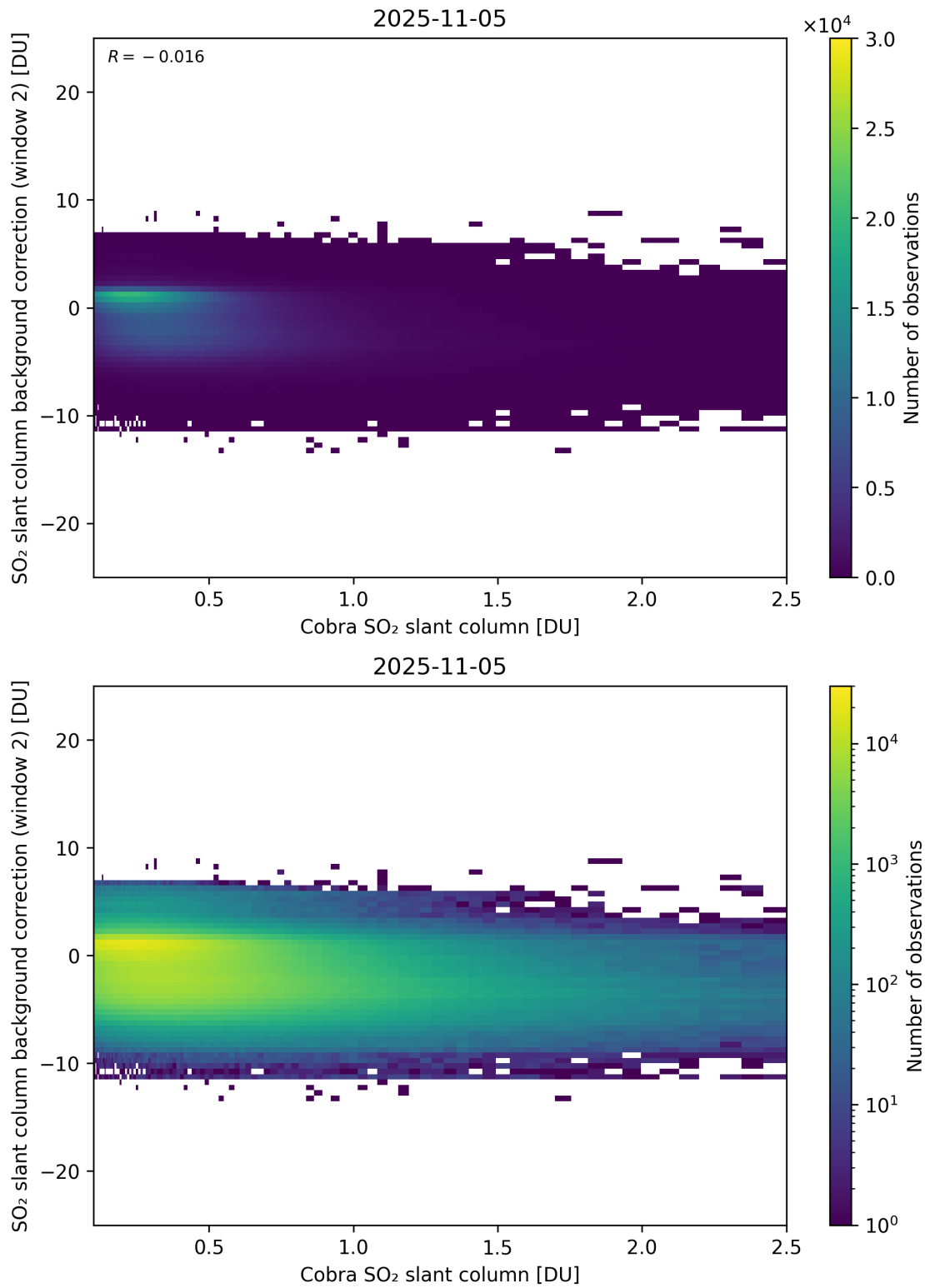
Figure 194: Scatter density plot of “Cobra SO 2 slant column” against “SO 2 slant column background correction (window 2)” for 2025-11-04 to 2025-11-06.
