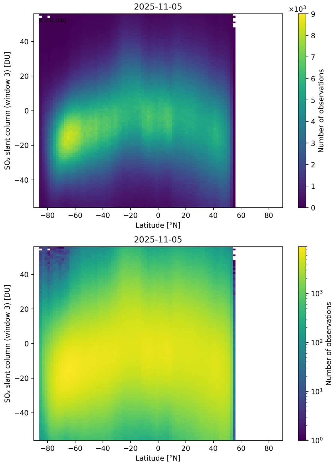
Figure 165: Scatter density plot of “Latitude” against “SO 2 slant column (window 3)” for 2025-11-04 to 2025-11-06.
