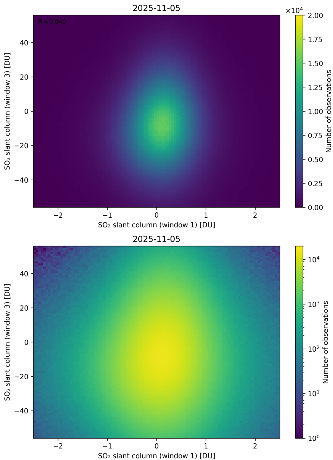
Figure 287: Scatter density plot of “SO 2 slant column (window 1)” against “SO 2 slant column (window 3)” for 2025-11-04 to 2025-11-06.
