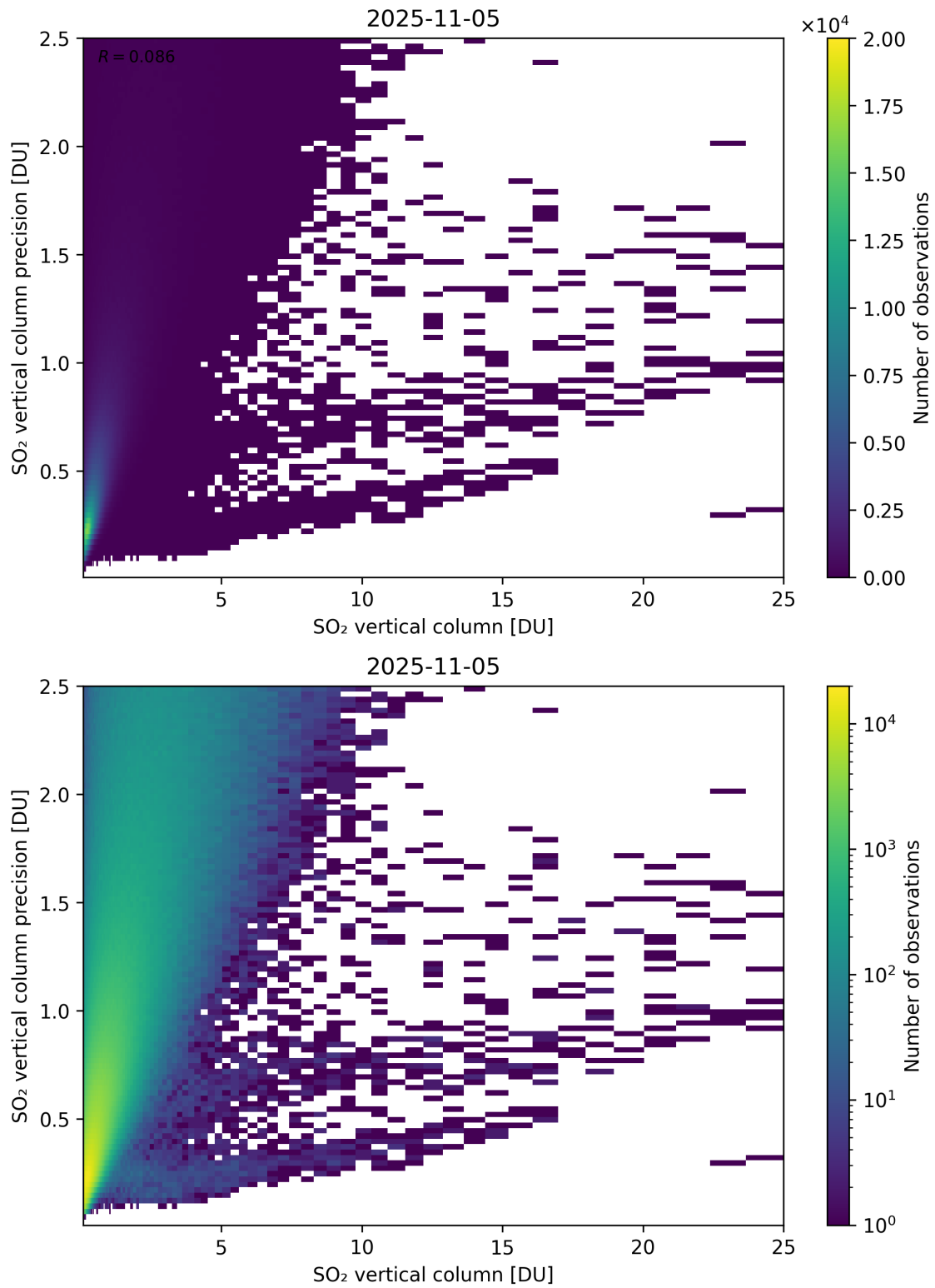
Figure 361: Scatter density plot of “SO 2 vertical column” against “SO 2 vertical column precision” for 2025-11-04 to 2025-11-06.
