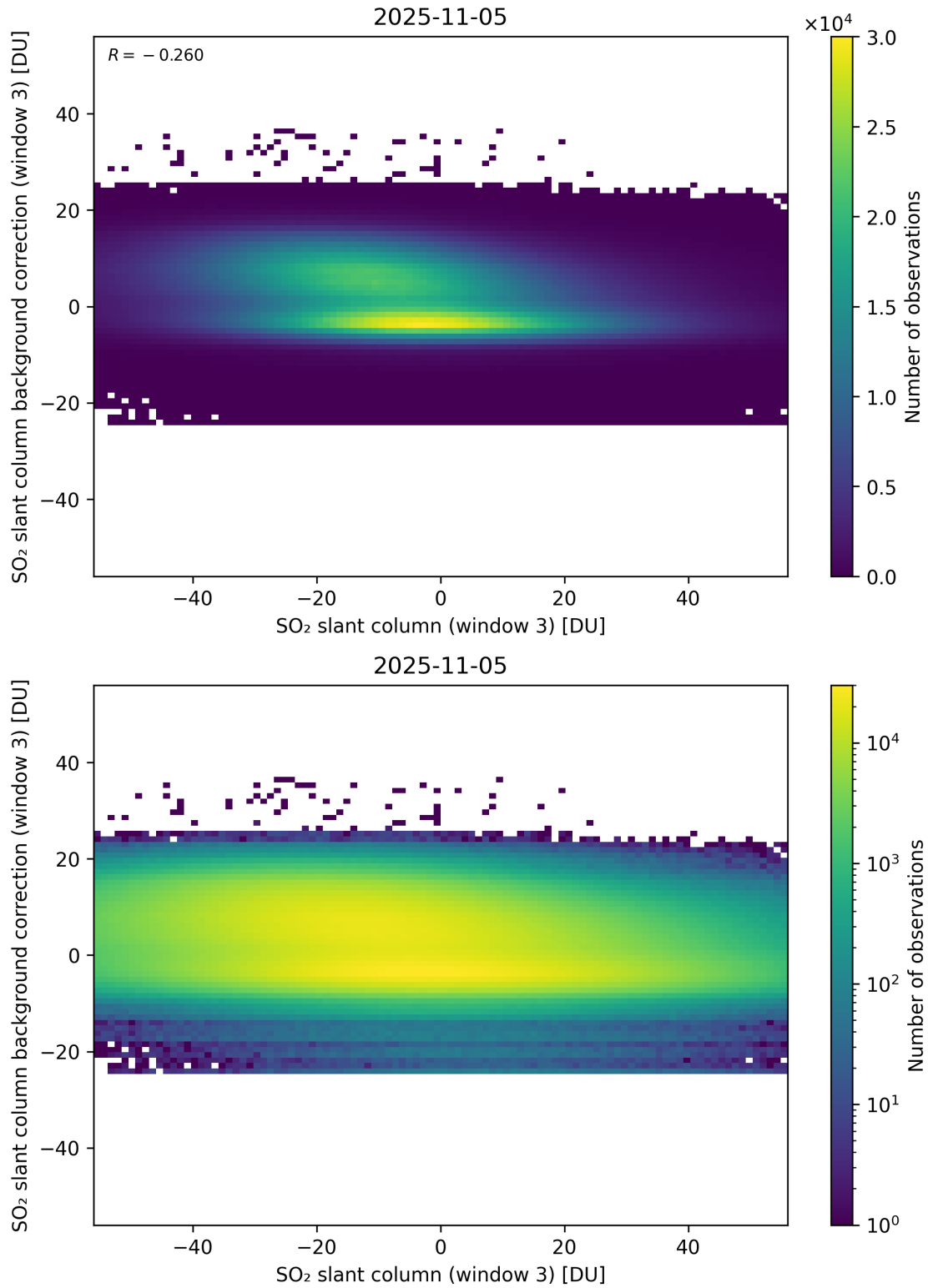
Figure 303: Scatter density plot of “SO 2 slant column (window 3)” against “SO 2 slant column background correction (window 3)” for 2025-11-04 to 2025-11-06.
