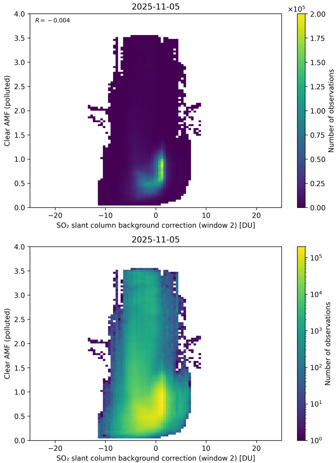
Figure 126: Scatter density plot of “SO 2 slant column background correction (window 2)” against “Clear AMF (polluted)” for 2025-11-04 to 2025-11-06.
