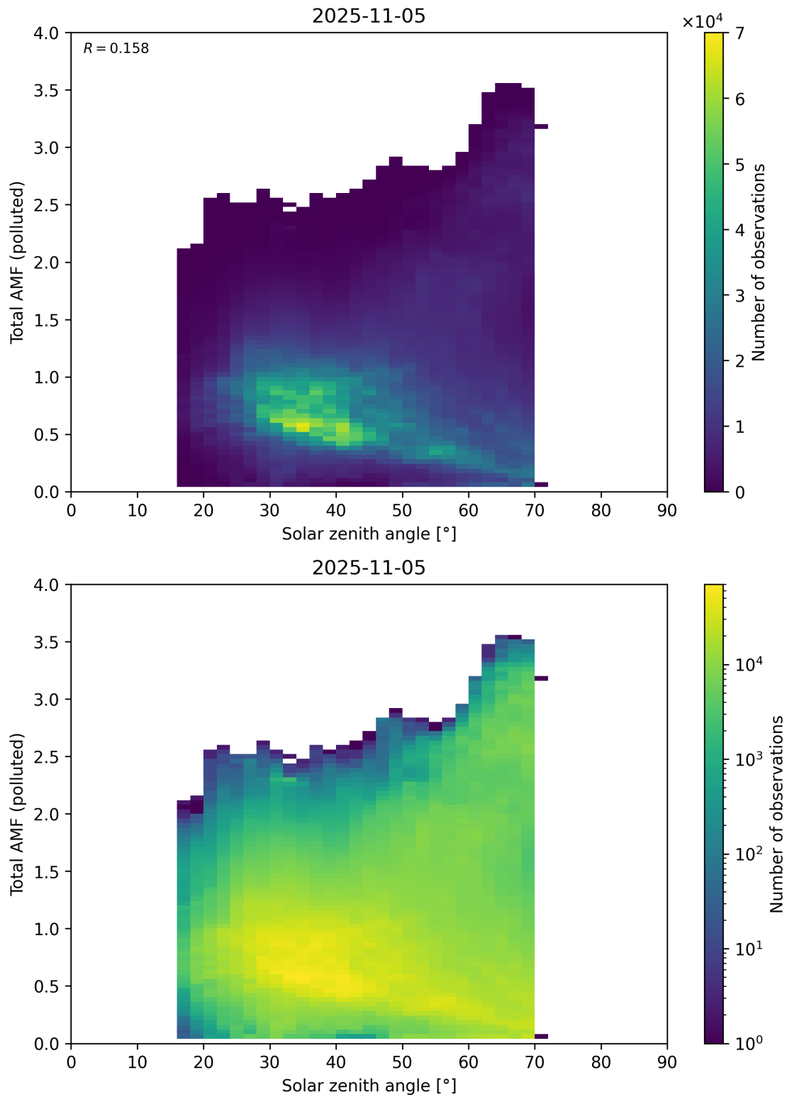
Figure 189: Scatter density plot of “Solar zenith angle” against “Total AMF (polluted)” for 2025-11-04 to 2025-11-06.
