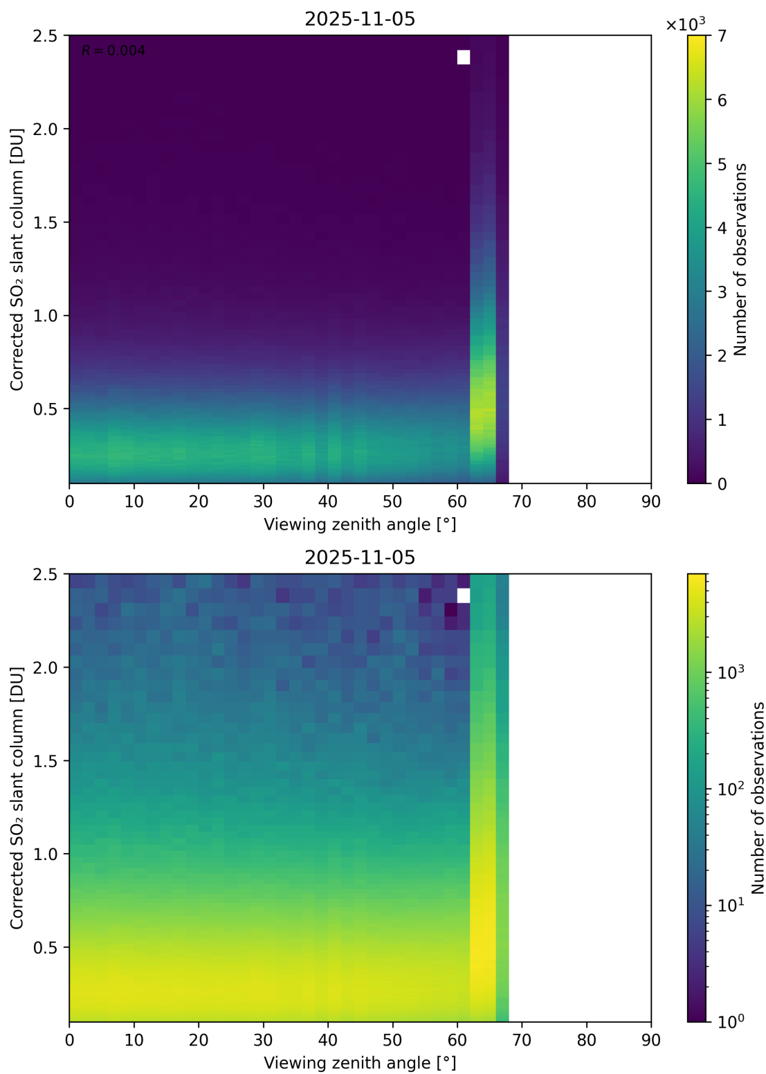
Figure 373: Scatter density plot of “Viewing zenith angle” against “Corrected SO 2 slant column” for 2025-11-04 to 2025-11-06.
