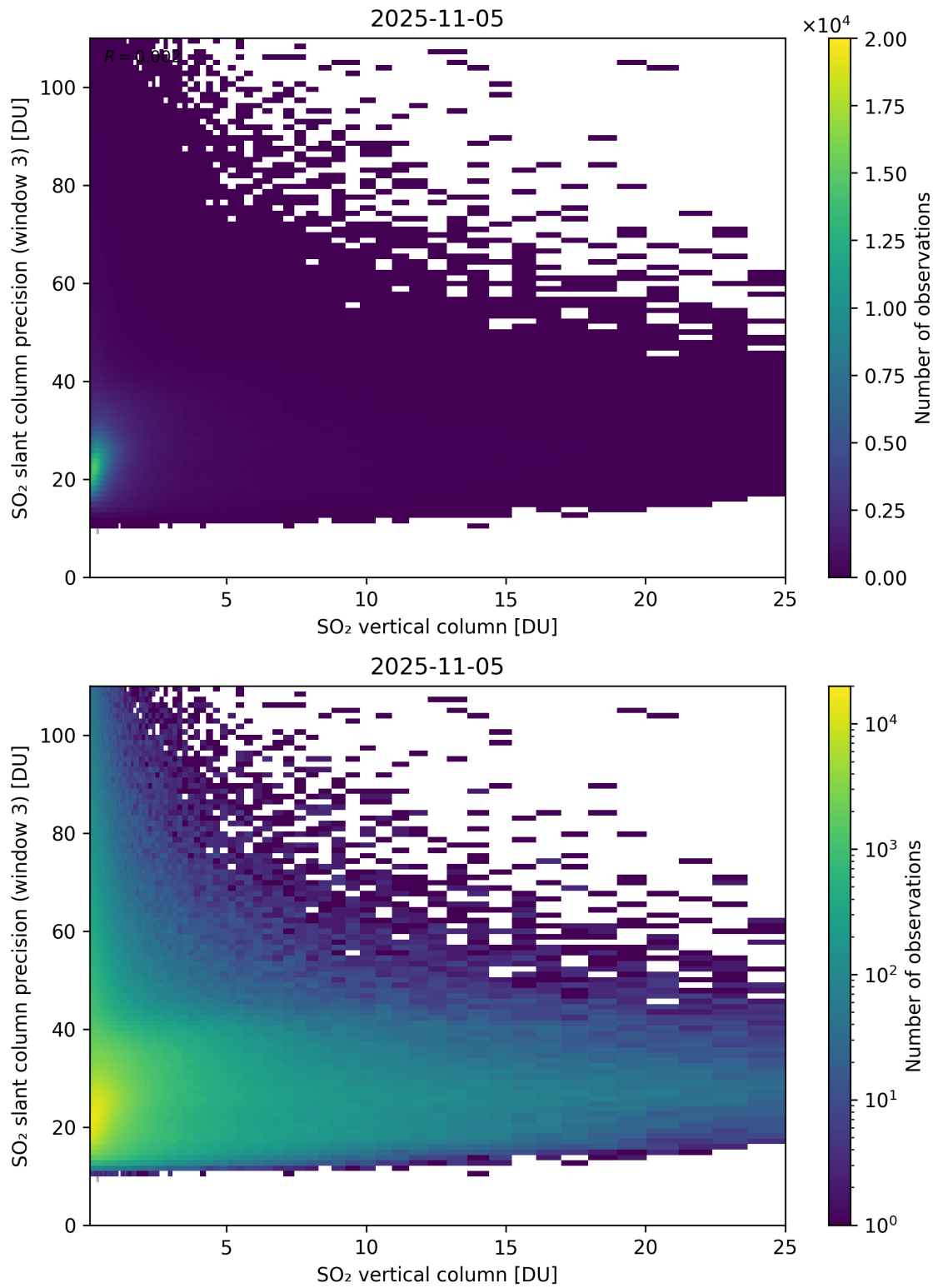
Figure 358: Scatter density plot of “SO 2 vertical column” against “SO 2 slant column precision (window 3)” for 2025-11-04 to 2025-11-06.
