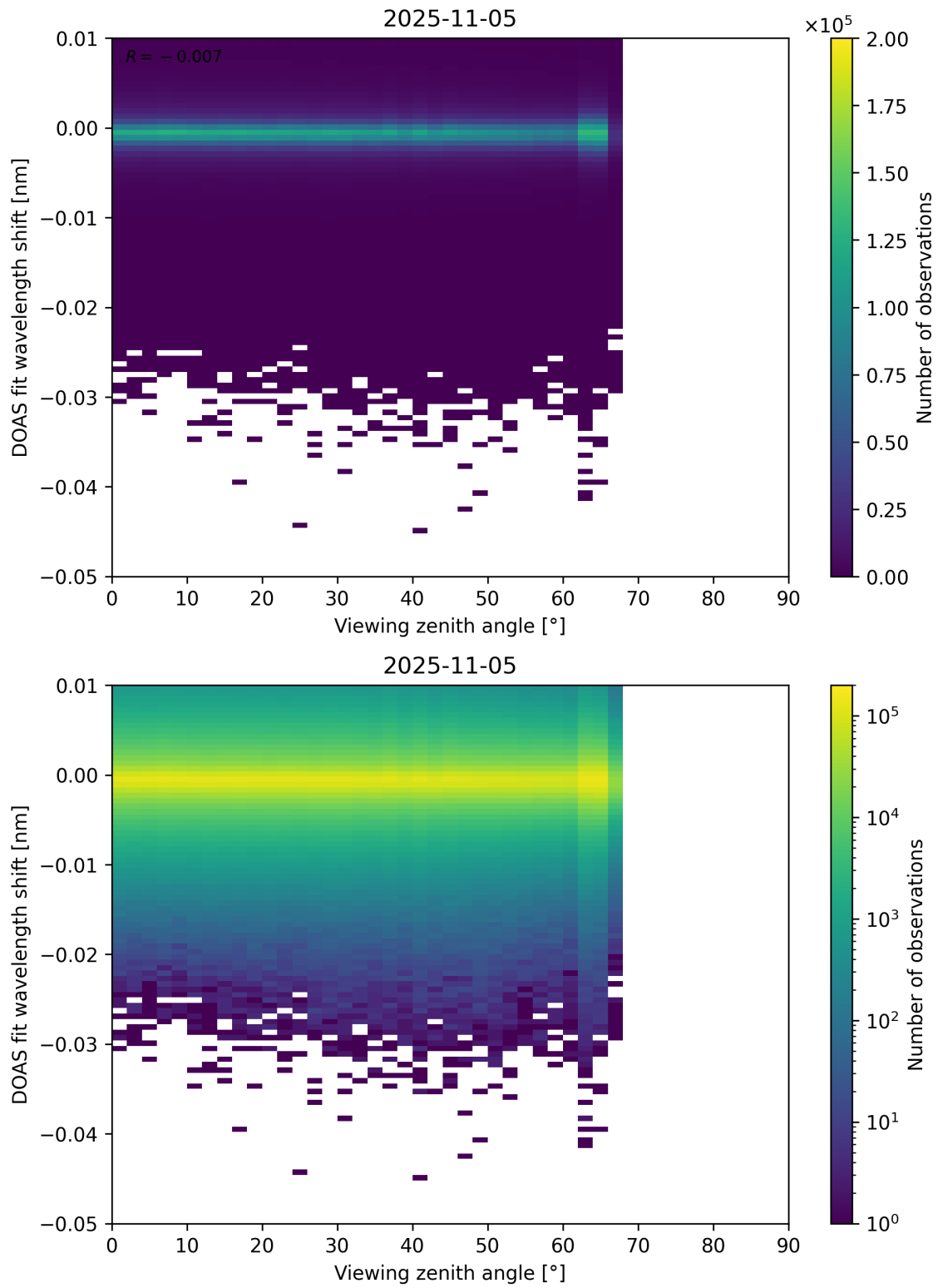
Figure 365: Scatter density plot of “Viewing zenith angle” against “DOAS fit wavelength shift” for 2025-11-04 to 2025-11-06.
