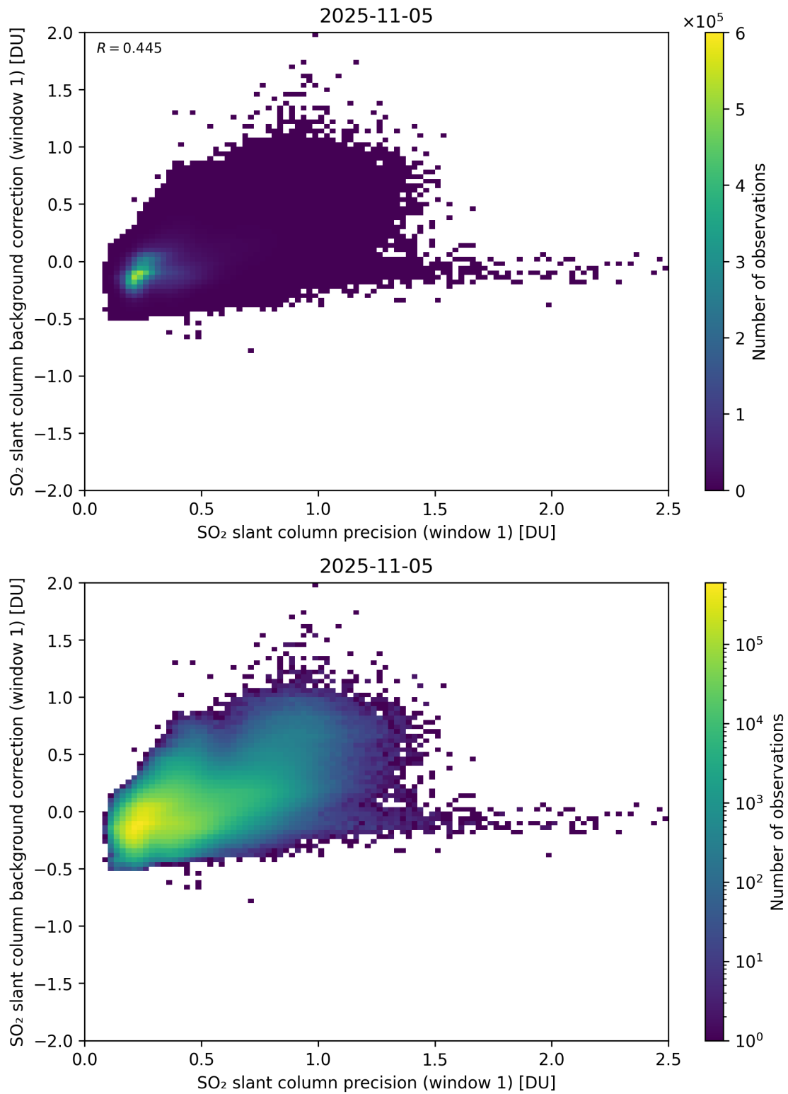
Figure 268: Scatter density plot of “SO 2 slant column precision (window 1)” against “SO 2 slant column background correction (window 1)” for 2025-11-04 to 2025-11-06.
