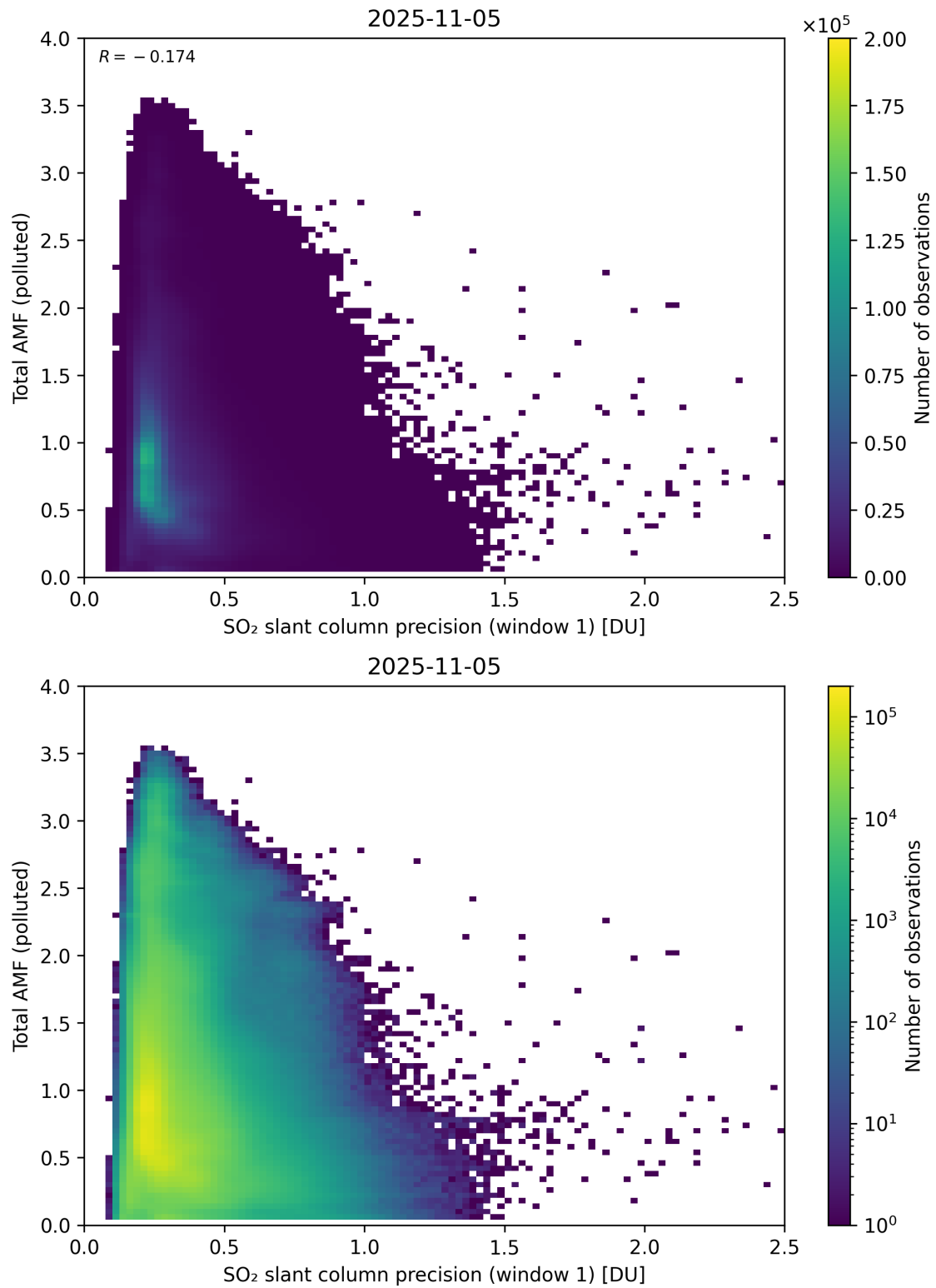
Figure 280: Scatter density plot of “SO 2 slant column precision (window 1)” against “Total AMF (polluted)” for 2025-11-04 to 2025-11-06.
