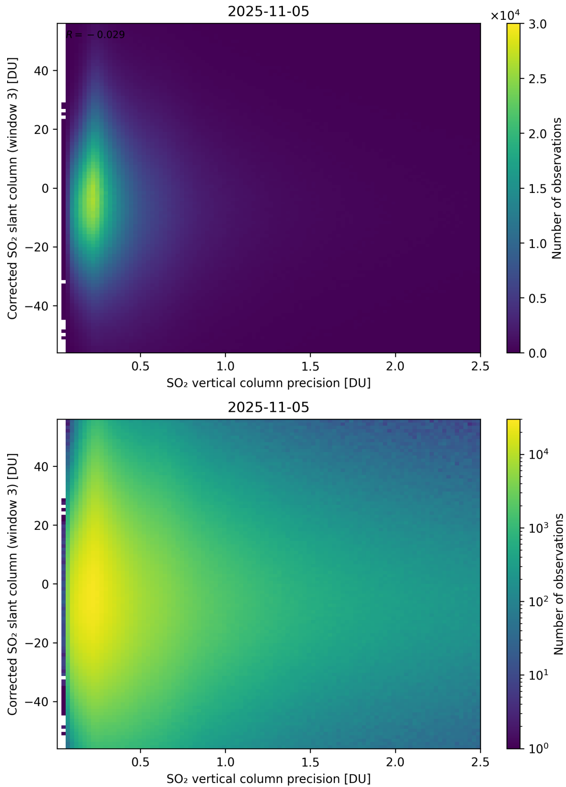
Figure 340: Scatter density plot of “SO 2 vertical column precision” against “Corrected SO 2 slant column (window 3)” for 2025-11-04 to 2025-11-06.
