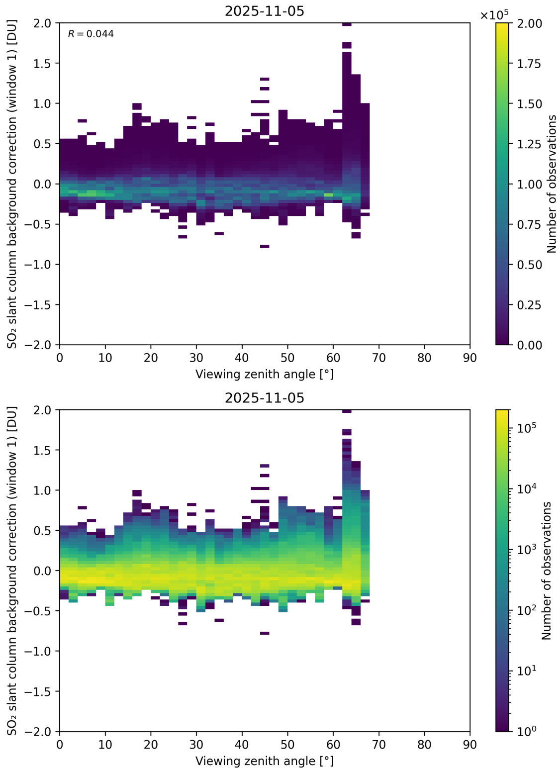
Figure 362: Scatter density plot of “Viewing zenith angle” against “SO 2 slant column background correction (window 1)” for 2025-11-04 to 2025-11-06.
