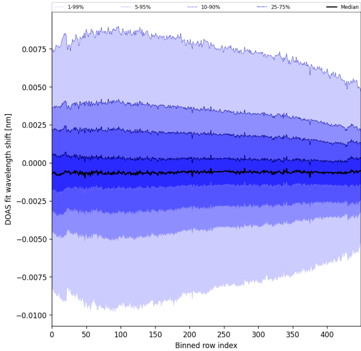
Figure 102: Along track statistics of “DOAS fit wavelength shift” for 2025-11-04 to 2025-11-06
