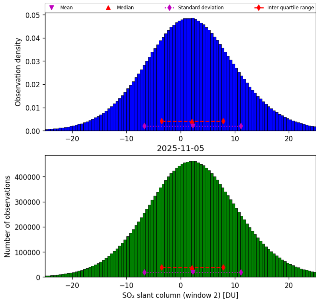
Figure 67: Histogram of “SO 2 slant column (window 2)” for 2025-11-04 to 2025-11-06
