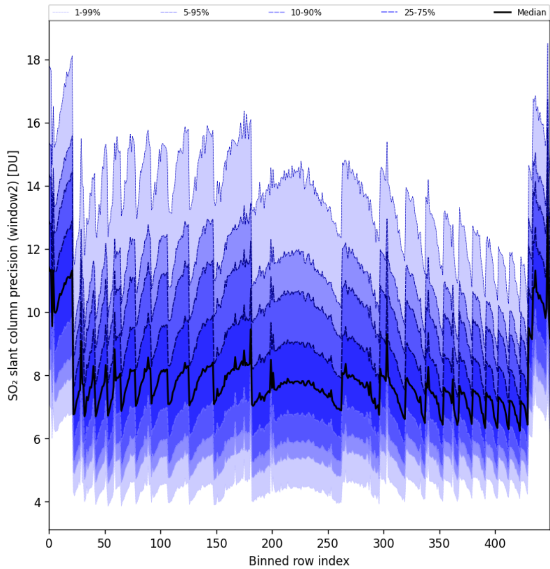
Figure 94: Along track statistics of “SO 2 slant column precision (window2)” for 2025-11-04 to 2025-11-06
