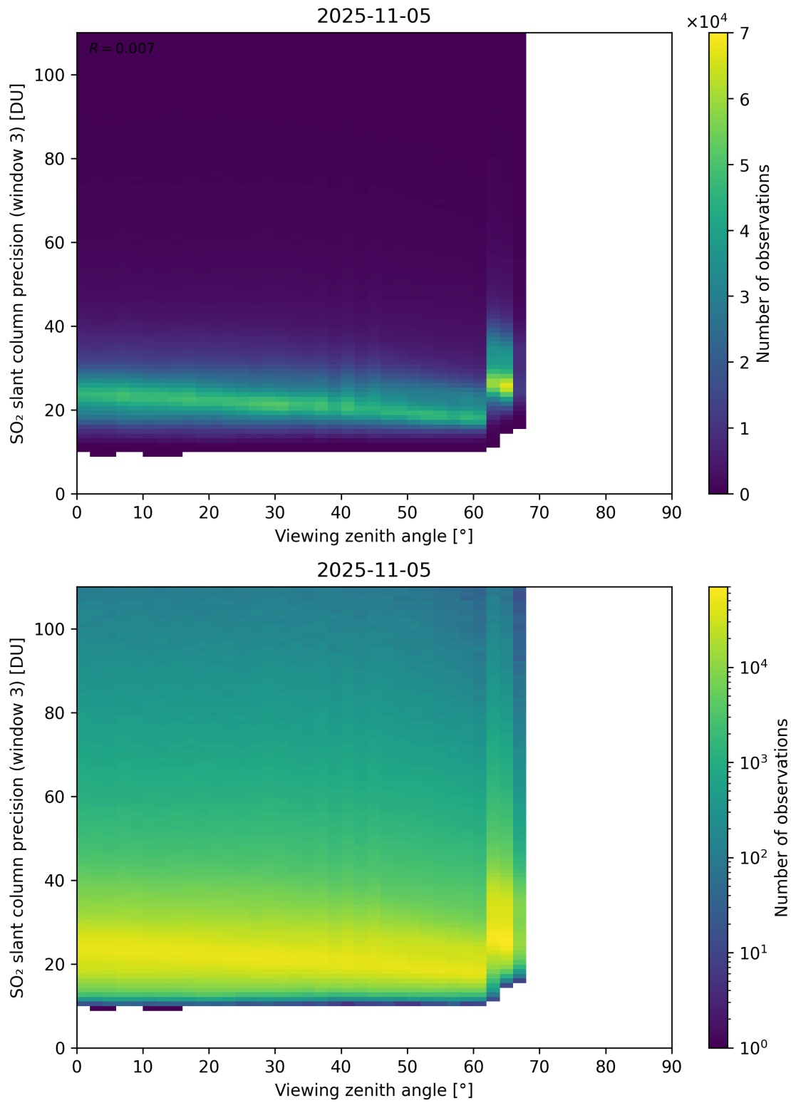
Figure 380: Scatter density plot of “Viewing zenith angle” against “SO 2 slant column precision (window 3)” for 2025-11-04 to 2025-11-06.
