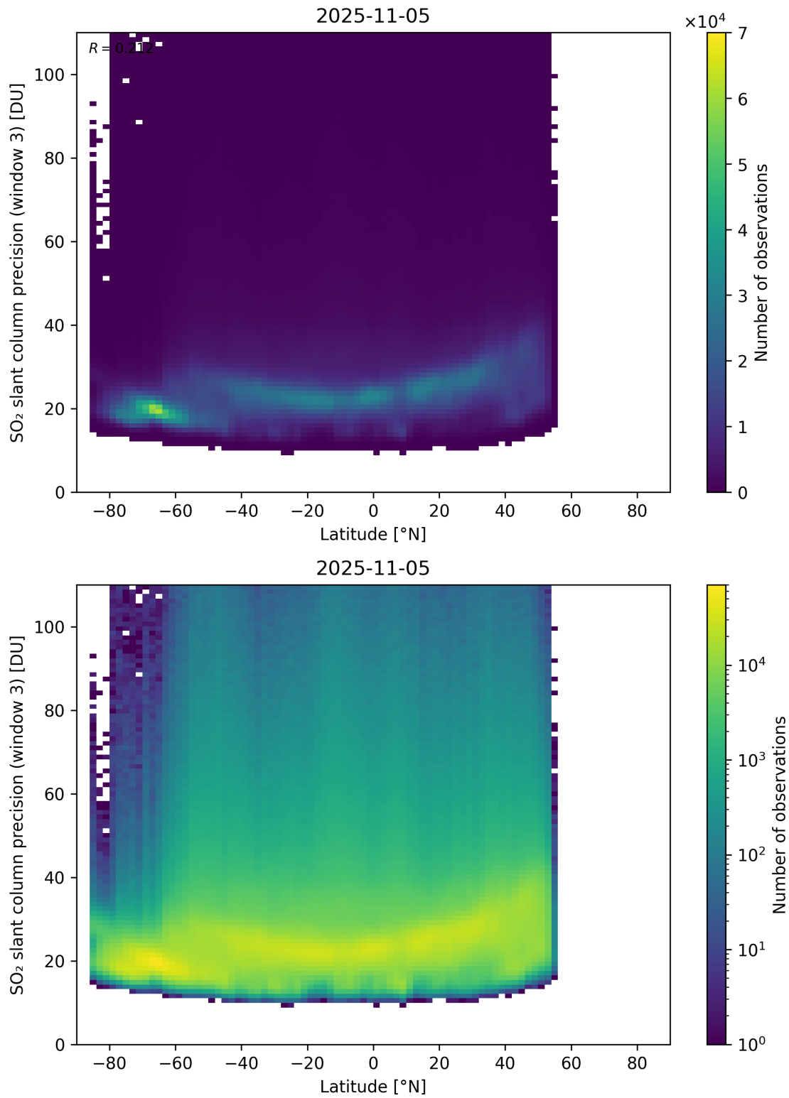
Figure 166: Scatter density plot of “Latitude” against “SO 2 slant column precision (window 3)” for 2025-11-04 to 2025-11-06.
