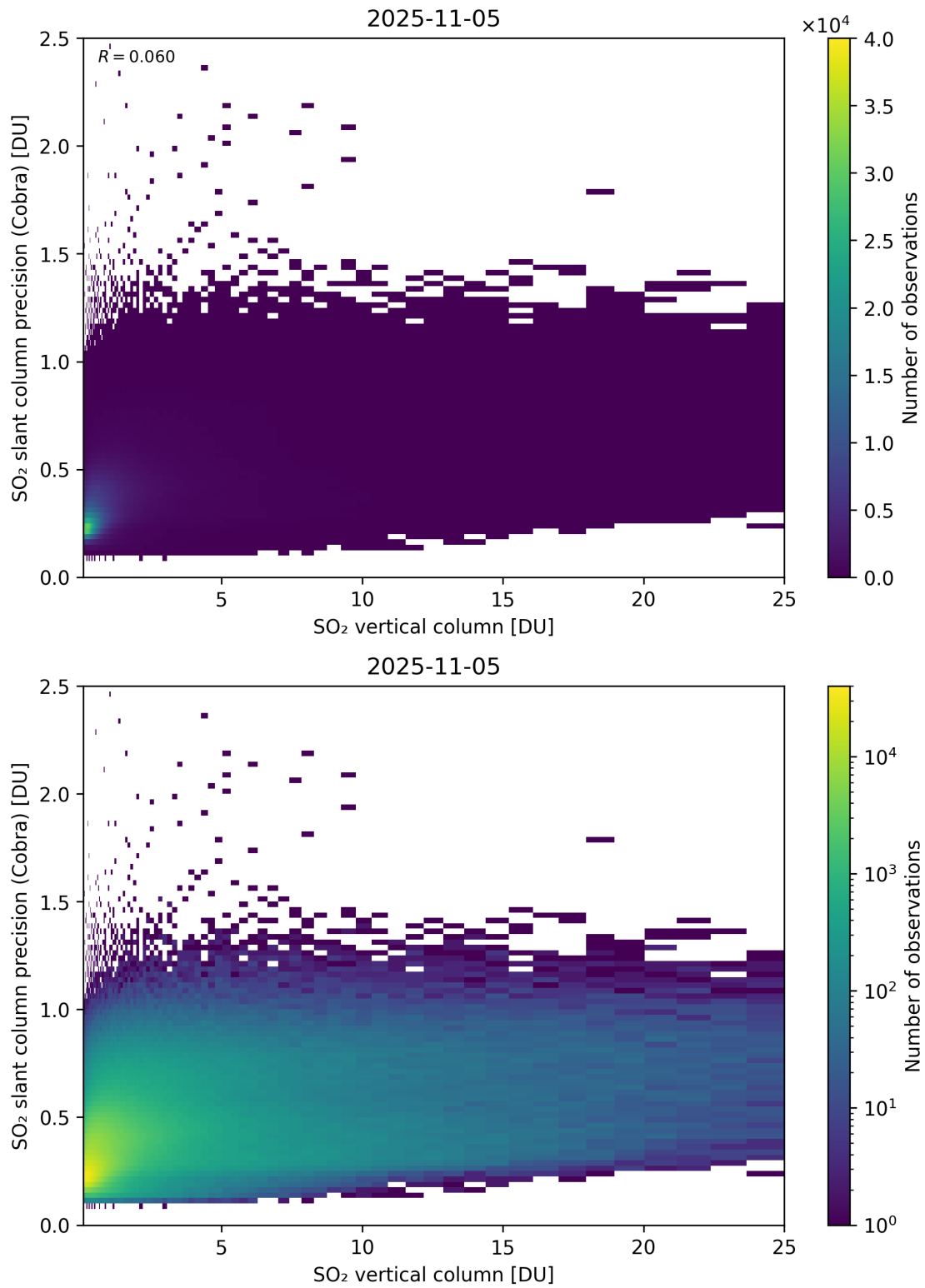
Figure 350: Scatter density plot of “SO 2 vertical column” against “SO 2 slant column precision (Cobra)” for 2025-11-04 to 2025-11-06.
