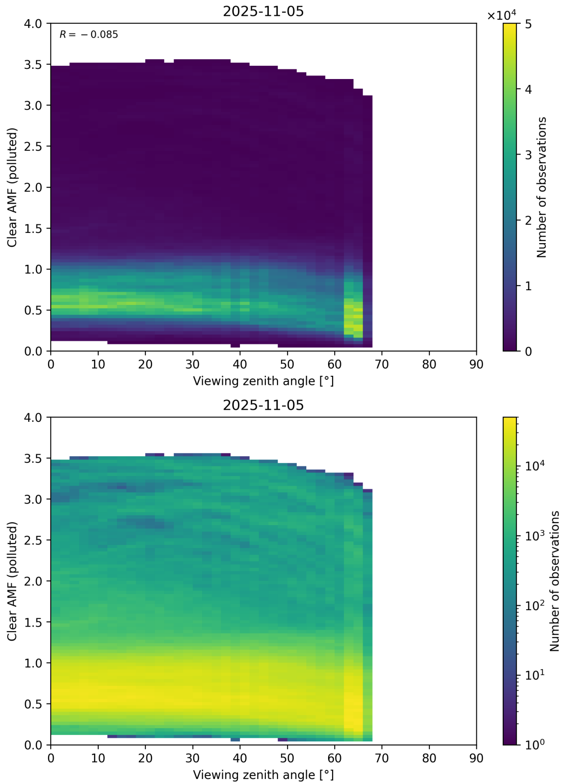
Figure 370: Scatter density plot of “Viewing zenith angle” against “Clear AMF (polluted)” for 2025-11-04 to 2025-11-06.
