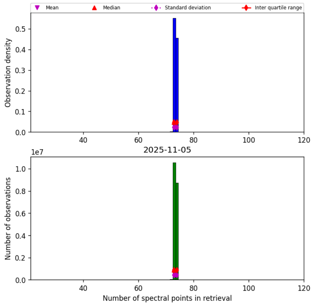
Figure 82: Histogram of “Number of spectral points in retrieval” for 2025-11-04 to 2025-11-06
