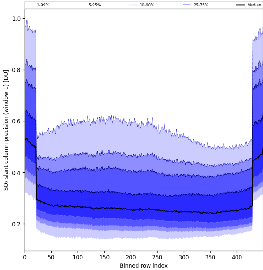
Figure 90: Along track statistics of “SO 2 slant column precision (window 1)” for 2025-11-04 to 2025-11-06
