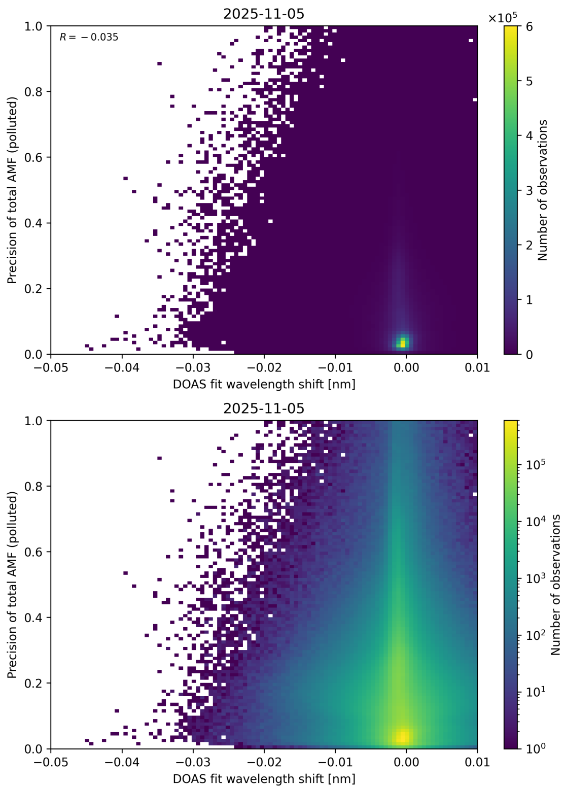
Figure 142: Scatter density plot of “DOAS fit wavelength shift” against “Precision of total AMF (polluted)” for 2025-11-04 to 2025-11-06.
