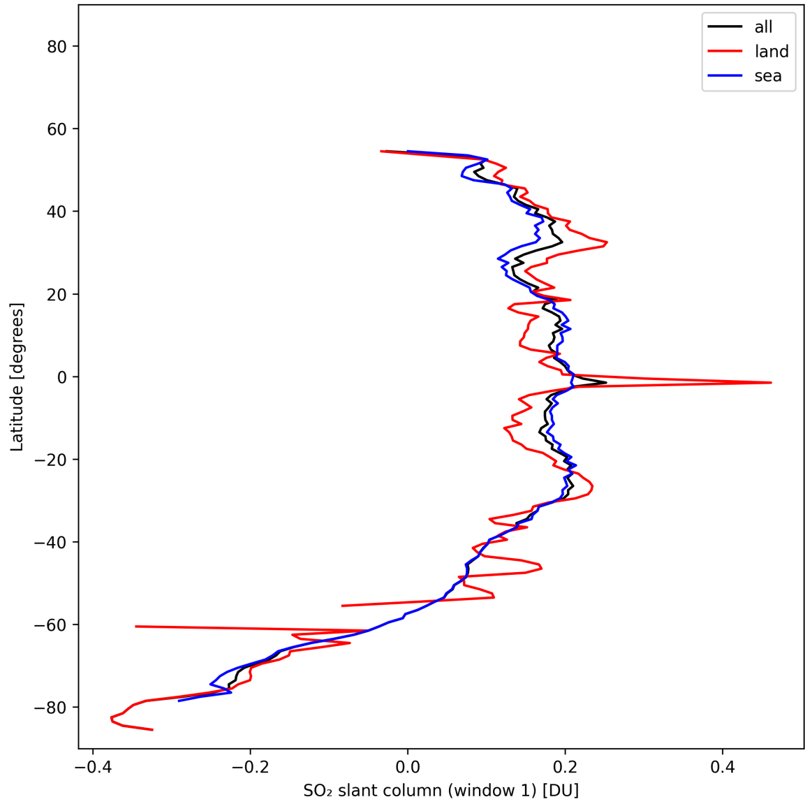
Figure 37: Zonal average of “SO 2 slant column (window 1)” for 2025-11-04 to 2025-11-06.
