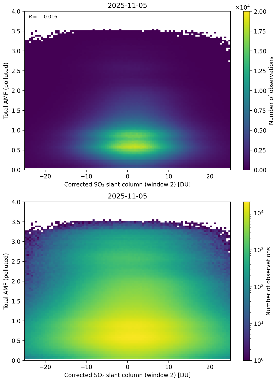
Figure 253: Scatter density plot of “Corrected SO 2 slant column (window 2)” against “Total AMF (polluted)” for 2025-11-04 to 2025-11-06.
