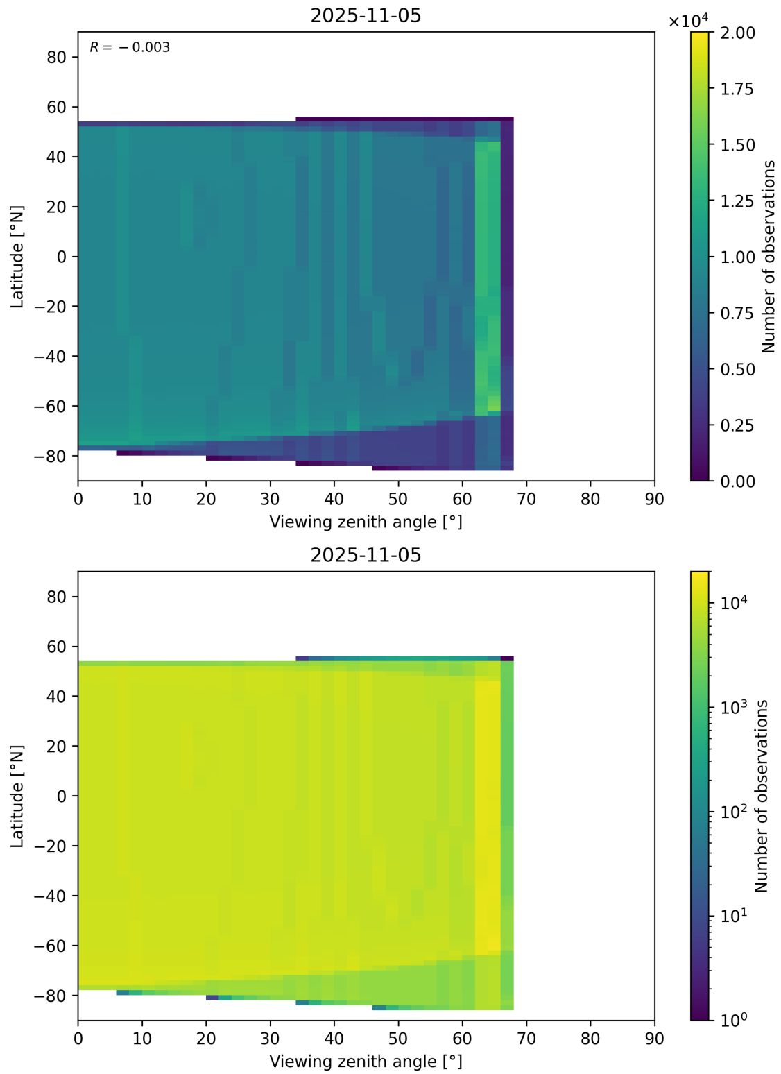
Figure 368: Scatter density plot of “Viewing zenith angle” against “Latitude” for 2025-11-04 to 2025-11-06.
