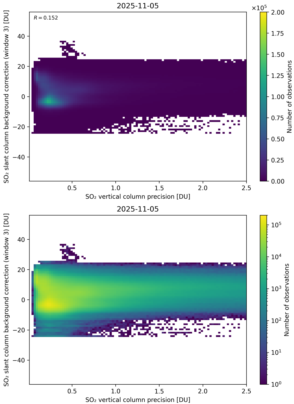
Figure 331: Scatter density plot of “SO 2 vertical column precision” against “SO 2 slant column background correction (window 3)” for 2025-11-04 to 2025-11-06.
