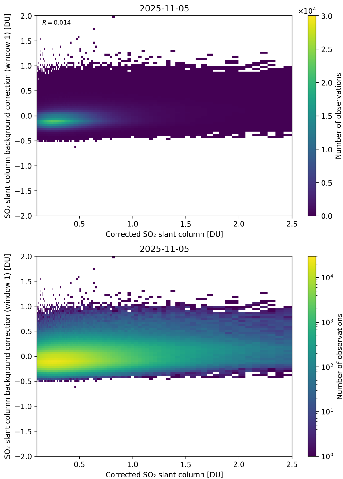
Figure 226: Scatter density plot of “Corrected SO 2 slant column” against “SO 2 slant column background correction (window 1)” for 2025-11-04 to 2025-11-06.
