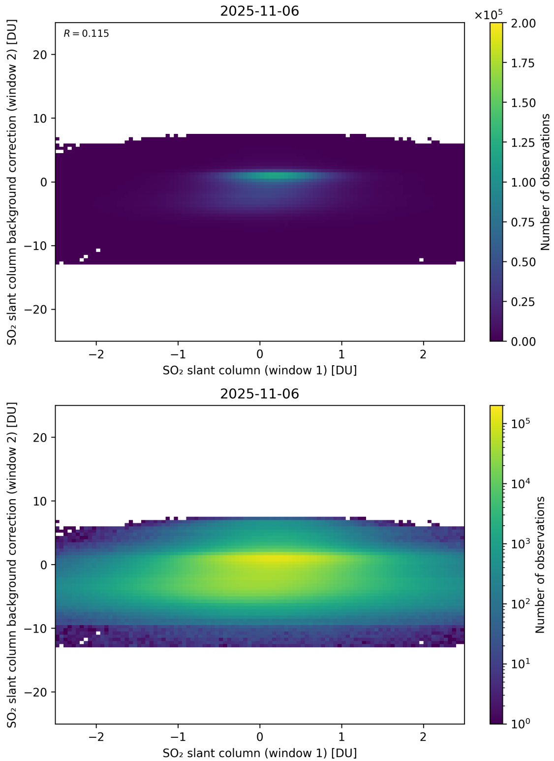
Figure 263: Scatter density plot of “SO 2 slant column (window 1)” against “SO 2 slant column background correction (window 2)” for 2025-11-05 to 2025-11-07.
