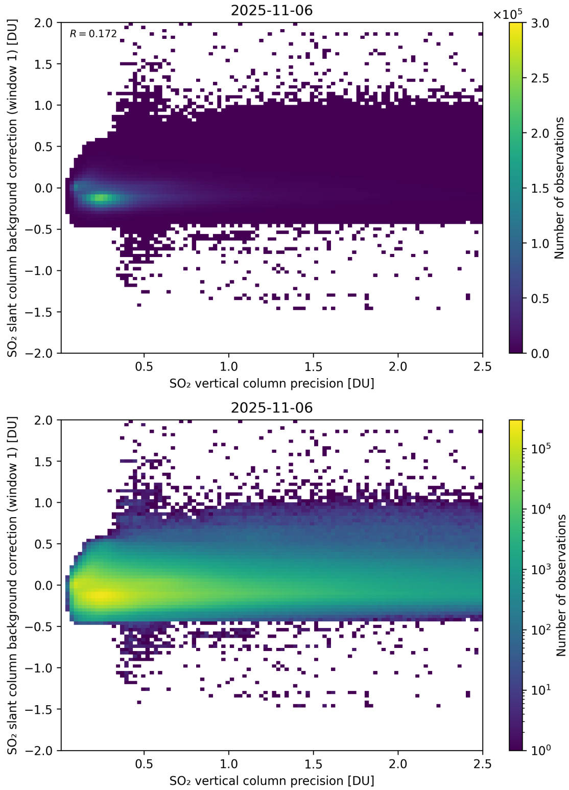
Figure 329: Scatter density plot of “SO 2 vertical column precision” against “SO 2 slant column background correction (window 1)” for 2025-11-05 to 2025-11-07.
