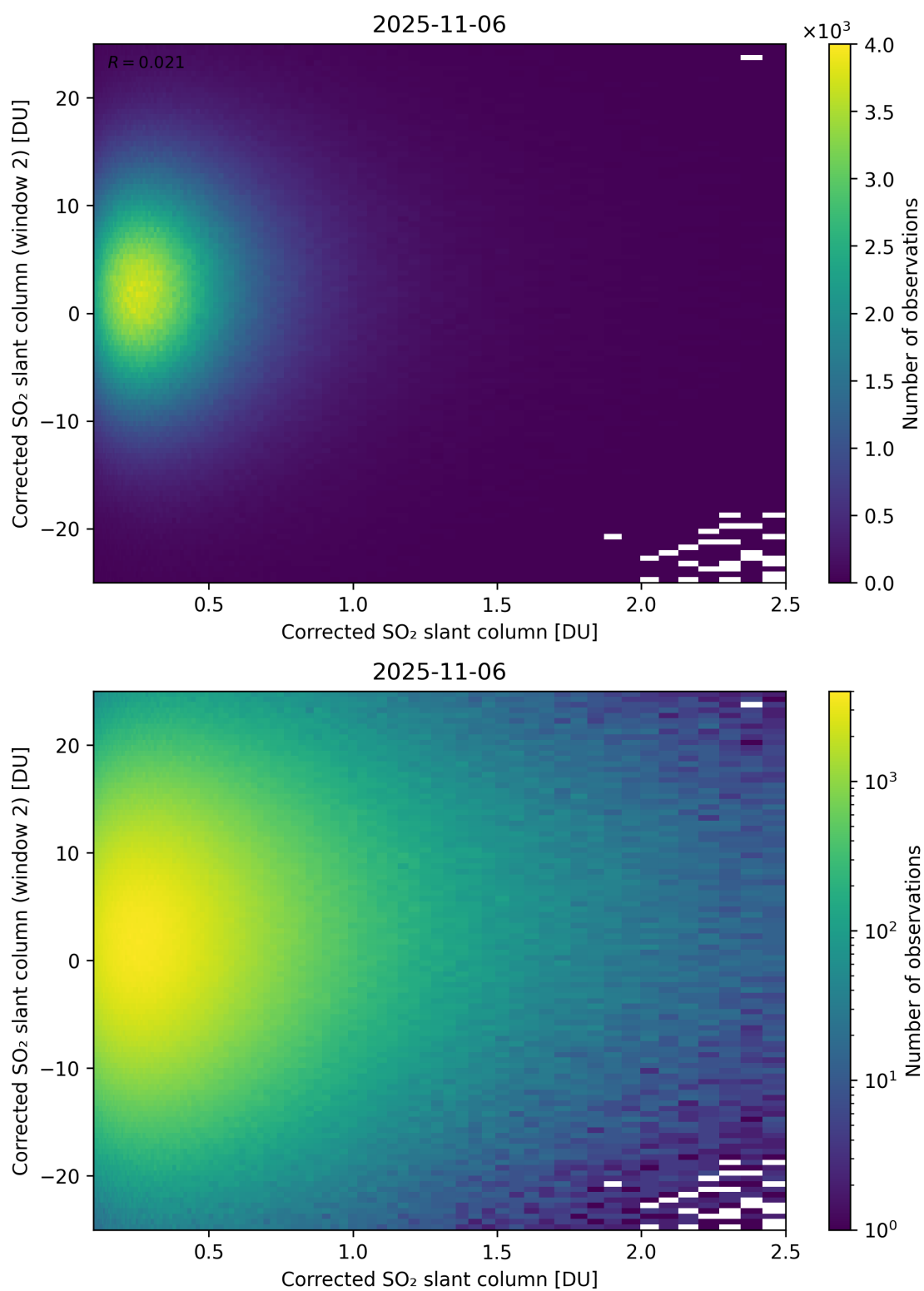
Figure 235: Scatter density plot of “Corrected SO 2 slant column” against “Corrected SO 2 slant column (window 2)” for 2025-11-05 to 2025-11-07.
