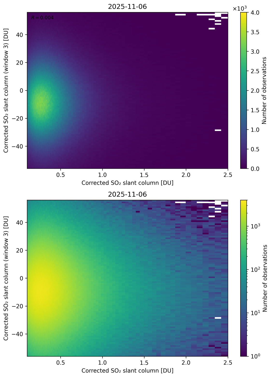
Figure 236: Scatter density plot of “Corrected SO 2 slant column” against “Corrected SO 2 slant column (window 3)” for 2025-11-05 to 2025-11-07.
