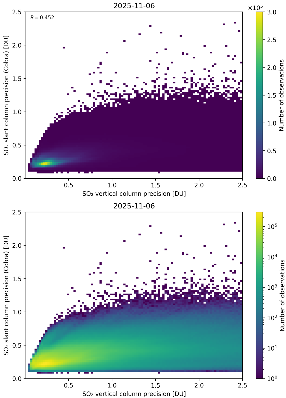
Figure 337: Scatter density plot of “SO 2 vertical column precision” against “SO 2 slant column precision (Cobra)” for 2025-11-05 to 2025-11-07.
