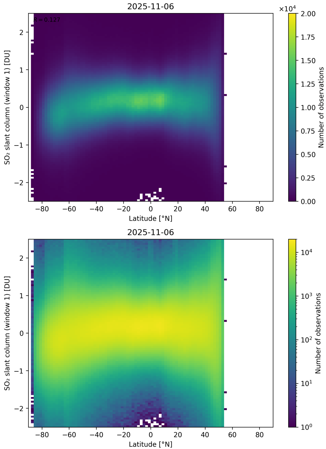
Figure 162: Scatter density plot of “Latitude” against “SO 2 slant column (window 1)” for 2025-11-05 to 2025-11-07.
