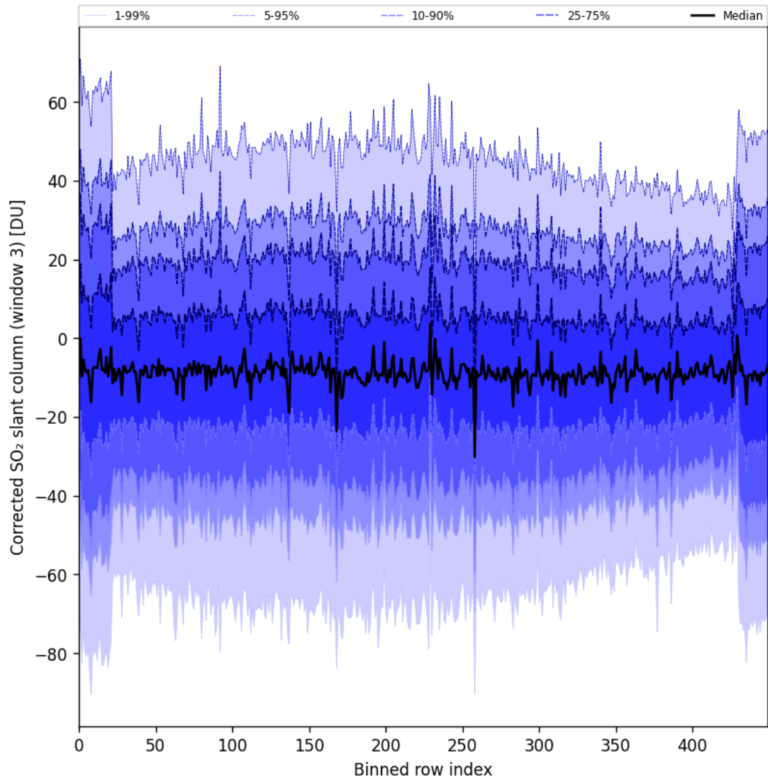
Figure 99: Along track statistics of “Corrected SO 2 slant column (window 3)” for 2025-11-05 to 2025-11-07
