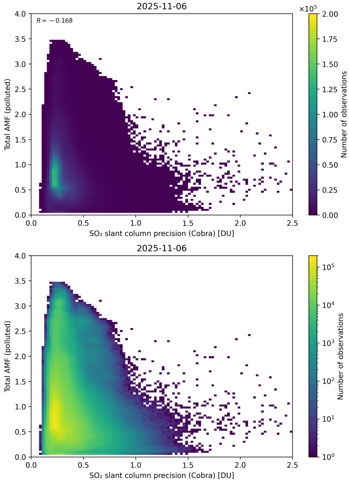
Figure 213: Scatter density plot of “SO 2 slant column precision (Cobra)” against “Total AMF (polluted)” for 2025-11-05 to 2025-11-07.
