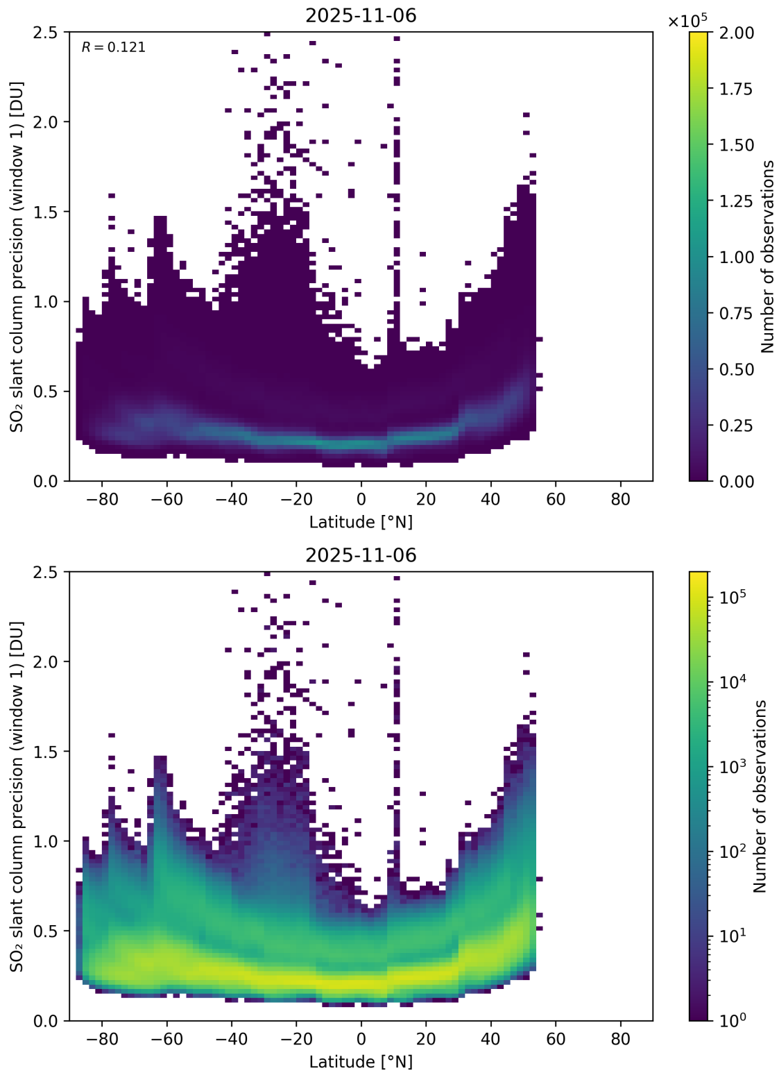
Figure 163: Scatter density plot of “Latitude” against “SO 2 slant column precision (window 1)” for 2025-11-05 to 2025-11-07.
