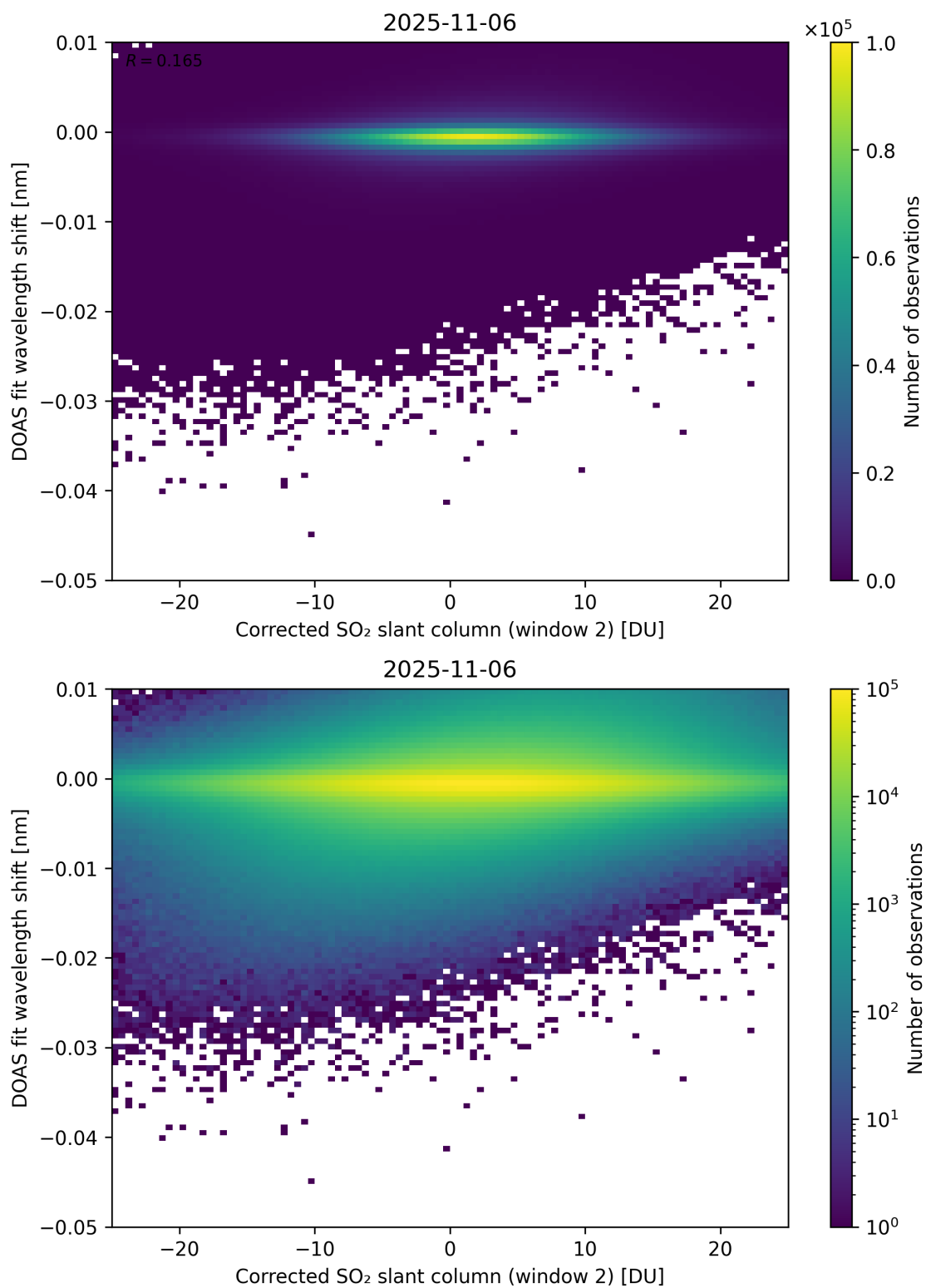
Figure 246: Scatter density plot of “Corrected SO 2 slant column (window 2)” against “DOAS fit wavelength shift” for 2025-11-05 to 2025-11-07.
