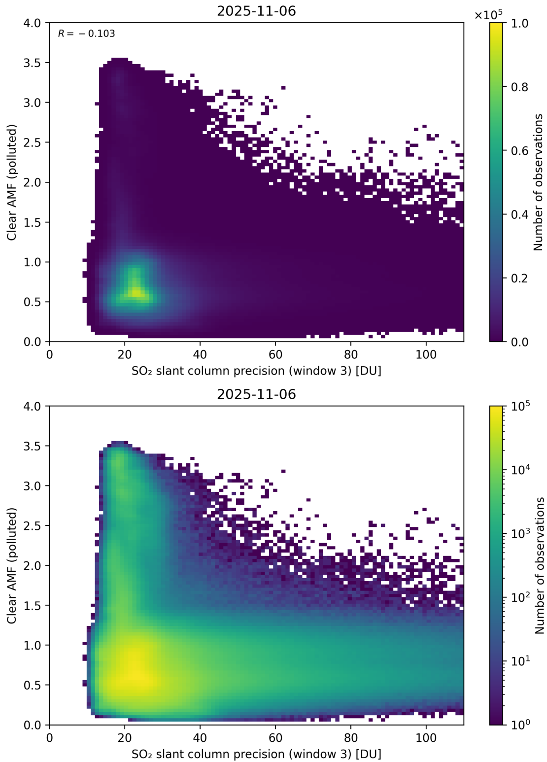
Figure 311: Scatter density plot of “SO 2 slant column precision (window 3)” against “Clear AMF (polluted)” for 2025-11-05 to 2025-11-07.
