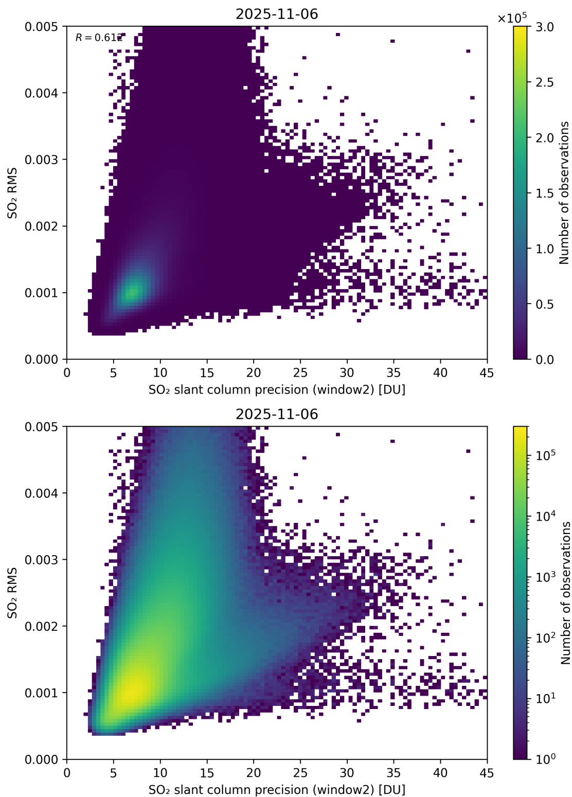
Figure 295: Scatter density plot of “SO 2 slant column precision (window2)” against “SO 2 RMS” for 2025-11-05 to 2025-11-07.
