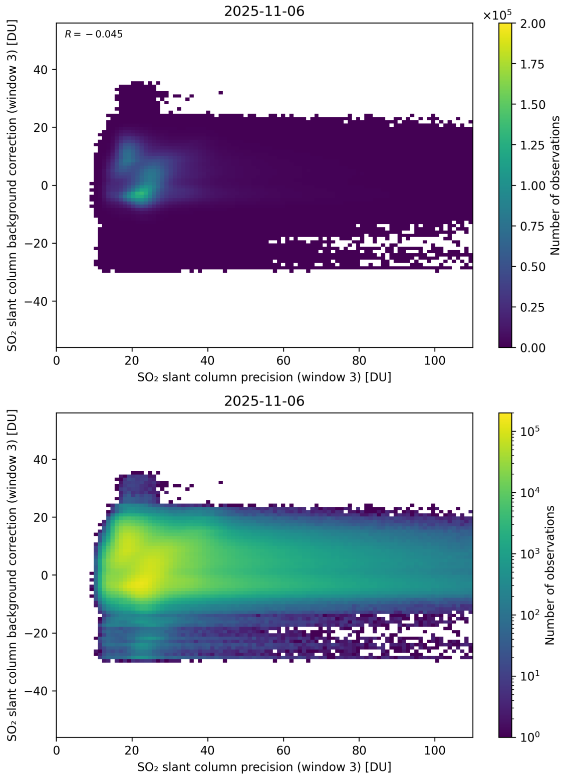
Figure 307: Scatter density plot of “SO 2 slant column precision (window 3)” against “SO 2 slant column background correction (window 3)” for 2025-11-05 to 2025-11-07.
