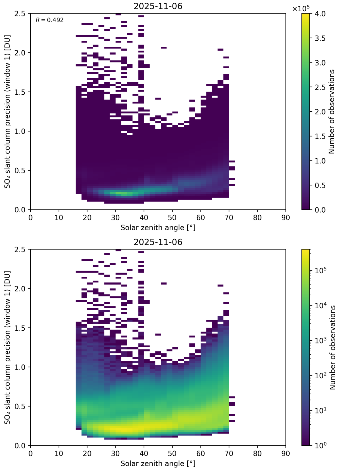
Figure 185: Scatter density plot of “Solar zenith angle” against “SO 2 slant column precision (window 1)” for 2025-11-05 to 2025-11-07.
