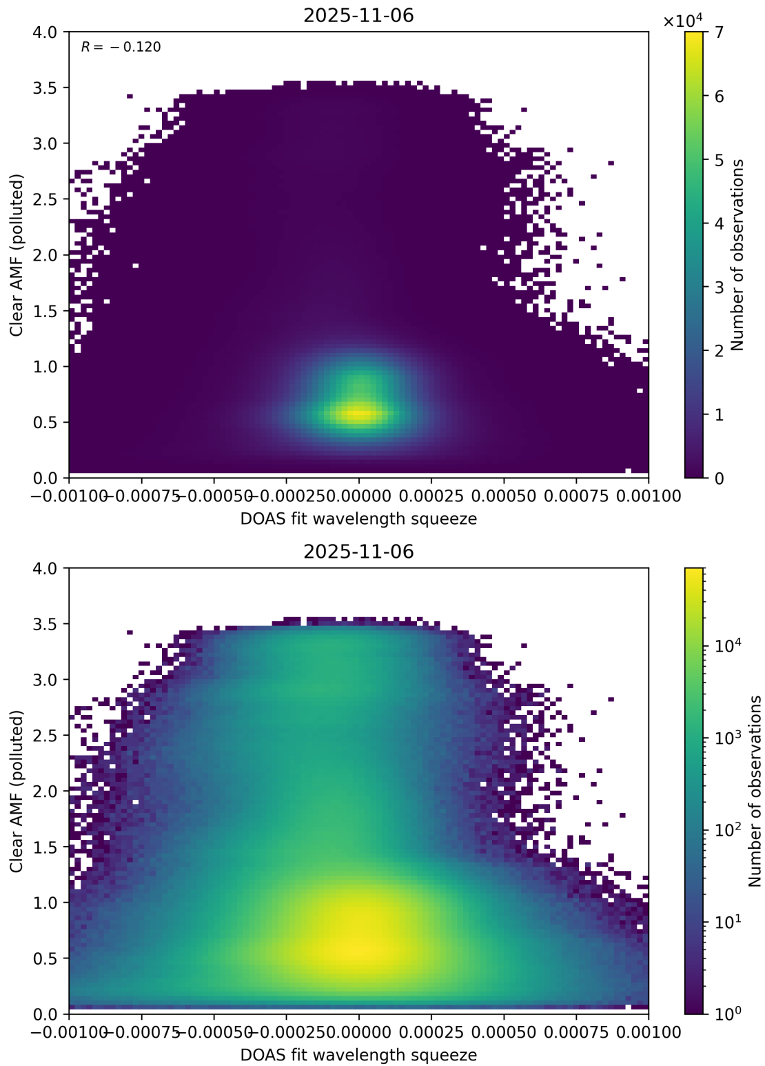
Figure 144: Scatter density plot of “DOAS fit wavelength squeeze” against “Clear AMF (polluted)” for 2025-11-05 to 2025-11-07.
