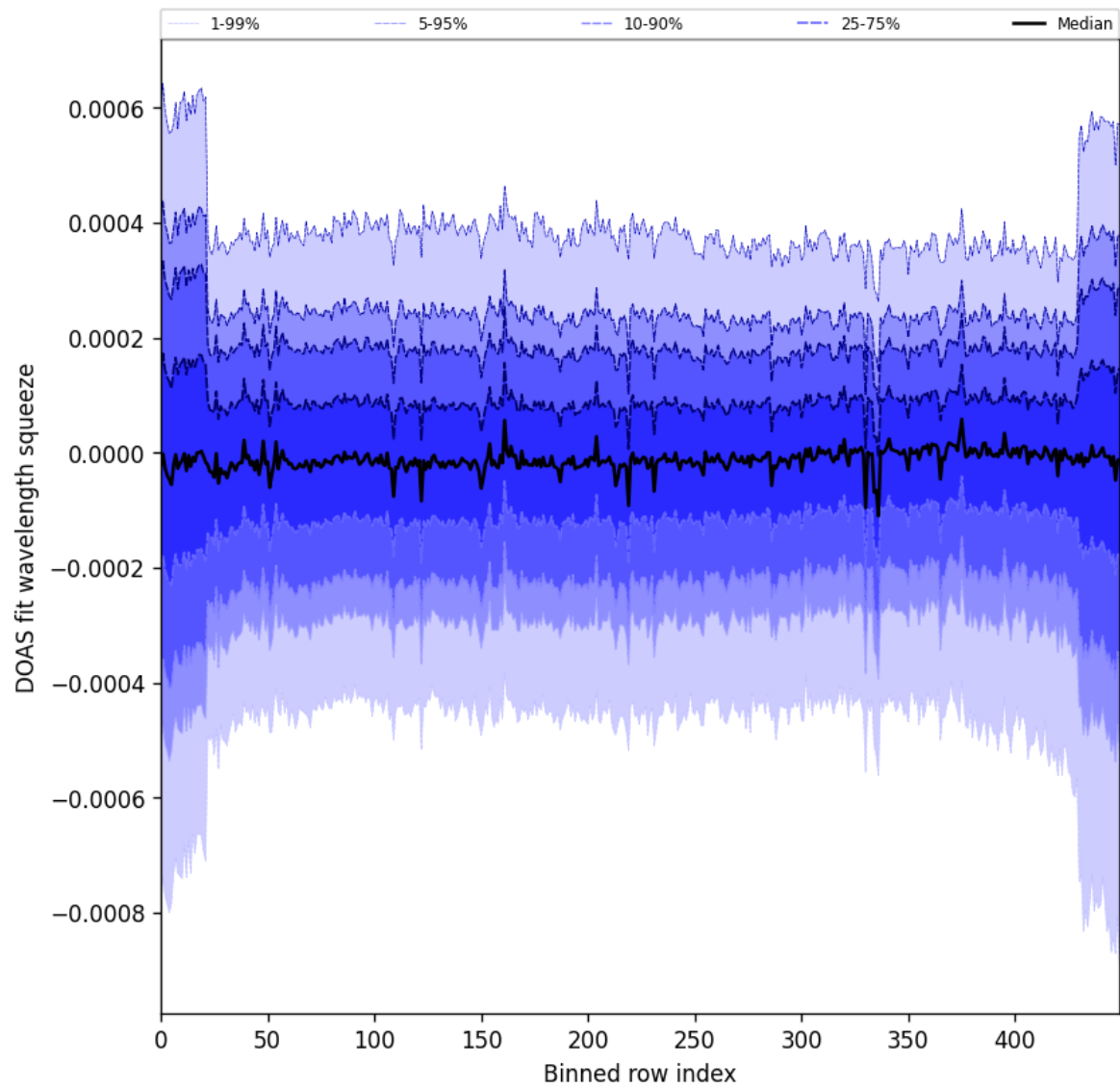
Figure 103: Along track statistics of “DOAS fit wavelength squeeze” for 2025-11-05 to 2025-11-07
