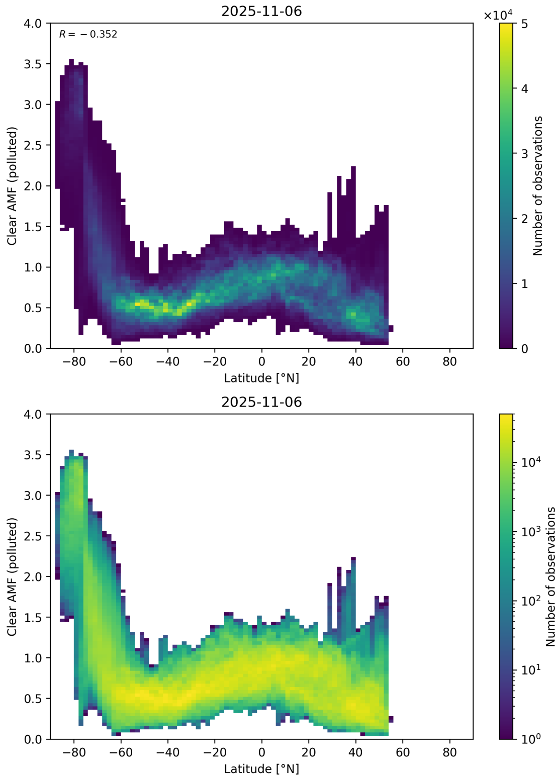
Figure 156: Scatter density plot of “Latitude” against “Clear AMF (polluted)” for 2025-11-05 to 2025-11-07.
