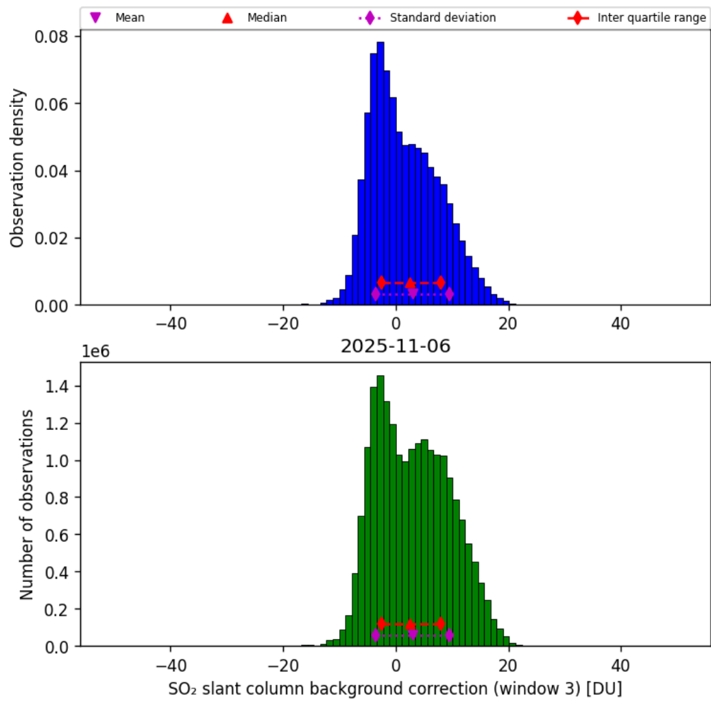
Figure 74: Histogram of “SO 2 slant column background correction (window 3)” for 2025-11-05 to 2025-11-07
