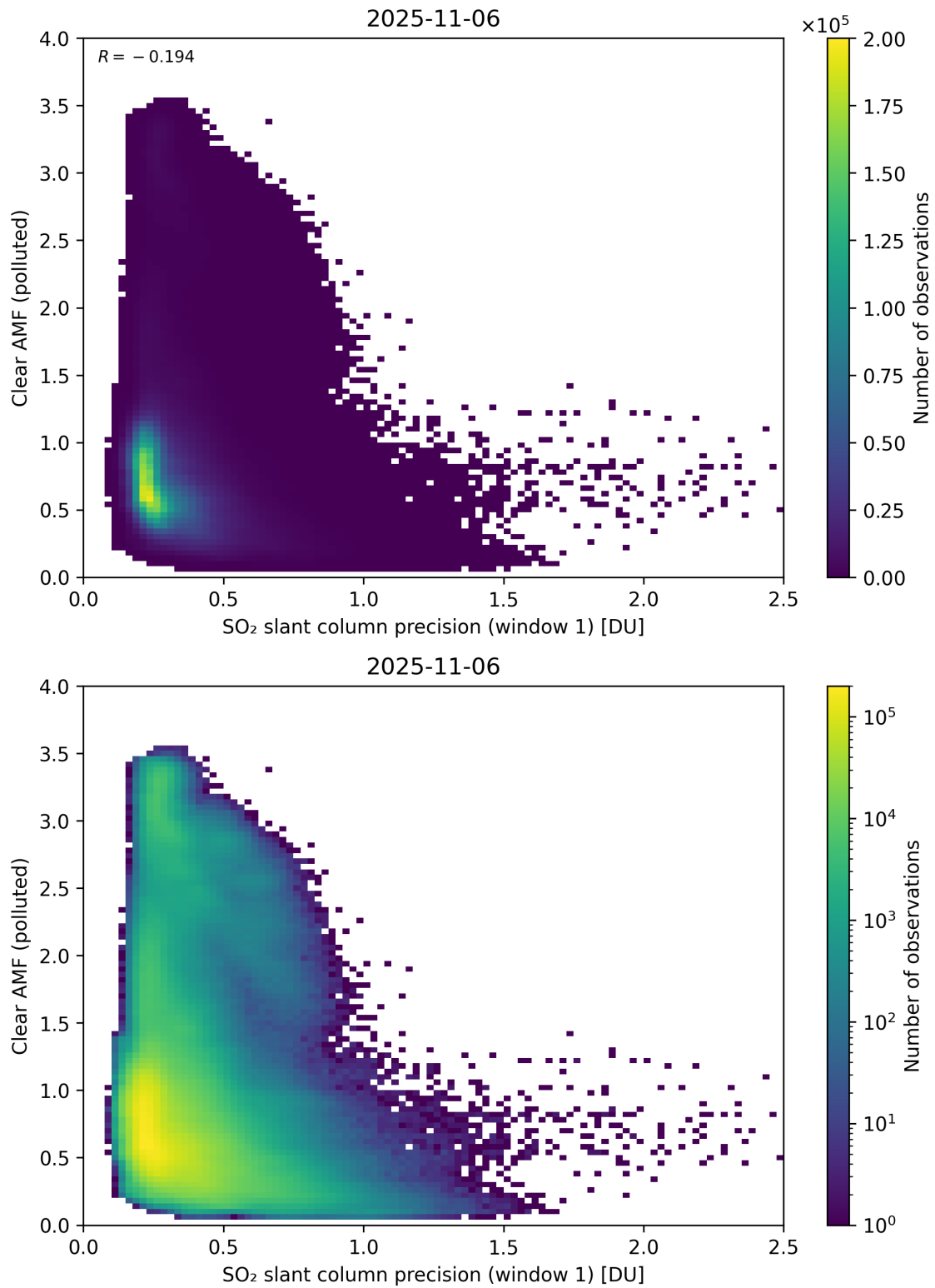
Figure 274: Scatter density plot of “SO 2 slant column precision (window 1)” against “Clear AMF (polluted)” for 2025-11-05 to 2025-11-07.
