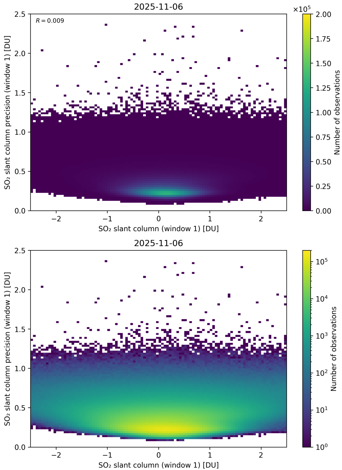
Figure 285: Scatter density plot of “SO 2 slant column (window 1)” against “SO 2 slant column precision (window 1)” for 2025-11-05 to 2025-11-07.
