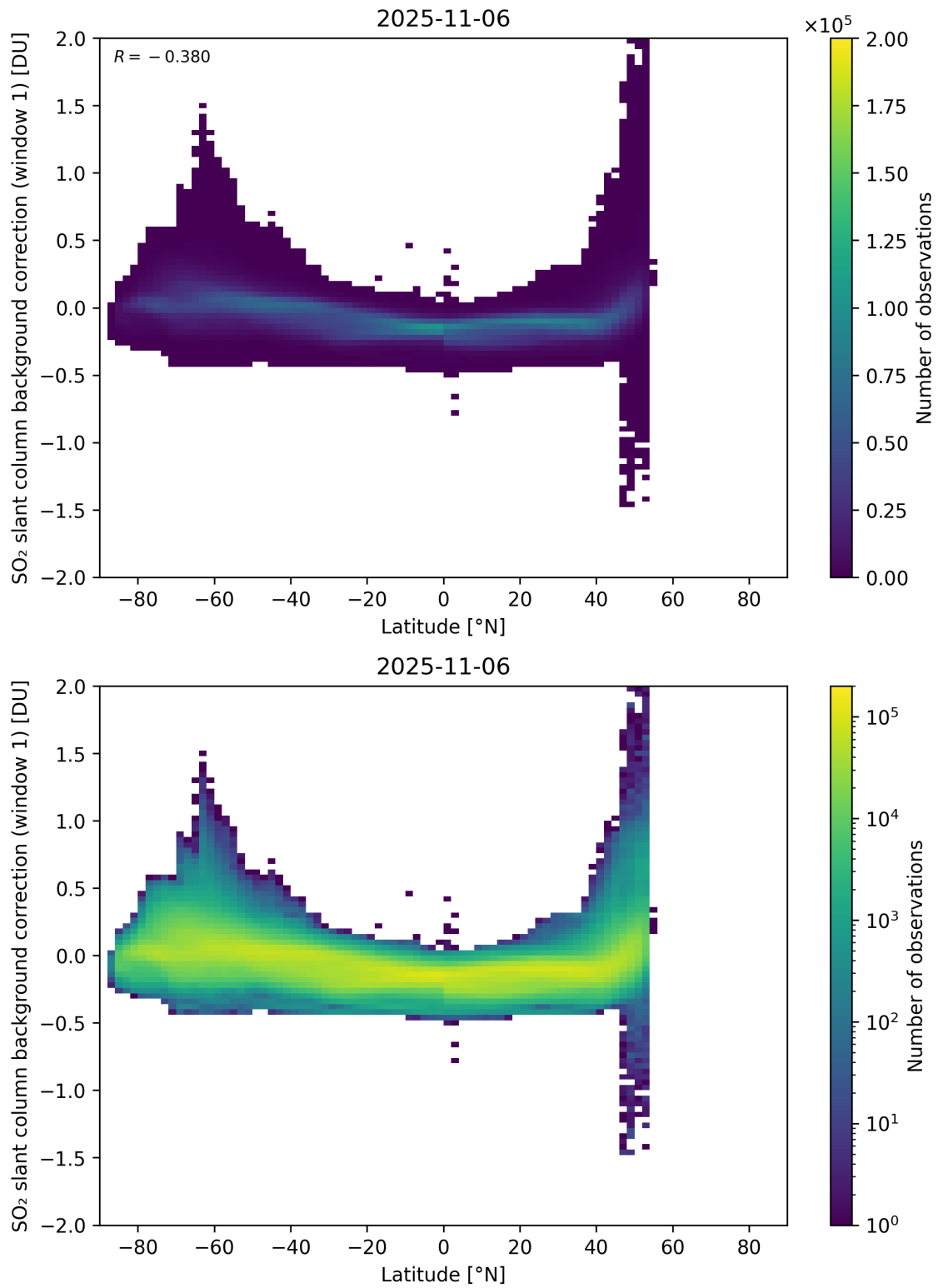
Figure 150: Scatter density plot of “Latitude” against “SO 2 slant column background correction (window 1)” for 2025-11-05 to 2025-11-07.
