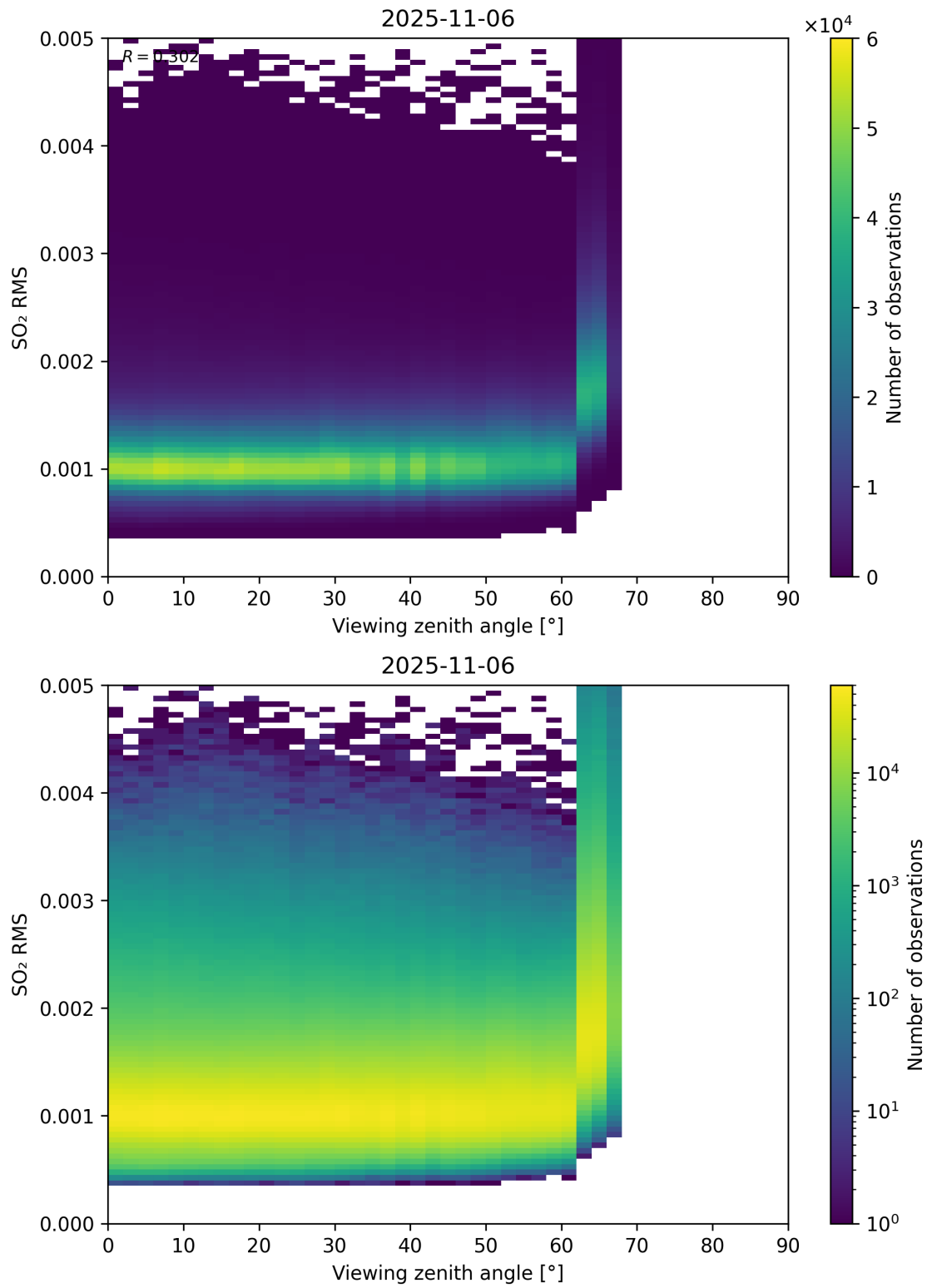
Figure 367: Scatter density plot of “Viewing zenith angle” against “SO 2 RMS” for 2025-11-05 to 2025-11-07.
