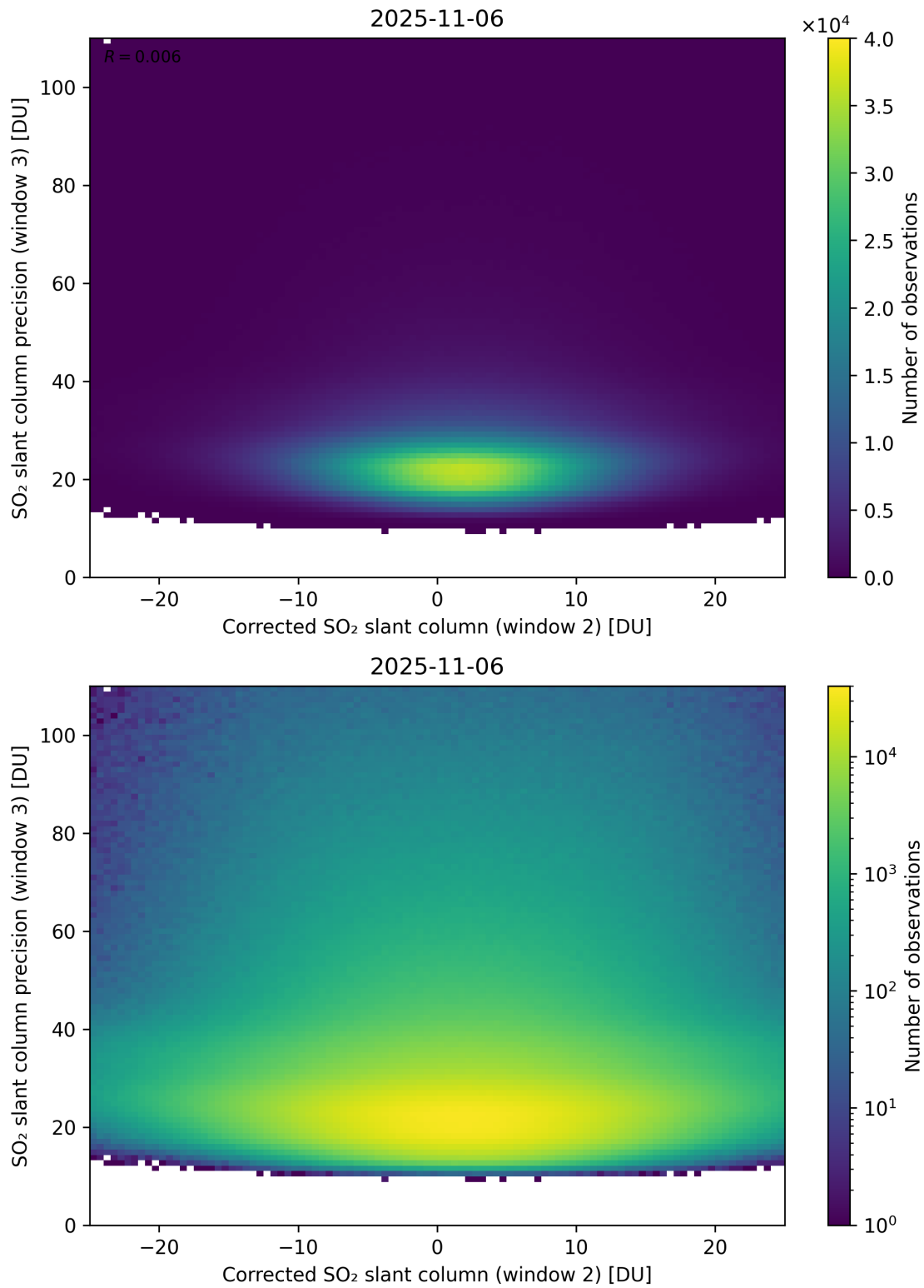
Figure 252: Scatter density plot of “Corrected SO 2 slant column (window 2)” against “SO 2 slant column precision (window 3)” for 2025-11-05 to 2025-11-07.
