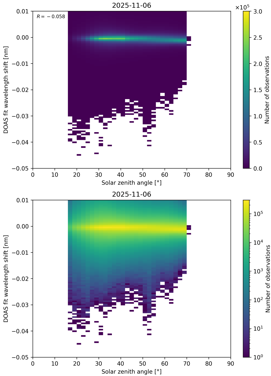
Figure 174: Scatter density plot of “Solar zenith angle” against “DOAS fit wavelength shift” for 2025-11-05 to 2025-11-07.
