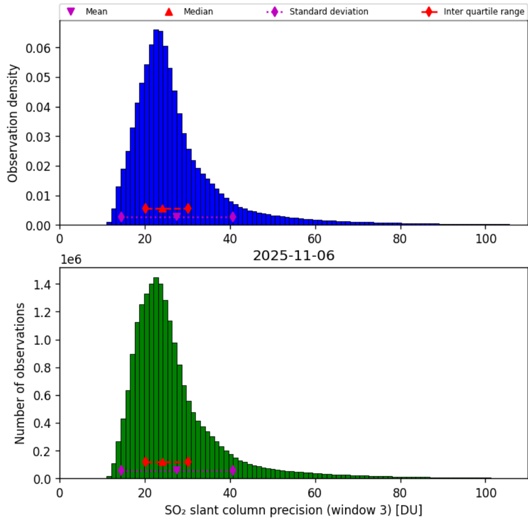
Figure 72: Histogram of “SO 2 slant column precision (window 3)” for 2025-11-05 to 2025-11-07
