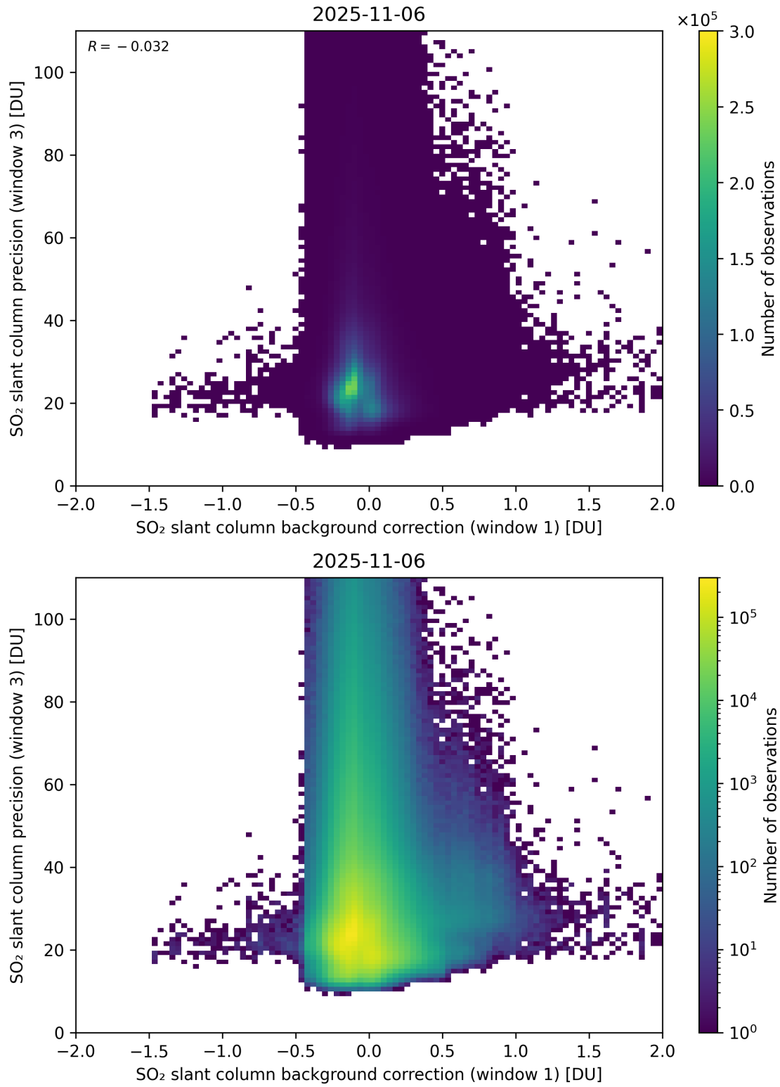
Figure 119: Scatter density plot of “SO 2 slant column background correction (window 1)” against “SO 2 slant column precision (window 3)” for 2025-11-05 to 2025-11-07.
