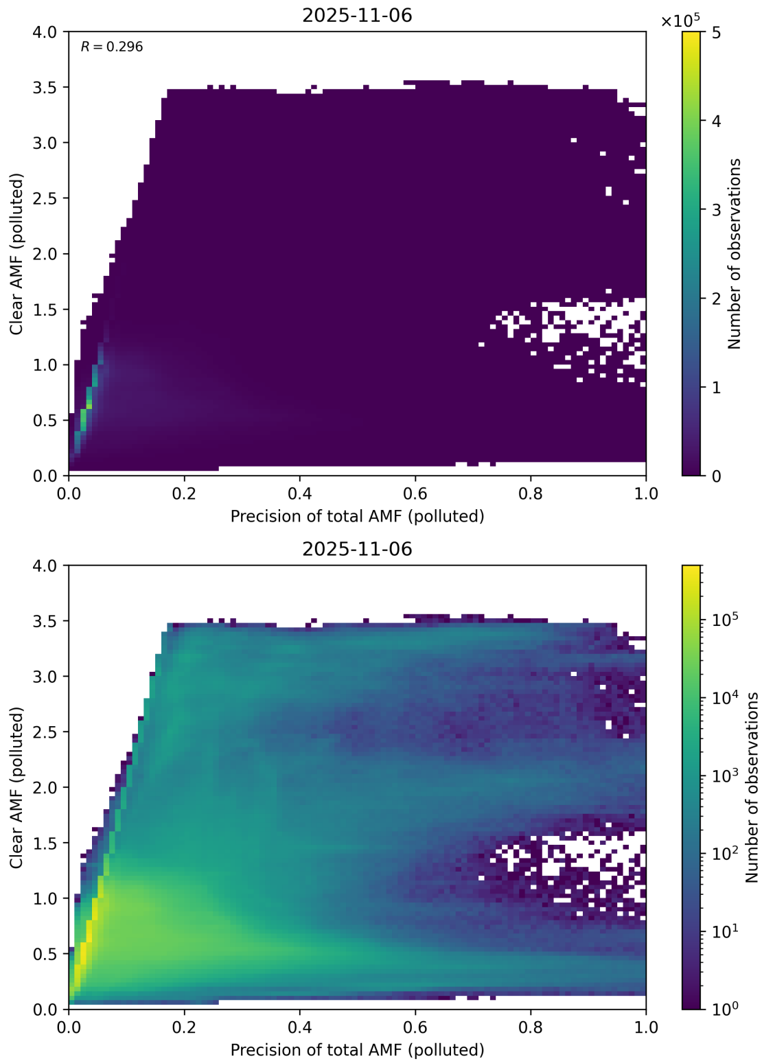
Figure 320: Scatter density plot of “Precision of total AMF (polluted)” against “Clear AMF (polluted)” for 2025-11-05 to 2025-11-07.
