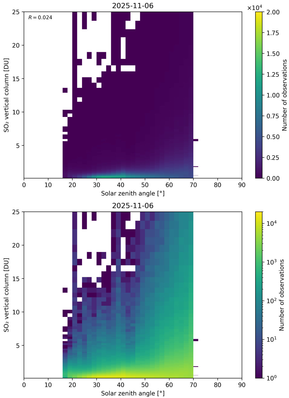
Figure 191: Scatter density plot of “Solar zenith angle” against “SO 2 vertical column” for 2025-11-05 to 2025-11-07.
