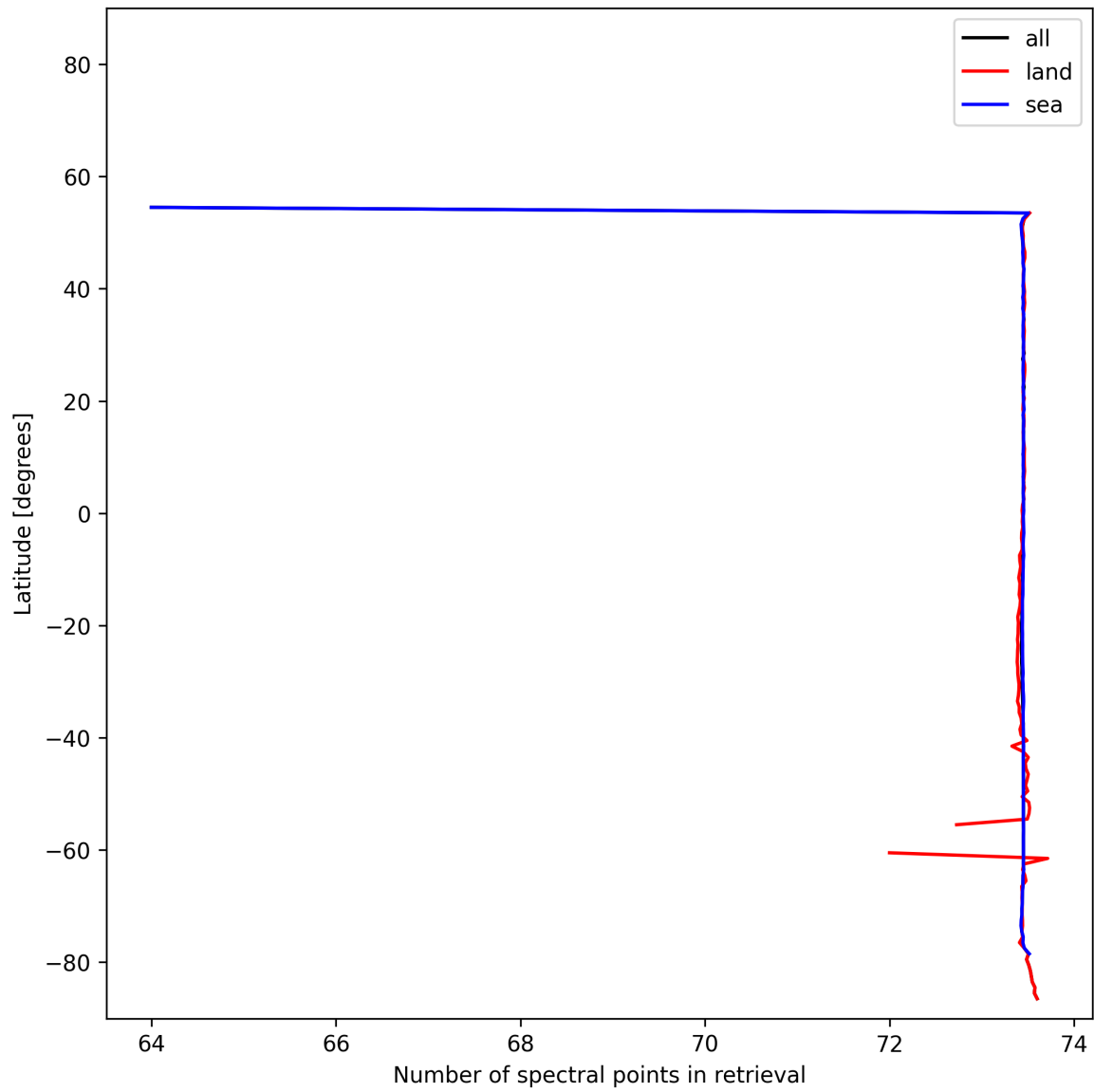
Figure 56: Zonal average of “Number of spectral points in retrieval” for 2025-11-05 to 2025-11-07.
