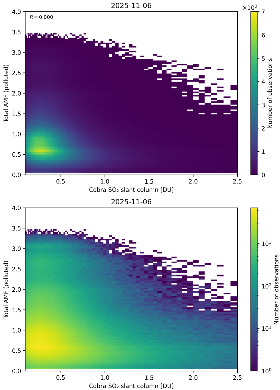
Figure 224: Scatter density plot of “Cobra SO 2 slant column” against “Total AMF (polluted)” for 2025-11-05 to 2025-11-07.
