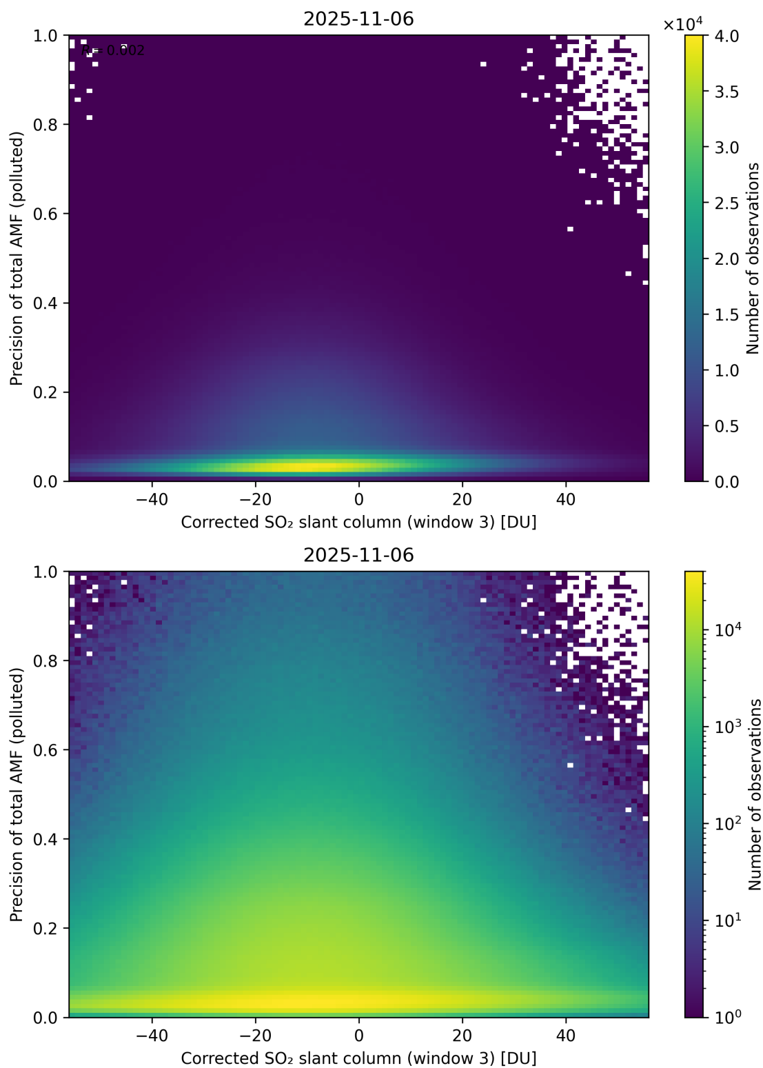
Figure 261: Scatter density plot of “Corrected SO 2 slant column (window 3)” against “Precision of total AMF (polluted)” for 2025-11-05 to 2025-11-07.
