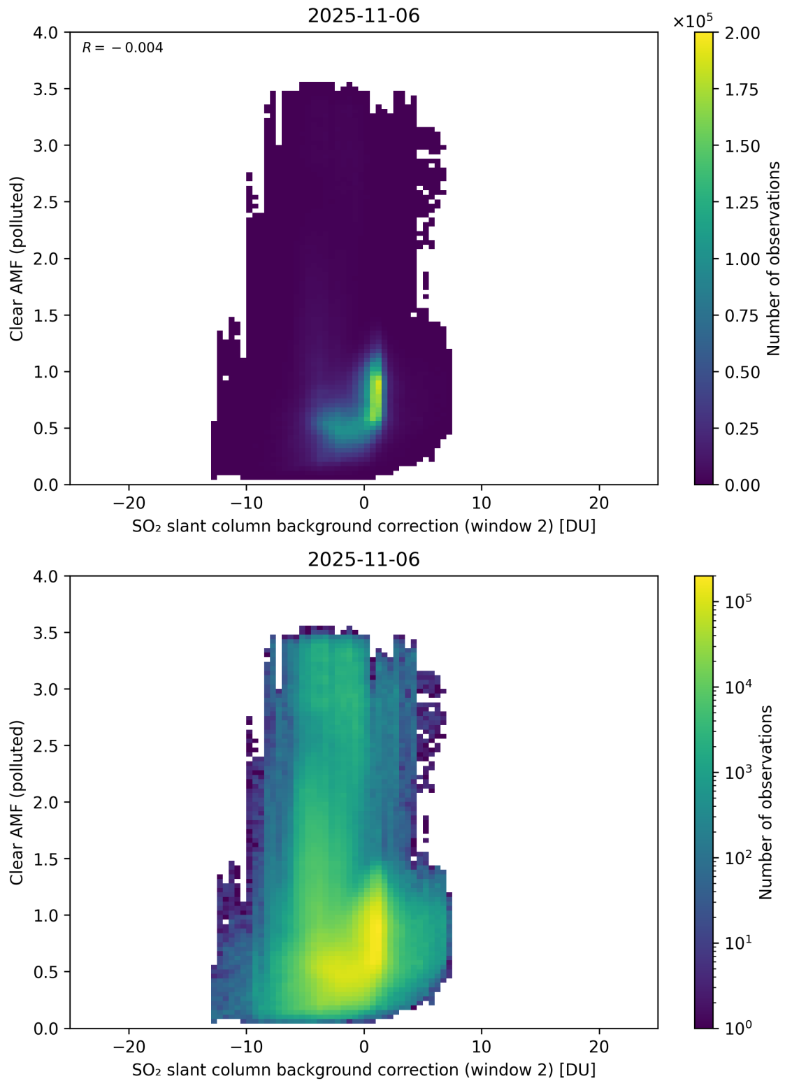
Figure 126: Scatter density plot of “SO 2 slant column background correction (window 2)” against “Clear AMF (polluted)” for 2025-11-05 to 2025-11-07.
