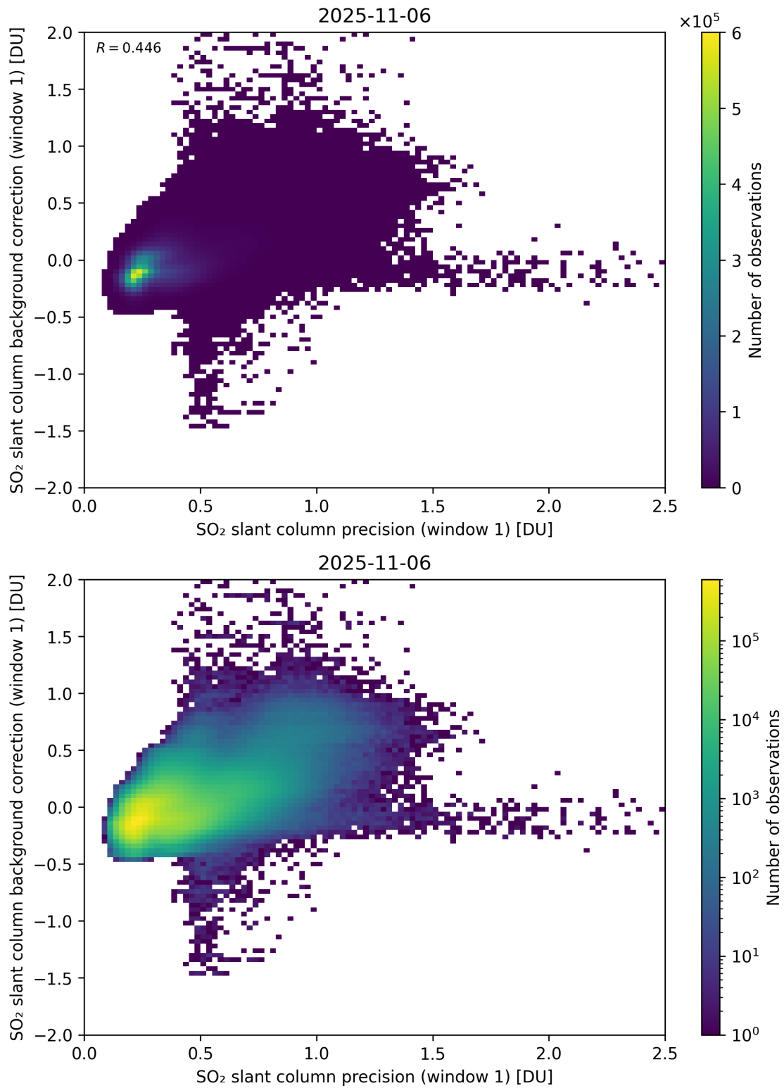
Figure 268: Scatter density plot of “SO 2 slant column precision (window 1)” against “SO 2 slant column background correction (window 1)” for 2025-11-05 to 2025-11-07.
