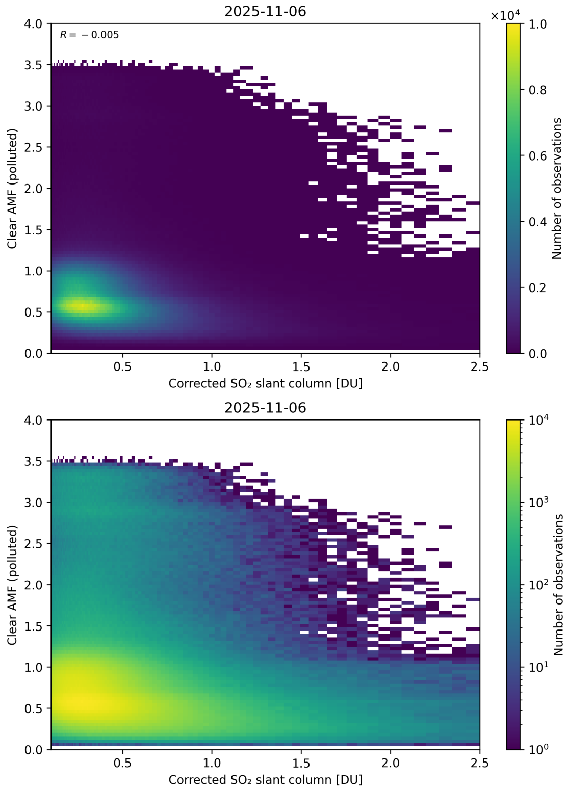
Figure 232: Scatter density plot of “Corrected SO 2 slant column” against “Clear AMF (polluted)” for 2025-11-05 to 2025-11-07.
