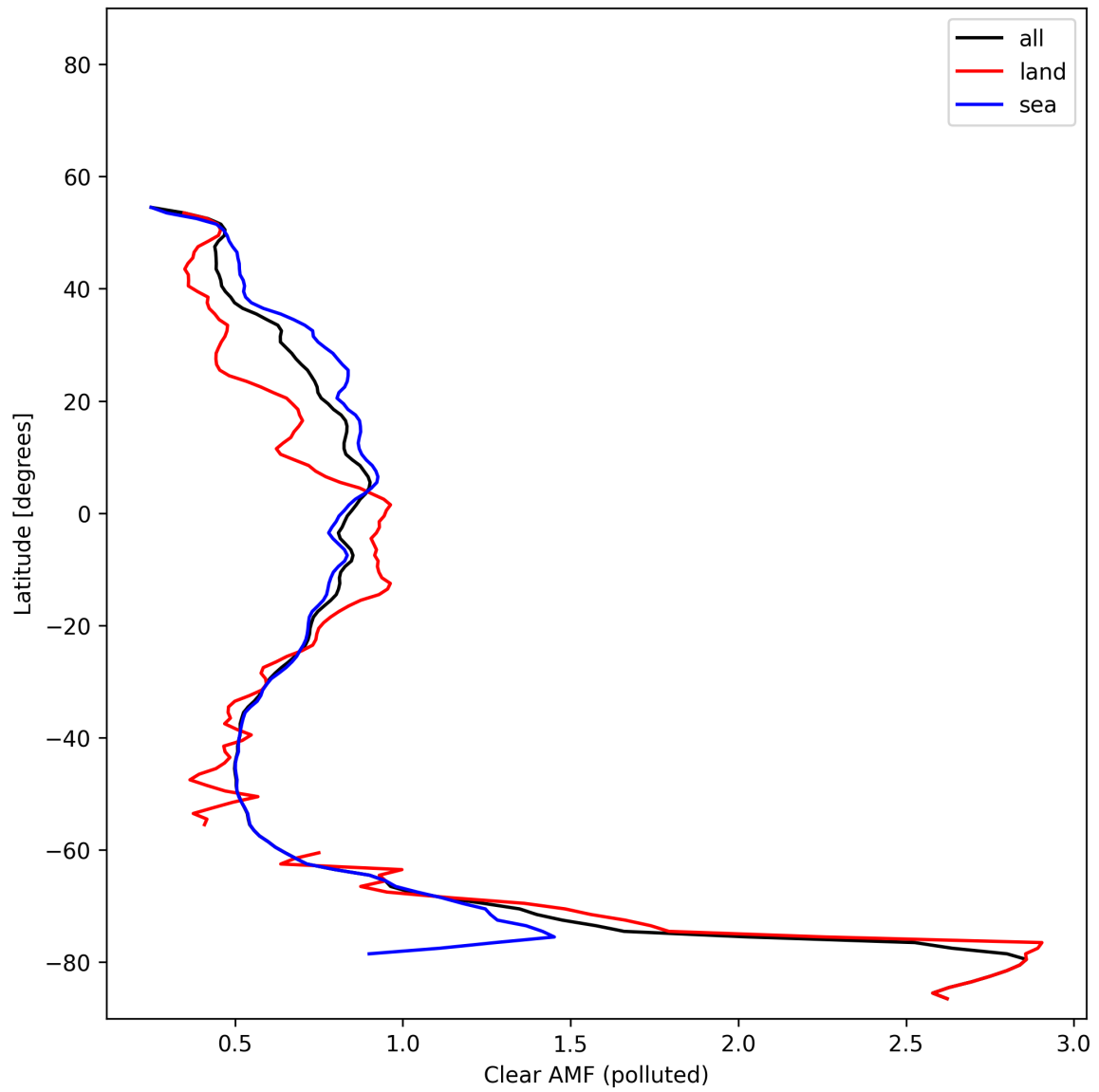
Figure 55: Zonal average of “Clear AMF (polluted)” for 2025-11-05 to 2025-11-07.
