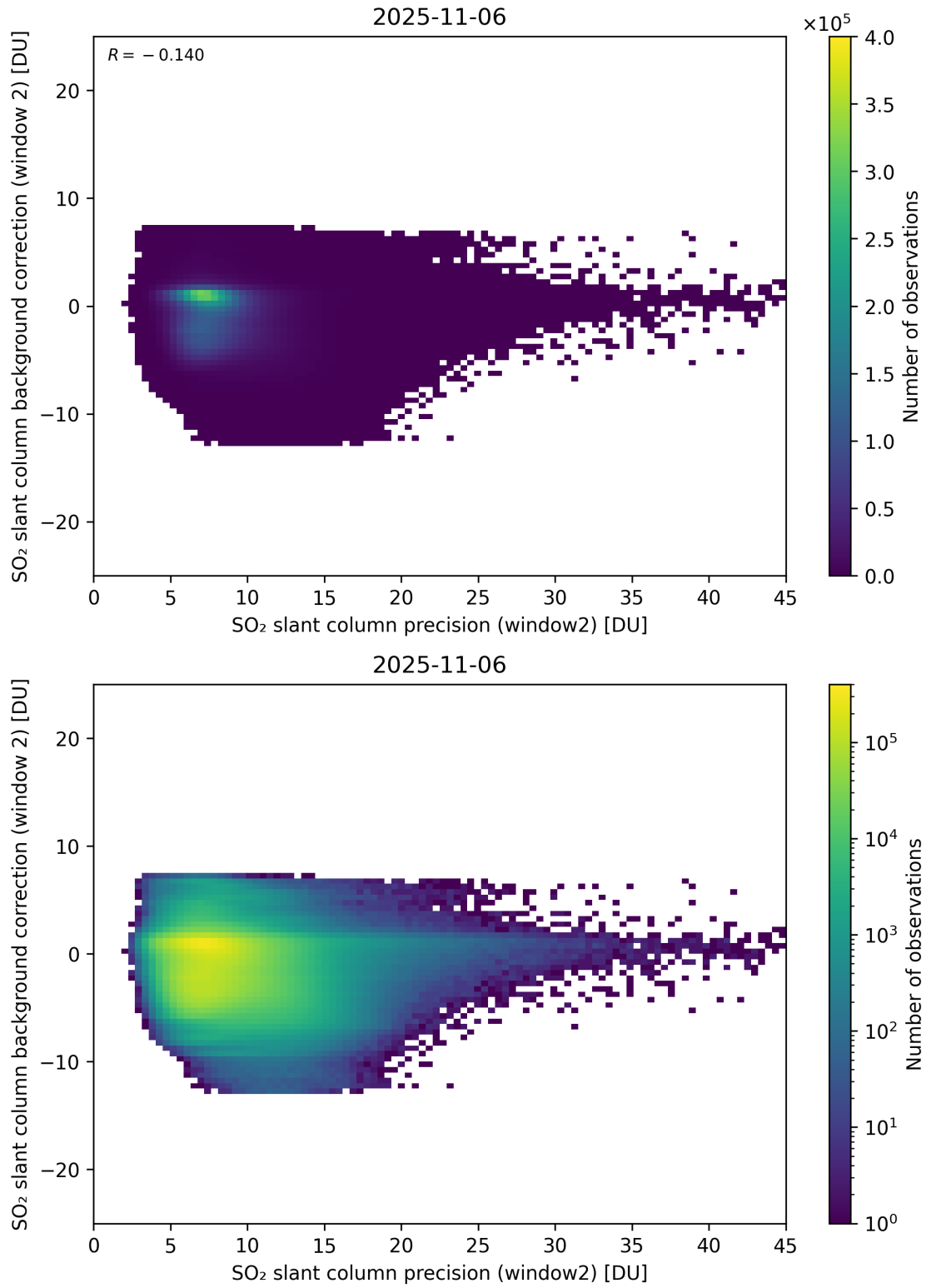
Figure 291: Scatter density plot of “SO 2 slant column precision (window2)” against “SO 2 slant column background correction (window 2)” for 2025-11-05 to 2025-11-07.
