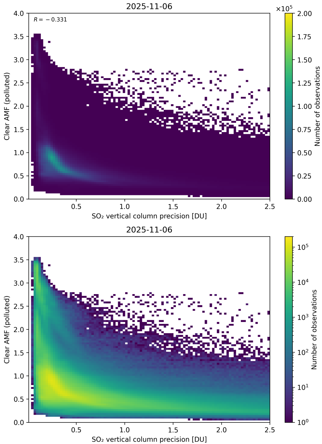
Figure 335: Scatter density plot of “SO 2 vertical column precision” against “Clear AMF (polluted)” for 2025-11-05 to 2025-11-07.
