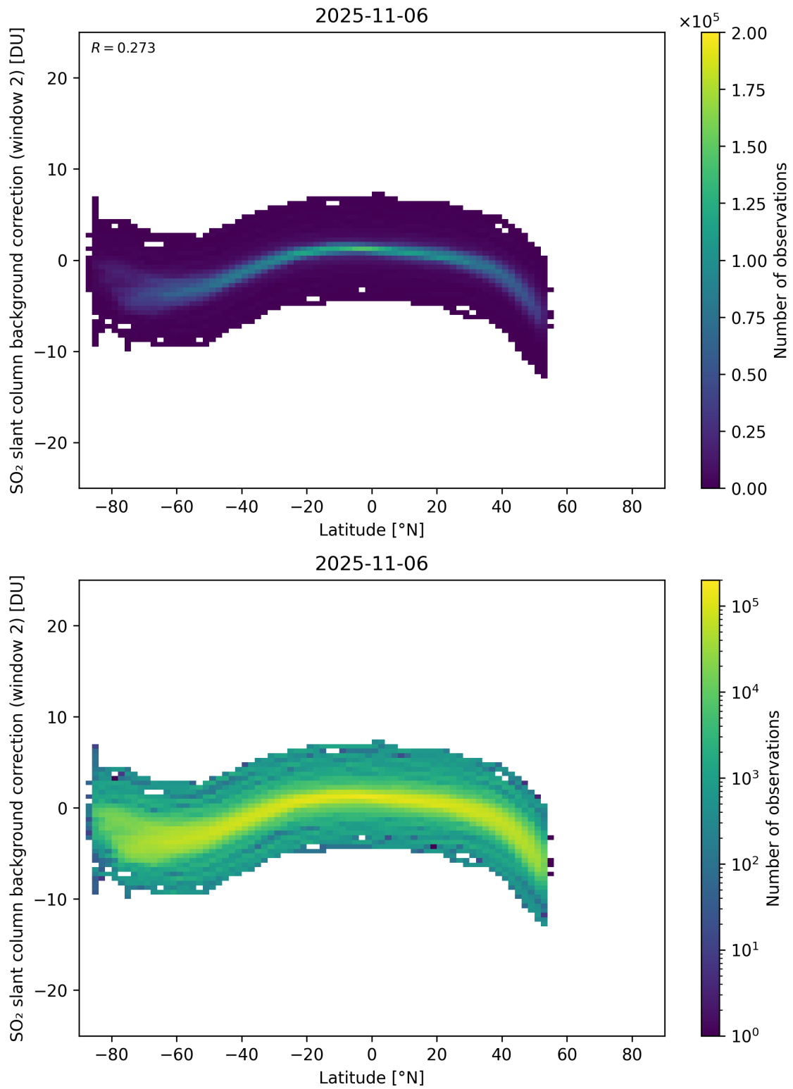
Figure 151: Scatter density plot of “Latitude” against “SO 2 slant column background correction (window 2)” for 2025-11-05 to 2025-11-07.
