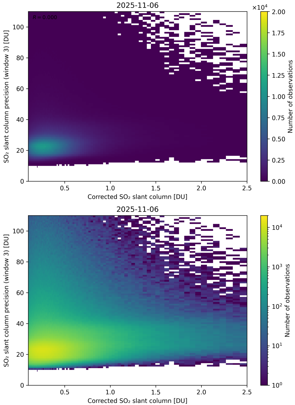
Figure 241: Scatter density plot of “Corrected SO 2 slant column” against “SO 2 slant column precision (window 3)” for 2025-11-05 to 2025-11-07.
