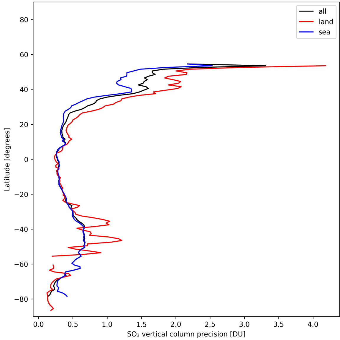
Figure 33: Zonal average of “SO 2 vertical column precision” for 2025-11-05 to 2025-11-07.
