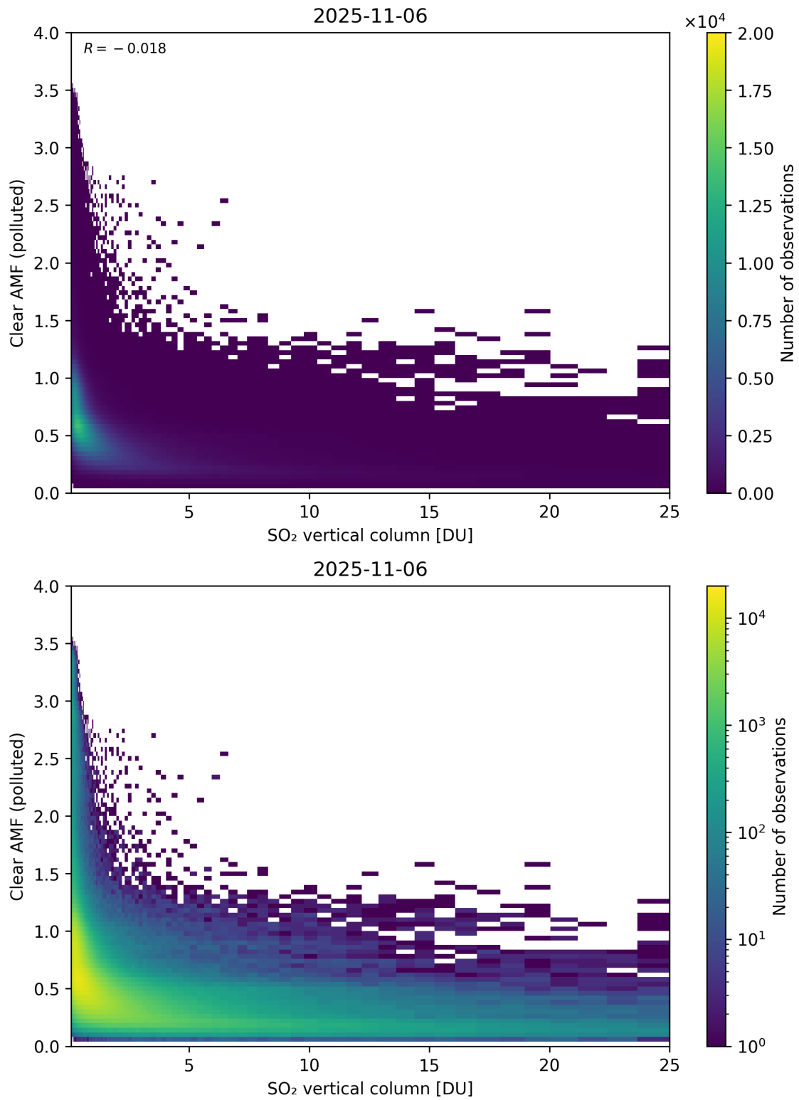
Figure 348: Scatter density plot of “SO 2 vertical column” against “Clear AMF (polluted)” for 2025-11-05 to 2025-11-07.
