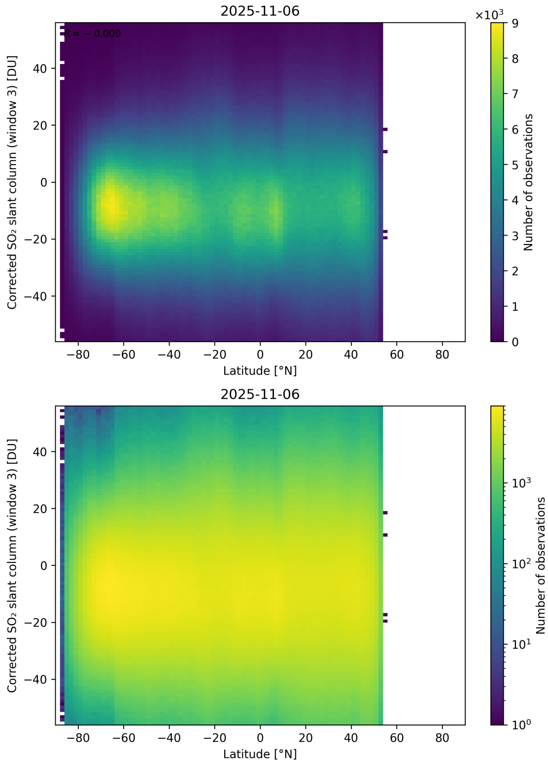
Figure 161: Scatter density plot of “Latitude” against “Corrected SO 2 slant column (window 3)” for 2025-11-05 to 2025-11-07.
