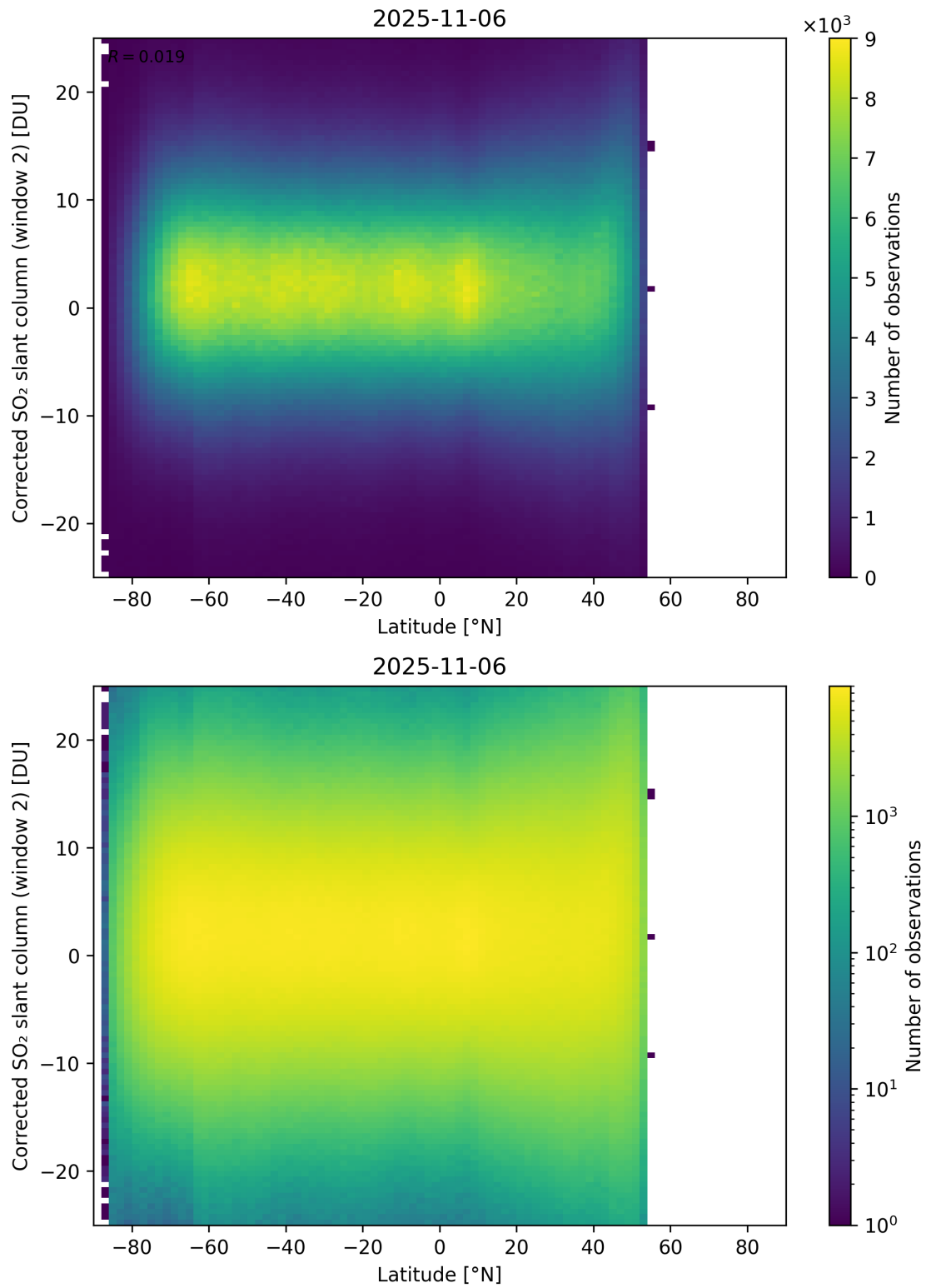
Figure 160: Scatter density plot of “Latitude” against “Corrected SO 2 slant column (window 2)” for 2025-11-05 to 2025-11-07.
