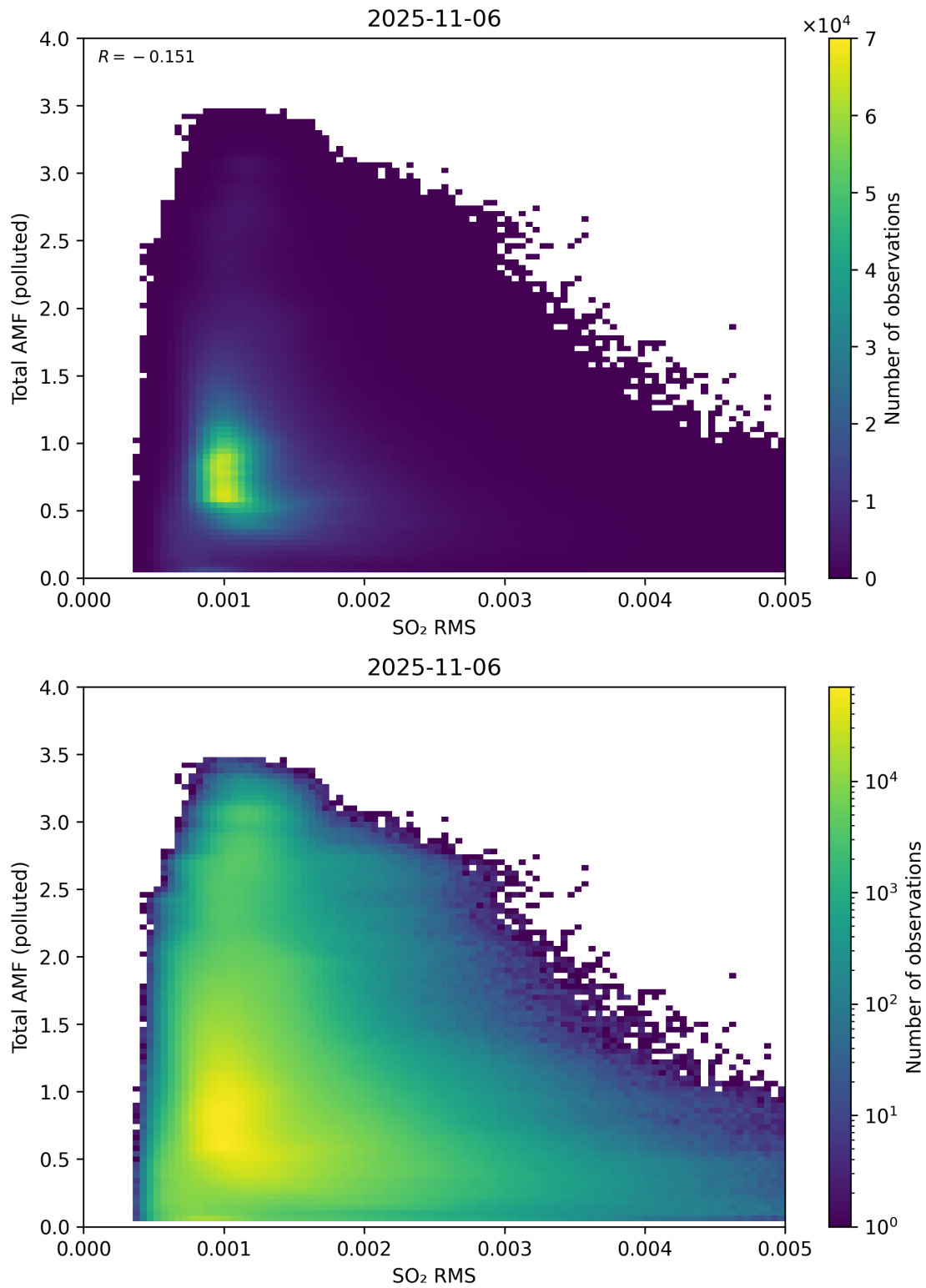
Figure 148: Scatter density plot of “SO 2 RMS” against “Total AMF (polluted)” for 2025-11-05 to 2025-11-07.
