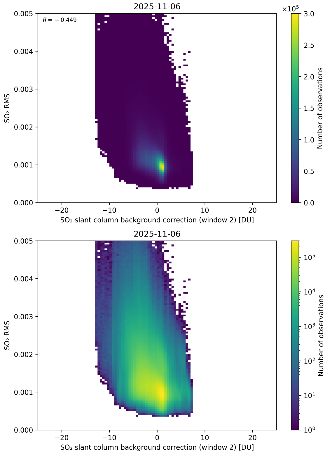
Figure 125: Scatter density plot of “SO 2 slant column background correction (window 2)” against “SO 2 RMS” for 2025-11-05 to 2025-11-07.
