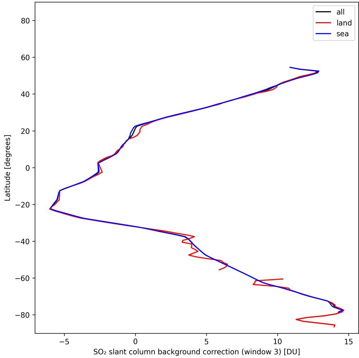
Figure 48: Zonal average of “SO 2 slant column background correction (window 3)” for 2025-11-05 to 2025-11-07.
