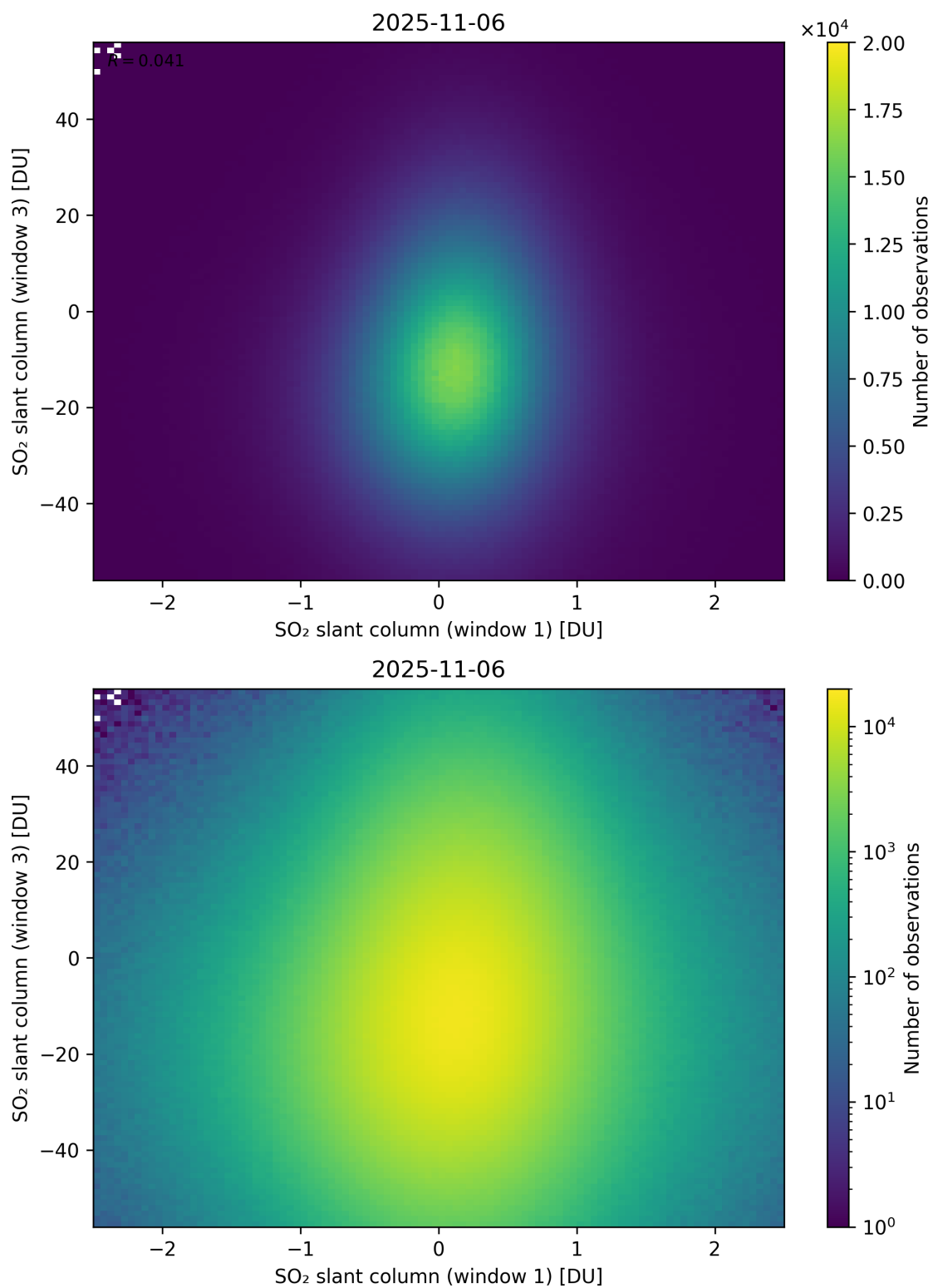
Figure 287: Scatter density plot of “SO 2 slant column (window 1)” against “SO 2 slant column (window 3)” for 2025-11-05 to 2025-11-07.
