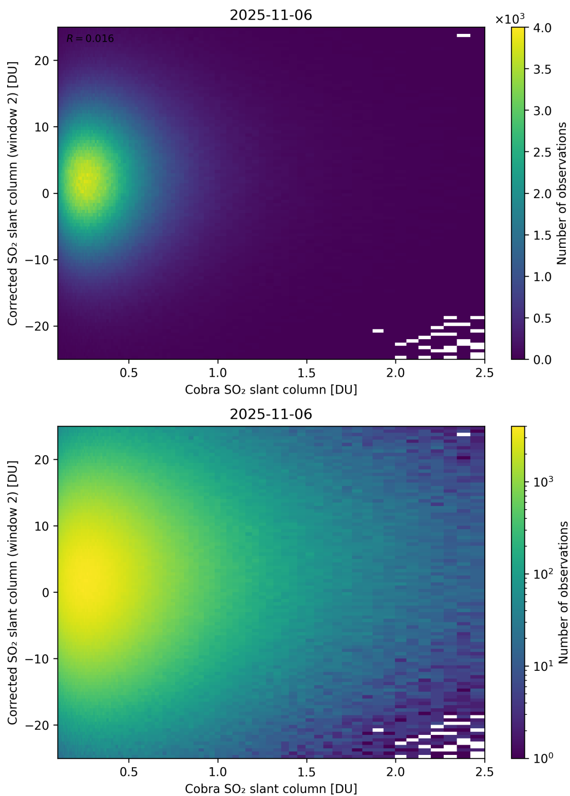
Figure 217: Scatter density plot of “Cobra SO 2 slant column” against “Corrected SO 2 slant column (window 2)” for 2025-11-05 to 2025-11-07.
