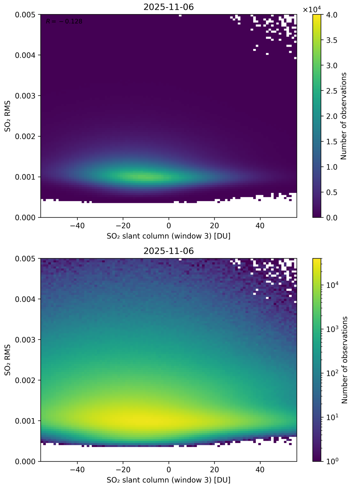
Figure 306: Scatter density plot of “SO 2 slant column (window 3)” against “SO 2 RMS” for 2025-11-05 to 2025-11-07.
