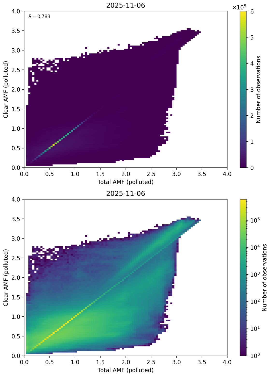
Figure 321: Scatter density plot of “Total AMF (polluted)” against “Clear AMF (polluted)” for 2025-11-05 to 2025-11-07.
