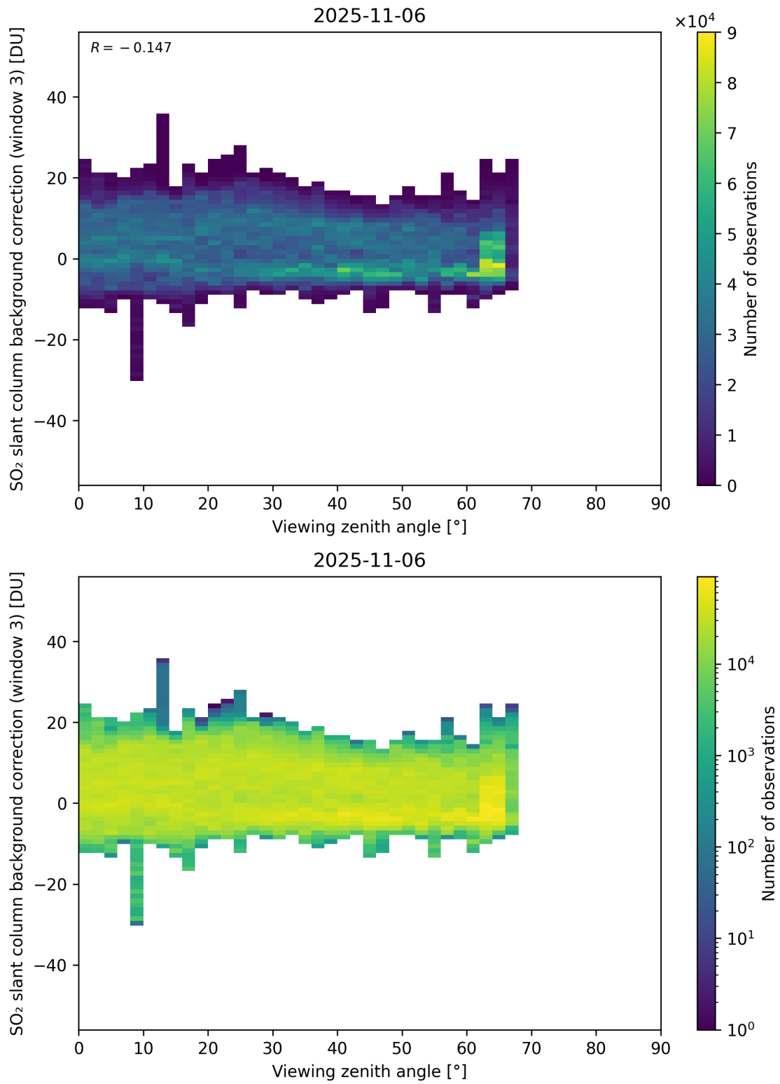
Figure 364: Scatter density plot of “Viewing zenith angle” against “SO 2 slant column background correction (window 3)” for 2025-11-05 to 2025-11-07.
