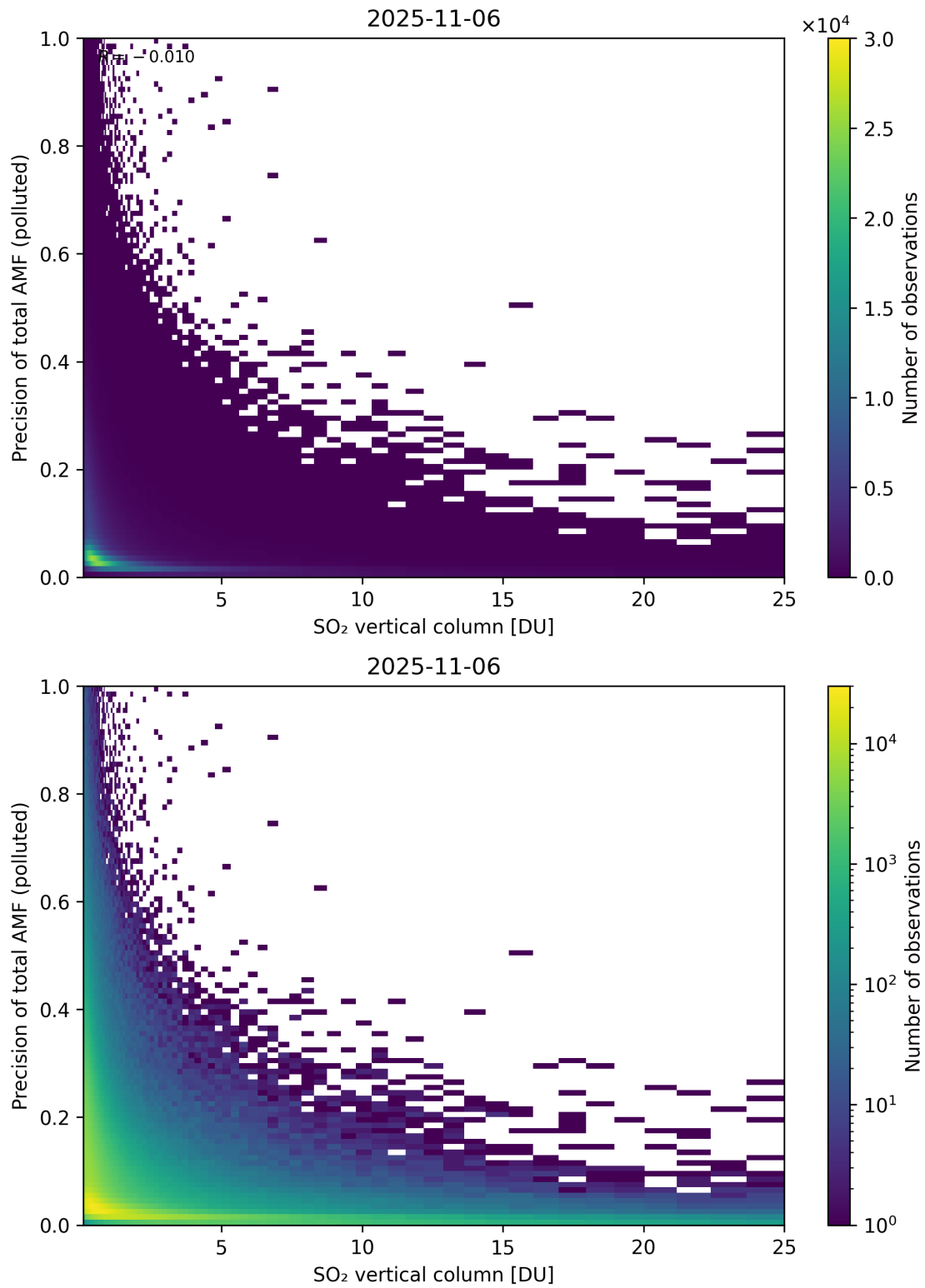
Figure 360: Scatter density plot of “SO 2 vertical column” against “Precision of total AMF (polluted)” for 2025-11-05 to 2025-11-07.
