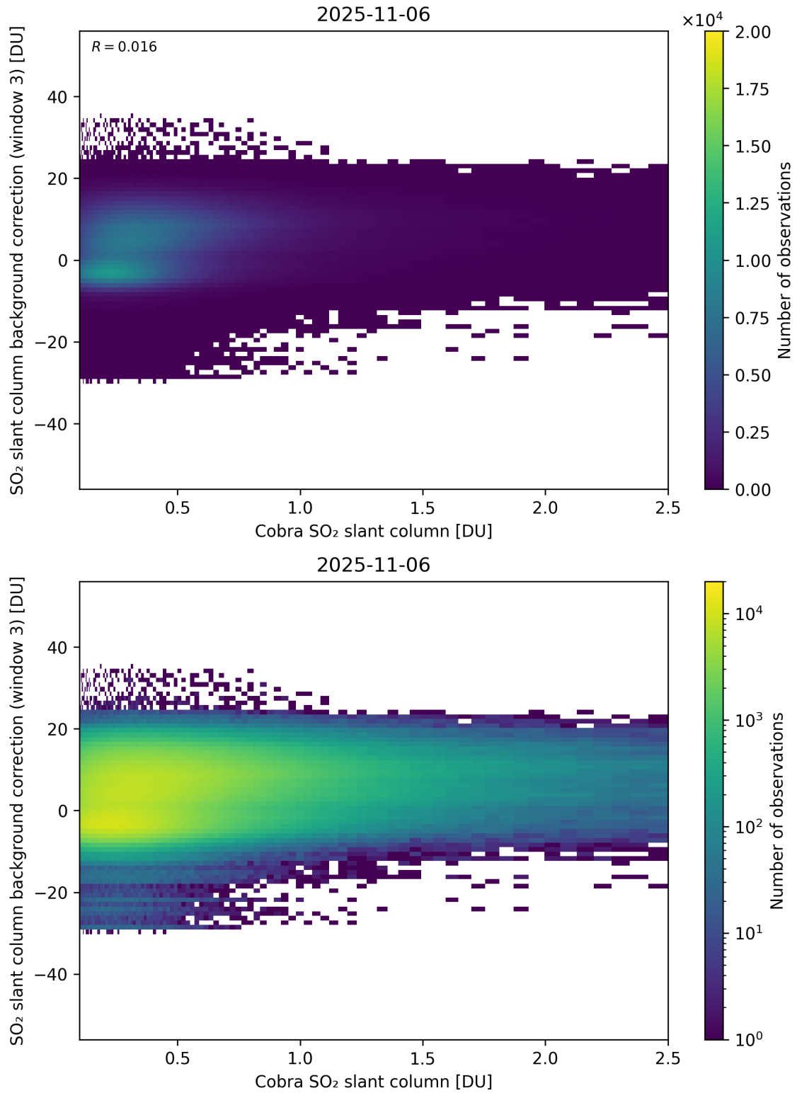
Figure 195: Scatter density plot of “Cobra SO 2 slant column” against “SO 2 slant column background correction (window 3)” for 2025-11-05 to 2025-11-07.
