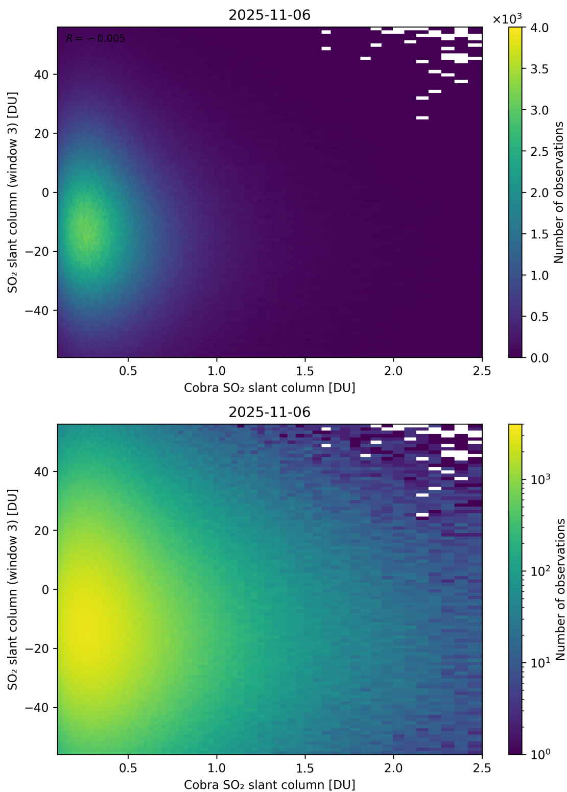
Figure 222: Scatter density plot of “Cobra SO 2 slant column” against “SO 2 slant column (window 3)” for 2025-11-05 to 2025-11-07.
