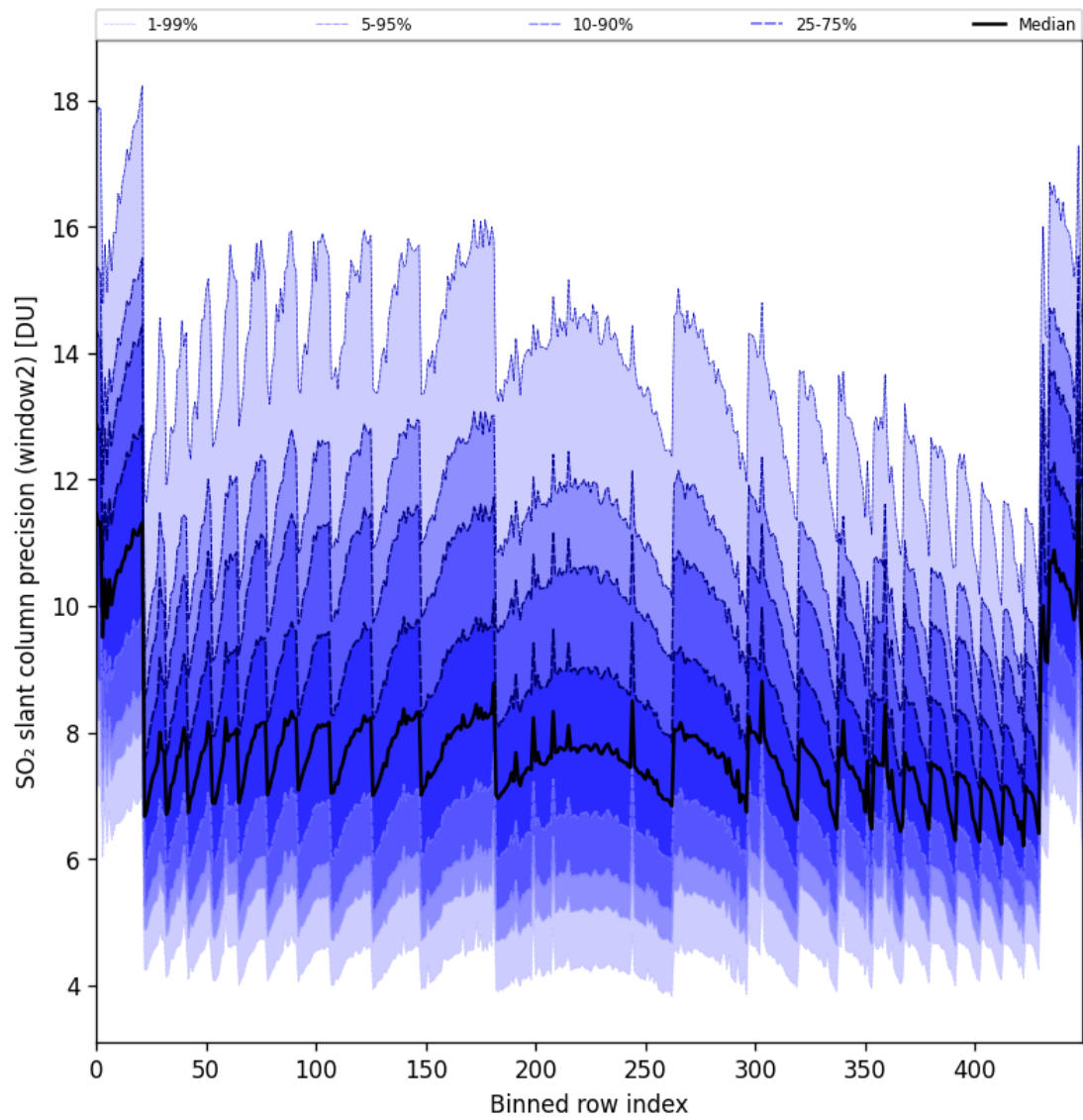
Figure 94: Along track statistics of “SO 2 slant column precision (window2)” for 2025-11-05 to 2025-11-07
