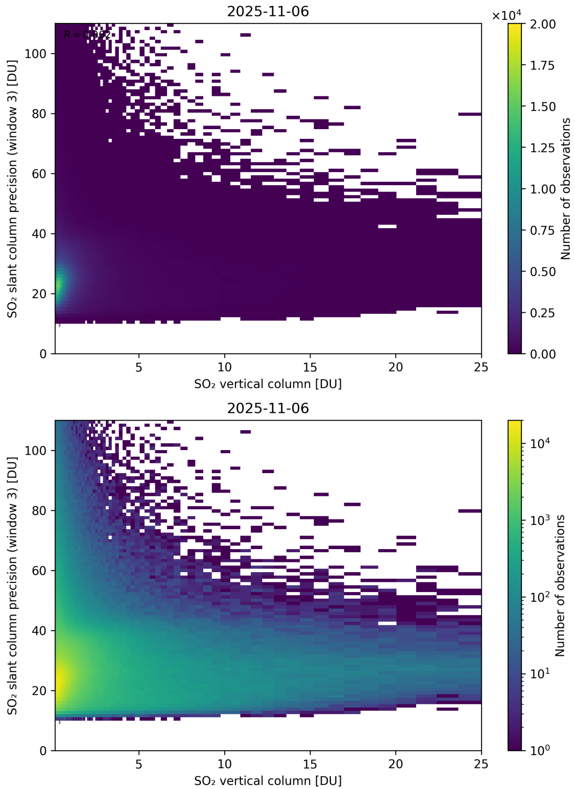
Figure 358: Scatter density plot of “SO 2 vertical column” against “SO 2 slant column precision (window 3)” for 2025-11-05 to 2025-11-07.
