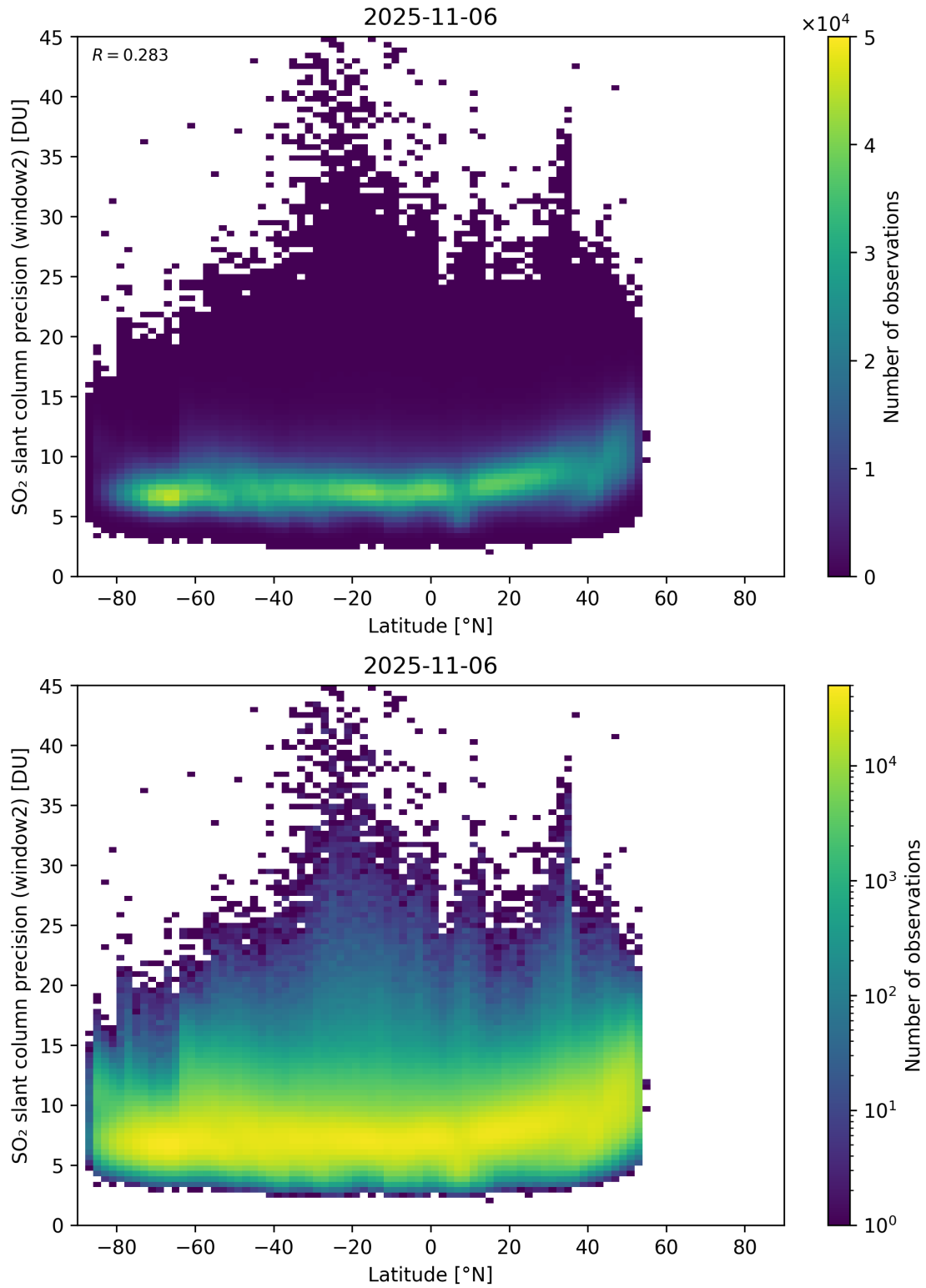
Figure 164: Scatter density plot of “Latitude” against “SO 2 slant column precision (window2)” for 2025-11-05 to 2025-11-07.
