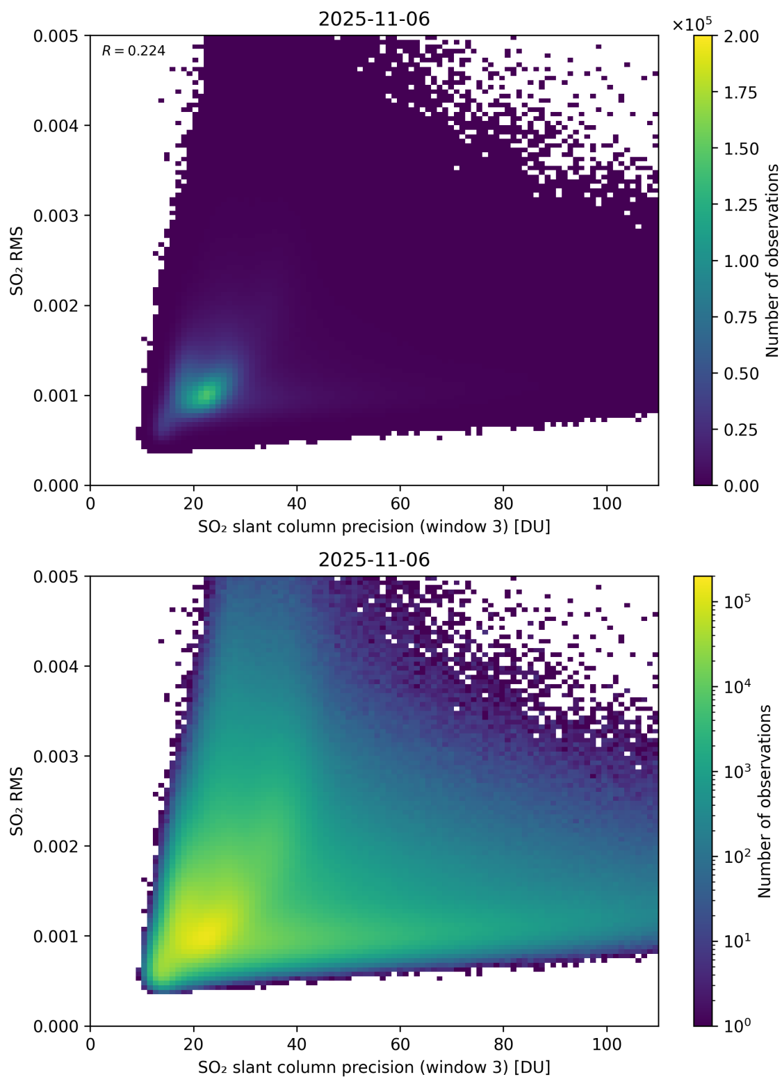
Figure 310: Scatter density plot of “SO 2 slant column precision (window 3)” against “SO 2 RMS” for 2025-11-05 to 2025-11-07.
