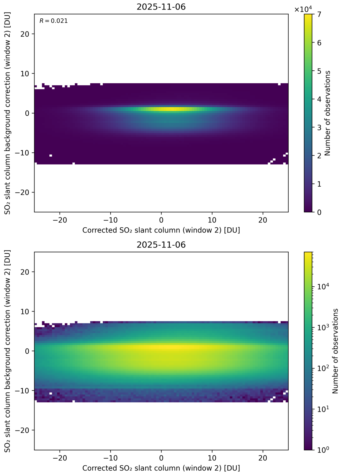
Figure 244: Scatter density plot of “Corrected SO 2 slant column (window 2)” against “SO 2 slant column background correction (window 2)” for 2025-11-05 to 2025-11-07.
