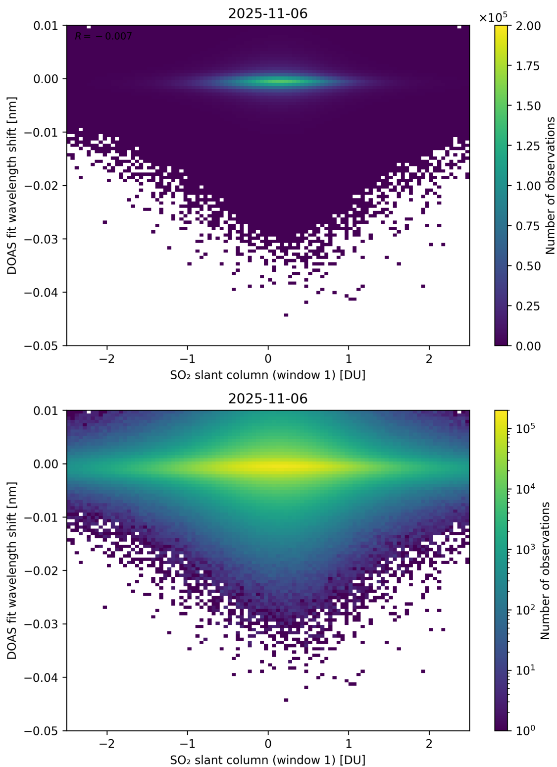
Figure 265: Scatter density plot of “SO 2 slant column (window 1)” against “DOAS fit wavelength shift” for 2025-11-05 to 2025-11-07.
