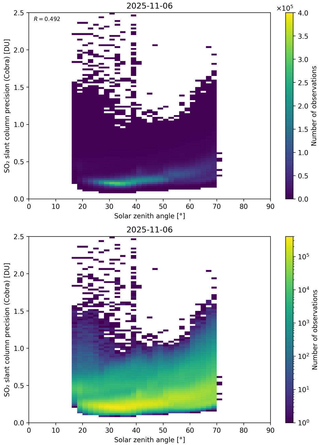
Figure 180: Scatter density plot of “Solar zenith angle” against “SO 2 slant column precision (Cobra)” for 2025-11-05 to 2025-11-07.
