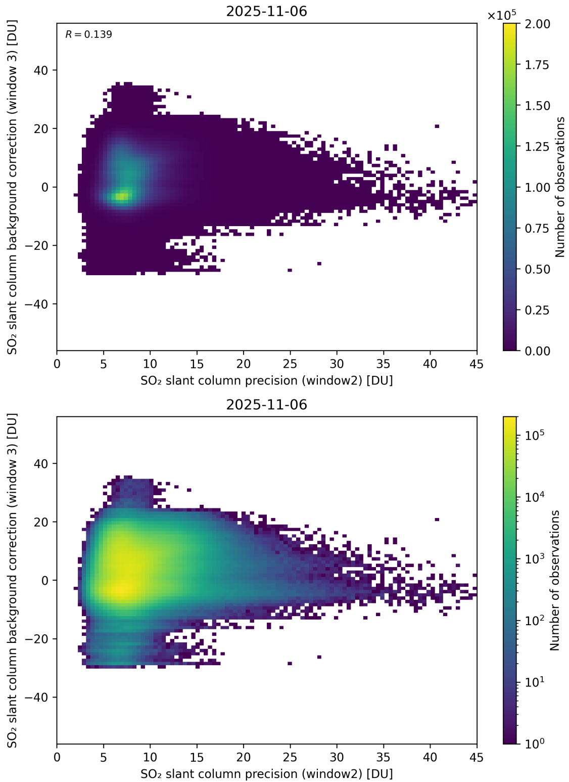
Figure 292: Scatter density plot of “SO 2 slant column precision (window2)” against “SO 2 slant column background correction (window 3)” for 2025-11-05 to 2025-11-07.
