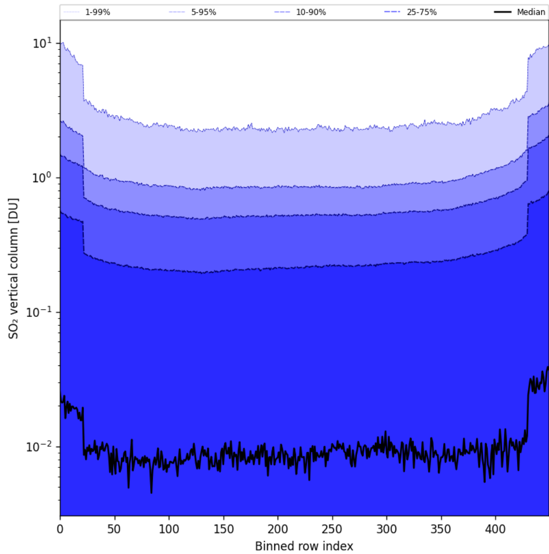
Figure 84: Along track statistics of “SO 2 vertical column” for 2025-11-05 to 2025-11-07
