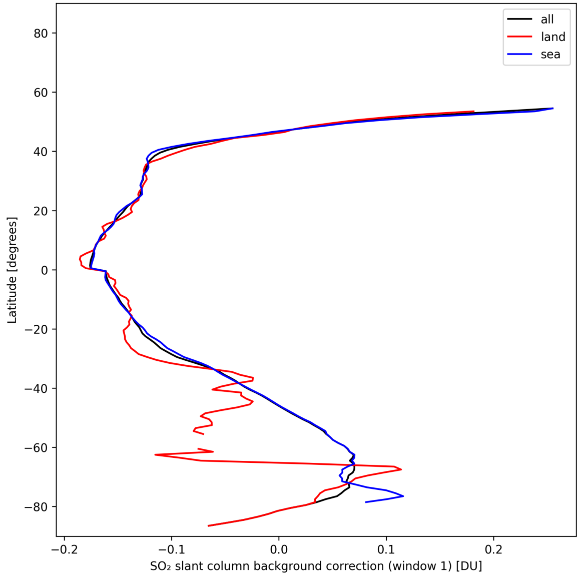
Figure 40: Zonal average of “SO 2 slant column background correction (window 1)” for 2025-11-05 to 2025-11-07.
