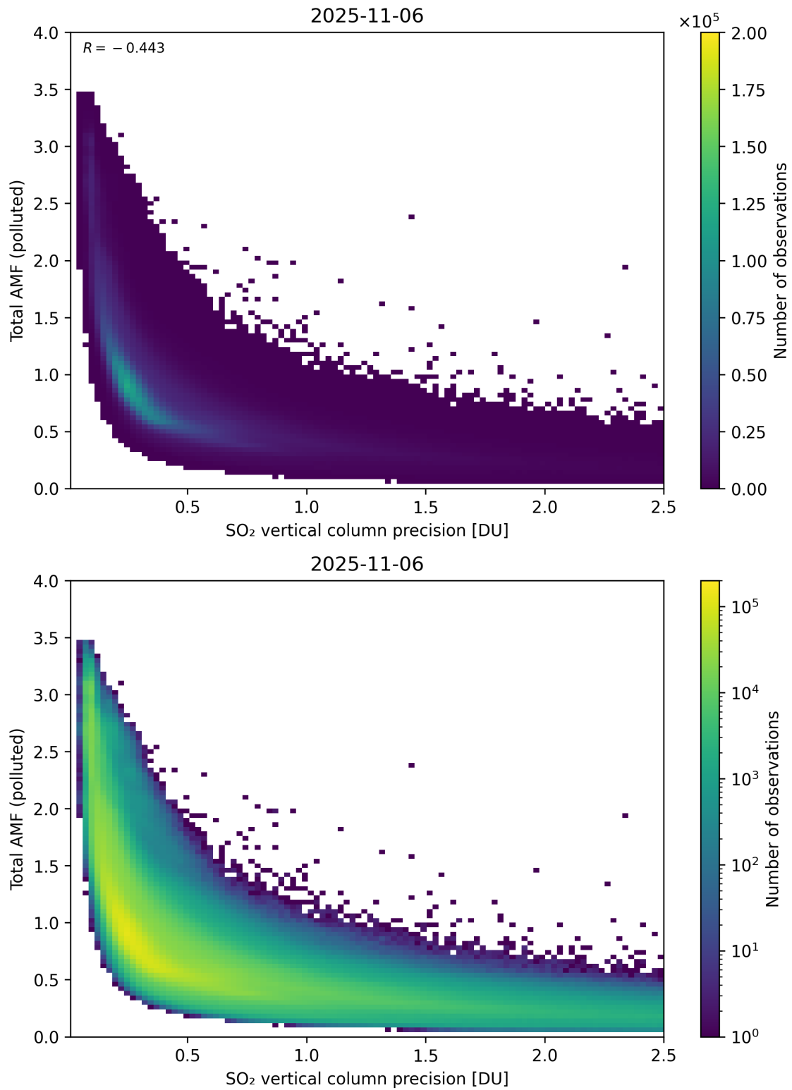
Figure 346: Scatter density plot of “SO 2 vertical column precision” against “Total AMF (polluted)” for 2025-11-05 to 2025-11-07.
