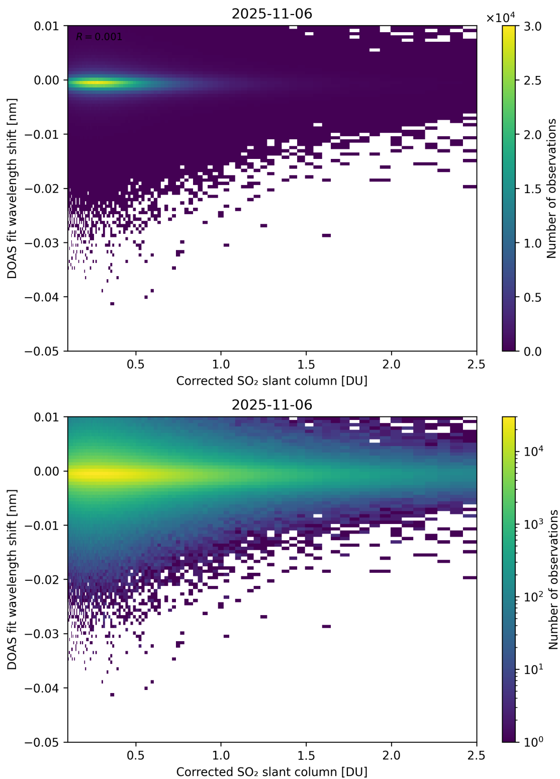
Figure 229: Scatter density plot of “Corrected SO 2 slant column” against “DOAS fit wavelength shift” for 2025-11-05 to 2025-11-07.
