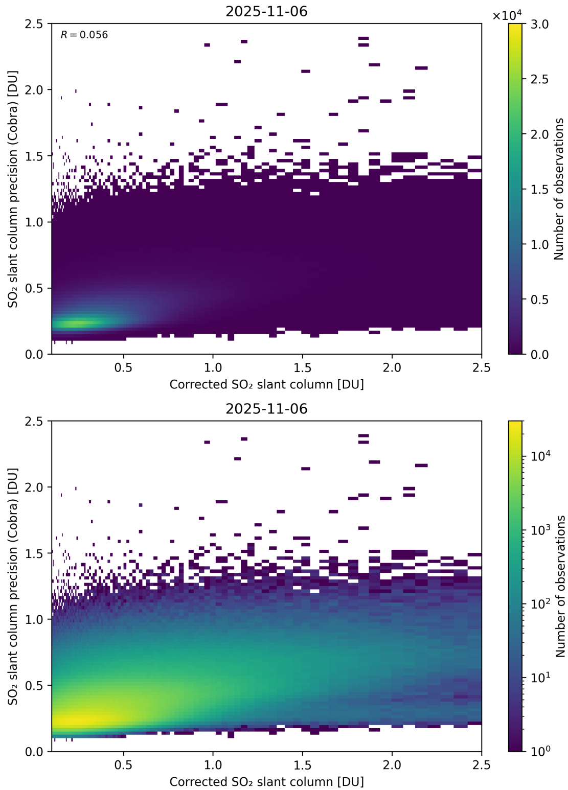
Figure 234: Scatter density plot of “Corrected SO 2 slant column” against “SO 2 slant column precision (Cobra)” for 2025-11-05 to 2025-11-07.
