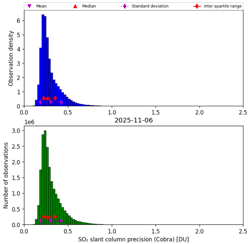
Figure 62: Histogram of “SO 2 slant column precision (Cobra)” for 2025-11-05 to 2025-11-07
