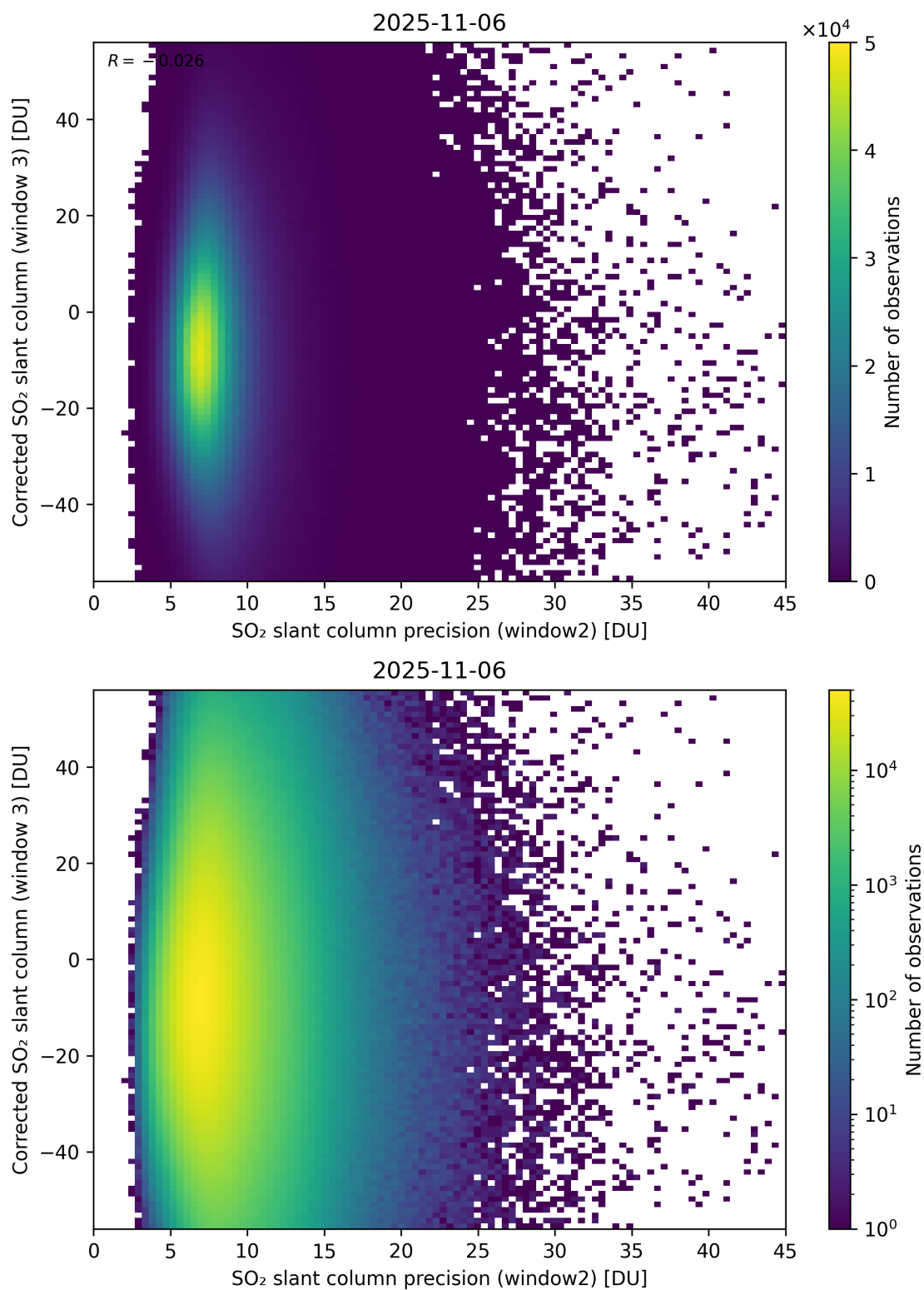
Figure 298: Scatter density plot of “SO 2 slant column precision (window2)” against “Corrected SO 2 slant column (window 3)” for 2025-11-05 to 2025-11-07.
