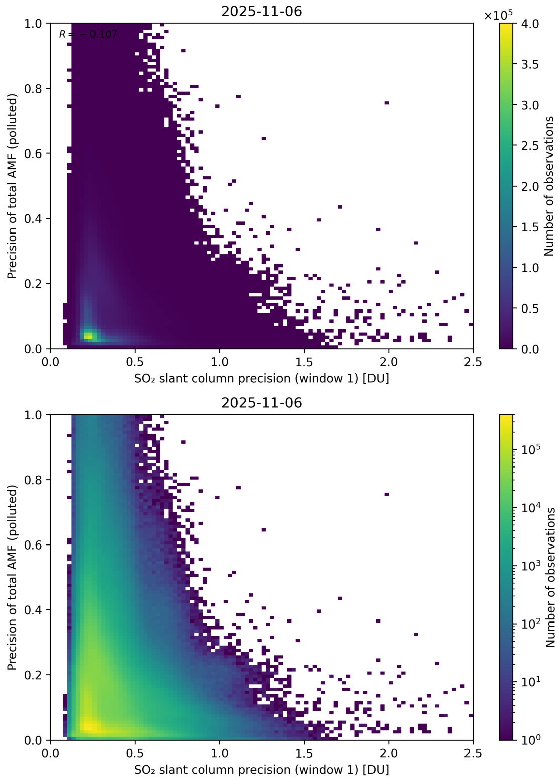
Figure 281: Scatter density plot of “SO 2 slant column precision (window 1)” against “Precision of total AMF (polluted)” for 2025-11-05 to 2025-11-07.
