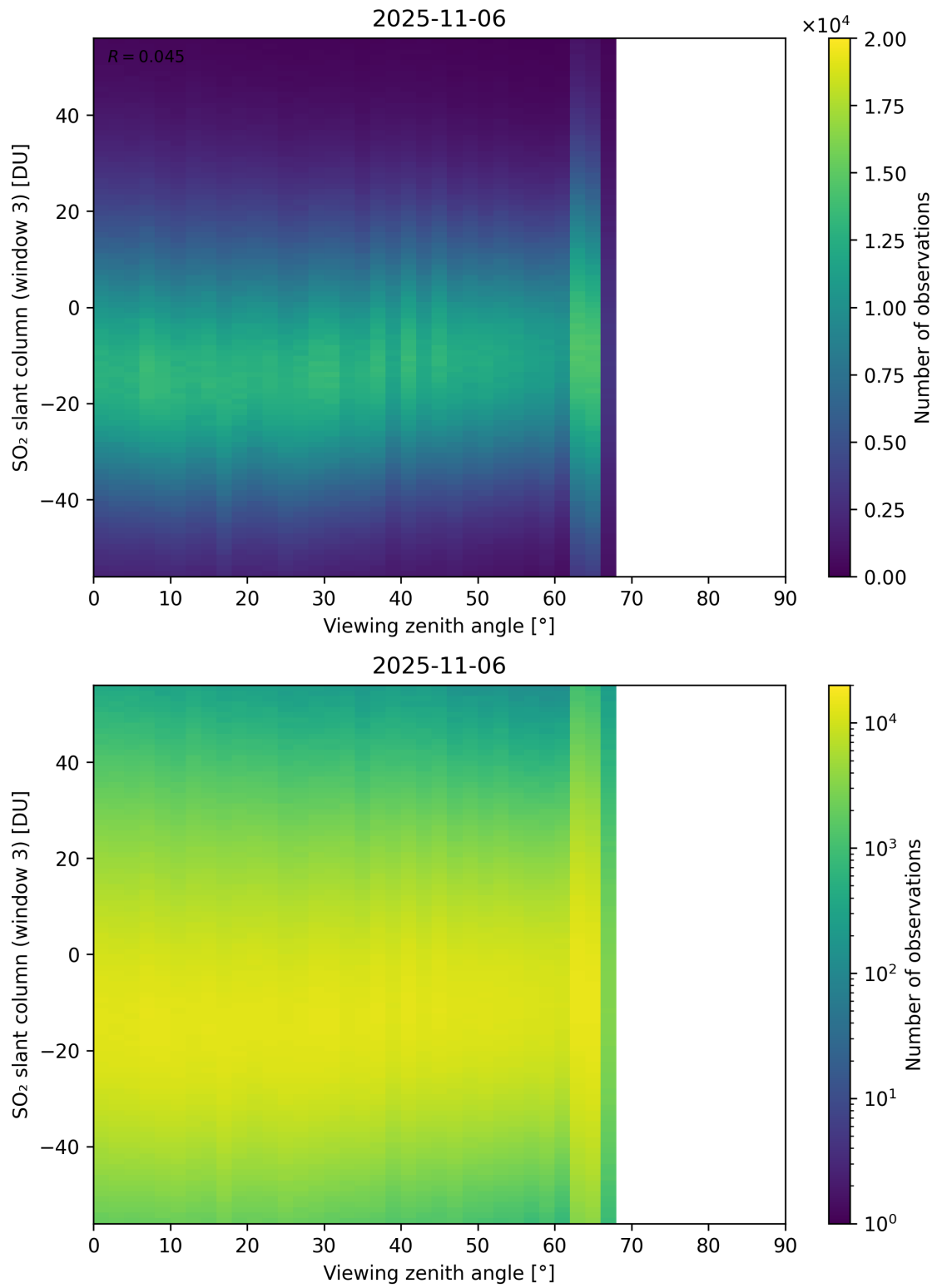
Figure 379: Scatter density plot of “Viewing zenith angle” against “SO 2 slant column (window 3)” for 2025-11-05 to 2025-11-07.
