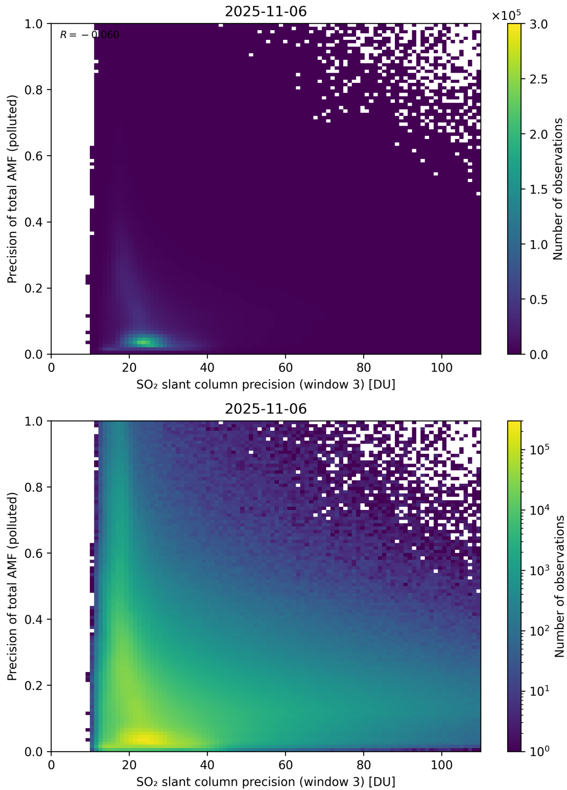
Figure 314: Scatter density plot of “SO 2 slant column precision (window 3)” against “Precision of total AMF (polluted)” for 2025-11-05 to 2025-11-07.
