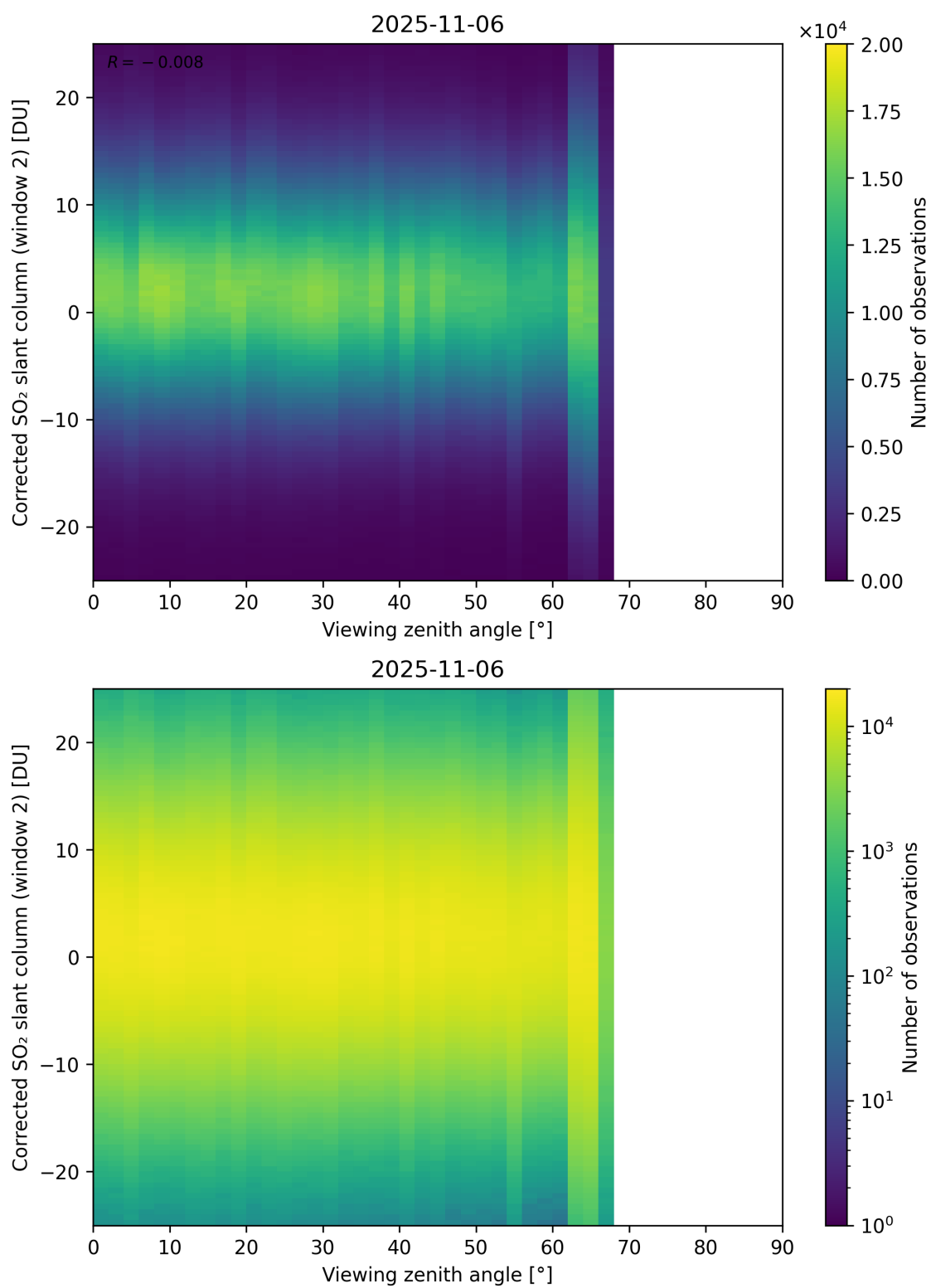
Figure 374: Scatter density plot of “Viewing zenith angle” against “Corrected SO 2 slant column (window 2)” for 2025-11-05 to 2025-11-07.
