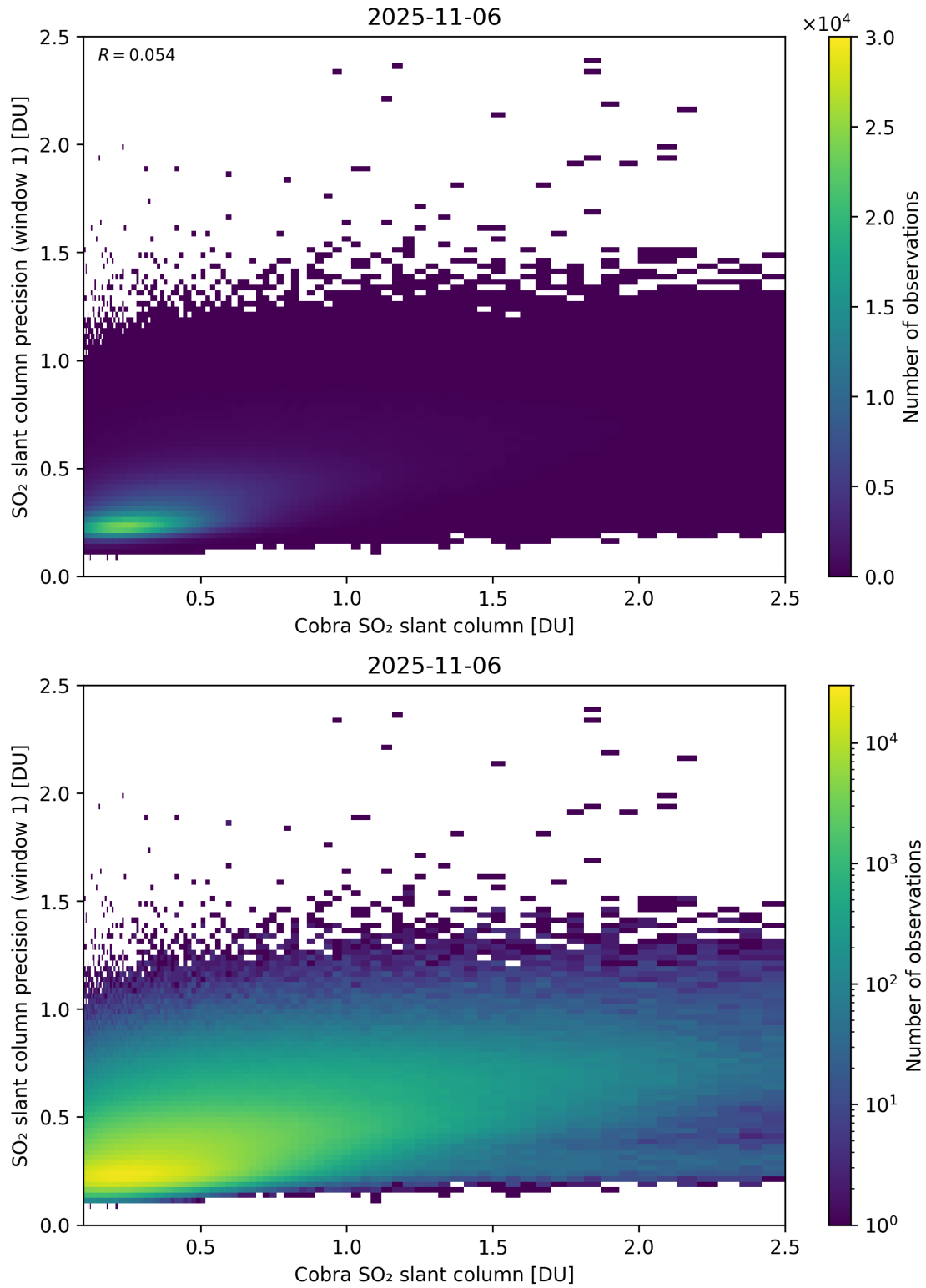
Figure 220: Scatter density plot of “Cobra SO 2 slant column” against “SO 2 slant column precision (window 1)” for 2025-11-05 to 2025-11-07.
