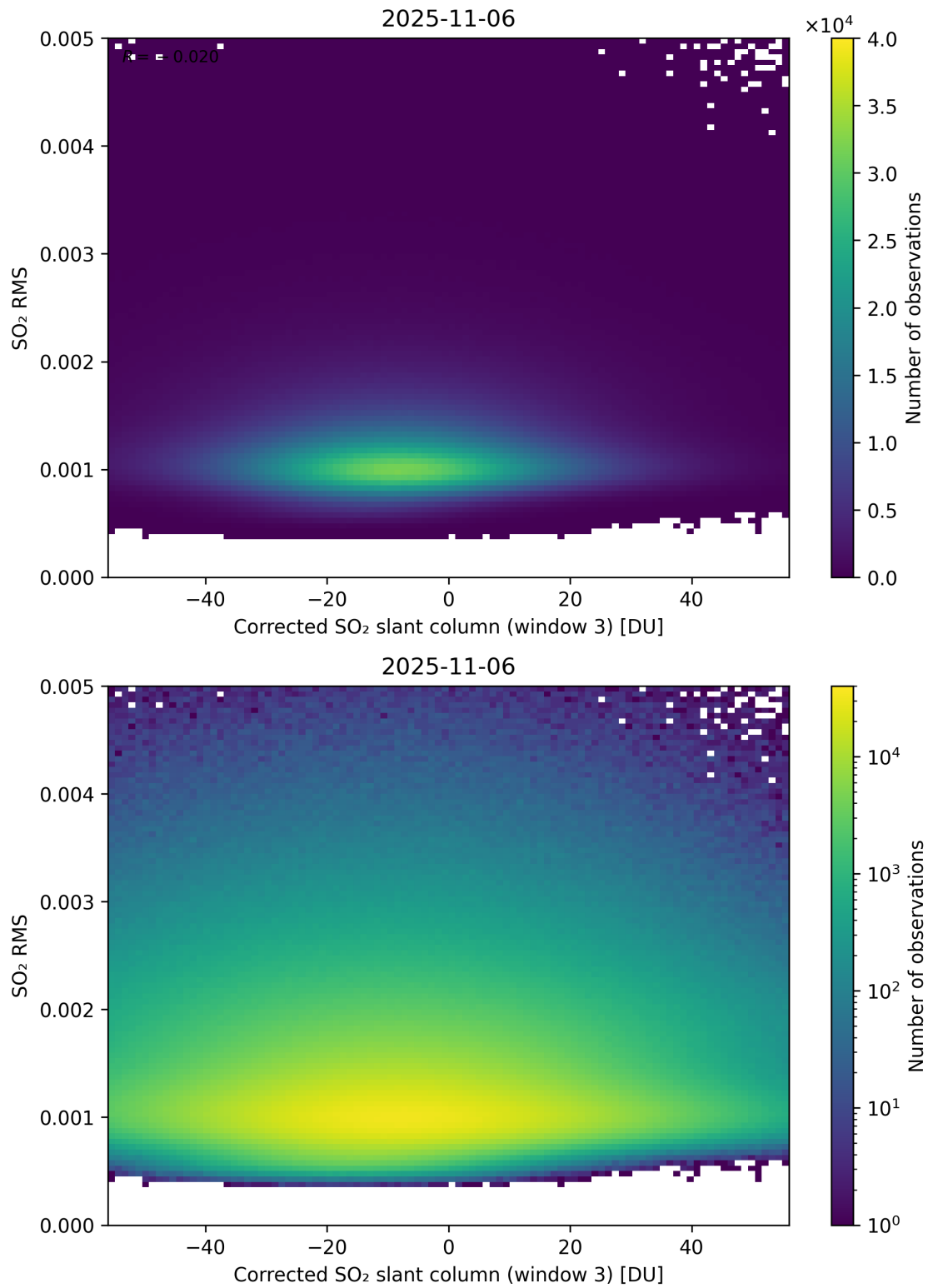
Figure 258: Scatter density plot of “Corrected SO 2 slant column (window 3)” against “SO 2 RMS” for 2025-11-05 to 2025-11-07.
