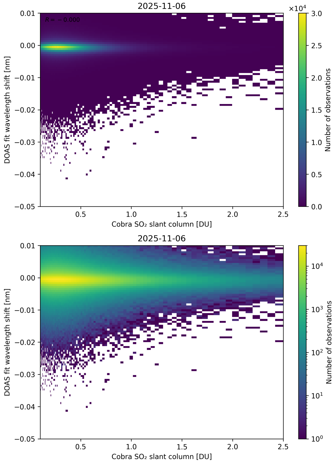
Figure 196: Scatter density plot of “Cobra SO 2 slant column” against “DOAS fit wavelength shift” for 2025-11-05 to 2025-11-07.
