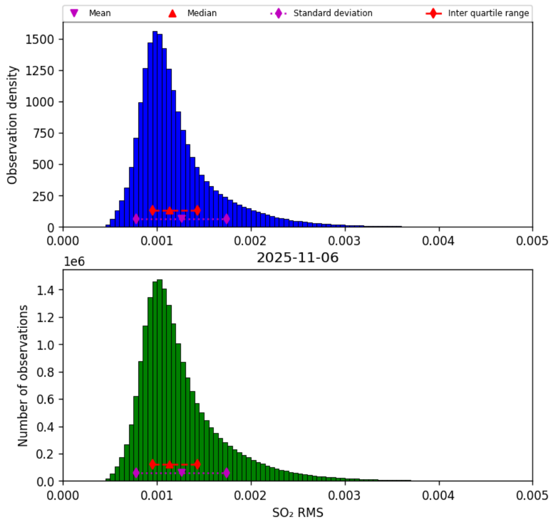
Figure 78: Histogram of “SO 2 RMS” for 2025-11-05 to 2025-11-07
