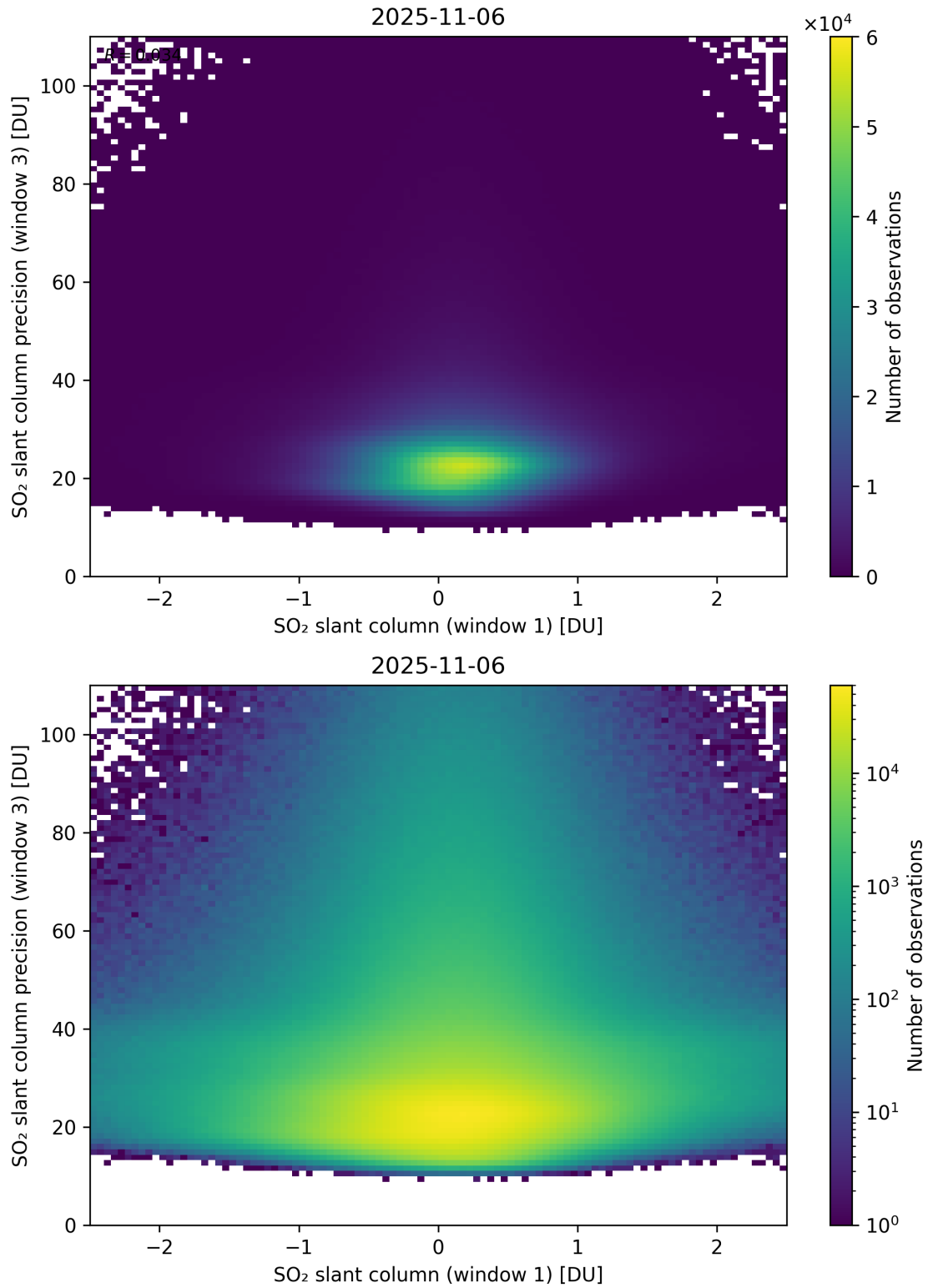
Figure 288: Scatter density plot of “SO 2 slant column (window 1)” against “SO 2 slant column precision (window 3)” for 2025-11-05 to 2025-11-07.
