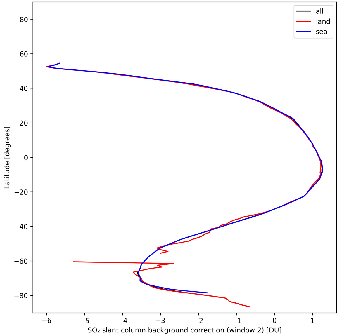
Figure 44: Zonal average of “SO 2 slant column background correction (window 2)” for 2025-11-05 to 2025-11-07.
