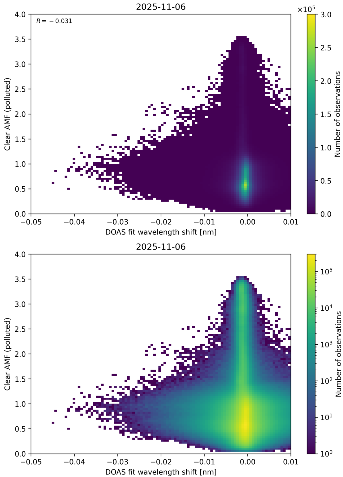
Figure 140: Scatter density plot of “DOAS fit wavelength shift” against “Clear AMF (polluted)” for 2025-11-05 to 2025-11-07.
