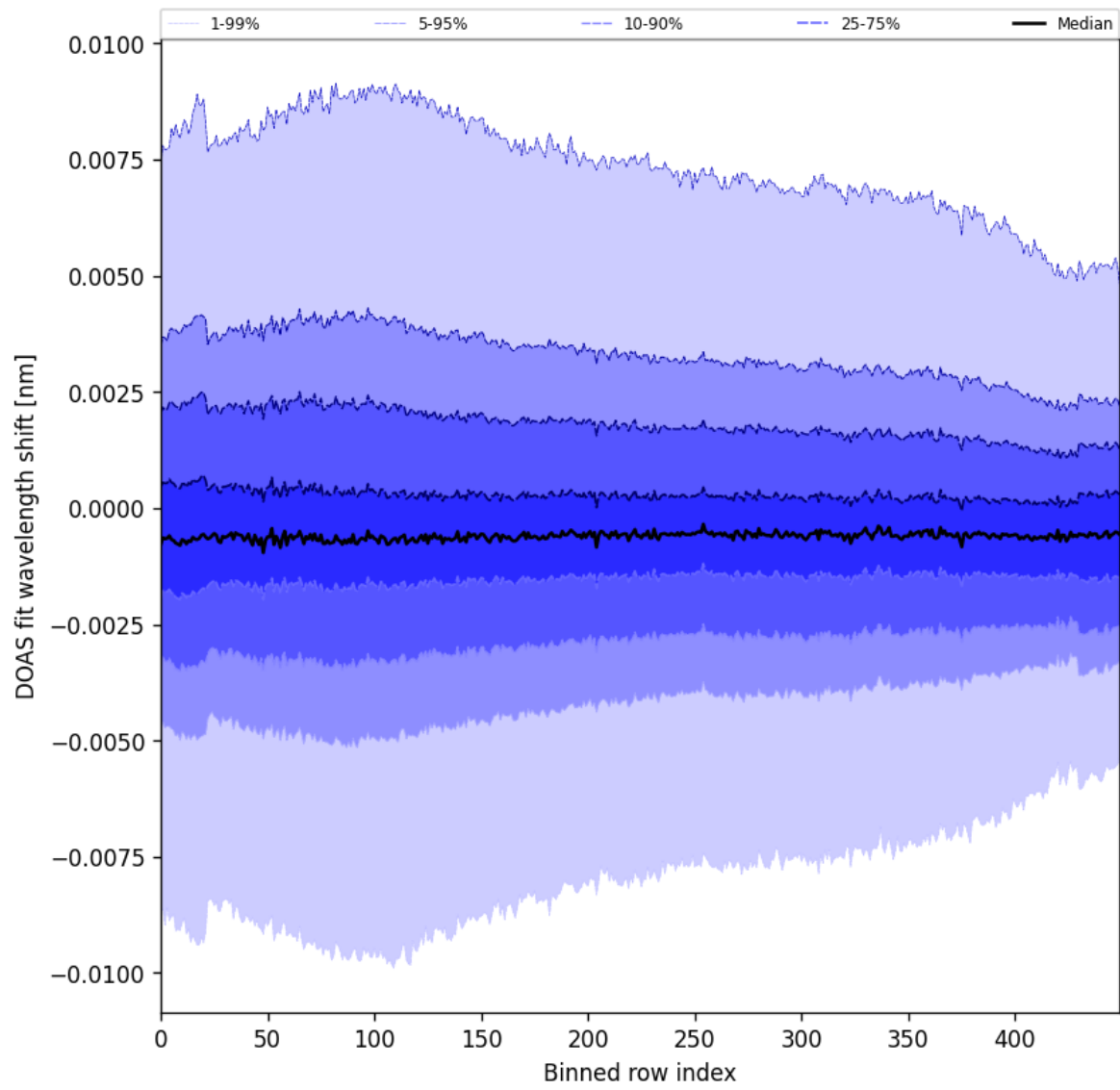
Figure 102: Along track statistics of “DOAS fit wavelength shift” for 2025-11-05 to 2025-11-07
