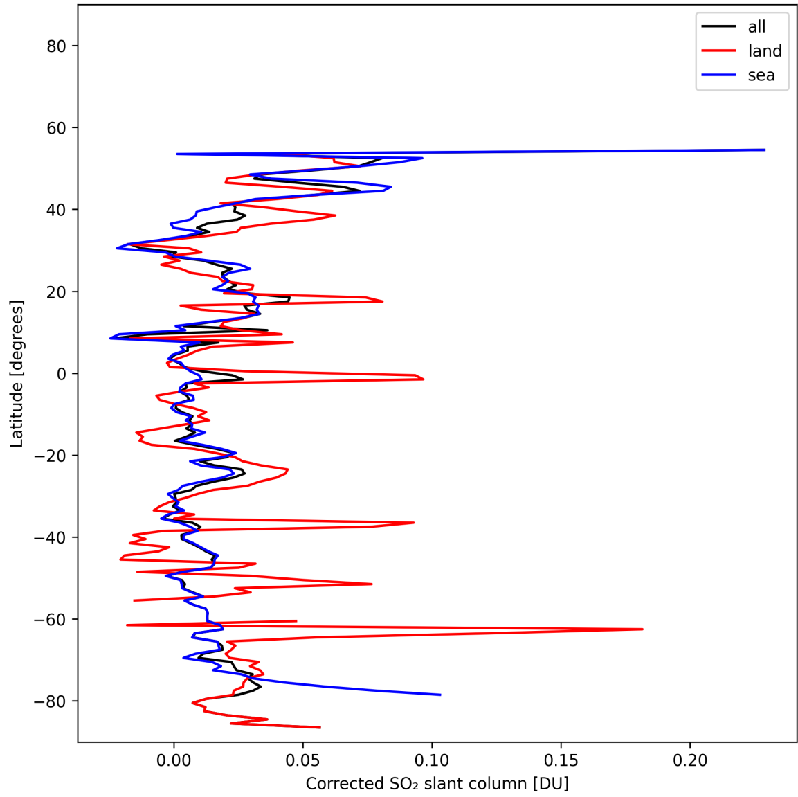
Figure 34: Zonal average of “Corrected SO 2 slant column” for 2025-11-05 to 2025-11-07.
