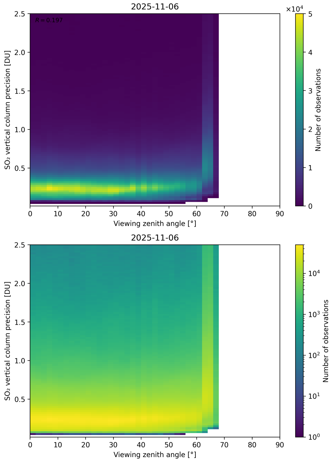
Figure 384: Scatter density plot of “Viewing zenith angle” against “SO 2 vertical column precision” for 2025-11-05 to 2025-11-07.
