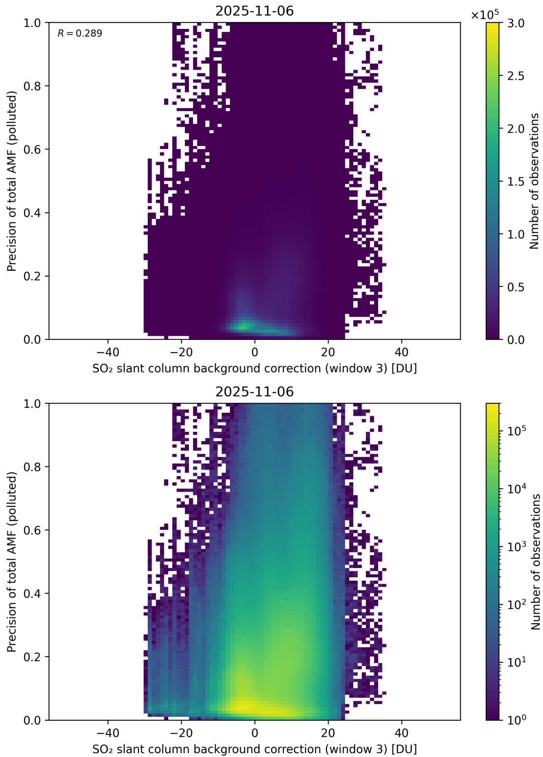
Figure 137: Scatter density plot of “SO 2 slant column background correction (window 3)” against “Precision of total AMF (polluted)” for 2025-11-05 to 2025-11-07.
