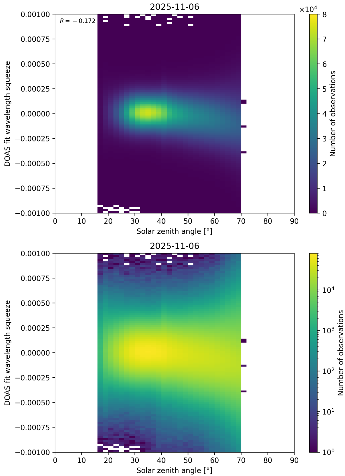
Figure 175: Scatter density plot of “Solar zenith angle” against “DOAS fit wavelength squeeze” for 2025-11-05 to 2025-11-07.
