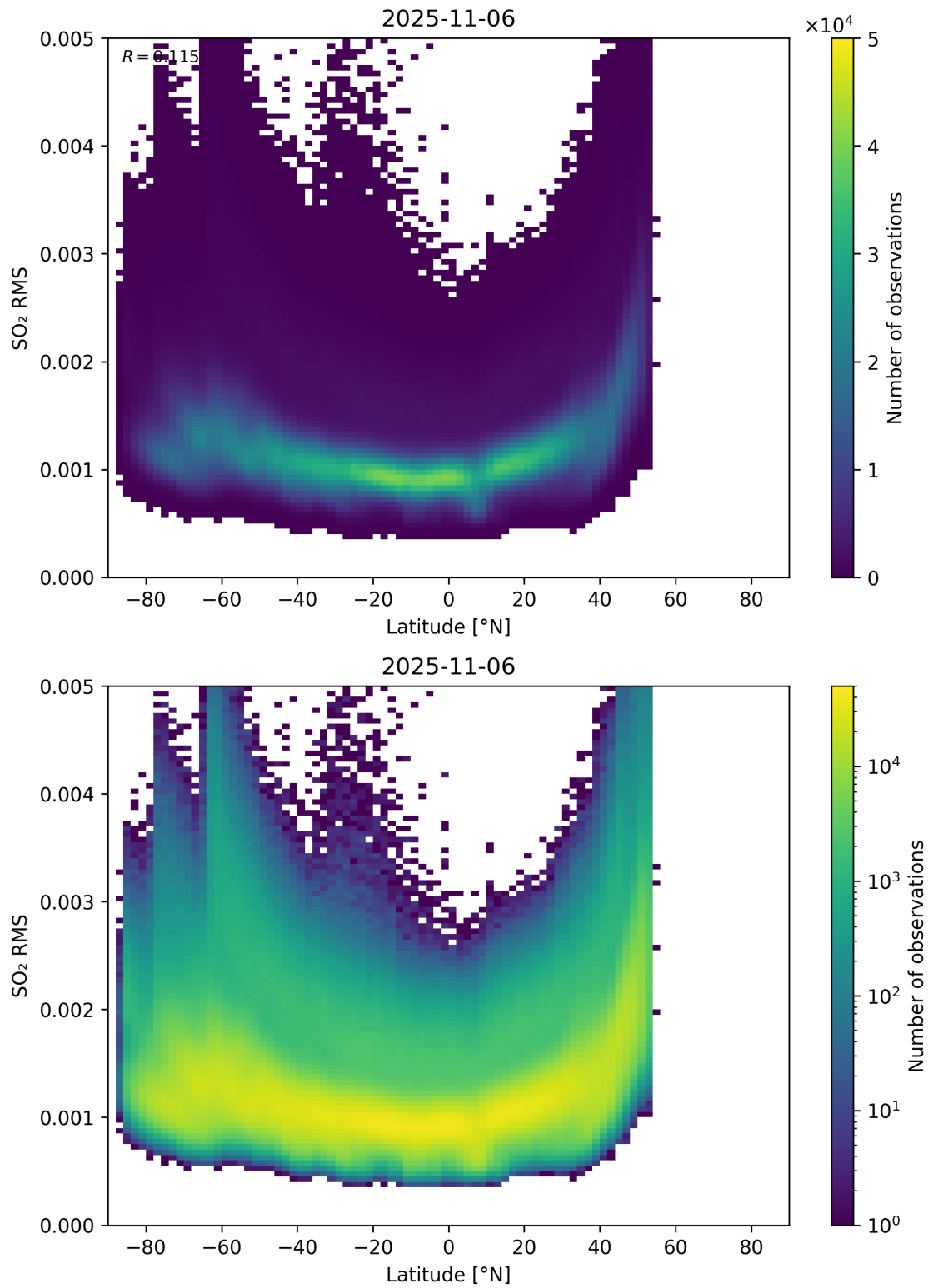
Figure 155: Scatter density plot of “Latitude” against “SO 2 RMS” for 2025-11-05 to 2025-11-07.
