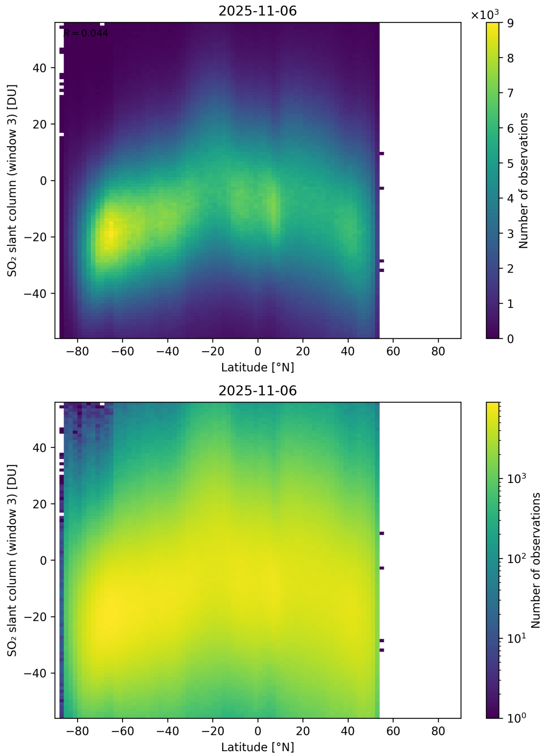
Figure 165: Scatter density plot of “Latitude” against “SO 2 slant column (window 3)” for 2025-11-05 to 2025-11-07.
