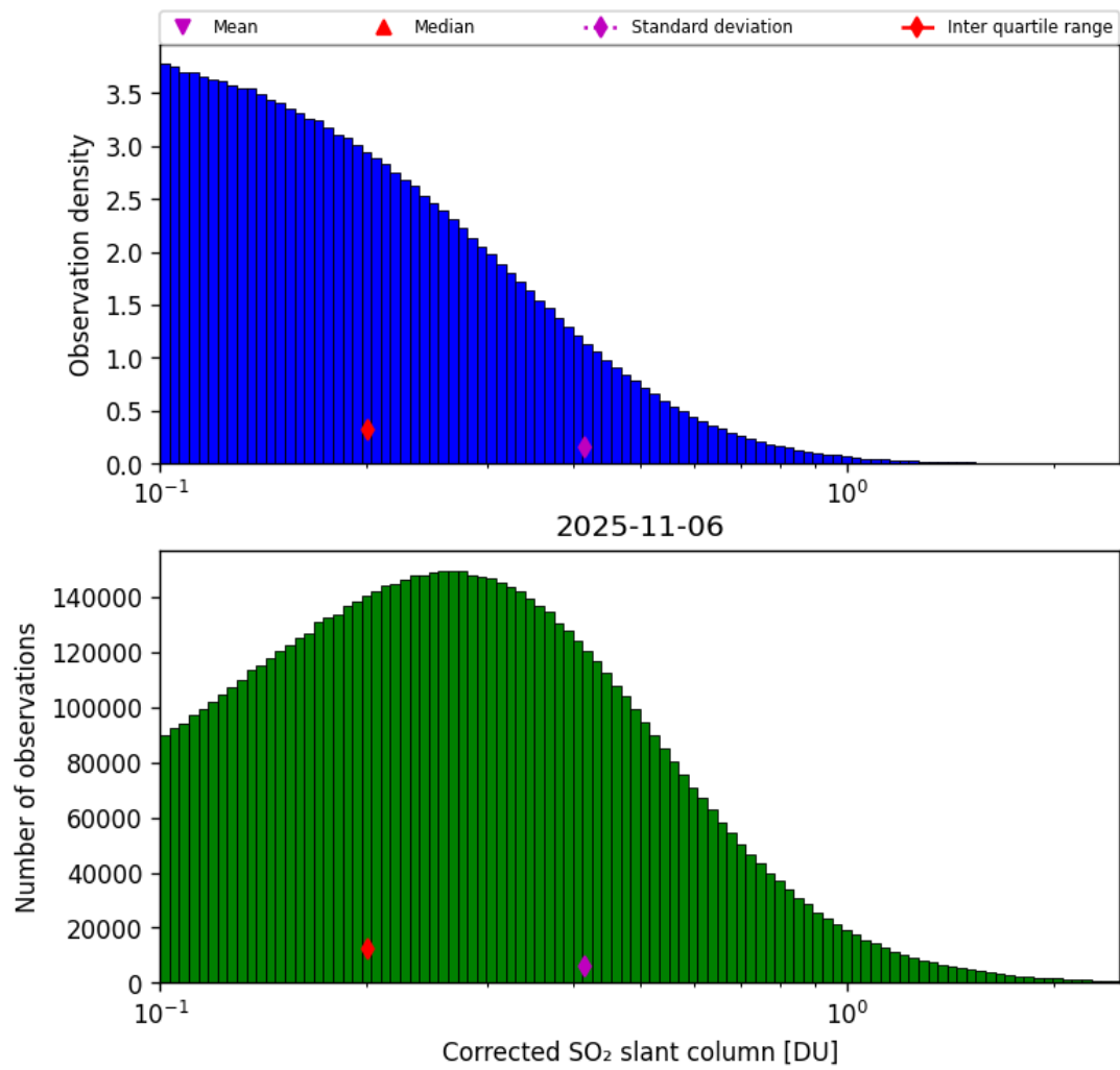
Figure 60: Histogram of “Corrected SO 2 slant column” for 2025-11-05 to 2025-11-07
