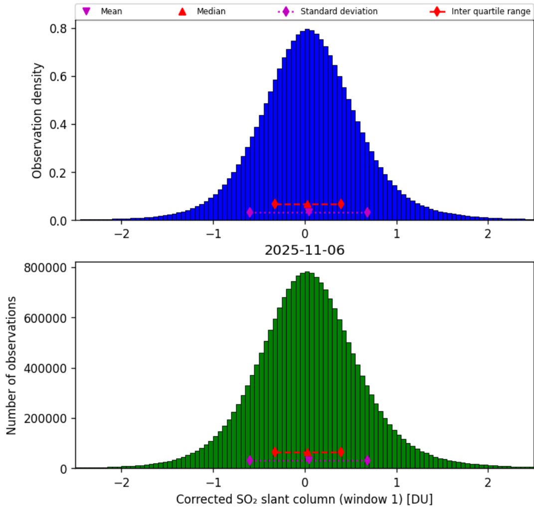
Figure 65: Histogram of “Corrected SO 2 slant column (window 1)” for 2025-11-05 to 2025-11-07
