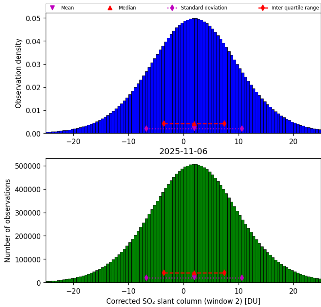
Figure 69: Histogram of “Corrected SO 2 slant column (window 2)” for 2025-11-05 to 2025-11-07
