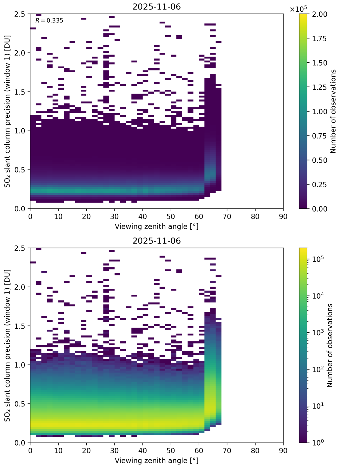
Figure 377: Scatter density plot of “Viewing zenith angle” against “SO 2 slant column precision (window 1)” for 2025-11-05 to 2025-11-07.
