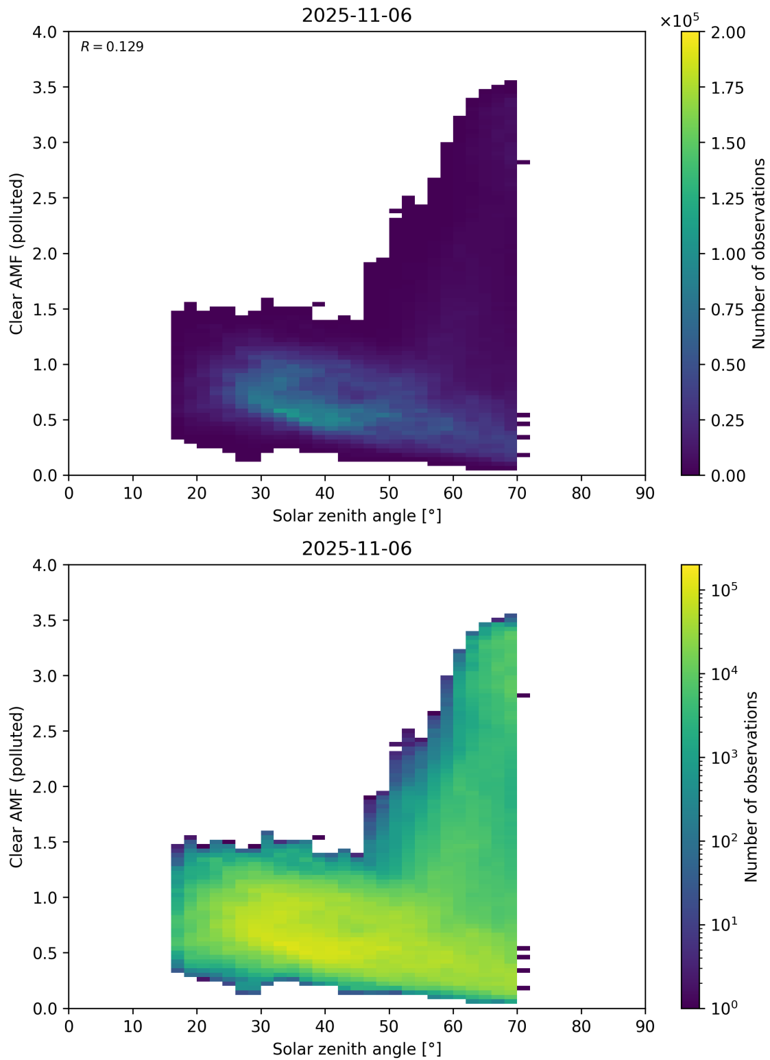
Figure 178: Scatter density plot of “Solar zenith angle” against “Clear AMF (polluted)” for 2025-11-05 to 2025-11-07.
