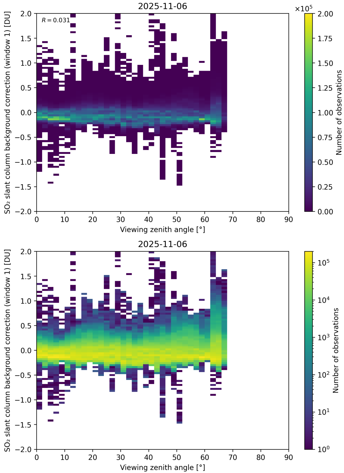
Figure 362: Scatter density plot of “Viewing zenith angle” against “SO 2 slant column background correction (window 1)” for 2025-11-05 to 2025-11-07.
