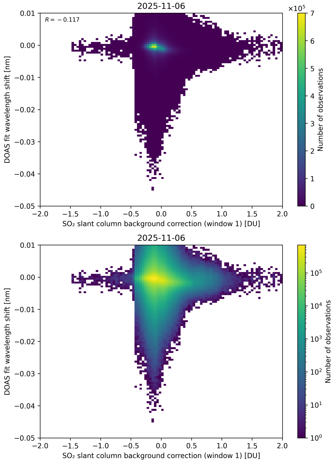
Figure 111: Scatter density plot of “SO 2 slant column background correction (window 1)” against “DOAS fit wavelength shift” for 2025-11-05 to 2025-11-07.
