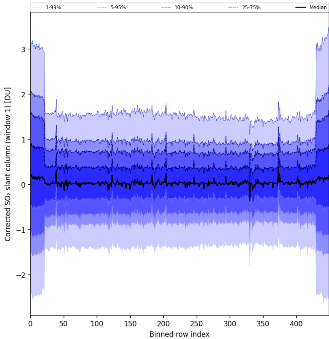
Figure 91: Along track statistics of “Corrected SO 2 slant column (window 1)” for 2025-11-05 to 2025-11-07
