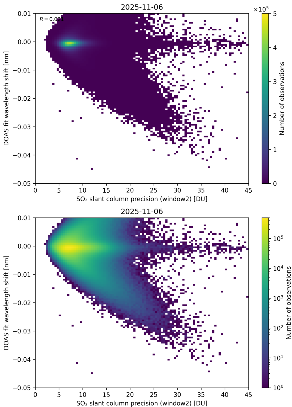
Figure 293: Scatter density plot of “SO 2 slant column precision (window2)” against “DOAS fit wavelength shift” for 2025-11-05 to 2025-11-07.
