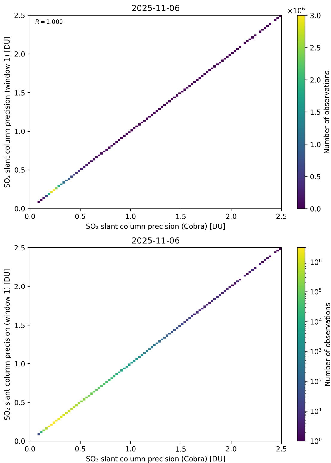
Figure 209: Scatter density plot of “SO 2 slant column precision (Cobra)” against “SO 2 slant column precision (window 1)” for 2025-11-05 to 2025-11-07.
