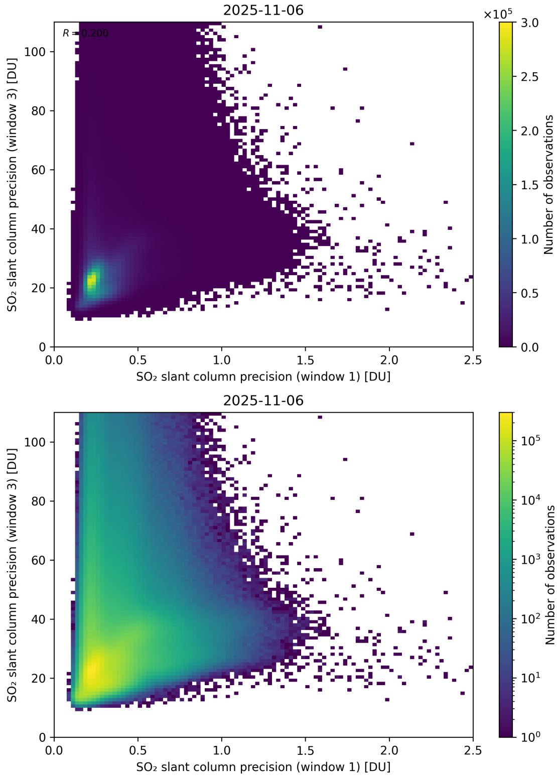
Figure 279: Scatter density plot of “SO 2 slant column precision (window 1)” against “SO 2 slant column precision (window 3)” for 2025-11-05 to 2025-11-07.
