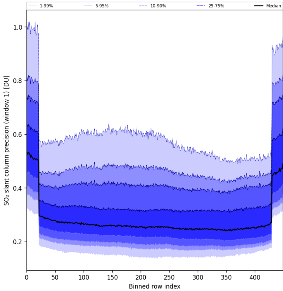
Figure 90: Along track statistics of “SO 2 slant column precision (window 1)” for 2025-11-05 to 2025-11-07
