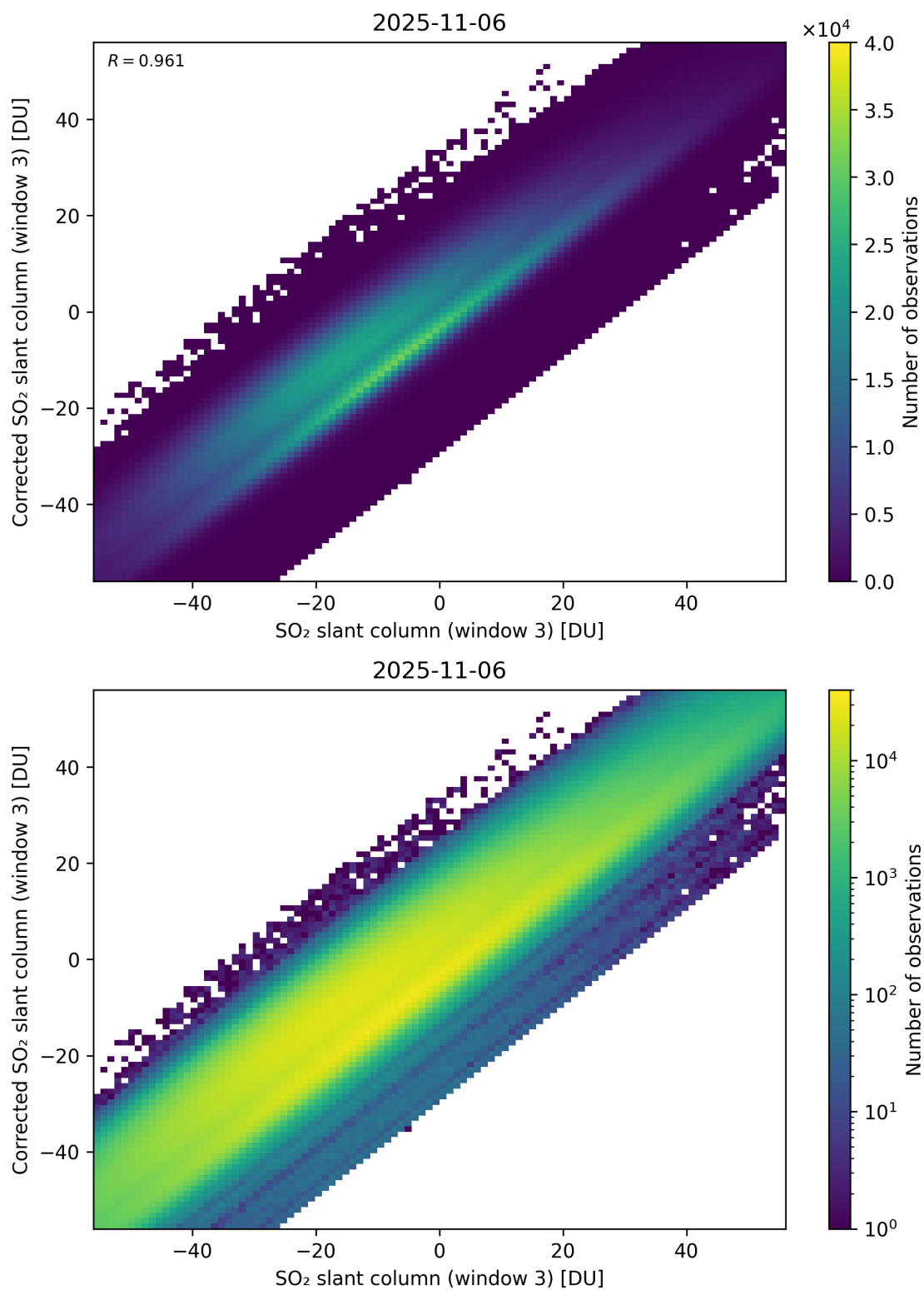
Figure 316: Scatter density plot of “SO 2 slant column (window 3)” against “Corrected SO 2 slant column (window 3)” for 2025-11-05 to 2025-11-07.
