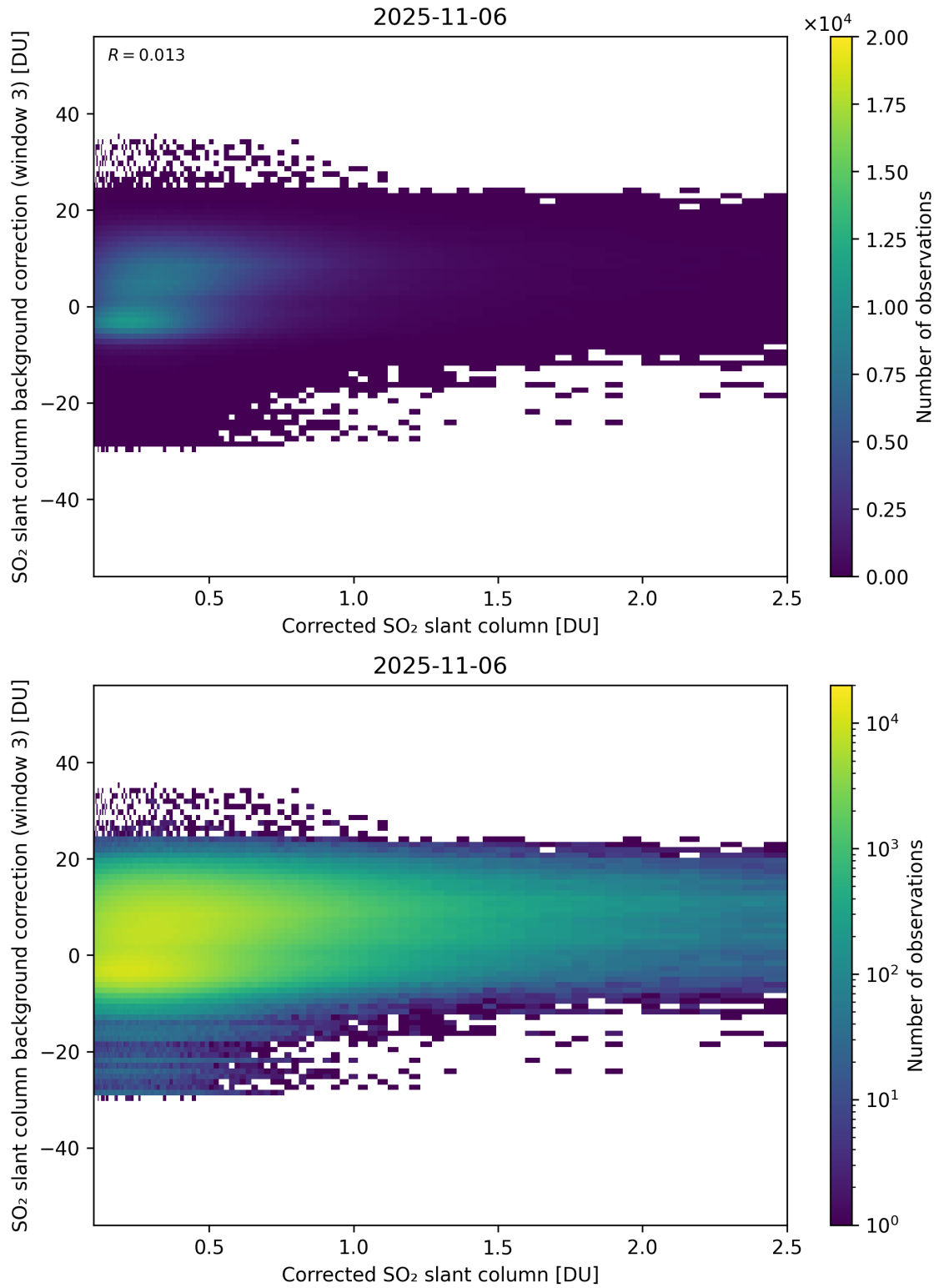
Figure 228: Scatter density plot of “Corrected SO 2 slant column” against “SO 2 slant column background correction (window 3)” for 2025-11-05 to 2025-11-07.
