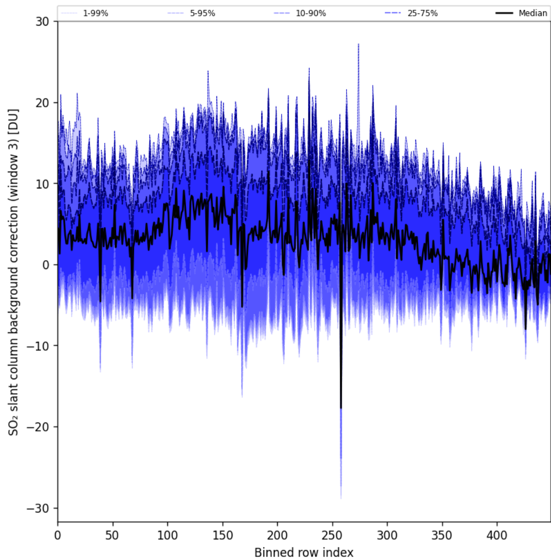
Figure 100: Along track statistics of “SO 2 slant column background correction (window 3)” for 2025-11-05 to 2025-11-07
