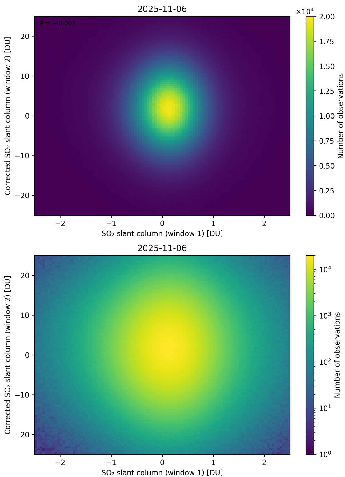
Figure 283: Scatter density plot of “SO 2 slant column (window 1)” against “Corrected SO 2 slant column (window 2)” for 2025-11-05 to 2025-11-07.
