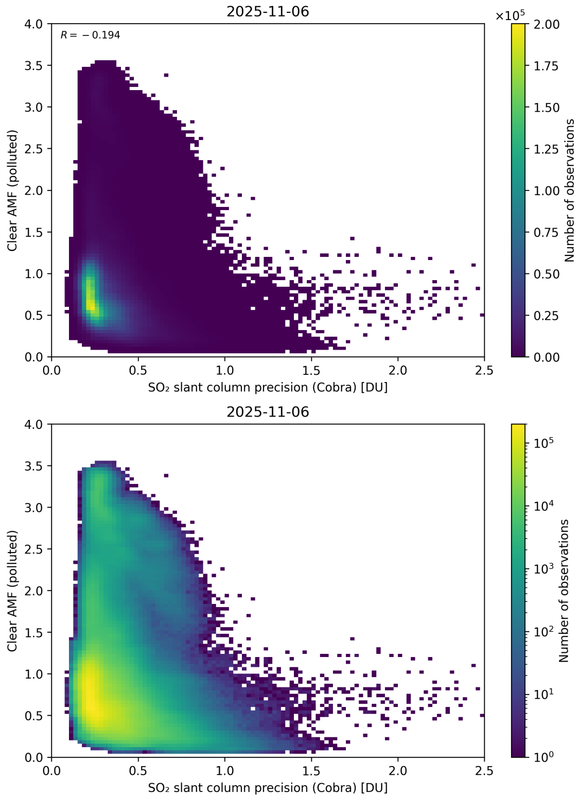
Figure 205: Scatter density plot of “SO 2 slant column precision (Cobra)” against “Clear AMF (polluted)” for 2025-11-05 to 2025-11-07.
