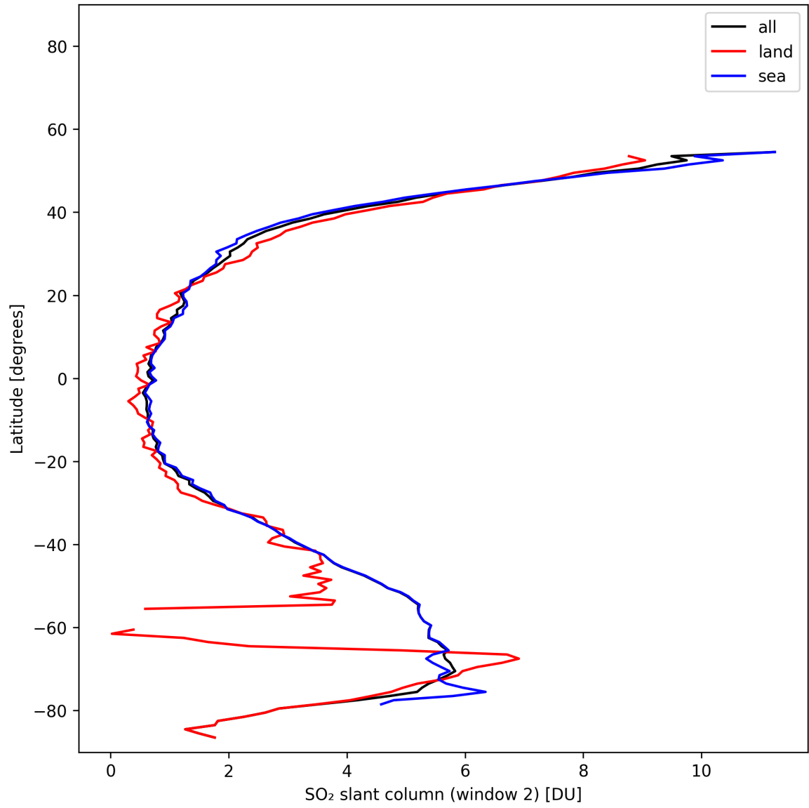
Figure 41: Zonal average of “SO 2 slant column (window 2)” for 2025-11-05 to 2025-11-07.
