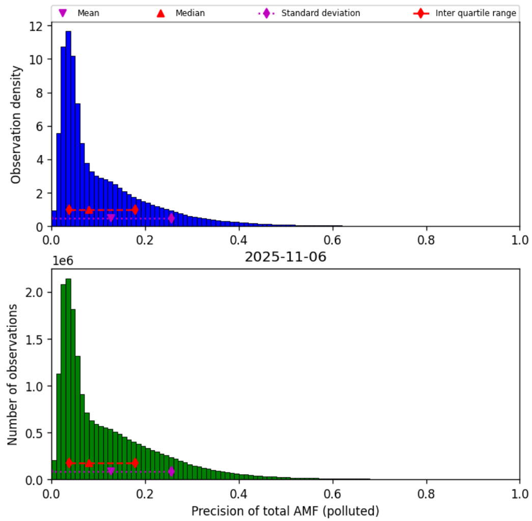
Figure 80: Histogram of “Precision of total AMF (polluted)” for 2025-11-05 to 2025-11-07
