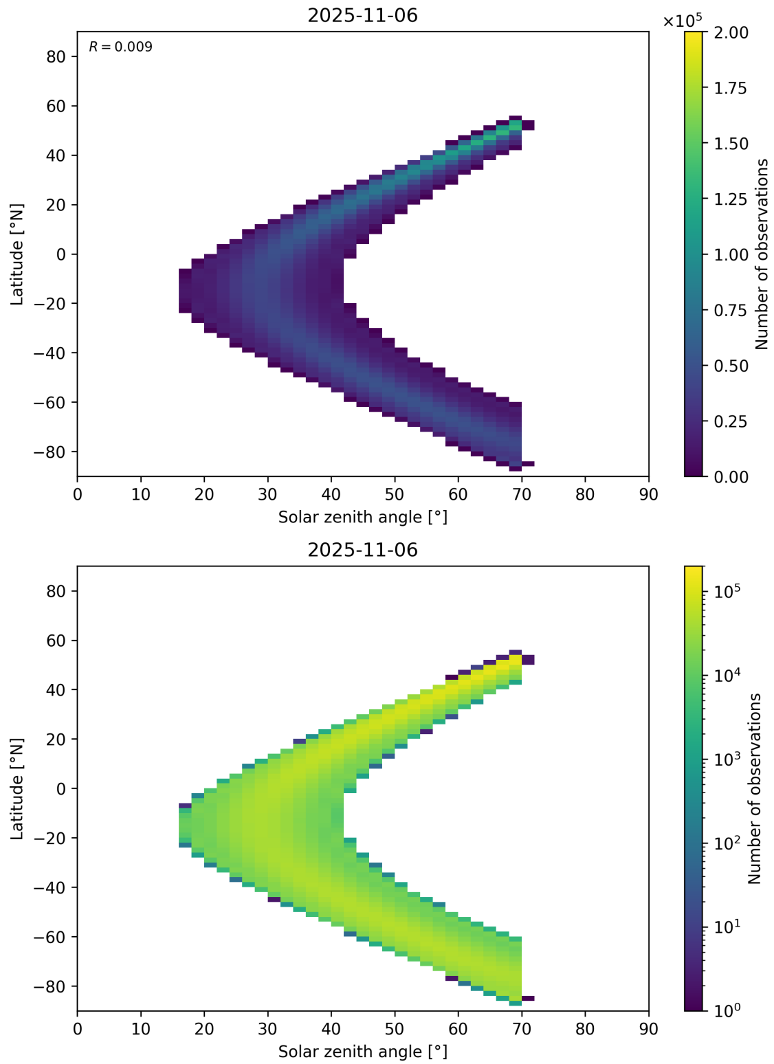
Figure 177: Scatter density plot of “Solar zenith angle” against “Latitude” for 2025-11-05 to 2025-11-07.
