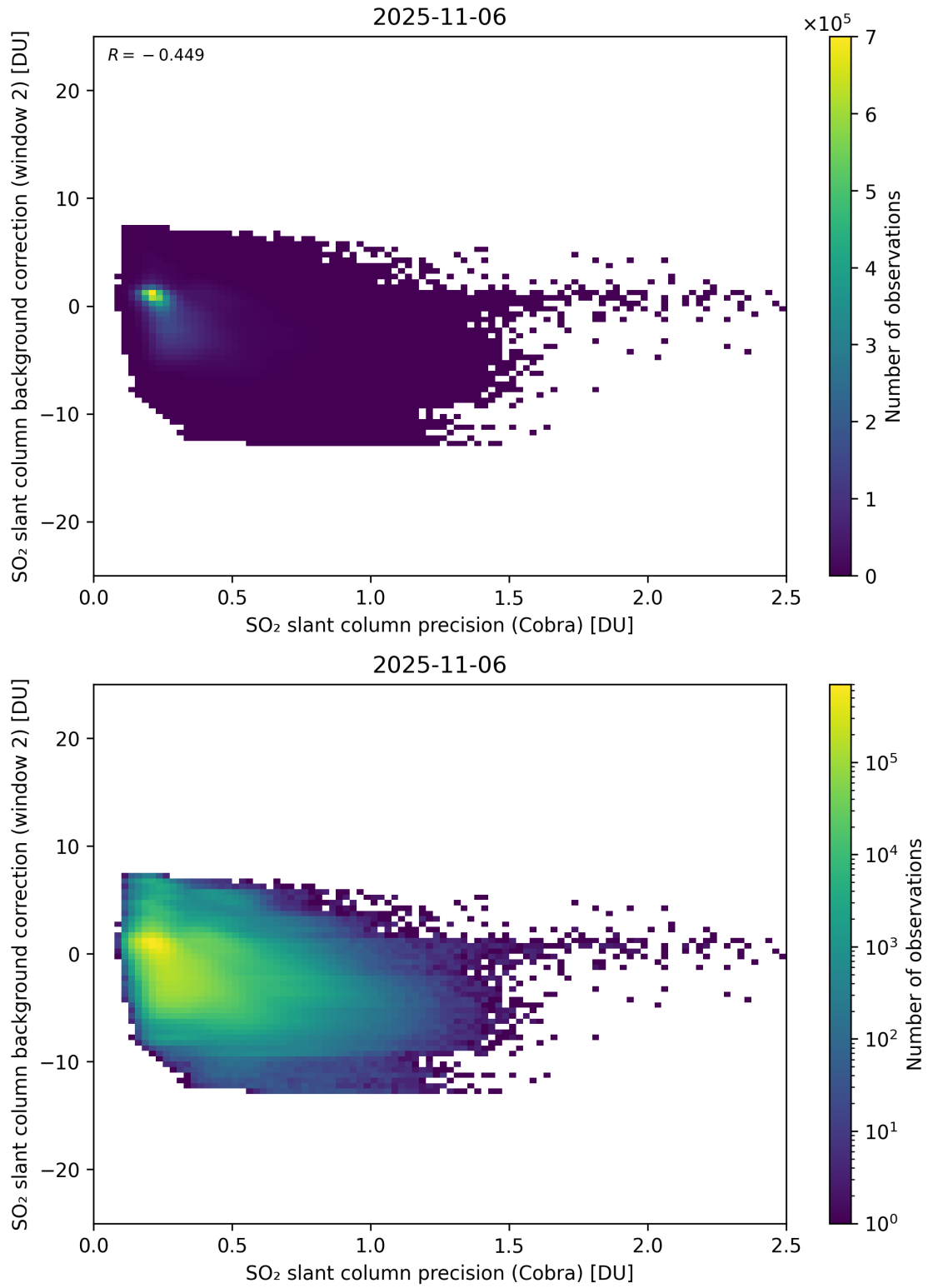
Figure 200: Scatter density plot of “SO 2 slant column precision (Cobra)” against “SO 2 slant column background correction (window 2)” for 2025-11-05 to 2025-11-07.
