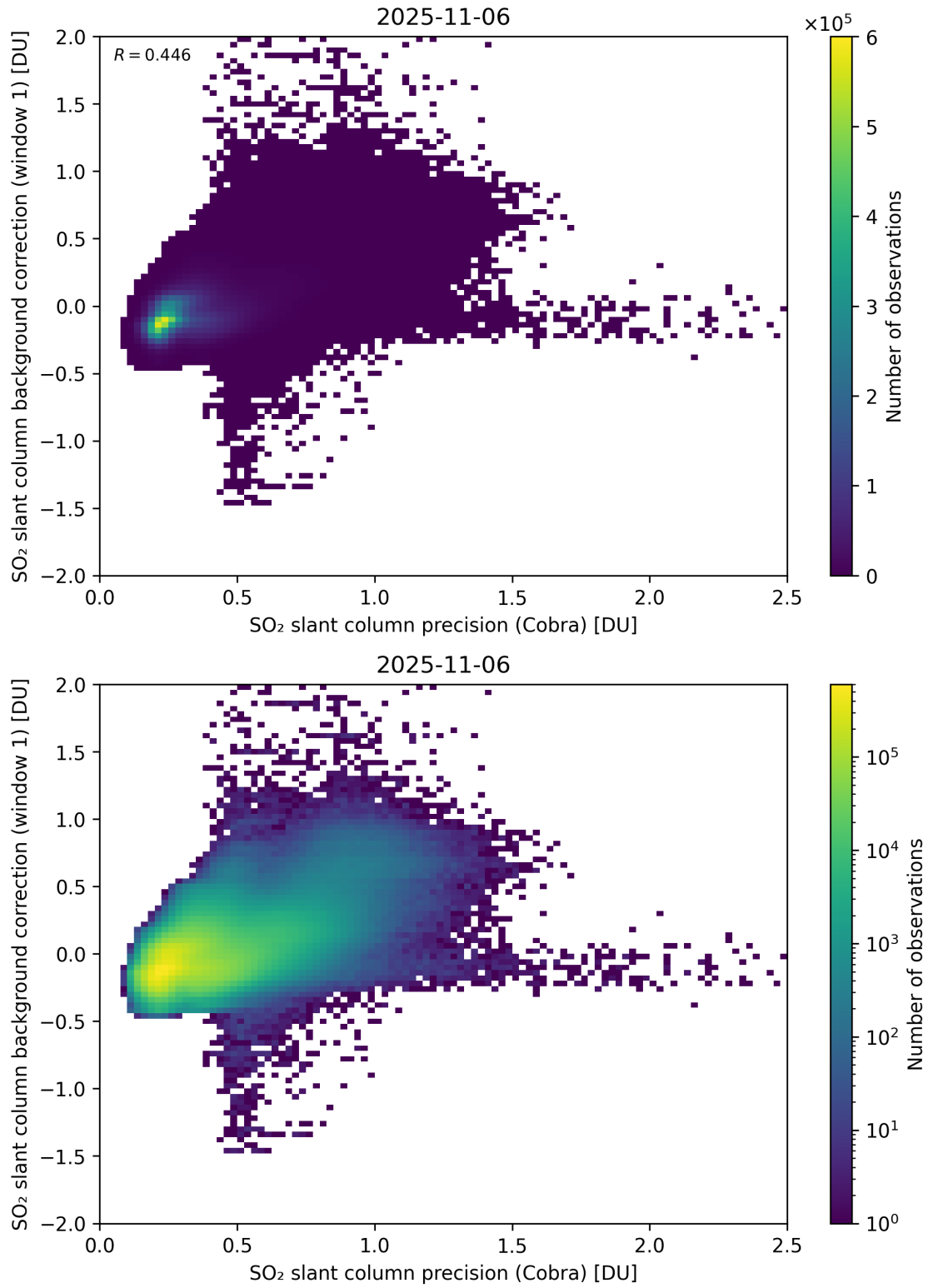
Figure 199: Scatter density plot of “SO 2 slant column precision (Cobra)” against “SO 2 slant column background correction (window 1)” for 2025-11-05 to 2025-11-07.
