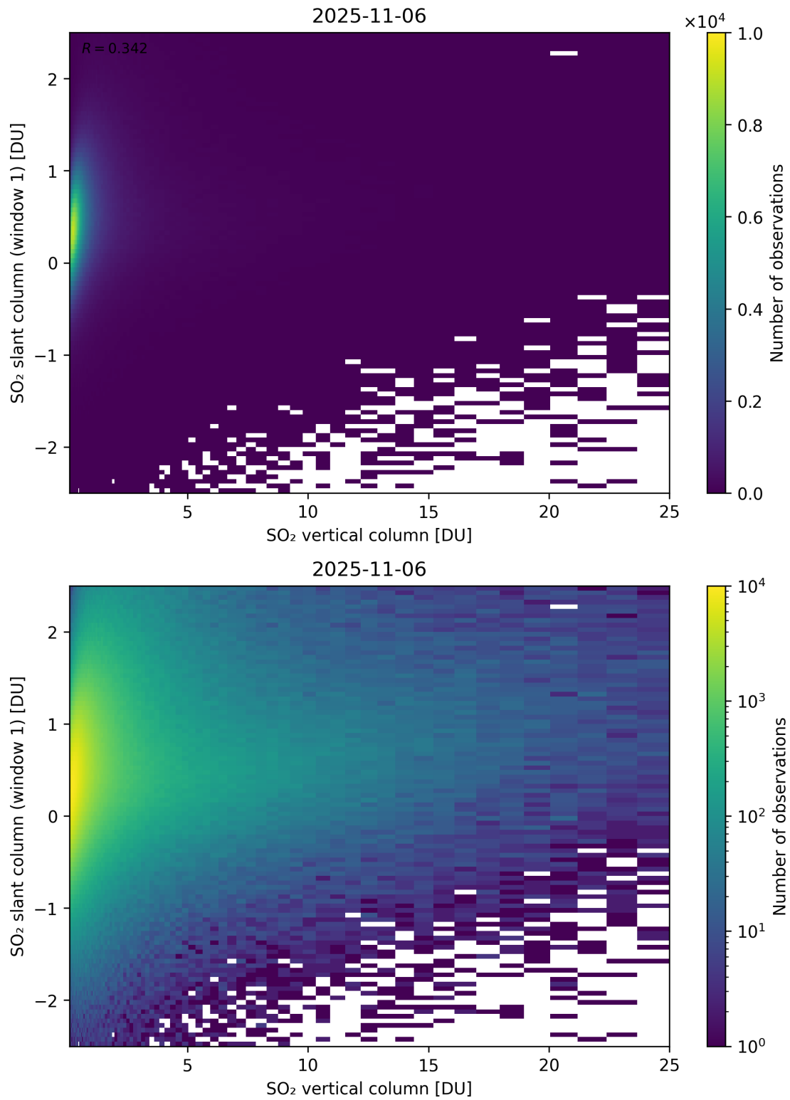
Figure 354: Scatter density plot of “SO 2 vertical column” against “SO 2 slant column (window 1)” for 2025-11-05 to 2025-11-07.
