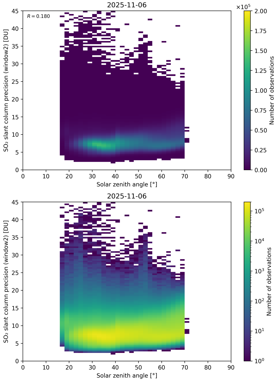
Figure 186: Scatter density plot of “Solar zenith angle” against “SO 2 slant column precision (window2)” for 2025-11-05 to 2025-11-07.
