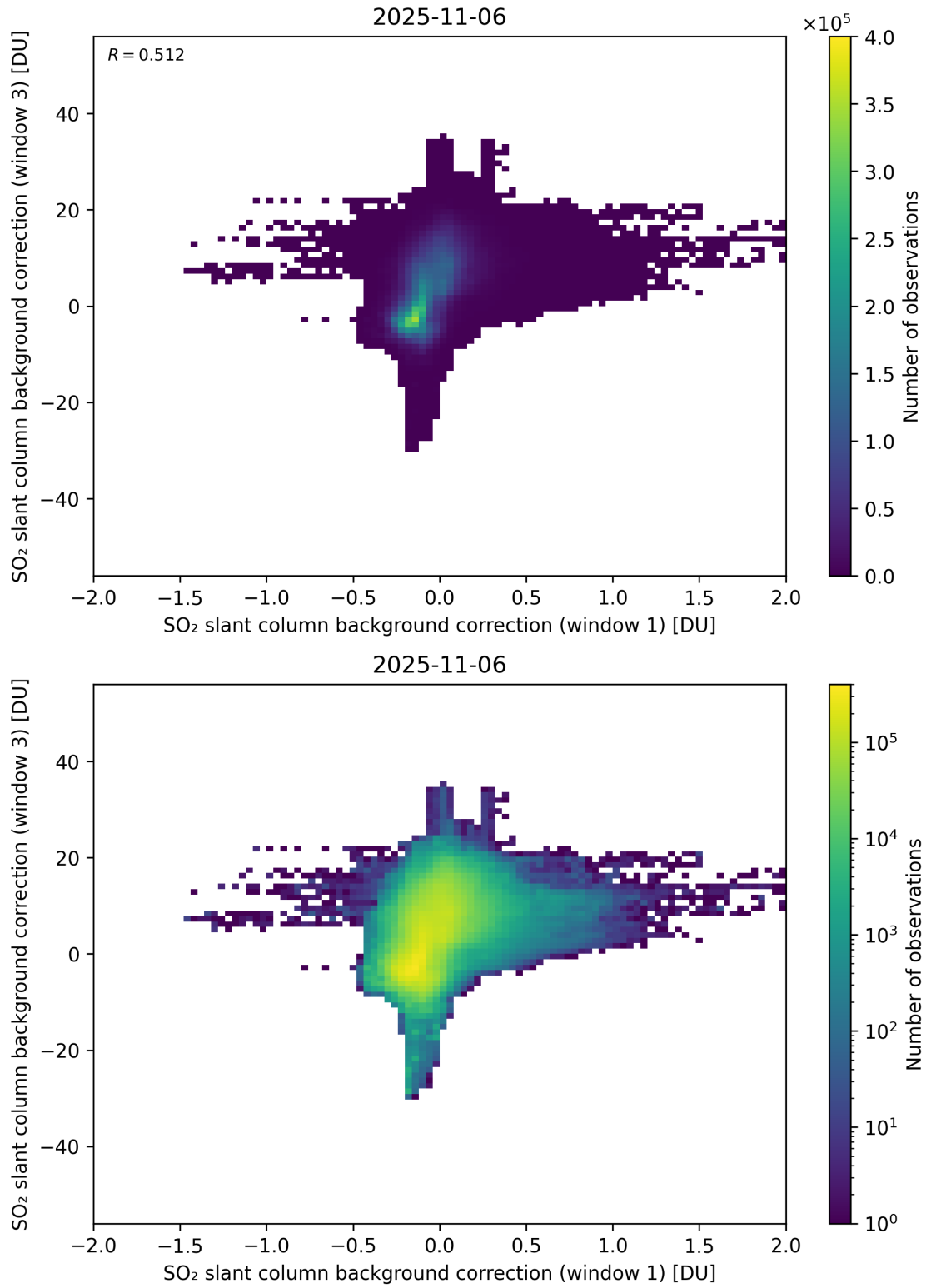
Figure 110: Scatter density plot of “SO 2 slant column background correction (window 1)” against “SO 2 slant column background correction (window 3)” for 2025-11-05 to 2025-11-07.
