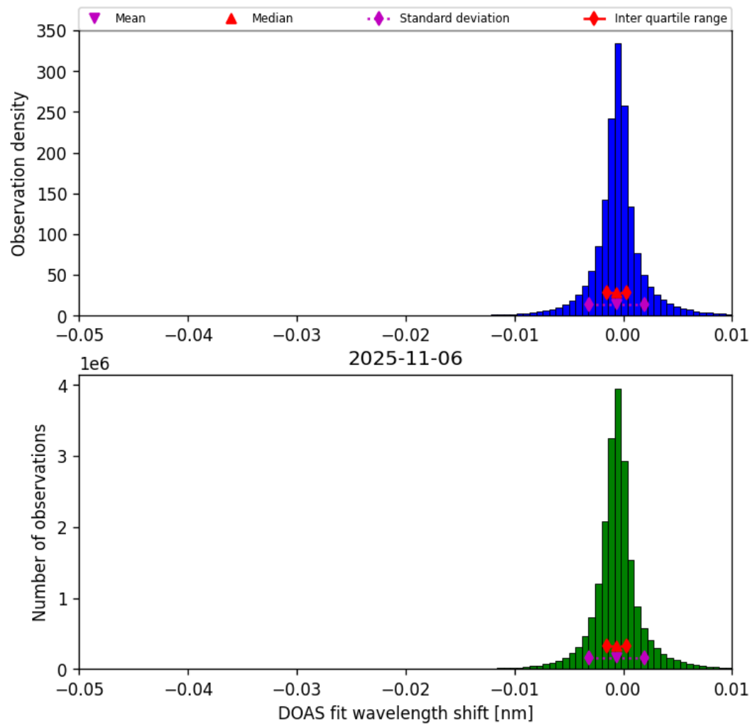
Figure 76: Histogram of “DOAS fit wavelength shift” for 2025-11-05 to 2025-11-07
