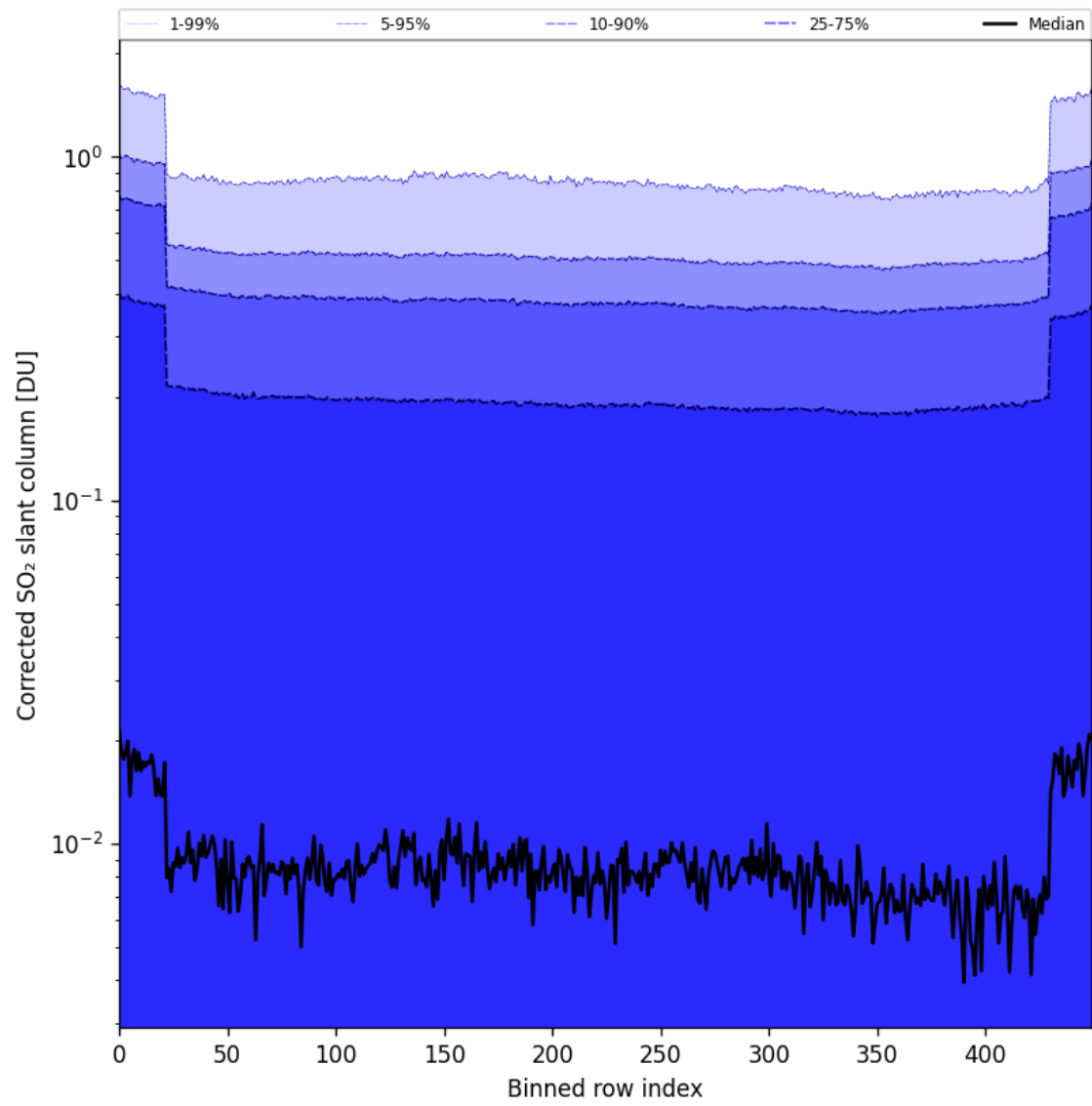
Figure 86: Along track statistics of “Corrected SO 2 slant column” for 2025-11-05 to 2025-11-07
