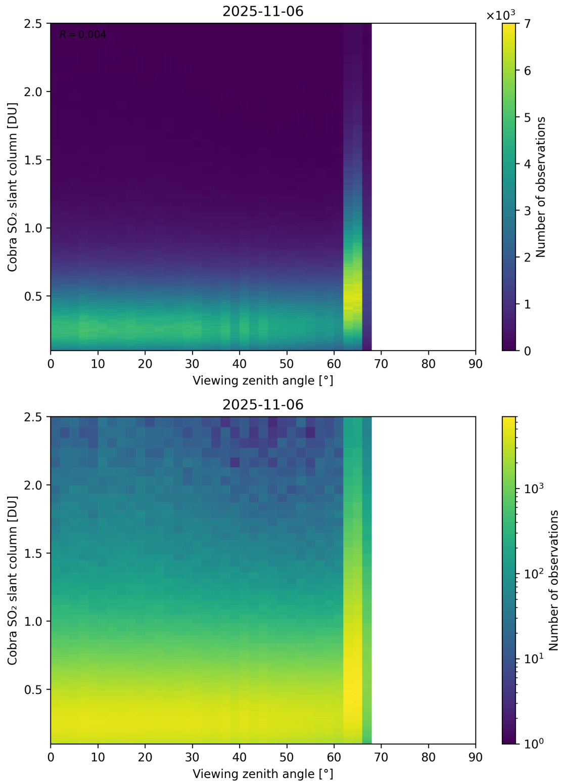
Figure 371: Scatter density plot of “Viewing zenith angle” against “Cobra SO 2 slant column” for 2025-11-05 to 2025-11-07.
