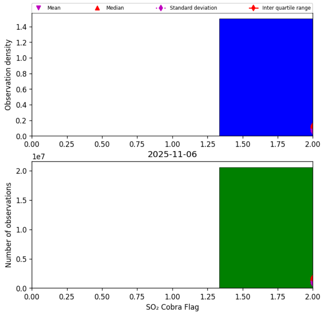
Figure 75: Histogram of “SO 2 Cobra Flag” for 2025-11-05 to 2025-11-07
