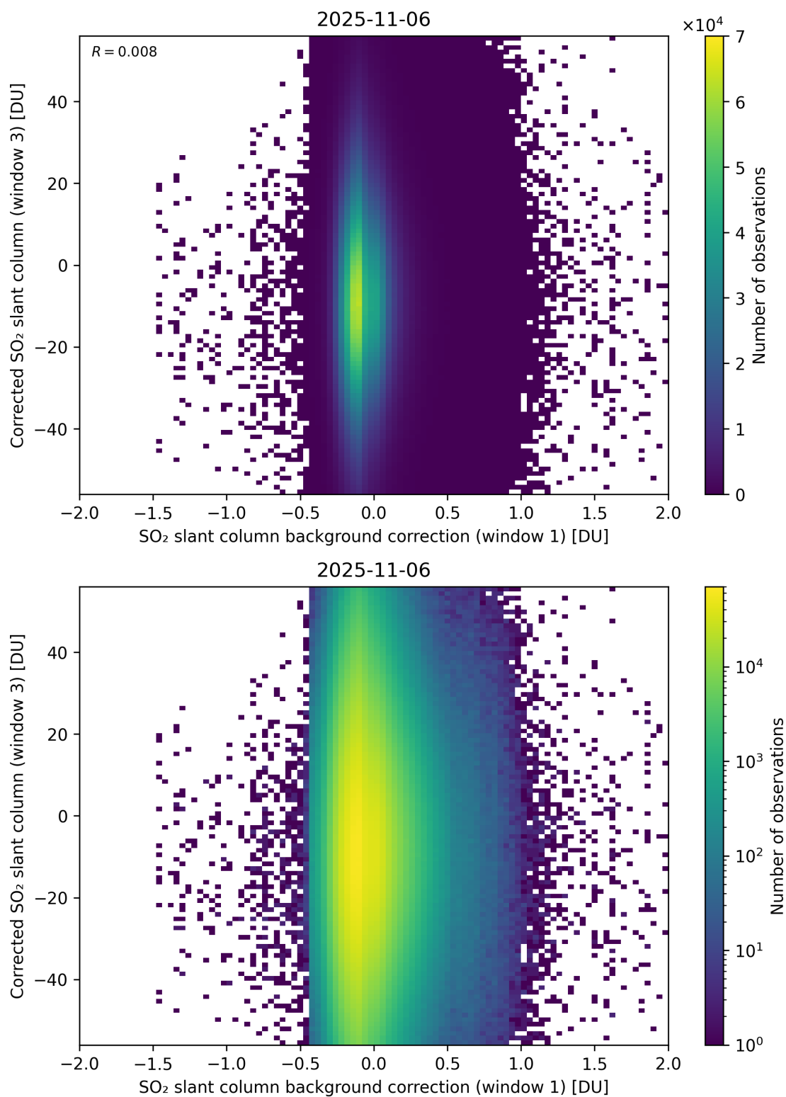
Figure 116: Scatter density plot of “SO 2 slant column background correction (window 1)” against “Corrected SO 2 slant column (window 3)” for 2025-11-05 to 2025-11-07.
