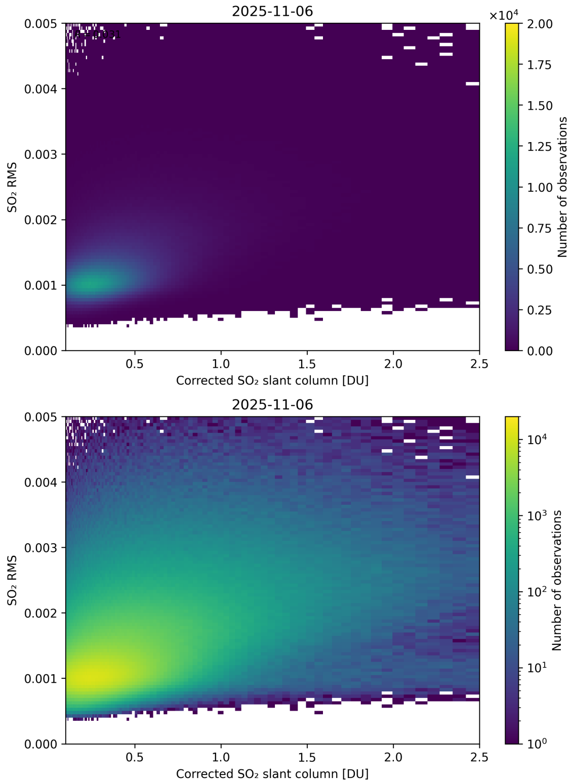
Figure 231: Scatter density plot of “Corrected SO 2 slant column” against “SO 2 RMS” for 2025-11-05 to 2025-11-07.
