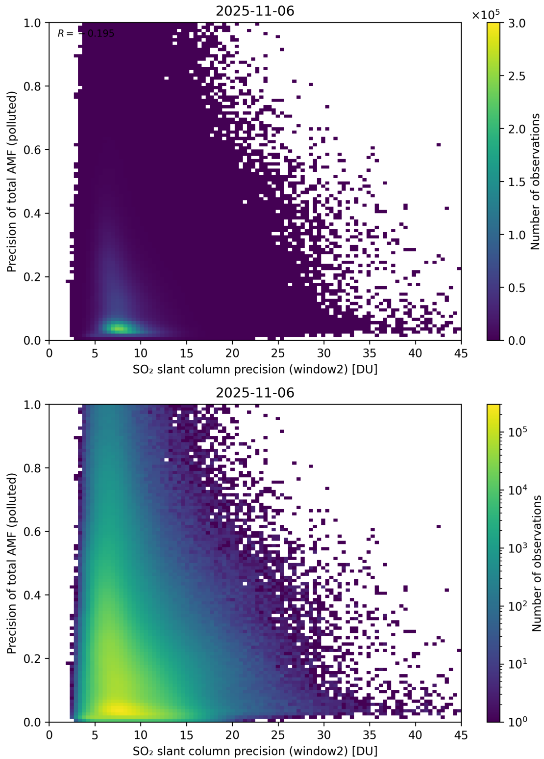
Figure 302: Scatter density plot of “SO 2 slant column precision (window2)” against “Precision of total AMF (polluted)” for 2025-11-05 to 2025-11-07.
