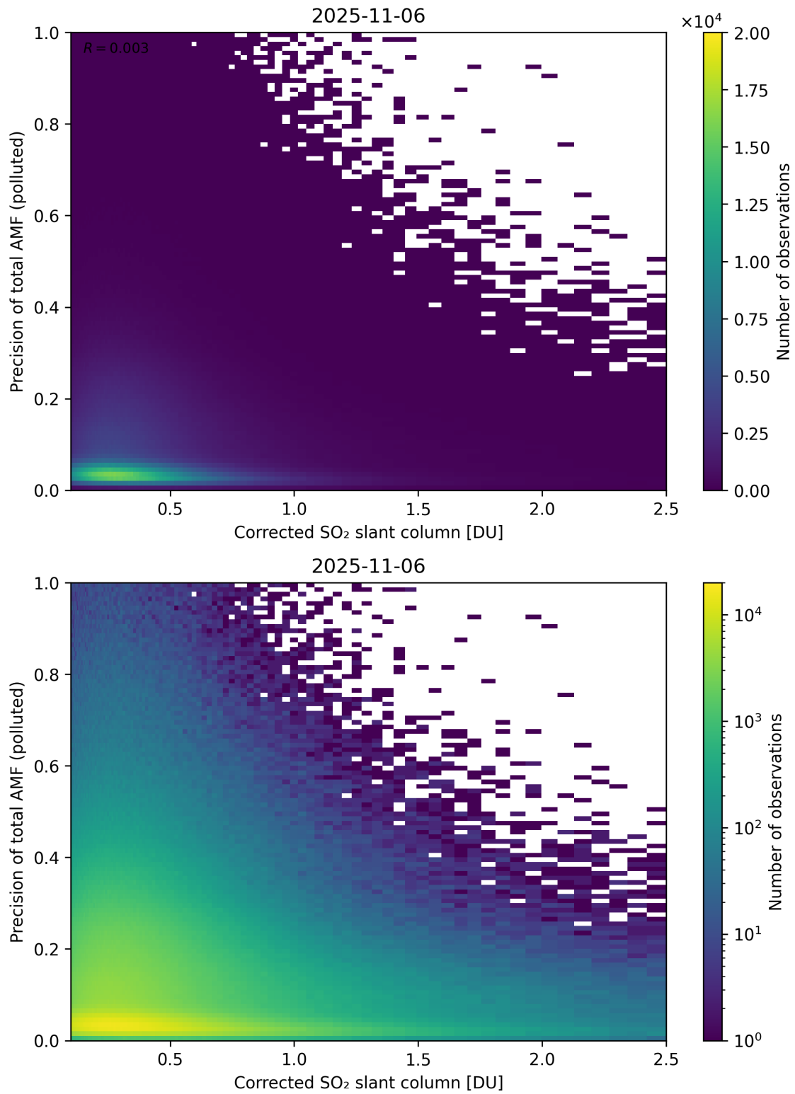
Figure 243: Scatter density plot of “Corrected SO 2 slant column” against “Precision of total AMF (polluted)” for 2025-11-05 to 2025-11-07.
