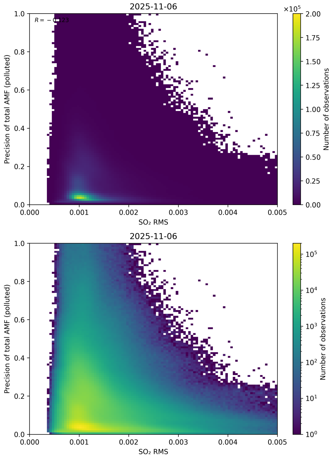
Figure 149: Scatter density plot of “SO 2 RMS” against “Precision of total AMF (polluted)” for 2025-11-05 to 2025-11-07.
