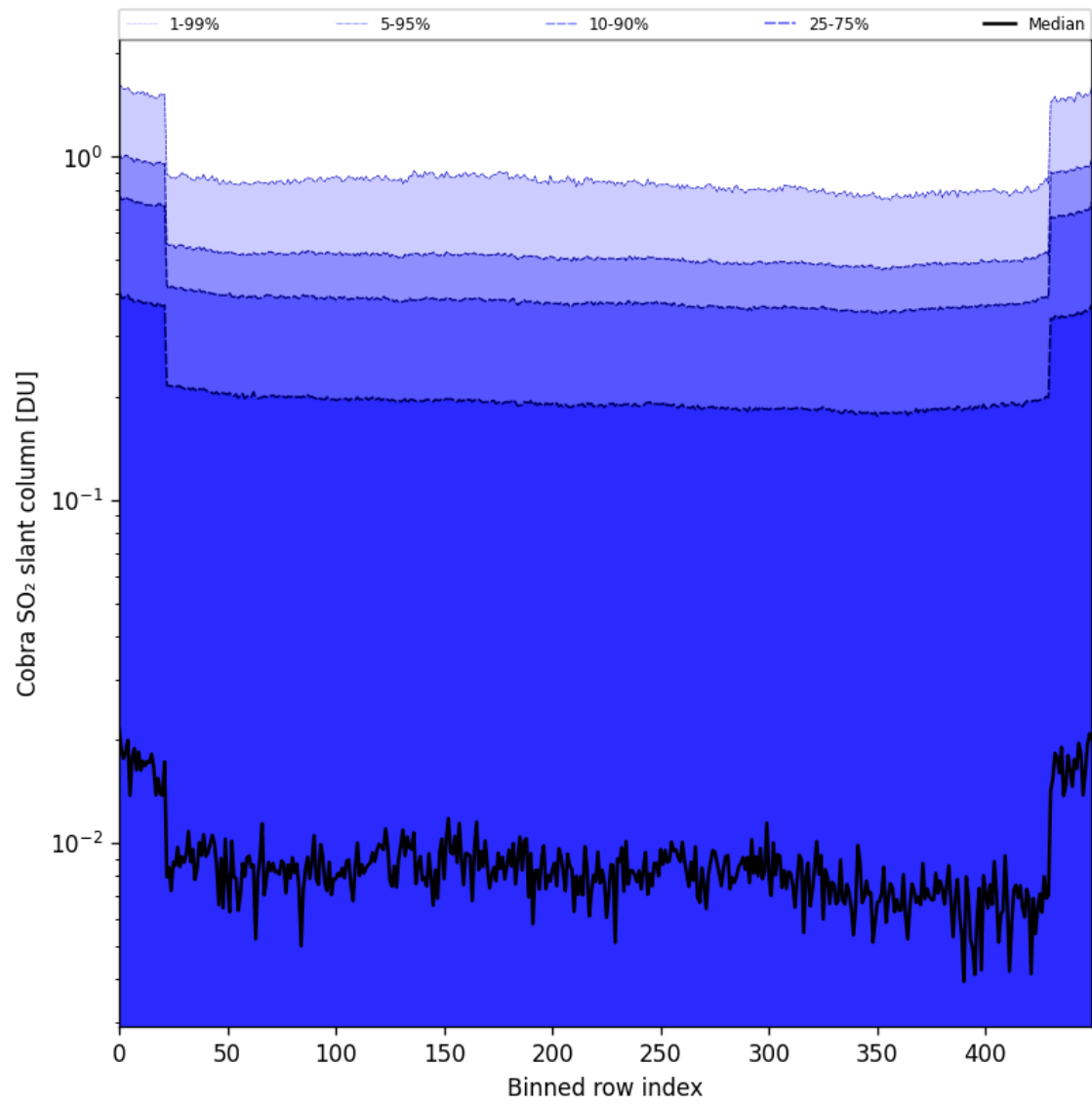
Figure 87: Along track statistics of "Cobra SO 2 slant column" for 2025-11-05 to 2025-11-07
