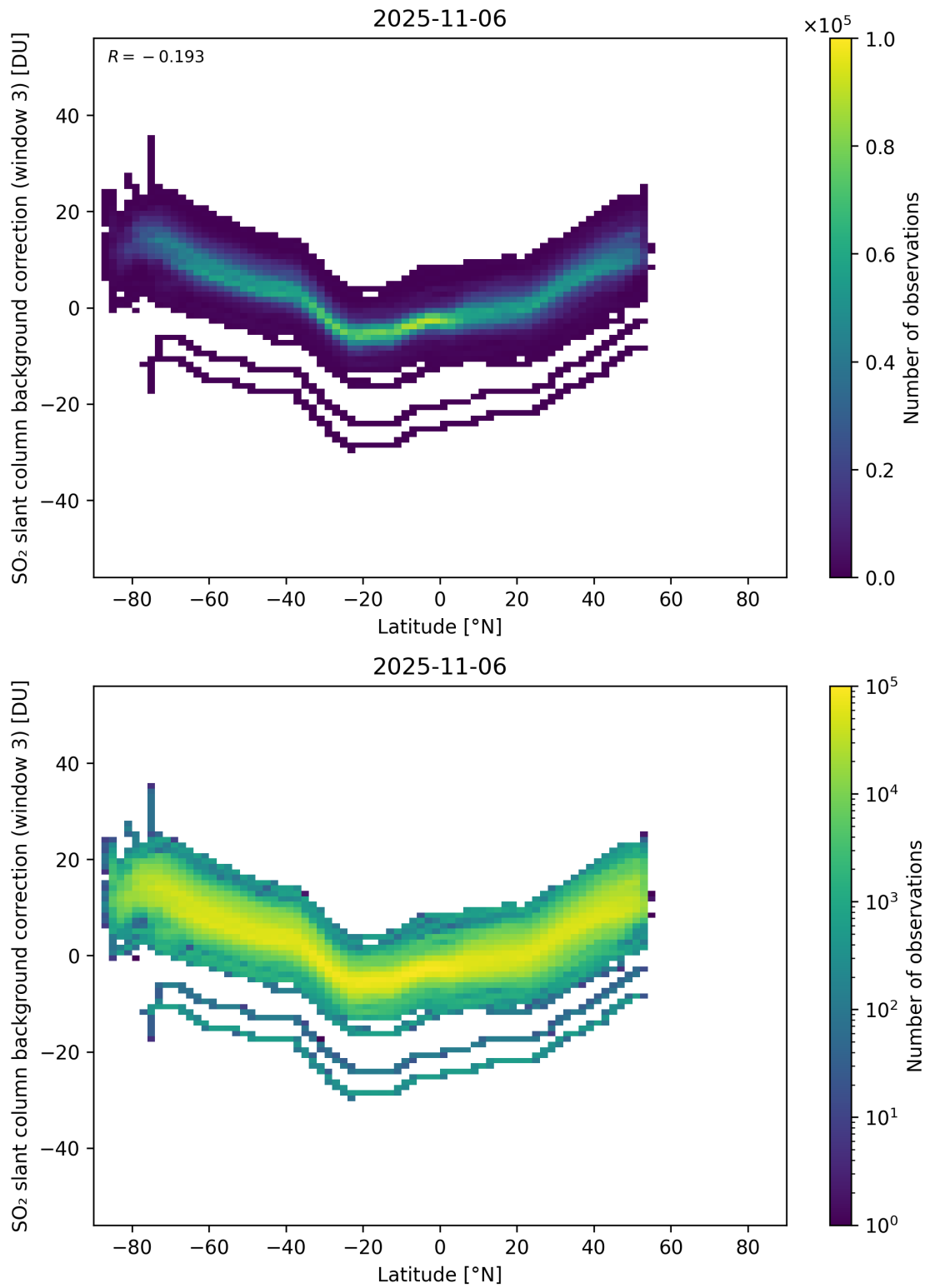
Figure 152: Scatter density plot of “Latitude” against “SO 2 slant column background correction (window 3)” for 2025-11-05 to 2025-11-07.
