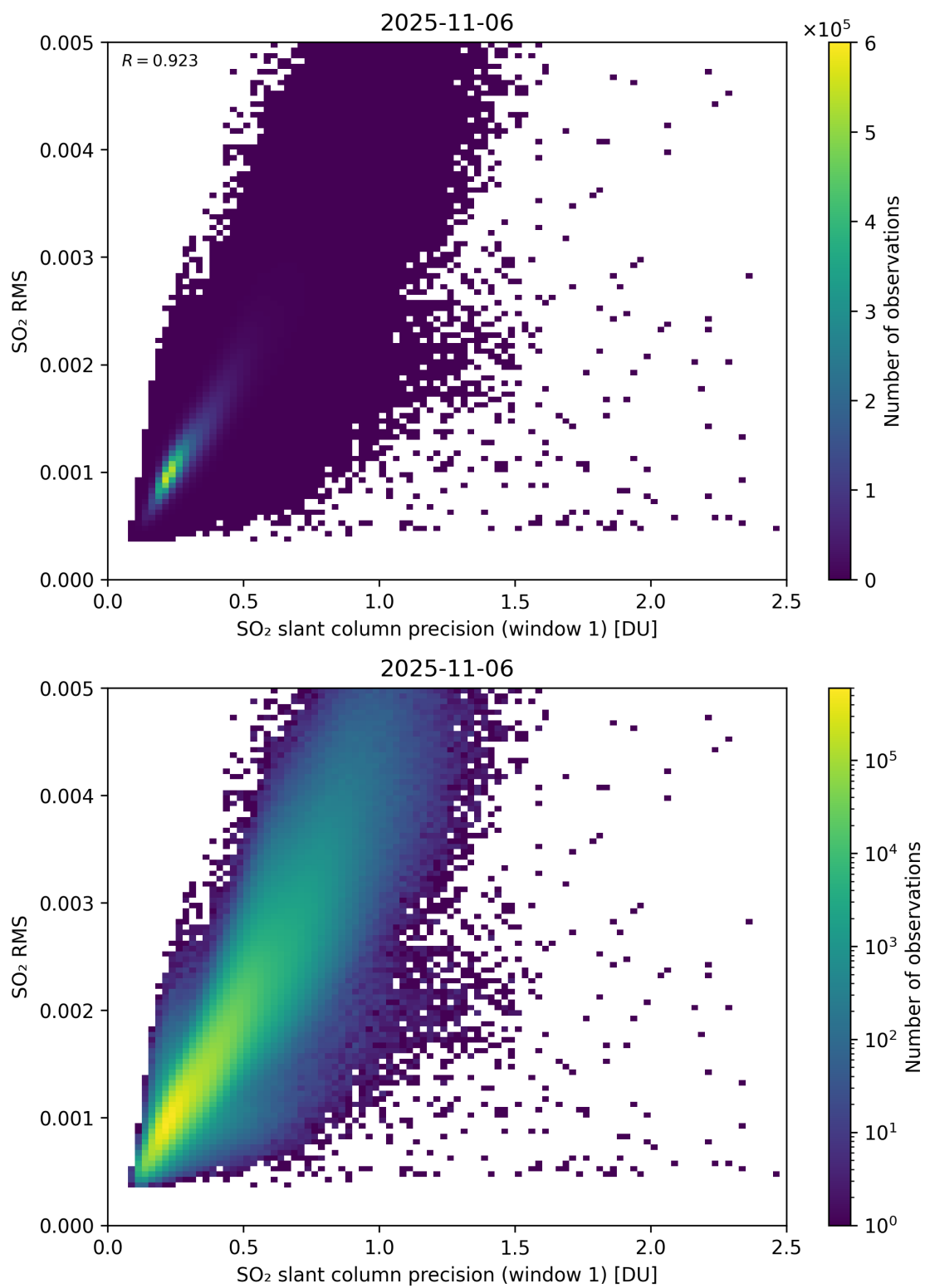
Figure 273: Scatter density plot of “SO 2 slant column precision (window 1)” against “SO 2 RMS” for 2025-11-05 to 2025-11-07.
