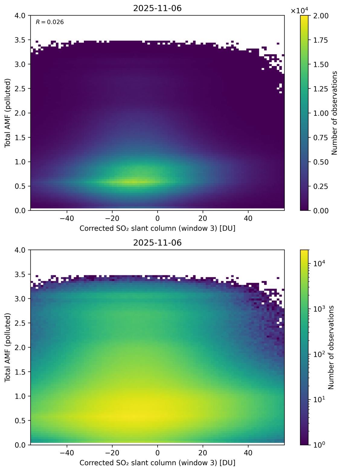
Figure 260: Scatter density plot of “Corrected SO 2 slant column (window 3)” against “Total AMF (polluted)” for 2025-11-05 to 2025-11-07.
