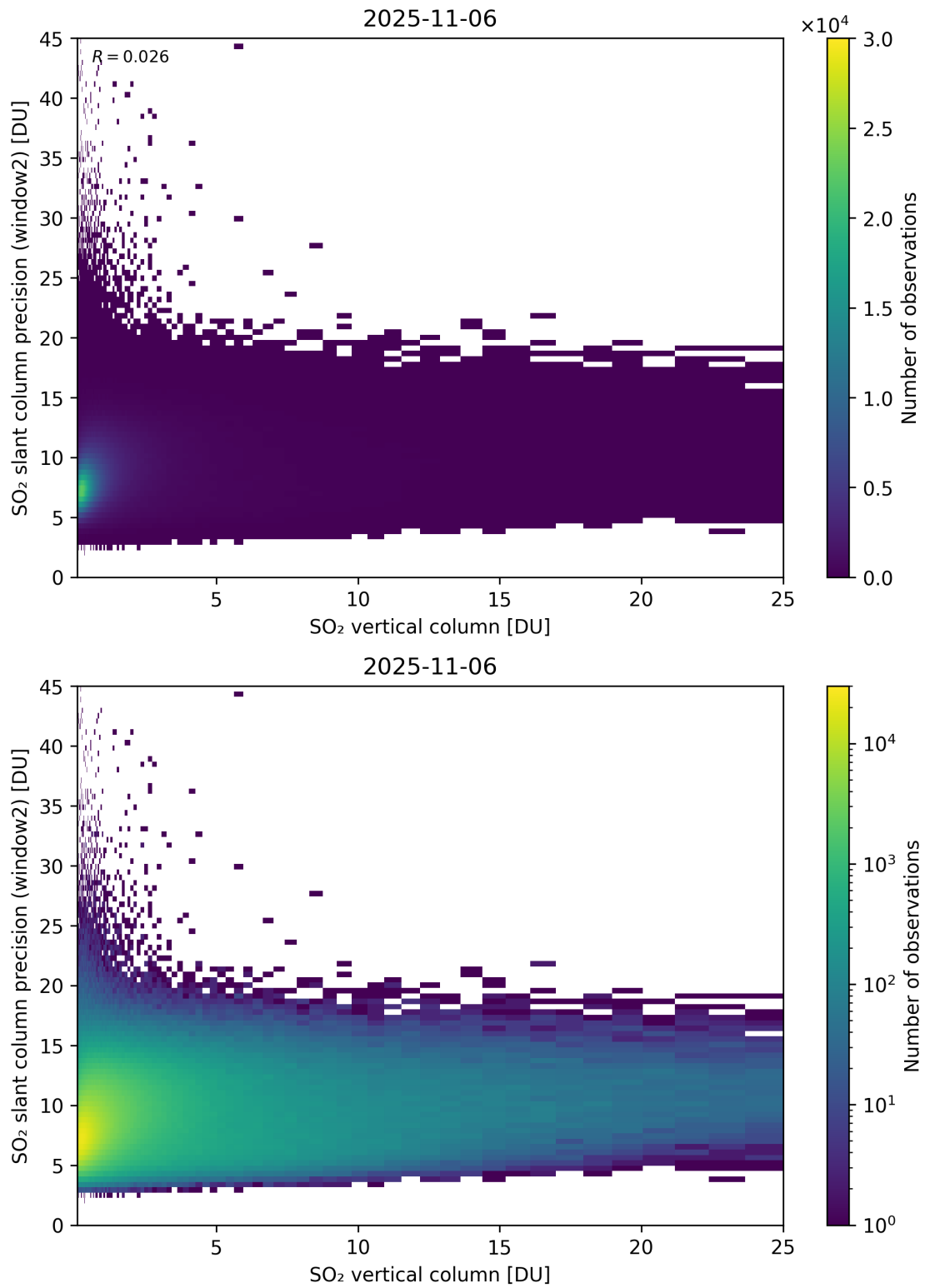
Figure 356: Scatter density plot of “SO 2 vertical column” against “SO 2 slant column precision (window2)” for 2025-11-05 to 2025-11-07.
