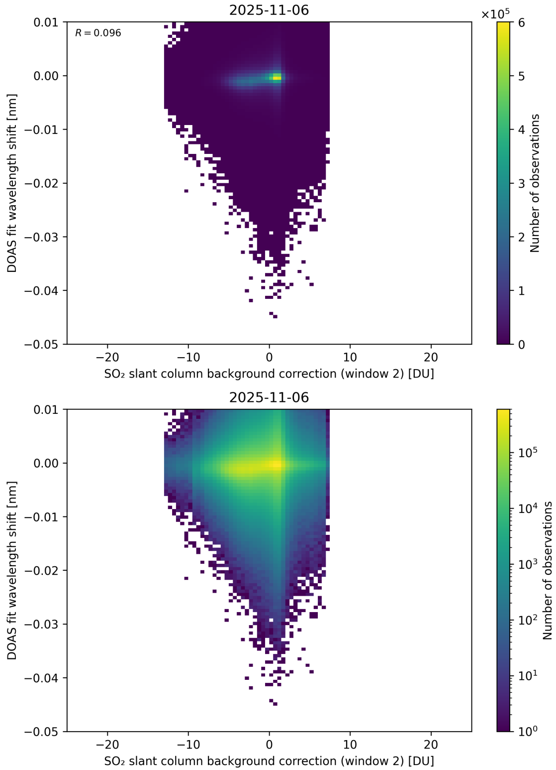
Figure 123: Scatter density plot of “SO 2 slant column background correction (window 2)” against “DOAS fit wavelength shift” for 2025-11-05 to 2025-11-07.
