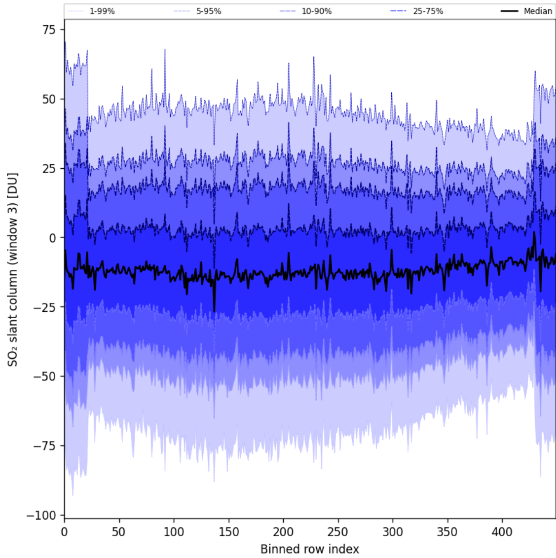
Figure 97: Along track statistics of “SO 2 slant column (window 3)” for 2025-11-05 to 2025-11-07
