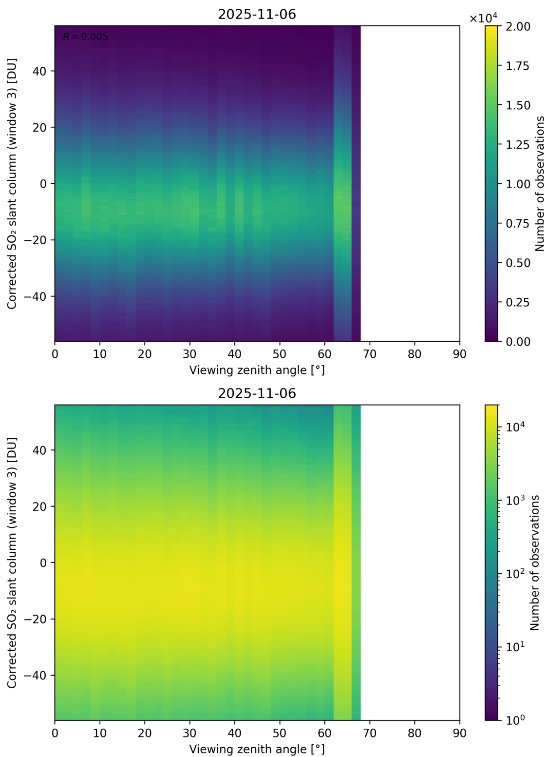
Figure 375: Scatter density plot of “Viewing zenith angle” against “Corrected SO 2 slant column (window 3)” for 2025-11-05 to 2025-11-07.
