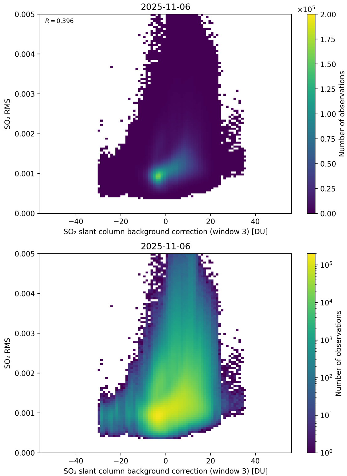
Figure 134: Scatter density plot of “SO 2 slant column background correction (window 3)” against “SO 2 RMS” for 2025-11-05 to 2025-11-07.
