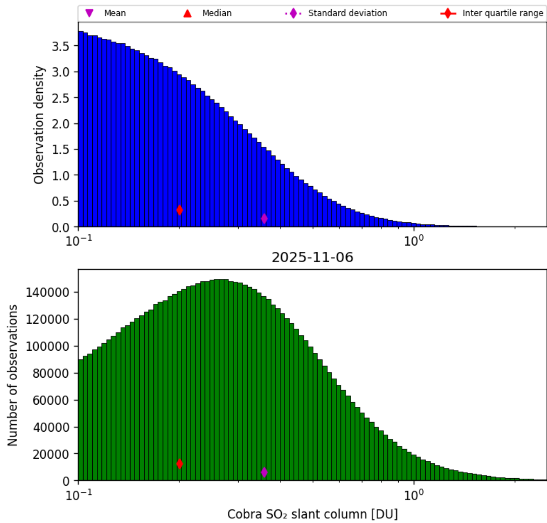
Figure 61: Histogram of “Cobra SO 2 slant column” for 2025-11-05 to 2025-11-07
