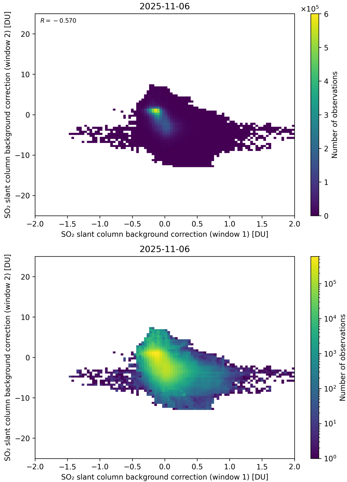
Figure 109: Scatter density plot of “SO 2 slant column background correction (window 1)” against “SO 2 slant column background correction (window 2)” for 2025-11-05 to 2025-11-07.
