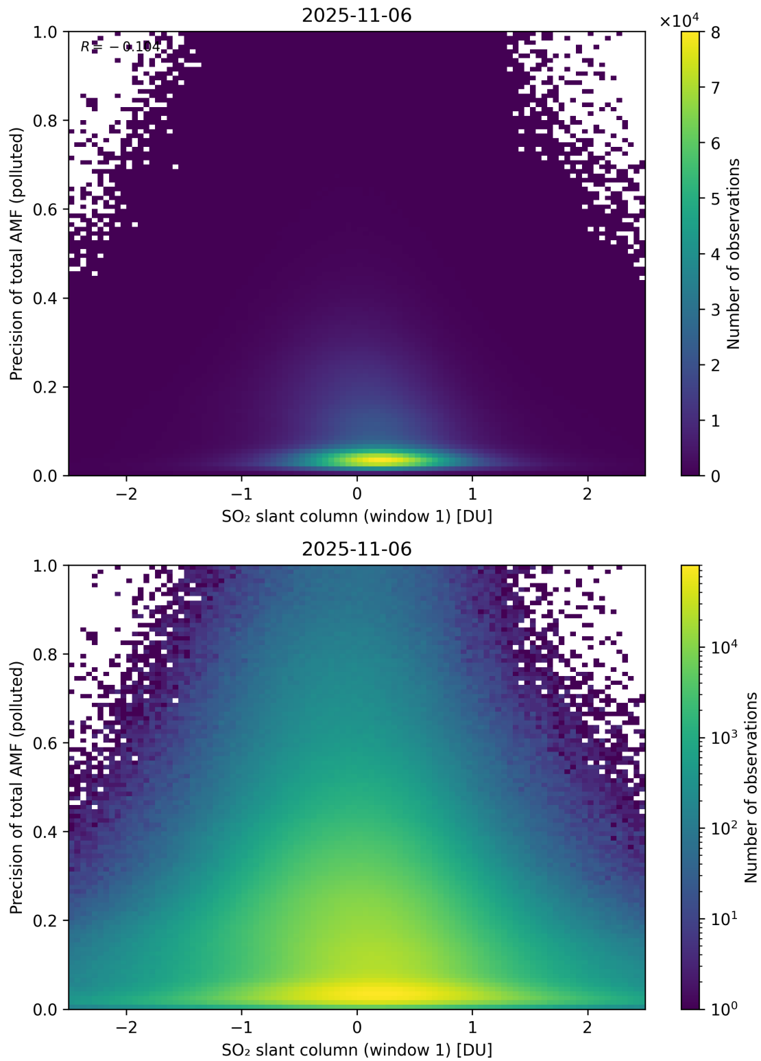
Figure 290: Scatter density plot of “SO 2 slant column (window 1)” against “Precision of total AMF (polluted)” for 2025-11-05 to 2025-11-07.
