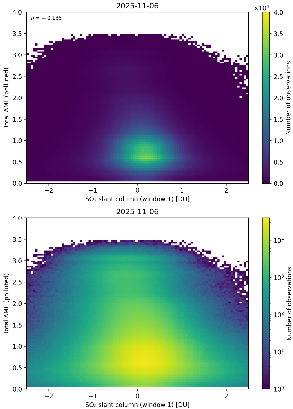
Figure 289: Scatter density plot of “SO 2 slant column (window 1)” against “Total AMF (polluted)” for 2025-11-05 to 2025-11-07.
