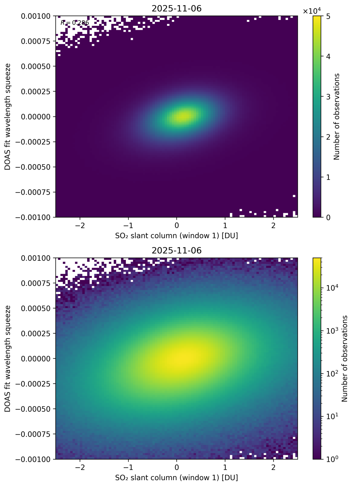
Figure 266: Scatter density plot of “SO 2 slant column (window 1)” against “DOAS fit wavelength squeeze” for 2025-11-05 to 2025-11-07.
