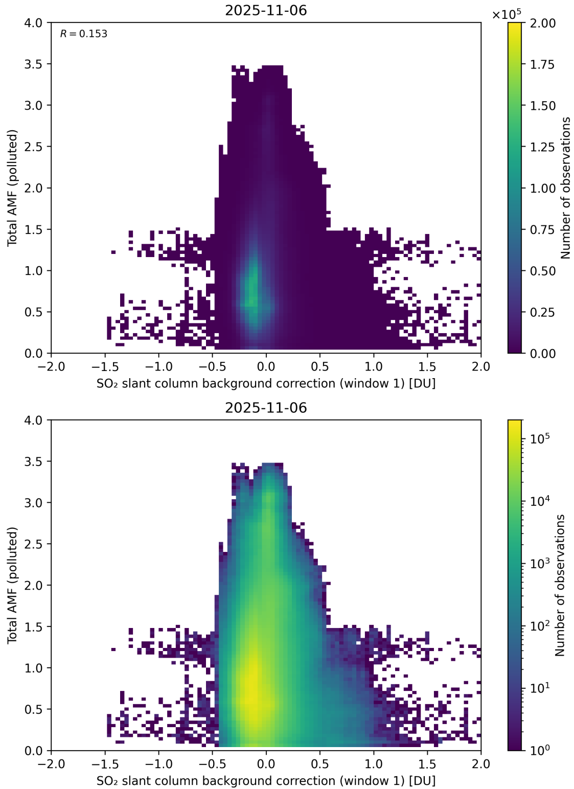
Figure 120: Scatter density plot of “SO 2 slant column background correction (window 1)” against “Total AMF (polluted)” for 2025-11-05 to 2025-11-07.
