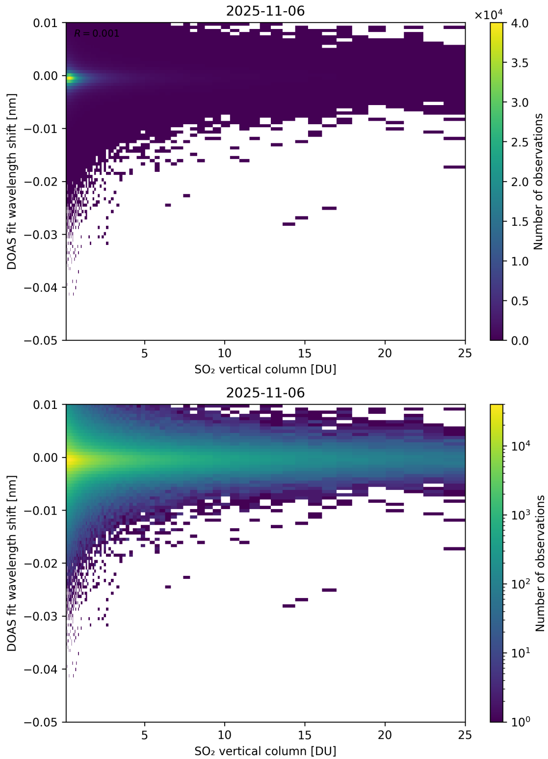
Figure 326: Scatter density plot of “SO 2 vertical column” against “DOAS fit wavelength shift” for 2025-11-05 to 2025-11-07.
