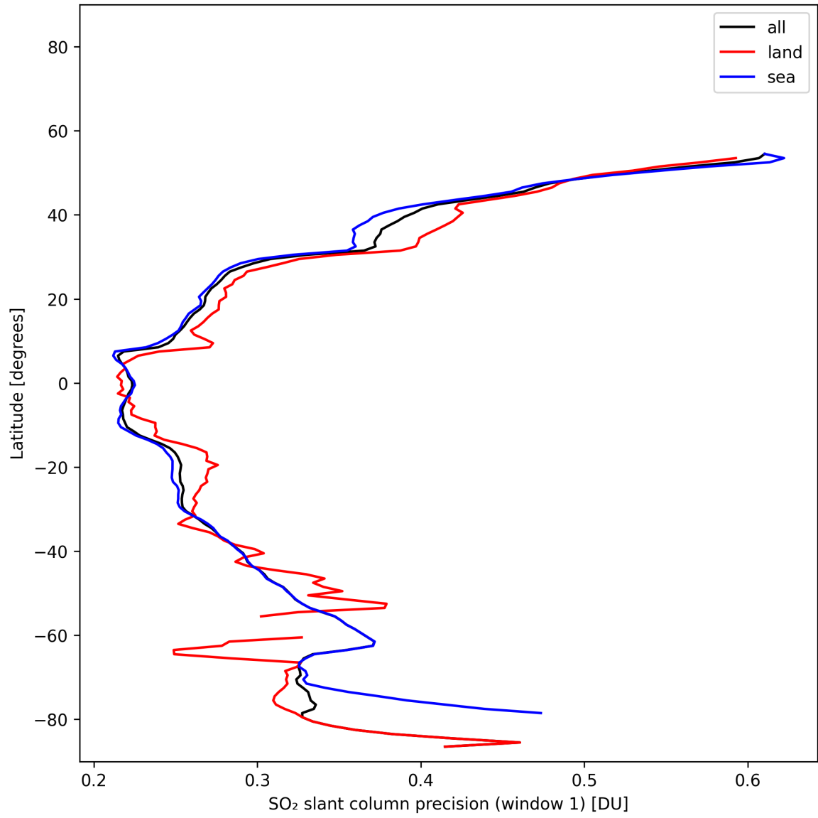
Figure 38: Zonal average of “SO 2 slant column precision (window 1)” for 2025-11-05 to 2025-11-07.
