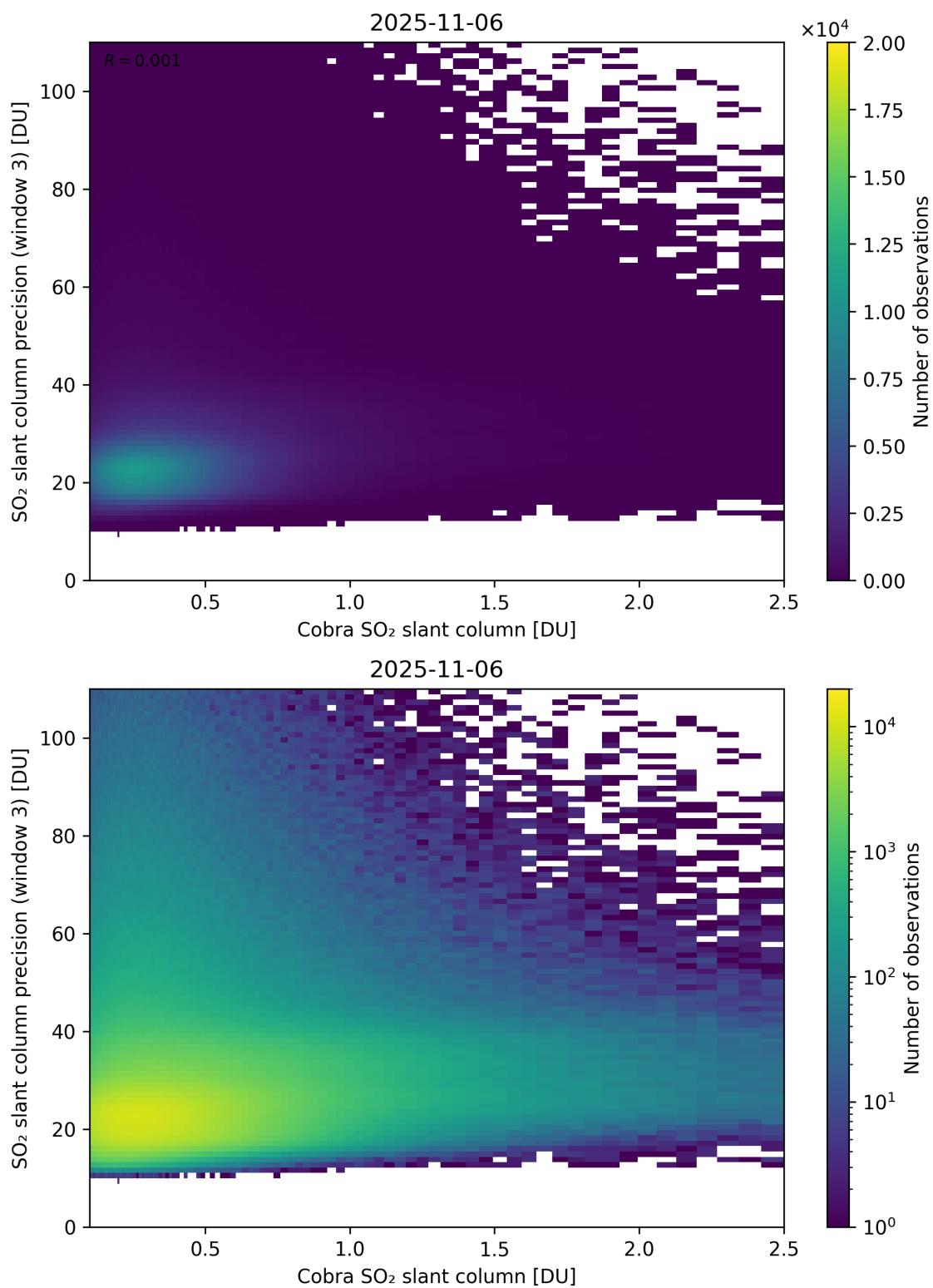
Figure 223: Scatter density plot of “Cobra SO 2 slant column” against “SO 2 slant column precision (window 3)” for 2025-11-05 to 2025-11-07.
