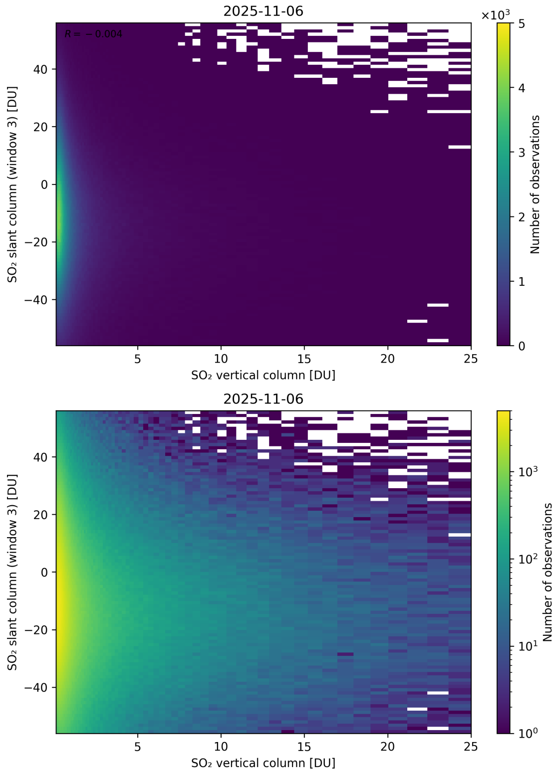
Figure 357: Scatter density plot of “SO 2 vertical column” against “SO 2 slant column (window 3)” for 2025-11-05 to 2025-11-07.
