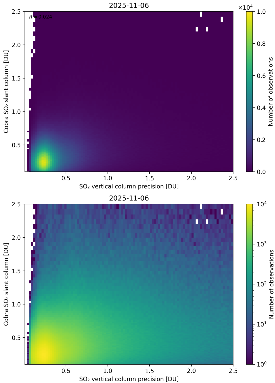
Figure 336: Scatter density plot of “SO 2 vertical column precision” against “Cobra SO 2 slant column” for 2025-11-05 to 2025-11-07.
