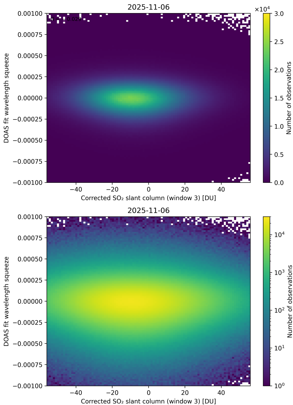
Figure 257: Scatter density plot of “Corrected SO 2 slant column (window 3)” against “DOAS fit wavelength squeeze” for 2025-11-05 to 2025-11-07.
