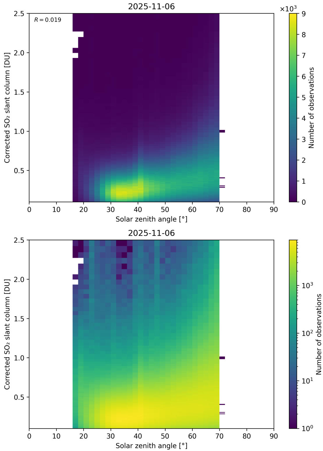
Figure 181: Scatter density plot of “Solar zenith angle” against “Corrected SO 2 slant column” for 2025-11-05 to 2025-11-07.
