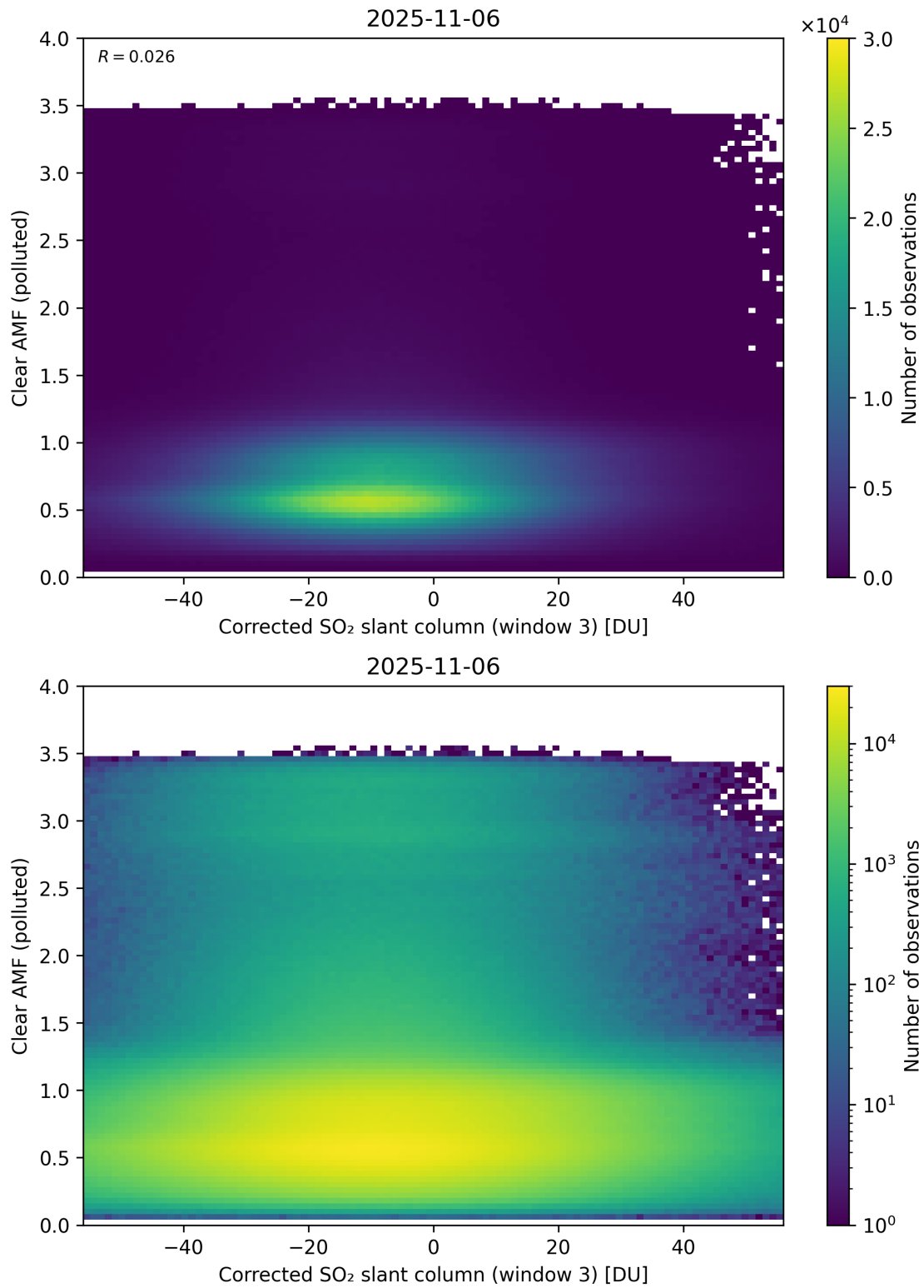
Figure 259: Scatter density plot of “Corrected SO 2 slant column (window 3)” against “Clear AMF (polluted)” for 2025-11-05 to 2025-11-07.
