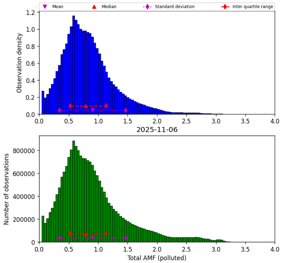
Figure 79: Histogram of “Total AMF (polluted)” for 2025-11-05 to 2025-11-07
