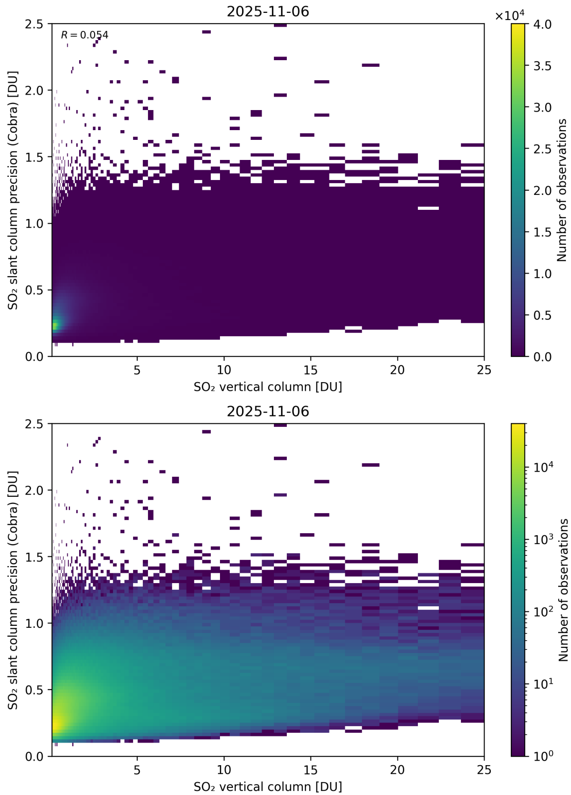
Figure 350: Scatter density plot of “SO 2 vertical column” against “SO 2 slant column precision (Cobra)” for 2025-11-05 to 2025-11-07.
