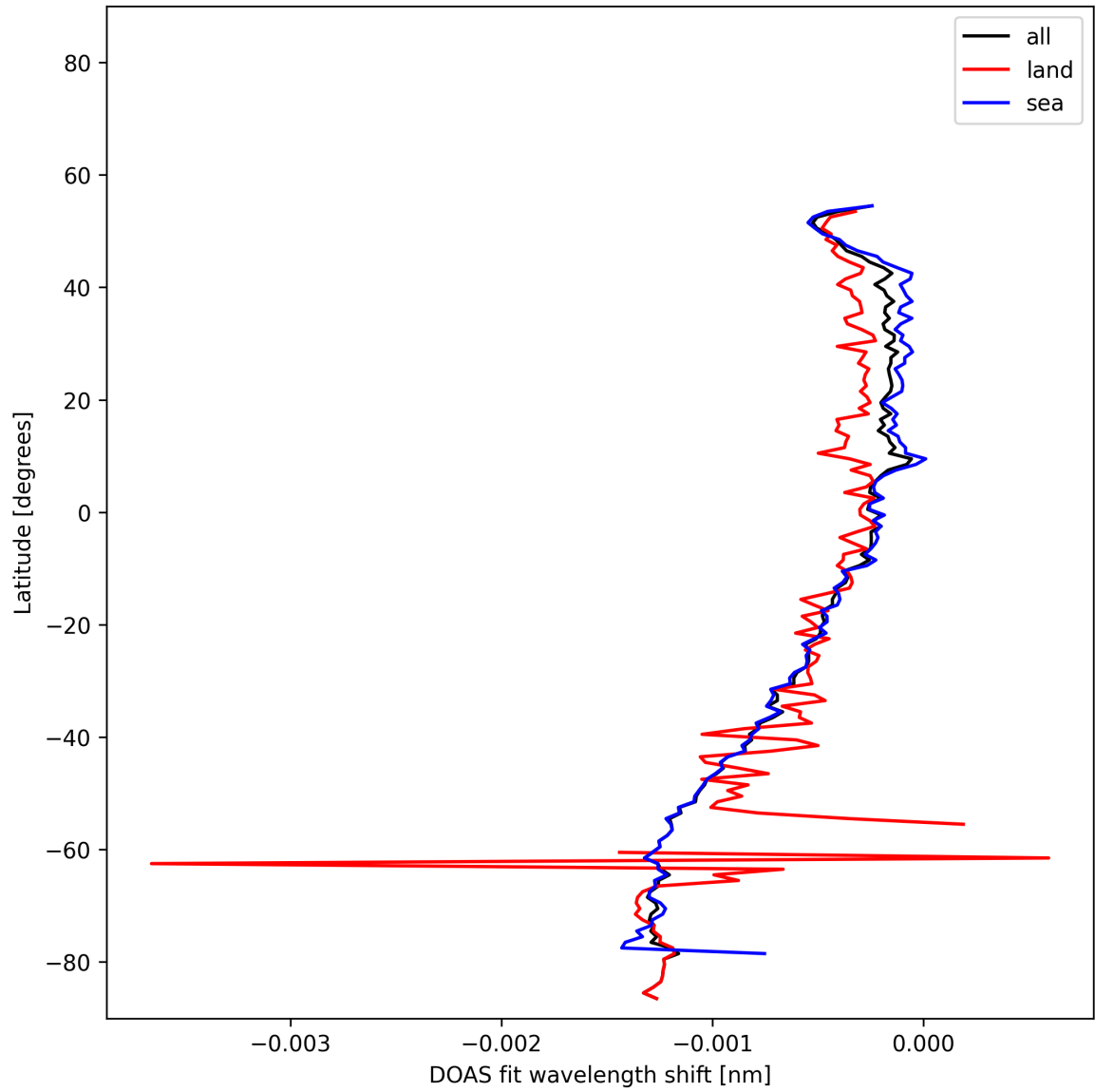
Figure 50: Zonal average of “DOAS fit wavelength shift” for 2025-11-05 to 2025-11-07.
