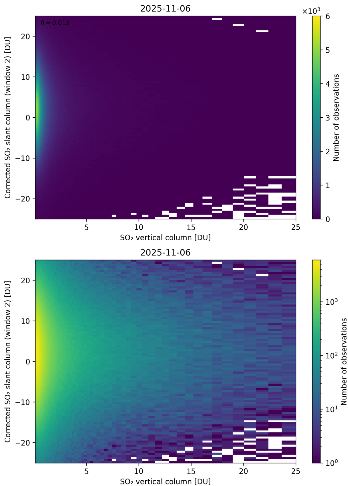
Figure 352: Scatter density plot of “SO 2 vertical column” against “Corrected SO 2 slant column (window 2)” for 2025-11-05 to 2025-11-07.
