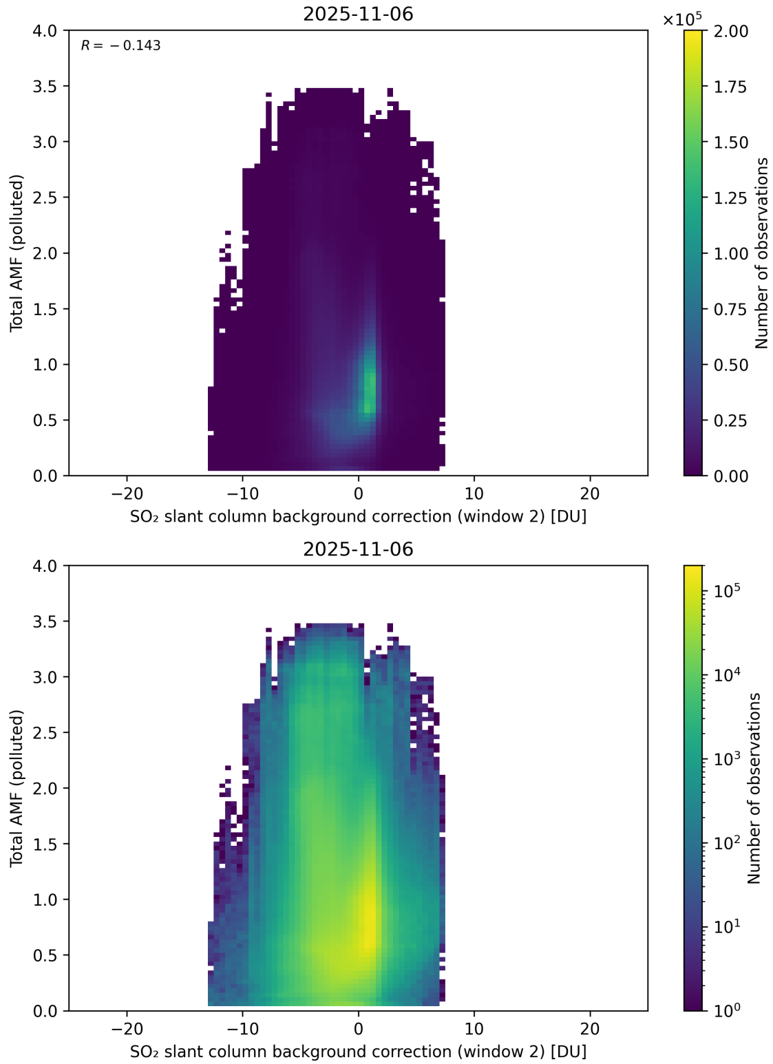
Figure 130: Scatter density plot of “SO 2 slant column background correction (window 2)” against “Total AMF (polluted)” for 2025-11-05 to 2025-11-07.
