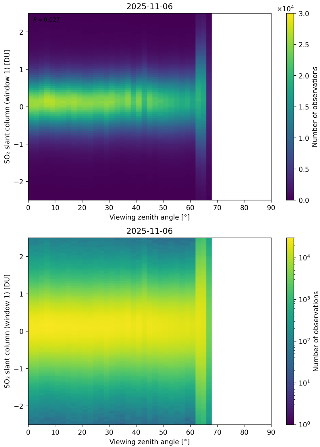
Figure 376: Scatter density plot of “Viewing zenith angle” against “SO 2 slant column (window 1)” for 2025-11-05 to 2025-11-07.
