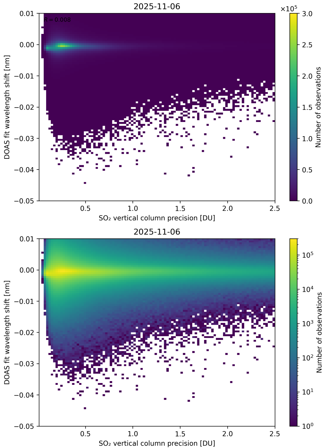
Figure 332: Scatter density plot of “SO 2 vertical column precision” against “DOAS fit wavelength shift” for 2025-11-05 to 2025-11-07.
