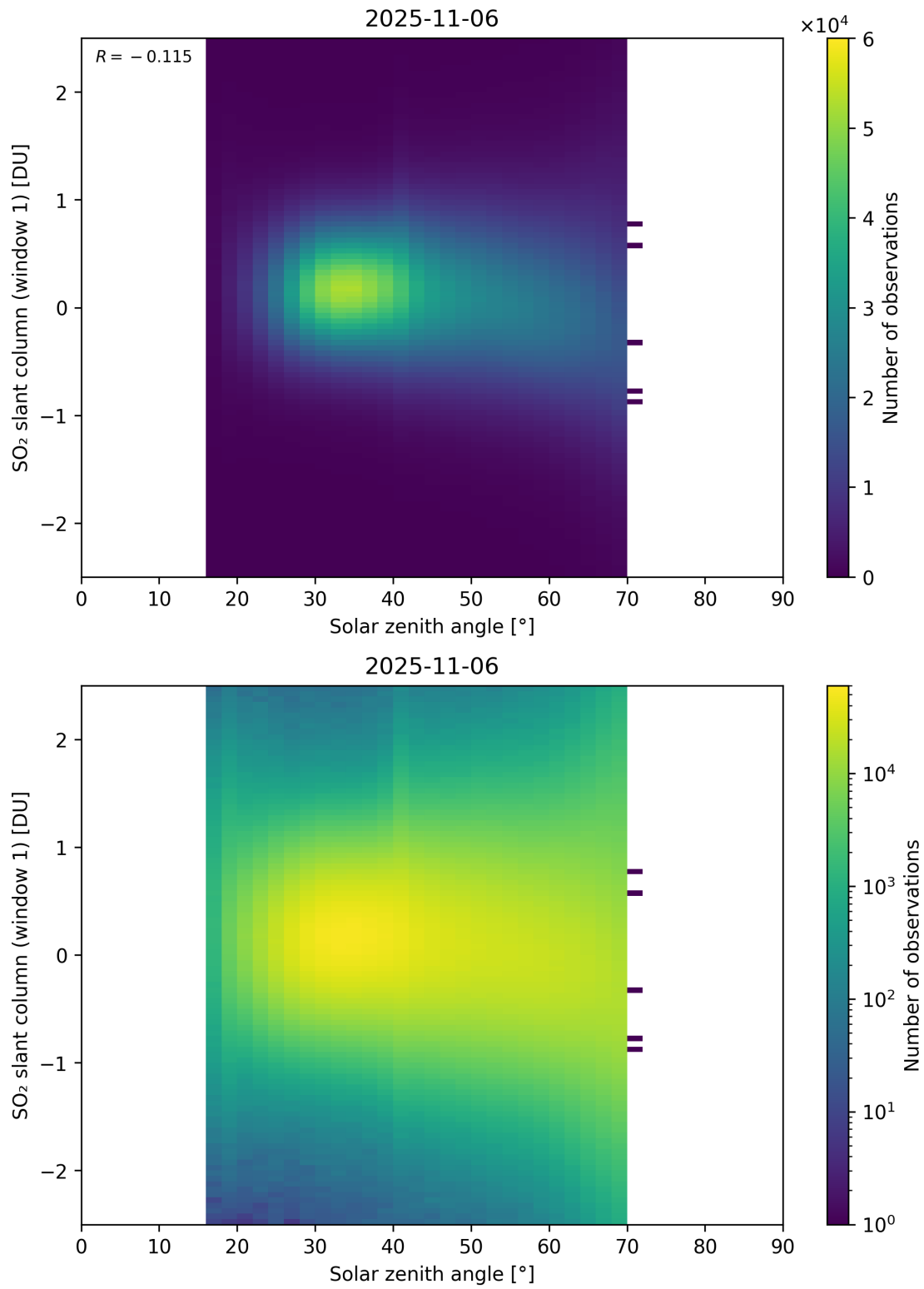
Figure 184: Scatter density plot of “Solar zenith angle” against “SO 2 slant column (window 1)” for 2025-11-05 to 2025-11-07.
