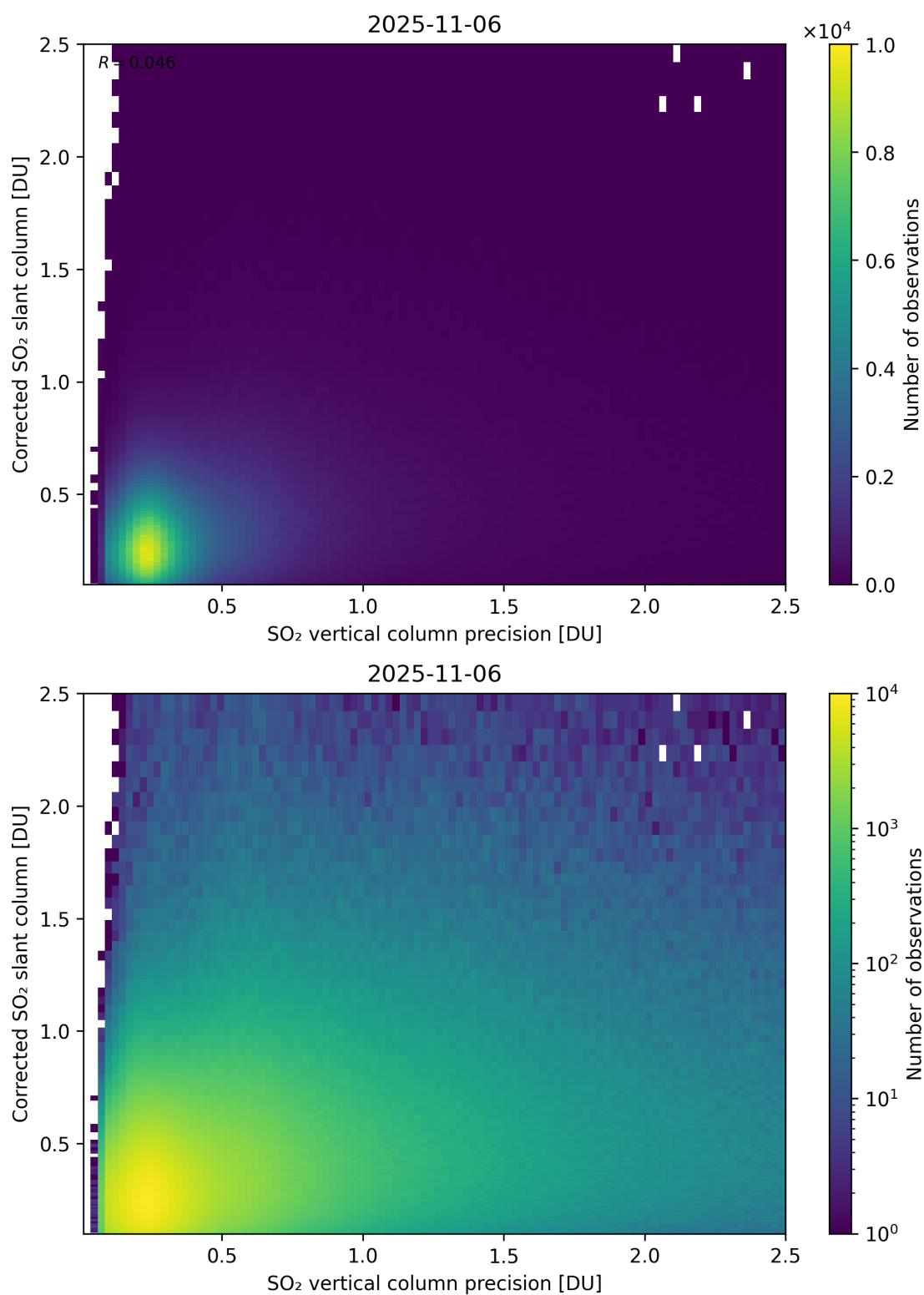
Figure 338: Scatter density plot of “SO 2 vertical column precision” against “Corrected SO 2 slant column” for 2025-11-05 to 2025-11-07.
