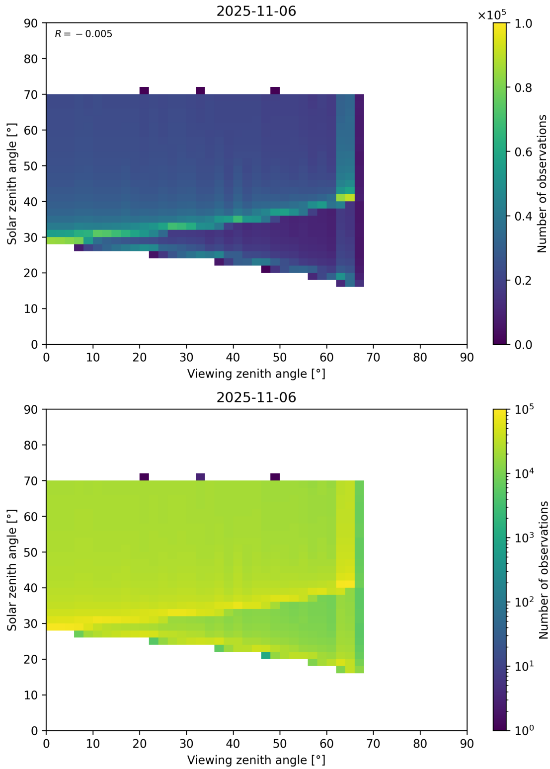
Figure 369: Scatter density plot of “Viewing zenith angle” against “Solar zenith angle” for 2025-11-05 to 2025-11-07.
