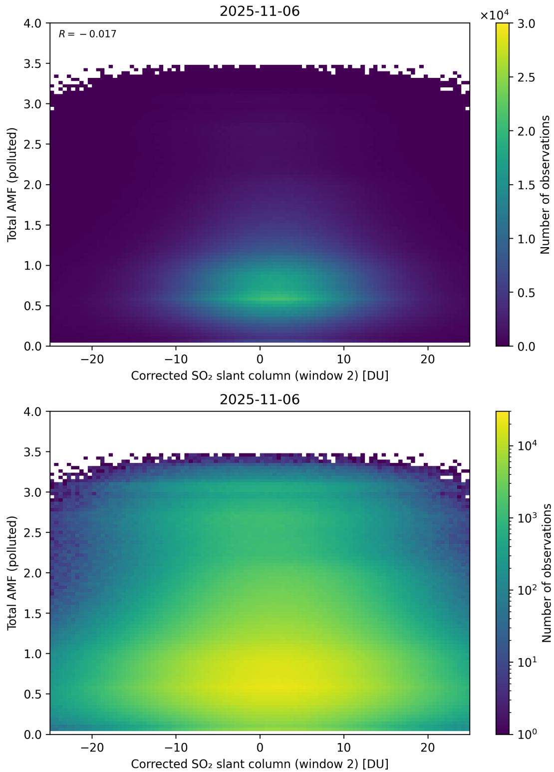
Figure 253: Scatter density plot of “Corrected SO 2 slant column (window 2)” against “Total AMF (polluted)” for 2025-11-05 to 2025-11-07.
