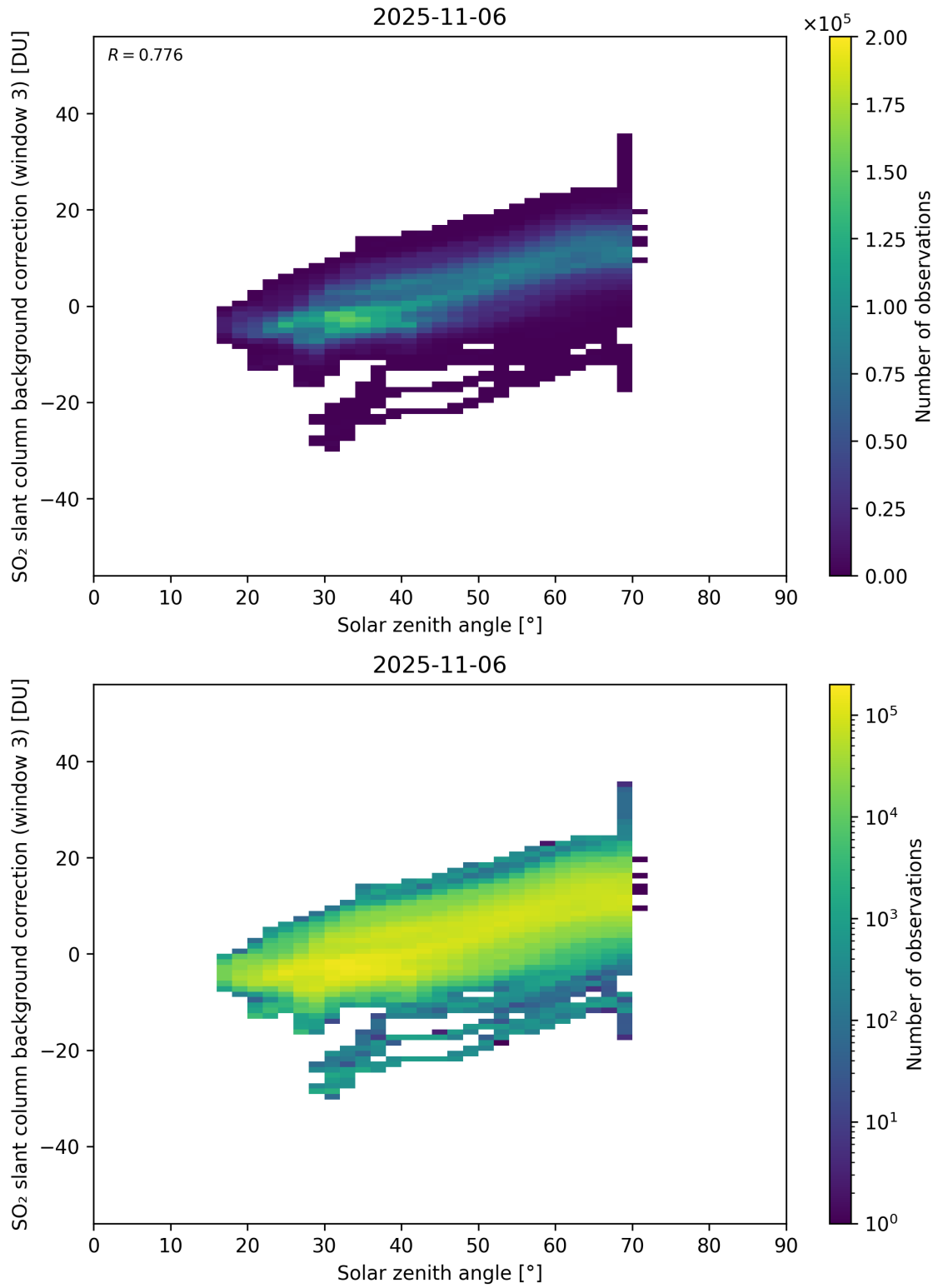
Figure 173: Scatter density plot of “Solar zenith angle” against “SO 2 slant column background correction (window 3)” for 2025-11-05 to 2025-11-07.
