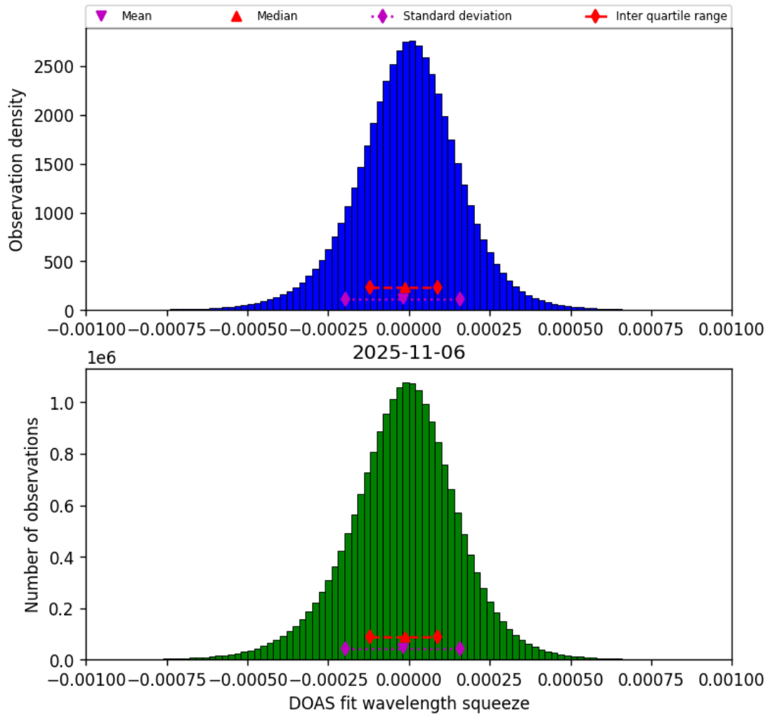
Figure 77: Histogram of “DOAS fit wavelength squeeze” for 2025-11-05 to 2025-11-07
