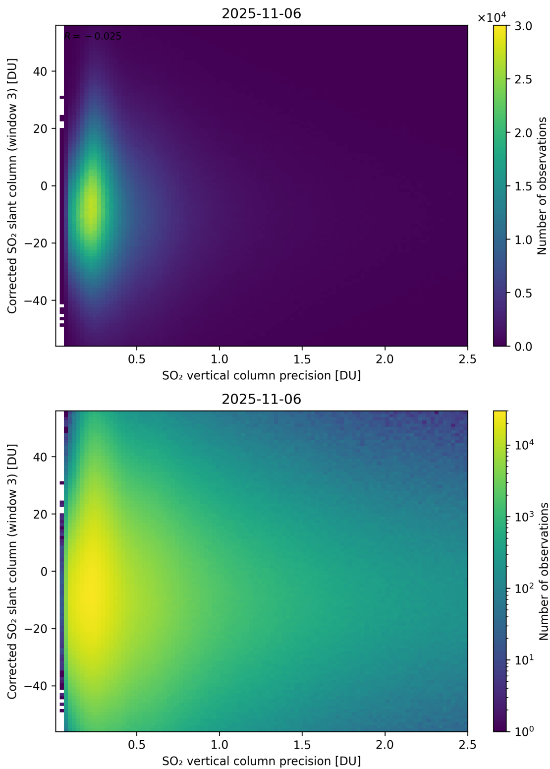
Figure 340: Scatter density plot of “SO 2 vertical column precision” against “Corrected SO 2 slant column (window 3)” for 2025-11-05 to 2025-11-07.
