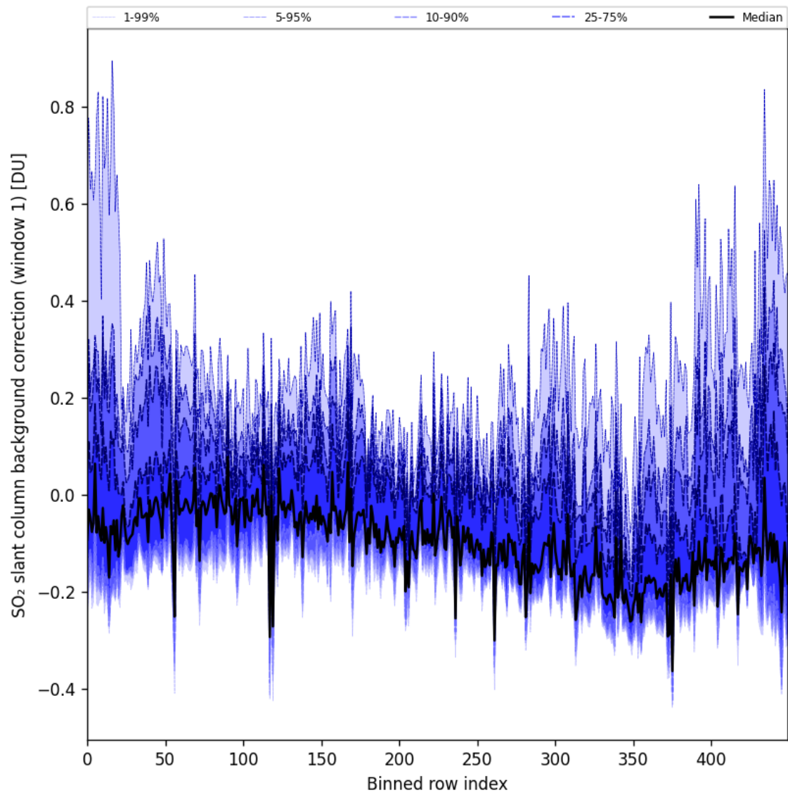
Figure 92: Along track statistics of “SO 2 slant column background correction (window 1)” for 2025-11-05 to 2025-11-07
