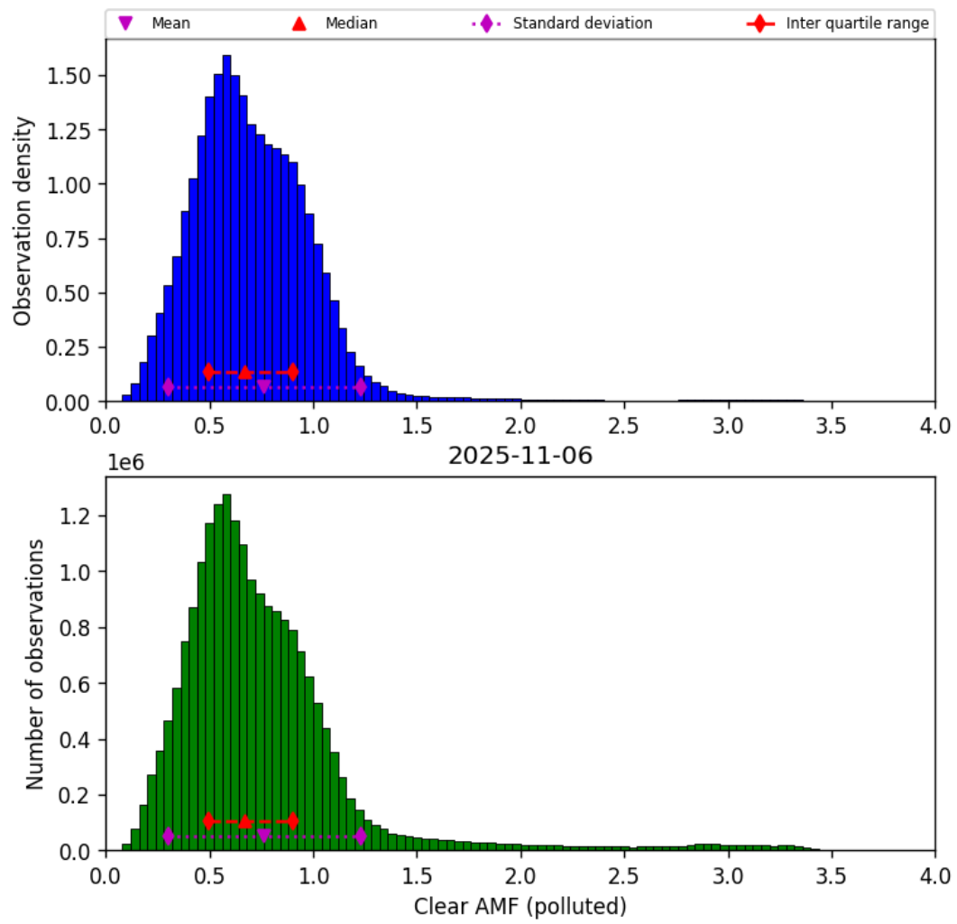
Figure 81: Histogram of “Clear AMF (polluted)” for 2025-11-05 to 2025-11-07
