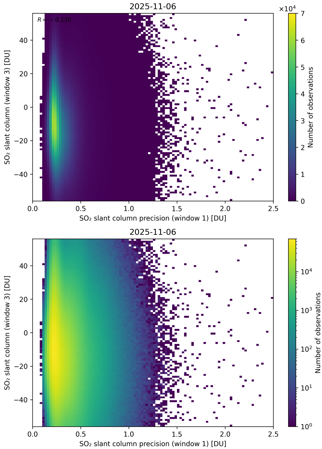
Figure 278: Scatter density plot of “SO 2 slant column precision (window 1)” against “SO 2 slant column (window 3)” for 2025-11-05 to 2025-11-07.
