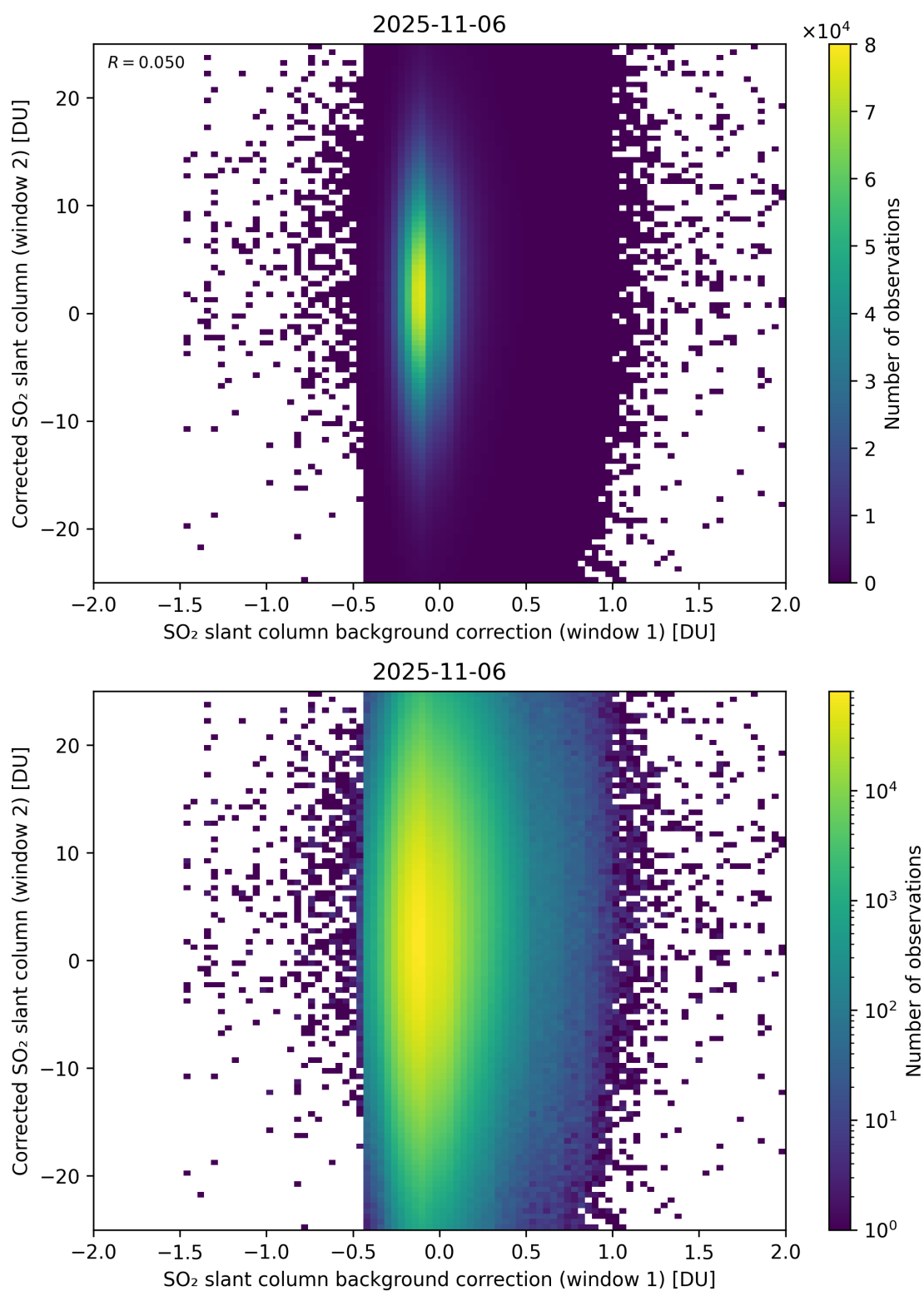
Figure 115: Scatter density plot of “SO 2 slant column background correction (window 1)” against “Corrected SO 2 slant column (window 2)” for 2025-11-05 to 2025-11-07.
