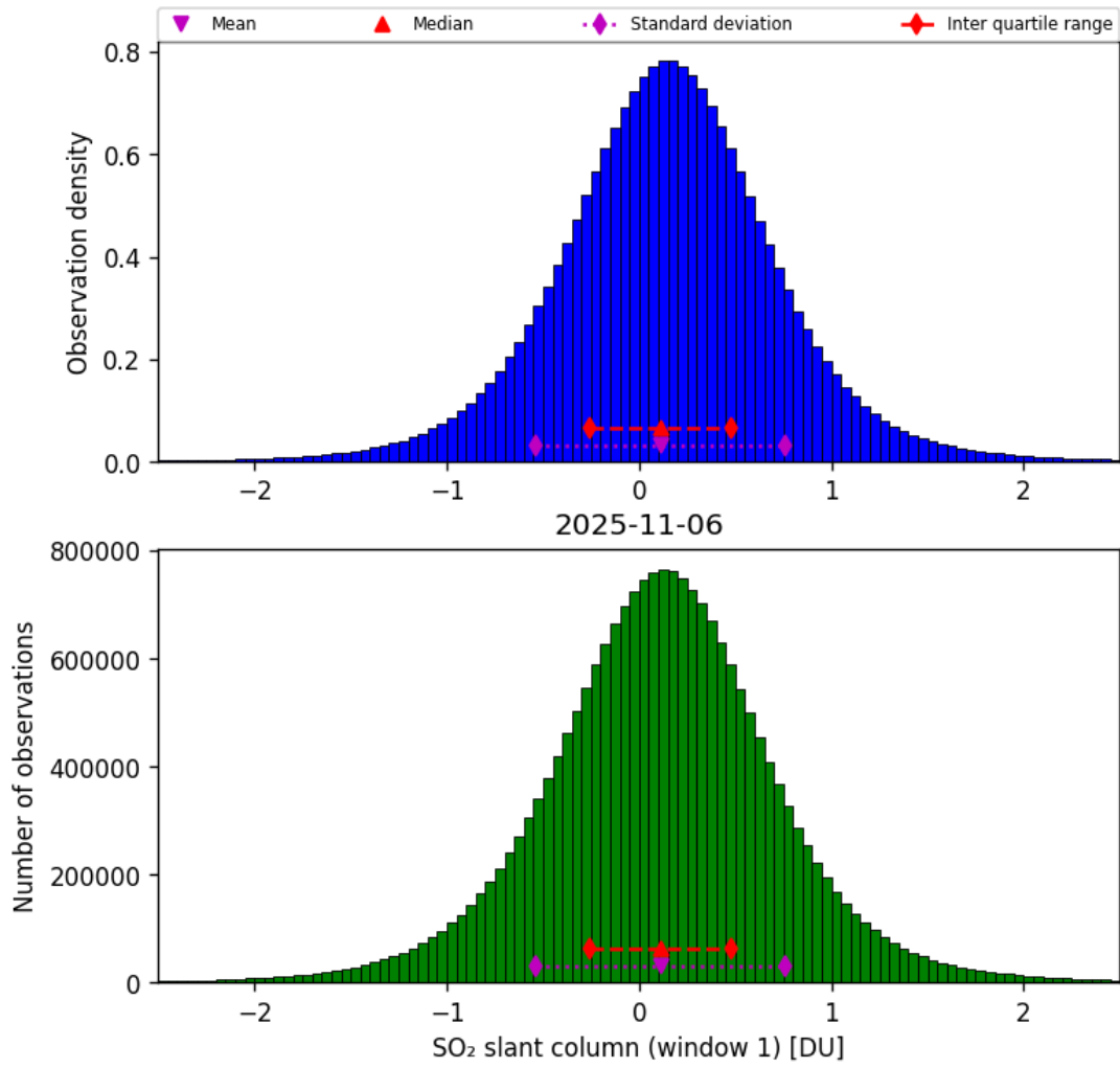
Figure 63: Histogram of “SO 2 slant column (window 1)” for 2025-11-05 to 2025-11-07
