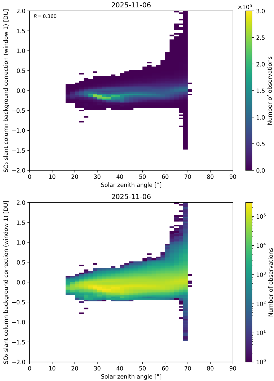
Figure 171: Scatter density plot of “Solar zenith angle” against “SO 2 slant column background correction (window 1)” for 2025-11-05 to 2025-11-07.
