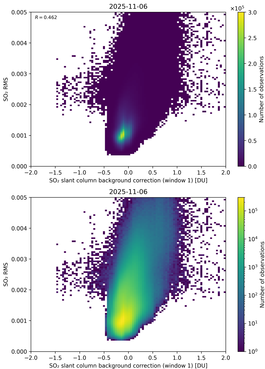
Figure 113: Scatter density plot of “SO 2 slant column background correction (window 1)” against “SO 2 RMS” for 2025-11-05 to 2025-11-07.
