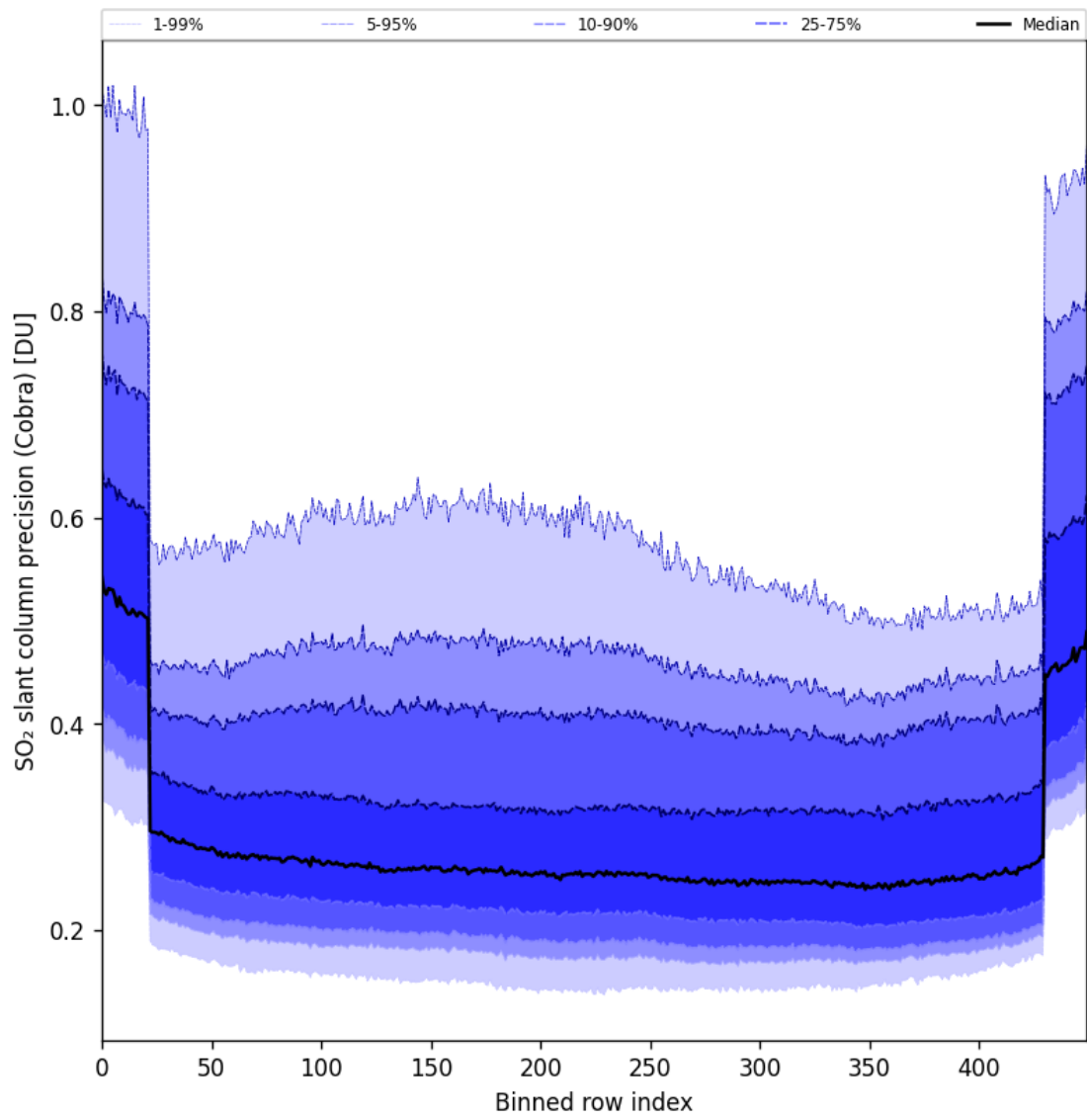
Figure 88: Along track statistics of “SO 2 slant column precision (Cobra)” for 2025-11-05 to 2025-11-07
