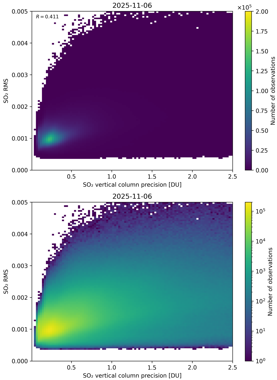
Figure 334: Scatter density plot of “SO 2 vertical column precision” against “SO 2 RMS” for 2025-11-05 to 2025-11-07.
