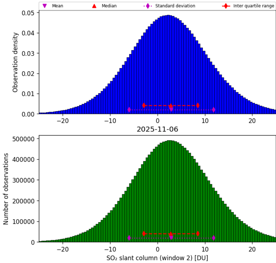
Figure 67: Histogram of “SO 2 slant column (window 2)” for 2025-11-05 to 2025-11-07
