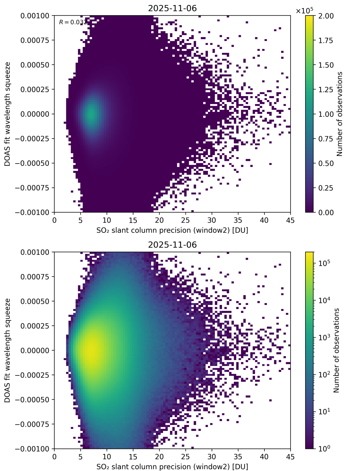
Figure 294: Scatter density plot of “SO 2 slant column precision (window2)” against “DOAS fit wavelength squeeze” for 2025-11-05 to 2025-11-07.
