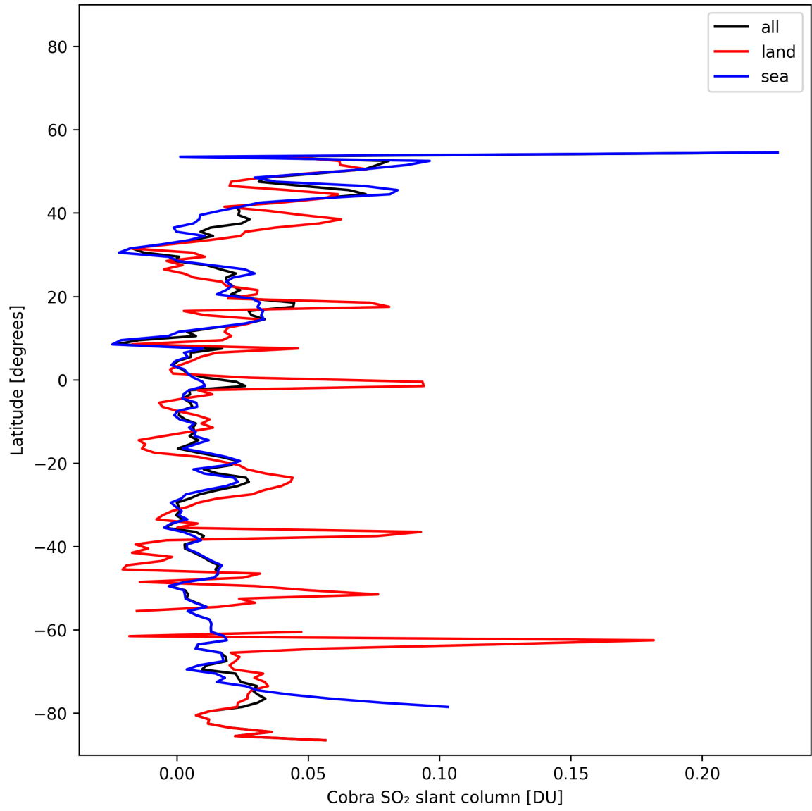
Figure 35: Zonal average of “Cobra SO 2 slant column” for 2025-11-05 to 2025-11-07.
