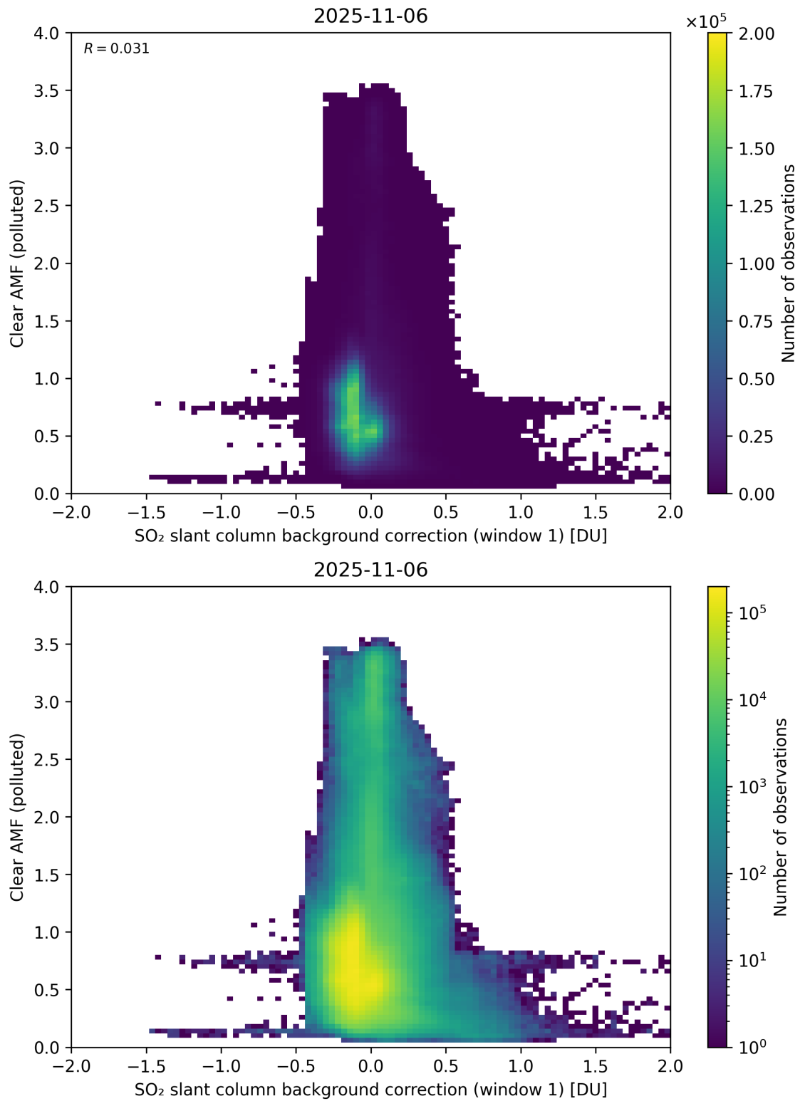
Figure 114: Scatter density plot of “SO 2 slant column background correction (window 1)” against “Clear AMF (polluted)” for 2025-11-05 to 2025-11-07.
