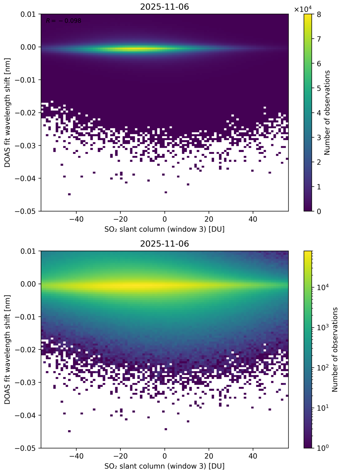
Figure 304: Scatter density plot of “SO 2 slant column (window 3)” against “DOAS fit wavelength shift” for 2025-11-05 to 2025-11-07.
