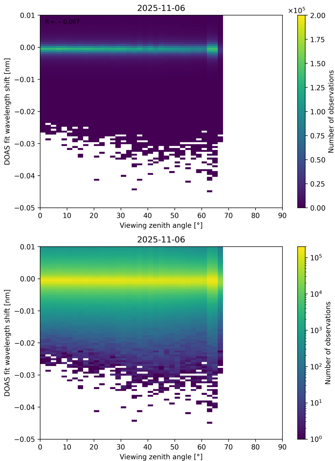
Figure 365: Scatter density plot of “Viewing zenith angle” against “DOAS fit wavelength shift” for 2025-11-05 to 2025-11-07.
