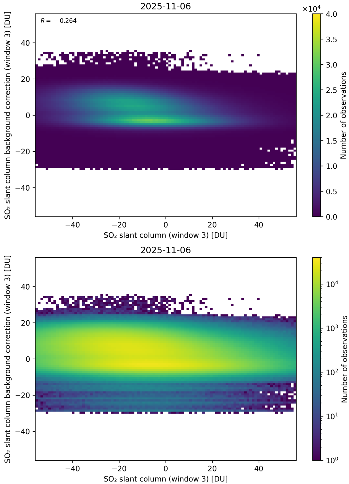
Figure 303: Scatter density plot of “SO 2 slant column (window 3)” against “SO 2 slant column background correction (window 3)” for 2025-11-05 to 2025-11-07.
