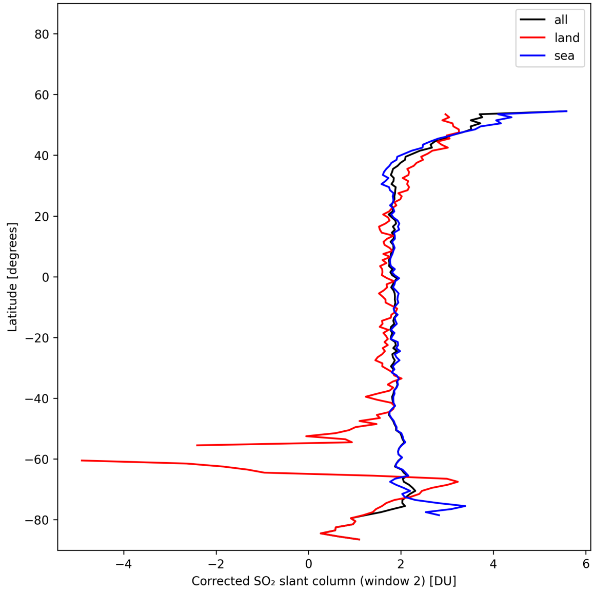
Figure 43: Zonal average of “Corrected SO 2 slant column (window 2)” for 2025-11-05 to 2025-11-07.
