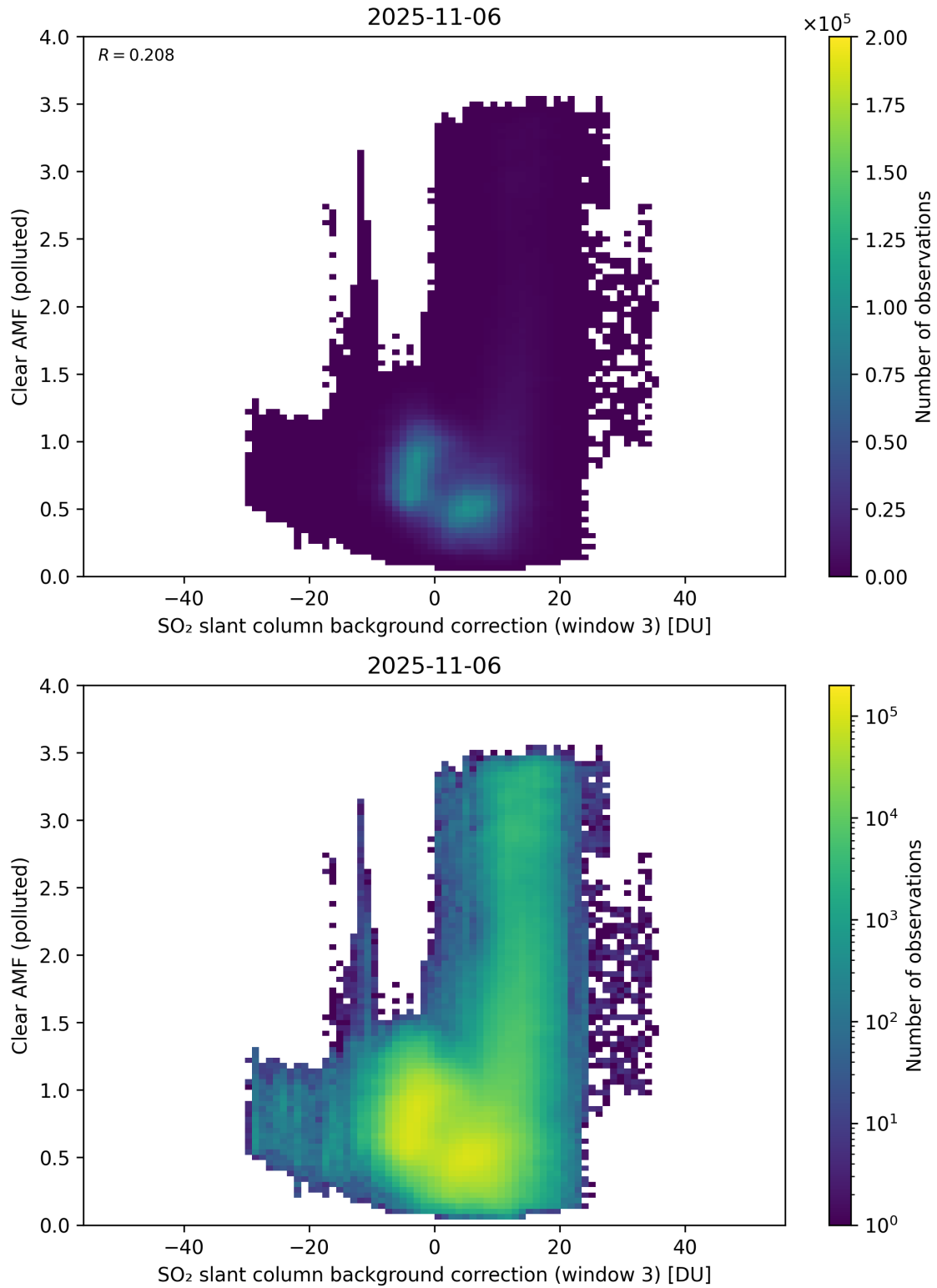
Figure 135: Scatter density plot of “SO 2 slant column background correction (window 3)” against “Clear AMF (polluted)” for 2025-11-05 to 2025-11-07.
