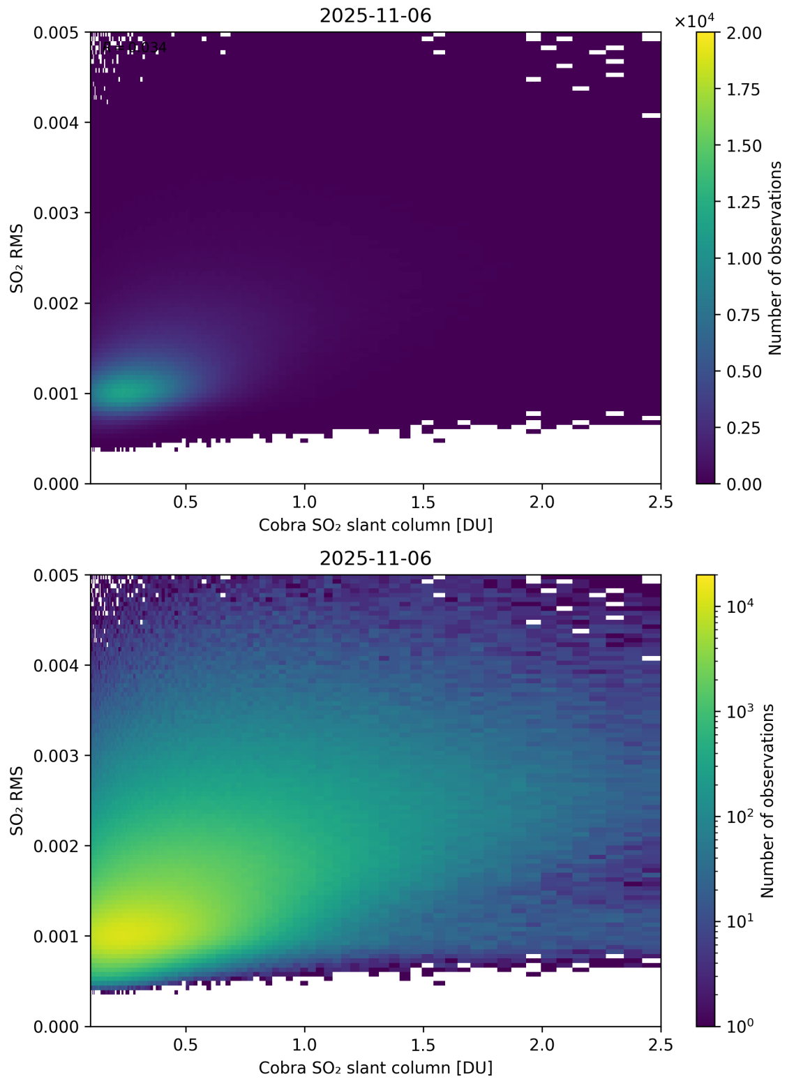
Figure 198: Scatter density plot of “Cobra SO 2 slant column” against “SO 2 RMS” for 2025-11-05 to 2025-11-07.
