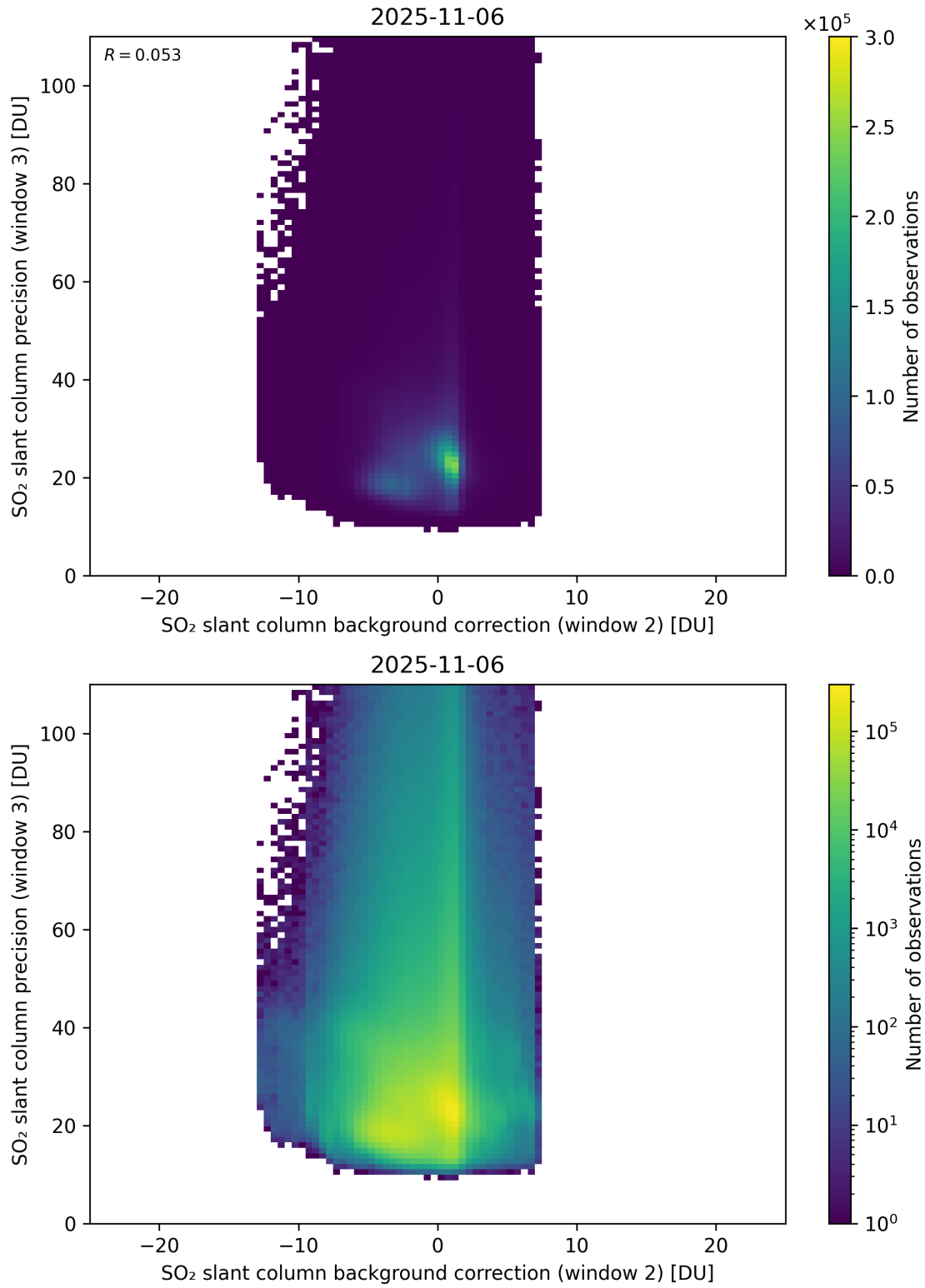
Figure 129: Scatter density plot of “SO 2 slant column background correction (window 2)” against “SO 2 slant column precision (window 3)” for 2025-11-05 to 2025-11-07.
