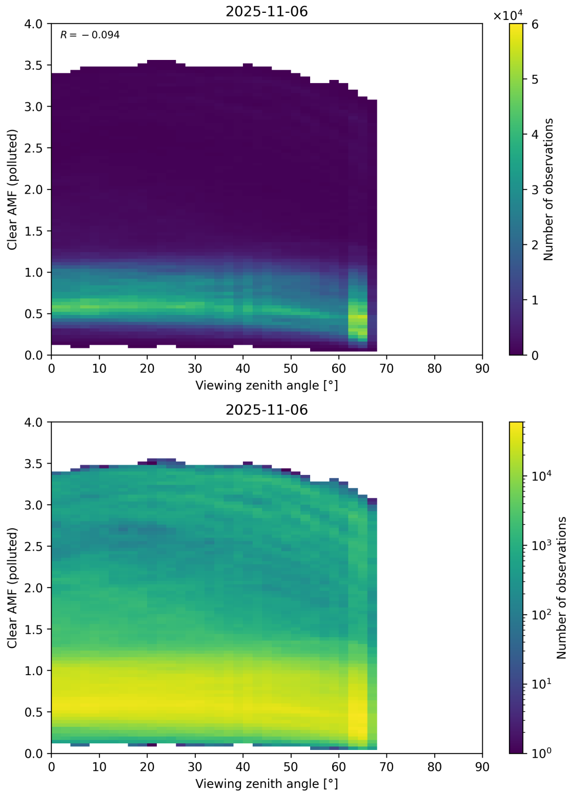
Figure 370: Scatter density plot of “Viewing zenith angle” against “Clear AMF (polluted)” for 2025-11-05 to 2025-11-07.
