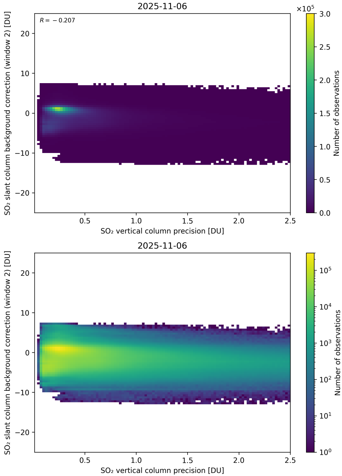
Figure 330: Scatter density plot of “SO 2 vertical column precision” against “SO 2 slant column background correction (window 2)” for 2025-11-05 to 2025-11-07.
