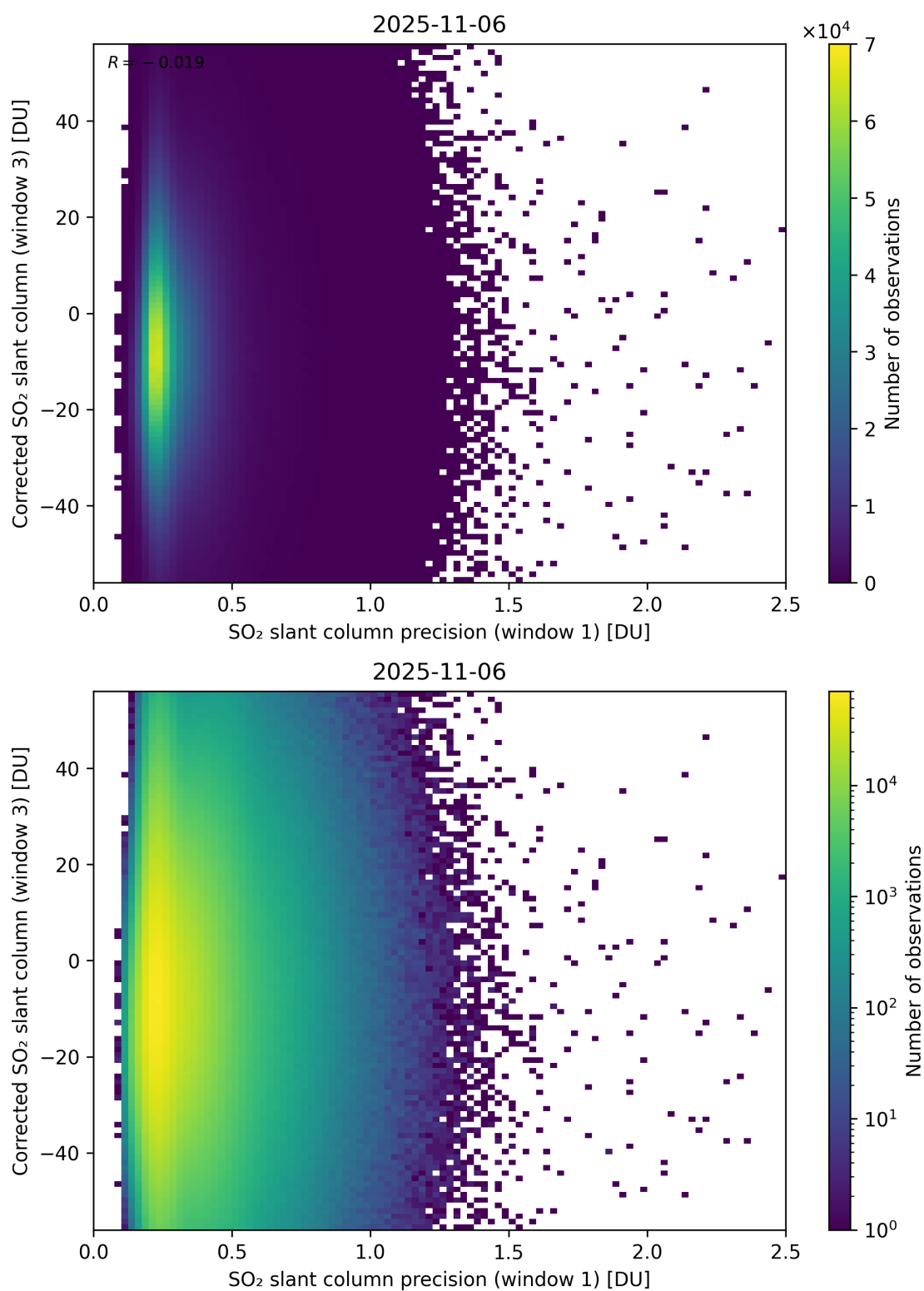
Figure 276: Scatter density plot of “SO 2 slant column precision (window 1)” against “Corrected SO 2 slant column (window 3)” for 2025-11-05 to 2025-11-07.
