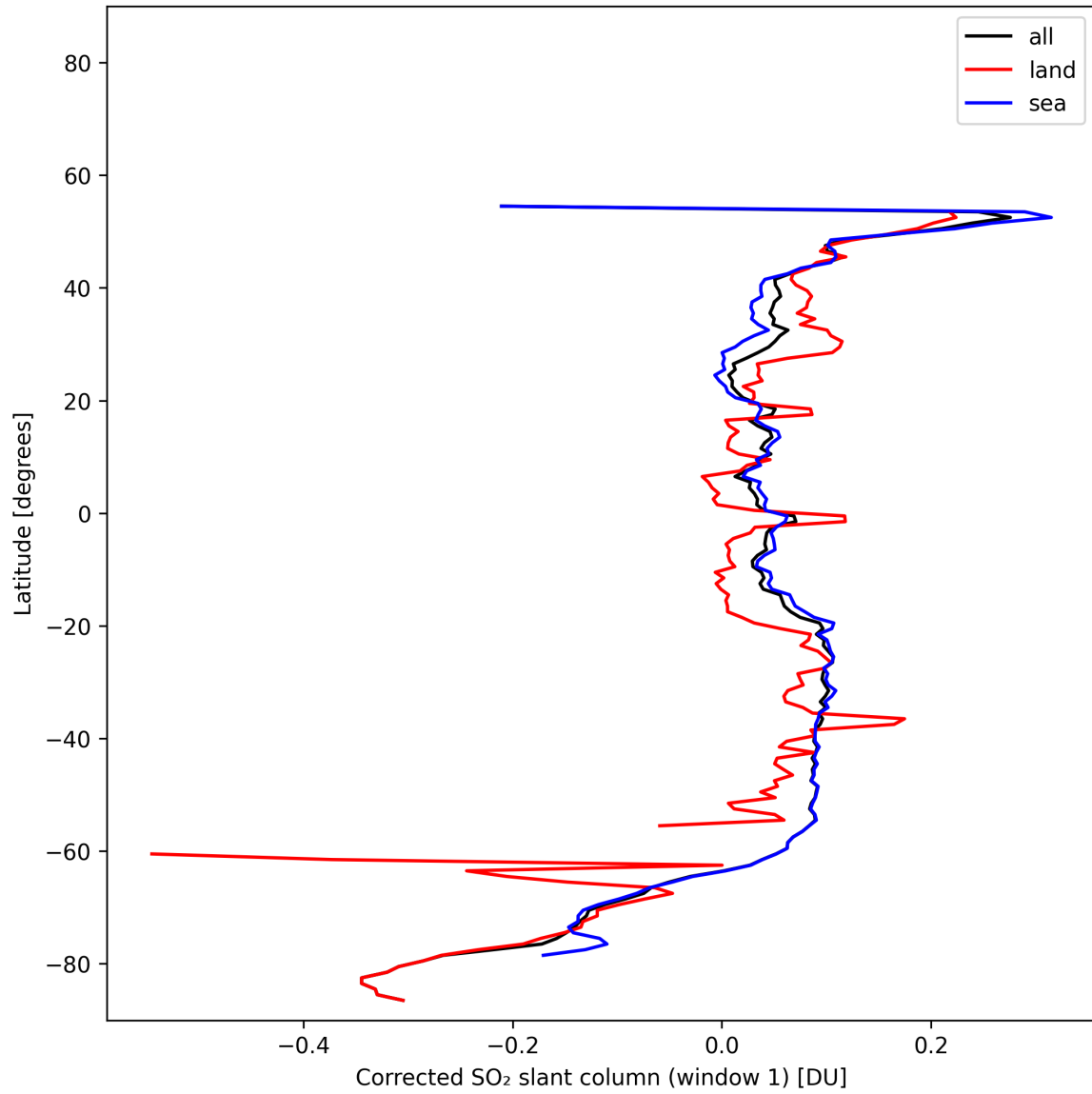
Figure 39: Zonal average of “Corrected SO 2 slant column (window 1)” for 2025-11-05 to 2025-11-07.
