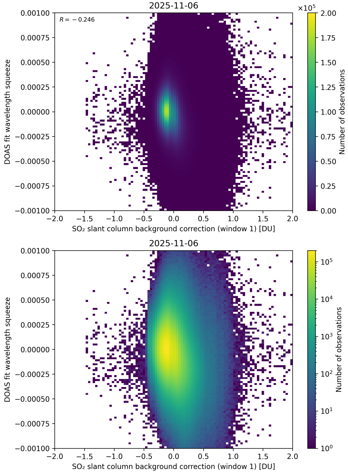
Figure 112: Scatter density plot of “SO 2 slant column background correction (window 1)” against “DOAS fit wavelength squeeze” for 2025-11-05 to 2025-11-07.
