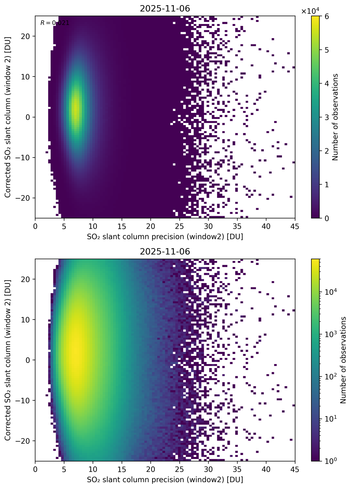
Figure 297: Scatter density plot of “SO 2 slant column precision (window2)” against “Corrected SO 2 slant column (window 2)” for 2025-11-05 to 2025-11-07.
