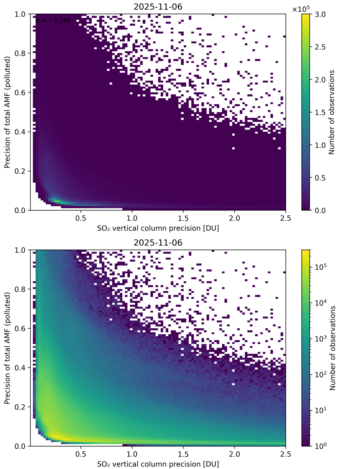
Figure 347: Scatter density plot of “SO 2 vertical column precision” against “Precision of total AMF (polluted)” for 2025-11-05 to 2025-11-07.
