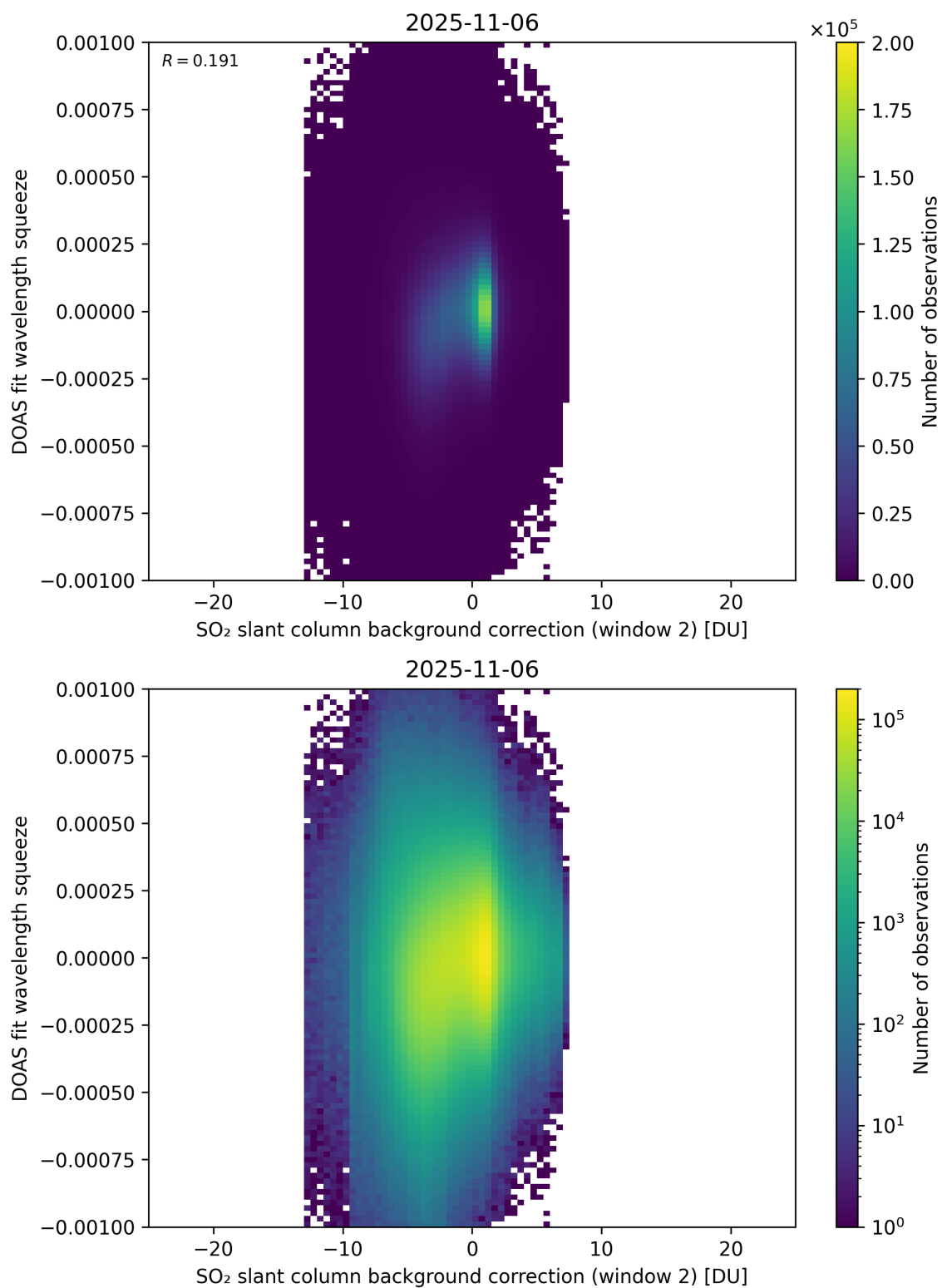
Figure 124: Scatter density plot of “SO 2 slant column background correction (window 2)” against “DOAS fit wavelength squeeze” for 2025-11-05 to 2025-11-07.
