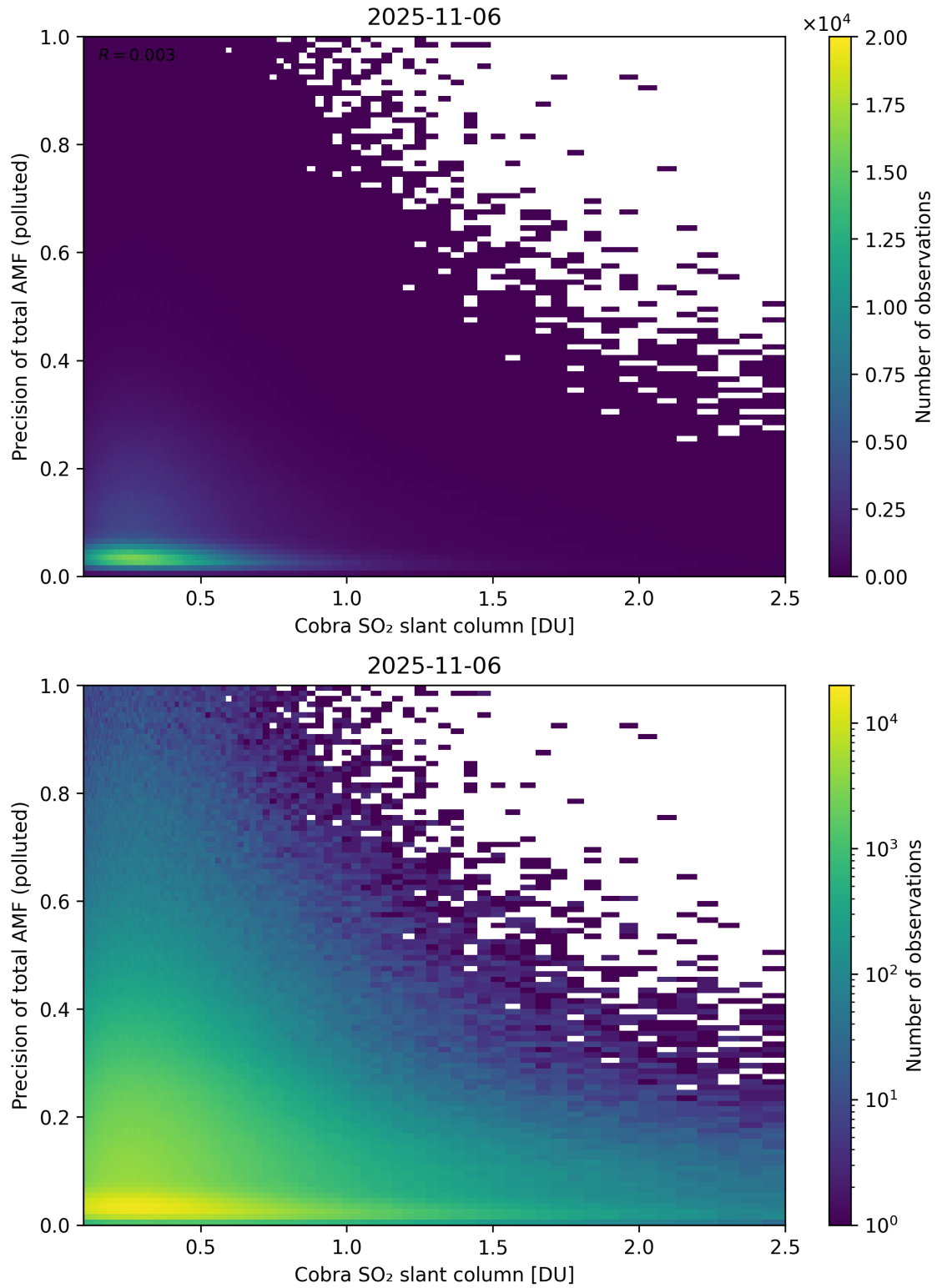
Figure 225: Scatter density plot of “Cobra SO 2 slant column” against “Precision of total AMF (polluted)” for 2025-11-05 to 2025-11-07.
