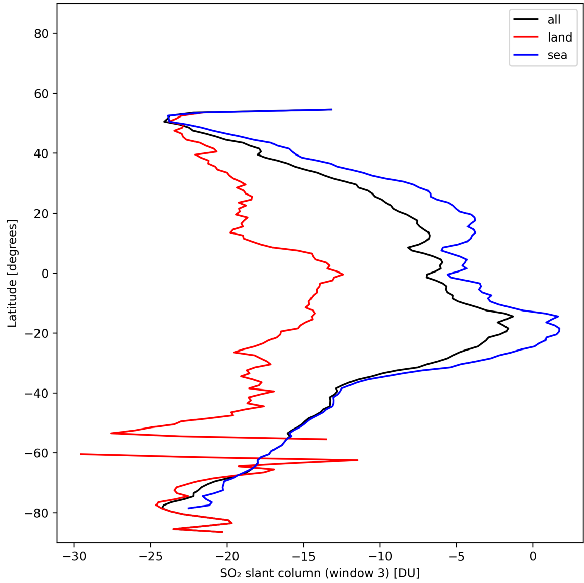
Figure 45: Zonal average of “SO 2 slant column (window 3)” for 2025-11-05 to 2025-11-07.
