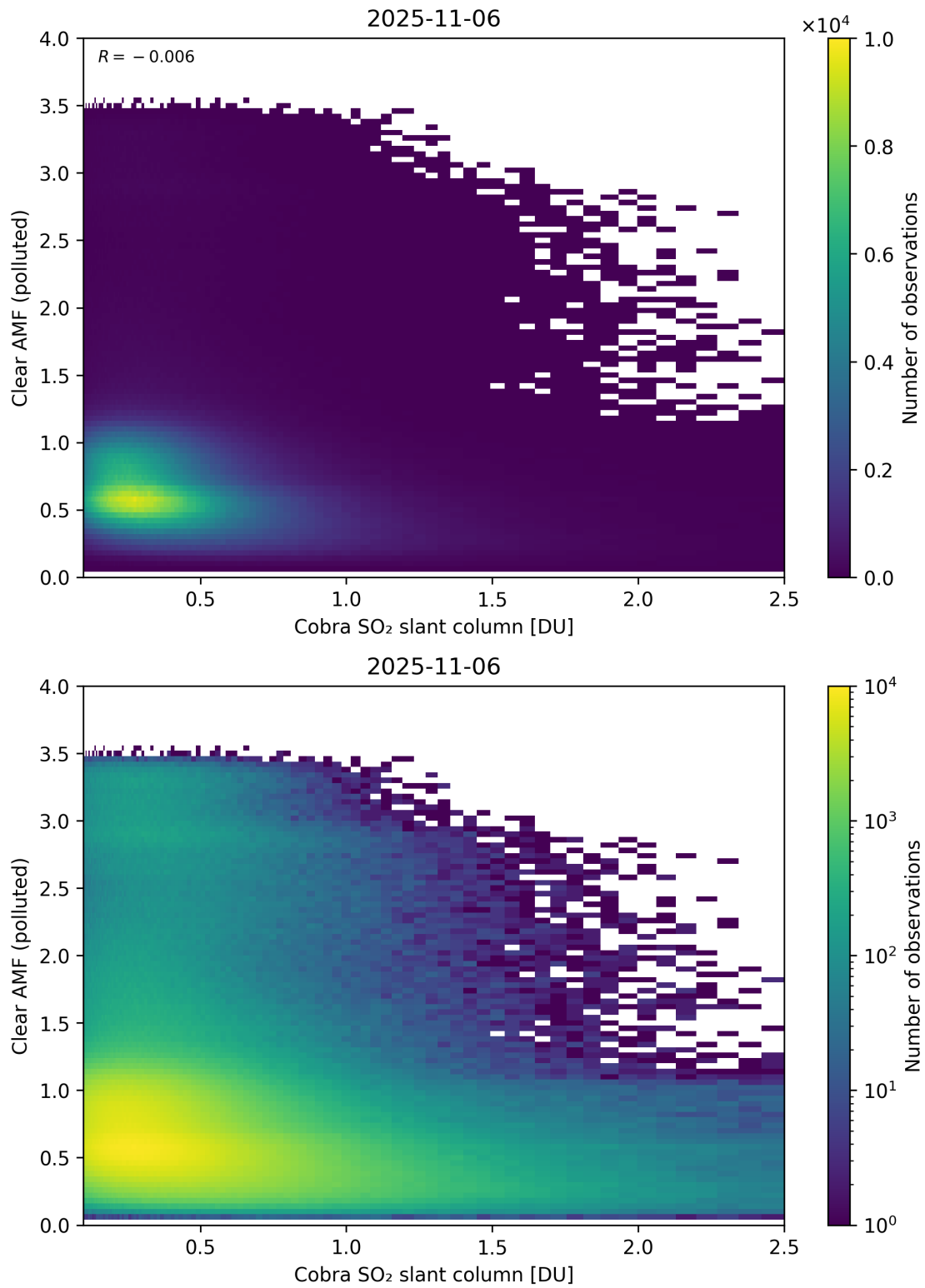
Figure 215: Scatter density plot of “Cobra SO 2 slant column” against “Clear AMF (polluted)” for 2025-11-05 to 2025-11-07.
