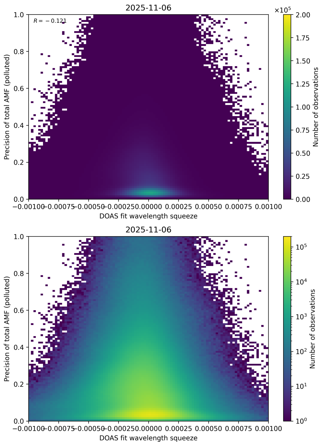
Figure 146: Scatter density plot of “DOAS fit wavelength squeeze” against “Precision of total AMF (polluted)” for 2025-11-05 to 2025-11-07.
