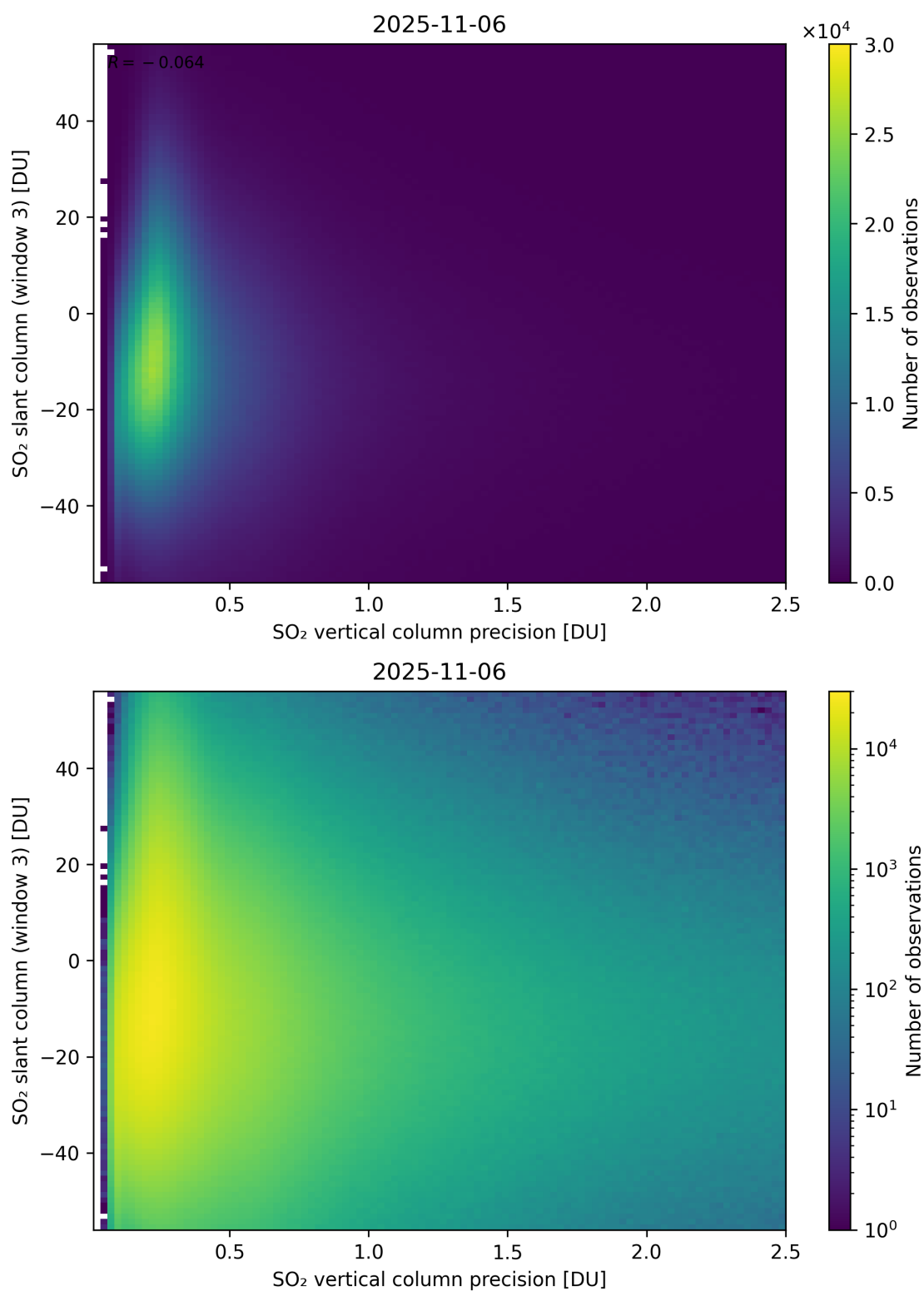
Figure 344: Scatter density plot of “SO 2 vertical column precision” against “SO 2 slant column (window 3)” for 2025-11-05 to 2025-11-07.
