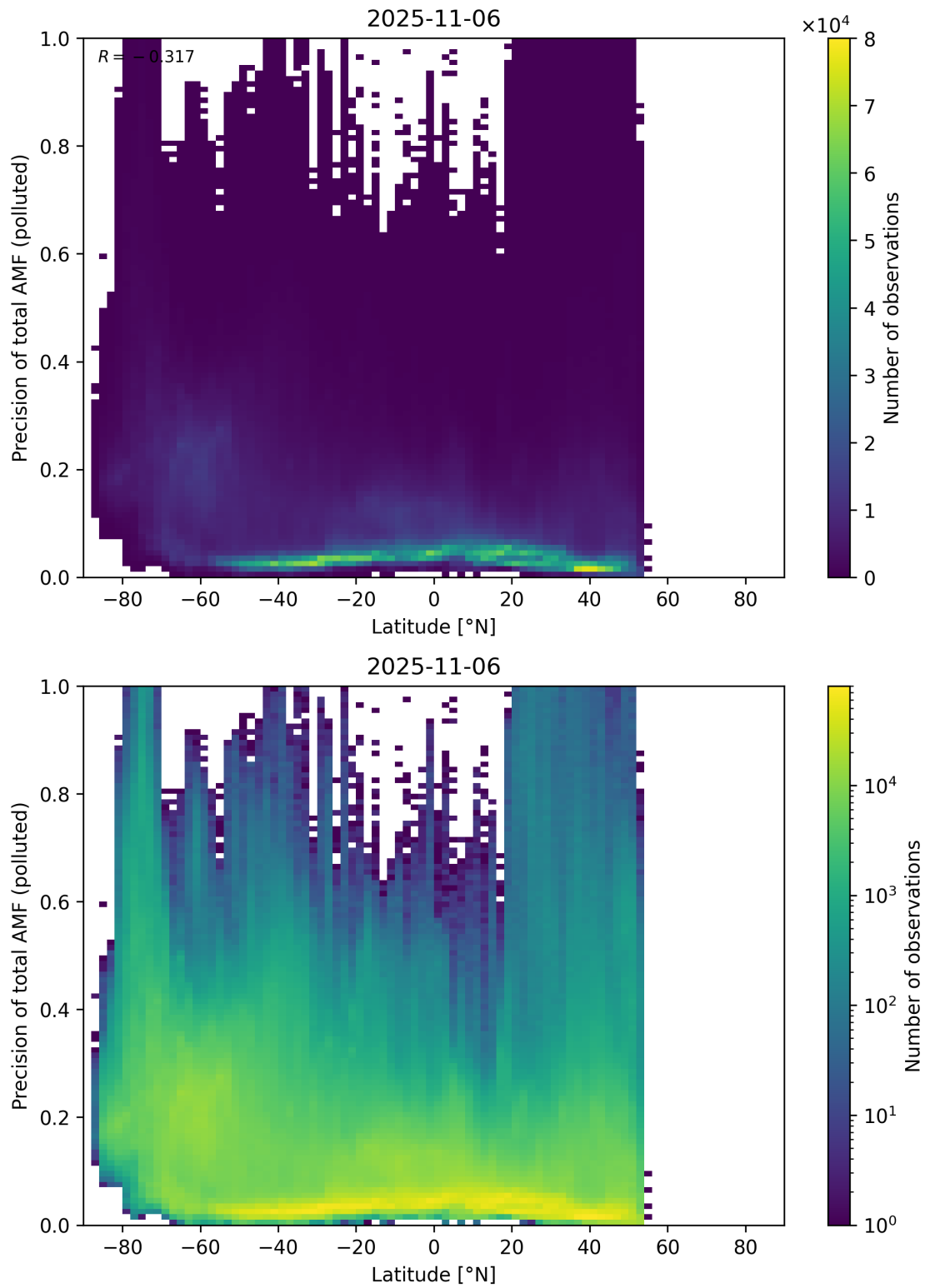
Figure 168: Scatter density plot of “Latitude” against “Precision of total AMF (polluted)” for 2025-11-05 to 2025-11-07.
