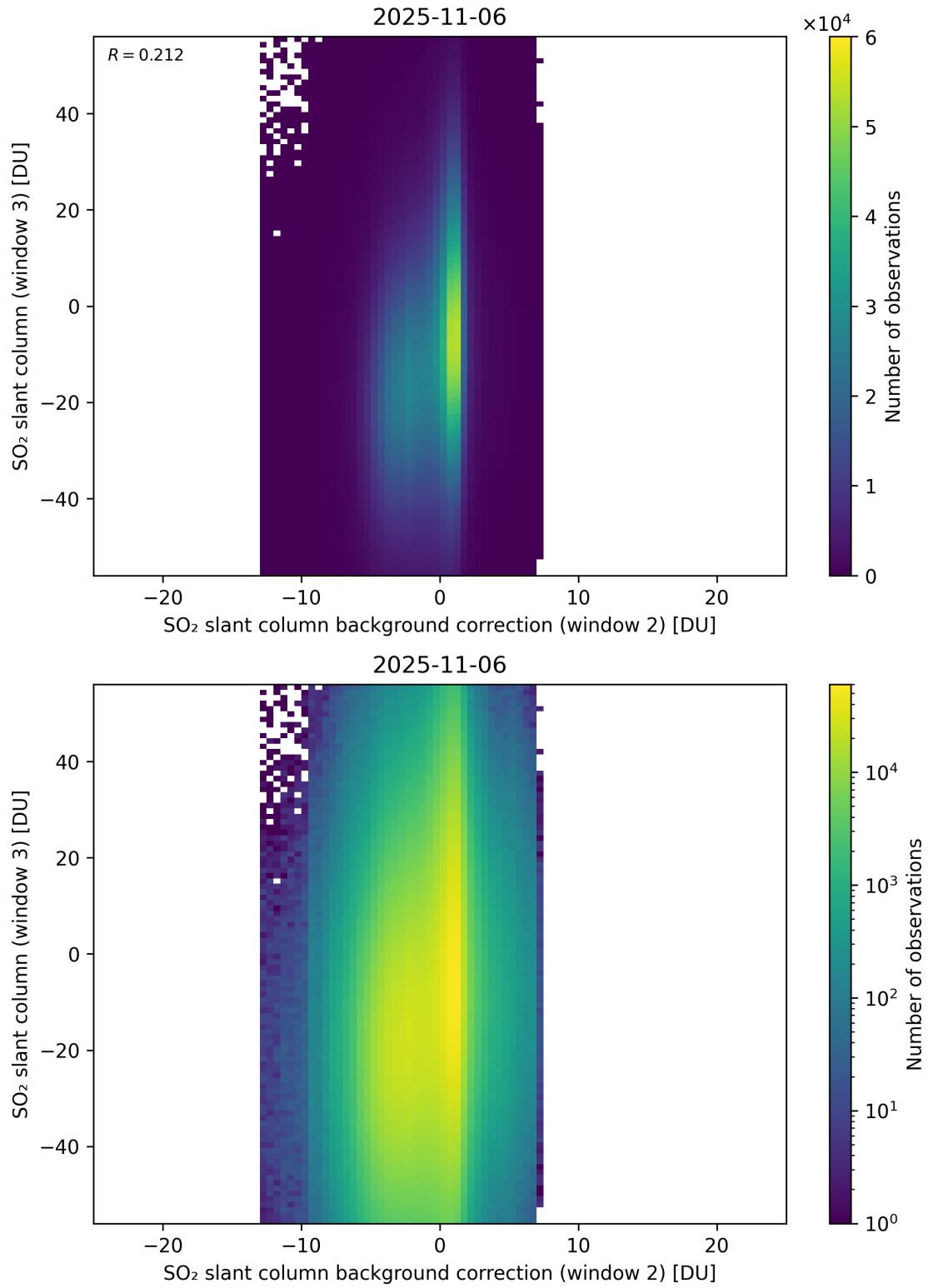
Figure 128: Scatter density plot of “SO 2 slant column background correction (window 2)” against “SO 2 slant column (window 3)” for 2025-11-05 to 2025-11-07.
