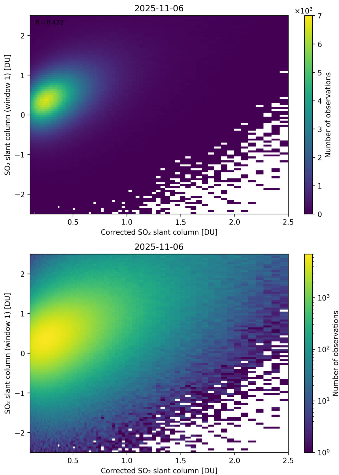
Figure 237: Scatter density plot of “Corrected SO 2 slant column” against “SO 2 slant column (window 1)” for 2025-11-05 to 2025-11-07.
