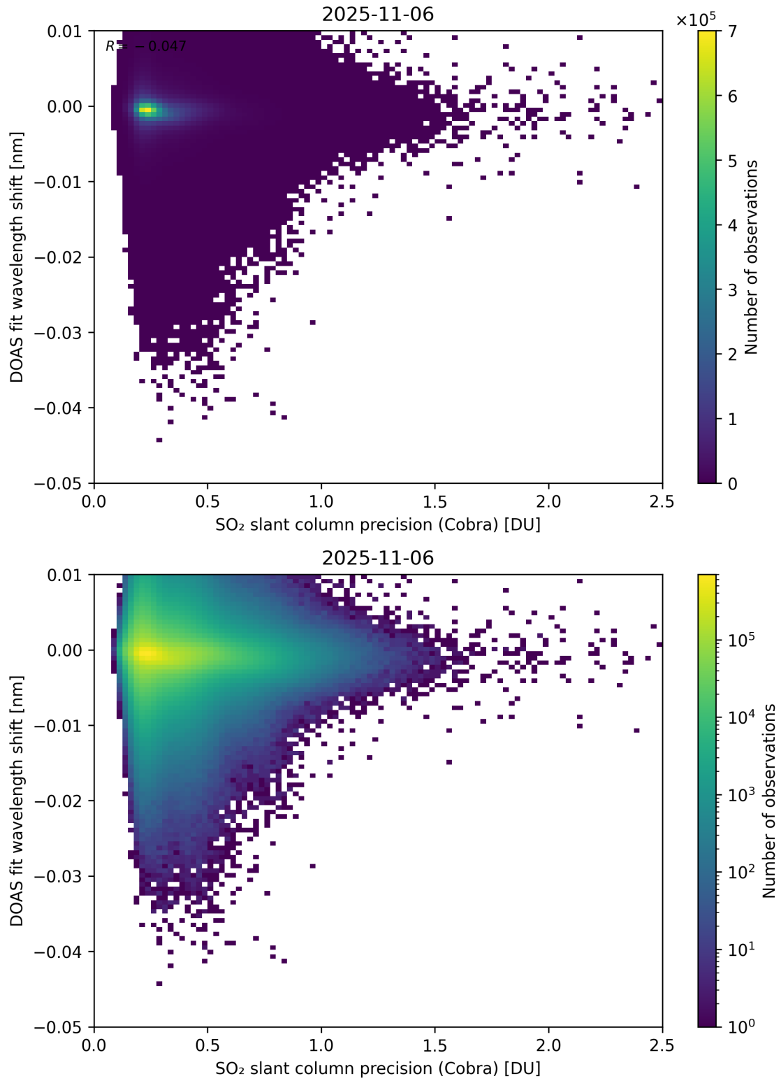
Figure 202: Scatter density plot of “SO 2 slant column precision (Cobra)” against “DOAS fit wavelength shift” for 2025-11-05 to 2025-11-07.
