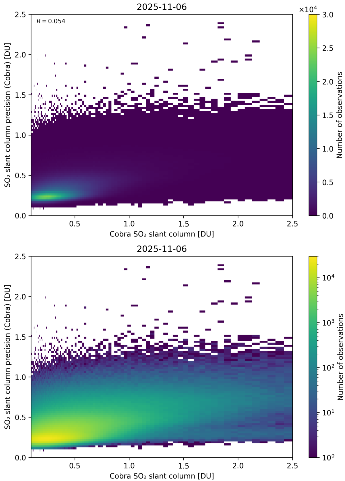
Figure 216: Scatter density plot of “Cobra SO 2 slant column” against “SO 2 slant column precision (Cobra)” for 2025-11-05 to 2025-11-07.
