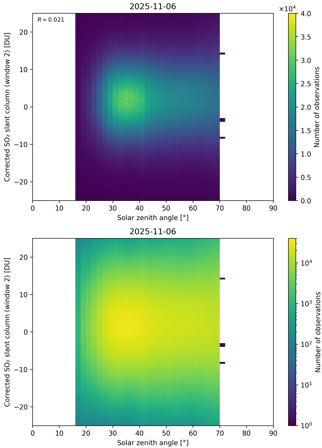
Figure 182: Scatter density plot of “Solar zenith angle” against “Corrected SO 2 slant column (window 2)” for 2025-11-05 to 2025-11-07.
