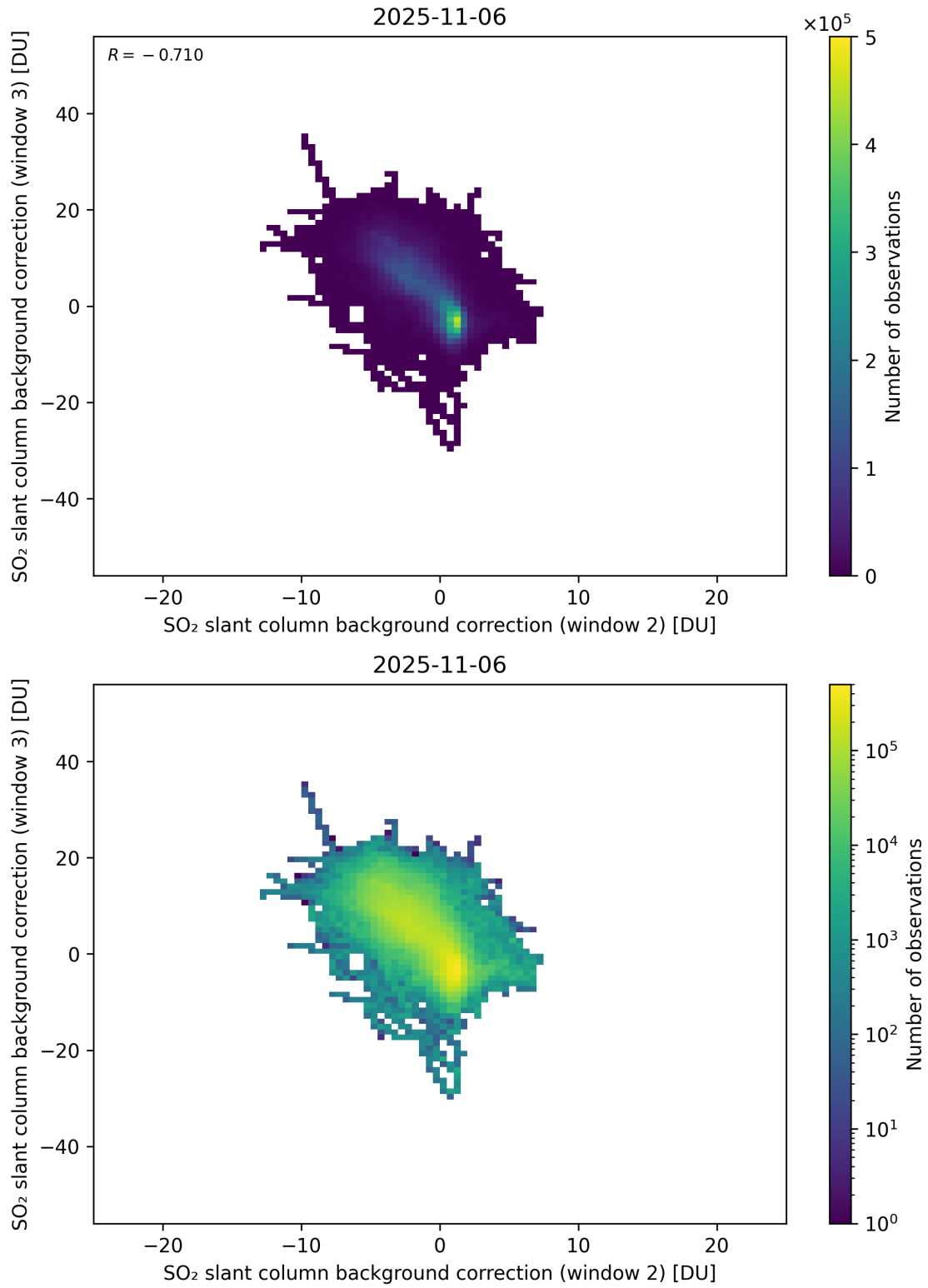
Figure 122: Scatter density plot of “SO 2 slant column background correction (window 2)” against “SO 2 slant column background correction (window 3)” for 2025-11-05 to 2025-11-07.
