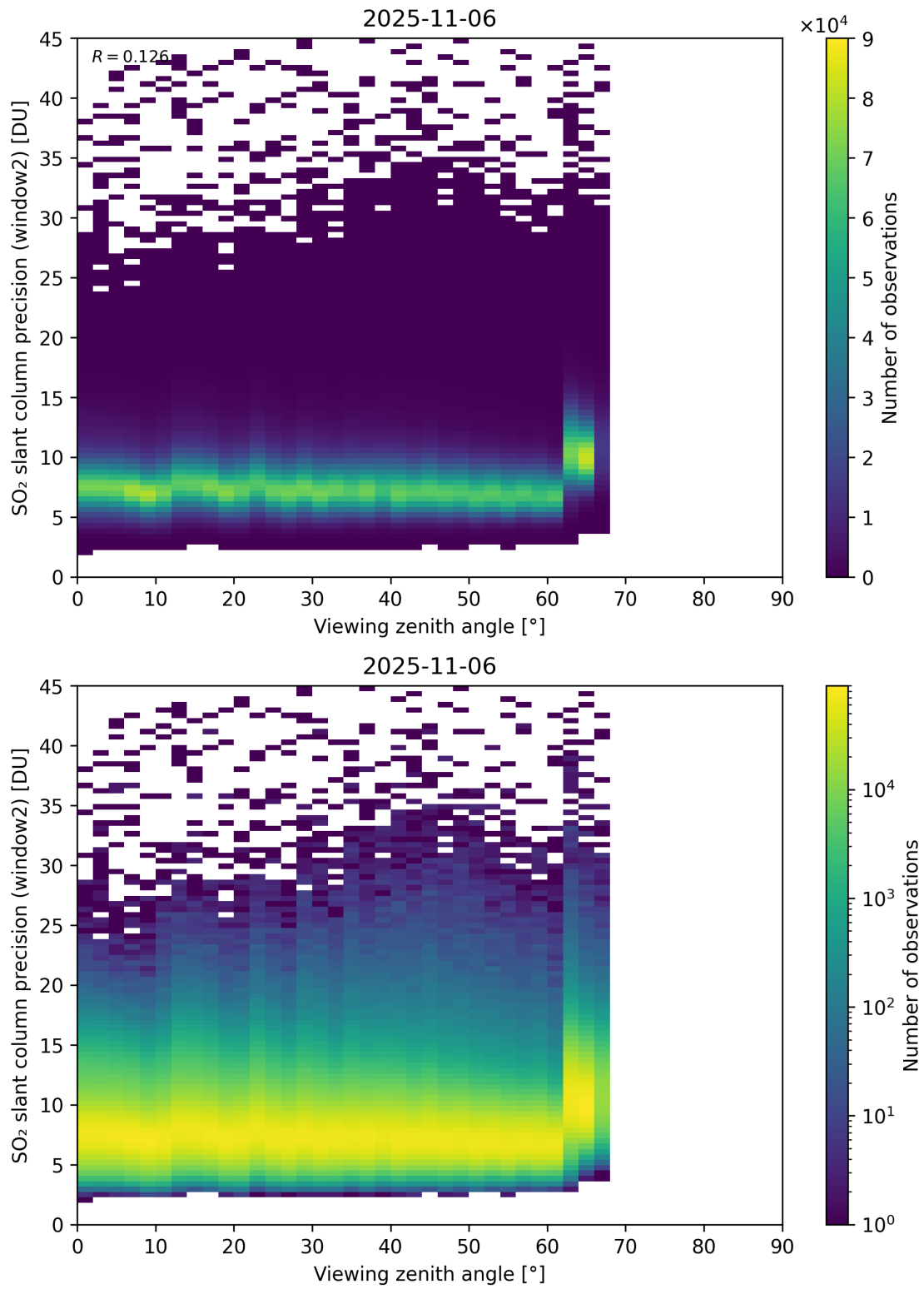
Figure 378: Scatter density plot of “Viewing zenith angle” against “SO 2 slant column precision (window2)” for 2025-11-05 to 2025-11-07.
