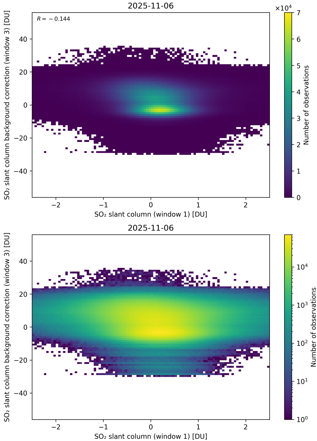
Figure 264: Scatter density plot of “SO 2 slant column (window 1)” against “SO 2 slant column background correction (window 3)” for 2025-11-05 to 2025-11-07.
