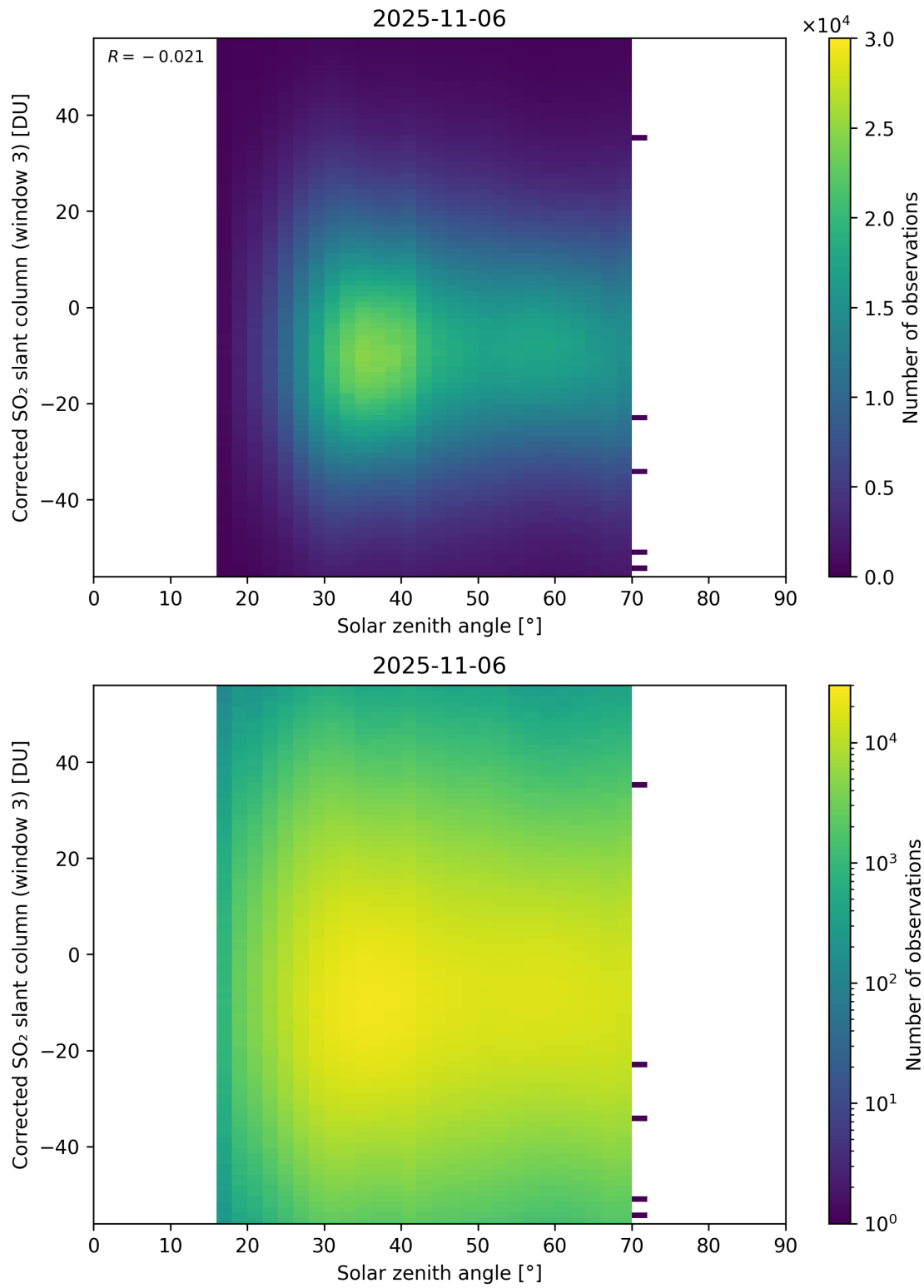
Figure 183: Scatter density plot of “Solar zenith angle” against “Corrected SO 2 slant column (window 3)” for 2025-11-05 to 2025-11-07.
