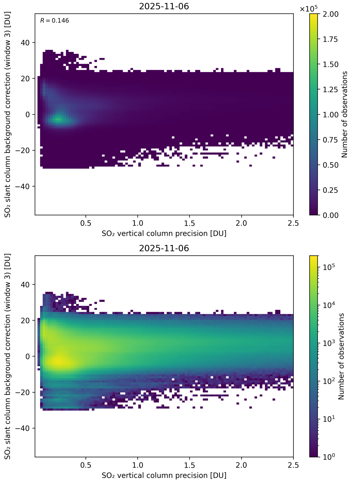
Figure 331: Scatter density plot of “SO 2 vertical column precision” against “SO 2 slant column background correction (window 3)” for 2025-11-05 to 2025-11-07.
