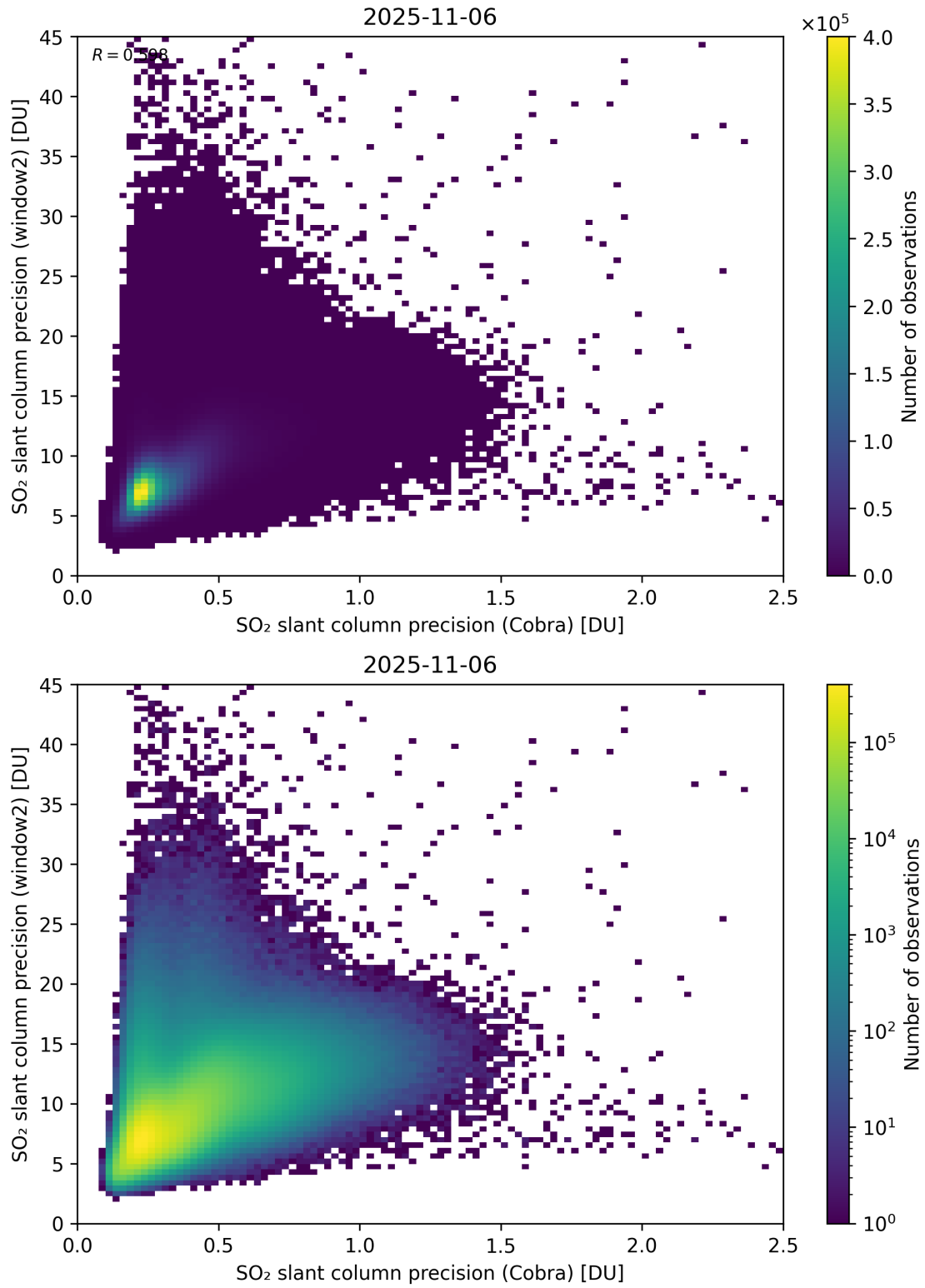
Figure 210: Scatter density plot of “SO 2 slant column precision (Cobra)” against “SO 2 slant column precision (window2)” for 2025-11-05 to 2025-11-07.
