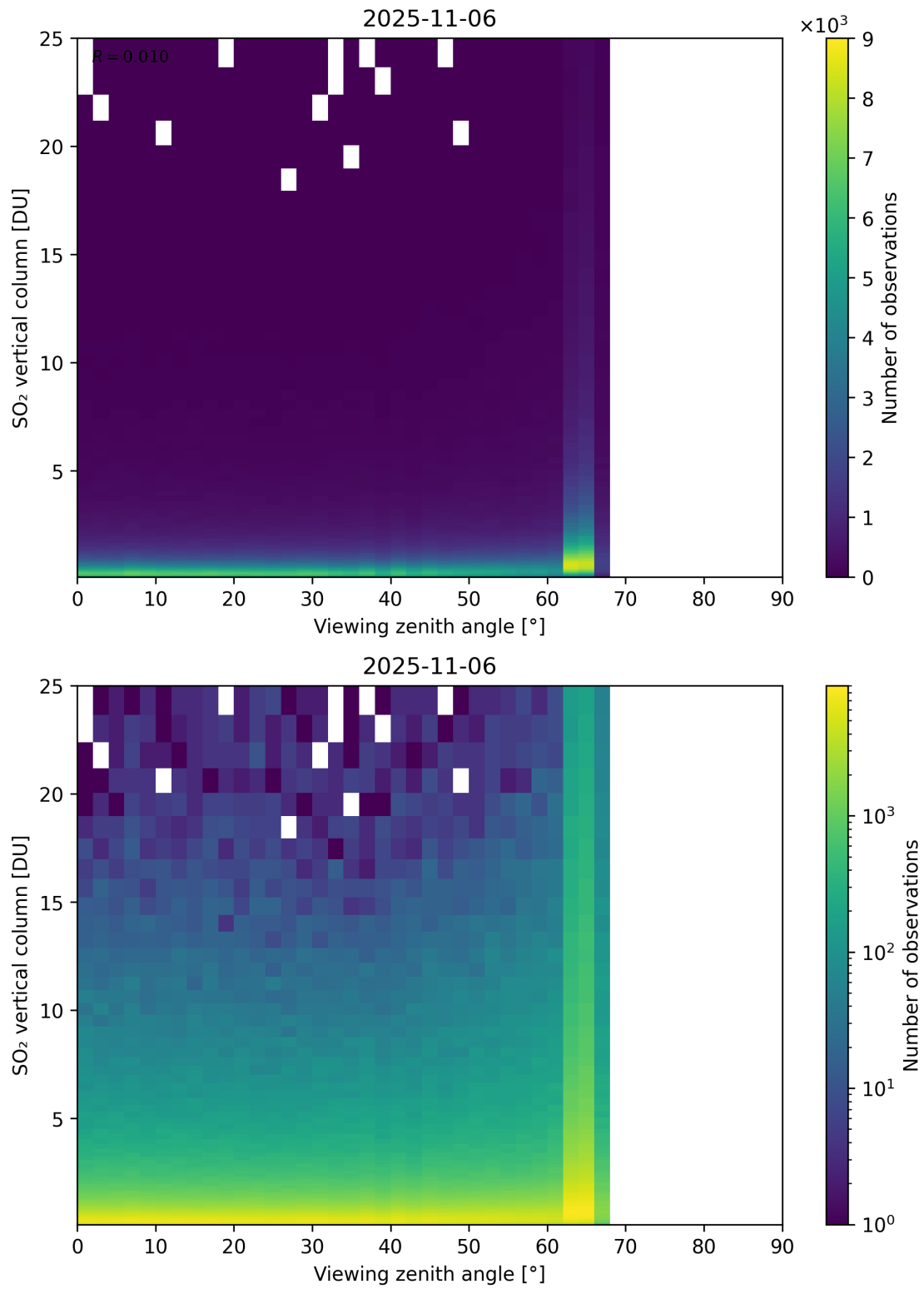
Figure 383: Scatter density plot of “Viewing zenith angle” against “SO 2 vertical column” for 2025-11-05 to 2025-11-07.
