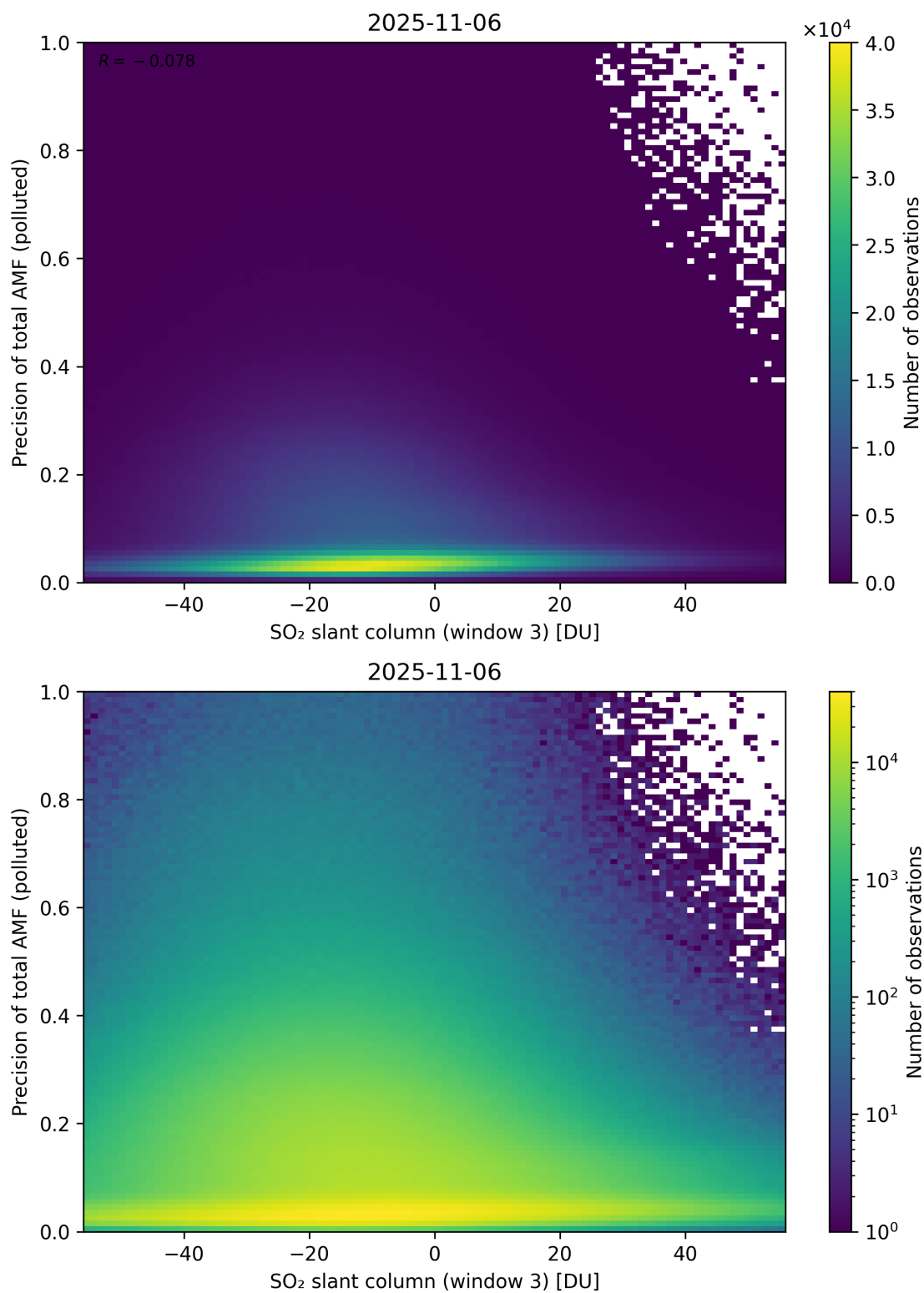
Figure 319: Scatter density plot of “SO 2 slant column (window 3)” against “Precision of total AMF (polluted)” for 2025-11-05 to 2025-11-07.
