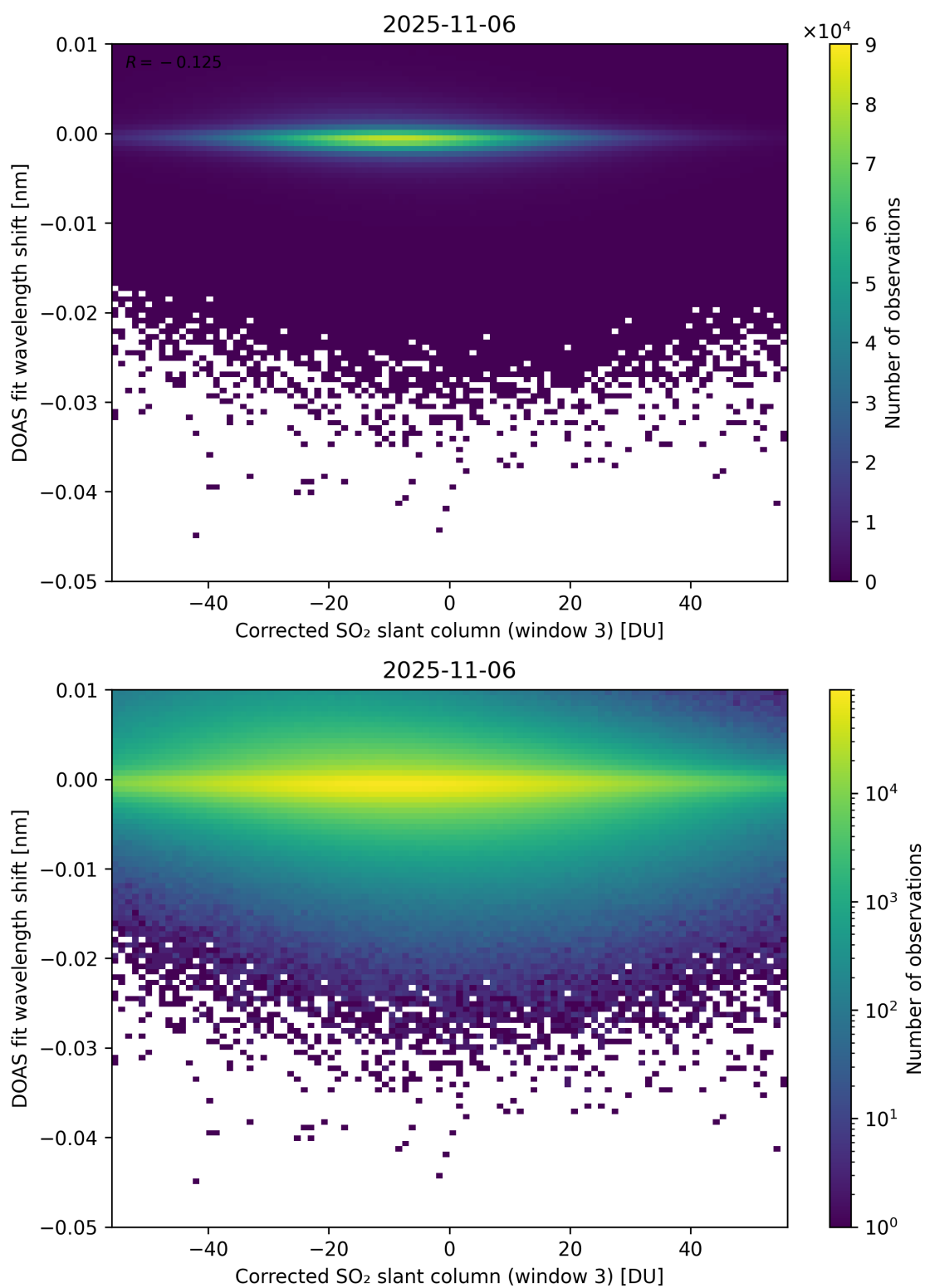
Figure 256: Scatter density plot of “Corrected SO 2 slant column (window 3)” against “DOAS fit wavelength shift” for 2025-11-05 to 2025-11-07.
