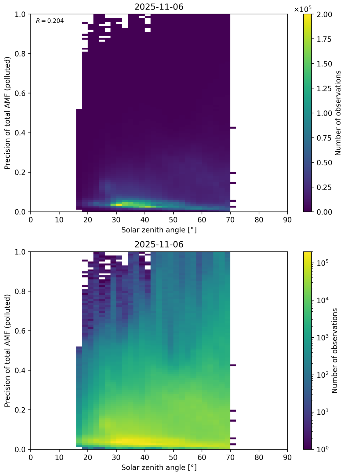
Figure 190: Scatter density plot of “Solar zenith angle” against “Precision of total AMF (polluted)” for 2025-11-05 to 2025-11-07.
