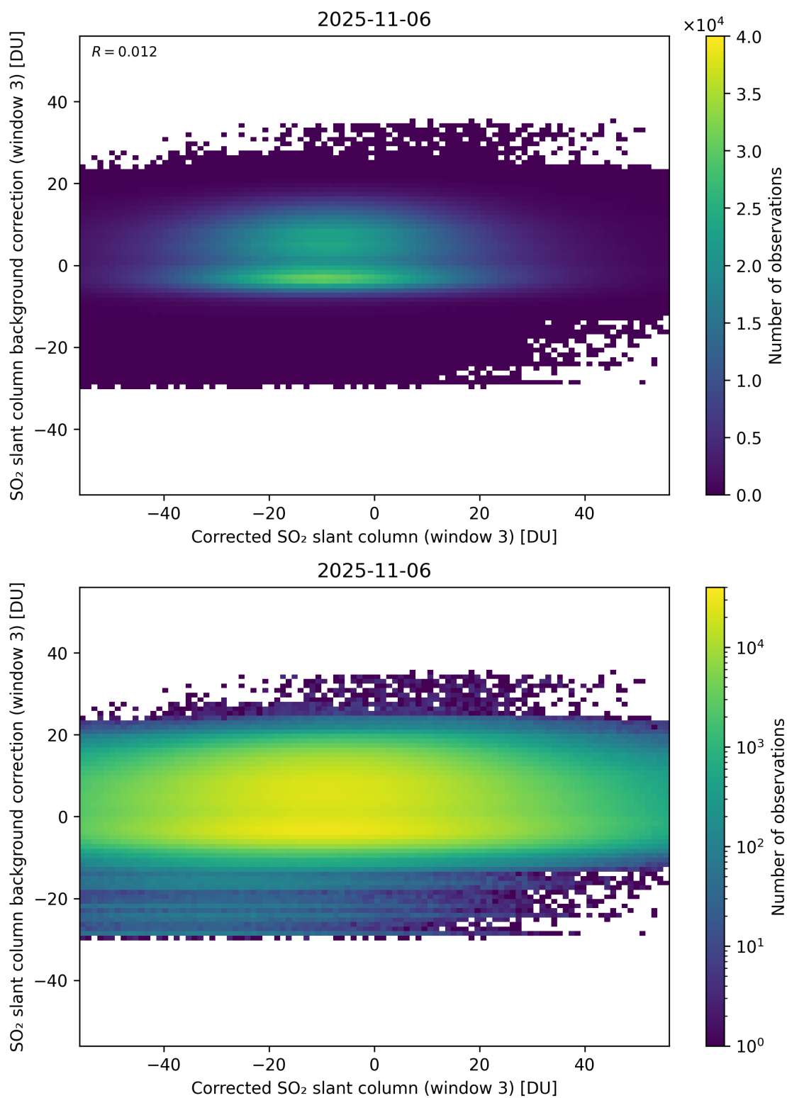
Figure 255: Scatter density plot of “Corrected SO 2 slant column (window 3)” against “SO 2 slant column background correction (window 3)” for 2025-11-05 to 2025-11-07.
