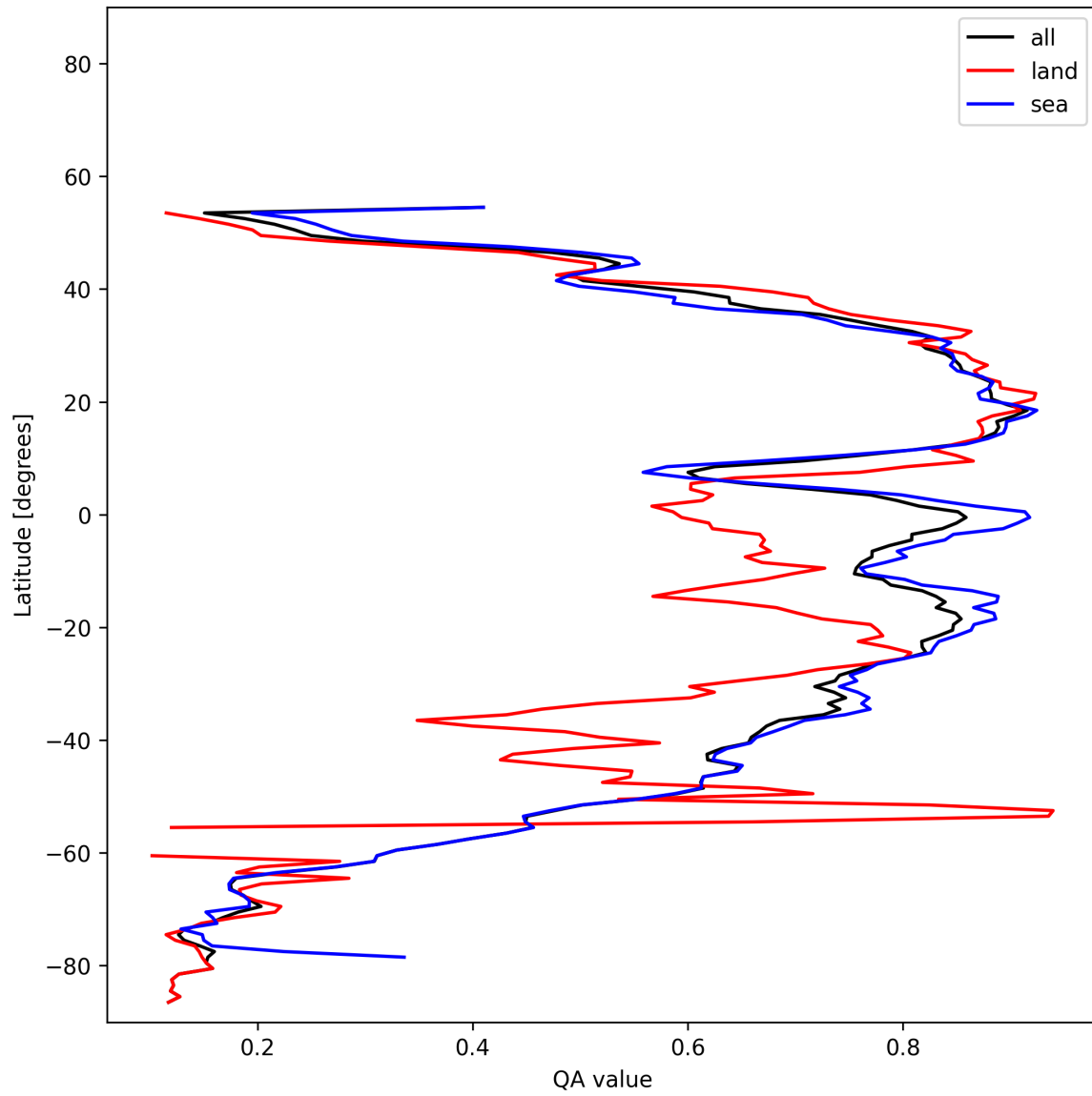
Figure 31: Zonal average of “QA value” for 2025-11-05 to 2025-11-07.
