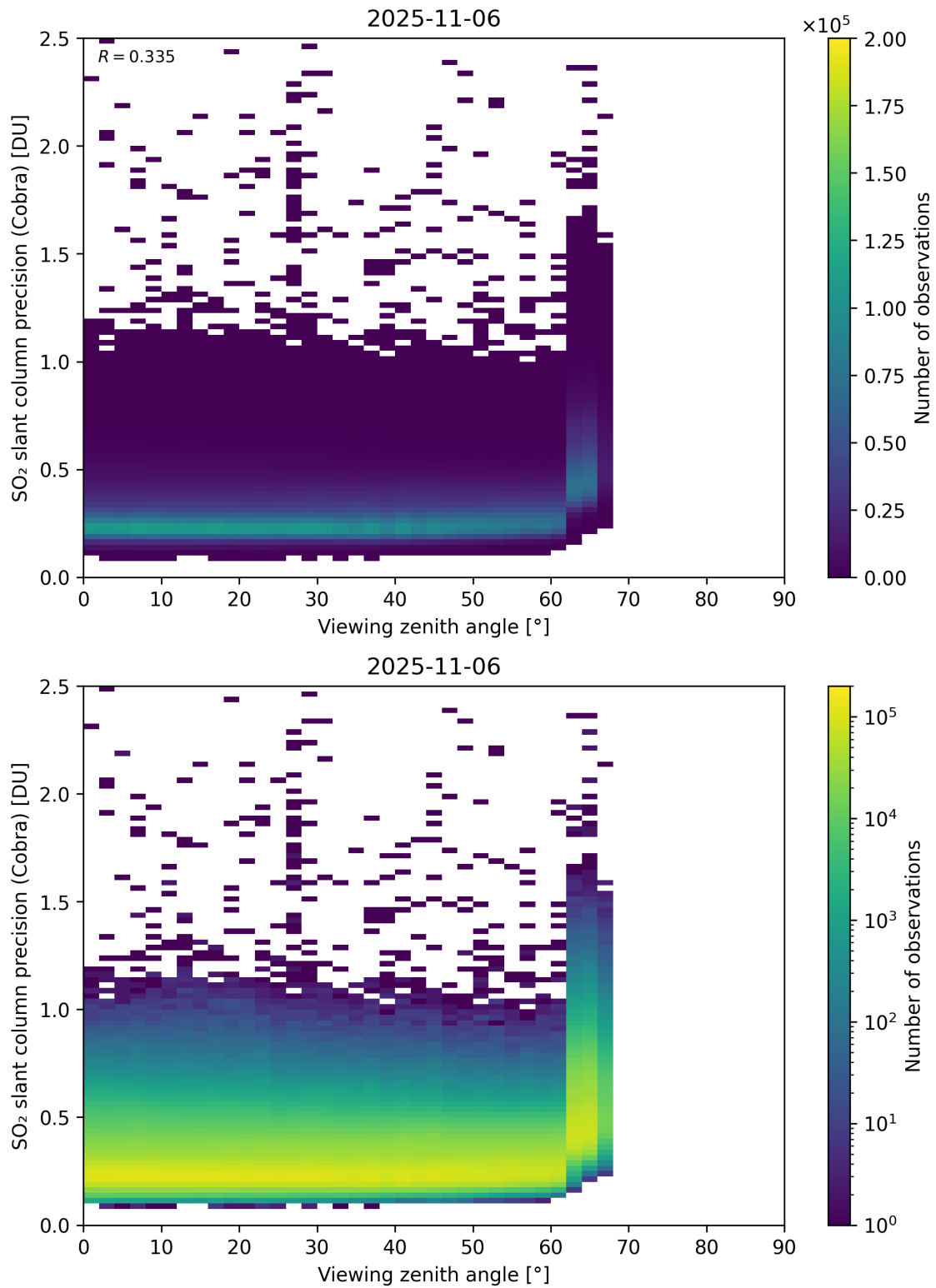
Figure 372: Scatter density plot of “Viewing zenith angle” against “SO 2 slant column precision (Cobra)” for 2025-11-05 to 2025-11-07.
