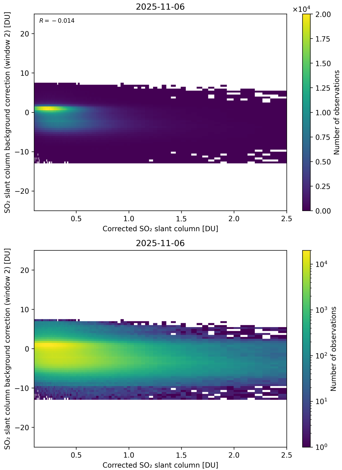
Figure 227: Scatter density plot of “Corrected SO 2 slant column” against “SO 2 slant column background correction (window 2)” for 2025-11-05 to 2025-11-07.
