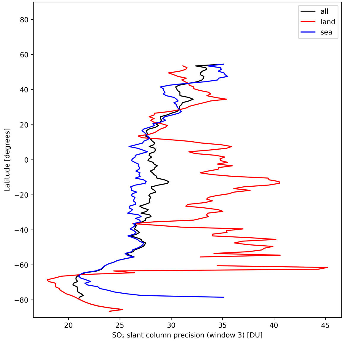
Figure 46: Zonal average of “SO 2 slant column precision (window 3)” for 2025-11-05 to 2025-11-07.
