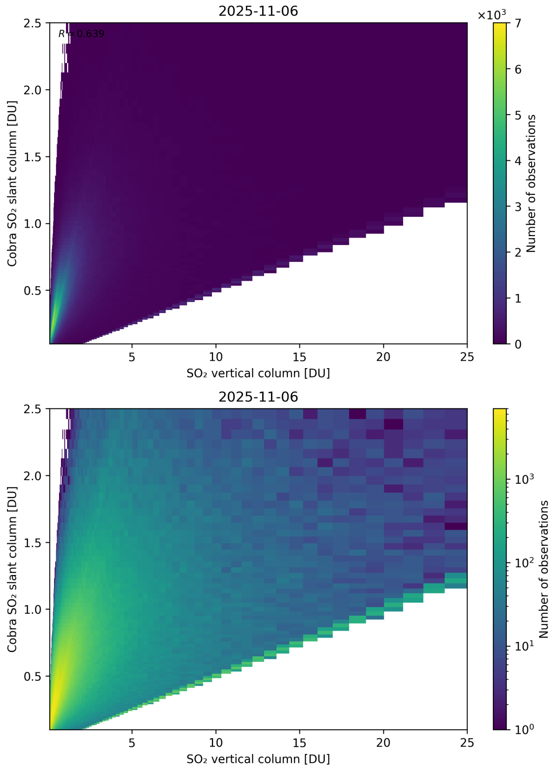
Figure 349: Scatter density plot of “SO 2 vertical column” against “Cobra SO 2 slant column” for 2025-11-05 to 2025-11-07.
