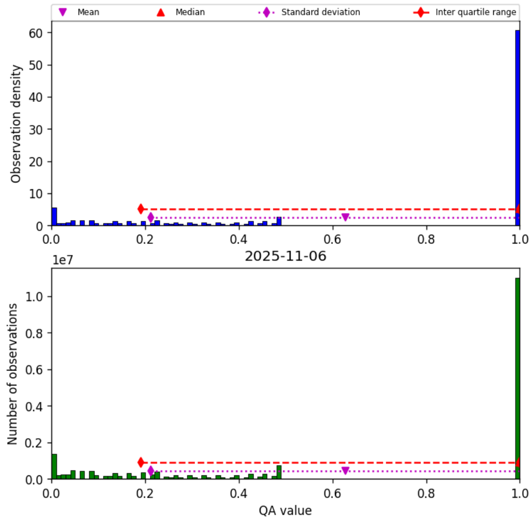
Figure 57: Histogram of “QA value” for 2025-11-05 to 2025-11-07
