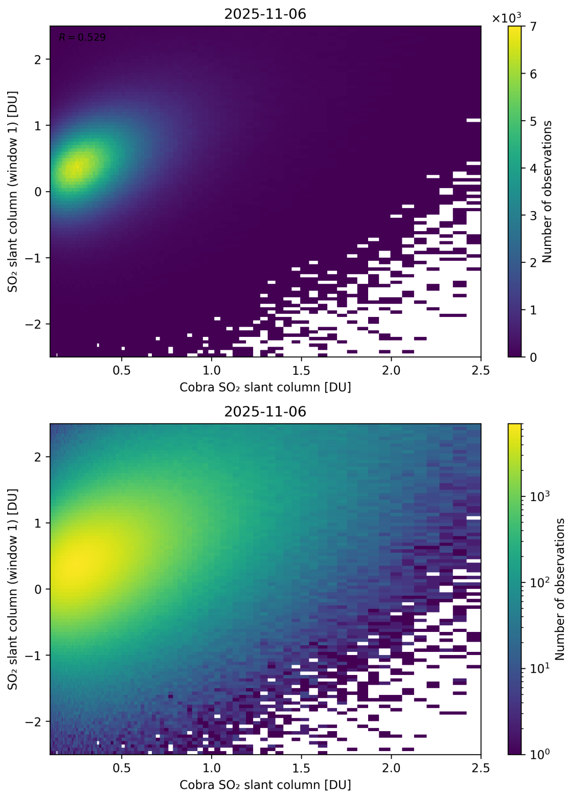
Figure 219: Scatter density plot of “Cobra SO 2 slant column” against “SO 2 slant column (window 1)” for 2025-11-05 to 2025-11-07.
