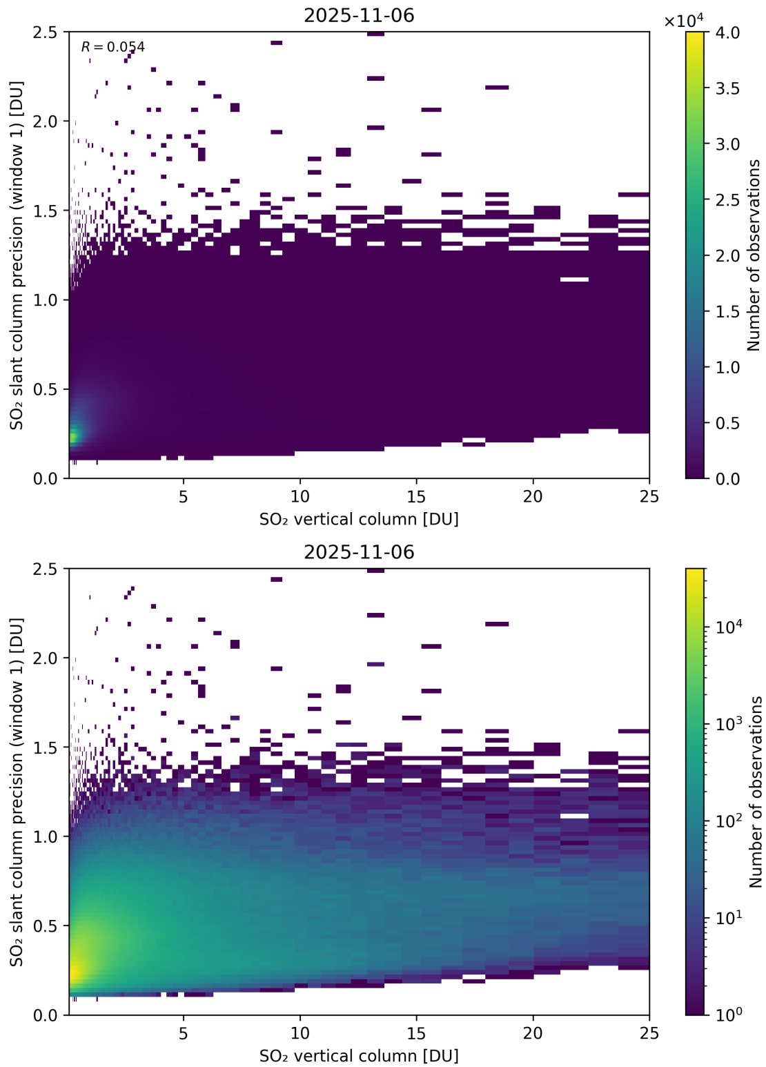
Figure 355: Scatter density plot of “SO 2 vertical column” against “SO 2 slant column precision (window 1)” for 2025-11-05 to 2025-11-07.
