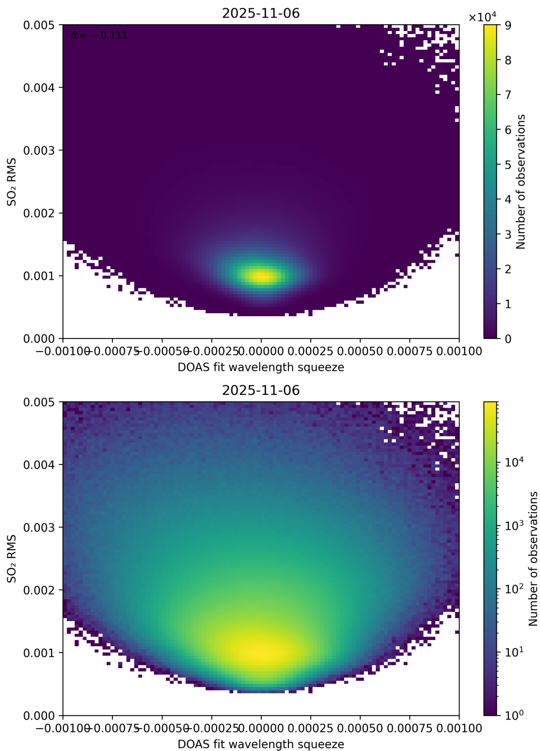
Figure 143: Scatter density plot of “DOAS fit wavelength squeeze” against “SO 2 RMS” for 2025-11-05 to 2025-11-07.
