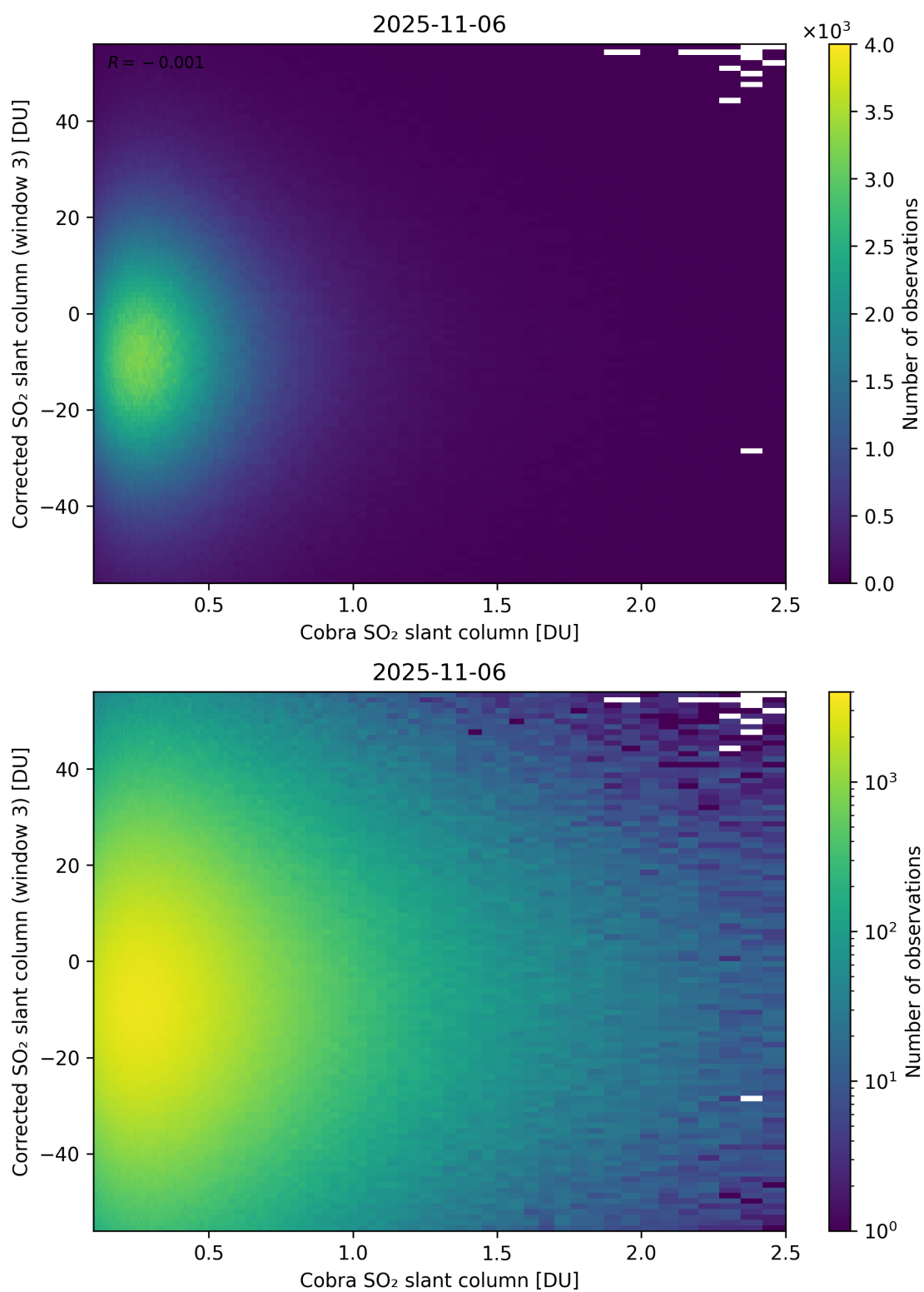
Figure 218: Scatter density plot of “Cobra SO 2 slant column” against “Corrected SO 2 slant column (window 3)” for 2025-11-05 to 2025-11-07.
