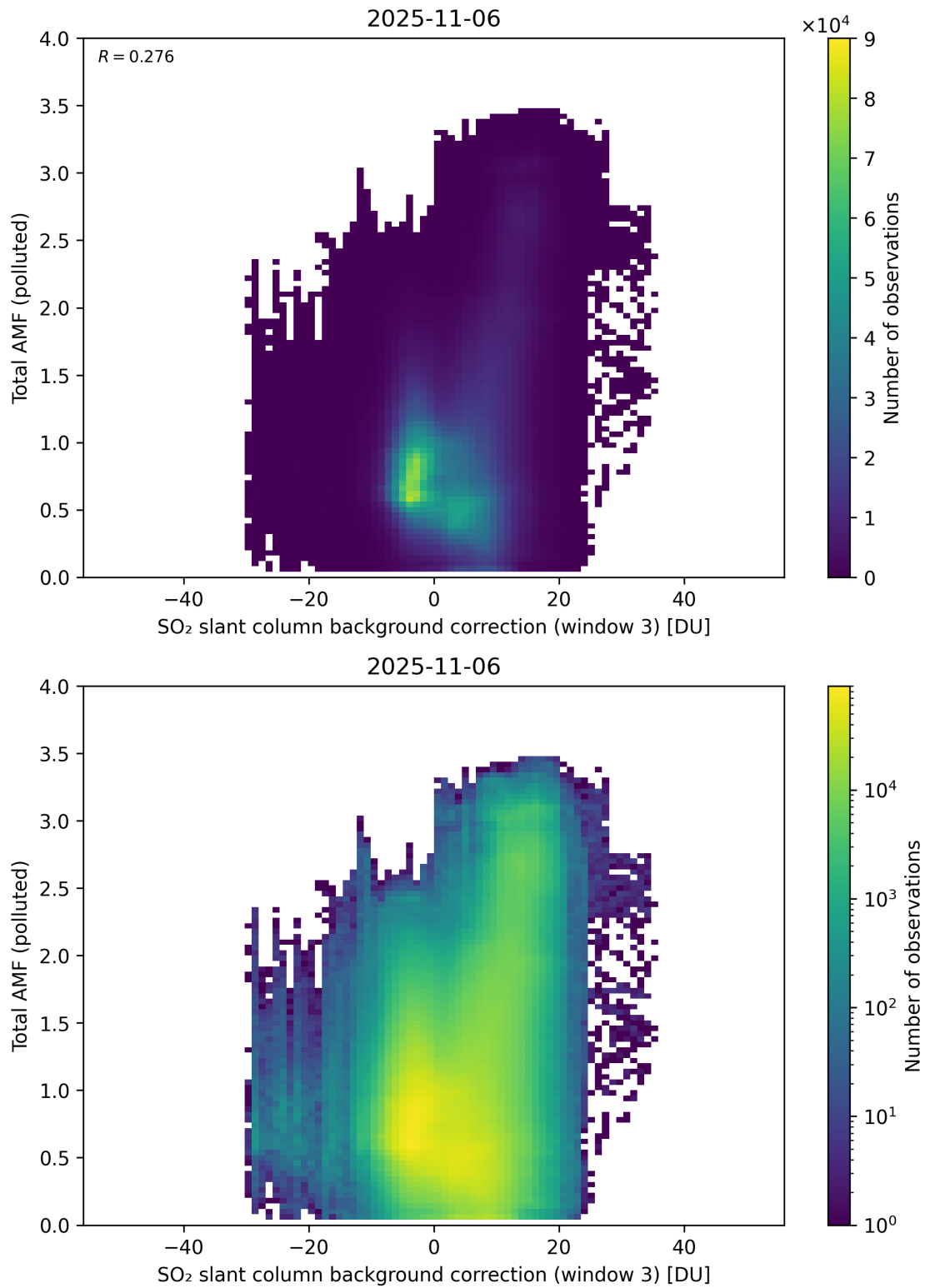
Figure 136: Scatter density plot of “SO 2 slant column background correction (window 3)” against “Total AMF (polluted)” for 2025-11-05 to 2025-11-07.
