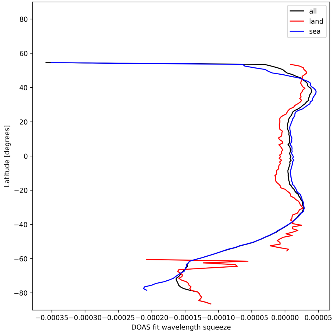
Figure 51: Zonal average of “DOAS fit wavelength squeeze” for 2025-11-05 to 2025-11-07.
