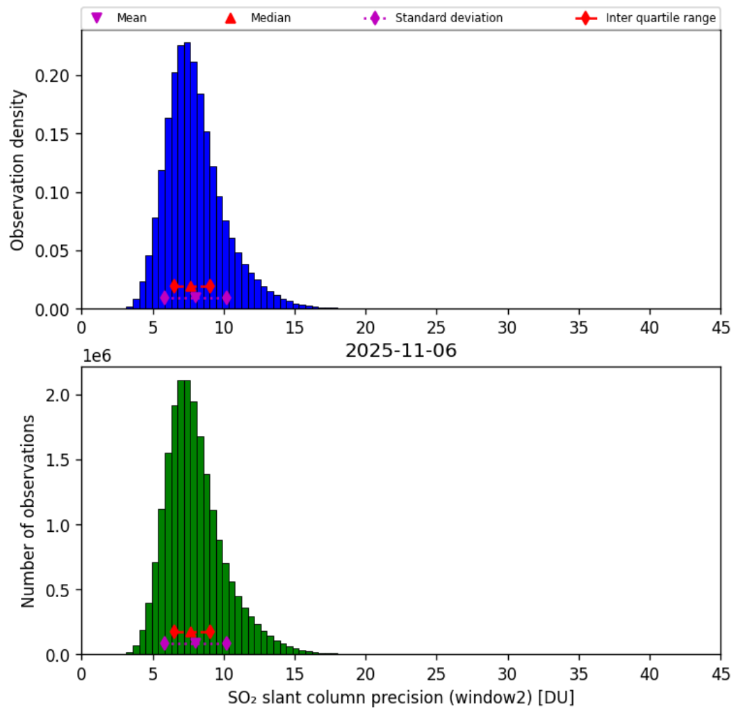
Figure 68: Histogram of “SO 2 slant column precision (window2)” for 2025-11-05 to 2025-11-07
