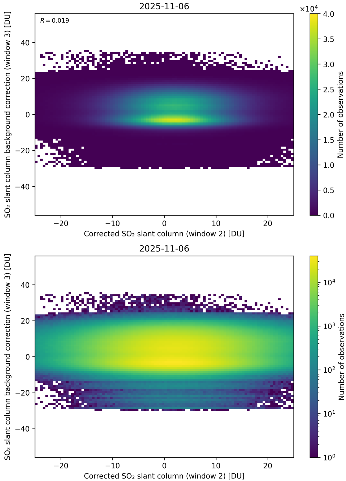
Figure 245: Scatter density plot of “Corrected SO 2 slant column (window 2)” against “SO 2 slant column background correction (window 3)” for 2025-11-05 to 2025-11-07.
