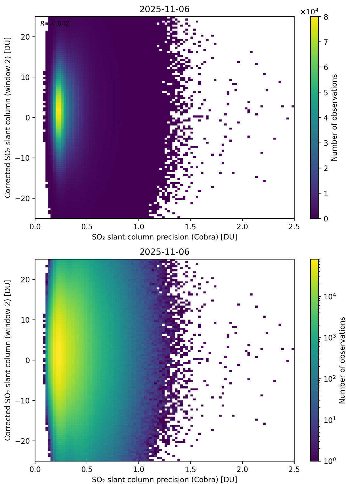
Figure 206: Scatter density plot of “SO 2 slant column precision (Cobra)” against “Corrected SO 2 slant column (window 2)” for 2025-11-05 to 2025-11-07.
