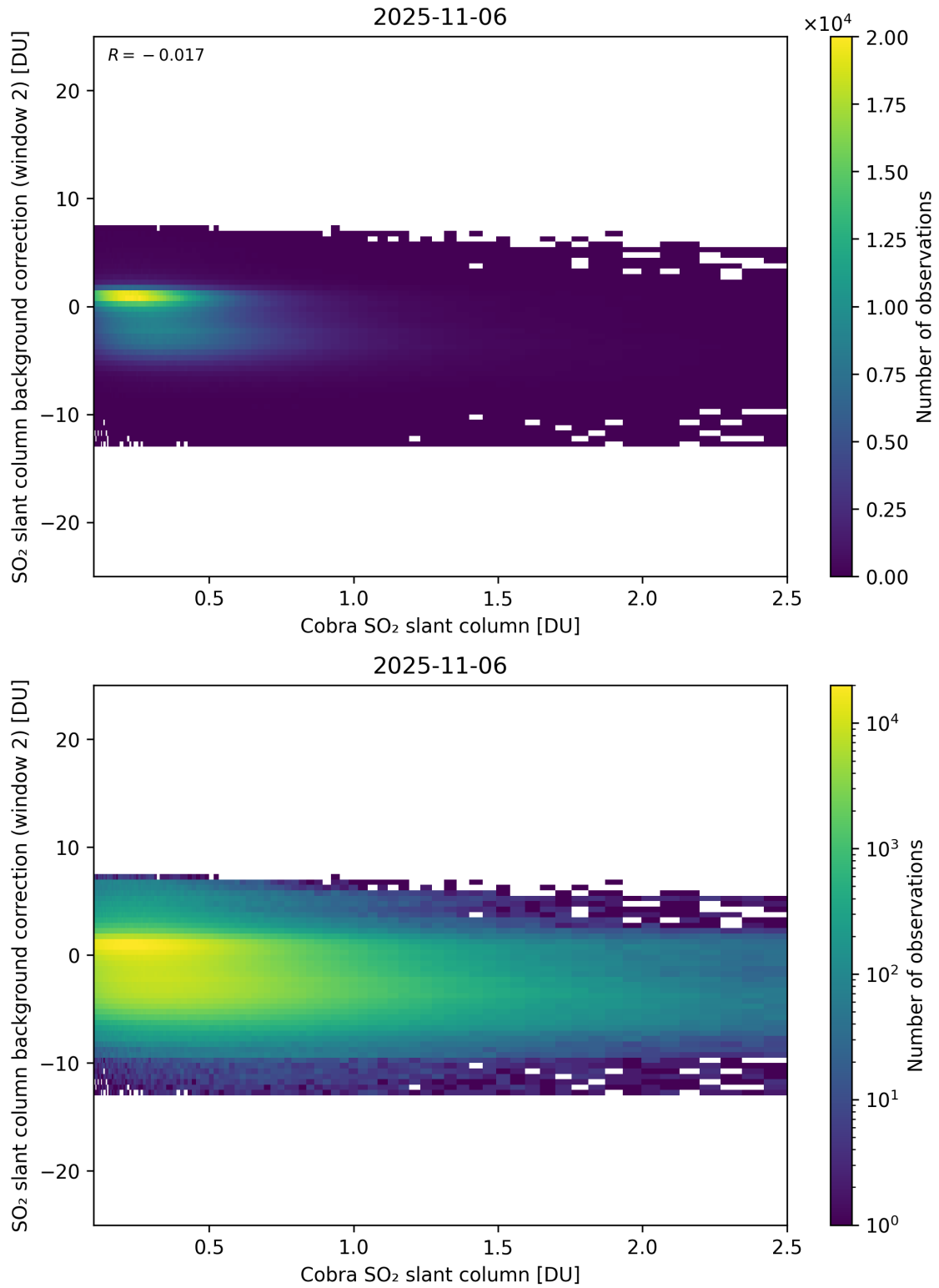
Figure 194: Scatter density plot of “Cobra SO 2 slant column” against “SO 2 slant column background correction (window 2)” for 2025-11-05 to 2025-11-07.
