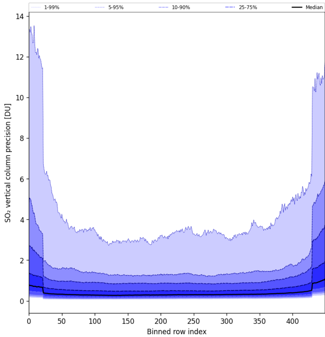
Figure 85: Along track statistics of “SO 2 vertical column precision” for 2025-11-05 to 2025-11-07
