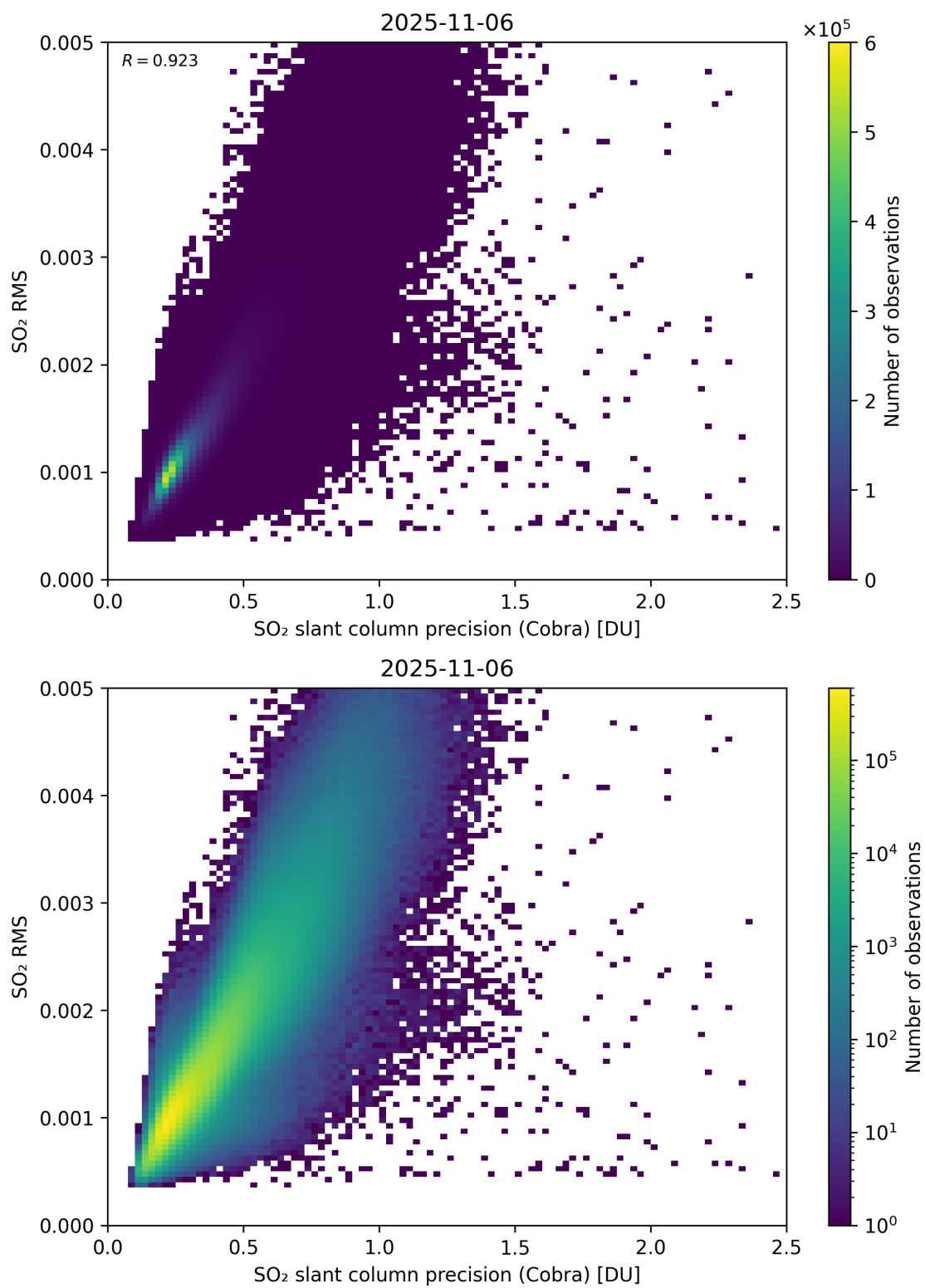
Figure 204: Scatter density plot of “SO 2 slant column precision (Cobra)” against “SO 2 RMS” for 2025-11-05 to 2025-11-07.
