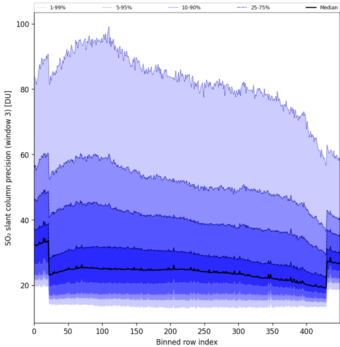
Figure 98: Along track statistics of “SO 2 slant column precision (window 3)” for 2025-11-05 to 2025-11-07
