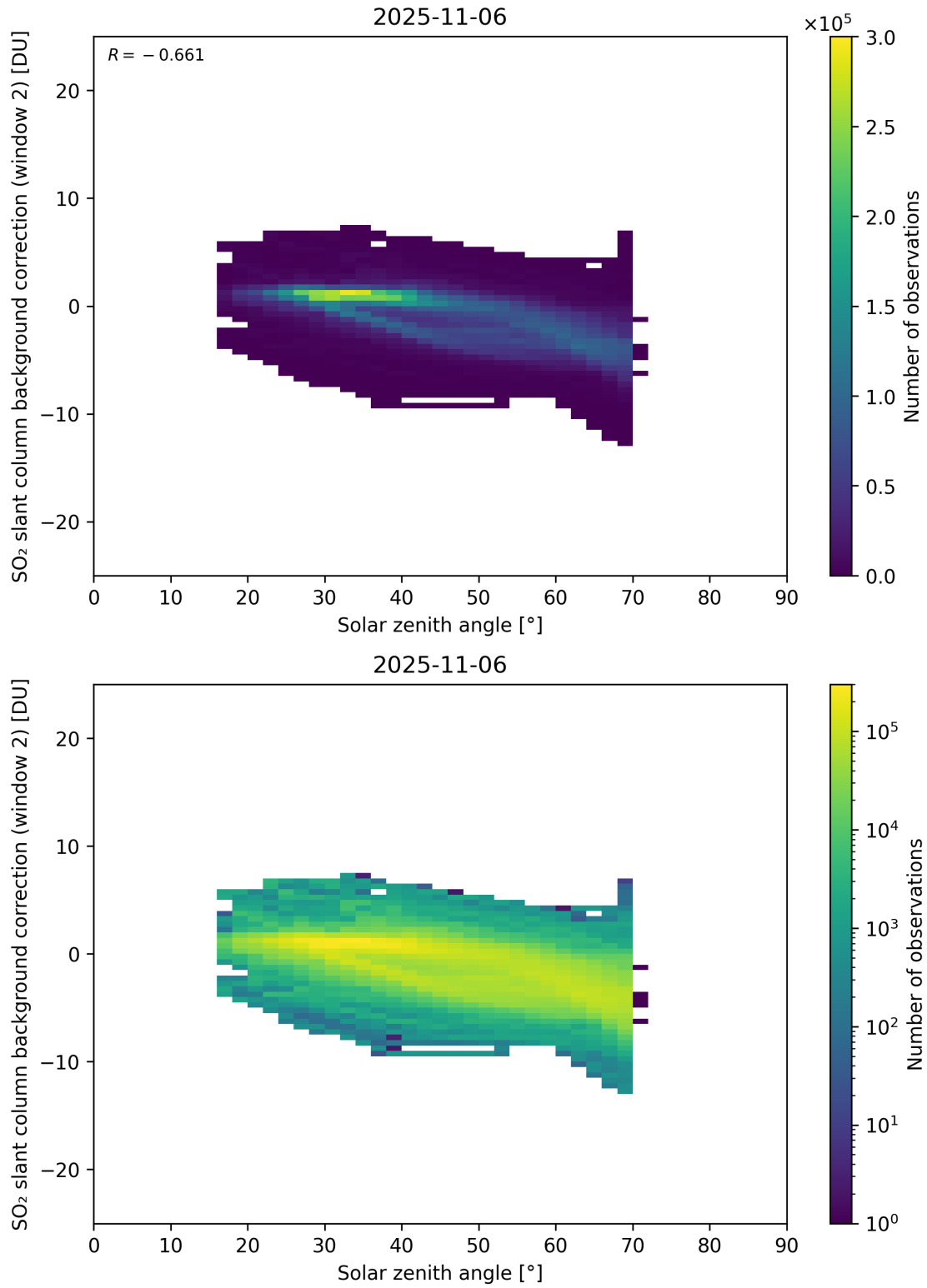
Figure 172: Scatter density plot of “Solar zenith angle” against “SO 2 slant column background correction (window 2)” for 2025-11-05 to 2025-11-07.
