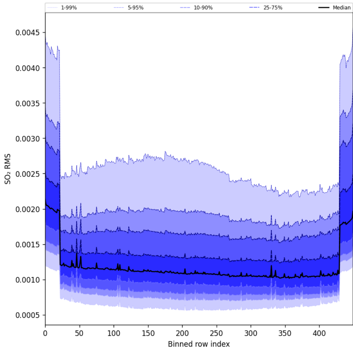
Figure 104: Along track statistics of “SO 2 RMS” for 2025-11-05 to 2025-11-07
