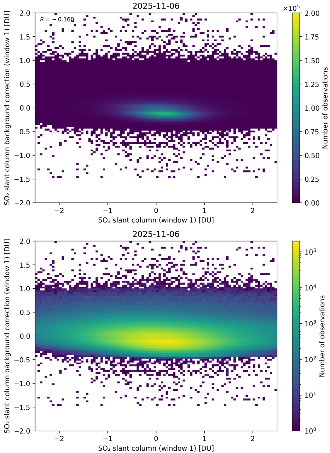
Figure 262: Scatter density plot of “SO 2 slant column (window 1)” against “SO 2 slant column background correction (window 1)” for 2025-11-05 to 2025-11-07.
