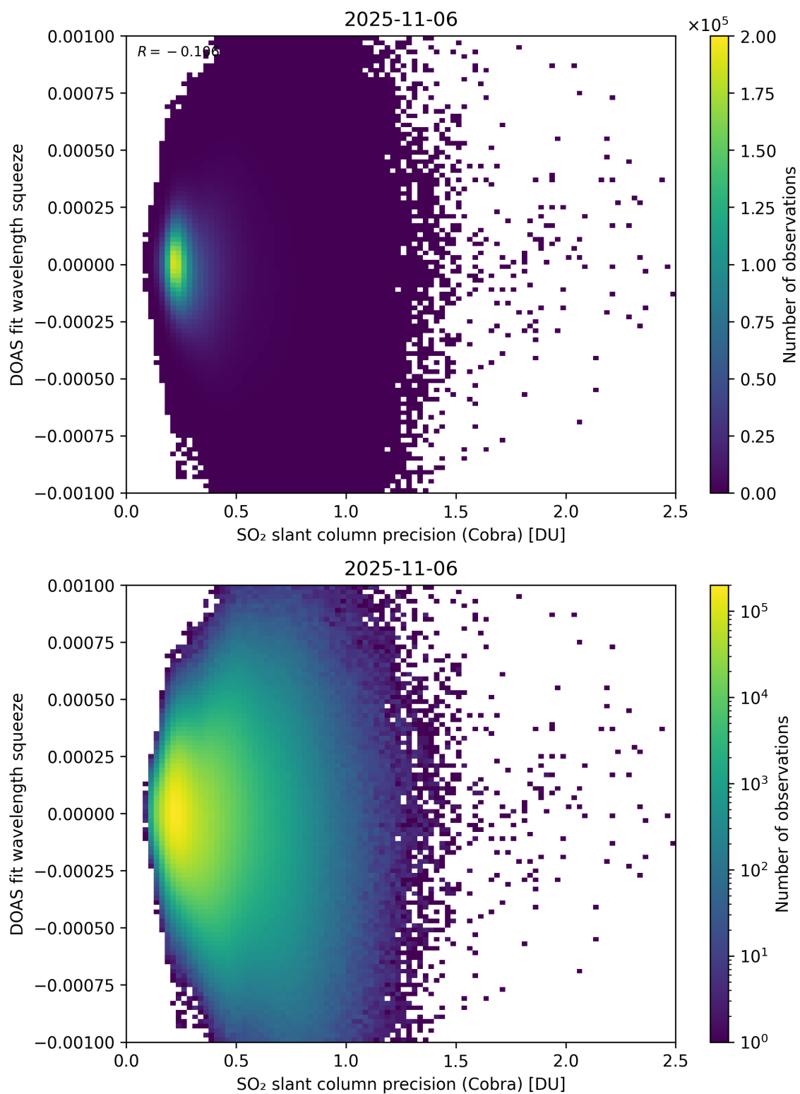
Figure 203: Scatter density plot of “SO 2 slant column precision (Cobra)” against “DOAS fit wavelength squeeze” for 2025-11-05 to 2025-11-07.
