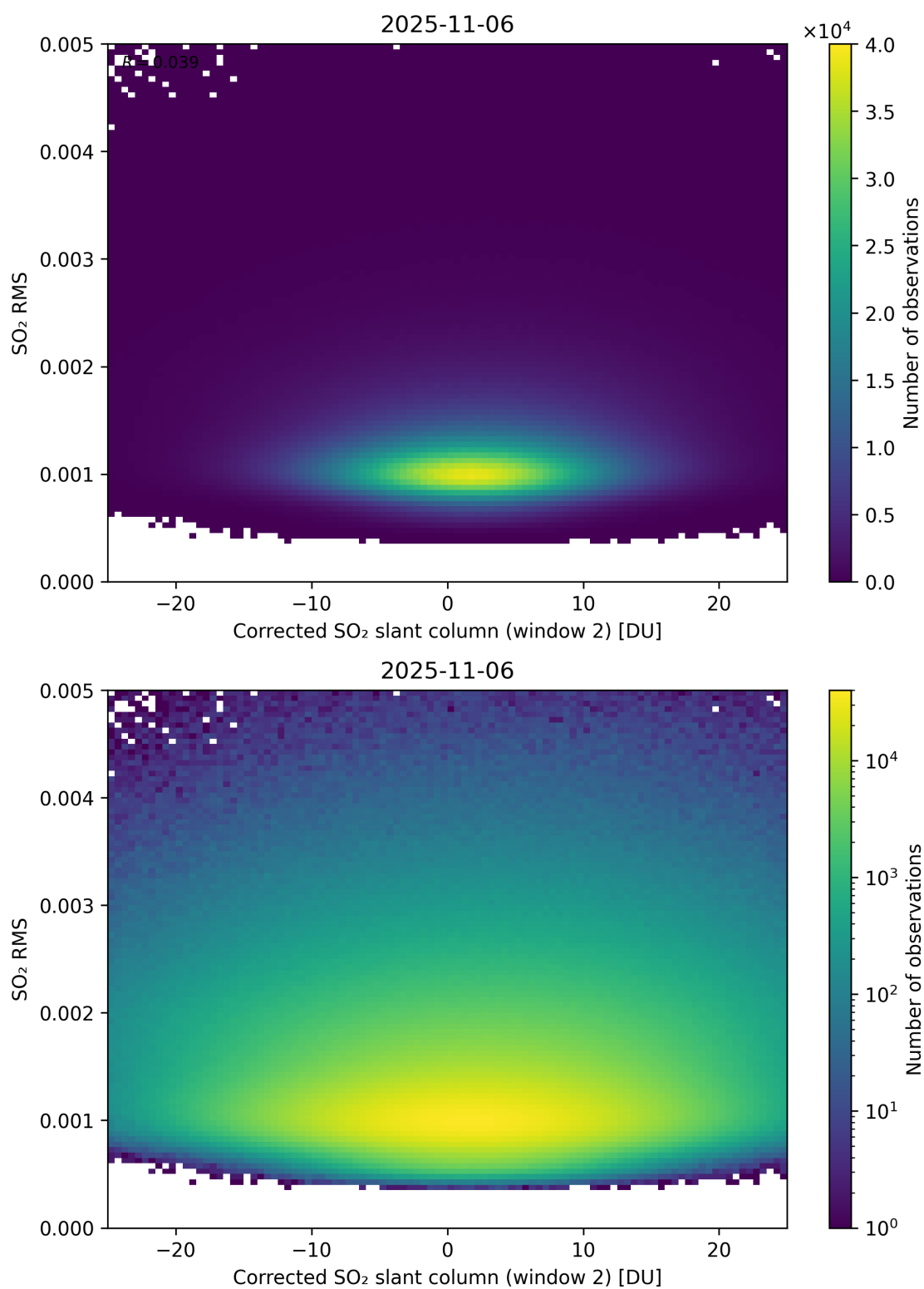
Figure 248: Scatter density plot of “Corrected SO 2 slant column (window 2)” against “SO 2 RMS” for 2025-11-05 to 2025-11-07.
