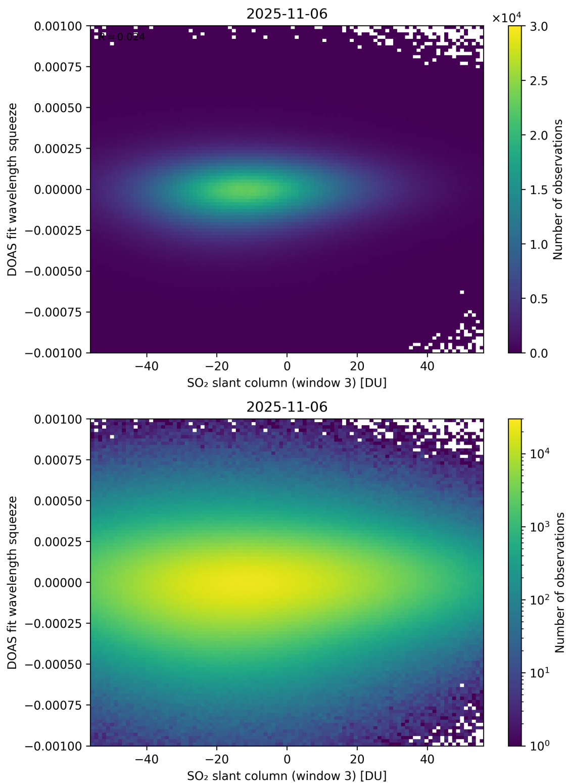
Figure 305: Scatter density plot of “SO 2 slant column (window 3)” against “DOAS fit wavelength squeeze” for 2025-11-05 to 2025-11-07.
