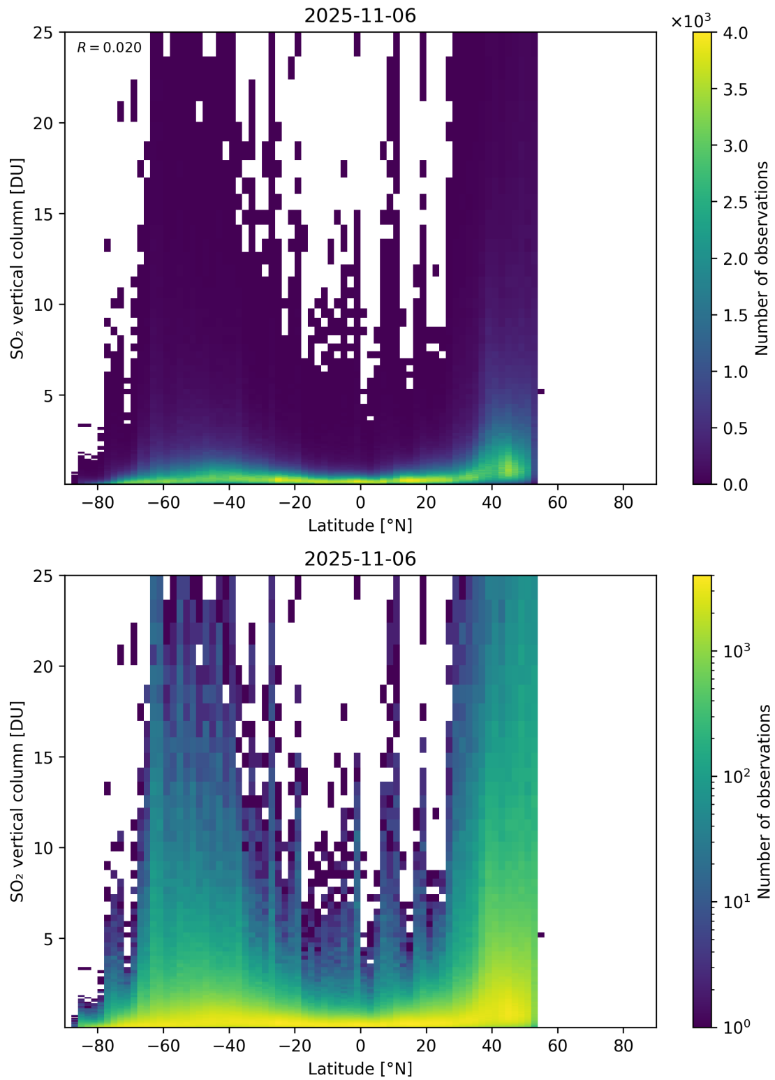
Figure 169: Scatter density plot of “Latitude” against “SO 2 vertical column” for 2025-11-05 to 2025-11-07.
