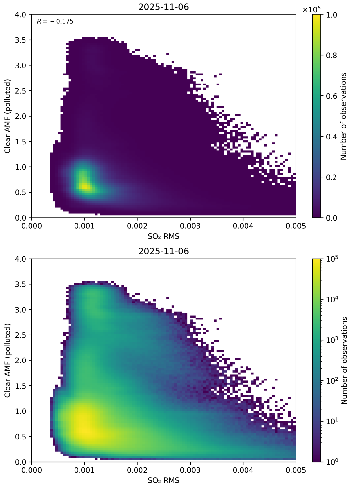
Figure 147: Scatter density plot of “SO 2 RMS” against “Clear AMF (polluted)” for 2025-11-05 to 2025-11-07.
