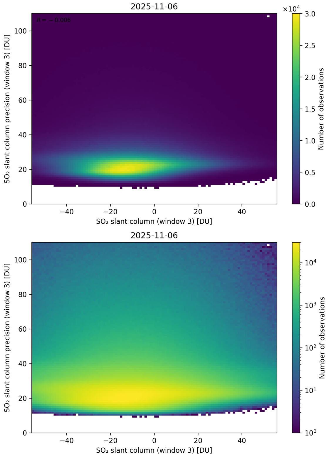
Figure 317: Scatter density plot of “SO 2 slant column (window 3)” against “SO 2 slant column precision (window 3)” for 2025-11-05 to 2025-11-07.
