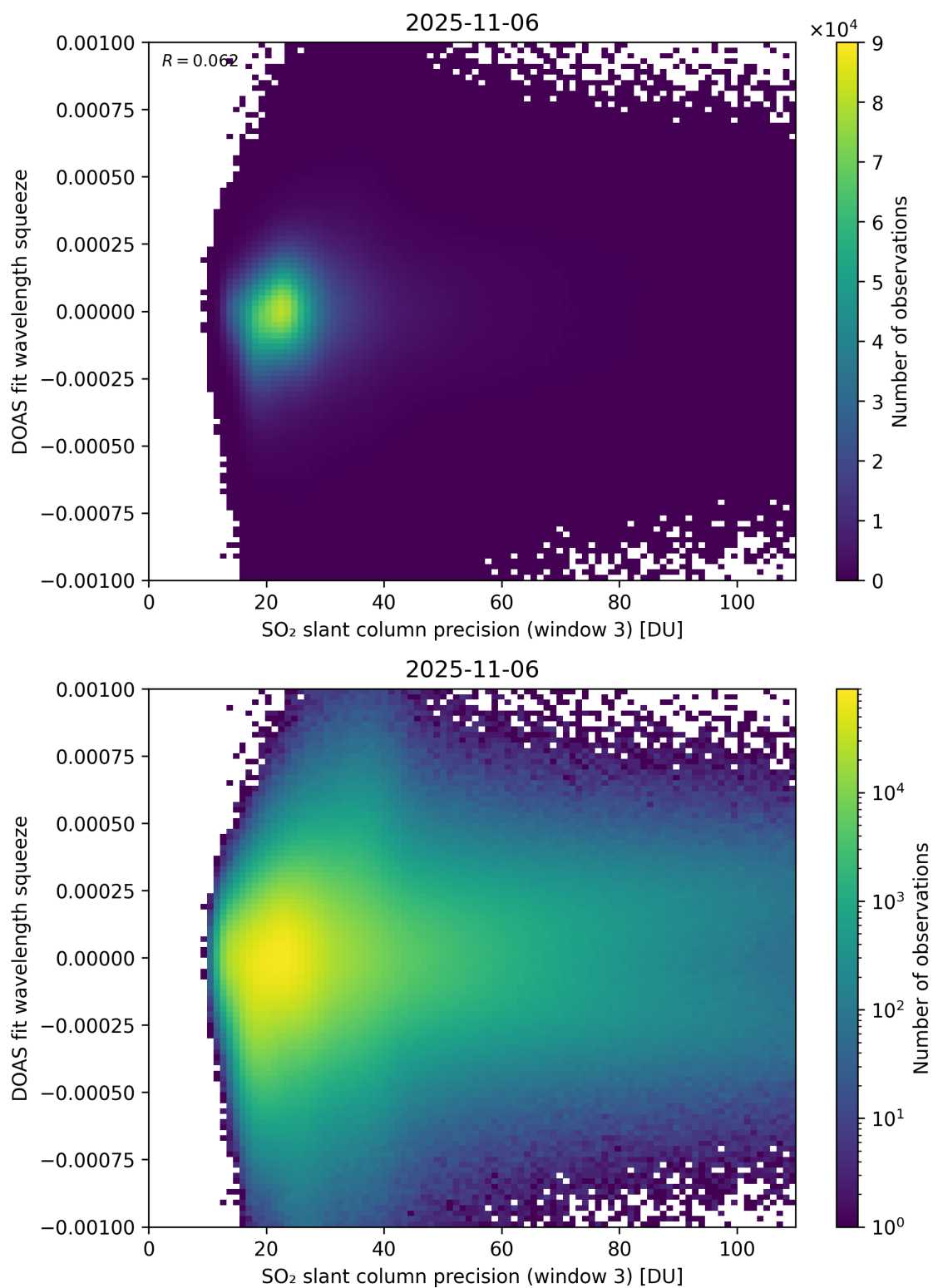
Figure 309: Scatter density plot of “SO 2 slant column precision (window 3)” against “DOAS fit wavelength squeeze” for 2025-11-05 to 2025-11-07.
