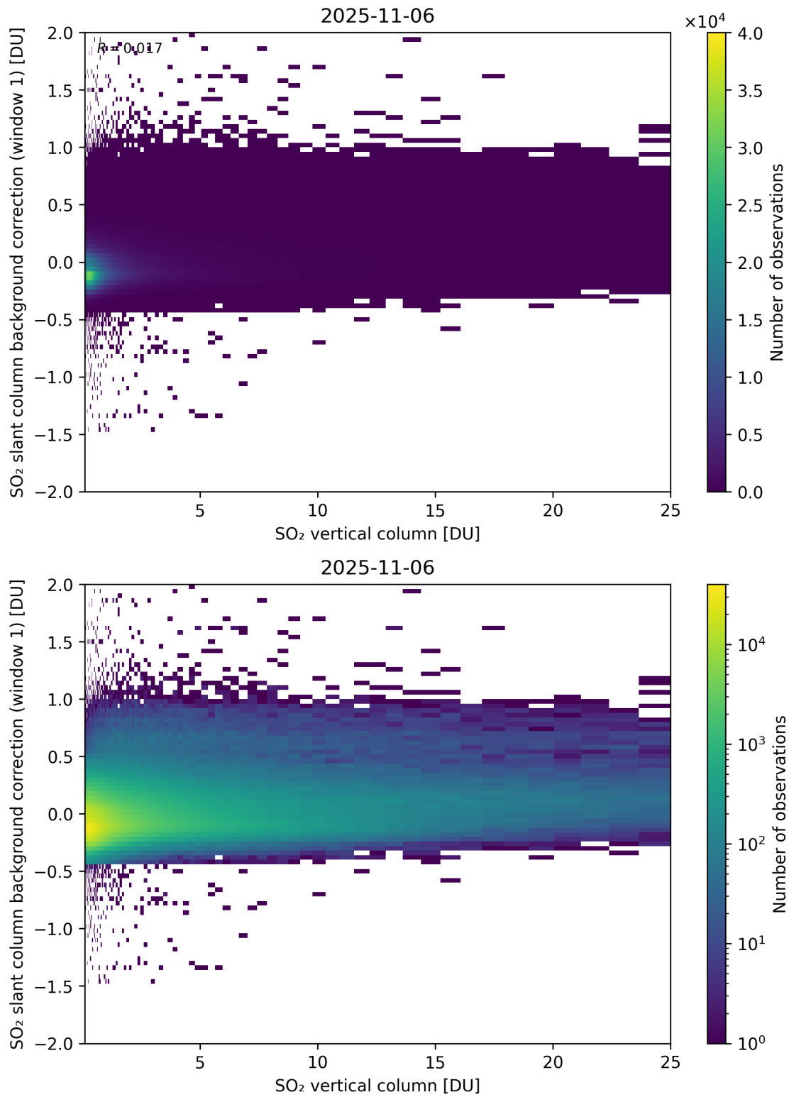
Figure 323: Scatter density plot of “SO 2 vertical column” against “SO 2 slant column background correction (window 1)” for 2025-11-05 to 2025-11-07.
