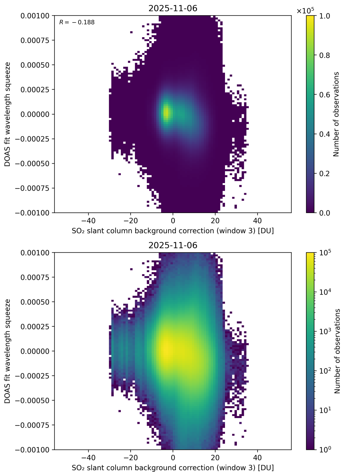
Figure 133: Scatter density plot of “SO 2 slant column background correction (window 3)” against “DOAS fit wavelength squeeze” for 2025-11-05 to 2025-11-07.
