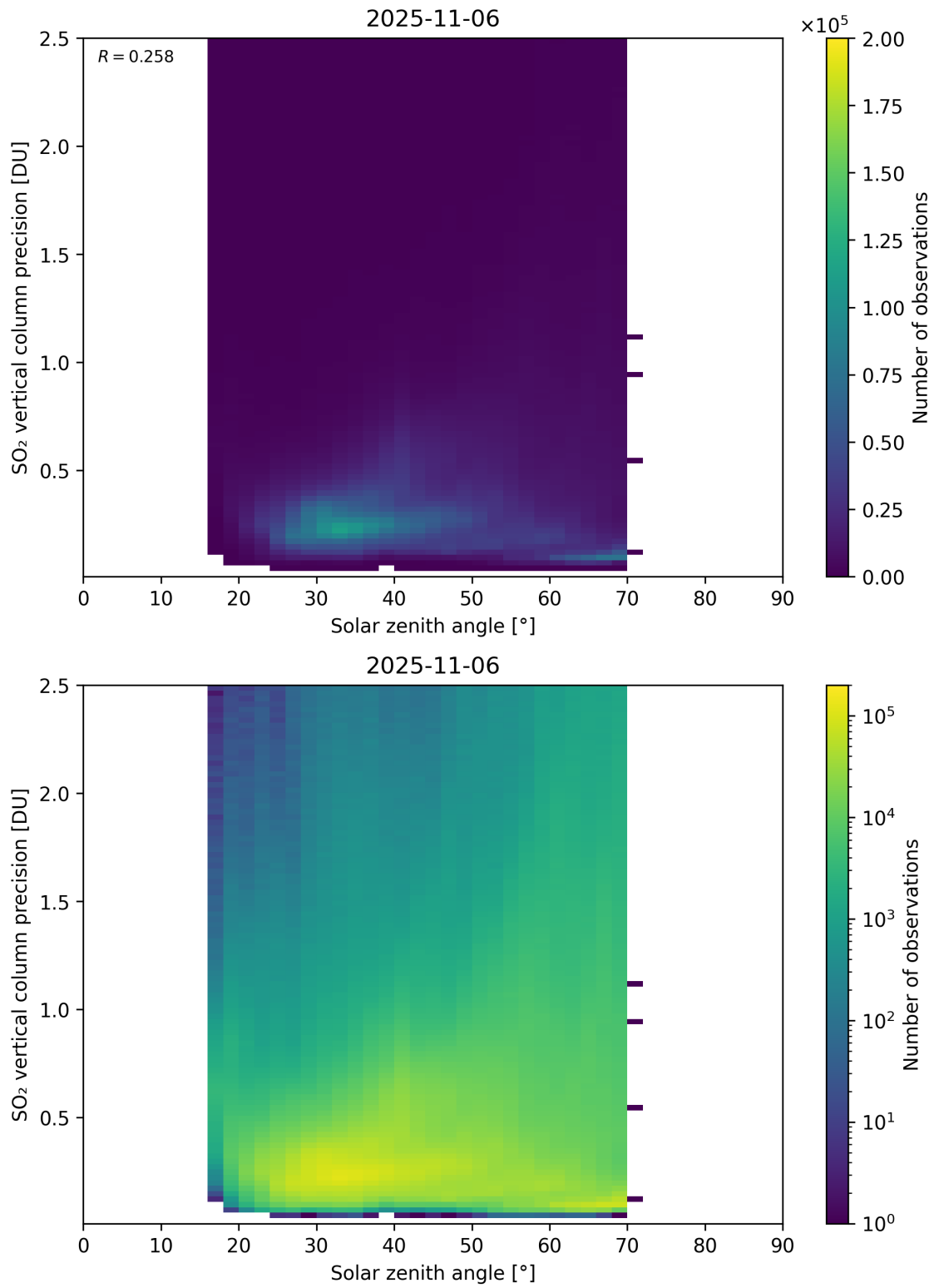
Figure 192: Scatter density plot of “Solar zenith angle” against “SO 2 vertical column precision” for 2025-11-05 to 2025-11-07.
