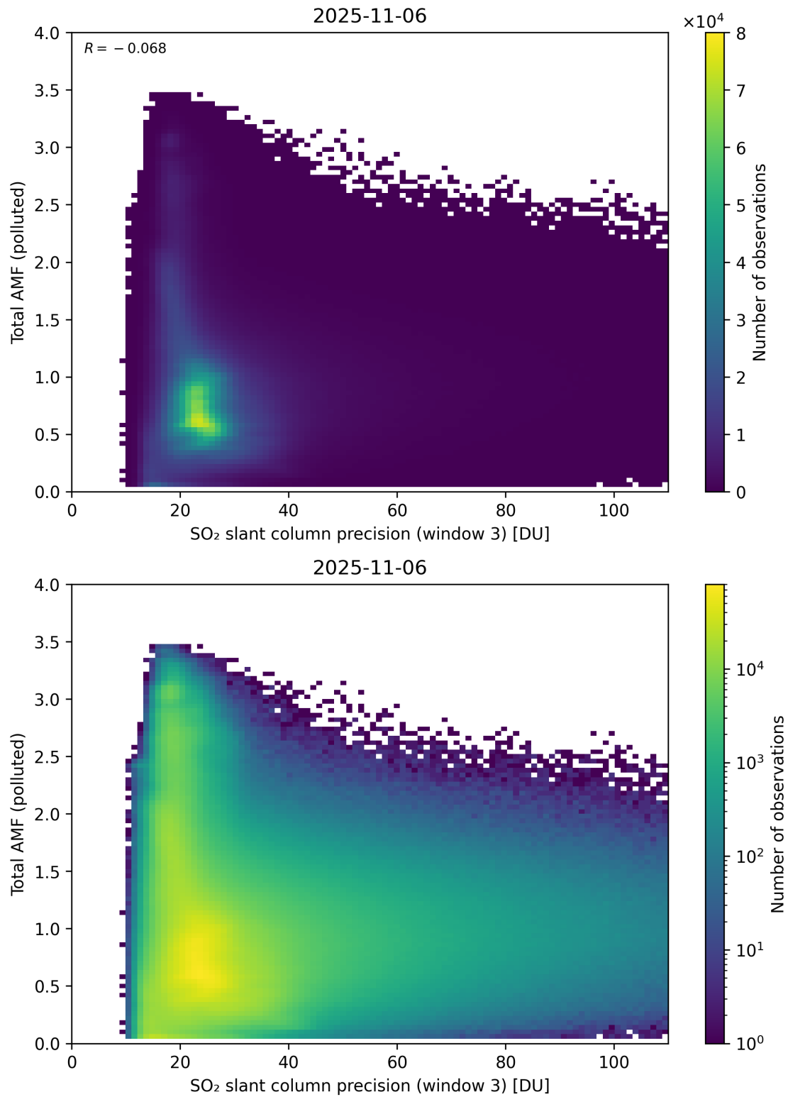
Figure 313: Scatter density plot of “SO 2 slant column precision (window 3)” against “Total AMF (polluted)” for 2025-11-05 to 2025-11-07.
