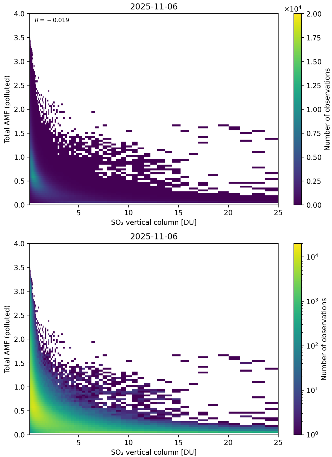
Figure 359: Scatter density plot of “SO 2 vertical column” against “Total AMF (polluted)” for 2025-11-05 to 2025-11-07.
