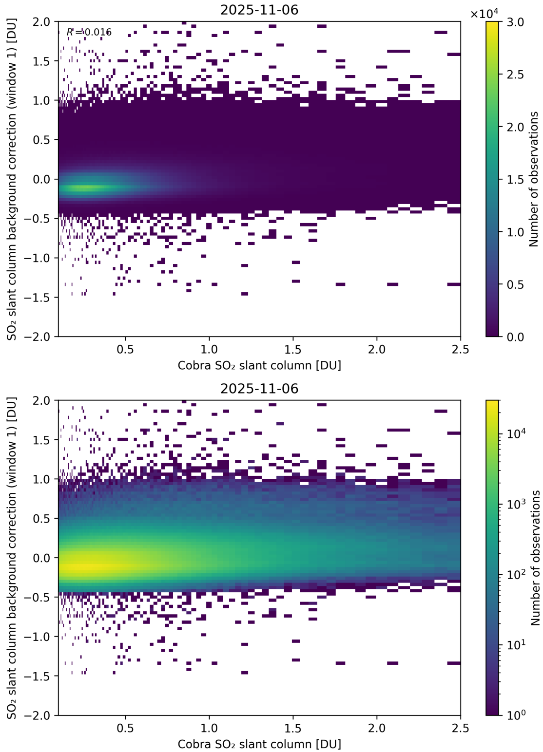
Figure 193: Scatter density plot of “Cobra SO 2 slant column” against “SO 2 slant column background correction (window 1)” for 2025-11-05 to 2025-11-07.
