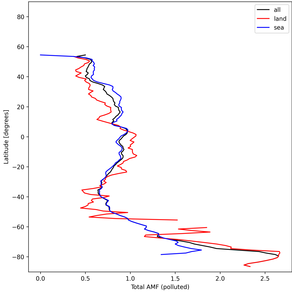
Figure 53: Zonal average of “Total AMF (polluted)” for 2025-11-05 to 2025-11-07.
