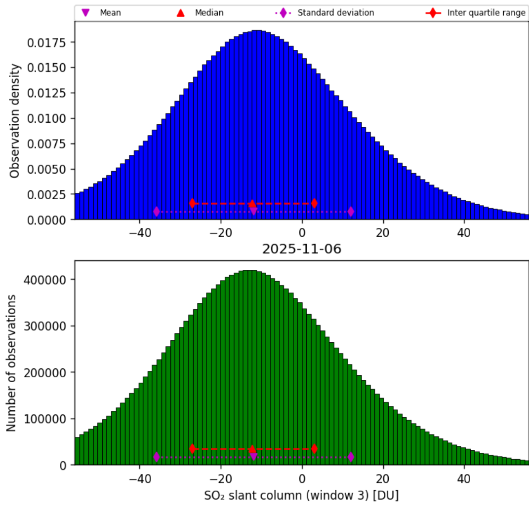
Figure 71: Histogram of “SO 2 slant column (window 3)” for 2025-11-05 to 2025-11-07
