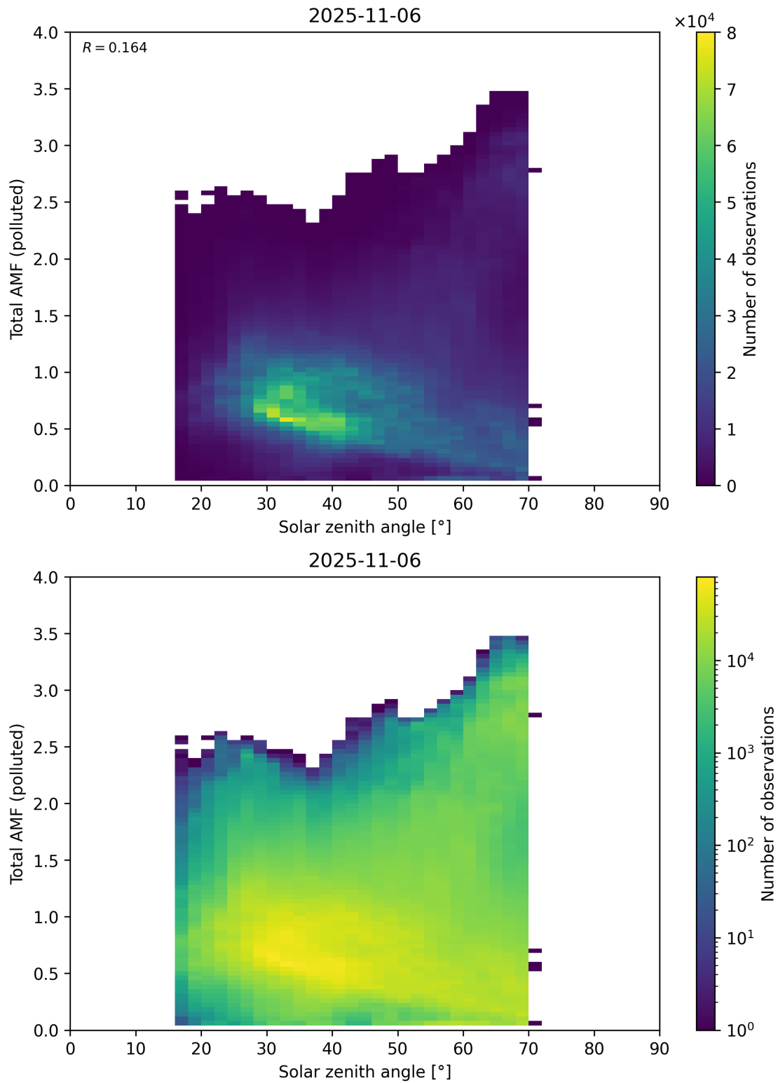
Figure 189: Scatter density plot of “Solar zenith angle” against “Total AMF (polluted)” for 2025-11-05 to 2025-11-07.
