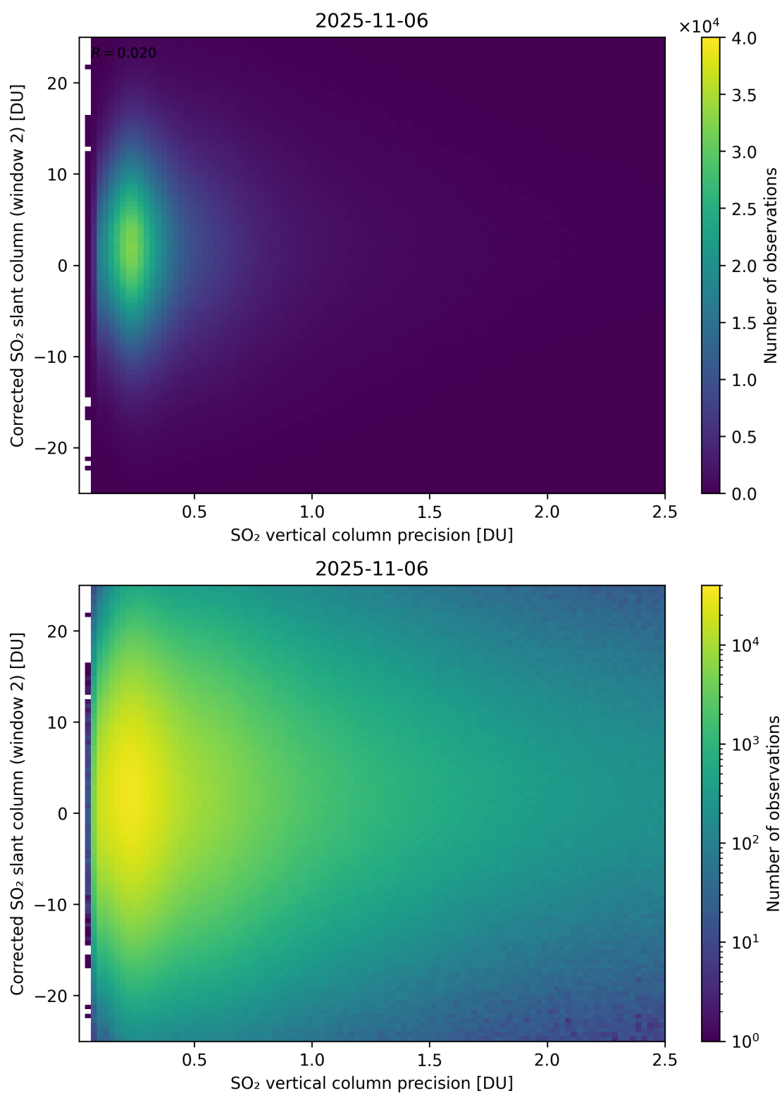
Figure 339: Scatter density plot of “SO 2 vertical column precision” against “Corrected SO 2 slant column (window 2)” for 2025-11-05 to 2025-11-07.
