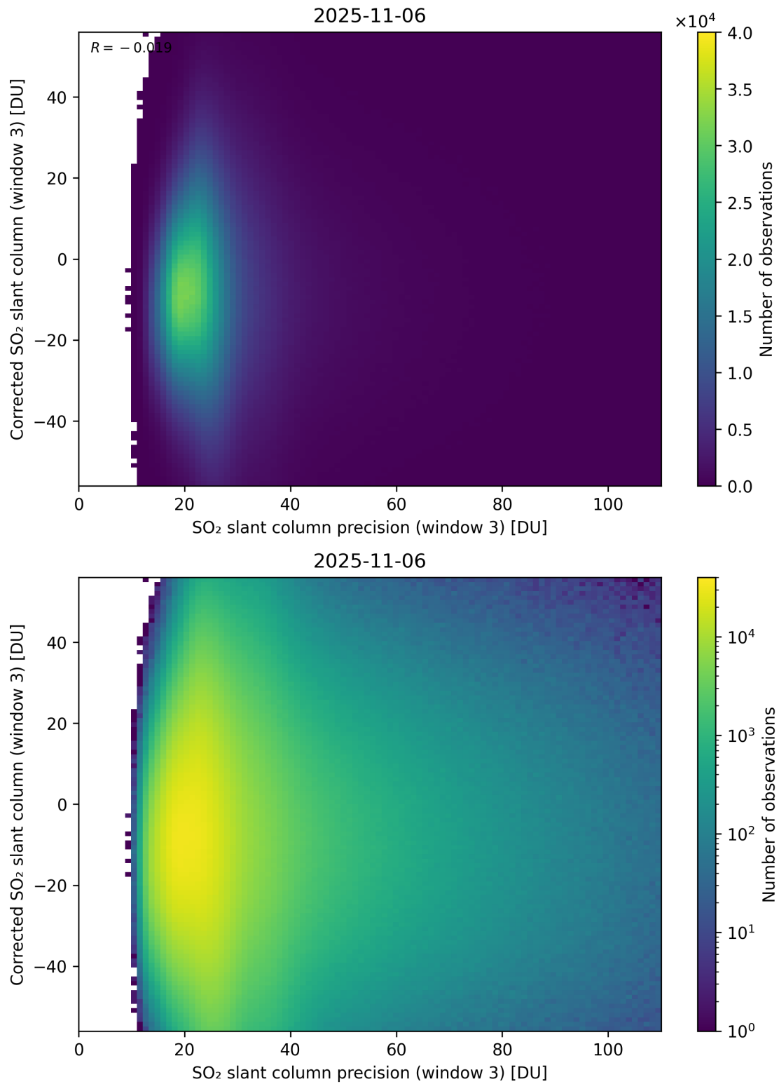
Figure 312: Scatter density plot of “SO 2 slant column precision (window 3)” against “Corrected SO 2 slant column (window 3)” for 2025-11-05 to 2025-11-07.
