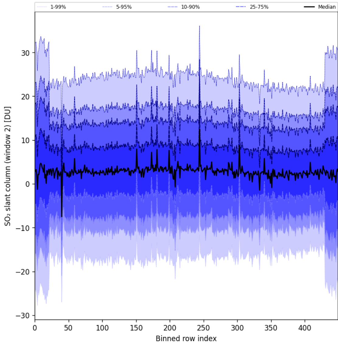
Figure 93: Along track statistics of “SO 2 slant column (window 2)” for 2025-11-05 to 2025-11-07
