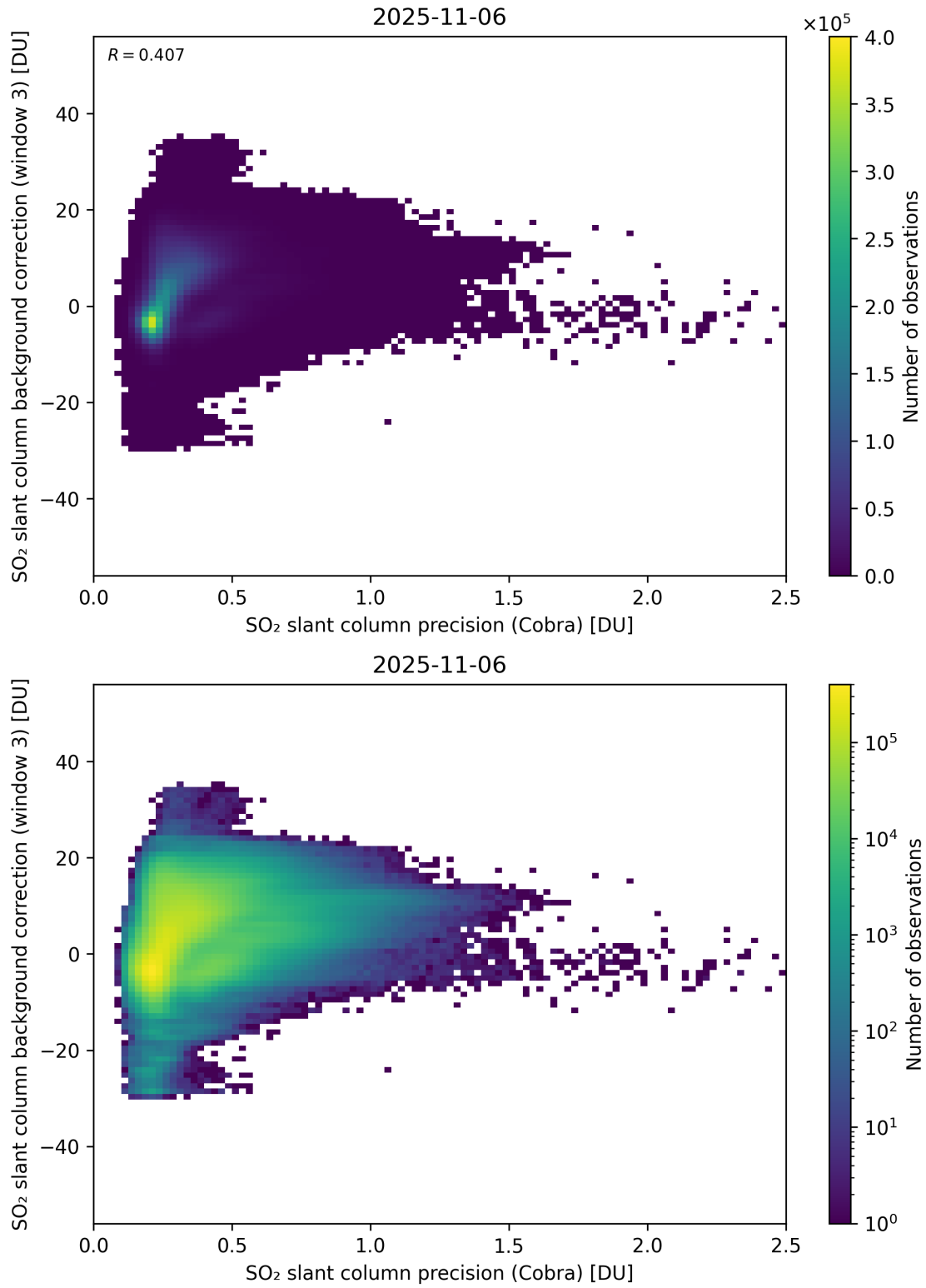
Figure 201: Scatter density plot of “SO 2 slant column precision (Cobra)” against “SO 2 slant column background correction (window 3)” for 2025-11-05 to 2025-11-07.
