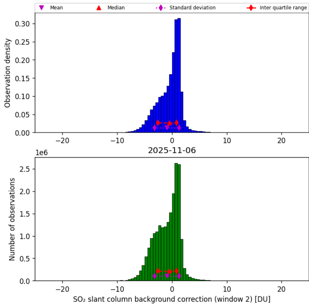
Figure 70: Histogram of “SO 2 slant column background correction (window 2)” for 2025-11-05 to 2025-11-07
