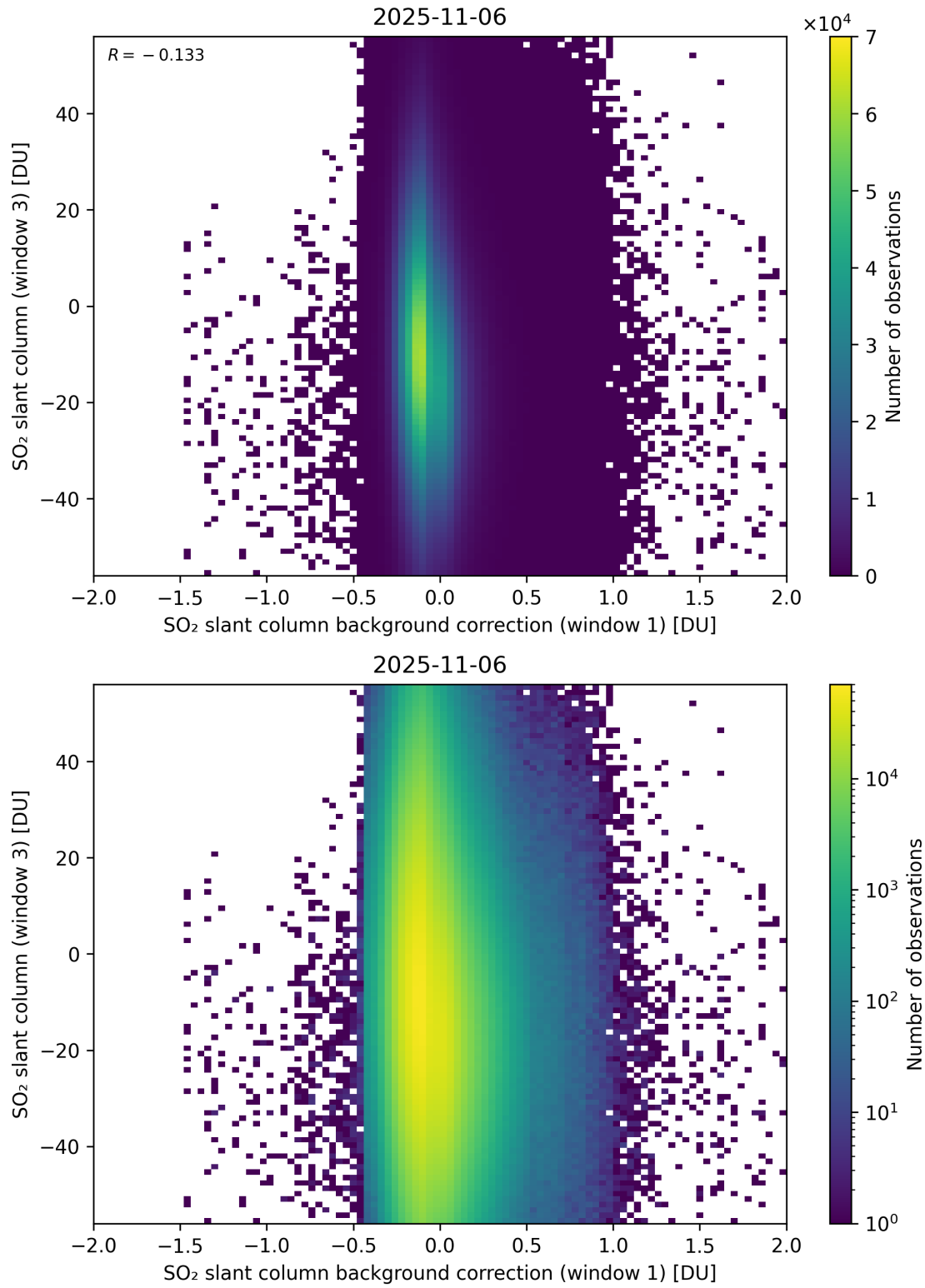
Figure 118: Scatter density plot of “SO 2 slant column background correction (window 1)” against “SO 2 slant column (window 3)” for 2025-11-05 to 2025-11-07.
