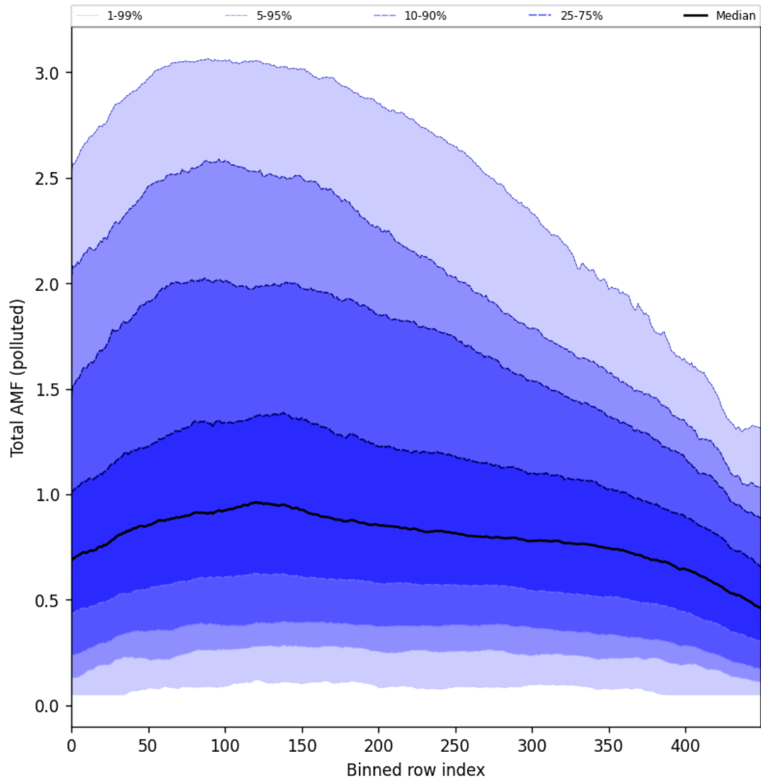
Figure 105: Along track statistics of “Total AMF (polluted)” for 2025-11-05 to 2025-11-07
