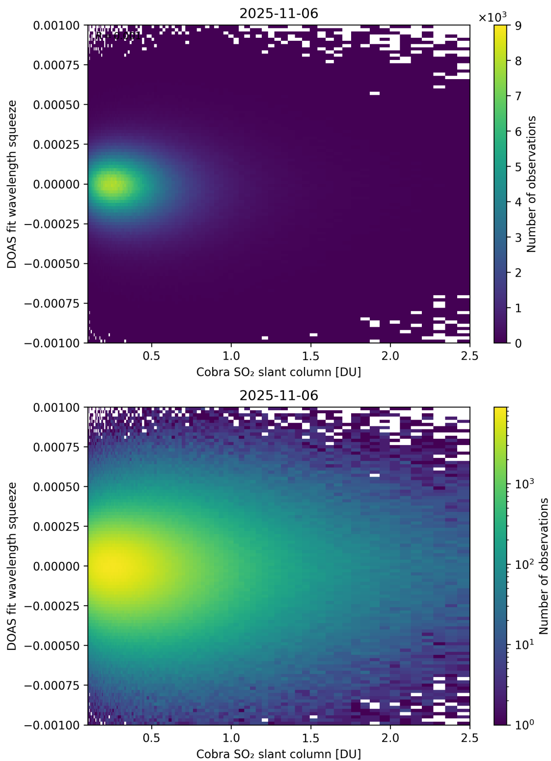
Figure 197: Scatter density plot of “Cobra SO 2 slant column” against “DOAS fit wavelength squeeze” for 2025-11-05 to 2025-11-07.
