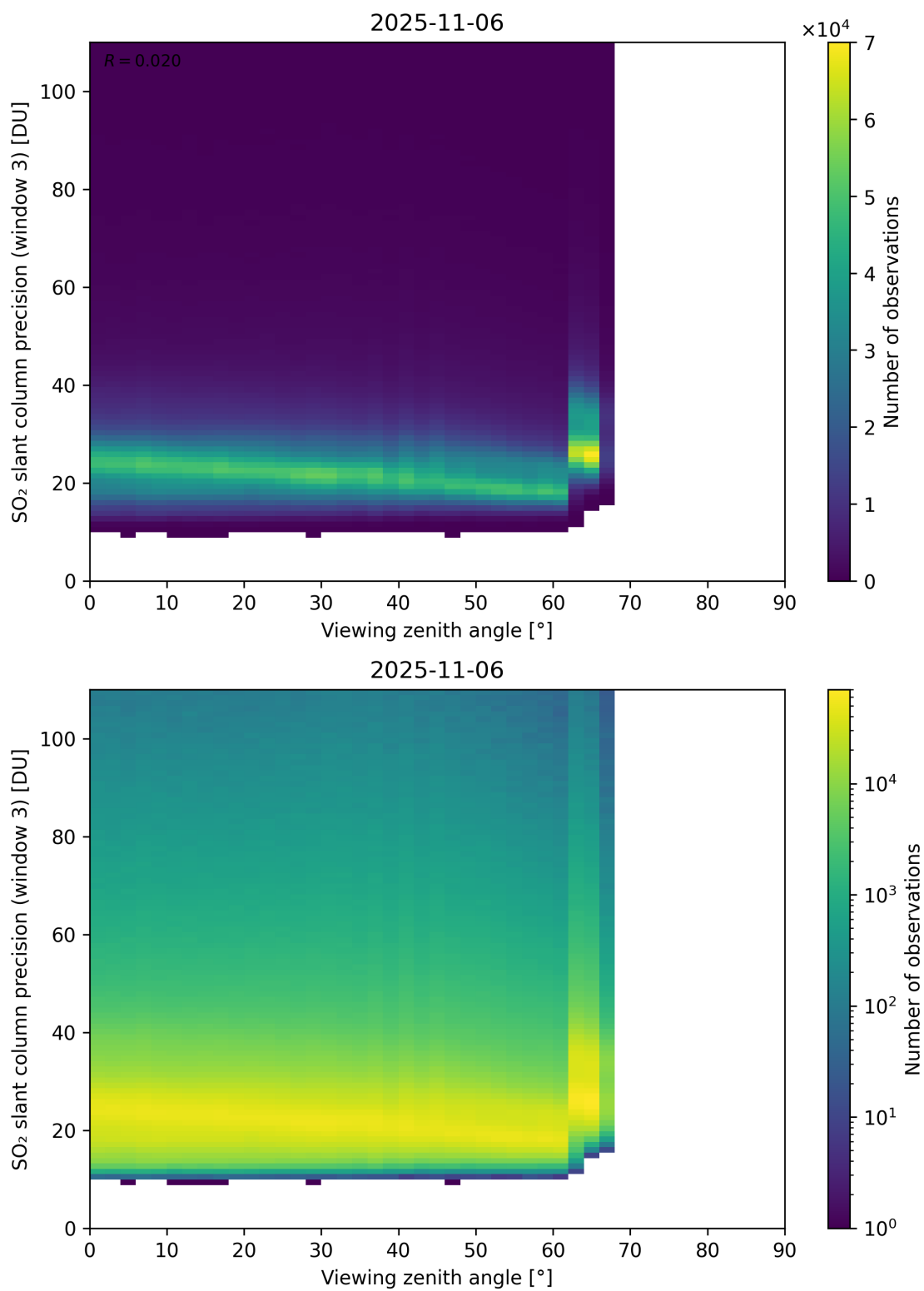
Figure 380: Scatter density plot of “Viewing zenith angle” against “SO 2 slant column precision (window 3)” for 2025-11-05 to 2025-11-07.
