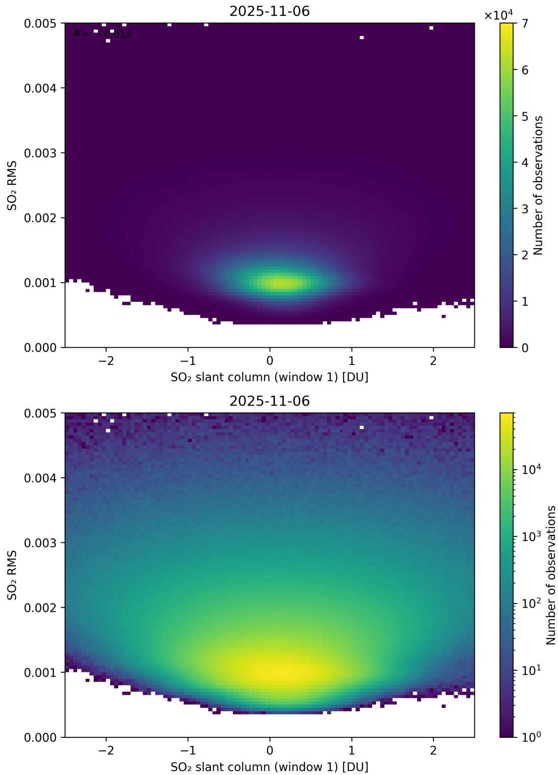
Figure 267: Scatter density plot of “SO 2 slant column (window 1)” against “SO 2 RMS” for 2025-11-05 to 2025-11-07.
