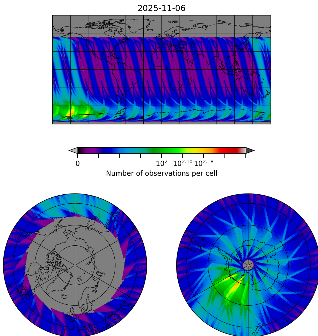
Figure 30: Map of the number of observations for 2025-11-05 to 2025-11-07
