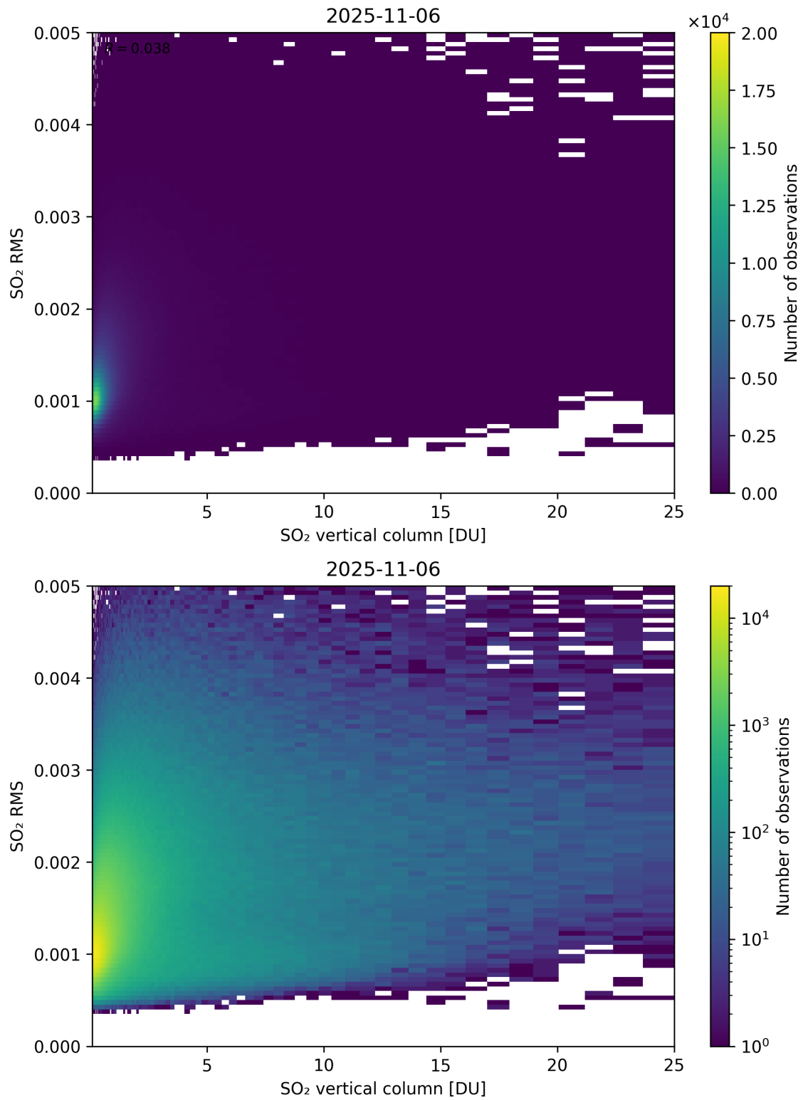
Figure 328: Scatter density plot of “SO 2 vertical column” against “SO 2 RMS” for 2025-11-05 to 2025-11-07.
