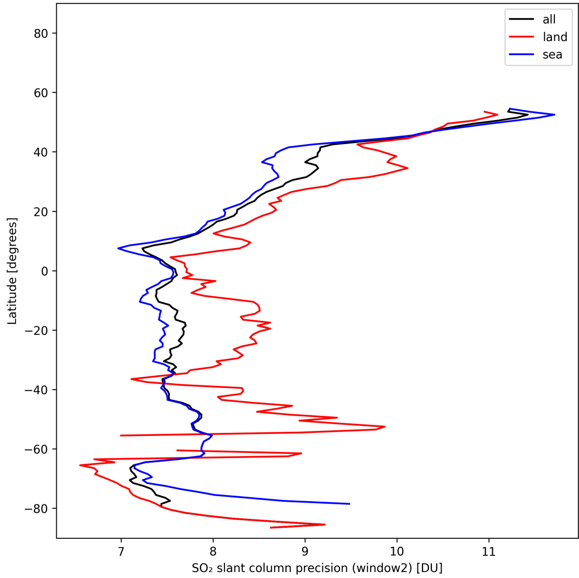
Figure 42: Zonal average of “SO 2 slant column precision (window2)” for 2025-11-05 to 2025-11-07.
