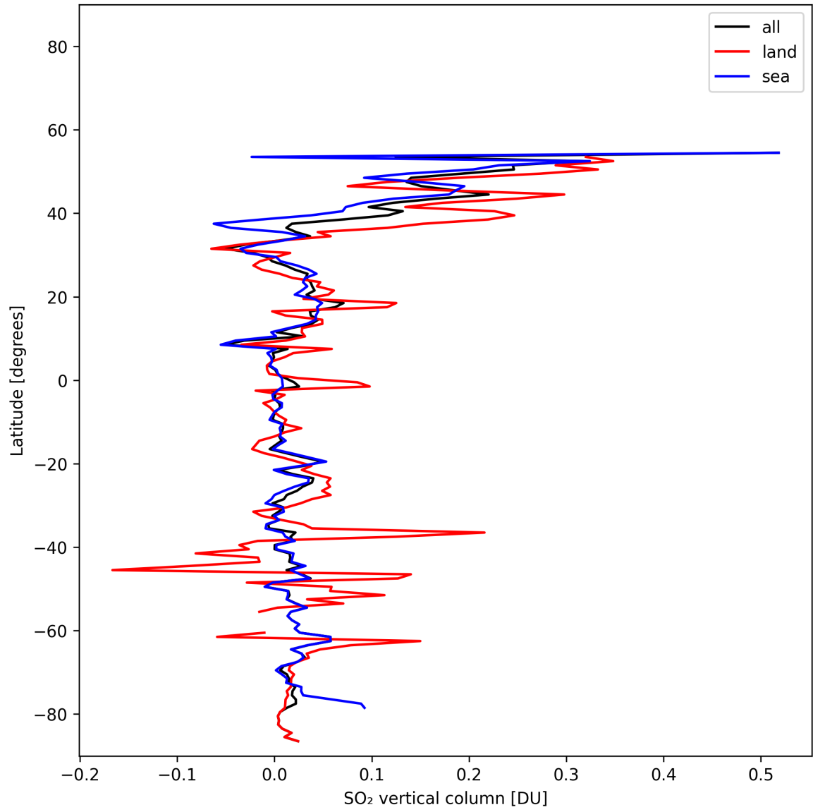
Figure 32: Zonal average of “SO 2 vertical column” for 2025-11-05 to 2025-11-07.
