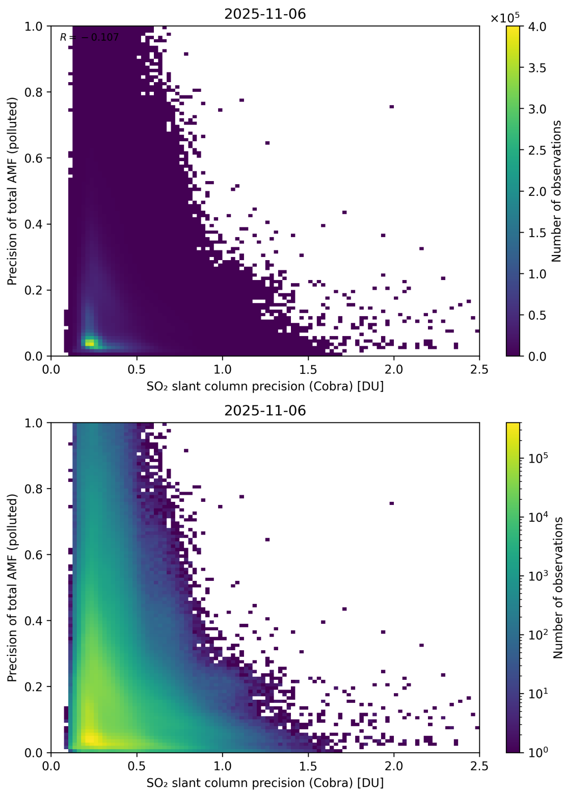
Figure 214: Scatter density plot of “SO 2 slant column precision (Cobra)” against “Precision of total AMF (polluted)” for 2025-11-05 to 2025-11-07.
