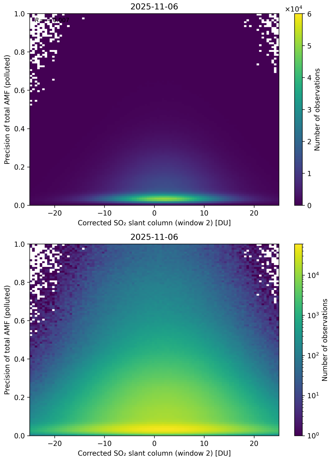
Figure 254: Scatter density plot of “Corrected SO 2 slant column (window 2)” against “Precision of total AMF (polluted)” for 2025-11-05 to 2025-11-07.
