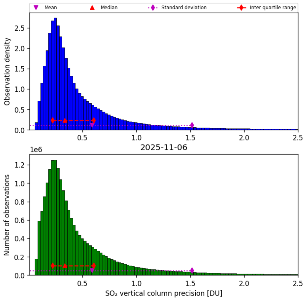
Figure 59: Histogram of “SO 2 vertical column precision” for 2025-11-05 to 2025-11-07
