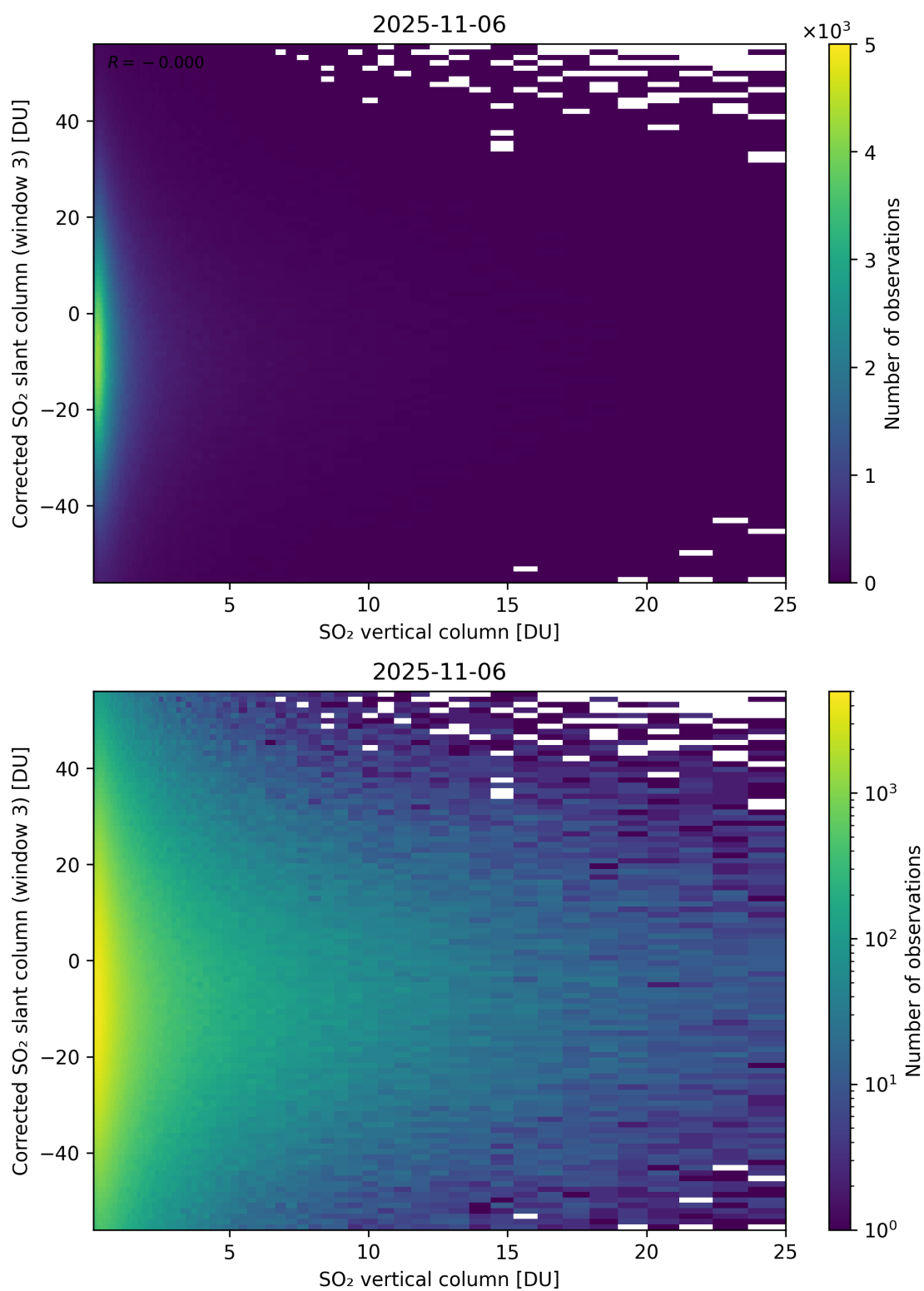
Figure 353: Scatter density plot of “SO 2 vertical column” against “Corrected SO 2 slant column (window 3)” for 2025-11-05 to 2025-11-07.
