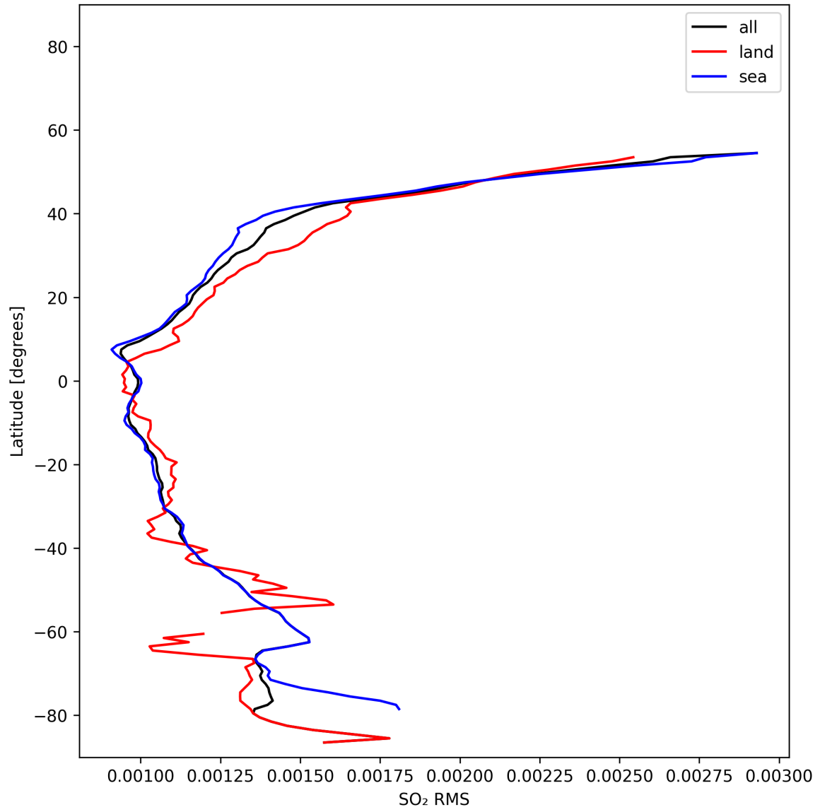
Figure 52: Zonal average of “SO 2 RMS” for 2025-11-05 to 2025-11-07.
