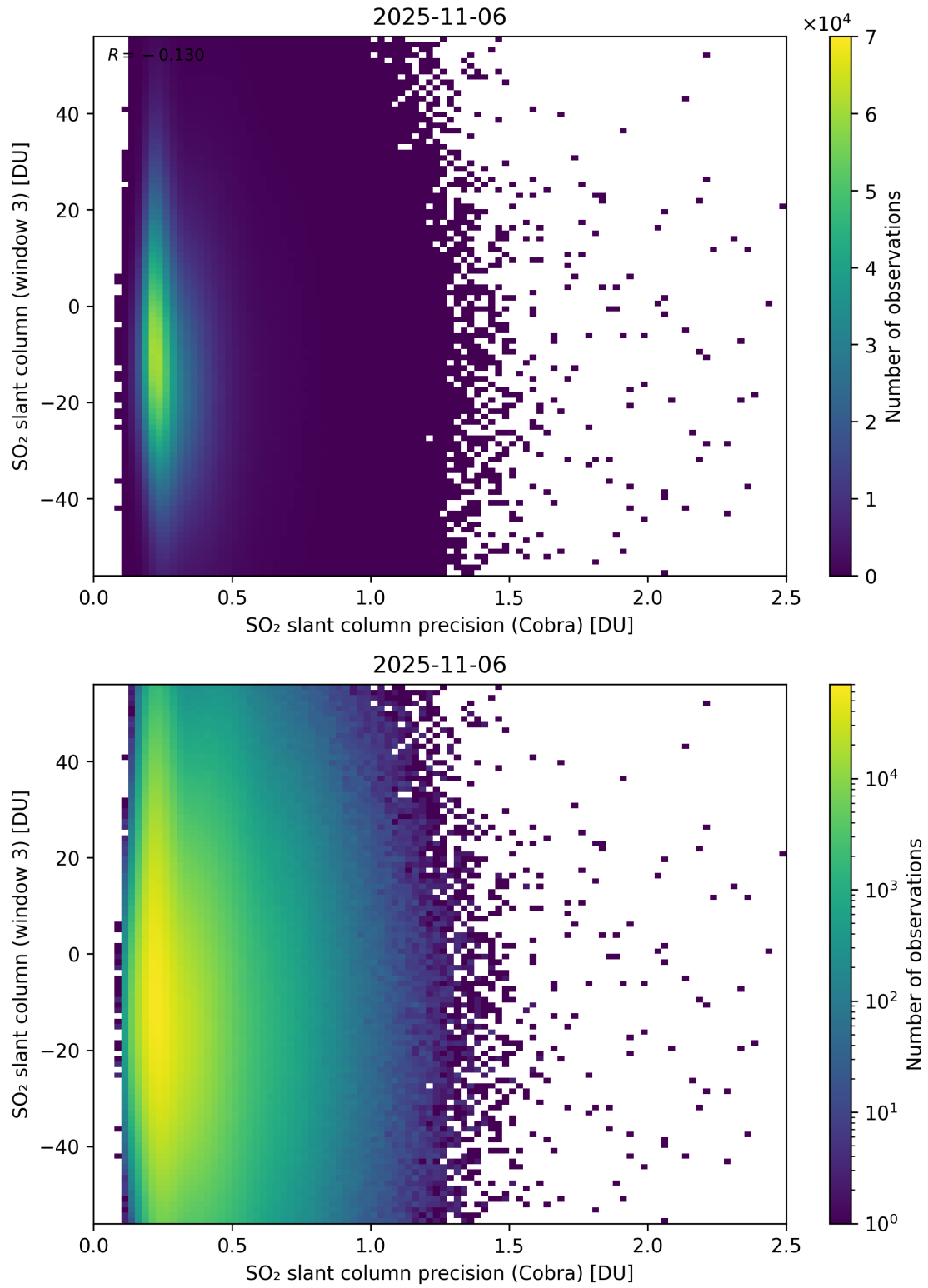
Figure 211: Scatter density plot of “SO 2 slant column precision (Cobra)” against “SO 2 slant column (window 3)” for 2025-11-05 to 2025-11-07.
