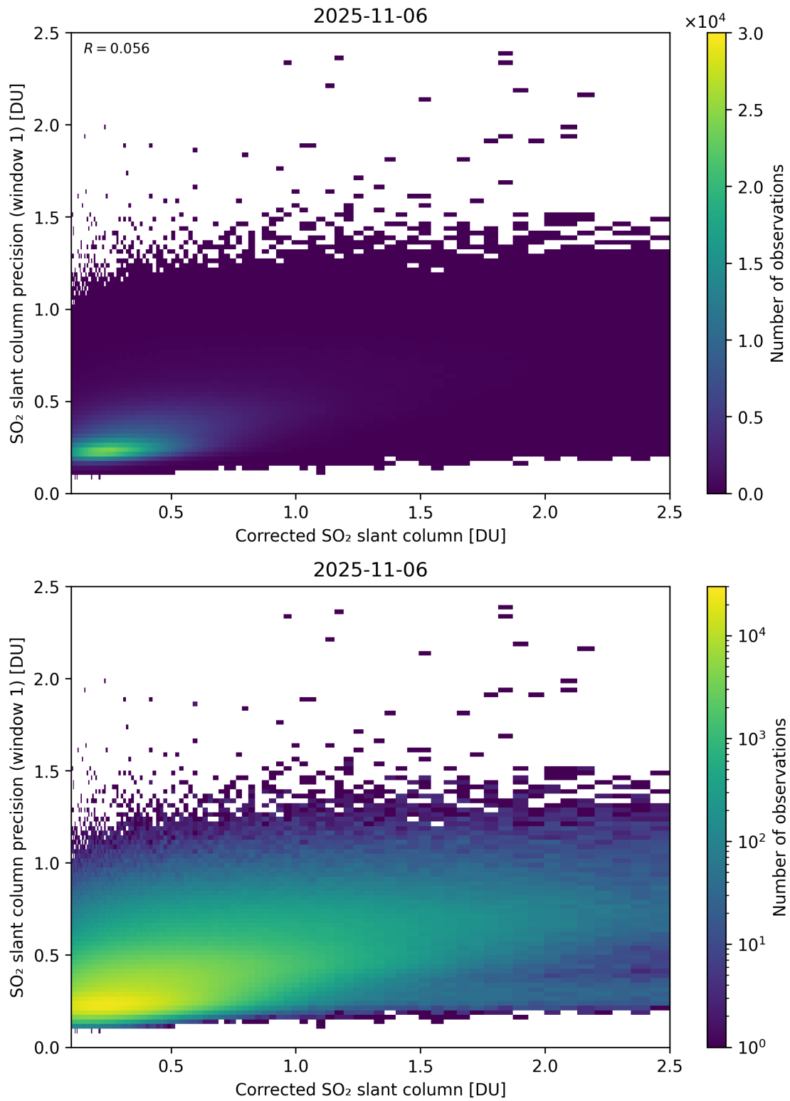
Figure 238: Scatter density plot of “Corrected SO 2 slant column” against “SO 2 slant column precision (window 1)” for 2025-11-05 to 2025-11-07.
