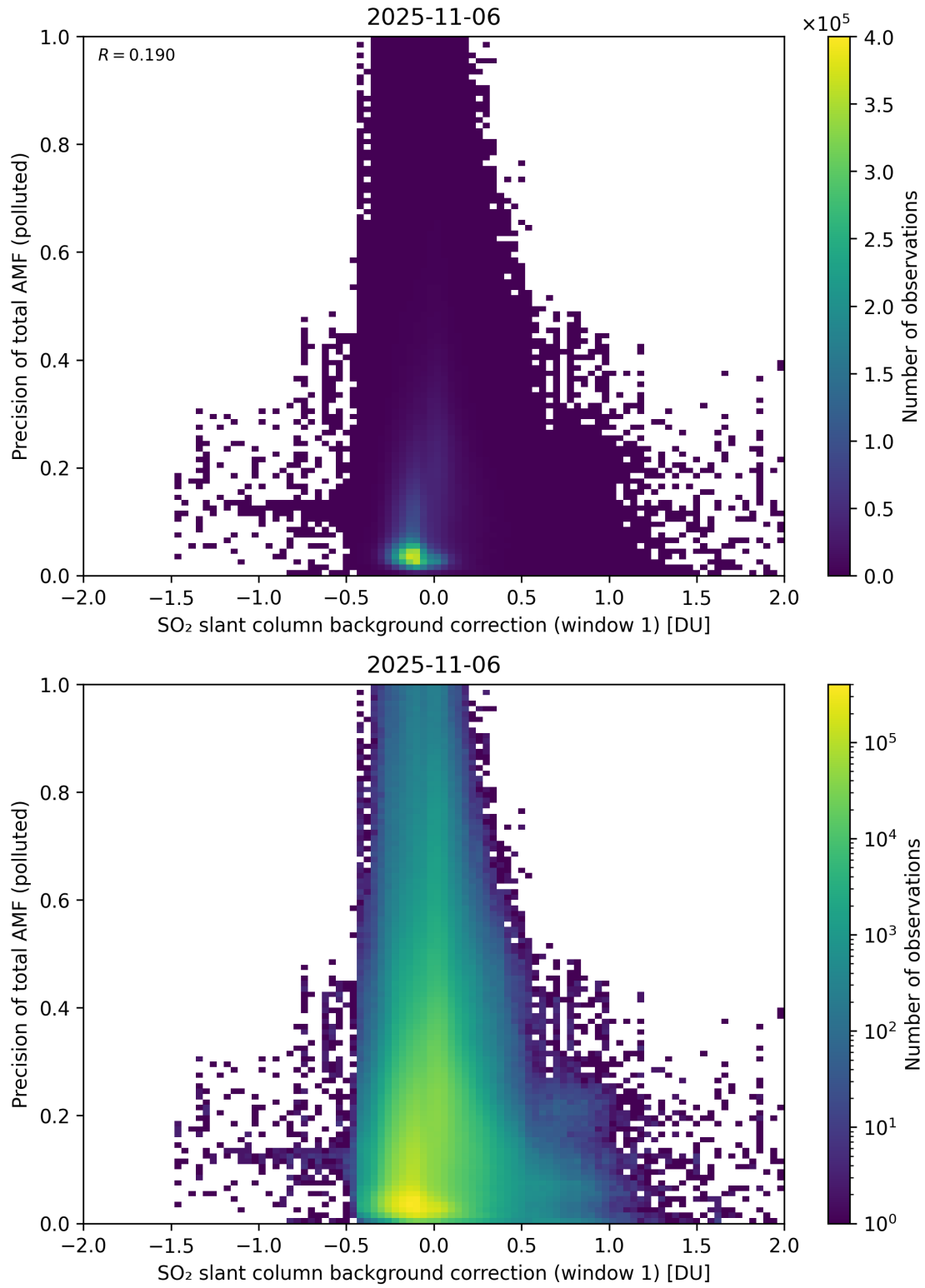
Figure 121: Scatter density plot of “SO 2 slant column background correction (window 1)” against “Precision of total AMF (polluted)” for 2025-11-05 to 2025-11-07.
