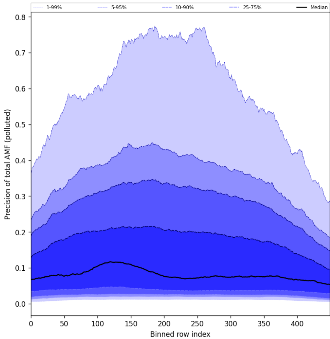
Figure 106: Along track statistics of “Precision of total AMF (polluted)” for 2025-11-05 to 2025-11-07
