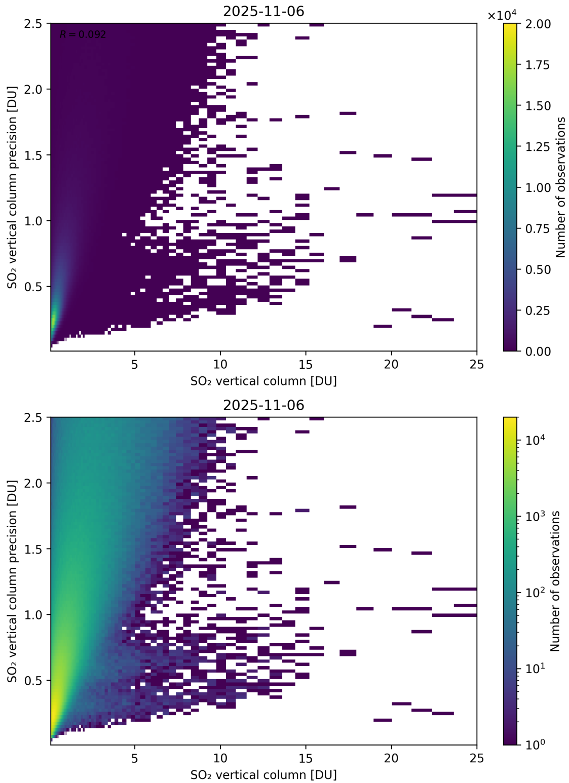
Figure 361: Scatter density plot of “SO 2 vertical column” against “SO 2 vertical column precision” for 2025-11-05 to 2025-11-07.
