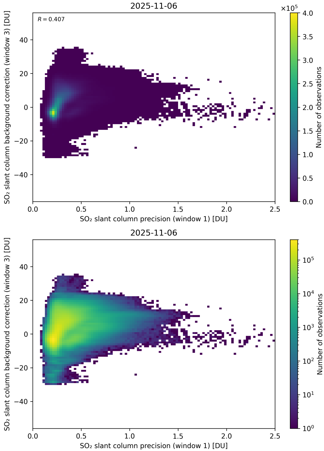
Figure 270: Scatter density plot of “SO 2 slant column precision (window 1)” against “SO 2 slant column background correction (window 3)” for 2025-11-05 to 2025-11-07.
