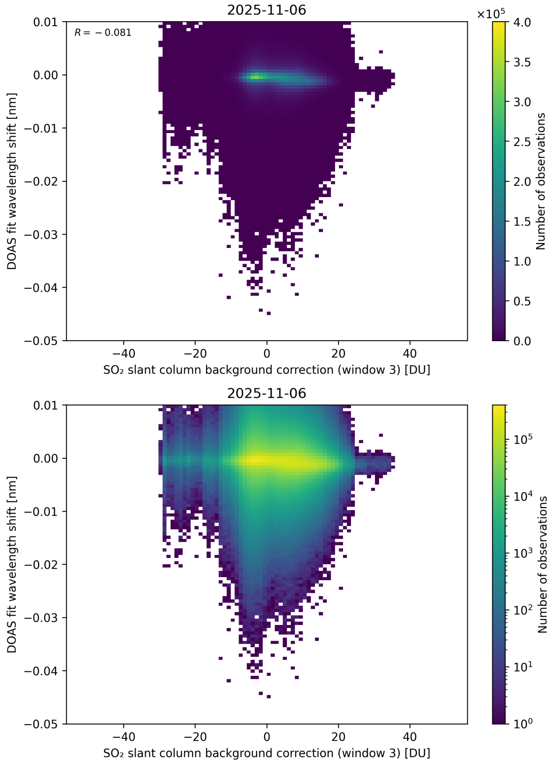
Figure 132: Scatter density plot of “SO 2 slant column background correction (window 3)” against “DOAS fit wavelength shift” for 2025-11-05 to 2025-11-07.
