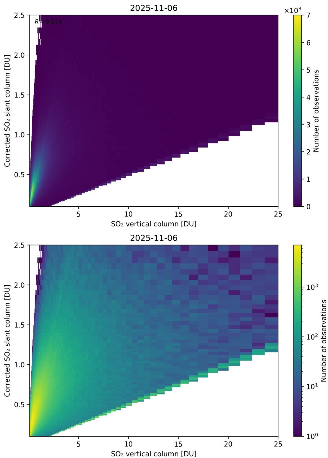
Figure 351: Scatter density plot of “SO 2 vertical column” against “Corrected SO 2 slant column” for 2025-11-05 to 2025-11-07.
