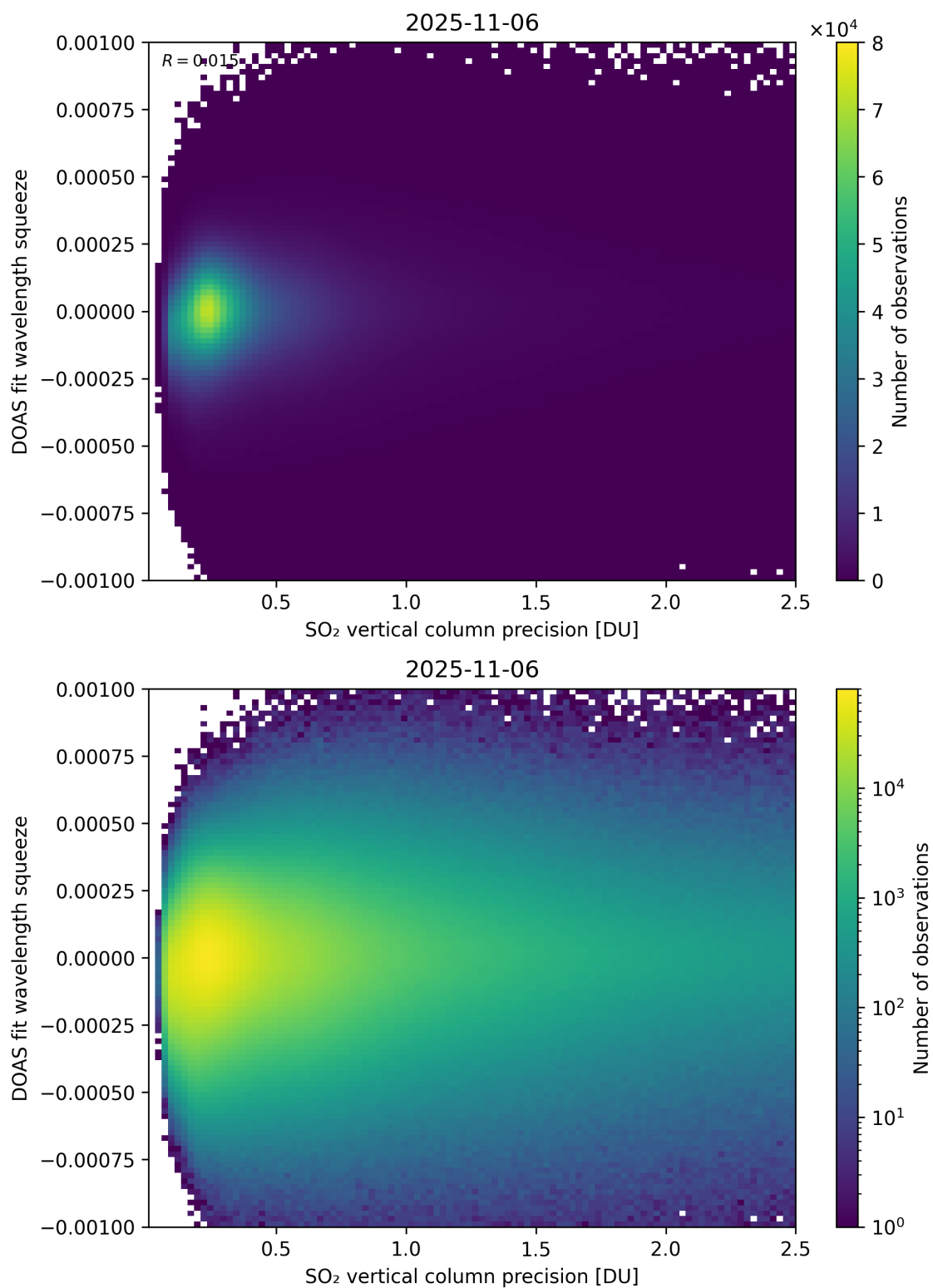
Figure 333: Scatter density plot of “SO 2 vertical column precision” against “DOAS fit wavelength squeeze” for 2025-11-05 to 2025-11-07.
