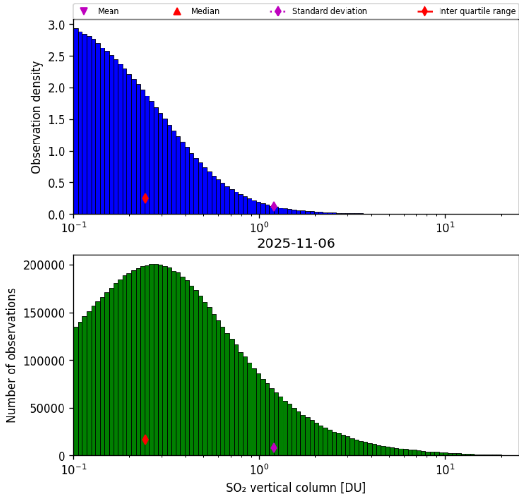
Figure 58: Histogram of “SO 2 vertical column” for 2025-11-05 to 2025-11-07
