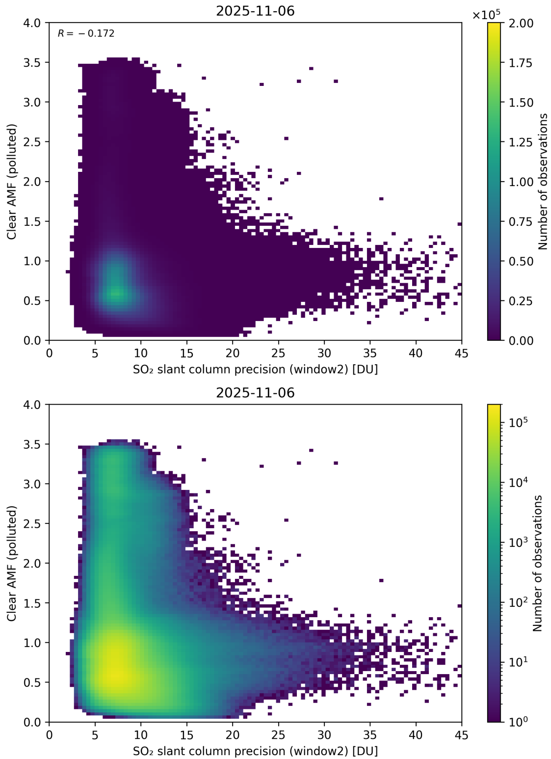
Figure 296: Scatter density plot of “SO 2 slant column precision (window2)” against “Clear AMF (polluted)” for 2025-11-05 to 2025-11-07.
