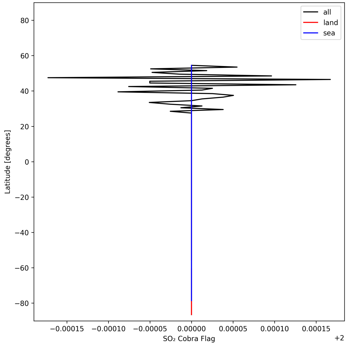
Figure 49: Zonal average of “SO 2 Cobra Flag” for 2025-11-05 to 2025-11-07.
