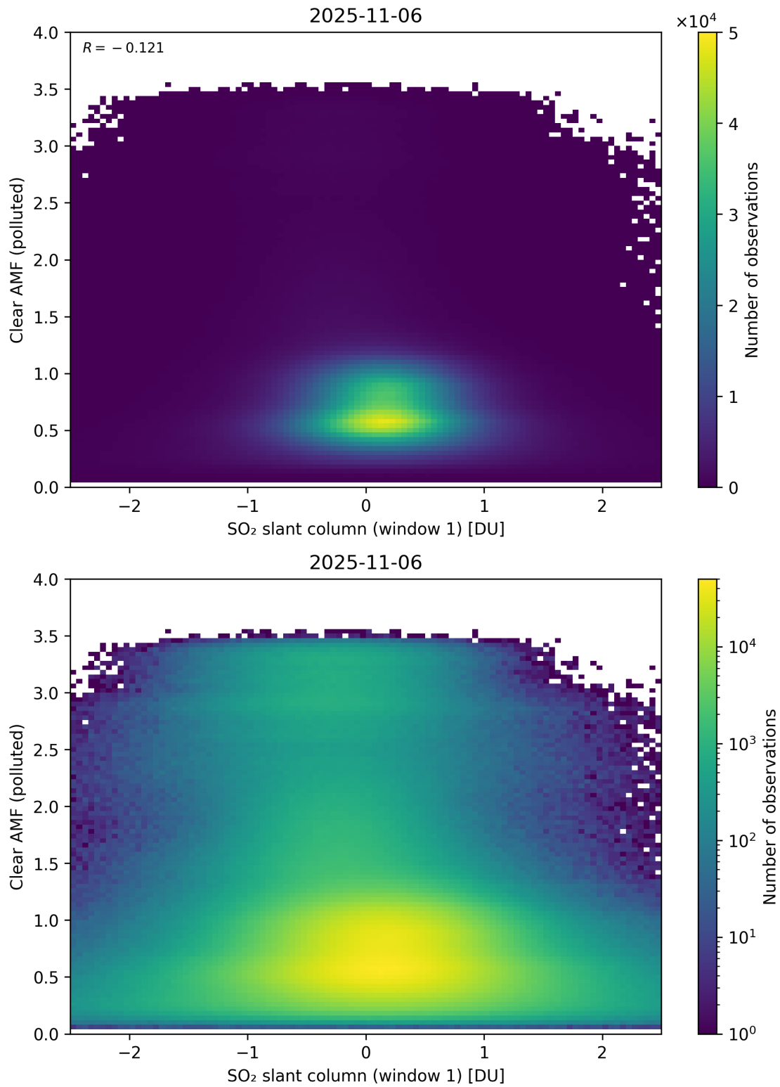
Figure 282: Scatter density plot of “SO 2 slant column (window 1)” against “Clear AMF (polluted)” for 2025-11-05 to 2025-11-07.
