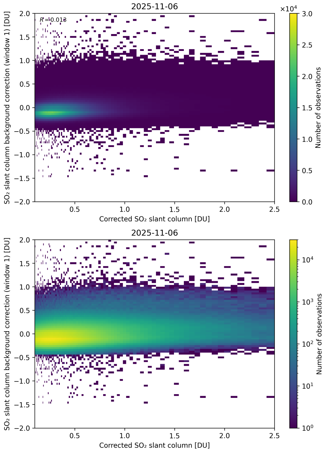
Figure 226: Scatter density plot of “Corrected SO 2 slant column” against “SO 2 slant column background correction (window 1)” for 2025-11-05 to 2025-11-07.
