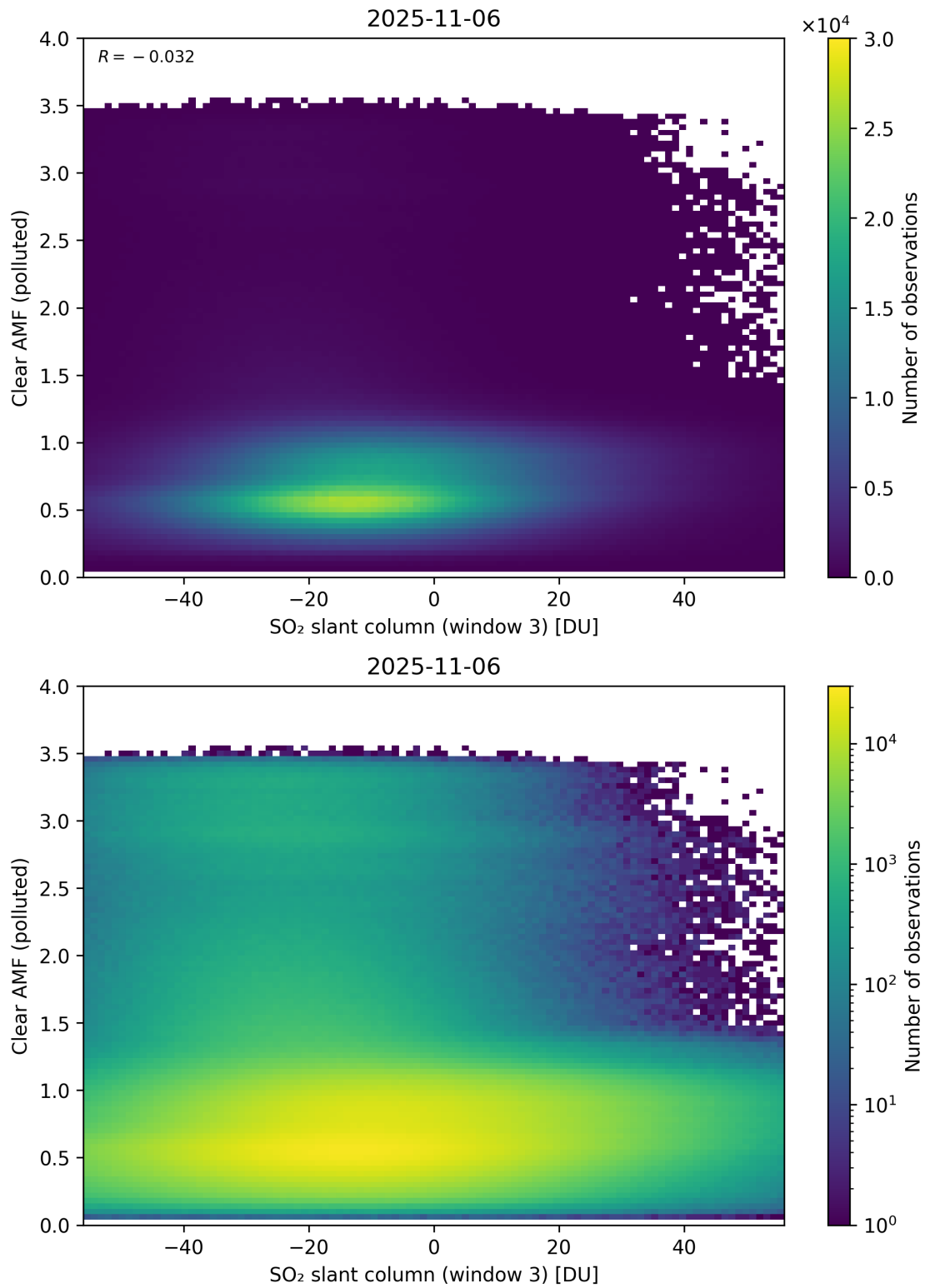
Figure 315: Scatter density plot of “SO 2 slant column (window 3)” against “Clear AMF (polluted)” for 2025-11-05 to 2025-11-07.
