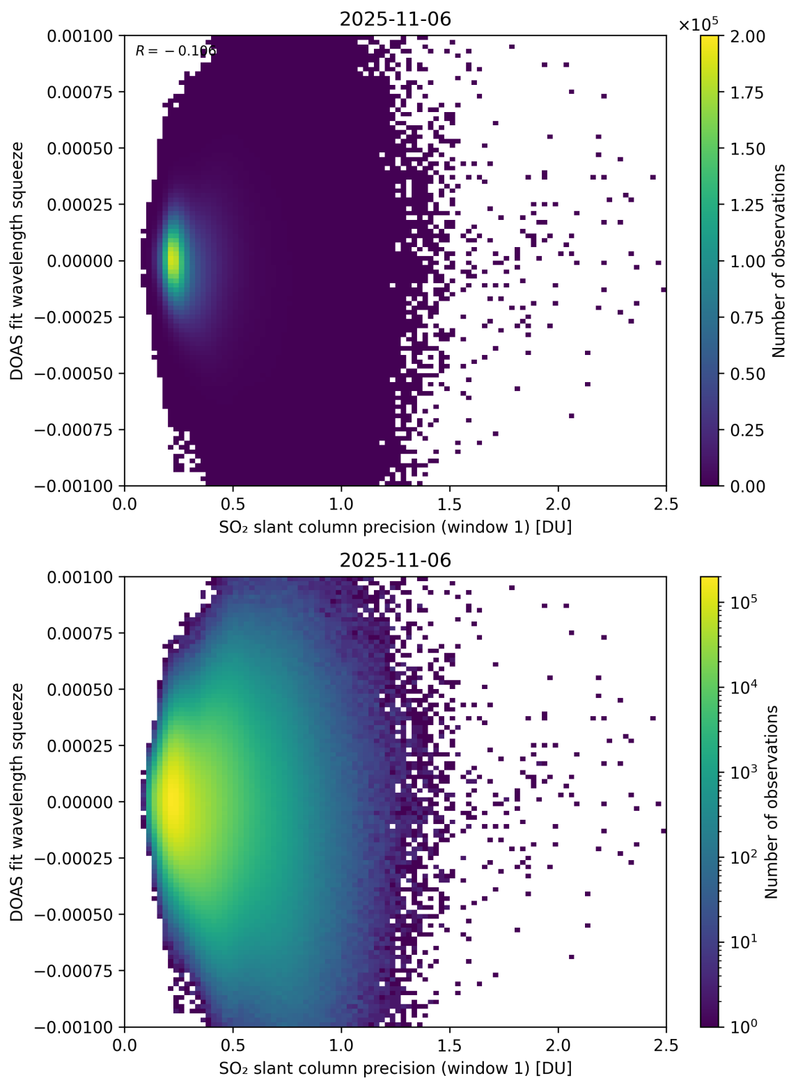
Figure 272: Scatter density plot of “SO 2 slant column precision (window 1)” against “DOAS fit wavelength squeeze” for 2025-11-05 to 2025-11-07.
