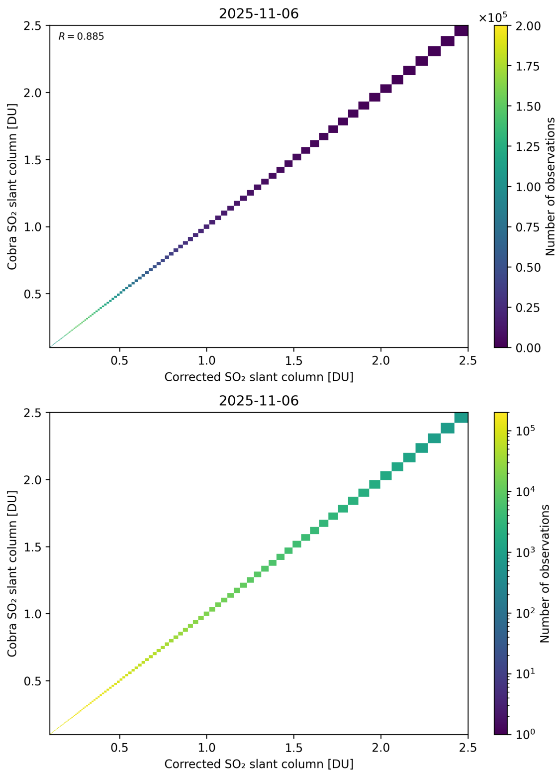
Figure 233: Scatter density plot of “Corrected SO 2 slant column” against “Cobra SO 2 slant column” for 2025-11-05 to 2025-11-07.
