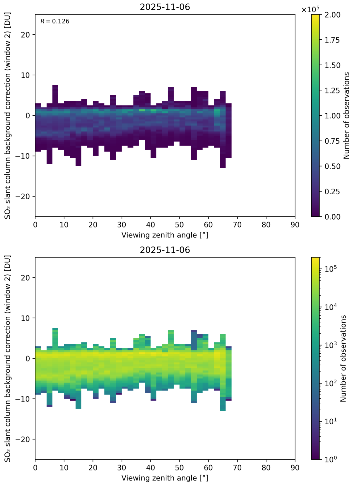
Figure 363: Scatter density plot of “Viewing zenith angle” against “SO 2 slant column background correction (window 2)” for 2025-11-05 to 2025-11-07.
