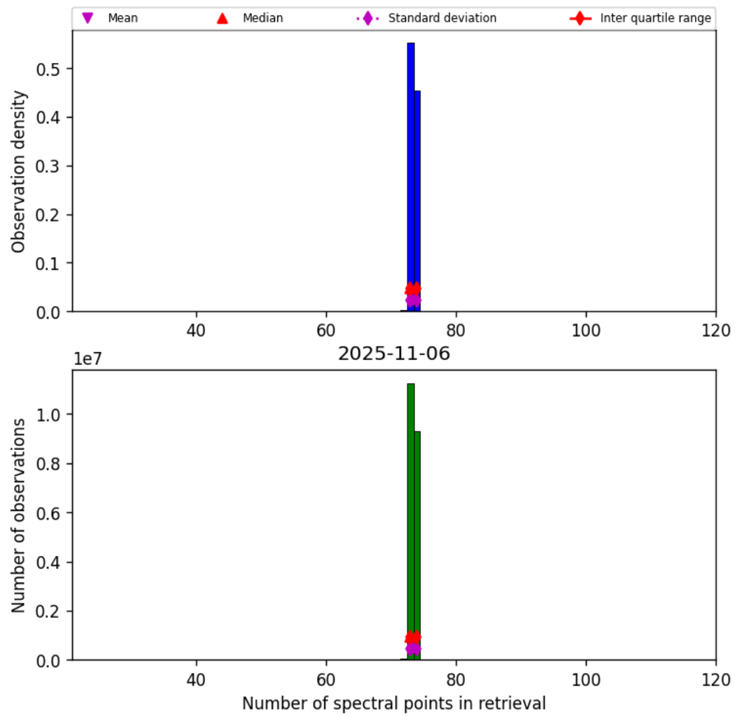
Figure 82: Histogram of “Number of spectral points in retrieval” for 2025-11-05 to 2025-11-07
