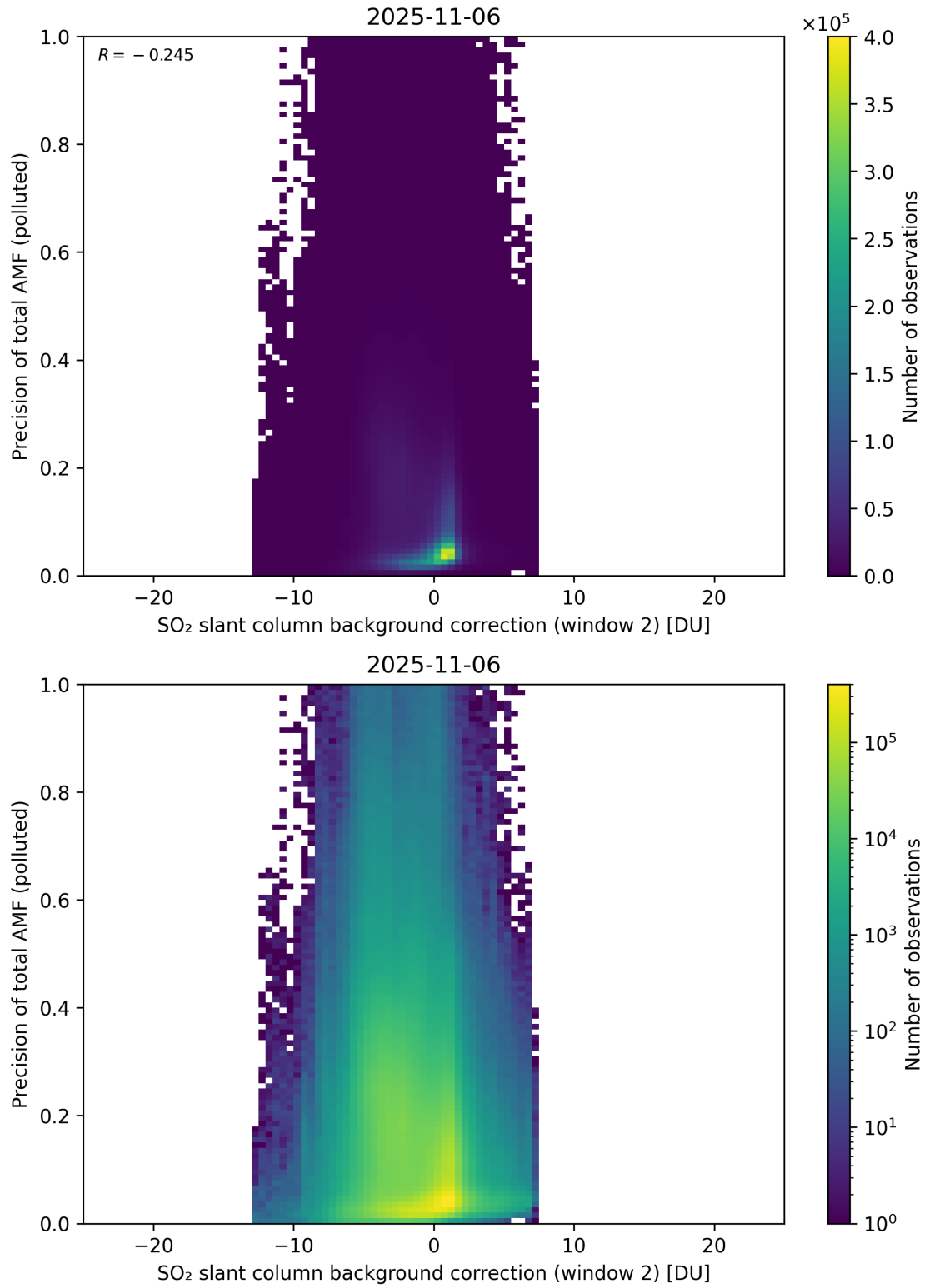
Figure 131: Scatter density plot of “SO 2 slant column background correction (window 2)” against “Precision of total AMF (polluted)” for 2025-11-05 to 2025-11-07.
