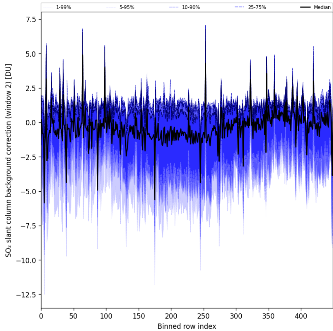
Figure 96: Along track statistics of "SO 2 slant column background correction (window 2)" for 2025-11-05 to 2025-11-07
