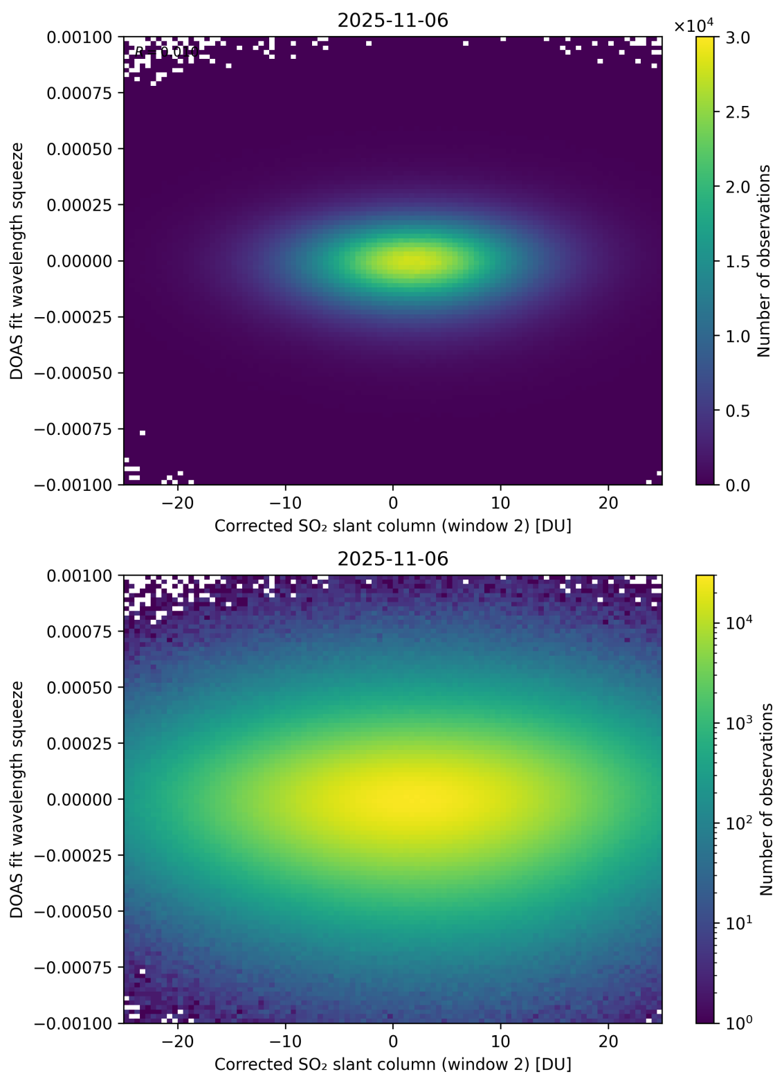
Figure 247: Scatter density plot of “Corrected SO 2 slant column (window 2)” against “DOAS fit wavelength squeeze” for 2025-11-05 to 2025-11-07.
