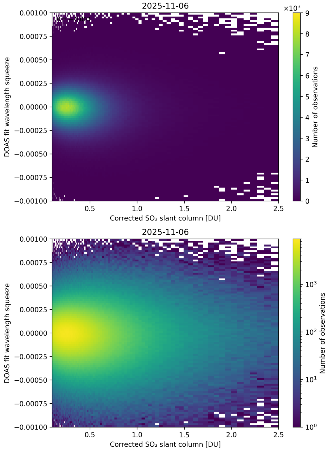
Figure 230: Scatter density plot of “Corrected SO 2 slant column” against “DOAS fit wavelength squeeze” for 2025-11-05 to 2025-11-07.
