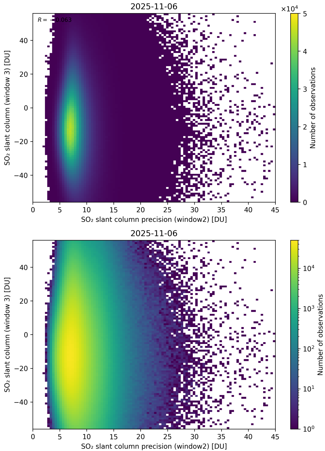
Figure 299: Scatter density plot of “SO 2 slant column precision (window2)” against “SO 2 slant column (window 3)” for 2025-11-05 to 2025-11-07.
