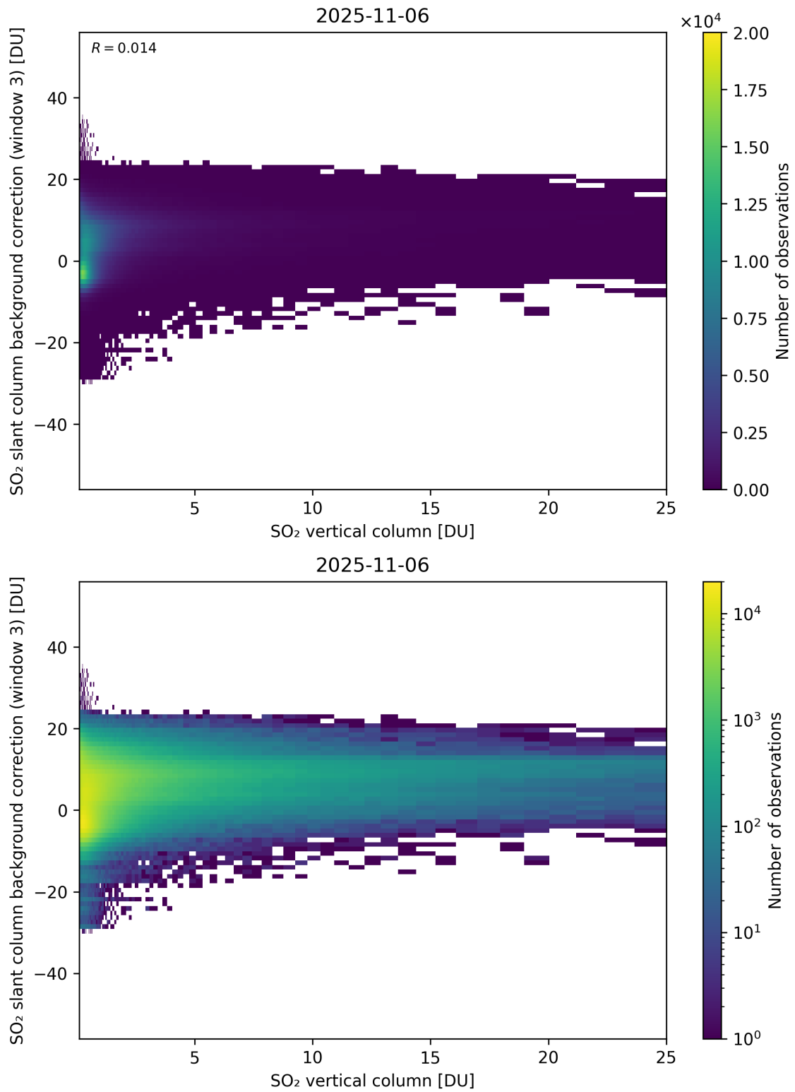
Figure 325: Scatter density plot of “SO 2 vertical column” against “SO 2 slant column background correction (window 3)” for 2025-11-05 to 2025-11-07.
