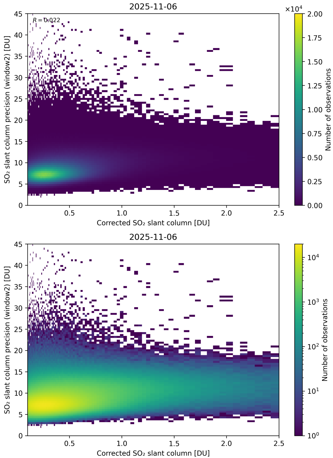
Figure 239: Scatter density plot of “Corrected SO 2 slant column” against “SO 2 slant column precision (window2)” for 2025-11-05 to 2025-11-07.
