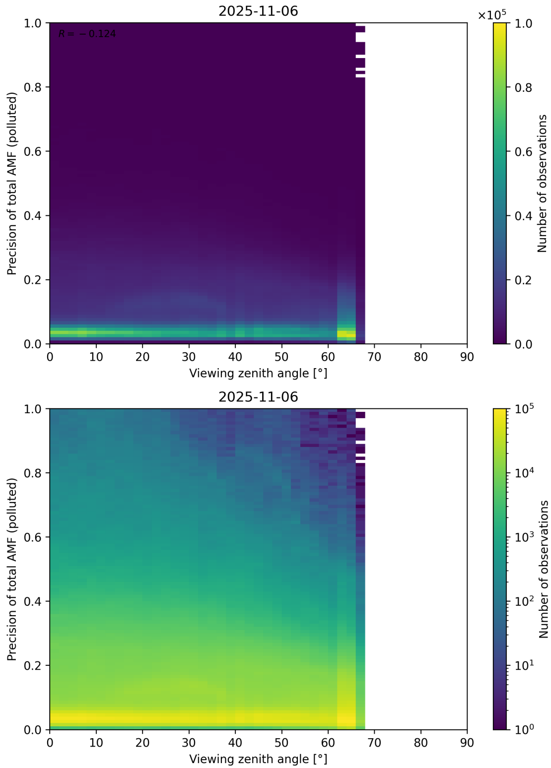
Figure 382: Scatter density plot of “Viewing zenith angle” against “Precision of total AMF (polluted)” for 2025-11-05 to 2025-11-07.
