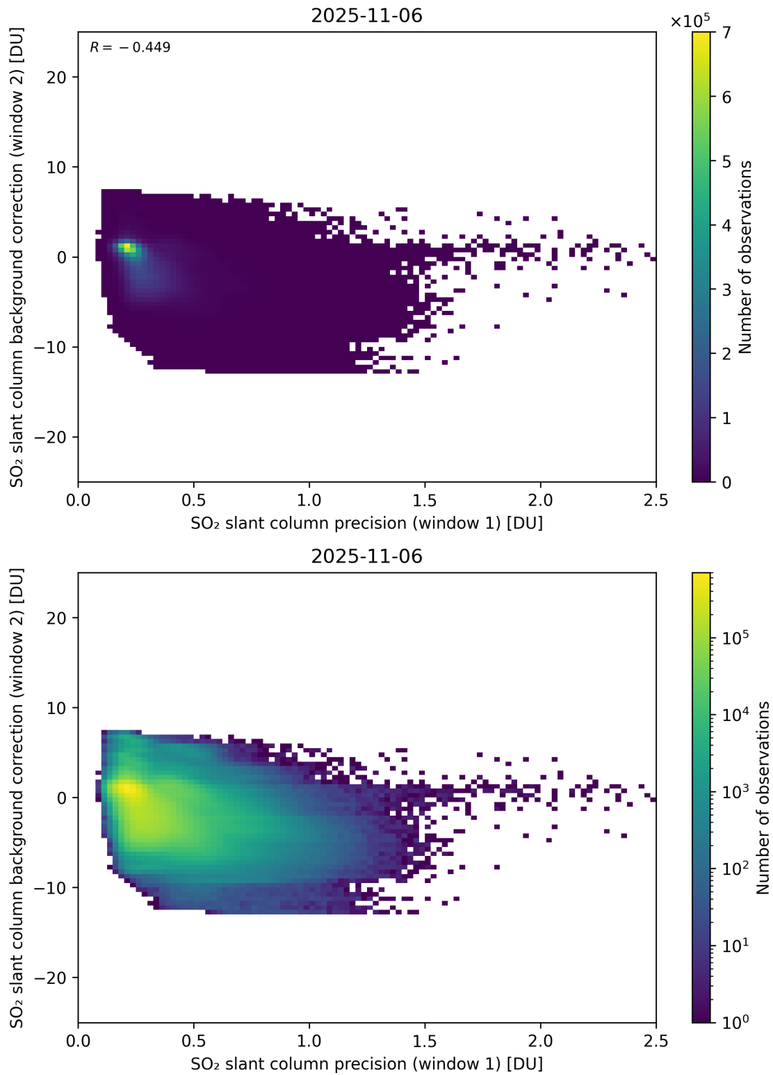
Figure 269: Scatter density plot of “SO 2 slant column precision (window 1)” against “SO 2 slant column background correction (window 2)” for 2025-11-05 to 2025-11-07.
