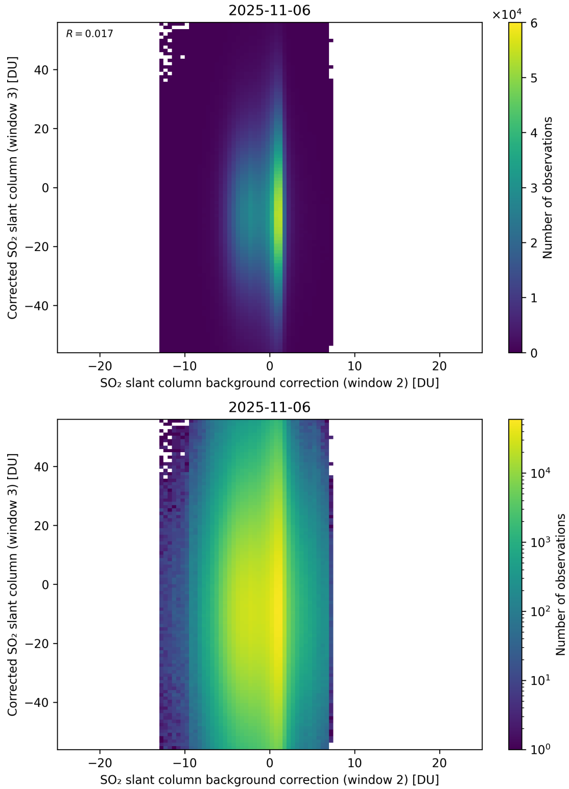
Figure 127: Scatter density plot of “SO 2 slant column background correction (window 2)” against “Corrected SO 2 slant column (window 3)” for 2025-11-05 to 2025-11-07.
