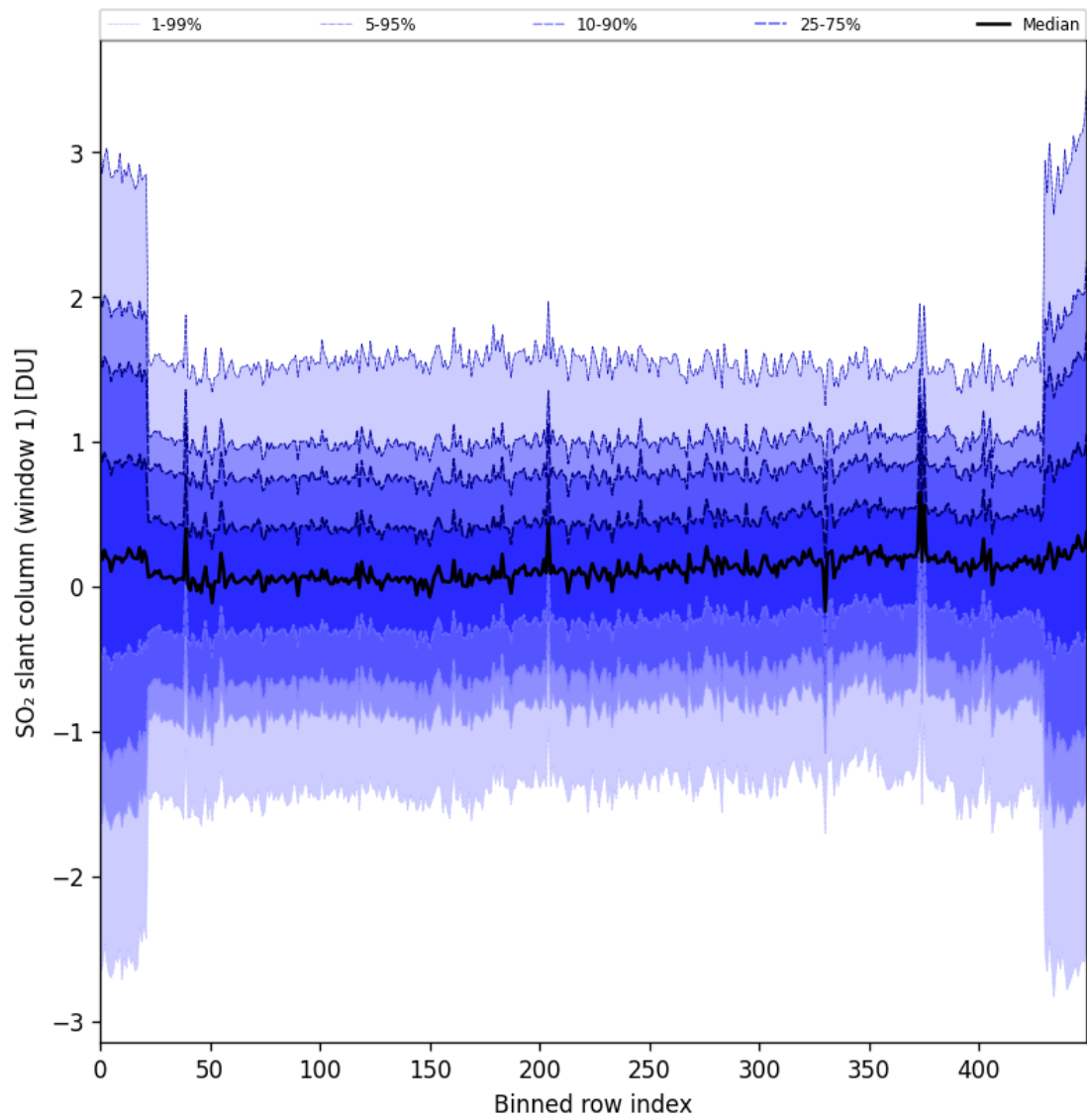
Figure 89: Along track statistics of “SO 2 slant column (window 1)” for 2025-11-05 to 2025-11-07
