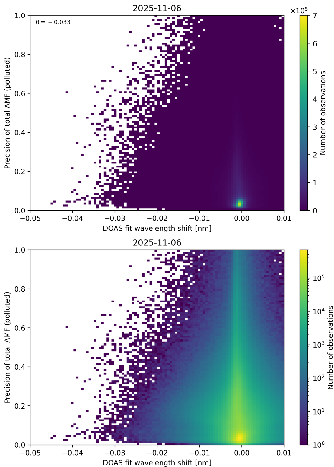
Figure 142: Scatter density plot of “DOAS fit wavelength shift” against “Precision of total AMF (polluted)” for 2025-11-05 to 2025-11-07.
