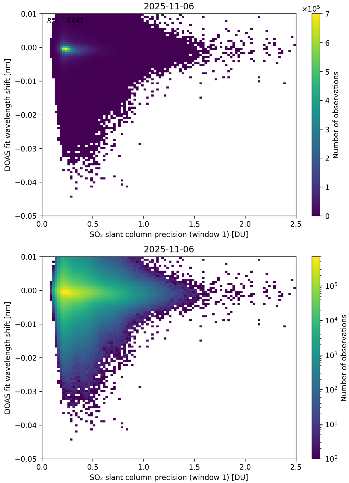
Figure 271: Scatter density plot of “SO 2 slant column precision (window 1)” against “DOAS fit wavelength shift” for 2025-11-05 to 2025-11-07.
