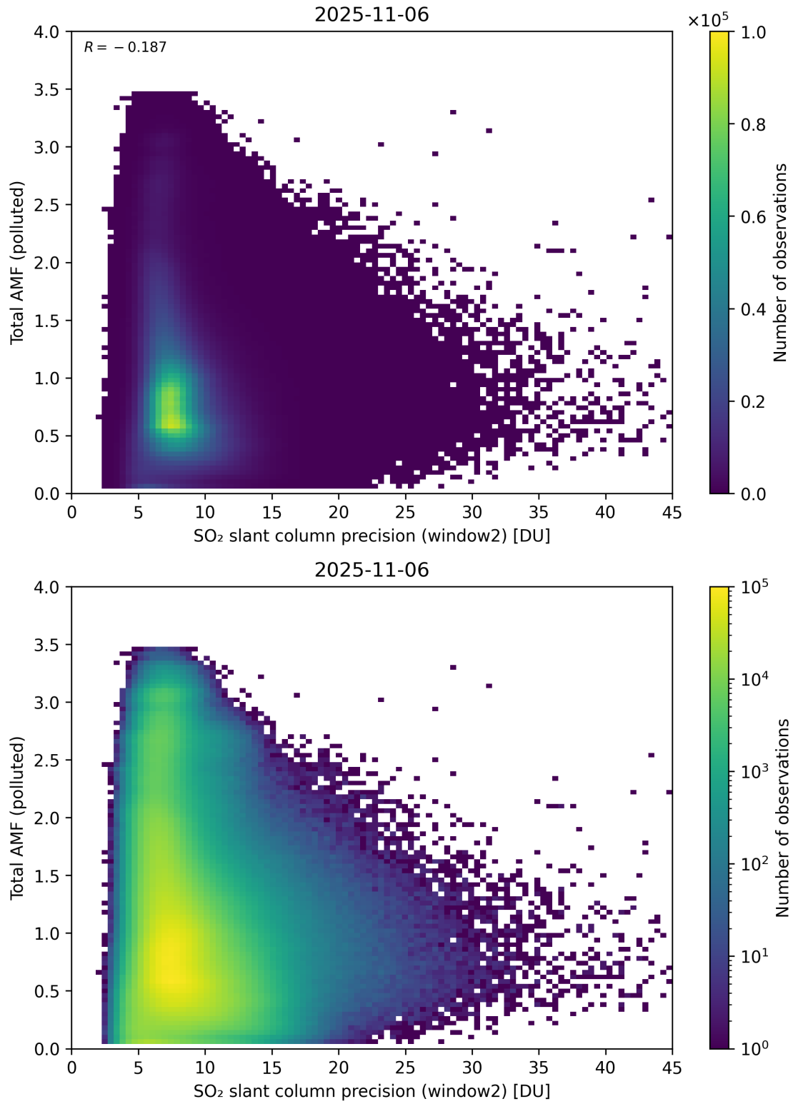
Figure 301: Scatter density plot of “SO 2 slant column precision (window2)” against “Total AMF (polluted)” for 2025-11-05 to 2025-11-07.
