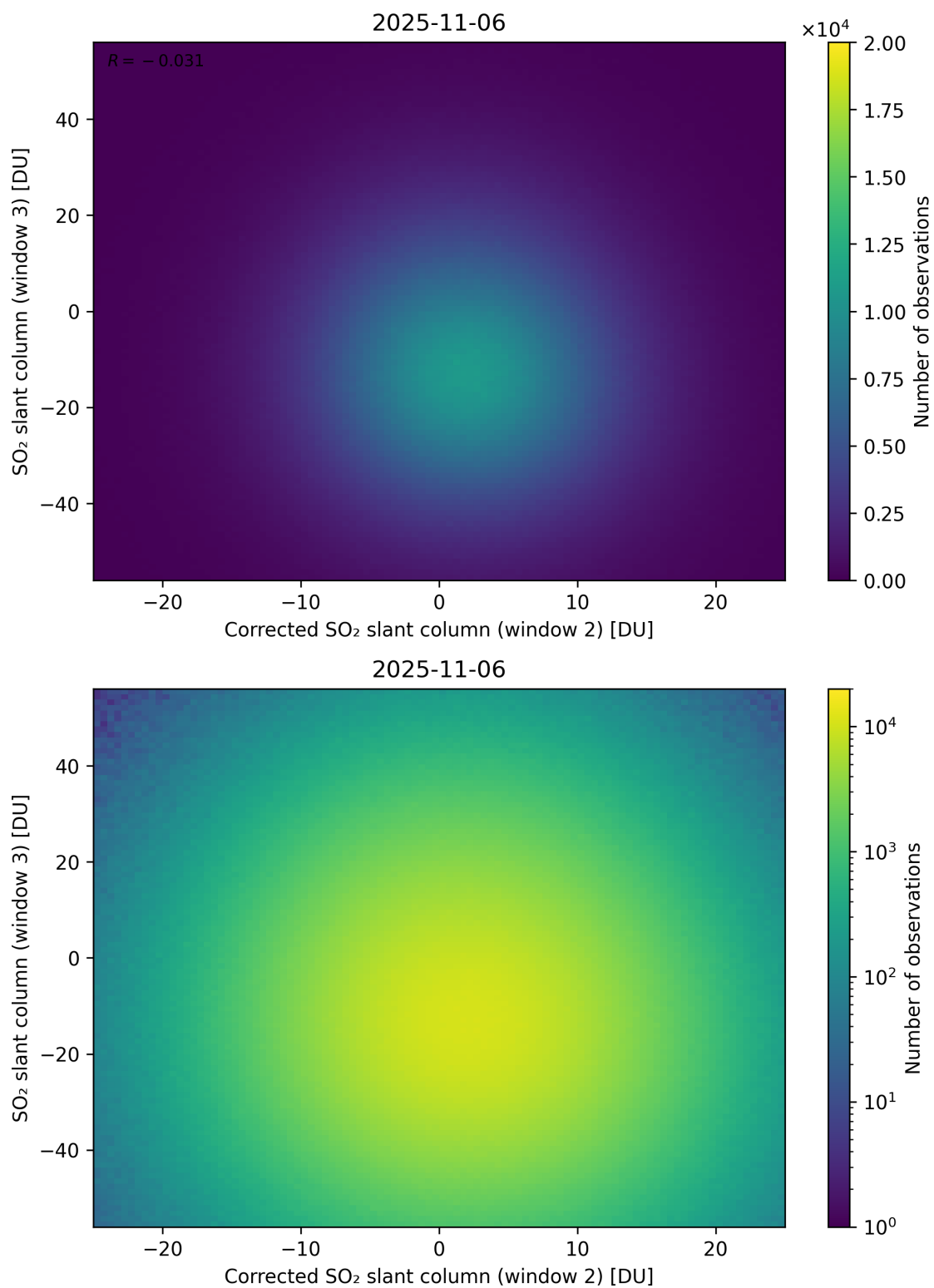
Figure 251: Scatter density plot of “Corrected SO 2 slant column (window 2)” against “SO 2 slant column (window 3)” for 2025-11-05 to 2025-11-07.
