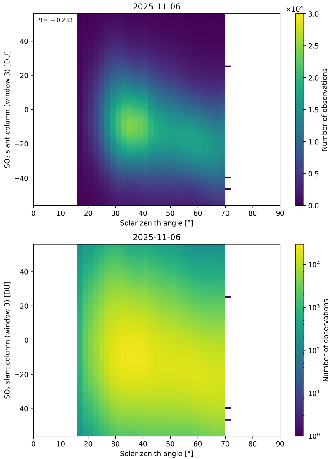
Figure 187: Scatter density plot of “Solar zenith angle” against “SO 2 slant column (window 3)” for 2025-11-05 to 2025-11-07.
