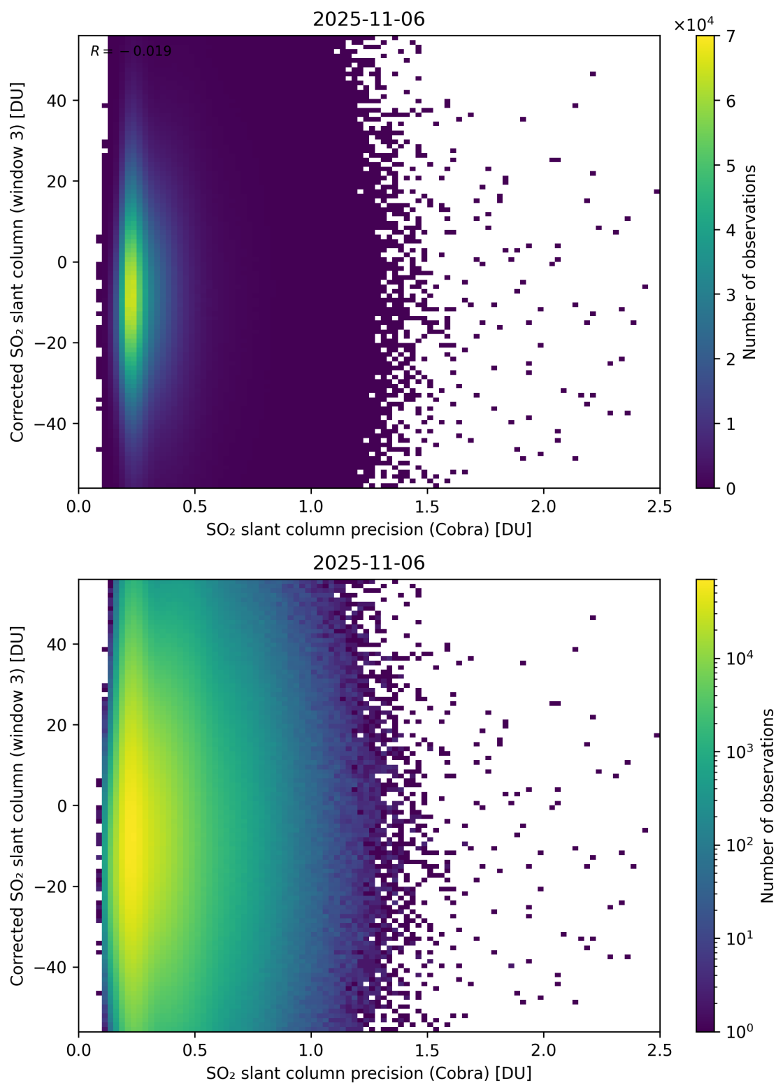
Figure 207: Scatter density plot of “SO 2 slant column precision (Cobra)” against “Corrected SO 2 slant column (window 3)” for 2025-11-05 to 2025-11-07.
