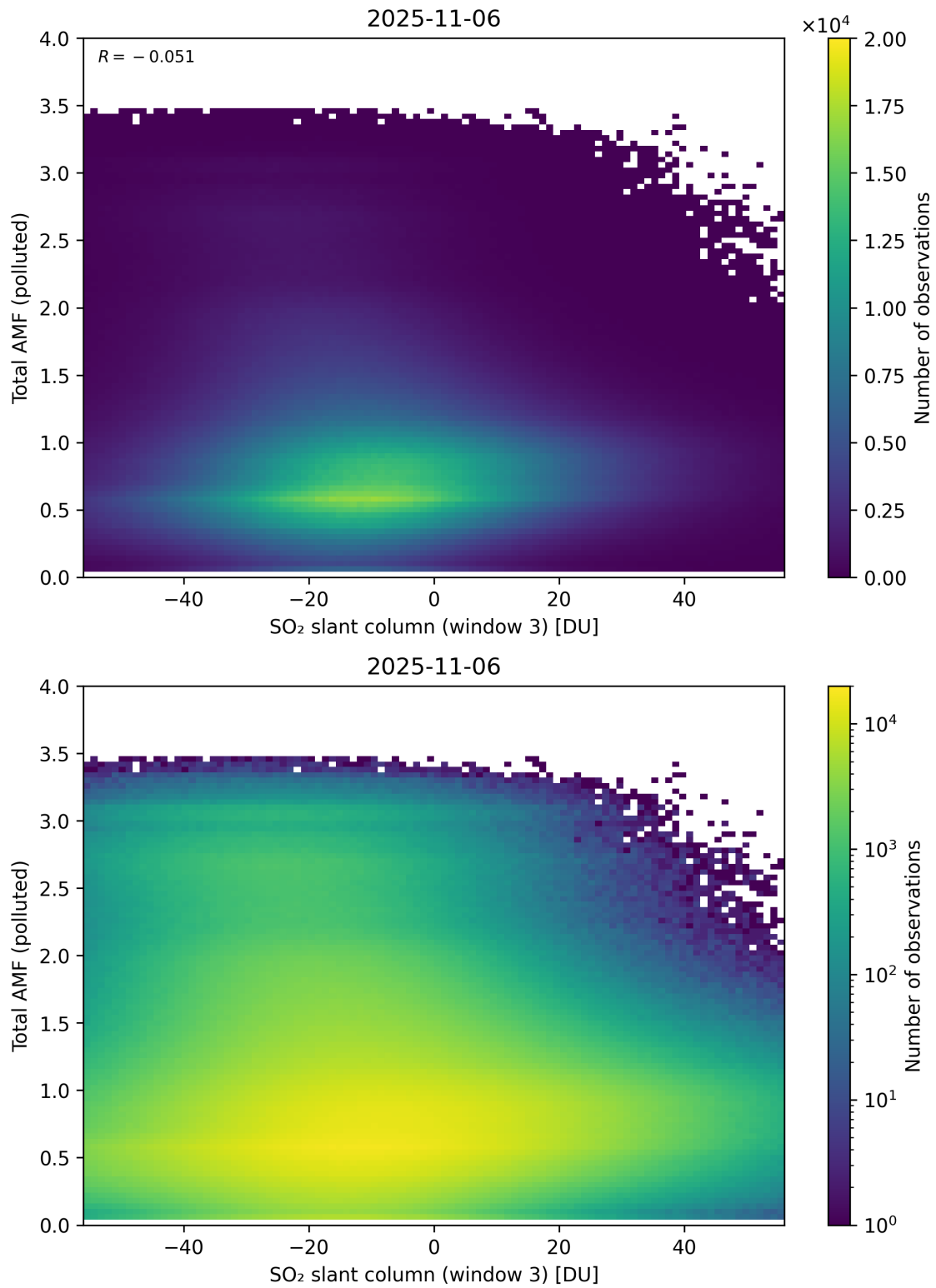
Figure 318: Scatter density plot of “SO 2 slant column (window 3)” against “Total AMF (polluted)” for 2025-11-05 to 2025-11-07.
