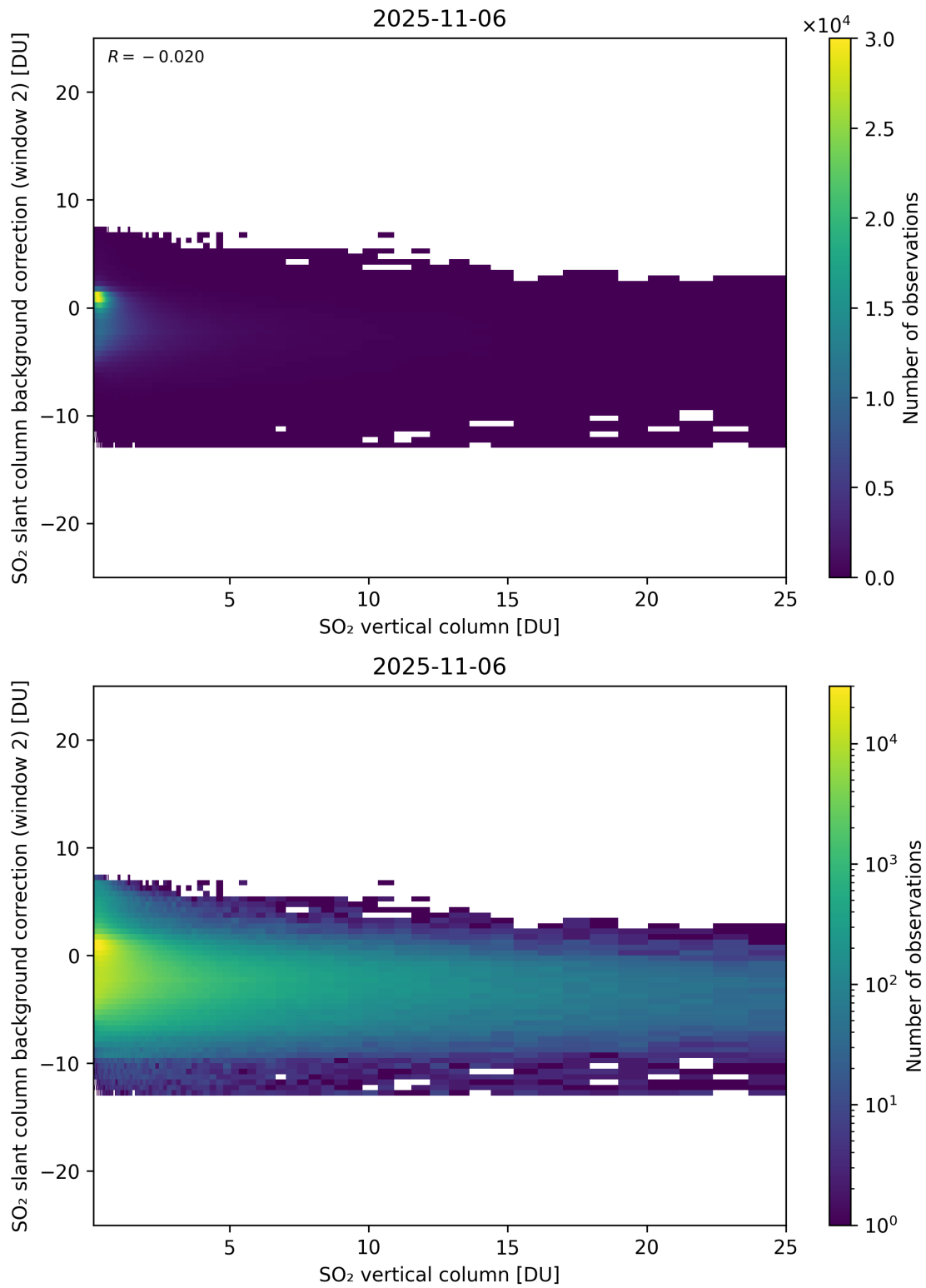
Figure 324: Scatter density plot of “SO 2 vertical column” against “SO 2 slant column background correction (window 2)” for 2025-11-05 to 2025-11-07.
