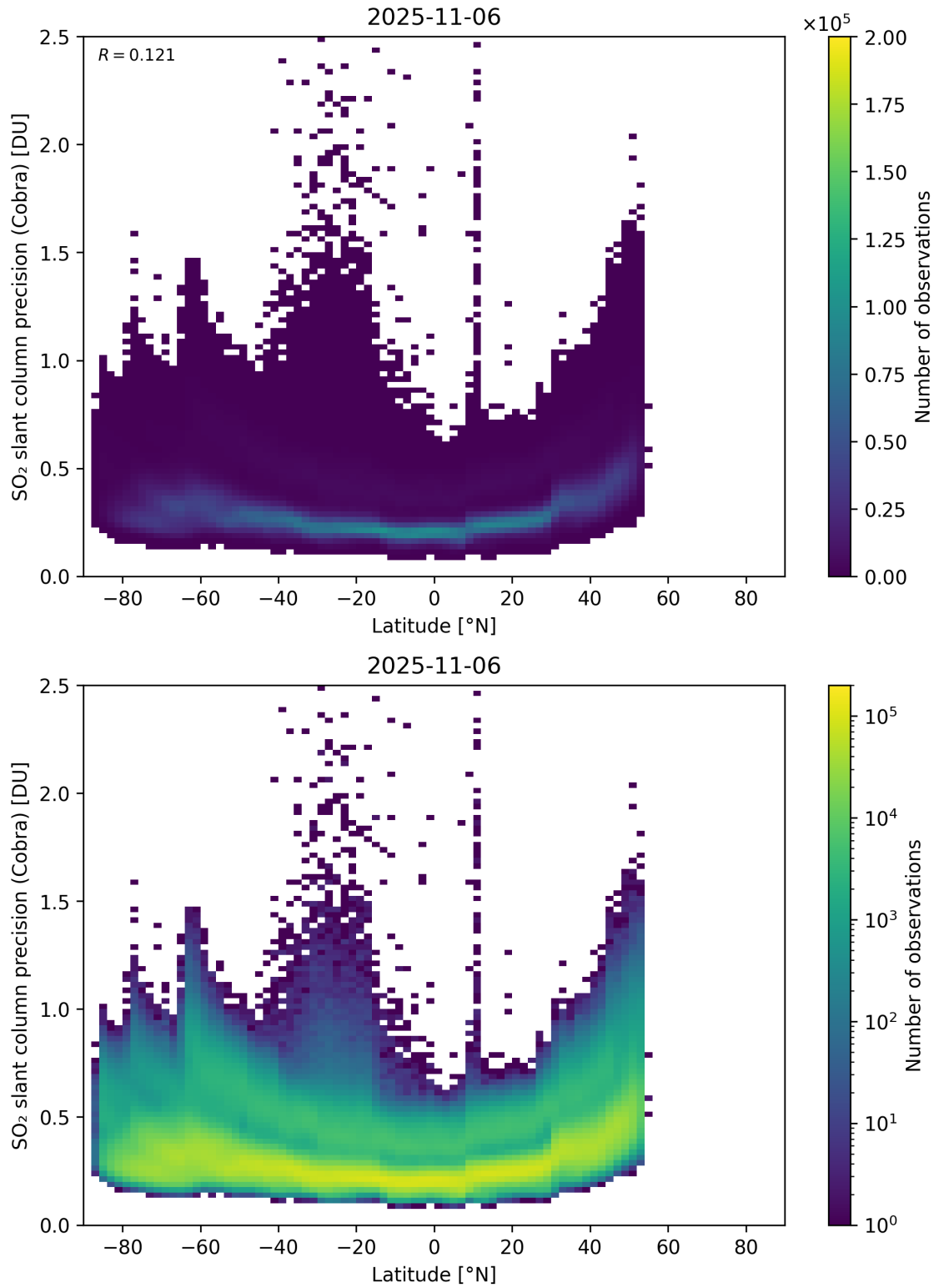
Figure 158: Scatter density plot of “Latitude” against “SO 2 slant column precision (Cobra)” for 2025-11-05 to 2025-11-07.
