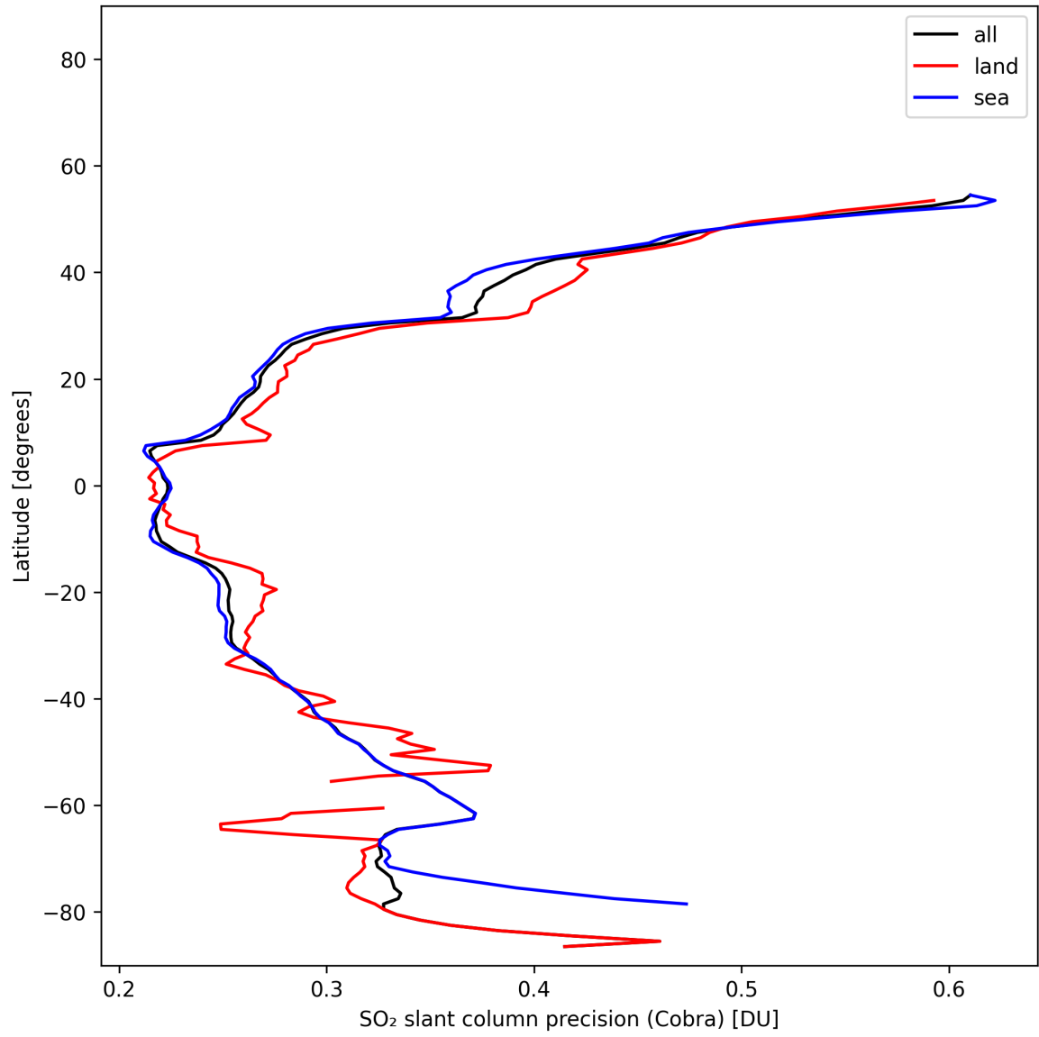
Figure 36: Zonal average of “SO 2 slant column precision (Cobra)” for 2025-11-05 to 2025-11-07.
