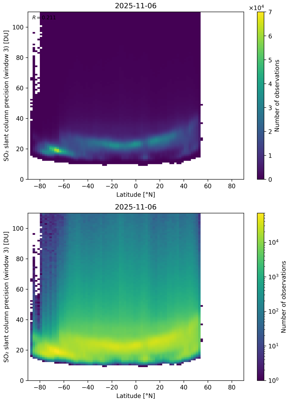
Figure 166: Scatter density plot of “Latitude” against “SO 2 slant column precision (window 3)” for 2025-11-05 to 2025-11-07.
