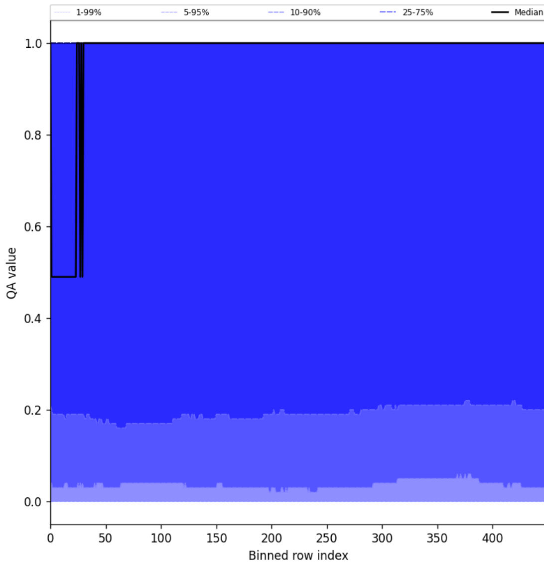
Figure 83: Along track statistics of “QA value” for 2025-11-05 to 2025-11-07
