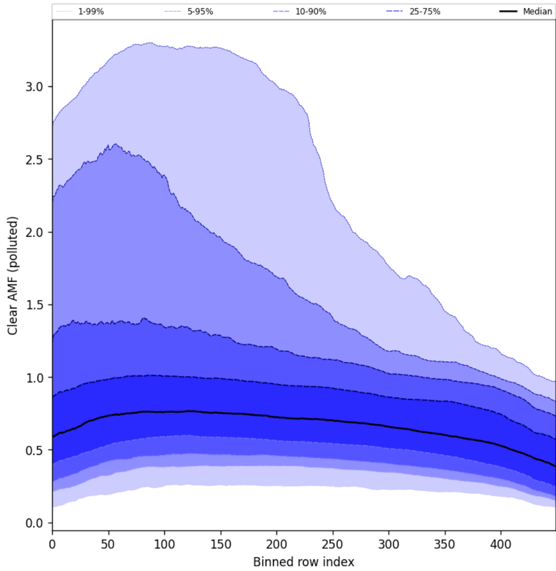
Figure 107: Along track statistics of “Clear AMF (polluted)” for 2025-11-05 to 2025-11-07
