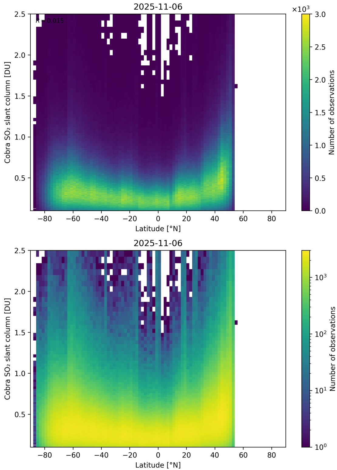
Figure 157: Scatter density plot of “Latitude” against “Cobra SO 2 slant column” for 2025-11-05 to 2025-11-07.
