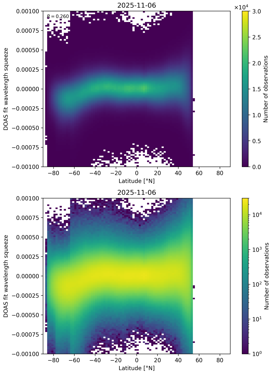
Figure 154: Scatter density plot of “Latitude” against “DOAS fit wavelength squeeze” for 2025-11-05 to 2025-11-07.
