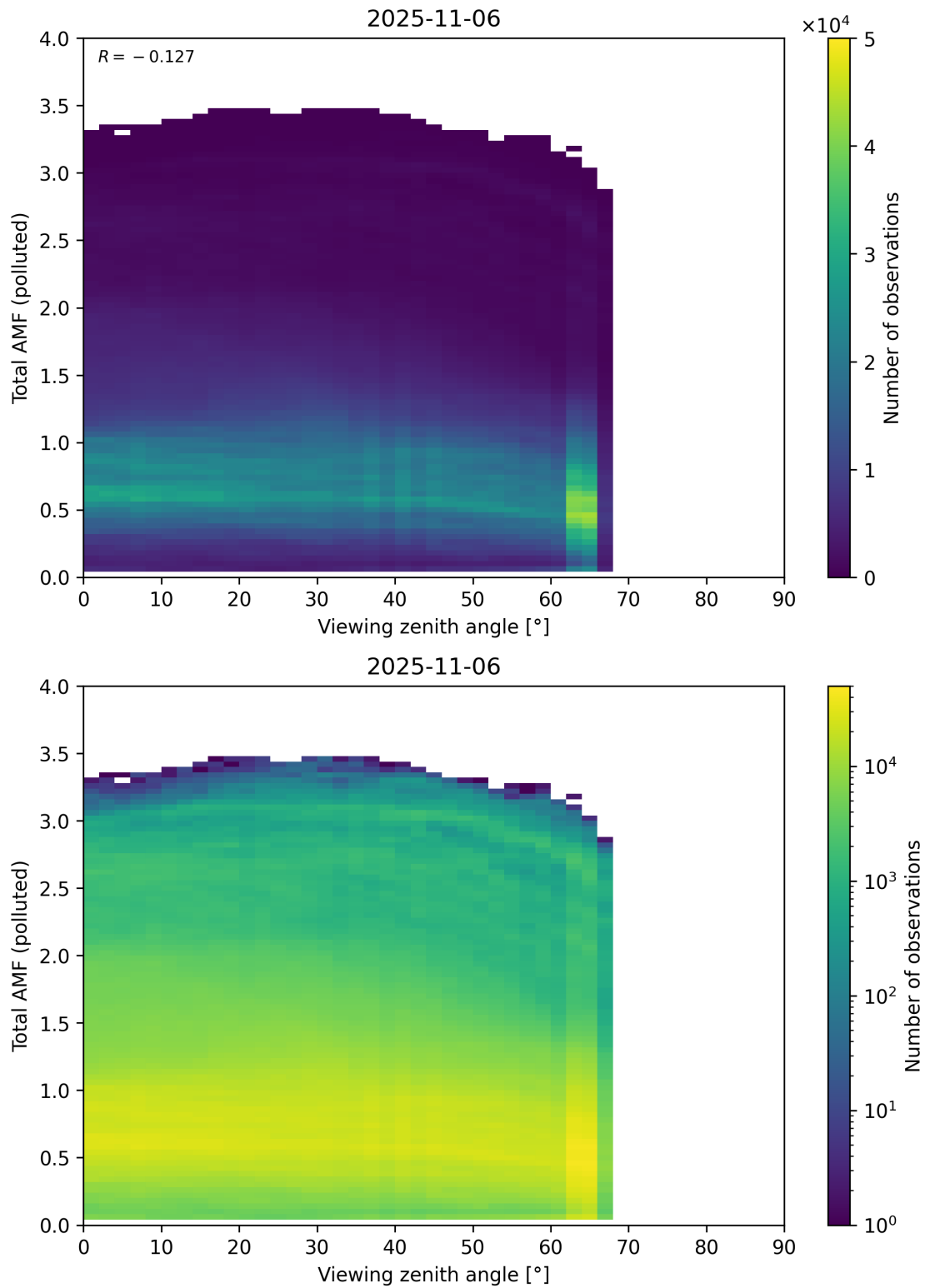
Figure 381: Scatter density plot of “Viewing zenith angle” against “Total AMF (polluted)” for 2025-11-05 to 2025-11-07.
