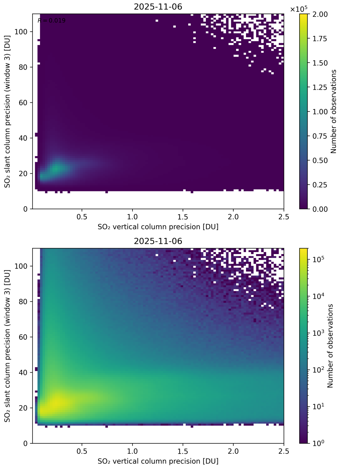
Figure 345: Scatter density plot of “SO 2 vertical column precision” against “SO 2 slant column precision (window 3)” for 2025-11-05 to 2025-11-07.
