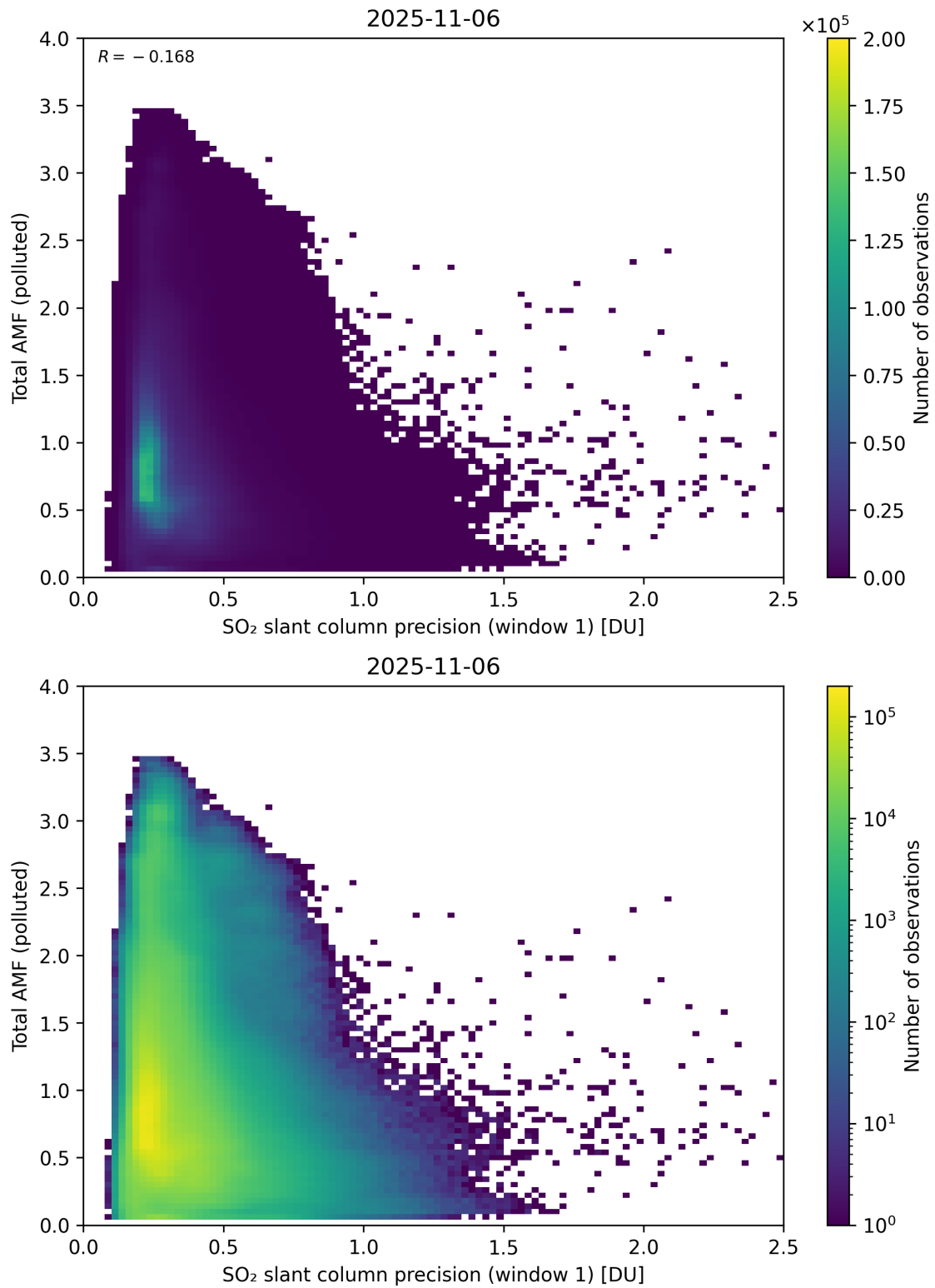
Figure 280: Scatter density plot of “SO 2 slant column precision (window 1)” against “Total AMF (polluted)” for 2025-11-05 to 2025-11-07.
