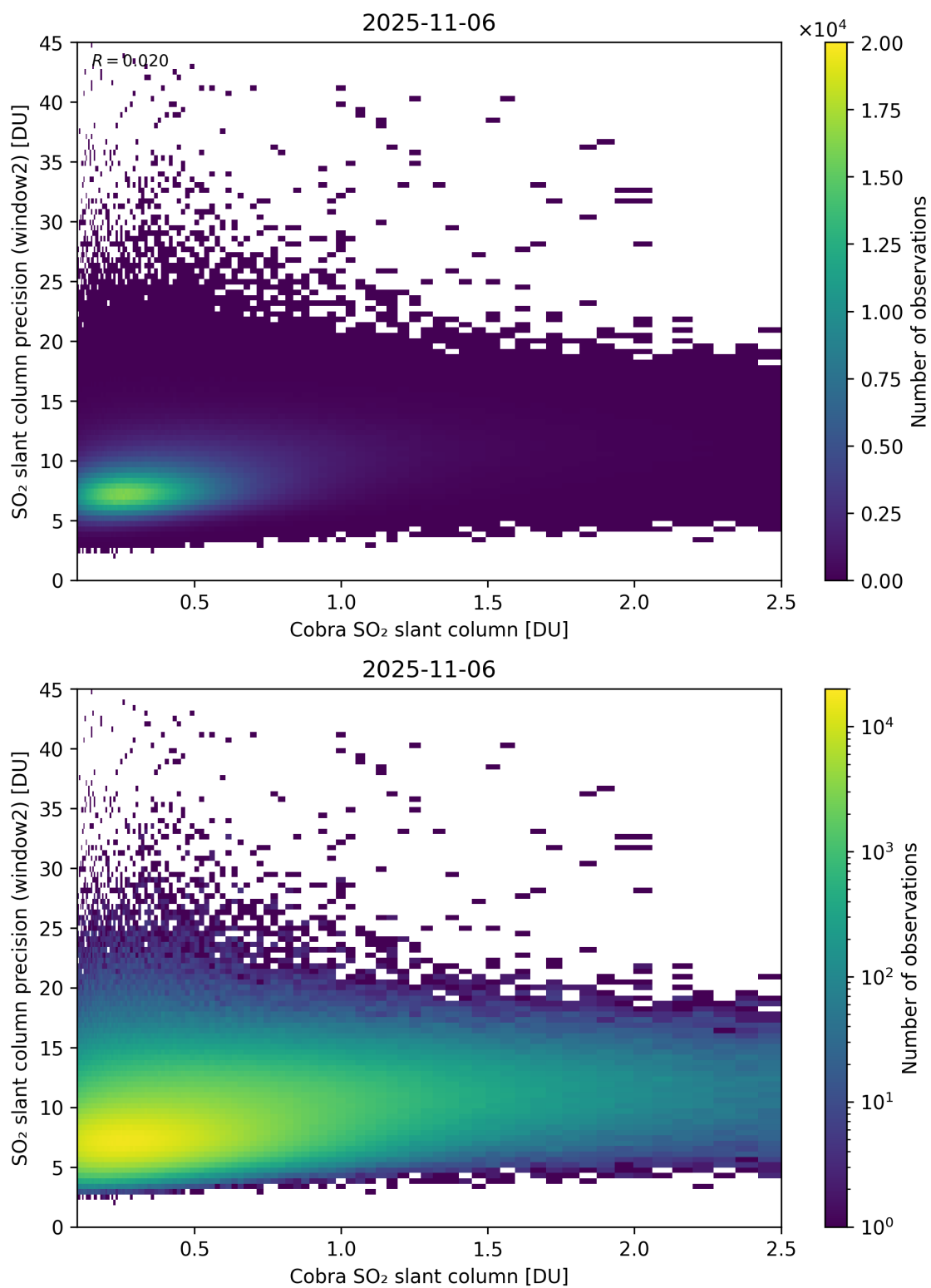
Figure 221: Scatter density plot of “Cobra SO 2 slant column” against “SO 2 slant column precision (window2)” for 2025-11-05 to 2025-11-07.
