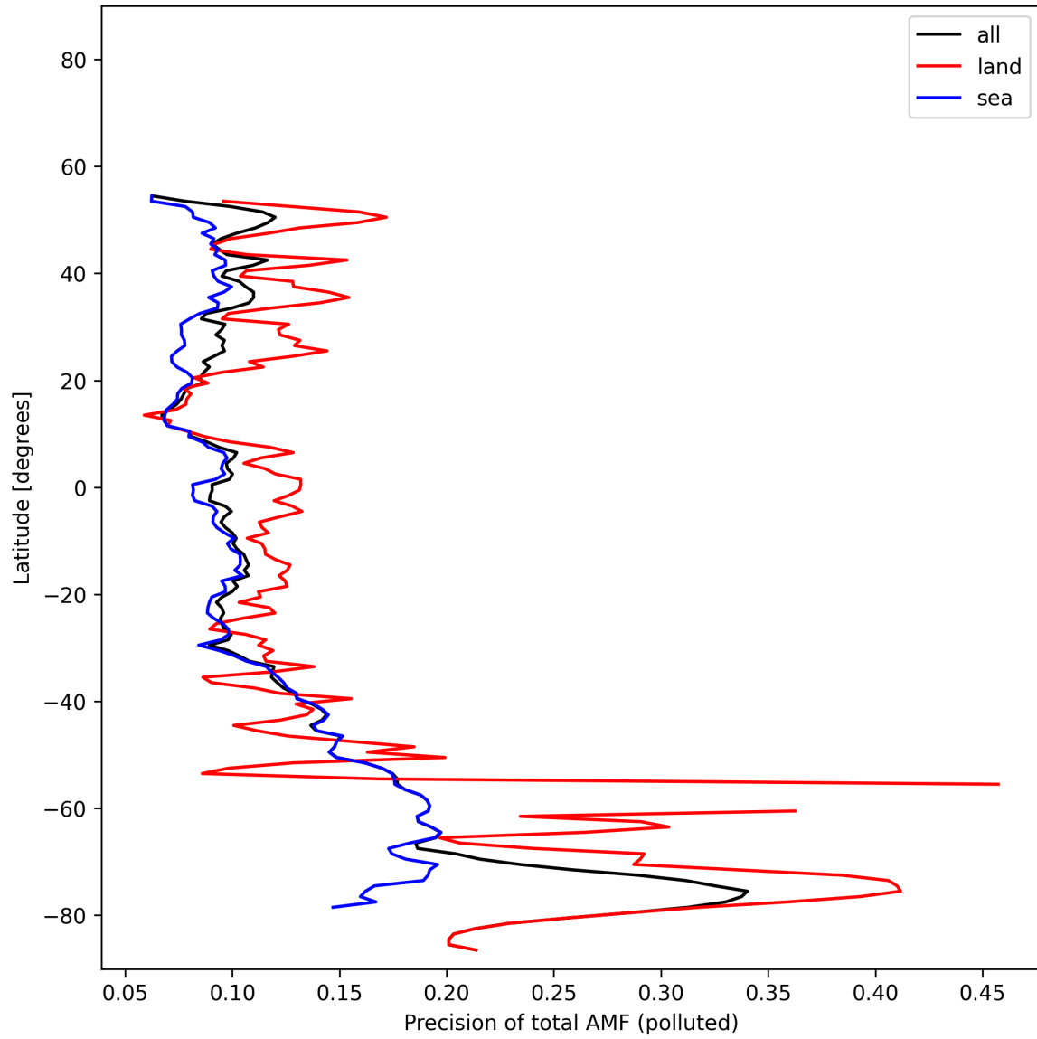
Figure 54: Zonal average of “Precision of total AMF (polluted)” for 2025-11-05 to 2025-11-07.
