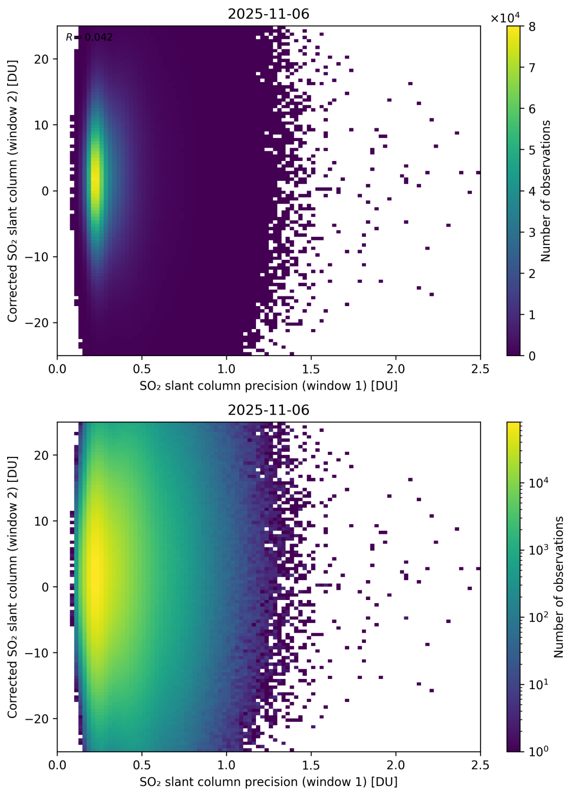
Figure 275: Scatter density plot of “SO 2 slant column precision (window 1)” against “Corrected SO 2 slant column (window 2)” for 2025-11-05 to 2025-11-07.
