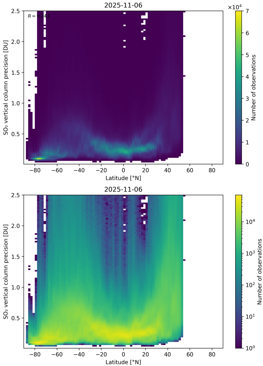
Figure 170: Scatter density plot of “Latitude” against “SO 2 vertical column precision” for 2025-11-05 to 2025-11-07.
