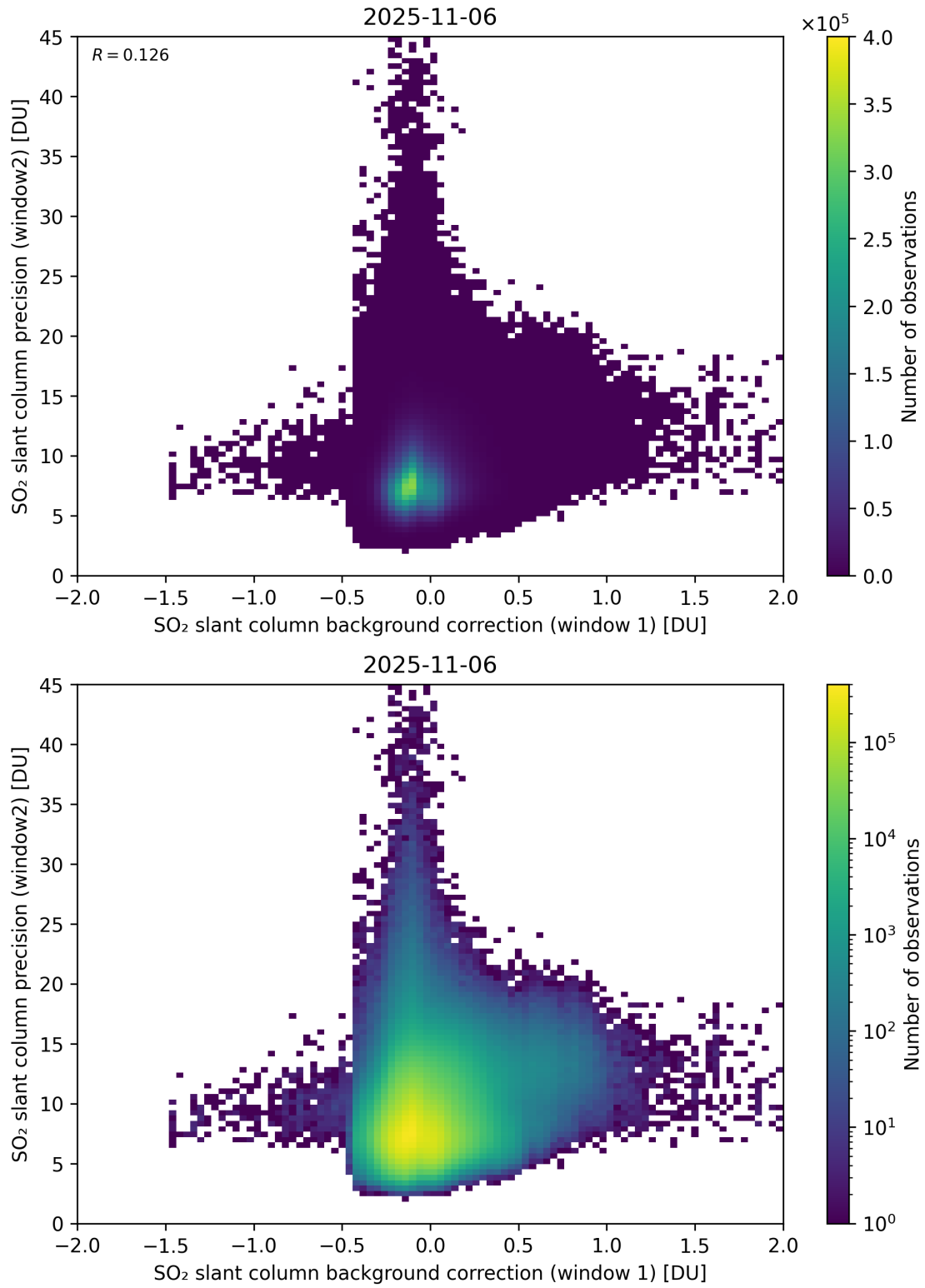
Figure 117: Scatter density plot of “SO 2 slant column background correction (window 1)” against “SO 2 slant column precision (window2)” for 2025-11-05 to 2025-11-07.
