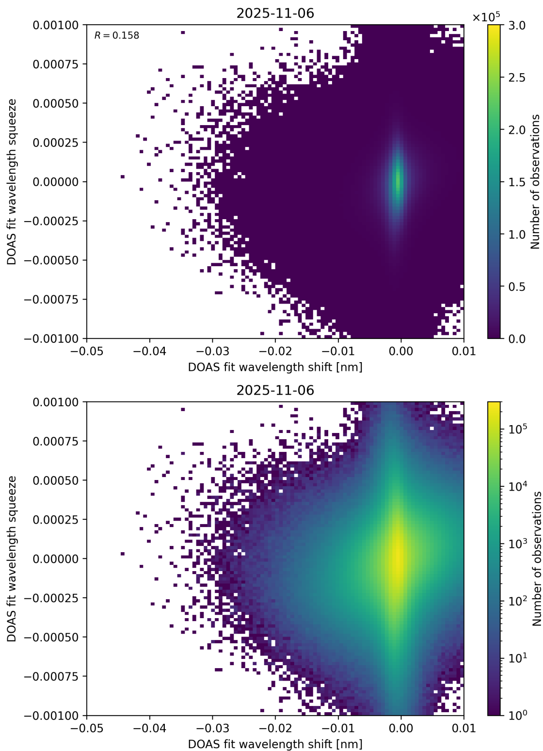
Figure 138: Scatter density plot of “DOAS fit wavelength shift” against “DOAS fit wavelength squeeze” for 2025-11-05 to 2025-11-07.
