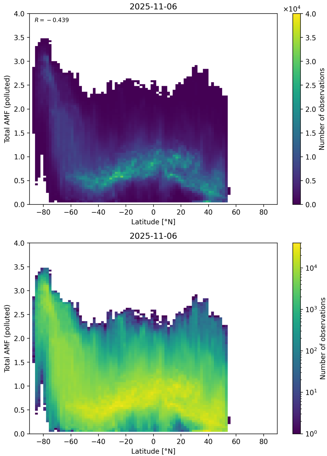
Figure 167: Scatter density plot of “Latitude” against “Total AMF (polluted)” for 2025-11-05 to 2025-11-07.
