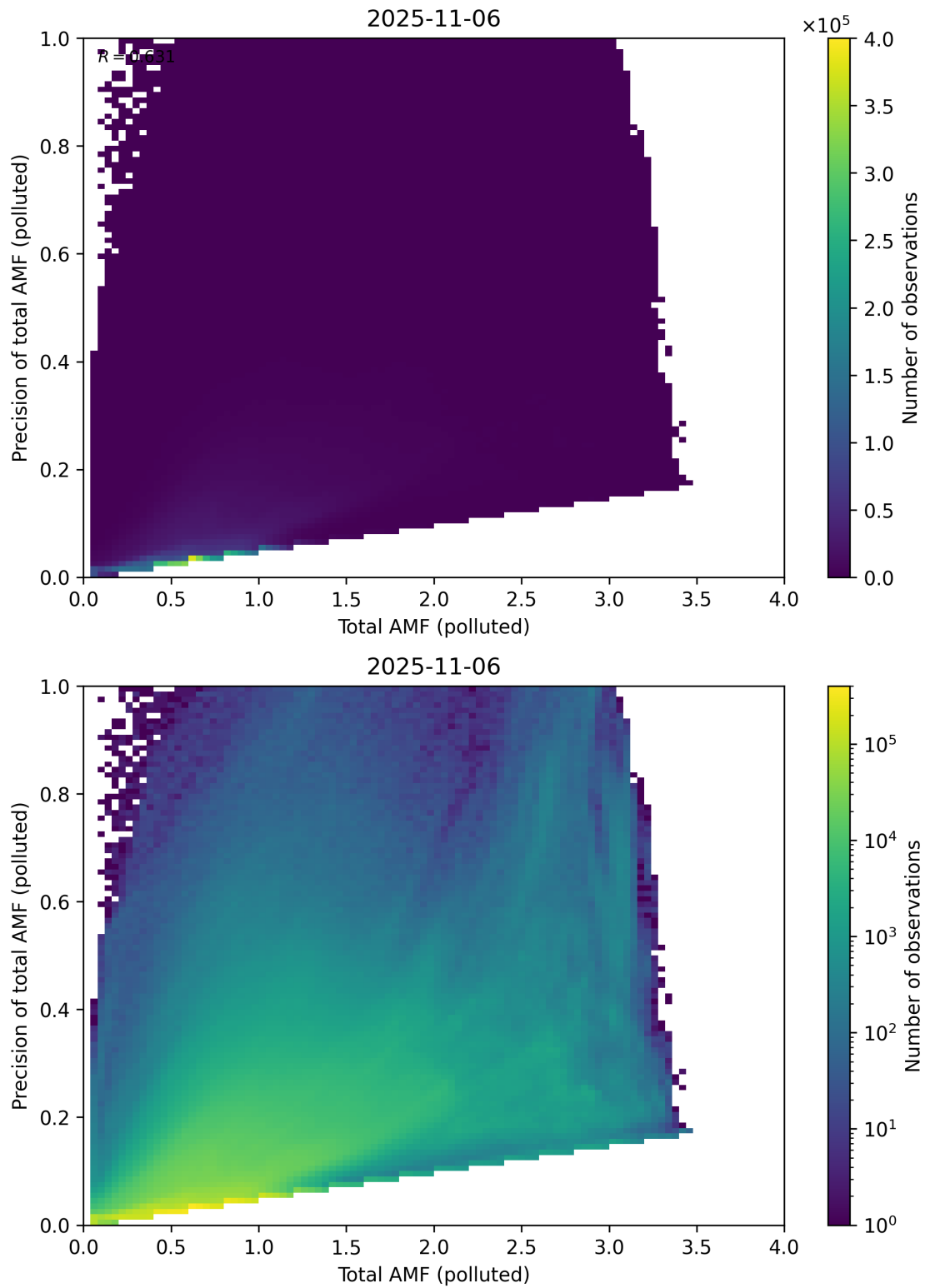
Figure 322: Scatter density plot of “Total AMF (polluted)” against “Precision of total AMF (polluted)” for 2025-11-05 to 2025-11-07.
