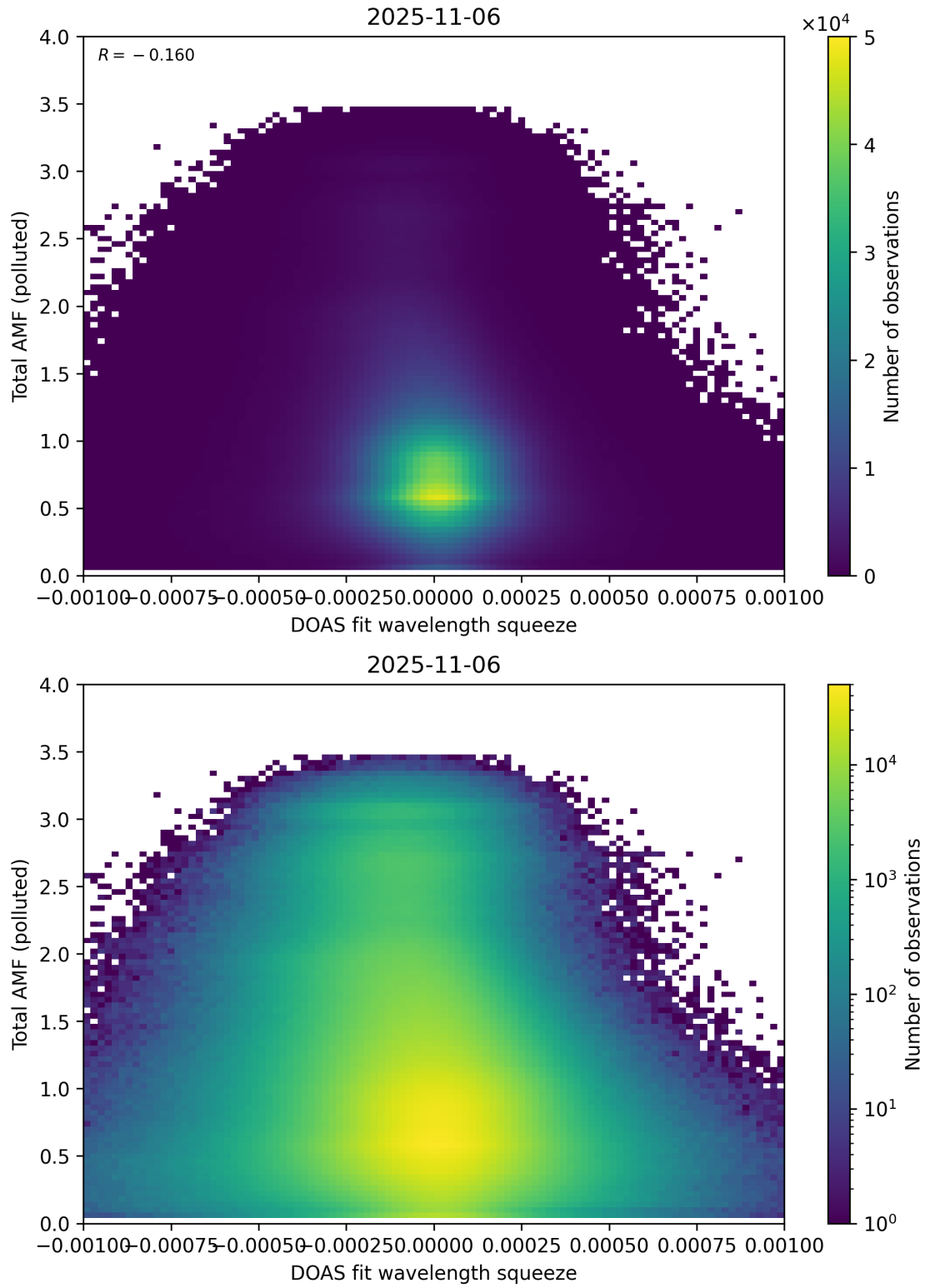
Figure 145: Scatter density plot of “DOAS fit wavelength squeeze” against “Total AMF (polluted)” for 2025-11-05 to 2025-11-07.
