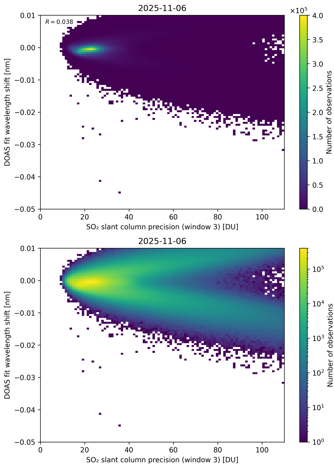
Figure 308: Scatter density plot of “SO 2 slant column precision (window 3)” against “DOAS fit wavelength shift” for 2025-11-05 to 2025-11-07.
