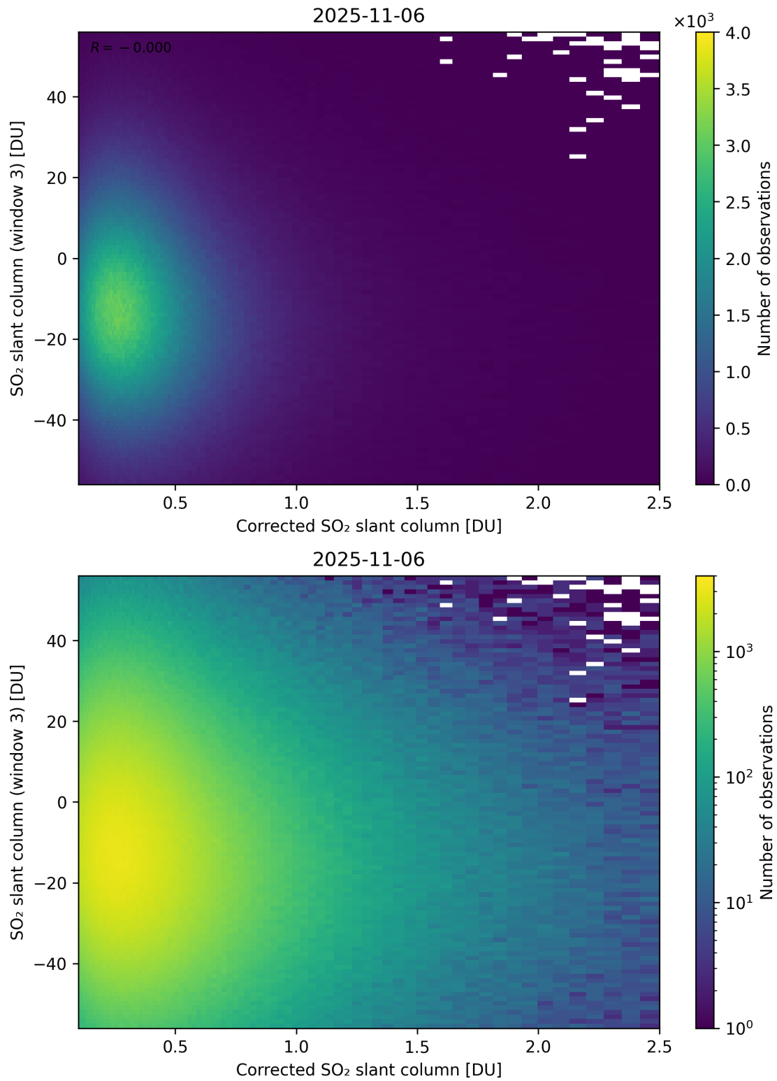
Figure 240: Scatter density plot of “Corrected SO 2 slant column” against “SO 2 slant column (window 3)” for 2025-11-05 to 2025-11-07.
