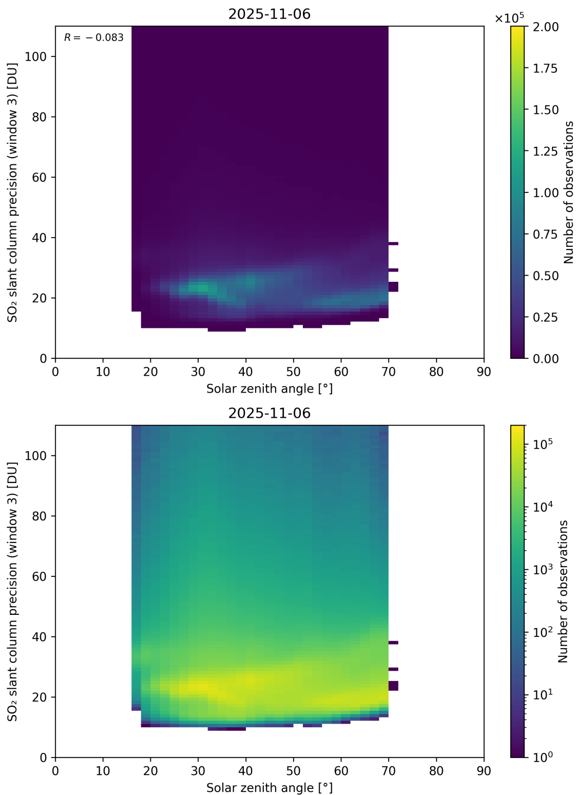
Figure 188: Scatter density plot of “Solar zenith angle” against “SO 2 slant column precision (window 3)” for 2025-11-05 to 2025-11-07.
