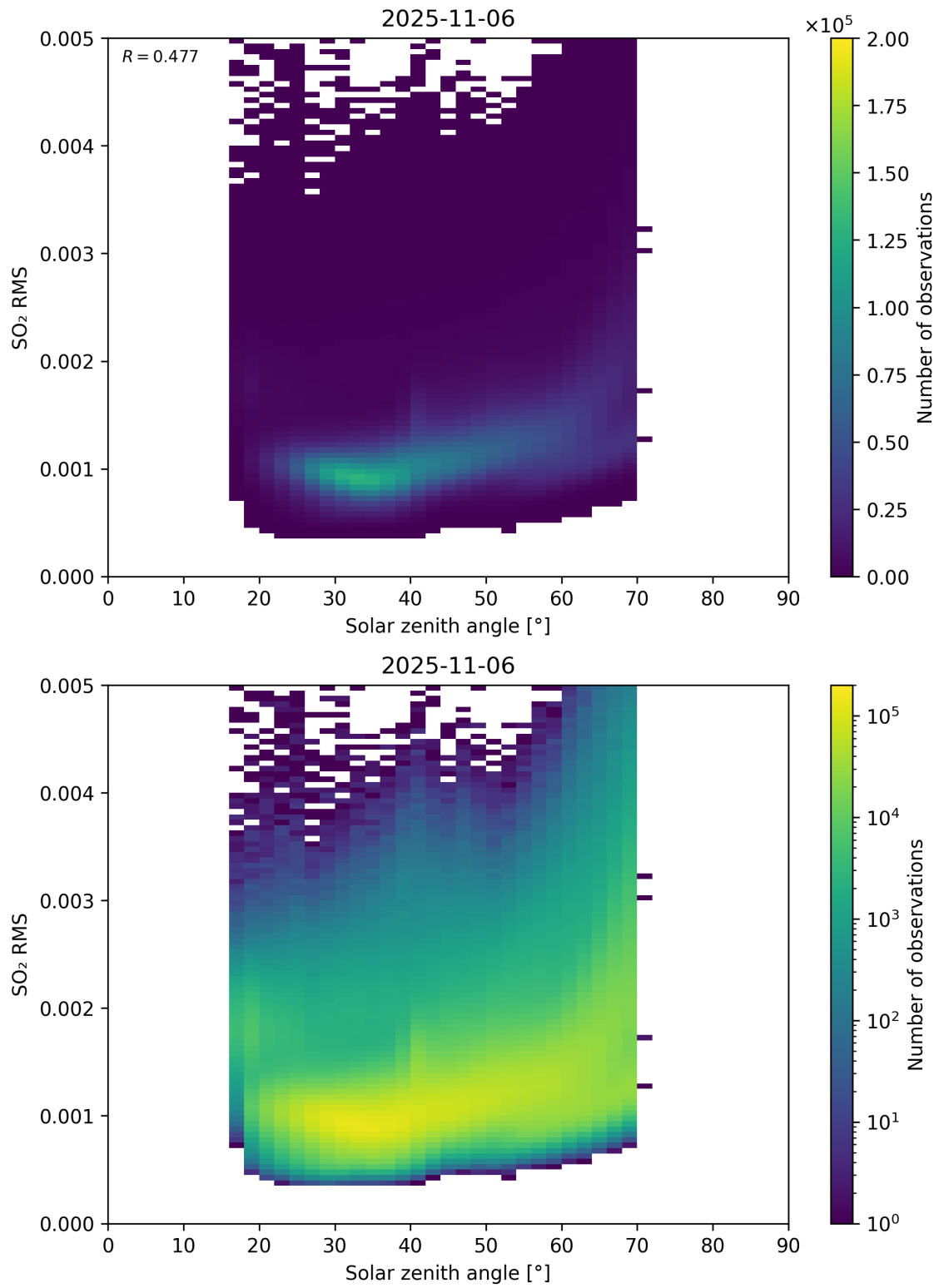
Figure 176: Scatter density plot of “Solar zenith angle” against “SO 2 RMS” for 2025-11-05 to 2025-11-07.
