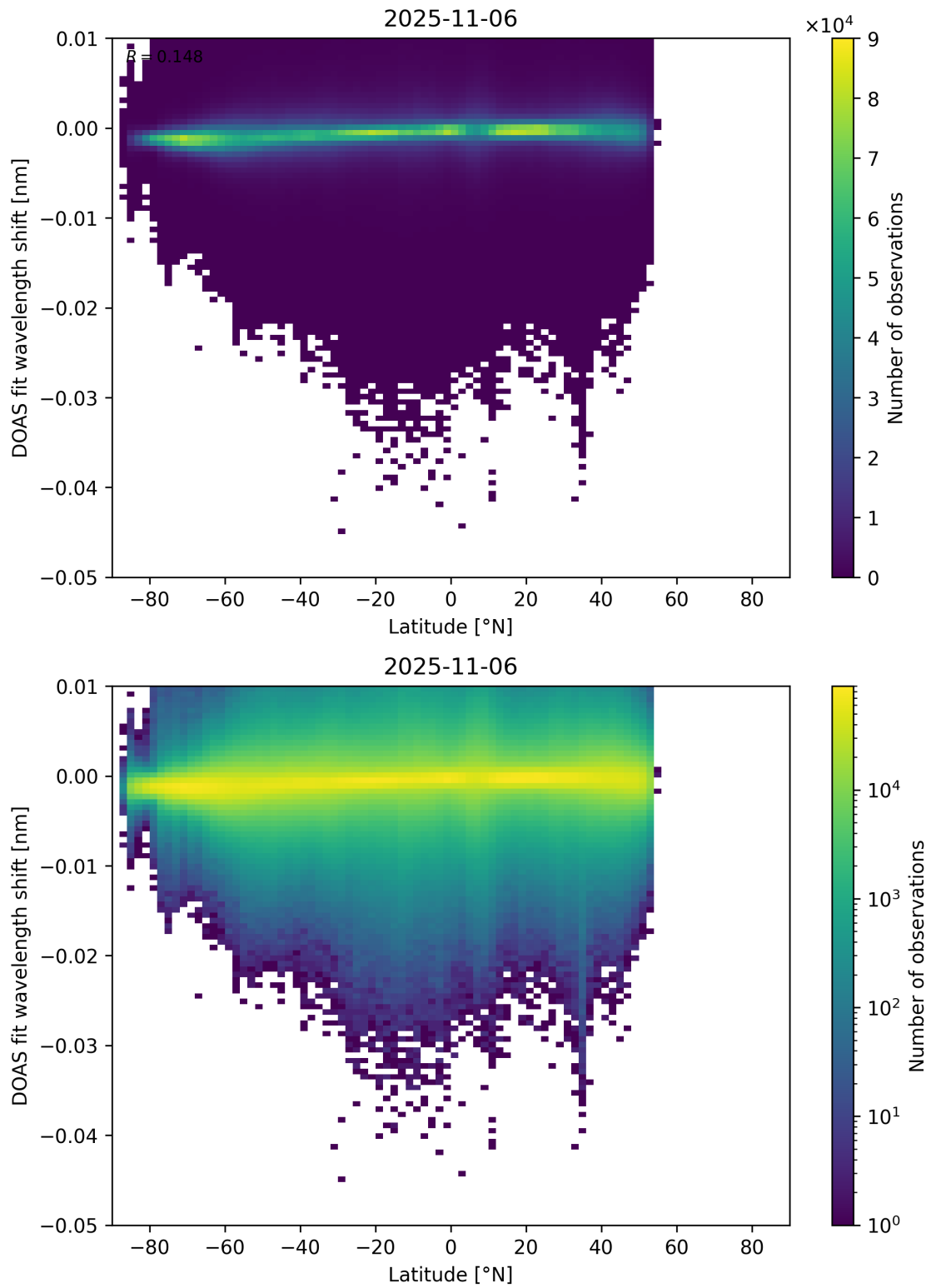
Figure 153: Scatter density plot of “Latitude” against “DOAS fit wavelength shift” for 2025-11-05 to 2025-11-07.
