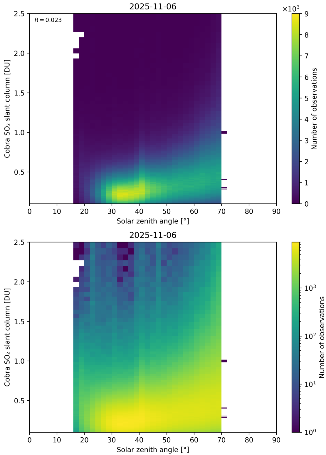
Figure 179: Scatter density plot of “Solar zenith angle” against “Cobra SO 2 slant column” for 2025-11-05 to 2025-11-07.
