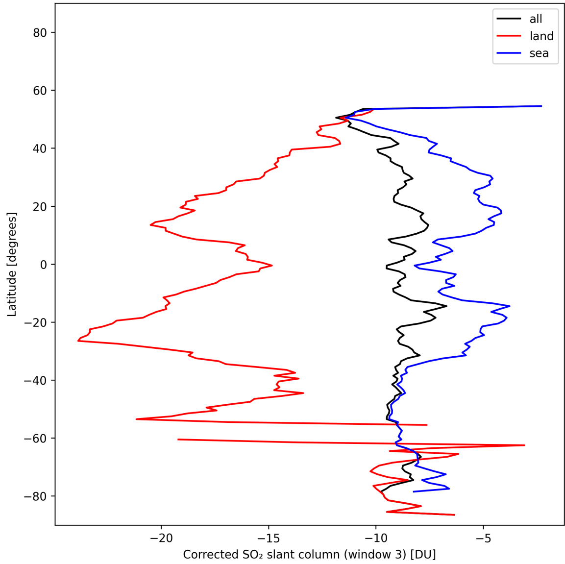
Figure 47: Zonal average of “Corrected SO 2 slant column (window 3)” for 2025-11-05 to 2025-11-07.
