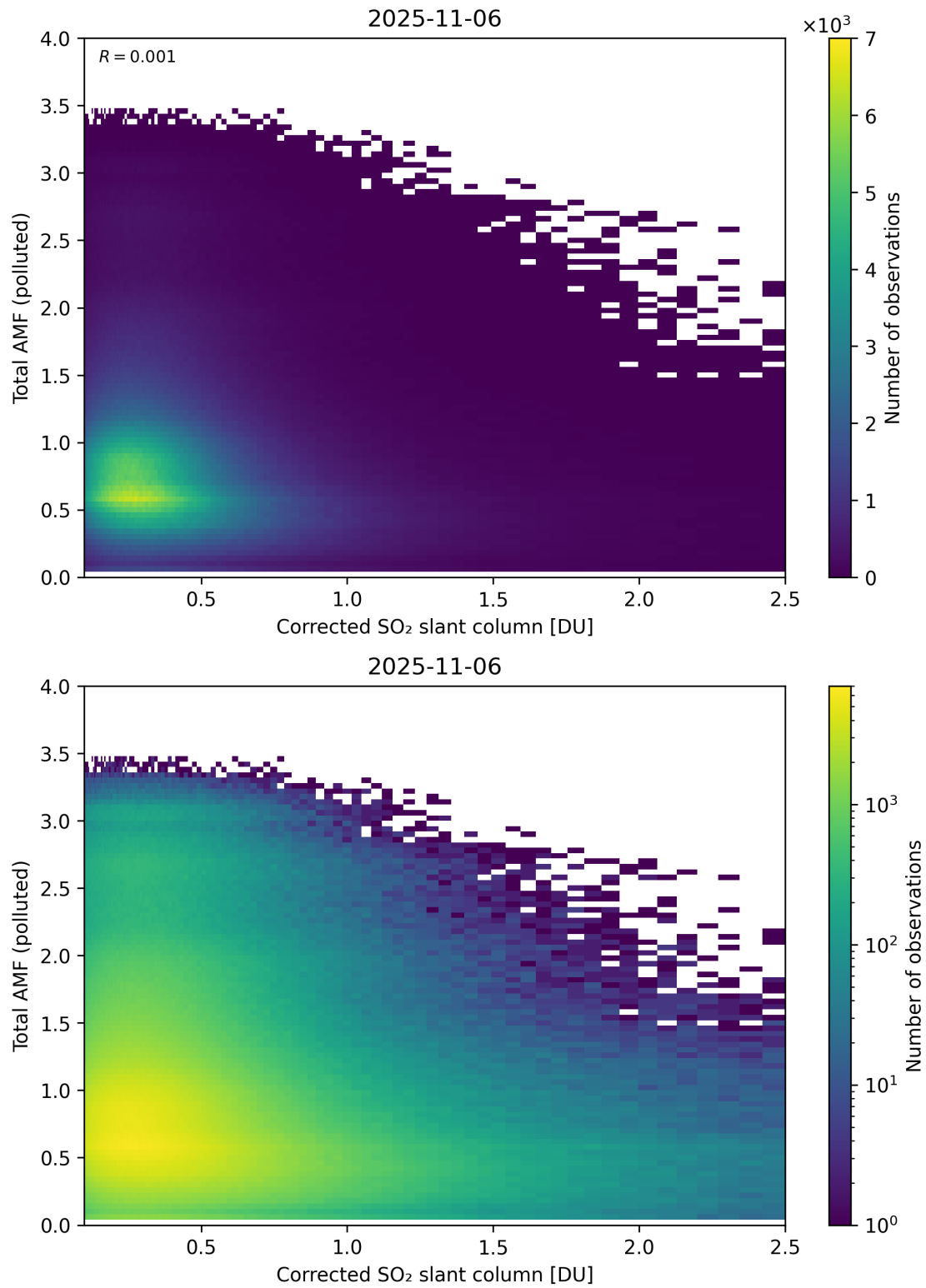
Figure 242: Scatter density plot of “Corrected SO 2 slant column” against “Total AMF (polluted)” for 2025-11-05 to 2025-11-07.
