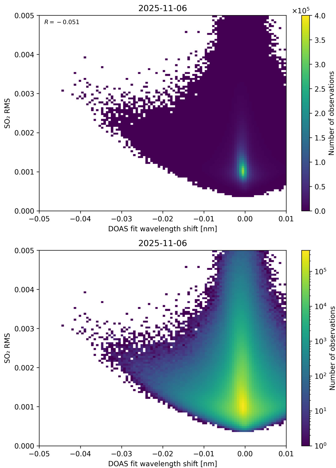
Figure 139: Scatter density plot of “DOAS fit wavelength shift” against “SO 2 RMS” for 2025-11-05 to 2025-11-07.
