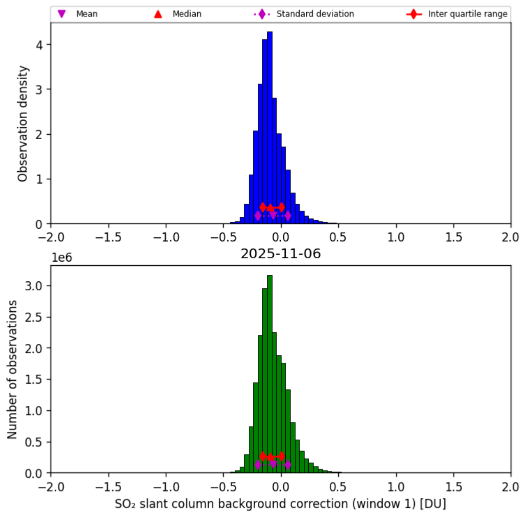
Figure 66: Histogram of “SO 2 slant column background correction (window 1)” for 2025-11-05 to 2025-11-07
