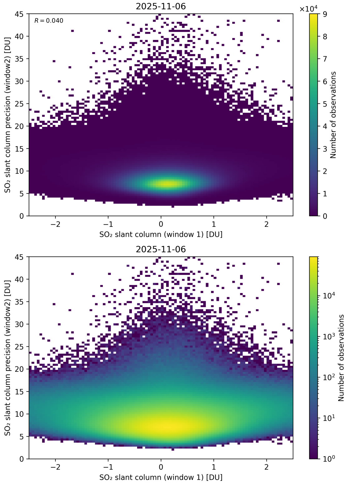
Figure 286: Scatter density plot of “SO 2 slant column (window 1)” against “SO 2 slant column precision (window2)” for 2025-11-05 to 2025-11-07.
