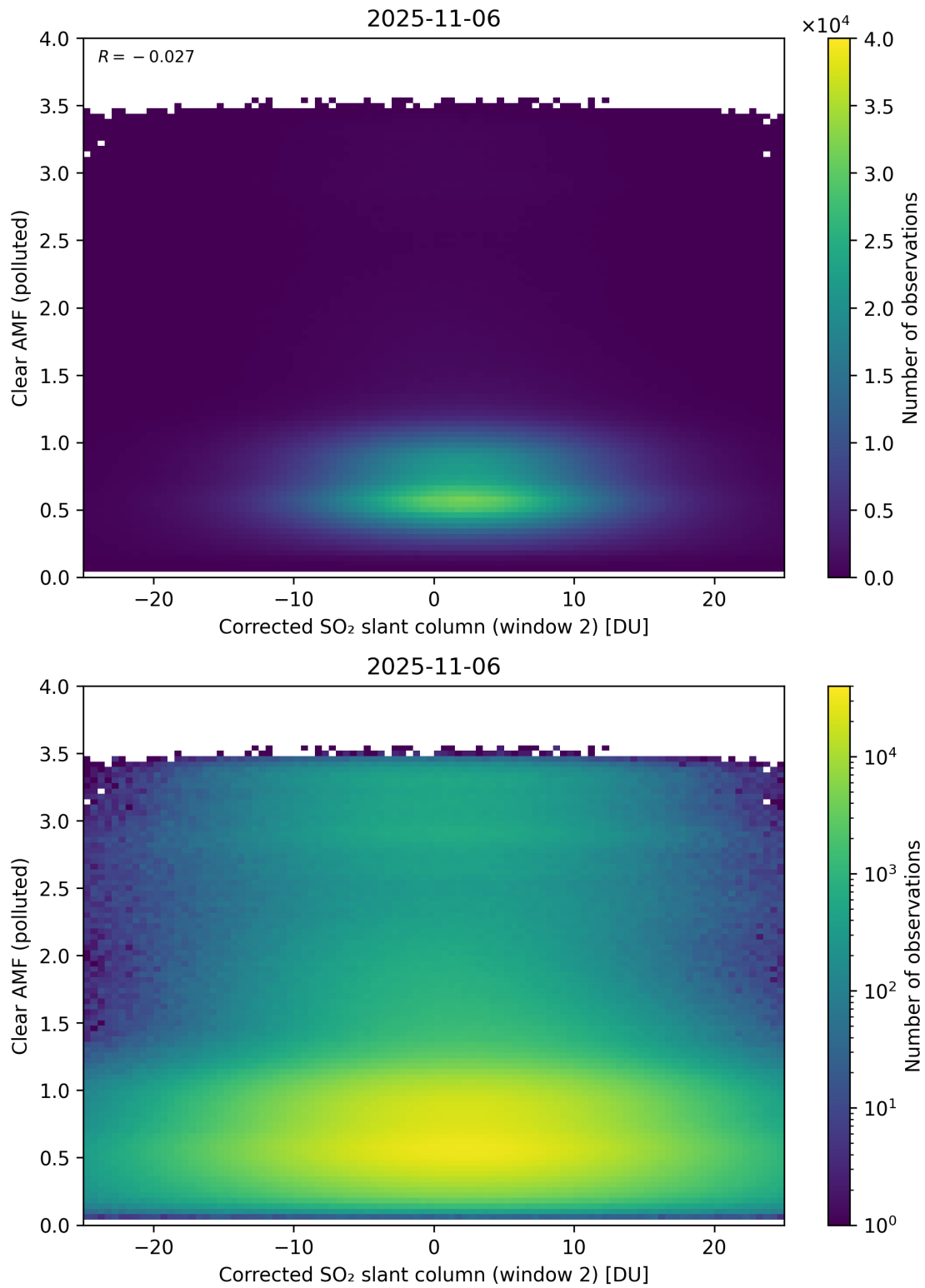
Figure 249: Scatter density plot of “Corrected SO 2 slant column (window 2)” against “Clear AMF (polluted)” for 2025-11-05 to 2025-11-07.
