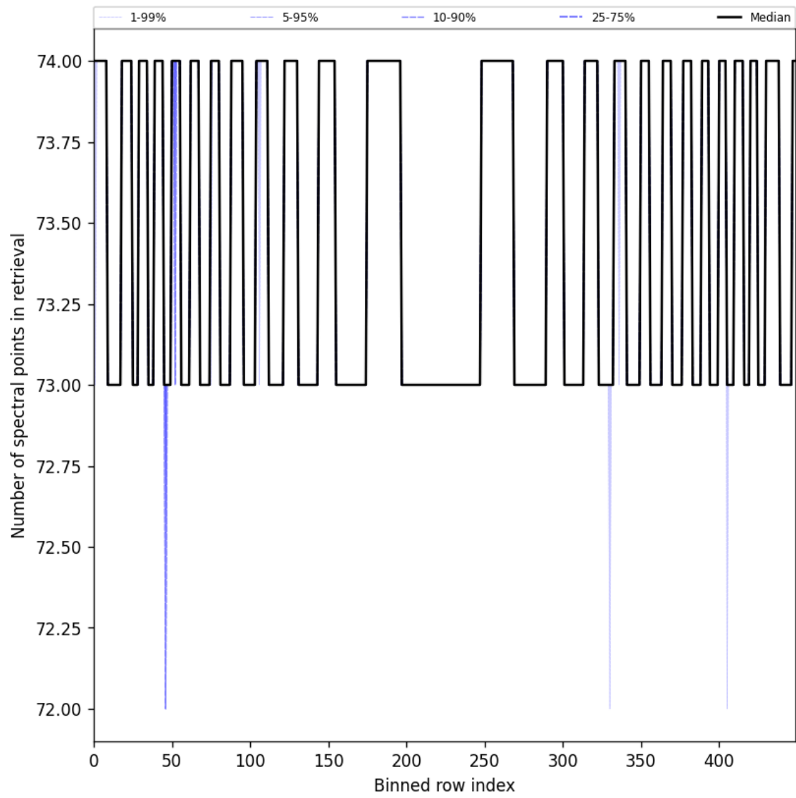
Figure 108: Along track statistics of “Number of spectral points in retrieval” for 2025-11-05 to 2025-11-07
