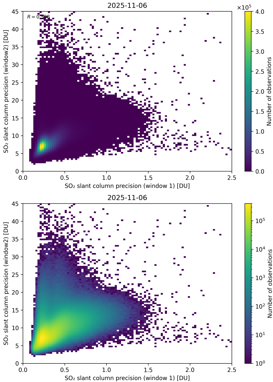
Figure 277: Scatter density plot of “SO 2 slant column precision (window 1)” against “SO 2 slant column precision (window2)” for 2025-11-05 to 2025-11-07.
