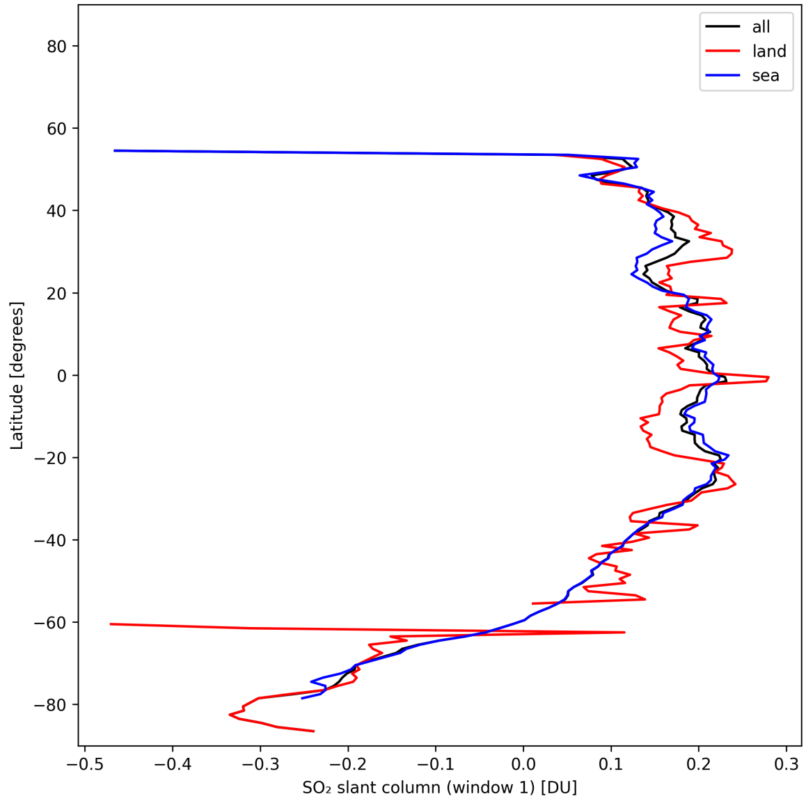
Figure 37: Zonal average of “SO 2 slant column (window 1)” for 2025-11-05 to 2025-11-07.
