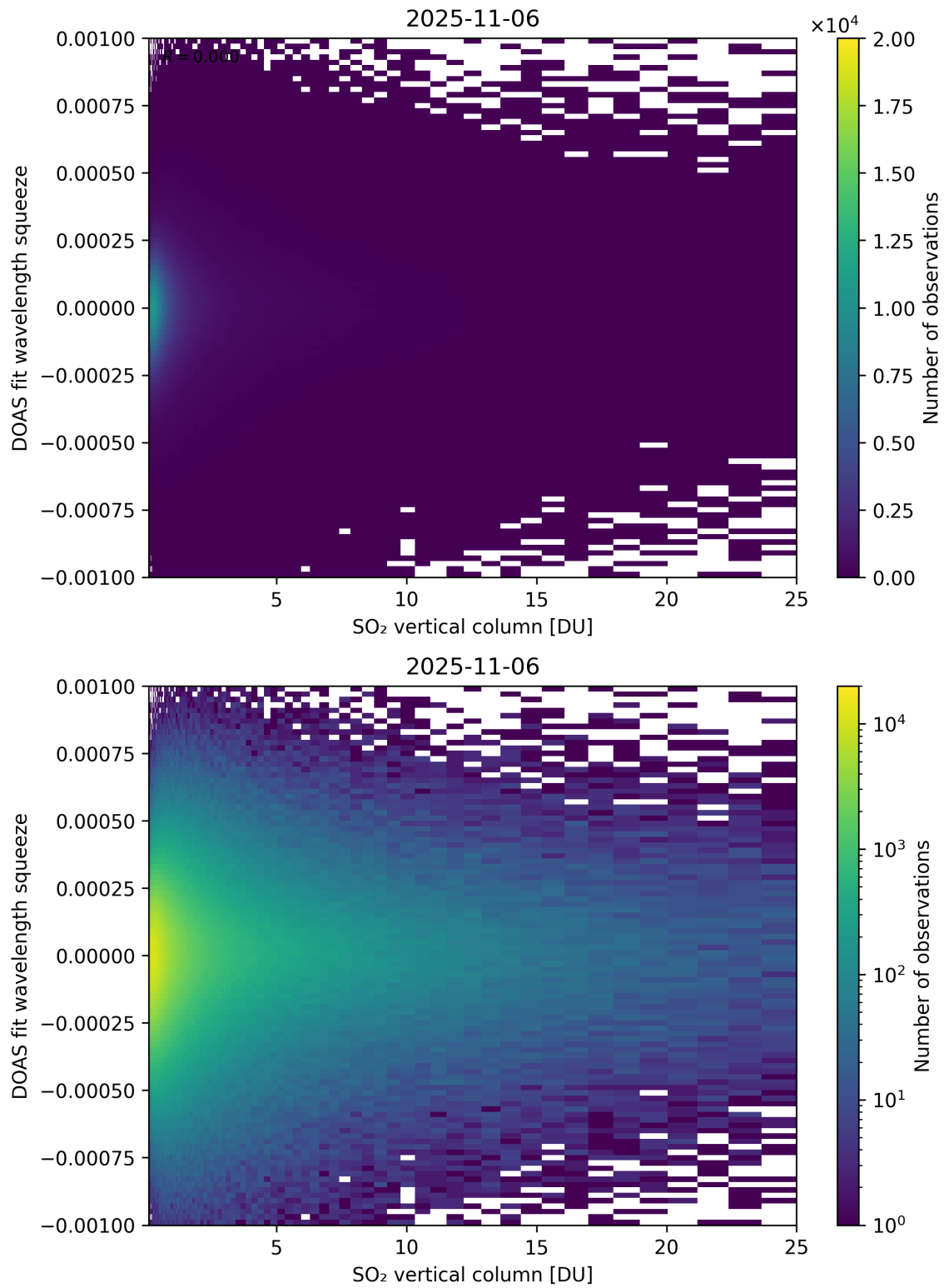
Figure 327: Scatter density plot of “SO 2 vertical column” against “DOAS fit wavelength squeeze” for 2025-11-05 to 2025-11-07.
