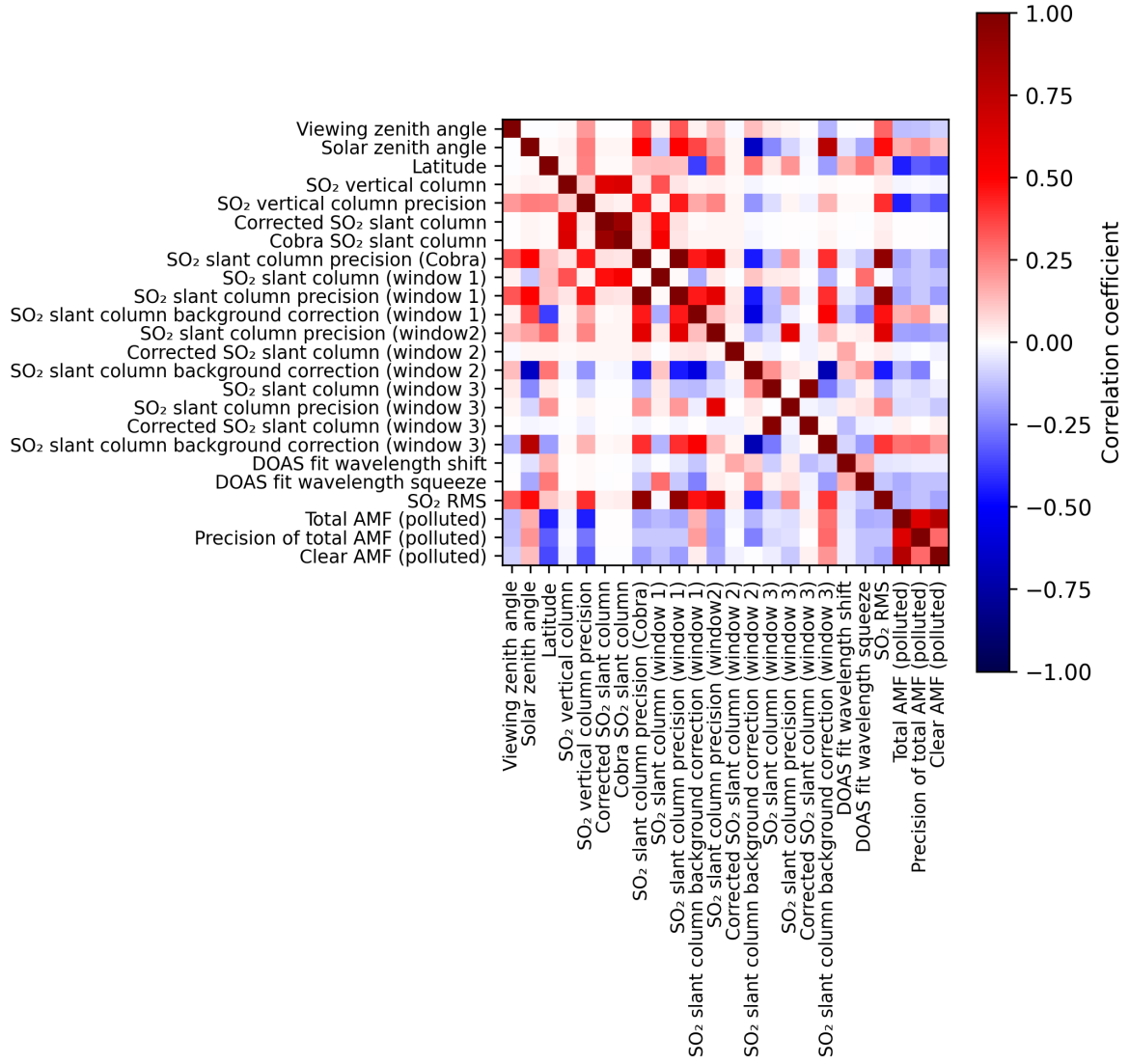
Figure 2: Map of correlation matrix for 2025-11-05 to 2025-11-07.
