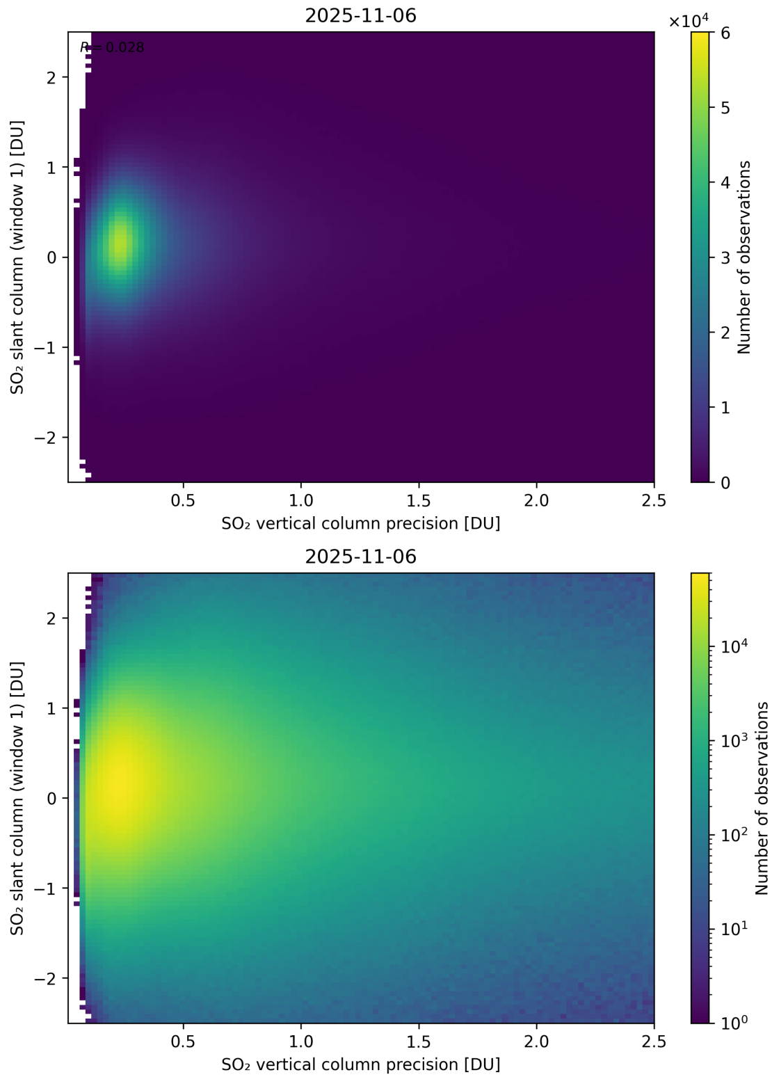
Figure 341: Scatter density plot of “SO 2 vertical column precision” against “SO 2 slant column (window 1)” for 2025-11-05 to 2025-11-07.
