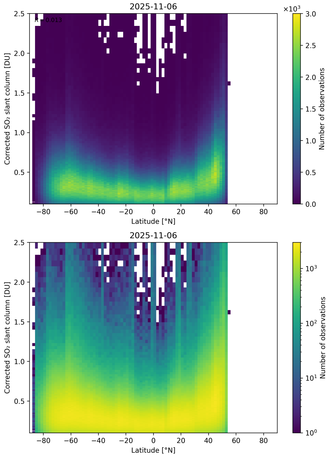
Figure 159: Scatter density plot of “Latitude” against “Corrected SO 2 slant column” for 2025-11-05 to 2025-11-07.
