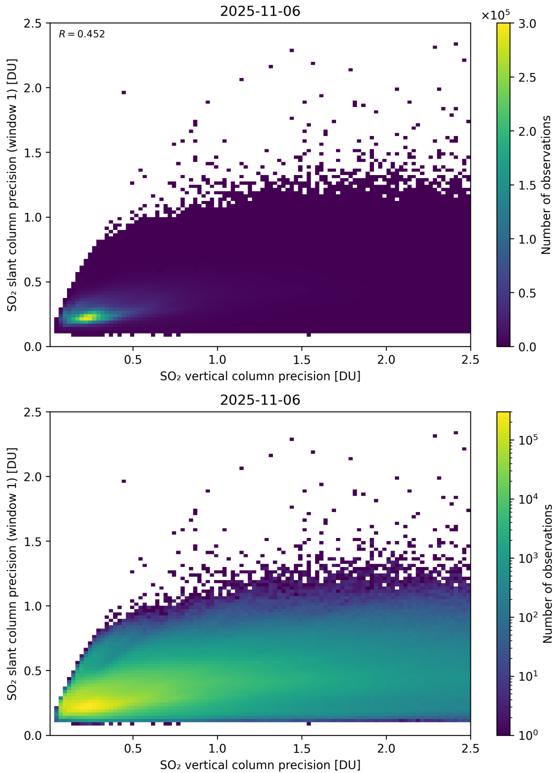
Figure 342: Scatter density plot of “SO 2 vertical column precision” against “SO 2 slant column precision (window 1)” for 2025-11-05 to 2025-11-07.
