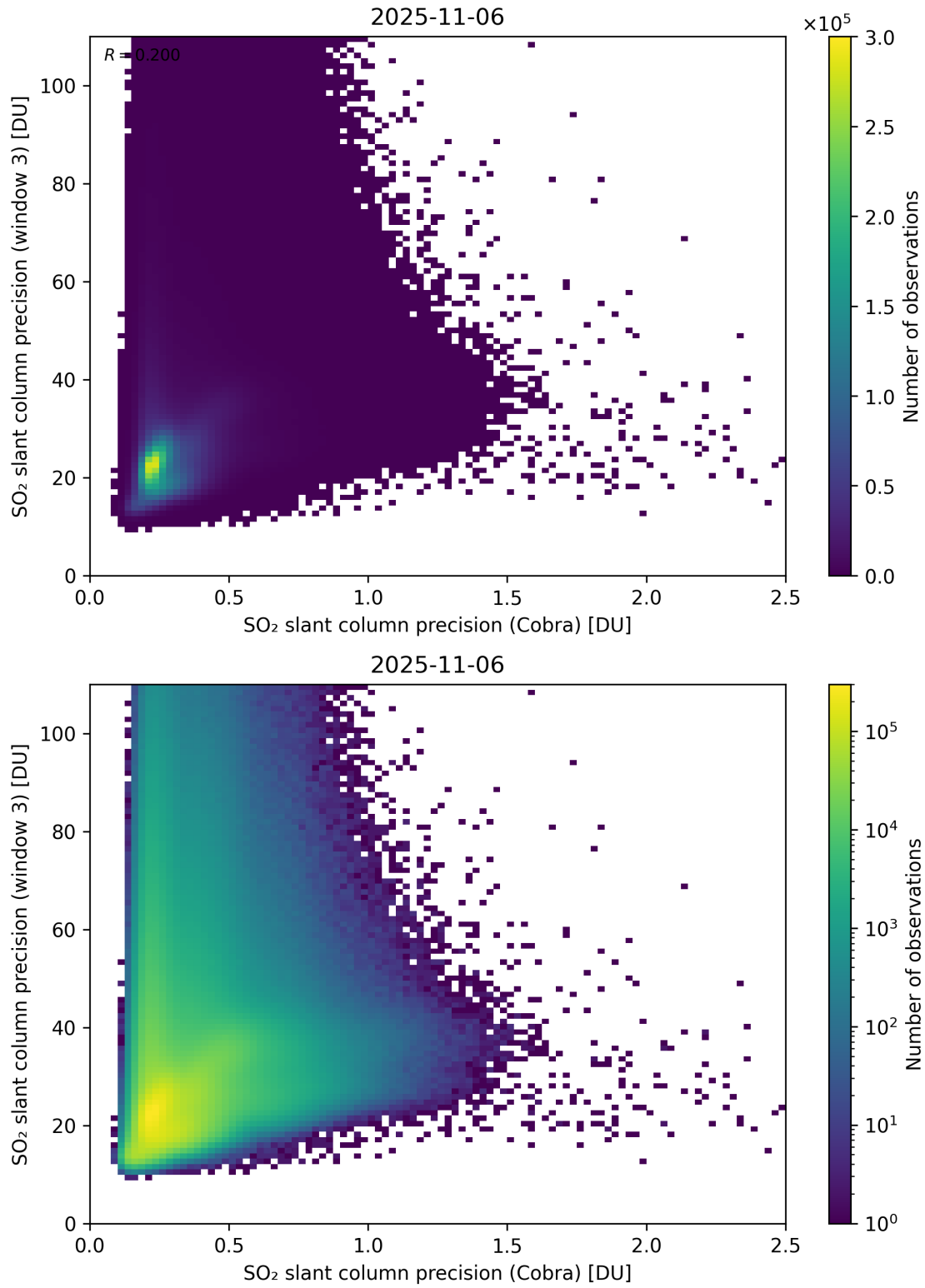
Figure 212: Scatter density plot of “SO 2 slant column precision (Cobra)” against “SO 2 slant column precision (window 3)” for 2025-11-05 to 2025-11-07.
