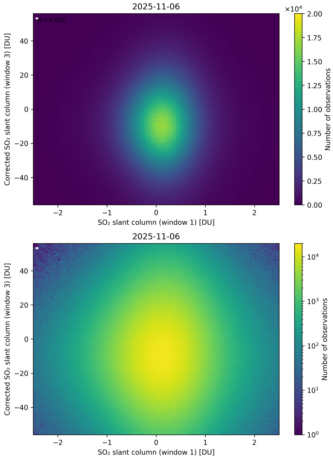
Figure 284: Scatter density plot of “SO 2 slant column (window 1)” against “Corrected SO 2 slant column (window 3)” for 2025-11-05 to 2025-11-07.
