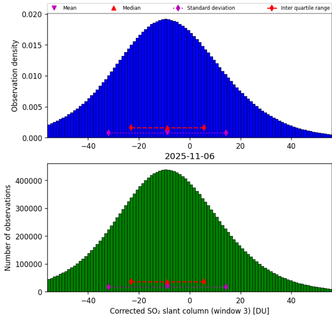
Figure 73: Histogram of “Corrected SO 2 slant column (window 3)” for 2025-11-05 to 2025-11-07
