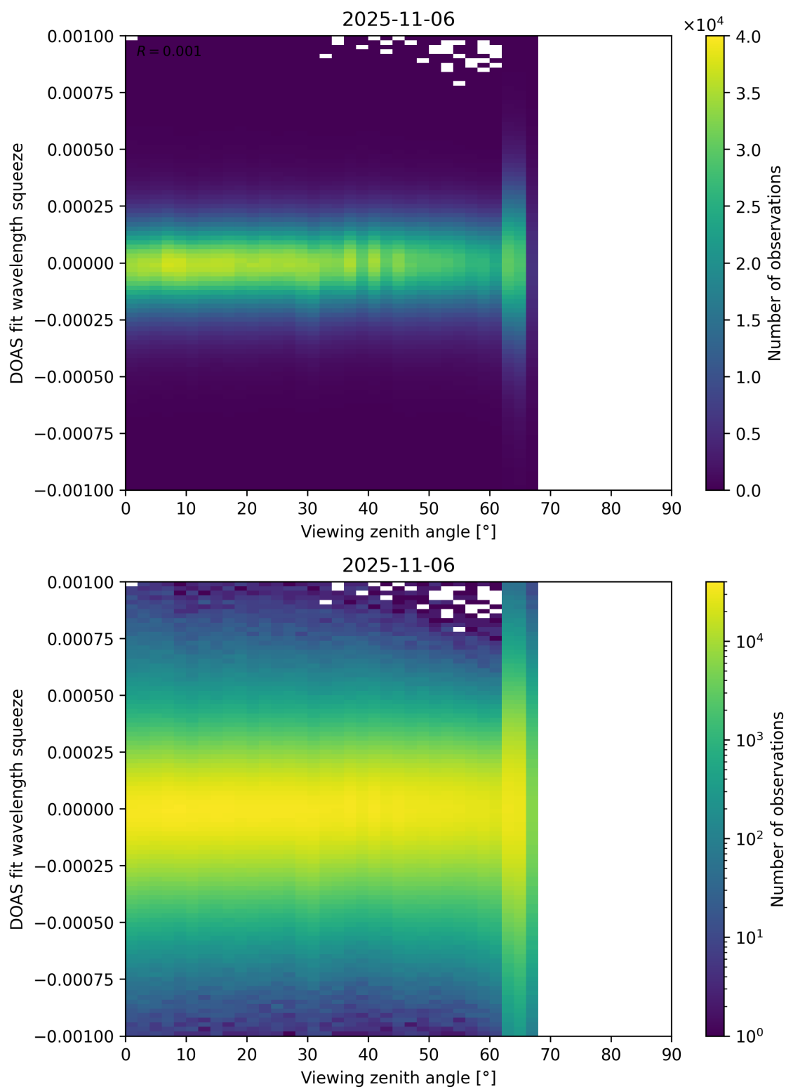
Figure 366: Scatter density plot of “Viewing zenith angle” against “DOAS fit wavelength squeeze” for 2025-11-05 to 2025-11-07.
