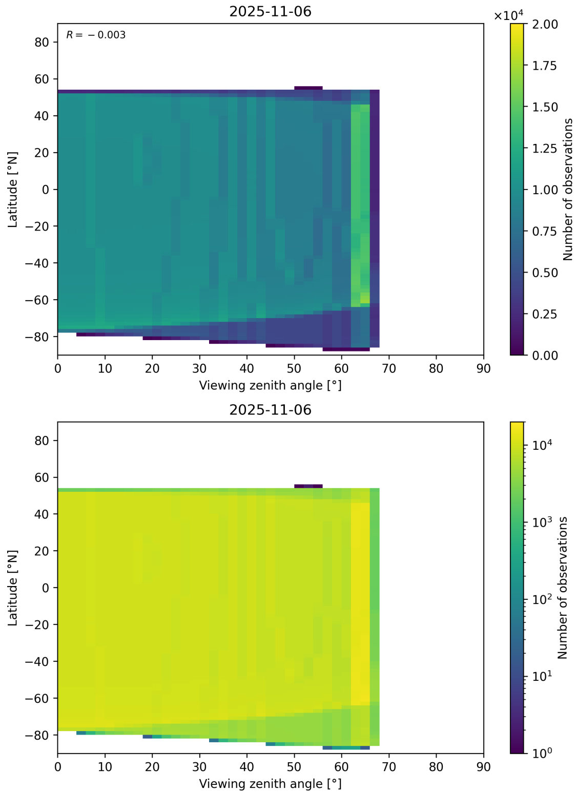
Figure 368: Scatter density plot of “Viewing zenith angle” against “Latitude” for 2025-11-05 to 2025-11-07.
