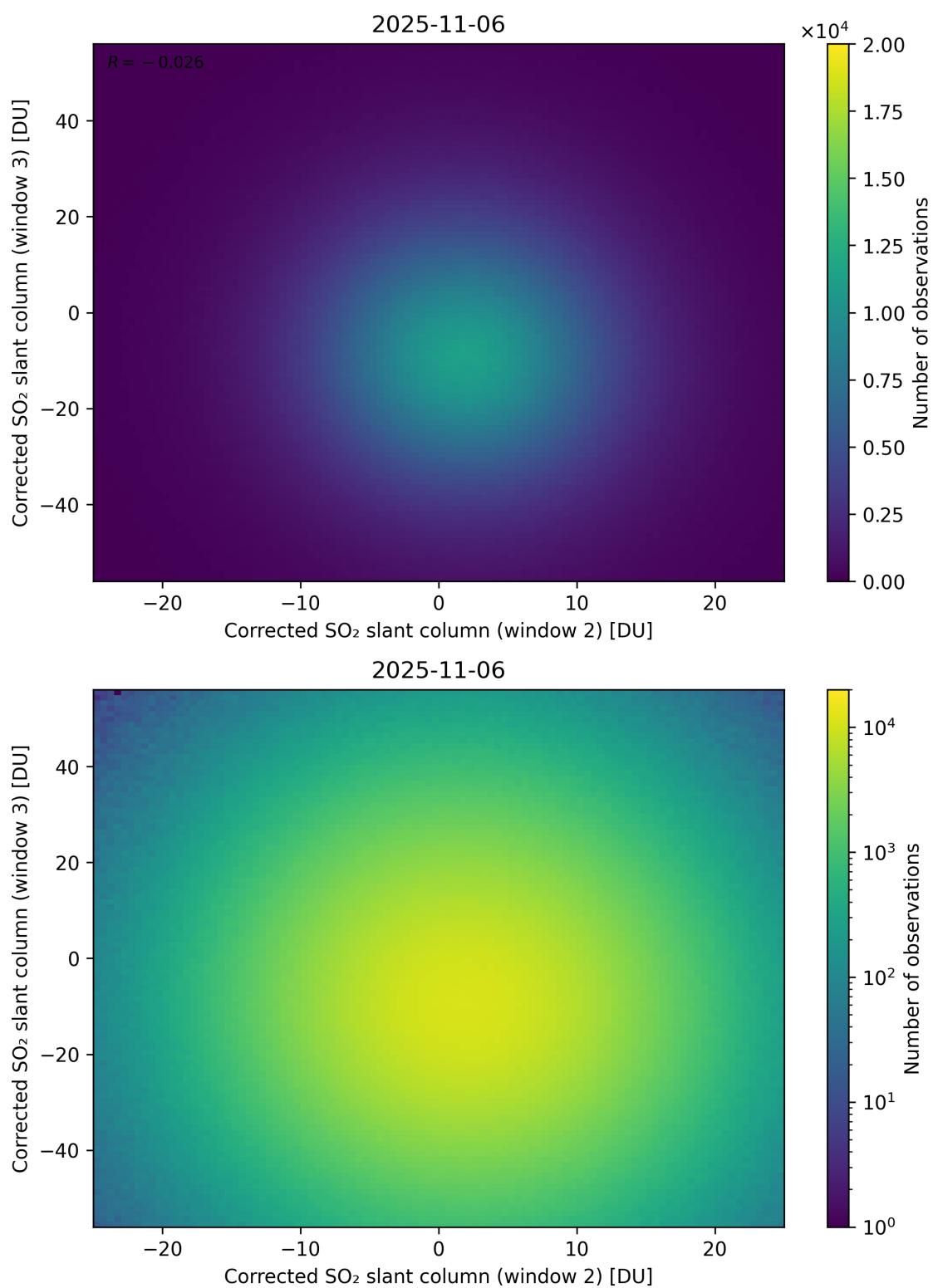
Figure 250: Scatter density plot of “Corrected SO 2 slant column (window 2)” against “Corrected SO 2 slant column (window 3)” for 2025-11-05 to 2025-11-07.
