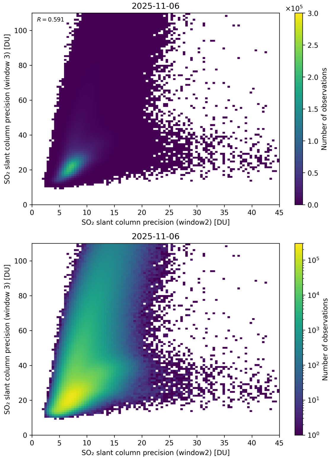
Figure 300: Scatter density plot of “SO 2 slant column precision (window2)” against “SO 2 slant column precision (window 3)” for 2025-11-05 to 2025-11-07.
