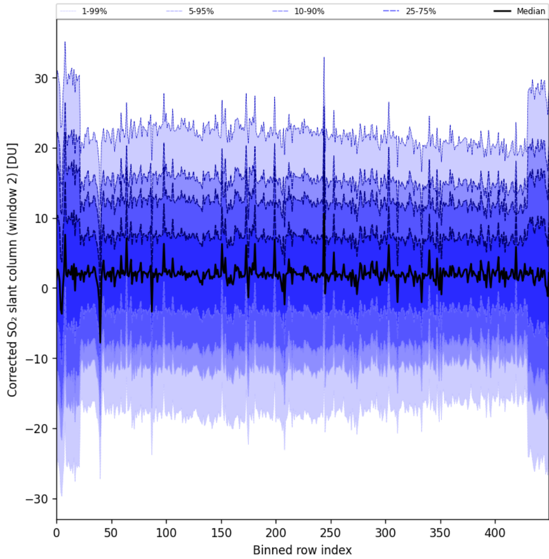
Figure 95: Along track statistics of “Corrected SO 2 slant column (window 2)” for 2025-11-05 to 2025-11-07
