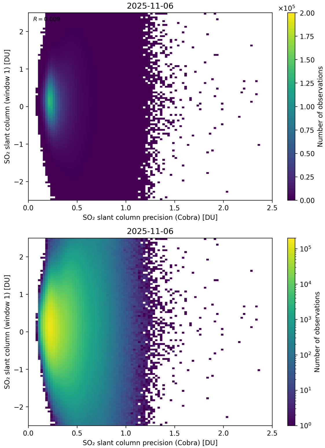
Figure 208: Scatter density plot of “SO 2 slant column precision (Cobra)” against “SO 2 slant column (window 1)” for 2025-11-05 to 2025-11-07.
