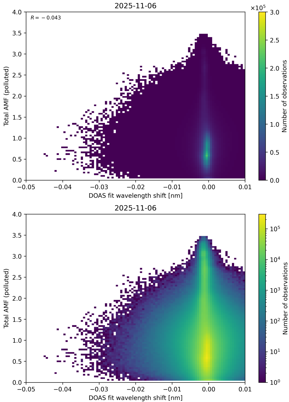
Figure 141: Scatter density plot of “DOAS fit wavelength shift” against “Total AMF (polluted)” for 2025-11-05 to 2025-11-07.
