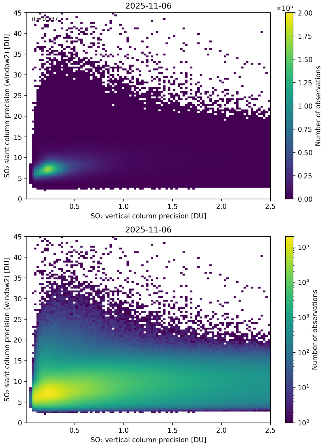
Figure 343: Scatter density plot of “SO 2 vertical column precision” against “SO 2 slant column precision (window2)” for 2025-11-05 to 2025-11-07.
