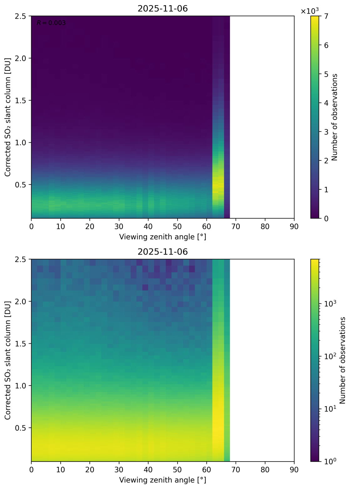
Figure 373: Scatter density plot of “Viewing zenith angle” against “Corrected SO 2 slant column” for 2025-11-05 to 2025-11-07.
