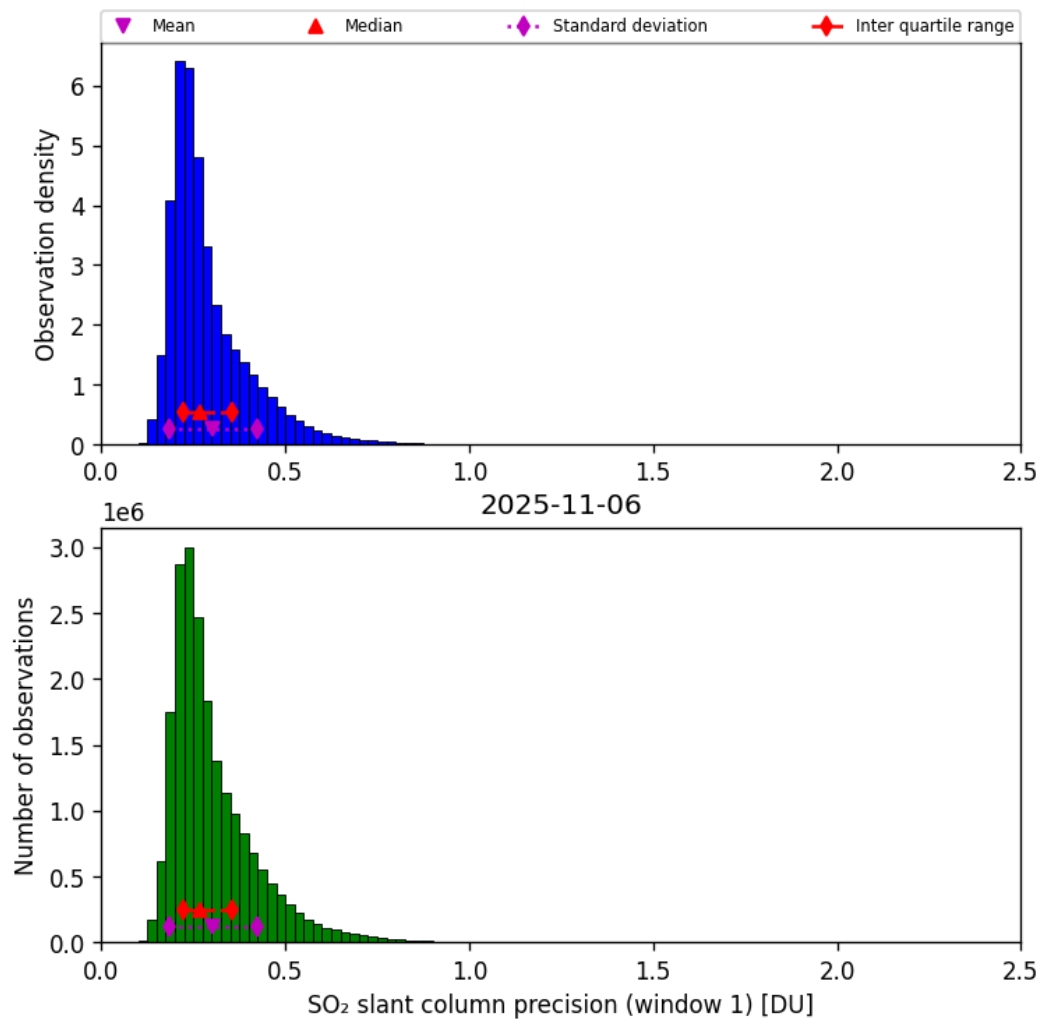
Figure 64: Histogram of “SO 2 slant column precision (window 1)” for 2025-11-05 to 2025-11-07
