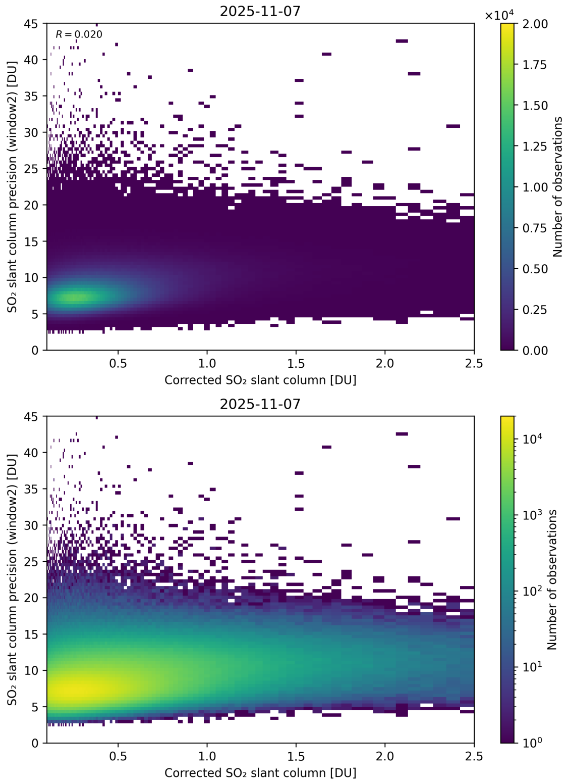
Figure 239: Scatter density plot of “Corrected SO 2 slant column” against “SO 2 slant column precision (window2)” for 2025-11-07 to 2025-11-08.
