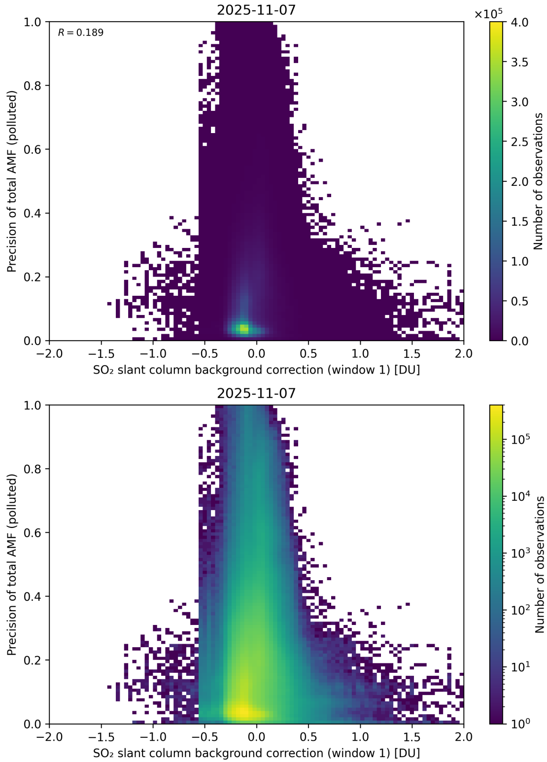
Figure 121: Scatter density plot of “SO 2 slant column background correction (window 1)” against “Precision of total AMF (polluted)” for 2025-11-07 to 2025-11-08.
