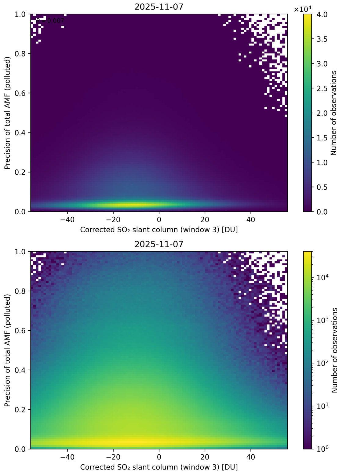
Figure 261: Scatter density plot of “Corrected SO 2 slant column (window 3)” against “Precision of total AMF (polluted)” for 2025-11-07 to 2025-11-08.
