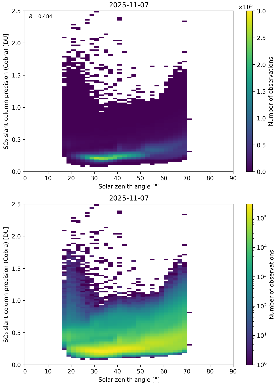
Figure 180: Scatter density plot of “Solar zenith angle” against “SO 2 slant column precision (Cobra)” for 2025-11-07 to 2025-11-08.
