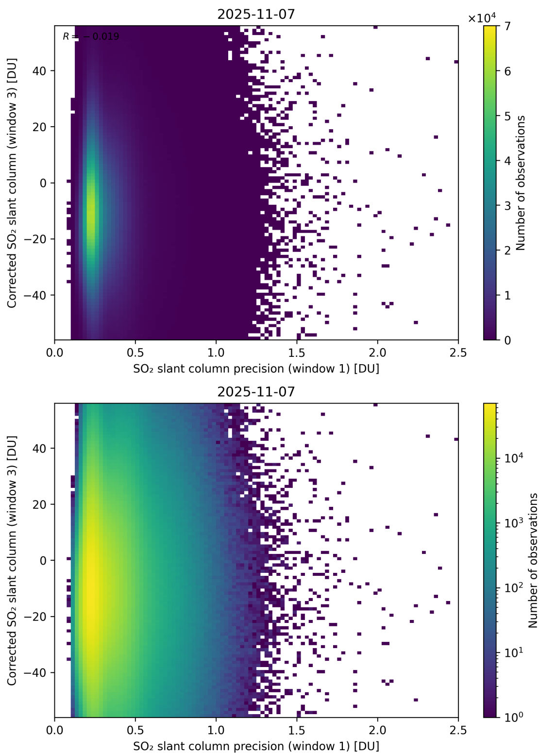
Figure 276: Scatter density plot of “SO 2 slant column precision (window 1)” against “Corrected SO 2 slant column (window 3)” for 2025-11-07 to 2025-11-08.
