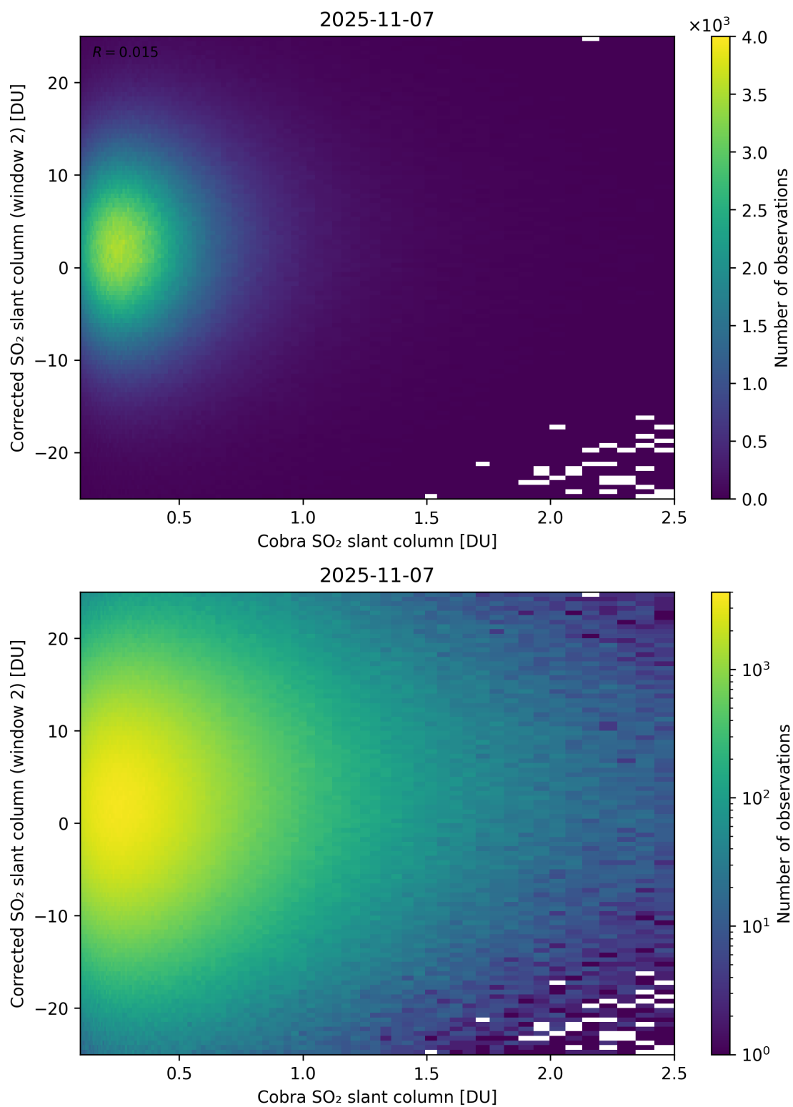
Figure 217: Scatter density plot of “Cobra SO 2 slant column” against “Corrected SO 2 slant column (window 2)” for 2025-11-07 to 2025-11-08.
