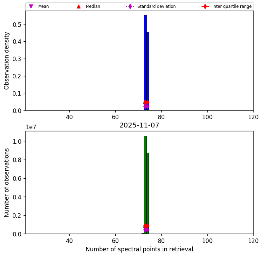
Figure 82: Histogram of “Number of spectral points in retrieval” for 2025-11-07 to 2025-11-08
