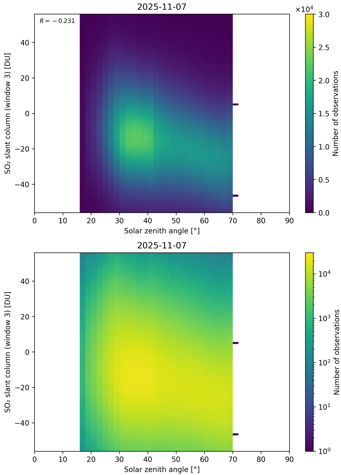
Figure 187: Scatter density plot of “Solar zenith angle” against “SO 2 slant column (window 3)” for 2025-11-07 to 2025-11-08.
