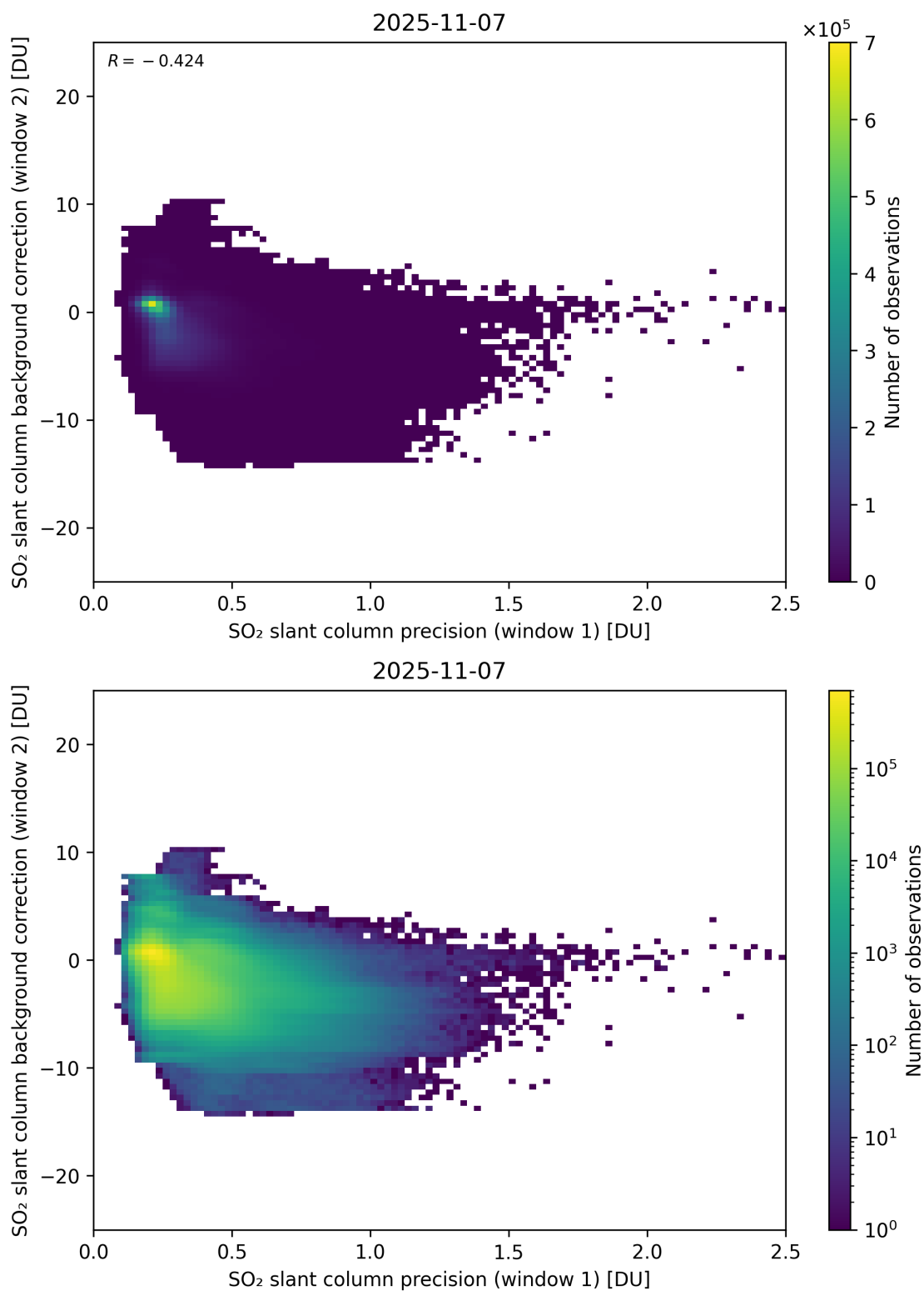
Figure 269: Scatter density plot of “SO 2 slant column precision (window 1)” against “SO 2 slant column background correction (window 2)” for 2025-11-07 to 2025-11-08.
