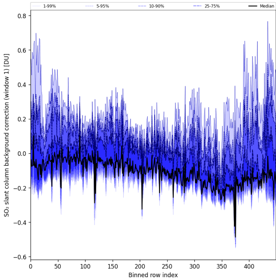
Figure 92: Along track statistics of “SO 2 slant column background correction (window 1)” for 2025-11-07 to 2025-11-08
