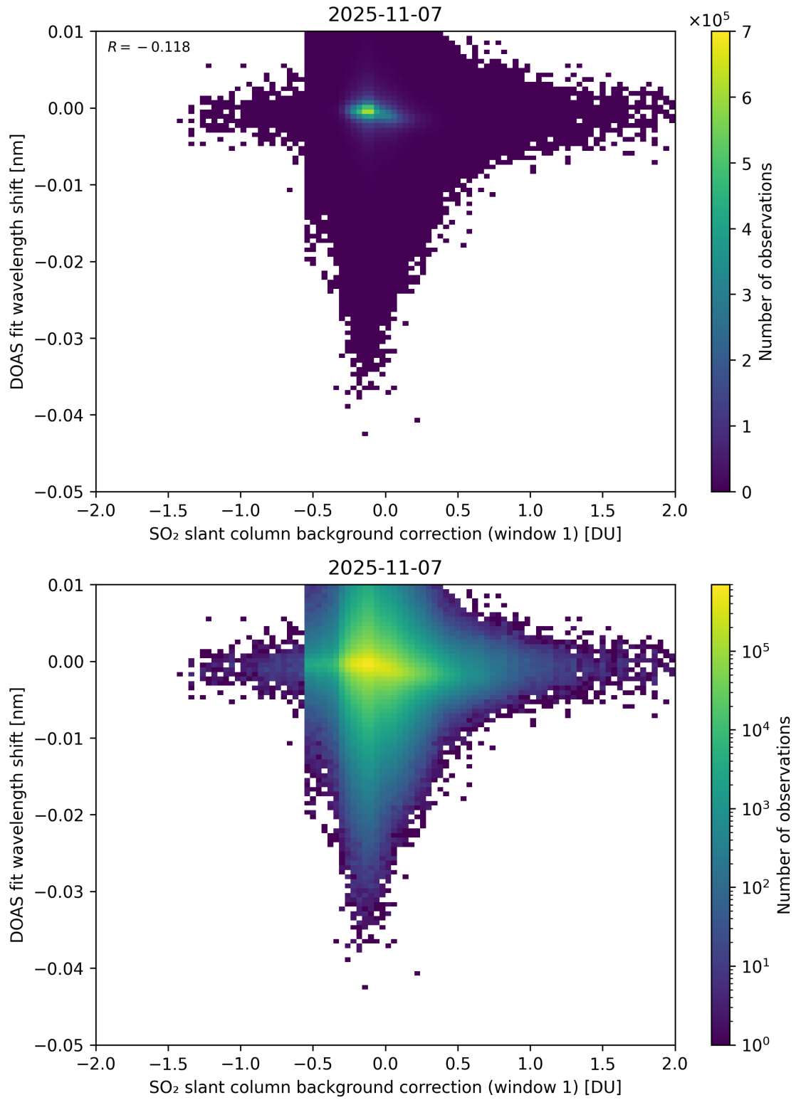
Figure 111: Scatter density plot of “SO 2 slant column background correction (window 1)” against “DOAS fit wavelength shift” for 2025-11-07 to 2025-11-08.
