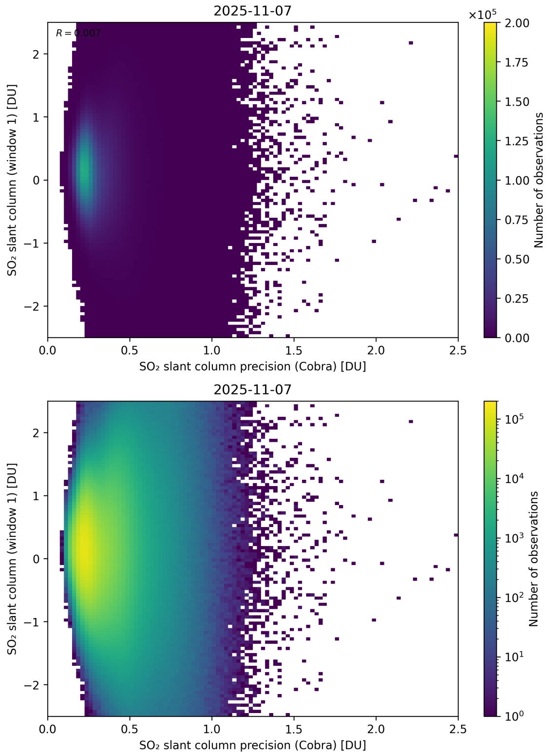
Figure 208: Scatter density plot of “SO 2 slant column precision (Cobra)” against “SO 2 slant column (window 1)” for 2025-11-07 to 2025-11-08.
