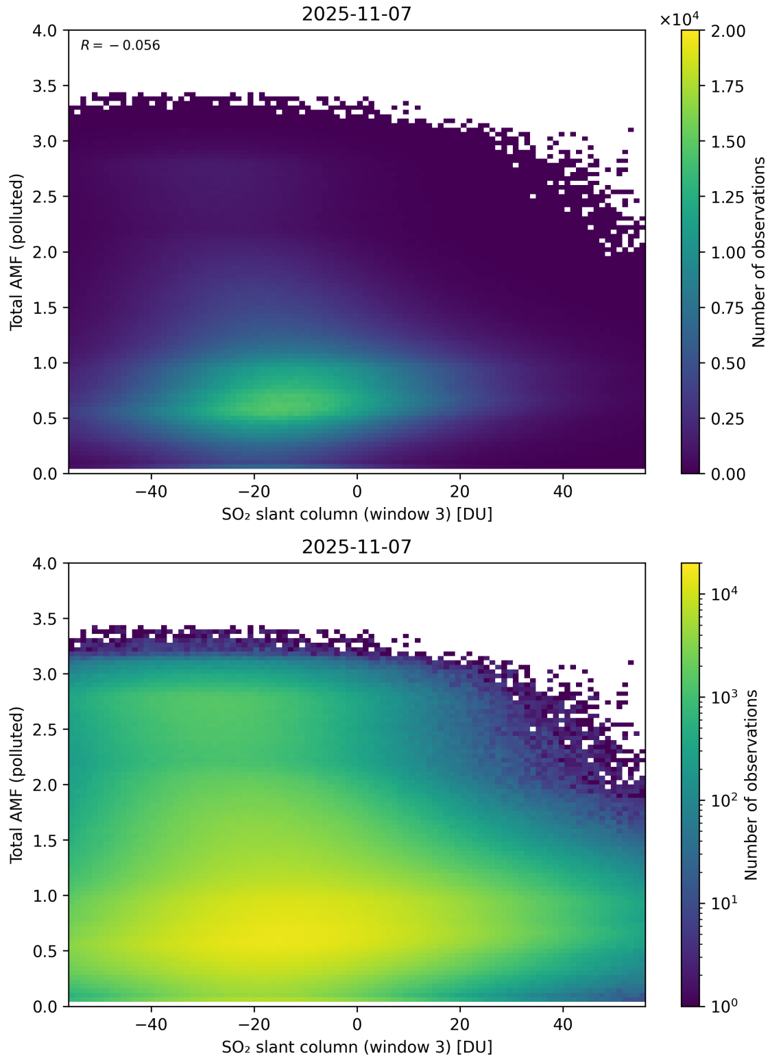
Figure 318: Scatter density plot of “SO 2 slant column (window 3)” against “Total AMF (polluted)” for 2025-11-07 to 2025-11-08.
