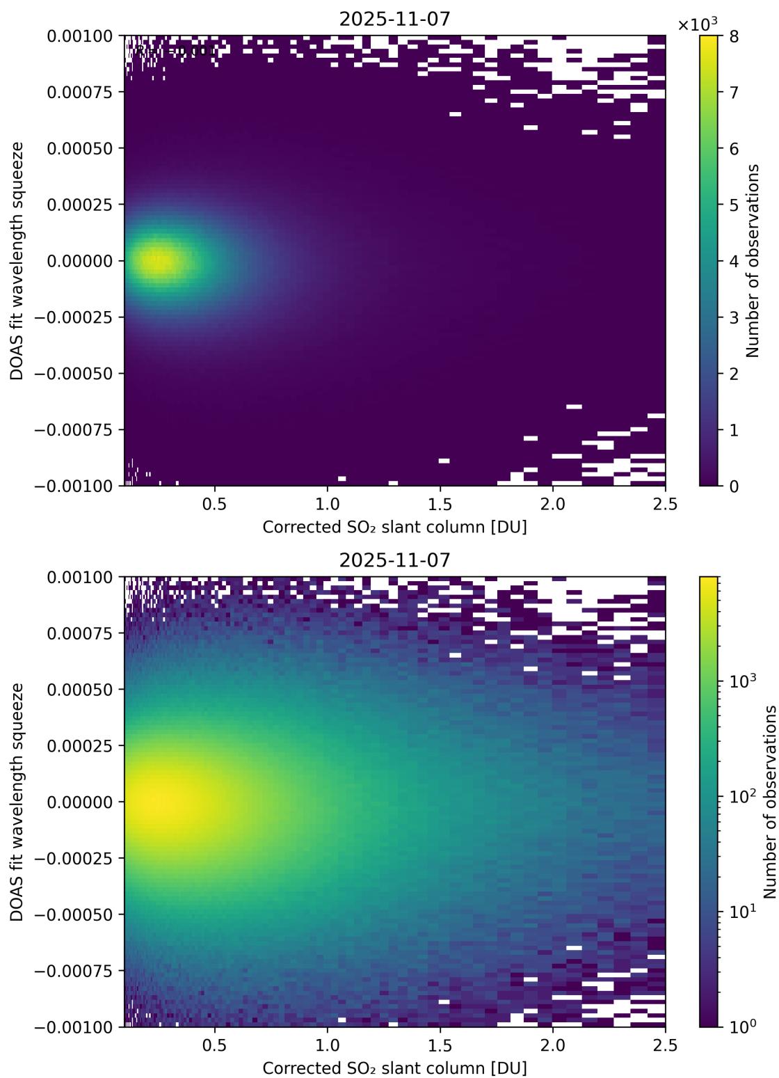
Figure 230: Scatter density plot of “Corrected SO 2 slant column” against “DOAS fit wavelength squeeze” for 2025-11-07 to 2025-11-08.
