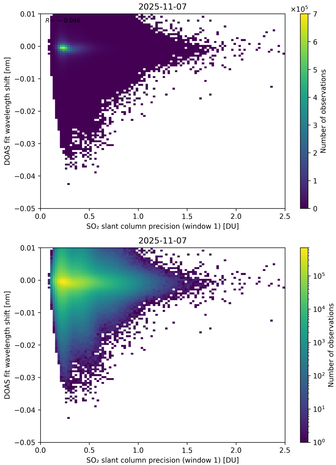
Figure 271: Scatter density plot of “SO 2 slant column precision (window 1)” against “DOAS fit wavelength shift” for 2025-11-07 to 2025-11-08.
