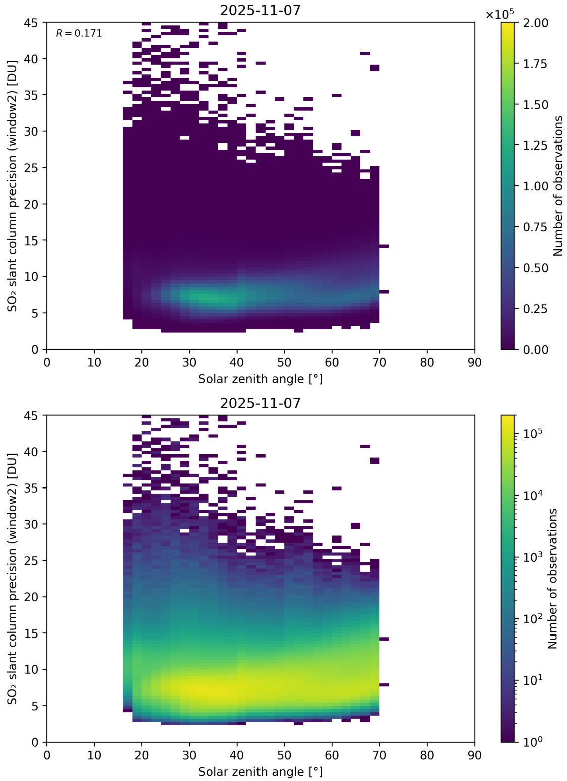
Figure 186: Scatter density plot of “Solar zenith angle” against “SO 2 slant column precision (window2)” for 2025-11-07 to 2025-11-08.
