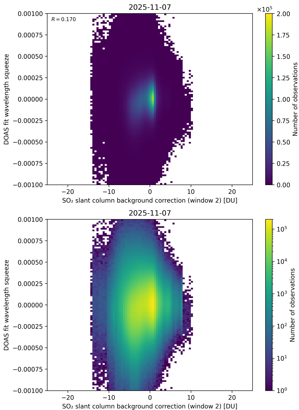
Figure 124: Scatter density plot of “SO 2 slant column background correction (window 2)” against “DOAS fit wavelength squeeze” for 2025-11-07 to 2025-11-08.
