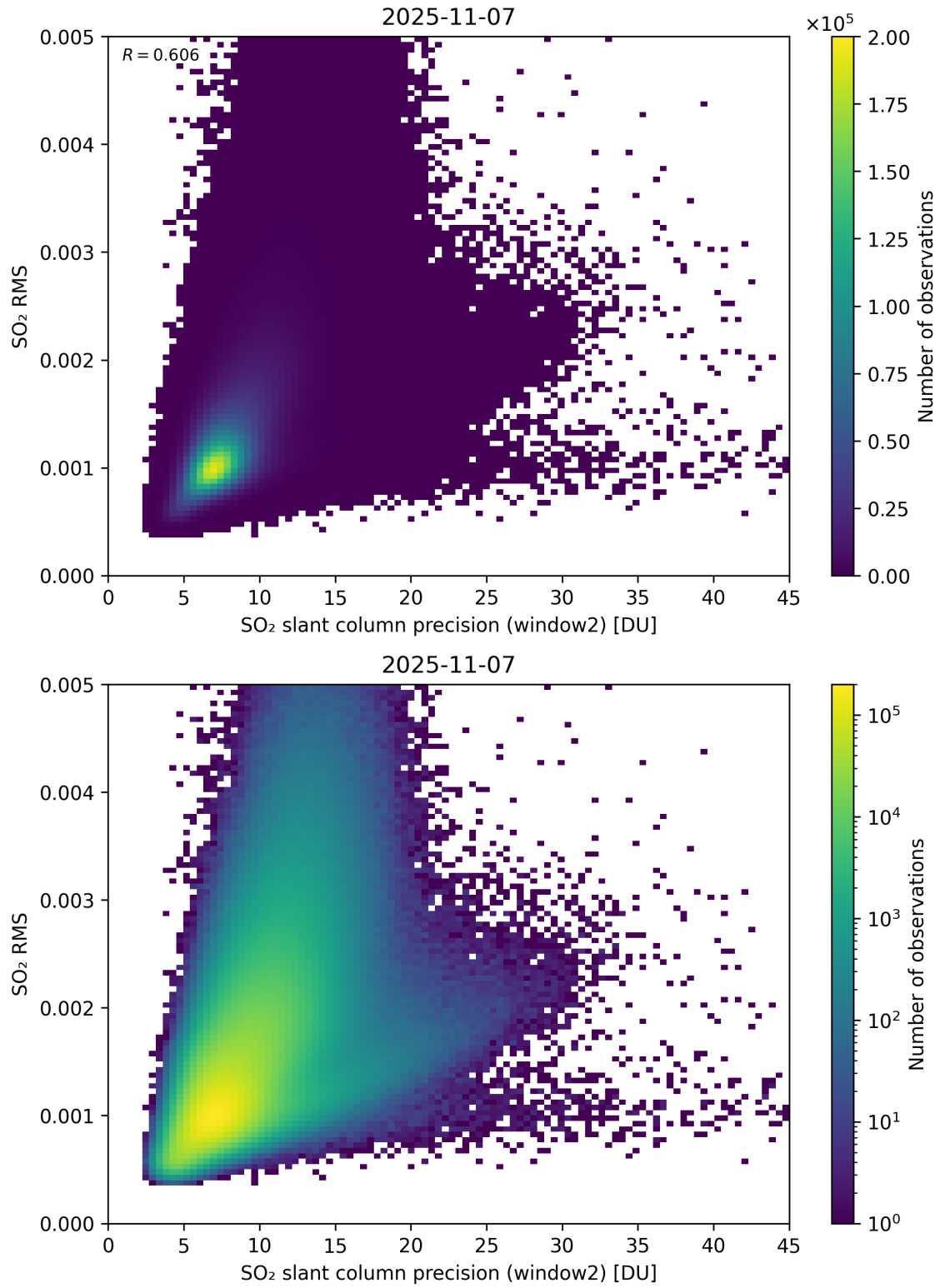
Figure 295: Scatter density plot of “SO 2 slant column precision (window2)” against “SO 2 RMS” for 2025-11-07 to 2025-11-08.
