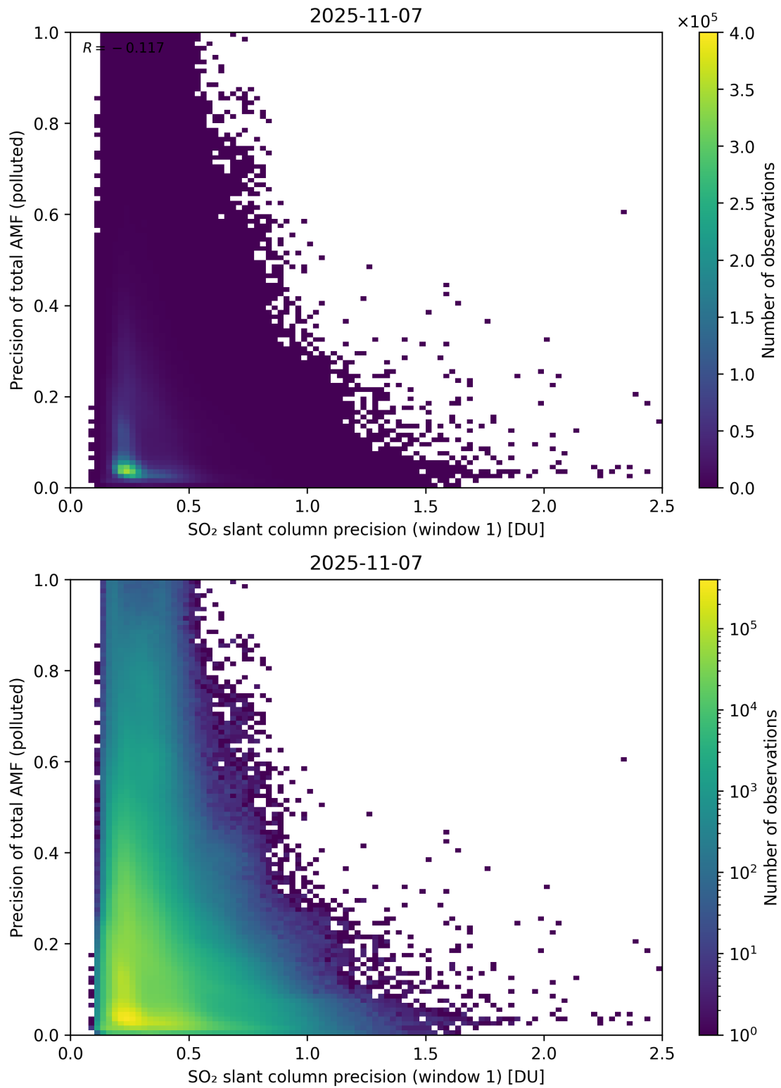
Figure 281: Scatter density plot of “SO 2 slant column precision (window 1)” against “Precision of total AMF (polluted)” for 2025-11-07 to 2025-11-08.
