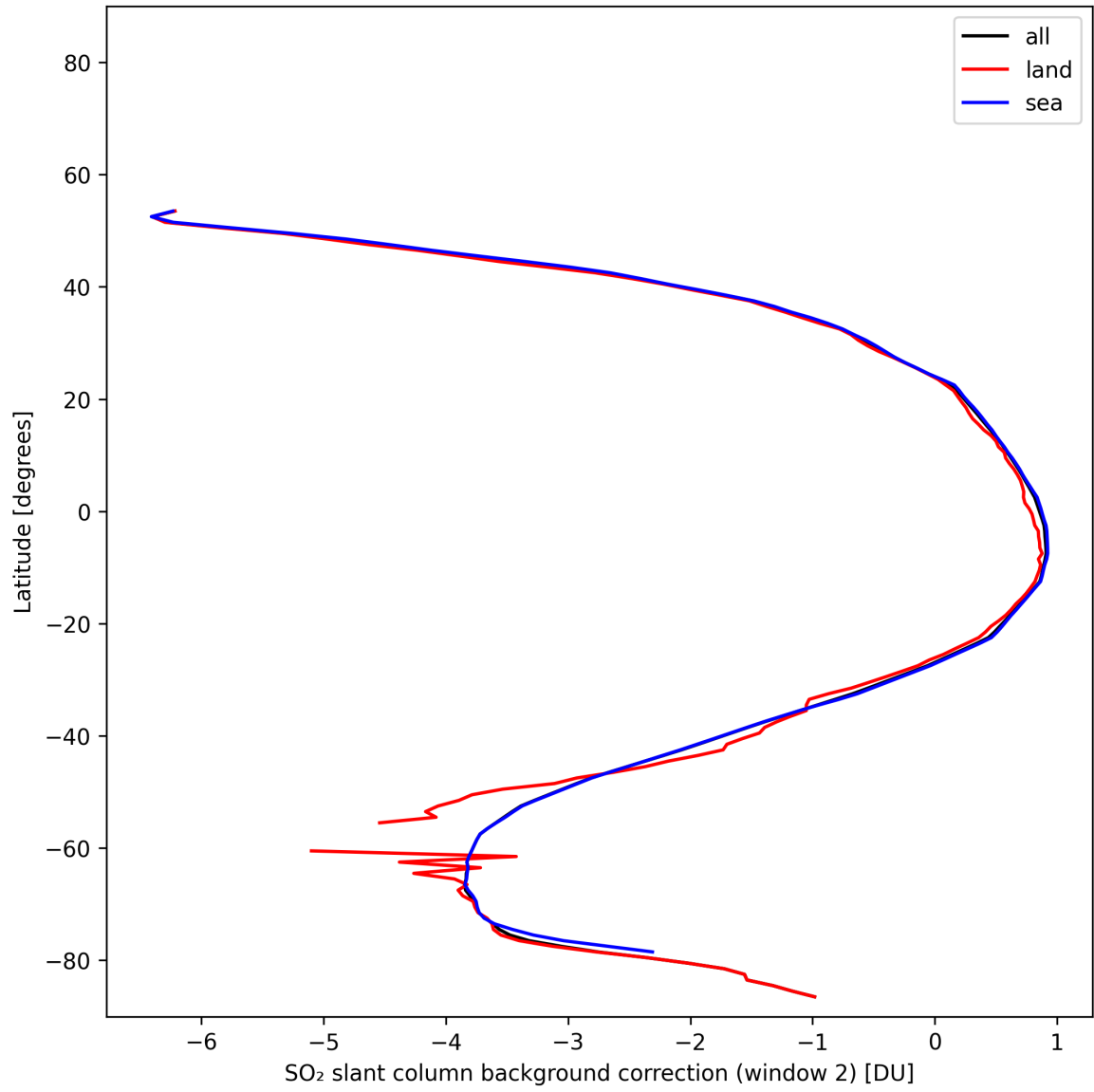
Figure 44: Zonal average of “SO 2 slant column background correction (window 2)” for 2025-11-07 to 2025-11-08.
