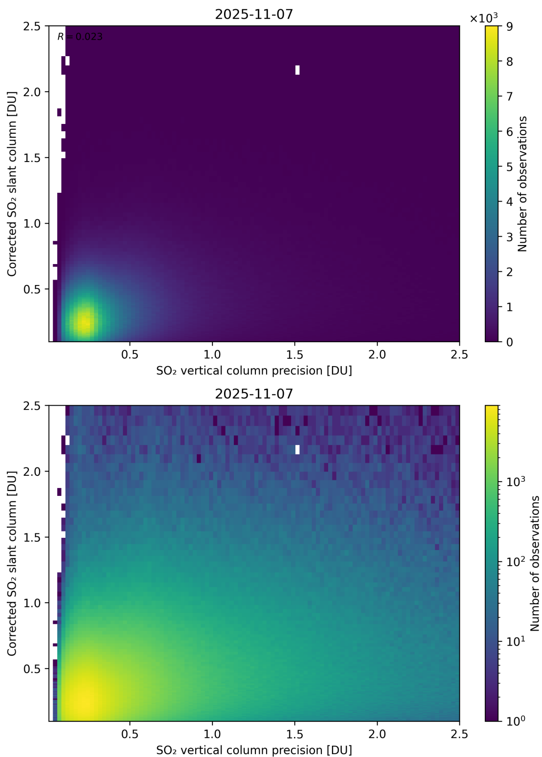
Figure 338: Scatter density plot of “SO 2 vertical column precision” against “Corrected SO 2 slant column” for 2025-11-07 to 2025-11-08.
