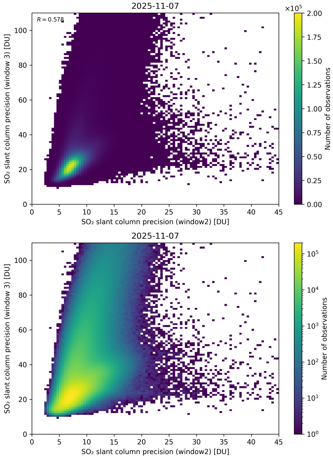
Figure 300: Scatter density plot of “SO 2 slant column precision (window2)” against “SO 2 slant column precision (window 3)” for 2025-11-07 to 2025-11-08.
