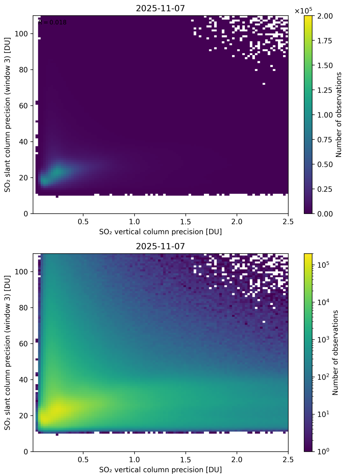
Figure 345: Scatter density plot of “SO 2 vertical column precision” against “SO 2 slant column precision (window 3)” for 2025-11-07 to 2025-11-08.
