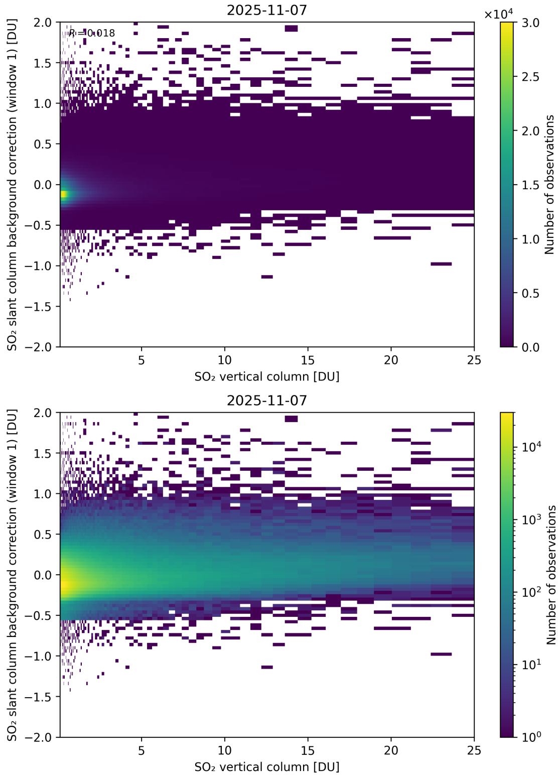
Figure 323: Scatter density plot of “SO 2 vertical column” against “SO 2 slant column background correction (window 1)” for 2025-11-07 to 2025-11-08.
