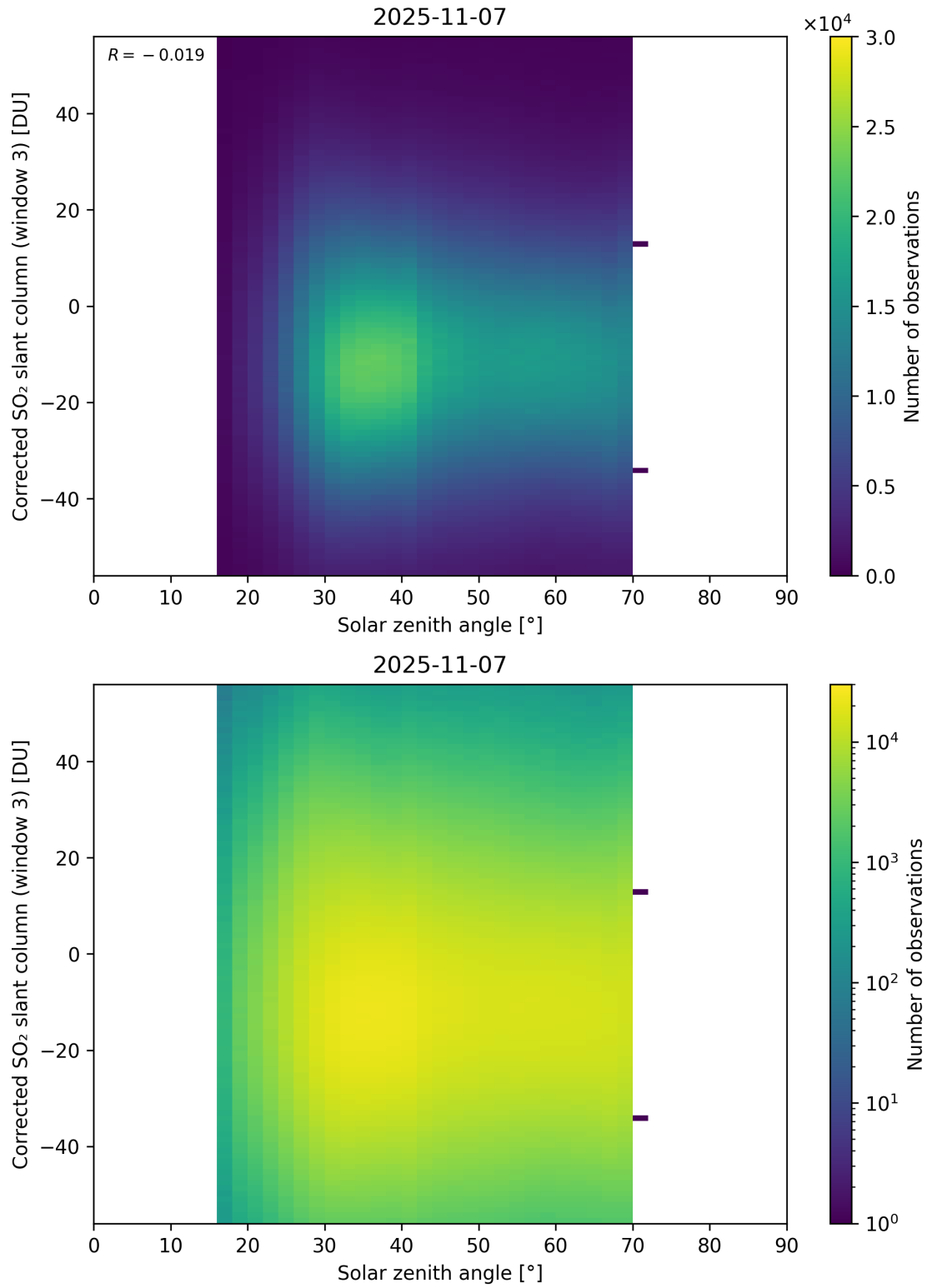
Figure 183: Scatter density plot of “Solar zenith angle” against “Corrected SO 2 slant column (window 3)” for 2025-11-07 to 2025-11-08.
