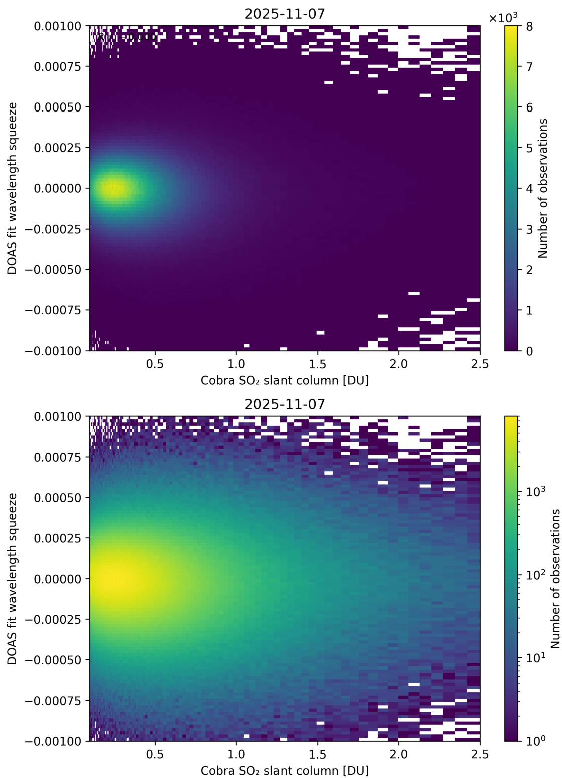
Figure 197: Scatter density plot of “Cobra SO 2 slant column” against “DOAS fit wavelength squeeze” for 2025-11-07 to 2025-11-08.
