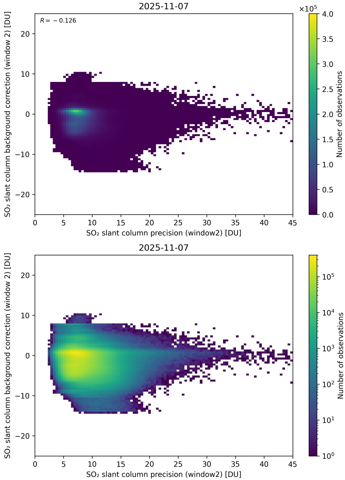
Figure 291: Scatter density plot of “SO 2 slant column precision (window2)” against “SO 2 slant column background correction (window 2)” for 2025-11-07 to 2025-11-08.
