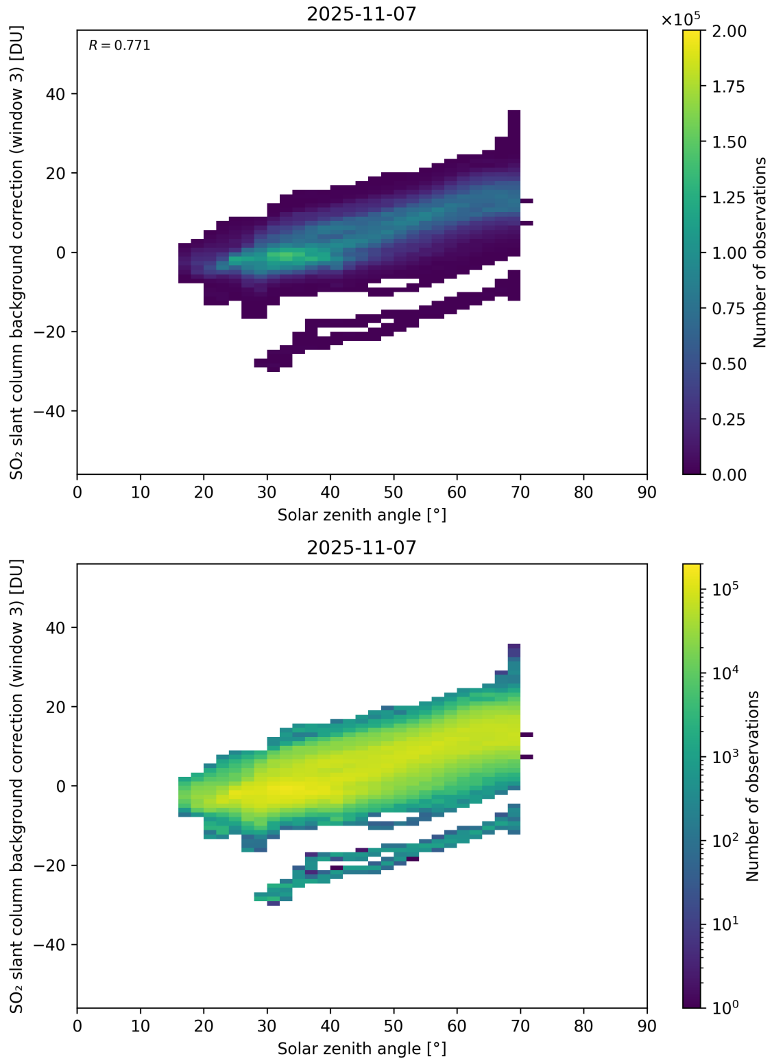
Figure 173: Scatter density plot of “Solar zenith angle” against “SO 2 slant column background correction (window 3)” for 2025-11-07 to 2025-11-08.
