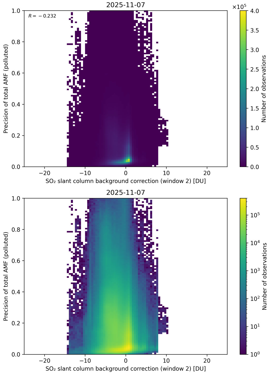
Figure 131: Scatter density plot of “SO 2 slant column background correction (window 2)” against “Precision of total AMF (polluted)” for 2025-11-07 to 2025-11-08.
