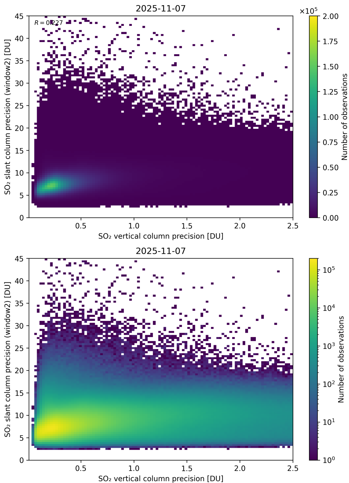
Figure 343: Scatter density plot of “SO 2 vertical column precision” against “SO 2 slant column precision (window2)” for 2025-11-07 to 2025-11-08.
