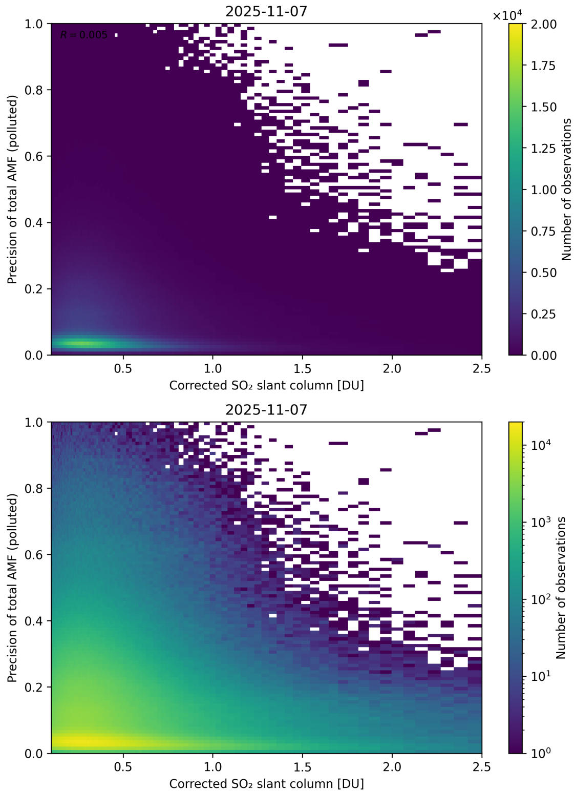
Figure 243: Scatter density plot of “Corrected SO 2 slant column” against “Precision of total AMF (polluted)” for 2025-11-07 to 2025-11-08.
