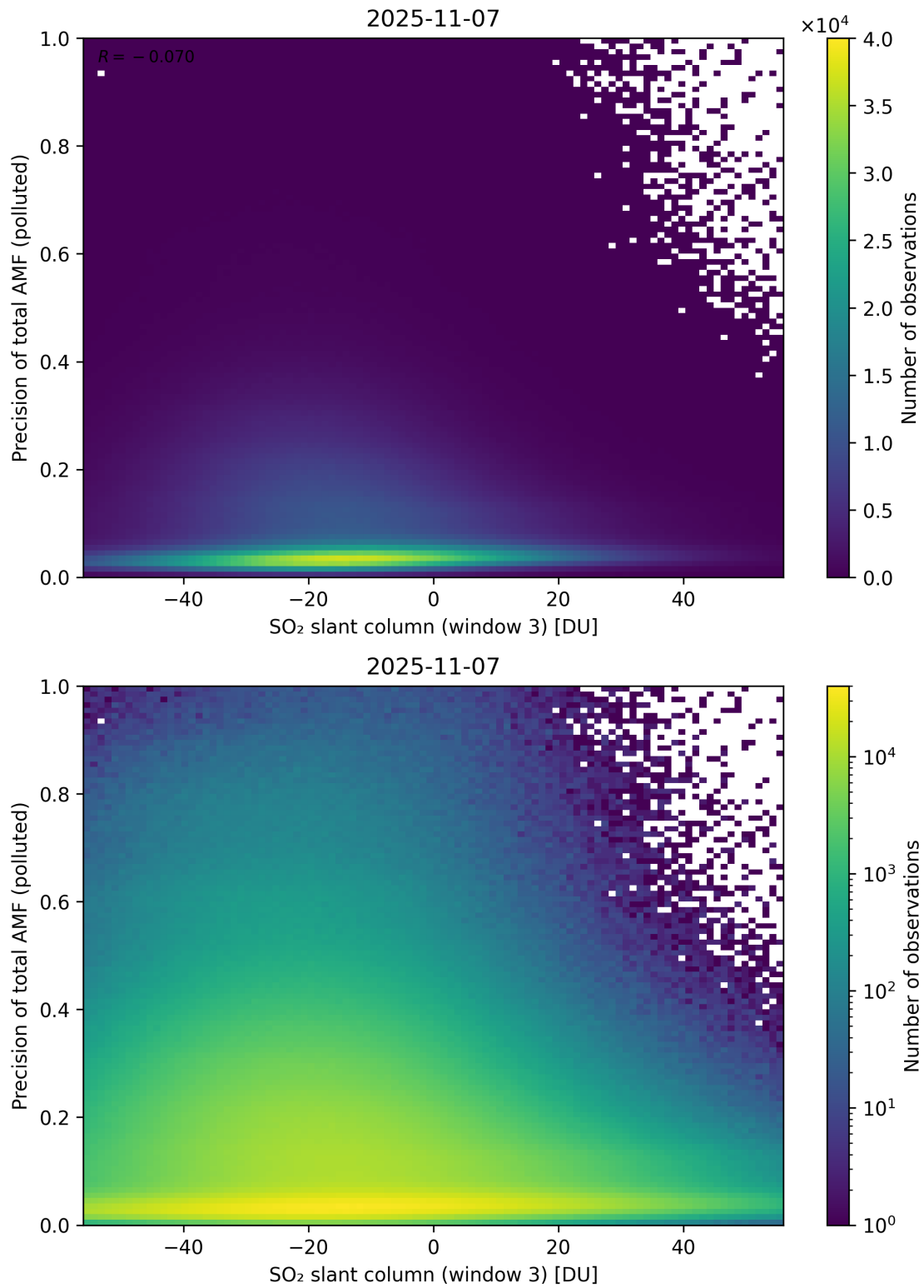
Figure 319: Scatter density plot of “SO 2 slant column (window 3)” against “Precision of total AMF (polluted)” for 2025-11-07 to 2025-11-08.
