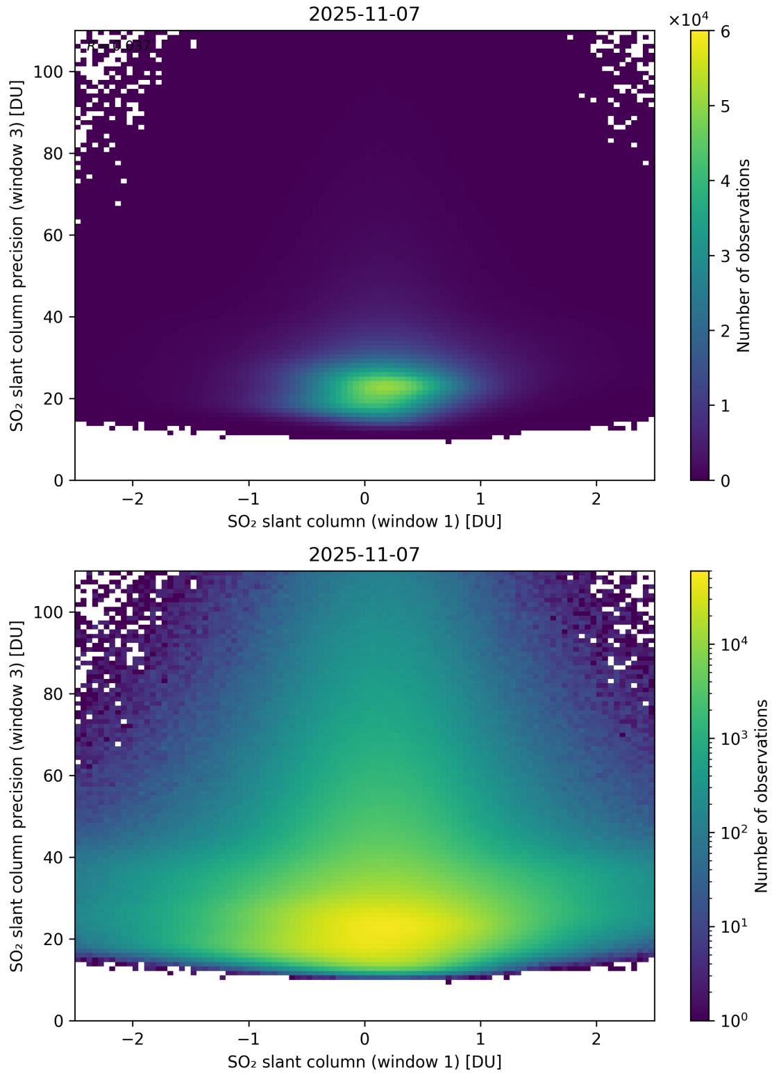
Figure 288: Scatter density plot of “SO 2 slant column (window 1)” against “SO 2 slant column precision (window 3)” for 2025-11-07 to 2025-11-08.
