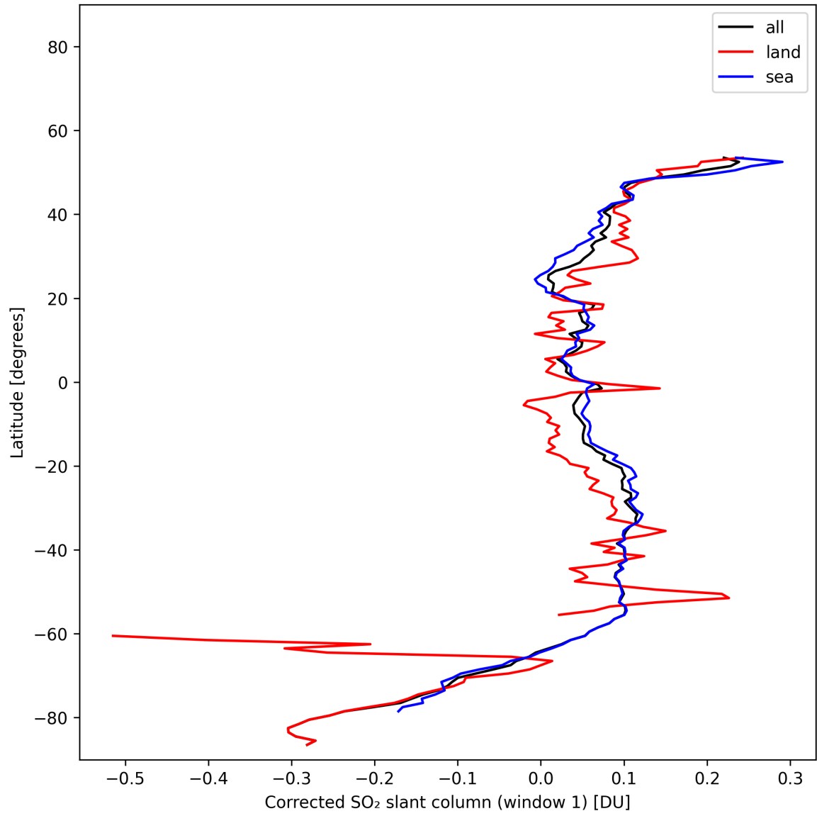
Figure 39: Zonal average of “Corrected SO 2 slant column (window 1)” for 2025-11-07 to 2025-11-08.
