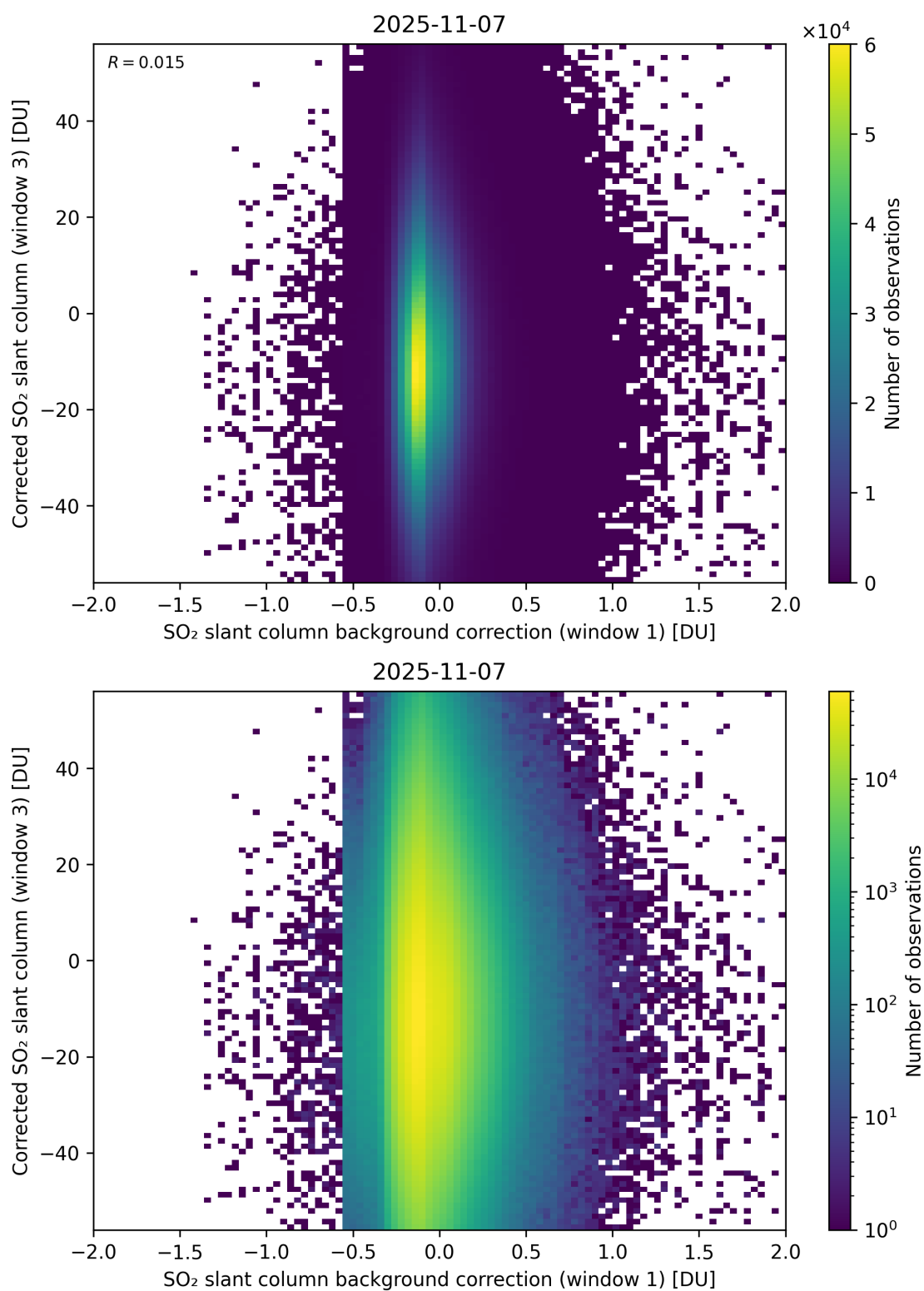
Figure 116: Scatter density plot of “SO 2 slant column background correction (window 1)” against “Corrected SO 2 slant column (window 3)” for 2025-11-07 to 2025-11-08.
