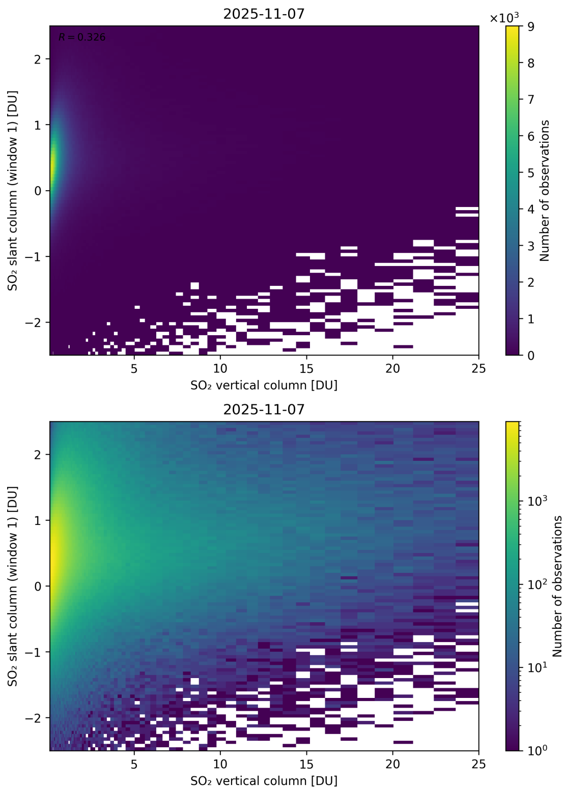
Figure 354: Scatter density plot of “SO 2 vertical column” against “SO 2 slant column (window 1)” for 2025-11-07 to 2025-11-08.
