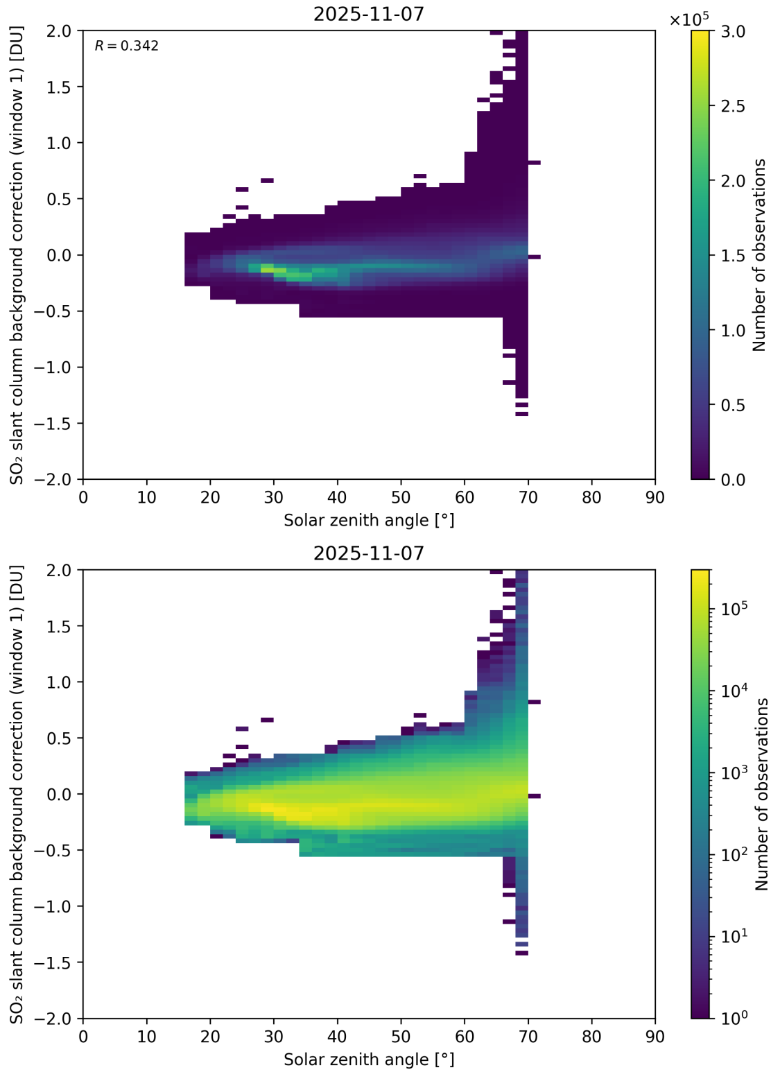
Figure 171: Scatter density plot of “Solar zenith angle” against “SO 2 slant column background correction (window 1)” for 2025-11-07 to 2025-11-08.
