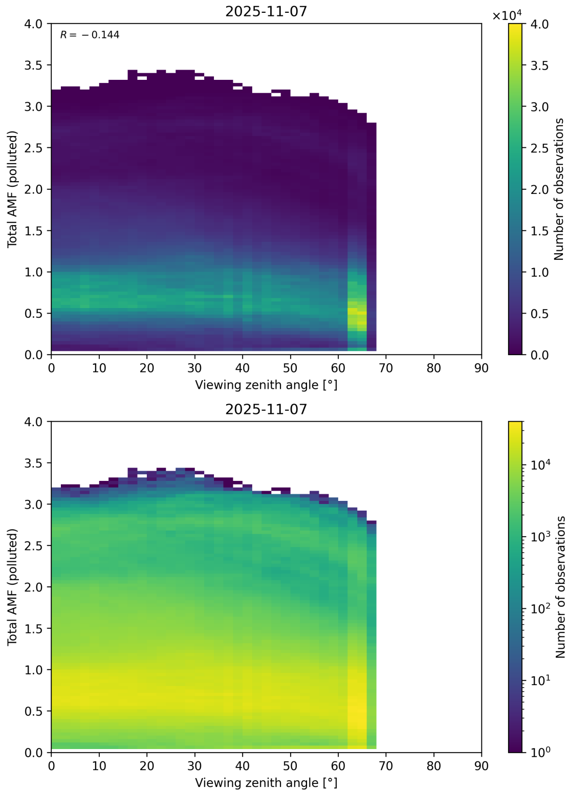
Figure 381: Scatter density plot of “Viewing zenith angle” against “Total AMF (polluted)” for 2025-11-07 to 2025-11-08.
