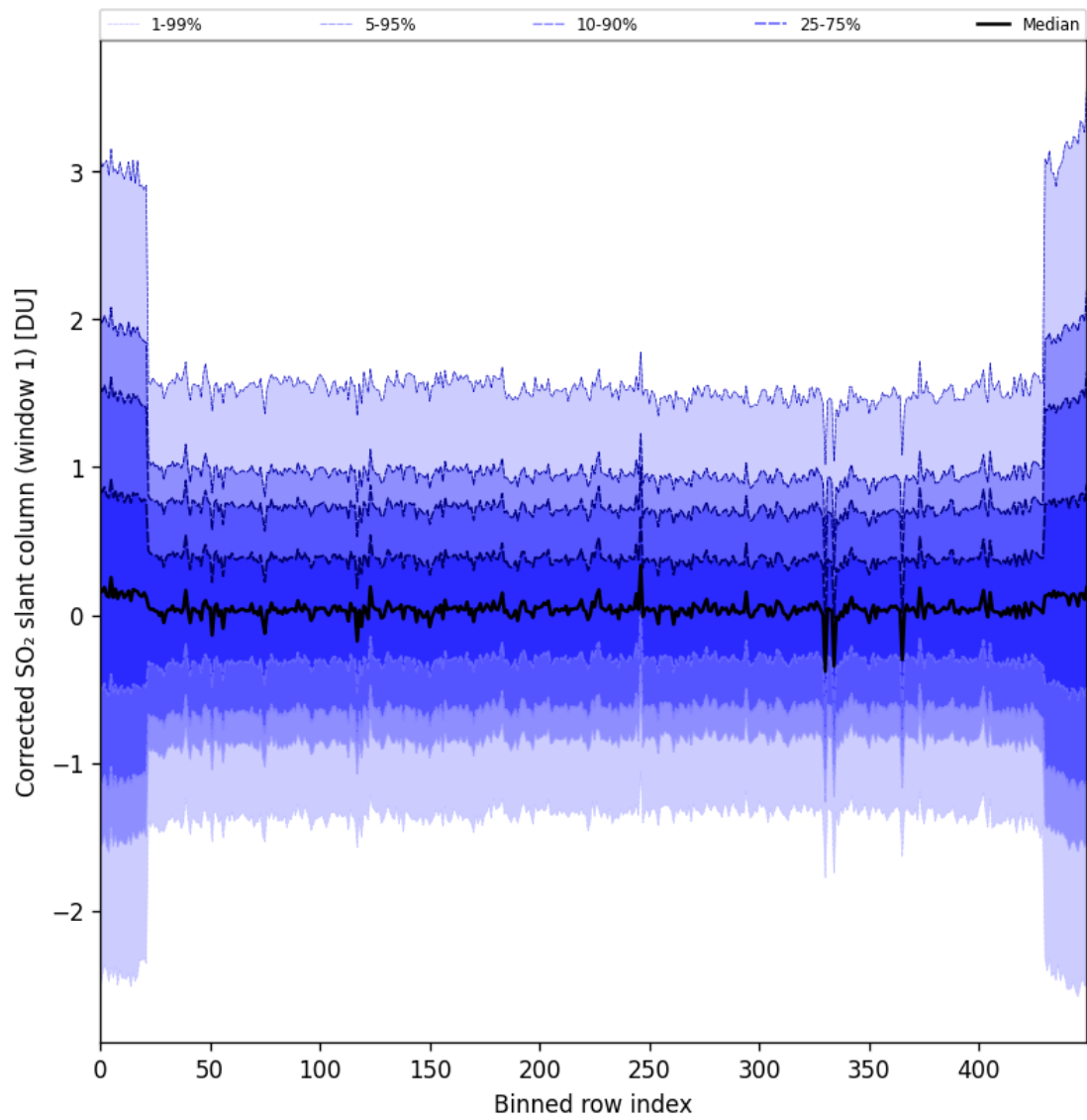
Figure 91: Along track statistics of “Corrected SO 2 slant column (window 1)” for 2025-11-07 to 2025-11-08
