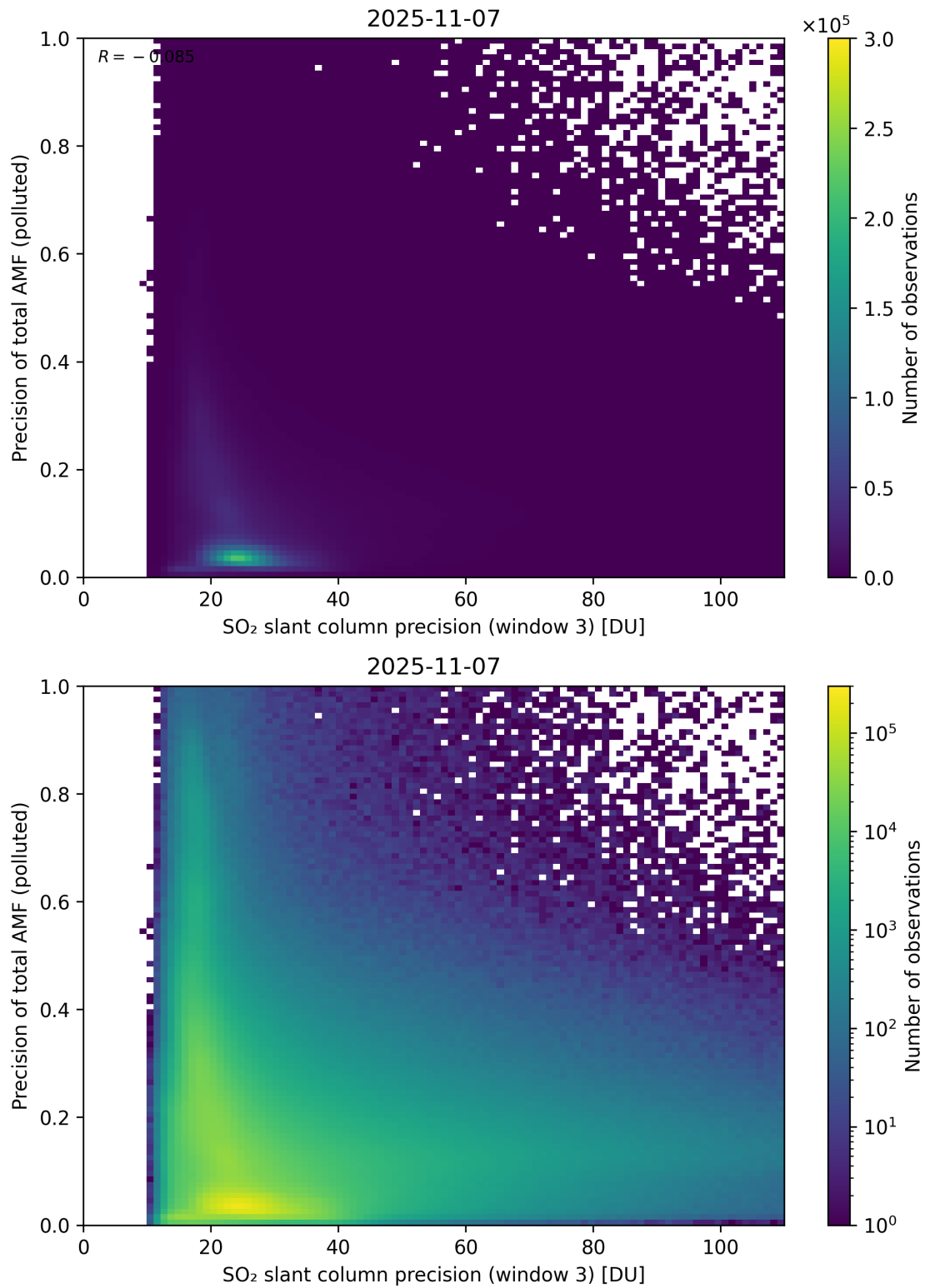
Figure 314: Scatter density plot of “SO 2 slant column precision (window 3)” against “Precision of total AMF (polluted)” for 2025-11-07 to 2025-11-08.
