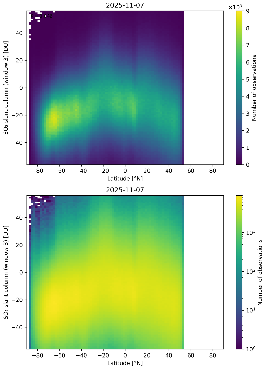
Figure 165: Scatter density plot of “Latitude” against “SO 2 slant column (window 3)” for 2025-11-07 to 2025-11-08.
