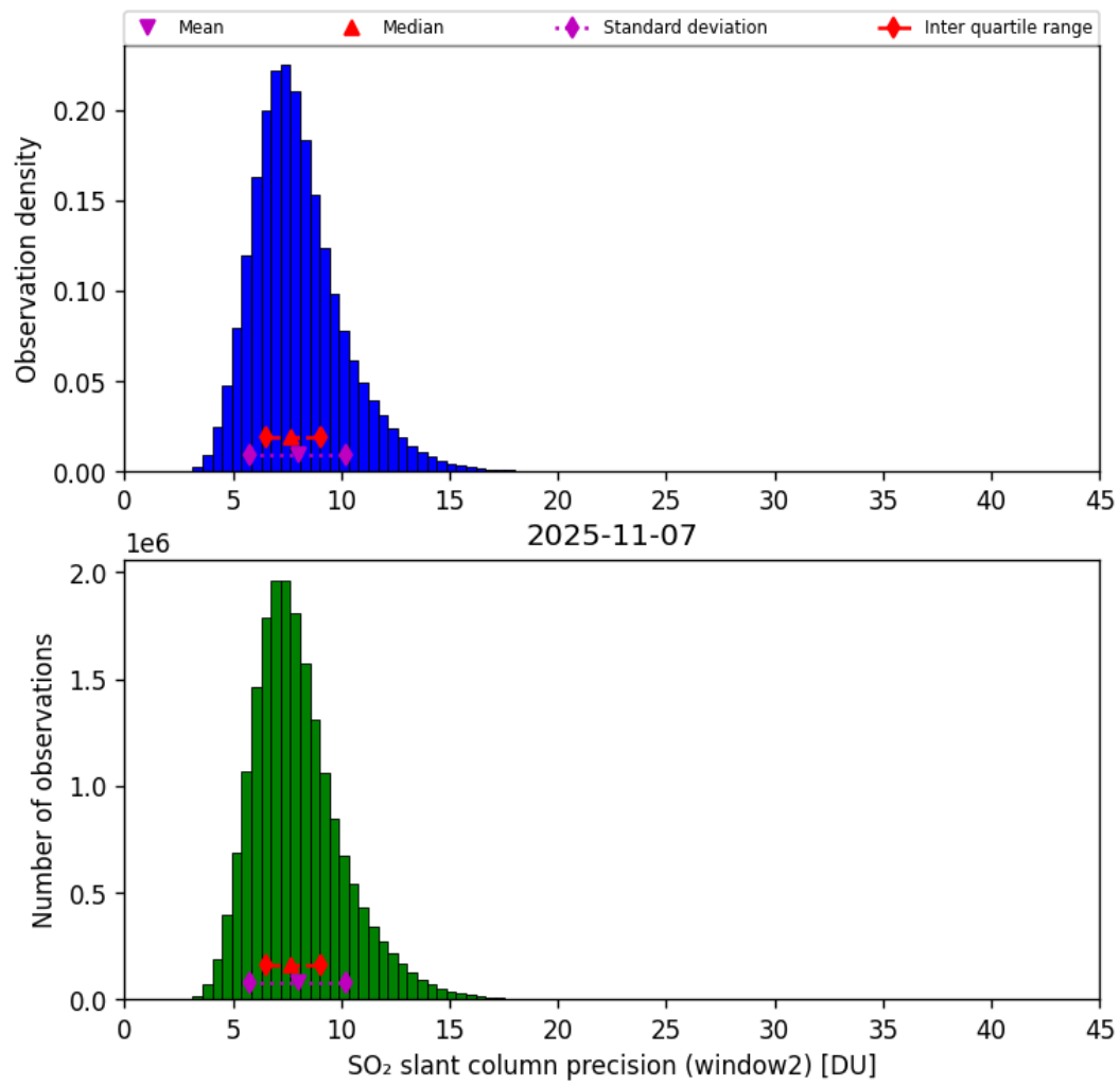
Figure 68: Histogram of “SO 2 slant column precision (window2)” for 2025-11-07 to 2025-11-08
