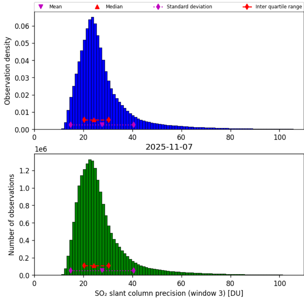
Figure 72: Histogram of “SO 2 slant column precision (window 3)” for 2025-11-07 to 2025-11-08
