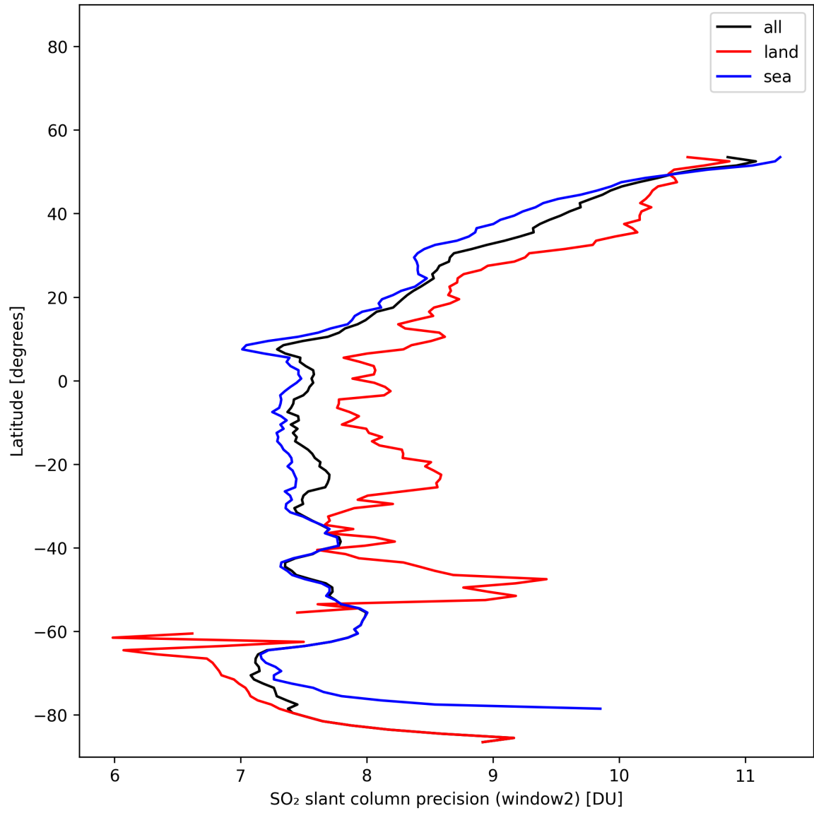
Figure 42: Zonal average of “SO 2 slant column precision (window2)” for 2025-11-07 to 2025-11-08.
