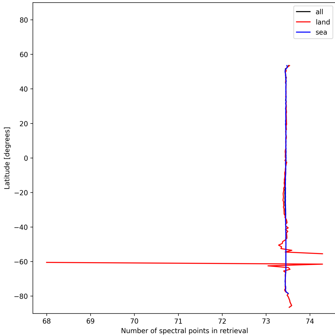
Figure 56: Zonal average of “Number of spectral points in retrieval” for 2025-11-07 to 2025-11-08.
