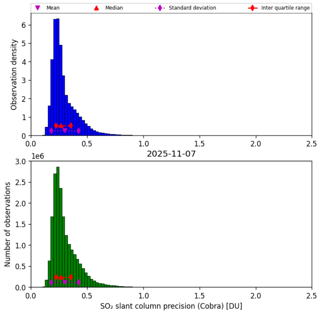
Figure 62: Histogram of “SO 2 slant column precision (Cobra)” for 2025-11-07 to 2025-11-08
