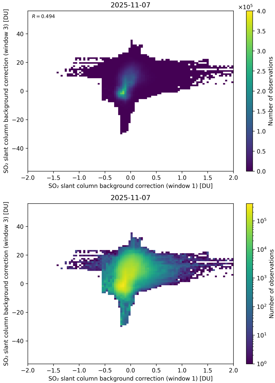
Figure 110: Scatter density plot of “SO 2 slant column background correction (window 1)” against “SO 2 slant column background correction (window 3)” for 2025-11-07 to 2025-11-08.
