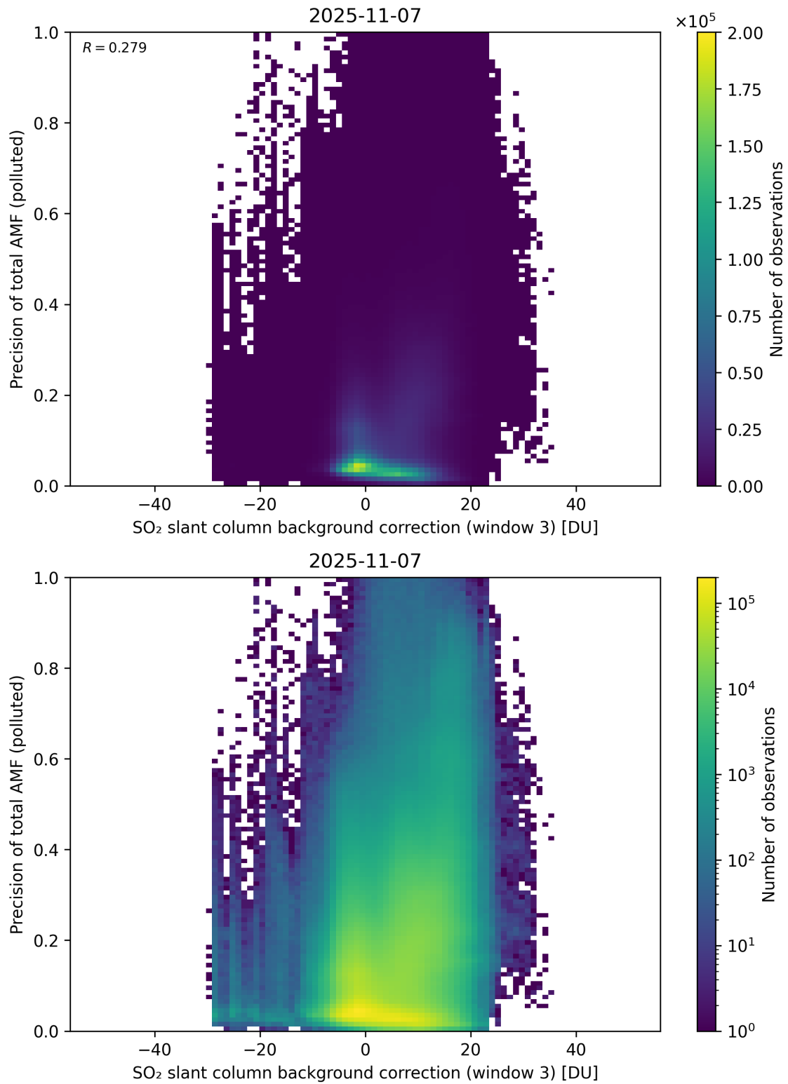
Figure 137: Scatter density plot of “SO 2 slant column background correction (window 3)” against “Precision of total AMF (polluted)” for 2025-11-07 to 2025-11-08.
