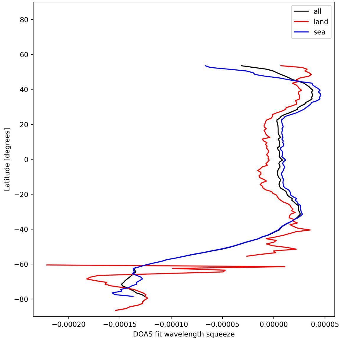
Figure 51: Zonal average of “DOAS fit wavelength squeeze” for 2025-11-07 to 2025-11-08.
