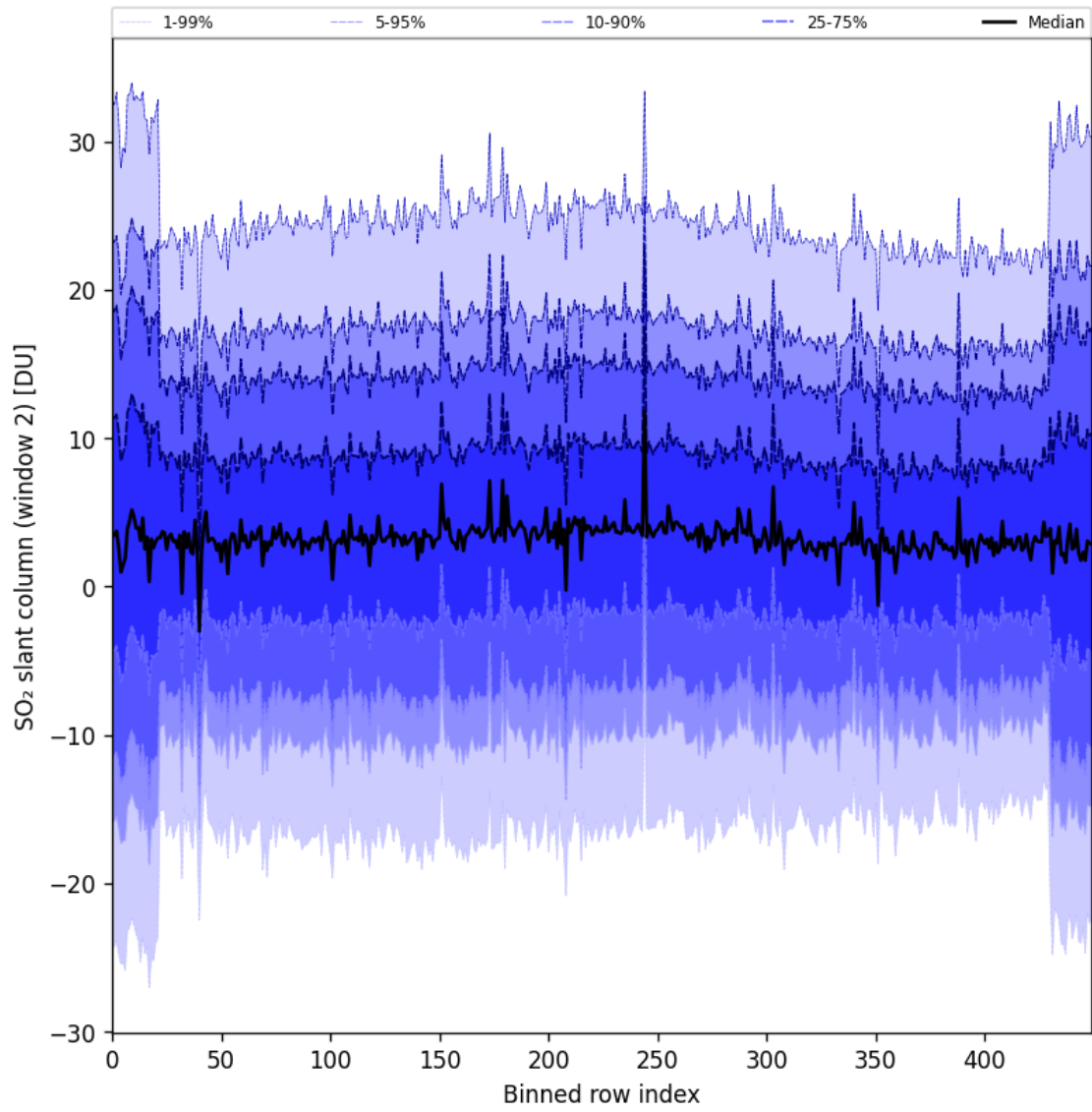
Figure 93: Along track statistics of “SO 2 slant column (window 2)” for 2025-11-07 to 2025-11-08
