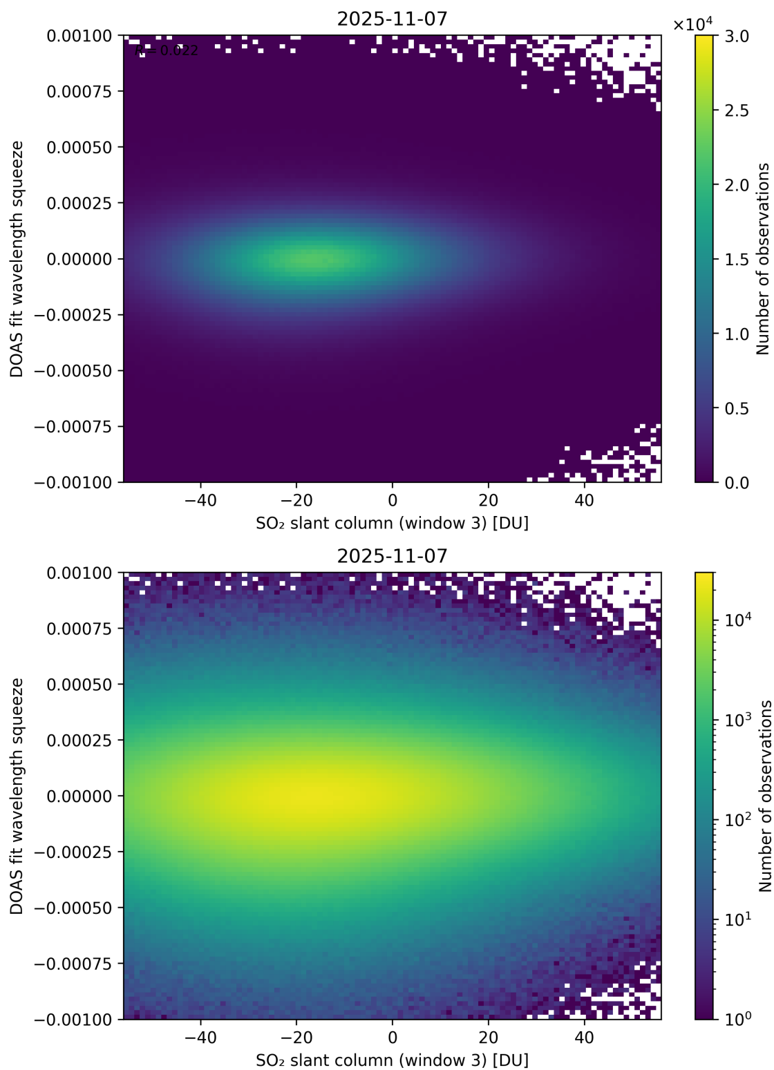
Figure 305: Scatter density plot of “SO 2 slant column (window 3)” against “DOAS fit wavelength squeeze” for 2025-11-07 to 2025-11-08.
