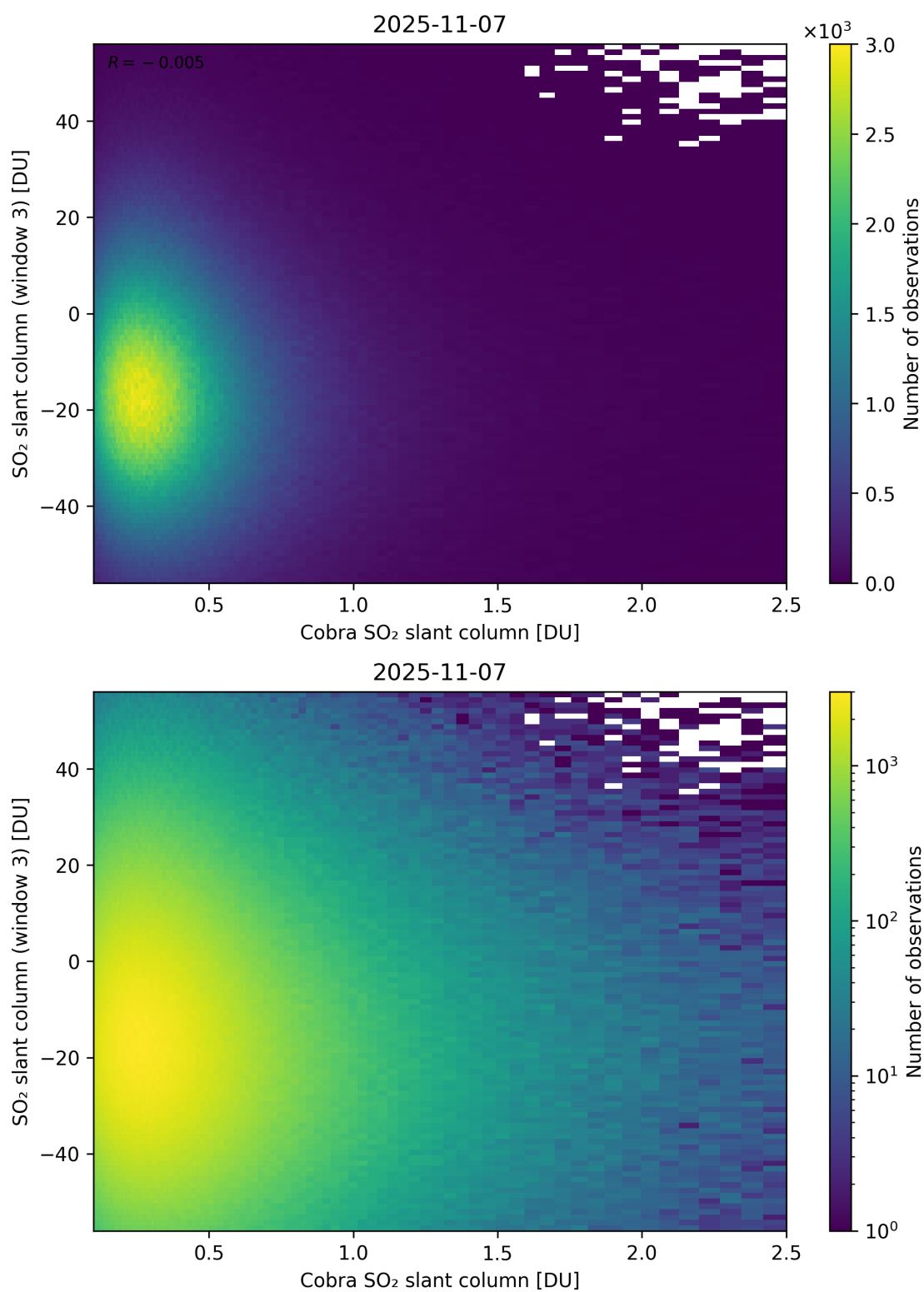
Figure 222: Scatter density plot of “Cobra SO 2 slant column” against “SO 2 slant column (window 3)” for 2025-11-07 to 2025-11-08.
