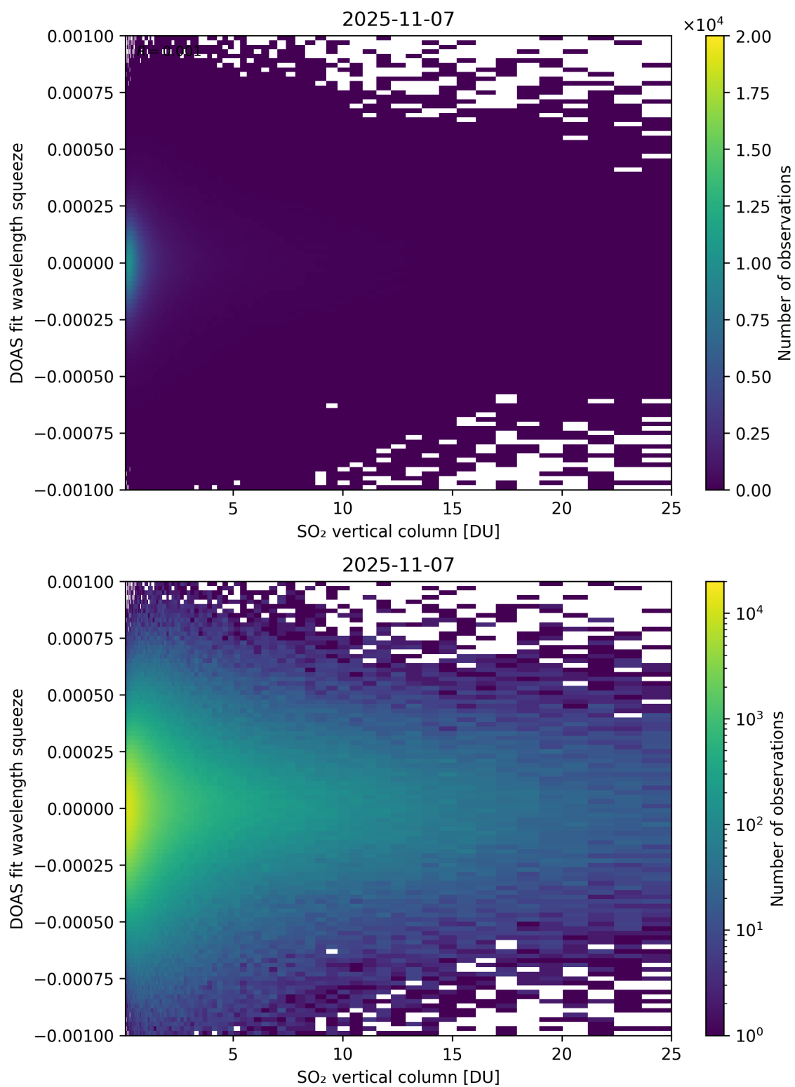
Figure 327: Scatter density plot of “SO 2 vertical column” against “DOAS fit wavelength squeeze” for 2025-11-07 to 2025-11-08.
