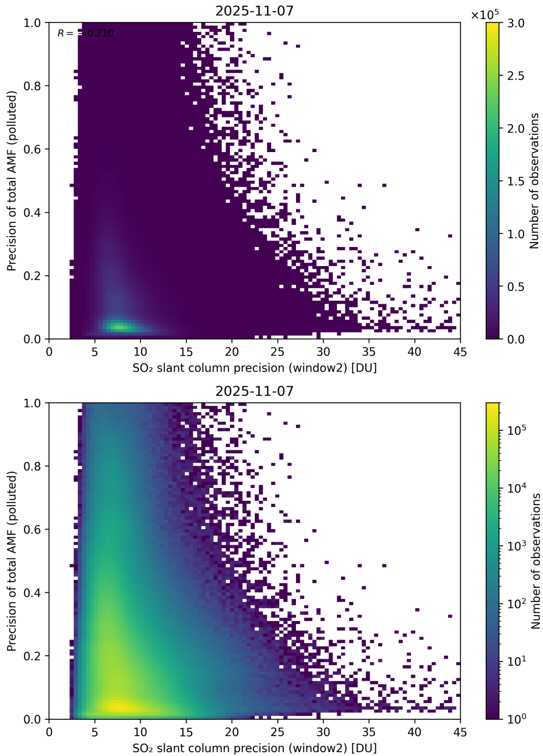
Figure 302: Scatter density plot of “SO 2 slant column precision (window2)” against “Precision of total AMF (polluted)” for 2025-11-07 to 2025-11-08.
