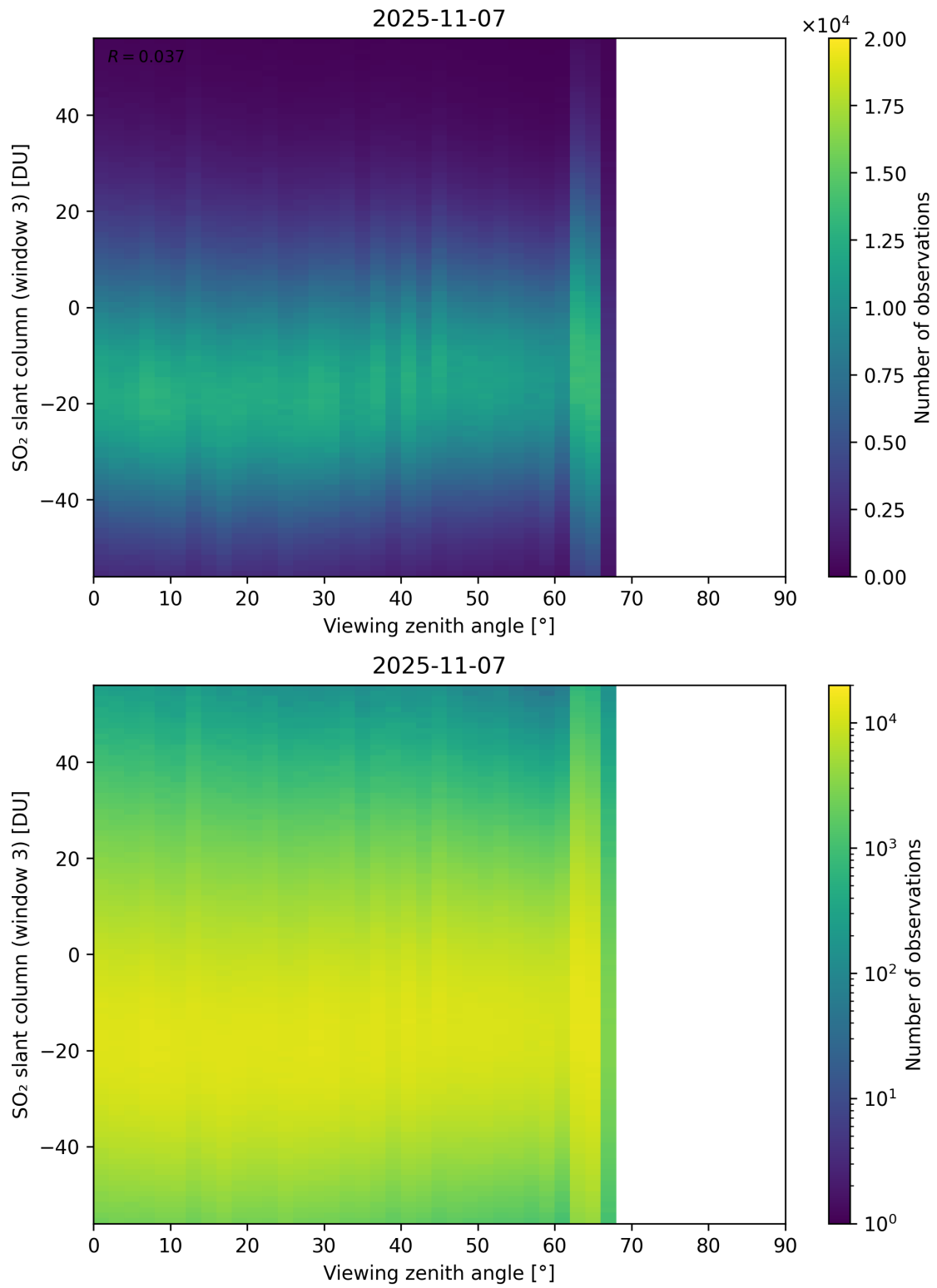
Figure 379: Scatter density plot of “Viewing zenith angle” against “SO 2 slant column (window 3)” for 2025-11-07 to 2025-11-08.
