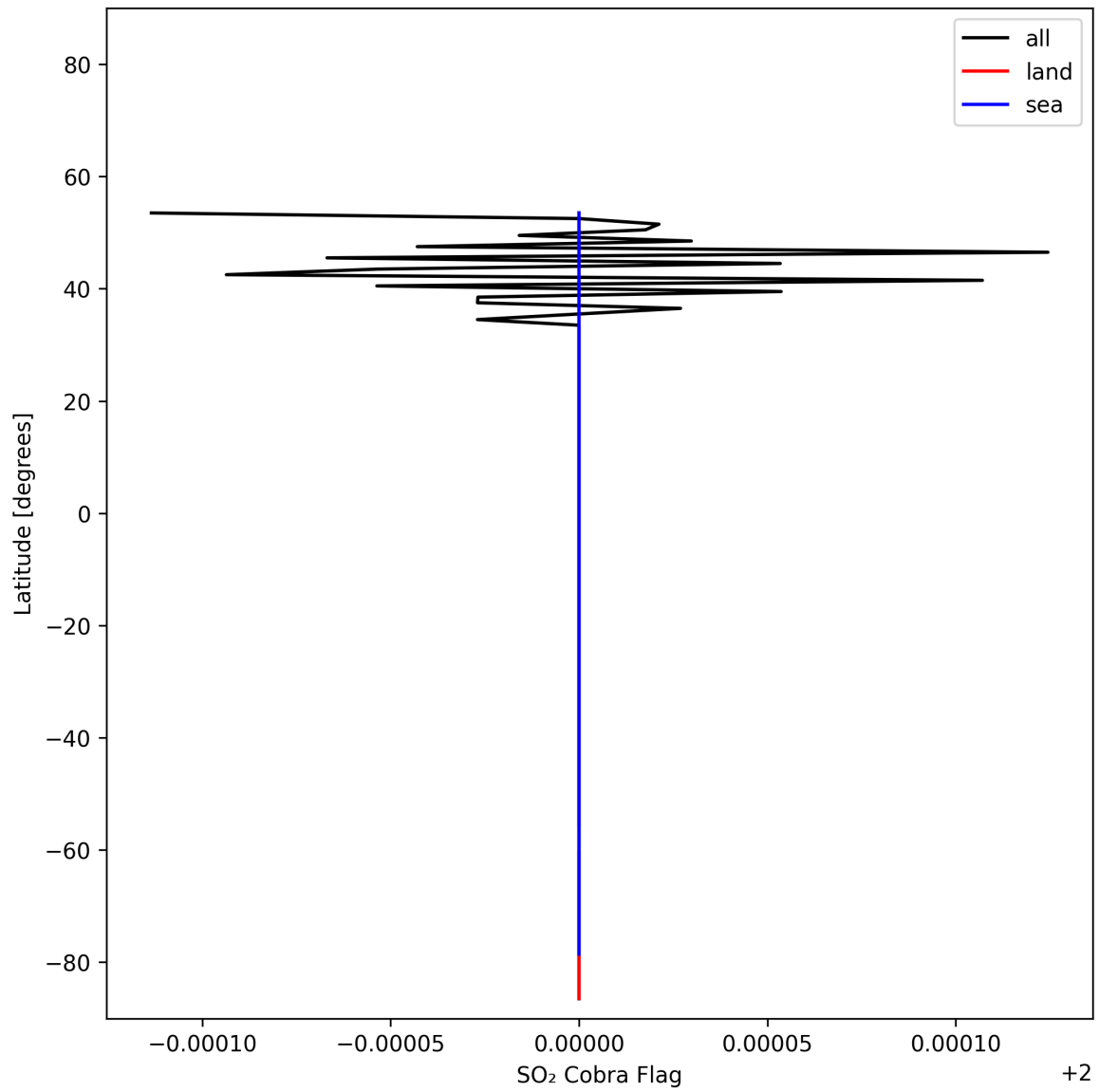
Figure 49: Zonal average of "SO 2 Cobra Flag" for 2025-11-07 to 2025-11-08.
