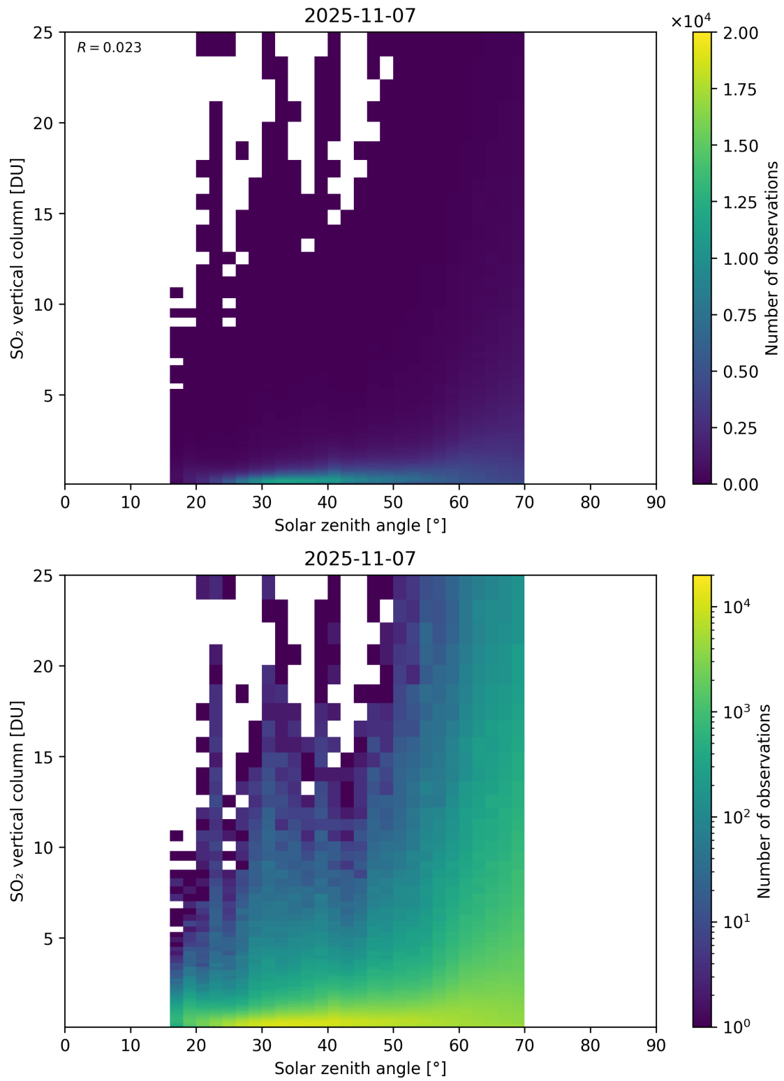
Figure 191: Scatter density plot of “Solar zenith angle” against “SO 2 vertical column” for 2025-11-07 to 2025-11-08.
