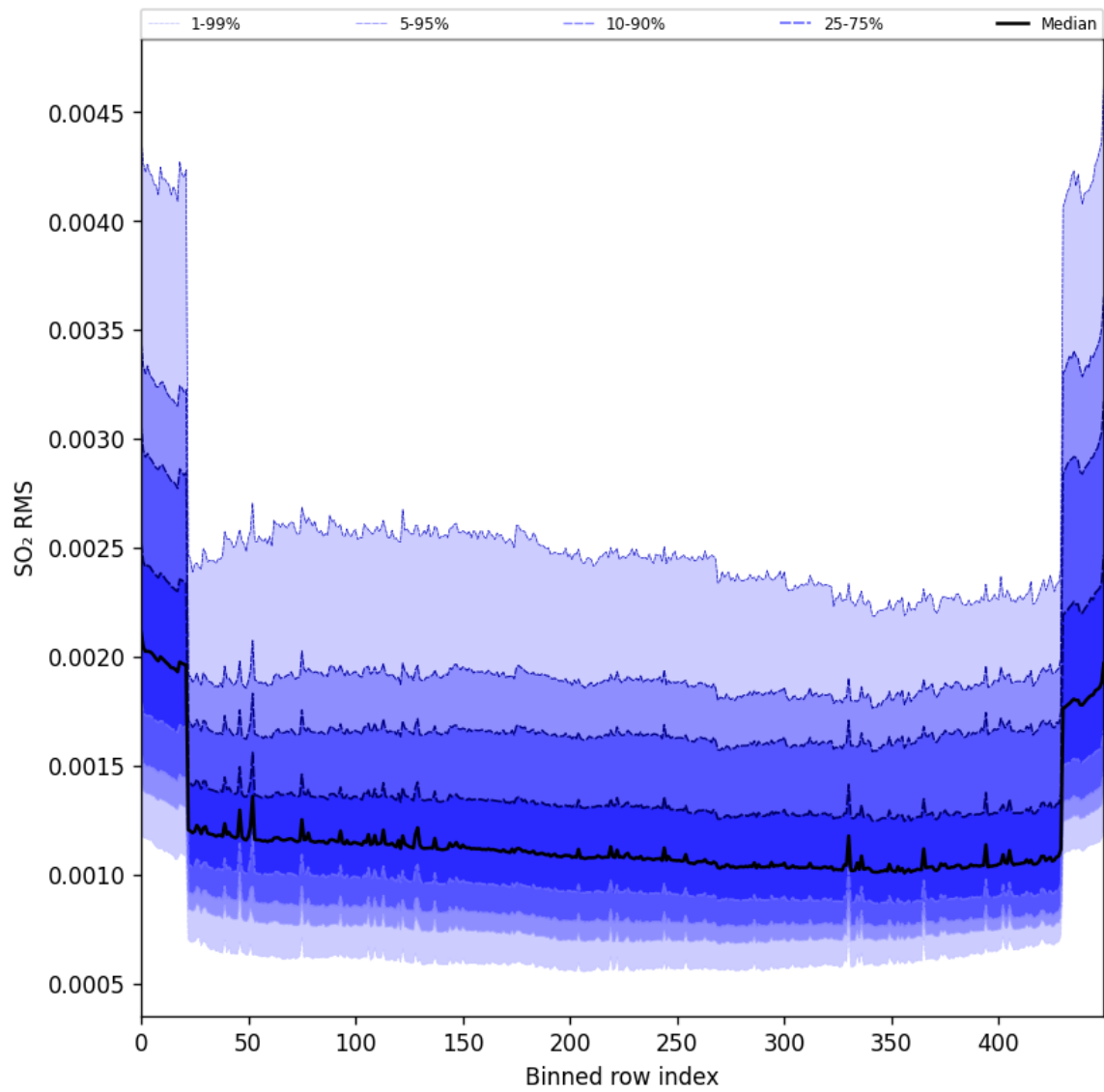
Figure 104: Along track statistics of “SO 2 RMS” for 2025-11-07 to 2025-11-08
