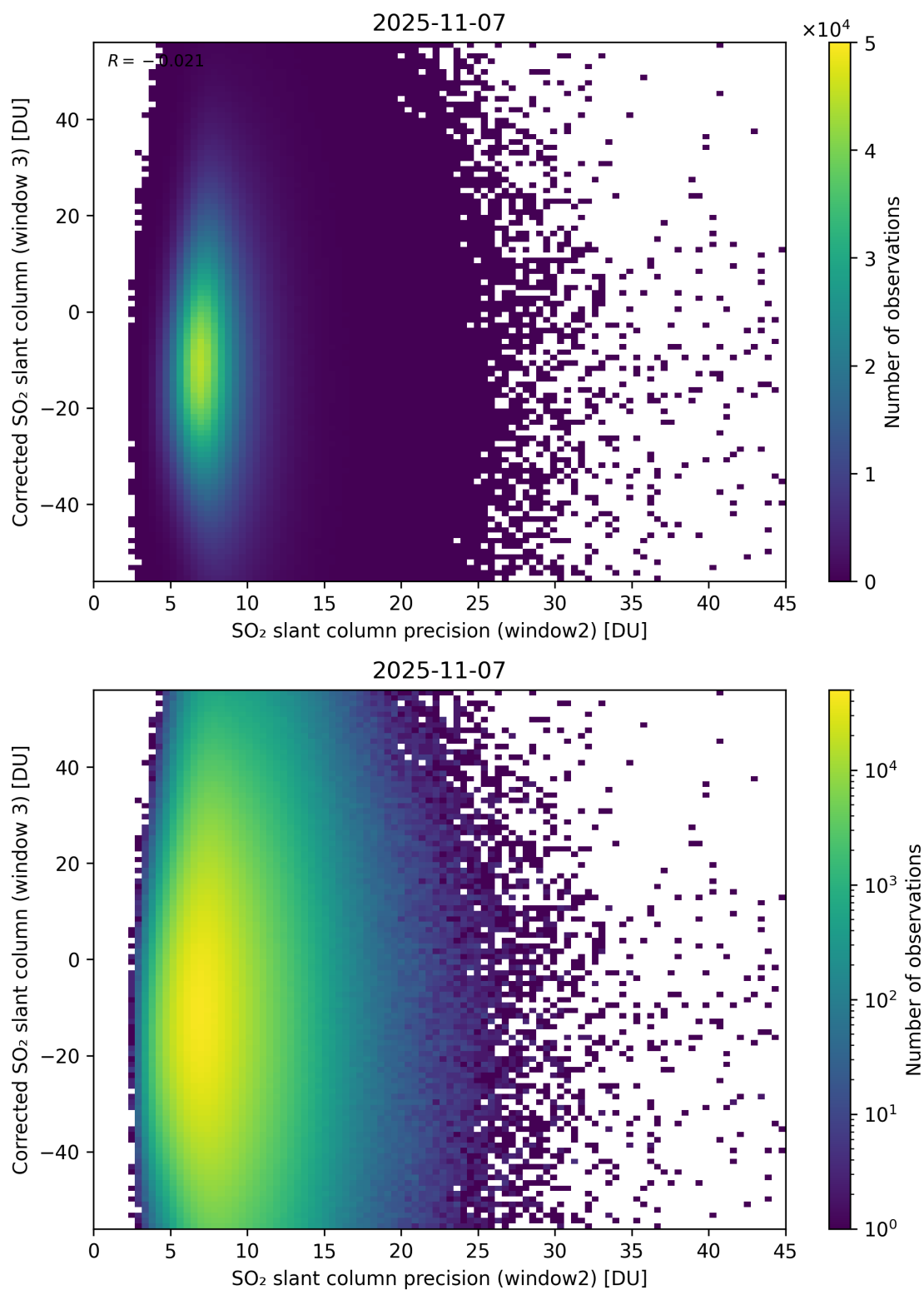
Figure 298: Scatter density plot of “SO 2 slant column precision (window2)” against “Corrected SO 2 slant column (window 3)” for 2025-11-07 to 2025-11-08.
