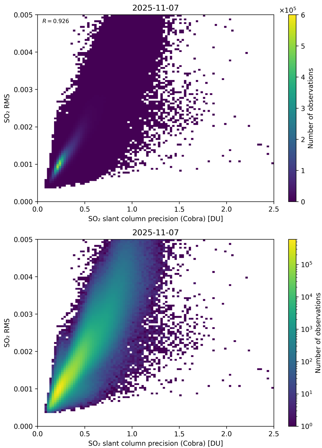
Figure 204: Scatter density plot of “SO 2 slant column precision (Cobra)” against “SO 2 RMS” for 2025-11-07 to 2025-11-08.
