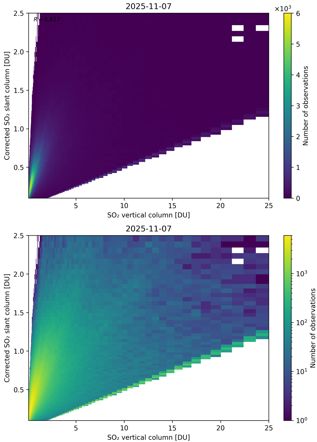
Figure 351: Scatter density plot of “SO 2 vertical column” against “Corrected SO 2 slant column” for 2025-11-07 to 2025-11-08.
