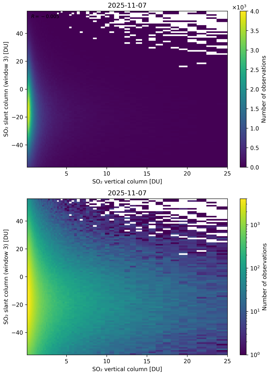
Figure 357: Scatter density plot of “SO 2 vertical column” against “SO 2 slant column (window 3)” for 2025-11-07 to 2025-11-08.
