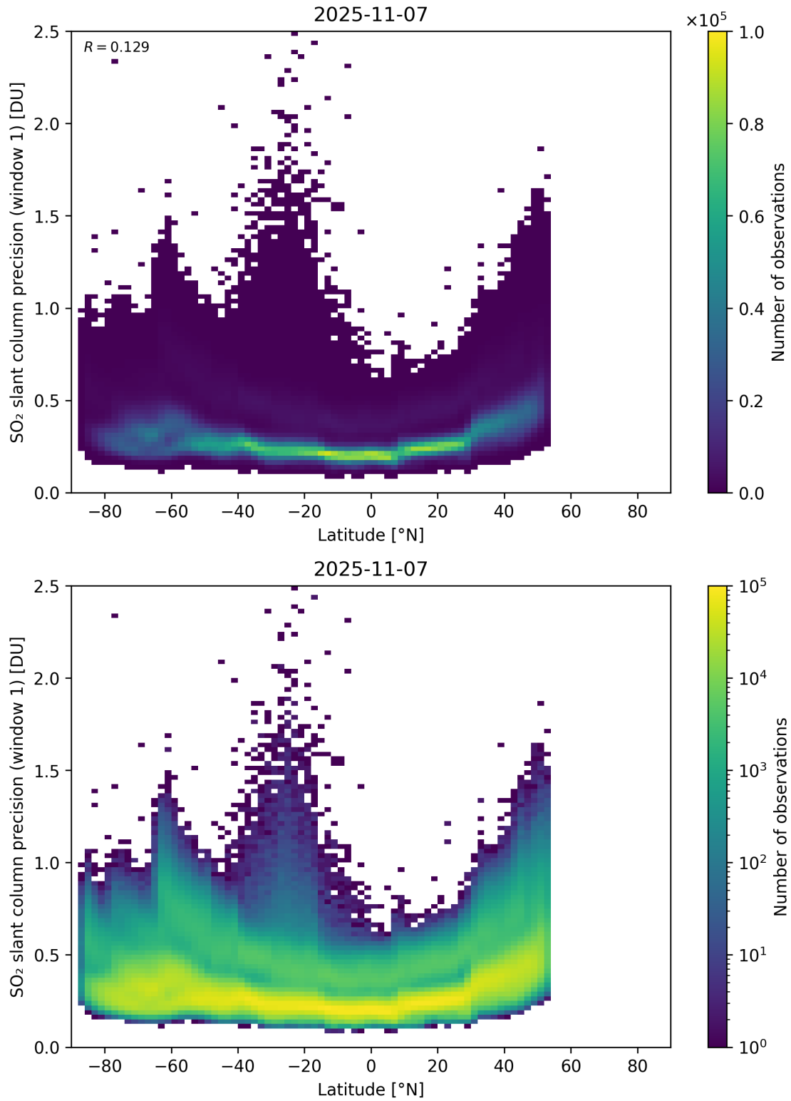
Figure 163: Scatter density plot of “Latitude” against “SO 2 slant column precision (window 1)” for 2025-11-07 to 2025-11-08.
