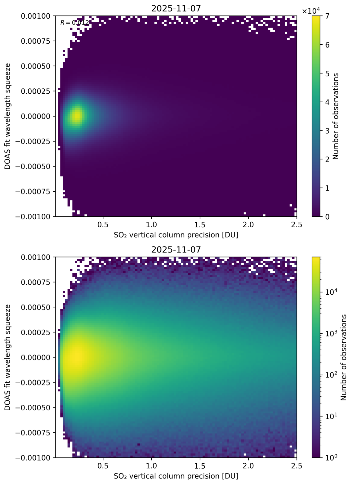
Figure 333: Scatter density plot of “SO 2 vertical column precision” against “DOAS fit wavelength squeeze” for 2025-11-07 to 2025-11-08.
