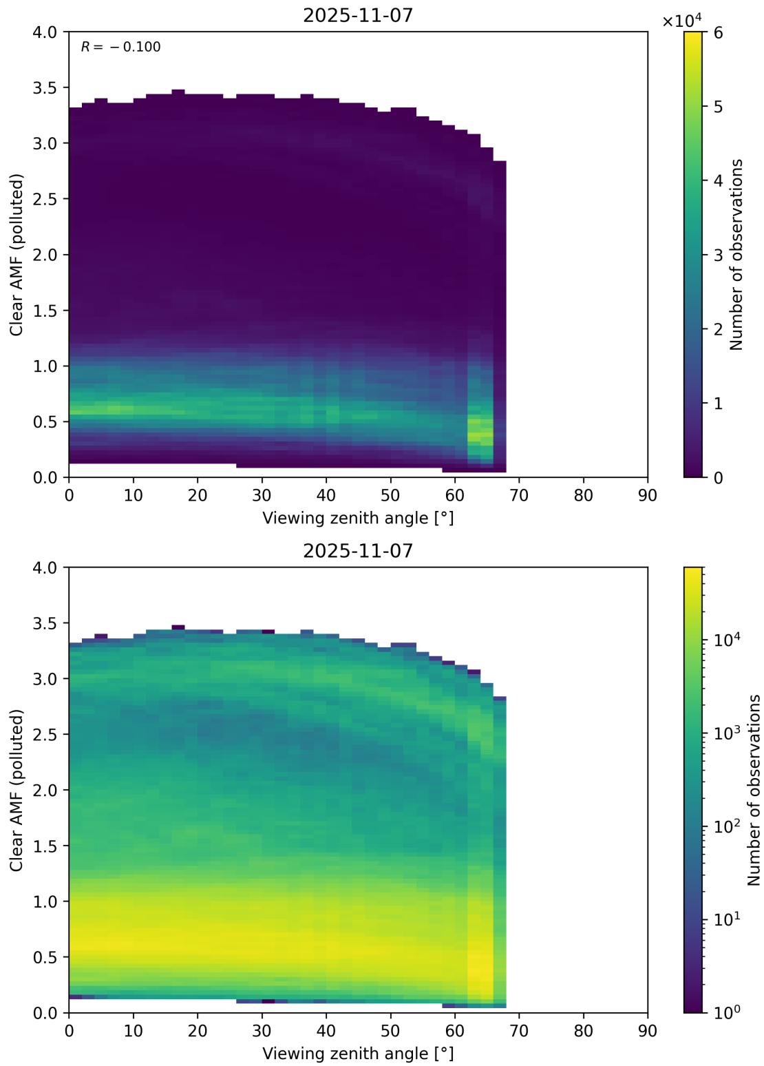
Figure 370: Scatter density plot of “Viewing zenith angle” against “Clear AMF (polluted)” for 2025-11-07 to 2025-11-08.
