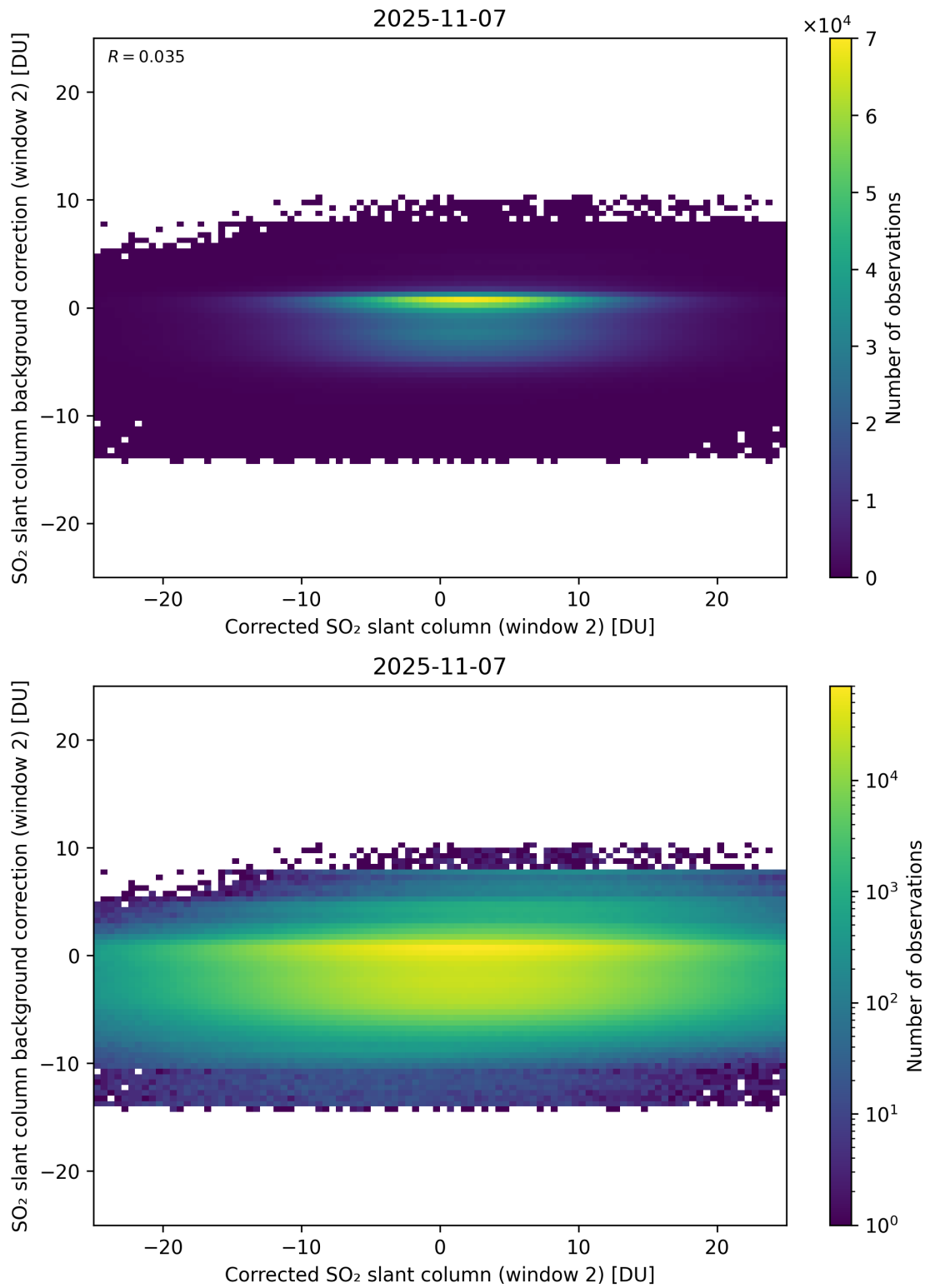
Figure 244: Scatter density plot of “Corrected SO 2 slant column (window 2)” against “SO 2 slant column background correction (window 2)” for 2025-11-07 to 2025-11-08.
