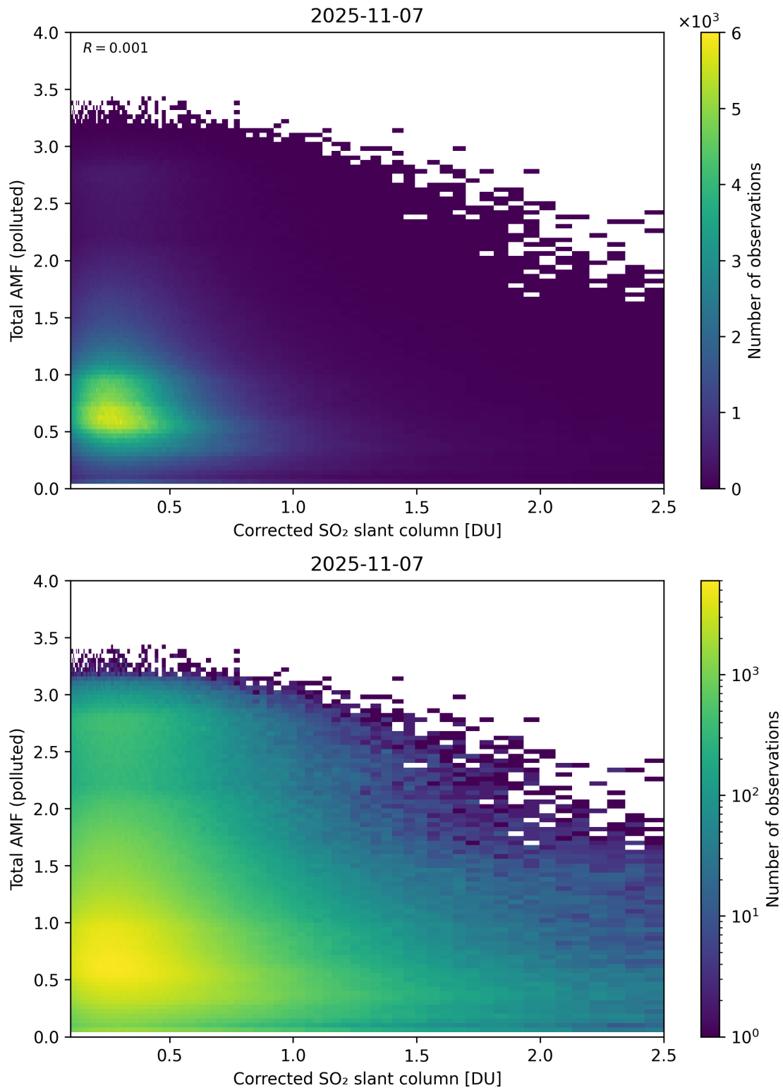
Figure 242: Scatter density plot of “Corrected SO 2 slant column” against “Total AMF (polluted)” for 2025-11-07 to 2025-11-08.
