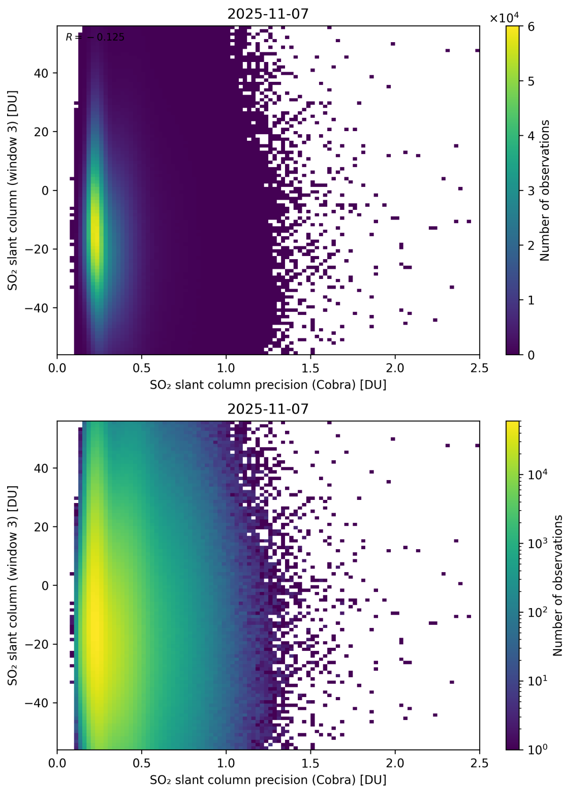
Figure 211: Scatter density plot of “SO 2 slant column precision (Cobra)” against “SO 2 slant column (window 3)” for 2025-11-07 to 2025-11-08.
