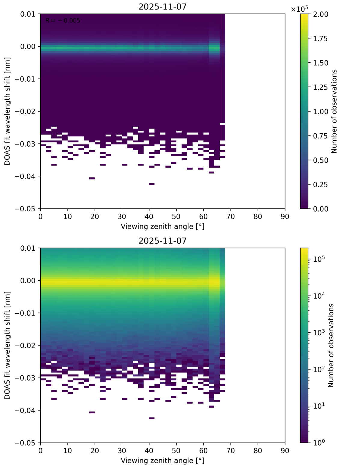
Figure 365: Scatter density plot of “Viewing zenith angle” against “DOAS fit wavelength shift” for 2025-11-07 to 2025-11-08.
