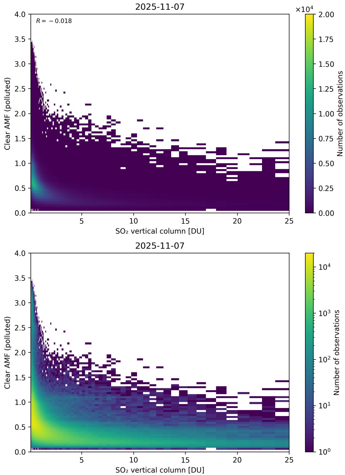
Figure 348: Scatter density plot of “SO 2 vertical column” against “Clear AMF (polluted)” for 2025-11-07 to 2025-11-08.
