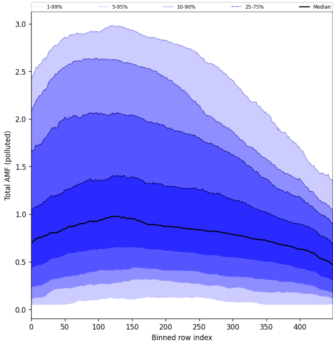
Figure 105: Along track statistics of “Total AMF (polluted)” for 2025-11-07 to 2025-11-08
