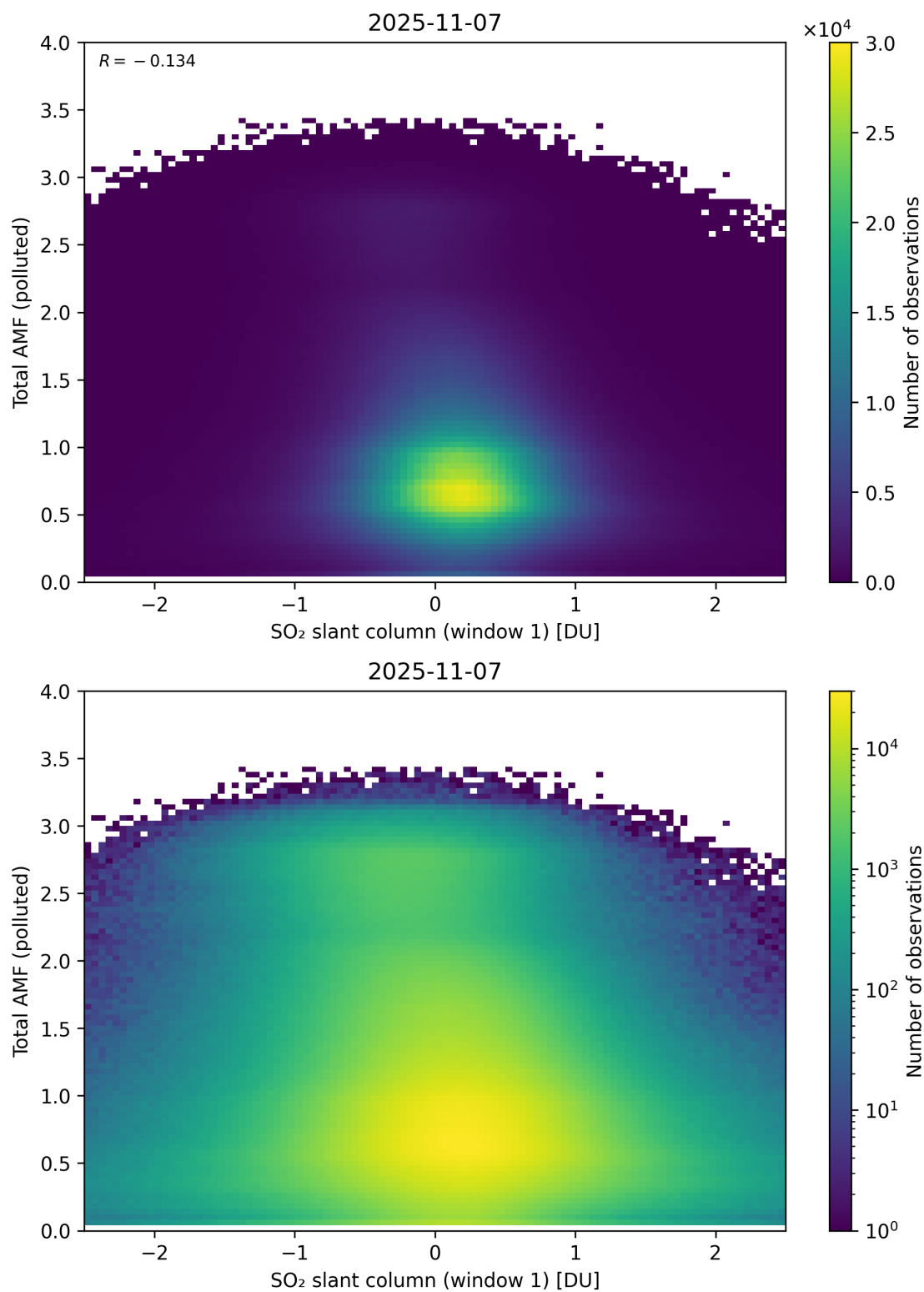
Figure 289: Scatter density plot of “SO 2 slant column (window 1)” against “Total AMF (polluted)” for 2025-11-07 to 2025-11-08.
