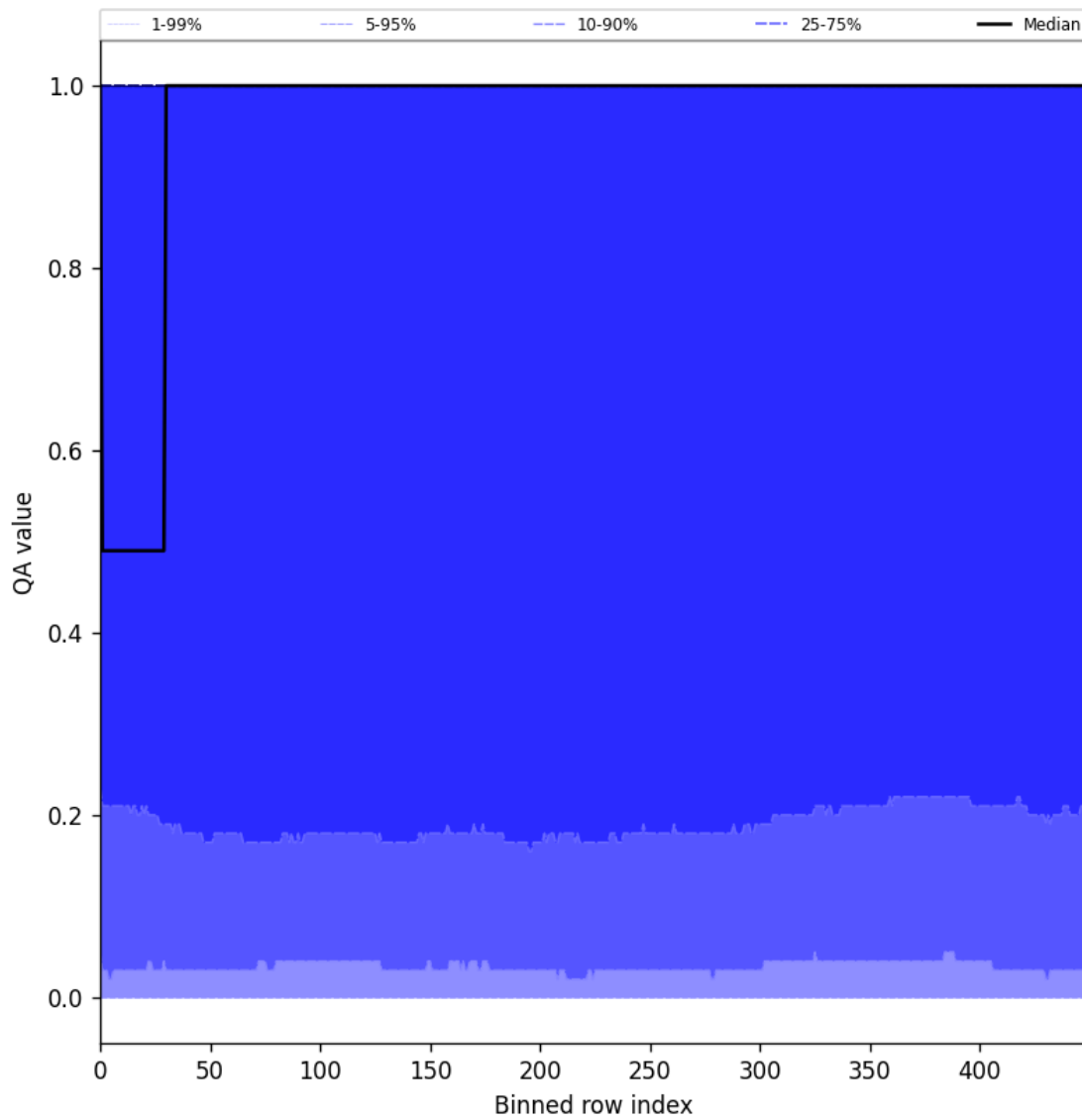
Figure 83: Along track statistics of “QA value” for 2025-11-07 to 2025-11-08
