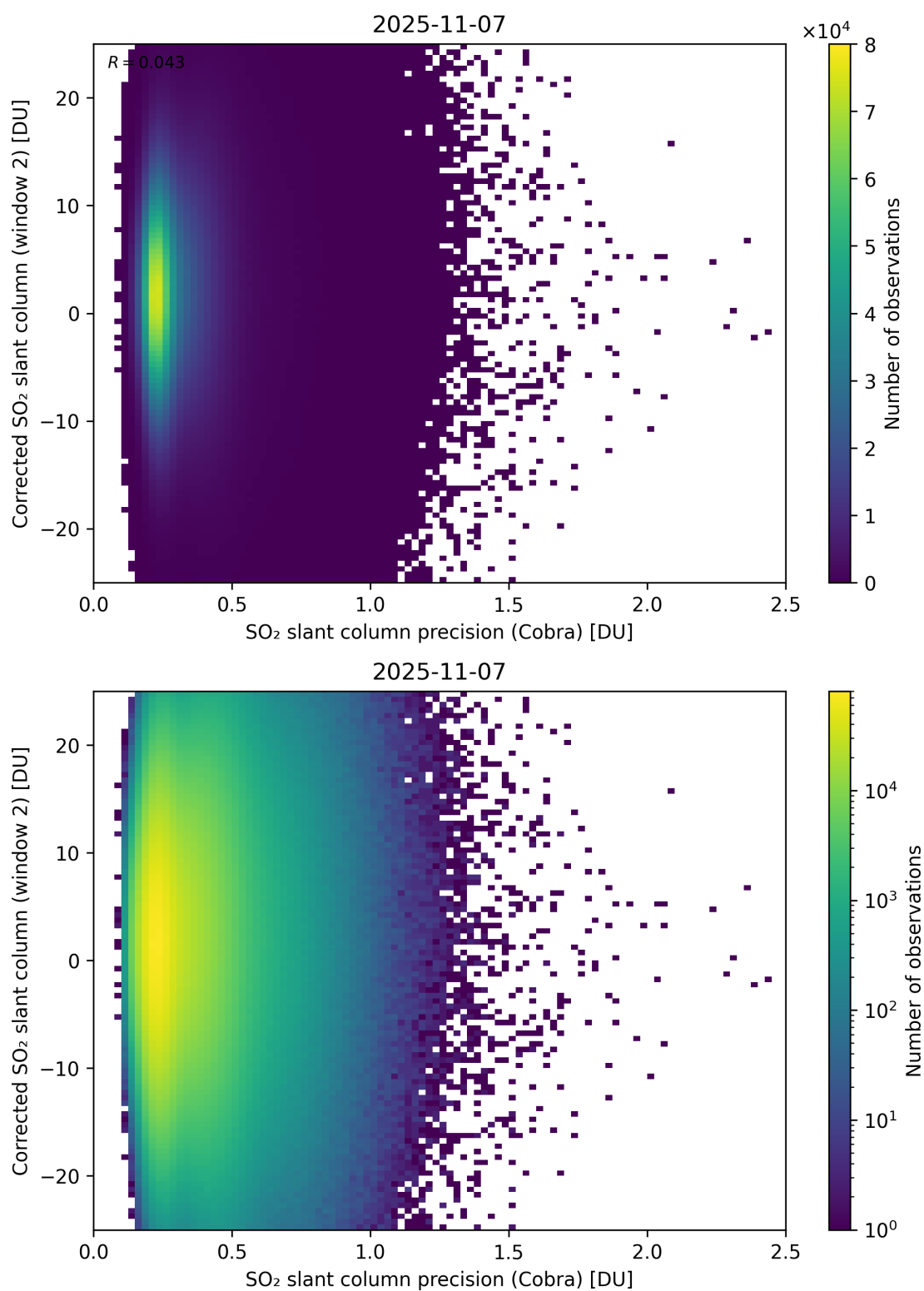
Figure 206: Scatter density plot of “SO 2 slant column precision (Cobra)” against “Corrected SO 2 slant column (window 2)” for 2025-11-07 to 2025-11-08.
