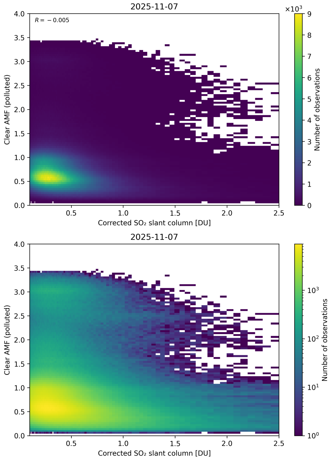
Figure 232: Scatter density plot of “Corrected SO 2 slant column” against “Clear AMF (polluted)” for 2025-11-07 to 2025-11-08.
