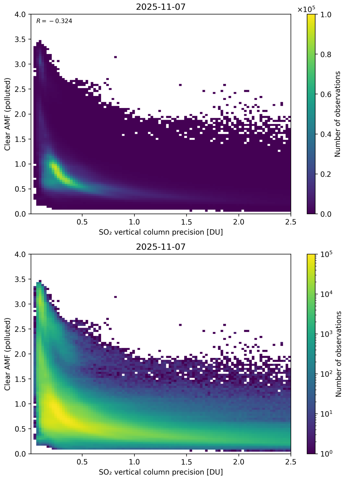
Figure 335: Scatter density plot of “SO 2 vertical column precision” against “Clear AMF (polluted)” for 2025-11-07 to 2025-11-08.
