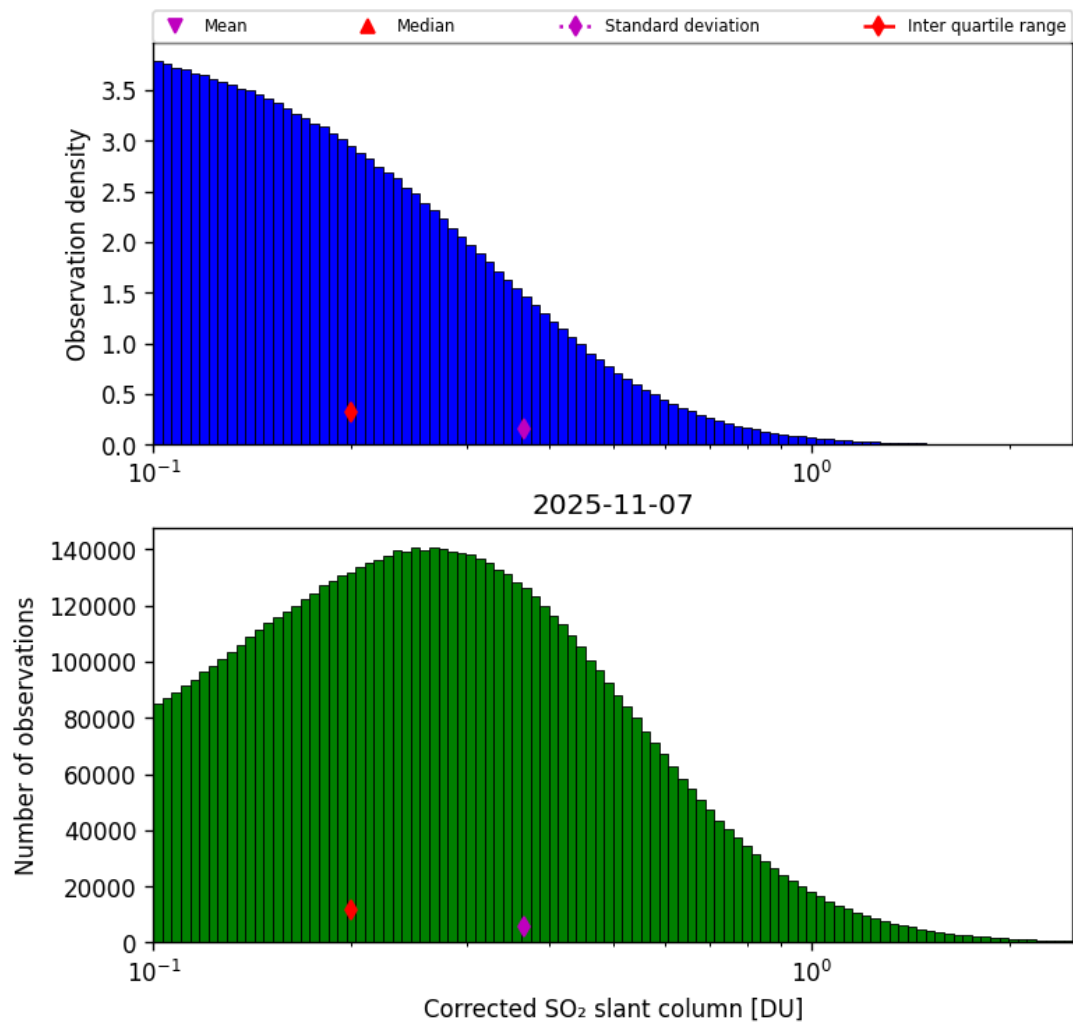
Figure 60: Histogram of “Corrected SO 2 slant column” for 2025-11-07 to 2025-11-08
