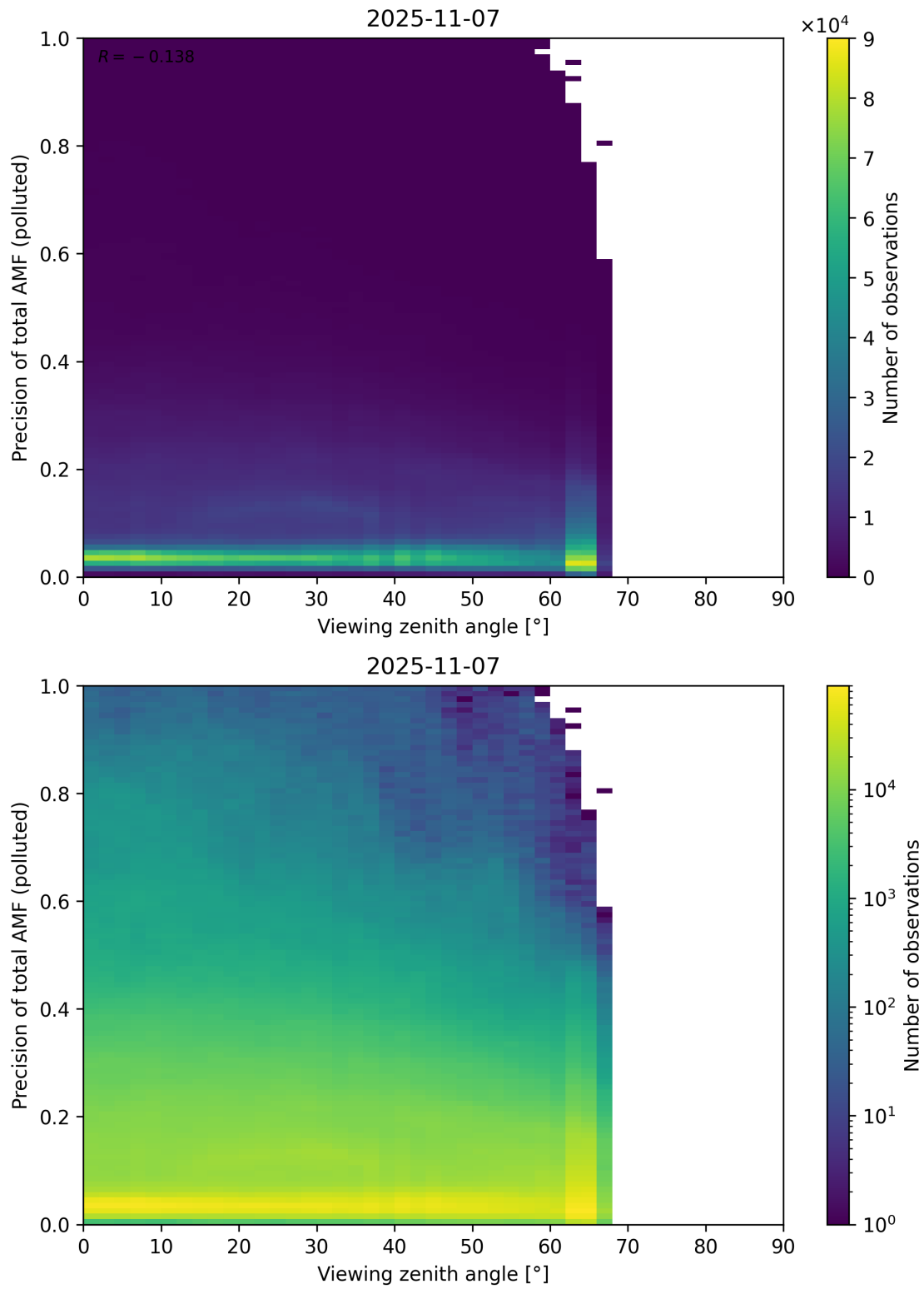
Figure 382: Scatter density plot of “Viewing zenith angle” against “Precision of total AMF (polluted)” for 2025-11-07 to 2025-11-08.
