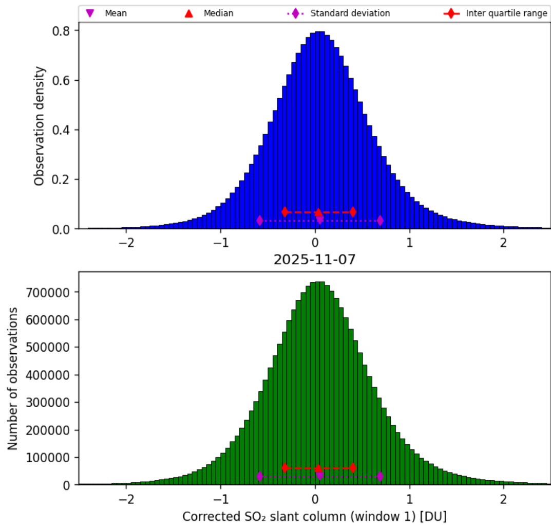
Figure 65: Histogram of “Corrected SO 2 slant column (window 1)” for 2025-11-07 to 2025-11-08
