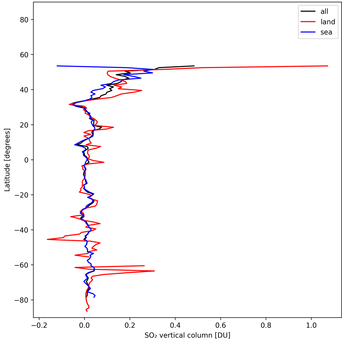
Figure 32: Zonal average of “SO 2 vertical column” for 2025-11-07 to 2025-11-08.
