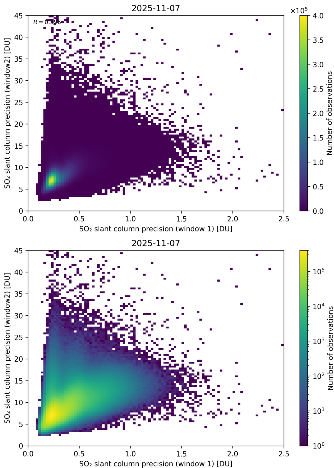
Figure 277: Scatter density plot of “SO 2 slant column precision (window 1)” against “SO 2 slant column precision (window2)” for 2025-11-07 to 2025-11-08.
