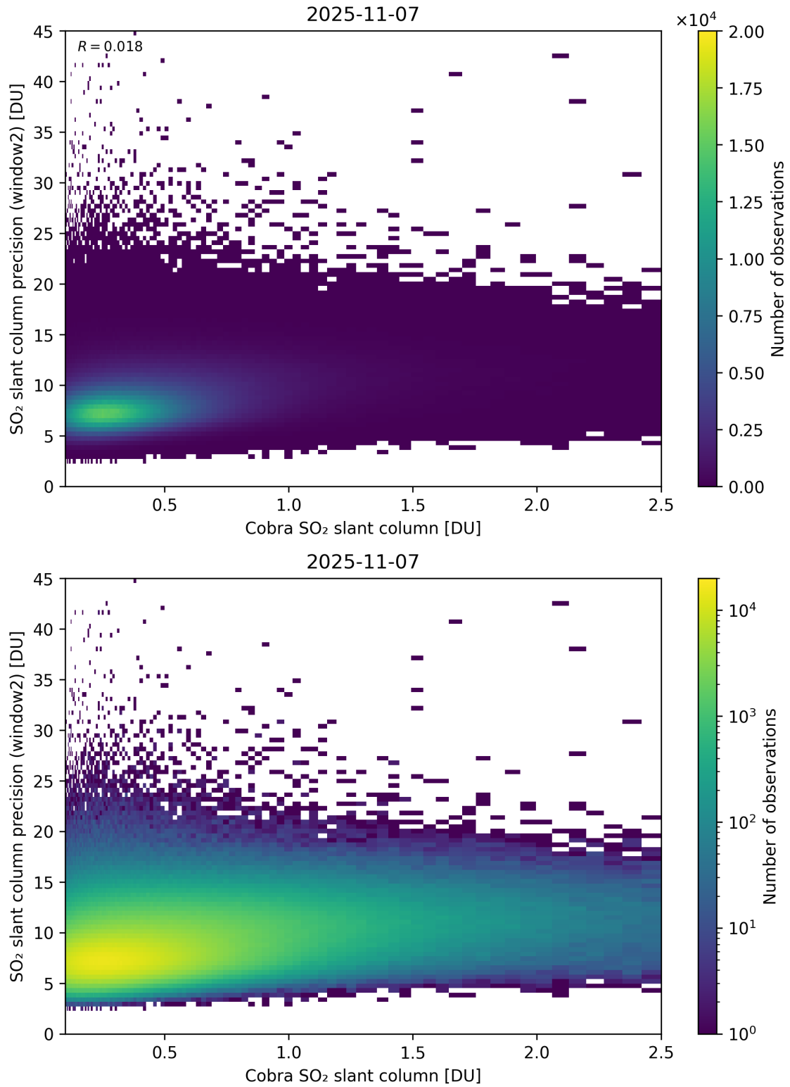
Figure 221: Scatter density plot of “Cobra SO 2 slant column” against “SO 2 slant column precision (window2)” for 2025-11-07 to 2025-11-08.
