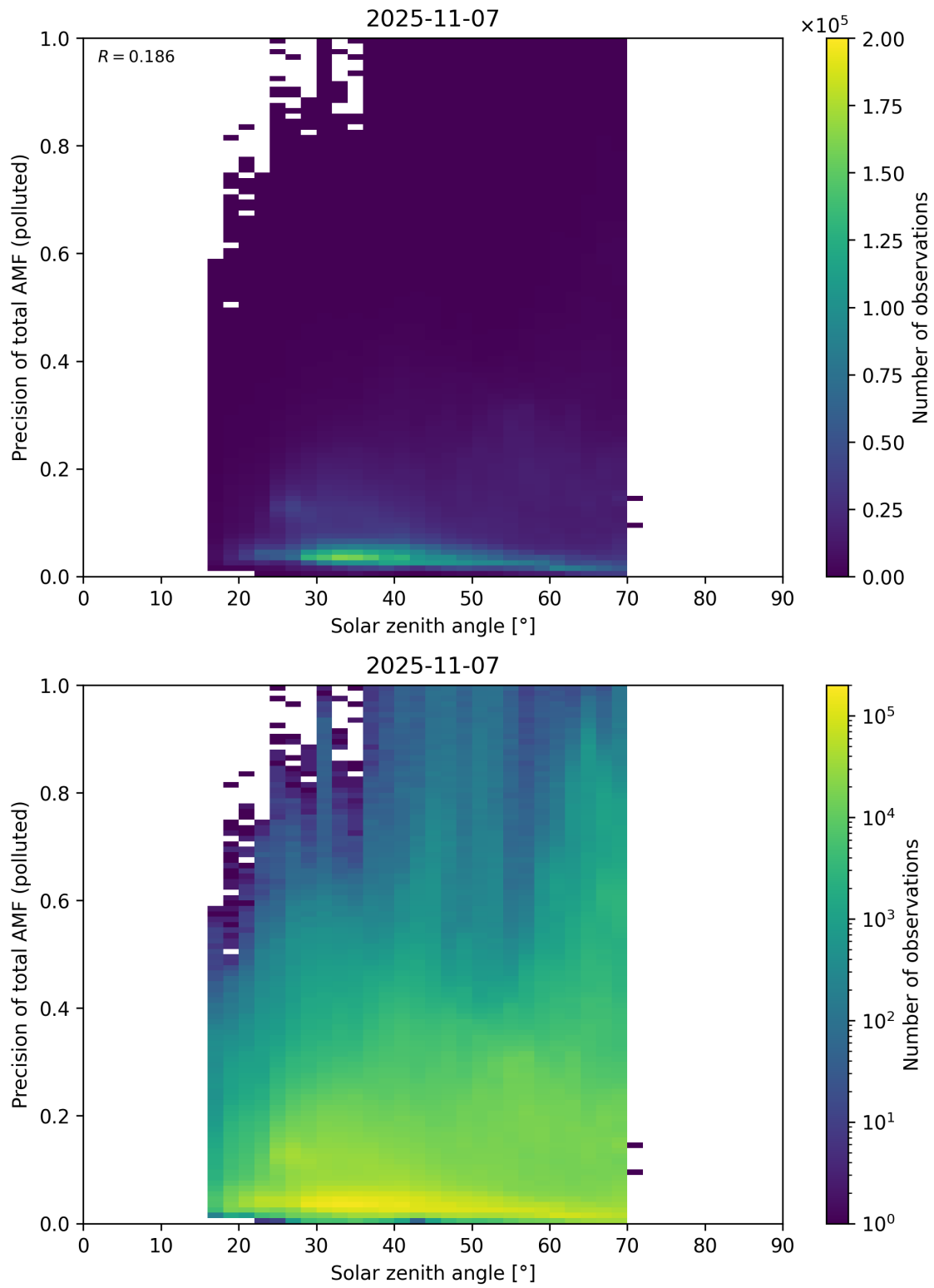
Figure 190: Scatter density plot of “Solar zenith angle” against “Precision of total AMF (polluted)” for 2025-11-07 to 2025-11-08.
