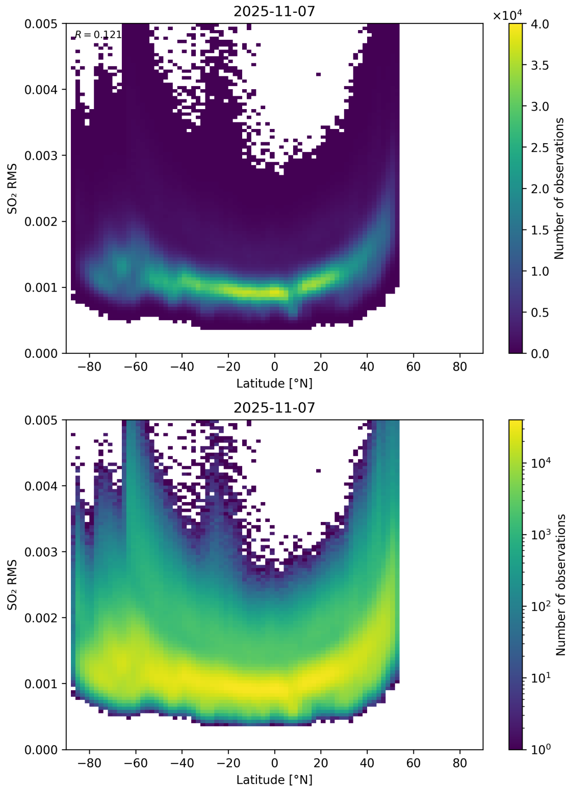
Figure 155: Scatter density plot of “Latitude” against “SO 2 RMS” for 2025-11-07 to 2025-11-08.
