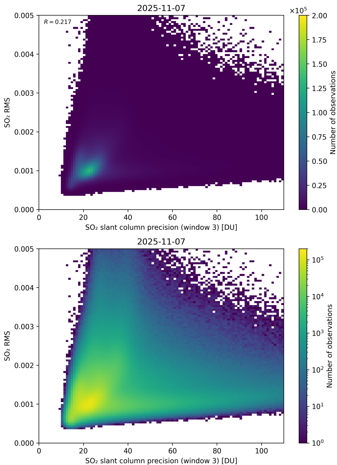
Figure 310: Scatter density plot of “SO 2 slant column precision (window 3)” against “SO 2 RMS” for 2025-11-07 to 2025-11-08.
