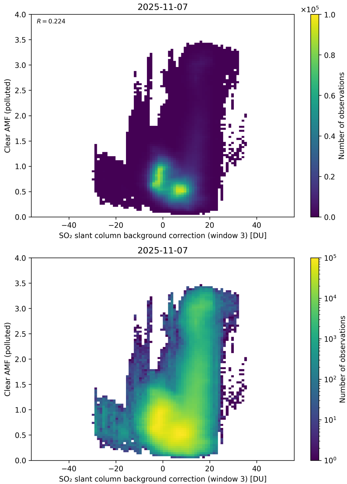
Figure 135: Scatter density plot of “SO 2 slant column background correction (window 3)” against “Clear AMF (polluted)” for 2025-11-07 to 2025-11-08.
