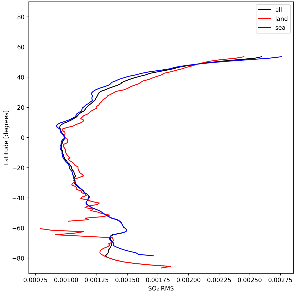
Figure 52: Zonal average of “SO 2 RMS” for 2025-11-07 to 2025-11-08.
