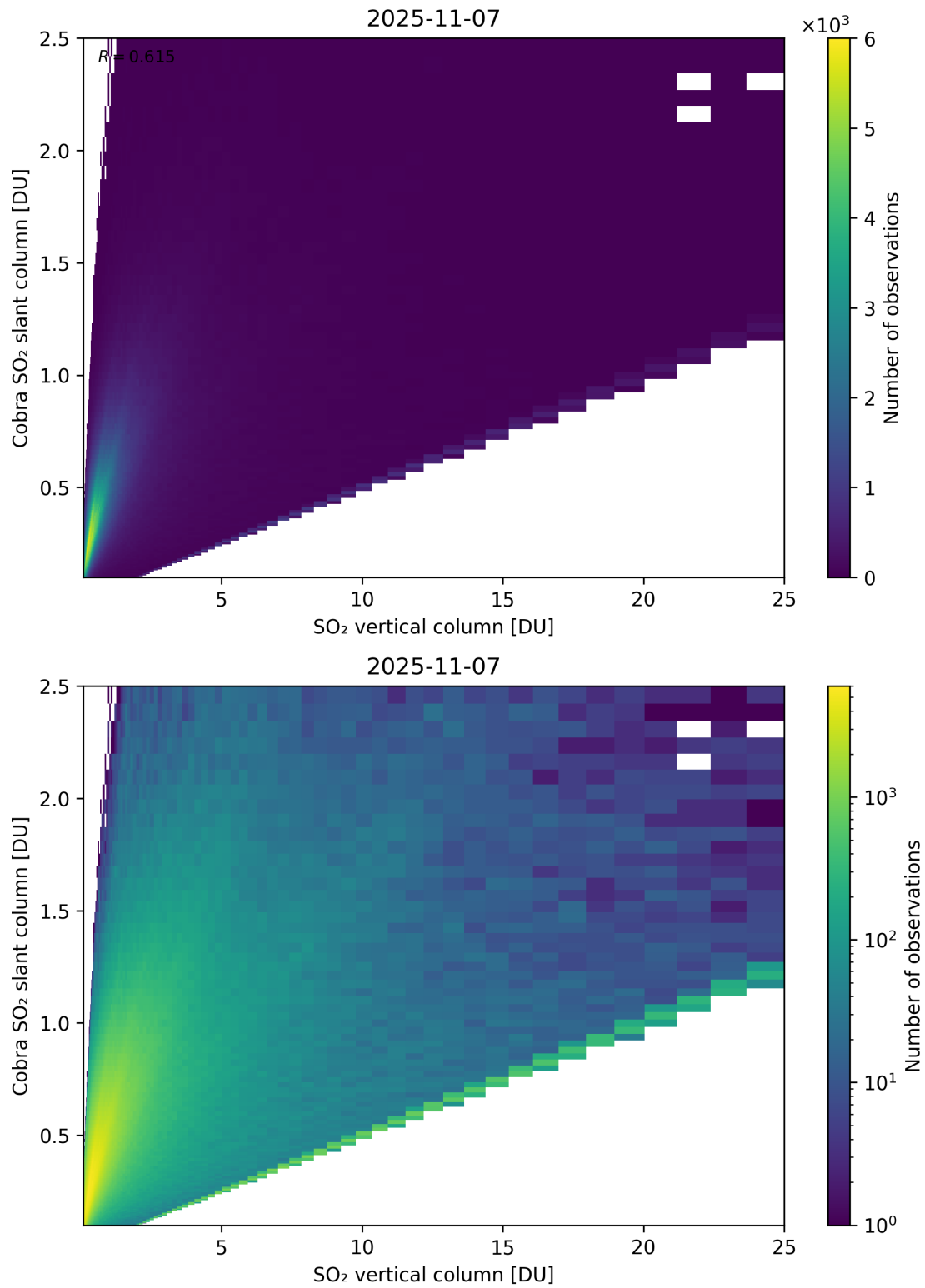
Figure 349: Scatter density plot of “SO 2 vertical column” against “Cobra SO 2 slant column” for 2025-11-07 to 2025-11-08.
