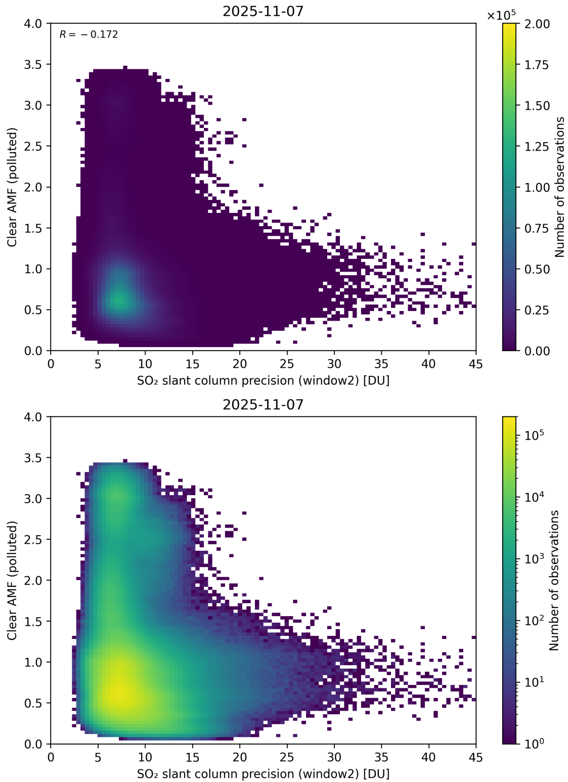
Figure 296: Scatter density plot of “SO 2 slant column precision (window2)” against “Clear AMF (polluted)” for 2025-11-07 to 2025-11-08.
