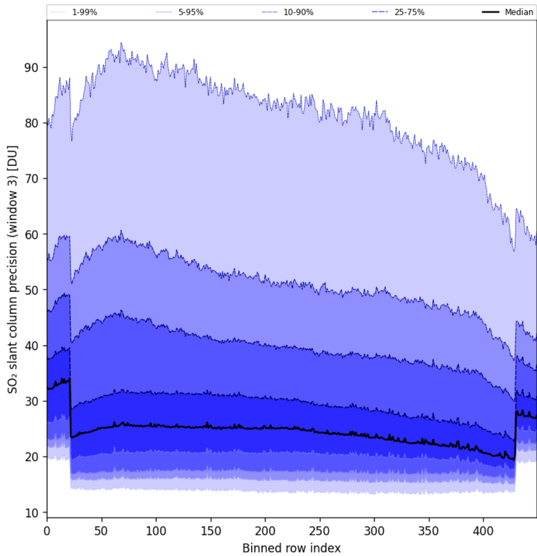
Figure 98: Along track statistics of “SO 2 slant column precision (window 3)” for 2025-11-07 to 2025-11-08
