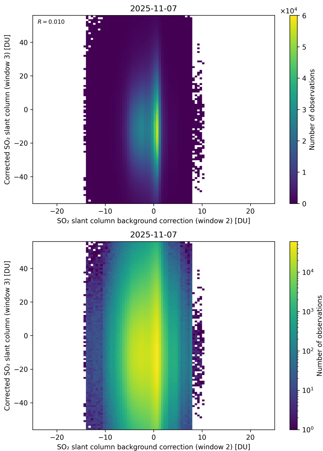
Figure 127: Scatter density plot of “SO 2 slant column background correction (window 2)” against “Corrected SO 2 slant column (window 3)” for 2025-11-07 to 2025-11-08.
