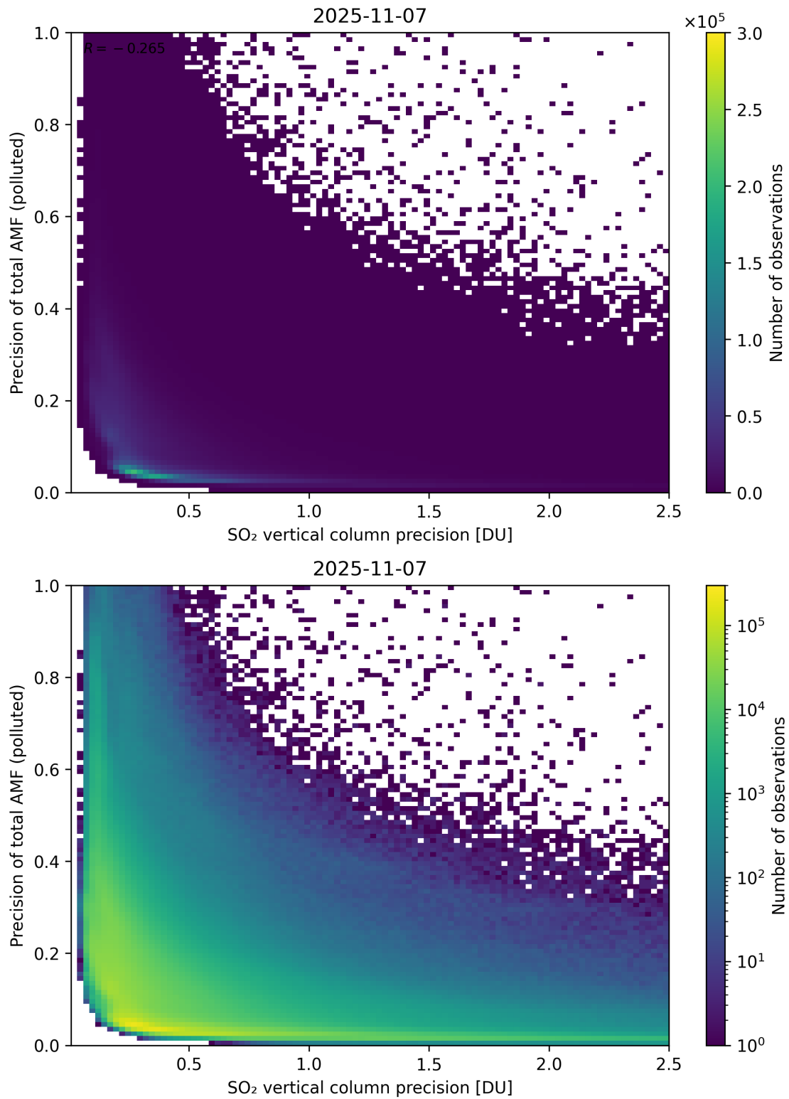
Figure 347: Scatter density plot of “SO 2 vertical column precision” against “Precision of total AMF (polluted)” for 2025-11-07 to 2025-11-08.
