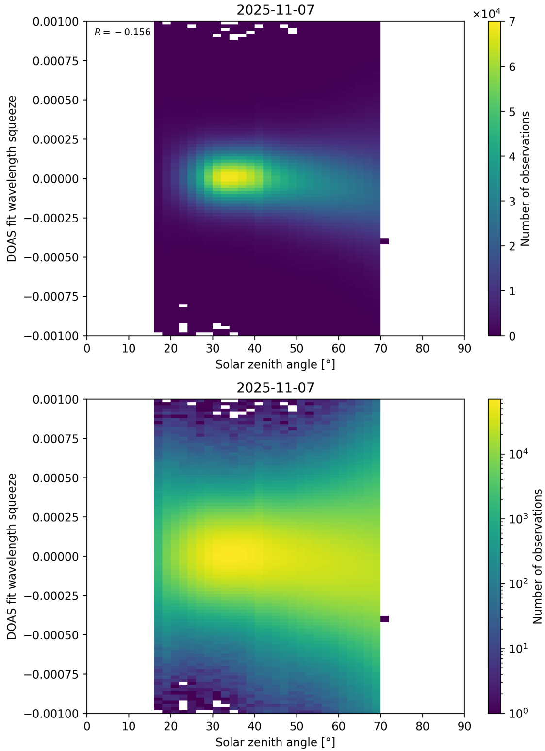
Figure 175: Scatter density plot of “Solar zenith angle” against “DOAS fit wavelength squeeze” for 2025-11-07 to 2025-11-08.
