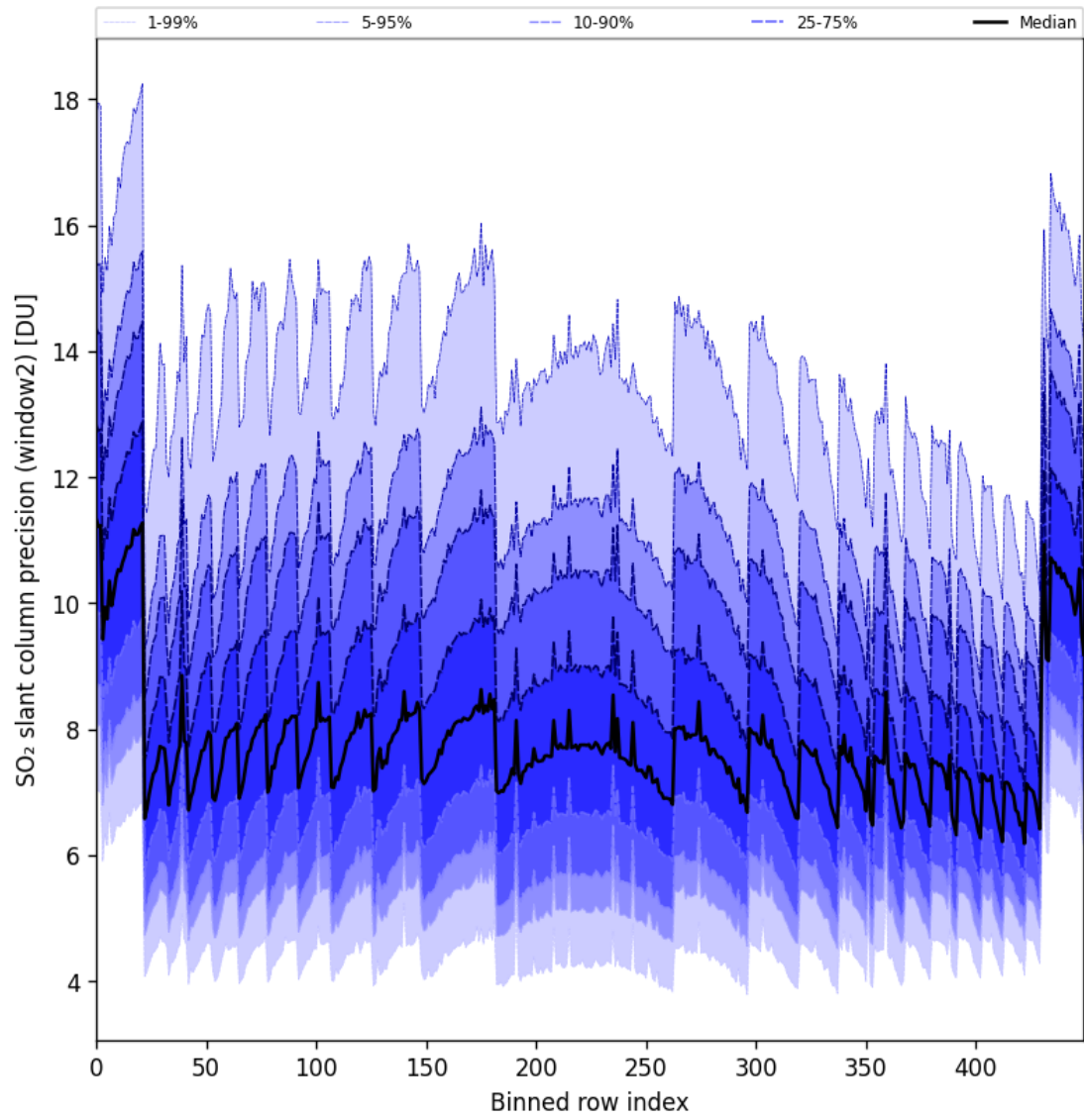
Figure 94: Along track statistics of “SO 2 slant column precision (window2)” for 2025-11-07 to 2025-11-08
