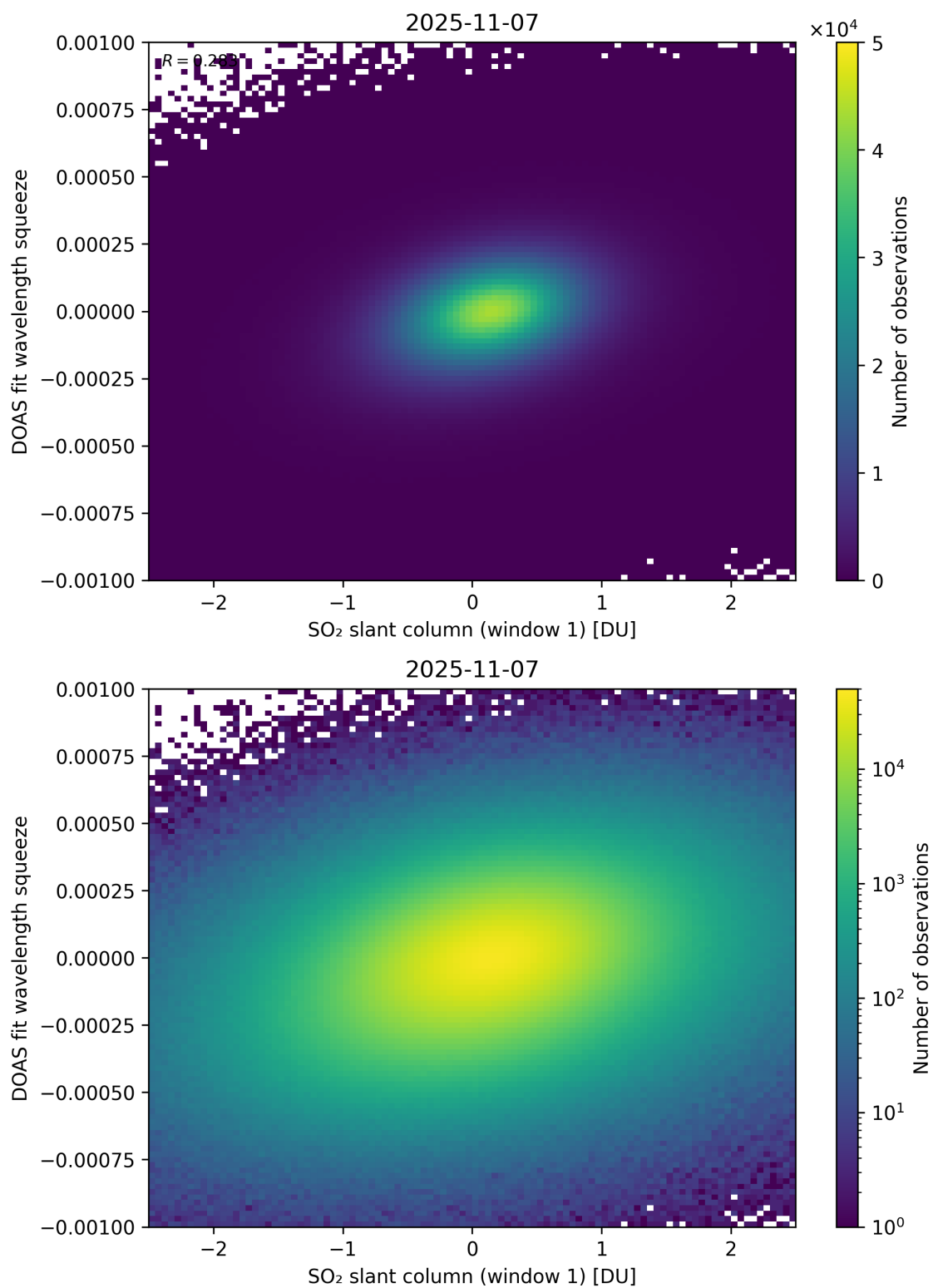
Figure 266: Scatter density plot of “SO 2 slant column (window 1)” against “DOAS fit wavelength squeeze” for 2025-11-07 to 2025-11-08.
