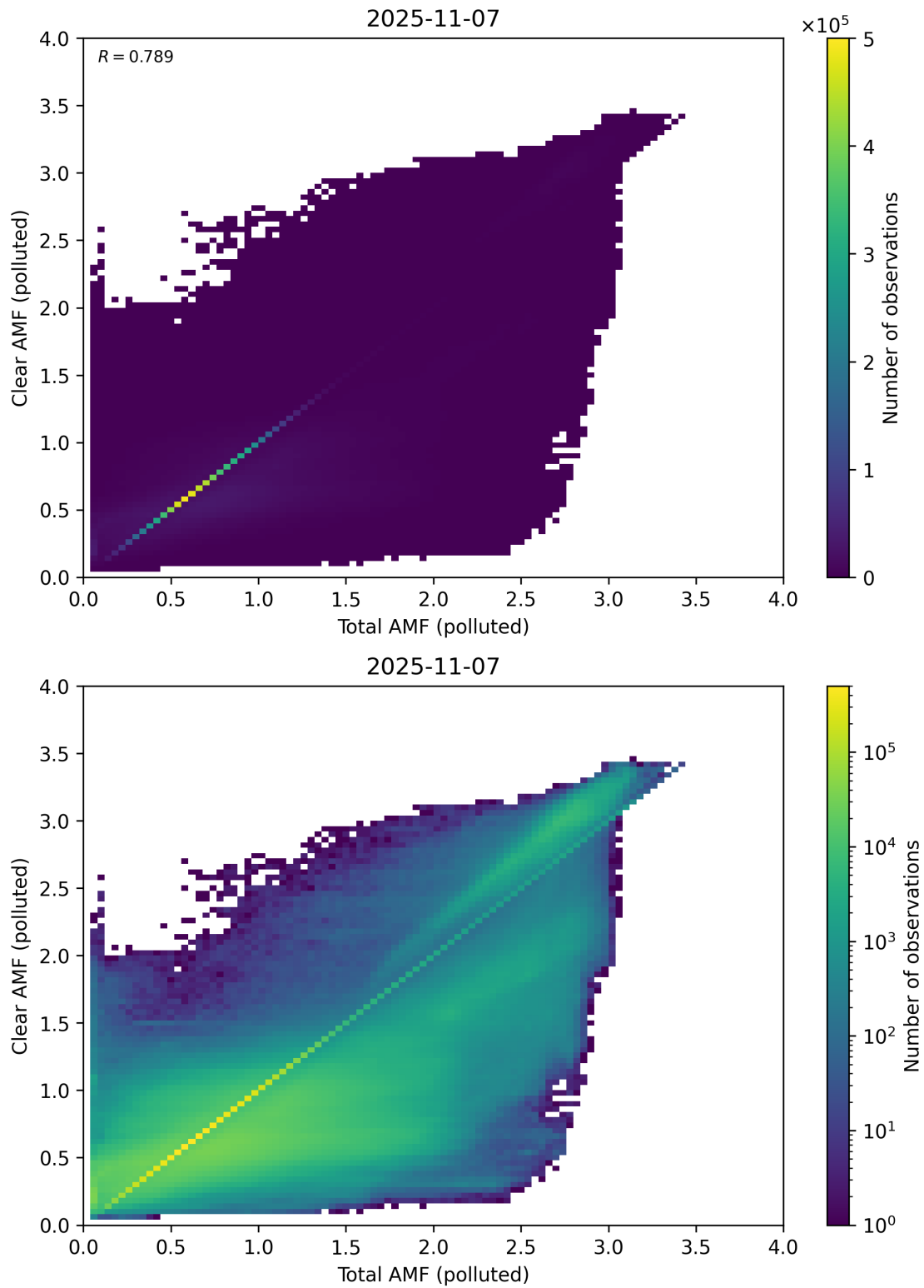
Figure 321: Scatter density plot of “Total AMF (polluted)” against “Clear AMF (polluted)” for 2025-11-07 to 2025-11-08.
