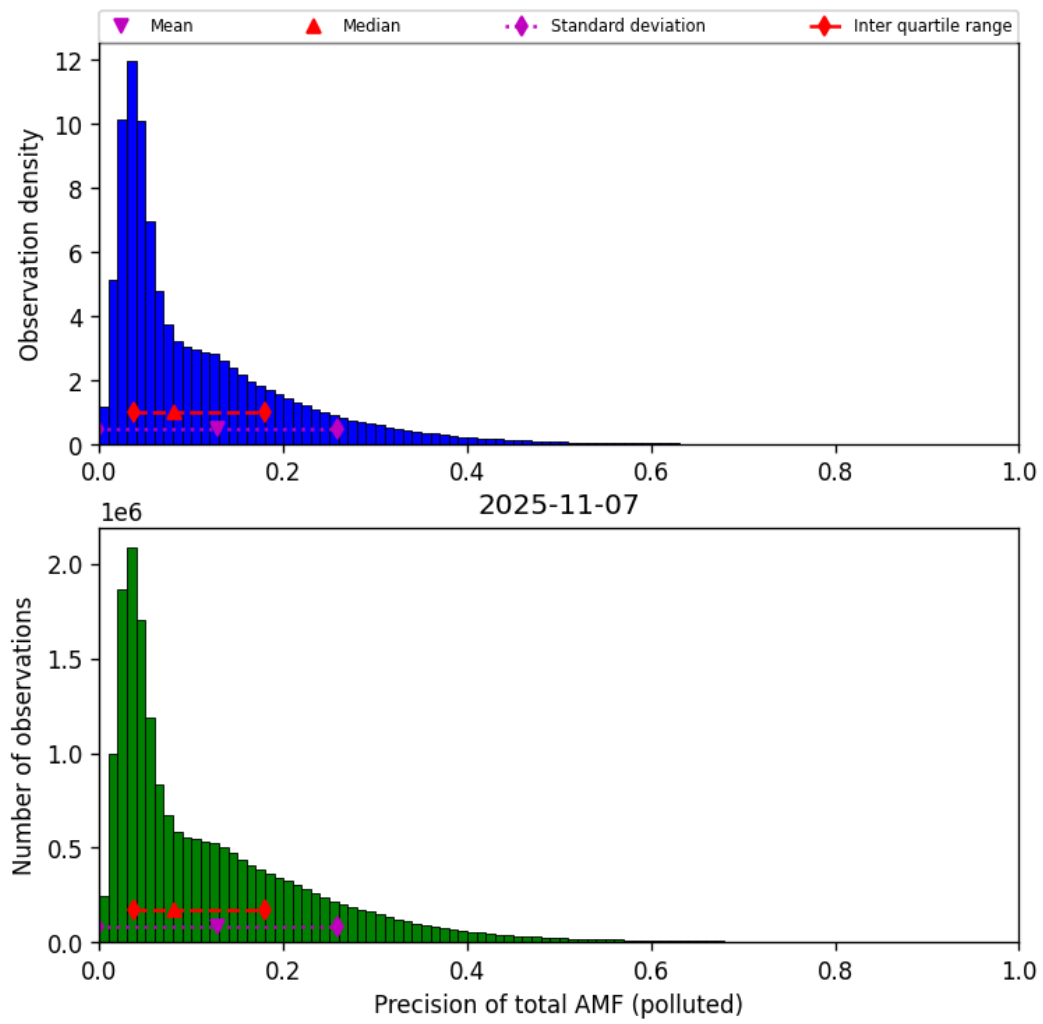
Figure 80: Histogram of “Precision of total AMF (polluted)” for 2025-11-07 to 2025-11-08
