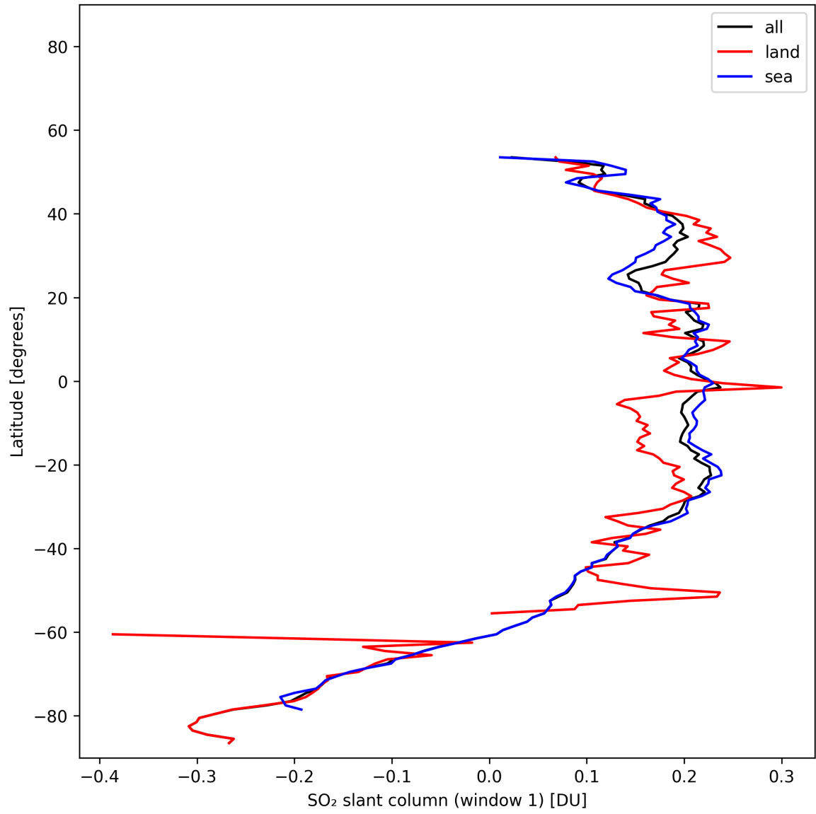
Figure 37: Zonal average of “SO 2 slant column (window 1)” for 2025-11-07 to 2025-11-08.
