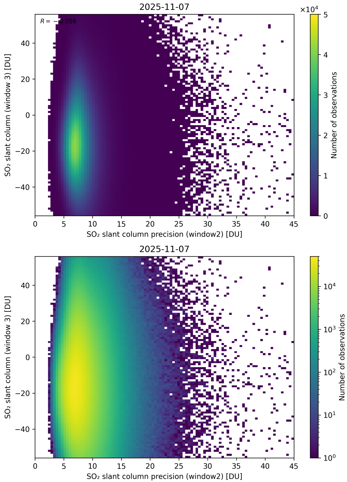
Figure 299: Scatter density plot of “SO 2 slant column precision (window2)” against “SO 2 slant column (window 3)” for 2025-11-07 to 2025-11-08.
