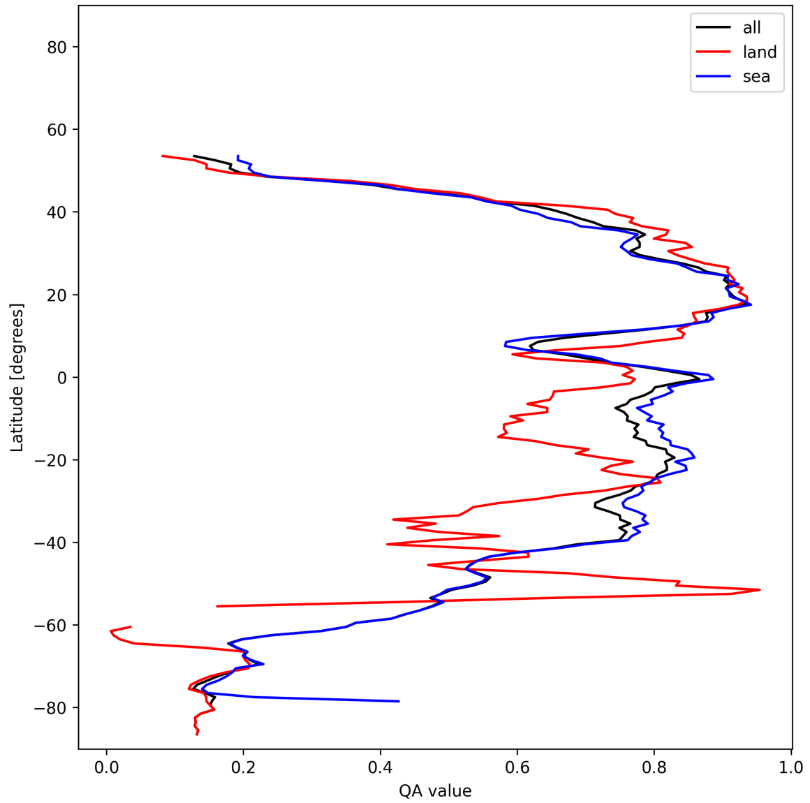
Figure 31: Zonal average of “QA value” for 2025-11-07 to 2025-11-08.
