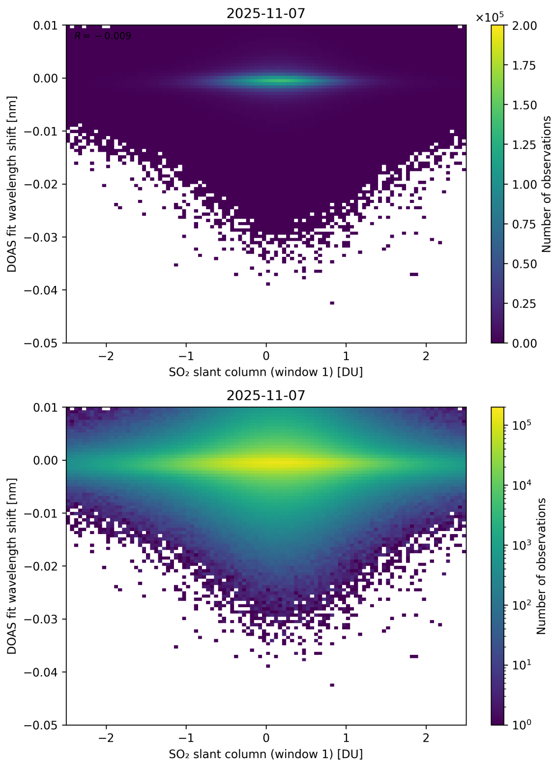
Figure 265: Scatter density plot of “SO 2 slant column (window 1)” against “DOAS fit wavelength shift” for 2025-11-07 to 2025-11-08.
