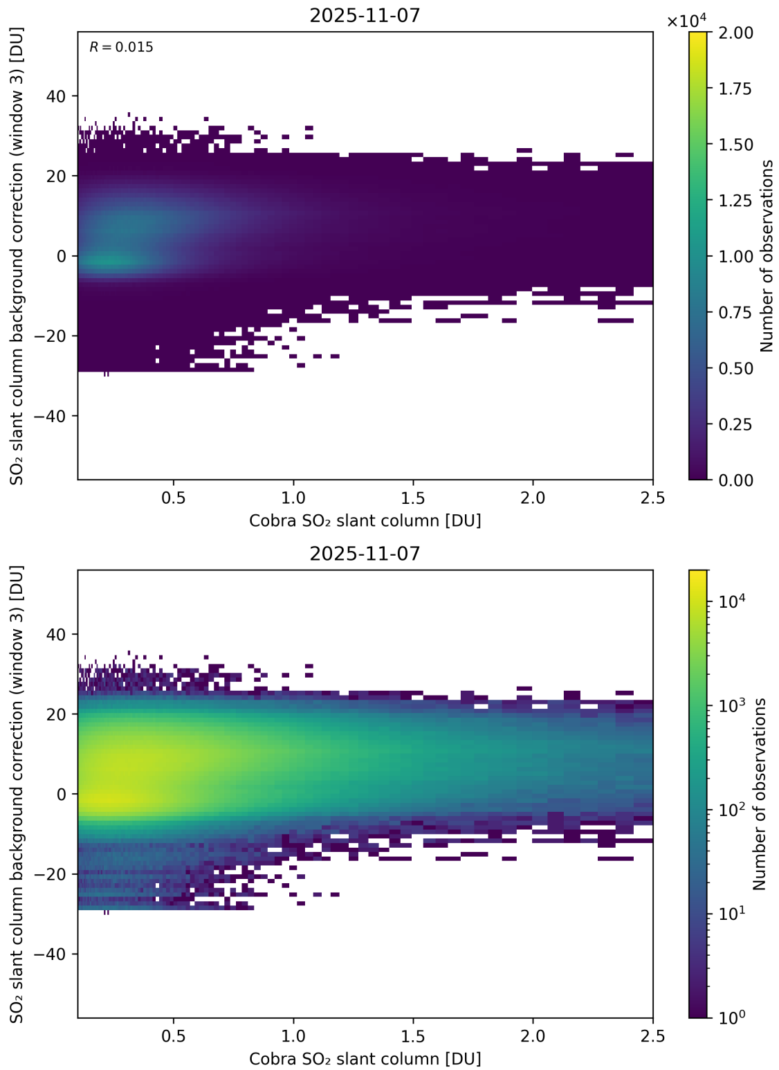
Figure 195: Scatter density plot of “Cobra SO 2 slant column” against “SO 2 slant column background correction (window 3)” for 2025-11-07 to 2025-11-08.
