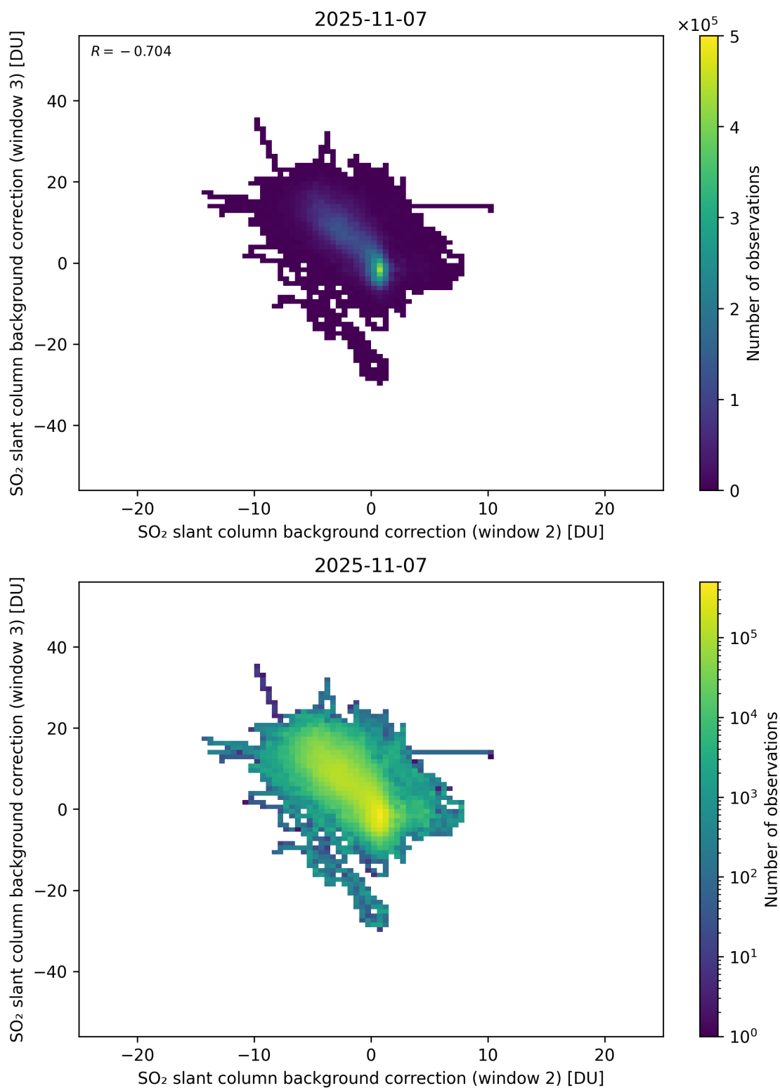
Figure 122: Scatter density plot of “SO 2 slant column background correction (window 2)” against “SO 2 slant column background correction (window 3)” for 2025-11-07 to 2025-11-08.
