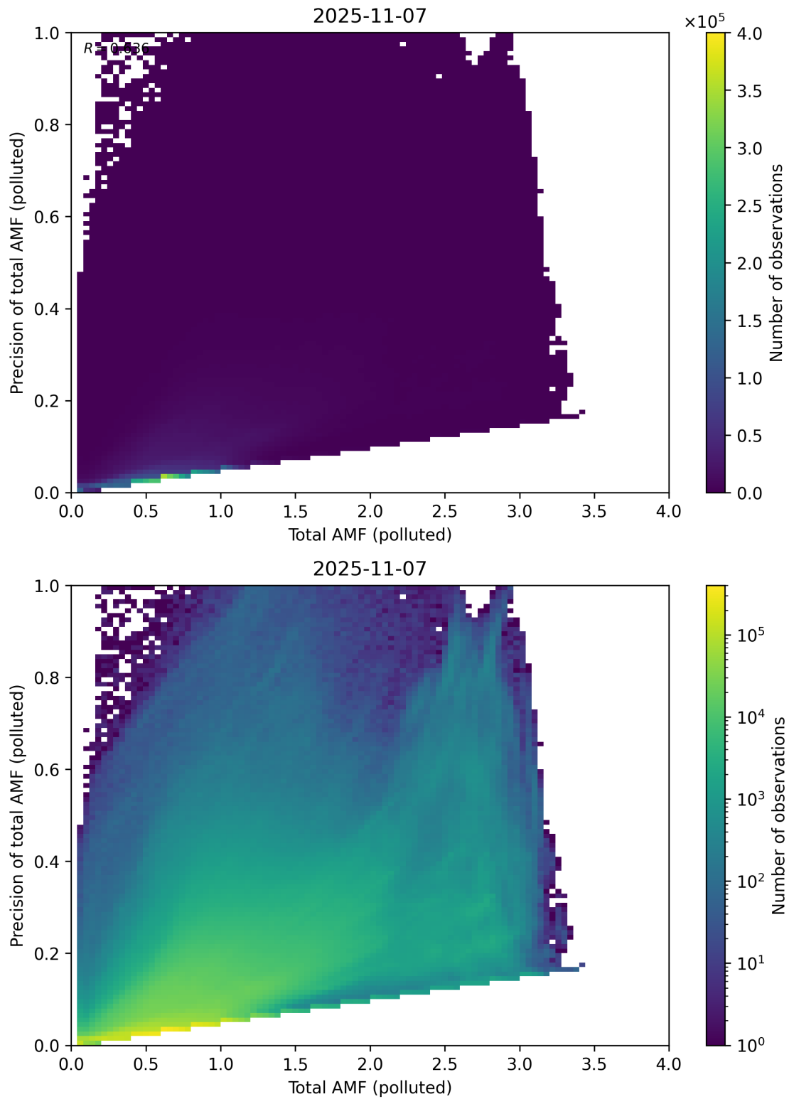
Figure 322: Scatter density plot of “Total AMF (polluted)” against “Precision of total AMF (polluted)” for 2025-11-07 to 2025-11-08.
