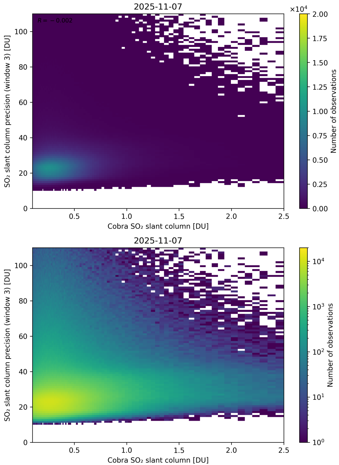
Figure 223: Scatter density plot of “Cobra SO 2 slant column” against “SO 2 slant column precision (window 3)” for 2025-11-07 to 2025-11-08.
