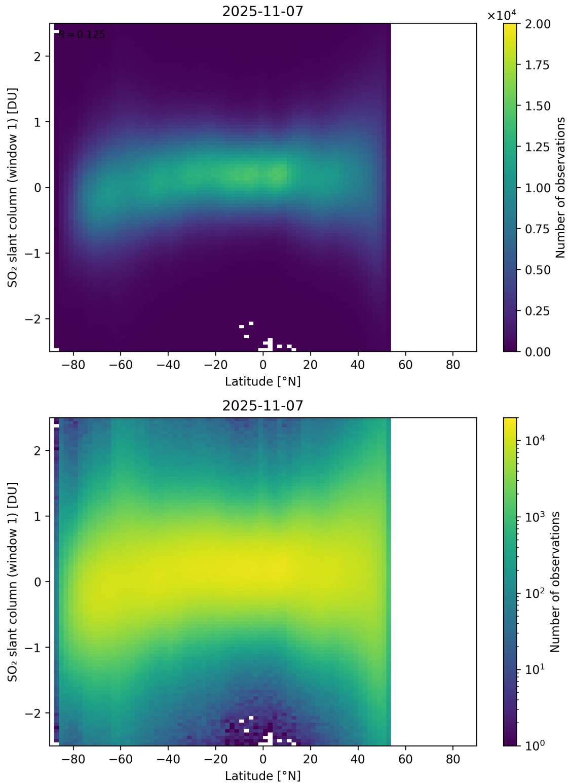
Figure 162: Scatter density plot of “Latitude” against “SO 2 slant column (window 1)” for 2025-11-07 to 2025-11-08.
