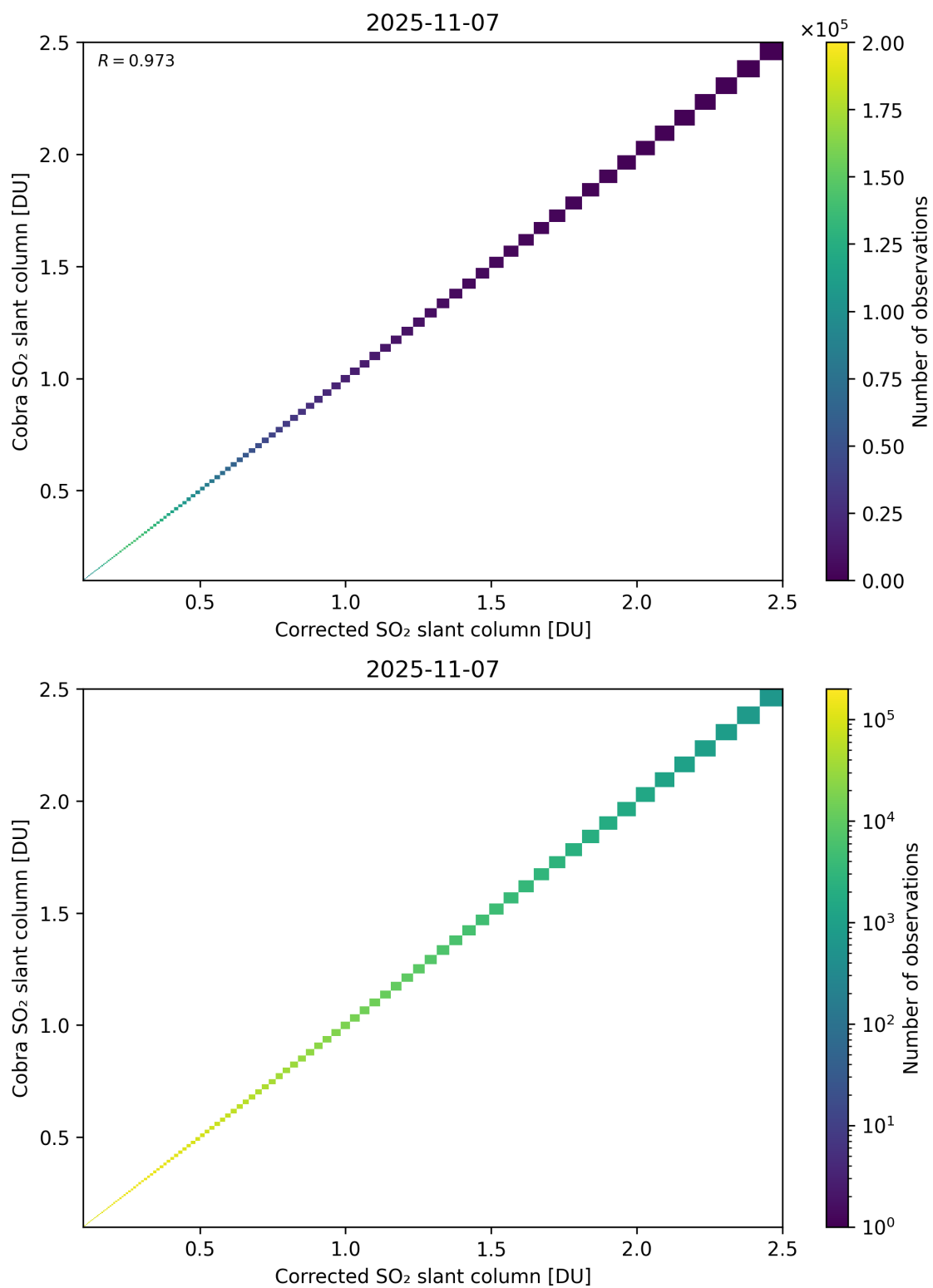
Figure 233: Scatter density plot of “Corrected SO 2 slant column” against “Cobra SO 2 slant column” for 2025-11-07 to 2025-11-08.
