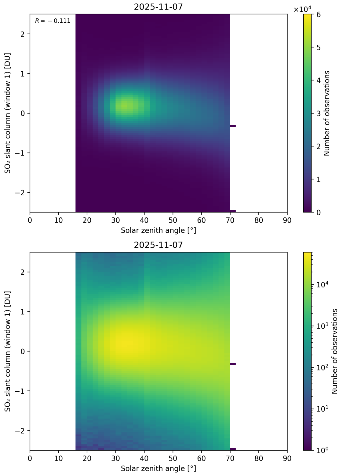
Figure 184: Scatter density plot of “Solar zenith angle” against “SO 2 slant column (window 1)” for 2025-11-07 to 2025-11-08.
