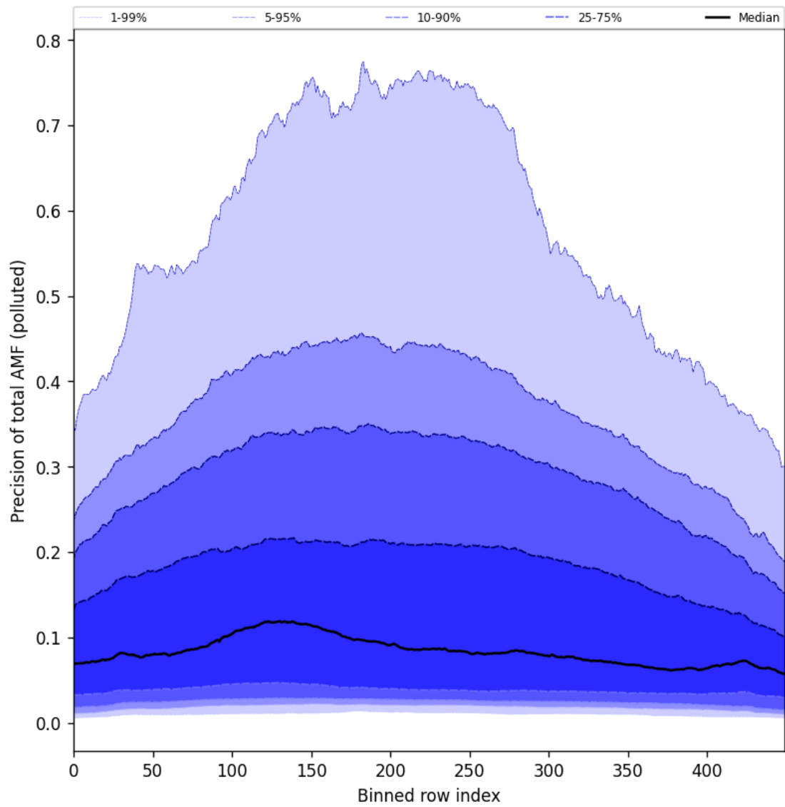
Figure 106: Along track statistics of “Precision of total AMF (polluted)” for 2025-11-07 to 2025-11-08
