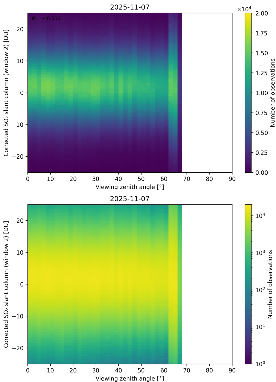
Figure 374: Scatter density plot of “Viewing zenith angle” against “Corrected SO 2 slant column (window 2)” for 2025-11-07 to 2025-11-08.
