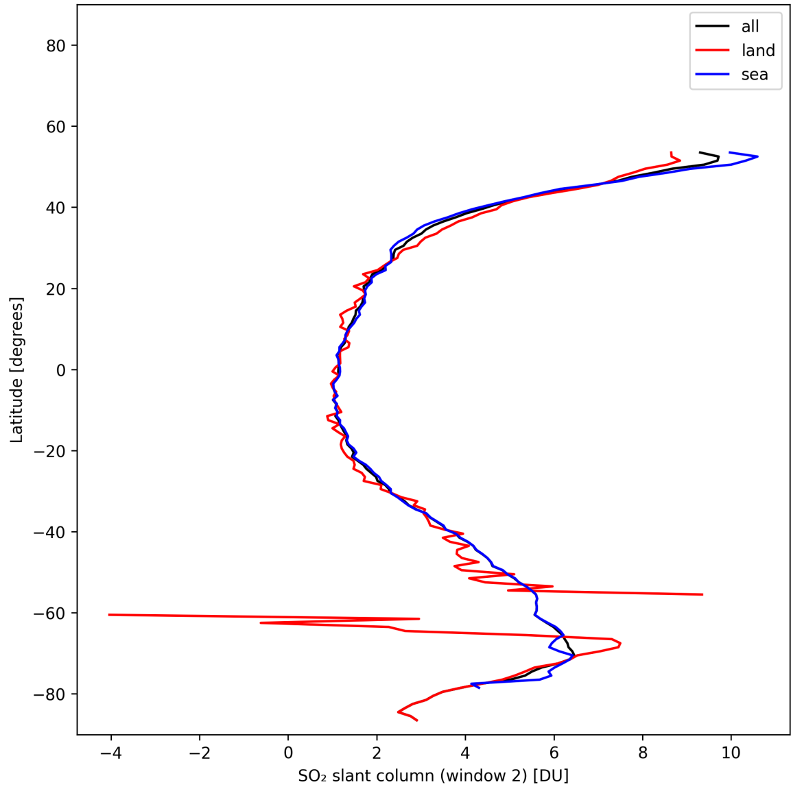
Figure 41: Zonal average of “SO 2 slant column (window 2)” for 2025-11-07 to 2025-11-08.
