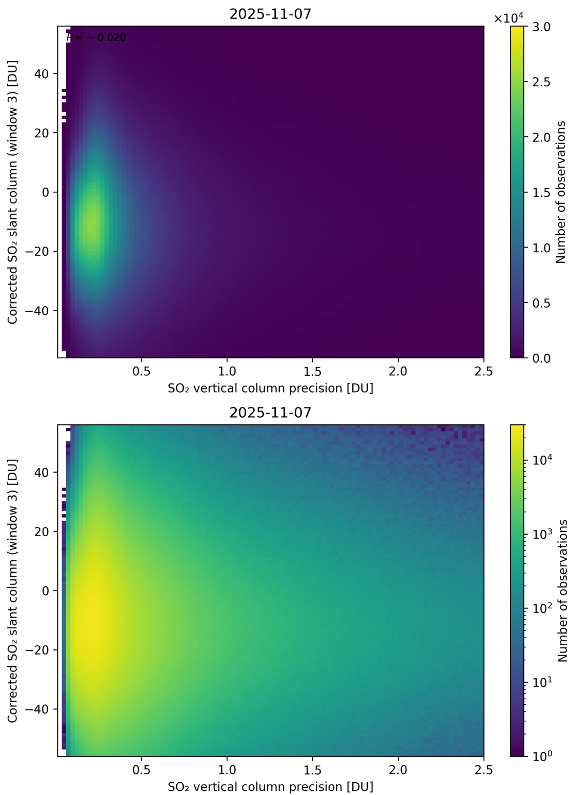
Figure 340: Scatter density plot of “SO 2 vertical column precision” against “Corrected SO 2 slant column (window 3)” for 2025-11-07 to 2025-11-08.
