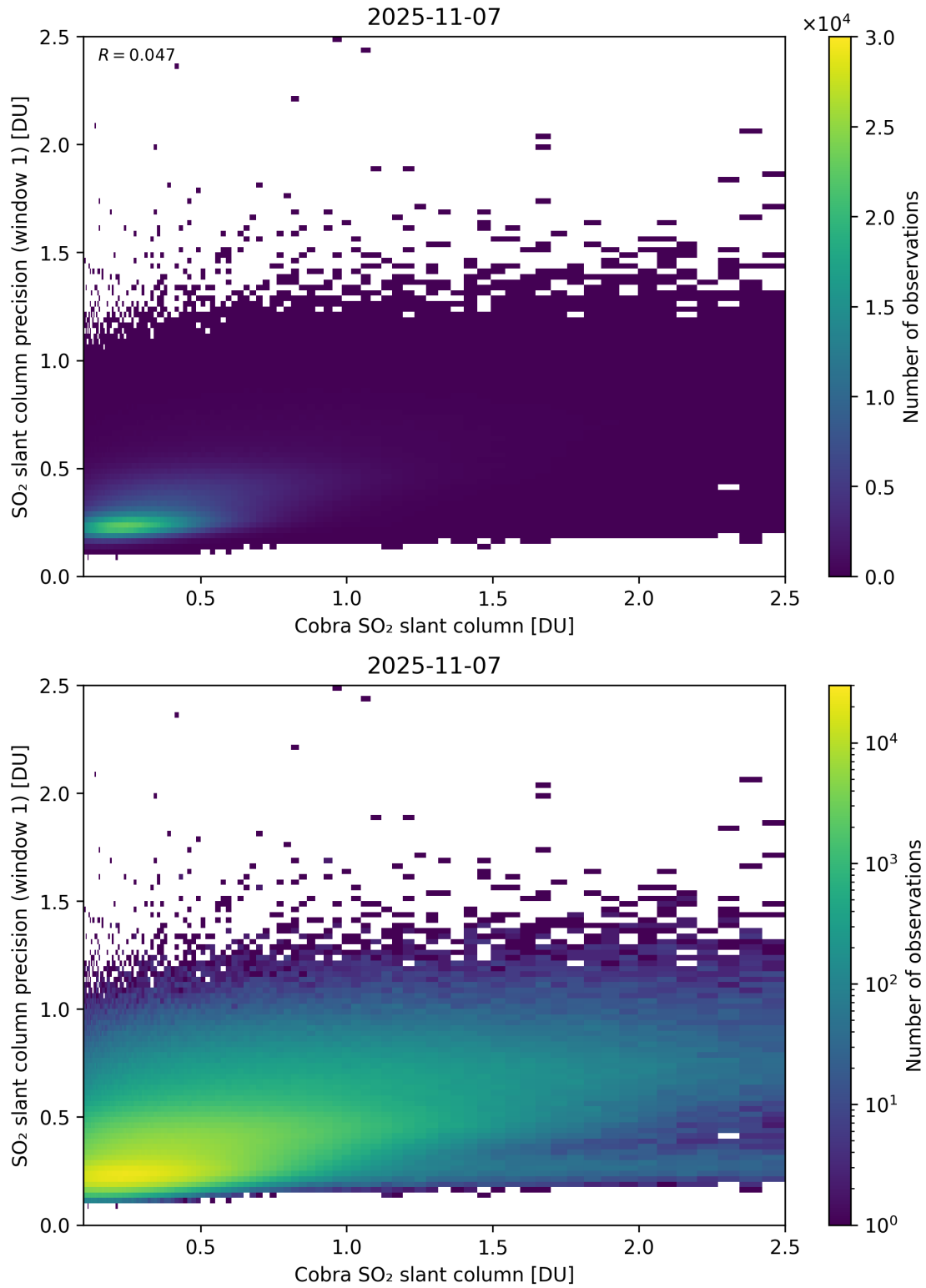
Figure 220: Scatter density plot of “Cobra SO 2 slant column” against “SO 2 slant column precision (window 1)” for 2025-11-07 to 2025-11-08.
