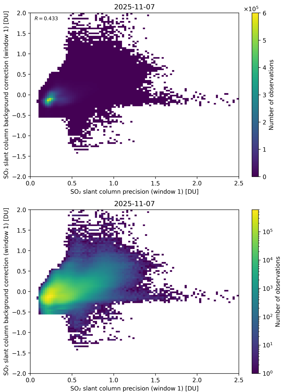
Figure 268: Scatter density plot of “SO 2 slant column precision (window 1)” against “SO 2 slant column background correction (window 1)” for 2025-11-07 to 2025-11-08.
