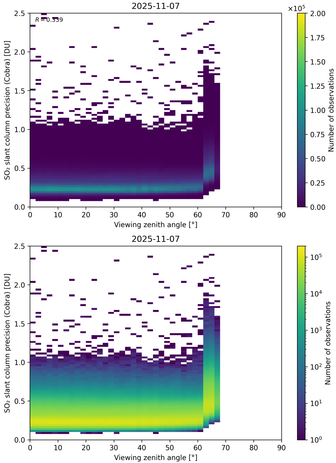
Figure 372: Scatter density plot of “Viewing zenith angle” against “SO 2 slant column precision (Cobra)” for 2025-11-07 to 2025-11-08.
