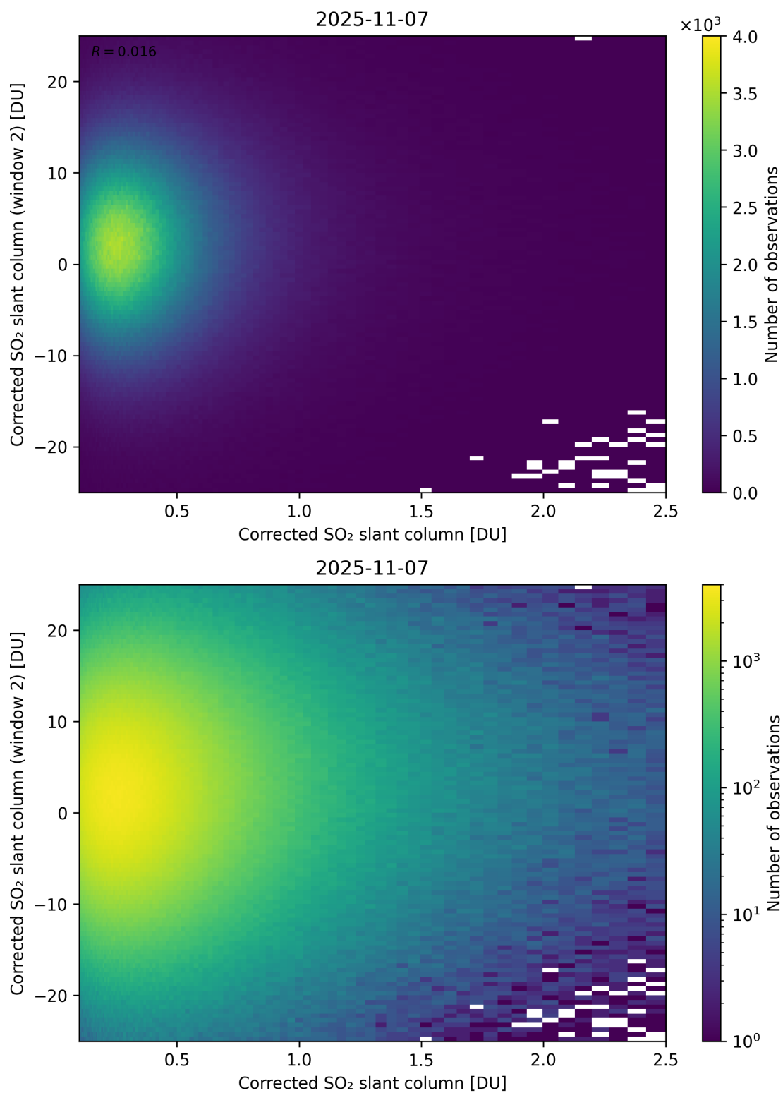
Figure 235: Scatter density plot of “Corrected SO 2 slant column” against “Corrected SO 2 slant column (window 2)” for 2025-11-07 to 2025-11-08.
