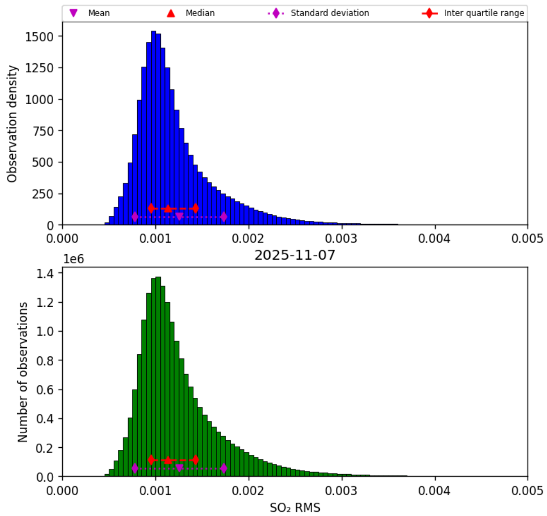
Figure 78: Histogram of “SO 2 RMS” for 2025-11-07 to 2025-11-08
