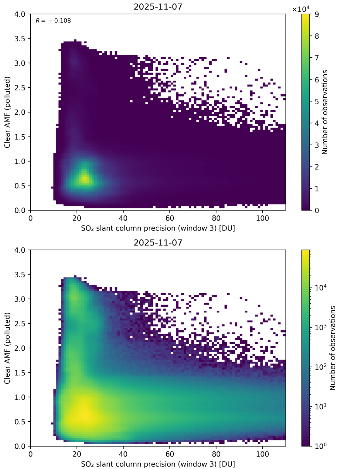
Figure 311: Scatter density plot of “SO 2 slant column precision (window 3)” against “Clear AMF (polluted)” for 2025-11-07 to 2025-11-08.
