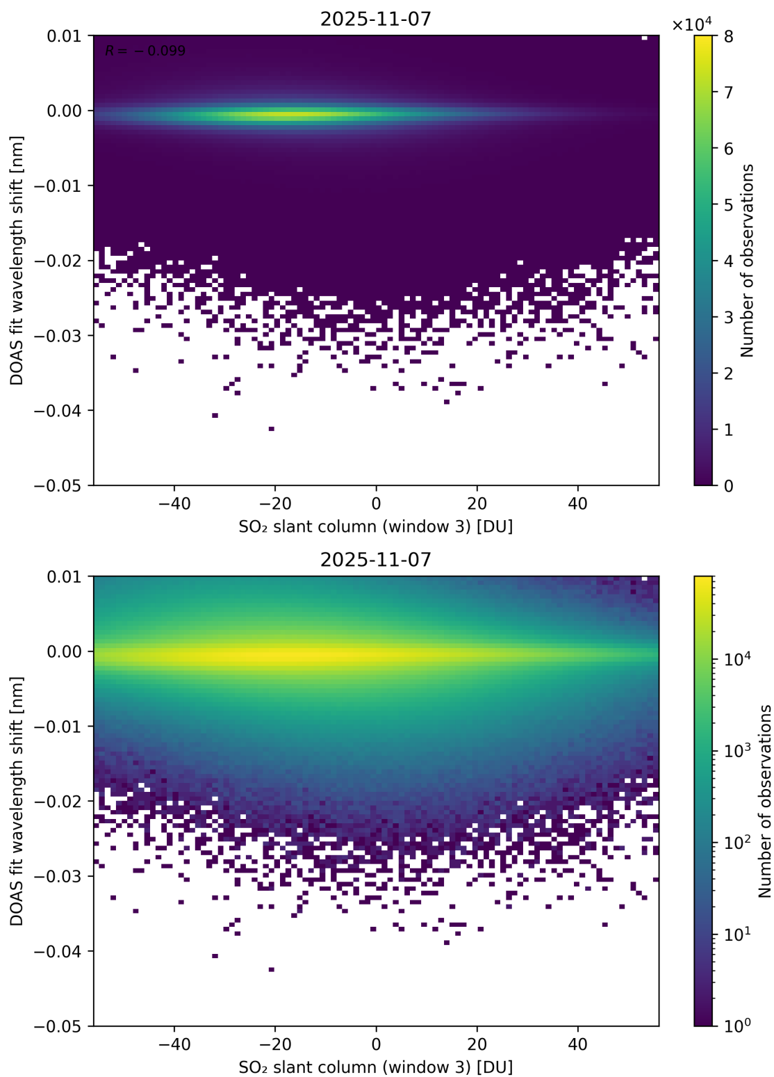
Figure 304: Scatter density plot of “SO 2 slant column (window 3)” against “DOAS fit wavelength shift” for 2025-11-07 to 2025-11-08.
