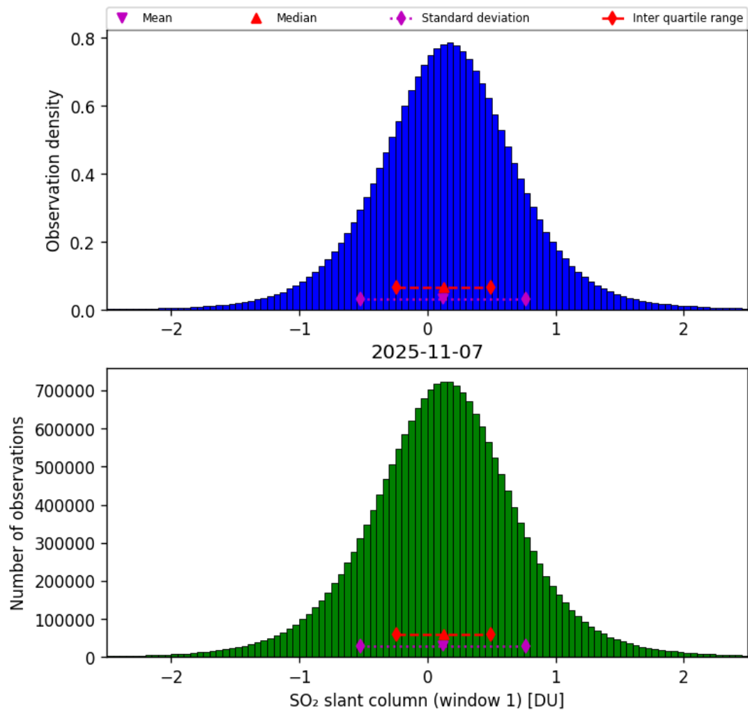
Figure 63: Histogram of “SO 2 slant column (window 1)” for 2025-11-07 to 2025-11-08
