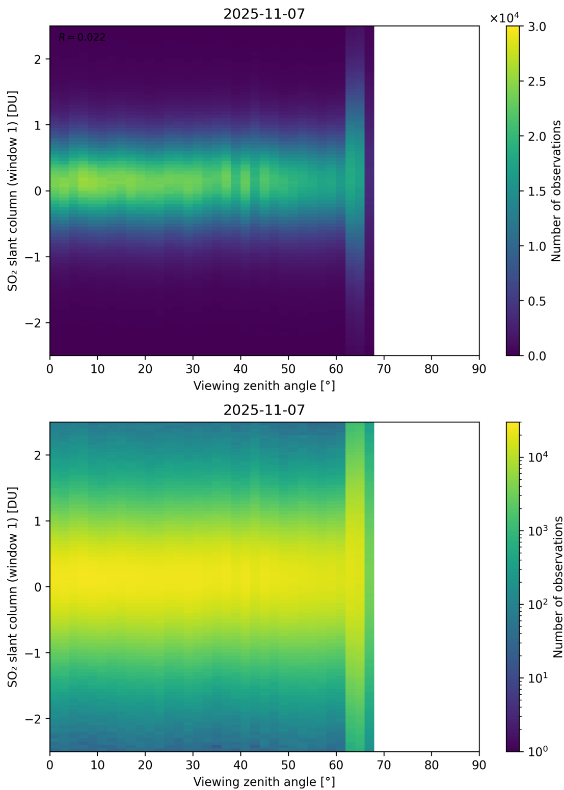
Figure 376: Scatter density plot of “Viewing zenith angle” against “SO 2 slant column (window 1)” for 2025-11-07 to 2025-11-08.
