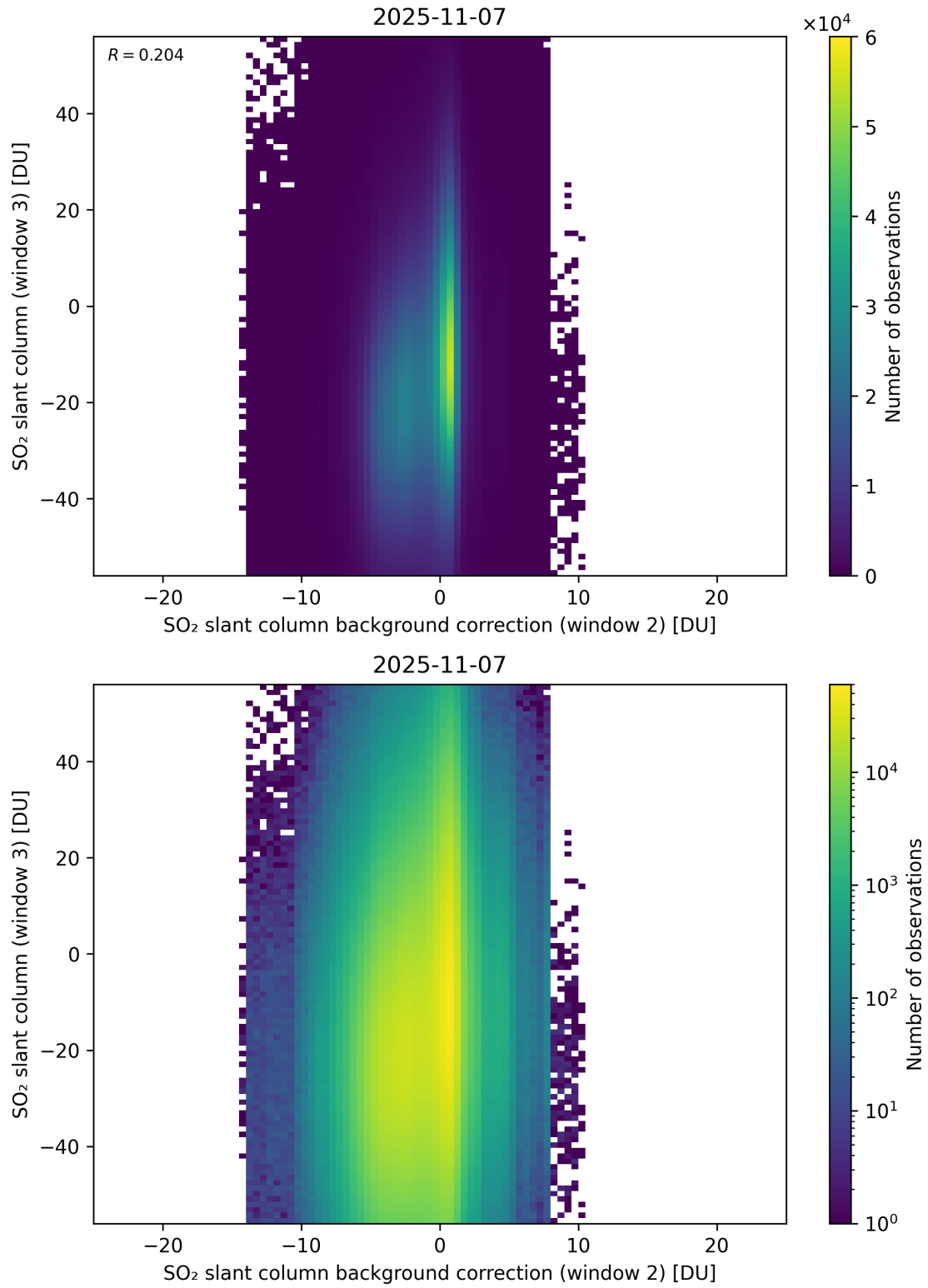
Figure 128: Scatter density plot of “SO 2 slant column background correction (window 2)” against “SO 2 slant column (window 3)” for 2025-11-07 to 2025-11-08.
