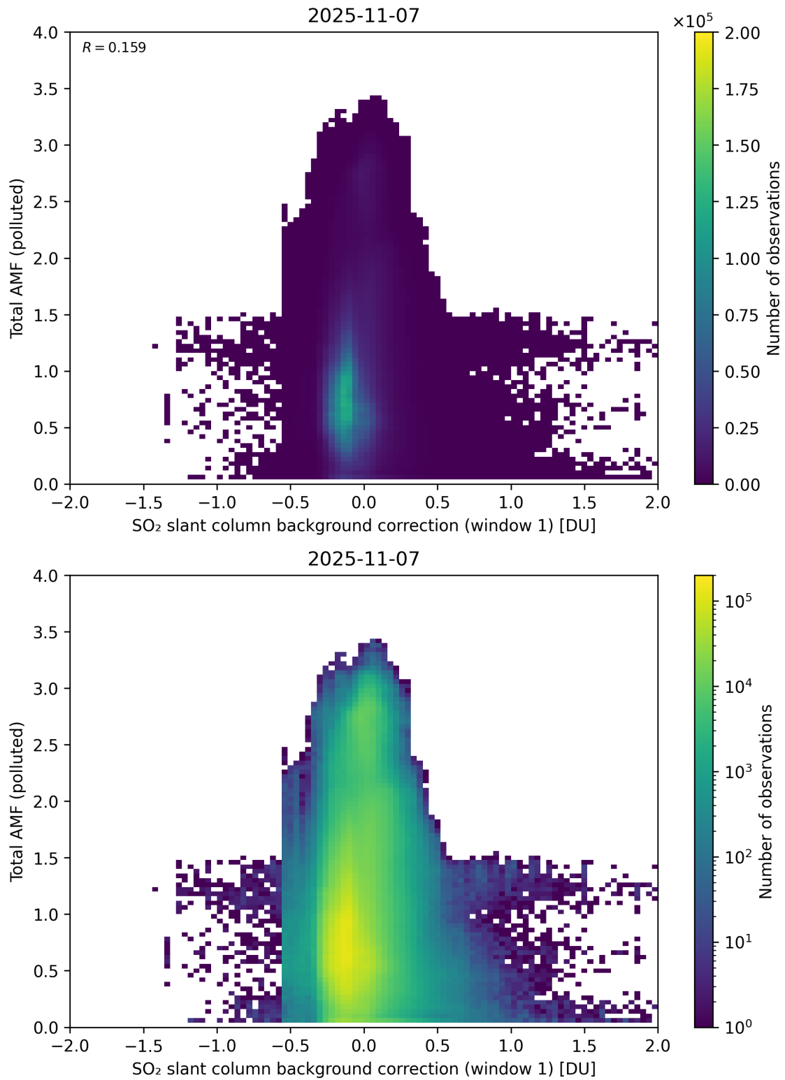
Figure 120: Scatter density plot of “SO 2 slant column background correction (window 1)” against “Total AMF (polluted)” for 2025-11-07 to 2025-11-08.
