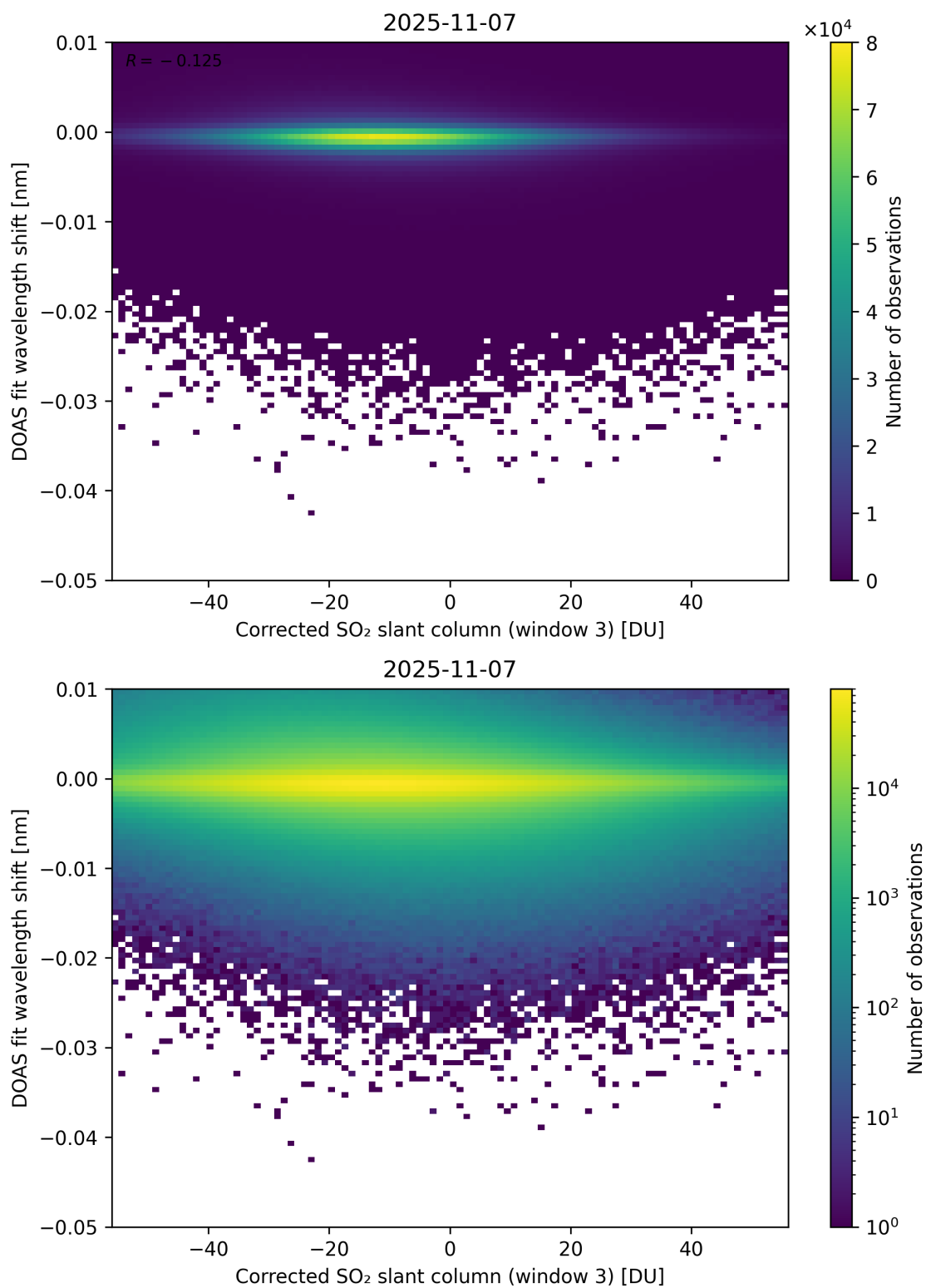
Figure 256: Scatter density plot of “Corrected SO 2 slant column (window 3)” against “DOAS fit wavelength shift” for 2025-11-07 to 2025-11-08.
