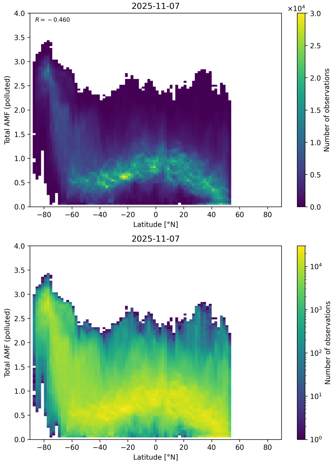
Figure 167: Scatter density plot of “Latitude” against “Total AMF (polluted)” for 2025-11-07 to 2025-11-08.
