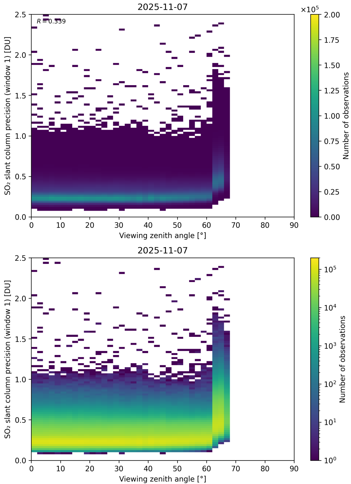
Figure 377: Scatter density plot of “Viewing zenith angle” against “SO 2 slant column precision (window 1)” for 2025-11-07 to 2025-11-08.
