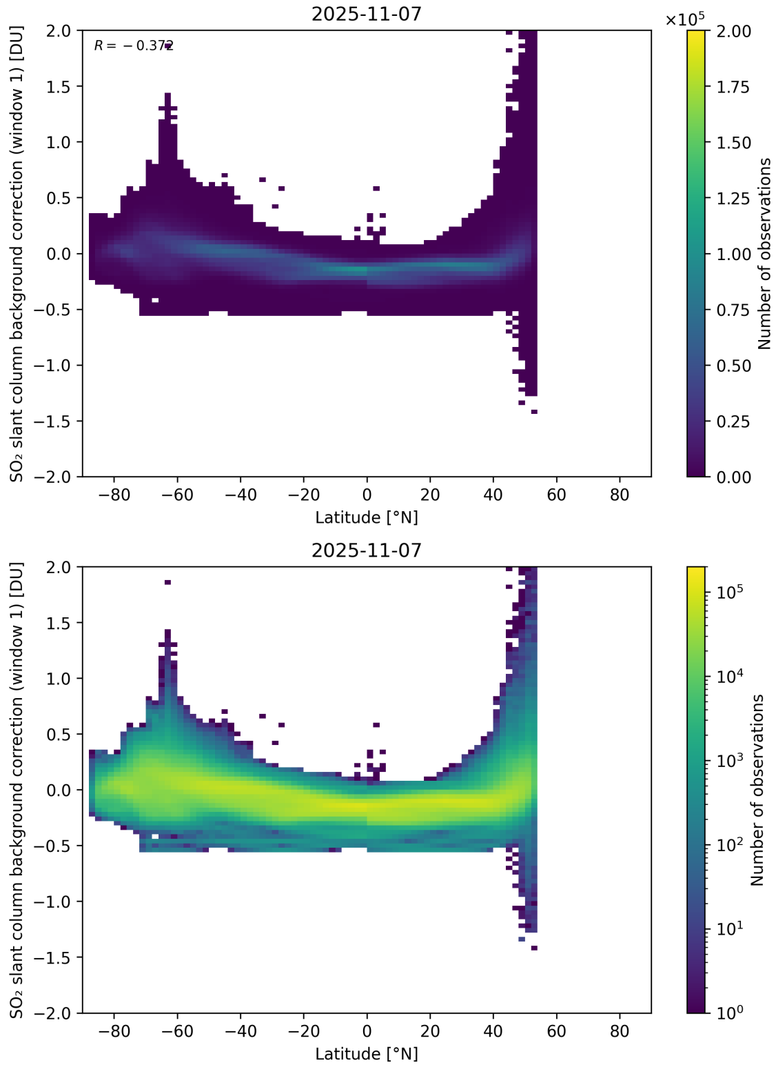
Figure 150: Scatter density plot of “Latitude” against “SO 2 slant column background correction (window 1)” for 2025-11-07 to 2025-11-08.
