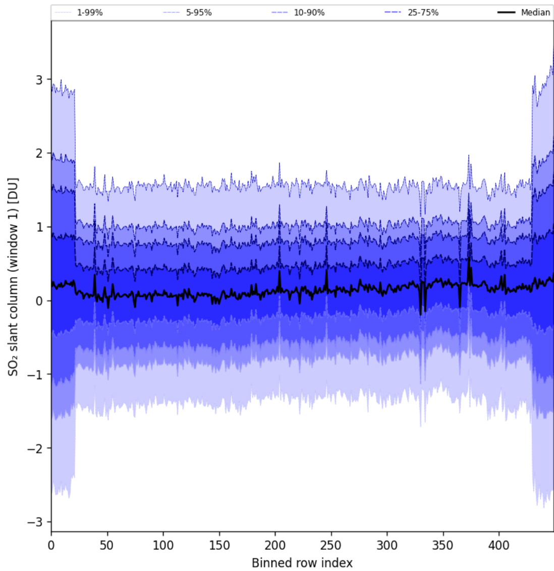
Figure 89: Along track statistics of “SO 2 slant column (window 1)” for 2025-11-07 to 2025-11-08
