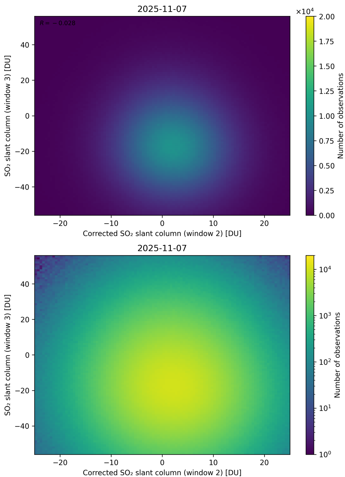
Figure 251: Scatter density plot of “Corrected SO 2 slant column (window 2)” against “SO 2 slant column (window 3)” for 2025-11-07 to 2025-11-08.
