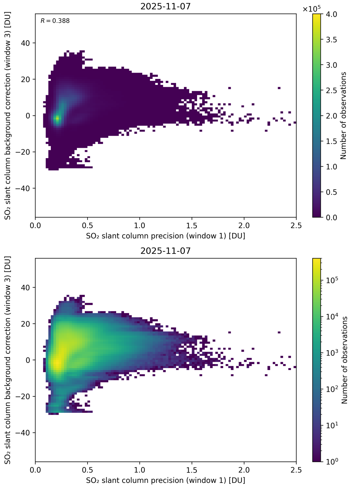
Figure 270: Scatter density plot of “SO 2 slant column precision (window 1)” against “SO 2 slant column background correction (window 3)” for 2025-11-07 to 2025-11-08.
