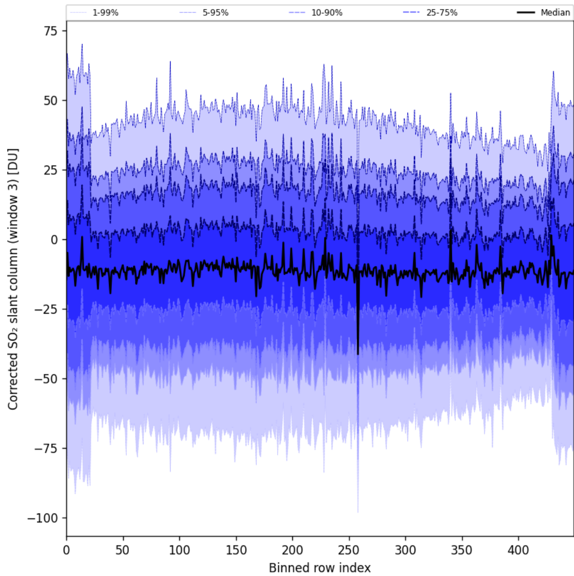
Figure 99: Along track statistics of “Corrected SO 2 slant column (window 3)” for 2025-11-07 to 2025-11-08
