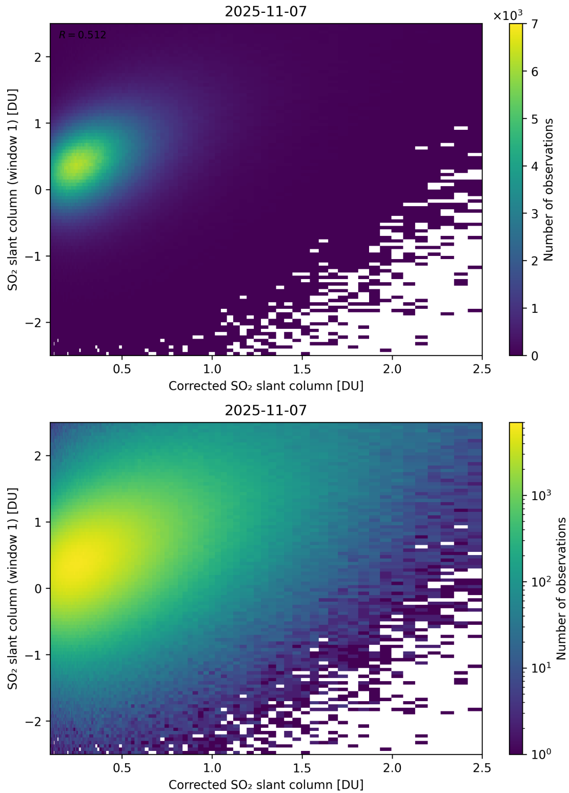
Figure 237: Scatter density plot of “Corrected SO 2 slant column” against “SO 2 slant column (window 1)” for 2025-11-07 to 2025-11-08.
