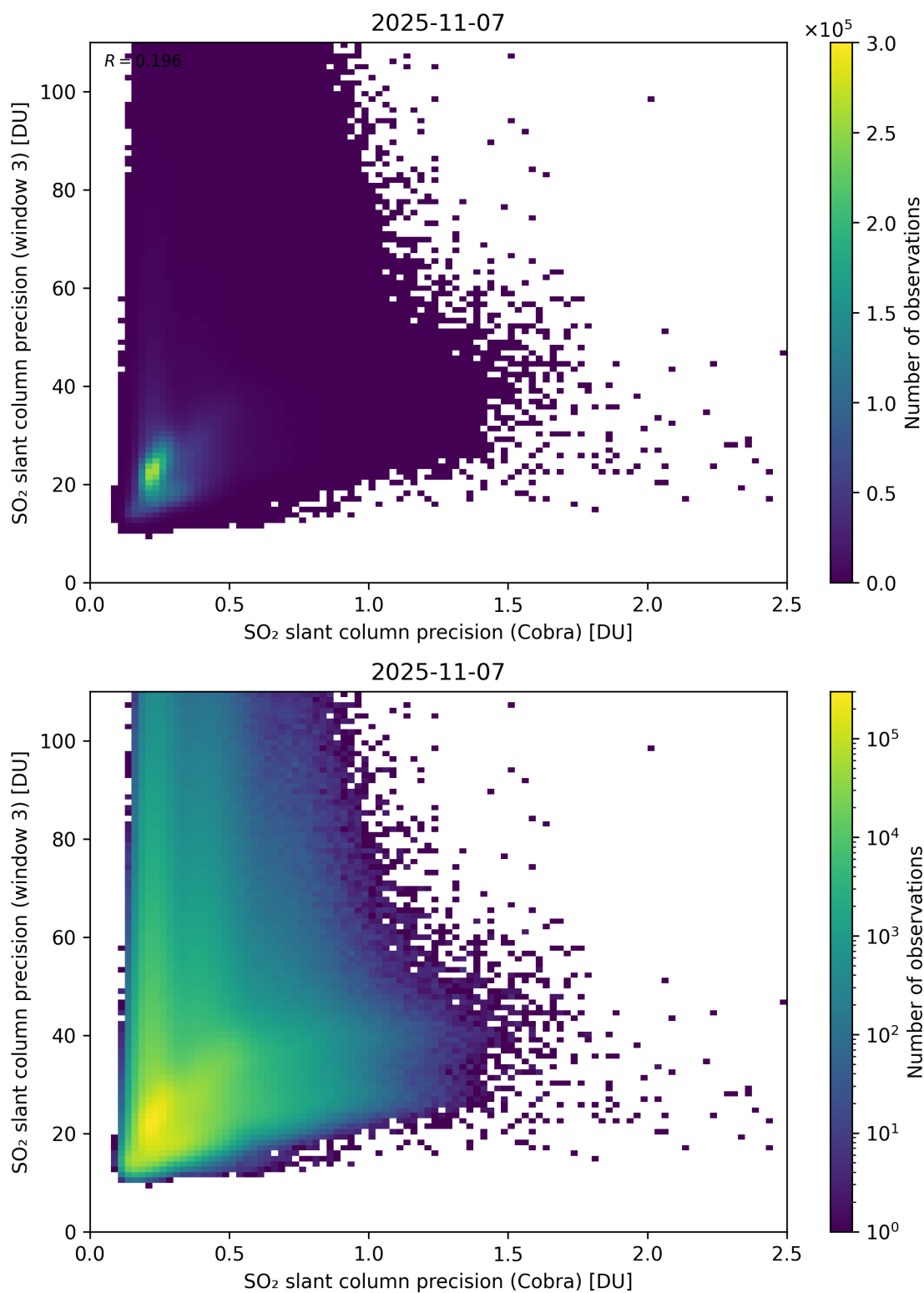
Figure 212: Scatter density plot of “SO 2 slant column precision (Cobra)” against “SO 2 slant column precision (window 3)” for 2025-11-07 to 2025-11-08.
