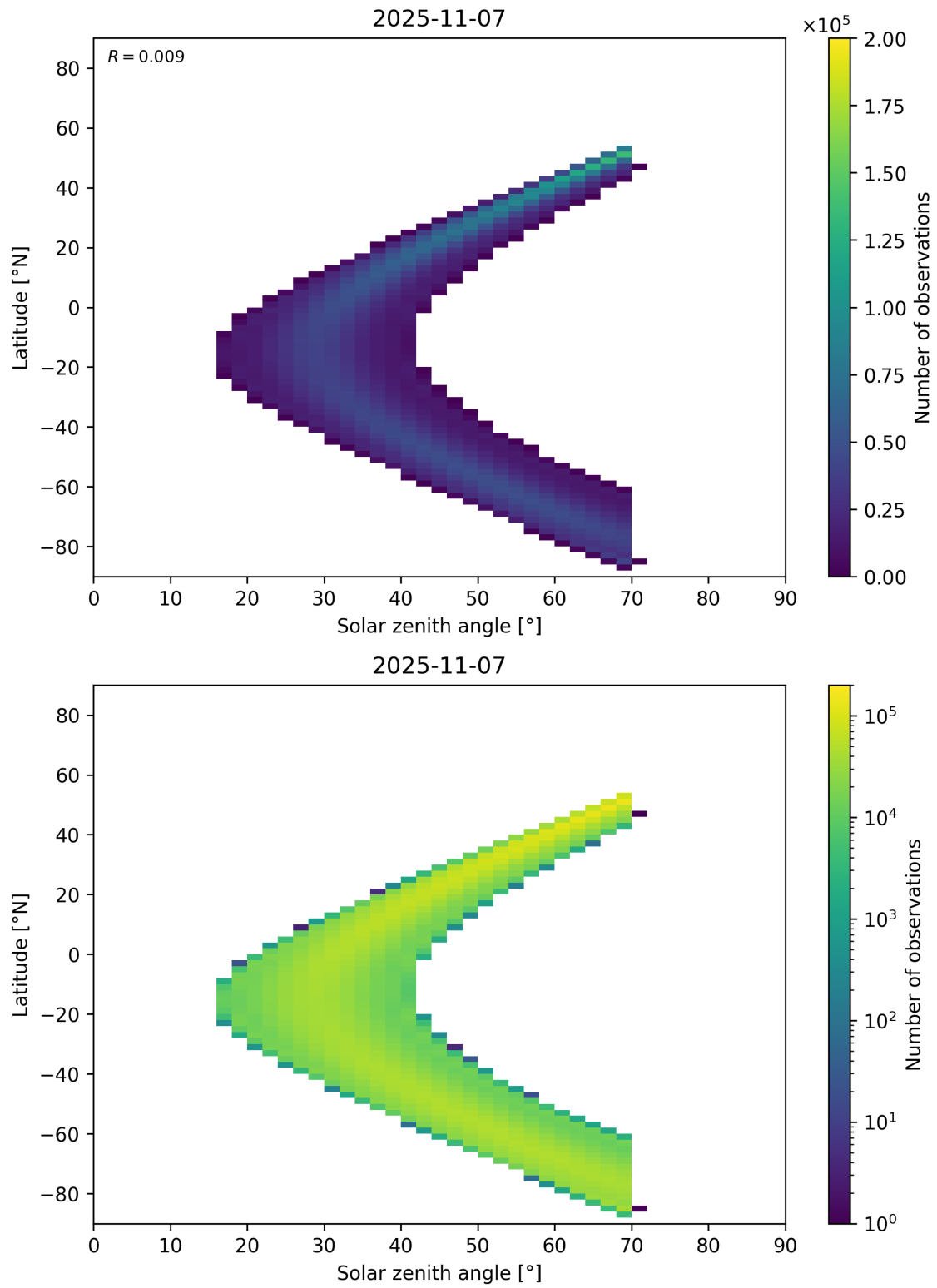
Figure 177: Scatter density plot of “Solar zenith angle” against “Latitude” for 2025-11-07 to 2025-11-08.
