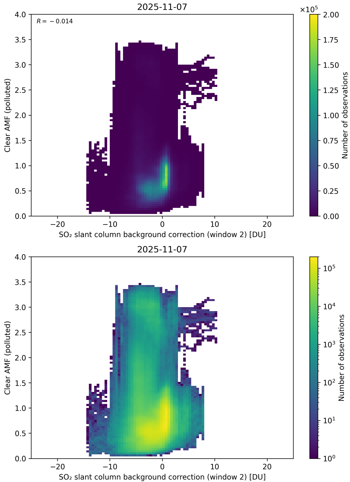
Figure 126: Scatter density plot of “SO 2 slant column background correction (window 2)” against “Clear AMF (polluted)” for 2025-11-07 to 2025-11-08.
