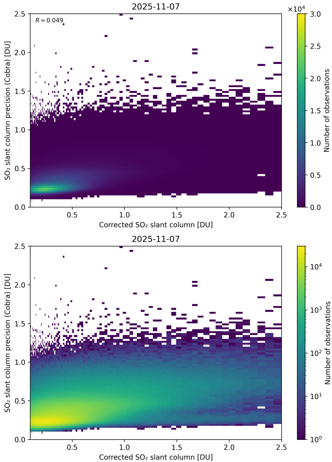
Figure 234: Scatter density plot of “Corrected SO 2 slant column” against “SO 2 slant column precision (Cobra)” for 2025-11-07 to 2025-11-08.
