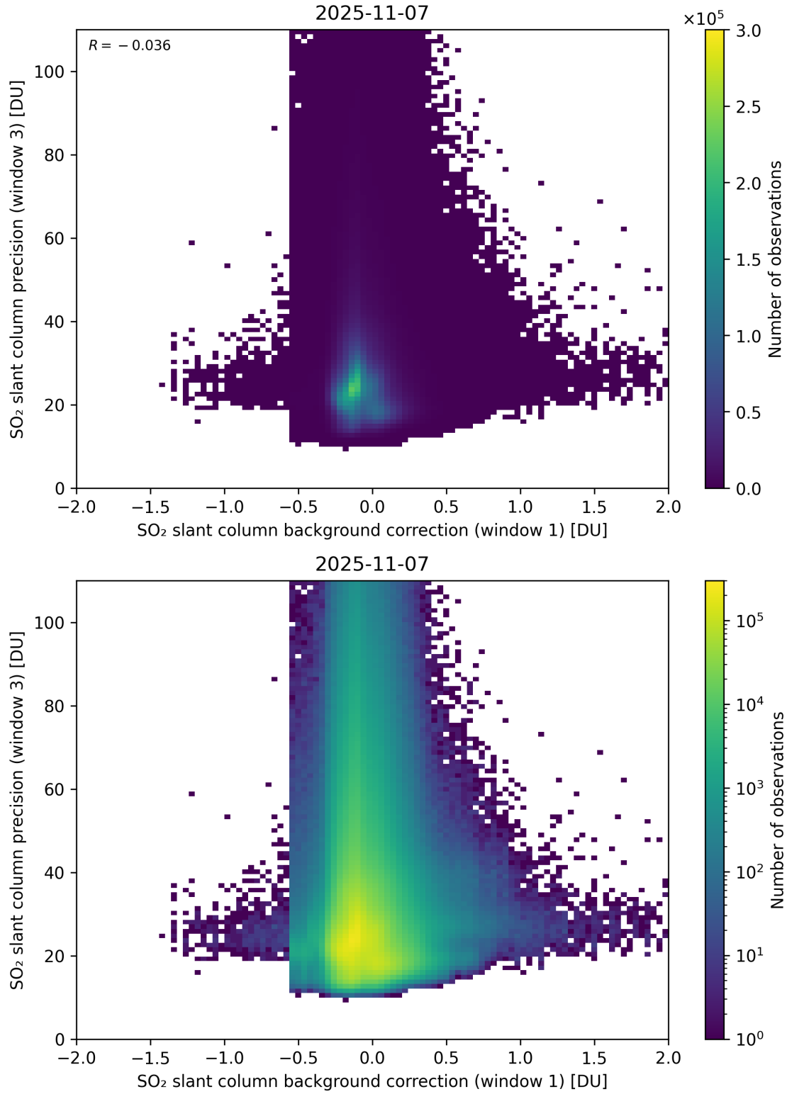
Figure 119: Scatter density plot of “SO 2 slant column background correction (window 1)” against “SO 2 slant column precision (window 3)” for 2025-11-07 to 2025-11-08.
