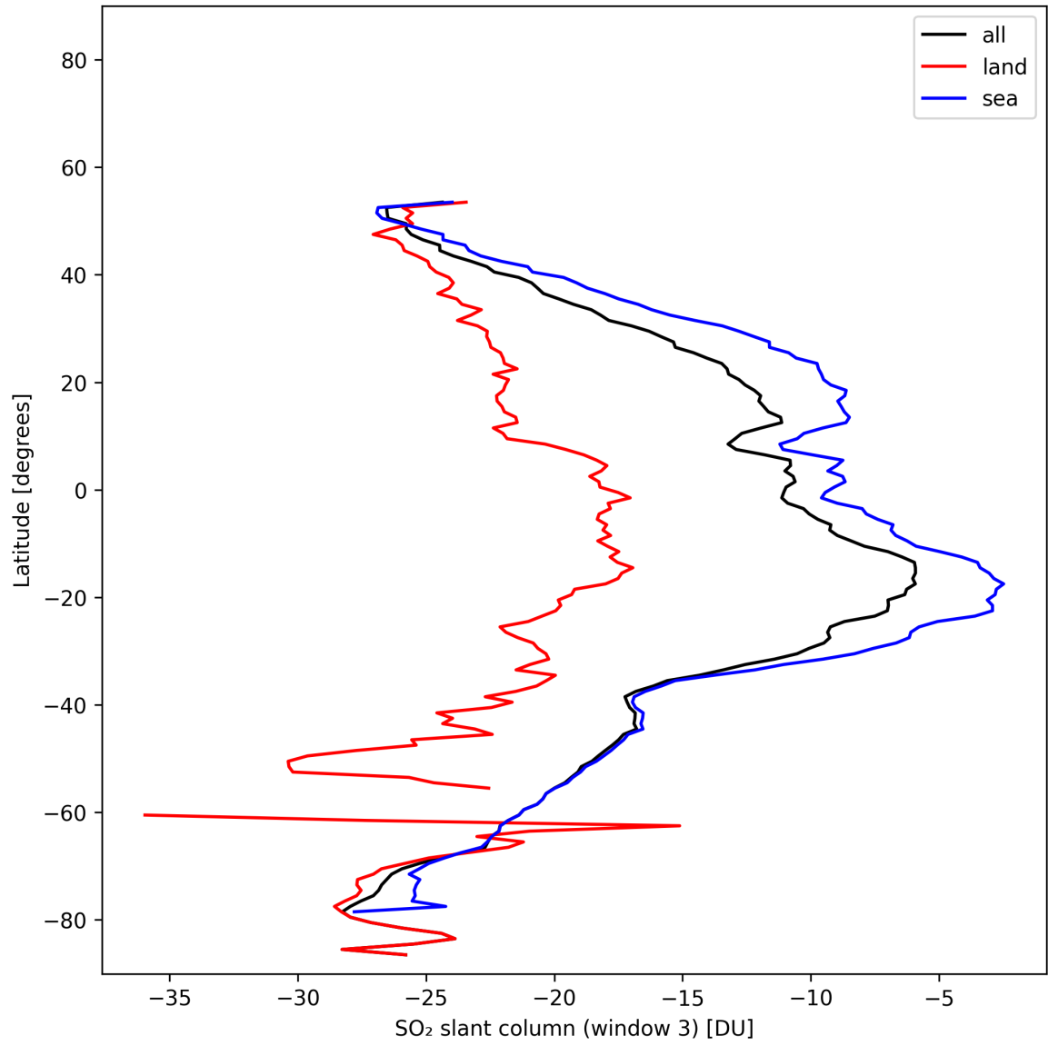
Figure 45: Zonal average of “SO 2 slant column (window 3)” for 2025-11-07 to 2025-11-08.
