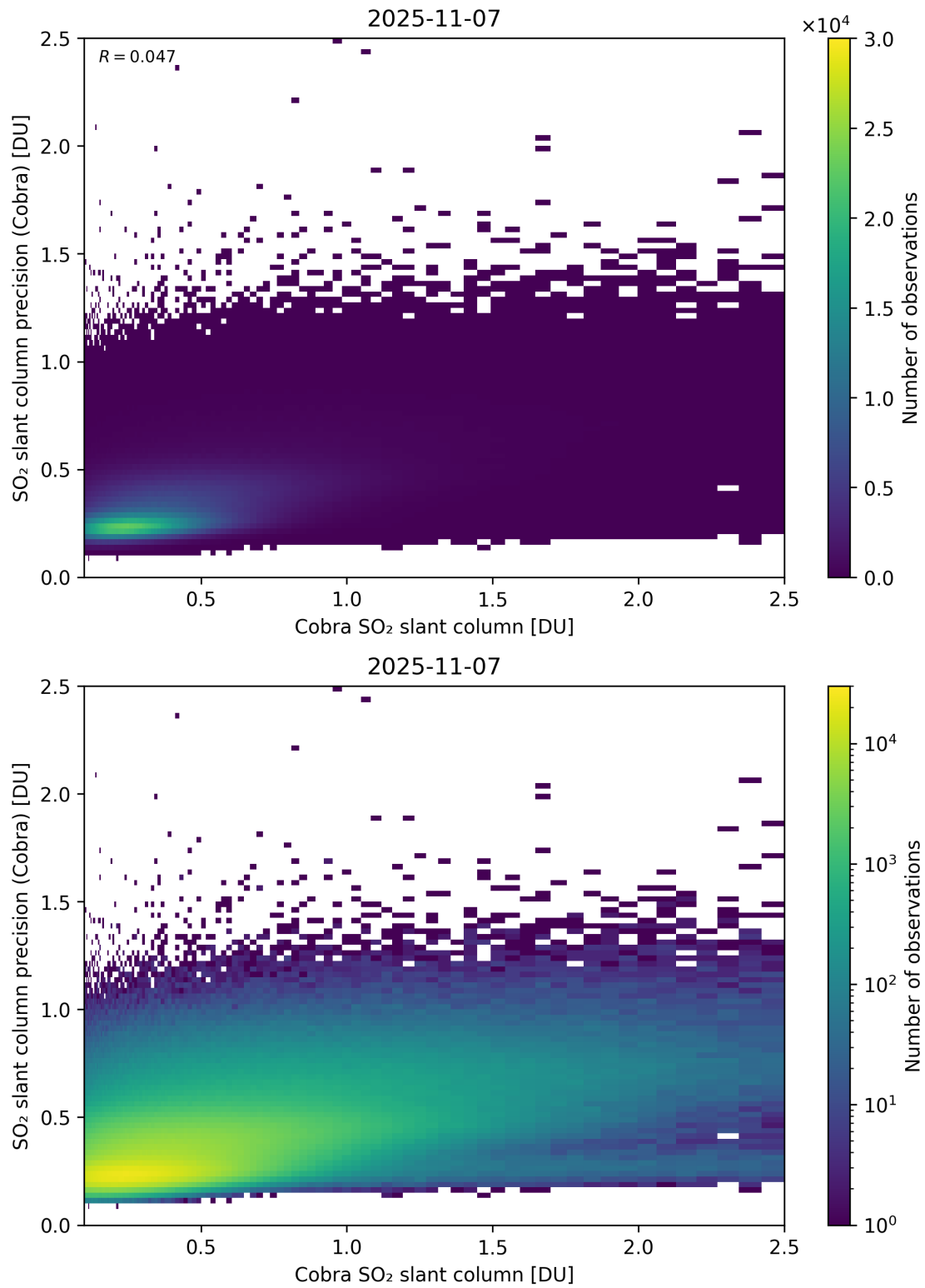
Figure 216: Scatter density plot of “Cobra SO 2 slant column” against “SO 2 slant column precision (Cobra)” for 2025-11-07 to 2025-11-08.
