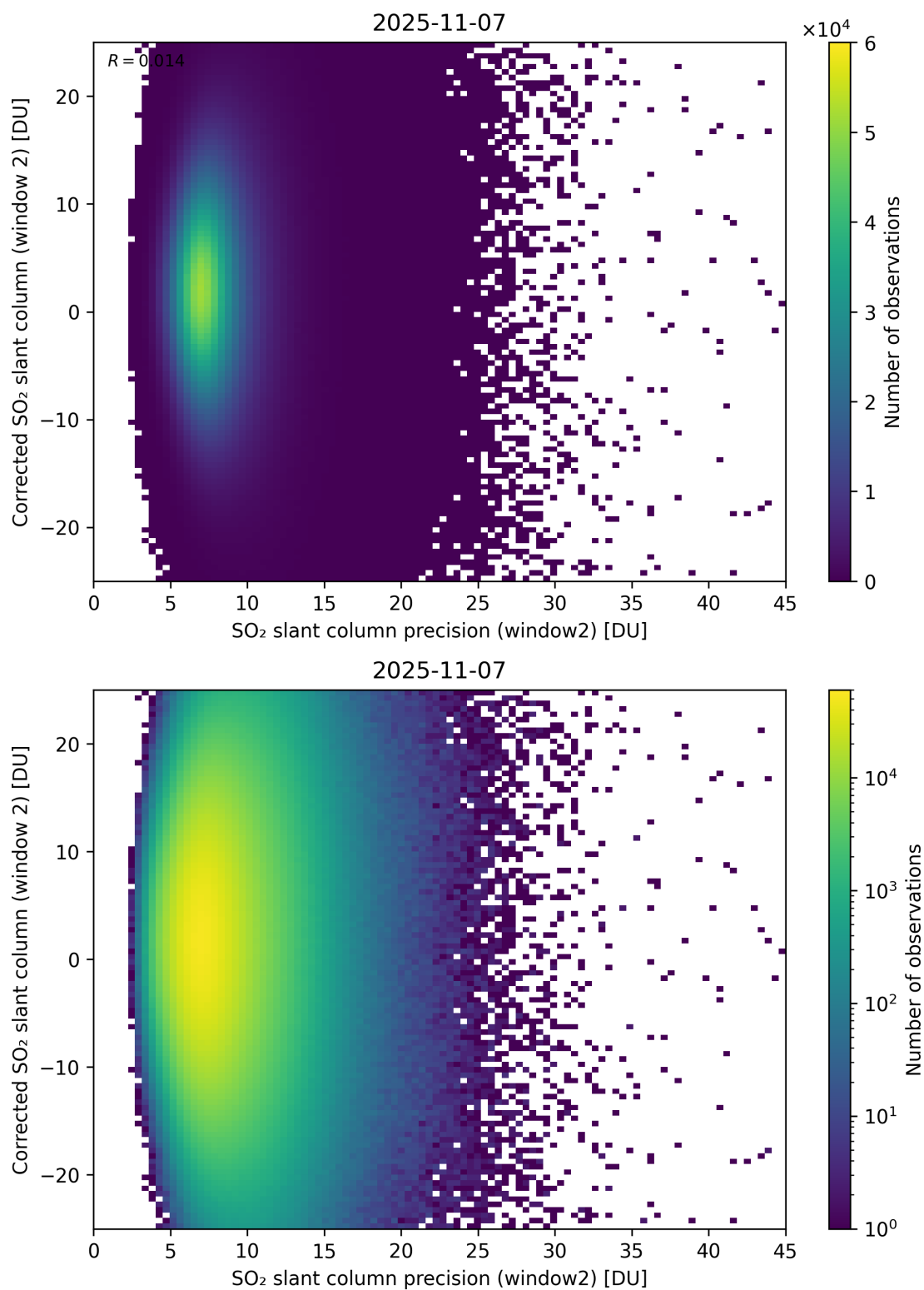
Figure 297: Scatter density plot of “SO 2 slant column precision (window2)” against “Corrected SO 2 slant column (window 2)” for 2025-11-07 to 2025-11-08.
