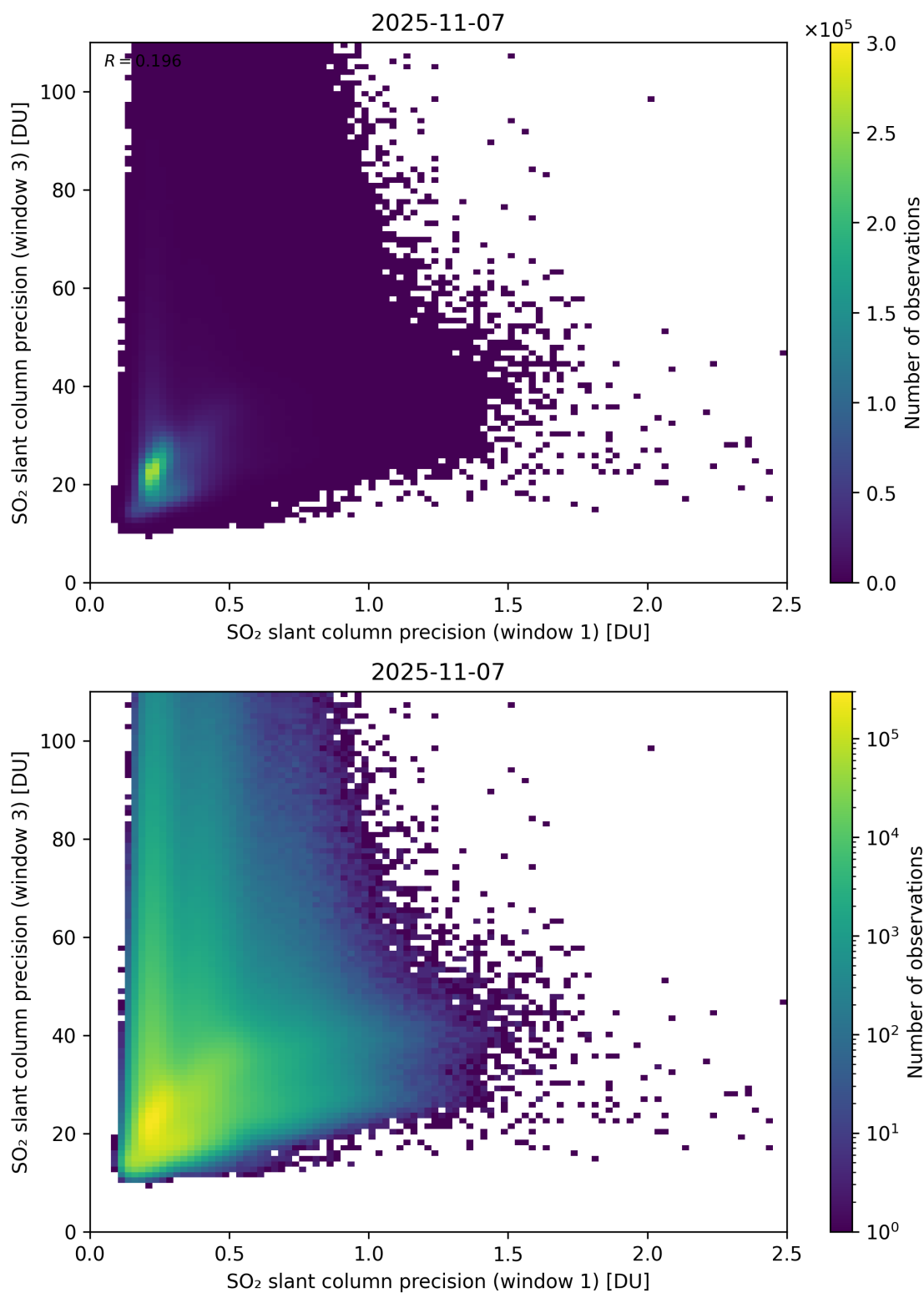
Figure 279: Scatter density plot of “SO 2 slant column precision (window 1)” against “SO 2 slant column precision (window 3)” for 2025-11-07 to 2025-11-08.
