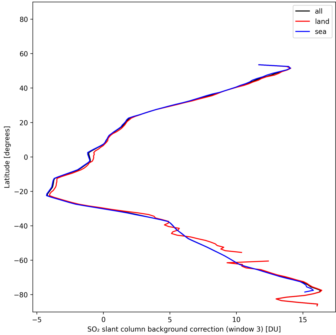
Figure 48: Zonal average of “SO 2 slant column background correction (window 3)” for 2025-11-07 to 2025-11-08.
