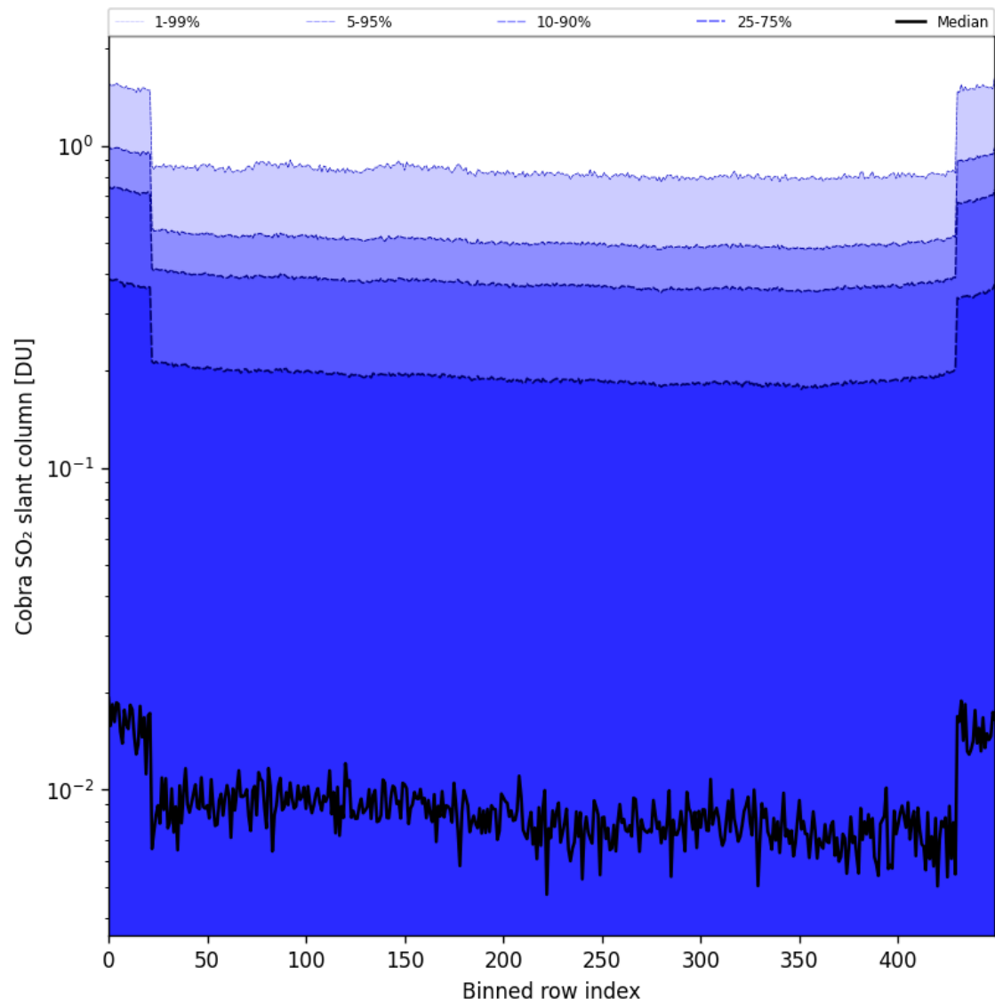
Figure 87: Along track statistics of "Cobra SO 2 slant column" for 2025-11-07 to 2025-11-08
