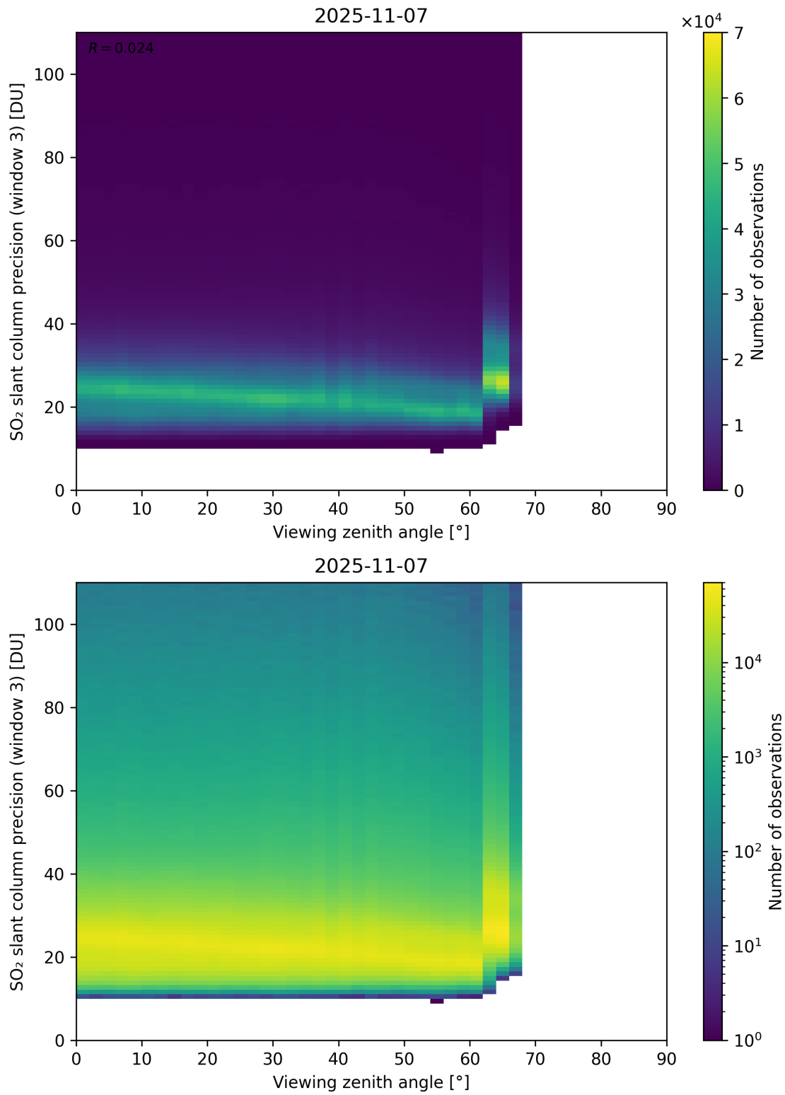
Figure 380: Scatter density plot of “Viewing zenith angle” against “SO 2 slant column precision (window 3)” for 2025-11-07 to 2025-11-08.
