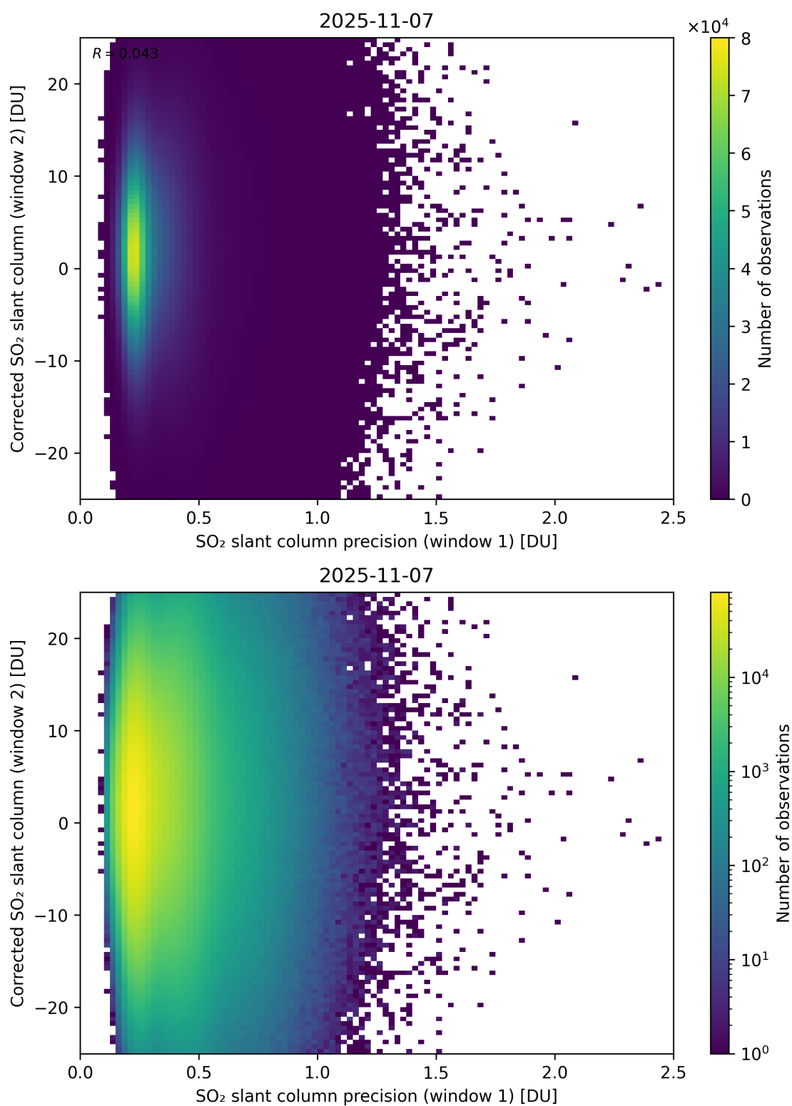
Figure 275: Scatter density plot of “SO 2 slant column precision (window 1)” against “Corrected SO 2 slant column (window 2)” for 2025-11-07 to 2025-11-08.
