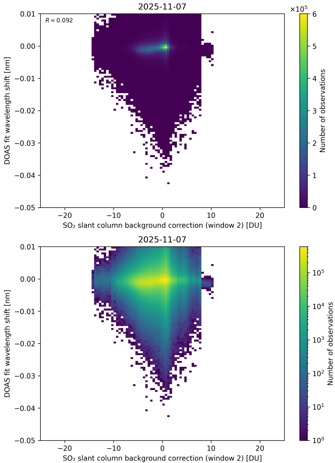
Figure 123: Scatter density plot of “SO 2 slant column background correction (window 2)” against “DOAS fit wavelength shift” for 2025-11-07 to 2025-11-08.
