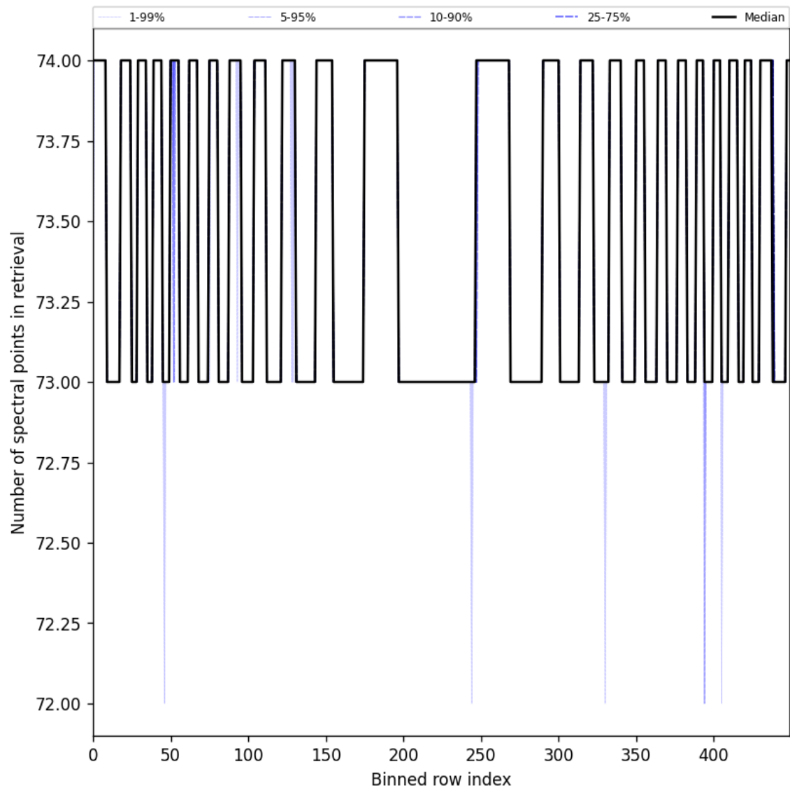
Figure 108: Along track statistics of “Number of spectral points in retrieval” for 2025-11-07 to 2025-11-08
