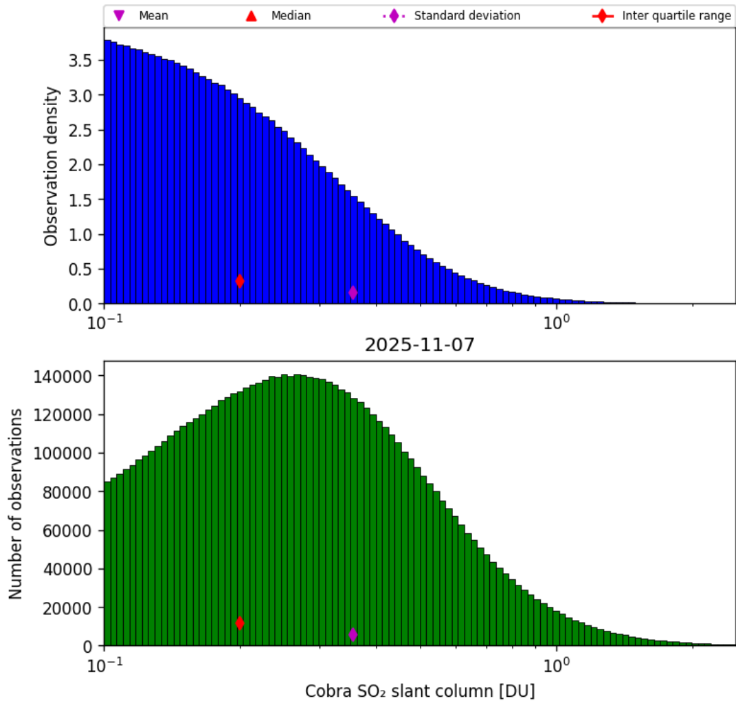
Figure 61: Histogram of “Cobra SO 2 slant column” for 2025-11-07 to 2025-11-08
