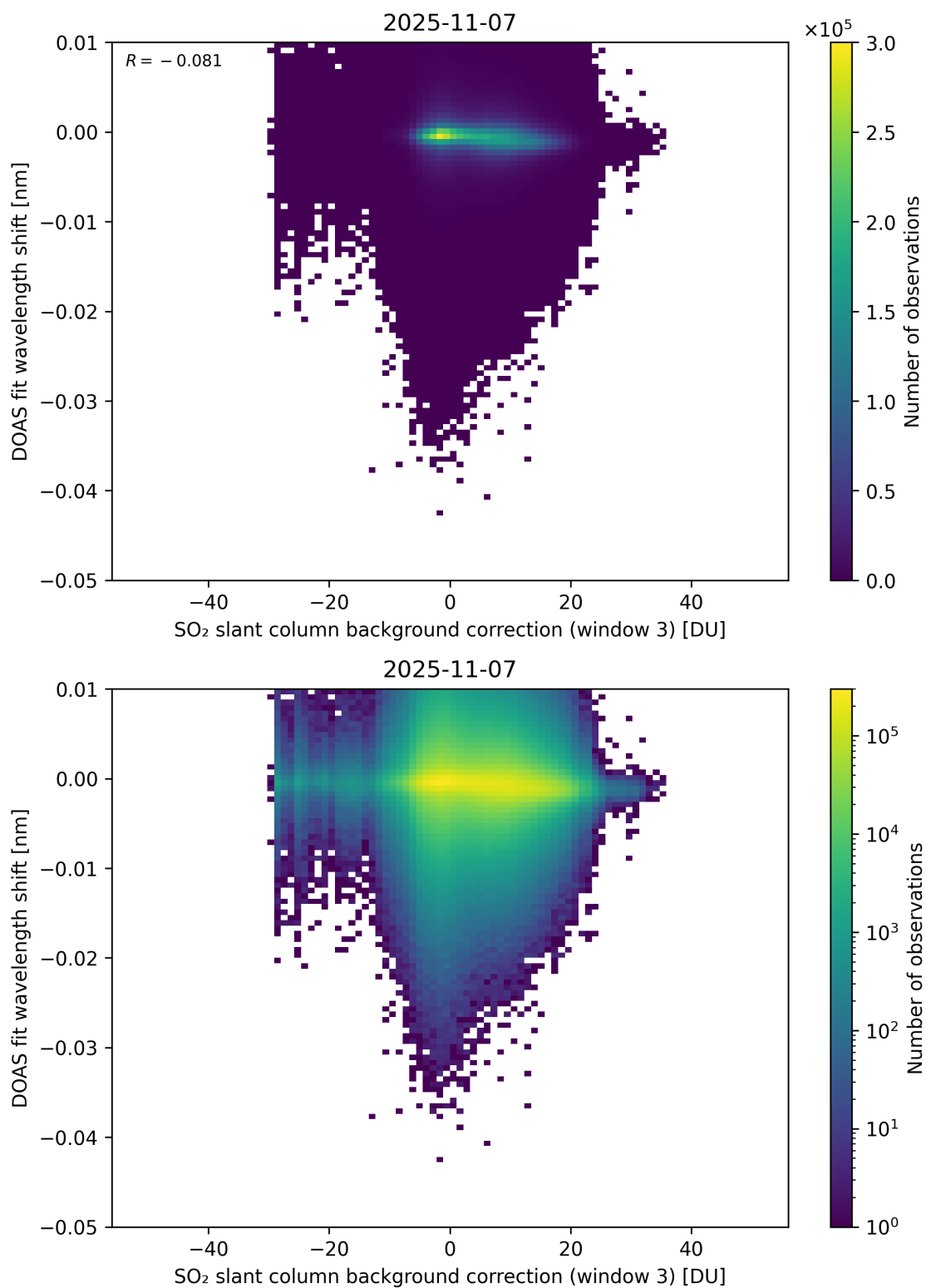
Figure 132: Scatter density plot of “SO 2 slant column background correction (window 3)” against “DOAS fit wavelength shift” for 2025-11-07 to 2025-11-08.
