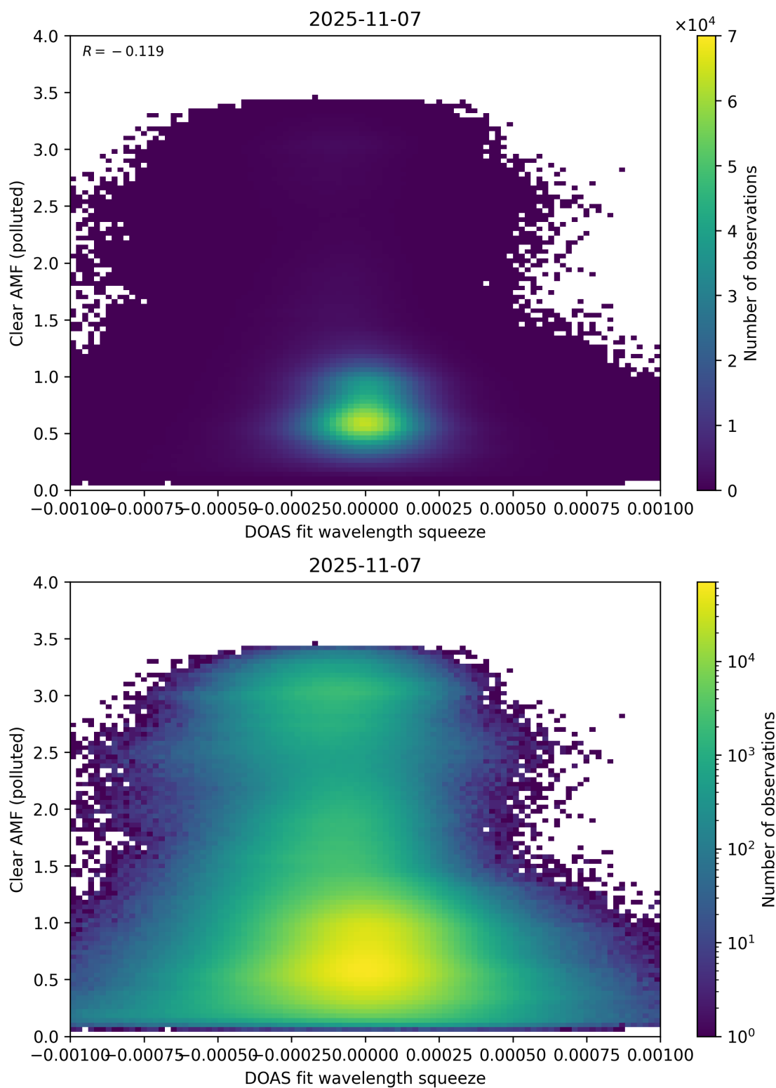
Figure 144: Scatter density plot of “DOAS fit wavelength squeeze” against “Clear AMF (polluted)” for 2025-11-07 to 2025-11-08.
