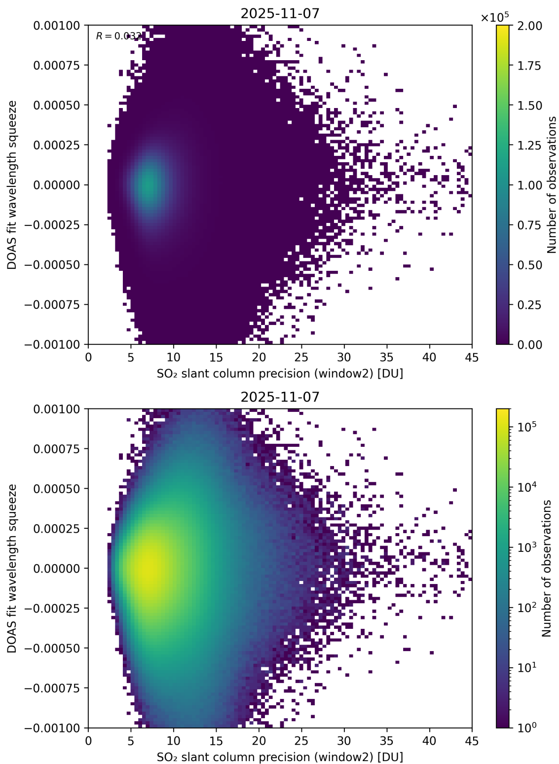
Figure 294: Scatter density plot of “SO 2 slant column precision (window2)” against “DOAS fit wavelength squeeze” for 2025-11-07 to 2025-11-08.
