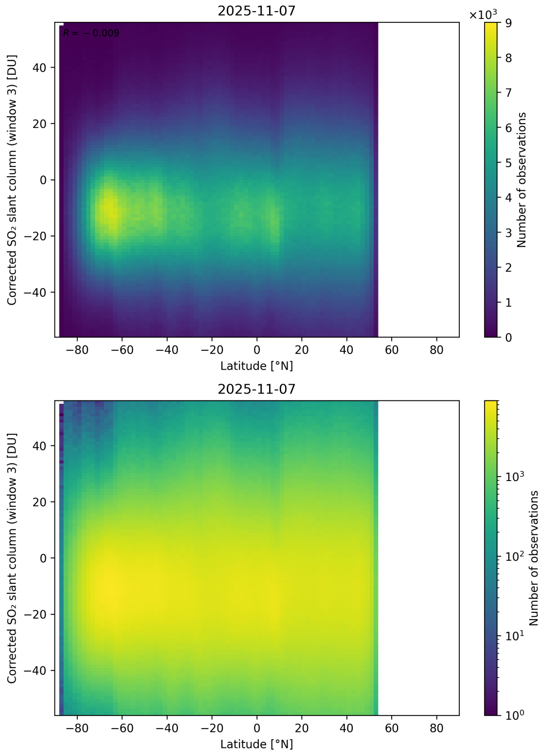
Figure 161: Scatter density plot of “Latitude” against “Corrected SO 2 slant column (window 3)” for 2025-11-07 to 2025-11-08.
