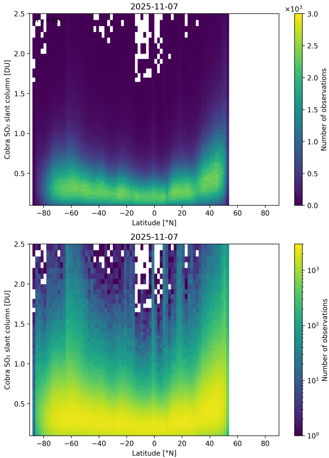
Figure 157: Scatter density plot of “Latitude” against “Cobra SO 2 slant column” for 2025-11-07 to 2025-11-08.
