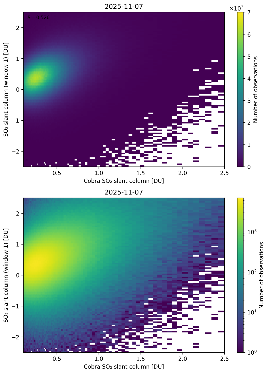
Figure 219: Scatter density plot of “Cobra SO 2 slant column” against “SO 2 slant column (window 1)” for 2025-11-07 to 2025-11-08.
