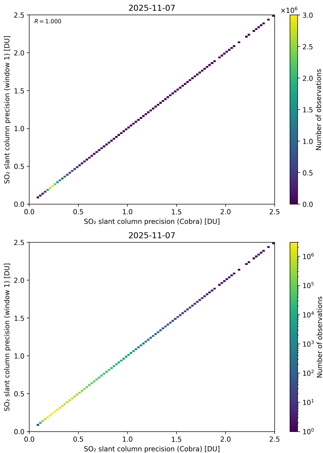
Figure 209: Scatter density plot of “SO 2 slant column precision (Cobra)” against “SO 2 slant column precision (window 1)” for 2025-11-07 to 2025-11-08.
