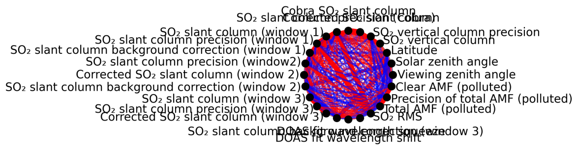
Figure 1: Map of correlation graph for 2025-11-07 to 2025-11-08.
