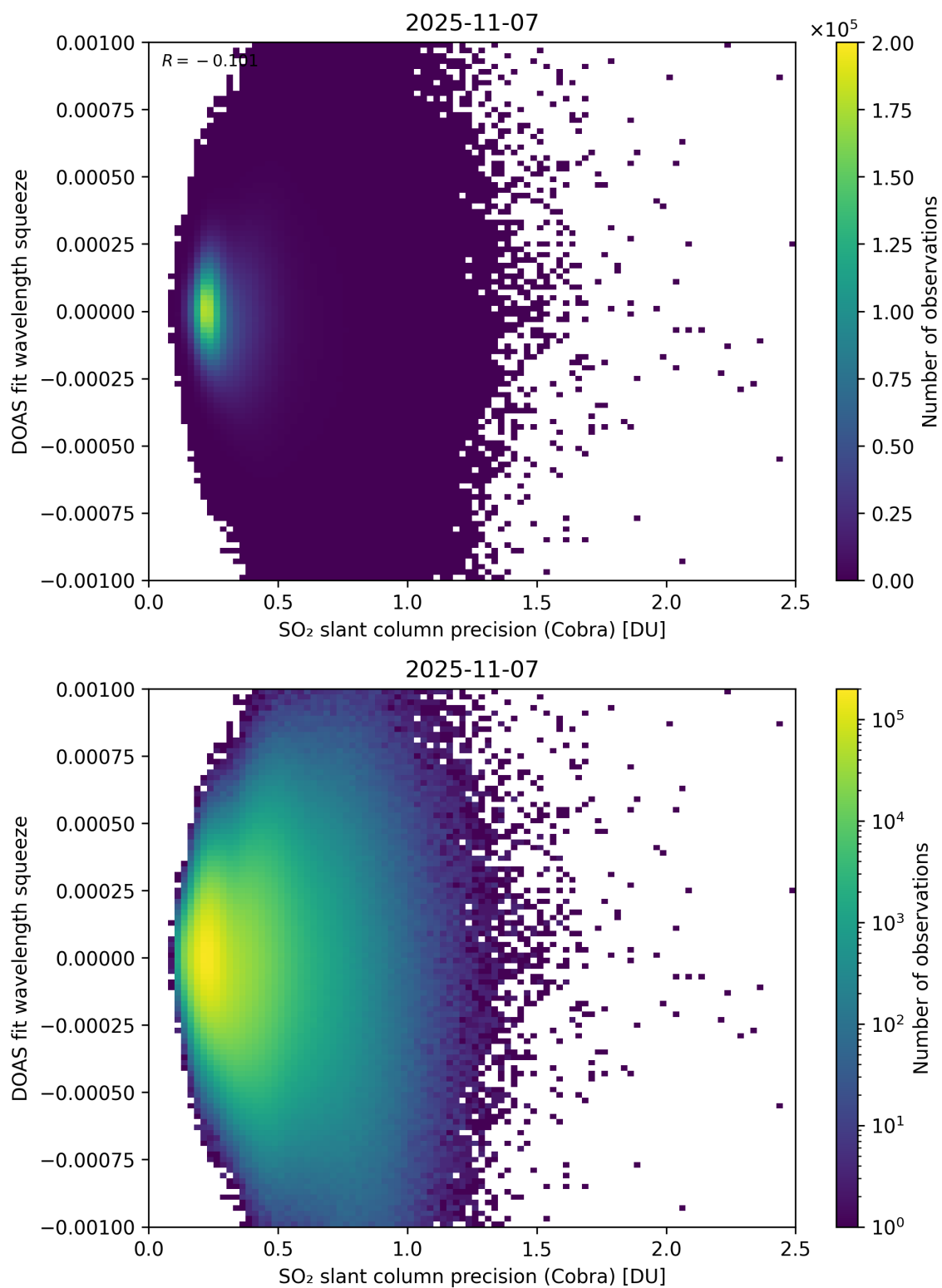
Figure 203: Scatter density plot of “SO 2 slant column precision (Cobra)” against “DOAS fit wavelength squeeze” for 2025-11-07 to 2025-11-08.
