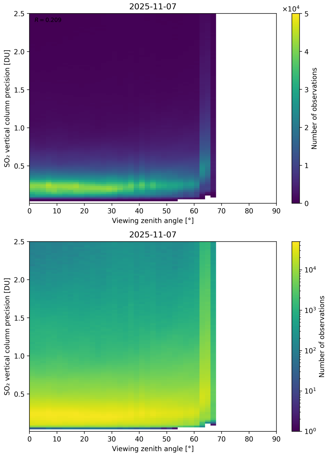
Figure 384: Scatter density plot of “Viewing zenith angle” against “SO 2 vertical column precision” for 2025-11-07 to 2025-11-08.
