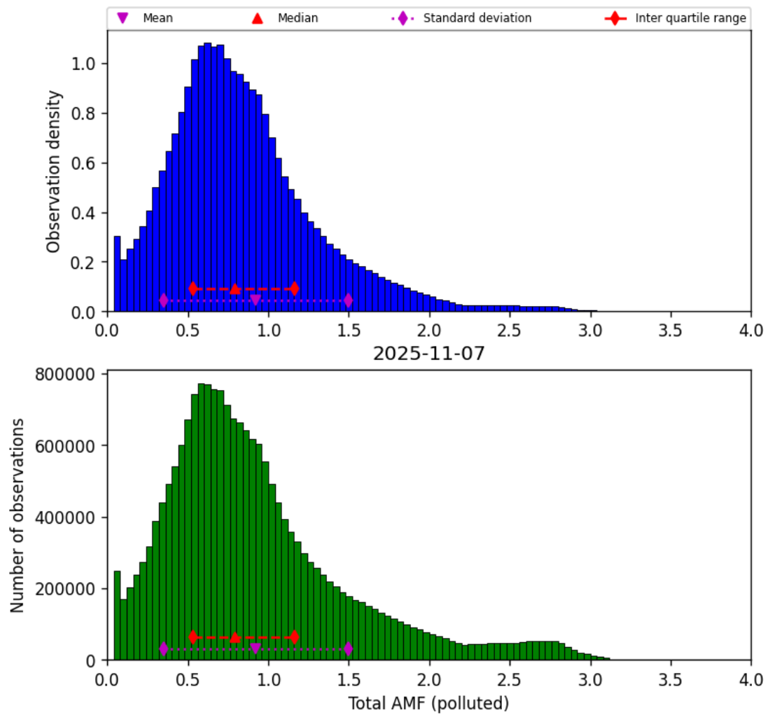
Figure 79: Histogram of “Total AMF (polluted)” for 2025-11-07 to 2025-11-08
