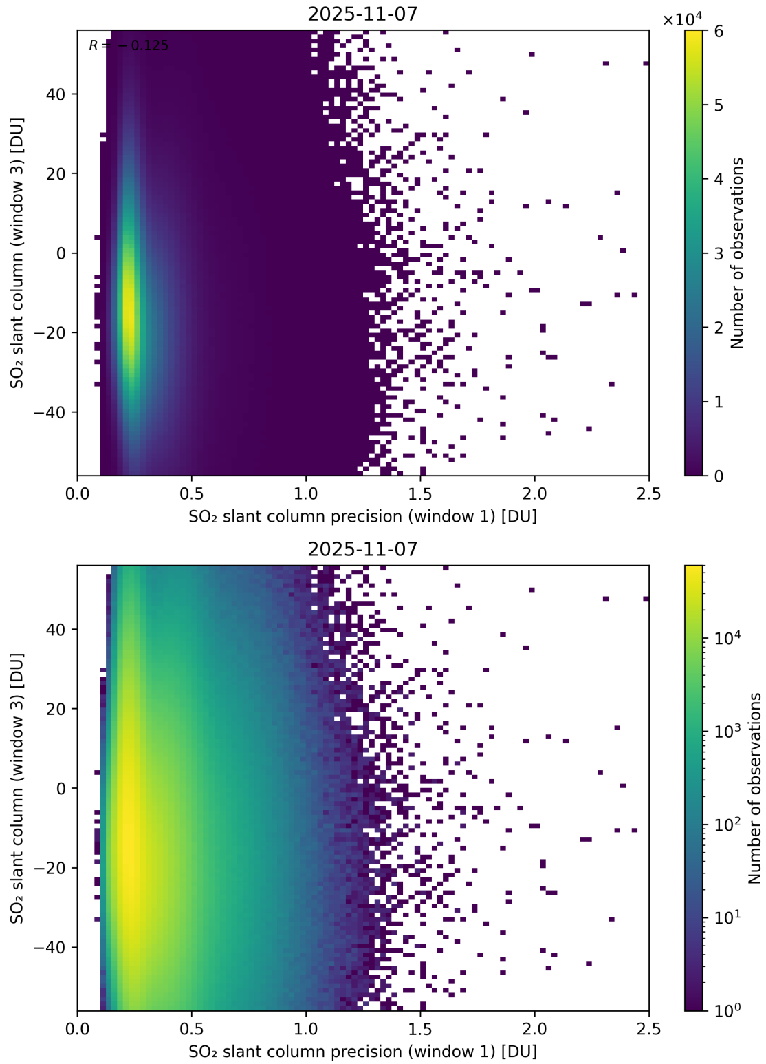
Figure 278: Scatter density plot of “SO 2 slant column precision (window 1)” against “SO 2 slant column (window 3)” for 2025-11-07 to 2025-11-08.
