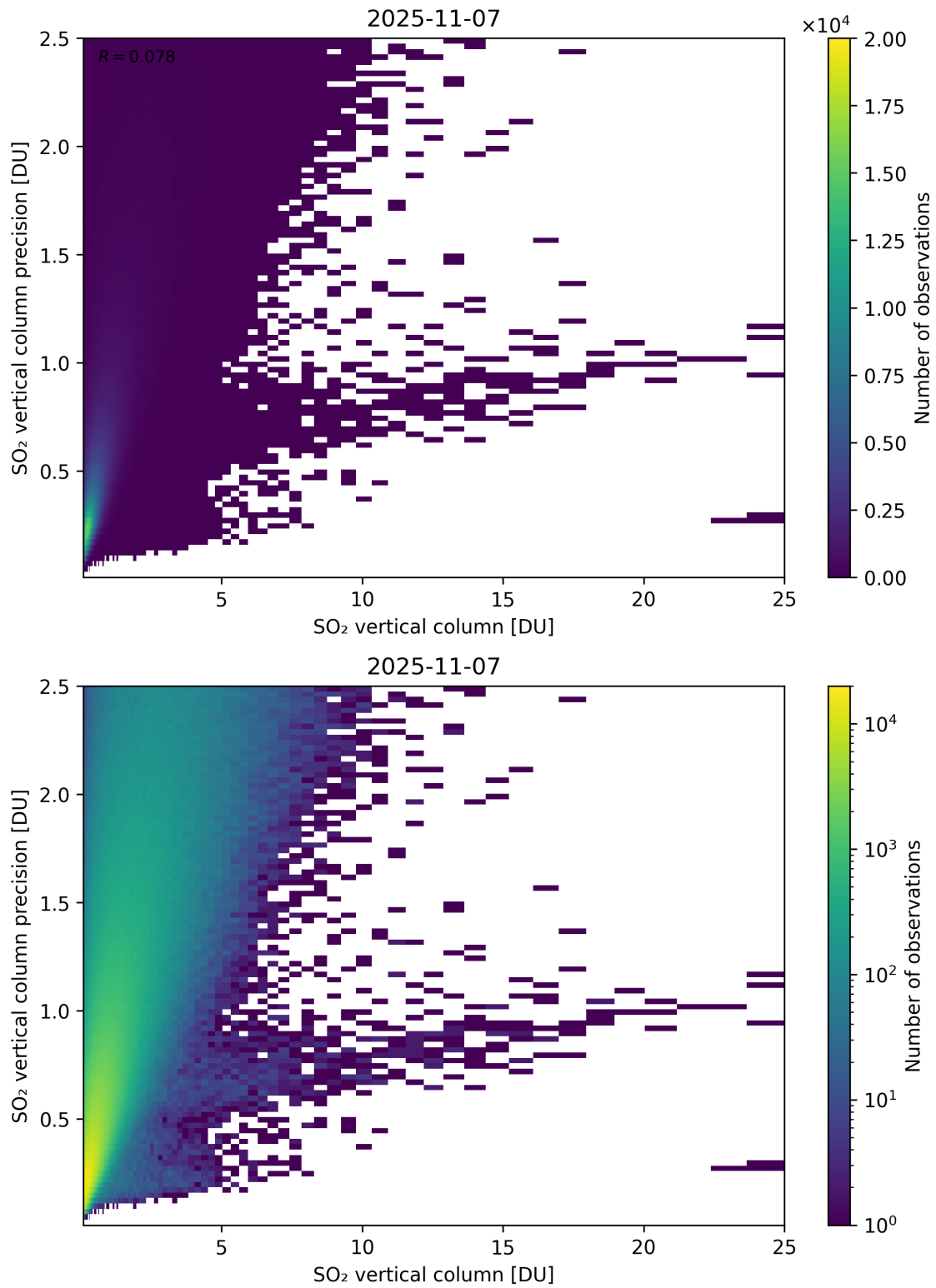
Figure 361: Scatter density plot of “SO 2 vertical column” against “SO 2 vertical column precision” for 2025-11-07 to 2025-11-08.
