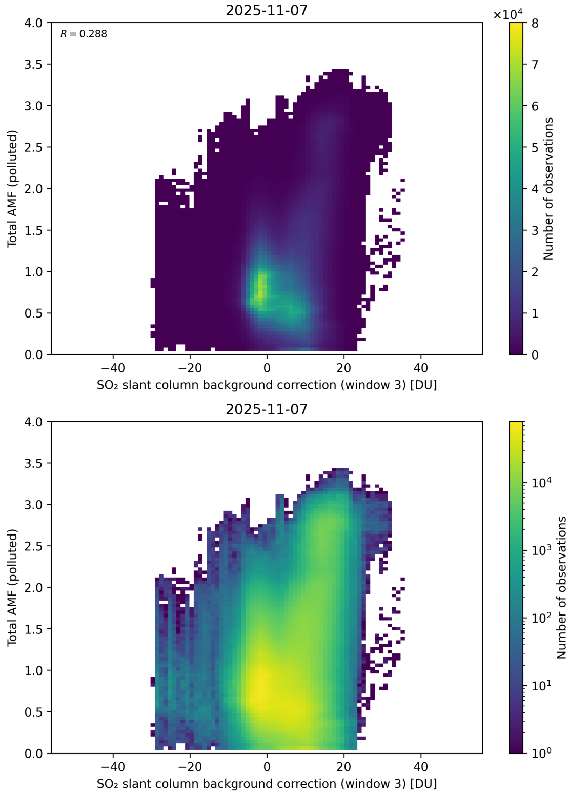
Figure 136: Scatter density plot of “SO 2 slant column background correction (window 3)” against “Total AMF (polluted)” for 2025-11-07 to 2025-11-08.
