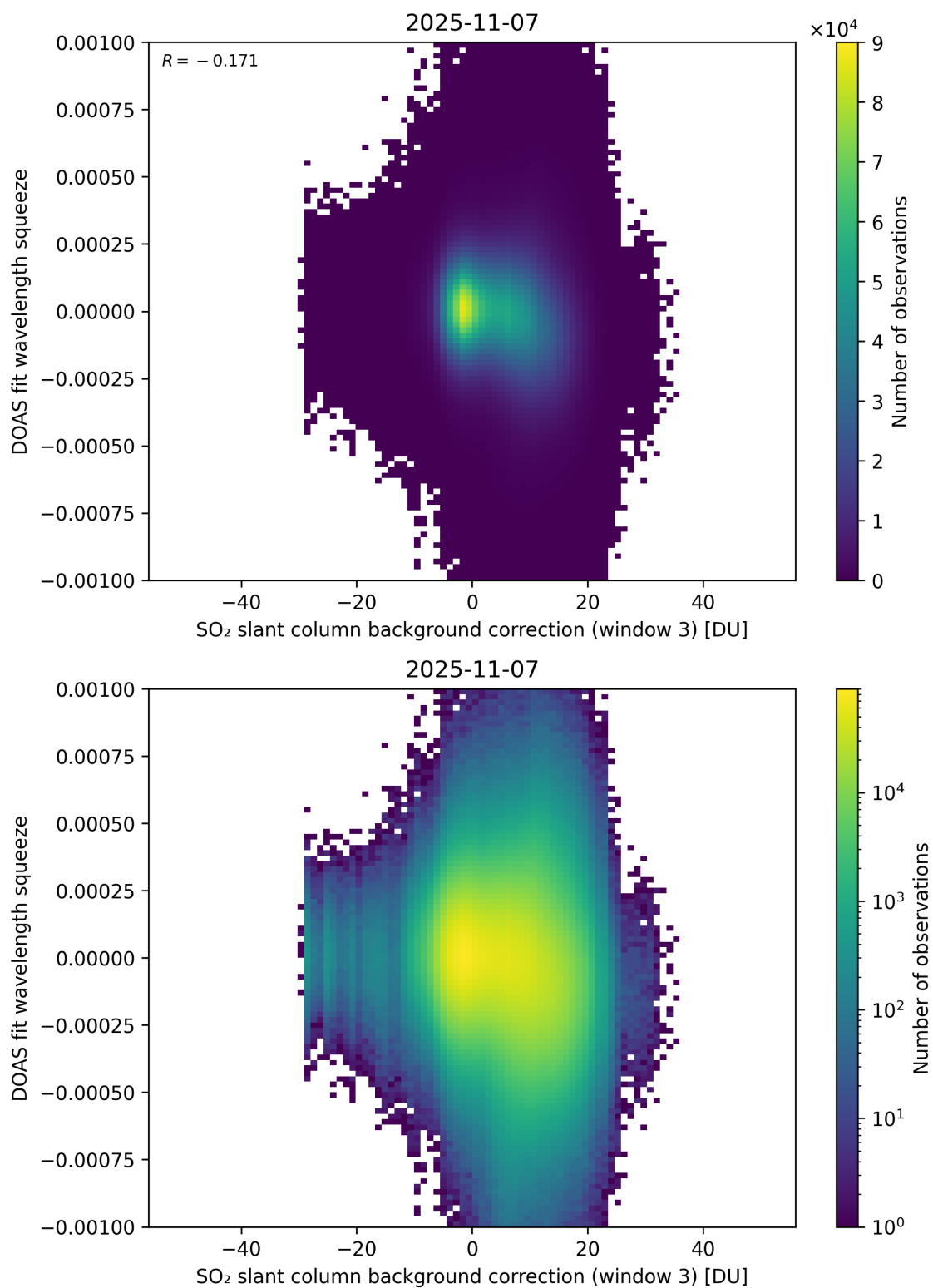
Figure 133: Scatter density plot of “SO 2 slant column background correction (window 3)” against “DOAS fit wavelength squeeze” for 2025-11-07 to 2025-11-08.
