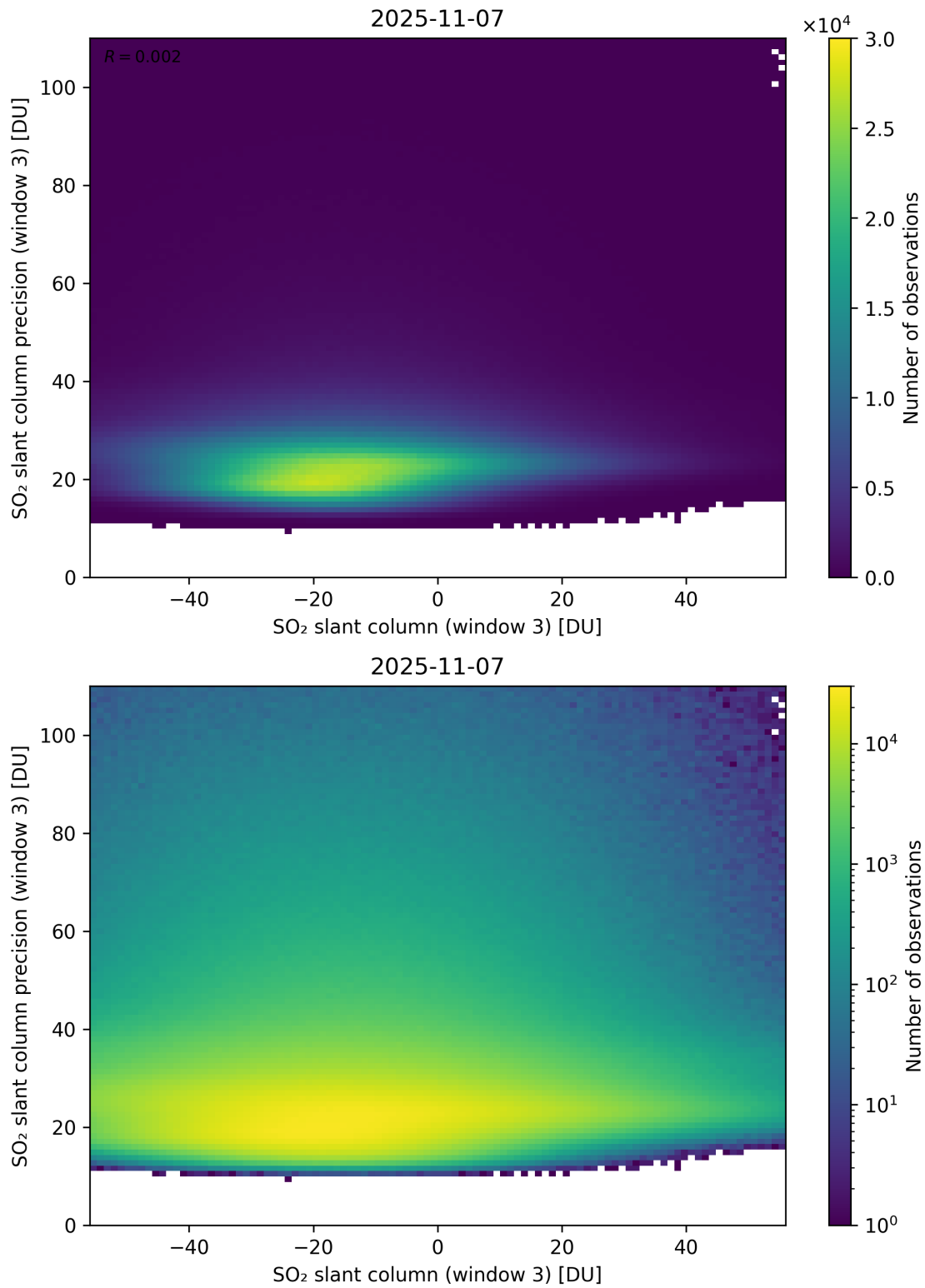
Figure 317: Scatter density plot of “SO 2 slant column (window 3)” against “SO 2 slant column precision (window 3)” for 2025-11-07 to 2025-11-08.
