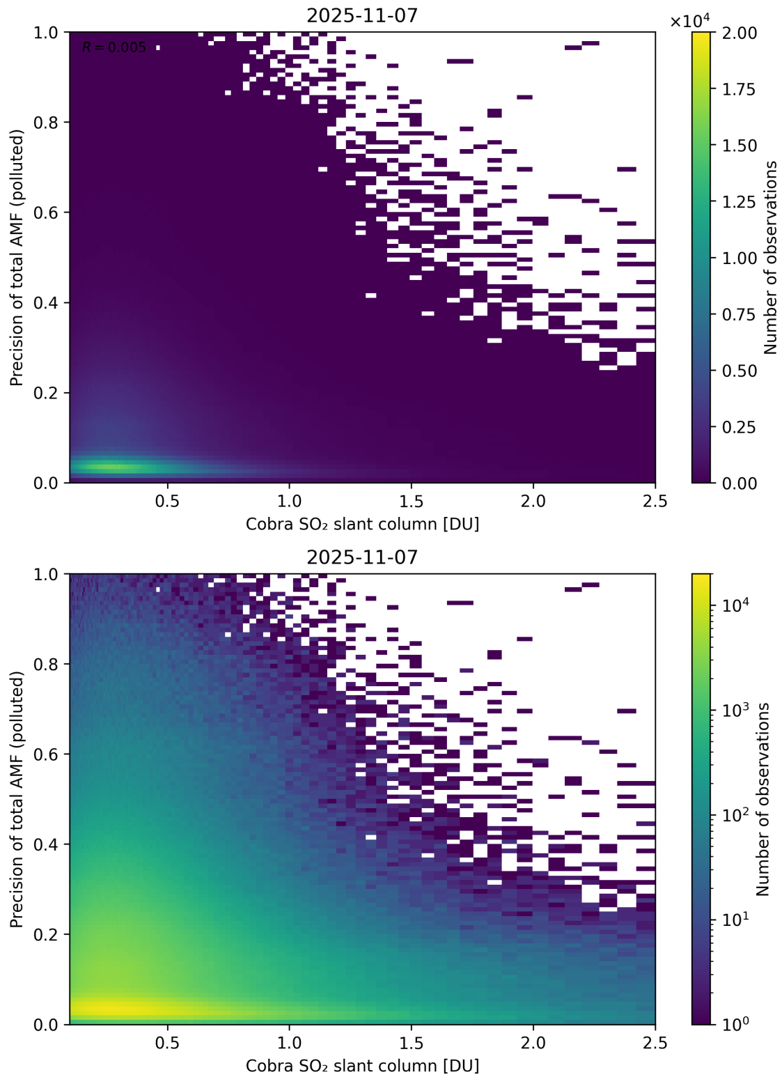
Figure 225: Scatter density plot of “Cobra SO 2 slant column” against “Precision of total AMF (polluted)” for 2025-11-07 to 2025-11-08.
