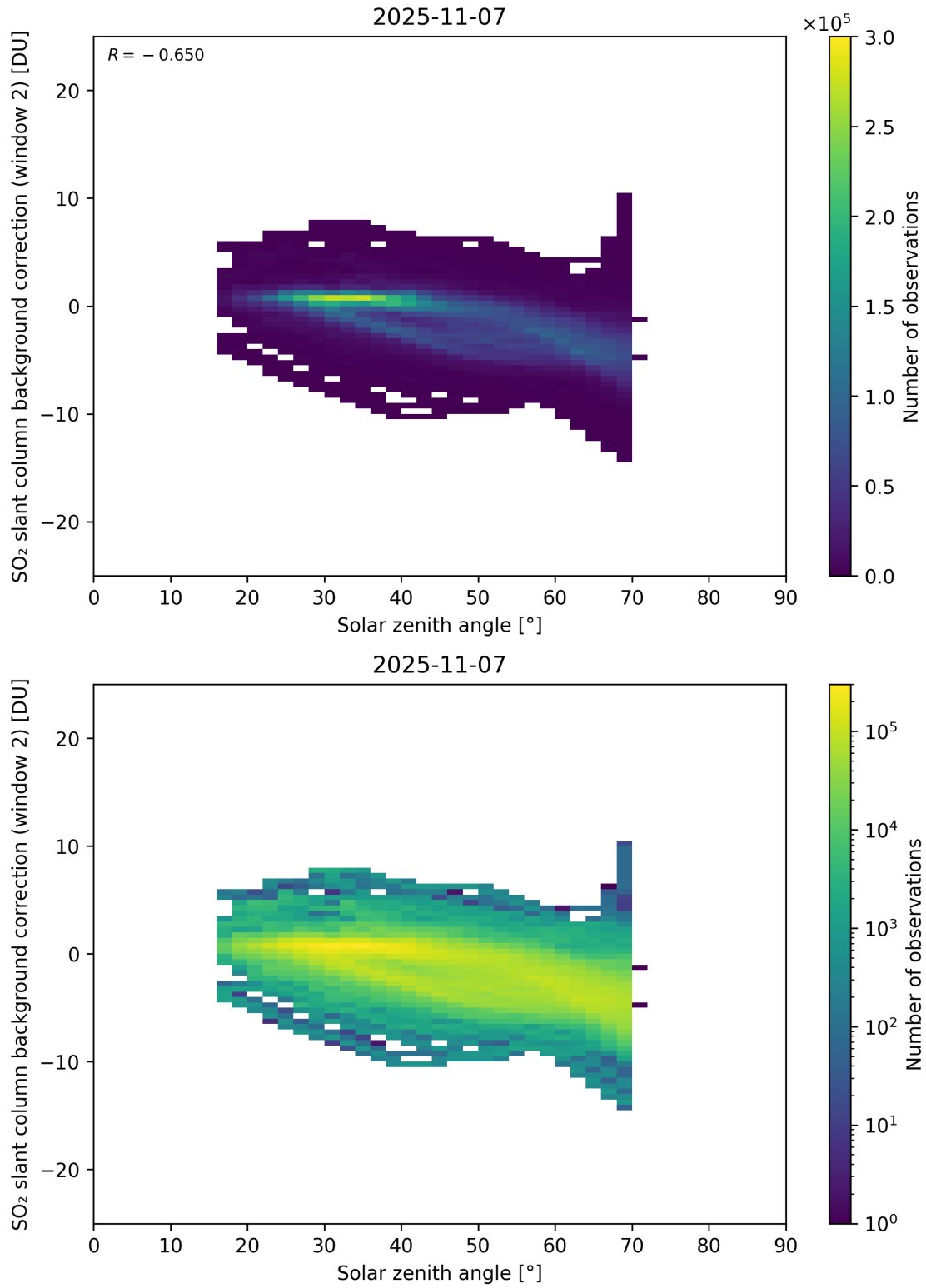
Figure 172: Scatter density plot of “Solar zenith angle” against “SO 2 slant column background correction (window 2)” for 2025-11-07 to 2025-11-08.
