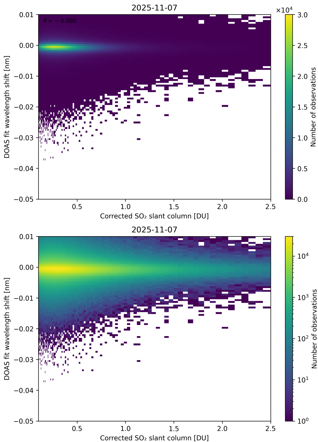
Figure 229: Scatter density plot of “Corrected SO 2 slant column” against “DOAS fit wavelength shift” for 2025-11-07 to 2025-11-08.
