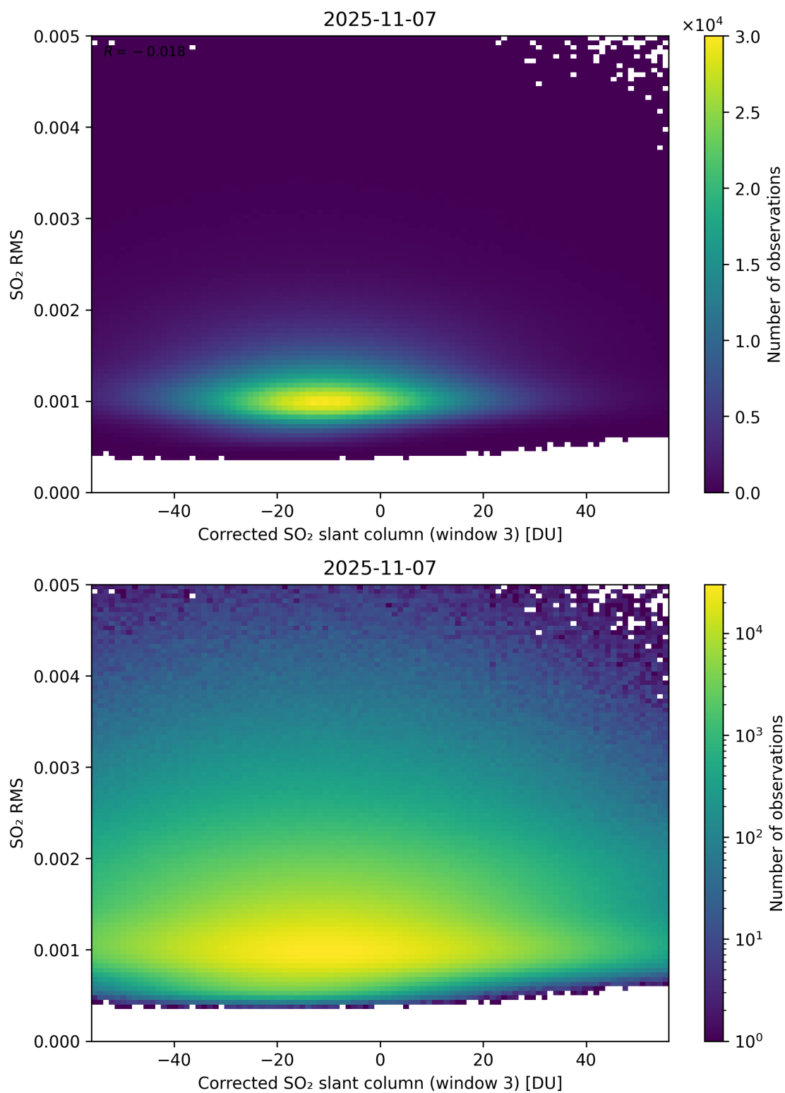
Figure 258: Scatter density plot of “Corrected SO 2 slant column (window 3)” against “SO 2 RMS” for 2025-11-07 to 2025-11-08.
