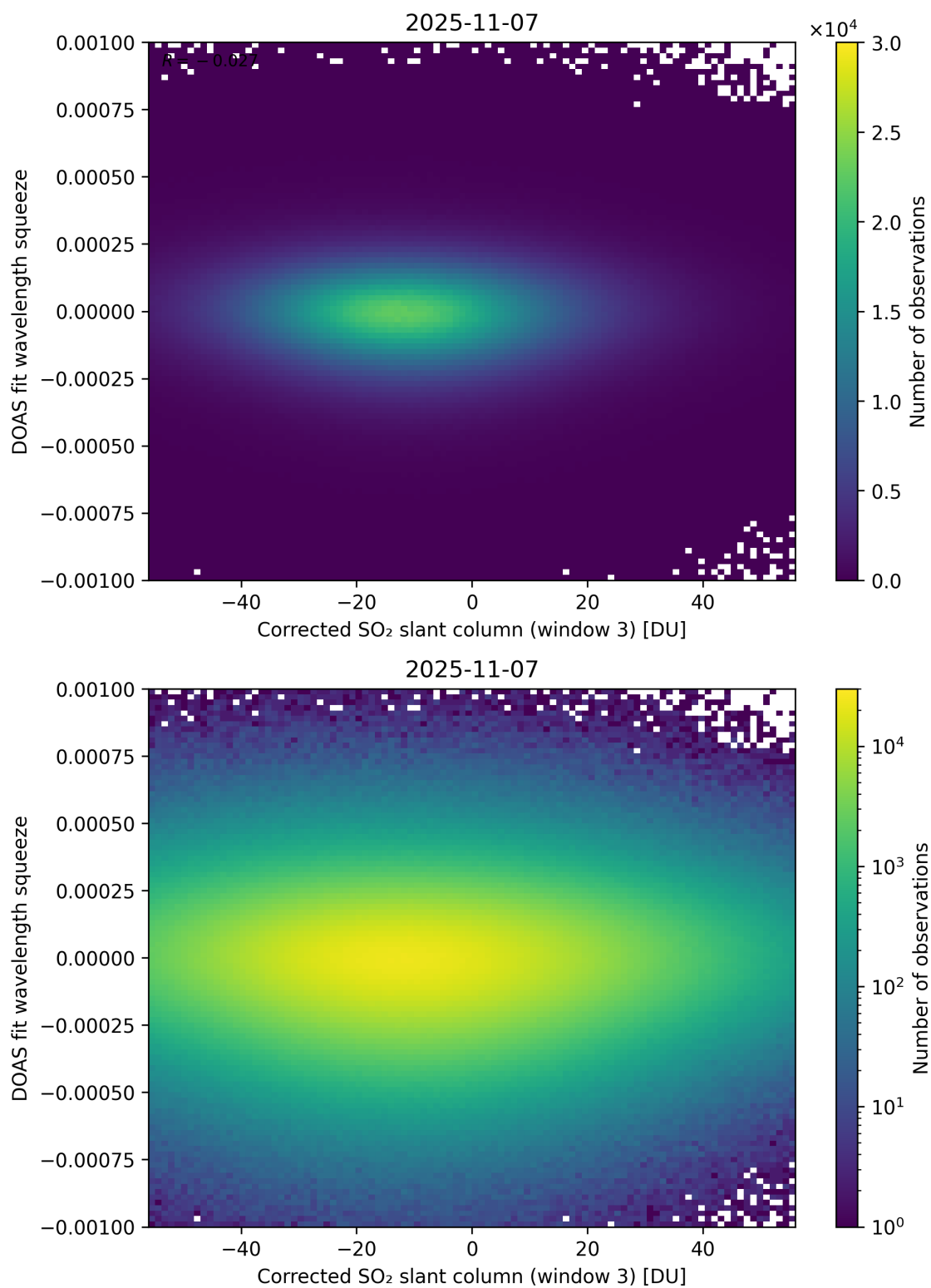
Figure 257: Scatter density plot of “Corrected SO 2 slant column (window 3)” against “DOAS fit wavelength squeeze” for 2025-11-07 to 2025-11-08.
