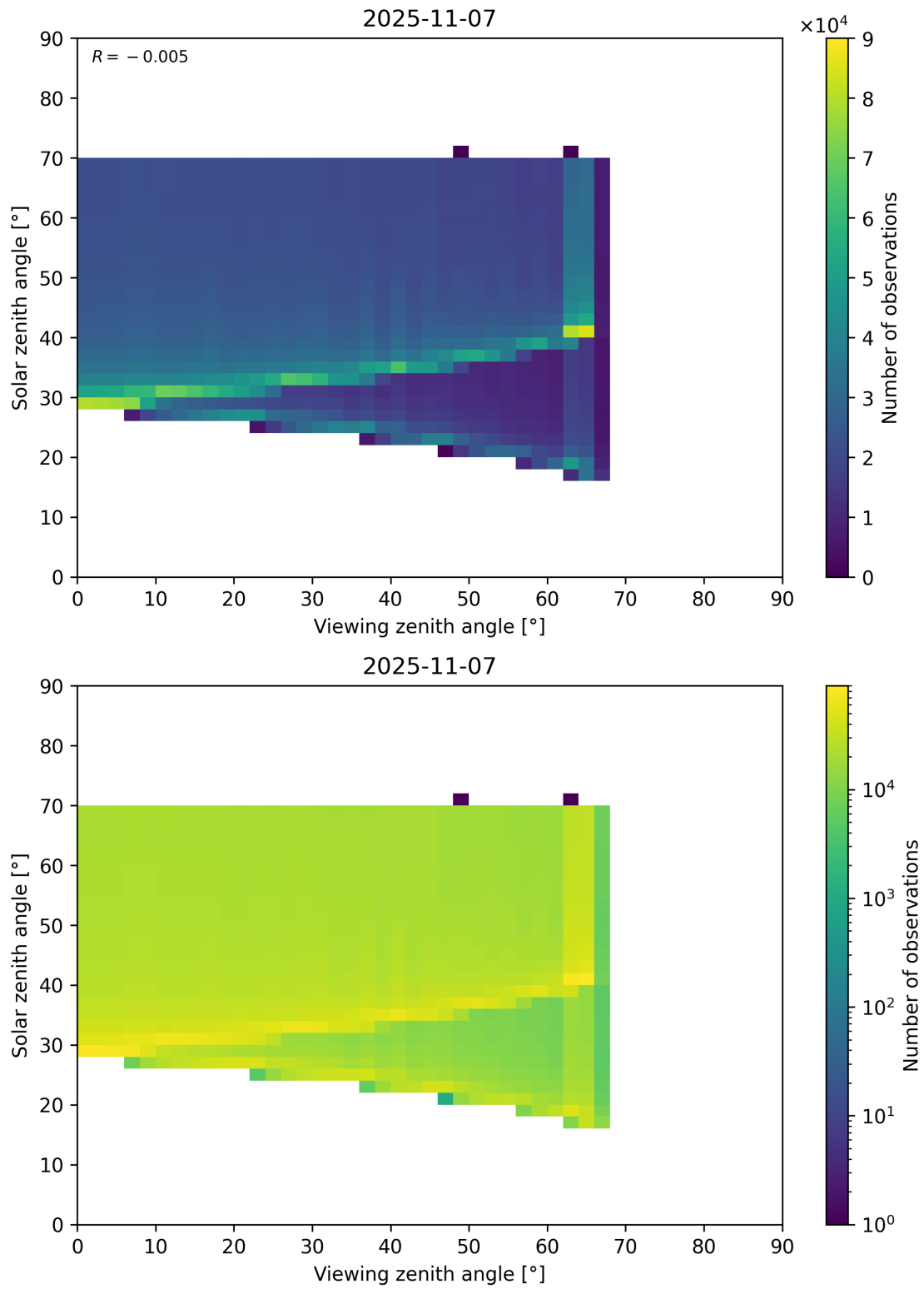
Figure 369: Scatter density plot of “Viewing zenith angle” against “Solar zenith angle” for 2025-11-07 to 2025-11-08.
