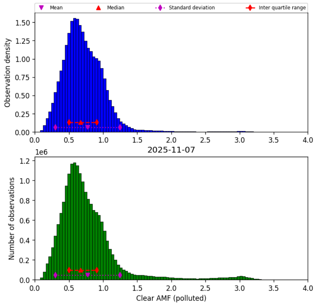
Figure 81: Histogram of “Clear AMF (polluted)” for 2025-11-07 to 2025-11-08
