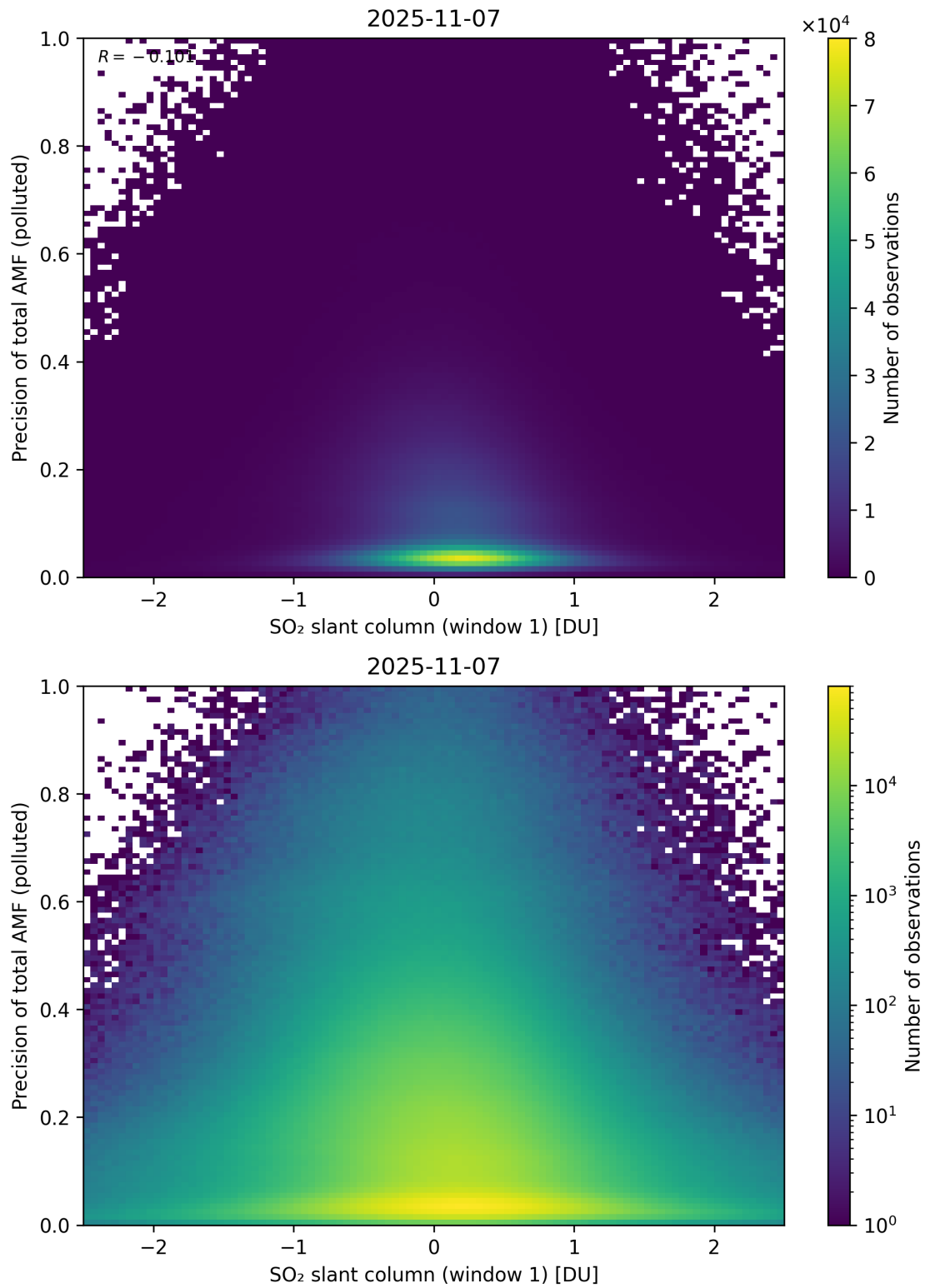
Figure 290: Scatter density plot of “SO 2 slant column (window 1)” against “Precision of total AMF (polluted)” for 2025-11-07 to 2025-11-08.
