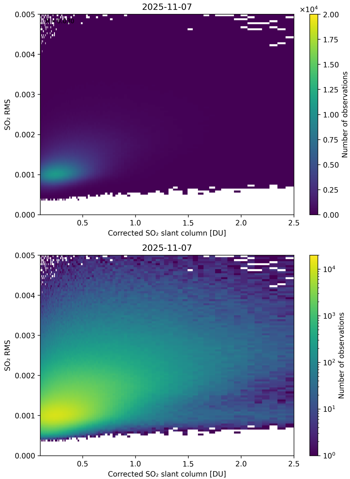
Figure 231: Scatter density plot of “Corrected SO 2 slant column” against “SO 2 RMS” for 2025-11-07 to 2025-11-08.
