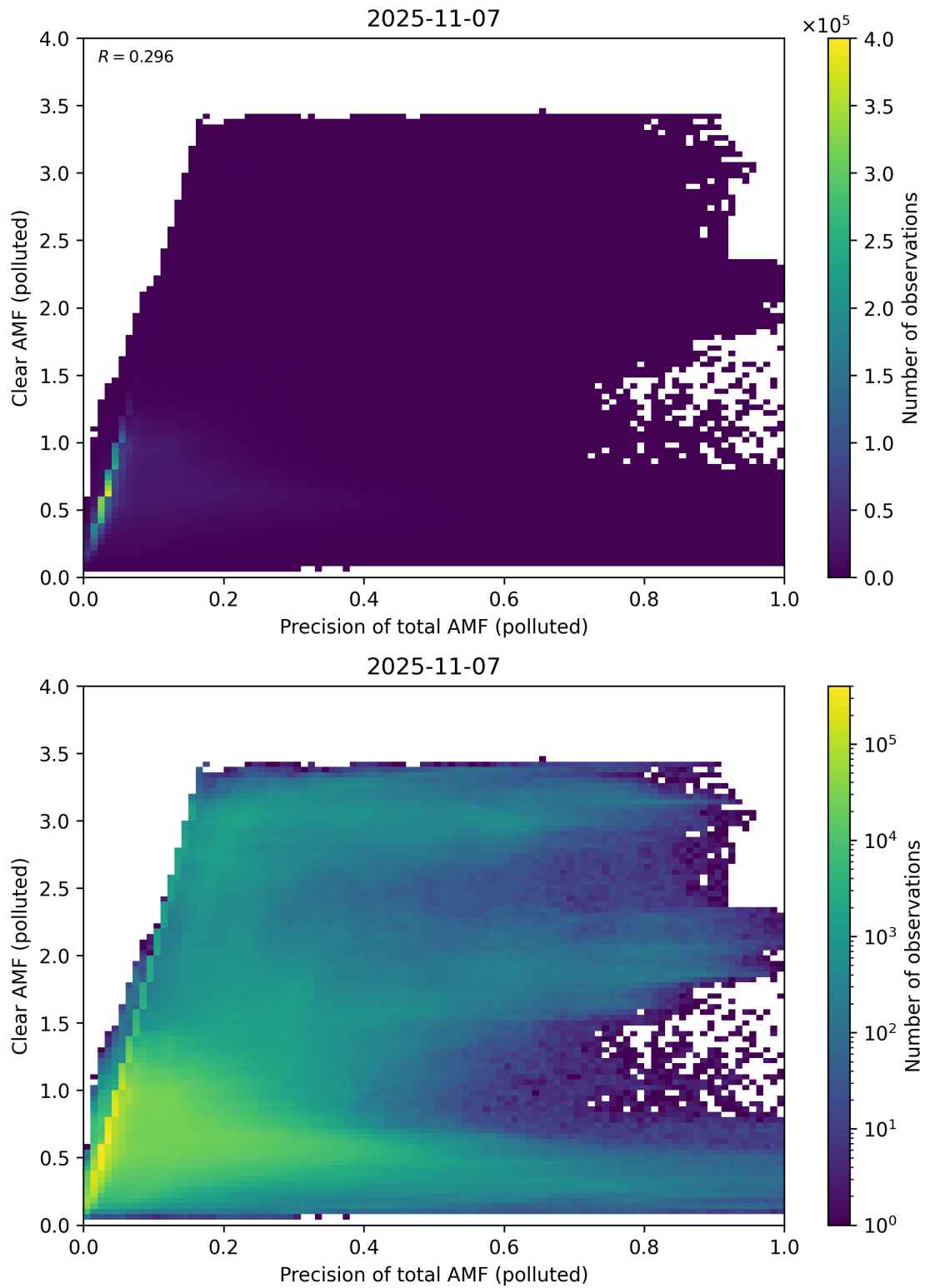
Figure 320: Scatter density plot of “Precision of total AMF (polluted)” against “Clear AMF (polluted)” for 2025-11-07 to 2025-11-08.
