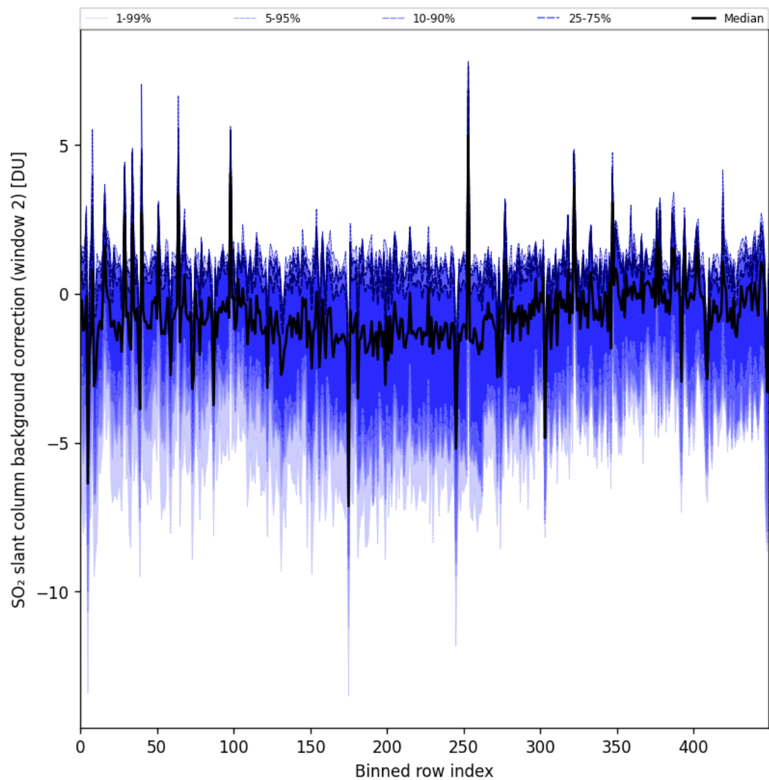
Figure 96: Along track statistics of “SO 2 slant column background correction (window 2)” for 2025-11-07 to 2025-11-08
