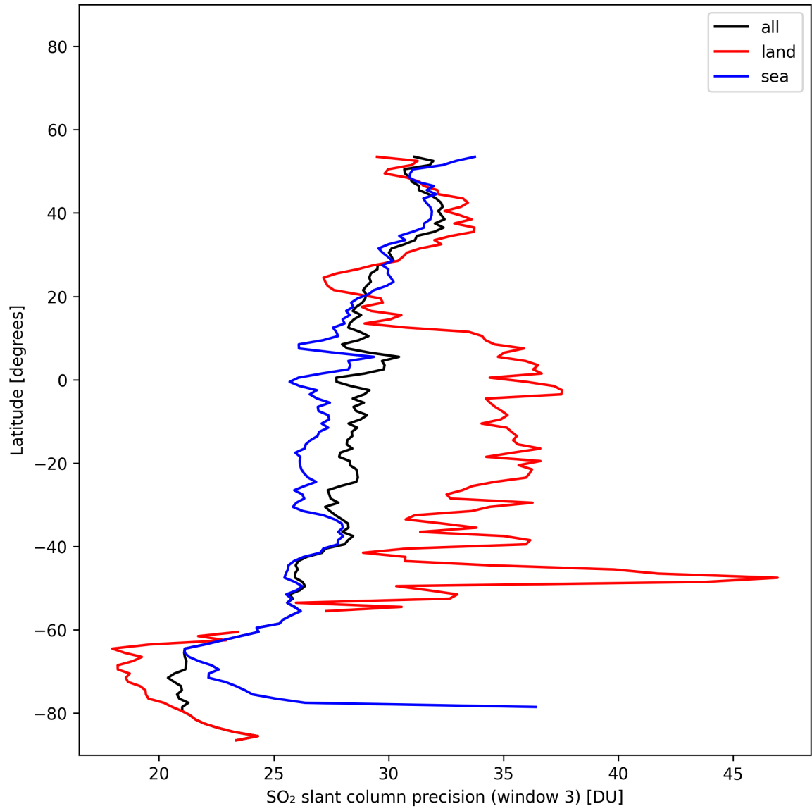
Figure 46: Zonal average of “SO 2 slant column precision (window 3)” for 2025-11-07 to 2025-11-08.
