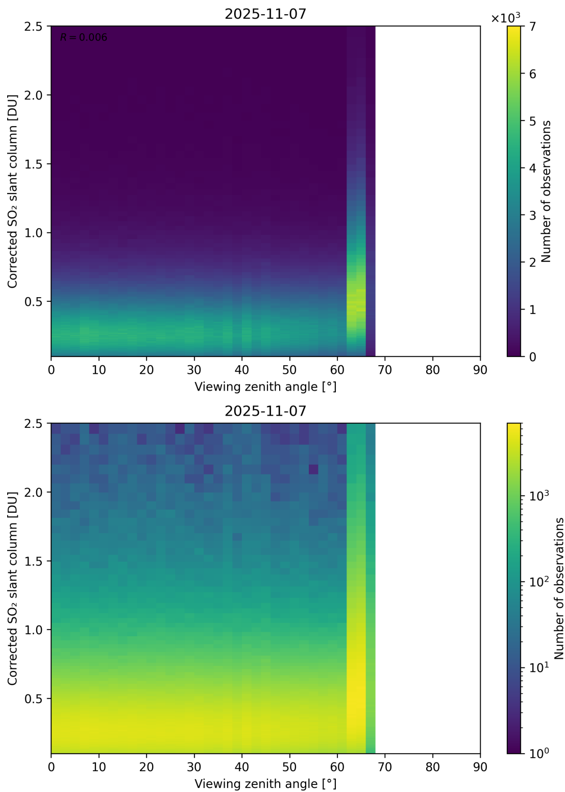
Figure 373: Scatter density plot of “Viewing zenith angle” against “Corrected SO 2 slant column” for 2025-11-07 to 2025-11-08.
