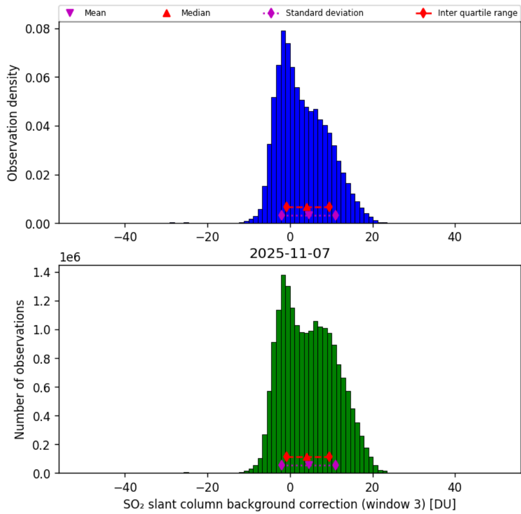
Figure 74: Histogram of “SO 2 slant column background correction (window 3)” for 2025-11-07 to 2025-11-08
