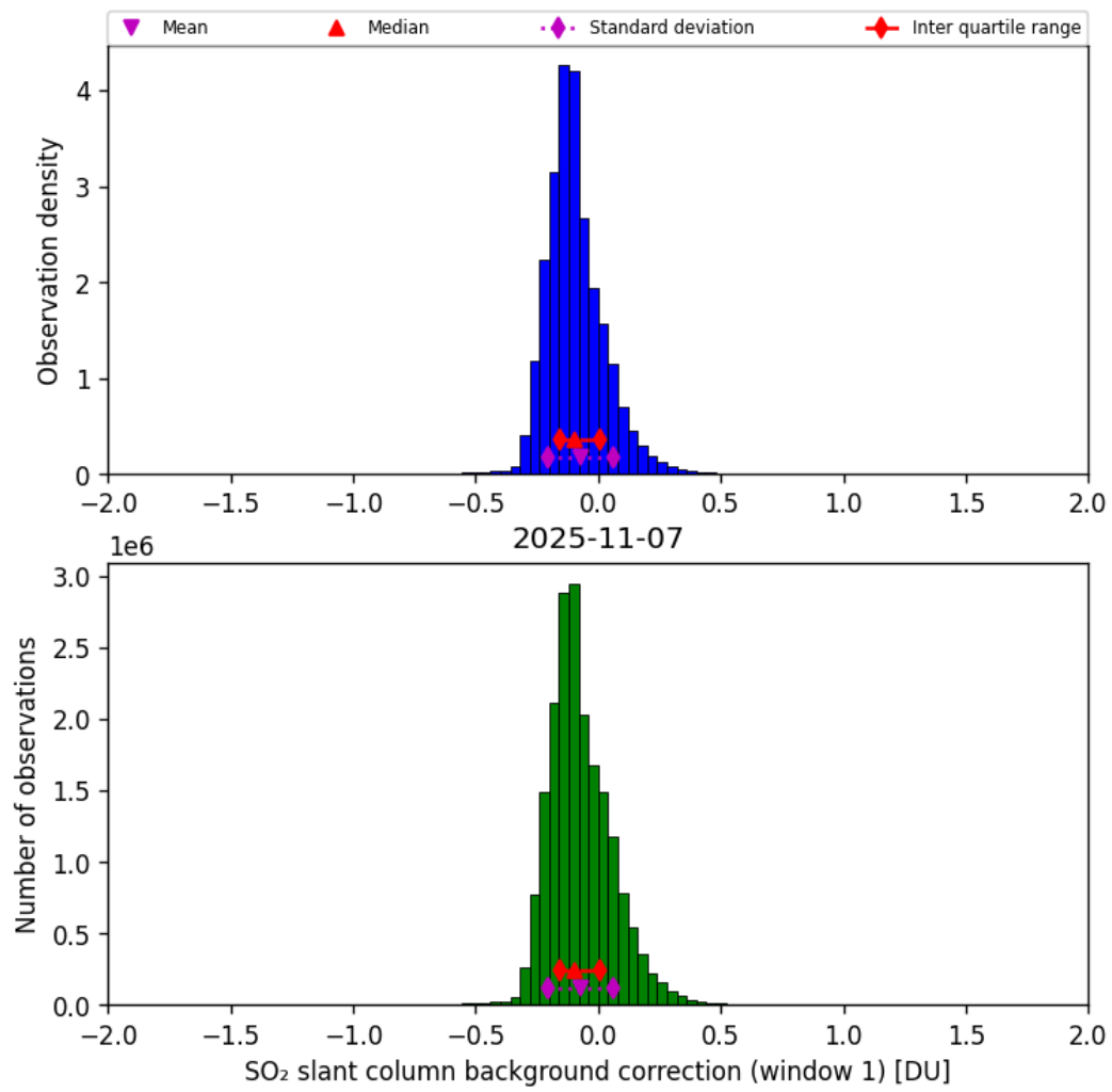
Figure 66: Histogram of “SO 2 slant column background correction (window 1)” for 2025-11-07 to 2025-11-08
