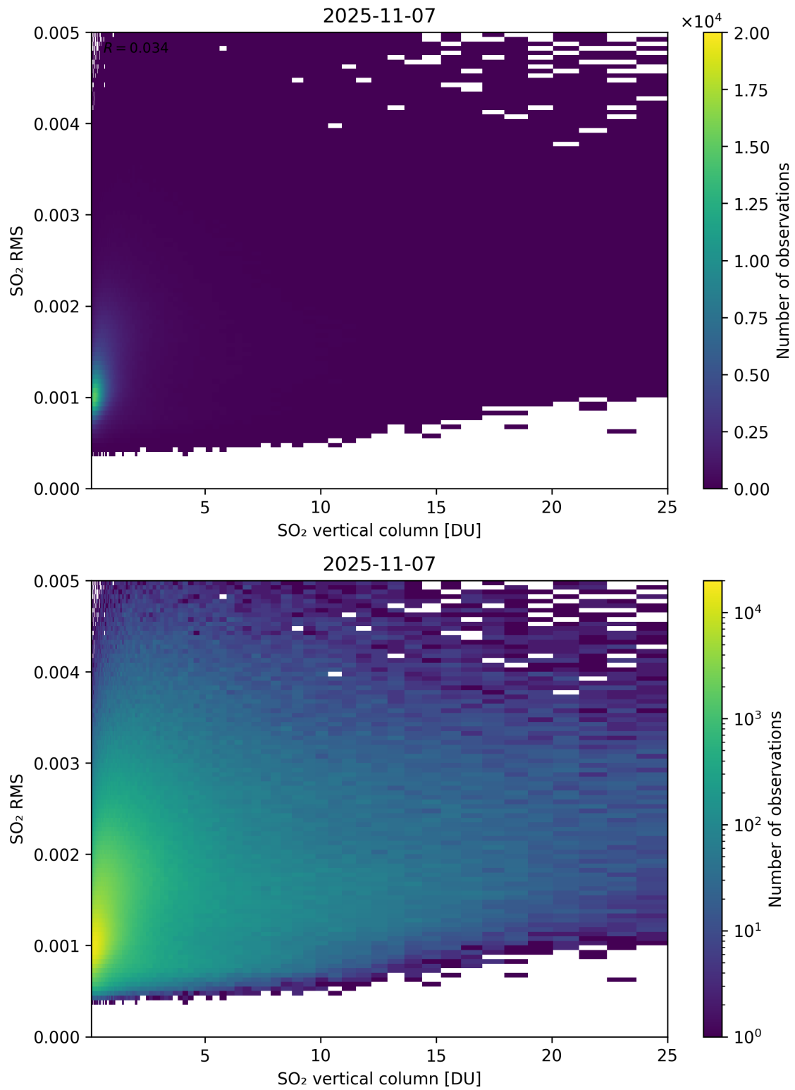
Figure 328: Scatter density plot of “SO 2 vertical column” against “SO 2 RMS” for 2025-11-07 to 2025-11-08.
