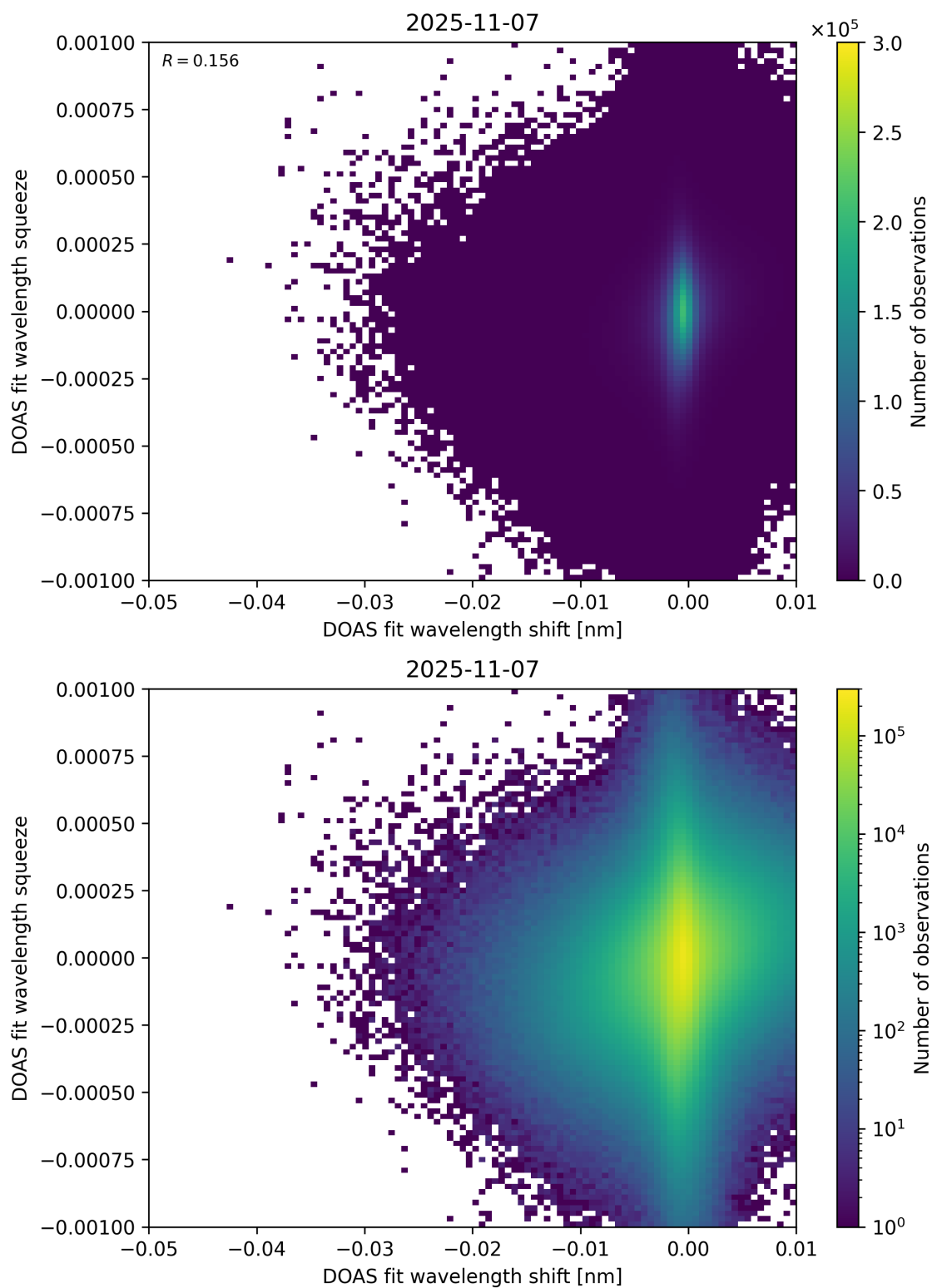
Figure 138: Scatter density plot of “DOAS fit wavelength shift” against “DOAS fit wavelength squeeze” for 2025-11-07 to 2025-11-08.
