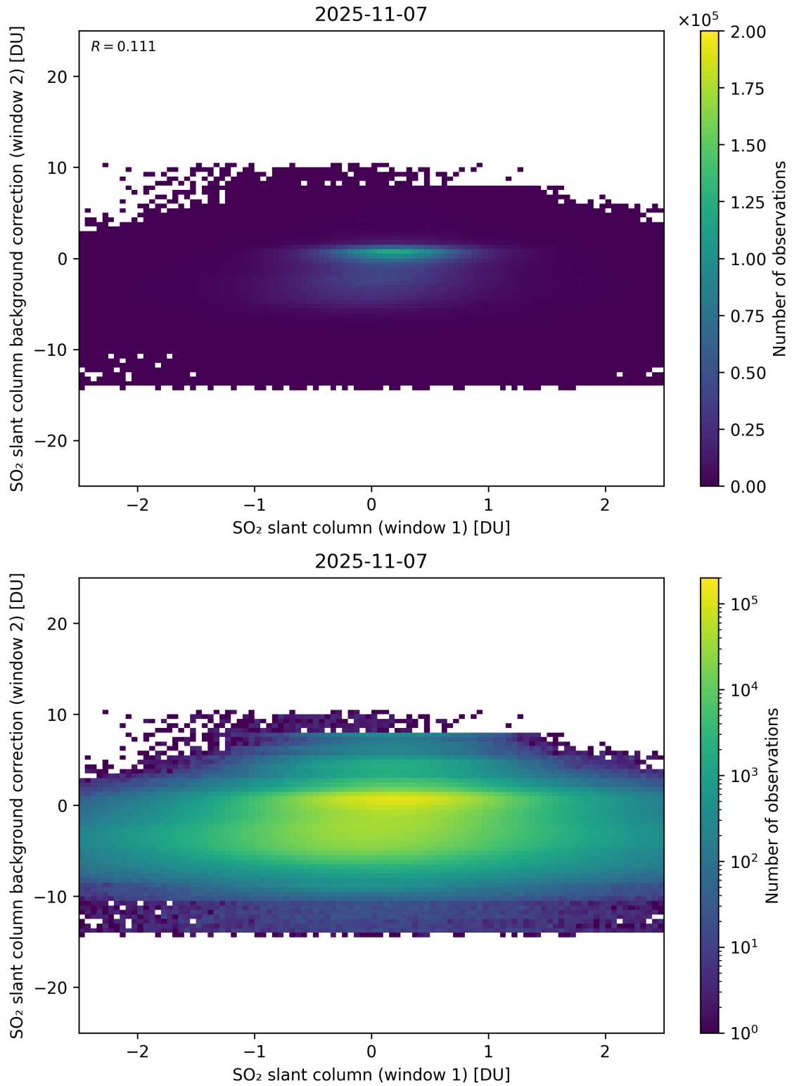
Figure 263: Scatter density plot of “SO 2 slant column (window 1)” against “SO 2 slant column background correction (window 2)” for 2025-11-07 to 2025-11-08.
