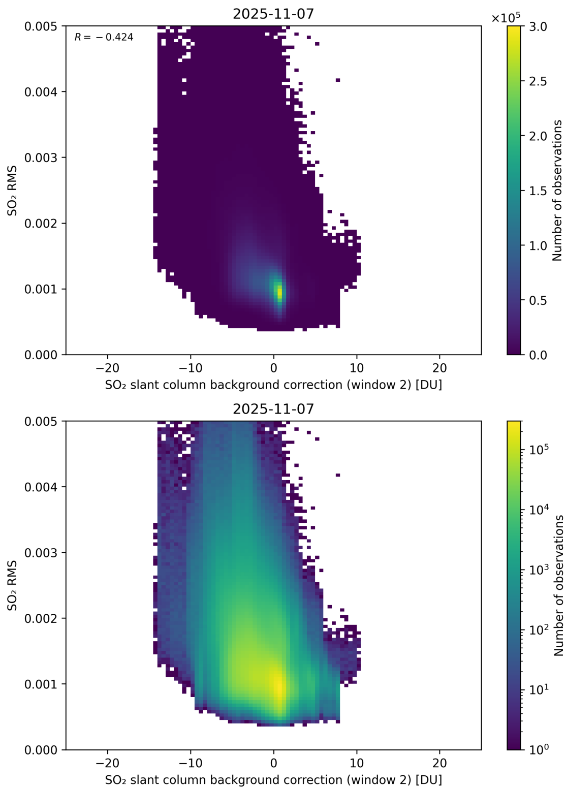
Figure 125: Scatter density plot of “SO 2 slant column background correction (window 2)” against “SO 2 RMS” for 2025-11-07 to 2025-11-08.
