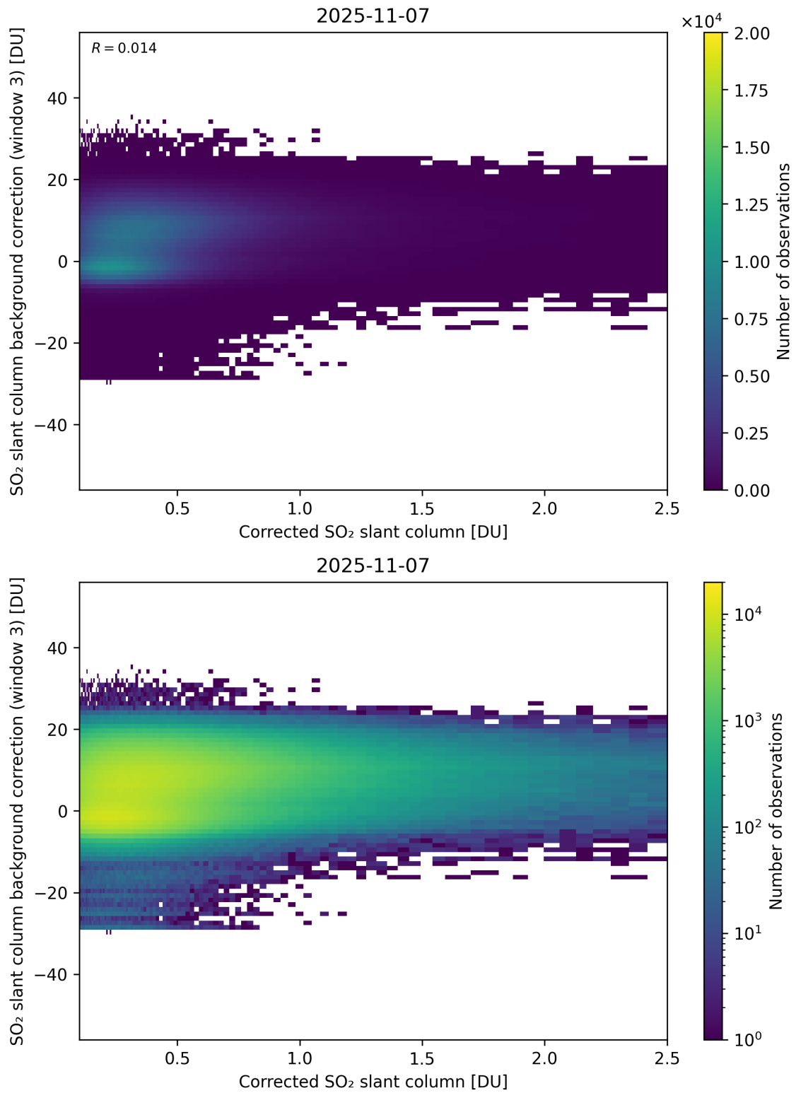
Figure 228: Scatter density plot of “Corrected SO 2 slant column” against “SO 2 slant column background correction (window 3)” for 2025-11-07 to 2025-11-08.
