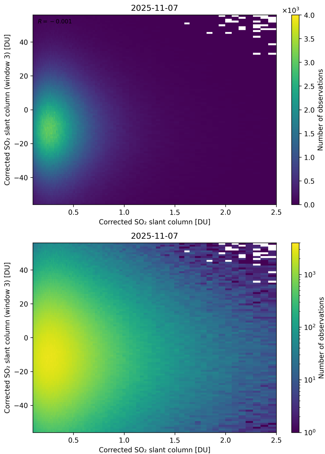
Figure 236: Scatter density plot of “Corrected SO 2 slant column” against “Corrected SO 2 slant column (window 3)” for 2025-11-07 to 2025-11-08.
