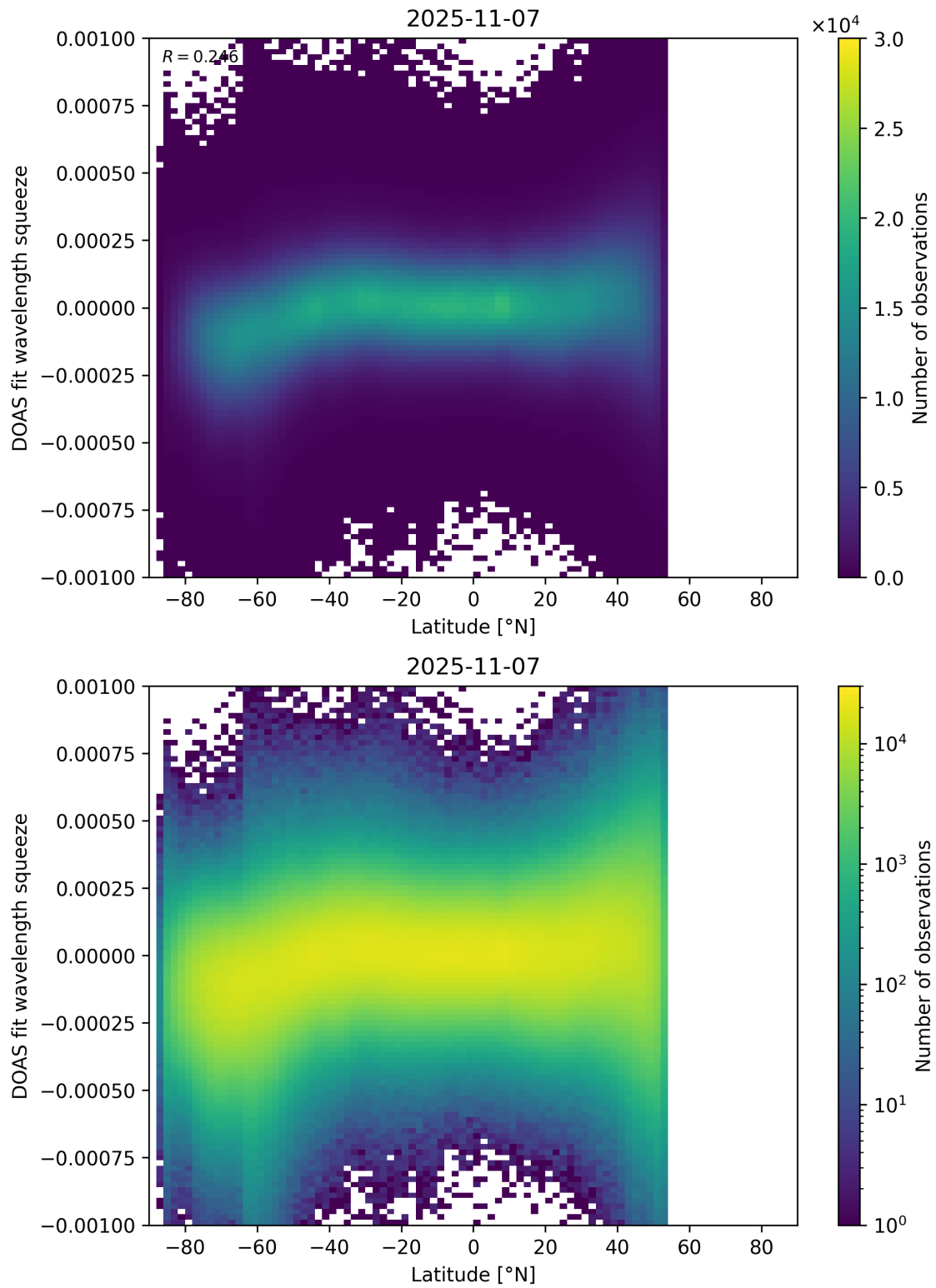
Figure 154: Scatter density plot of “Latitude” against “DOAS fit wavelength squeeze” for 2025-11-07 to 2025-11-08.
