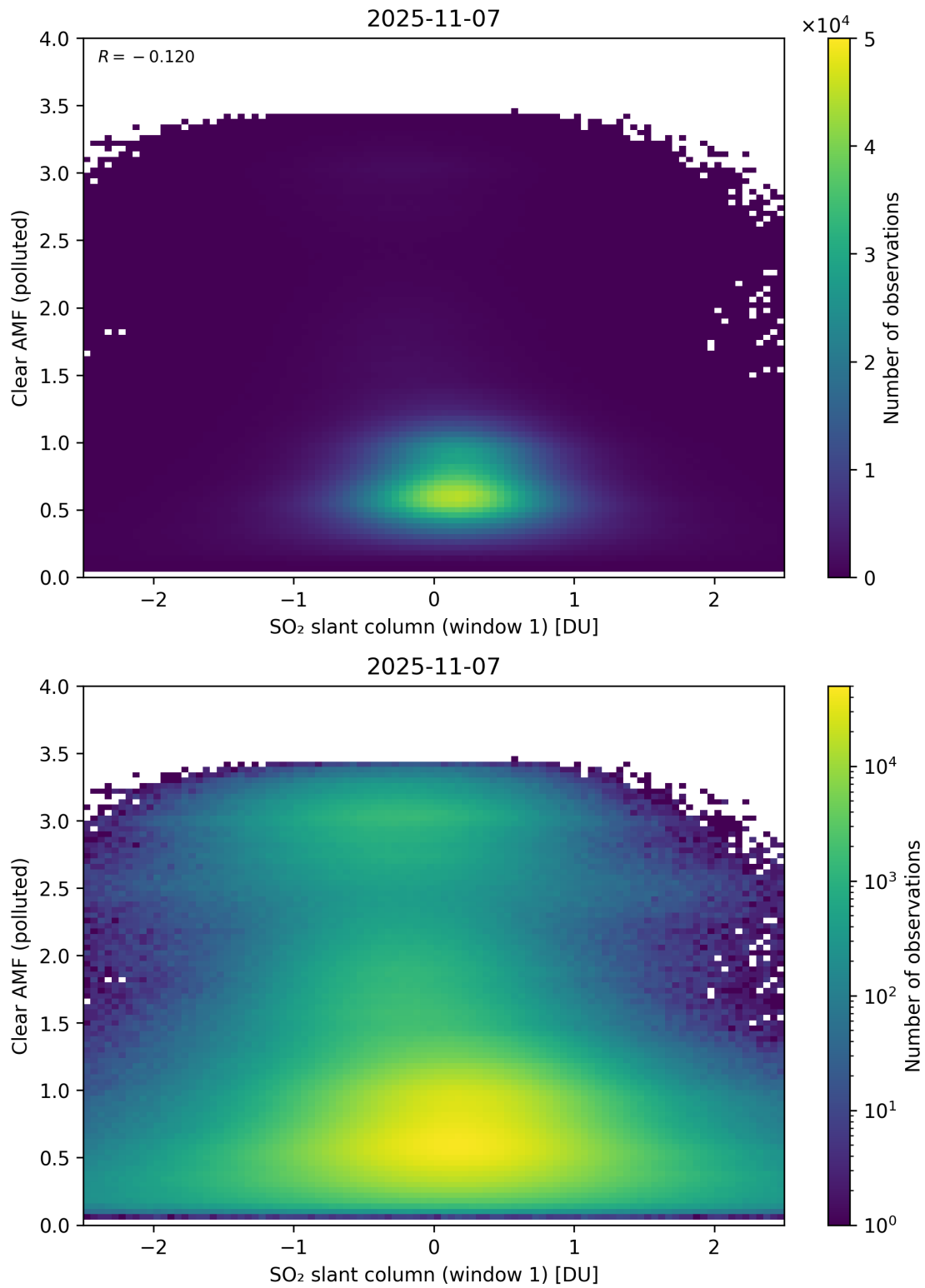
Figure 282: Scatter density plot of “SO 2 slant column (window 1)” against “Clear AMF (polluted)” for 2025-11-07 to 2025-11-08.
