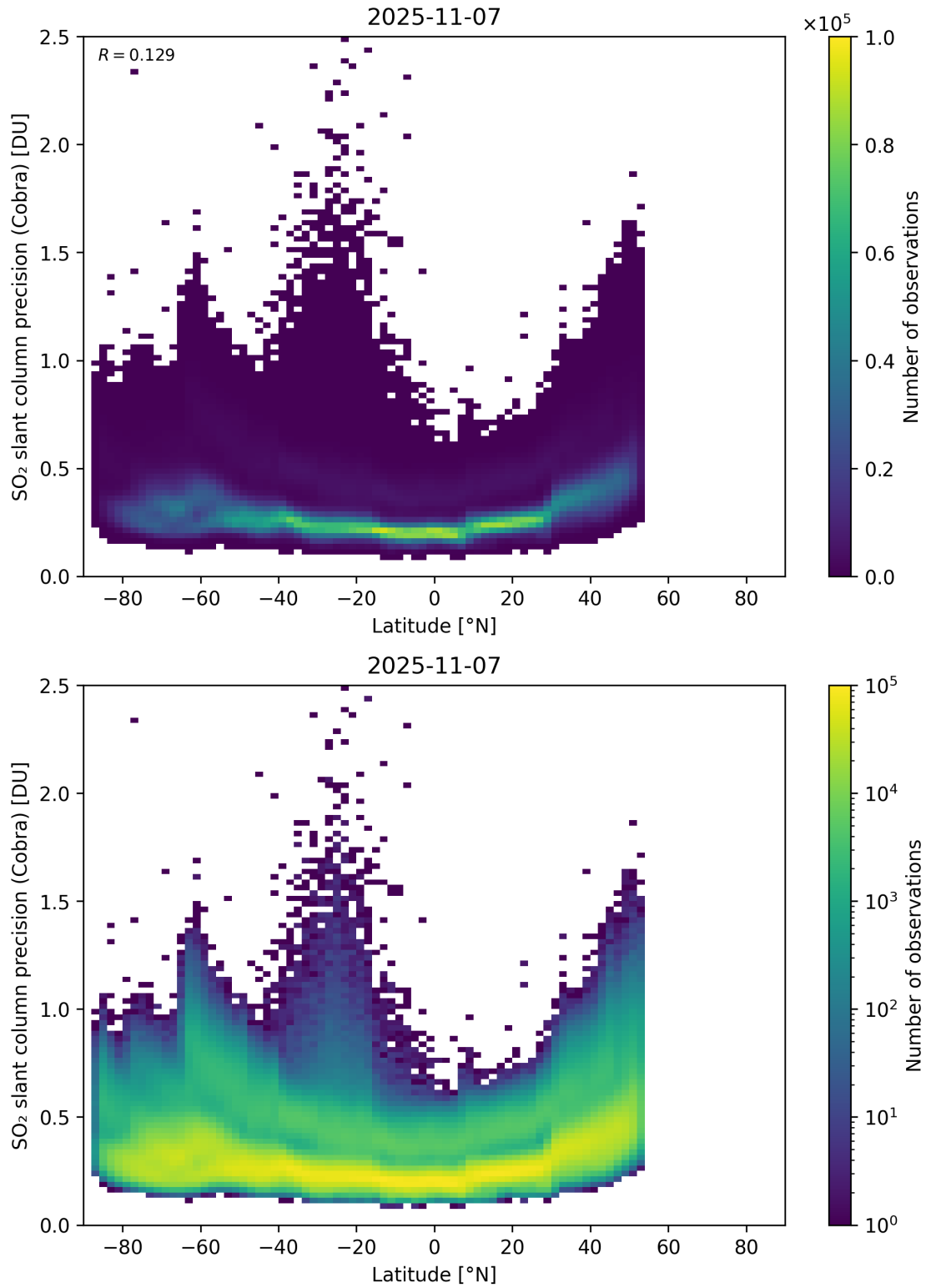
Figure 158: Scatter density plot of “Latitude” against “SO 2 slant column precision (Cobra)” for 2025-11-07 to 2025-11-08.
