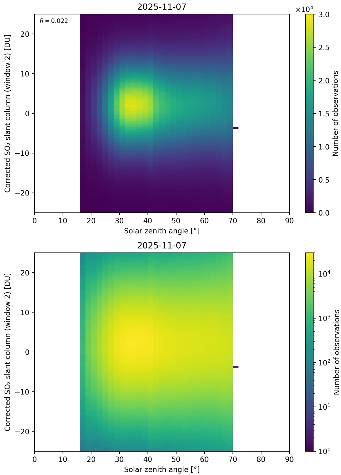
Figure 182: Scatter density plot of “Solar zenith angle” against “Corrected SO 2 slant column (window 2)” for 2025-11-07 to 2025-11-08.
