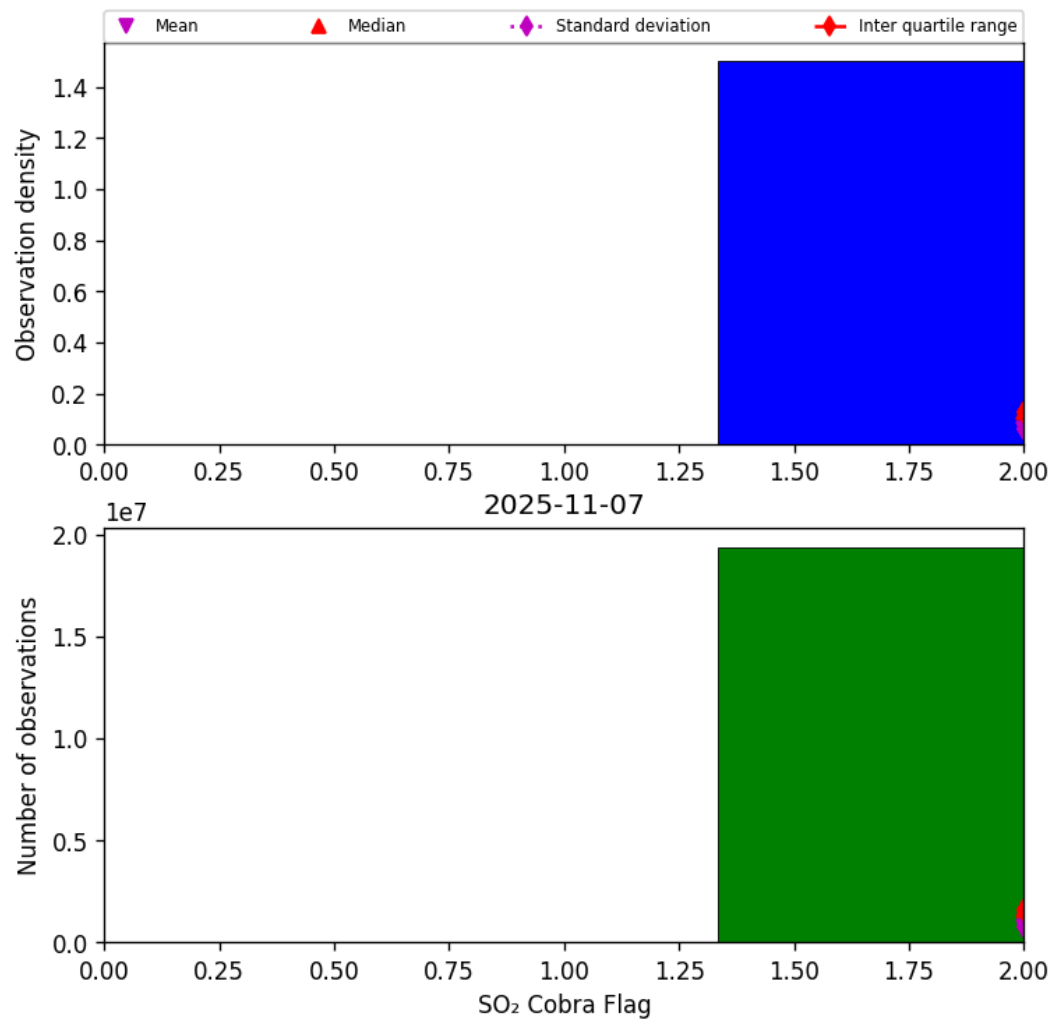
Figure 75: Histogram of “SO 2 Cobra Flag” for 2025-11-07 to 2025-11-08
