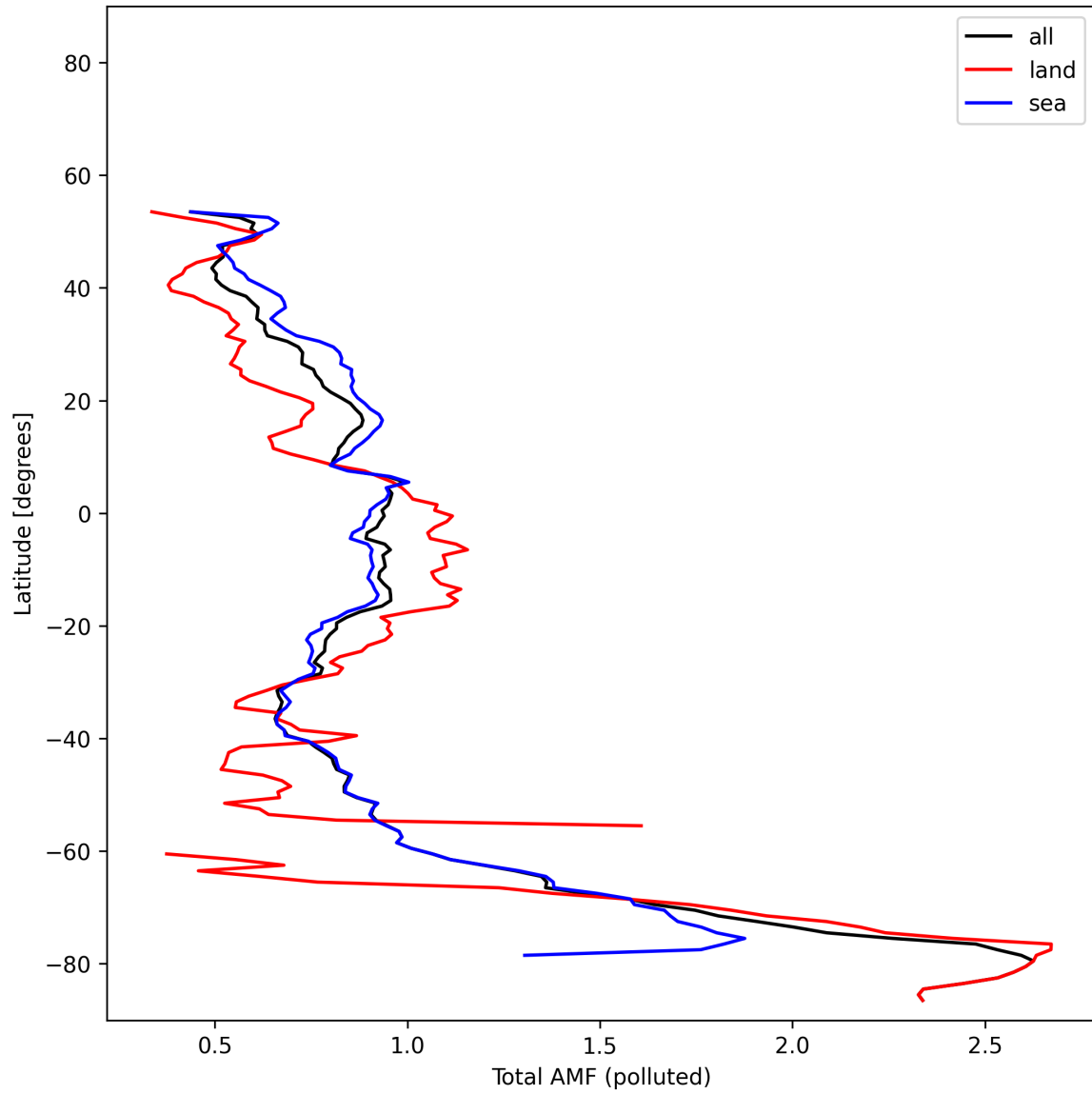
Figure 53: Zonal average of “Total AMF (polluted)” for 2025-11-07 to 2025-11-08.
