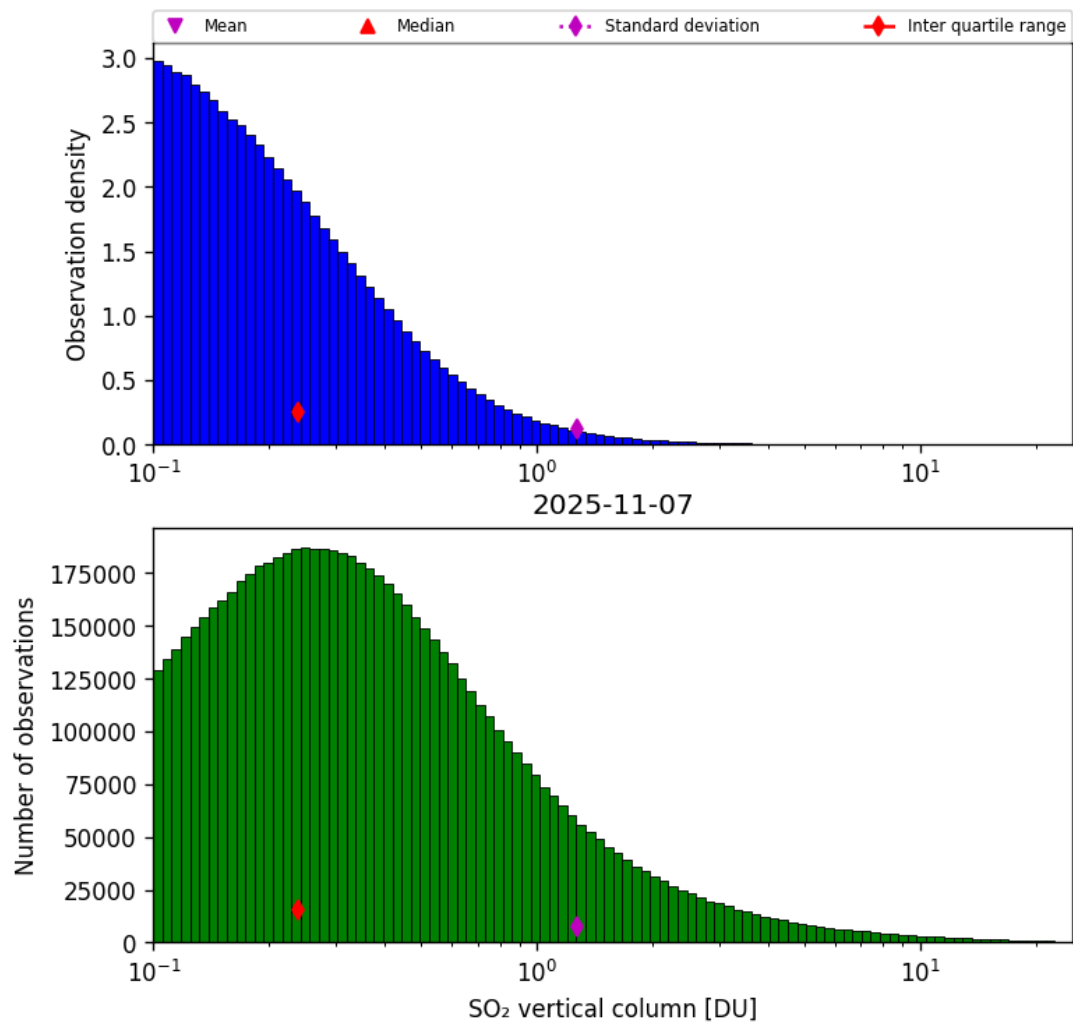
Figure 58: Histogram of “SO 2 vertical column” for 2025-11-07 to 2025-11-08
