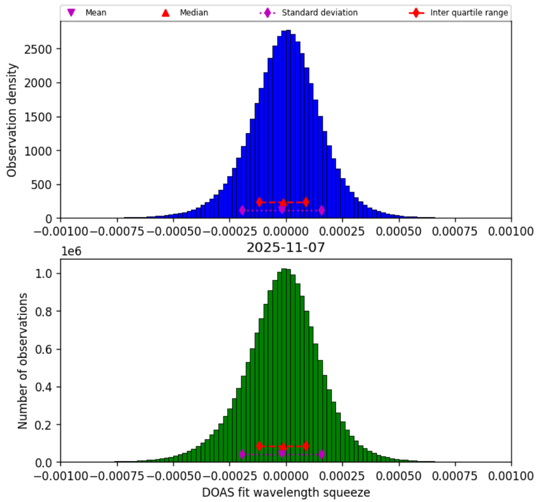
Figure 77: Histogram of “DOAS fit wavelength squeeze” for 2025-11-07 to 2025-11-08
