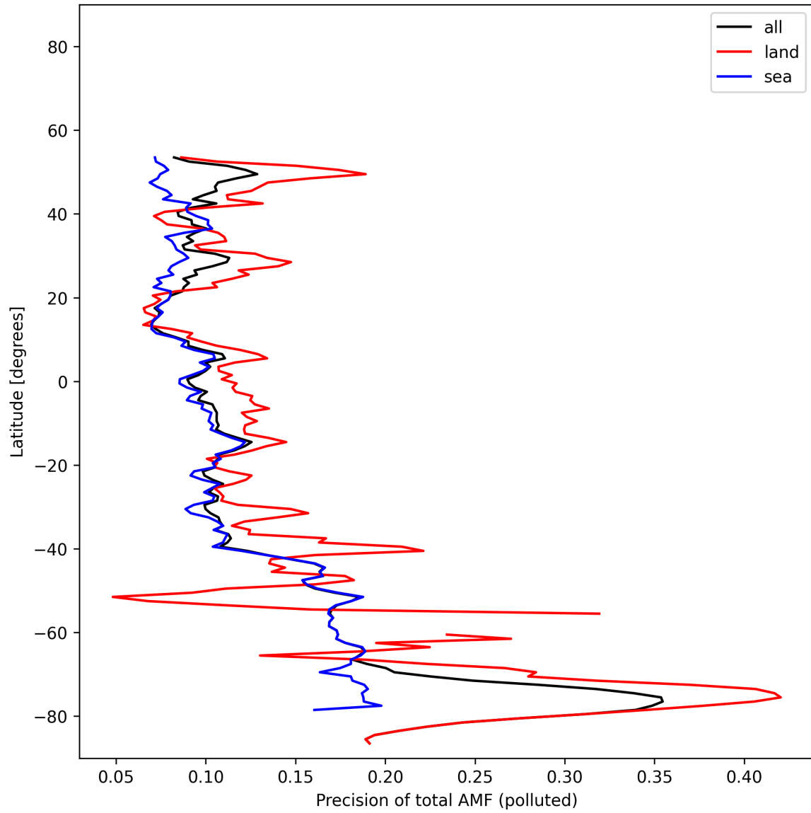
Figure 54: Zonal average of “Precision of total AMF (polluted)” for 2025-11-07 to 2025-11-08.
