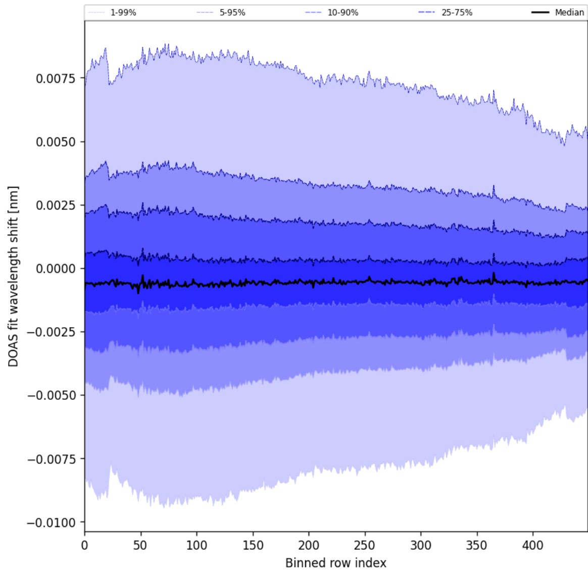
Figure 102: Along track statistics of “DOAS fit wavelength shift” for 2025-11-07 to 2025-11-08
