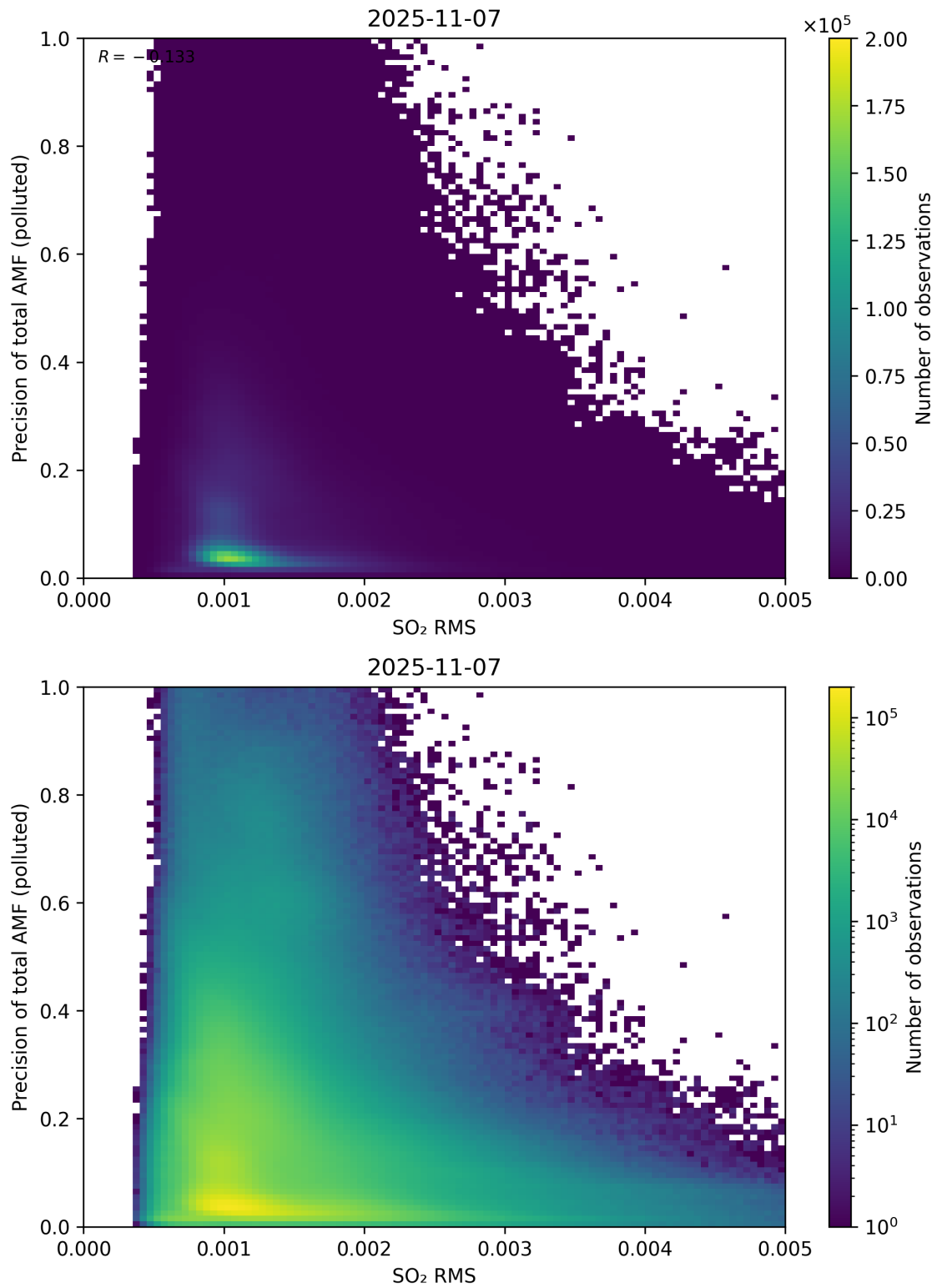
Figure 149: Scatter density plot of “SO 2 RMS” against “Precision of total AMF (polluted)” for 2025-11-07 to 2025-11-08.
