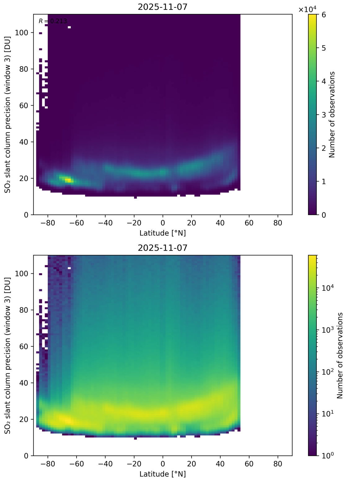
Figure 166: Scatter density plot of “Latitude” against “SO 2 slant column precision (window 3)” for 2025-11-07 to 2025-11-08.
