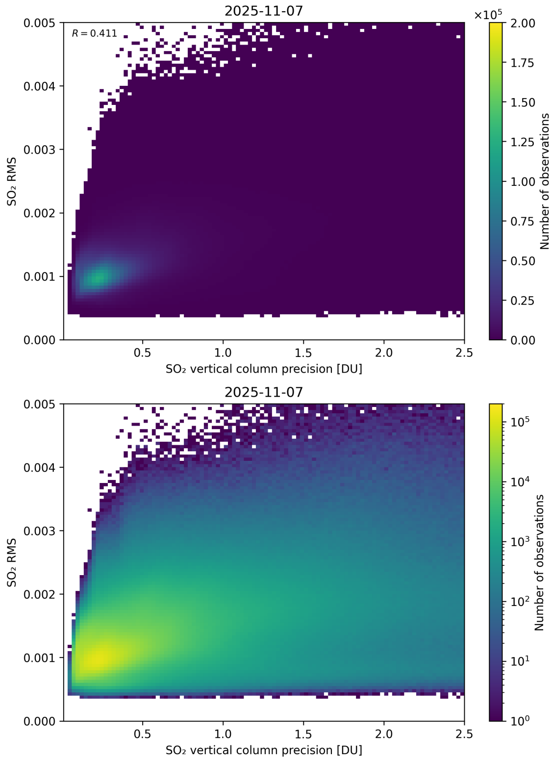
Figure 334: Scatter density plot of “SO 2 vertical column precision” against “SO 2 RMS” for 2025-11-07 to 2025-11-08.
