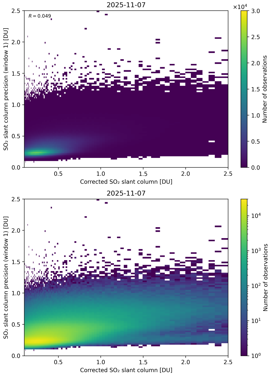
Figure 238: Scatter density plot of “Corrected SO 2 slant column” against “SO 2 slant column precision (window 1)” for 2025-11-07 to 2025-11-08.
