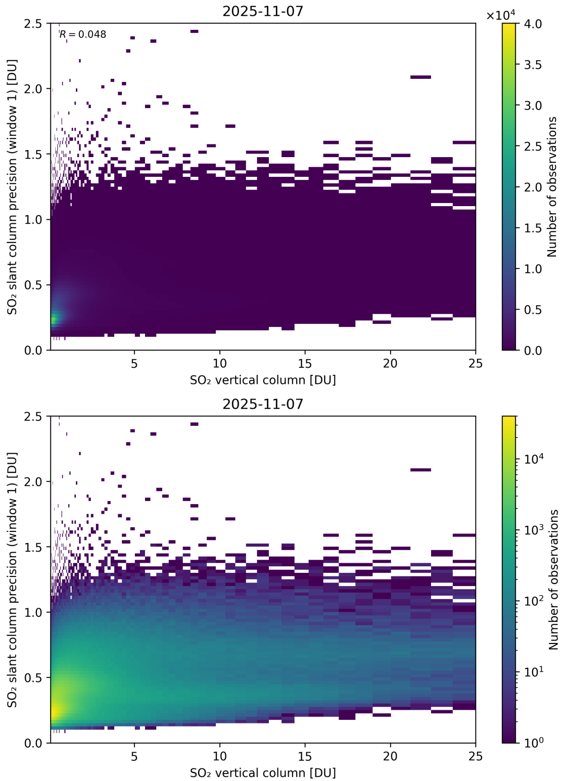
Figure 355: Scatter density plot of “SO 2 vertical column” against “SO 2 slant column precision (window 1)” for 2025-11-07 to 2025-11-08.
