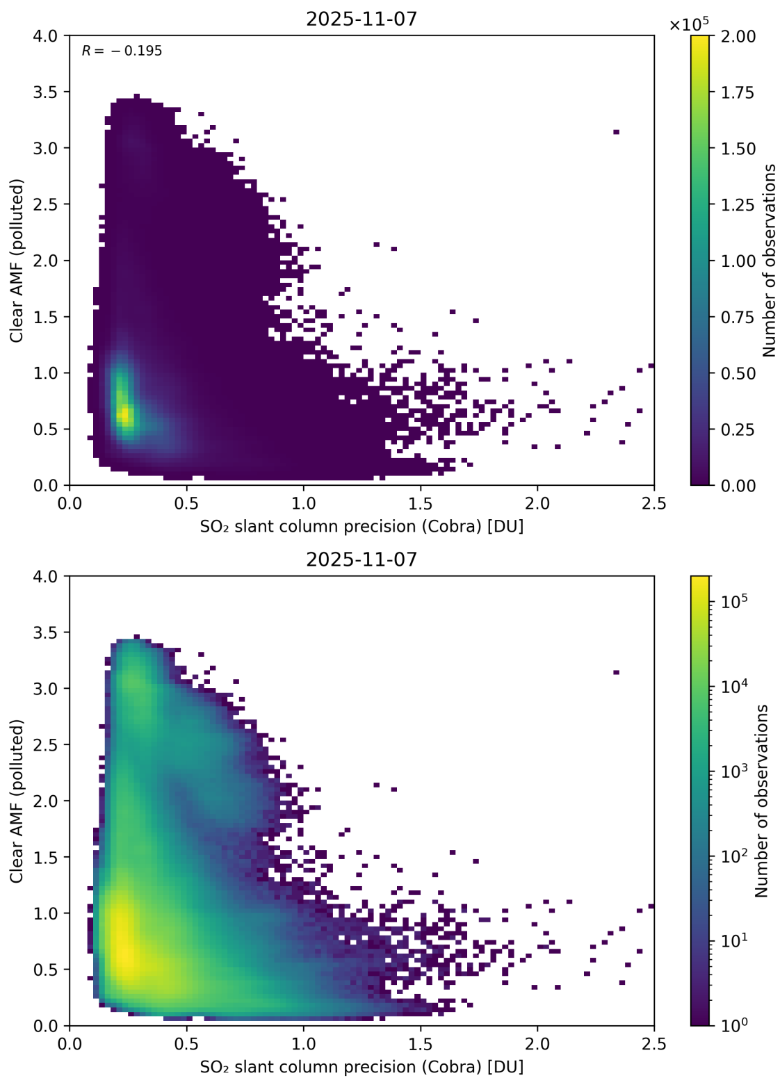
Figure 205: Scatter density plot of “SO 2 slant column precision (Cobra)” against “Clear AMF (polluted)” for 2025-11-07 to 2025-11-08.
