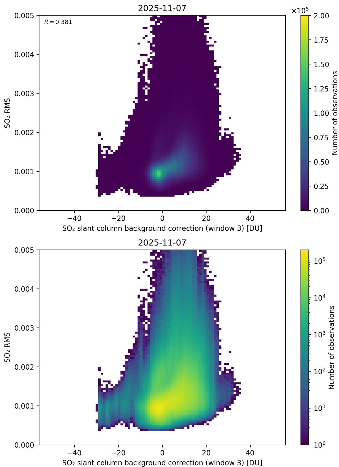
Figure 134: Scatter density plot of “SO 2 slant column background correction (window 3)” against “SO 2 RMS” for 2025-11-07 to 2025-11-08.
