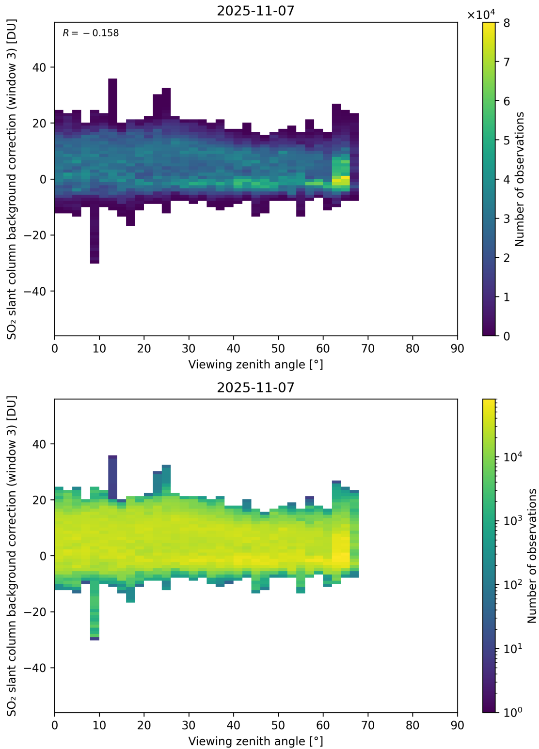
Figure 364: Scatter density plot of “Viewing zenith angle” against “SO 2 slant column background correction (window 3)” for 2025-11-07 to 2025-11-08.
