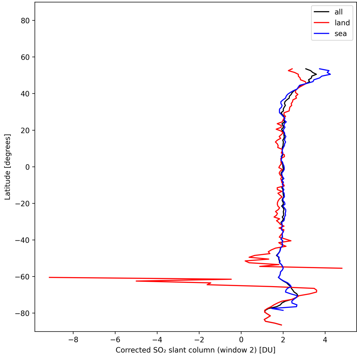
Figure 43: Zonal average of “Corrected SO 2 slant column (window 2)” for 2025-11-07 to 2025-11-08.
