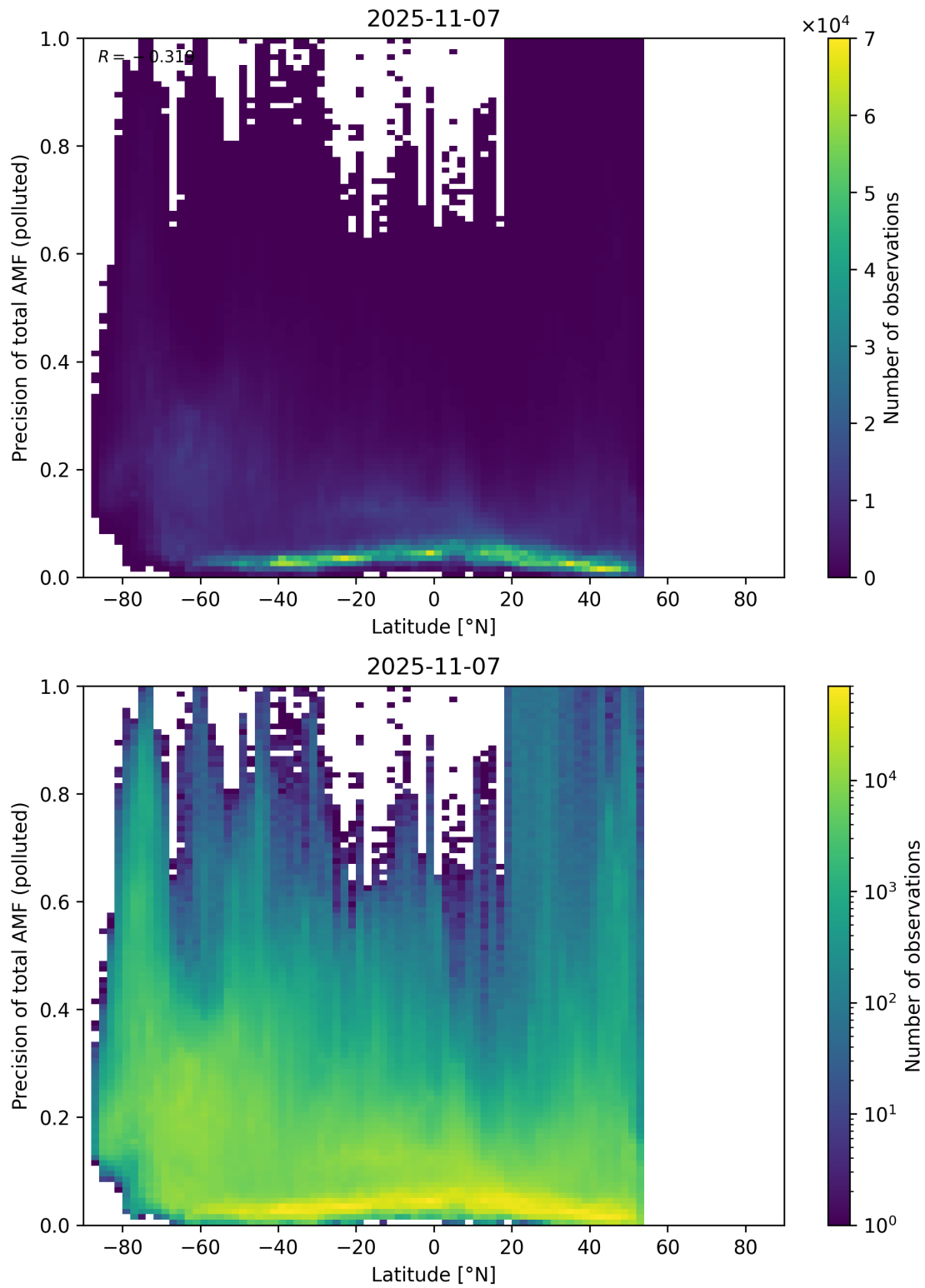
Figure 168: Scatter density plot of “Latitude” against “Precision of total AMF (polluted)” for 2025-11-07 to 2025-11-08.
