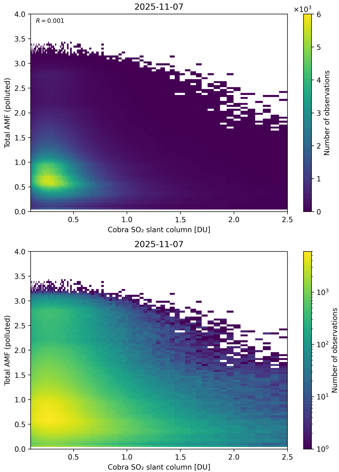
Figure 224: Scatter density plot of “Cobra SO 2 slant column” against “Total AMF (polluted)” for 2025-11-07 to 2025-11-08.
