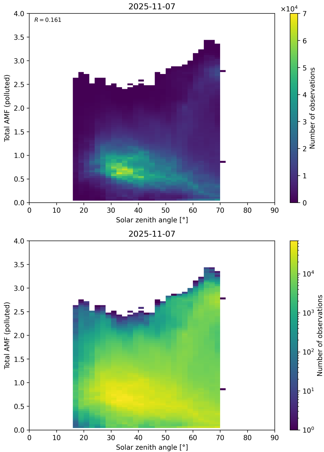
Figure 189: Scatter density plot of “Solar zenith angle” against “Total AMF (polluted)” for 2025-11-07 to 2025-11-08.
