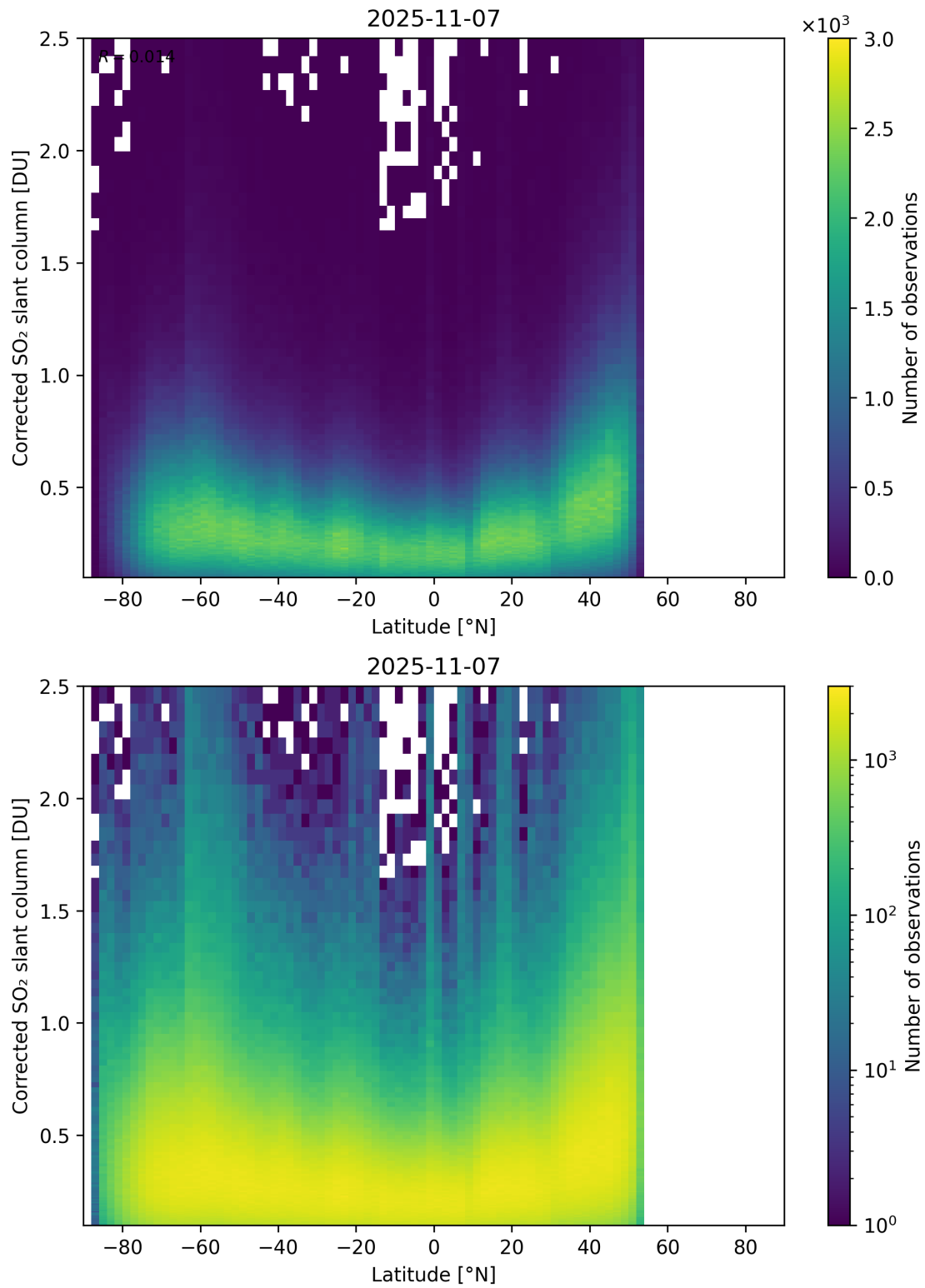
Figure 159: Scatter density plot of “Latitude” against “Corrected SO 2 slant column” for 2025-11-07 to 2025-11-08.
