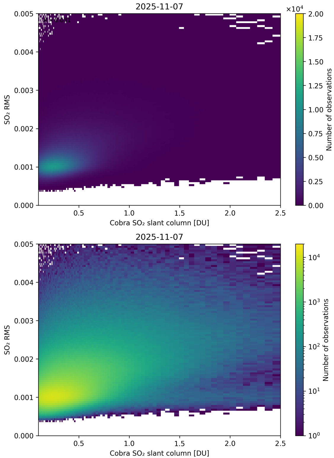
Figure 198: Scatter density plot of “Cobra SO 2 slant column” against “SO 2 RMS” for 2025-11-07 to 2025-11-08.
