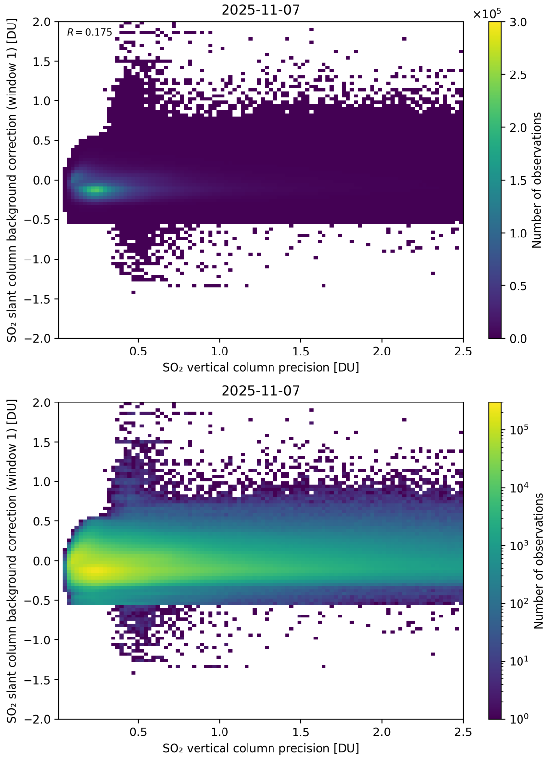
Figure 329: Scatter density plot of “SO 2 vertical column precision” against “SO 2 slant column background correction (window 1)” for 2025-11-07 to 2025-11-08.
