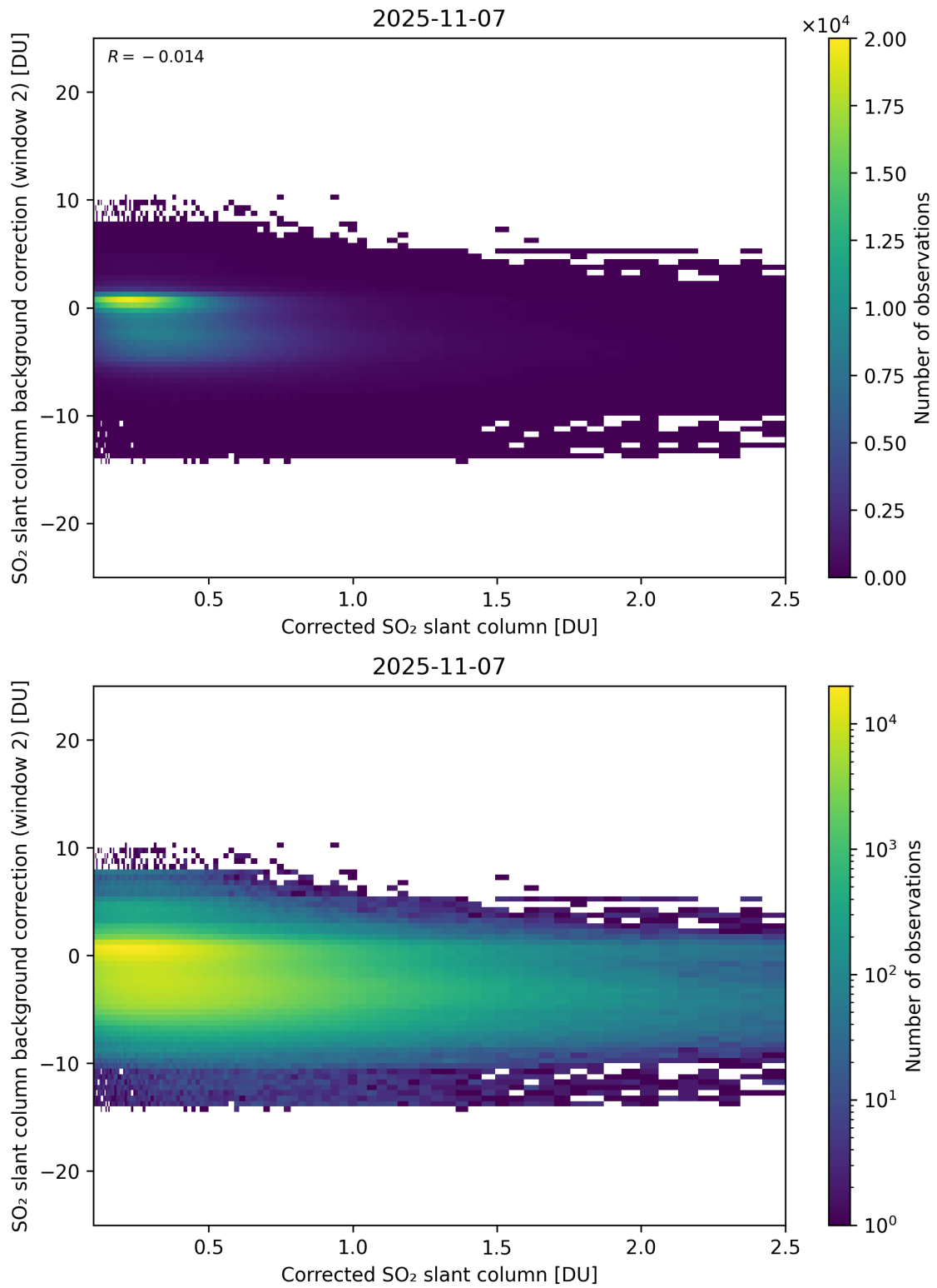
Figure 227: Scatter density plot of “Corrected SO 2 slant column” against “SO 2 slant column background correction (window 2)” for 2025-11-07 to 2025-11-08.
