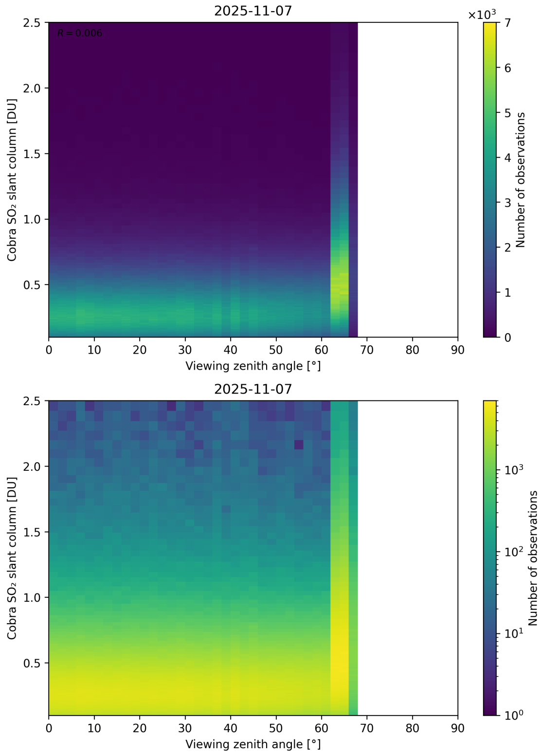
Figure 371: Scatter density plot of “Viewing zenith angle” against “Cobra SO 2 slant column” for 2025-11-07 to 2025-11-08.
