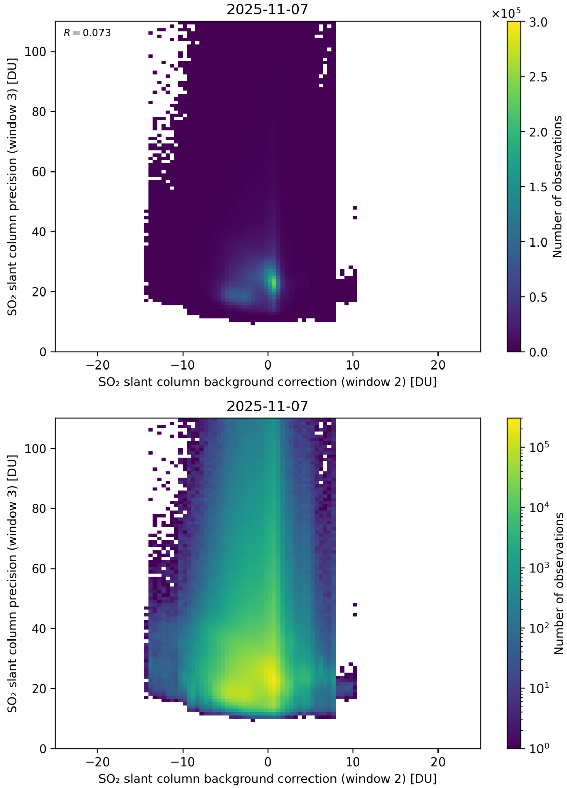
Figure 129: Scatter density plot of “SO 2 slant column background correction (window 2)” against “SO 2 slant column precision (window 3)” for 2025-11-07 to 2025-11-08.
