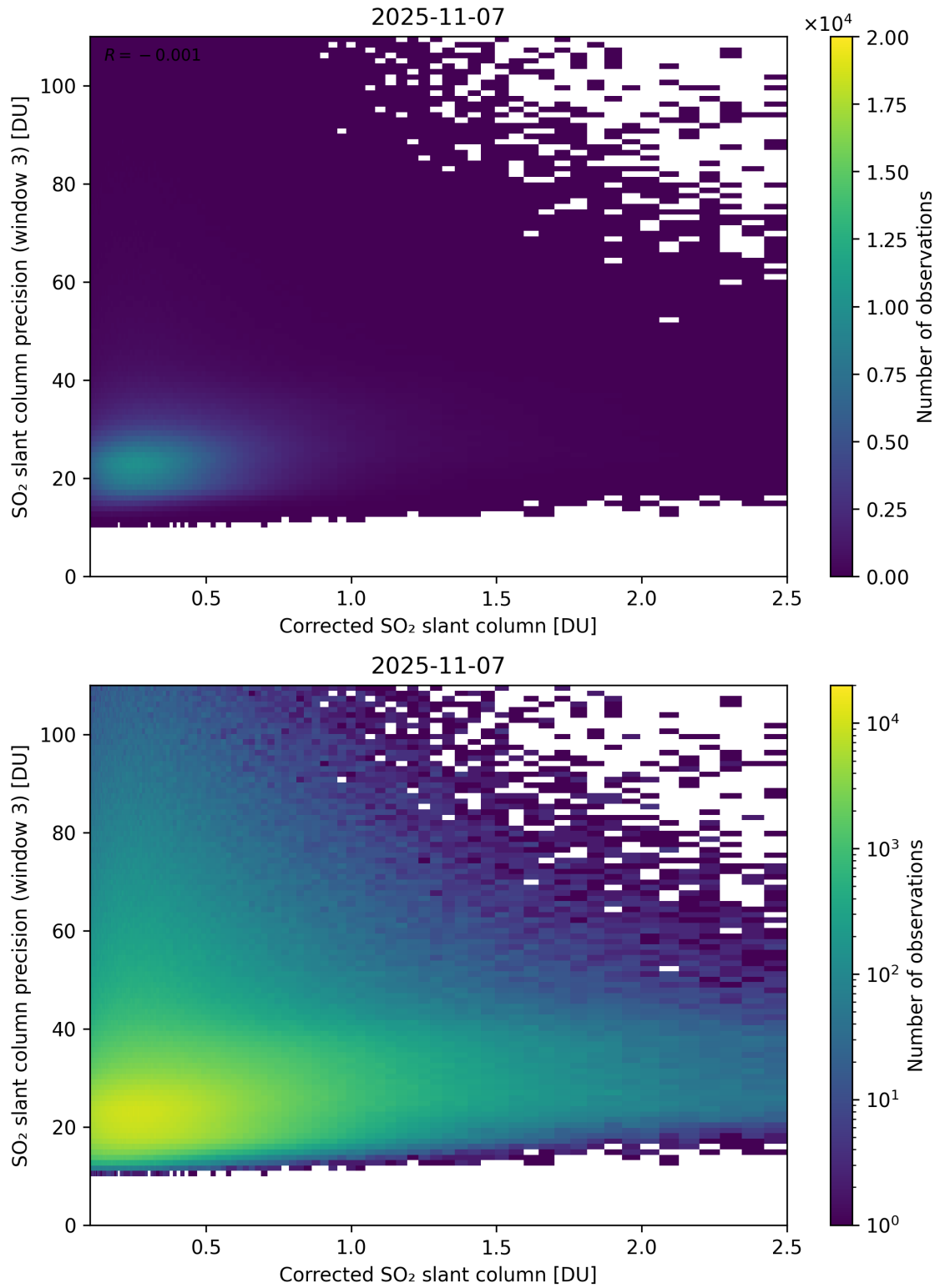
Figure 241: Scatter density plot of “Corrected SO 2 slant column” against “SO 2 slant column precision (window 3)” for 2025-11-07 to 2025-11-08.
