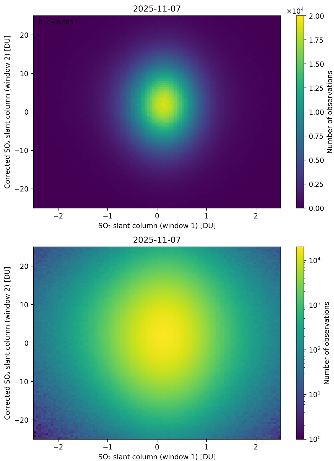
Figure 283: Scatter density plot of “SO 2 slant column (window 1)” against “Corrected SO 2 slant column (window 2)” for 2025-11-07 to 2025-11-08.
