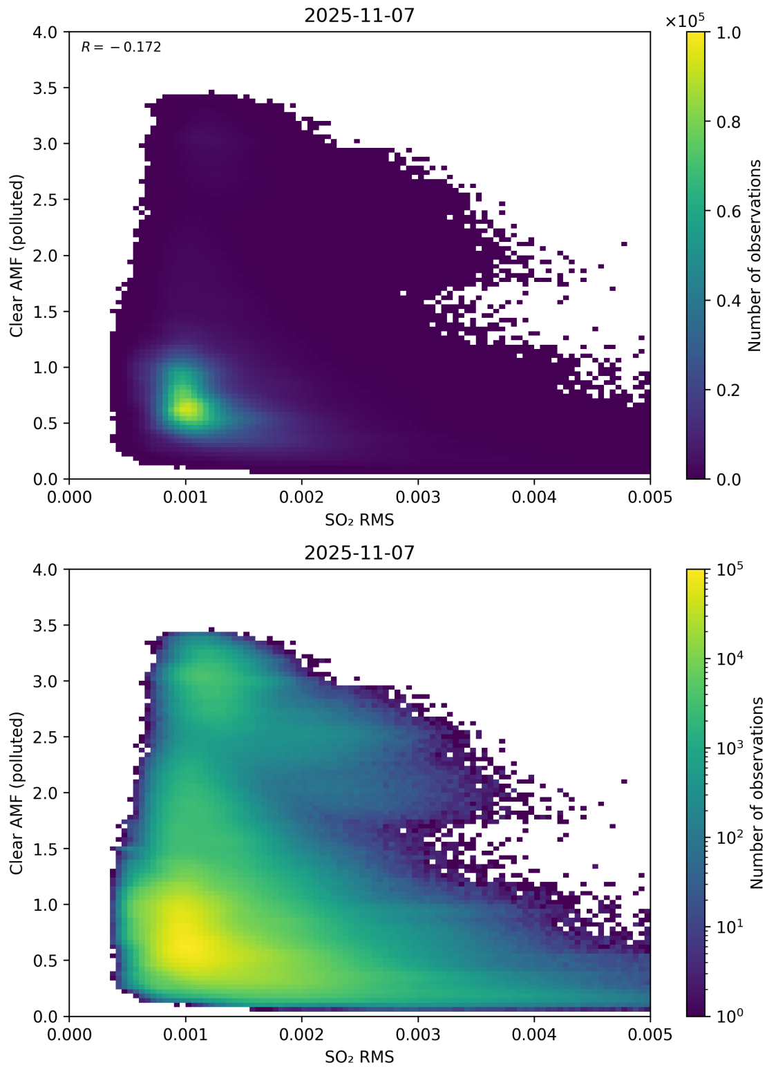
Figure 147: Scatter density plot of “SO 2 RMS” against “Clear AMF (polluted)” for 2025-11-07 to 2025-11-08.
