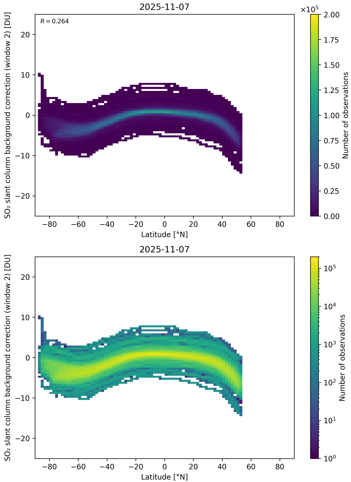
Figure 151: Scatter density plot of “Latitude” against “SO 2 slant column background correction (window 2)” for 2025-11-07 to 2025-11-08.
