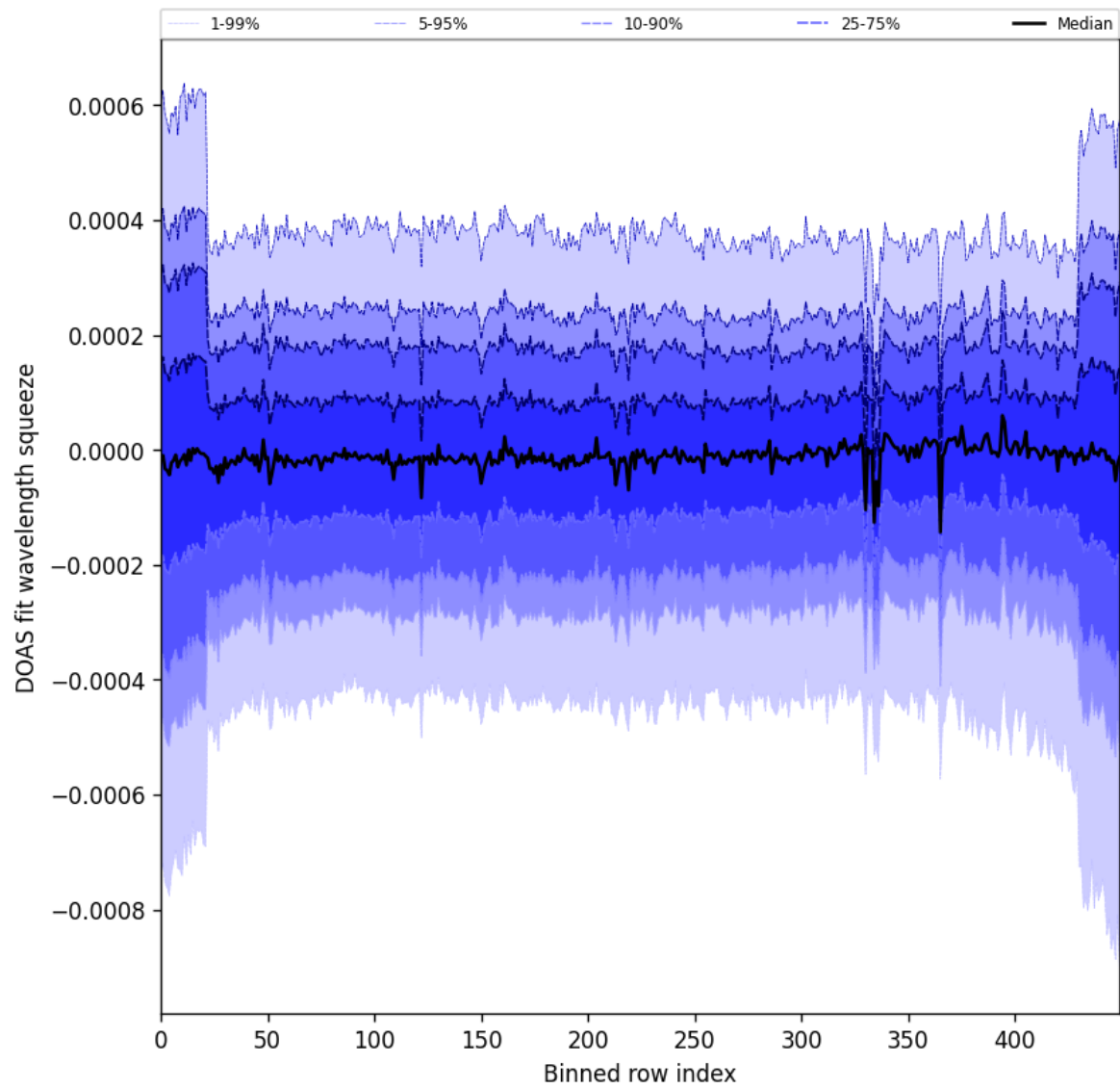
Figure 103: Along track statistics of “DOAS fit wavelength squeeze” for 2025-11-07 to 2025-11-08
