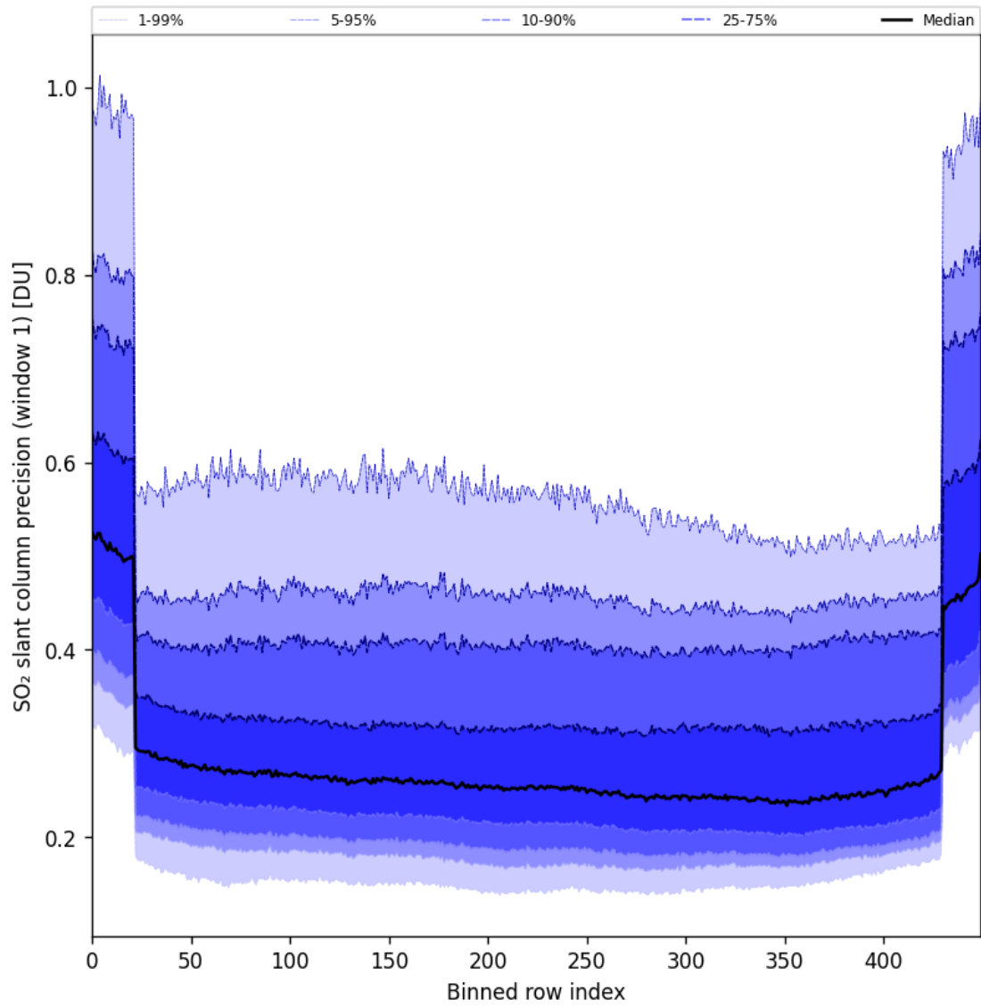
Figure 90: Along track statistics of “SO 2 slant column precision (window 1)” for 2025-11-07 to 2025-11-08
