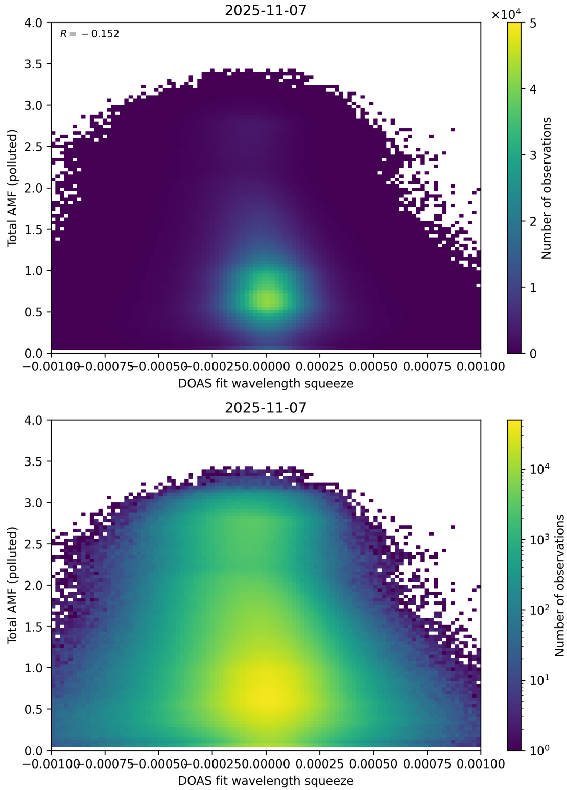
Figure 145: Scatter density plot of “DOAS fit wavelength squeeze” against “Total AMF (polluted)” for 2025-11-07 to 2025-11-08.
