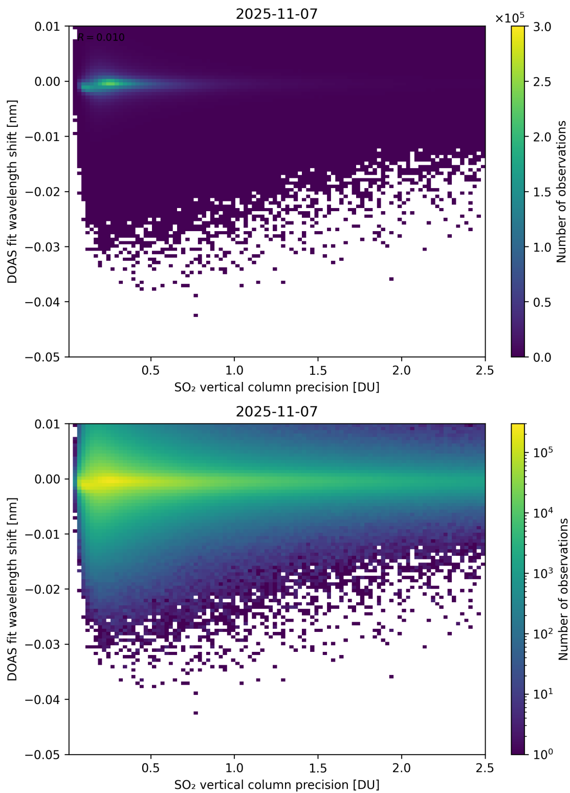
Figure 332: Scatter density plot of “SO 2 vertical column precision” against “DOAS fit wavelength shift” for 2025-11-07 to 2025-11-08.
