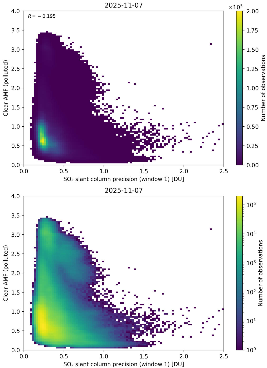
Figure 274: Scatter density plot of “SO 2 slant column precision (window 1)” against “Clear AMF (polluted)” for 2025-11-07 to 2025-11-08.
