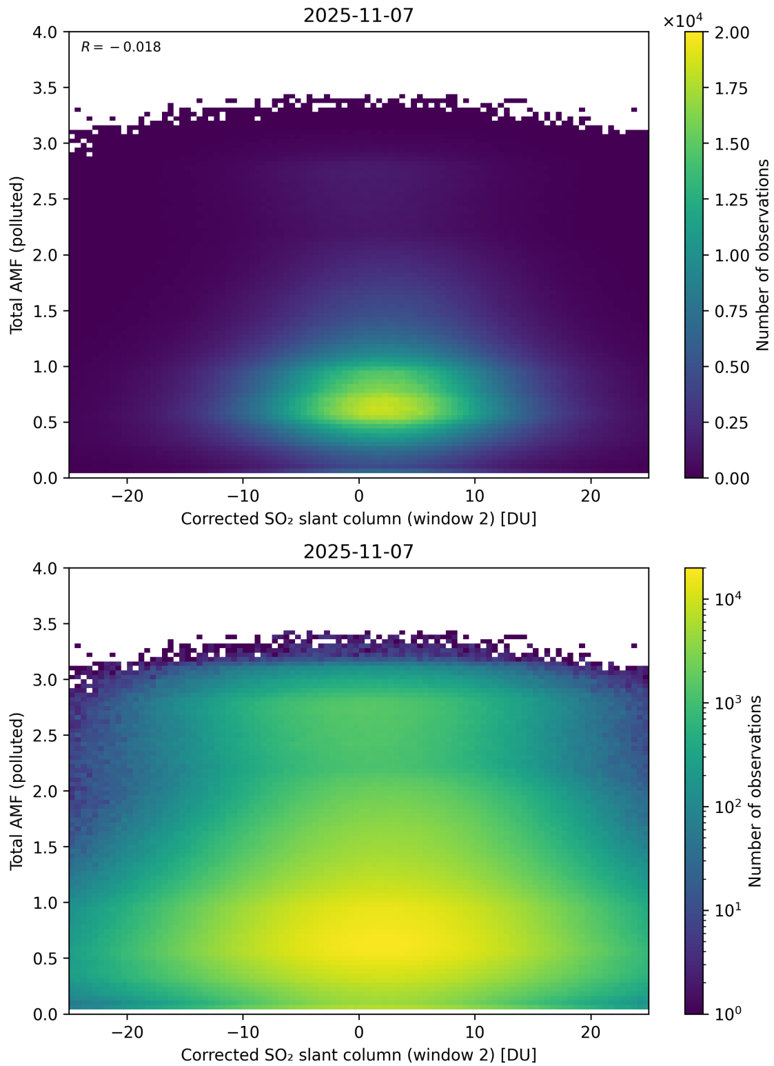
Figure 253: Scatter density plot of “Corrected SO 2 slant column (window 2)” against “Total AMF (polluted)” for 2025-11-07 to 2025-11-08.
