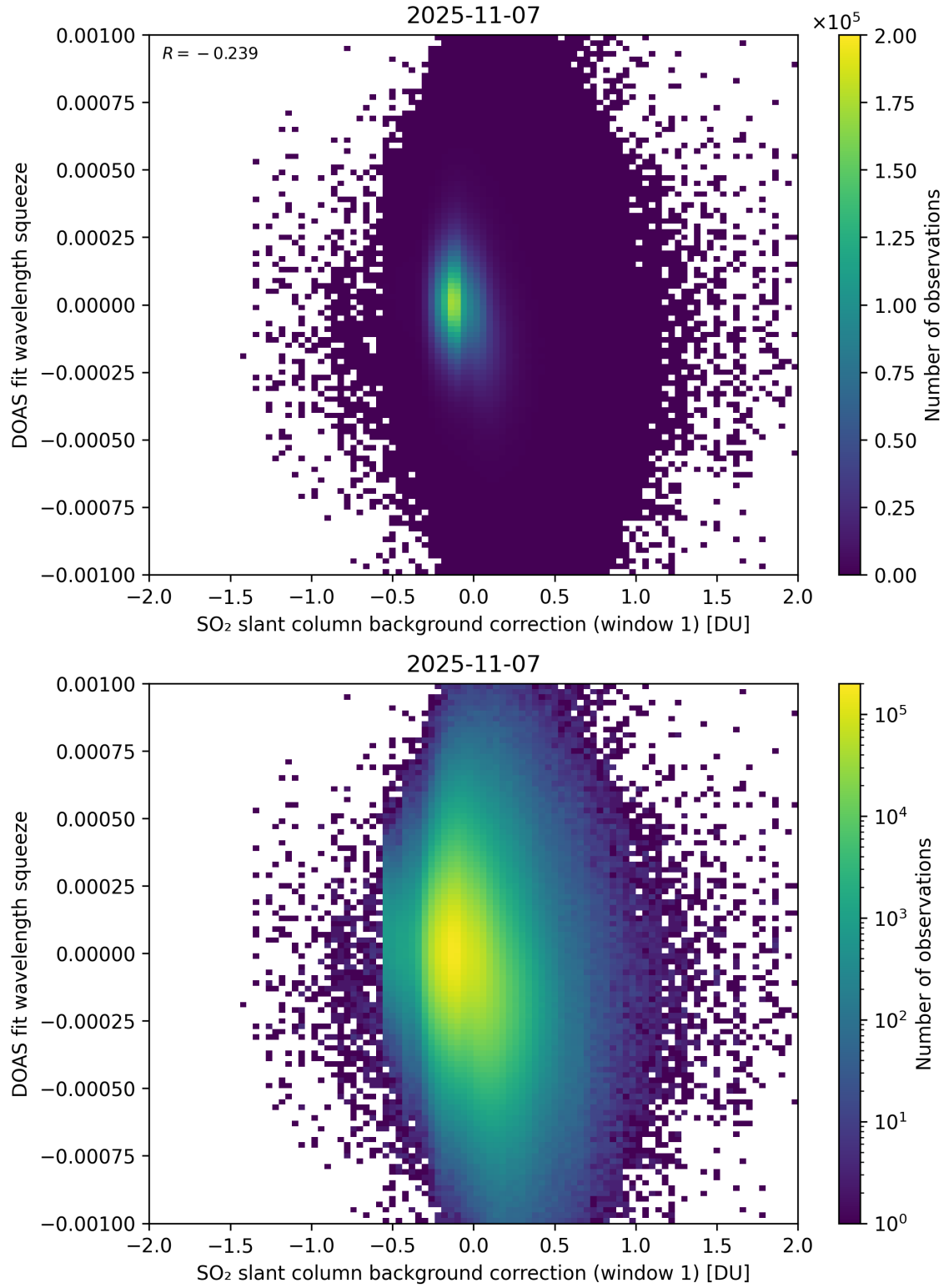
Figure 112: Scatter density plot of “SO 2 slant column background correction (window 1)” against “DOAS fit wavelength squeeze” for 2025-11-07 to 2025-11-08.
