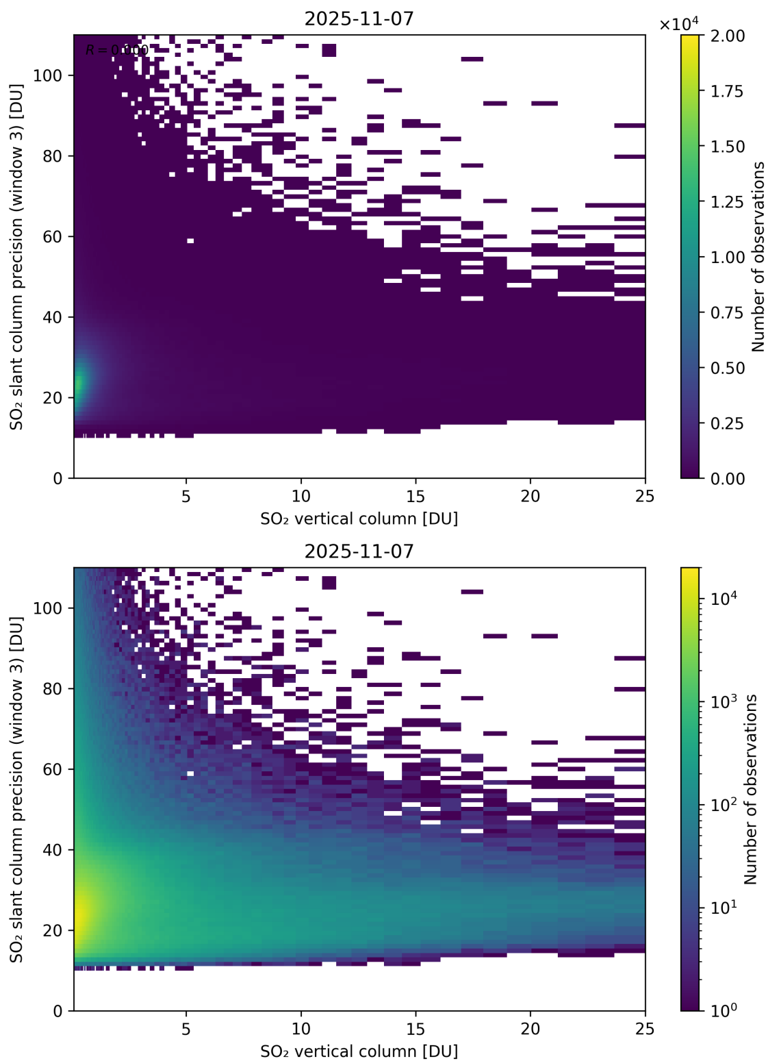
Figure 358: Scatter density plot of “SO 2 vertical column” against “SO 2 slant column precision (window 3)” for 2025-11-07 to 2025-11-08.
