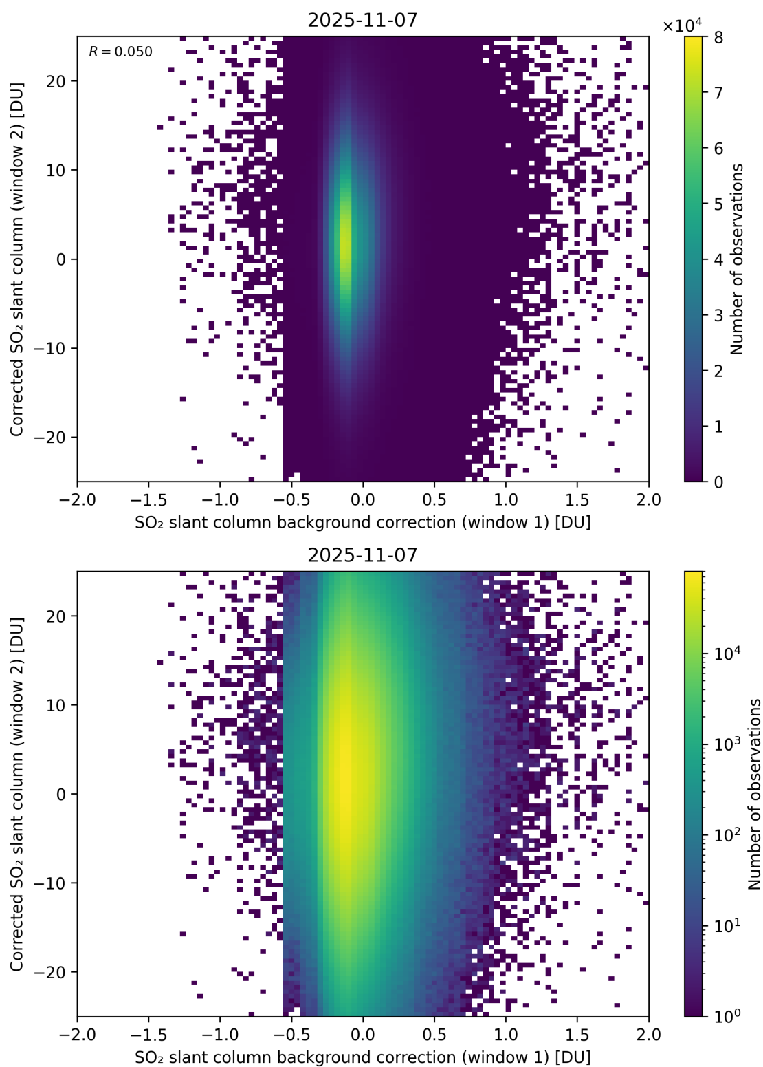
Figure 115: Scatter density plot of “SO 2 slant column background correction (window 1)” against “Corrected SO 2 slant column (window 2)” for 2025-11-07 to 2025-11-08.
