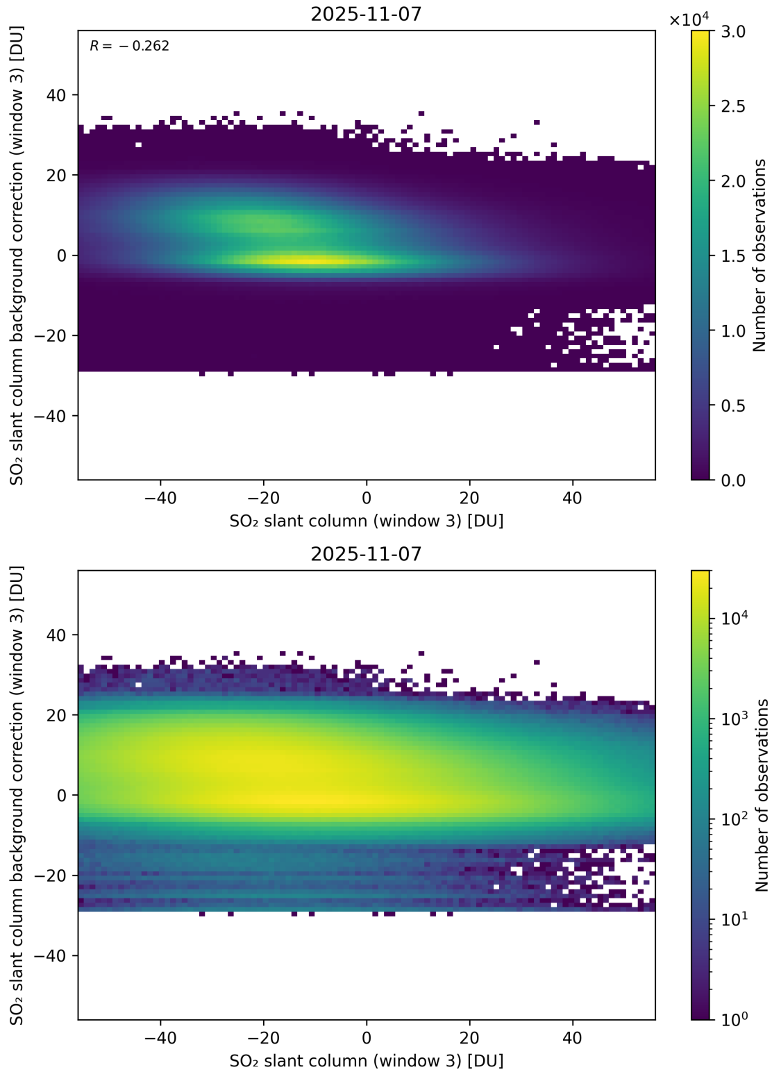
Figure 303: Scatter density plot of “SO 2 slant column (window 3)” against “SO 2 slant column background correction (window 3)” for 2025-11-07 to 2025-11-08.
