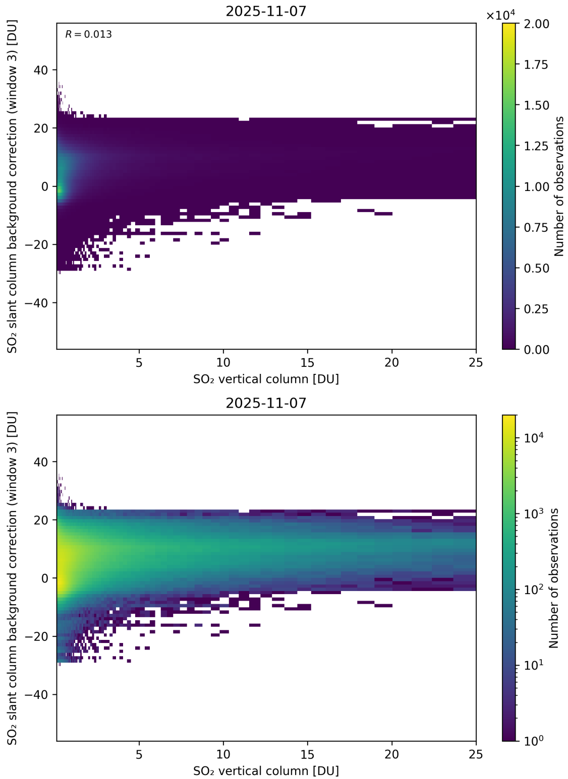
Figure 325: Scatter density plot of “SO 2 vertical column” against “SO 2 slant column background correction (window 3)” for 2025-11-07 to 2025-11-08.
