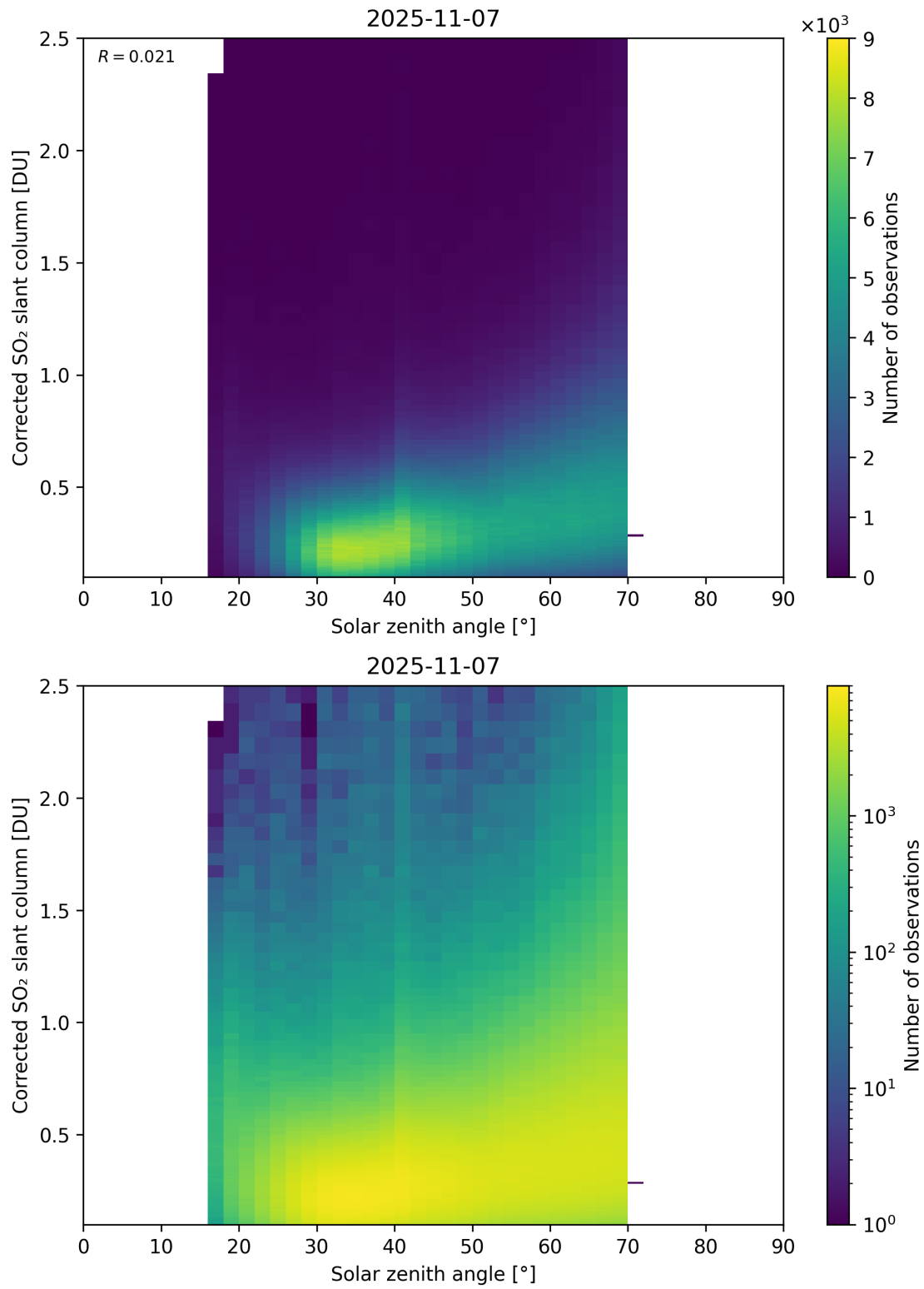
Figure 181: Scatter density plot of “Solar zenith angle” against “Corrected SO 2 slant column” for 2025-11-07 to 2025-11-08.
