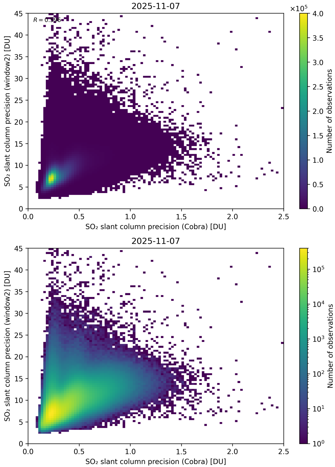
Figure 210: Scatter density plot of “SO 2 slant column precision (Cobra)” against “SO 2 slant column precision (window2)” for 2025-11-07 to 2025-11-08.
