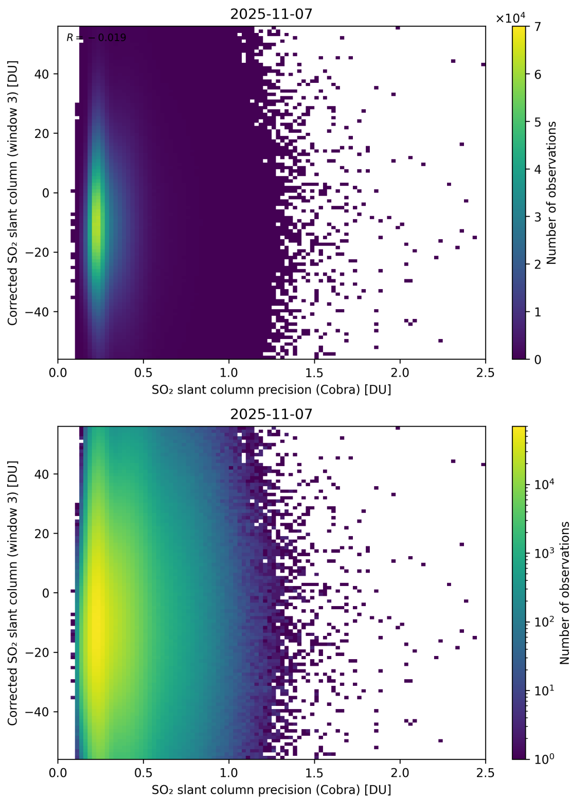
Figure 207: Scatter density plot of “SO 2 slant column precision (Cobra)” against “Corrected SO 2 slant column (window 3)” for 2025-11-07 to 2025-11-08.
