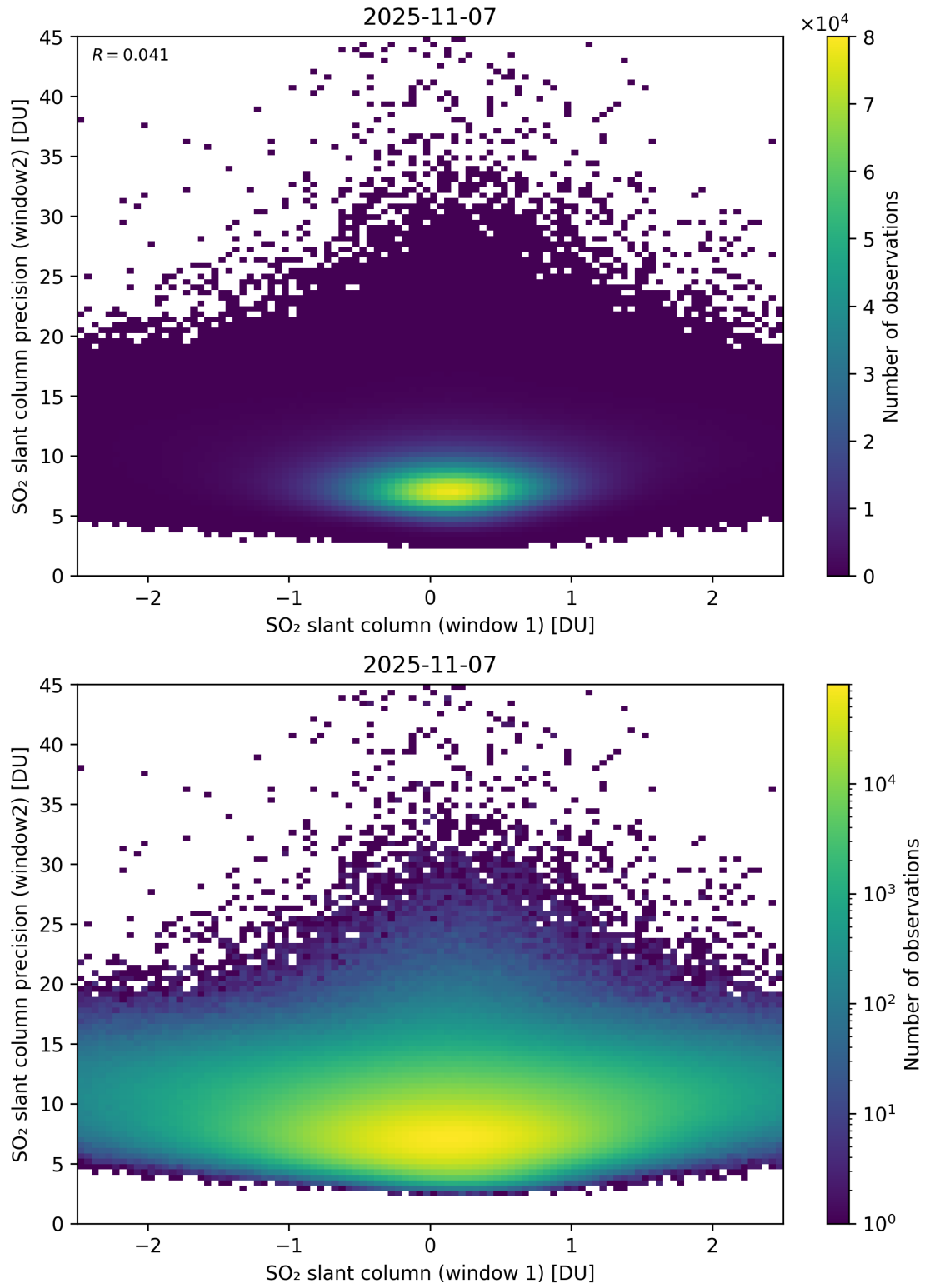
Figure 286: Scatter density plot of “SO 2 slant column (window 1)” against “SO 2 slant column precision (window2)” for 2025-11-07 to 2025-11-08.
