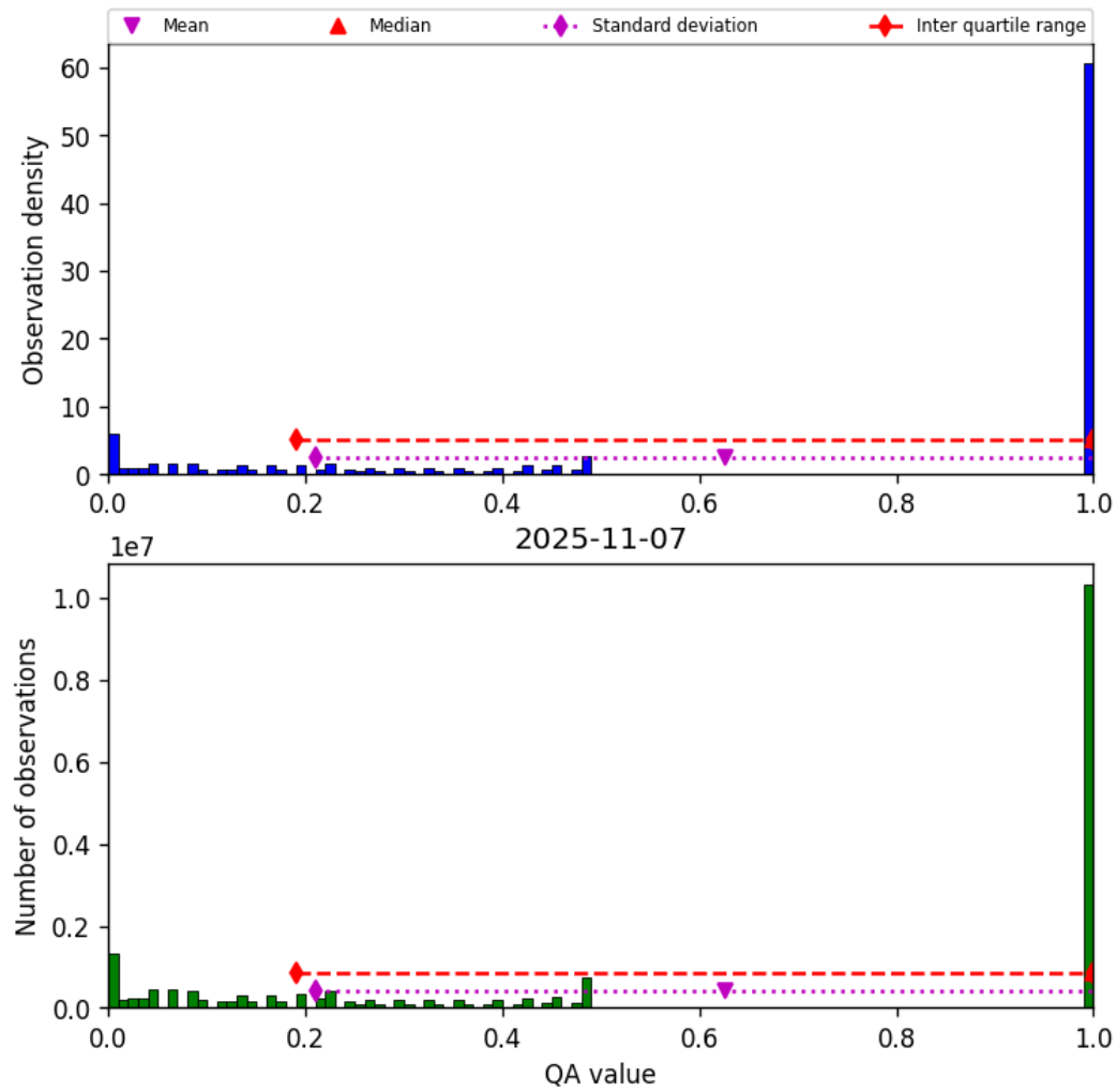
Figure 57: Histogram of “QA value” for 2025-11-07 to 2025-11-08
