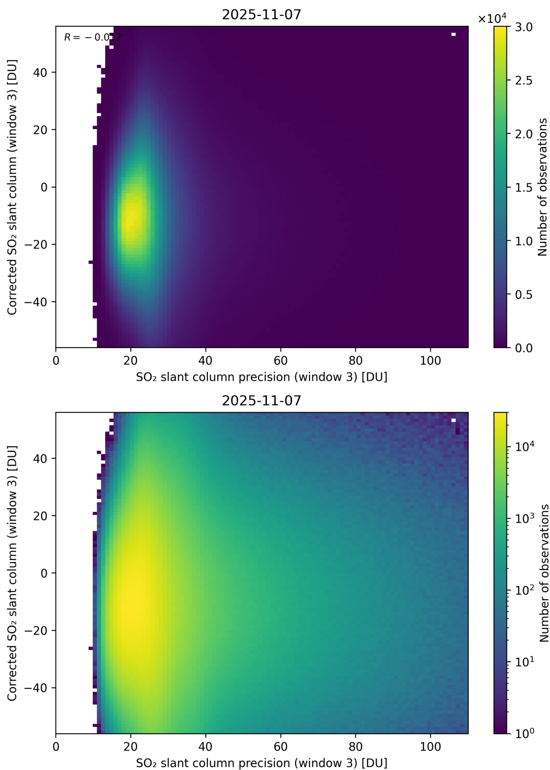
Figure 312: Scatter density plot of “SO 2 slant column precision (window 3)” against “Corrected SO 2 slant column (window 3)” for 2025-11-07 to 2025-11-08.
