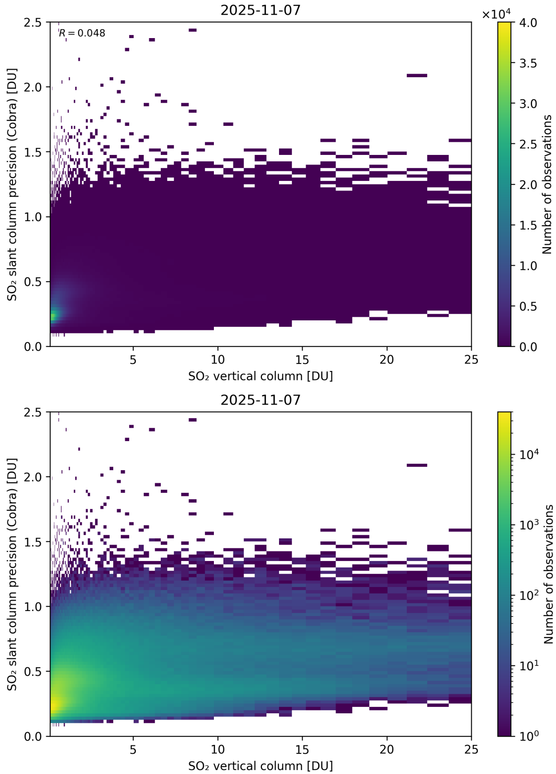
Figure 350: Scatter density plot of “SO 2 vertical column” against “SO 2 slant column precision (Cobra)” for 2025-11-07 to 2025-11-08.
