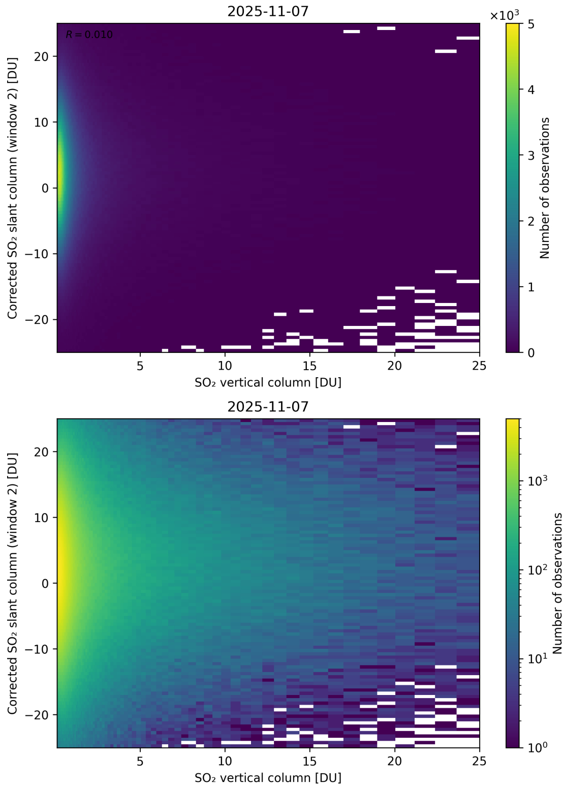
Figure 352: Scatter density plot of “SO 2 vertical column” against “Corrected SO 2 slant column (window 2)” for 2025-11-07 to 2025-11-08.
