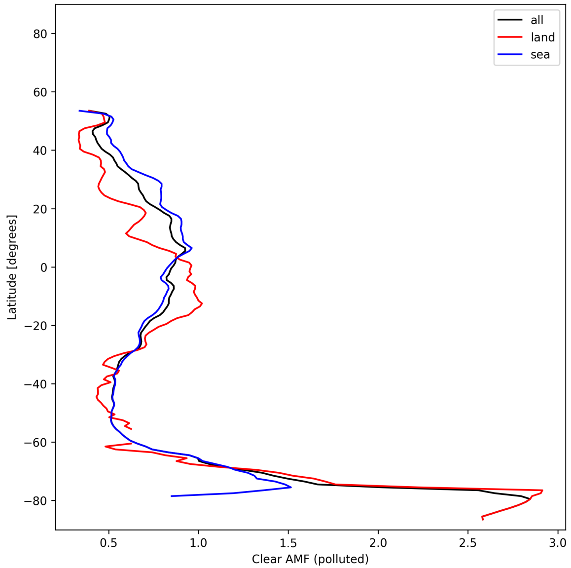
Figure 55: Zonal average of “Clear AMF (polluted)” for 2025-11-07 to 2025-11-08.
