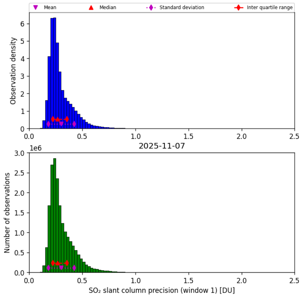
Figure 64: Histogram of “SO 2 slant column precision (window 1)” for 2025-11-07 to 2025-11-08
