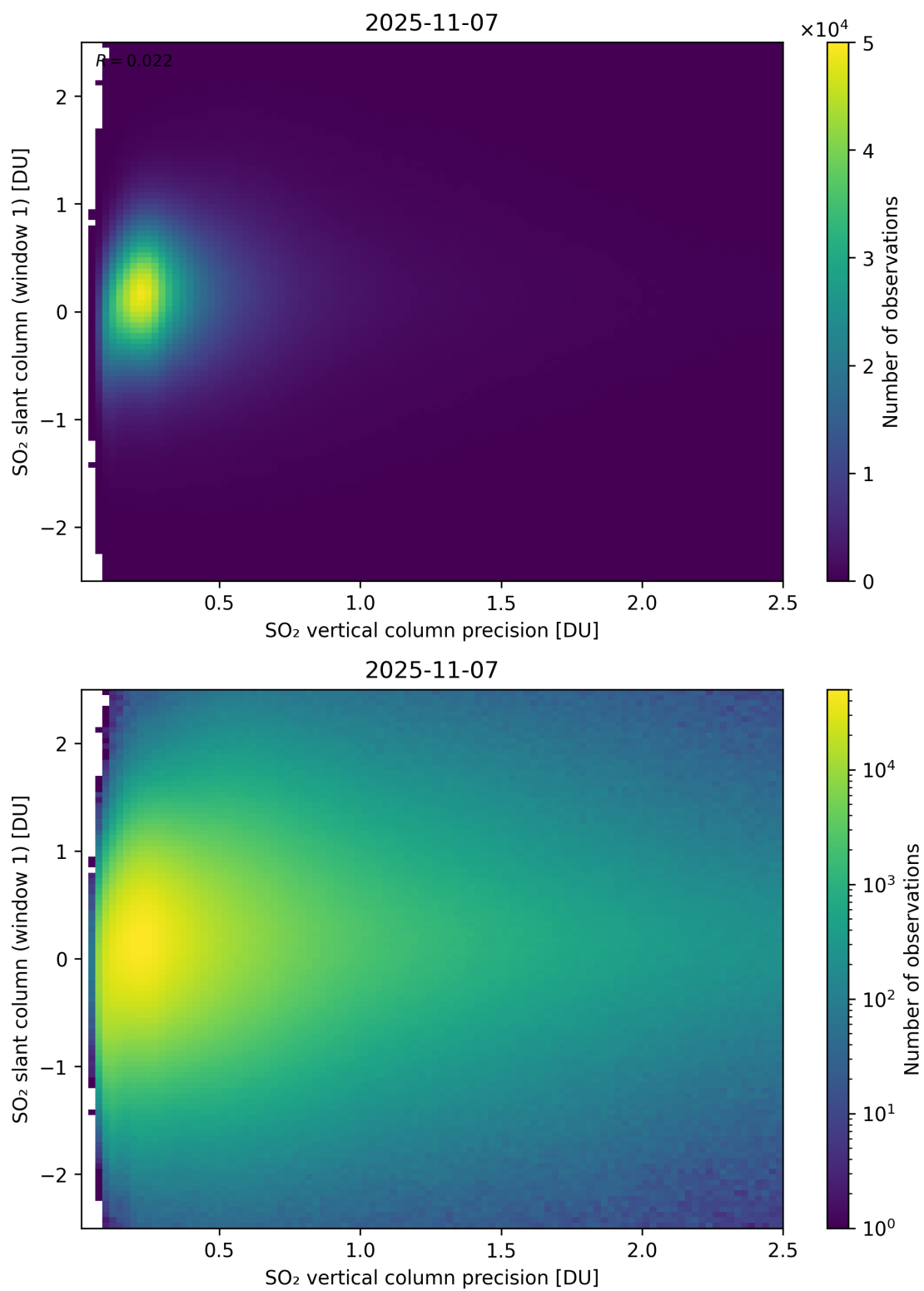
Figure 341: Scatter density plot of “SO 2 vertical column precision” against “SO 2 slant column (window 1)” for 2025-11-07 to 2025-11-08.
