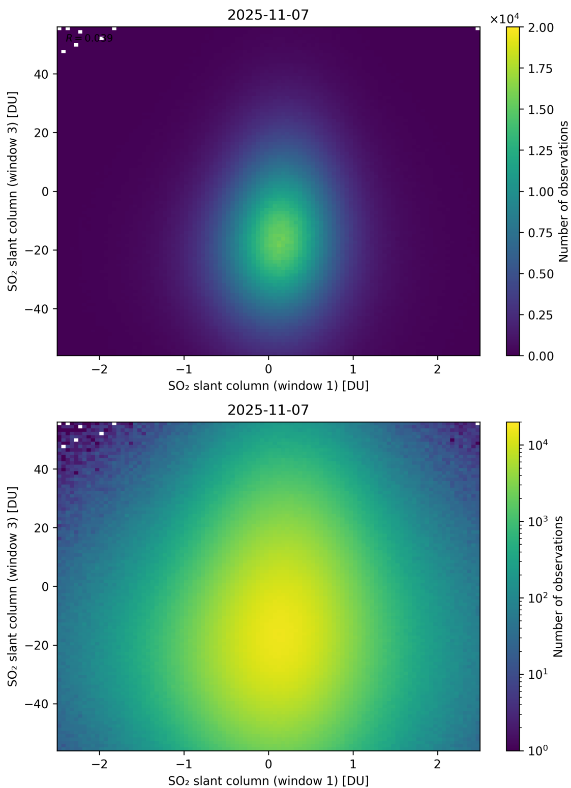
Figure 287: Scatter density plot of “SO 2 slant column (window 1)” against “SO 2 slant column (window 3)” for 2025-11-07 to 2025-11-08.
