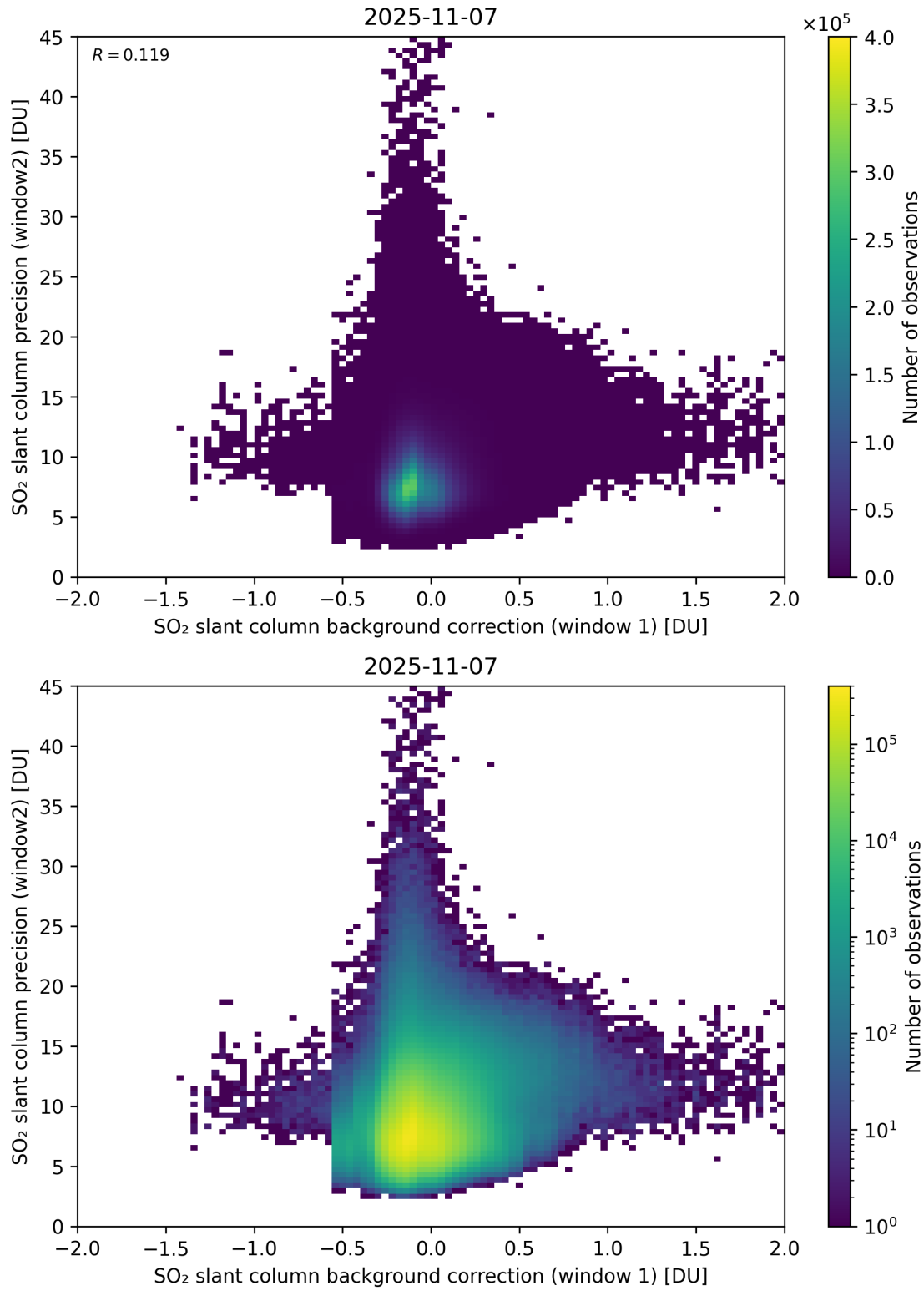
Figure 117: Scatter density plot of “SO 2 slant column background correction (window 1)” against “SO 2 slant column precision (window2)” for 2025-11-07 to 2025-11-08.
