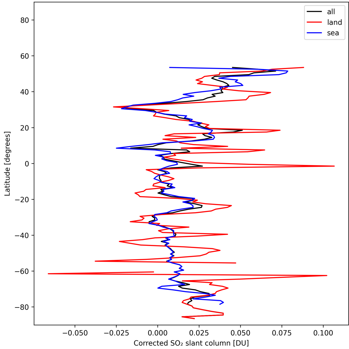
Figure 34: Zonal average of “Corrected SO 2 slant column” for 2025-11-07 to 2025-11-08.
