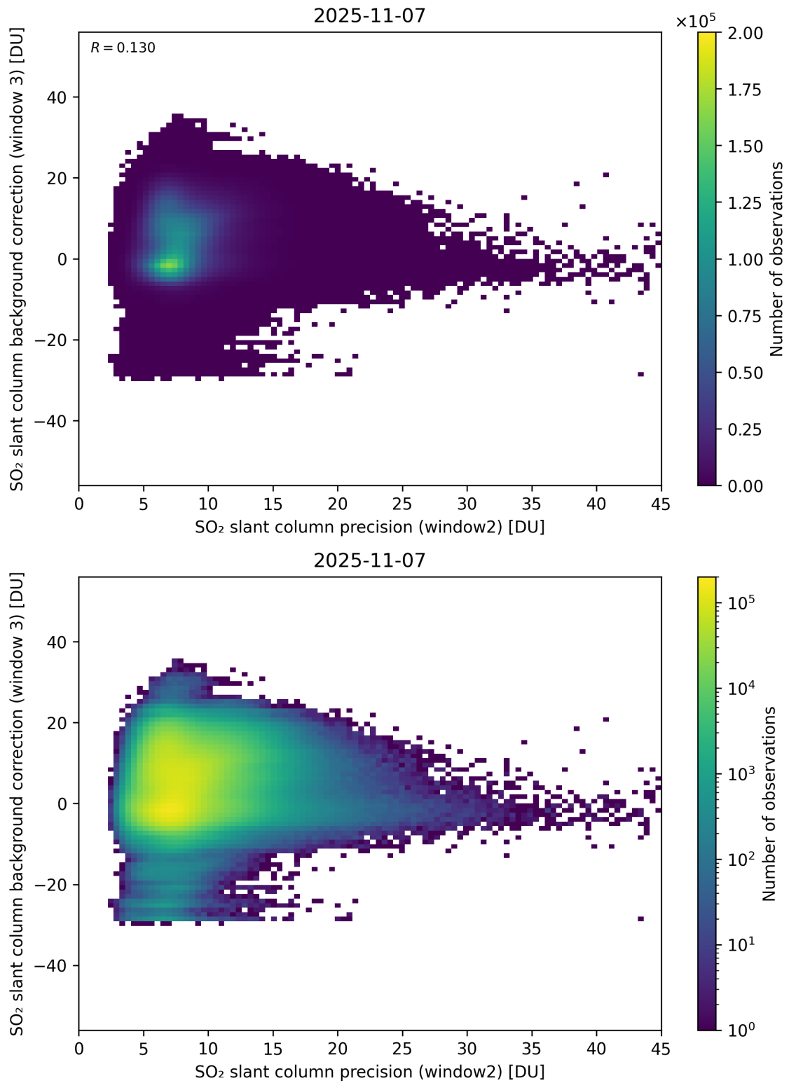
Figure 292: Scatter density plot of “SO 2 slant column precision (window2)” against “SO 2 slant column background correction (window 3)” for 2025-11-07 to 2025-11-08.
