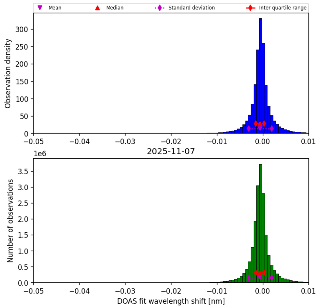
Figure 76: Histogram of “DOAS fit wavelength shift” for 2025-11-07 to 2025-11-08
