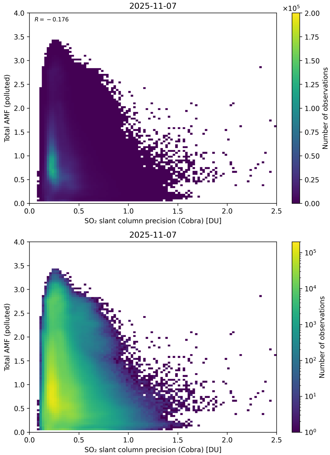
Figure 213: Scatter density plot of “SO 2 slant column precision (Cobra)” against “Total AMF (polluted)” for 2025-11-07 to 2025-11-08.
