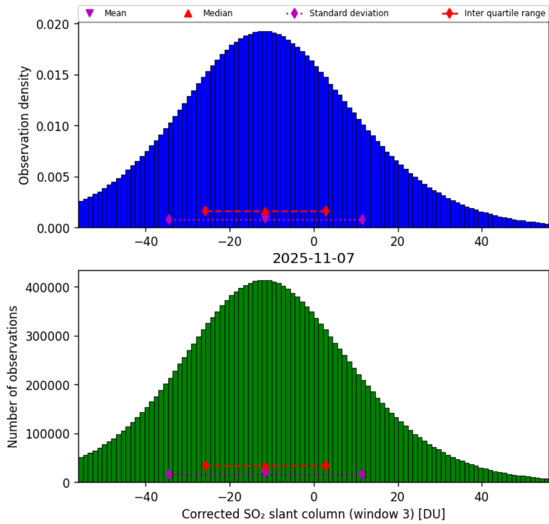
Figure 73: Histogram of “Corrected SO 2 slant column (window 3)” for 2025-11-07 to 2025-11-08
