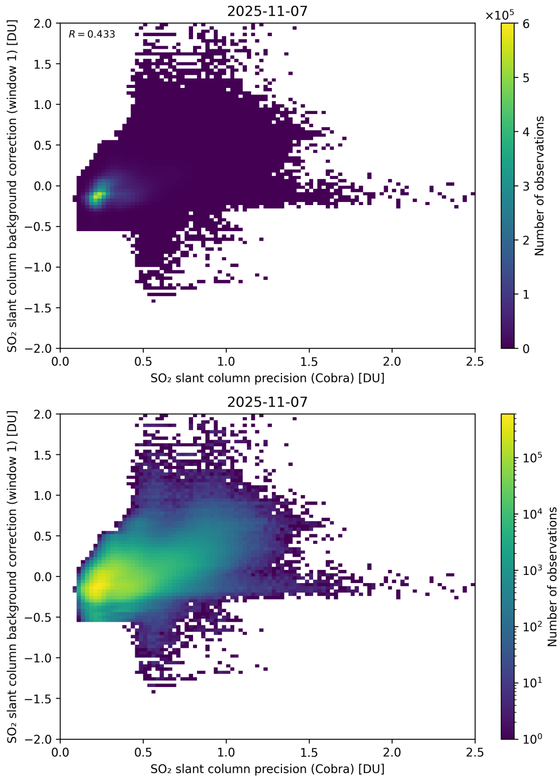
Figure 199: Scatter density plot of “SO 2 slant column precision (Cobra)” against “SO 2 slant column background correction (window 1)” for 2025-11-07 to 2025-11-08.
