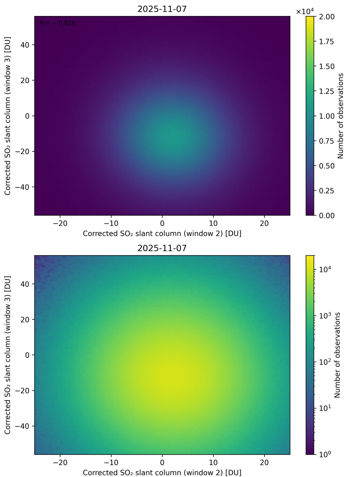
Figure 250: Scatter density plot of “Corrected SO 2 slant column (window 2)” against “Corrected SO 2 slant column (window 3)” for 2025-11-07 to 2025-11-08.
