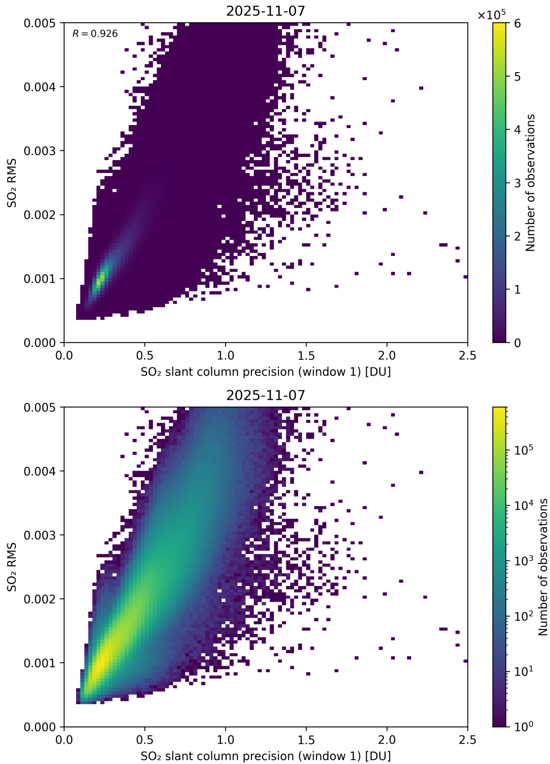
Figure 273: Scatter density plot of “SO 2 slant column precision (window 1)” against “SO 2 RMS” for 2025-11-07 to 2025-11-08.
