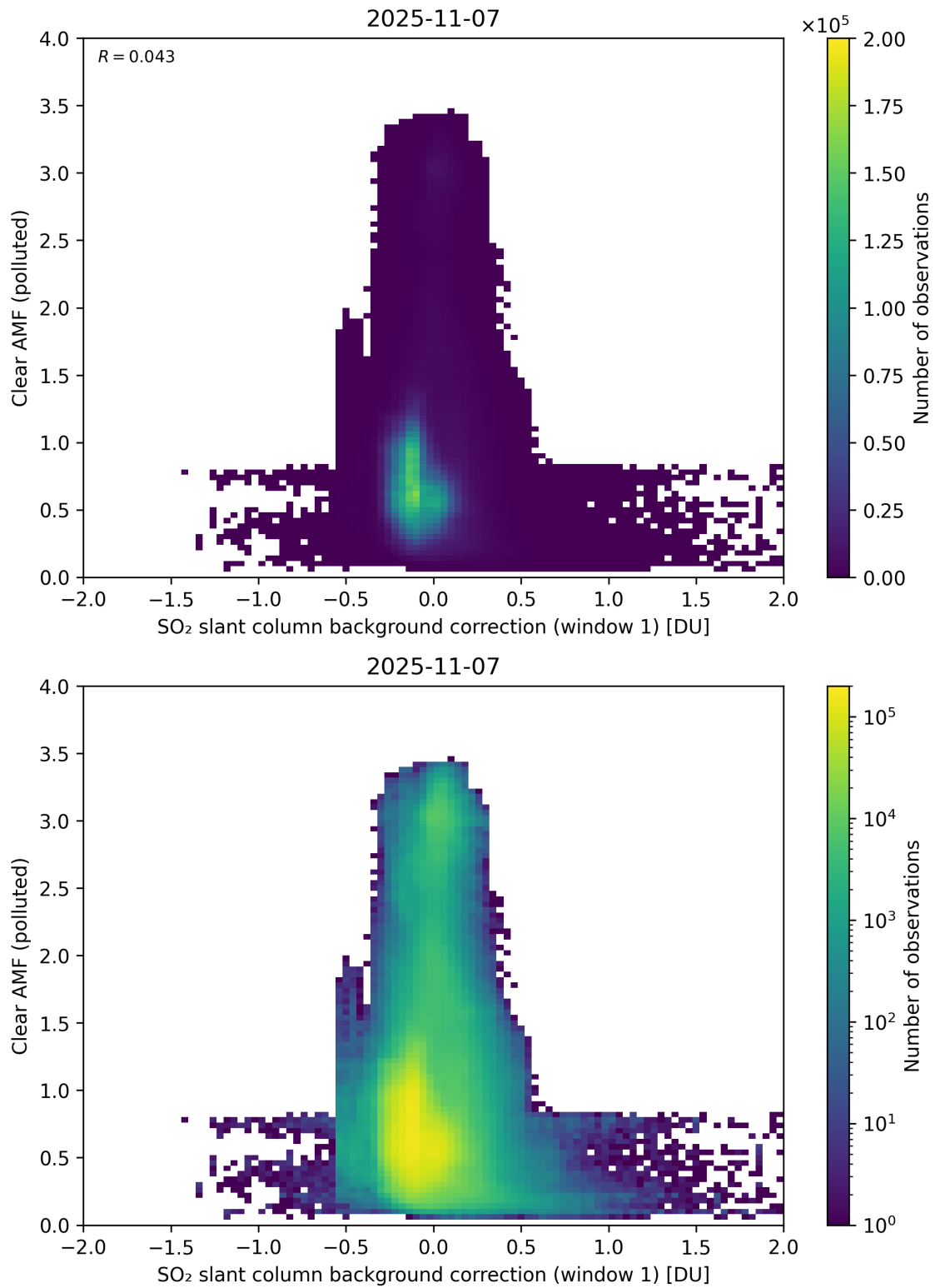
Figure 114: Scatter density plot of “SO 2 slant column background correction (window 1)” against “Clear AMF (polluted)” for 2025-11-07 to 2025-11-08.
