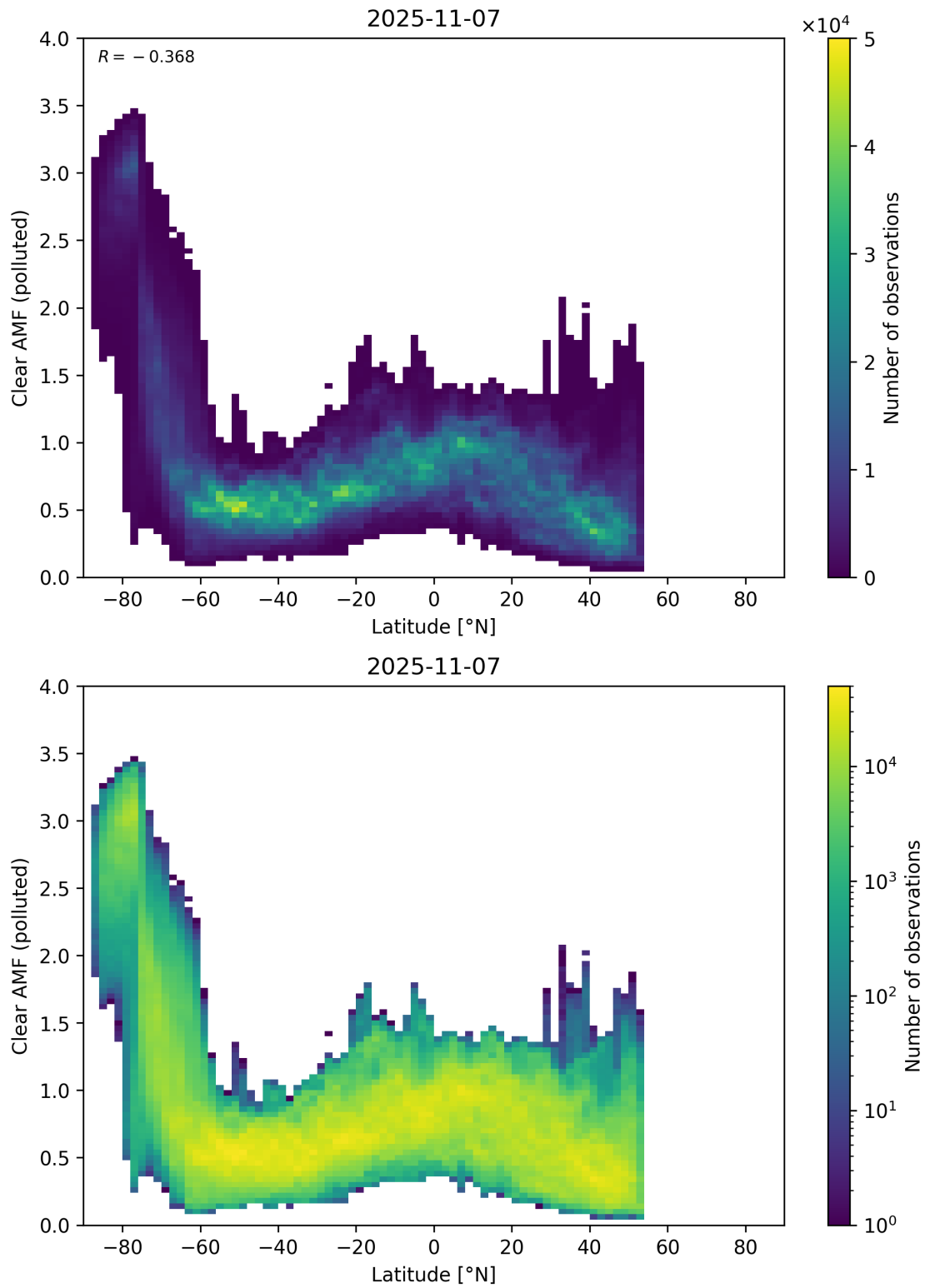
Figure 156: Scatter density plot of “Latitude” against “Clear AMF (polluted)” for 2025-11-07 to 2025-11-08.
