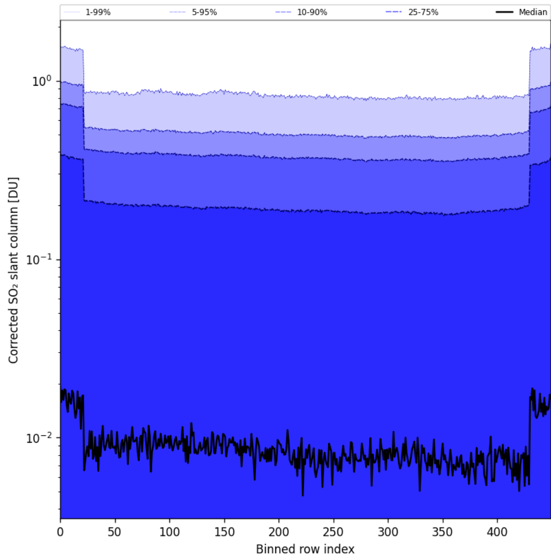
Figure 86: Along track statistics of “Corrected SO 2 slant column” for 2025-11-07 to 2025-11-08
