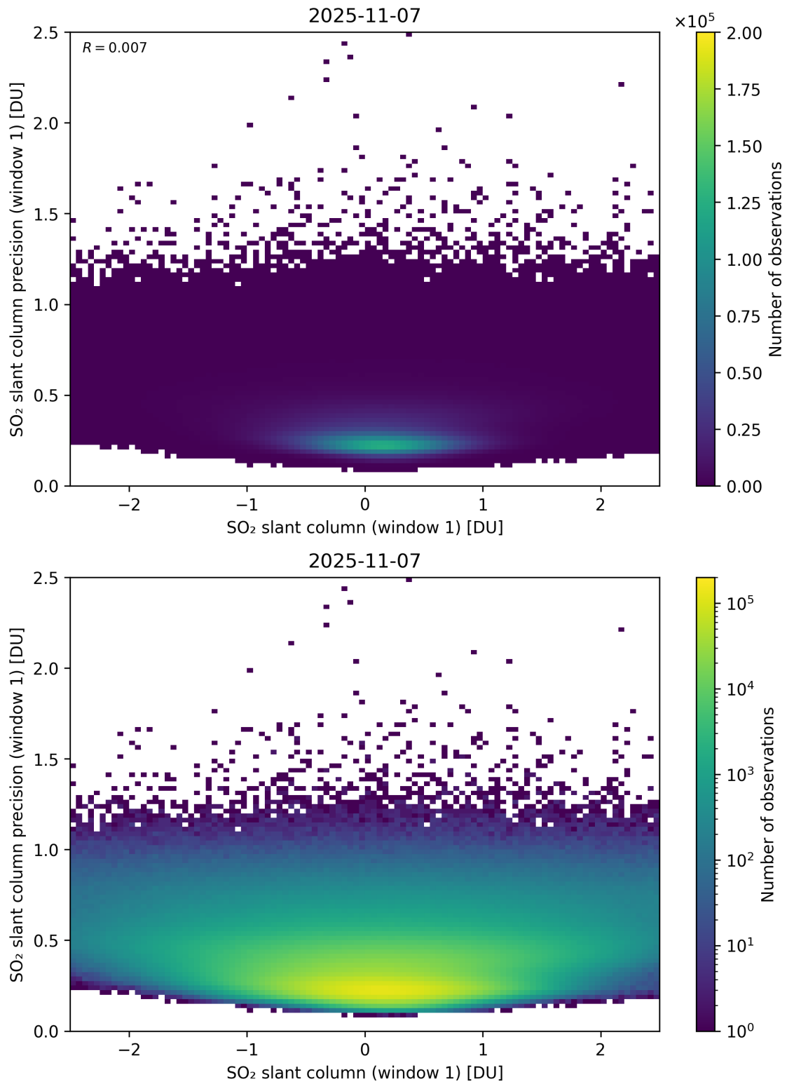
Figure 285: Scatter density plot of “SO 2 slant column (window 1)” against “SO 2 slant column precision (window 1)” for 2025-11-07 to 2025-11-08.
