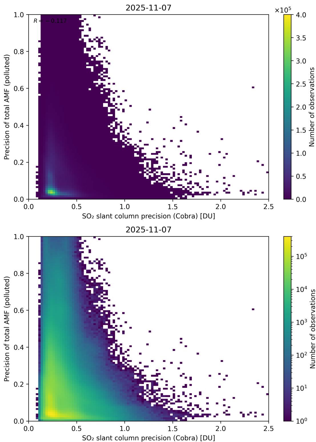
Figure 214: Scatter density plot of “SO 2 slant column precision (Cobra)” against “Precision of total AMF (polluted)” for 2025-11-07 to 2025-11-08.
