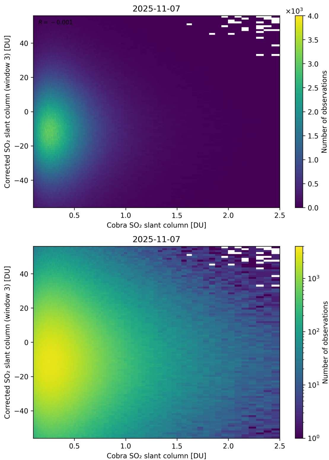
Figure 218: Scatter density plot of “Cobra SO 2 slant column” against “Corrected SO 2 slant column (window 3)” for 2025-11-07 to 2025-11-08.
