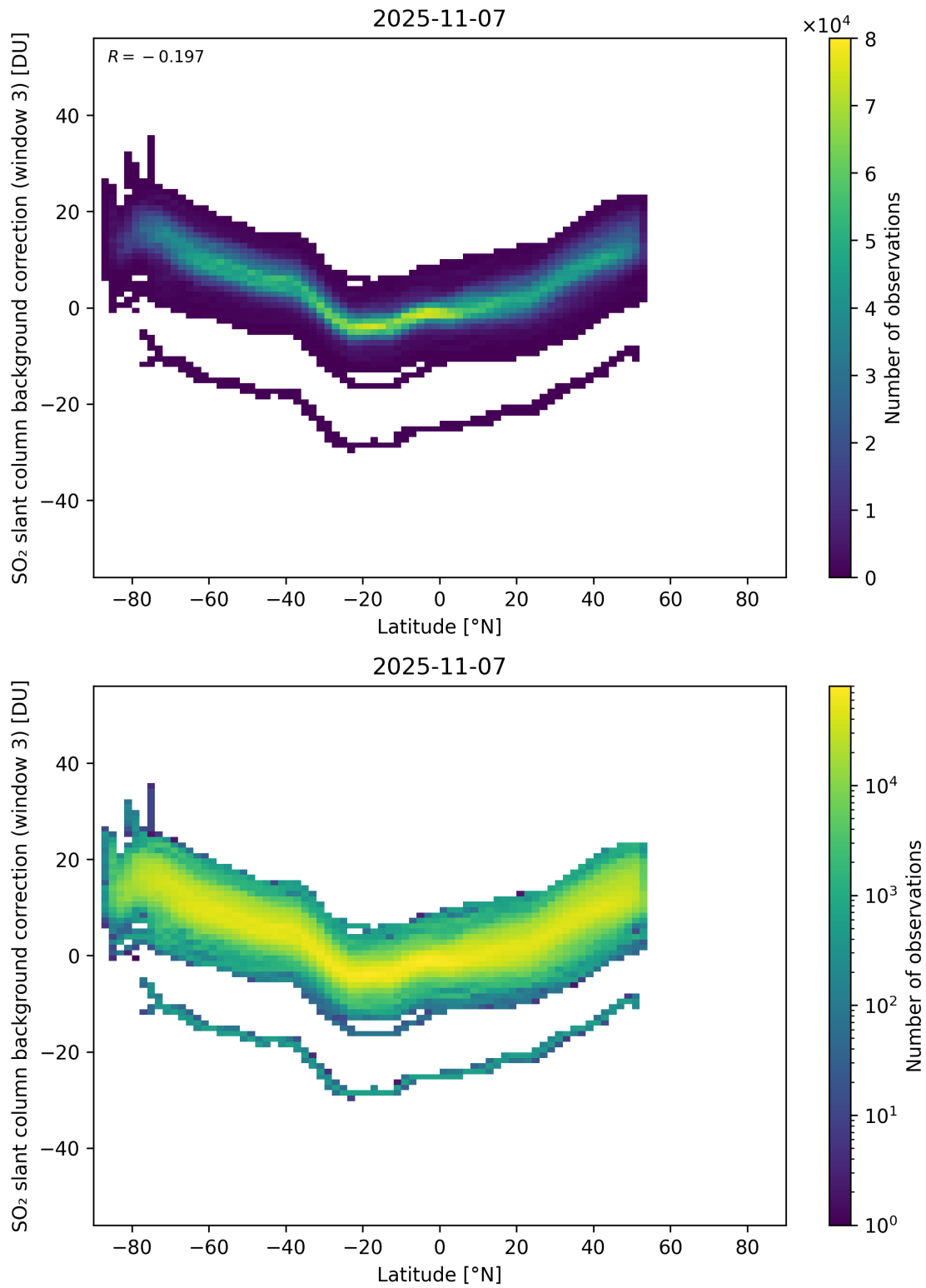
Figure 152: Scatter density plot of “Latitude” against “SO 2 slant column background correction (window 3)” for 2025-11-07 to 2025-11-08.
