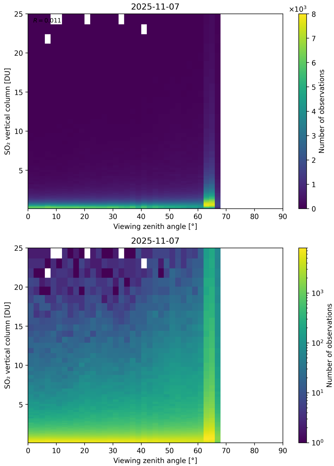
Figure 383: Scatter density plot of “Viewing zenith angle” against “SO 2 vertical column” for 2025-11-07 to 2025-11-08.
