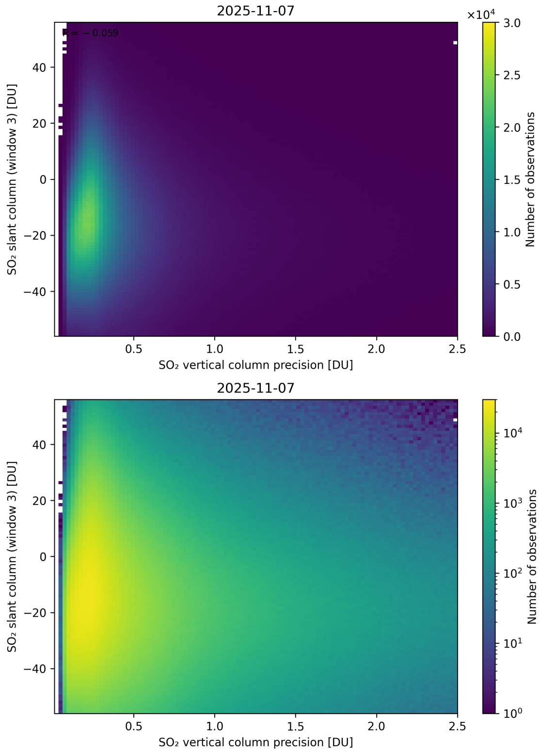
Figure 344: Scatter density plot of “SO 2 vertical column precision” against “SO 2 slant column (window 3)” for 2025-11-07 to 2025-11-08.
