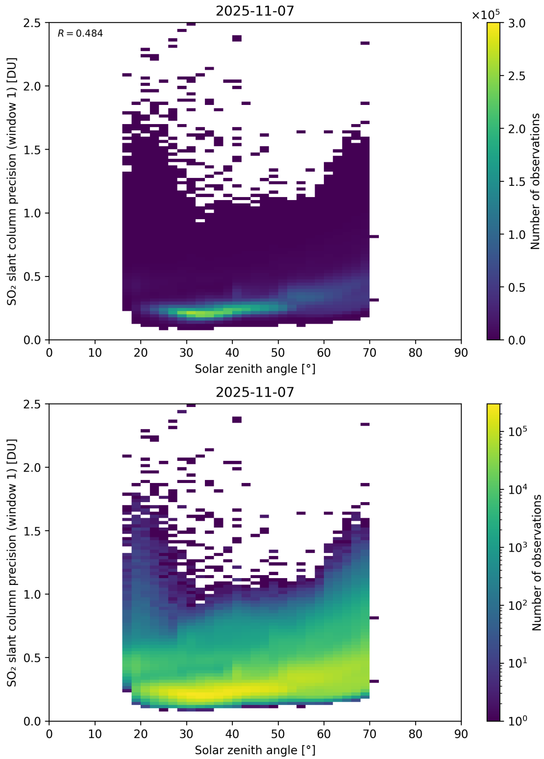
Figure 185: Scatter density plot of “Solar zenith angle” against “SO 2 slant column precision (window 1)” for 2025-11-07 to 2025-11-08.
