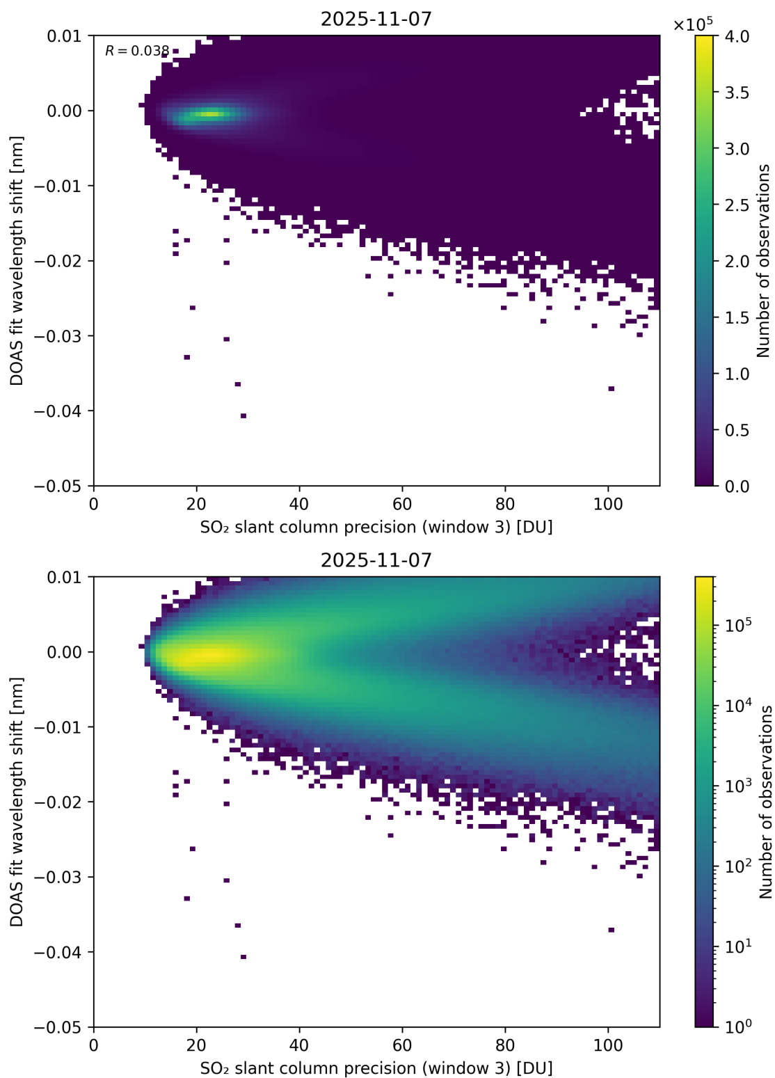
Figure 308: Scatter density plot of “SO 2 slant column precision (window 3)” against “DOAS fit wavelength shift” for 2025-11-07 to 2025-11-08.
