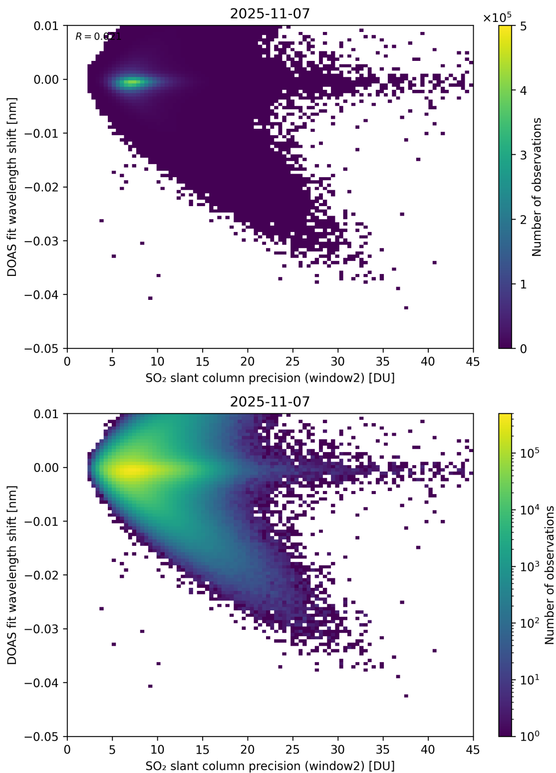
Figure 293: Scatter density plot of “SO 2 slant column precision (window2)” against “DOAS fit wavelength shift” for 2025-11-07 to 2025-11-08.
