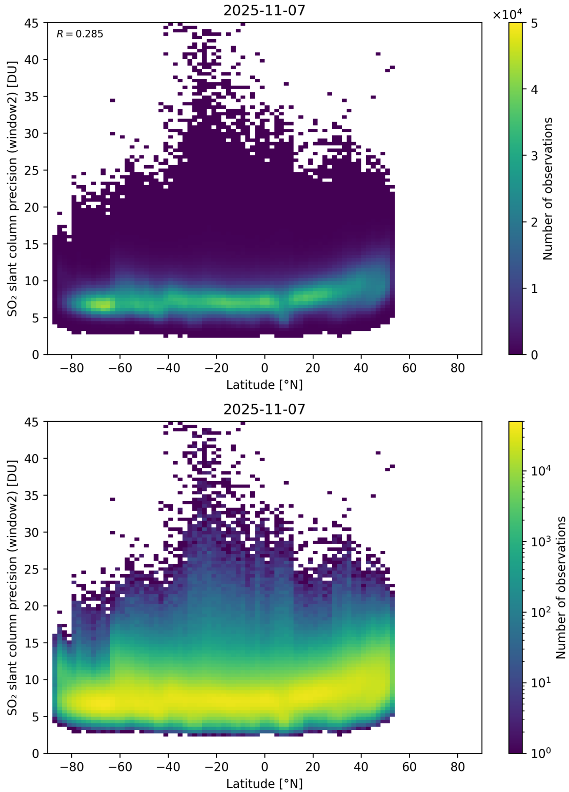
Figure 164: Scatter density plot of “Latitude” against “SO 2 slant column precision (window2)” for 2025-11-07 to 2025-11-08.
