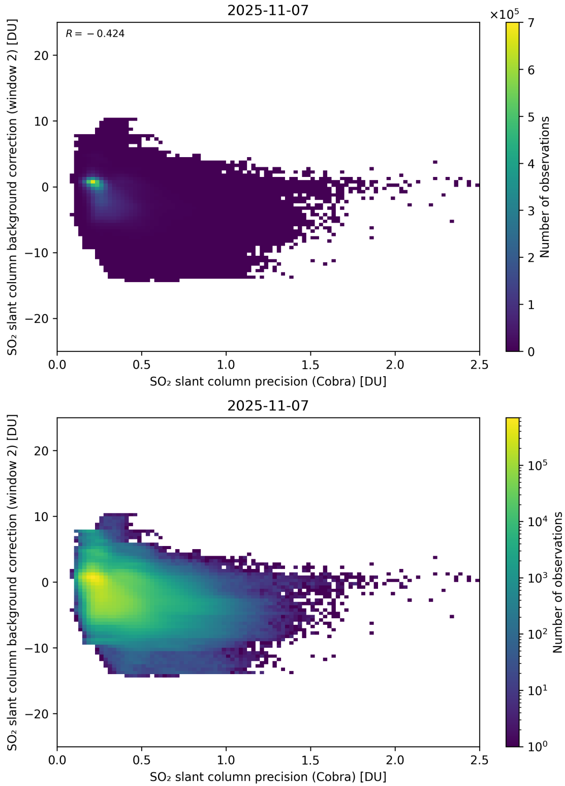
Figure 200: Scatter density plot of “SO 2 slant column precision (Cobra)” against “SO 2 slant column background correction (window 2)” for 2025-11-07 to 2025-11-08.
