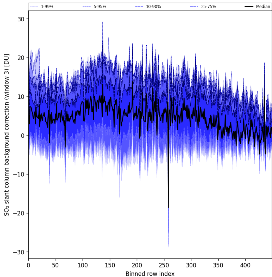
Figure 100: Along track statistics of “SO 2 slant column background correction (window 3)” for 2025-11-07 to 2025-11-08
