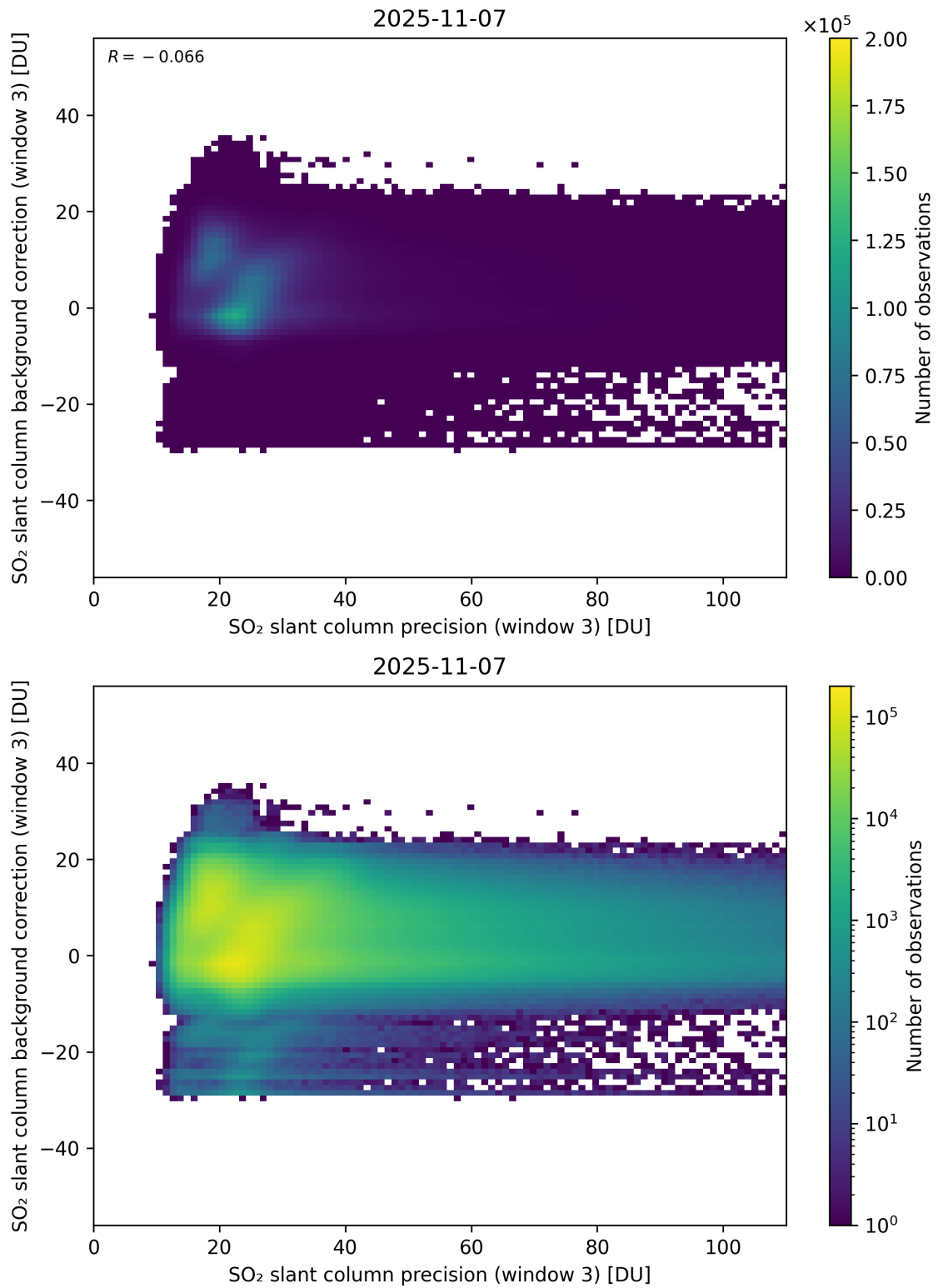
Figure 307: Scatter density plot of “SO 2 slant column precision (window 3)” against “SO 2 slant column background correction (window 3)” for 2025-11-07 to 2025-11-08.
