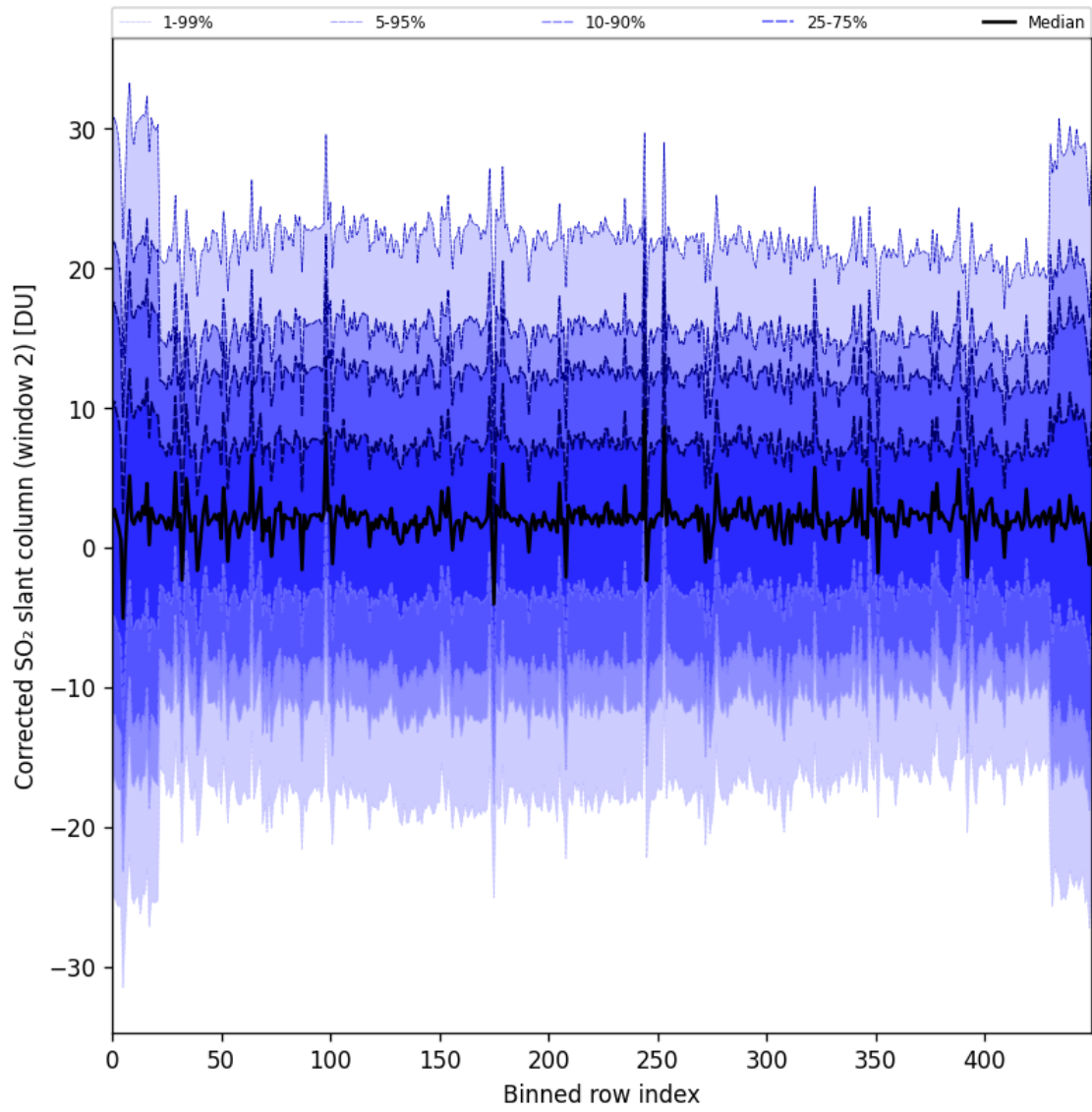
Figure 95: Along track statistics of “Corrected SO 2 slant column (window 2)” for 2025-11-07 to 2025-11-08
