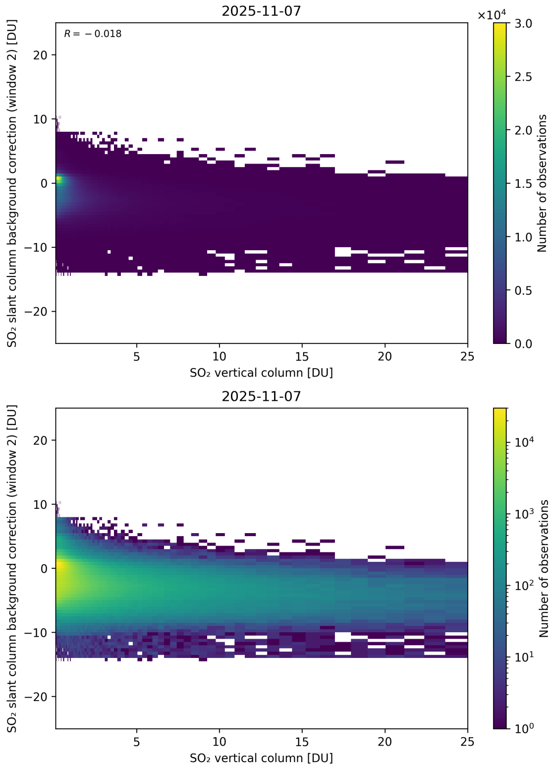
Figure 324: Scatter density plot of “SO 2 vertical column” against “SO 2 slant column background correction (window 2)” for 2025-11-07 to 2025-11-08.
