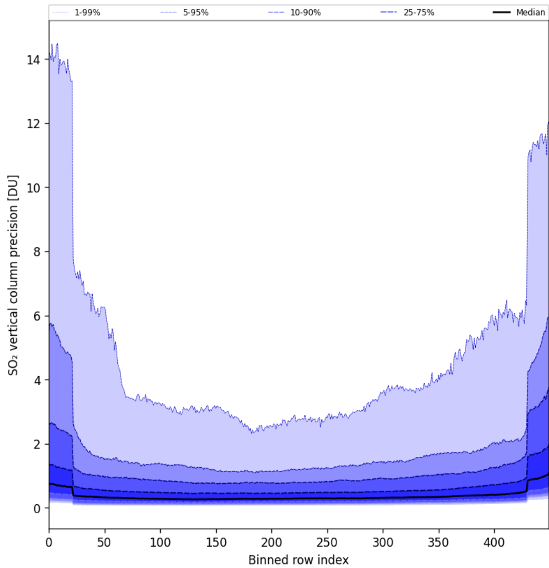
Figure 85: Along track statistics of “SO 2 vertical column precision” for 2025-11-07 to 2025-11-08
