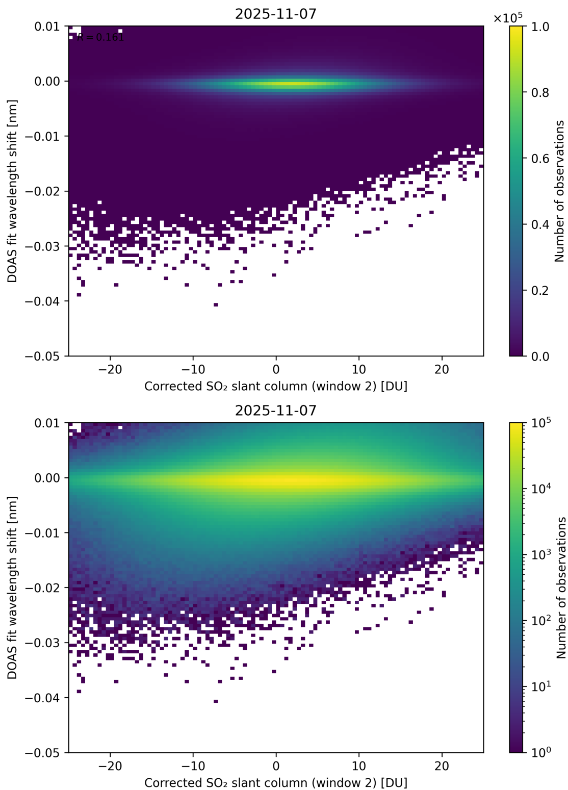
Figure 246: Scatter density plot of “Corrected SO 2 slant column (window 2)” against “DOAS fit wavelength shift” for 2025-11-07 to 2025-11-08.
