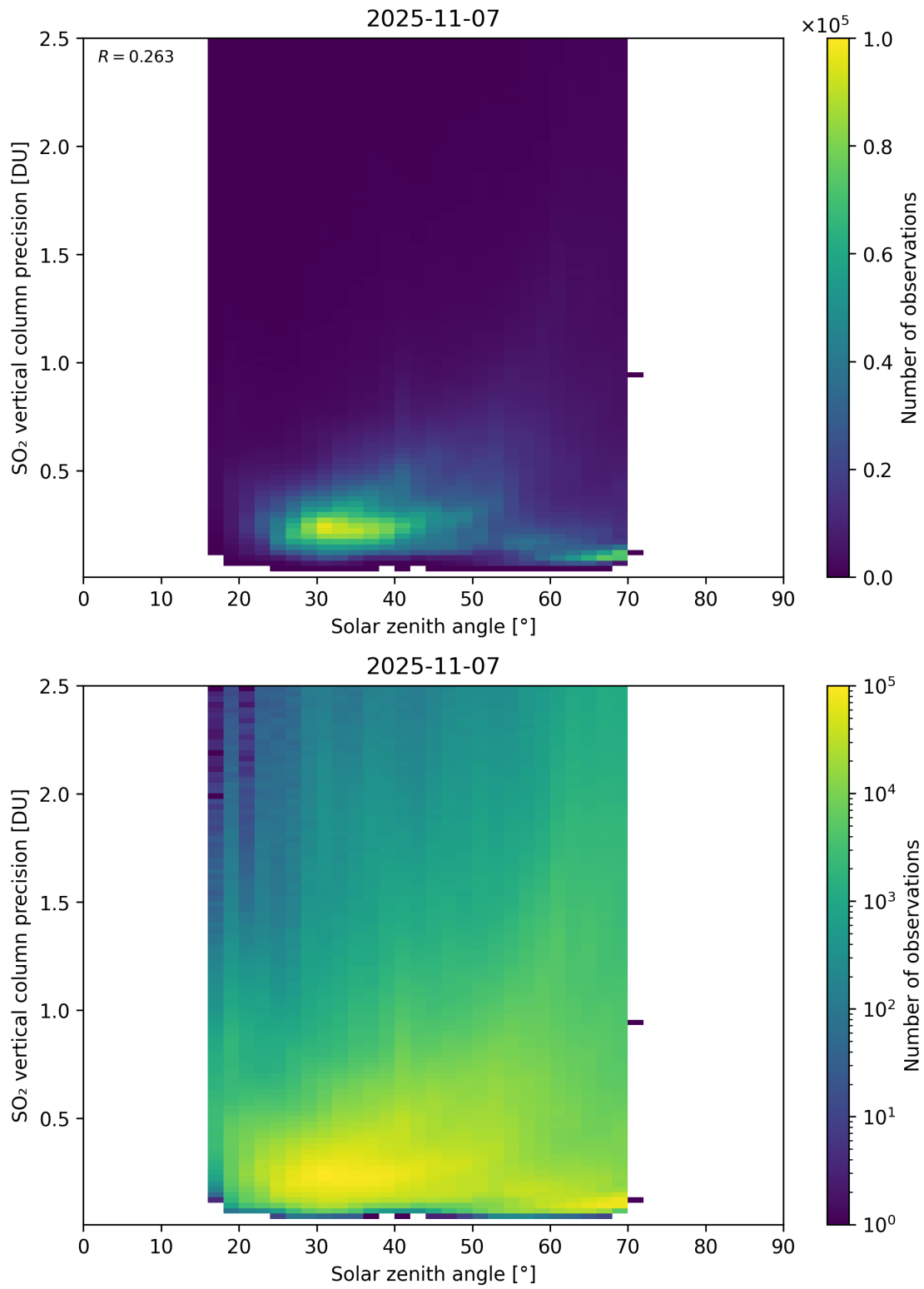
Figure 192: Scatter density plot of “Solar zenith angle” against “SO 2 vertical column precision” for 2025-11-07 to 2025-11-08.
