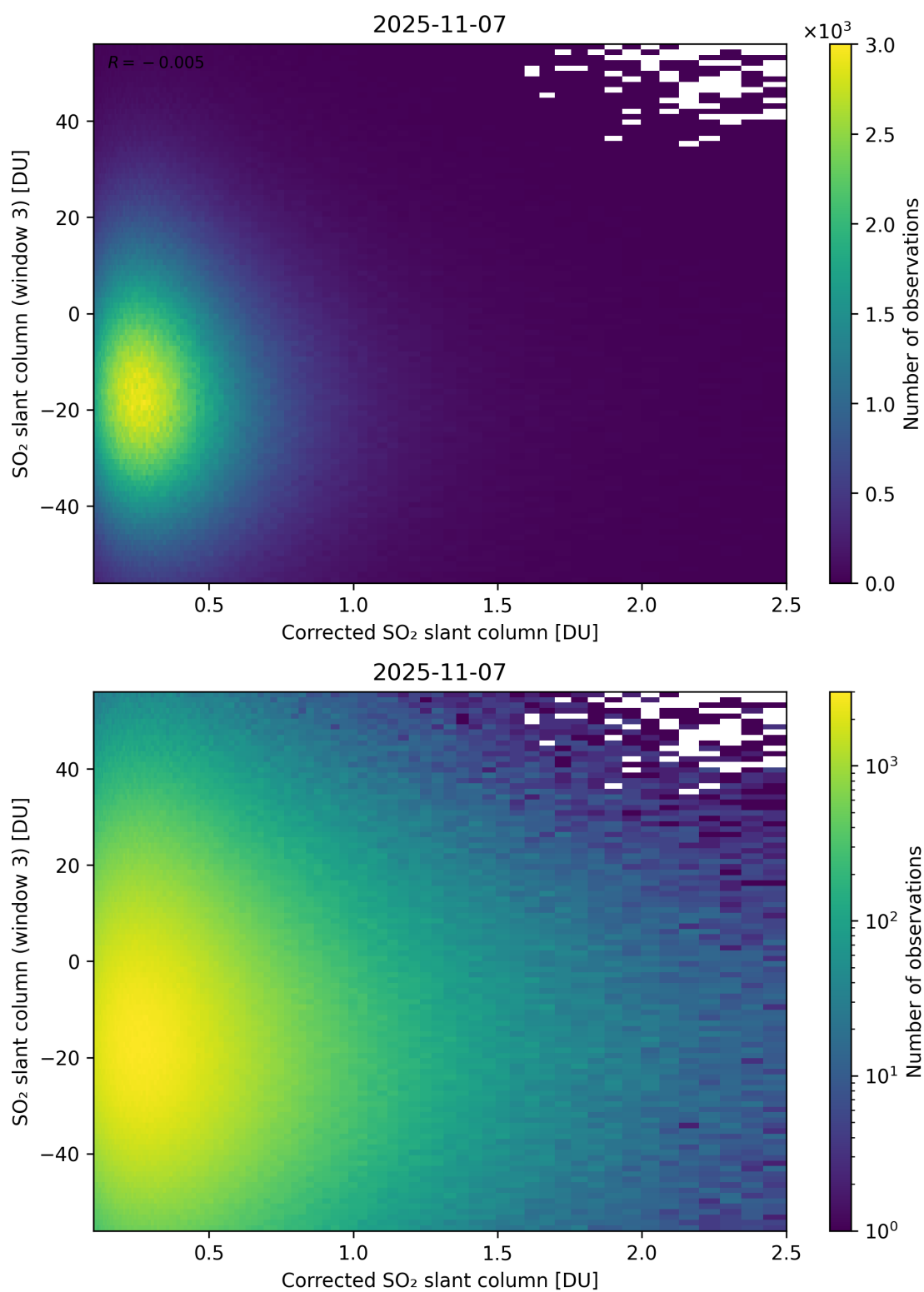
Figure 240: Scatter density plot of “Corrected SO 2 slant column” against “SO 2 slant column (window 3)” for 2025-11-07 to 2025-11-08.
