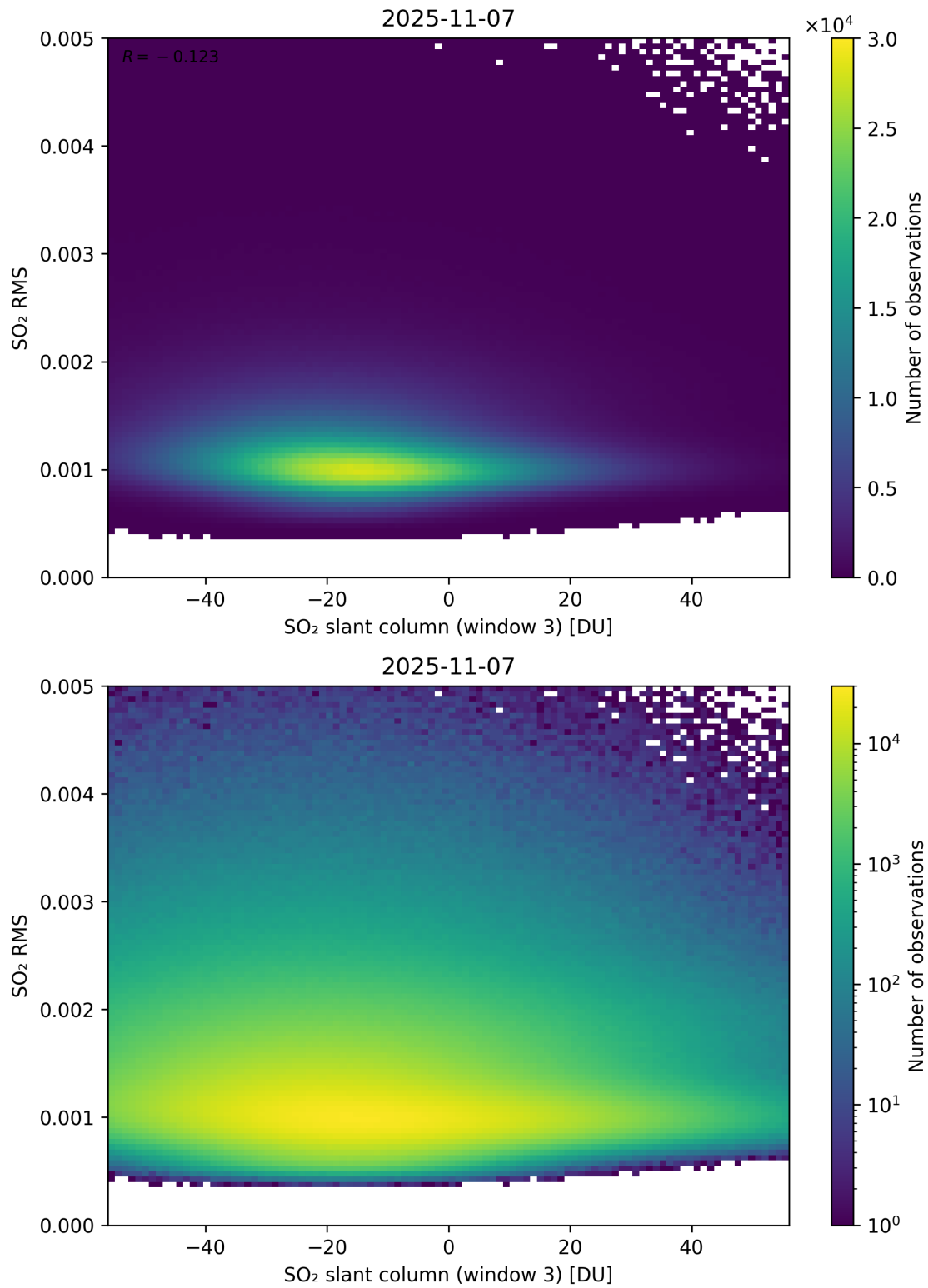
Figure 306: Scatter density plot of “SO 2 slant column (window 3)” against “SO 2 RMS” for 2025-11-07 to 2025-11-08.
