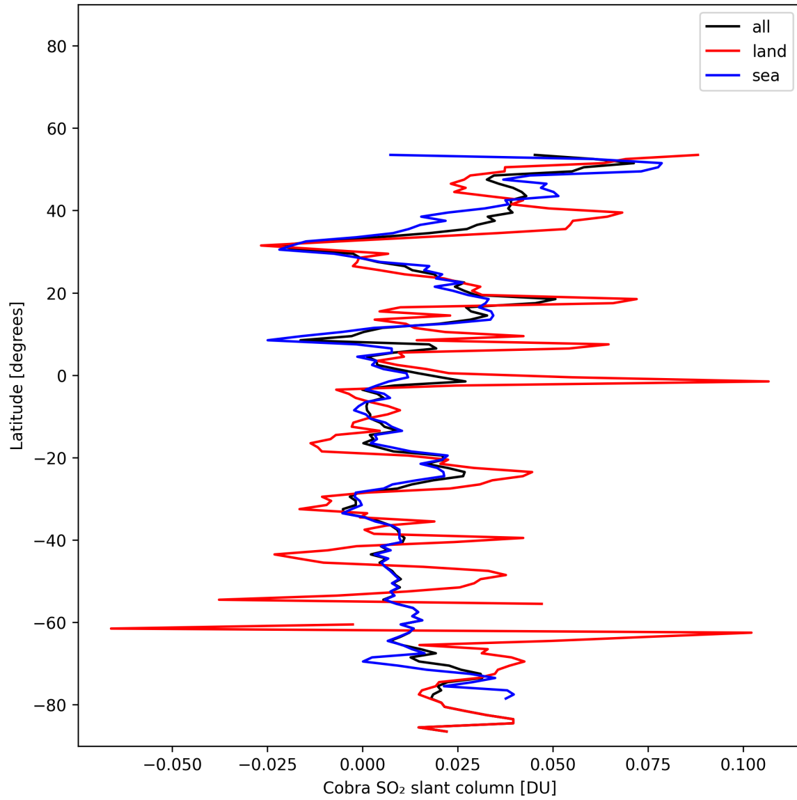
Figure 35: Zonal average of “Cobra SO 2 slant column” for 2025-11-07 to 2025-11-08.
