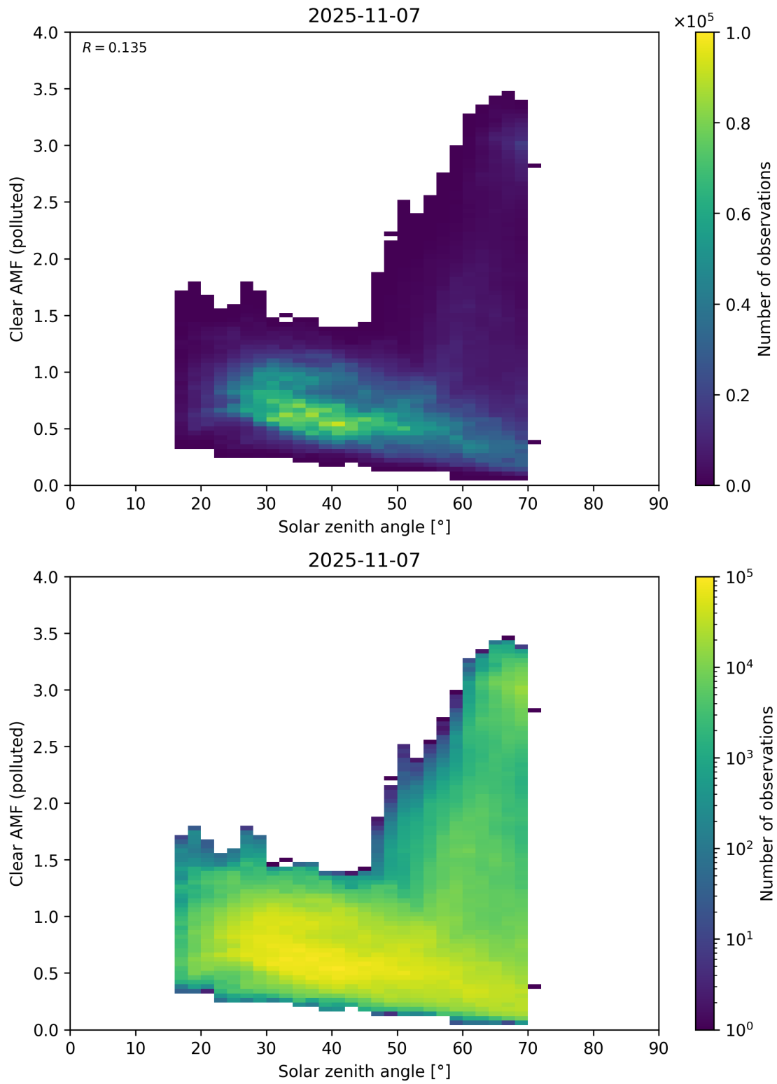
Figure 178: Scatter density plot of “Solar zenith angle” against “Clear AMF (polluted)” for 2025-11-07 to 2025-11-08.
