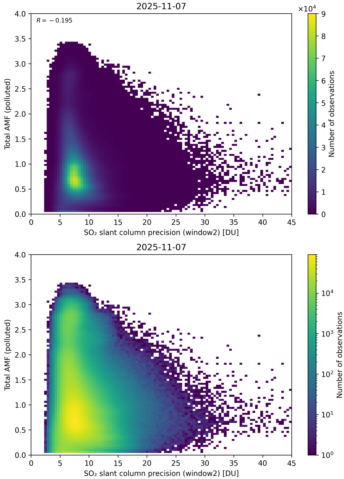
Figure 301: Scatter density plot of “SO 2 slant column precision (window2)” against “Total AMF (polluted)” for 2025-11-07 to 2025-11-08.
