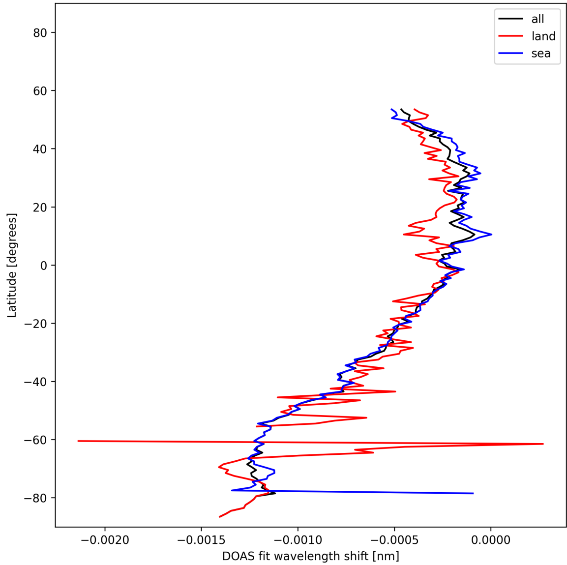
Figure 50: Zonal average of “DOAS fit wavelength shift” for 2025-11-07 to 2025-11-08.
