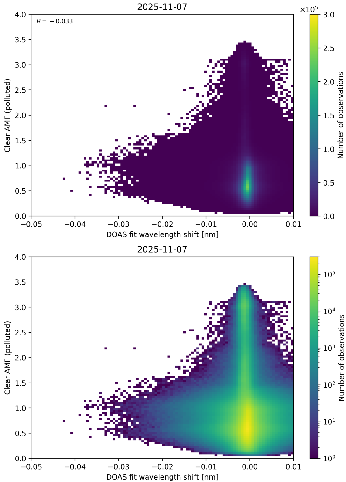
Figure 140: Scatter density plot of “DOAS fit wavelength shift” against “Clear AMF (polluted)” for 2025-11-07 to 2025-11-08.
