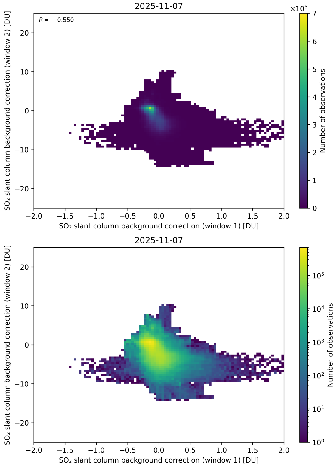
Figure 109: Scatter density plot of “SO 2 slant column background correction (window 1)” against “SO 2 slant column background correction (window 2)” for 2025-11-07 to 2025-11-08.
