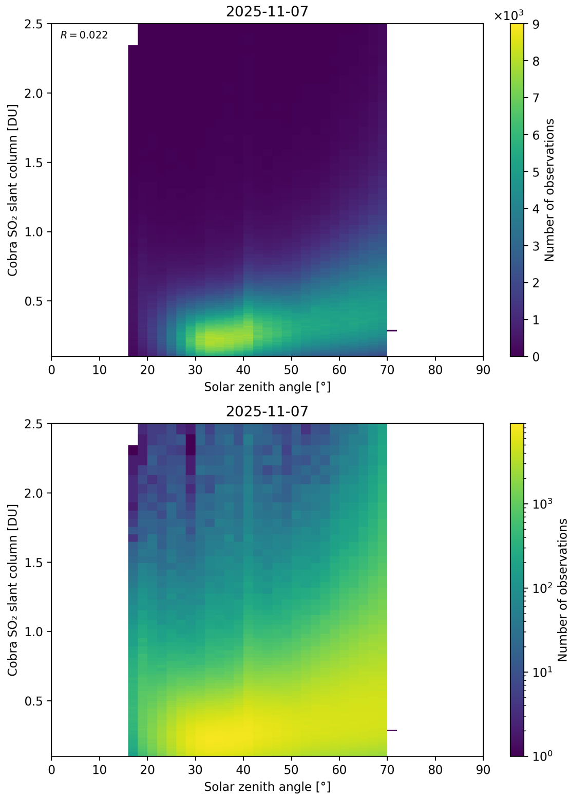
Figure 179: Scatter density plot of “Solar zenith angle” against “Cobra SO 2 slant column” for 2025-11-07 to 2025-11-08.
