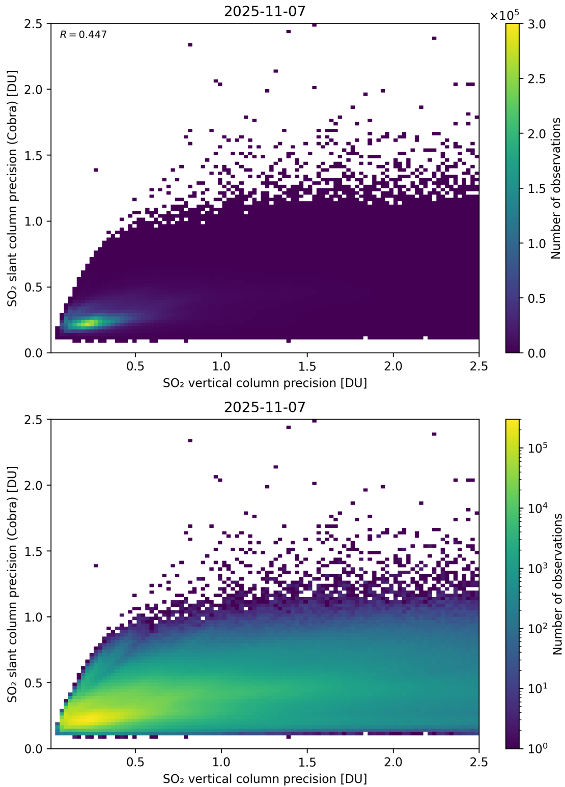
Figure 337: Scatter density plot of “SO 2 vertical column precision” against “SO 2 slant column precision (Cobra)” for 2025-11-07 to 2025-11-08.
