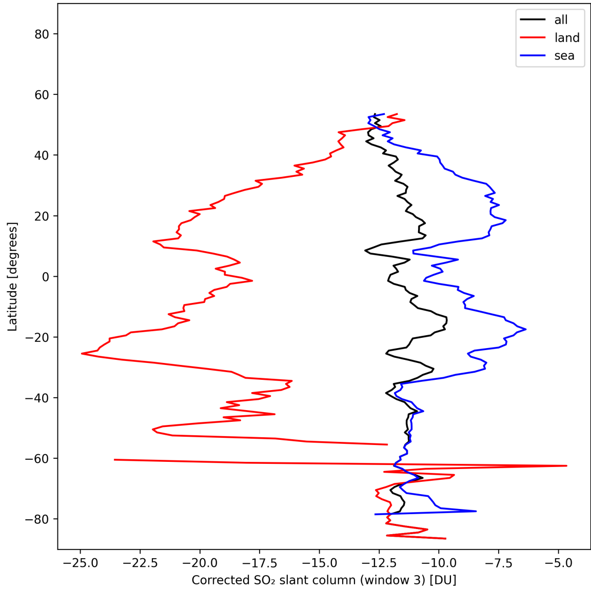
Figure 47: Zonal average of “Corrected SO 2 slant column (window 3)” for 2025-11-07 to 2025-11-08.
