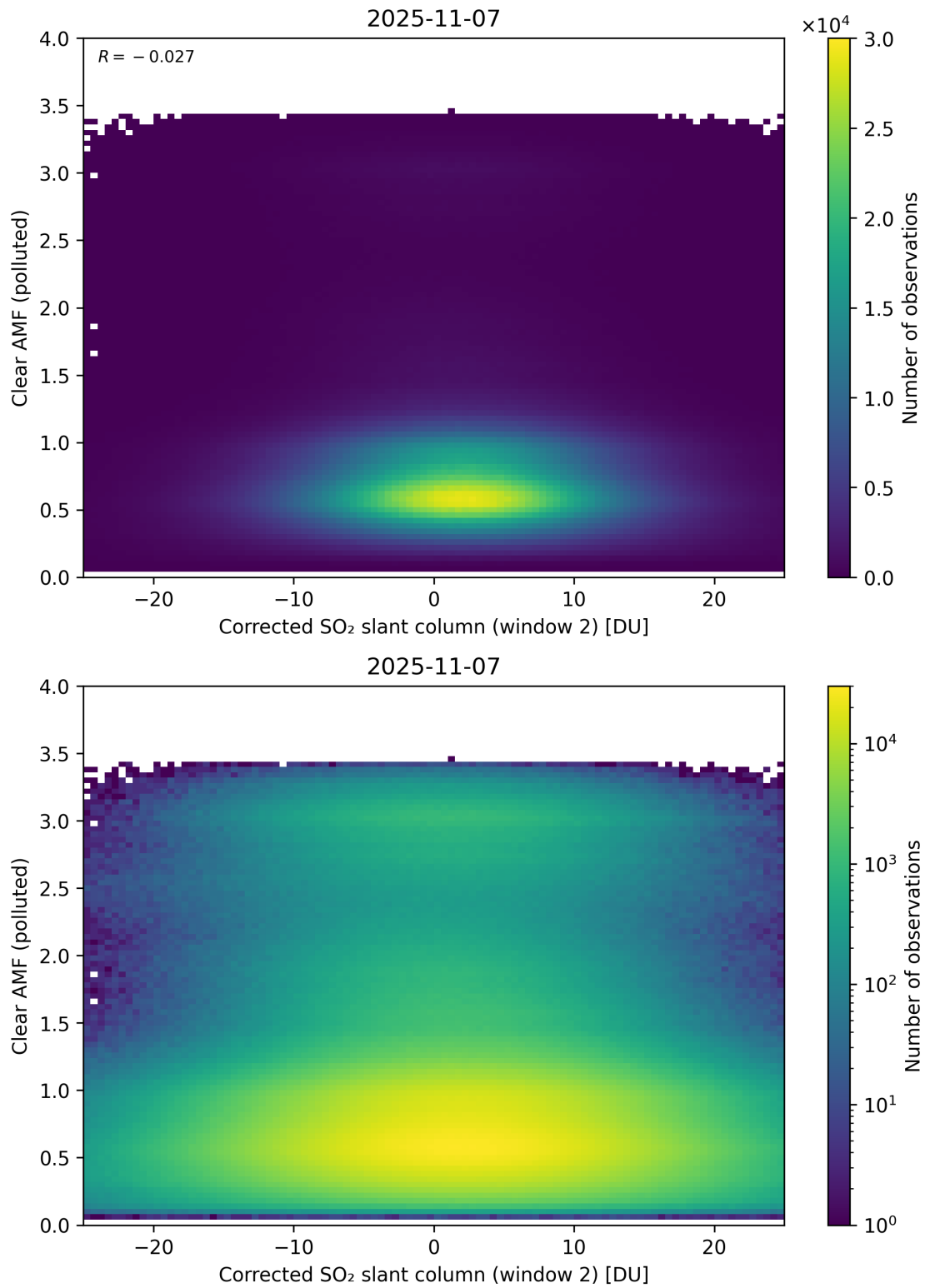
Figure 249: Scatter density plot of “Corrected SO 2 slant column (window 2)” against “Clear AMF (polluted)” for 2025-11-07 to 2025-11-08.
