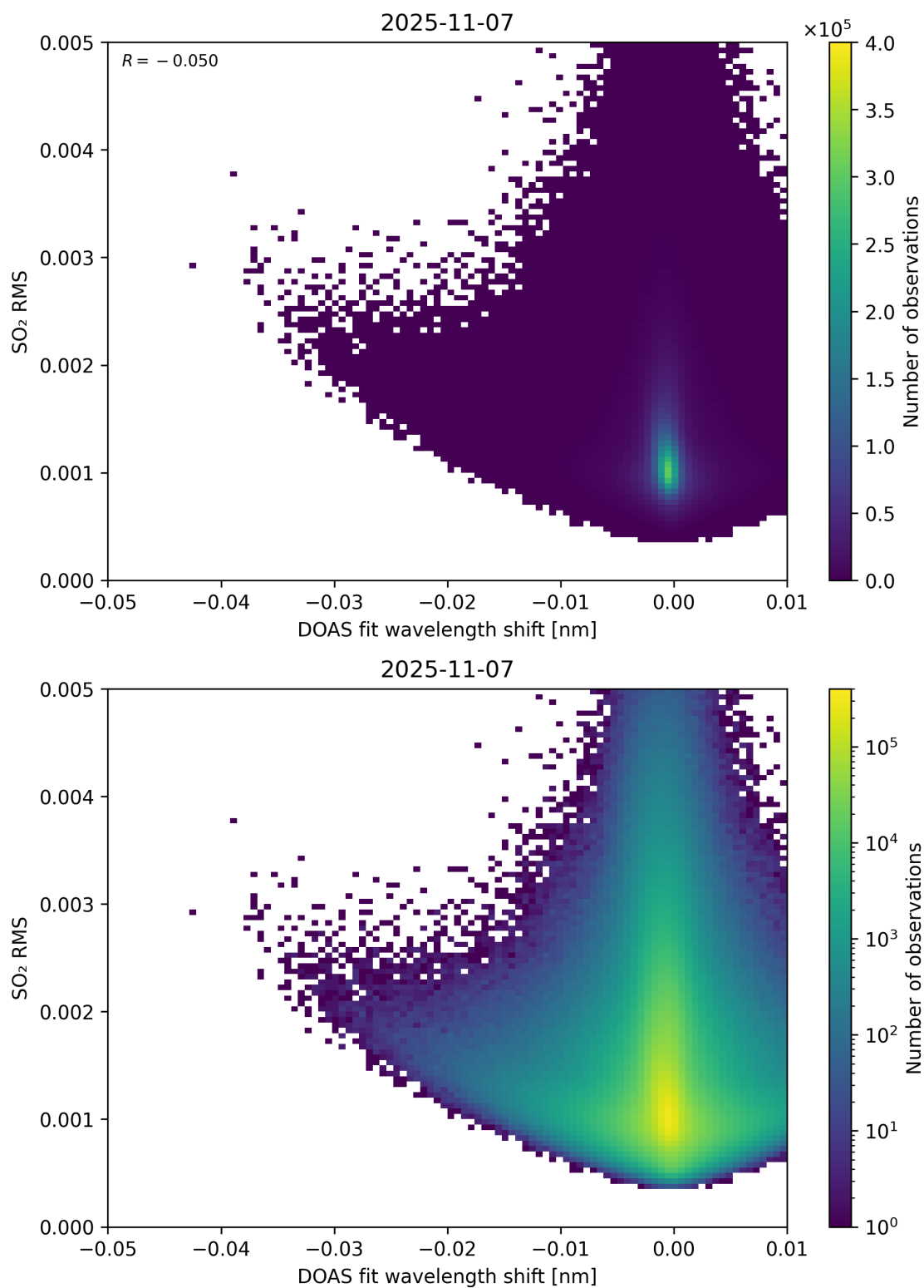
Figure 139: Scatter density plot of “DOAS fit wavelength shift” against “SO 2 RMS” for 2025-11-07 to 2025-11-08.
