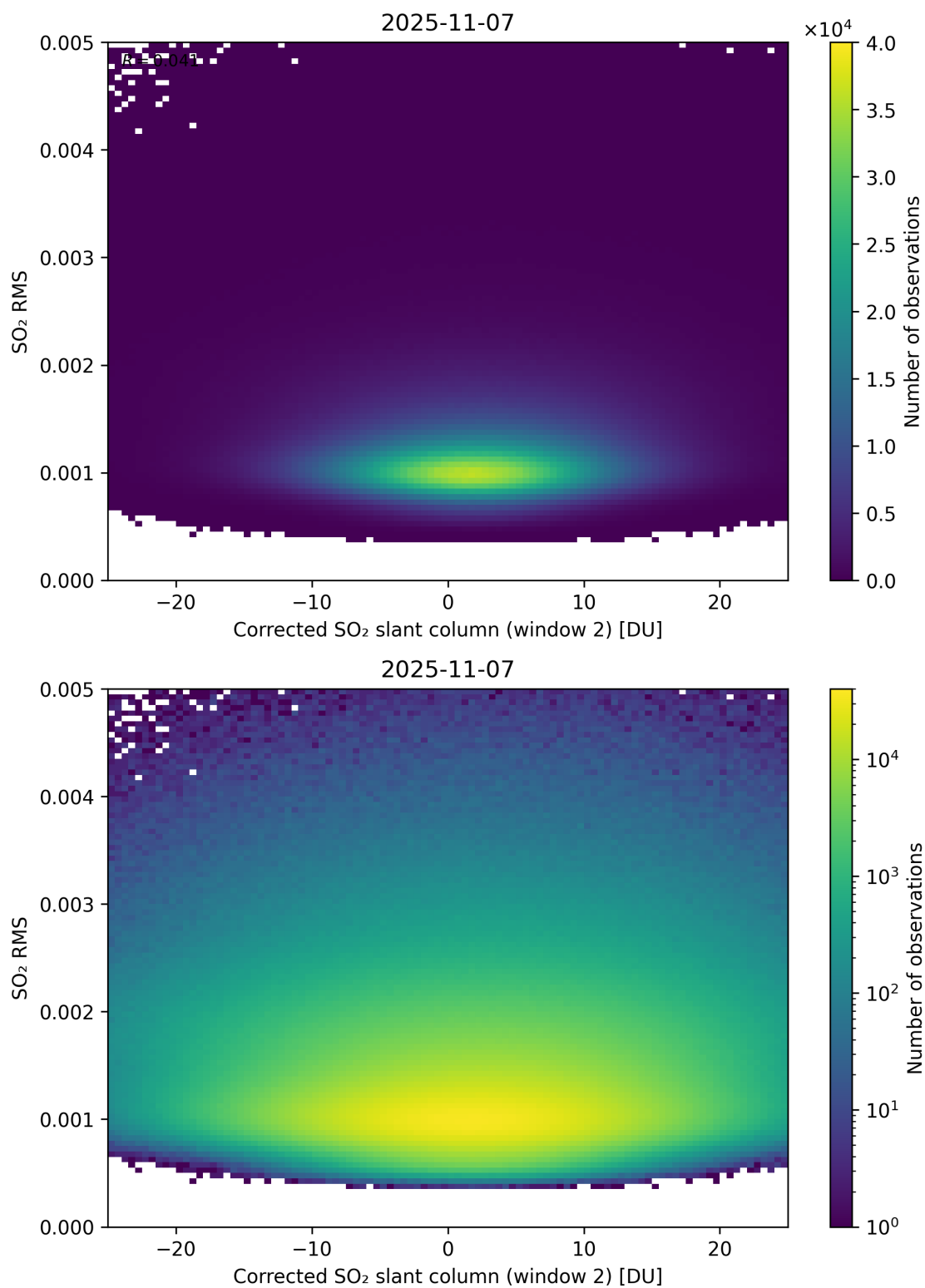
Figure 248: Scatter density plot of “Corrected SO 2 slant column (window 2)” against “SO 2 RMS” for 2025-11-07 to 2025-11-08.
