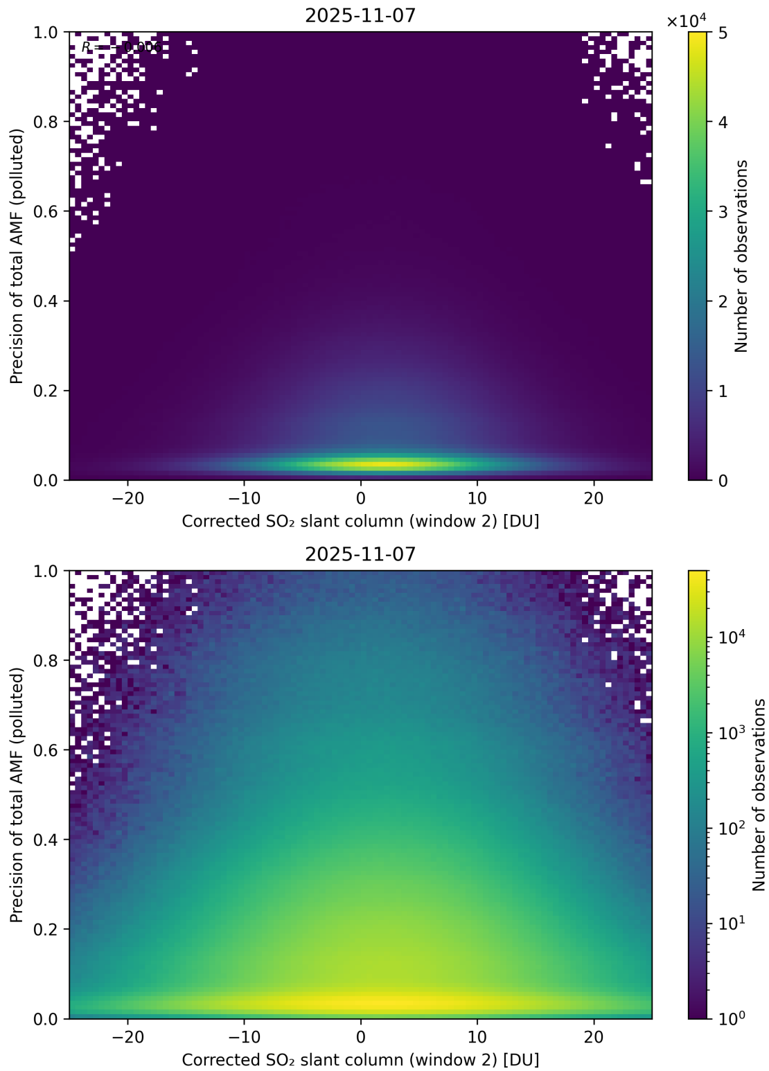
Figure 254: Scatter density plot of “Corrected SO 2 slant column (window 2)” against “Precision of total AMF (polluted)” for 2025-11-07 to 2025-11-08.
