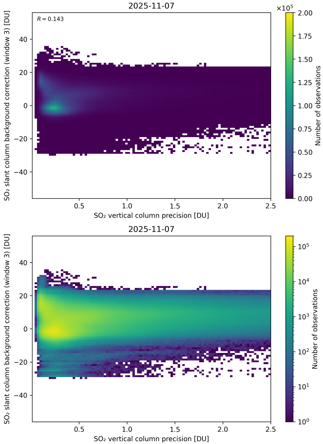
Figure 331: Scatter density plot of “SO 2 vertical column precision” against “SO 2 slant column background correction (window 3)” for 2025-11-07 to 2025-11-08.
