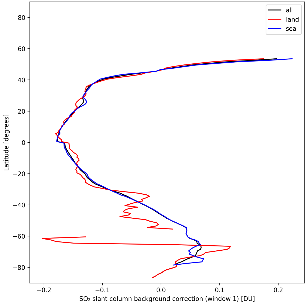
Figure 40: Zonal average of “SO 2 slant column background correction (window 1)” for 2025-11-07 to 2025-11-08.
