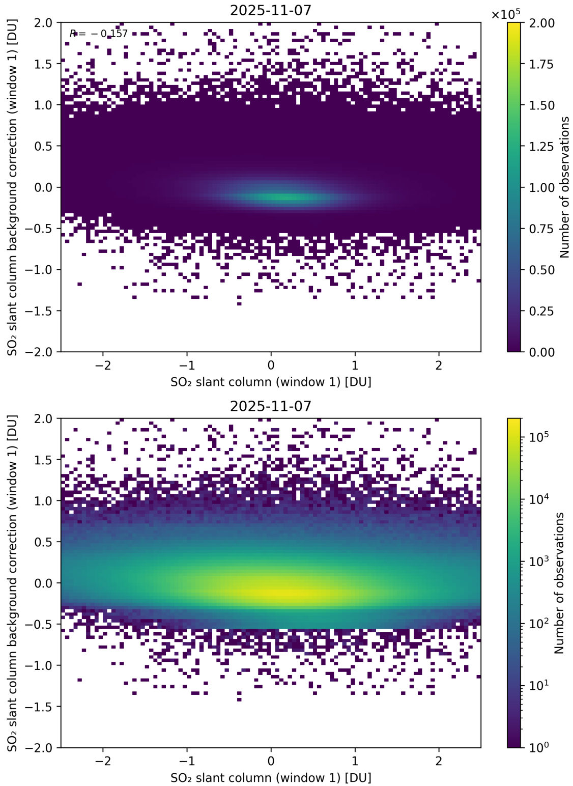
Figure 262: Scatter density plot of “SO 2 slant column (window 1)” against “SO 2 slant column background correction (window 1)” for 2025-11-07 to 2025-11-08.
