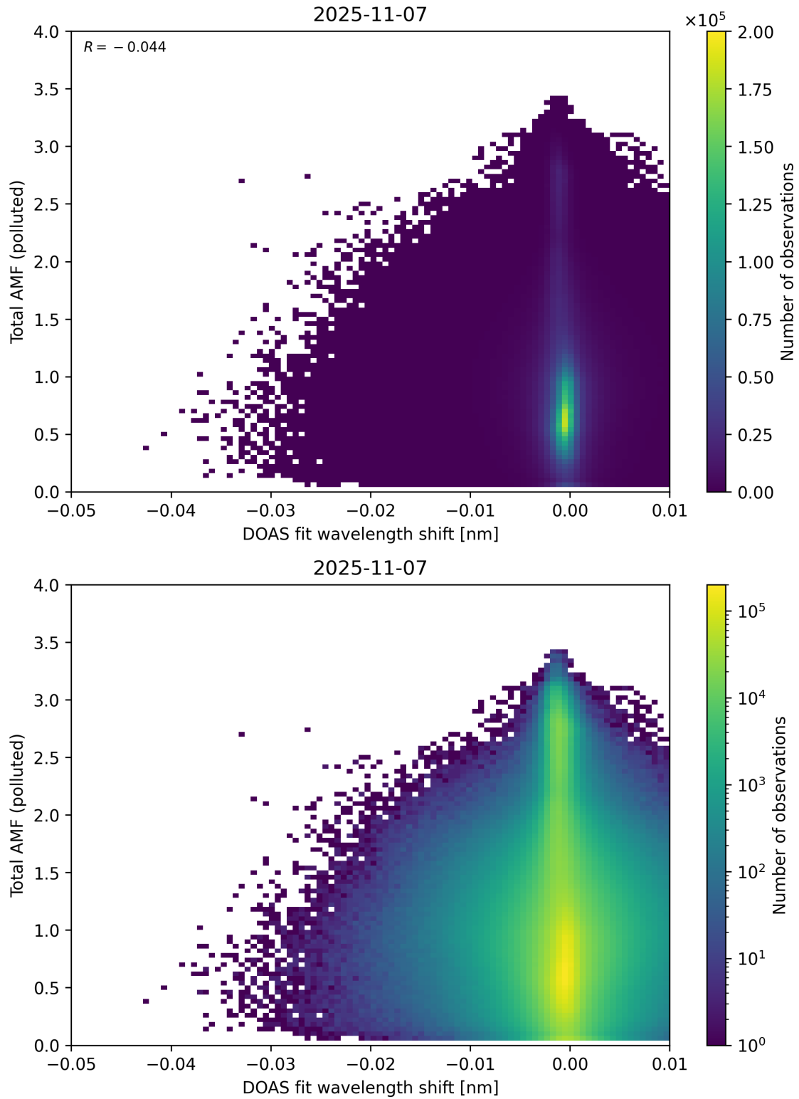
Figure 141: Scatter density plot of “DOAS fit wavelength shift” against “Total AMF (polluted)” for 2025-11-07 to 2025-11-08.
