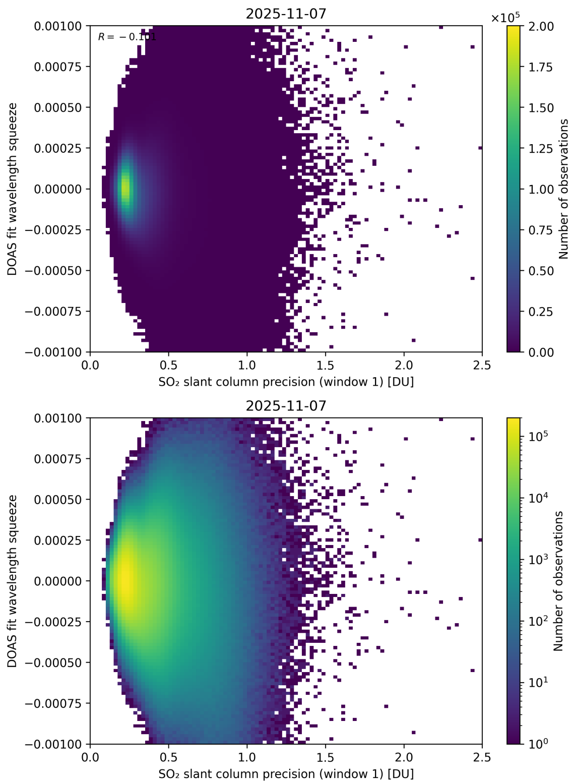
Figure 272: Scatter density plot of “SO 2 slant column precision (window 1)” against “DOAS fit wavelength squeeze” for 2025-11-07 to 2025-11-08.
