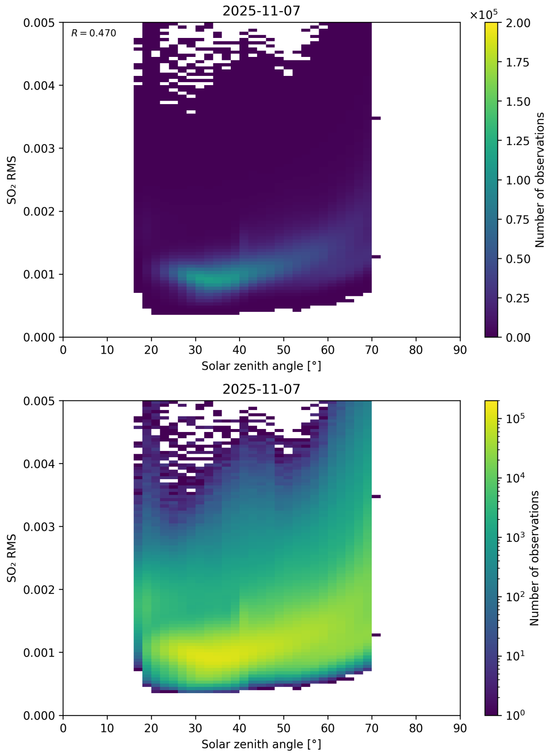
Figure 176: Scatter density plot of “Solar zenith angle” against “SO 2 RMS” for 2025-11-07 to 2025-11-08.
