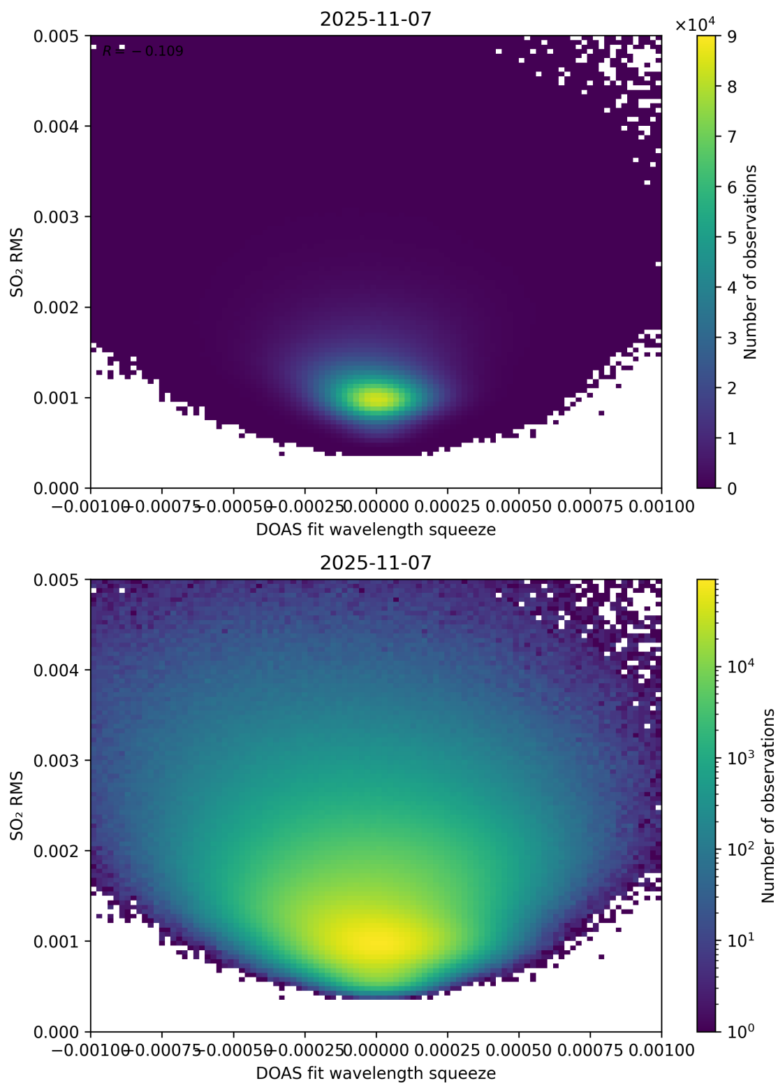
Figure 143: Scatter density plot of “DOAS fit wavelength squeeze” against “SO 2 RMS” for 2025-11-07 to 2025-11-08.
