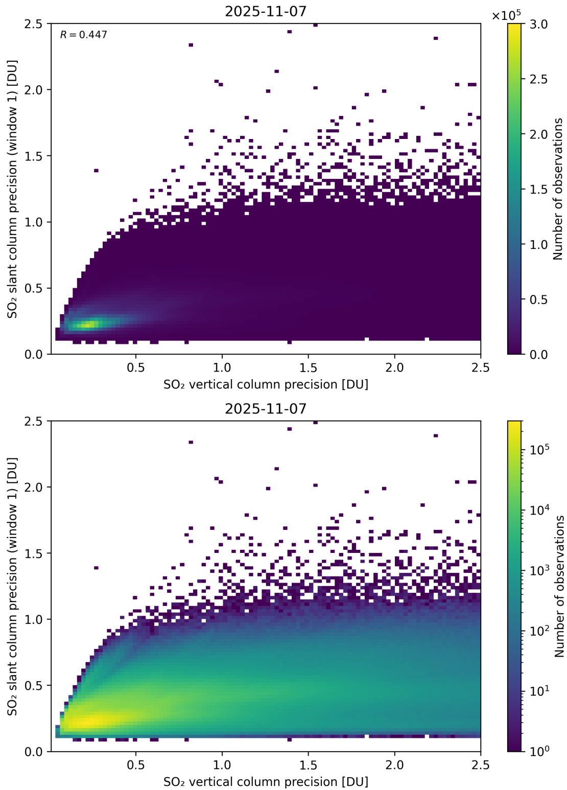
Figure 342: Scatter density plot of “SO 2 vertical column precision” against “SO 2 slant column precision (window 1)” for 2025-11-07 to 2025-11-08.
