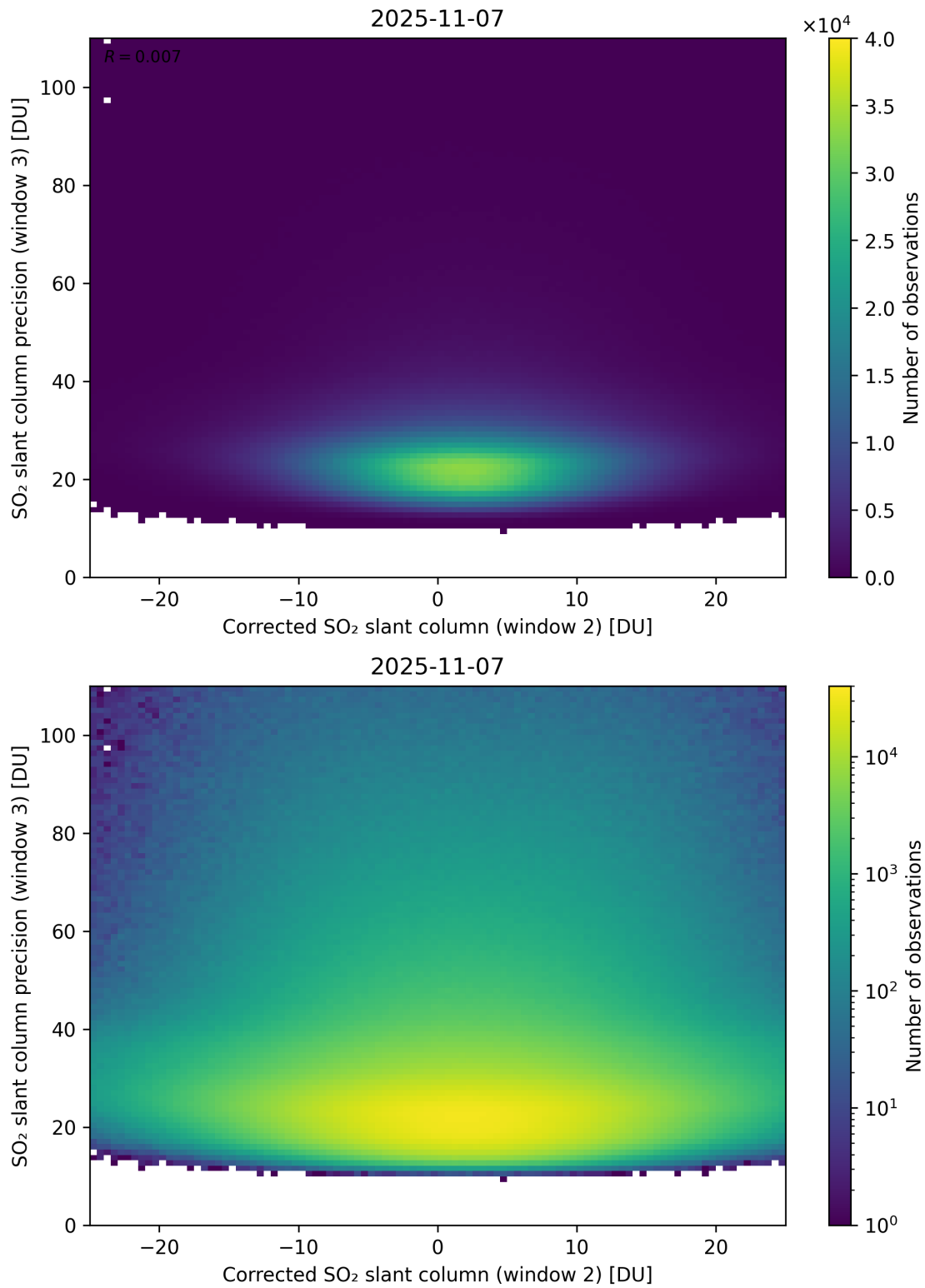
Figure 252: Scatter density plot of “Corrected SO 2 slant column (window 2)” against “SO 2 slant column precision (window 3)” for 2025-11-07 to 2025-11-08.
