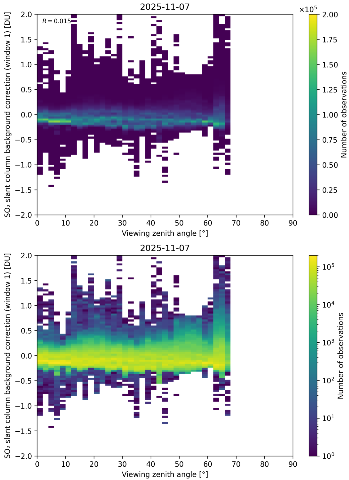
Figure 362: Scatter density plot of “Viewing zenith angle” against “SO 2 slant column background correction (window 1)” for 2025-11-07 to 2025-11-08.
