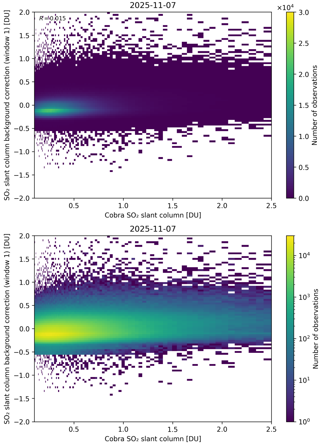
Figure 193: Scatter density plot of “Cobra SO 2 slant column” against “SO 2 slant column background correction (window 1)” for 2025-11-07 to 2025-11-08.
