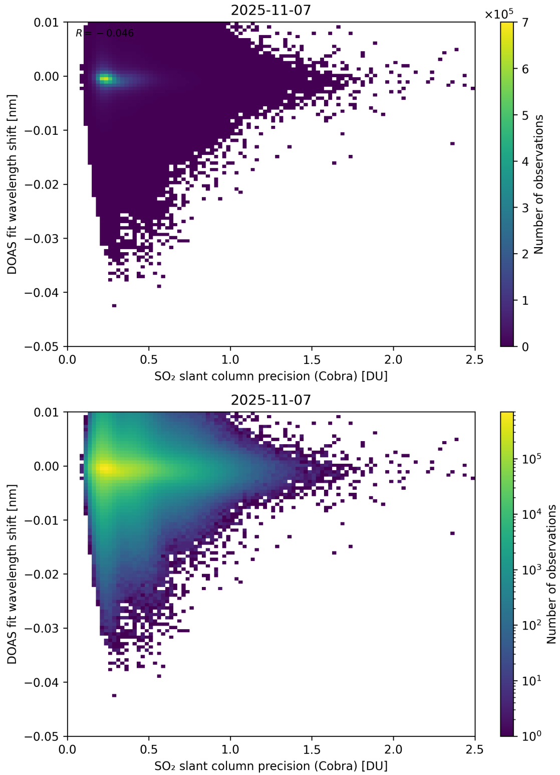
Figure 202: Scatter density plot of “SO 2 slant column precision (Cobra)” against “DOAS fit wavelength shift” for 2025-11-07 to 2025-11-08.
