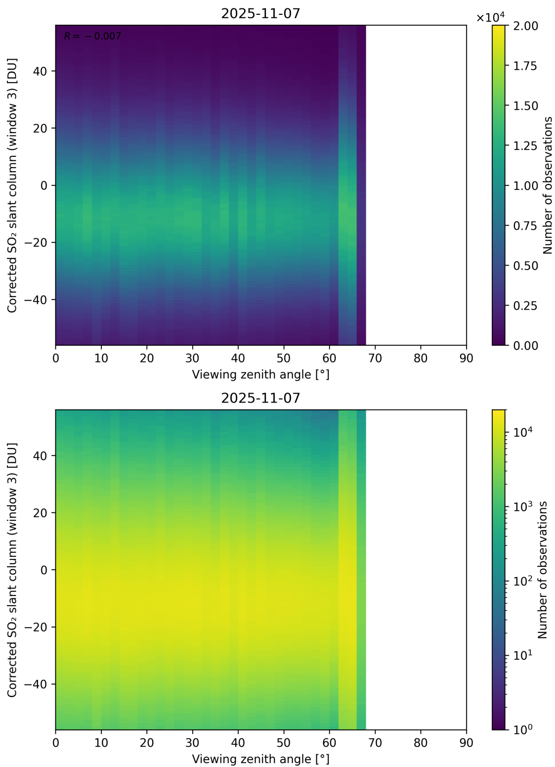
Figure 375: Scatter density plot of “Viewing zenith angle” against “Corrected SO 2 slant column (window 3)” for 2025-11-07 to 2025-11-08.
