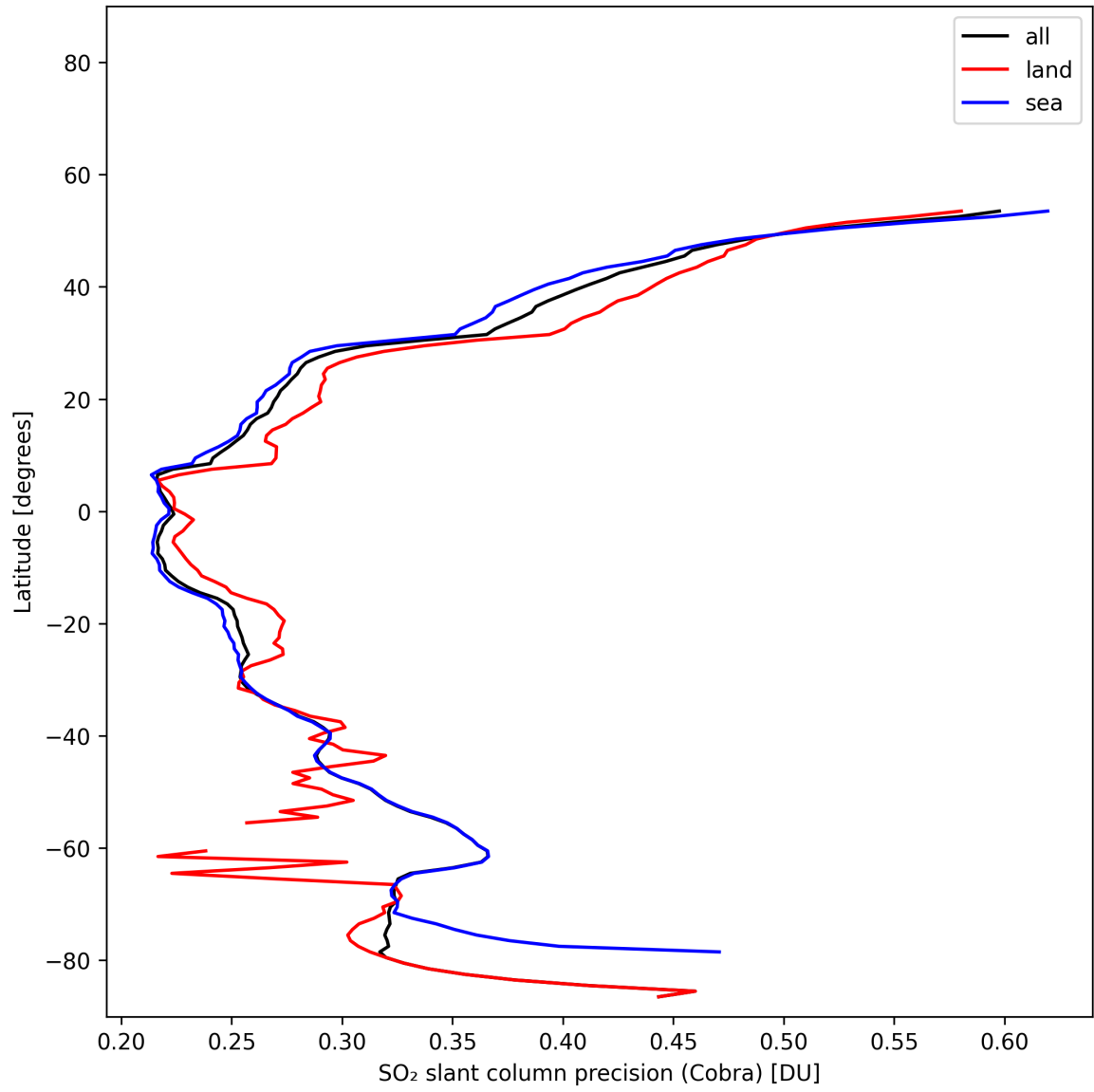
Figure 36: Zonal average of “SO 2 slant column precision (Cobra)” for 2025-11-07 to 2025-11-08.
