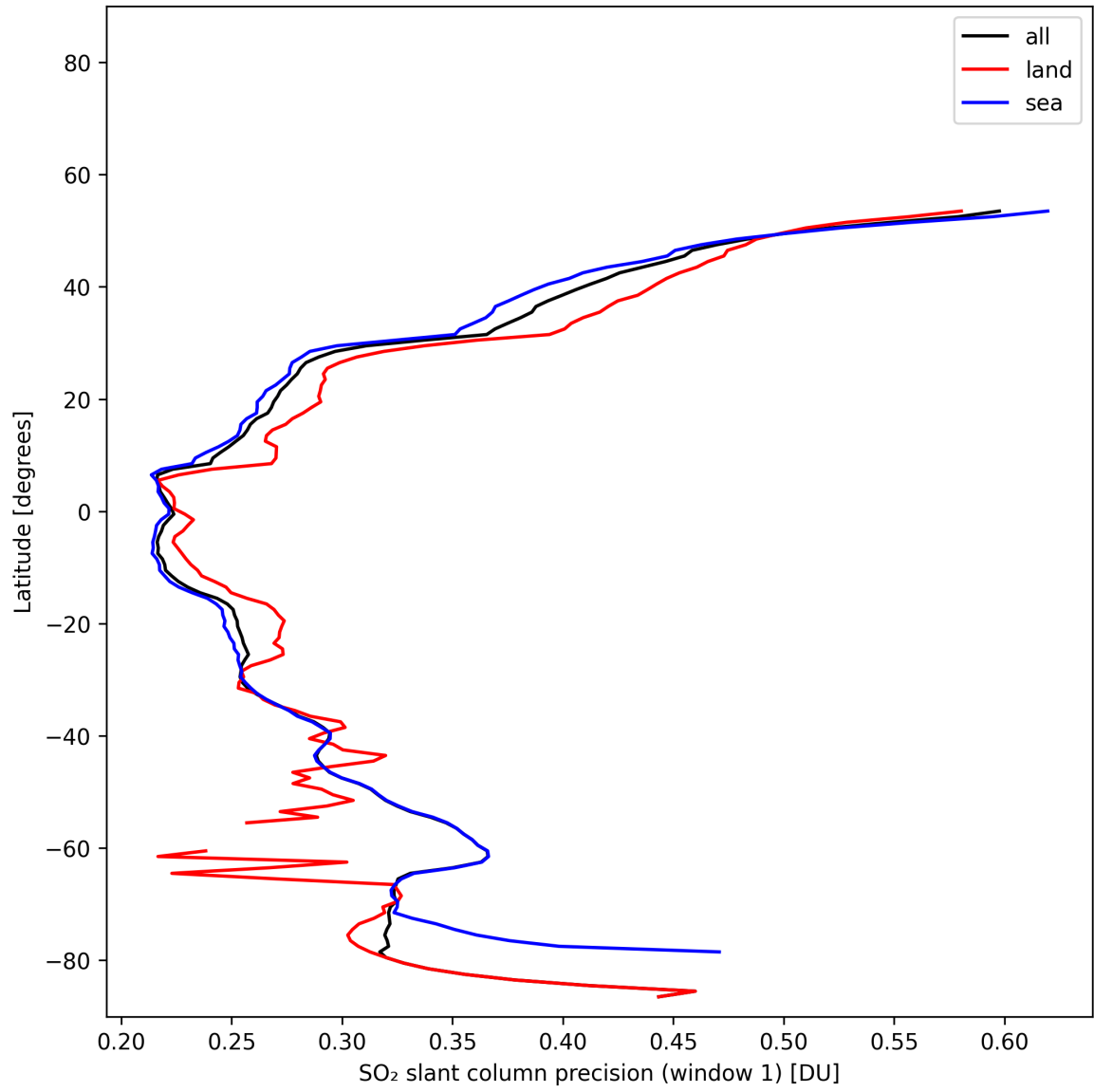
Figure 38: Zonal average of “SO 2 slant column precision (window 1)” for 2025-11-07 to 2025-11-08.
