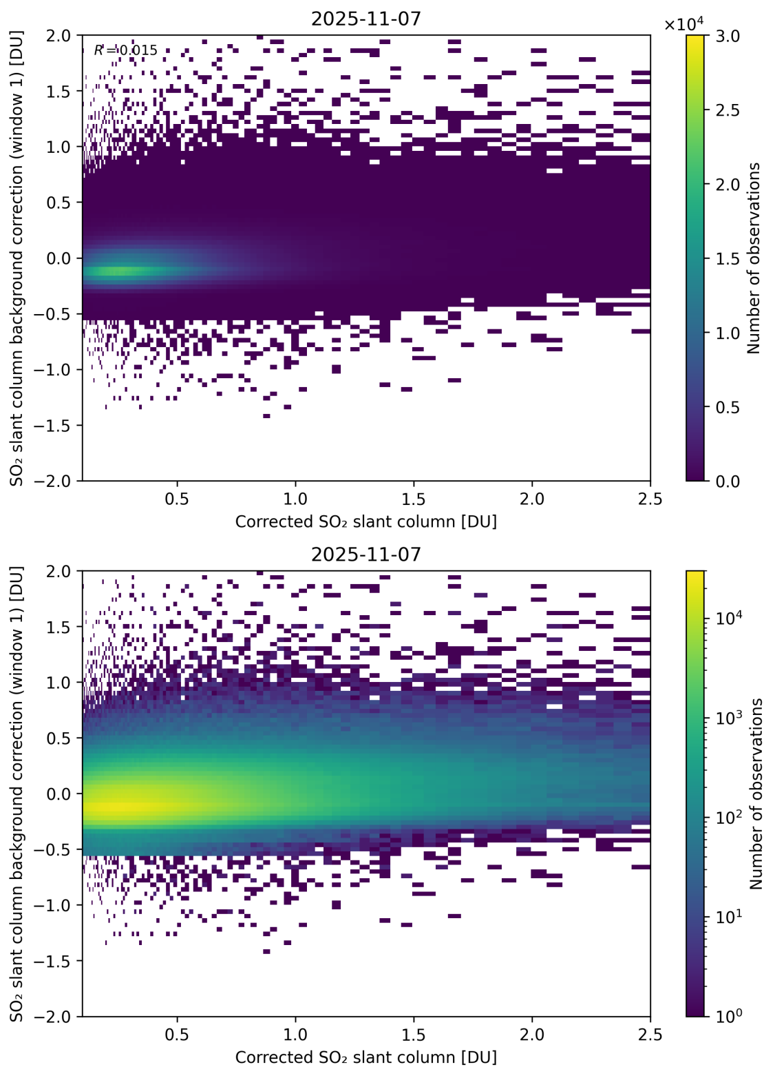
Figure 226: Scatter density plot of “Corrected SO 2 slant column” against “SO 2 slant column background correction (window 1)” for 2025-11-07 to 2025-11-08.
