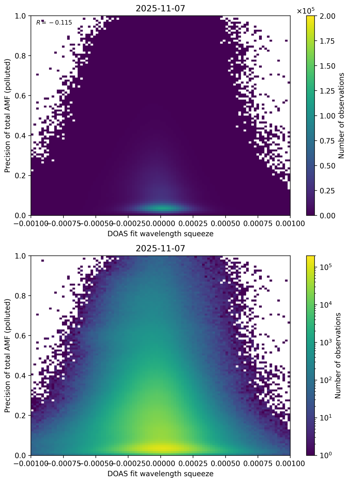
Figure 146: Scatter density plot of “DOAS fit wavelength squeeze” against “Precision of total AMF (polluted)” for 2025-11-07 to 2025-11-08.
