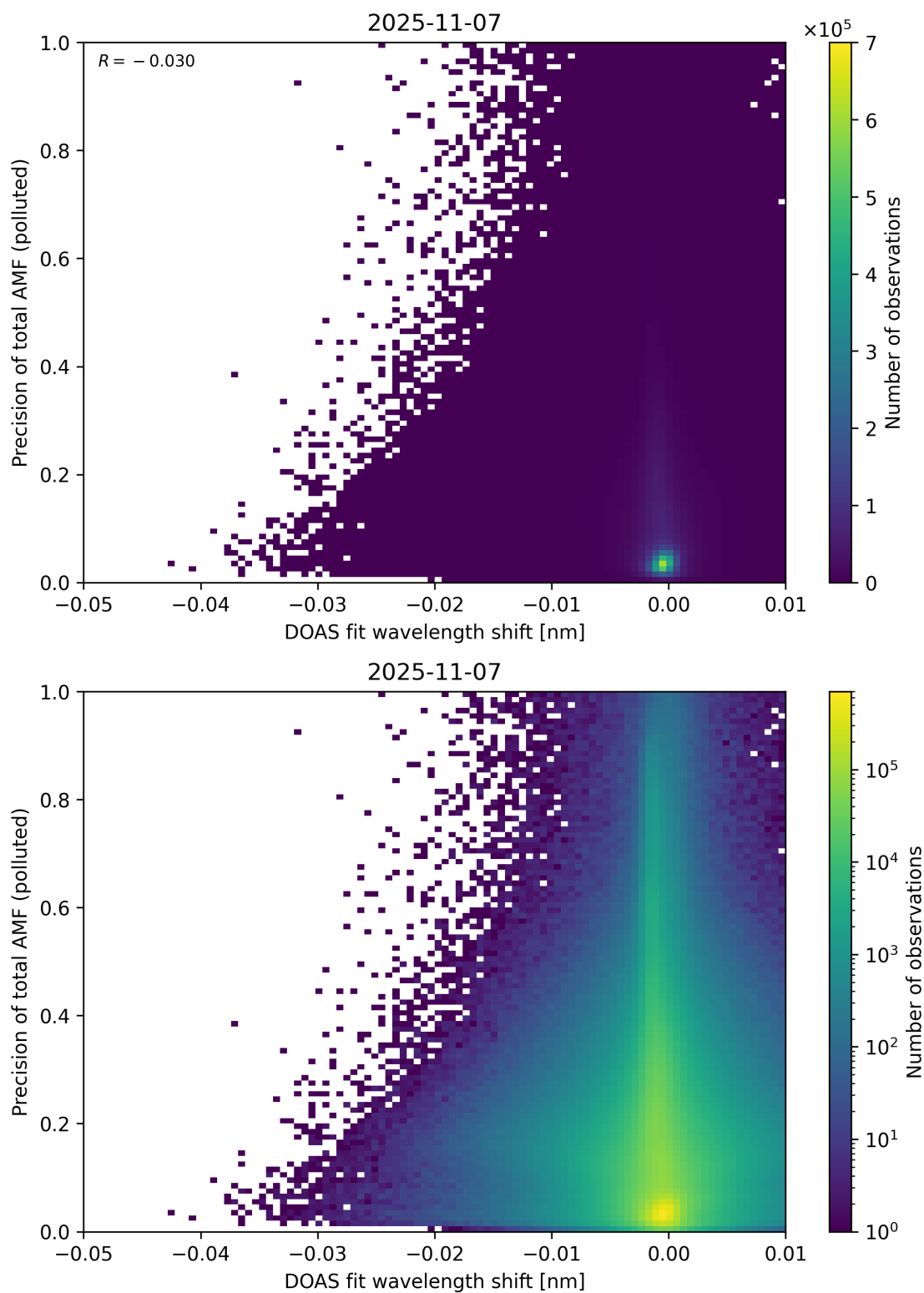
Figure 142: Scatter density plot of “DOAS fit wavelength shift” against “Precision of total AMF (polluted)” for 2025-11-07 to 2025-11-08.
