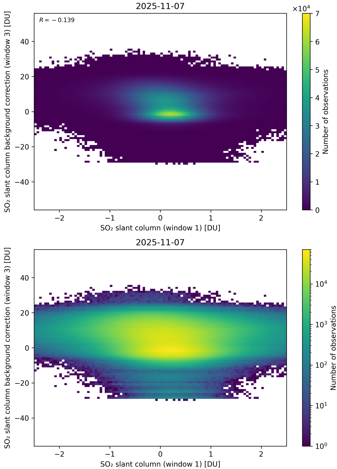
Figure 264: Scatter density plot of “SO 2 slant column (window 1)” against “SO 2 slant column background correction (window 3)” for 2025-11-07 to 2025-11-08.
