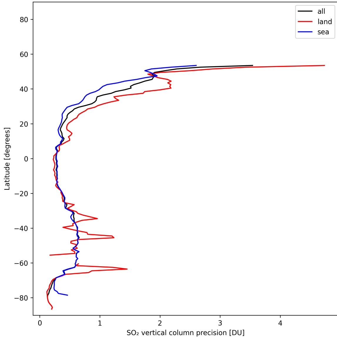
Figure 33: Zonal average of “SO 2 vertical column precision” for 2025-11-07 to 2025-11-08.
