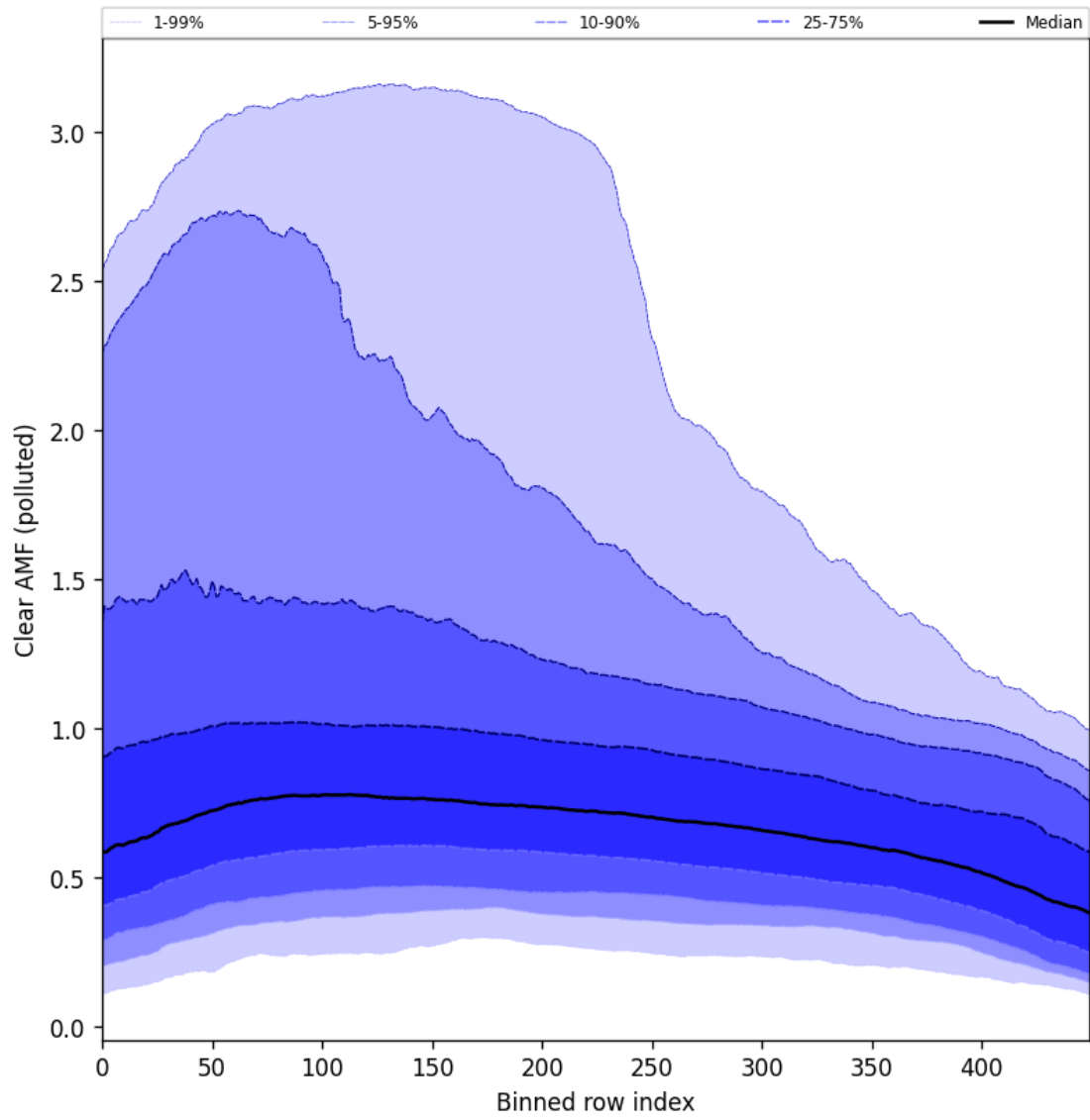
Figure 107: Along track statistics of “Clear AMF (polluted)” for 2025-11-07 to 2025-11-08
