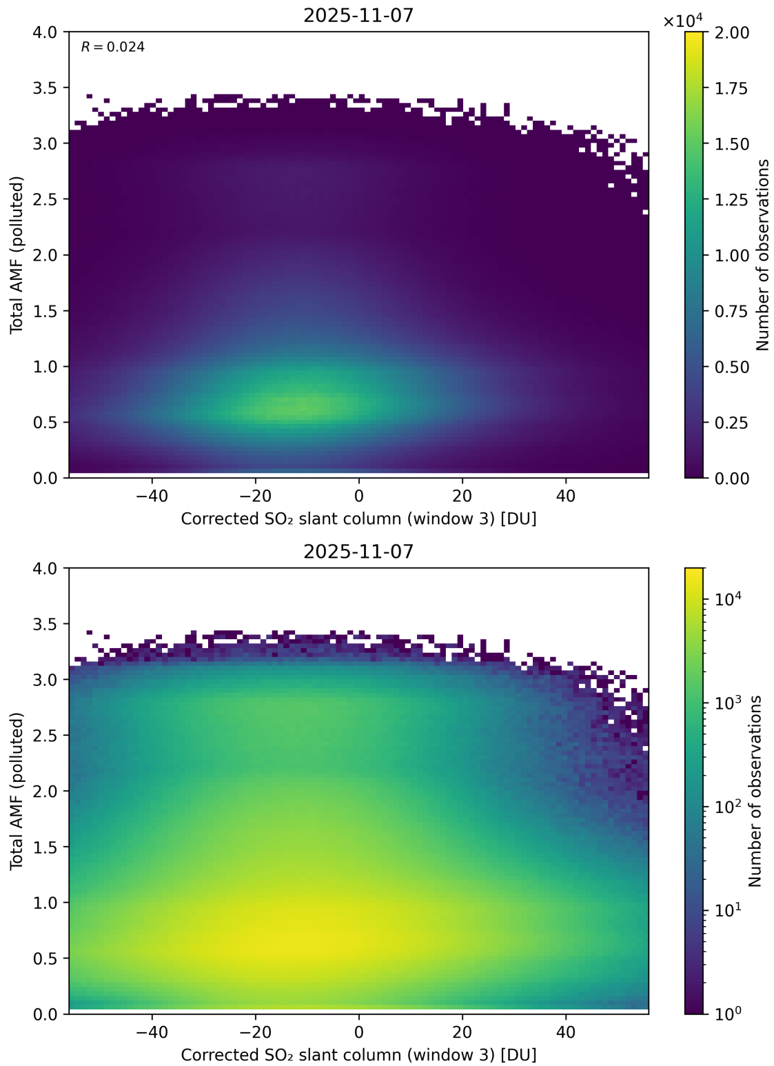
Figure 260: Scatter density plot of “Corrected SO 2 slant column (window 3)” against “Total AMF (polluted)” for 2025-11-07 to 2025-11-08.
