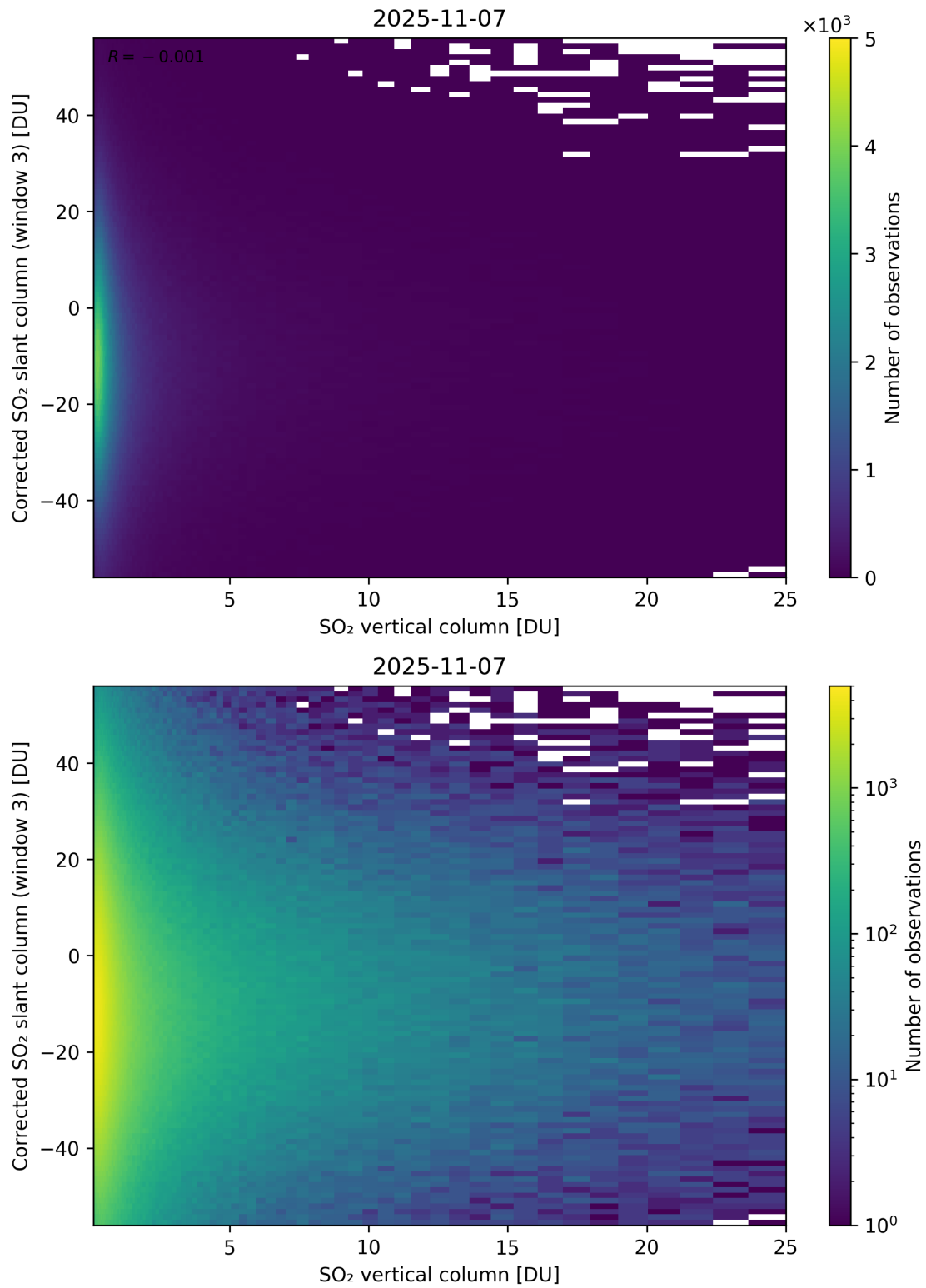
Figure 353: Scatter density plot of “SO 2 vertical column” against “Corrected SO 2 slant column (window 3)” for 2025-11-07 to 2025-11-08.
