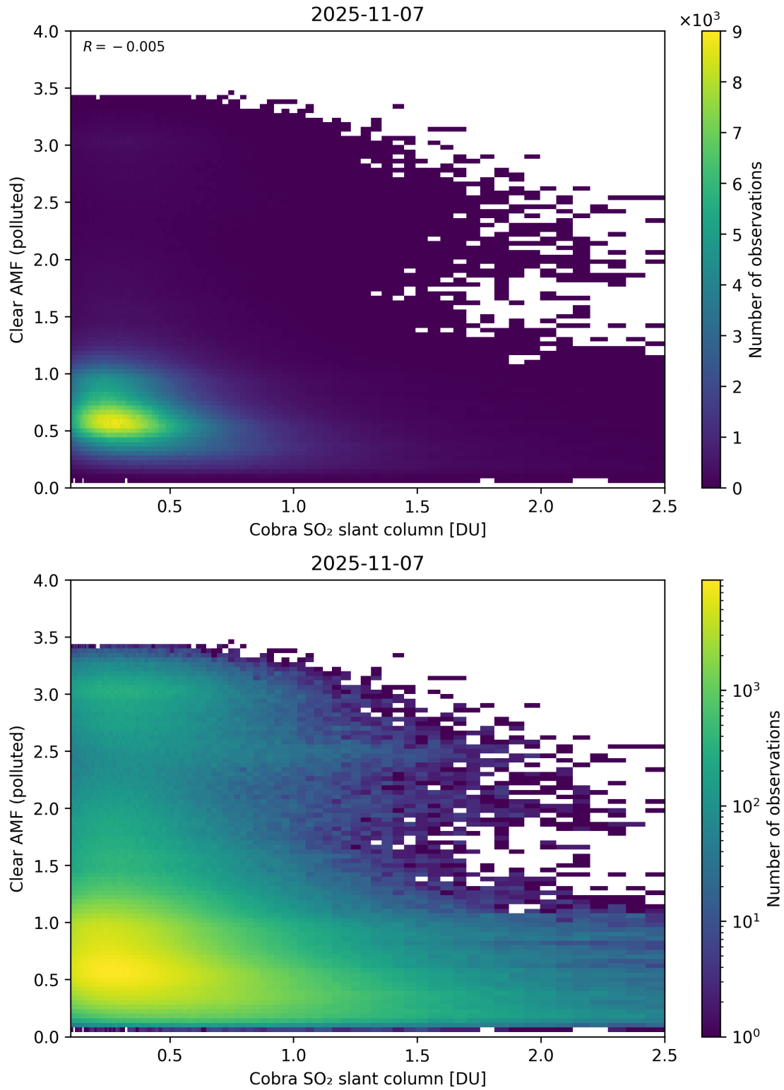
Figure 215: Scatter density plot of “Cobra SO 2 slant column” against “Clear AMF (polluted)” for 2025-11-07 to 2025-11-08.
