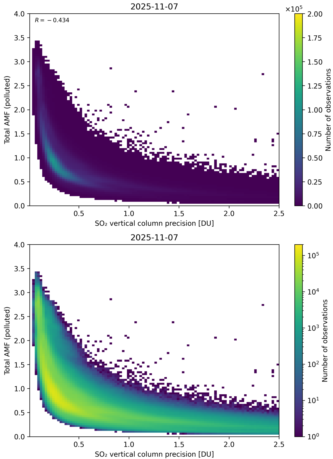
Figure 346: Scatter density plot of “SO 2 vertical column precision” against “Total AMF (polluted)” for 2025-11-07 to 2025-11-08.
