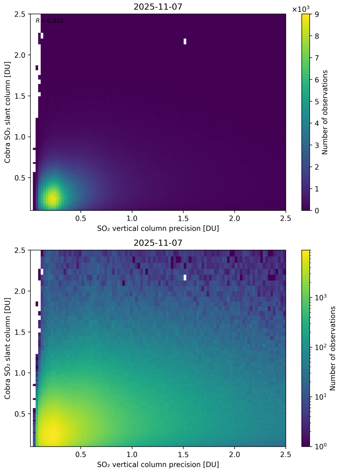
Figure 336: Scatter density plot of “SO 2 vertical column precision” against “Cobra SO 2 slant column” for 2025-11-07 to 2025-11-08.
