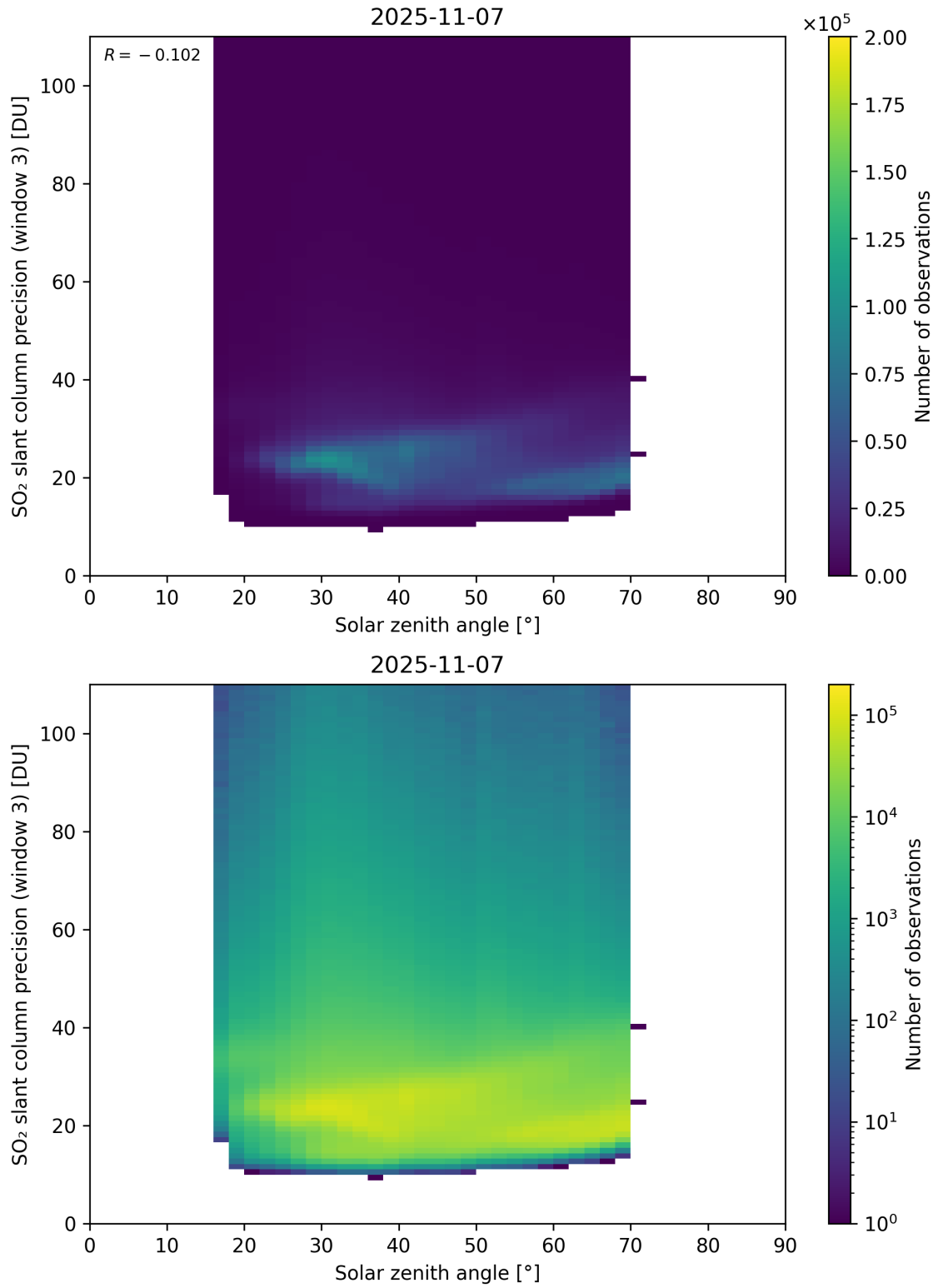
Figure 188: Scatter density plot of “Solar zenith angle” against “SO 2 slant column precision (window 3)” for 2025-11-07 to 2025-11-08.
