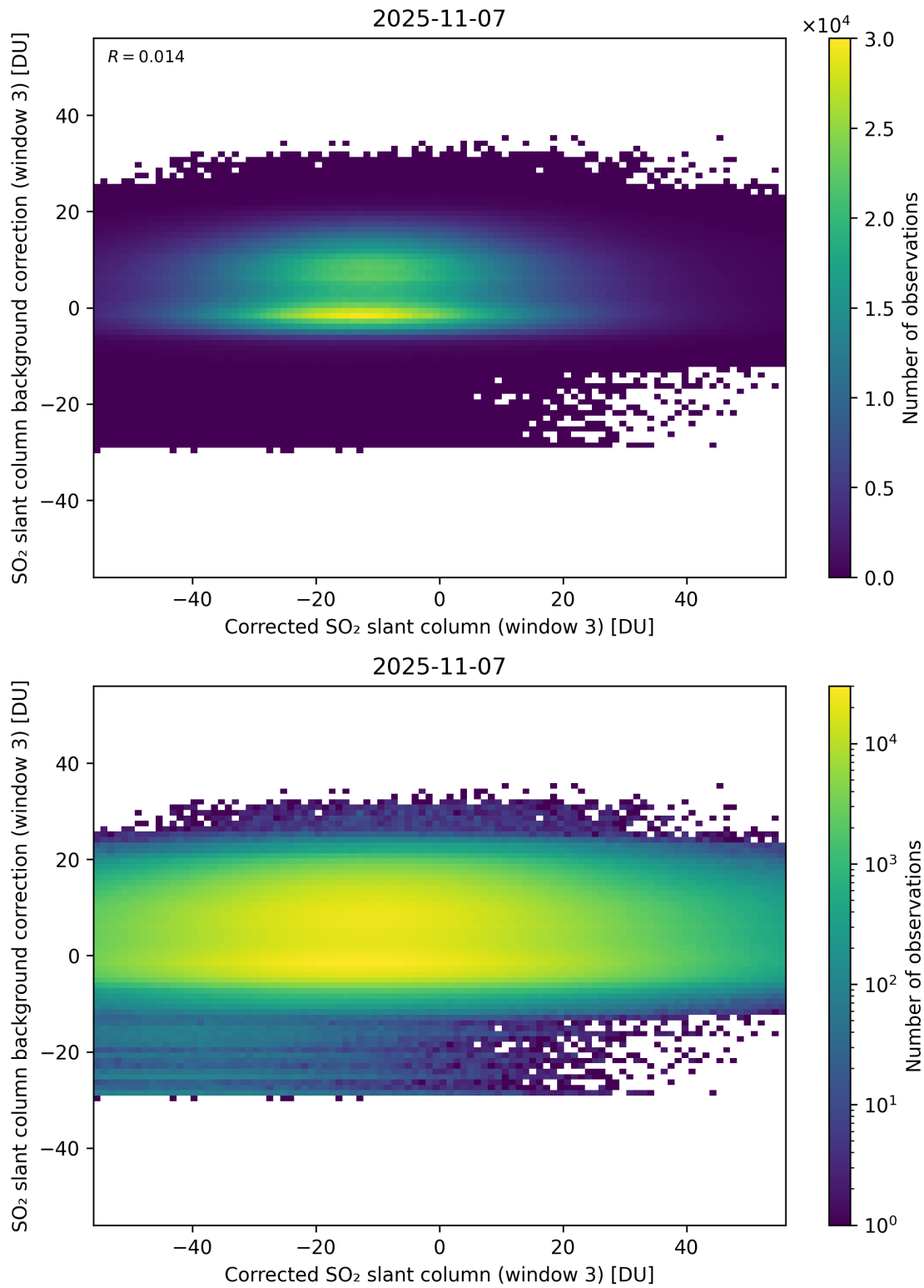
Figure 255: Scatter density plot of “Corrected SO 2 slant column (window 3)” against “SO 2 slant column background correction (window 3)” for 2025-11-07 to 2025-11-08.
