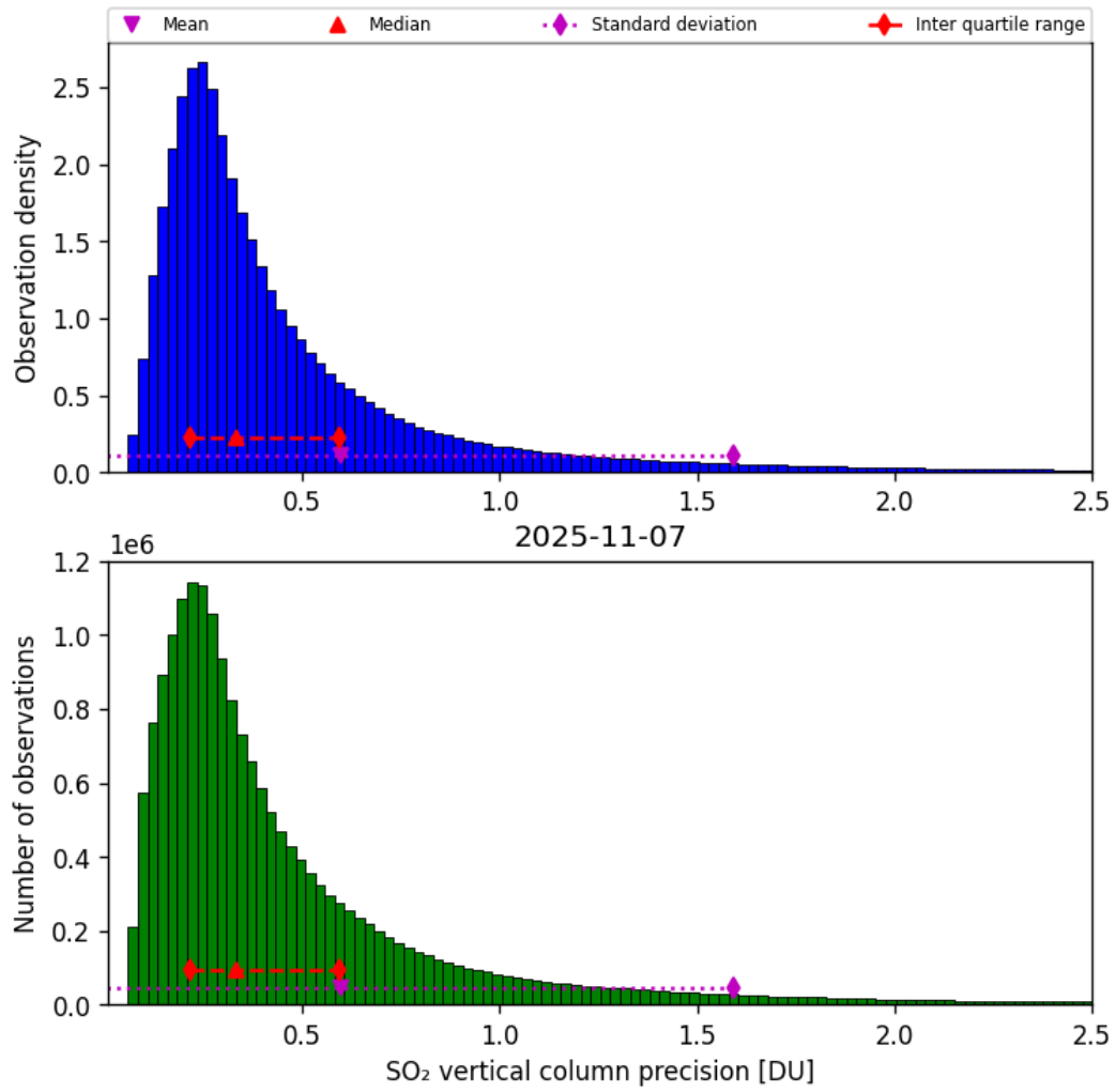
Figure 59: Histogram of “SO 2 vertical column precision” for 2025-11-07 to 2025-11-08
