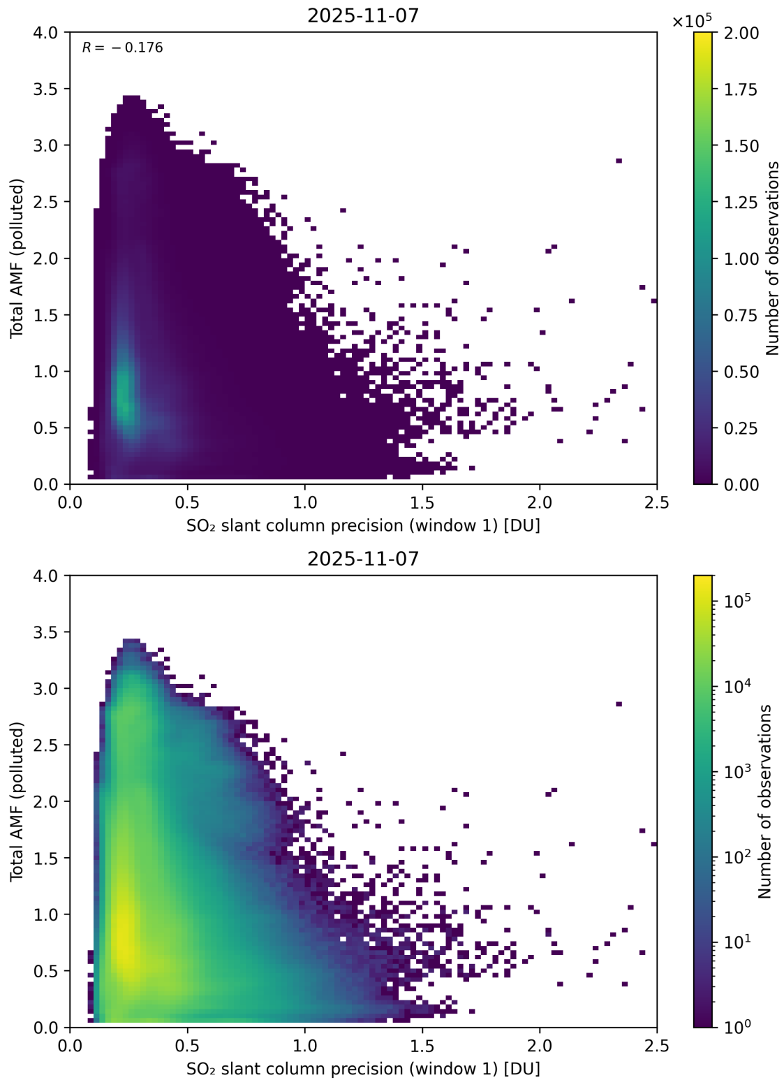
Figure 280: Scatter density plot of “SO 2 slant column precision (window 1)” against “Total AMF (polluted)” for 2025-11-07 to 2025-11-08.
