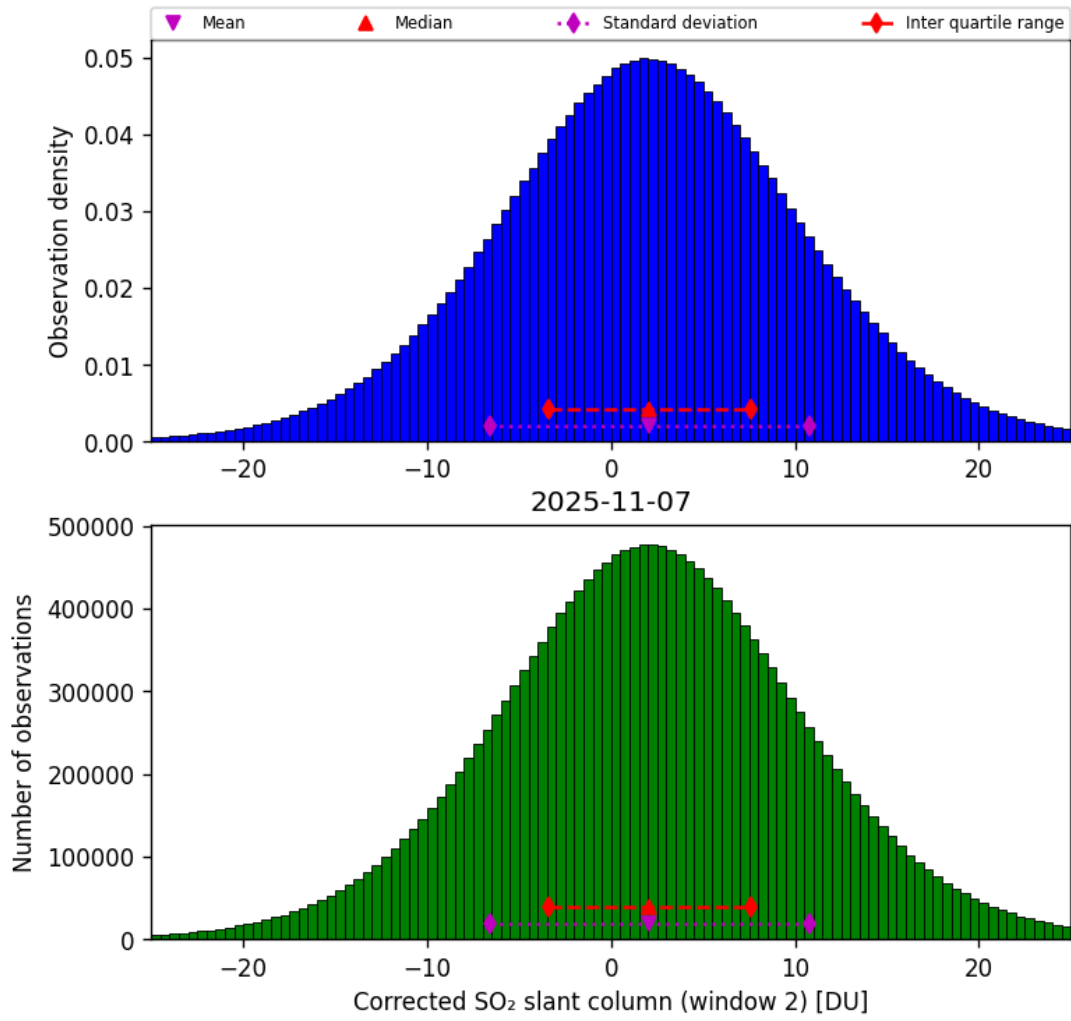
Figure 69: Histogram of “Corrected SO 2 slant column (window 2)” for 2025-11-07 to 2025-11-08
