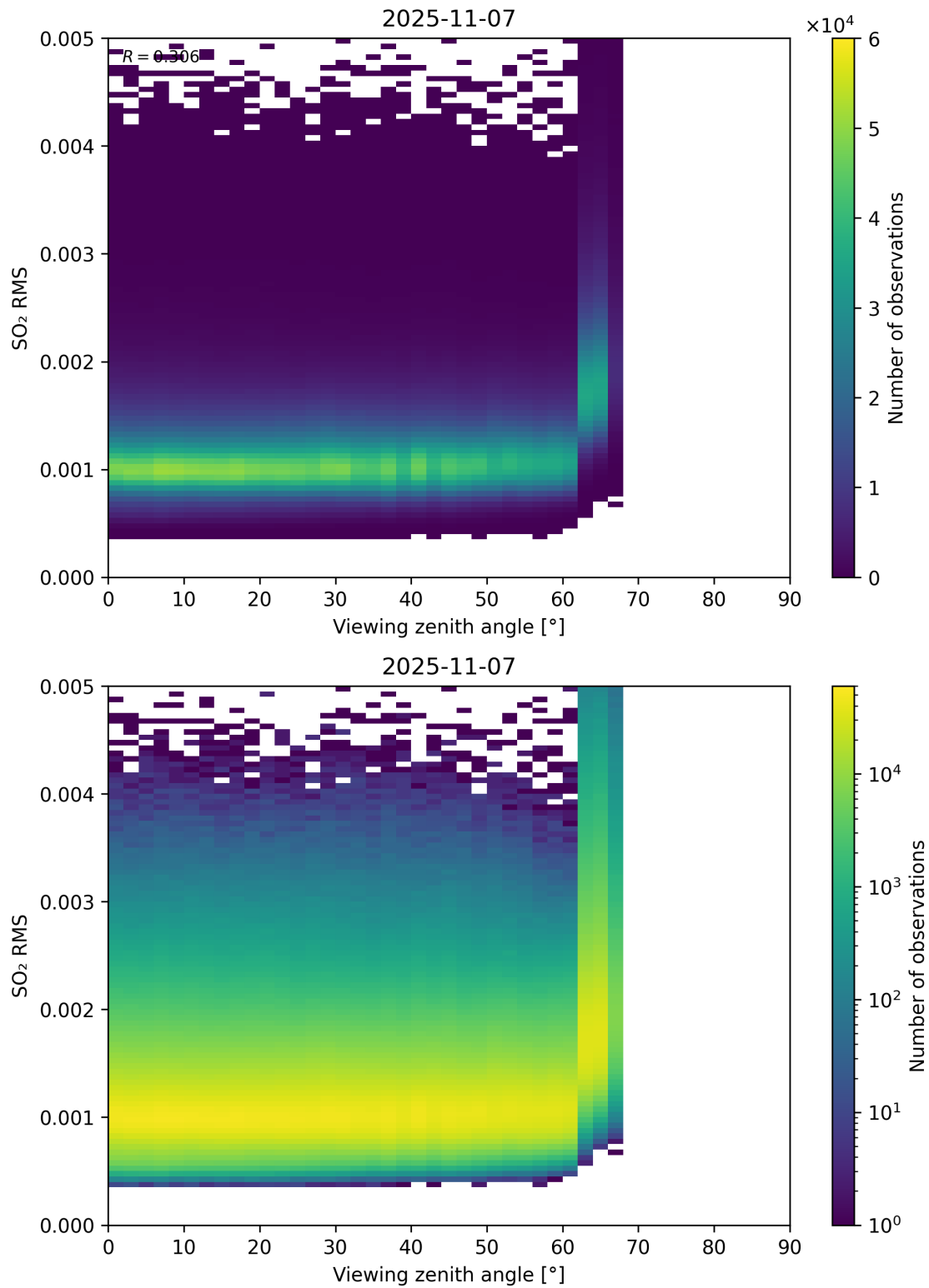
Figure 367: Scatter density plot of “Viewing zenith angle” against “SO 2 RMS” for 2025-11-07 to 2025-11-08.
