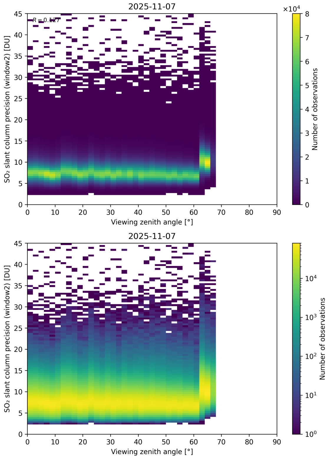
Figure 378: Scatter density plot of “Viewing zenith angle” against “SO 2 slant column precision (window2)” for 2025-11-07 to 2025-11-08.
