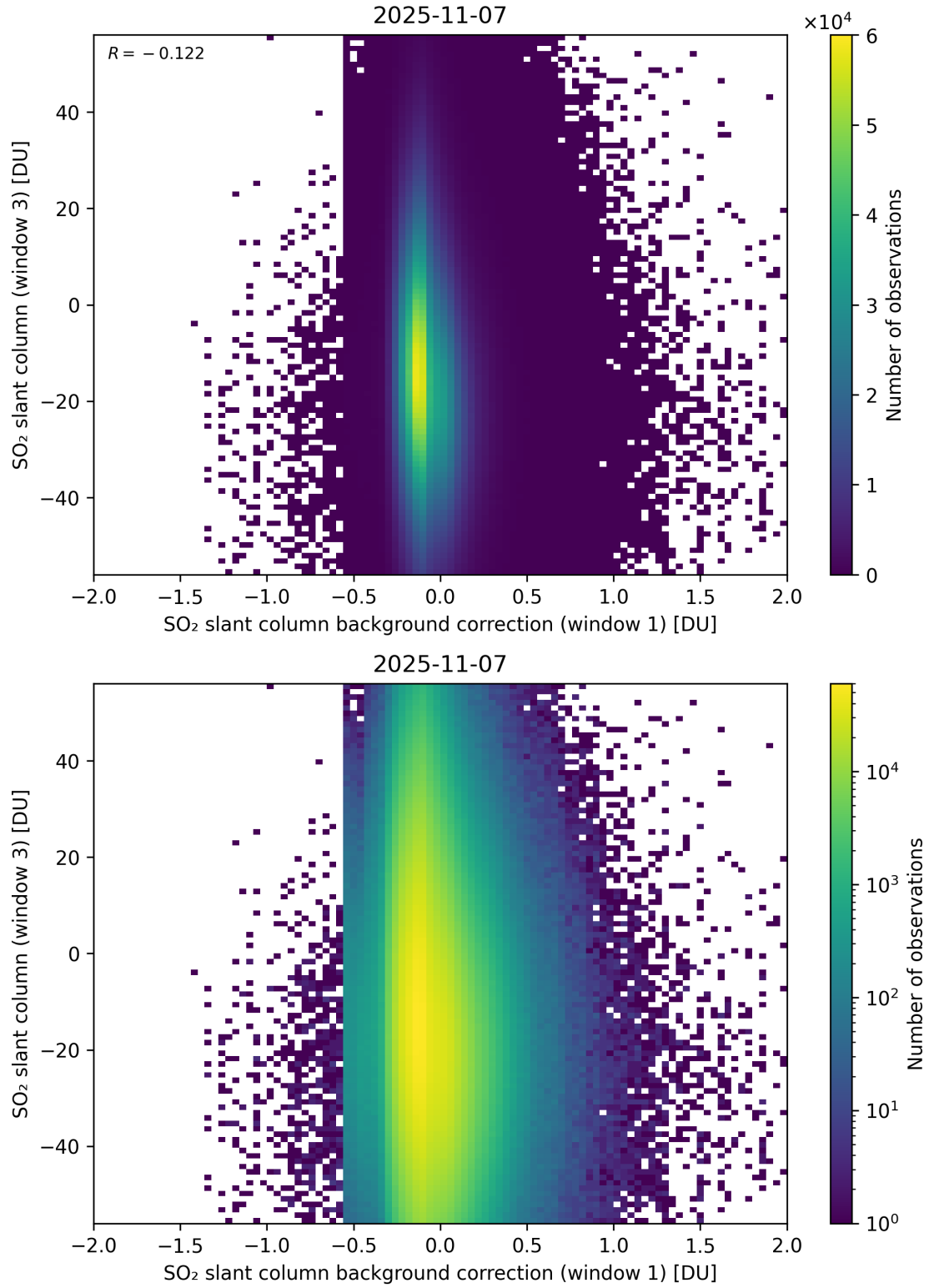
Figure 118: Scatter density plot of “SO 2 slant column background correction (window 1)” against “SO 2 slant column (window 3)” for 2025-11-07 to 2025-11-08.
