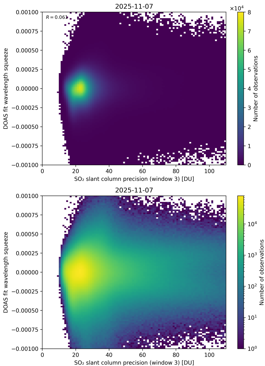
Figure 309: Scatter density plot of “SO 2 slant column precision (window 3)” against “DOAS fit wavelength squeeze” for 2025-11-07 to 2025-11-08.
