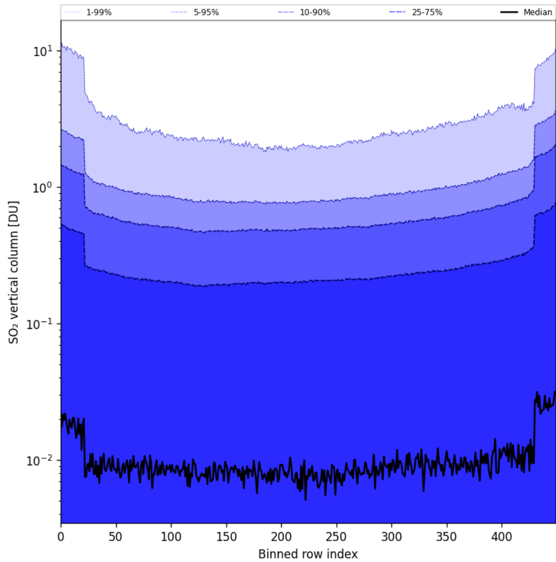
Figure 84: Along track statistics of “SO 2 vertical column” for 2025-11-07 to 2025-11-08
