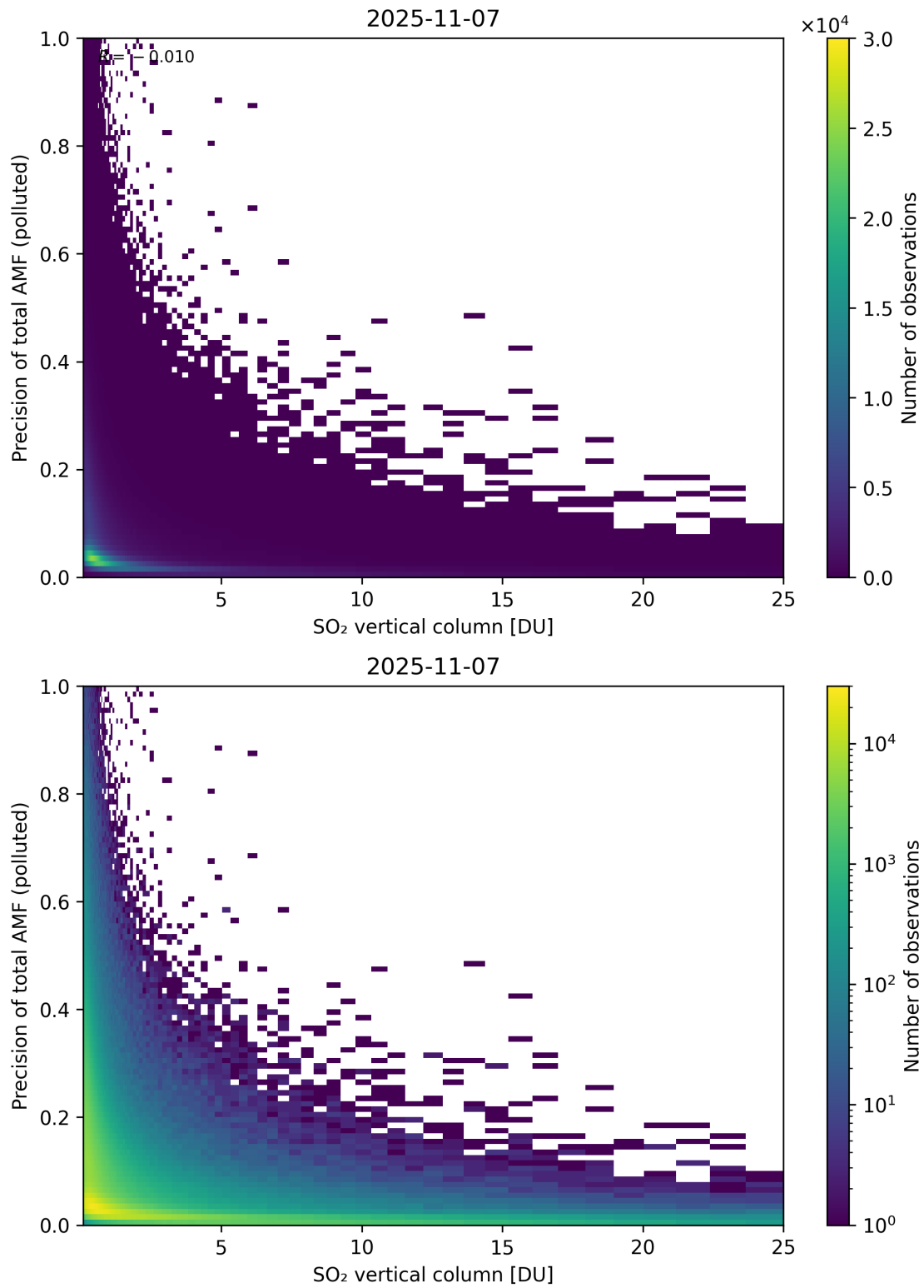
Figure 360: Scatter density plot of “SO 2 vertical column” against “Precision of total AMF (polluted)” for 2025-11-07 to 2025-11-08.
