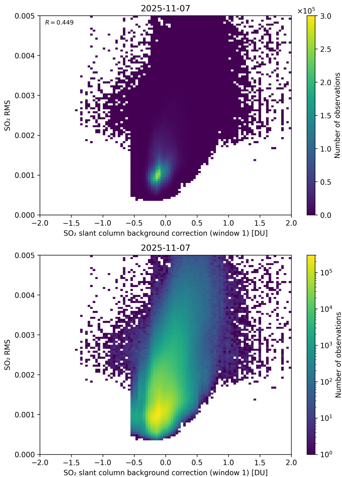
Figure 113: Scatter density plot of “SO 2 slant column background correction (window 1)” against “SO 2 RMS” for 2025-11-07 to 2025-11-08.
