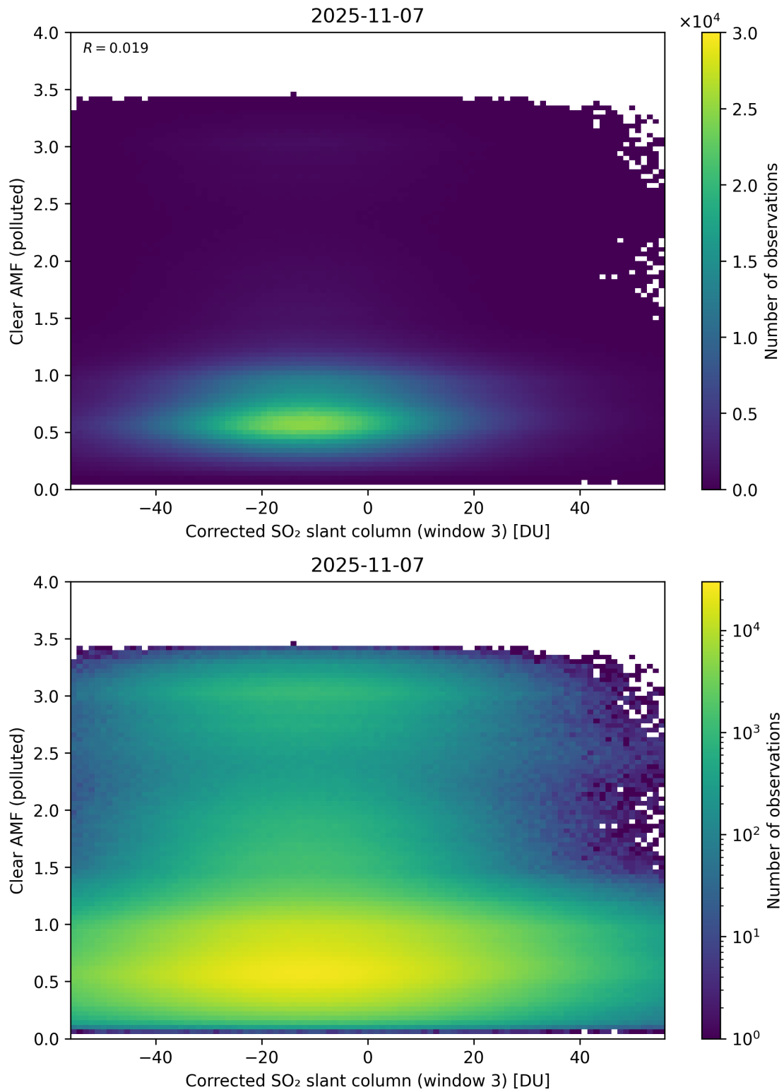
Figure 259: Scatter density plot of “Corrected SO 2 slant column (window 3)” against “Clear AMF (polluted)” for 2025-11-07 to 2025-11-08.
