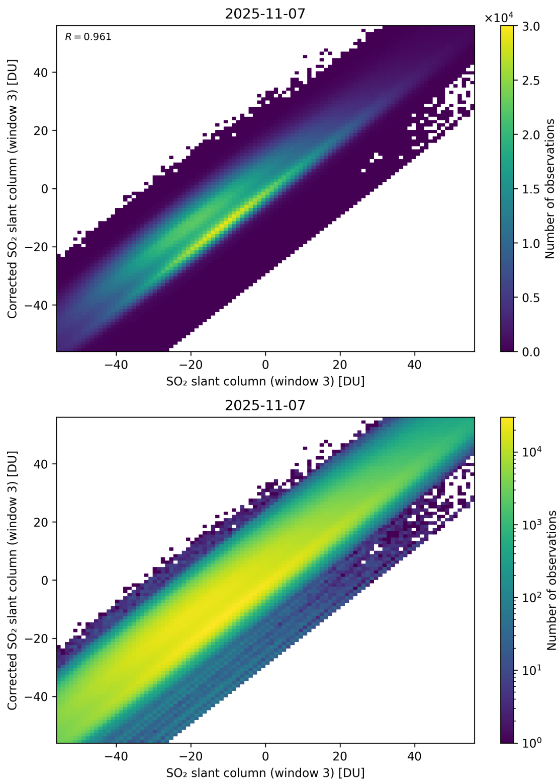
Figure 316: Scatter density plot of “SO 2 slant column (window 3)” against “Corrected SO 2 slant column (window 3)” for 2025-11-07 to 2025-11-08.
