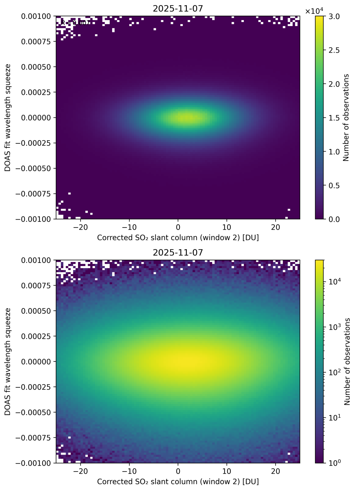
Figure 247: Scatter density plot of “Corrected SO 2 slant column (window 2)” against “DOAS fit wavelength squeeze” for 2025-11-07 to 2025-11-08.
