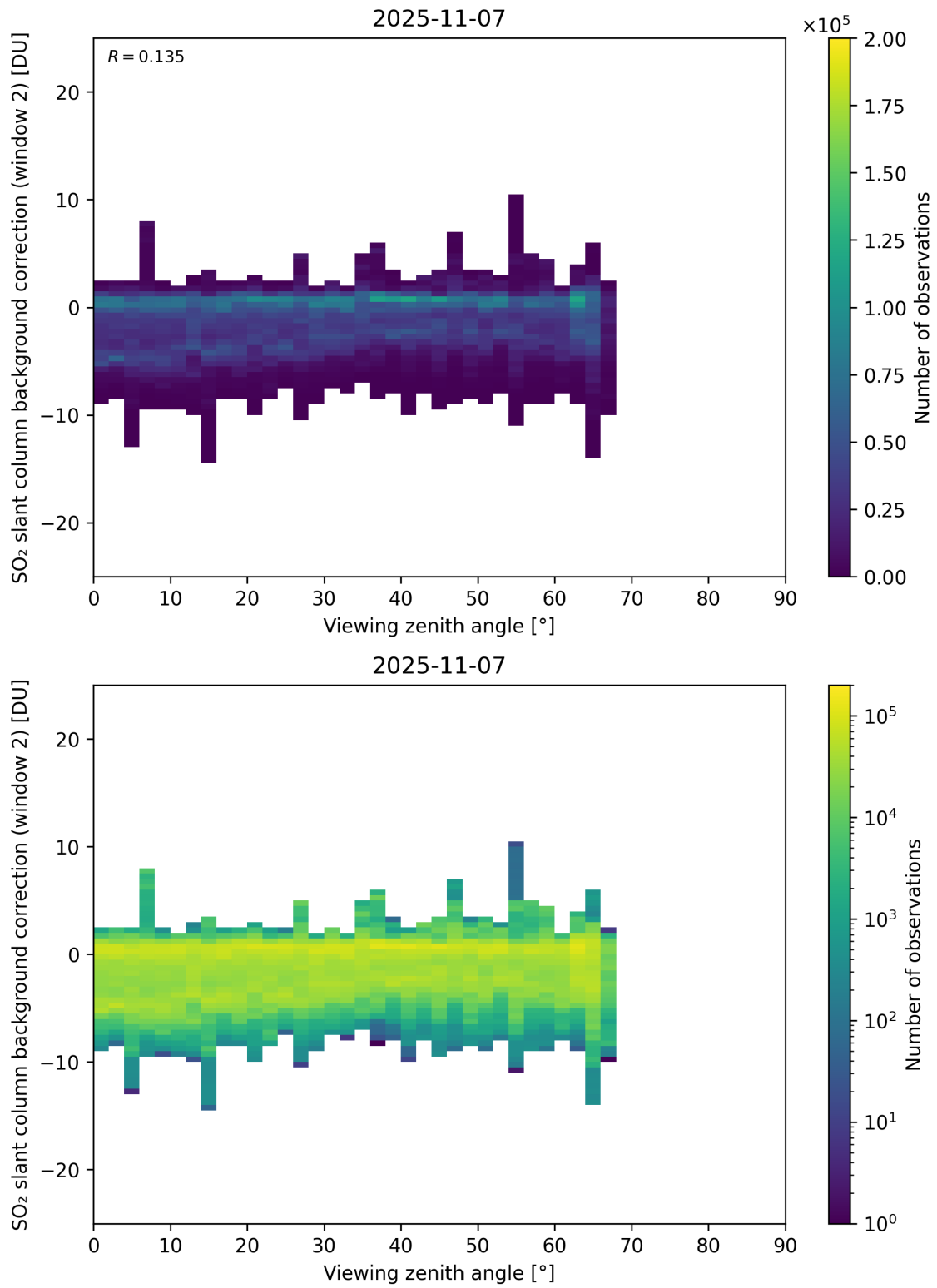
Figure 363: Scatter density plot of “Viewing zenith angle” against “SO 2 slant column background correction (window 2)” for 2025-11-07 to 2025-11-08.
