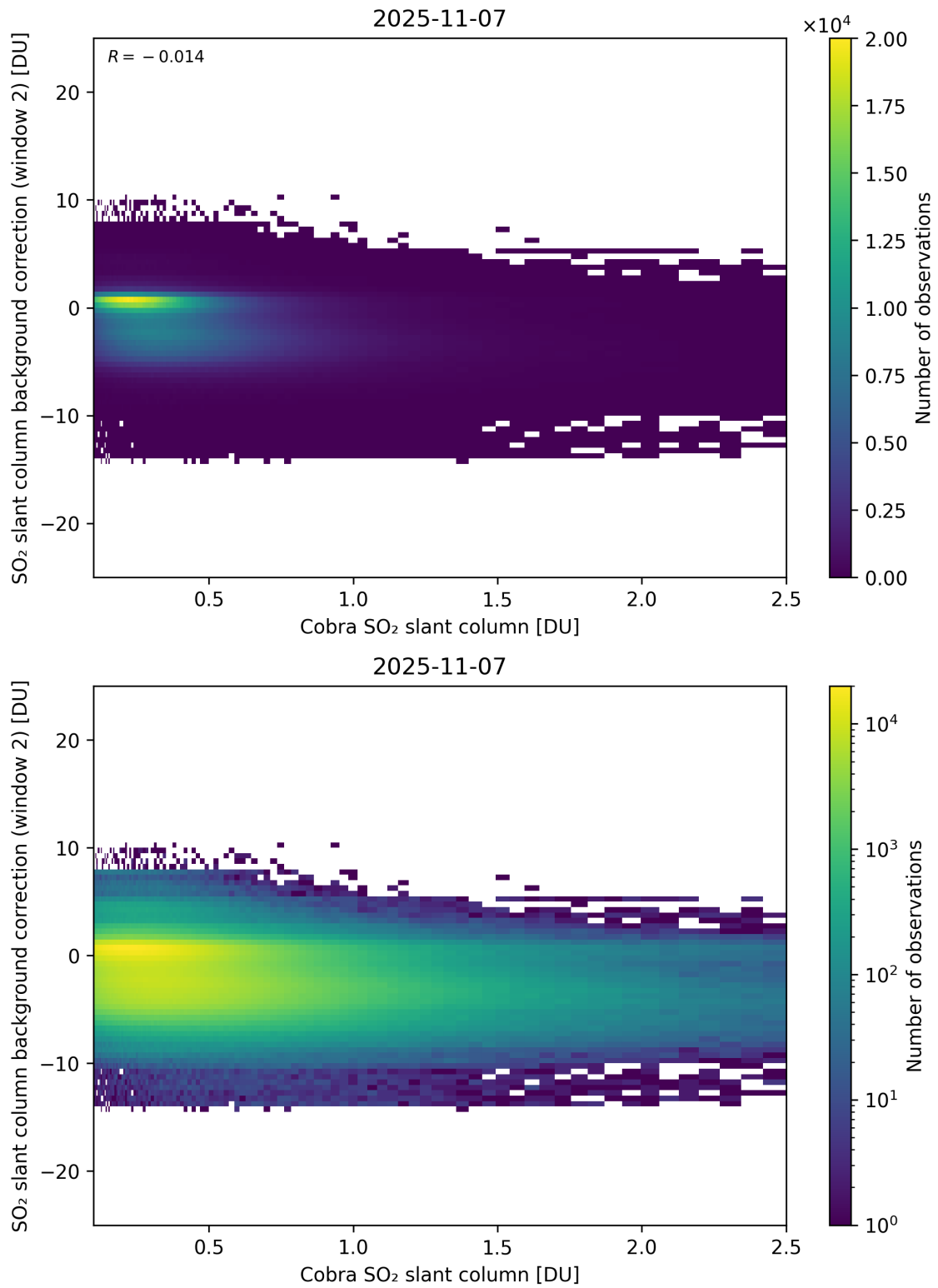
Figure 194: Scatter density plot of “Cobra SO 2 slant column” against “SO 2 slant column background correction (window 2)” for 2025-11-07 to 2025-11-08.
