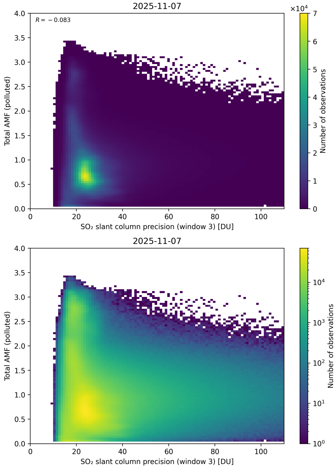
Figure 313: Scatter density plot of “SO 2 slant column precision (window 3)” against “Total AMF (polluted)” for 2025-11-07 to 2025-11-08.
