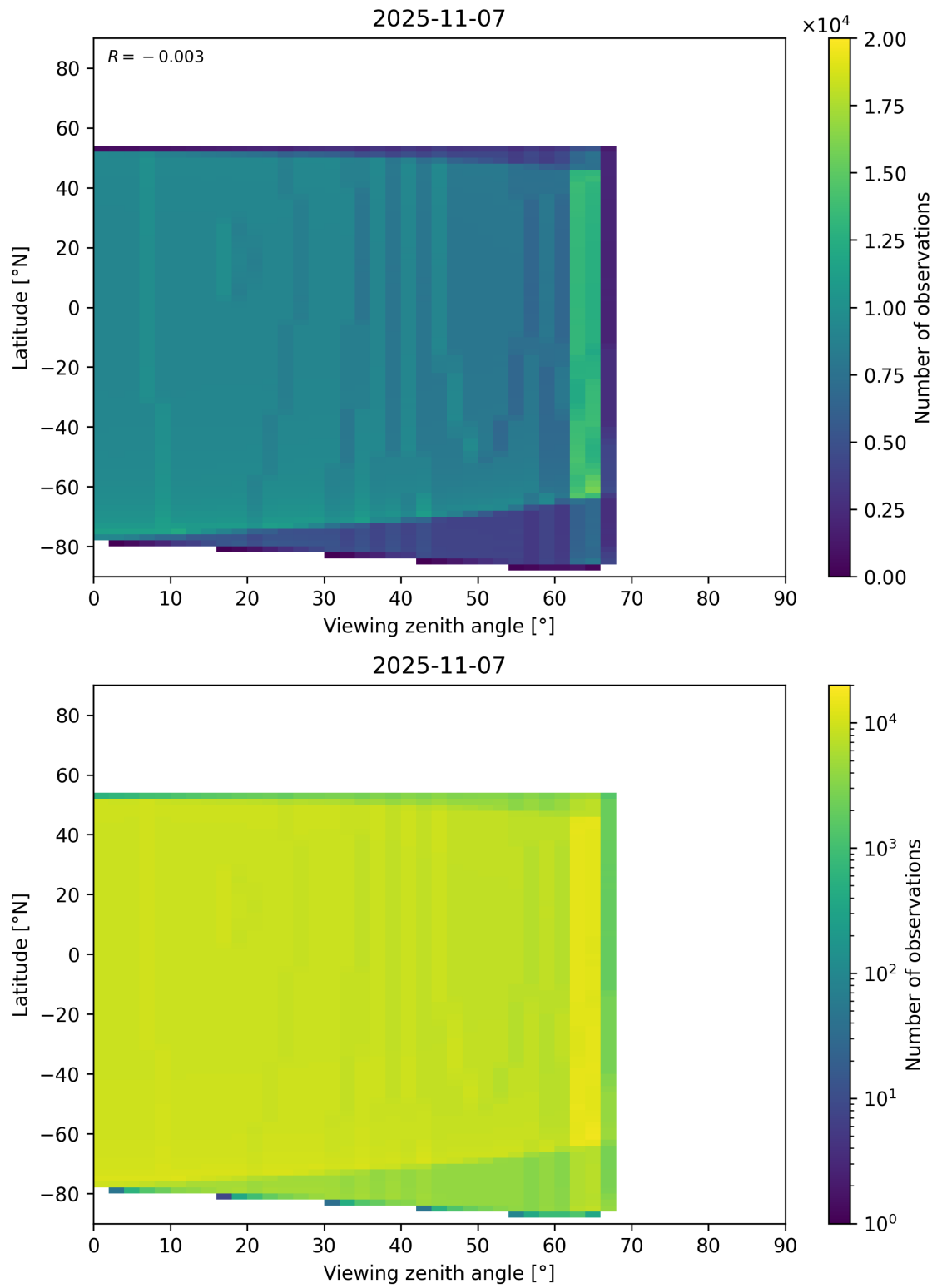
Figure 368: Scatter density plot of “Viewing zenith angle” against “Latitude” for 2025-11-07 to 2025-11-08.
