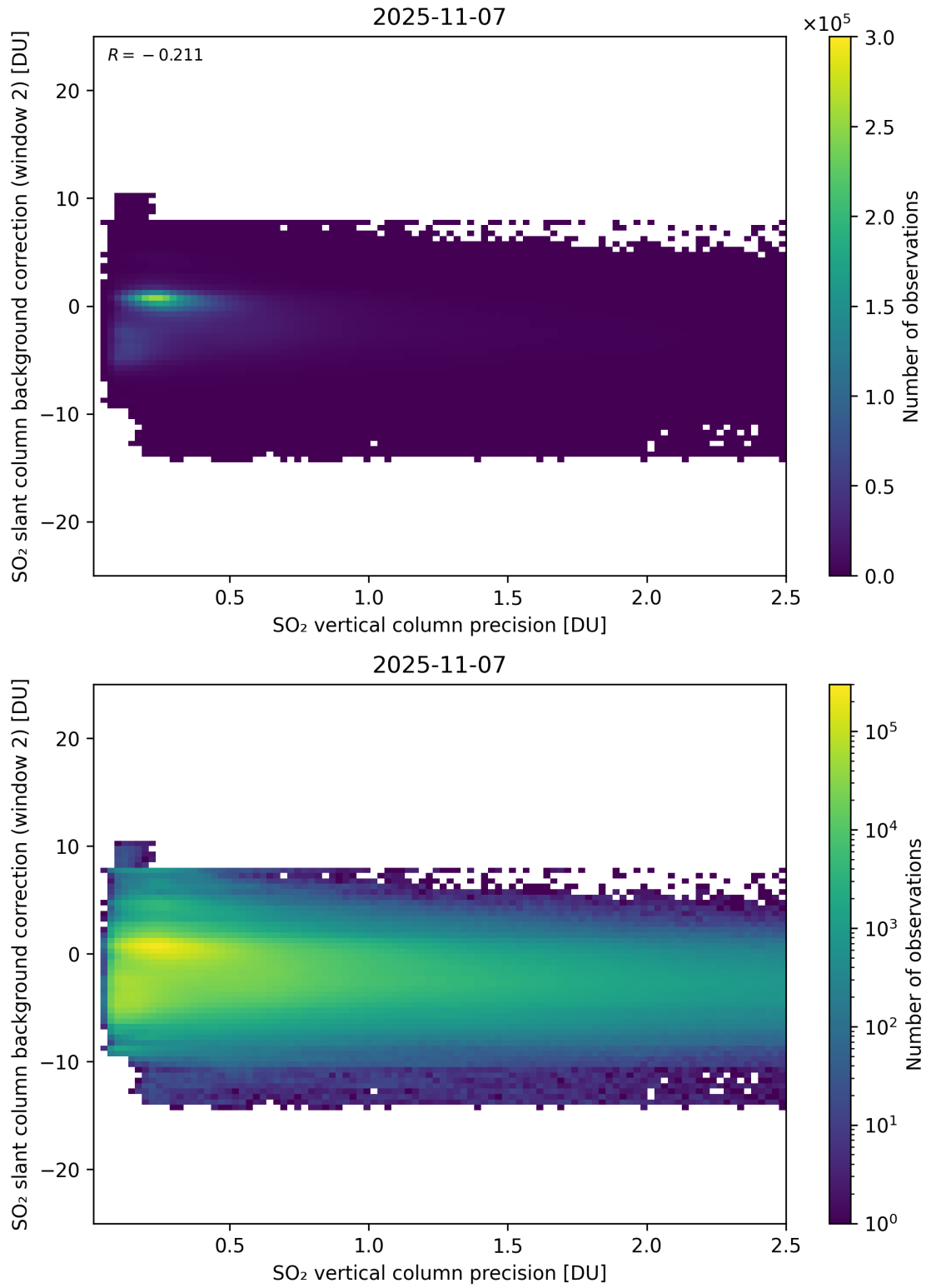
Figure 330: Scatter density plot of “SO 2 vertical column precision” against “SO 2 slant column background correction (window 2)” for 2025-11-07 to 2025-11-08.
