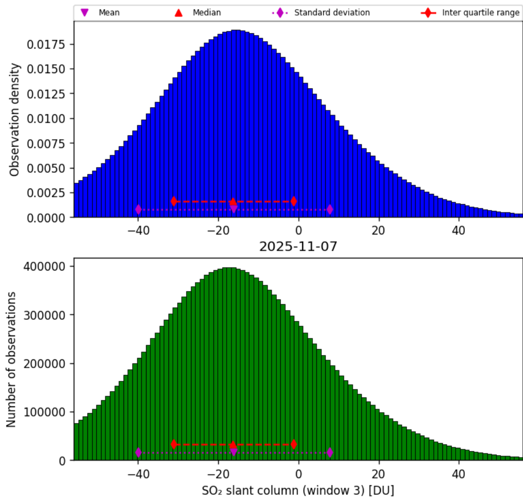
Figure 71: Histogram of “SO 2 slant column (window 3)” for 2025-11-07 to 2025-11-08
