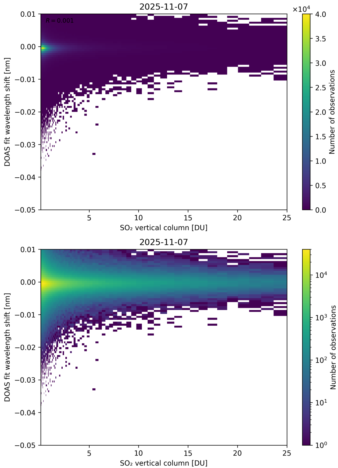
Figure 326: Scatter density plot of “SO 2 vertical column” against “DOAS fit wavelength shift” for 2025-11-07 to 2025-11-08.
