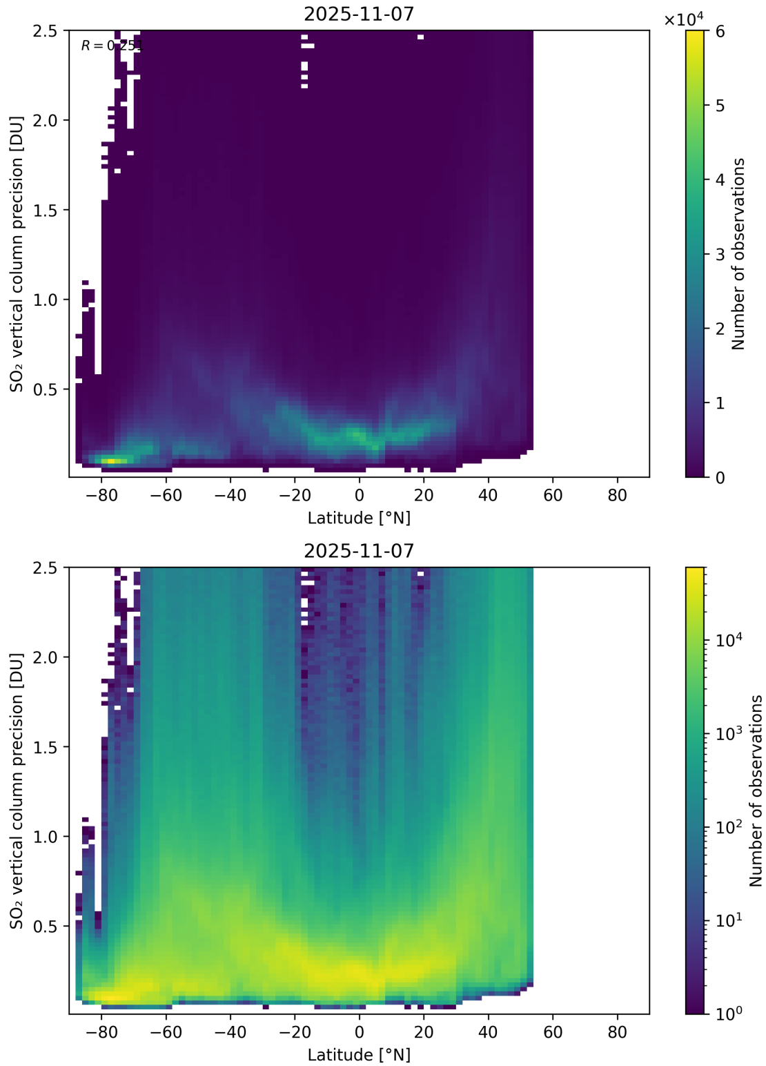
Figure 170: Scatter density plot of “Latitude” against “SO 2 vertical column precision” for 2025-11-07 to 2025-11-08.
