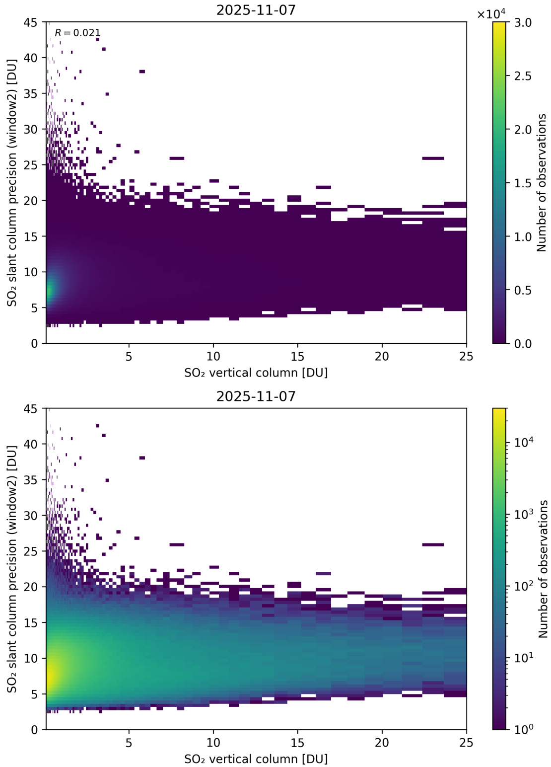
Figure 356: Scatter density plot of “SO 2 vertical column” against “SO 2 slant column precision (window2)” for 2025-11-07 to 2025-11-08.
