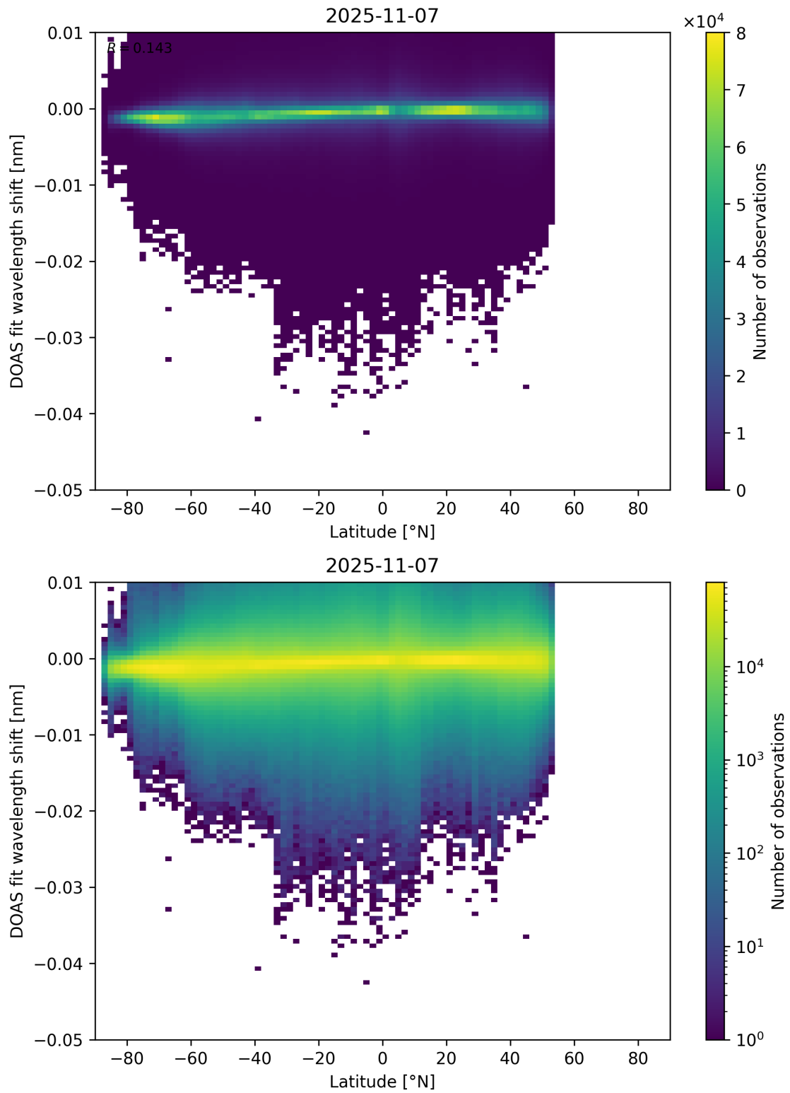
Figure 153: Scatter density plot of “Latitude” against “DOAS fit wavelength shift” for 2025-11-07 to 2025-11-08.
