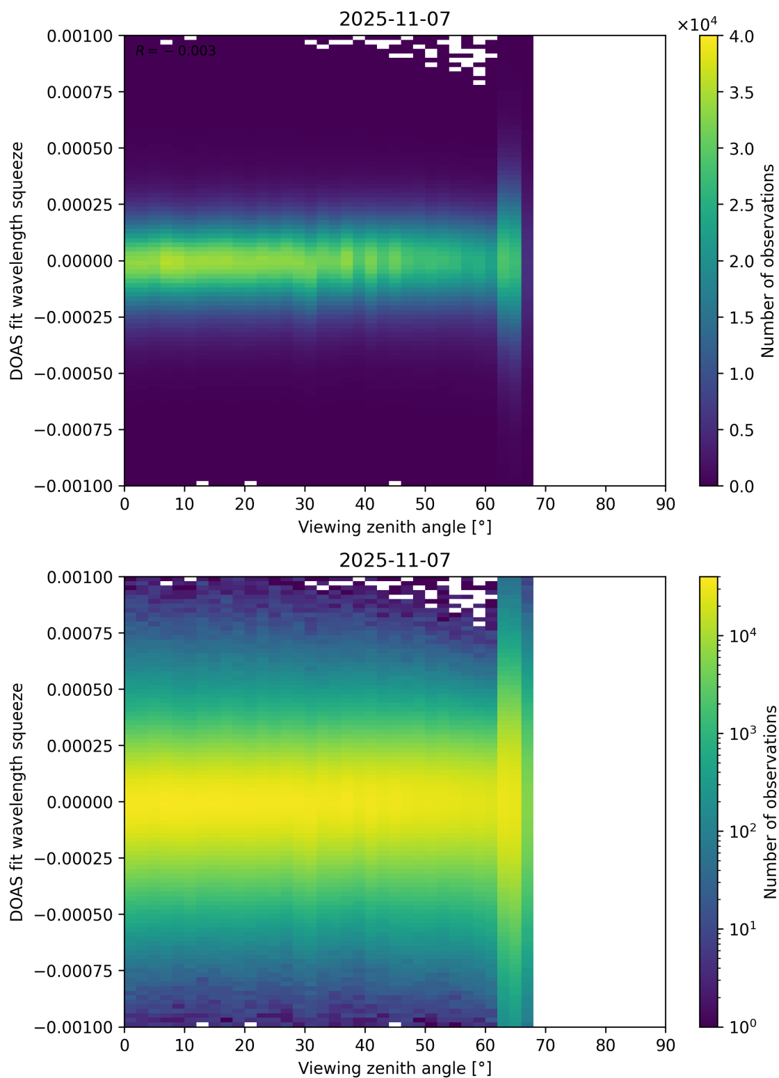
Figure 366: Scatter density plot of “Viewing zenith angle” against “DOAS fit wavelength squeeze” for 2025-11-07 to 2025-11-08.
