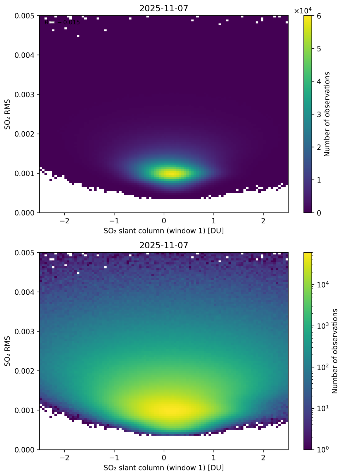
Figure 267: Scatter density plot of “SO 2 slant column (window 1)” against “SO 2 RMS” for 2025-11-07 to 2025-11-08.
