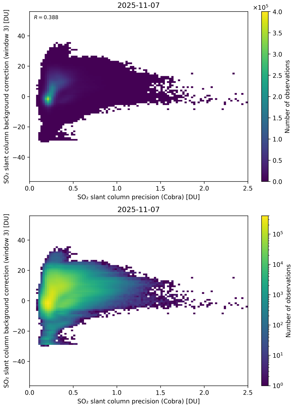
Figure 201: Scatter density plot of “SO 2 slant column precision (Cobra)” against “SO 2 slant column background correction (window 3)” for 2025-11-07 to 2025-11-08.
