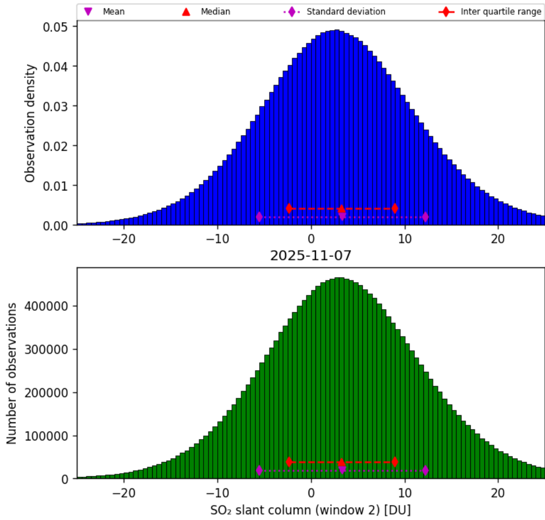
Figure 67: Histogram of “SO 2 slant column (window 2)” for 2025-11-07 to 2025-11-08
