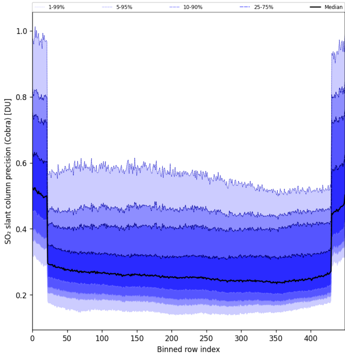
Figure 88: Along track statistics of “SO 2 slant column precision (Cobra)” for 2025-11-07 to 2025-11-08
