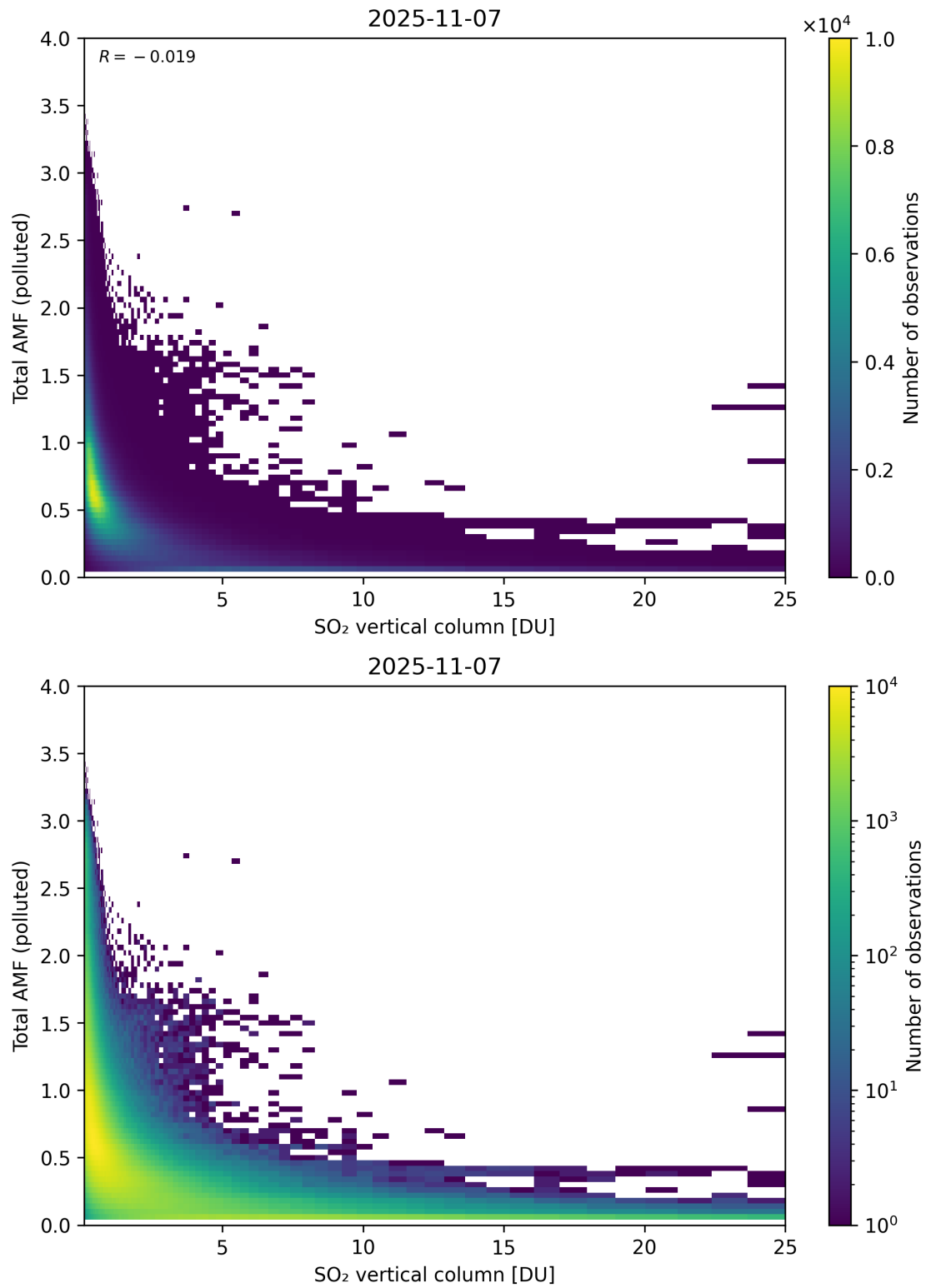
Figure 359: Scatter density plot of “SO 2 vertical column” against “Total AMF (polluted)” for 2025-11-07 to 2025-11-08.
