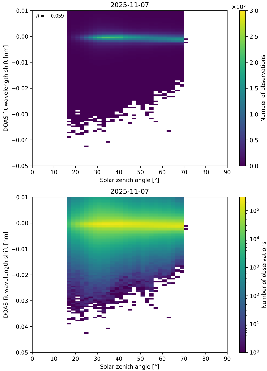
Figure 174: Scatter density plot of “Solar zenith angle” against “DOAS fit wavelength shift” for 2025-11-07 to 2025-11-08.
