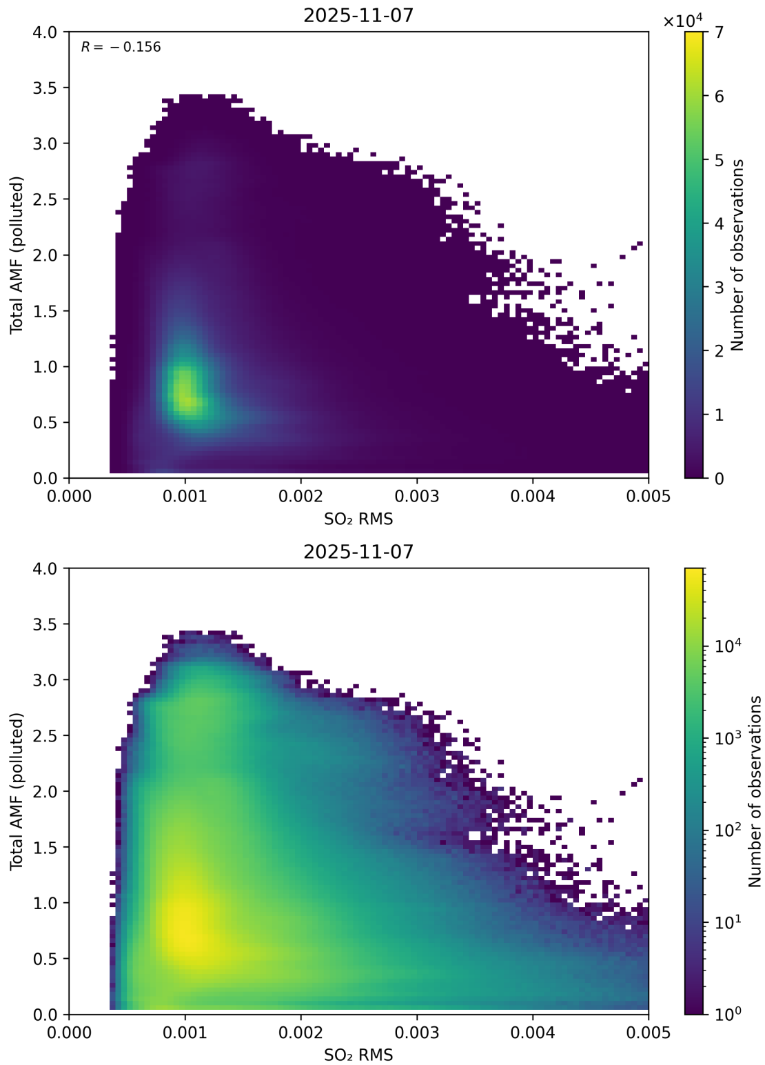
Figure 148: Scatter density plot of “SO 2 RMS” against “Total AMF (polluted)” for 2025-11-07 to 2025-11-08.
