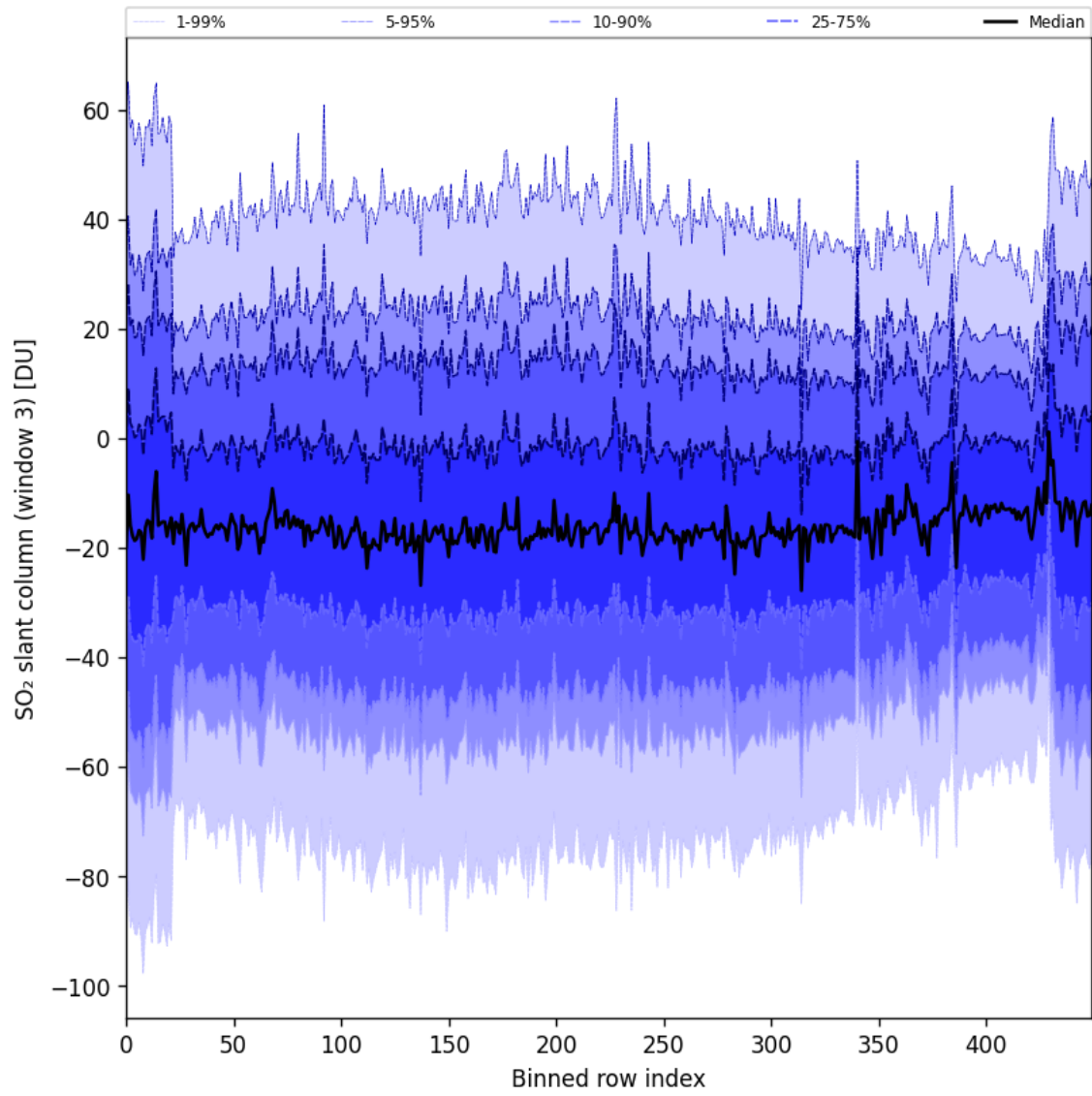
Figure 97: Along track statistics of “SO 2 slant column (window 3)” for 2025-11-07 to 2025-11-08
