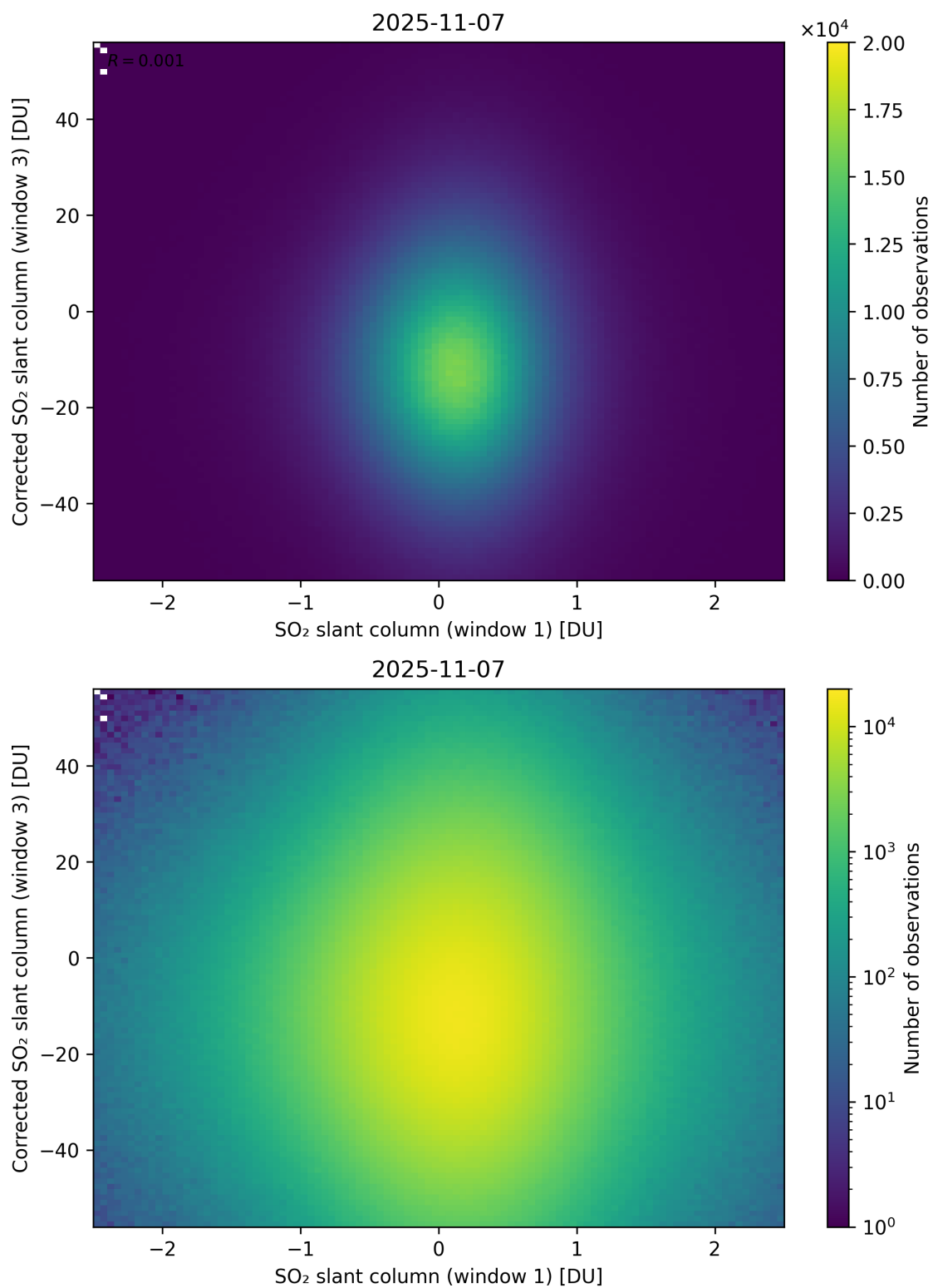
Figure 284: Scatter density plot of “SO 2 slant column (window 1)” against “Corrected SO 2 slant column (window 3)” for 2025-11-07 to 2025-11-08.
