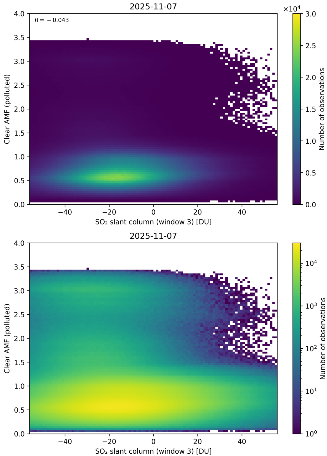
Figure 315: Scatter density plot of “SO 2 slant column (window 3)” against “Clear AMF (polluted)” for 2025-11-07 to 2025-11-08.
