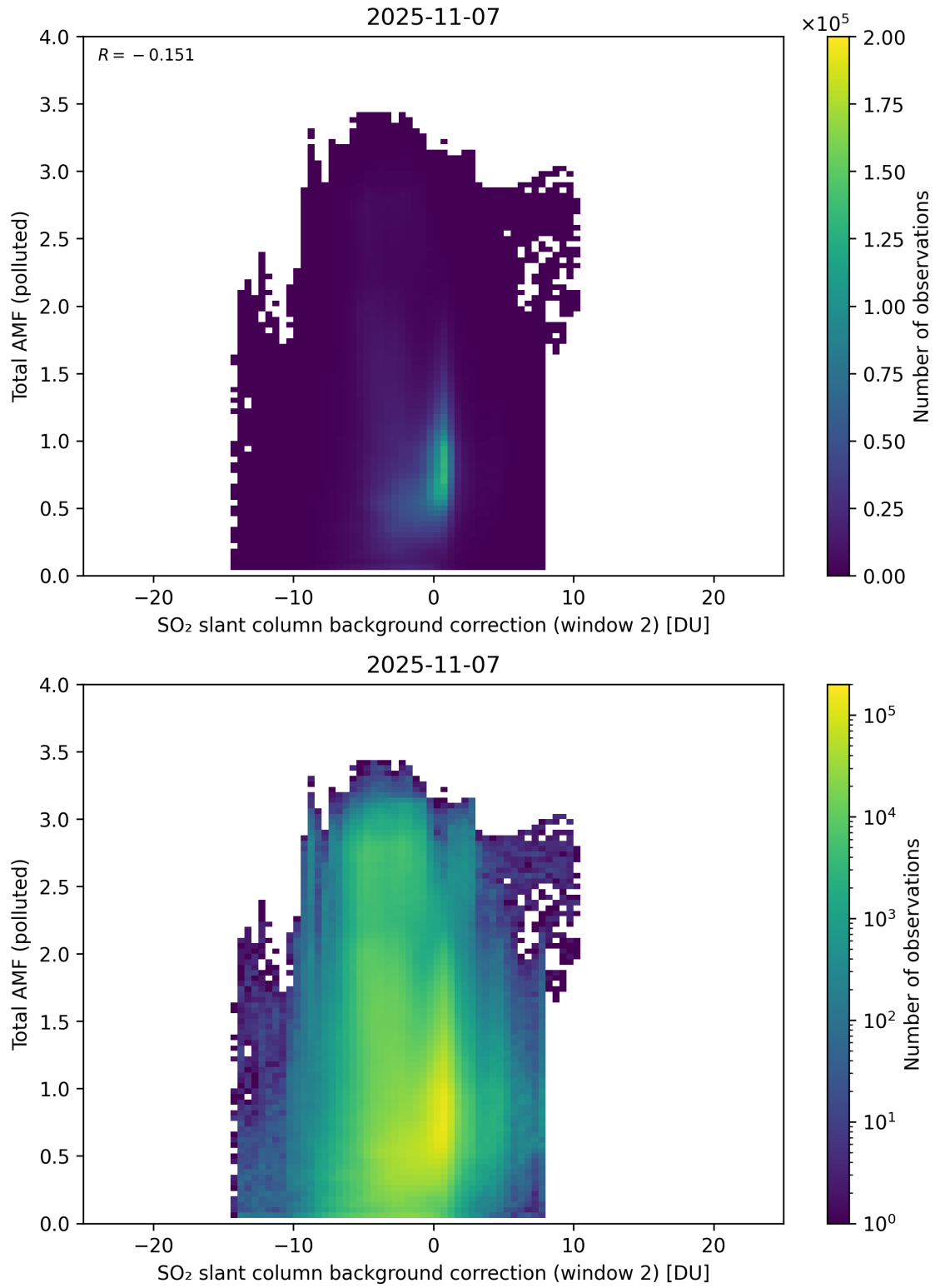
Figure 130: Scatter density plot of “SO 2 slant column background correction (window 2)” against “Total AMF (polluted)” for 2025-11-07 to 2025-11-08.
