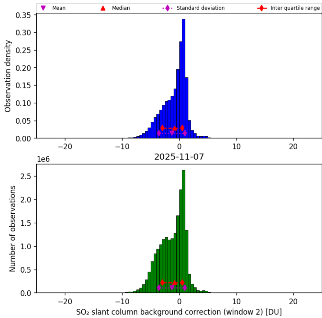
Figure 70: Histogram of “SO 2 slant column background correction (window 2)” for 2025-11-07 to 2025-11-08
