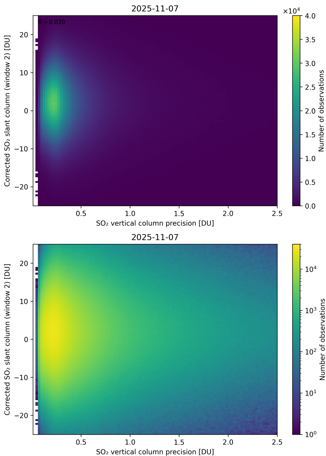
Figure 339: Scatter density plot of “SO 2 vertical column precision” against “Corrected SO 2 slant column (window 2)” for 2025-11-07 to 2025-11-08.
