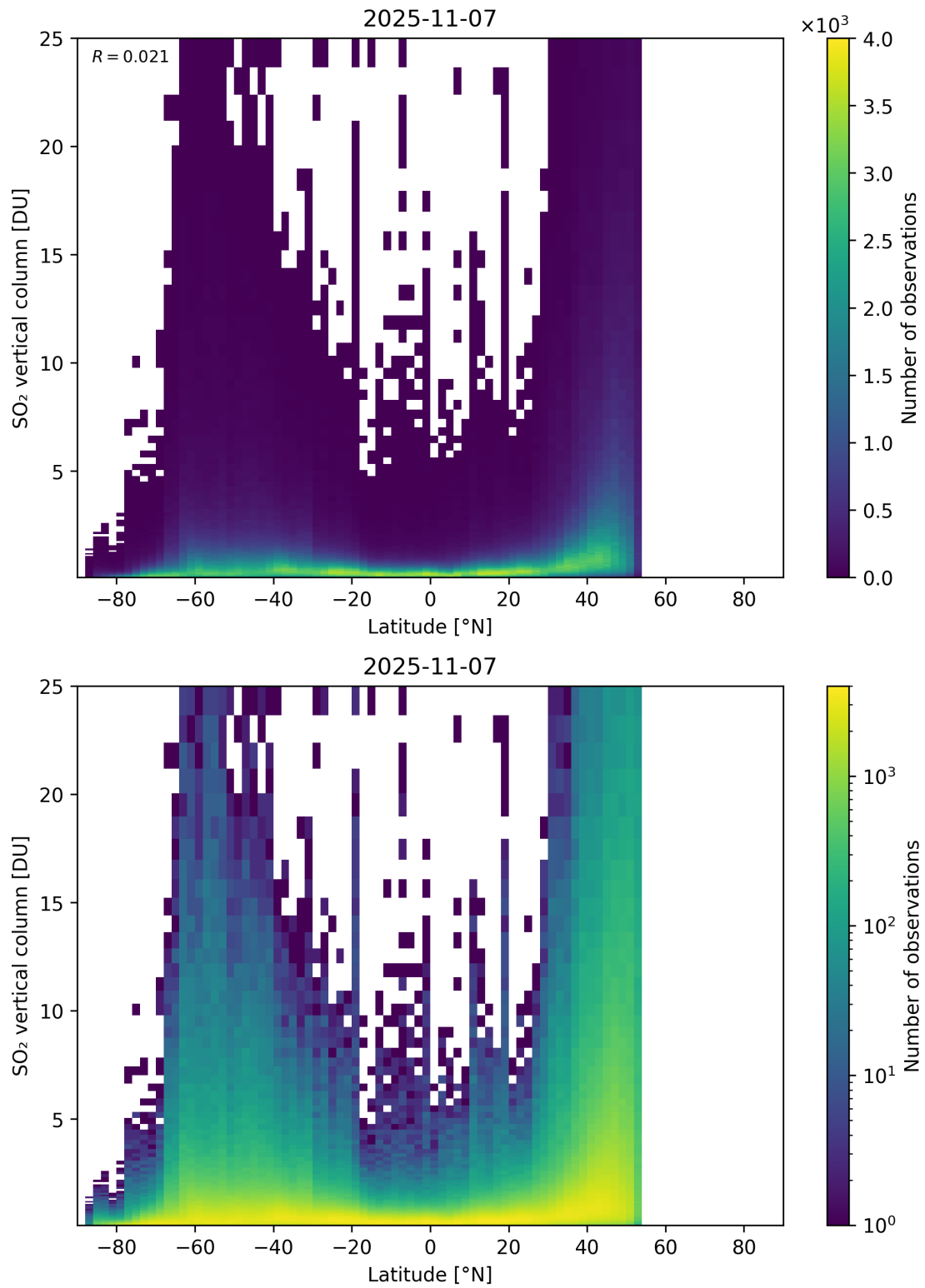
Figure 169: Scatter density plot of “Latitude” against “SO 2 vertical column” for 2025-11-07 to 2025-11-08.
