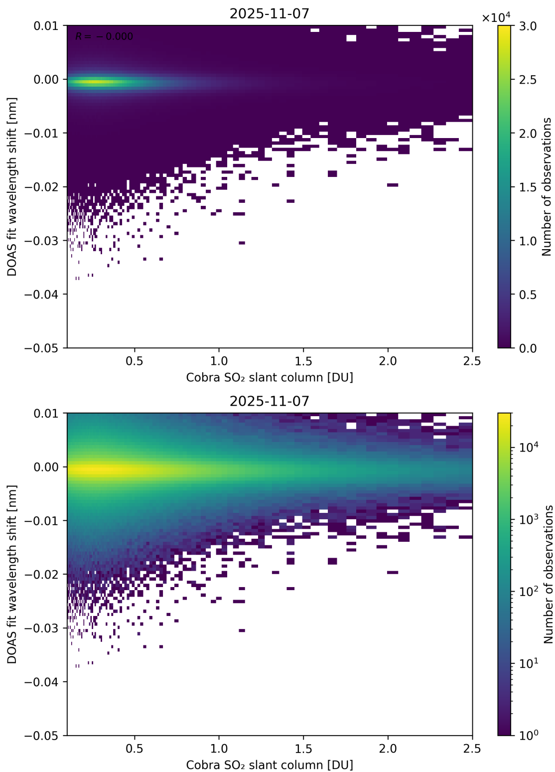
Figure 196: Scatter density plot of “Cobra SO 2 slant column” against “DOAS fit wavelength shift” for 2025-11-07 to 2025-11-08.
