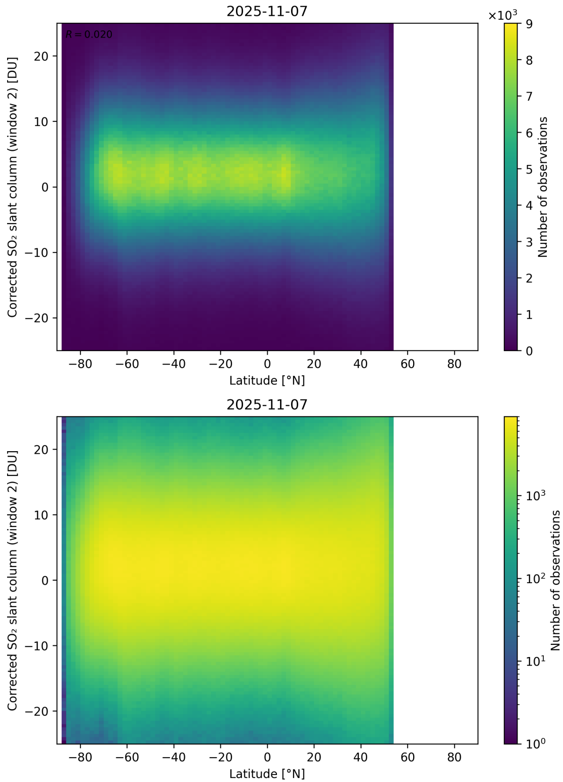
Figure 160: Scatter density plot of “Latitude” against “Corrected SO 2 slant column (window 2)” for 2025-11-07 to 2025-11-08.
