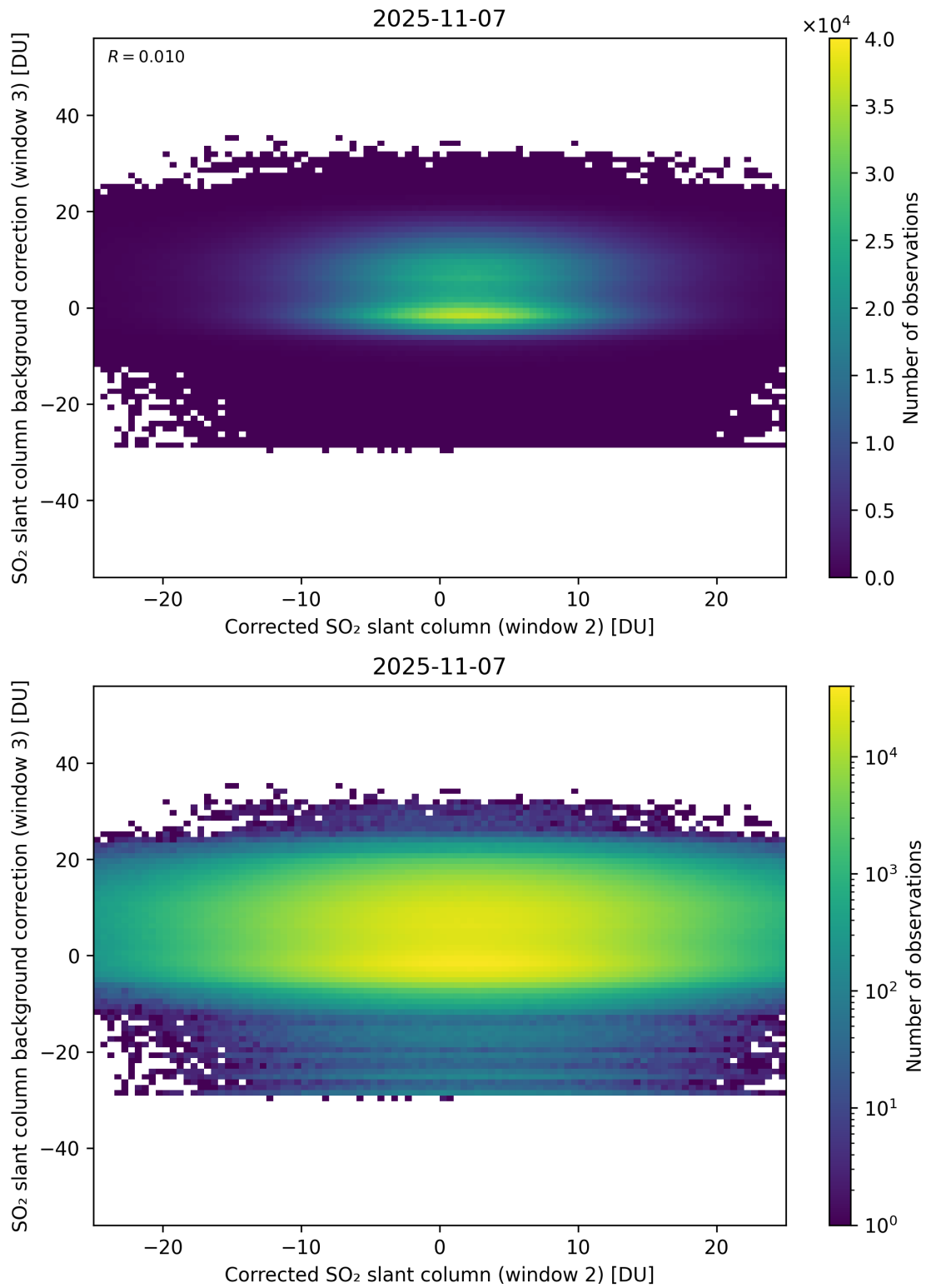
Figure 245: Scatter density plot of “Corrected SO 2 slant column (window 2)” against “SO 2 slant column background correction (window 3)” for 2025-11-07 to 2025-11-08.
