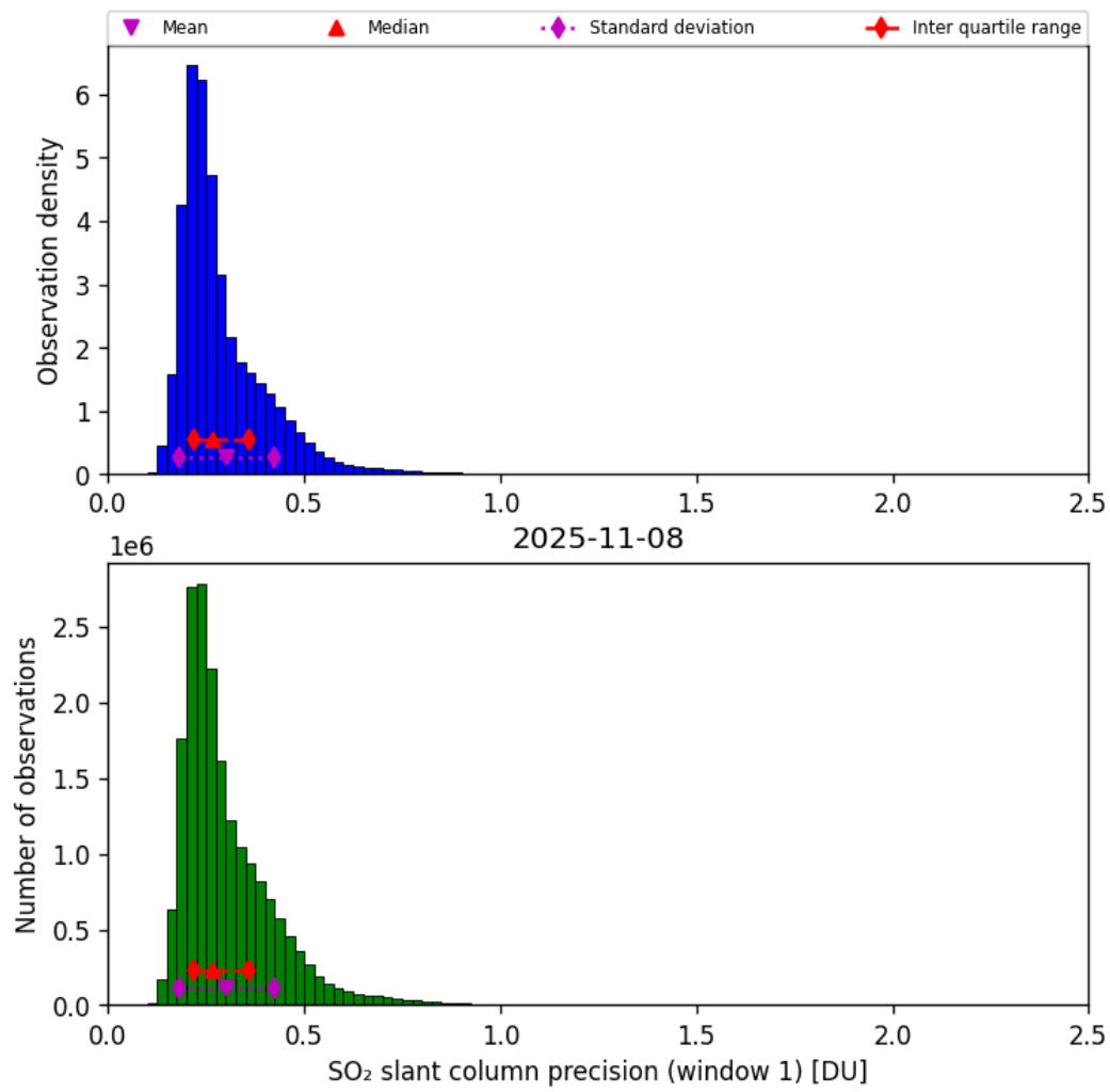
Figure 64: Histogram of “SO 2 slant column precision (window 1)” for 2025-11-07 to 2025-11-09
