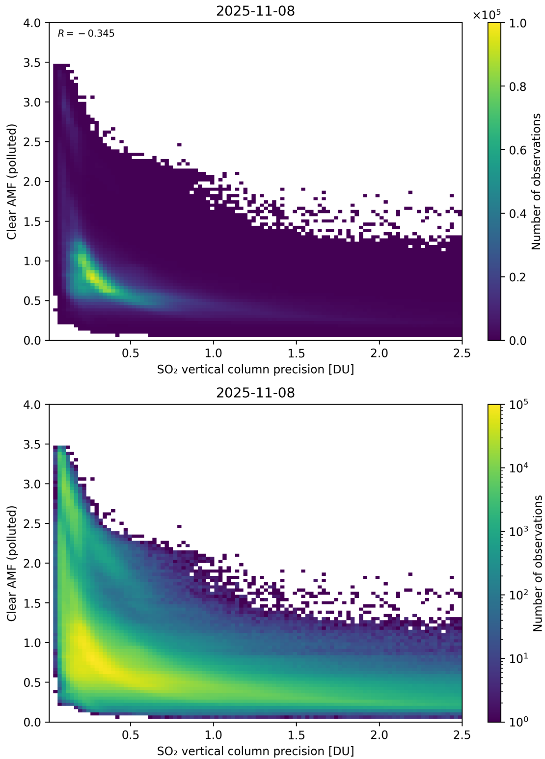
Figure 335: Scatter density plot of “SO 2 vertical column precision” against “Clear AMF (polluted)” for 2025-11-07 to 2025-11-09.
