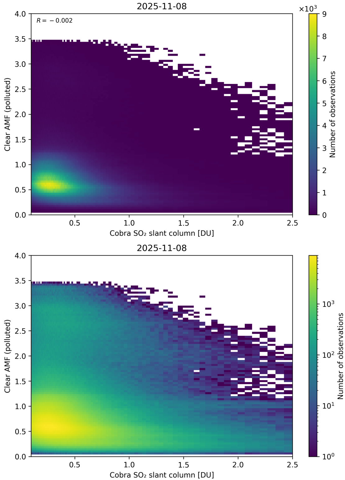
Figure 215: Scatter density plot of “Cobra SO 2 slant column” against “Clear AMF (polluted)” for 2025-11-07 to 2025-11-09.
