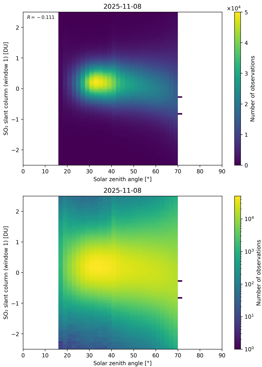
Figure 184: Scatter density plot of “Solar zenith angle” against “SO 2 slant column (window 1)” for 2025-11-07 to 2025-11-09.
