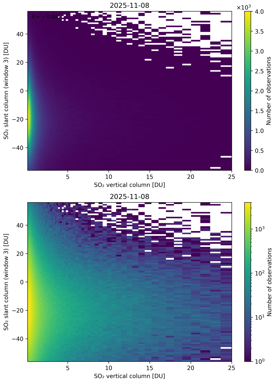
Figure 357: Scatter density plot of “SO 2 vertical column” against “SO 2 slant column (window 3)” for 2025-11-07 to 2025-11-09.
