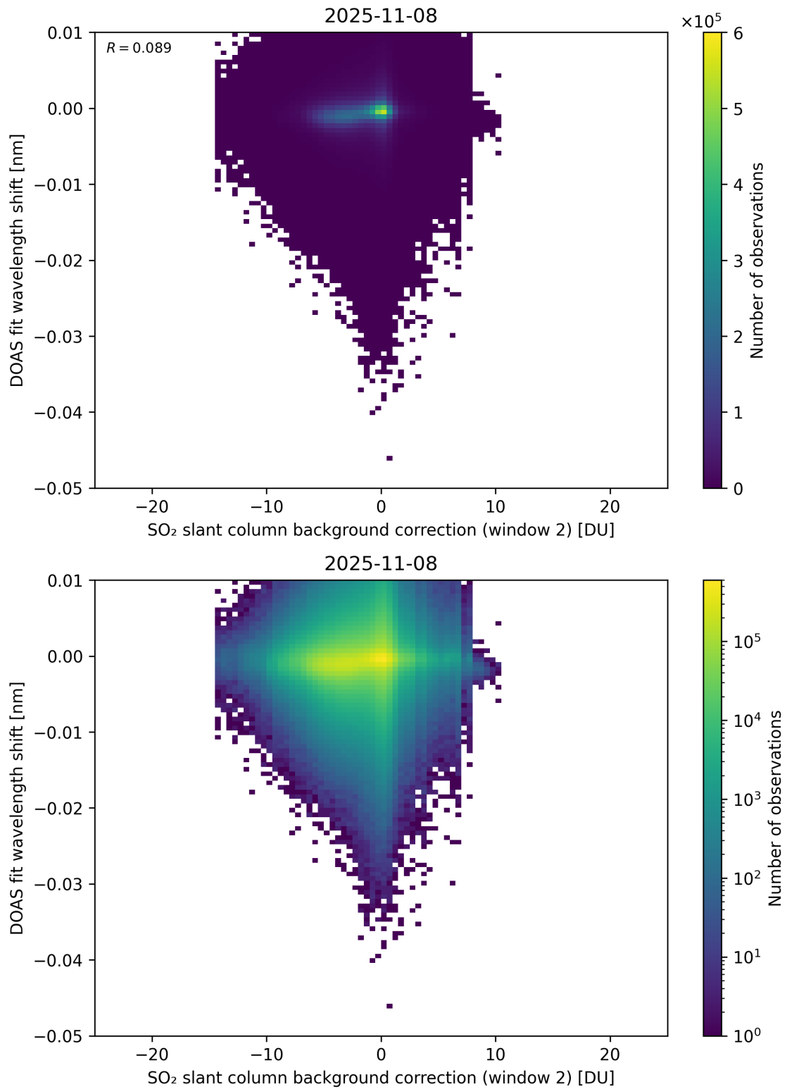
Figure 123: Scatter density plot of “SO 2 slant column background correction (window 2)” against “DOAS fit wavelength shift” for 2025-11-07 to 2025-11-09.
