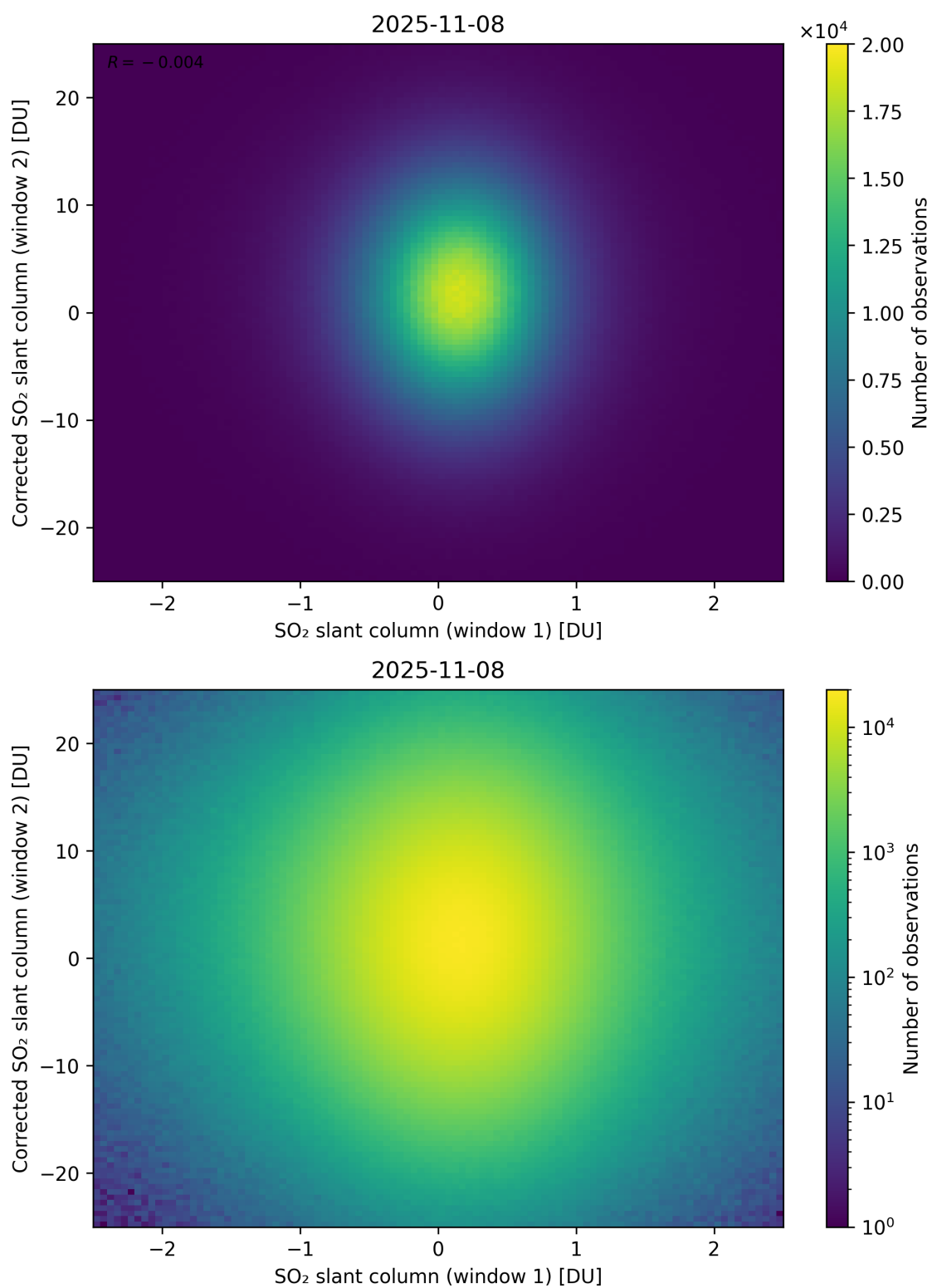
Figure 283: Scatter density plot of “SO 2 slant column (window 1)” against “Corrected SO 2 slant column (window 2)” for 2025-11-07 to 2025-11-09.
