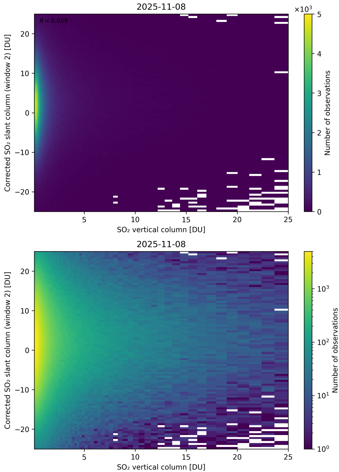
Figure 352: Scatter density plot of “SO 2 vertical column” against “Corrected SO 2 slant column (window 2)” for 2025-11-07 to 2025-11-09.
