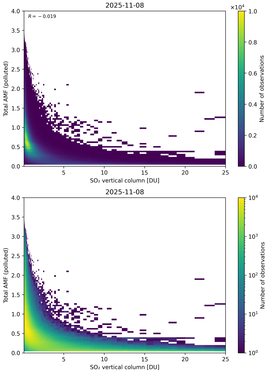
Figure 359: Scatter density plot of “SO 2 vertical column” against “Total AMF (polluted)” for 2025-11-07 to 2025-11-09.
