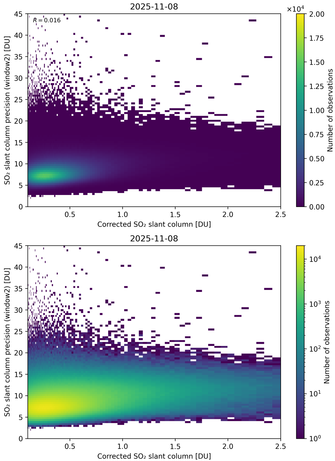
Figure 239: Scatter density plot of “Corrected SO 2 slant column” against “SO 2 slant column precision (window2)” for 2025-11-07 to 2025-11-09.
