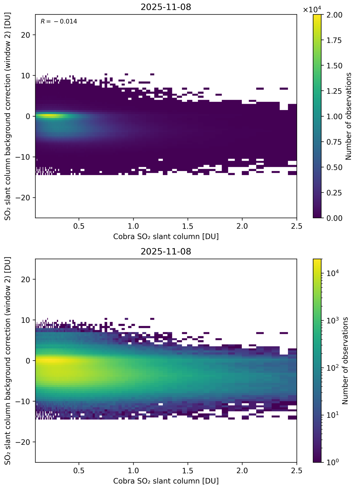
Figure 194: Scatter density plot of “Cobra SO 2 slant column” against “SO 2 slant column background correction (window 2)” for 2025-11-07 to 2025-11-09.
