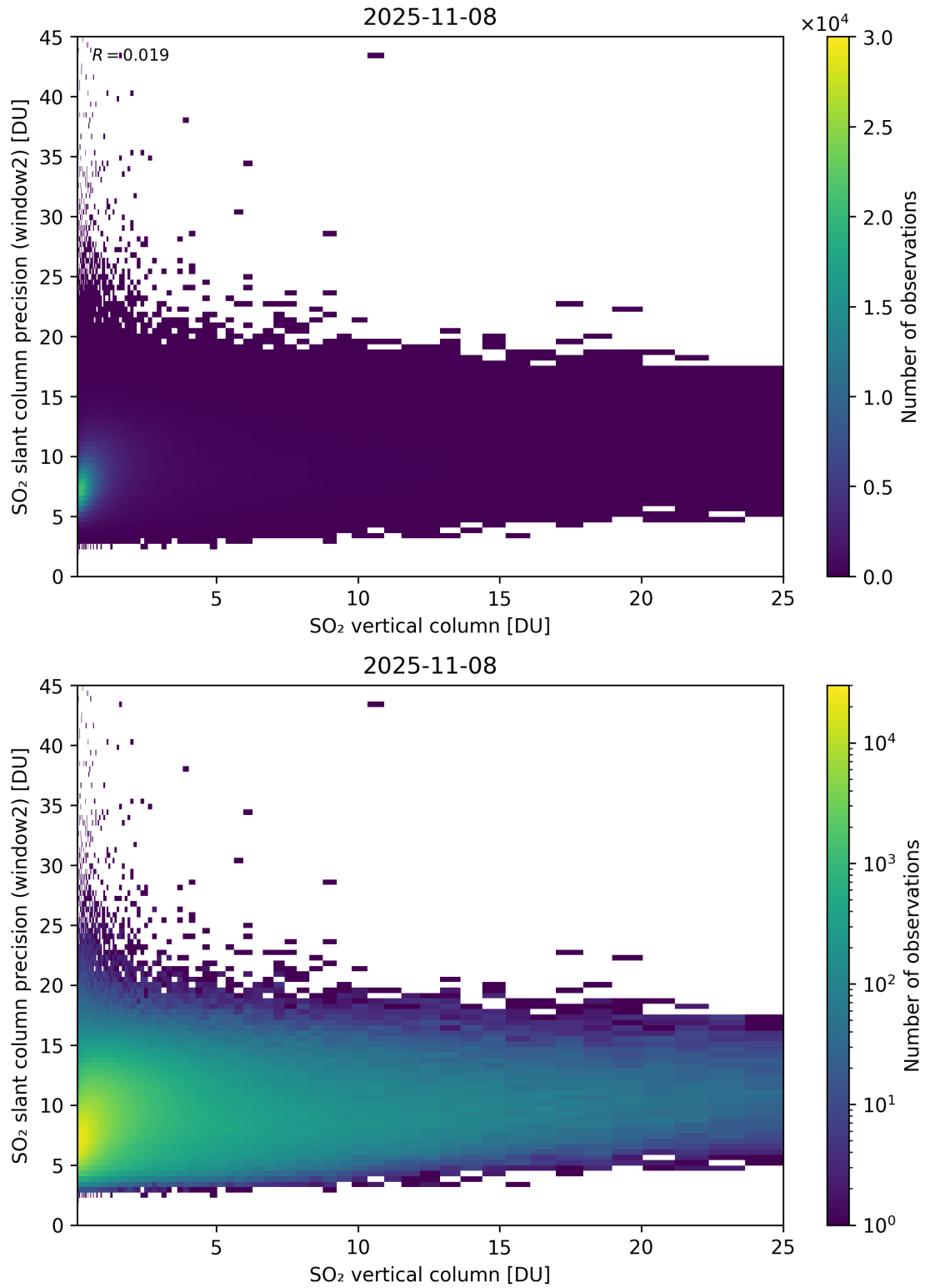
Figure 356: Scatter density plot of “SO 2 vertical column” against “SO 2 slant column precision (window2)” for 2025-11-07 to 2025-11-09.
