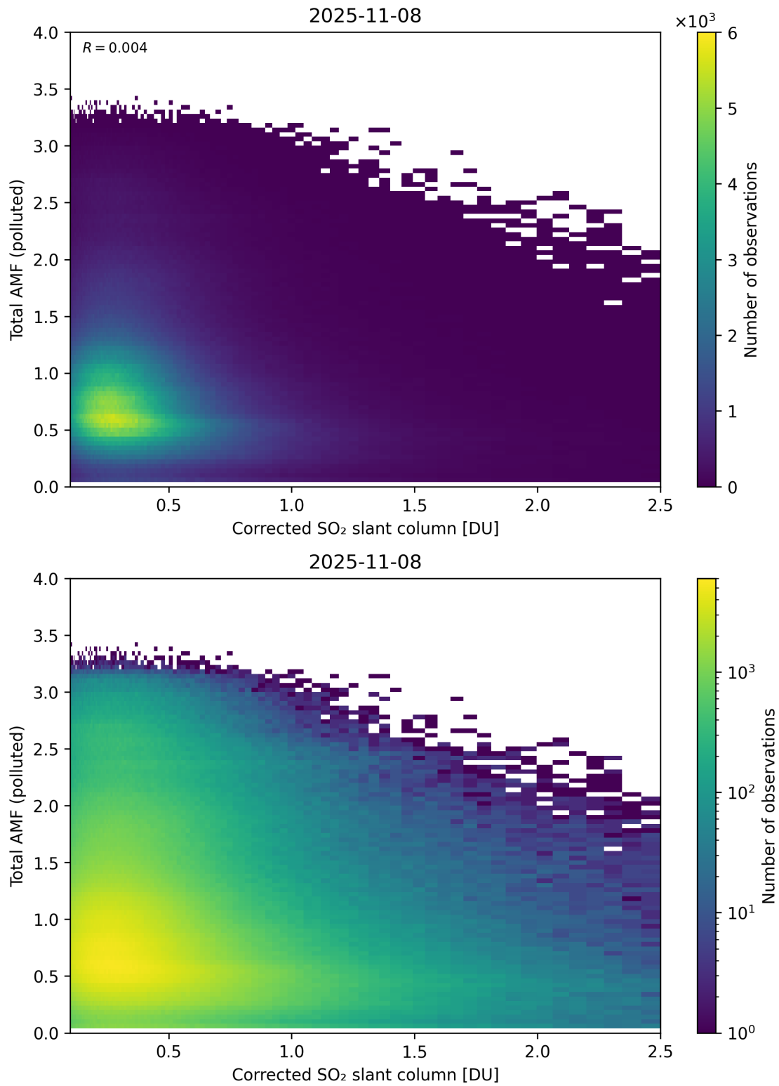
Figure 242: Scatter density plot of “Corrected SO 2 slant column” against “Total AMF (polluted)” for 2025-11-07 to 2025-11-09.
