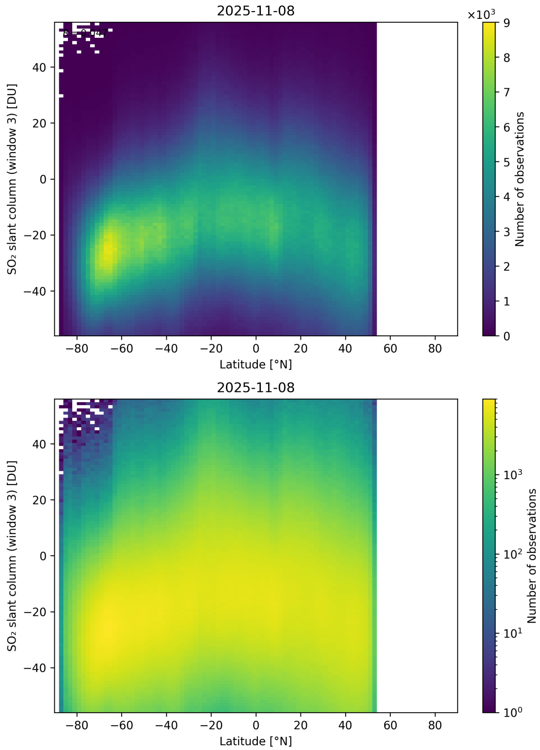
Figure 165: Scatter density plot of “Latitude” against “SO 2 slant column (window 3)” for 2025-11-07 to 2025-11-09.
