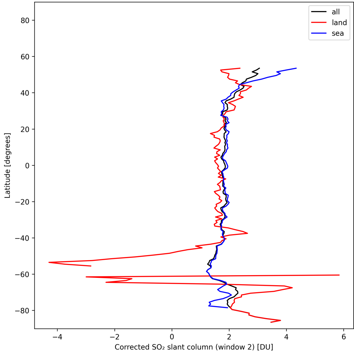
Figure 43: Zonal average of “Corrected SO 2 slant column (window 2)” for 2025-11-07 to 2025-11-09.
