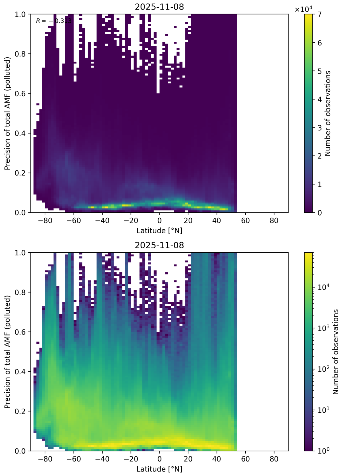
Figure 168: Scatter density plot of “Latitude” against “Precision of total AMF (polluted)” for 2025-11-07 to 2025-11-09.
