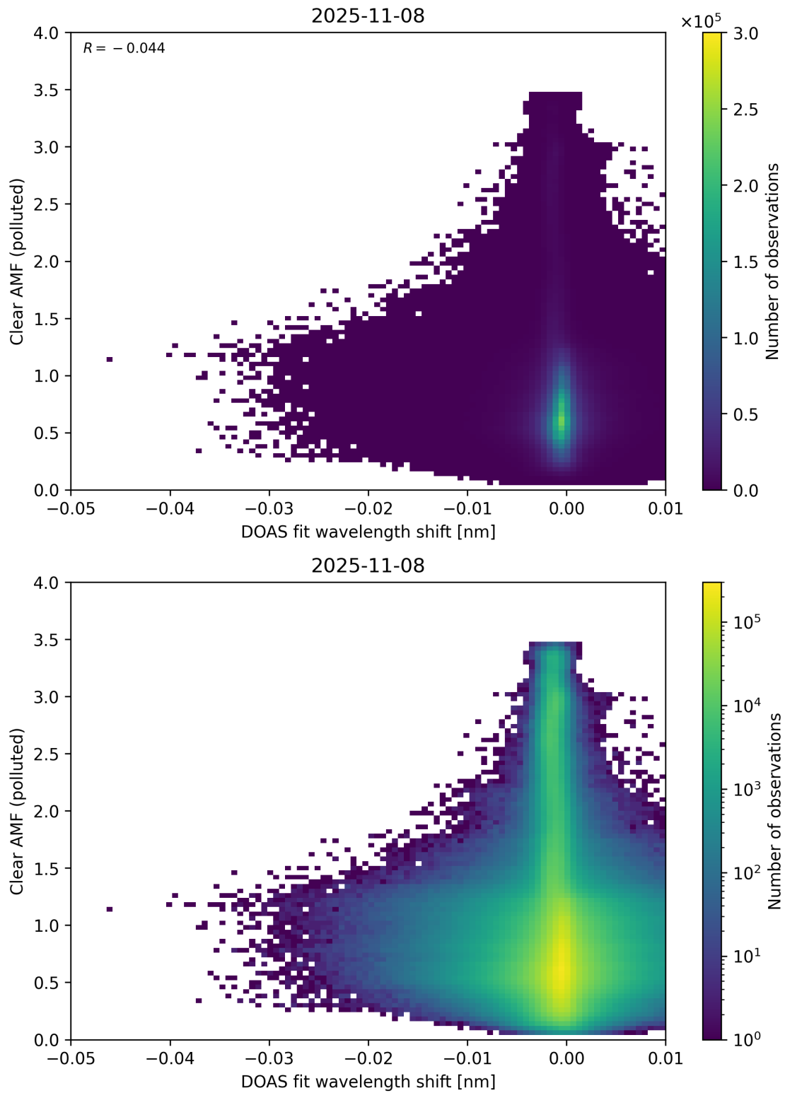
Figure 140: Scatter density plot of “DOAS fit wavelength shift” against “Clear AMF (polluted)” for 2025-11-07 to 2025-11-09.
