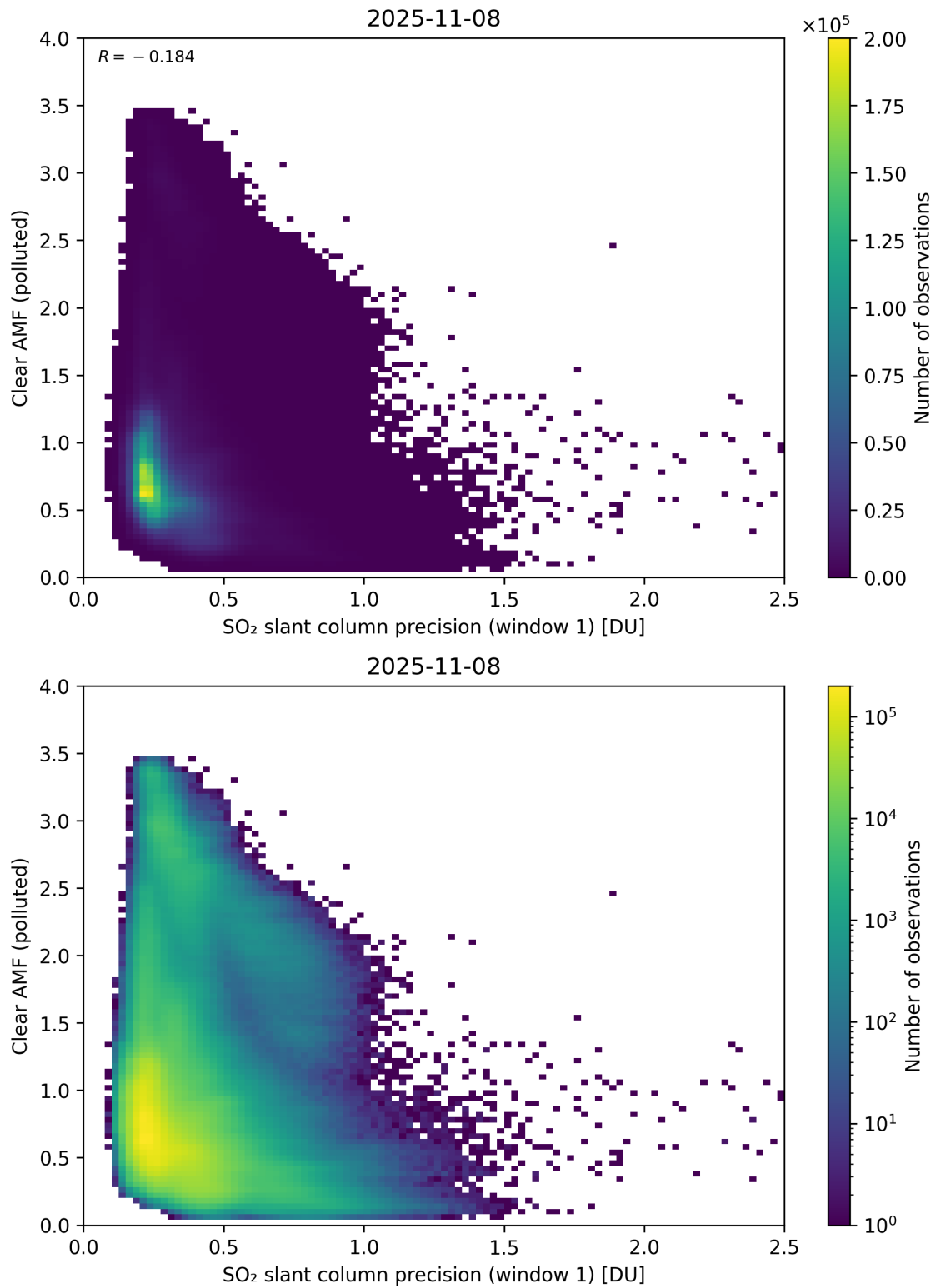
Figure 274: Scatter density plot of “SO 2 slant column precision (window 1)” against “Clear AMF (polluted)” for 2025-11-07 to 2025-11-09.
