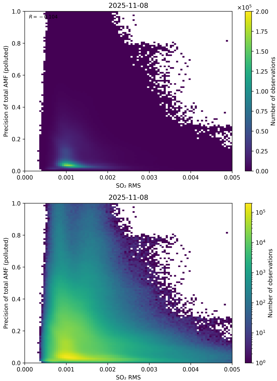
Figure 149: Scatter density plot of “SO 2 RMS” against “Precision of total AMF (polluted)” for 2025-11-07 to 2025-11-09.
