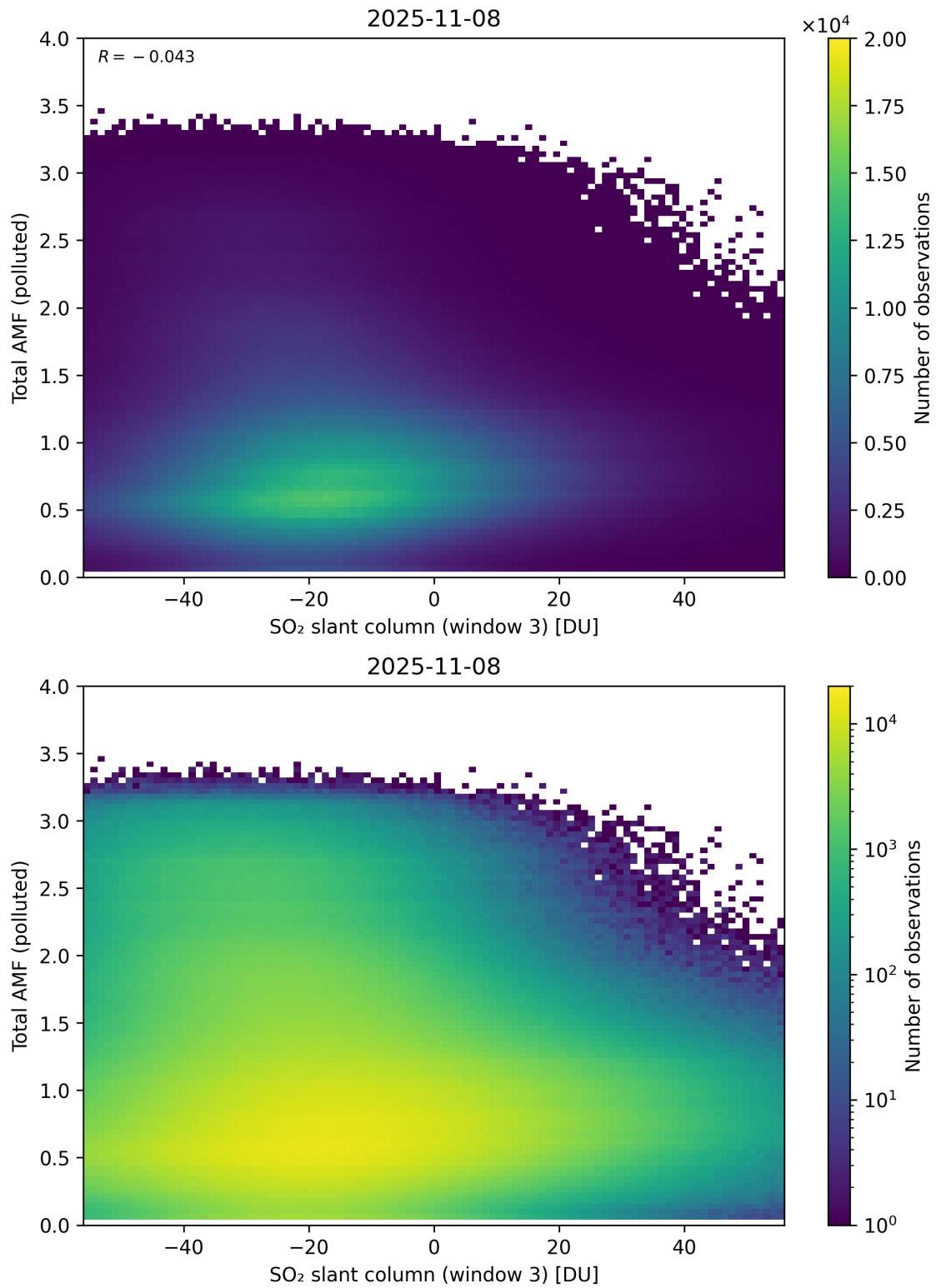
Figure 318: Scatter density plot of “SO 2 slant column (window 3)” against “Total AMF (polluted)” for 2025-11-07 to 2025-11-09.
