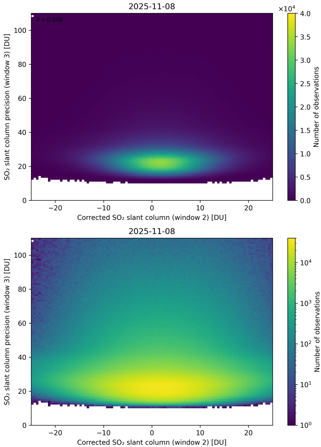
Figure 252: Scatter density plot of “Corrected SO 2 slant column (window 2)” against “SO 2 slant column precision (window 3)” for 2025-11-07 to 2025-11-09.
