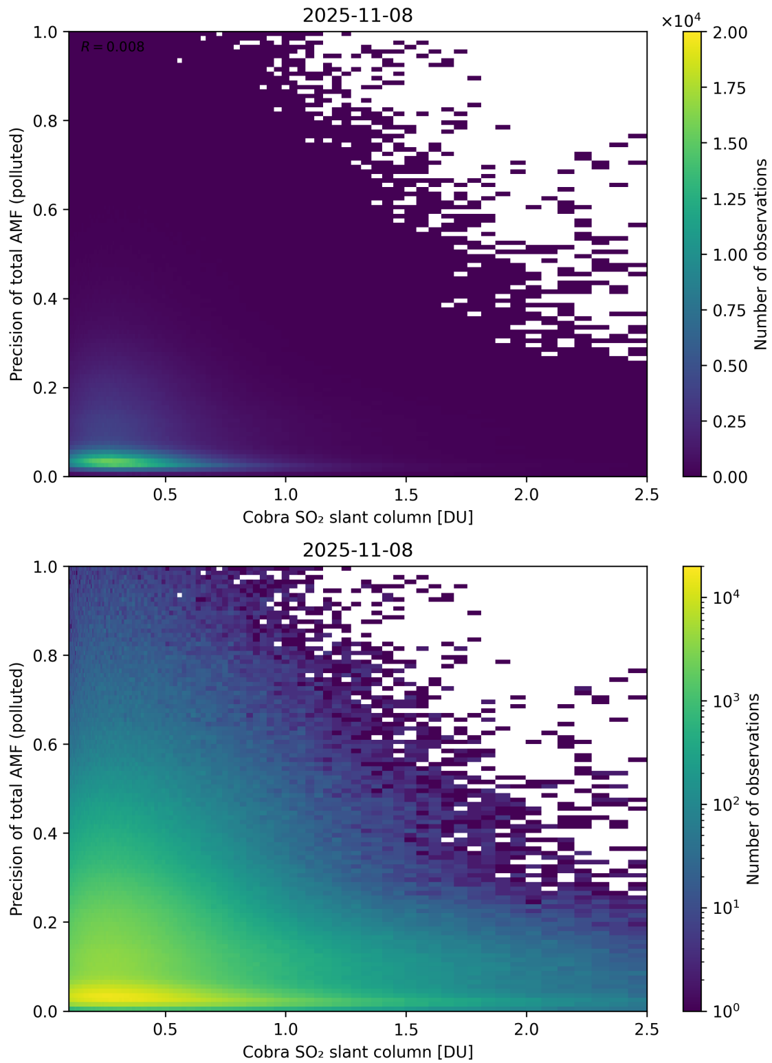
Figure 225: Scatter density plot of “Cobra SO 2 slant column” against “Precision of total AMF (polluted)” for 2025-11-07 to 2025-11-09.
