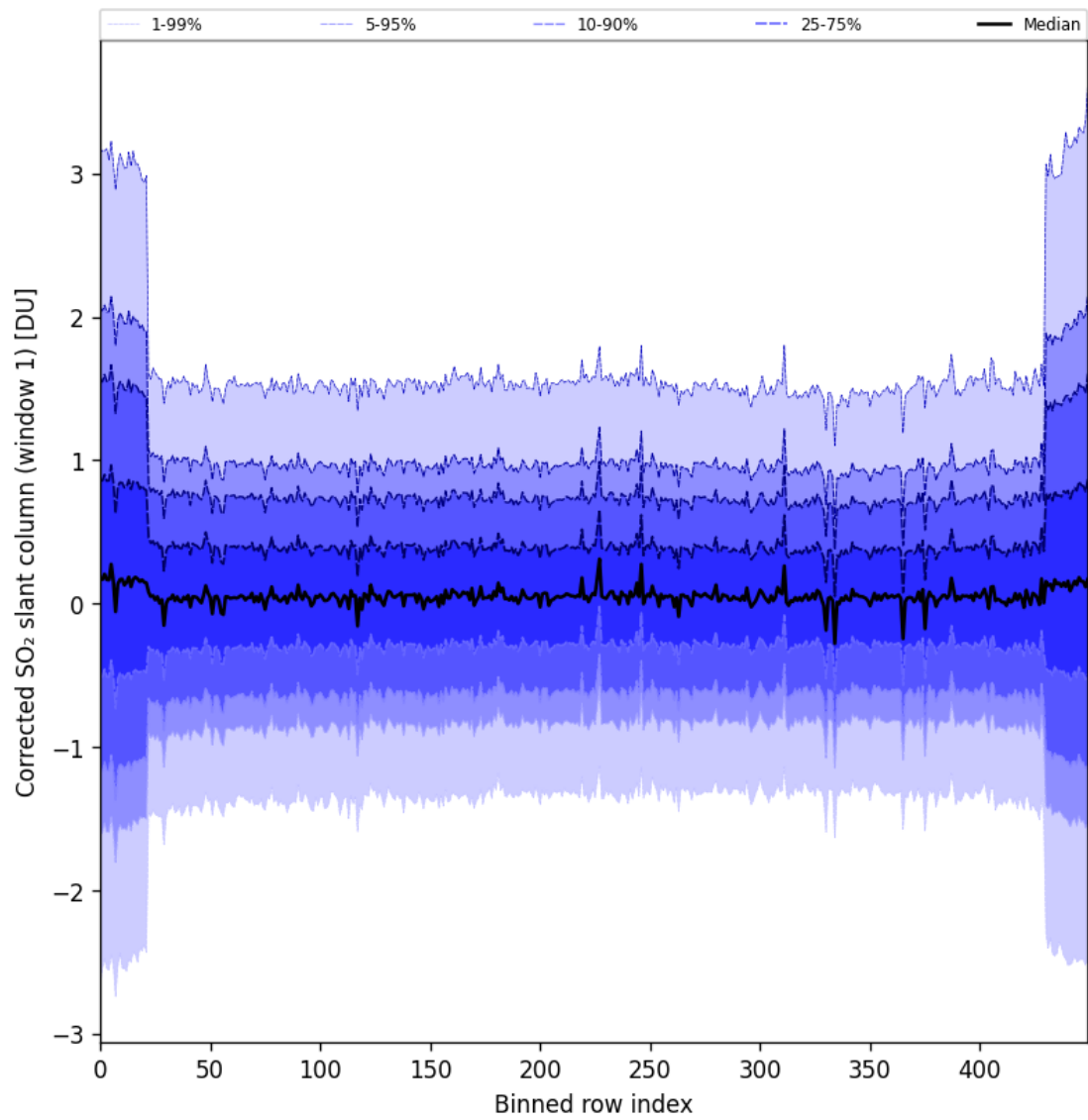
Figure 91: Along track statistics of “Corrected SO 2 slant column (window 1)” for 2025-11-07 to 2025-11-09
