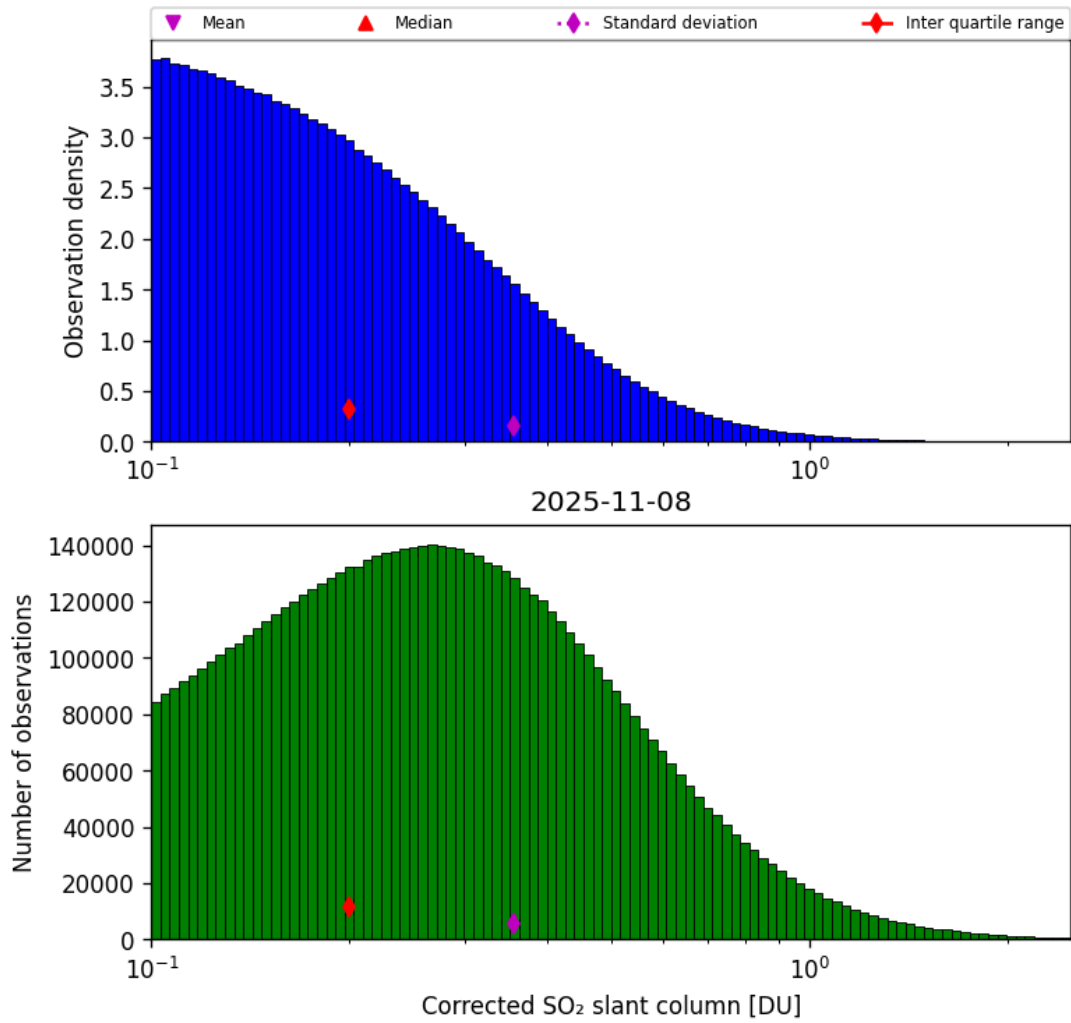
Figure 60: Histogram of “Corrected SO 2 slant column” for 2025-11-07 to 2025-11-09
