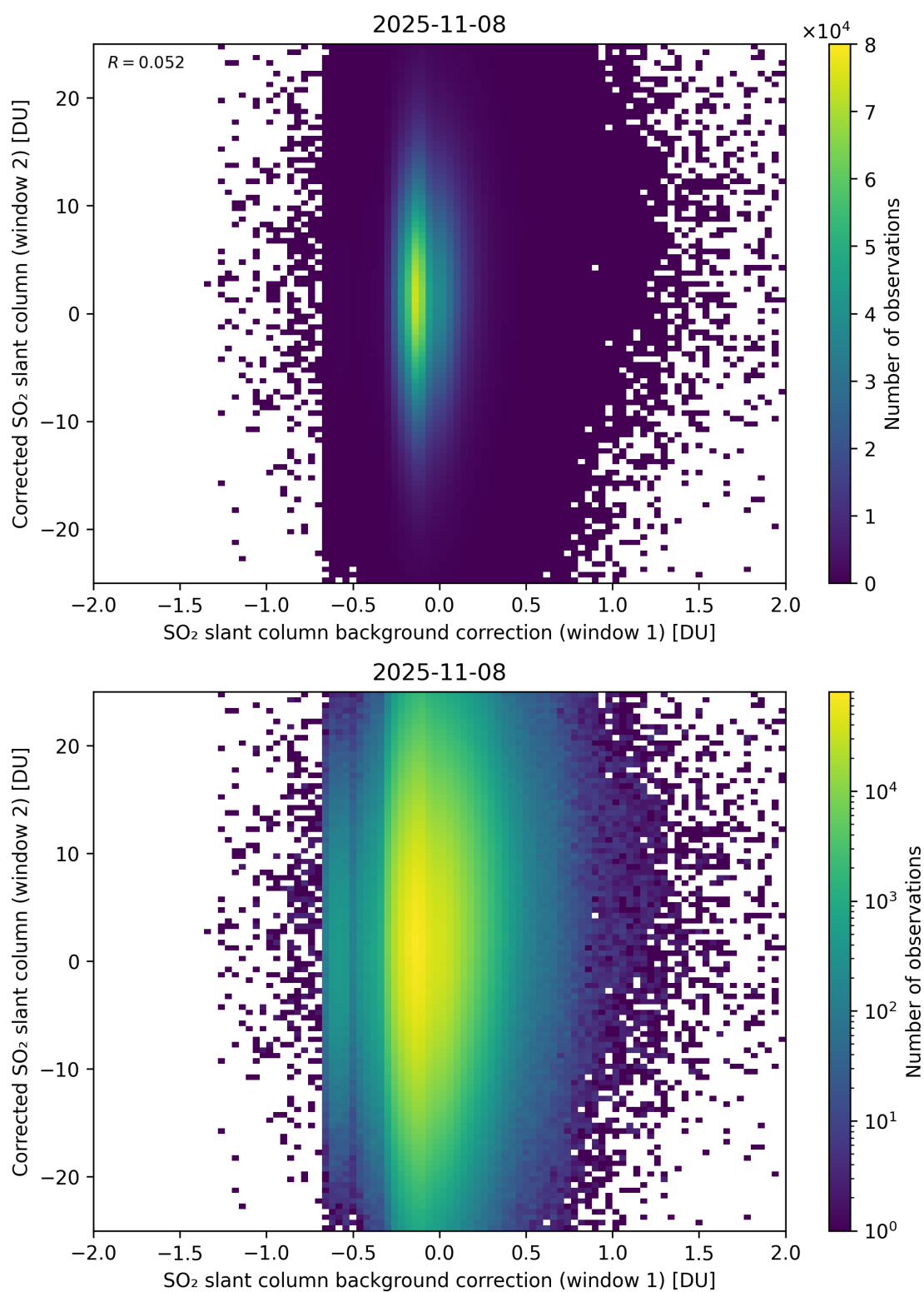
Figure 115: Scatter density plot of “SO 2 slant column background correction (window 1)” against “Corrected SO 2 slant column (window 2)” for 2025-11-07 to 2025-11-09.
