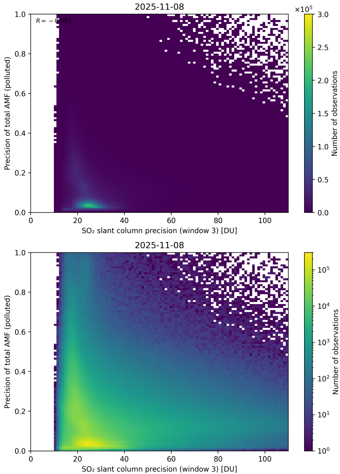
Figure 314: Scatter density plot of “SO 2 slant column precision (window 3)” against “Precision of total AMF (polluted)” for 2025-11-07 to 2025-11-09.
