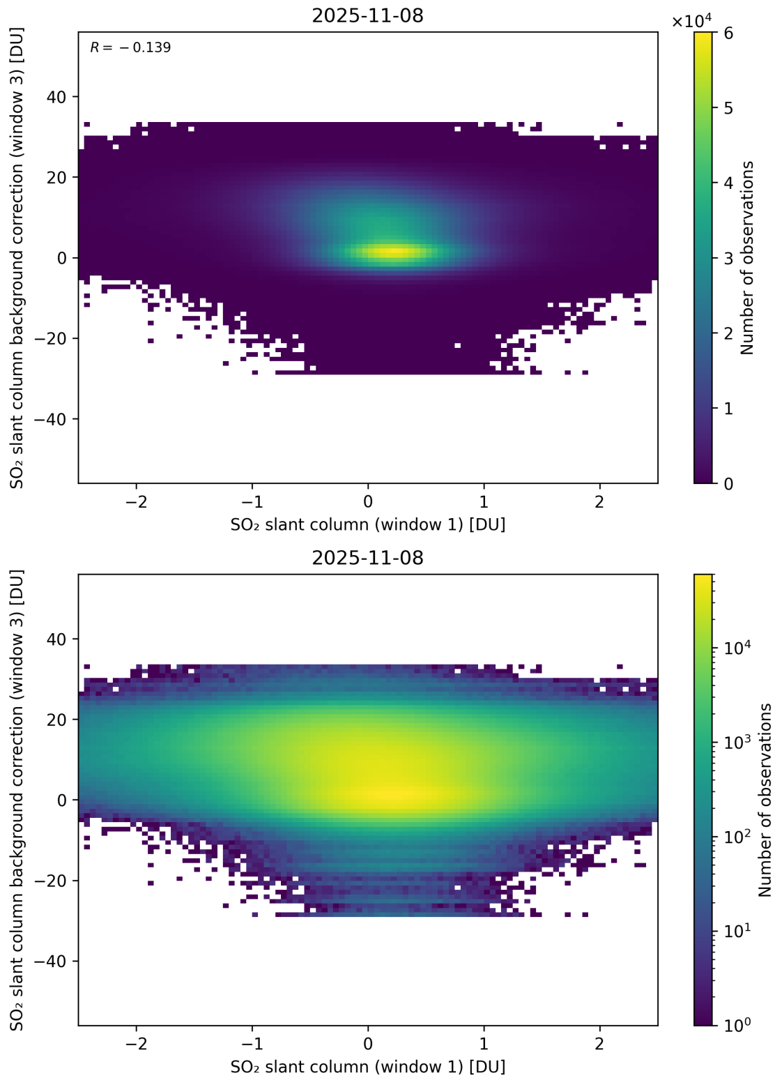
Figure 264: Scatter density plot of “SO 2 slant column (window 1)” against “SO 2 slant column background correction (window 3)” for 2025-11-07 to 2025-11-09.
