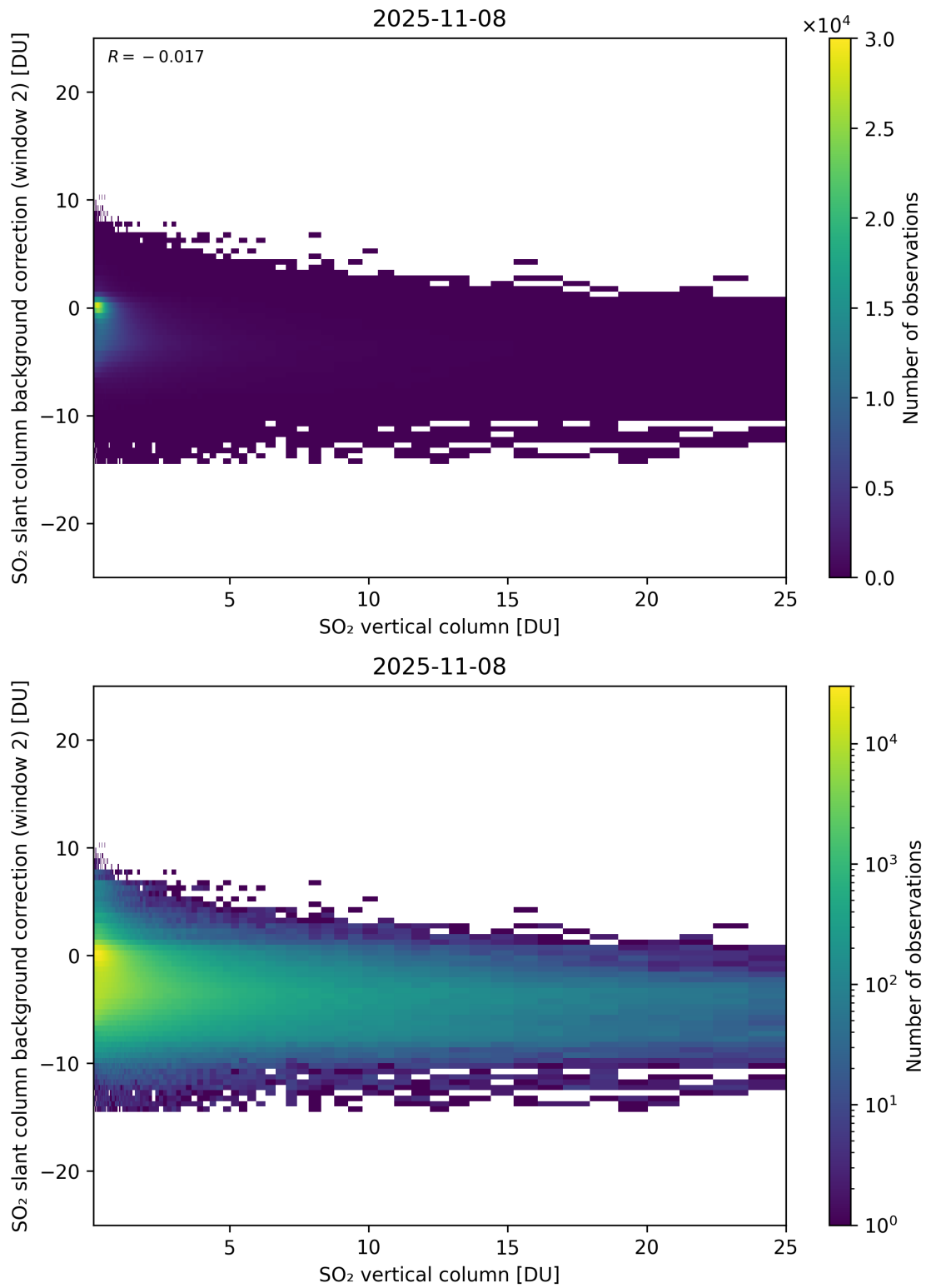
Figure 324: Scatter density plot of “SO 2 vertical column” against “SO 2 slant column background correction (window 2)” for 2025-11-07 to 2025-11-09.
