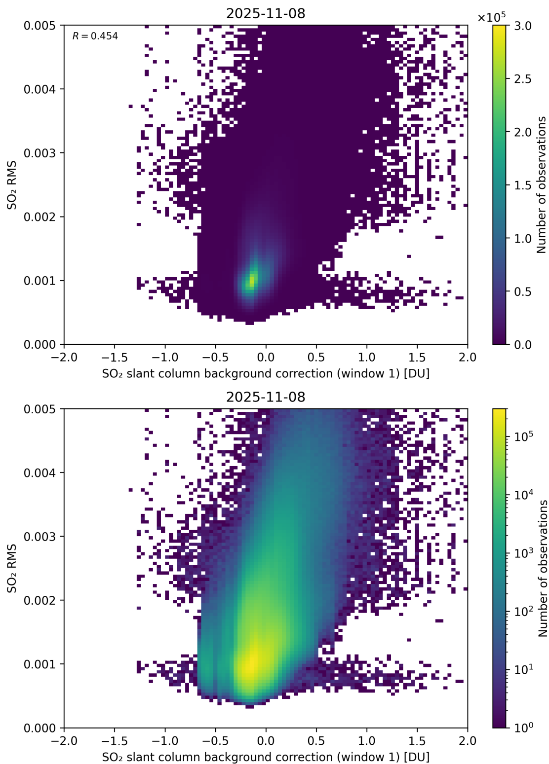
Figure 113: Scatter density plot of “SO 2 slant column background correction (window 1)” against “SO 2 RMS” for 2025-11-07 to 2025-11-09.
