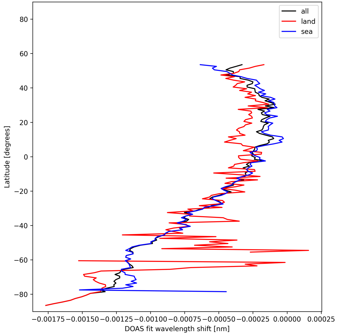
Figure 50: Zonal average of "DOAS fit wavelength shift" for 2025-11-07 to 2025-11-09.
