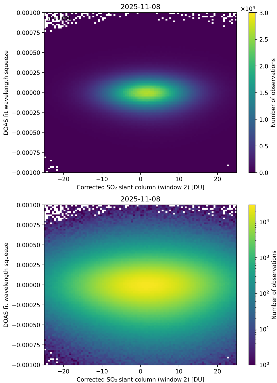
Figure 247: Scatter density plot of “Corrected SO 2 slant column (window 2)” against “DOAS fit wavelength squeeze” for 2025-11-07 to 2025-11-09.
