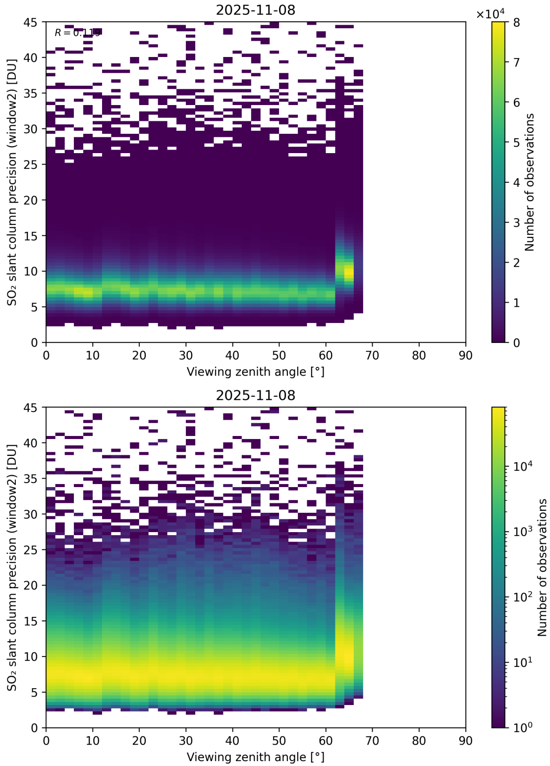
Figure 378: Scatter density plot of “Viewing zenith angle” against “SO 2 slant column precision (window2)” for 2025-11-07 to 2025-11-09.
