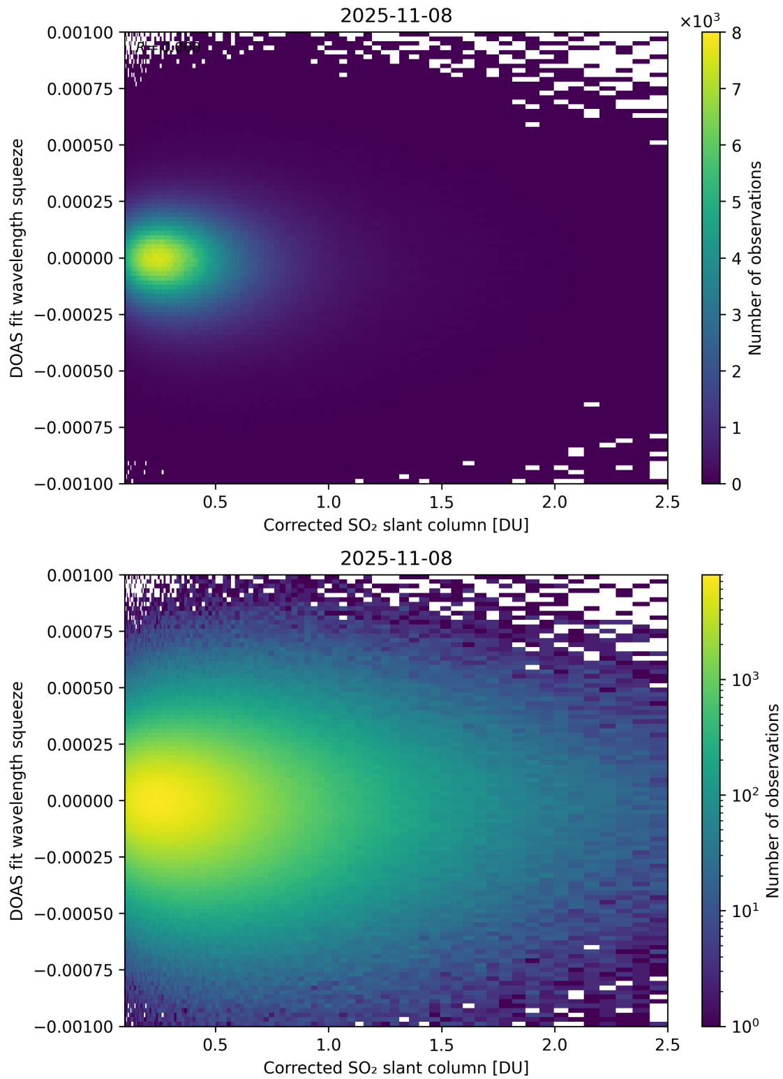
Figure 230: Scatter density plot of “Corrected SO 2 slant column” against “DOAS fit wavelength squeeze” for 2025-11-07 to 2025-11-09.
