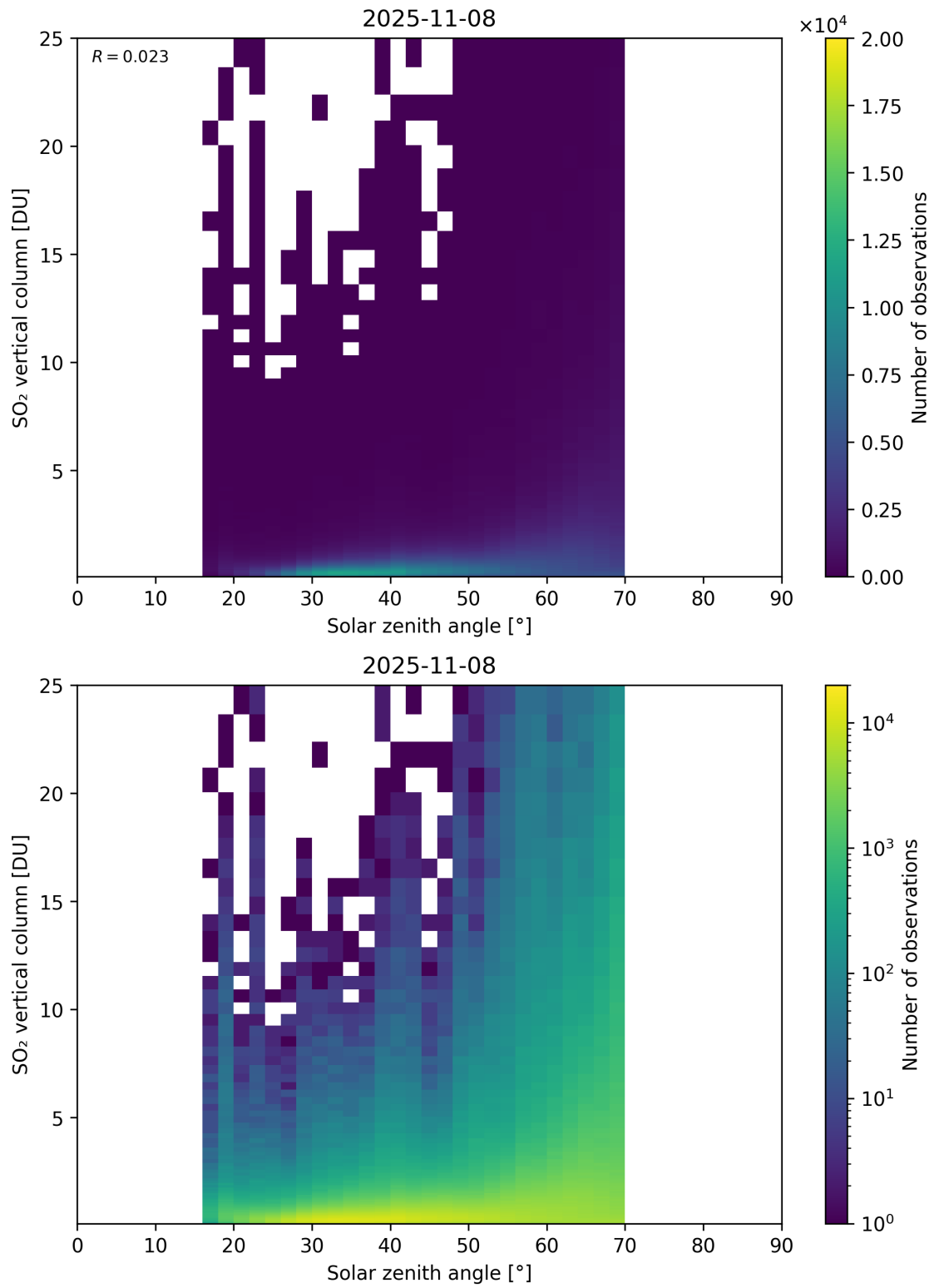
Figure 191: Scatter density plot of “Solar zenith angle” against “SO 2 vertical column” for 2025-11-07 to 2025-11-09.
