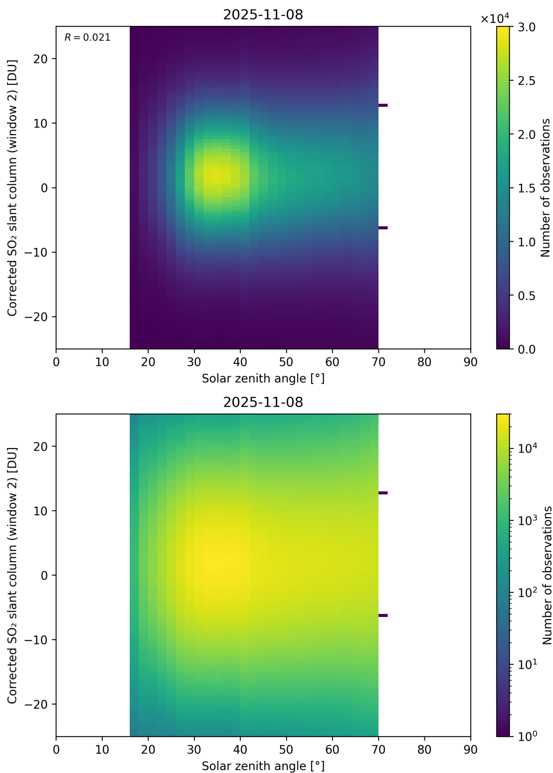
Figure 182: Scatter density plot of “Solar zenith angle” against “Corrected SO 2 slant column (window 2)” for 2025-11-07 to 2025-11-09.
