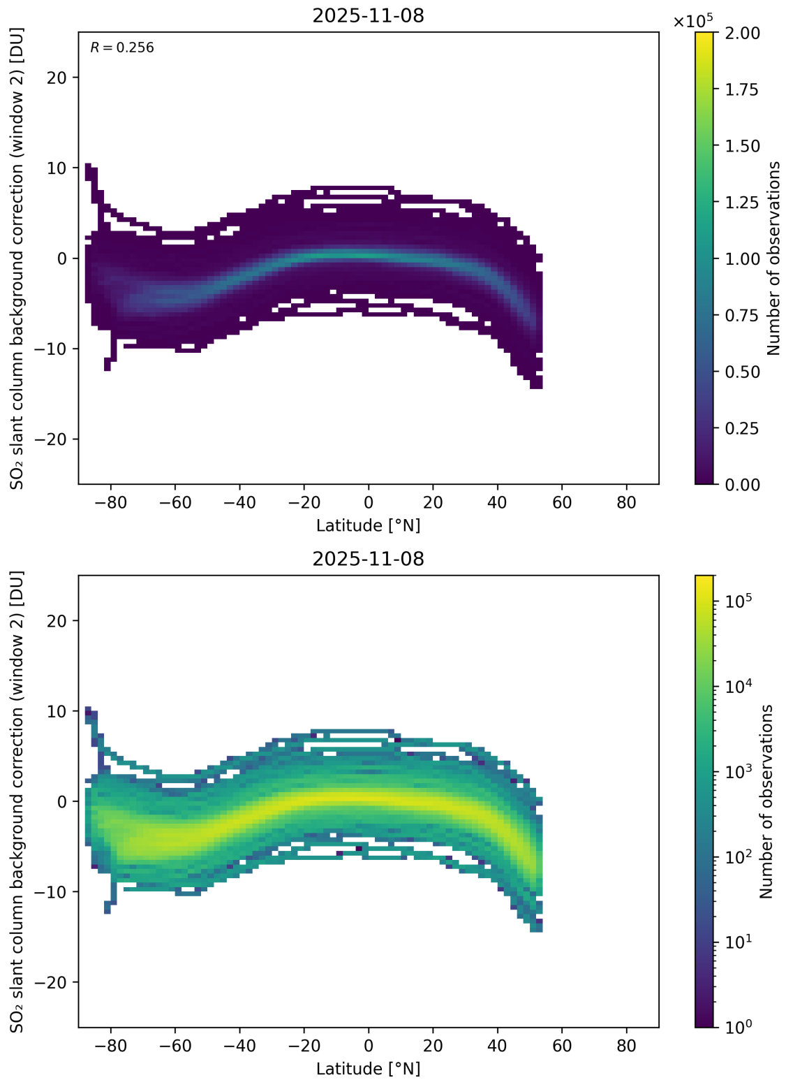
Figure 151: Scatter density plot of “Latitude” against “SO 2 slant column background correction (window 2)” for 2025-11-07 to 2025-11-09.
