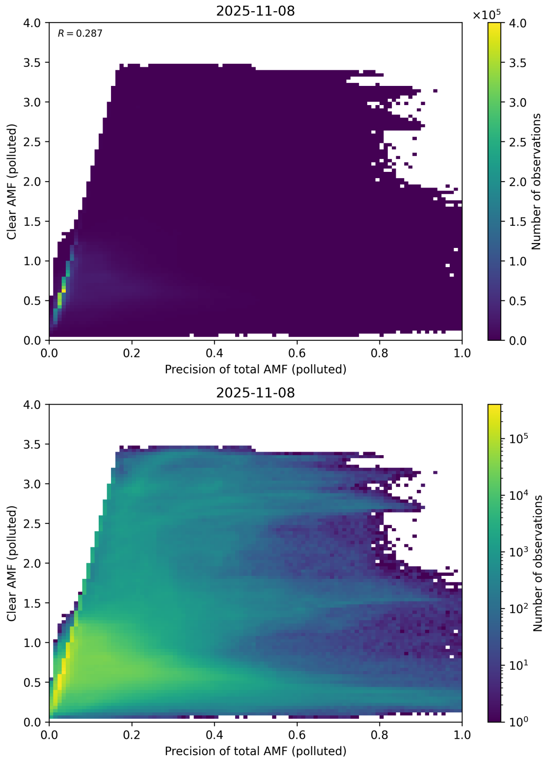
Figure 320: Scatter density plot of “Precision of total AMF (polluted)” against “Clear AMF (polluted)” for 2025-11-07 to 2025-11-09.
