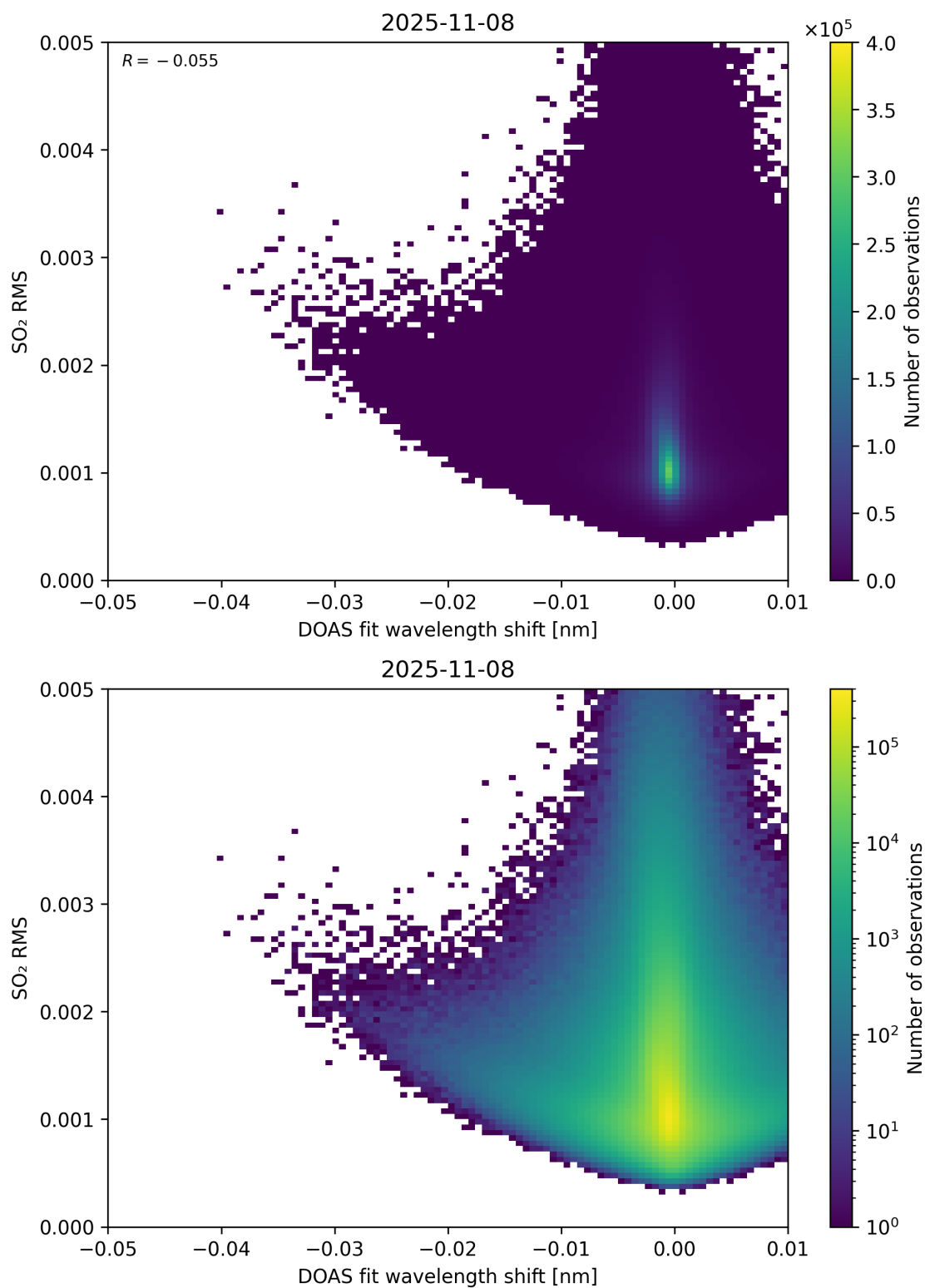
Figure 139: Scatter density plot of “DOAS fit wavelength shift” against “SO 2 RMS” for 2025-11-07 to 2025-11-09.
