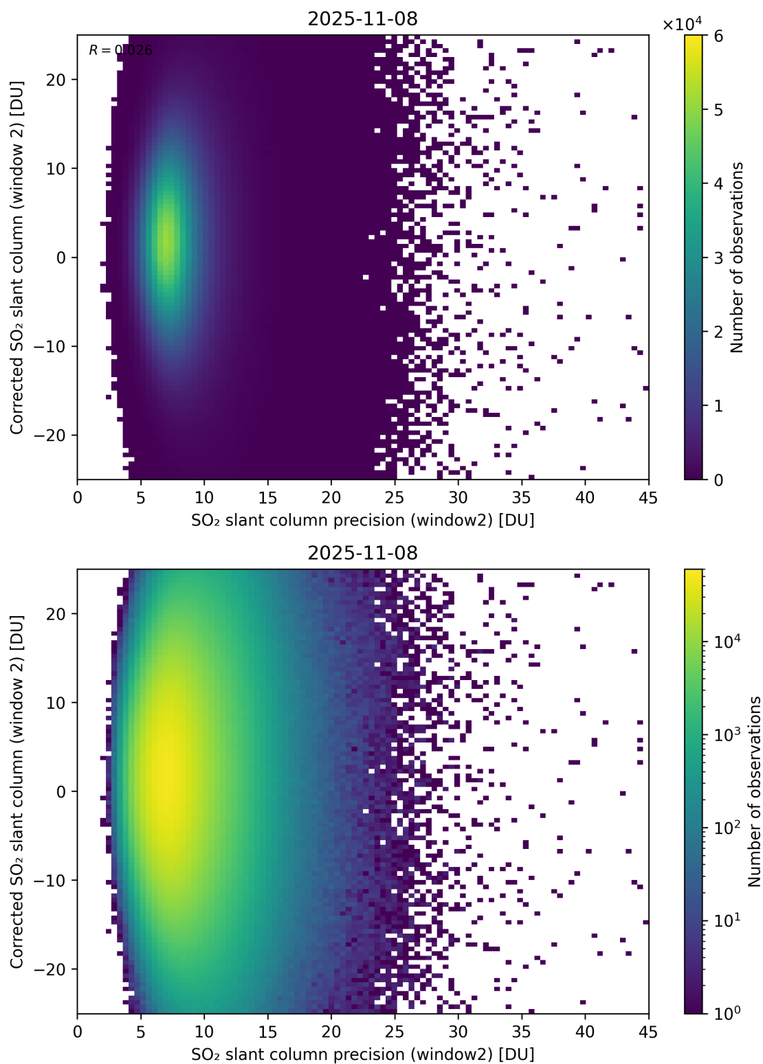
Figure 297: Scatter density plot of “SO 2 slant column precision (window2)” against “Corrected SO 2 slant column (window 2)” for 2025-11-07 to 2025-11-09.
