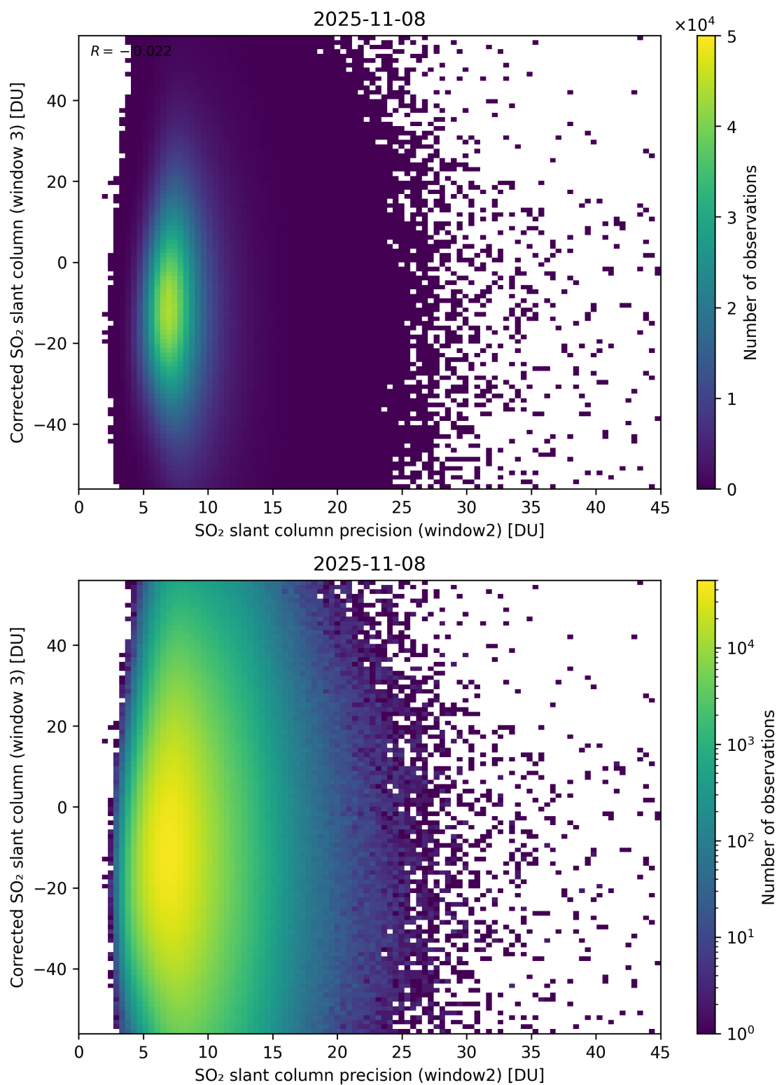
Figure 298: Scatter density plot of “SO 2 slant column precision (window2)” against “Corrected SO 2 slant column (window 3)” for 2025-11-07 to 2025-11-09.
