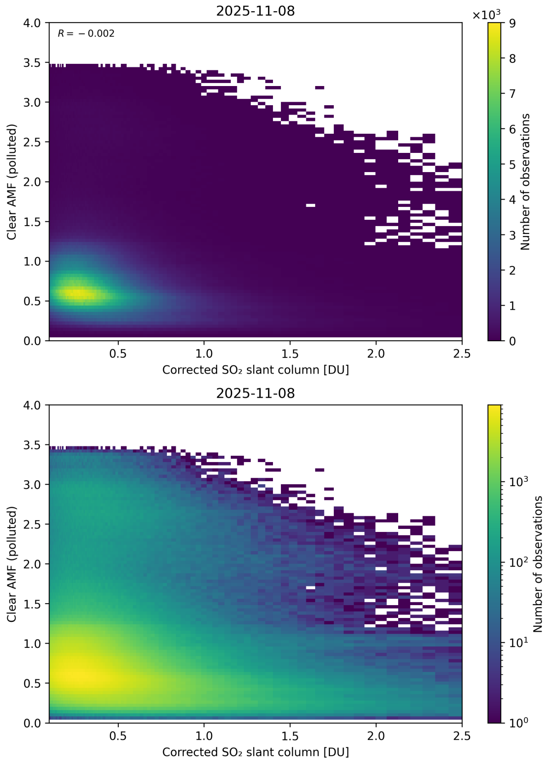
Figure 232: Scatter density plot of “Corrected SO 2 slant column” against “Clear AMF (polluted)” for 2025-11-07 to 2025-11-09.
