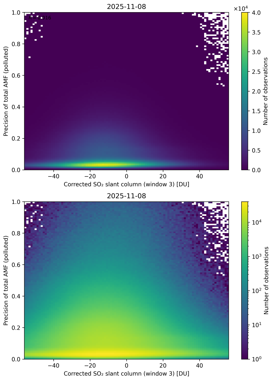
Figure 261: Scatter density plot of “Corrected SO 2 slant column (window 3)” against “Precision of total AMF (polluted)” for 2025-11-07 to 2025-11-09.
