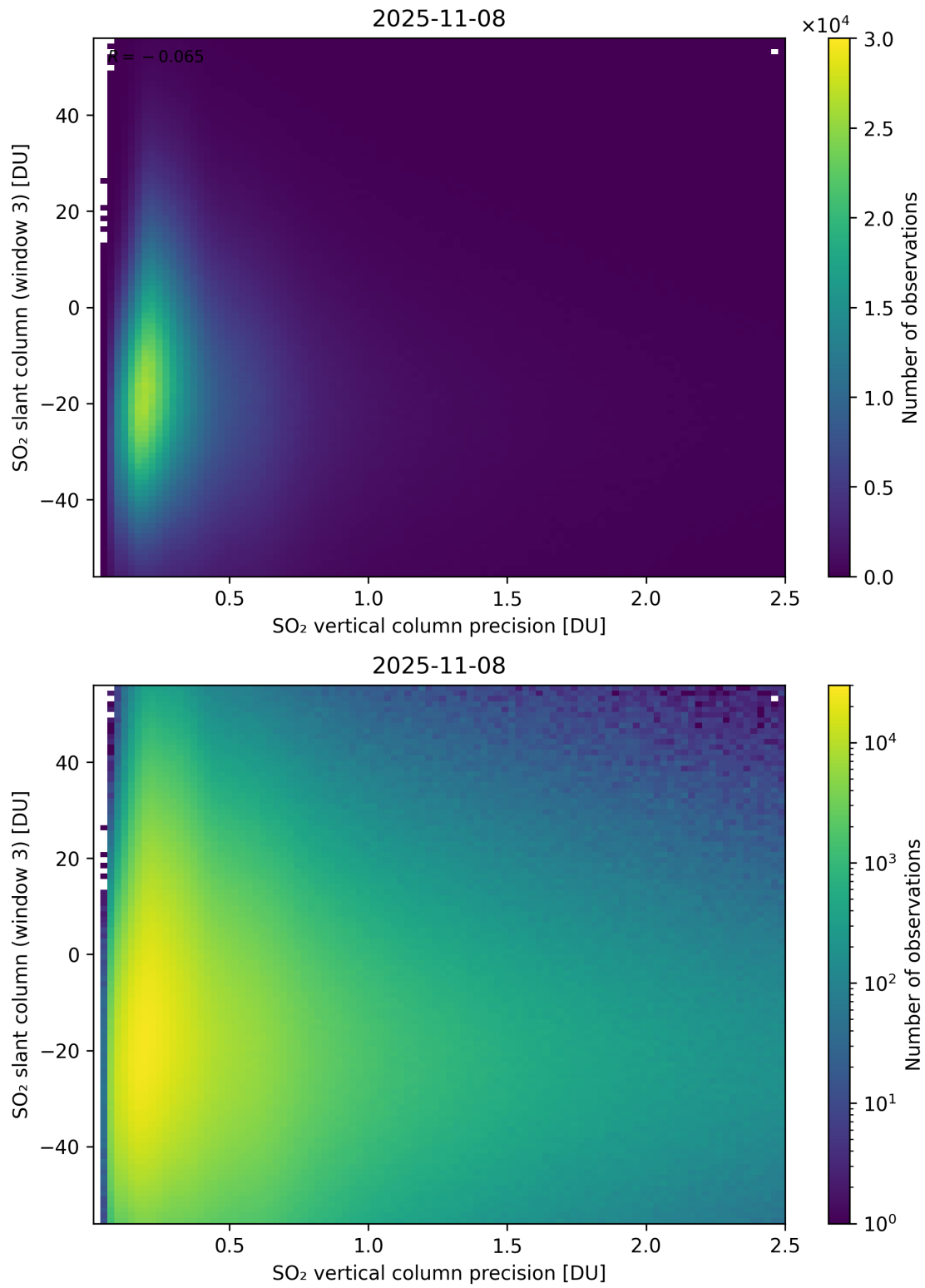
Figure 344: Scatter density plot of “SO 2 vertical column precision” against “SO 2 slant column (window 3)” for 2025-11-07 to 2025-11-09.
