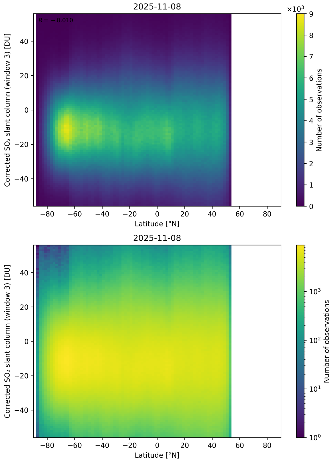
Figure 161: Scatter density plot of “Latitude” against “Corrected SO 2 slant column (window 3)” for 2025-11-07 to 2025-11-09.
