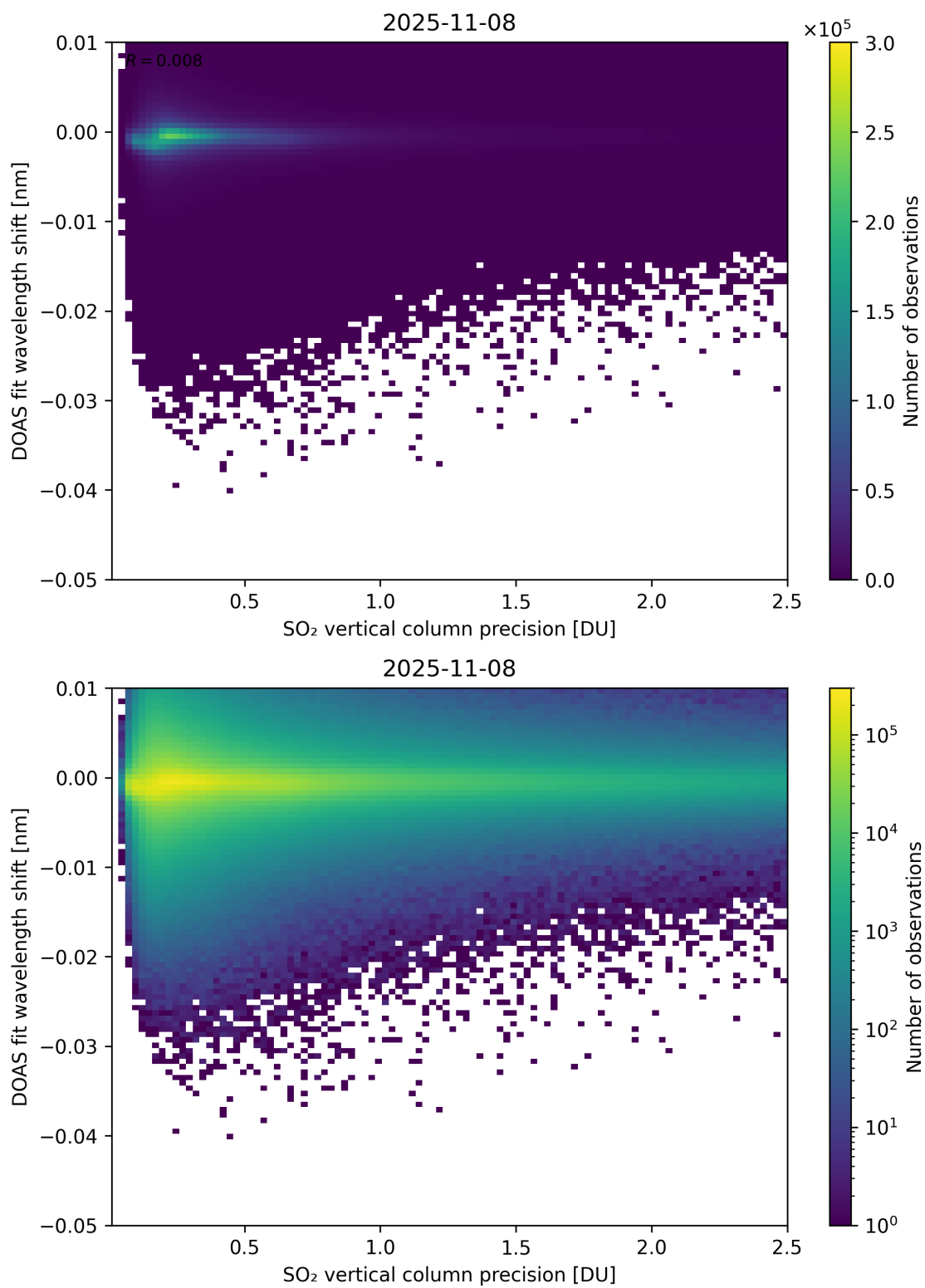
Figure 332: Scatter density plot of “SO 2 vertical column precision” against “DOAS fit wavelength shift” for 2025-11-07 to 2025-11-09.
