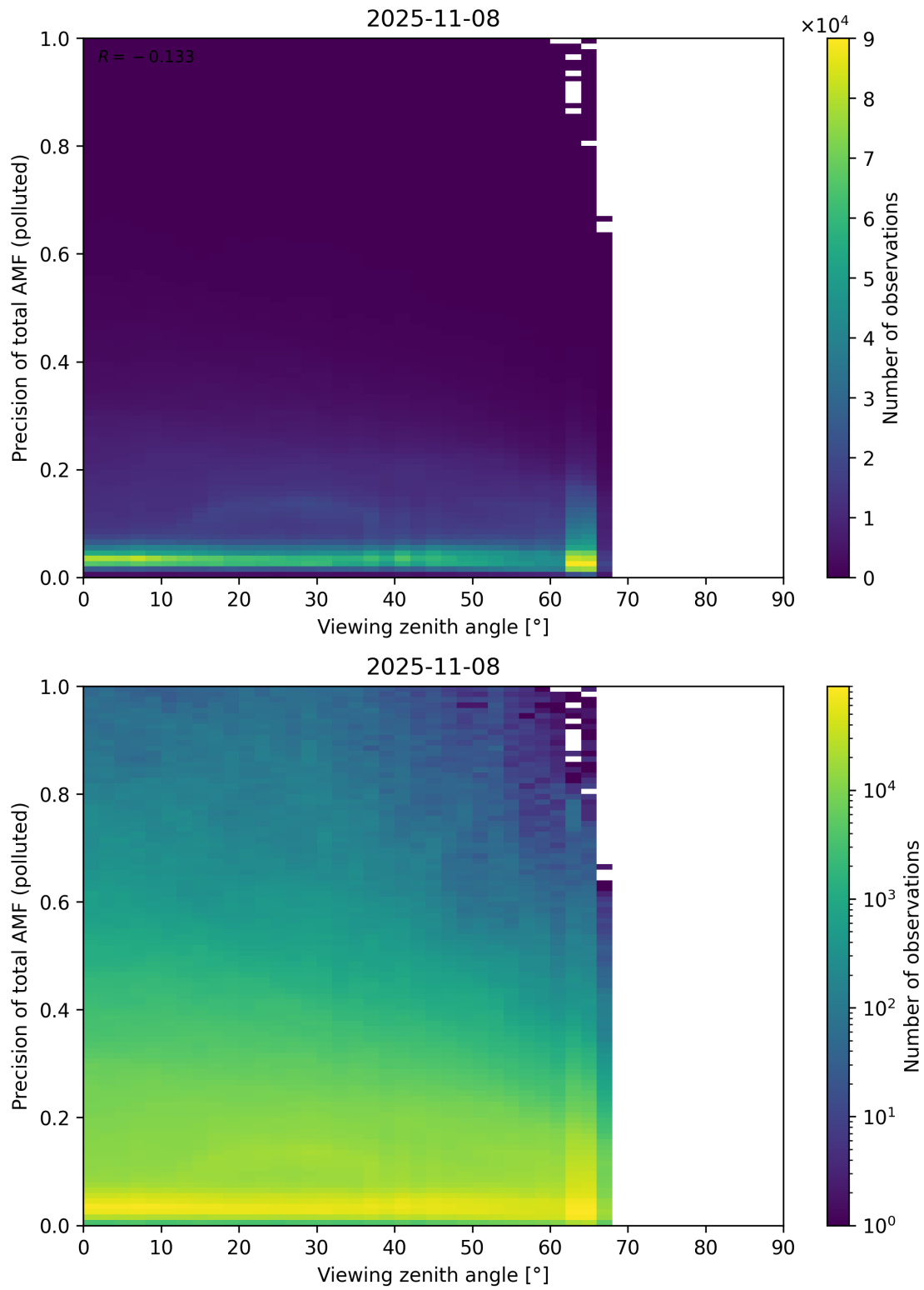
Figure 382: Scatter density plot of “Viewing zenith angle” against “Precision of total AMF (polluted)” for 2025-11-07 to 2025-11-09.
