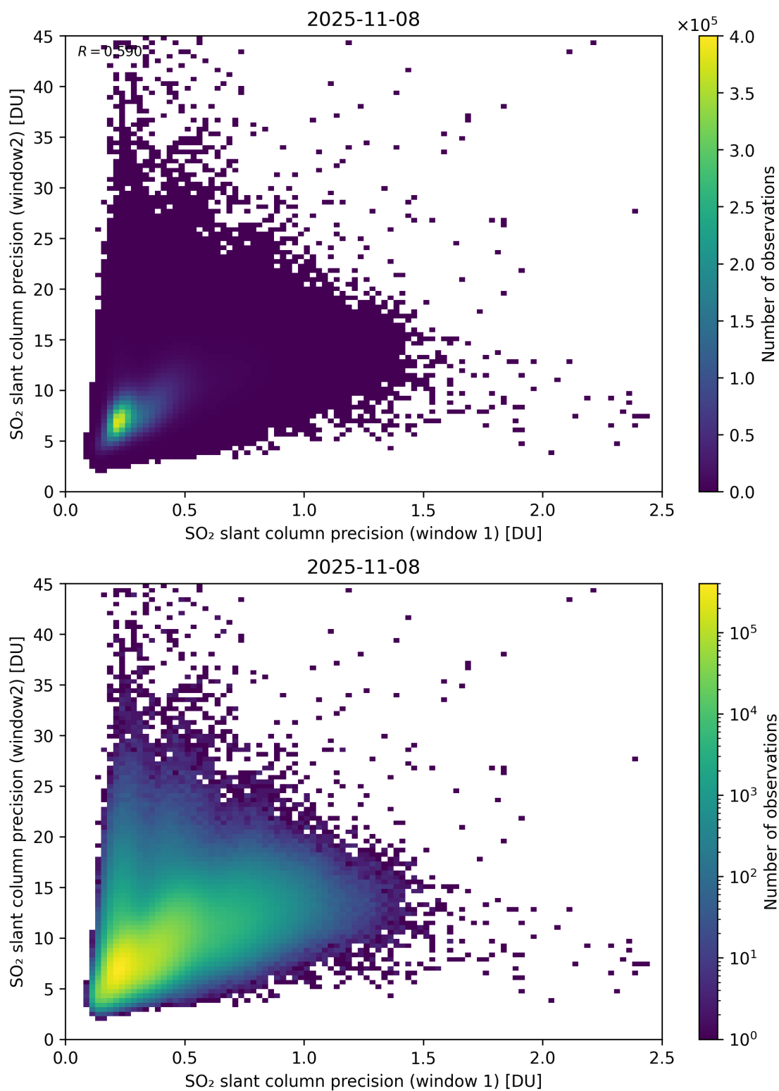
Figure 277: Scatter density plot of “SO 2 slant column precision (window 1)” against “SO 2 slant column precision (window2)” for 2025-11-07 to 2025-11-09.
