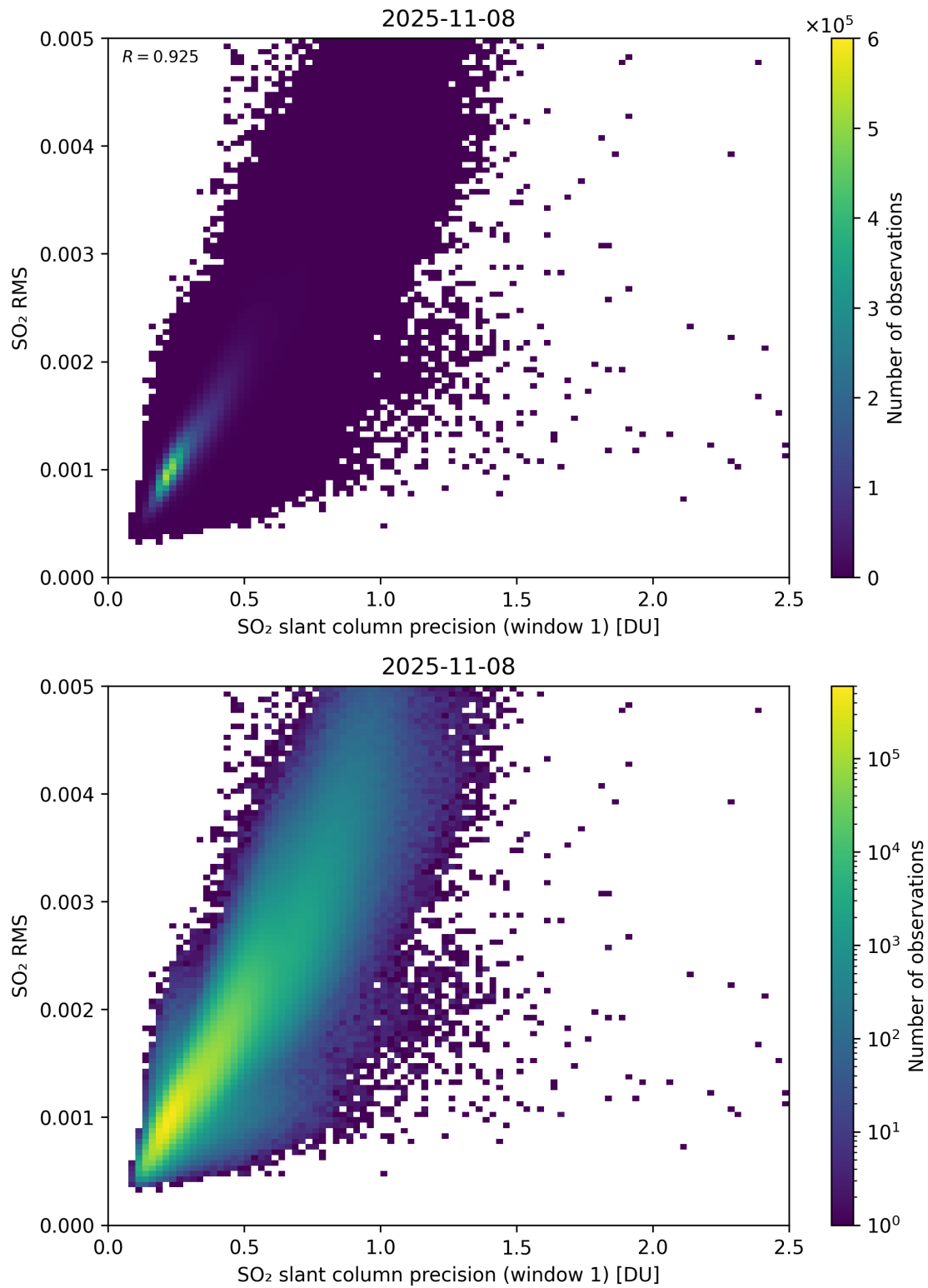
Figure 273: Scatter density plot of “SO 2 slant column precision (window 1)” against “SO 2 RMS” for 2025-11-07 to 2025-11-09.
