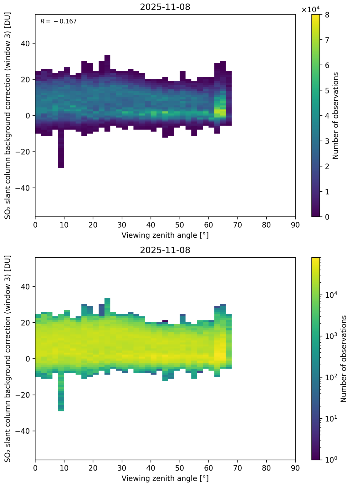
Figure 364: Scatter density plot of “Viewing zenith angle” against “SO 2 slant column background correction (window 3)” for 2025-11-07 to 2025-11-09.
