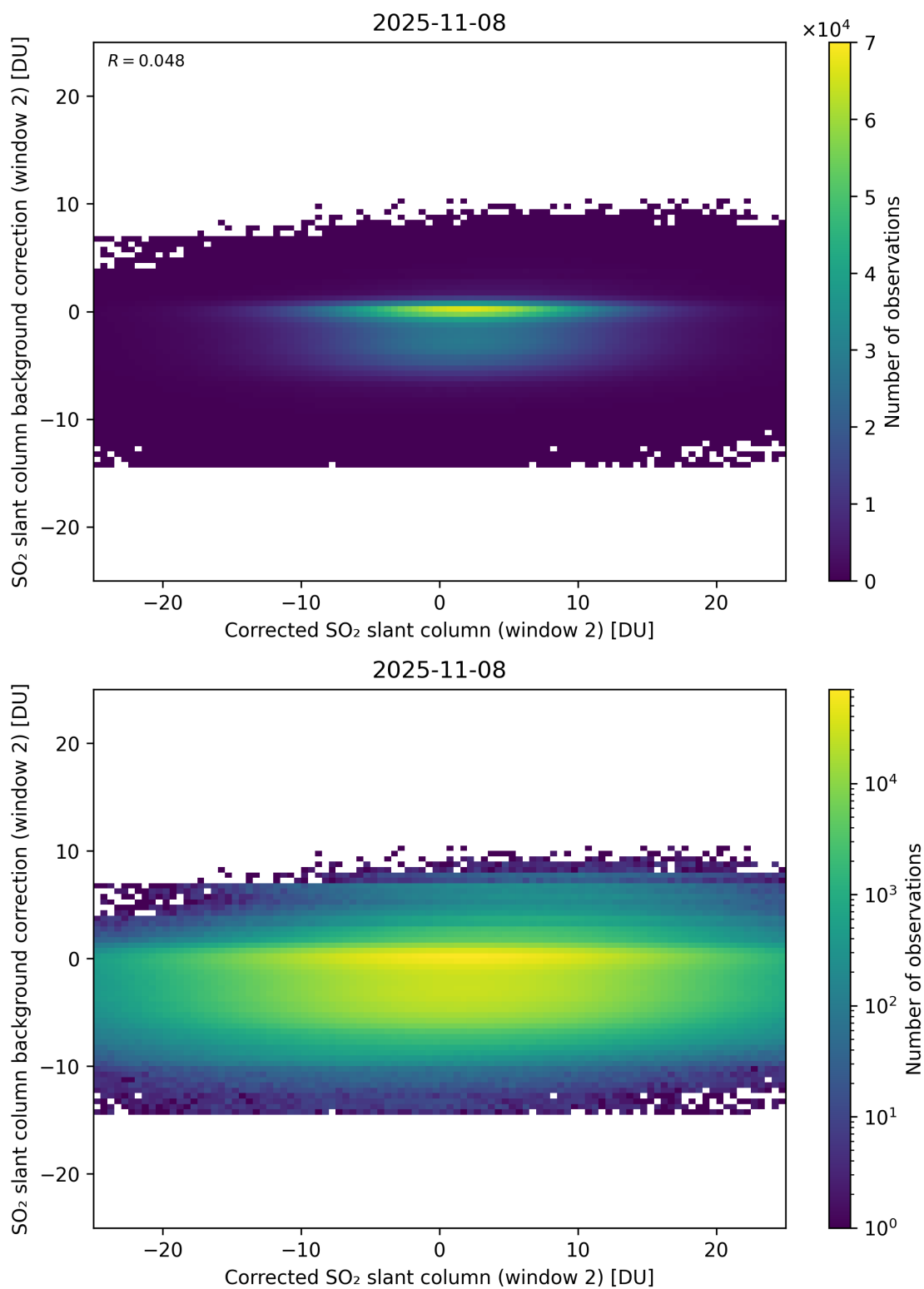
Figure 244: Scatter density plot of “Corrected SO 2 slant column (window 2)” against “SO 2 slant column background correction (window 2)” for 2025-11-07 to 2025-11-09.
