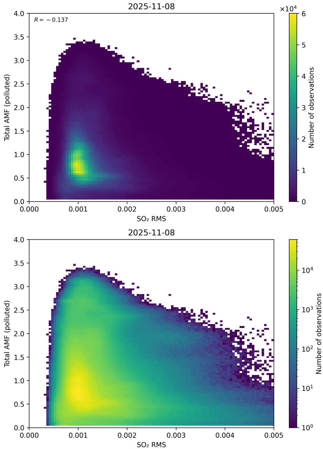
Figure 148: Scatter density plot of “SO 2 RMS” against “Total AMF (polluted)” for 2025-11-07 to 2025-11-09.
