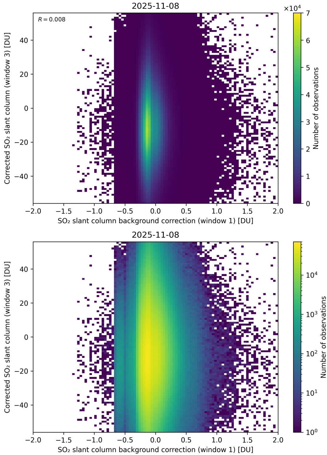
Figure 116: Scatter density plot of “SO 2 slant column background correction (window 1)” against “Corrected SO 2 slant column (window 3)” for 2025-11-07 to 2025-11-09.
