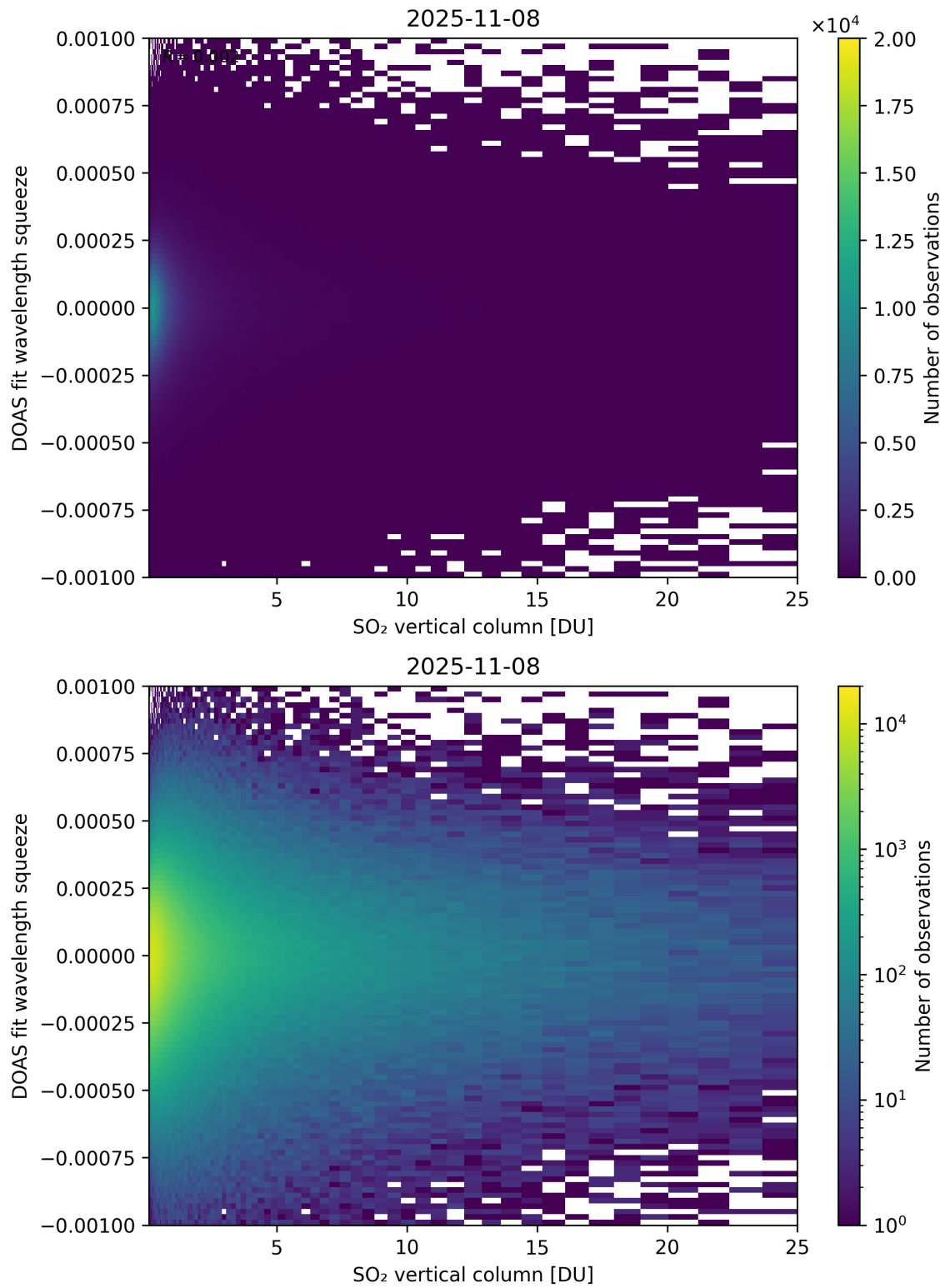
Figure 327: Scatter density plot of “SO 2 vertical column” against “DOAS fit wavelength squeeze” for 2025-11-07 to 2025-11-09.
