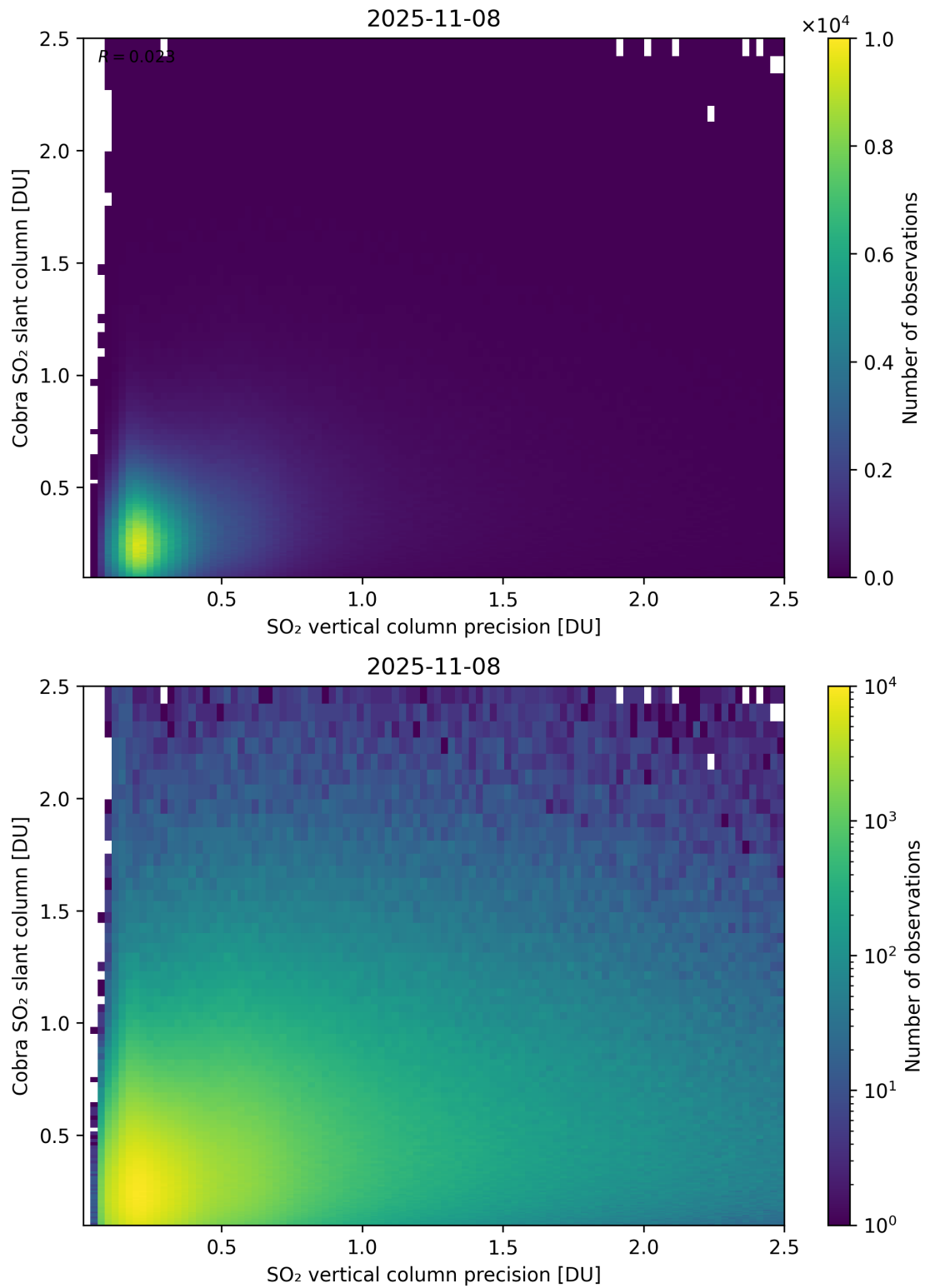
Figure 336: Scatter density plot of “SO 2 vertical column precision” against “Cobra SO 2 slant column” for 2025-11-07 to 2025-11-09.
