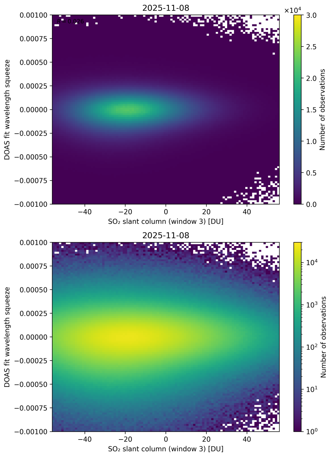
Figure 305: Scatter density plot of “SO 2 slant column (window 3)” against “DOAS fit wavelength squeeze” for 2025-11-07 to 2025-11-09.
