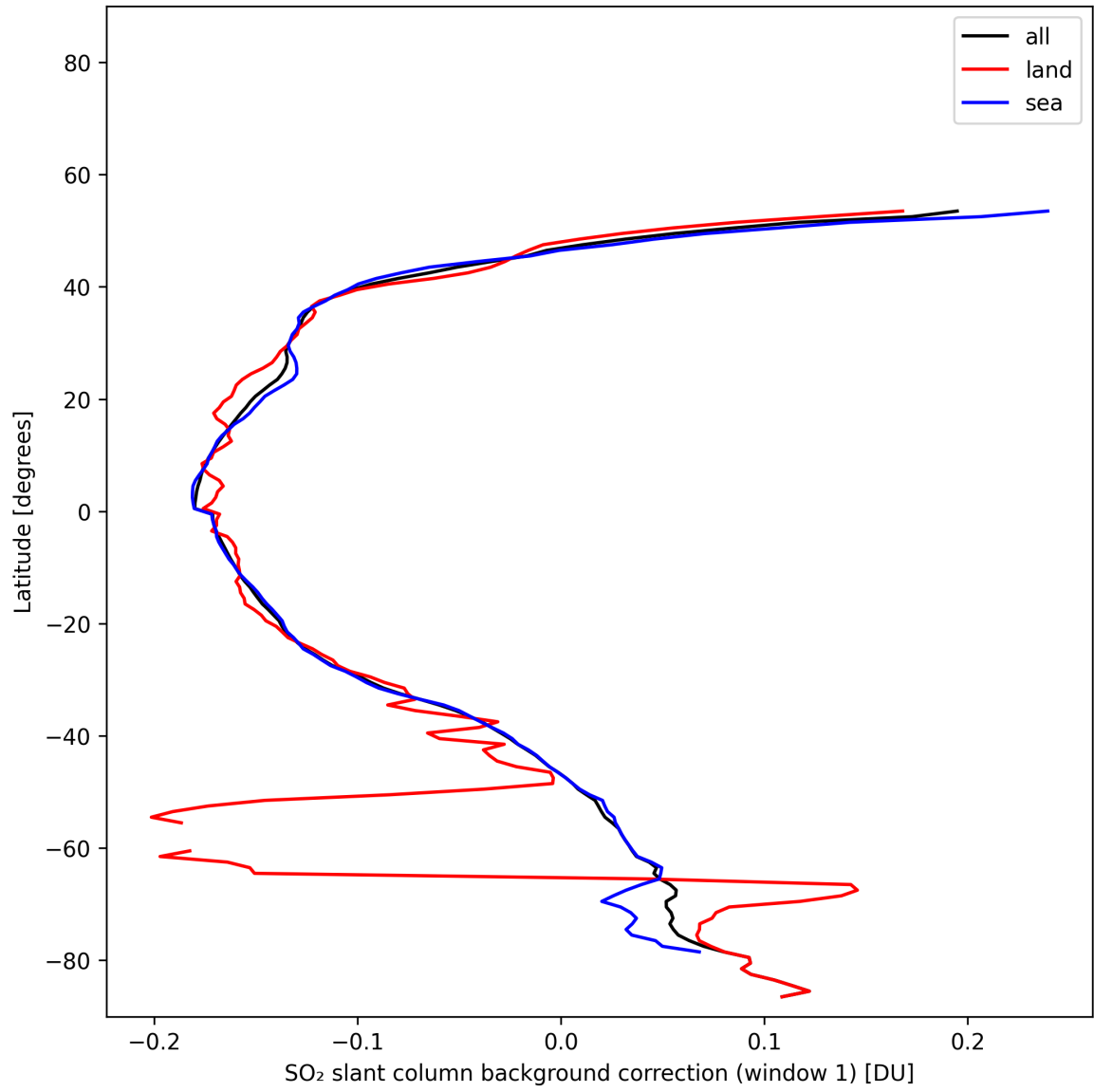
Figure 40: Zonal average of “SO 2 slant column background correction (window 1)” for 2025-11-07 to 2025-11-09.
