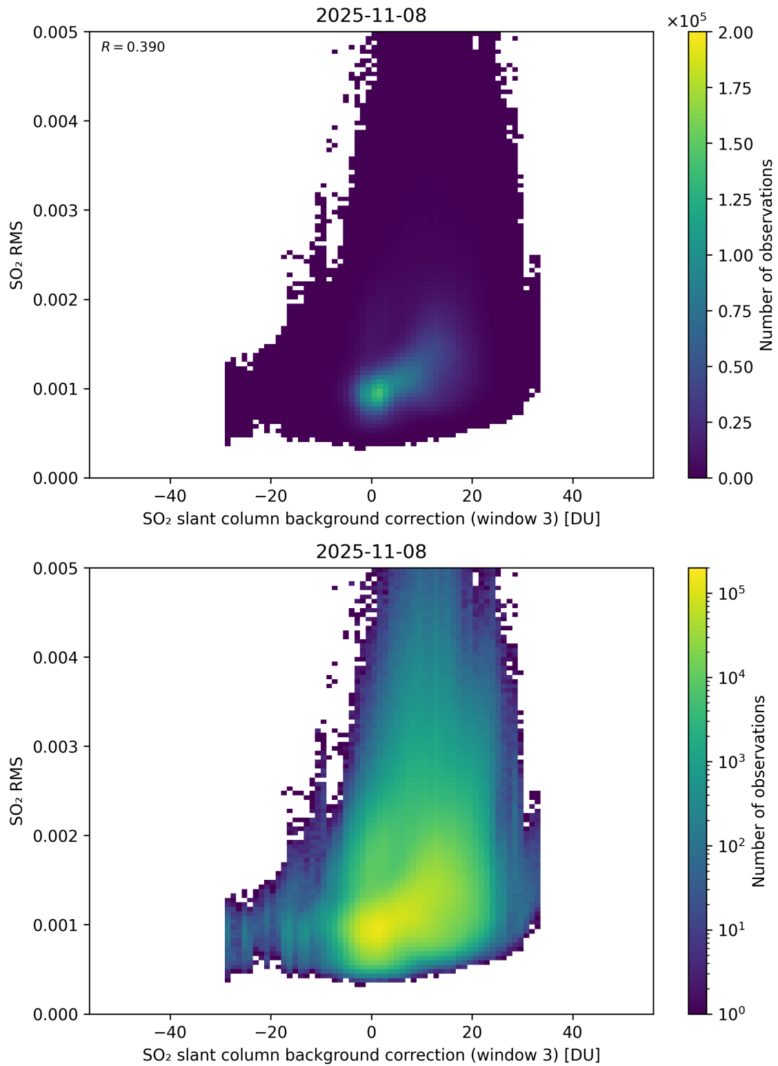
Figure 134: Scatter density plot of “SO 2 slant column background correction (window 3)” against “SO 2 RMS” for 2025-11-07 to 2025-11-09.
