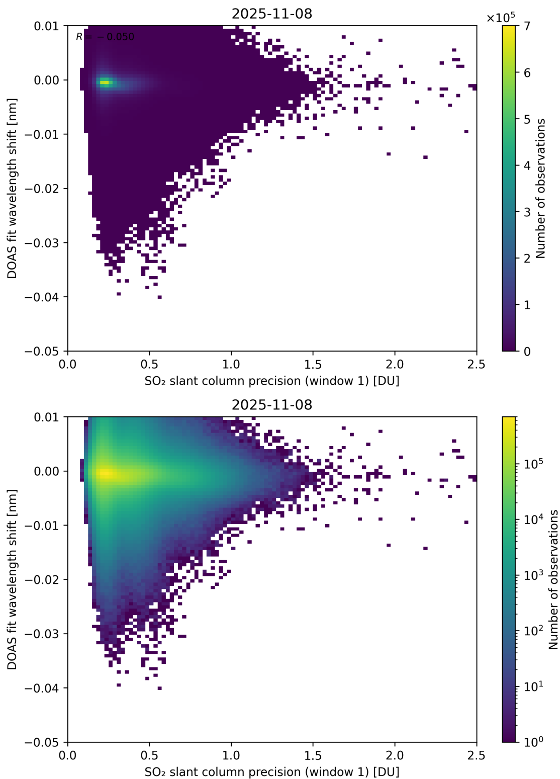
Figure 271: Scatter density plot of “SO 2 slant column precision (window 1)” against “DOAS fit wavelength shift” for 2025-11-07 to 2025-11-09.
