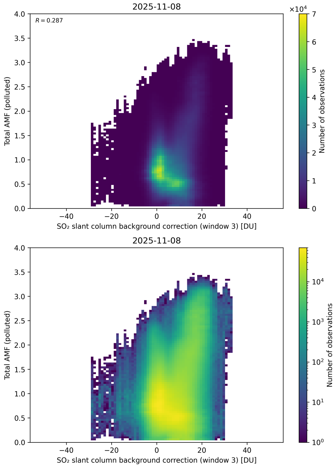
Figure 136: Scatter density plot of “SO 2 slant column background correction (window 3)” against “Total AMF (polluted)” for 2025-11-07 to 2025-11-09.
