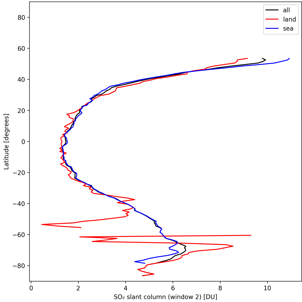
Figure 41: Zonal average of “SO 2 slant column (window 2)” for 2025-11-07 to 2025-11-09.
