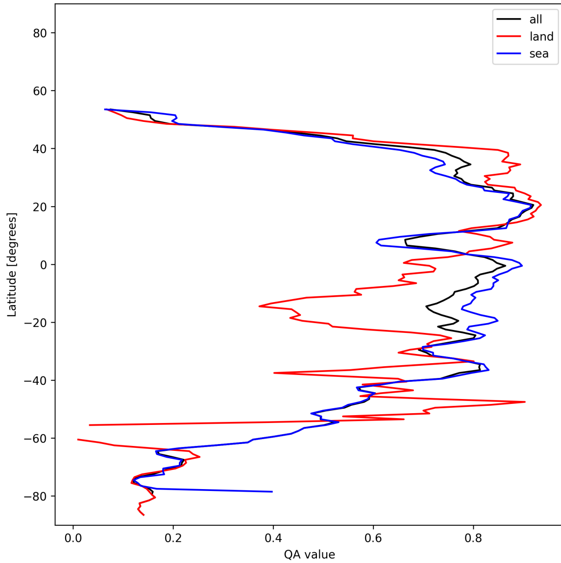
Figure 31: Zonal average of “QA value” for 2025-11-07 to 2025-11-09.
