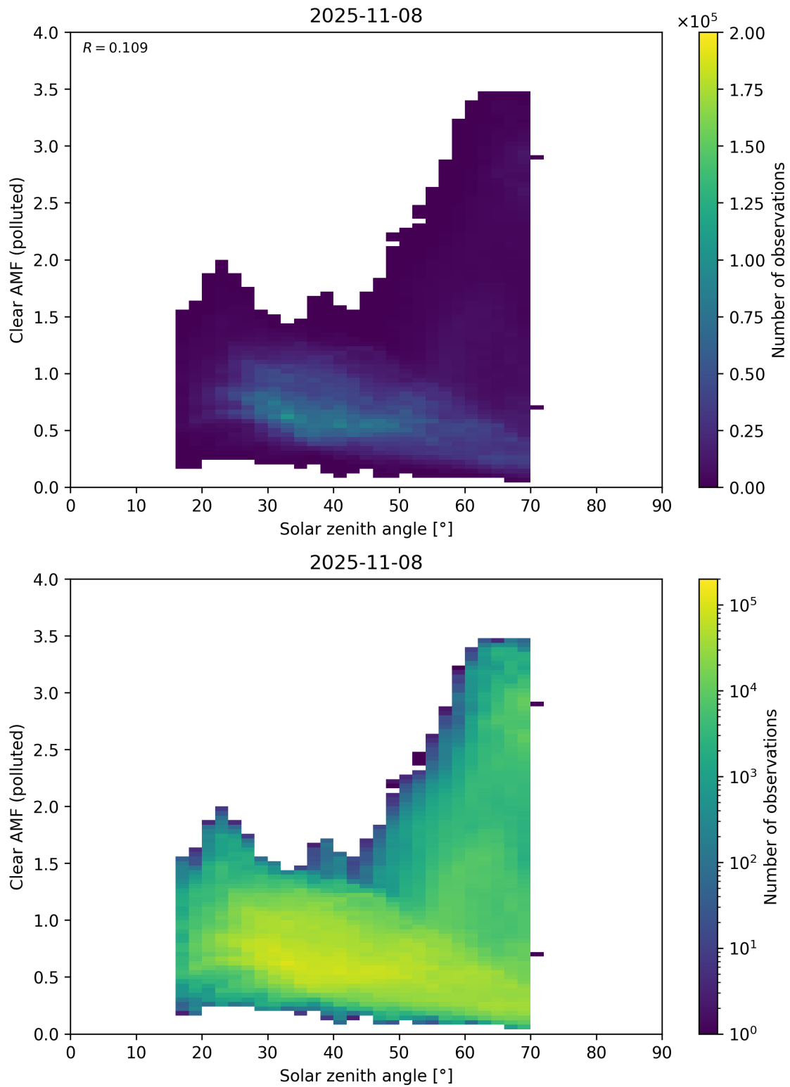
Figure 178: Scatter density plot of “Solar zenith angle” against “Clear AMF (polluted)” for 2025-11-07 to 2025-11-09.
