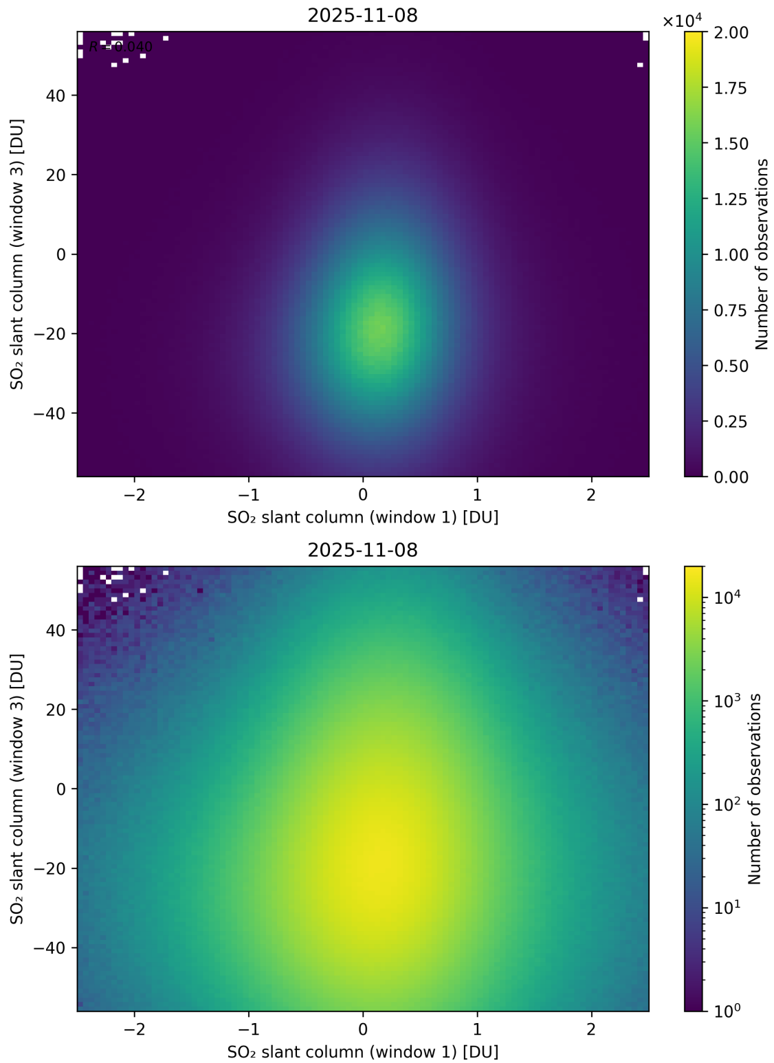
Figure 287: Scatter density plot of “SO 2 slant column (window 1)” against “SO 2 slant column (window 3)” for 2025-11-07 to 2025-11-09.
