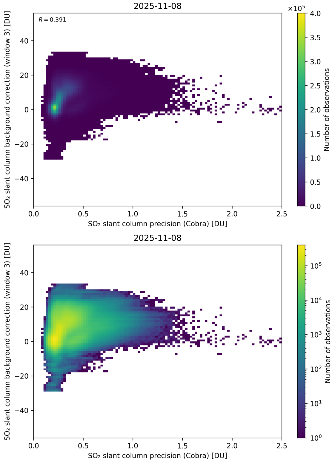
Figure 201: Scatter density plot of “SO 2 slant column precision (Cobra)” against “SO 2 slant column background correction (window 3)” for 2025-11-07 to 2025-11-09.
