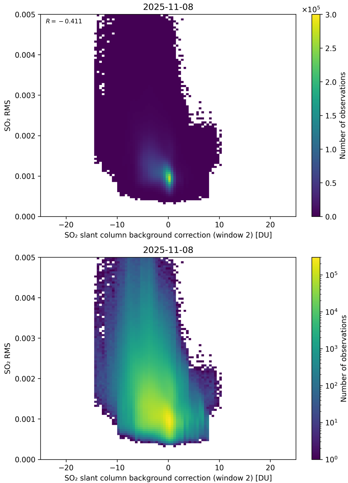
Figure 125: Scatter density plot of “SO 2 slant column background correction (window 2)” against “SO 2 RMS” for 2025-11-07 to 2025-11-09.
