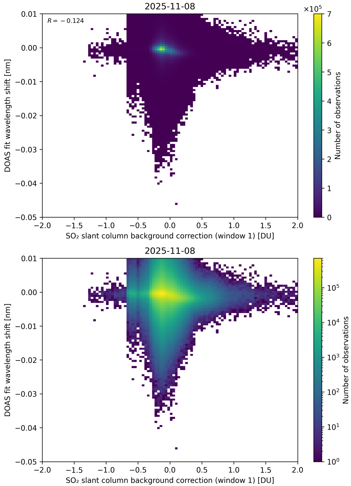
Figure 111: Scatter density plot of “SO 2 slant column background correction (window 1)” against “DOAS fit wavelength shift” for 2025-11-07 to 2025-11-09.
