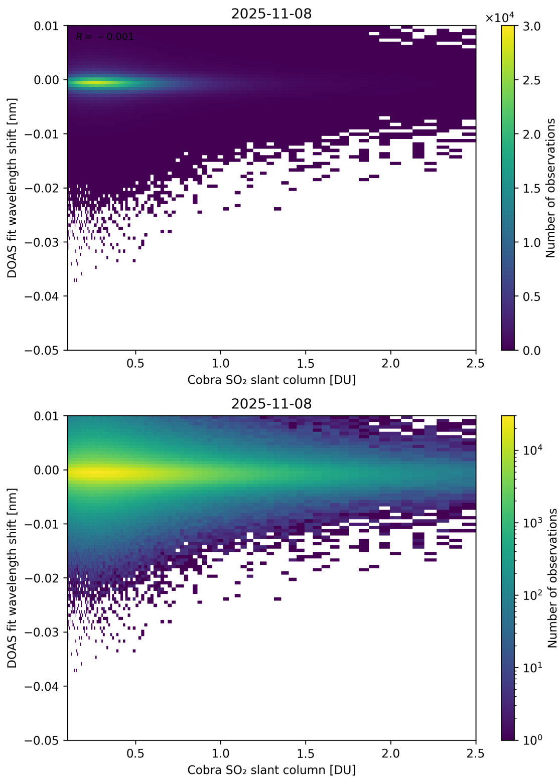
Figure 196: Scatter density plot of “Cobra SO 2 slant column” against “DOAS fit wavelength shift” for 2025-11-07 to 2025-11-09.
