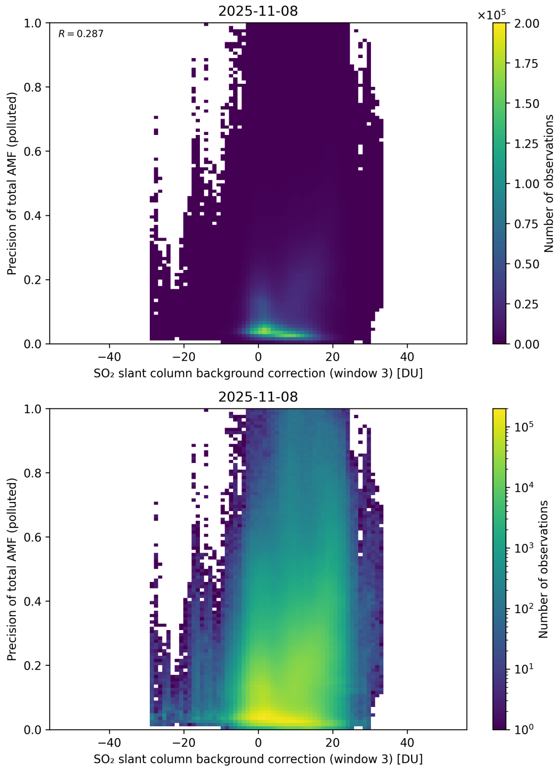
Figure 137: Scatter density plot of “SO 2 slant column background correction (window 3)” against “Precision of total AMF (polluted)” for 2025-11-07 to 2025-11-09.
