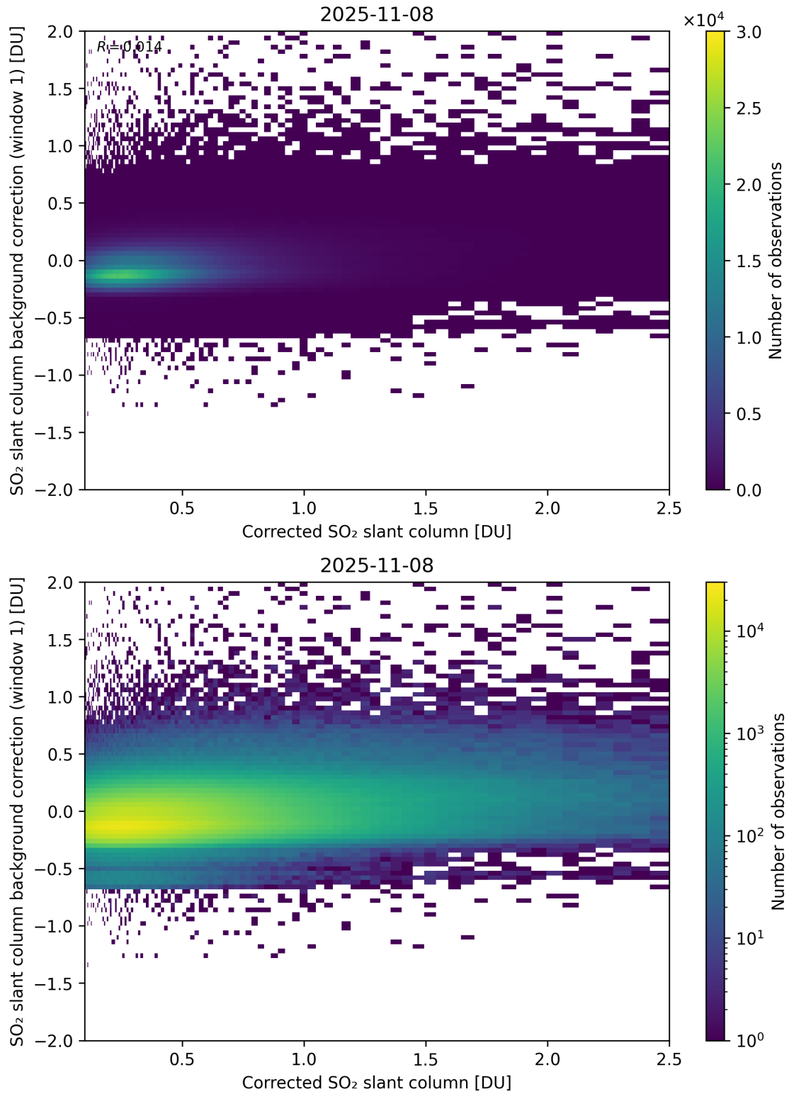
Figure 226: Scatter density plot of “Corrected SO 2 slant column” against “SO 2 slant column background correction (window 1)” for 2025-11-07 to 2025-11-09.
