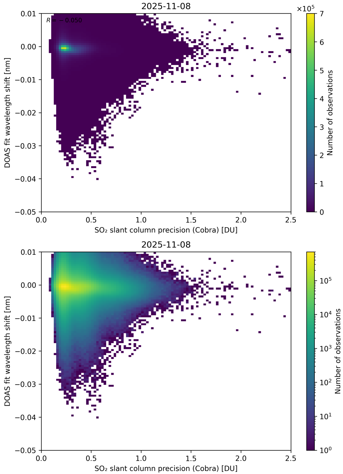
Figure 202: Scatter density plot of “SO 2 slant column precision (Cobra)” against “DOAS fit wavelength shift” for 2025-11-07 to 2025-11-09.
