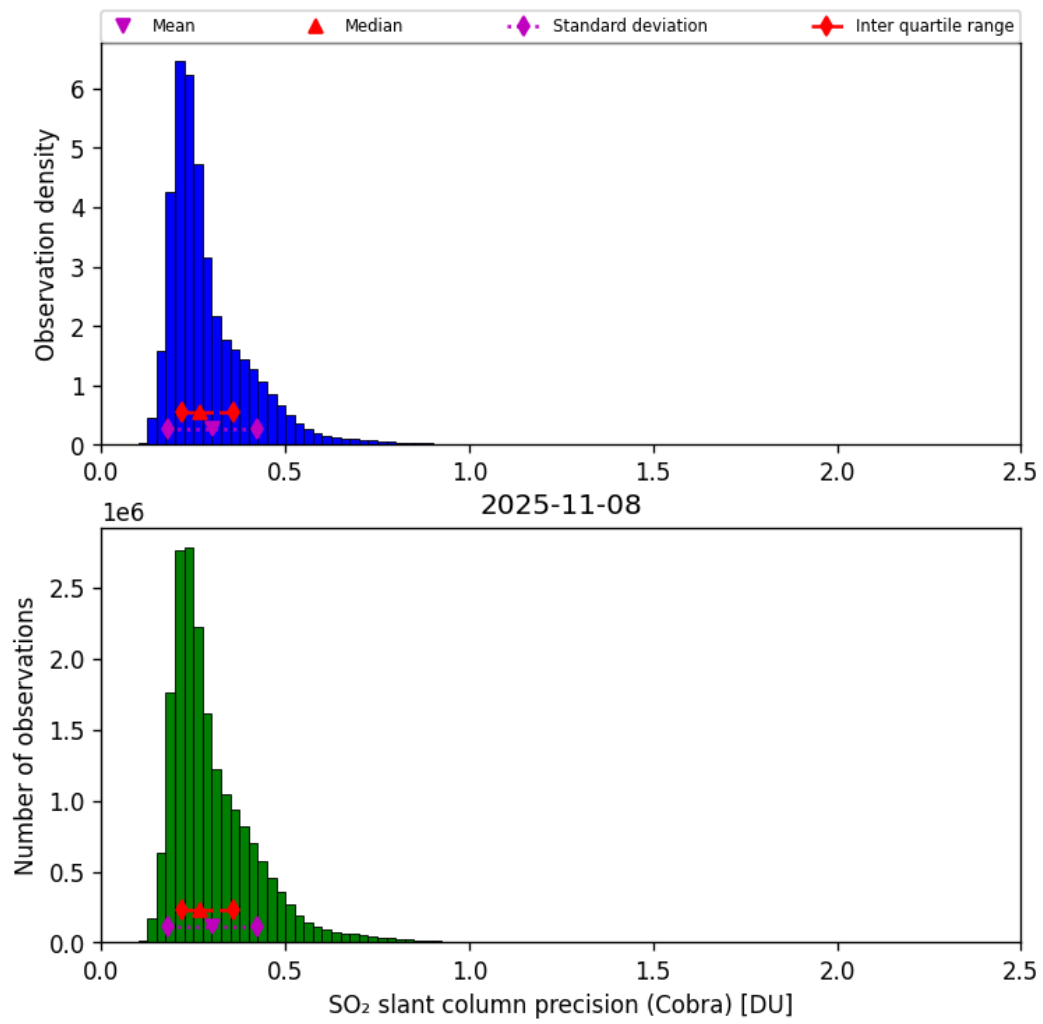
Figure 62: Histogram of “SO 2 slant column precision (Cobra)” for 2025-11-07 to 2025-11-09
