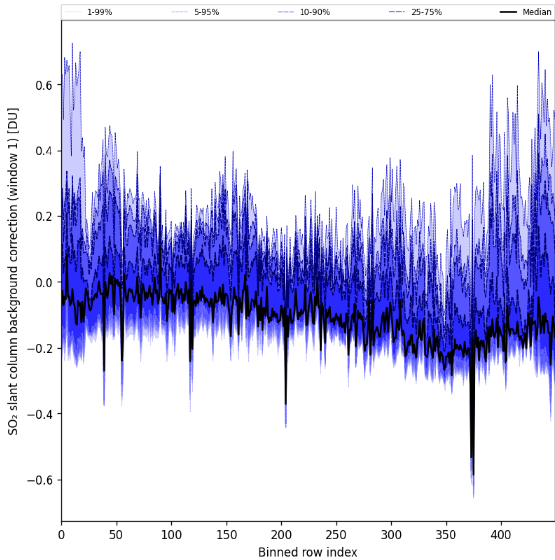
Figure 92: Along track statistics of “SO 2 slant column background correction (window 1)” for 2025-11-07 to 2025-11-09
