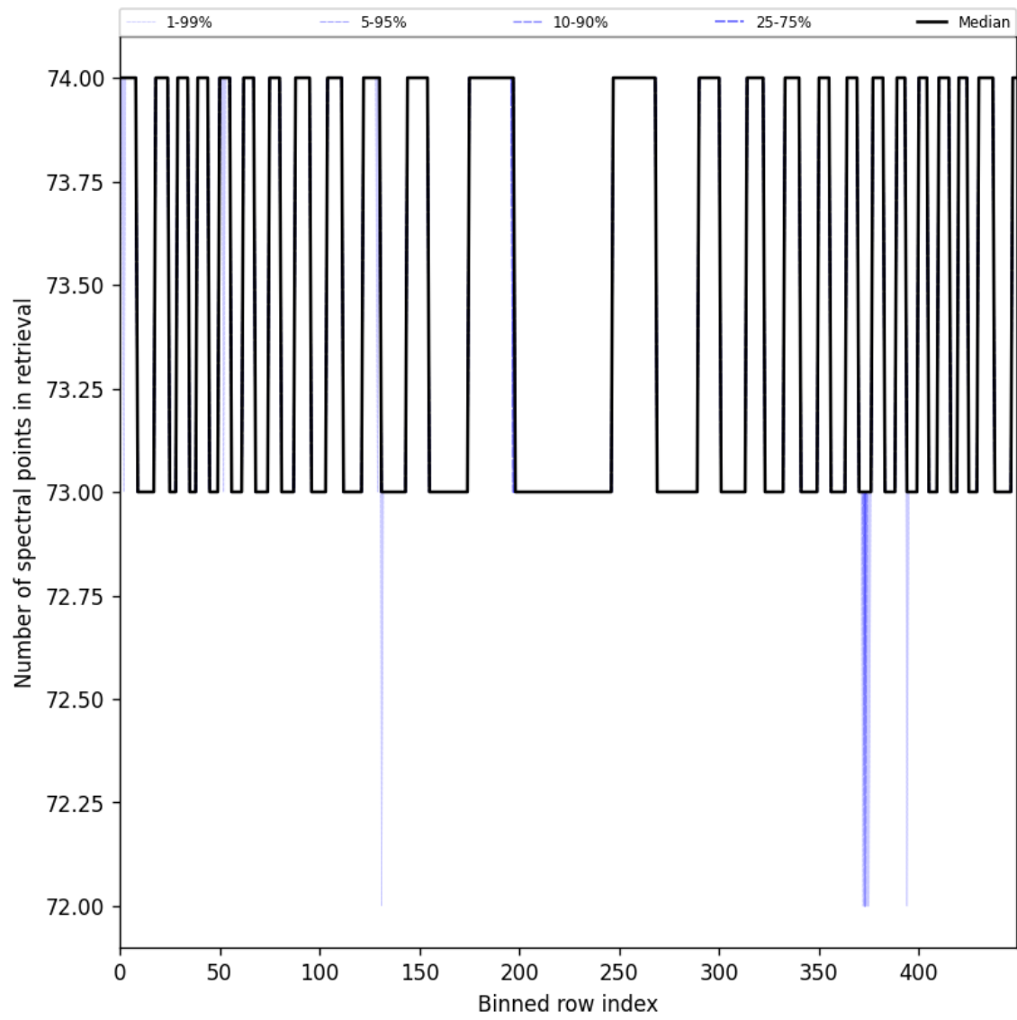
Figure 108: Along track statistics of “Number of spectral points in retrieval” for 2025-11-07 to 2025-11-09
