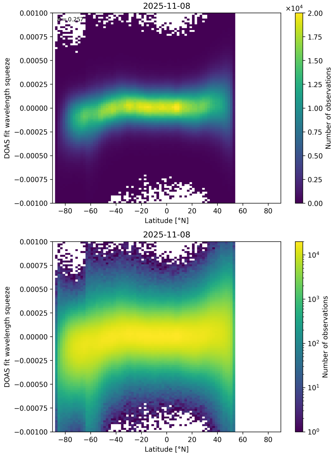
Figure 154: Scatter density plot of “Latitude” against “DOAS fit wavelength squeeze” for 2025-11-07 to 2025-11-09.
