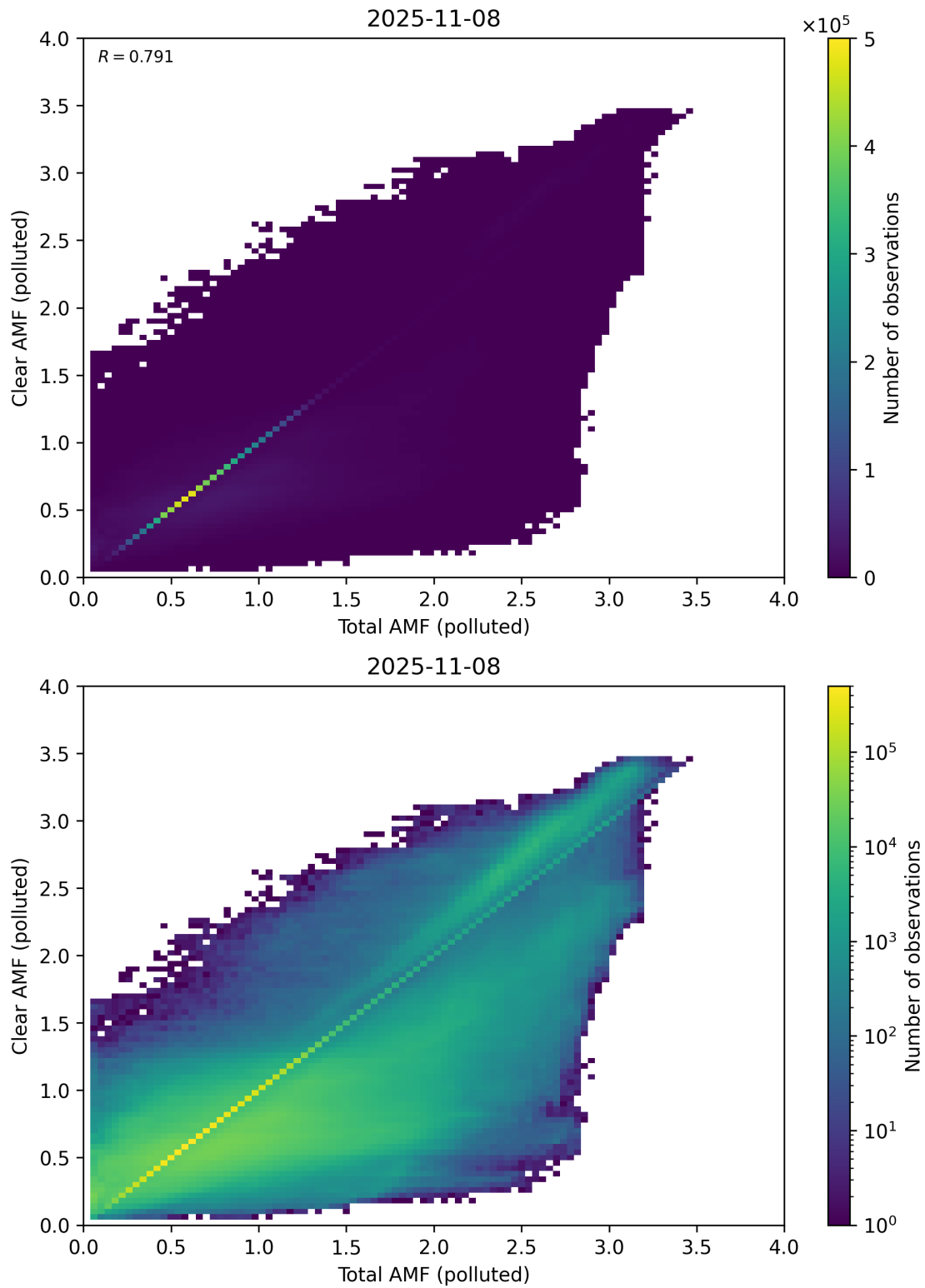
Figure 321: Scatter density plot of “Total AMF (polluted)” against “Clear AMF (polluted)” for 2025-11-07 to 2025-11-09.
