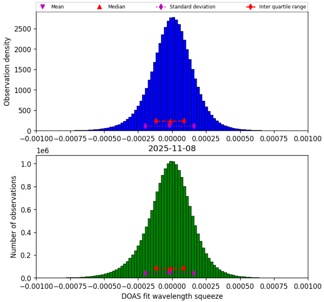
Figure 77: Histogram of “DOAS fit wavelength squeeze” for 2025-11-07 to 2025-11-09
