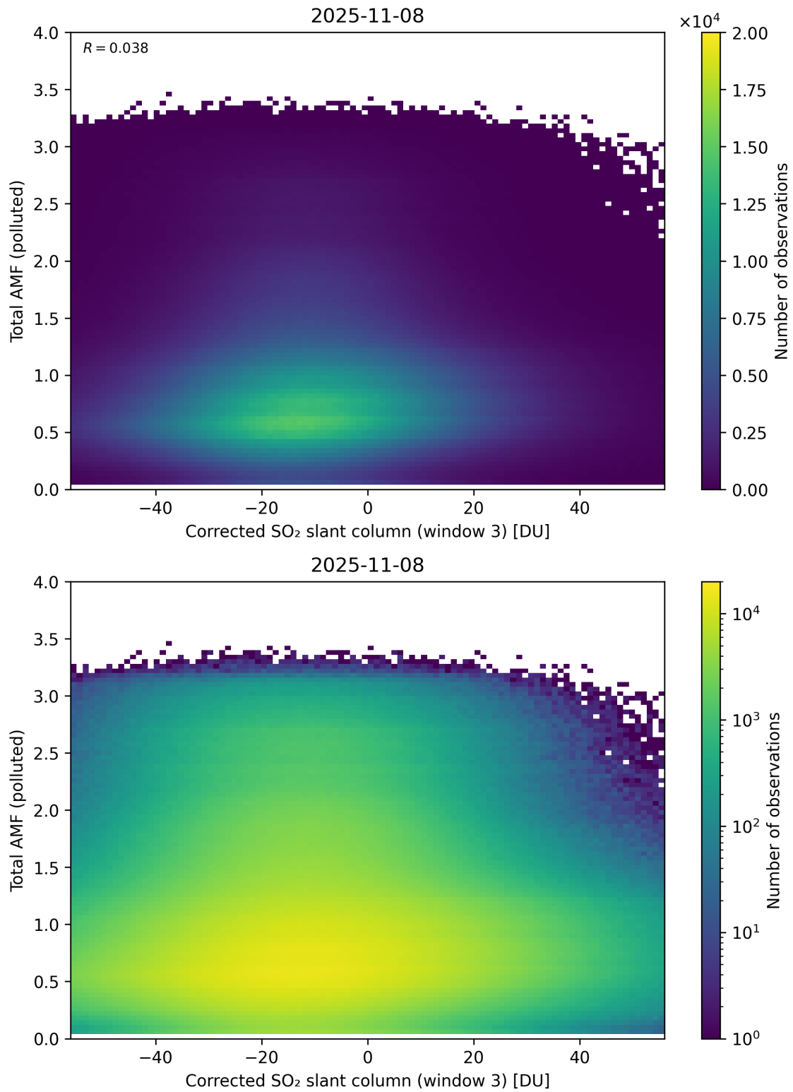
Figure 260: Scatter density plot of “Corrected SO 2 slant column (window 3)” against “Total AMF (polluted)” for 2025-11-07 to 2025-11-09.
