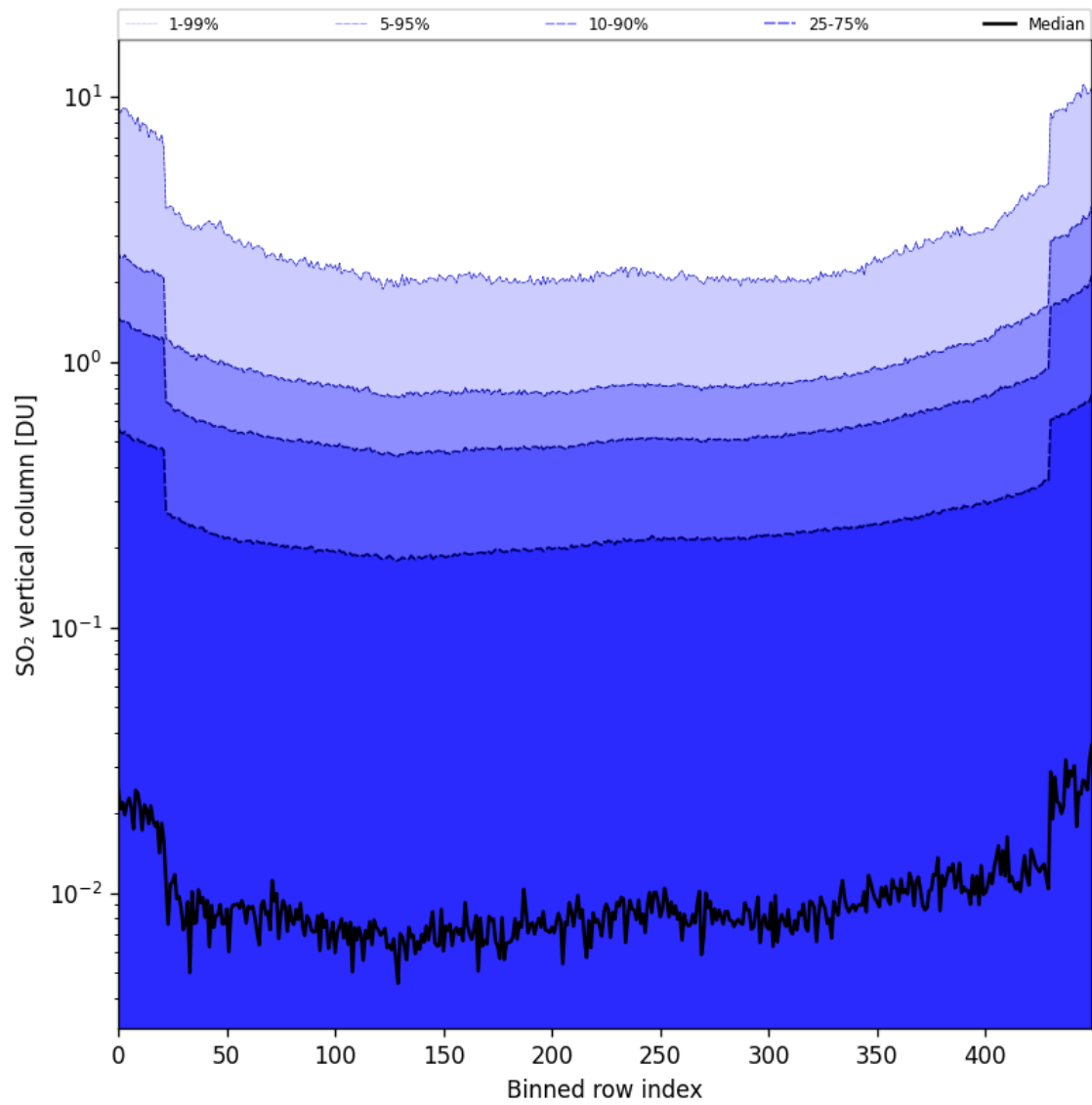
Figure 84: Along track statistics of “SO 2 vertical column” for 2025-11-07 to 2025-11-09
