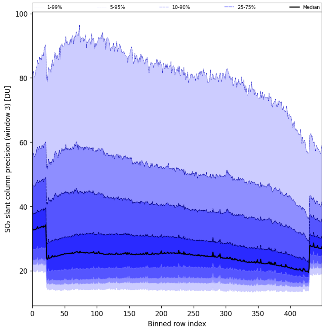
Figure 98: Along track statistics of “SO 2 slant column precision (window 3)” for 2025-11-07 to 2025-11-09
