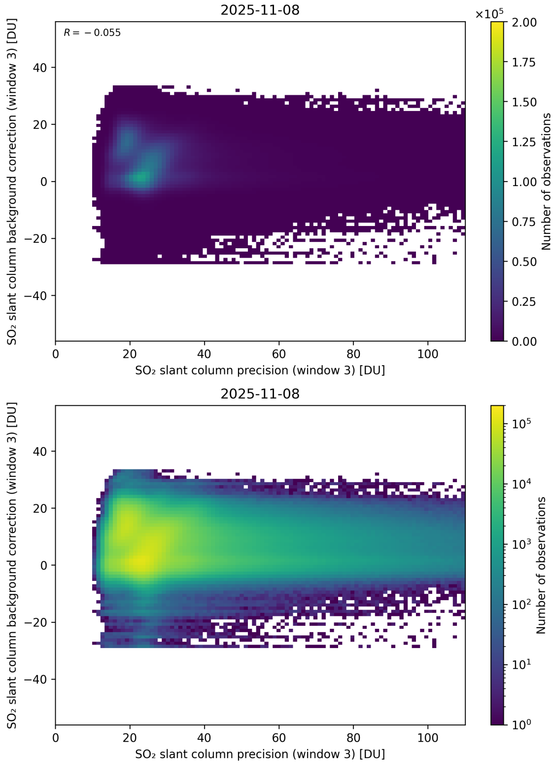
Figure 307: Scatter density plot of “SO 2 slant column precision (window 3)” against “SO 2 slant column background correction (window 3)” for 2025-11-07 to 2025-11-09.
