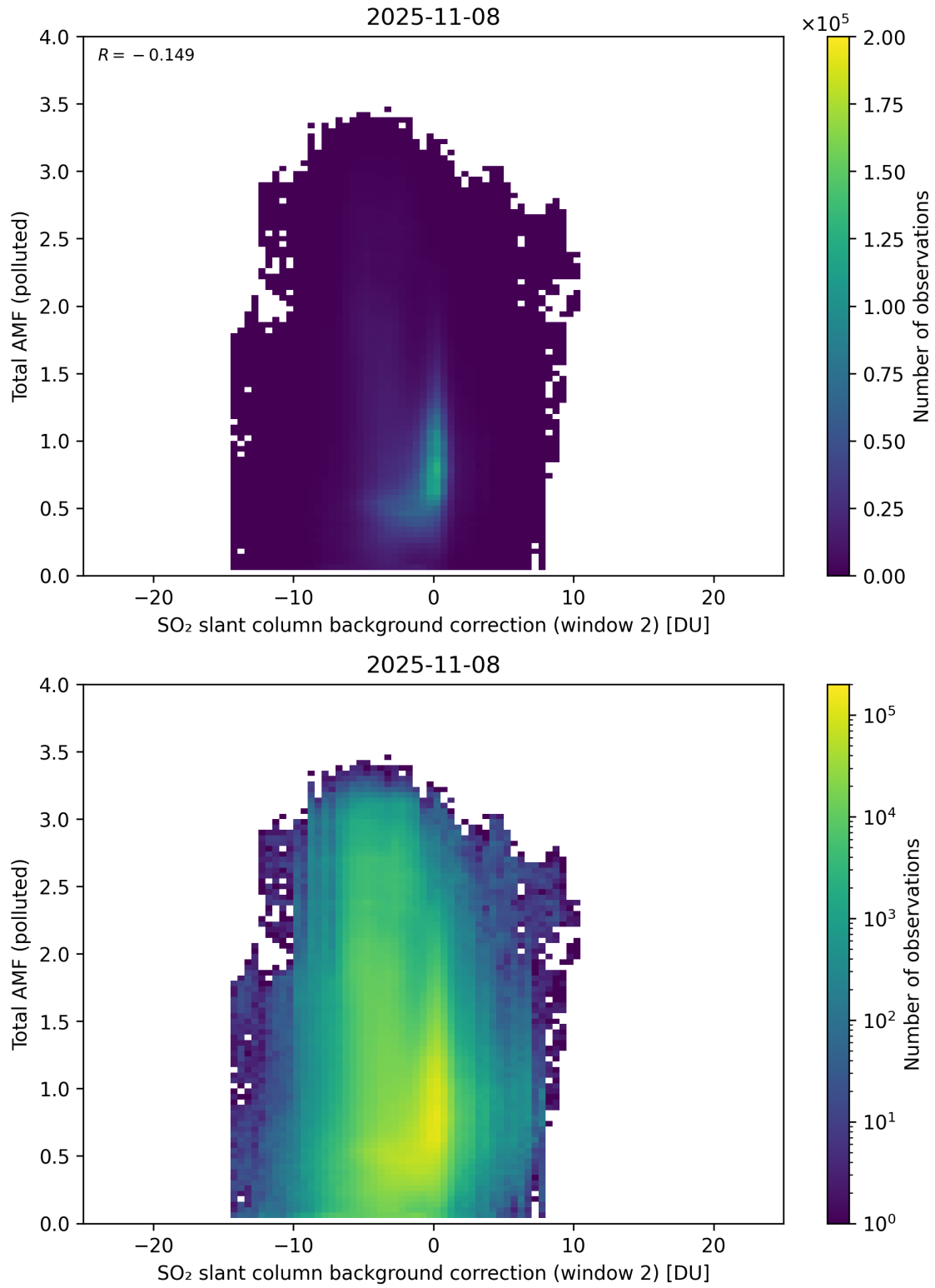
Figure 130: Scatter density plot of “SO 2 slant column background correction (window 2)” against “Total AMF (polluted)” for 2025-11-07 to 2025-11-09.
