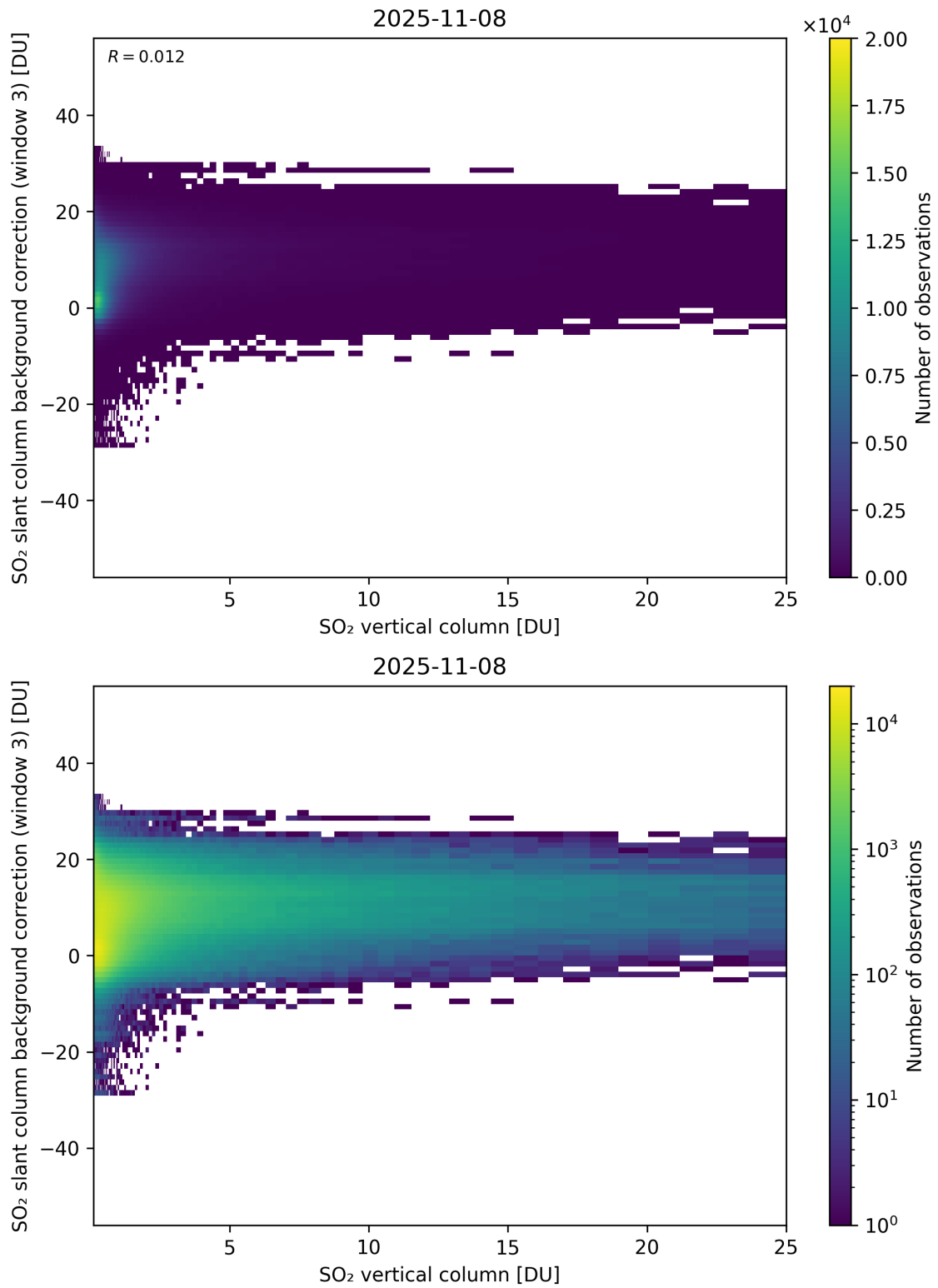
Figure 325: Scatter density plot of “SO 2 vertical column” against “SO 2 slant column background correction (window 3)” for 2025-11-07 to 2025-11-09.
