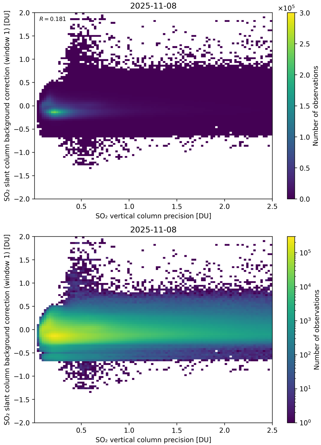
Figure 329: Scatter density plot of “SO 2 vertical column precision” against “SO 2 slant column background correction (window 1)” for 2025-11-07 to 2025-11-09.
