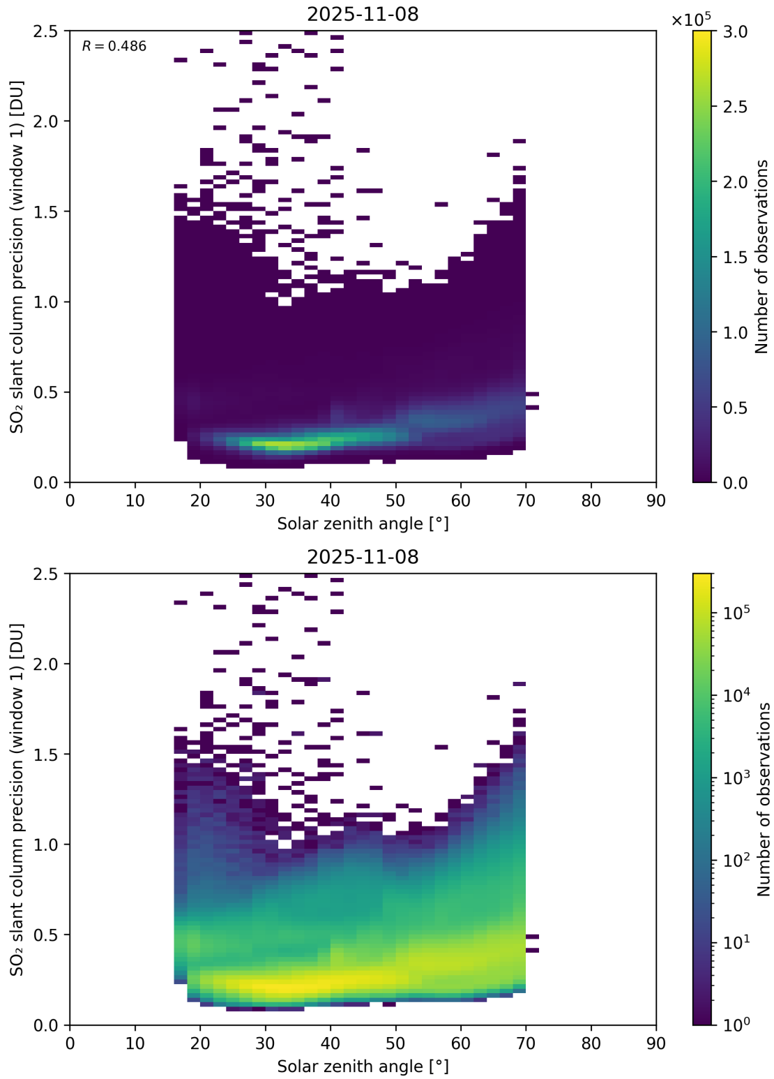
Figure 185: Scatter density plot of “Solar zenith angle” against “SO 2 slant column precision (window 1)” for 2025-11-07 to 2025-11-09.
