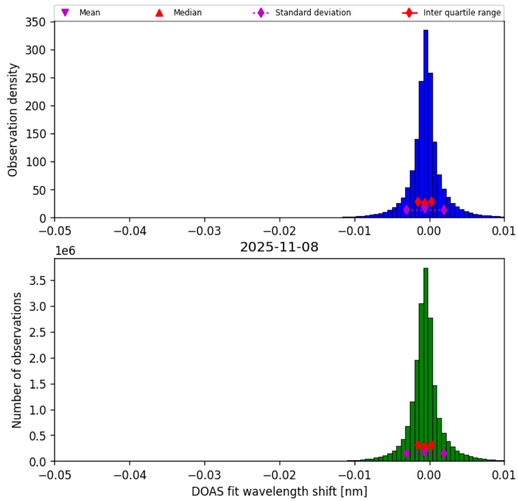
Figure 76: Histogram of “DOAS fit wavelength shift” for 2025-11-07 to 2025-11-09
