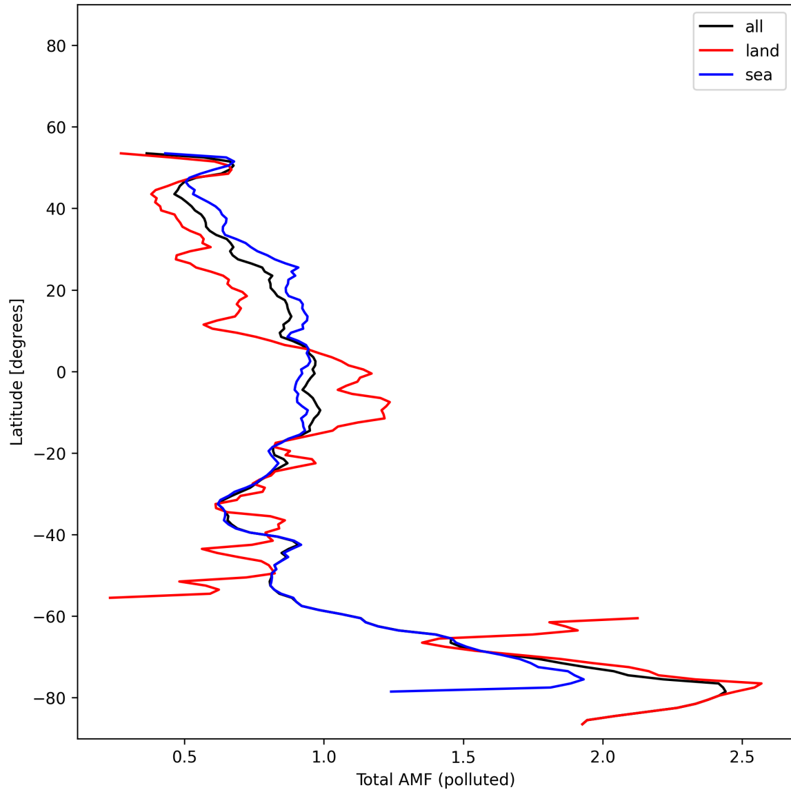
Figure 53: Zonal average of “Total AMF (polluted)” for 2025-11-07 to 2025-11-09.
