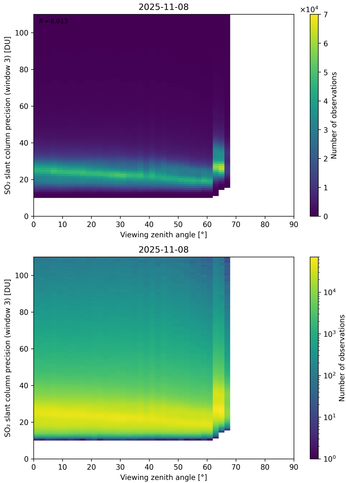
Figure 380: Scatter density plot of “Viewing zenith angle” against “SO 2 slant column precision (window 3)” for 2025-11-07 to 2025-11-09.
