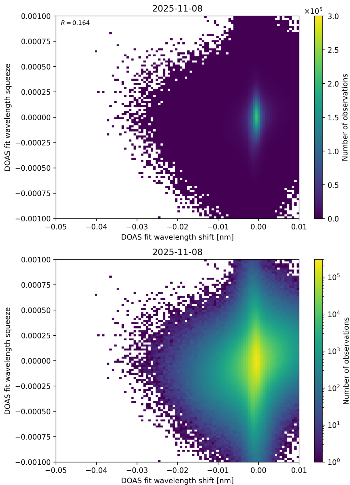
Figure 138: Scatter density plot of “DOAS fit wavelength shift” against “DOAS fit wavelength squeeze” for 2025-11-07 to 2025-11-09.
