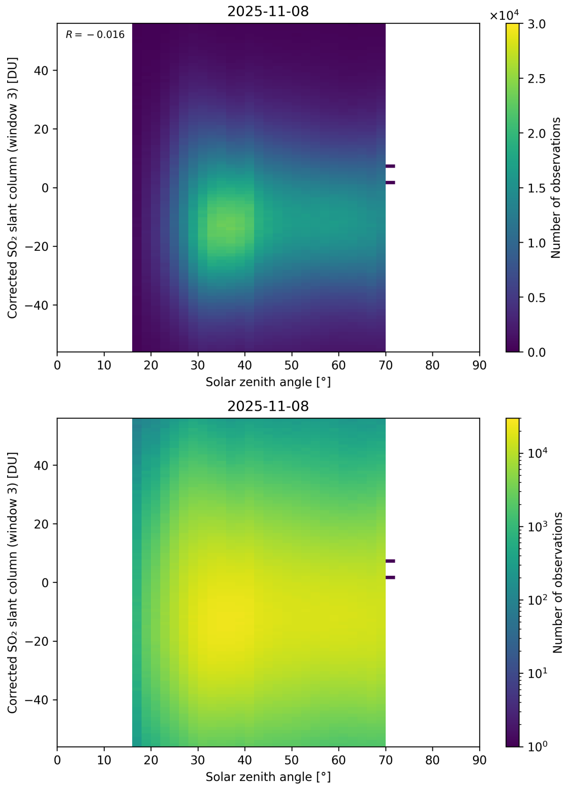
Figure 183: Scatter density plot of “Solar zenith angle” against “Corrected SO 2 slant column (window 3)” for 2025-11-07 to 2025-11-09.
