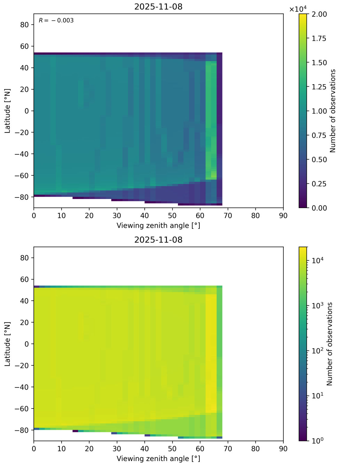
Figure 368: Scatter density plot of “Viewing zenith angle” against “Latitude” for 2025-11-07 to 2025-11-09.
