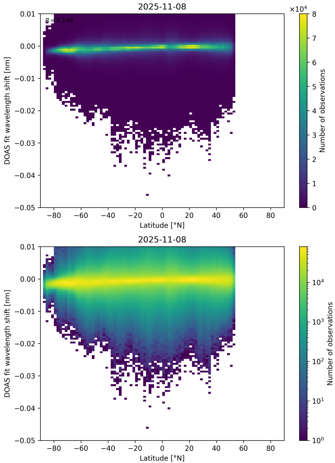
Figure 153: Scatter density plot of “Latitude” against “DOAS fit wavelength shift” for 2025-11-07 to 2025-11-09.
