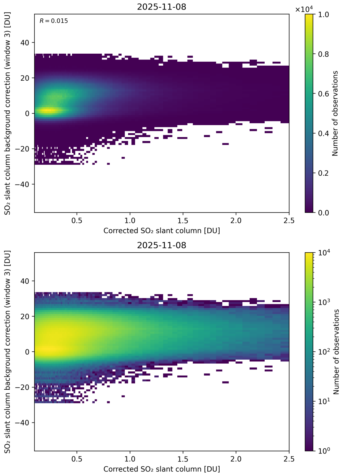
Figure 228: Scatter density plot of “Corrected SO 2 slant column” against “SO 2 slant column background correction (window 3)” for 2025-11-07 to 2025-11-09.
