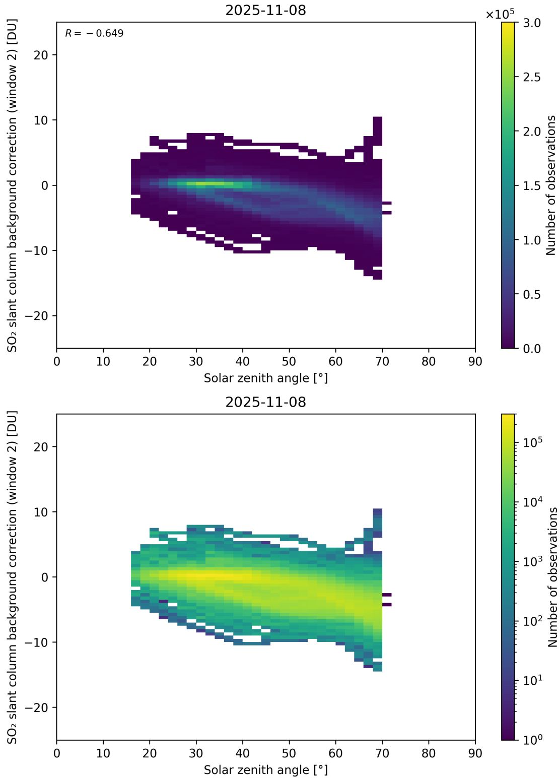
Figure 172: Scatter density plot of “Solar zenith angle” against “SO 2 slant column background correction (window 2)” for 2025-11-07 to 2025-11-09.
