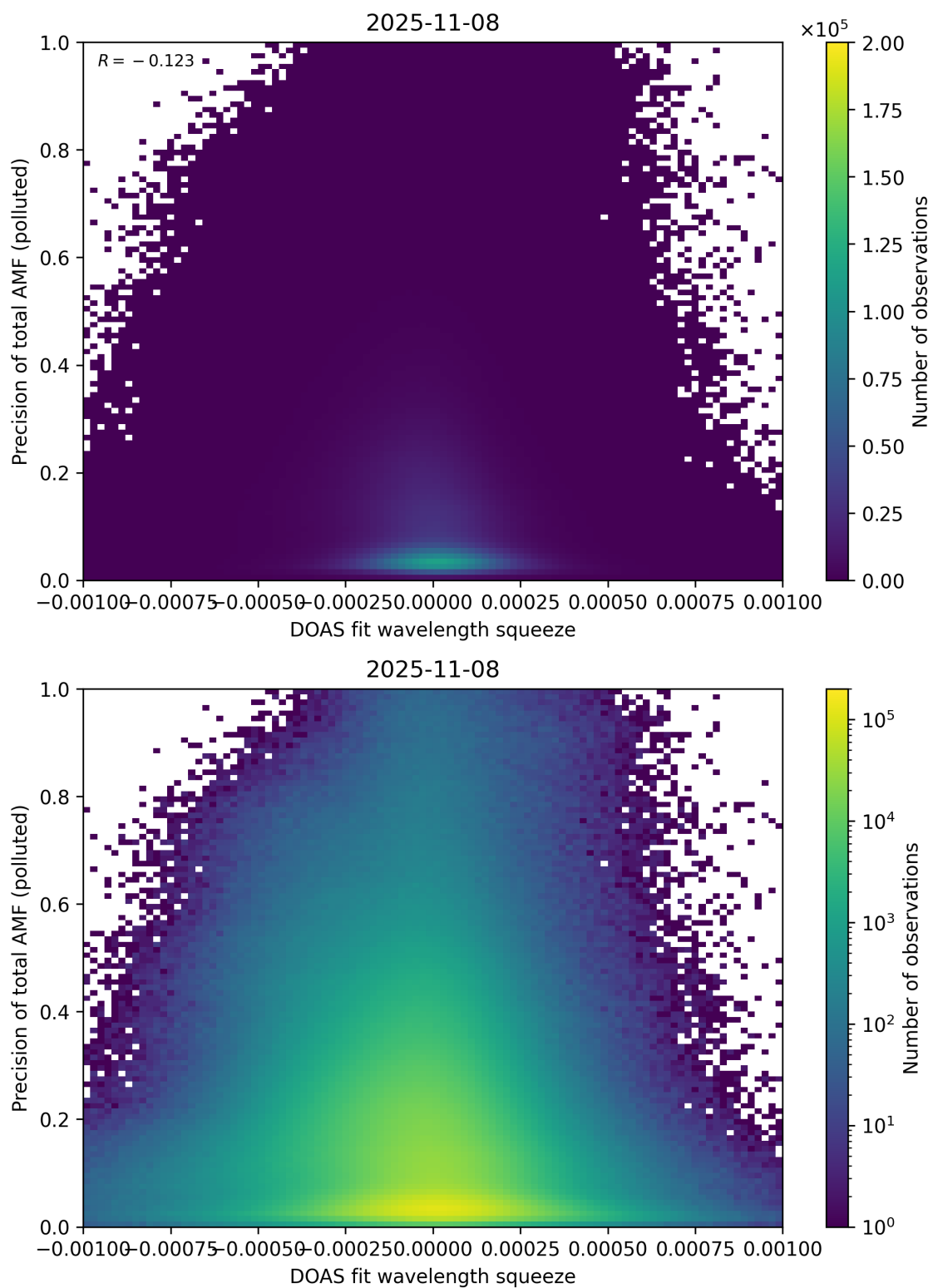
Figure 146: Scatter density plot of “DOAS fit wavelength squeeze” against “Precision of total AMF (polluted)” for 2025-11-07 to 2025-11-09.
