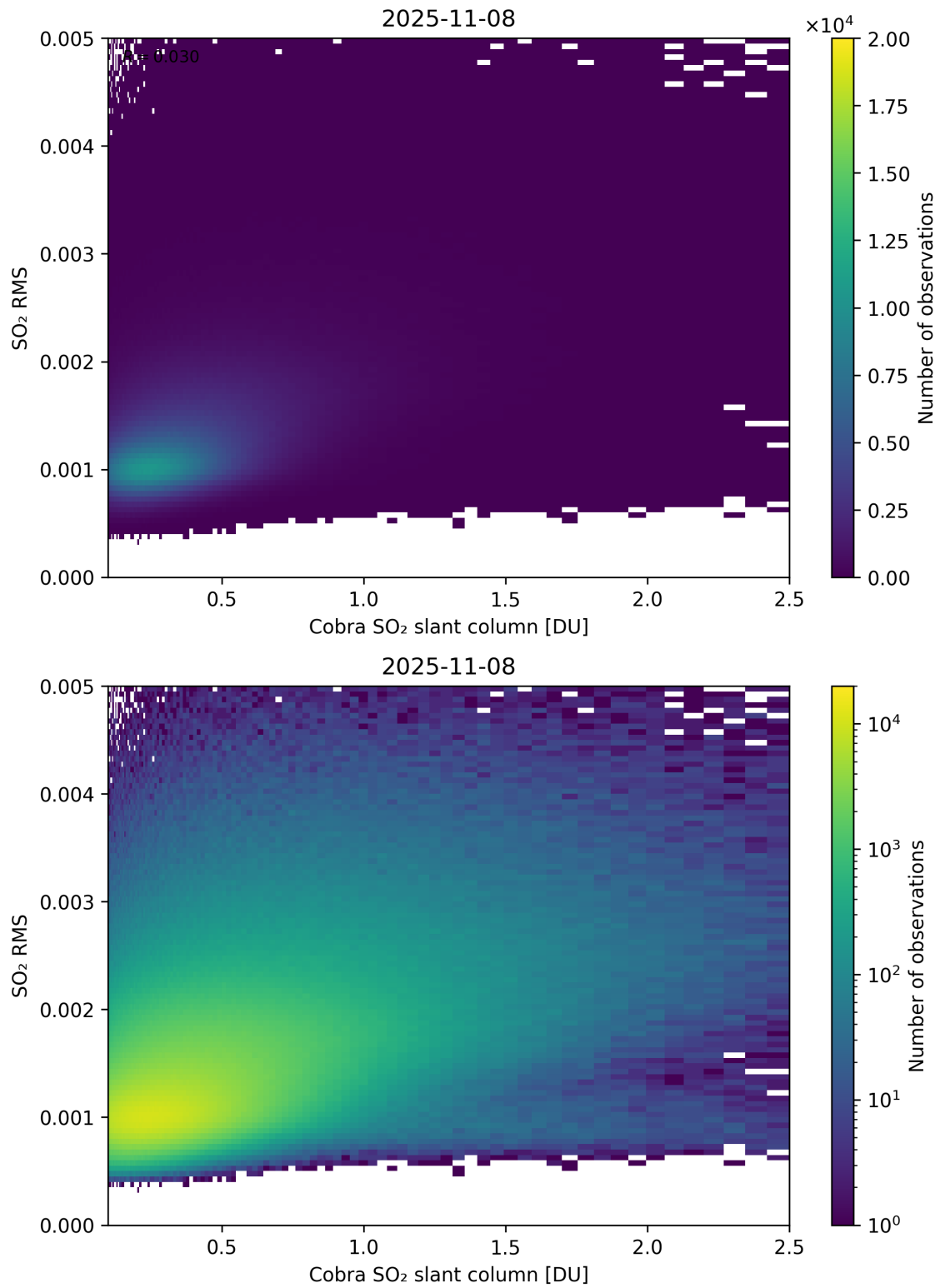
Figure 198: Scatter density plot of “Cobra SO 2 slant column” against “SO 2 RMS” for 2025-11-07 to 2025-11-09.
