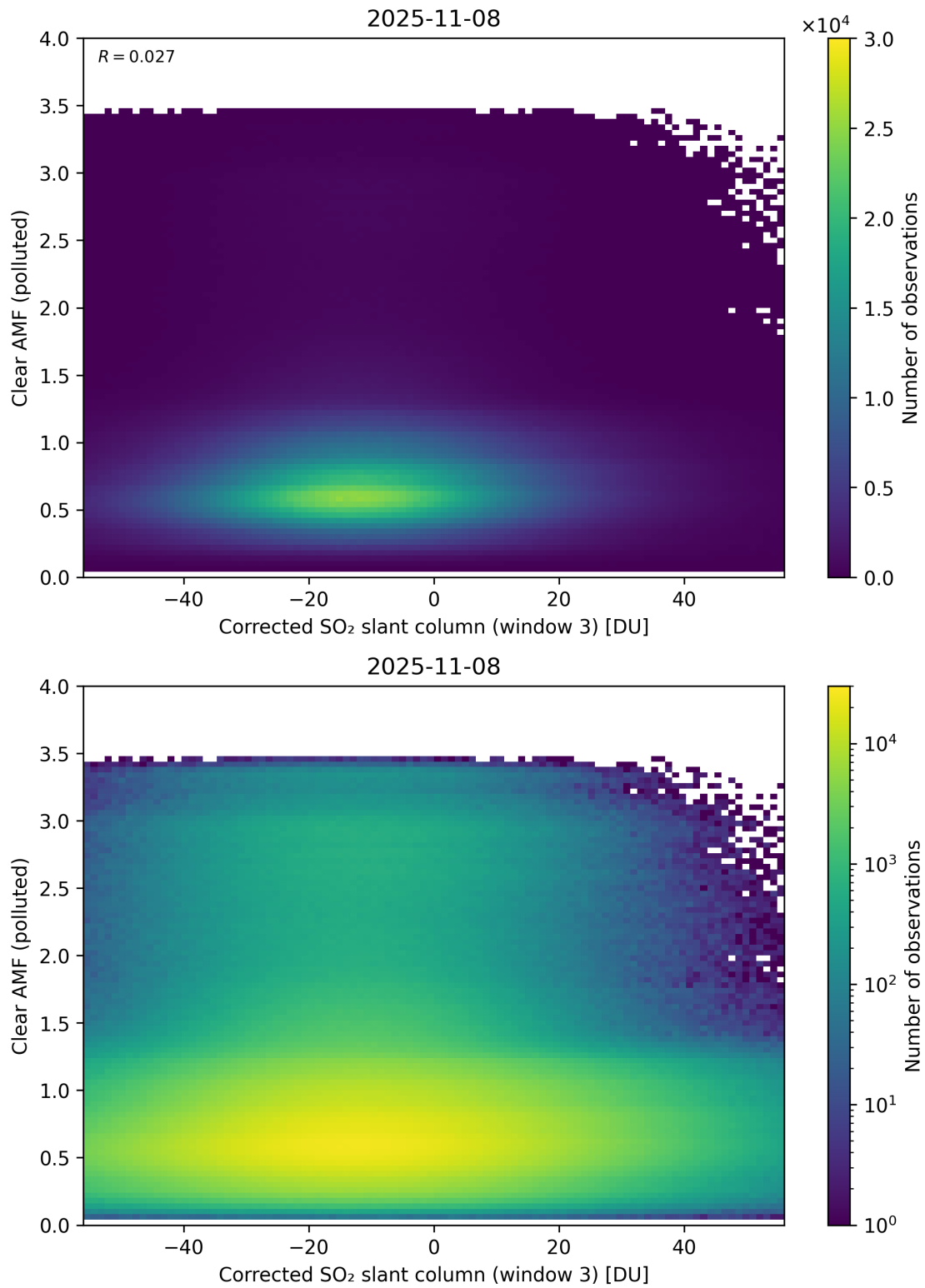
Figure 259: Scatter density plot of “Corrected SO 2 slant column (window 3)” against “Clear AMF (polluted)” for 2025-11-07 to 2025-11-09.
