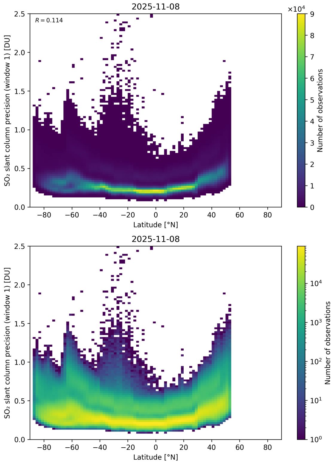
Figure 163: Scatter density plot of “Latitude” against “SO 2 slant column precision (window 1)” for 2025-11-07 to 2025-11-09.
