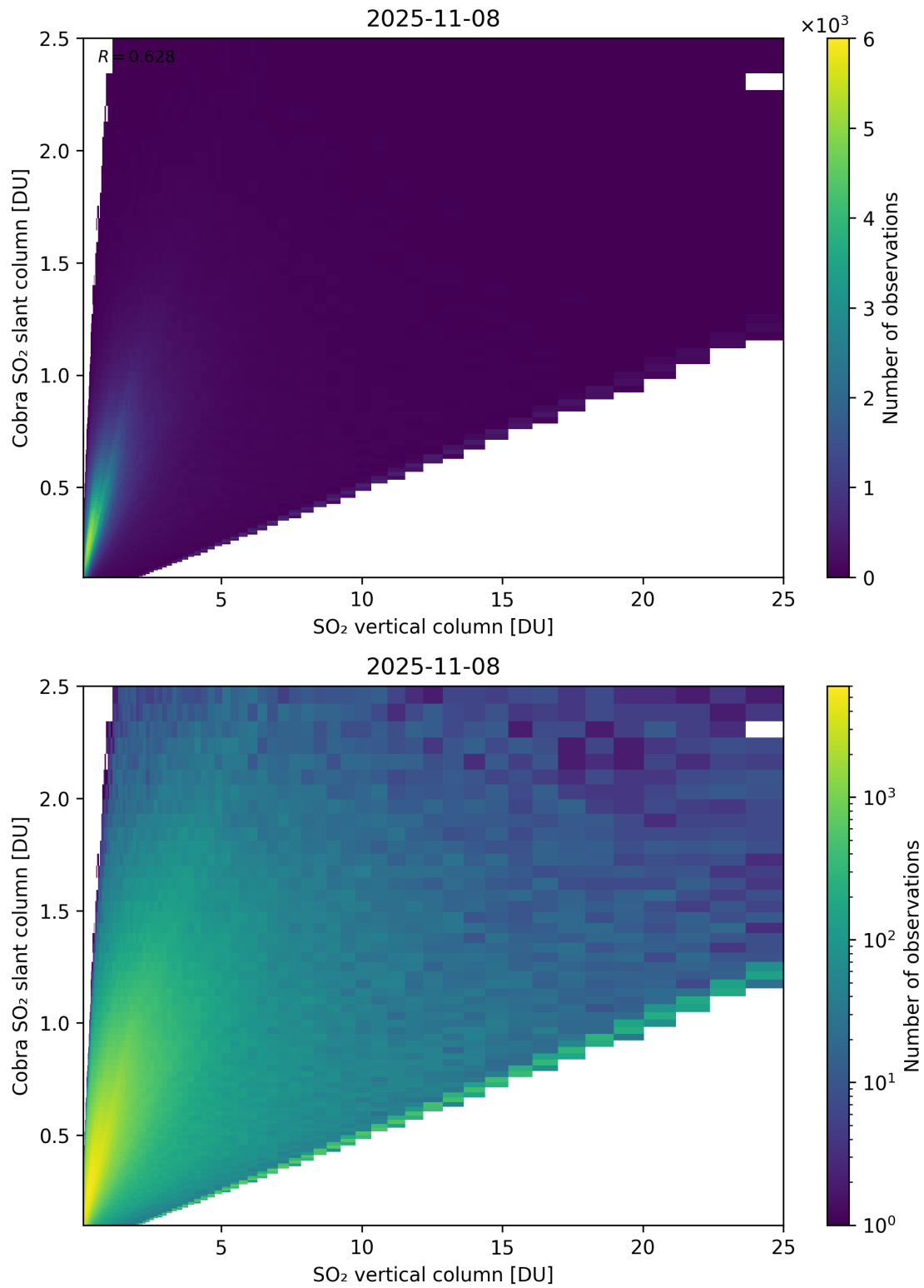
Figure 349: Scatter density plot of “SO 2 vertical column” against “Cobra SO 2 slant column” for 2025-11-07 to 2025-11-09.
