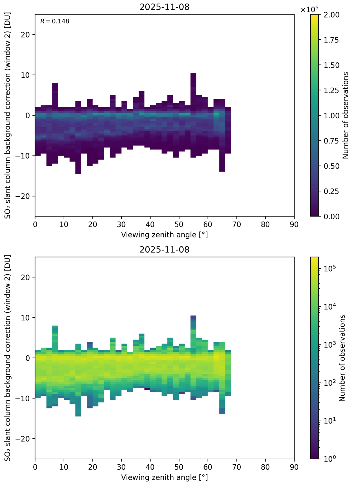
Figure 363: Scatter density plot of “Viewing zenith angle” against “SO 2 slant column background correction (window 2)” for 2025-11-07 to 2025-11-09.
