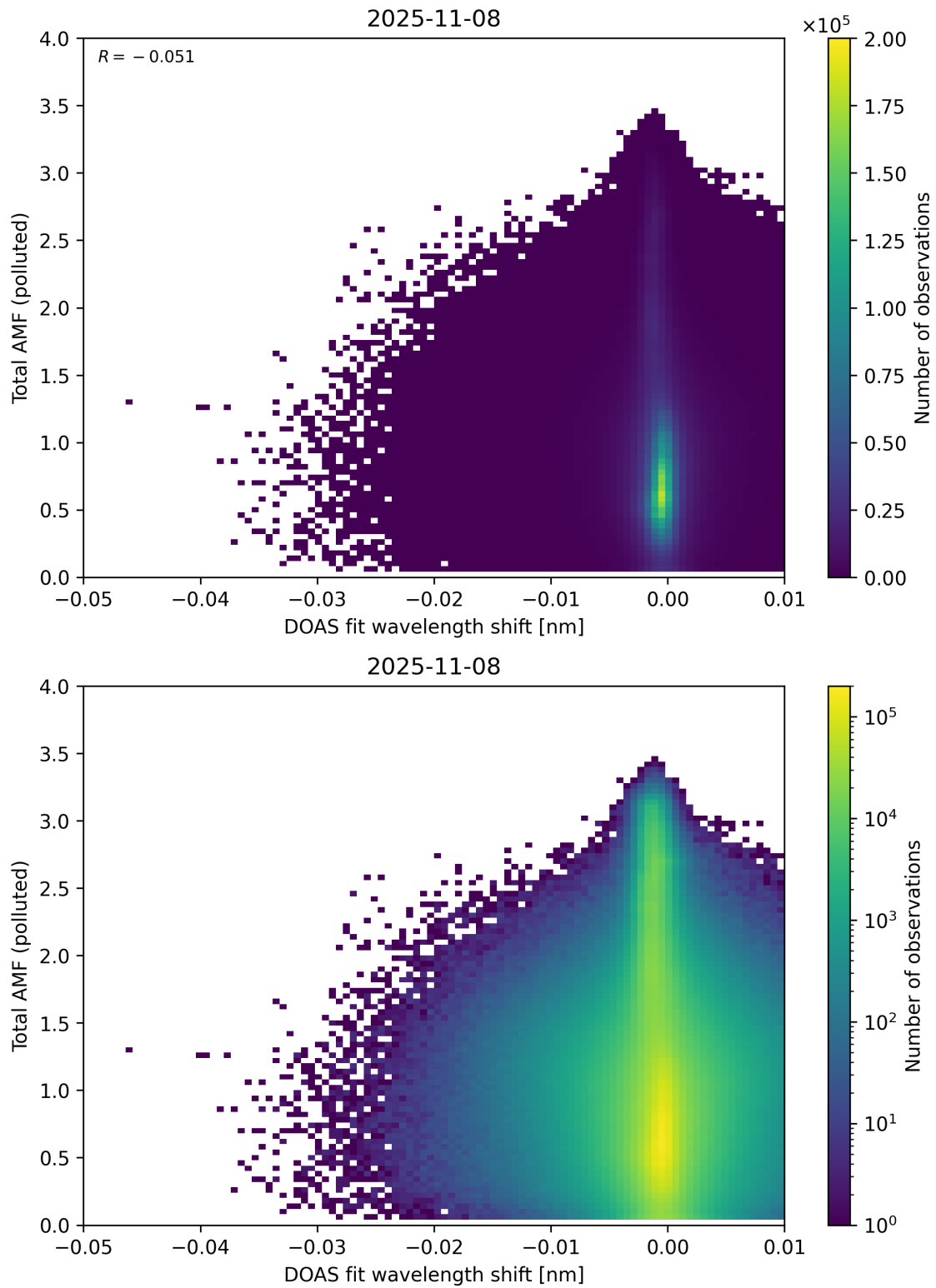
Figure 141: Scatter density plot of “DOAS fit wavelength shift” against “Total AMF (polluted)” for 2025-11-07 to 2025-11-09.
