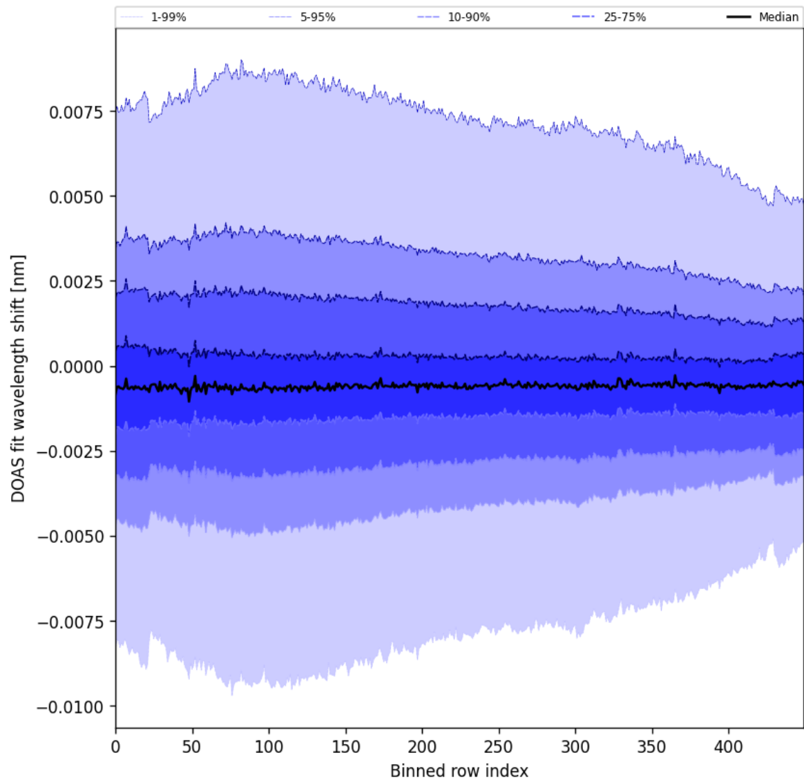
Figure 102: Along track statistics of “DOAS fit wavelength shift” for 2025-11-07 to 2025-11-09
