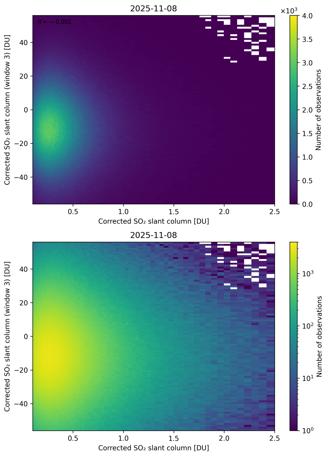
Figure 236: Scatter density plot of “Corrected SO 2 slant column” against “Corrected SO 2 slant column (window 3)” for 2025-11-07 to 2025-11-09.
