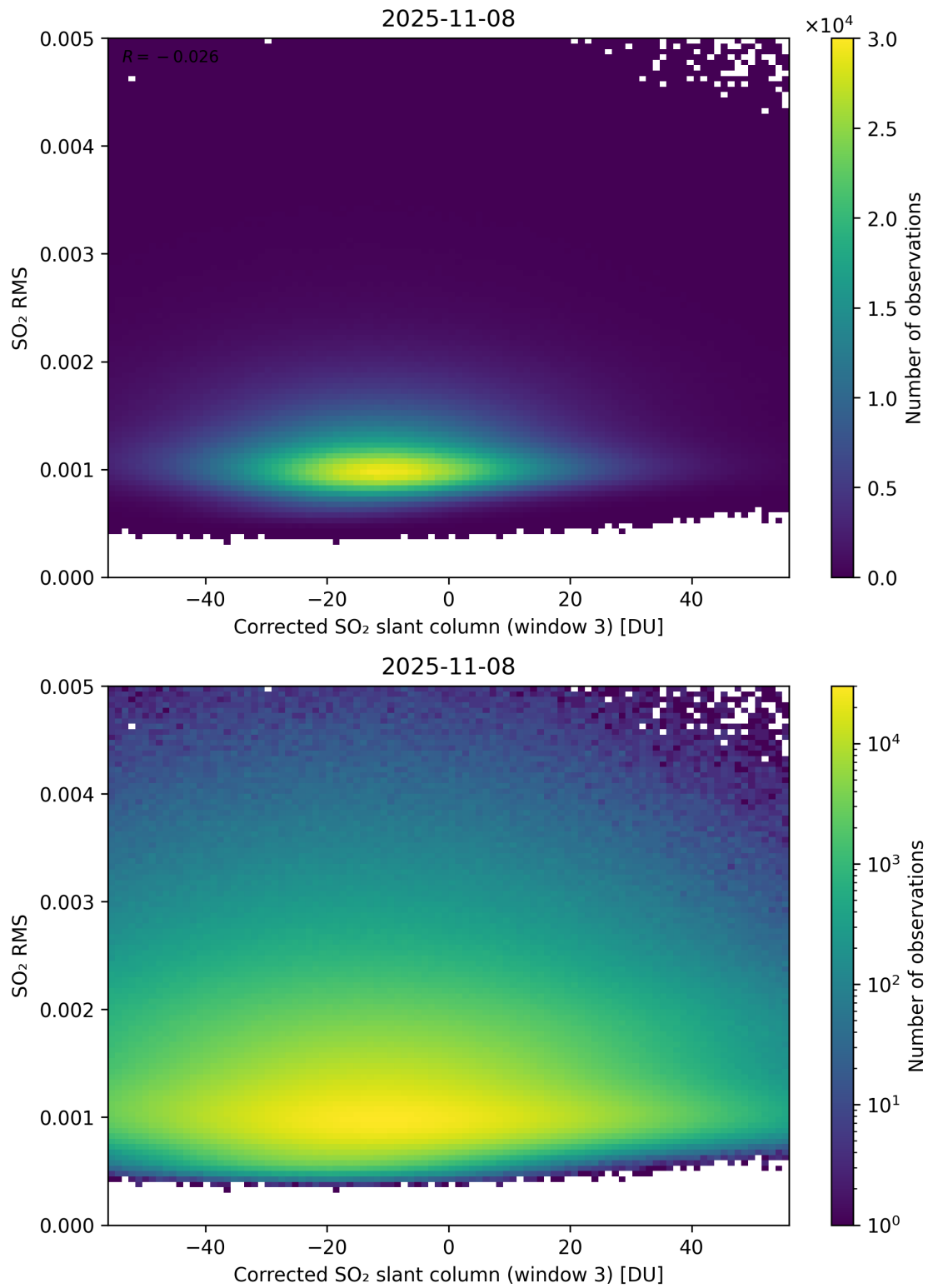
Figure 258: Scatter density plot of “Corrected SO 2 slant column (window 3)” against “SO 2 RMS” for 2025-11-07 to 2025-11-09.
