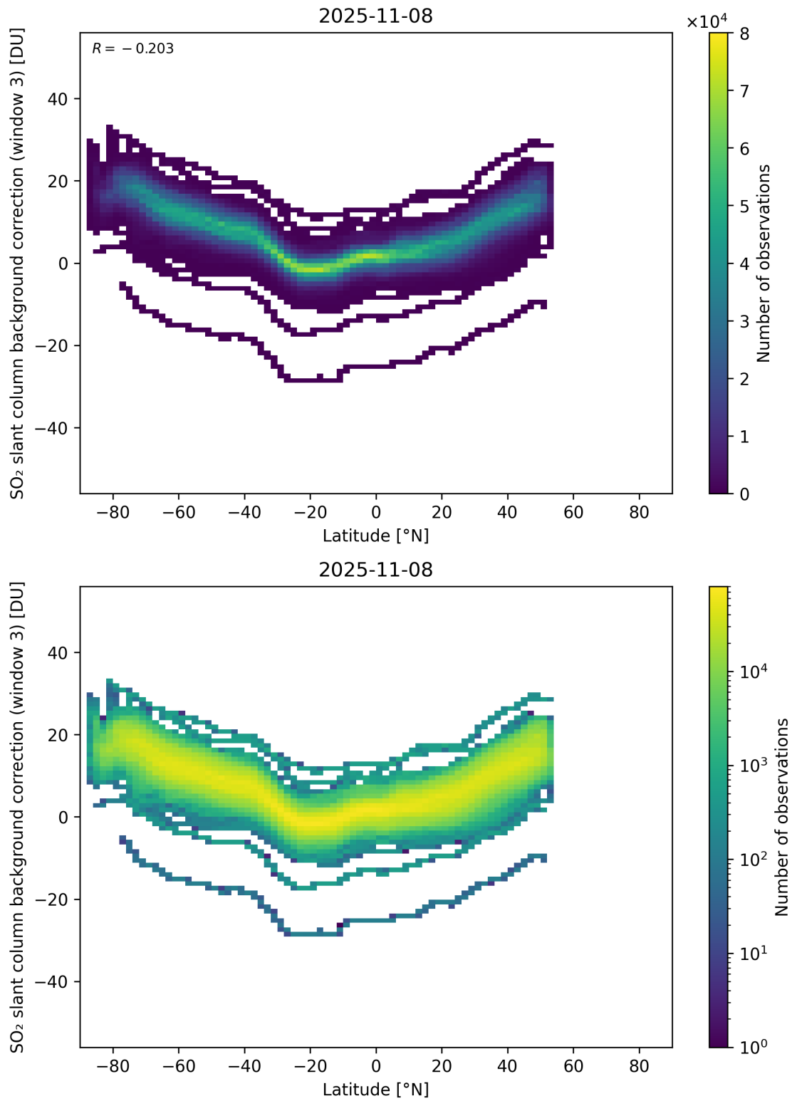
Figure 152: Scatter density plot of “Latitude” against “SO 2 slant column background correction (window 3)” for 2025-11-07 to 2025-11-09.
