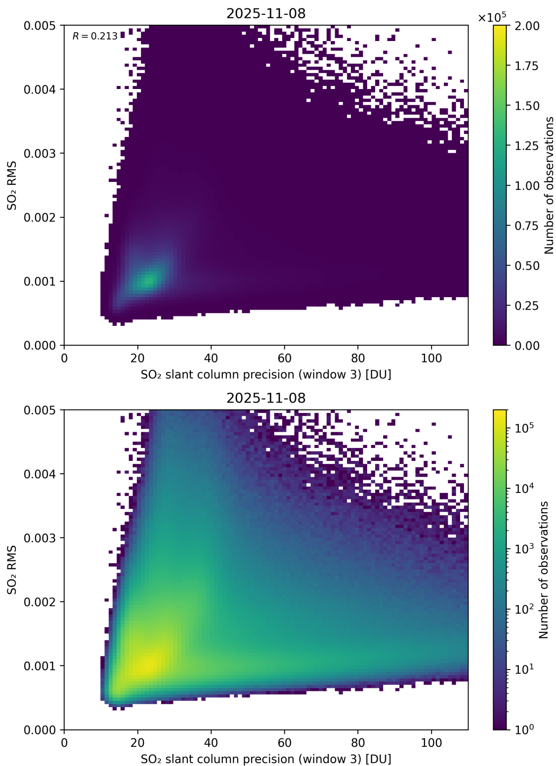
Figure 310: Scatter density plot of “SO 2 slant column precision (window 3)” against “SO 2 RMS” for 2025-11-07 to 2025-11-09.
