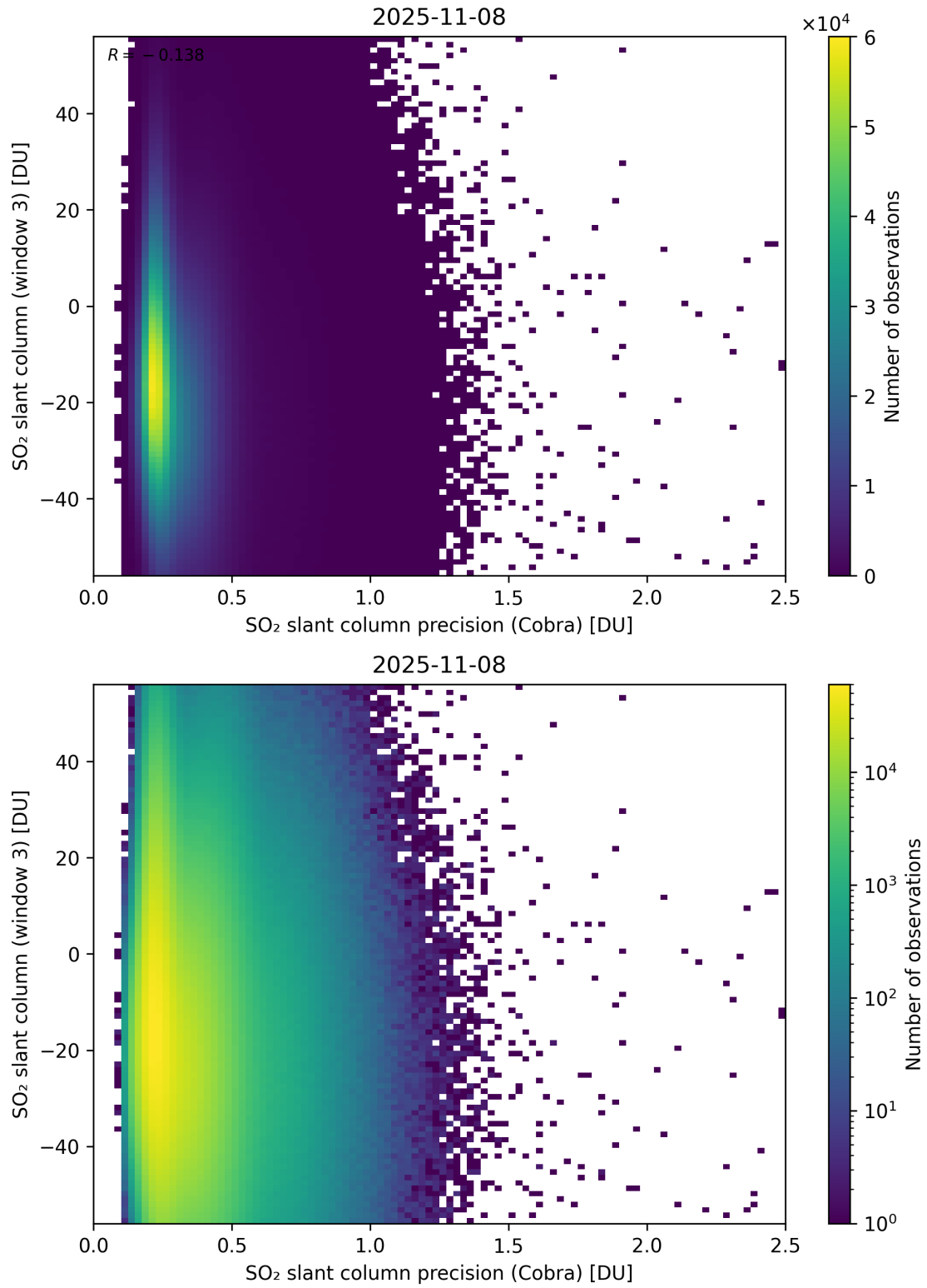
Figure 211: Scatter density plot of “SO 2 slant column precision (Cobra)” against “SO 2 slant column (window 3)” for 2025-11-07 to 2025-11-09.
