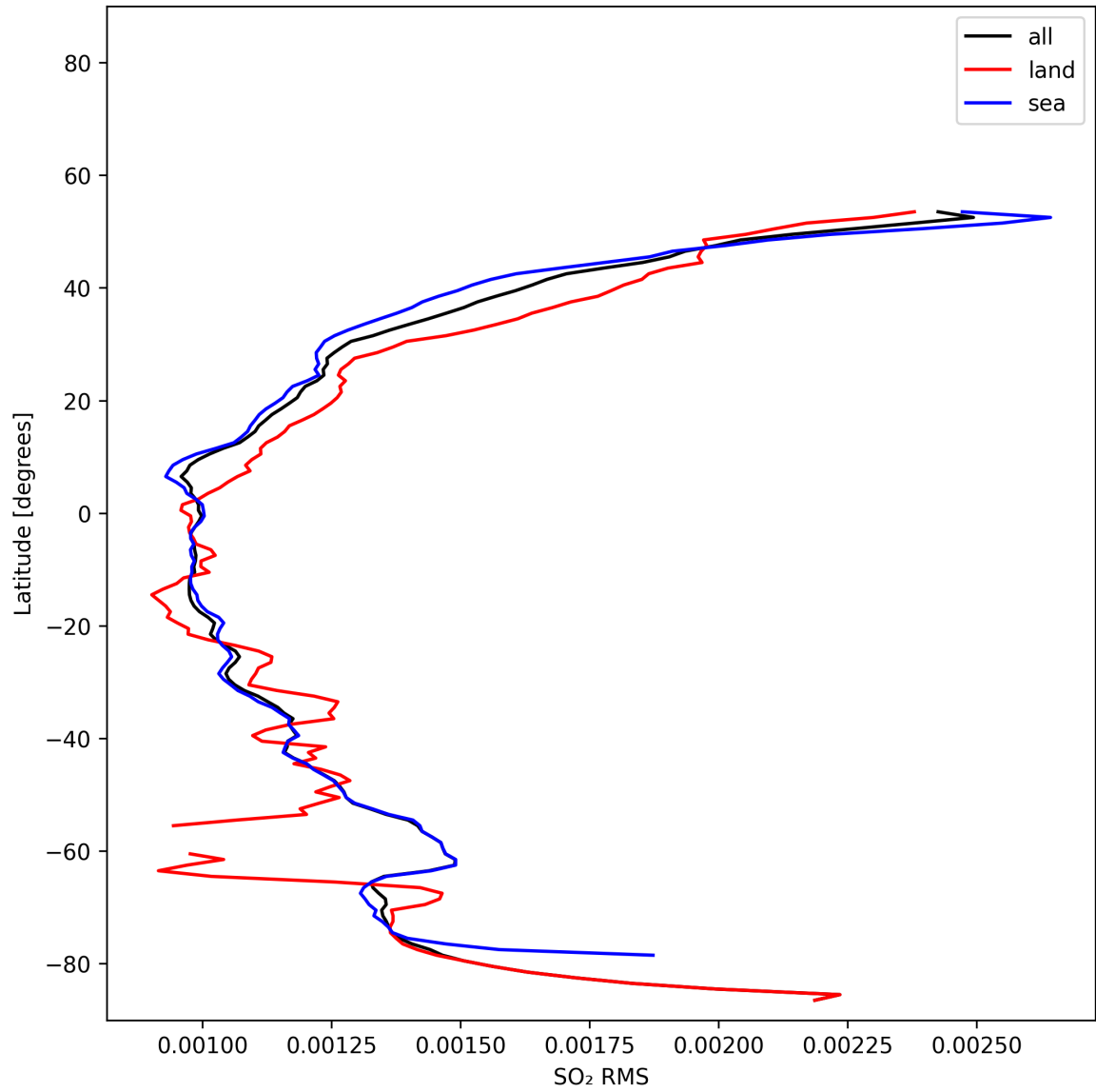
Figure 52: Zonal average of “SO 2 RMS” for 2025-11-07 to 2025-11-09.
