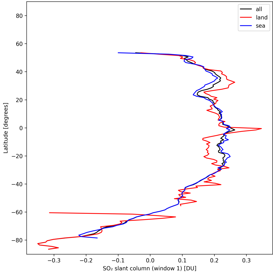
Figure 37: Zonal average of “SO 2 slant column (window 1)” for 2025-11-07 to 2025-11-09.
