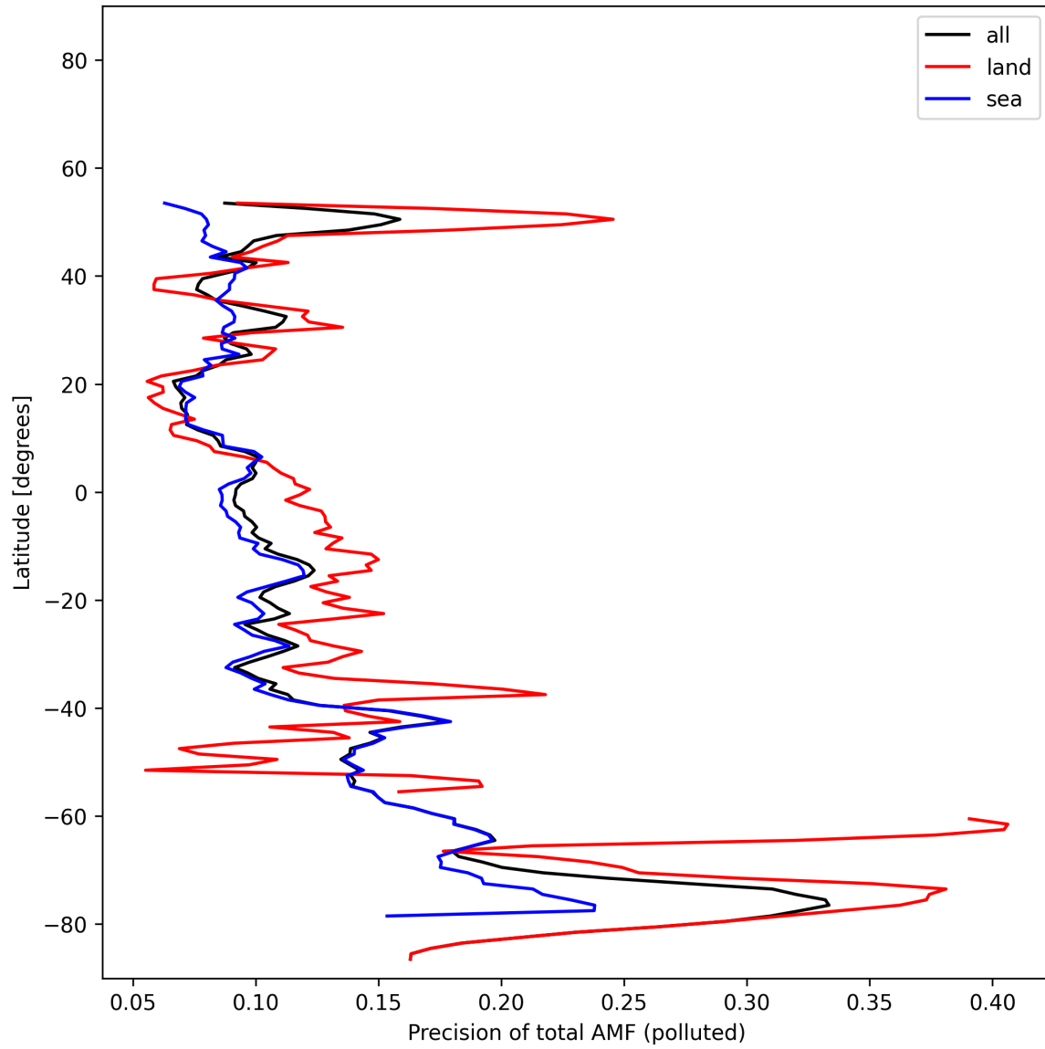
Figure 54: Zonal average of “Precision of total AMF (polluted)” for 2025-11-07 to 2025-11-09.
