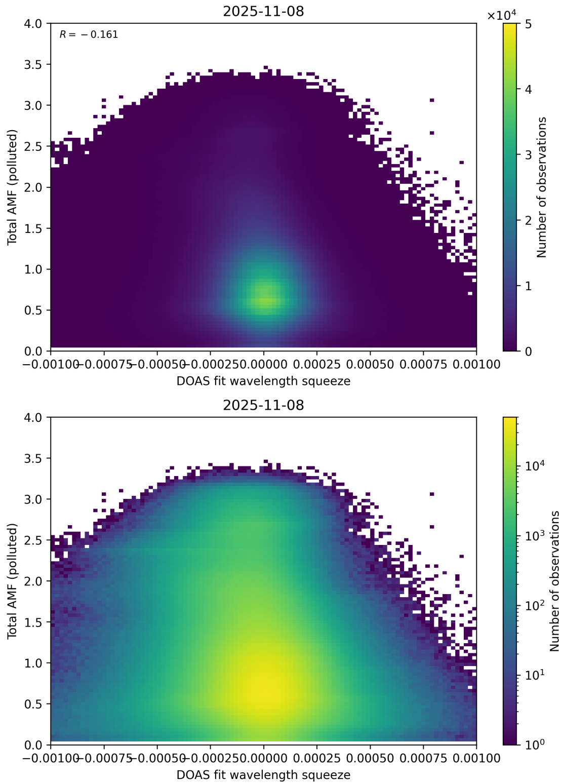
Figure 145: Scatter density plot of “DOAS fit wavelength squeeze” against “Total AMF (polluted)” for 2025-11-07 to 2025-11-09.
