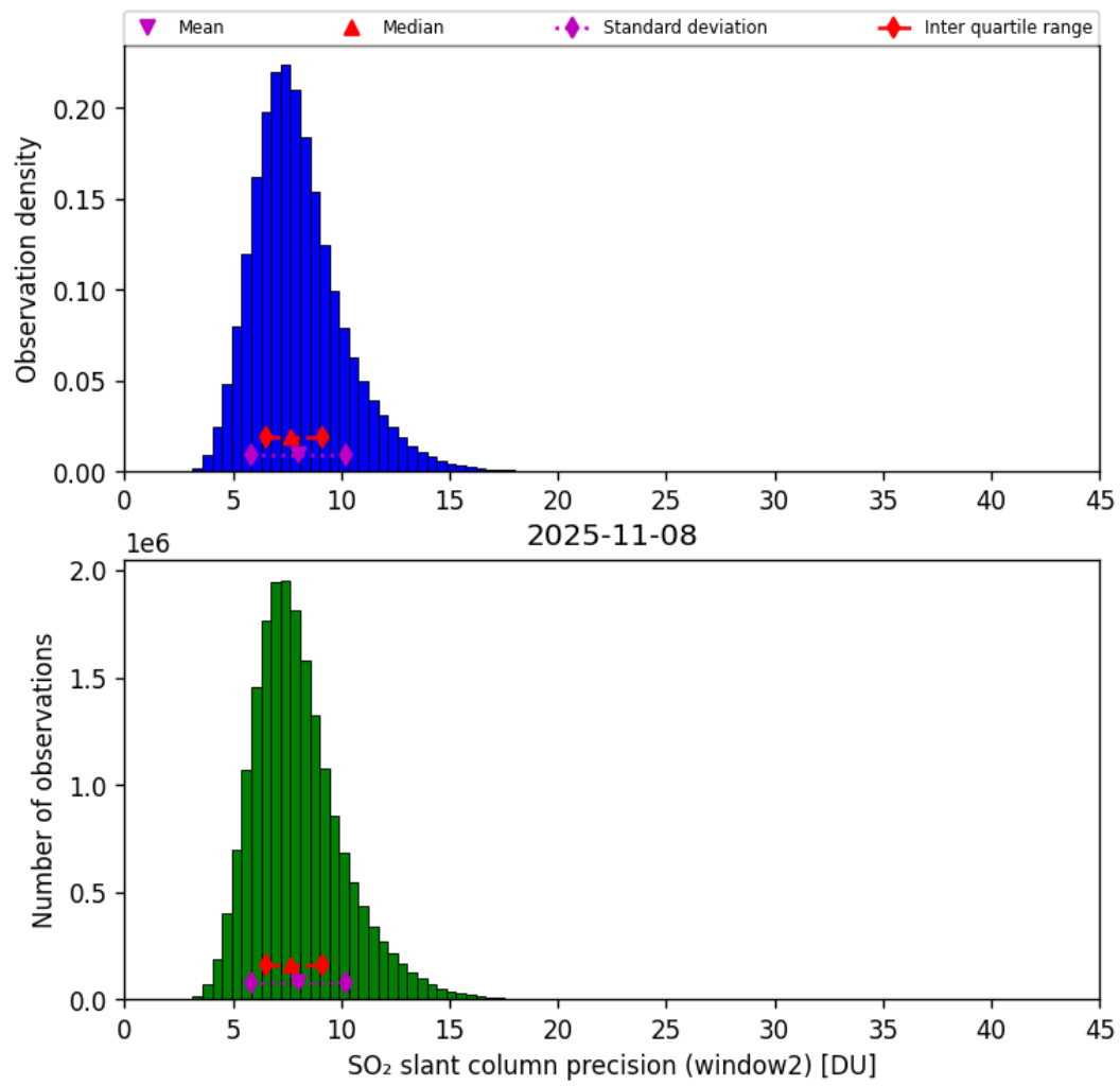
Figure 68: Histogram of “SO 2 slant column precision (window2)” for 2025-11-07 to 2025-11-09
