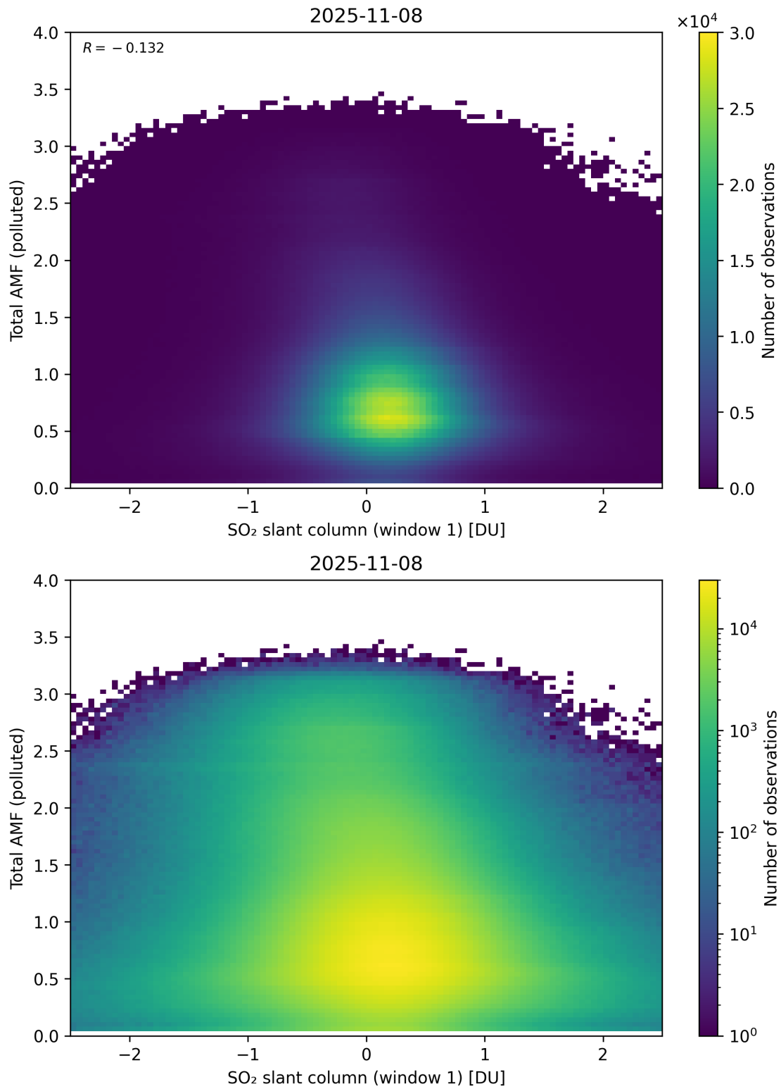
Figure 289: Scatter density plot of “SO 2 slant column (window 1)” against “Total AMF (polluted)” for 2025-11-07 to 2025-11-09.
