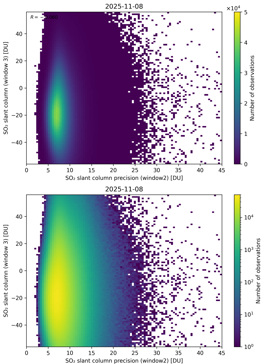
Figure 299: Scatter density plot of “SO 2 slant column precision (window2)” against “SO 2 slant column (window 3)” for 2025-11-07 to 2025-11-09.
