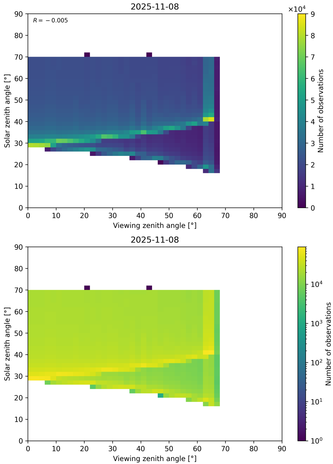
Figure 369: Scatter density plot of “Viewing zenith angle” against “Solar zenith angle” for 2025-11-07 to 2025-11-09.
