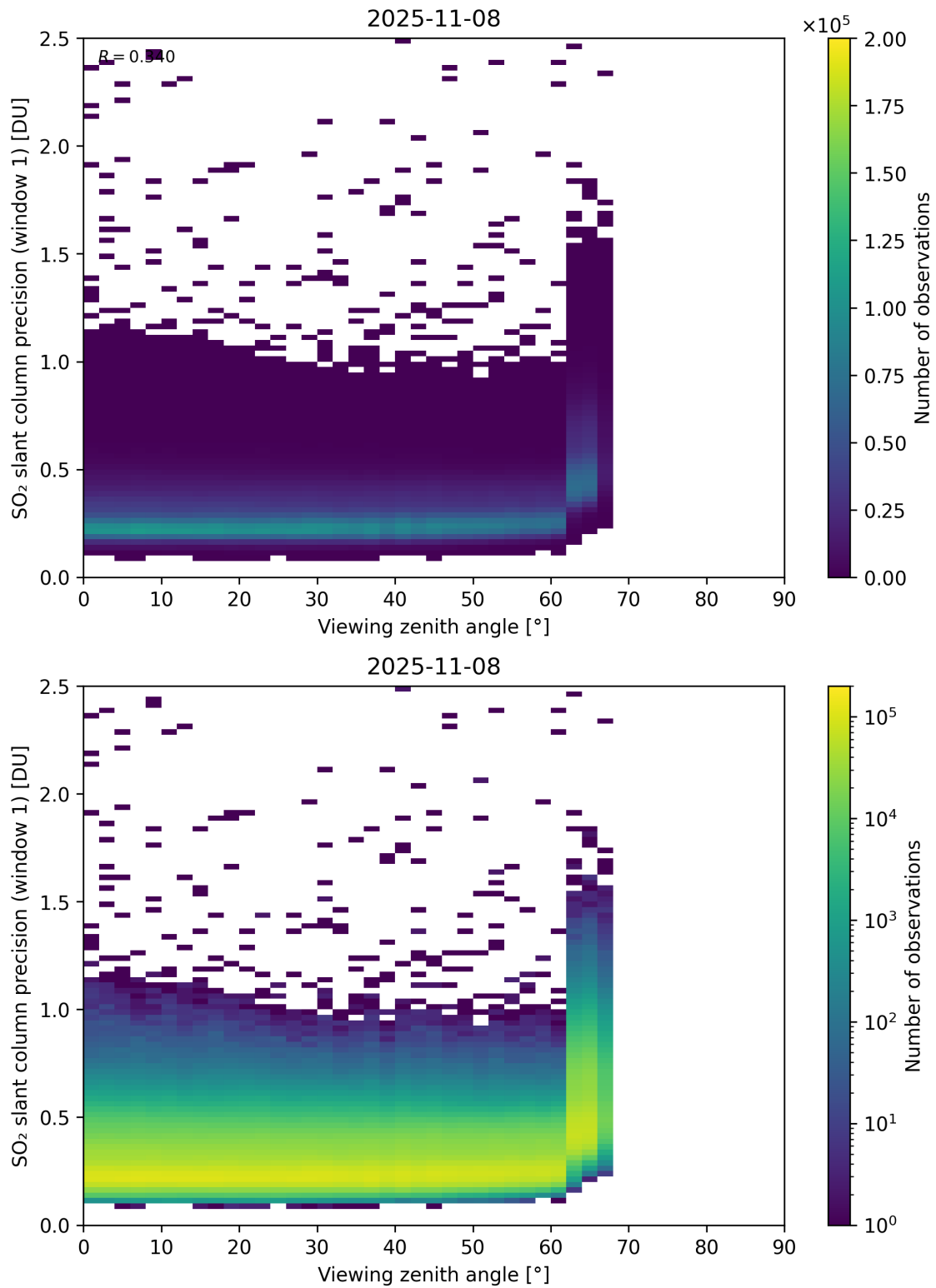
Figure 377: Scatter density plot of “Viewing zenith angle” against “SO 2 slant column precision (window 1)” for 2025-11-07 to 2025-11-09.
