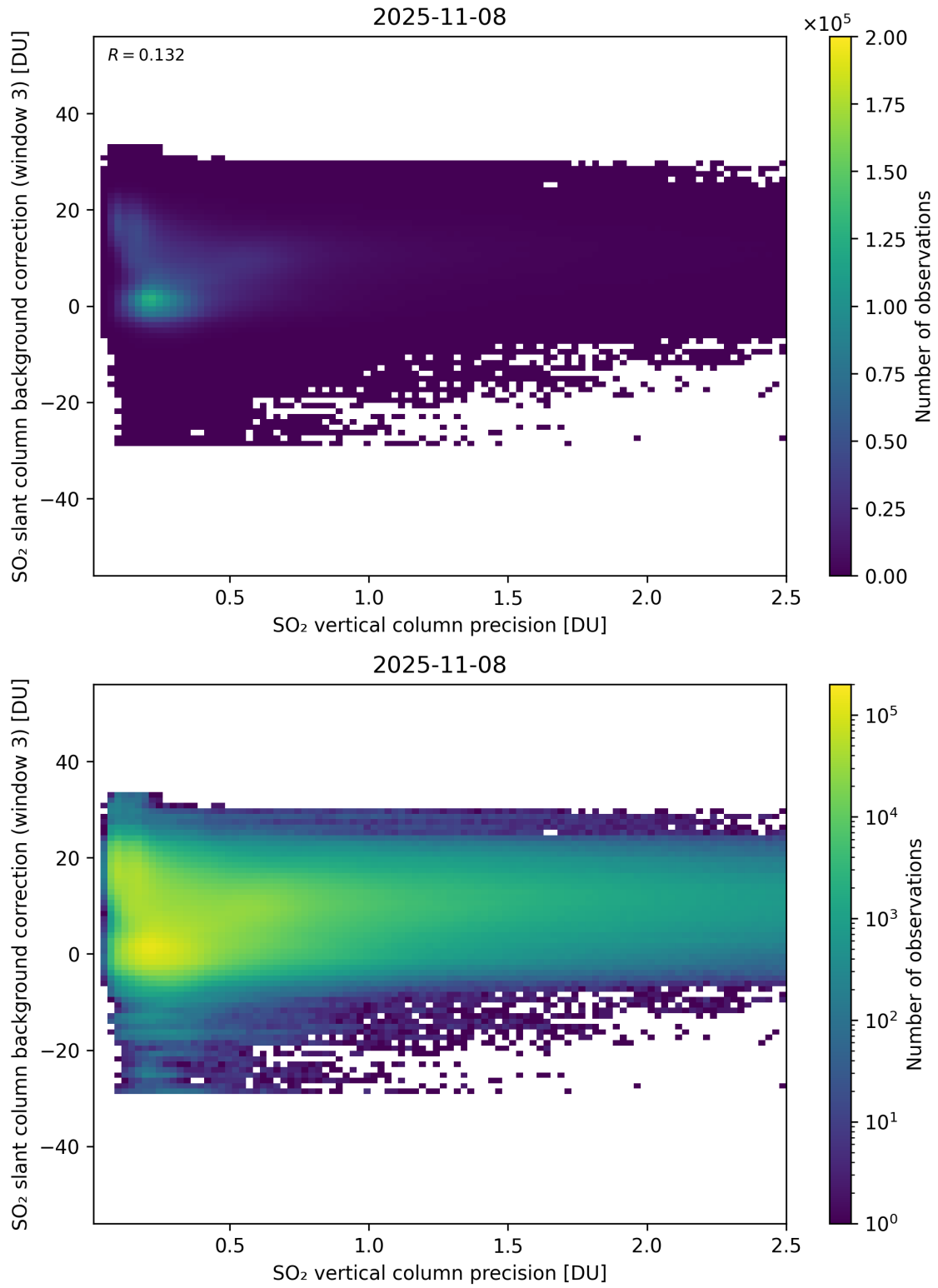
Figure 331: Scatter density plot of “SO 2 vertical column precision” against “SO 2 slant column background correction (window 3)” for 2025-11-07 to 2025-11-09.
