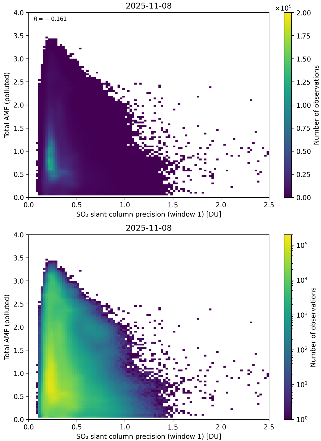
Figure 280: Scatter density plot of “SO 2 slant column precision (window 1)” against “Total AMF (polluted)” for 2025-11-07 to 2025-11-09.
