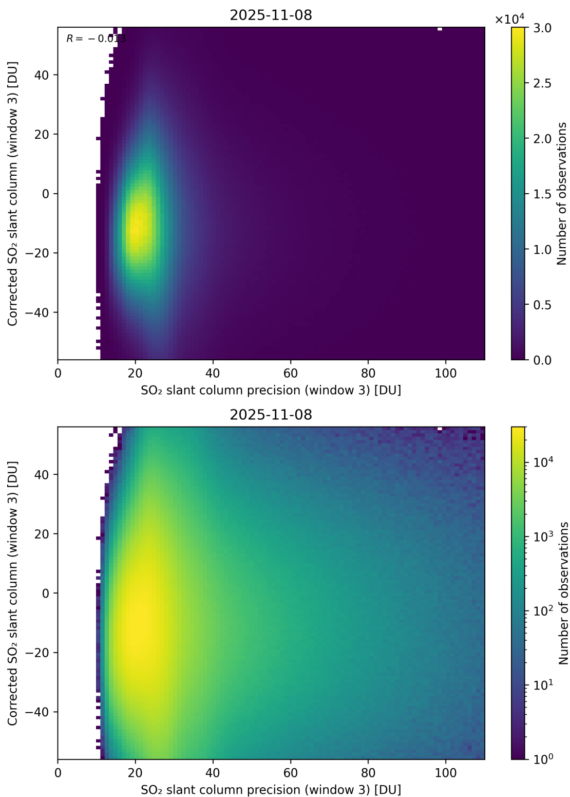
Figure 312: Scatter density plot of “SO 2 slant column precision (window 3)” against “Corrected SO 2 slant column (window 3)” for 2025-11-07 to 2025-11-09.
