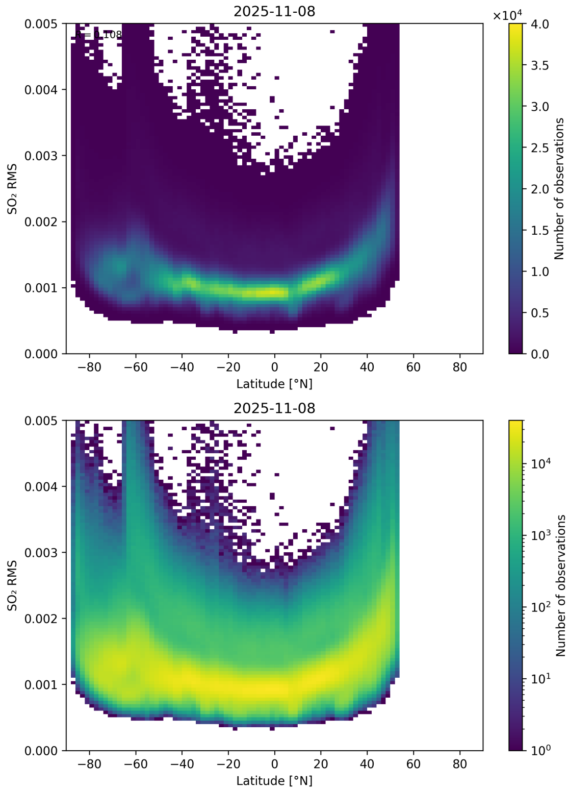
Figure 155: Scatter density plot of “Latitude” against “SO 2 RMS” for 2025-11-07 to 2025-11-09.
