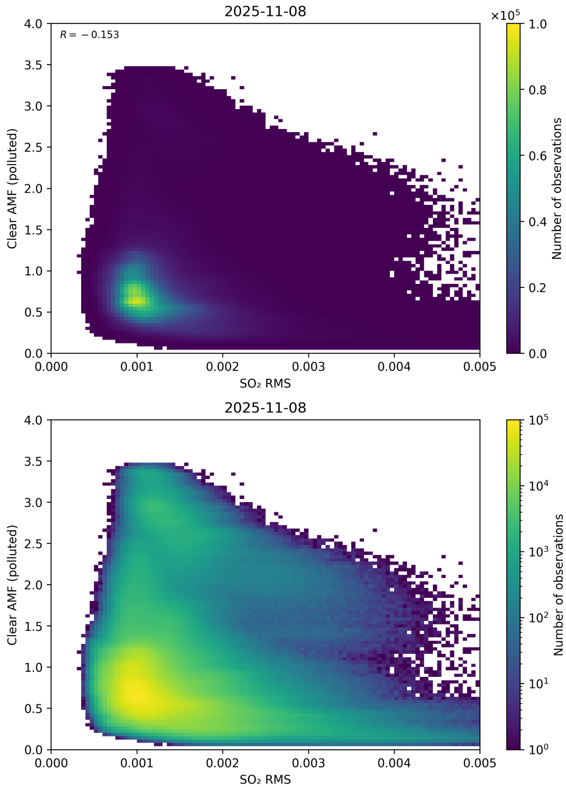
Figure 147: Scatter density plot of “SO 2 RMS” against “Clear AMF (polluted)” for 2025-11-07 to 2025-11-09.
