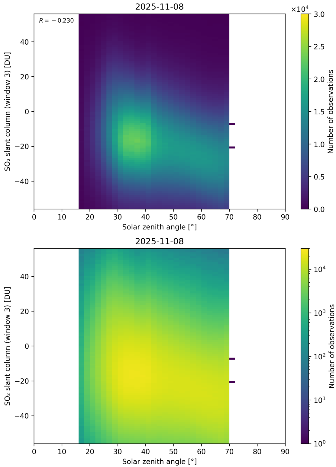
Figure 187: Scatter density plot of “Solar zenith angle” against “SO 2 slant column (window 3)” for 2025-11-07 to 2025-11-09.
