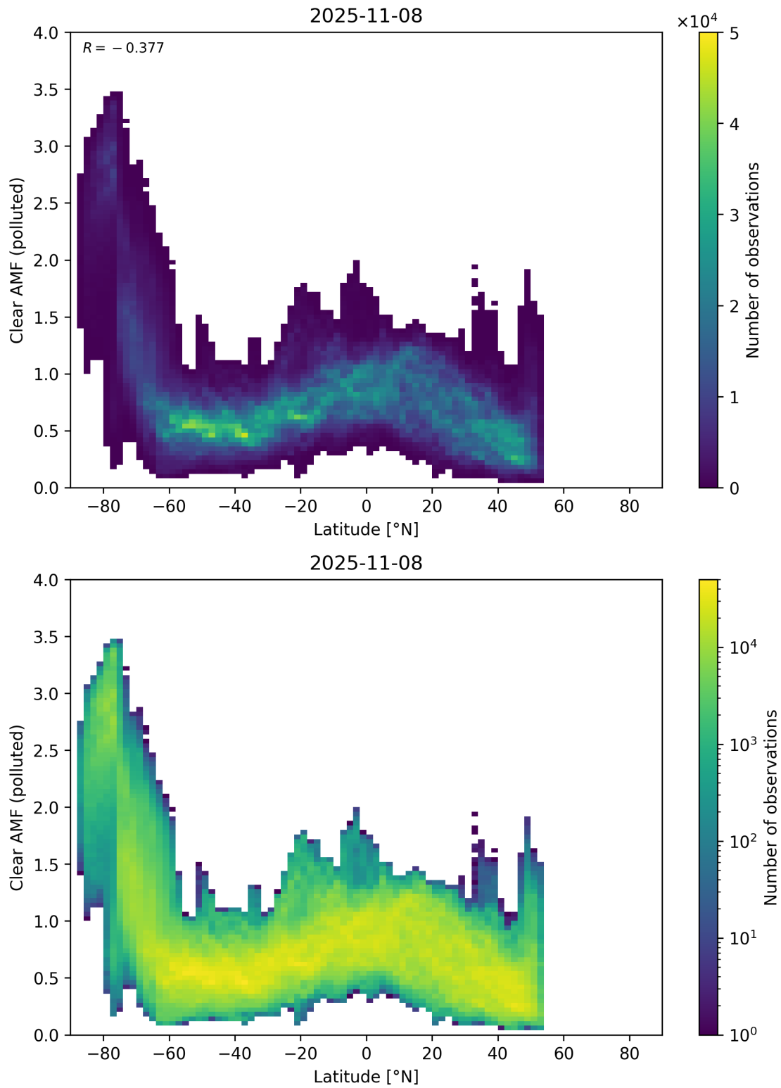
Figure 156: Scatter density plot of “Latitude” against “Clear AMF (polluted)” for 2025-11-07 to 2025-11-09.
