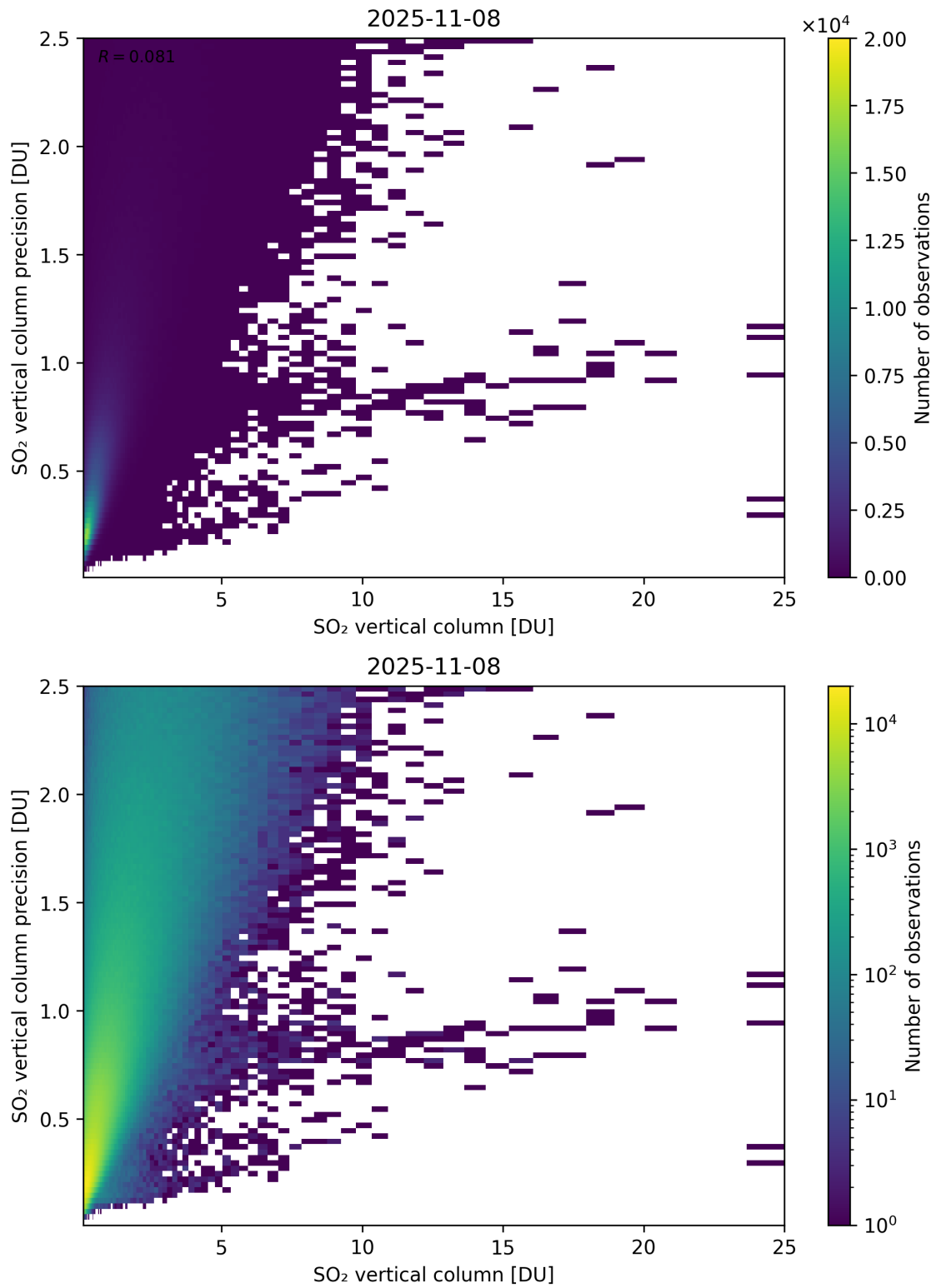
Figure 361: Scatter density plot of “SO 2 vertical column” against “SO 2 vertical column precision” for 2025-11-07 to 2025-11-09.
