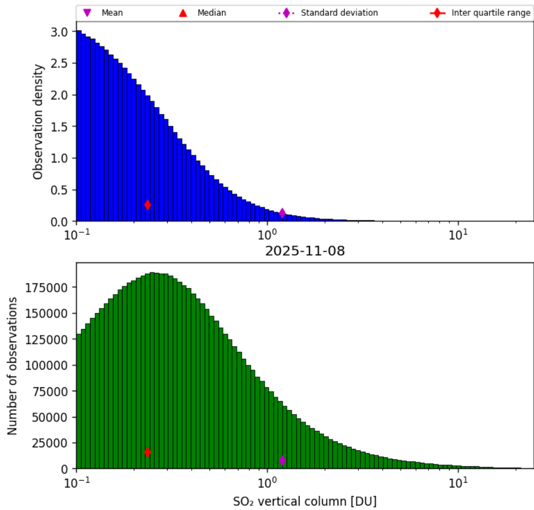
Figure 58: Histogram of “SO 2 vertical column” for 2025-11-07 to 2025-11-09
