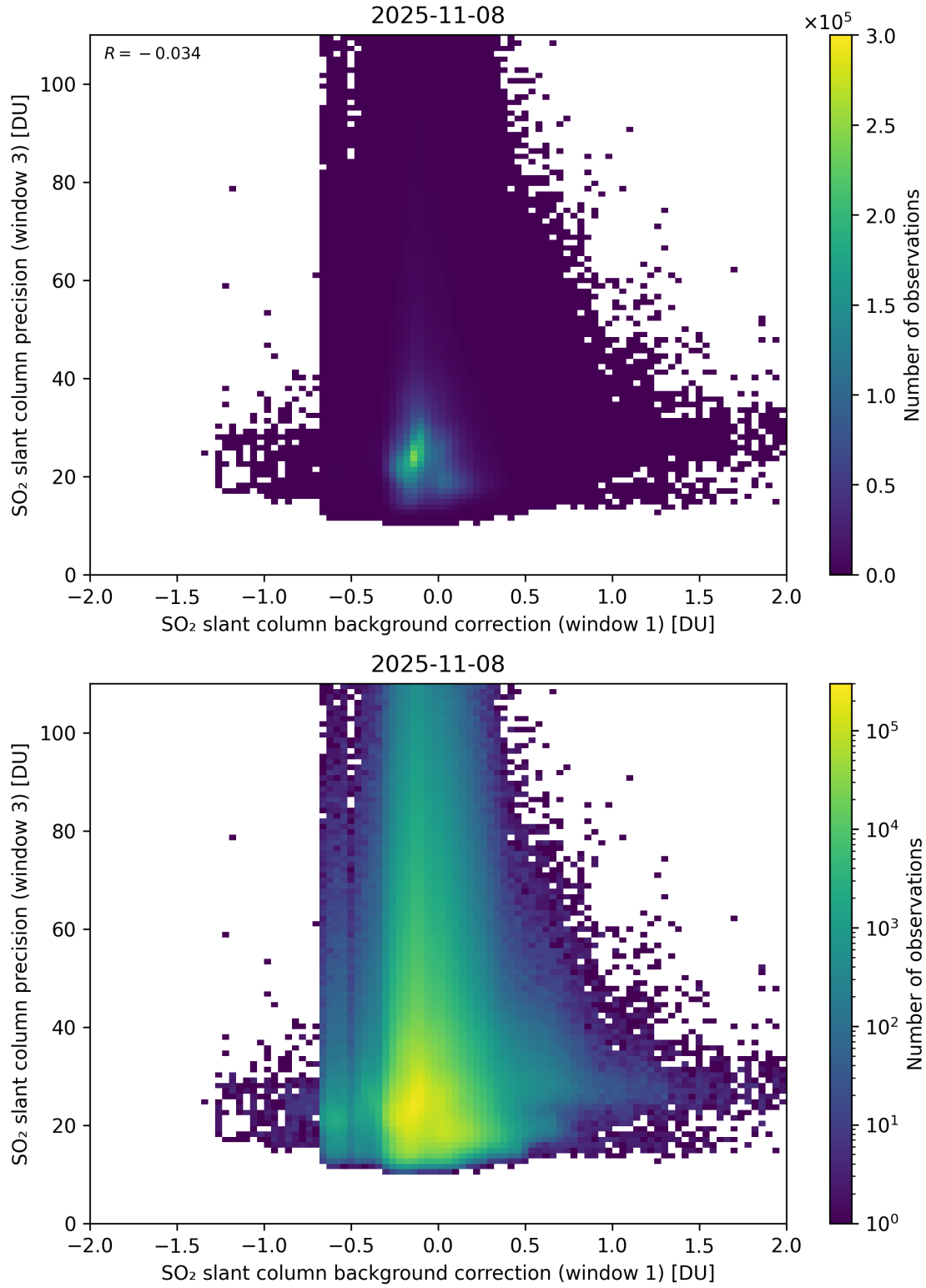
Figure 119: Scatter density plot of “SO 2 slant column background correction (window 1)” against “SO 2 slant column precision (window 3)” for 2025-11-07 to 2025-11-09.
