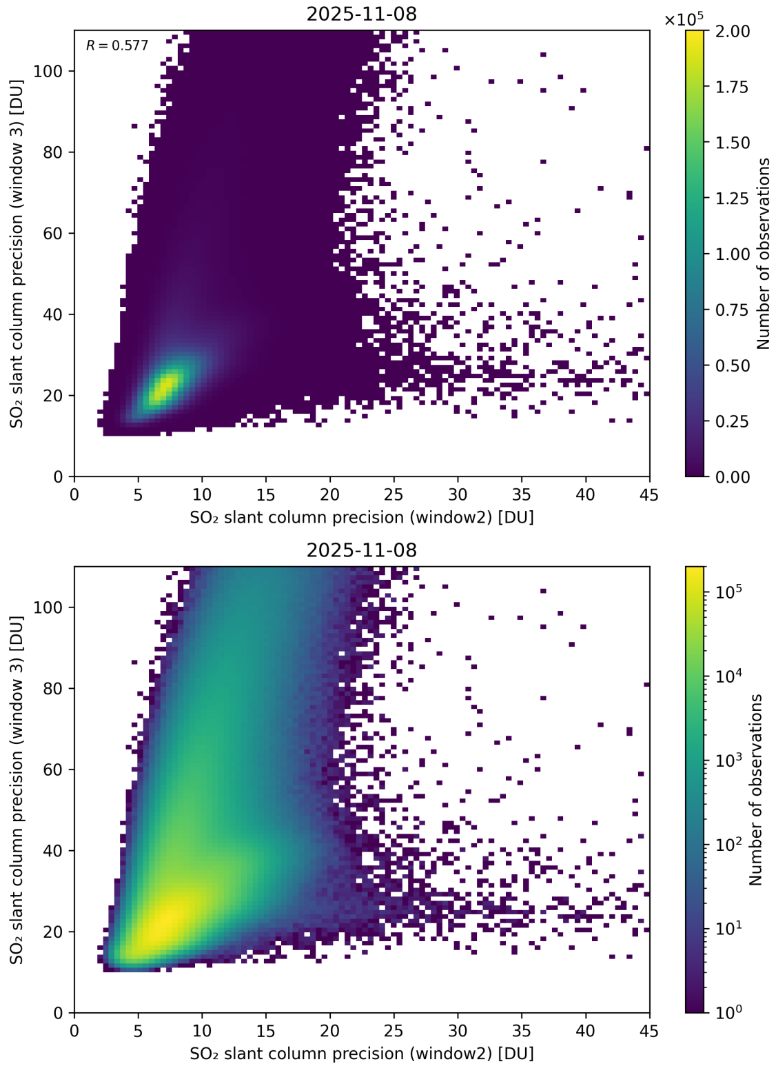
Figure 300: Scatter density plot of “SO 2 slant column precision (window2)” against “SO 2 slant column precision (window 3)” for 2025-11-07 to 2025-11-09.
