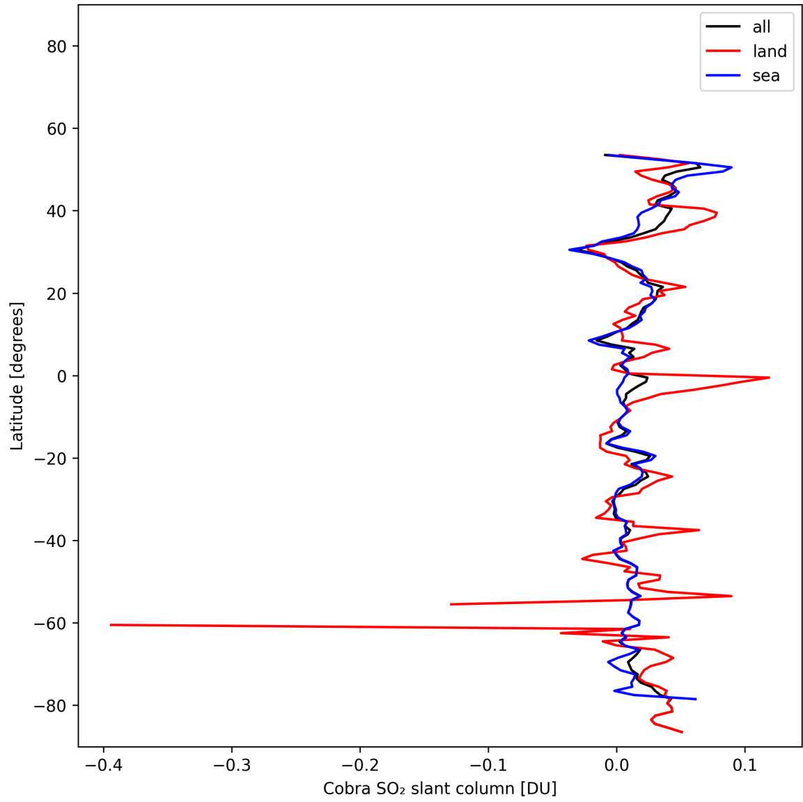
Figure 35: Zonal average of “Cobra SO 2 slant column” for 2025-11-07 to 2025-11-09.
