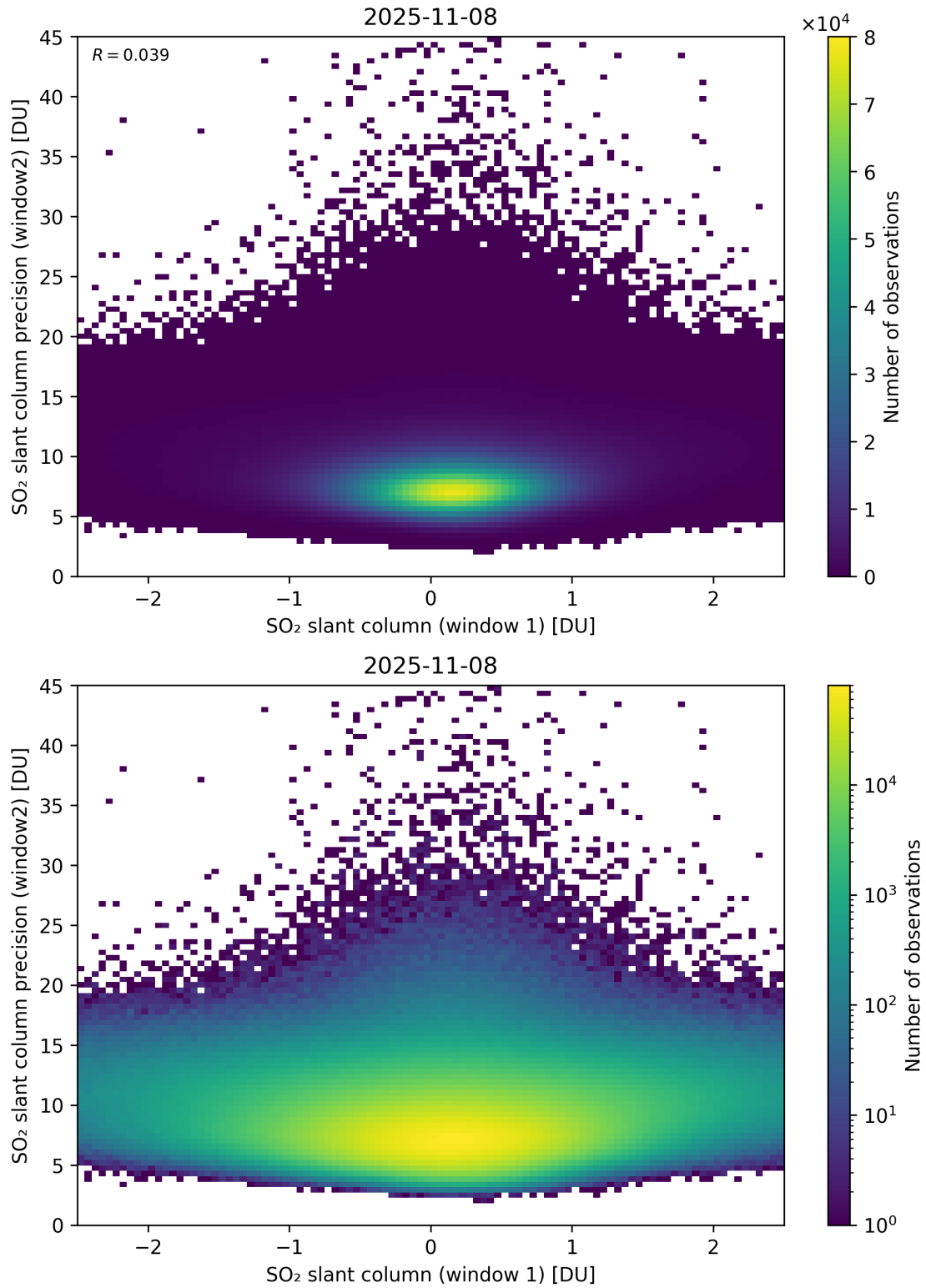
Figure 286: Scatter density plot of “SO 2 slant column (window 1)” against “SO 2 slant column precision (window2)” for 2025-11-07 to 2025-11-09.
