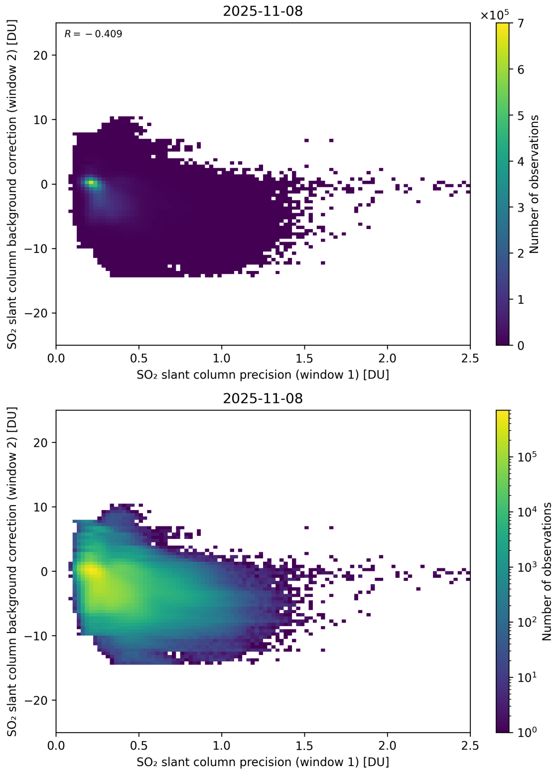
Figure 269: Scatter density plot of “SO 2 slant column precision (window 1)” against “SO 2 slant column background correction (window 2)” for 2025-11-07 to 2025-11-09.
