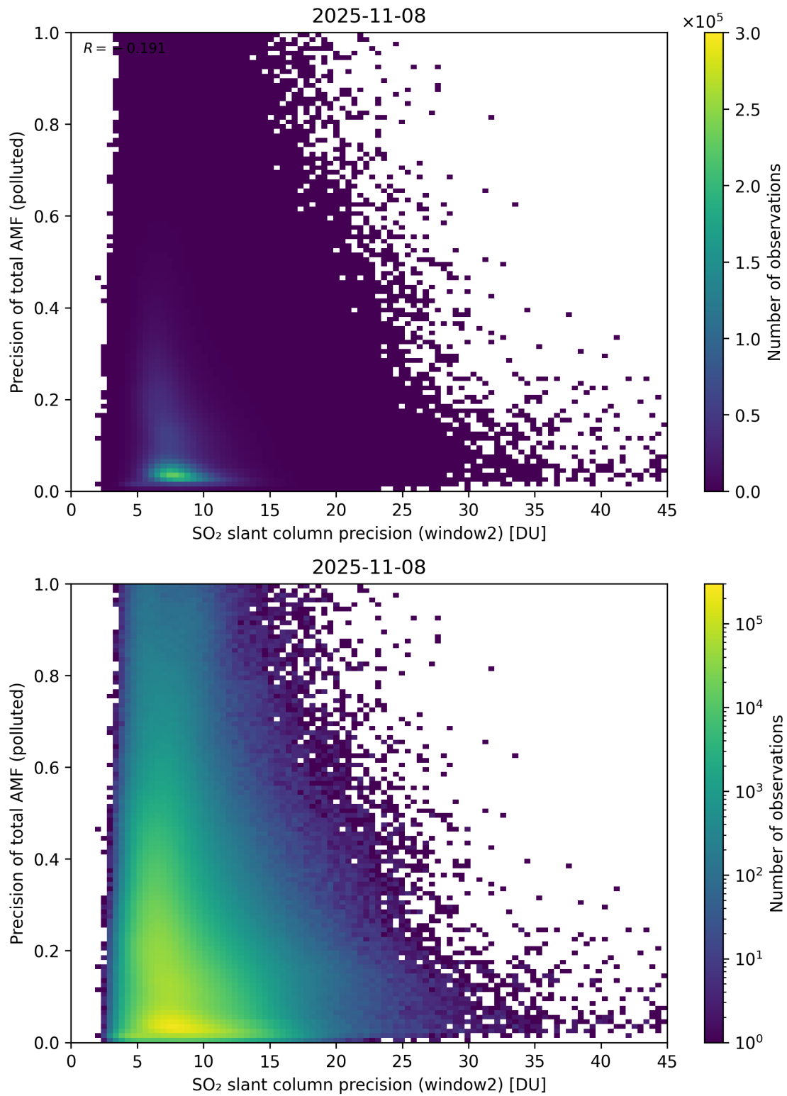
Figure 302: Scatter density plot of “SO 2 slant column precision (window2)” against “Precision of total AMF (polluted)” for 2025-11-07 to 2025-11-09.
