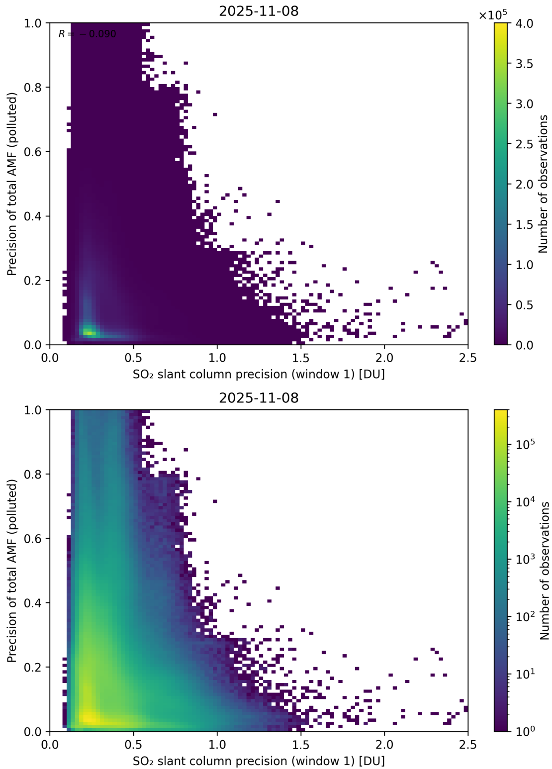
Figure 281: Scatter density plot of “SO 2 slant column precision (window 1)” against “Precision of total AMF (polluted)” for 2025-11-07 to 2025-11-09.
