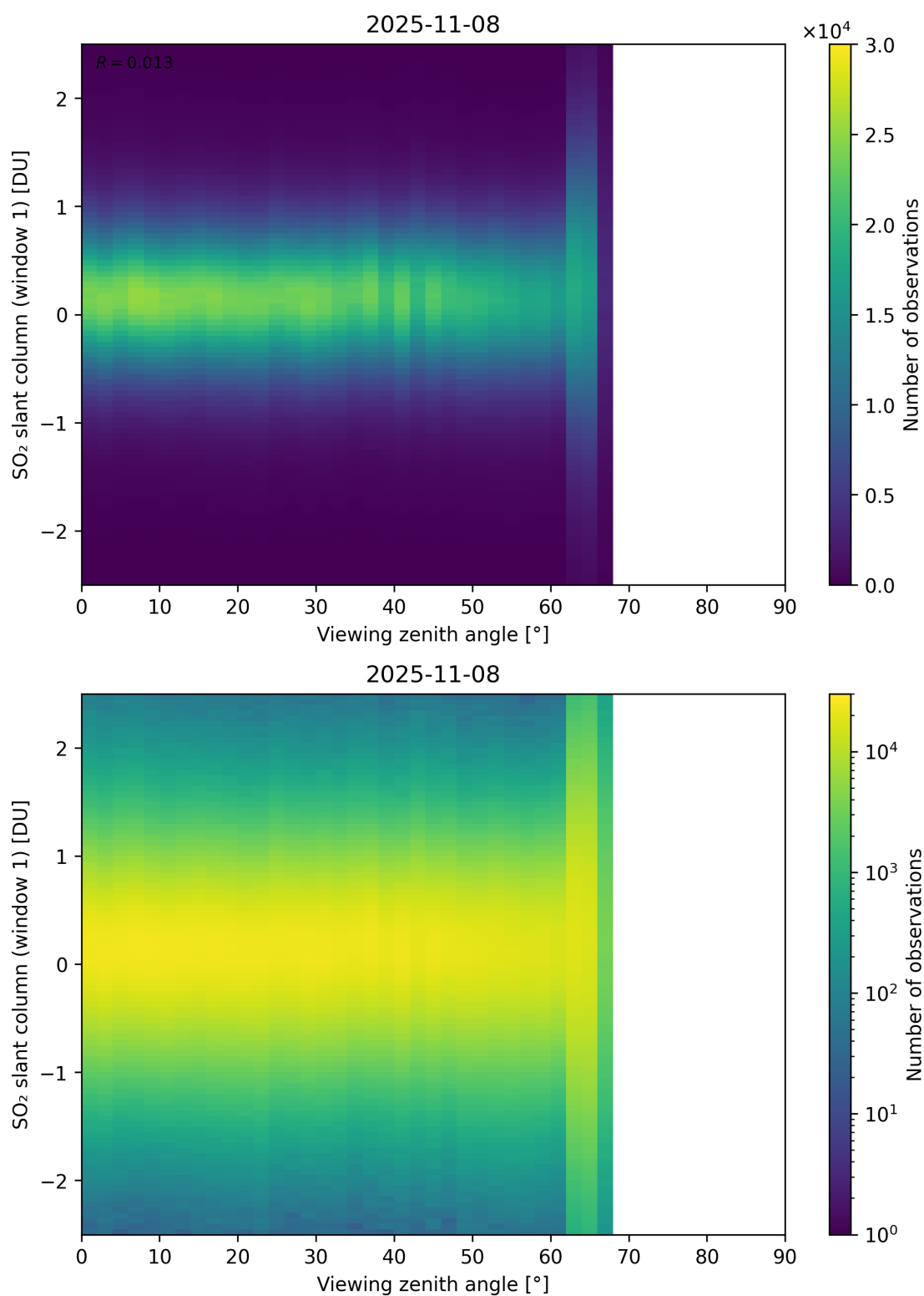
Figure 376: Scatter density plot of “Viewing zenith angle” against “SO 2 slant column (window 1)” for 2025-11-07 to 2025-11-09.
