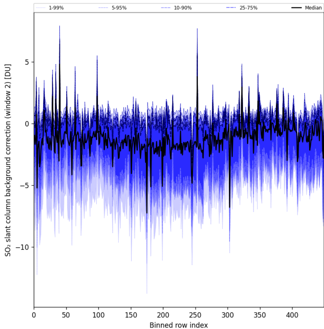
Figure 96: Along track statistics of “SO 2 slant column background correction (window 2)” for 2025-11-07 to 2025-11-09
