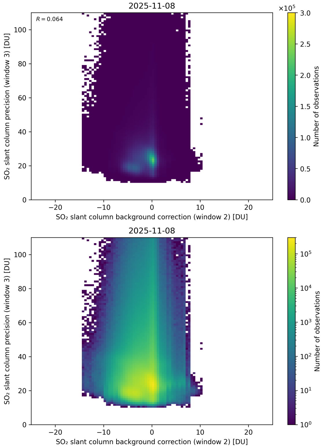
Figure 129: Scatter density plot of “SO 2 slant column background correction (window 2)” against “SO 2 slant column precision (window 3)” for 2025-11-07 to 2025-11-09.
