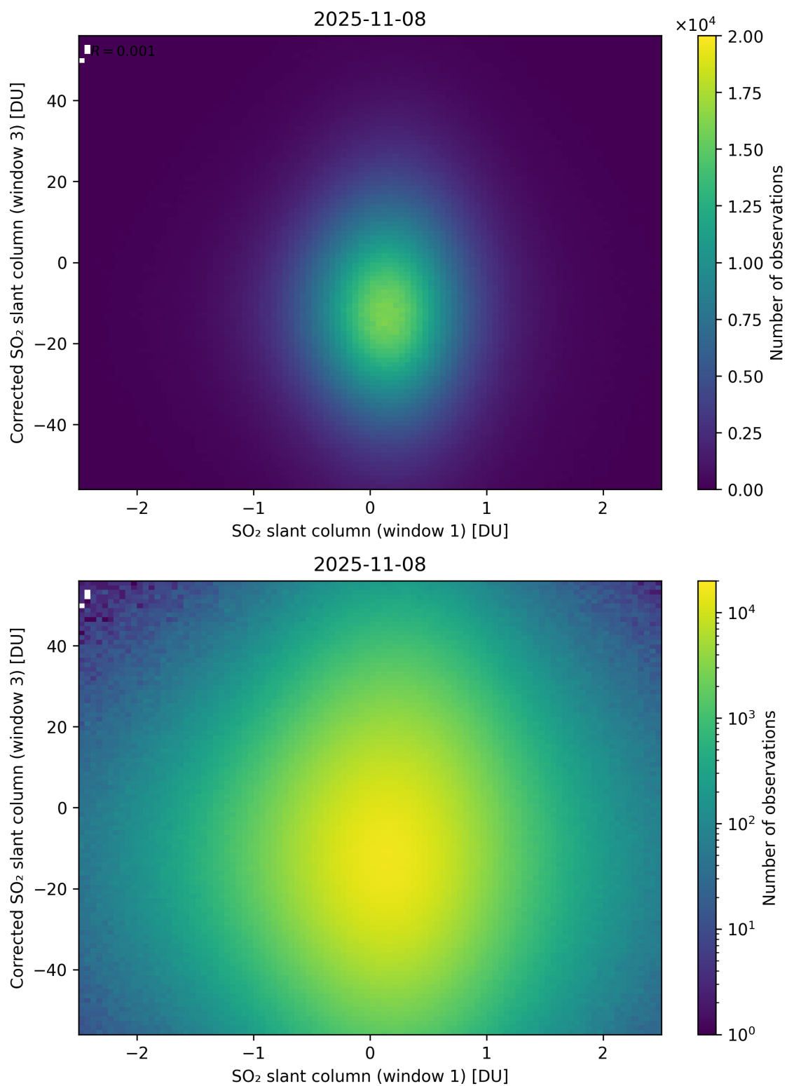
Figure 284: Scatter density plot of “SO 2 slant column (window 1)” against “Corrected SO 2 slant column (window 3)” for 2025-11-07 to 2025-11-09.
