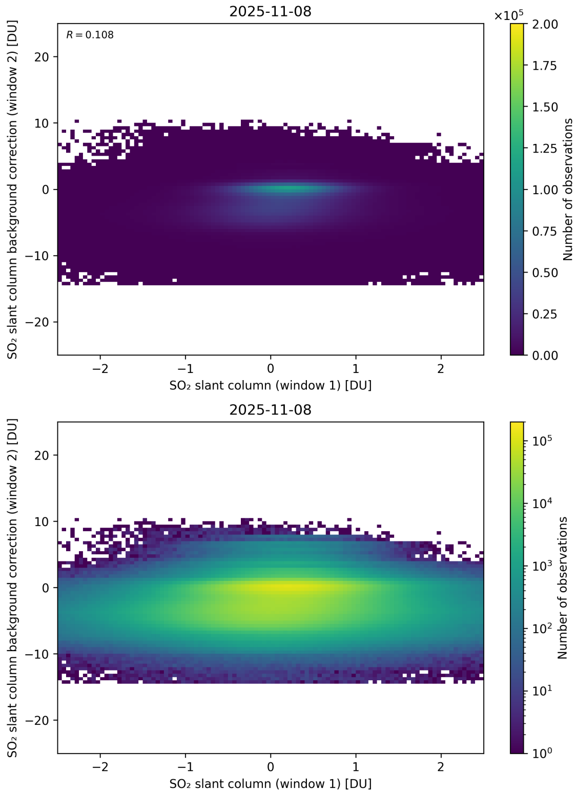
Figure 263: Scatter density plot of “SO 2 slant column (window 1)” against “SO 2 slant column background correction (window 2)” for 2025-11-07 to 2025-11-09.
