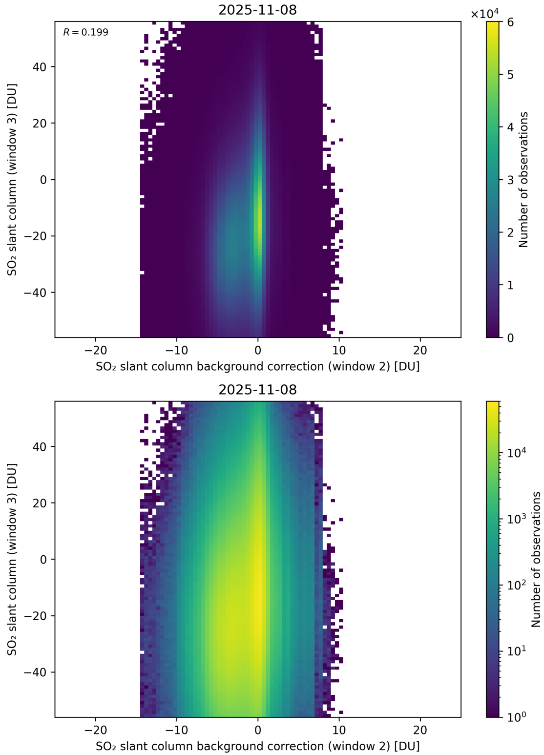
Figure 128: Scatter density plot of “SO 2 slant column background correction (window 2)” against “SO 2 slant column (window 3)” for 2025-11-07 to 2025-11-09.
