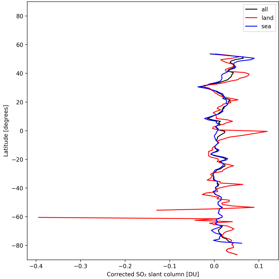
Figure 34: Zonal average of “Corrected SO 2 slant column” for 2025-11-07 to 2025-11-09.
