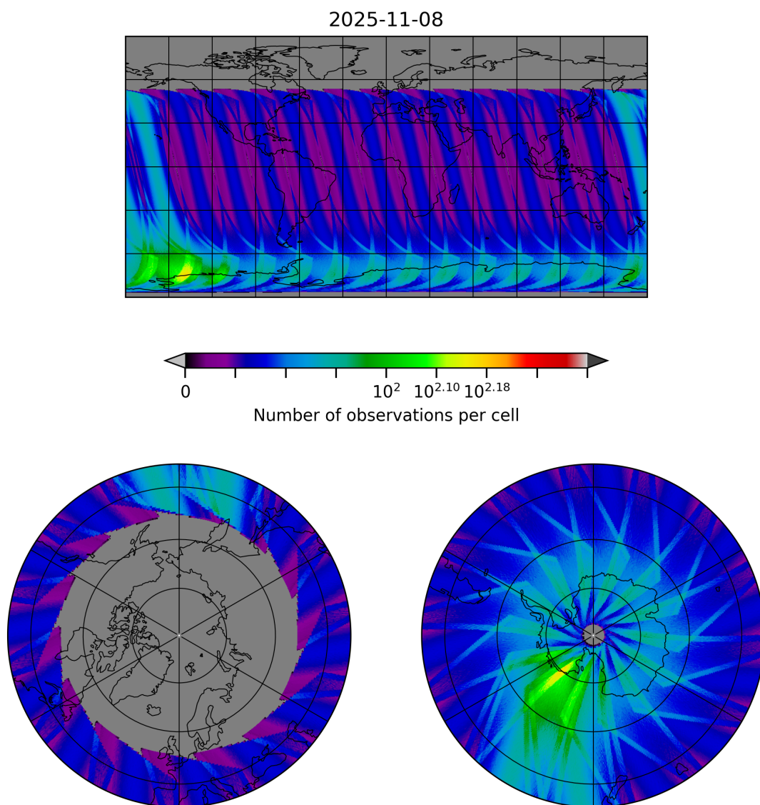
Figure 30: Map of the number of observations for 2025-11-07 to 2025-11-09
