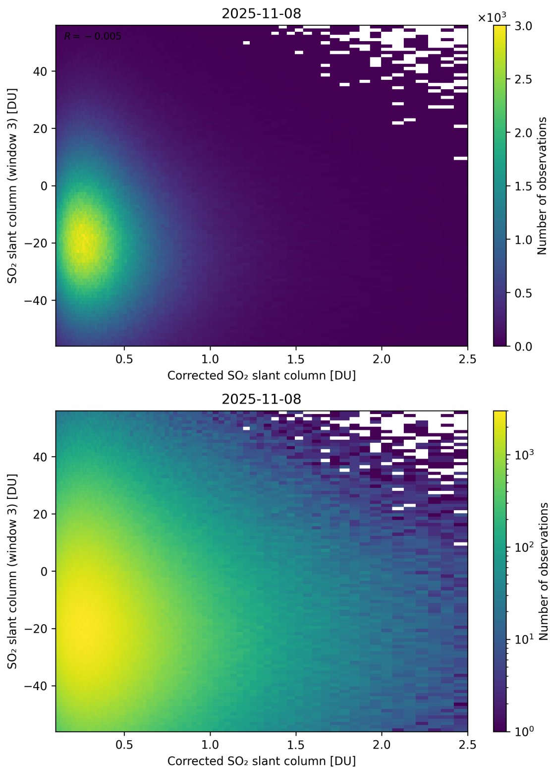
Figure 240: Scatter density plot of “Corrected SO 2 slant column” against “SO 2 slant column (window 3)” for 2025-11-07 to 2025-11-09.
