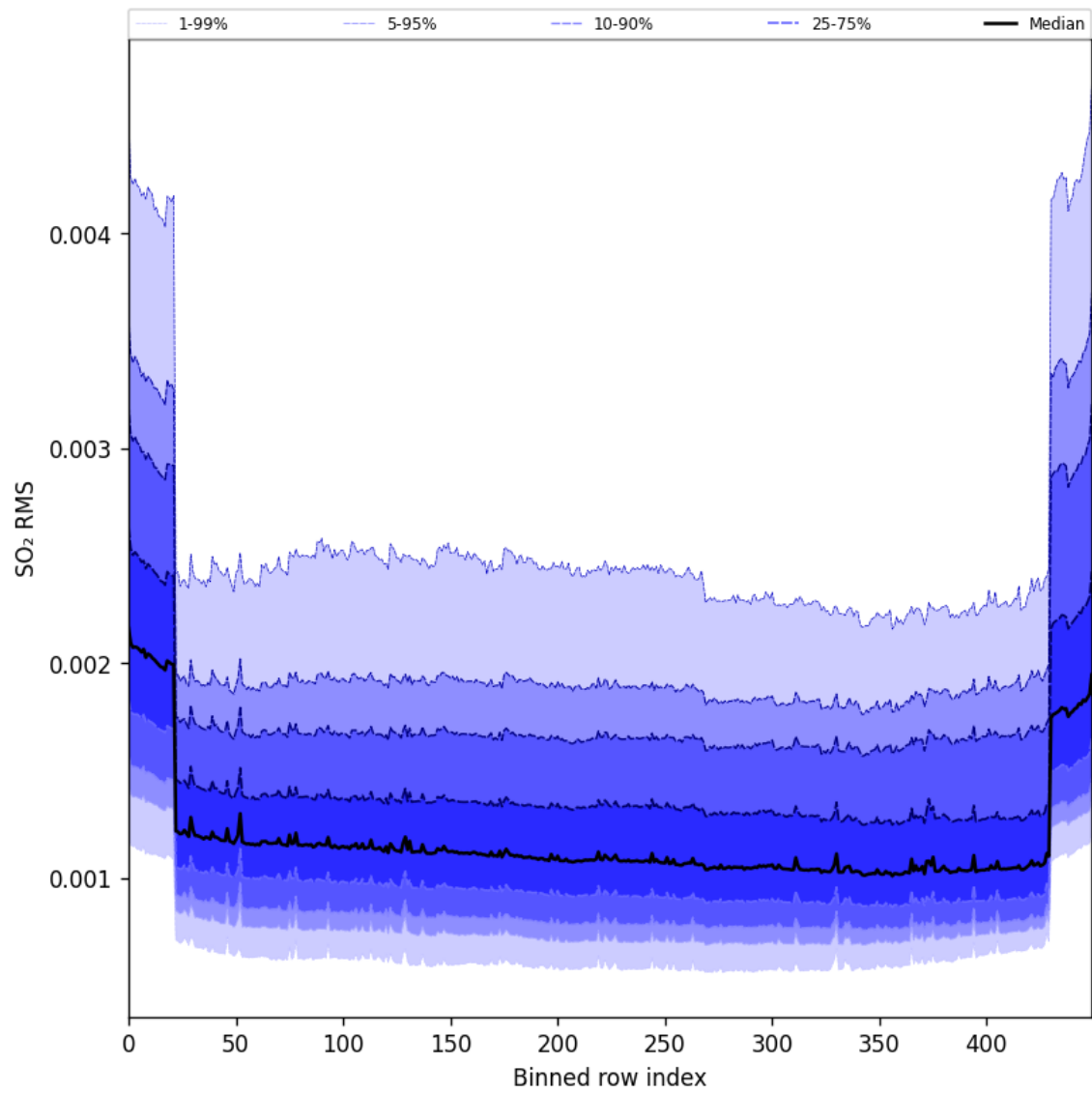
Figure 104: Along track statistics of “SO 2 RMS” for 2025-11-07 to 2025-11-09
