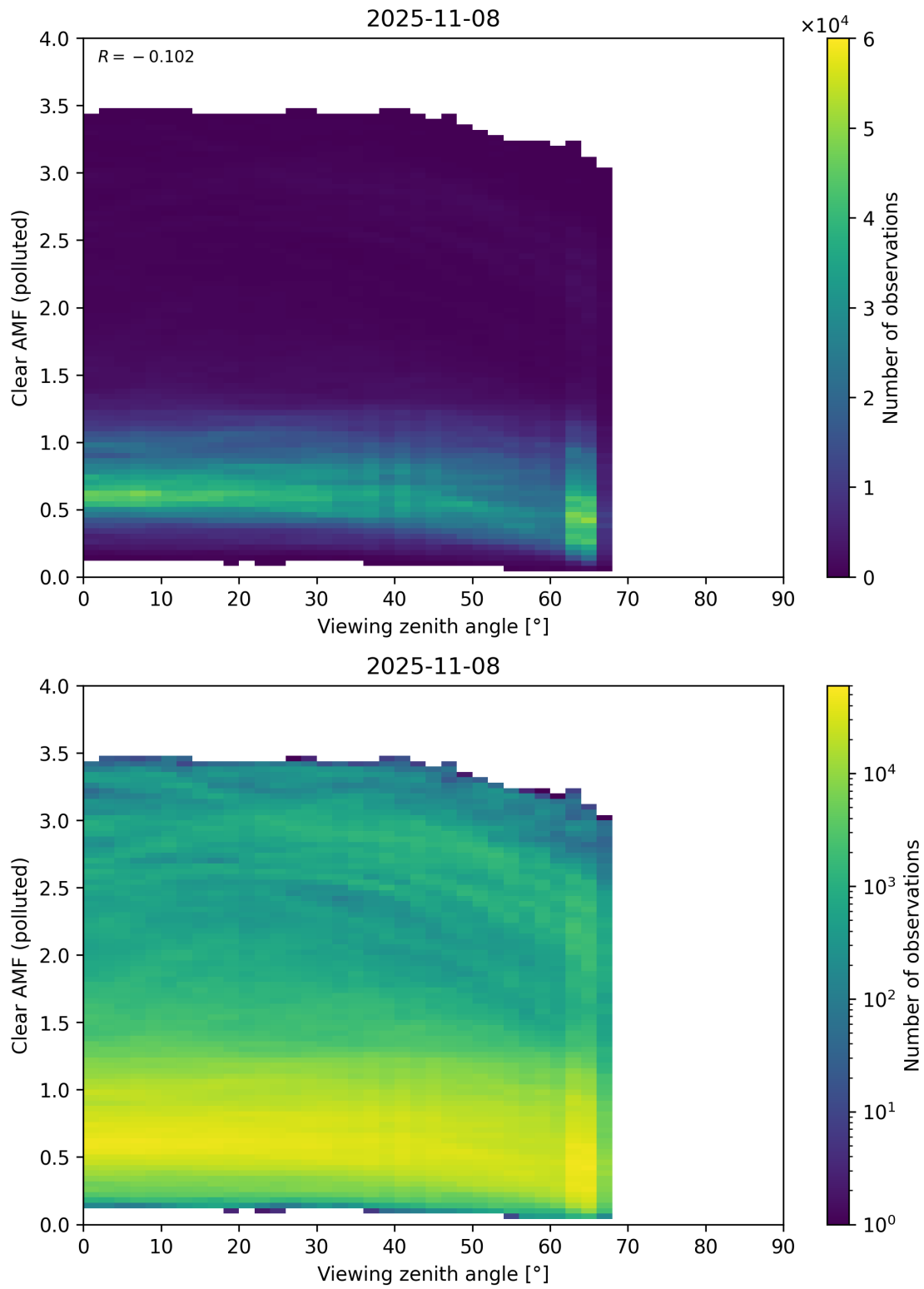
Figure 370: Scatter density plot of “Viewing zenith angle” against “Clear AMF (polluted)” for 2025-11-07 to 2025-11-09.
