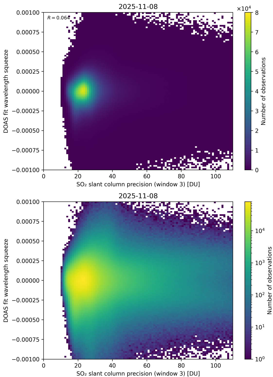
Figure 309: Scatter density plot of “SO 2 slant column precision (window 3)” against “DOAS fit wavelength squeeze” for 2025-11-07 to 2025-11-09.
