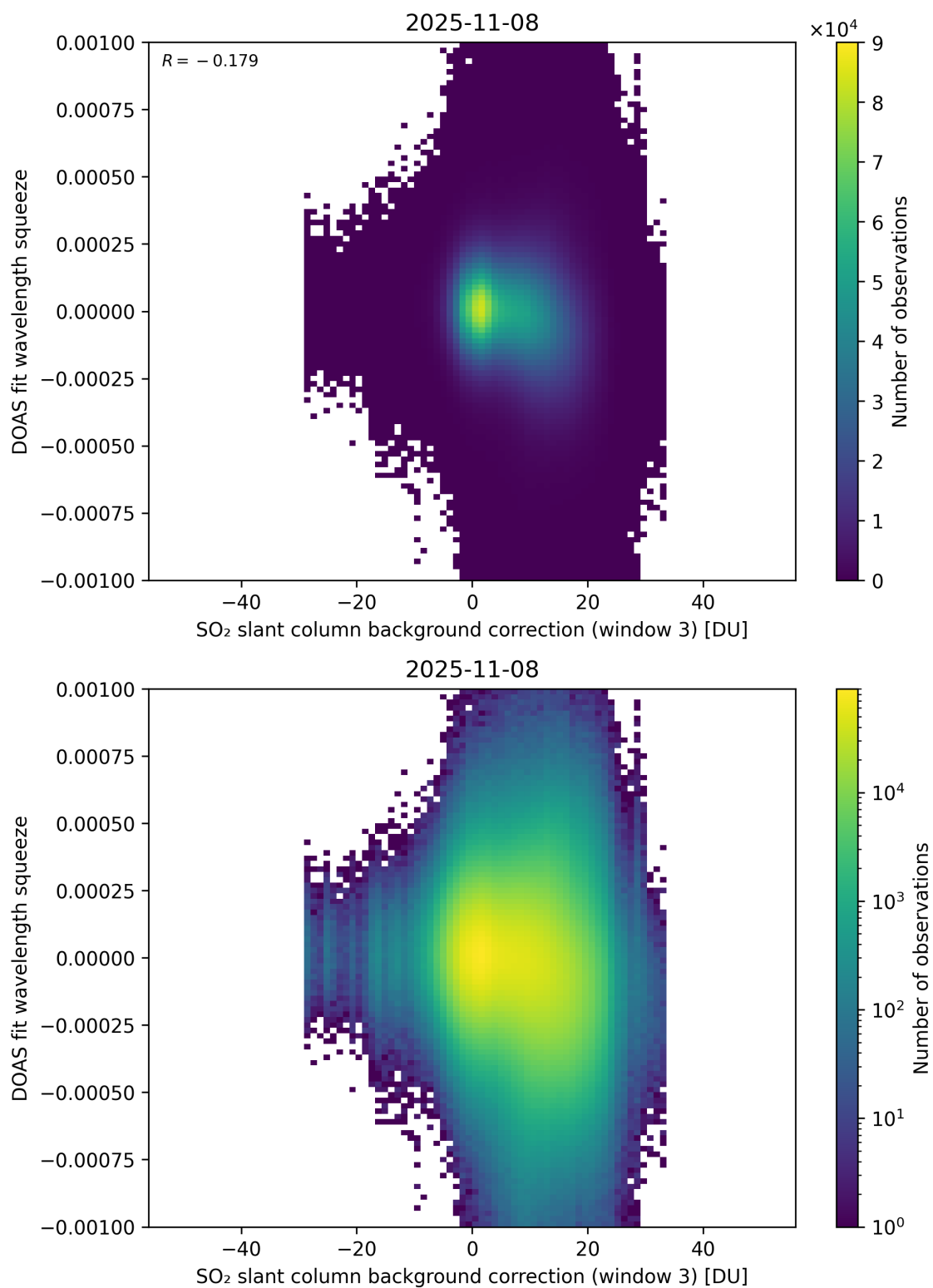
Figure 133: Scatter density plot of “SO 2 slant column background correction (window 3)” against “DOAS fit wavelength squeeze” for 2025-11-07 to 2025-11-09.
