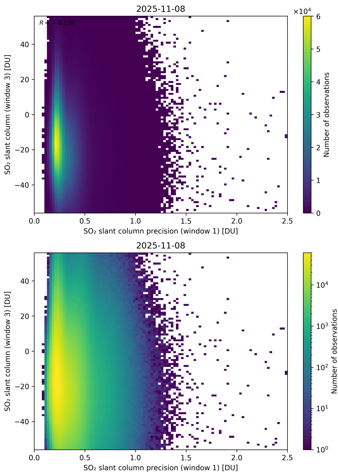
Figure 278: Scatter density plot of “SO 2 slant column precision (window 1)” against “SO 2 slant column (window 3)” for 2025-11-07 to 2025-11-09.
