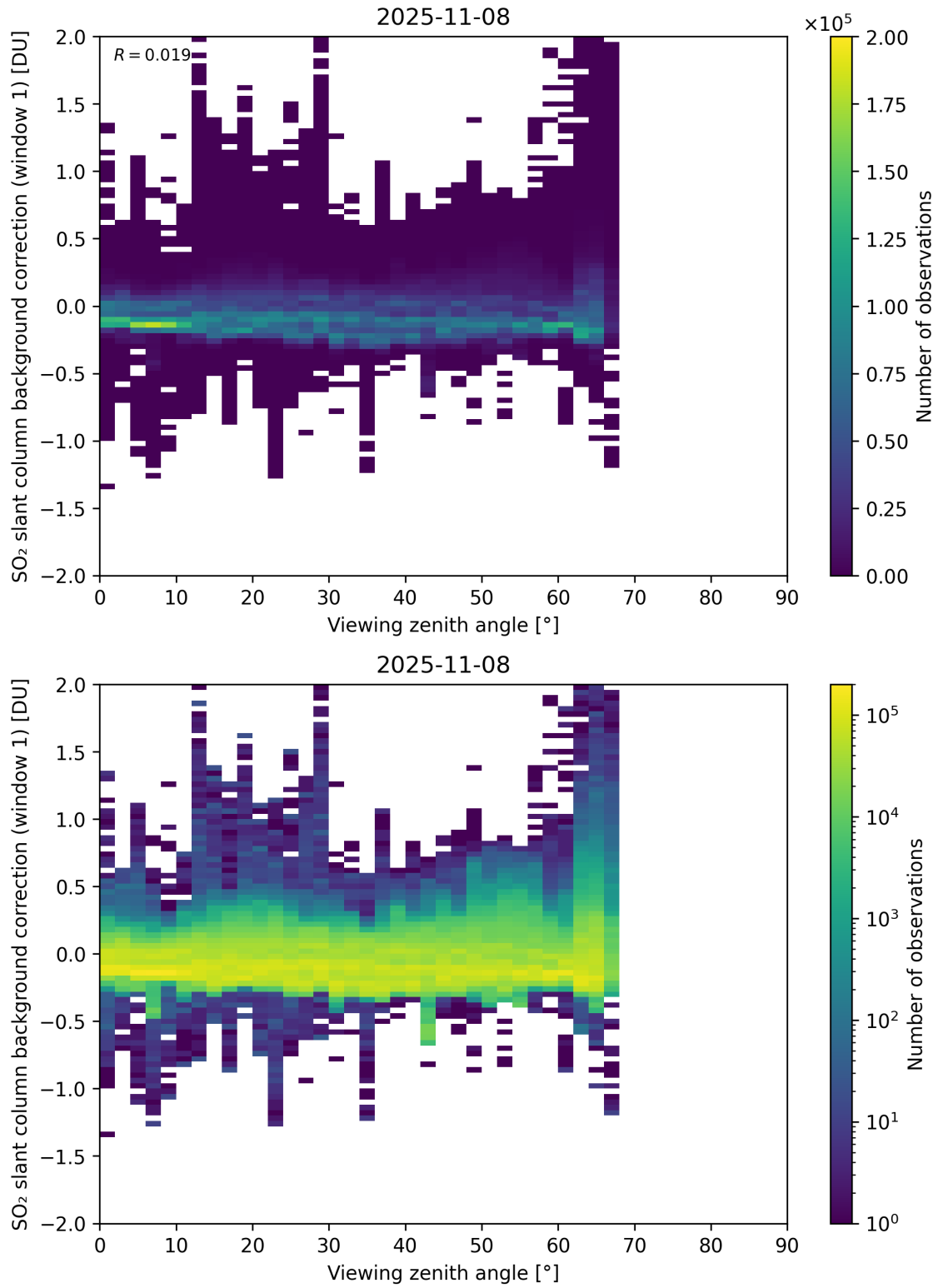
Figure 362: Scatter density plot of “Viewing zenith angle” against “SO 2 slant column background correction (window 1)” for 2025-11-07 to 2025-11-09.
