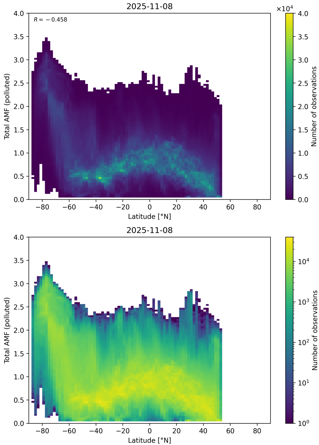
Figure 167: Scatter density plot of “Latitude” against “Total AMF (polluted)” for 2025-11-07 to 2025-11-09.
