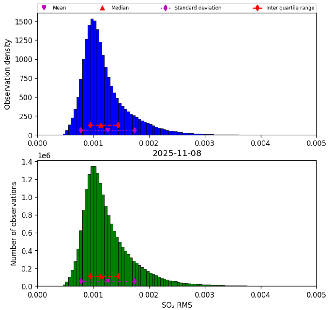
Figure 78: Histogram of “SO 2 RMS” for 2025-11-07 to 2025-11-09
