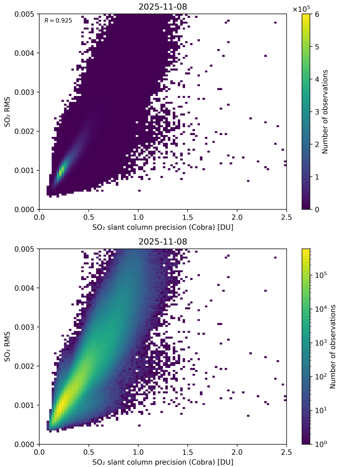
Figure 204: Scatter density plot of “SO 2 slant column precision (Cobra)” against “SO 2 RMS” for 2025-11-07 to 2025-11-09.
