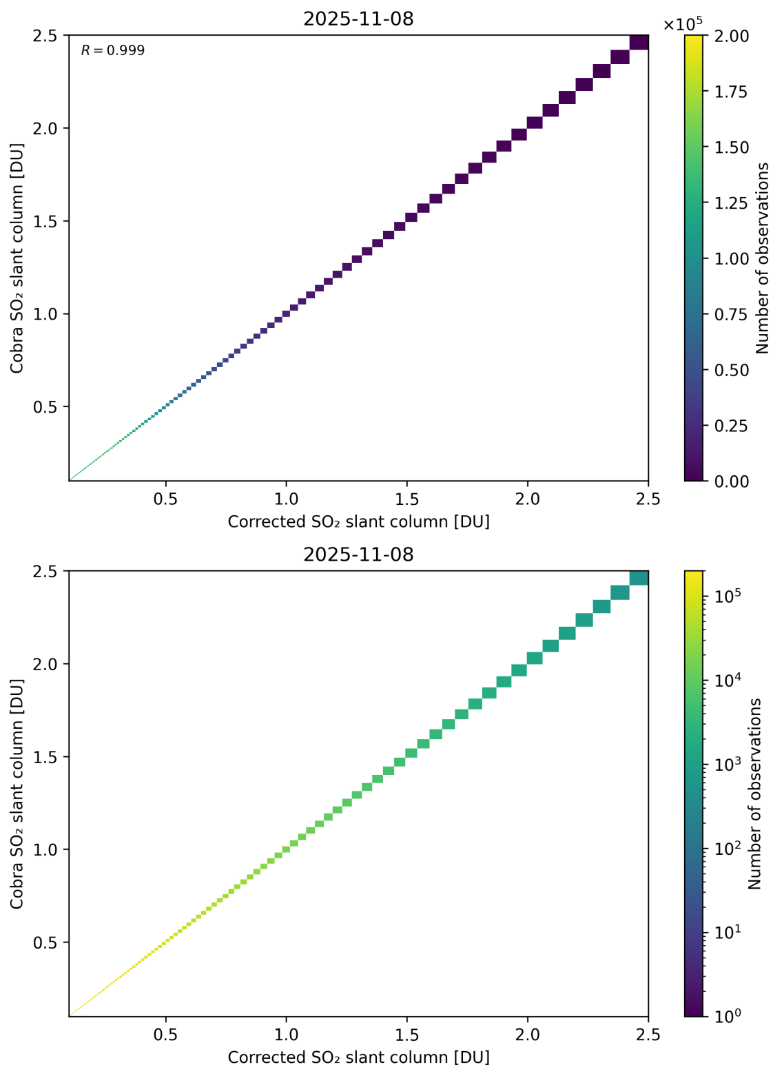
Figure 233: Scatter density plot of “Corrected SO 2 slant column” against “Cobra SO 2 slant column” for 2025-11-07 to 2025-11-09.
