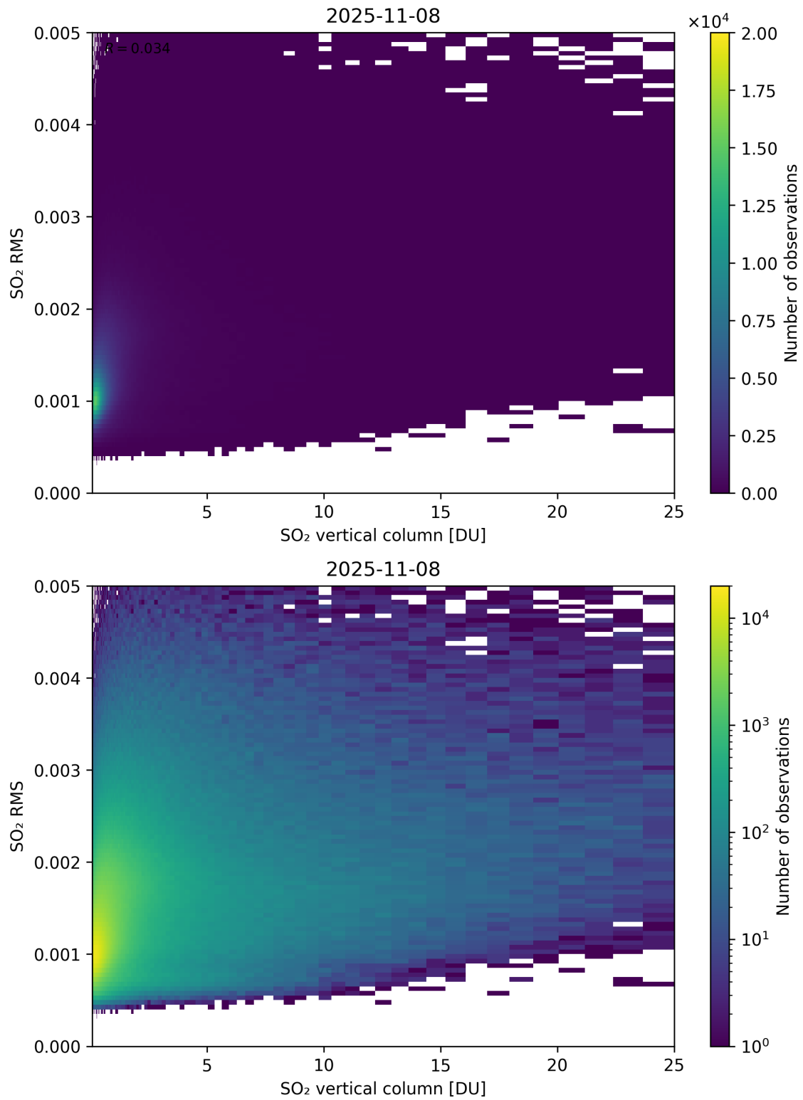
Figure 328: Scatter density plot of “SO 2 vertical column” against “SO 2 RMS” for 2025-11-07 to 2025-11-09.
