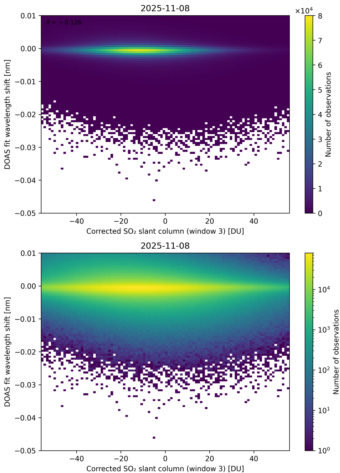
Figure 256: Scatter density plot of “Corrected SO 2 slant column (window 3)” against “DOAS fit wavelength shift” for 2025-11-07 to 2025-11-09.
