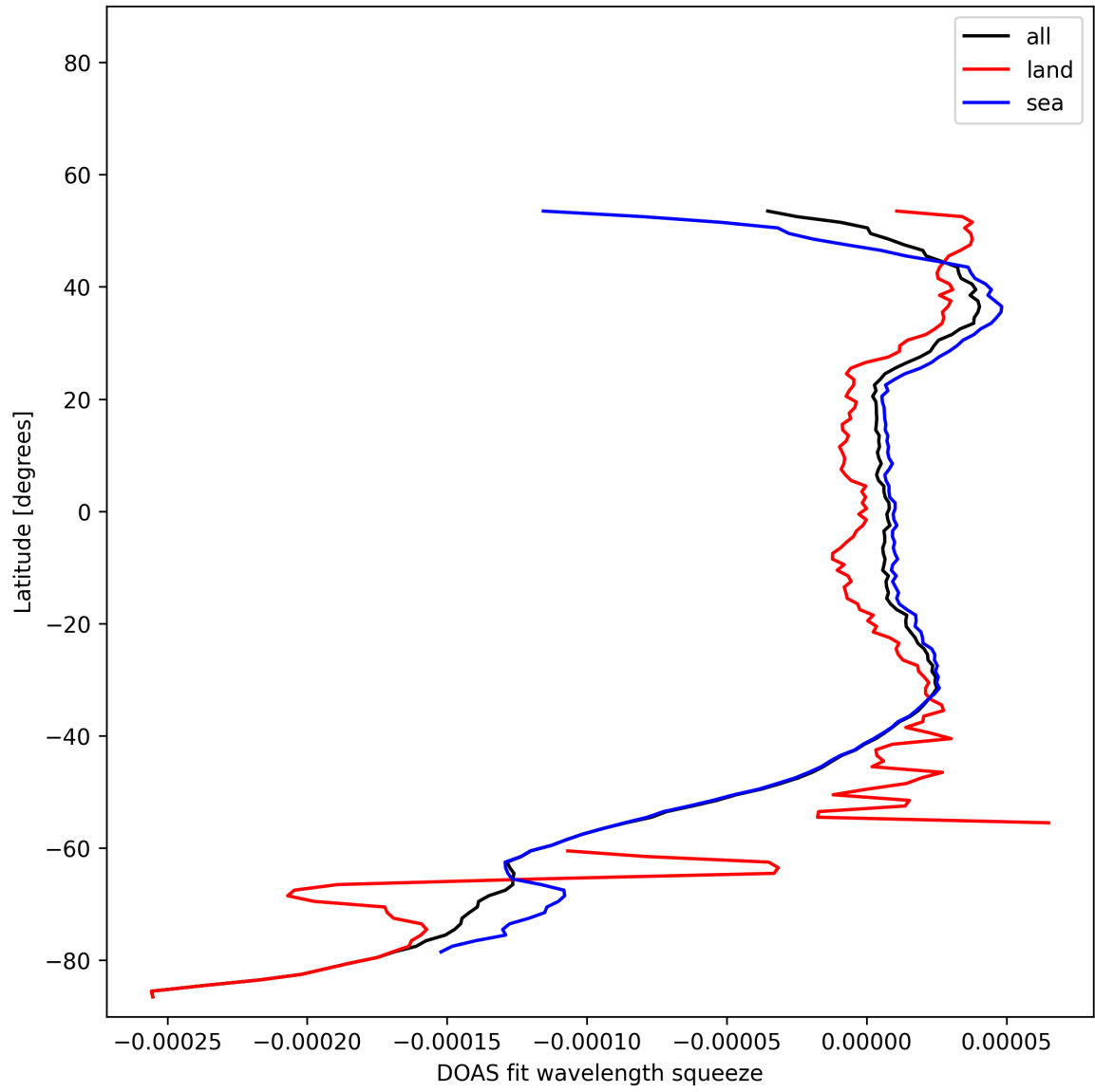
Figure 51: Zonal average of “DOAS fit wavelength squeeze” for 2025-11-07 to 2025-11-09.
