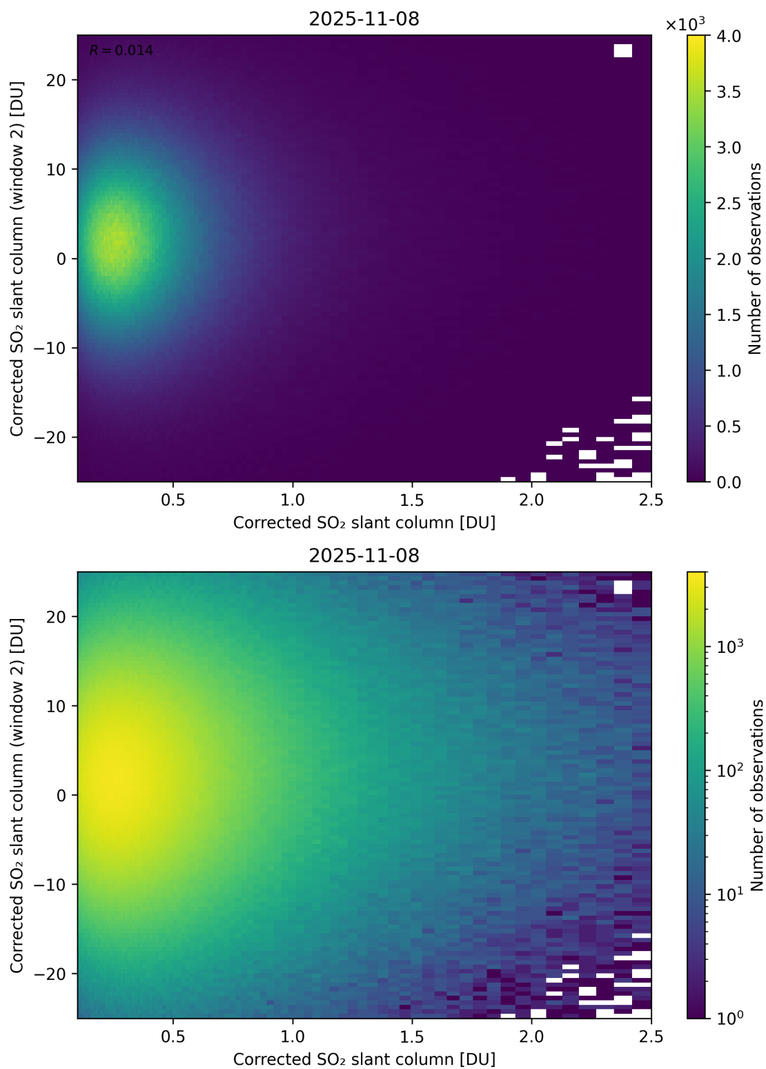
Figure 235: Scatter density plot of “Corrected SO 2 slant column” against “Corrected SO 2 slant column (window 2)” for 2025-11-07 to 2025-11-09.
