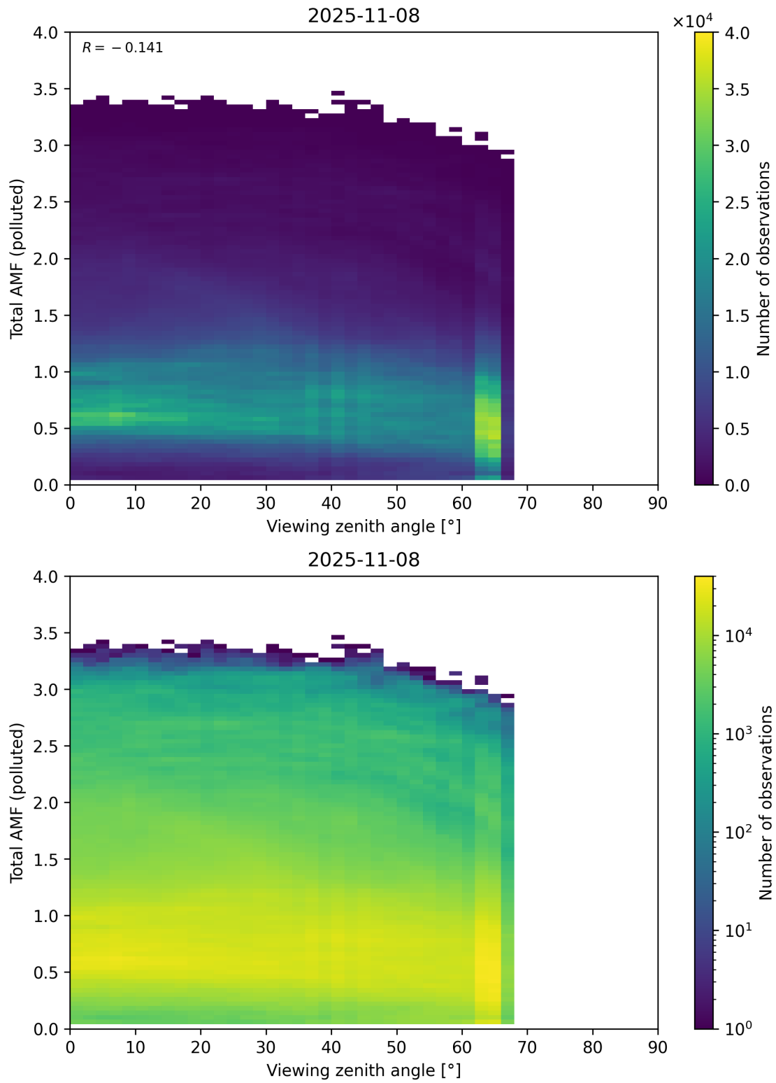
Figure 381: Scatter density plot of “Viewing zenith angle” against “Total AMF (polluted)” for 2025-11-07 to 2025-11-09.
