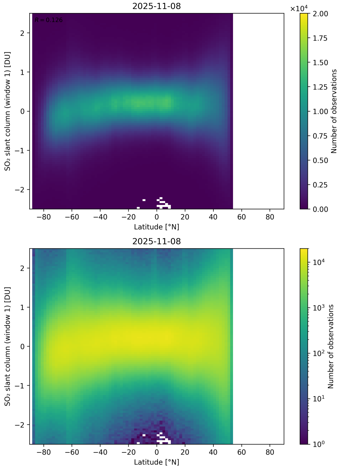
Figure 162: Scatter density plot of “Latitude” against “SO 2 slant column (window 1)” for 2025-11-07 to 2025-11-09.
