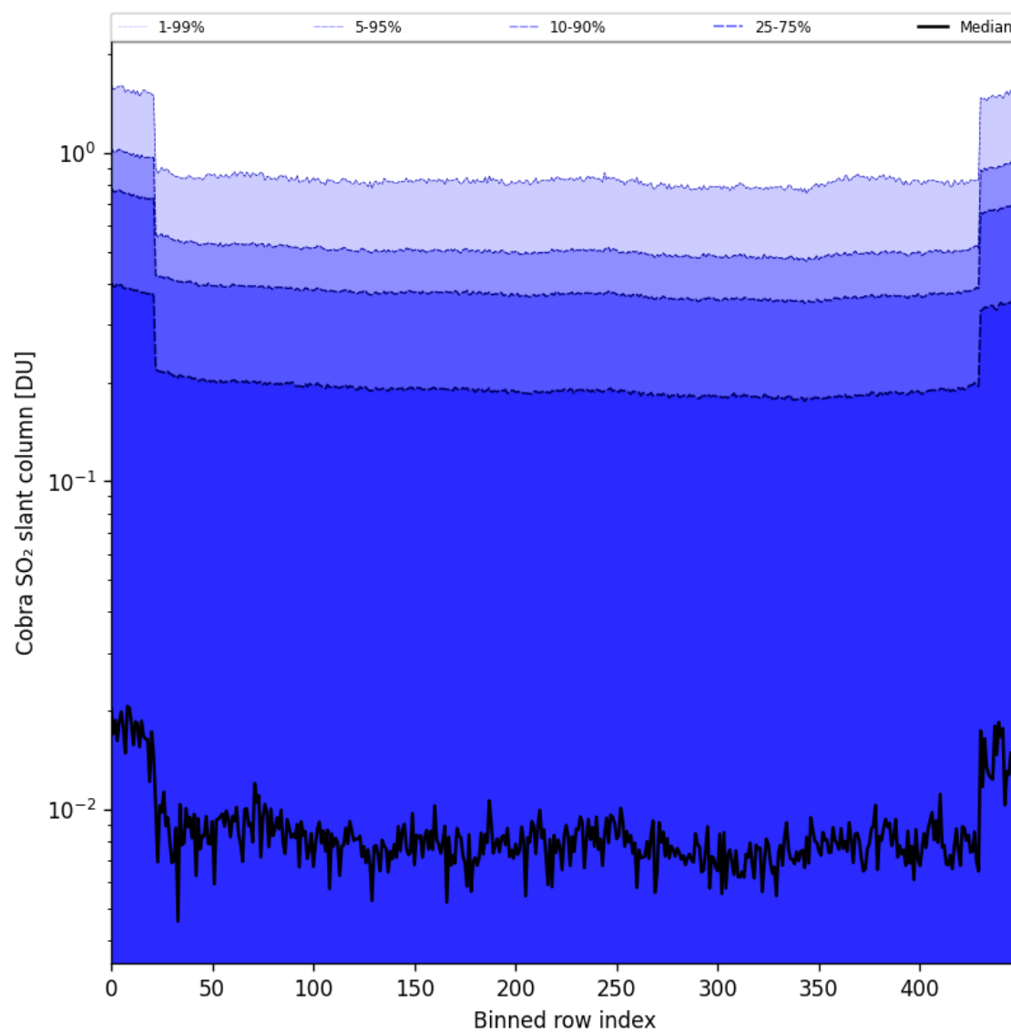
Figure 87: Along track statistics of "Cobra SO 2 slant column" for 2025-11-07 to 2025-11-09
