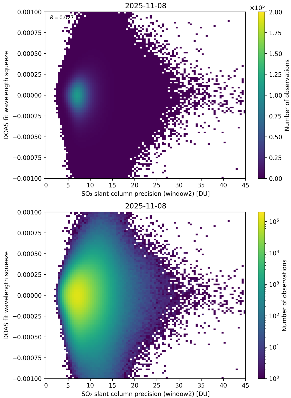
Figure 294: Scatter density plot of “SO 2 slant column precision (window2)” against “DOAS fit wavelength squeeze” for 2025-11-07 to 2025-11-09.
