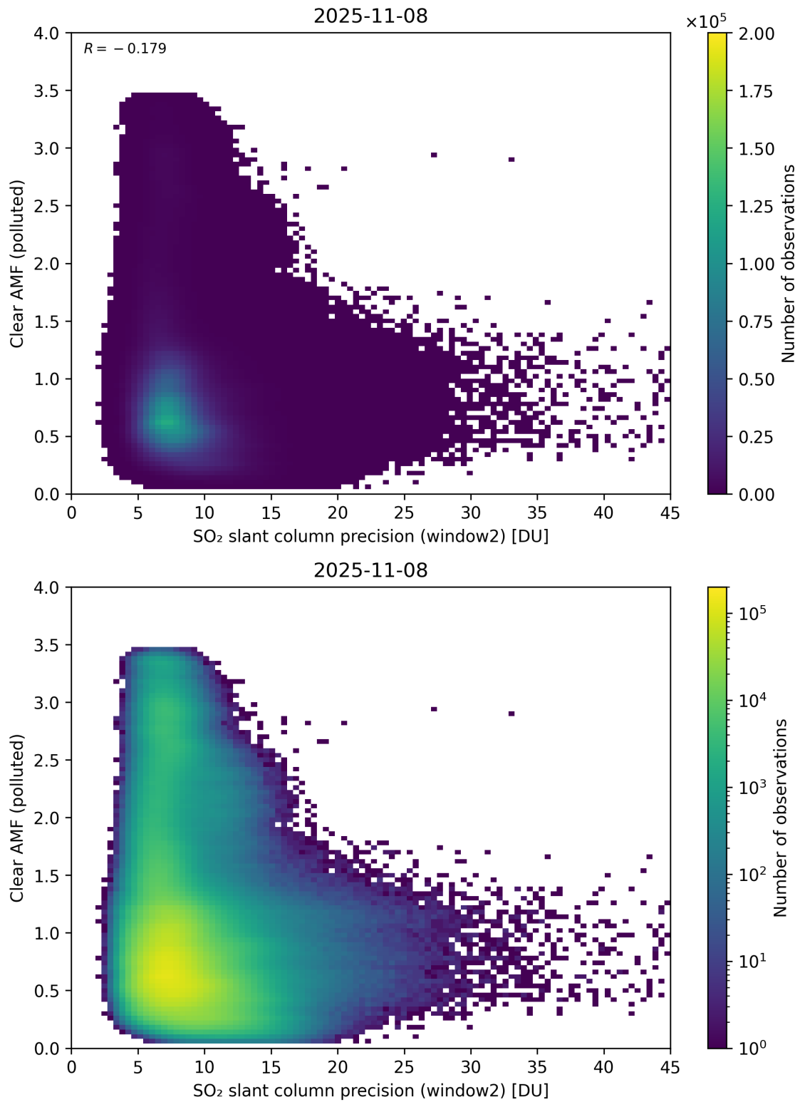
Figure 296: Scatter density plot of “SO 2 slant column precision (window2)” against “Clear AMF (polluted)” for 2025-11-07 to 2025-11-09.
