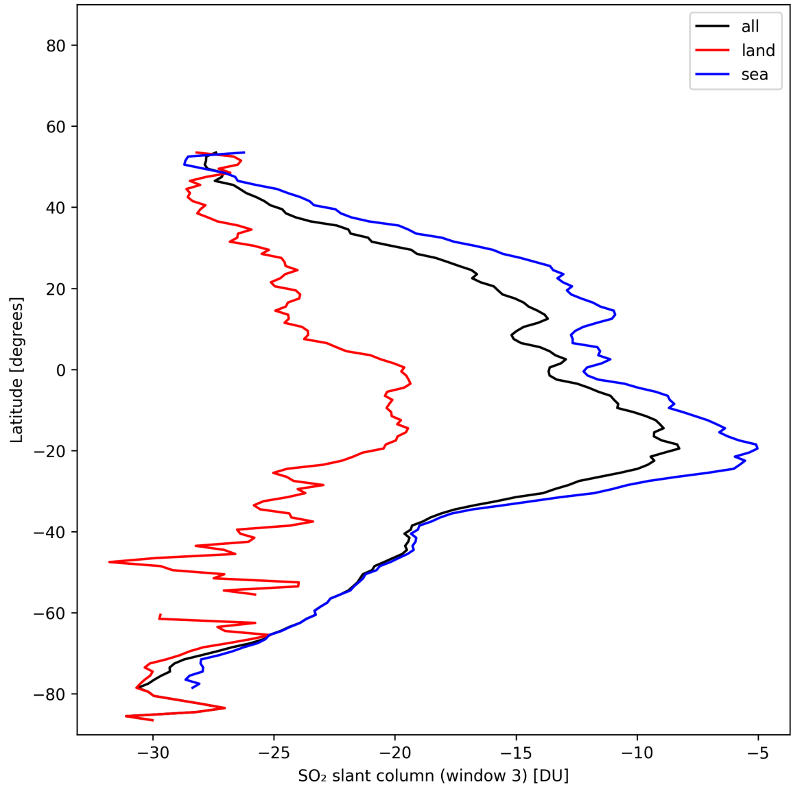
Figure 45: Zonal average of “SO 2 slant column (window 3)” for 2025-11-07 to 2025-11-09.
