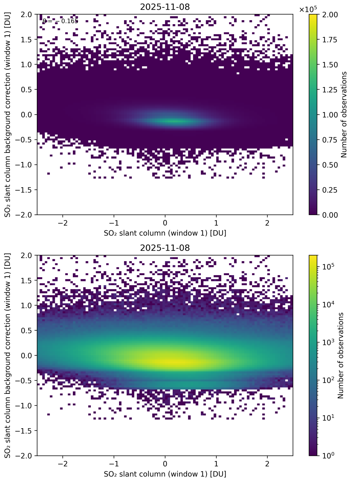
Figure 262: Scatter density plot of “SO 2 slant column (window 1)” against “SO 2 slant column background correction (window 1)” for 2025-11-07 to 2025-11-09.
