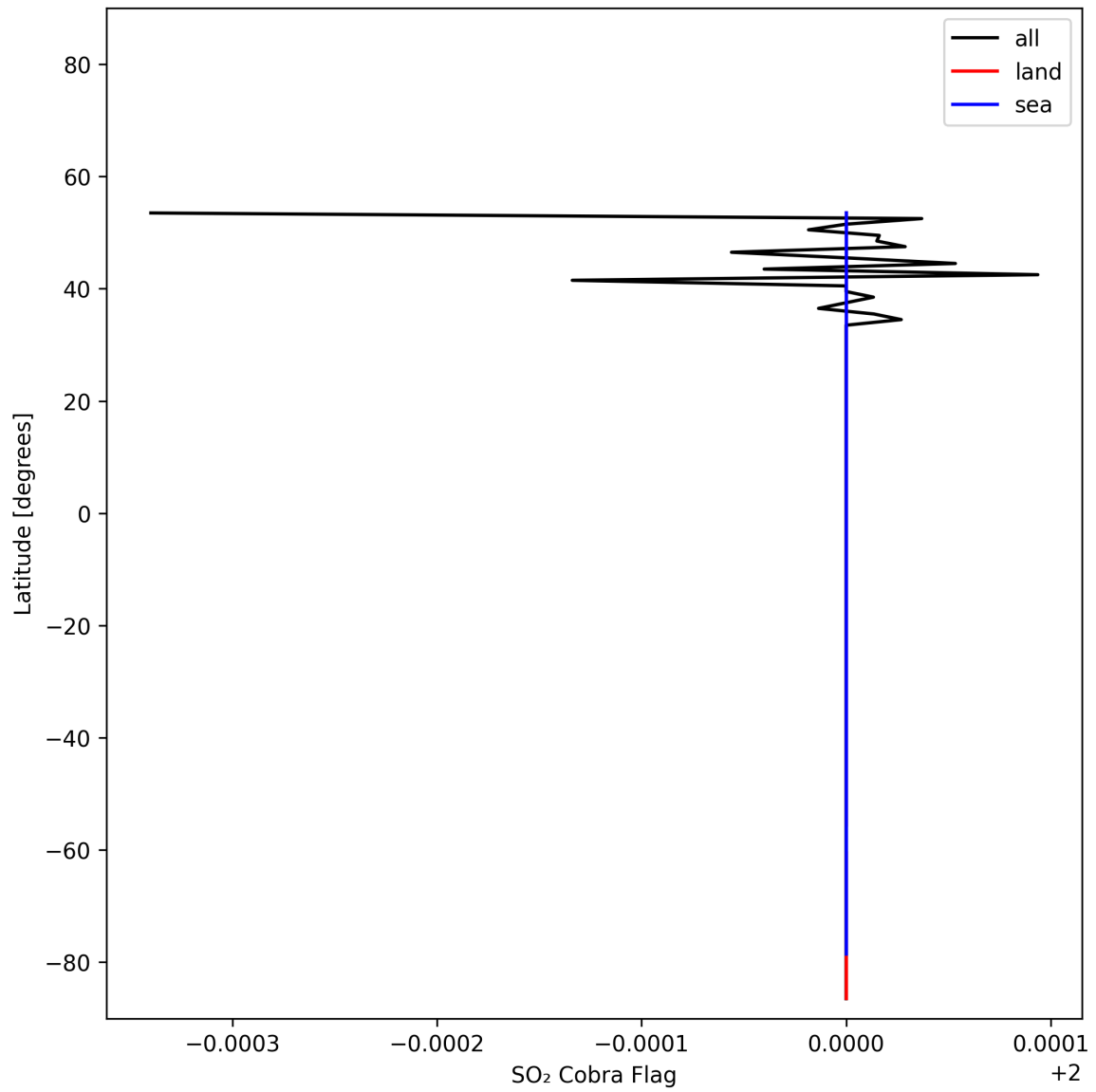
Figure 49: Zonal average of "SO 2 Cobra Flag" for 2025-11-07 to 2025-11-09.
