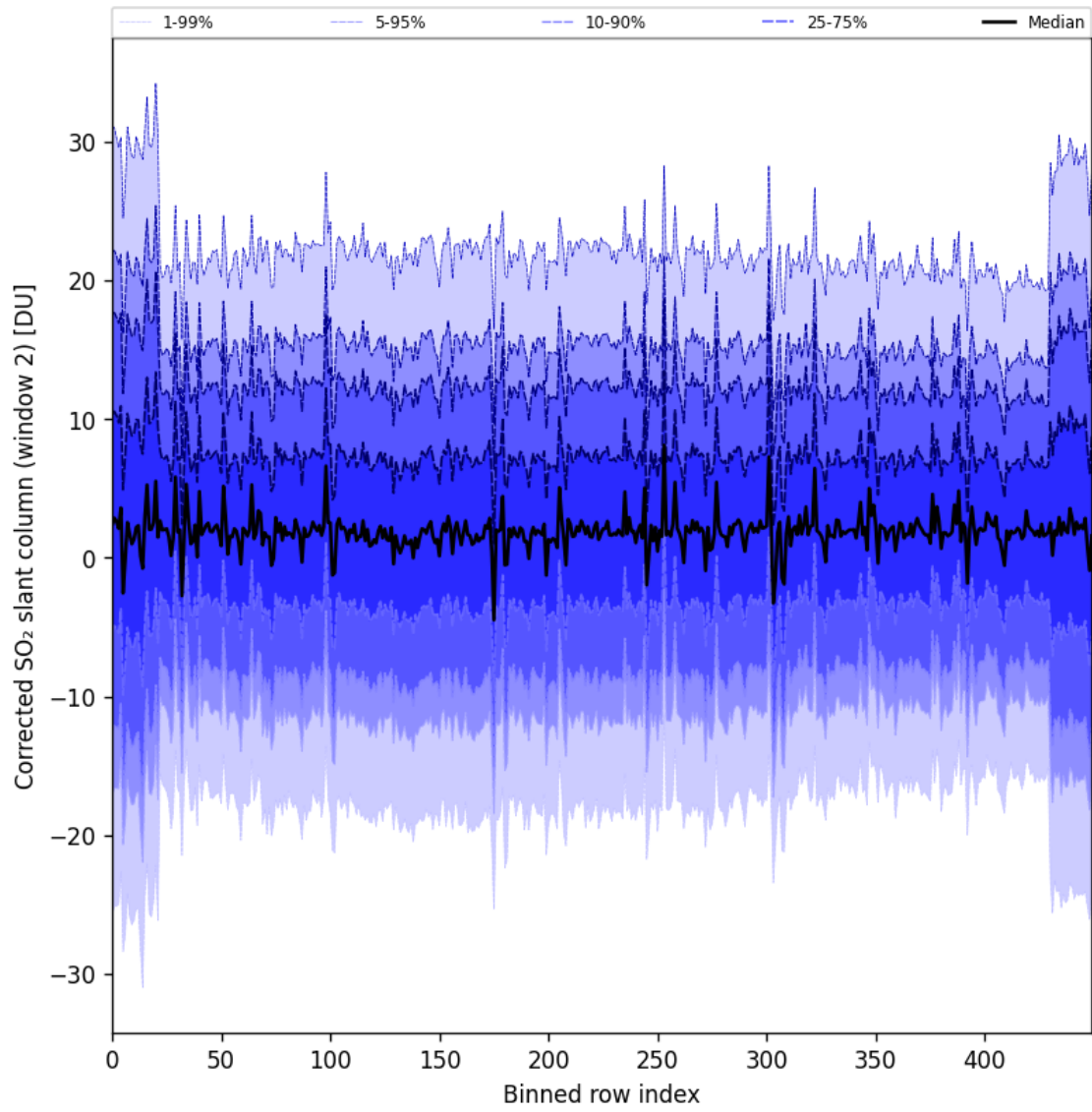
Figure 95: Along track statistics of “Corrected SO 2 slant column (window 2)” for 2025-11-07 to 2025-11-09
