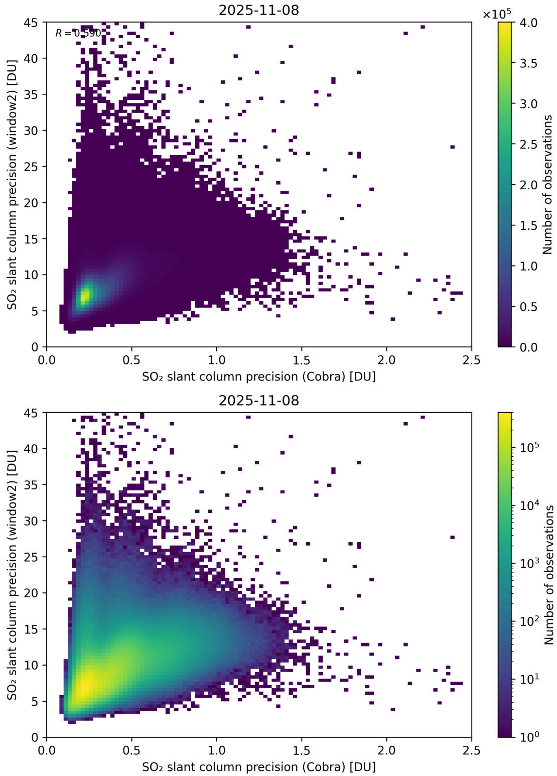
Figure 210: Scatter density plot of “SO 2 slant column precision (Cobra)” against “SO 2 slant column precision (window2)” for 2025-11-07 to 2025-11-09.
