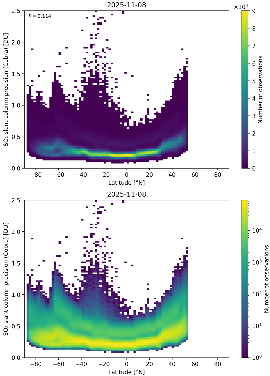
Figure 158: Scatter density plot of “Latitude” against “SO 2 slant column precision (Cobra)” for 2025-11-07 to 2025-11-09.
