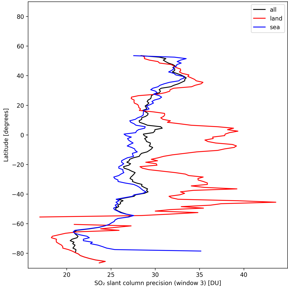
Figure 46: Zonal average of “SO 2 slant column precision (window 3)” for 2025-11-07 to 2025-11-09.
