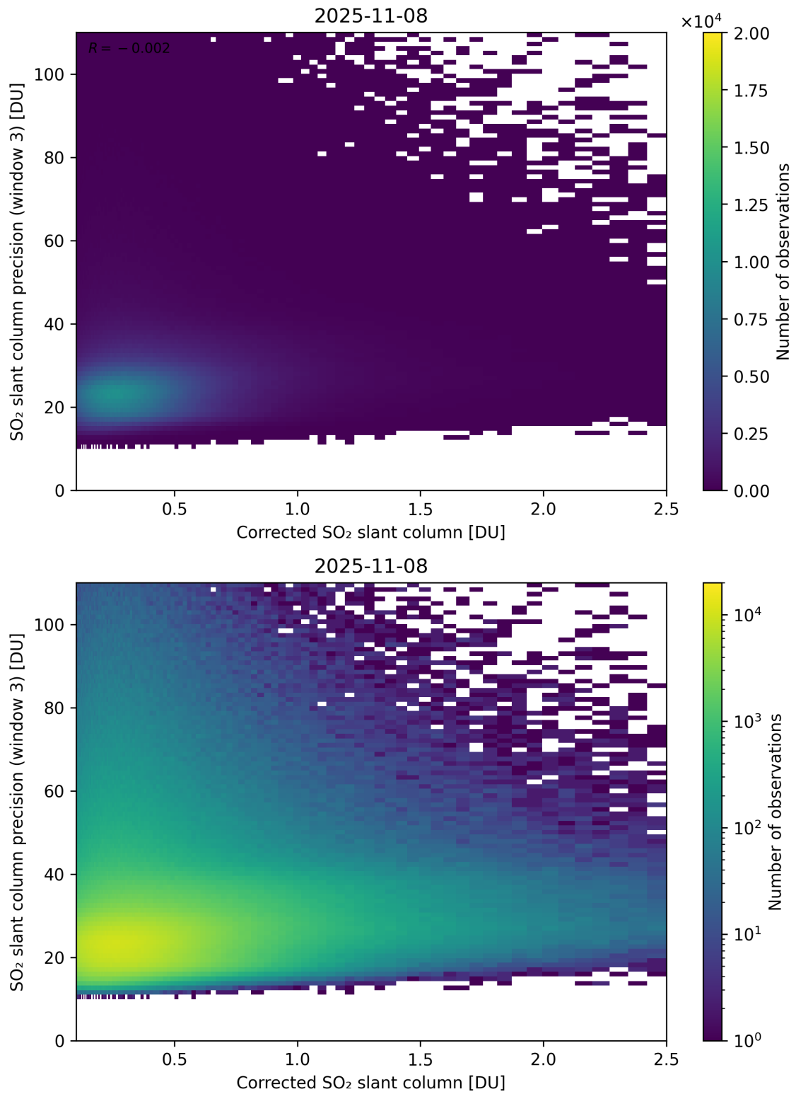
Figure 241: Scatter density plot of “Corrected SO 2 slant column” against “SO 2 slant column precision (window 3)” for 2025-11-07 to 2025-11-09.
