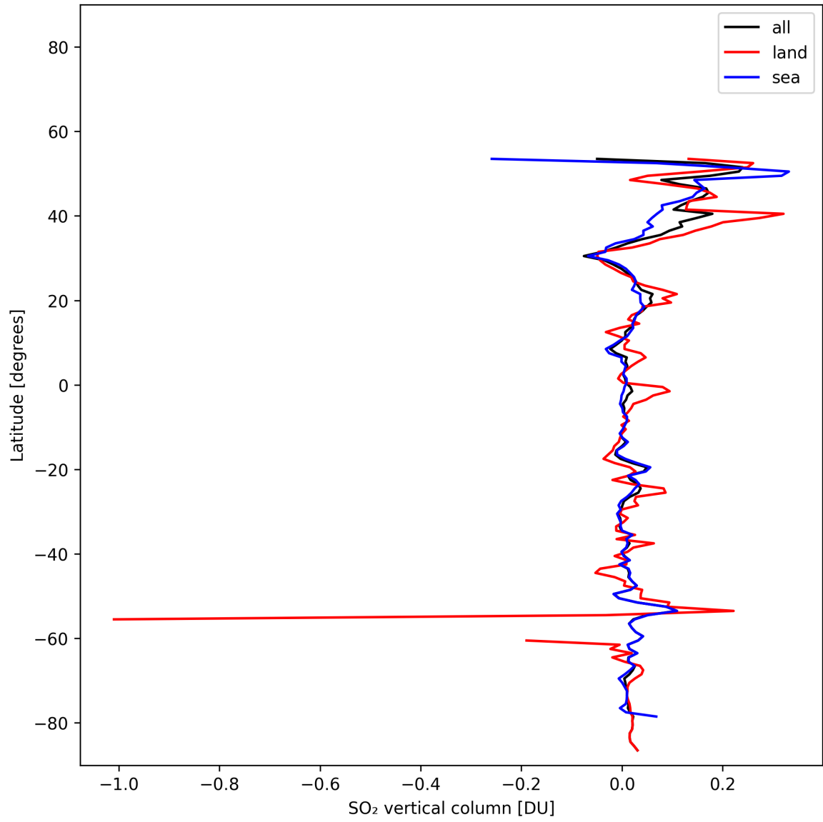
Figure 32: Zonal average of “SO 2 vertical column” for 2025-11-07 to 2025-11-09.
