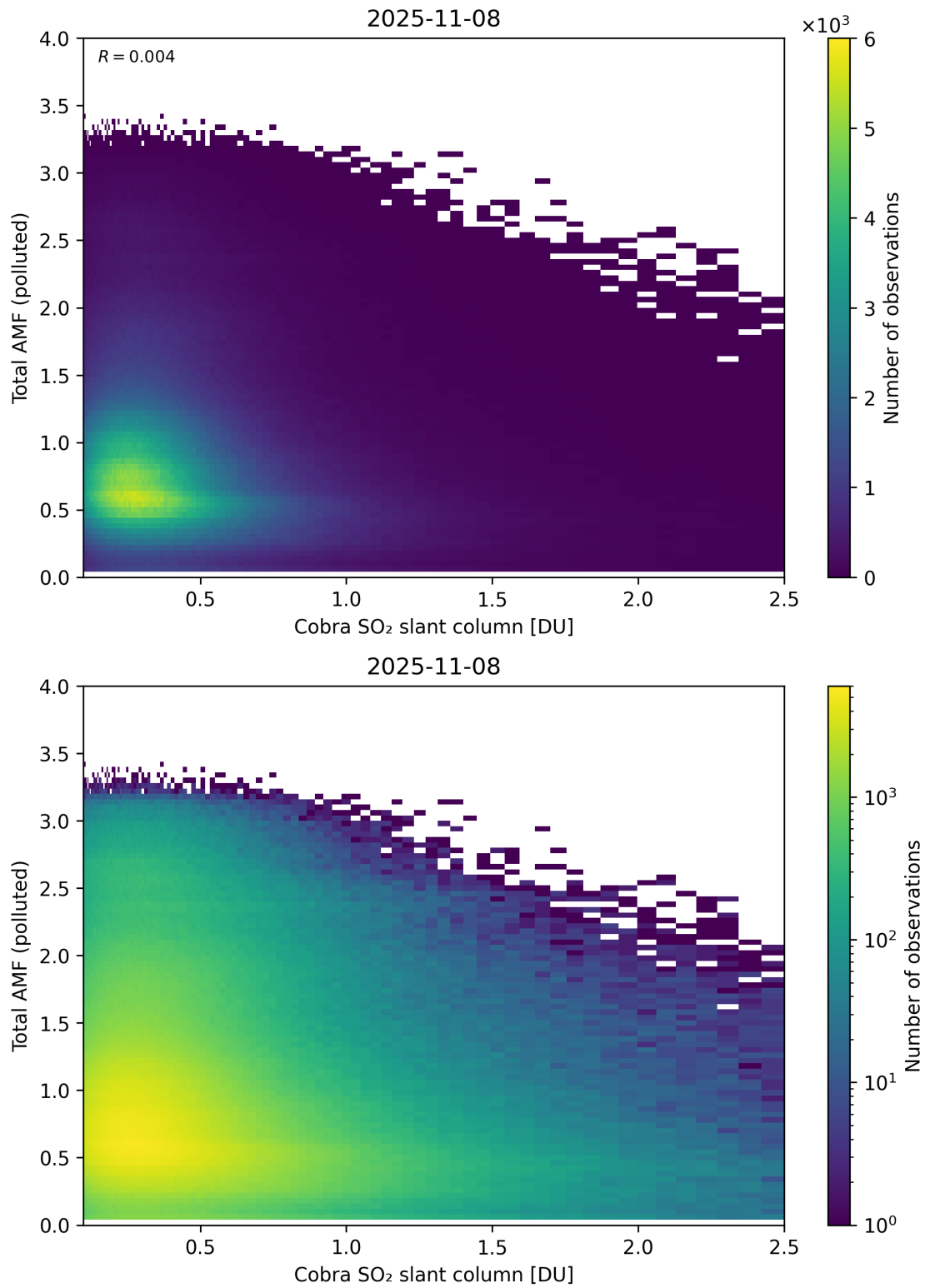
Figure 224: Scatter density plot of “Cobra SO 2 slant column” against “Total AMF (polluted)” for 2025-11-07 to 2025-11-09.
