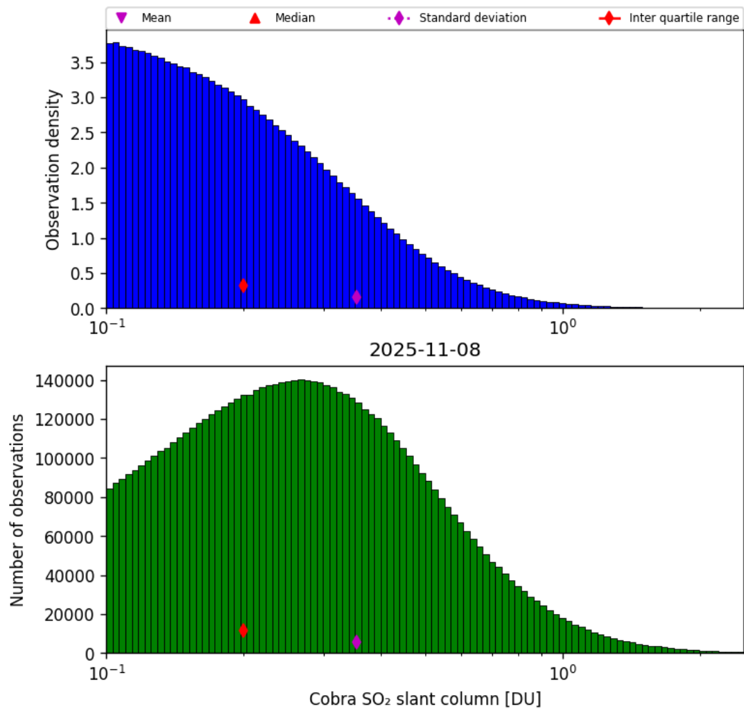
Figure 61: Histogram of “Cobra SO 2 slant column” for 2025-11-07 to 2025-11-09
