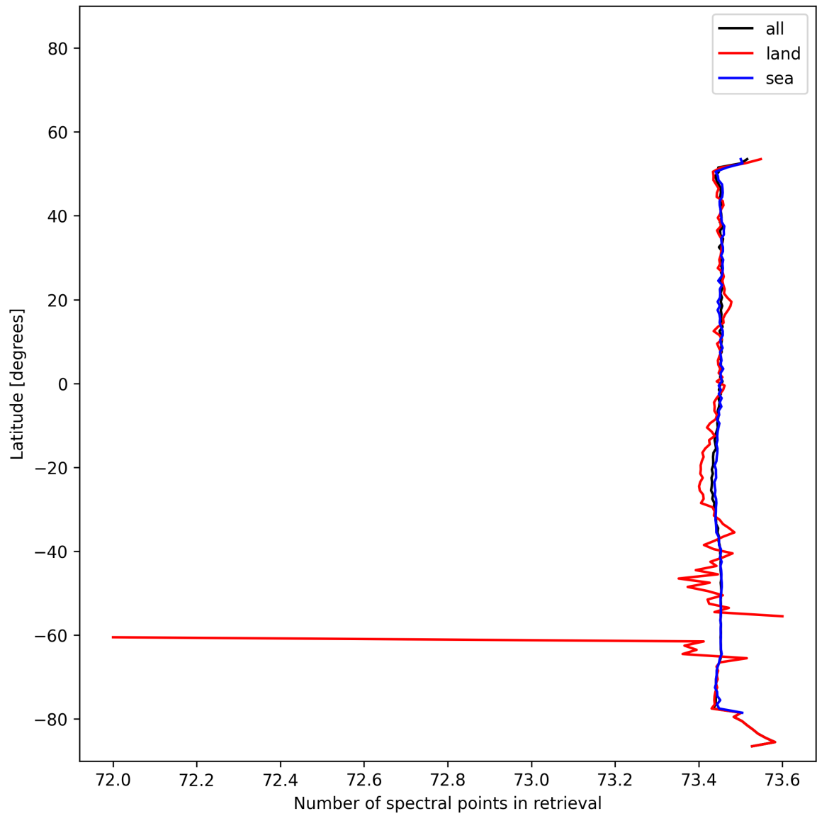
Figure 56: Zonal average of “Number of spectral points in retrieval” for 2025-11-07 to 2025-11-09.
