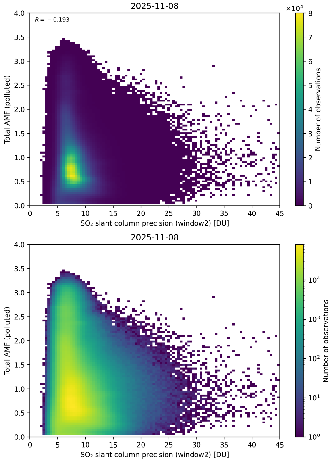
Figure 301: Scatter density plot of “SO 2 slant column precision (window2)” against “Total AMF (polluted)” for 2025-11-07 to 2025-11-09.
