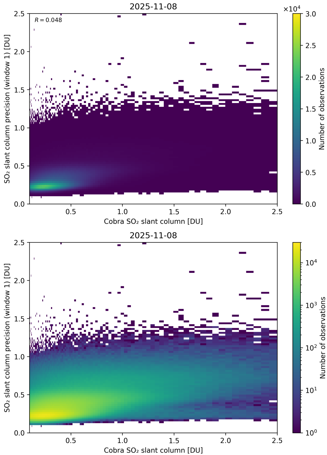
Figure 220: Scatter density plot of “Cobra SO 2 slant column” against “SO 2 slant column precision (window 1)” for 2025-11-07 to 2025-11-09.
