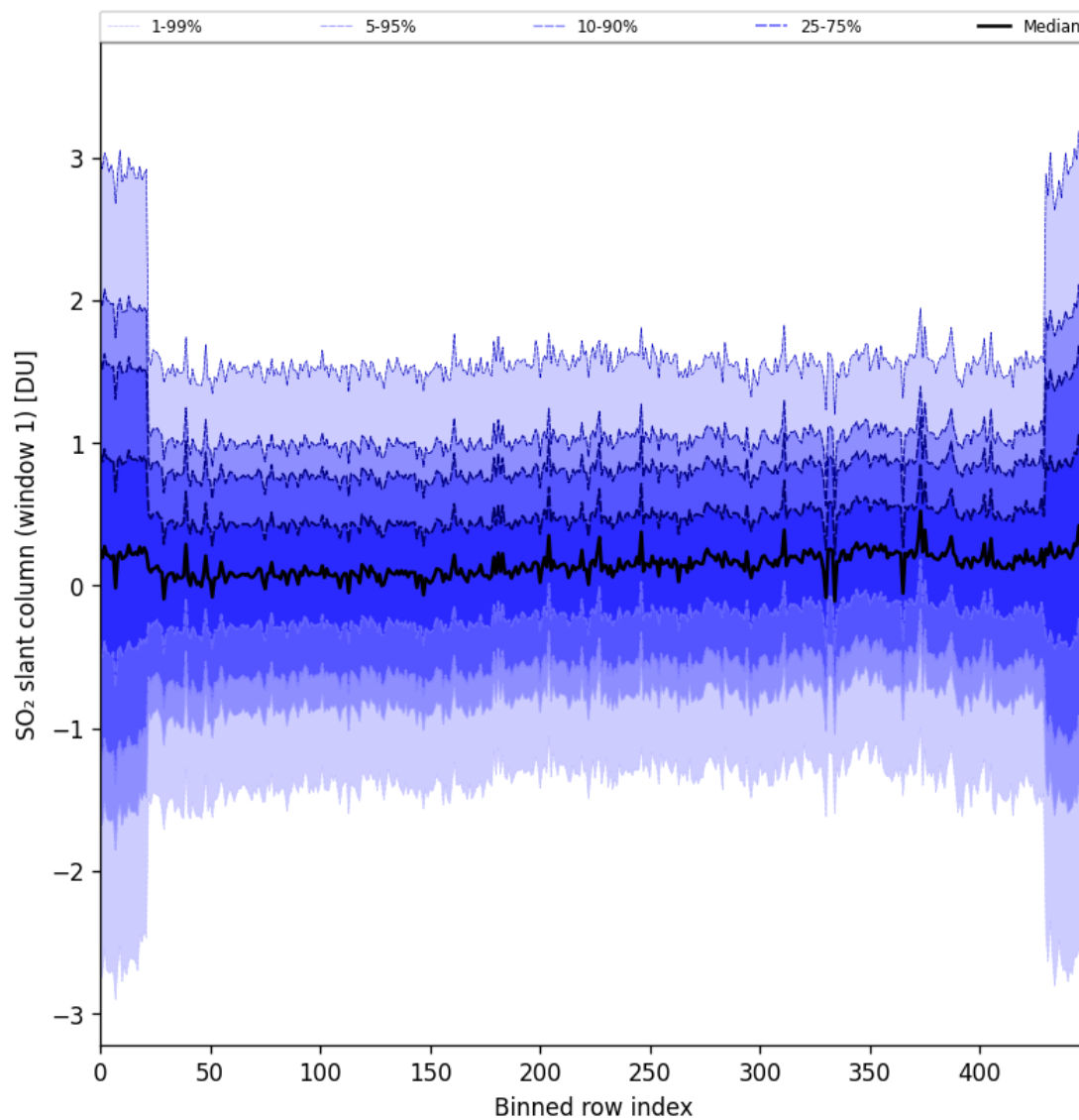
Figure 89: Along track statistics of “SO 2 slant column (window 1)” for 2025-11-07 to 2025-11-09
