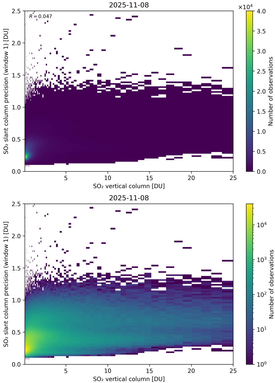
Figure 355: Scatter density plot of “SO 2 vertical column” against “SO 2 slant column precision (window 1)” for 2025-11-07 to 2025-11-09.
