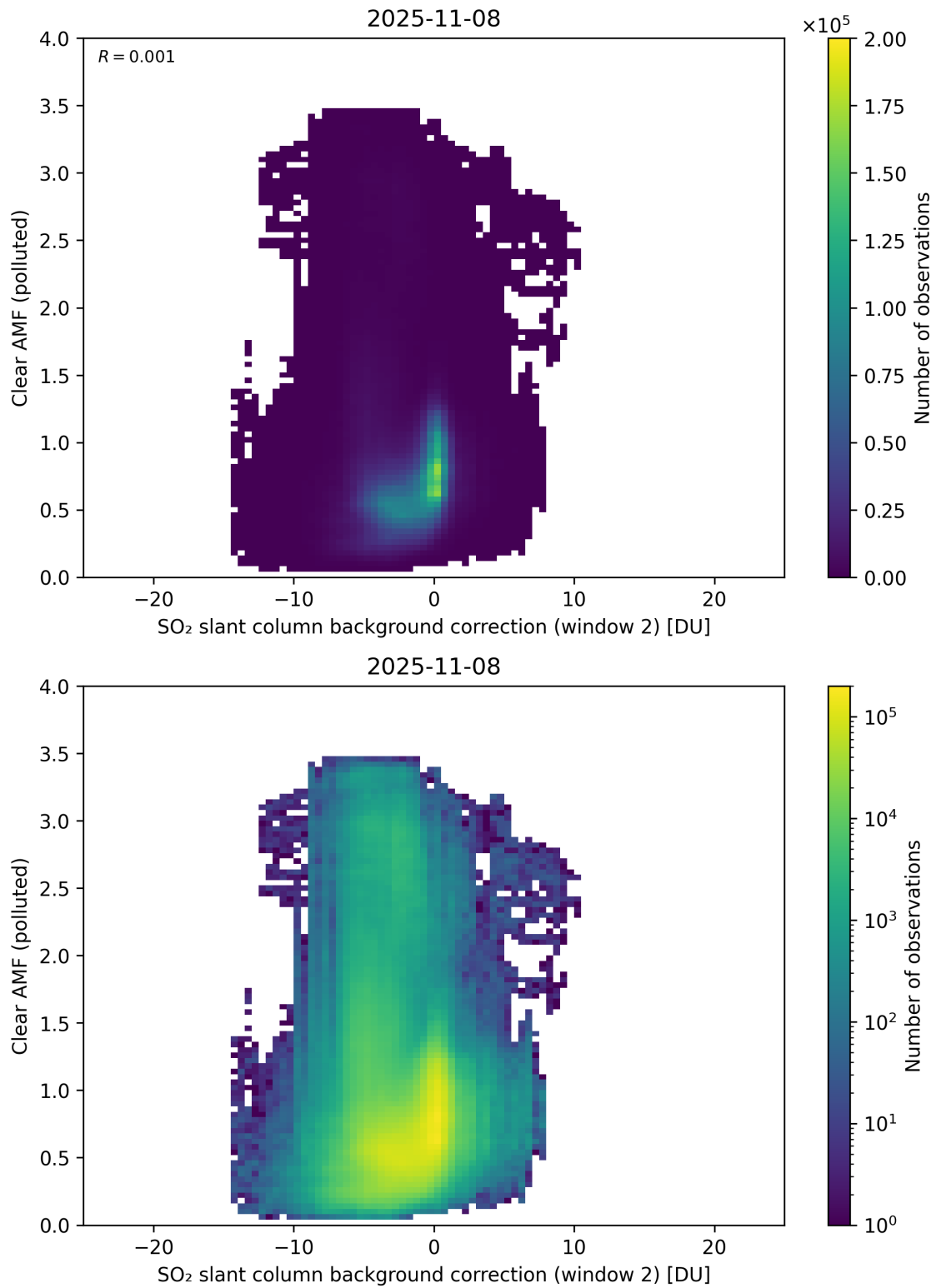
Figure 126: Scatter density plot of “SO 2 slant column background correction (window 2)” against “Clear AMF (polluted)” for 2025-11-07 to 2025-11-09.
