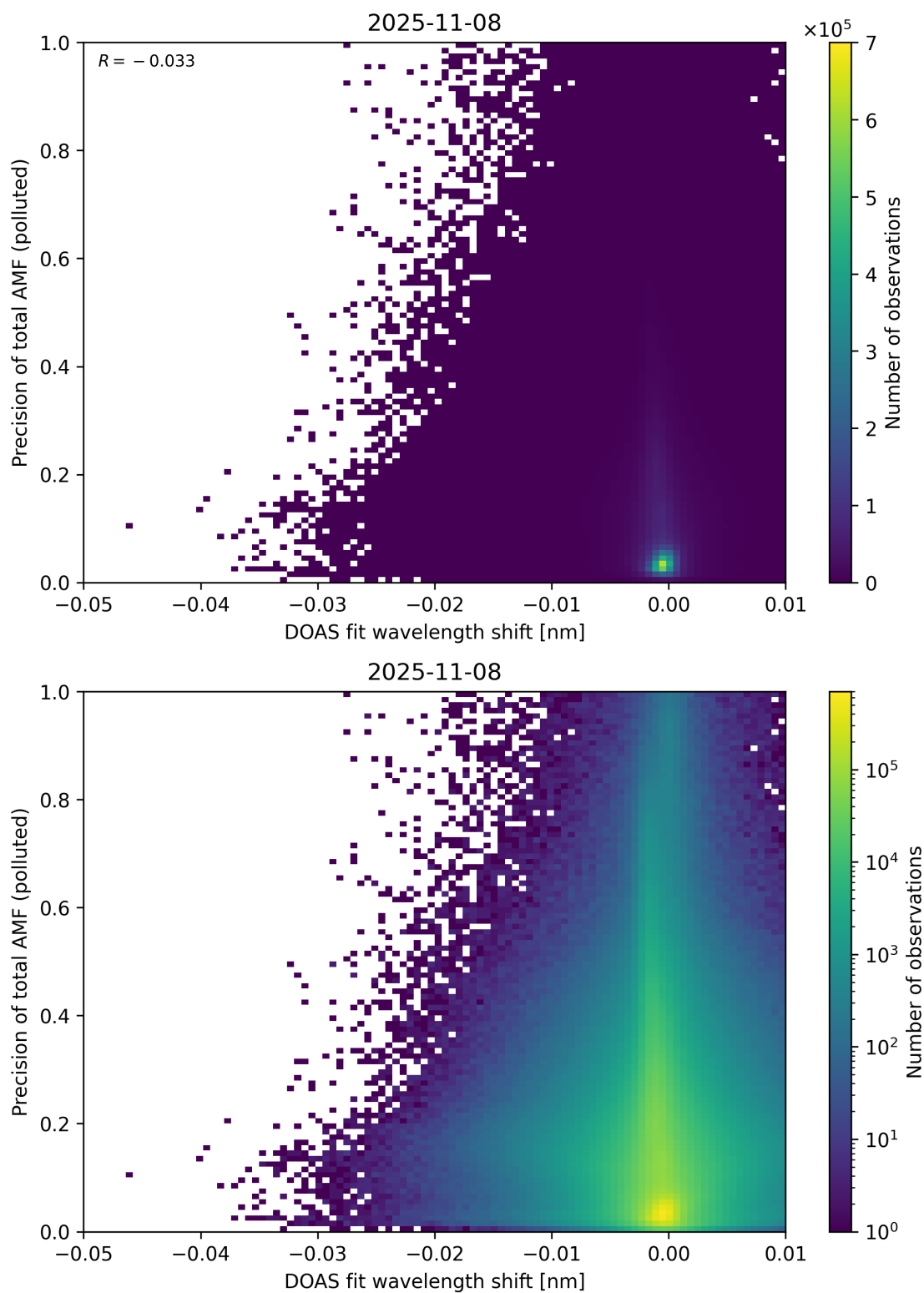
Figure 142: Scatter density plot of “DOAS fit wavelength shift” against “Precision of total AMF (polluted)” for 2025-11-07 to 2025-11-09.
