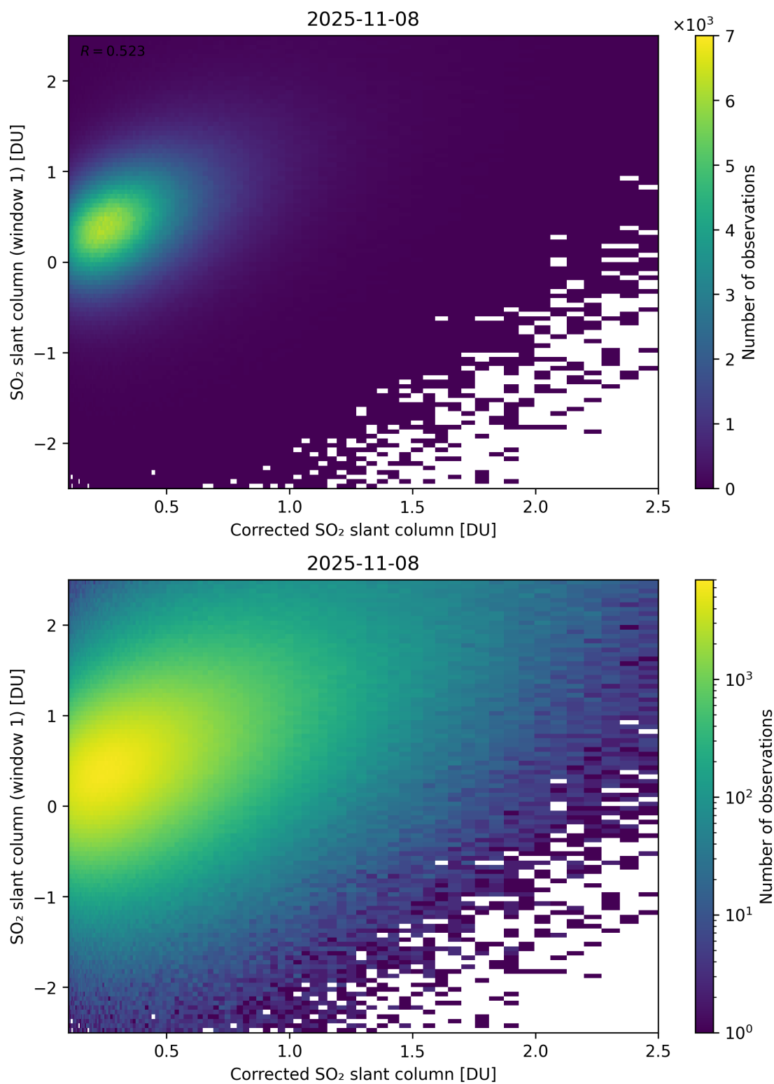
Figure 237: Scatter density plot of “Corrected SO 2 slant column” against “SO 2 slant column (window 1)” for 2025-11-07 to 2025-11-09.
