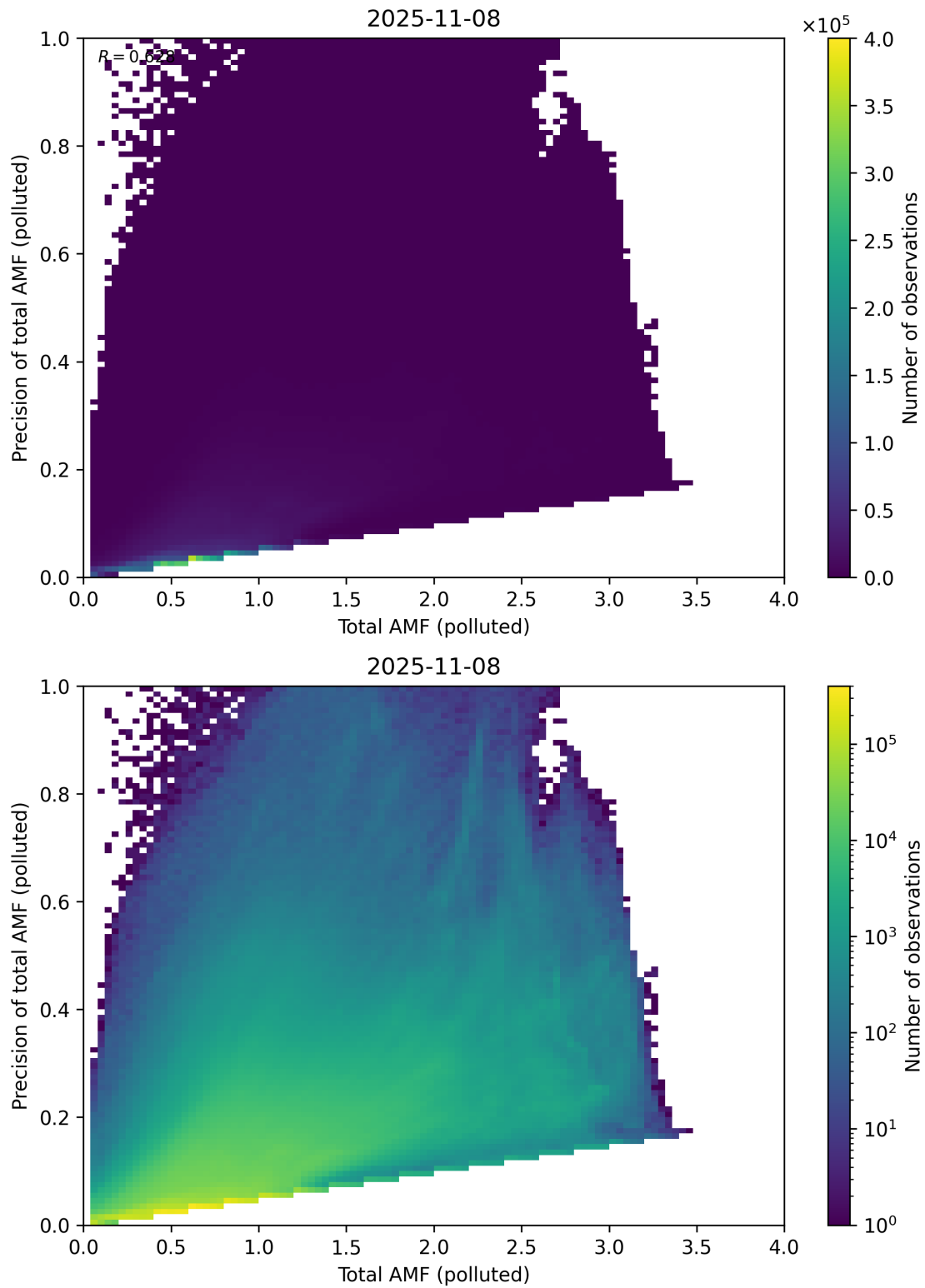
Figure 322: Scatter density plot of “Total AMF (polluted)” against “Precision of total AMF (polluted)” for 2025-11-07 to 2025-11-09.
