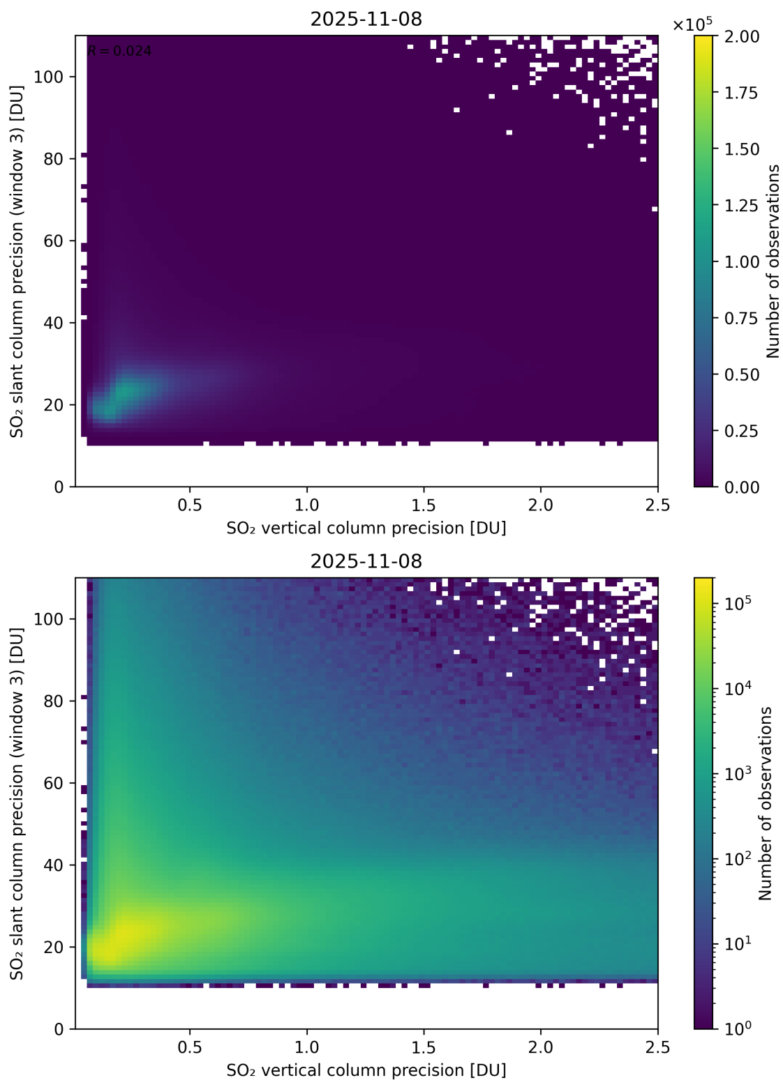
Figure 345: Scatter density plot of “SO 2 vertical column precision” against “SO 2 slant column precision (window 3)” for 2025-11-07 to 2025-11-09.
