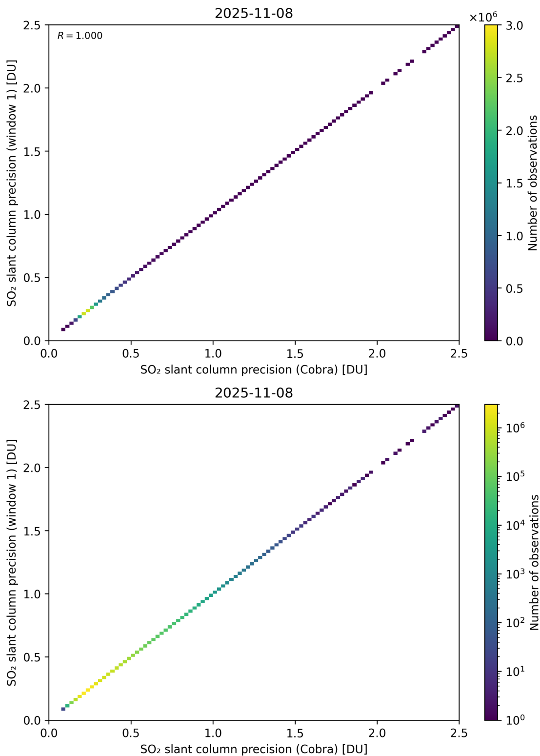
Figure 209: Scatter density plot of “SO 2 slant column precision (Cobra)” against “SO 2 slant column precision (window 1)” for 2025-11-07 to 2025-11-09.
