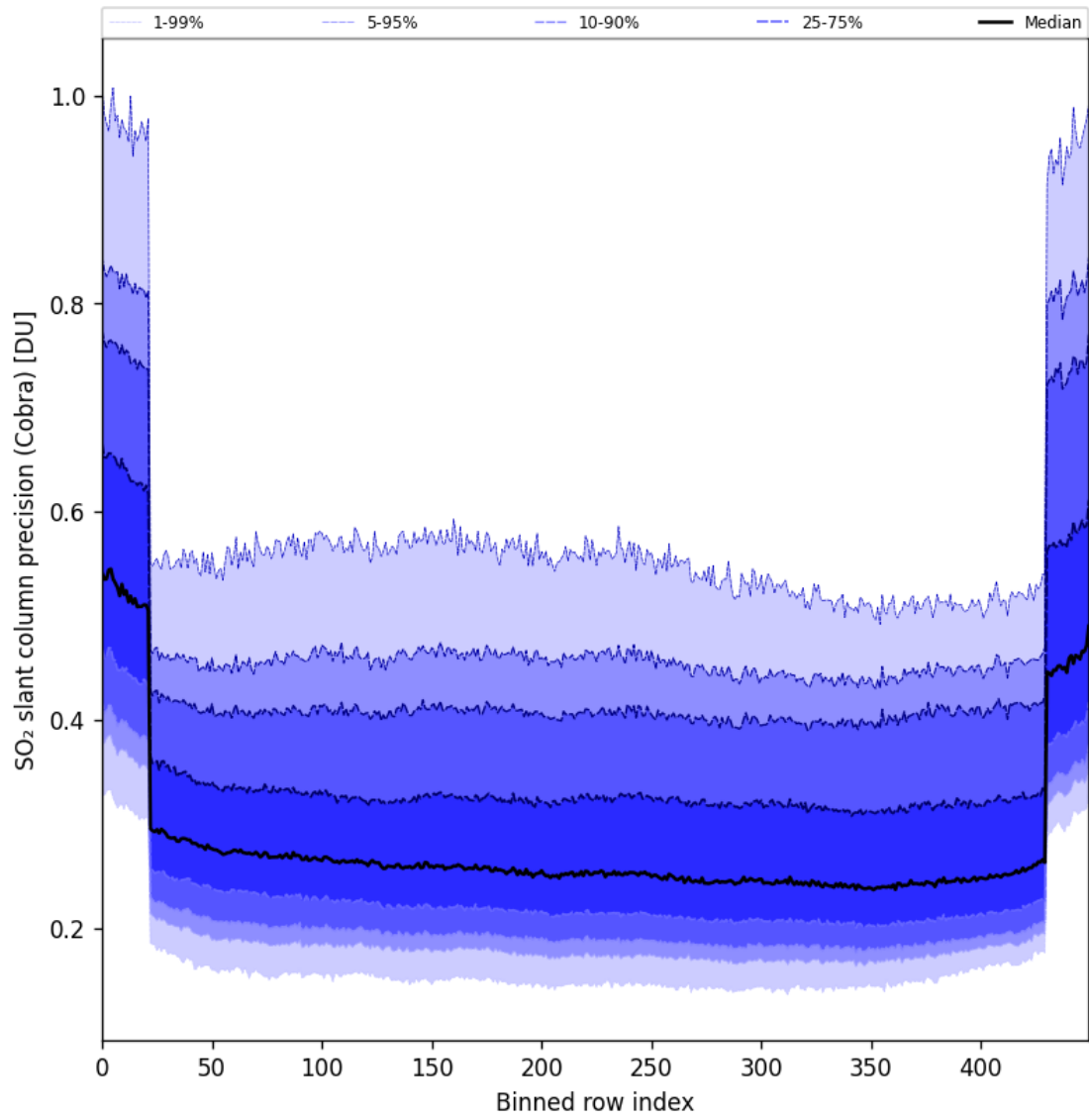
Figure 88: Along track statistics of “SO 2 slant column precision (Cobra)” for 2025-11-07 to 2025-11-09
