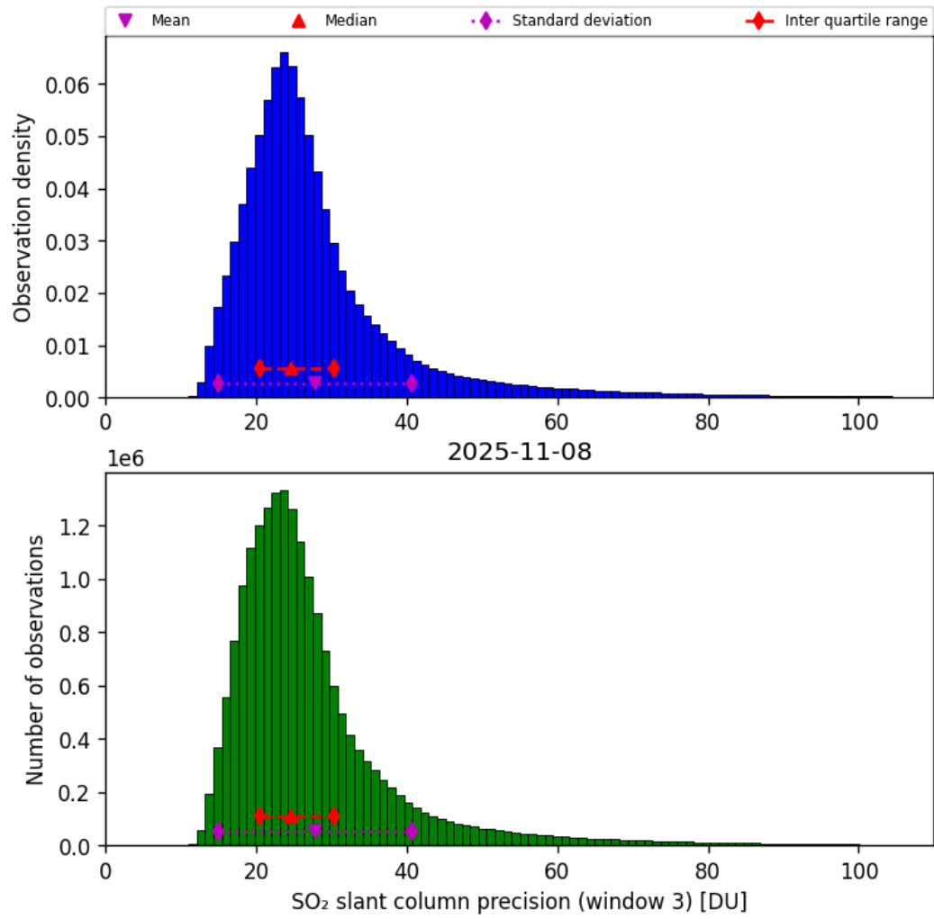
Figure 72: Histogram of “SO 2 slant column precision (window 3)” for 2025-11-07 to 2025-11-09
