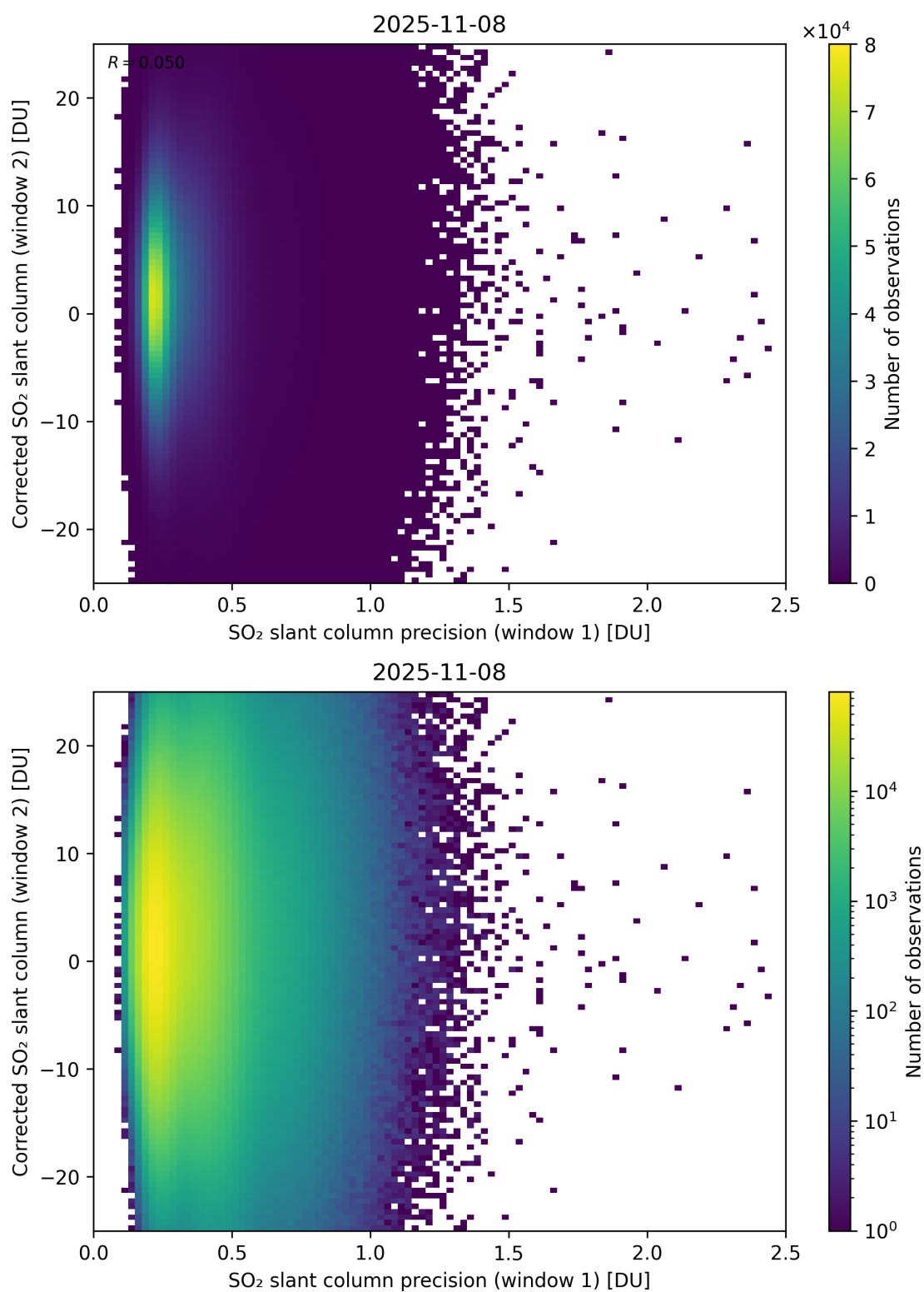
Figure 275: Scatter density plot of “SO 2 slant column precision (window 1)” against “Corrected SO 2 slant column (window 2)” for 2025-11-07 to 2025-11-09.
