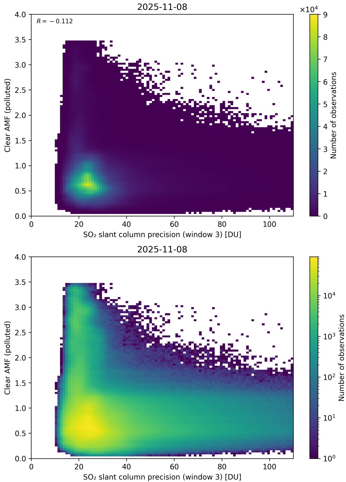
Figure 311: Scatter density plot of “SO 2 slant column precision (window 3)” against “Clear AMF (polluted)” for 2025-11-07 to 2025-11-09.
