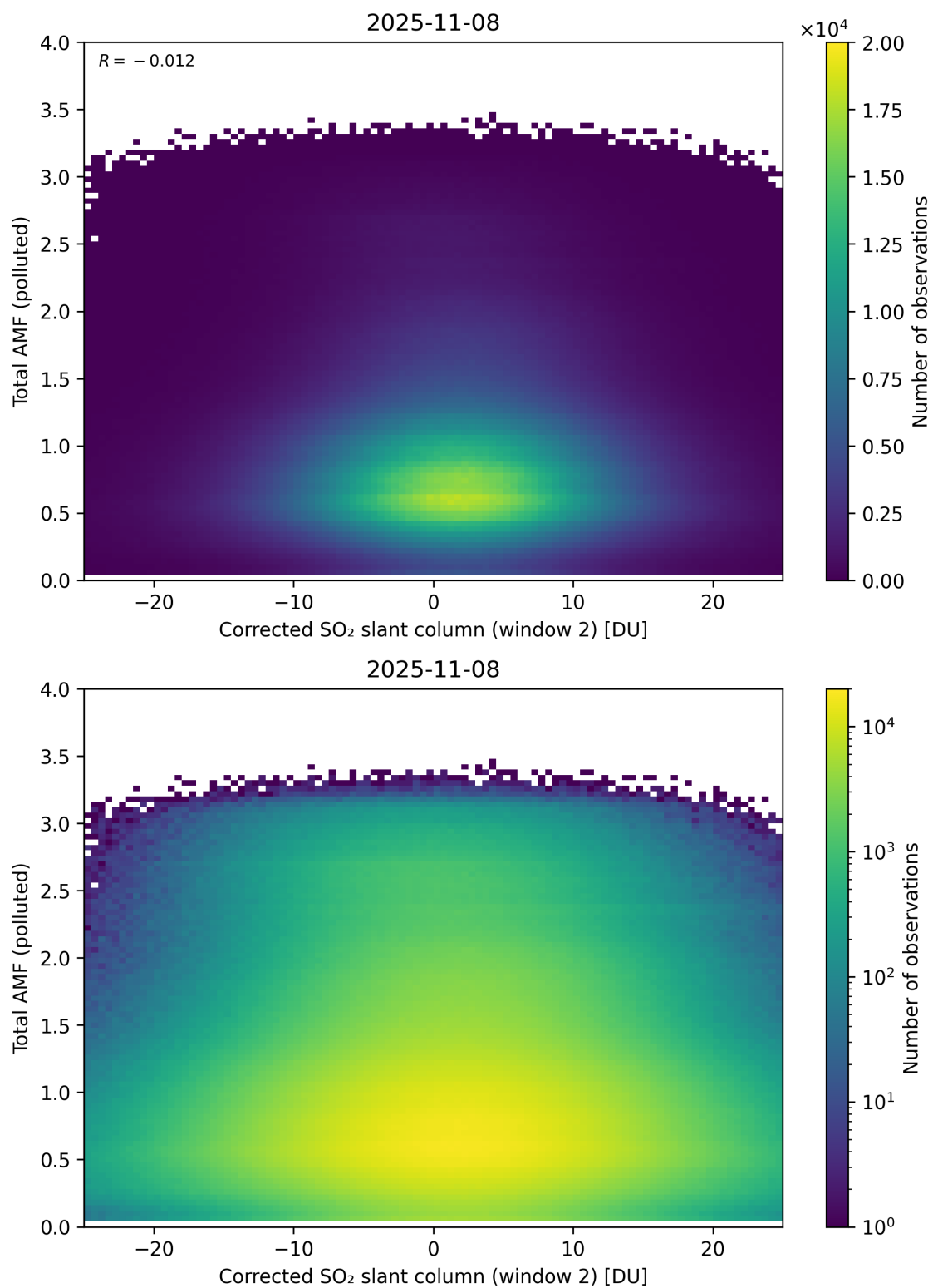
Figure 253: Scatter density plot of “Corrected SO 2 slant column (window 2)” against “Total AMF (polluted)” for 2025-11-07 to 2025-11-09.
