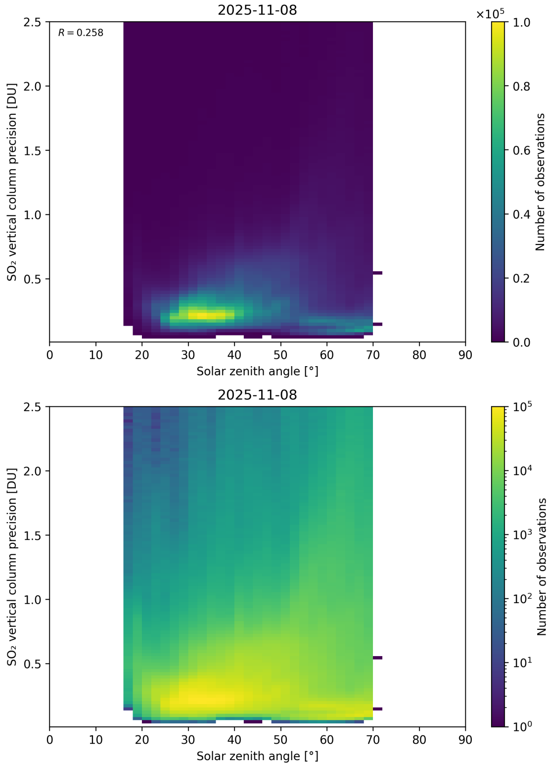
Figure 192: Scatter density plot of “Solar zenith angle” against “SO 2 vertical column precision” for 2025-11-07 to 2025-11-09.
