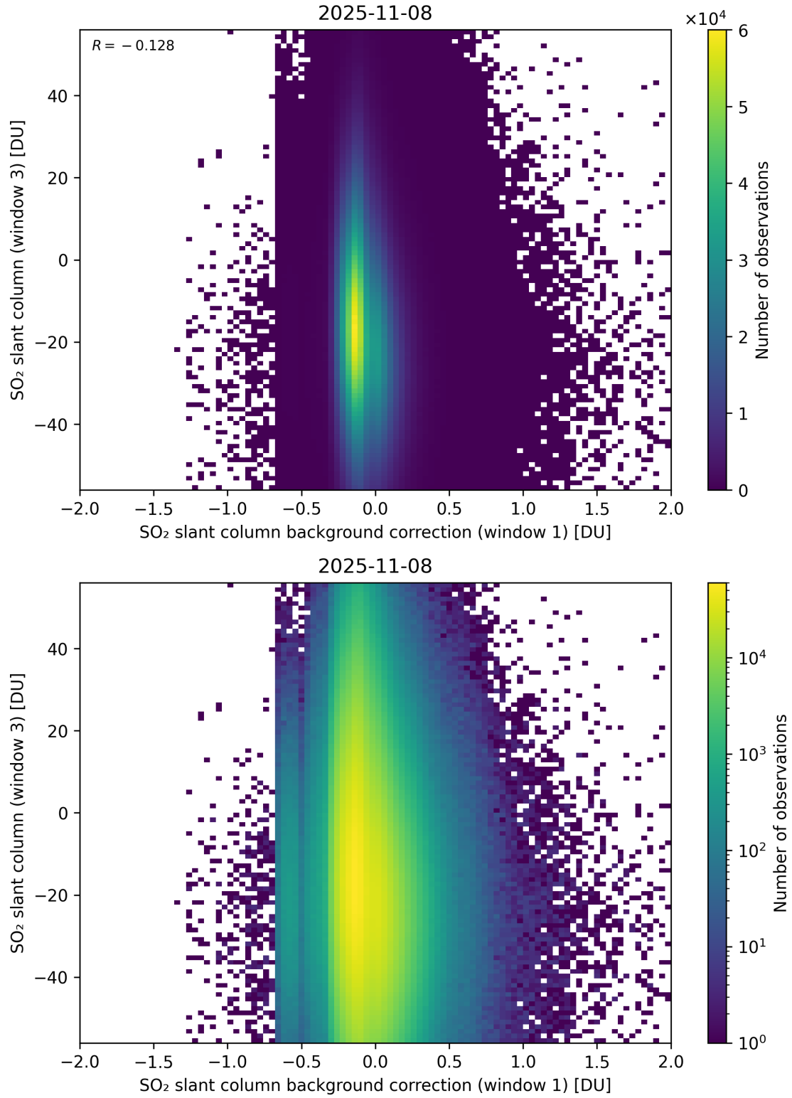
Figure 118: Scatter density plot of “SO 2 slant column background correction (window 1)” against “SO 2 slant column (window 3)” for 2025-11-07 to 2025-11-09.
