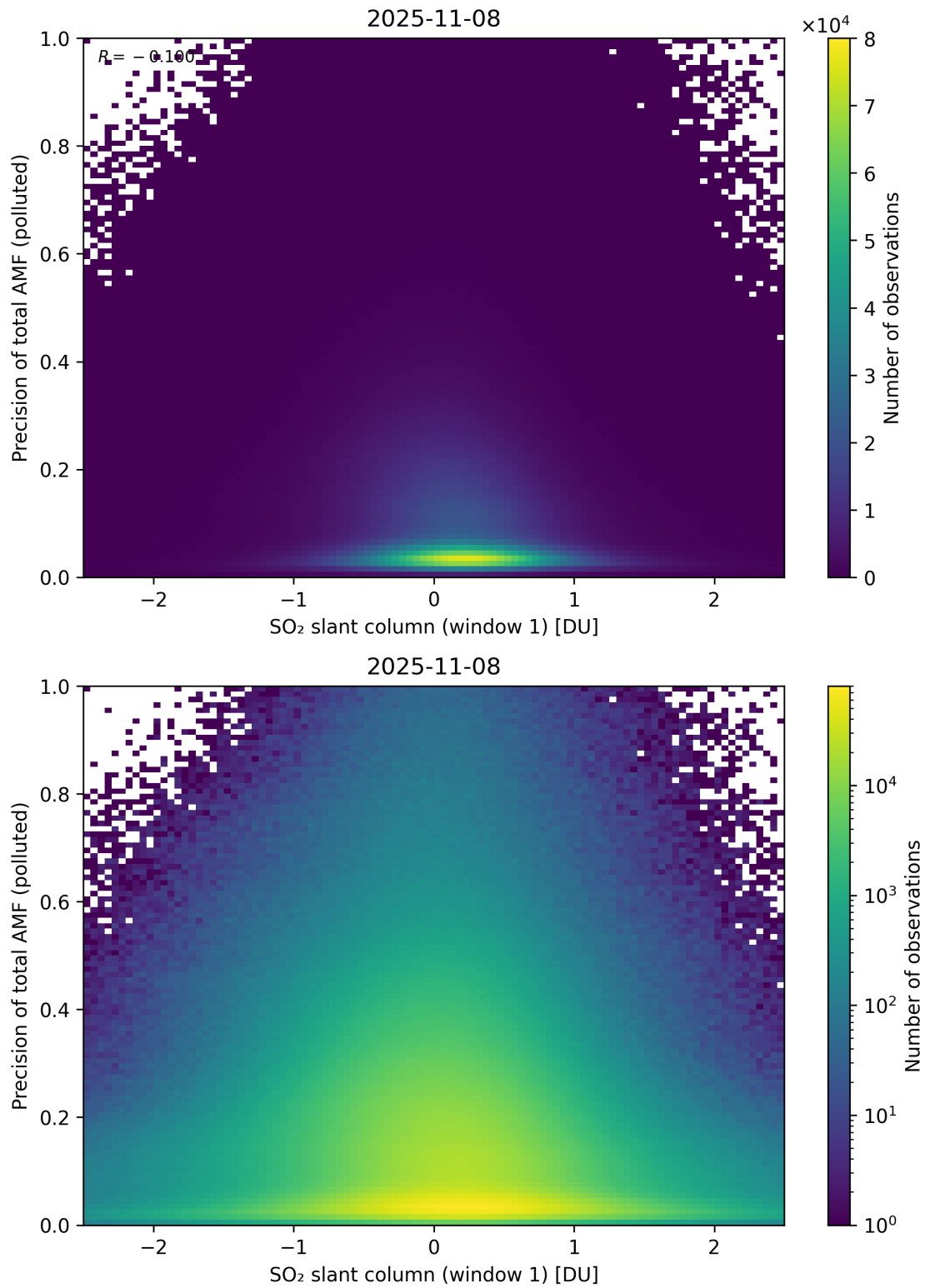
Figure 290: Scatter density plot of “SO 2 slant column (window 1)” against “Precision of total AMF (polluted)” for 2025-11-07 to 2025-11-09.
