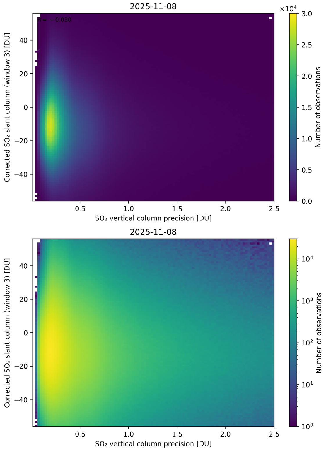
Figure 340: Scatter density plot of “SO 2 vertical column precision” against “Corrected SO 2 slant column (window 3)” for 2025-11-07 to 2025-11-09.
