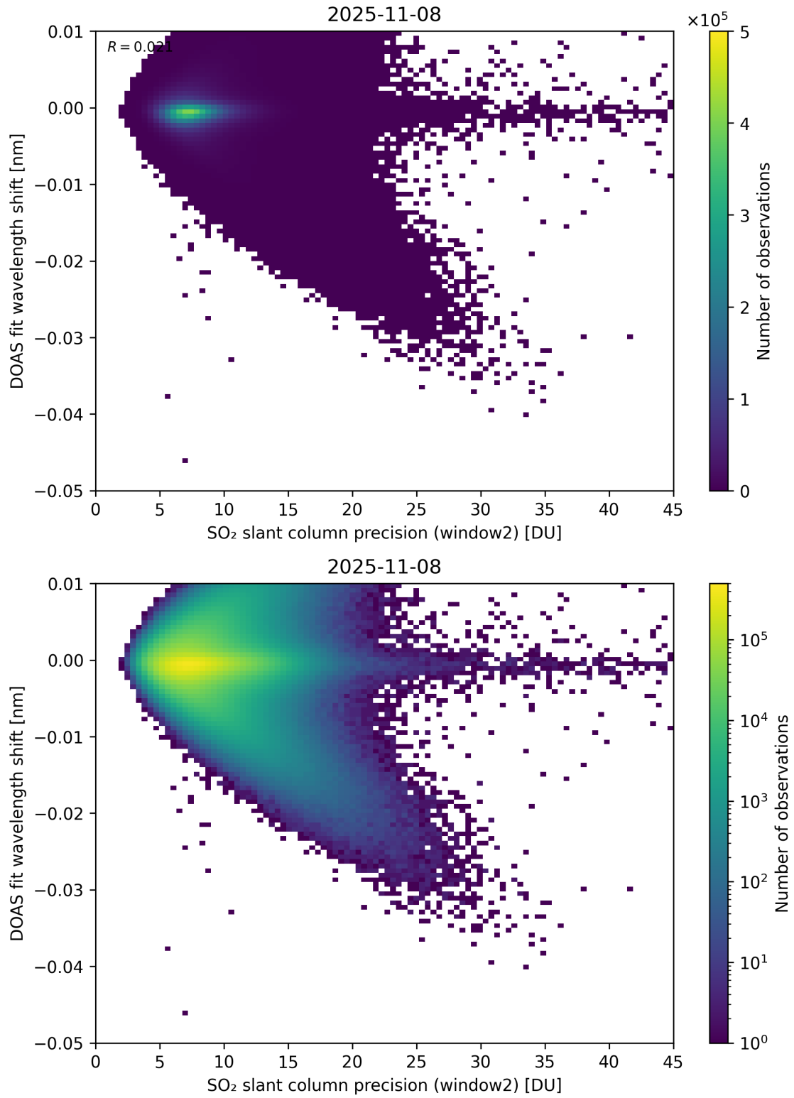
Figure 293: Scatter density plot of “SO 2 slant column precision (window2)” against “DOAS fit wavelength shift” for 2025-11-07 to 2025-11-09.
