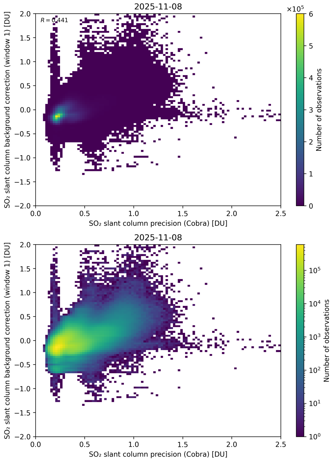
Figure 199: Scatter density plot of “SO 2 slant column precision (Cobra)” against “SO 2 slant column background correction (window 1)” for 2025-11-07 to 2025-11-09.
