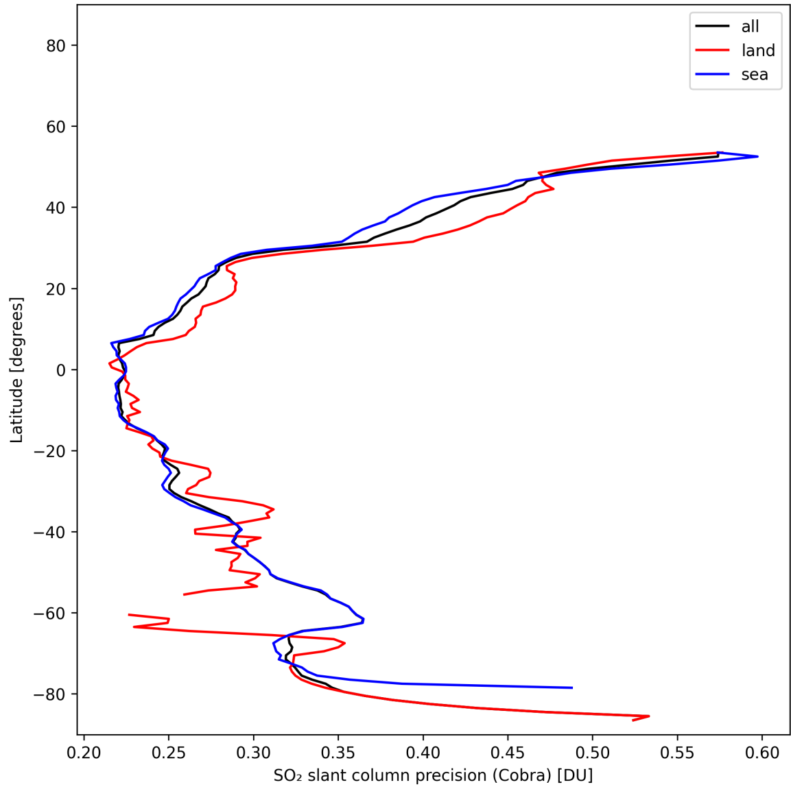
Figure 36: Zonal average of “SO 2 slant column precision (Cobra)” for 2025-11-07 to 2025-11-09.
