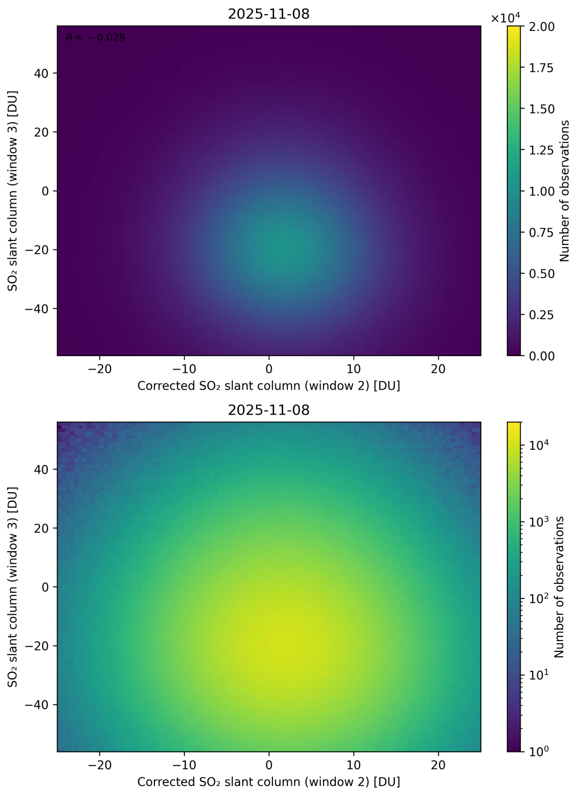
Figure 251: Scatter density plot of “Corrected SO 2 slant column (window 2)” against “SO 2 slant column (window 3)” for 2025-11-07 to 2025-11-09.
