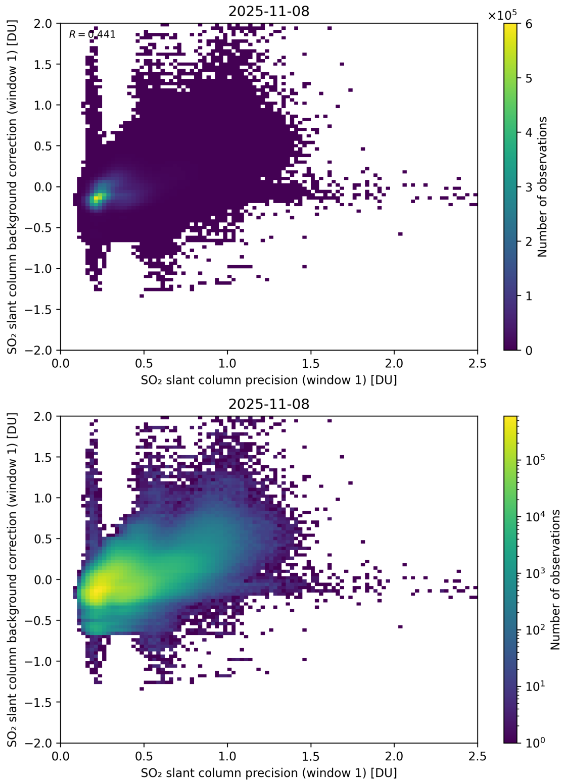
Figure 268: Scatter density plot of “SO 2 slant column precision (window 1)” against “SO 2 slant column background correction (window 1)” for 2025-11-07 to 2025-11-09.
