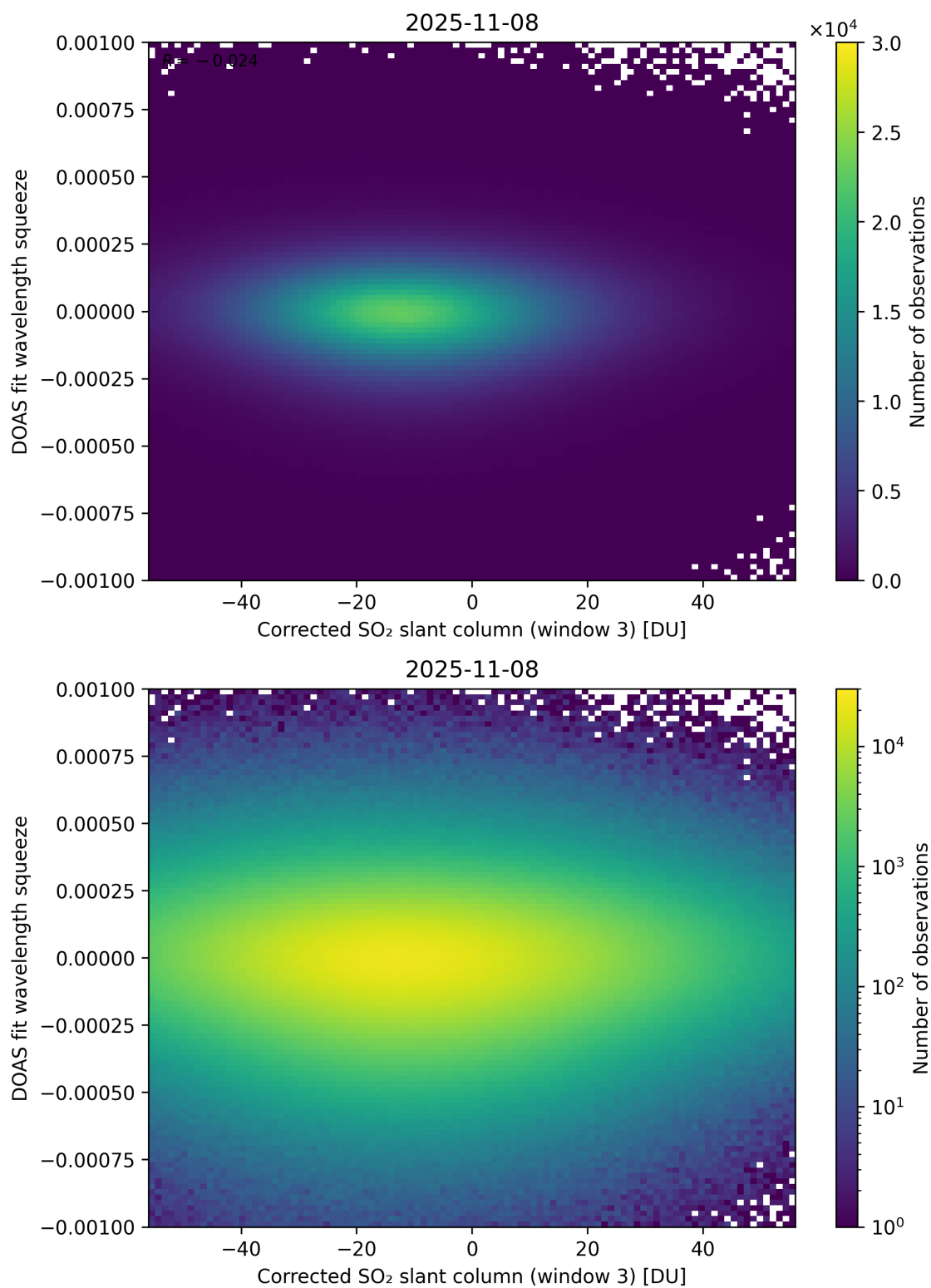
Figure 257: Scatter density plot of “Corrected SO 2 slant column (window 3)” against “DOAS fit wavelength squeeze” for 2025-11-07 to 2025-11-09.
