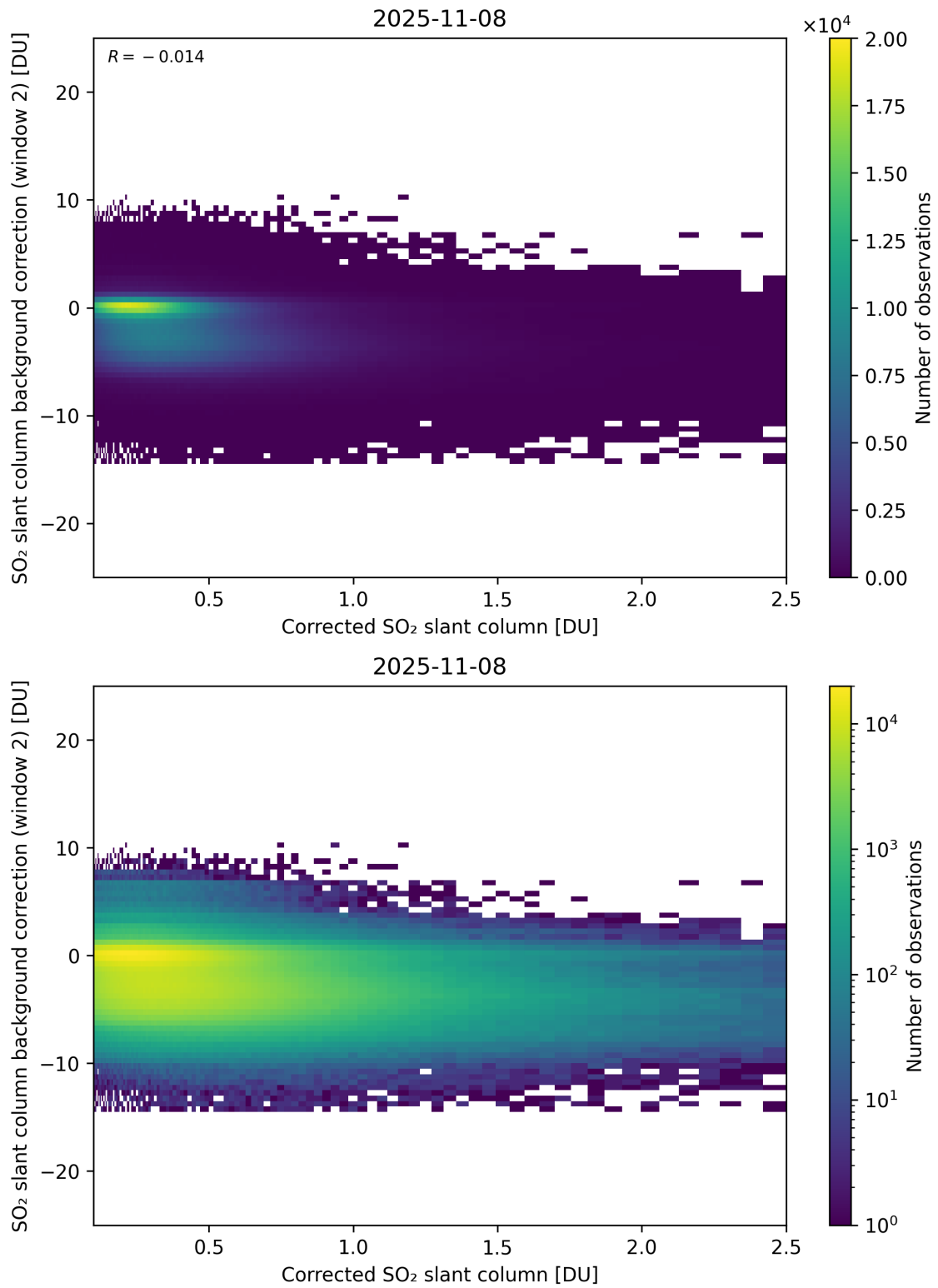
Figure 227: Scatter density plot of “Corrected SO 2 slant column” against “SO 2 slant column background correction (window 2)” for 2025-11-07 to 2025-11-09.
