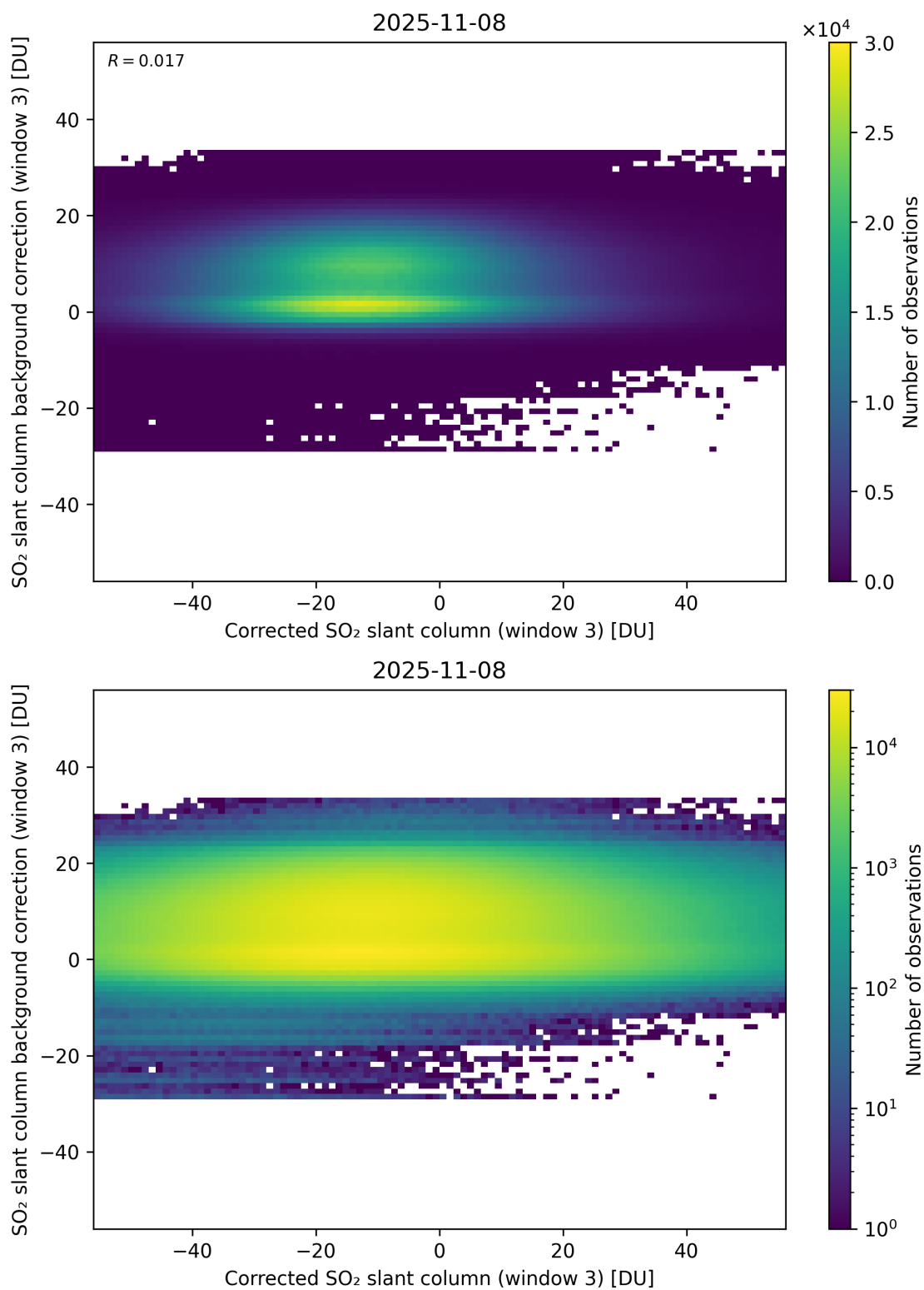
Figure 255: Scatter density plot of “Corrected SO 2 slant column (window 3)” against “SO 2 slant column background correction (window 3)” for 2025-11-07 to 2025-11-09.
