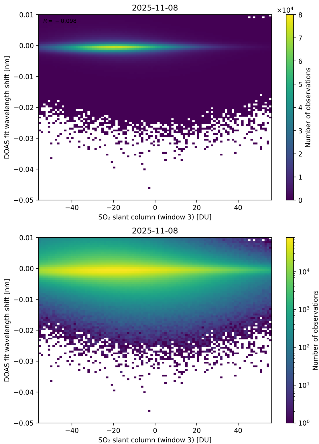
Figure 304: Scatter density plot of “SO 2 slant column (window 3)” against “DOAS fit wavelength shift” for 2025-11-07 to 2025-11-09.
