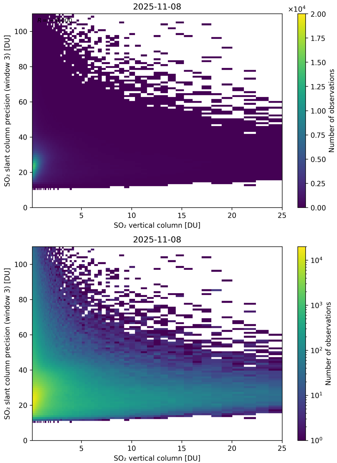
Figure 358: Scatter density plot of “SO 2 vertical column” against “SO 2 slant column precision (window 3)” for 2025-11-07 to 2025-11-09.
