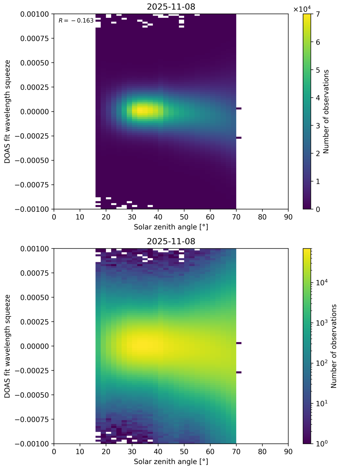
Figure 175: Scatter density plot of “Solar zenith angle” against “DOAS fit wavelength squeeze” for 2025-11-07 to 2025-11-09.
