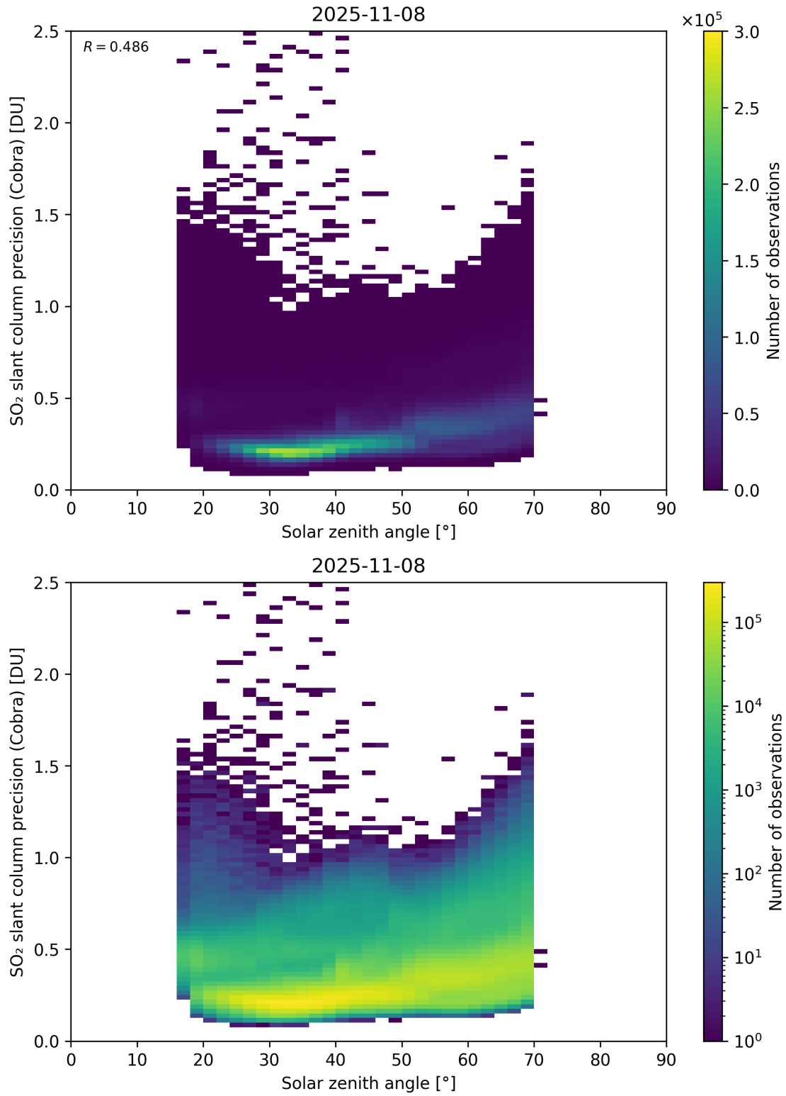
Figure 180: Scatter density plot of “Solar zenith angle” against “SO 2 slant column precision (Cobra)” for 2025-11-07 to 2025-11-09.
