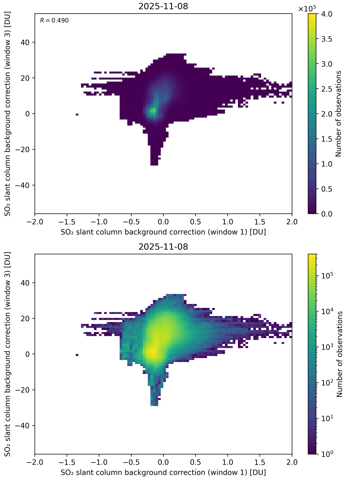
Figure 110: Scatter density plot of “SO 2 slant column background correction (window 1)” against “SO 2 slant column background correction (window 3)” for 2025-11-07 to 2025-11-09.
