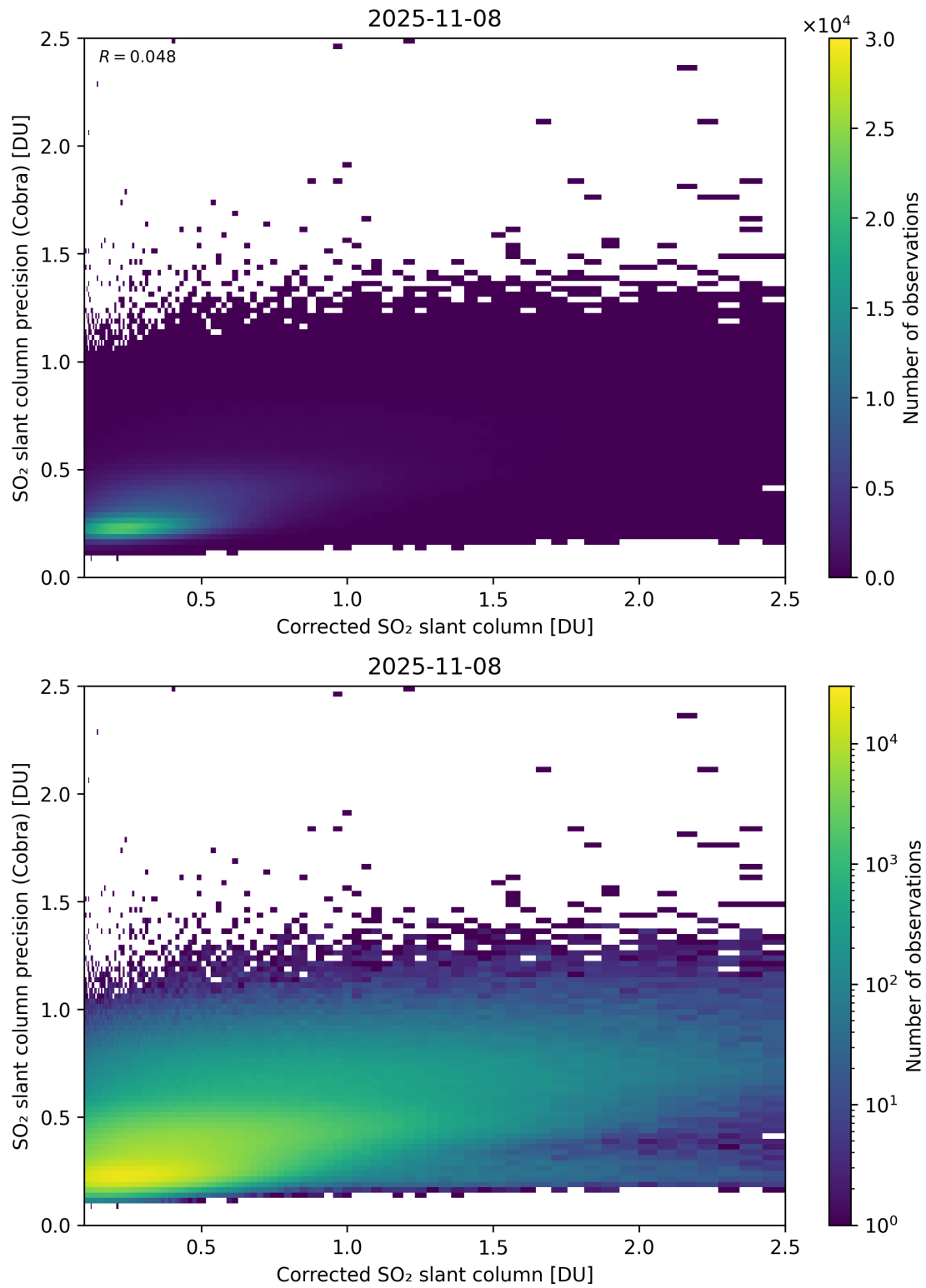
Figure 234: Scatter density plot of “Corrected SO 2 slant column” against “SO 2 slant column precision (Cobra)” for 2025-11-07 to 2025-11-09.
