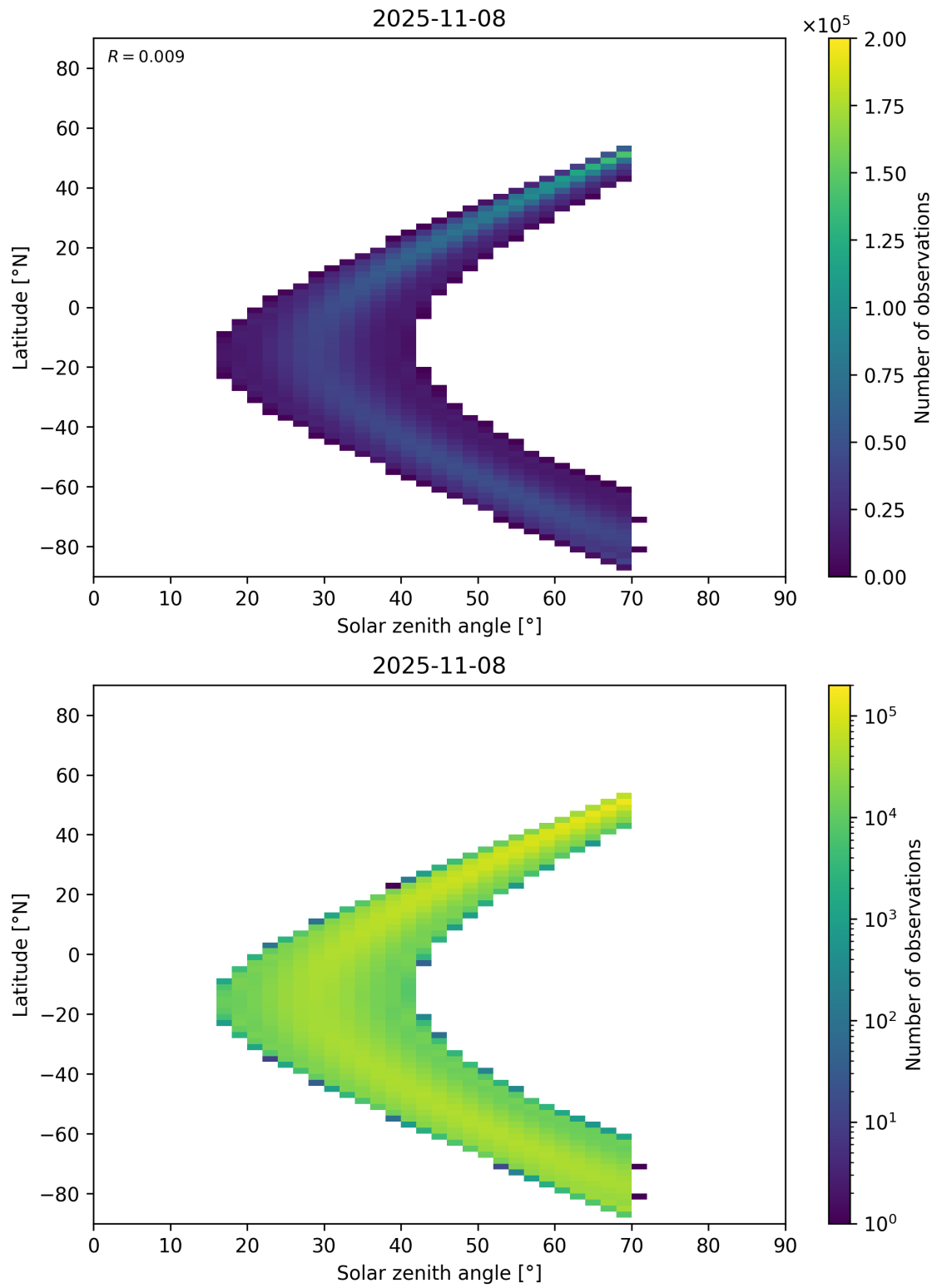
Figure 177: Scatter density plot of “Solar zenith angle” against “Latitude” for 2025-11-07 to 2025-11-09.
