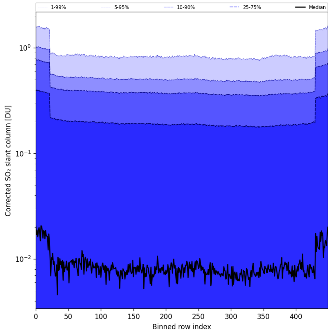
Figure 86: Along track statistics of "Corrected SO 2 slant column" for 2025-11-07 to 2025-11-09
