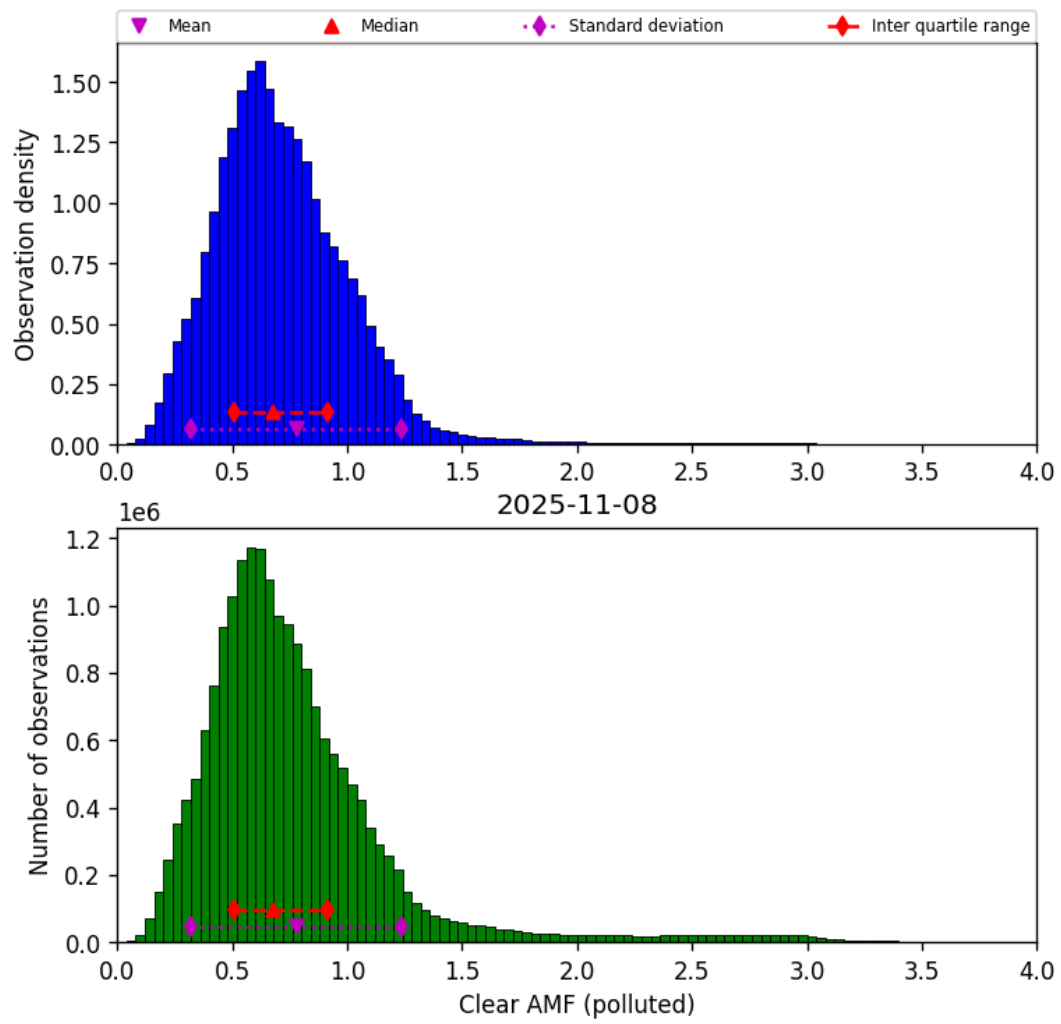
Figure 81: Histogram of “Clear AMF (polluted)” for 2025-11-07 to 2025-11-09
