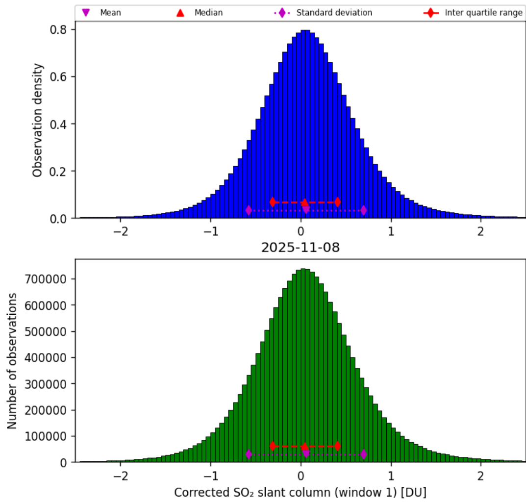
Figure 65: Histogram of “Corrected SO 2 slant column (window 1)” for 2025-11-07 to 2025-11-09
