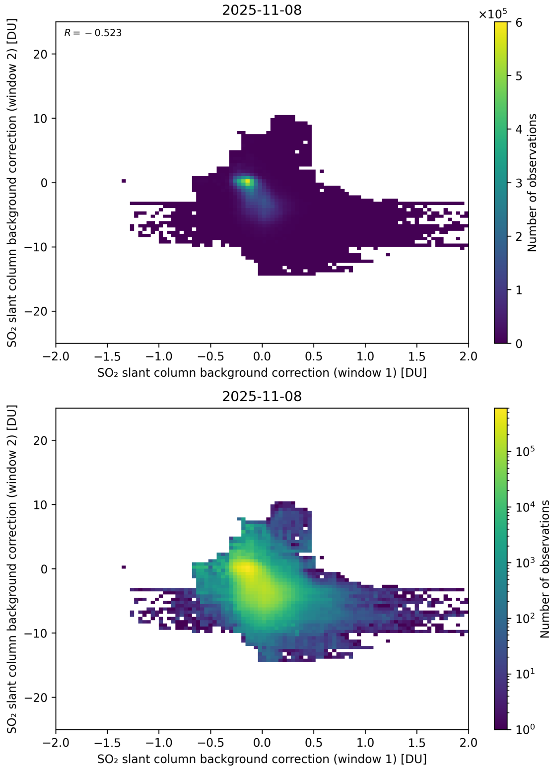
Figure 109: Scatter density plot of “SO 2 slant column background correction (window 1)” against “SO 2 slant column background correction (window 2)” for 2025-11-07 to 2025-11-09.
