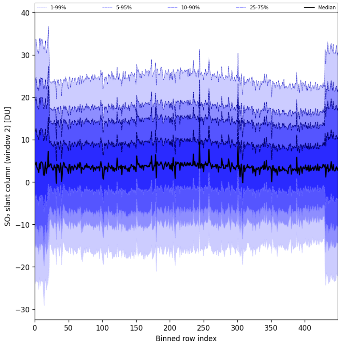
Figure 93: Along track statistics of “SO 2 slant column (window 2)” for 2025-11-07 to 2025-11-09
