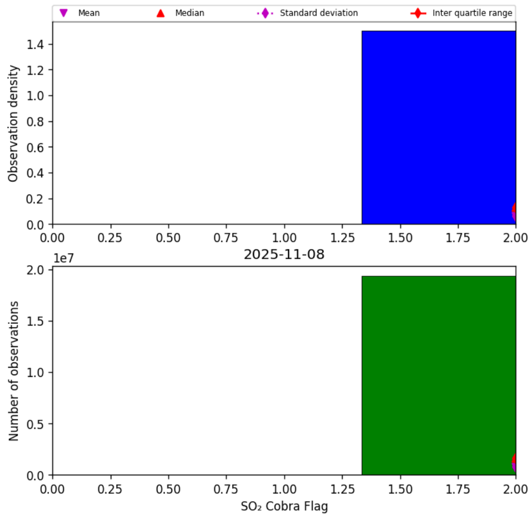
Figure 75: Histogram of “SO 2 Cobra Flag” for 2025-11-07 to 2025-11-09
