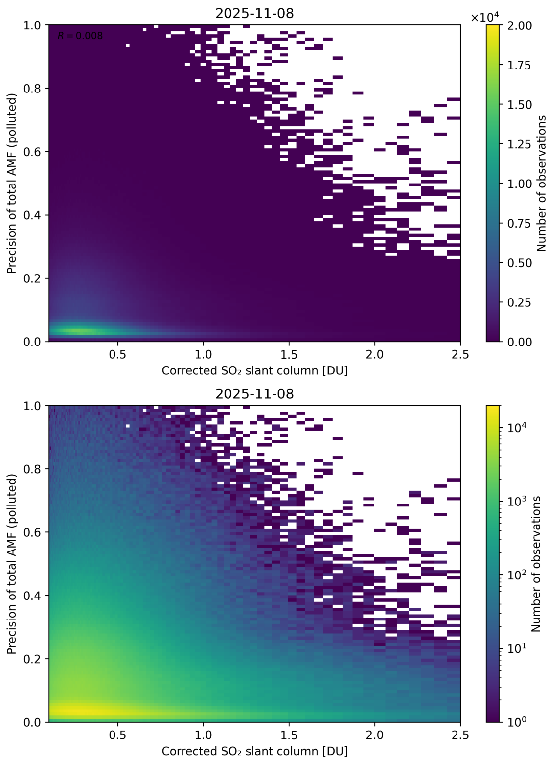
Figure 243: Scatter density plot of “Corrected SO 2 slant column” against “Precision of total AMF (polluted)” for 2025-11-07 to 2025-11-09.
