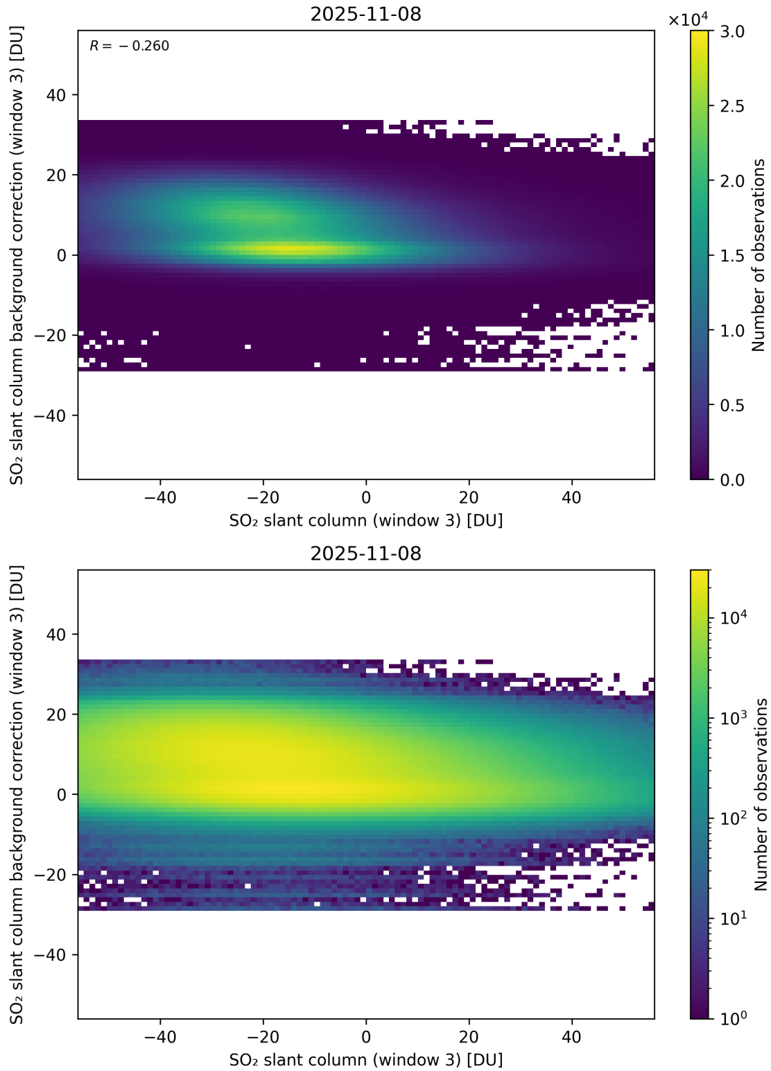
Figure 303: Scatter density plot of “SO 2 slant column (window 3)” against “SO 2 slant column background correction (window 3)” for 2025-11-07 to 2025-11-09.
