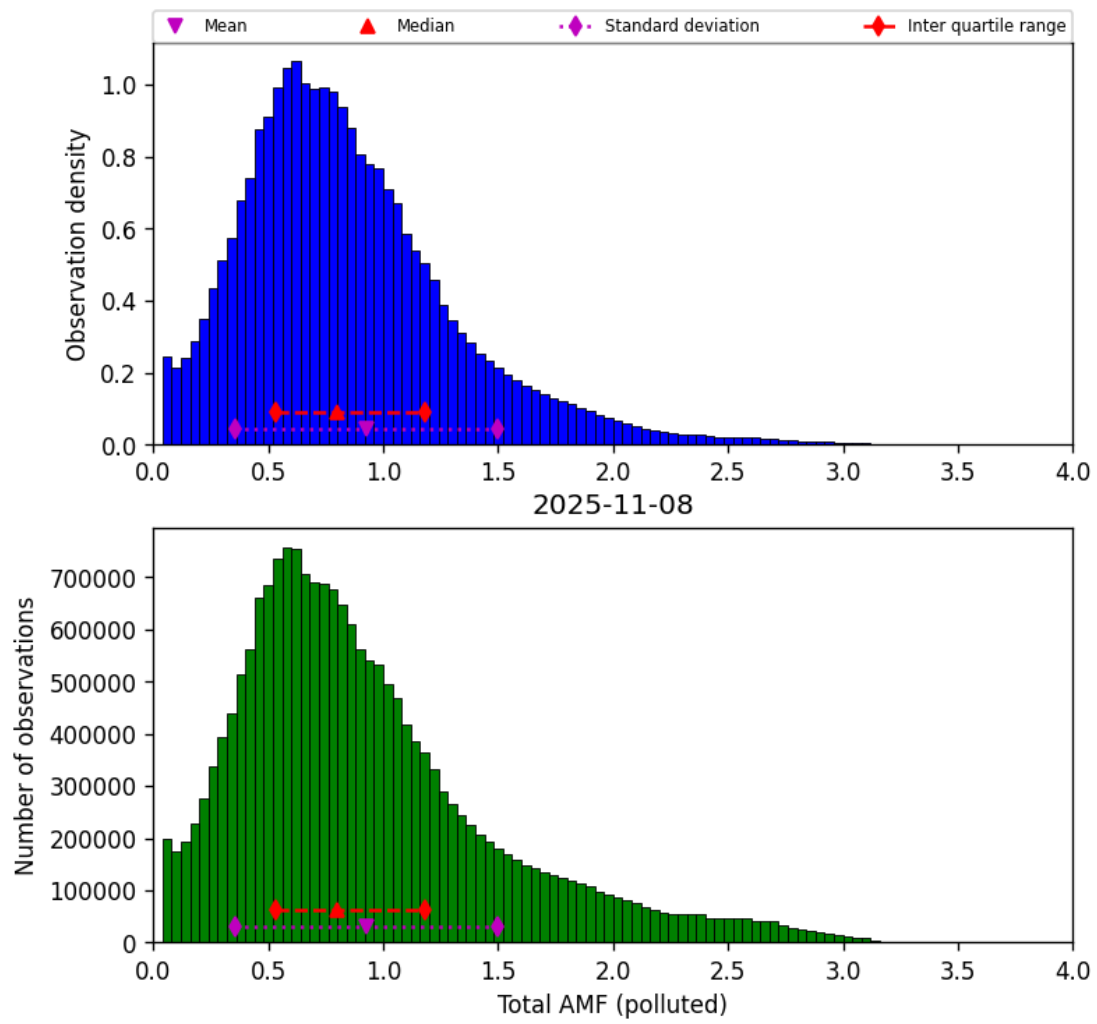
Figure 79: Histogram of “Total AMF (polluted)” for 2025-11-07 to 2025-11-09
