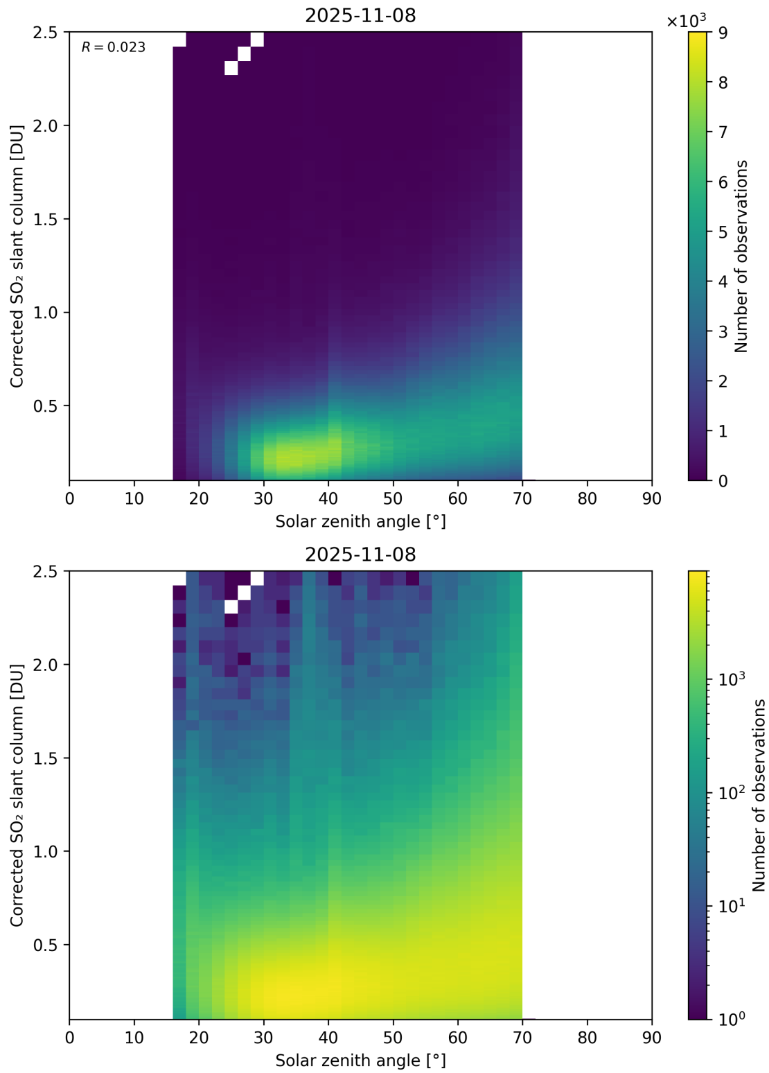
Figure 181: Scatter density plot of “Solar zenith angle” against “Corrected SO 2 slant column” for 2025-11-07 to 2025-11-09.
