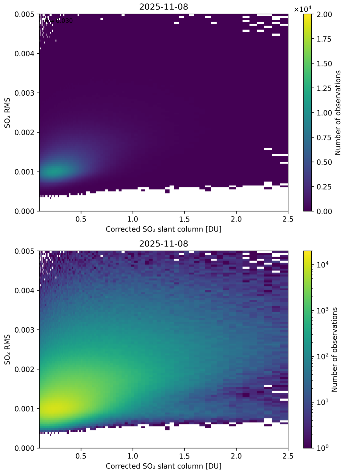
Figure 231: Scatter density plot of “Corrected SO 2 slant column” against “SO 2 RMS” for 2025-11-07 to 2025-11-09.
