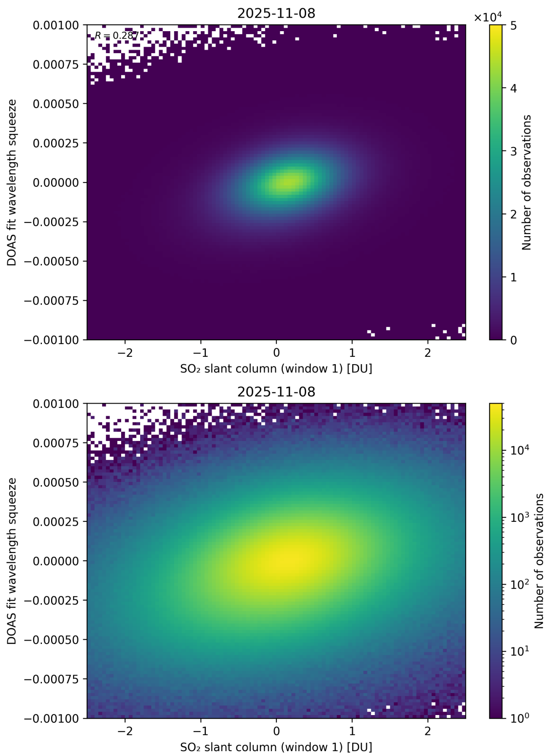
Figure 266: Scatter density plot of “SO 2 slant column (window 1)” against “DOAS fit wavelength squeeze” for 2025-11-07 to 2025-11-09.
