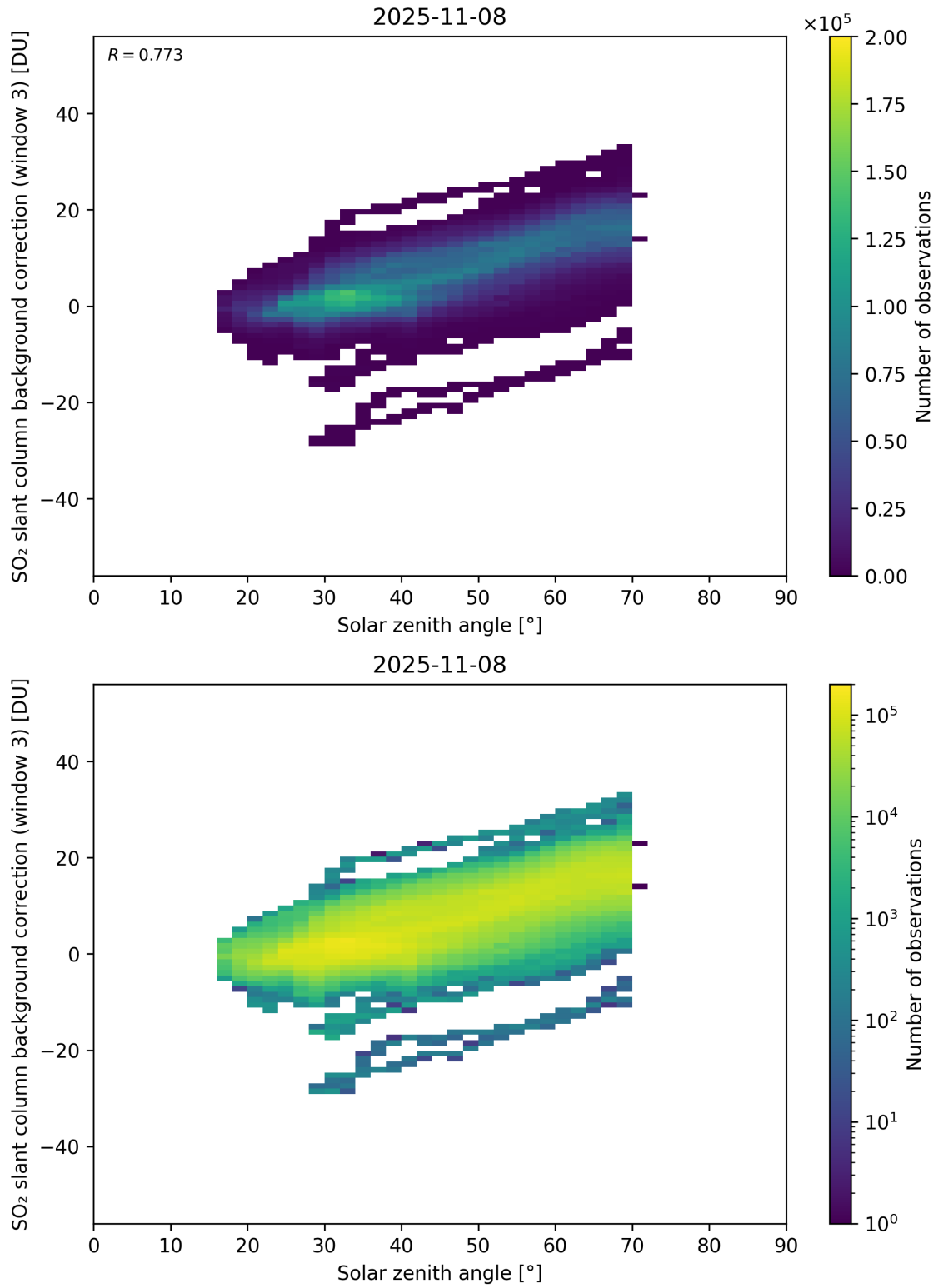
Figure 173: Scatter density plot of “Solar zenith angle” against “SO 2 slant column background correction (window 3)” for 2025-11-07 to 2025-11-09.
