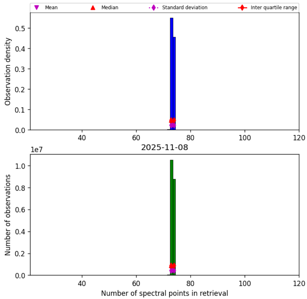
Figure 82: Histogram of “Number of spectral points in retrieval” for 2025-11-07 to 2025-11-09
