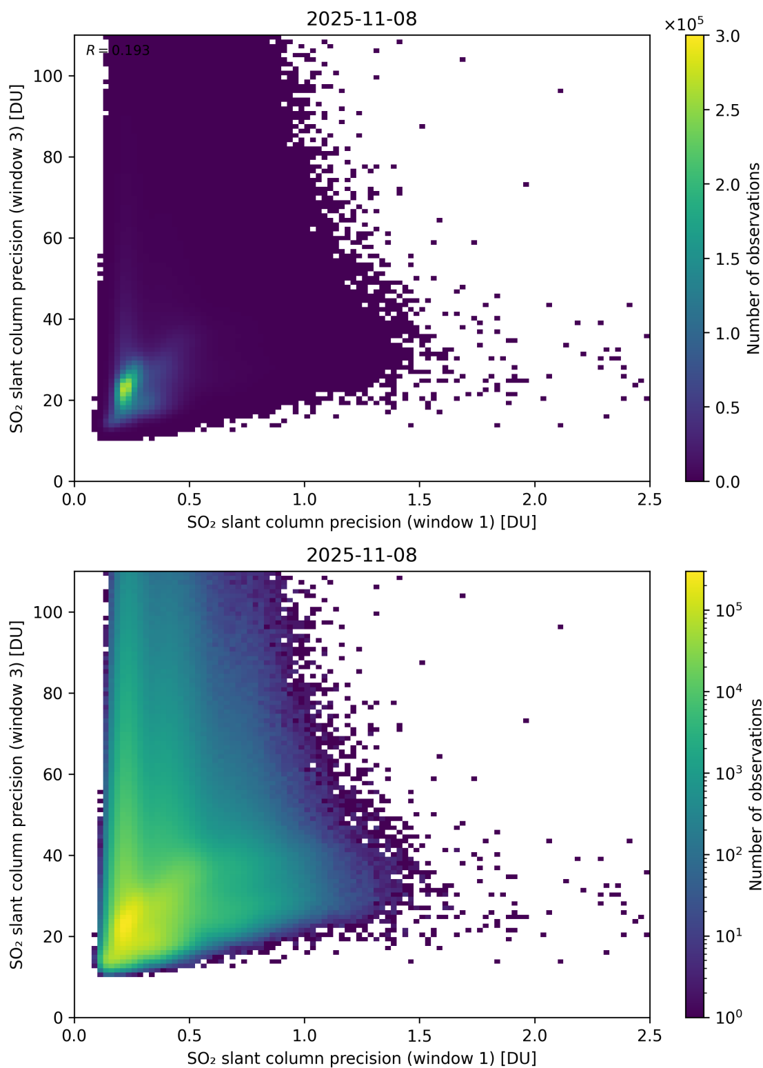
Figure 279: Scatter density plot of “SO 2 slant column precision (window 1)” against “SO 2 slant column precision (window 3)” for 2025-11-07 to 2025-11-09.
