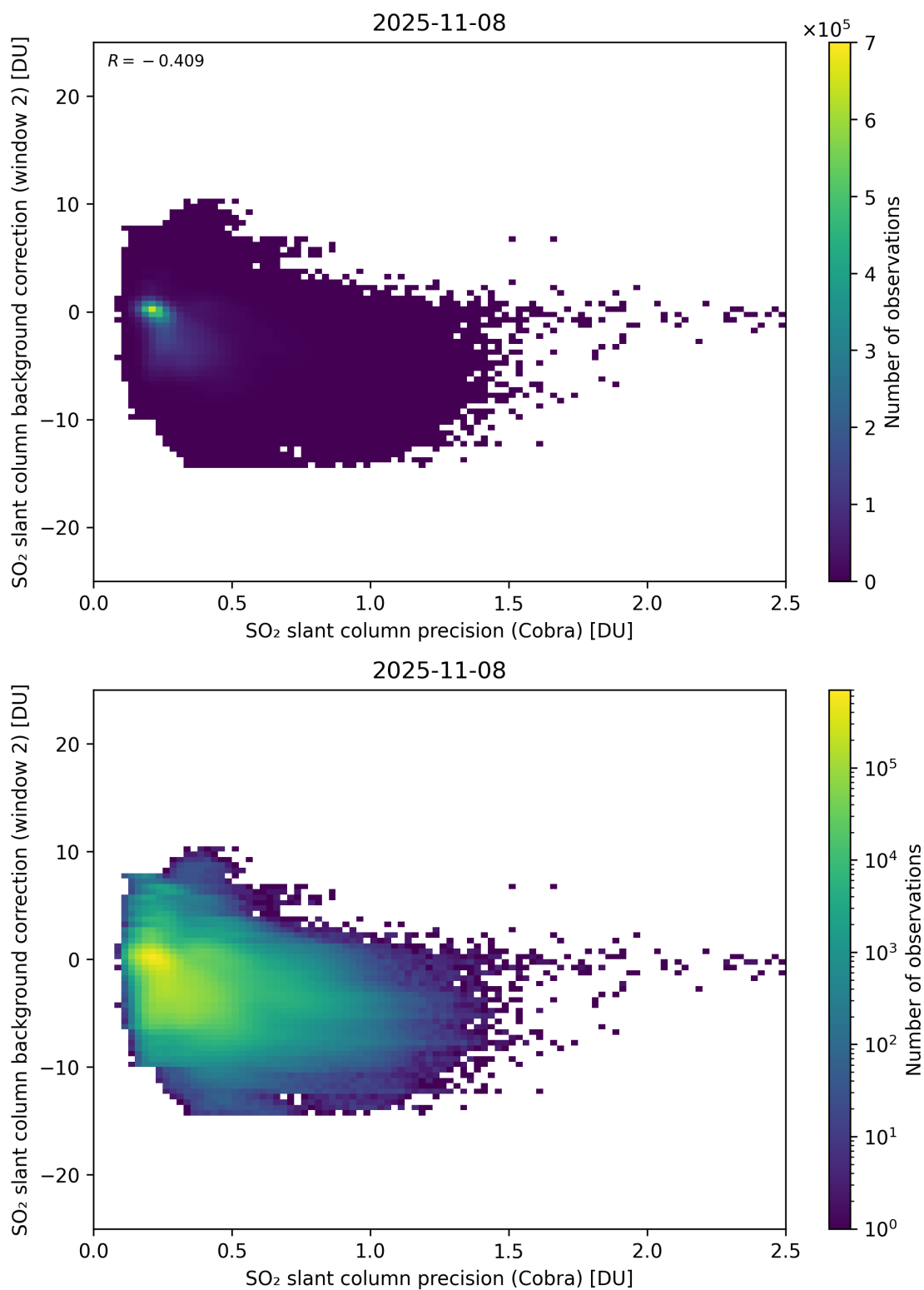
Figure 200: Scatter density plot of “SO 2 slant column precision (Cobra)” against “SO 2 slant column background correction (window 2)” for 2025-11-07 to 2025-11-09.
