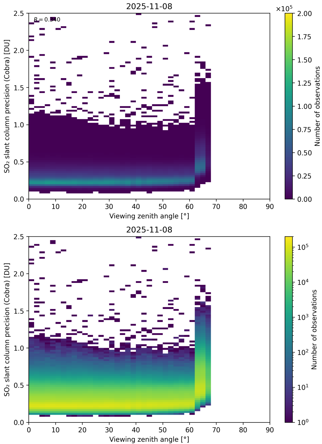
Figure 372: Scatter density plot of “Viewing zenith angle” against “SO 2 slant column precision (Cobra)” for 2025-11-07 to 2025-11-09.
