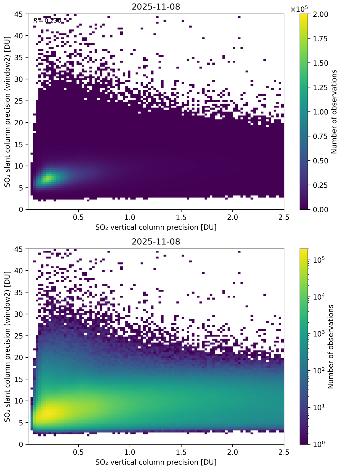
Figure 343: Scatter density plot of “SO 2 vertical column precision” against “SO 2 slant column precision (window2)” for 2025-11-07 to 2025-11-09.
