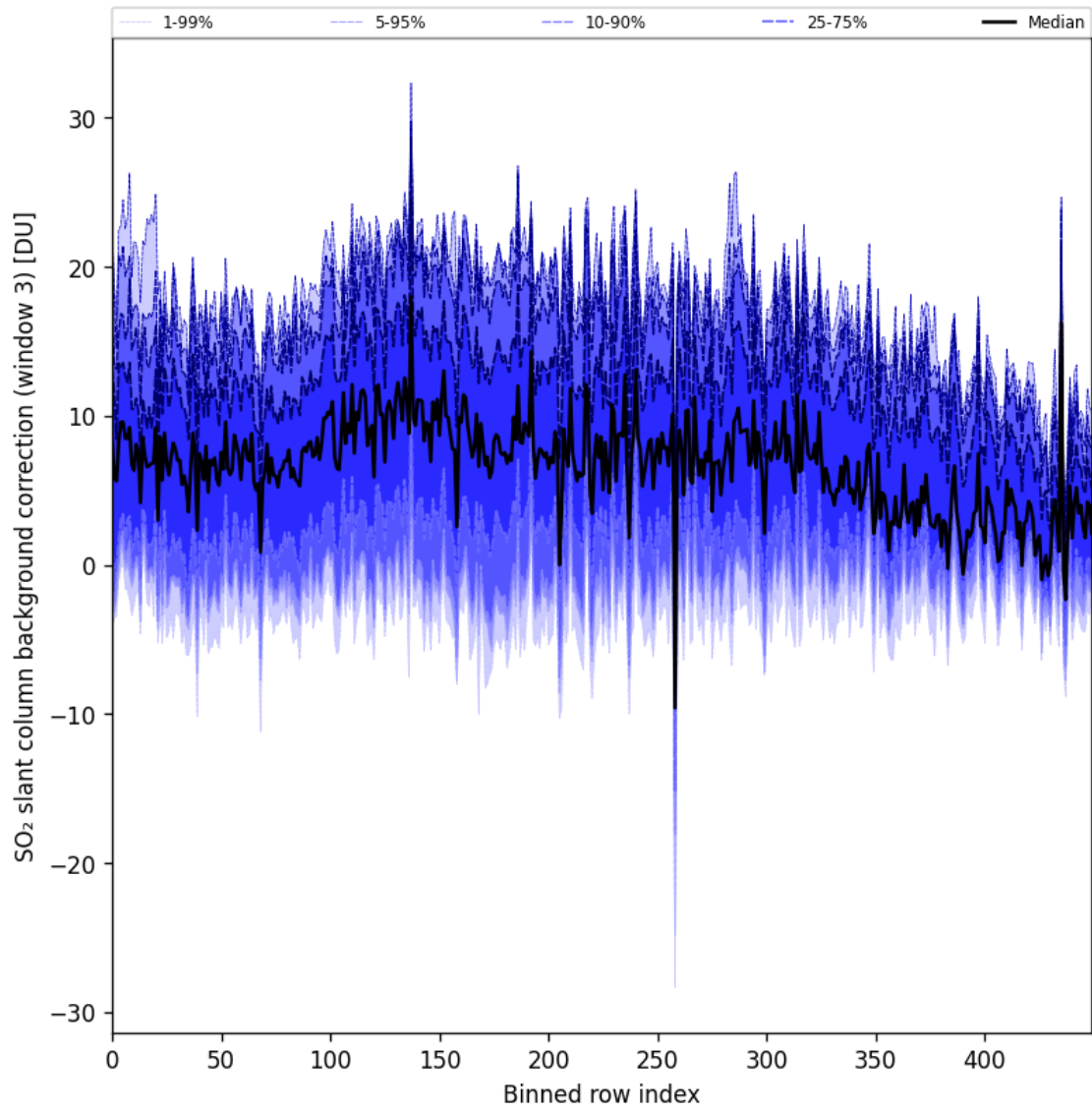
Figure 100: Along track statistics of “SO 2 slant column background correction (window 3)” for 2025-11-07 to 2025-11-09
