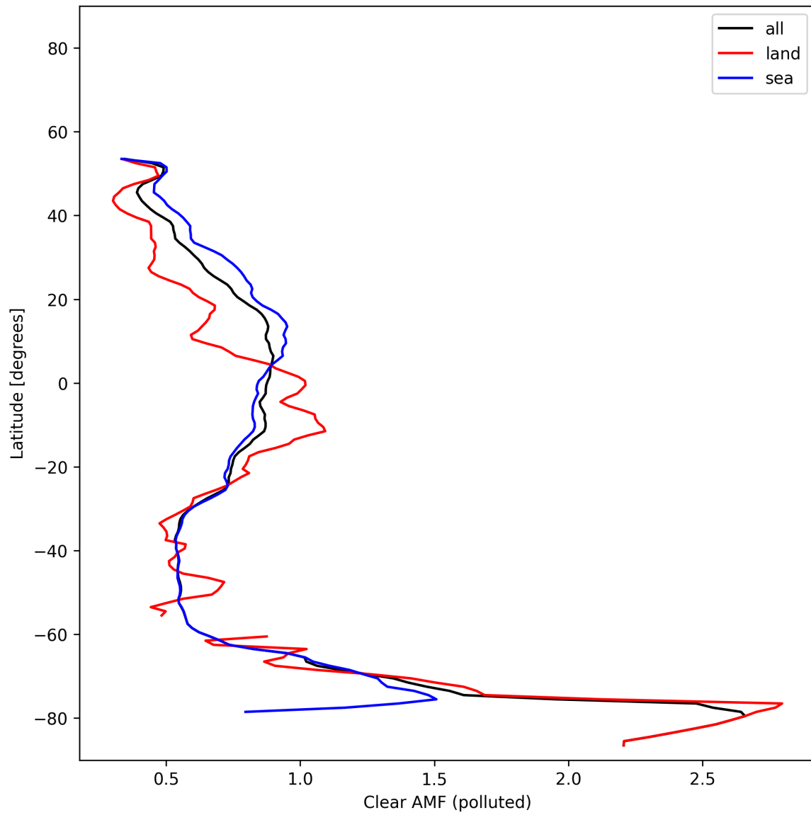
Figure 55: Zonal average of “Clear AMF (polluted)” for 2025-11-07 to 2025-11-09.
