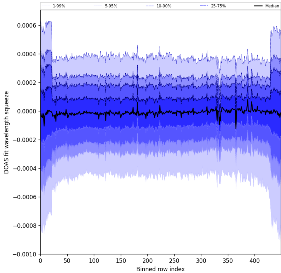
Figure 103: Along track statistics of “DOAS fit wavelength squeeze” for 2025-11-07 to 2025-11-09
