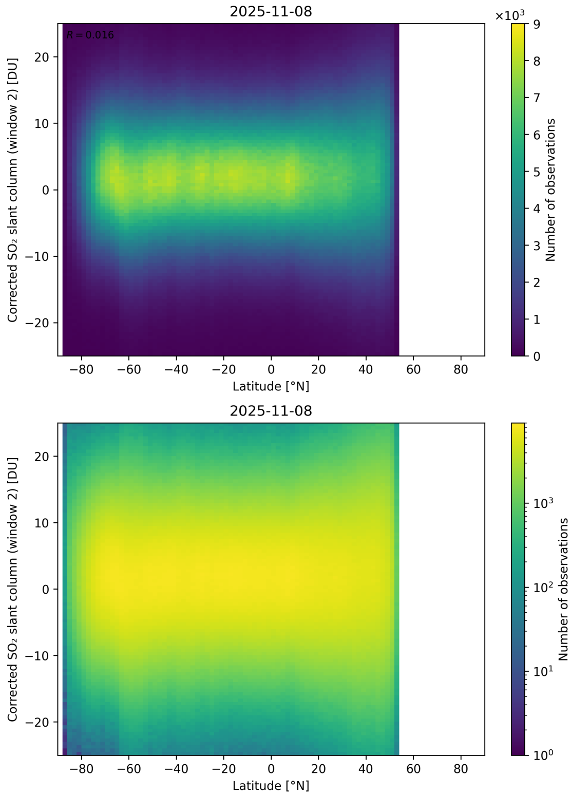
Figure 160: Scatter density plot of “Latitude” against “Corrected SO 2 slant column (window 2)” for 2025-11-07 to 2025-11-09.
