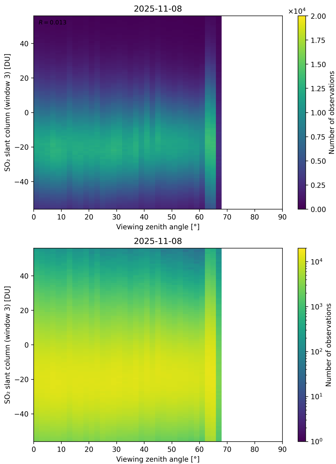
Figure 379: Scatter density plot of “Viewing zenith angle” against “SO 2 slant column (window 3)” for 2025-11-07 to 2025-11-09.
