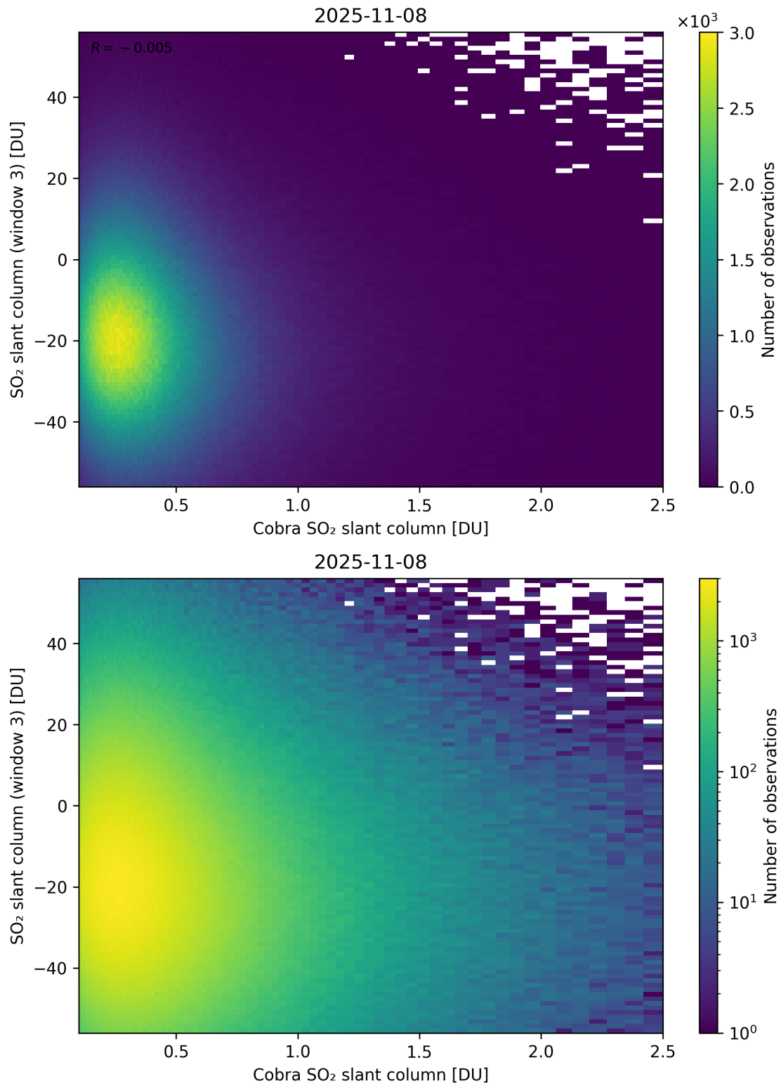
Figure 222: Scatter density plot of “Cobra SO 2 slant column” against “SO 2 slant column (window 3)” for 2025-11-07 to 2025-11-09.
