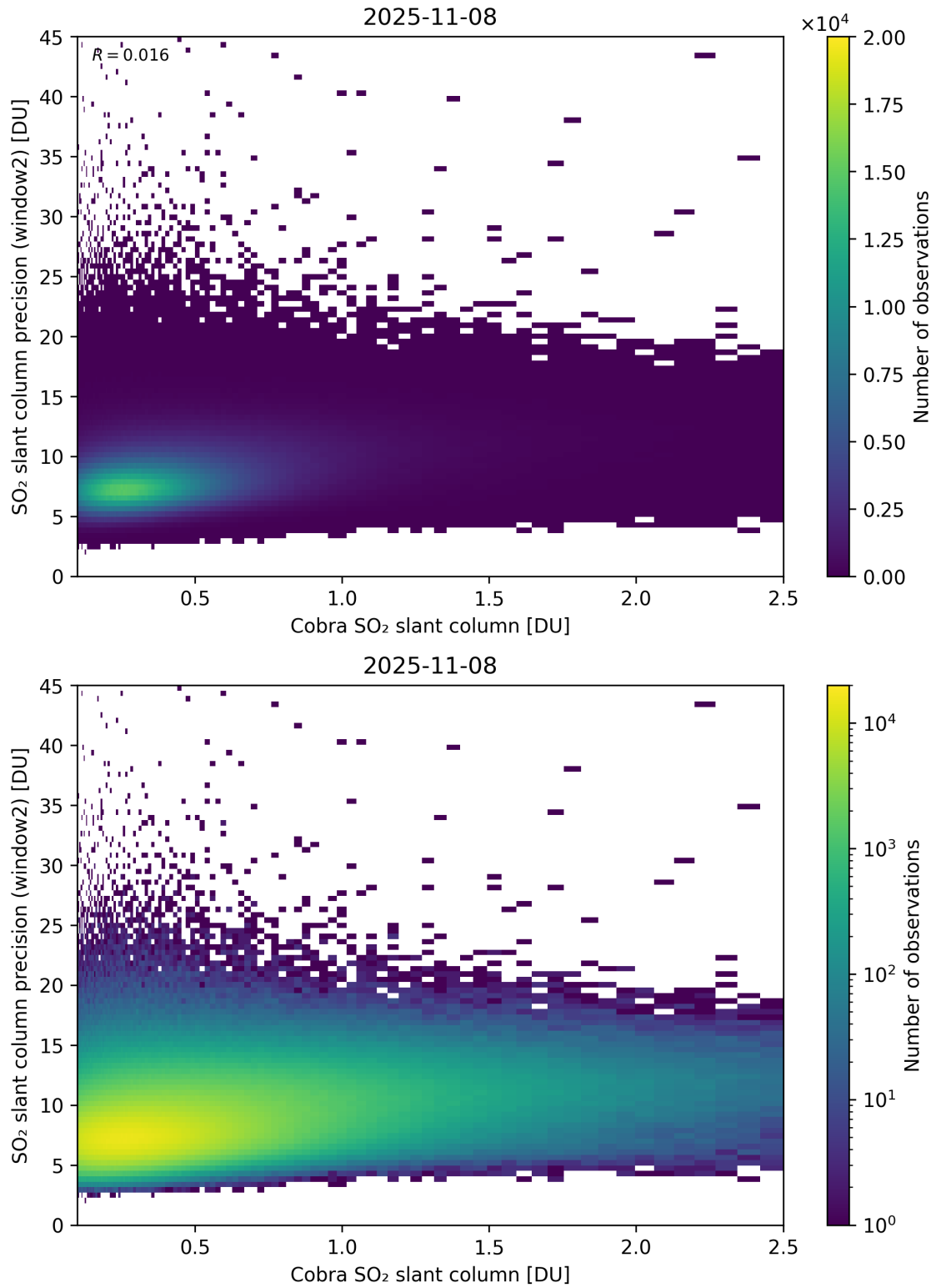
Figure 221: Scatter density plot of “Cobra SO 2 slant column” against “SO 2 slant column precision (window2)” for 2025-11-07 to 2025-11-09.
