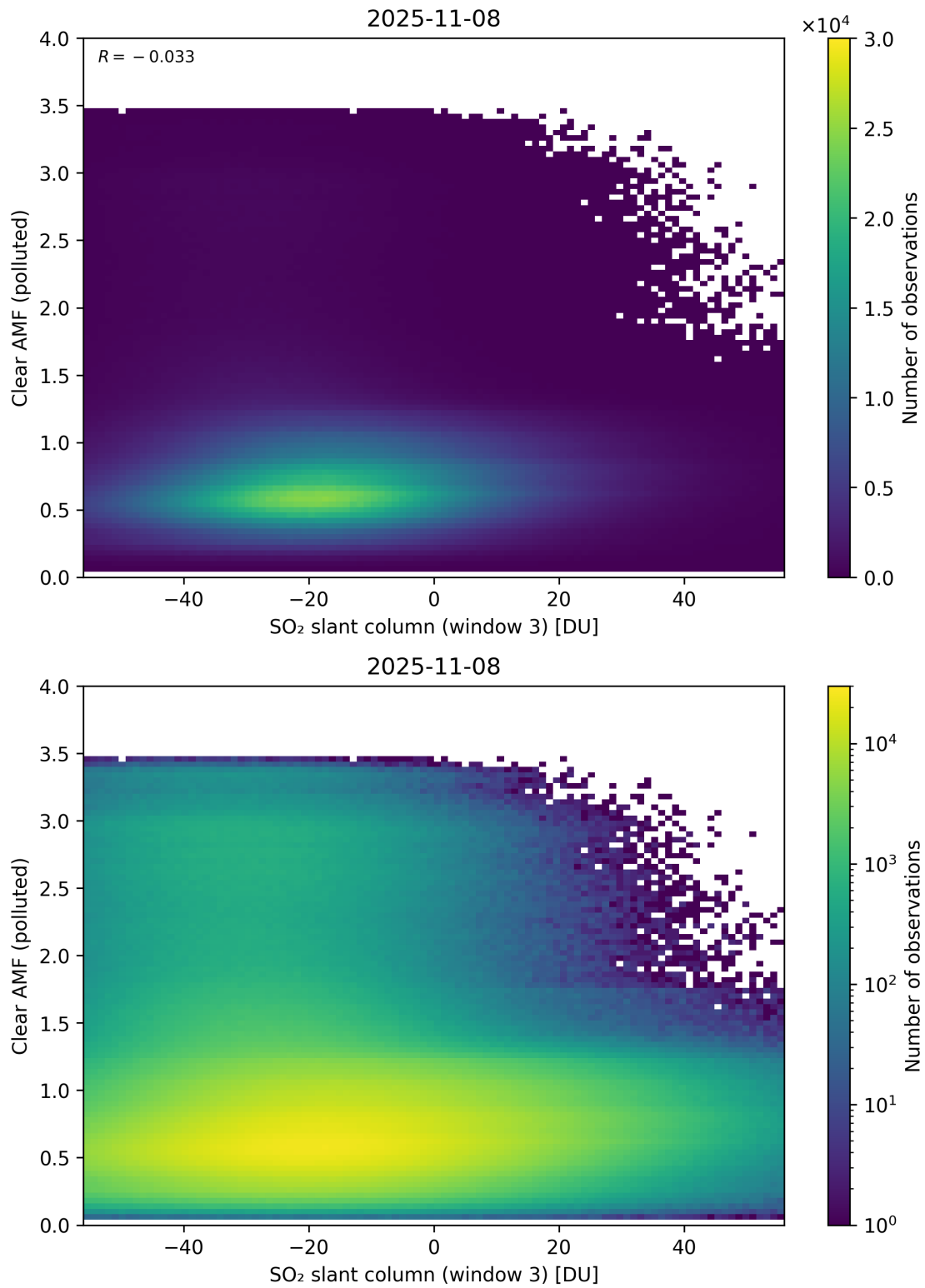
Figure 315: Scatter density plot of “SO 2 slant column (window 3)” against “Clear AMF (polluted)” for 2025-11-07 to 2025-11-09.
