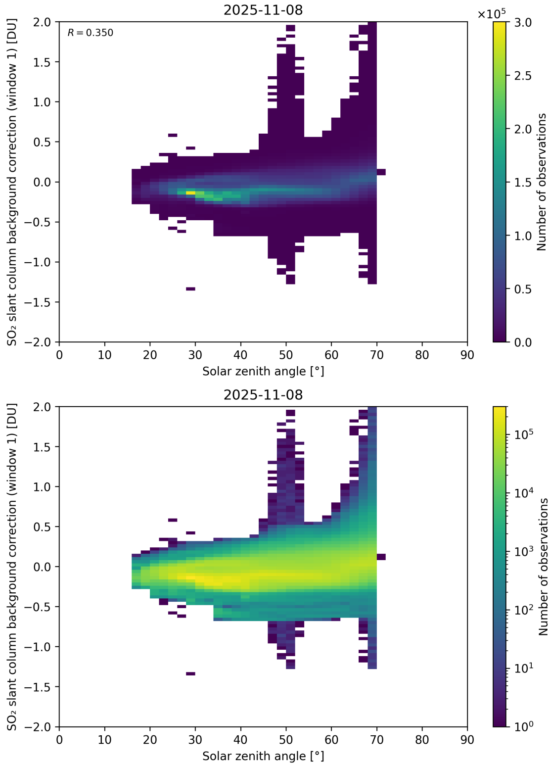
Figure 171: Scatter density plot of “Solar zenith angle” against “SO 2 slant column background correction (window 1)” for 2025-11-07 to 2025-11-09.
