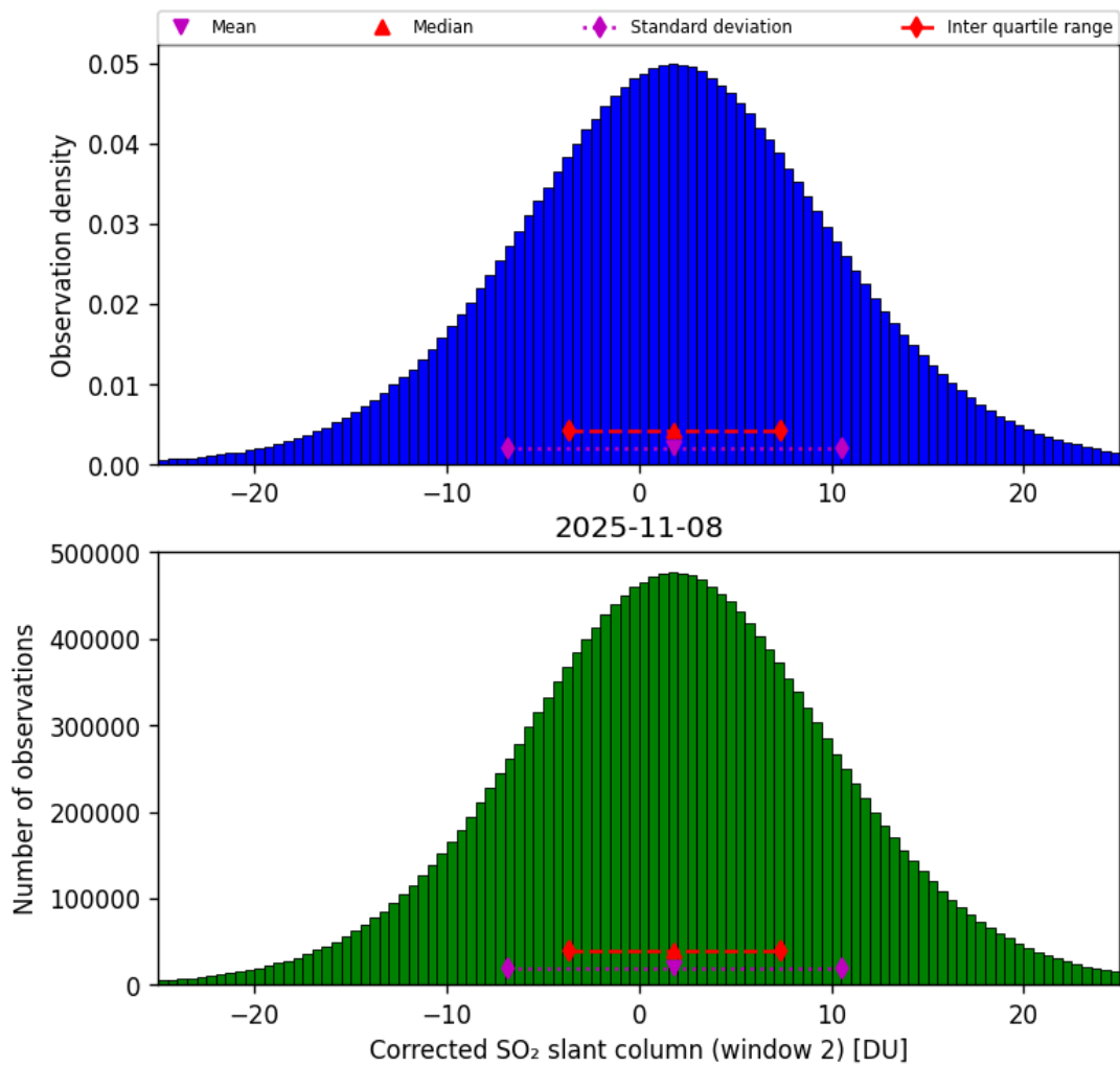
Figure 69: Histogram of “Corrected SO 2 slant column (window 2)” for 2025-11-07 to 2025-11-09
