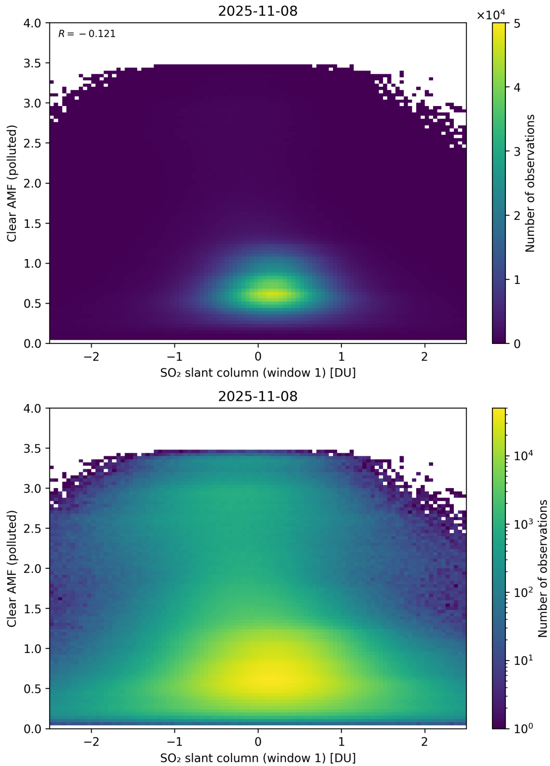
Figure 282: Scatter density plot of “SO 2 slant column (window 1)” against “Clear AMF (polluted)” for 2025-11-07 to 2025-11-09.
