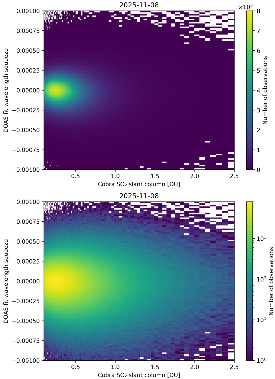
Figure 197: Scatter density plot of “Cobra SO 2 slant column” against “DOAS fit wavelength squeeze” for 2025-11-07 to 2025-11-09.
