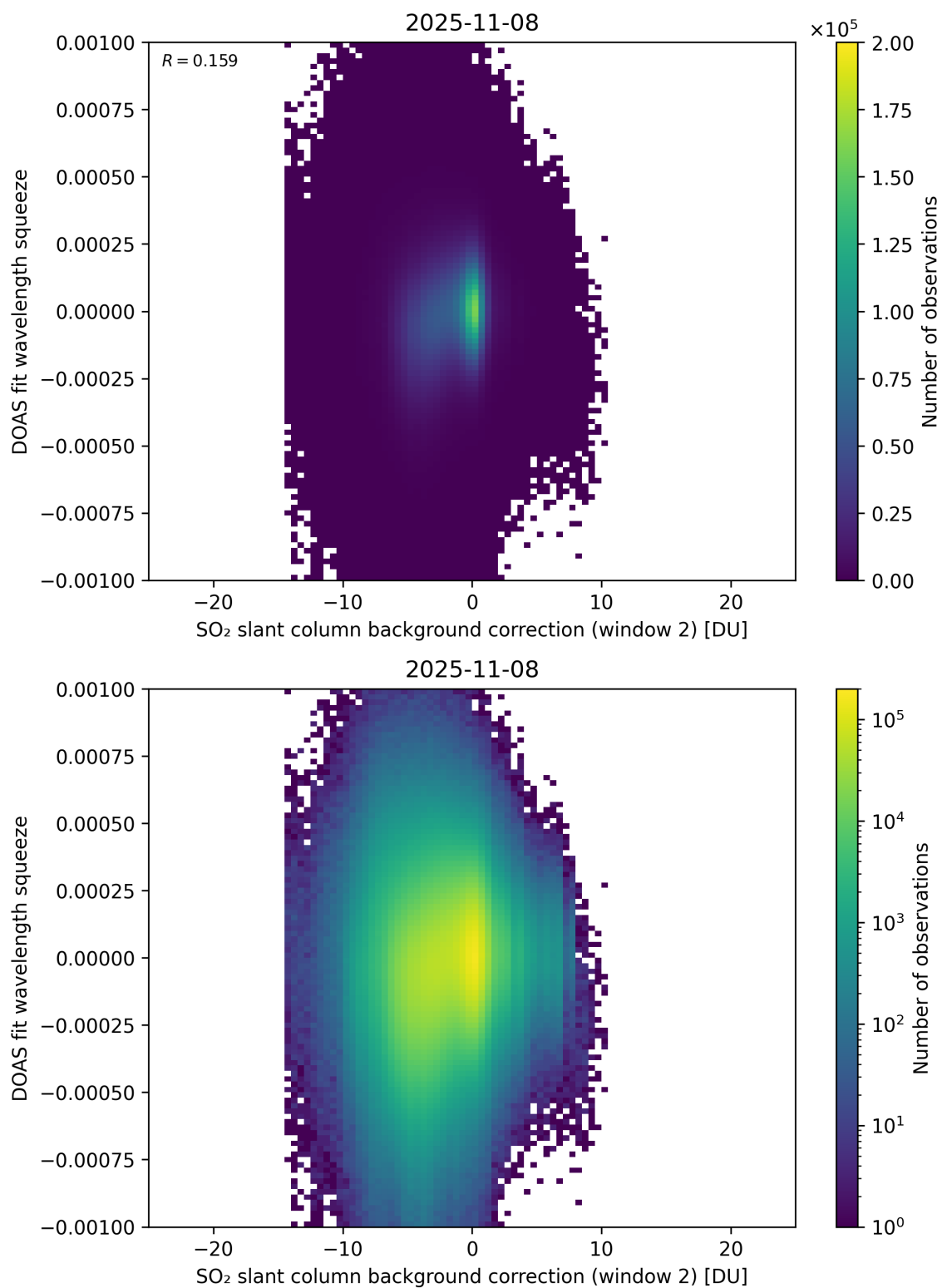
Figure 124: Scatter density plot of “SO 2 slant column background correction (window 2)” against “DOAS fit wavelength squeeze” for 2025-11-07 to 2025-11-09.
