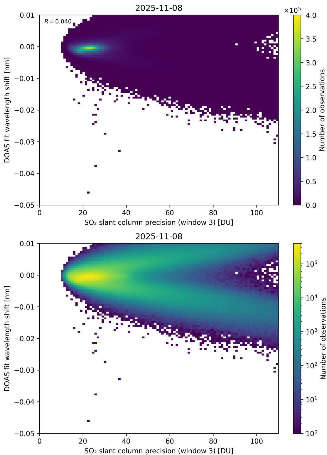
Figure 308: Scatter density plot of “SO 2 slant column precision (window 3)” against “DOAS fit wavelength shift” for 2025-11-07 to 2025-11-09.
