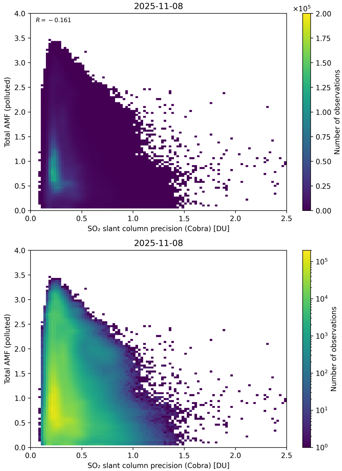
Figure 213: Scatter density plot of “SO 2 slant column precision (Cobra)” against “Total AMF (polluted)” for 2025-11-07 to 2025-11-09.
