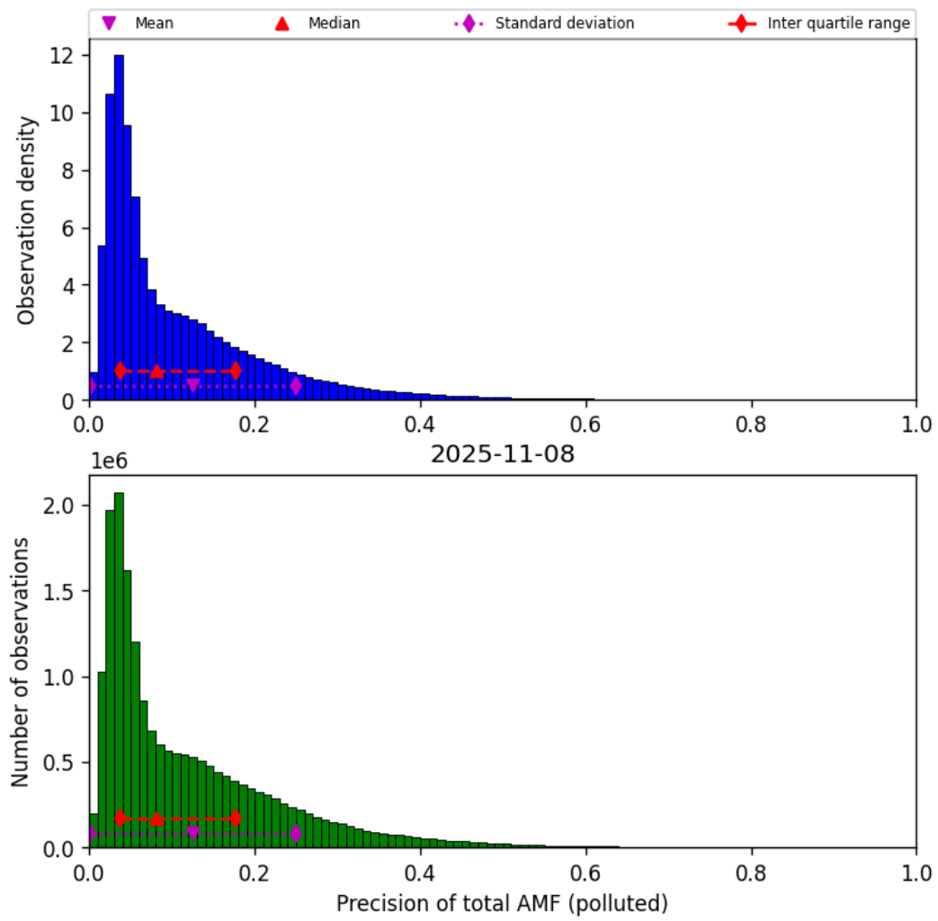
Figure 80: Histogram of “Precision of total AMF (polluted)” for 2025-11-07 to 2025-11-09
