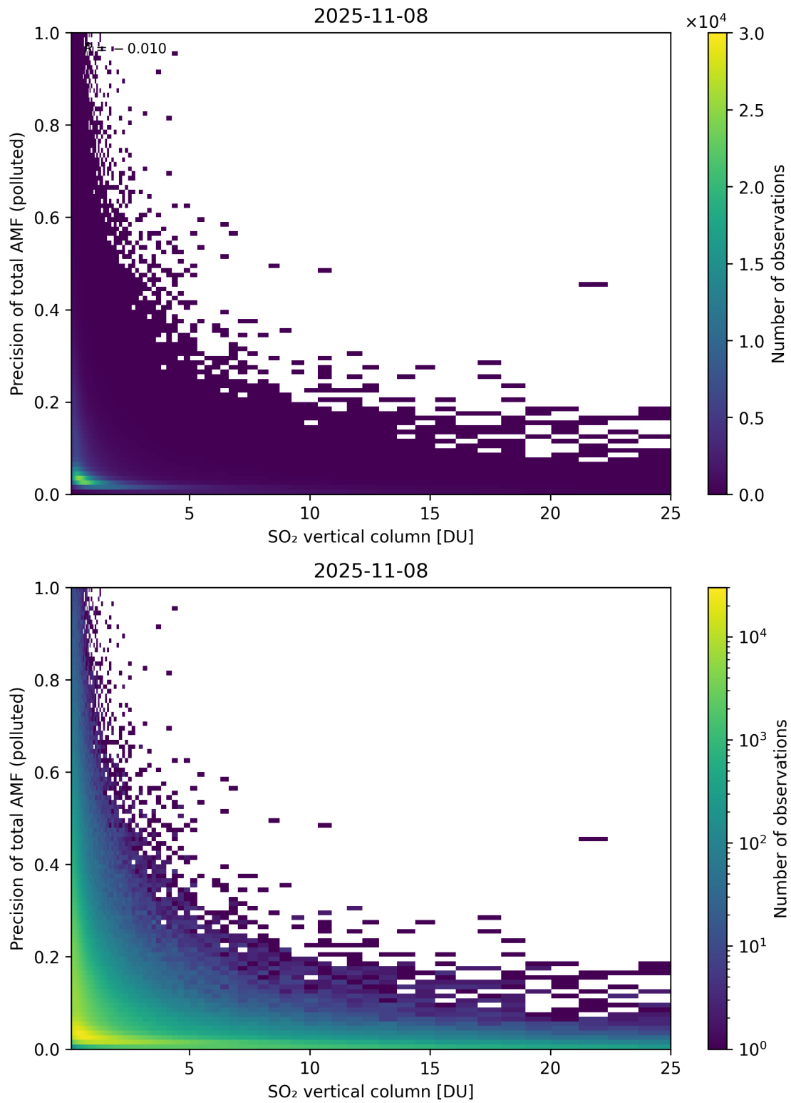
Figure 360: Scatter density plot of “SO 2 vertical column” against “Precision of total AMF (polluted)” for 2025-11-07 to 2025-11-09.
