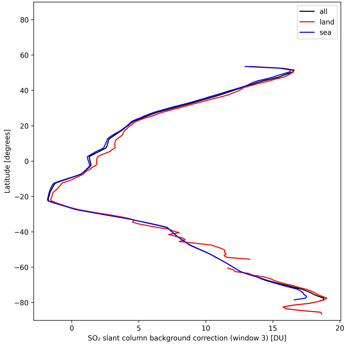
Figure 48: Zonal average of “SO 2 slant column background correction (window 3)” for 2025-11-07 to 2025-11-09.
