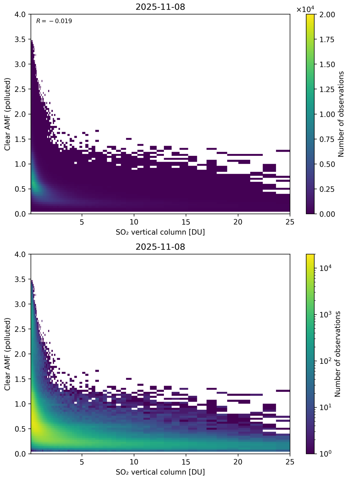
Figure 348: Scatter density plot of “SO 2 vertical column” against “Clear AMF (polluted)” for 2025-11-07 to 2025-11-09.
