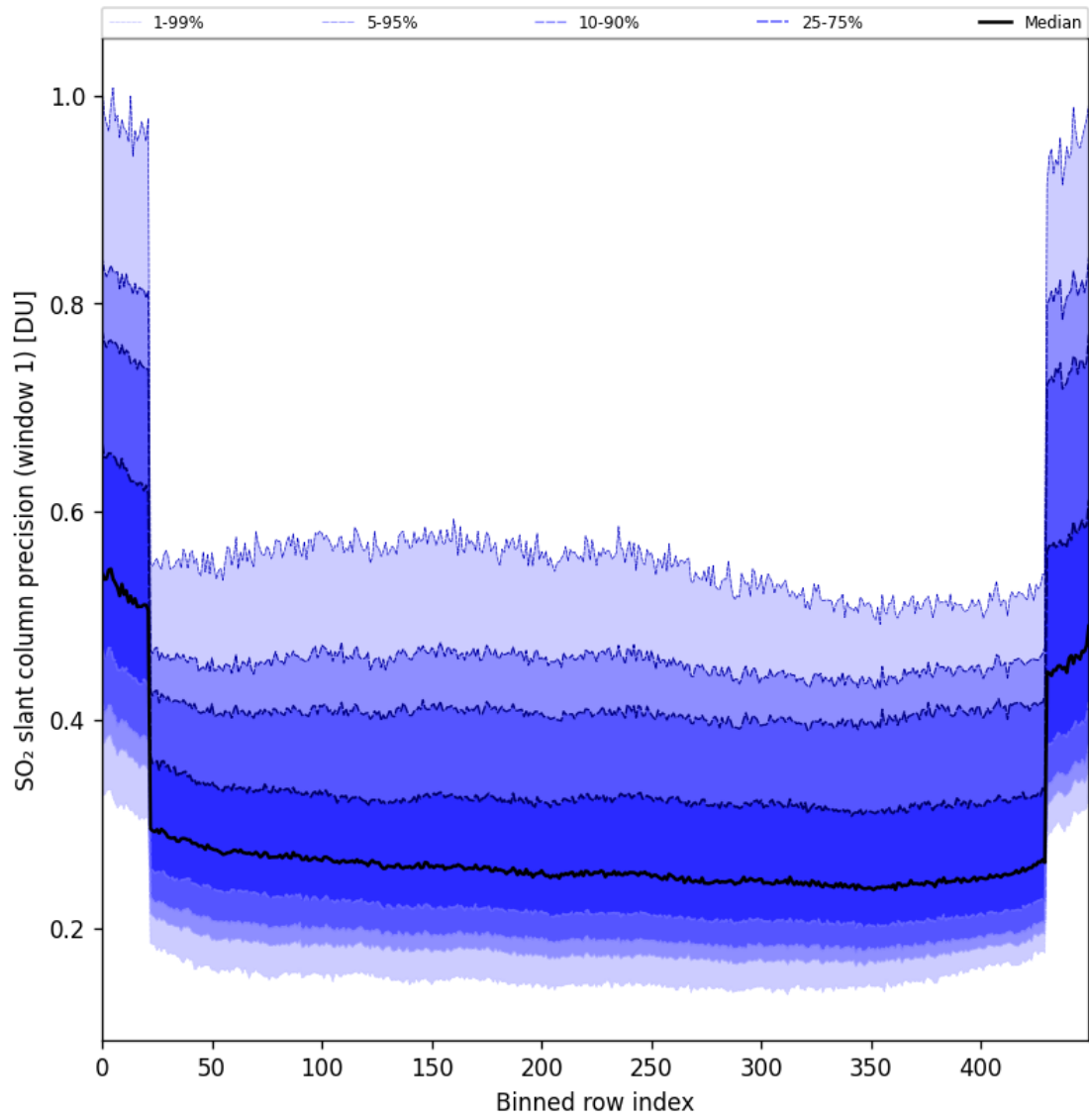
Figure 90: Along track statistics of “SO 2 slant column precision (window 1)” for 2025-11-07 to 2025-11-09
