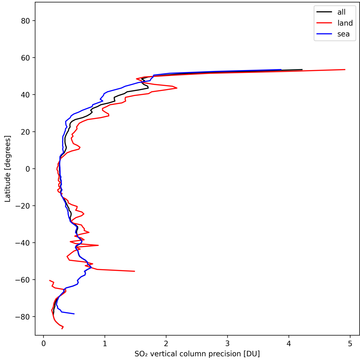
Figure 33: Zonal average of “SO 2 vertical column precision” for 2025-11-07 to 2025-11-09.
