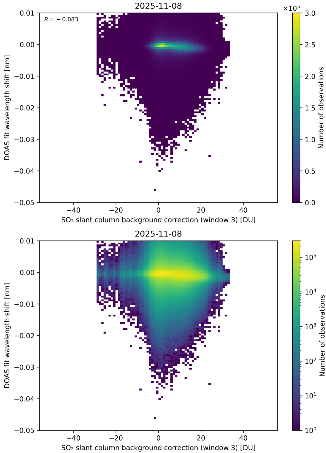
Figure 132: Scatter density plot of “SO 2 slant column background correction (window 3)” against “DOAS fit wavelength shift” for 2025-11-07 to 2025-11-09.
