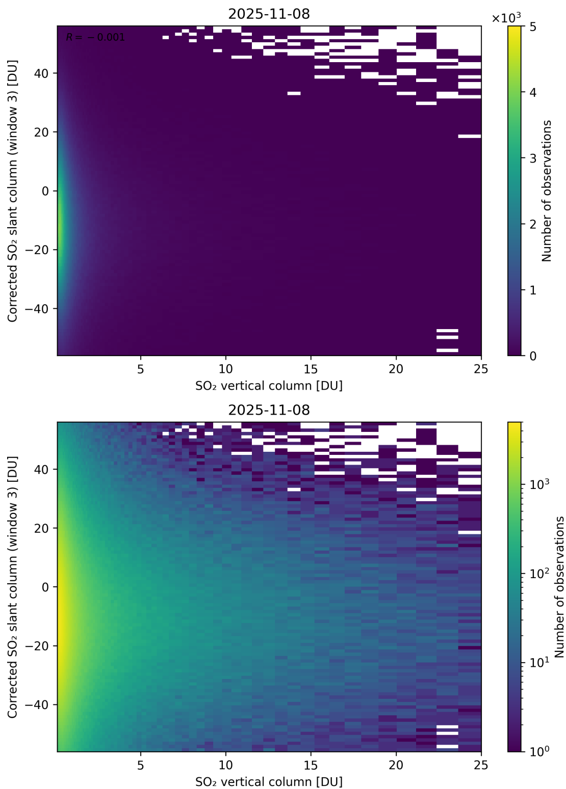
Figure 353: Scatter density plot of “SO 2 vertical column” against “Corrected SO 2 slant column (window 3)” for 2025-11-07 to 2025-11-09.
