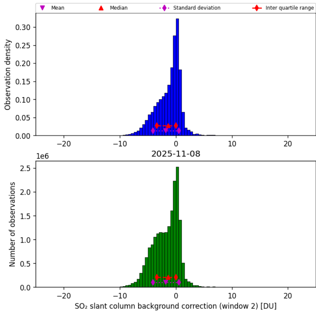
Figure 70: Histogram of “SO 2 slant column background correction (window 2)” for 2025-11-07 to 2025-11-09
