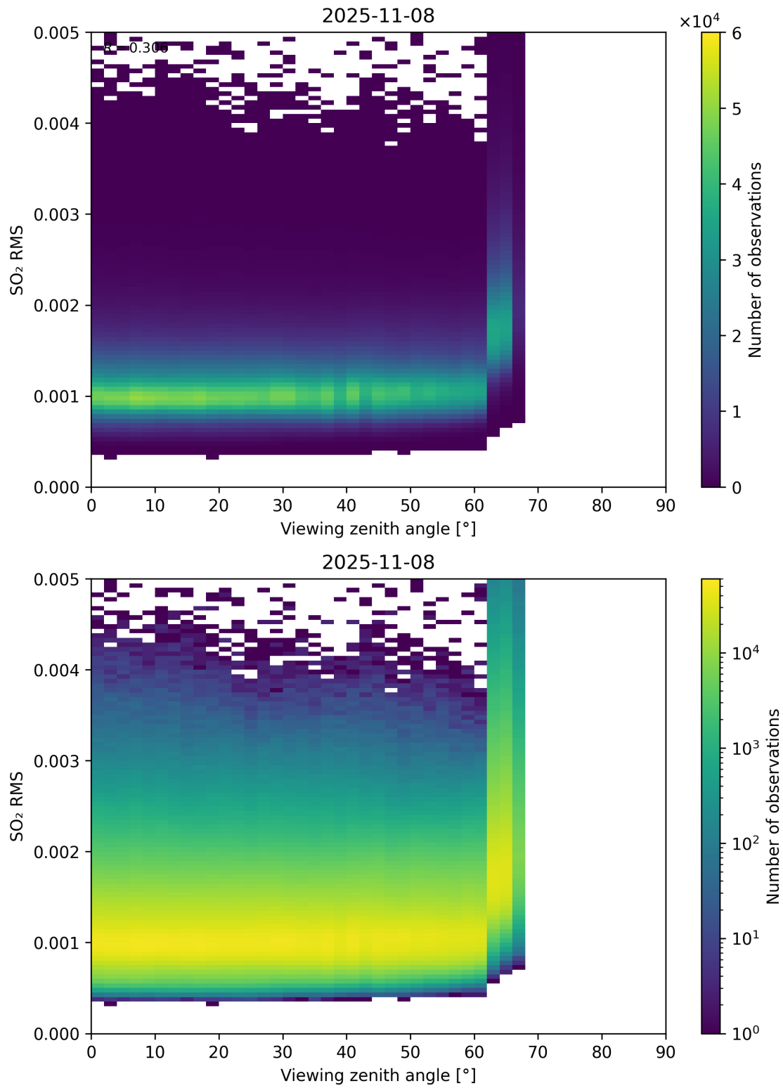
Figure 367: Scatter density plot of “Viewing zenith angle” against “SO 2 RMS” for 2025-11-07 to 2025-11-09.
