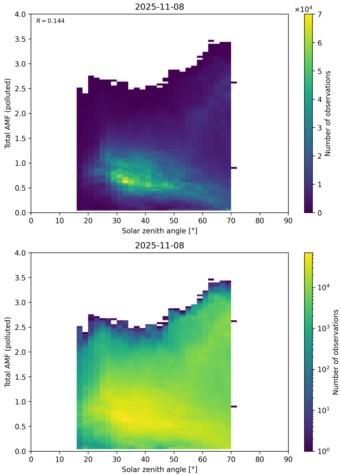
Figure 189: Scatter density plot of “Solar zenith angle” against “Total AMF (polluted)” for 2025-11-07 to 2025-11-09.
