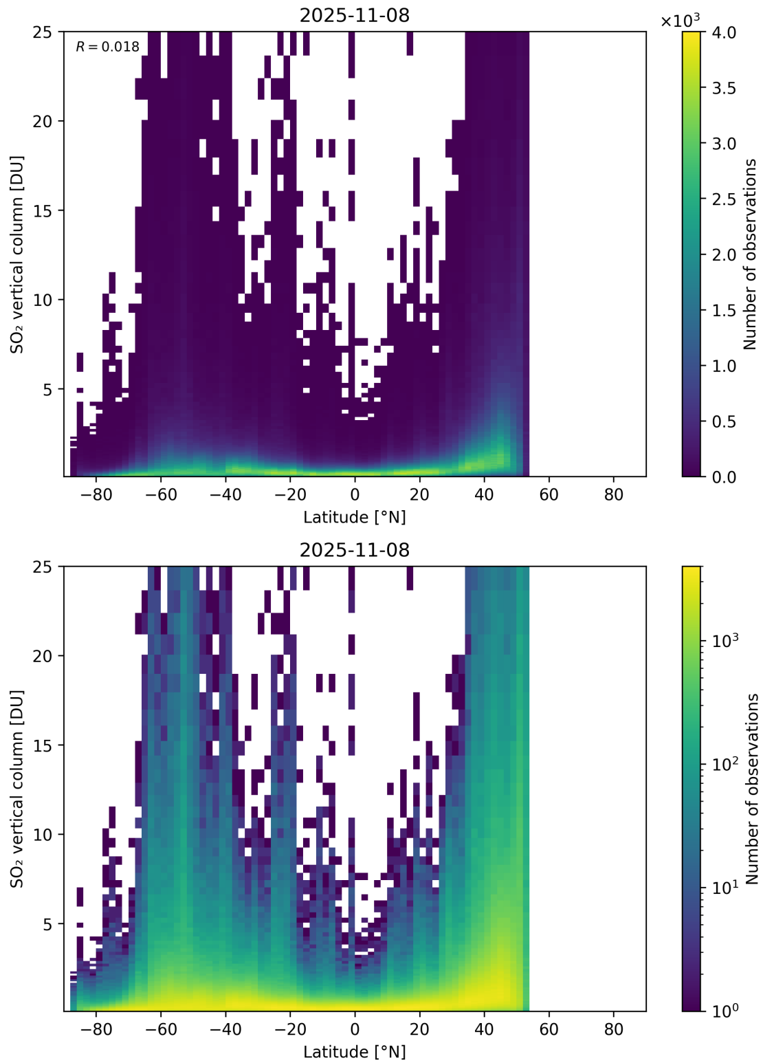
Figure 169: Scatter density plot of “Latitude” against “SO 2 vertical column” for 2025-11-07 to 2025-11-09.
