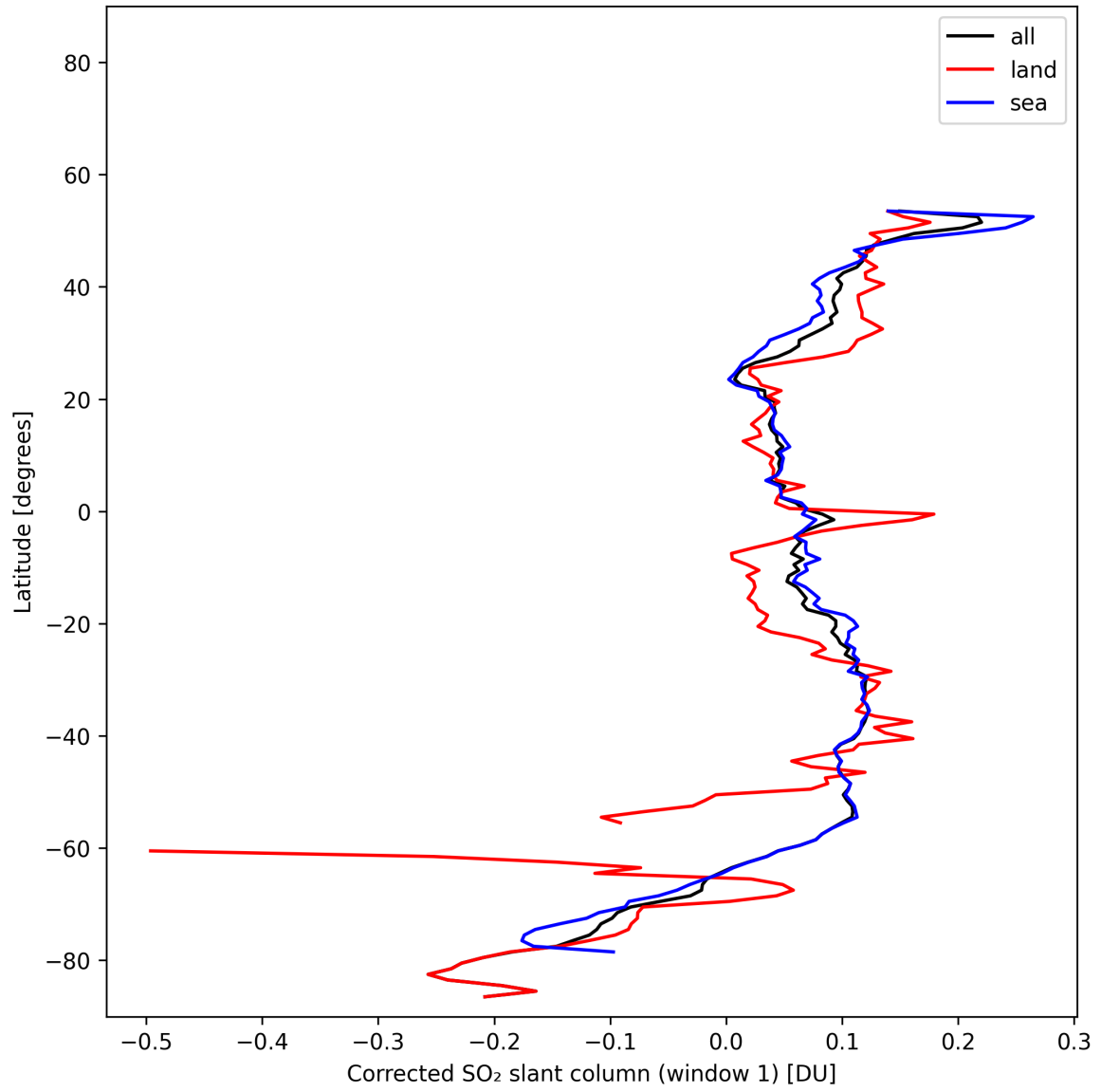
Figure 39: Zonal average of “Corrected SO 2 slant column (window 1)” for 2025-11-07 to 2025-11-09.
