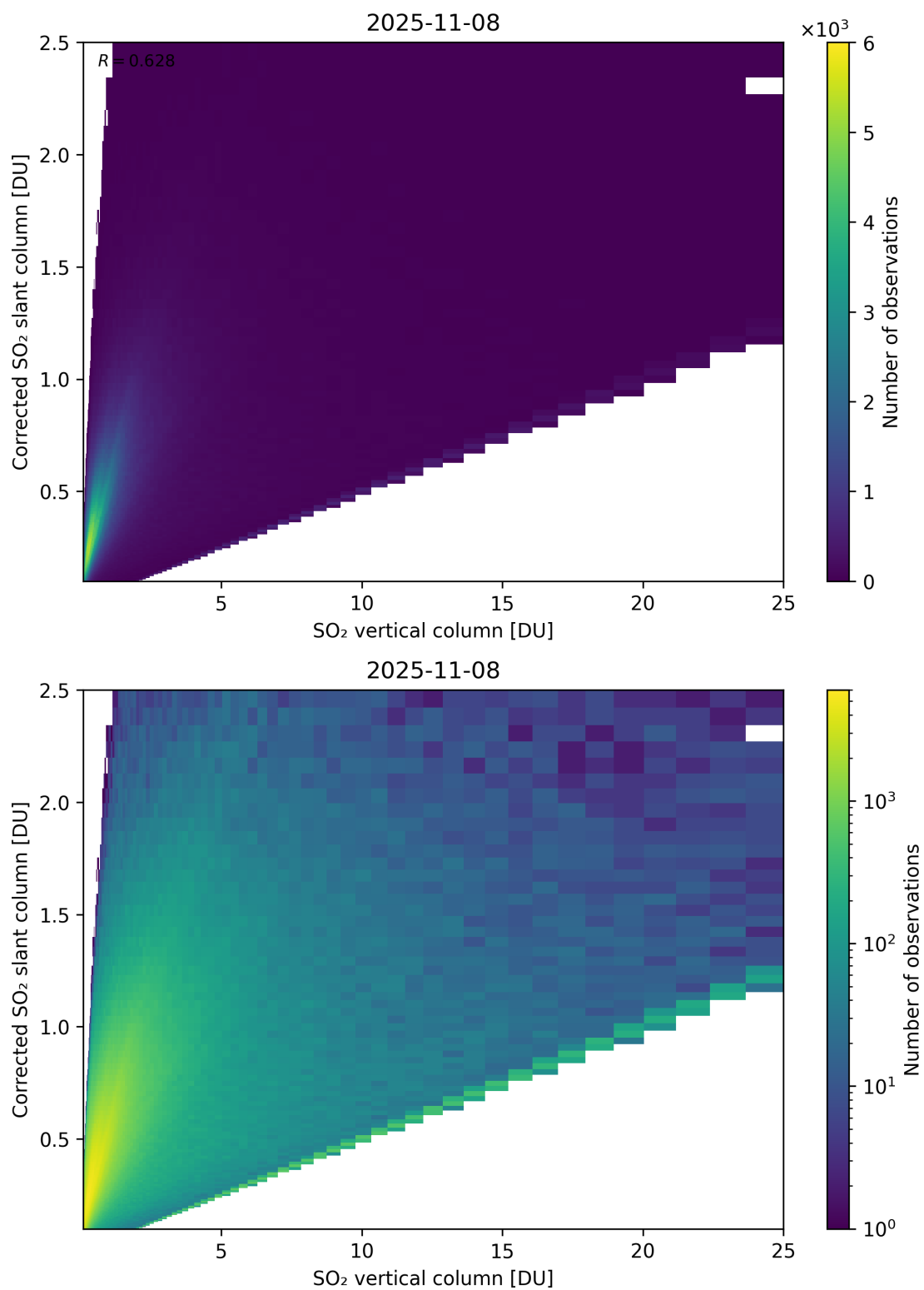
Figure 351: Scatter density plot of “SO 2 vertical column” against “Corrected SO 2 slant column” for 2025-11-07 to 2025-11-09.
