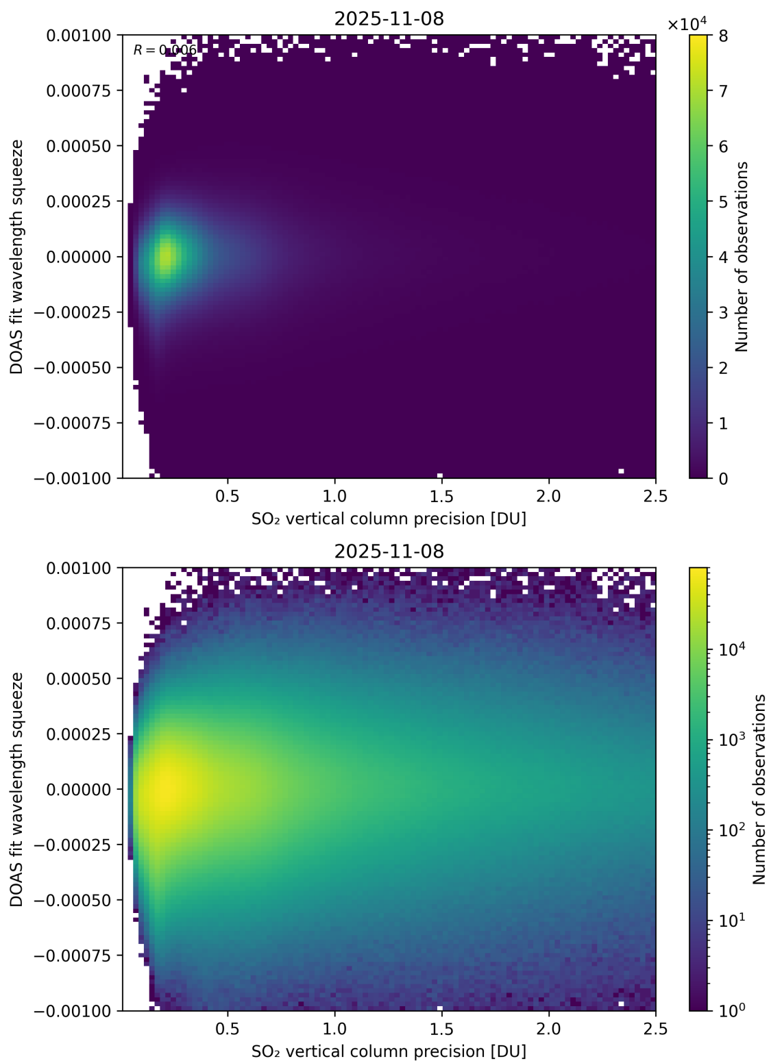
Figure 333: Scatter density plot of “SO 2 vertical column precision” against “DOAS fit wavelength squeeze” for 2025-11-07 to 2025-11-09.
