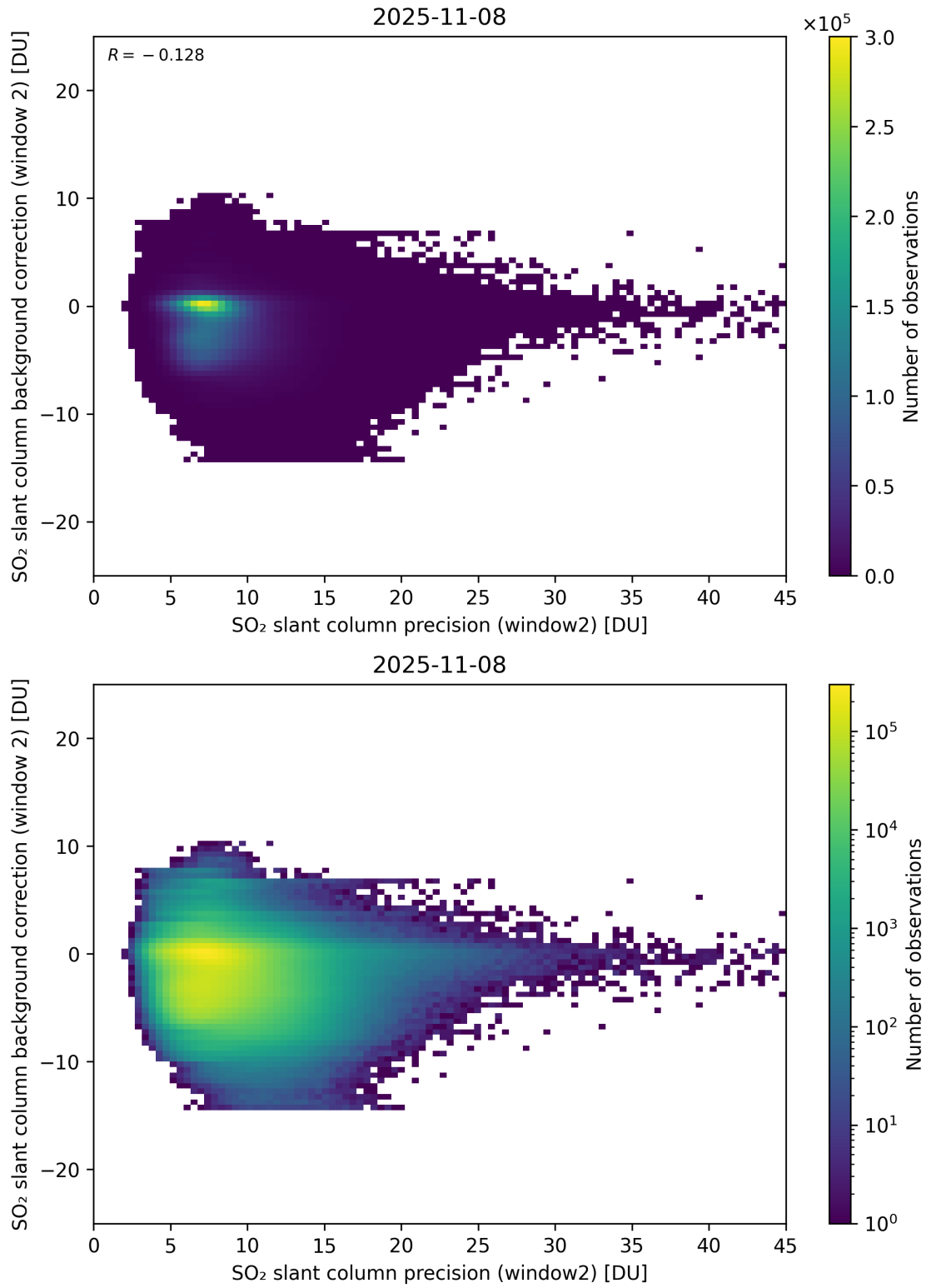
Figure 291: Scatter density plot of “SO 2 slant column precision (window2)” against “SO 2 slant column background correction (window 2)” for 2025-11-07 to 2025-11-09.
