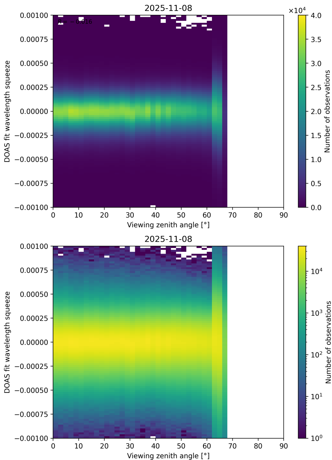
Figure 366: Scatter density plot of “Viewing zenith angle” against “DOAS fit wavelength squeeze” for 2025-11-07 to 2025-11-09.
