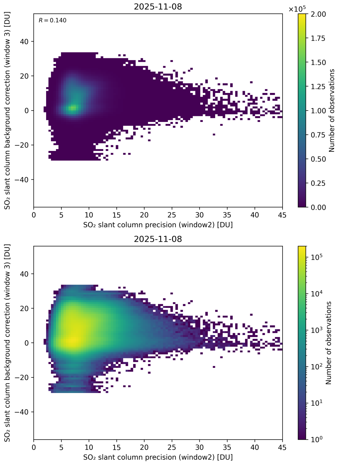
Figure 292: Scatter density plot of “SO 2 slant column precision (window2)” against “SO 2 slant column background correction (window 3)” for 2025-11-07 to 2025-11-09.
