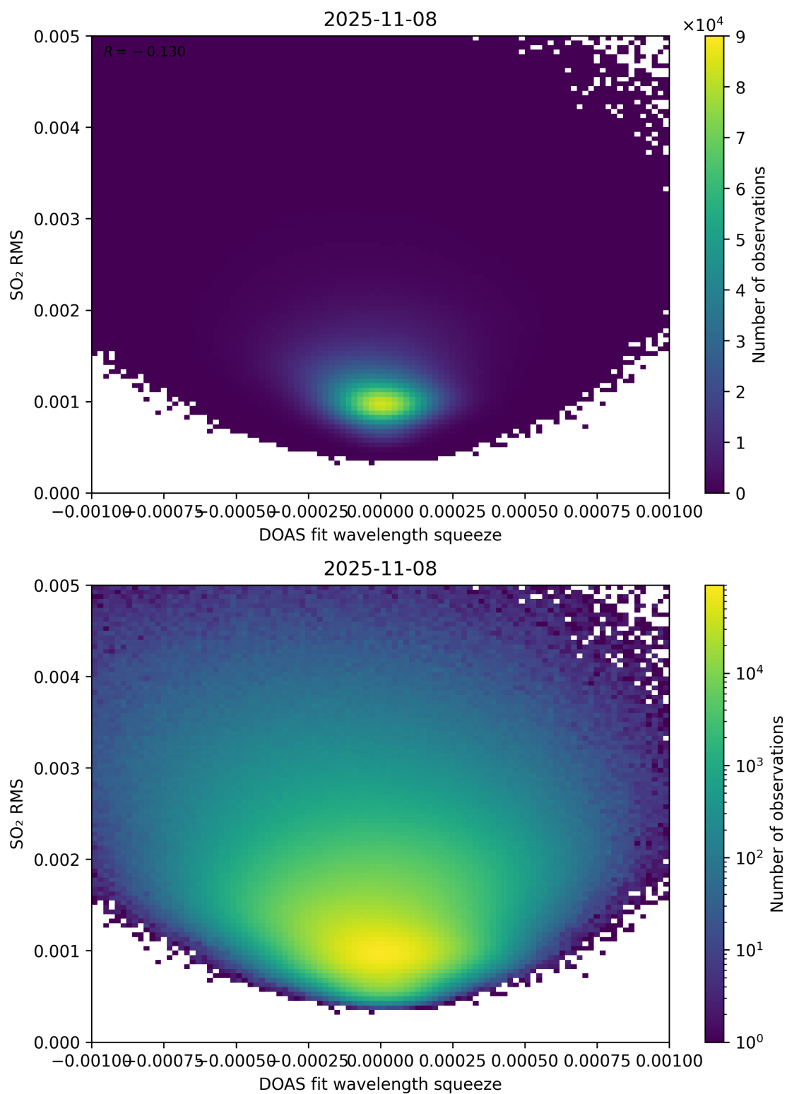
Figure 143: Scatter density plot of “DOAS fit wavelength squeeze” against “SO 2 RMS” for 2025-11-07 to 2025-11-09.
