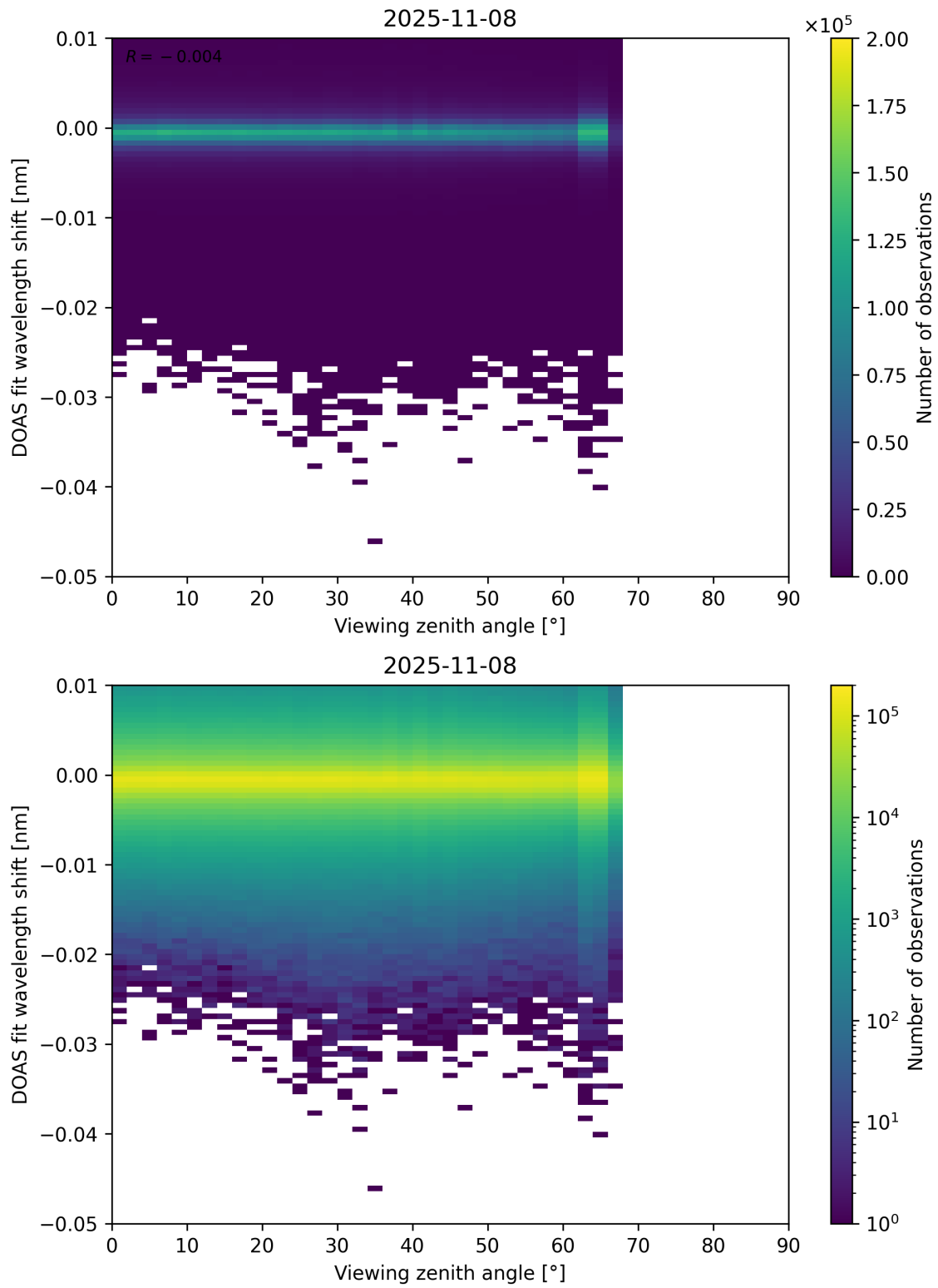
Figure 365: Scatter density plot of “Viewing zenith angle” against “DOAS fit wavelength shift” for 2025-11-07 to 2025-11-09.
