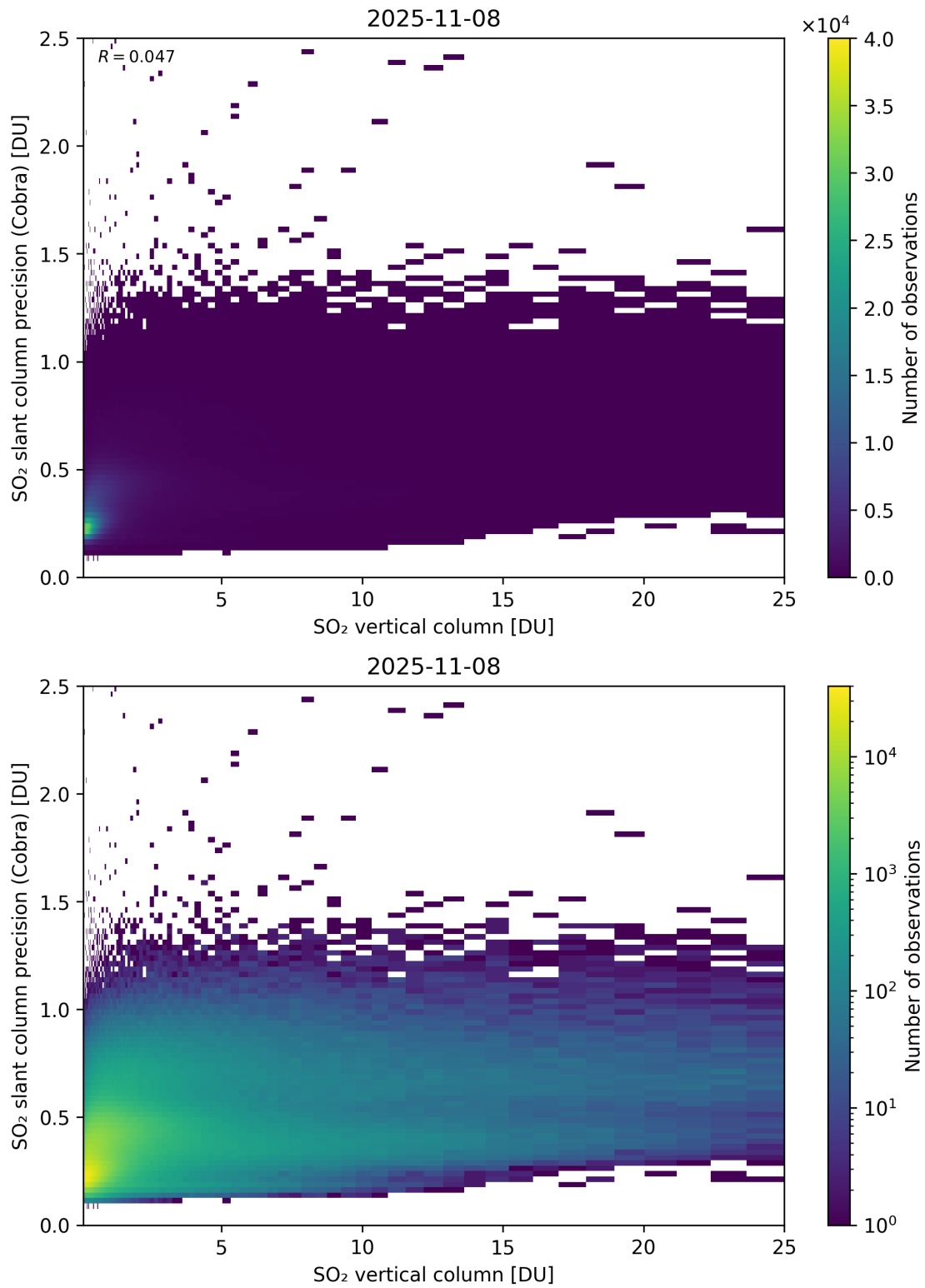
Figure 350: Scatter density plot of “SO 2 vertical column” against “SO 2 slant column precision (Cobra)” for 2025-11-07 to 2025-11-09.
