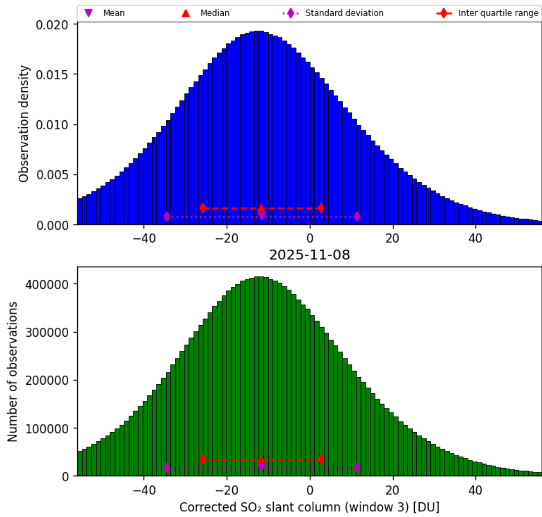
Figure 73: Histogram of “Corrected SO 2 slant column (window 3)” for 2025-11-07 to 2025-11-09
