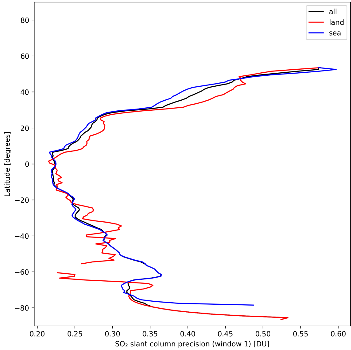
Figure 38: Zonal average of “SO 2 slant column precision (window 1)” for 2025-11-07 to 2025-11-09.
