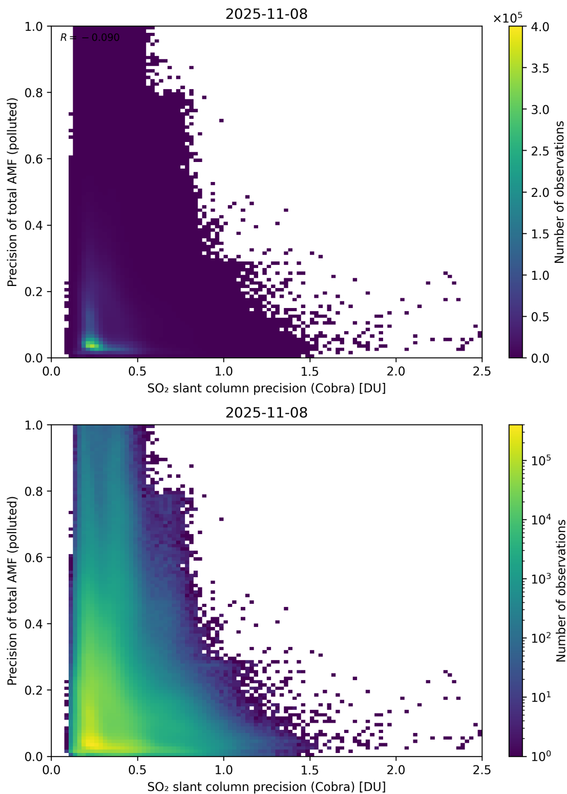
Figure 214: Scatter density plot of “SO 2 slant column precision (Cobra)” against “Precision of total AMF (polluted)” for 2025-11-07 to 2025-11-09.
