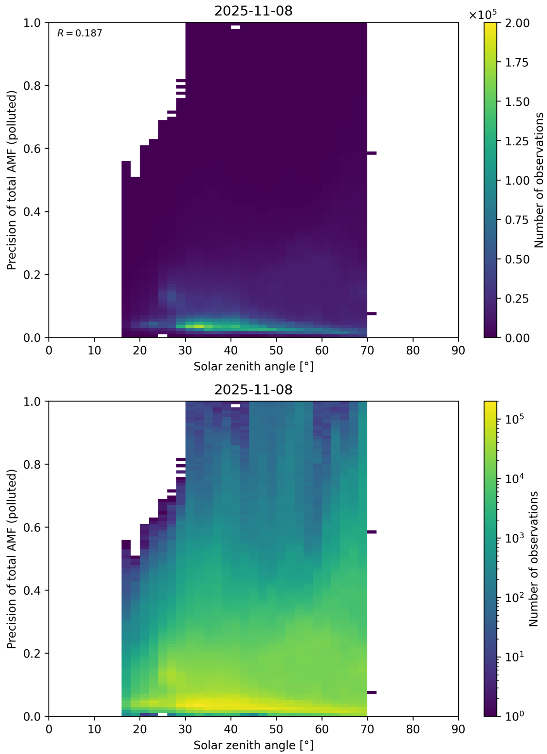
Figure 190: Scatter density plot of “Solar zenith angle” against “Precision of total AMF (polluted)” for 2025-11-07 to 2025-11-09.
