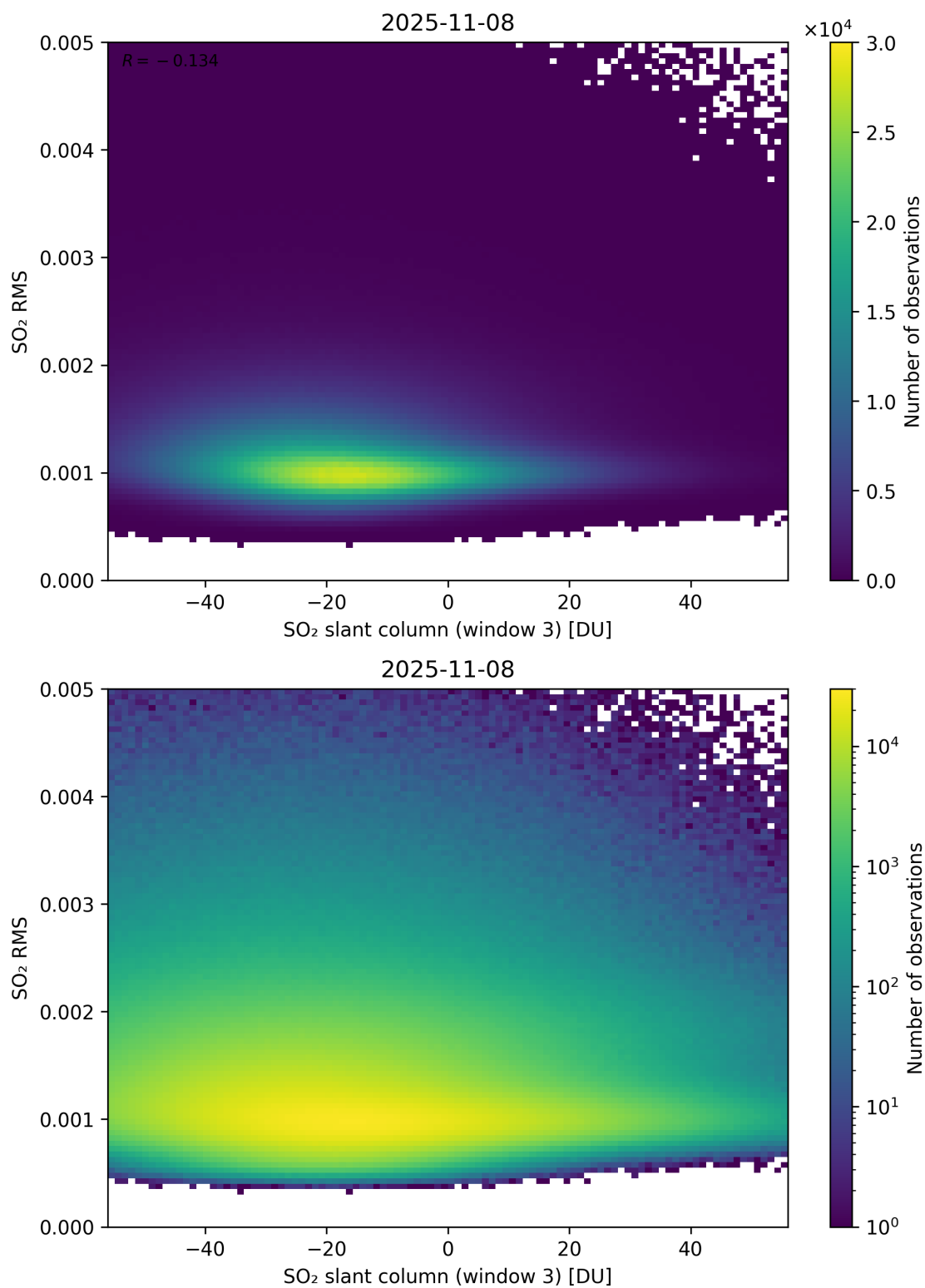
Figure 306: Scatter density plot of “SO 2 slant column (window 3)” against “SO 2 RMS” for 2025-11-07 to 2025-11-09.
