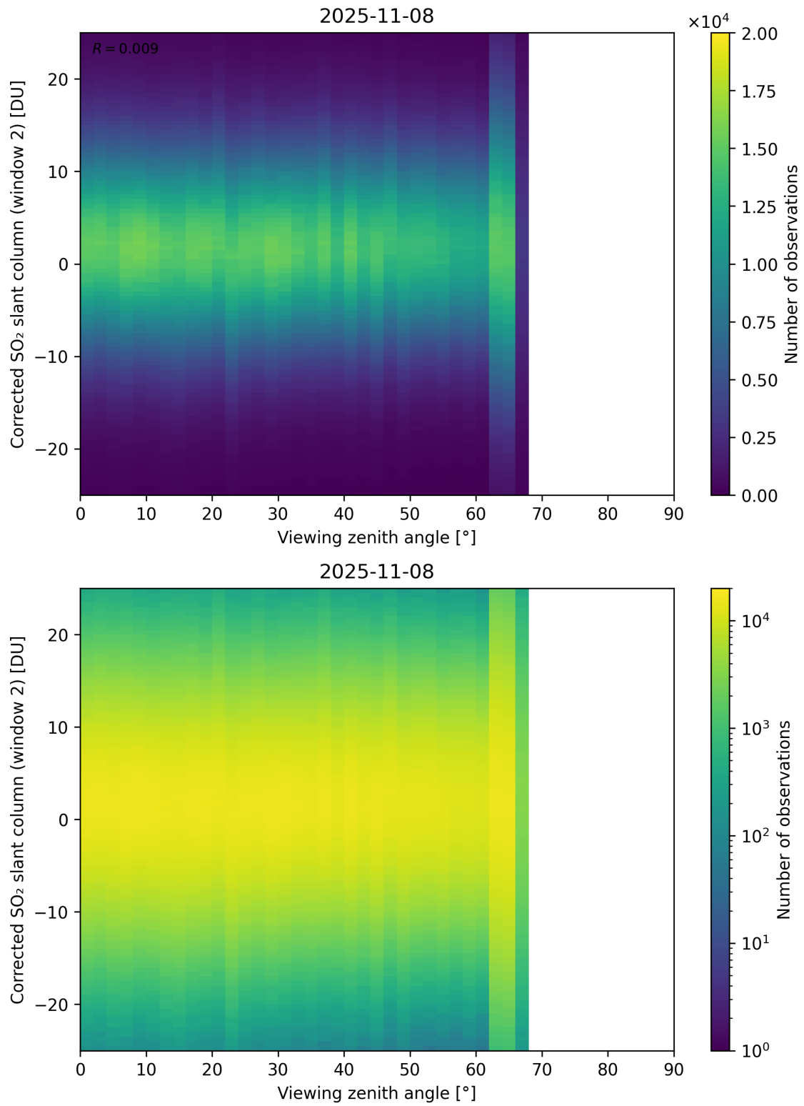
Figure 374: Scatter density plot of “Viewing zenith angle” against “Corrected SO 2 slant column (window 2)” for 2025-11-07 to 2025-11-09.
