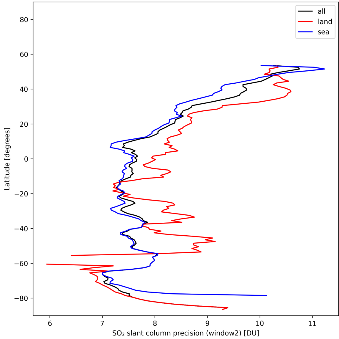
Figure 42: Zonal average of “SO 2 slant column precision (window2)” for 2025-11-07 to 2025-11-09.
