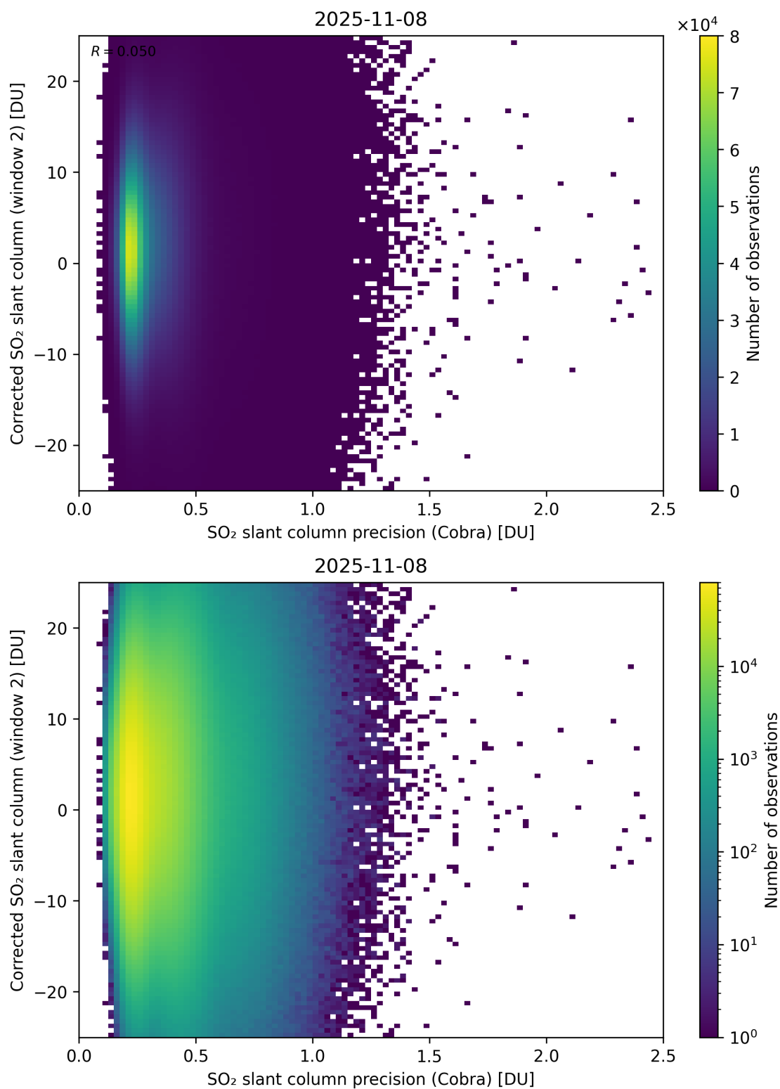
Figure 206: Scatter density plot of “SO 2 slant column precision (Cobra)” against “Corrected SO 2 slant column (window 2)” for 2025-11-07 to 2025-11-09.
