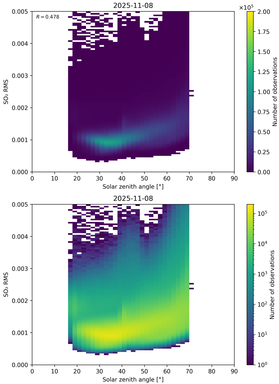
Figure 176: Scatter density plot of “Solar zenith angle” against “SO 2 RMS” for 2025-11-07 to 2025-11-09.
