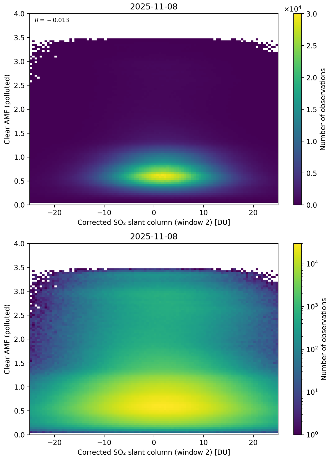
Figure 249: Scatter density plot of “Corrected SO 2 slant column (window 2)” against “Clear AMF (polluted)” for 2025-11-07 to 2025-11-09.
