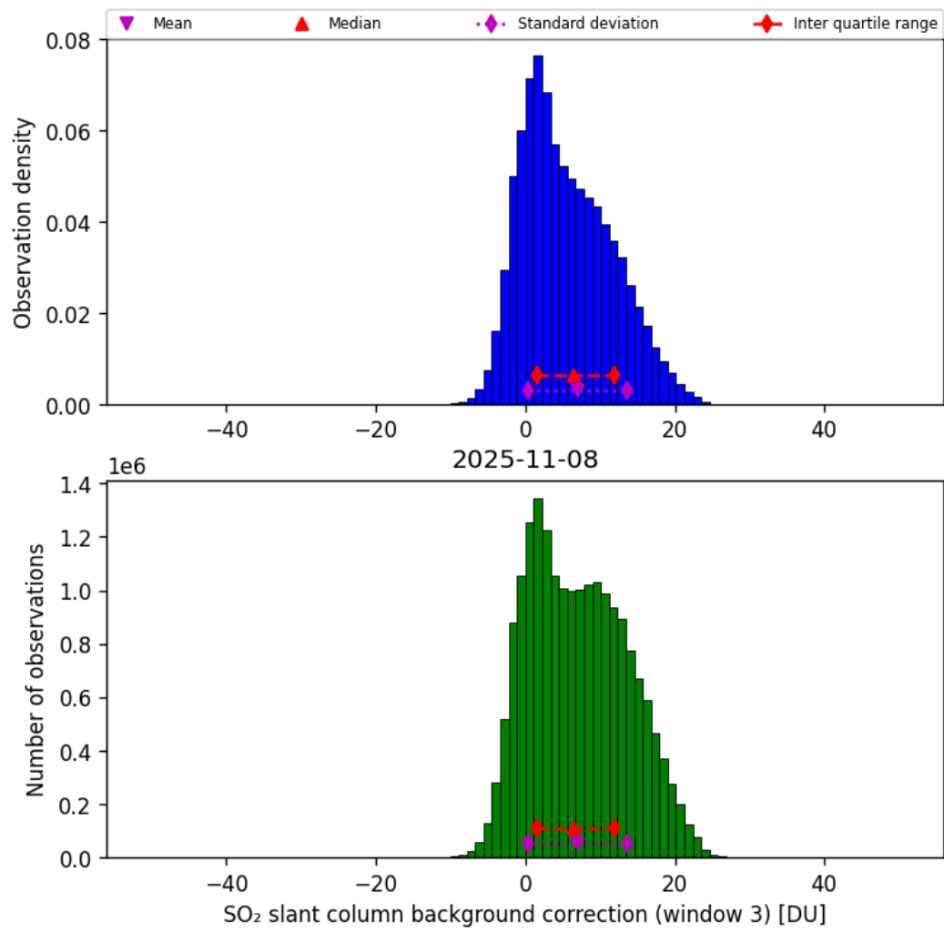
Figure 74: Histogram of “SO 2 slant column background correction (window 3)” for 2025-11-07 to 2025-11-09
