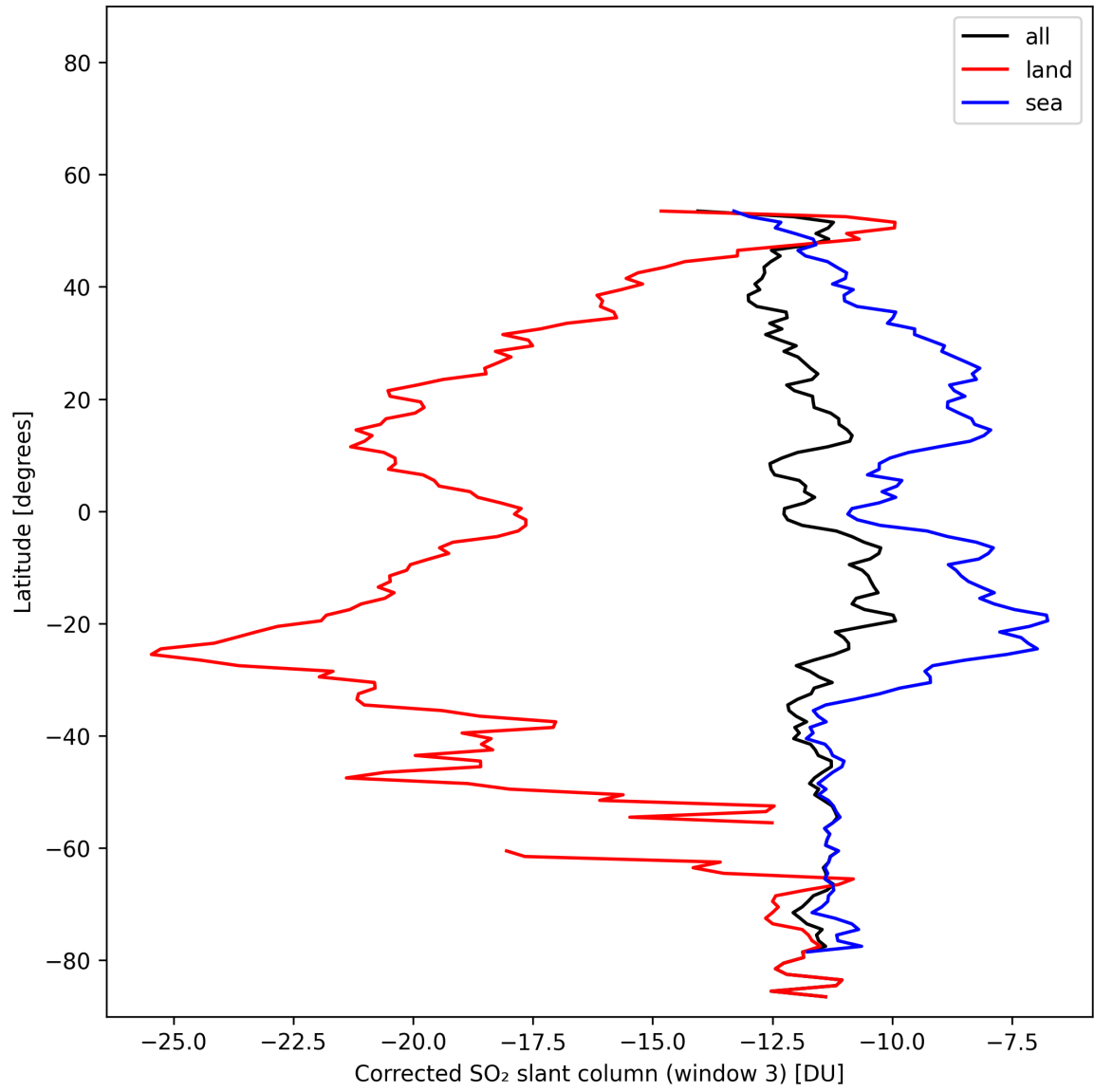
Figure 47: Zonal average of "Corrected SO 2 slant column (window 3)" for 2025-11-07 to 2025-11-09.
