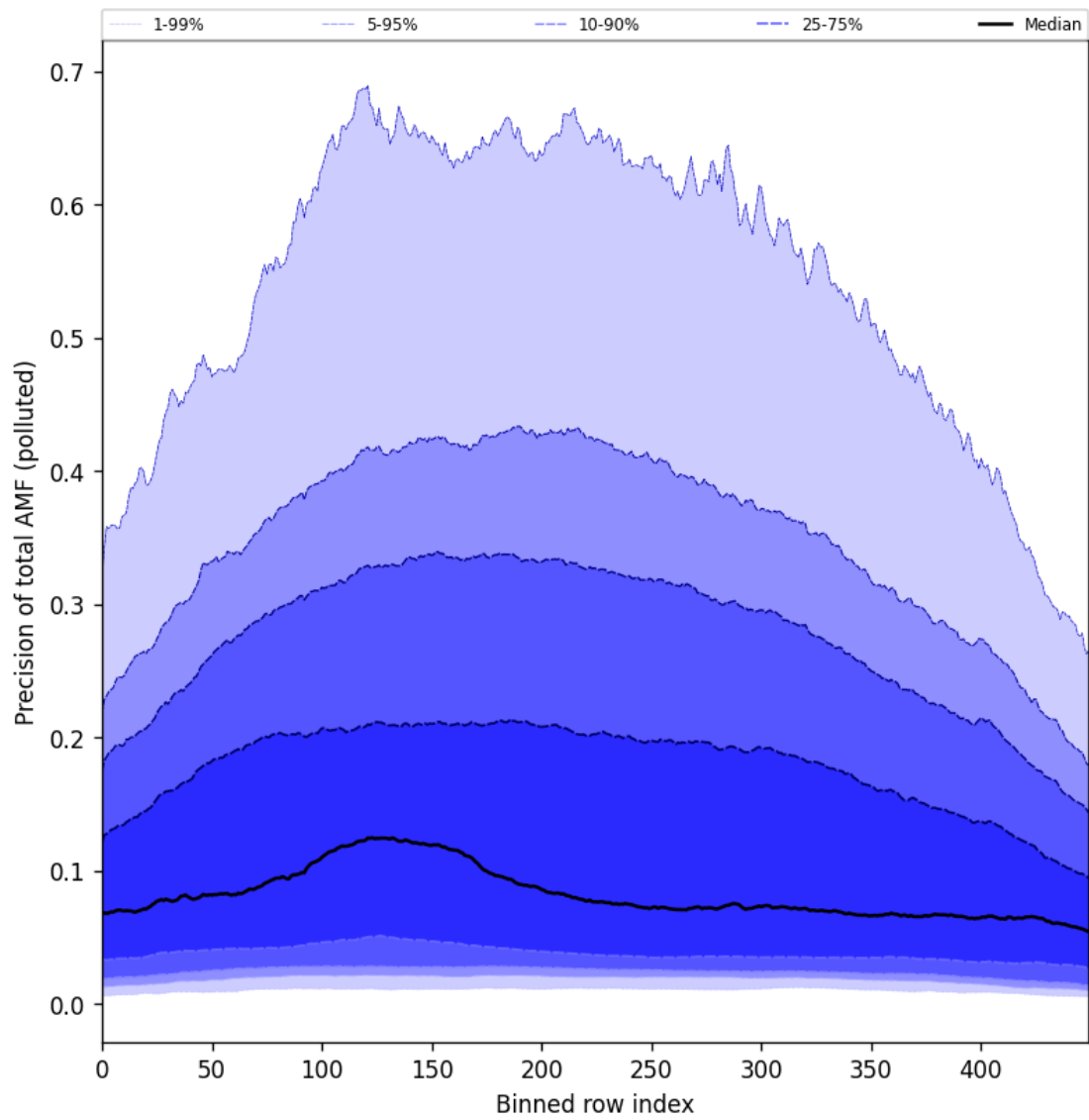
Figure 106: Along track statistics of “Precision of total AMF (polluted)” for 2025-11-07 to 2025-11-09
