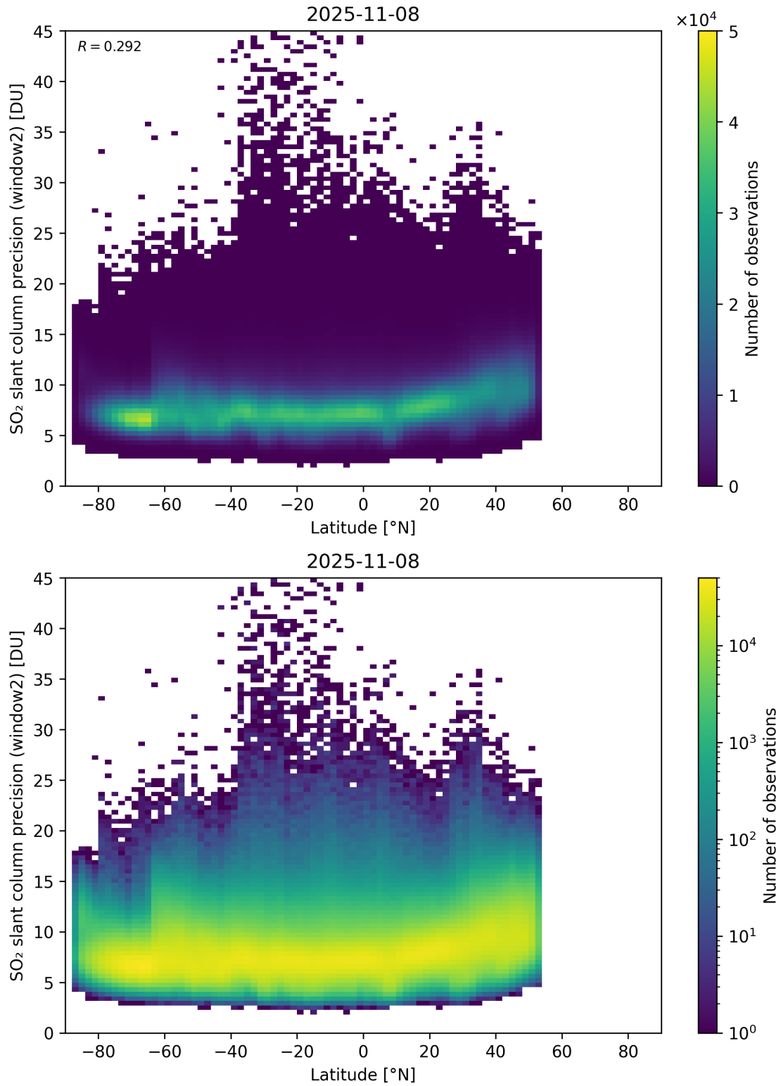
Figure 164: Scatter density plot of “Latitude” against “SO 2 slant column precision (window2)” for 2025-11-07 to 2025-11-09.
