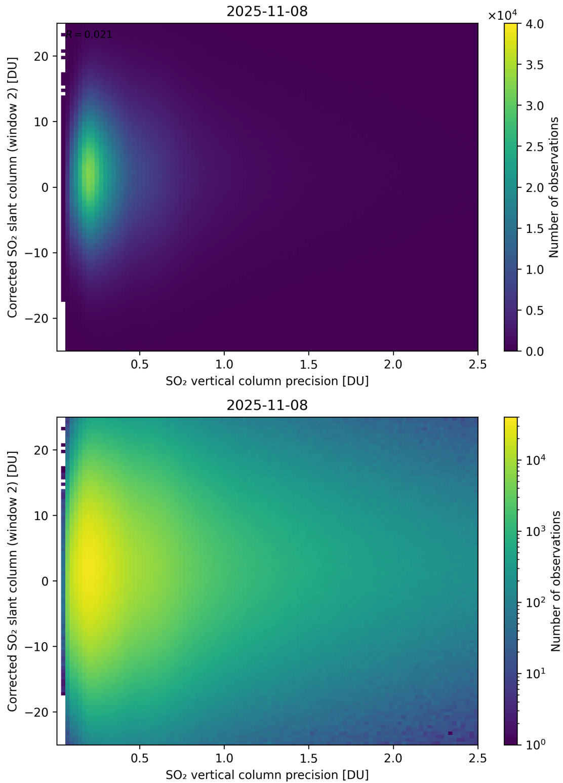
Figure 339: Scatter density plot of “SO 2 vertical column precision” against “Corrected SO 2 slant column (window 2)” for 2025-11-07 to 2025-11-09.
