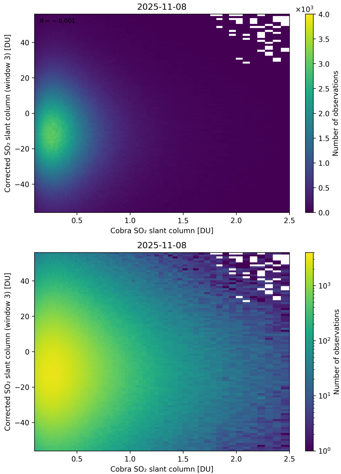
Figure 218: Scatter density plot of “Cobra SO 2 slant column” against “Corrected SO 2 slant column (window 3)” for 2025-11-07 to 2025-11-09.
