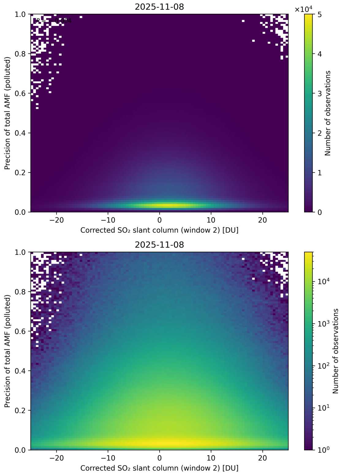
Figure 254: Scatter density plot of “Corrected SO 2 slant column (window 2)” against “Precision of total AMF (polluted)” for 2025-11-07 to 2025-11-09.
