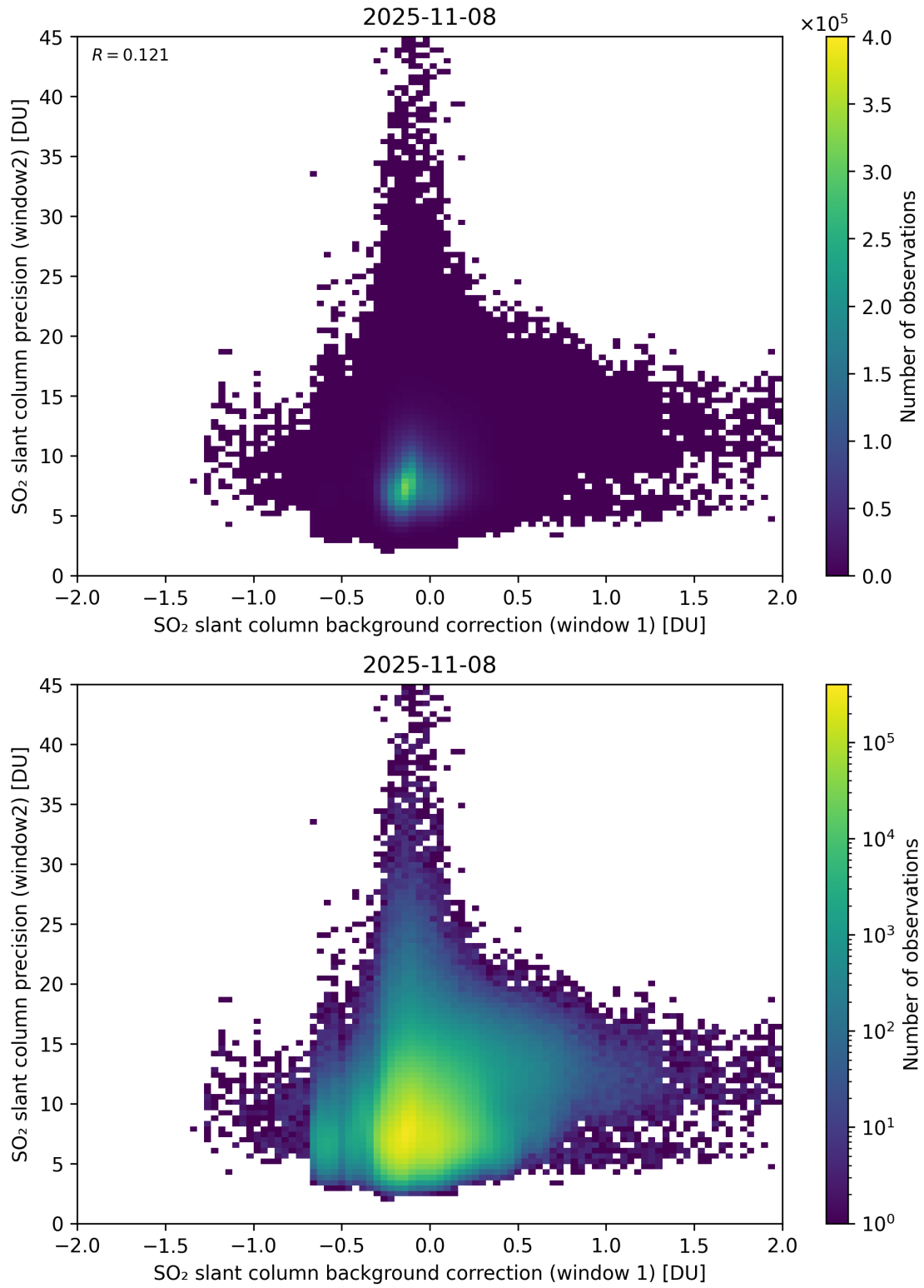
Figure 117: Scatter density plot of “SO 2 slant column background correction (window 1)” against “SO 2 slant column precision (window2)” for 2025-11-07 to 2025-11-09.
