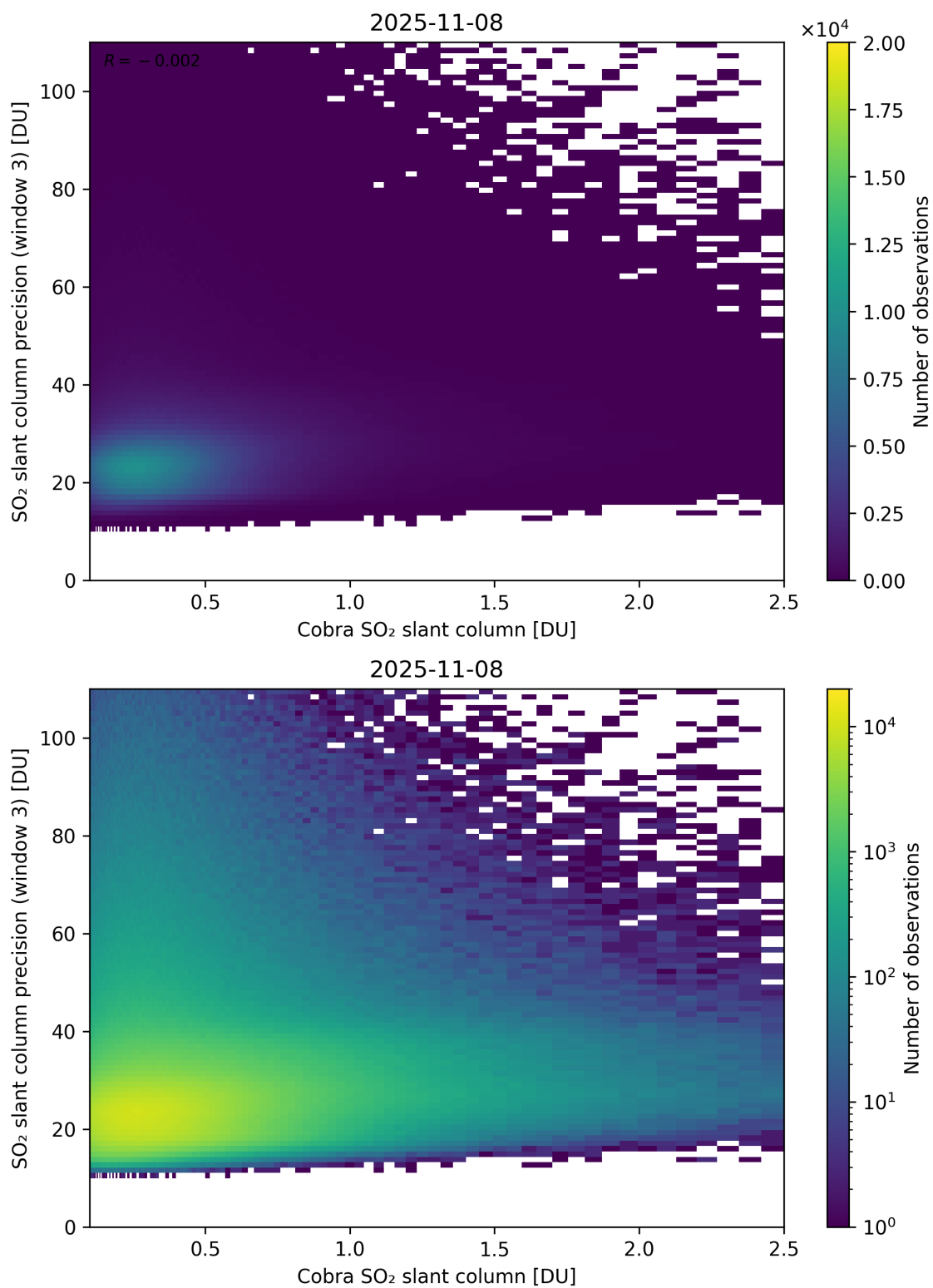
Figure 223: Scatter density plot of “Cobra SO 2 slant column” against “SO 2 slant column precision (window 3)” for 2025-11-07 to 2025-11-09.
