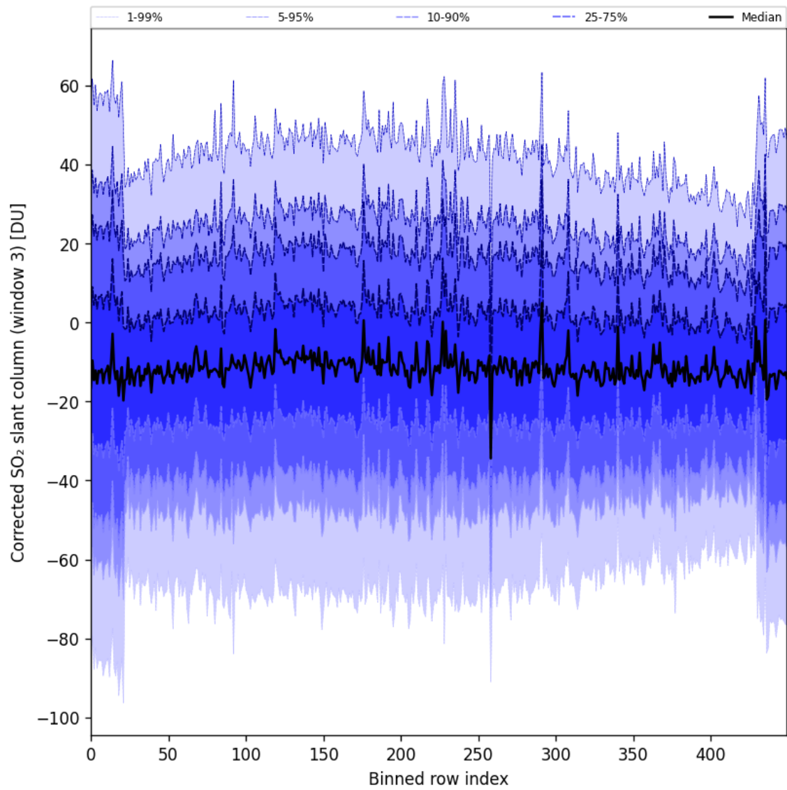
Figure 99: Along track statistics of “Corrected SO 2 slant column (window 3)” for 2025-11-07 to 2025-11-09
