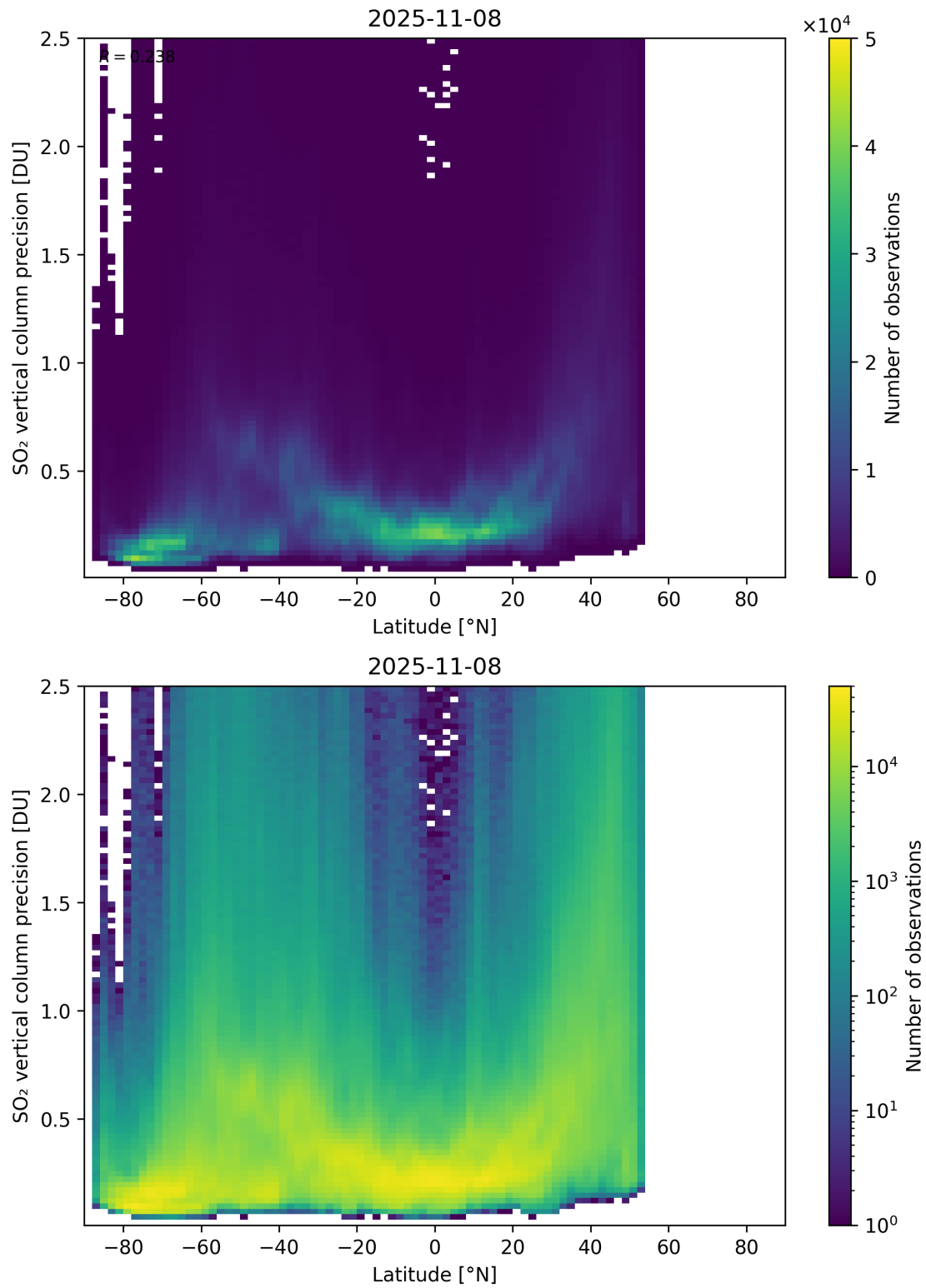
Figure 170: Scatter density plot of “Latitude” against “SO 2 vertical column precision” for 2025-11-07 to 2025-11-09.
