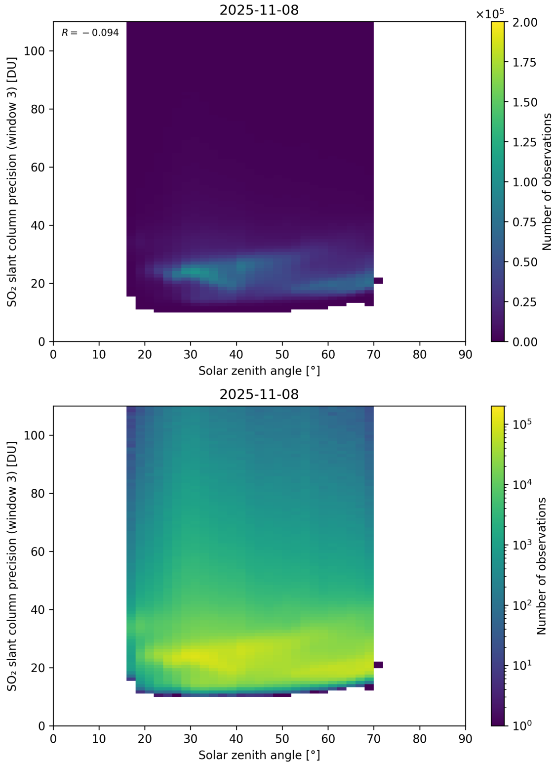
Figure 188: Scatter density plot of “Solar zenith angle” against “SO 2 slant column precision (window 3)” for 2025-11-07 to 2025-11-09.
