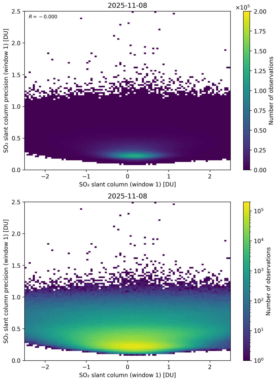
Figure 285: Scatter density plot of “SO 2 slant column (window 1)” against “SO 2 slant column precision (window 1)” for 2025-11-07 to 2025-11-09.
