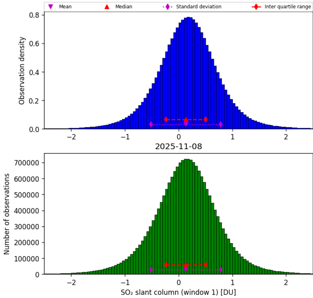
Figure 63: Histogram of “SO 2 slant column (window 1)” for 2025-11-07 to 2025-11-09
