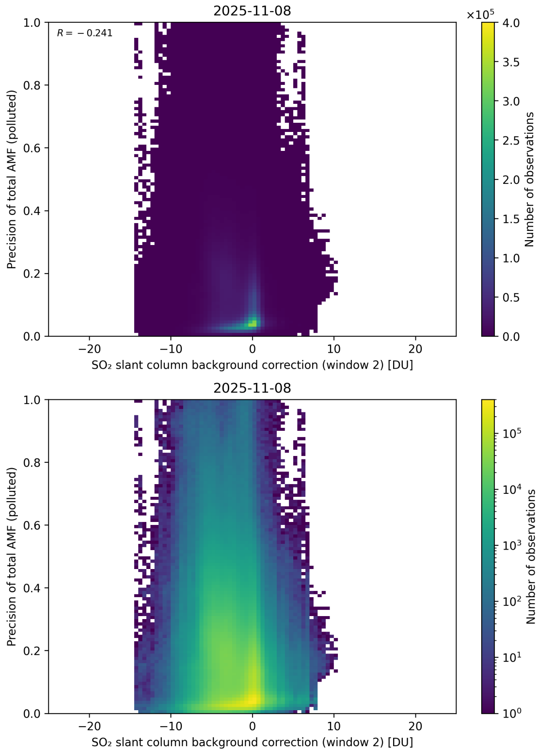
Figure 131: Scatter density plot of “SO 2 slant column background correction (window 2)” against “Precision of total AMF (polluted)” for 2025-11-07 to 2025-11-09.
