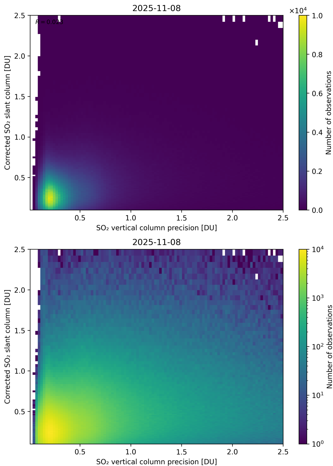
Figure 338: Scatter density plot of “SO 2 vertical column precision” against “Corrected SO 2 slant column” for 2025-11-07 to 2025-11-09.
