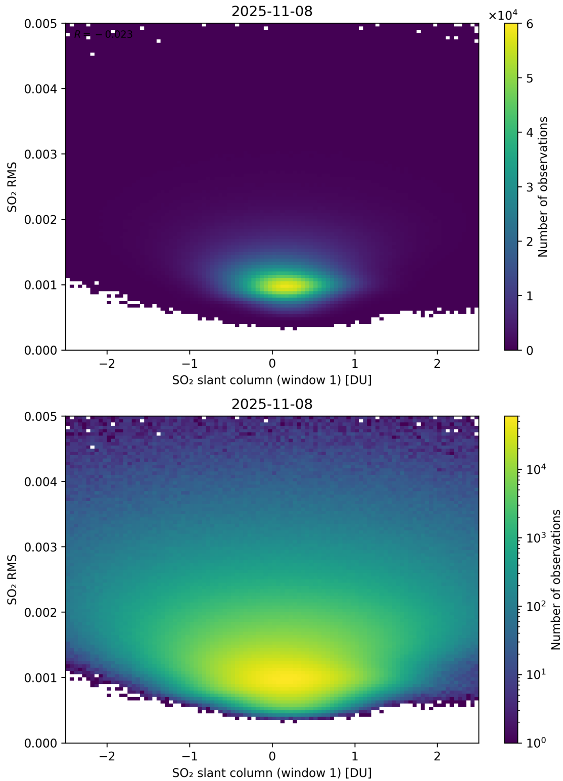
Figure 267: Scatter density plot of “SO 2 slant column (window 1)” against “SO 2 RMS” for 2025-11-07 to 2025-11-09.
