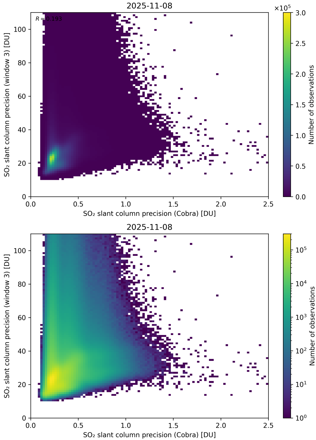
Figure 212: Scatter density plot of “SO 2 slant column precision (Cobra)” against “SO 2 slant column precision (window 3)” for 2025-11-07 to 2025-11-09.
