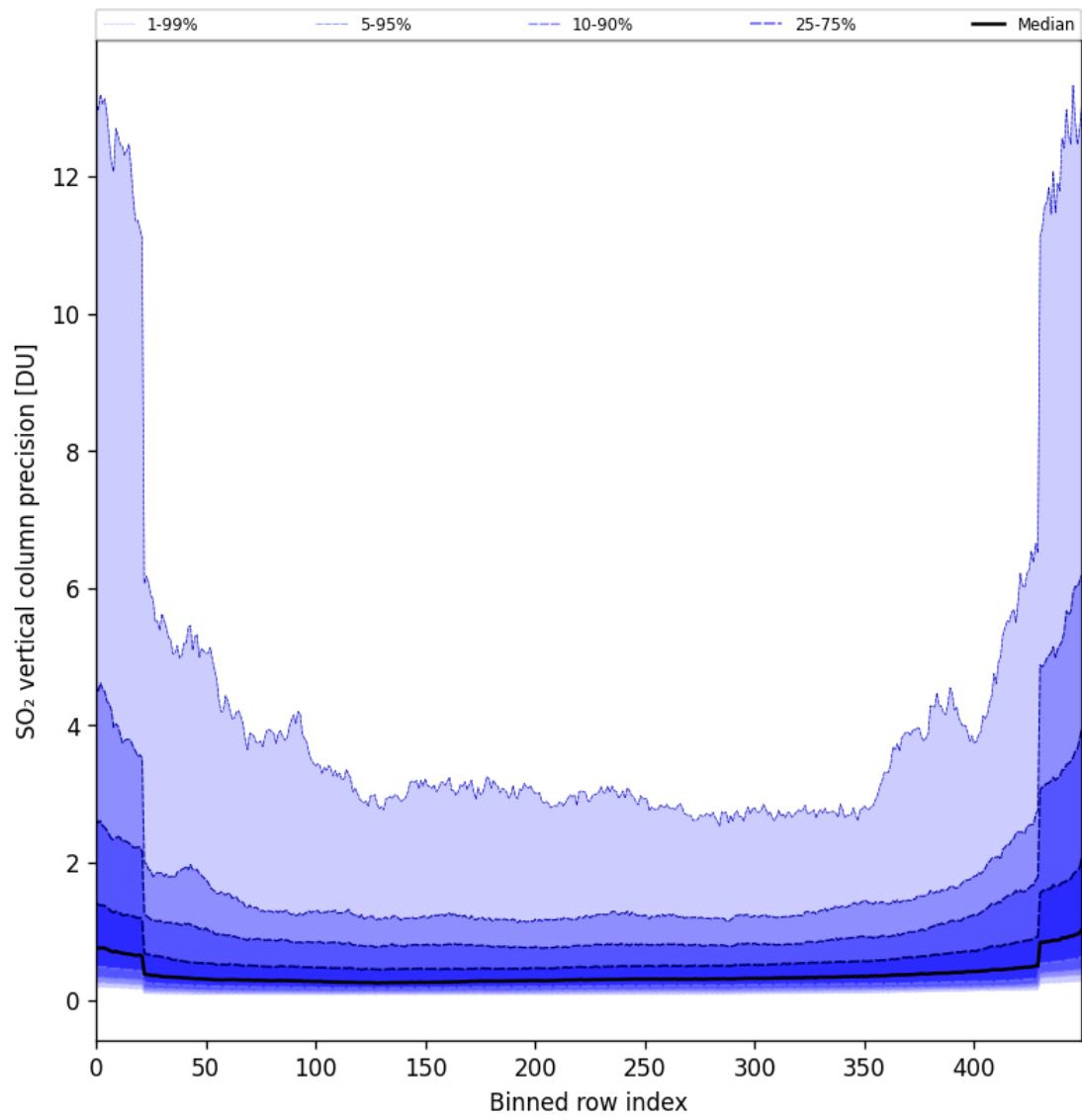
Figure 85: Along track statistics of “SO 2 vertical column precision” for 2025-11-07 to 2025-11-09
