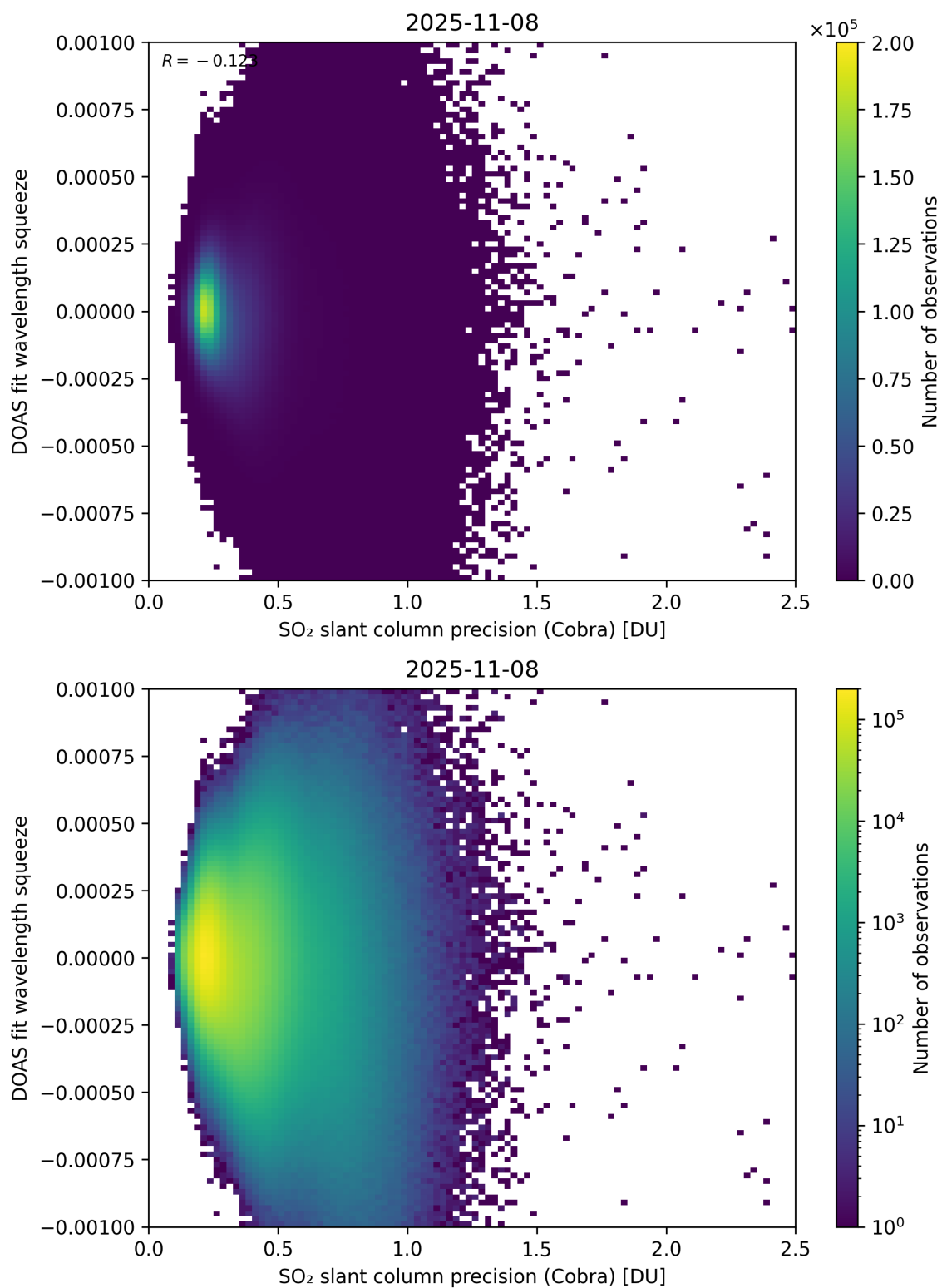
Figure 203: Scatter density plot of “SO 2 slant column precision (Cobra)” against “DOAS fit wavelength squeeze” for 2025-11-07 to 2025-11-09.
