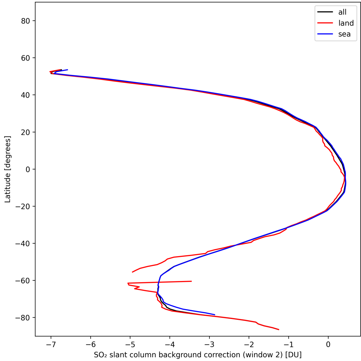
Figure 44: Zonal average of “SO 2 slant column background correction (window 2)” for 2025-11-07 to 2025-11-09.
