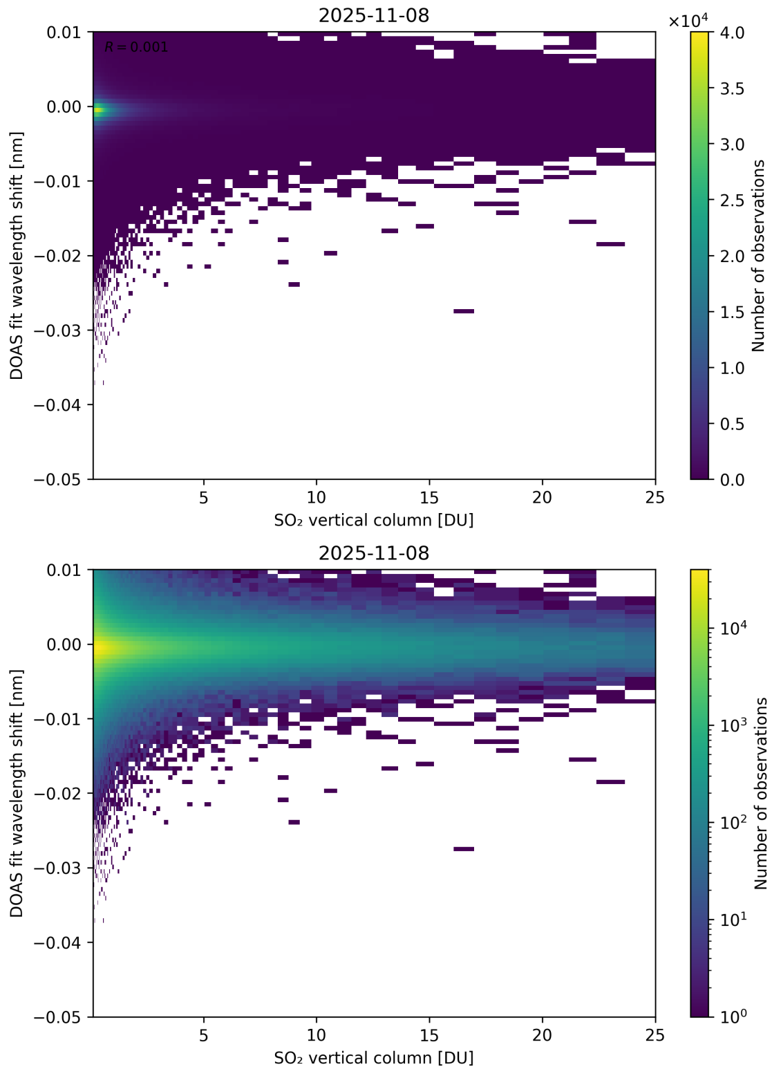
Figure 326: Scatter density plot of “SO 2 vertical column” against “DOAS fit wavelength shift” for 2025-11-07 to 2025-11-09.
