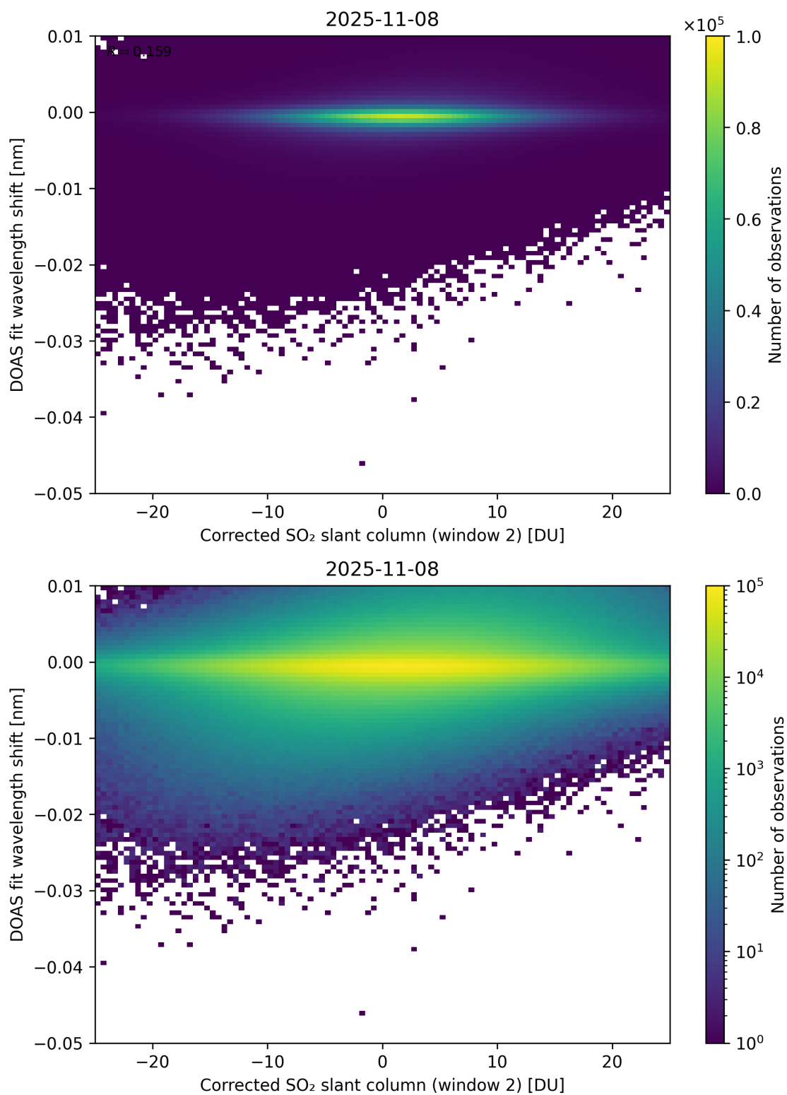
Figure 246: Scatter density plot of “Corrected SO 2 slant column (window 2)” against “DOAS fit wavelength shift” for 2025-11-07 to 2025-11-09.
