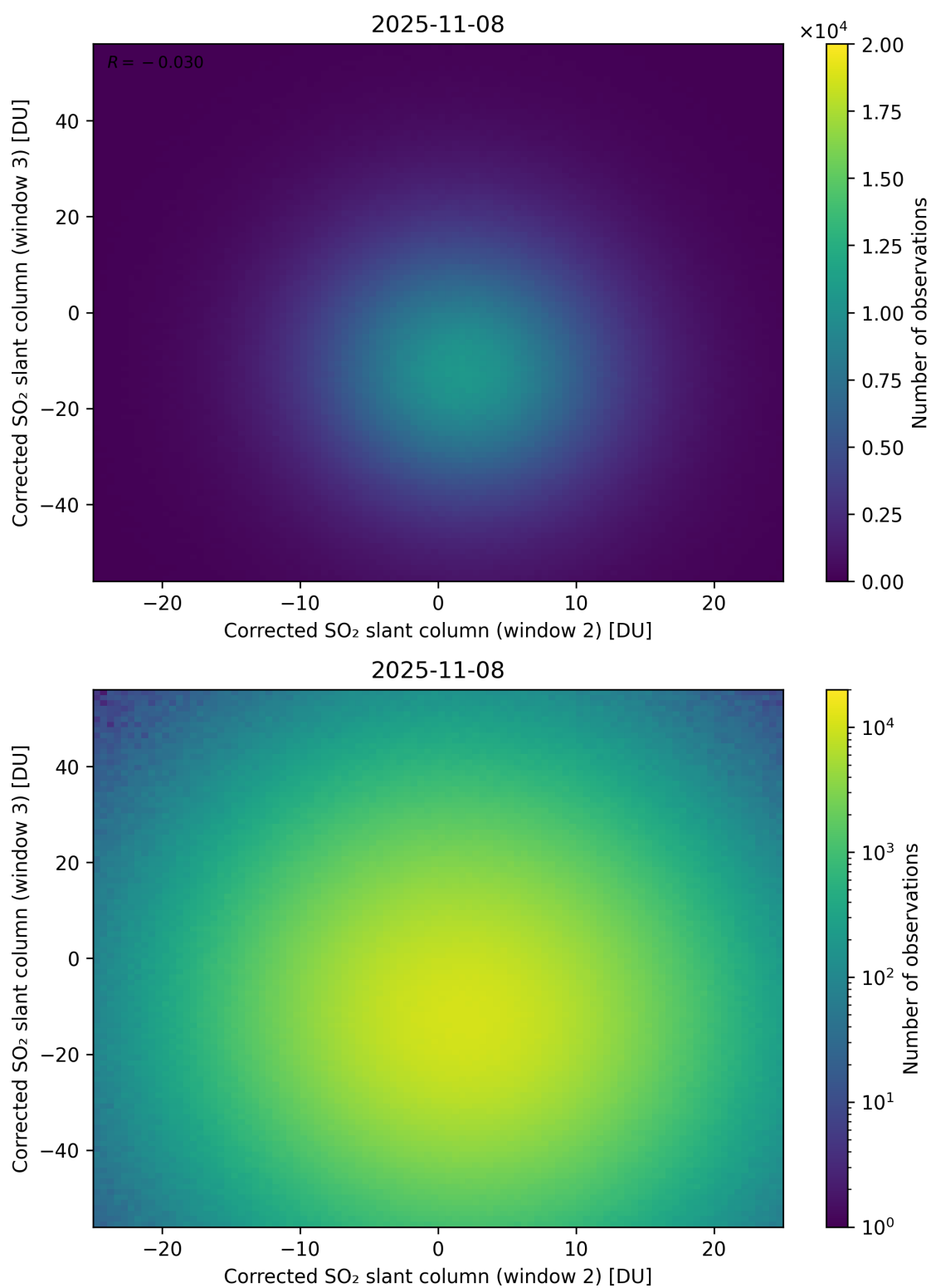
Figure 250: Scatter density plot of “Corrected SO 2 slant column (window 2)” against “Corrected SO 2 slant column (window 3)” for 2025-11-07 to 2025-11-09.
