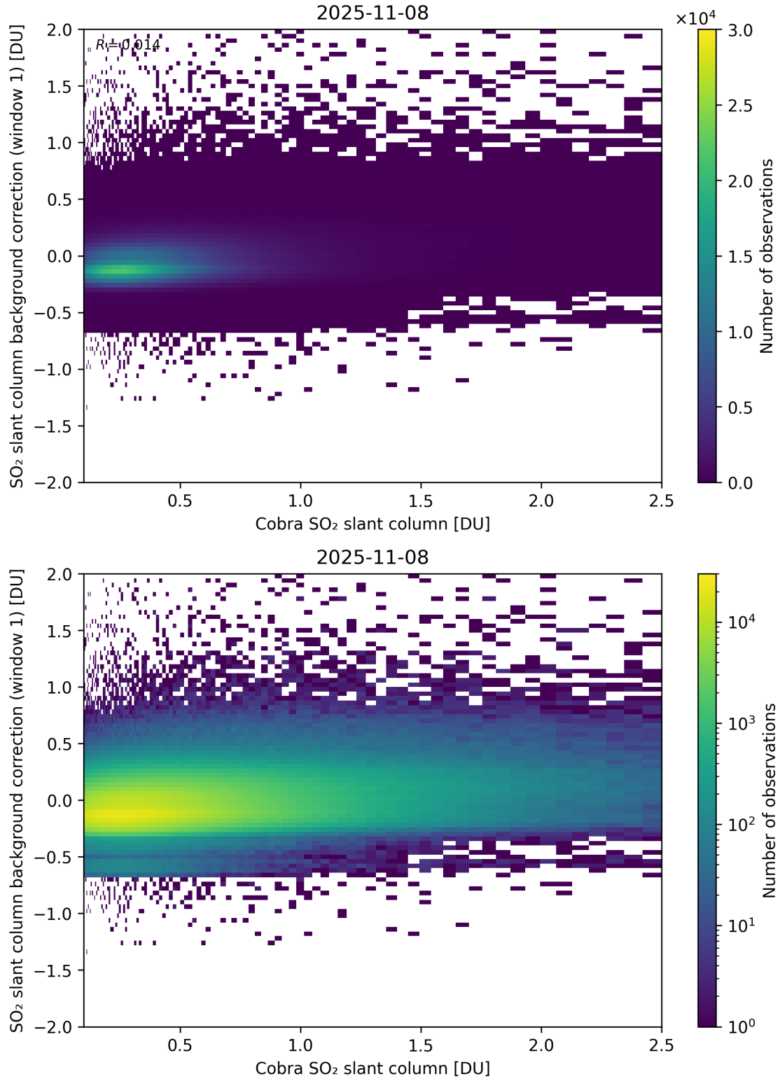
Figure 193: Scatter density plot of “Cobra SO 2 slant column” against “SO 2 slant column background correction (window 1)” for 2025-11-07 to 2025-11-09.
