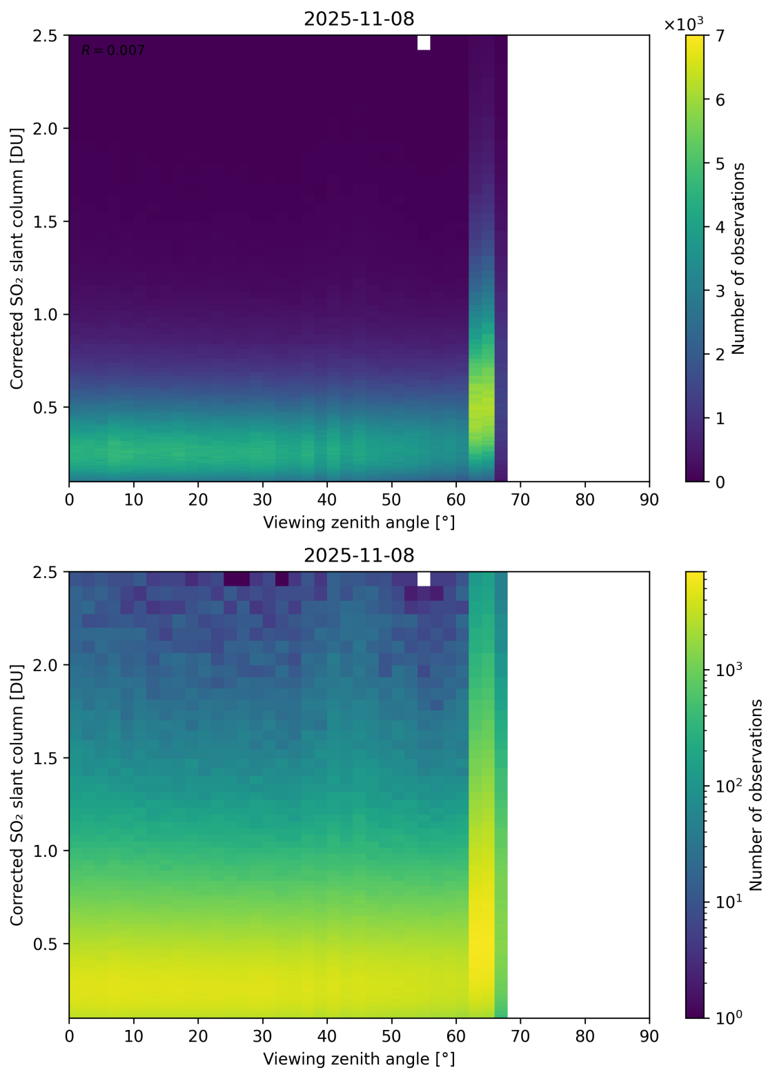
Figure 373: Scatter density plot of “Viewing zenith angle” against “Corrected SO 2 slant column” for 2025-11-07 to 2025-11-09.
