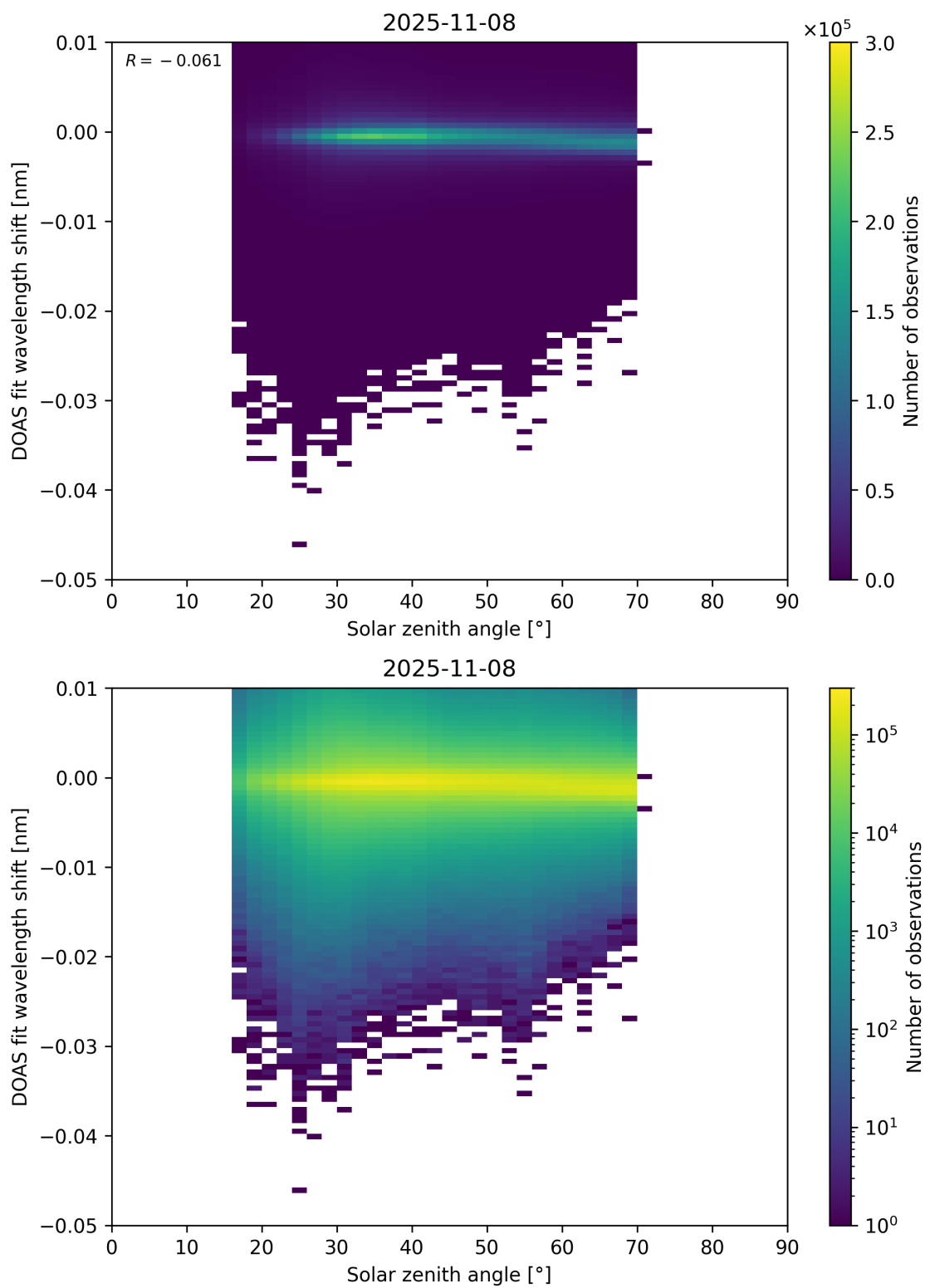
Figure 174: Scatter density plot of “Solar zenith angle” against “DOAS fit wavelength shift” for 2025-11-07 to 2025-11-09.
