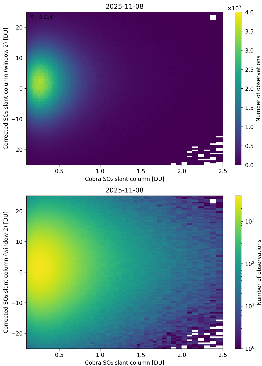
Figure 217: Scatter density plot of “Cobra SO 2 slant column” against “Corrected SO 2 slant column (window 2)” for 2025-11-07 to 2025-11-09.
