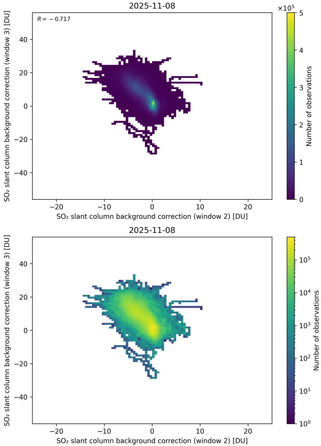
Figure 122: Scatter density plot of “SO 2 slant column background correction (window 2)” against “SO 2 slant column background correction (window 3)” for 2025-11-07 to 2025-11-09.
