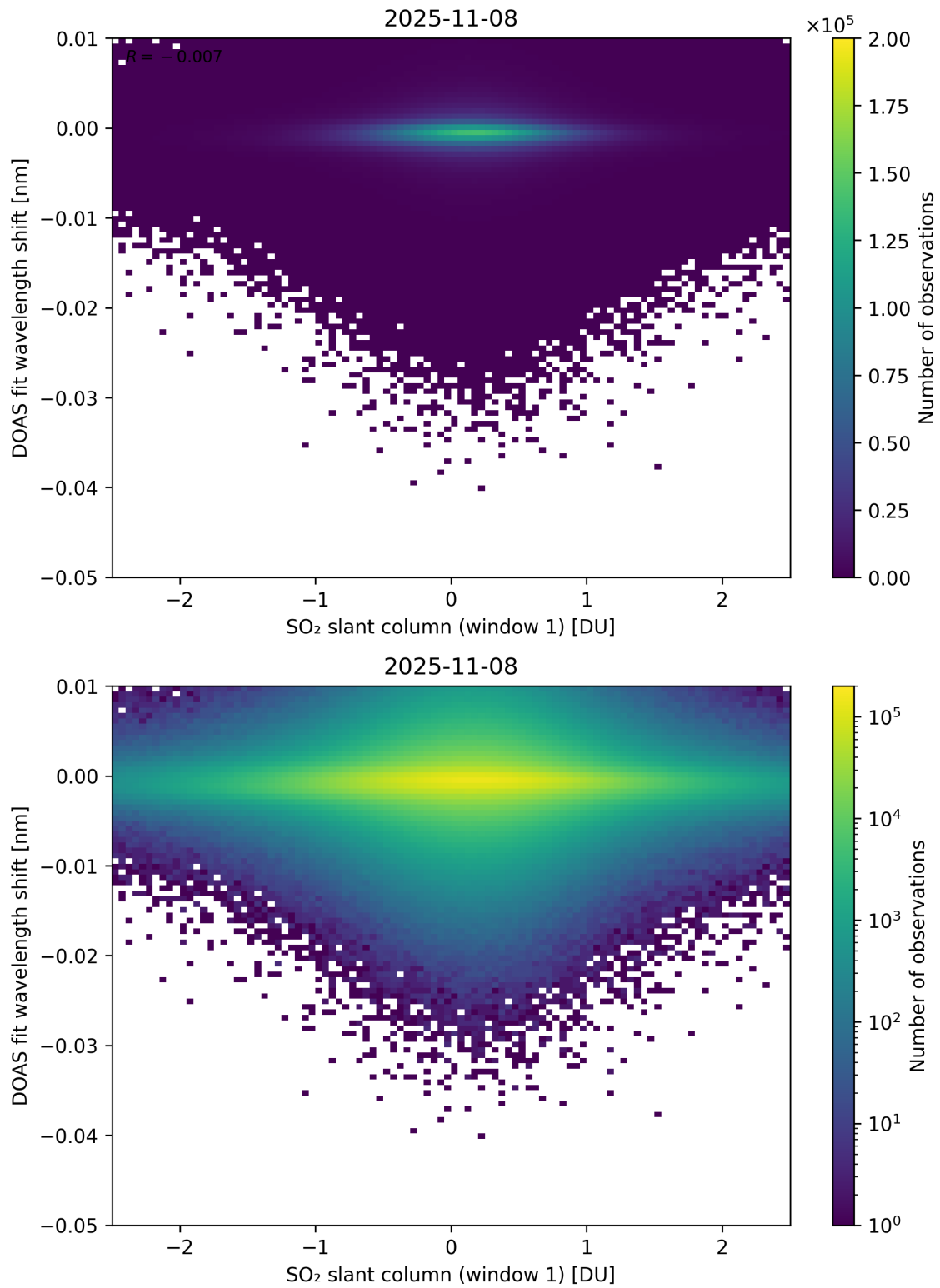
Figure 265: Scatter density plot of “SO 2 slant column (window 1)” against “DOAS fit wavelength shift” for 2025-11-07 to 2025-11-09.
