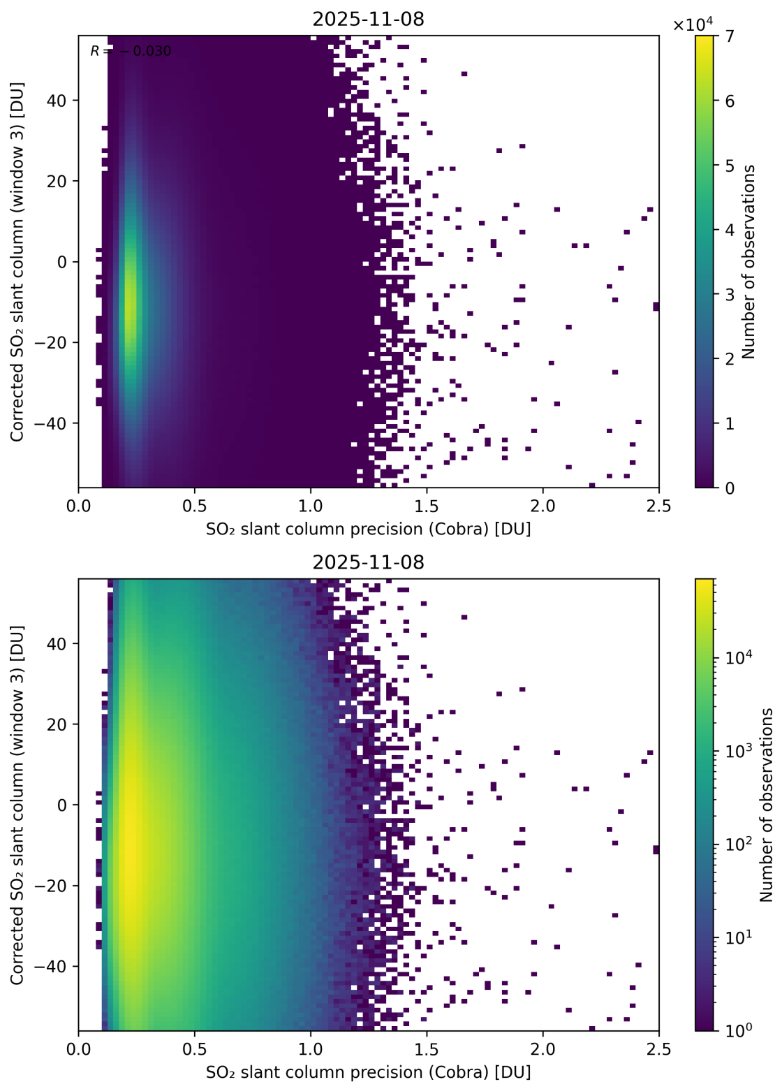
Figure 207: Scatter density plot of “SO 2 slant column precision (Cobra)” against “Corrected SO 2 slant column (window 3)” for 2025-11-07 to 2025-11-09.
