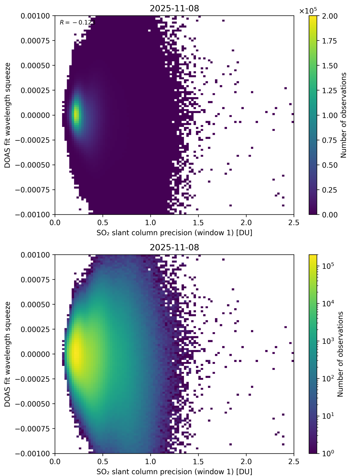
Figure 272: Scatter density plot of “SO 2 slant column precision (window 1)” against “DOAS fit wavelength squeeze” for 2025-11-07 to 2025-11-09.
