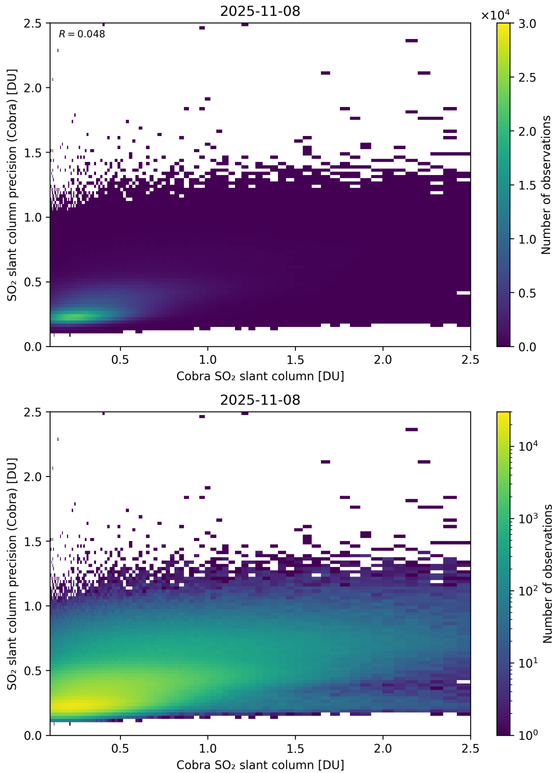
Figure 216: Scatter density plot of “Cobra SO 2 slant column” against “SO 2 slant column precision (Cobra)” for 2025-11-07 to 2025-11-09.
