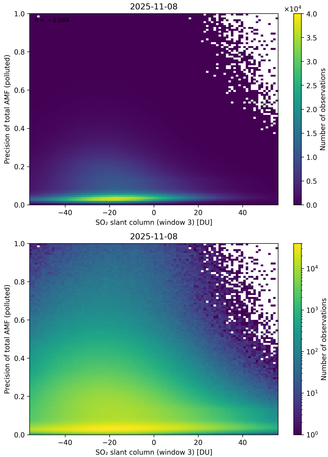
Figure 319: Scatter density plot of “SO 2 slant column (window 3)” against “Precision of total AMF (polluted)” for 2025-11-07 to 2025-11-09.
