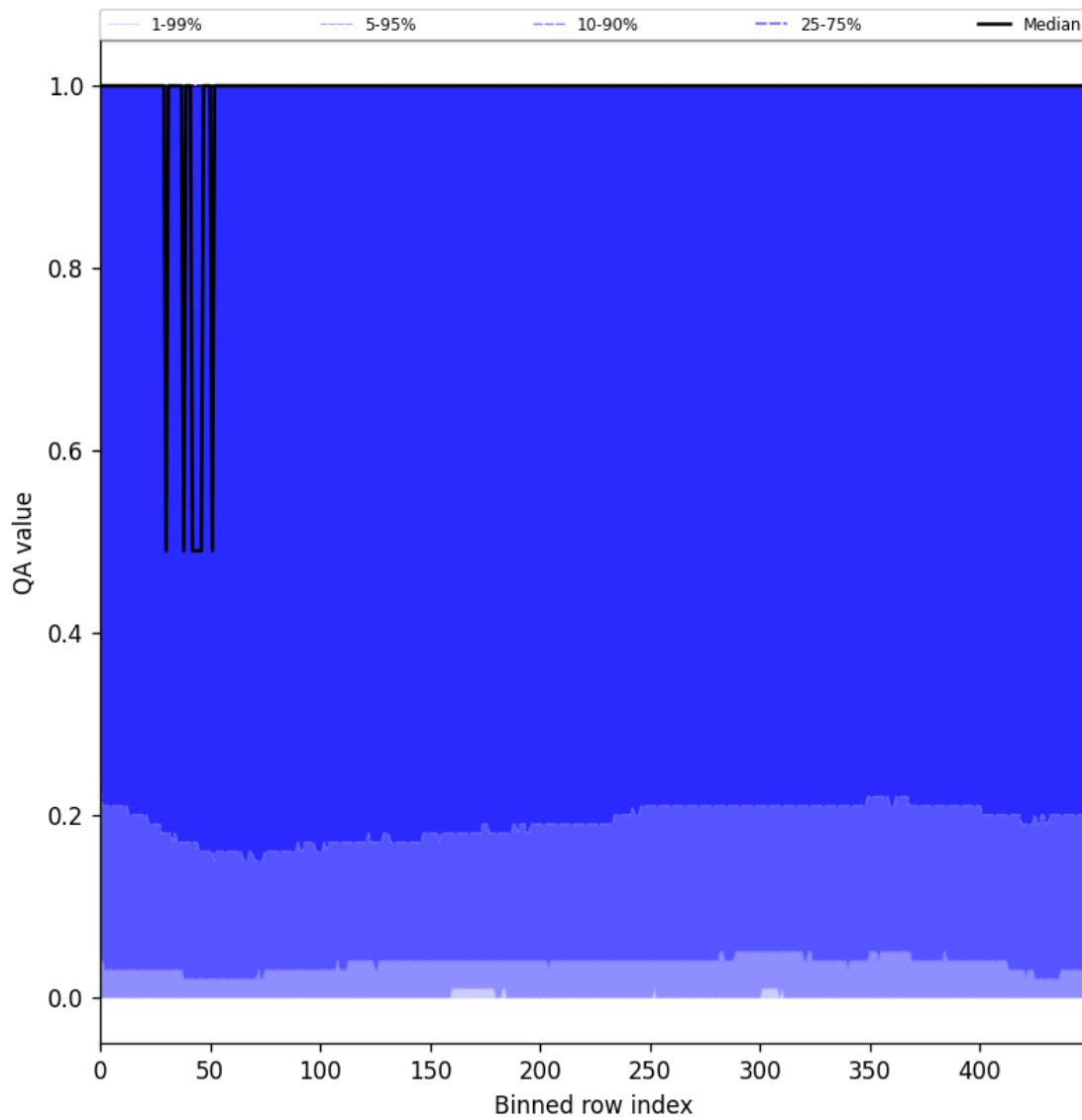
Figure 83: Along track statistics of “QA value” for 2025-11-07 to 2025-11-09
