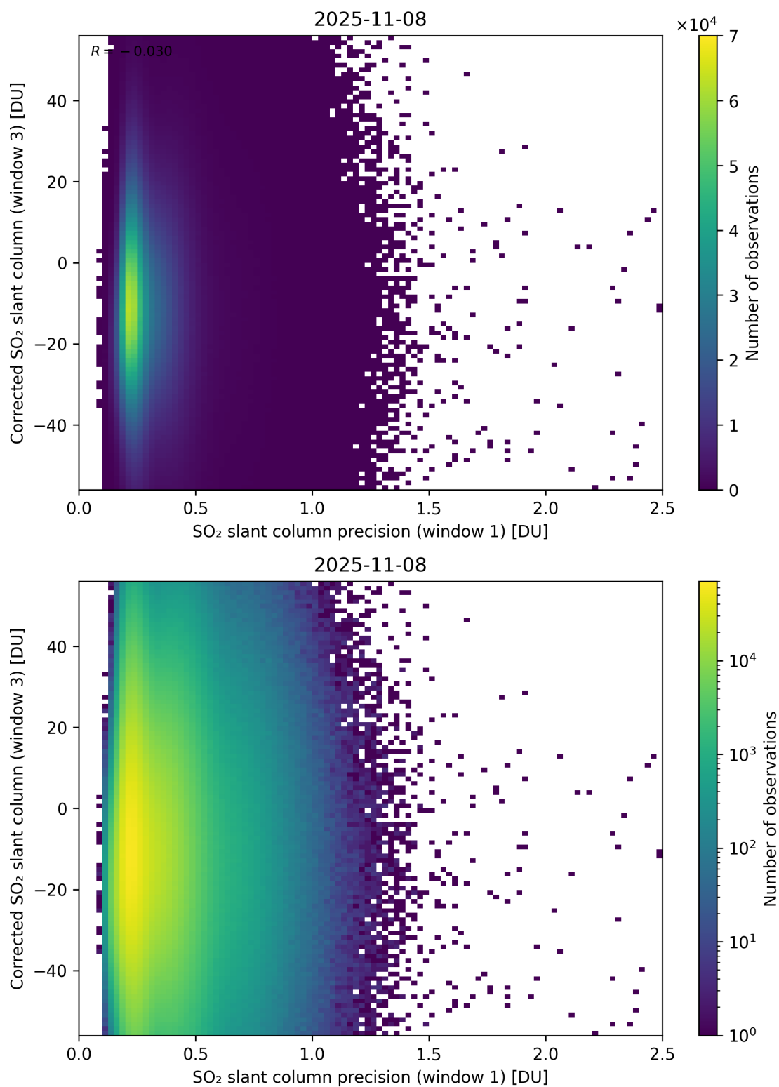
Figure 276: Scatter density plot of “SO 2 slant column precision (window 1)” against “Corrected SO 2 slant column (window 3)” for 2025-11-07 to 2025-11-09.
