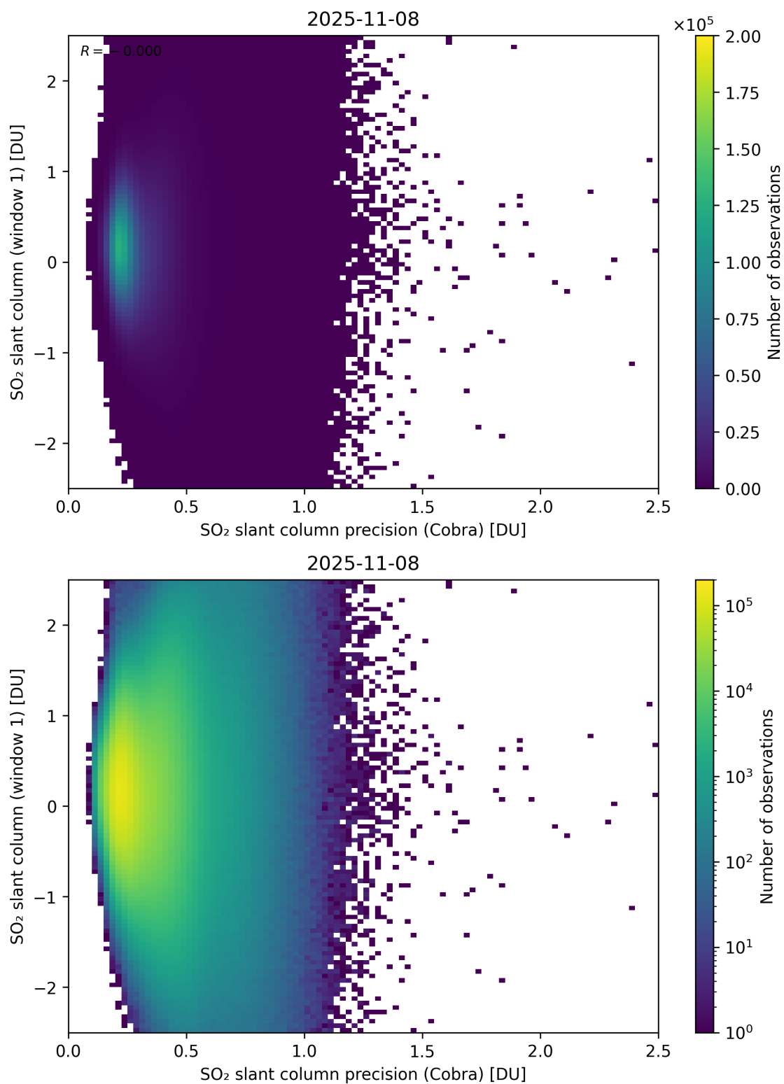
Figure 208: Scatter density plot of “SO 2 slant column precision (Cobra)” against “SO 2 slant column (window 1)” for 2025-11-07 to 2025-11-09.
