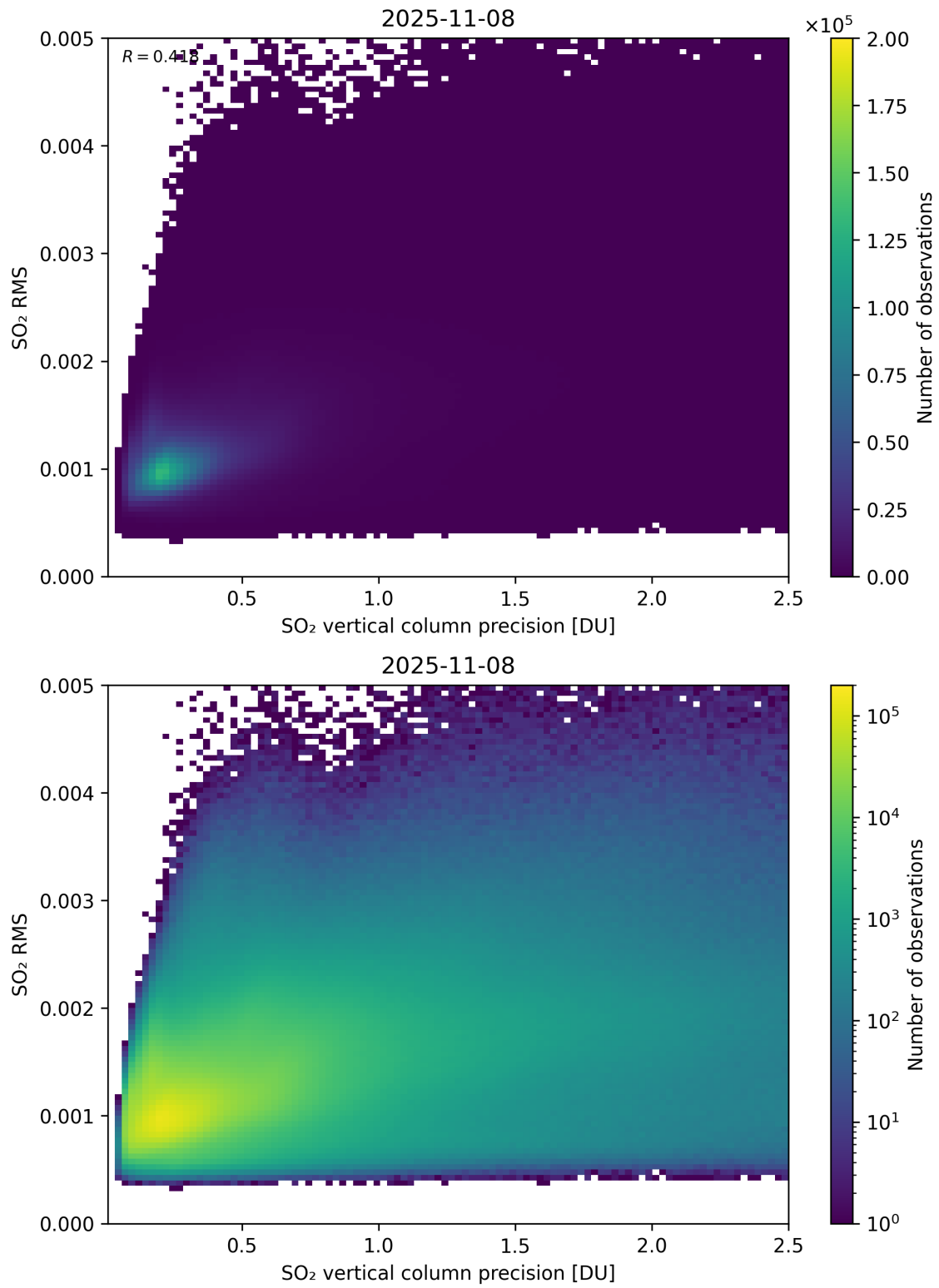
Figure 334: Scatter density plot of “SO 2 vertical column precision” against “SO 2 RMS” for 2025-11-07 to 2025-11-09.
