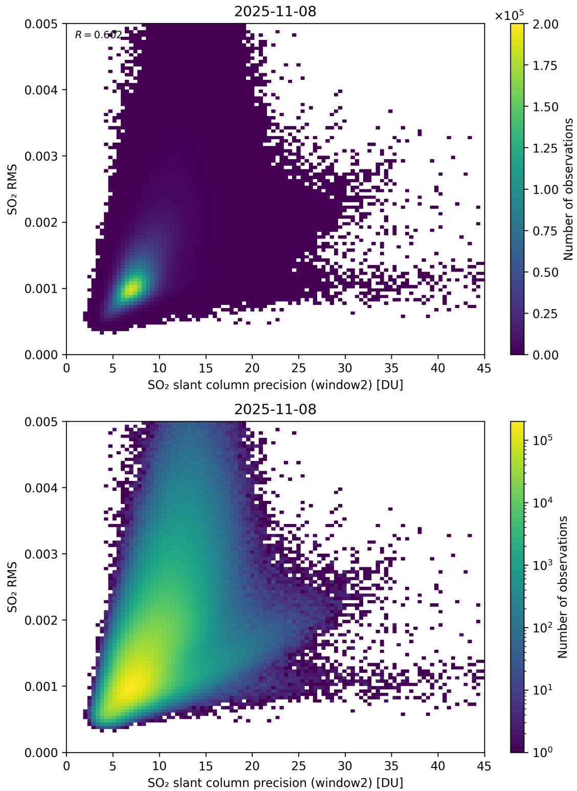
Figure 295: Scatter density plot of “SO 2 slant column precision (window2)” against “SO 2 RMS” for 2025-11-07 to 2025-11-09.
