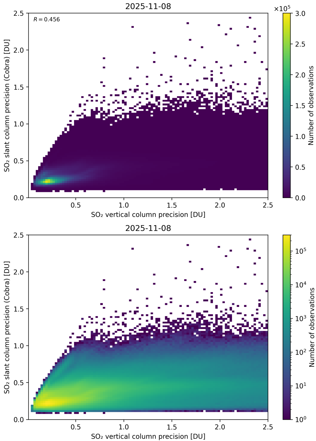
Figure 337: Scatter density plot of “SO 2 vertical column precision” against “SO 2 slant column precision (Cobra)” for 2025-11-07 to 2025-11-09.
