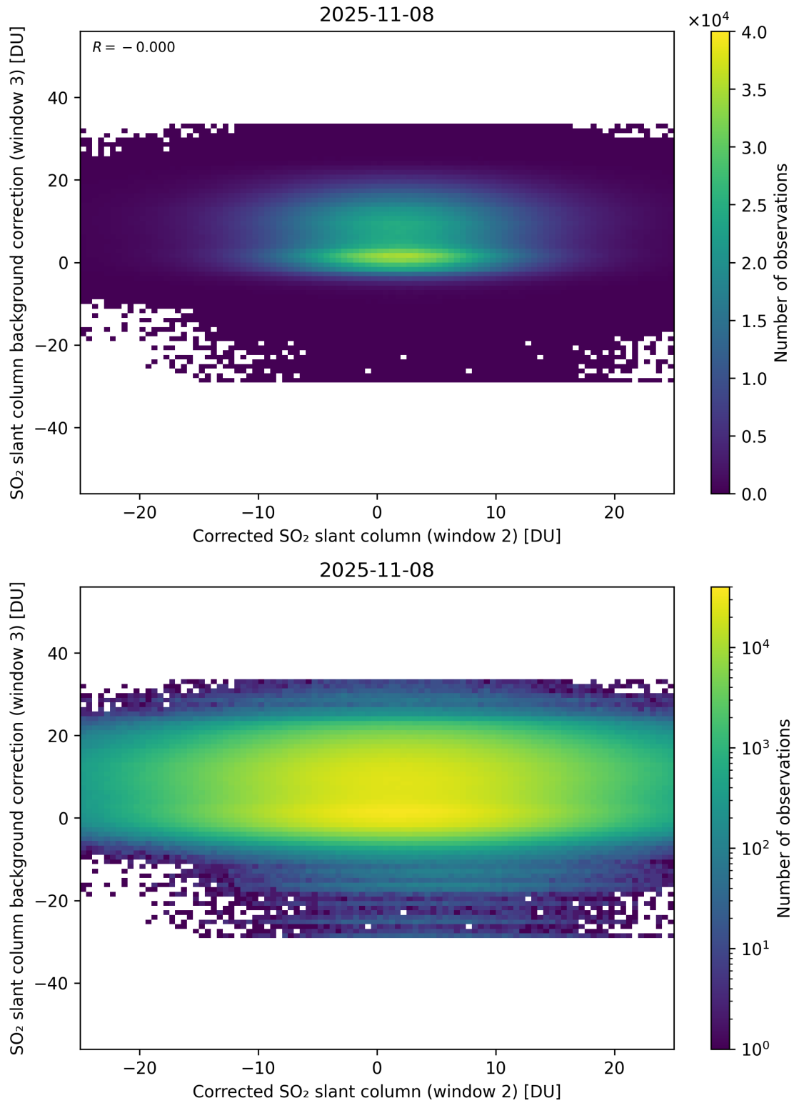
Figure 245: Scatter density plot of “Corrected SO 2 slant column (window 2)” against “SO 2 slant column background correction (window 3)” for 2025-11-07 to 2025-11-09.
