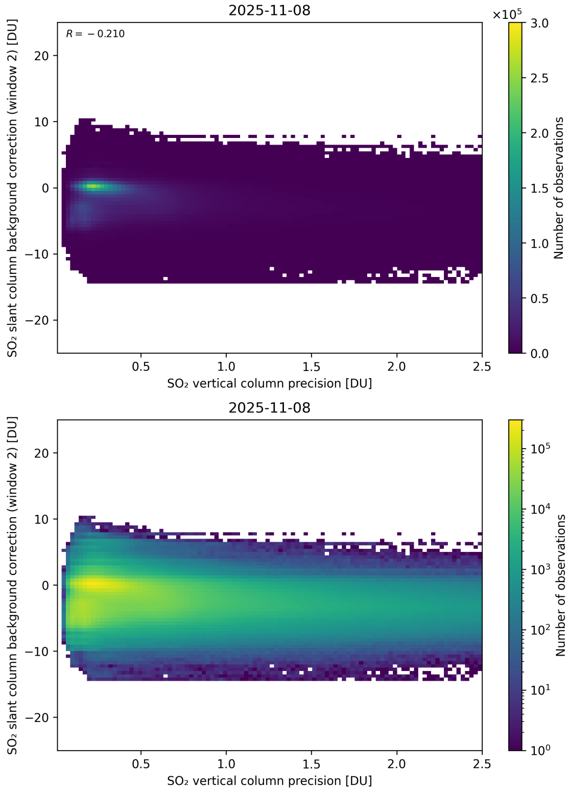
Figure 330: Scatter density plot of “SO 2 vertical column precision” against “SO 2 slant column background correction (window 2)” for 2025-11-07 to 2025-11-09.
