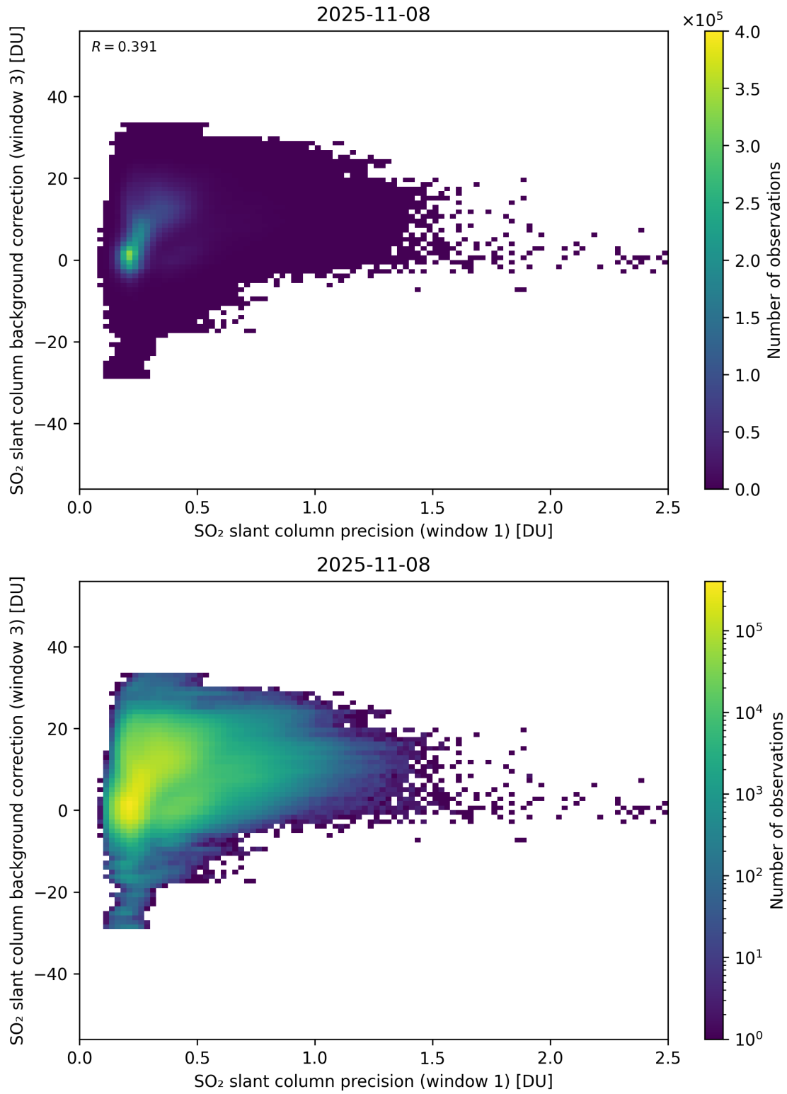
Figure 270: Scatter density plot of “SO 2 slant column precision (window 1)” against “SO 2 slant column background correction (window 3)” for 2025-11-07 to 2025-11-09.
