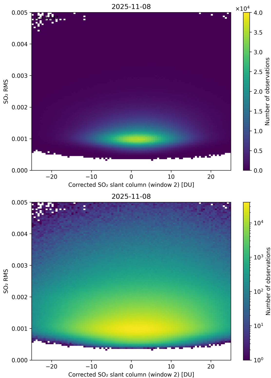
Figure 248: Scatter density plot of “Corrected SO 2 slant column (window 2)” against “SO 2 RMS” for 2025-11-07 to 2025-11-09.
