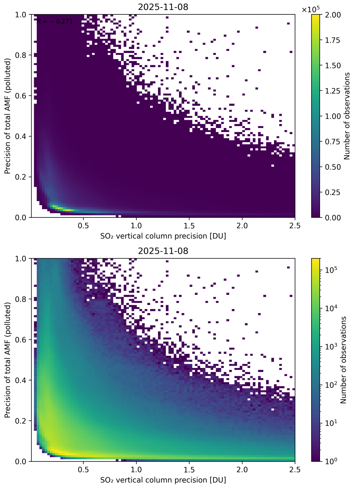
Figure 347: Scatter density plot of “SO 2 vertical column precision” against “Precision of total AMF (polluted)” for 2025-11-07 to 2025-11-09.
