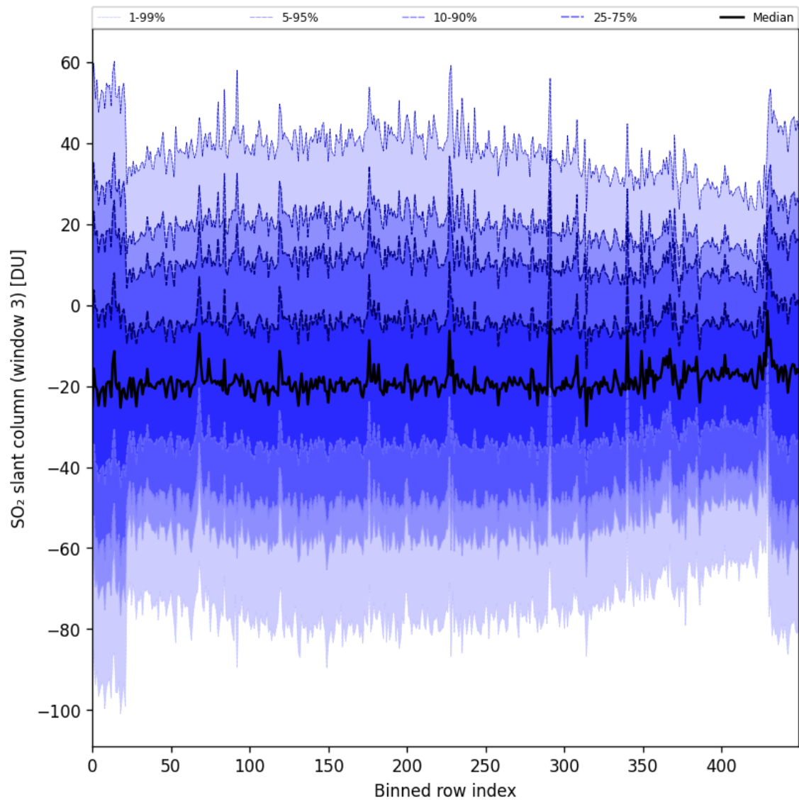
Figure 97: Along track statistics of “SO 2 slant column (window 3)” for 2025-11-07 to 2025-11-09
