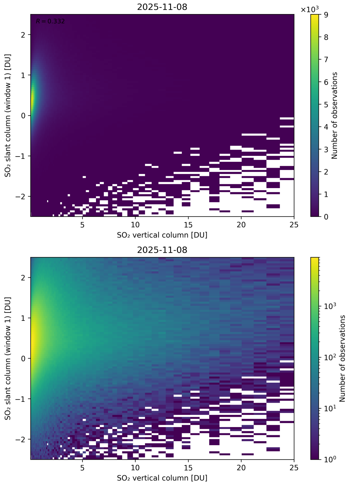
Figure 354: Scatter density plot of “SO 2 vertical column” against “SO 2 slant column (window 1)” for 2025-11-07 to 2025-11-09.
