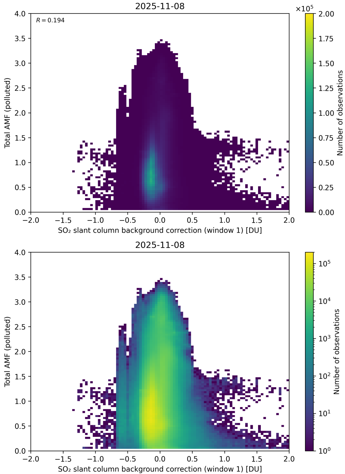
Figure 120: Scatter density plot of “SO 2 slant column background correction (window 1)” against “Total AMF (polluted)” for 2025-11-07 to 2025-11-09.
