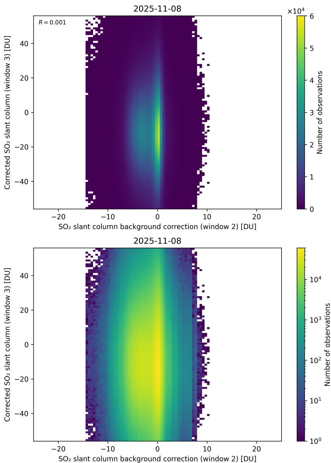
Figure 127: Scatter density plot of “SO 2 slant column background correction (window 2)” against “Corrected SO 2 slant column (window 3)” for 2025-11-07 to 2025-11-09.
