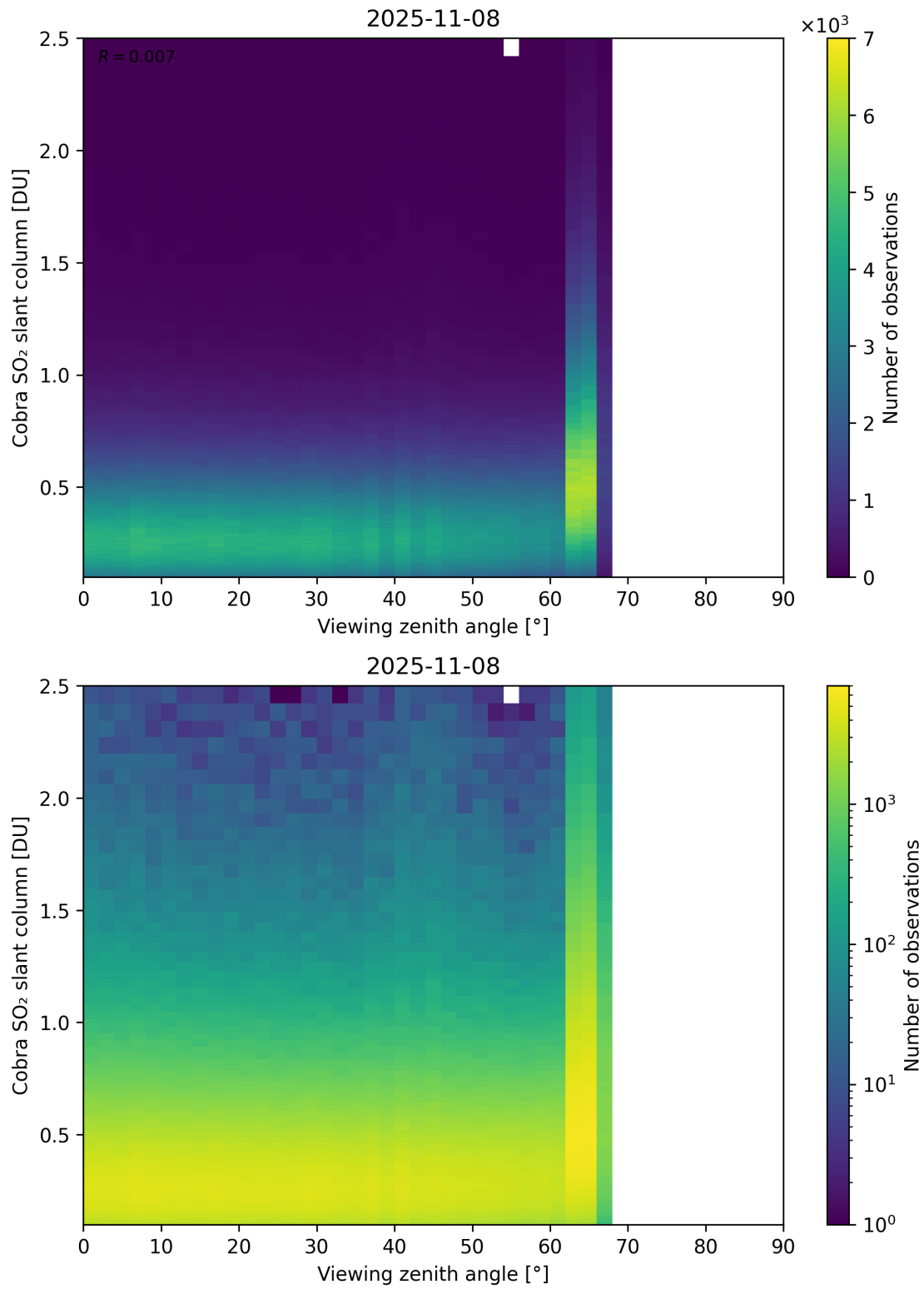
Figure 371: Scatter density plot of “Viewing zenith angle” against “Cobra SO 2 slant column” for 2025-11-07 to 2025-11-09.
