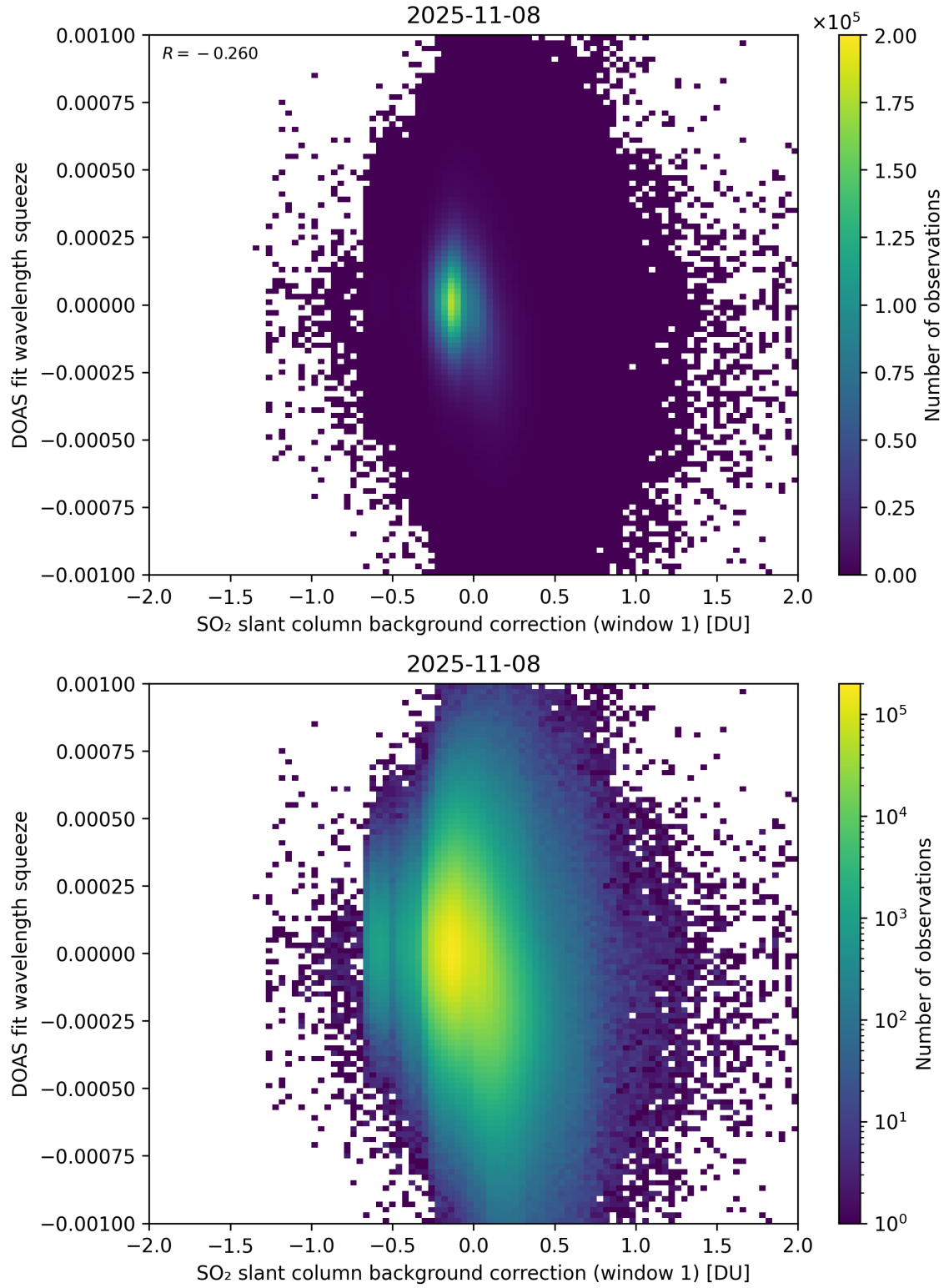
Figure 112: Scatter density plot of “SO 2 slant column background correction (window 1)” against “DOAS fit wavelength squeeze” for 2025-11-07 to 2025-11-09.
