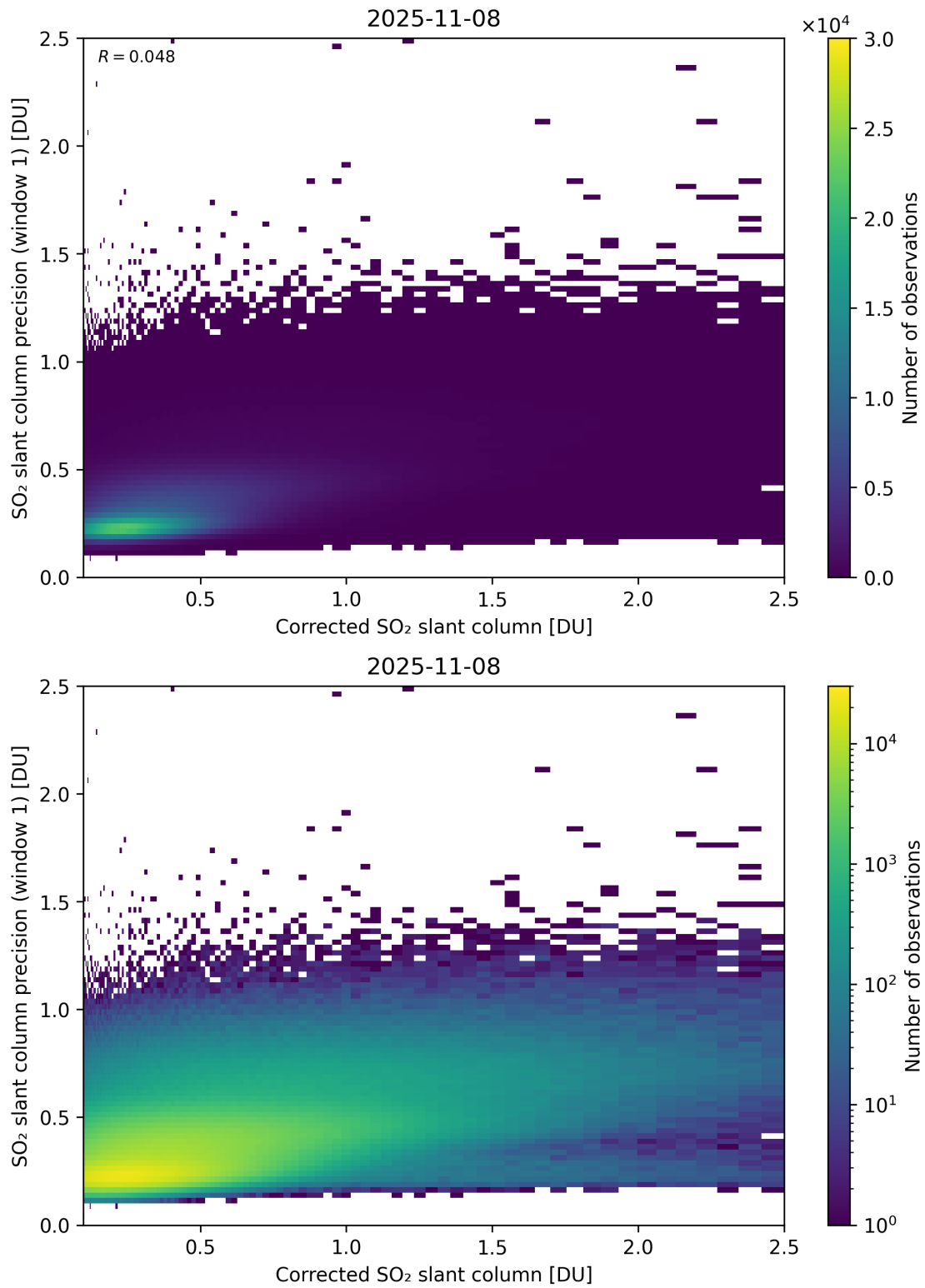
Figure 238: Scatter density plot of “Corrected SO 2 slant column” against “SO 2 slant column precision (window 1)” for 2025-11-07 to 2025-11-09.
