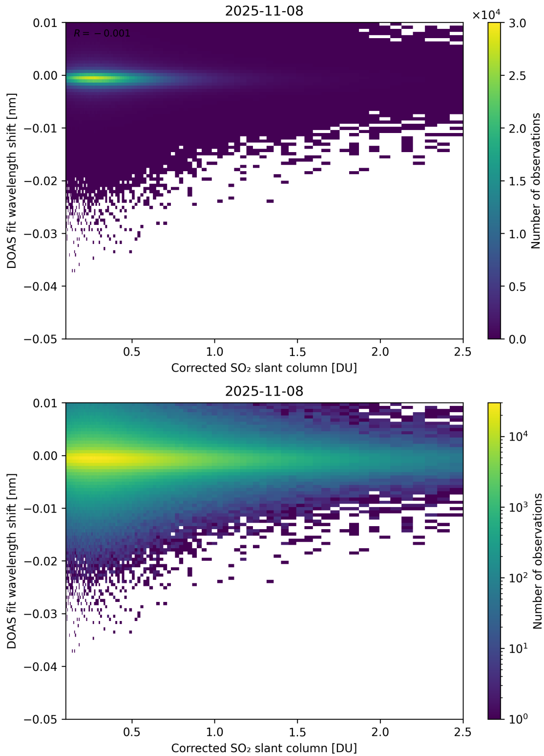
Figure 229: Scatter density plot of “Corrected SO 2 slant column” against “DOAS fit wavelength shift” for 2025-11-07 to 2025-11-09.
