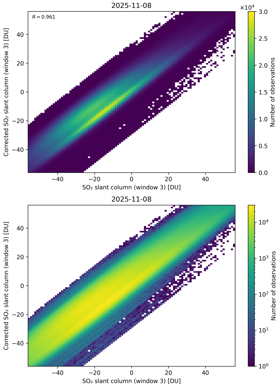
Figure 316: Scatter density plot of “SO 2 slant column (window 3)” against “Corrected SO 2 slant column (window 3)” for 2025-11-07 to 2025-11-09.
