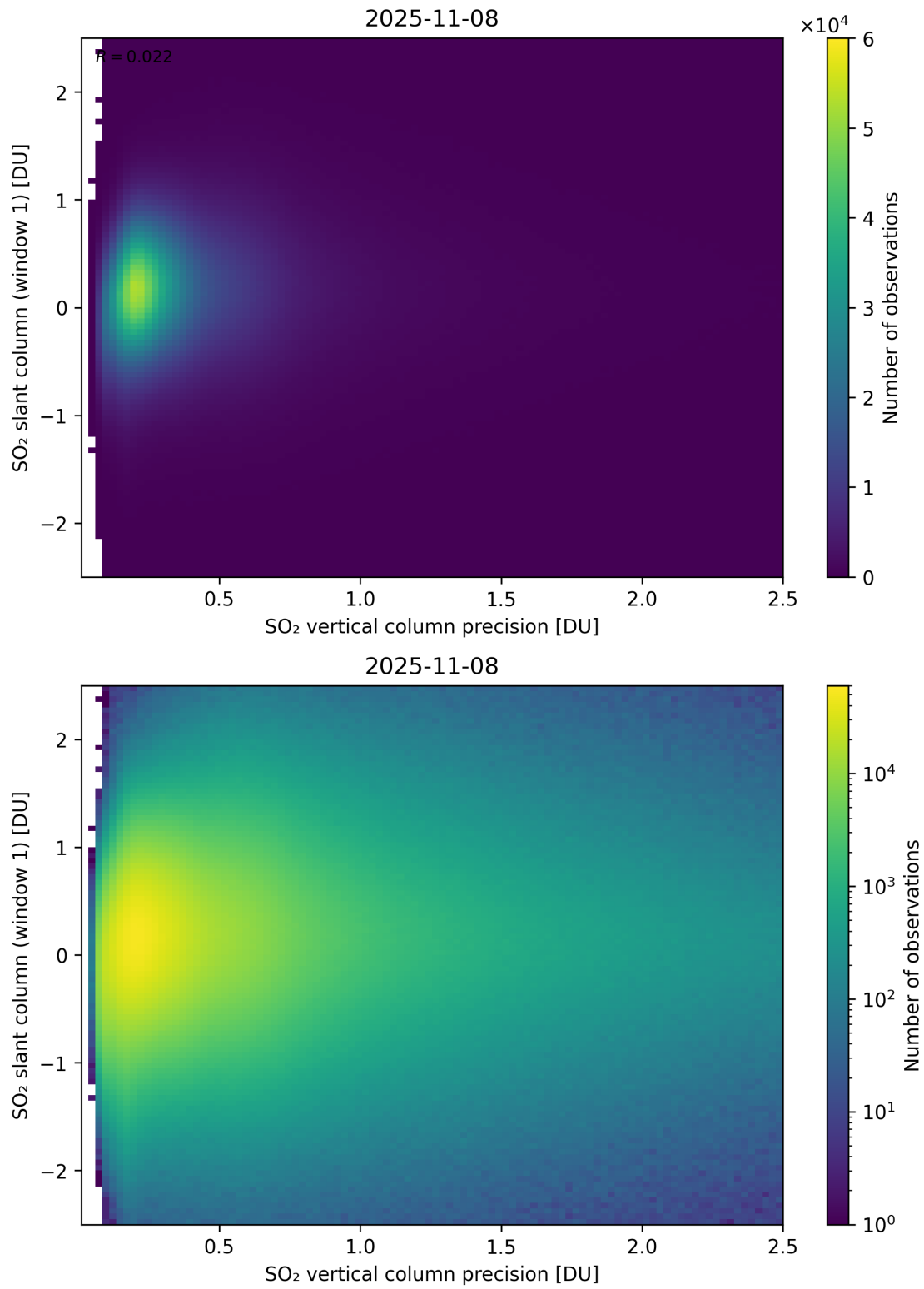
Figure 341: Scatter density plot of “SO 2 vertical column precision” against “SO 2 slant column (window 1)” for 2025-11-07 to 2025-11-09.
