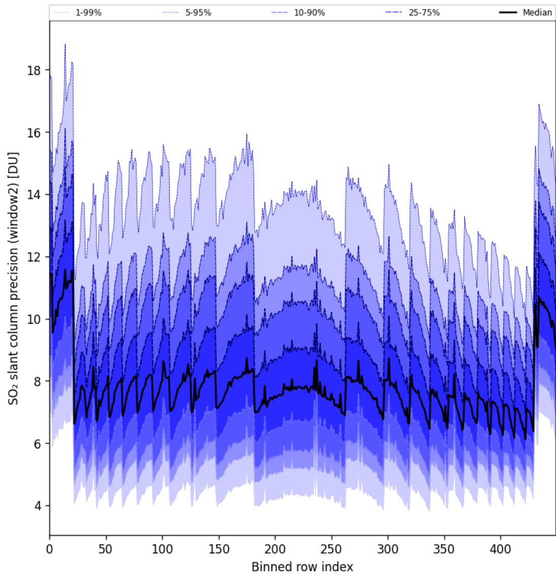
Figure 94: Along track statistics of “SO 2 slant column precision (window2)” for 2025-11-07 to 2025-11-09
