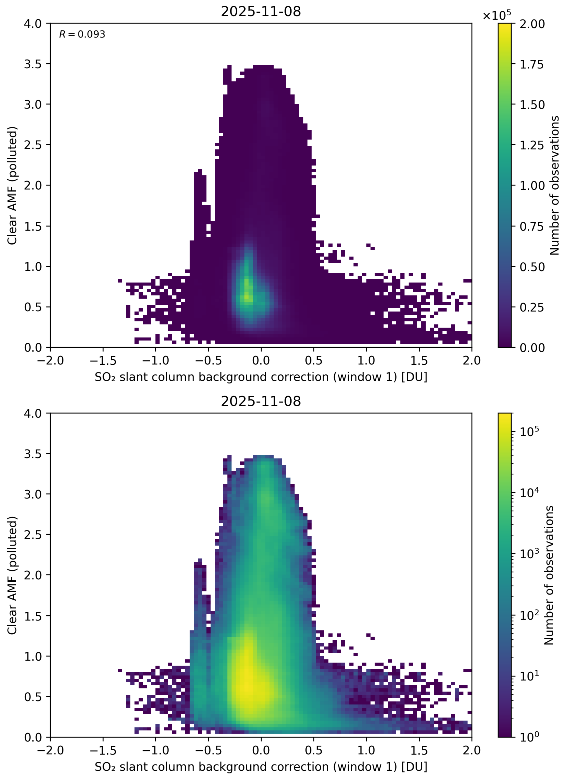
Figure 114: Scatter density plot of “SO 2 slant column background correction (window 1)” against “Clear AMF (polluted)” for 2025-11-07 to 2025-11-09.
