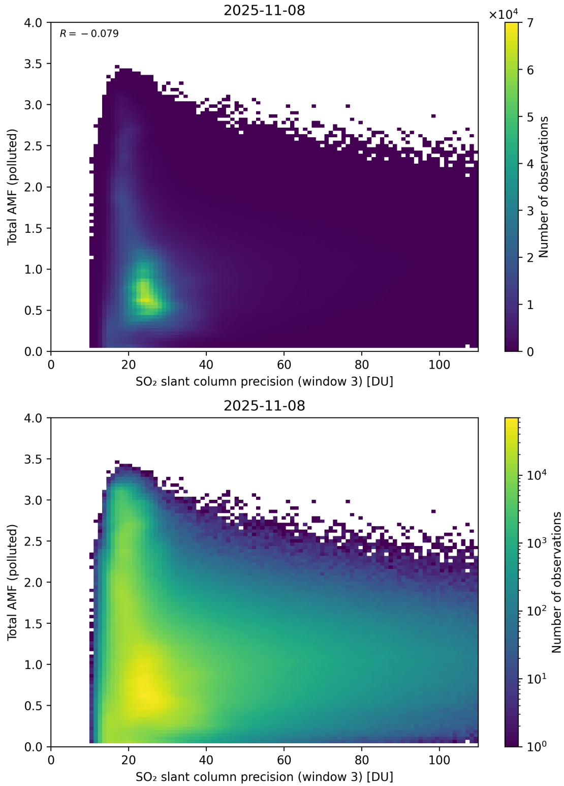
Figure 313: Scatter density plot of “SO 2 slant column precision (window 3)” against “Total AMF (polluted)” for 2025-11-07 to 2025-11-09.
