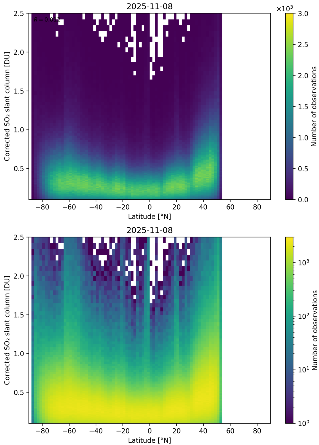
Figure 159: Scatter density plot of “Latitude” against “Corrected SO 2 slant column” for 2025-11-07 to 2025-11-09.
