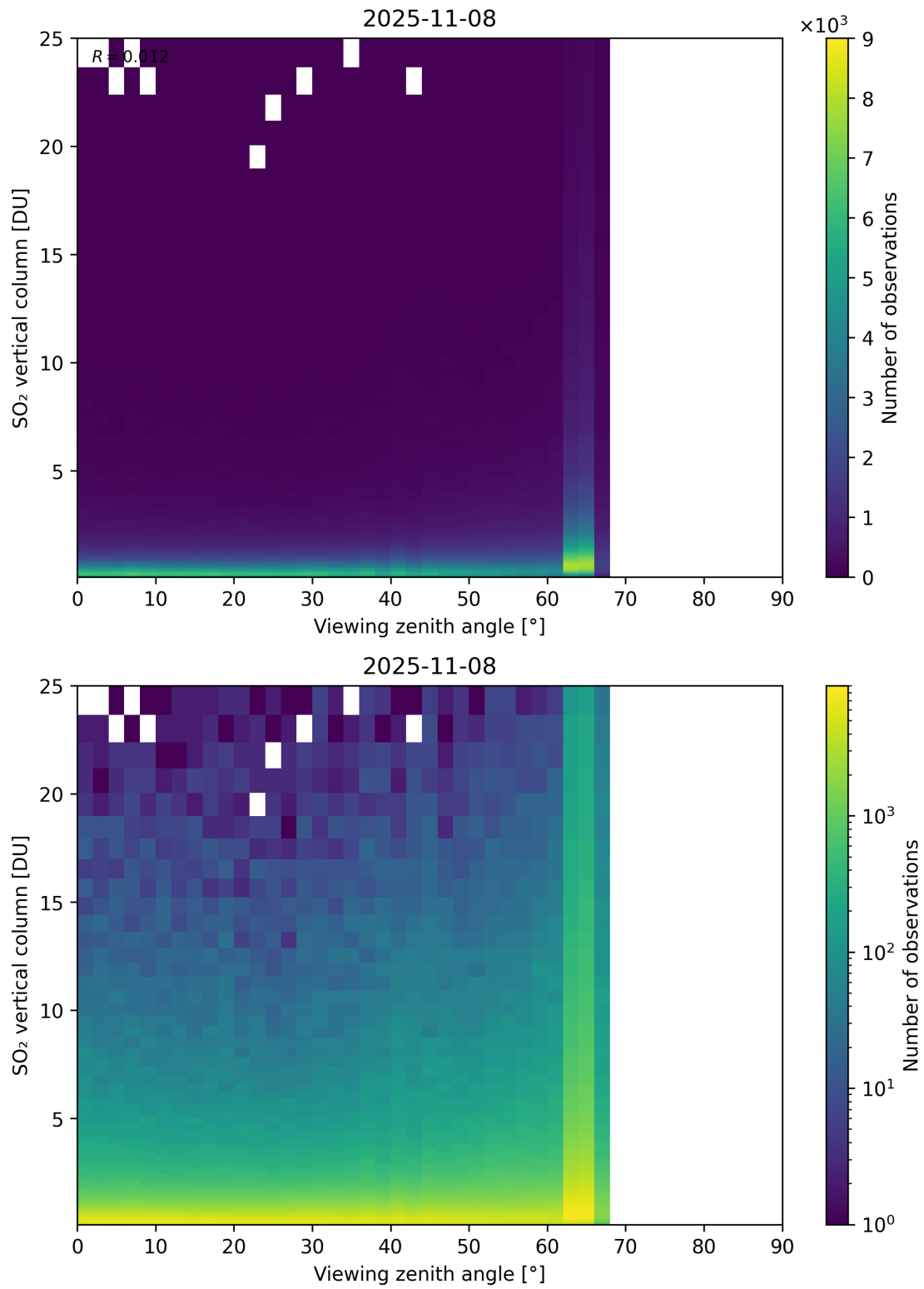
Figure 383: Scatter density plot of “Viewing zenith angle” against “SO 2 vertical column” for 2025-11-07 to 2025-11-09.
