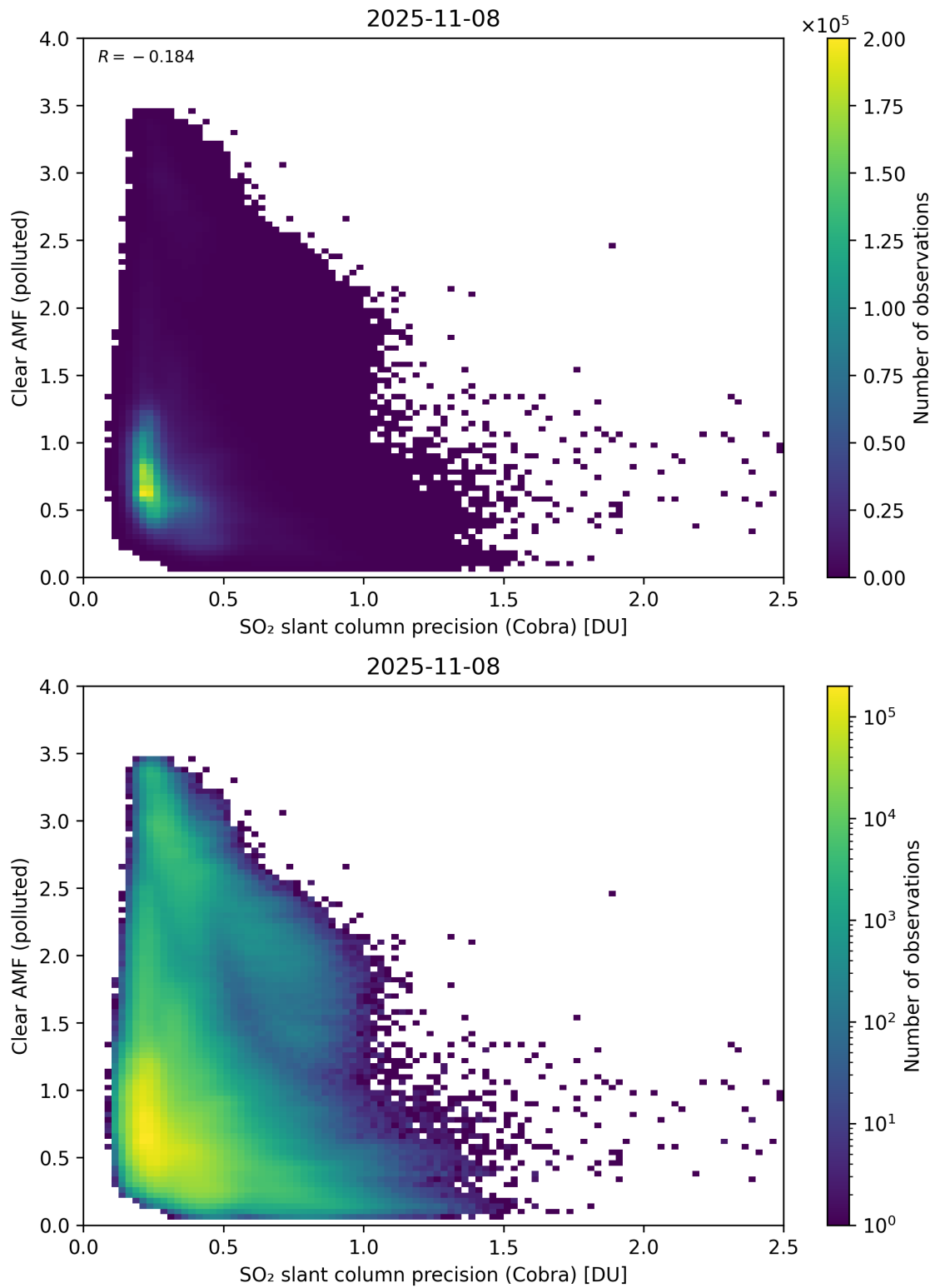
Figure 205: Scatter density plot of “SO 2 slant column precision (Cobra)” against “Clear AMF (polluted)” for 2025-11-07 to 2025-11-09.
