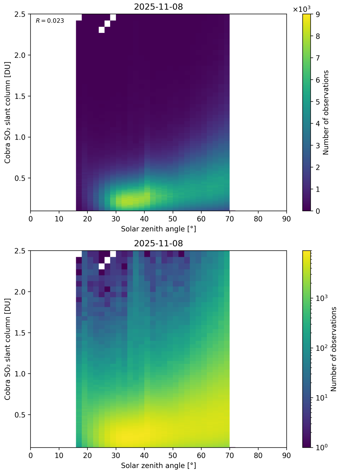
Figure 179: Scatter density plot of “Solar zenith angle” against “Cobra SO 2 slant column” for 2025-11-07 to 2025-11-09.
