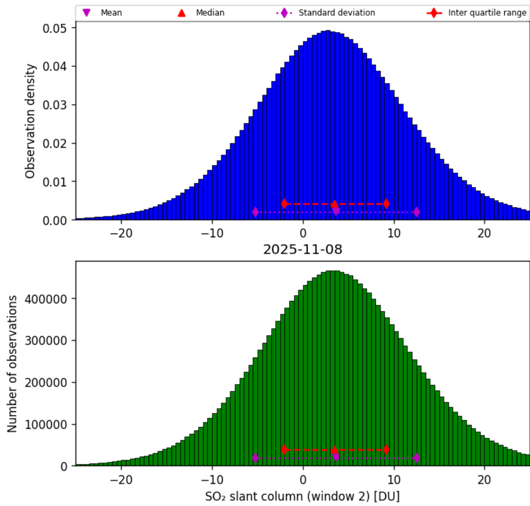
Figure 67: Histogram of “SO 2 slant column (window 2)” for 2025-11-07 to 2025-11-09
