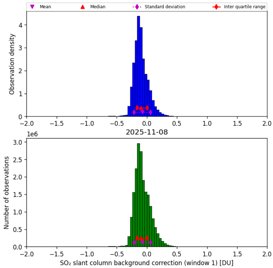
Figure 66: Histogram of “SO 2 slant column background correction (window 1)” for 2025-11-07 to 2025-11-09
