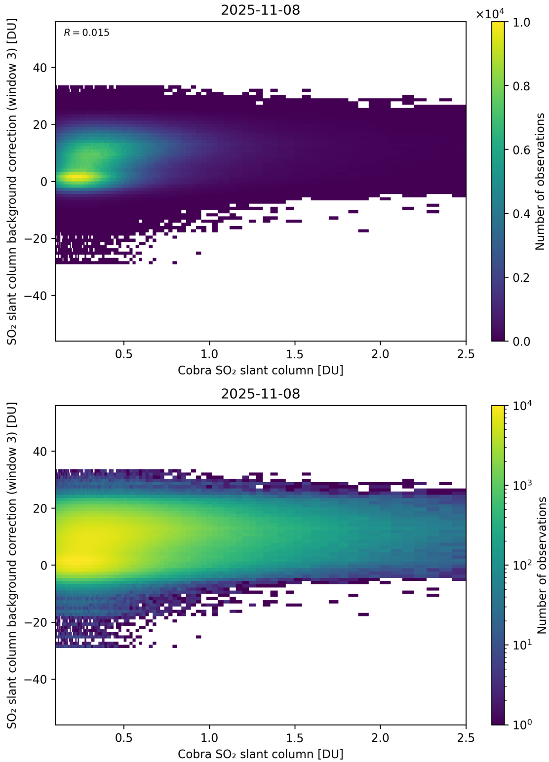
Figure 195: Scatter density plot of “Cobra SO 2 slant column” against “SO 2 slant column background correction (window 3)” for 2025-11-07 to 2025-11-09.
