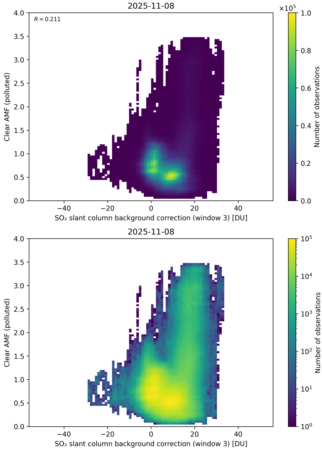
Figure 135: Scatter density plot of “SO 2 slant column background correction (window 3)” against “Clear AMF (polluted)” for 2025-11-07 to 2025-11-09.
