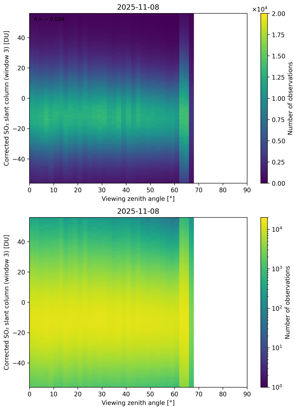
Figure 375: Scatter density plot of “Viewing zenith angle” against “Corrected SO 2 slant column (window 3)” for 2025-11-07 to 2025-11-09.
