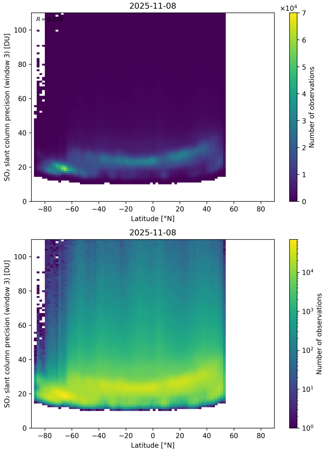
Figure 166: Scatter density plot of “Latitude” against “SO 2 slant column precision (window 3)” for 2025-11-07 to 2025-11-09.
