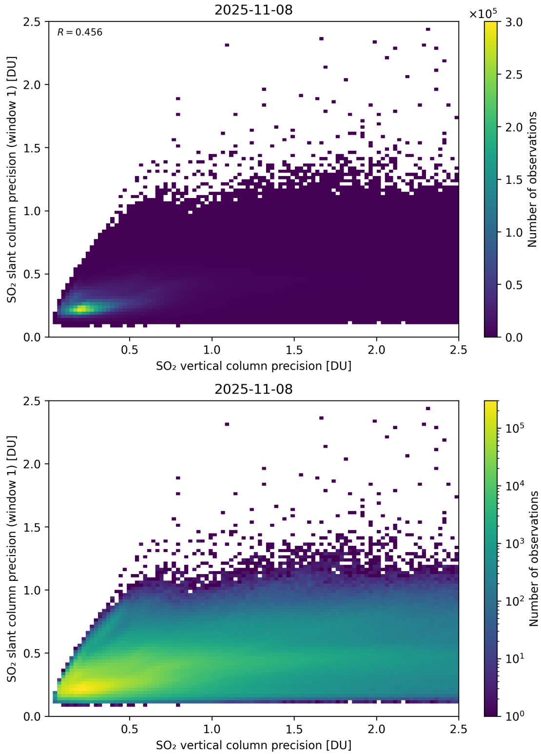
Figure 342: Scatter density plot of “SO 2 vertical column precision” against “SO 2 slant column precision (window 1)” for 2025-11-07 to 2025-11-09.
