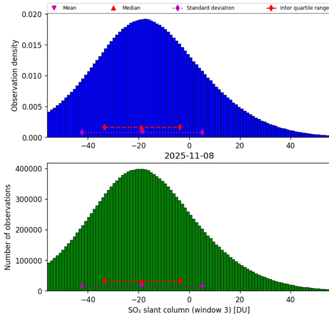
Figure 71: Histogram of “SO 2 slant column (window 3)” for 2025-11-07 to 2025-11-09
