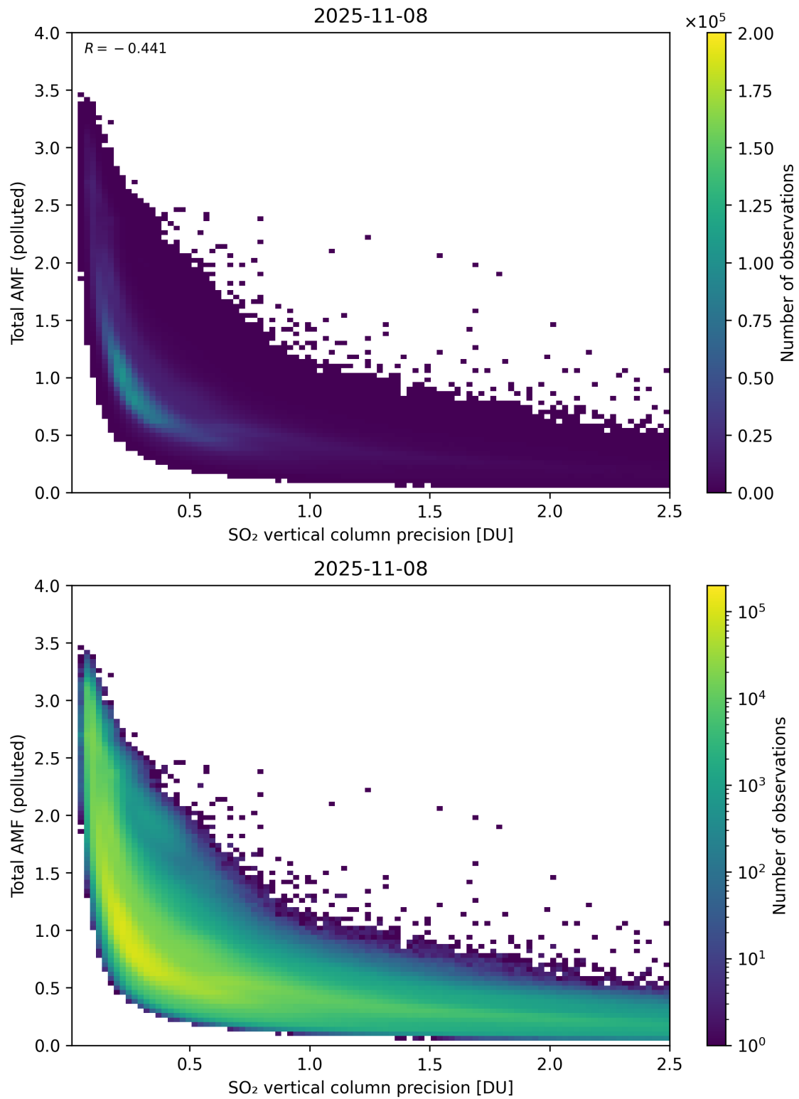
Figure 346: Scatter density plot of “SO 2 vertical column precision” against “Total AMF (polluted)” for 2025-11-07 to 2025-11-09.
