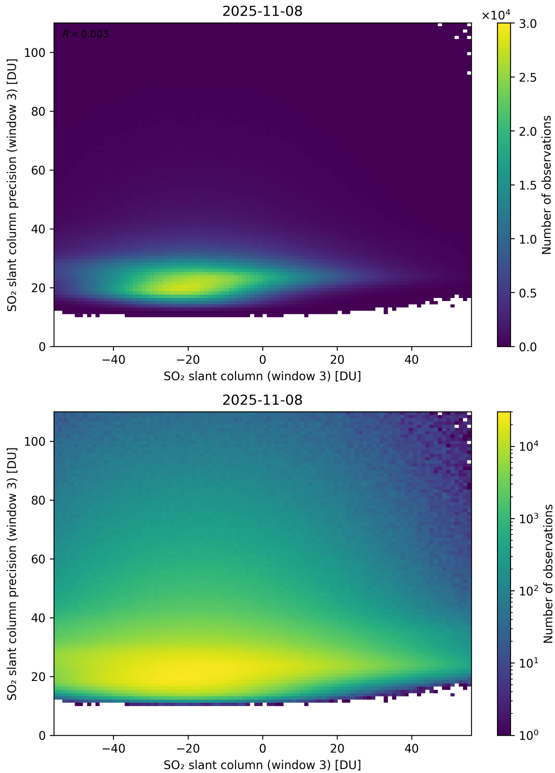
Figure 317: Scatter density plot of “SO 2 slant column (window 3)” against “SO 2 slant column precision (window 3)” for 2025-11-07 to 2025-11-09.
