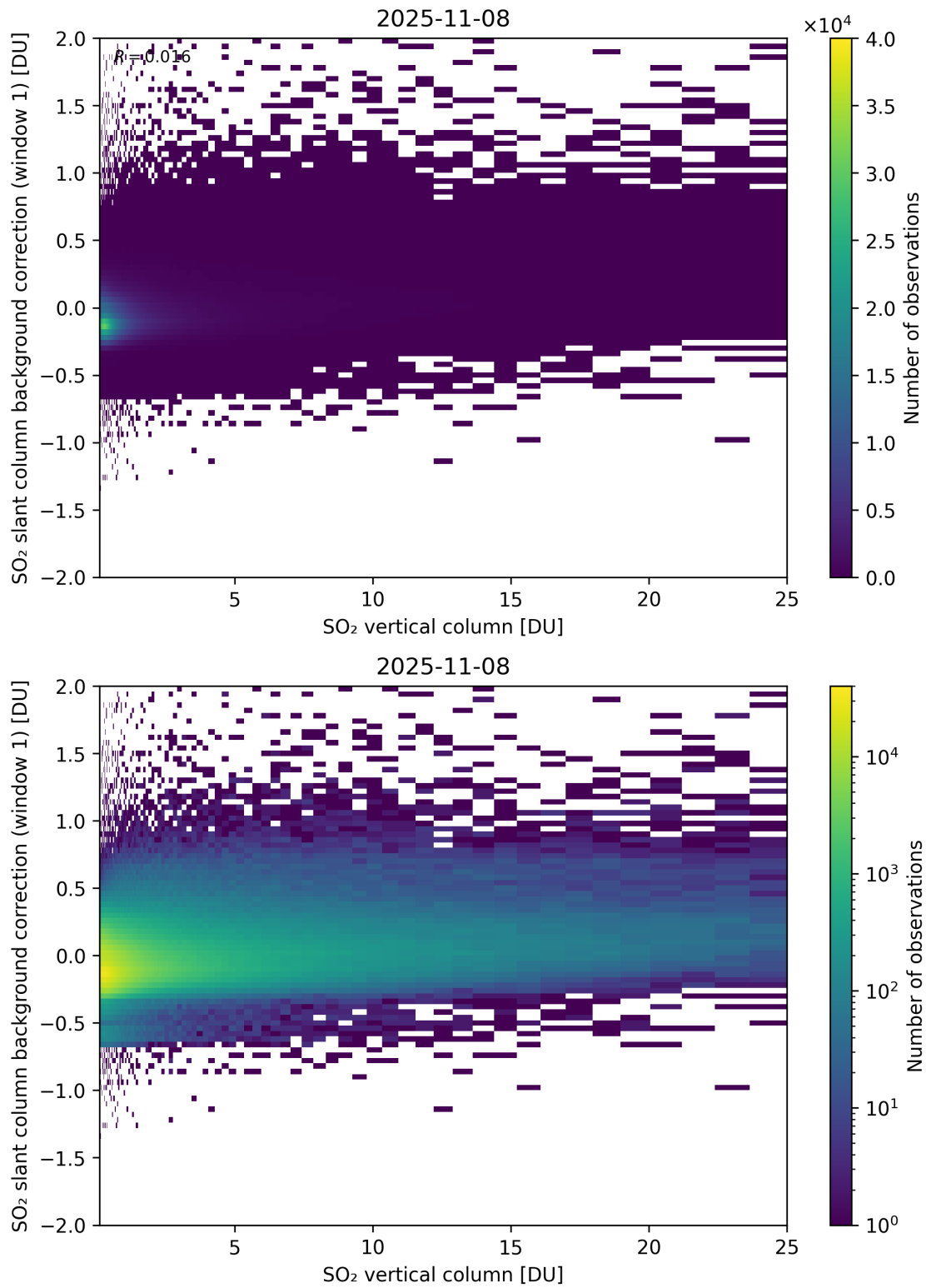
Figure 323: Scatter density plot of “SO 2 vertical column” against “SO 2 slant column background correction (window 1)” for 2025-11-07 to 2025-11-09.
