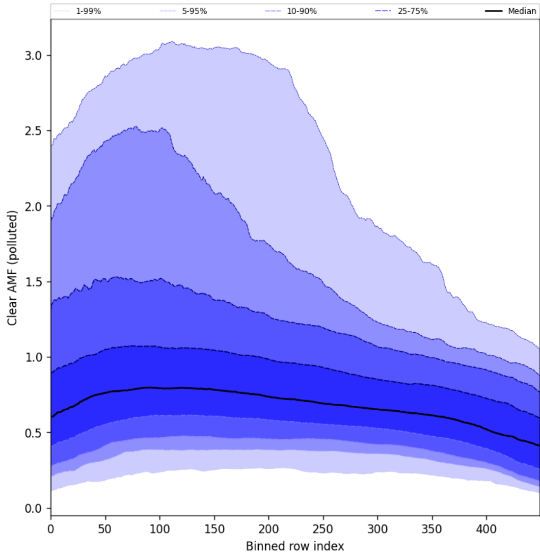
Figure 107: Along track statistics of “Clear AMF (polluted)” for 2025-11-07 to 2025-11-09
