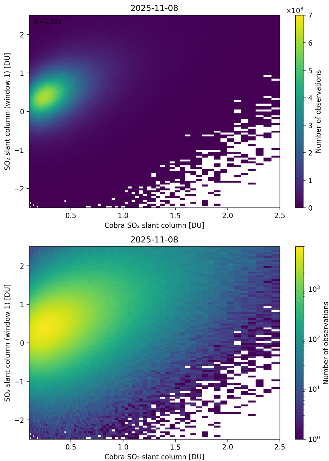
Figure 219: Scatter density plot of “Cobra SO 2 slant column” against “SO 2 slant column (window 1)” for 2025-11-07 to 2025-11-09.
