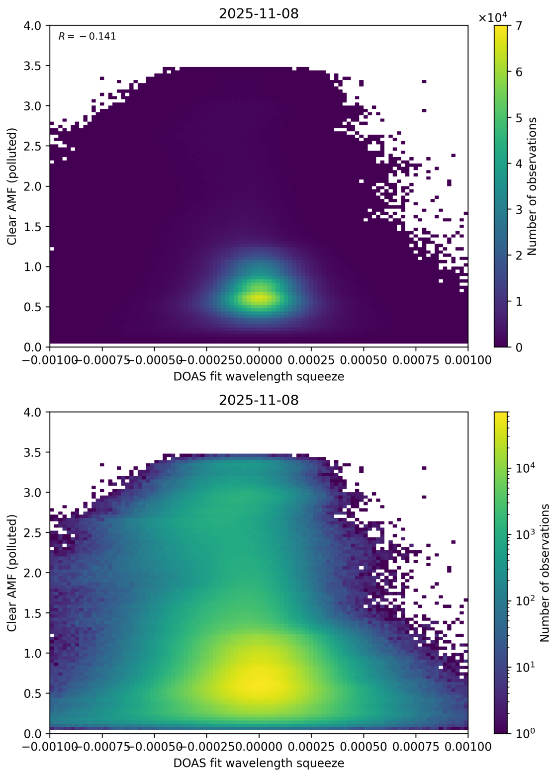
Figure 144: Scatter density plot of “DOAS fit wavelength squeeze” against “Clear AMF (polluted)” for 2025-11-07 to 2025-11-09.
