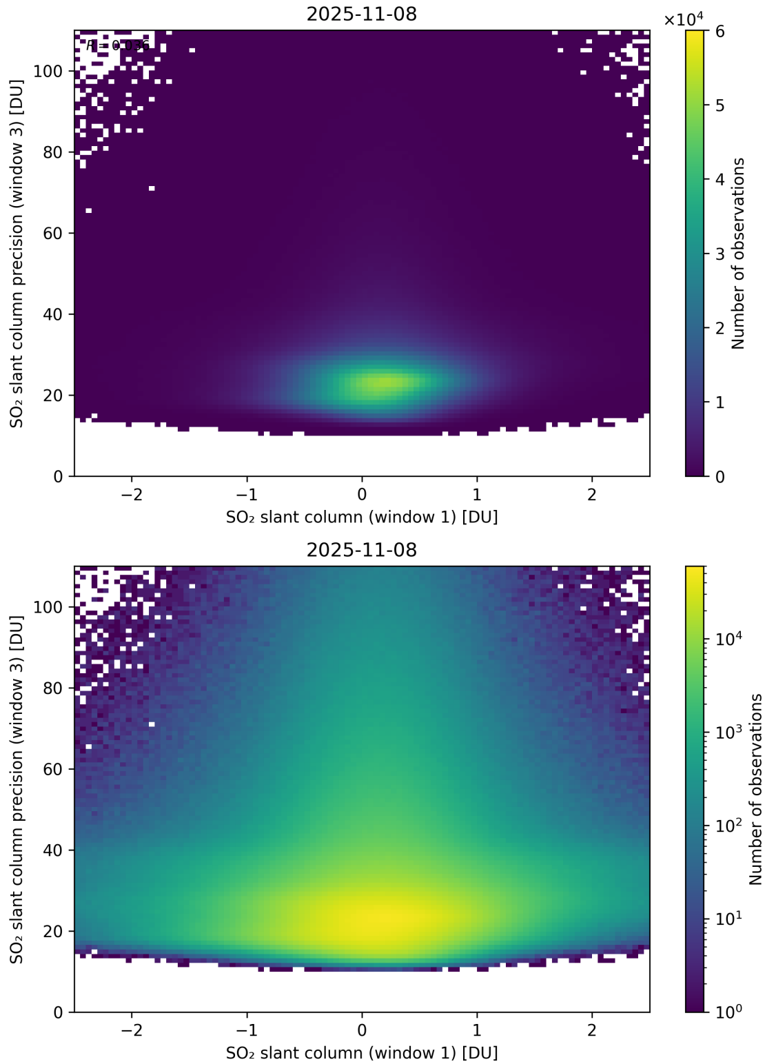
Figure 288: Scatter density plot of “SO 2 slant column (window 1)” against “SO 2 slant column precision (window 3)” for 2025-11-07 to 2025-11-09.
