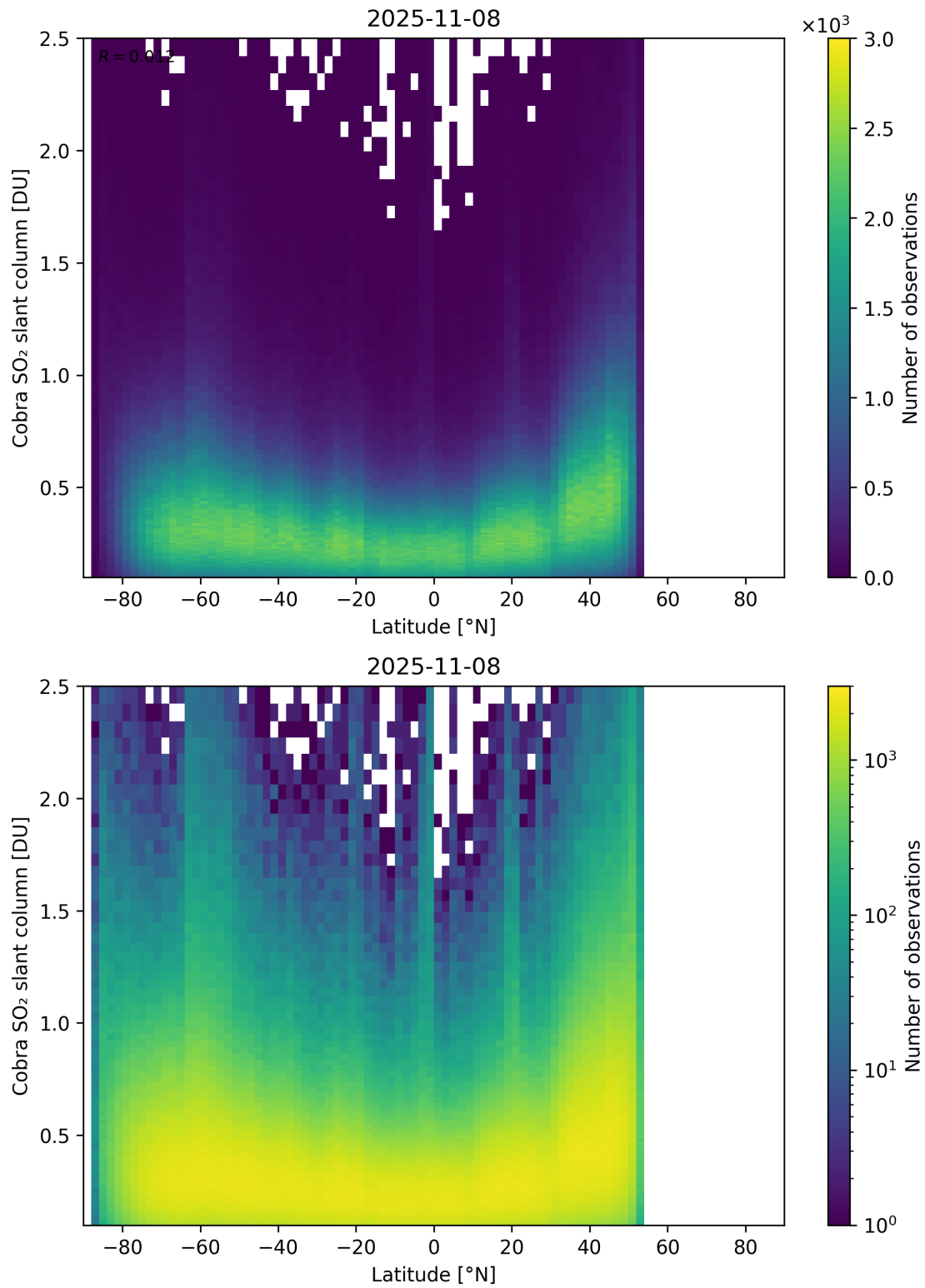
Figure 157: Scatter density plot of “Latitude” against “Cobra SO 2 slant column” for 2025-11-07 to 2025-11-09.
