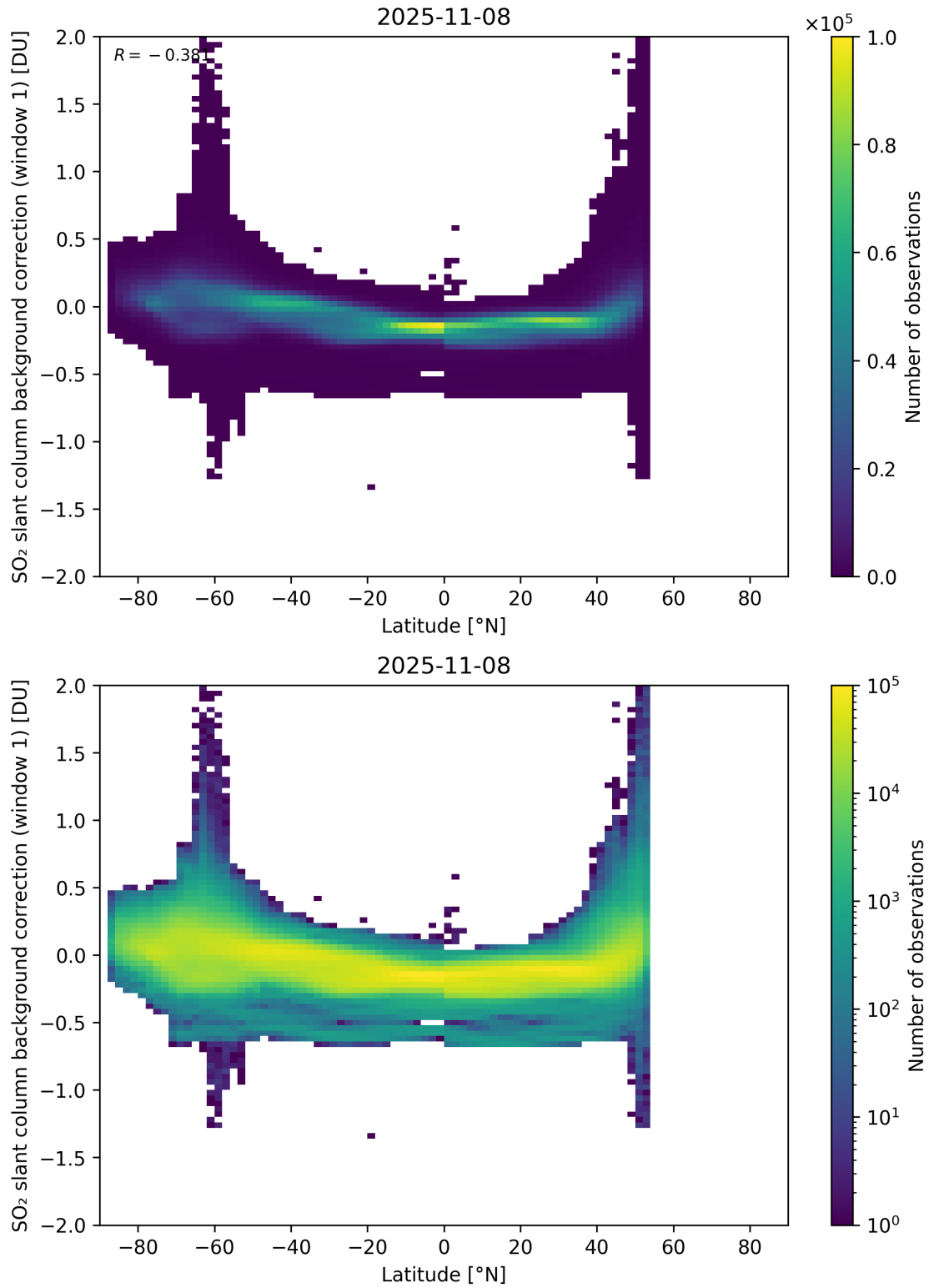
Figure 150: Scatter density plot of “Latitude” against “SO 2 slant column background correction (window 1)” for 2025-11-07 to 2025-11-09.
