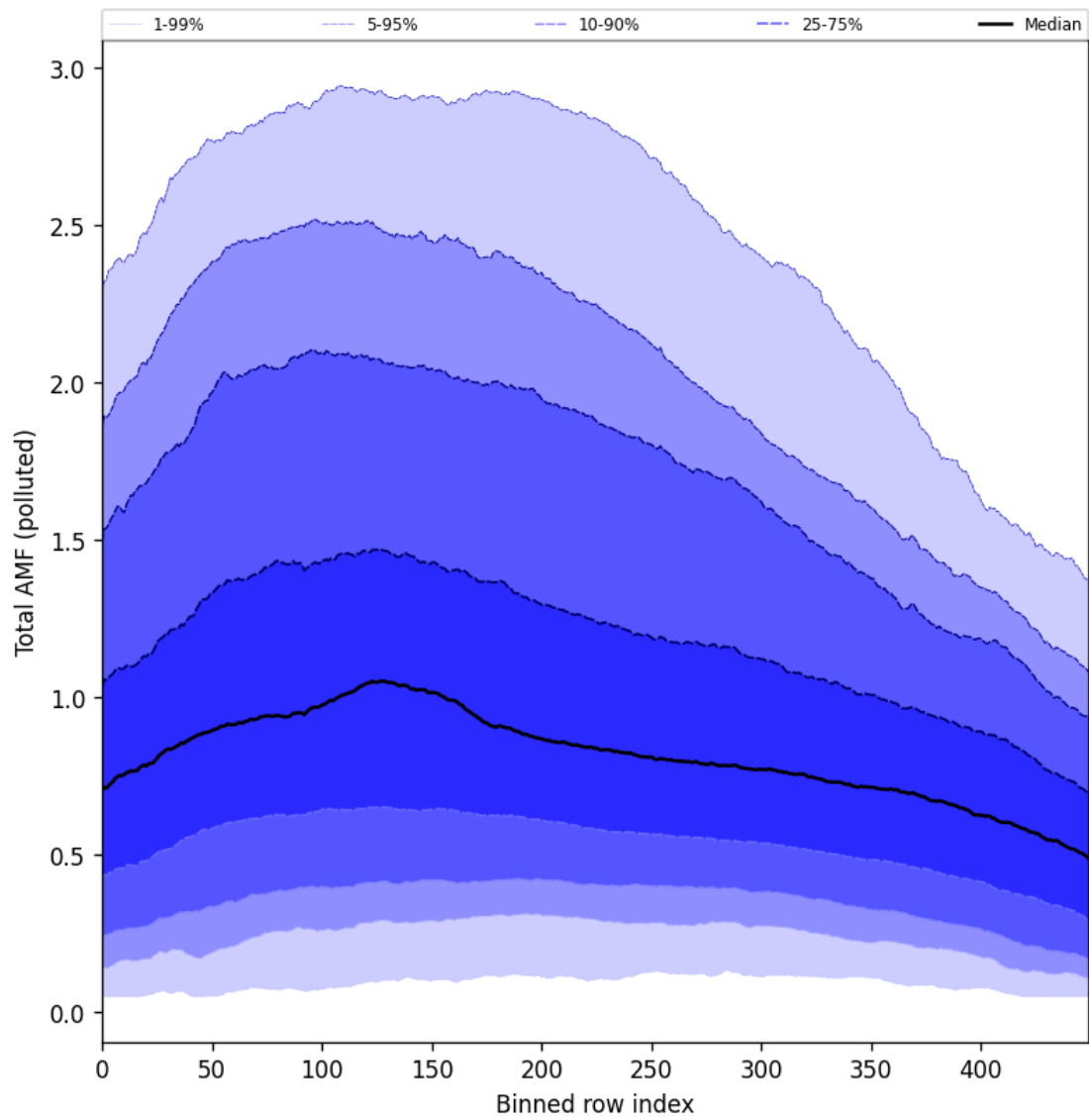
Figure 105: Along track statistics of “Total AMF (polluted)” for 2025-11-07 to 2025-11-09
