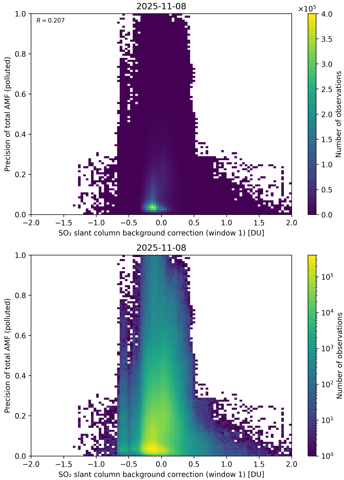
Figure 121: Scatter density plot of “SO 2 slant column background correction (window 1)” against “Precision of total AMF (polluted)” for 2025-11-07 to 2025-11-09.
