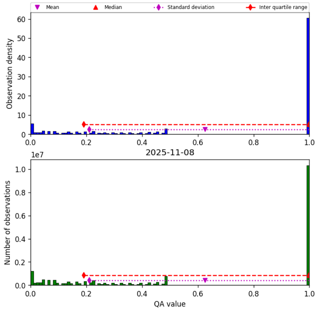
Figure 57: Histogram of “QA value” for 2025-11-07 to 2025-11-09
