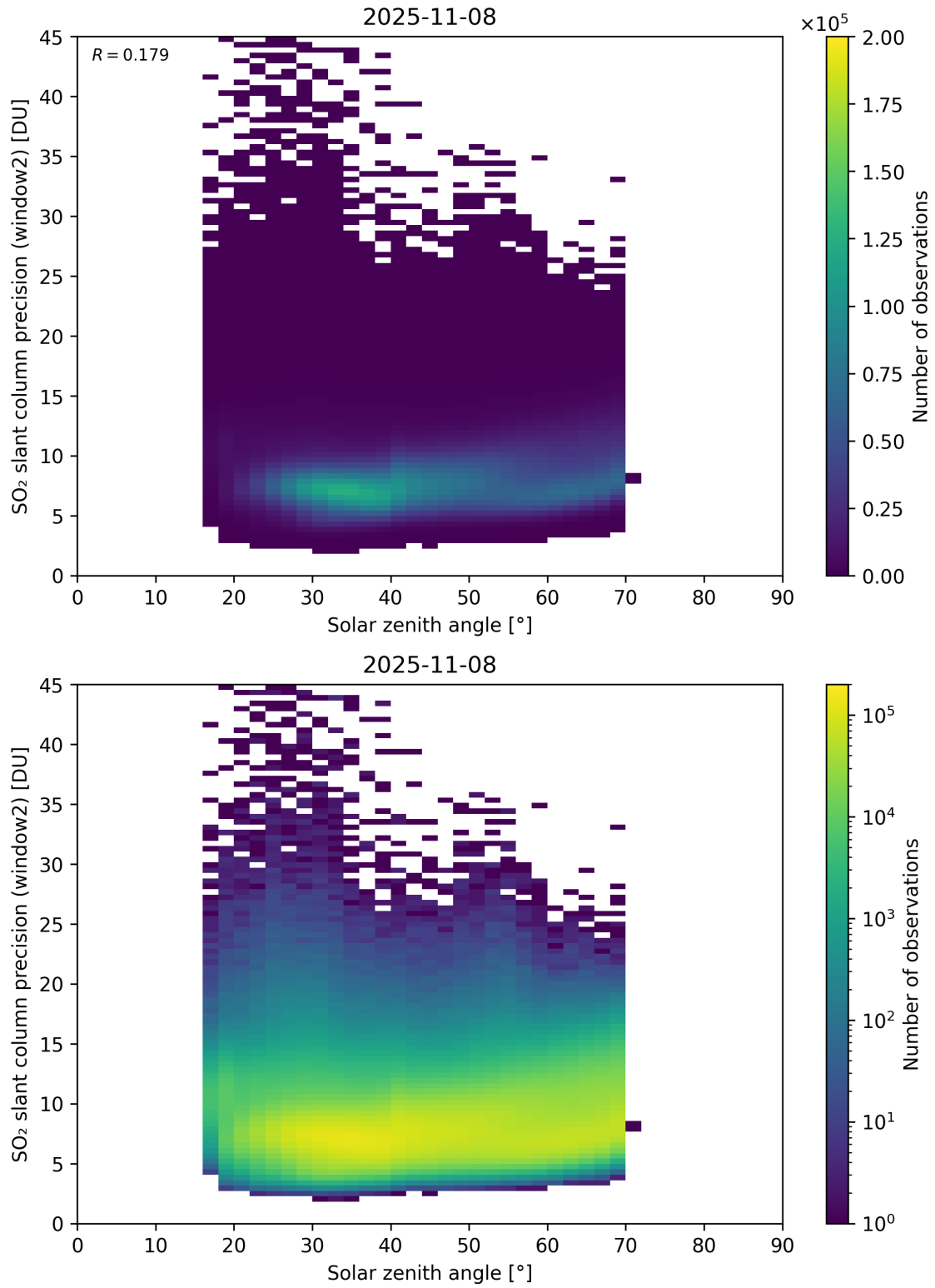
Figure 186: Scatter density plot of “Solar zenith angle” against “SO 2 slant column precision (window2)” for 2025-11-07 to 2025-11-09.
