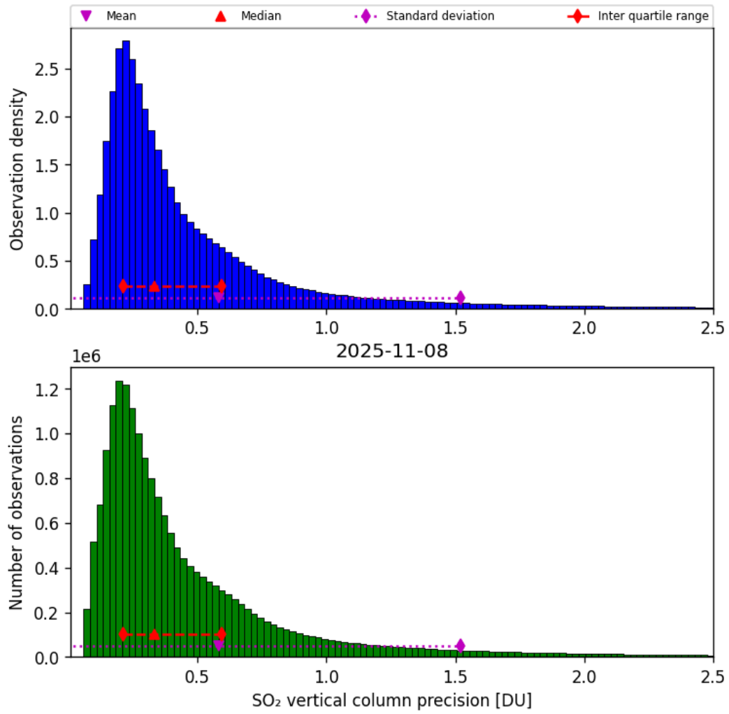
Figure 59: Histogram of “SO 2 vertical column precision” for 2025-11-07 to 2025-11-09
