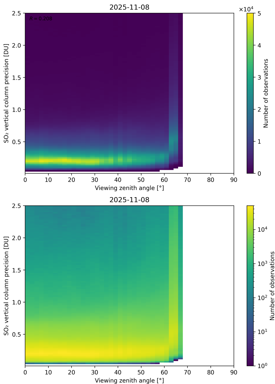
Figure 384: Scatter density plot of “Viewing zenith angle” against “SO 2 vertical column precision” for 2025-11-07 to 2025-11-09.
