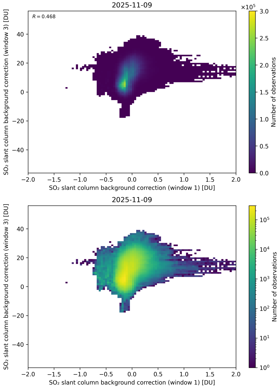
Figure 110: Scatter density plot of “SO 2 slant column background correction (window 1)” against “SO 2 slant column background correction (window 3)” for 2025-11-08 to 2025-11-10.
