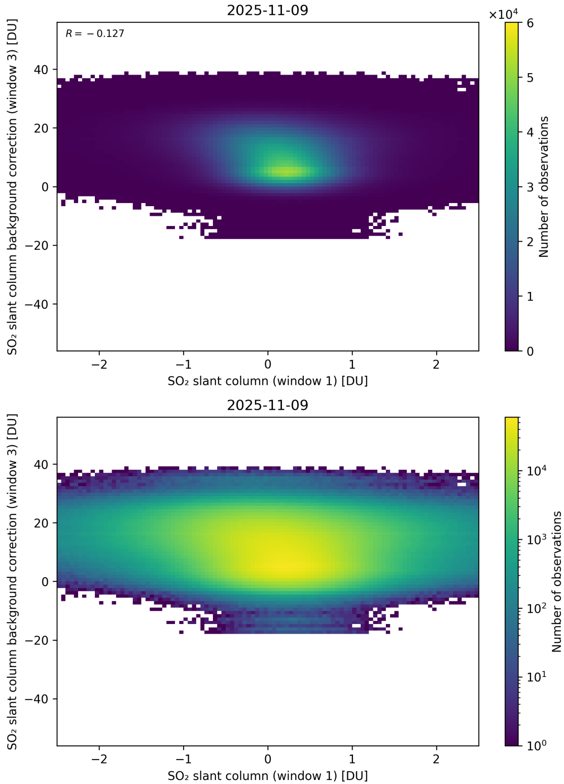
Figure 264: Scatter density plot of “SO 2 slant column (window 1)” against “SO 2 slant column background correction (window 3)” for 2025-11-08 to 2025-11-10.
