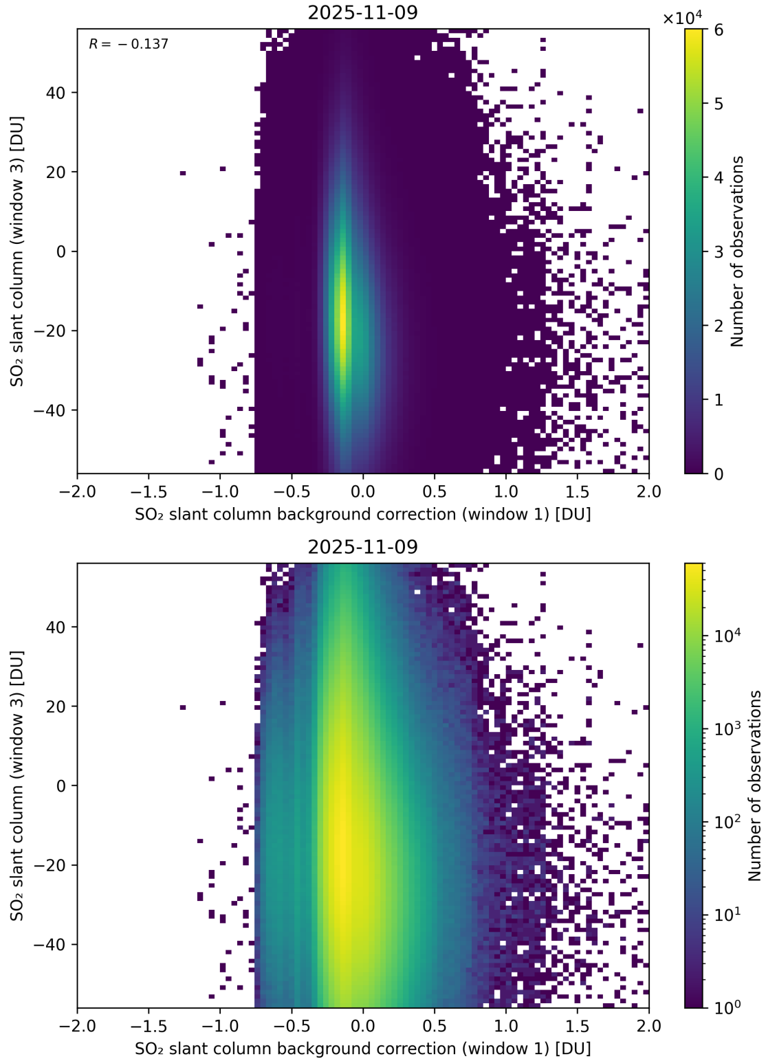
Figure 118: Scatter density plot of “SO 2 slant column background correction (window 1)” against “SO 2 slant column (window 3)” for 2025-11-08 to 2025-11-10.
