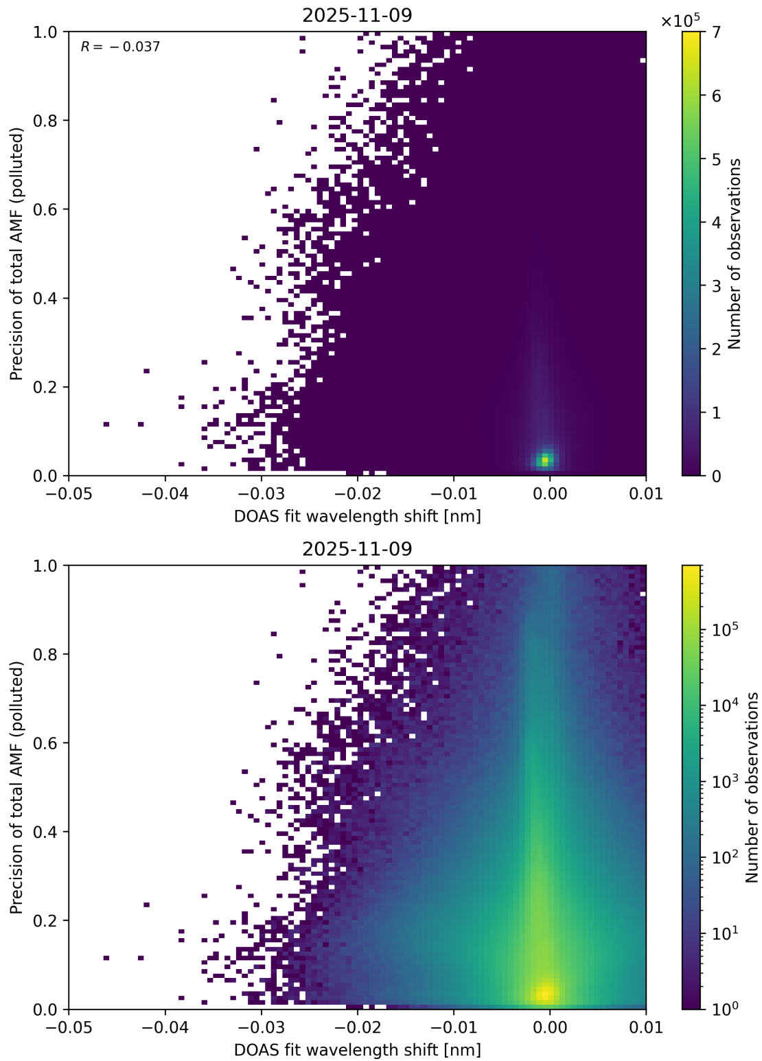
Figure 142: Scatter density plot of “DOAS fit wavelength shift” against “Precision of total AMF (polluted)” for 2025-11-08 to 2025-11-10.
