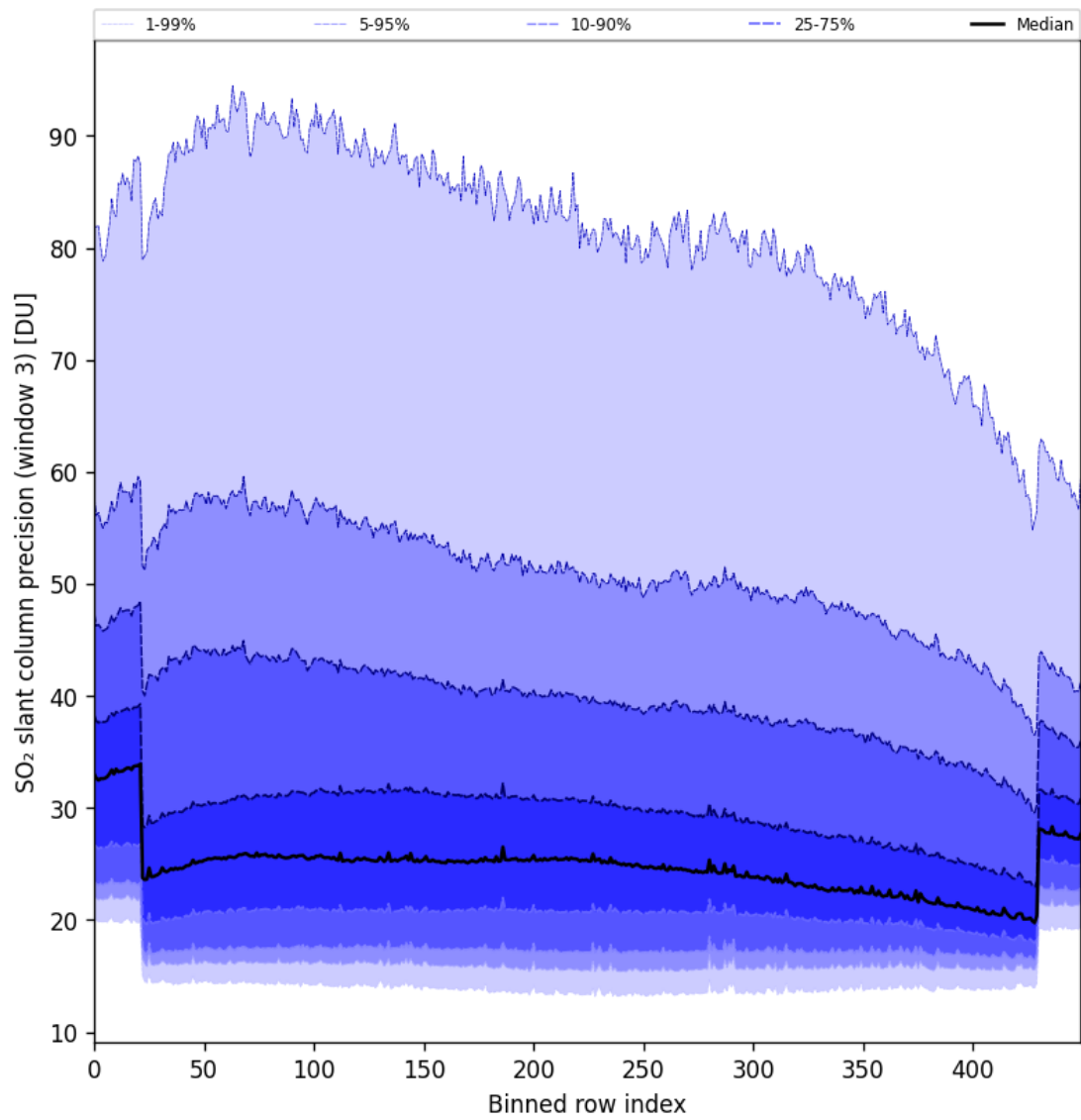
Figure 98: Along track statistics of “SO 2 slant column precision (window 3)” for 2025-11-08 to 2025-11-10
