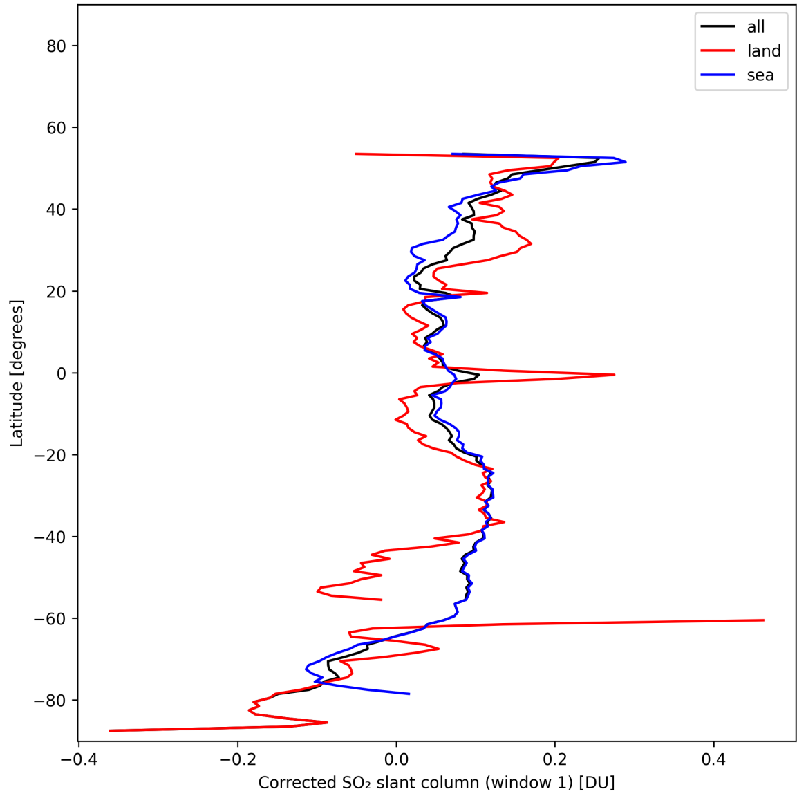
Figure 39: Zonal average of “Corrected SO 2 slant column (window 1)” for 2025-11-08 to 2025-11-10.
