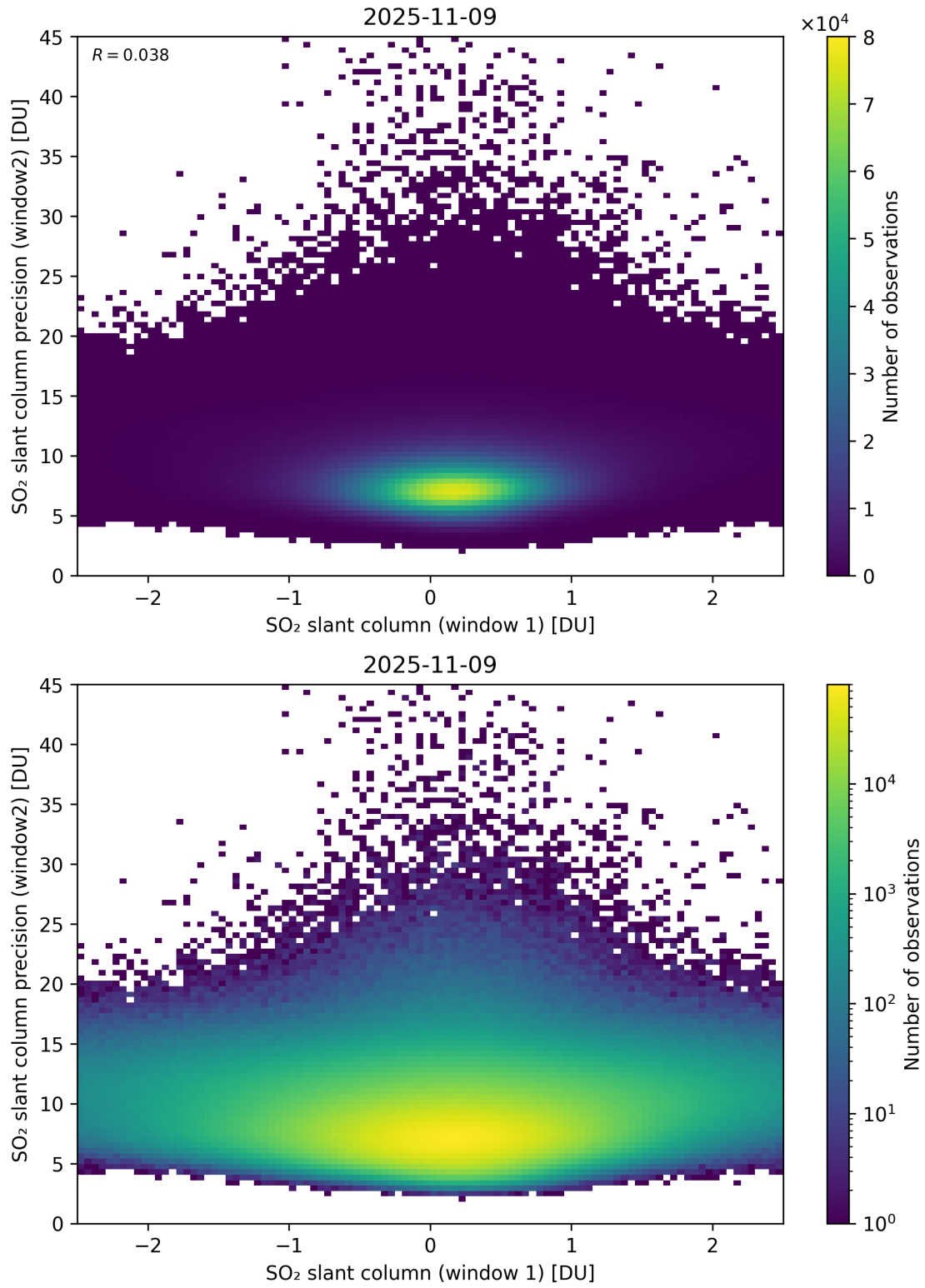
Figure 286: Scatter density plot of “SO 2 slant column (window 1)” against “SO 2 slant column precision (window2)” for 2025-11-08 to 2025-11-10.
