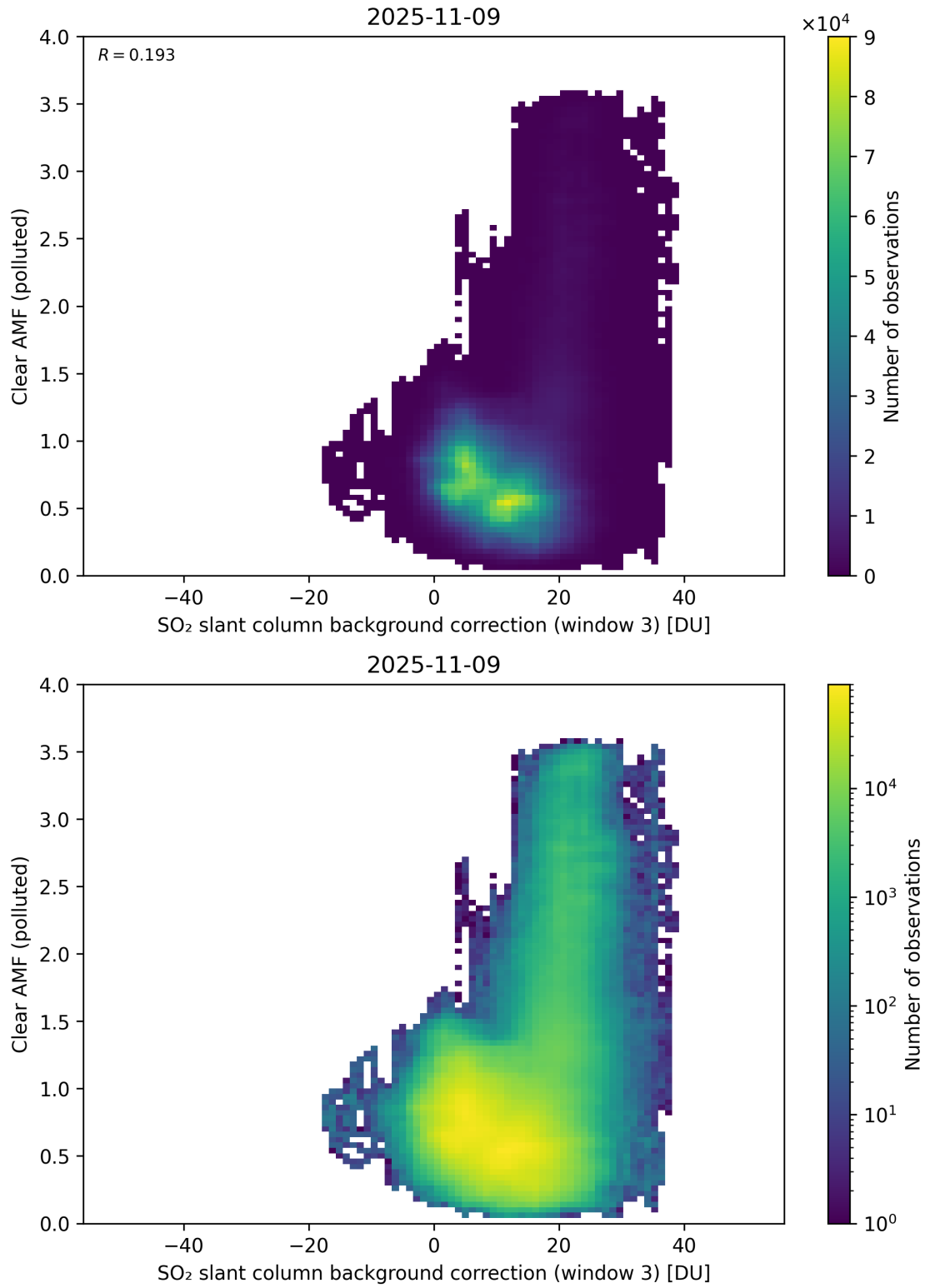
Figure 135: Scatter density plot of “SO 2 slant column background correction (window 3)” against “Clear AMF (polluted)” for 2025-11-08 to 2025-11-10.
