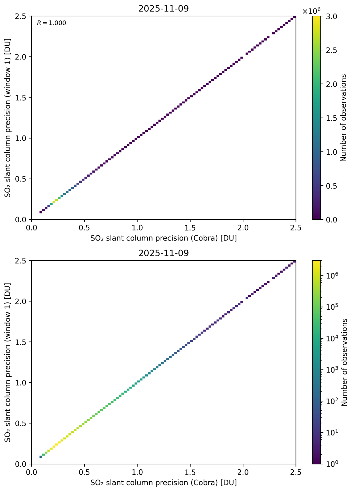
Figure 209: Scatter density plot of “SO 2 slant column precision (Cobra)” against “SO 2 slant column precision (window 1)” for 2025-11-08 to 2025-11-10.
