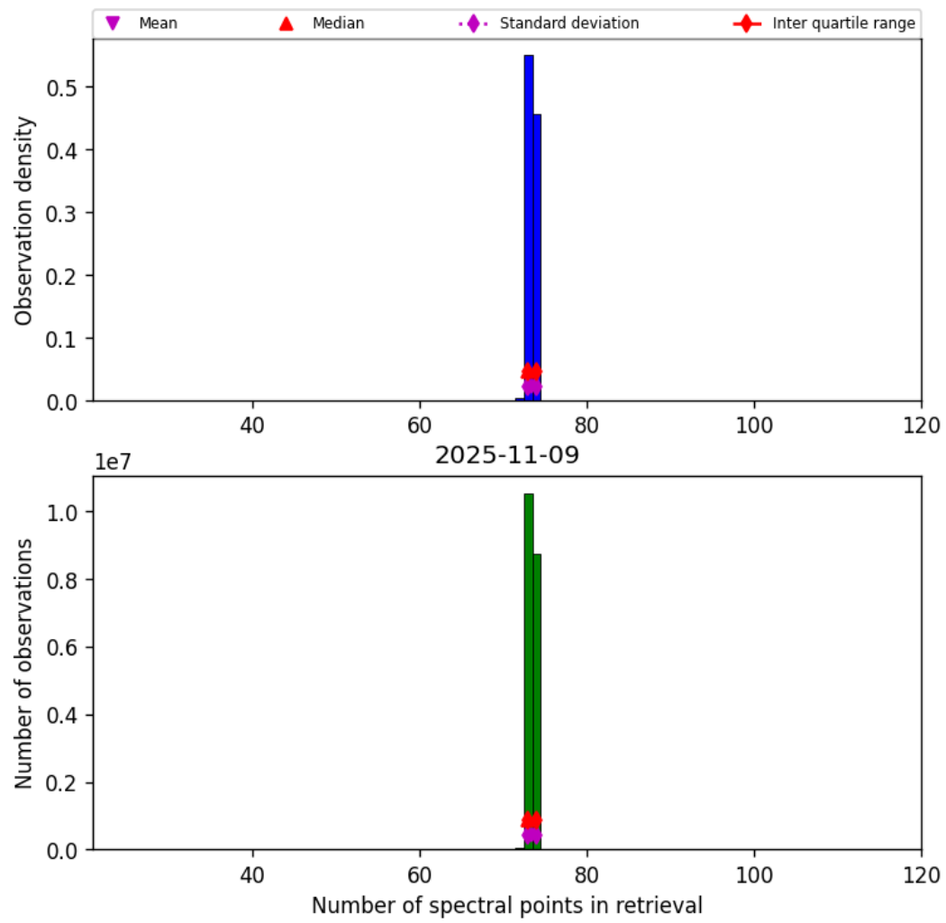
Figure 82: Histogram of “Number of spectral points in retrieval” for 2025-11-08 to 2025-11-10
