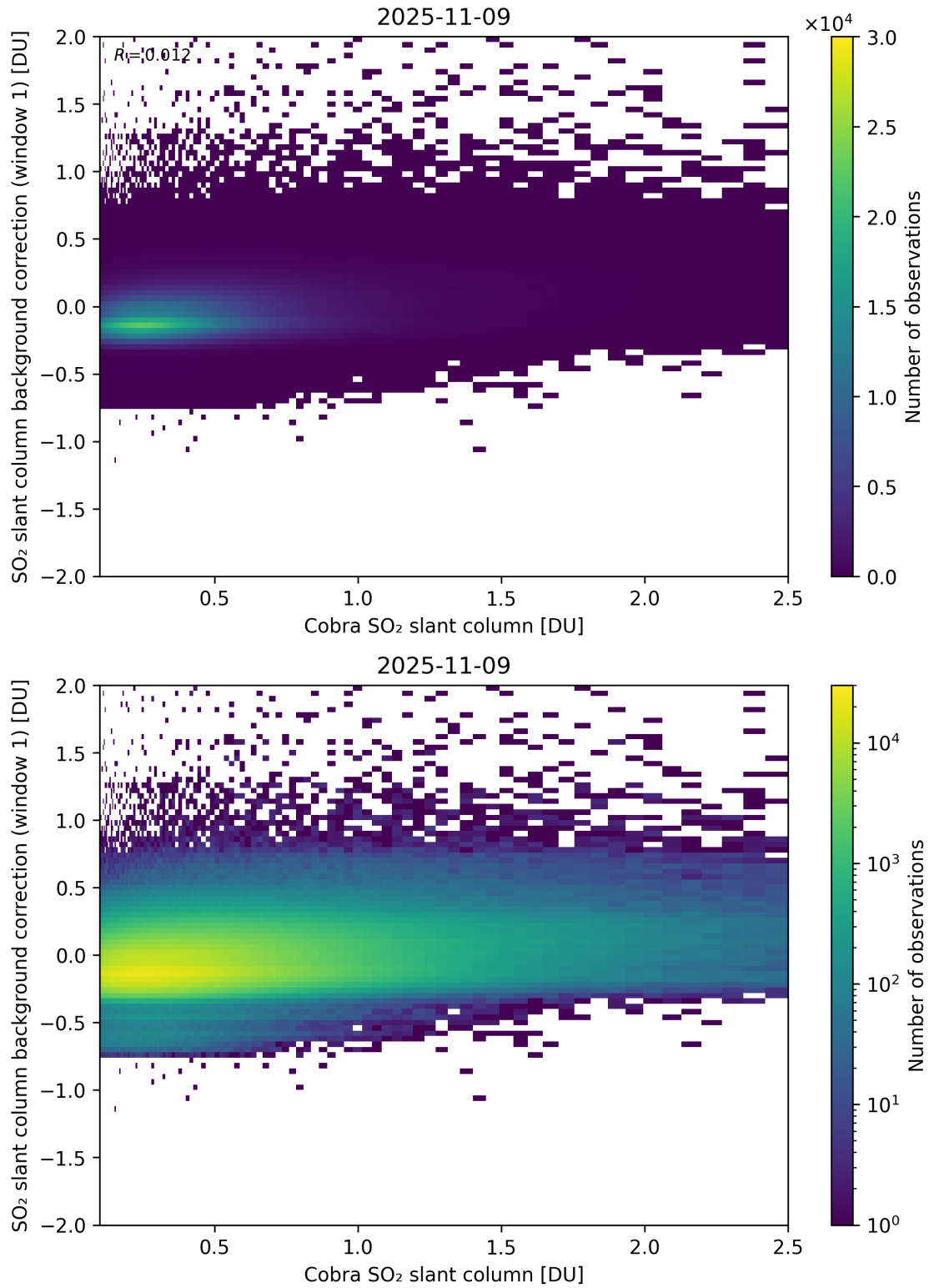
Figure 193: Scatter density plot of “Cobra SO 2 slant column” against “SO 2 slant column background correction (window 1)” for 2025-11-08 to 2025-11-10.
