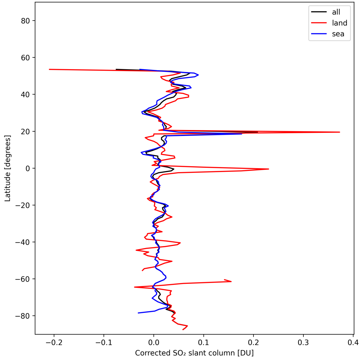
Figure 34: Zonal average of “Corrected SO 2 slant column” for 2025-11-08 to 2025-11-10.
