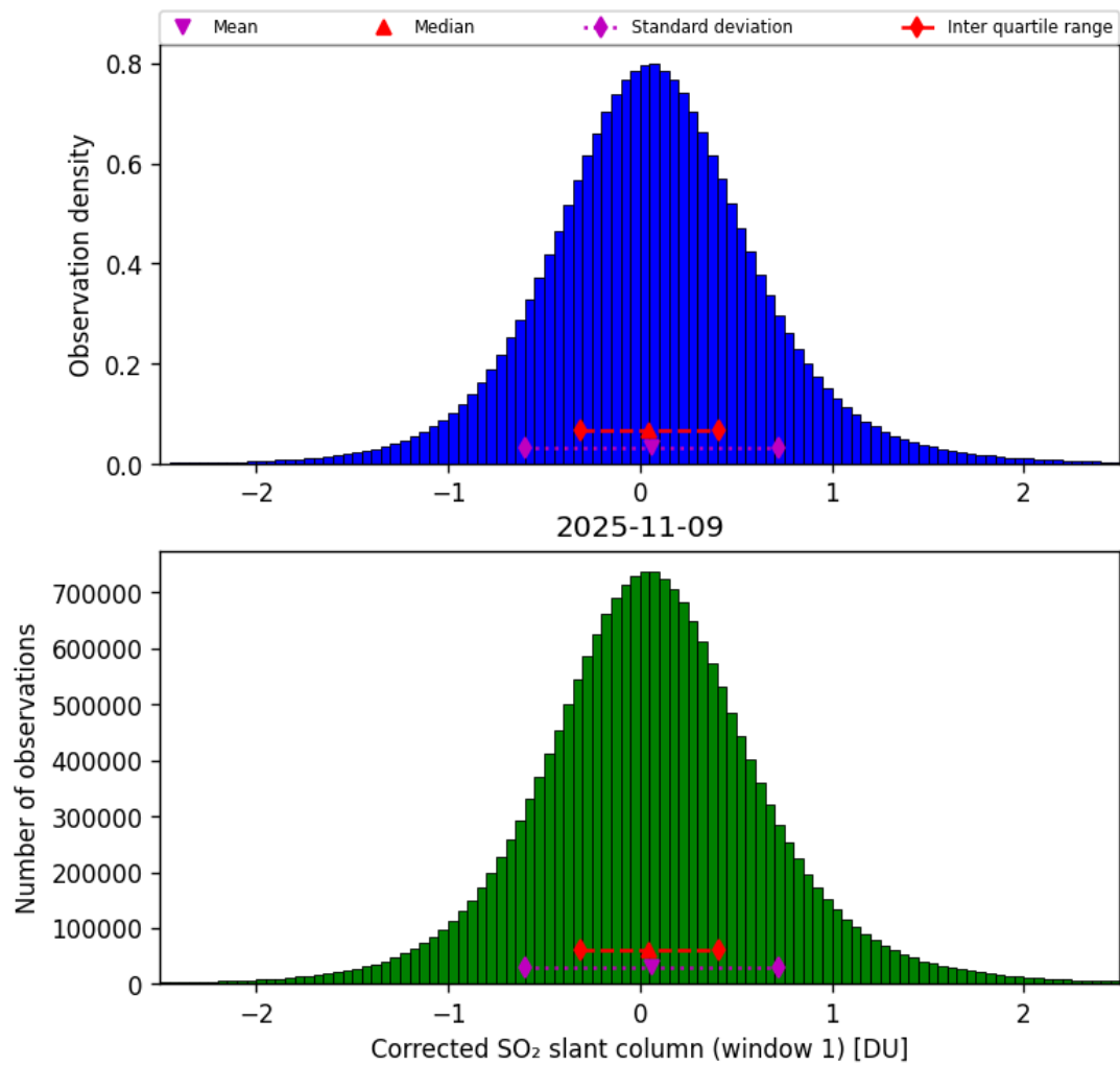
Figure 65: Histogram of “Corrected SO 2 slant column (window 1)” for 2025-11-08 to 2025-11-10
