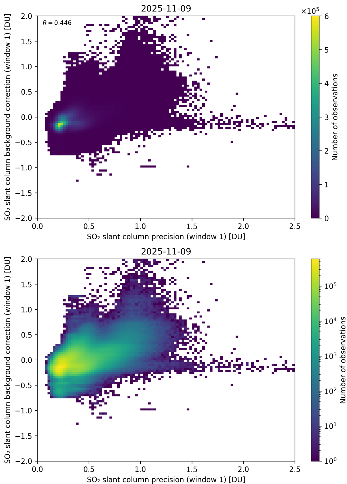
Figure 268: Scatter density plot of “SO 2 slant column precision (window 1)” against “SO 2 slant column background correction (window 1)” for 2025-11-08 to 2025-11-10.
