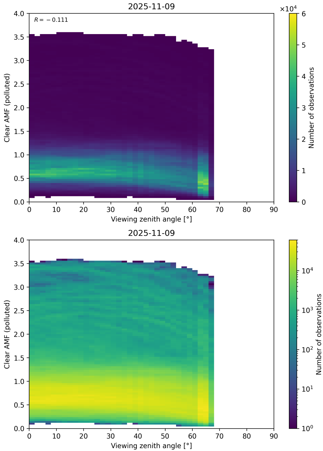
Figure 370: Scatter density plot of “Viewing zenith angle” against “Clear AMF (polluted)” for 2025-11-08 to 2025-11-10.
