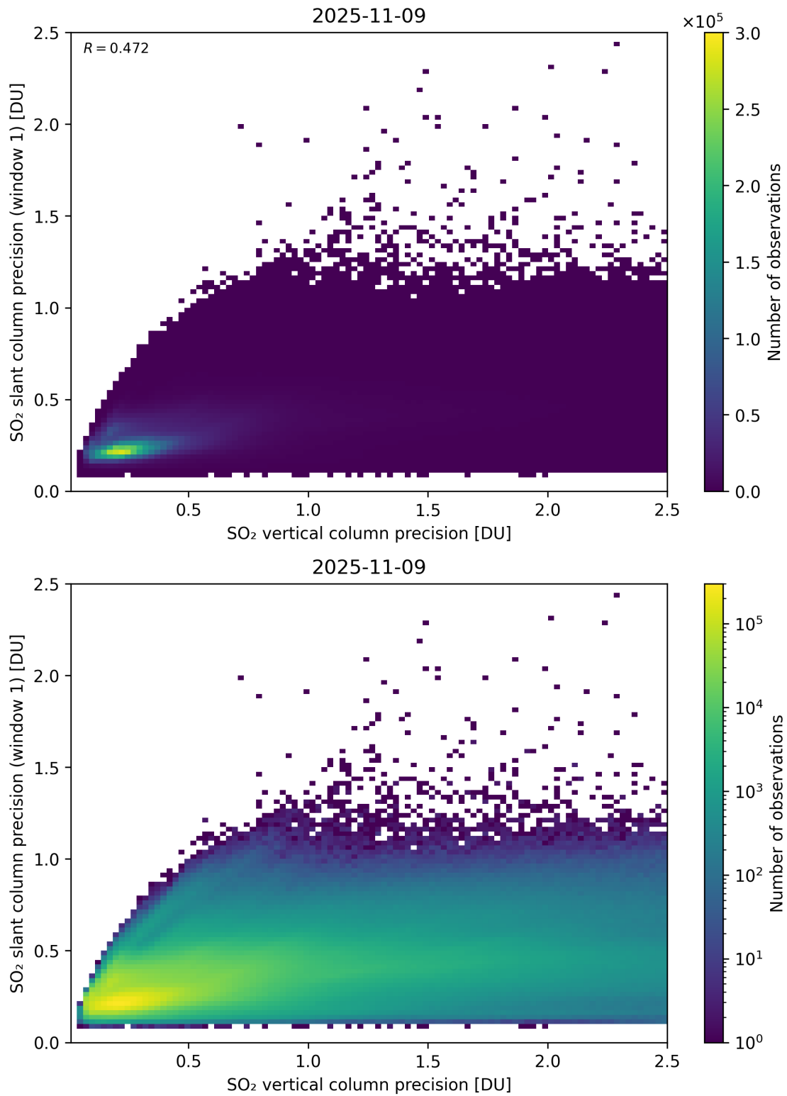
Figure 342: Scatter density plot of “SO 2 vertical column precision” against “SO 2 slant column precision (window 1)” for 2025-11-08 to 2025-11-10.
