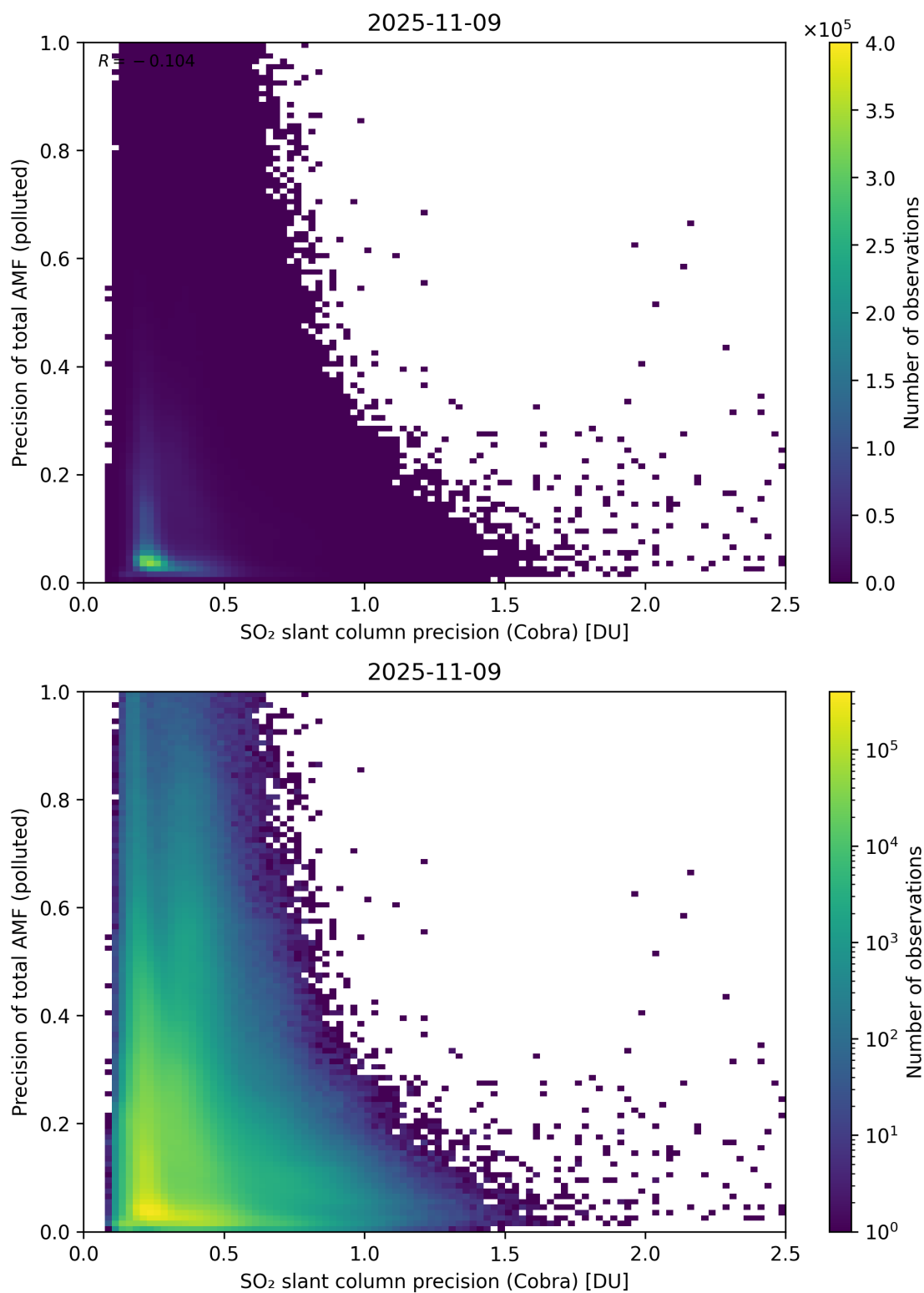
Figure 214: Scatter density plot of “SO 2 slant column precision (Cobra)” against “Precision of total AMF (polluted)” for 2025-11-08 to 2025-11-10.
