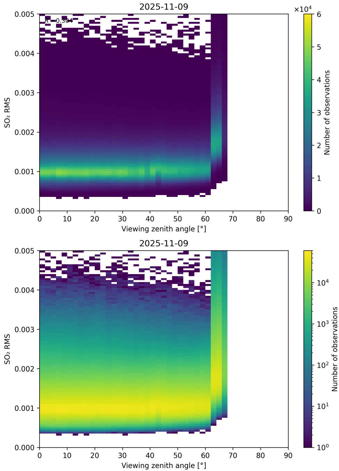
Figure 367: Scatter density plot of “Viewing zenith angle” against “SO 2 RMS” for 2025-11-08 to 2025-11-10.
