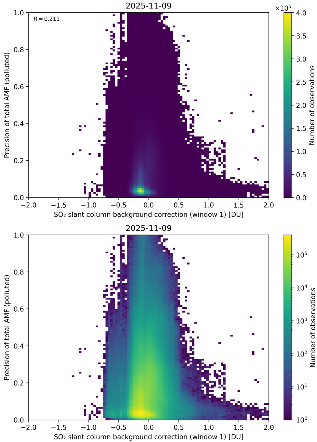
Figure 121: Scatter density plot of “SO 2 slant column background correction (window 1)” against “Precision of total AMF (polluted)” for 2025-11-08 to 2025-11-10.
