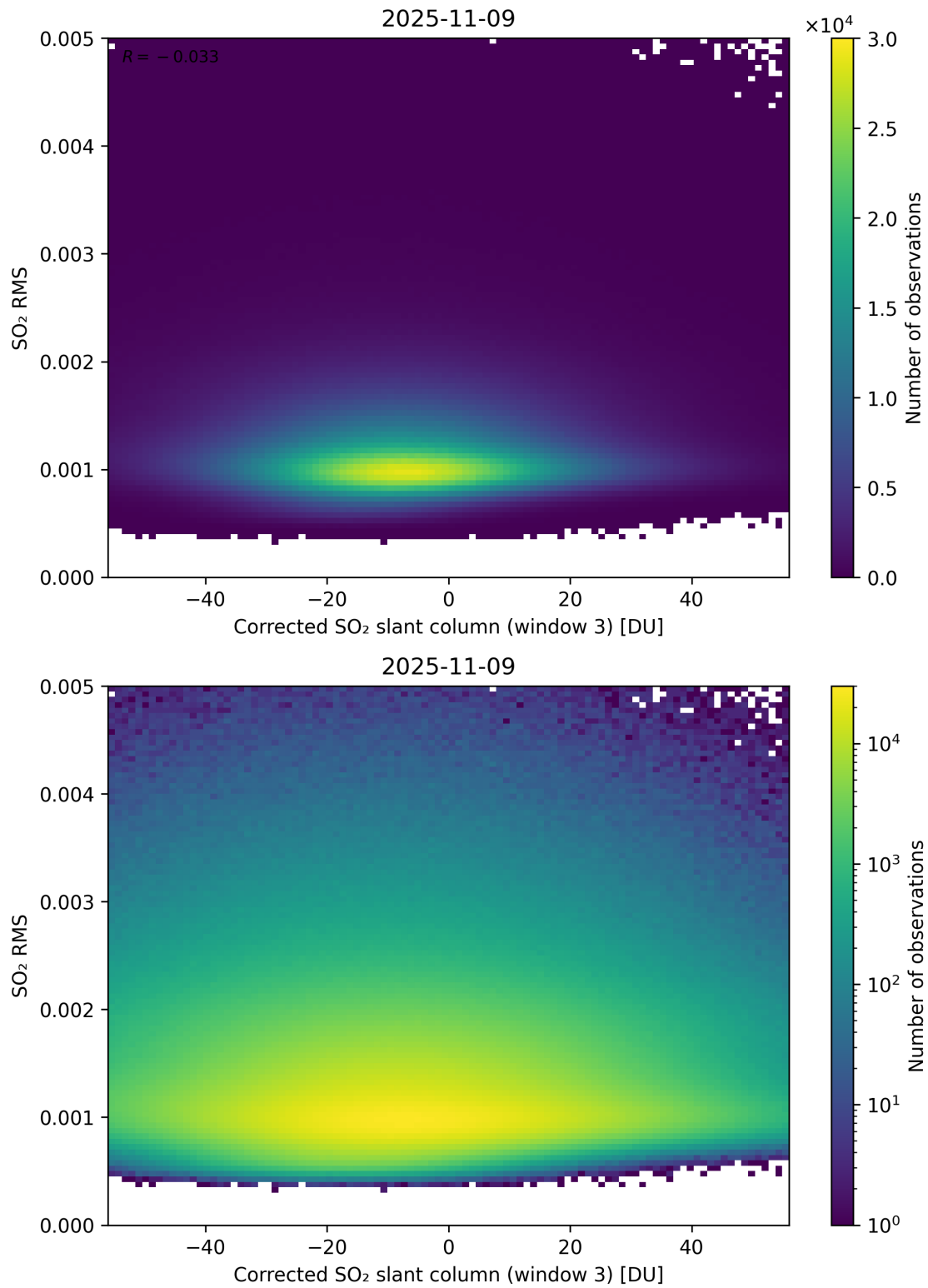
Figure 258: Scatter density plot of “Corrected SO 2 slant column (window 3)” against “SO 2 RMS” for 2025-11-08 to 2025-11-10.
