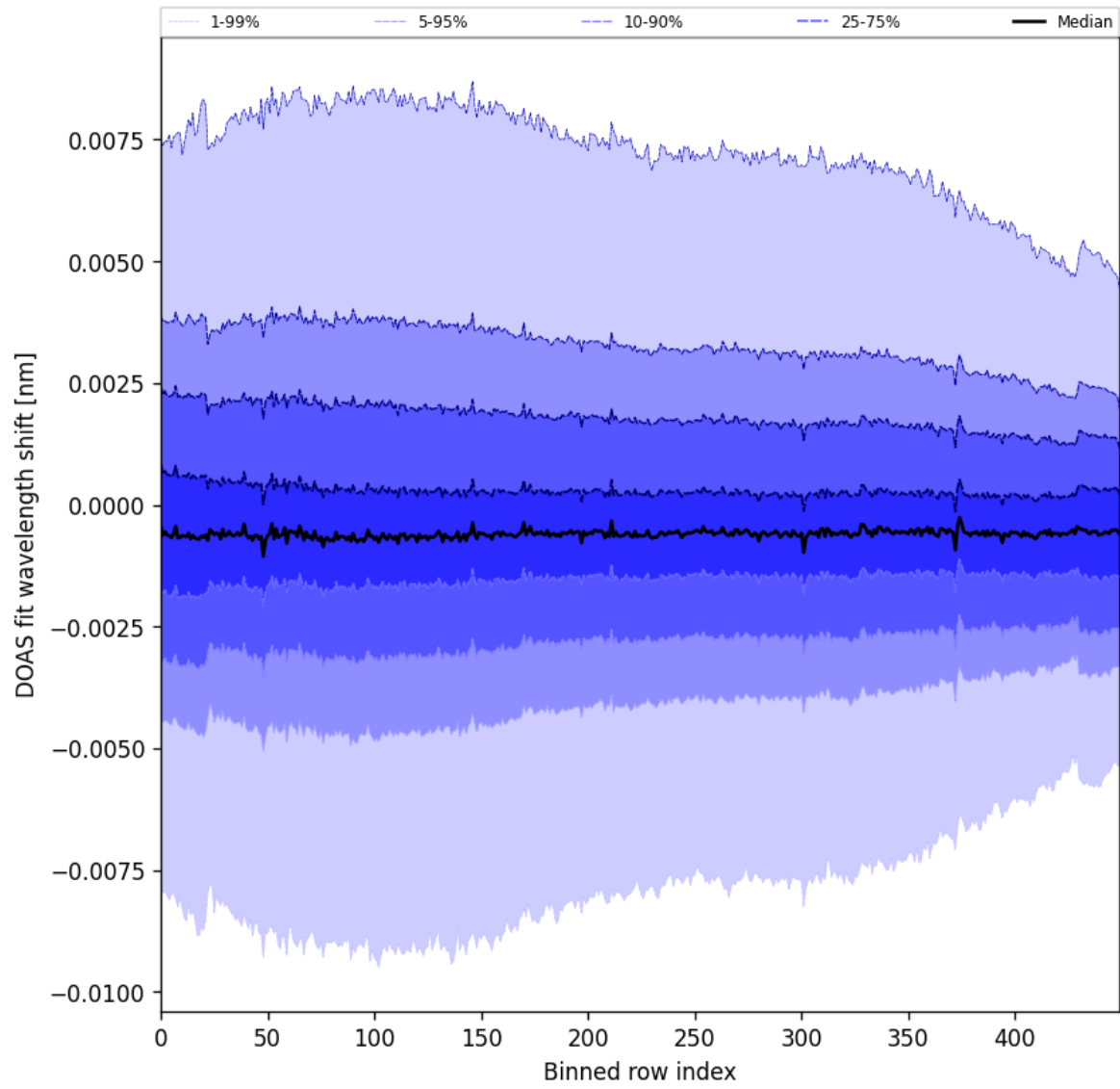
Figure 102: Along track statistics of “DOAS fit wavelength shift” for 2025-11-08 to 2025-11-10
