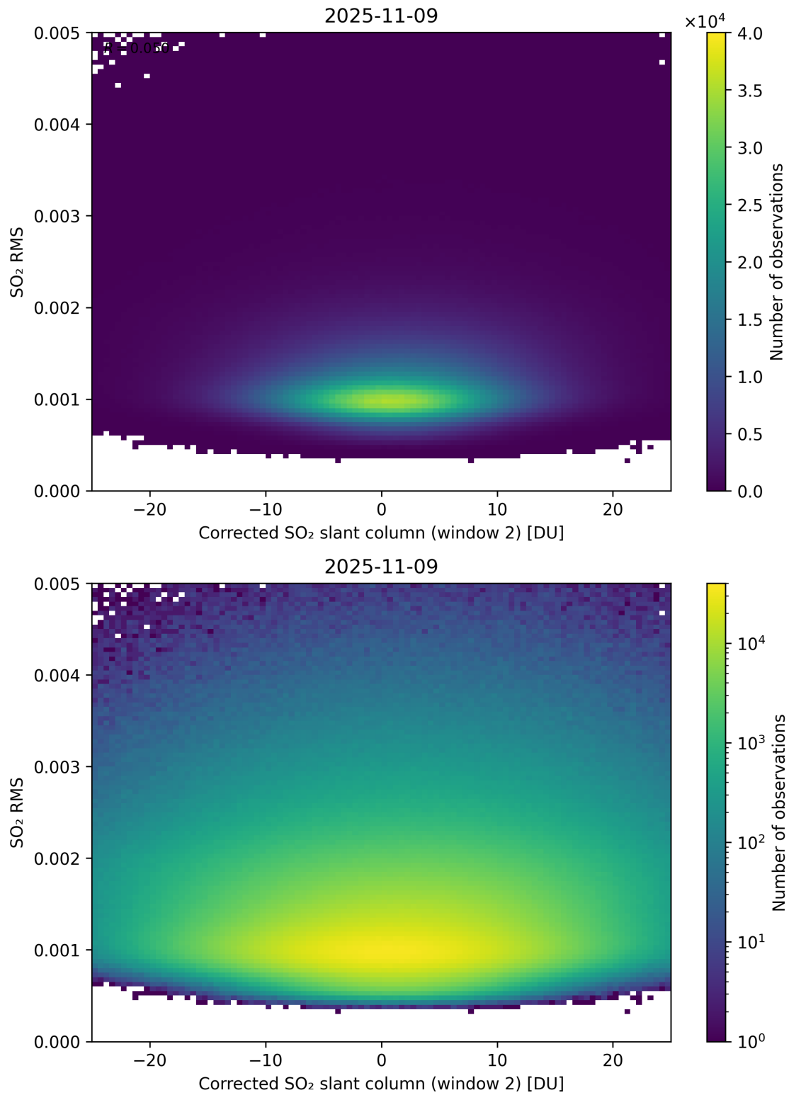
Figure 248: Scatter density plot of “Corrected SO 2 slant column (window 2)” against “SO 2 RMS” for 2025-11-08 to 2025-11-10.
