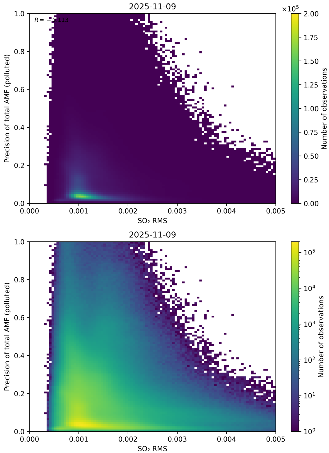
Figure 149: Scatter density plot of “SO 2 RMS” against “Precision of total AMF (polluted)” for 2025-11-08 to 2025-11-10.
