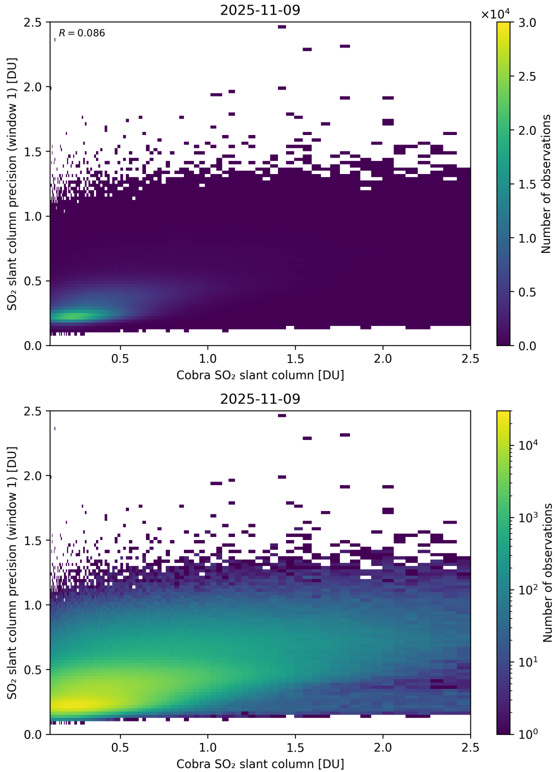
Figure 220: Scatter density plot of “Cobra SO 2 slant column” against “SO 2 slant column precision (window 1)” for 2025-11-08 to 2025-11-10.
