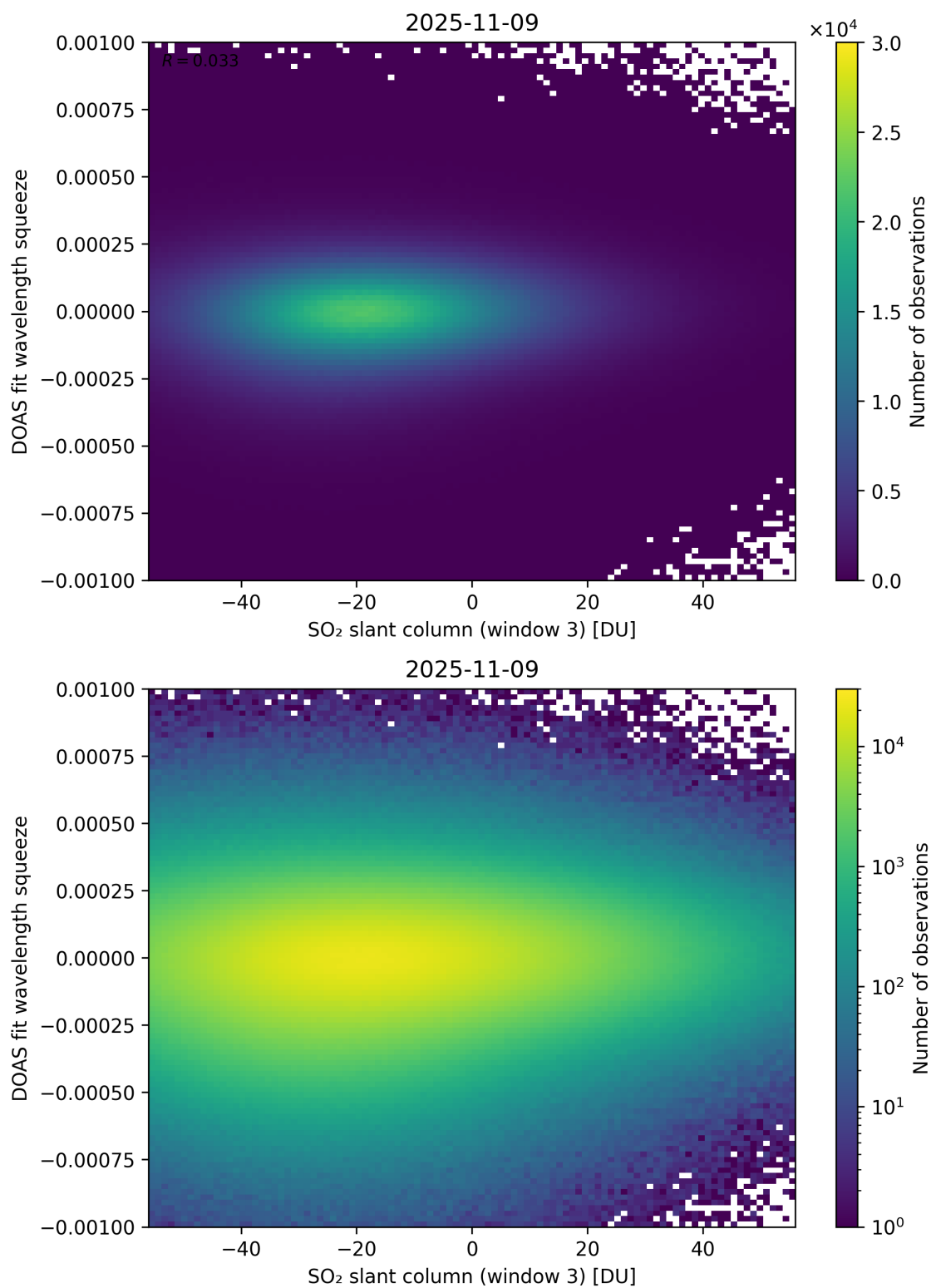
Figure 305: Scatter density plot of “SO 2 slant column (window 3)” against “DOAS fit wavelength squeeze” for 2025-11-08 to 2025-11-10.
