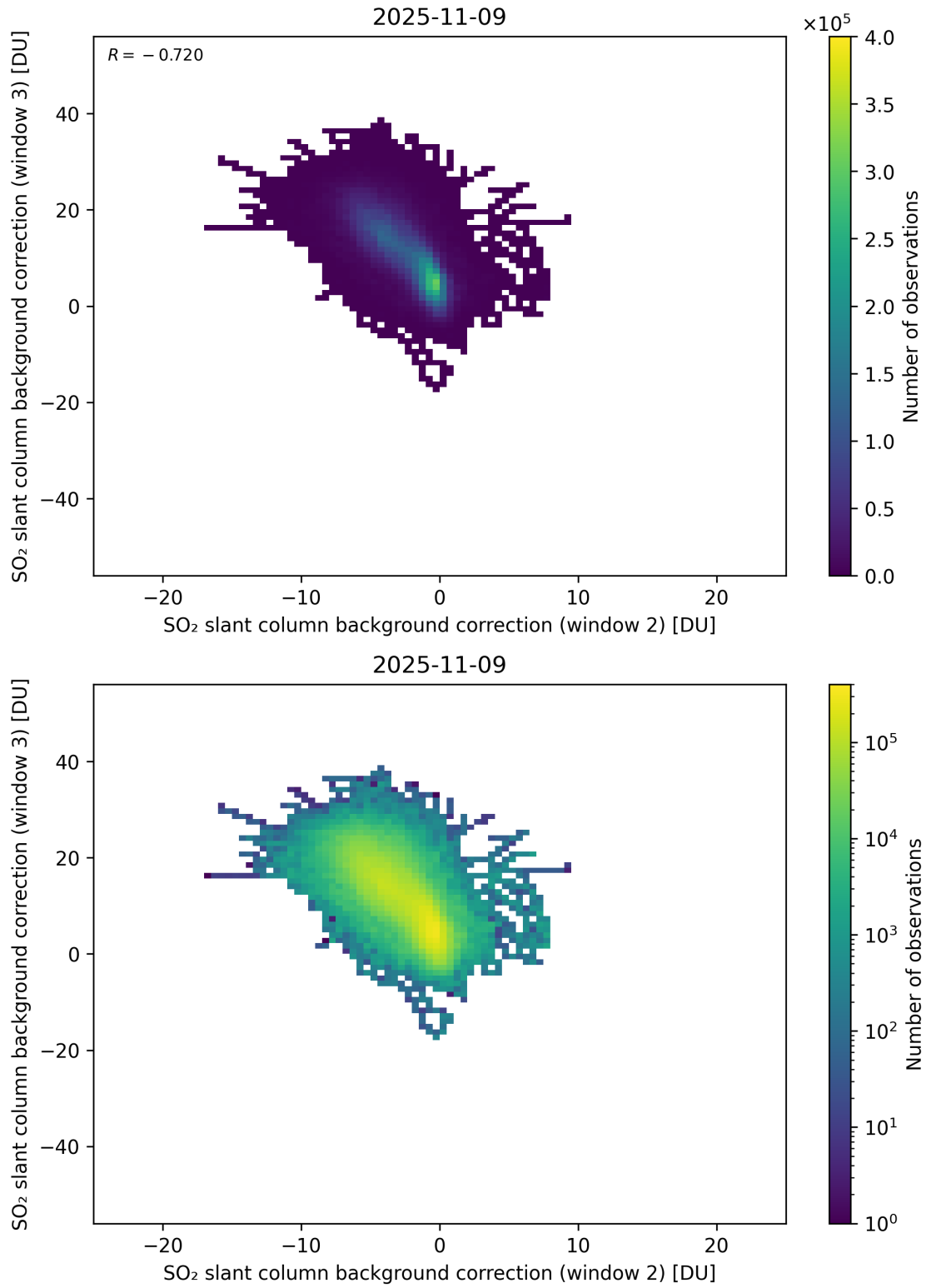
Figure 122: Scatter density plot of “SO 2 slant column background correction (window 2)” against “SO 2 slant column background correction (window 3)” for 2025-11-08 to 2025-11-10.
