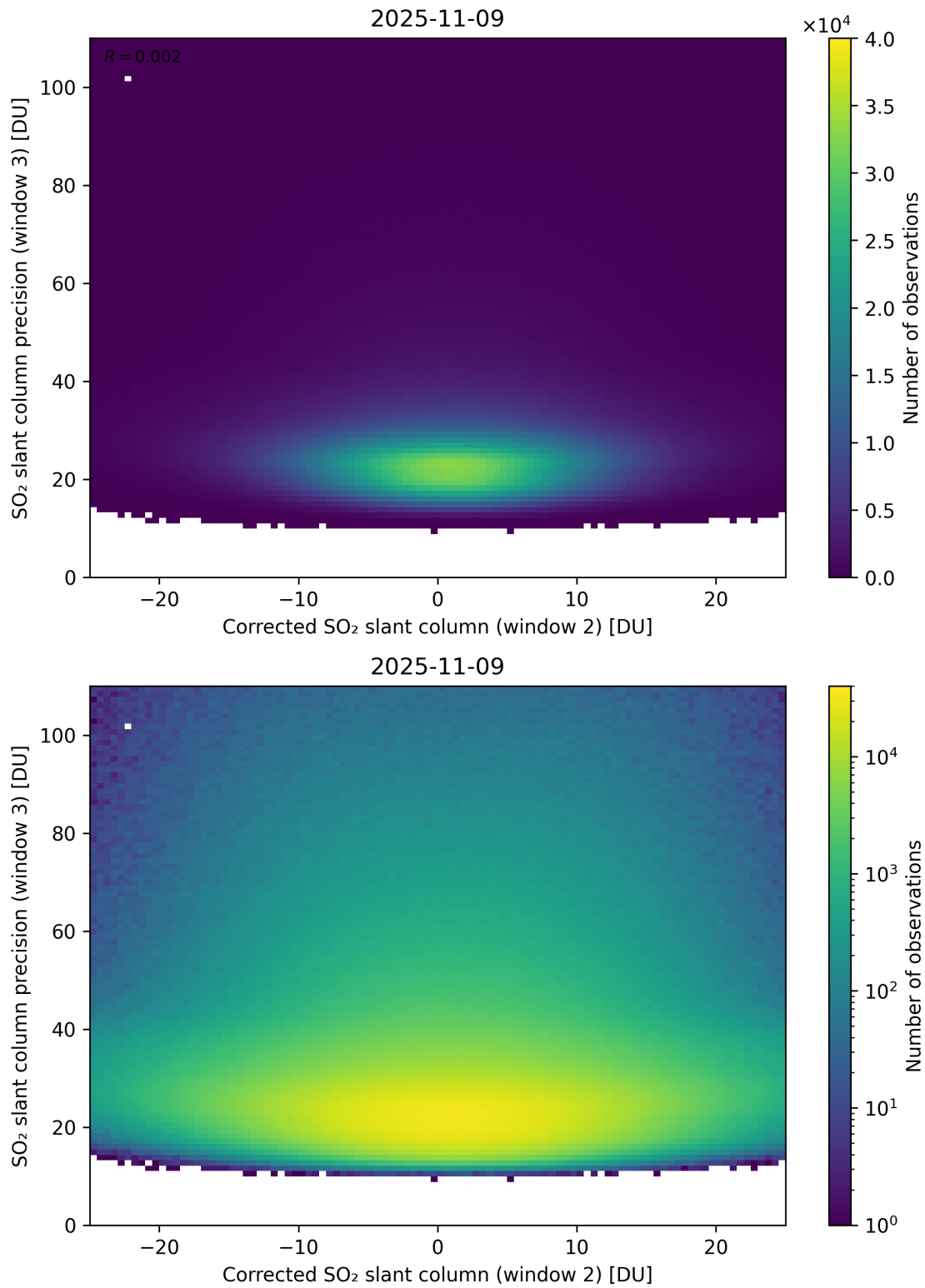
Figure 252: Scatter density plot of “Corrected SO 2 slant column (window 2)” against “SO 2 slant column precision (window 3)” for 2025-11-08 to 2025-11-10.
