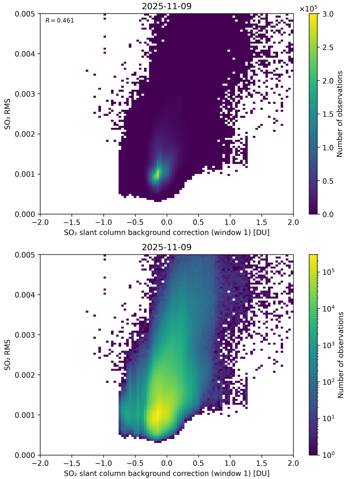
Figure 113: Scatter density plot of “SO 2 slant column background correction (window 1)” against “SO 2 RMS” for 2025-11-08 to 2025-11-10.
