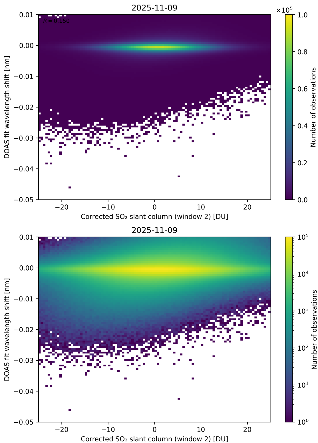
Figure 246: Scatter density plot of “Corrected SO 2 slant column (window 2)” against “DOAS fit wavelength shift” for 2025-11-08 to 2025-11-10.
