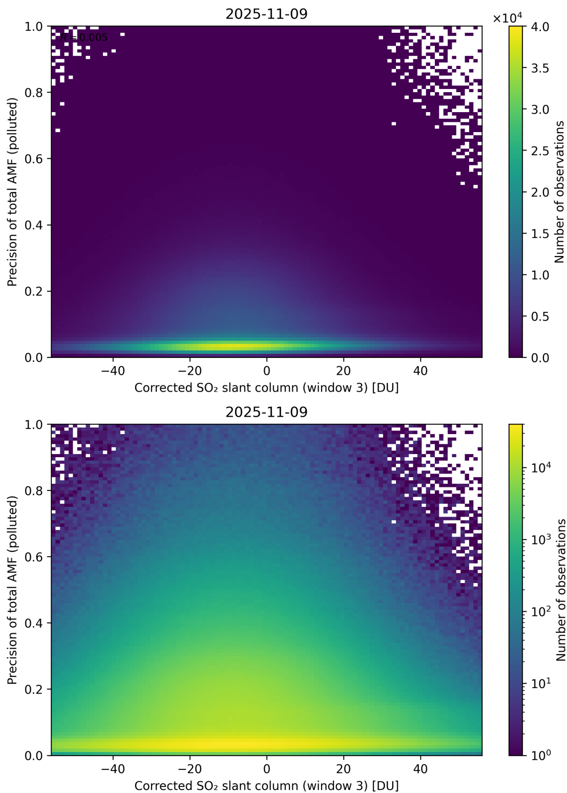
Figure 261: Scatter density plot of “Corrected SO 2 slant column (window 3)” against “Precision of total AMF (polluted)” for 2025-11-08 to 2025-11-10.
