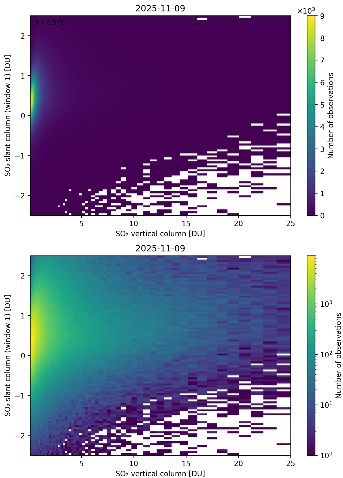
Figure 354: Scatter density plot of “SO 2 vertical column” against “SO 2 slant column (window 1)” for 2025-11-08 to 2025-11-10.
