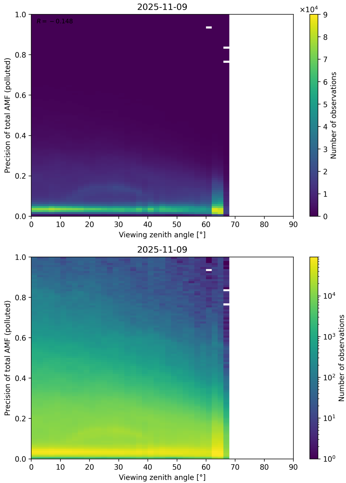
Figure 382: Scatter density plot of “Viewing zenith angle” against “Precision of total AMF (polluted)” for 2025-11-08 to 2025-11-10.
