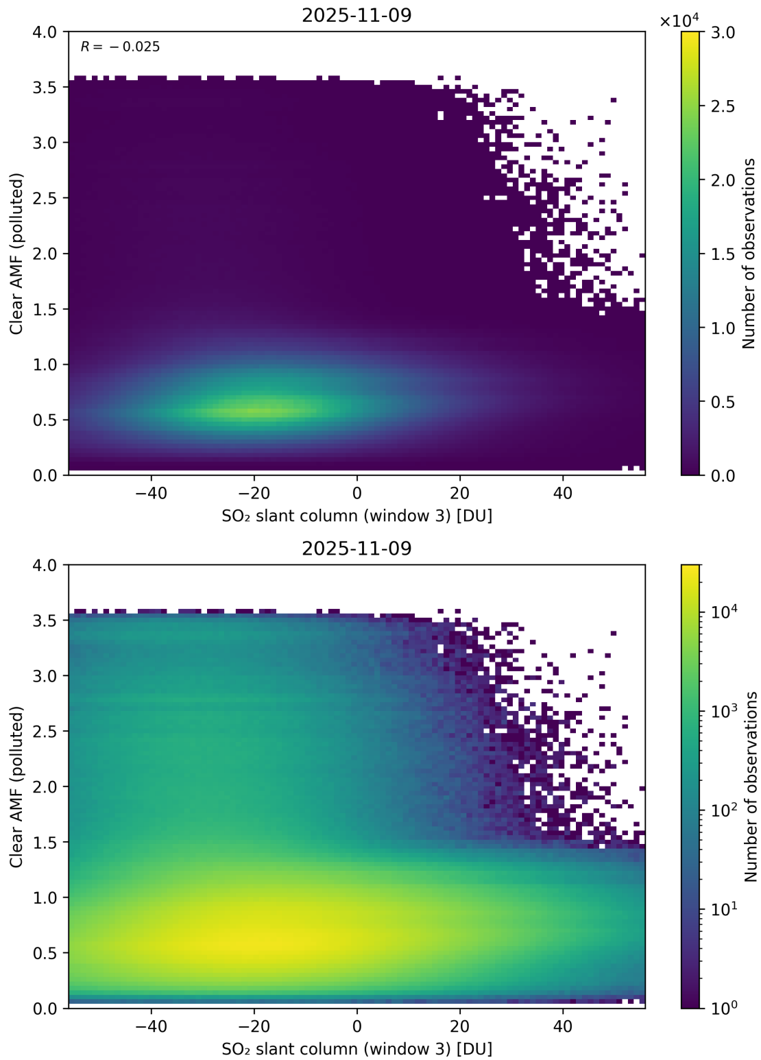
Figure 315: Scatter density plot of “SO 2 slant column (window 3)” against “Clear AMF (polluted)” for 2025-11-08 to 2025-11-10.
