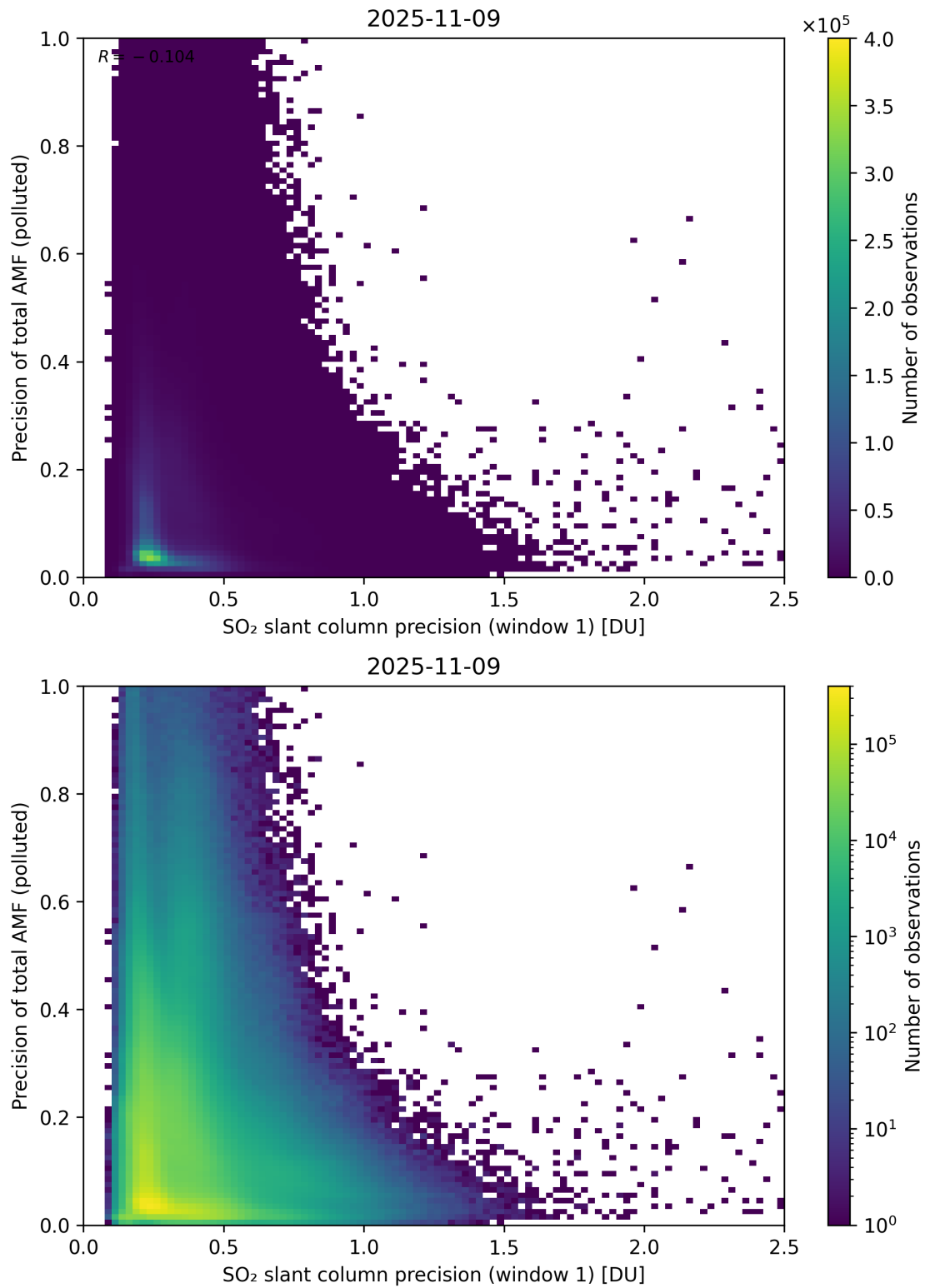
Figure 281: Scatter density plot of “SO 2 slant column precision (window 1)” against “Precision of total AMF (polluted)” for 2025-11-08 to 2025-11-10.
