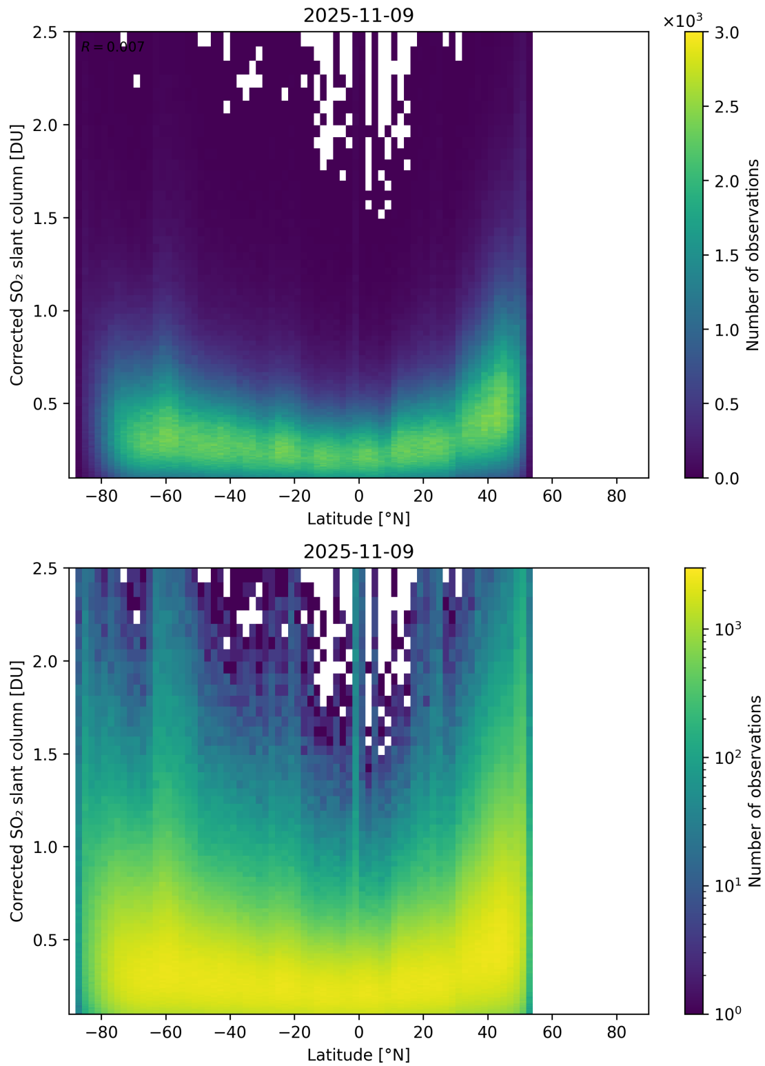
Figure 159: Scatter density plot of “Latitude” against “Corrected SO 2 slant column” for 2025-11-08 to 2025-11-10.
