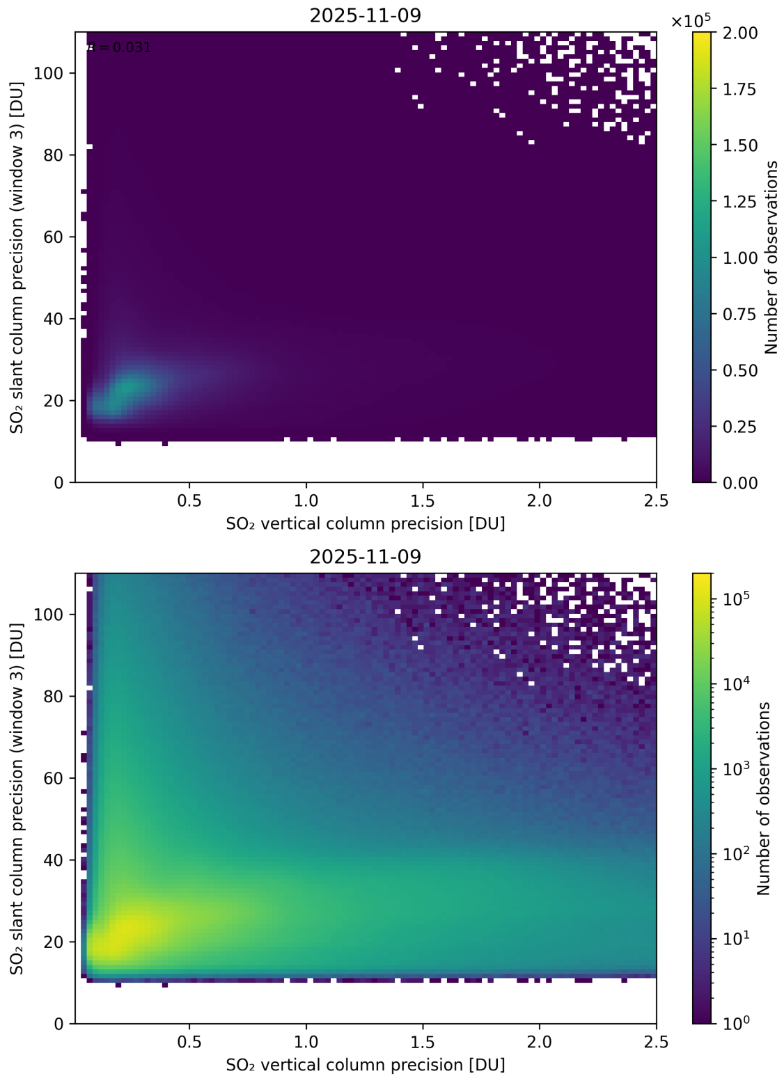
Figure 345: Scatter density plot of “SO 2 vertical column precision” against “SO 2 slant column precision (window 3)” for 2025-11-08 to 2025-11-10.
