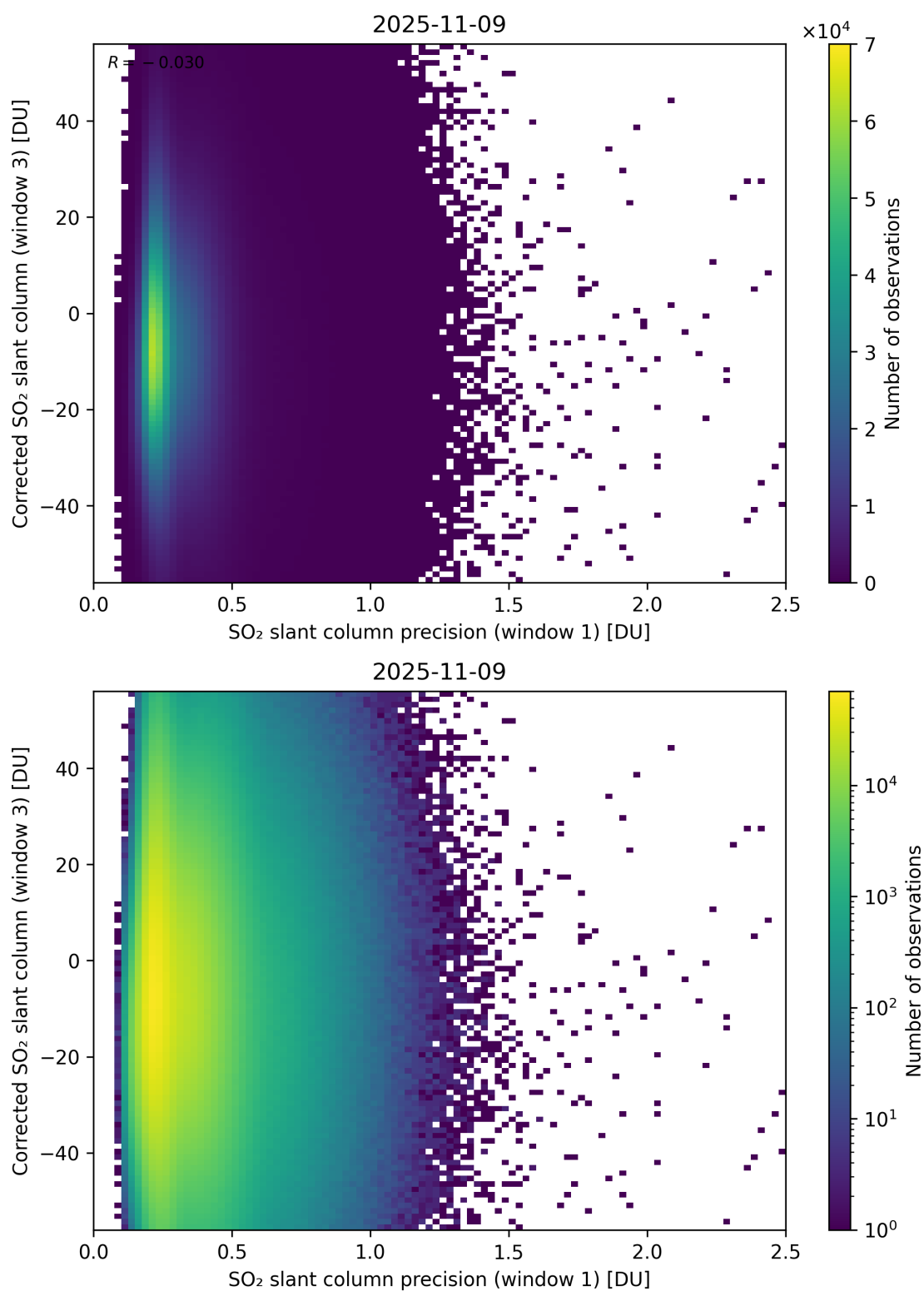
Figure 276: Scatter density plot of “SO 2 slant column precision (window 1)” against “Corrected SO 2 slant column (window 3)” for 2025-11-08 to 2025-11-10.
