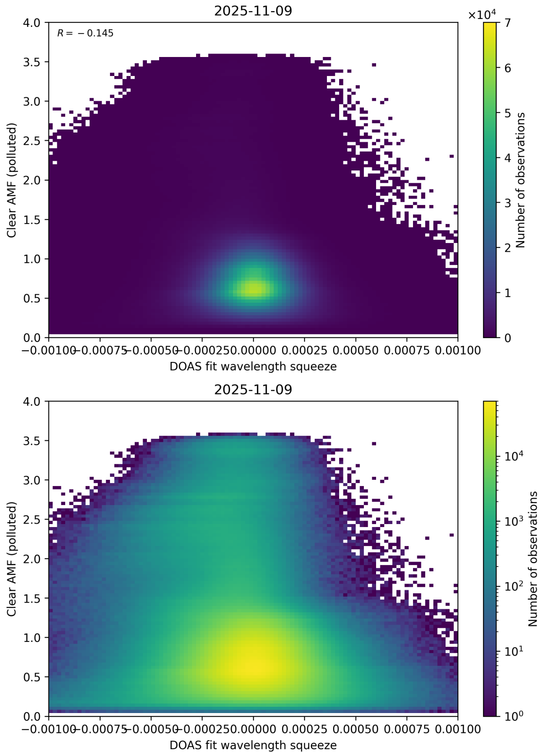
Figure 144: Scatter density plot of “DOAS fit wavelength squeeze” against “Clear AMF (polluted)” for 2025-11-08 to 2025-11-10.
