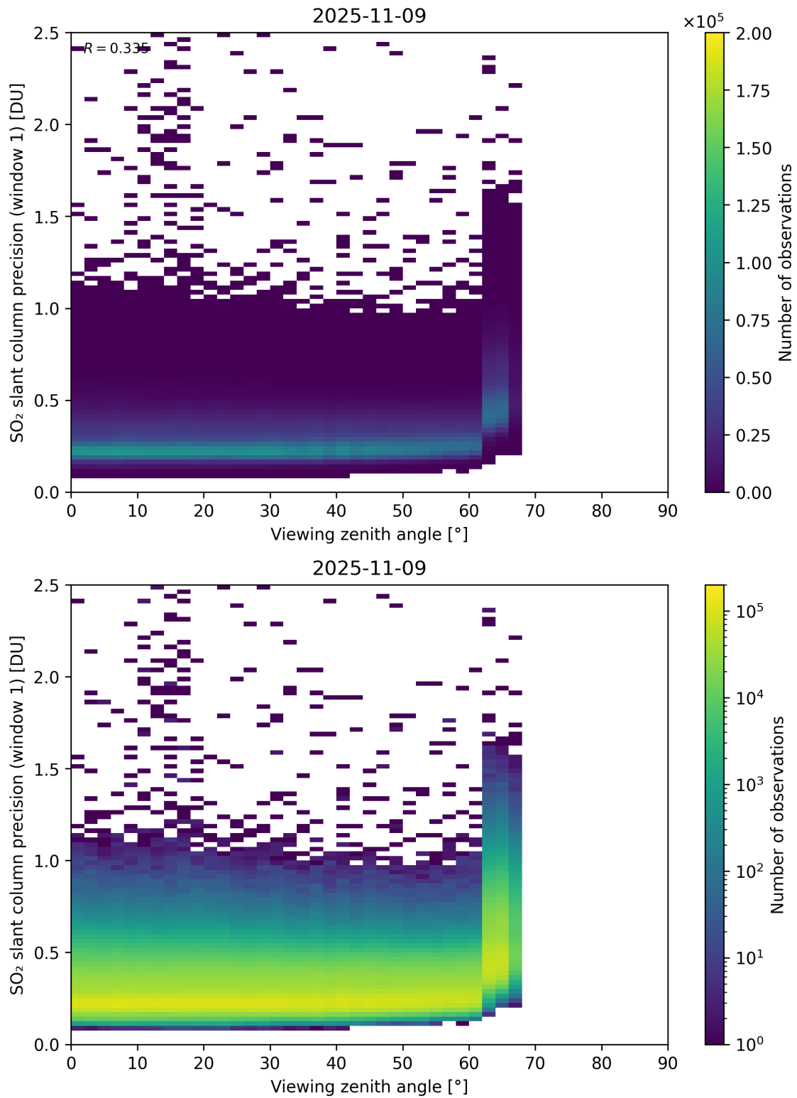
Figure 377: Scatter density plot of “Viewing zenith angle” against “SO 2 slant column precision (window 1)” for 2025-11-08 to 2025-11-10.
