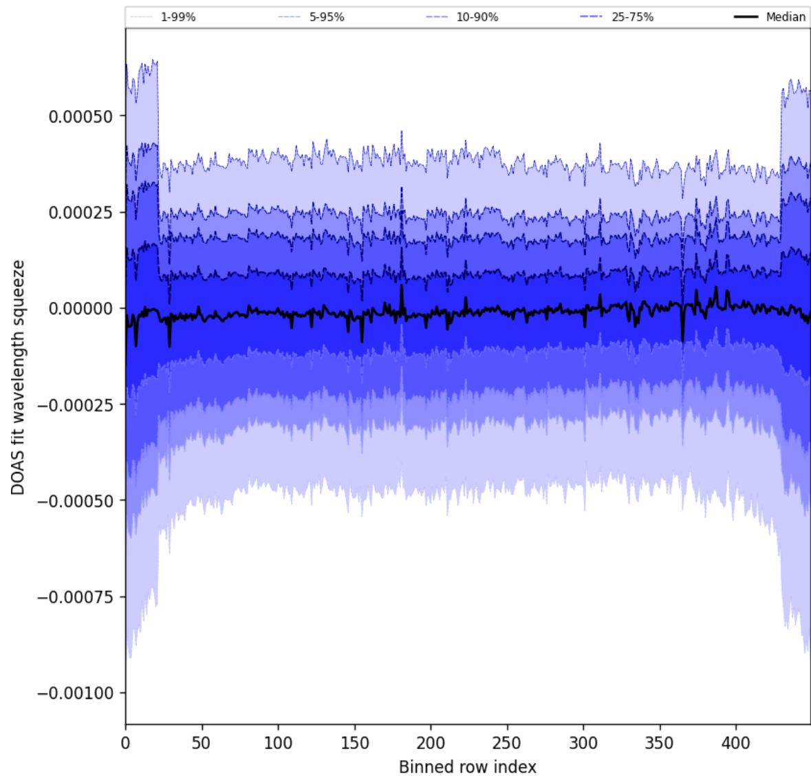
Figure 103: Along track statistics of “DOAS fit wavelength squeeze” for 2025-11-08 to 2025-11-10
