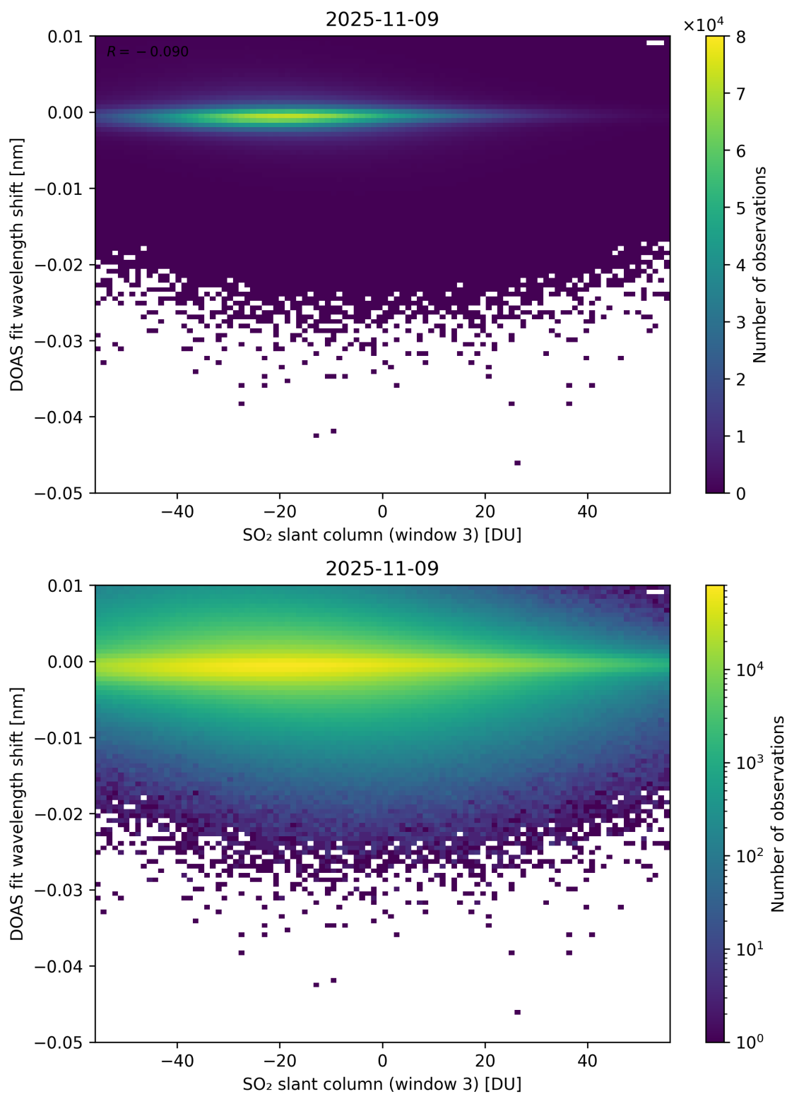
Figure 304: Scatter density plot of “SO 2 slant column (window 3)” against “DOAS fit wavelength shift” for 2025-11-08 to 2025-11-10.
