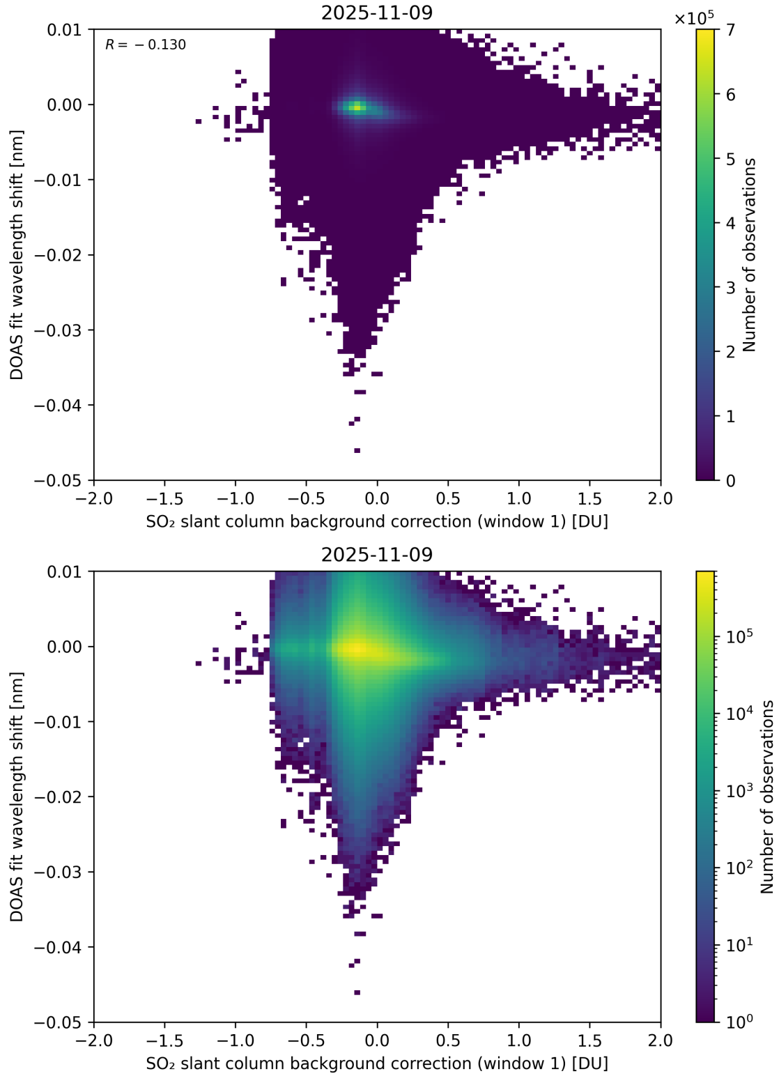
Figure 111: Scatter density plot of “SO 2 slant column background correction (window 1)” against “DOAS fit wavelength shift” for 2025-11-08 to 2025-11-10.
