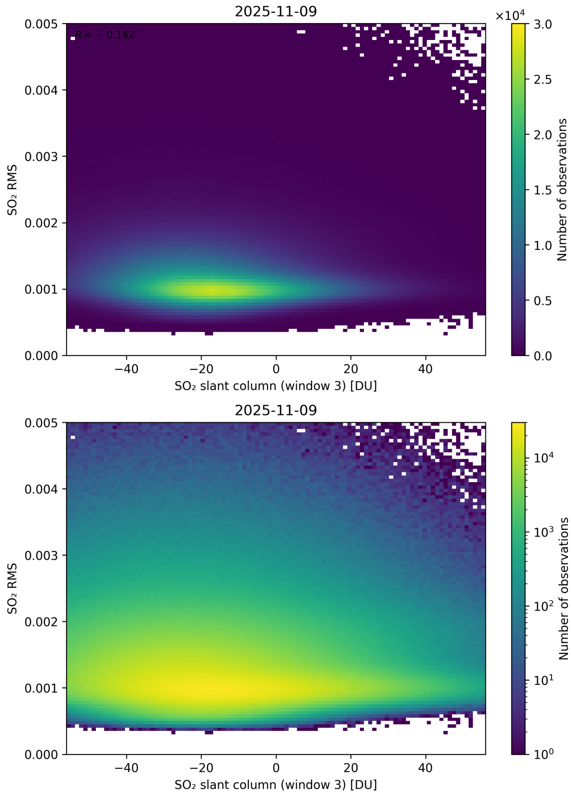
Figure 306: Scatter density plot of “SO 2 slant column (window 3)” against “SO 2 RMS” for 2025-11-08 to 2025-11-10.
