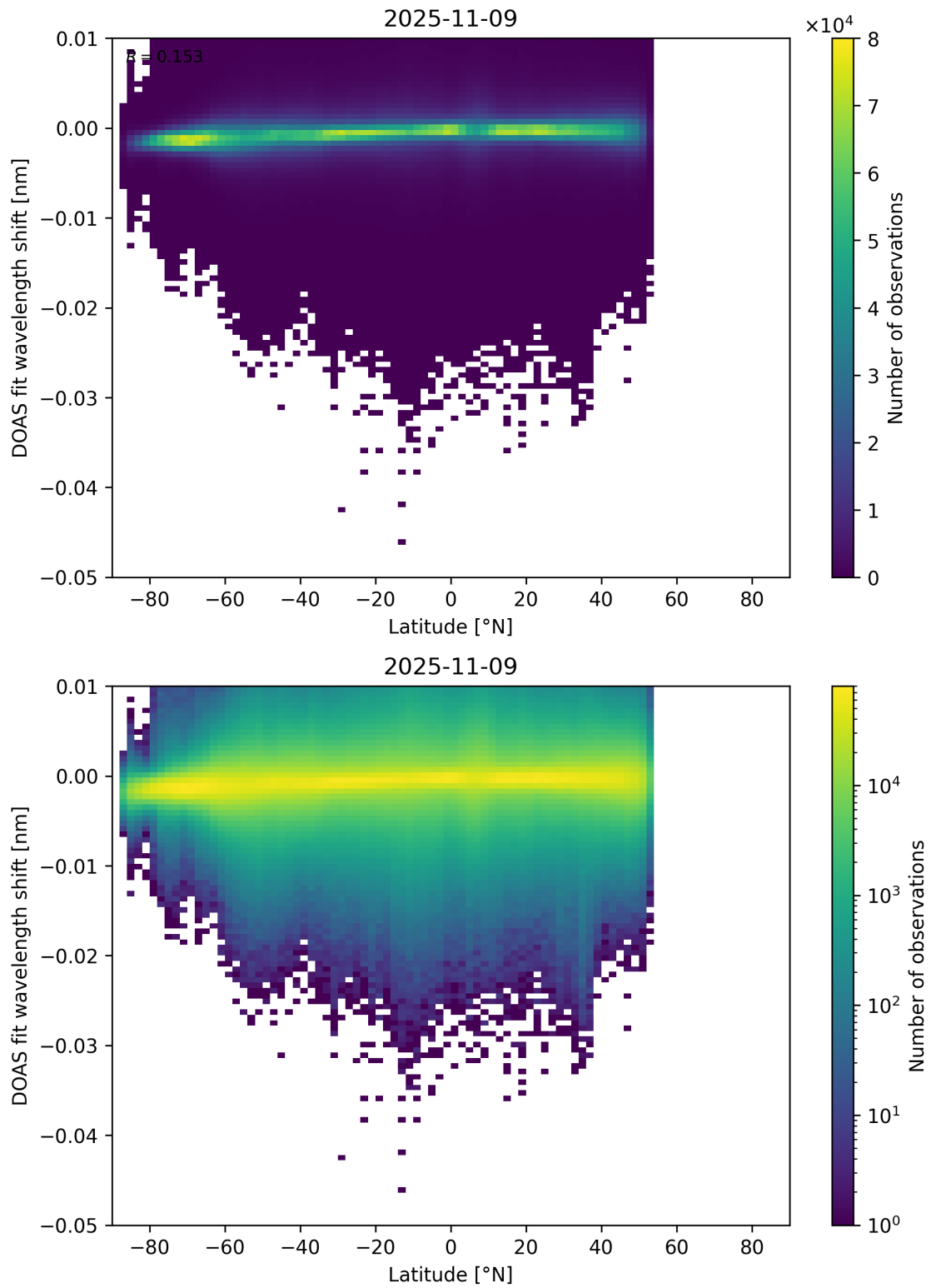
Figure 153: Scatter density plot of “Latitude” against “DOAS fit wavelength shift” for 2025-11-08 to 2025-11-10.
