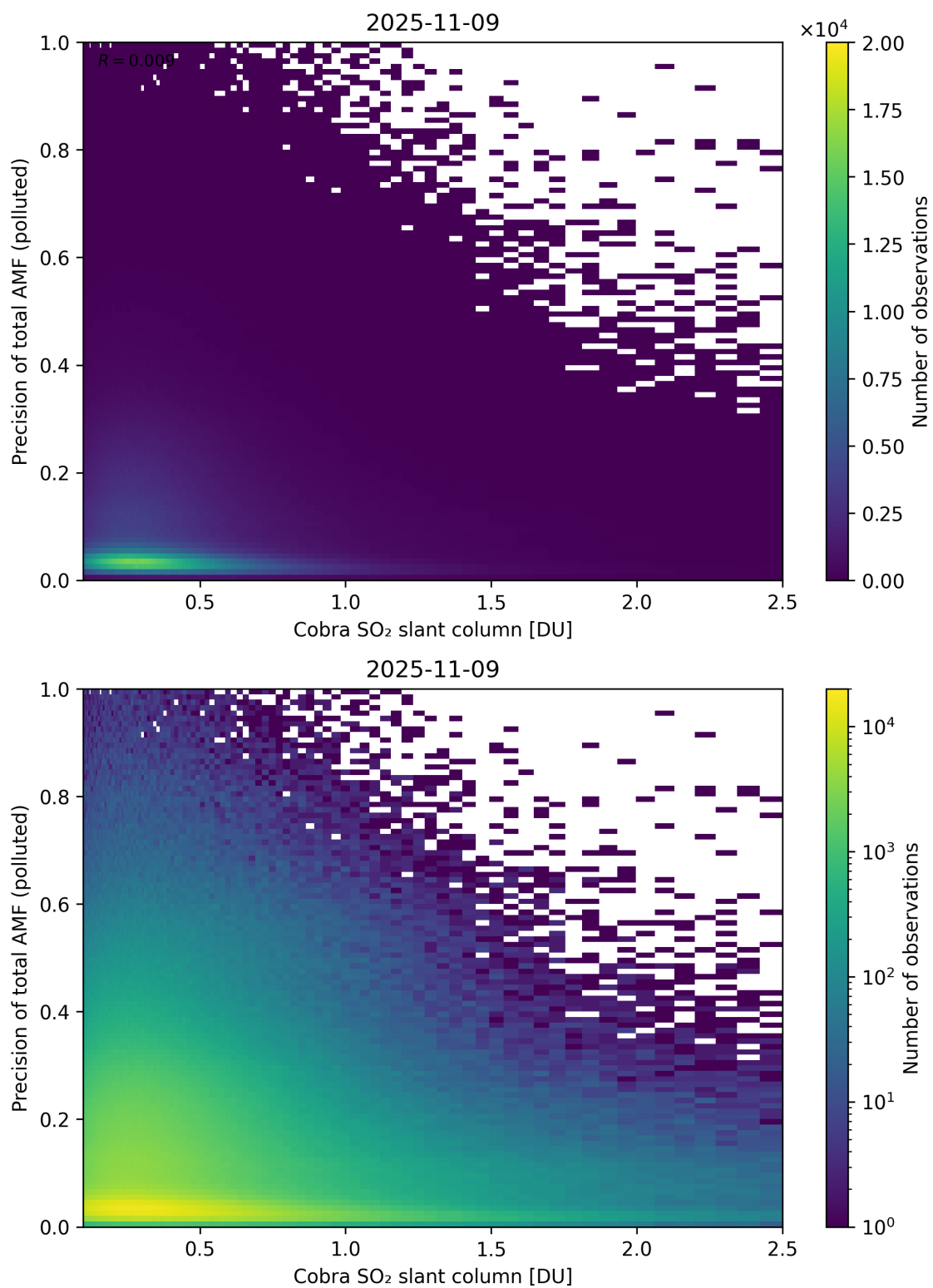
Figure 225: Scatter density plot of “Cobra SO 2 slant column” against “Precision of total AMF (polluted)” for 2025-11-08 to 2025-11-10.
