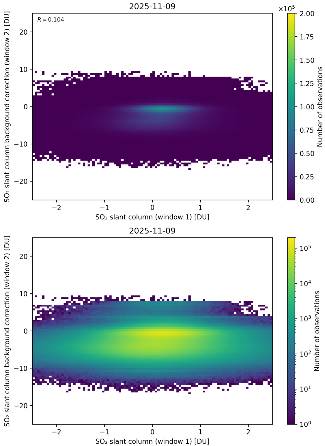
Figure 263: Scatter density plot of “SO 2 slant column (window 1)” against “SO 2 slant column background correction (window 2)” for 2025-11-08 to 2025-11-10.
