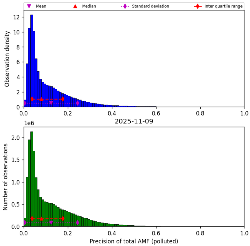
Figure 80: Histogram of “Precision of total AMF (polluted)” for 2025-11-08 to 2025-11-10
