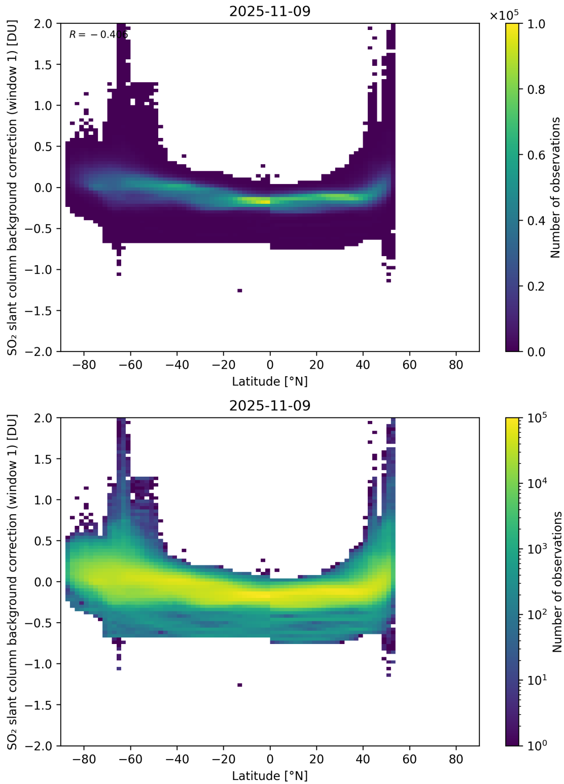
Figure 150: Scatter density plot of “Latitude” against “SO 2 slant column background correction (window 1)” for 2025-11-08 to 2025-11-10.
