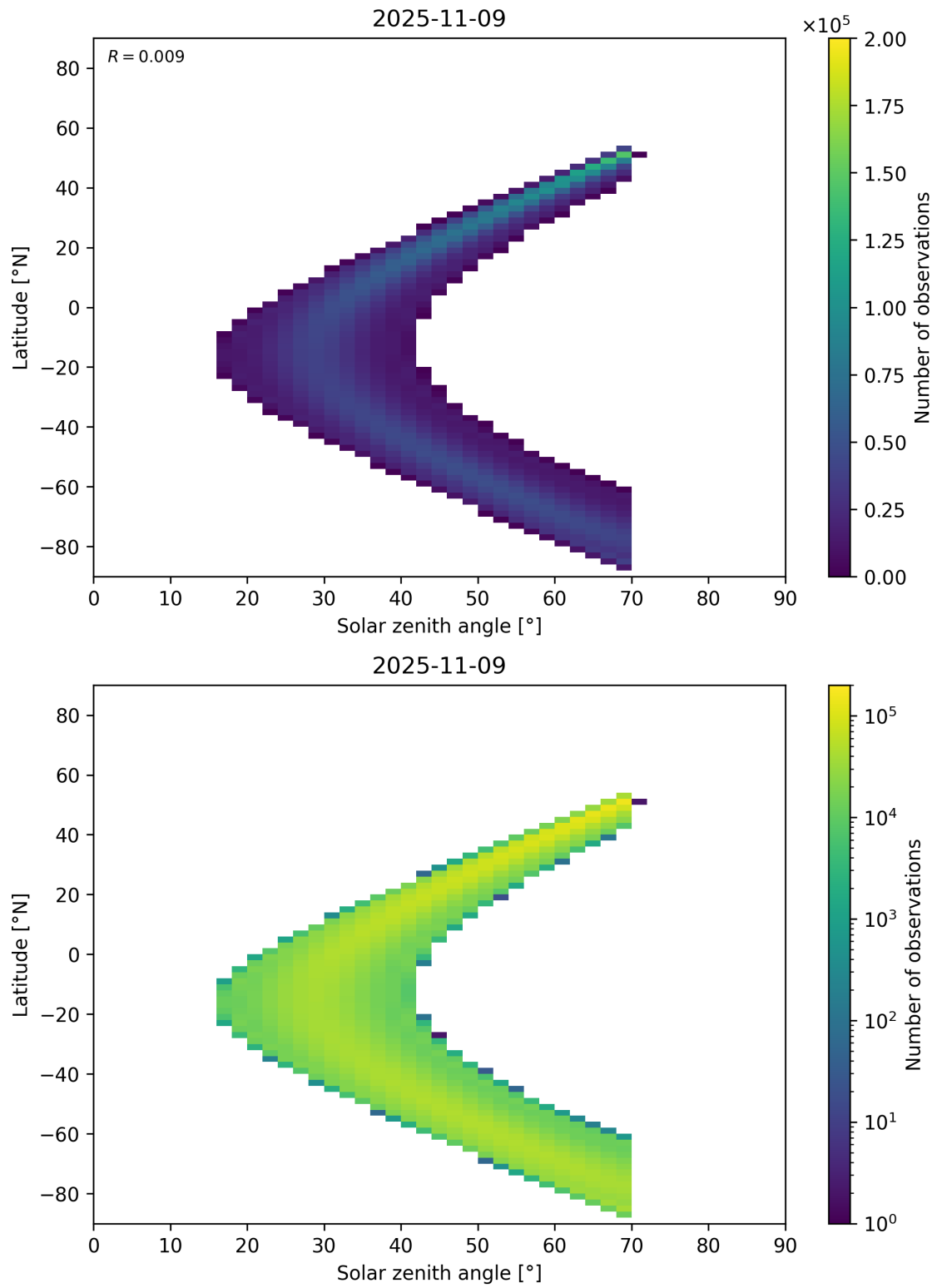
Figure 177: Scatter density plot of “Solar zenith angle” against “Latitude” for 2025-11-08 to 2025-11-10.
