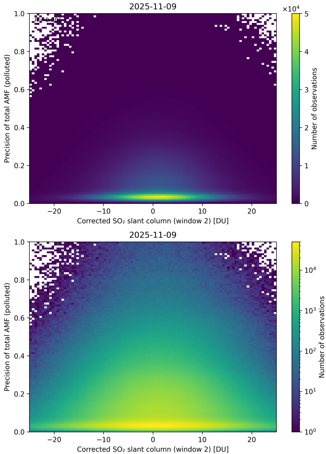
Figure 254: Scatter density plot of “Corrected SO 2 slant column (window 2)” against “Precision of total AMF (polluted)” for 2025-11-08 to 2025-11-10.
