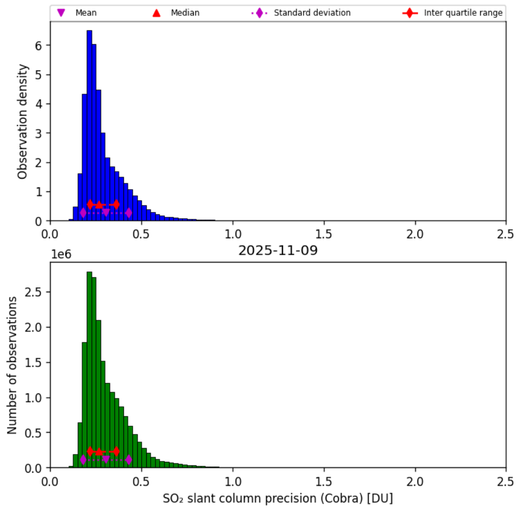
Figure 62: Histogram of “SO 2 slant column precision (Cobra)” for 2025-11-08 to 2025-11-10
