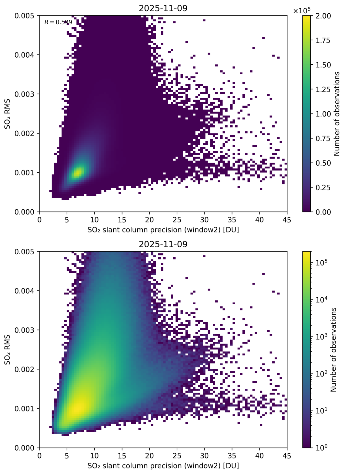
Figure 295: Scatter density plot of “SO 2 slant column precision (window2)” against “SO 2 RMS” for 2025-11-08 to 2025-11-10.
