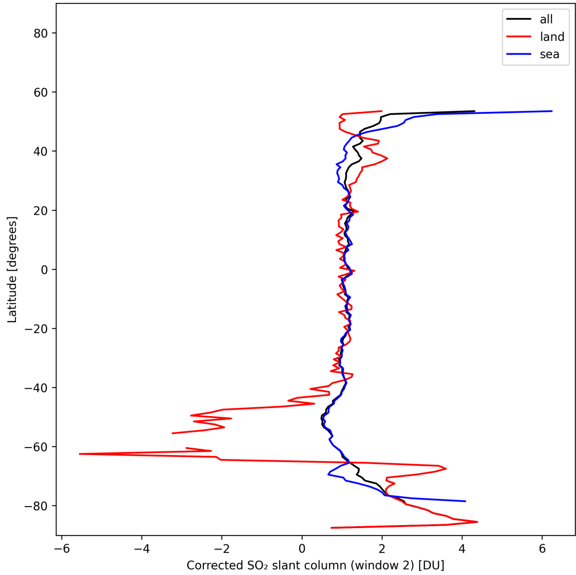
Figure 43: Zonal average of “Corrected SO 2 slant column (window 2)” for 2025-11-08 to 2025-11-10.
