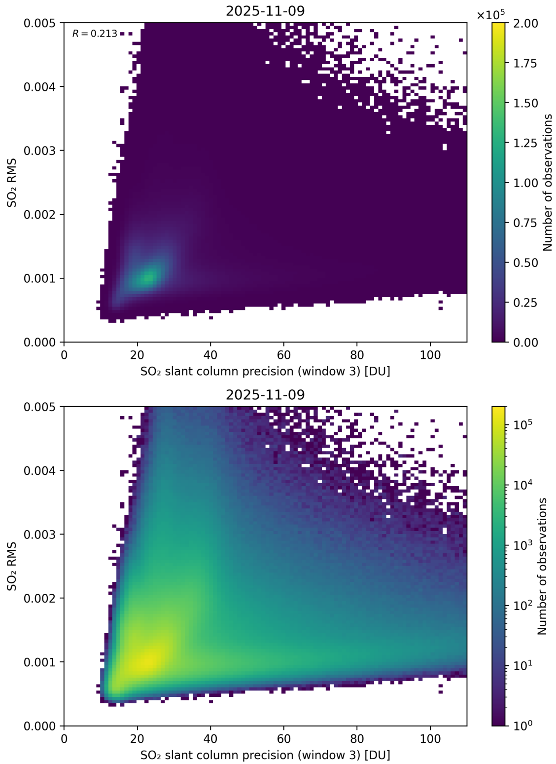
Figure 310: Scatter density plot of “SO 2 slant column precision (window 3)” against “SO 2 RMS” for 2025-11-08 to 2025-11-10.
