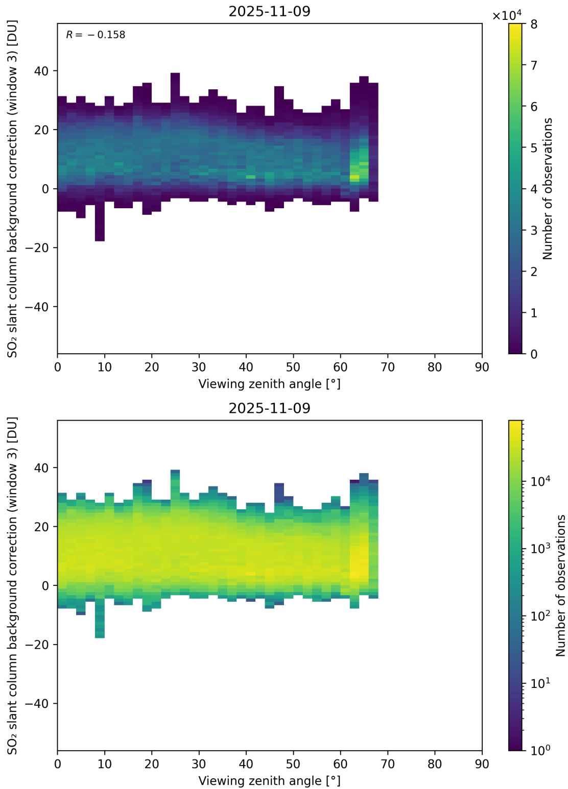
Figure 364: Scatter density plot of “Viewing zenith angle” against “SO 2 slant column background correction (window 3)” for 2025-11-08 to 2025-11-10.
