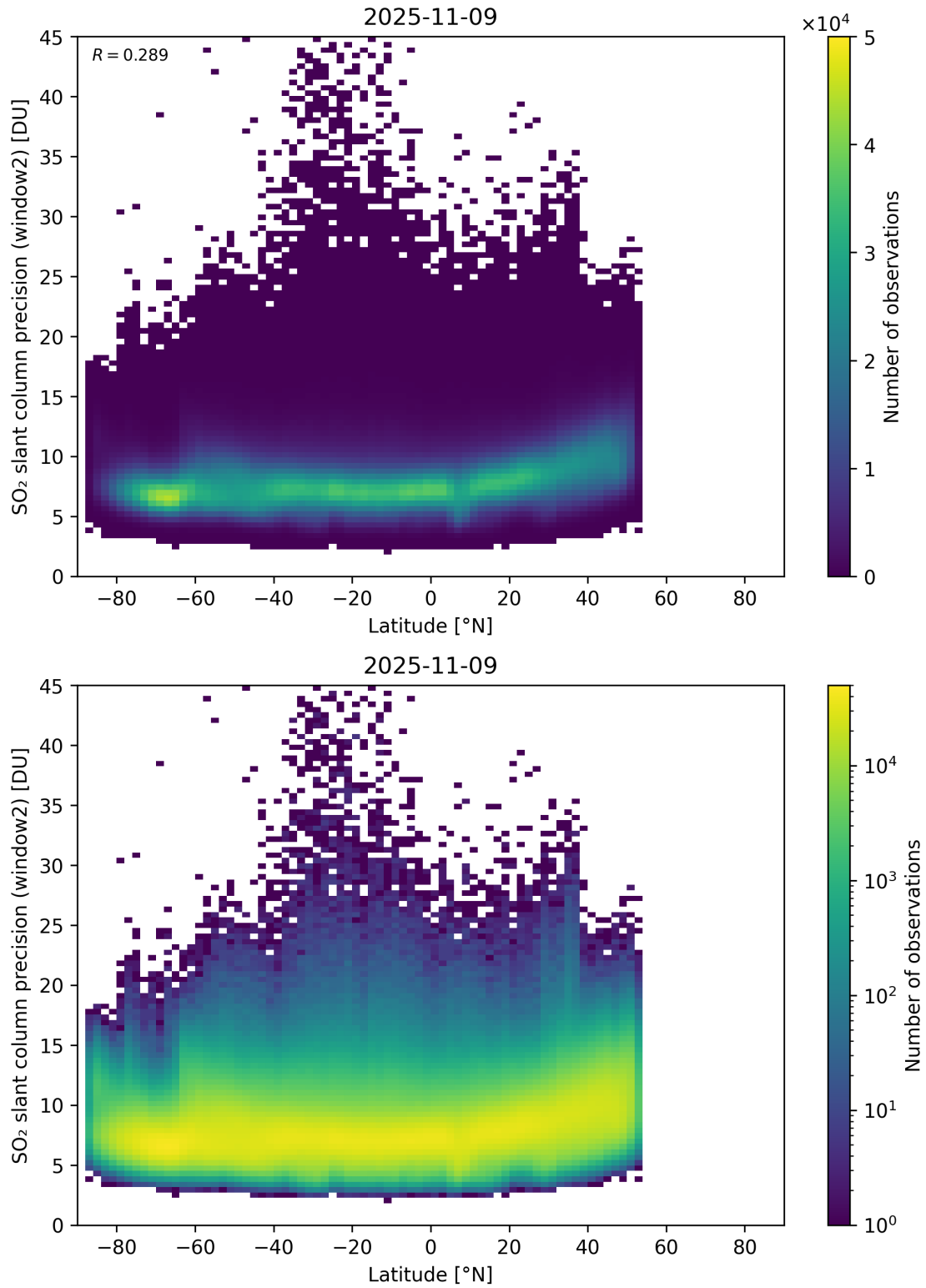
Figure 164: Scatter density plot of “Latitude” against “SO 2 slant column precision (window2)” for 2025-11-08 to 2025-11-10.
