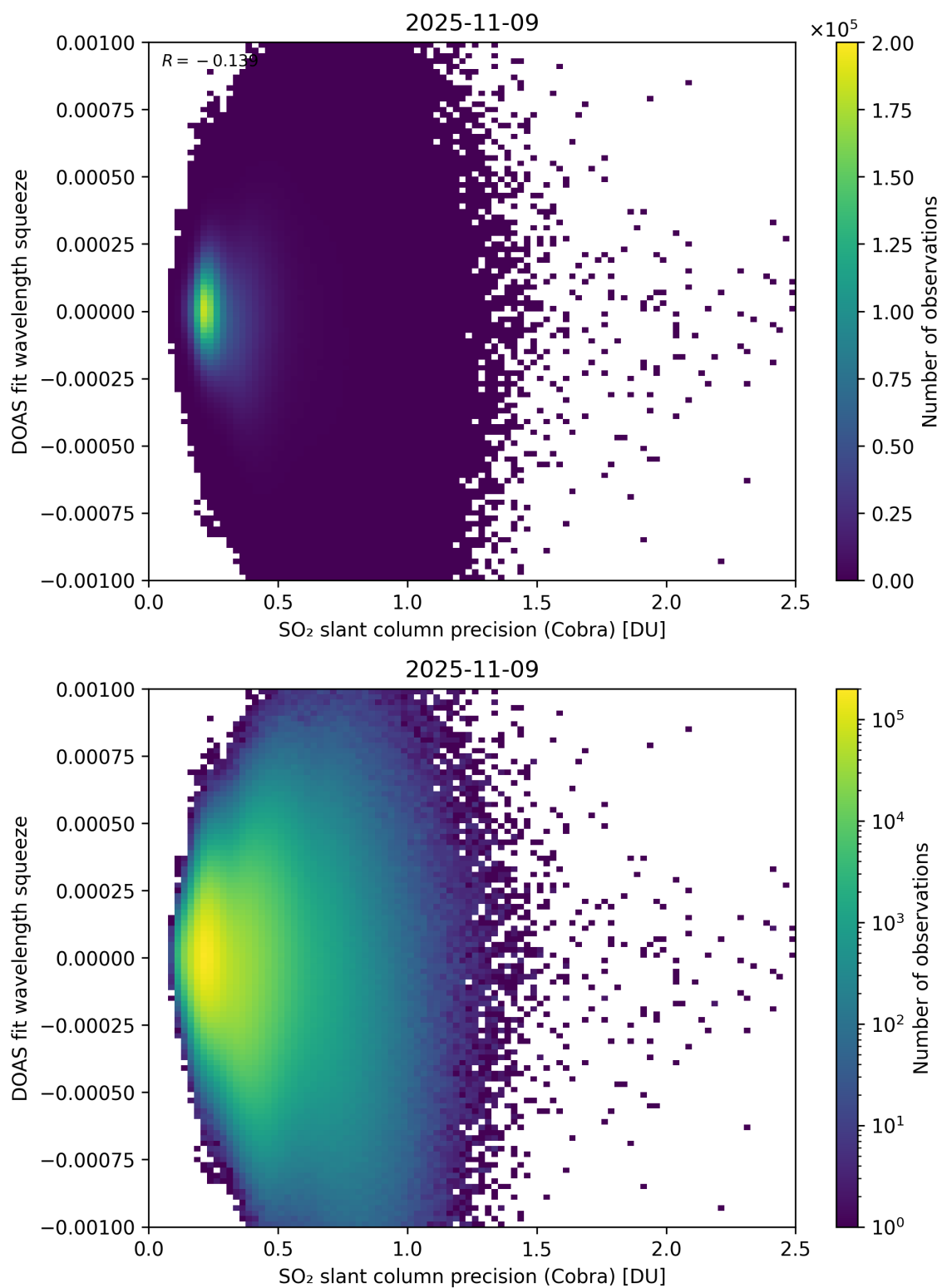
Figure 203: Scatter density plot of “SO 2 slant column precision (Cobra)” against “DOAS fit wavelength squeeze” for 2025-11-08 to 2025-11-10.
