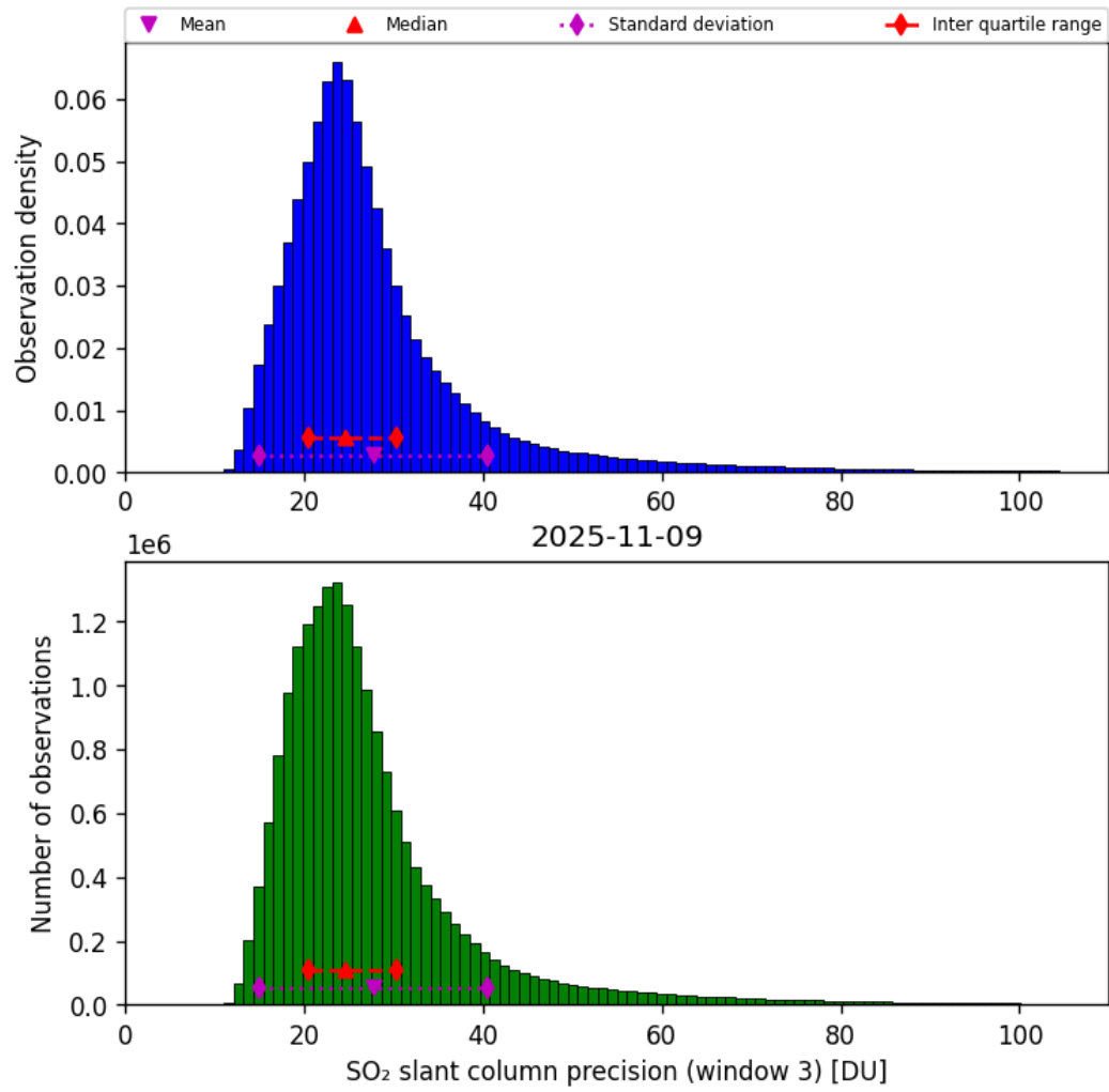
Figure 72: Histogram of “SO 2 slant column precision (window 3)” for 2025-11-08 to 2025-11-10
