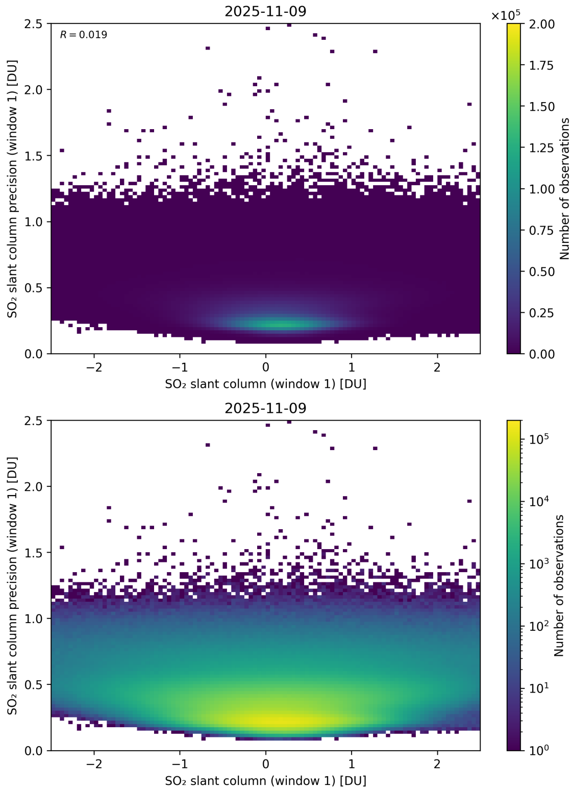
Figure 285: Scatter density plot of “SO 2 slant column (window 1)” against “SO 2 slant column precision (window 1)” for 2025-11-08 to 2025-11-10.
