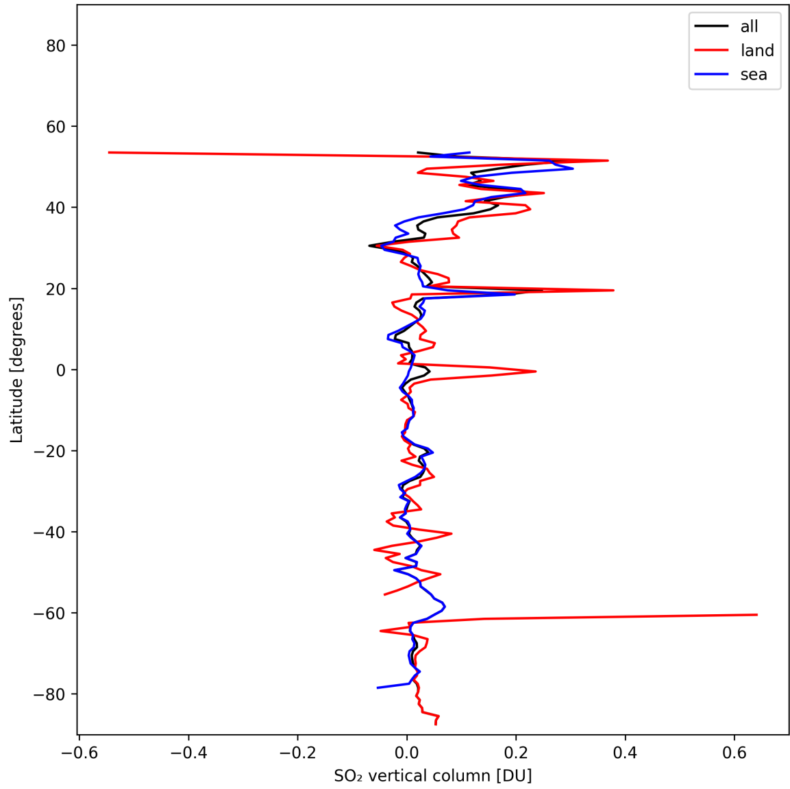
Figure 32: Zonal average of “SO 2 vertical column” for 2025-11-08 to 2025-11-10.
