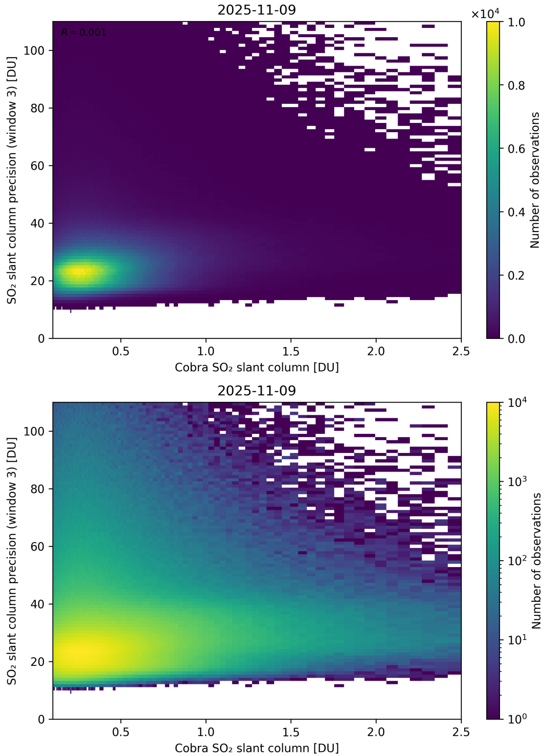
Figure 223: Scatter density plot of “Cobra SO 2 slant column” against “SO 2 slant column precision (window 3)” for 2025-11-08 to 2025-11-10.
