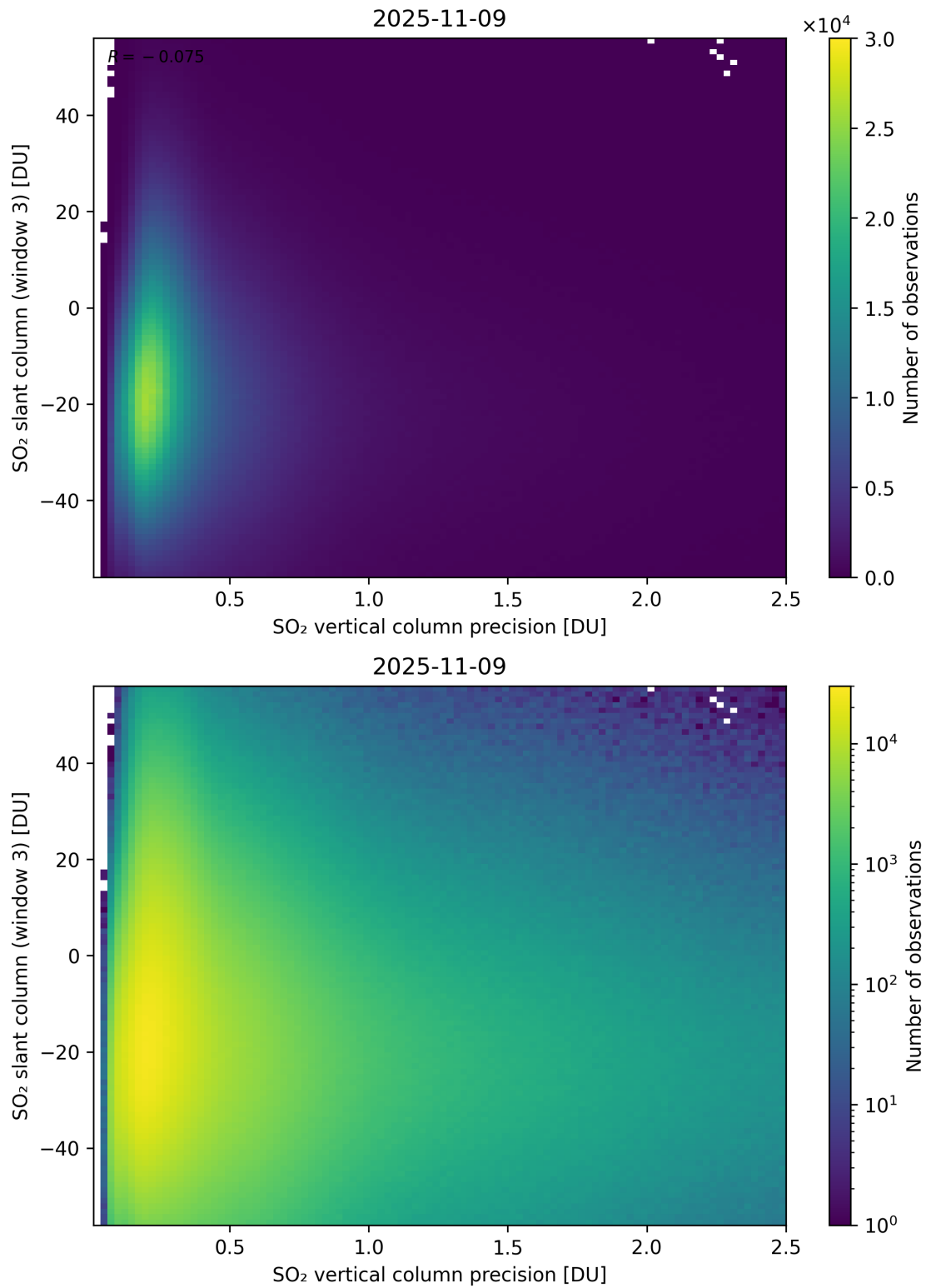
Figure 344: Scatter density plot of “SO 2 vertical column precision” against “SO 2 slant column (window 3)” for 2025-11-08 to 2025-11-10.
