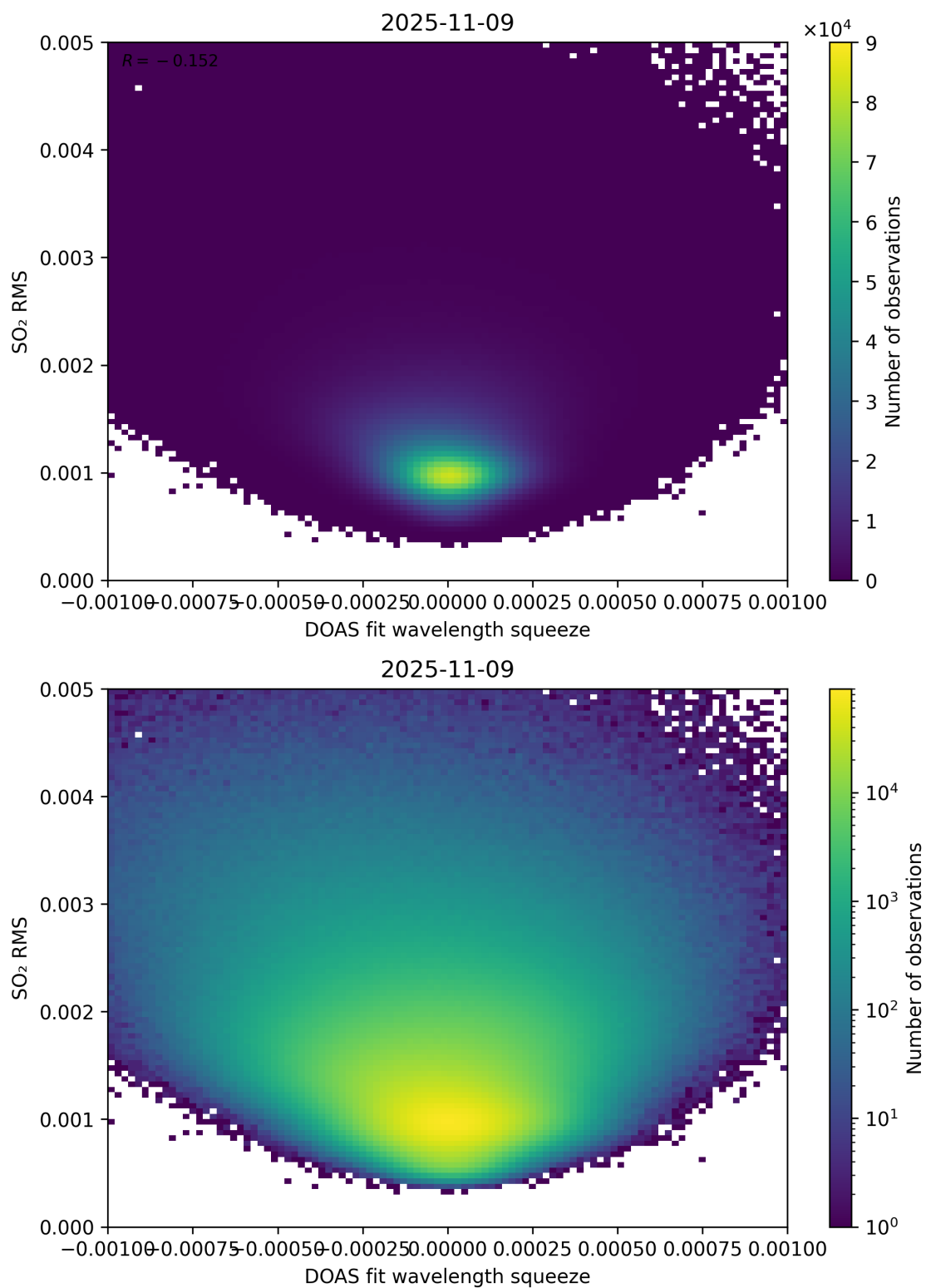
Figure 143: Scatter density plot of “DOAS fit wavelength squeeze” against “SO 2 RMS” for 2025-11-08 to 2025-11-10.
