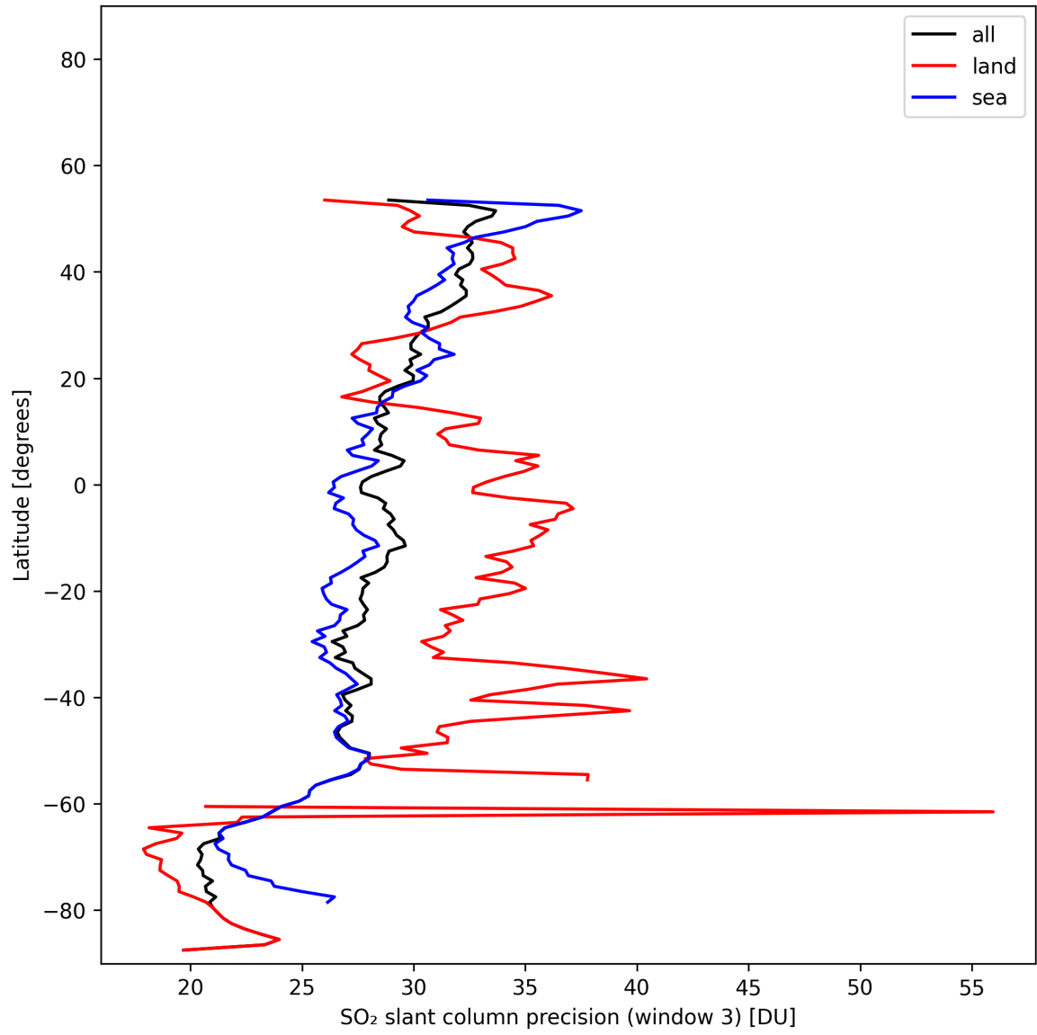
Figure 46: Zonal average of “SO 2 slant column precision (window 3)” for 2025-11-08 to 2025-11-10.
