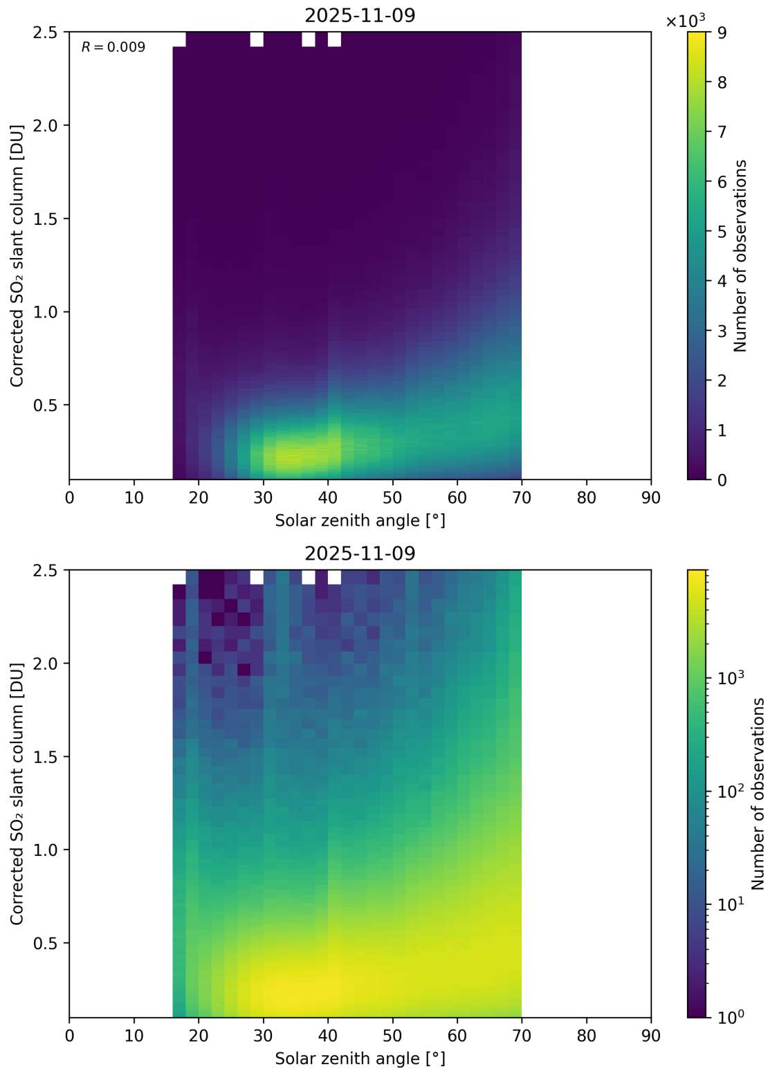
Figure 181: Scatter density plot of “Solar zenith angle” against “Corrected SO 2 slant column” for 2025-11-08 to 2025-11-10.
