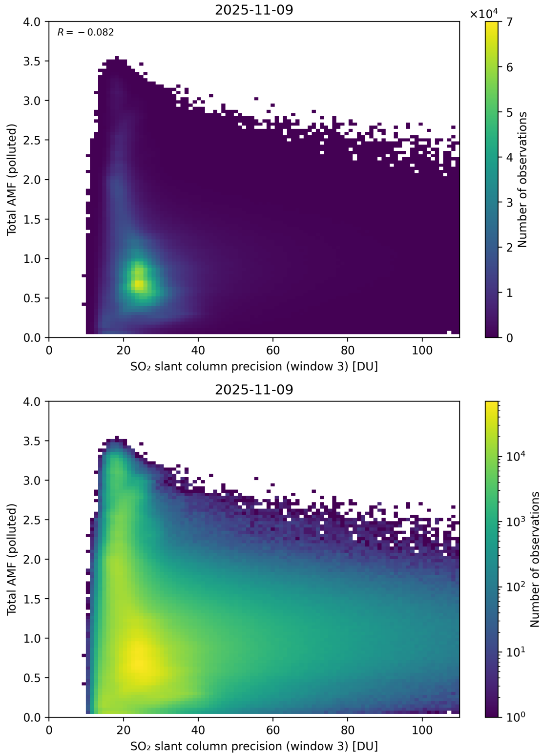
Figure 313: Scatter density plot of “SO 2 slant column precision (window 3)” against “Total AMF (polluted)” for 2025-11-08 to 2025-11-10.
