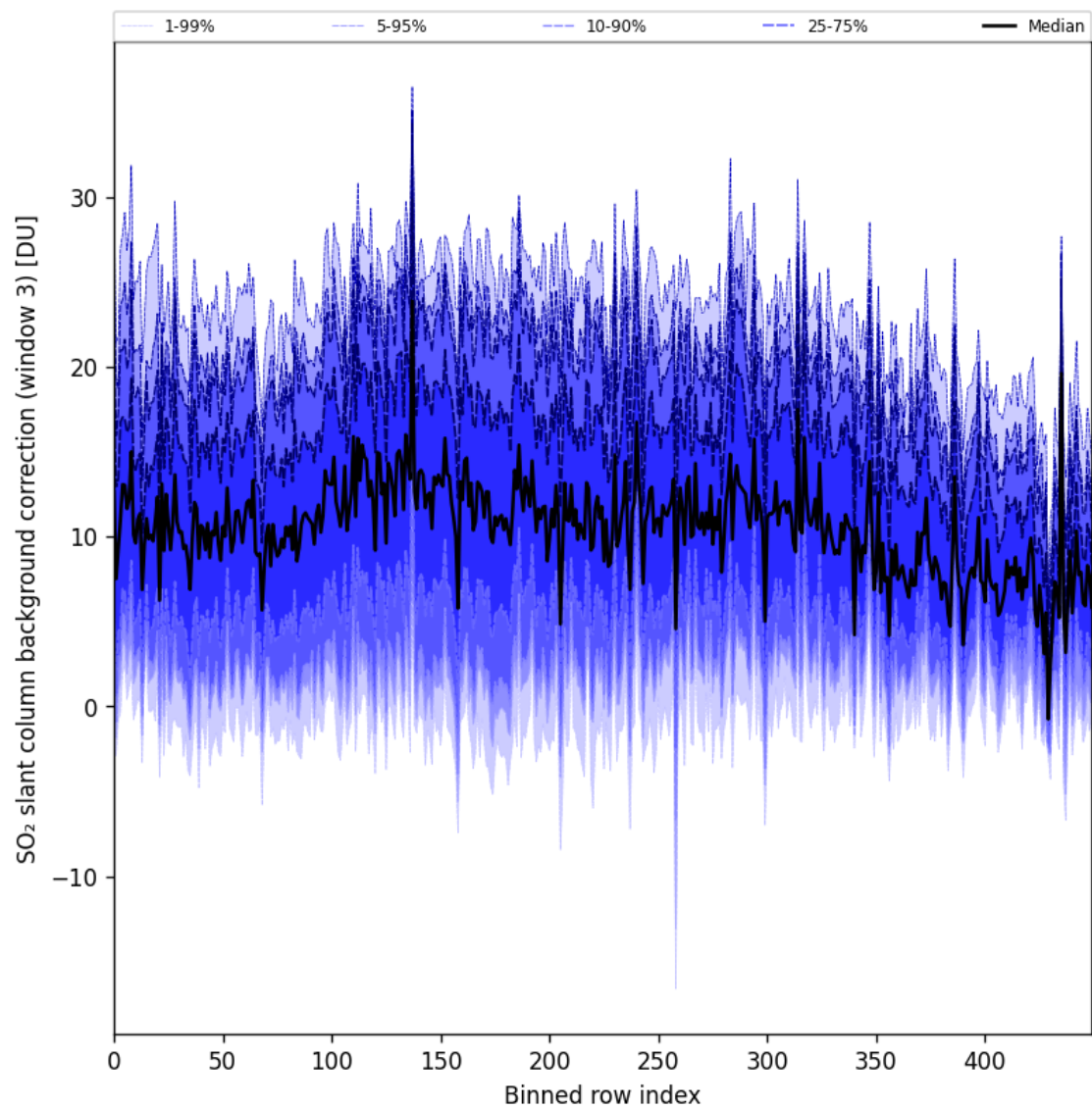
Figure 100: Along track statistics of “SO 2 slant column background correction (window 3)” for 2025-11-08 to 2025-11-10
