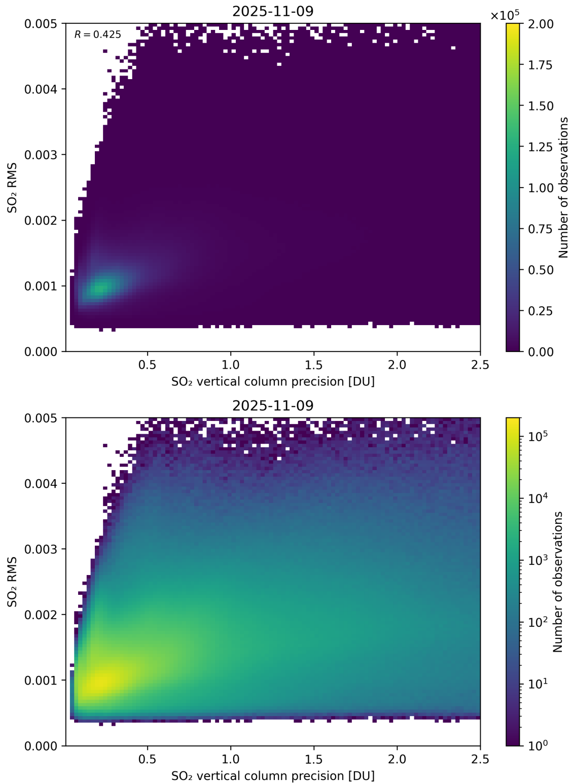
Figure 334: Scatter density plot of “SO 2 vertical column precision” against “SO 2 RMS” for 2025-11-08 to 2025-11-10.
