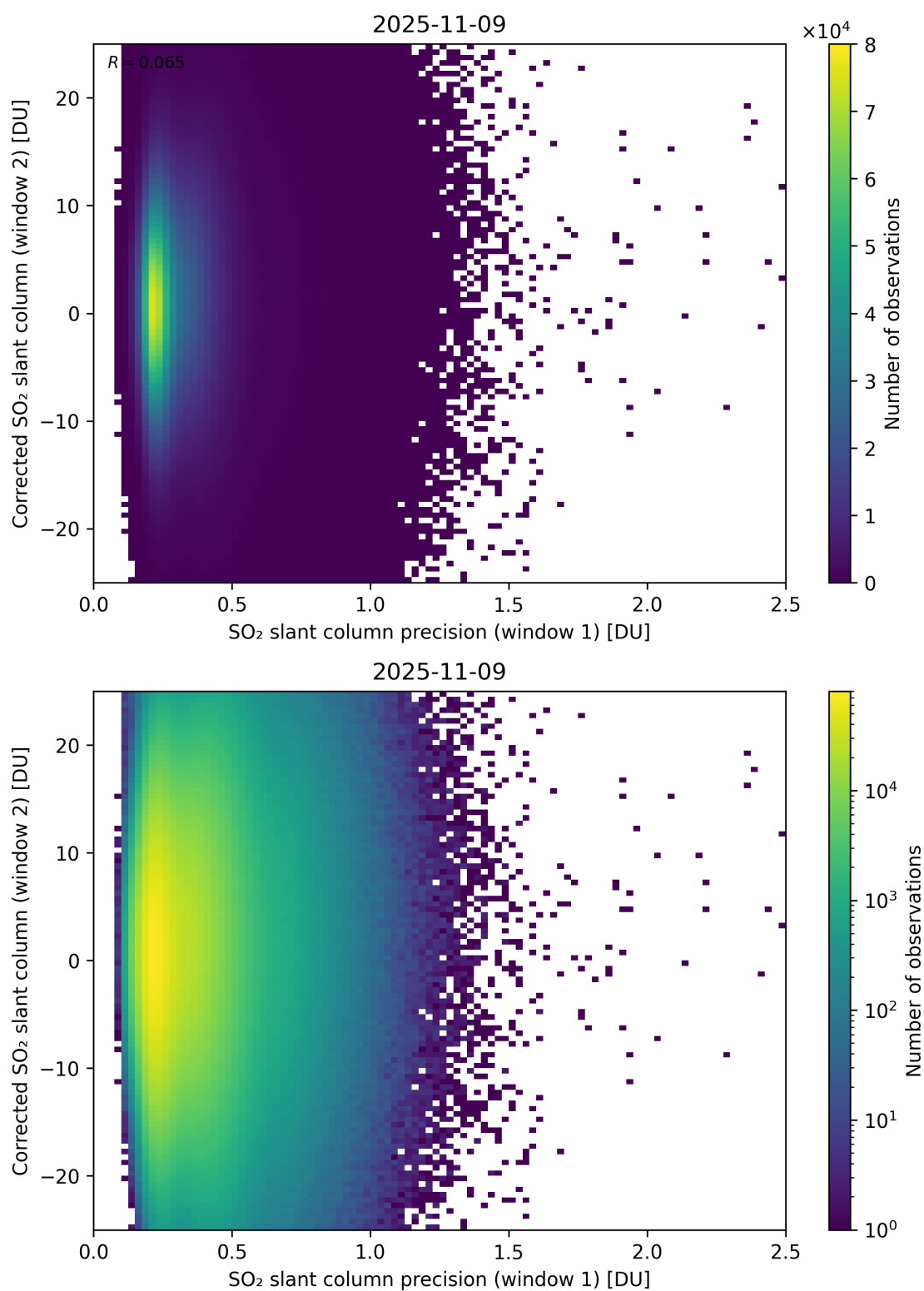
Figure 275: Scatter density plot of “SO 2 slant column precision (window 1)” against “Corrected SO 2 slant column (window 2)” for 2025-11-08 to 2025-11-10.
