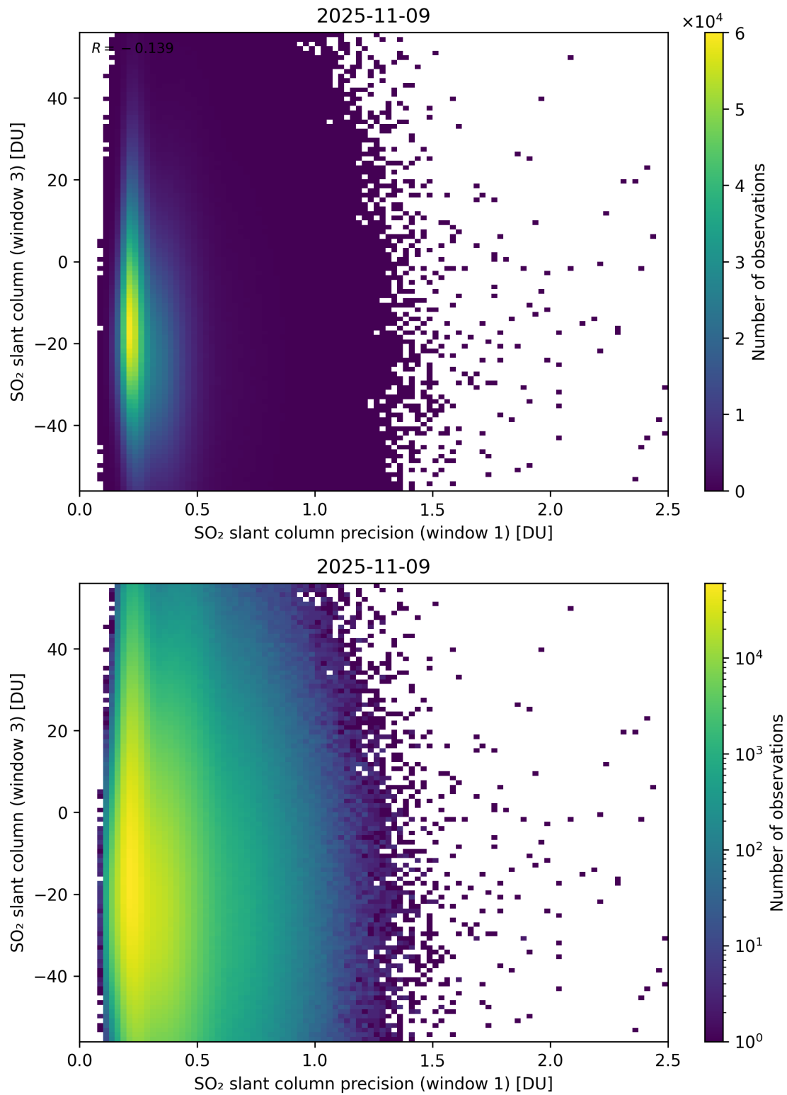
Figure 278: Scatter density plot of “SO 2 slant column precision (window 1)” against “SO 2 slant column (window 3)” for 2025-11-08 to 2025-11-10.
