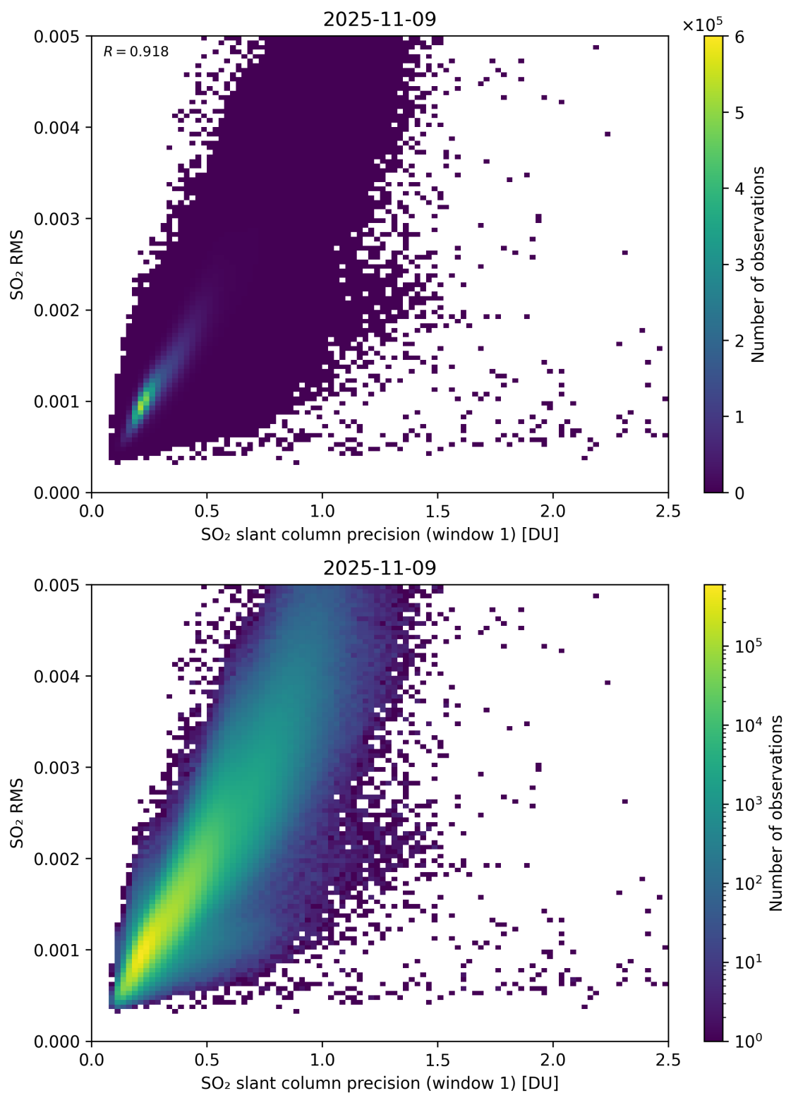
Figure 273: Scatter density plot of “SO 2 slant column precision (window 1)” against “SO 2 RMS” for 2025-11-08 to 2025-11-10.
