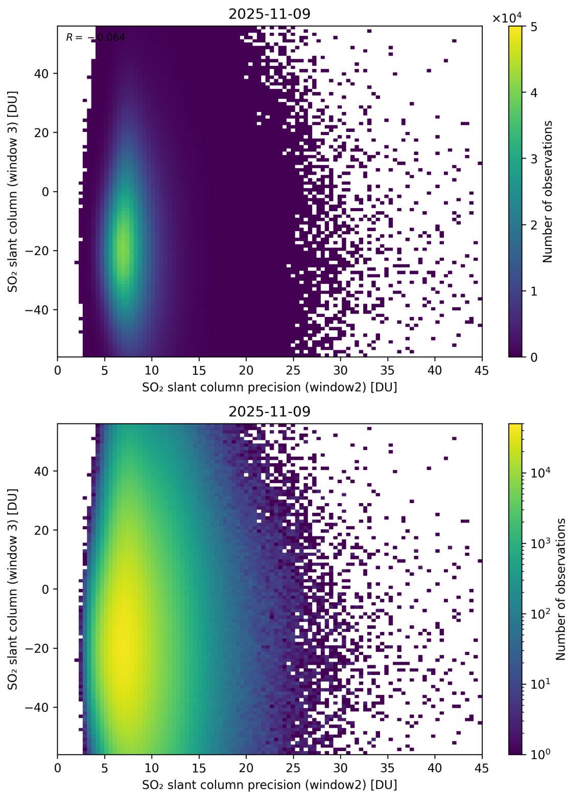
Figure 299: Scatter density plot of “SO 2 slant column precision (window2)” against “SO 2 slant column (window 3)” for 2025-11-08 to 2025-11-10.
