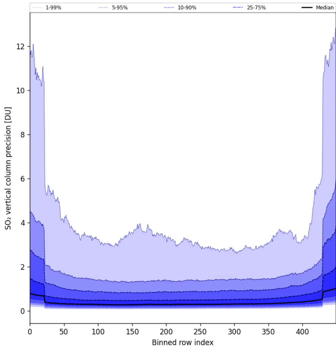
Figure 85: Along track statistics of “SO 2 vertical column precision” for 2025-11-08 to 2025-11-10
