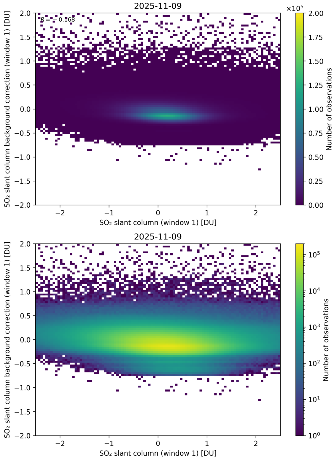
Figure 262: Scatter density plot of “SO 2 slant column (window 1)” against “SO 2 slant column background correction (window 1)” for 2025-11-08 to 2025-11-10.
