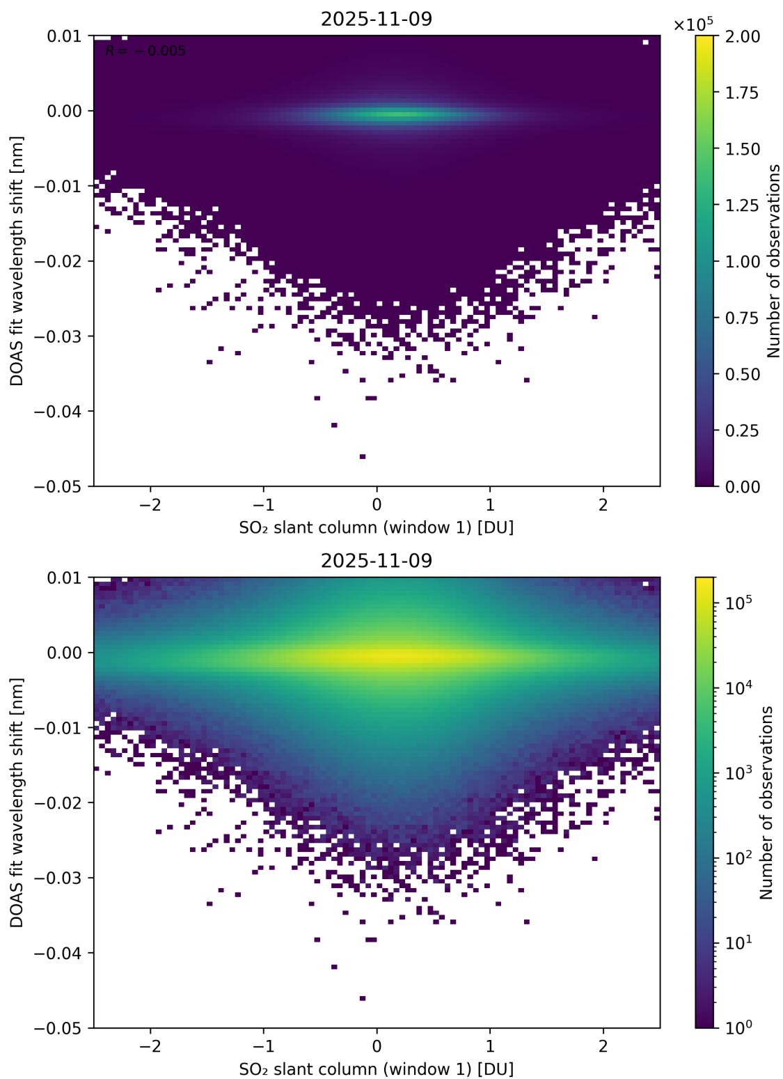
Figure 265: Scatter density plot of “SO 2 slant column (window 1)” against “DOAS fit wavelength shift” for 2025-11-08 to 2025-11-10.
