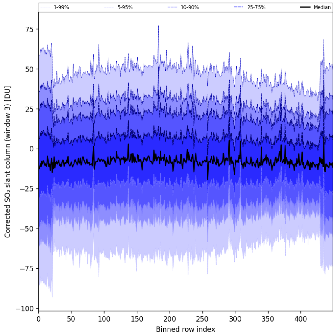
Figure 99: Along track statistics of “Corrected SO 2 slant column (window 3)” for 2025-11-08 to 2025-11-10
