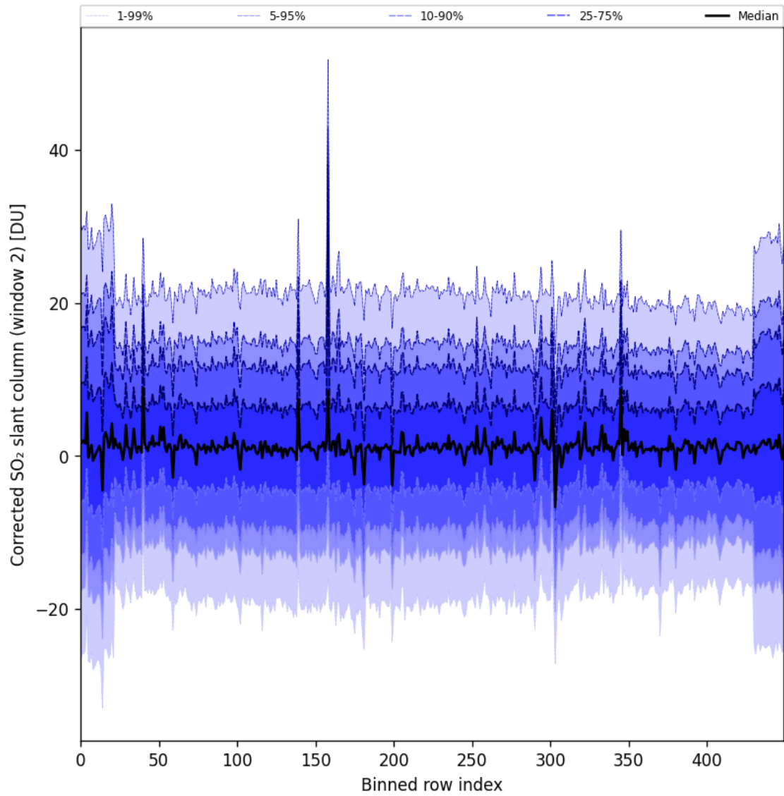
Figure 95: Along track statistics of “Corrected SO 2 slant column (window 2)” for 2025-11-08 to 2025-11-10
