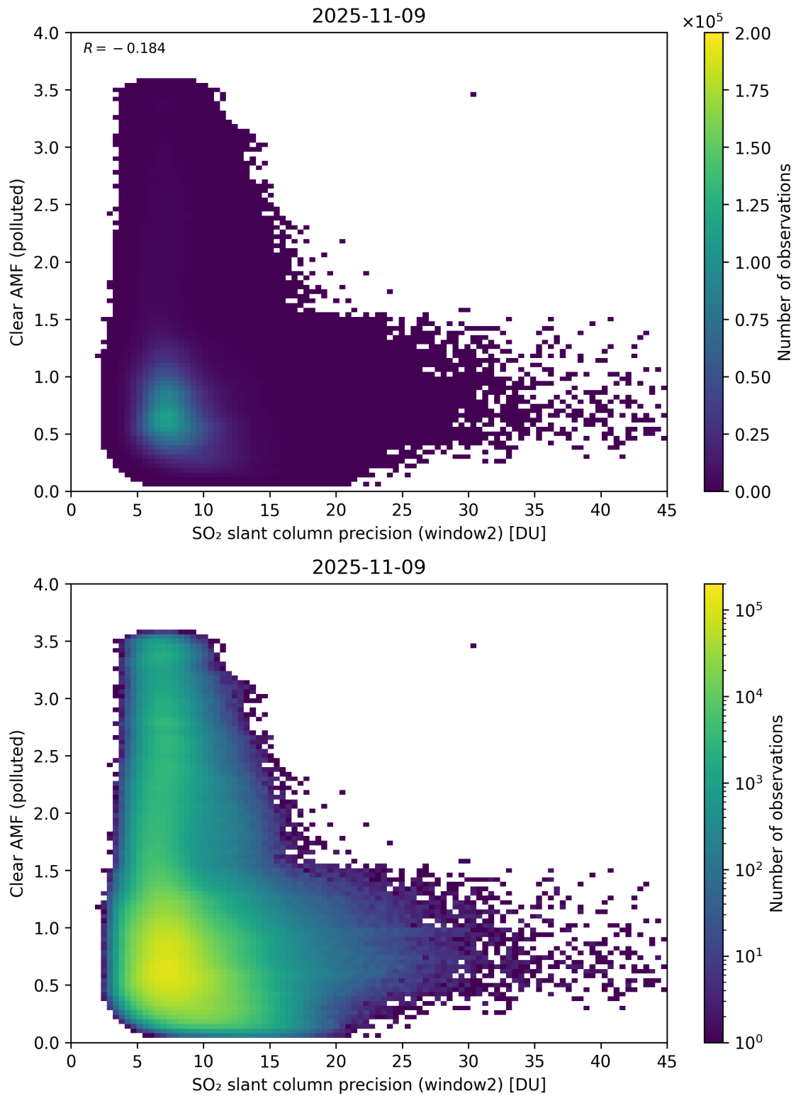
Figure 296: Scatter density plot of “SO 2 slant column precision (window2)” against “Clear AMF (polluted)” for 2025-11-08 to 2025-11-10.
