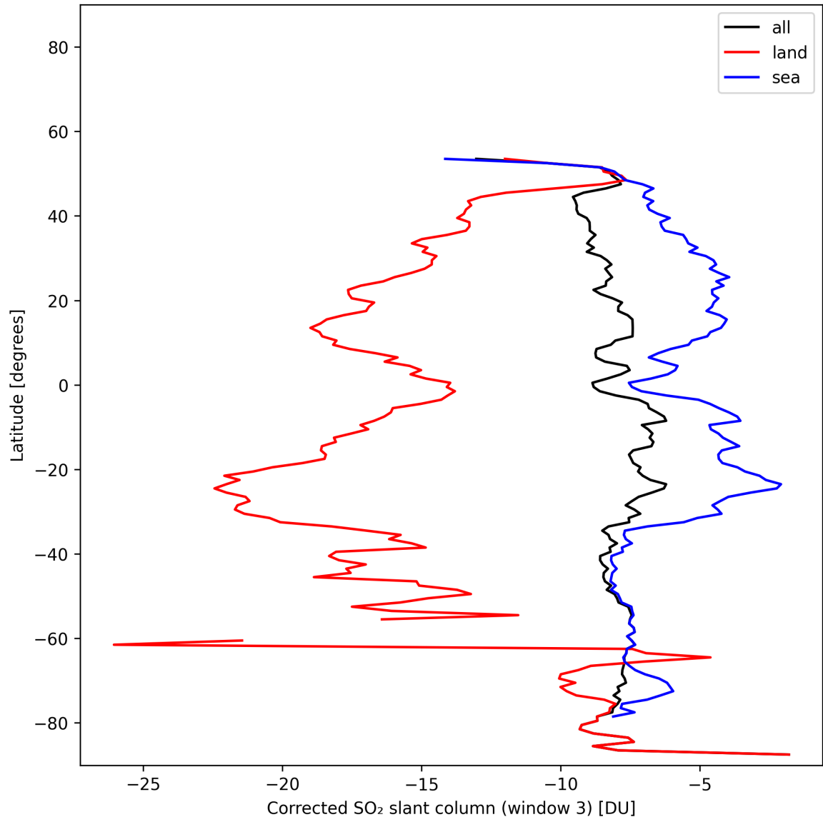
Figure 47: Zonal average of “Corrected SO 2 slant column (window 3)” for 2025-11-08 to 2025-11-10.
