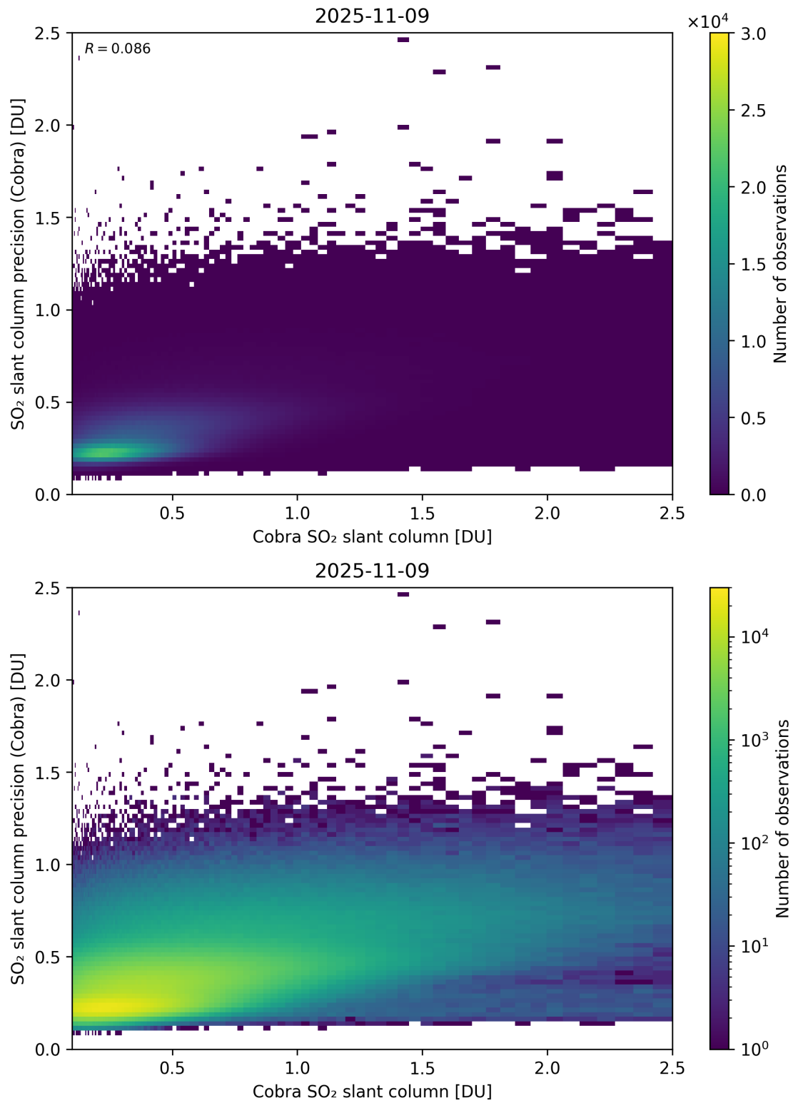
Figure 216: Scatter density plot of “Cobra SO 2 slant column” against “SO 2 slant column precision (Cobra)” for 2025-11-08 to 2025-11-10.
