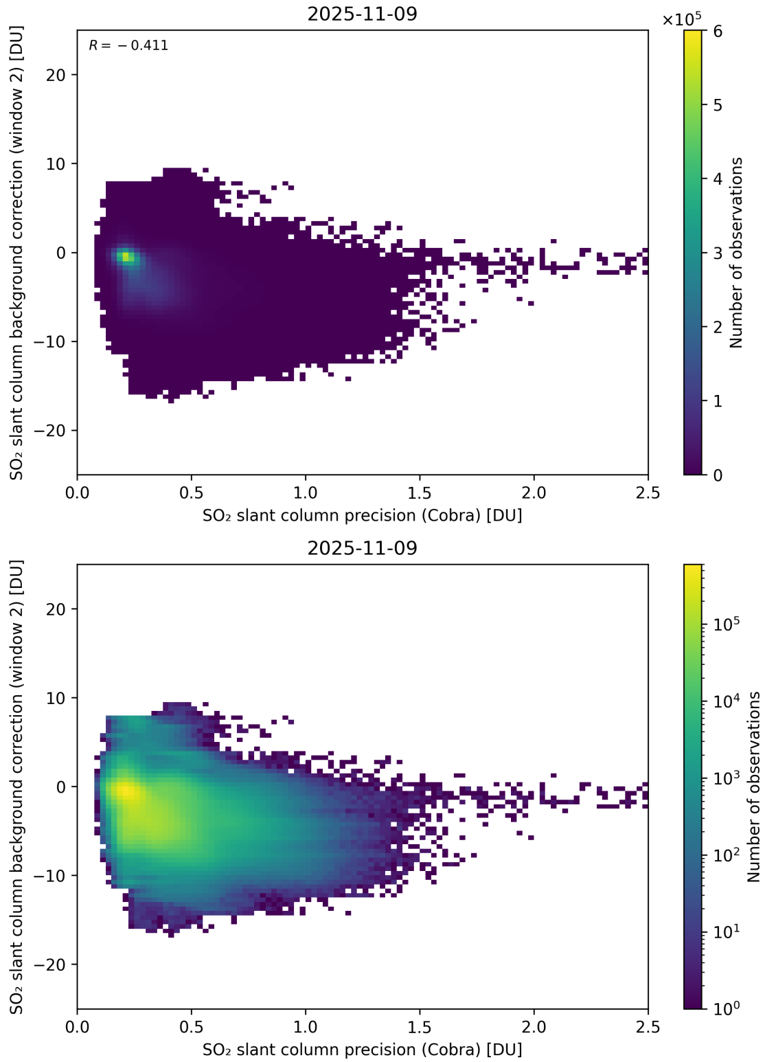
Figure 200: Scatter density plot of “SO 2 slant column precision (Cobra)” against “SO 2 slant column background correction (window 2)” for 2025-11-08 to 2025-11-10.
