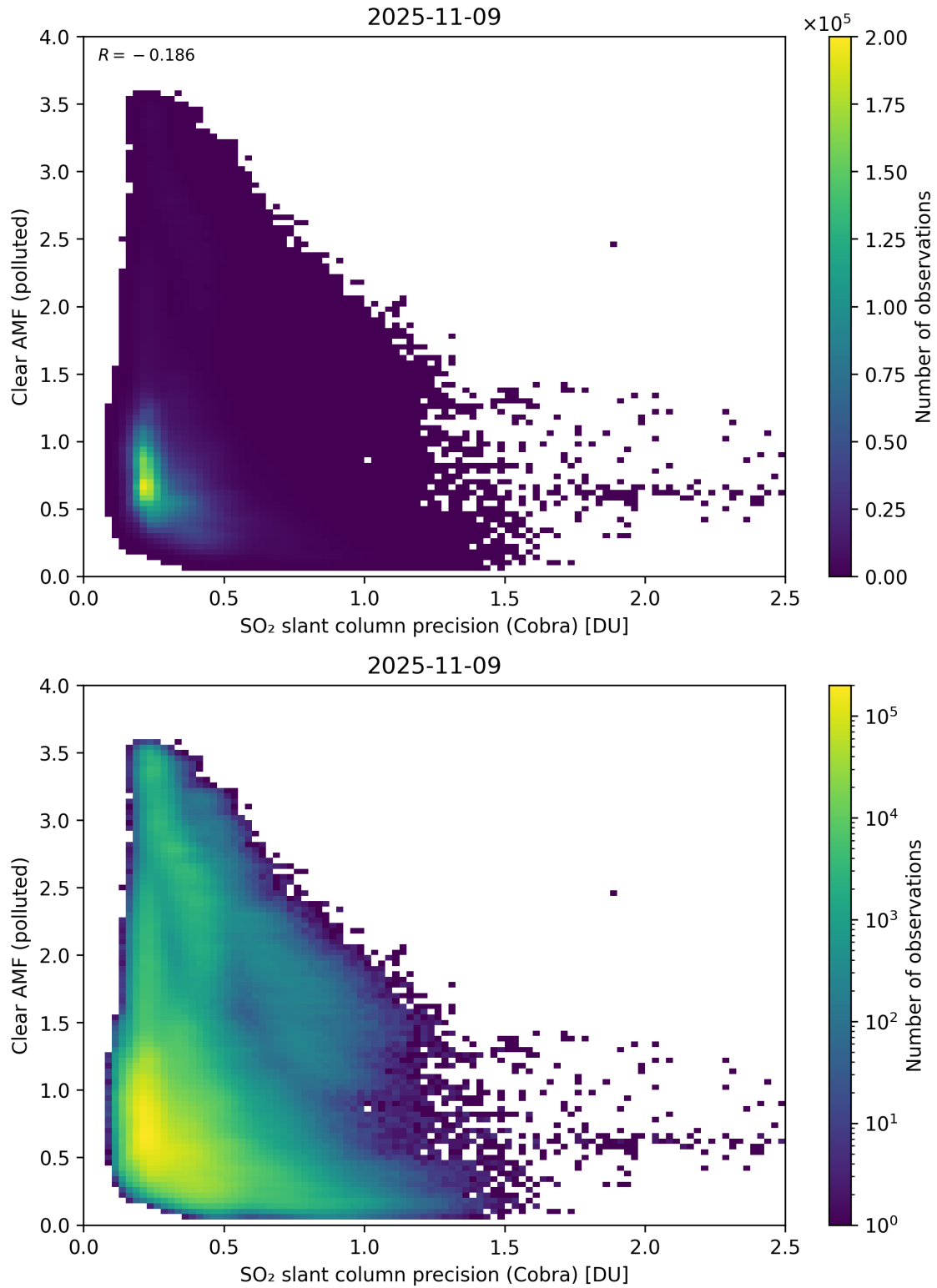
Figure 205: Scatter density plot of “SO 2 slant column precision (Cobra)” against “Clear AMF (polluted)” for 2025-11-08 to 2025-11-10.
