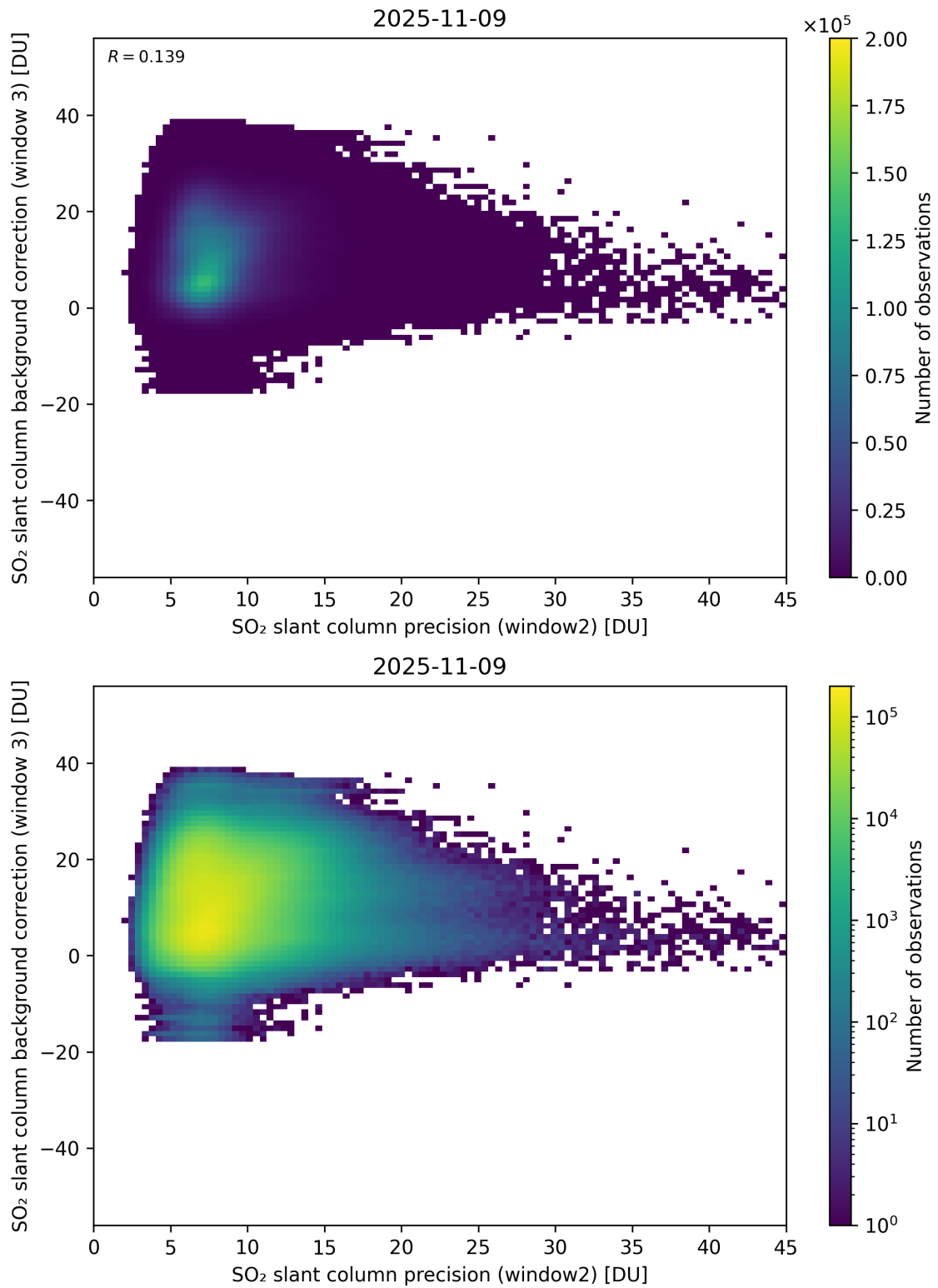
Figure 292: Scatter density plot of “SO 2 slant column precision (window2)” against “SO 2 slant column background correction (window 3)” for 2025-11-08 to 2025-11-10.
