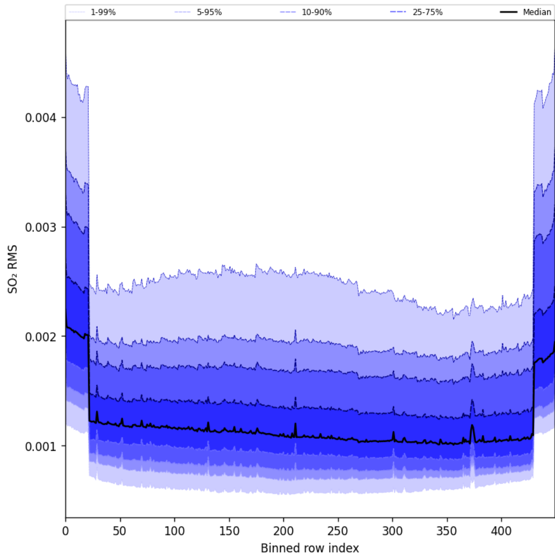
Figure 104: Along track statistics of “SO 2 RMS” for 2025-11-08 to 2025-11-10
