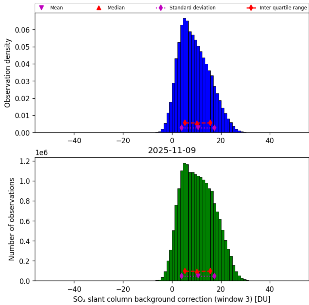
Figure 74: Histogram of “SO 2 slant column background correction (window 3)” for 2025-11-08 to 2025-11-10
