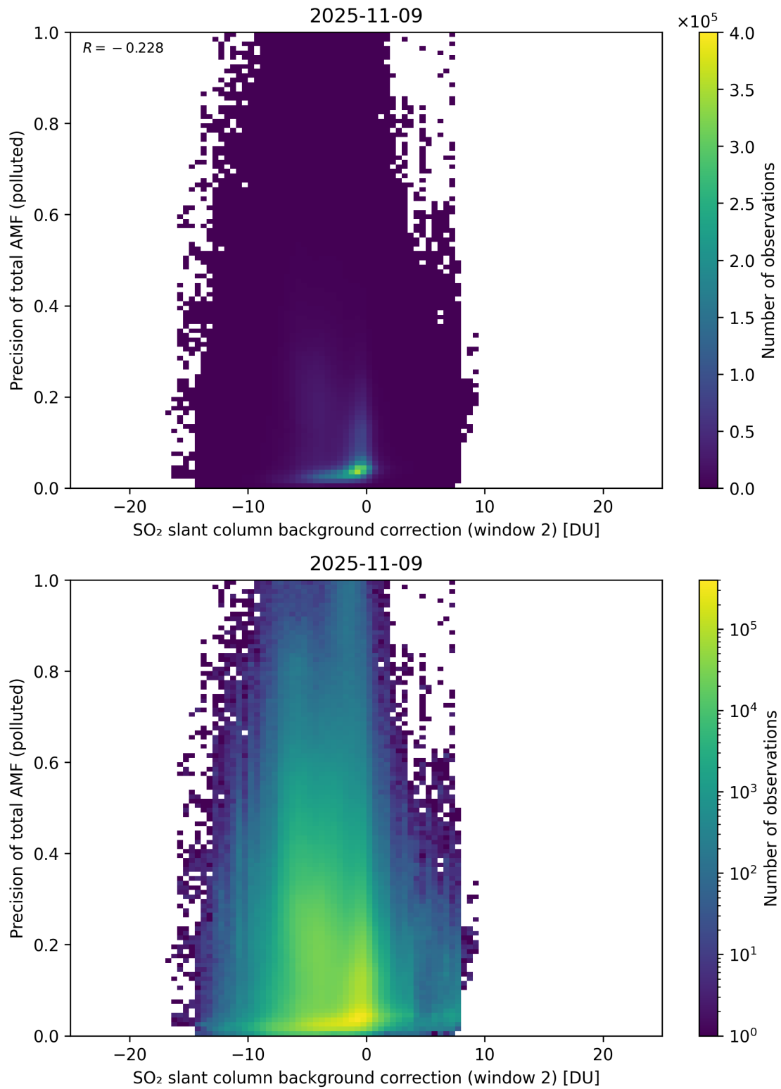
Figure 131: Scatter density plot of “SO 2 slant column background correction (window 2)” against “Precision of total AMF (polluted)” for 2025-11-08 to 2025-11-10.
