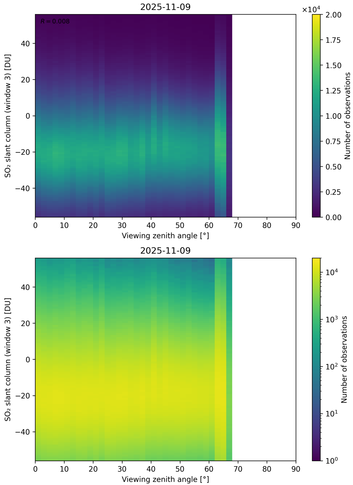
Figure 379: Scatter density plot of “Viewing zenith angle” against “SO 2 slant column (window 3)” for 2025-11-08 to 2025-11-10.
