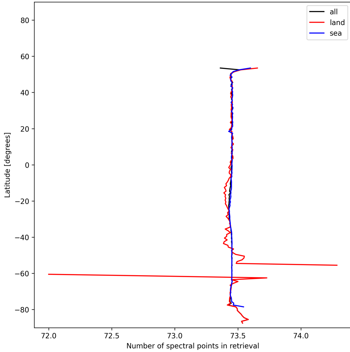
Figure 56: Zonal average of “Number of spectral points in retrieval” for 2025-11-08 to 2025-11-10.
