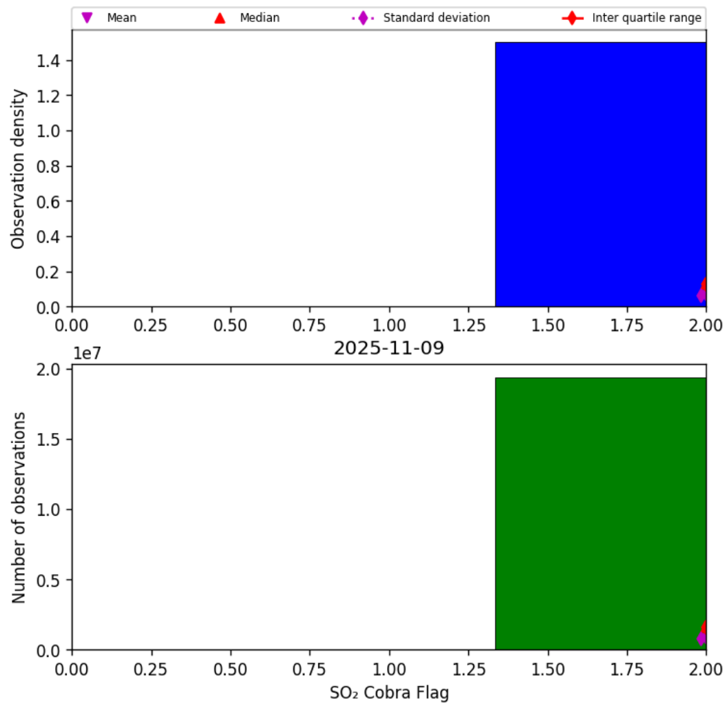
Figure 75: Histogram of “SO 2 Cobra Flag” for 2025-11-08 to 2025-11-10
