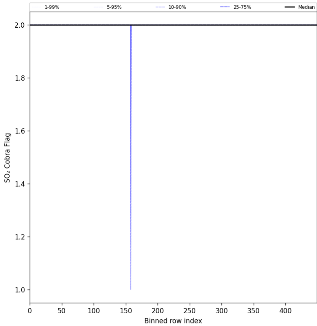
Figure 101: Along track statistics of “SO 2 Cobra Flag” for 2025-11-08 to 2025-11-10
