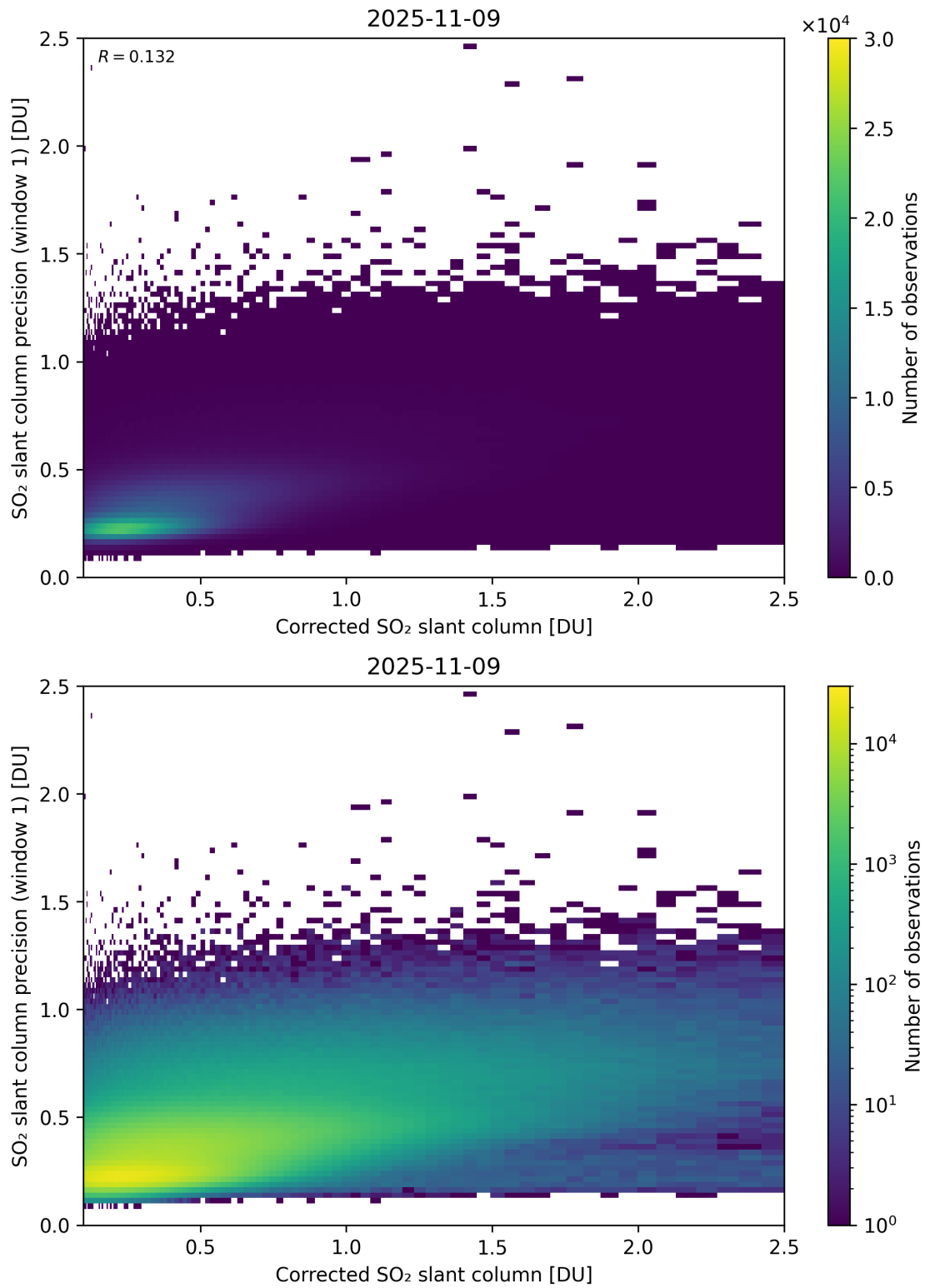
Figure 238: Scatter density plot of “Corrected SO 2 slant column” against “SO 2 slant column precision (window 1)” for 2025-11-08 to 2025-11-10.
