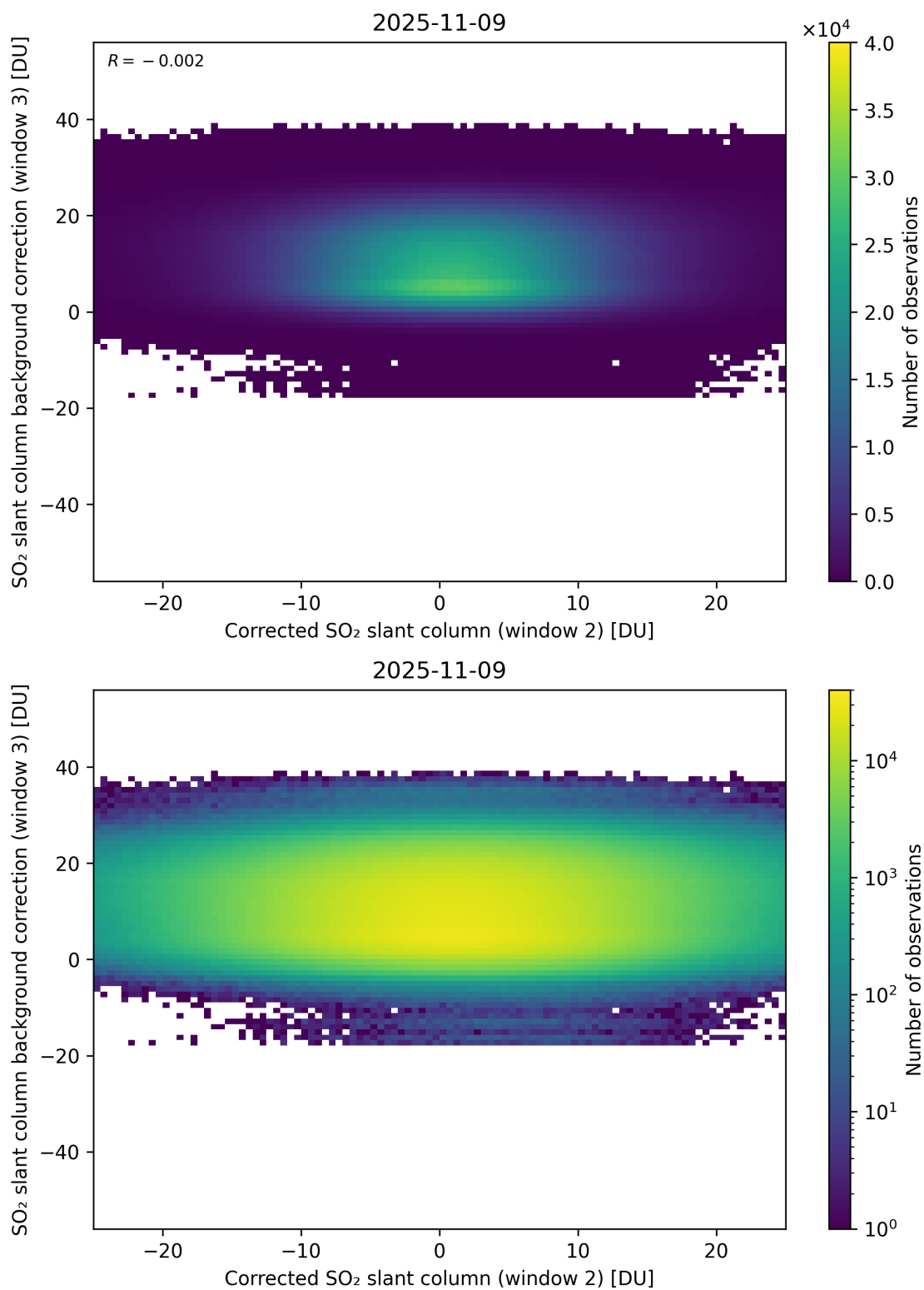
Figure 245: Scatter density plot of “Corrected SO 2 slant column (window 2)” against “SO 2 slant column background correction (window 3)” for 2025-11-08 to 2025-11-10.
