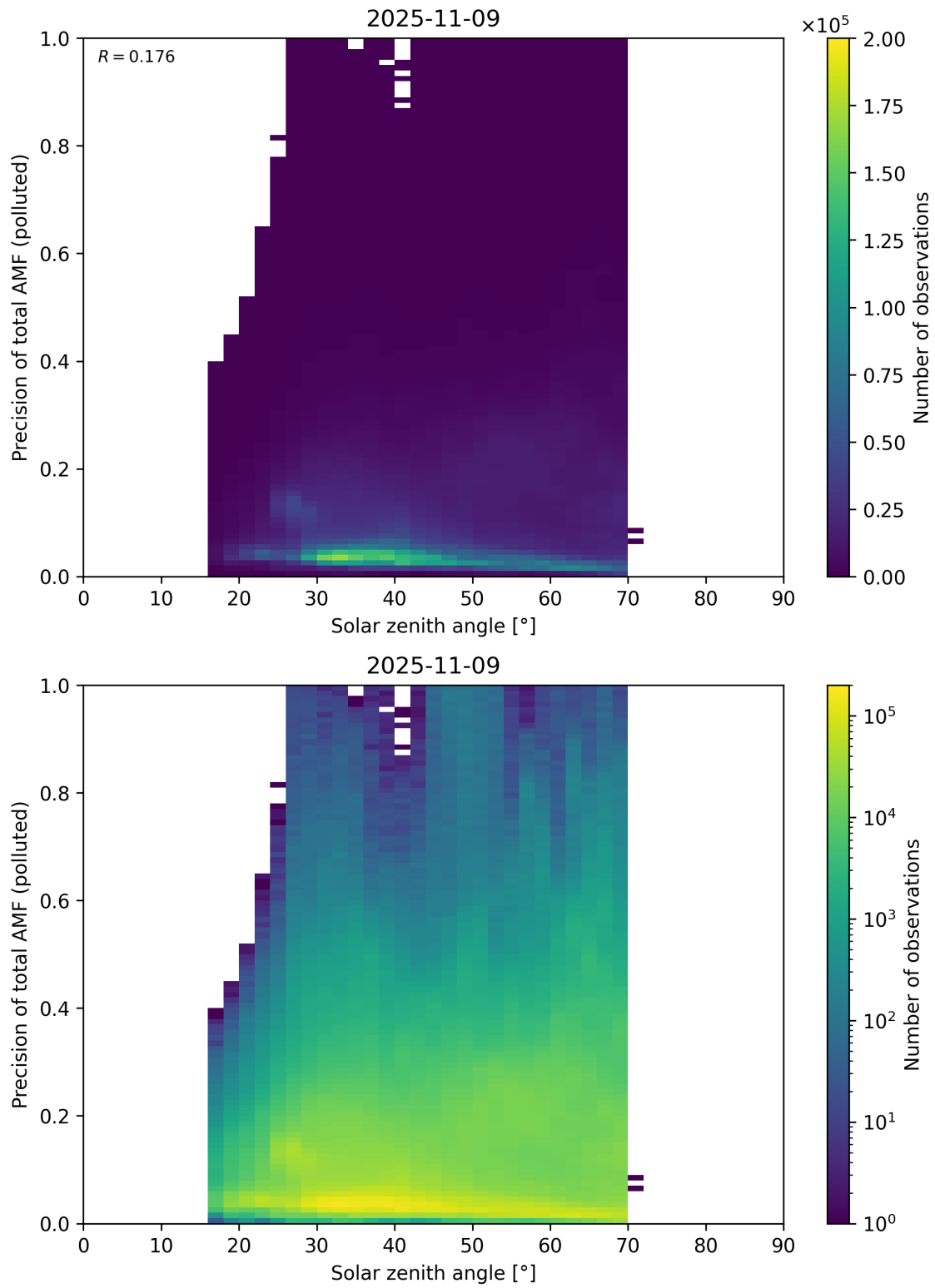
Figure 190: Scatter density plot of “Solar zenith angle” against “Precision of total AMF (polluted)” for 2025-11-08 to 2025-11-10.
