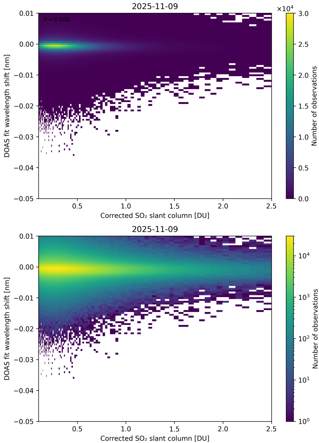
Figure 229: Scatter density plot of “Corrected SO 2 slant column” against “DOAS fit wavelength shift” for 2025-11-08 to 2025-11-10.
