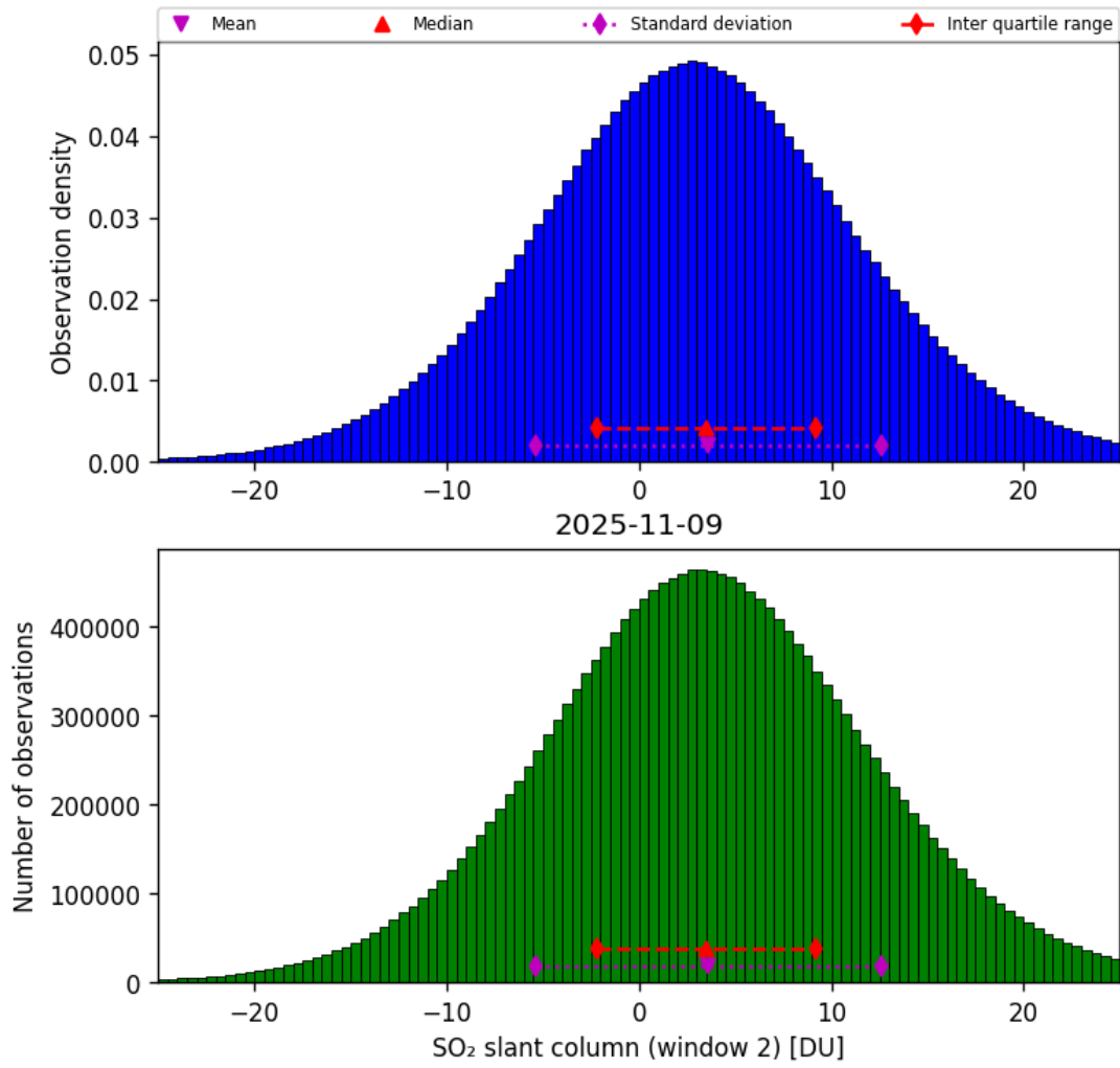
Figure 67: Histogram of “SO 2 slant column (window 2)” for 2025-11-08 to 2025-11-10
