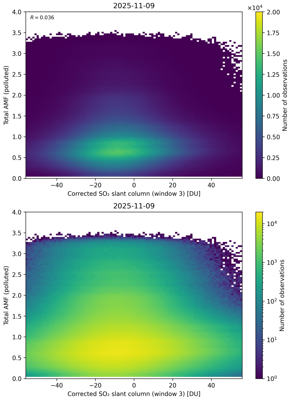
Figure 260: Scatter density plot of “Corrected SO 2 slant column (window 3)” against “Total AMF (polluted)” for 2025-11-08 to 2025-11-10.
