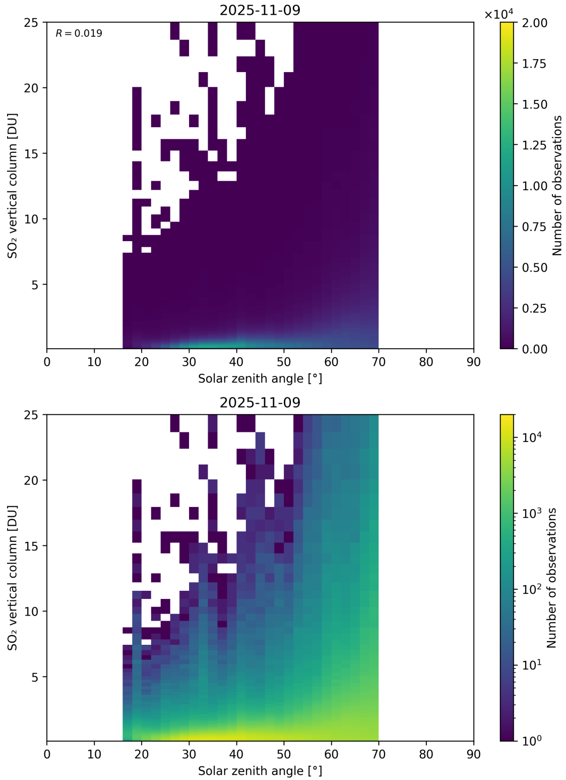
Figure 191: Scatter density plot of “Solar zenith angle” against “SO 2 vertical column” for 2025-11-08 to 2025-11-10.
