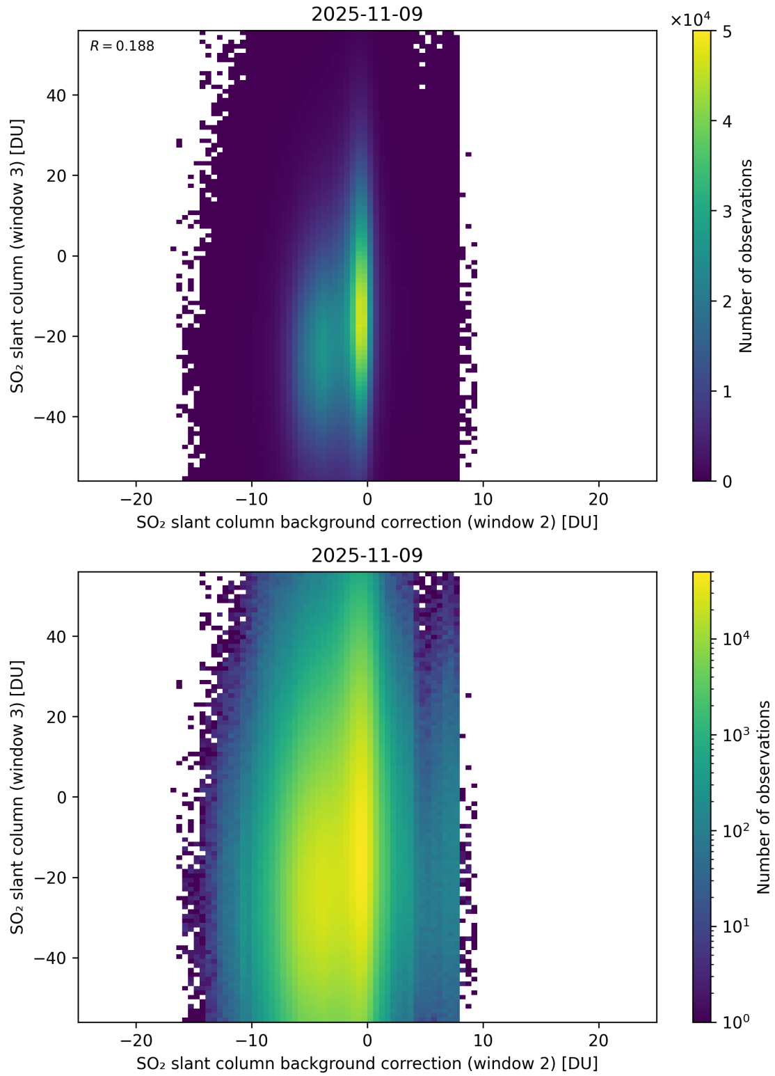
Figure 128: Scatter density plot of “SO 2 slant column background correction (window 2)” against “SO 2 slant column (window 3)” for 2025-11-08 to 2025-11-10.
