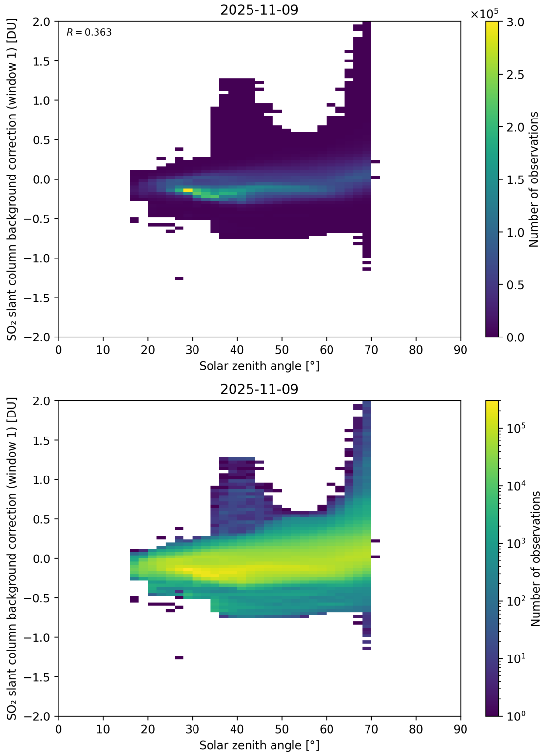
Figure 171: Scatter density plot of “Solar zenith angle” against “SO 2 slant column background correction (window 1)” for 2025-11-08 to 2025-11-10.
