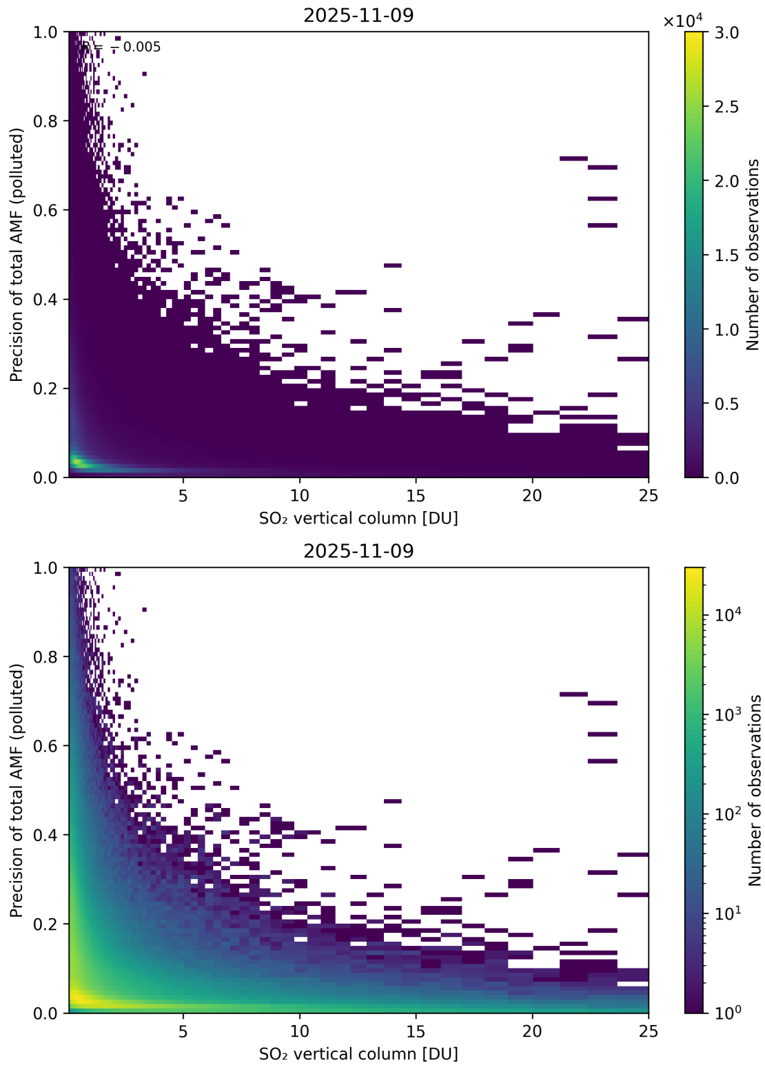
Figure 360: Scatter density plot of “SO 2 vertical column” against “Precision of total AMF (polluted)” for 2025-11-08 to 2025-11-10.
