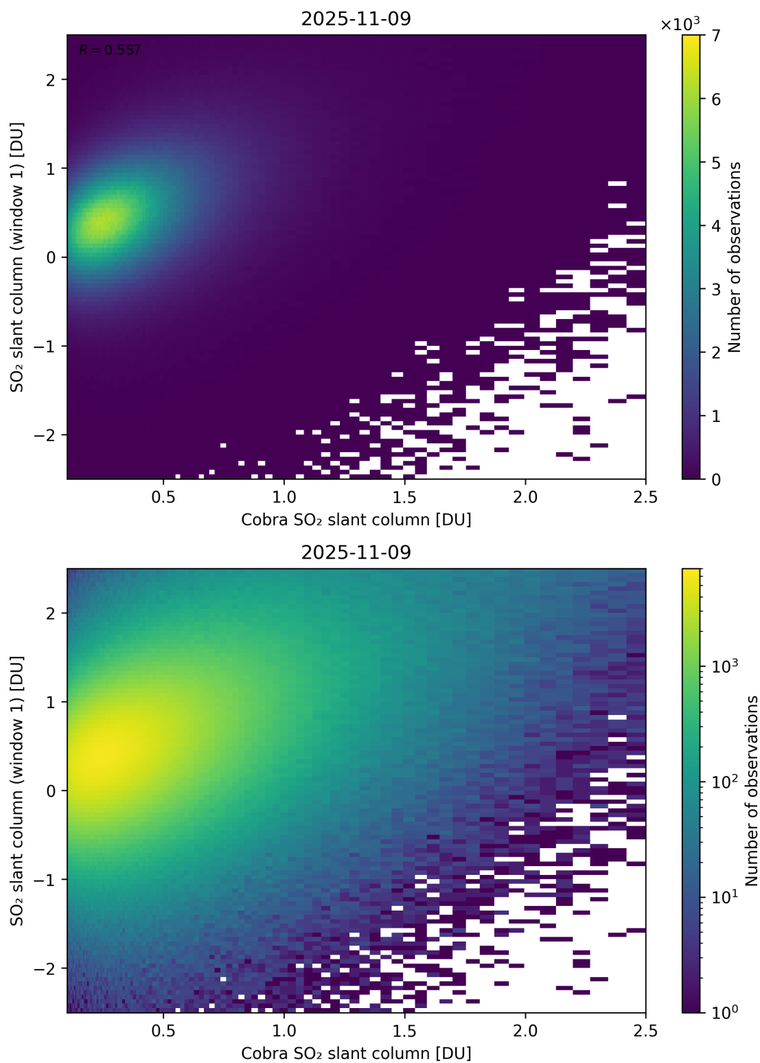
Figure 219: Scatter density plot of “Cobra SO 2 slant column” against “SO 2 slant column (window 1)” for 2025-11-08 to 2025-11-10.
