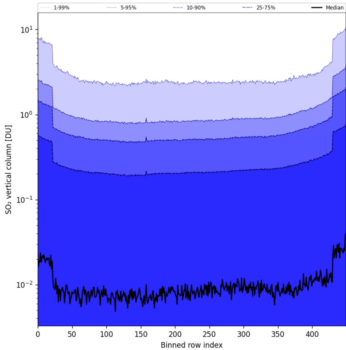
Figure 84: Along track statistics of “SO 2 vertical column” for 2025-11-08 to 2025-11-10
