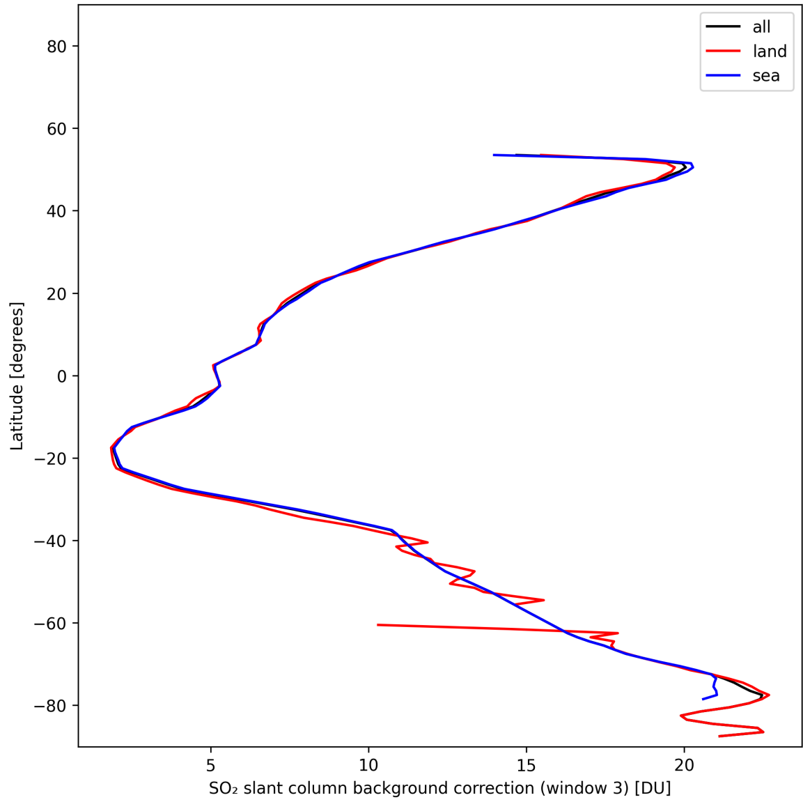
Figure 48: Zonal average of “SO 2 slant column background correction (window 3)” for 2025-11-08 to 2025-11-10.
