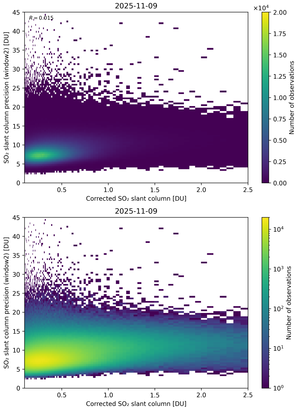
Figure 239: Scatter density plot of “Corrected SO 2 slant column” against “SO 2 slant column precision (window2)” for 2025-11-08 to 2025-11-10.
