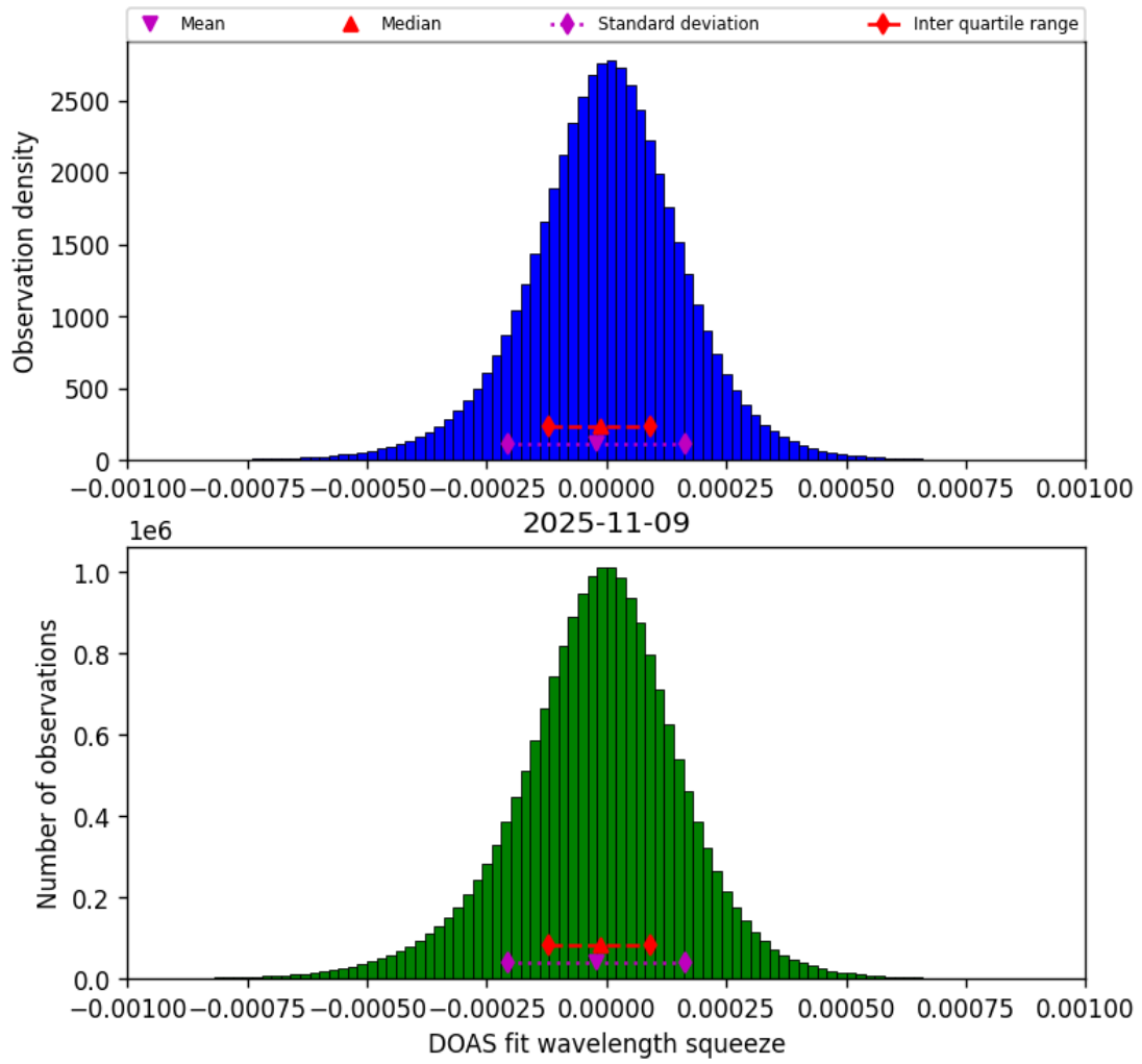
Figure 77: Histogram of “DOAS fit wavelength squeeze” for 2025-11-08 to 2025-11-10
