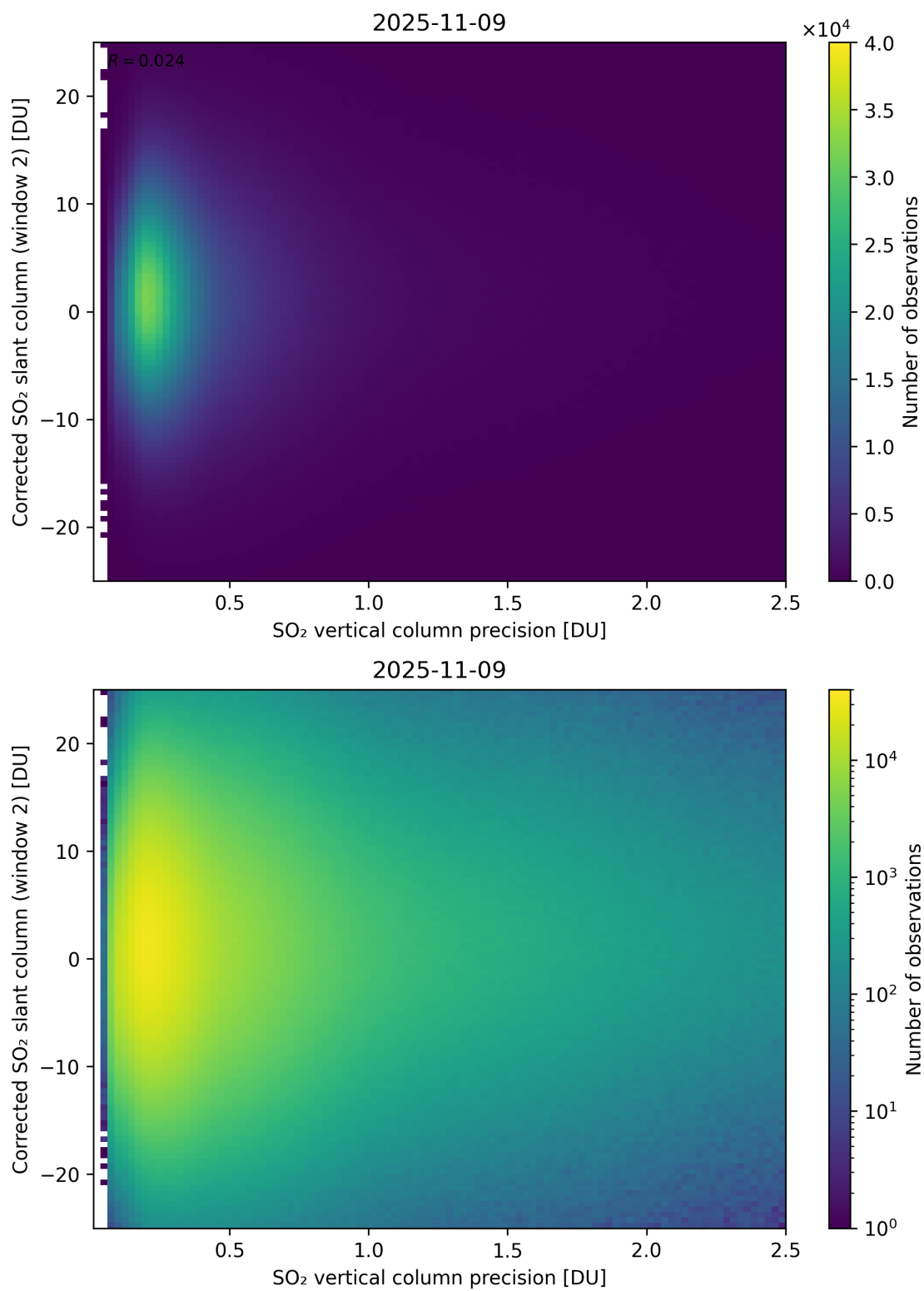
Figure 339: Scatter density plot of “SO 2 vertical column precision” against “Corrected SO 2 slant column (window 2)” for 2025-11-08 to 2025-11-10.
