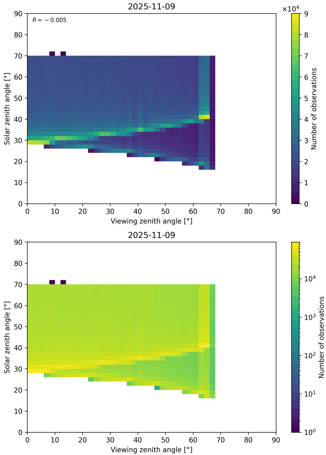
Figure 369: Scatter density plot of “Viewing zenith angle” against “Solar zenith angle” for 2025-11-08 to 2025-11-10.
