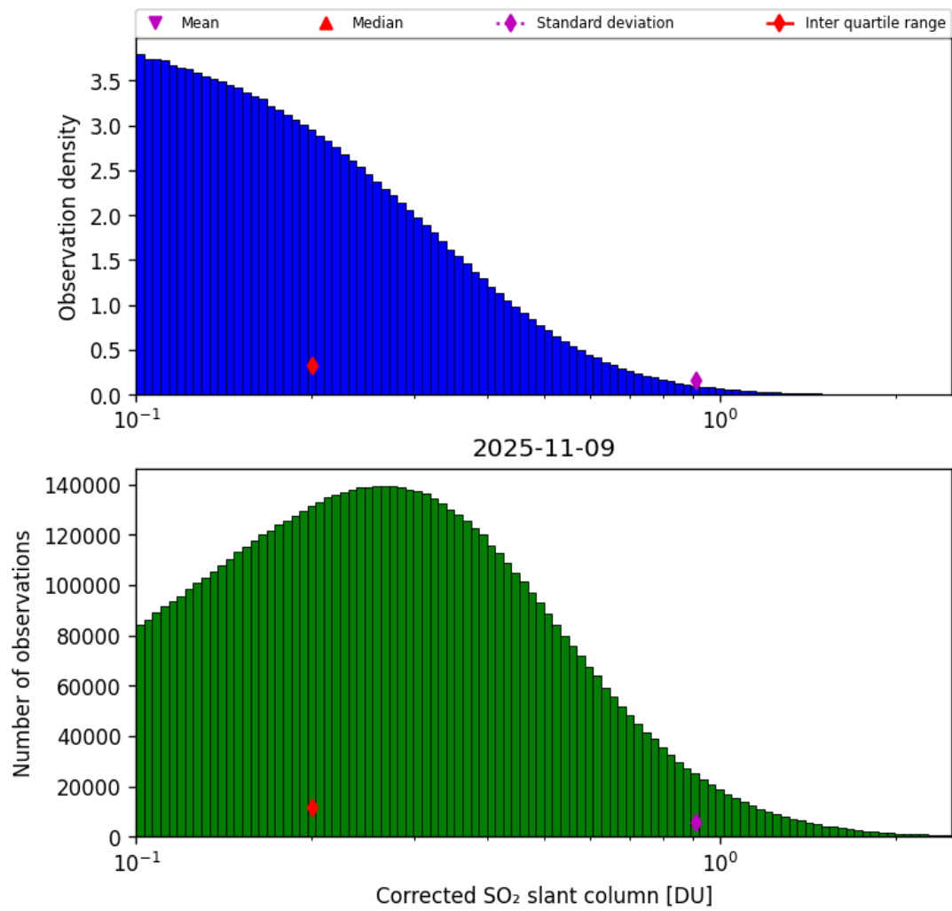
Figure 60: Histogram of “Corrected SO 2 slant column” for 2025-11-08 to 2025-11-10
