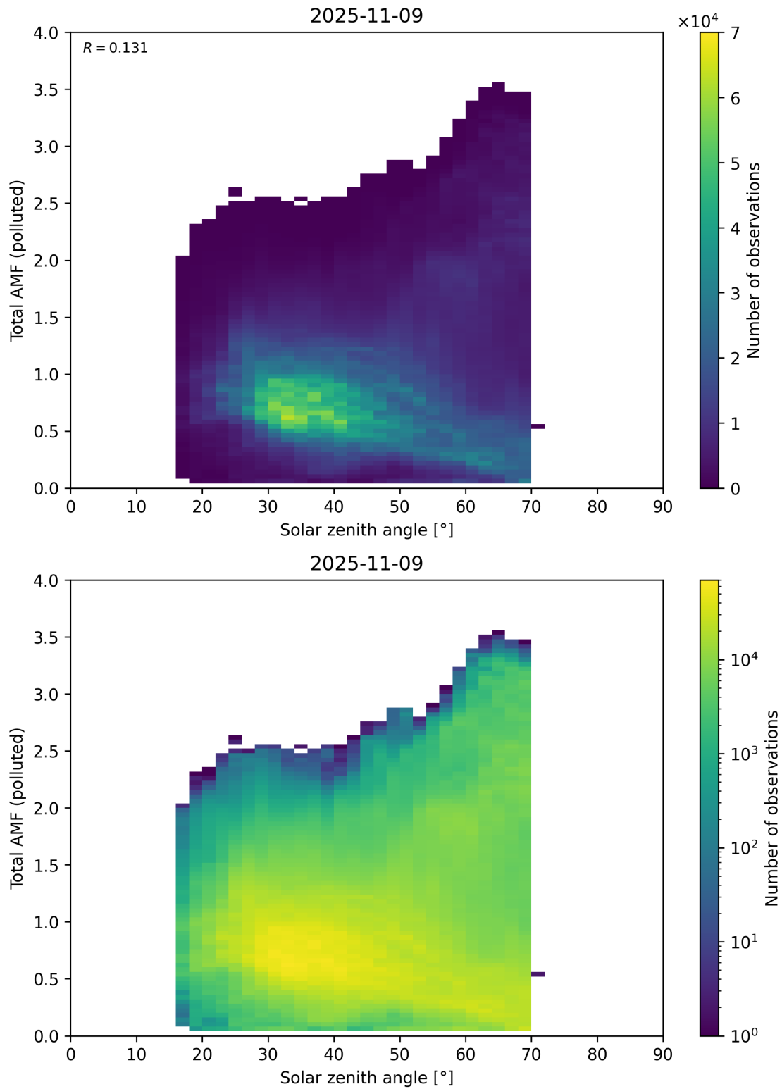
Figure 189: Scatter density plot of “Solar zenith angle” against “Total AMF (polluted)” for 2025-11-08 to 2025-11-10.
