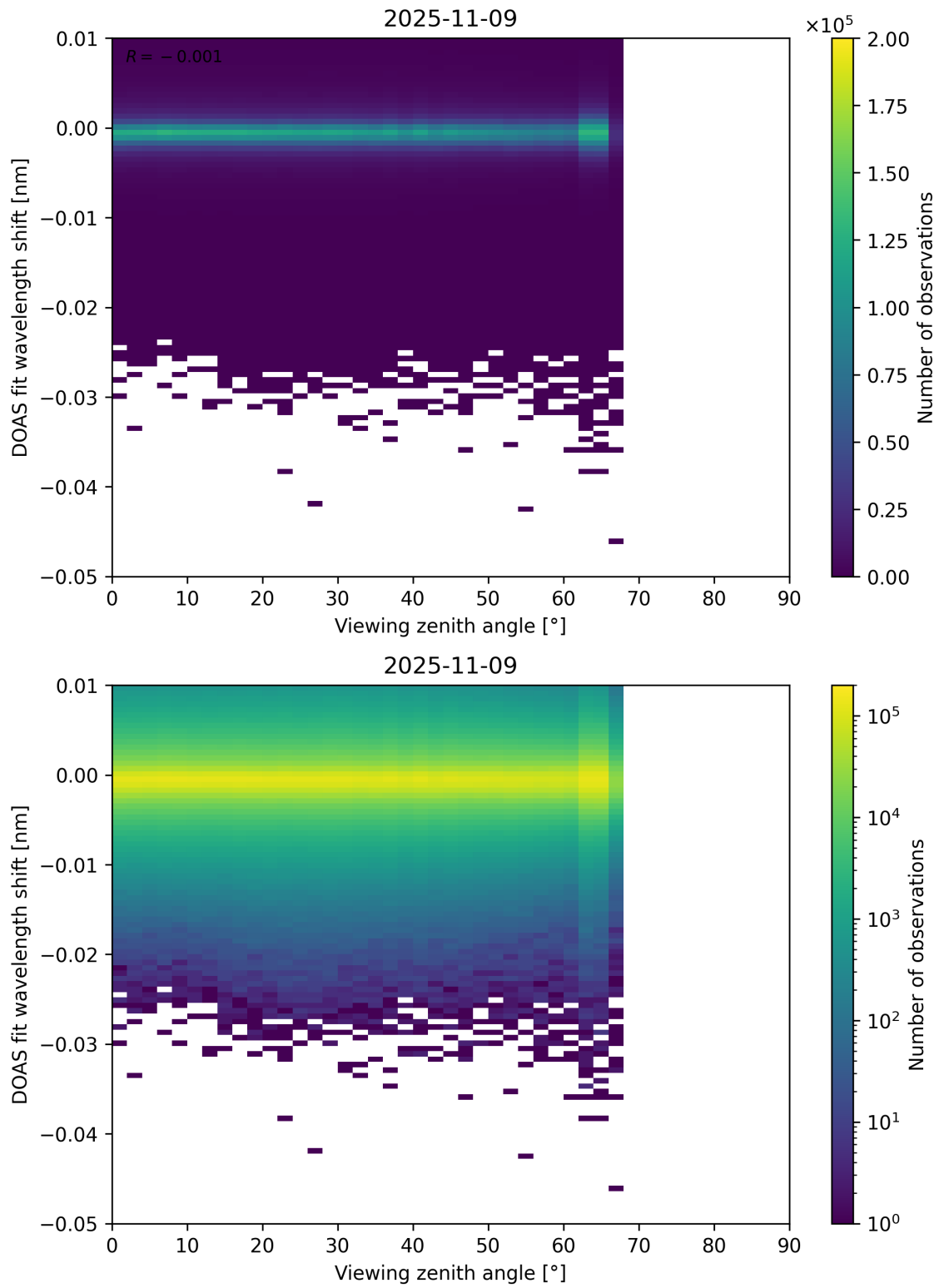
Figure 365: Scatter density plot of “Viewing zenith angle” against “DOAS fit wavelength shift” for 2025-11-08 to 2025-11-10.
