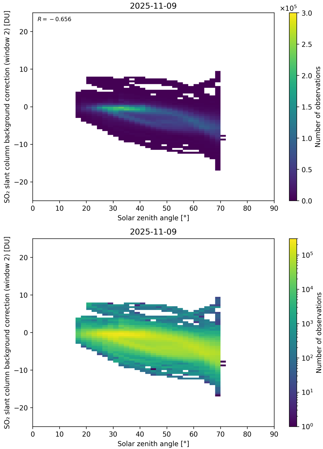
Figure 172: Scatter density plot of “Solar zenith angle” against “SO 2 slant column background correction (window 2)” for 2025-11-08 to 2025-11-10.
