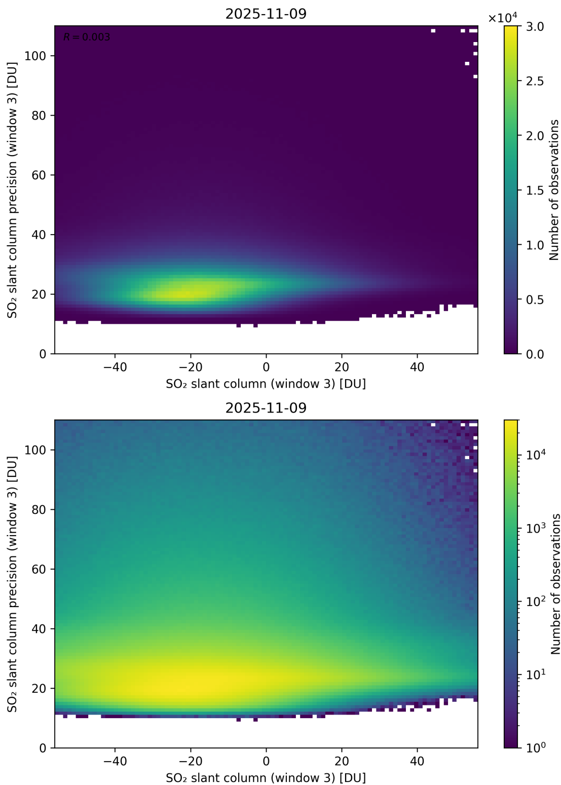
Figure 317: Scatter density plot of “SO 2 slant column (window 3)” against “SO 2 slant column precision (window 3)” for 2025-11-08 to 2025-11-10.
