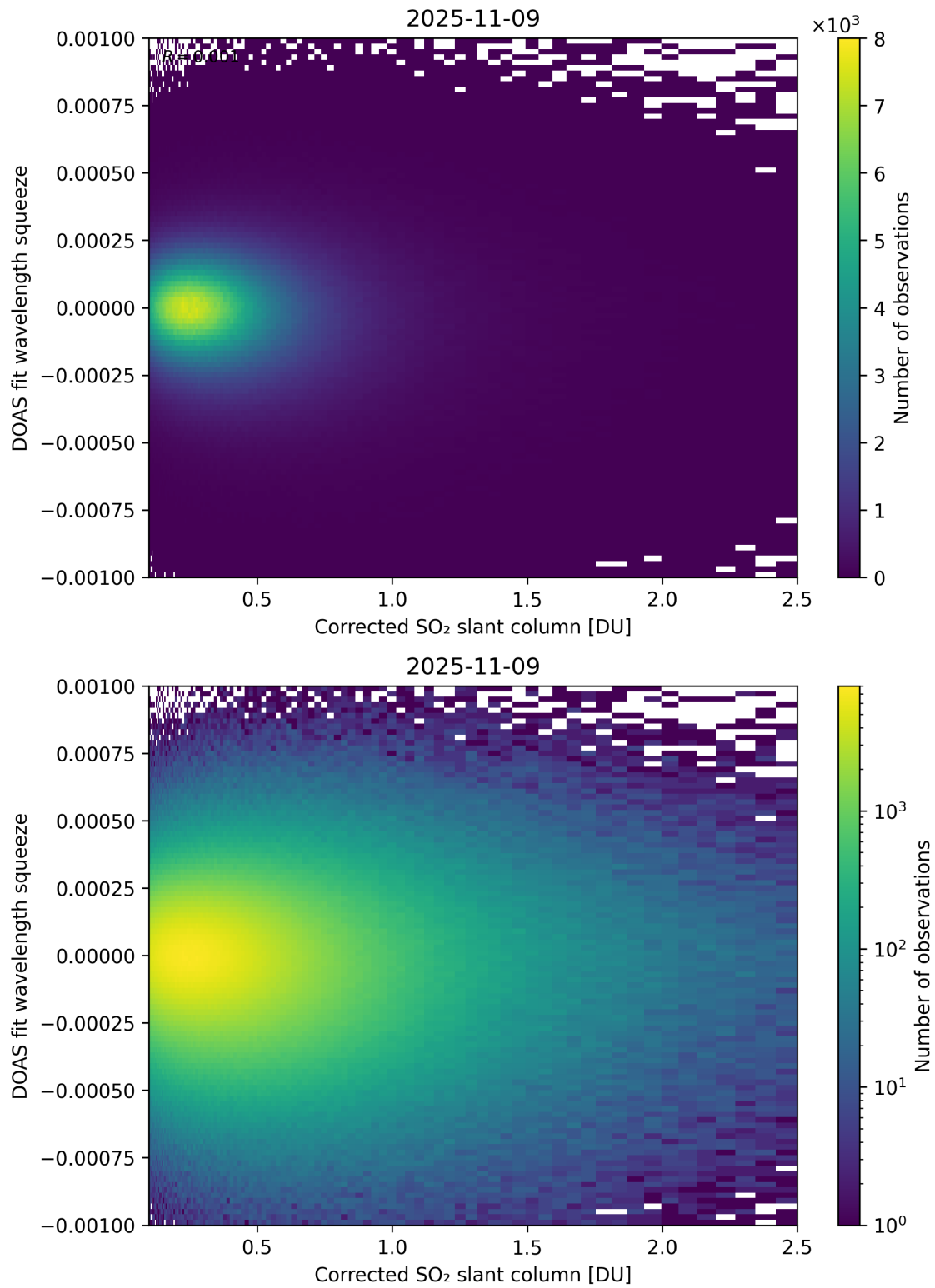
Figure 230: Scatter density plot of "Corrected SO 2 slant column" against "DOAS fit wavelength squeeze" for 2025-11-08 to 2025-11-10.
