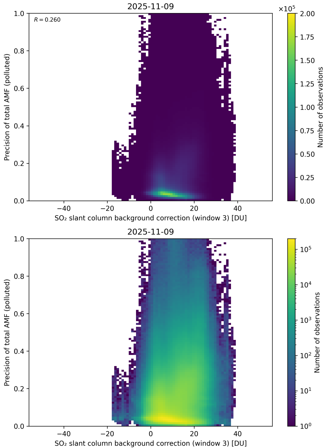
Figure 137: Scatter density plot of “SO 2 slant column background correction (window 3)” against “Precision of total AMF (polluted)” for 2025-11-08 to 2025-11-10.
