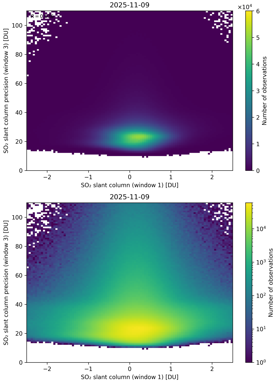
Figure 288: Scatter density plot of “SO 2 slant column (window 1)” against “SO 2 slant column precision (window 3)” for 2025-11-08 to 2025-11-10.
