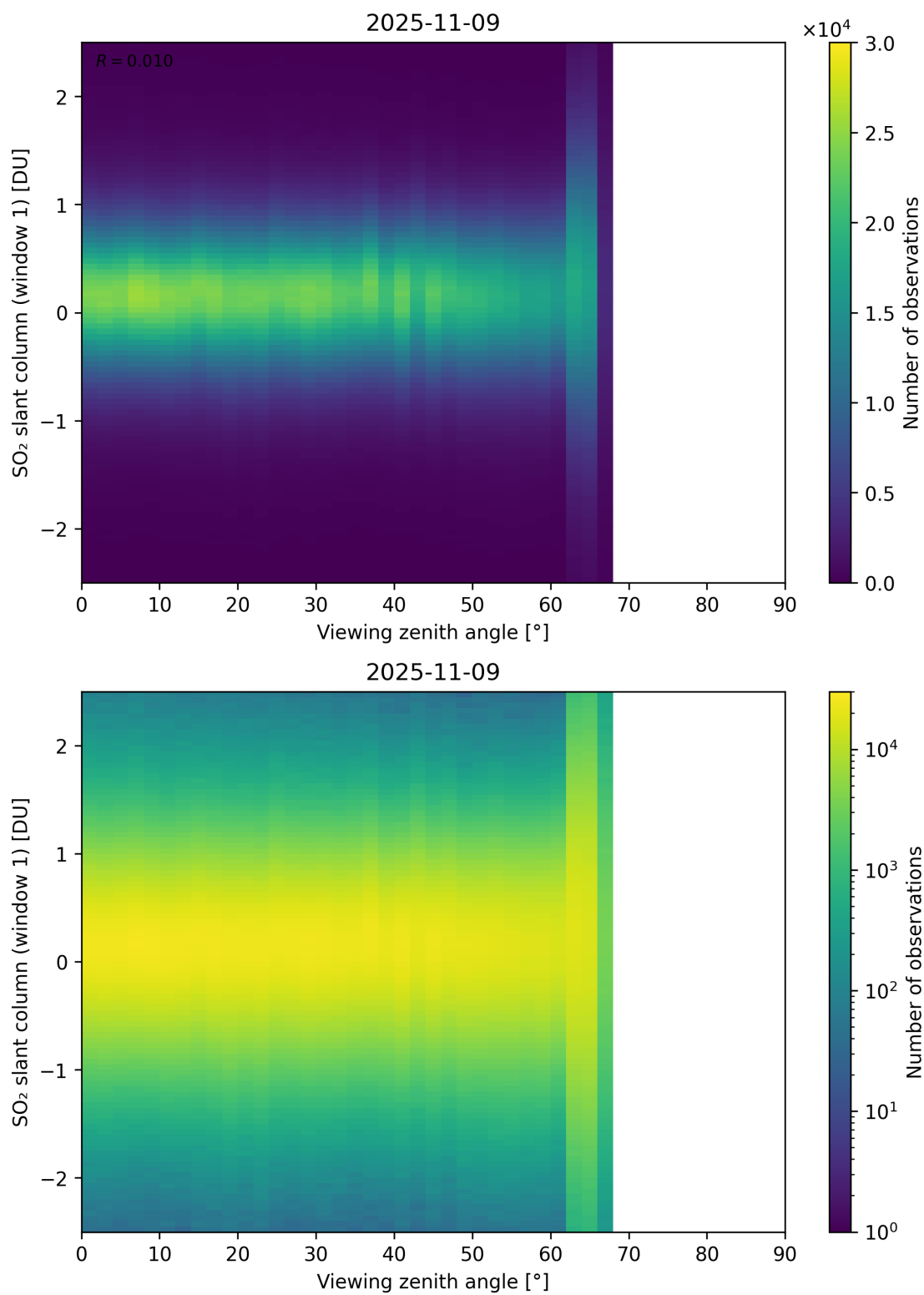
Figure 376: Scatter density plot of “Viewing zenith angle” against “SO 2 slant column (window 1)” for 2025-11-08 to 2025-11-10.
