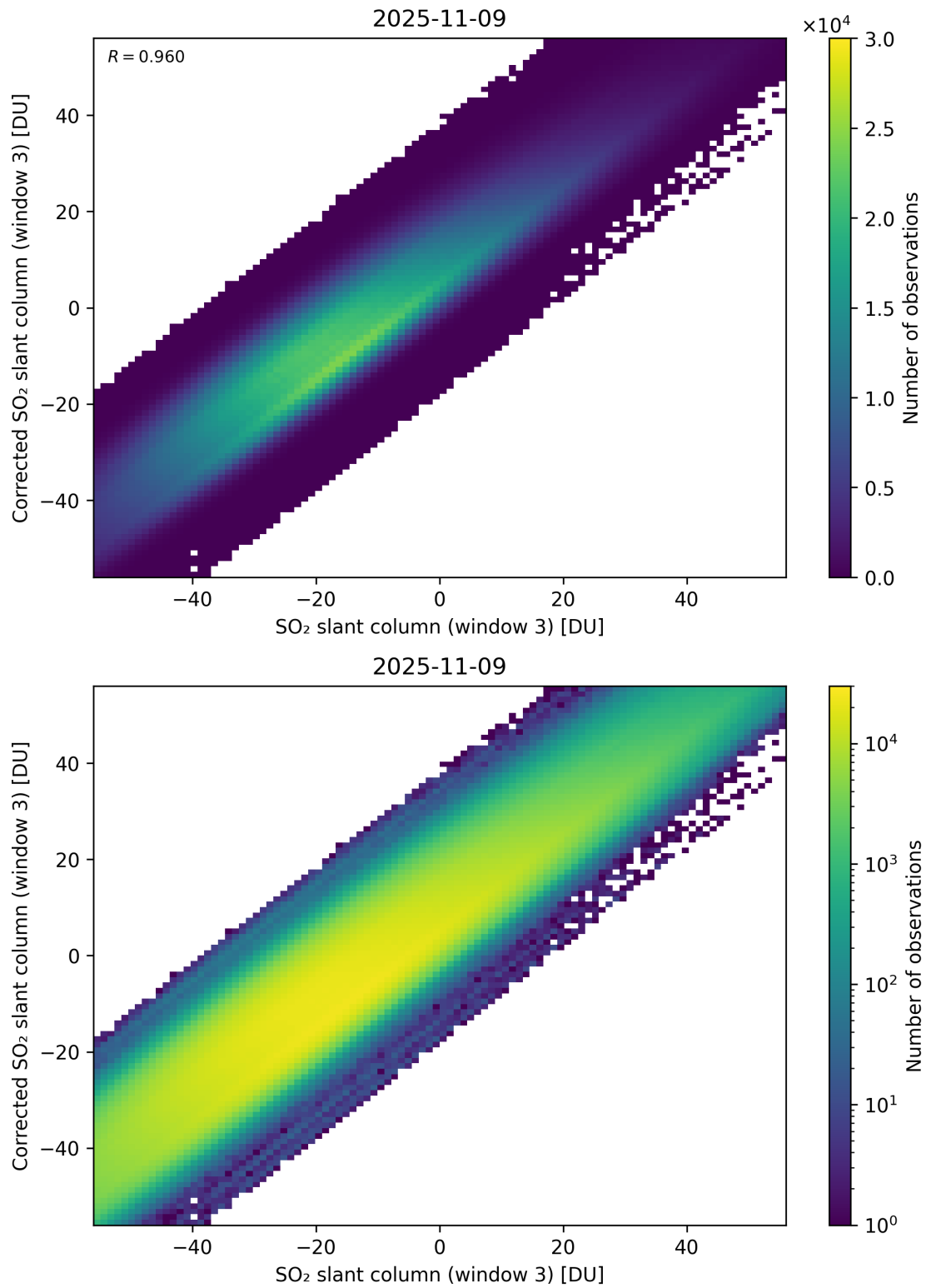
Figure 316: Scatter density plot of “SO 2 slant column (window 3)” against “Corrected SO 2 slant column (window 3)” for 2025-11-08 to 2025-11-10.
