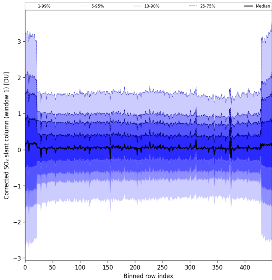
Figure 91: Along track statistics of “Corrected SO 2 slant column (window 1)” for 2025-11-08 to 2025-11-10
