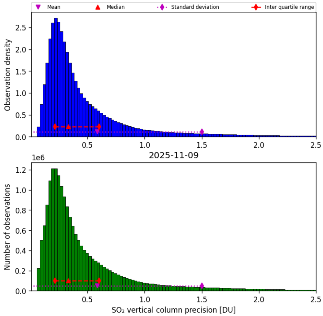
Figure 59: Histogram of “SO 2 vertical column precision” for 2025-11-08 to 2025-11-10
