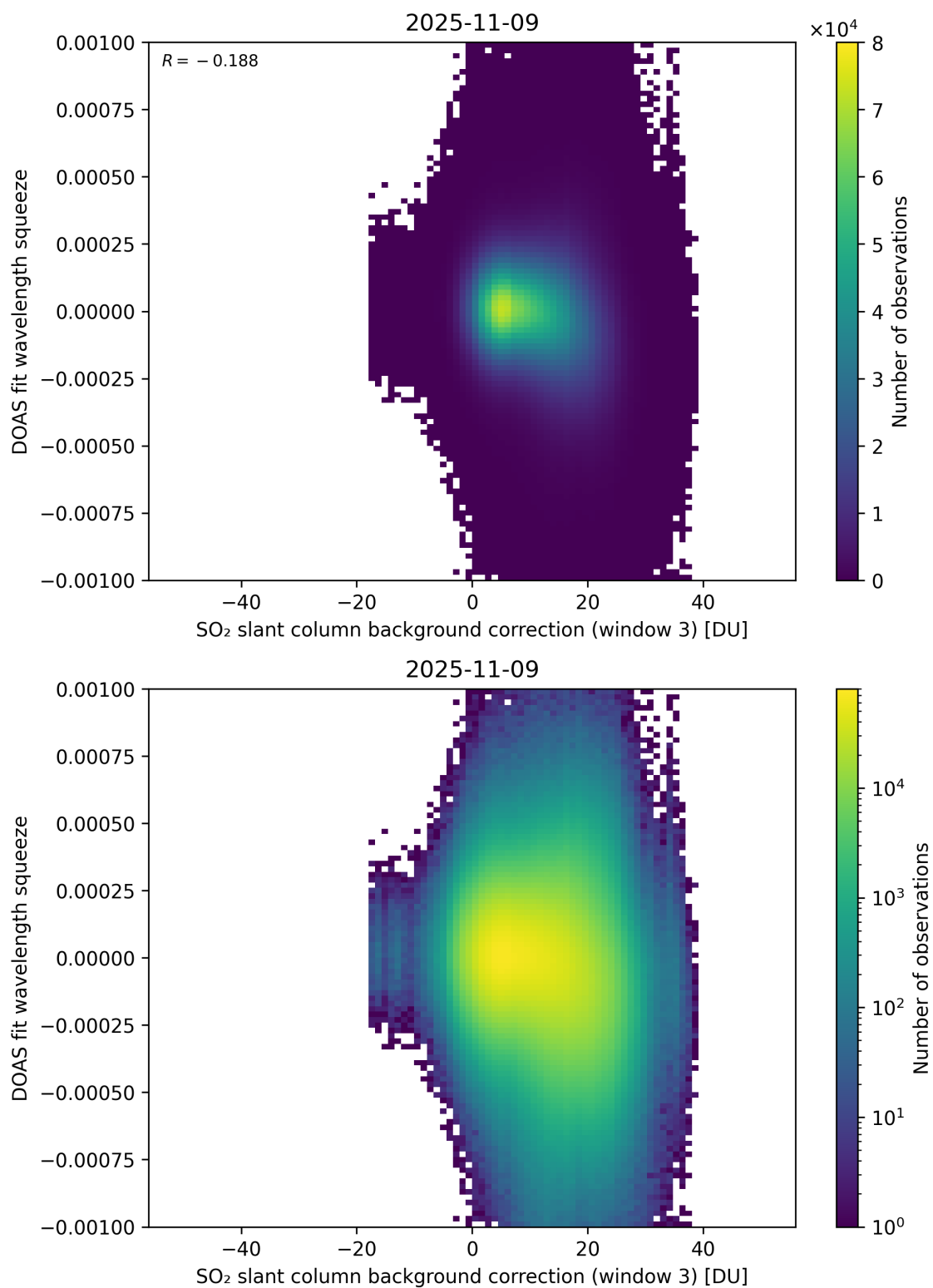
Figure 133: Scatter density plot of “SO 2 slant column background correction (window 3)” against “DOAS fit wavelength squeeze” for 2025-11-08 to 2025-11-10.
