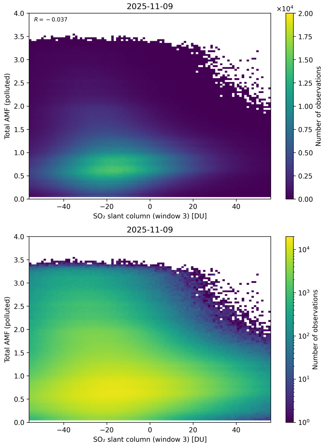
Figure 318: Scatter density plot of “SO 2 slant column (window 3)” against “Total AMF (polluted)” for 2025-11-08 to 2025-11-10.
