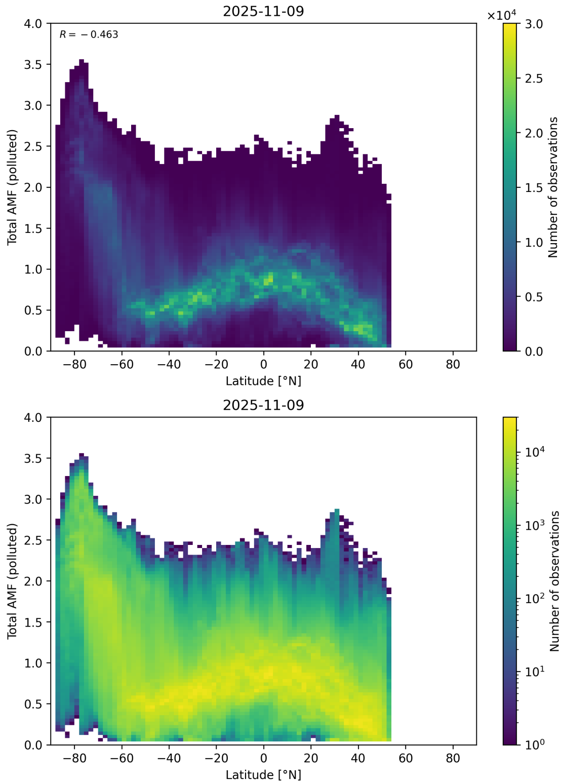
Figure 167: Scatter density plot of “Latitude” against “Total AMF (polluted)” for 2025-11-08 to 2025-11-10.
