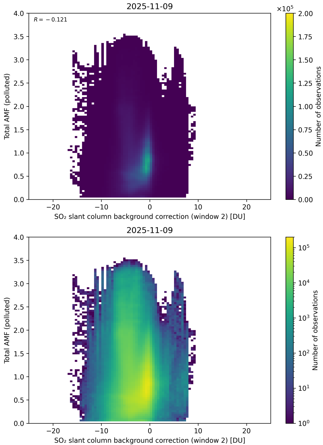
Figure 130: Scatter density plot of “SO 2 slant column background correction (window 2)” against “Total AMF (polluted)” for 2025-11-08 to 2025-11-10.
