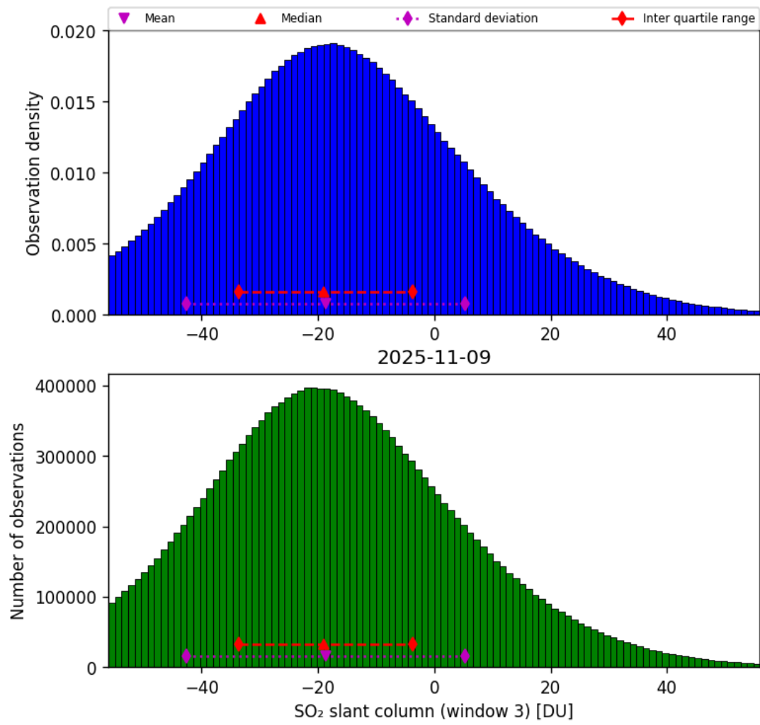
Figure 71: Histogram of “SO 2 slant column (window 3)” for 2025-11-08 to 2025-11-10
