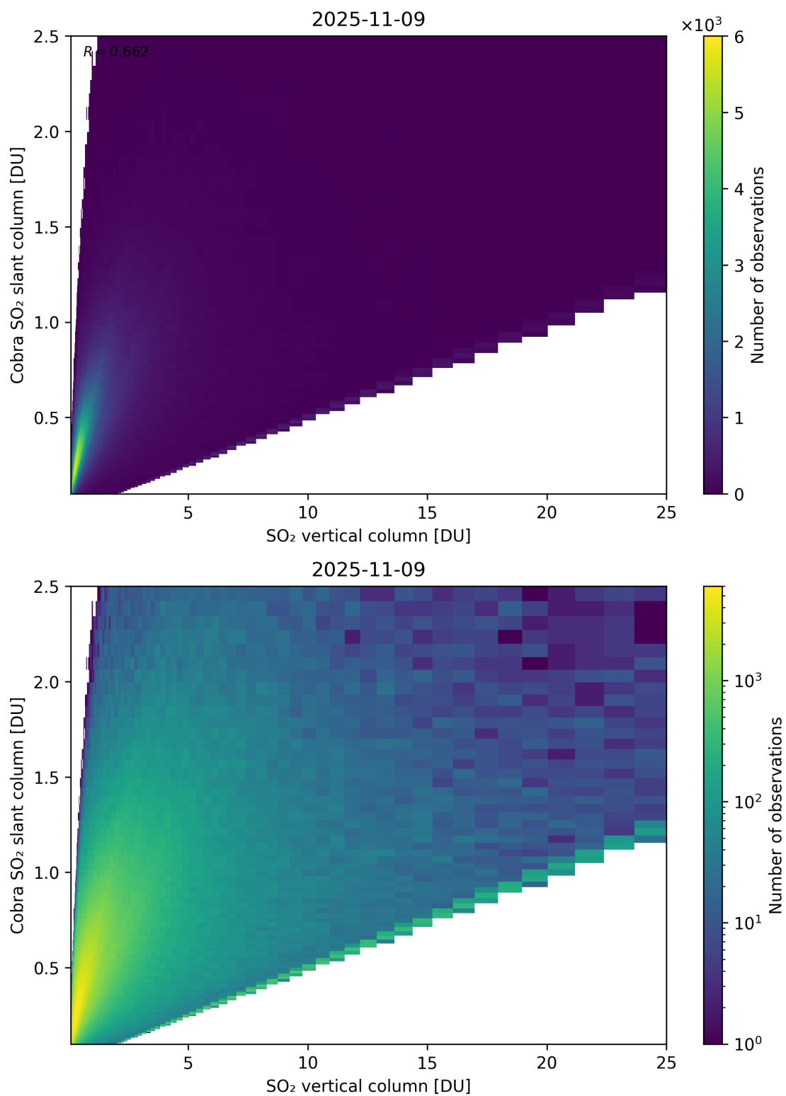
Figure 349: Scatter density plot of “SO 2 vertical column” against “Cobra SO 2 slant column” for 2025-11-08 to 2025-11-10.
