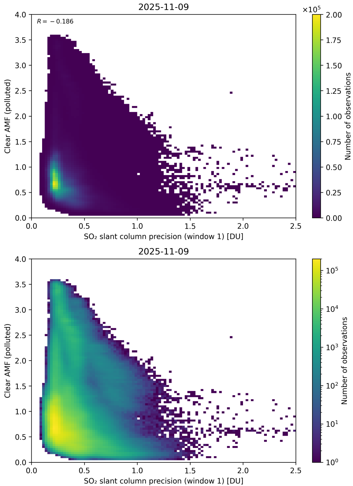
Figure 274: Scatter density plot of “SO 2 slant column precision (window 1)” against “Clear AMF (polluted)” for 2025-11-08 to 2025-11-10.
