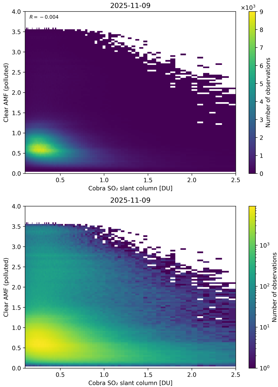
Figure 215: Scatter density plot of “Cobra SO 2 slant column” against “Clear AMF (polluted)” for 2025-11-08 to 2025-11-10.
