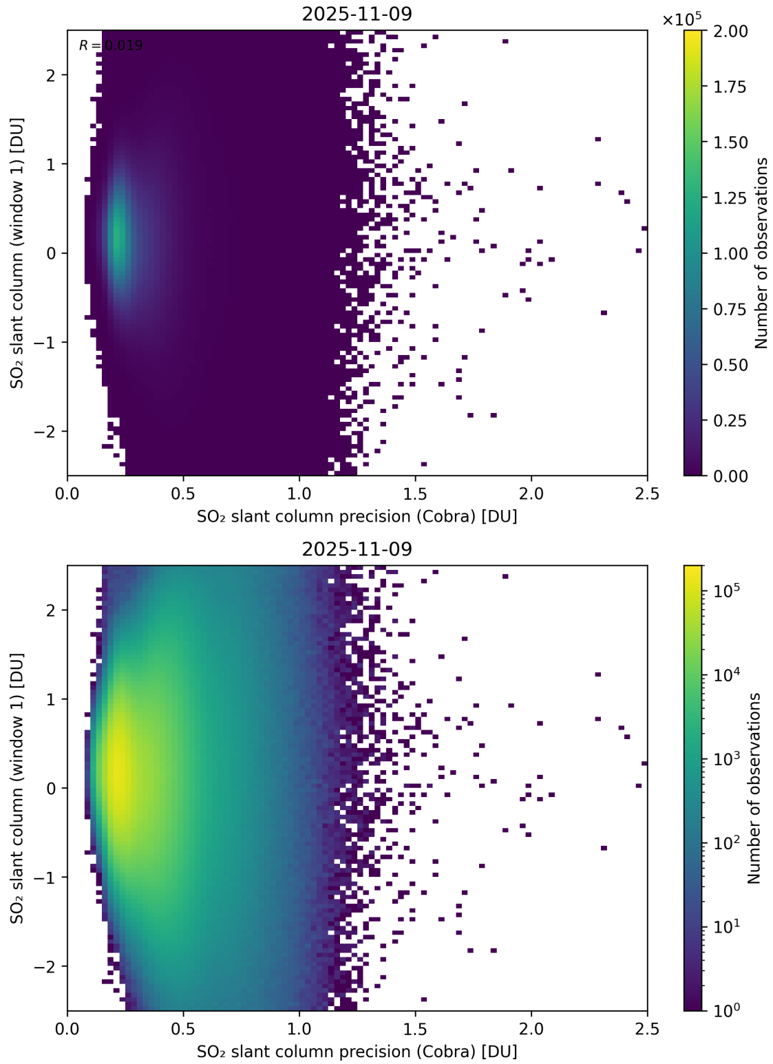
Figure 208: Scatter density plot of “SO 2 slant column precision (Cobra)” against “SO 2 slant column (window 1)” for 2025-11-08 to 2025-11-10.
