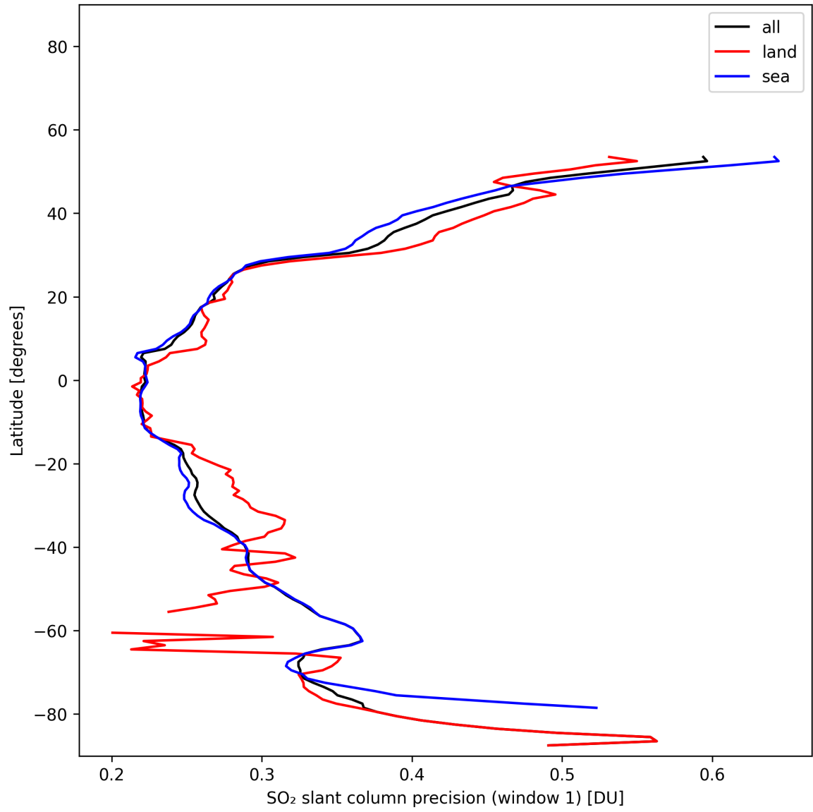
Figure 38: Zonal average of “SO 2 slant column precision (window 1)” for 2025-11-08 to 2025-11-10.
