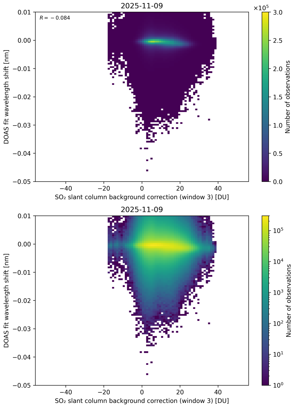
Figure 132: Scatter density plot of “SO 2 slant column background correction (window 3)” against “DOAS fit wavelength shift” for 2025-11-08 to 2025-11-10.
