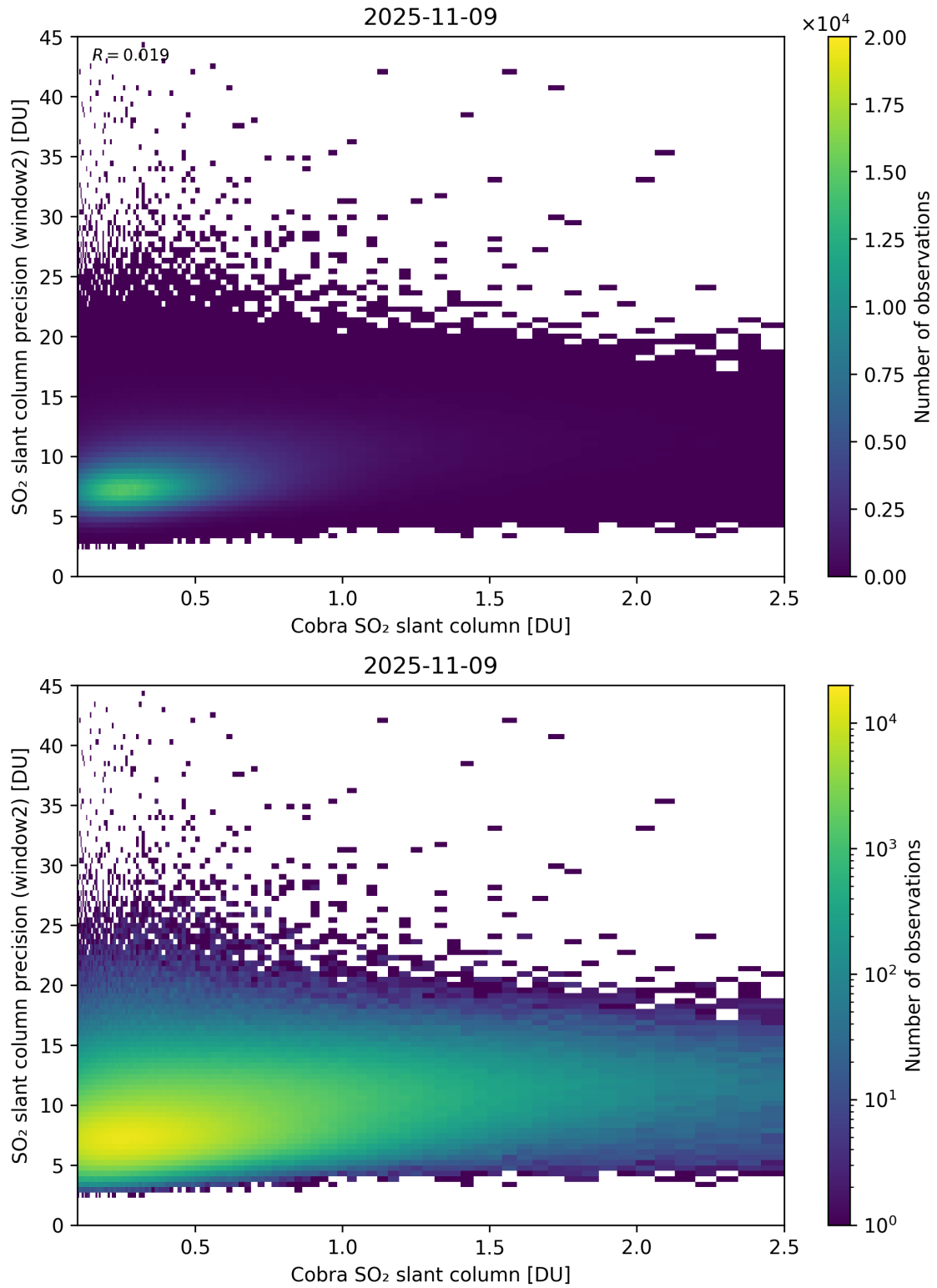
Figure 221: Scatter density plot of “Cobra SO 2 slant column” against “SO 2 slant column precision (window2)” for 2025-11-08 to 2025-11-10.
