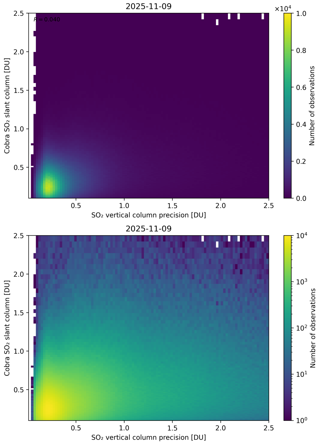
Figure 336: Scatter density plot of “SO 2 vertical column precision” against “Cobra SO 2 slant column” for 2025-11-08 to 2025-11-10.
