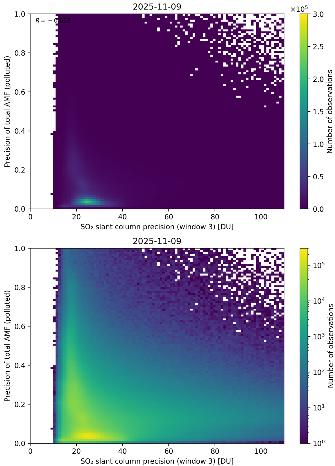
Figure 314: Scatter density plot of “SO 2 slant column precision (window 3)” against “Precision of total AMF (polluted)” for 2025-11-08 to 2025-11-10.
