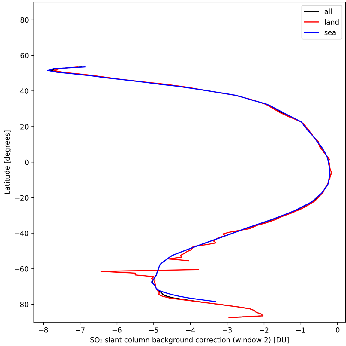
Figure 44: Zonal average of “SO 2 slant column background correction (window 2)” for 2025-11-08 to 2025-11-10.
