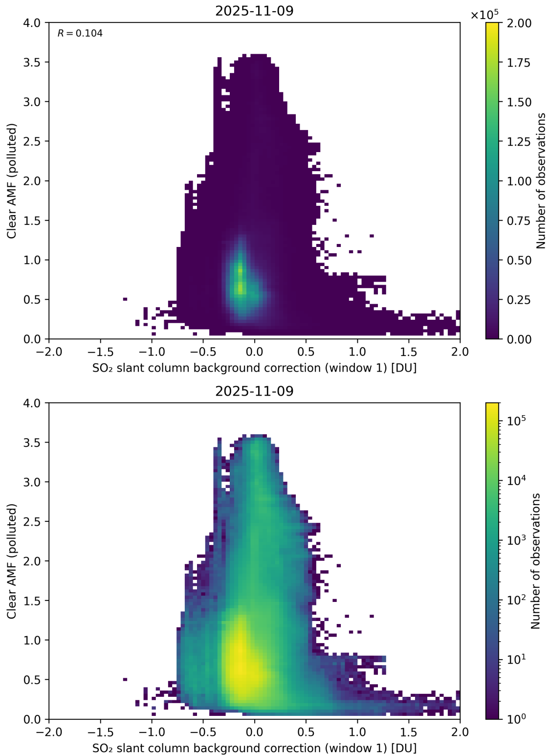
Figure 114: Scatter density plot of “SO 2 slant column background correction (window 1)” against “Clear AMF (polluted)” for 2025-11-08 to 2025-11-10.
