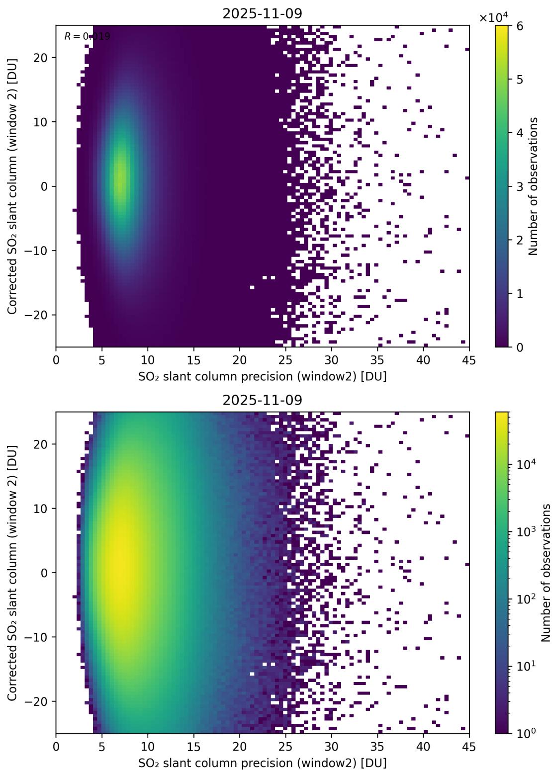
Figure 297: Scatter density plot of “SO 2 slant column precision (window2)” against “Corrected SO 2 slant column (window 2)” for 2025-11-08 to 2025-11-10.
