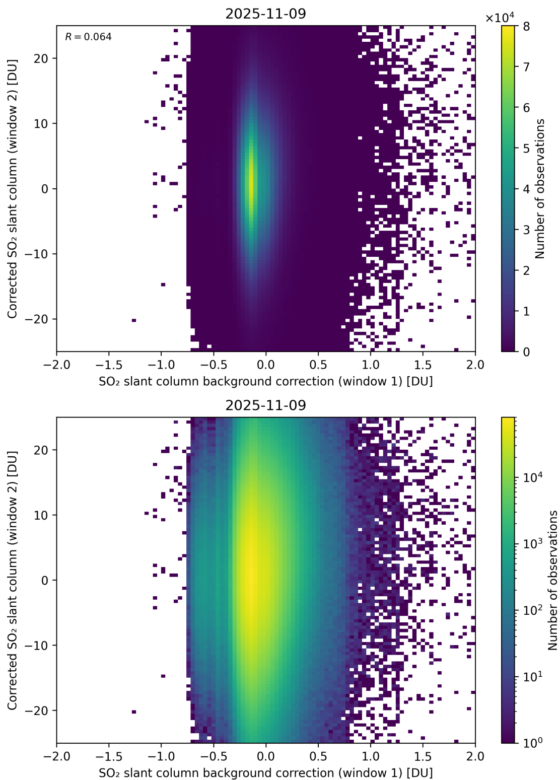
Figure 115: Scatter density plot of “SO 2 slant column background correction (window 1)” against “Corrected SO 2 slant column (window 2)” for 2025-11-08 to 2025-11-10.
