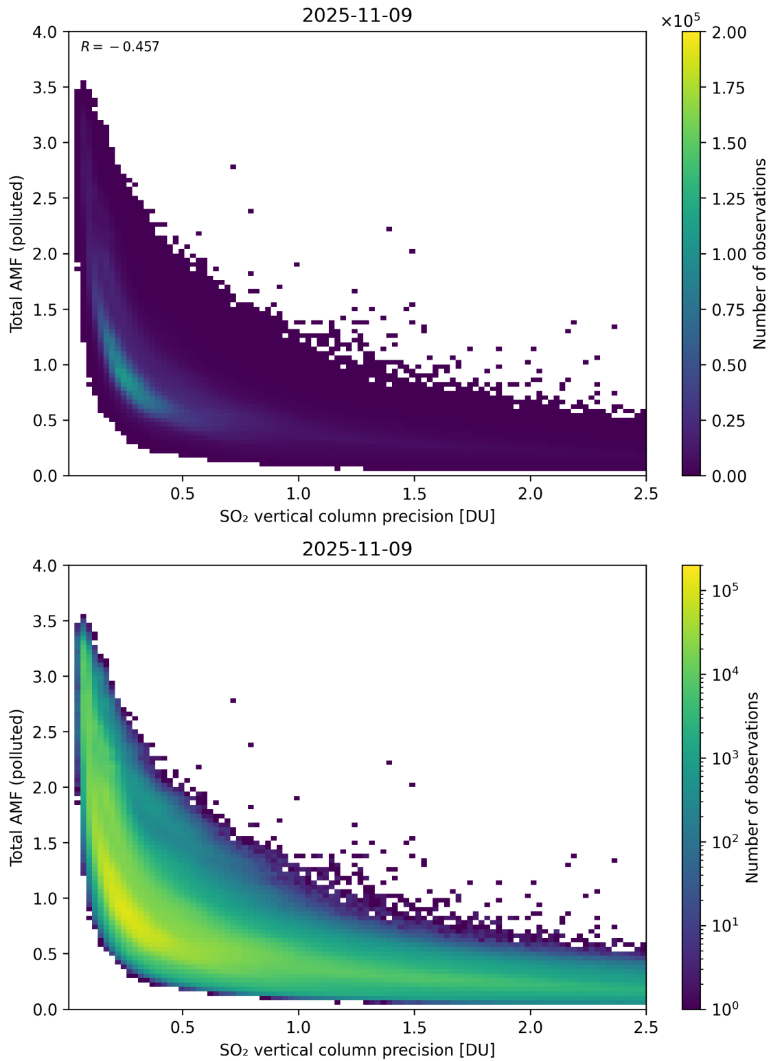
Figure 346: Scatter density plot of “SO 2 vertical column precision” against “Total AMF (polluted)” for 2025-11-08 to 2025-11-10.
