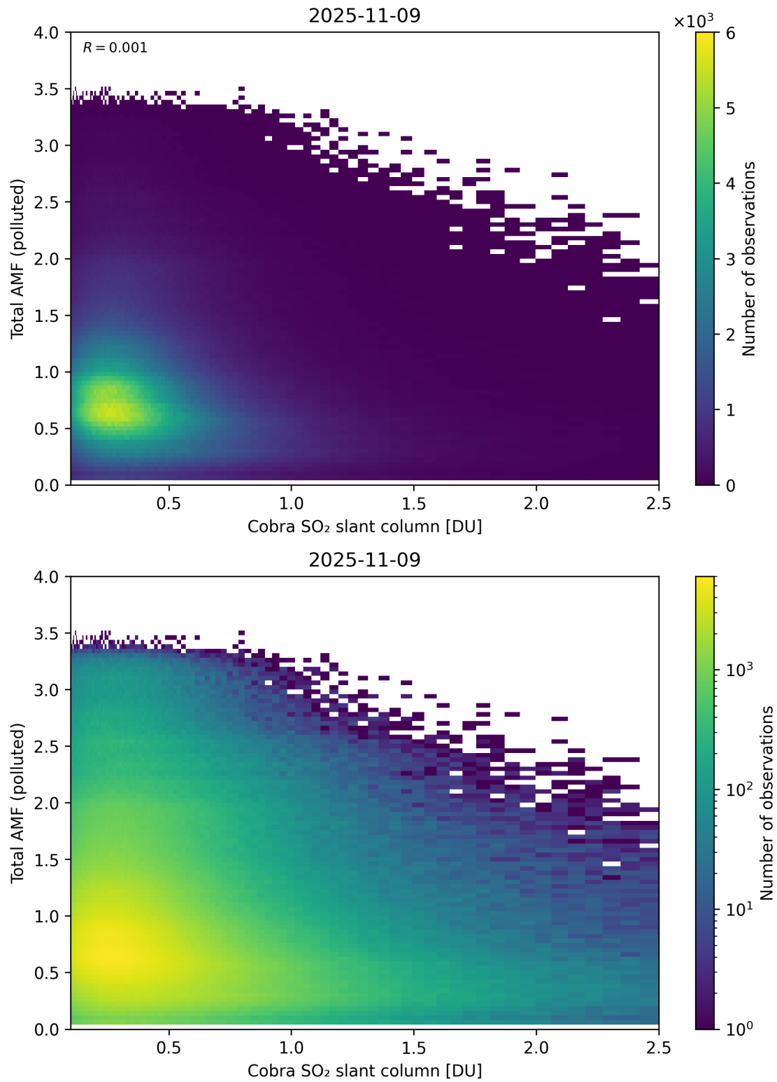
Figure 224: Scatter density plot of “Cobra SO 2 slant column” against “Total AMF (polluted)” for 2025-11-08 to 2025-11-10.
