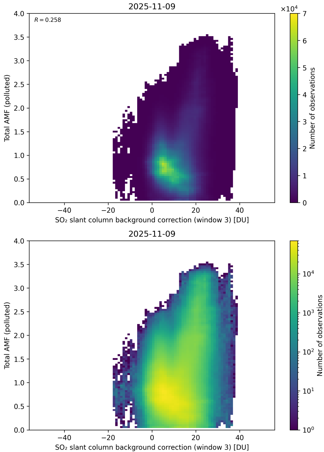
Figure 136: Scatter density plot of “SO 2 slant column background correction (window 3)” against “Total AMF (polluted)” for 2025-11-08 to 2025-11-10.
