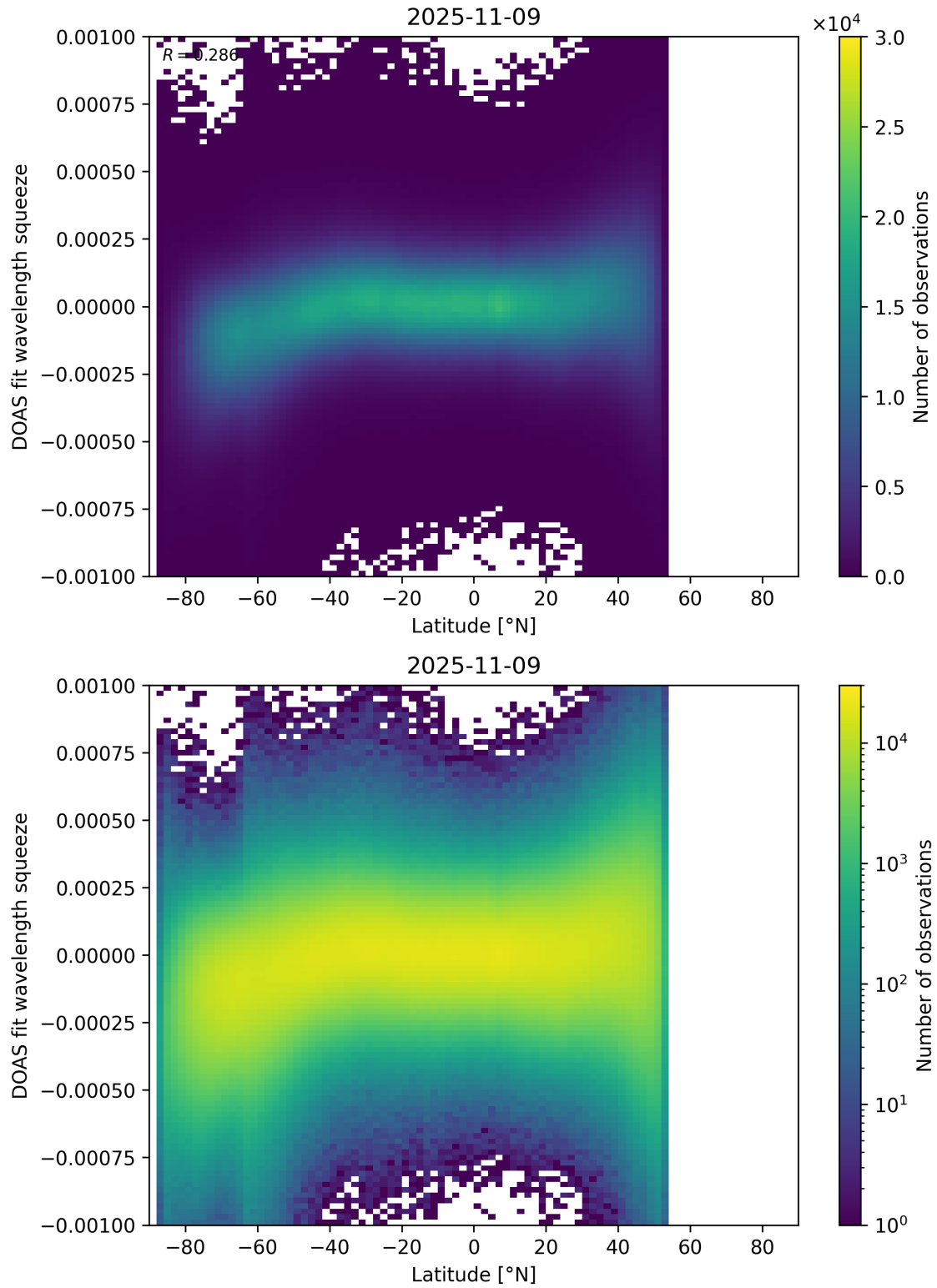
Figure 154: Scatter density plot of “Latitude” against “DOAS fit wavelength squeeze” for 2025-11-08 to 2025-11-10.
