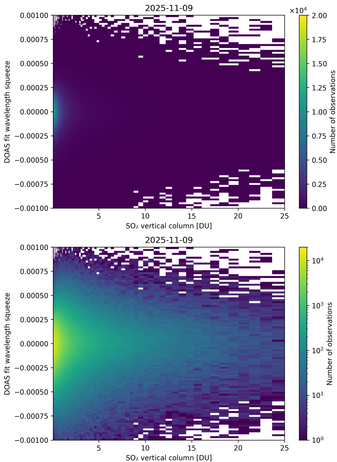
Figure 327: Scatter density plot of “SO 2 vertical column” against “DOAS fit wavelength squeeze” for 2025-11-08 to 2025-11-10.
