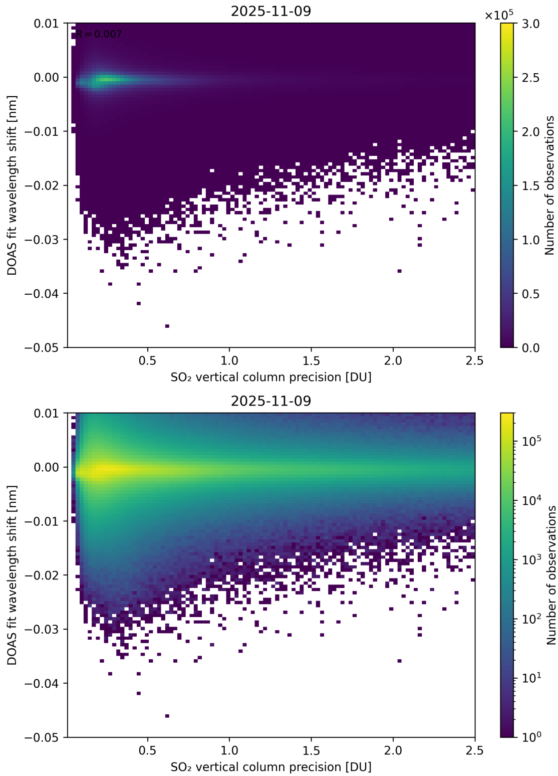
Figure 332: Scatter density plot of “SO 2 vertical column precision” against “DOAS fit wavelength shift” for 2025-11-08 to 2025-11-10.
