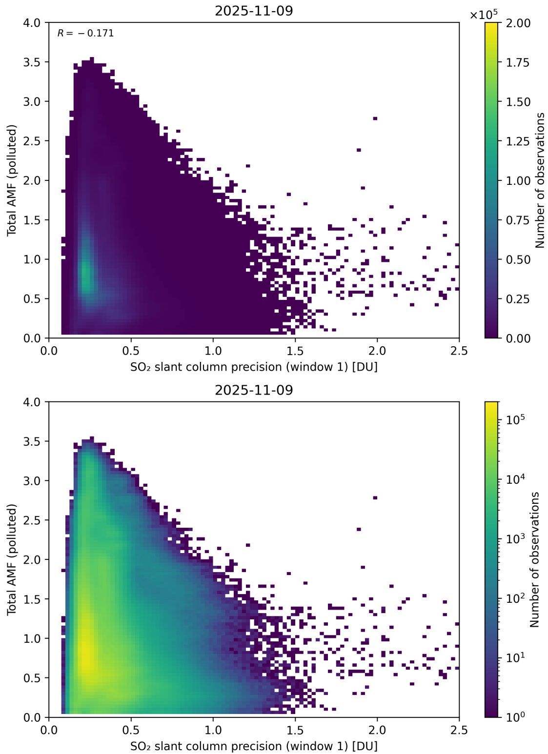
Figure 280: Scatter density plot of “SO 2 slant column precision (window 1)” against “Total AMF (polluted)” for 2025-11-08 to 2025-11-10.
