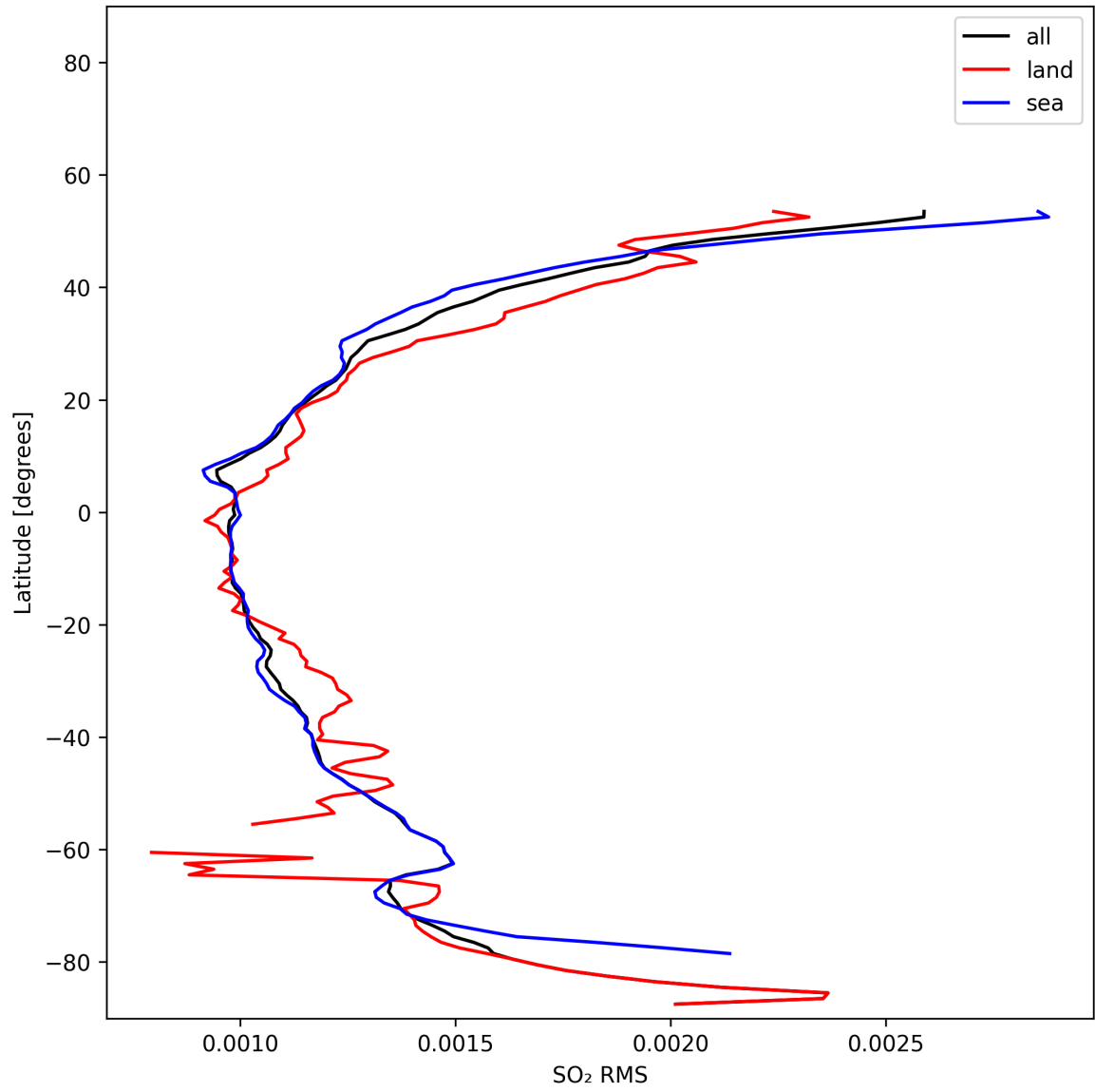
Figure 52: Zonal average of “SO 2 RMS” for 2025-11-08 to 2025-11-10.
