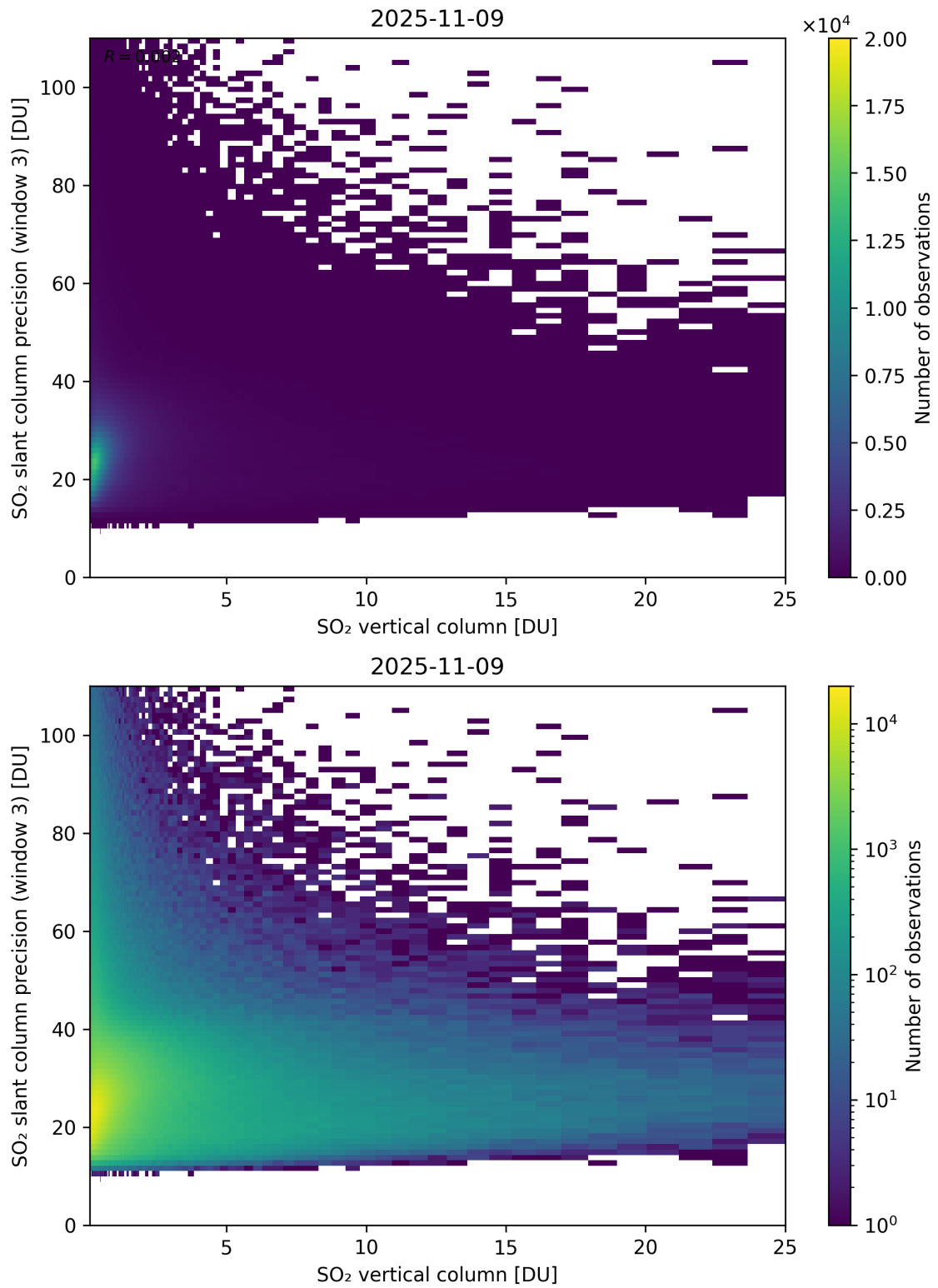
Figure 358: Scatter density plot of “SO 2 vertical column” against “SO 2 slant column precision (window 3)” for 2025-11-08 to 2025-11-10.
