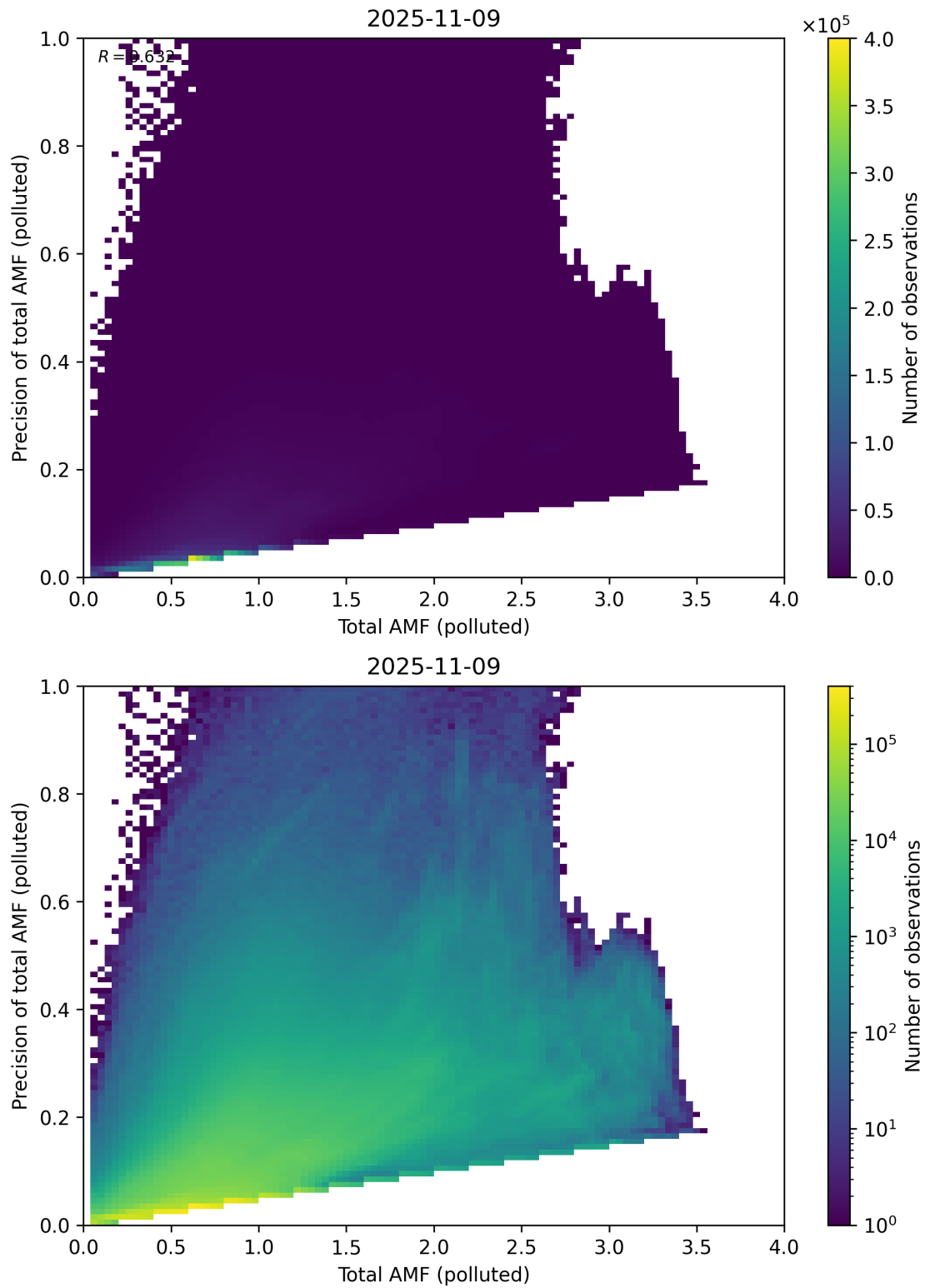
Figure 322: Scatter density plot of “Total AMF (polluted)” against “Precision of total AMF (polluted)” for 2025-11-08 to 2025-11-10.
