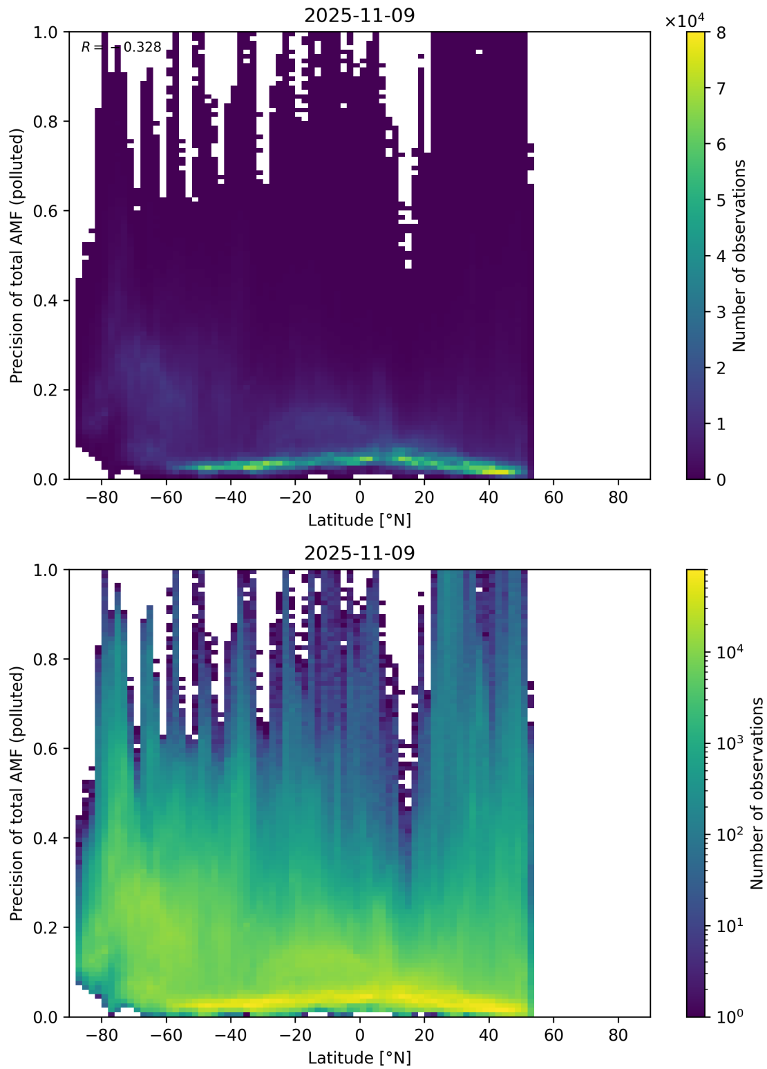
Figure 168: Scatter density plot of “Latitude” against “Precision of total AMF (polluted)” for 2025-11-08 to 2025-11-10.
