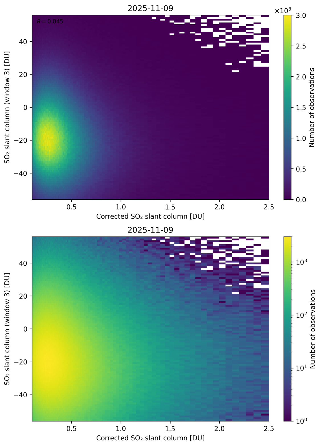
Figure 240: Scatter density plot of “Corrected SO 2 slant column” against “SO 2 slant column (window 3)” for 2025-11-08 to 2025-11-10.
