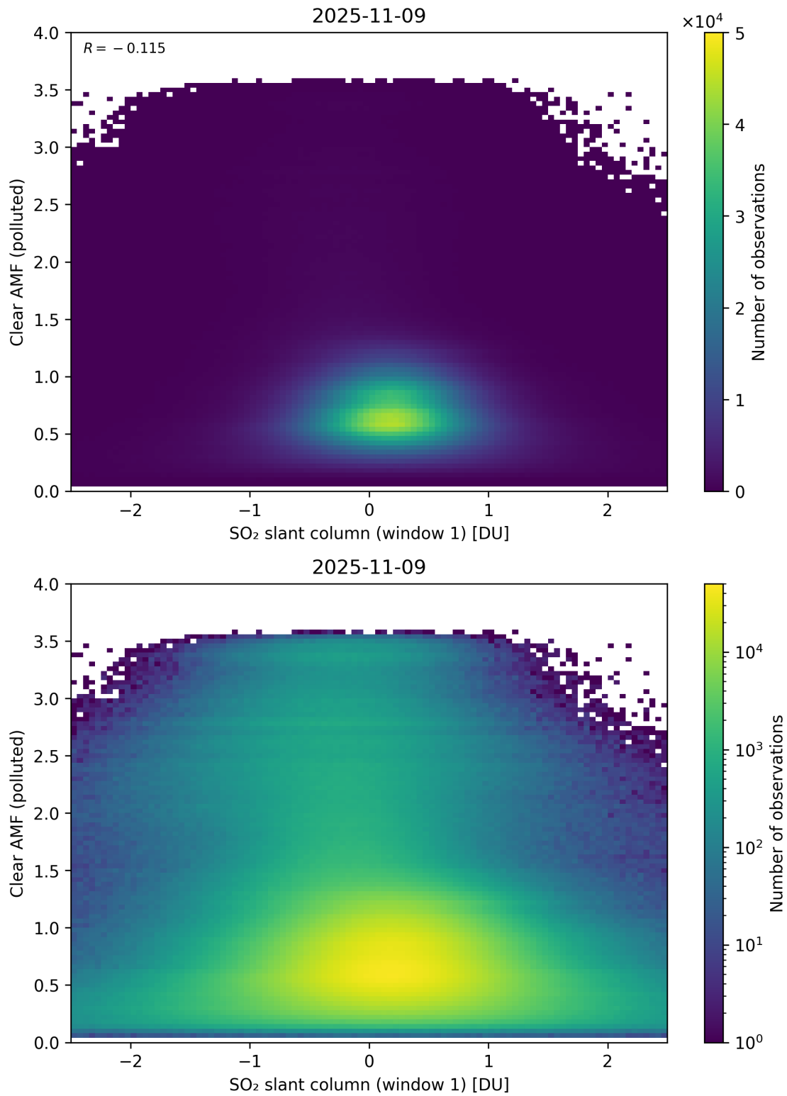
Figure 282: Scatter density plot of “SO 2 slant column (window 1)” against “Clear AMF (polluted)” for 2025-11-08 to 2025-11-10.
