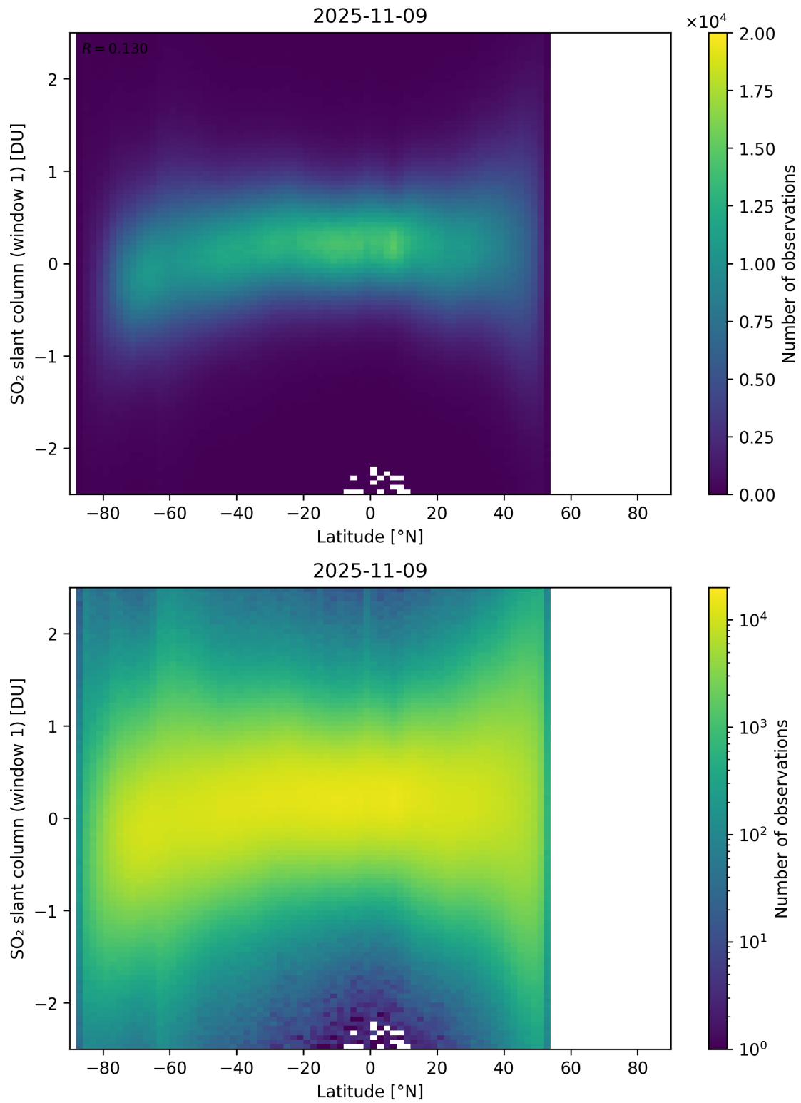
Figure 162: Scatter density plot of “Latitude” against “SO 2 slant column (window 1)” for 2025-11-08 to 2025-11-10.
