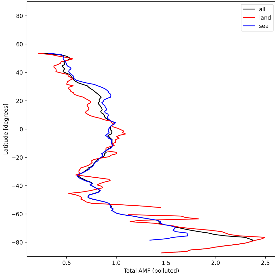
Figure 53: Zonal average of “Total AMF (polluted)” for 2025-11-08 to 2025-11-10.
