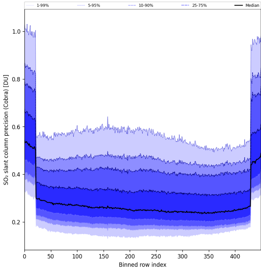
Figure 88: Along track statistics of “SO 2 slant column precision (Cobra)” for 2025-11-08 to 2025-11-10
