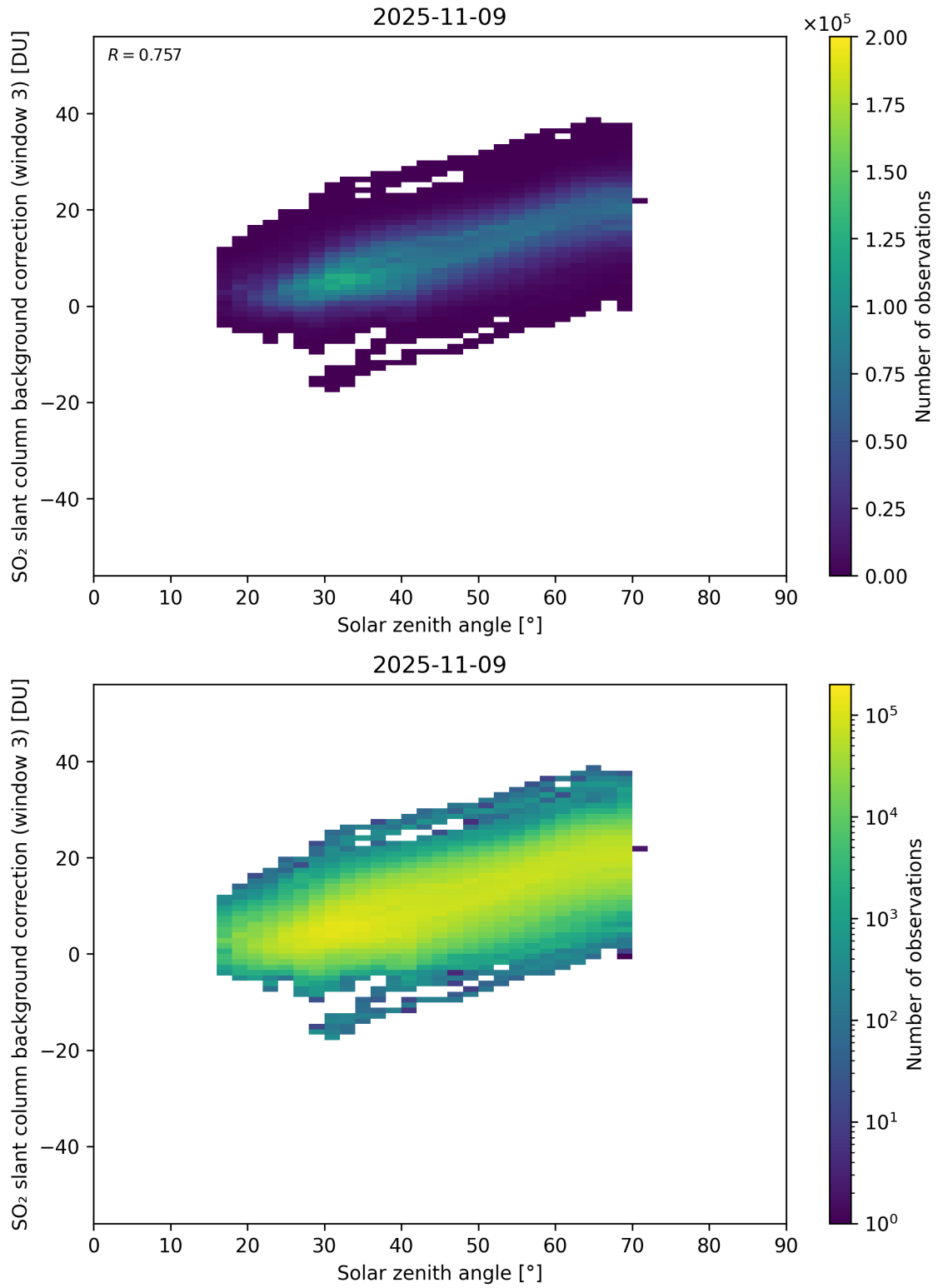
Figure 173: Scatter density plot of “Solar zenith angle” against “SO 2 slant column background correction (window 3)” for 2025-11-08 to 2025-11-10.
