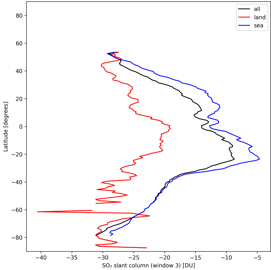
Figure 45: Zonal average of “SO 2 slant column (window 3)” for 2025-11-08 to 2025-11-10.
