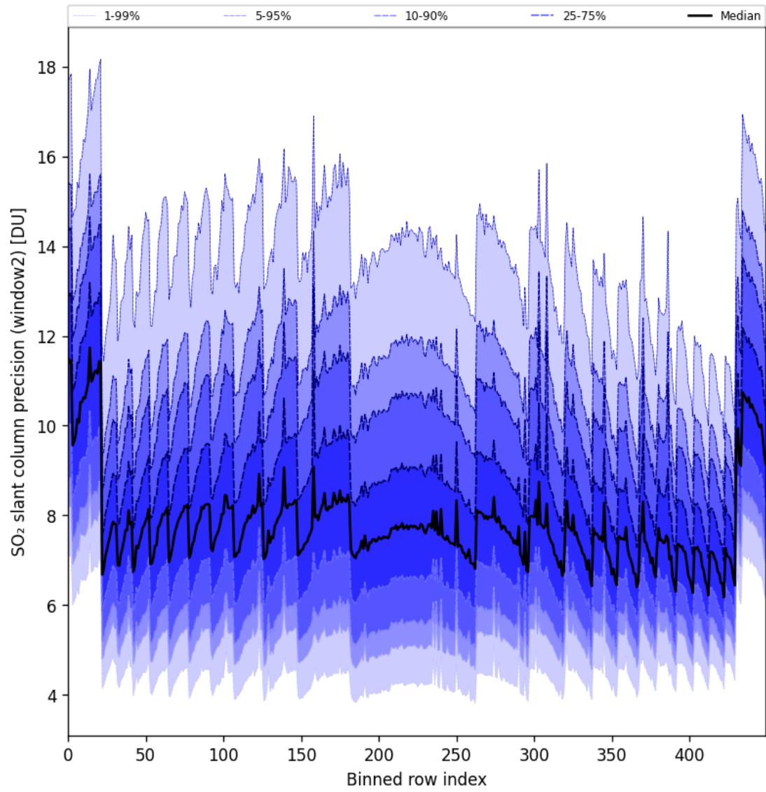
Figure 94: Along track statistics of “SO 2 slant column precision (window2)” for 2025-11-08 to 2025-11-10
