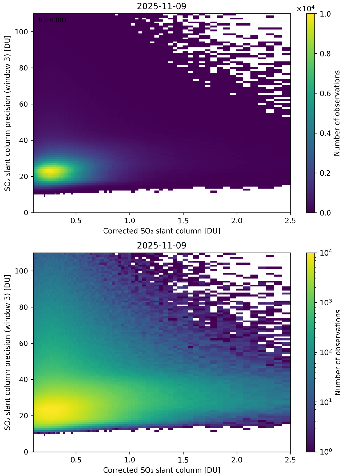
Figure 241: Scatter density plot of “Corrected SO 2 slant column” against “SO 2 slant column precision (window 3)” for 2025-11-08 to 2025-11-10.
