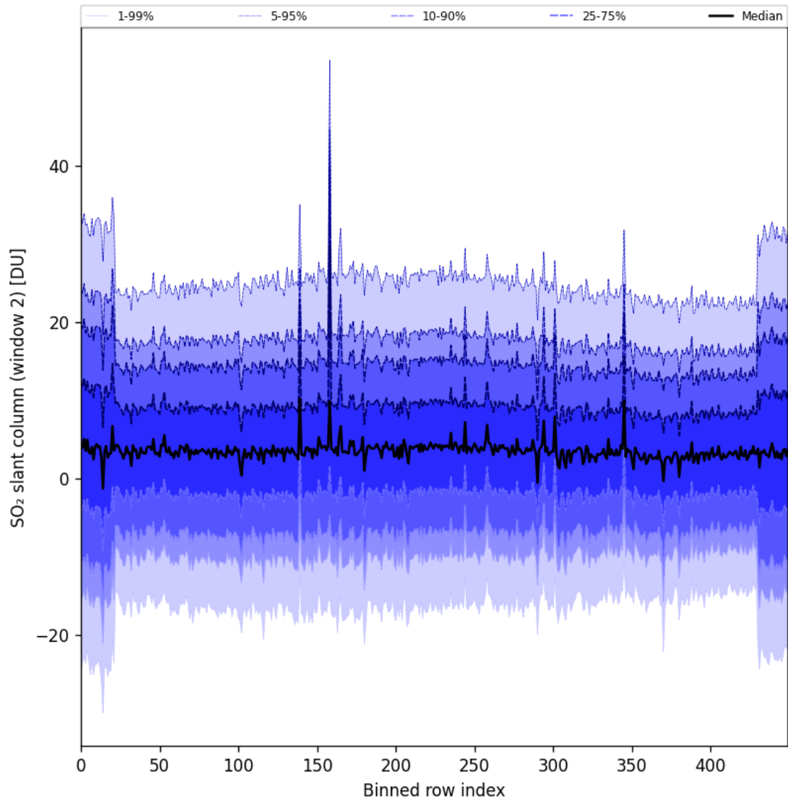
Figure 93: Along track statistics of “SO 2 slant column (window 2)” for 2025-11-08 to 2025-11-10
