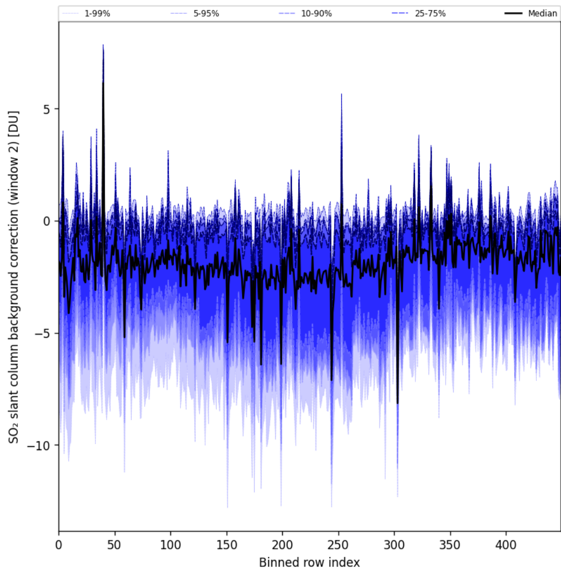
Figure 96: Along track statistics of “SO 2 slant column background correction (window 2)” for 2025-11-08 to 2025-11-10
