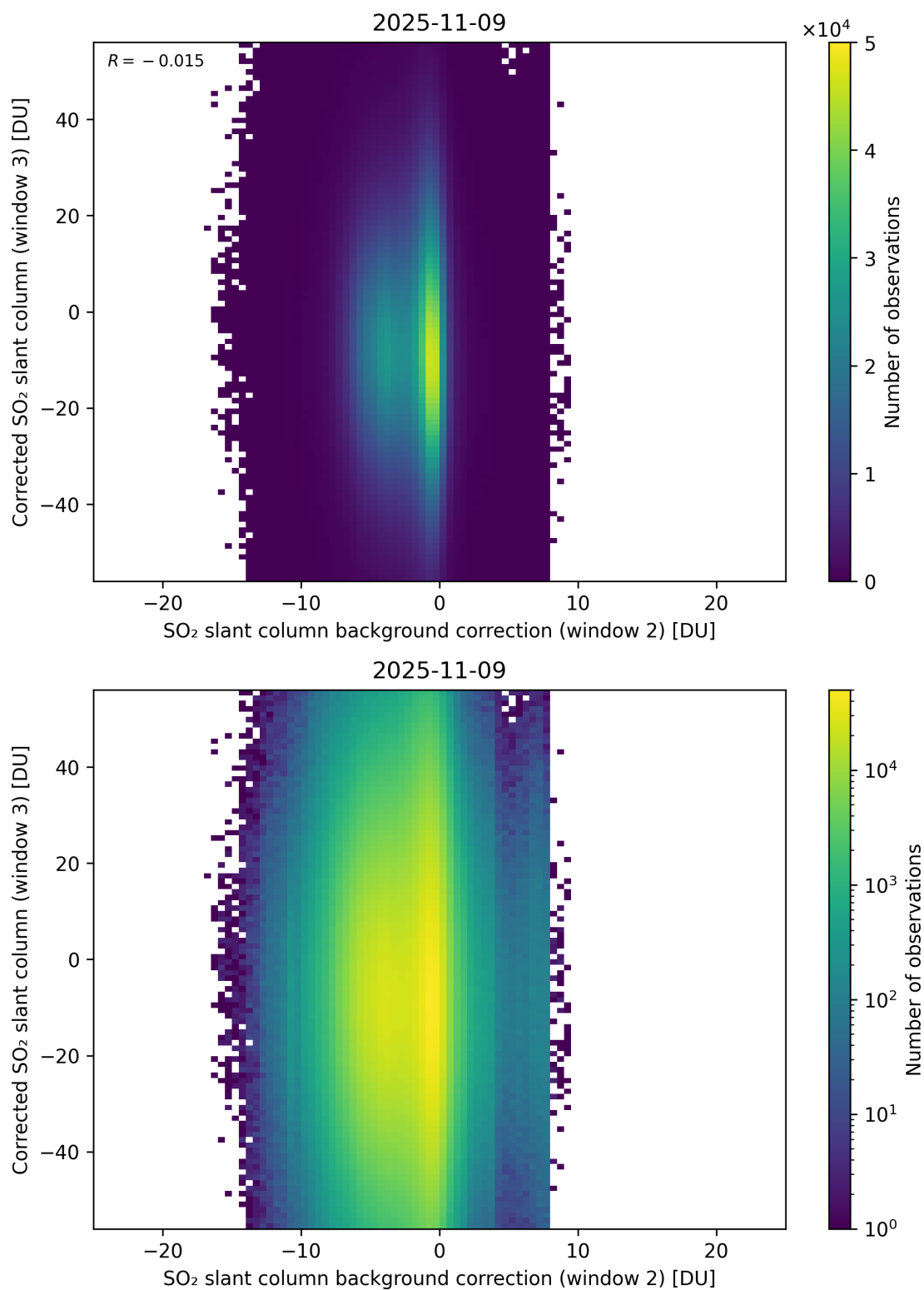
Figure 127: Scatter density plot of “SO 2 slant column background correction (window 2)” against “Corrected SO 2 slant column (window 3)” for 2025-11-08 to 2025-11-10.
