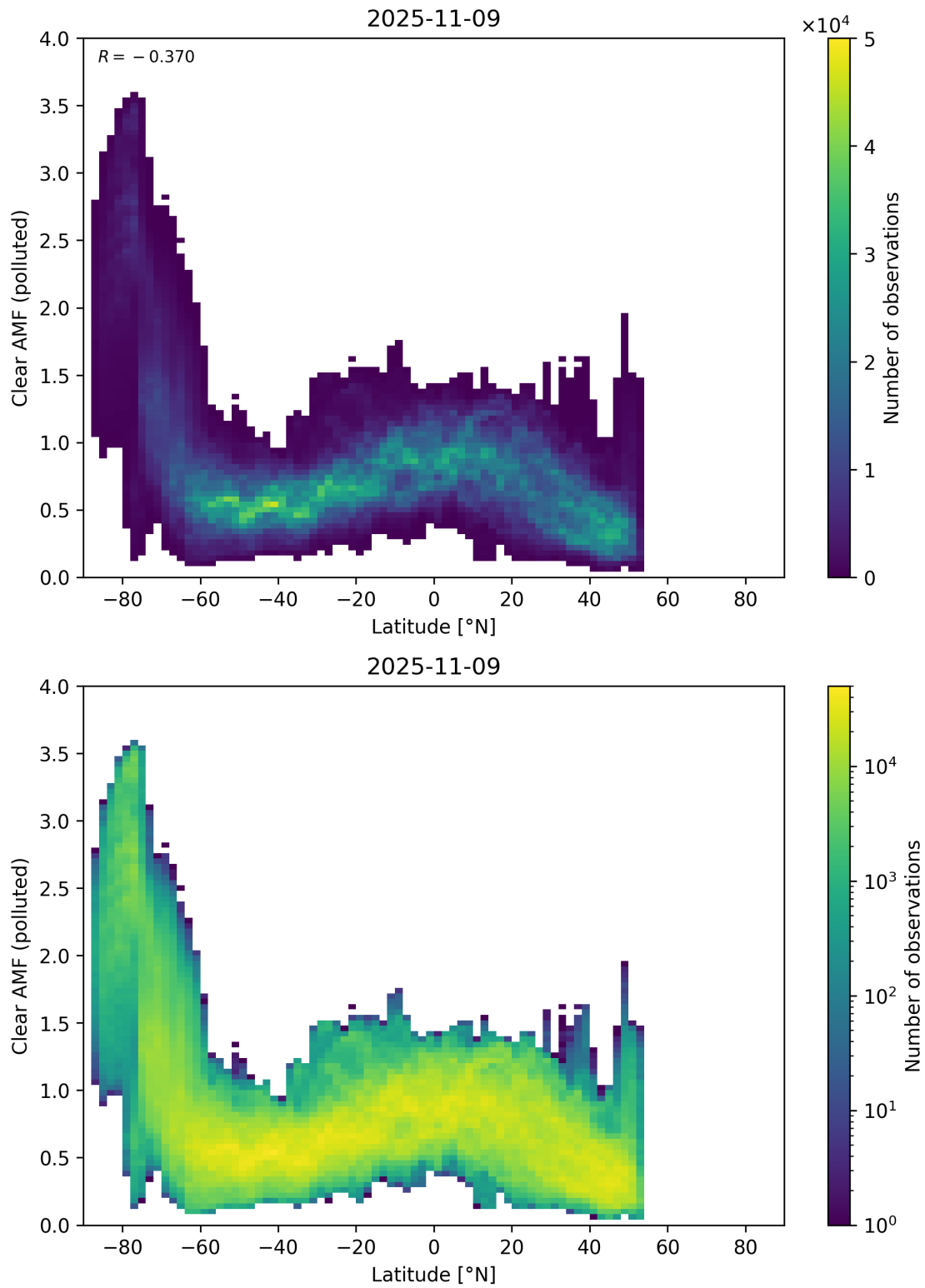
Figure 156: Scatter density plot of “Latitude” against “Clear AMF (polluted)” for 2025-11-08 to 2025-11-10.
