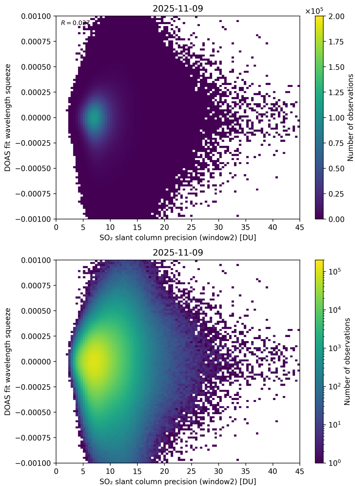
Figure 294: Scatter density plot of “SO 2 slant column precision (window2)” against “DOAS fit wavelength squeeze” for 2025-11-08 to 2025-11-10.
