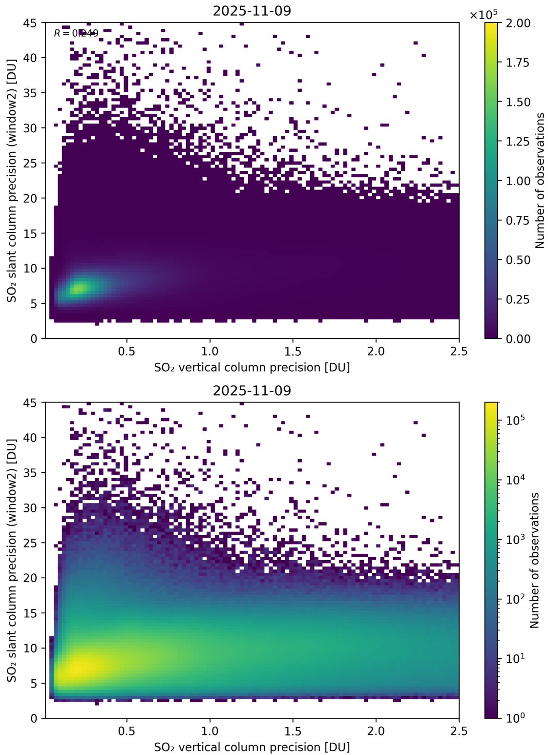
Figure 343: Scatter density plot of “SO 2 vertical column precision” against “SO 2 slant column precision (window2)” for 2025-11-08 to 2025-11-10.
