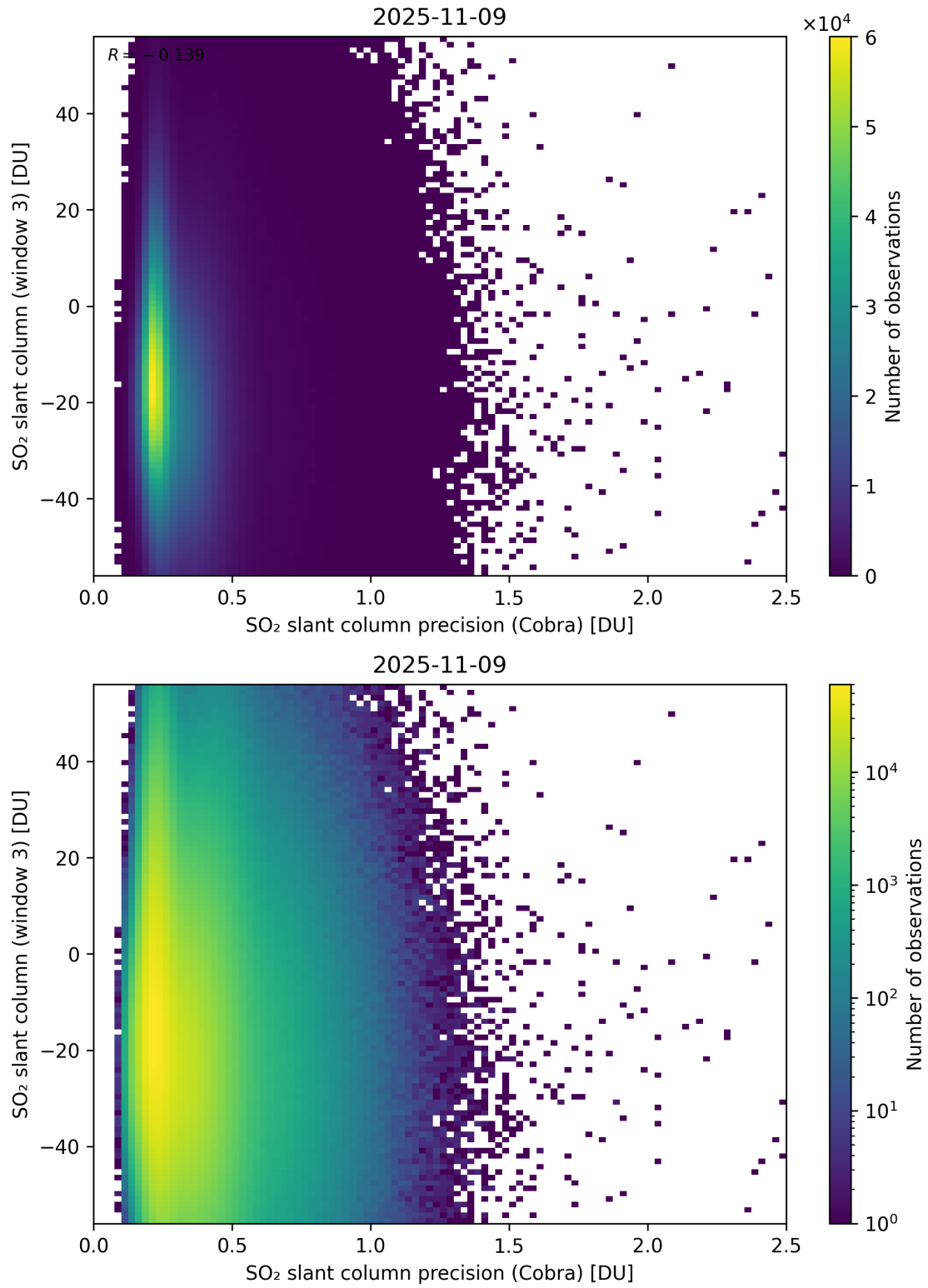
Figure 211: Scatter density plot of “SO 2 slant column precision (Cobra)” against “SO 2 slant column (window 3)” for 2025-11-08 to 2025-11-10.
