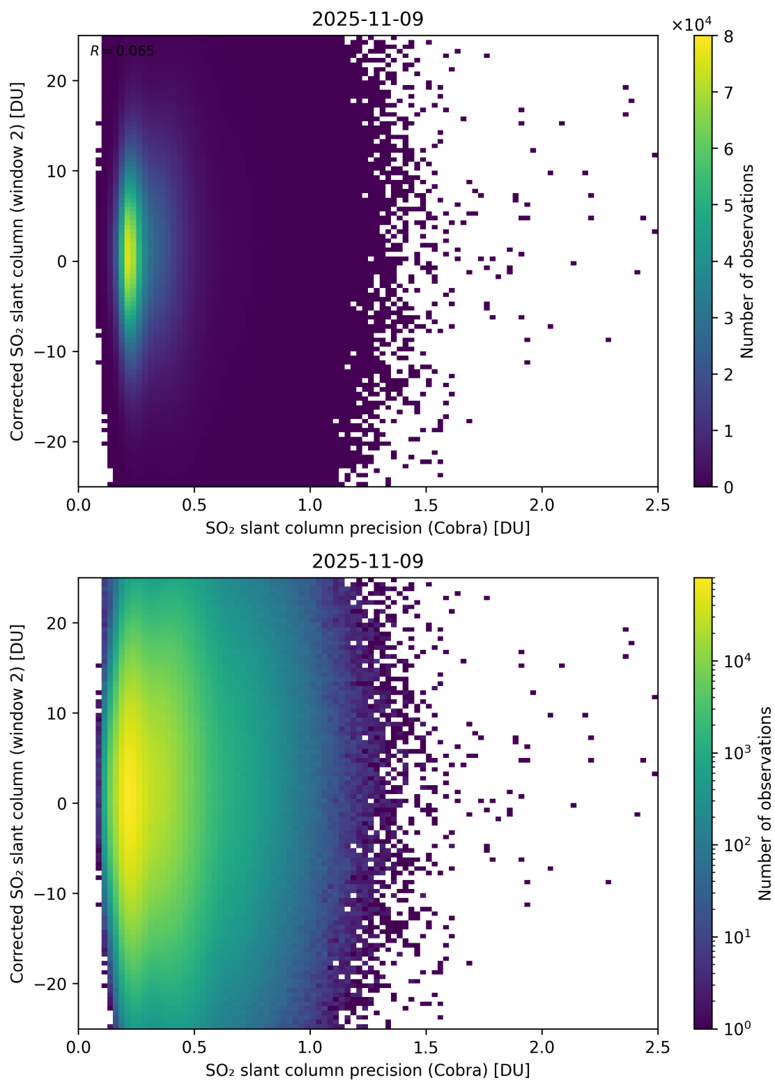
Figure 206: Scatter density plot of “SO 2 slant column precision (Cobra)” against “Corrected SO 2 slant column (window 2)” for 2025-11-08 to 2025-11-10.
