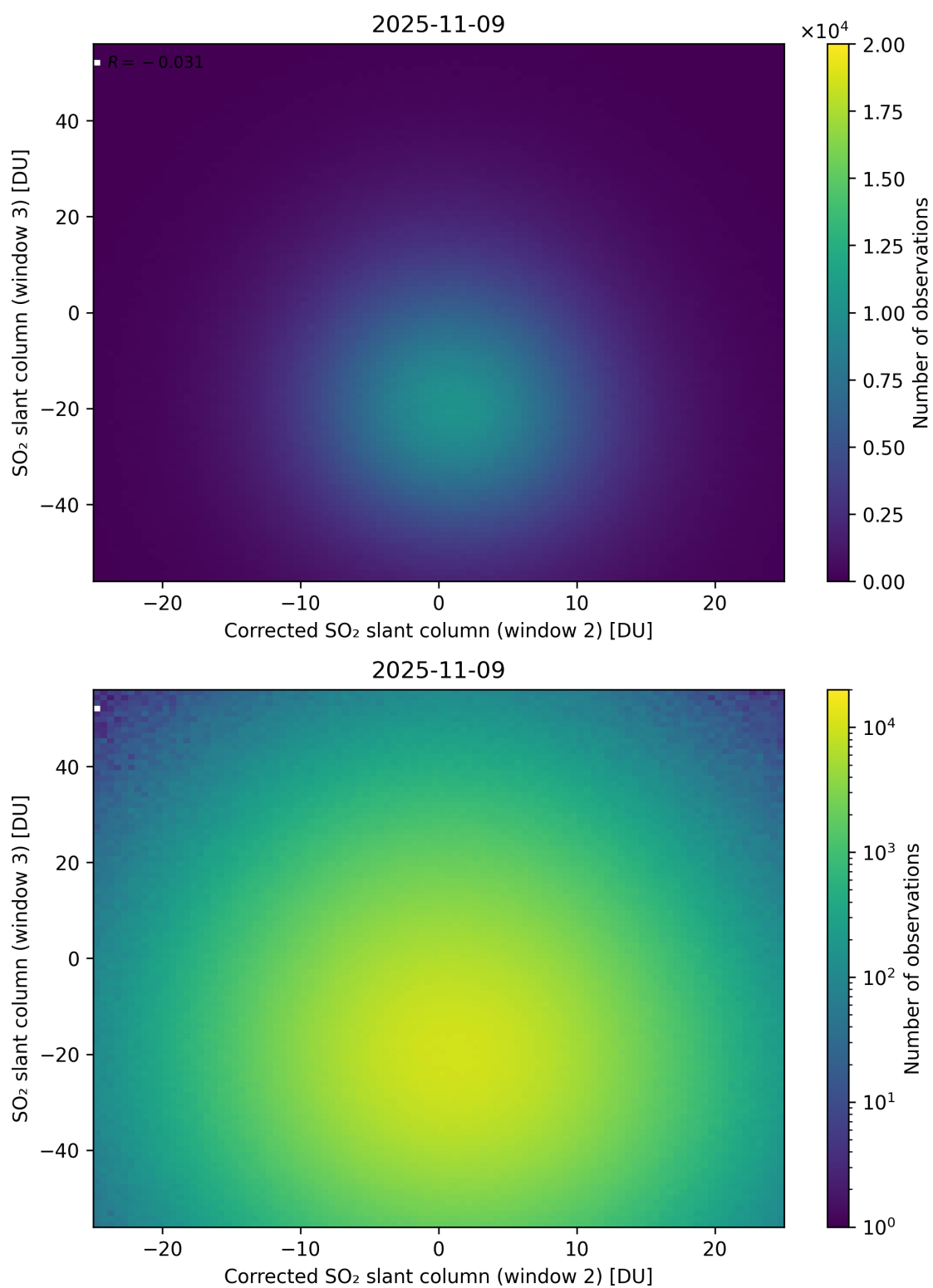
Figure 251: Scatter density plot of “Corrected SO 2 slant column (window 2)” against “SO 2 slant column (window 3)” for 2025-11-08 to 2025-11-10.
