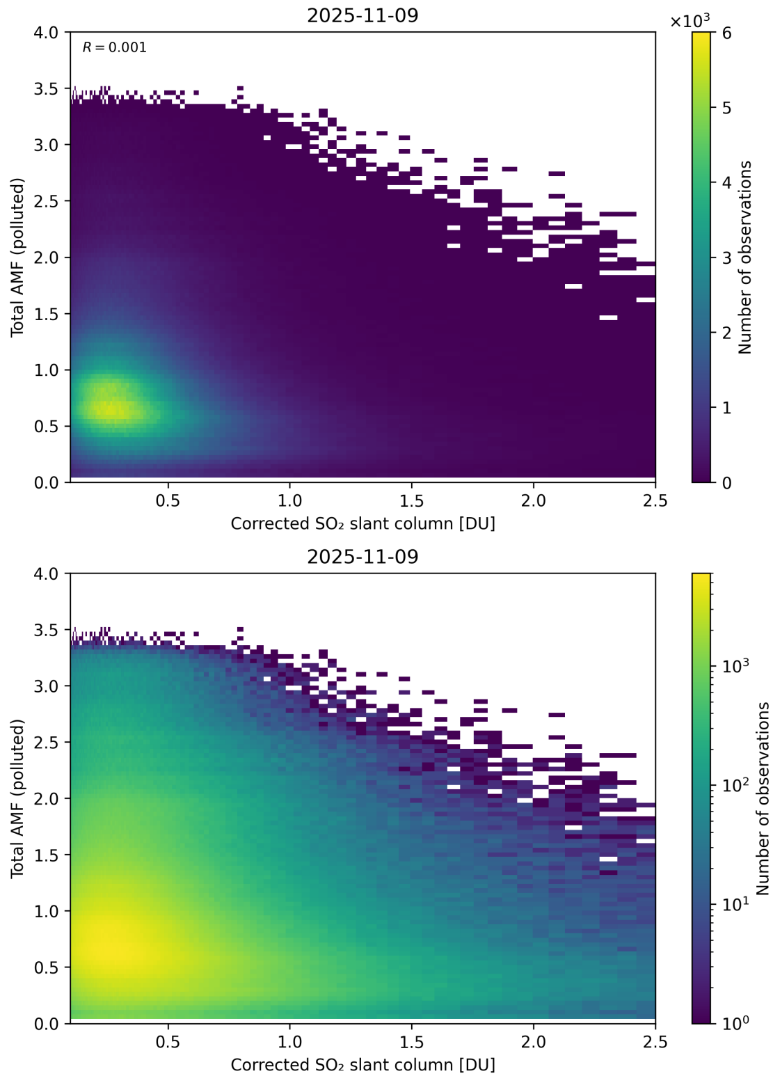
Figure 242: Scatter density plot of “Corrected SO 2 slant column” against “Total AMF (polluted)” for 2025-11-08 to 2025-11-10.
