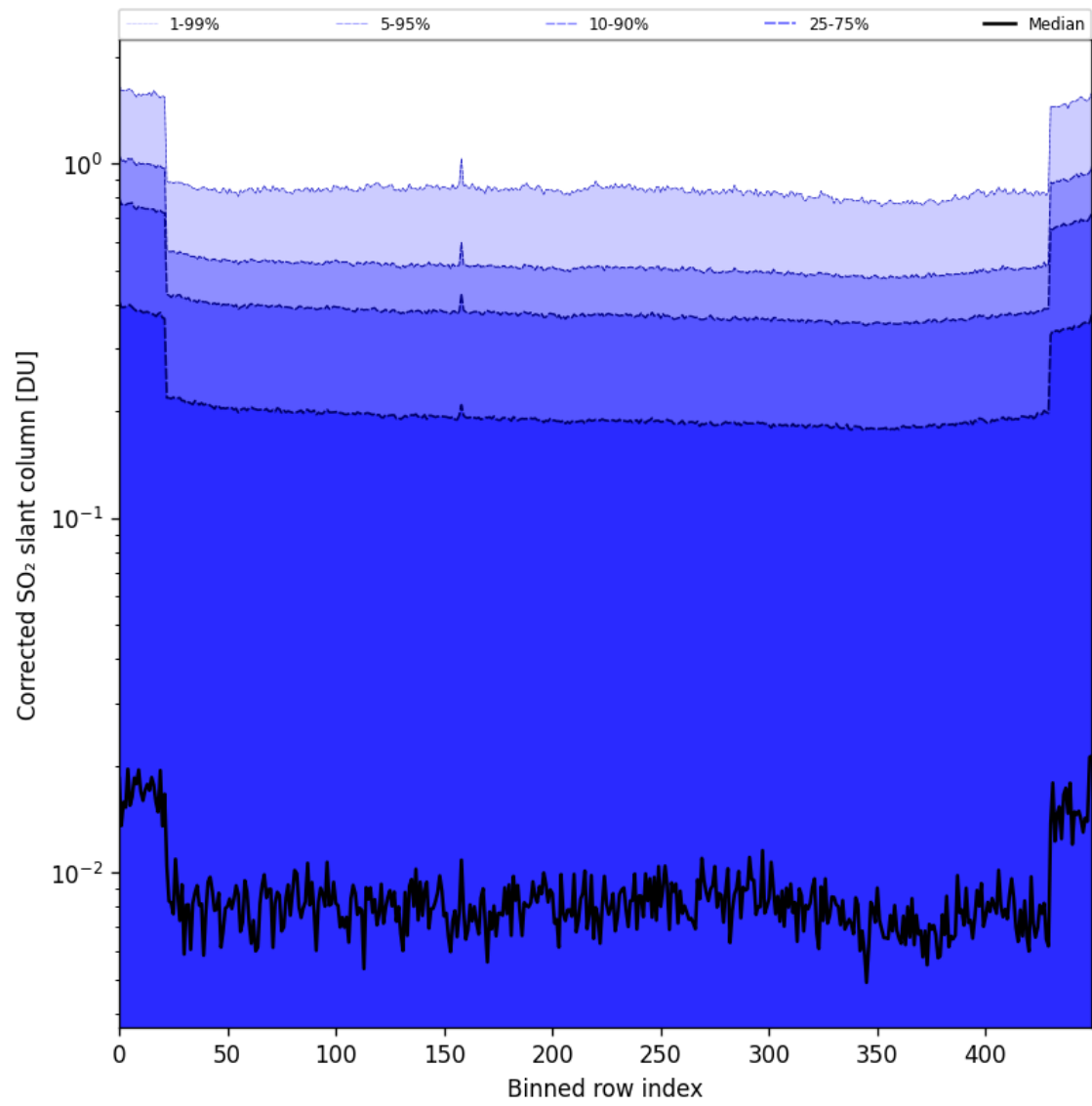
Figure 86: Along track statistics of “Corrected SO 2 slant column” for 2025-11-08 to 2025-11-10
