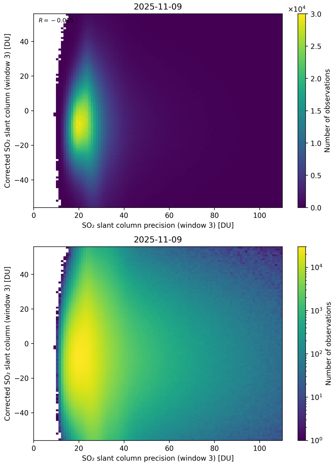
Figure 312: Scatter density plot of “SO 2 slant column precision (window 3)” against “Corrected SO 2 slant column (window 3)” for 2025-11-08 to 2025-11-10.
