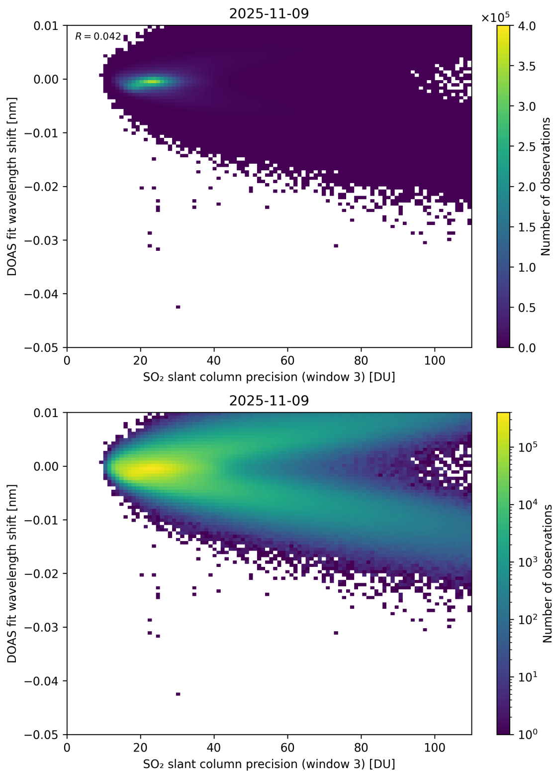
Figure 308: Scatter density plot of “SO 2 slant column precision (window 3)” against “DOAS fit wavelength shift” for 2025-11-08 to 2025-11-10.
