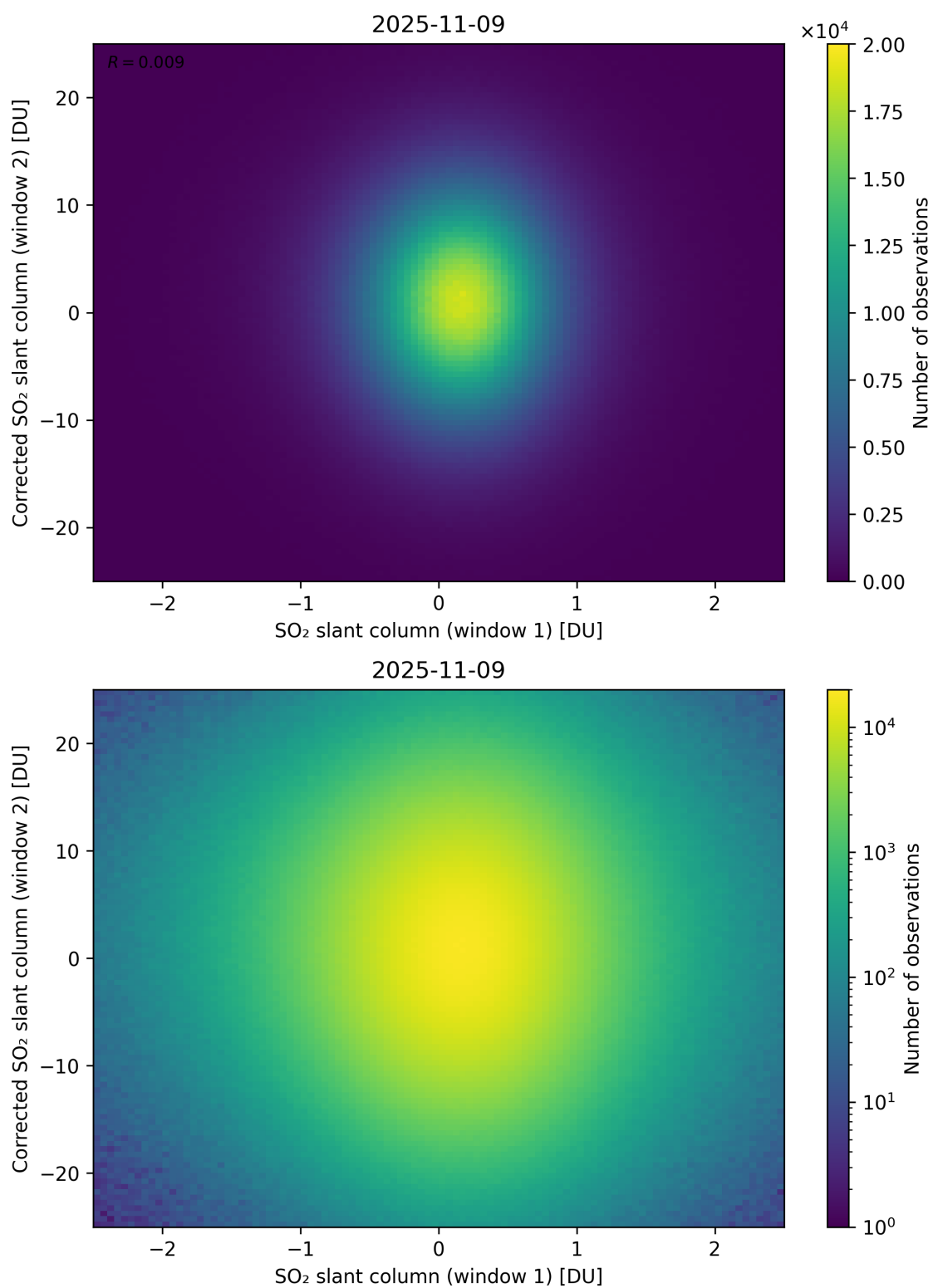
Figure 283: Scatter density plot of “SO 2 slant column (window 1)” against “Corrected SO 2 slant column (window 2)” for 2025-11-08 to 2025-11-10.
