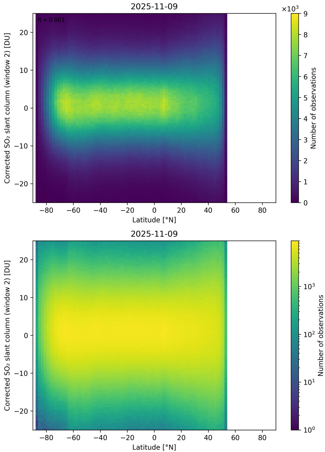
Figure 160: Scatter density plot of “Latitude” against “Corrected SO 2 slant column (window 2)” for 2025-11-08 to 2025-11-10.
