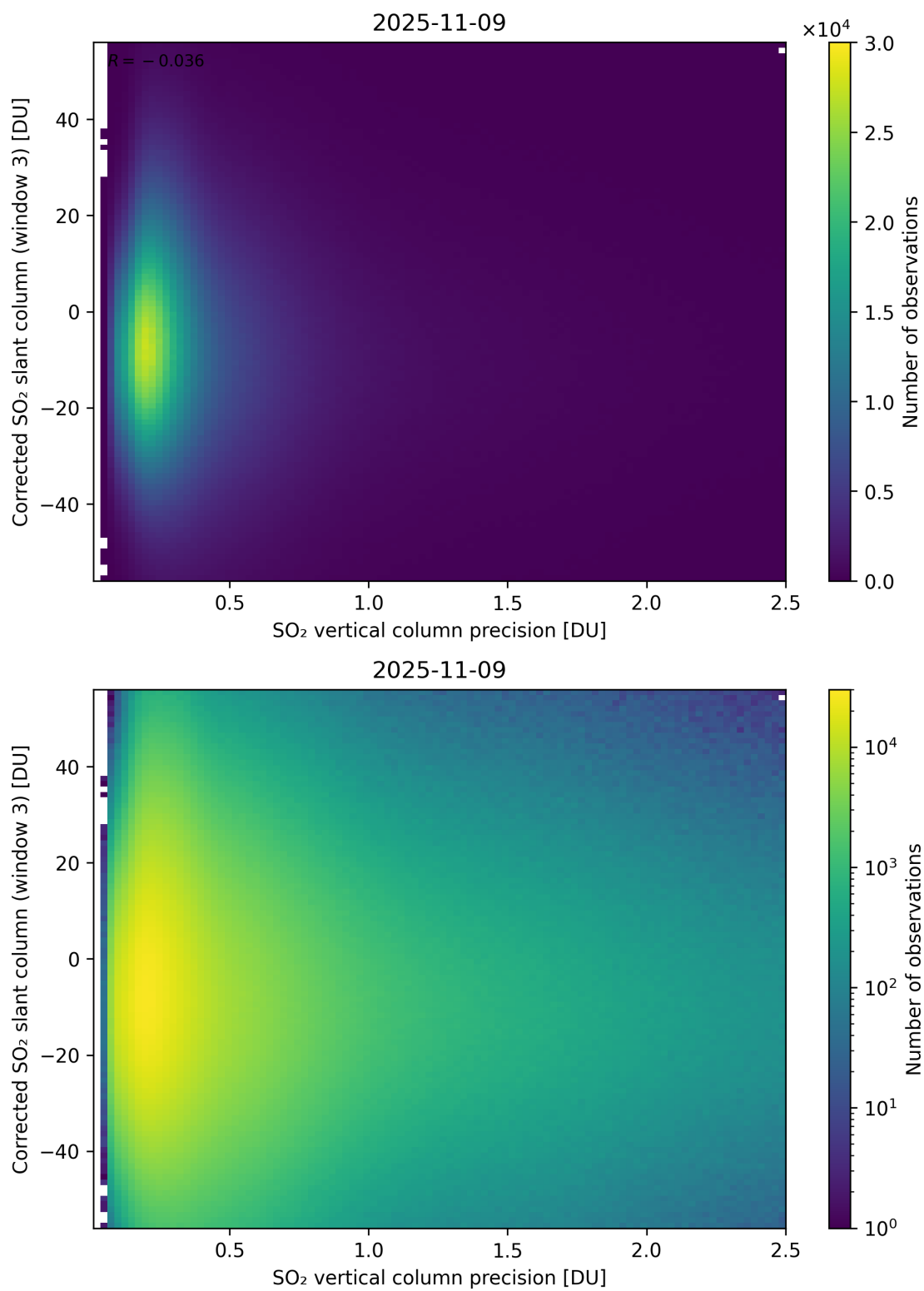
Figure 340: Scatter density plot of “SO 2 vertical column precision” against “Corrected SO 2 slant column (window 3)” for 2025-11-08 to 2025-11-10.
