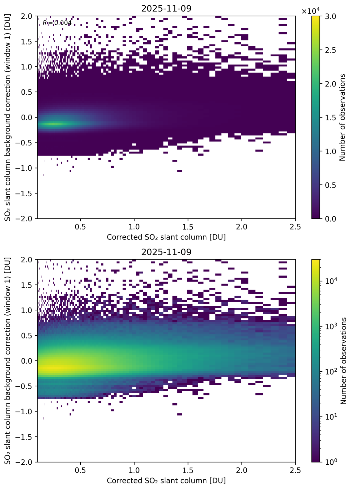
Figure 226: Scatter density plot of “Corrected SO 2 slant column” against “SO 2 slant column background correction (window 1)” for 2025-11-08 to 2025-11-10.
