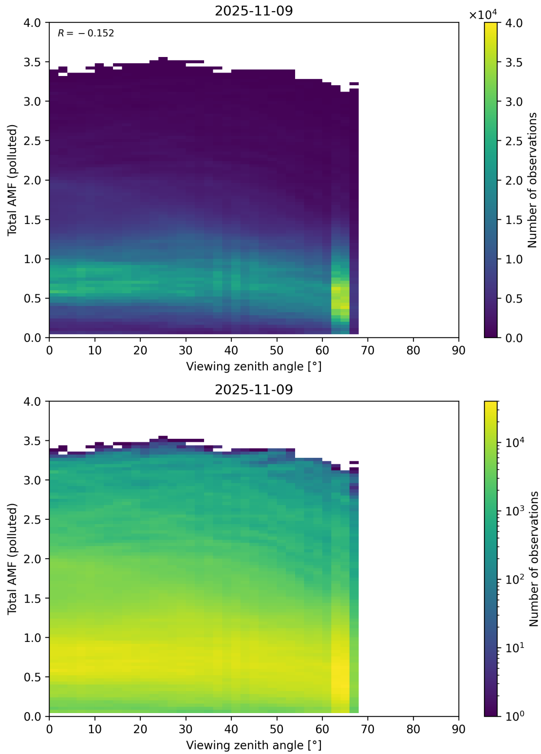
Figure 381: Scatter density plot of “Viewing zenith angle” against “Total AMF (polluted)” for 2025-11-08 to 2025-11-10.
