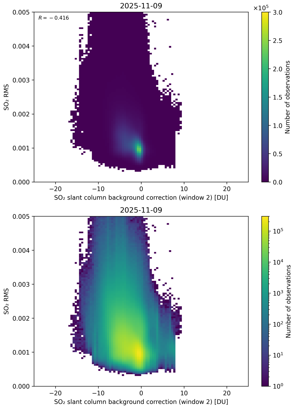
Figure 125: Scatter density plot of “SO 2 slant column background correction (window 2)” against “SO 2 RMS” for 2025-11-08 to 2025-11-10.
