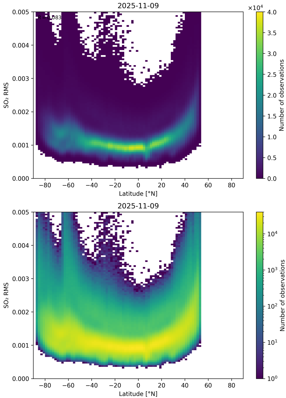
Figure 155: Scatter density plot of “Latitude” against “SO 2 RMS” for 2025-11-08 to 2025-11-10.
