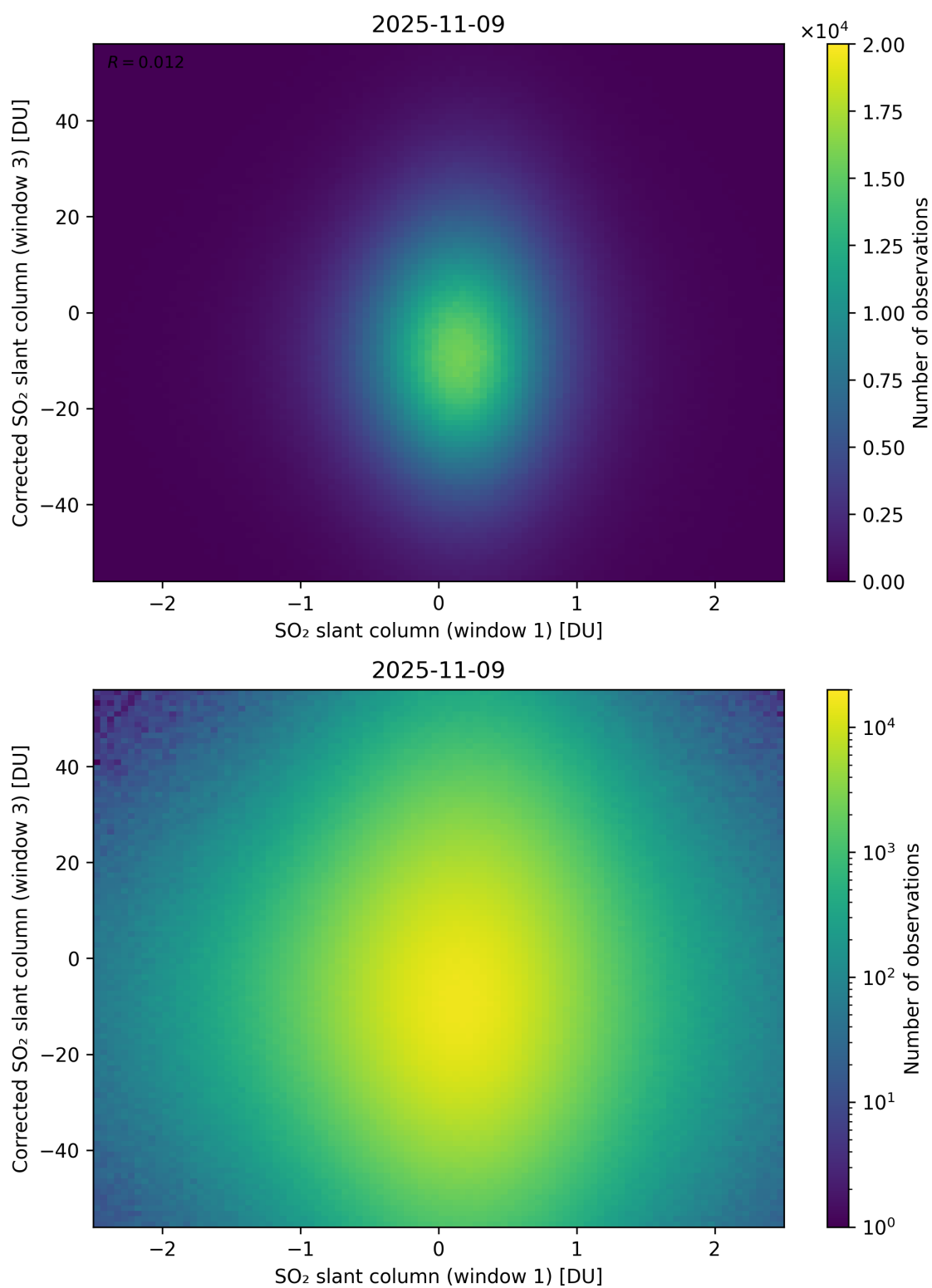
Figure 284: Scatter density plot of “SO 2 slant column (window 1)” against “Corrected SO 2 slant column (window 3)” for 2025-11-08 to 2025-11-10.
