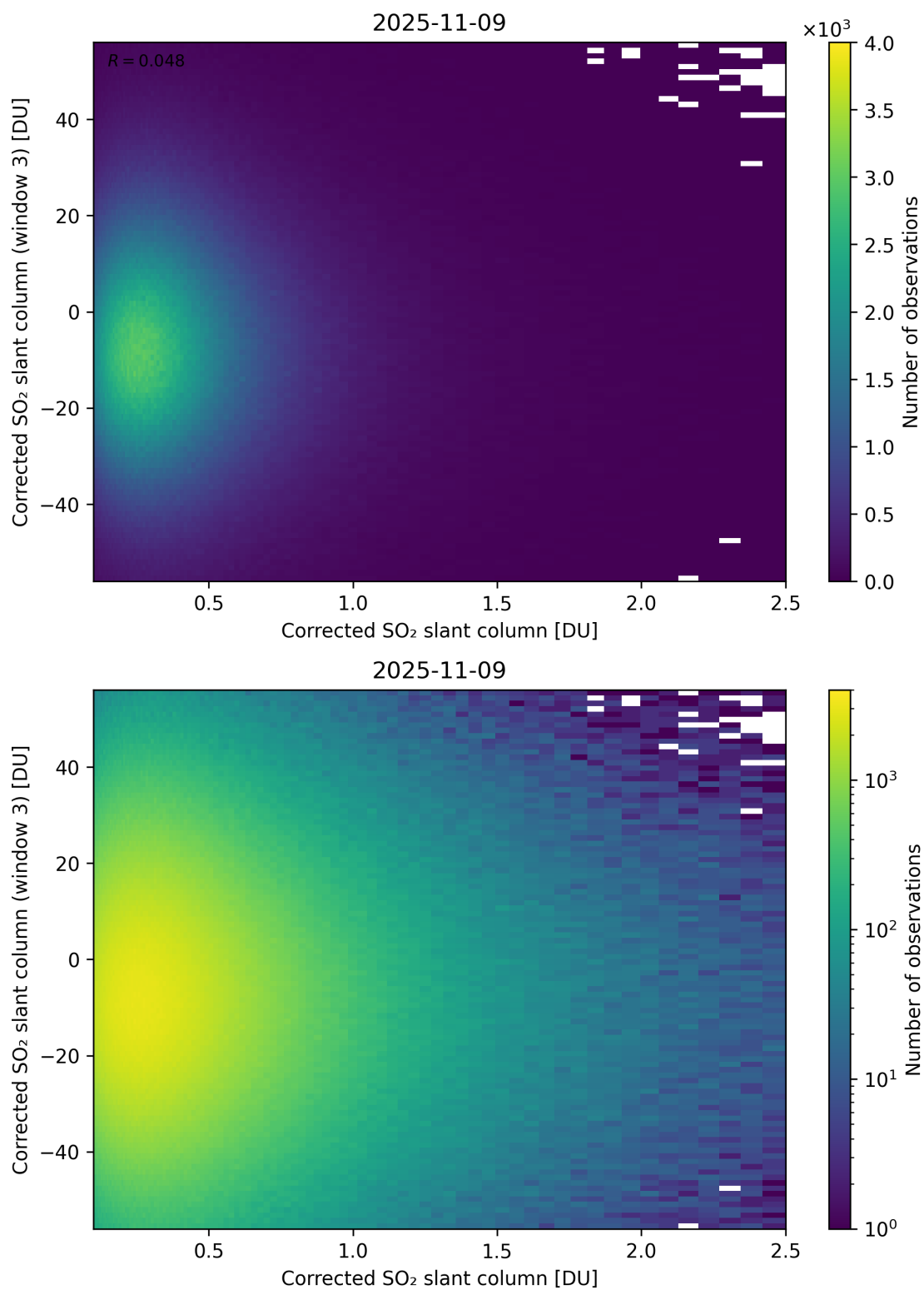
Figure 236: Scatter density plot of “Corrected SO 2 slant column” against “Corrected SO 2 slant column (window 3)” for 2025-11-08 to 2025-11-10.
