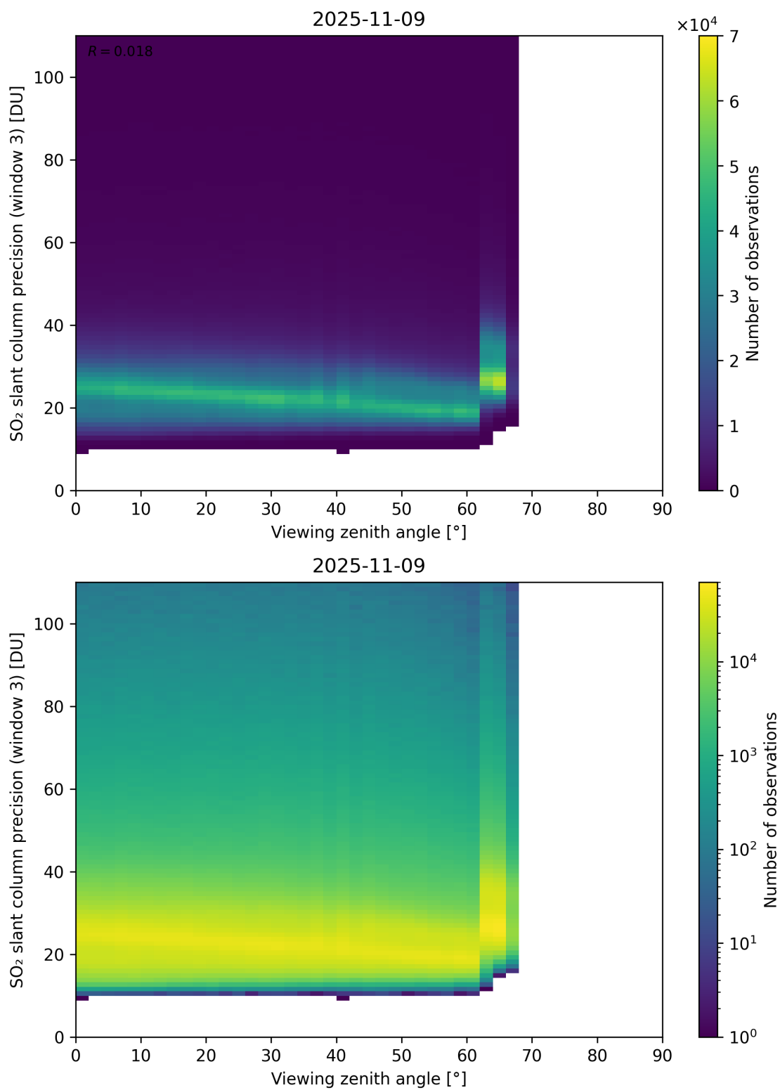
Figure 380: Scatter density plot of “Viewing zenith angle” against “SO 2 slant column precision (window 3)” for 2025-11-08 to 2025-11-10.
