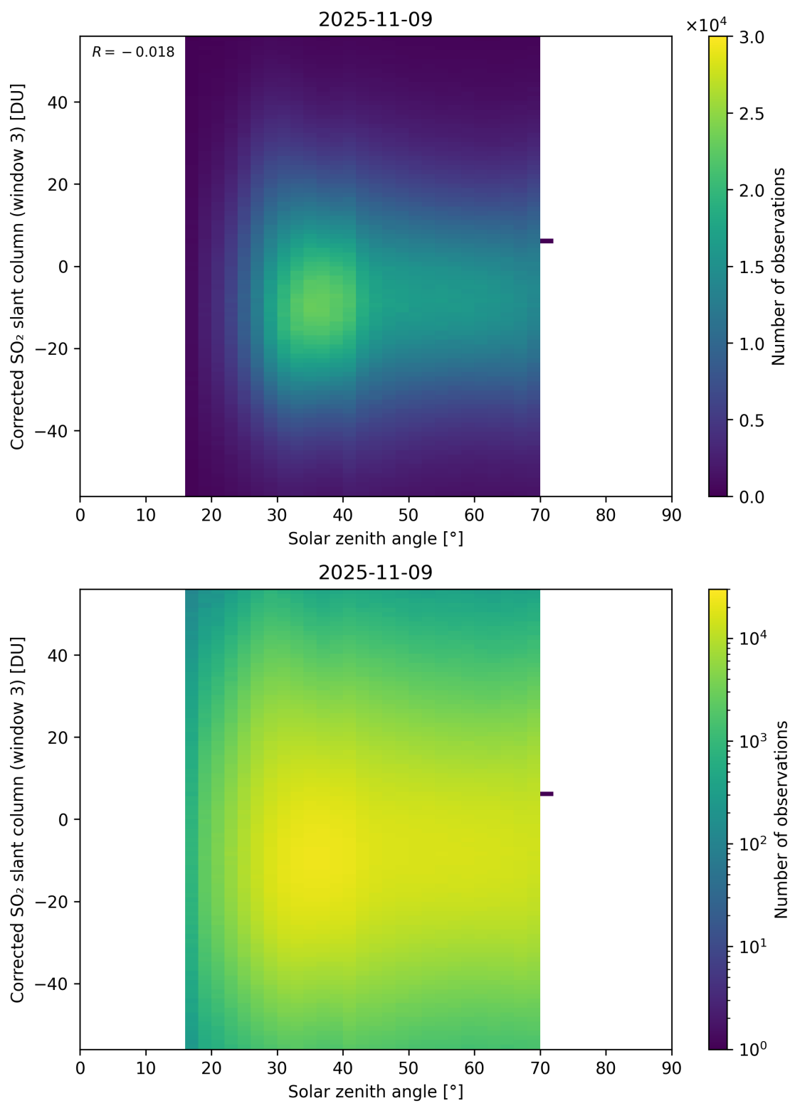
Figure 183: Scatter density plot of “Solar zenith angle” against “Corrected SO 2 slant column (window 3)” for 2025-11-08 to 2025-11-10.
