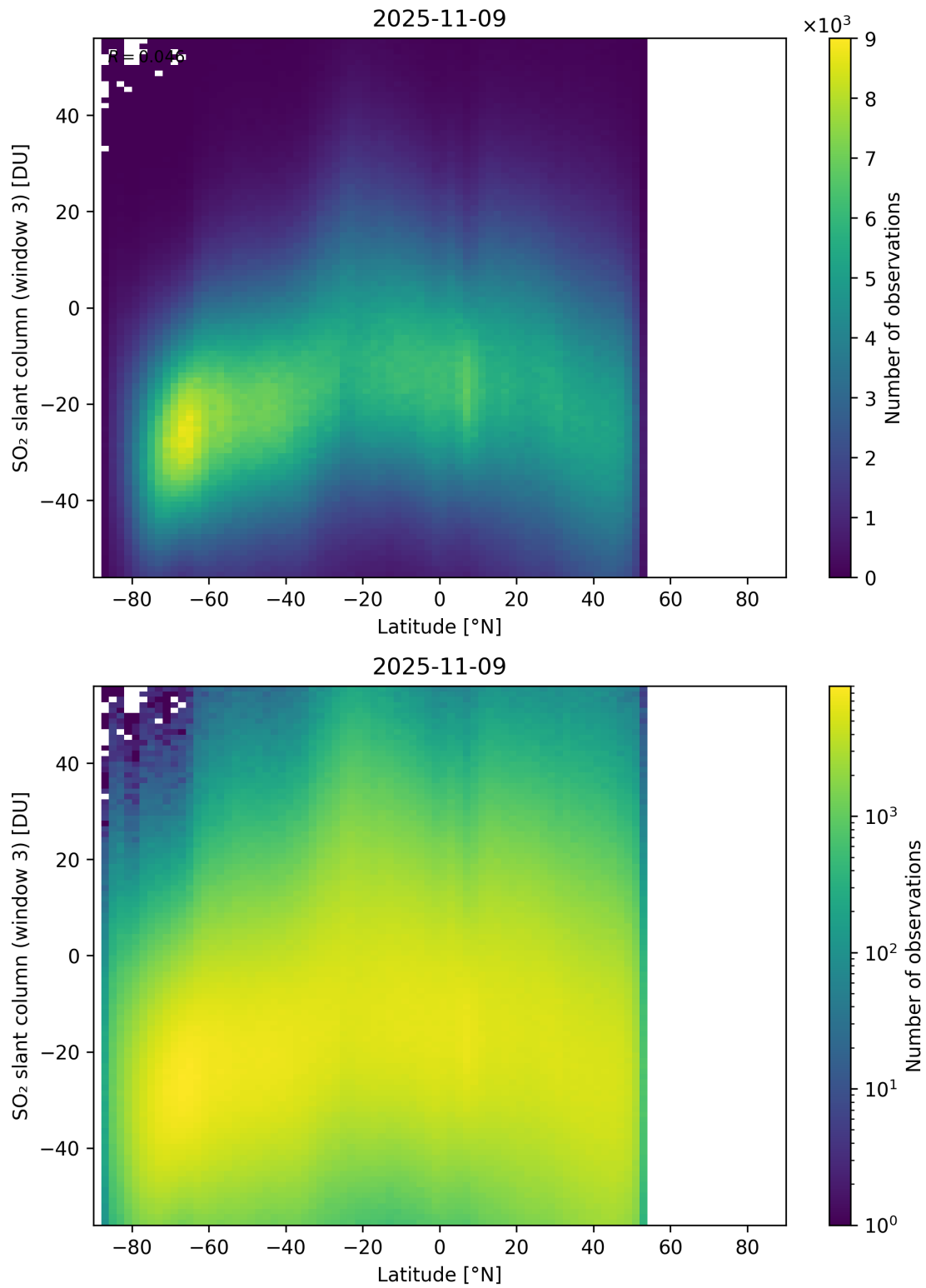
Figure 165: Scatter density plot of “Latitude” against “SO 2 slant column (window 3)” for 2025-11-08 to 2025-11-10.
