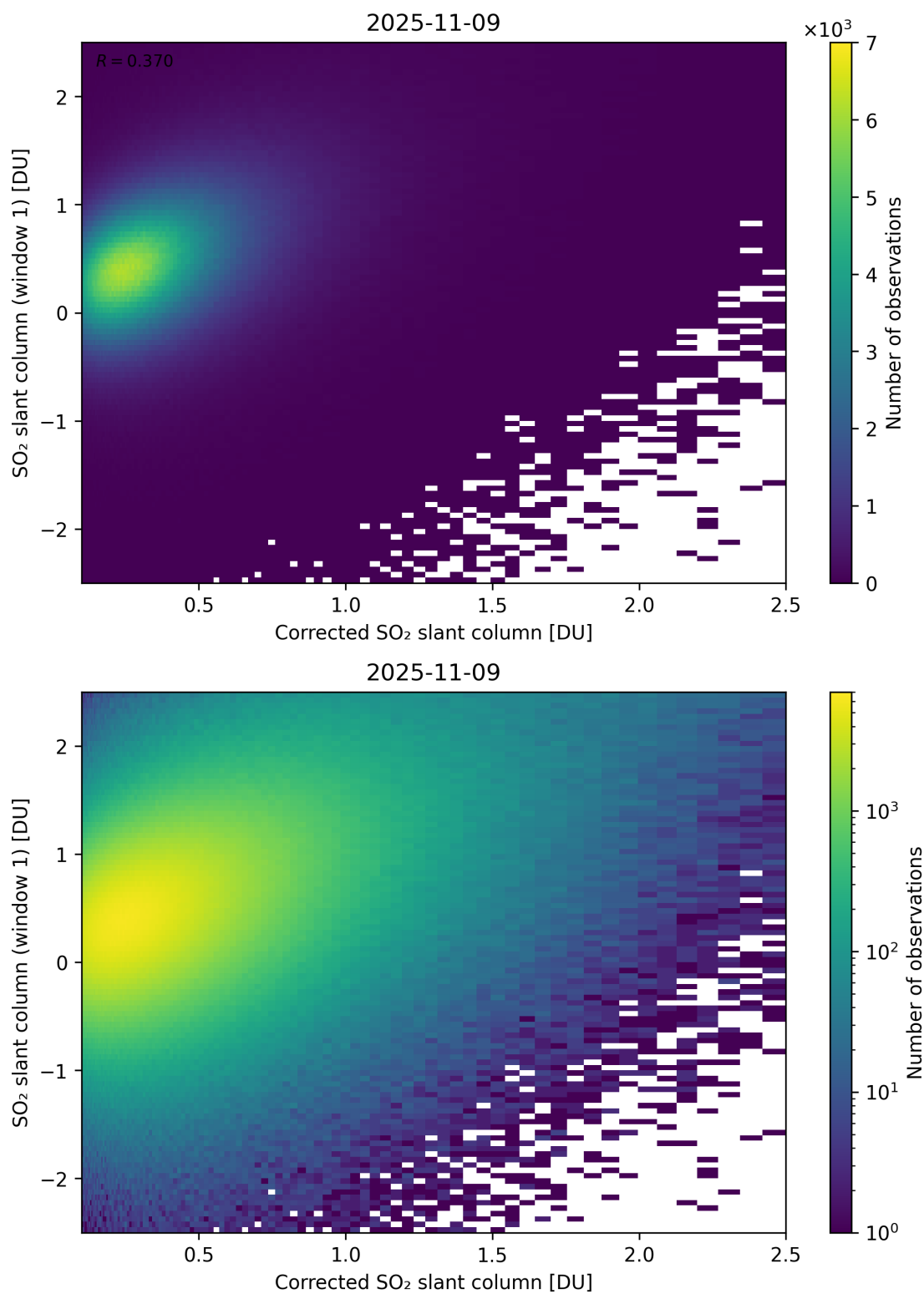
Figure 237: Scatter density plot of “Corrected SO 2 slant column” against “SO 2 slant column (window 1)” for 2025-11-08 to 2025-11-10.
