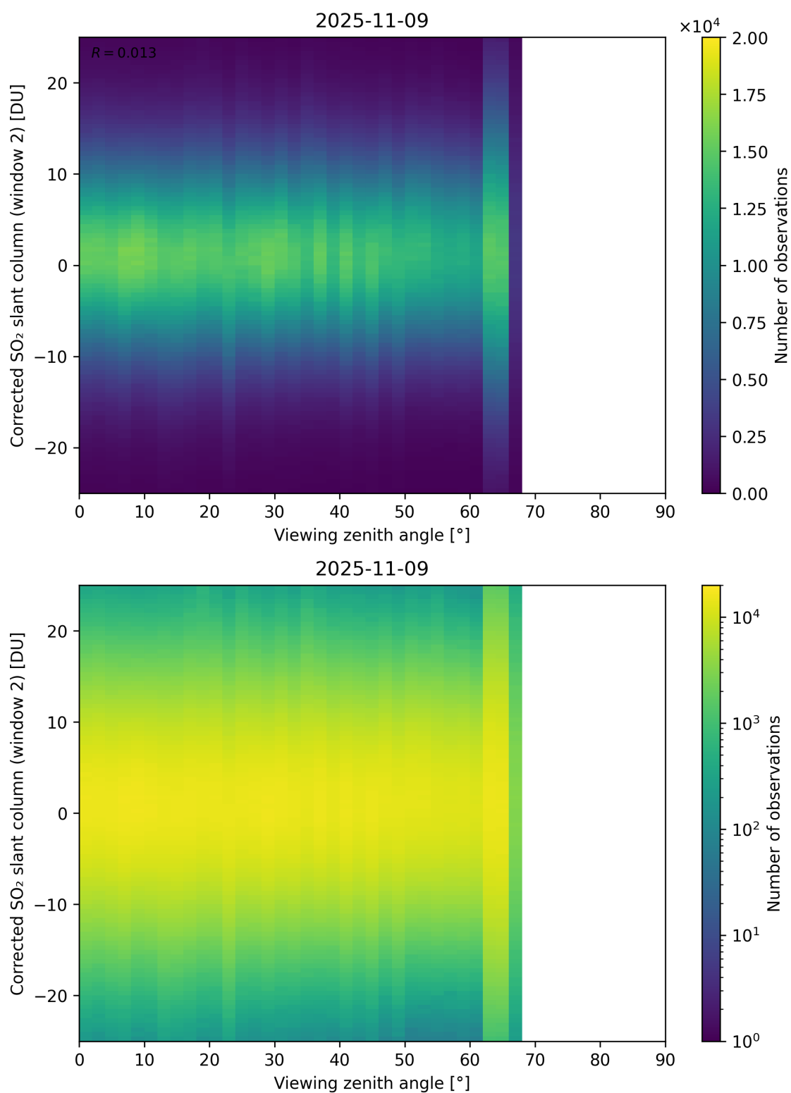
Figure 374: Scatter density plot of “Viewing zenith angle” against “Corrected SO 2 slant column (window 2)” for 2025-11-08 to 2025-11-10.
