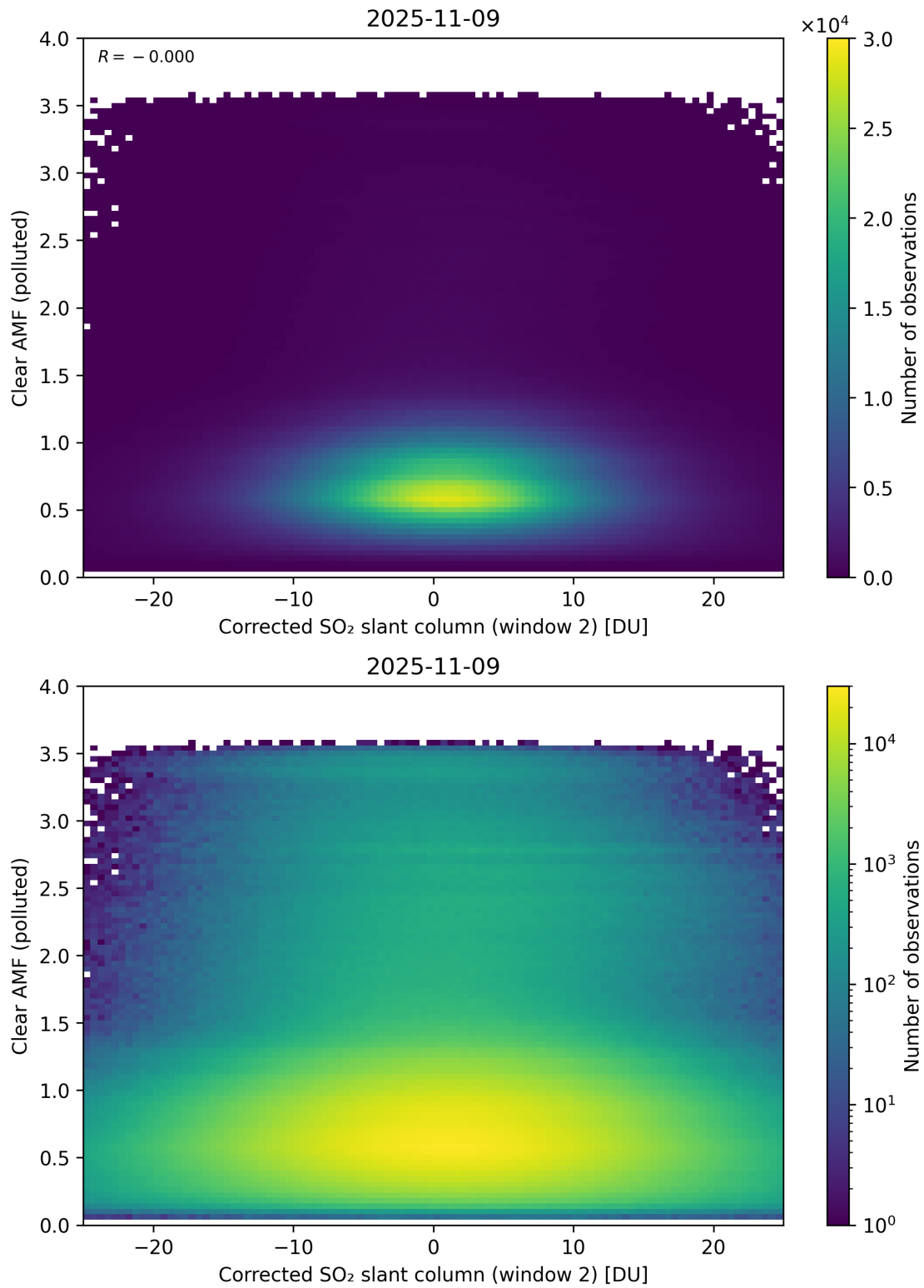
Figure 249: Scatter density plot of “Corrected SO 2 slant column (window 2)” against “Clear AMF (polluted)” for 2025-11-08 to 2025-11-10.
