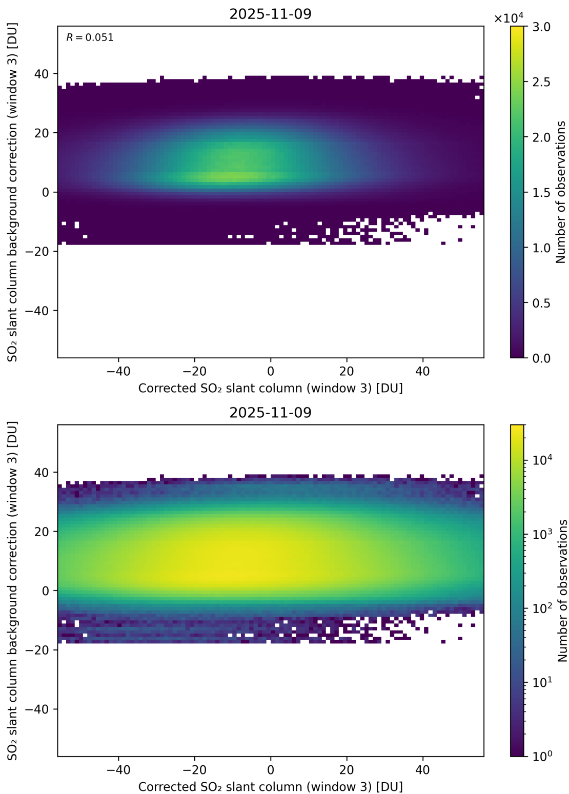
Figure 255: Scatter density plot of “Corrected SO 2 slant column (window 3)” against “SO 2 slant column background correction (window 3)” for 2025-11-08 to 2025-11-10.
