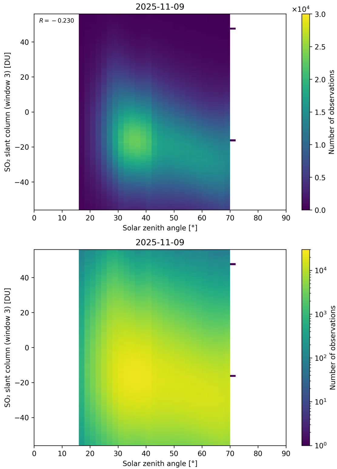
Figure 187: Scatter density plot of “Solar zenith angle” against “SO 2 slant column (window 3)” for 2025-11-08 to 2025-11-10.
