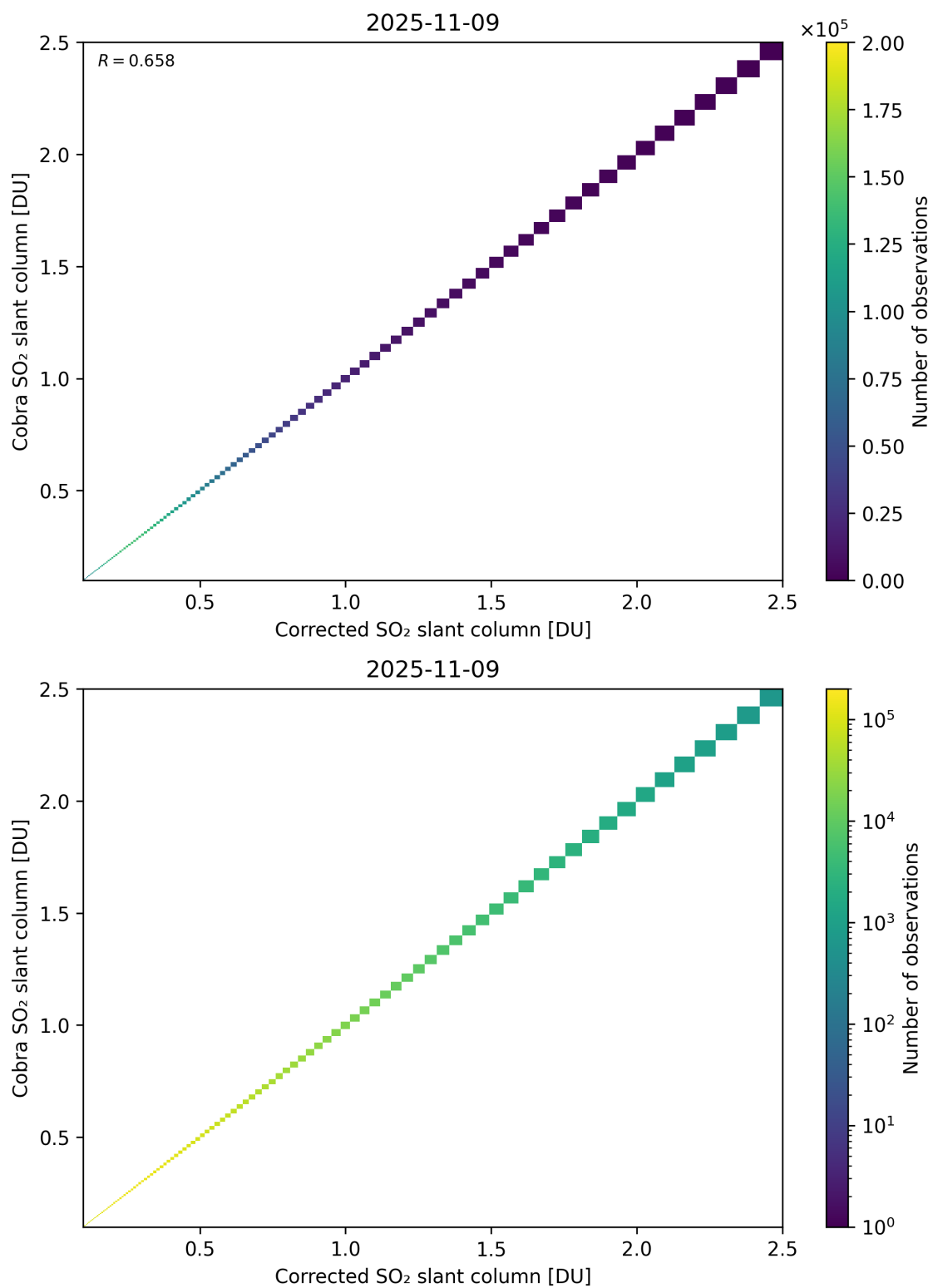
Figure 233: Scatter density plot of “Corrected SO 2 slant column” against “Cobra SO 2 slant column” for 2025-11-08 to 2025-11-10.
