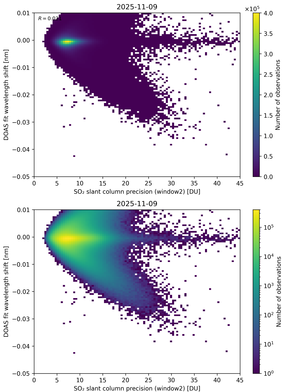
Figure 293: Scatter density plot of “SO 2 slant column precision (window2)” against “DOAS fit wavelength shift” for 2025-11-08 to 2025-11-10.
