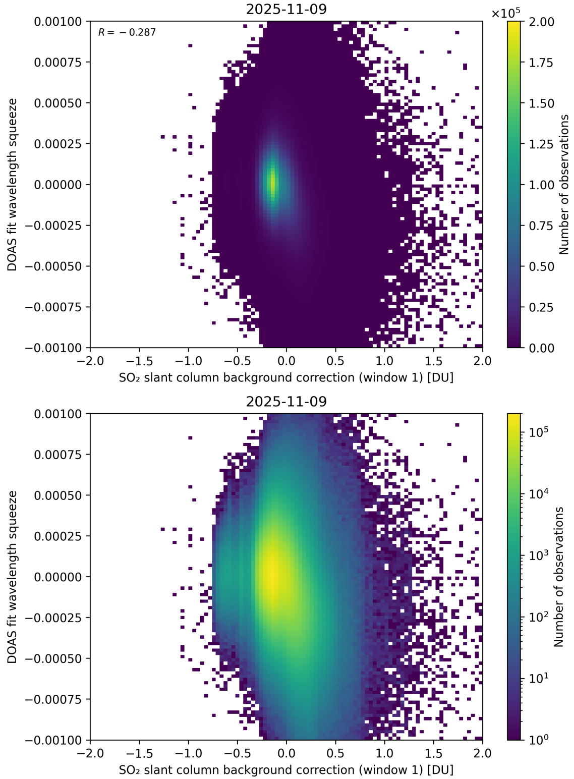
Figure 112: Scatter density plot of “SO 2 slant column background correction (window 1)” against “DOAS fit wavelength squeeze” for 2025-11-08 to 2025-11-10.
