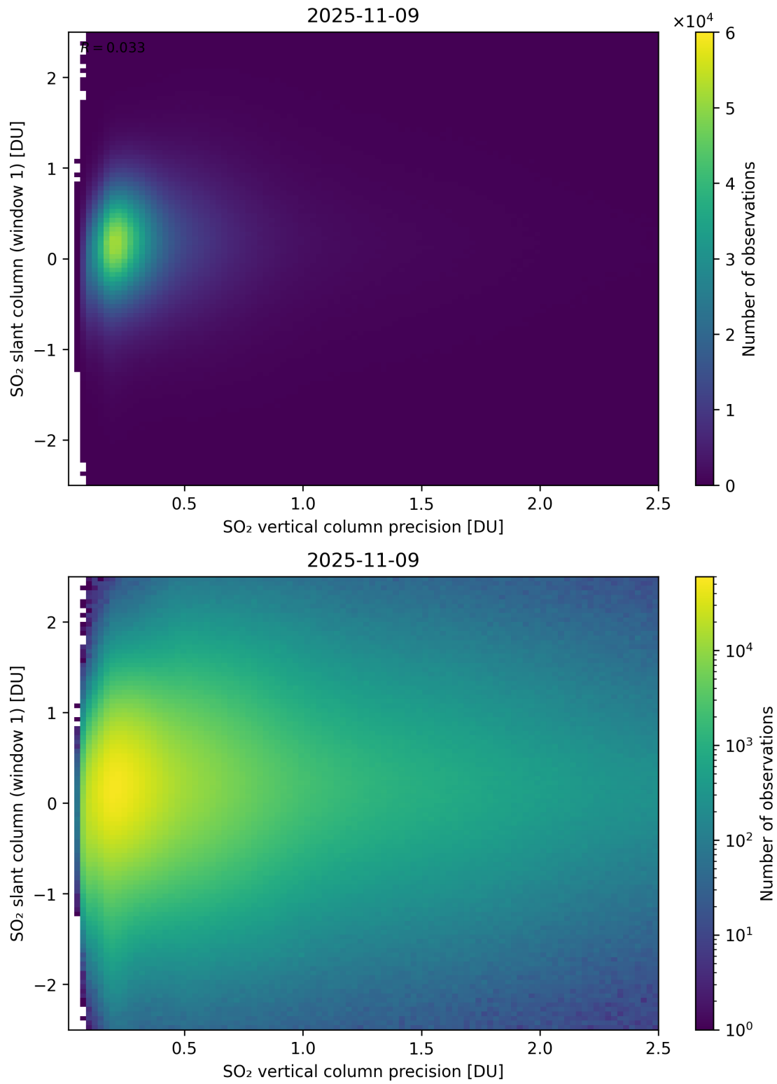
Figure 341: Scatter density plot of “SO 2 vertical column precision” against “SO 2 slant column (window 1)” for 2025-11-08 to 2025-11-10.
