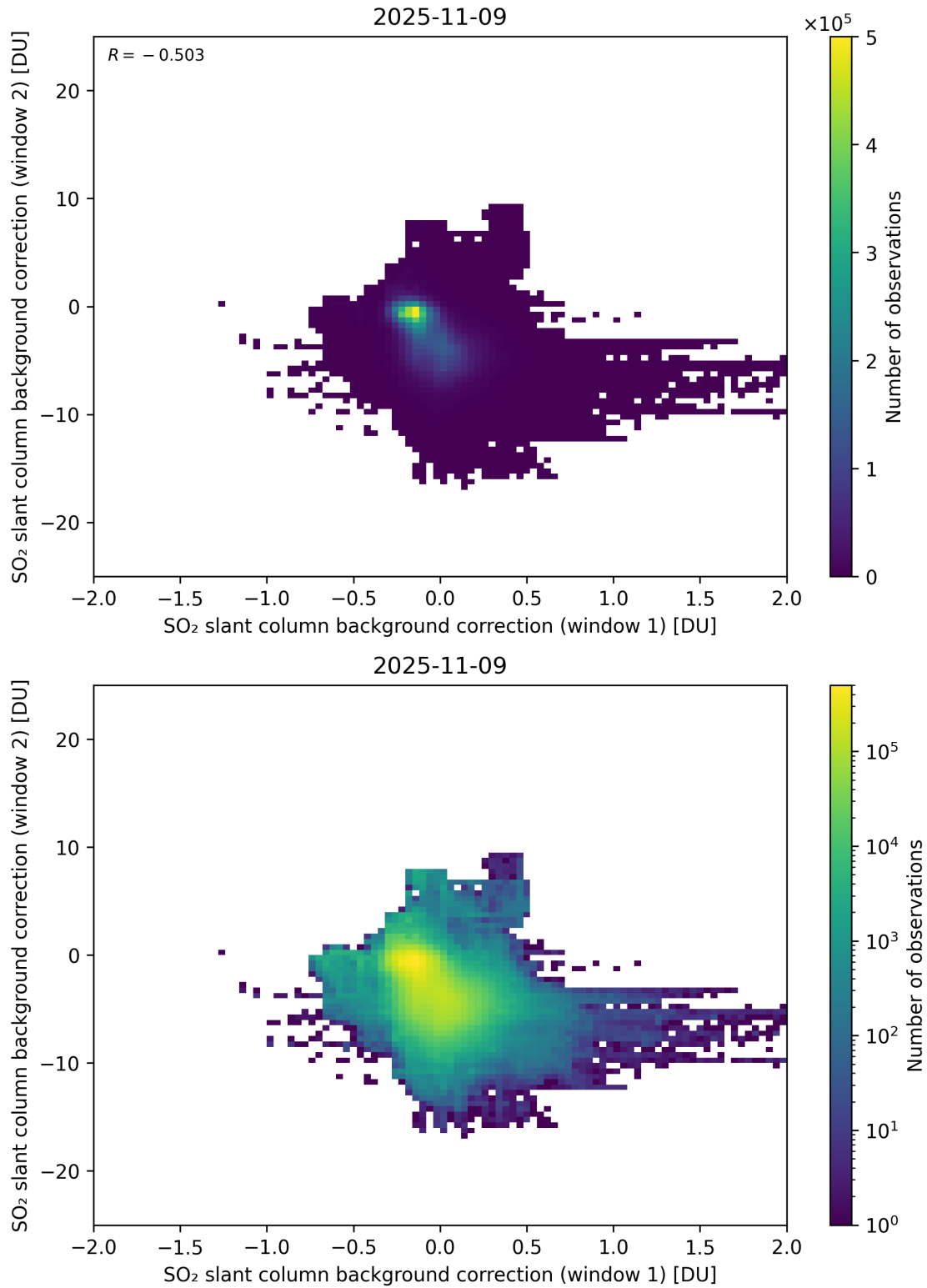
Figure 109: Scatter density plot of “SO 2 slant column background correction (window 1)” against “SO 2 slant column background correction (window 2)” for 2025-11-08 to 2025-11-10.
