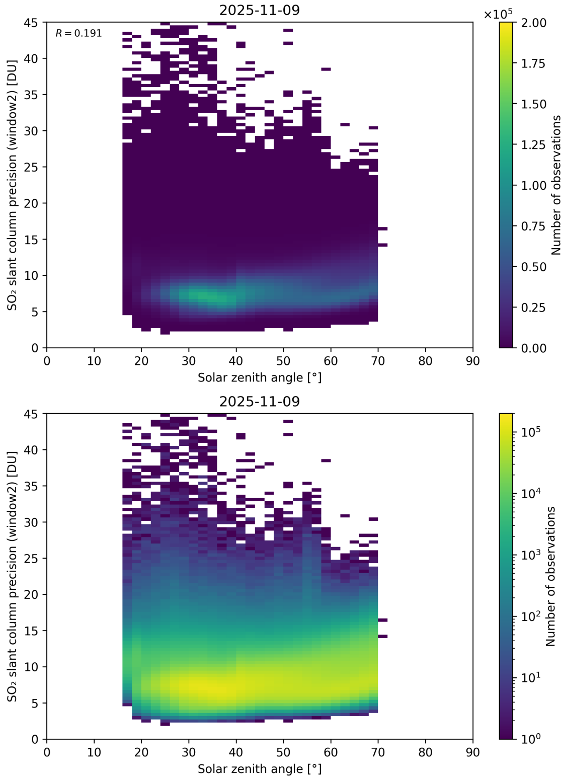
Figure 186: Scatter density plot of “Solar zenith angle” against “SO 2 slant column precision (window2)” for 2025-11-08 to 2025-11-10.
