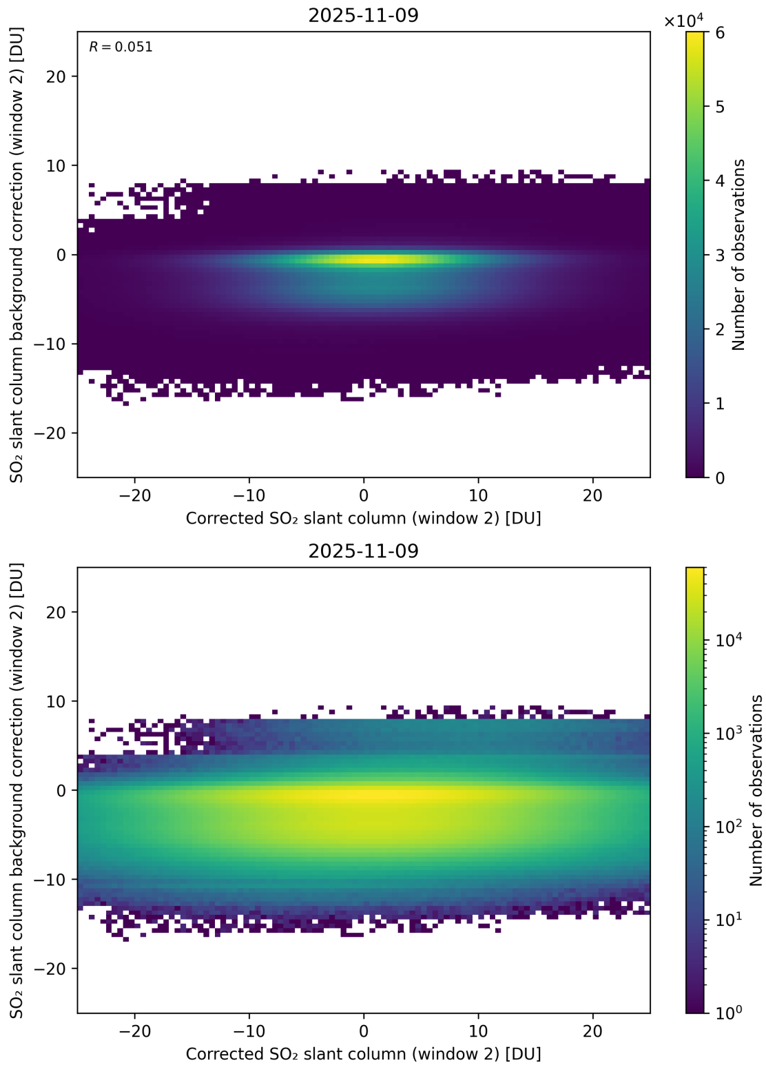
Figure 244: Scatter density plot of “Corrected SO 2 slant column (window 2)” against “SO 2 slant column background correction (window 2)” for 2025-11-08 to 2025-11-10.
