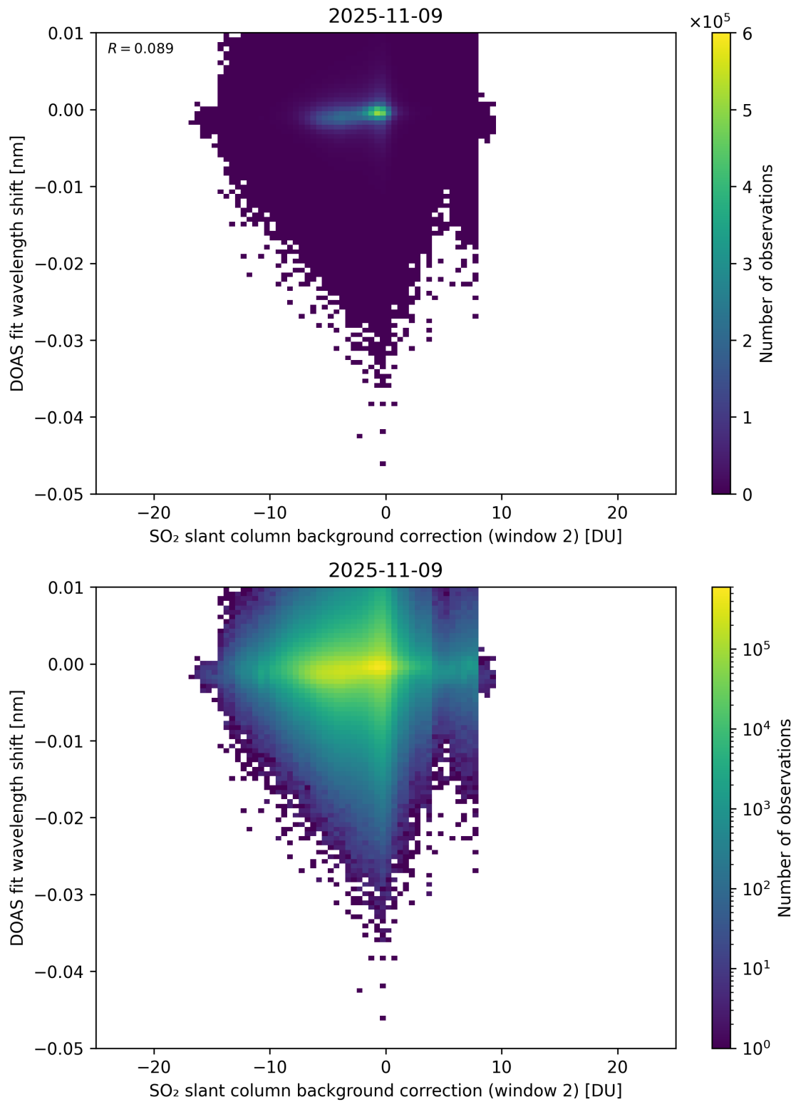
Figure 123: Scatter density plot of “SO 2 slant column background correction (window 2)” against “DOAS fit wavelength shift” for 2025-11-08 to 2025-11-10.
