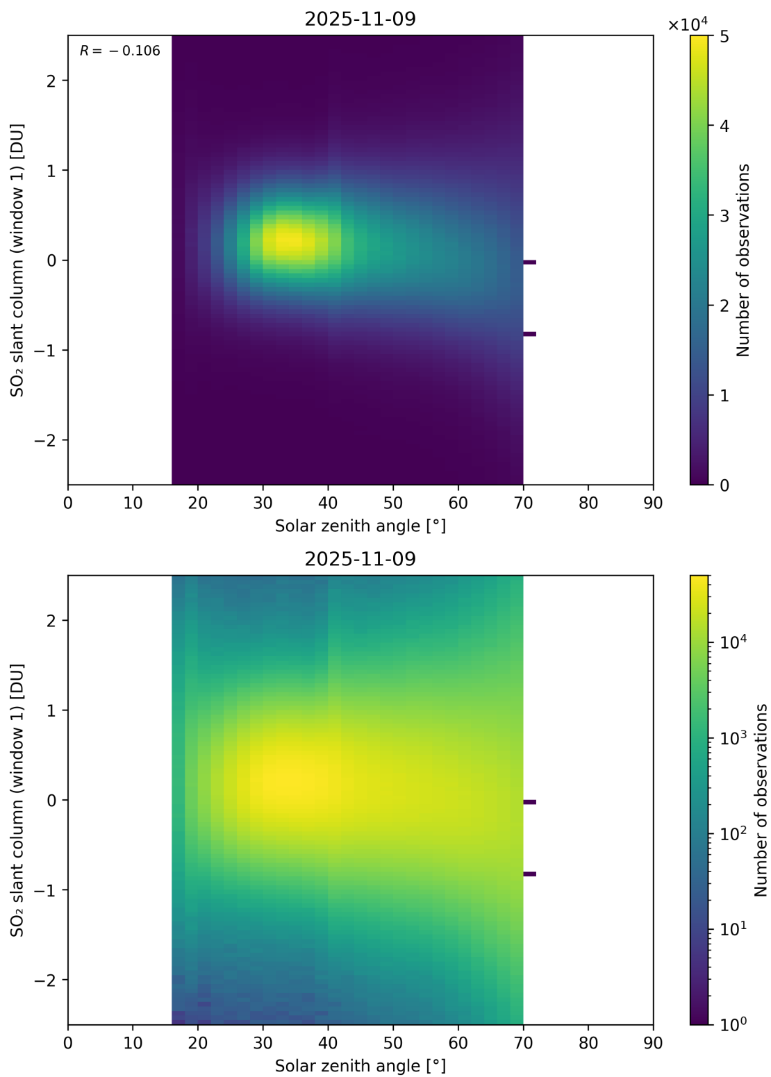
Figure 184: Scatter density plot of “Solar zenith angle” against “SO 2 slant column (window 1)” for 2025-11-08 to 2025-11-10.
