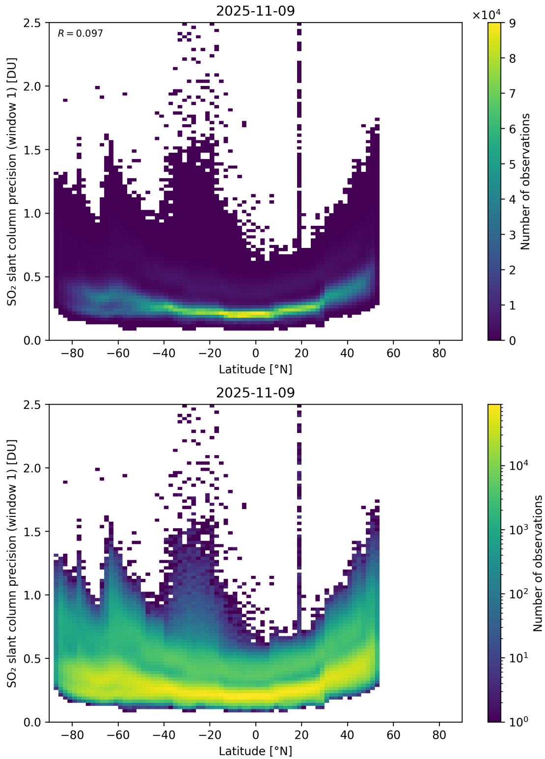
Figure 163: Scatter density plot of “Latitude” against “SO 2 slant column precision (window 1)” for 2025-11-08 to 2025-11-10.
