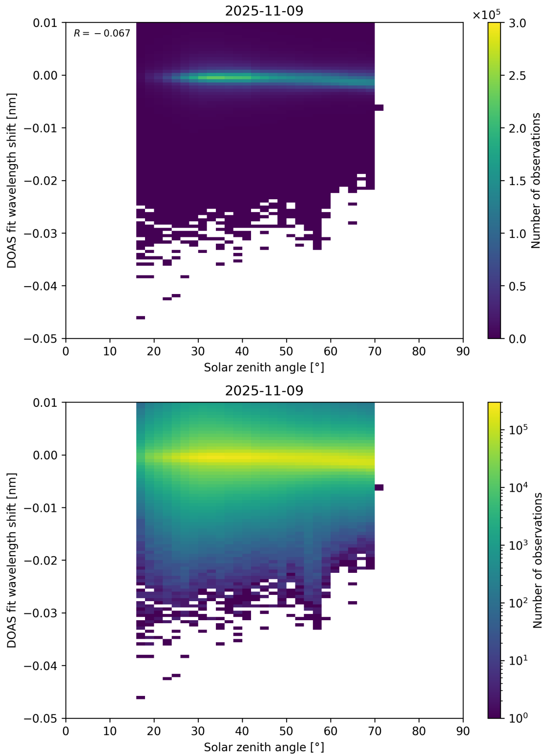
Figure 174: Scatter density plot of “Solar zenith angle” against “DOAS fit wavelength shift” for 2025-11-08 to 2025-11-10.
