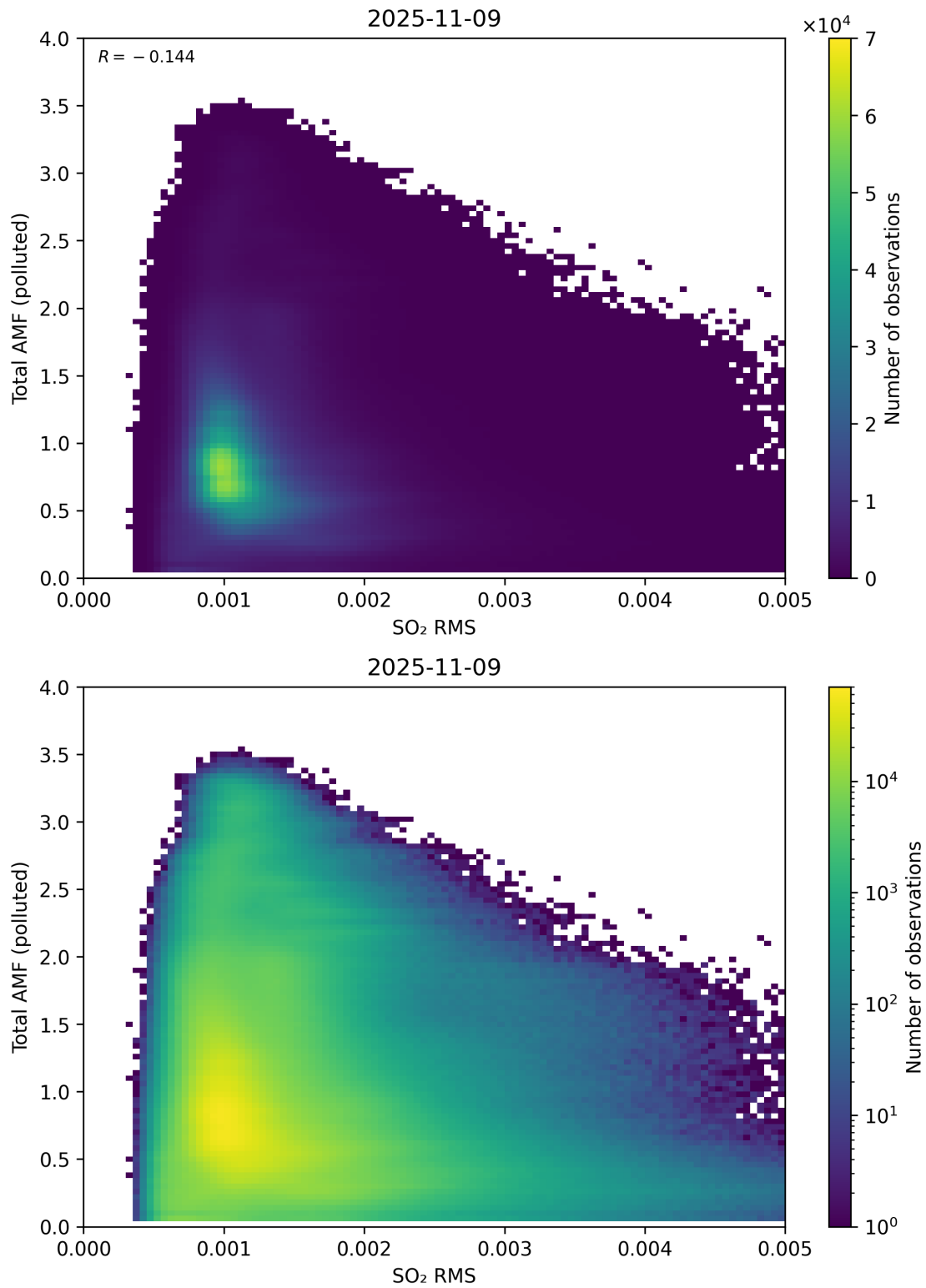
Figure 148: Scatter density plot of “SO 2 RMS” against “Total AMF (polluted)” for 2025-11-08 to 2025-11-10.
