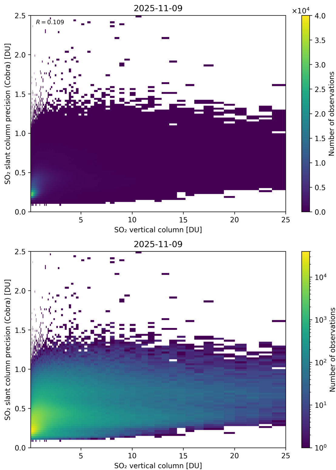
Figure 350: Scatter density plot of “SO 2 vertical column” against “SO 2 slant column precision (Cobra)” for 2025-11-08 to 2025-11-10.
