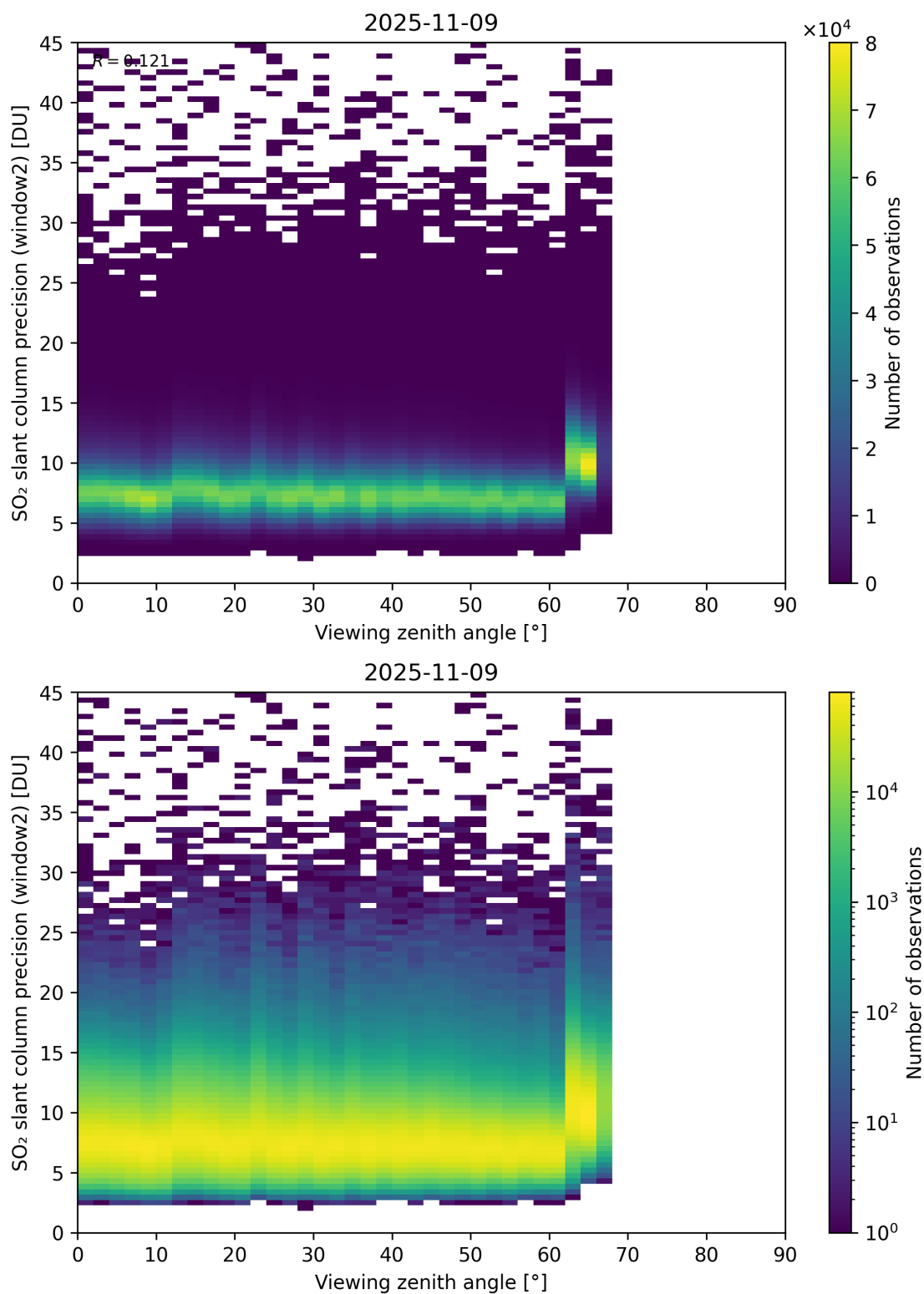
Figure 378: Scatter density plot of “Viewing zenith angle” against “SO 2 slant column precision (window2)” for 2025-11-08 to 2025-11-10.
