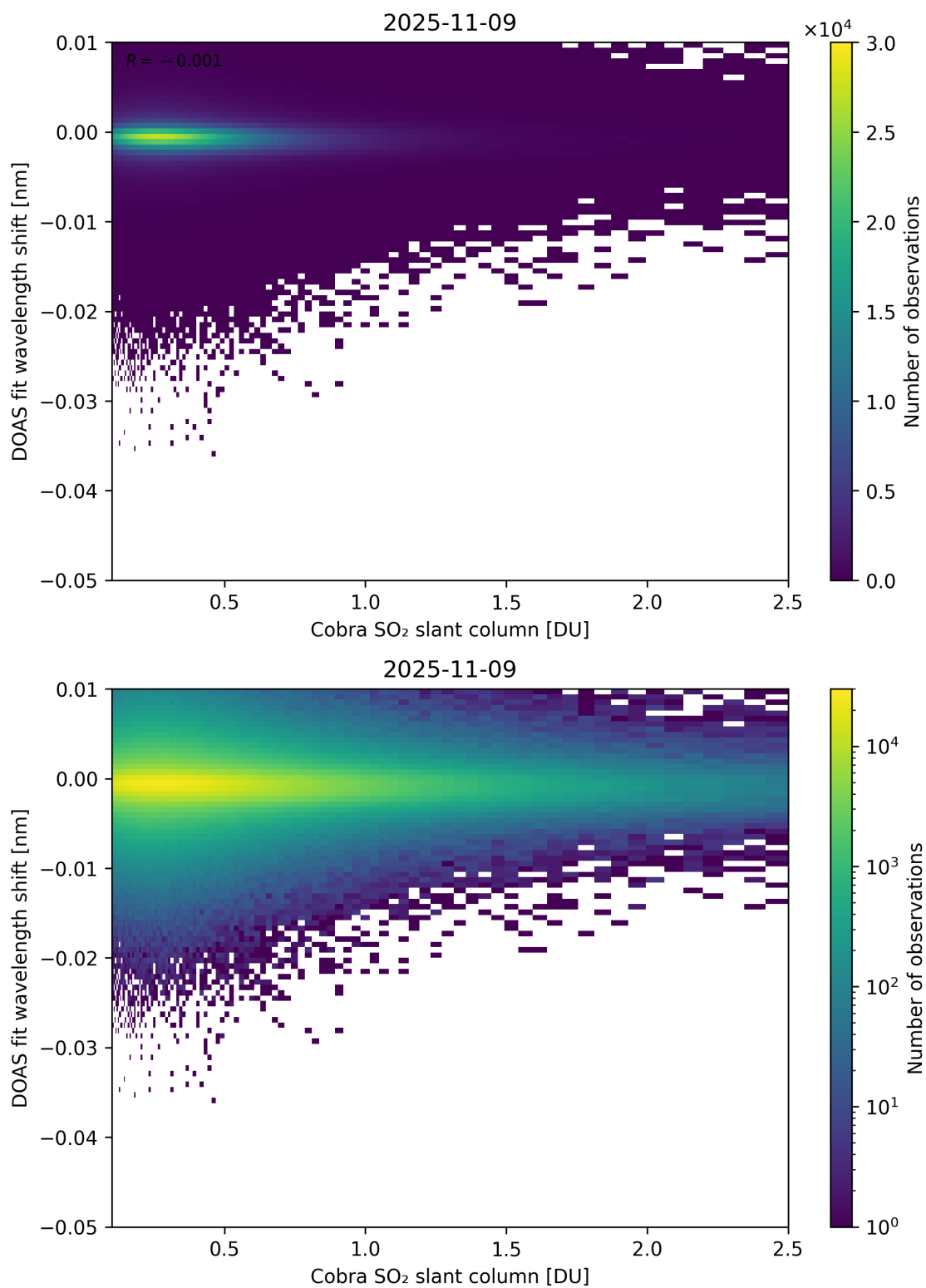
Figure 196: Scatter density plot of “Cobra SO 2 slant column” against “DOAS fit wavelength shift” for 2025-11-08 to 2025-11-10.
