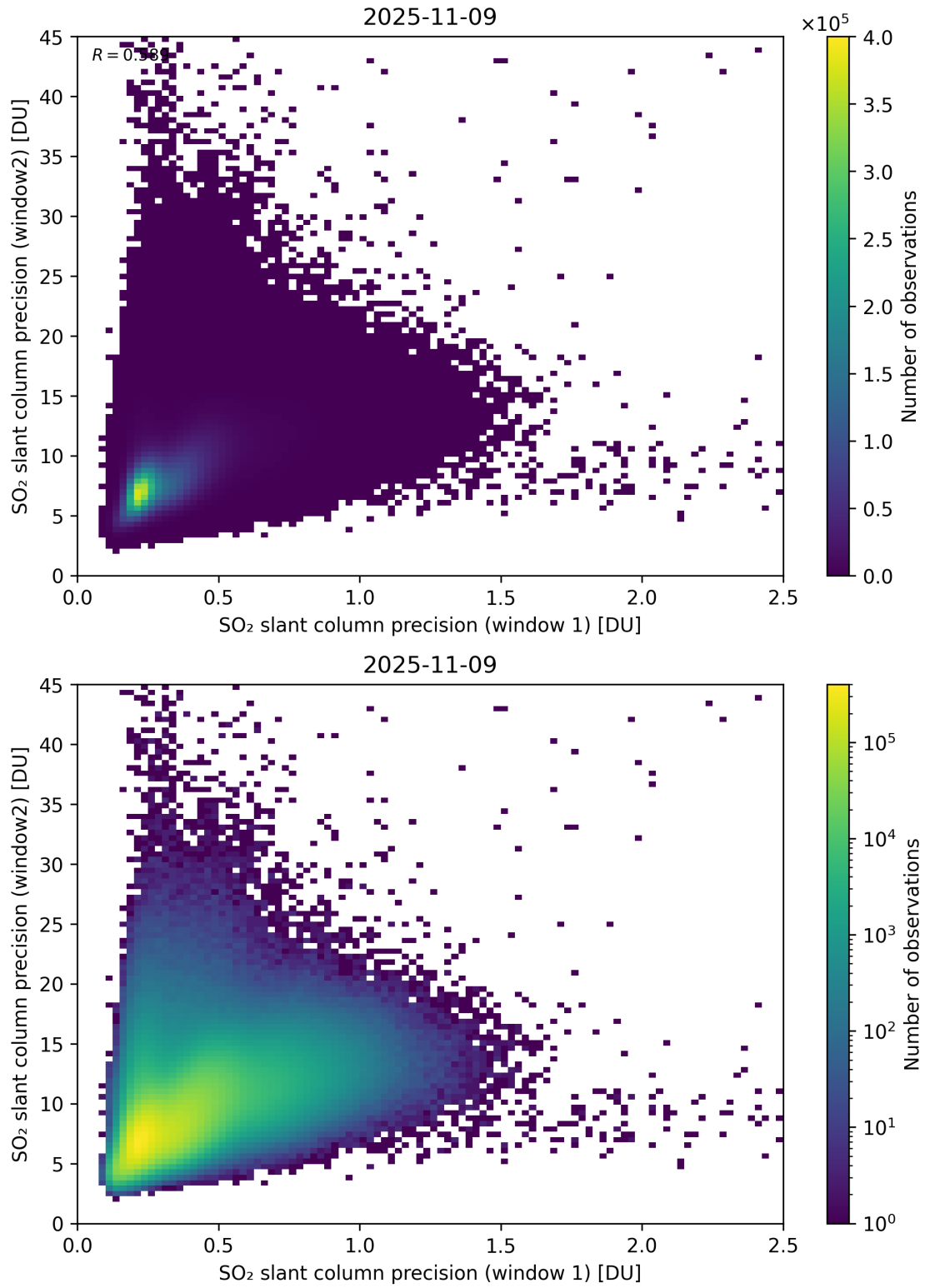
Figure 277: Scatter density plot of “SO 2 slant column precision (window 1)” against “SO 2 slant column precision (window2)” for 2025-11-08 to 2025-11-10.
