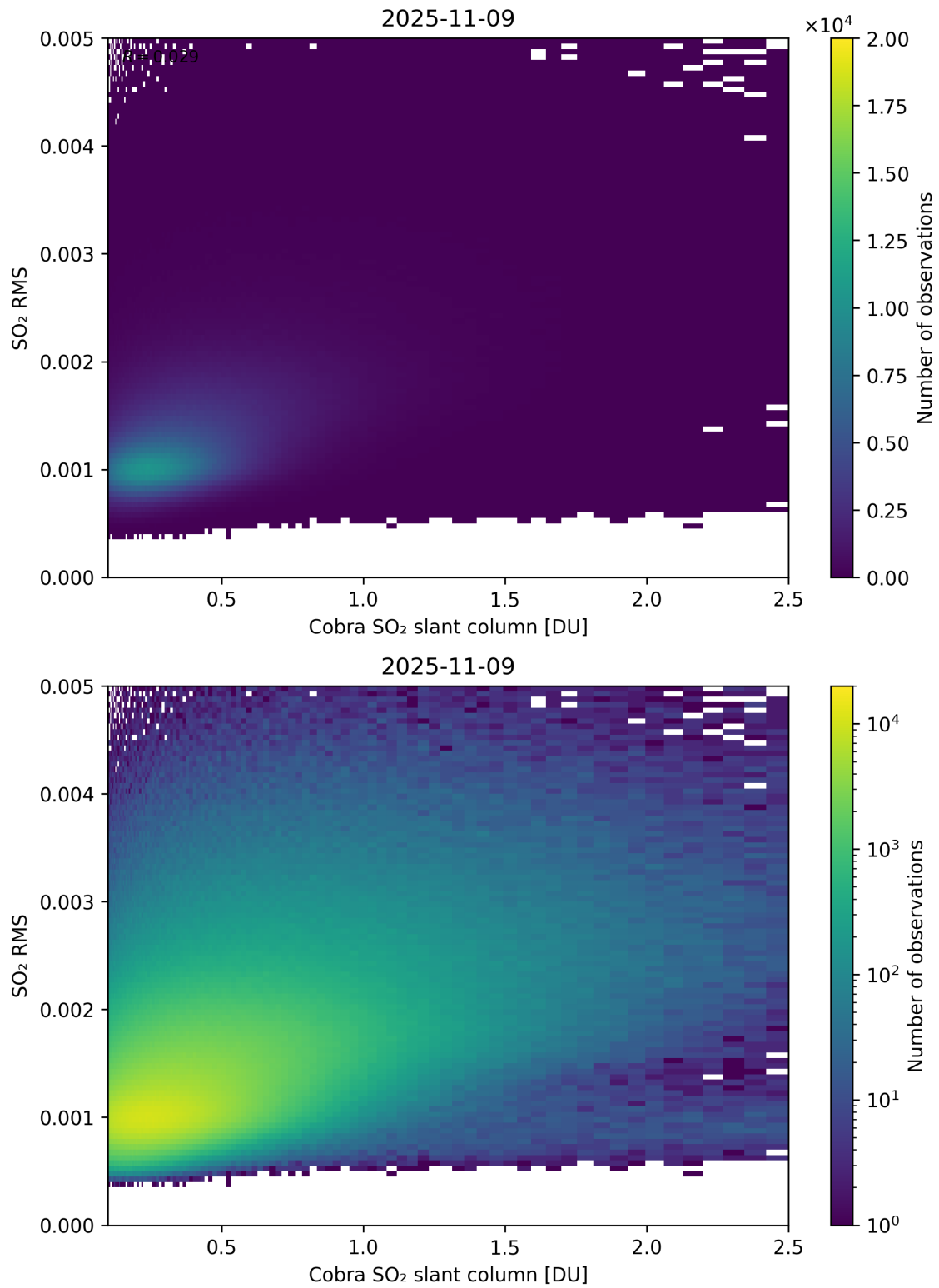
Figure 198: Scatter density plot of “Cobra SO 2 slant column” against “SO 2 RMS” for 2025-11-08 to 2025-11-10.
