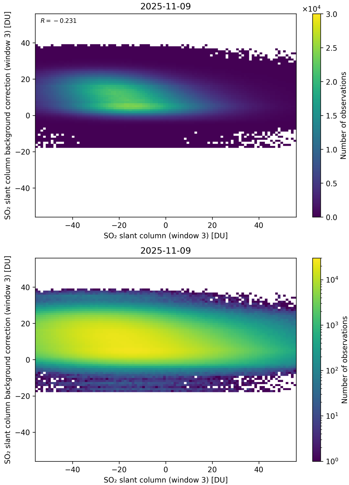
Figure 303: Scatter density plot of “SO 2 slant column (window 3)” against “SO 2 slant column background correction (window 3)” for 2025-11-08 to 2025-11-10.
