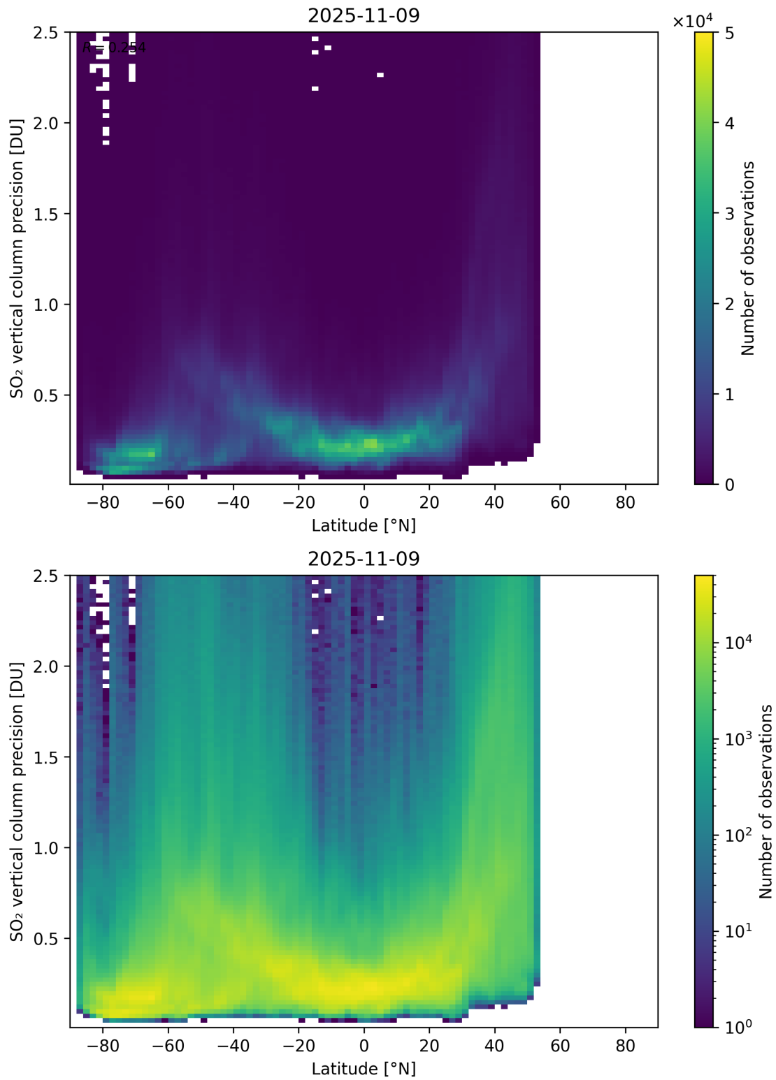
Figure 170: Scatter density plot of “Latitude” against “SO 2 vertical column precision” for 2025-11-08 to 2025-11-10.
