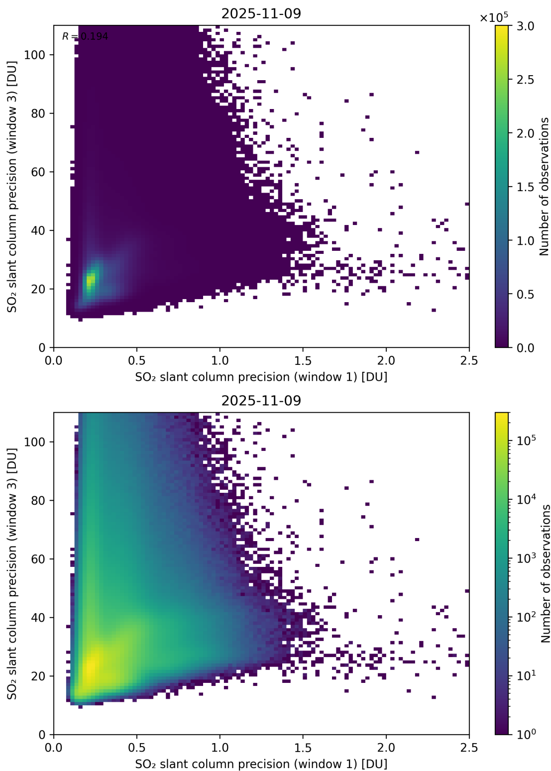
Figure 279: Scatter density plot of “SO 2 slant column precision (window 1)” against “SO 2 slant column precision (window 3)” for 2025-11-08 to 2025-11-10.
