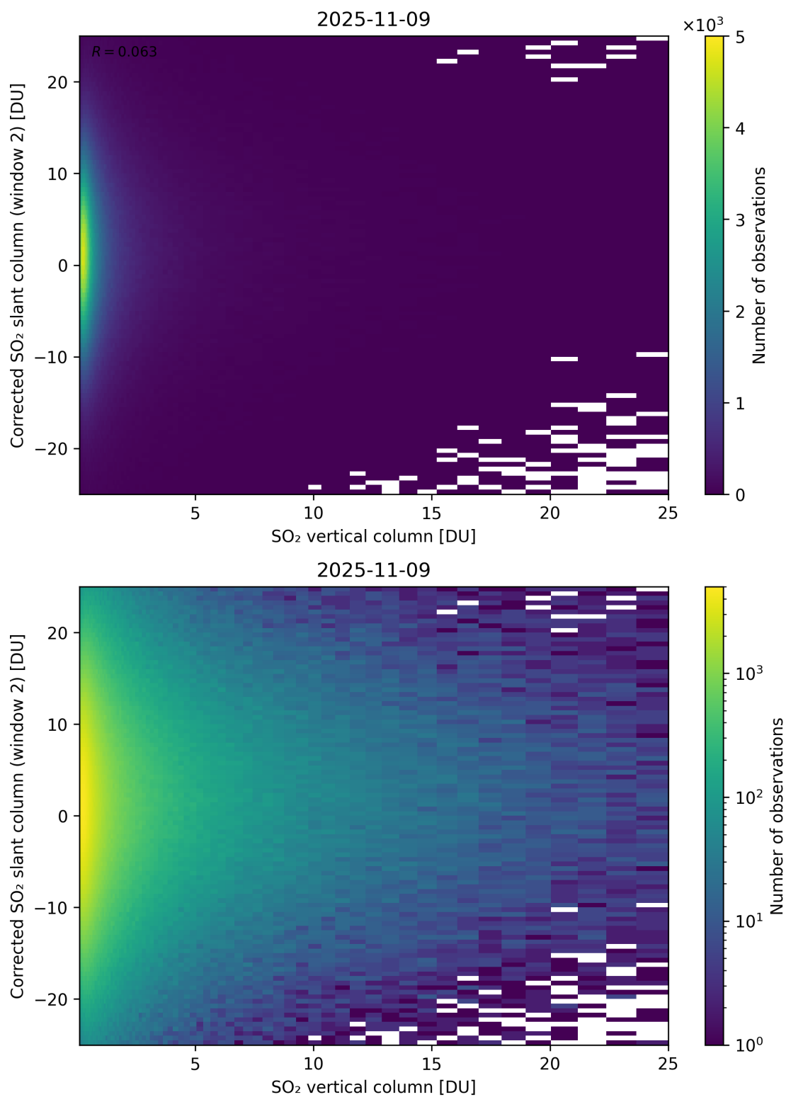
Figure 352: Scatter density plot of “SO 2 vertical column” against “Corrected SO 2 slant column (window 2)” for 2025-11-08 to 2025-11-10.
