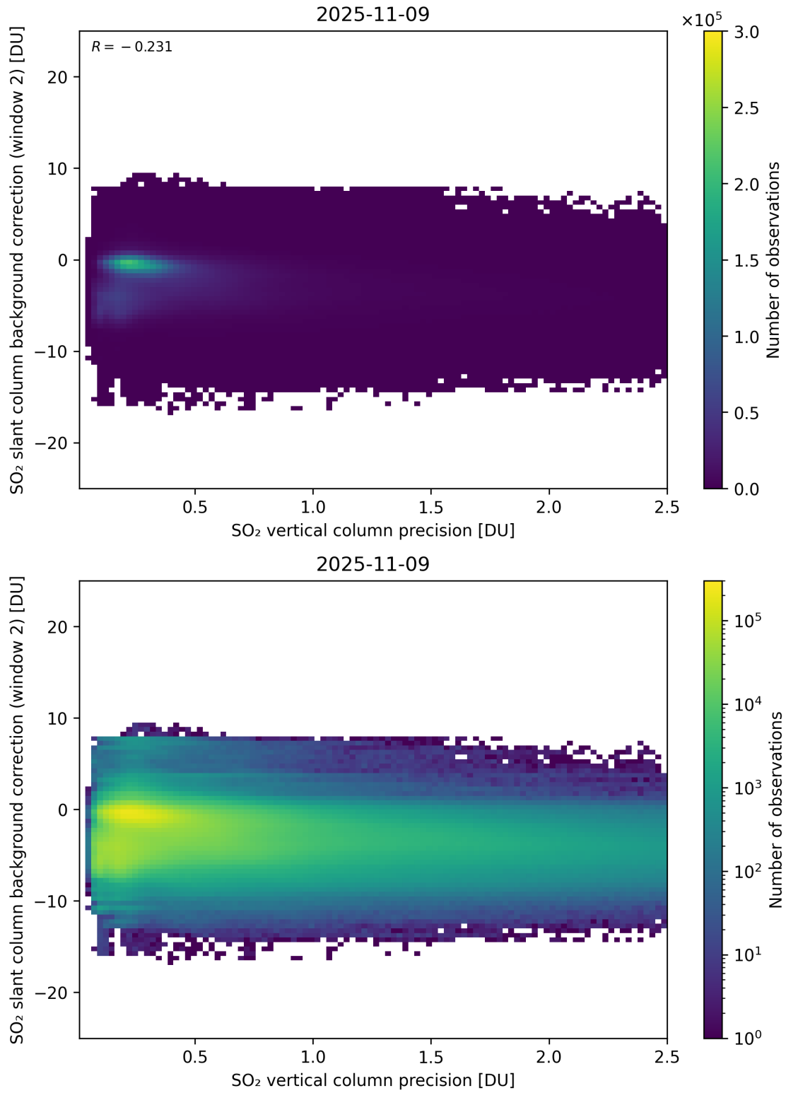
Figure 330: Scatter density plot of “SO 2 vertical column precision” against “SO 2 slant column background correction (window 2)” for 2025-11-08 to 2025-11-10.
