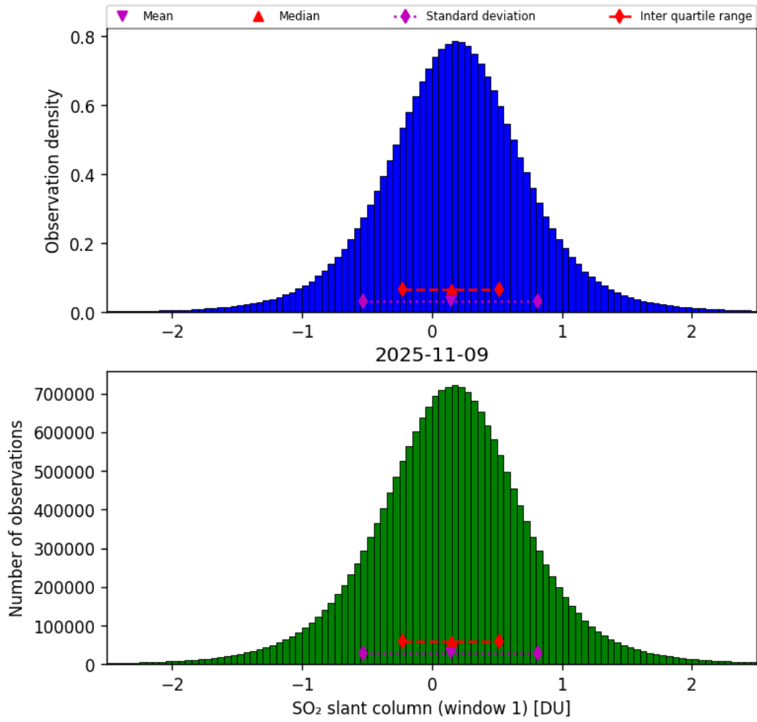
Figure 63: Histogram of “SO 2 slant column (window 1)” for 2025-11-08 to 2025-11-10
