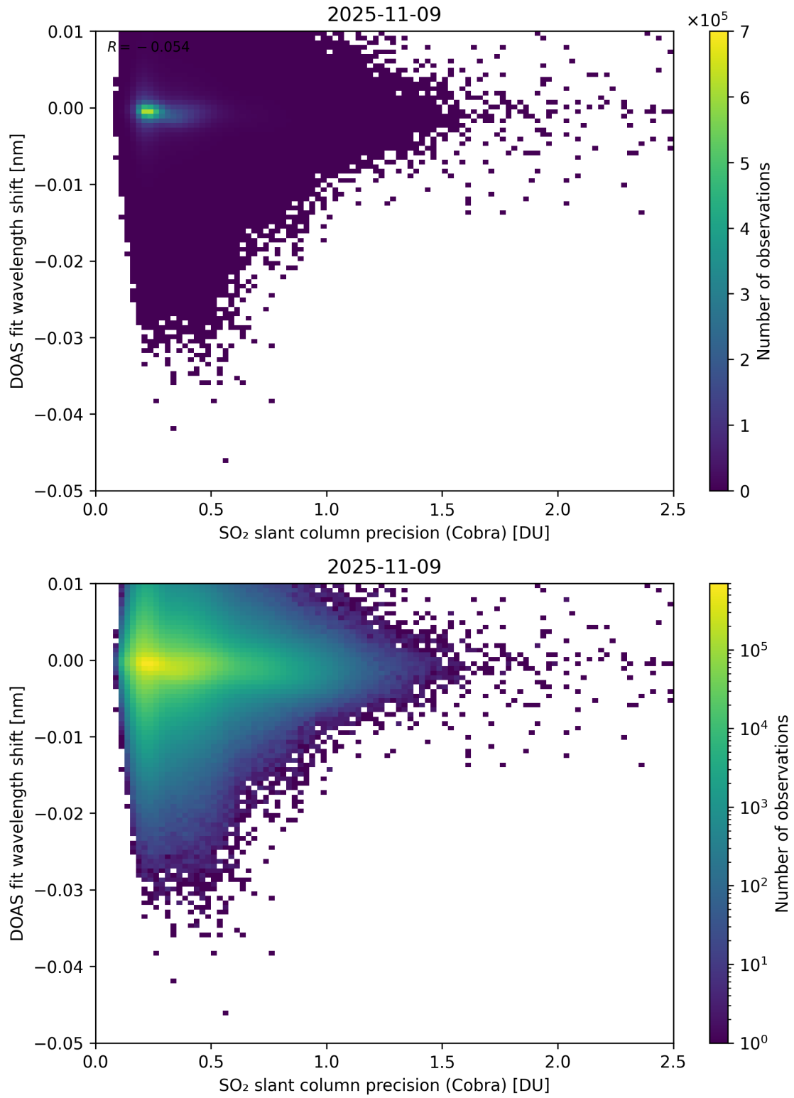
Figure 202: Scatter density plot of “SO 2 slant column precision (Cobra)” against “DOAS fit wavelength shift” for 2025-11-08 to 2025-11-10.
