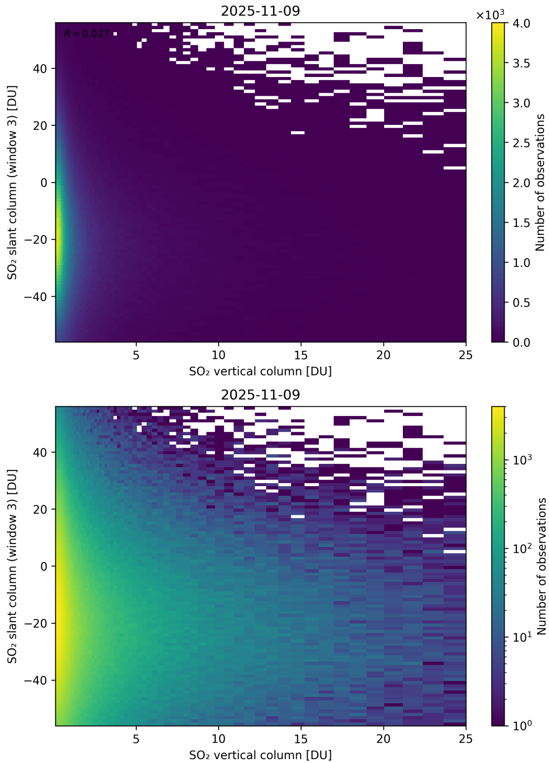
Figure 357: Scatter density plot of “SO 2 vertical column” against “SO 2 slant column (window 3)” for 2025-11-08 to 2025-11-10.
