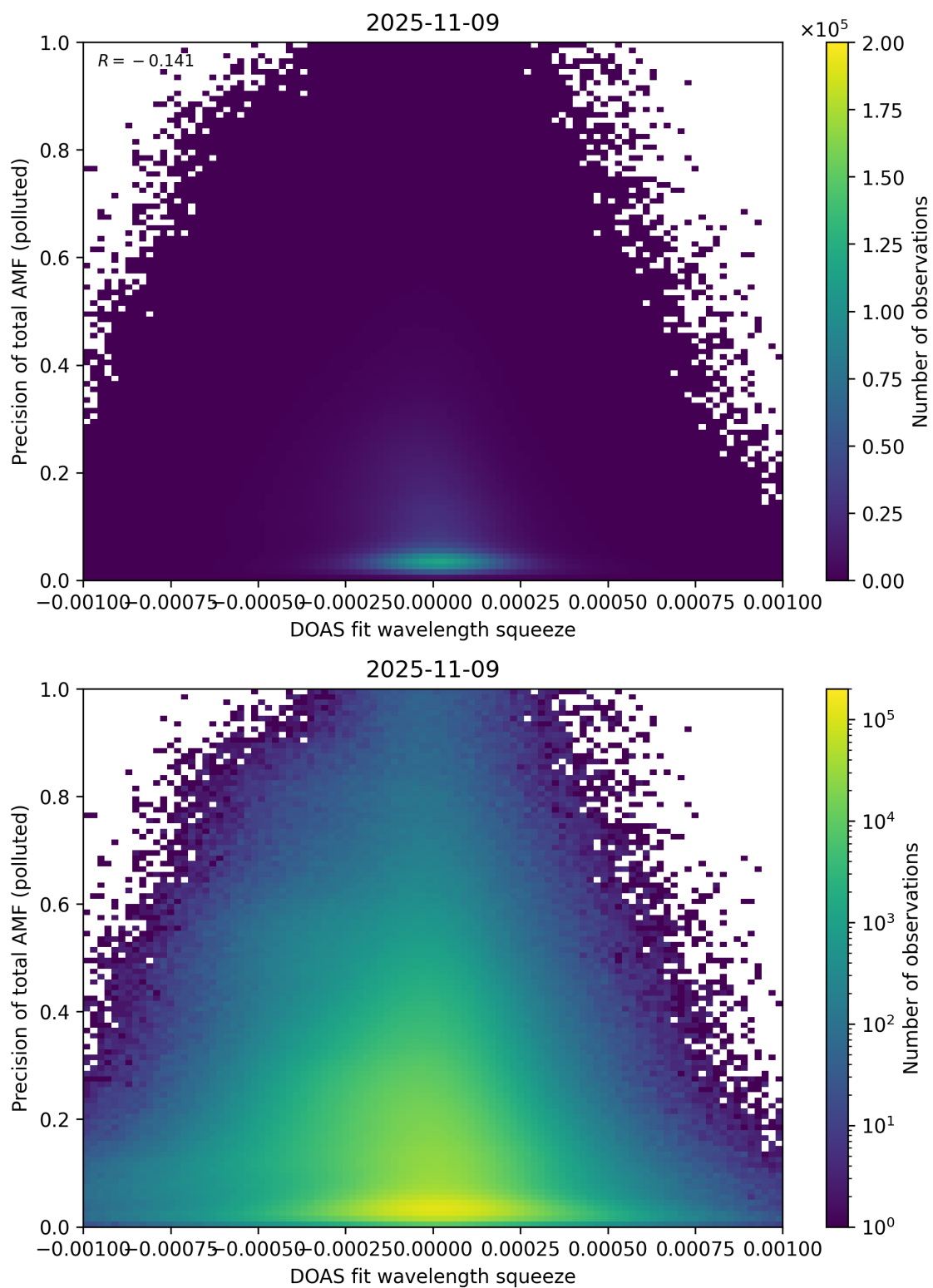
Figure 146: Scatter density plot of “DOAS fit wavelength squeeze” against “Precision of total AMF (polluted)” for 2025-11-08 to 2025-11-10.
