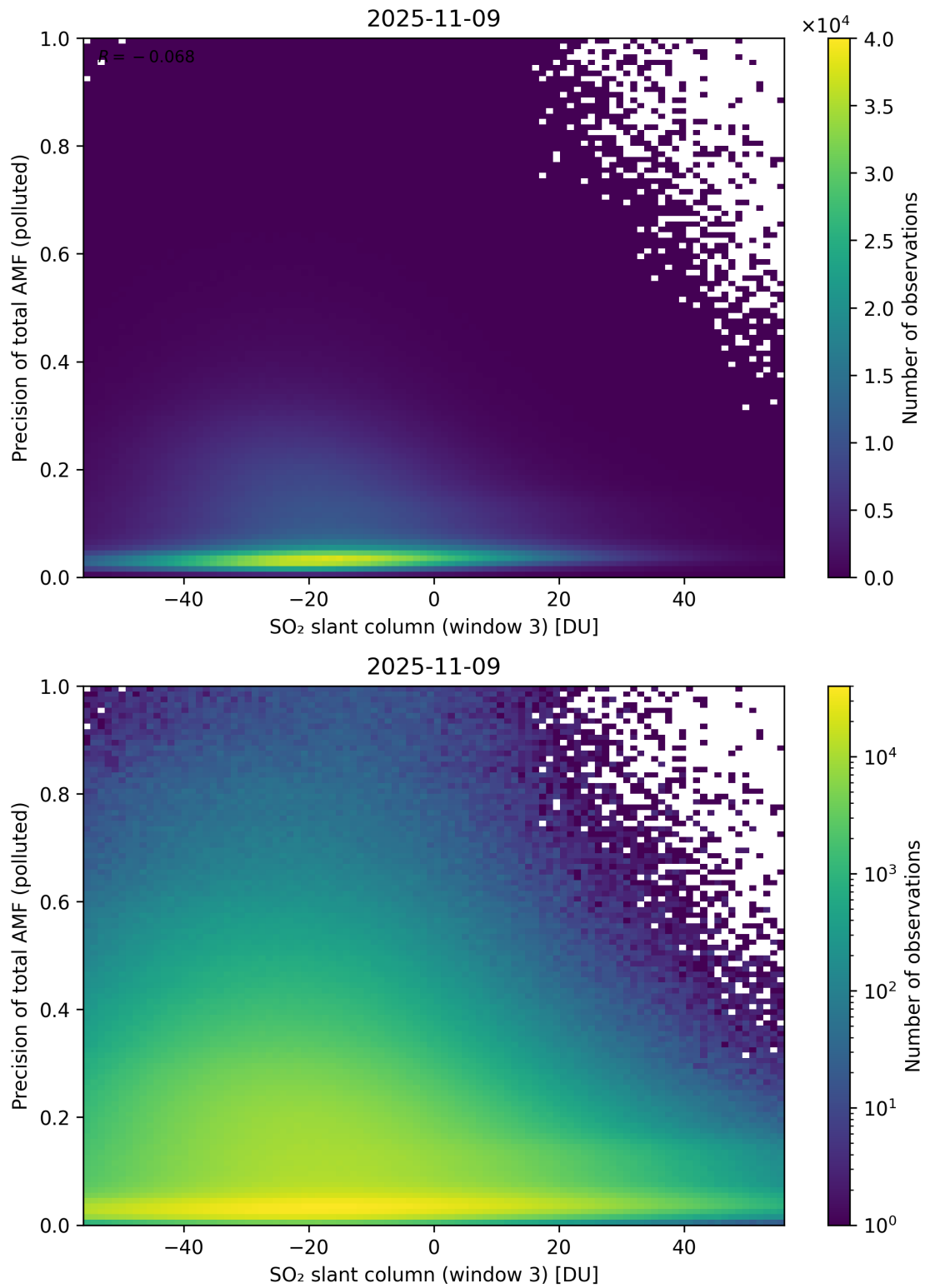
Figure 319: Scatter density plot of “SO 2 slant column (window 3)” against “Precision of total AMF (polluted)” for 2025-11-08 to 2025-11-10.
