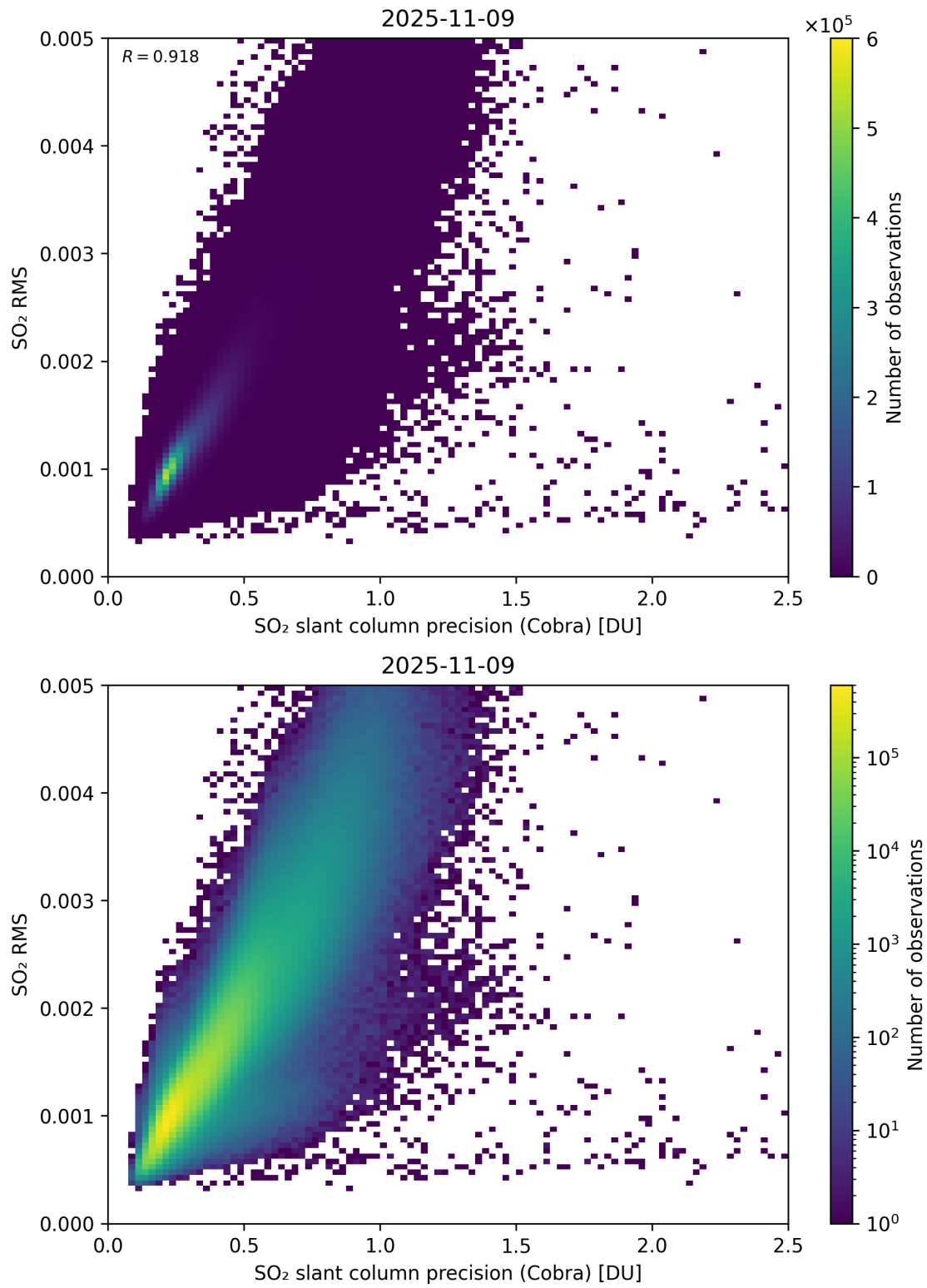
Figure 204: Scatter density plot of “SO 2 slant column precision (Cobra)” against “SO 2 RMS” for 2025-11-08 to 2025-11-10.
