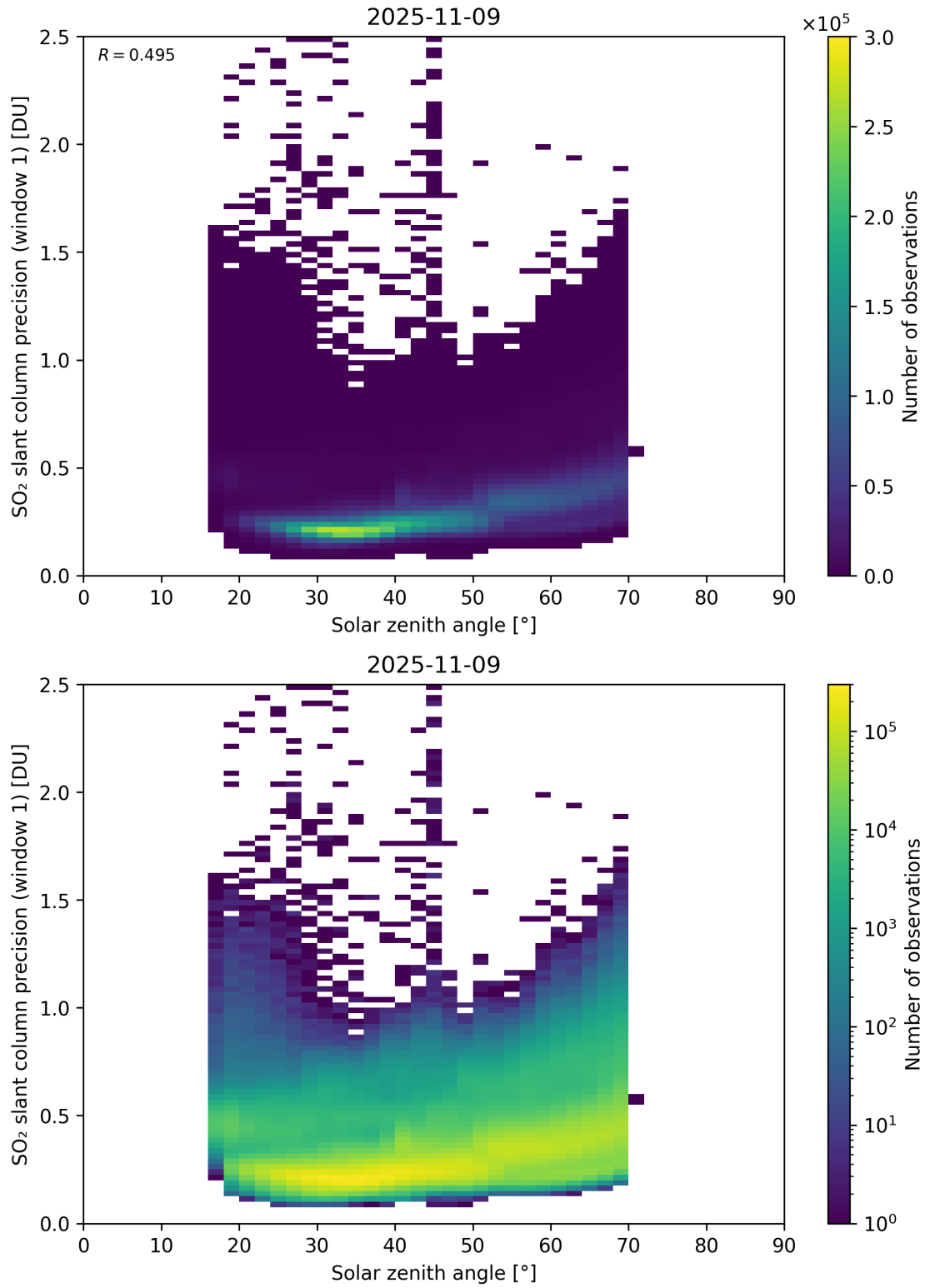
Figure 185: Scatter density plot of “Solar zenith angle” against “SO 2 slant column precision (window 1)” for 2025-11-08 to 2025-11-10.
