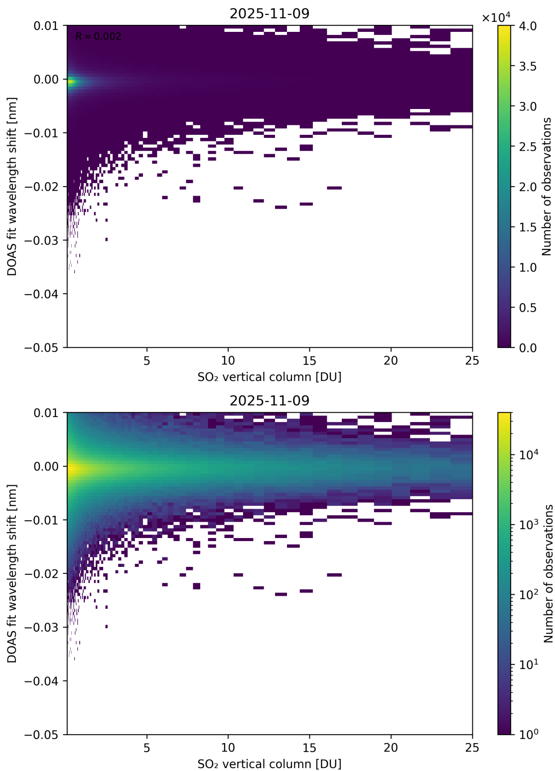
Figure 326: Scatter density plot of “SO 2 vertical column” against “DOAS fit wavelength shift” for 2025-11-08 to 2025-11-10.
