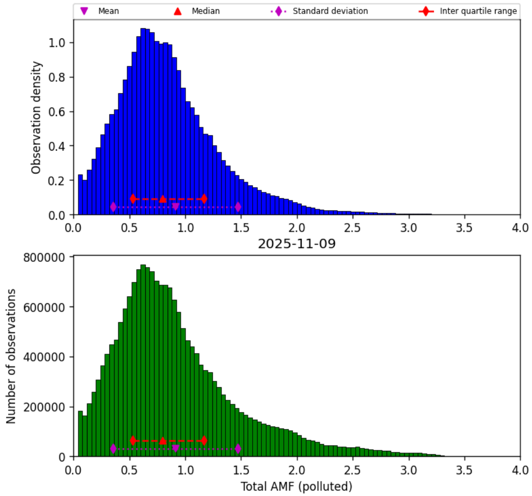
Figure 79: Histogram of “Total AMF (polluted)” for 2025-11-08 to 2025-11-10
