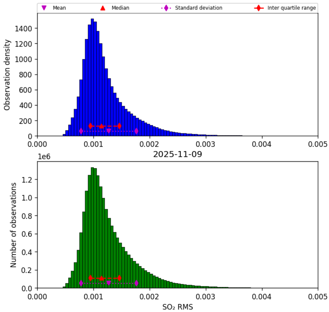
Figure 78: Histogram of “SO 2 RMS” for 2025-11-08 to 2025-11-10
