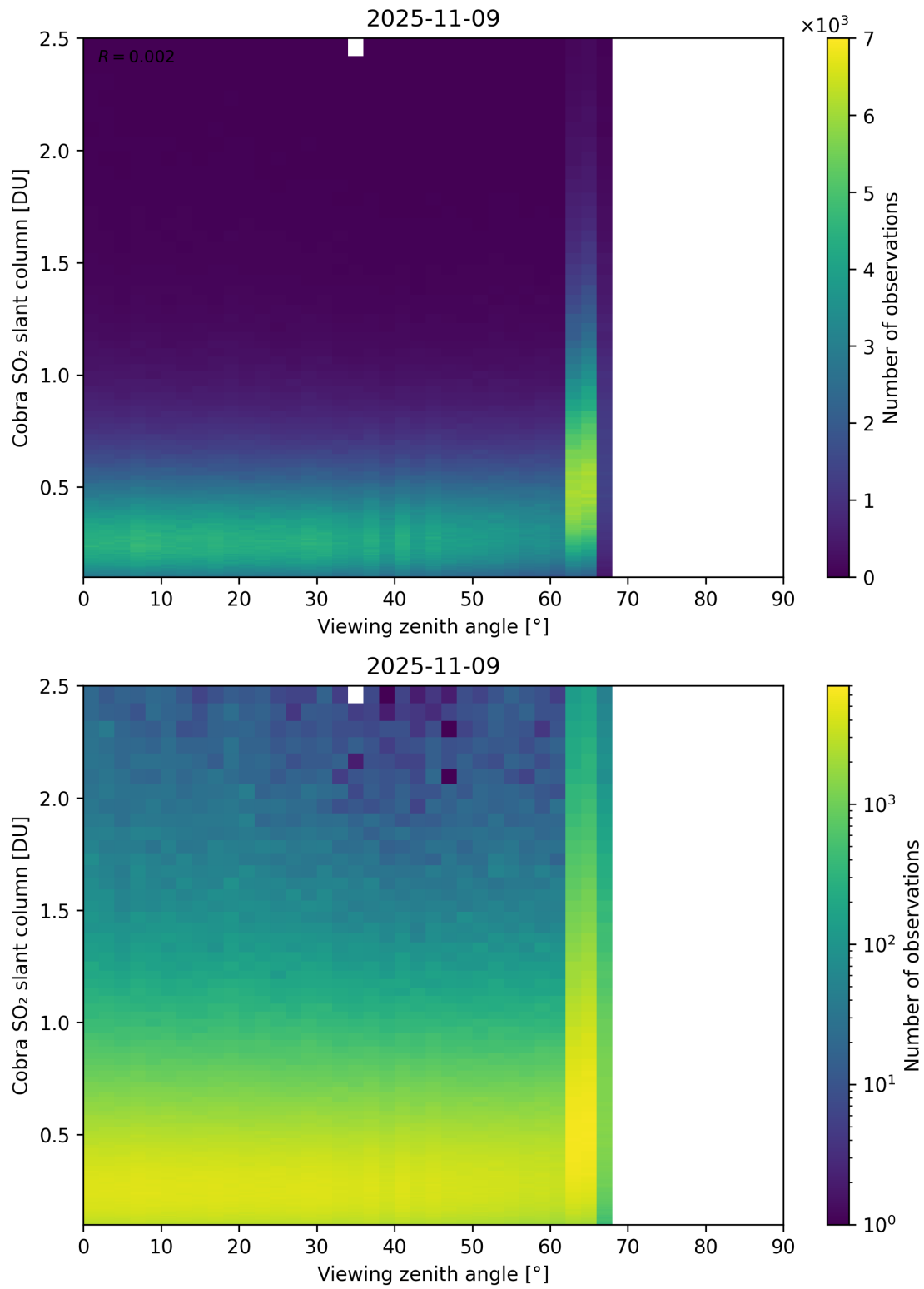
Figure 371: Scatter density plot of “Viewing zenith angle” against “Cobra SO 2 slant column” for 2025-11-08 to 2025-11-10.
