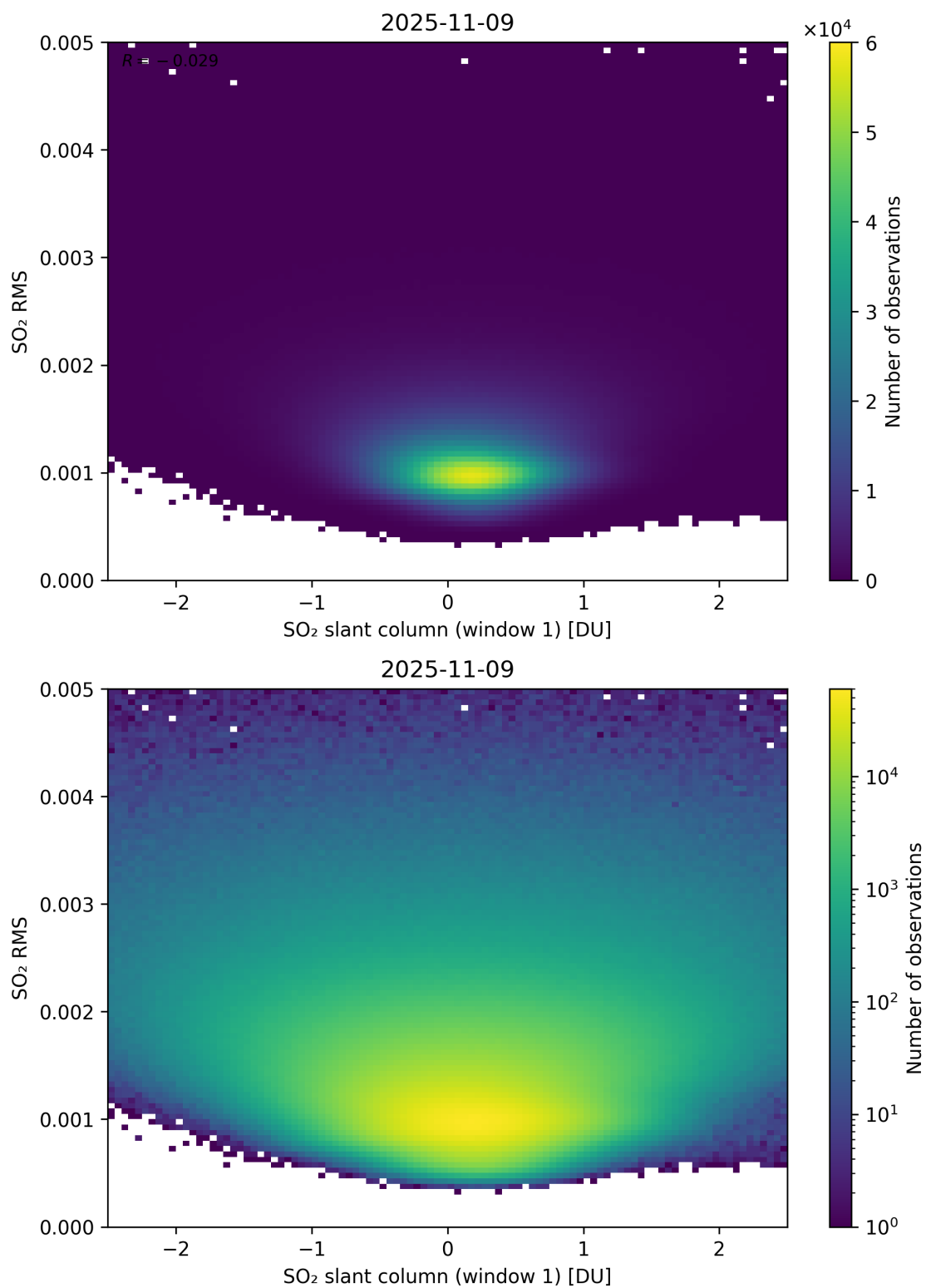
Figure 267: Scatter density plot of “SO 2 slant column (window 1)” against “SO 2 RMS” for 2025-11-08 to 2025-11-10.
