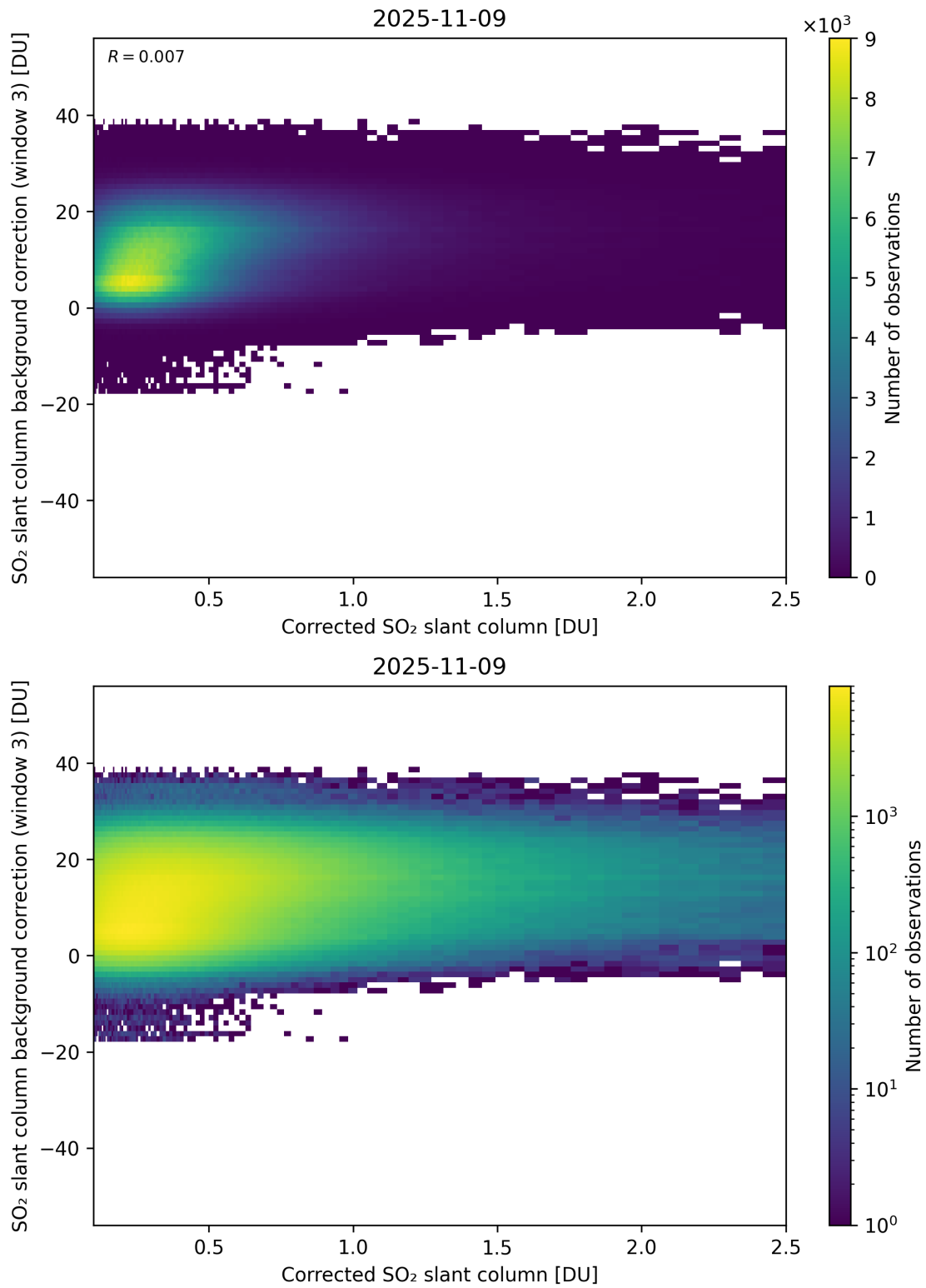
Figure 228: Scatter density plot of “Corrected SO 2 slant column” against “SO 2 slant column background correction (window 3)” for 2025-11-08 to 2025-11-10.
