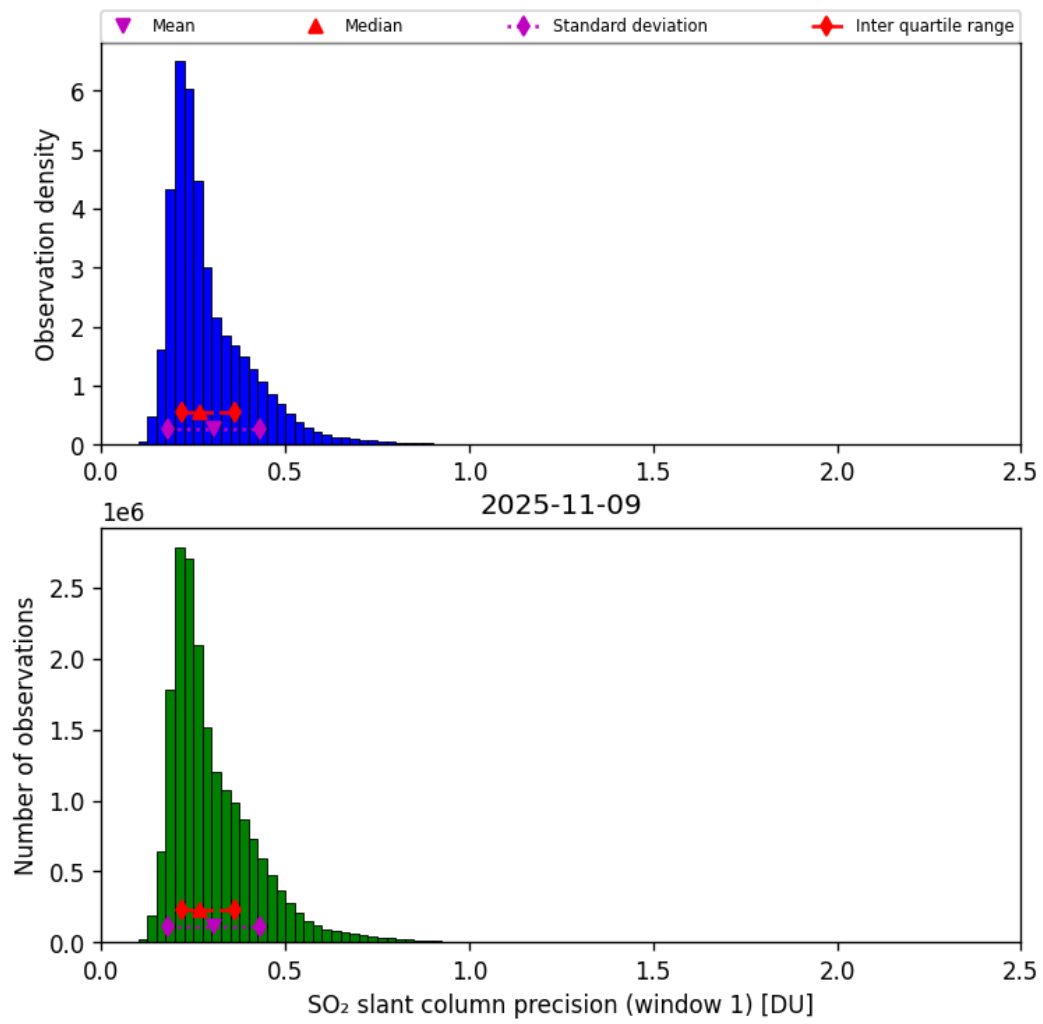
Figure 64: Histogram of “SO 2 slant column precision (window 1)” for 2025-11-08 to 2025-11-10
