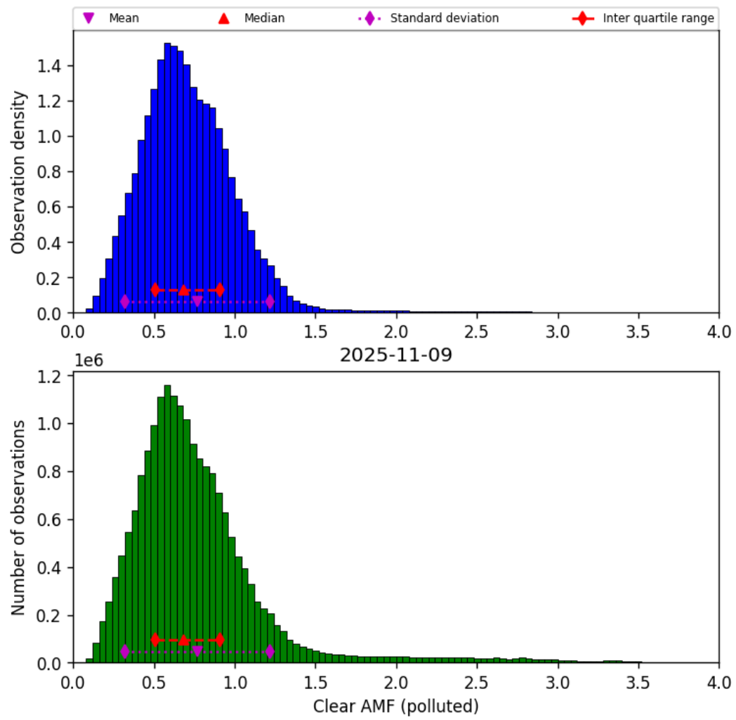
Figure 81: Histogram of "Clear AMF (polluted)" for 2025-11-08 to 2025-11-10
