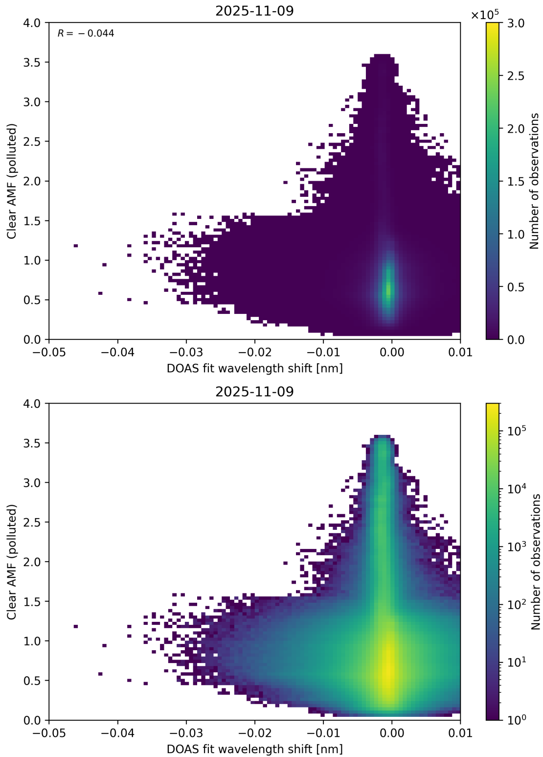
Figure 140: Scatter density plot of “DOAS fit wavelength shift” against “Clear AMF (polluted)” for 2025-11-08 to 2025-11-10.
