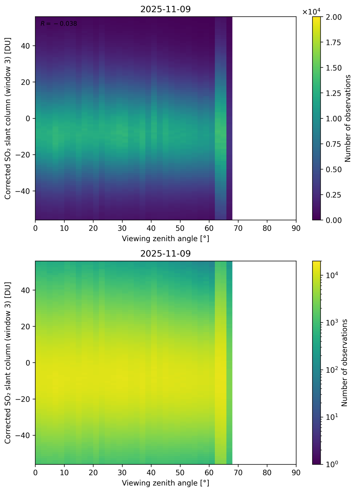
Figure 375: Scatter density plot of “Viewing zenith angle” against “Corrected SO 2 slant column (window 3)” for 2025-11-08 to 2025-11-10.
