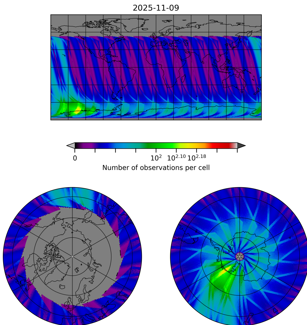
Figure 30: Map of the number of observations for 2025-11-08 to 2025-11-10
