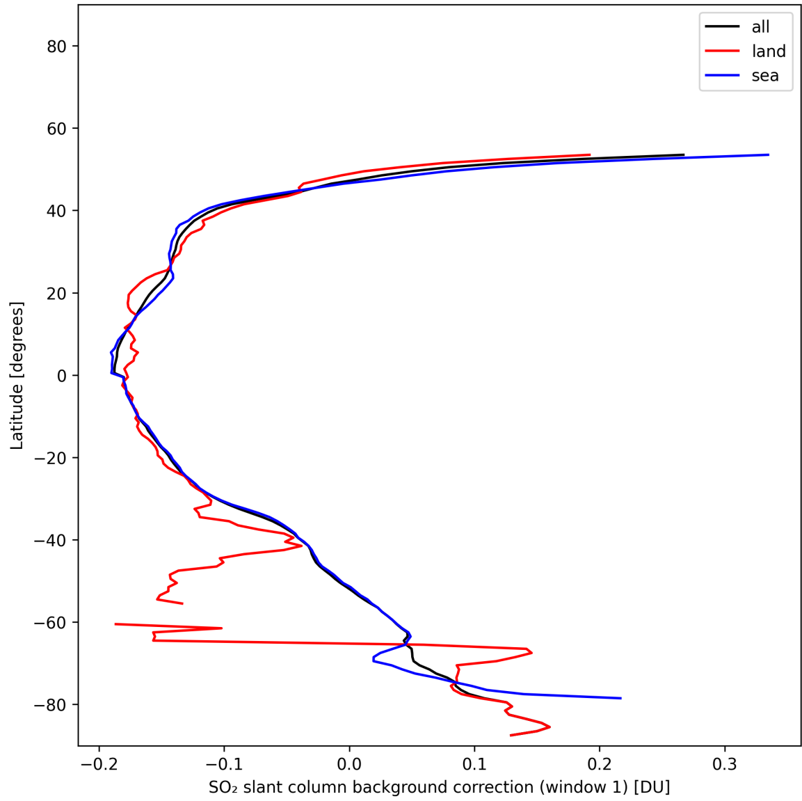
Figure 40: Zonal average of “SO 2 slant column background correction (window 1)” for 2025-11-08 to 2025-11-10.
