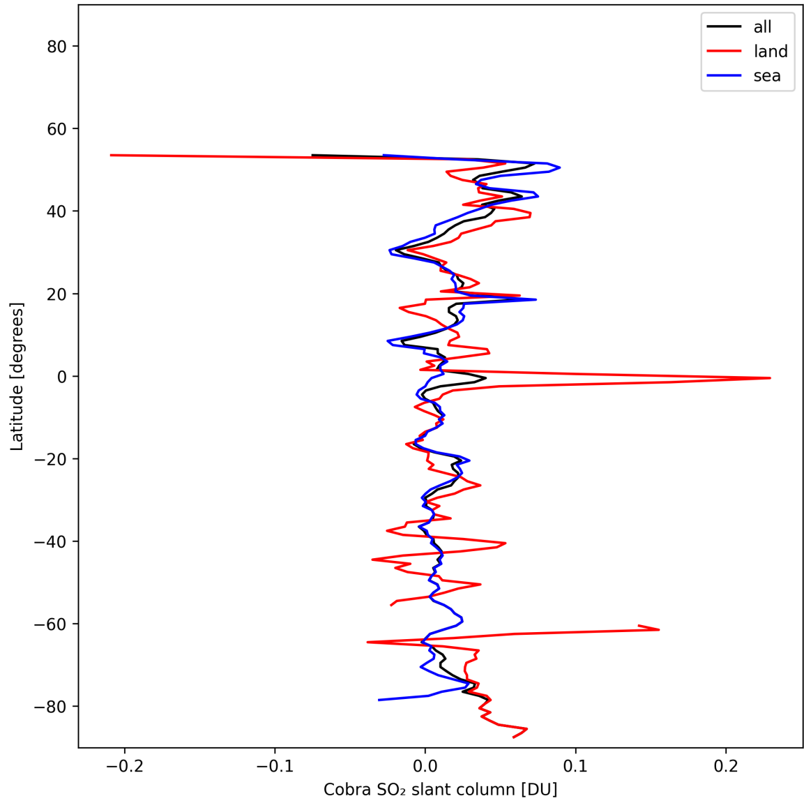
Figure 35: Zonal average of “Cobra SO 2 slant column” for 2025-11-08 to 2025-11-10.
