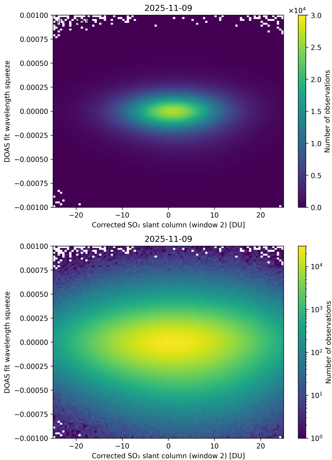
Figure 247: Scatter density plot of “Corrected SO 2 slant column (window 2)” against “DOAS fit wavelength squeeze” for 2025-11-08 to 2025-11-10.
