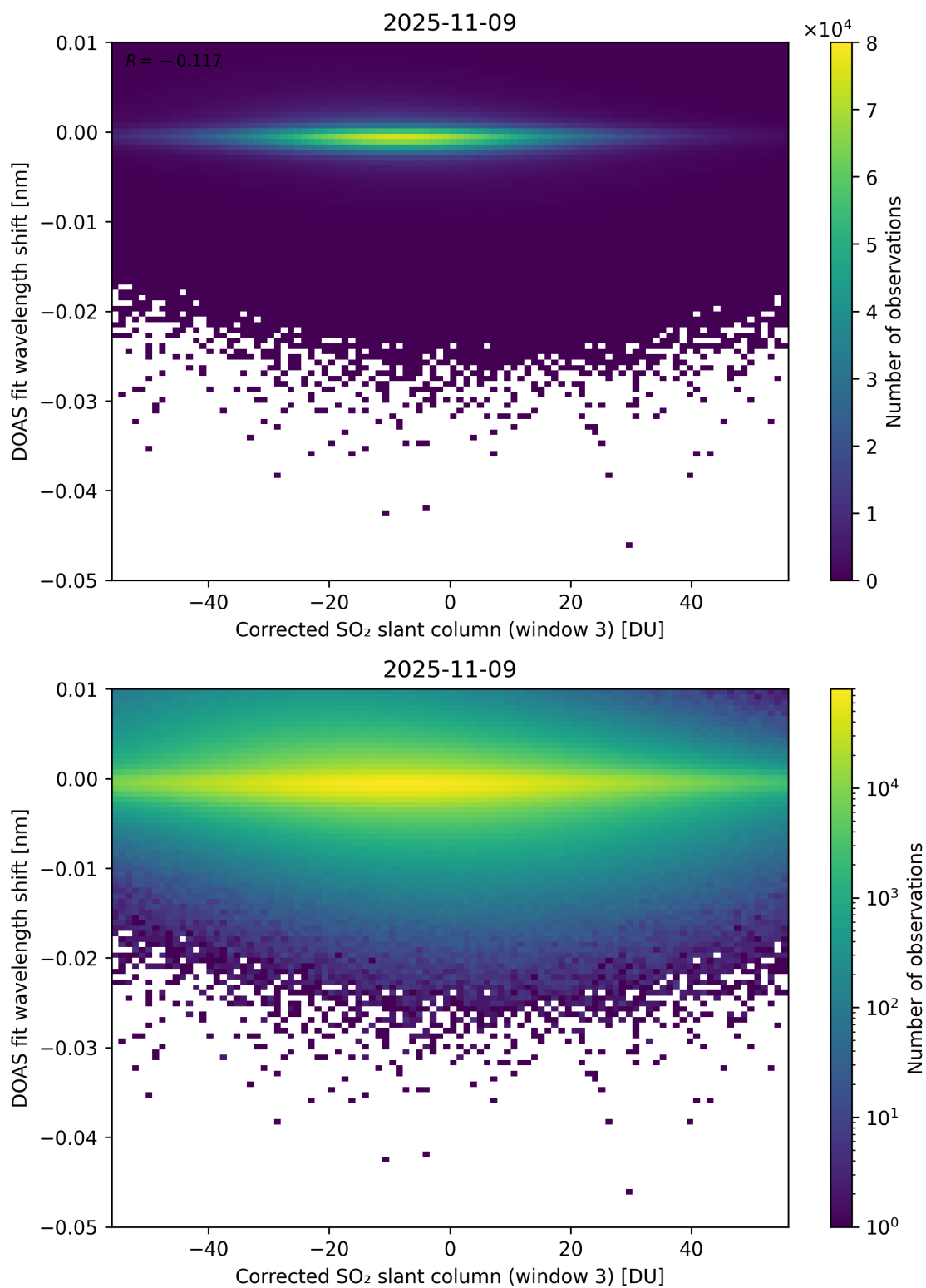
Figure 256: Scatter density plot of “Corrected SO 2 slant column (window 3)” against “DOAS fit wavelength shift” for 2025-11-08 to 2025-11-10.
