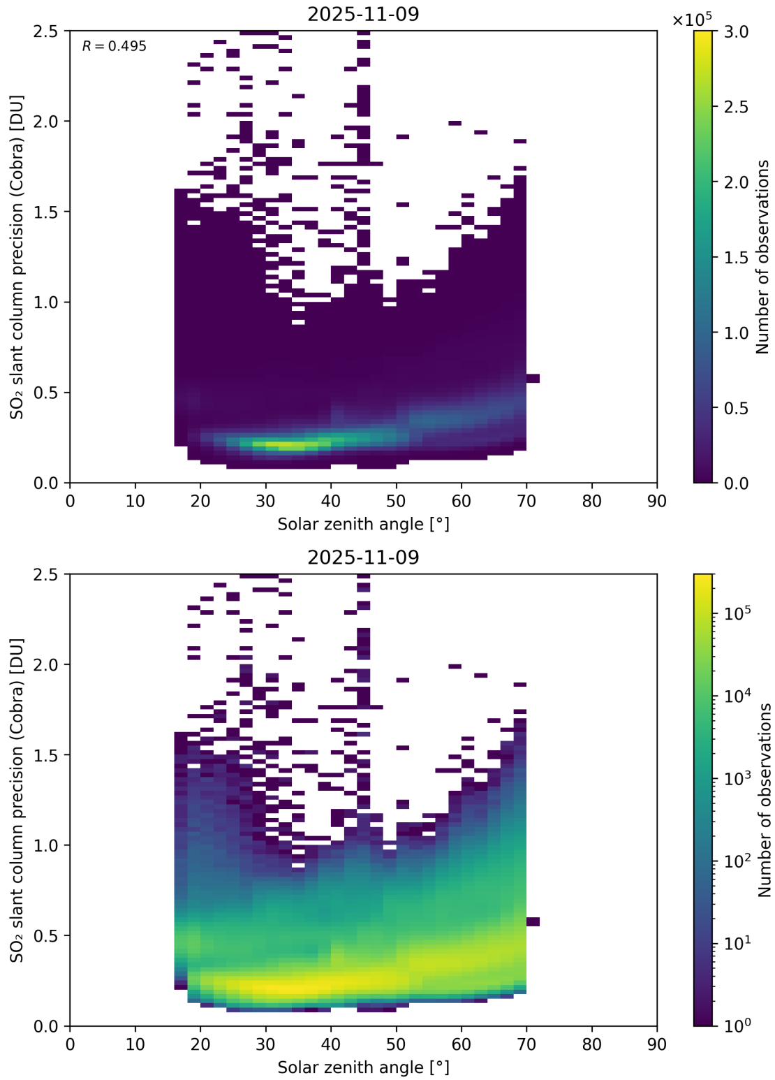
Figure 180: Scatter density plot of “Solar zenith angle” against “SO 2 slant column precision (Cobra)” for 2025-11-08 to 2025-11-10.
