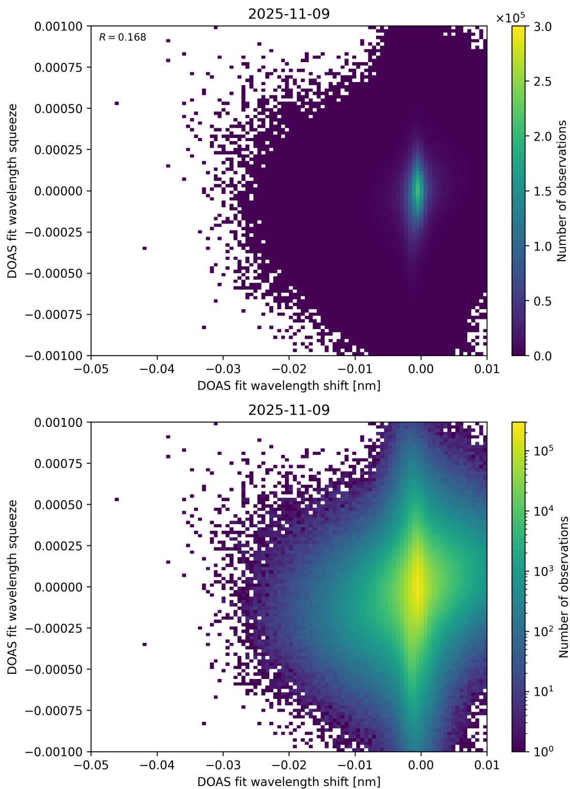
Figure 138: Scatter density plot of “DOAS fit wavelength shift” against “DOAS fit wavelength squeeze” for 2025-11-08 to 2025-11-10.
