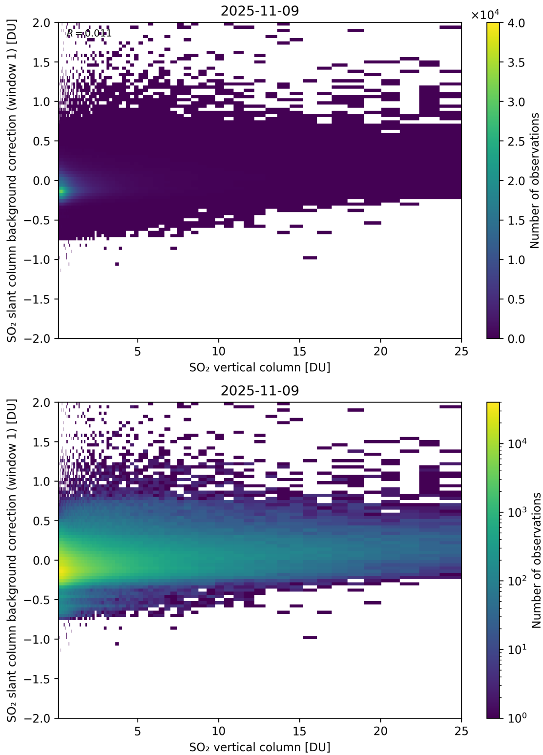
Figure 323: Scatter density plot of “SO 2 vertical column” against “SO 2 slant column background correction (window 1)” for 2025-11-08 to 2025-11-10.
