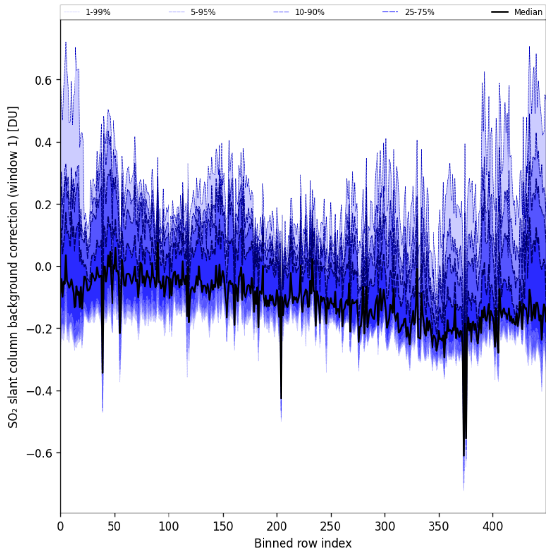
Figure 92: Along track statistics of “SO 2 slant column background correction (window 1)” for 2025-11-08 to 2025-11-10
