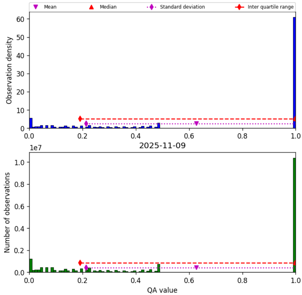
Figure 57: Histogram of “QA value” for 2025-11-08 to 2025-11-10
