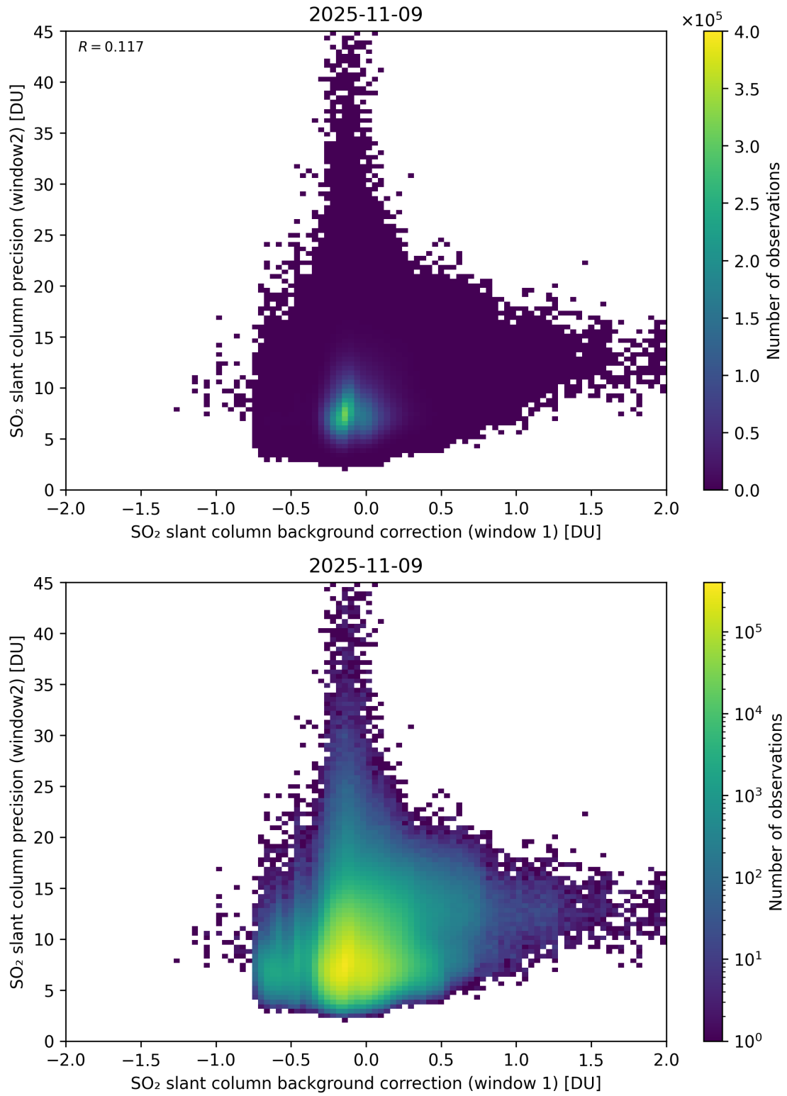
Figure 117: Scatter density plot of “SO 2 slant column background correction (window 1)” against “SO 2 slant column precision (window2)” for 2025-11-08 to 2025-11-10.
