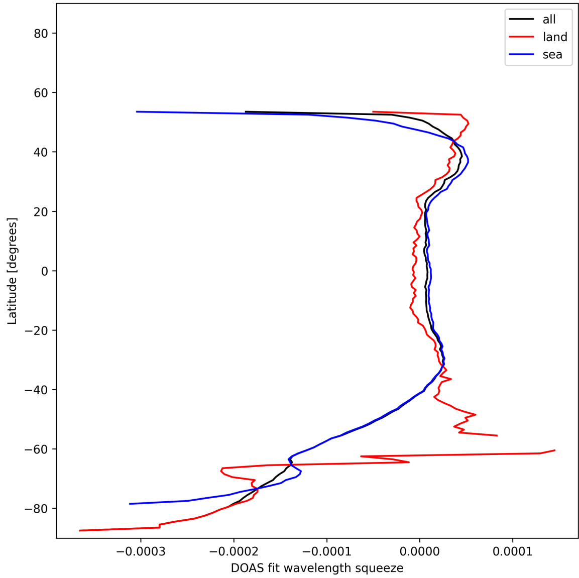
Figure 51: Zonal average of “DOAS fit wavelength squeeze” for 2025-11-08 to 2025-11-10.
