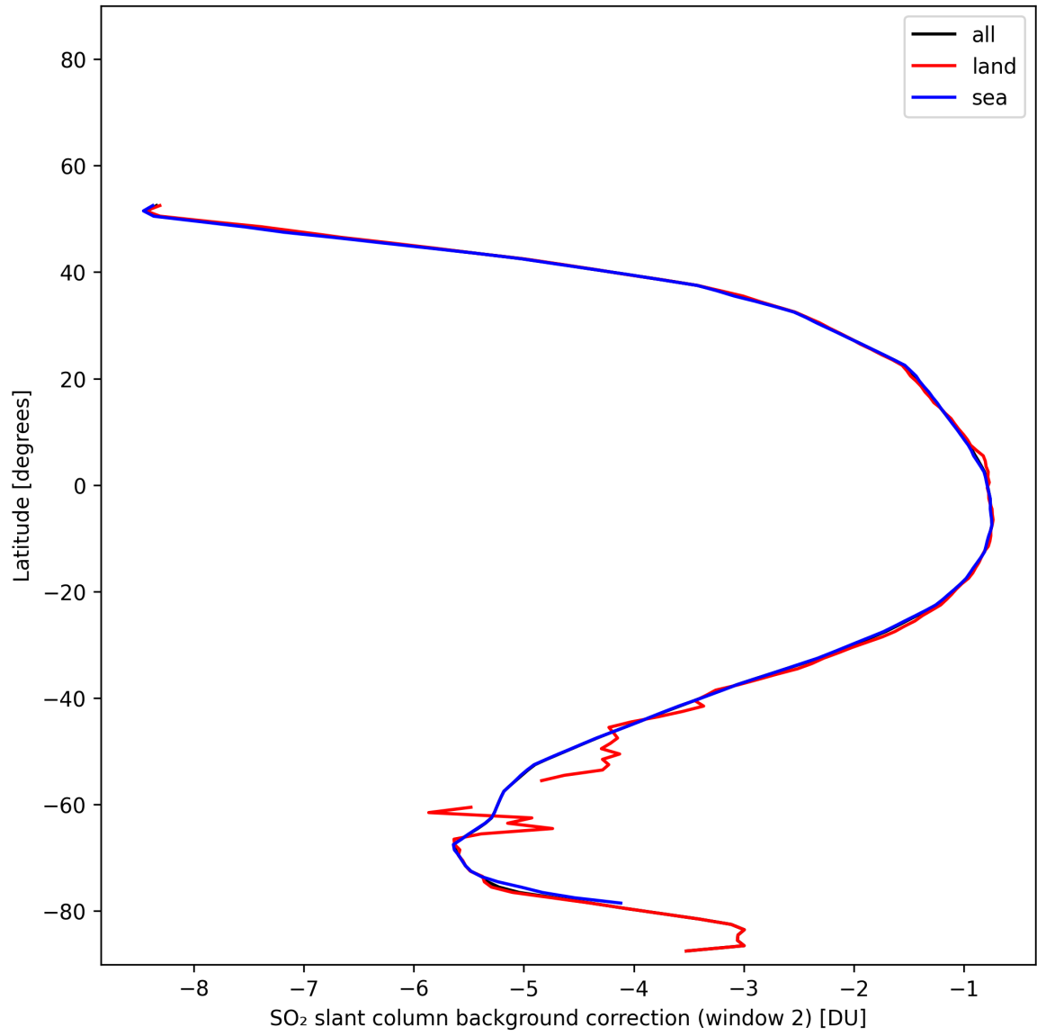
Figure 44: Zonal average of “SO 2 slant column background correction (window 2)” for 2025-11-09 to 2025-11-11.
