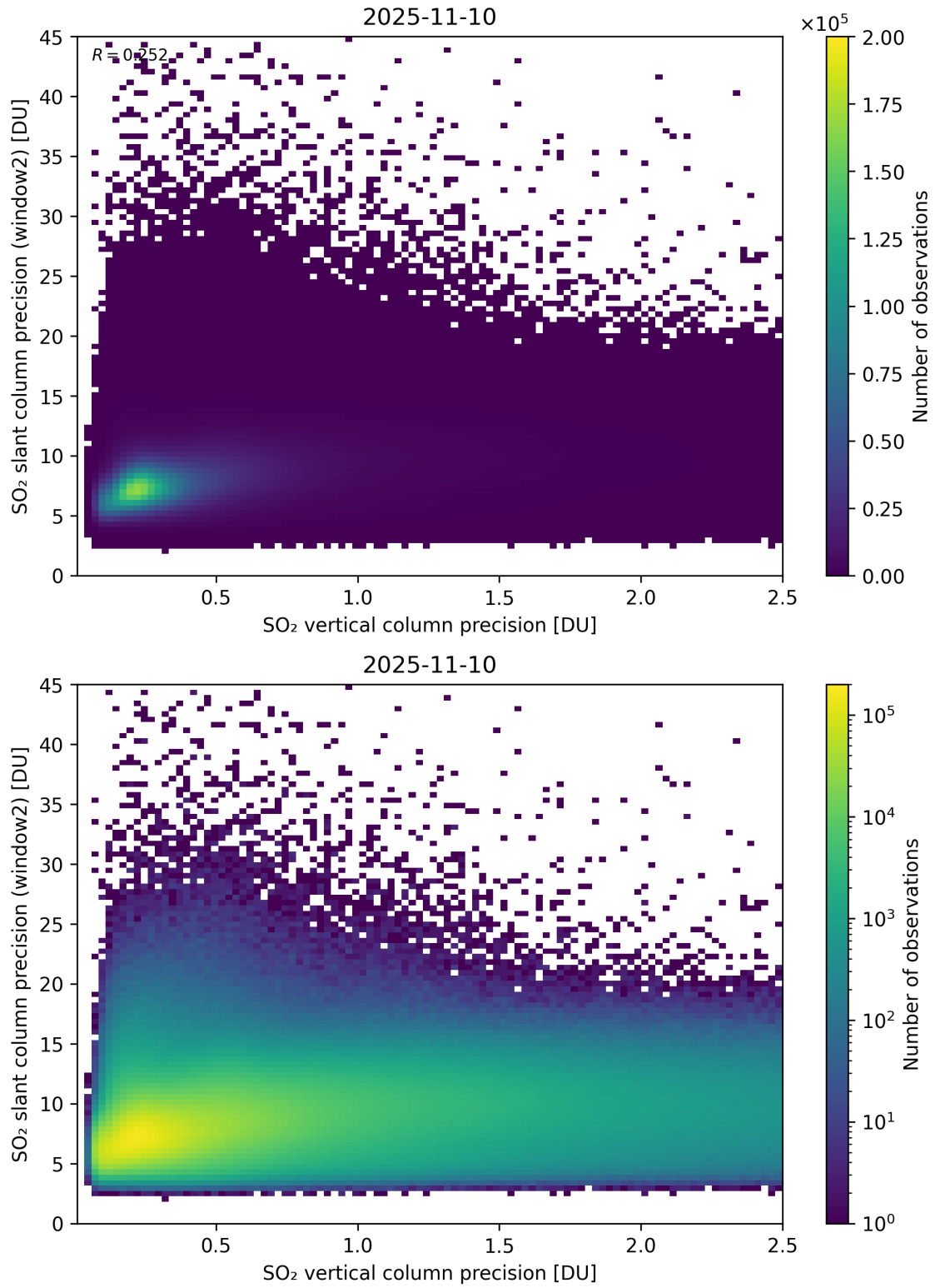
Figure 343: Scatter density plot of “SO 2 vertical column precision” against “SO 2 slant column precision (window2)” for 2025-11-09 to 2025-11-11.
