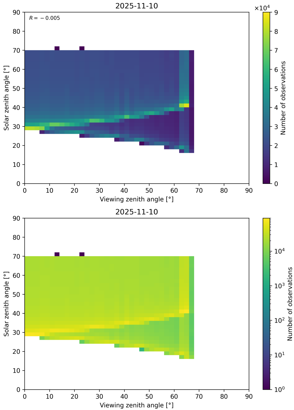
Figure 369: Scatter density plot of “Viewing zenith angle” against “Solar zenith angle” for 2025-11-09 to 2025-11-11.
