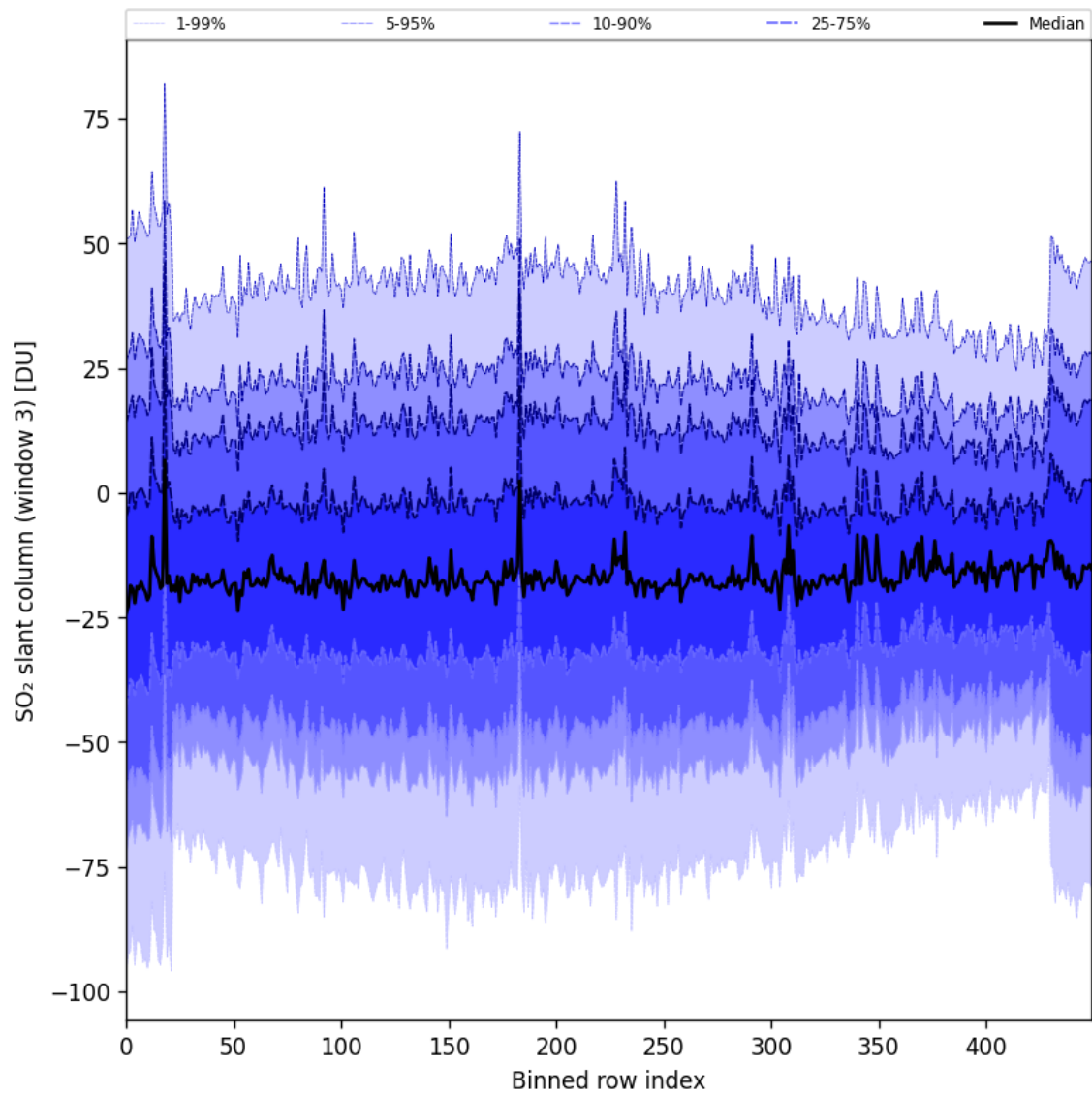
Figure 97: Along track statistics of “SO 2 slant column (window 3)” for 2025-11-09 to 2025-11-11
