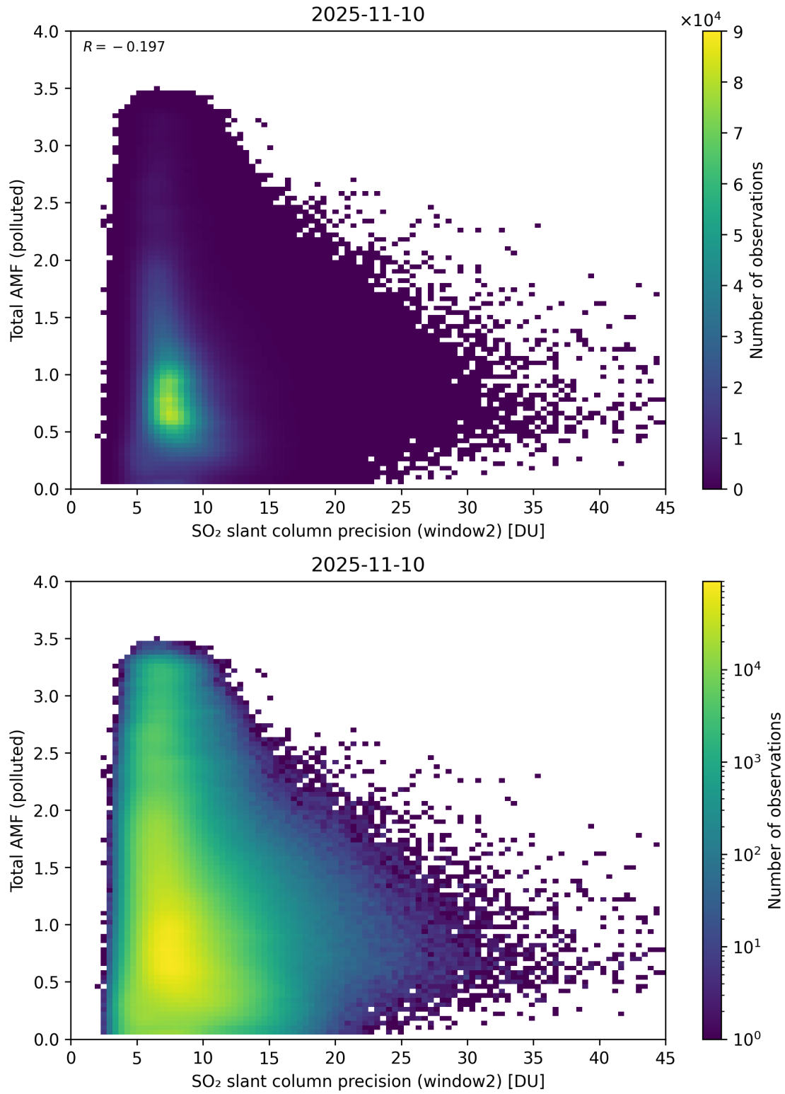
Figure 301: Scatter density plot of “SO 2 slant column precision (window2)” against “Total AMF (polluted)” for 2025-11-09 to 2025-11-11.
