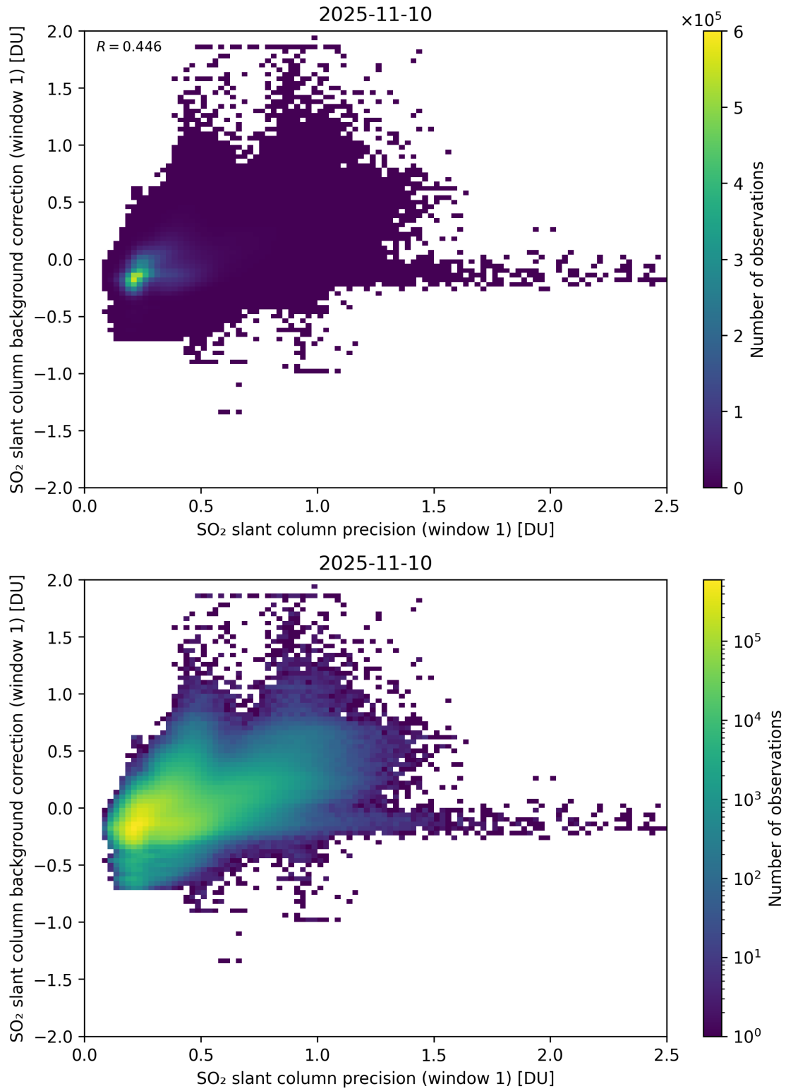
Figure 268: Scatter density plot of “SO 2 slant column precision (window 1)” against “SO 2 slant column background correction (window 1)” for 2025-11-09 to 2025-11-11.
