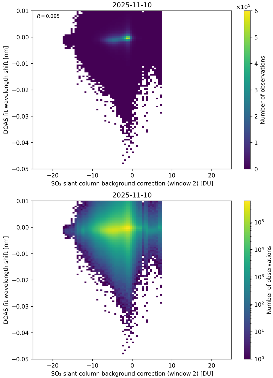
Figure 123: Scatter density plot of “SO 2 slant column background correction (window 2)” against “DOAS fit wavelength shift” for 2025-11-09 to 2025-11-11.
