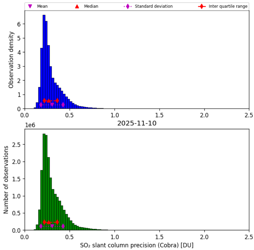
Figure 62: Histogram of “SO 2 slant column precision (Cobra)” for 2025-11-09 to 2025-11-11
