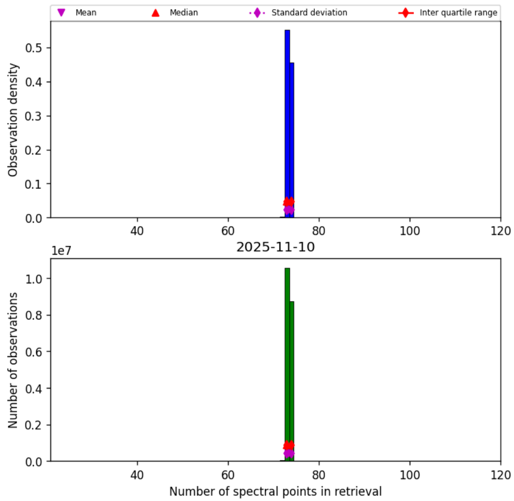
Figure 82: Histogram of “Number of spectral points in retrieval” for 2025-11-09 to 2025-11-11
