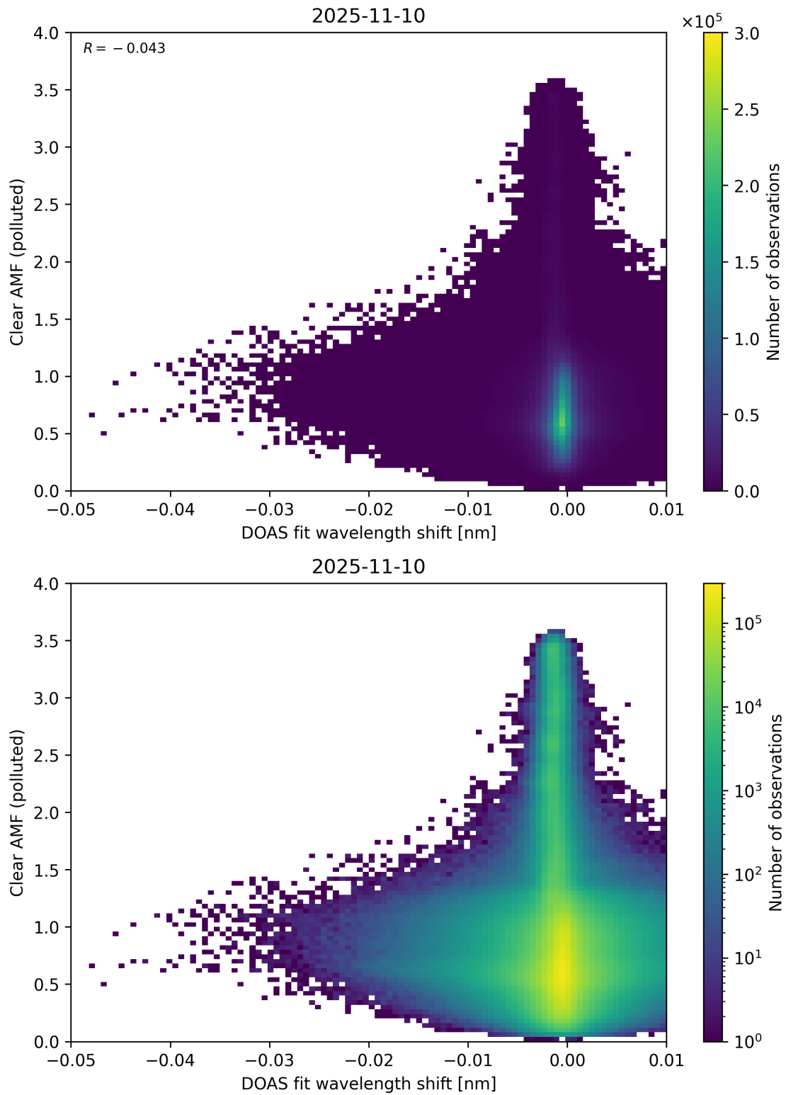
Figure 140: Scatter density plot of “DOAS fit wavelength shift” against “Clear AMF (polluted)” for 2025-11-09 to 2025-11-11.
