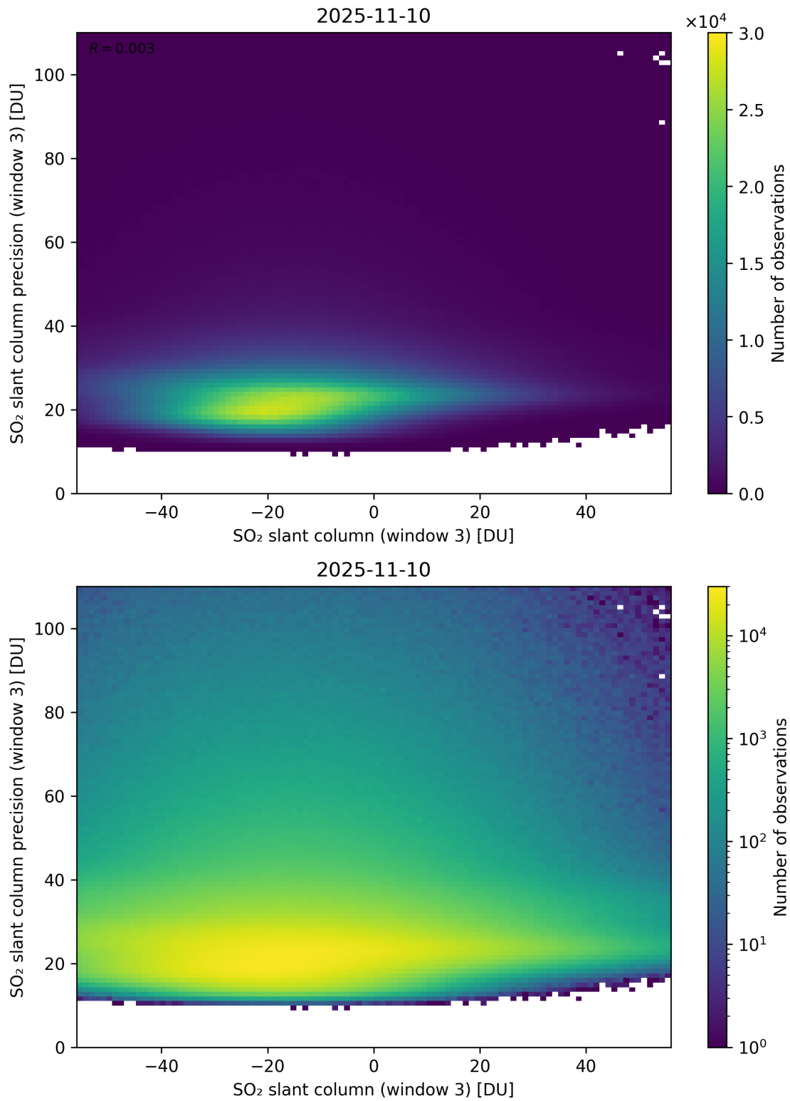
Figure 317: Scatter density plot of “SO 2 slant column (window 3)” against “SO 2 slant column precision (window 3)” for 2025-11-09 to 2025-11-11.
