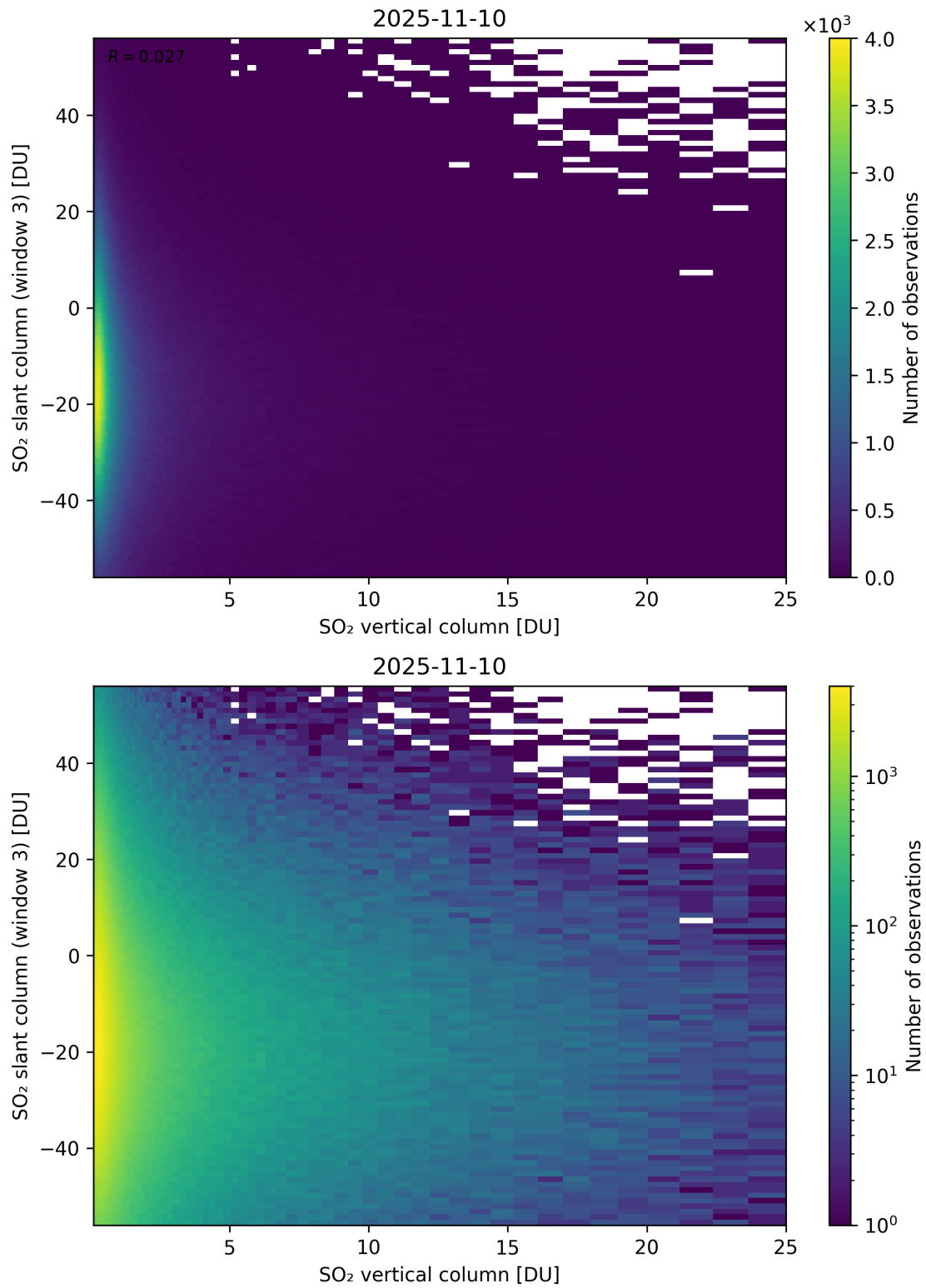
Figure 357: Scatter density plot of “SO 2 vertical column” against “SO 2 slant column (window 3)” for 2025-11-09 to 2025-11-11.
