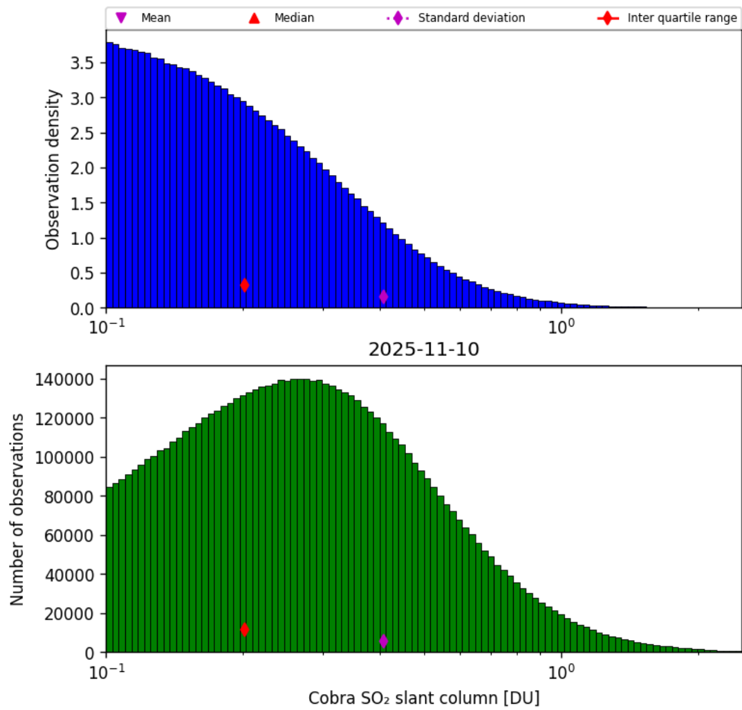
Figure 61: Histogram of “Cobra SO 2 slant column” for 2025-11-09 to 2025-11-11
