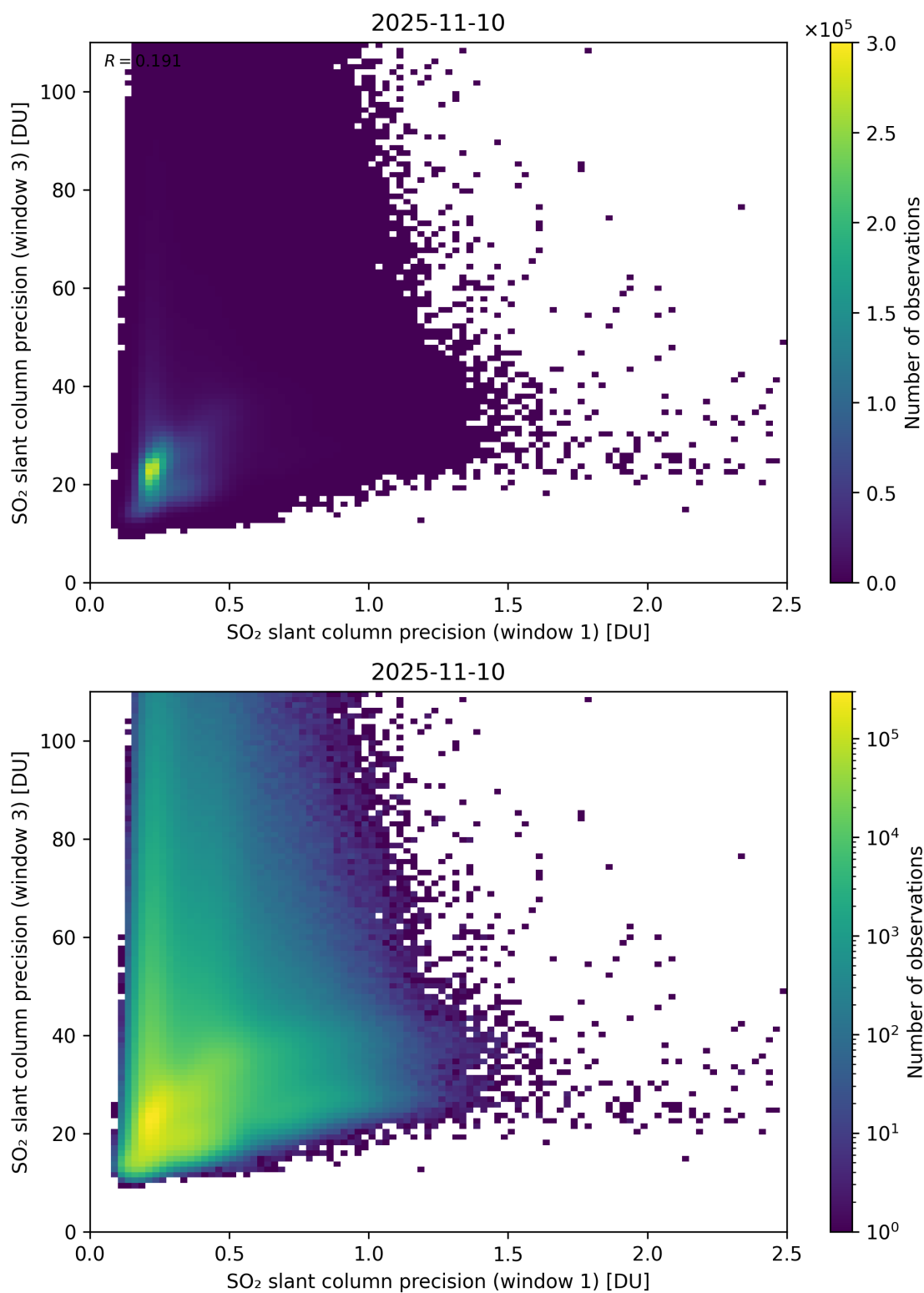
Figure 279: Scatter density plot of “SO 2 slant column precision (window 1)” against “SO 2 slant column precision (window 3)” for 2025-11-09 to 2025-11-11.
