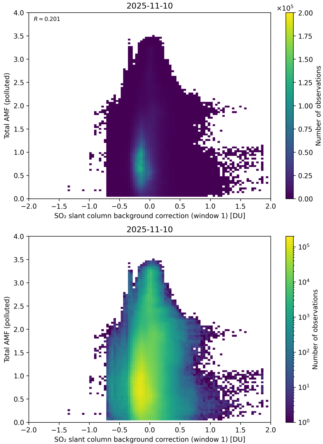
Figure 120: Scatter density plot of “SO 2 slant column background correction (window 1)” against “Total AMF (polluted)” for 2025-11-09 to 2025-11-11.
