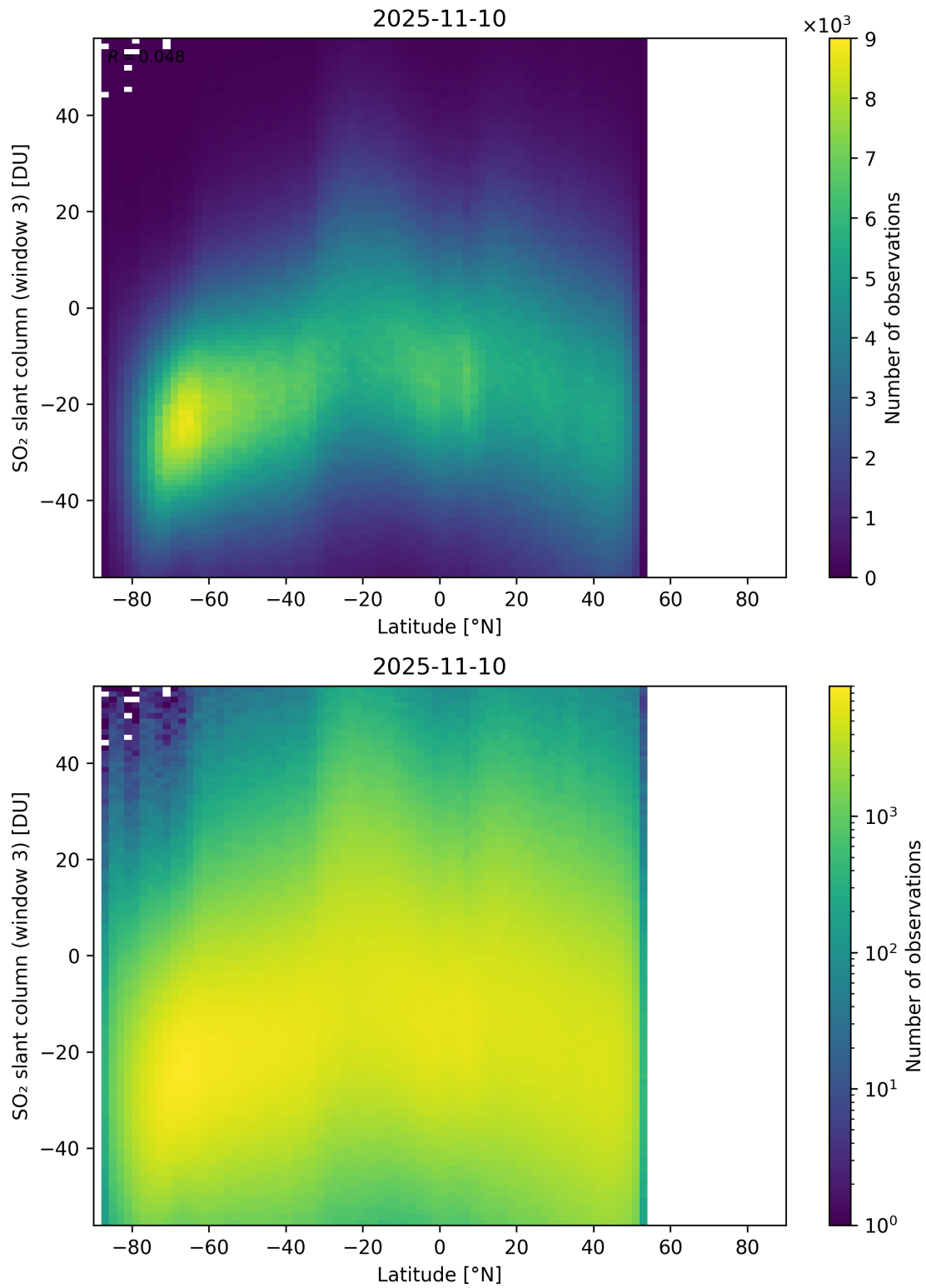
Figure 165: Scatter density plot of “Latitude” against “SO 2 slant column (window 3)” for 2025-11-09 to 2025-11-11.
