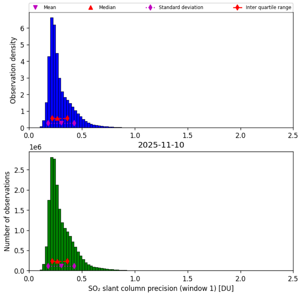
Figure 64: Histogram of “SO 2 slant column precision (window 1)” for 2025-11-09 to 2025-11-11
