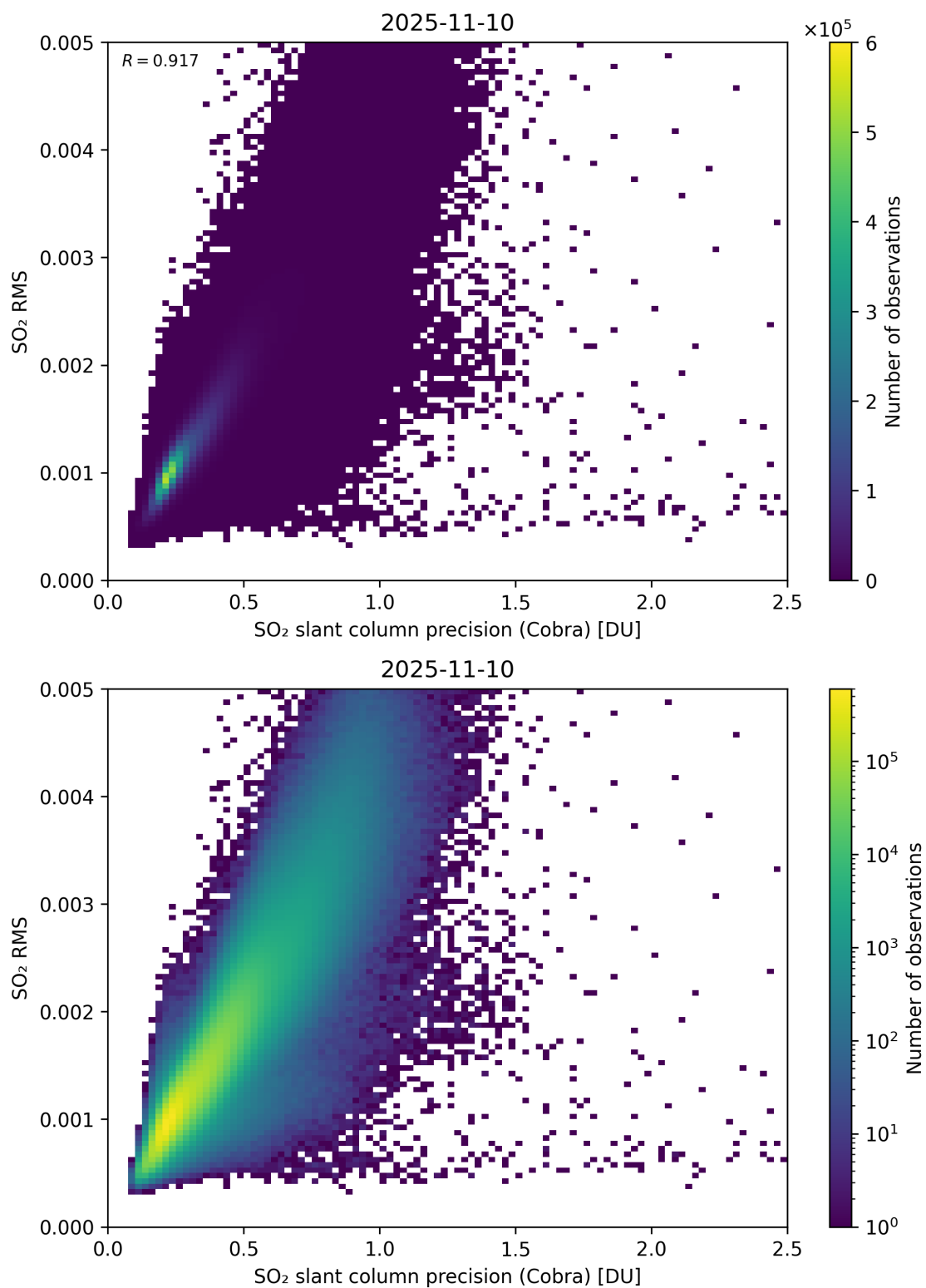
Figure 204: Scatter density plot of “SO 2 slant column precision (Cobra)” against “SO 2 RMS” for 2025-11-09 to 2025-11-11.
