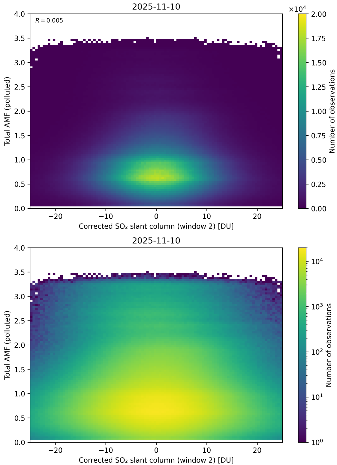
Figure 253: Scatter density plot of “Corrected SO 2 slant column (window 2)” against “Total AMF (polluted)” for 2025-11-09 to 2025-11-11.
