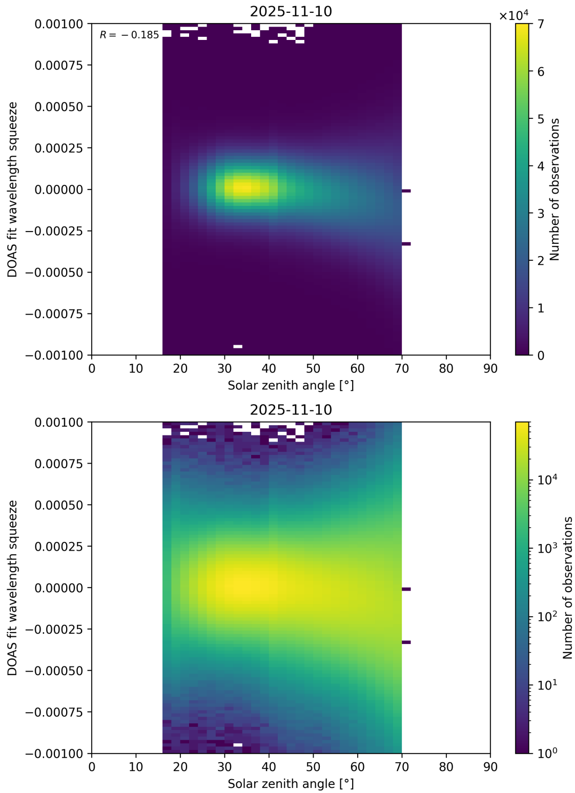
Figure 175: Scatter density plot of “Solar zenith angle” against “DOAS fit wavelength squeeze” for 2025-11-09 to 2025-11-11.
