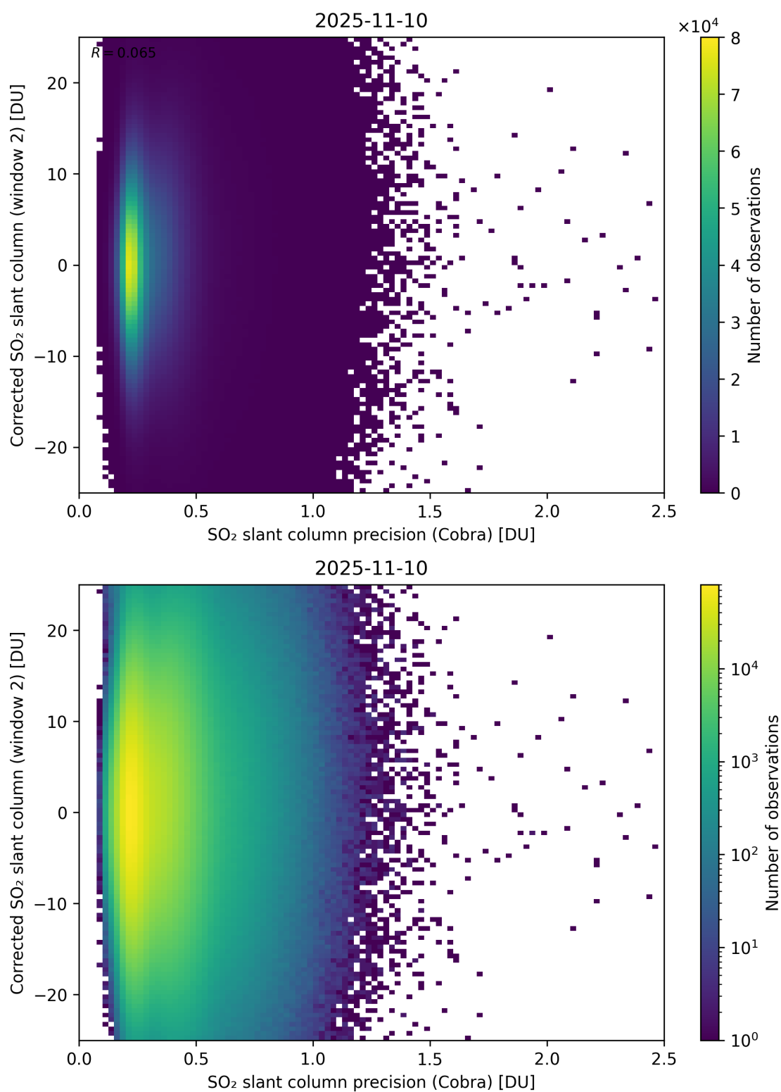
Figure 206: Scatter density plot of “SO 2 slant column precision (Cobra)” against “Corrected SO 2 slant column (window 2)” for 2025-11-09 to 2025-11-11.
