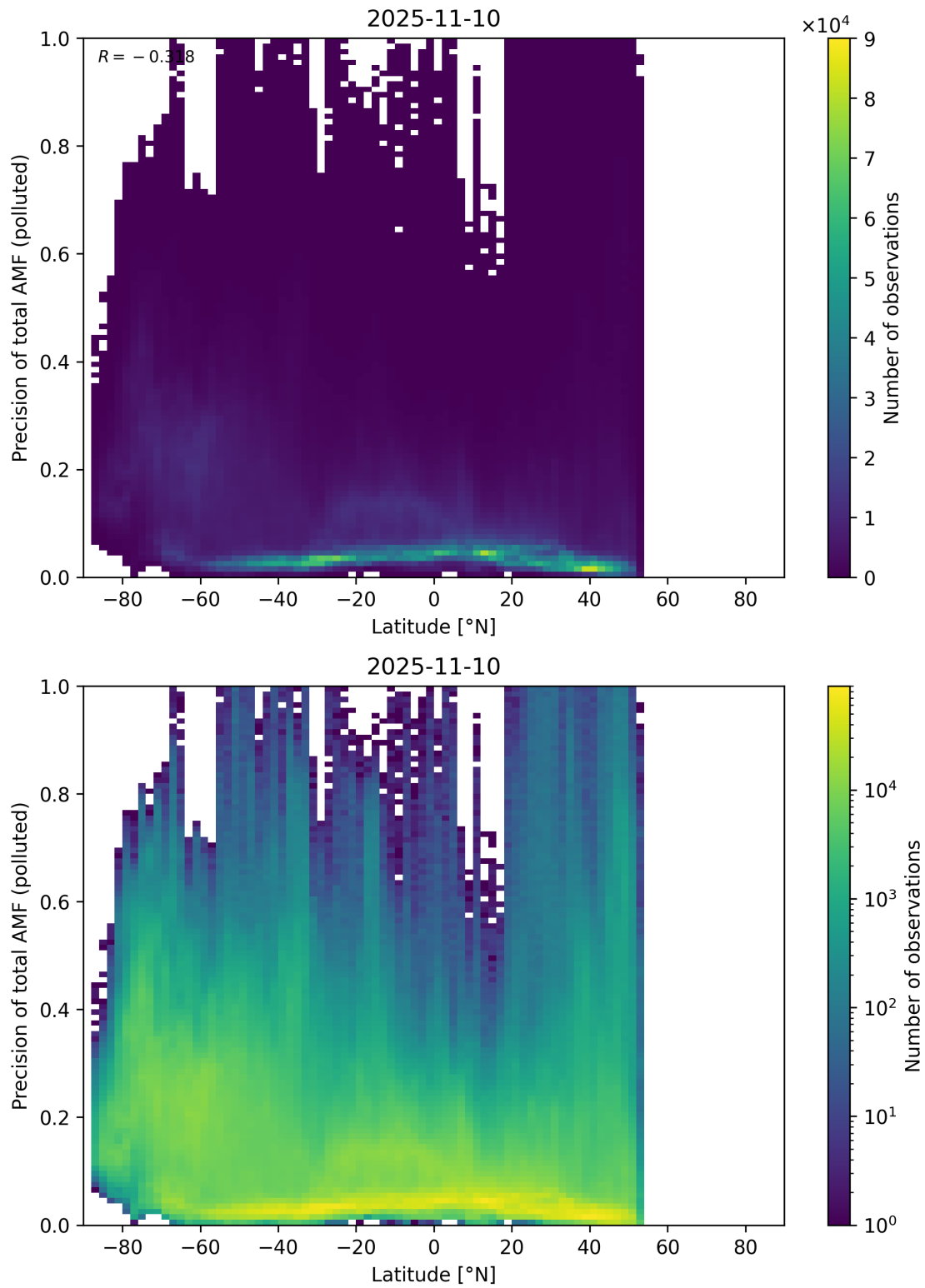
Figure 168: Scatter density plot of “Latitude” against “Precision of total AMF (polluted)” for 2025-11-09 to 2025-11-11.
