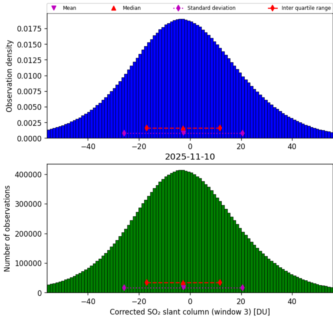
Figure 73: Histogram of “Corrected SO 2 slant column (window 3)” for 2025-11-09 to 2025-11-11
