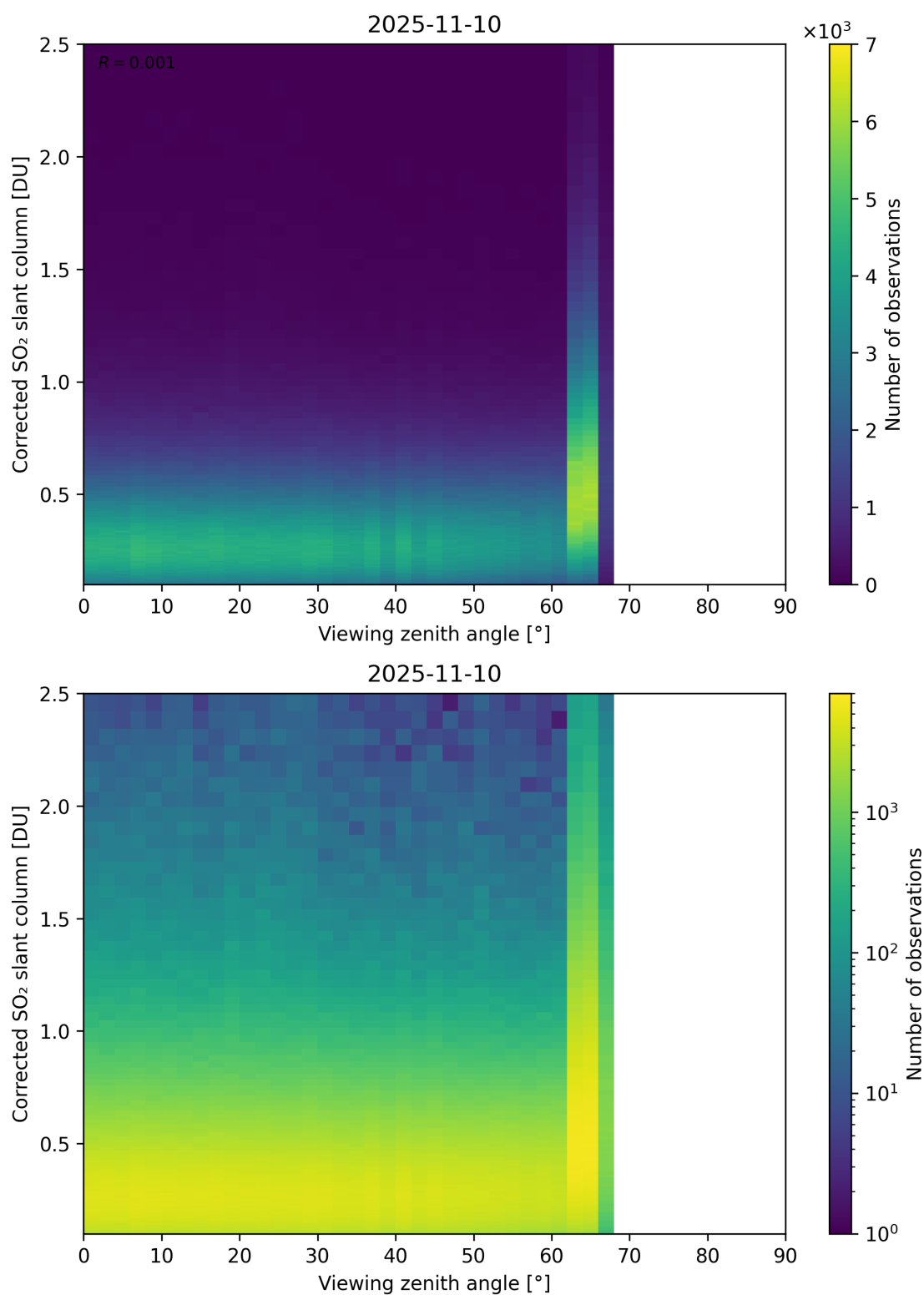
Figure 373: Scatter density plot of “Viewing zenith angle” against “Corrected SO 2 slant column” for 2025-11-09 to 2025-11-11.
