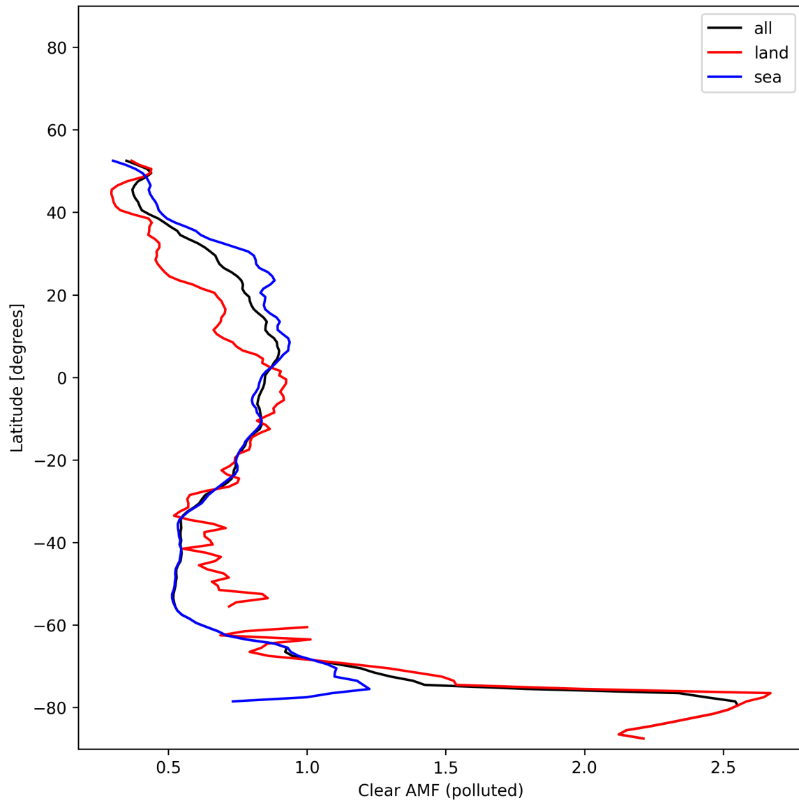
Figure 55: Zonal average of “Clear AMF (polluted)” for 2025-11-09 to 2025-11-11.
