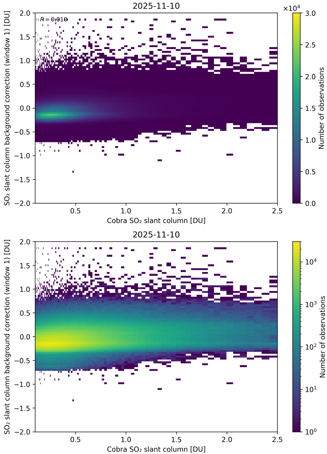
Figure 193: Scatter density plot of “Cobra SO 2 slant column” against “SO 2 slant column background correction (window 1)” for 2025-11-09 to 2025-11-11.
