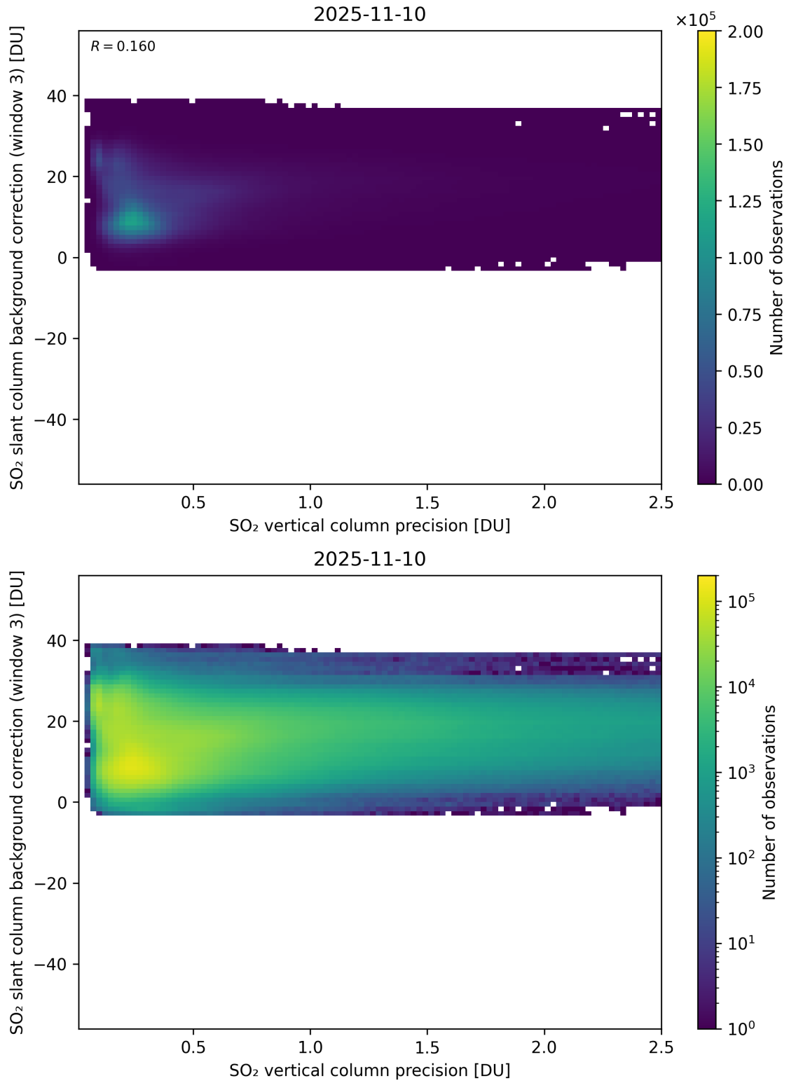
Figure 331: Scatter density plot of “SO 2 vertical column precision” against “SO 2 slant column background correction (window 3)” for 2025-11-09 to 2025-11-11.
