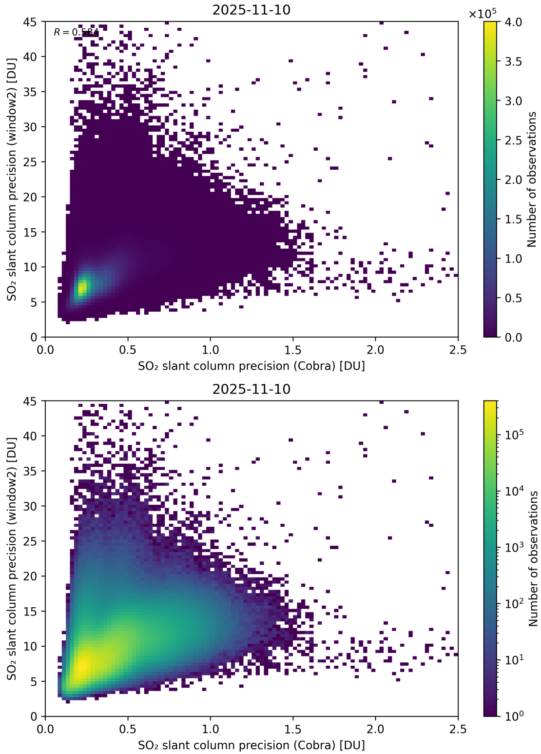
Figure 210: Scatter density plot of “SO 2 slant column precision (Cobra)” against “SO 2 slant column precision (window2)” for 2025-11-09 to 2025-11-11.
