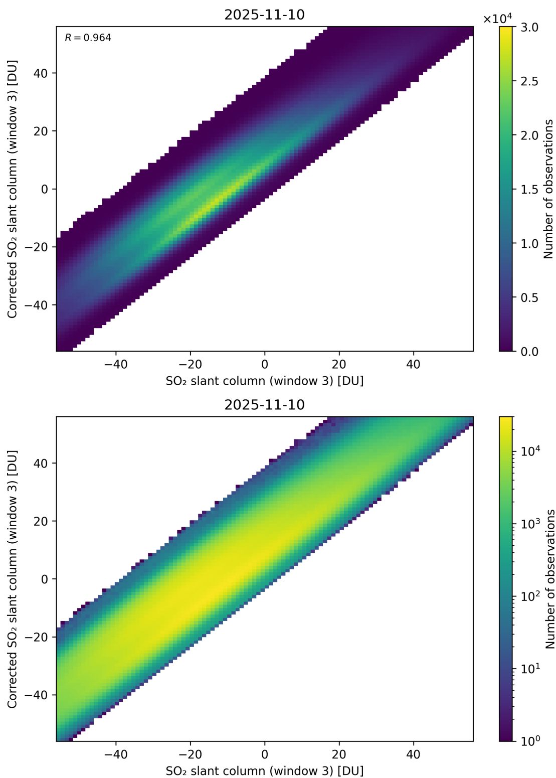
Figure 316: Scatter density plot of “SO 2 slant column (window 3)” against “Corrected SO 2 slant column (window 3)” for 2025-11-09 to 2025-11-11.
