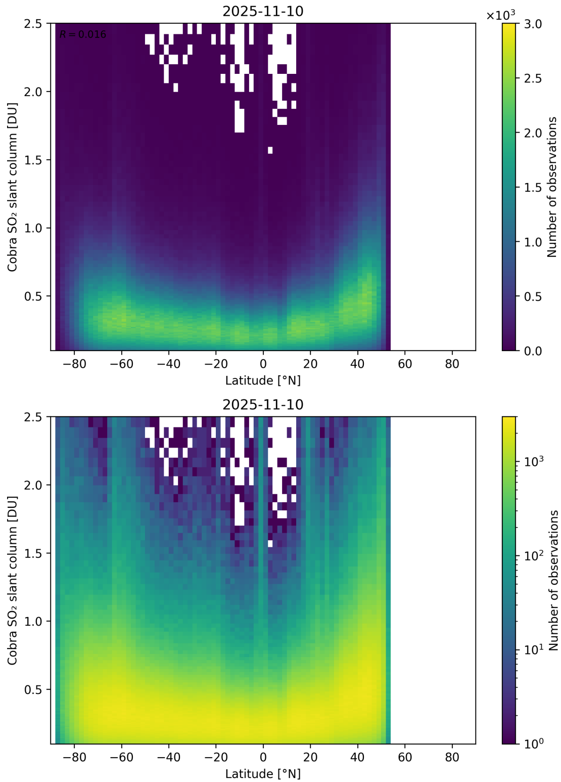
Figure 157: Scatter density plot of “Latitude” against “Cobra SO 2 slant column” for 2025-11-09 to 2025-11-11.
