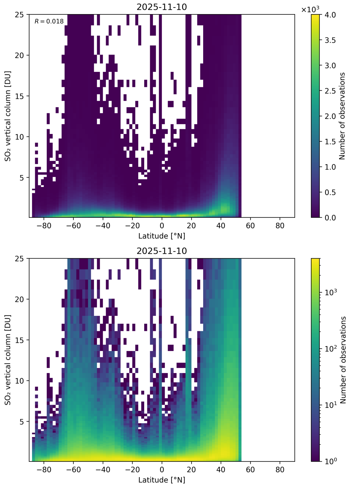
Figure 169: Scatter density plot of “Latitude” against “SO 2 vertical column” for 2025-11-09 to 2025-11-11.
