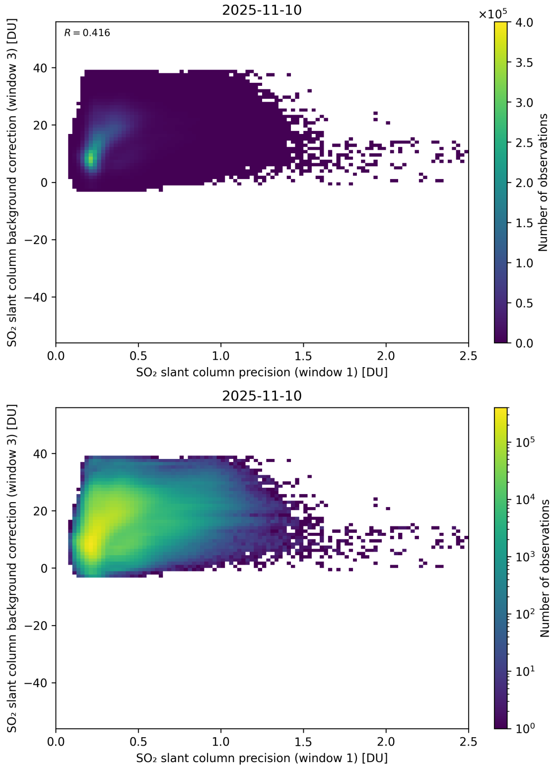
Figure 270: Scatter density plot of “SO 2 slant column precision (window 1)” against “SO 2 slant column background correction (window 3)” for 2025-11-09 to 2025-11-11.
