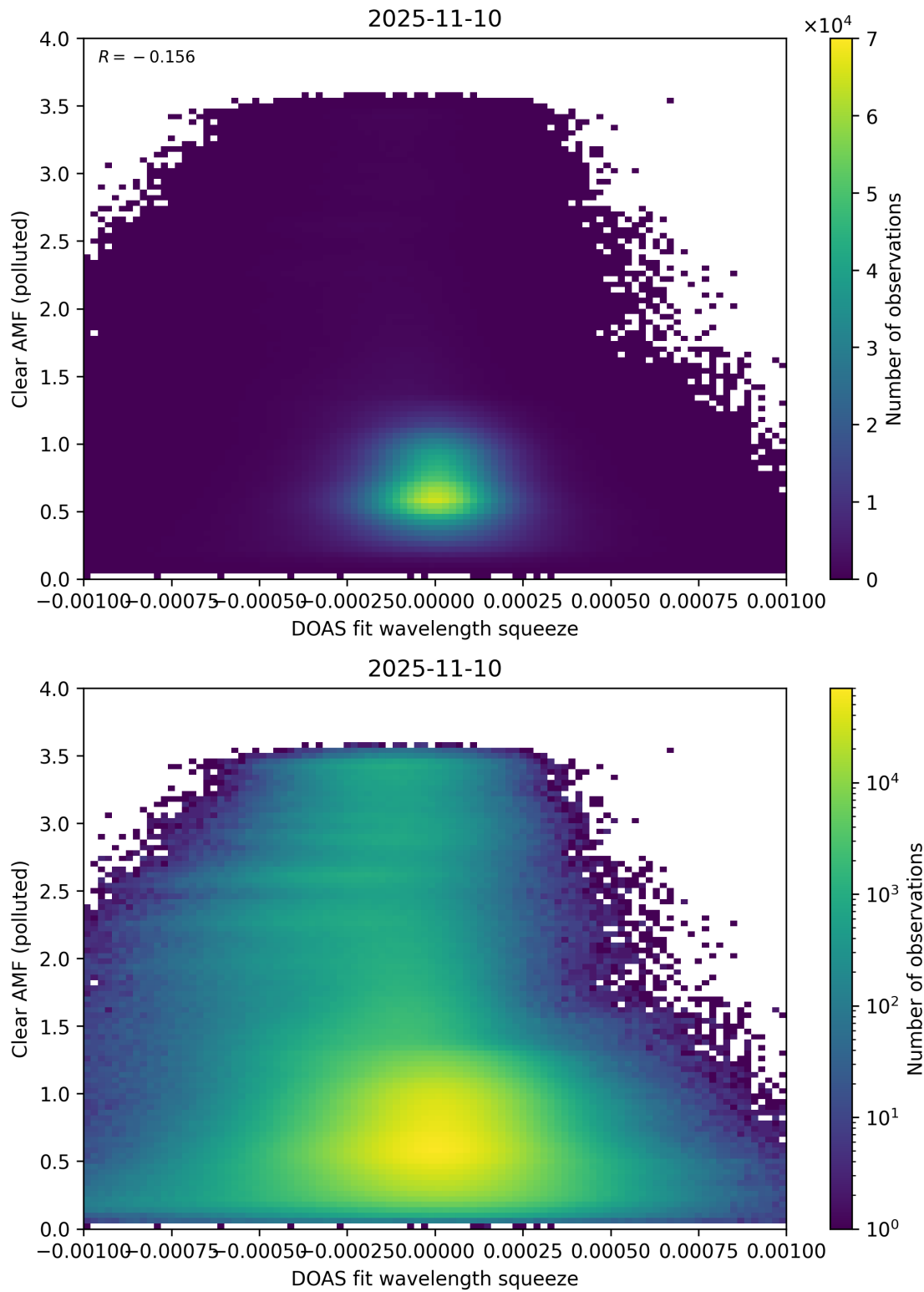
Figure 144: Scatter density plot of “DOAS fit wavelength squeeze” against “Clear AMF (polluted)” for 2025-11-09 to 2025-11-11.
