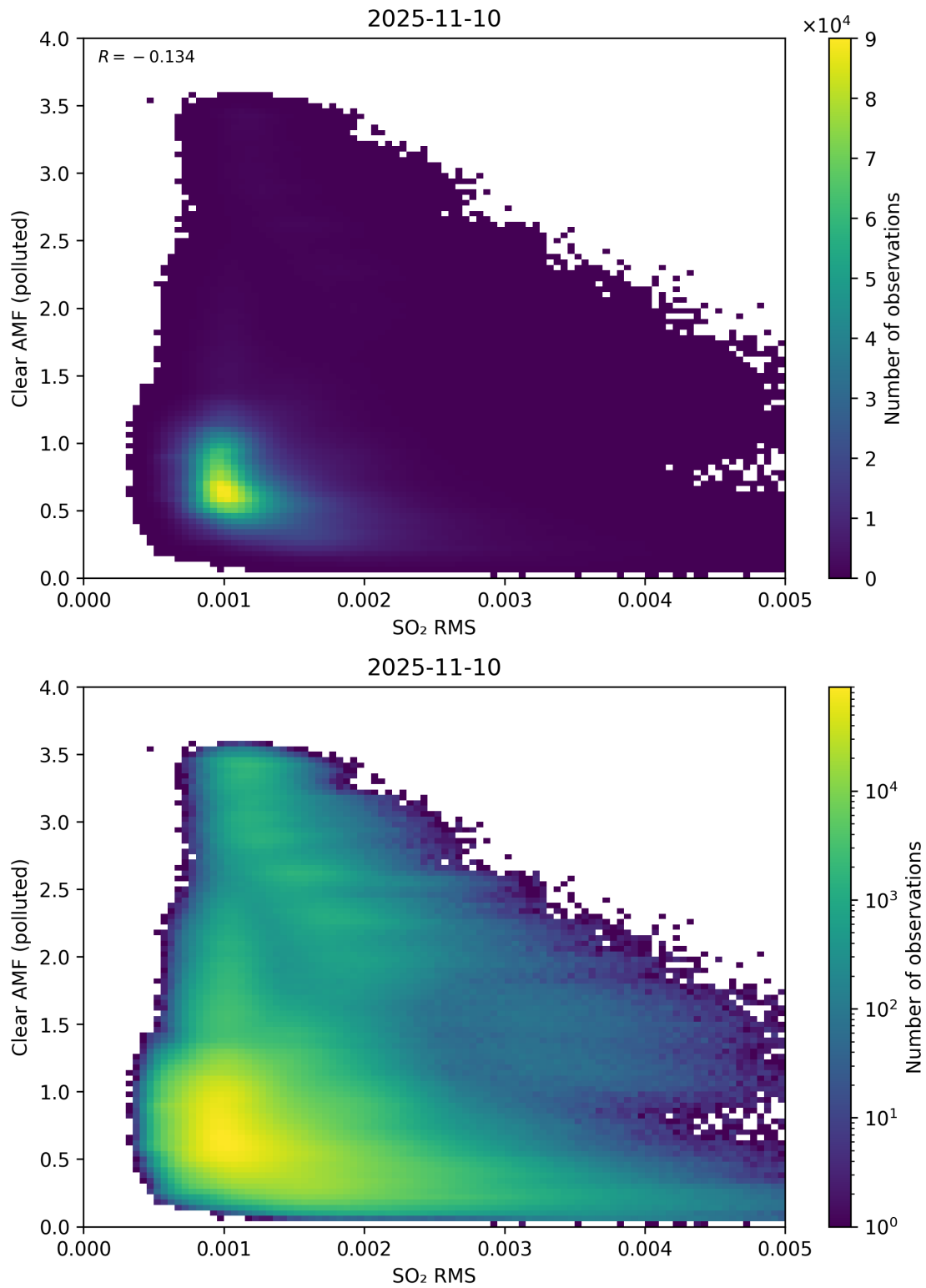
Figure 147: Scatter density plot of “SO 2 RMS” against “Clear AMF (polluted)” for 2025-11-09 to 2025-11-11.
