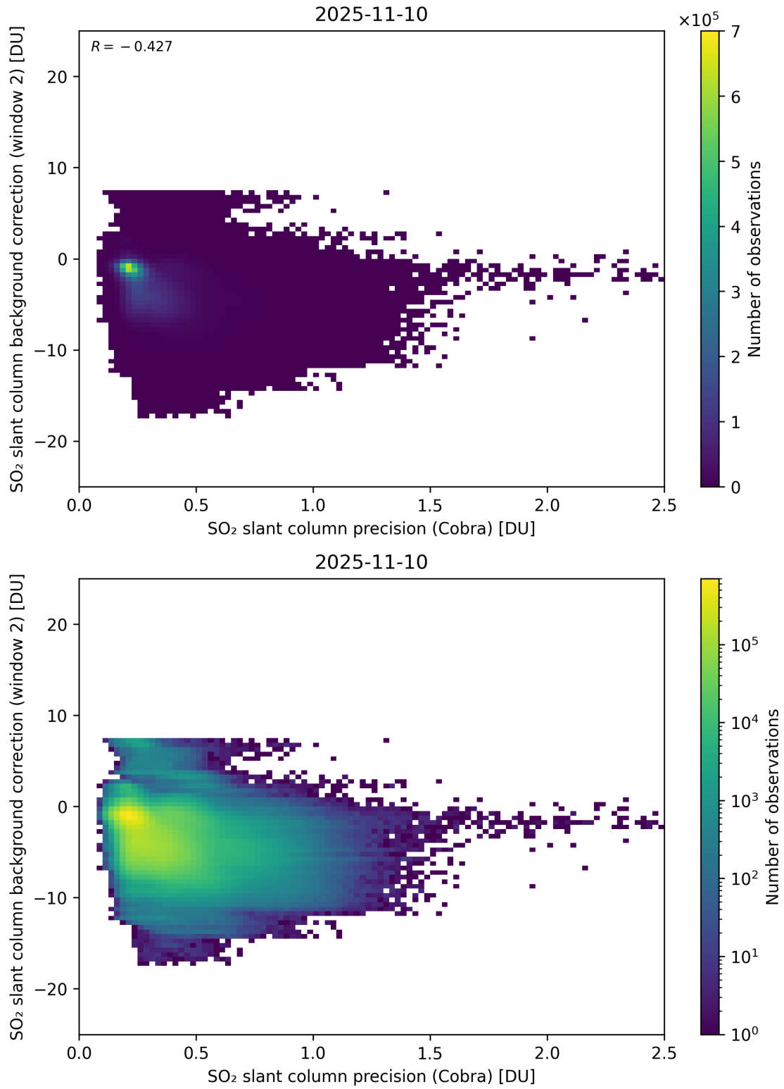
Figure 200: Scatter density plot of “SO 2 slant column precision (Cobra)” against “SO 2 slant column background correction (window 2)” for 2025-11-09 to 2025-11-11.
