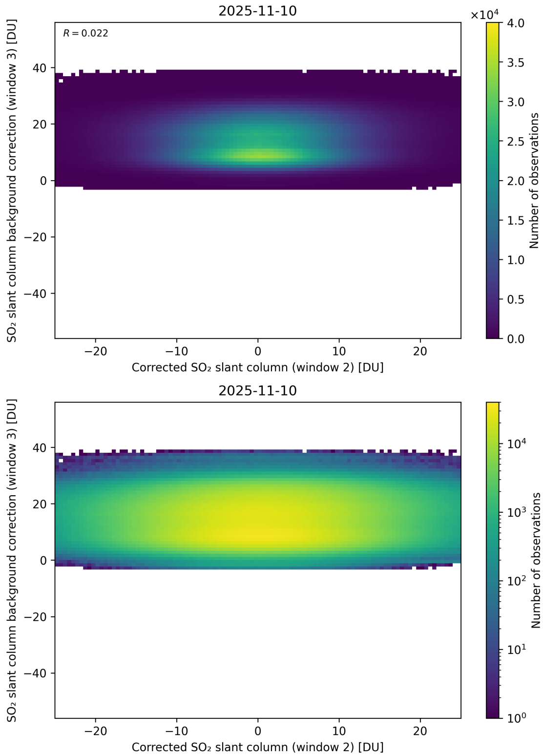
Figure 245: Scatter density plot of “Corrected SO 2 slant column (window 2)” against “SO 2 slant column background correction (window 3)” for 2025-11-09 to 2025-11-11.
