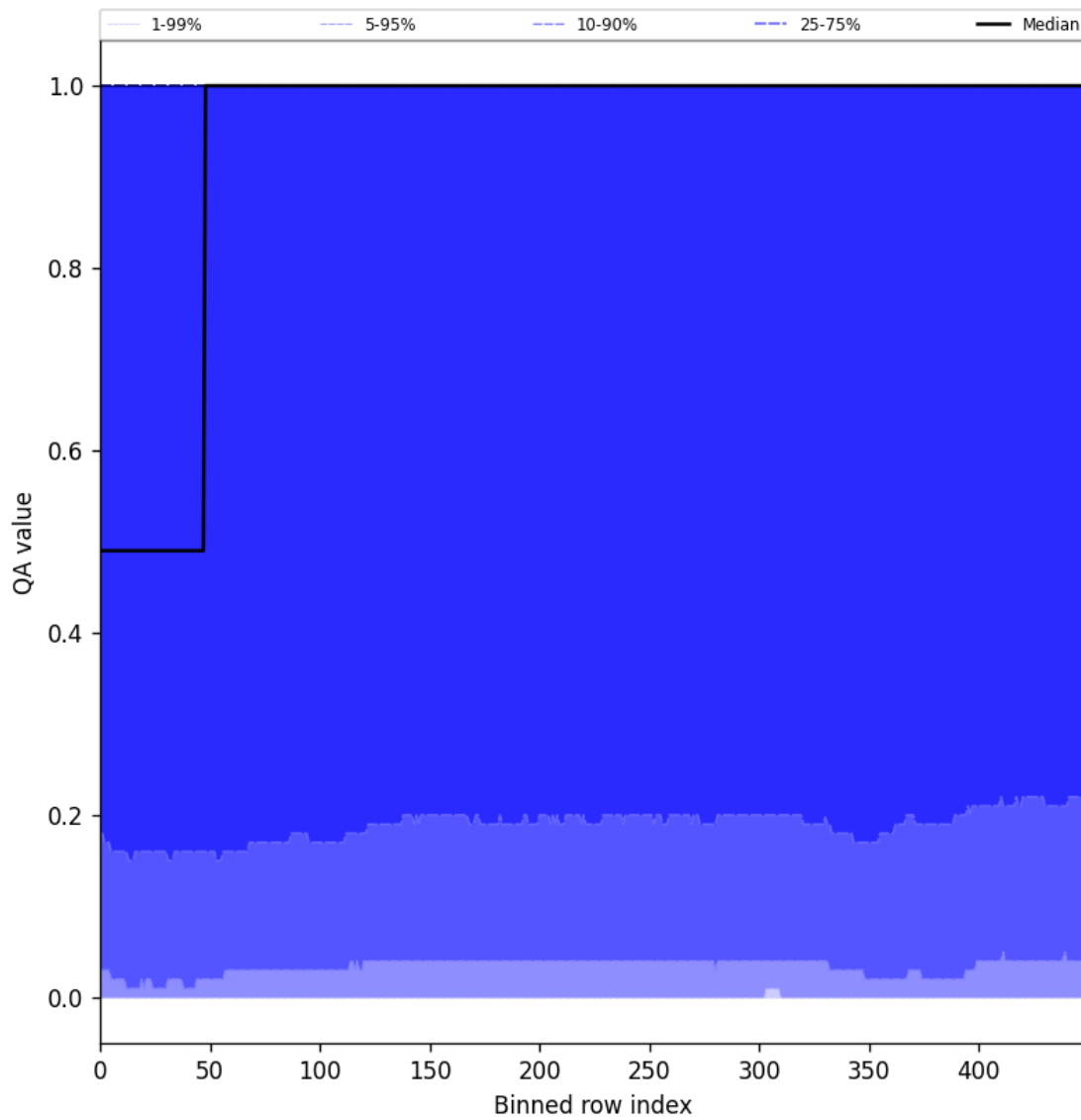
Figure 83: Along track statistics of “QA value” for 2025-11-09 to 2025-11-11
