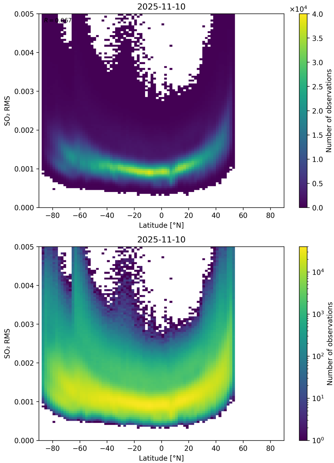
Figure 155: Scatter density plot of “Latitude” against “SO 2 RMS” for 2025-11-09 to 2025-11-11.
