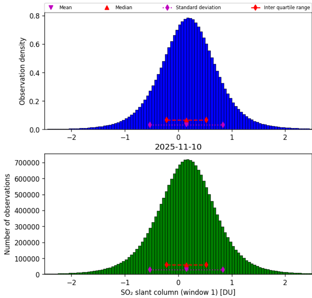
Figure 63: Histogram of “SO 2 slant column (window 1)” for 2025-11-09 to 2025-11-11
