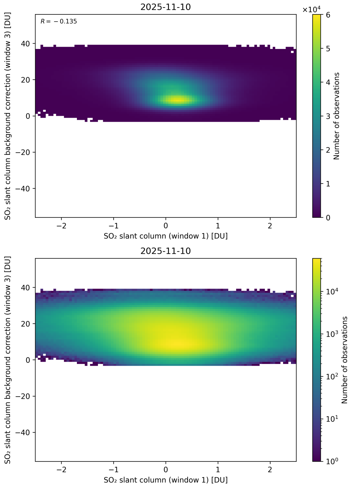
Figure 264: Scatter density plot of “SO 2 slant column (window 1)” against “SO 2 slant column background correction (window 3)” for 2025-11-09 to 2025-11-11.
