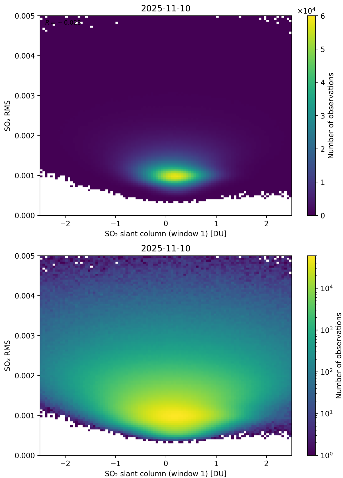
Figure 267: Scatter density plot of “SO 2 slant column (window 1)” against “SO 2 RMS” for 2025-11-09 to 2025-11-11.
