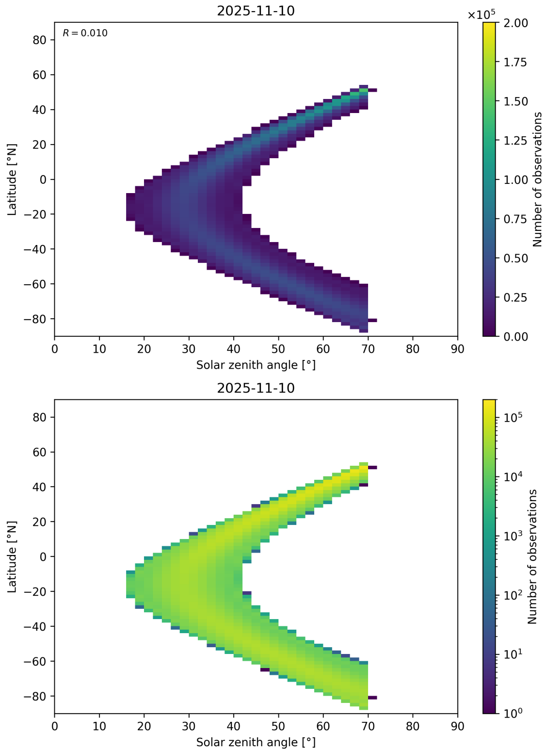
Figure 177: Scatter density plot of “Solar zenith angle” against “Latitude” for 2025-11-09 to 2025-11-11.
