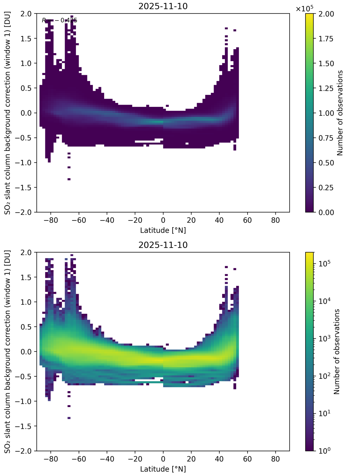
Figure 150: Scatter density plot of “Latitude” against “SO 2 slant column background correction (window 1)” for 2025-11-09 to 2025-11-11.
