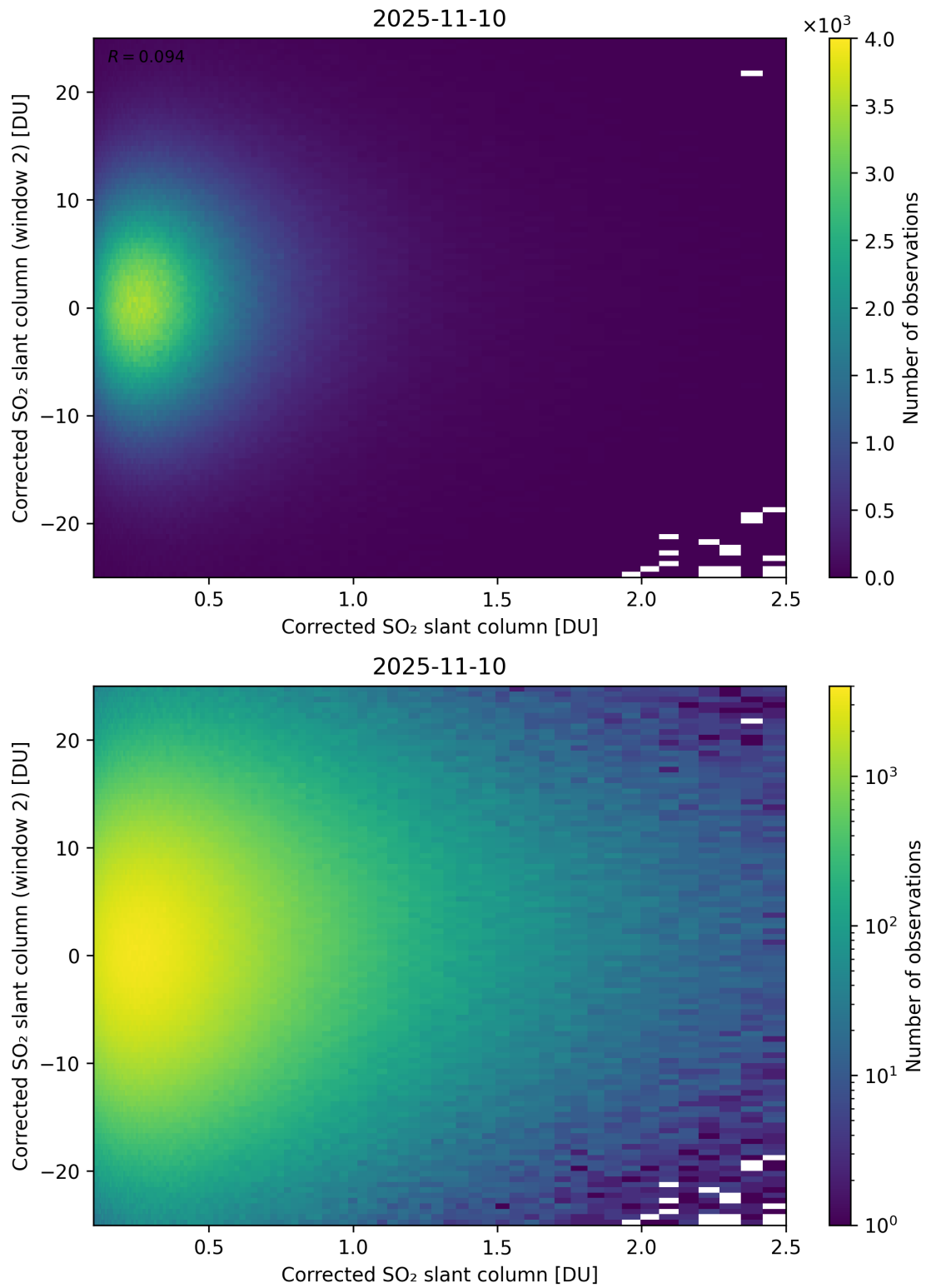
Figure 235: Scatter density plot of “Corrected SO 2 slant column” against “Corrected SO 2 slant column (window 2)” for 2025-11-09 to 2025-11-11.
