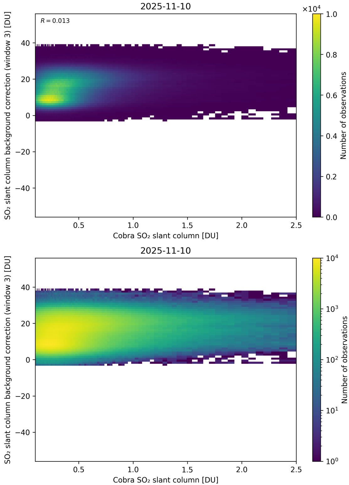
Figure 195: Scatter density plot of “Cobra SO 2 slant column” against “SO 2 slant column background correction (window 3)” for 2025-11-09 to 2025-11-11.
