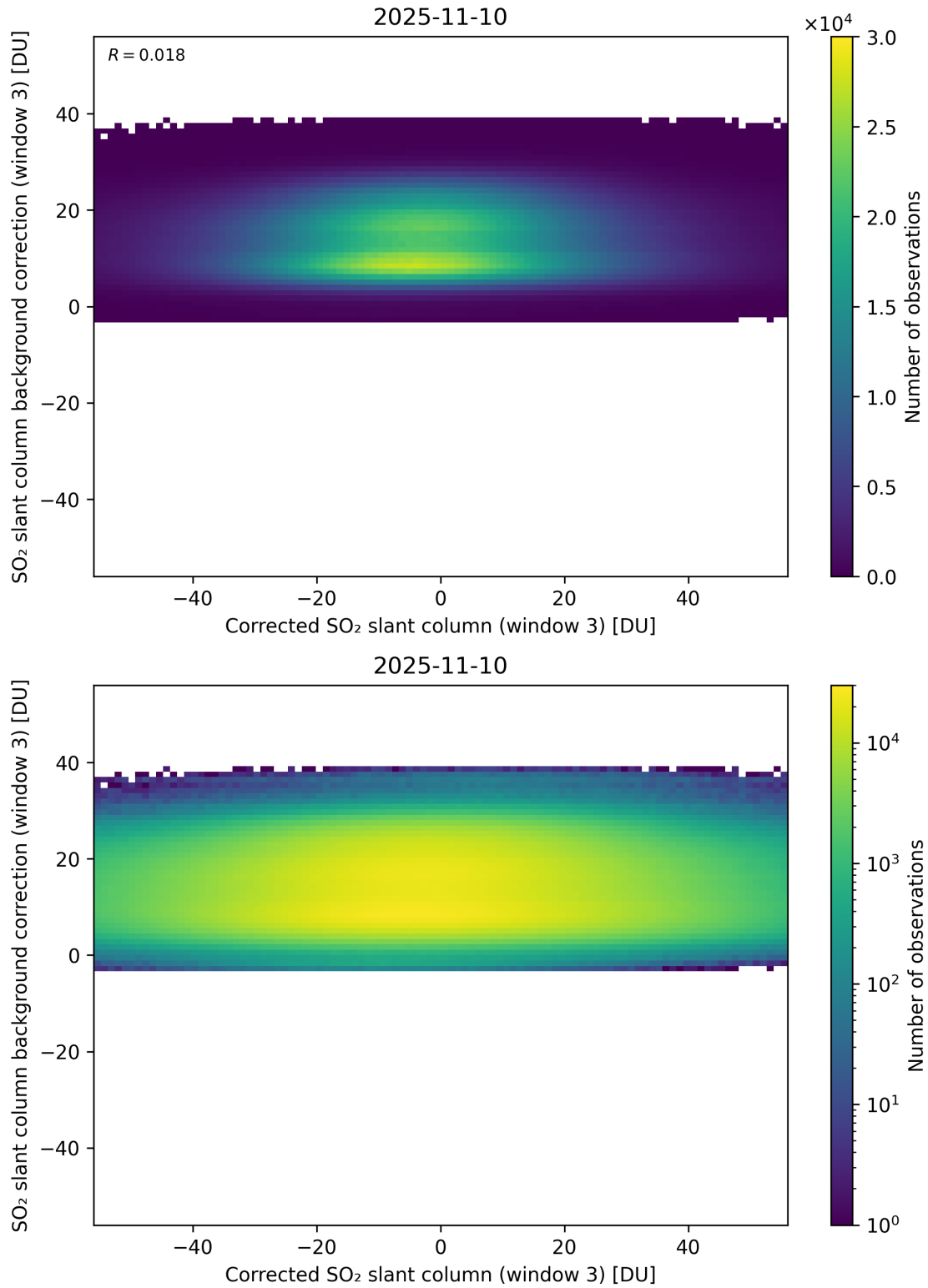
Figure 255: Scatter density plot of “Corrected SO 2 slant column (window 3)” against “SO 2 slant column background correction (window 3)” for 2025-11-09 to 2025-11-11.
