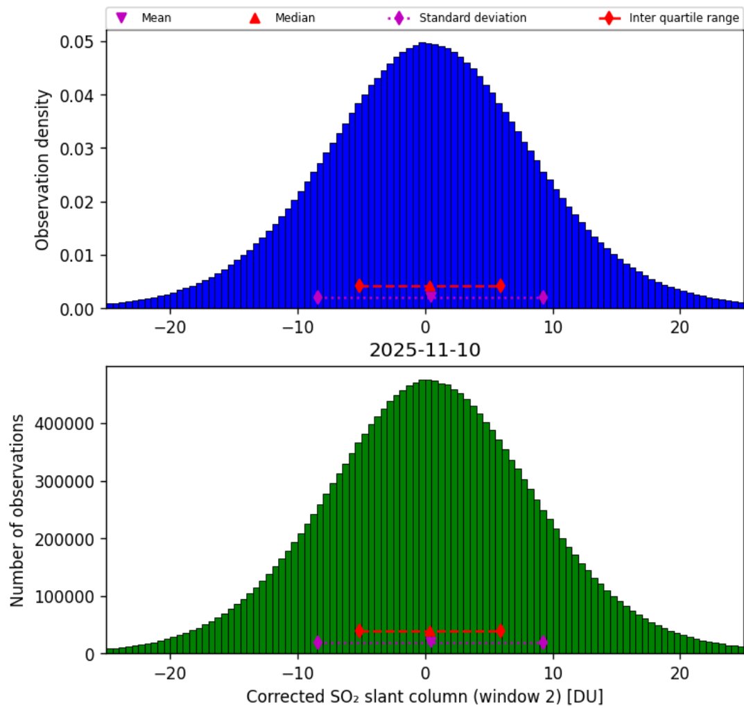
Figure 69: Histogram of “Corrected SO 2 slant column (window 2)” for 2025-11-09 to 2025-11-11
