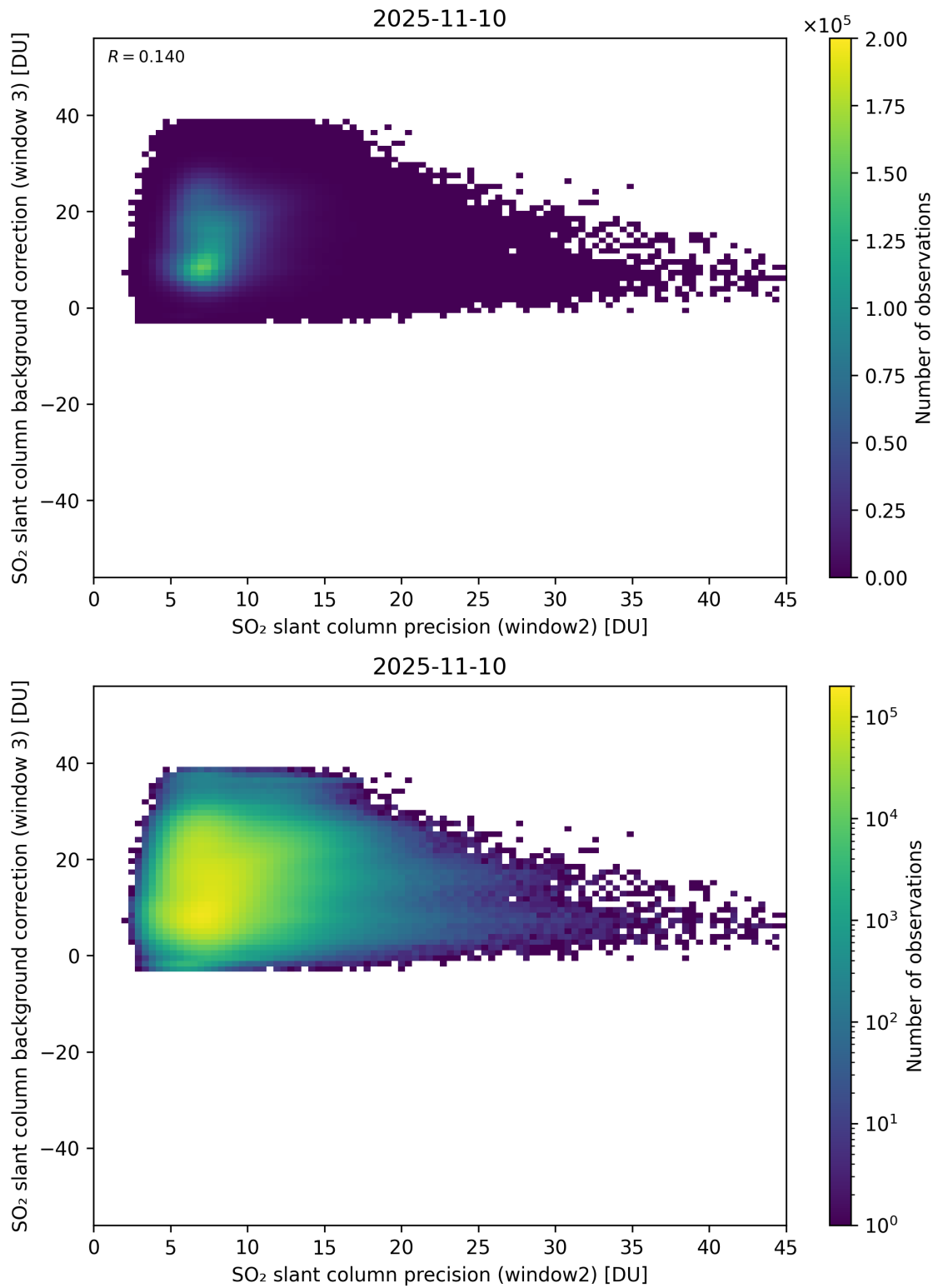
Figure 292: Scatter density plot of “SO 2 slant column precision (window2)” against “SO 2 slant column background correction (window 3)” for 2025-11-09 to 2025-11-11.
