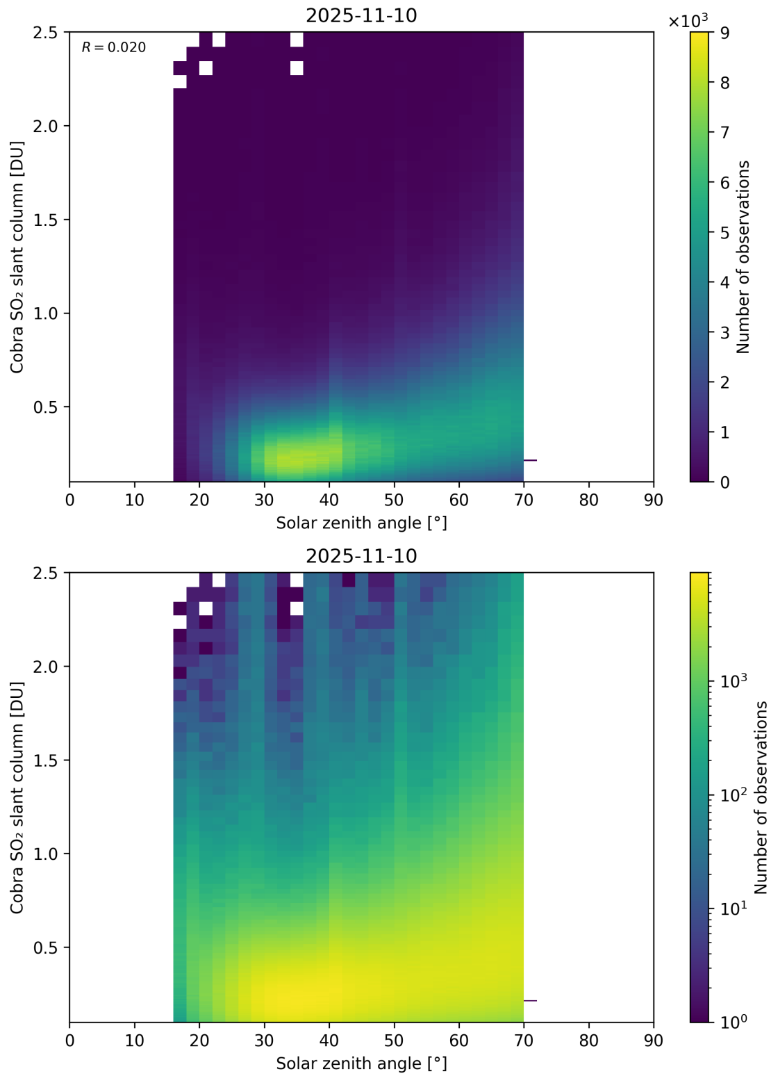
Figure 179: Scatter density plot of “Solar zenith angle” against “Cobra SO 2 slant column” for 2025-11-09 to 2025-11-11.
