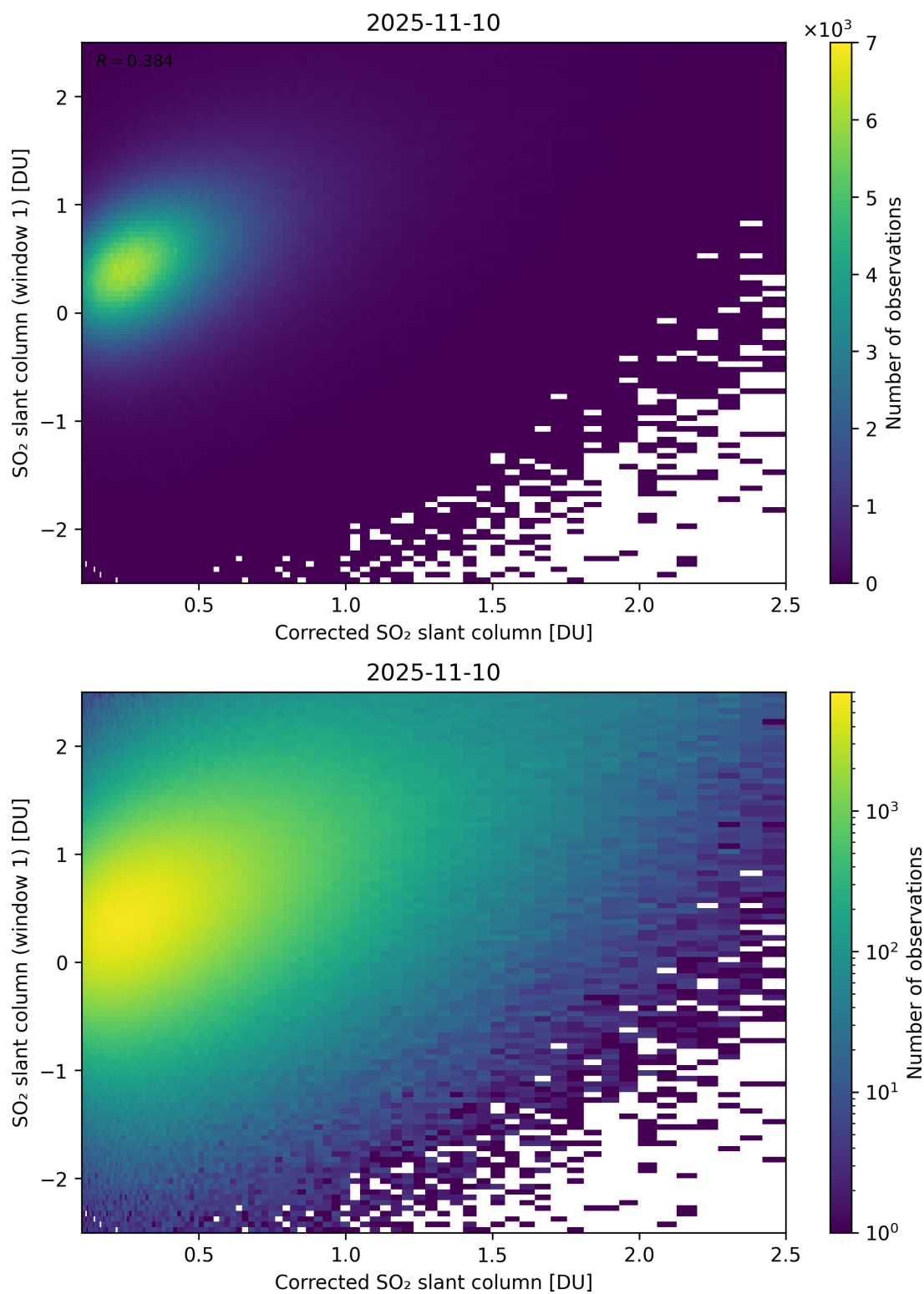
Figure 237: Scatter density plot of “Corrected SO 2 slant column” against “SO 2 slant column (window 1)” for 2025-11-09 to 2025-11-11.
