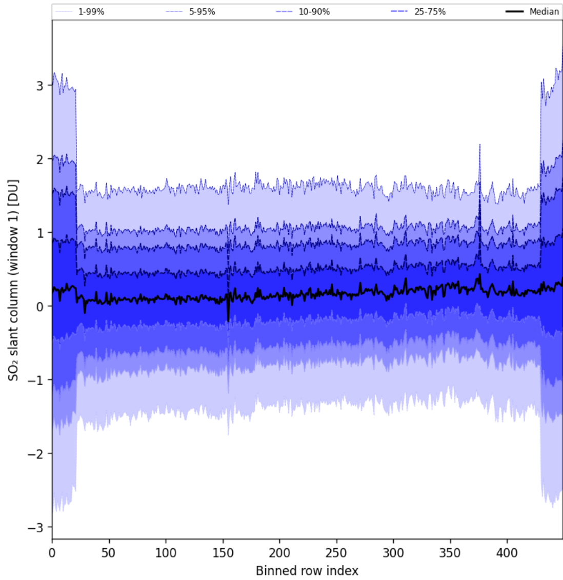
Figure 89: Along track statistics of “SO 2 slant column (window 1)” for 2025-11-09 to 2025-11-11
