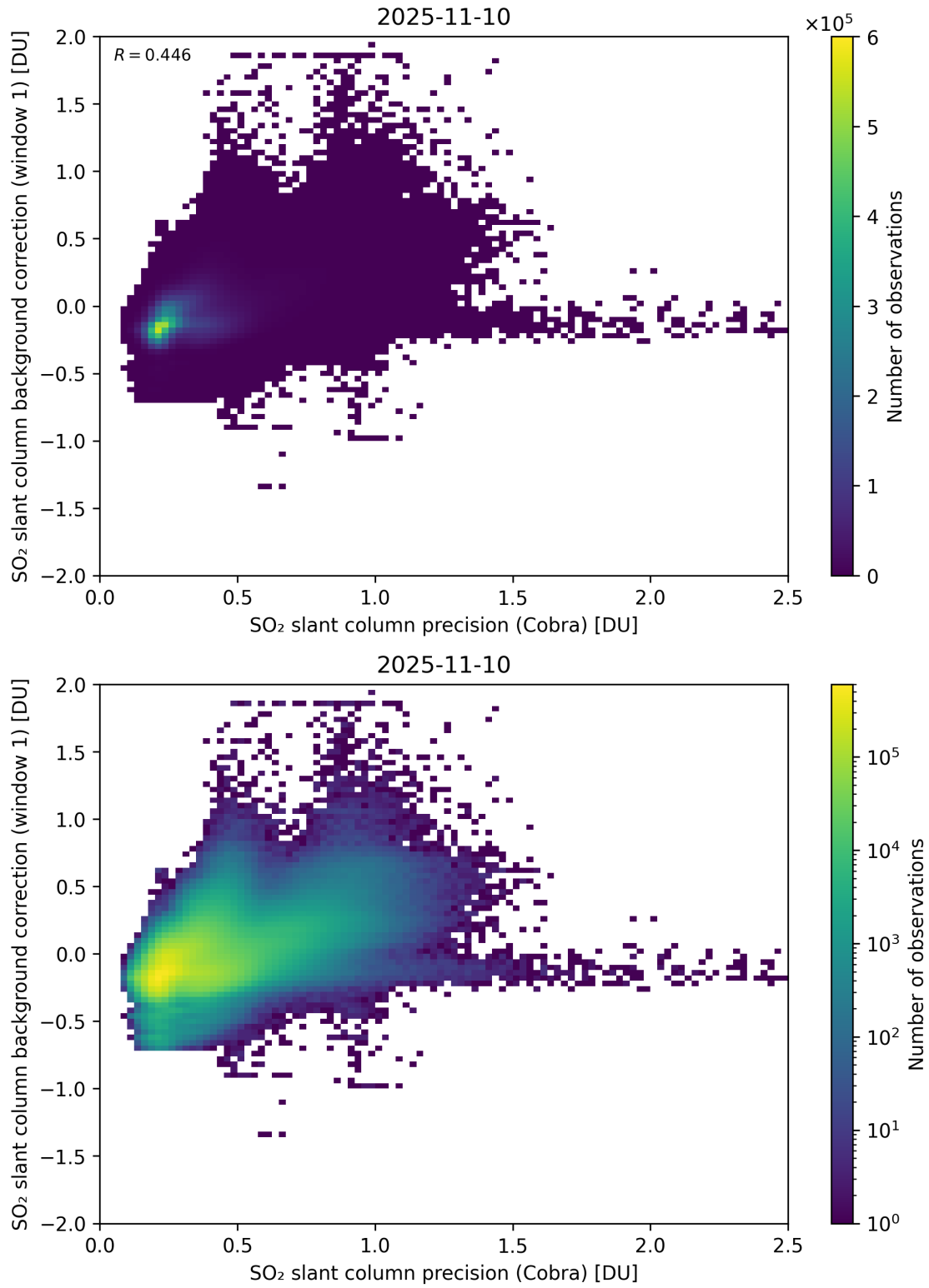
Figure 199: Scatter density plot of “SO 2 slant column precision (Cobra)” against “SO 2 slant column background correction (window 1)” for 2025-11-09 to 2025-11-11.
