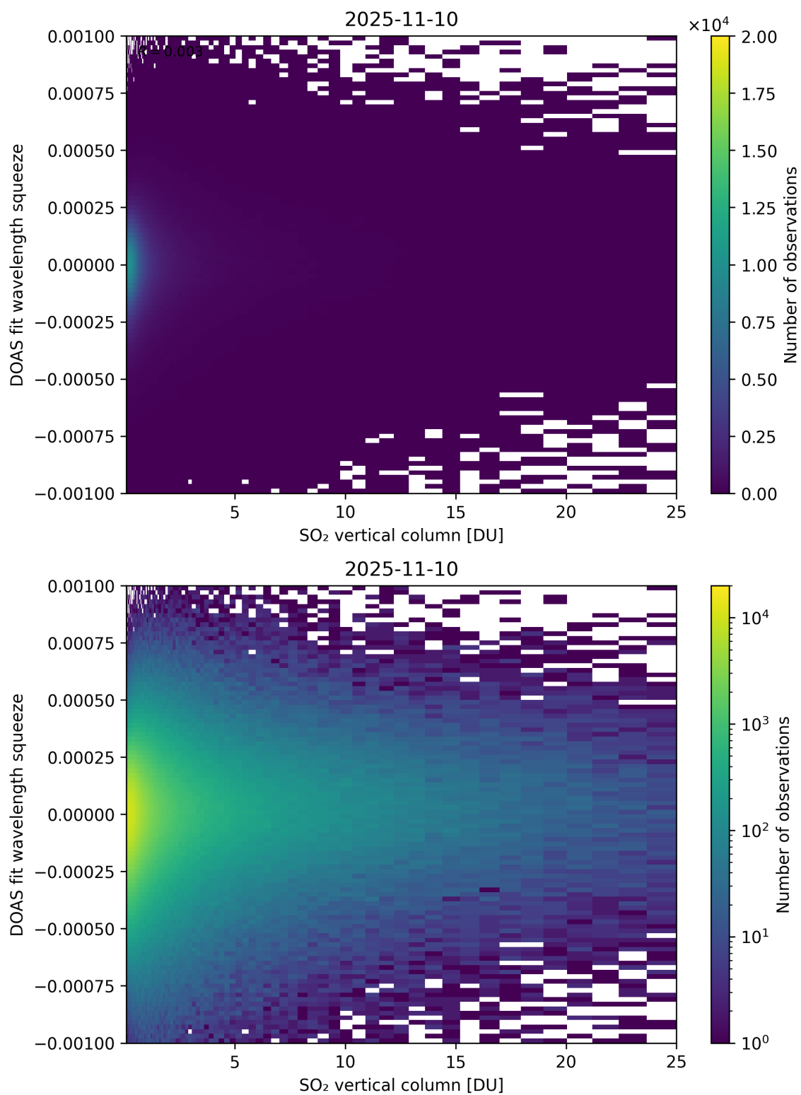
Figure 327: Scatter density plot of “SO 2 vertical column” against “DOAS fit wavelength squeeze” for 2025-11-09 to 2025-11-11.
