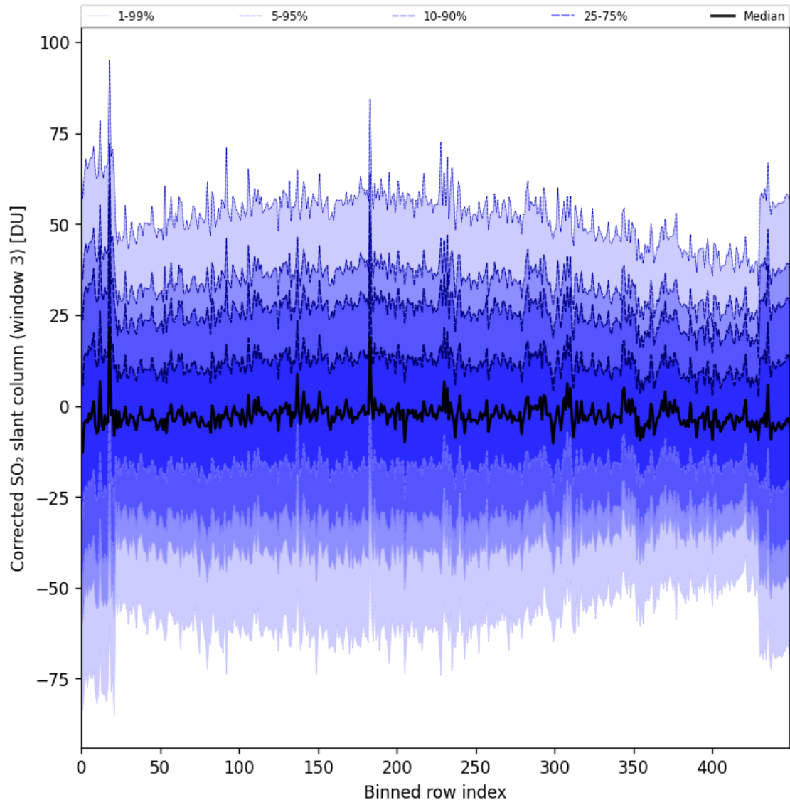
Figure 99: Along track statistics of “Corrected SO 2 slant column (window 3)” for 2025-11-09 to 2025-11-11
