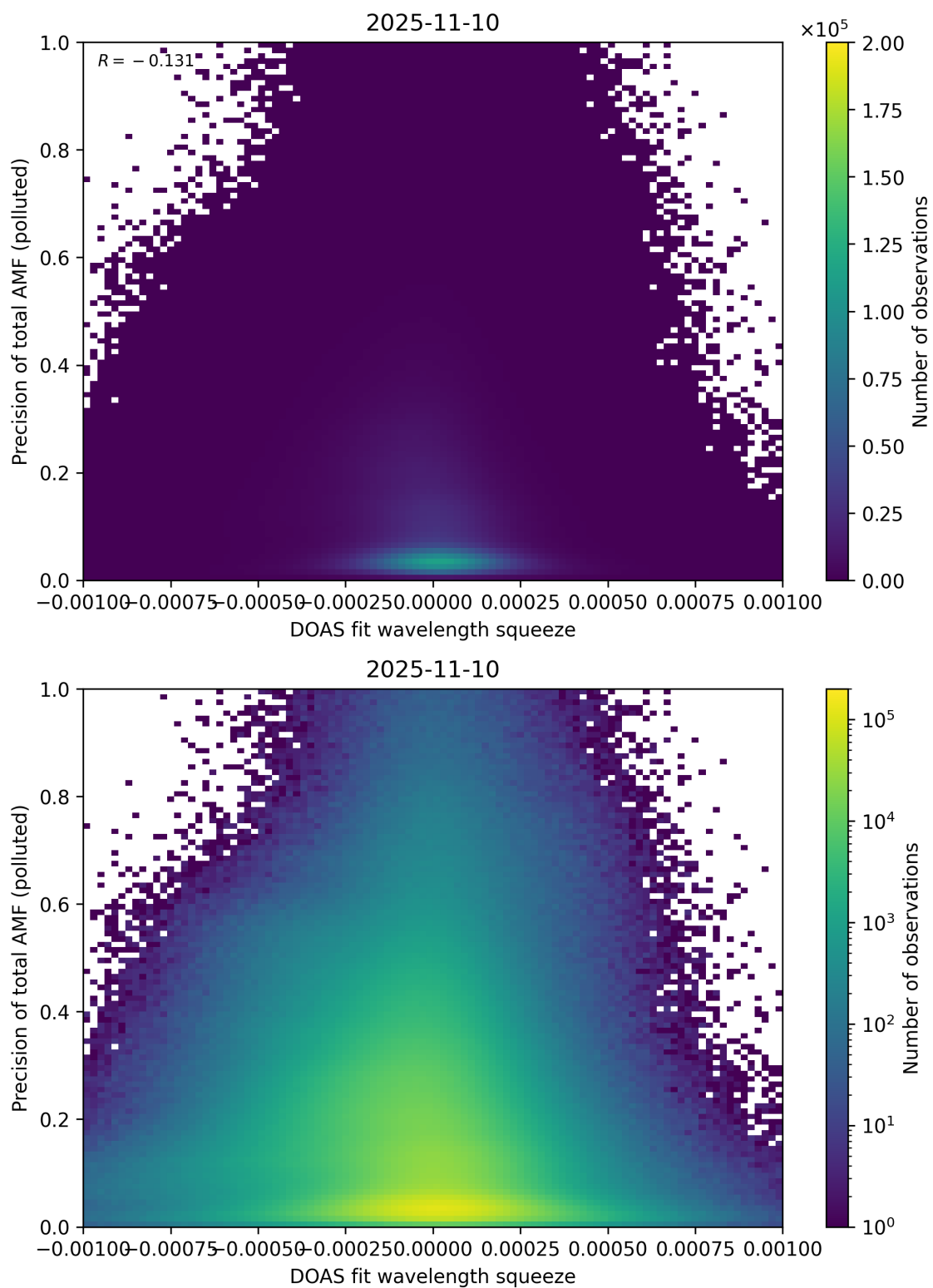
Figure 146: Scatter density plot of “DOAS fit wavelength squeeze” against “Precision of total AMF (polluted)” for 2025-11-09 to 2025-11-11.
