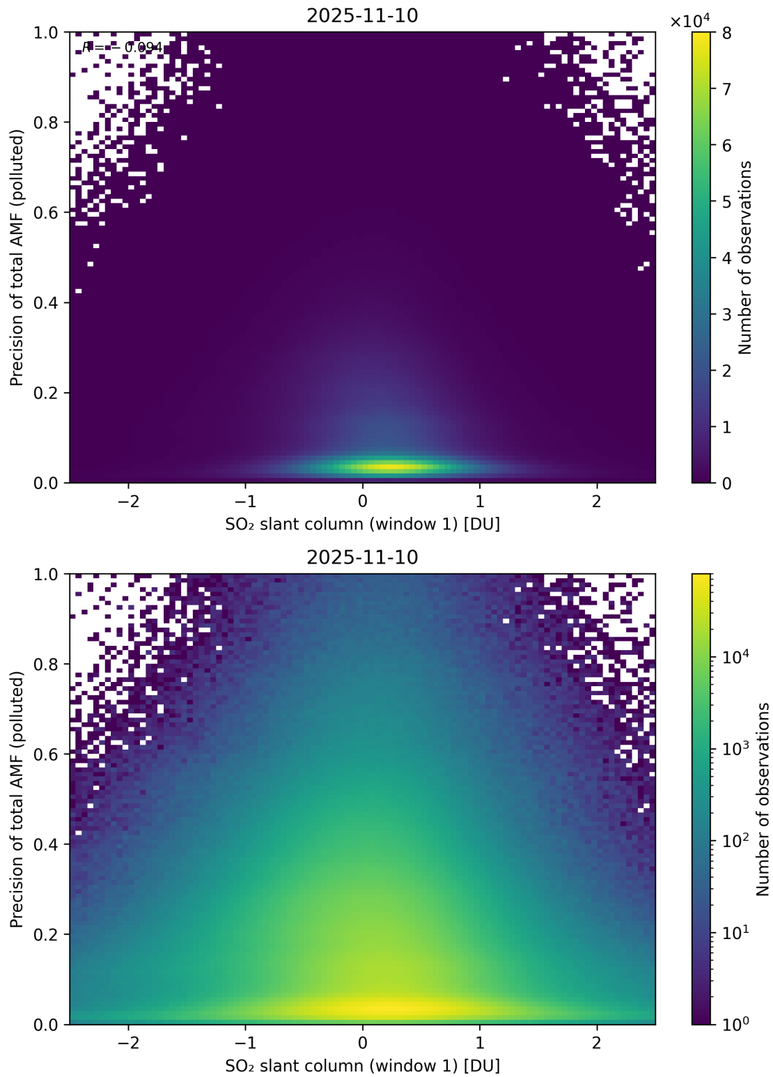
Figure 290: Scatter density plot of “SO 2 slant column (window 1)” against “Precision of total AMF (polluted)” for 2025-11-09 to 2025-11-11.
