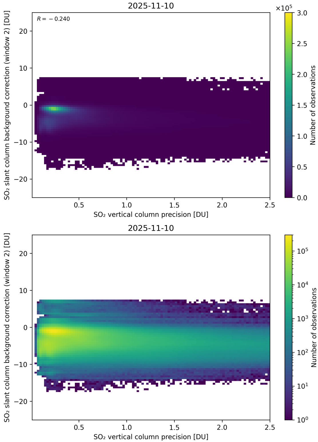
Figure 330: Scatter density plot of “SO 2 vertical column precision” against “SO 2 slant column background correction (window 2)” for 2025-11-09 to 2025-11-11.
