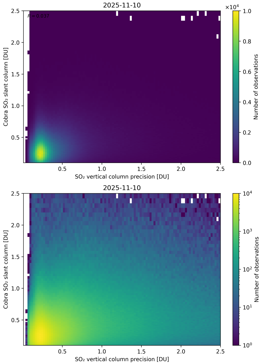
Figure 336: Scatter density plot of “SO 2 vertical column precision” against “Cobra SO 2 slant column” for 2025-11-09 to 2025-11-11.
