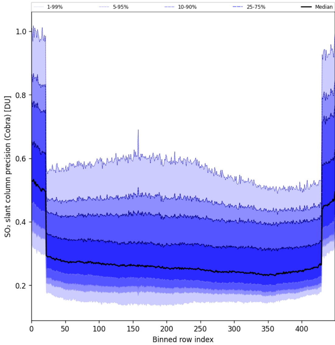
Figure 88: Along track statistics of “SO 2 slant column precision (Cobra)” for 2025-11-09 to 2025-11-11
