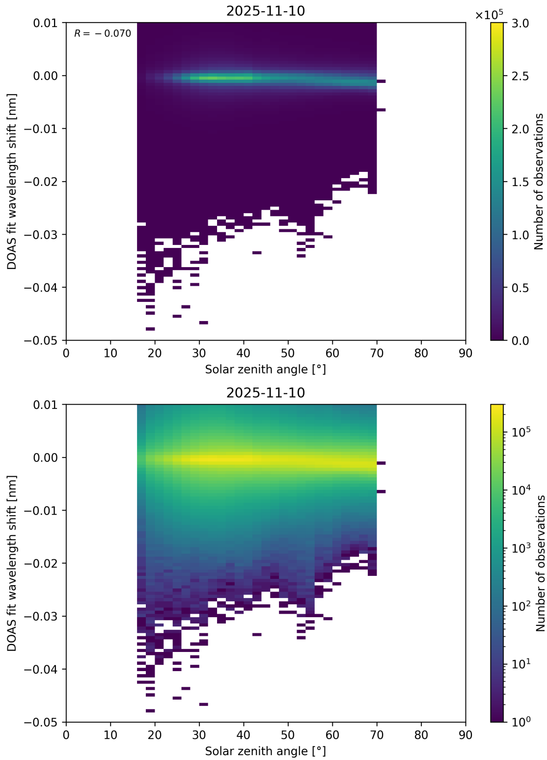
Figure 174: Scatter density plot of “Solar zenith angle” against “DOAS fit wavelength shift” for 2025-11-09 to 2025-11-11.
