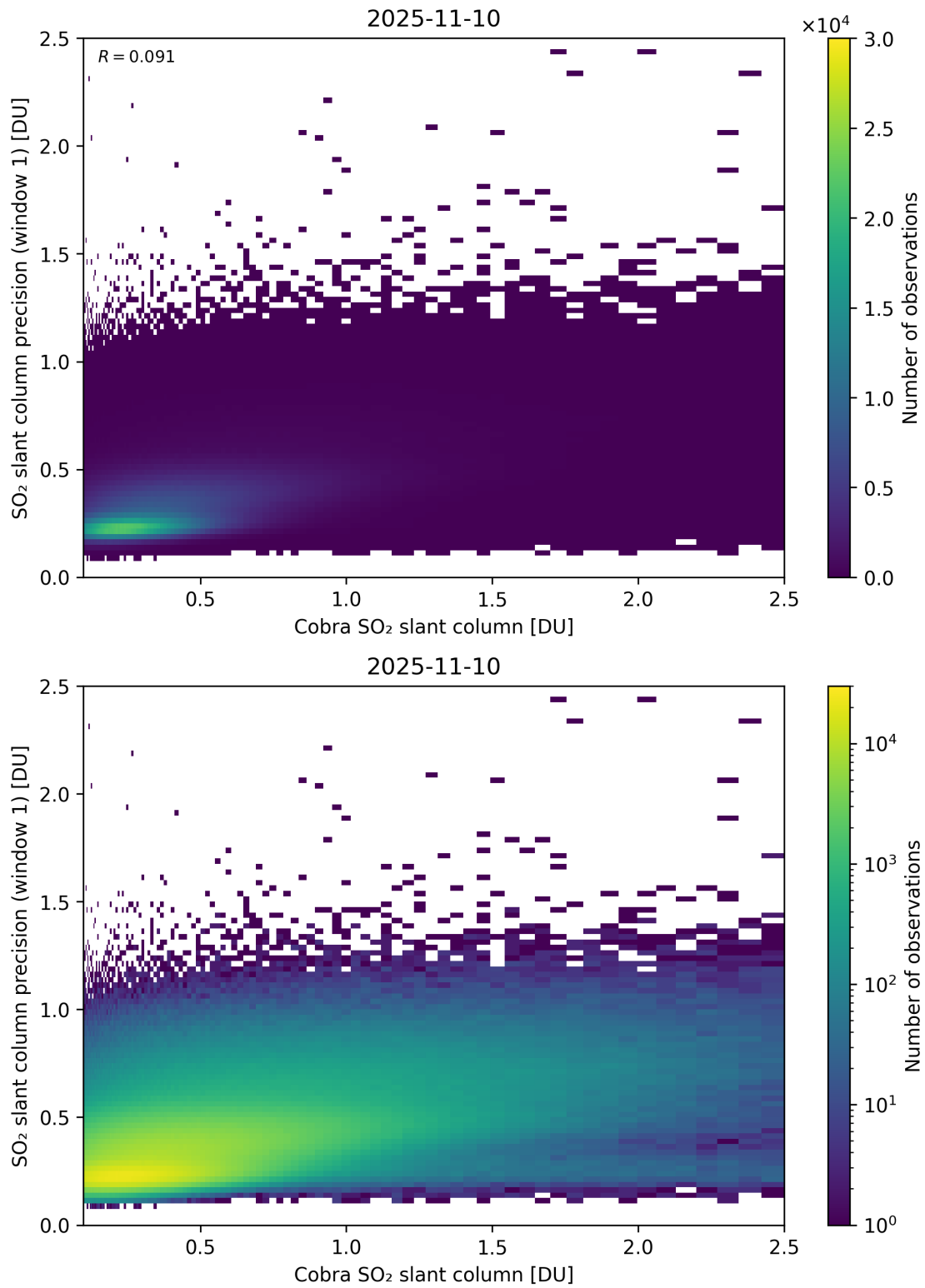
Figure 220: Scatter density plot of “Cobra SO 2 slant column” against “SO 2 slant column precision (window 1)” for 2025-11-09 to 2025-11-11.
