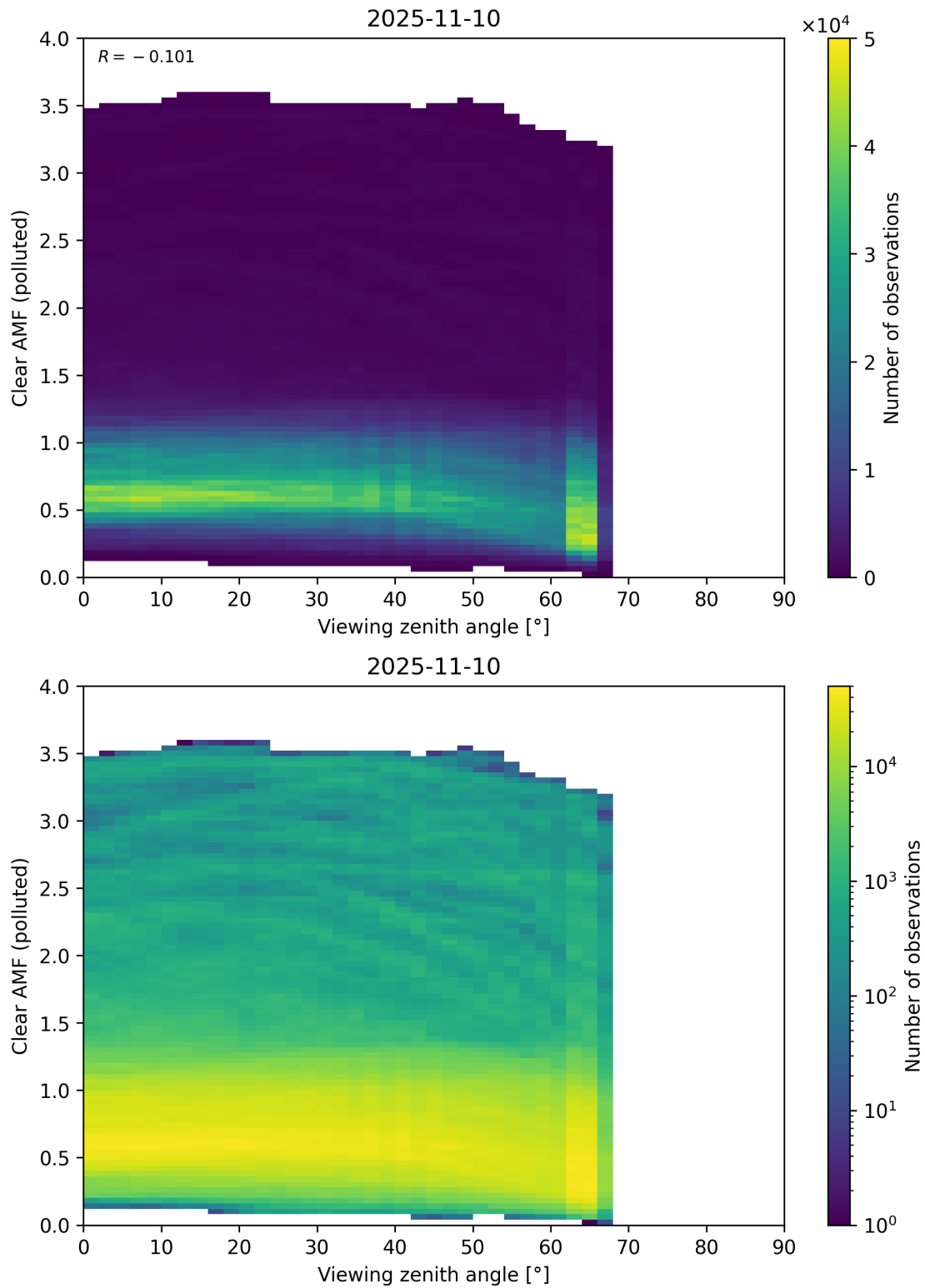
Figure 370: Scatter density plot of “Viewing zenith angle” against “Clear AMF (polluted)” for 2025-11-09 to 2025-11-11.
