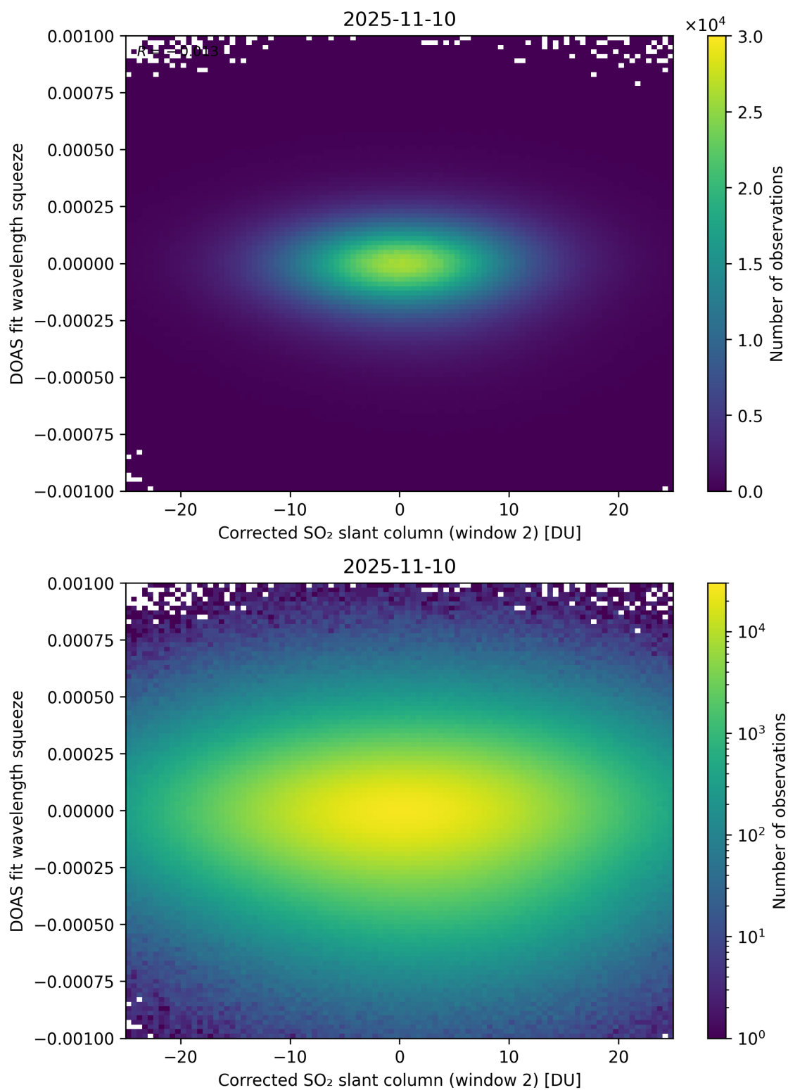
Figure 247: Scatter density plot of “Corrected SO 2 slant column (window 2)” against “DOAS fit wavelength squeeze” for 2025-11-09 to 2025-11-11.
