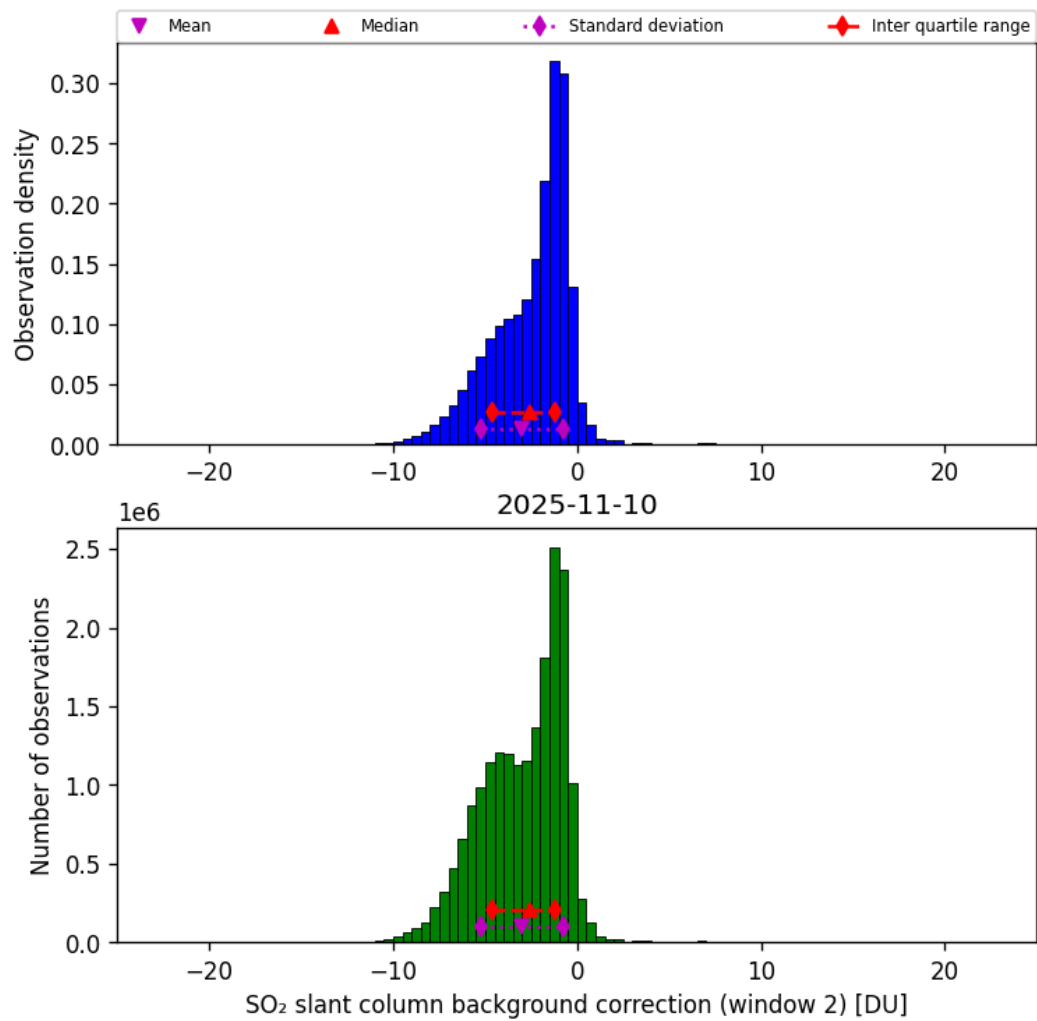
Figure 70: Histogram of “SO 2 slant column background correction (window 2)” for 2025-11-09 to 2025-11-11
