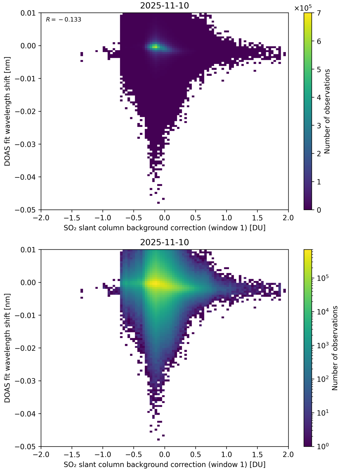
Figure 111: Scatter density plot of “SO 2 slant column background correction (window 1)” against “DOAS fit wavelength shift” for 2025-11-09 to 2025-11-11.
