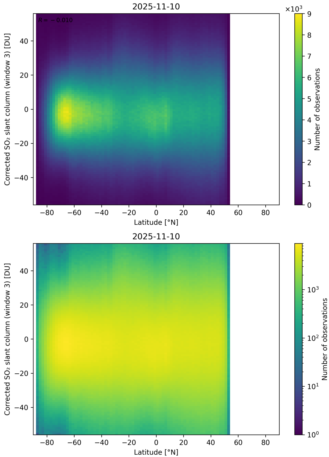
Figure 161: Scatter density plot of “Latitude” against “Corrected SO 2 slant column (window 3)” for 2025-11-09 to 2025-11-11.
