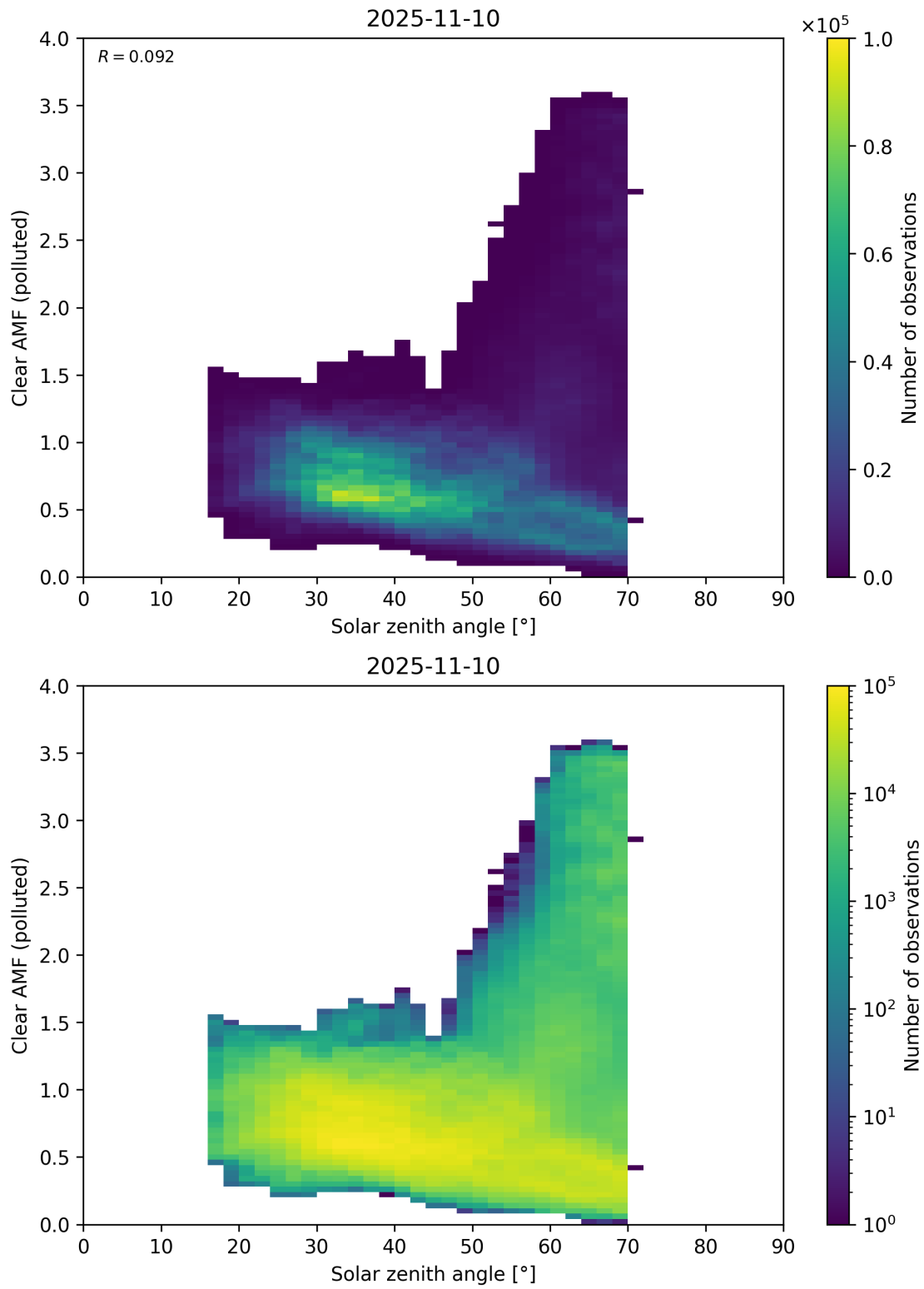
Figure 178: Scatter density plot of “Solar zenith angle” against “Clear AMF (polluted)” for 2025-11-09 to 2025-11-11.
