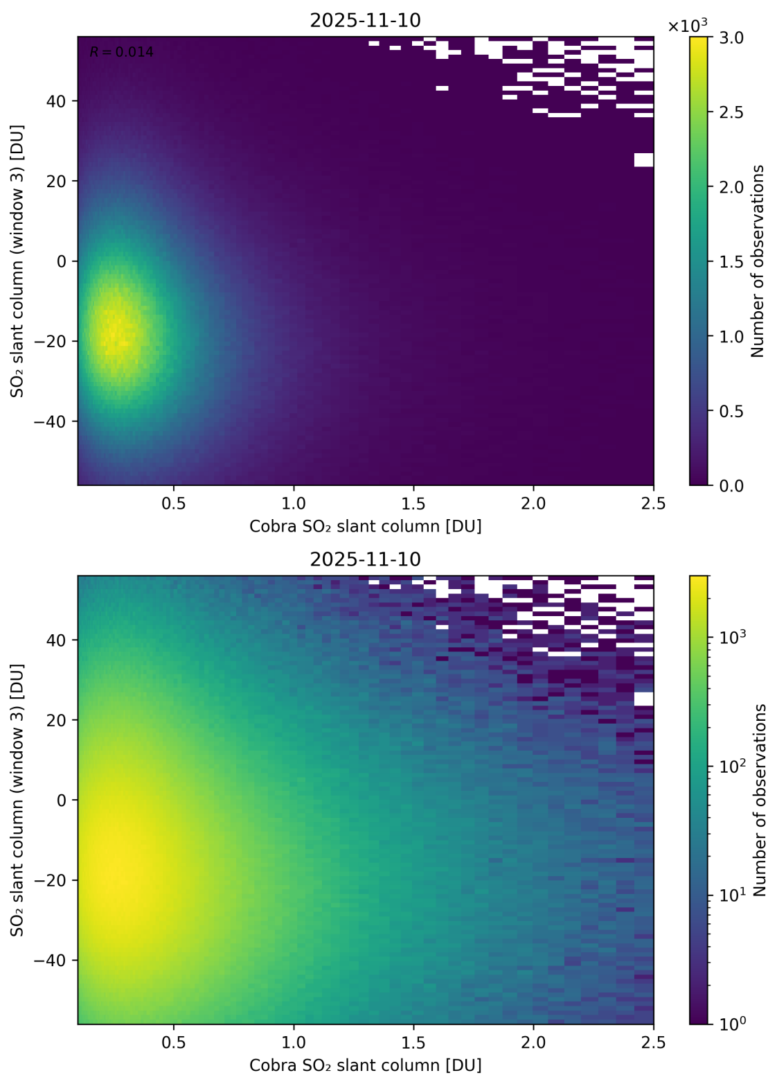
Figure 222: Scatter density plot of “Cobra SO 2 slant column” against “SO 2 slant column (window 3)” for 2025-11-09 to 2025-11-11.
