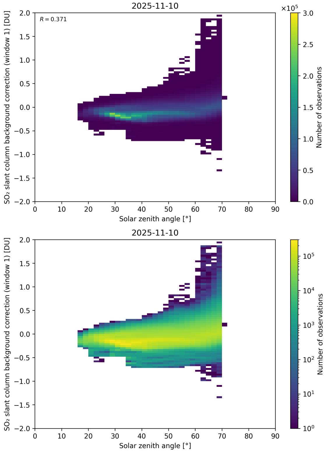
Figure 171: Scatter density plot of “Solar zenith angle” against “SO 2 slant column background correction (window 1)” for 2025-11-09 to 2025-11-11.
