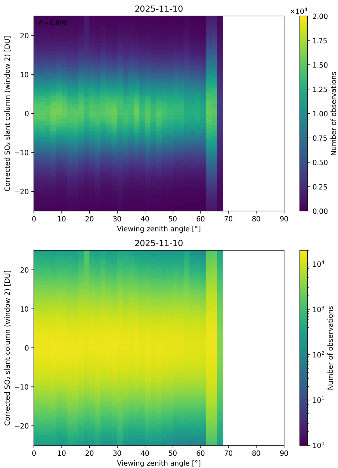
Figure 374: Scatter density plot of “Viewing zenith angle” against “Corrected SO 2 slant column (window 2)” for 2025-11-09 to 2025-11-11.
