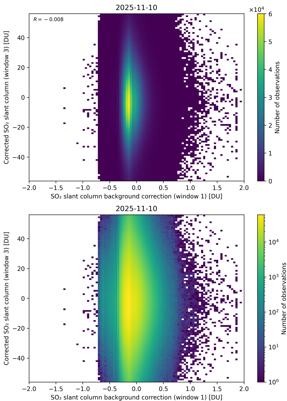
Figure 116: Scatter density plot of “SO 2 slant column background correction (window 1)” against “Corrected SO 2 slant column (window 3)” for 2025-11-09 to 2025-11-11.
