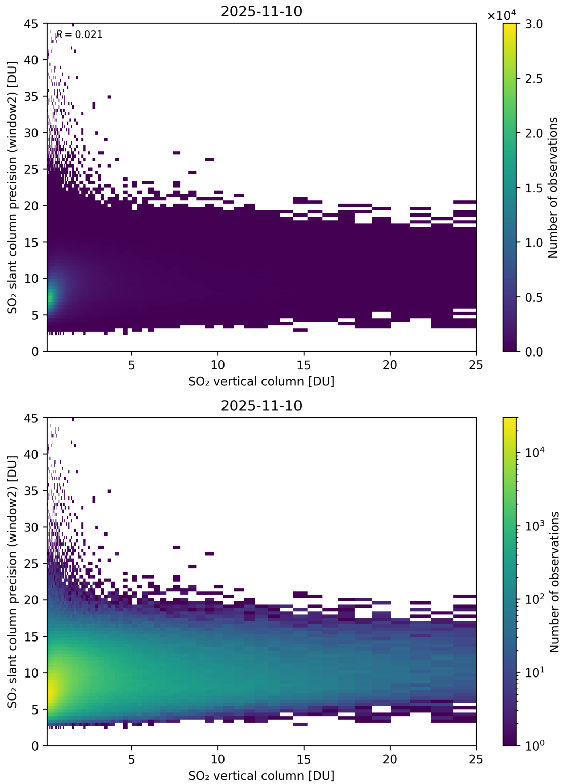
Figure 356: Scatter density plot of “SO 2 vertical column” against “SO 2 slant column precision (window2)” for 2025-11-09 to 2025-11-11.
