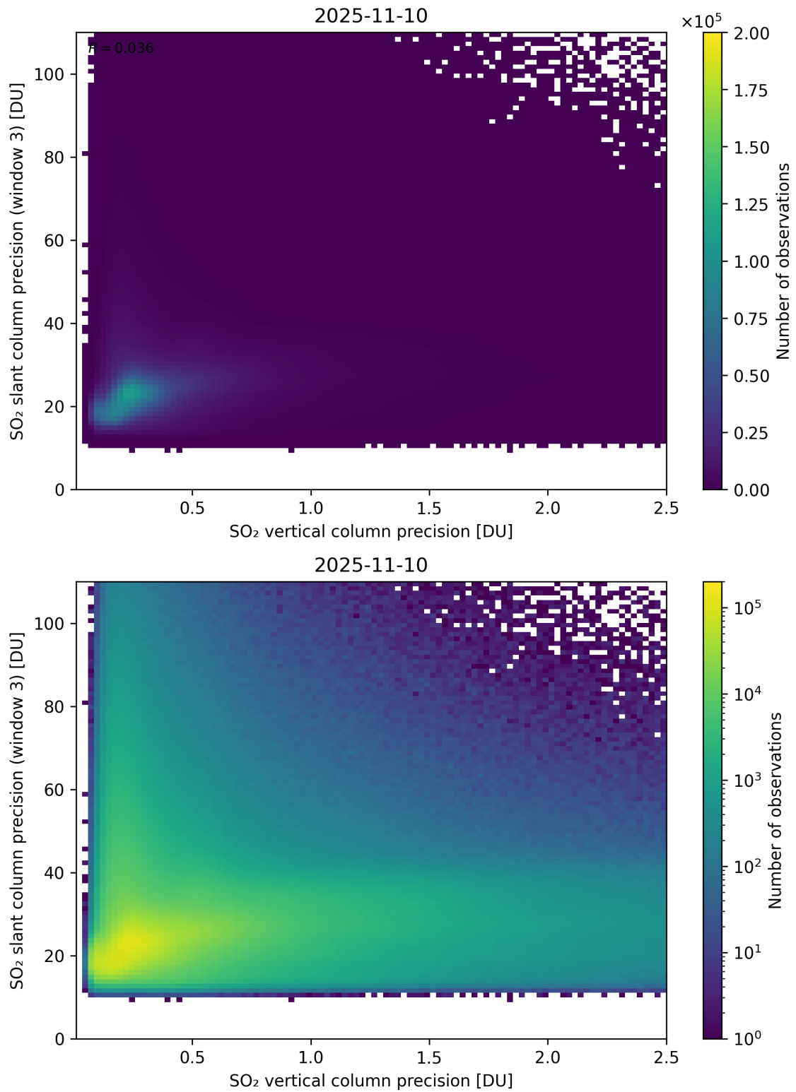
Figure 345: Scatter density plot of “SO 2 vertical column precision” against “SO 2 slant column precision (window 3)” for 2025-11-09 to 2025-11-11.
