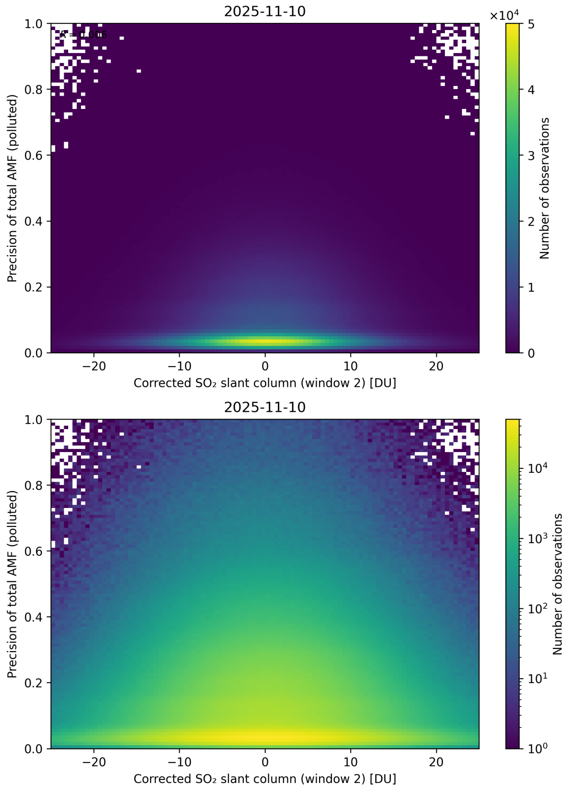
Figure 254: Scatter density plot of “Corrected SO 2 slant column (window 2)” against “Precision of total AMF (polluted)” for 2025-11-09 to 2025-11-11.
