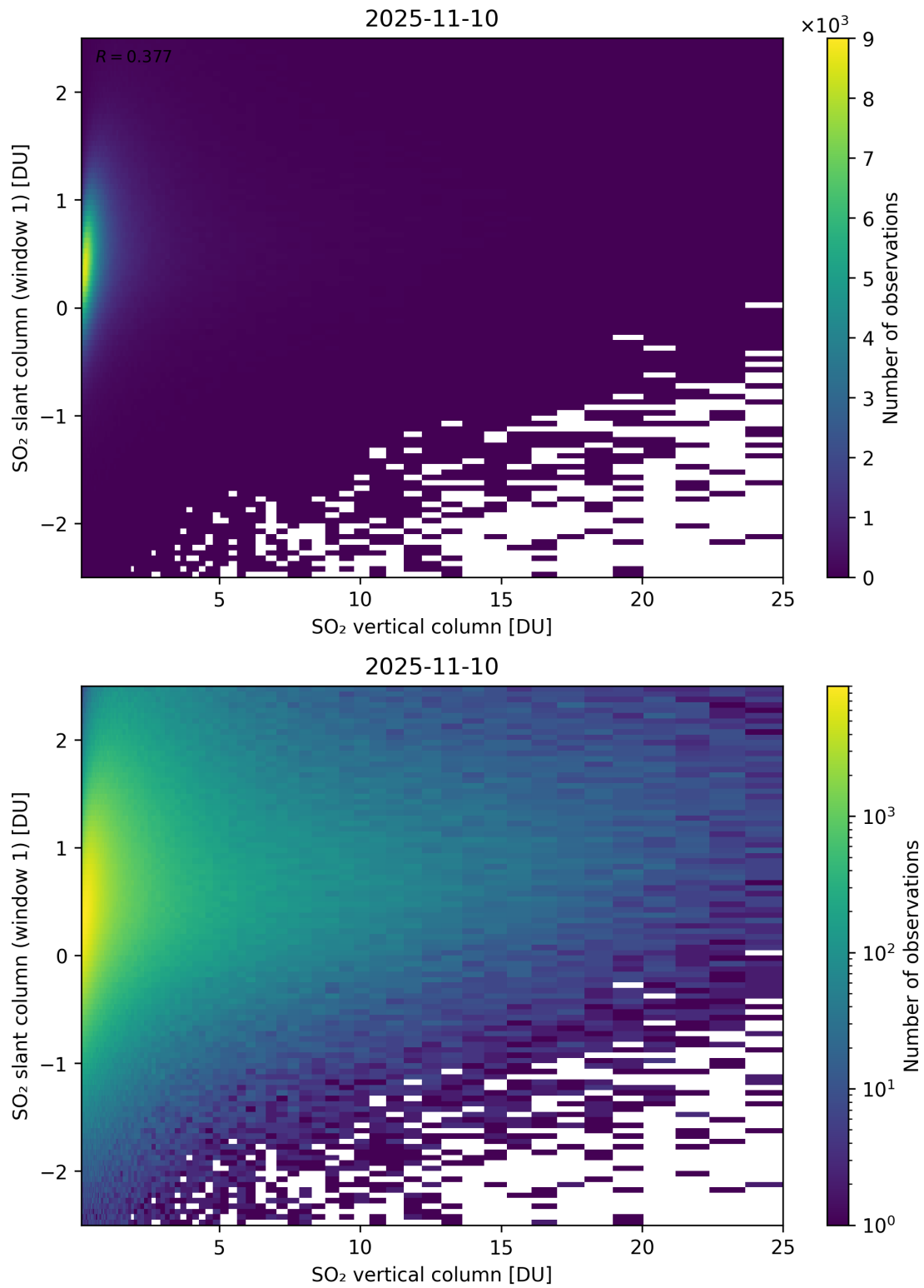
Figure 354: Scatter density plot of “SO 2 vertical column” against “SO 2 slant column (window 1)” for 2025-11-09 to 2025-11-11.
