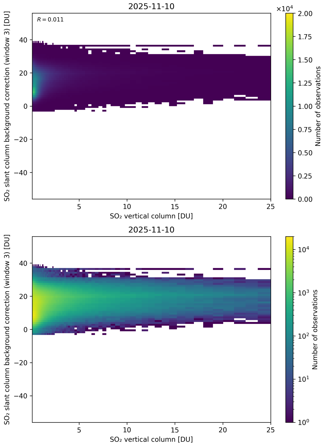
Figure 325: Scatter density plot of “SO 2 vertical column” against “SO 2 slant column background correction (window 3)” for 2025-11-09 to 2025-11-11.
