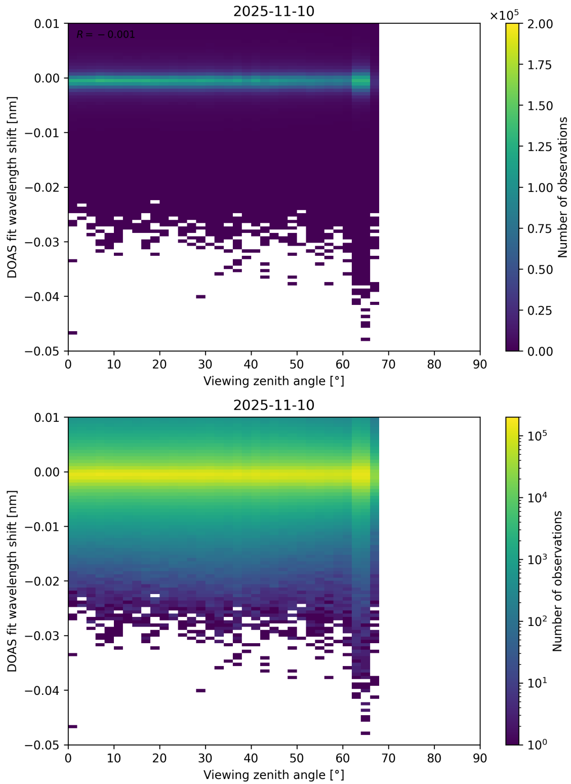
Figure 365: Scatter density plot of “Viewing zenith angle” against “DOAS fit wavelength shift” for 2025-11-09 to 2025-11-11.
