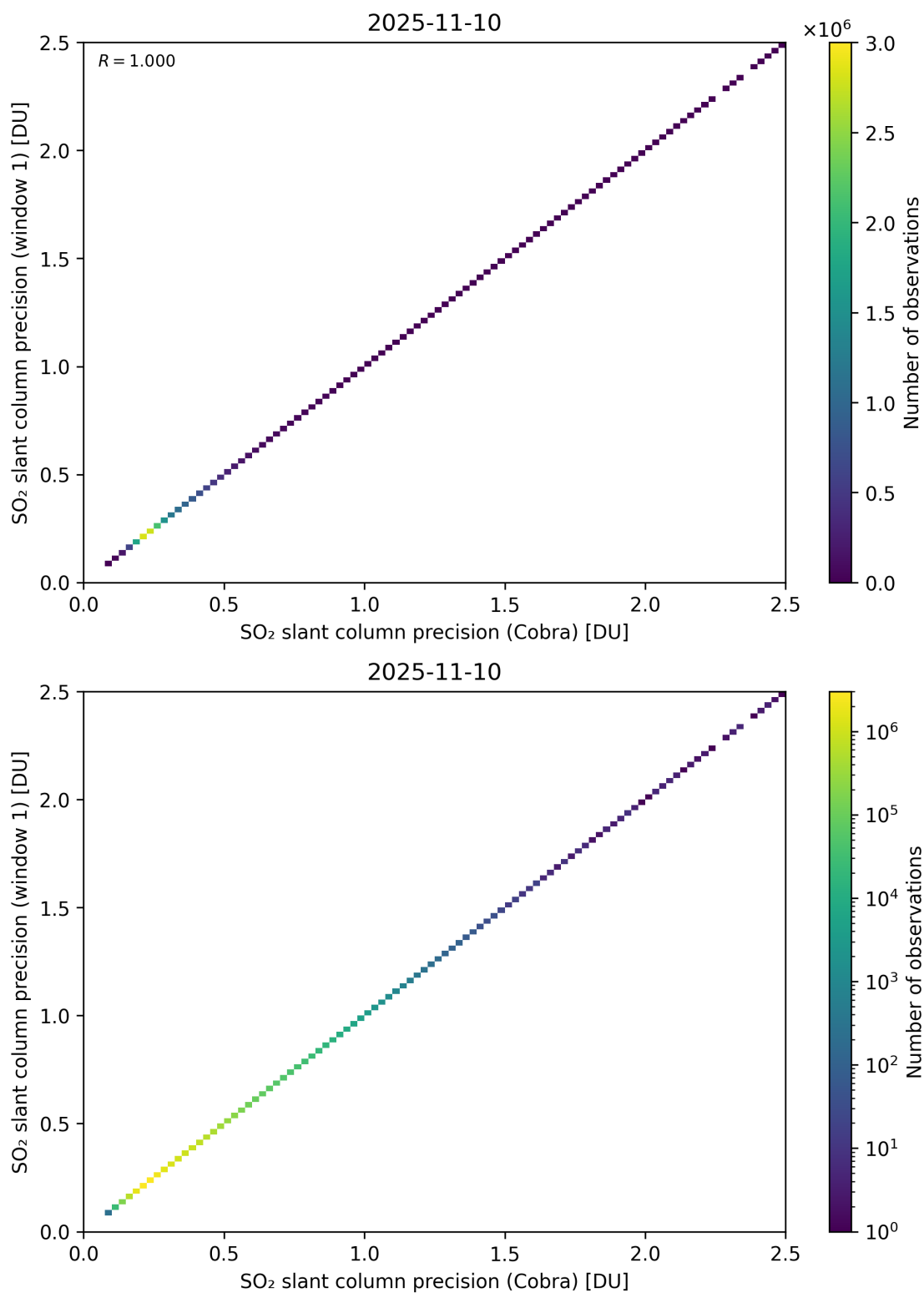
Figure 209: Scatter density plot of “SO 2 slant column precision (Cobra)” against “SO 2 slant column precision (window 1)” for 2025-11-09 to 2025-11-11.
