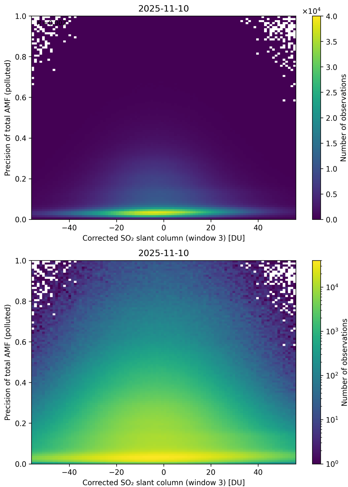
Figure 261: Scatter density plot of “Corrected SO 2 slant column (window 3)” against “Precision of total AMF (polluted)” for 2025-11-09 to 2025-11-11.
