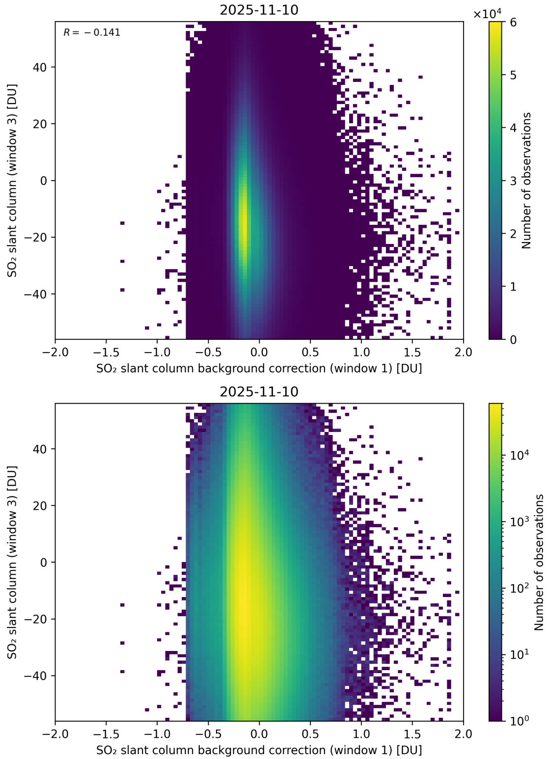
Figure 118: Scatter density plot of “SO 2 slant column background correction (window 1)” against “SO 2 slant column (window 3)” for 2025-11-09 to 2025-11-11.
