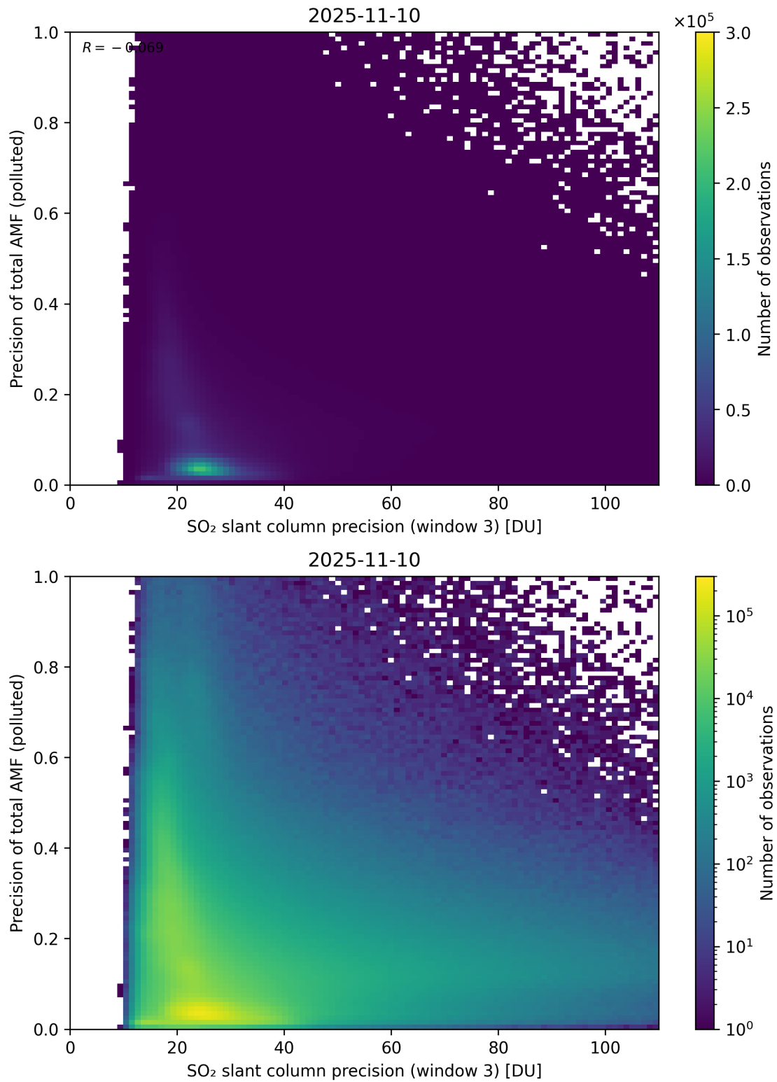
Figure 314: Scatter density plot of “SO 2 slant column precision (window 3)” against “Precision of total AMF (polluted)” for 2025-11-09 to 2025-11-11.
