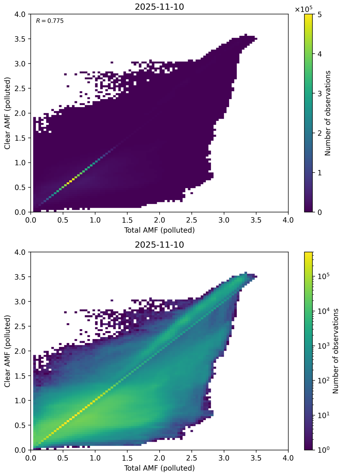
Figure 321: Scatter density plot of “Total AMF (polluted)” against “Clear AMF (polluted)” for 2025-11-09 to 2025-11-11.
