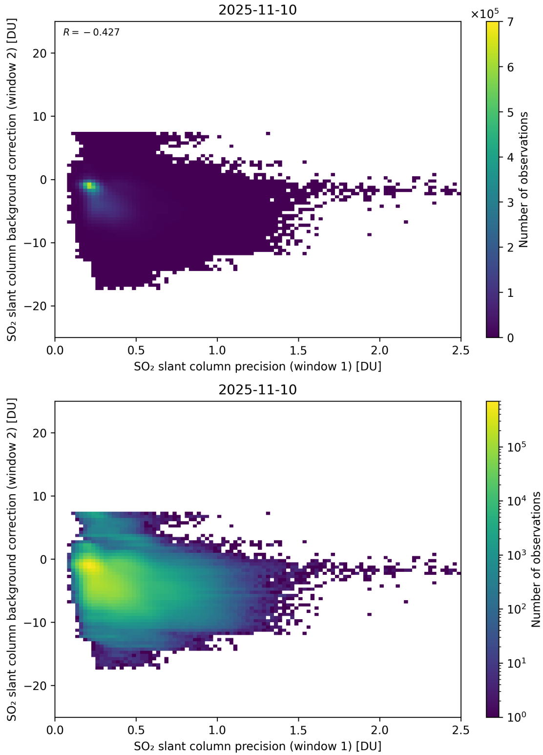
Figure 269: Scatter density plot of “SO 2 slant column precision (window 1)” against “SO 2 slant column background correction (window 2)” for 2025-11-09 to 2025-11-11.
