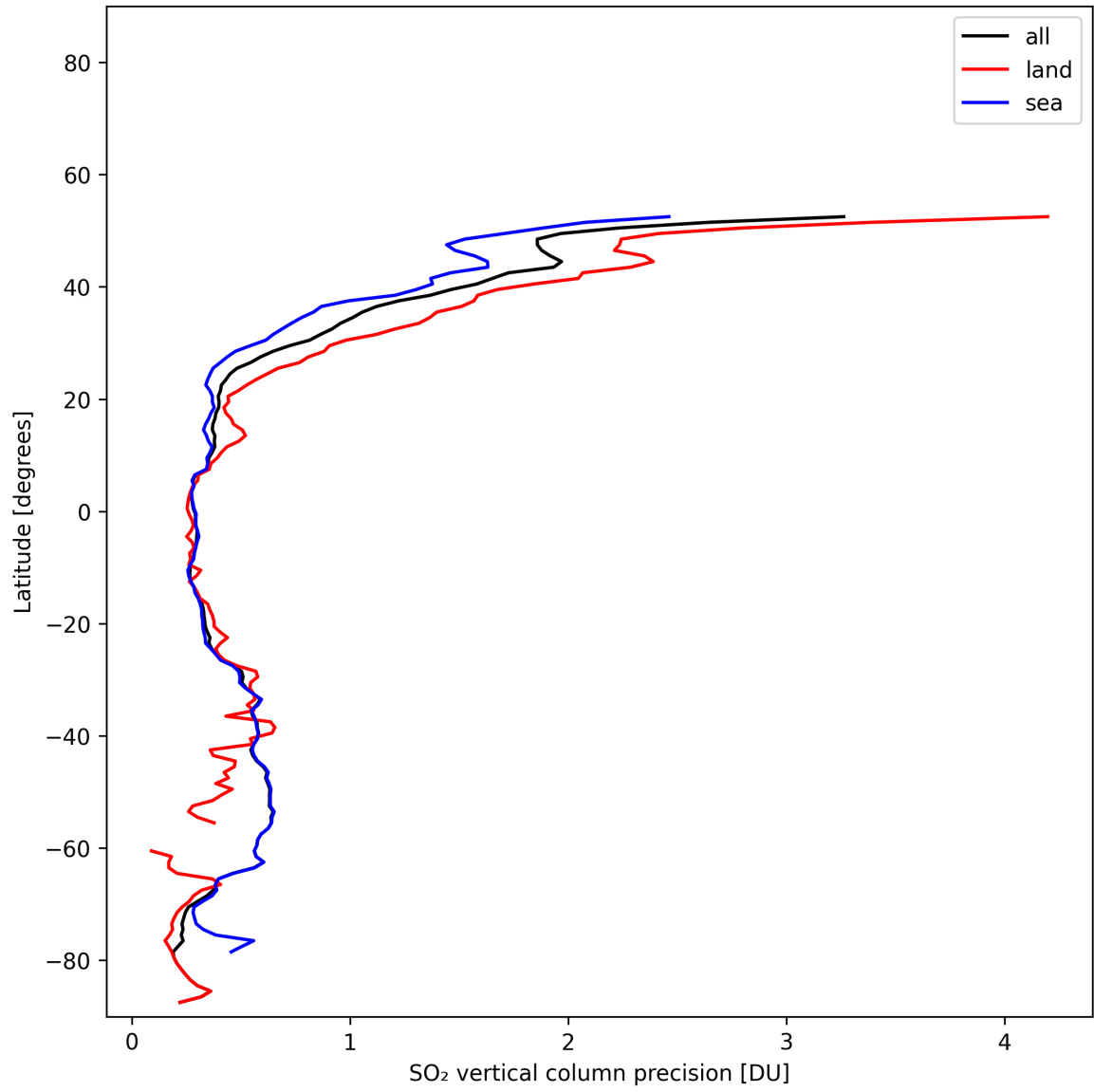
Figure 33: Zonal average of “SO 2 vertical column precision” for 2025-11-09 to 2025-11-11.
