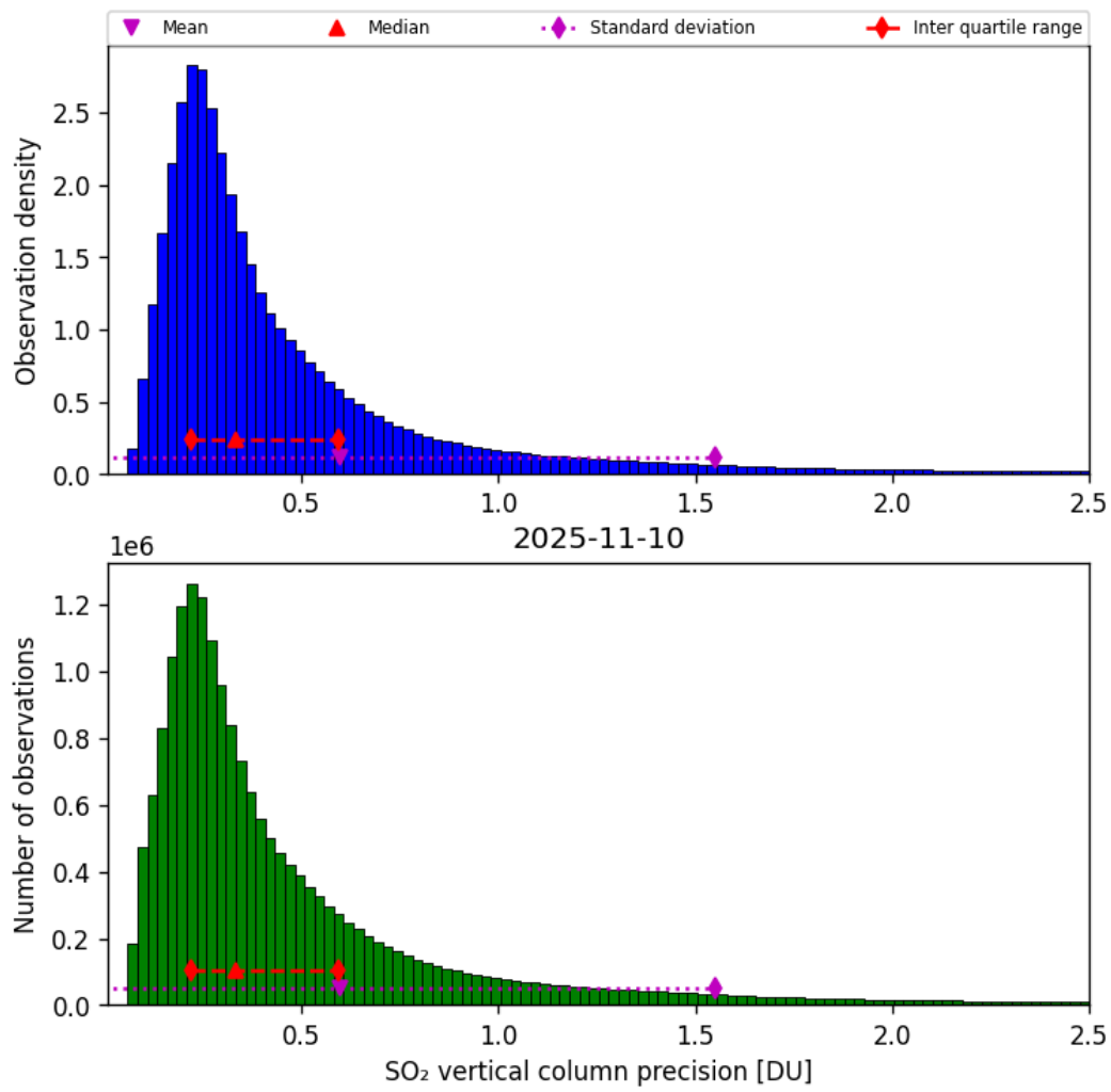
Figure 59: Histogram of “SO 2 vertical column precision” for 2025-11-09 to 2025-11-11
