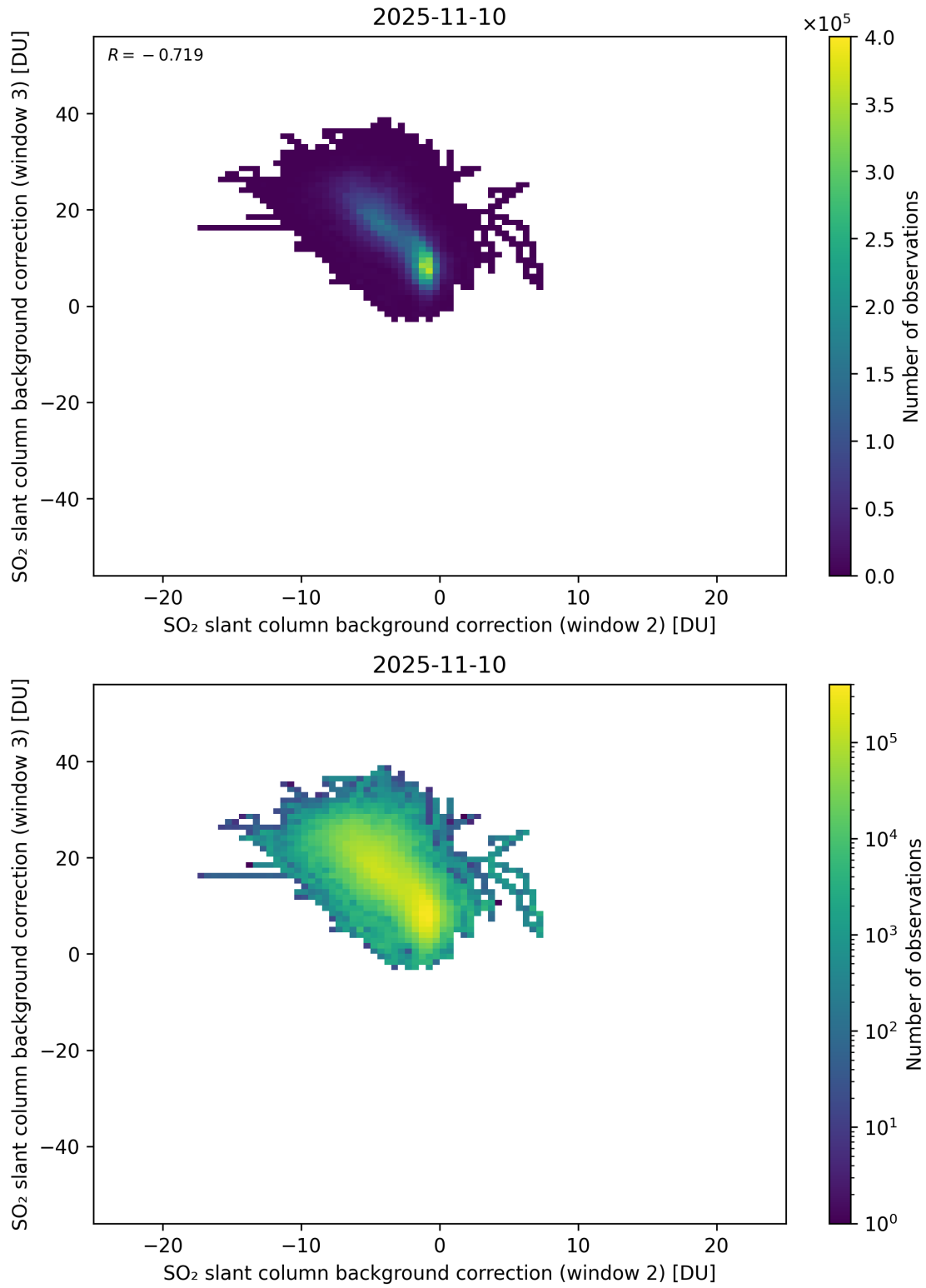
Figure 122: Scatter density plot of “SO 2 slant column background correction (window 2)” against “SO 2 slant column background correction (window 3)” for 2025-11-09 to 2025-11-11.
