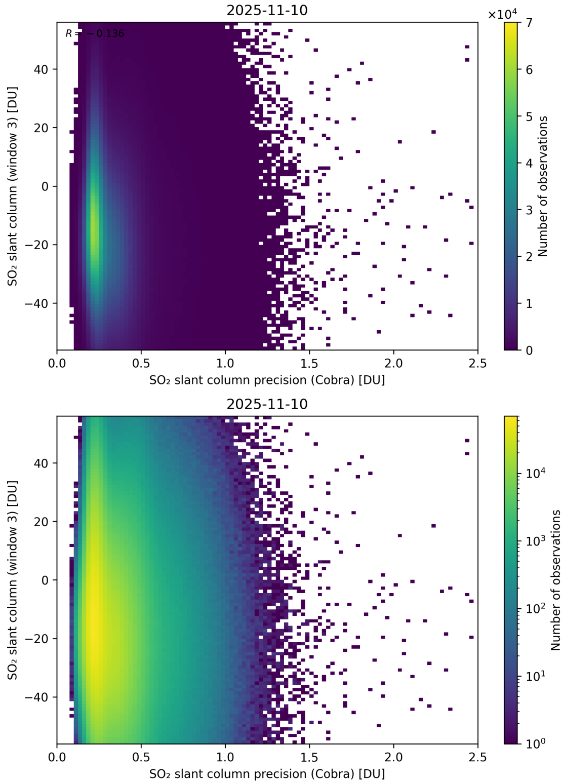
Figure 211: Scatter density plot of “SO 2 slant column precision (Cobra)” against “SO 2 slant column (window 3)” for 2025-11-09 to 2025-11-11.
