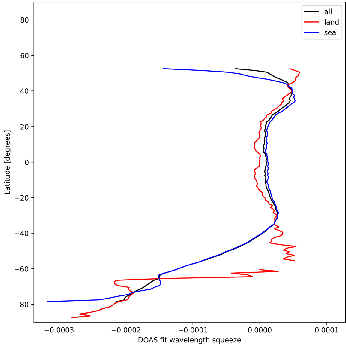
Figure 51: Zonal average of “DOAS fit wavelength squeeze” for 2025-11-09 to 2025-11-11.
