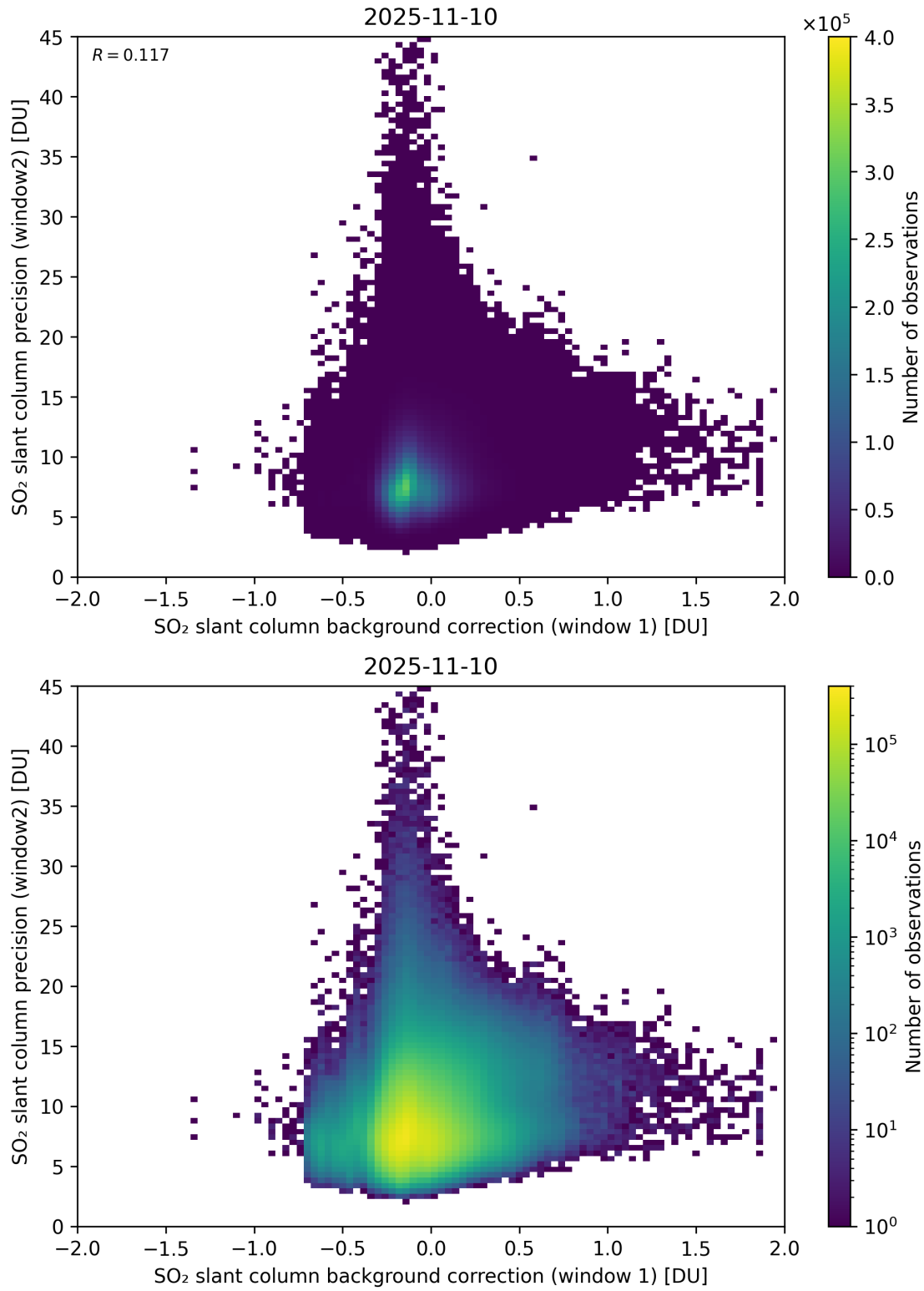
Figure 117: Scatter density plot of “SO 2 slant column background correction (window 1)” against “SO 2 slant column precision (window2)” for 2025-11-09 to 2025-11-11.
