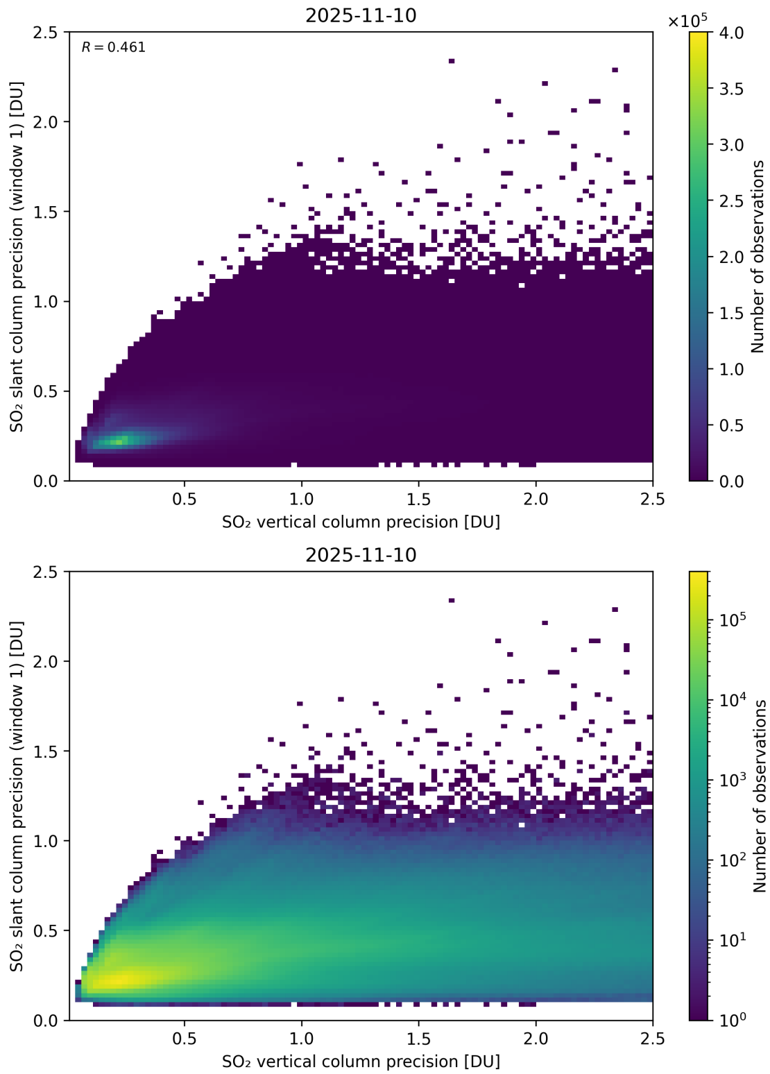
Figure 342: Scatter density plot of “SO 2 vertical column precision” against “SO 2 slant column precision (window 1)” for 2025-11-09 to 2025-11-11.
