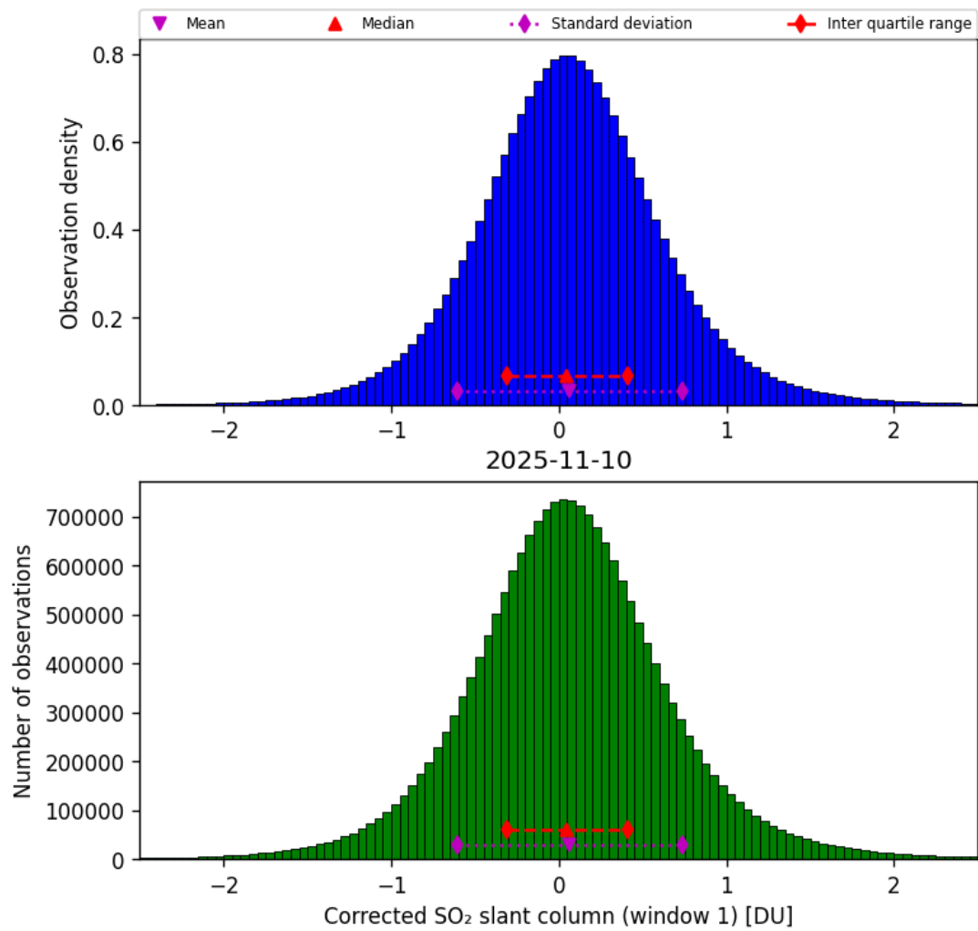
Figure 65: Histogram of “Corrected SO 2 slant column (window 1)” for 2025-11-09 to 2025-11-11
