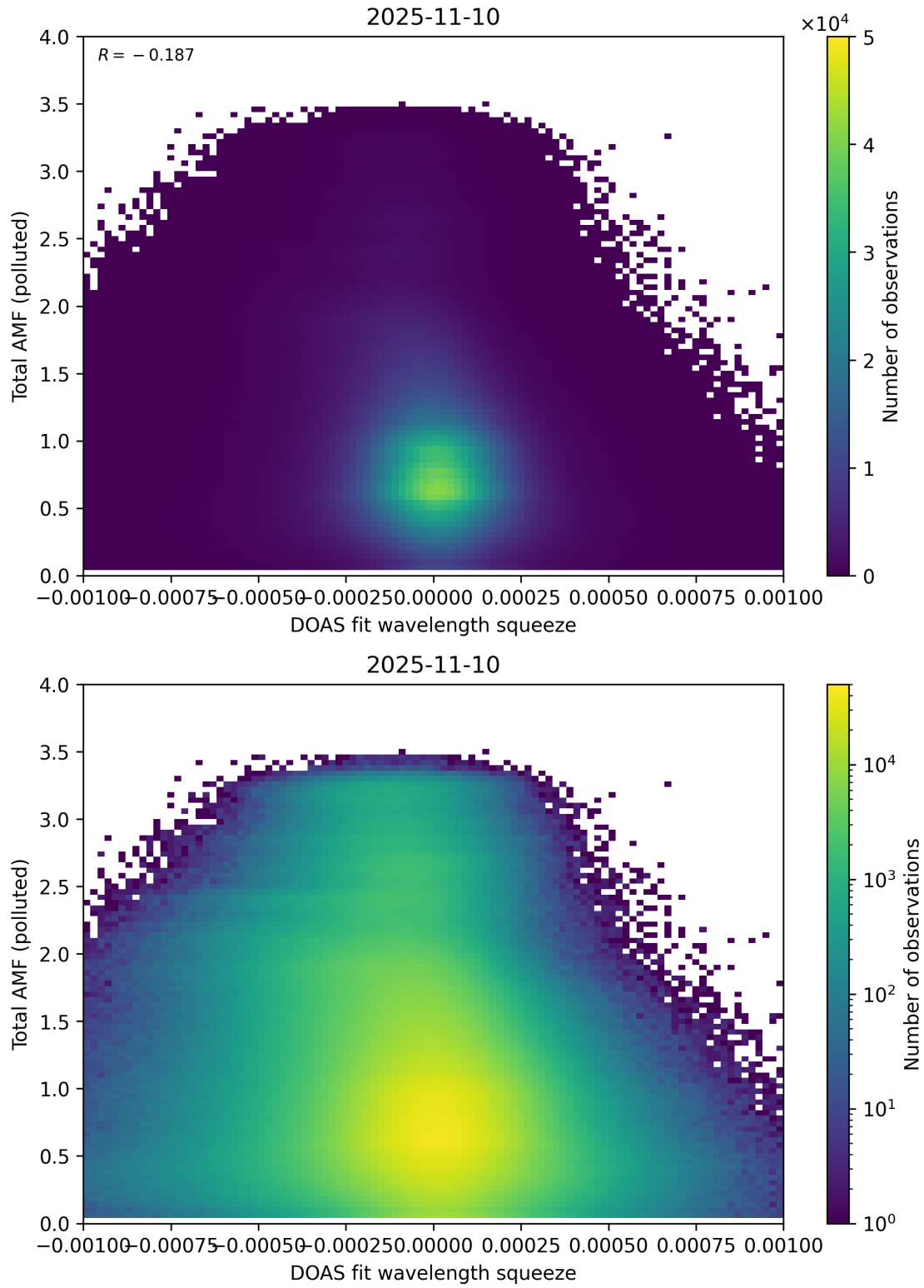
Figure 145: Scatter density plot of “DOAS fit wavelength squeeze” against “Total AMF (polluted)” for 2025-11-09 to 2025-11-11.
