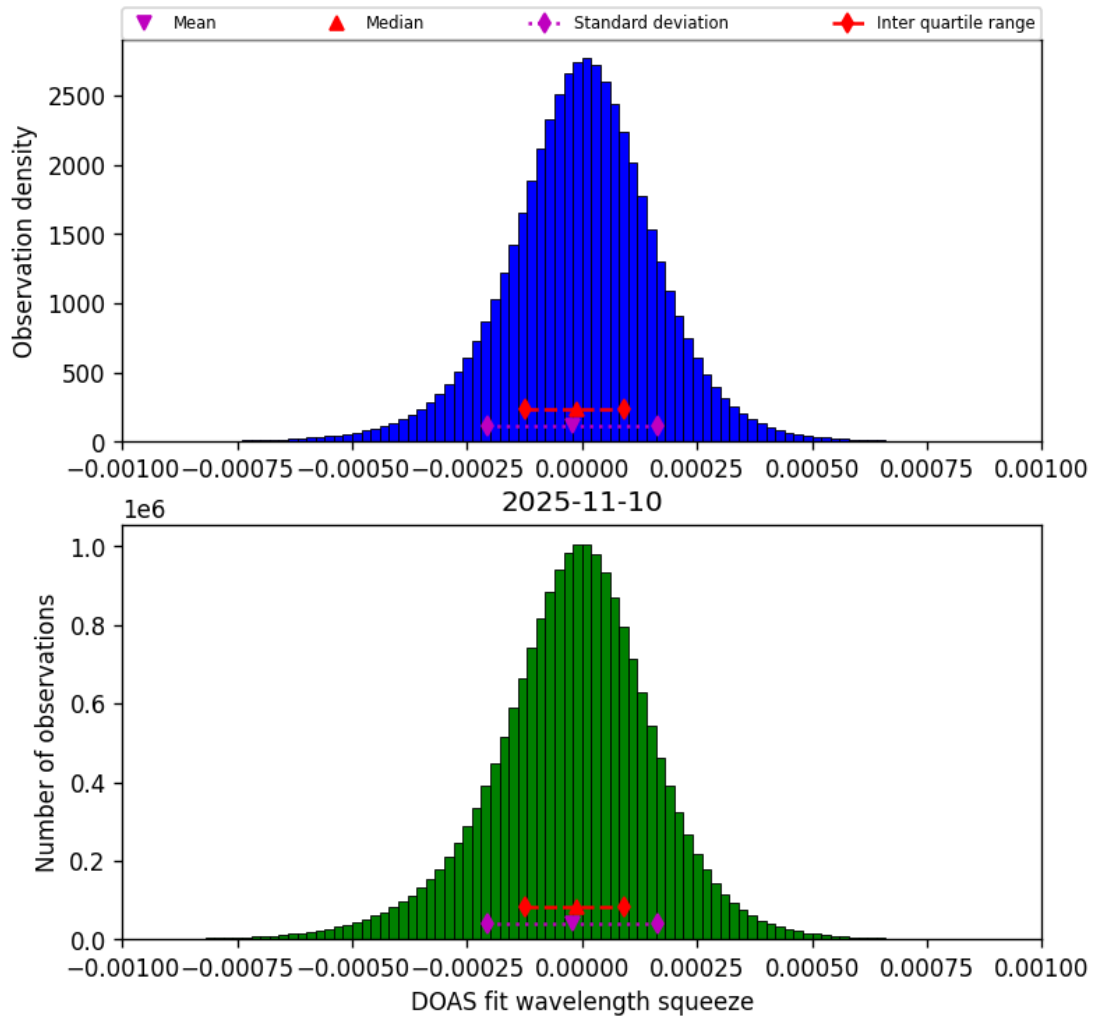
Figure 77: Histogram of “DOAS fit wavelength squeeze” for 2025-11-09 to 2025-11-11
