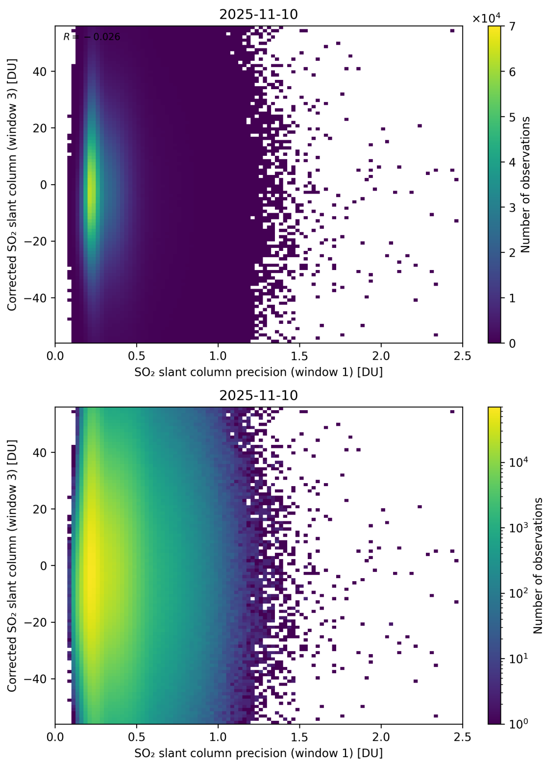
Figure 276: Scatter density plot of “SO 2 slant column precision (window 1)” against “Corrected SO 2 slant column (window 3)” for 2025-11-09 to 2025-11-11.
