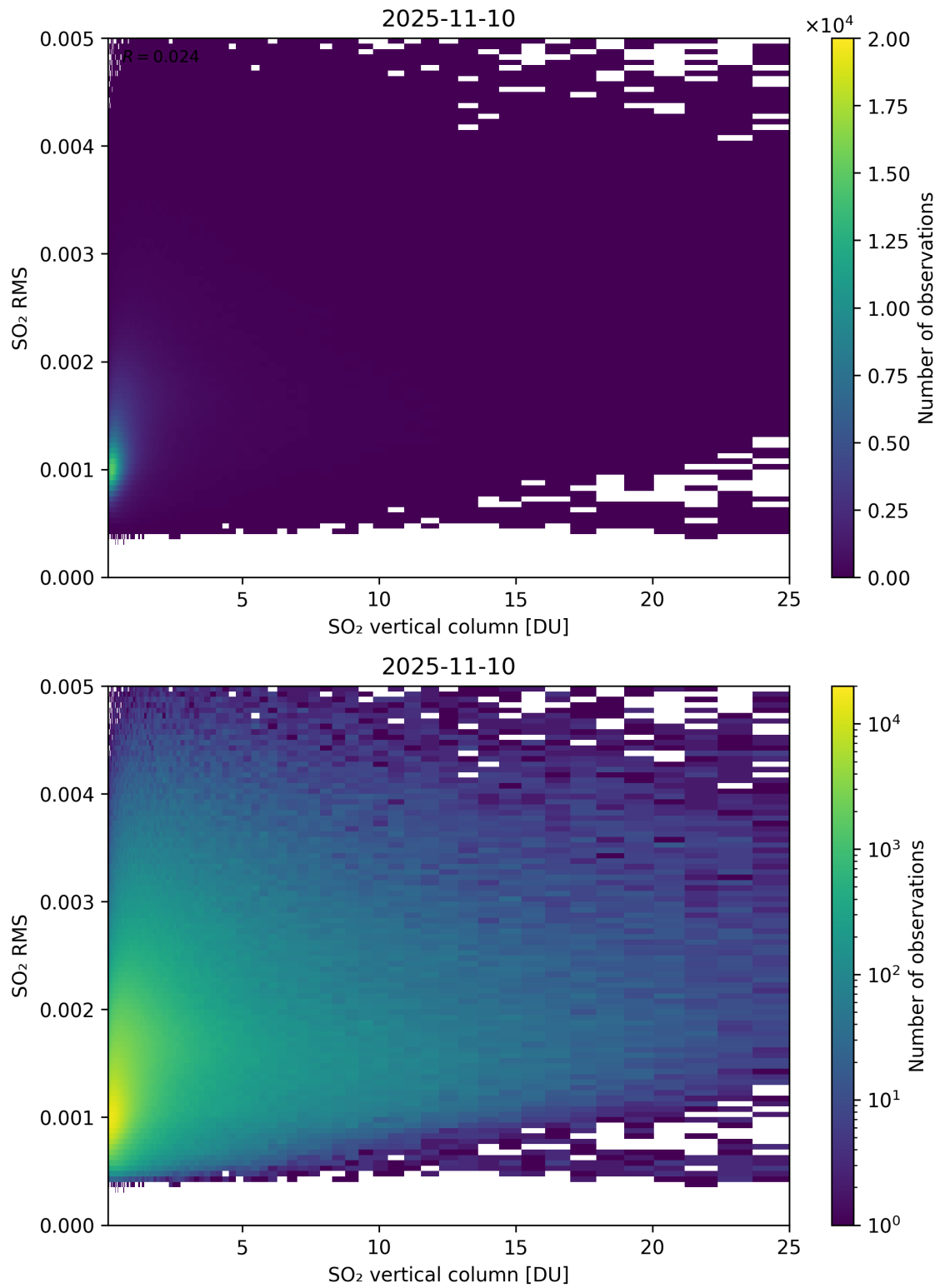
Figure 328: Scatter density plot of “SO 2 vertical column” against “SO 2 RMS” for 2025-11-09 to 2025-11-11.
