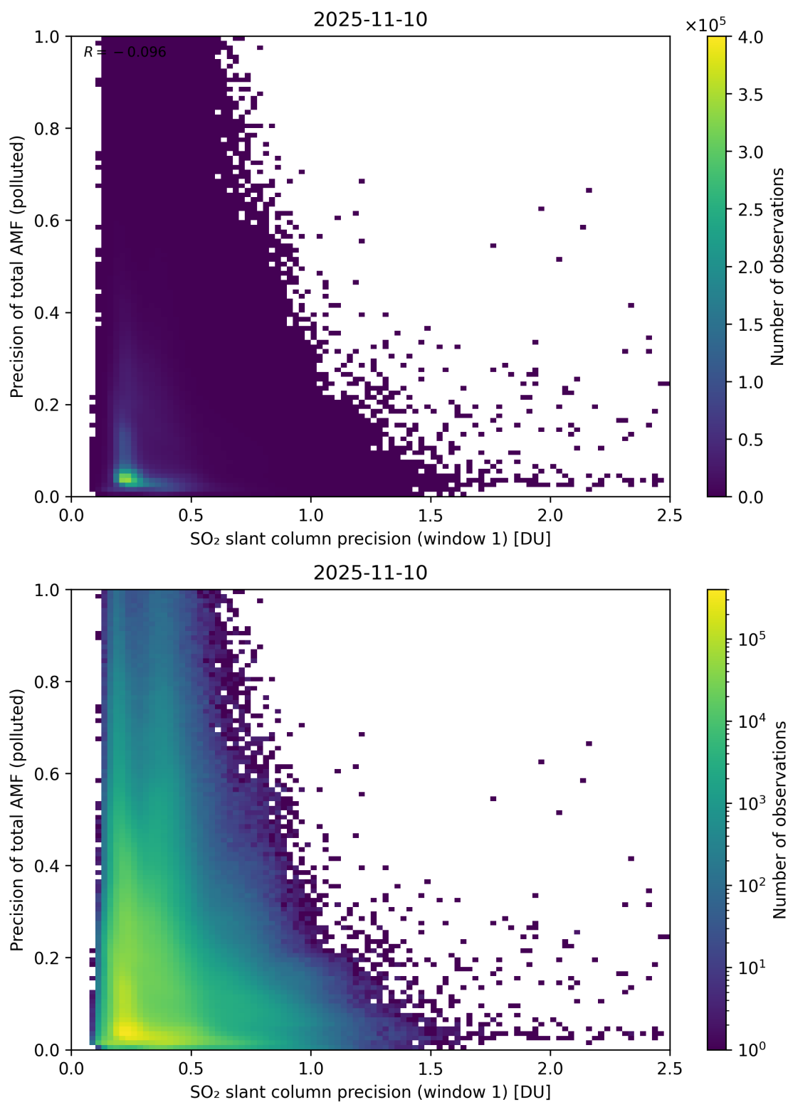
Figure 281: Scatter density plot of “SO 2 slant column precision (window 1)” against “Precision of total AMF (polluted)” for 2025-11-09 to 2025-11-11.
