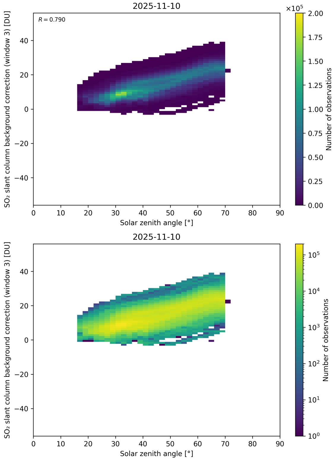
Figure 173: Scatter density plot of “Solar zenith angle” against “SO 2 slant column background correction (window 3)” for 2025-11-09 to 2025-11-11.
