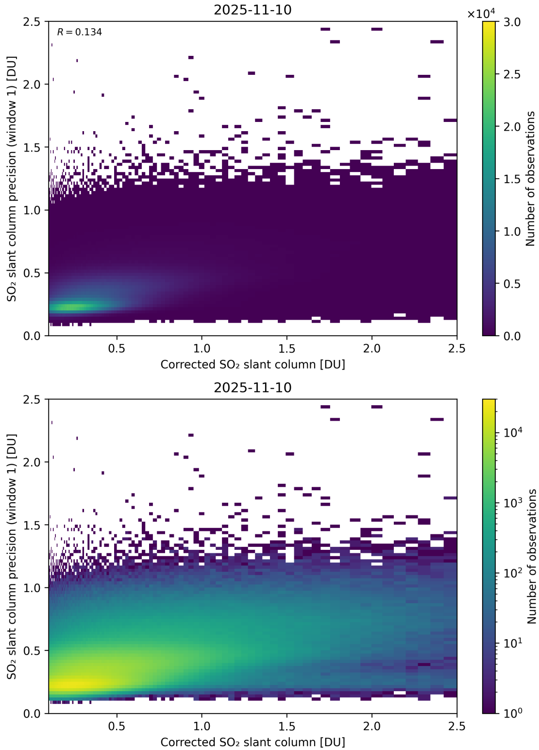
Figure 238: Scatter density plot of “Corrected SO 2 slant column” against “SO 2 slant column precision (window 1)” for 2025-11-09 to 2025-11-11.
