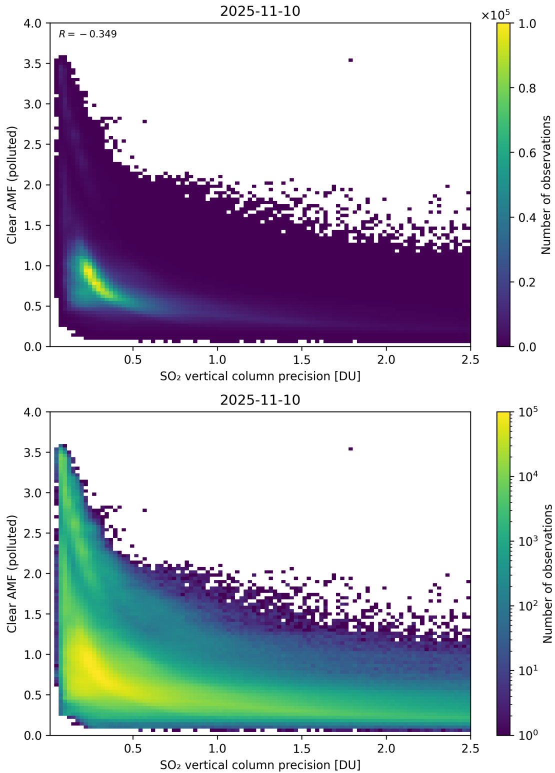
Figure 335: Scatter density plot of “SO 2 vertical column precision” against “Clear AMF (polluted)” for 2025-11-09 to 2025-11-11.
