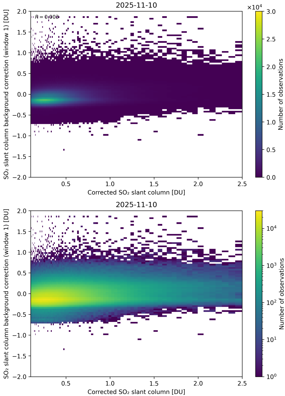
Figure 226: Scatter density plot of “Corrected SO 2 slant column” against “SO 2 slant column background correction (window 1)” for 2025-11-09 to 2025-11-11.
