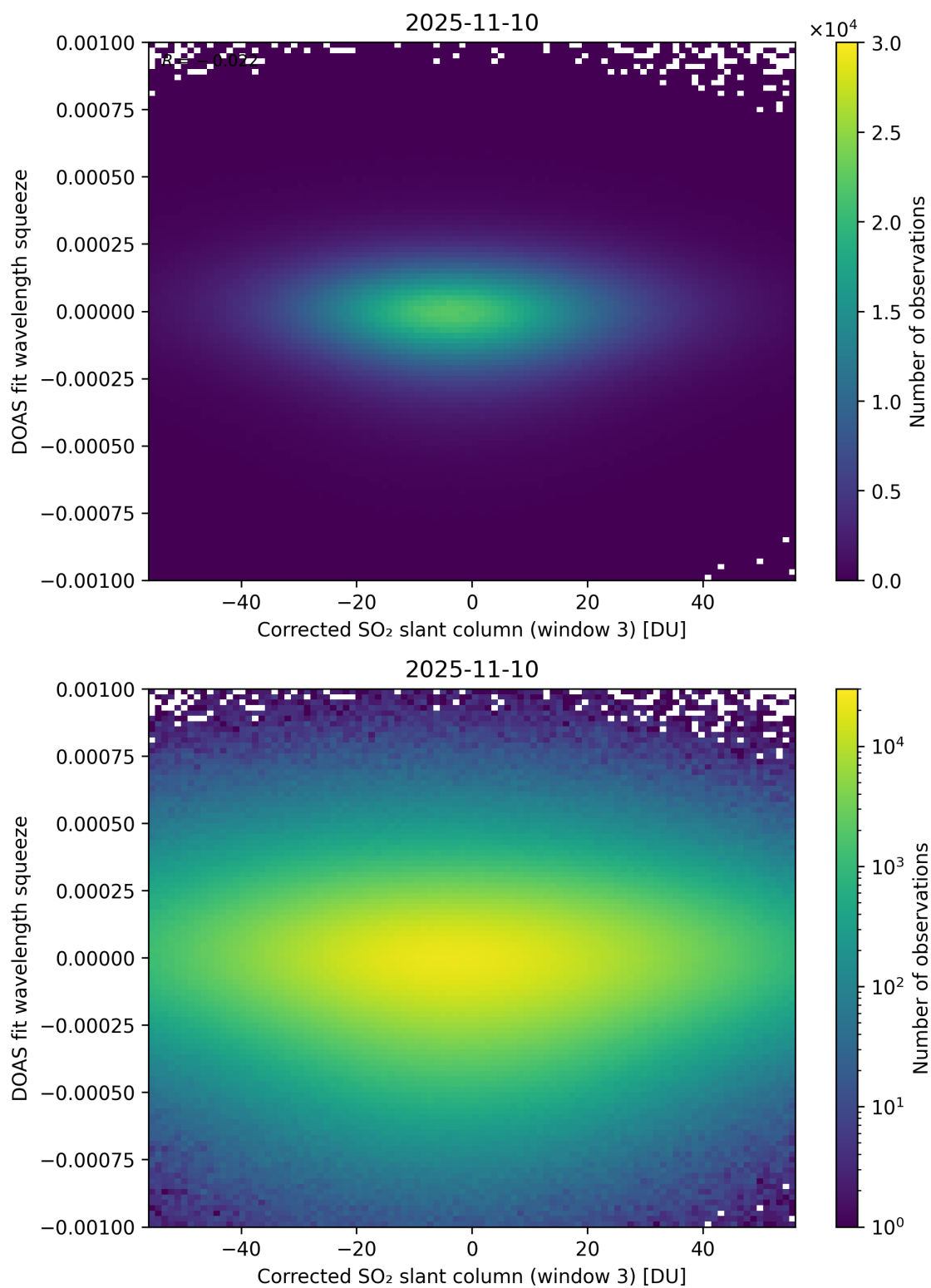
Figure 257: Scatter density plot of “Corrected SO 2 slant column (window 3)” against “DOAS fit wavelength squeeze” for 2025-11-09 to 2025-11-11.
