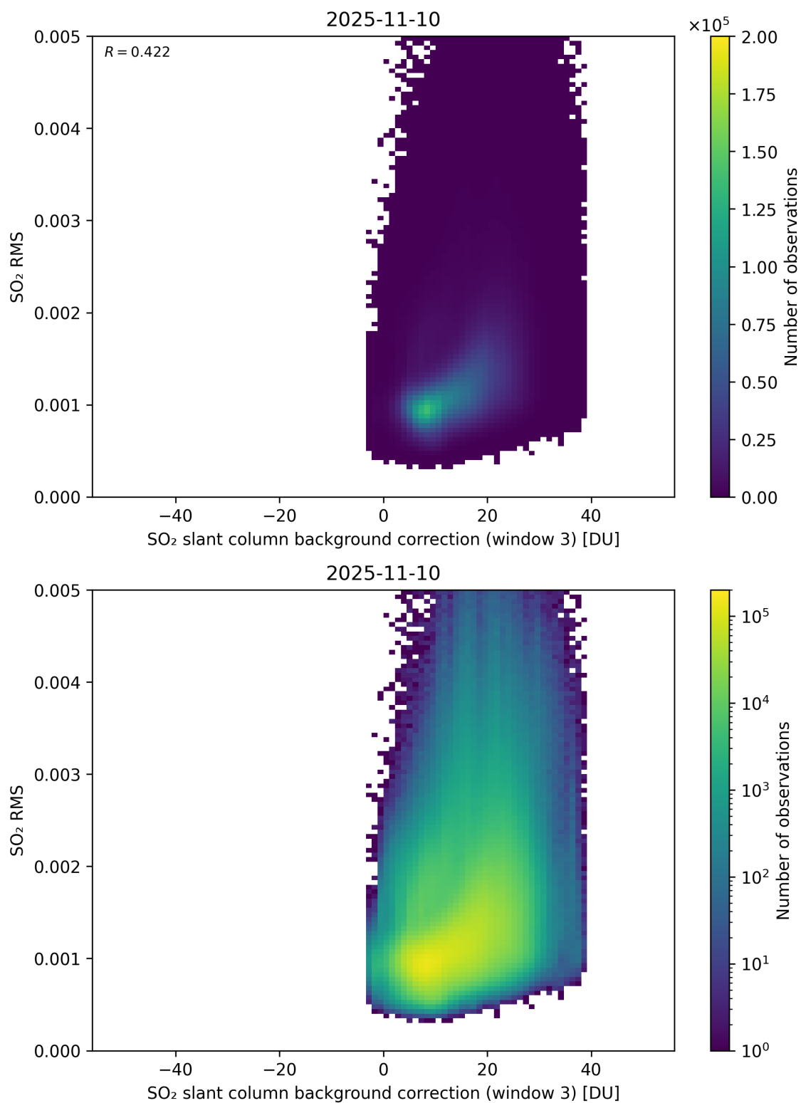
Figure 134: Scatter density plot of “SO 2 slant column background correction (window 3)” against “SO 2 RMS” for 2025-11-09 to 2025-11-11.
