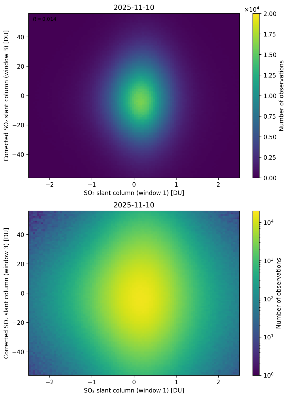
Figure 284: Scatter density plot of “SO 2 slant column (window 1)” against “Corrected SO 2 slant column (window 3)” for 2025-11-09 to 2025-11-11.
