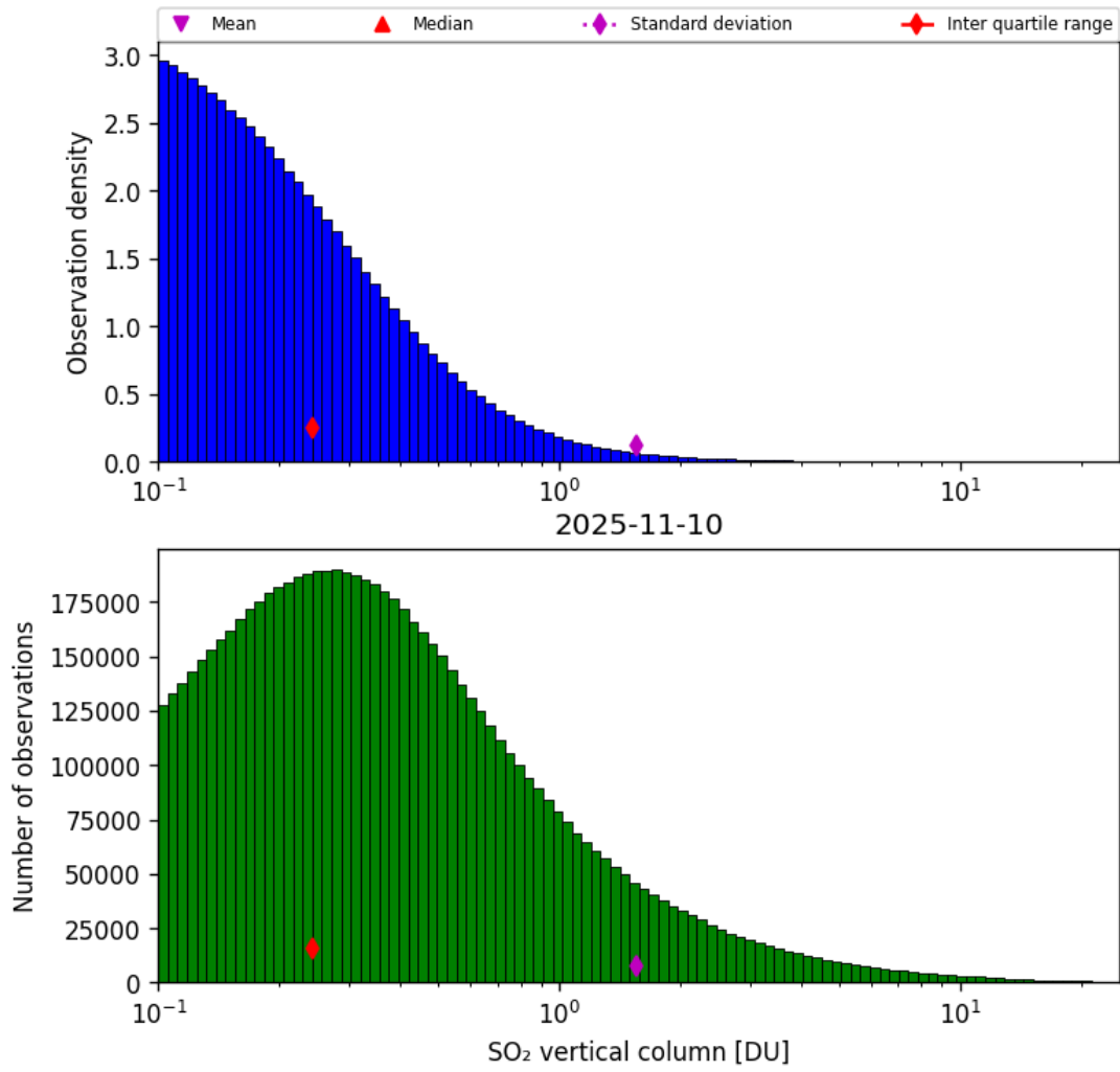
Figure 58: Histogram of “SO 2 vertical column” for 2025-11-09 to 2025-11-11
