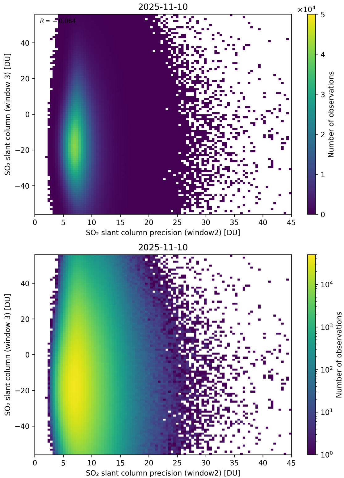
Figure 299: Scatter density plot of “SO 2 slant column precision (window2)” against “SO 2 slant column (window 3)” for 2025-11-09 to 2025-11-11.
