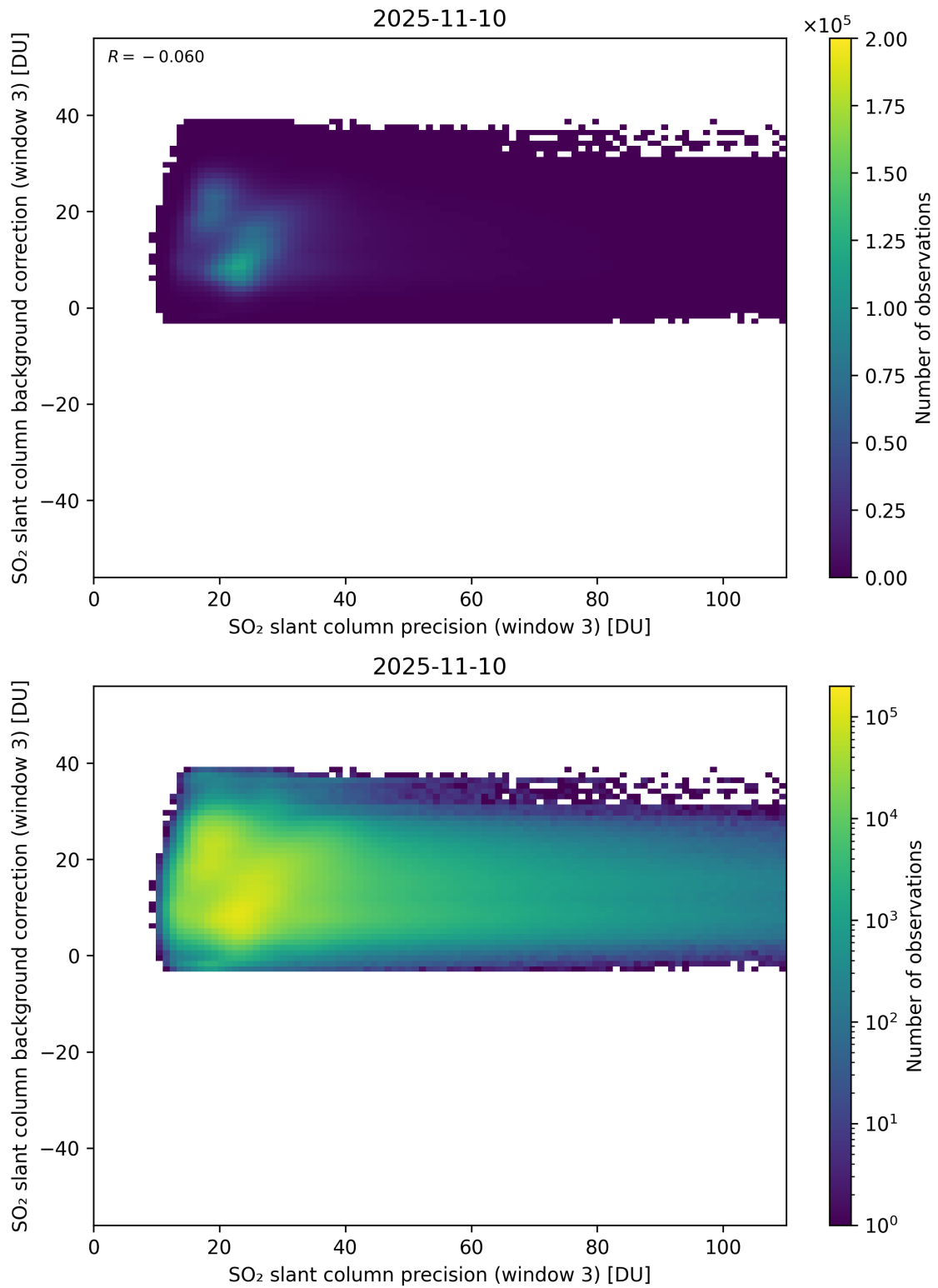
Figure 307: Scatter density plot of “SO 2 slant column precision (window 3)” against “SO 2 slant column background correction (window 3)” for 2025-11-09 to 2025-11-11.
