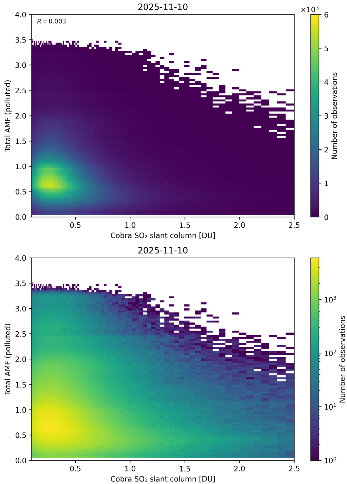
Figure 224: Scatter density plot of “Cobra SO 2 slant column” against “Total AMF (polluted)” for 2025-11-09 to 2025-11-11.
