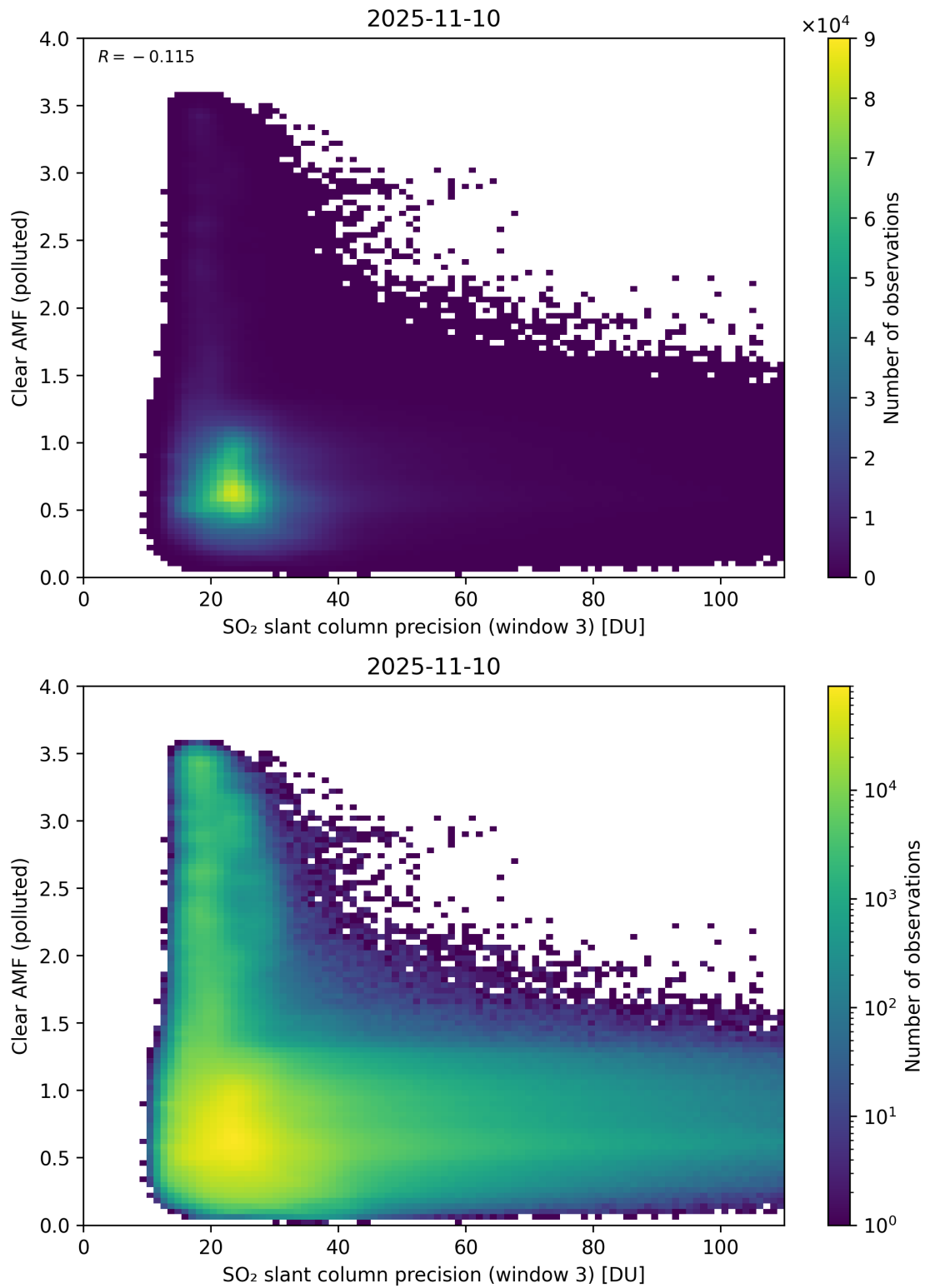
Figure 311: Scatter density plot of “SO 2 slant column precision (window 3)” against “Clear AMF (polluted)” for 2025-11-09 to 2025-11-11.
