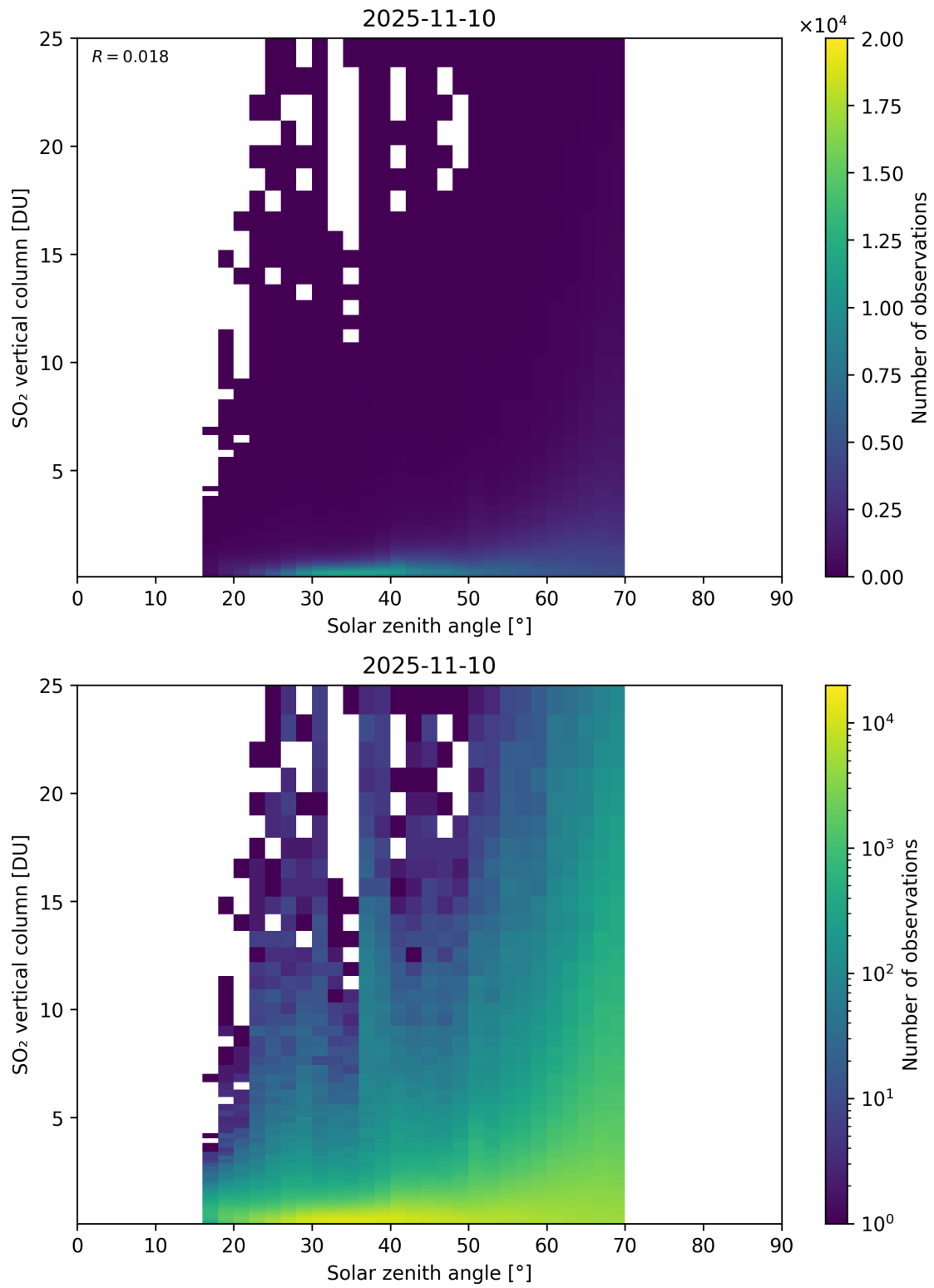
Figure 191: Scatter density plot of “Solar zenith angle” against “SO 2 vertical column” for 2025-11-09 to 2025-11-11.
