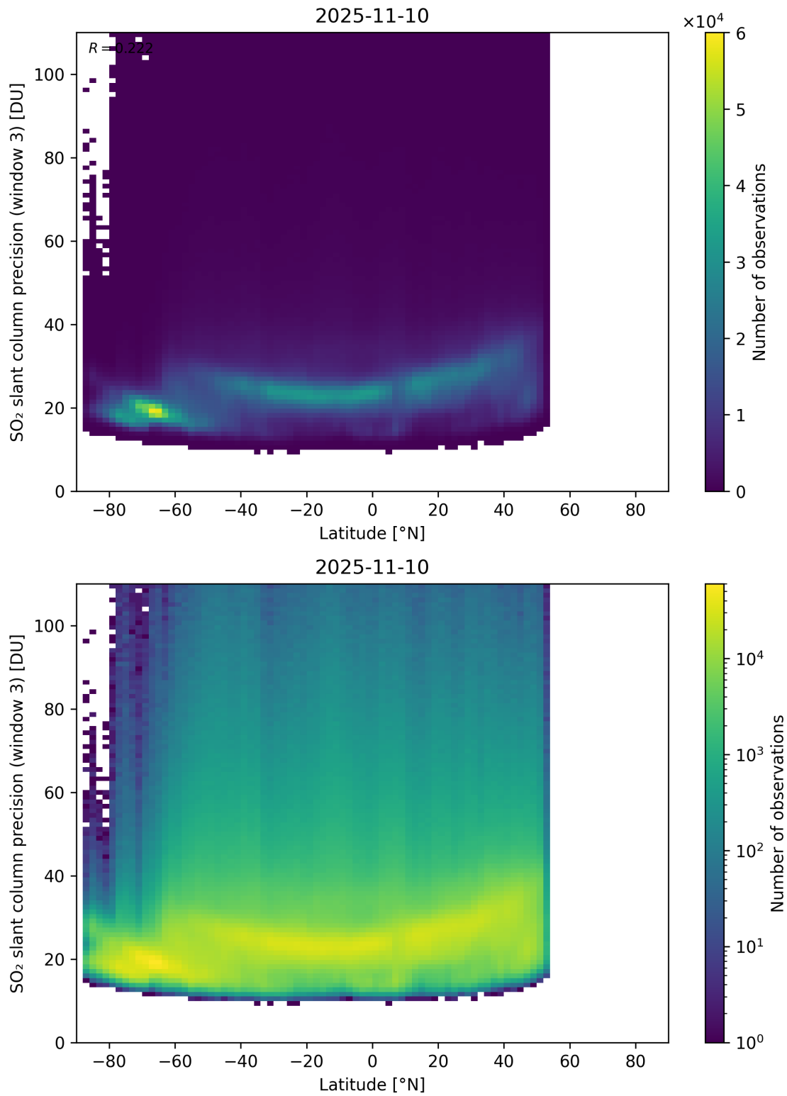
Figure 166: Scatter density plot of “Latitude” against “SO 2 slant column precision (window 3)” for 2025-11-09 to 2025-11-11.
