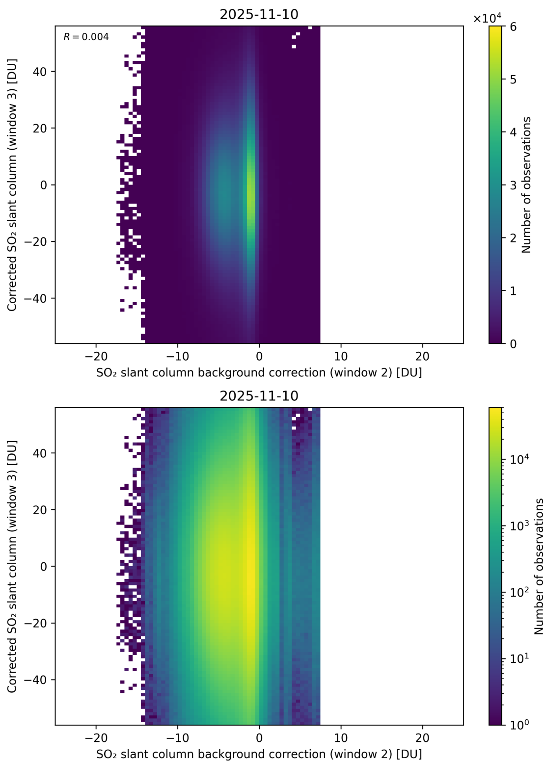
Figure 127: Scatter density plot of “SO 2 slant column background correction (window 2)” against “Corrected SO 2 slant column (window 3)” for 2025-11-09 to 2025-11-11.
