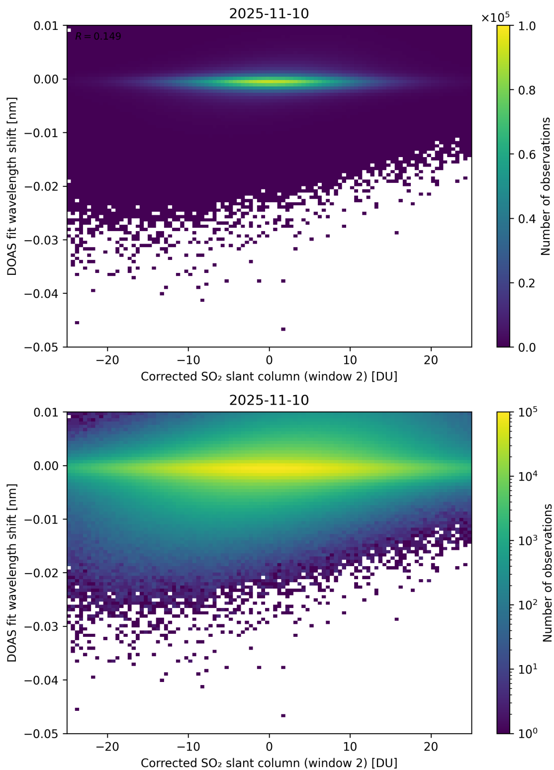
Figure 246: Scatter density plot of “Corrected SO 2 slant column (window 2)” against “DOAS fit wavelength shift” for 2025-11-09 to 2025-11-11.
