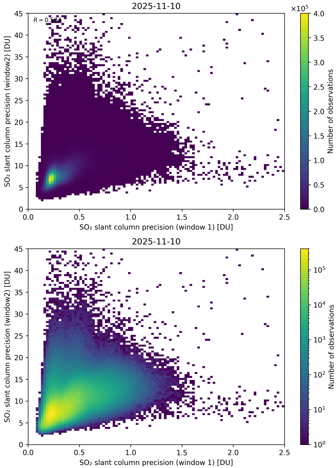
Figure 277: Scatter density plot of “SO 2 slant column precision (window 1)” against “SO 2 slant column precision (window2)” for 2025-11-09 to 2025-11-11.
