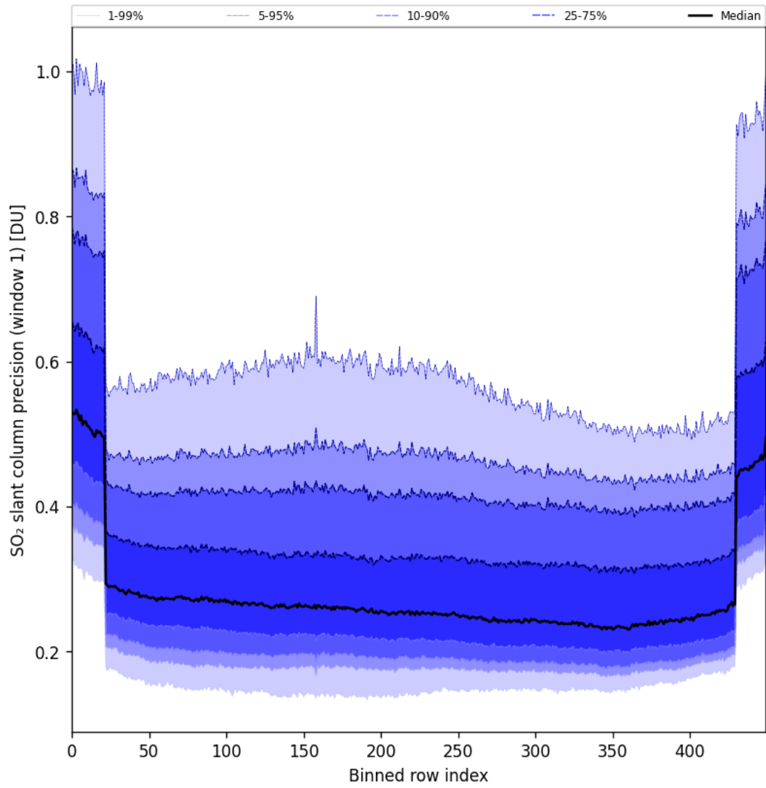
Figure 90: Along track statistics of “SO 2 slant column precision (window 1)” for 2025-11-09 to 2025-11-11
