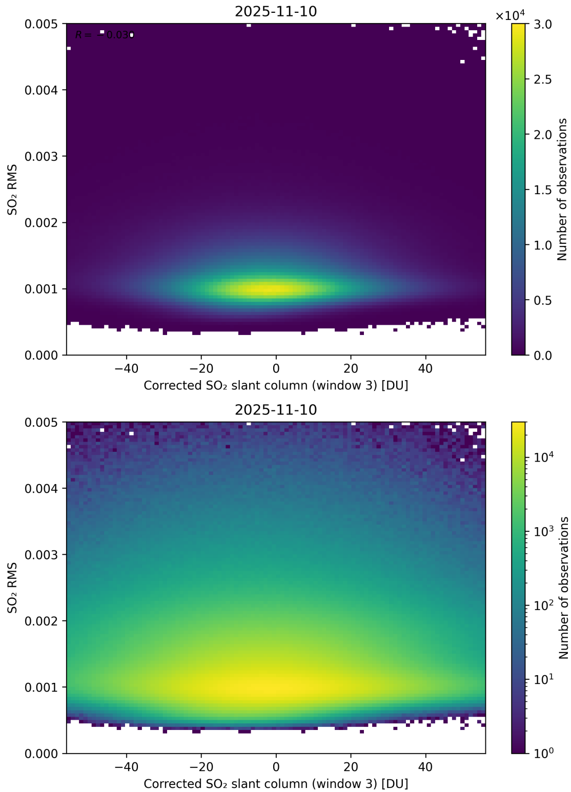
Figure 258: Scatter density plot of “Corrected SO 2 slant column (window 3)” against “SO 2 RMS” for 2025-11-09 to 2025-11-11.
