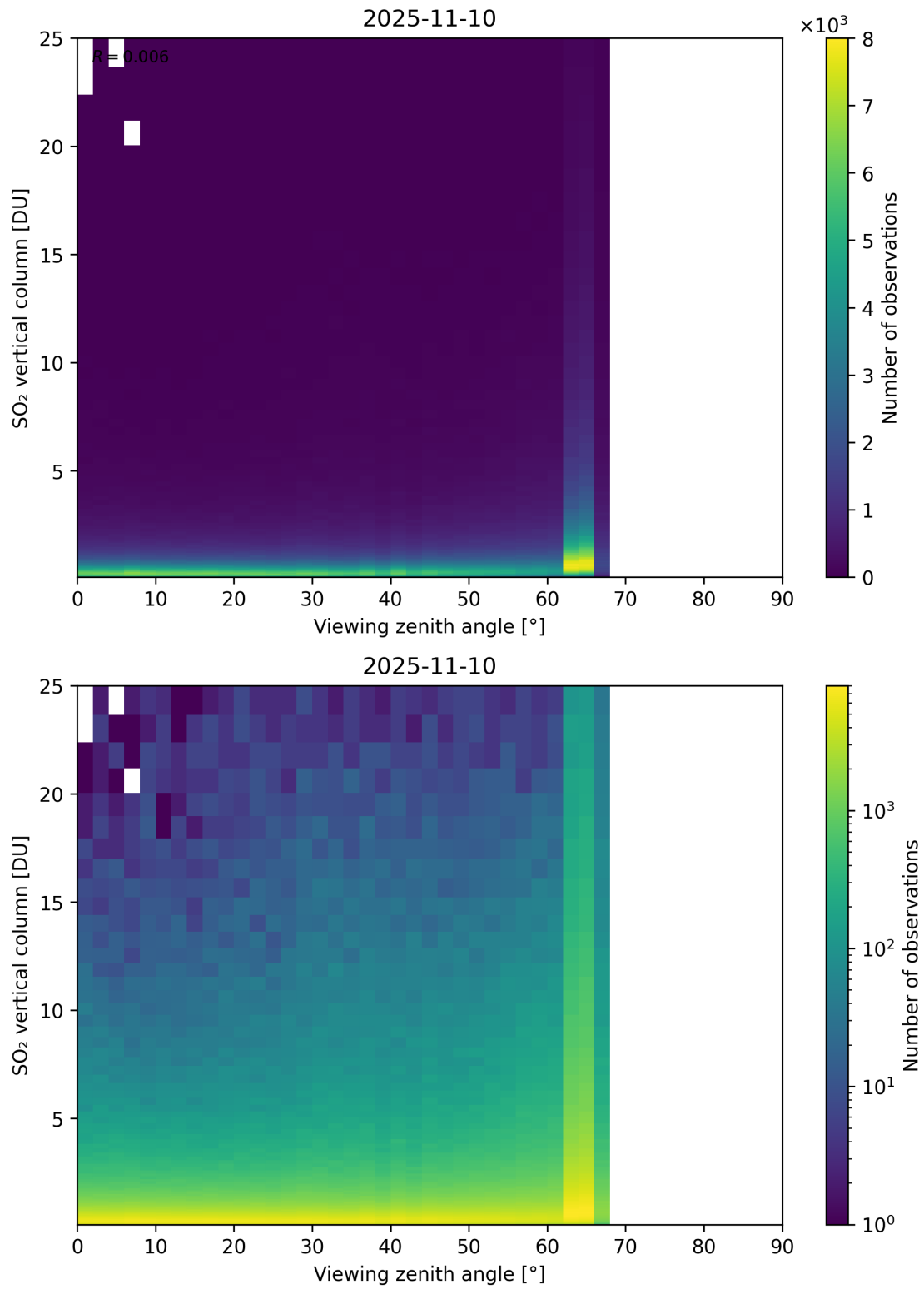
Figure 383: Scatter density plot of “Viewing zenith angle” against “SO 2 vertical column” for 2025-11-09 to 2025-11-11.
