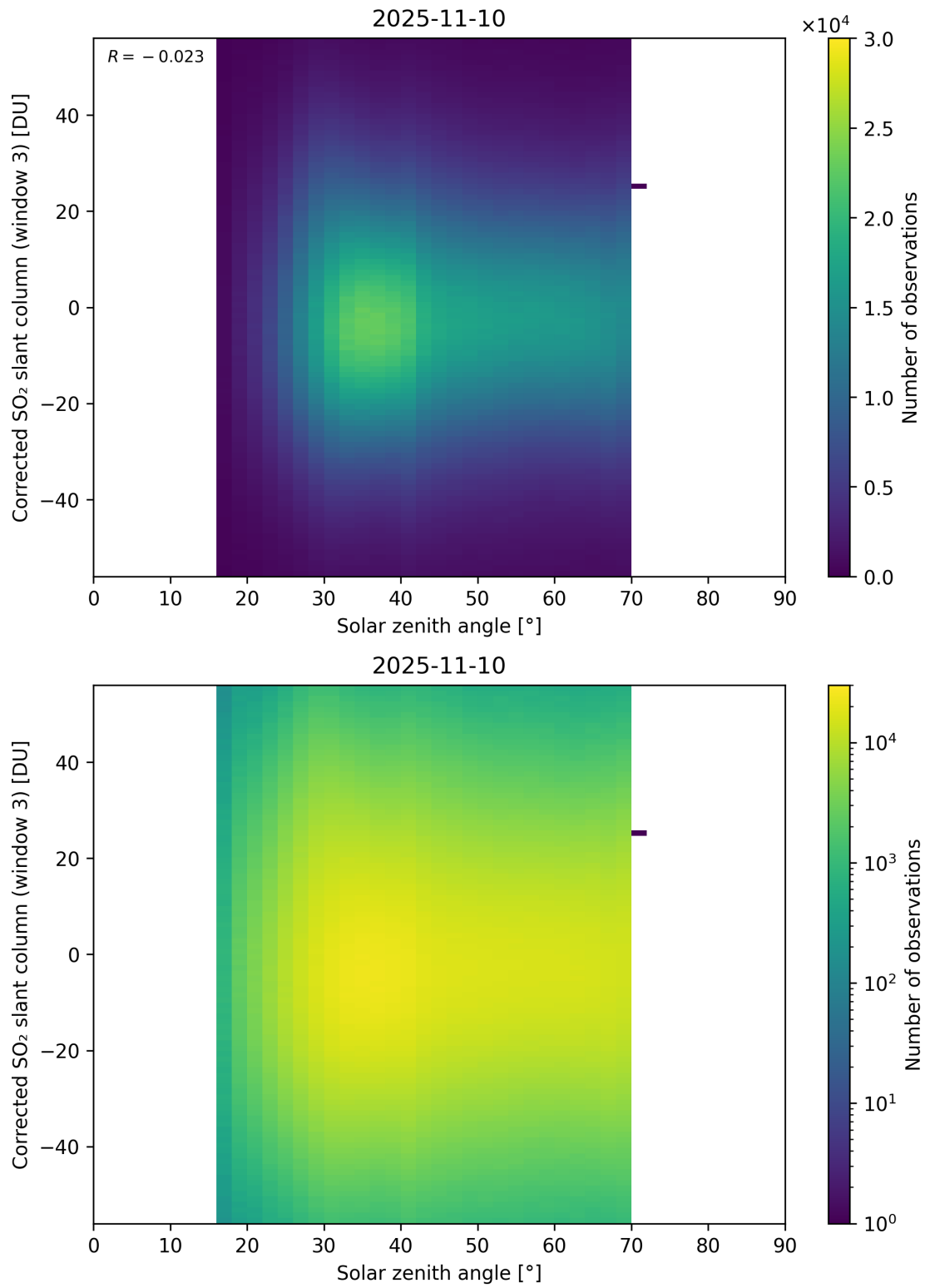
Figure 183: Scatter density plot of “Solar zenith angle” against “Corrected SO 2 slant column (window 3)” for 2025-11-09 to 2025-11-11.
