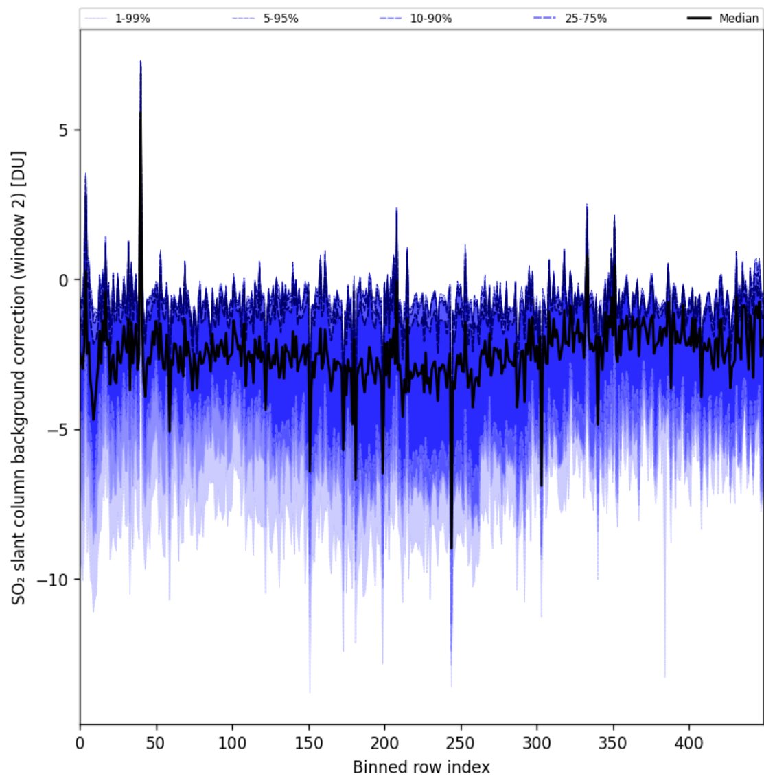
Figure 96: Along track statistics of “SO 2 slant column background correction (window 2)” for 2025-11-09 to 2025-11-11
