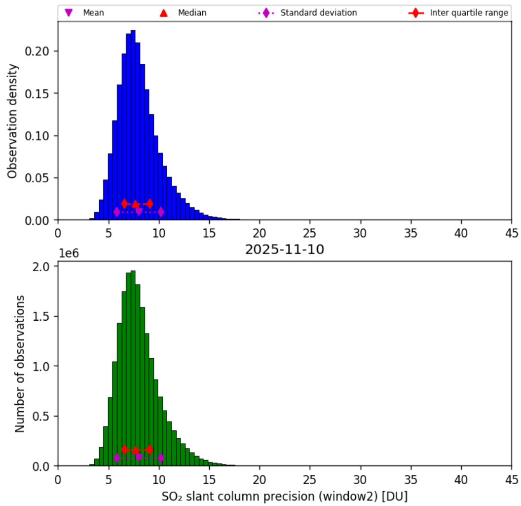
Figure 68: Histogram of “SO 2 slant column precision (window2)” for 2025-11-09 to 2025-11-11
