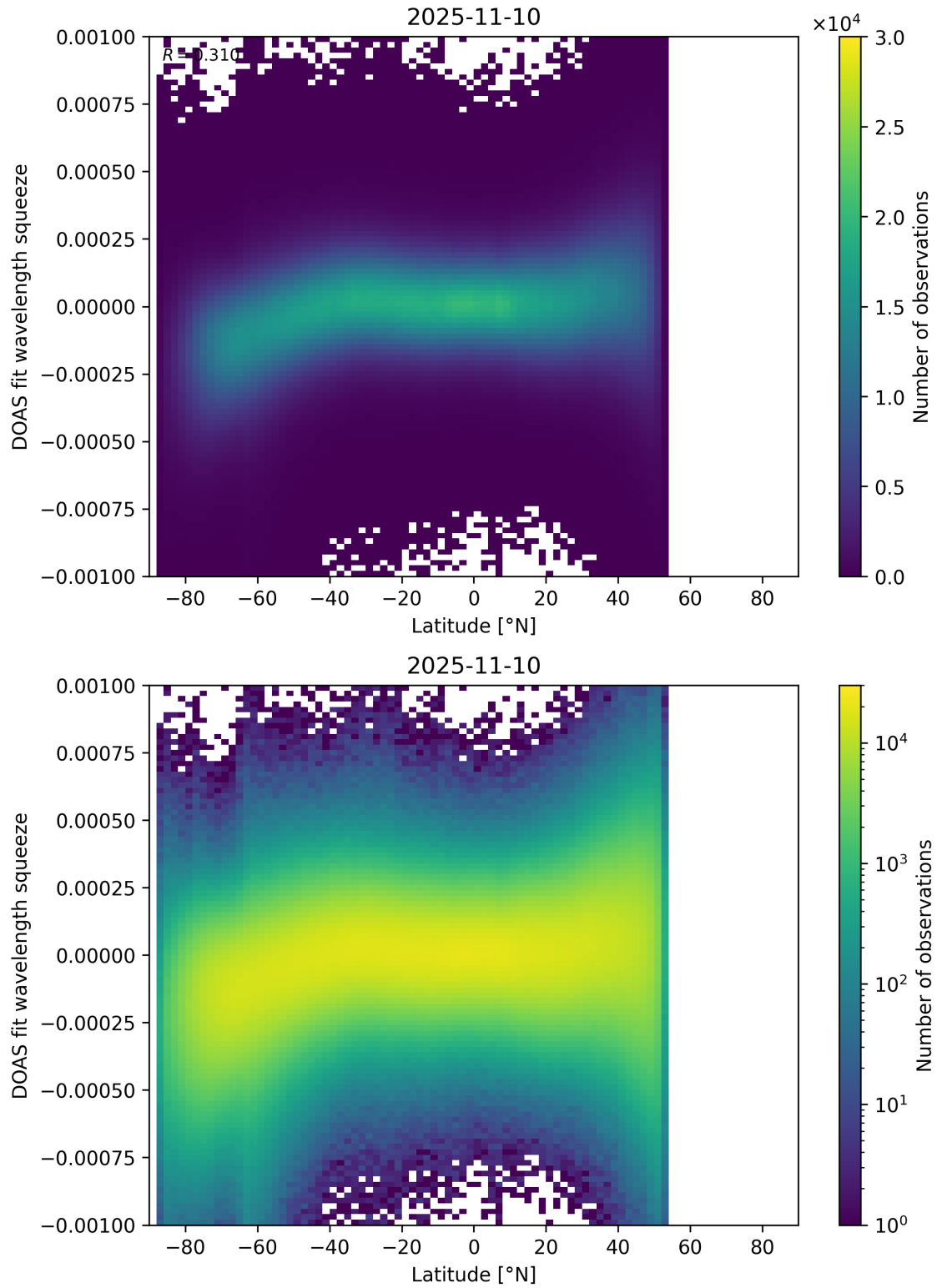
Figure 154: Scatter density plot of “Latitude” against “DOAS fit wavelength squeeze” for 2025-11-09 to 2025-11-11.
