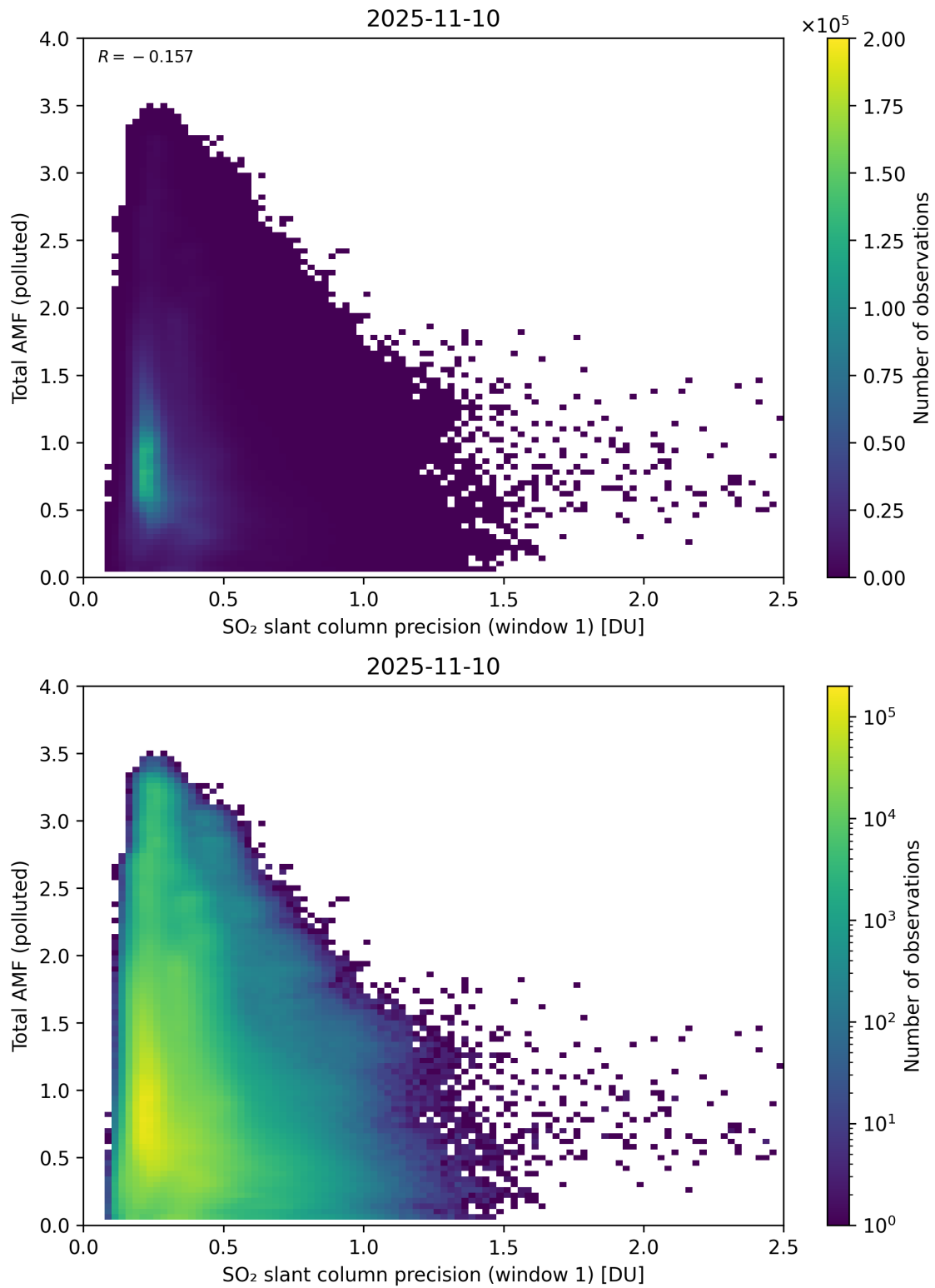
Figure 280: Scatter density plot of “SO 2 slant column precision (window 1)” against “Total AMF (polluted)” for 2025-11-09 to 2025-11-11.
