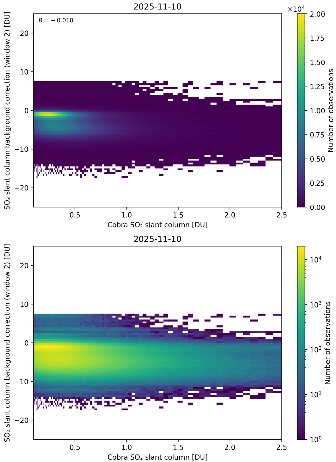
Figure 194: Scatter density plot of “Cobra SO 2 slant column” against “SO 2 slant column background correction (window 2)” for 2025-11-09 to 2025-11-11.
