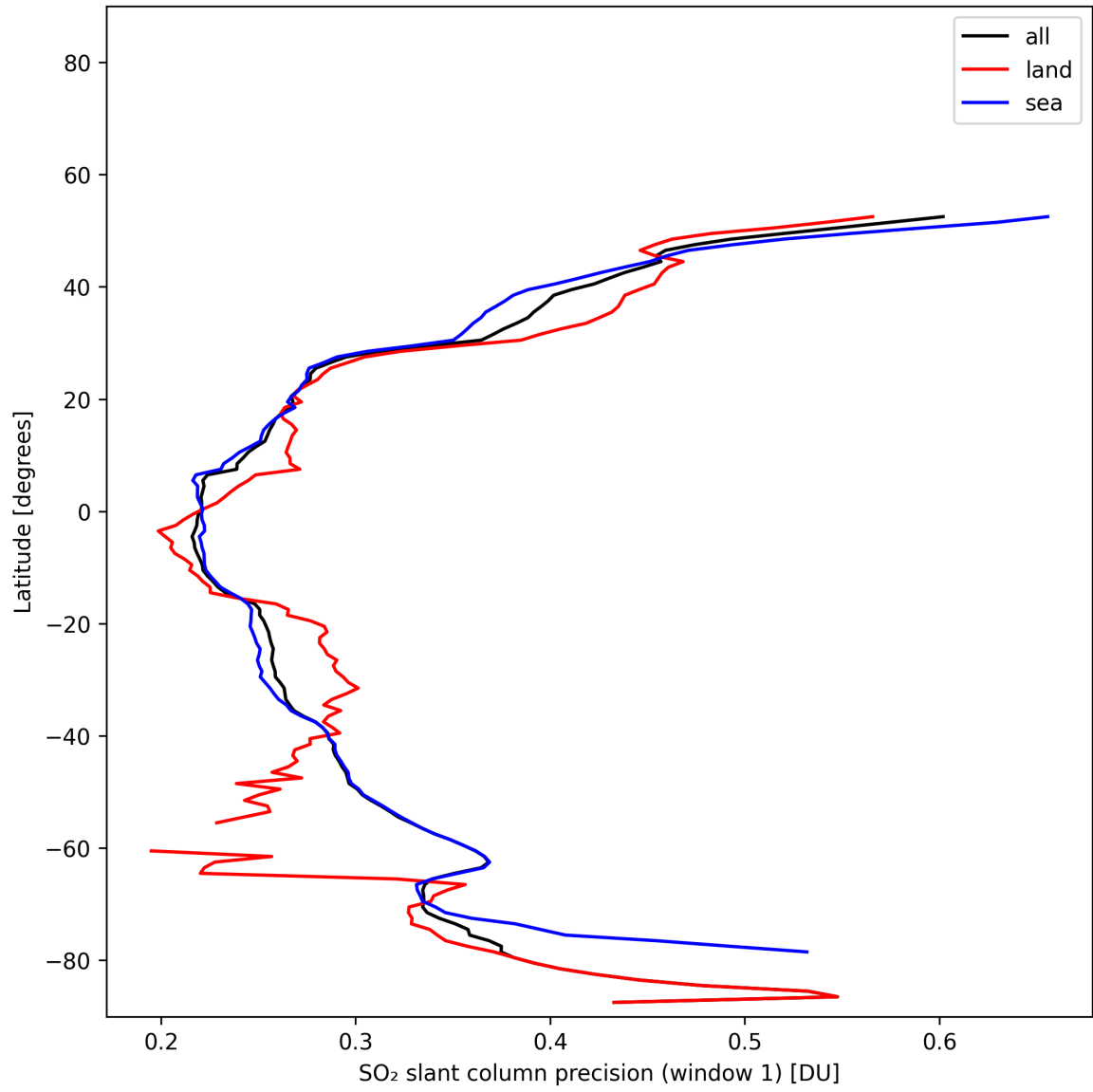
Figure 38: Zonal average of “SO 2 slant column precision (window 1)” for 2025-11-09 to 2025-11-11.
