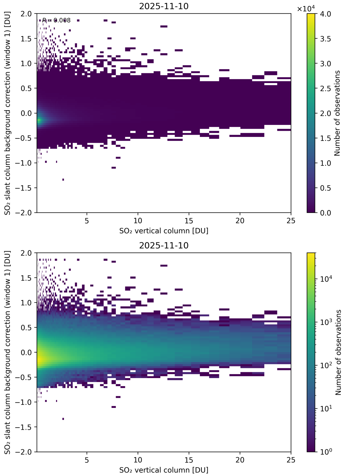
Figure 323: Scatter density plot of “SO 2 vertical column” against “SO 2 slant column background correction (window 1)” for 2025-11-09 to 2025-11-11.
