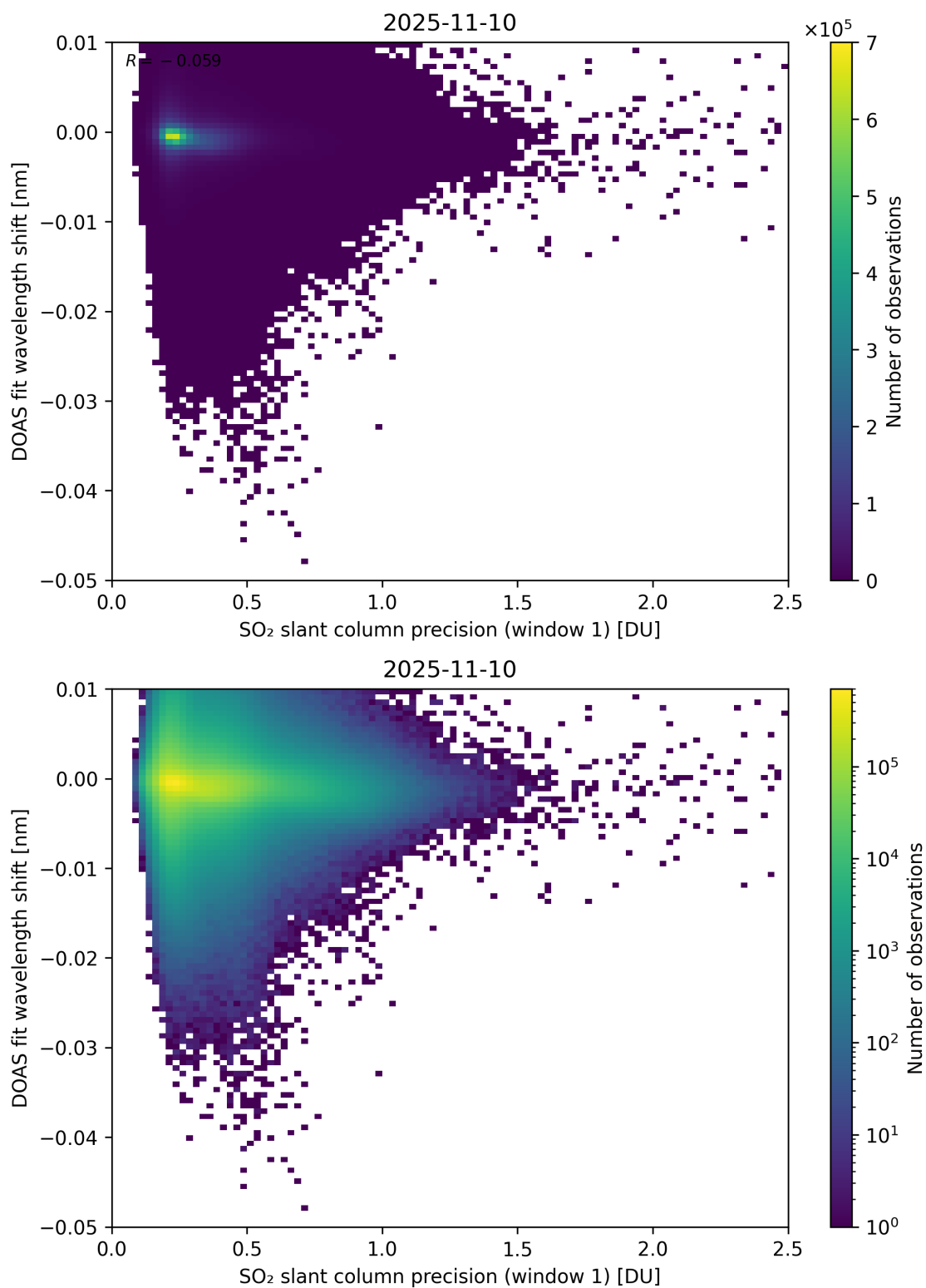
Figure 271: Scatter density plot of “SO 2 slant column precision (window 1)” against “DOAS fit wavelength shift” for 2025-11-09 to 2025-11-11.
