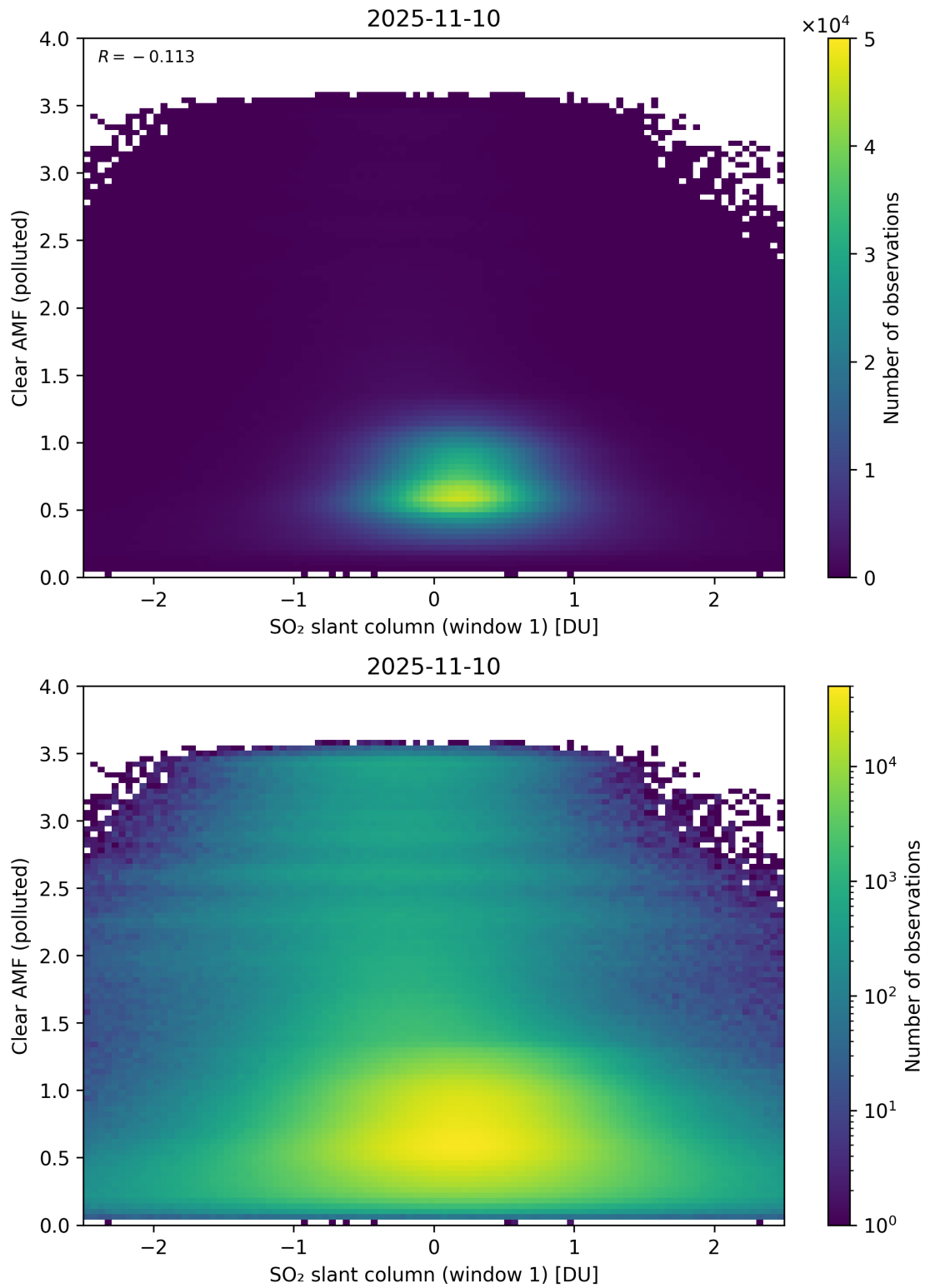
Figure 282: Scatter density plot of “SO 2 slant column (window 1)” against “Clear AMF (polluted)” for 2025-11-09 to 2025-11-11.
