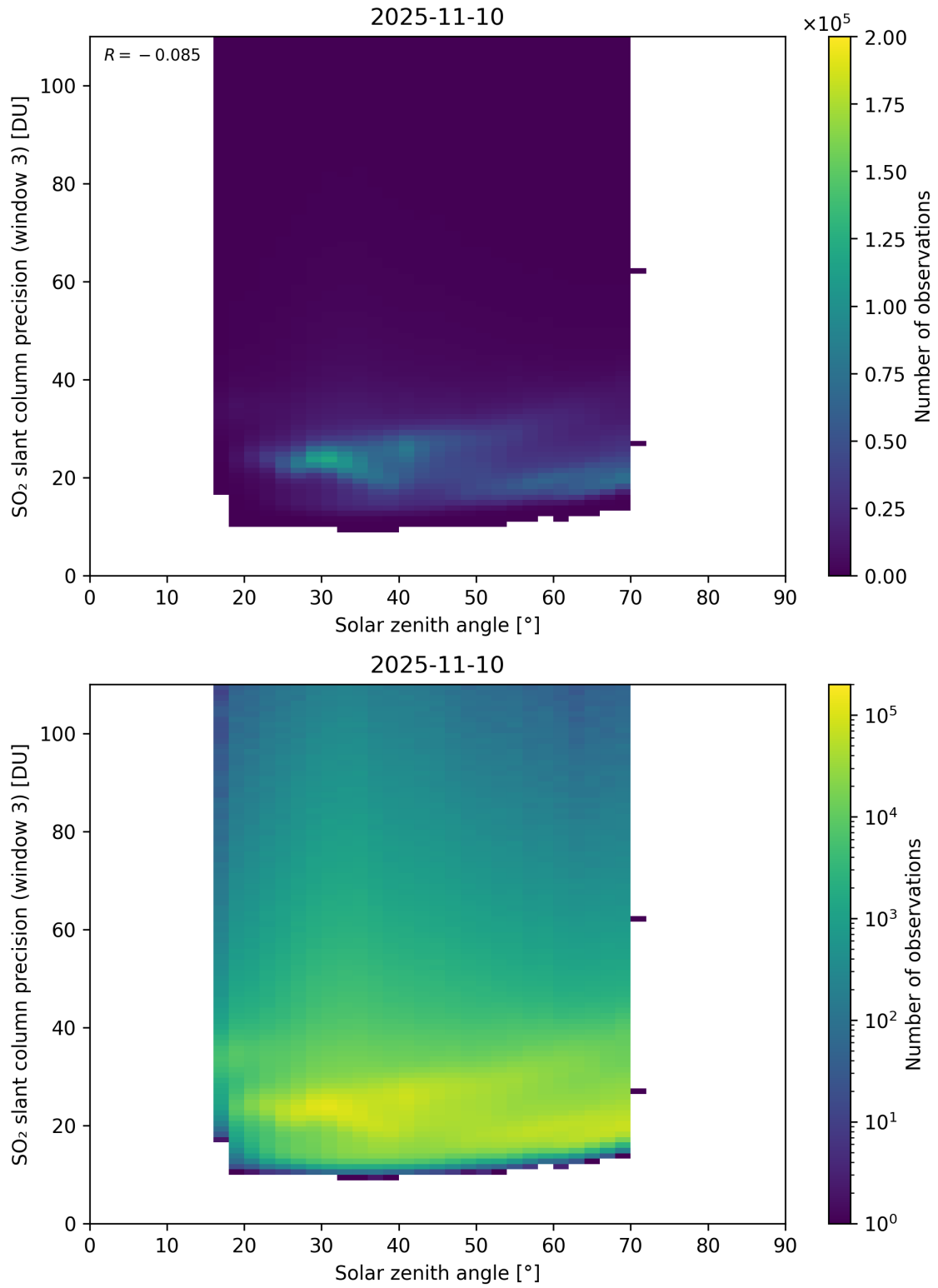
Figure 188: Scatter density plot of “Solar zenith angle” against “SO 2 slant column precision (window 3)” for 2025-11-09 to 2025-11-11.
