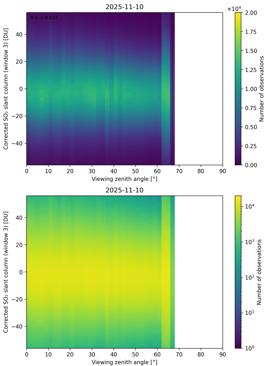
Figure 375: Scatter density plot of “Viewing zenith angle” against “Corrected SO 2 slant column (window 3)” for 2025-11-09 to 2025-11-11.
