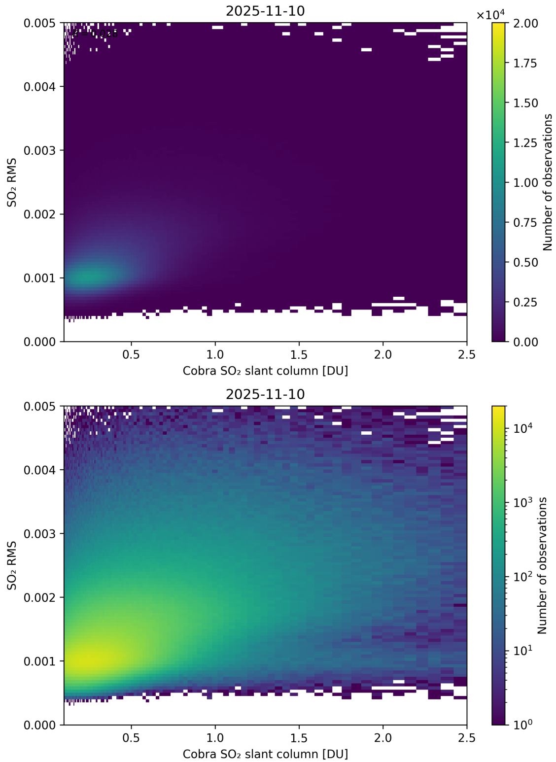
Figure 198: Scatter density plot of “Cobra SO 2 slant column” against “SO 2 RMS” for 2025-11-09 to 2025-11-11.
