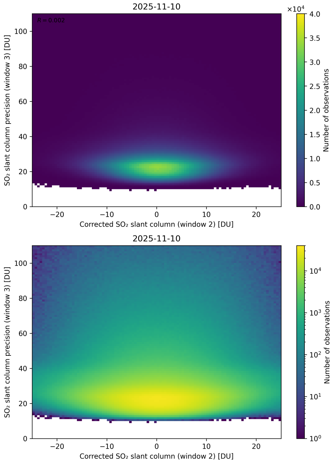
Figure 252: Scatter density plot of “Corrected SO 2 slant column (window 2)” against “SO 2 slant column precision (window 3)” for 2025-11-09 to 2025-11-11.
