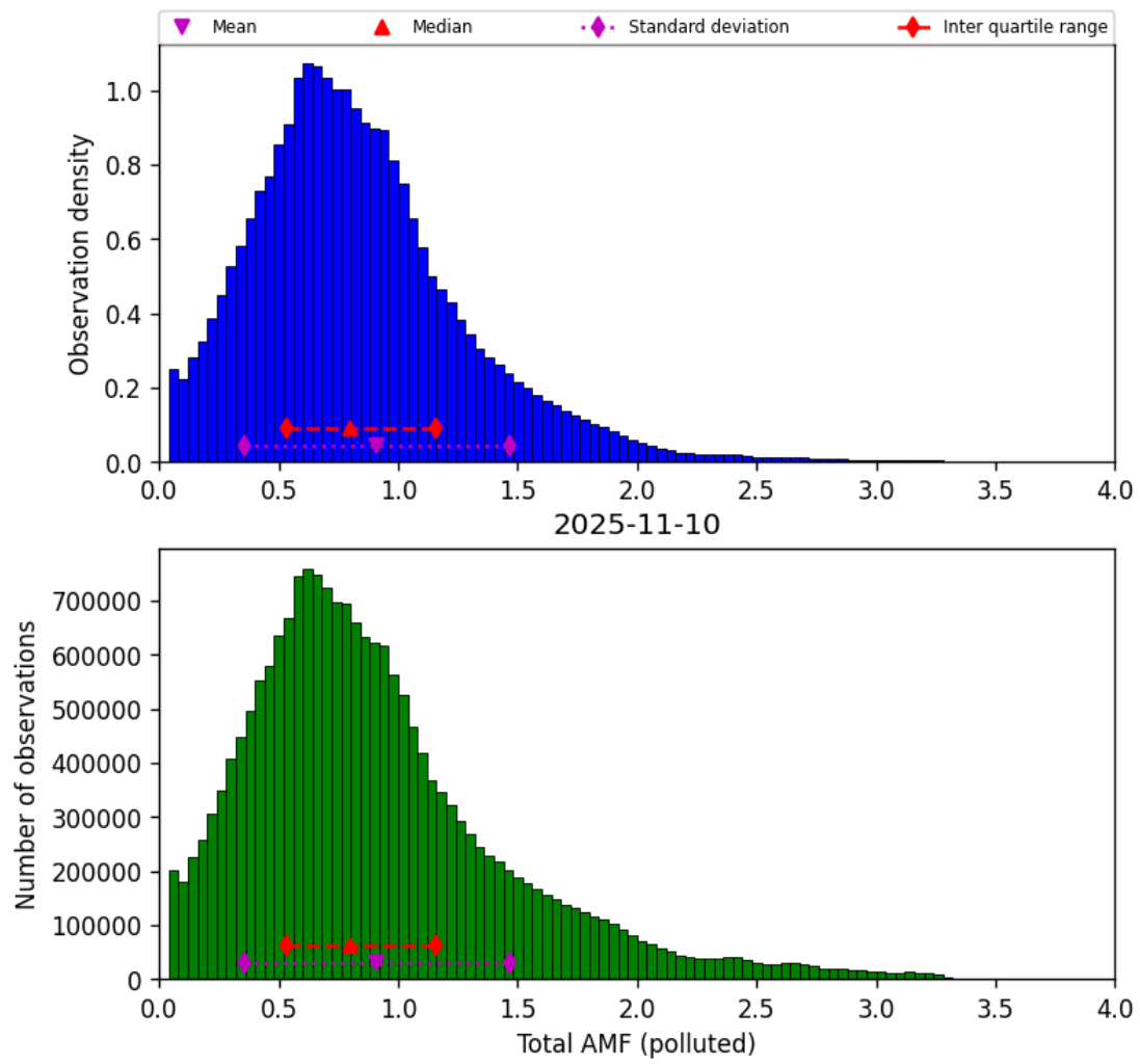
Figure 79: Histogram of “Total AMF (polluted)” for 2025-11-09 to 2025-11-11
