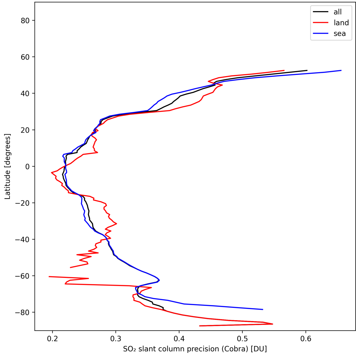
Figure 36: Zonal average of “SO 2 slant column precision (Cobra)” for 2025-11-09 to 2025-11-11.
