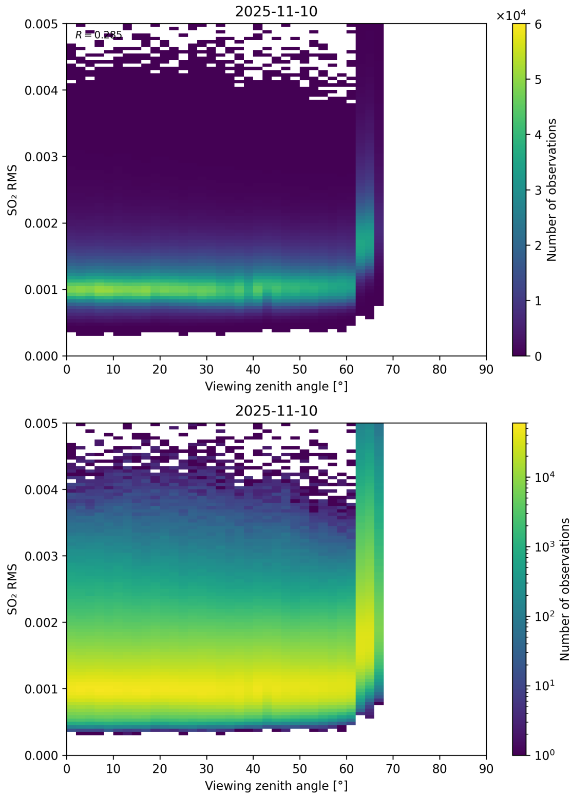
Figure 367: Scatter density plot of “Viewing zenith angle” against “SO 2 RMS” for 2025-11-09 to 2025-11-11.
