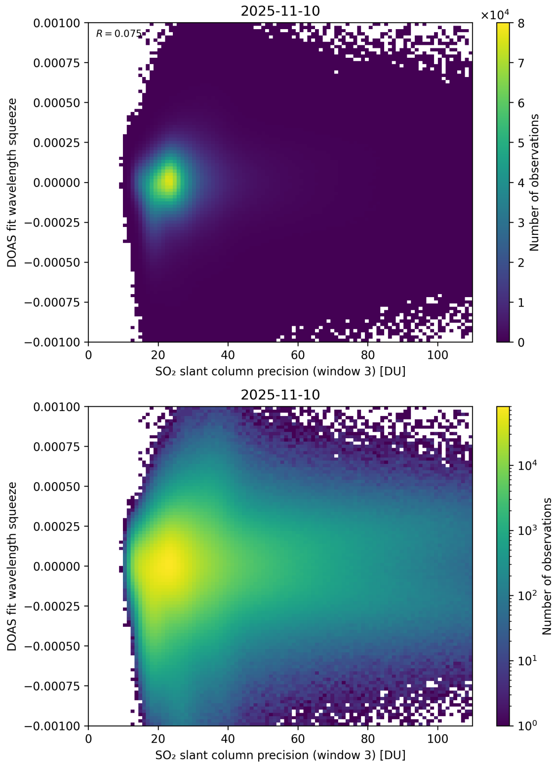
Figure 309: Scatter density plot of “SO 2 slant column precision (window 3)” against “DOAS fit wavelength squeeze” for 2025-11-09 to 2025-11-11.
