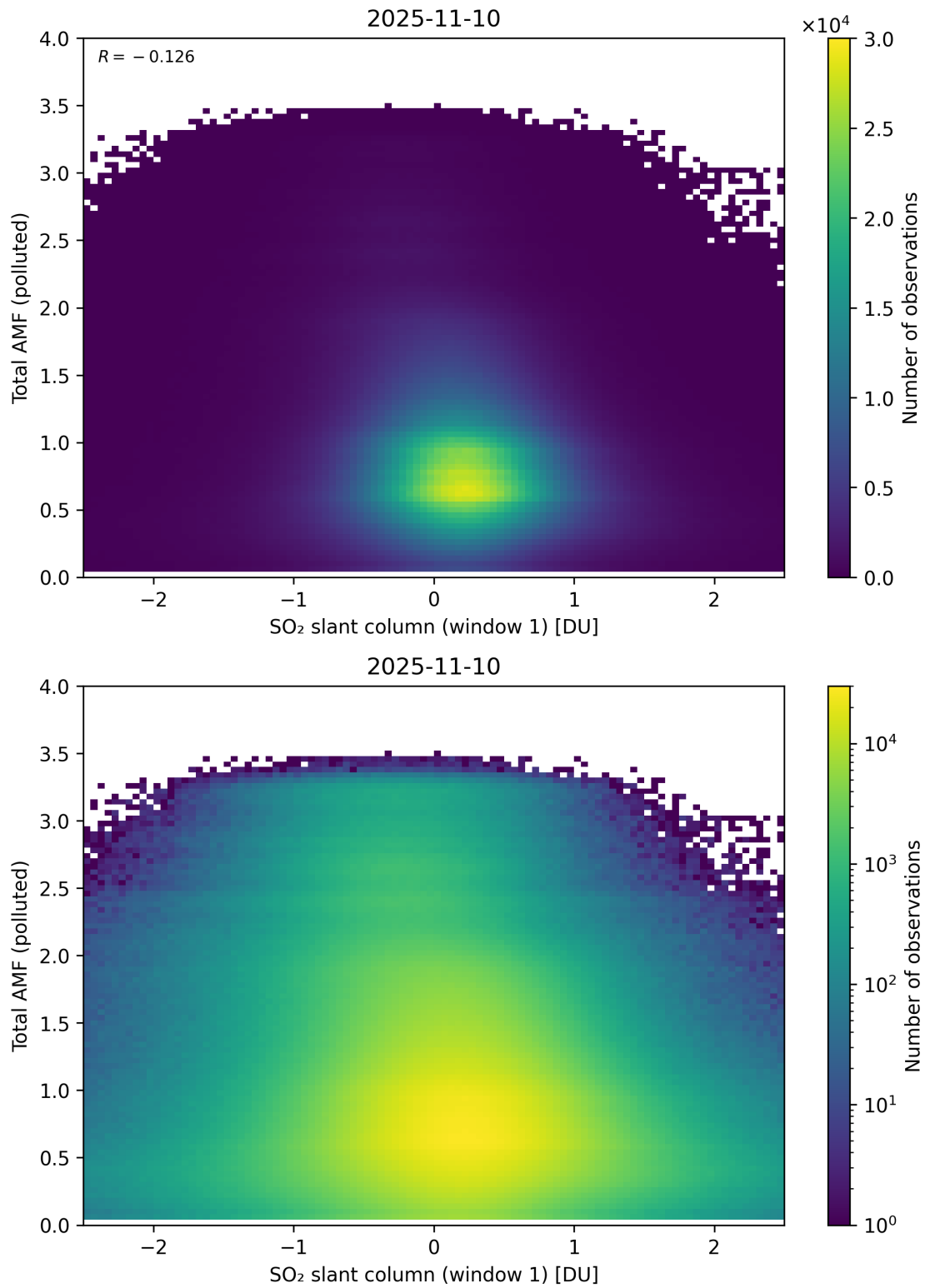
Figure 289: Scatter density plot of “SO 2 slant column (window 1)” against “Total AMF (polluted)” for 2025-11-09 to 2025-11-11.
