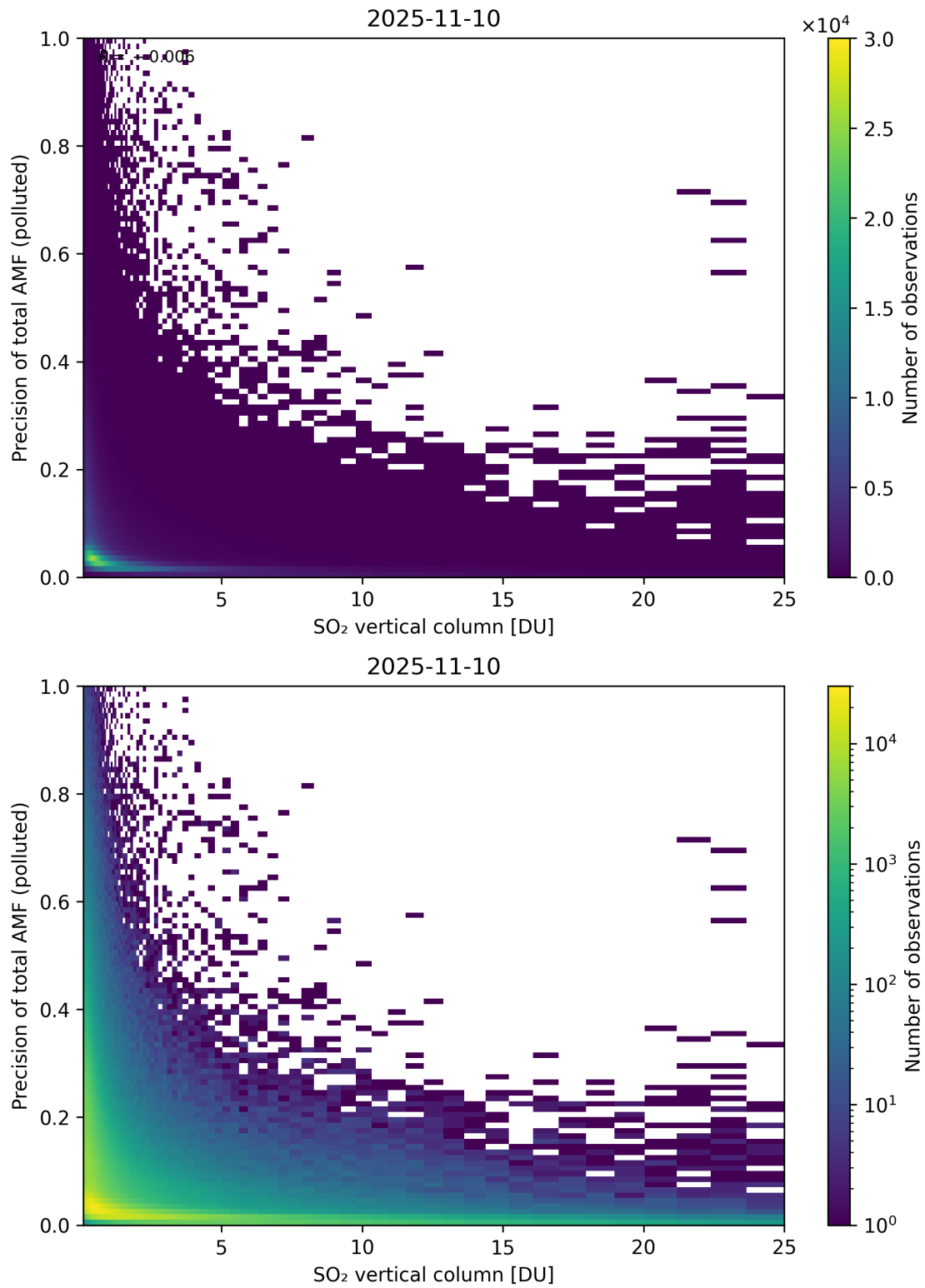
Figure 360: Scatter density plot of “SO 2 vertical column” against “Precision of total AMF (polluted)” for 2025-11-09 to 2025-11-11.
