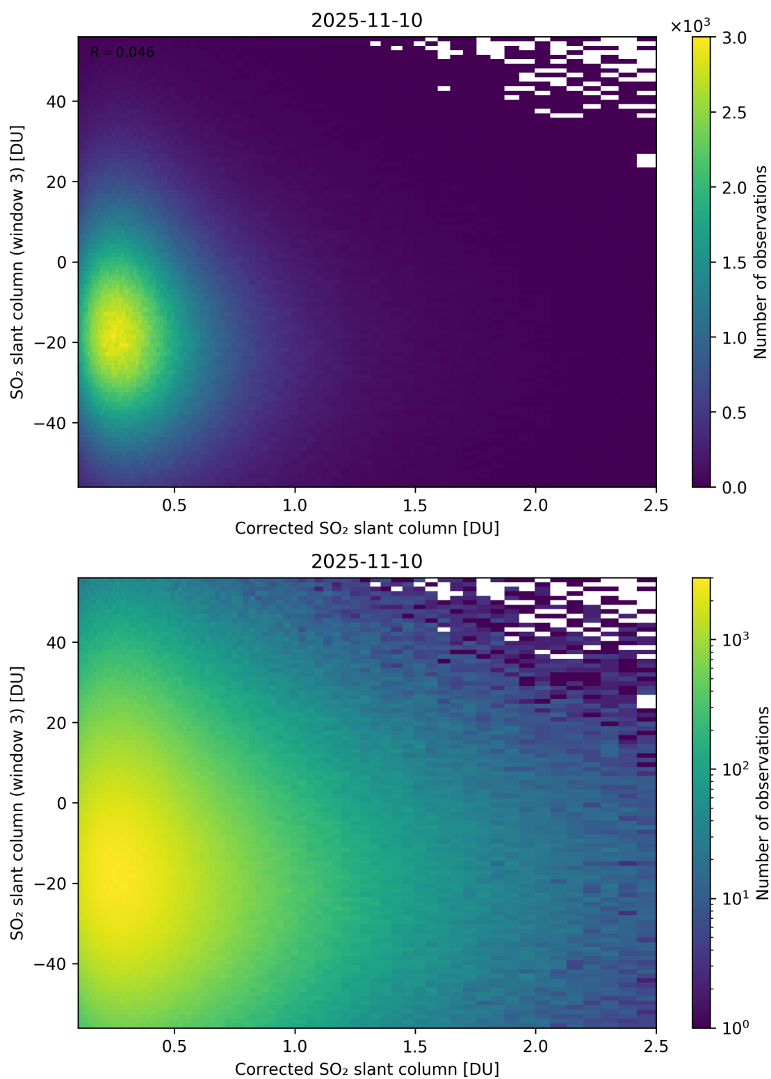
Figure 240: Scatter density plot of “Corrected SO 2 slant column” against “SO 2 slant column (window 3)” for 2025-11-09 to 2025-11-11.
