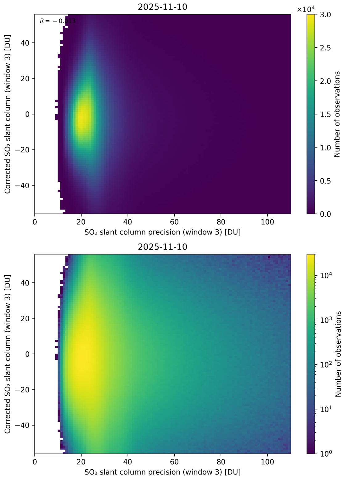
Figure 312: Scatter density plot of “SO 2 slant column precision (window 3)” against “Corrected SO 2 slant column (window 3)” for 2025-11-09 to 2025-11-11.
