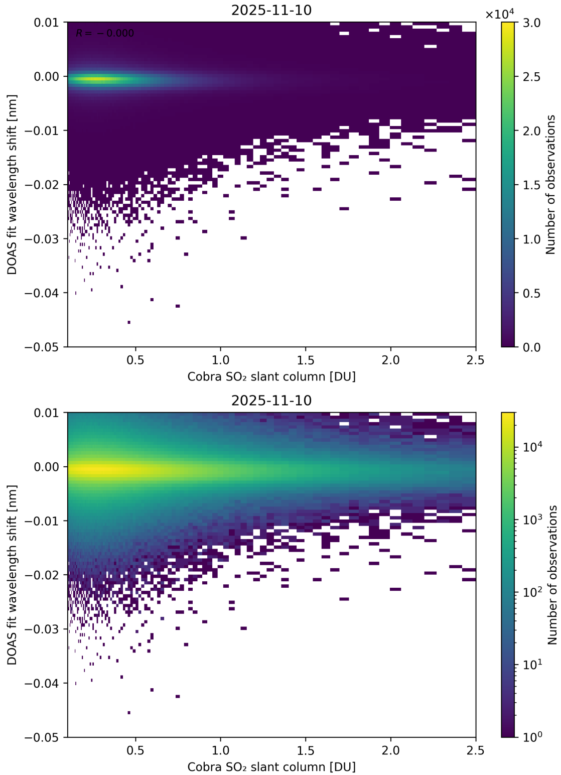
Figure 196: Scatter density plot of “Cobra SO 2 slant column” against “DOAS fit wavelength shift” for 2025-11-09 to 2025-11-11.
