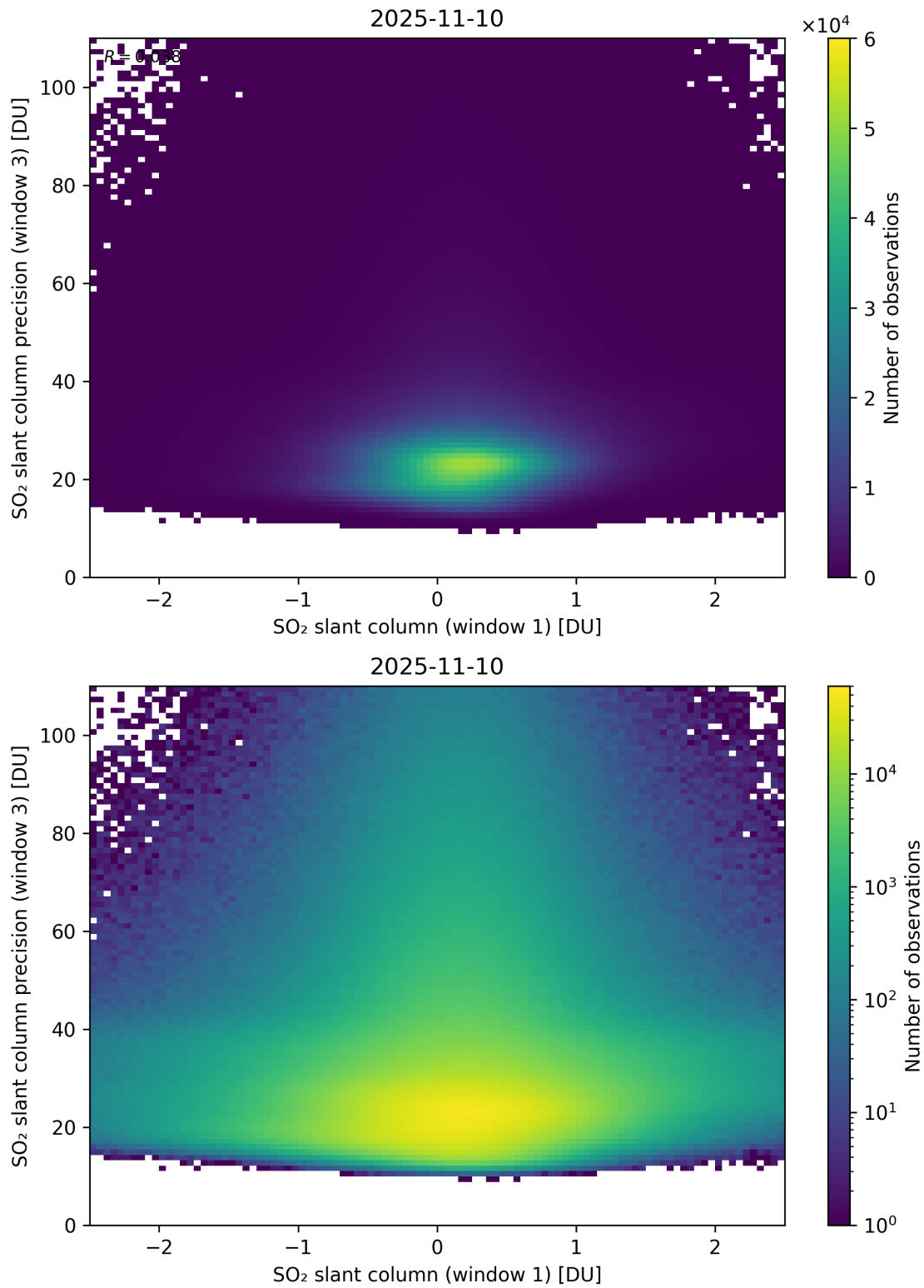
Figure 288: Scatter density plot of “SO 2 slant column (window 1)” against “SO 2 slant column precision (window 3)” for 2025-11-09 to 2025-11-11.
