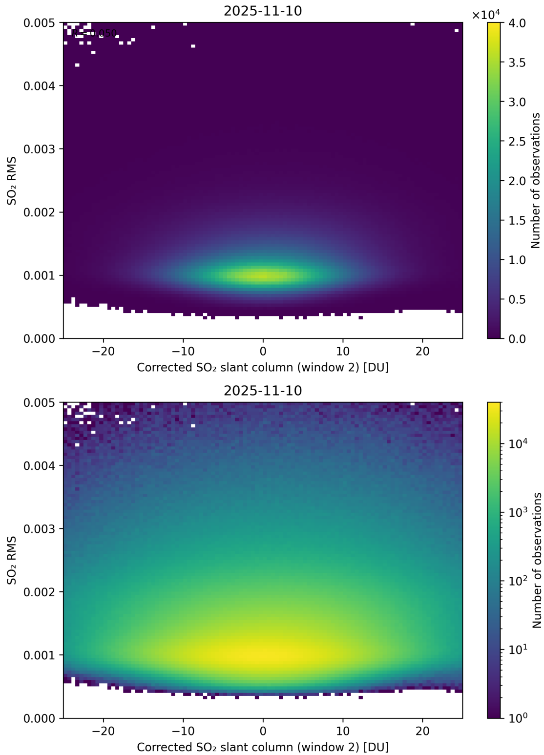
Figure 248: Scatter density plot of “Corrected SO 2 slant column (window 2)” against “SO 2 RMS” for 2025-11-09 to 2025-11-11.
