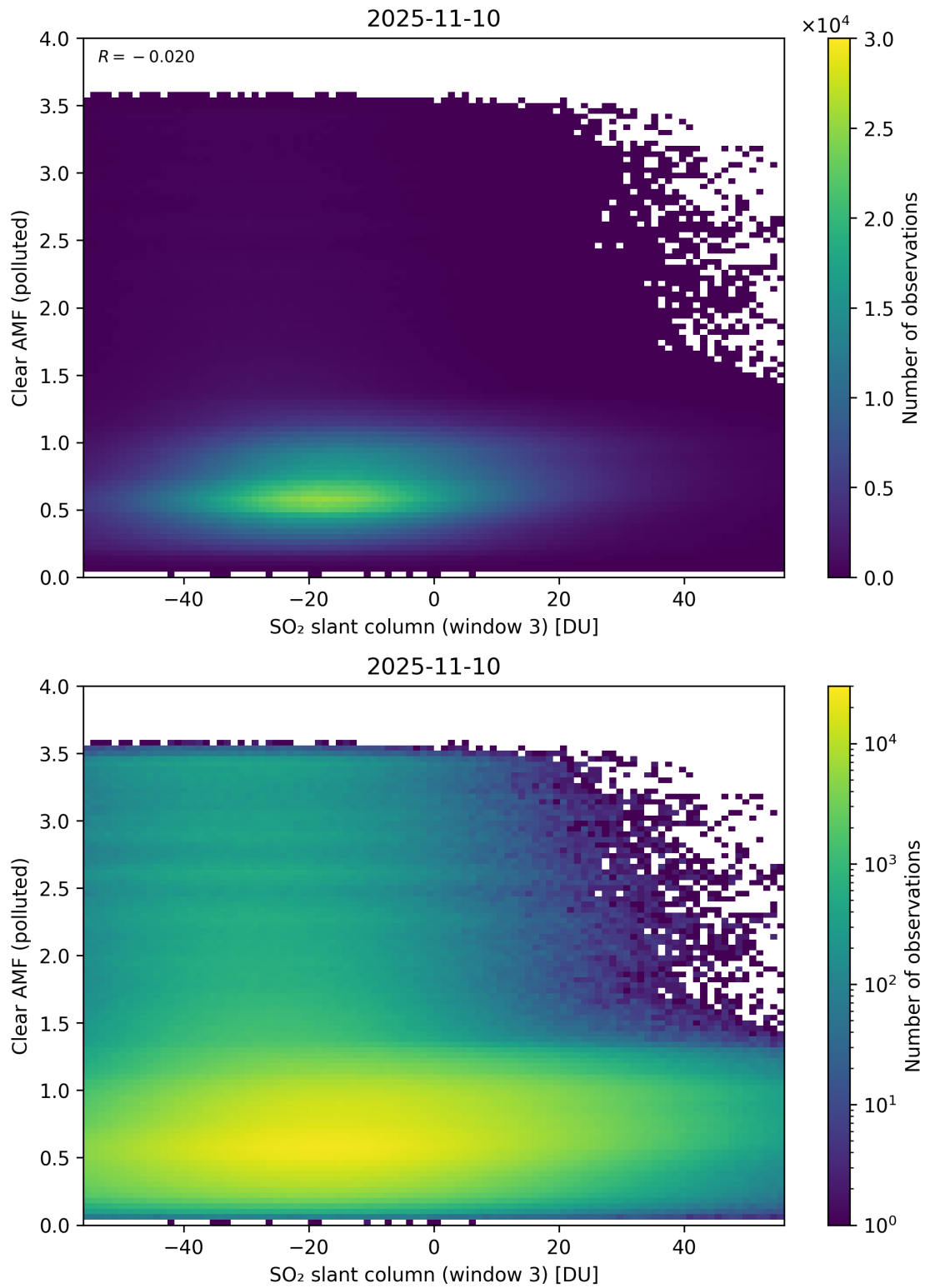
Figure 315: Scatter density plot of “SO 2 slant column (window 3)” against “Clear AMF (polluted)” for 2025-11-09 to 2025-11-11.
