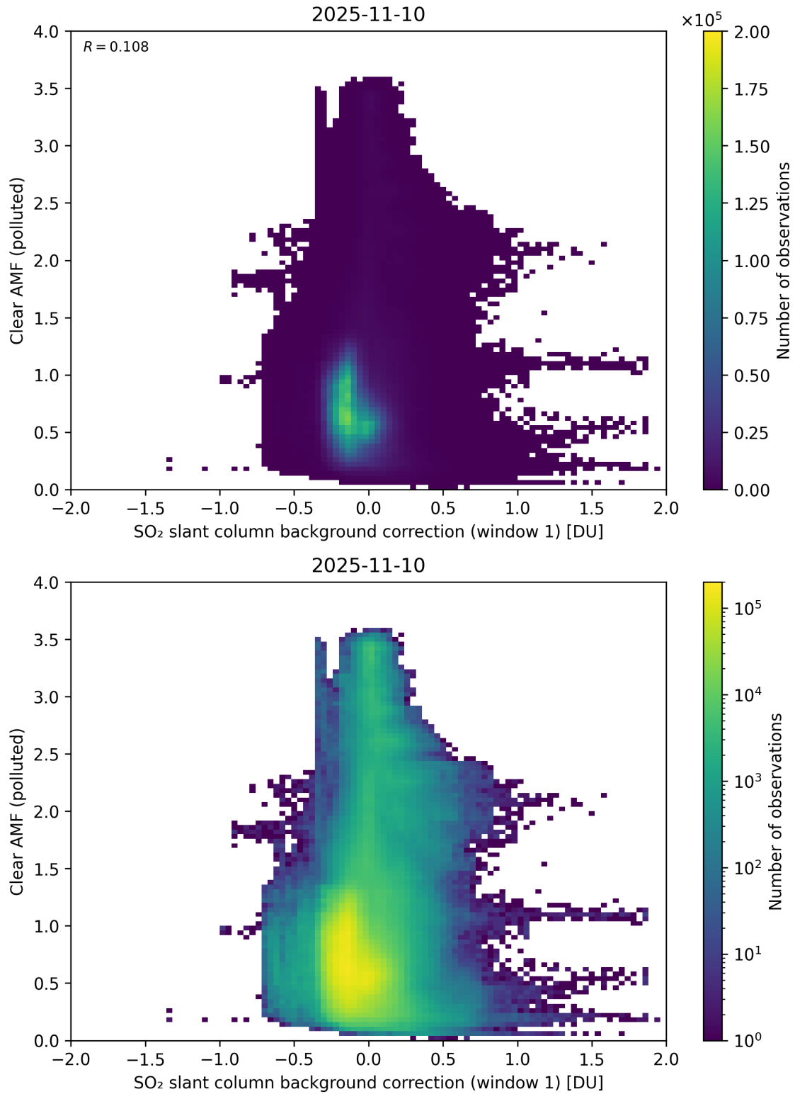
Figure 114: Scatter density plot of “SO 2 slant column background correction (window 1)” against “Clear AMF (polluted)” for 2025-11-09 to 2025-11-11.
