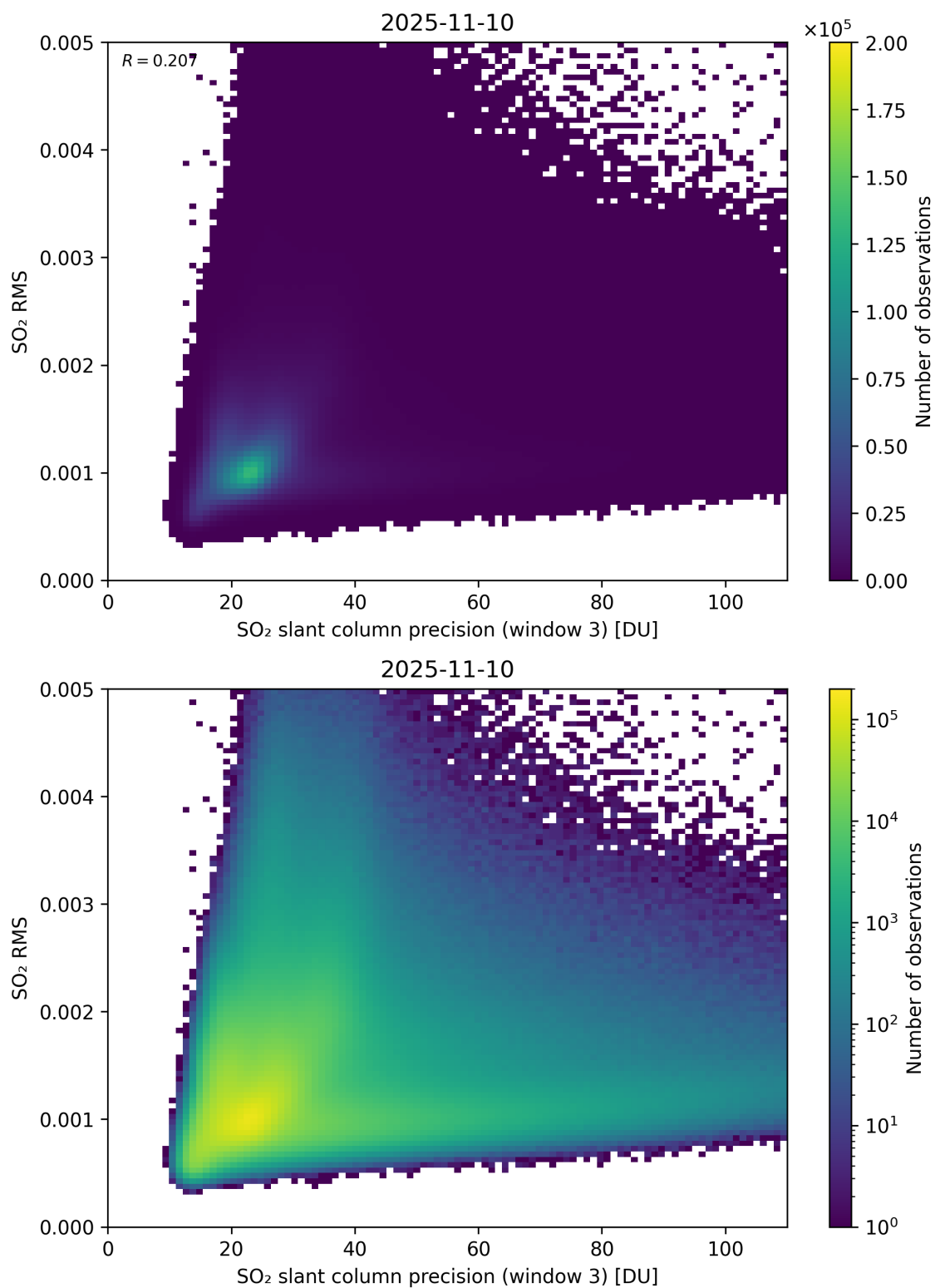
Figure 310: Scatter density plot of “SO 2 slant column precision (window 3)” against “SO 2 RMS” for 2025-11-09 to 2025-11-11.
