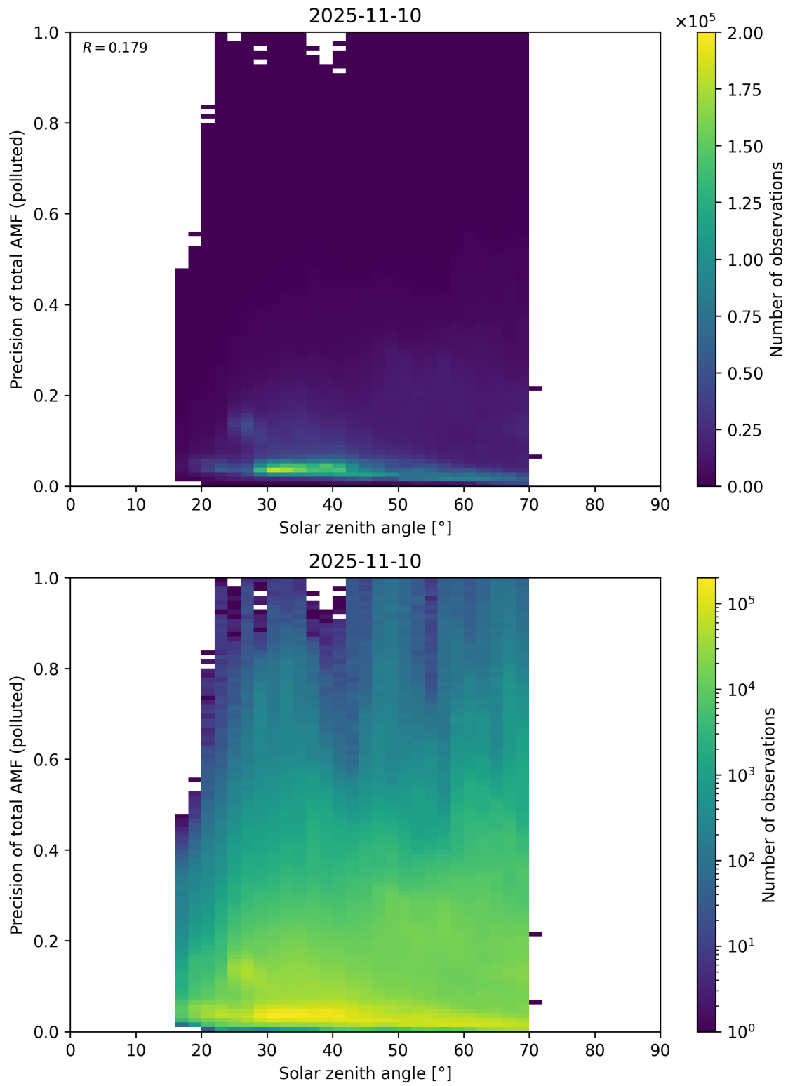
Figure 190: Scatter density plot of “Solar zenith angle” against “Precision of total AMF (polluted)” for 2025-11-09 to 2025-11-11.
