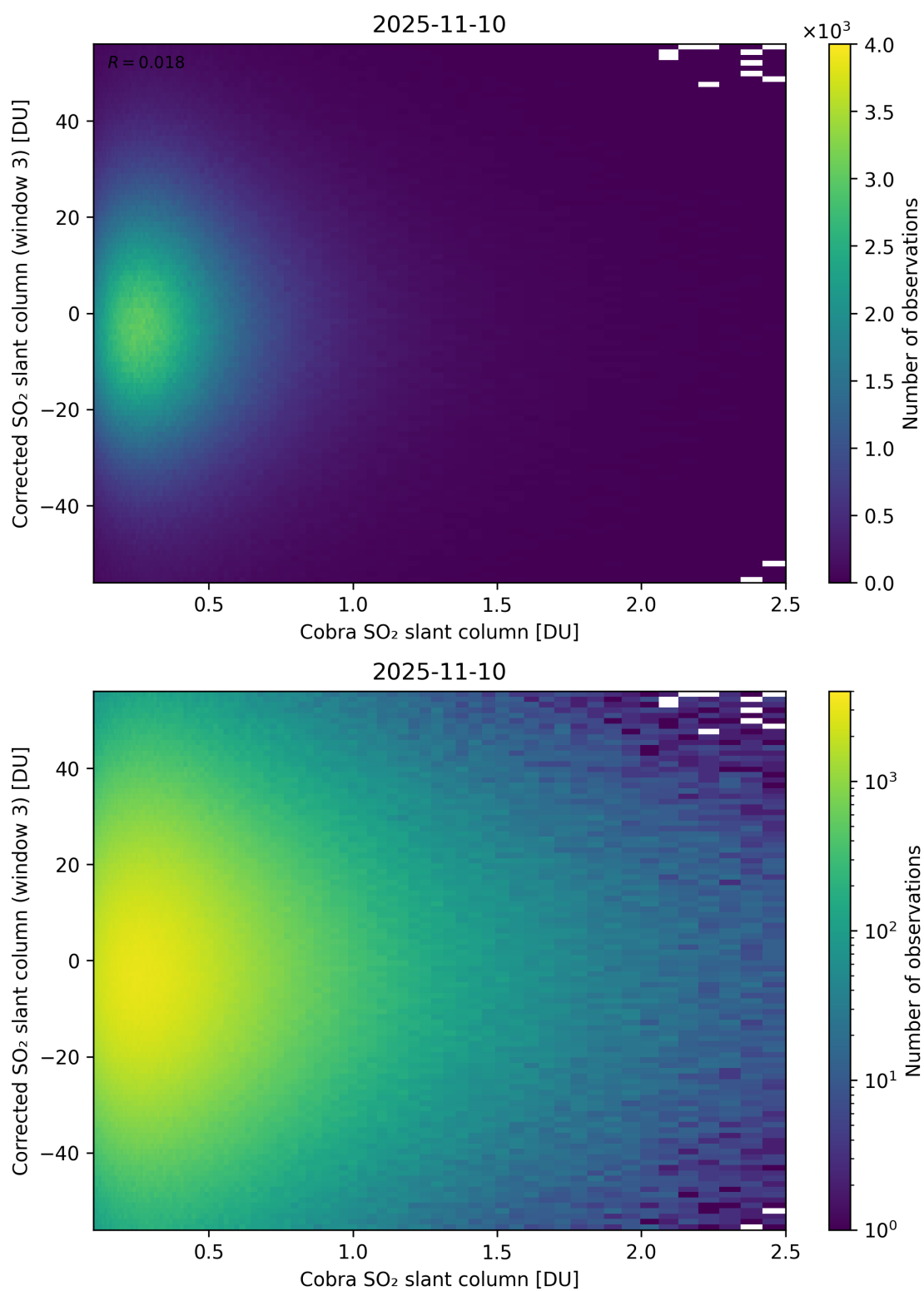
Figure 218: Scatter density plot of “Cobra SO 2 slant column” against “Corrected SO 2 slant column (window 3)” for 2025-11-09 to 2025-11-11.
