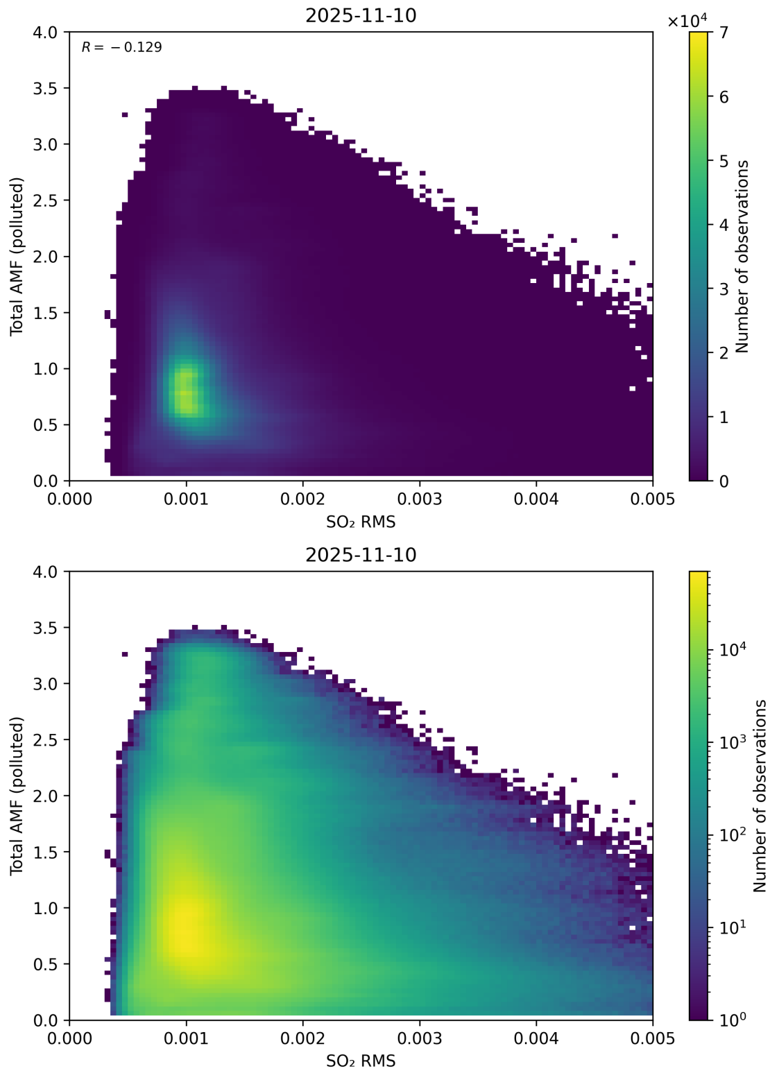
Figure 148: Scatter density plot of “SO 2 RMS” against “Total AMF (polluted)” for 2025-11-09 to 2025-11-11.
