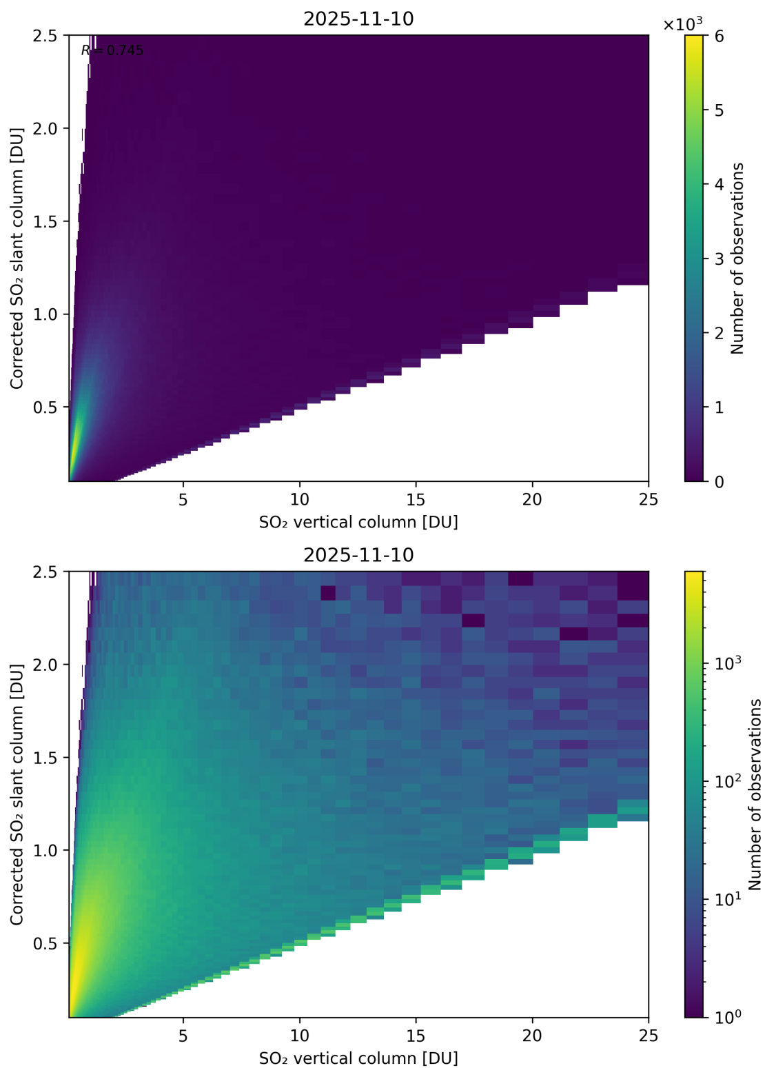
Figure 351: Scatter density plot of “SO 2 vertical column” against “Corrected SO 2 slant column” for 2025-11-09 to 2025-11-11.
