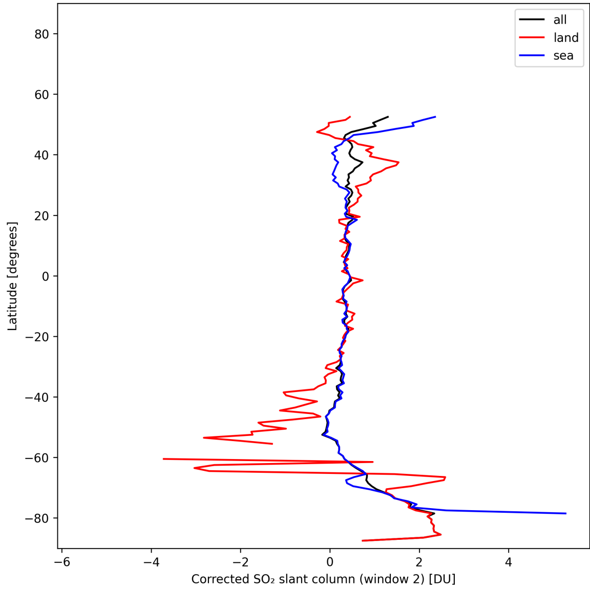
Figure 43: Zonal average of “Corrected SO 2 slant column (window 2)” for 2025-11-09 to 2025-11-11.
