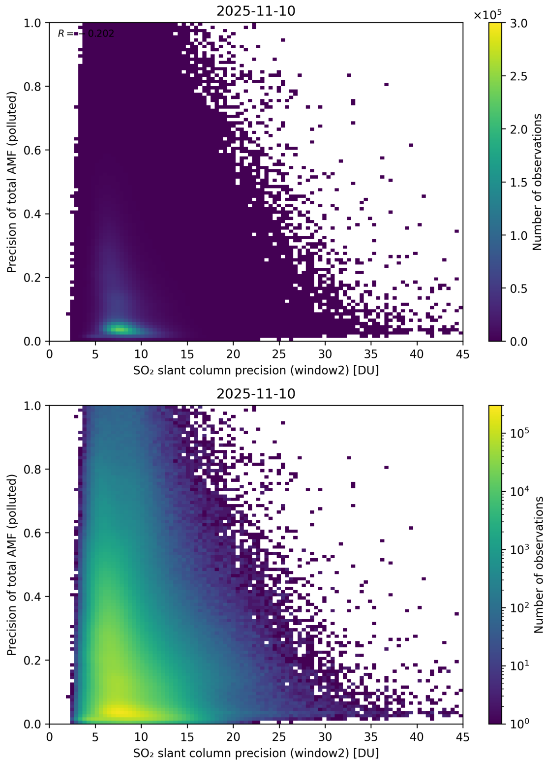
Figure 302: Scatter density plot of “SO 2 slant column precision (window2)” against “Precision of total AMF (polluted)” for 2025-11-09 to 2025-11-11.
