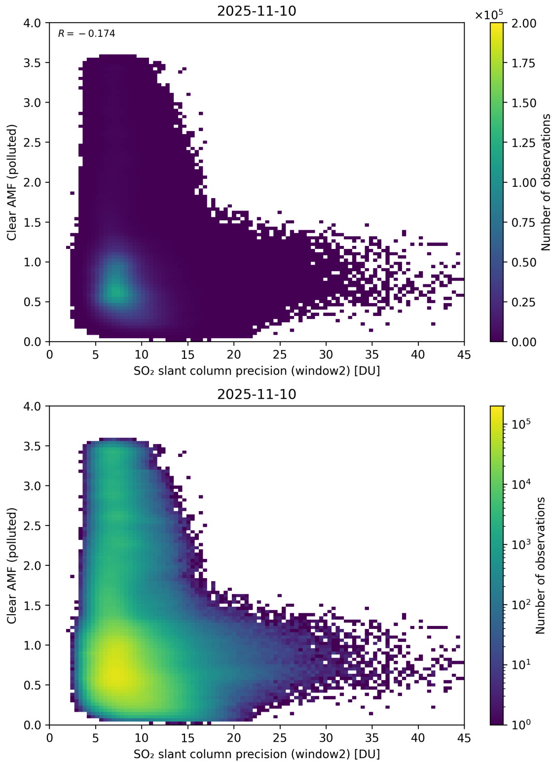
Figure 296: Scatter density plot of “SO 2 slant column precision (window2)” against “Clear AMF (polluted)” for 2025-11-09 to 2025-11-11.
