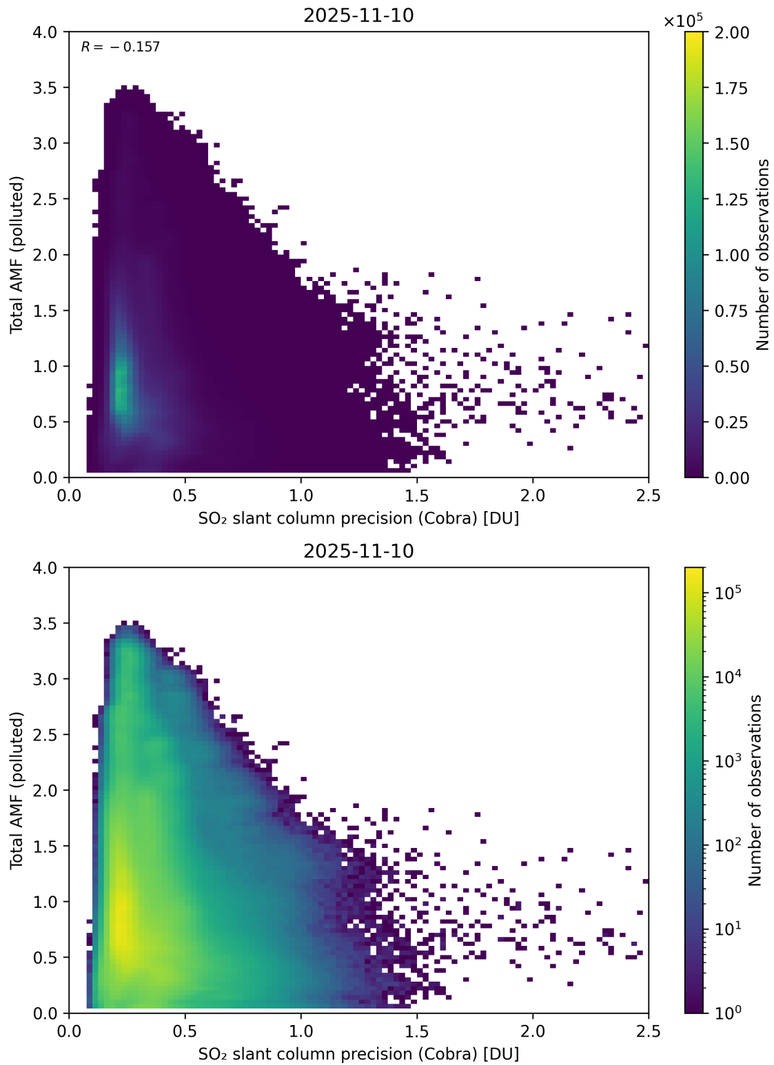
Figure 213: Scatter density plot of “SO 2 slant column precision (Cobra)” against “Total AMF (polluted)” for 2025-11-09 to 2025-11-11.
