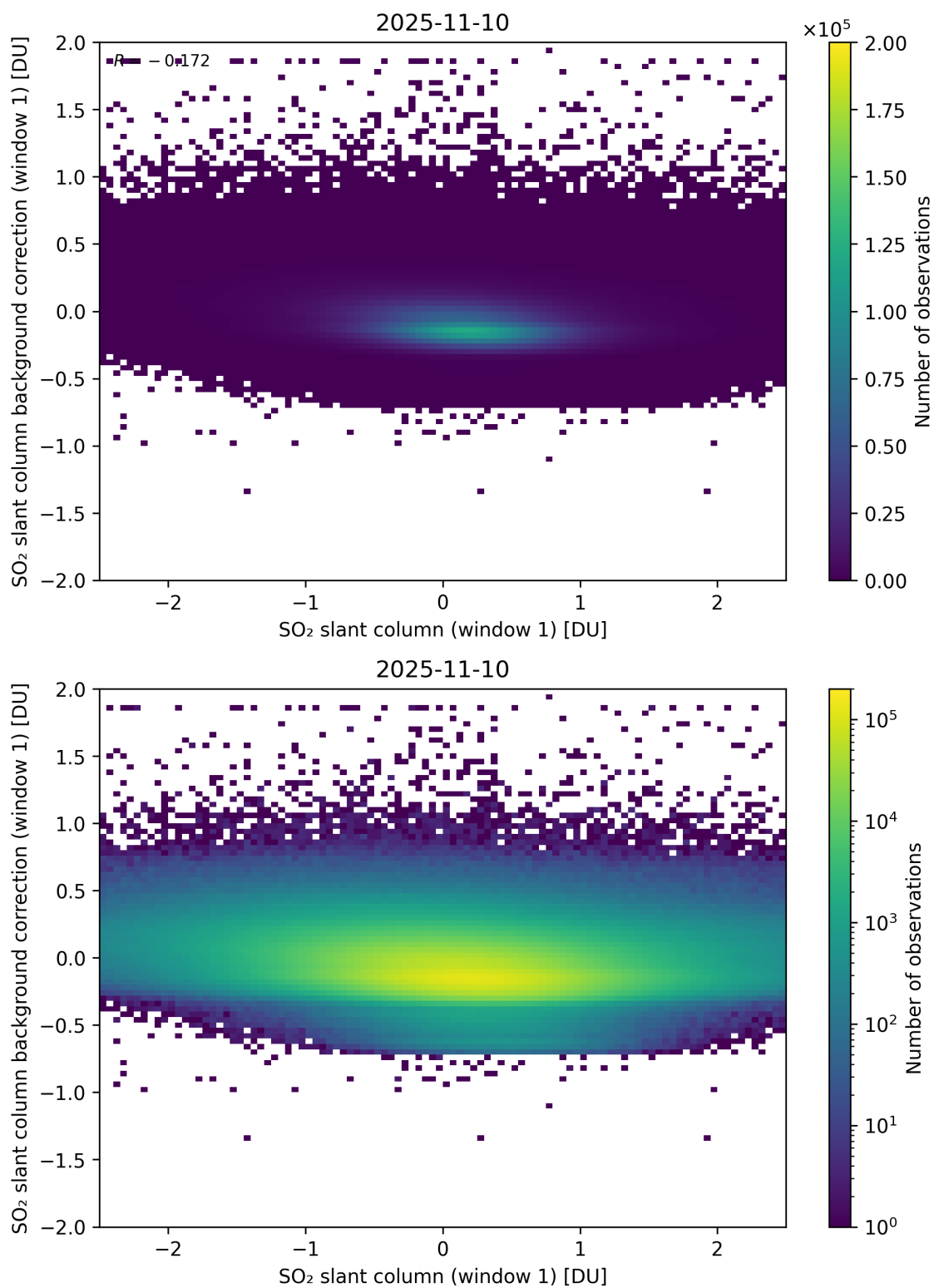
Figure 262: Scatter density plot of “SO 2 slant column (window 1)” against “SO 2 slant column background correction (window 1)” for 2025-11-09 to 2025-11-11.
