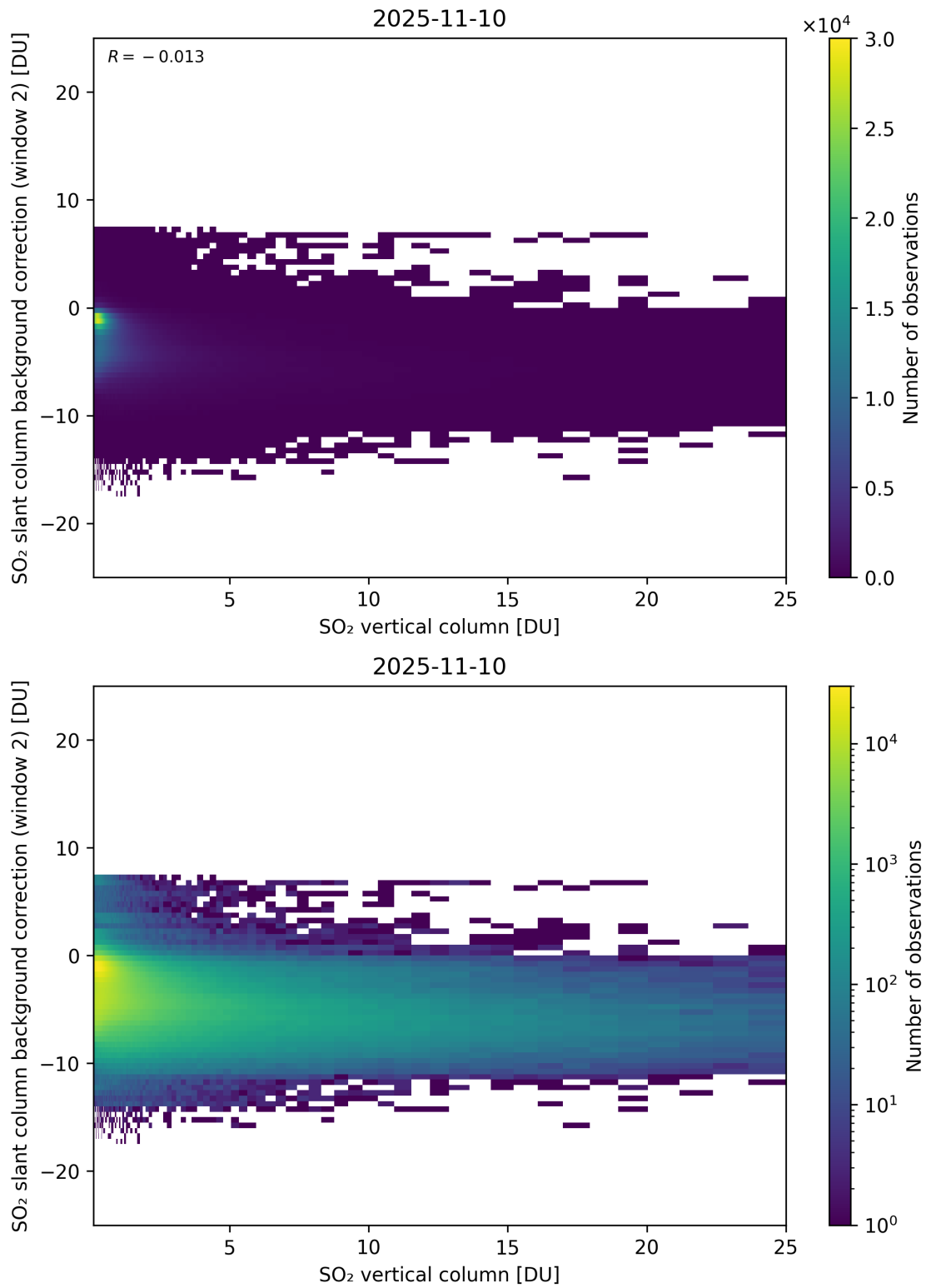
Figure 324: Scatter density plot of “SO 2 vertical column” against “SO 2 slant column background correction (window 2)” for 2025-11-09 to 2025-11-11.
