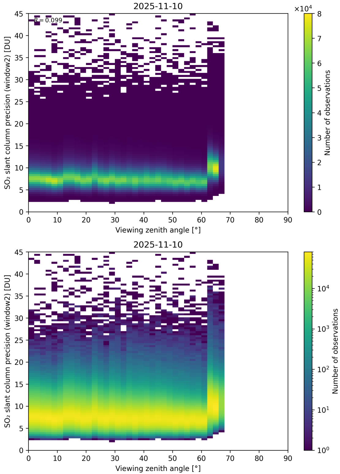
Figure 378: Scatter density plot of “Viewing zenith angle” against “SO 2 slant column precision (window2)” for 2025-11-09 to 2025-11-11.
