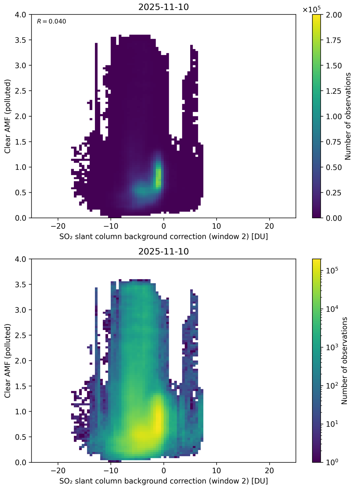
Figure 126: Scatter density plot of “SO 2 slant column background correction (window 2)” against “Clear AMF (polluted)” for 2025-11-09 to 2025-11-11.
