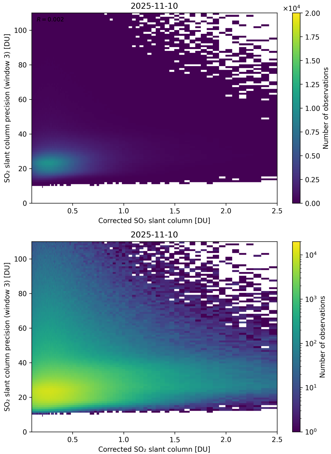
Figure 241: Scatter density plot of “Corrected SO 2 slant column” against “SO 2 slant column precision (window 3)” for 2025-11-09 to 2025-11-11.
