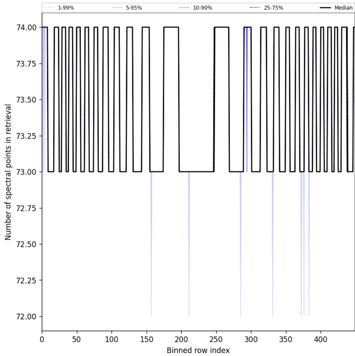
Figure 108: Along track statistics of “Number of spectral points in retrieval” for 2025-11-09 to 2025-11-11
