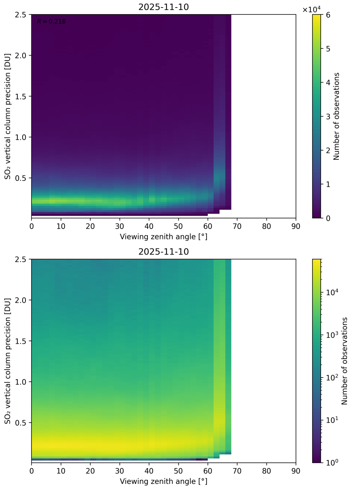
Figure 384: Scatter density plot of “Viewing zenith angle” against “SO 2 vertical column precision” for 2025-11-09 to 2025-11-11.
