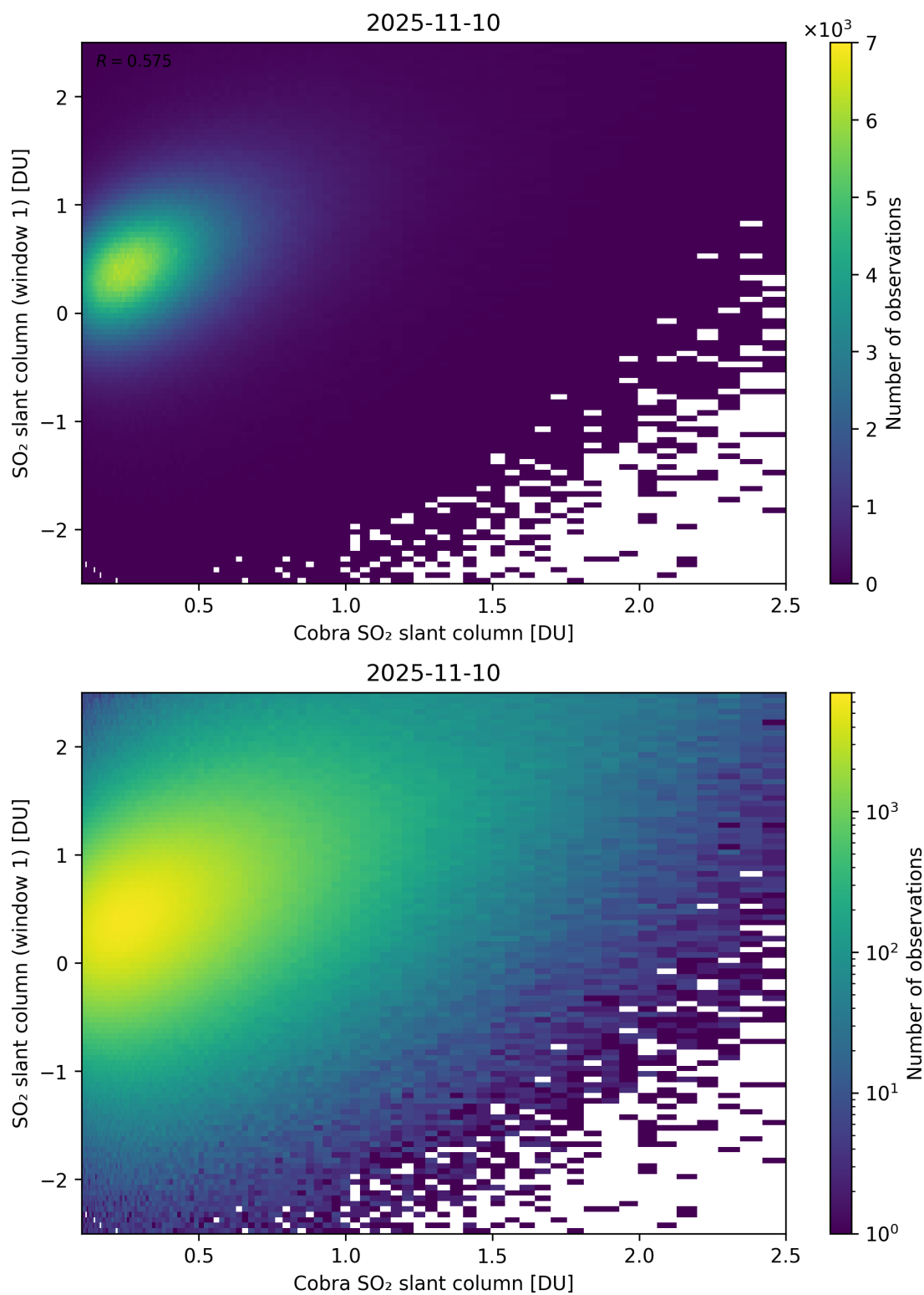
Figure 219: Scatter density plot of “Cobra SO 2 slant column” against “SO 2 slant column (window 1)” for 2025-11-09 to 2025-11-11.
