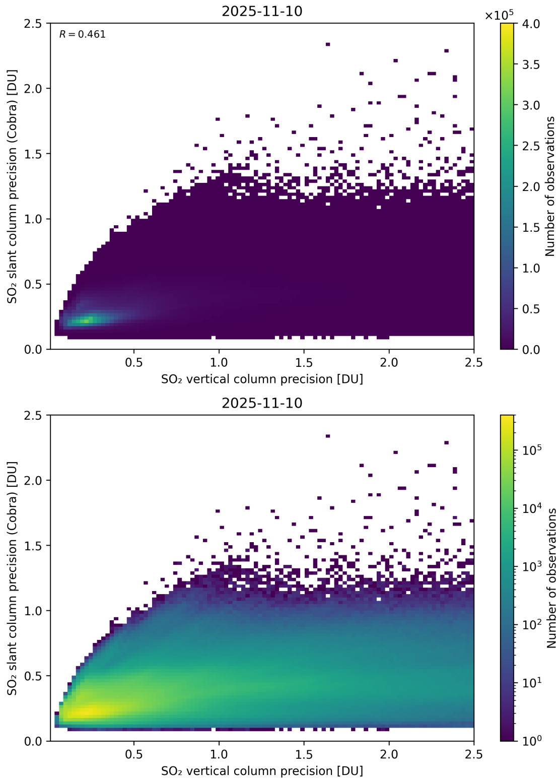
Figure 337: Scatter density plot of “SO 2 vertical column precision” against “SO 2 slant column precision (Cobra)” for 2025-11-09 to 2025-11-11.
