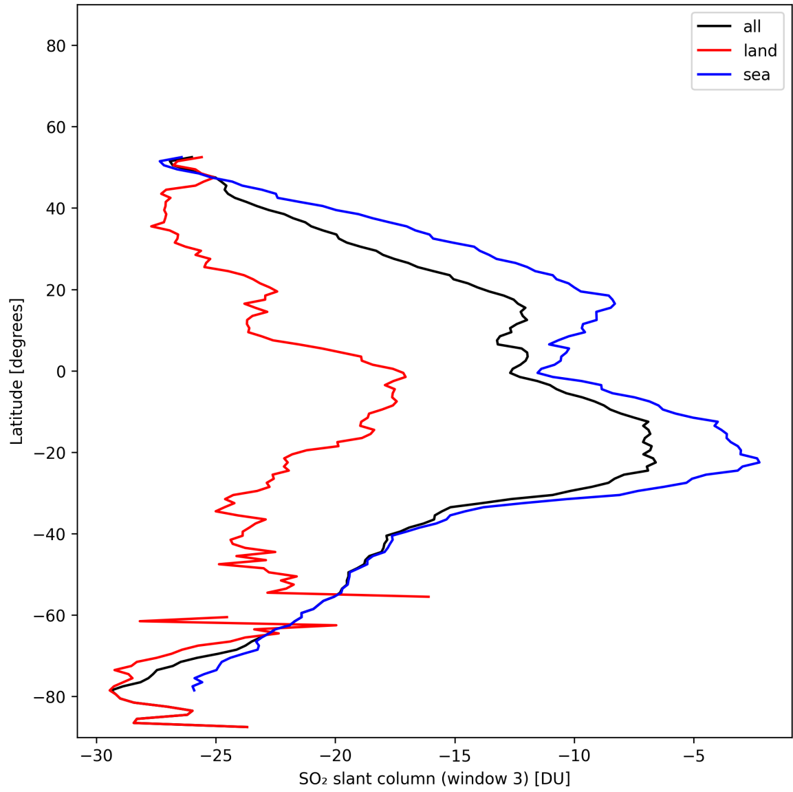
Figure 45: Zonal average of “SO 2 slant column (window 3)” for 2025-11-09 to 2025-11-11.
