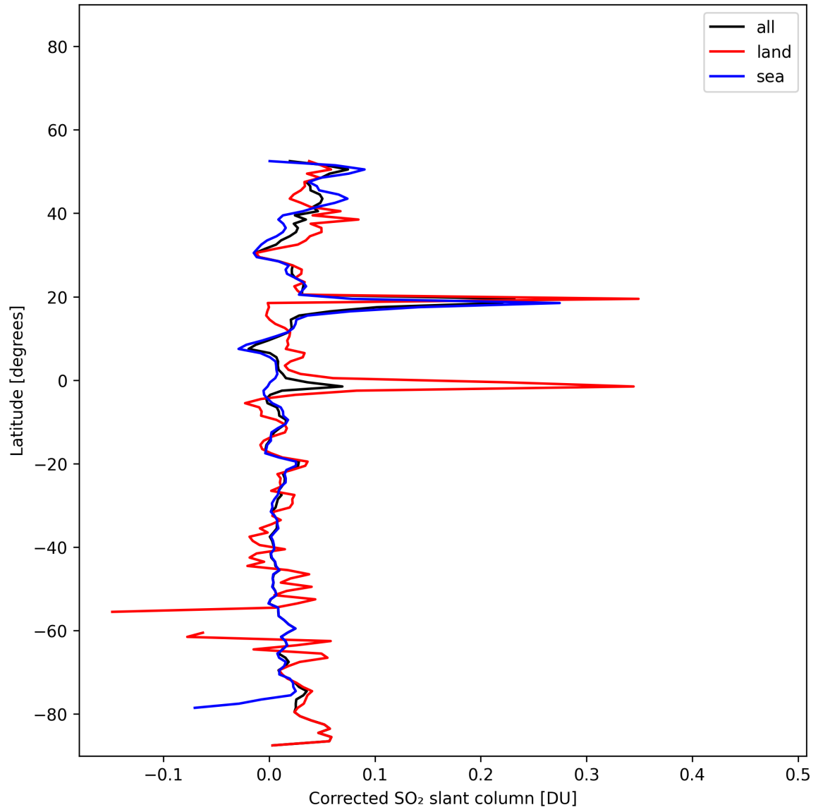
Figure 34: Zonal average of “Corrected SO 2 slant column” for 2025-11-09 to 2025-11-11.
