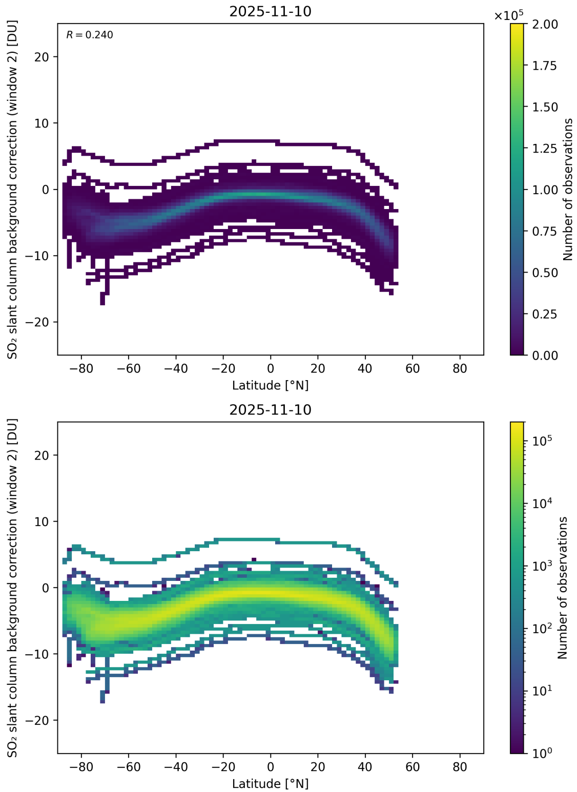
Figure 151: Scatter density plot of “Latitude” against “SO 2 slant column background correction (window 2)” for 2025-11-09 to 2025-11-11.
