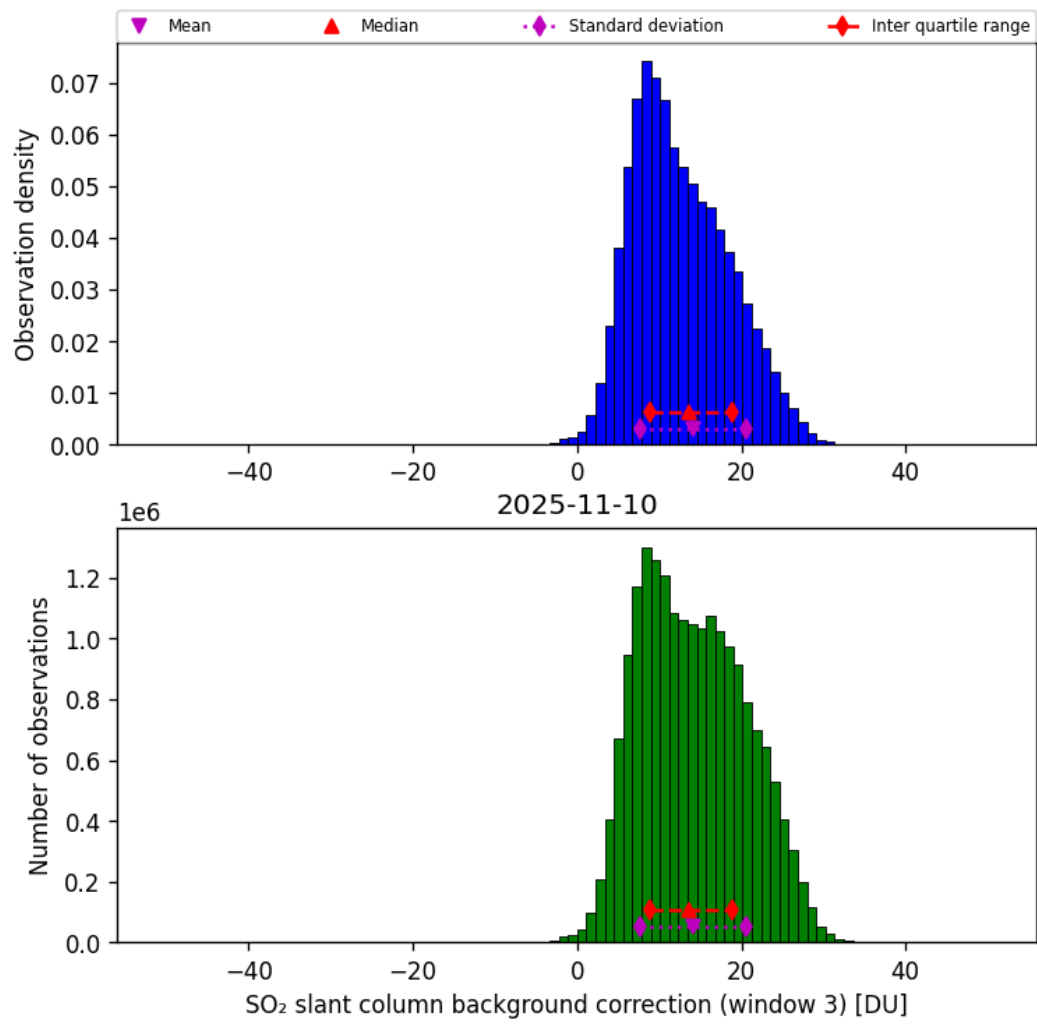
Figure 74: Histogram of “SO 2 slant column background correction (window 3)” for 2025-11-09 to 2025-11-11
