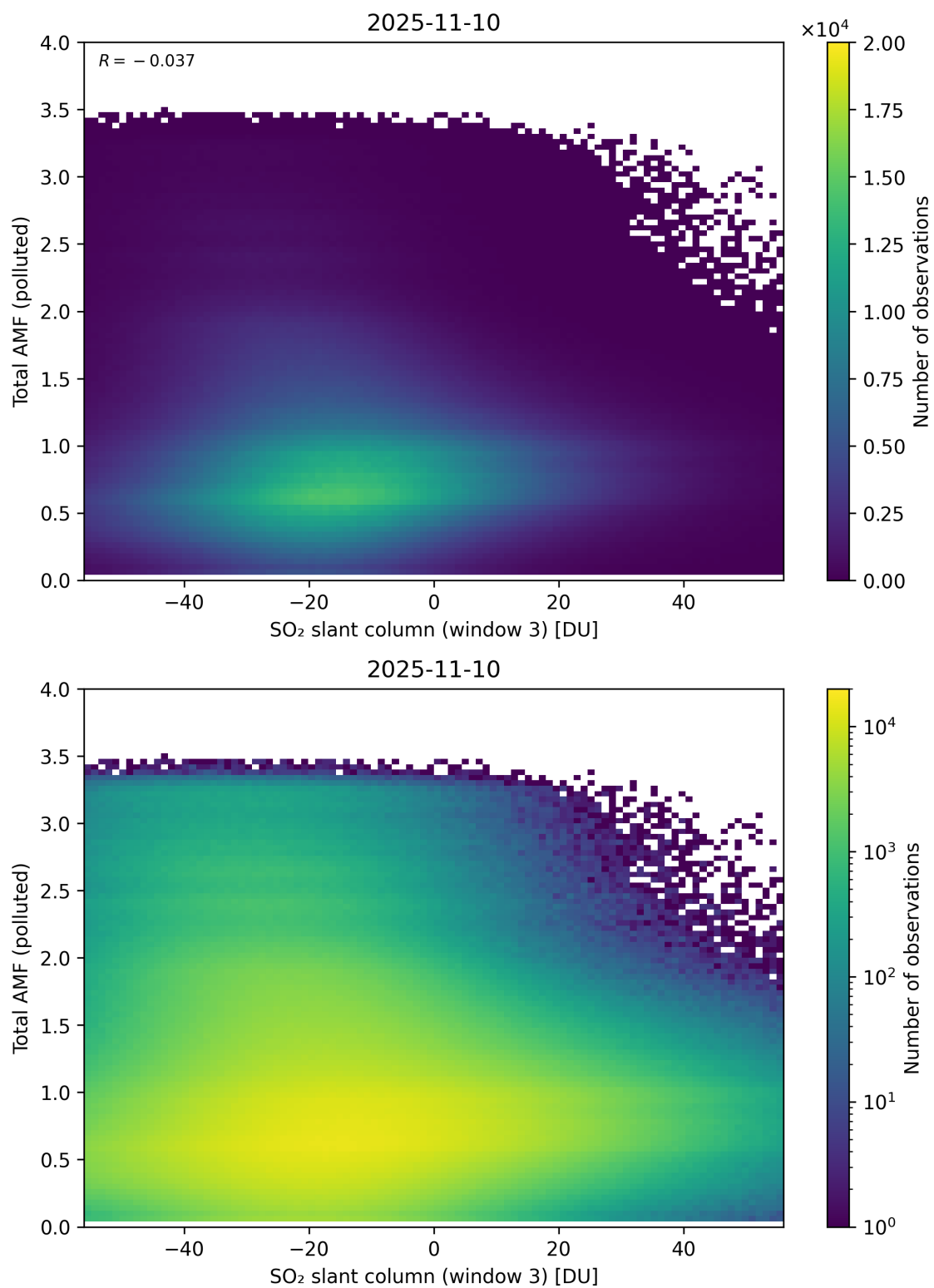
Figure 318: Scatter density plot of “SO 2 slant column (window 3)” against “Total AMF (polluted)” for 2025-11-09 to 2025-11-11.
