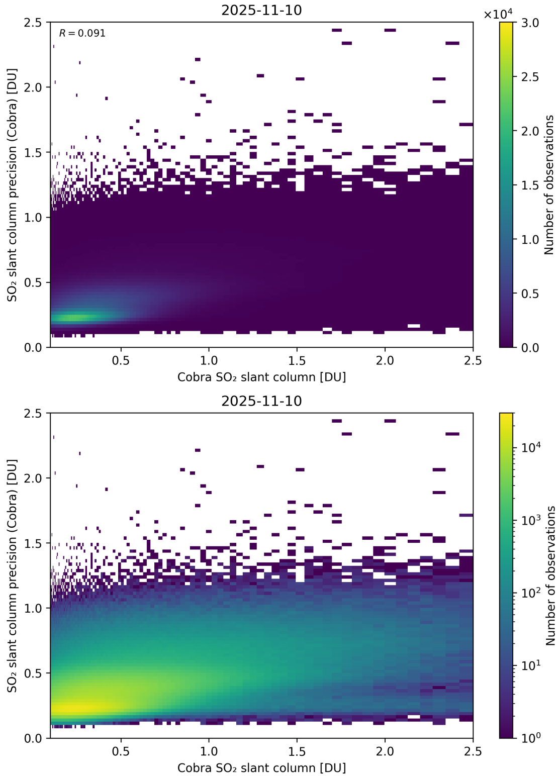
Figure 216: Scatter density plot of “Cobra SO 2 slant column” against “SO 2 slant column precision (Cobra)” for 2025-11-09 to 2025-11-11.
