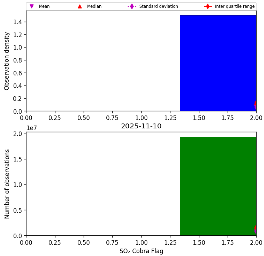
Figure 75: Histogram of “SO 2 Cobra Flag” for 2025-11-09 to 2025-11-11
