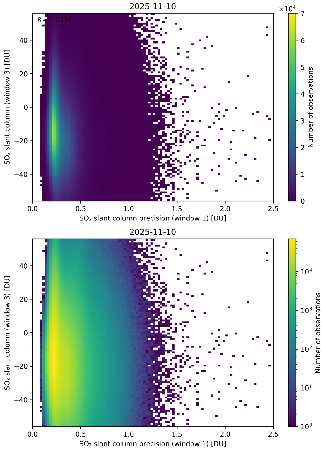
Figure 278: Scatter density plot of “SO 2 slant column precision (window 1)” against “SO 2 slant column (window 3)” for 2025-11-09 to 2025-11-11.
