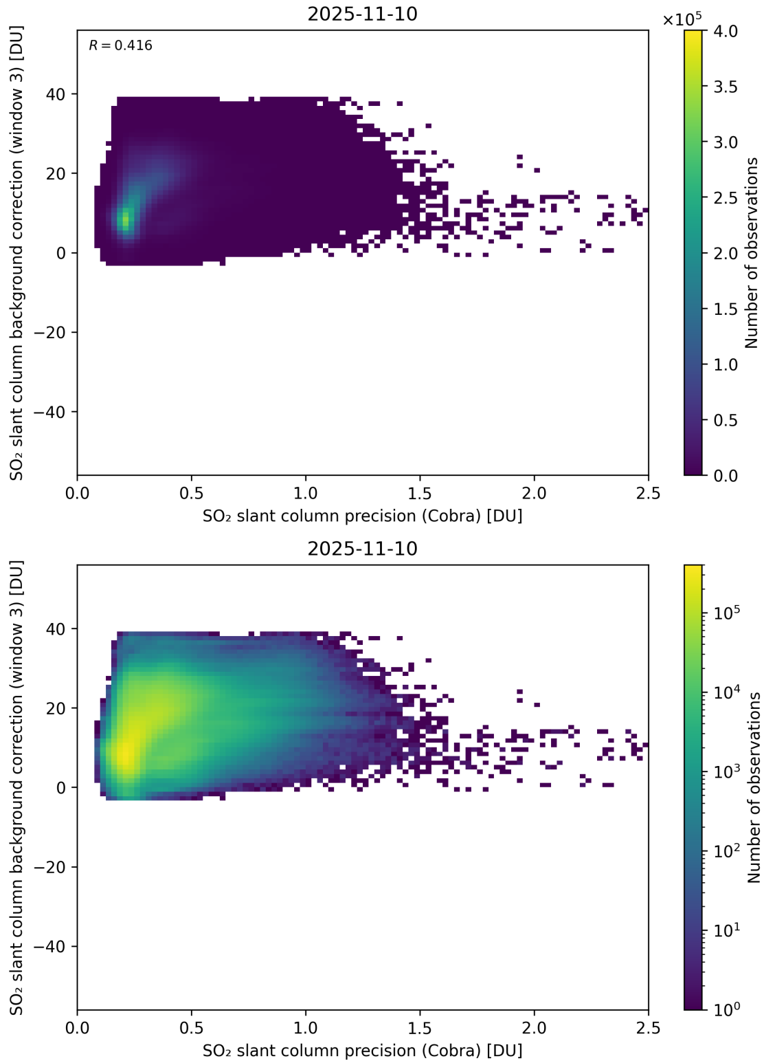
Figure 201: Scatter density plot of “SO 2 slant column precision (Cobra)” against “SO 2 slant column background correction (window 3)” for 2025-11-09 to 2025-11-11.
