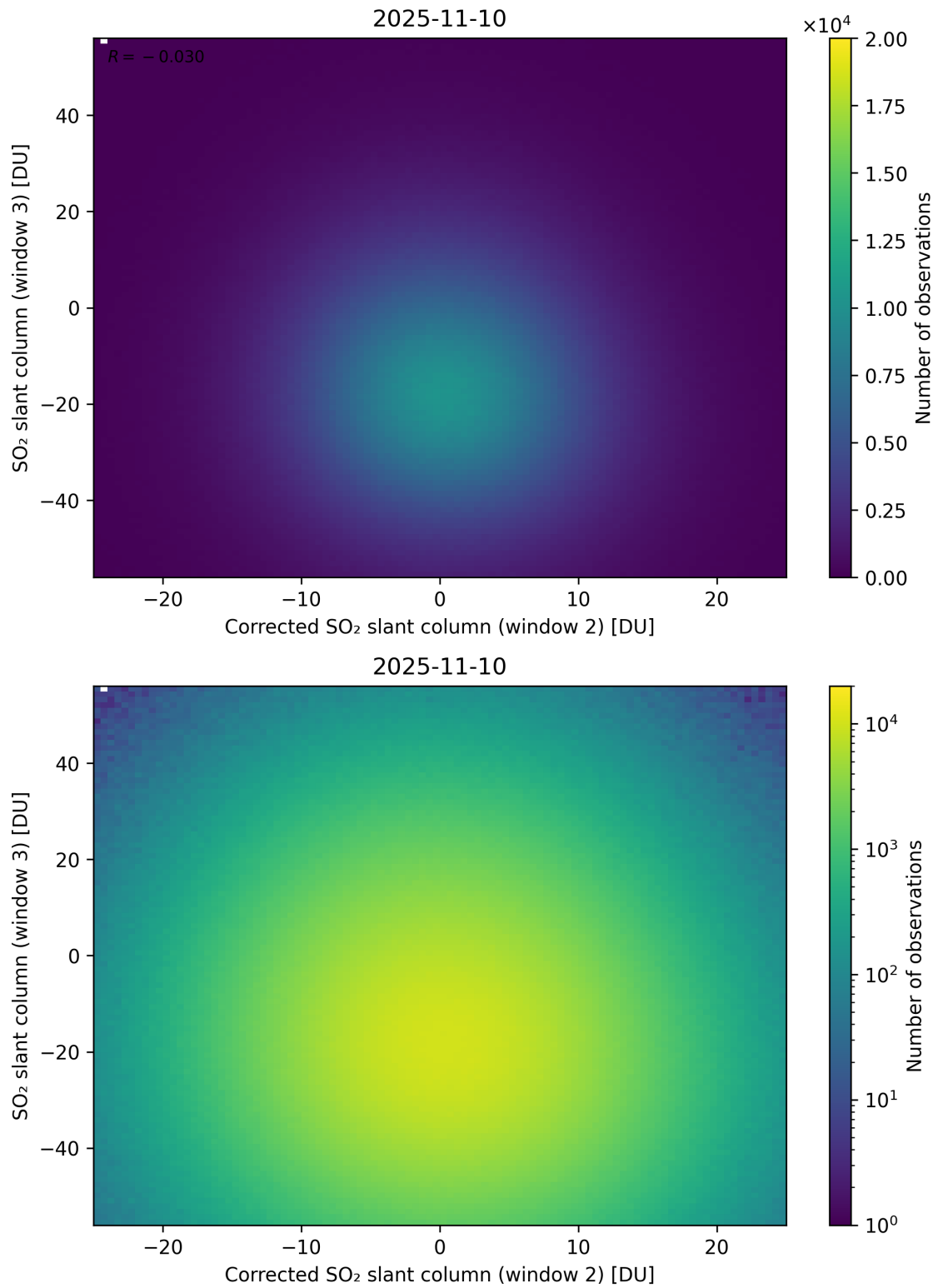
Figure 251: Scatter density plot of “Corrected SO 2 slant column (window 2)” against “SO 2 slant column (window 3)” for 2025-11-09 to 2025-11-11.
