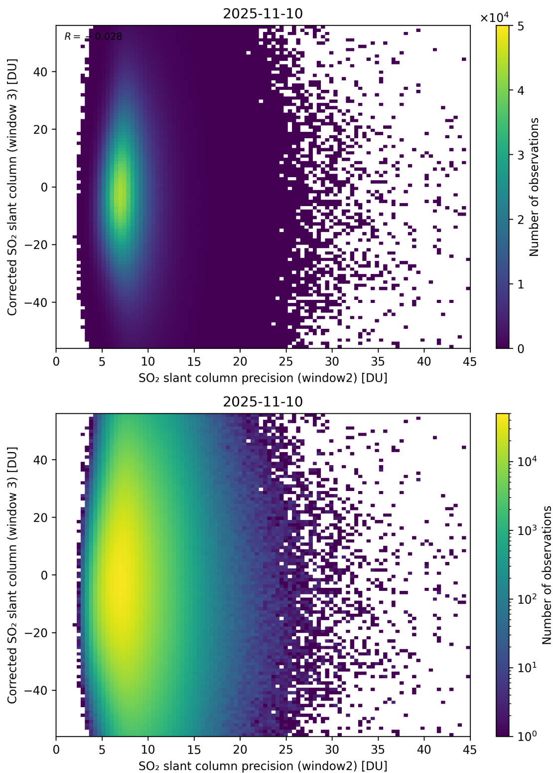
Figure 298: Scatter density plot of “SO 2 slant column precision (window2)” against “Corrected SO 2 slant column (window 3)” for 2025-11-09 to 2025-11-11.
