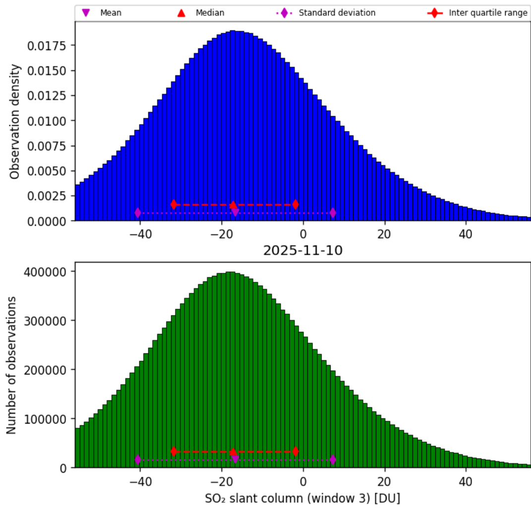
Figure 71: Histogram of “SO 2 slant column (window 3)” for 2025-11-09 to 2025-11-11
