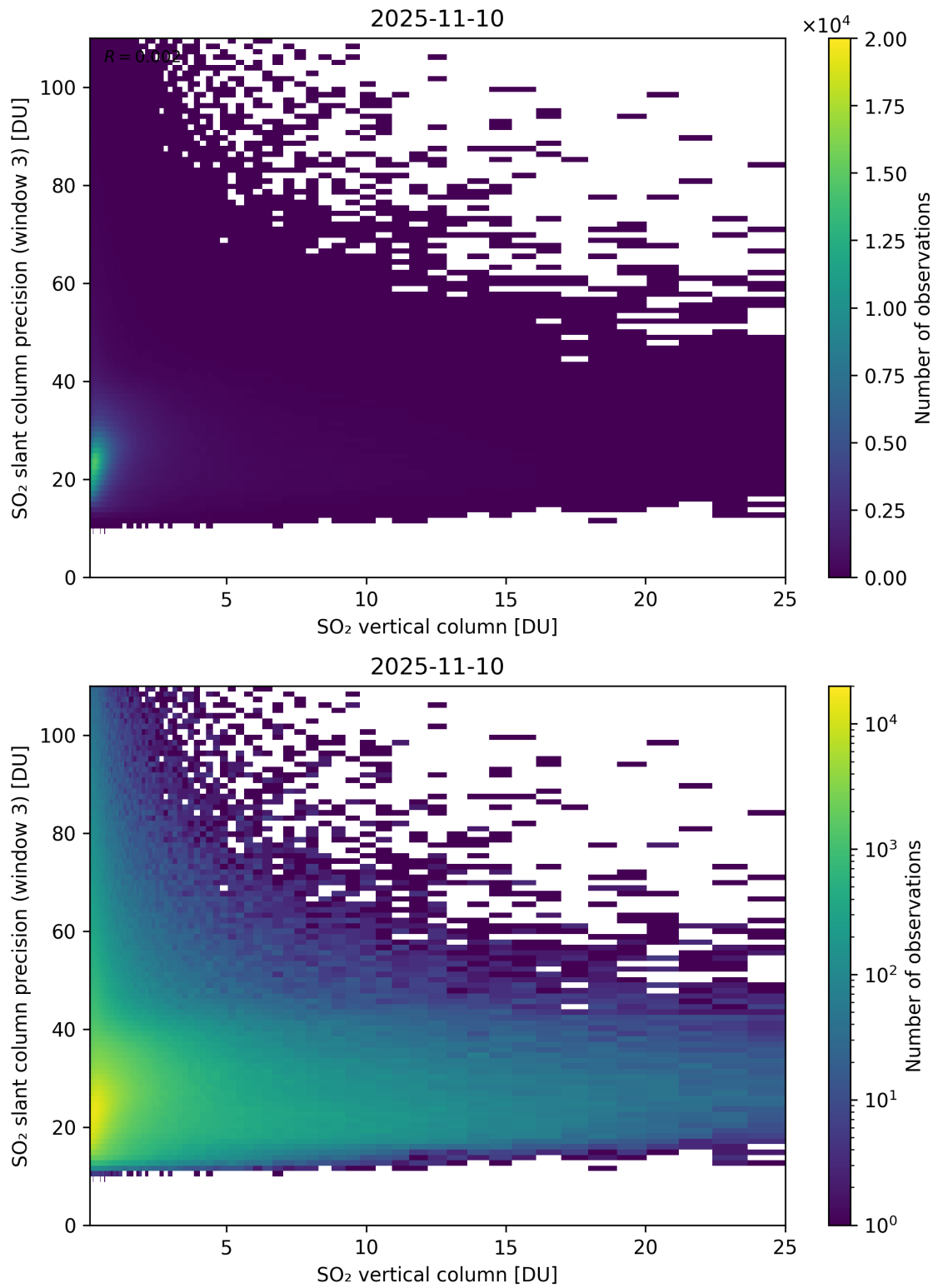
Figure 358: Scatter density plot of “SO 2 vertical column” against “SO 2 slant column precision (window 3)” for 2025-11-09 to 2025-11-11.
