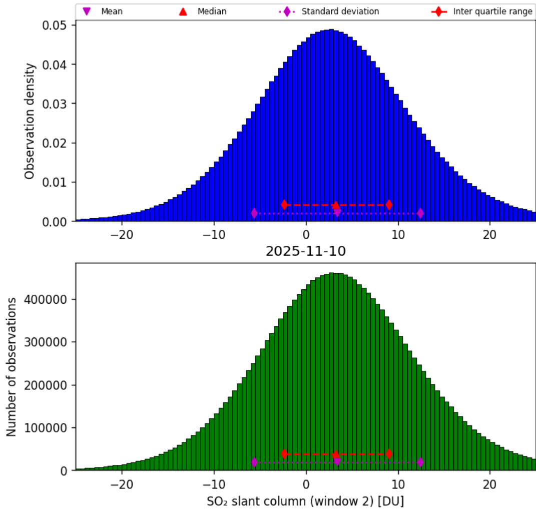
Figure 67: Histogram of “SO 2 slant column (window 2)” for 2025-11-09 to 2025-11-11
