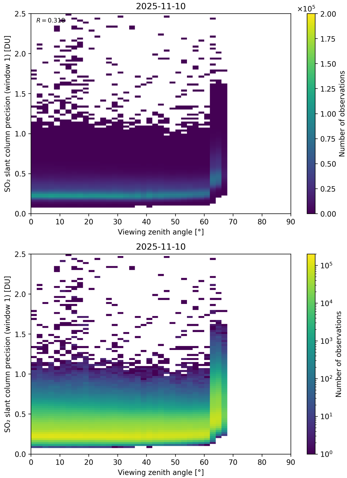
Figure 377: Scatter density plot of “Viewing zenith angle” against “SO 2 slant column precision (window 1)” for 2025-11-09 to 2025-11-11.
