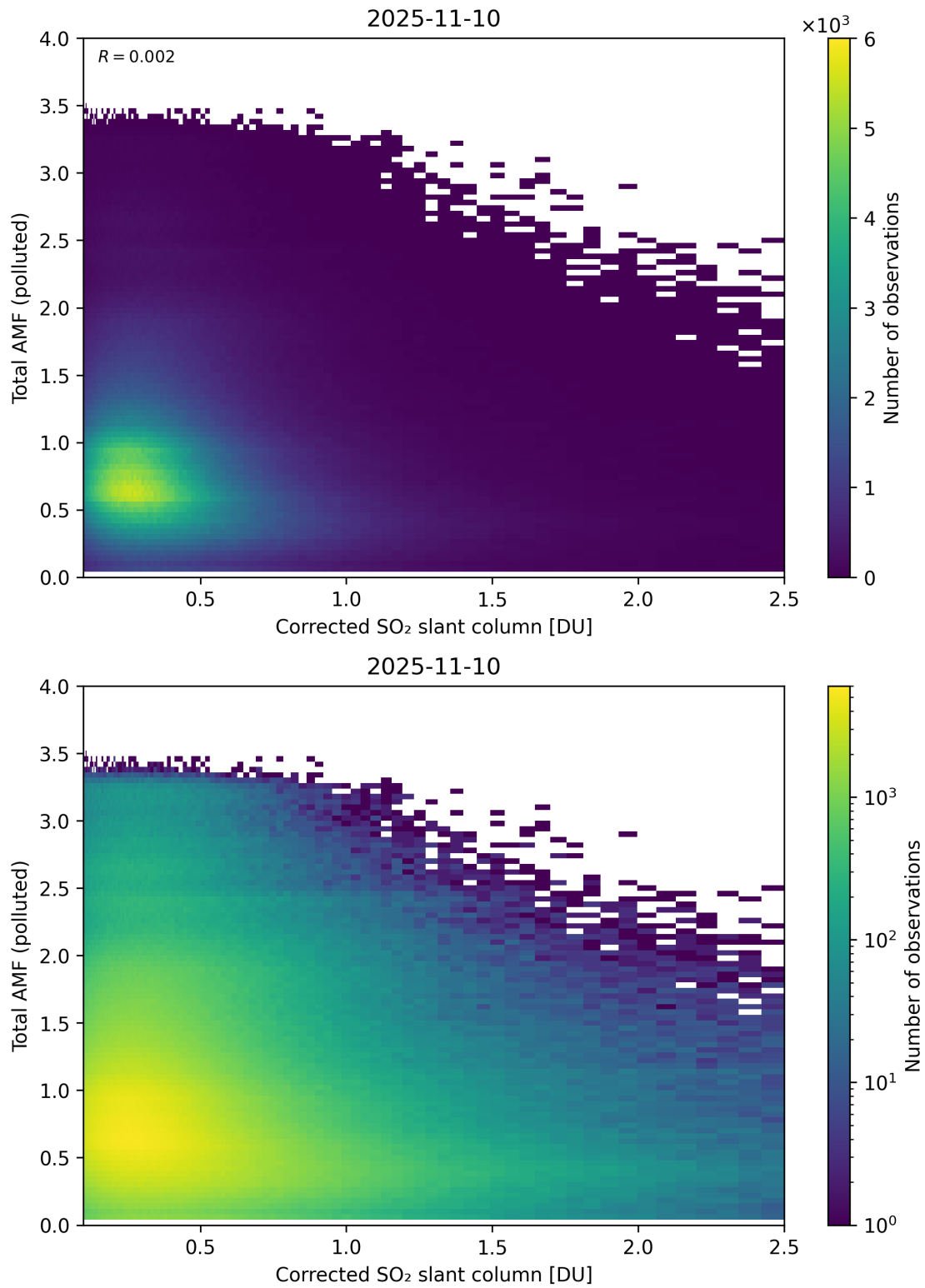
Figure 242: Scatter density plot of “Corrected SO 2 slant column” against “Total AMF (polluted)” for 2025-11-09 to 2025-11-11.
