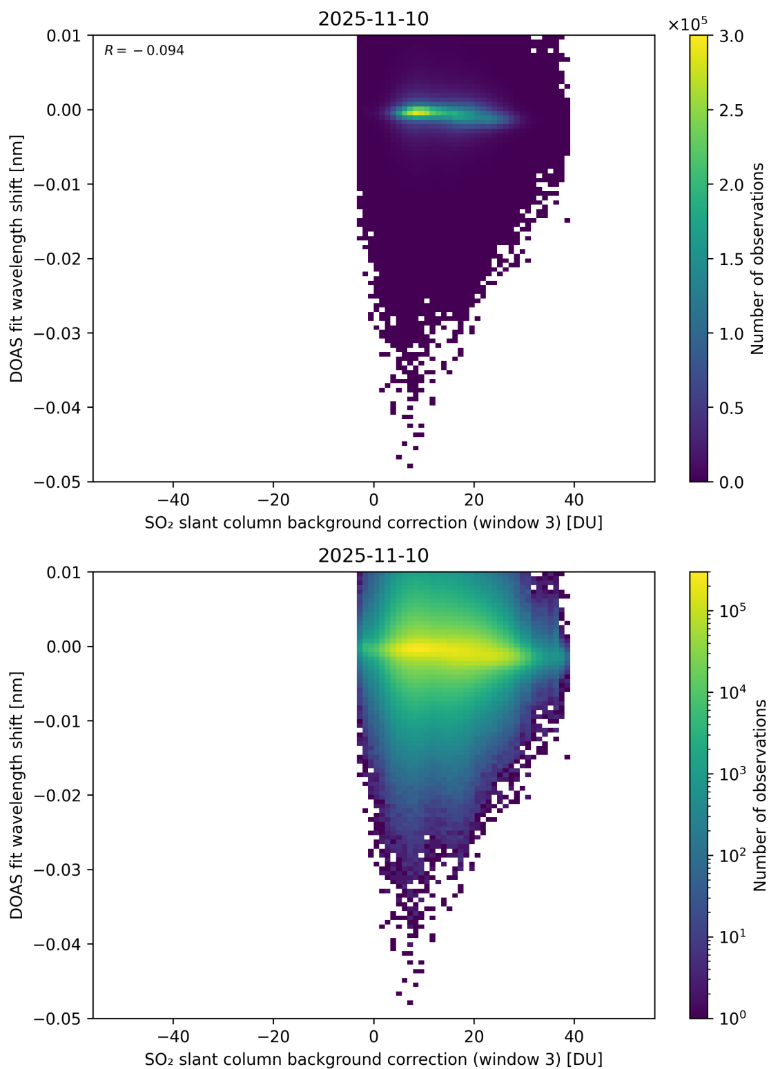
Figure 132: Scatter density plot of “SO 2 slant column background correction (window 3)” against “DOAS fit wavelength shift” for 2025-11-09 to 2025-11-11.
