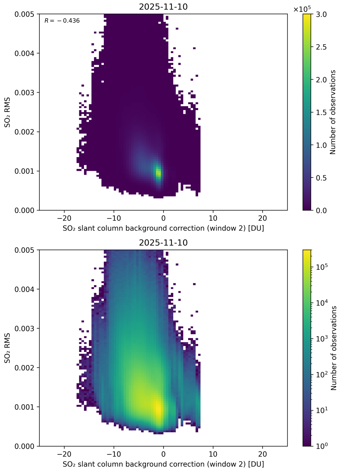
Figure 125: Scatter density plot of “SO 2 slant column background correction (window 2)” against “SO 2 RMS” for 2025-11-09 to 2025-11-11.
