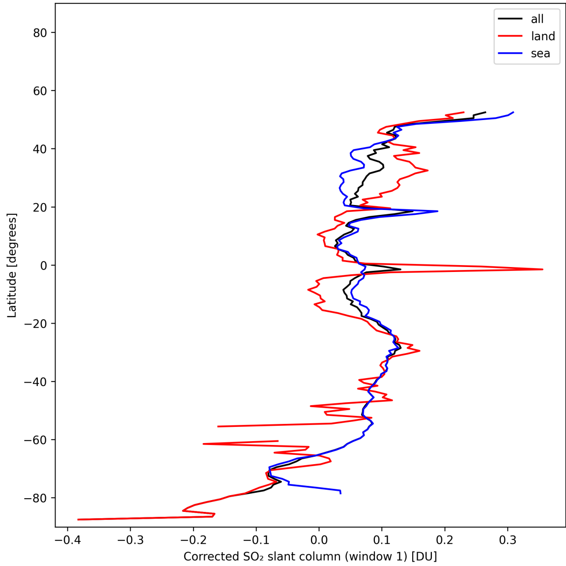
Figure 39: Zonal average of “Corrected SO 2 slant column (window 1)” for 2025-11-09 to 2025-11-11.
