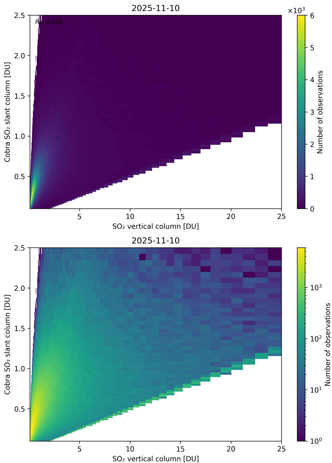
Figure 349: Scatter density plot of “SO 2 vertical column” against “Cobra SO 2 slant column” for 2025-11-09 to 2025-11-11.
