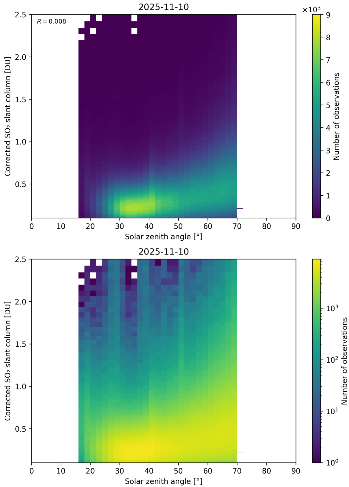
Figure 181: Scatter density plot of “Solar zenith angle” against “Corrected SO 2 slant column” for 2025-11-09 to 2025-11-11.
