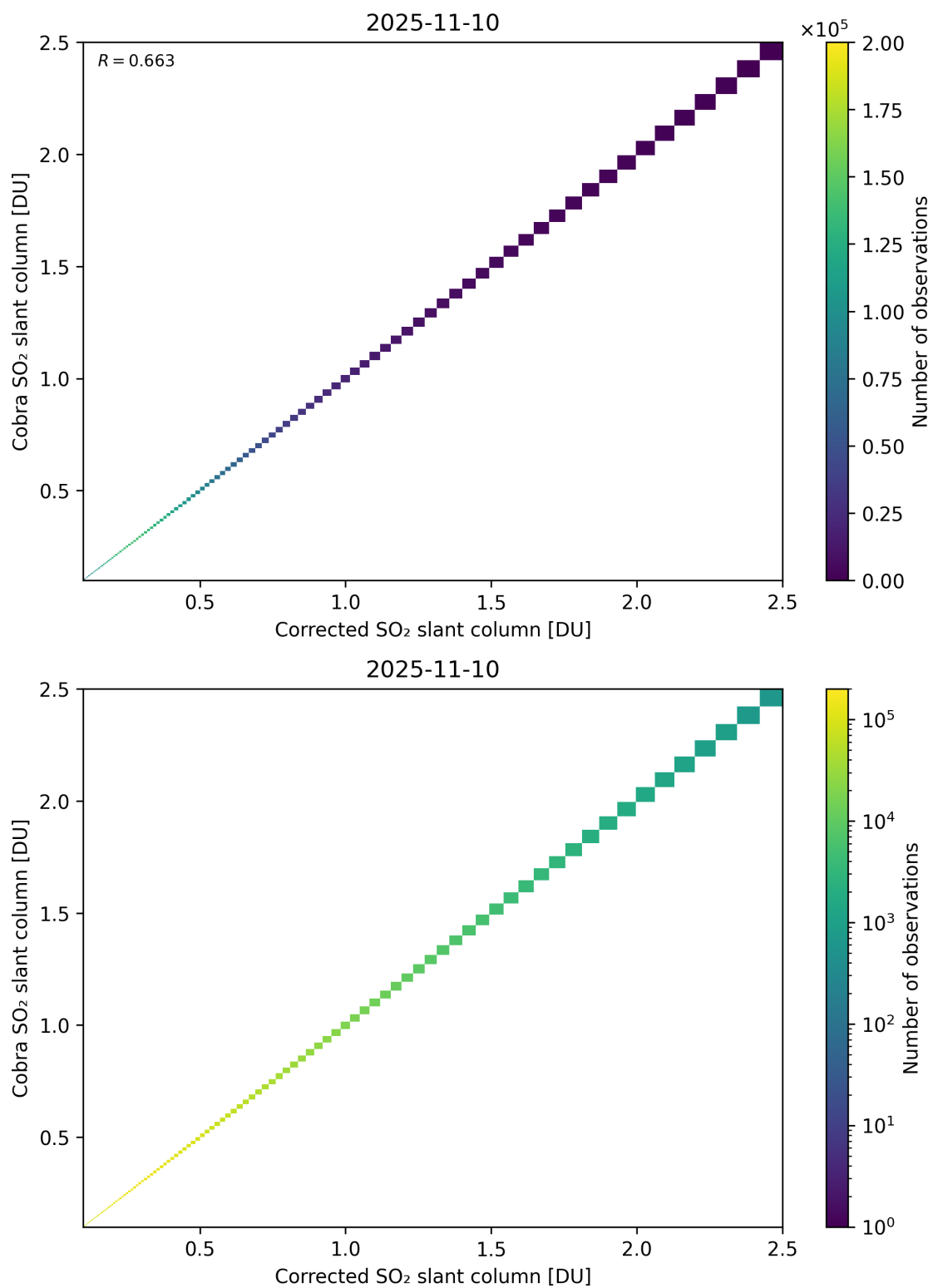
Figure 233: Scatter density plot of “Corrected SO 2 slant column” against “Cobra SO 2 slant column” for 2025-11-09 to 2025-11-11.
