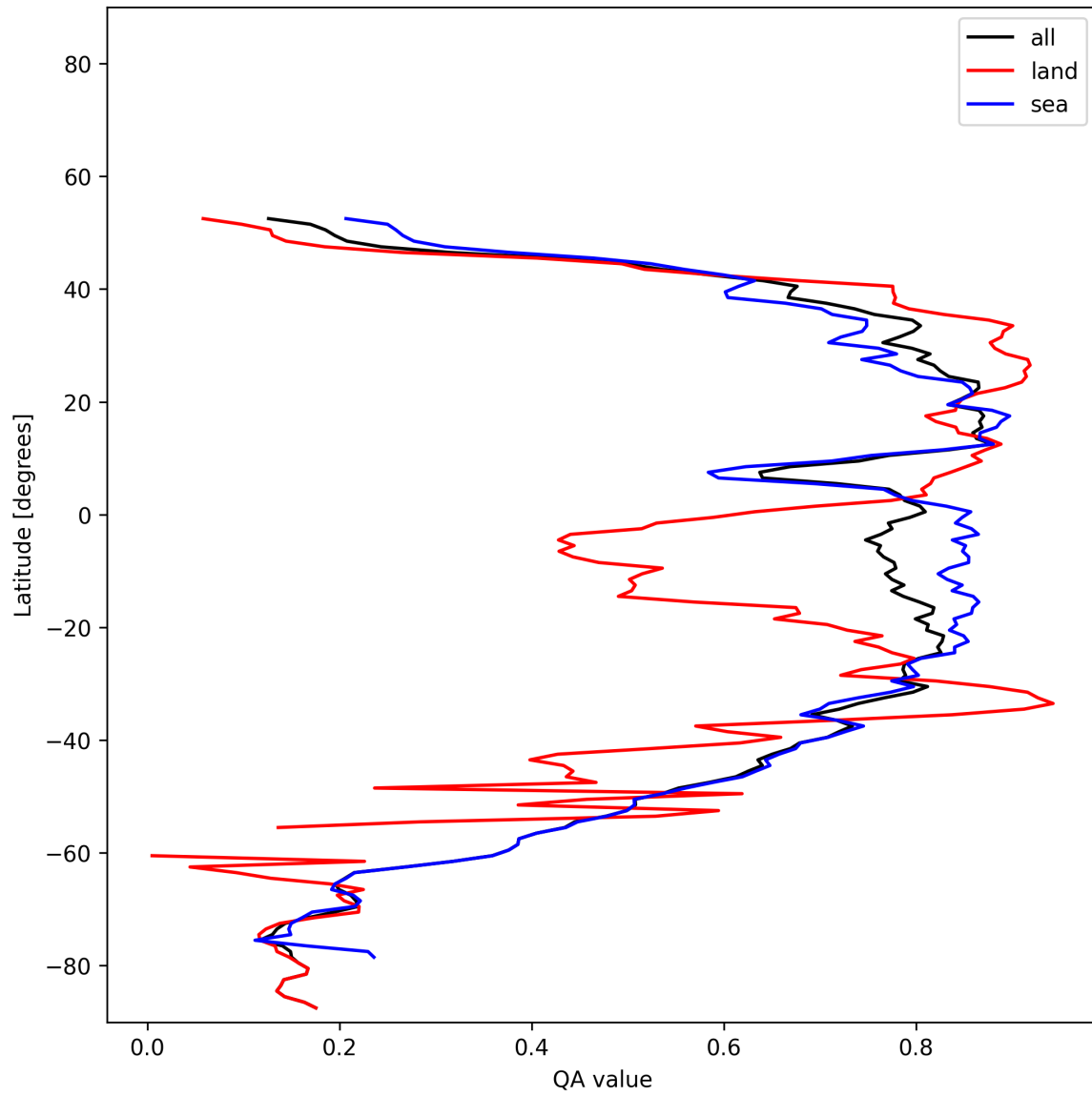
Figure 31: Zonal average of “QA value” for 2025-11-09 to 2025-11-11.
