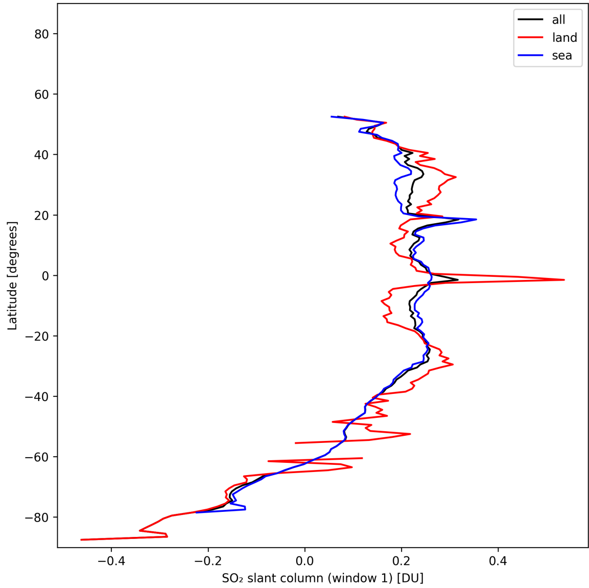
Figure 37: Zonal average of “SO 2 slant column (window 1)” for 2025-11-09 to 2025-11-11.
