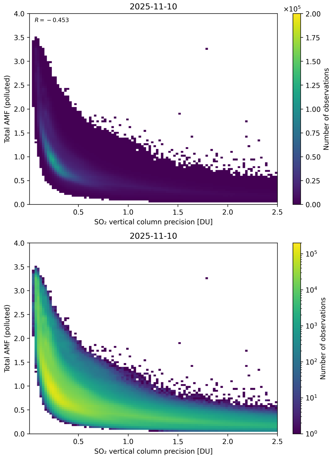
Figure 346: Scatter density plot of “SO 2 vertical column precision” against “Total AMF (polluted)” for 2025-11-09 to 2025-11-11.
