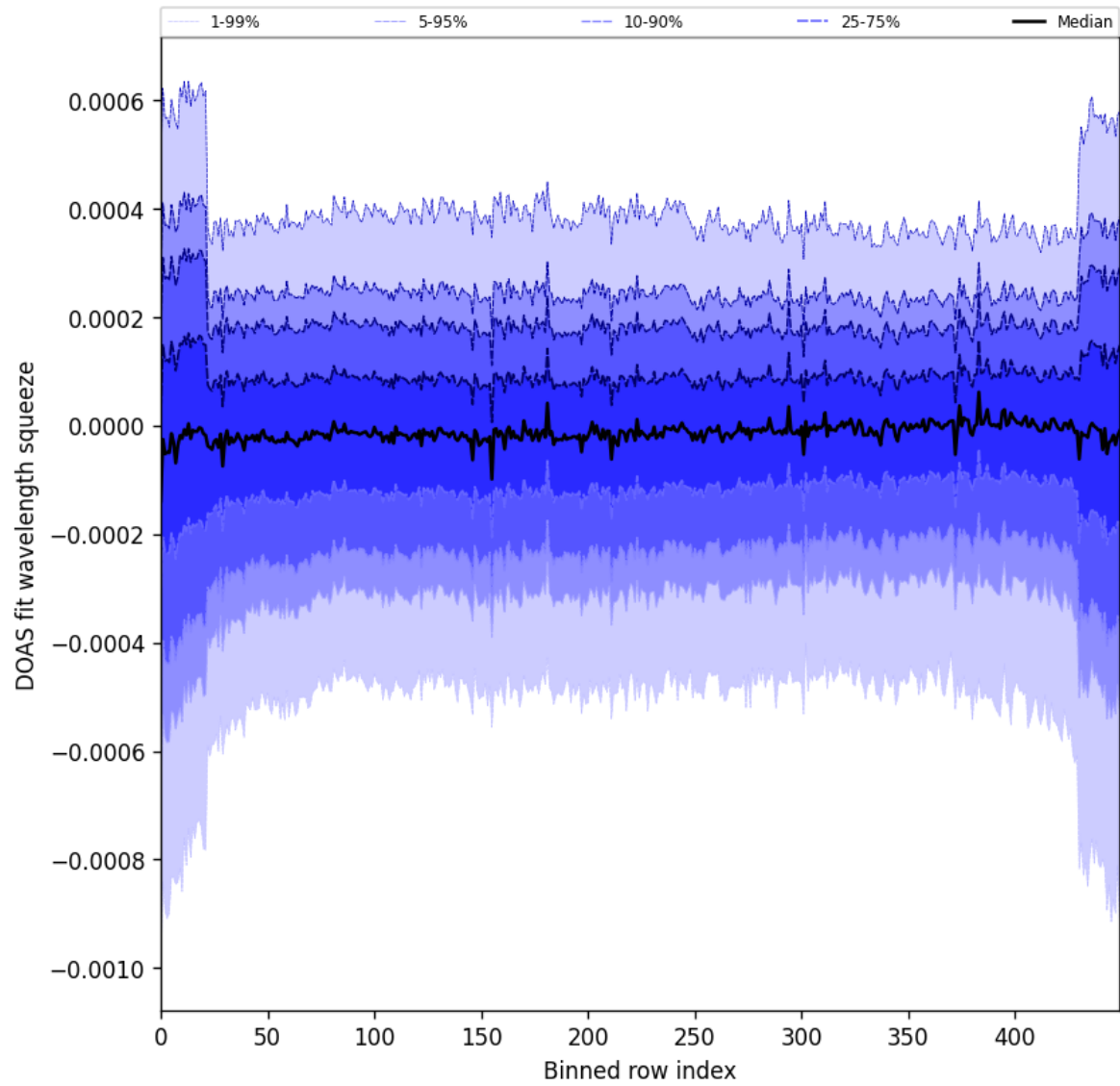
Figure 103: Along track statistics of “DOAS fit wavelength squeeze” for 2025-11-09 to 2025-11-11
