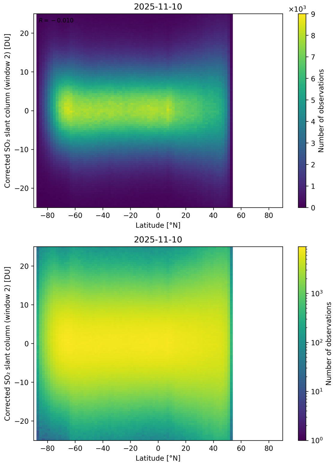
Figure 160: Scatter density plot of “Latitude” against “Corrected SO 2 slant column (window 2)” for 2025-11-09 to 2025-11-11.
