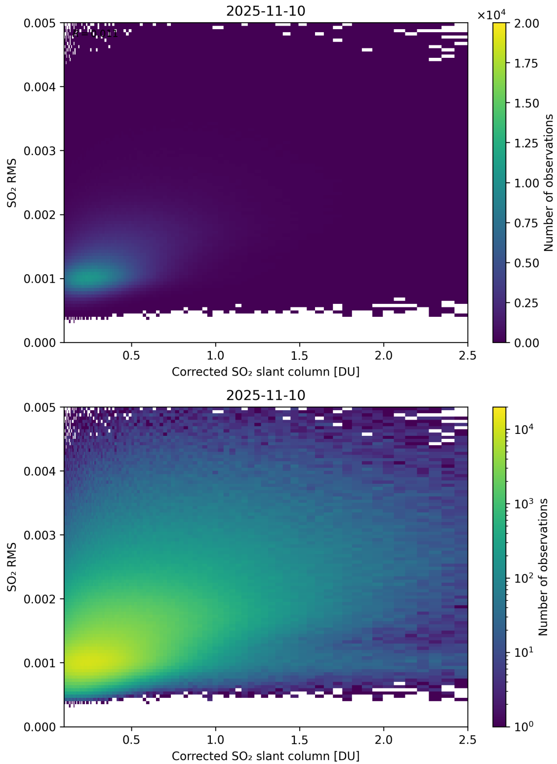
Figure 231: Scatter density plot of “Corrected SO 2 slant column” against “SO 2 RMS” for 2025-11-09 to 2025-11-11.
