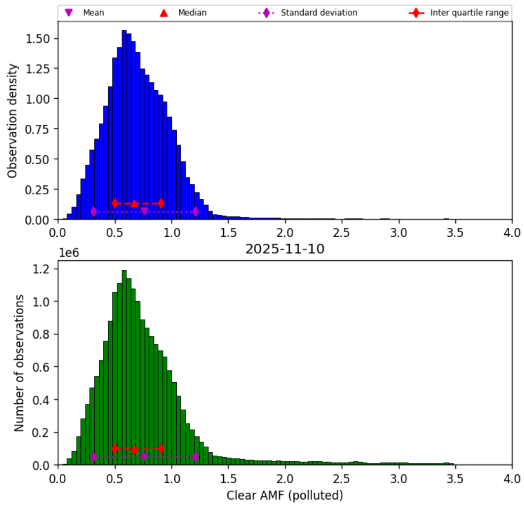
Figure 81: Histogram of “Clear AMF (polluted)” for 2025-11-09 to 2025-11-11
