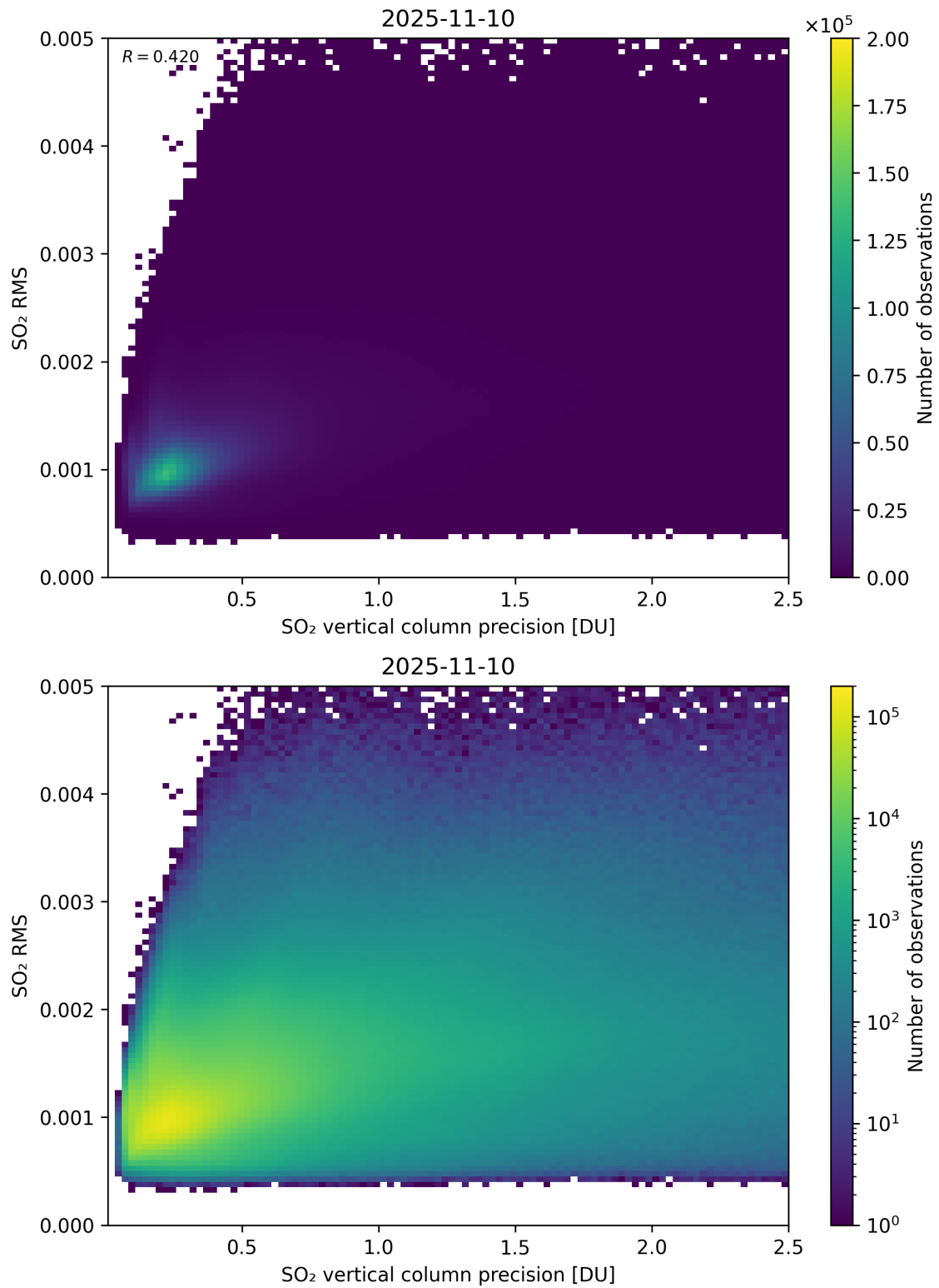
Figure 334: Scatter density plot of “SO 2 vertical column precision” against “SO 2 RMS” for 2025-11-09 to 2025-11-11.
