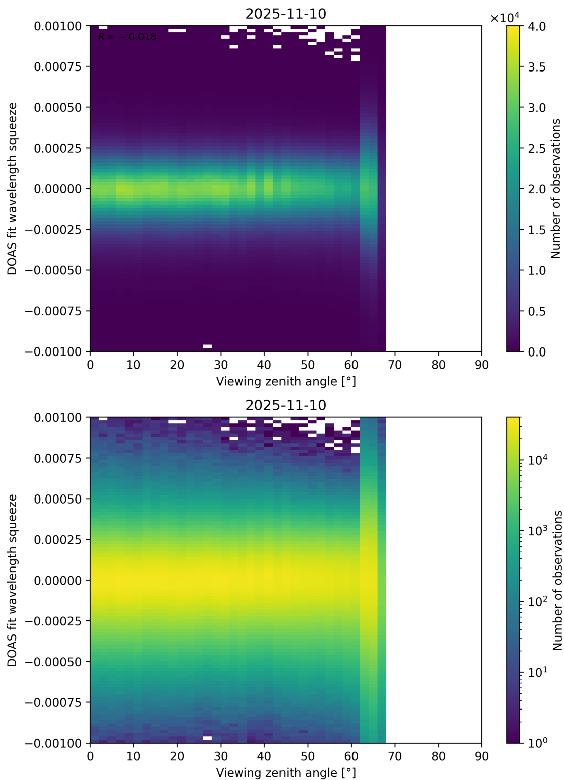
Figure 366: Scatter density plot of “Viewing zenith angle” against “DOAS fit wavelength squeeze” for 2025-11-09 to 2025-11-11.
