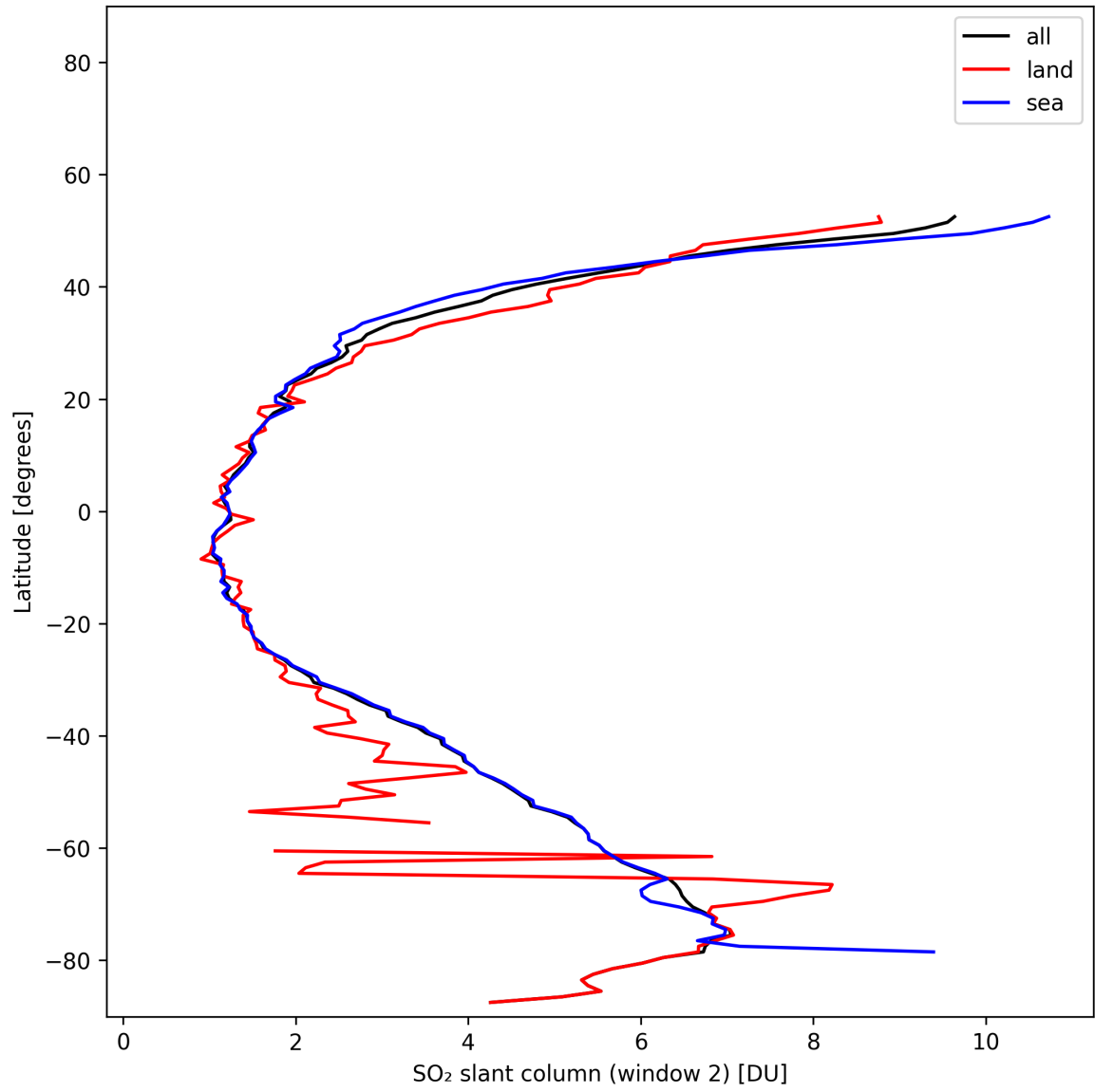
Figure 41: Zonal average of “SO 2 slant column (window 2)” for 2025-11-09 to 2025-11-11.
