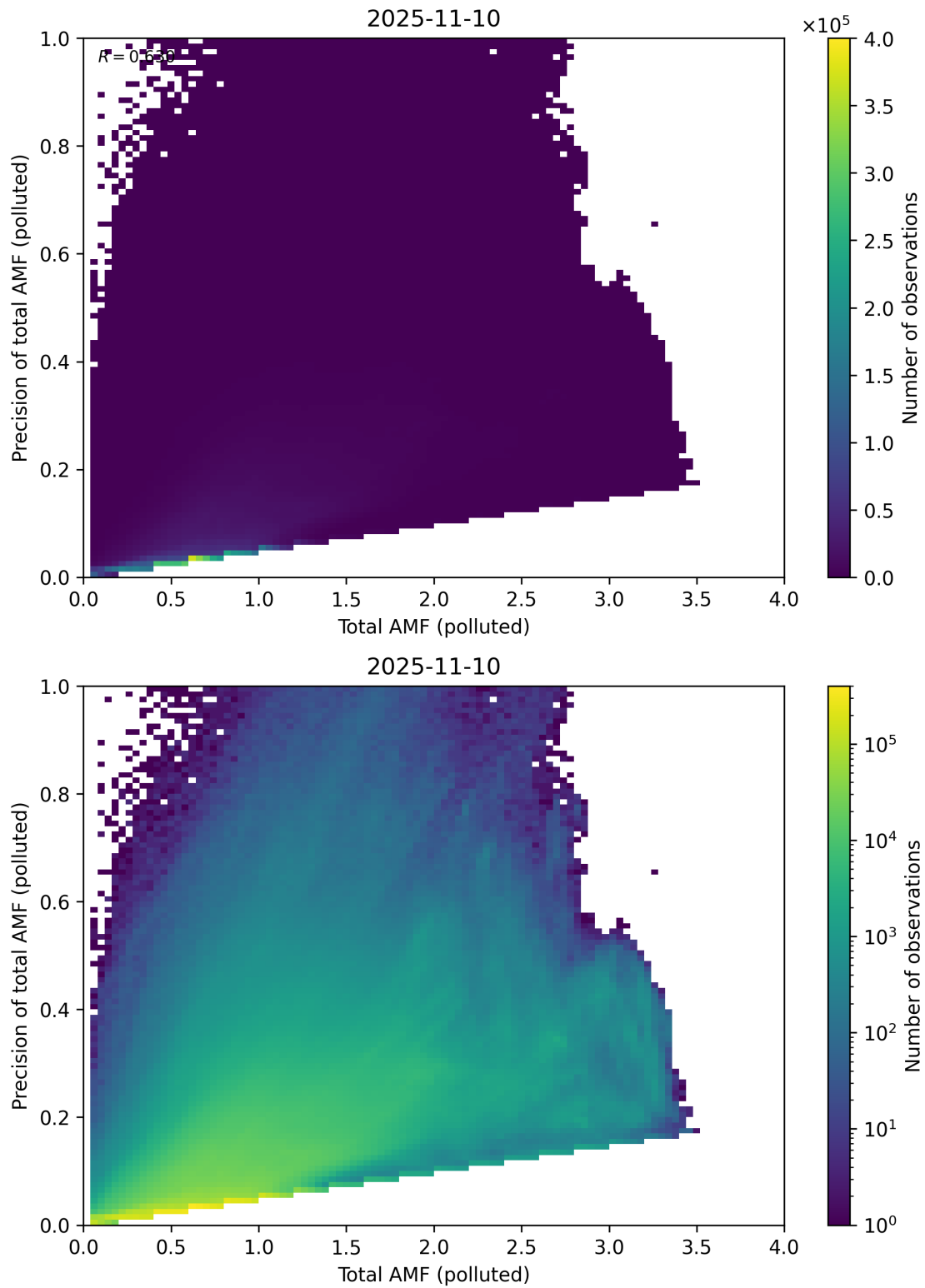
Figure 322: Scatter density plot of “Total AMF (polluted)” against “Precision of total AMF (polluted)” for 2025-11-09 to 2025-11-11.
