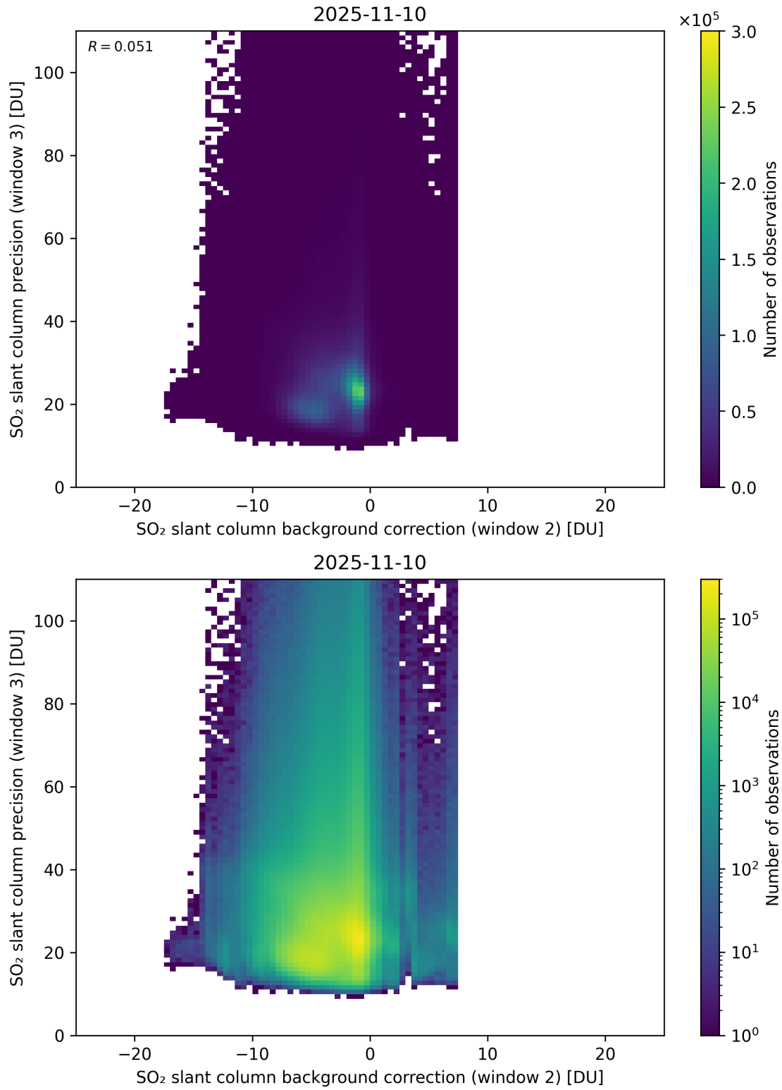
Figure 129: Scatter density plot of “SO 2 slant column background correction (window 2)” against “SO 2 slant column precision (window 3)” for 2025-11-09 to 2025-11-11.
