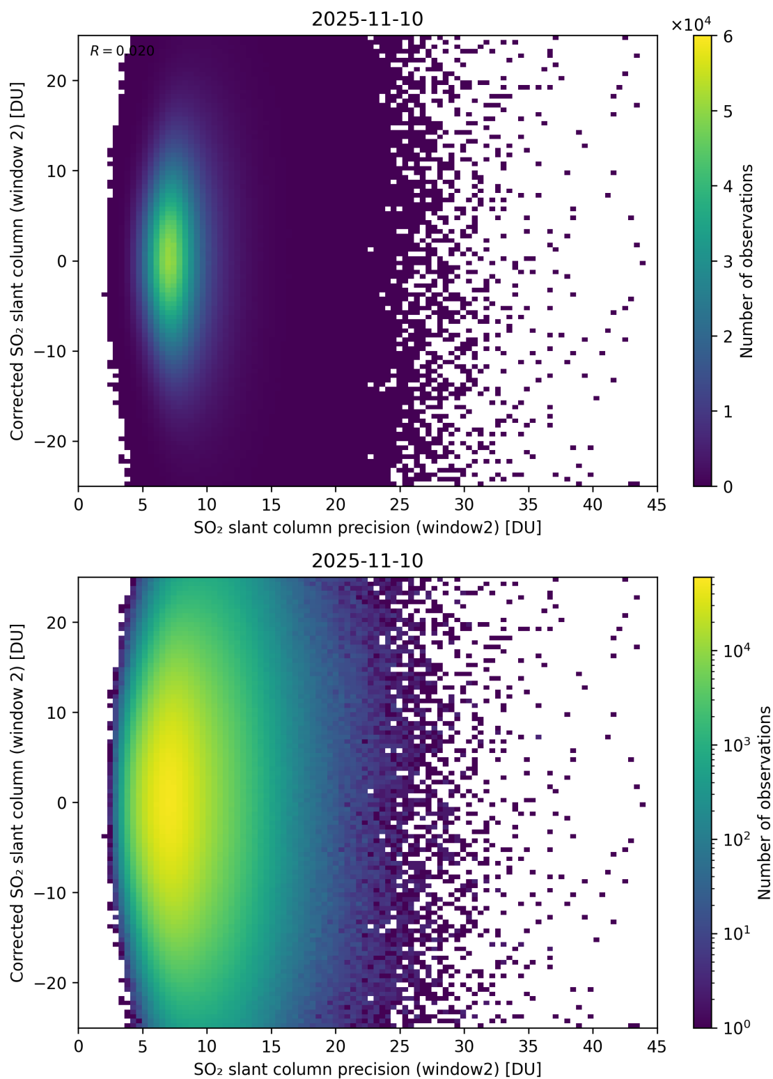
Figure 297: Scatter density plot of “SO 2 slant column precision (window2)” against “Corrected SO 2 slant column (window 2)” for 2025-11-09 to 2025-11-11.
