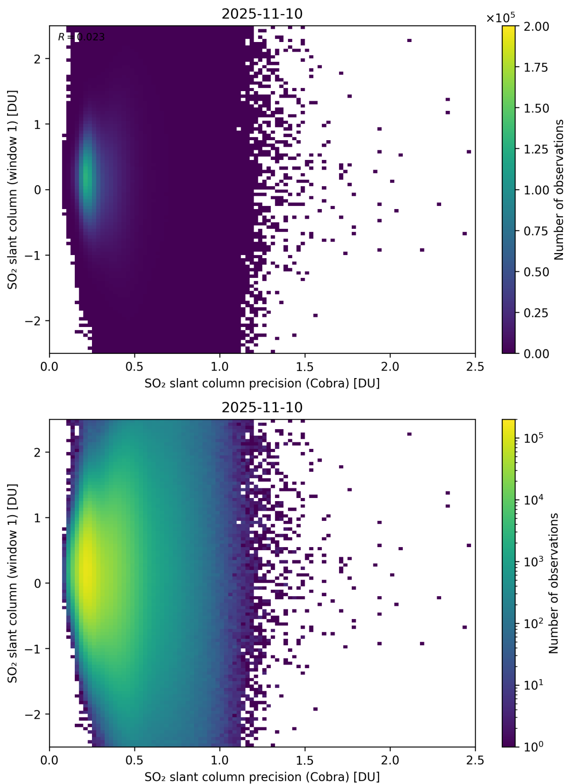
Figure 208: Scatter density plot of “SO 2 slant column precision (Cobra)” against “SO 2 slant column (window 1)” for 2025-11-09 to 2025-11-11.
