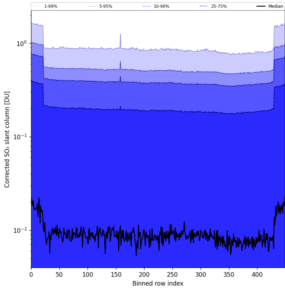
Figure 86: Along track statistics of “Corrected SO 2 slant column” for 2025-11-09 to 2025-11-11
