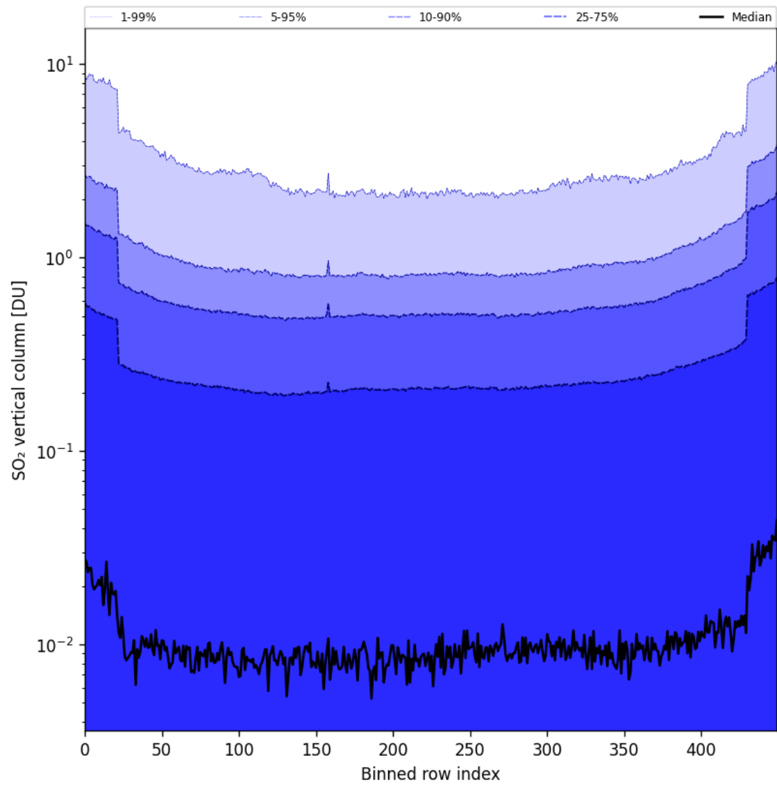
Figure 84: Along track statistics of “SO 2 vertical column” for 2025-11-09 to 2025-11-11
