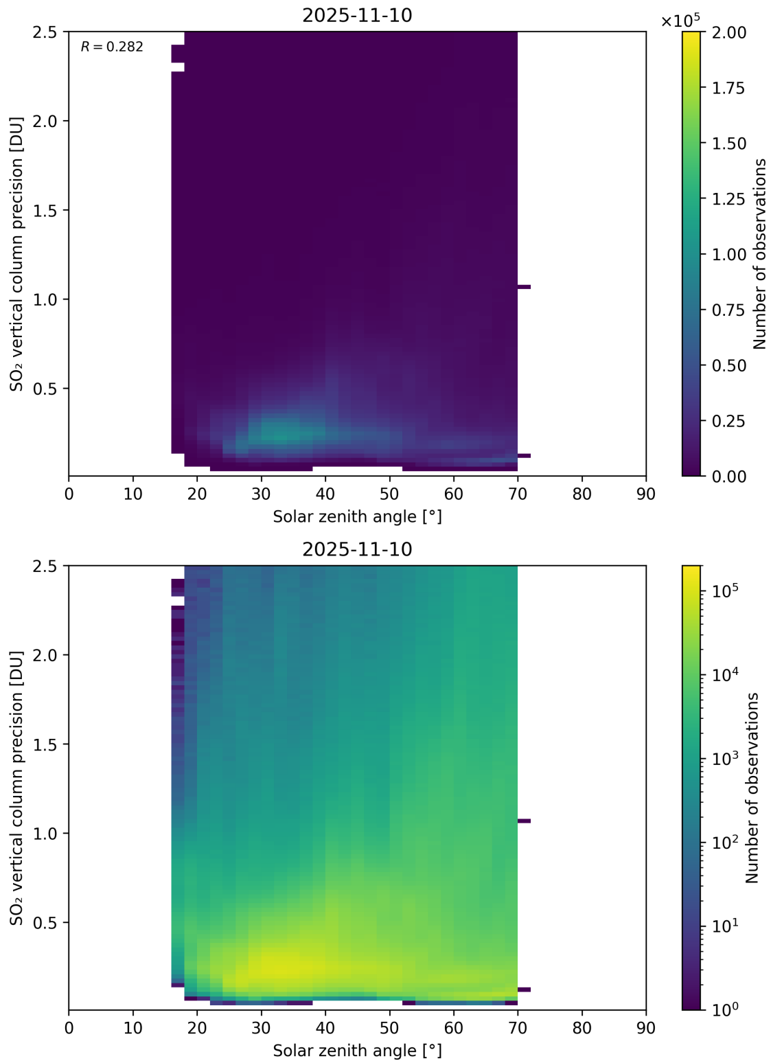
Figure 192: Scatter density plot of “Solar zenith angle” against “SO 2 vertical column precision” for 2025-11-09 to 2025-11-11.
