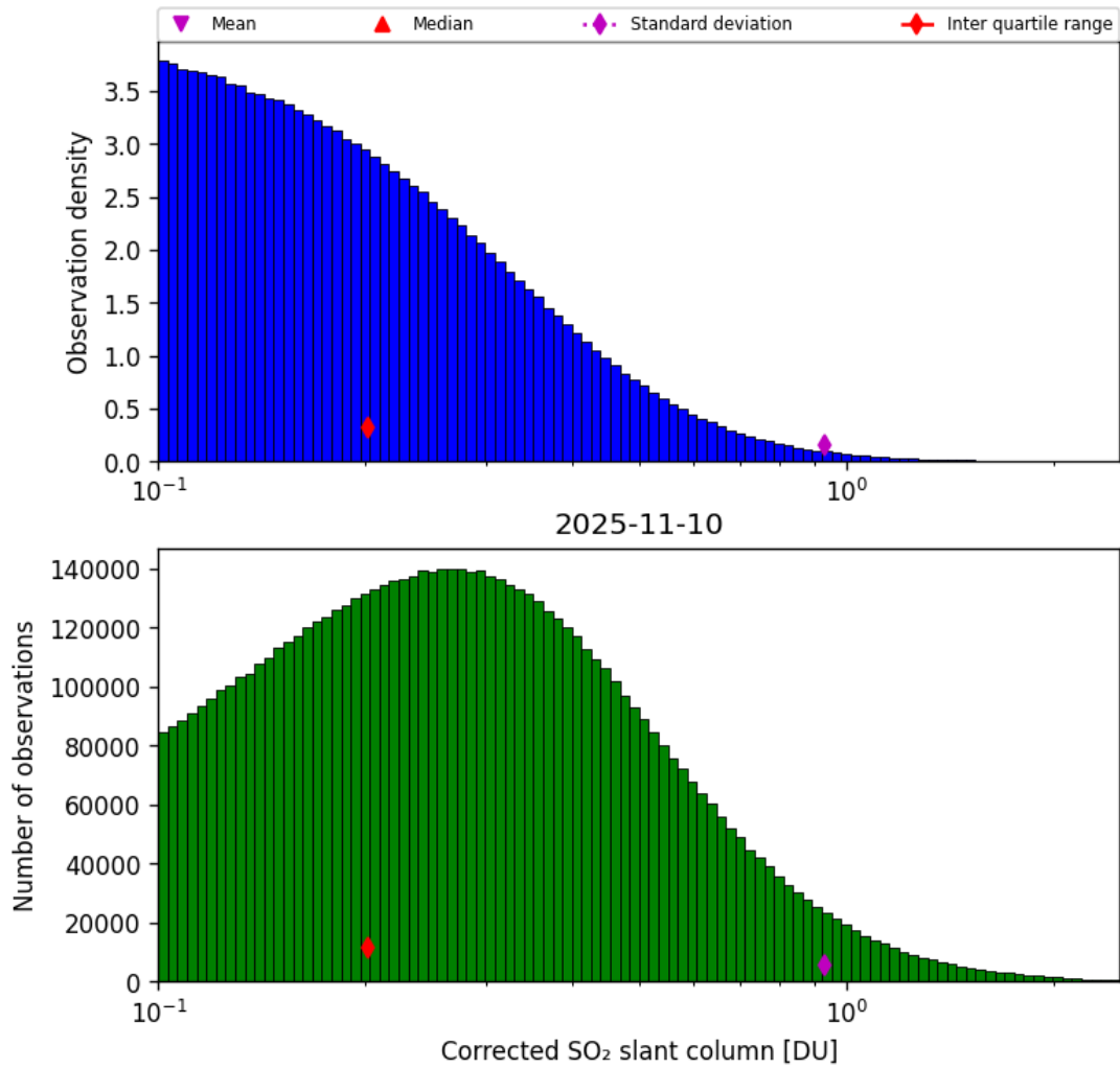
Figure 60: Histogram of “Corrected SO 2 slant column” for 2025-11-09 to 2025-11-11
