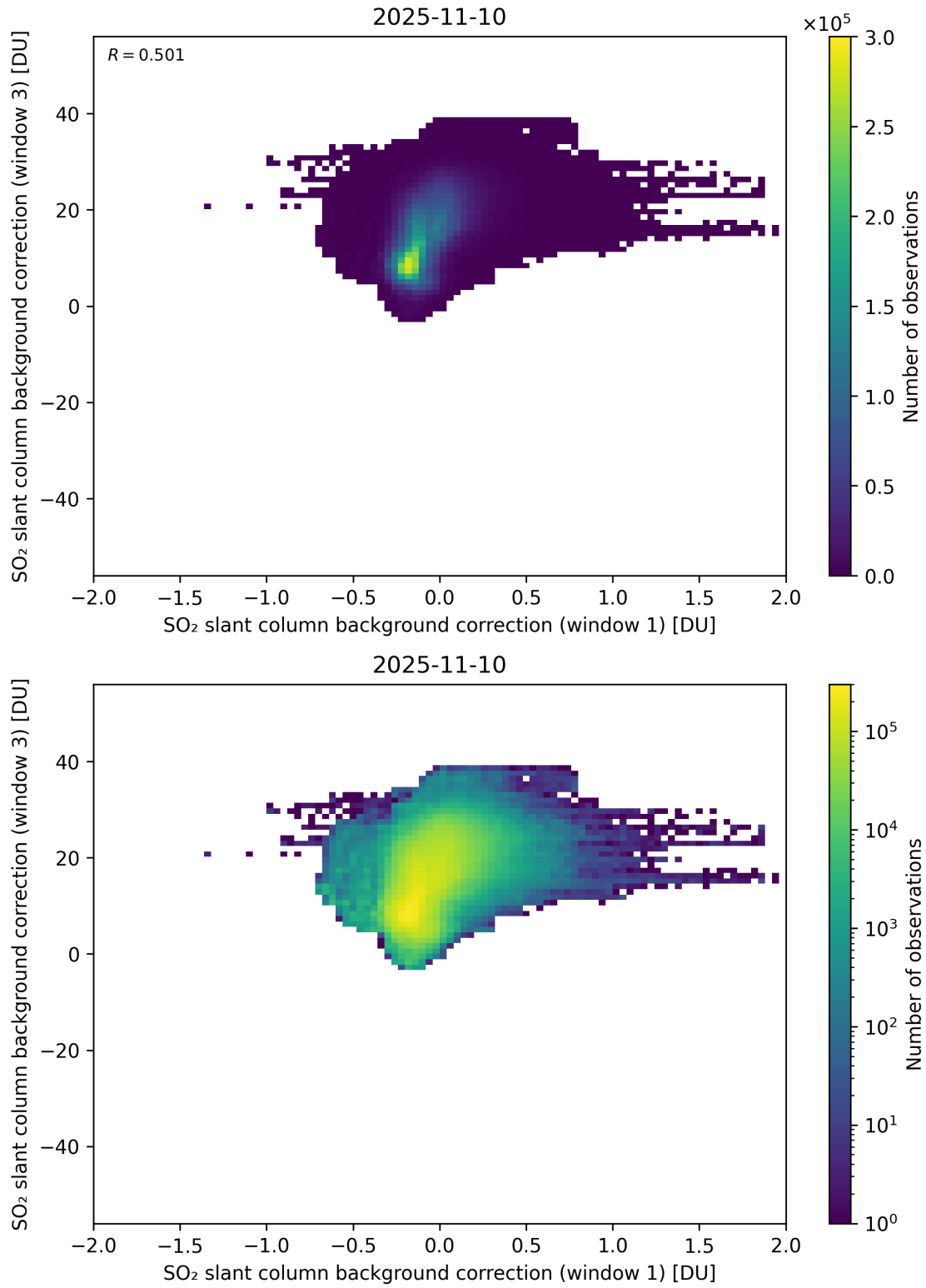
Figure 110: Scatter density plot of “SO 2 slant column background correction (window 1)” against “SO 2 slant column background correction (window 3)” for 2025-11-09 to 2025-11-11.
