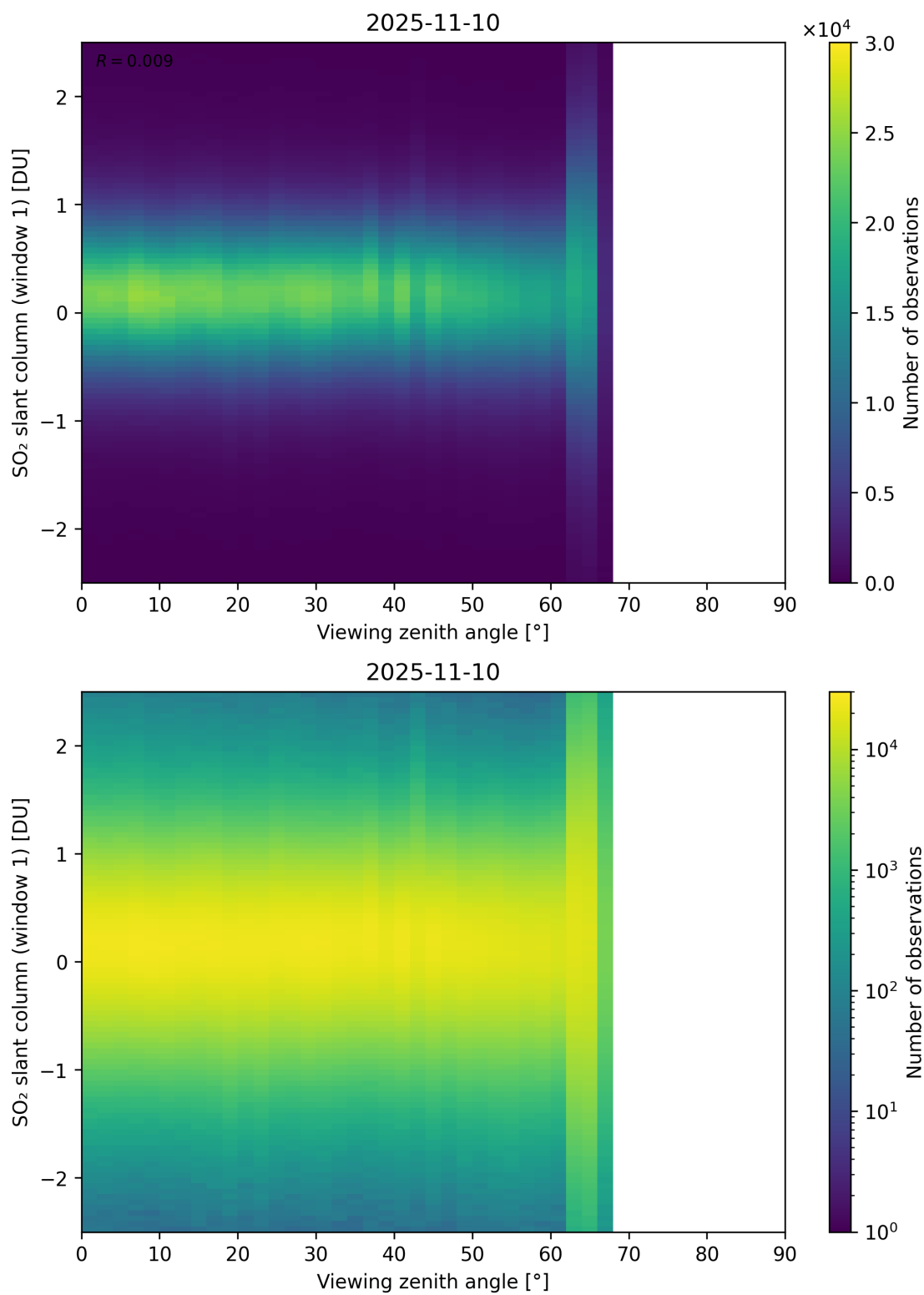
Figure 376: Scatter density plot of “Viewing zenith angle” against “SO 2 slant column (window 1)” for 2025-11-09 to 2025-11-11.
