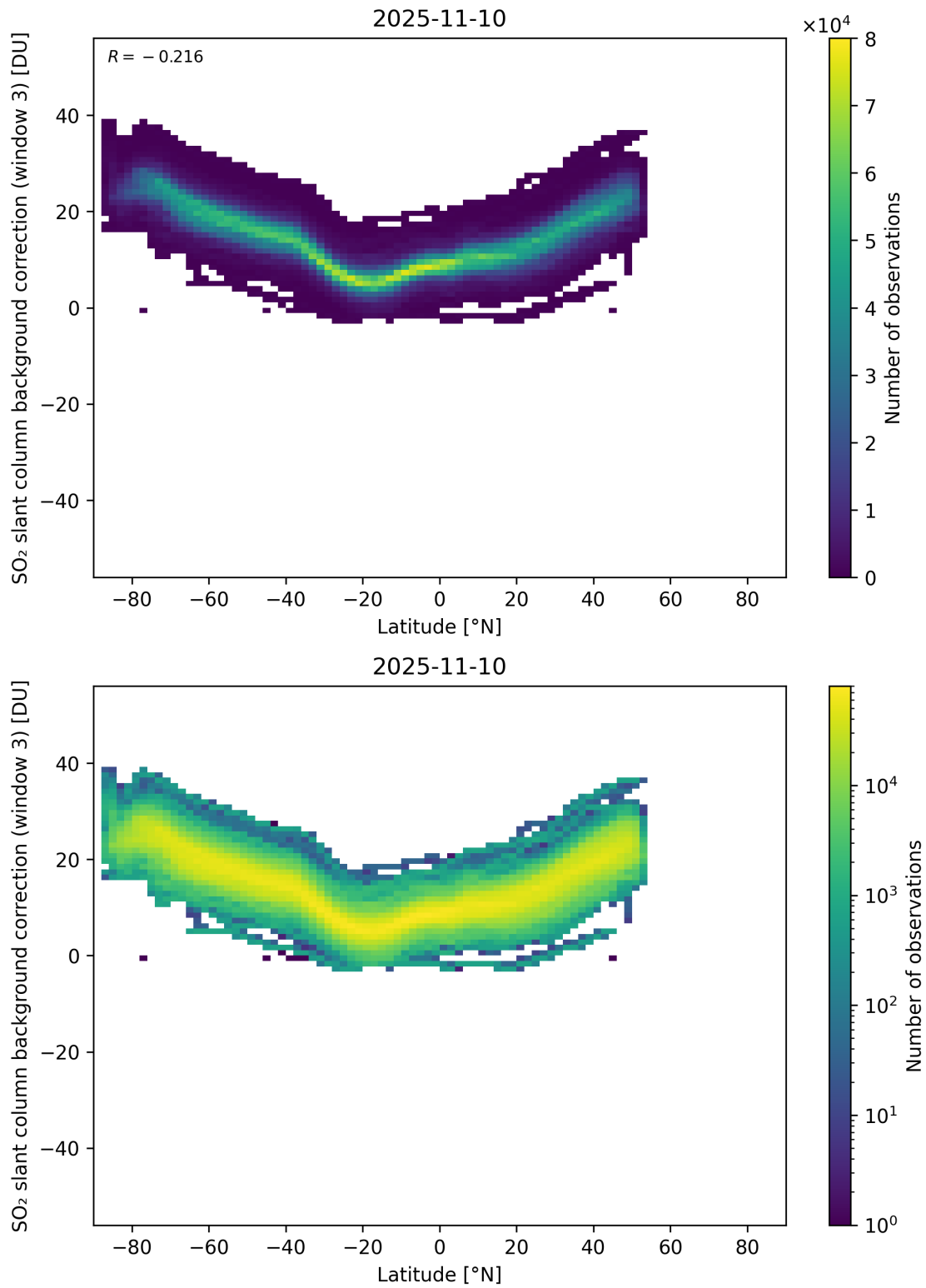
Figure 152: Scatter density plot of “Latitude” against “SO 2 slant column background correction (window 3)” for 2025-11-09 to 2025-11-11.
