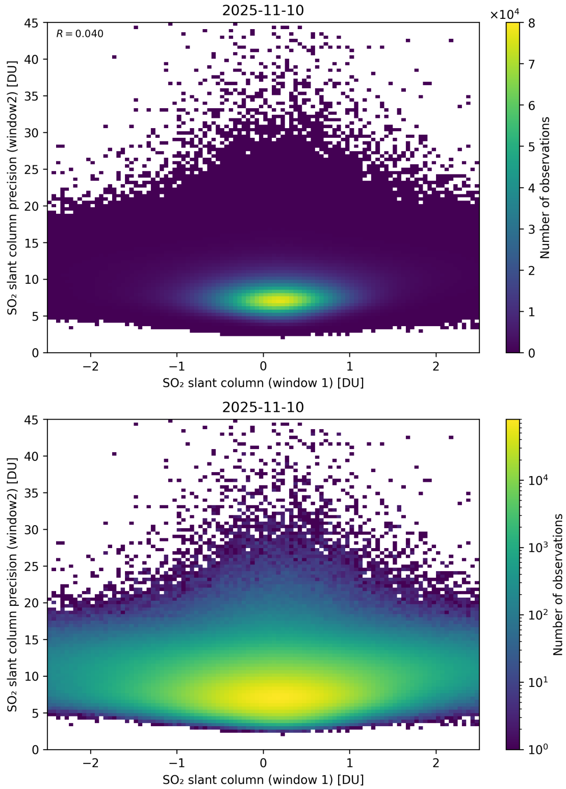
Figure 286: Scatter density plot of “SO 2 slant column (window 1)” against “SO 2 slant column precision (window2)” for 2025-11-09 to 2025-11-11.
