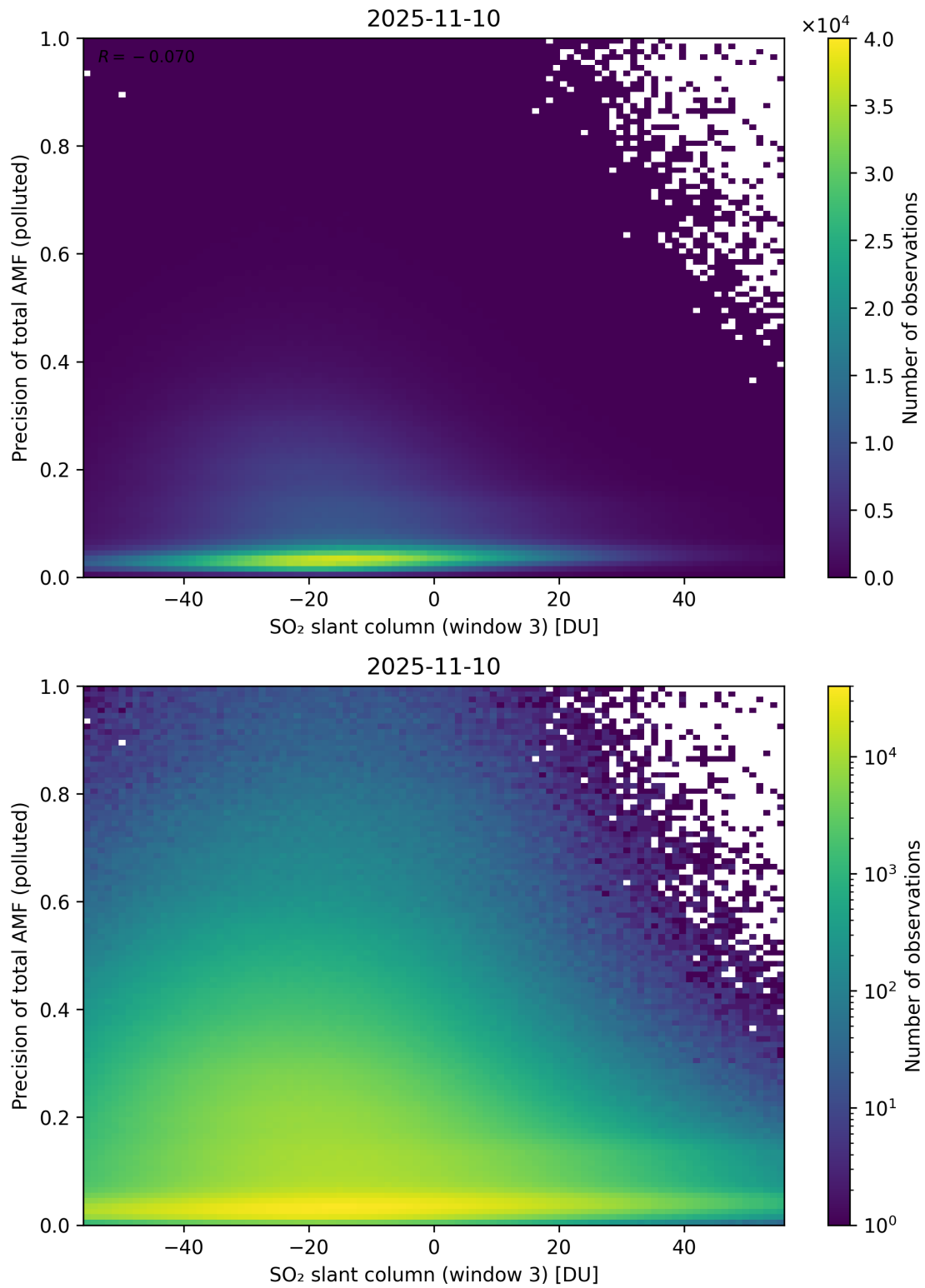
Figure 319: Scatter density plot of “SO 2 slant column (window 3)” against “Precision of total AMF (polluted)” for 2025-11-09 to 2025-11-11.
