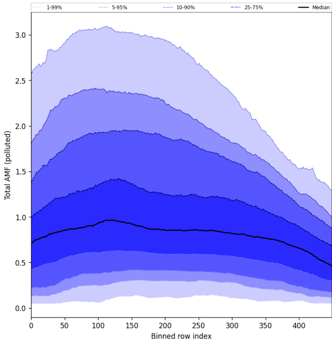
Figure 105: Along track statistics of “Total AMF (polluted)” for 2025-11-09 to 2025-11-11
