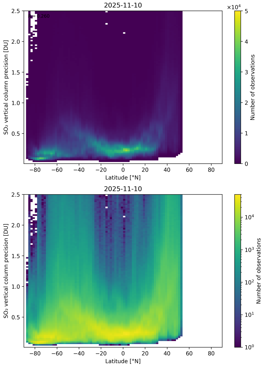
Figure 170: Scatter density plot of “Latitude” against “SO 2 vertical column precision” for 2025-11-09 to 2025-11-11.
