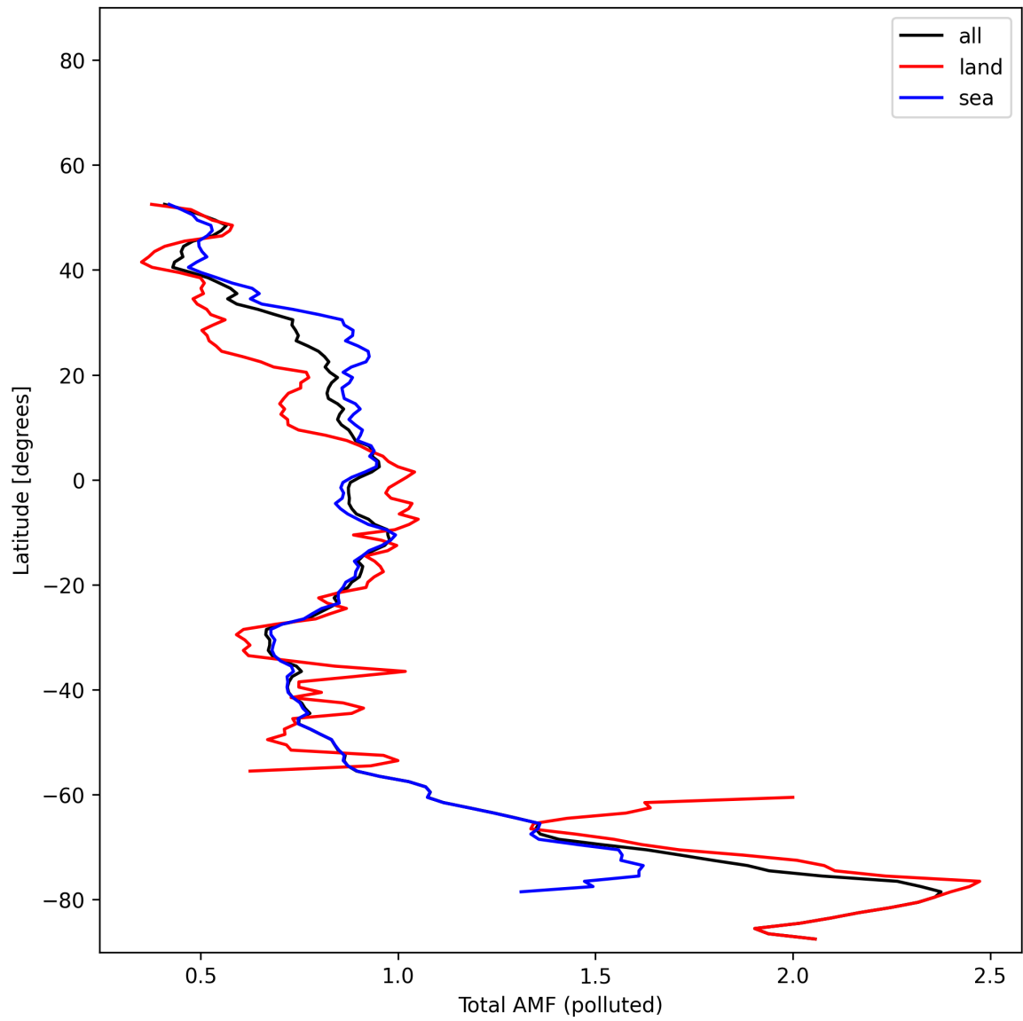
Figure 53: Zonal average of “Total AMF (polluted)” for 2025-11-09 to 2025-11-11.
