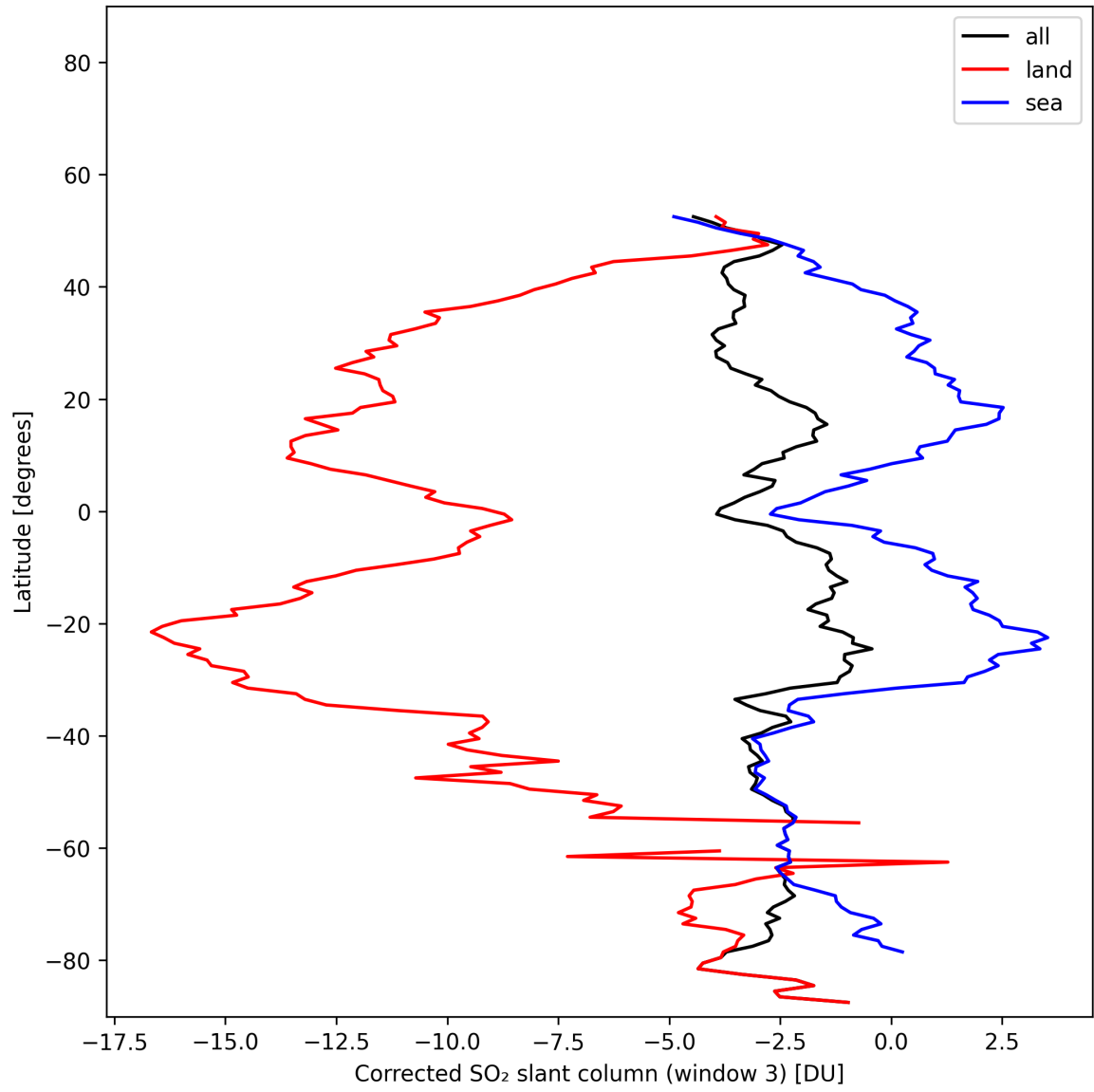
Figure 47: Zonal average of “Corrected SO 2 slant column (window 3)” for 2025-11-09 to 2025-11-11.
