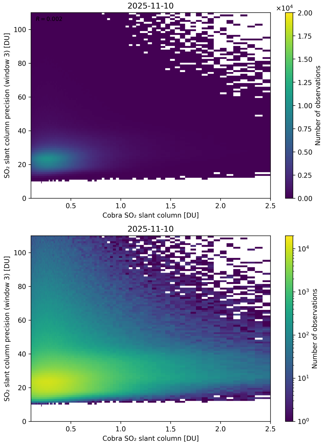
Figure 223: Scatter density plot of “Cobra SO 2 slant column” against “SO 2 slant column precision (window 3)” for 2025-11-09 to 2025-11-11.
