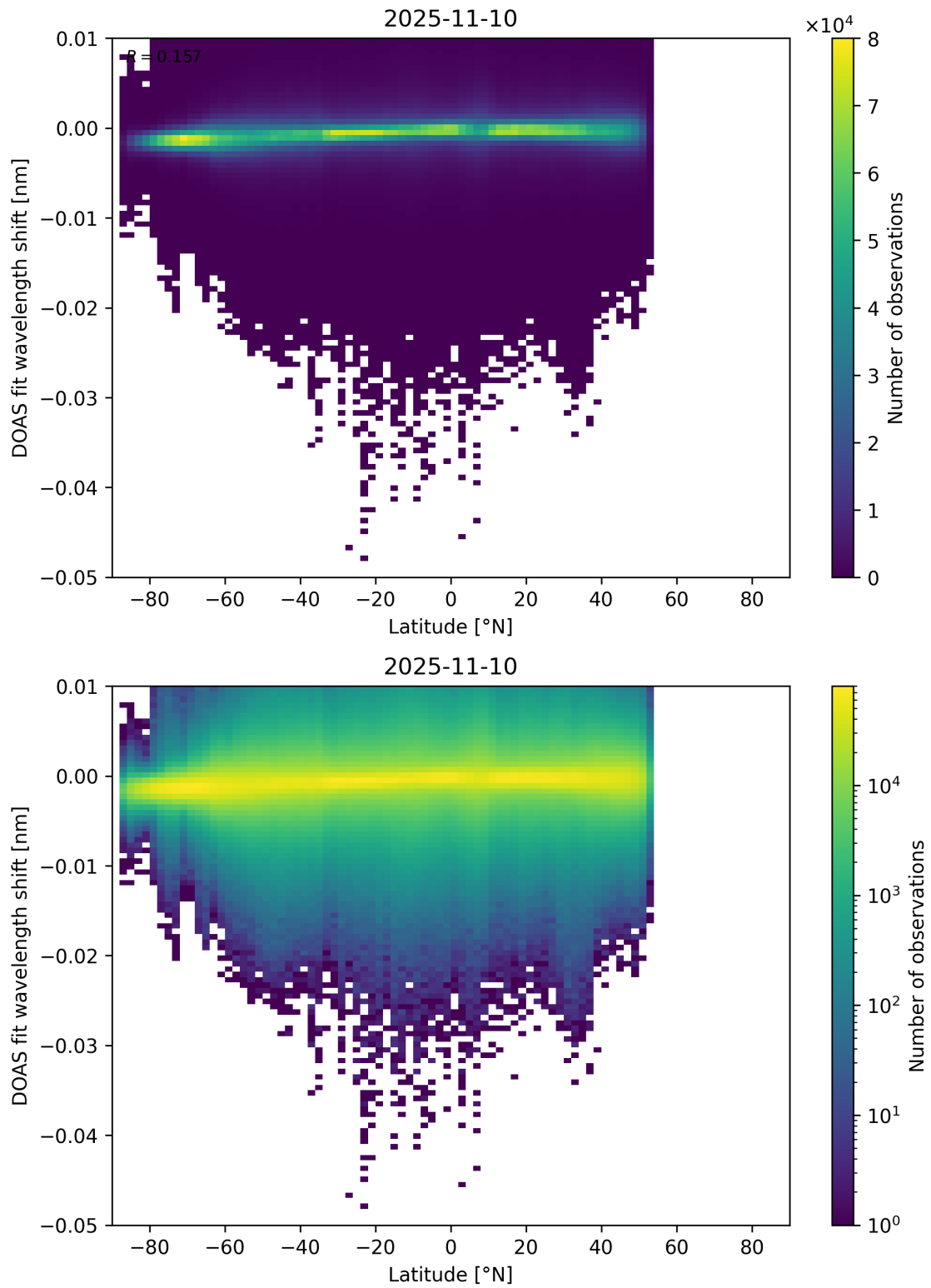
Figure 153: Scatter density plot of “Latitude” against “DOAS fit wavelength shift” for 2025-11-09 to 2025-11-11.
