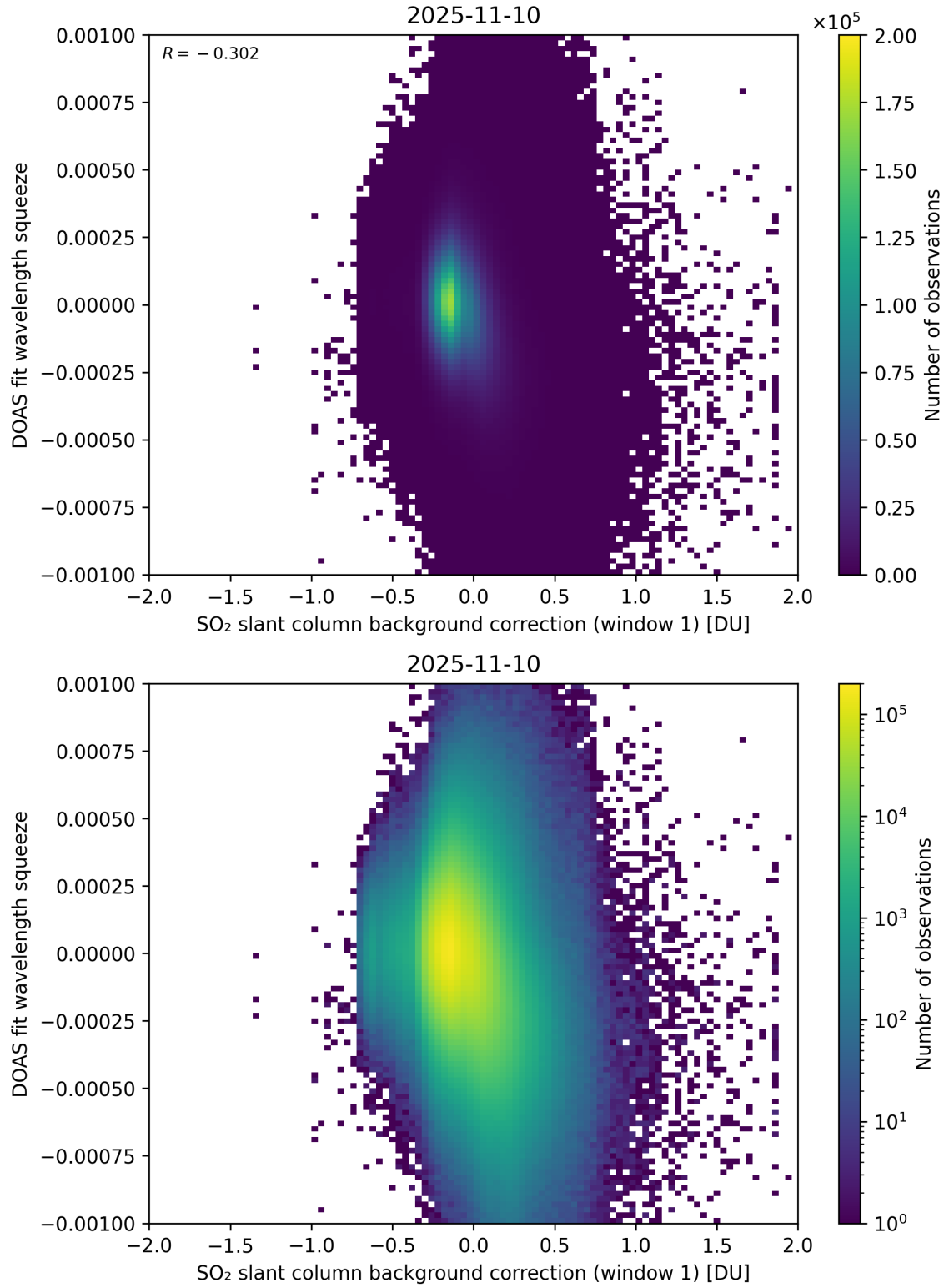
Figure 112: Scatter density plot of “SO 2 slant column background correction (window 1)” against “DOAS fit wavelength squeeze” for 2025-11-09 to 2025-11-11.
