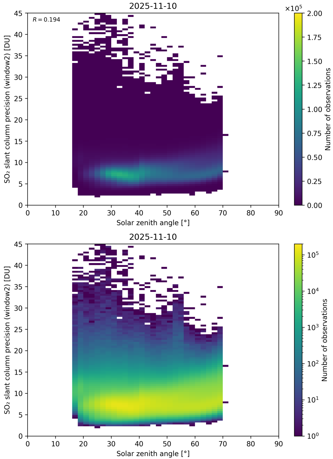
Figure 186: Scatter density plot of “Solar zenith angle” against “SO 2 slant column precision (window2)” for 2025-11-09 to 2025-11-11.
