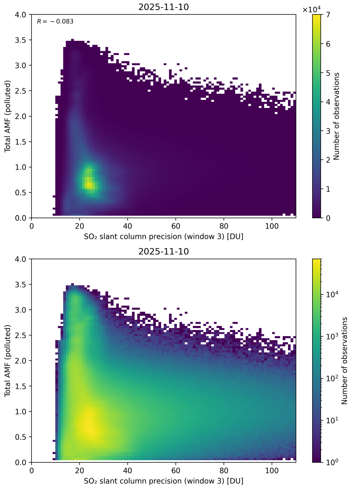
Figure 313: Scatter density plot of “SO 2 slant column precision (window 3)” against “Total AMF (polluted)” for 2025-11-09 to 2025-11-11.
