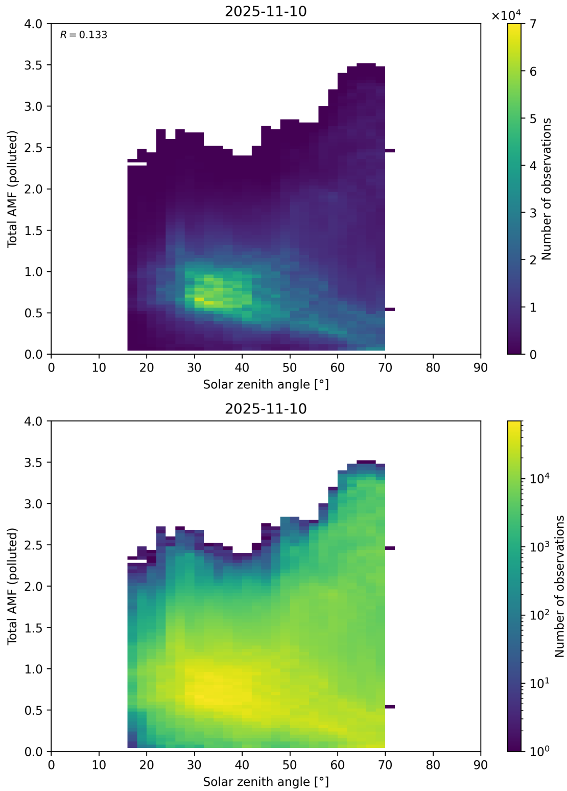
Figure 189: Scatter density plot of “Solar zenith angle” against “Total AMF (polluted)” for 2025-11-09 to 2025-11-11.
