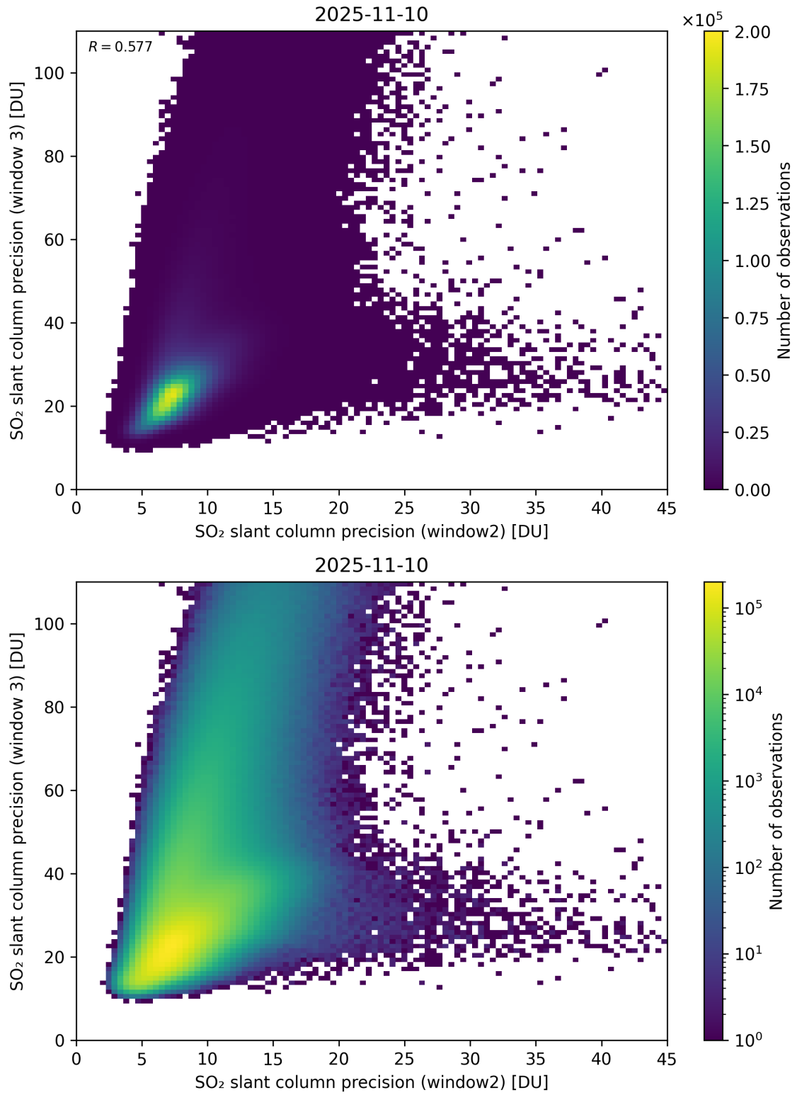
Figure 300: Scatter density plot of “SO 2 slant column precision (window2)” against “SO 2 slant column precision (window 3)” for 2025-11-09 to 2025-11-11.
