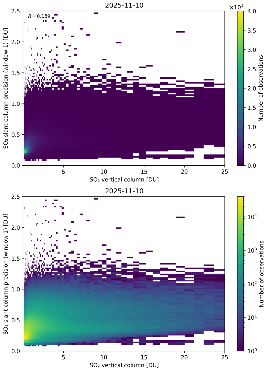
Figure 355: Scatter density plot of “SO 2 vertical column” against “SO 2 slant column precision (window 1)” for 2025-11-09 to 2025-11-11.
