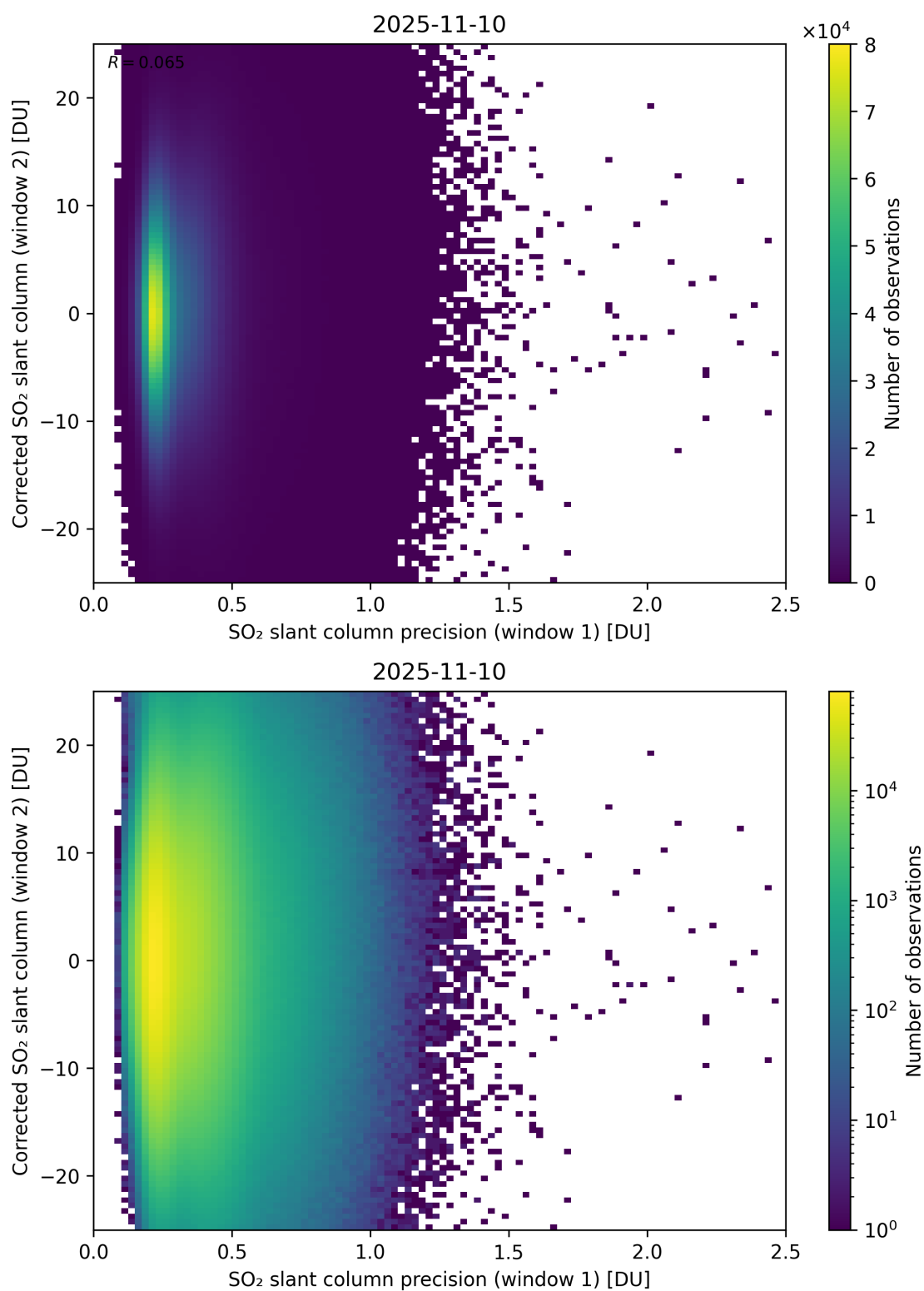
Figure 275: Scatter density plot of “SO 2 slant column precision (window 1)” against “Corrected SO 2 slant column (window 2)” for 2025-11-09 to 2025-11-11.
