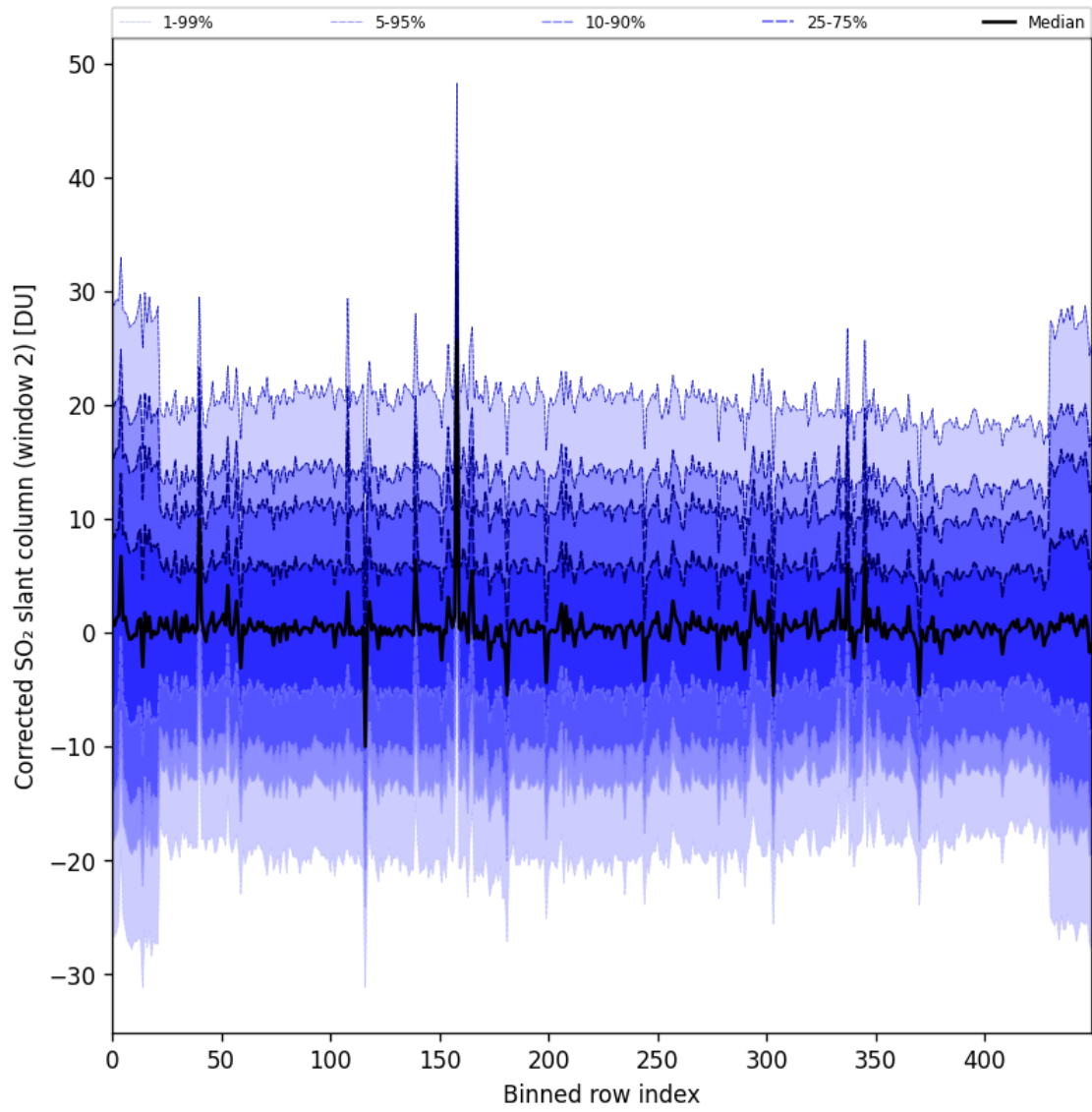
Figure 95: Along track statistics of "Corrected SO 2 slant column (window 2)" for 2025-11-09 to 2025-11-11
