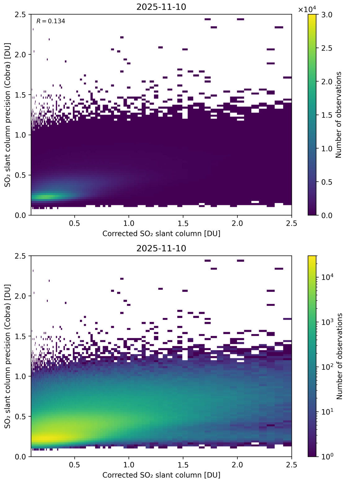
Figure 234: Scatter density plot of “Corrected SO 2 slant column” against “SO 2 slant column precision (Cobra)” for 2025-11-09 to 2025-11-11.
