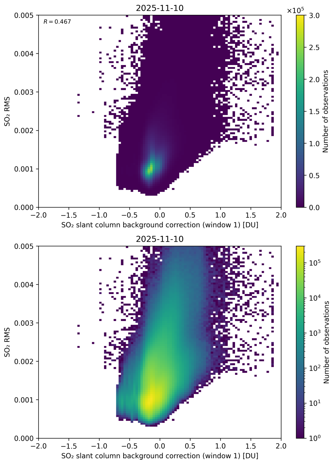
Figure 113: Scatter density plot of “SO 2 slant column background correction (window 1)” against “SO 2 RMS” for 2025-11-09 to 2025-11-11.
