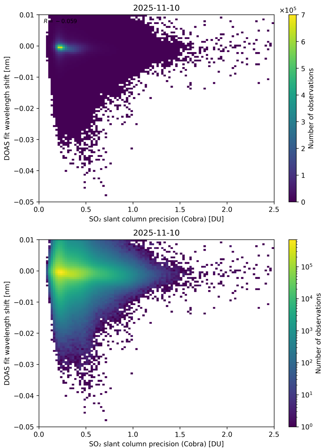
Figure 202: Scatter density plot of “SO 2 slant column precision (Cobra)” against “DOAS fit wavelength shift” for 2025-11-09 to 2025-11-11.
