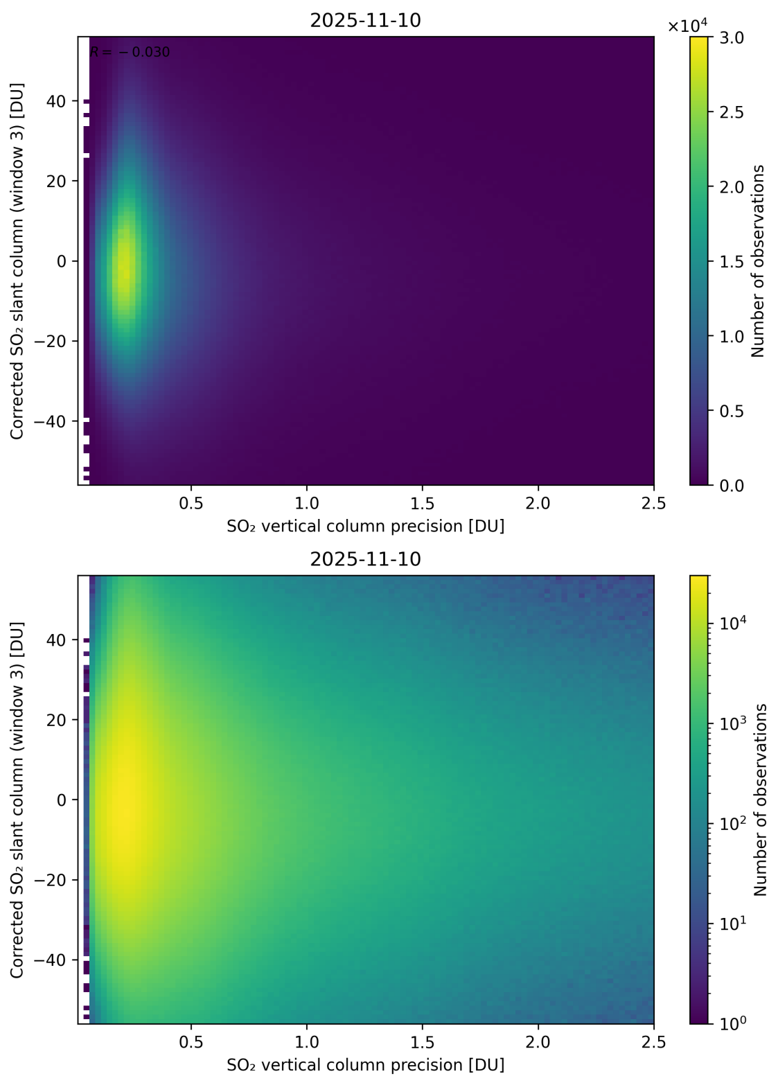
Figure 340: Scatter density plot of “SO 2 vertical column precision” against “Corrected SO 2 slant column (window 3)” for 2025-11-09 to 2025-11-11.
