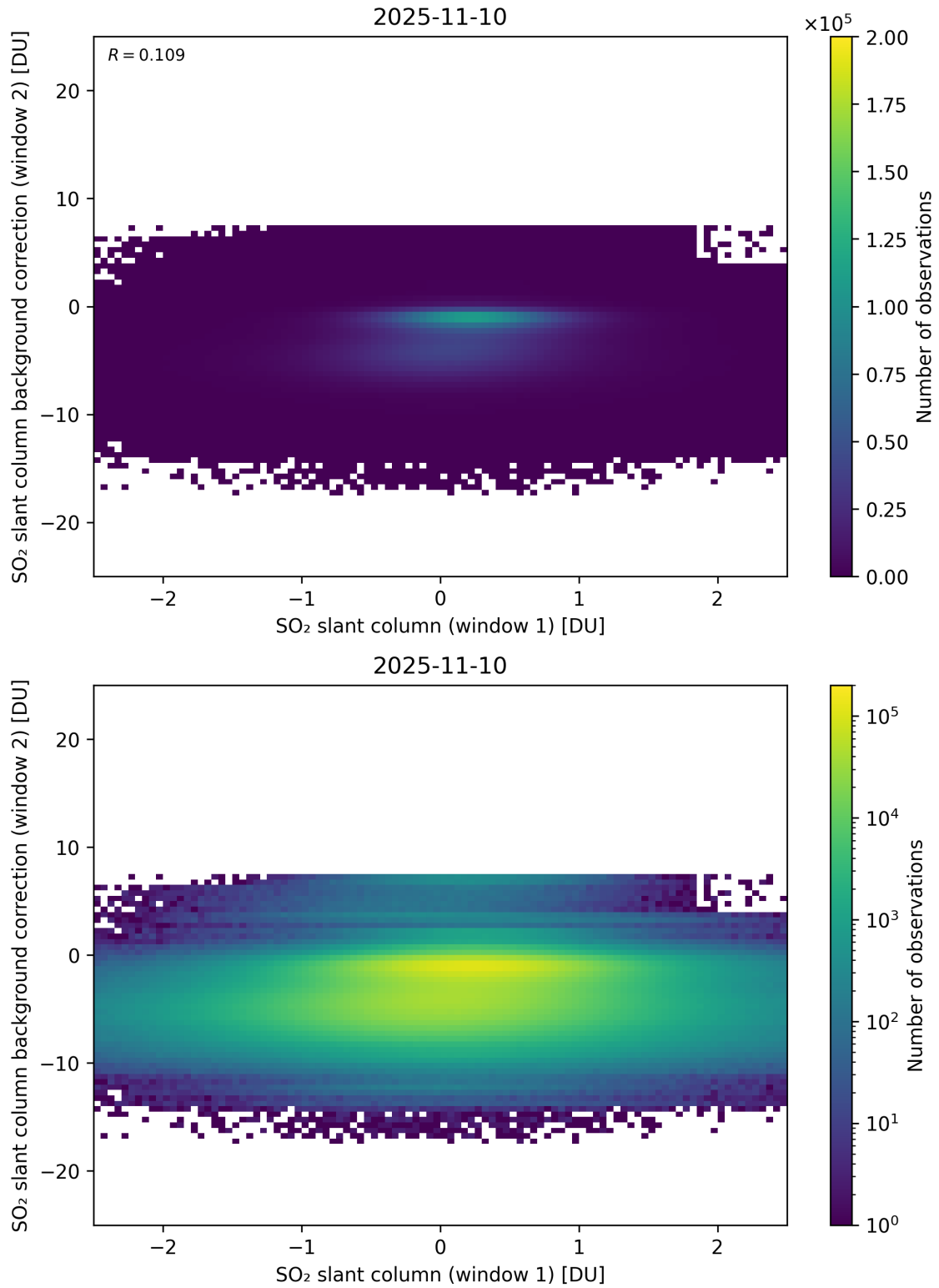
Figure 263: Scatter density plot of “SO 2 slant column (window 1)” against “SO 2 slant column background correction (window 2)” for 2025-11-09 to 2025-11-11.
