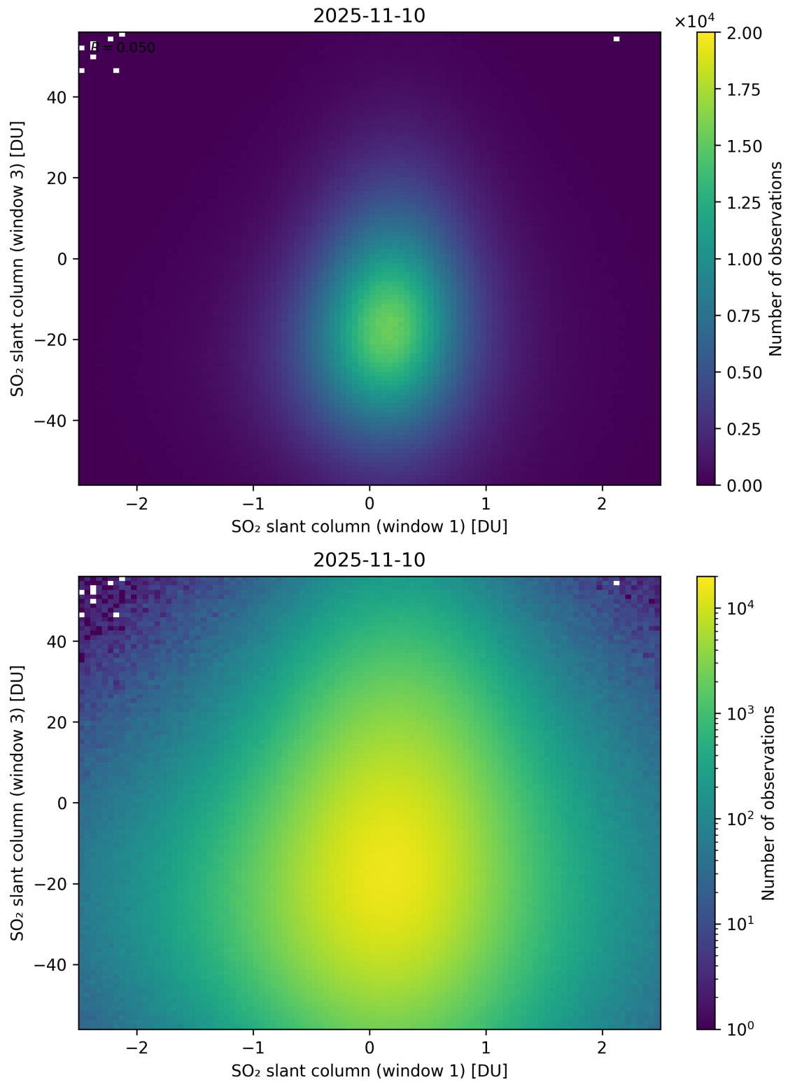
Figure 287: Scatter density plot of “SO 2 slant column (window 1)” against “SO 2 slant column (window 3)” for 2025-11-09 to 2025-11-11.
