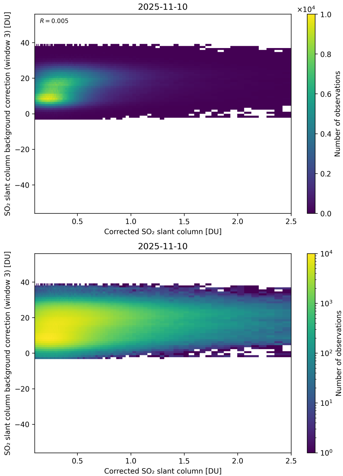
Figure 228: Scatter density plot of “Corrected SO 2 slant column” against “SO 2 slant column background correction (window 3)” for 2025-11-09 to 2025-11-11.
