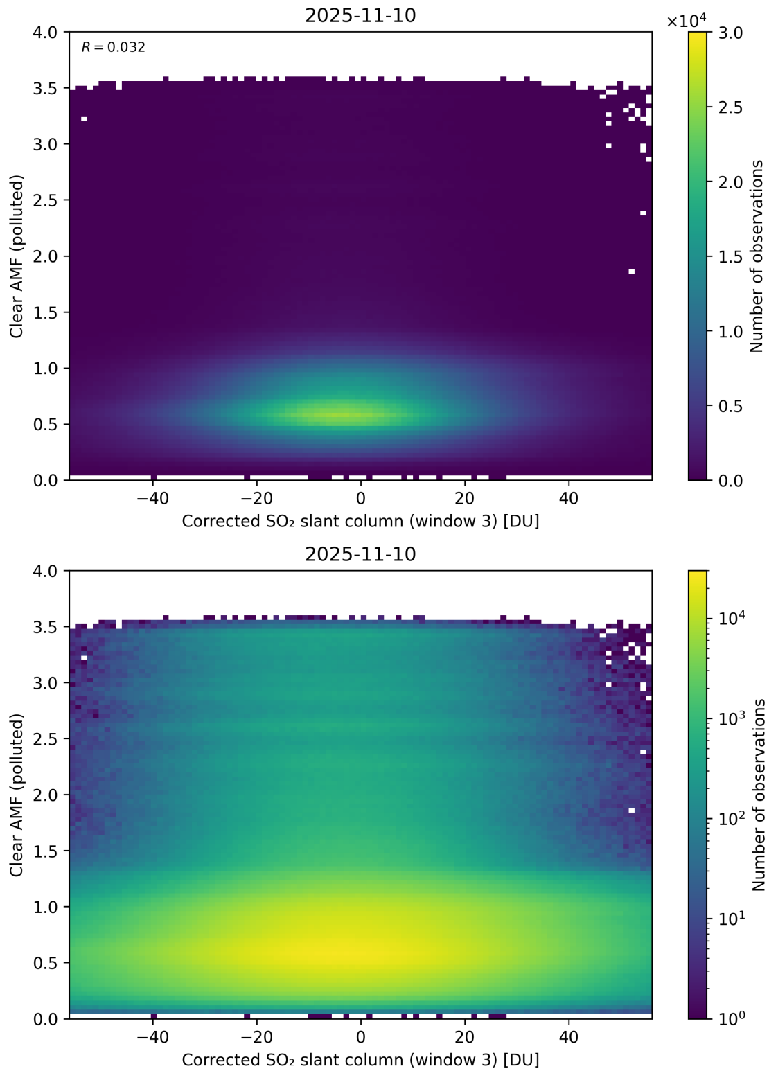
Figure 259: Scatter density plot of “Corrected SO 2 slant column (window 3)” against “Clear AMF (polluted)” for 2025-11-09 to 2025-11-11.
