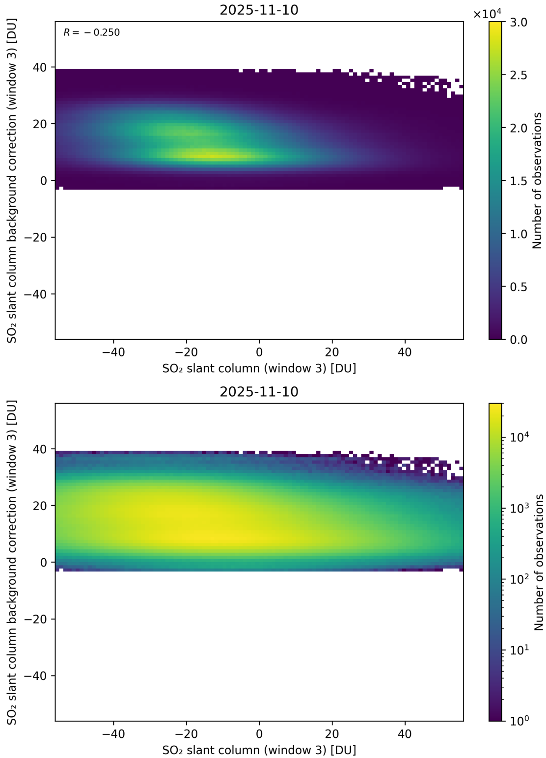
Figure 303: Scatter density plot of “SO 2 slant column (window 3)” against “SO 2 slant column background correction (window 3)” for 2025-11-09 to 2025-11-11.
