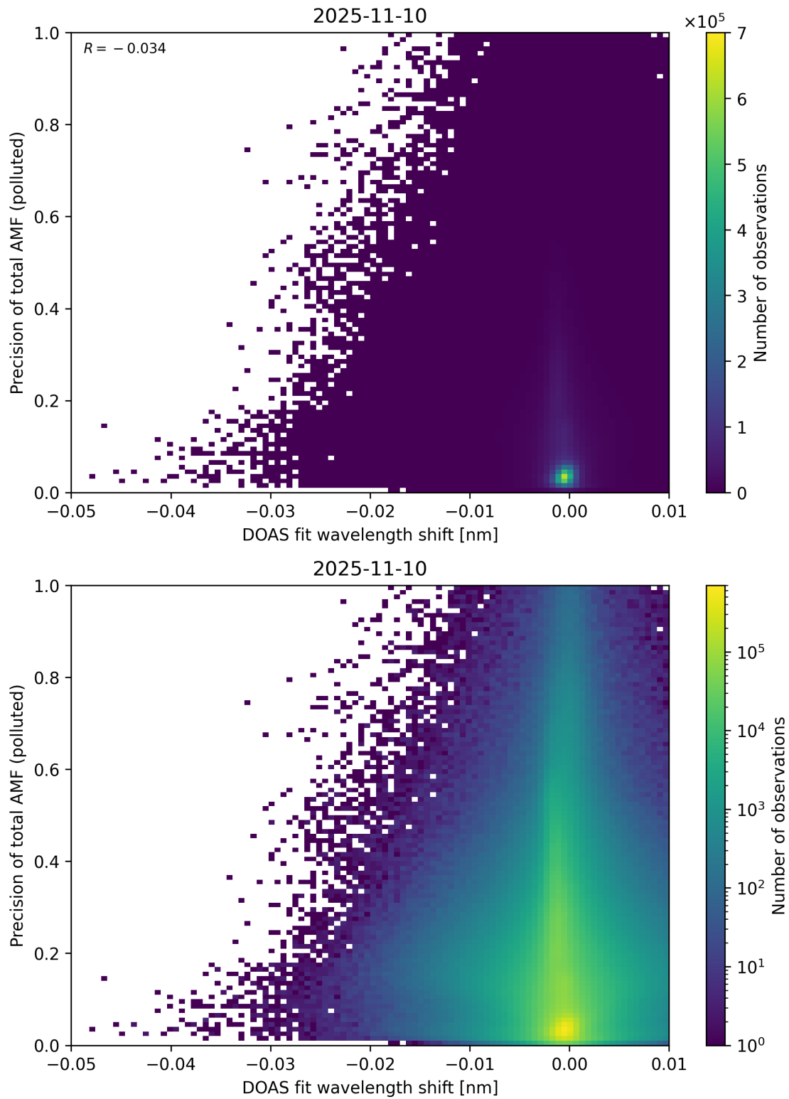
Figure 142: Scatter density plot of “DOAS fit wavelength shift” against “Precision of total AMF (polluted)” for 2025-11-09 to 2025-11-11.
