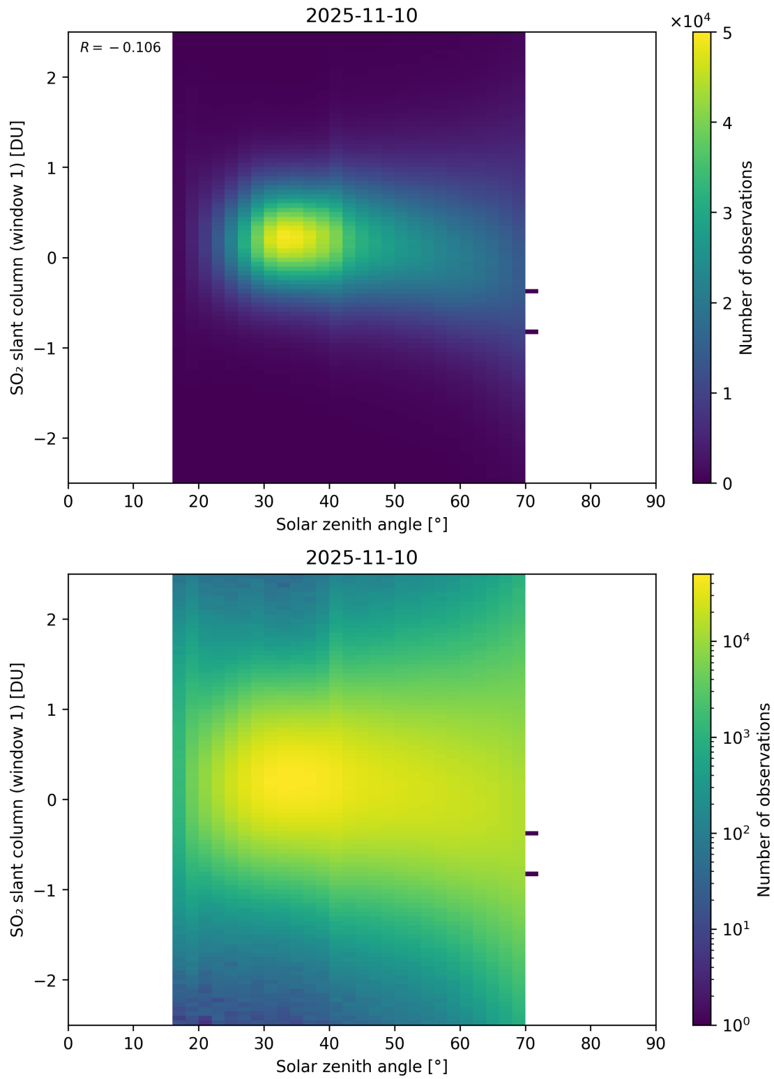
Figure 184: Scatter density plot of “Solar zenith angle” against “SO 2 slant column (window 1)” for 2025-11-09 to 2025-11-11.
