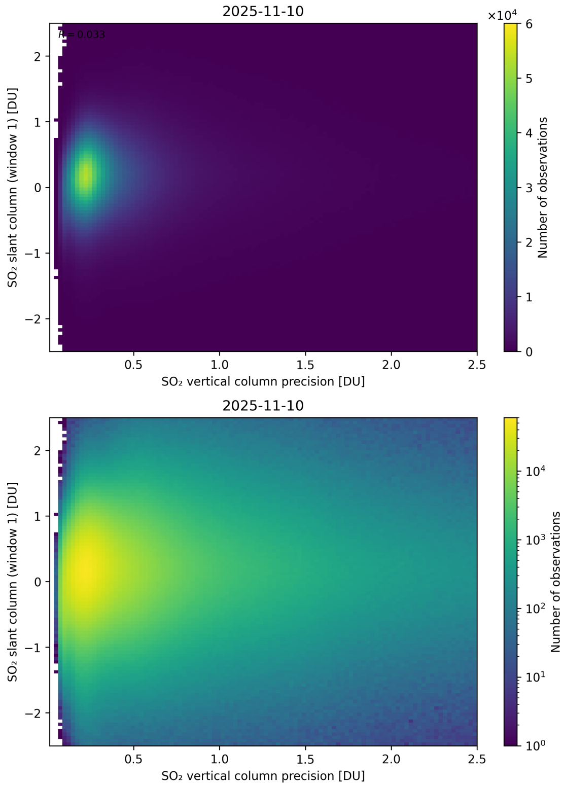
Figure 341: Scatter density plot of “SO 2 vertical column precision” against “SO 2 slant column (window 1)” for 2025-11-09 to 2025-11-11.
