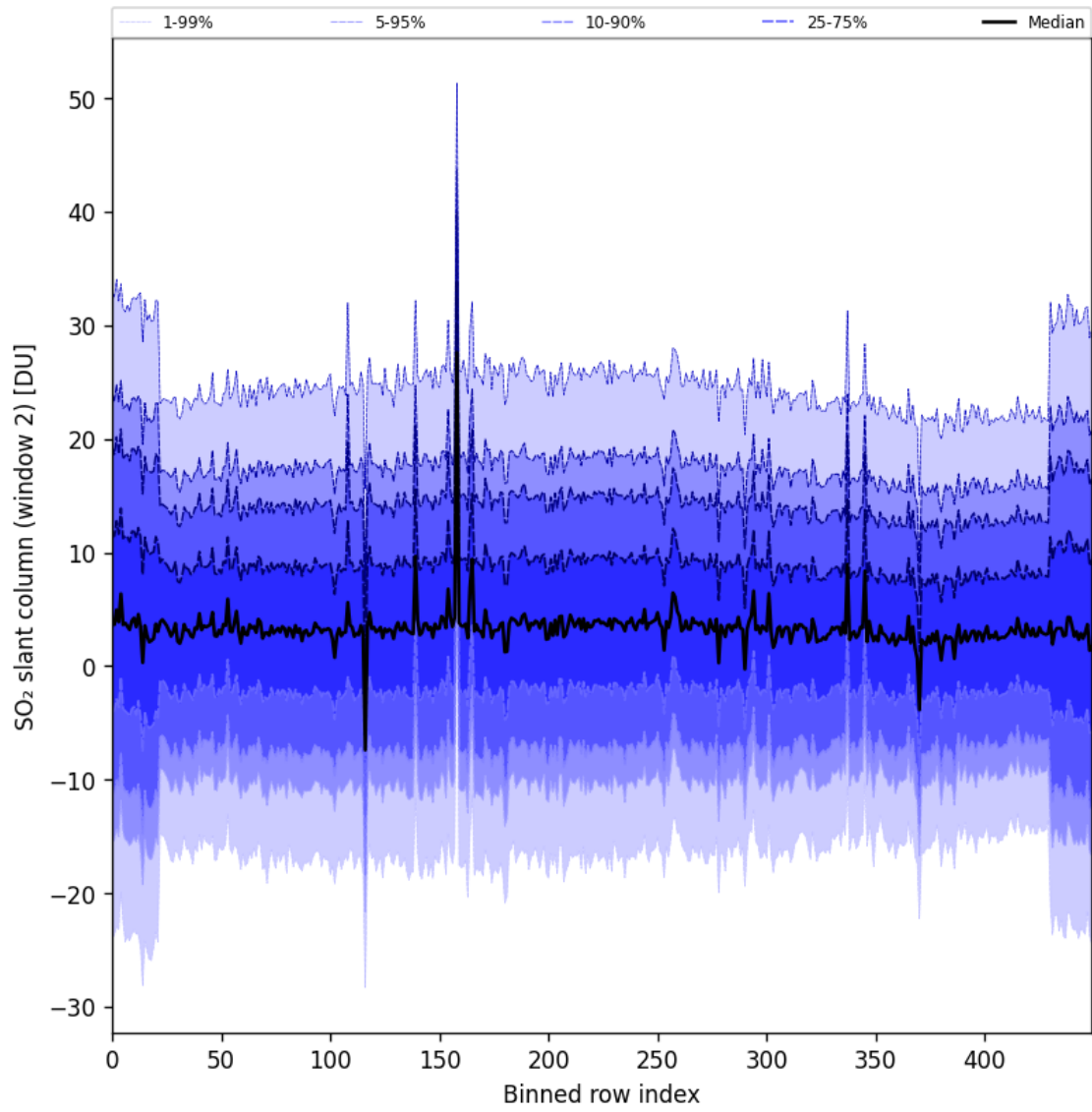
Figure 93: Along track statistics of “SO 2 slant column (window 2)” for 2025-11-09 to 2025-11-11
