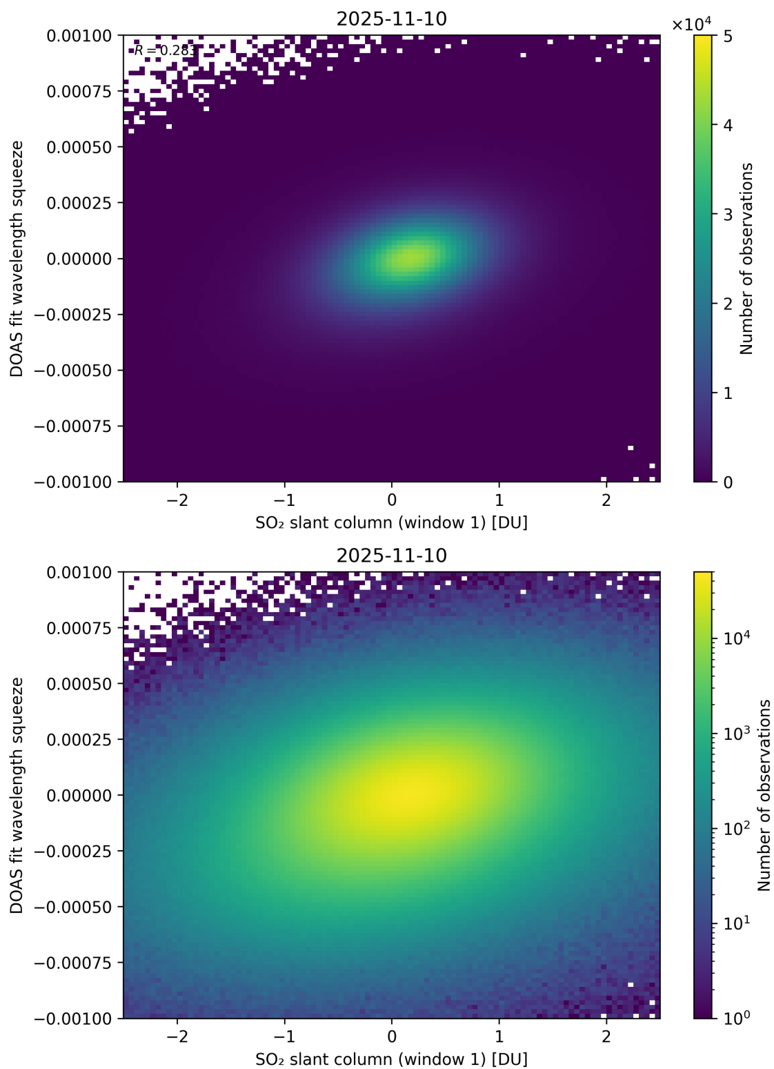
Figure 266: Scatter density plot of “SO 2 slant column (window 1)” against “DOAS fit wavelength squeeze” for 2025-11-09 to 2025-11-11.
