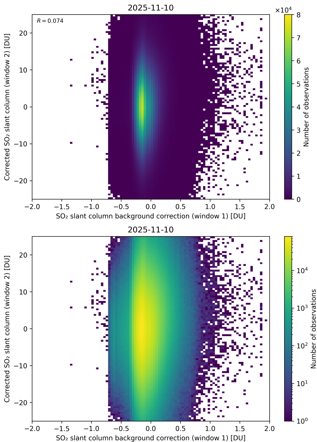
Figure 115: Scatter density plot of “SO 2 slant column background correction (window 1)” against “Corrected SO 2 slant column (window 2)” for 2025-11-09 to 2025-11-11.
