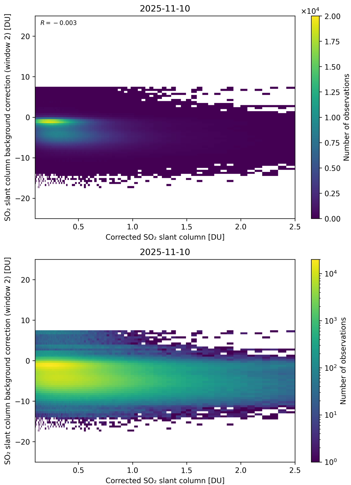
Figure 227: Scatter density plot of “Corrected SO 2 slant column” against “SO 2 slant column background correction (window 2)” for 2025-11-09 to 2025-11-11.
