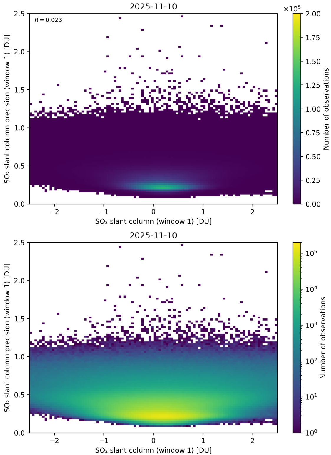
Figure 285: Scatter density plot of “SO 2 slant column (window 1)” against “SO 2 slant column precision (window 1)” for 2025-11-09 to 2025-11-11.
