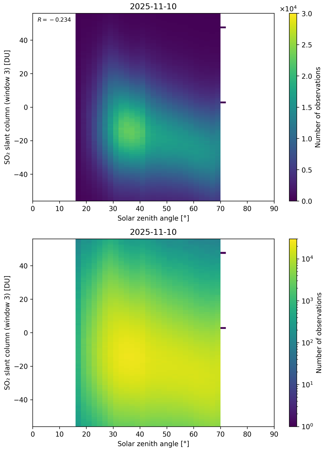
Figure 187: Scatter density plot of “Solar zenith angle” against “SO 2 slant column (window 3)” for 2025-11-09 to 2025-11-11.
