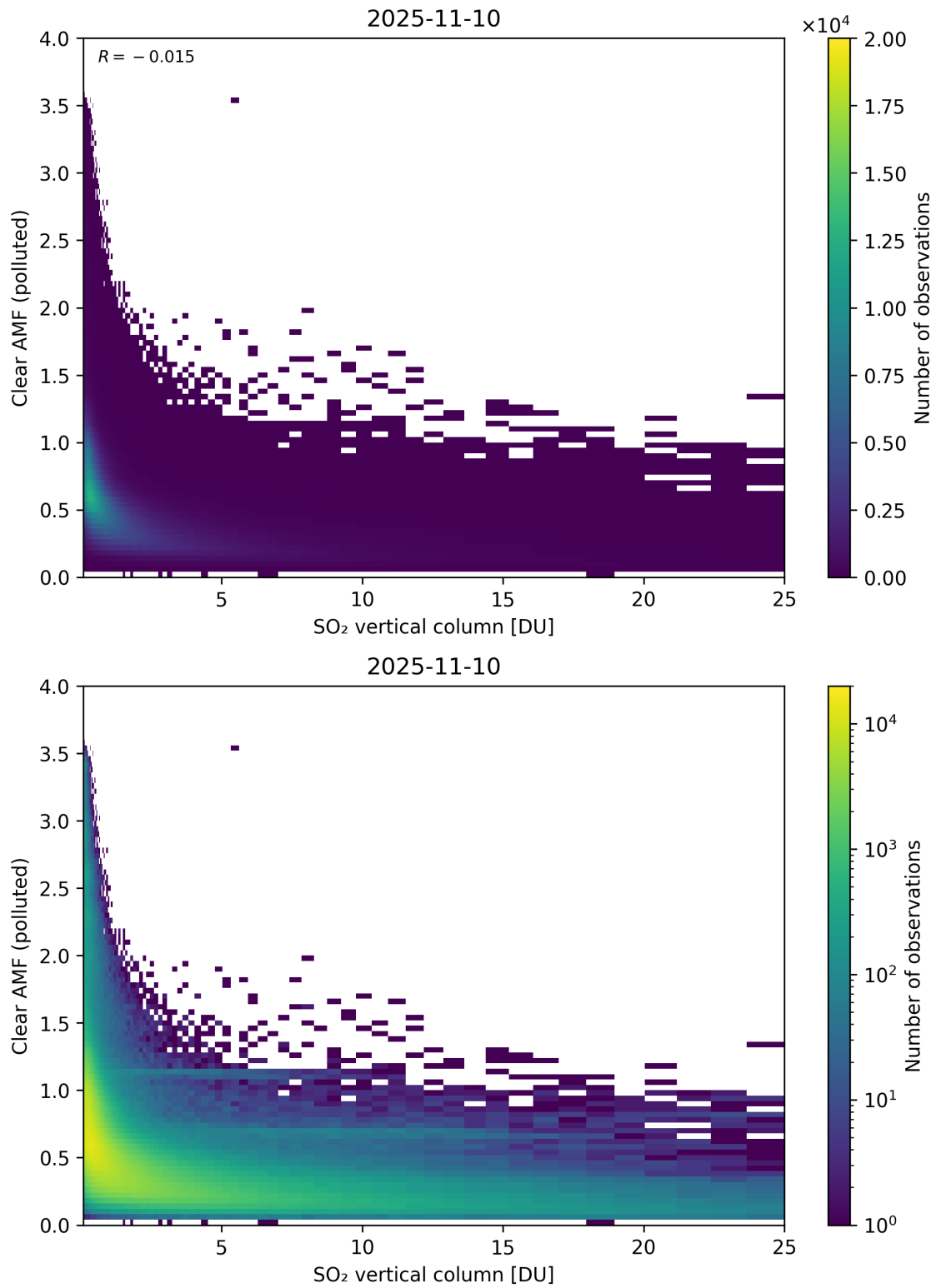
Figure 348: Scatter density plot of “SO 2 vertical column” against “Clear AMF (polluted)” for 2025-11-09 to 2025-11-11.
