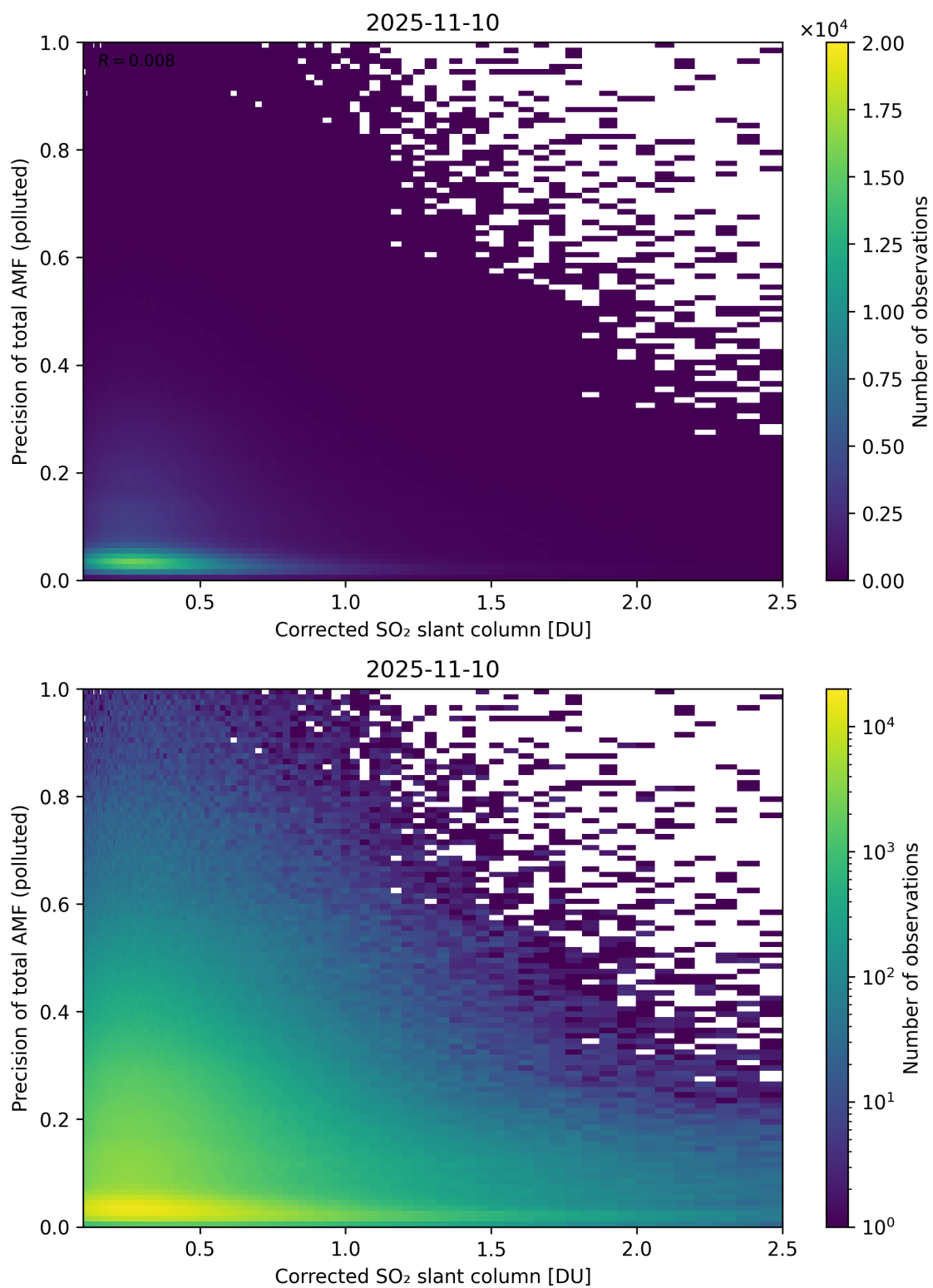
Figure 243: Scatter density plot of “Corrected SO 2 slant column” against “Precision of total AMF (polluted)” for 2025-11-09 to 2025-11-11.
