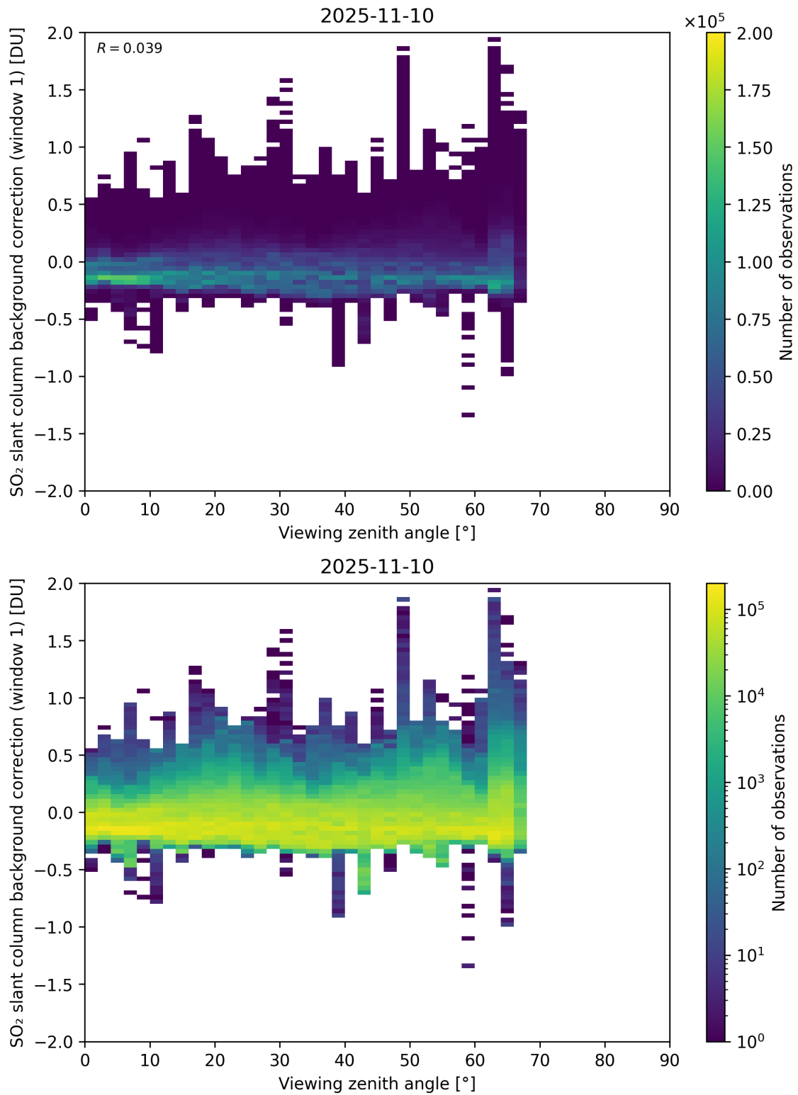
Figure 362: Scatter density plot of “Viewing zenith angle” against “SO 2 slant column background correction (window 1)” for 2025-11-09 to 2025-11-11.
