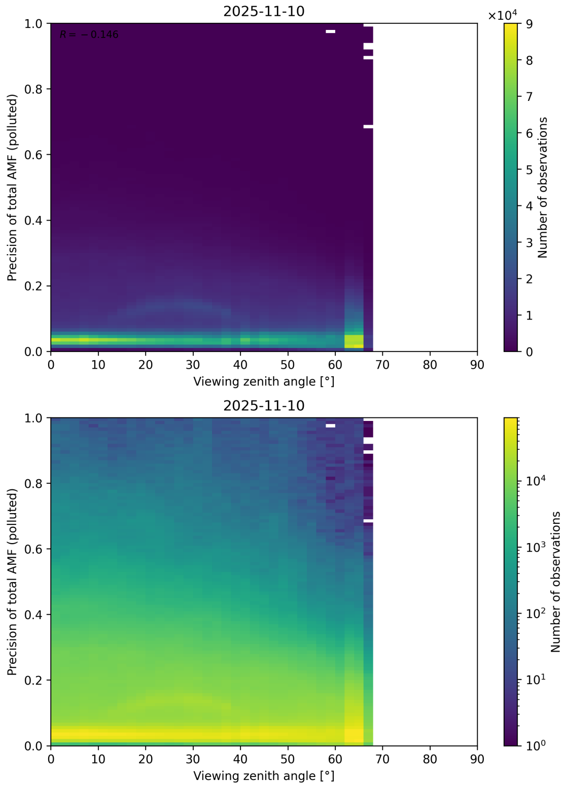
Figure 382: Scatter density plot of “Viewing zenith angle” against “Precision of total AMF (polluted)” for 2025-11-09 to 2025-11-11.
