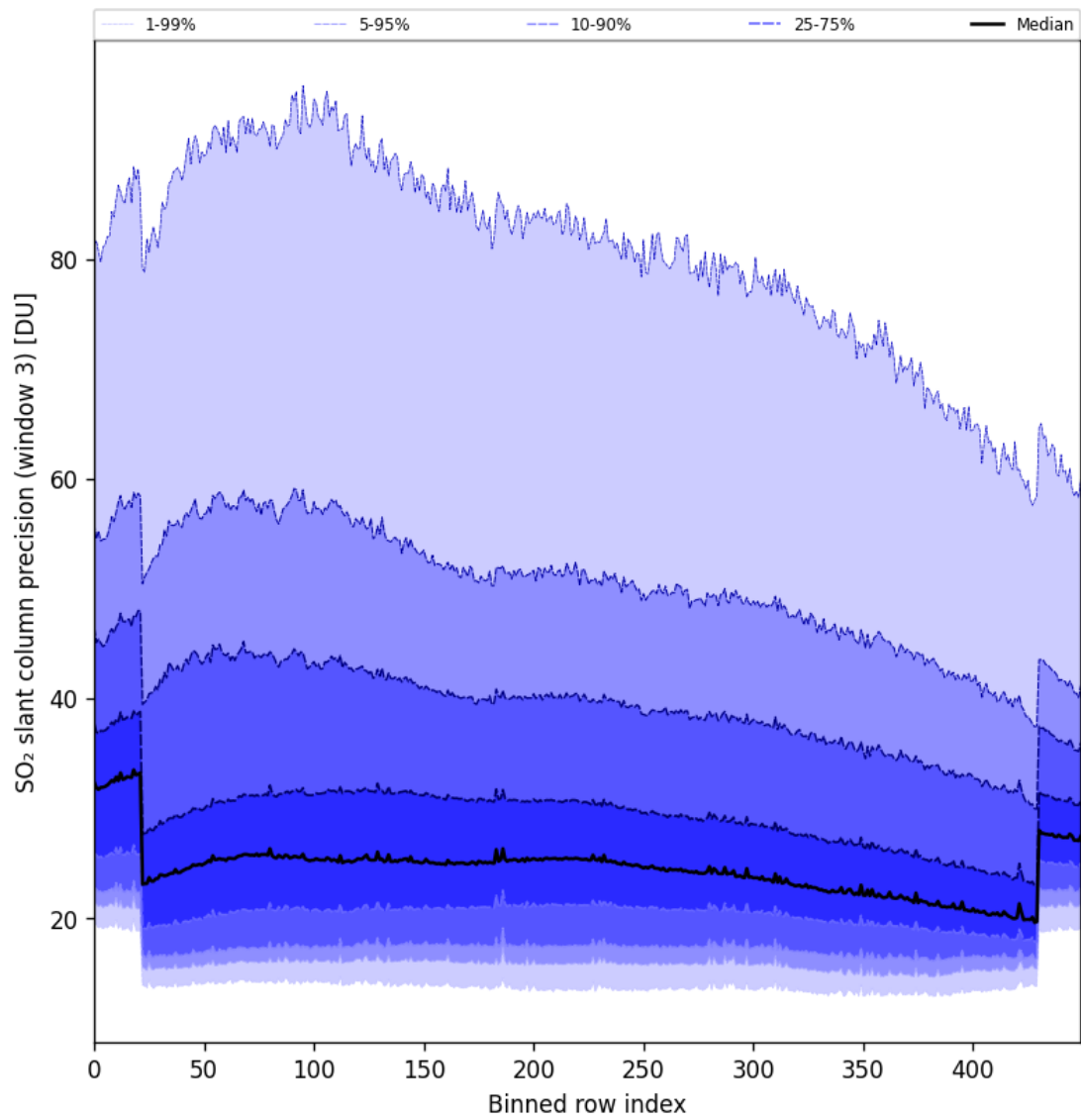
Figure 98: Along track statistics of “SO 2 slant column precision (window 3)” for 2025-11-09 to 2025-11-11
