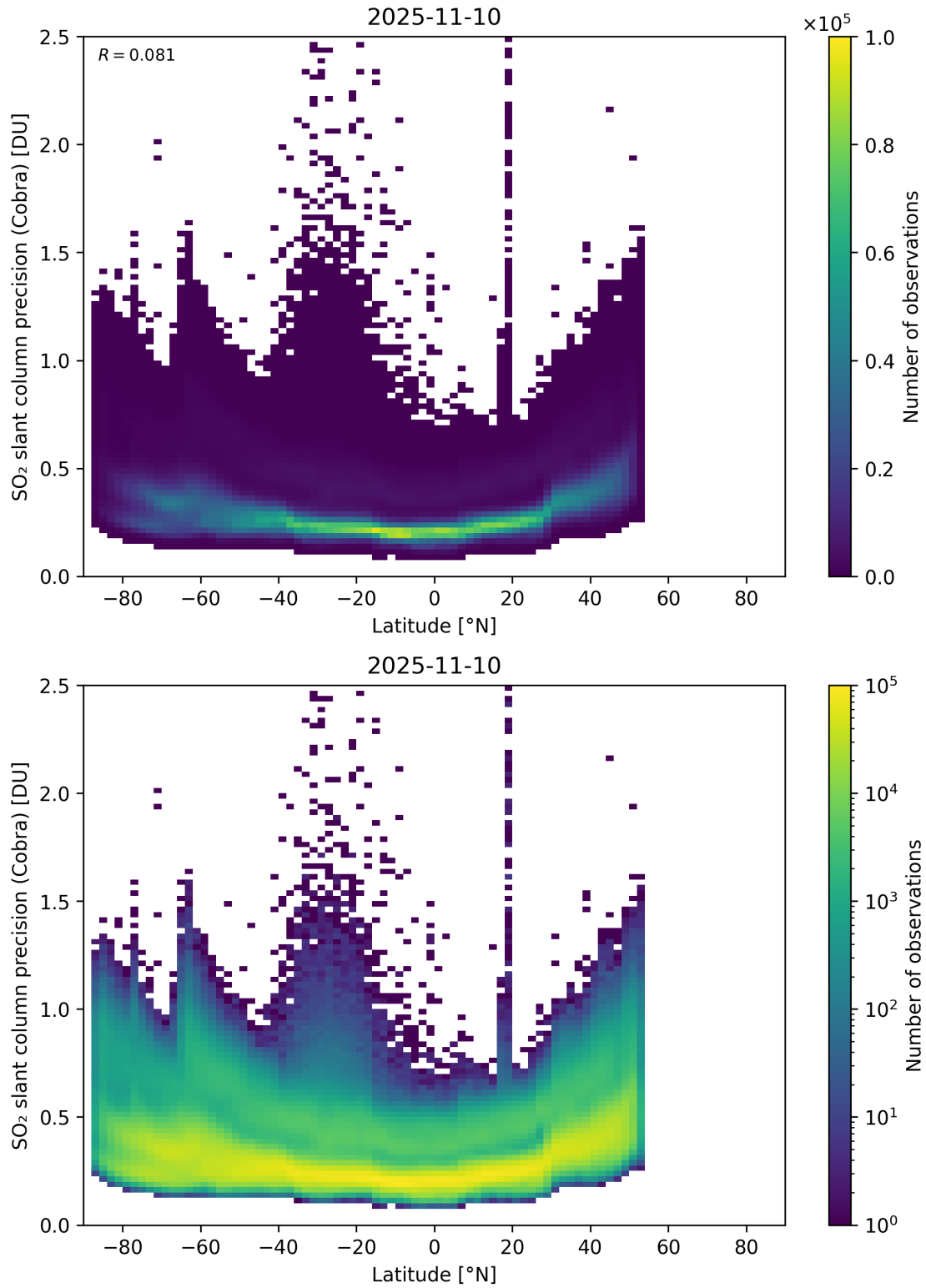
Figure 158: Scatter density plot of “Latitude” against “SO 2 slant column precision (Cobra)” for 2025-11-09 to 2025-11-11.
