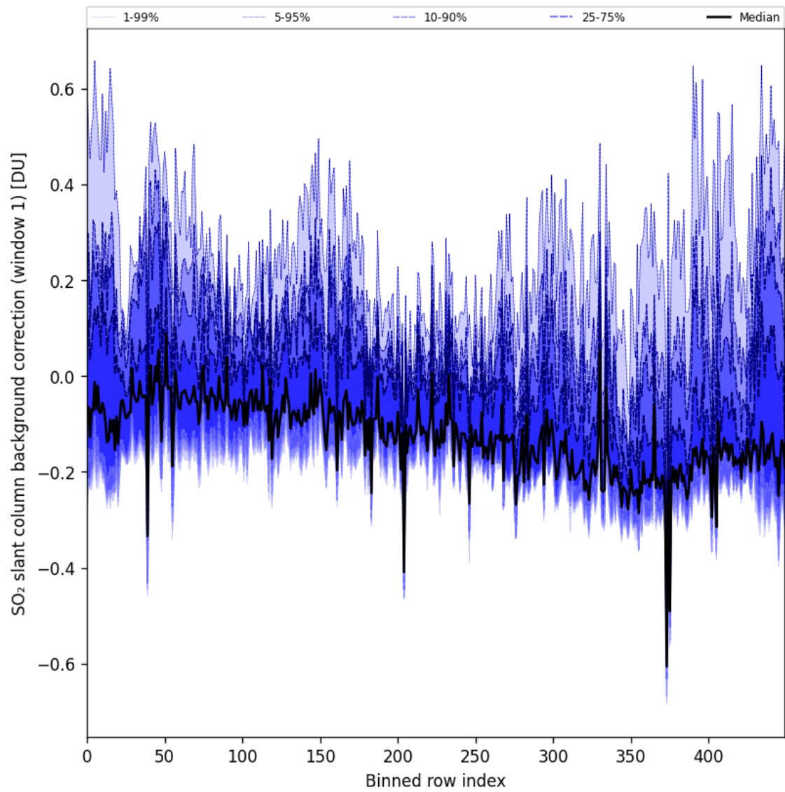
Figure 92: Along track statistics of “SO 2 slant column background correction (window 1)” for 2025-11-09 to 2025-11-11
