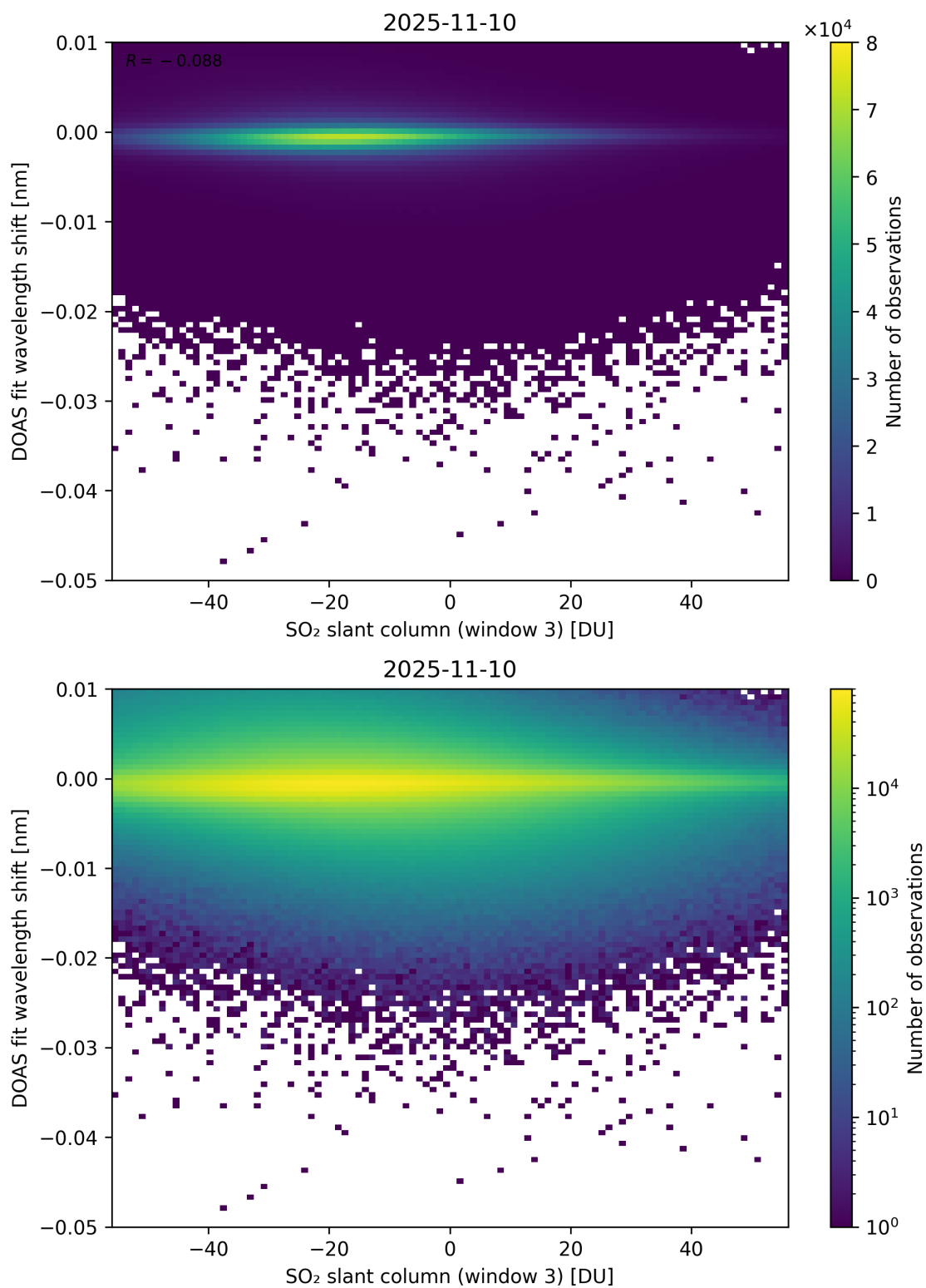
Figure 304: Scatter density plot of “SO 2 slant column (window 3)” against “DOAS fit wavelength shift” for 2025-11-09 to 2025-11-11.
