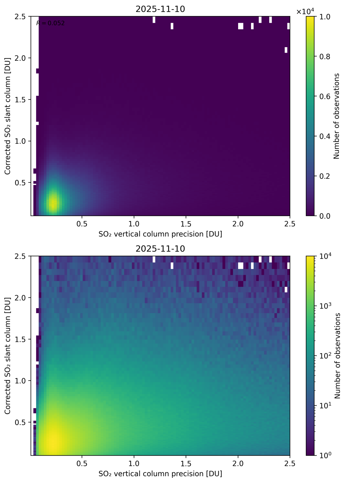
Figure 338: Scatter density plot of “SO 2 vertical column precision” against “Corrected SO 2 slant column” for 2025-11-09 to 2025-11-11.
