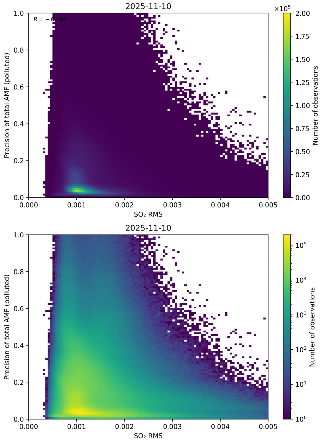
Figure 149: Scatter density plot of “SO 2 RMS” against “Precision of total AMF (polluted)” for 2025-11-09 to 2025-11-11.
