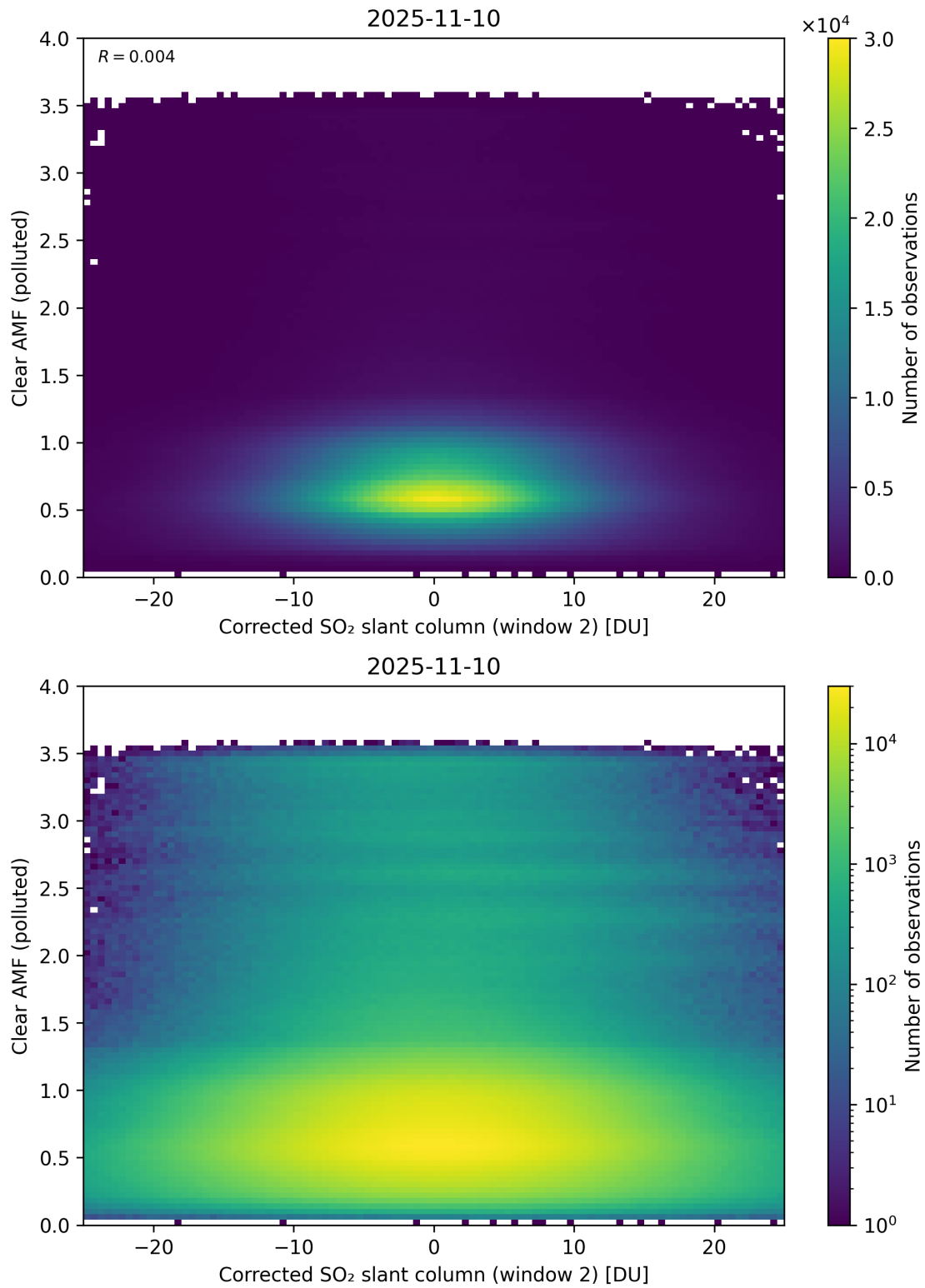
Figure 249: Scatter density plot of “Corrected SO 2 slant column (window 2)” against “Clear AMF (polluted)” for 2025-11-09 to 2025-11-11.
