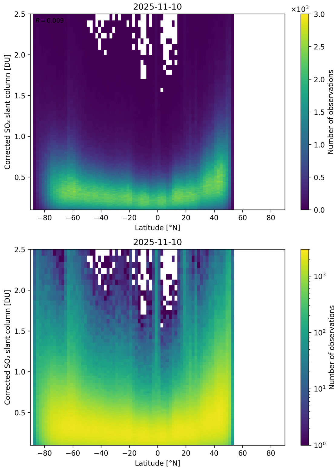
Figure 159: Scatter density plot of “Latitude” against “Corrected SO 2 slant column” for 2025-11-09 to 2025-11-11.
