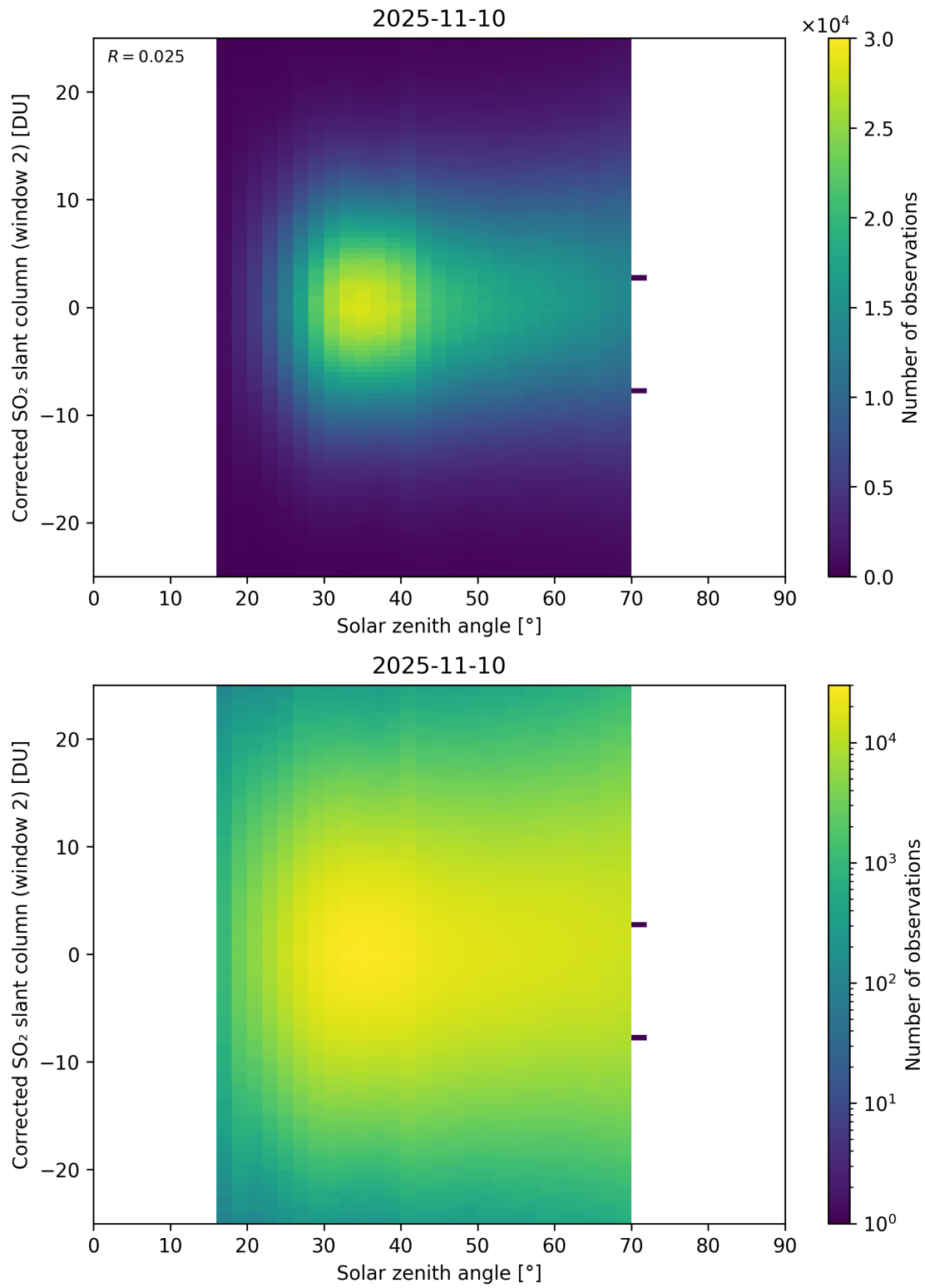
Figure 182: Scatter density plot of “Solar zenith angle” against “Corrected SO 2 slant column (window 2)” for 2025-11-09 to 2025-11-11.
