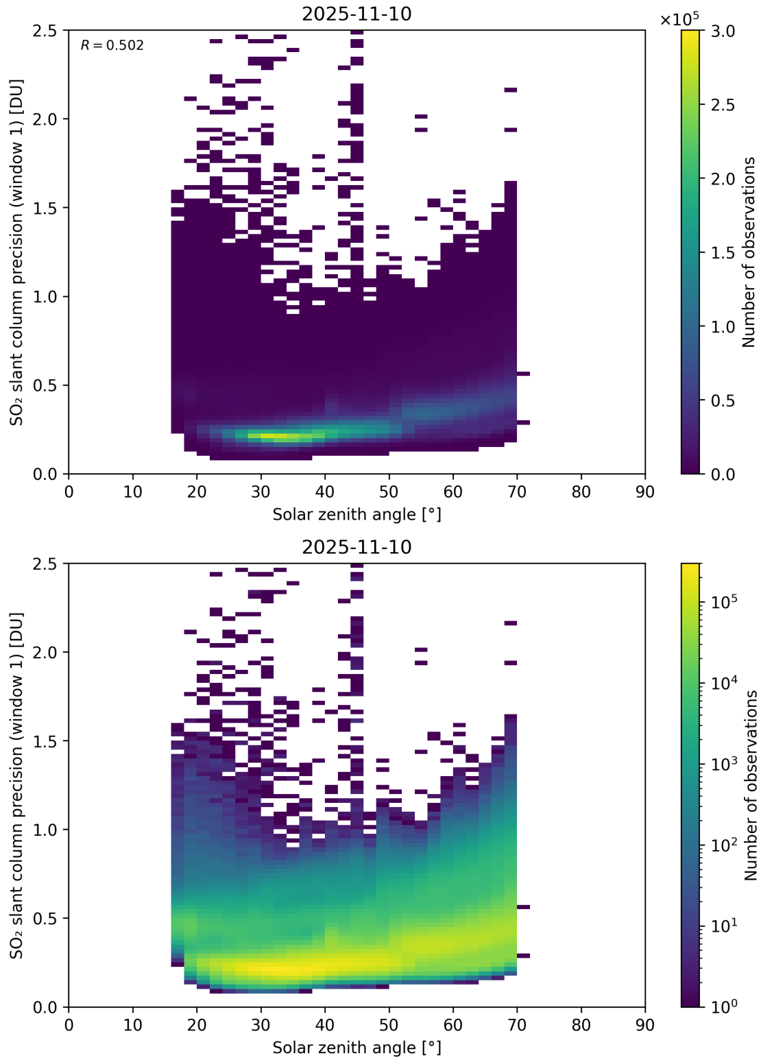
Figure 185: Scatter density plot of “Solar zenith angle” against “SO 2 slant column precision (window 1)” for 2025-11-09 to 2025-11-11.
