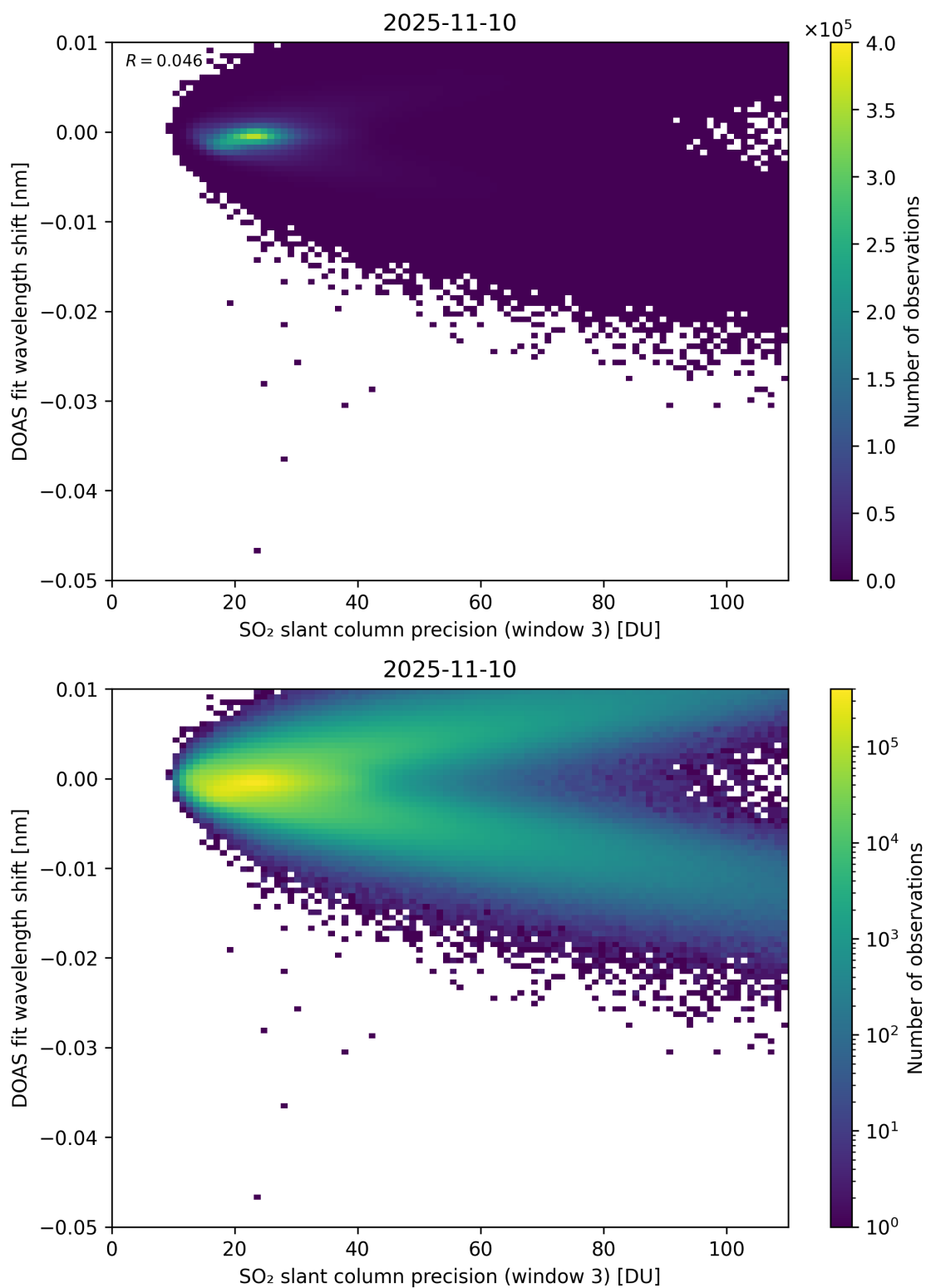
Figure 308: Scatter density plot of “SO 2 slant column precision (window 3)” against “DOAS fit wavelength shift” for 2025-11-09 to 2025-11-11.
