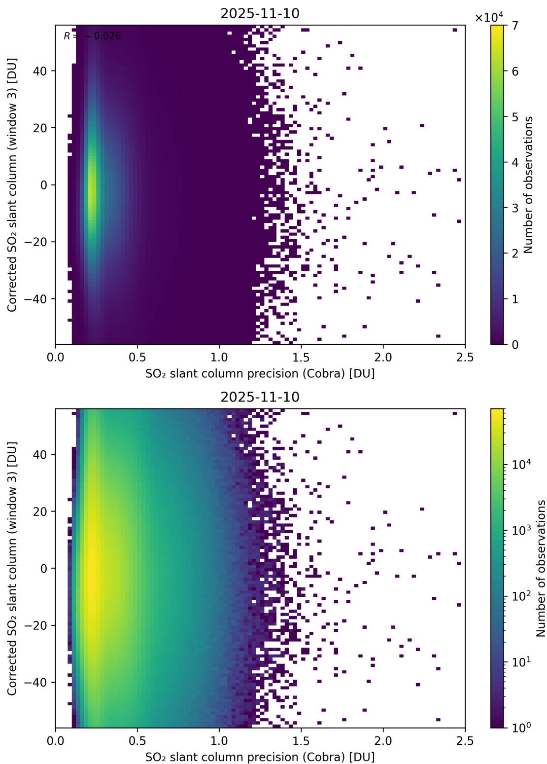
Figure 207: Scatter density plot of “SO 2 slant column precision (Cobra)” against “Corrected SO 2 slant column (window 3)” for 2025-11-09 to 2025-11-11.
