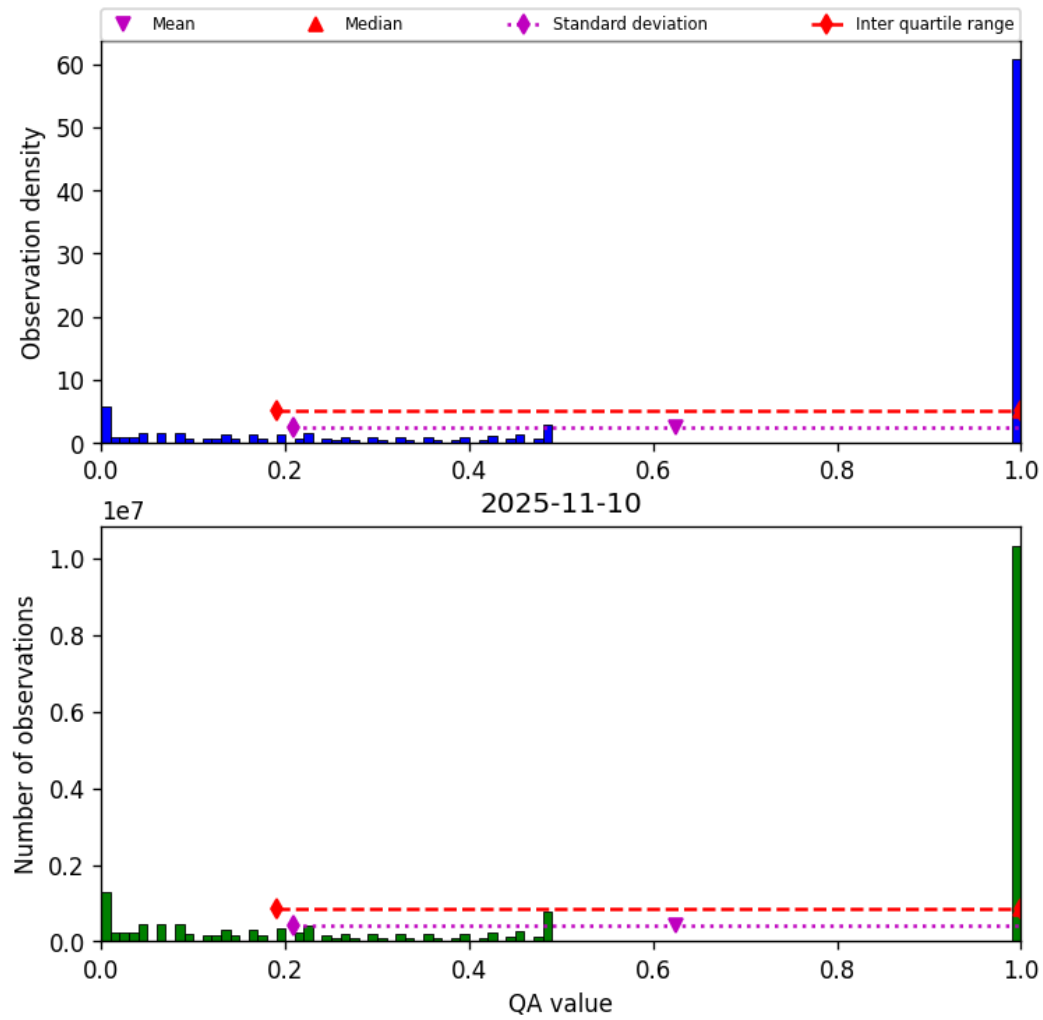
Figure 57: Histogram of “QA value” for 2025-11-09 to 2025-11-11
