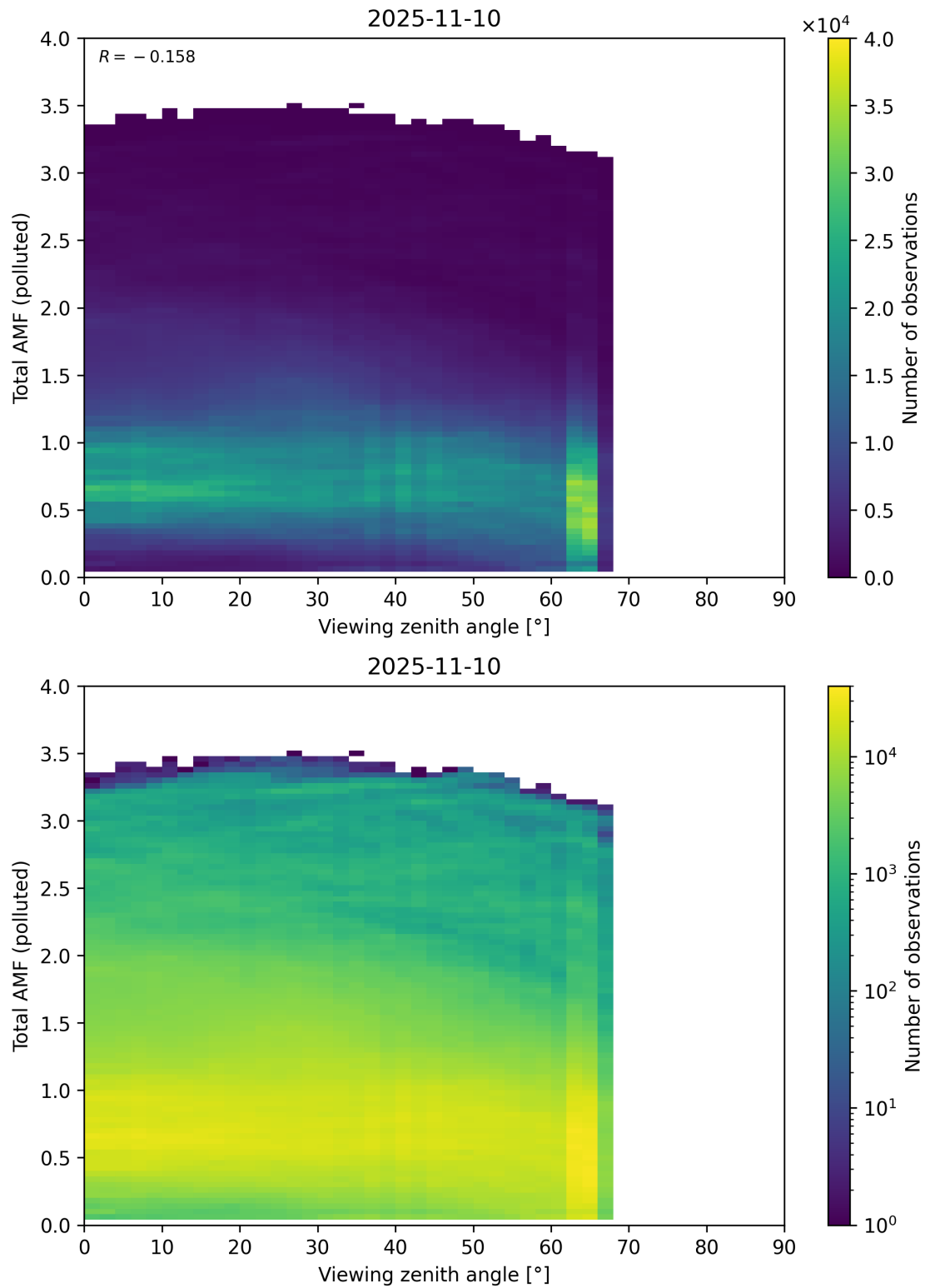
Figure 381: Scatter density plot of “Viewing zenith angle” against “Total AMF (polluted)” for 2025-11-09 to 2025-11-11.
