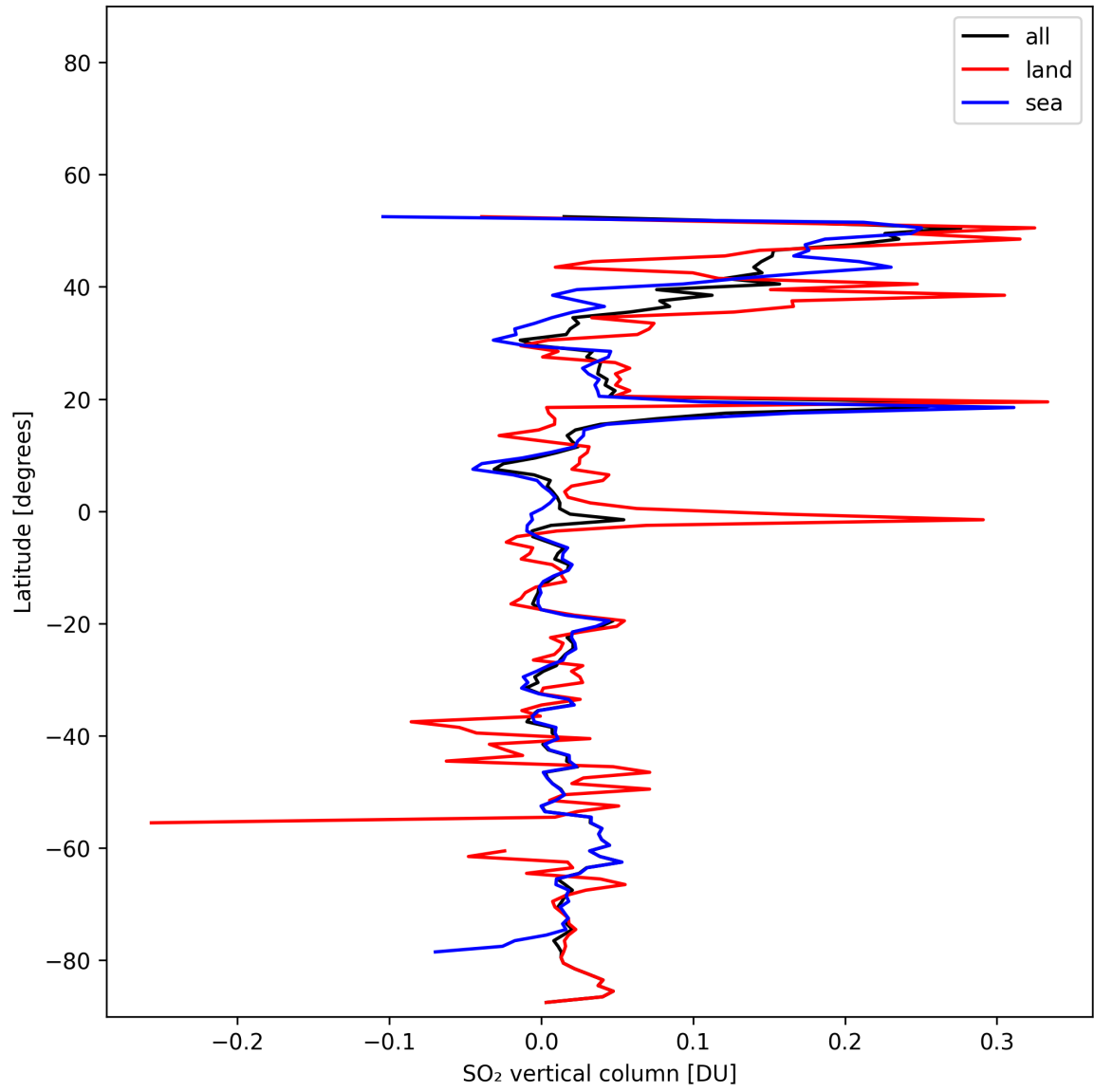
Figure 32: Zonal average of “SO 2 vertical column” for 2025-11-09 to 2025-11-11.
