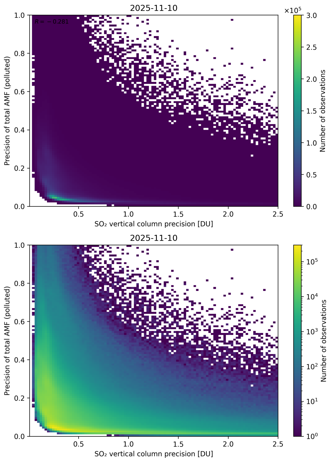
Figure 347: Scatter density plot of “SO 2 vertical column precision” against “Precision of total AMF (polluted)” for 2025-11-09 to 2025-11-11.
