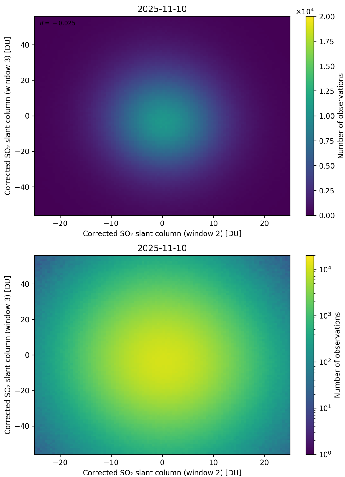
Figure 250: Scatter density plot of “Corrected SO 2 slant column (window 2)” against “Corrected SO 2 slant column (window 3)” for 2025-11-09 to 2025-11-11.
