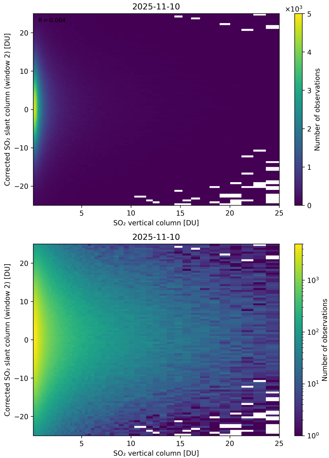
Figure 352: Scatter density plot of “SO 2 vertical column” against “Corrected SO 2 slant column (window 2)” for 2025-11-09 to 2025-11-11.
