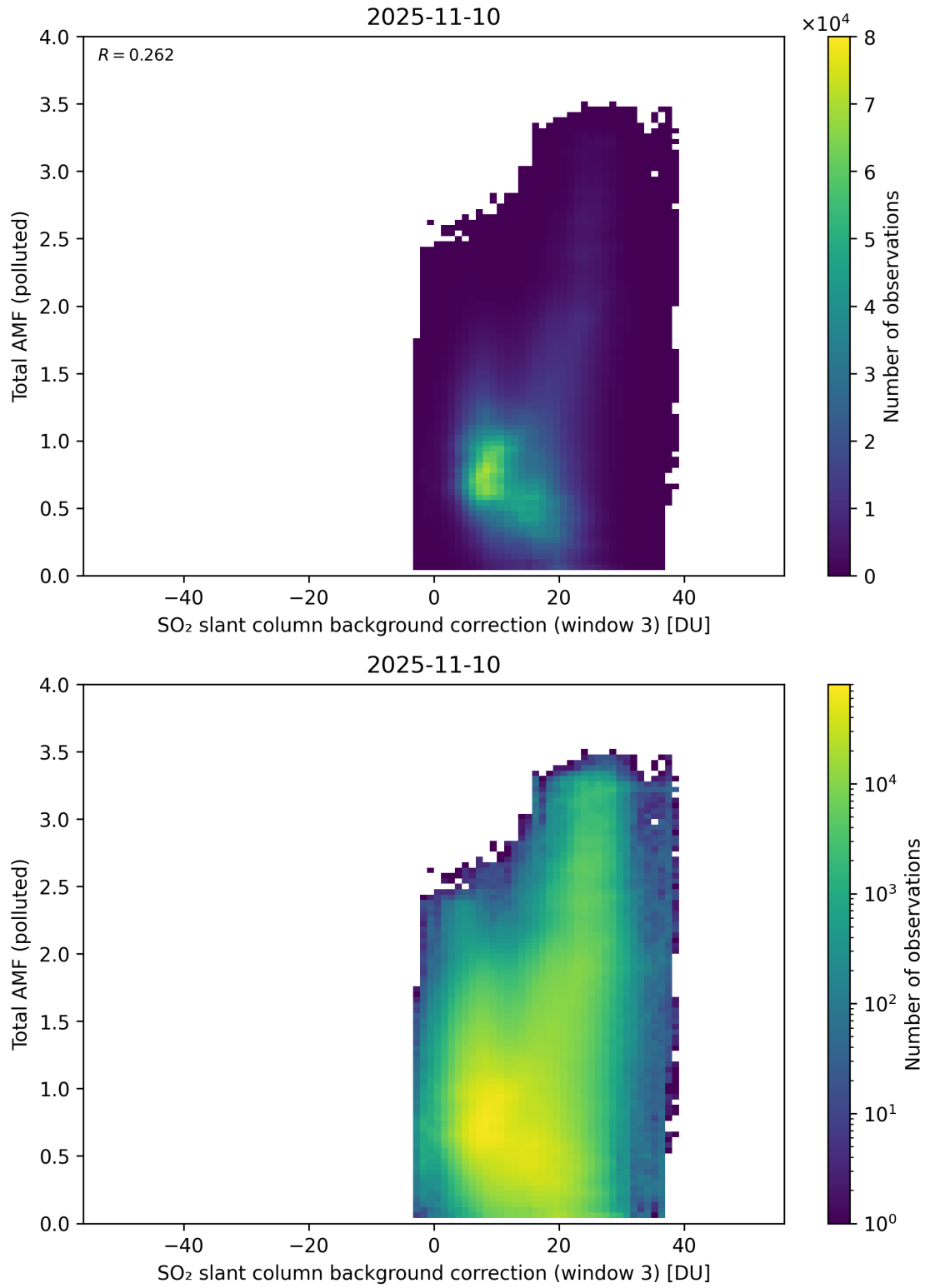
Figure 136: Scatter density plot of “SO 2 slant column background correction (window 3)” against “Total AMF (polluted)” for 2025-11-09 to 2025-11-11.
