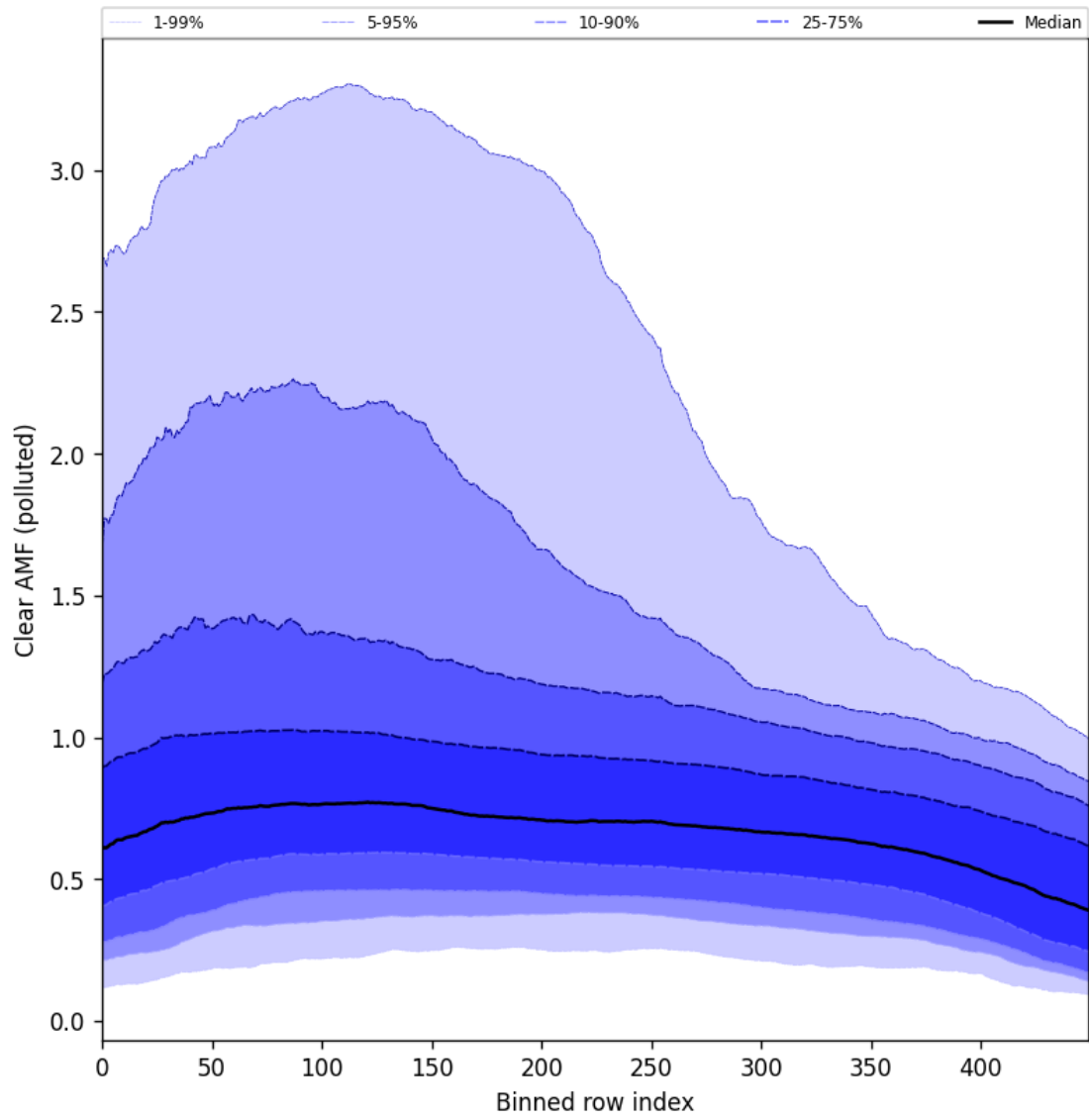
Figure 107: Along track statistics of “Clear AMF (polluted)” for 2025-11-09 to 2025-11-11
