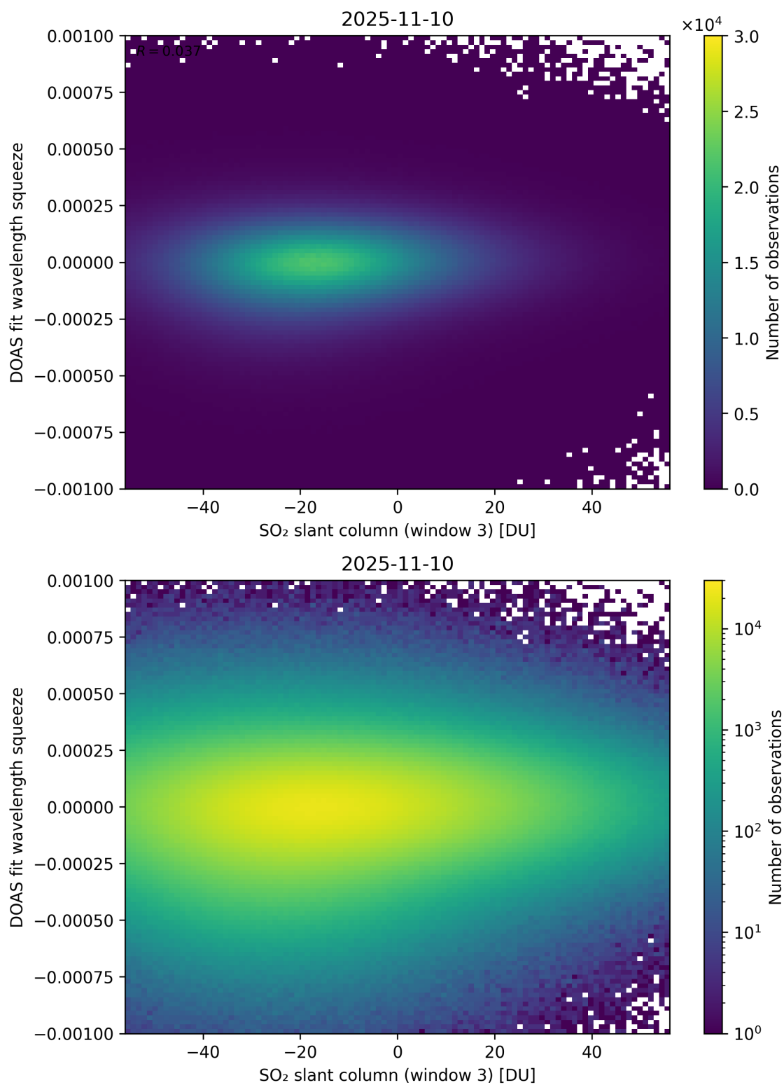
Figure 305: Scatter density plot of “SO 2 slant column (window 3)” against “DOAS fit wavelength squeeze” for 2025-11-09 to 2025-11-11.
