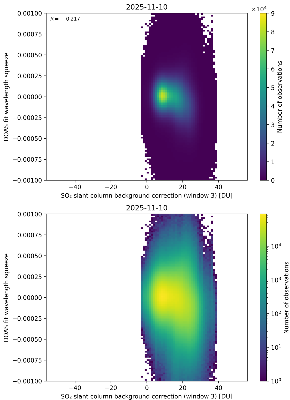
Figure 133: Scatter density plot of “SO 2 slant column background correction (window 3)” against “DOAS fit wavelength squeeze” for 2025-11-09 to 2025-11-11.
