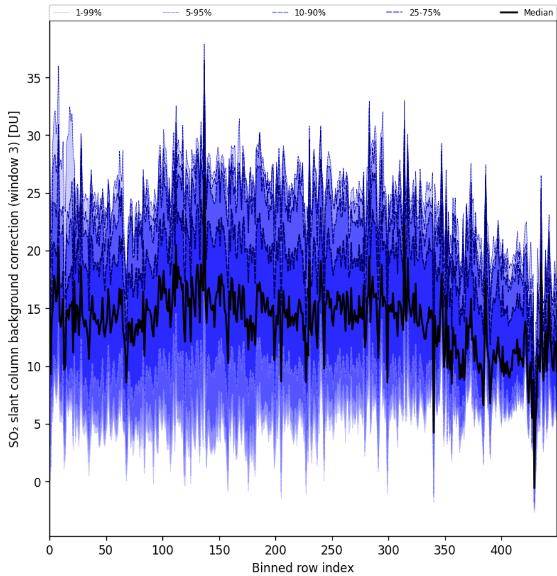
Figure 100: Along track statistics of “SO 2 slant column background correction (window 3)” for 2025-11-09 to 2025-11-11
