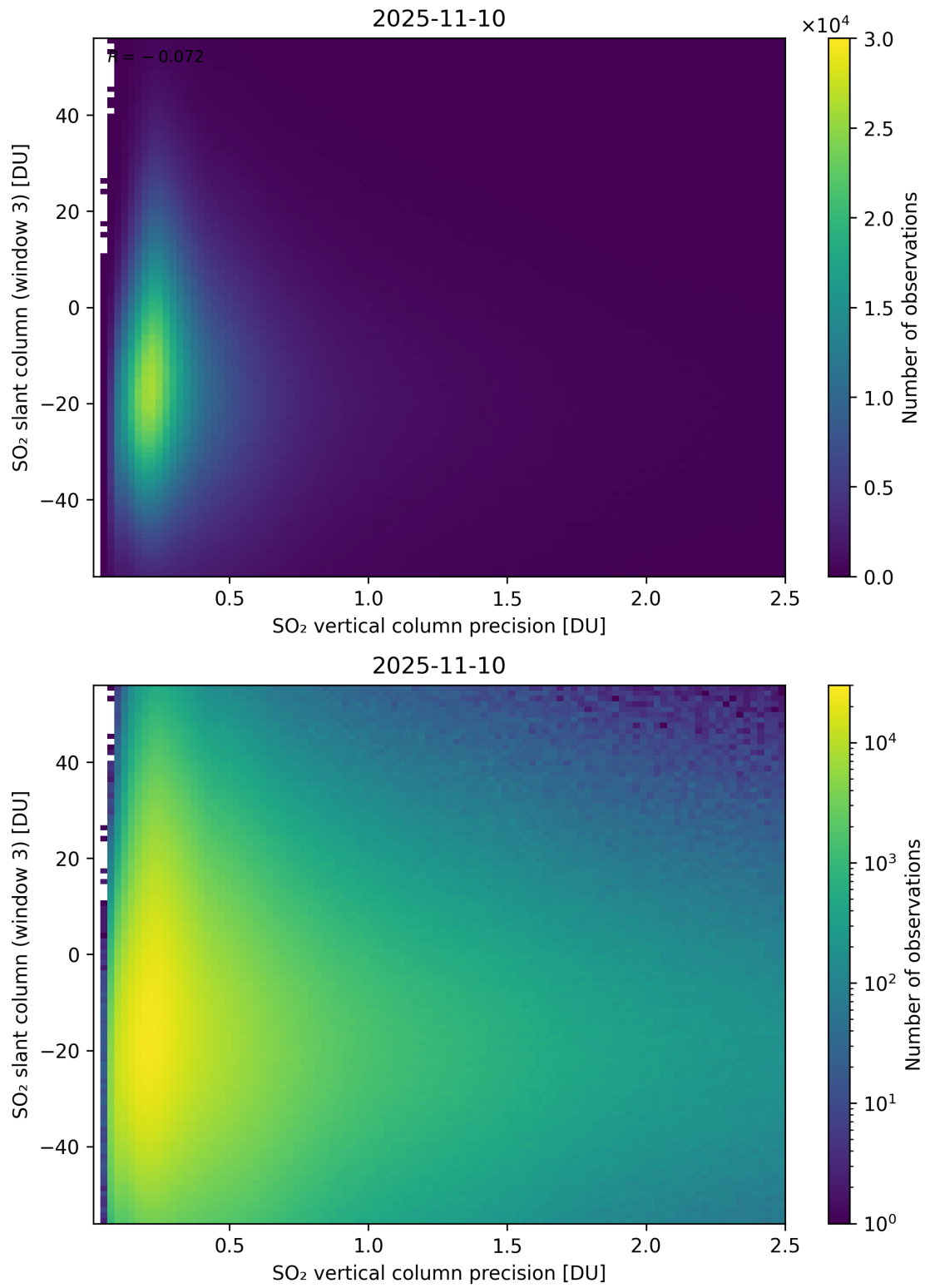
Figure 344: Scatter density plot of “SO 2 vertical column precision” against “SO 2 slant column (window 3)” for 2025-11-09 to 2025-11-11.
