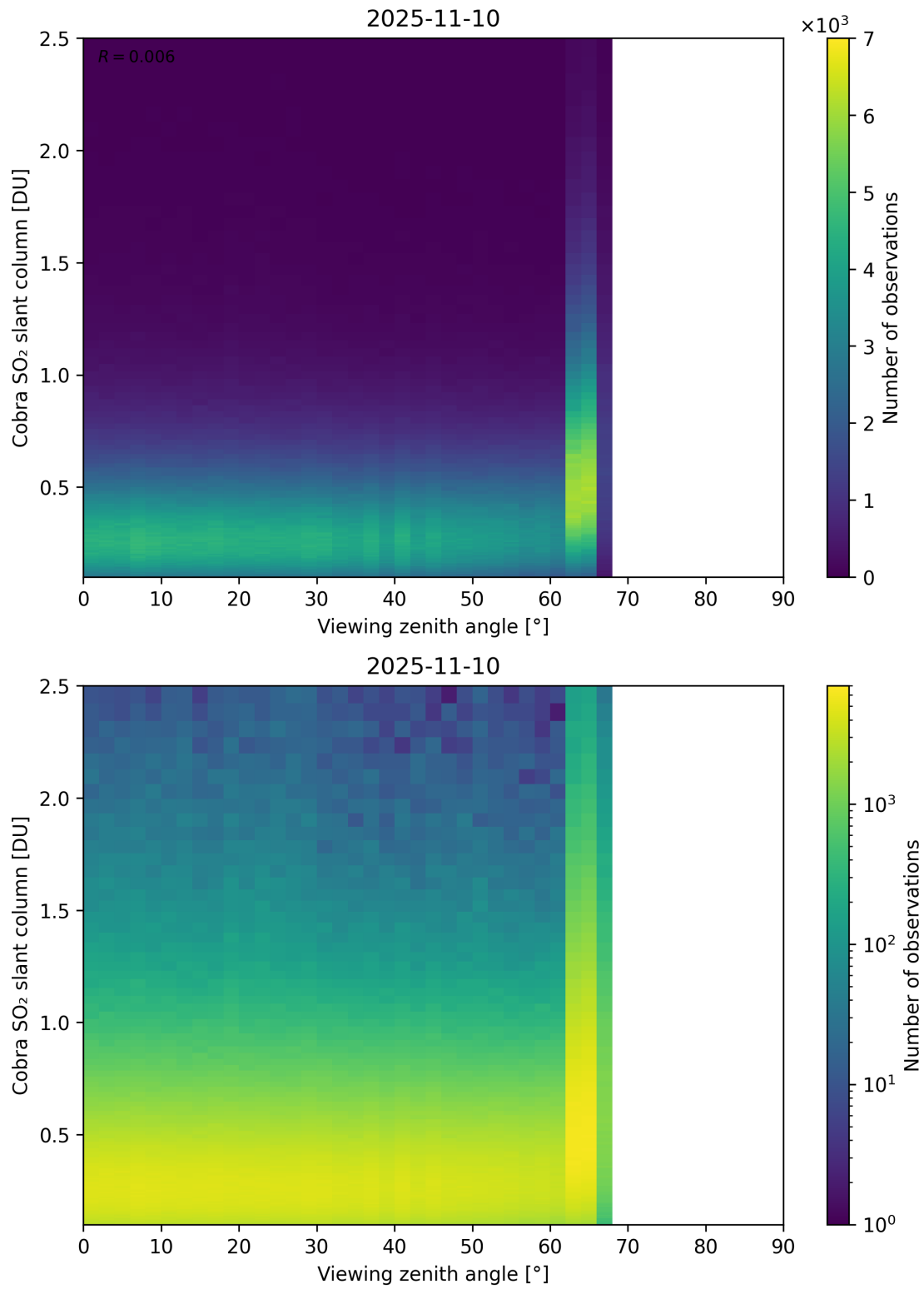
Figure 371: Scatter density plot of “Viewing zenith angle” against “Cobra SO 2 slant column” for 2025-11-09 to 2025-11-11.
