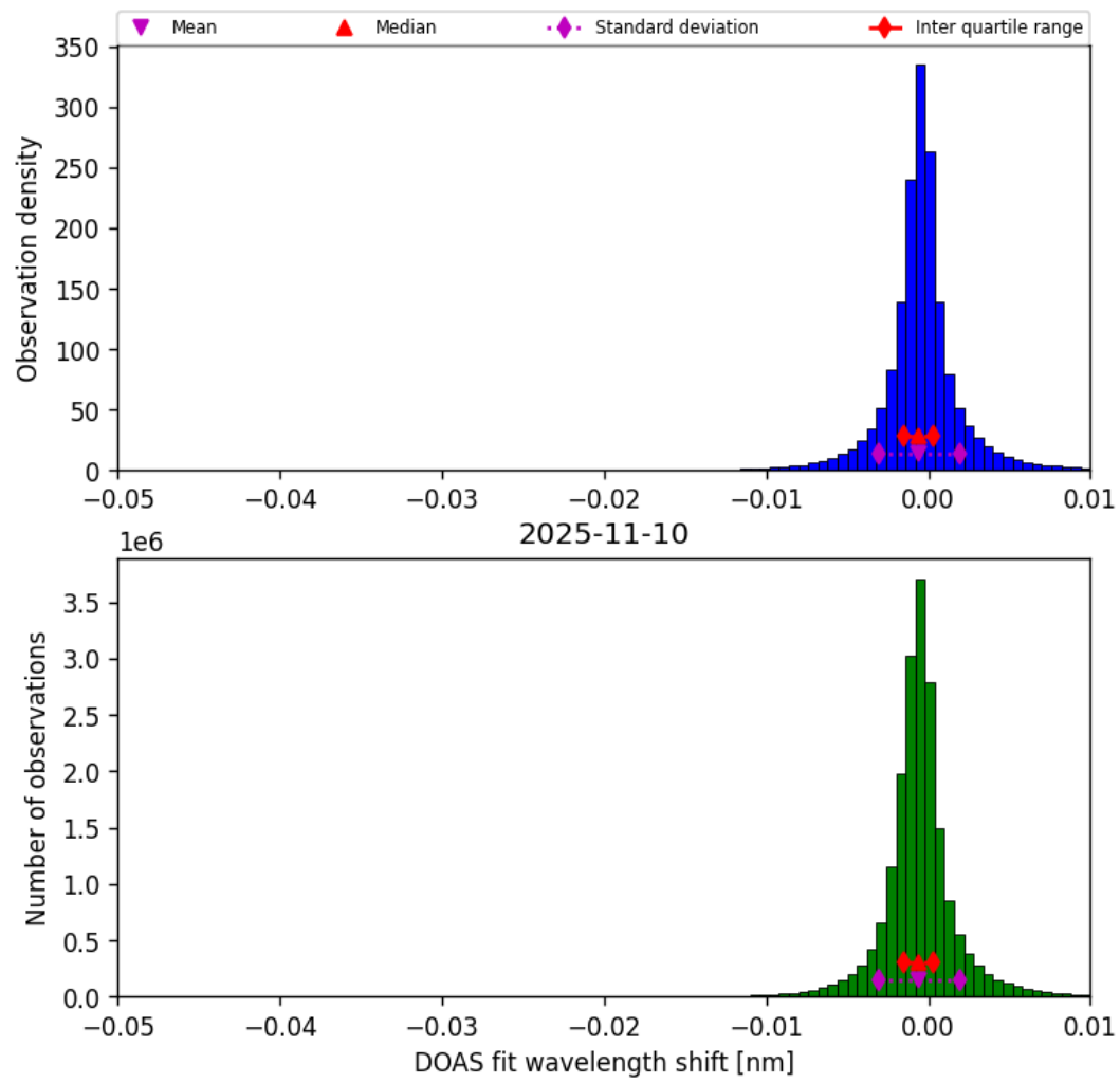
Figure 76: Histogram of “DOAS fit wavelength shift” for 2025-11-09 to 2025-11-11
