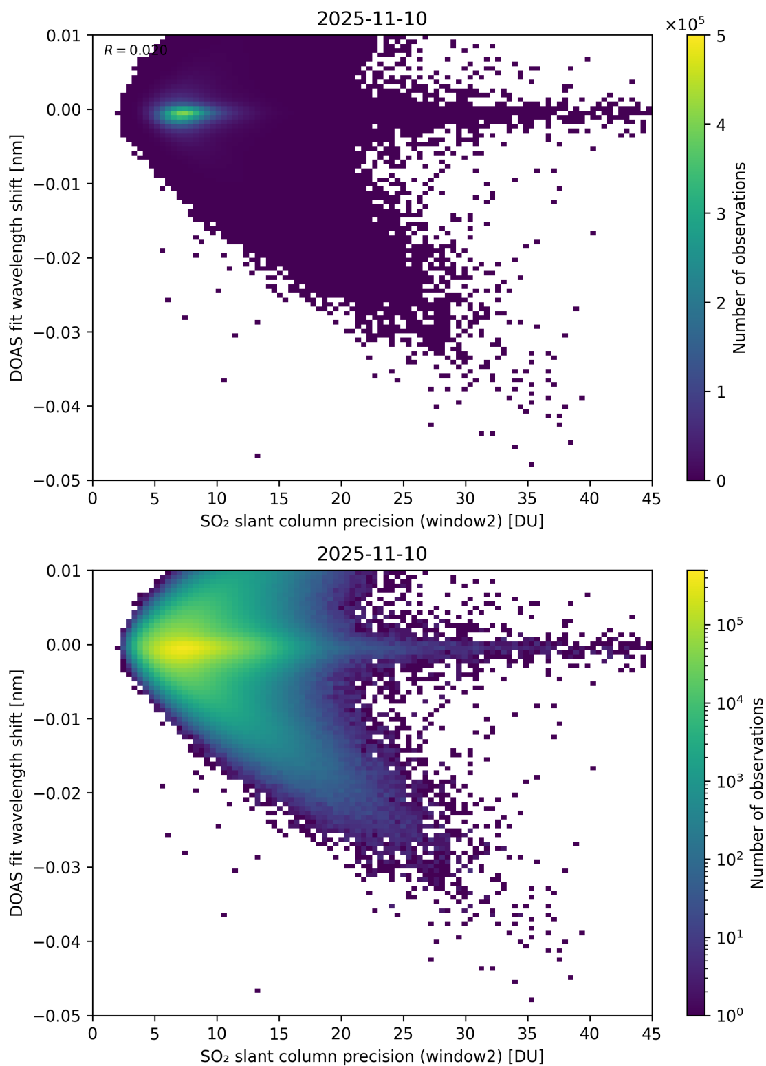
Figure 293: Scatter density plot of “SO 2 slant column precision (window2)” against “DOAS fit wavelength shift” for 2025-11-09 to 2025-11-11.
