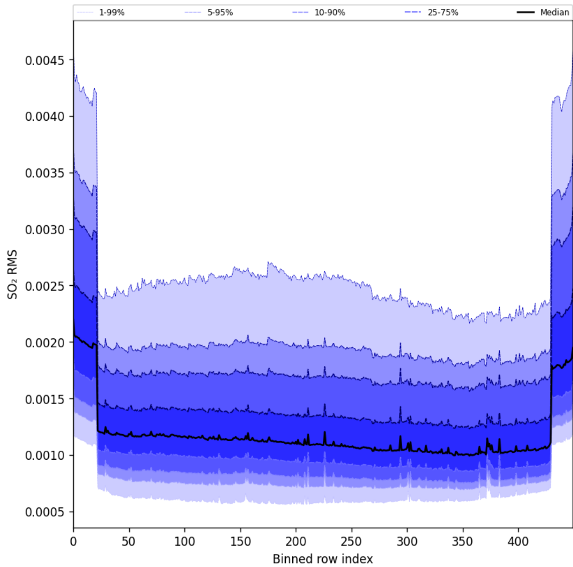
Figure 104: Along track statistics of “SO 2 RMS” for 2025-11-09 to 2025-11-11
