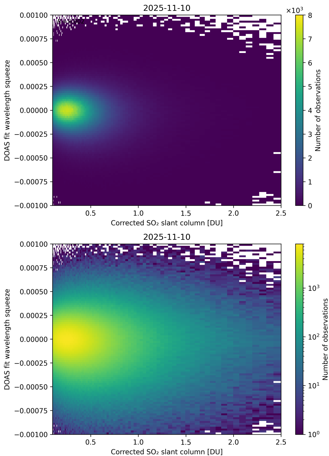
Figure 230: Scatter density plot of “Corrected SO 2 slant column” against “DOAS fit wavelength squeeze” for 2025-11-09 to 2025-11-11.
