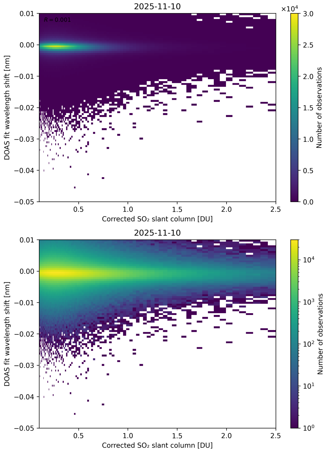
Figure 229: Scatter density plot of “Corrected SO 2 slant column” against “DOAS fit wavelength shift” for 2025-11-09 to 2025-11-11.
