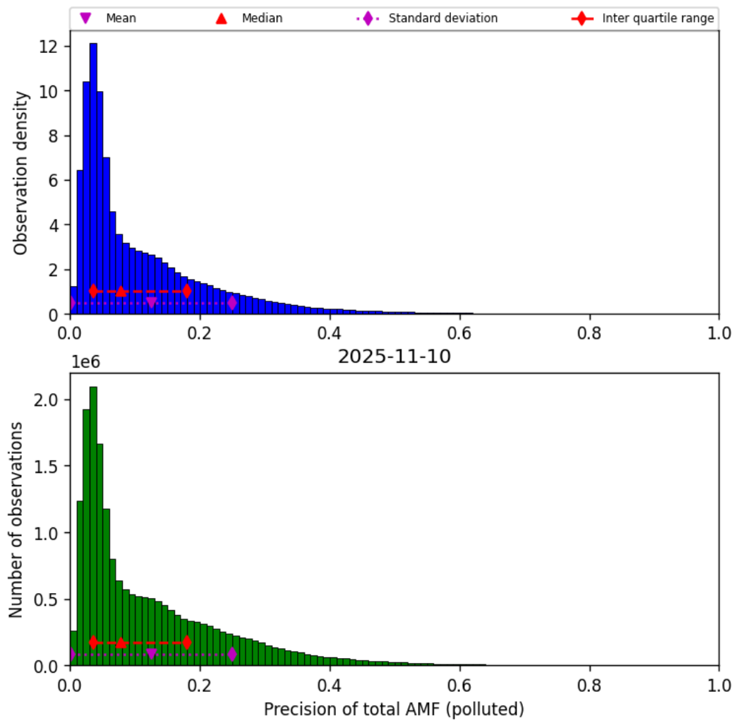
Figure 80: Histogram of “Precision of total AMF (polluted)” for 2025-11-09 to 2025-11-11
