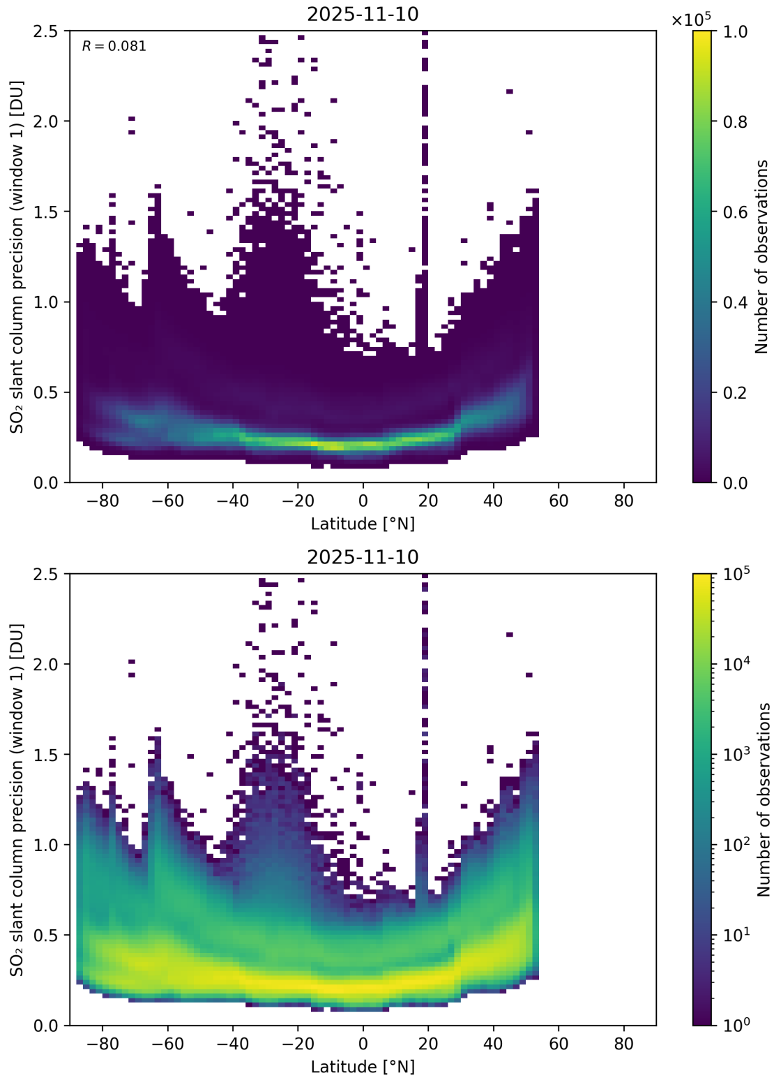
Figure 163: Scatter density plot of “Latitude” against “SO 2 slant column precision (window 1)” for 2025-11-09 to 2025-11-11.
