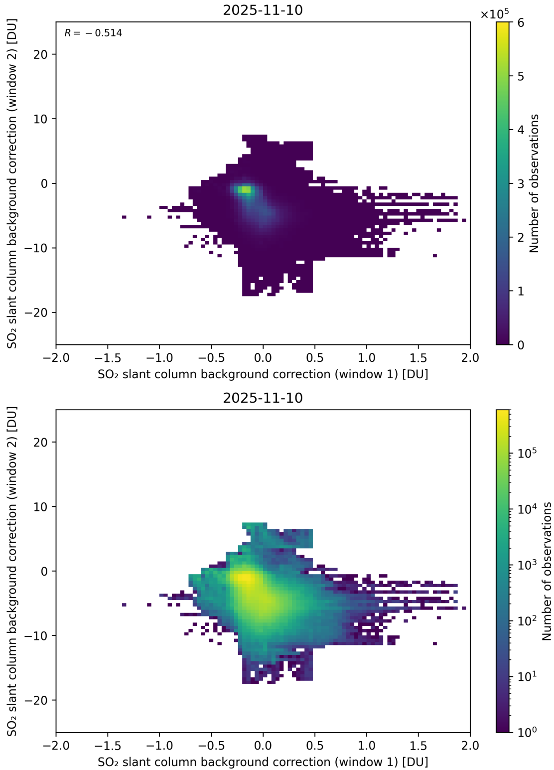
Figure 109: Scatter density plot of “SO 2 slant column background correction (window 1)” against “SO 2 slant column background correction (window 2)” for 2025-11-09 to 2025-11-11.
