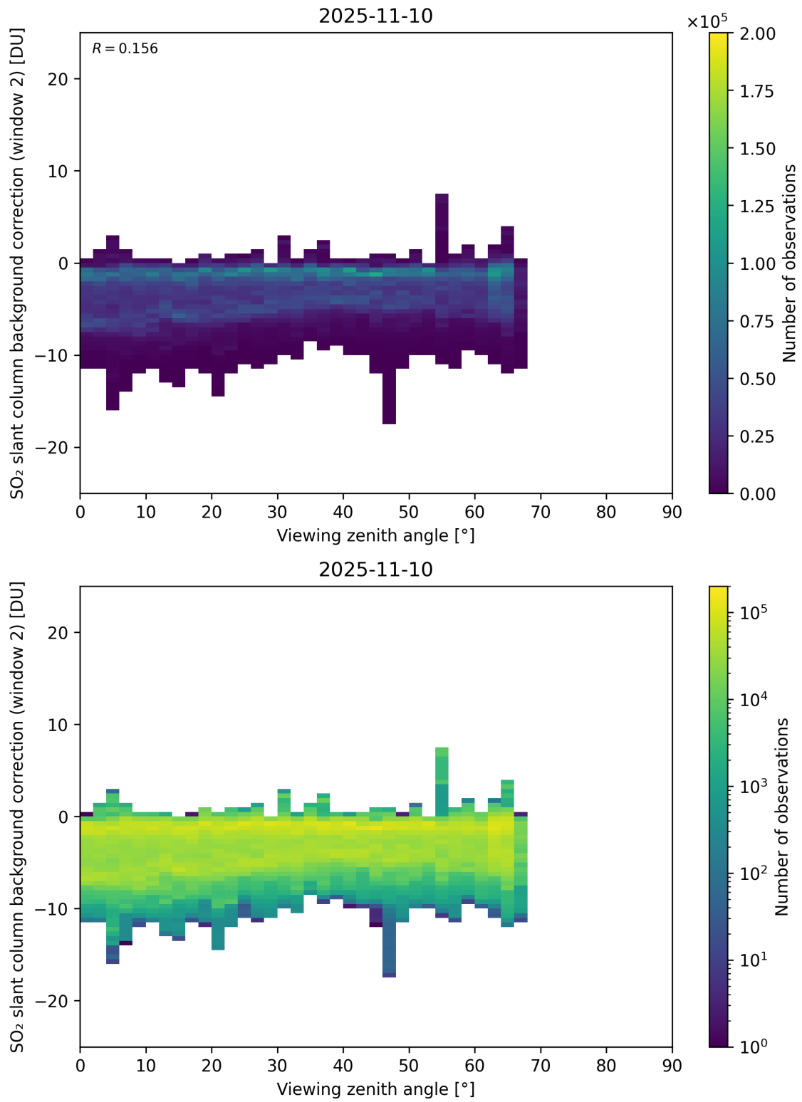
Figure 363: Scatter density plot of “Viewing zenith angle” against “SO 2 slant column background correction (window 2)” for 2025-11-09 to 2025-11-11.
