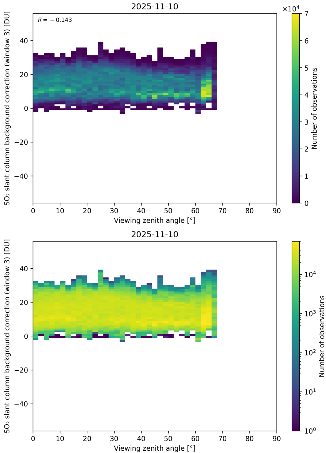
Figure 364: Scatter density plot of “Viewing zenith angle” against “SO 2 slant column background correction (window 3)” for 2025-11-09 to 2025-11-11.
