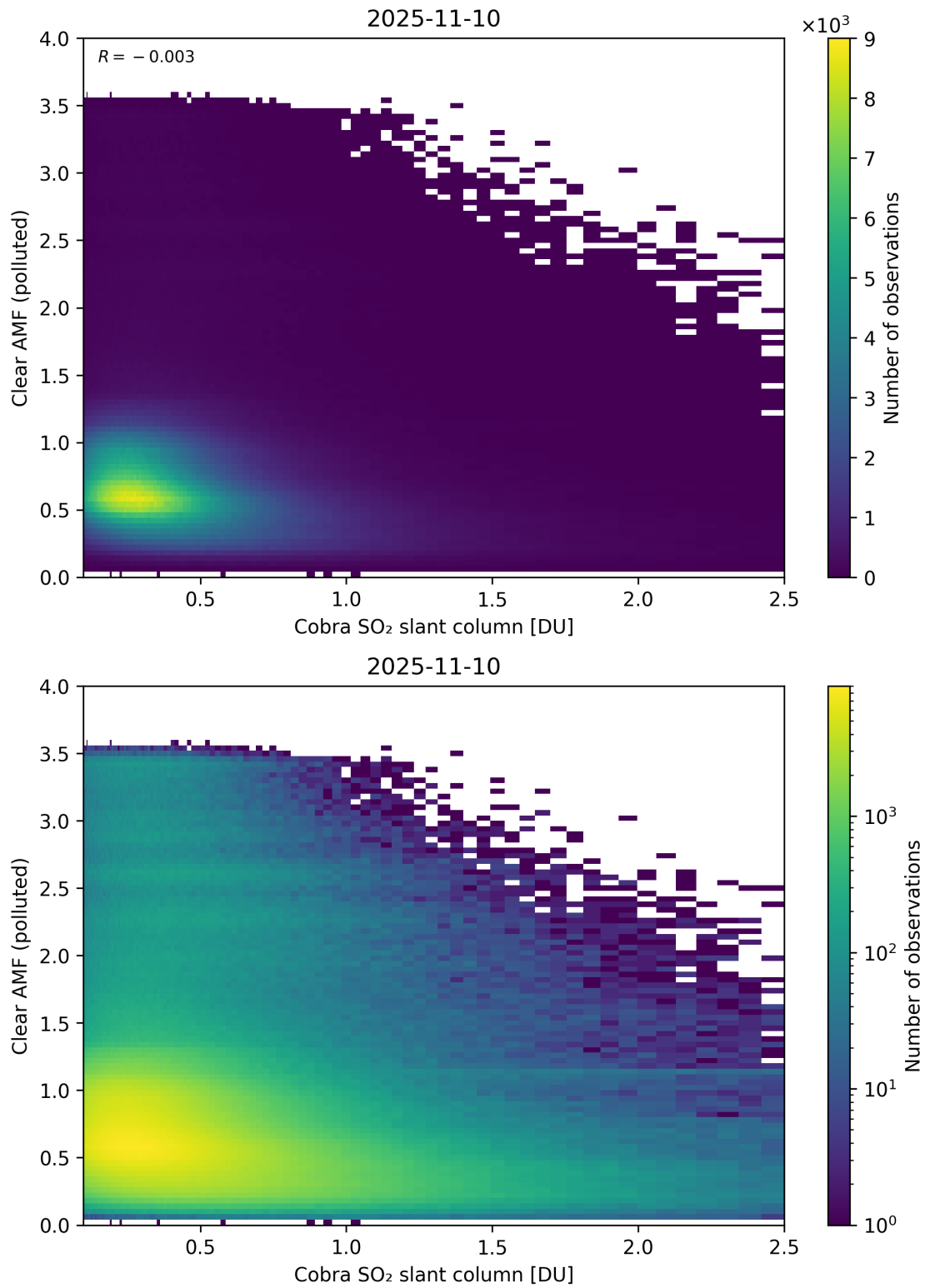
Figure 215: Scatter density plot of “Cobra SO 2 slant column” against “Clear AMF (polluted)” for 2025-11-09 to 2025-11-11.
