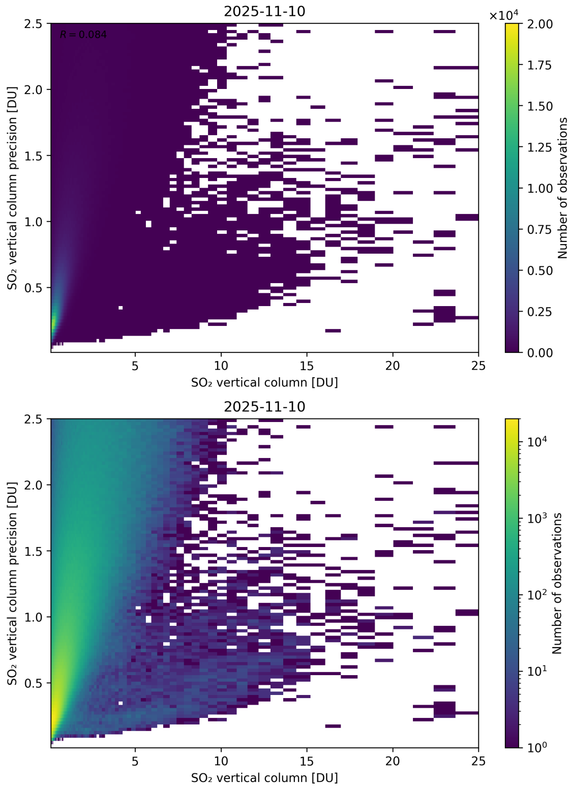
Figure 361: Scatter density plot of “SO 2 vertical column” against “SO 2 vertical column precision” for 2025-11-09 to 2025-11-11.
