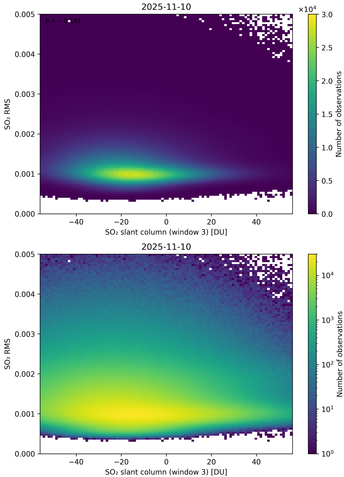
Figure 306: Scatter density plot of “SO 2 slant column (window 3)” against “SO 2 RMS” for 2025-11-09 to 2025-11-11.
