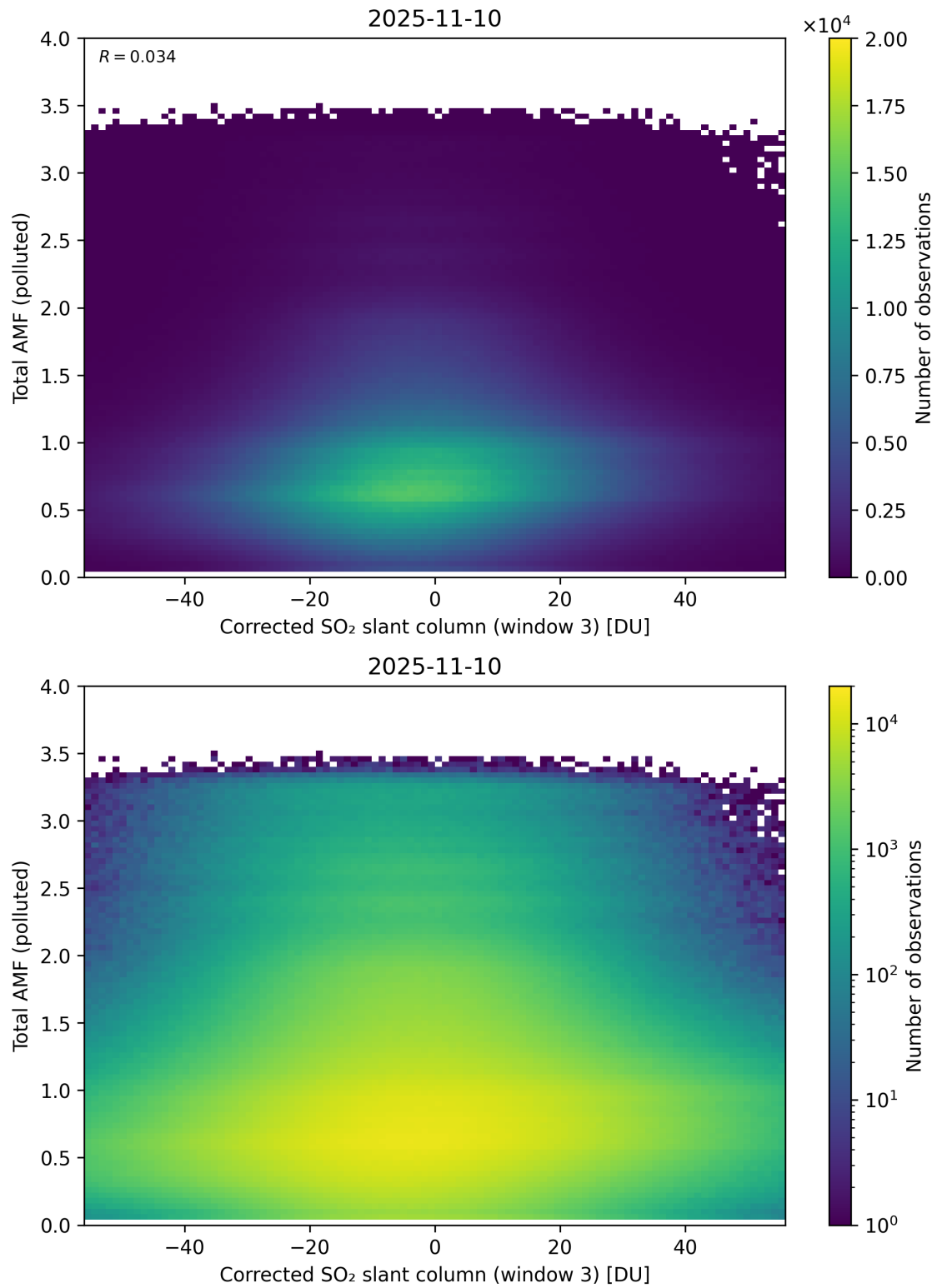
Figure 260: Scatter density plot of “Corrected SO 2 slant column (window 3)” against “Total AMF (polluted)” for 2025-11-09 to 2025-11-11.
