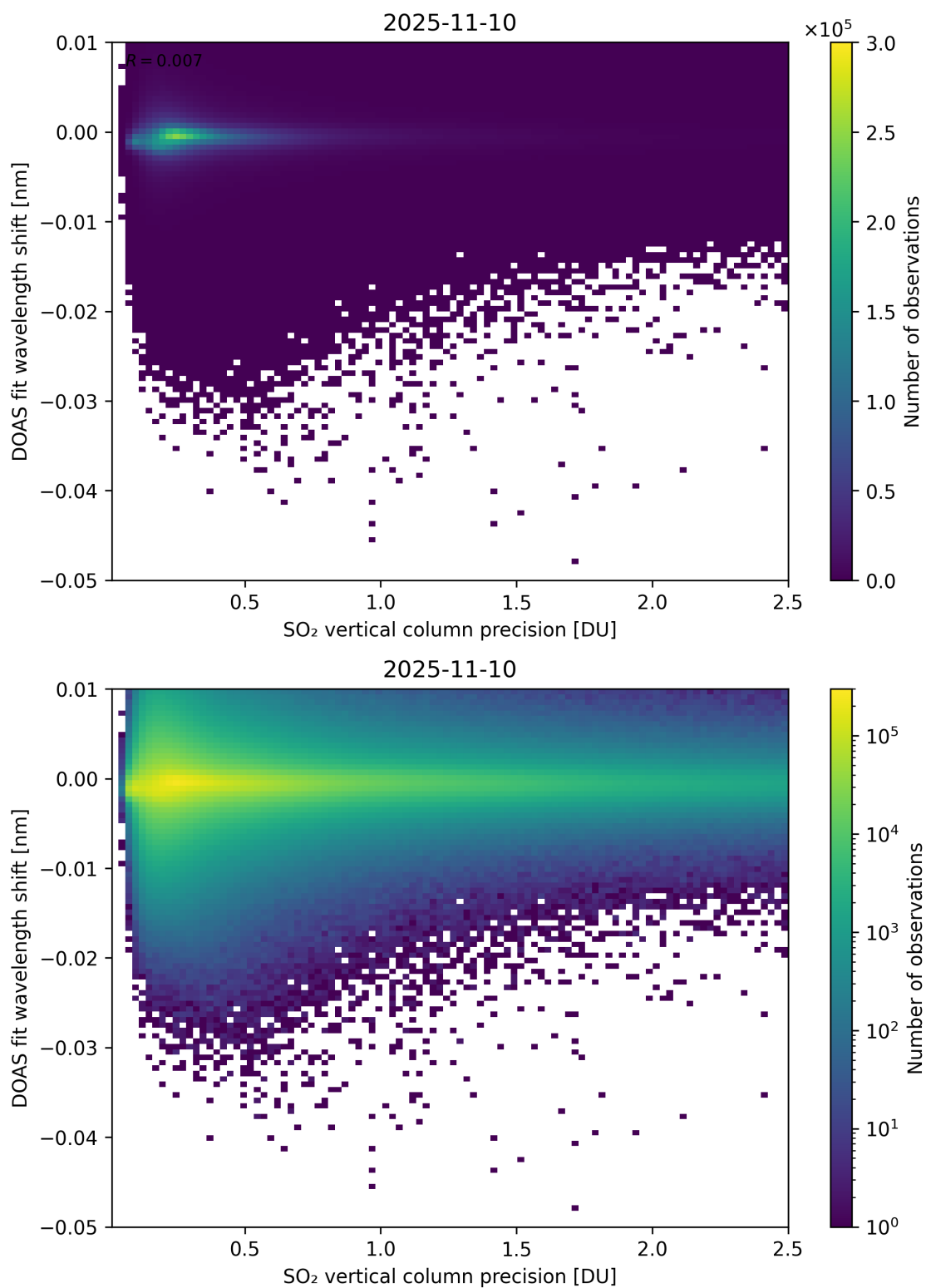
Figure 332: Scatter density plot of “SO 2 vertical column precision” against “DOAS fit wavelength shift” for 2025-11-09 to 2025-11-11.
