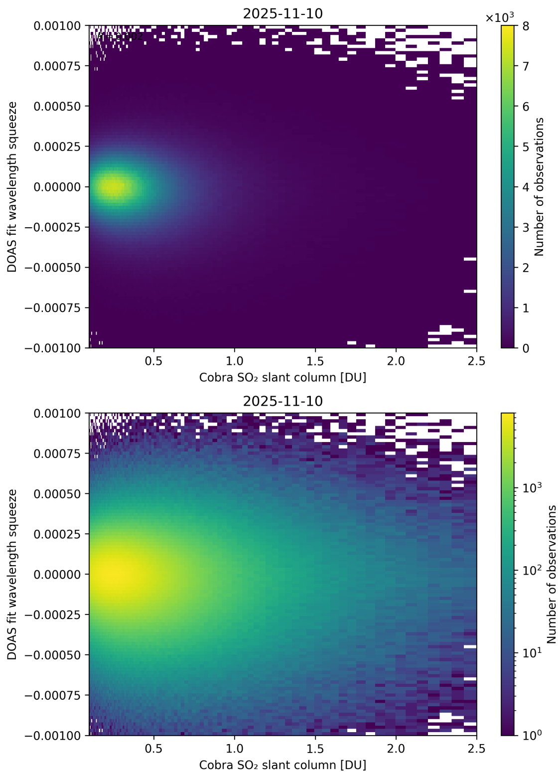
Figure 197: Scatter density plot of “Cobra SO 2 slant column” against “DOAS fit wavelength squeeze” for 2025-11-09 to 2025-11-11.
