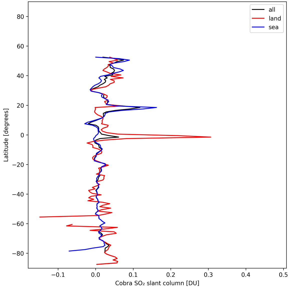
Figure 35: Zonal average of “Cobra SO 2 slant column” for 2025-11-09 to 2025-11-11.
