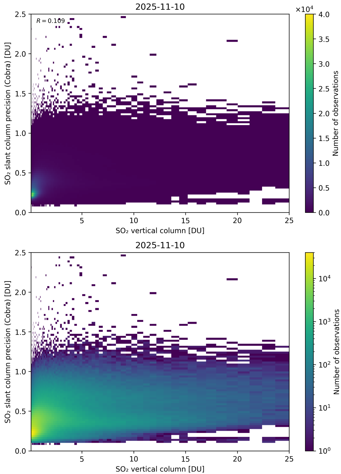
Figure 350: Scatter density plot of “SO 2 vertical column” against “SO 2 slant column precision (Cobra)” for 2025-11-09 to 2025-11-11.
