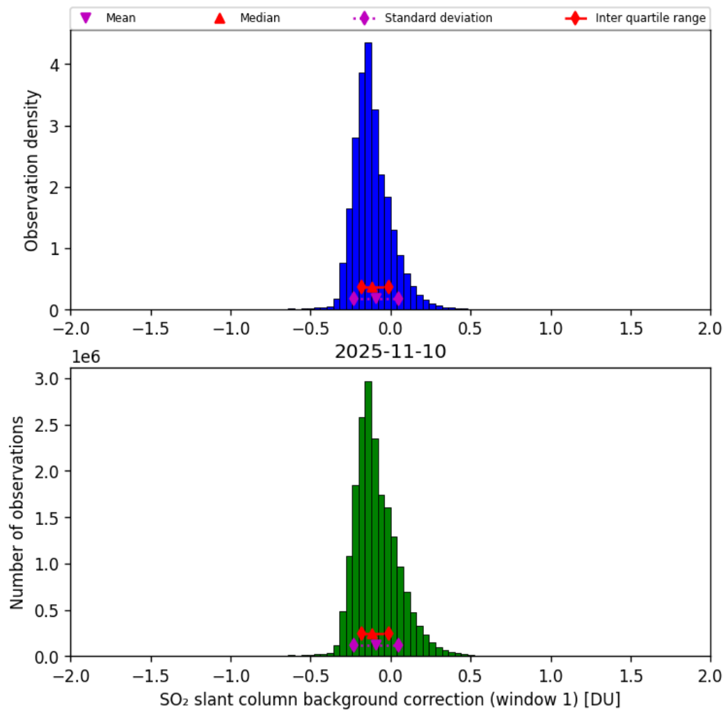
Figure 66: Histogram of “SO 2 slant column background correction (window 1)” for 2025-11-09 to 2025-11-11
