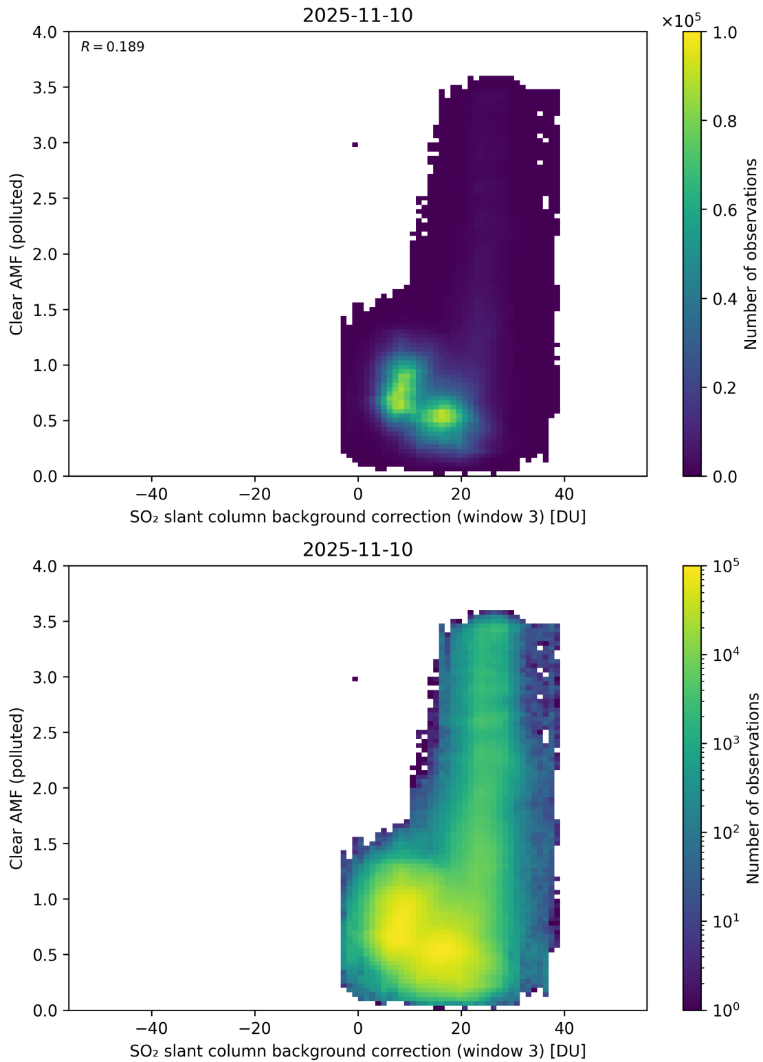
Figure 135: Scatter density plot of “SO 2 slant column background correction (window 3)” against “Clear AMF (polluted)” for 2025-11-09 to 2025-11-11.
