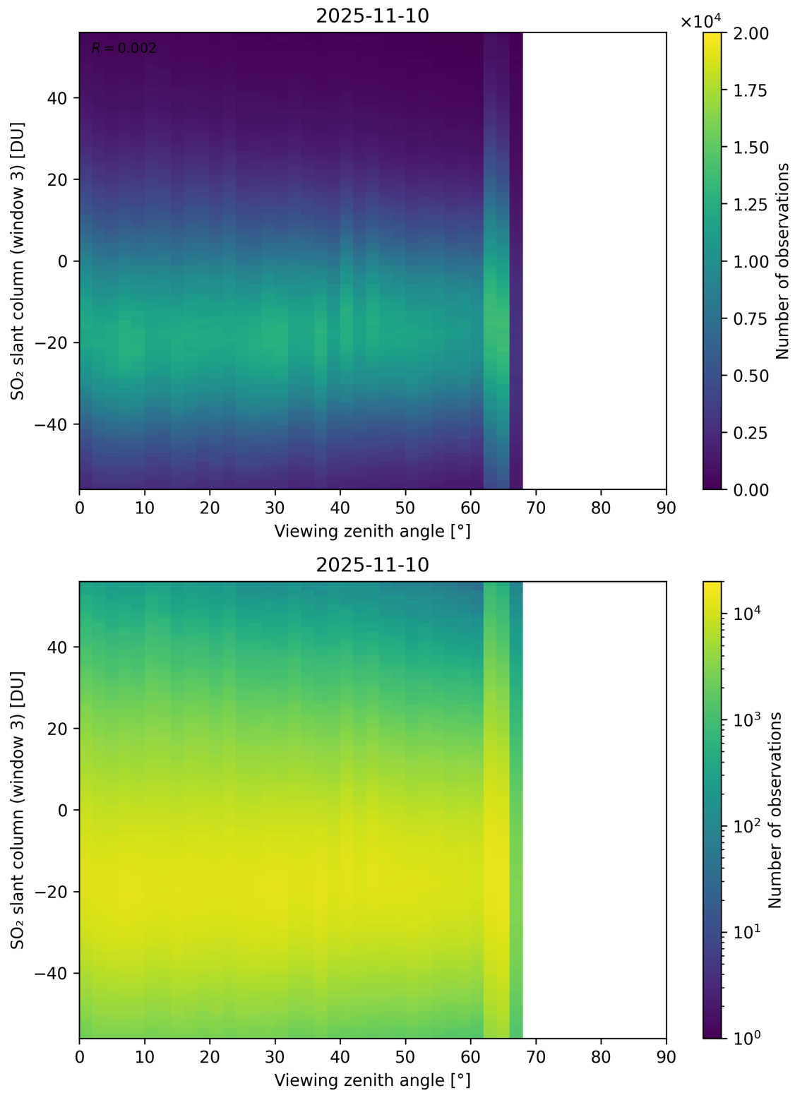
Figure 379: Scatter density plot of “Viewing zenith angle” against “SO 2 slant column (window 3)” for 2025-11-09 to 2025-11-11.
