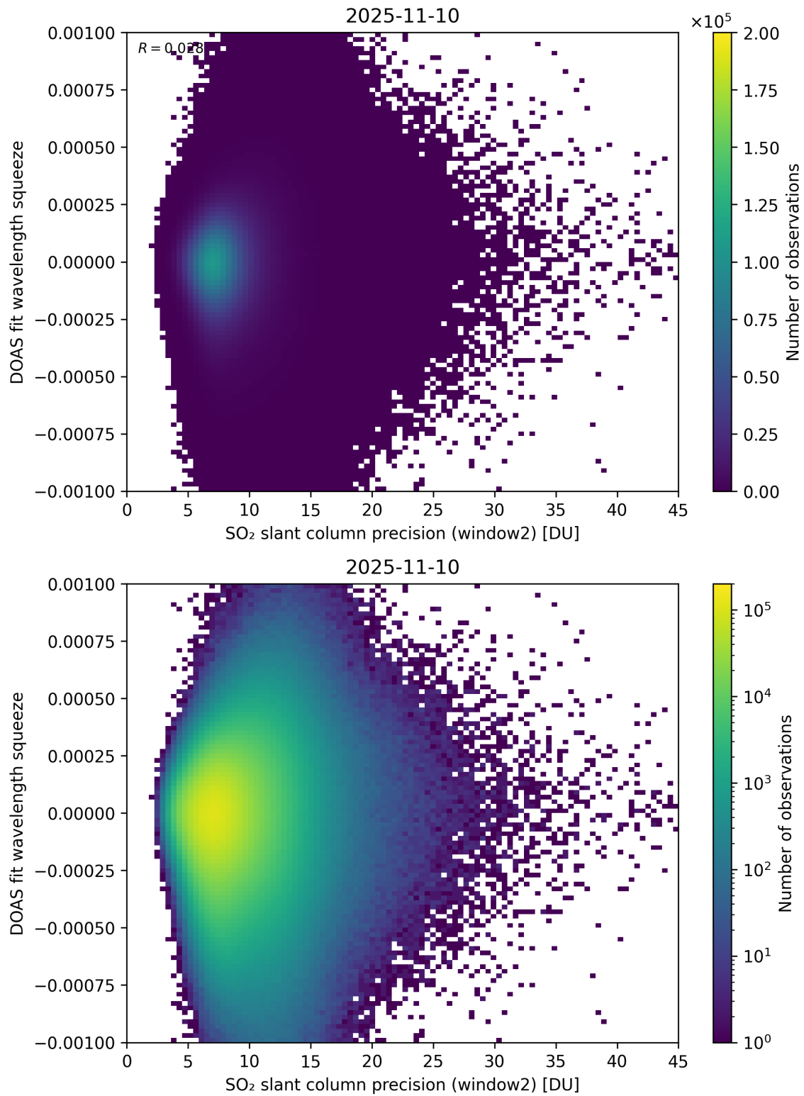
Figure 294: Scatter density plot of “SO 2 slant column precision (window2)” against “DOAS fit wavelength squeeze” for 2025-11-09 to 2025-11-11.
