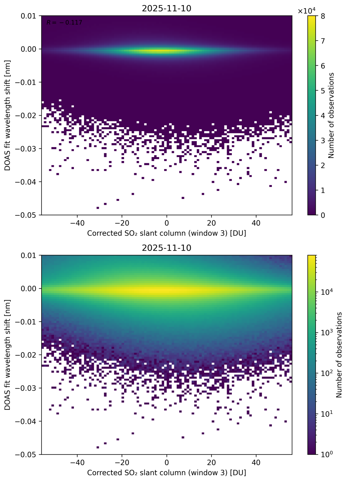
Figure 256: Scatter density plot of “Corrected SO 2 slant column (window 3)” against “DOAS fit wavelength shift” for 2025-11-09 to 2025-11-11.
