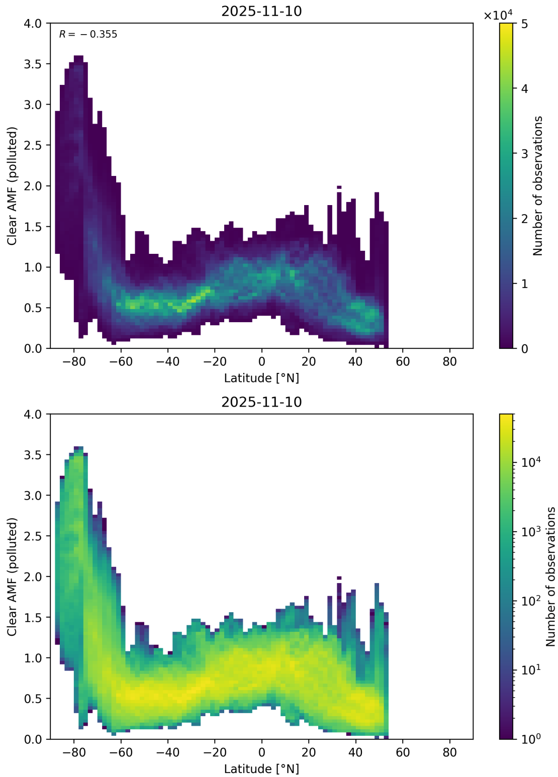
Figure 156: Scatter density plot of “Latitude” against “Clear AMF (polluted)” for 2025-11-09 to 2025-11-11.
