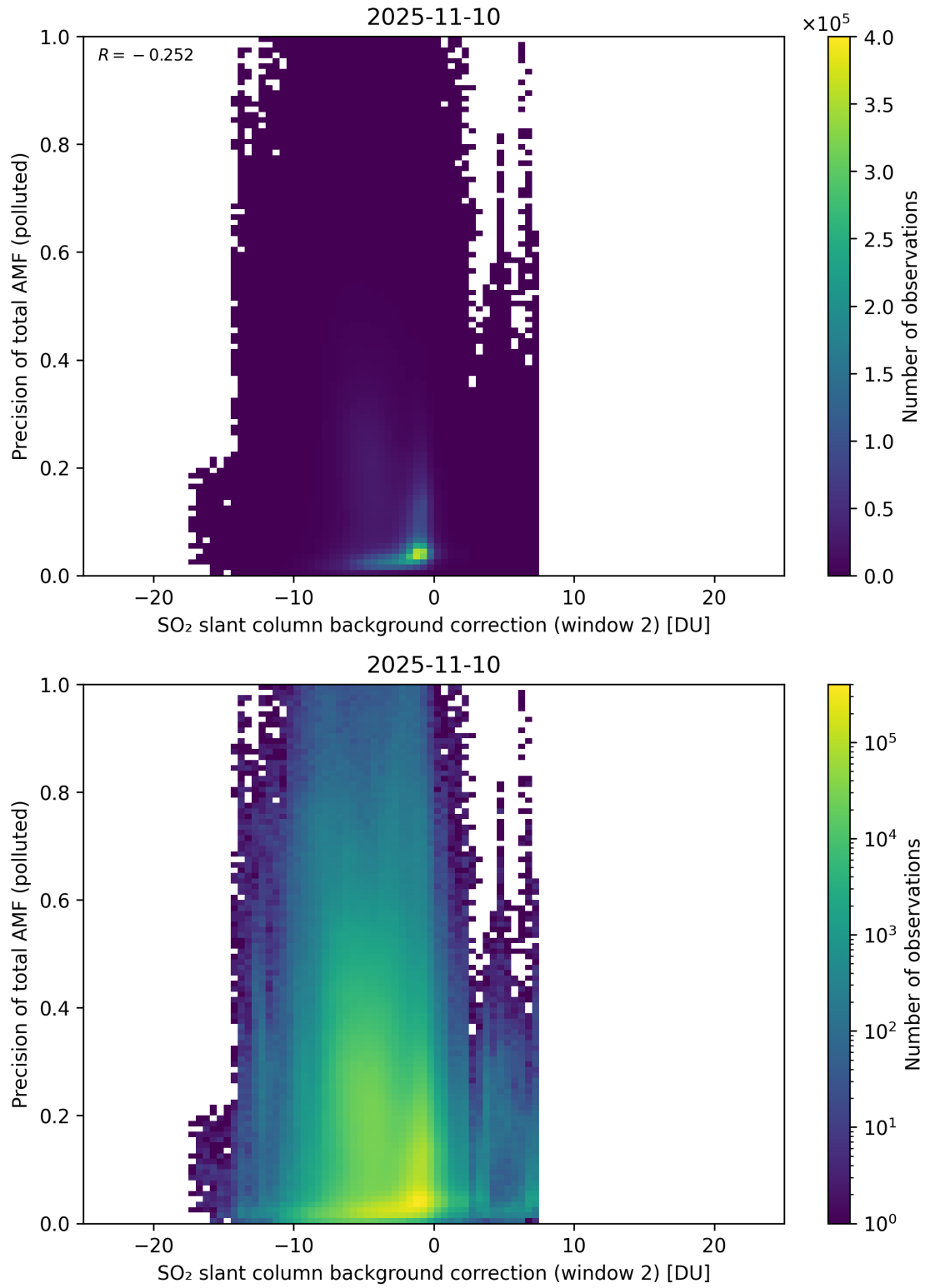
Figure 131: Scatter density plot of “SO 2 slant column background correction (window 2)” against “Precision of total AMF (polluted)” for 2025-11-09 to 2025-11-11.
