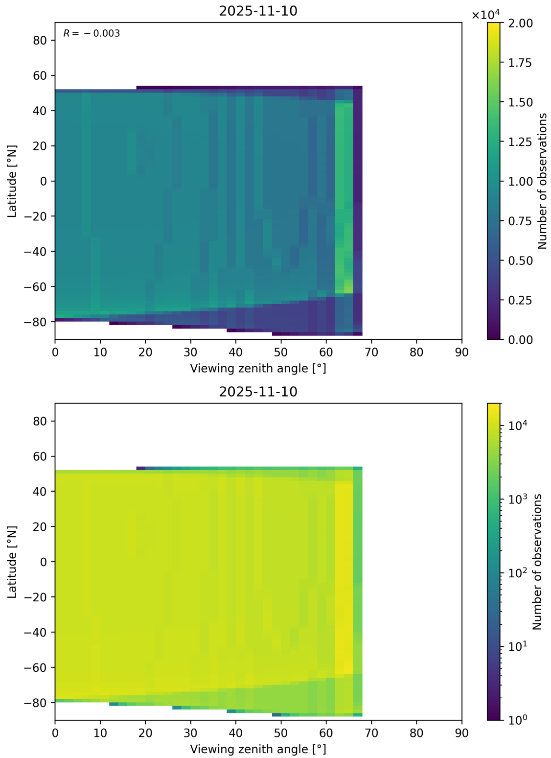
Figure 368: Scatter density plot of “Viewing zenith angle” against “Latitude” for 2025-11-09 to 2025-11-11.
