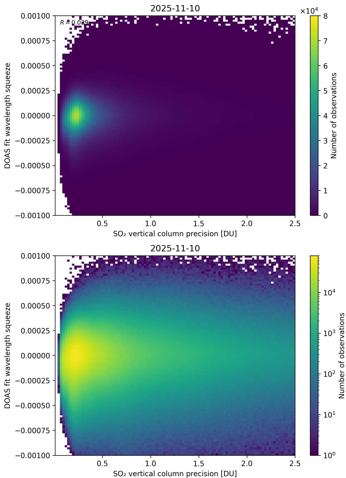
Figure 333: Scatter density plot of “SO 2 vertical column precision” against “DOAS fit wavelength squeeze” for 2025-11-09 to 2025-11-11.
