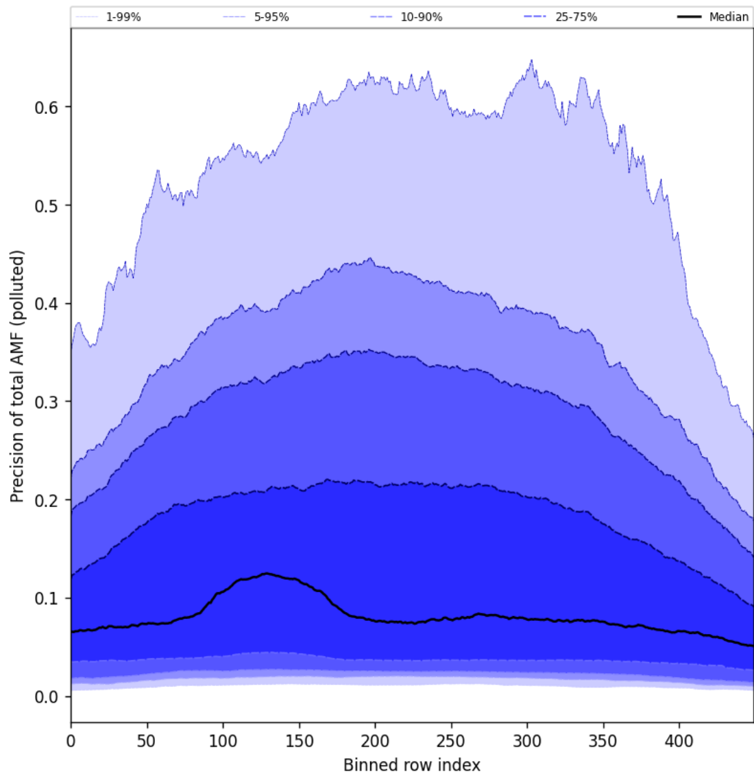
Figure 106: Along track statistics of “Precision of total AMF (polluted)” for 2025-11-09 to 2025-11-11
