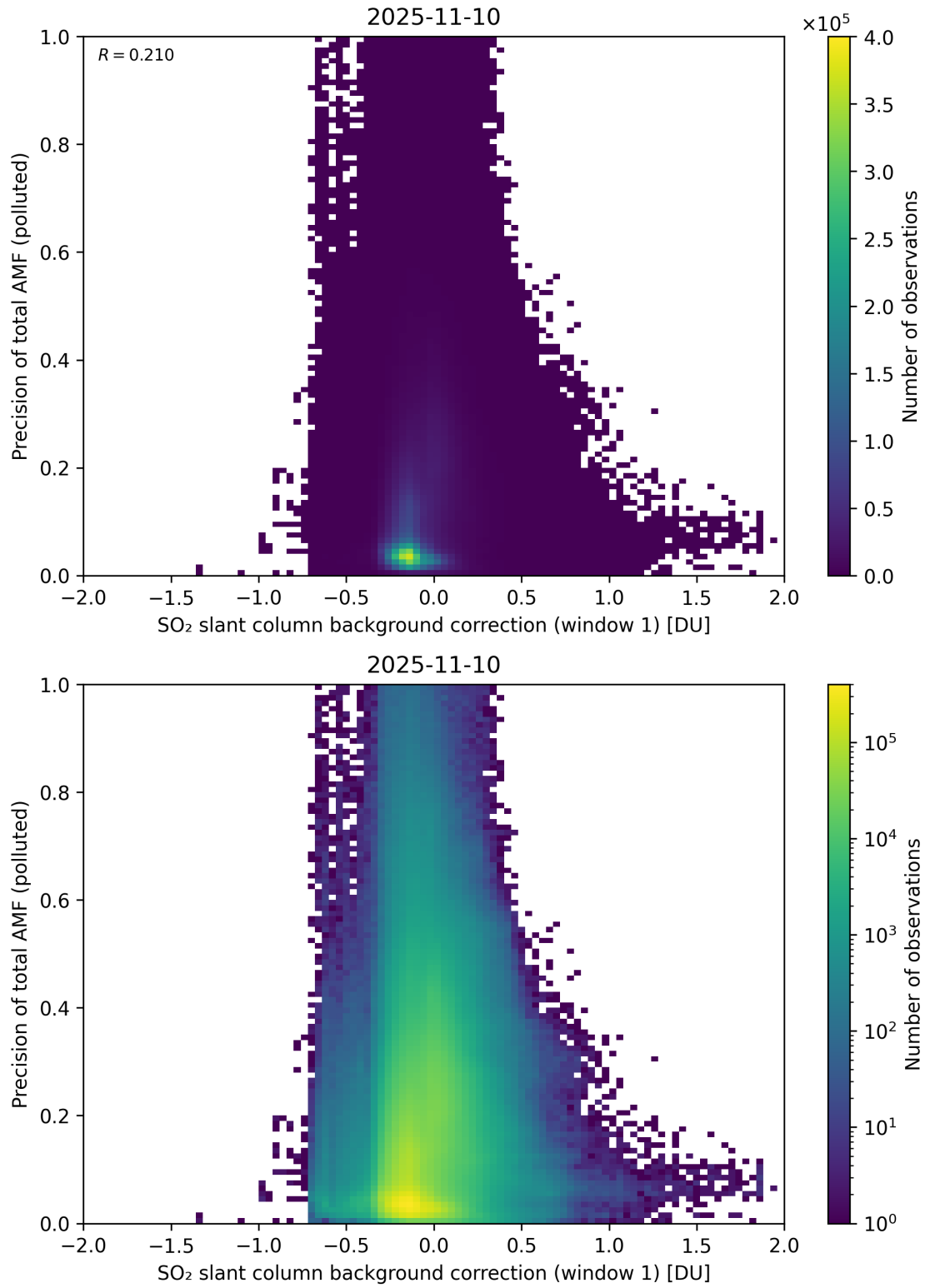
Figure 121: Scatter density plot of “SO 2 slant column background correction (window 1)” against “Precision of total AMF (polluted)” for 2025-11-09 to 2025-11-11.
