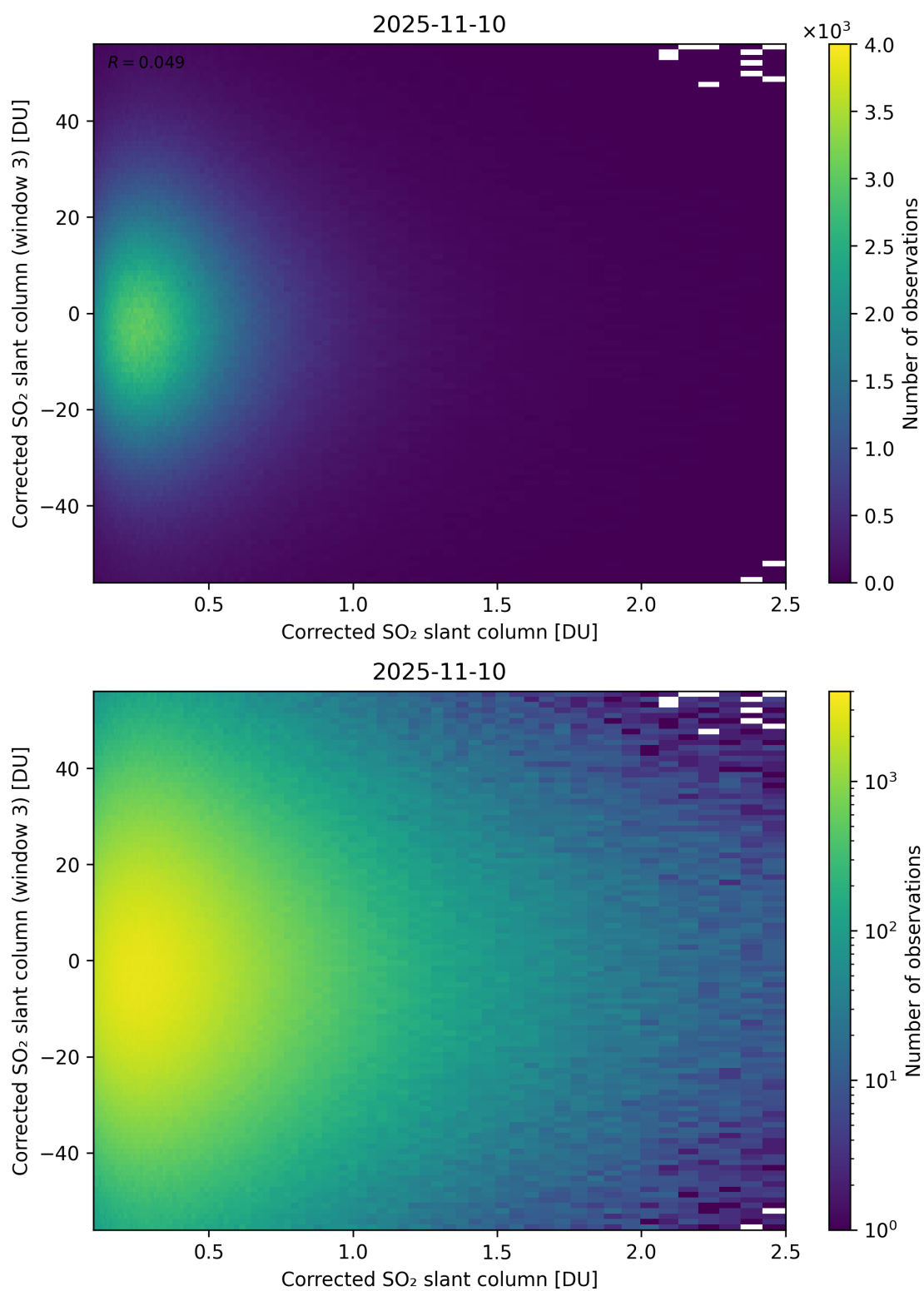
Figure 236: Scatter density plot of “Corrected SO 2 slant column” against “Corrected SO 2 slant column (window 3)” for 2025-11-09 to 2025-11-11.
