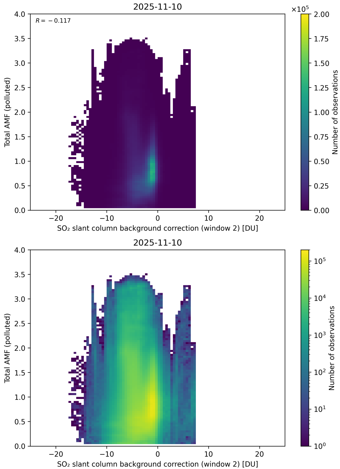
Figure 130: Scatter density plot of “SO 2 slant column background correction (window 2)” against “Total AMF (polluted)” for 2025-11-09 to 2025-11-11.
