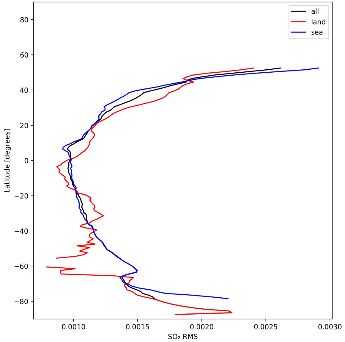
Figure 52: Zonal average of “SO 2 RMS” for 2025-11-09 to 2025-11-11.
