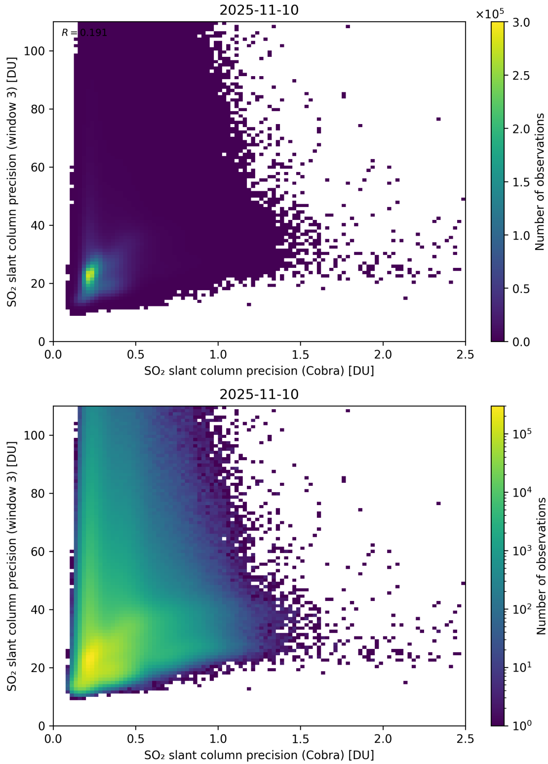
Figure 212: Scatter density plot of “SO 2 slant column precision (Cobra)” against “SO 2 slant column precision (window 3)” for 2025-11-09 to 2025-11-11.
