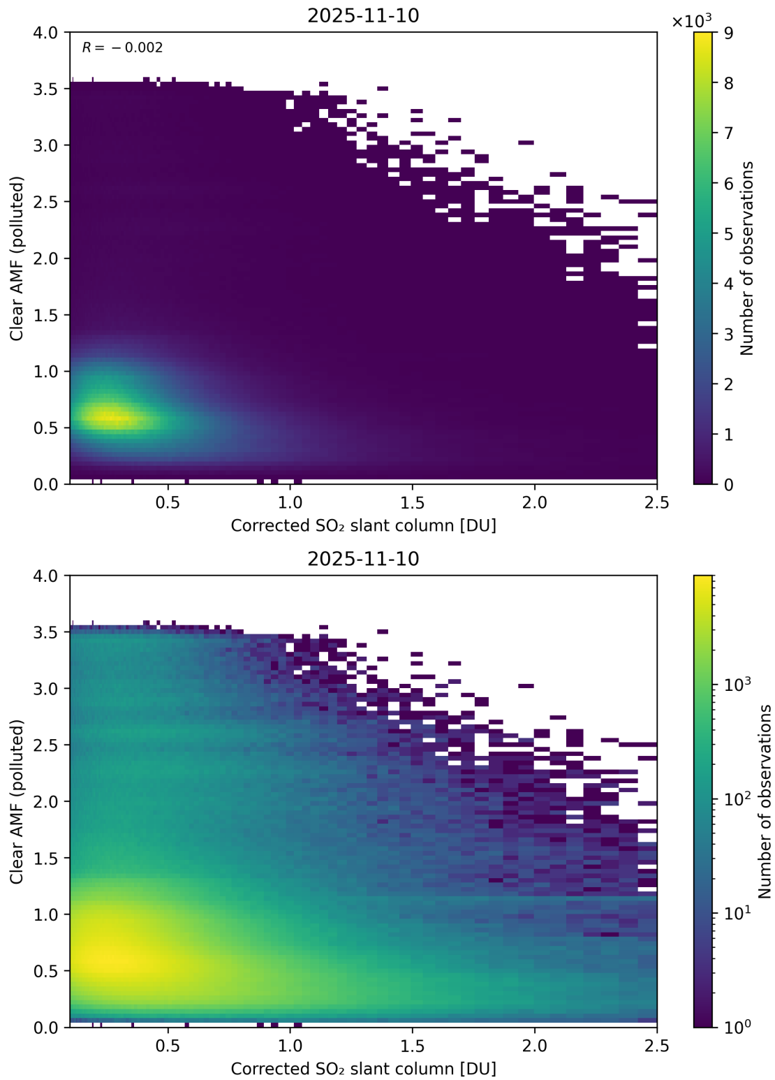
Figure 232: Scatter density plot of “Corrected SO 2 slant column” against “Clear AMF (polluted)” for 2025-11-09 to 2025-11-11.
