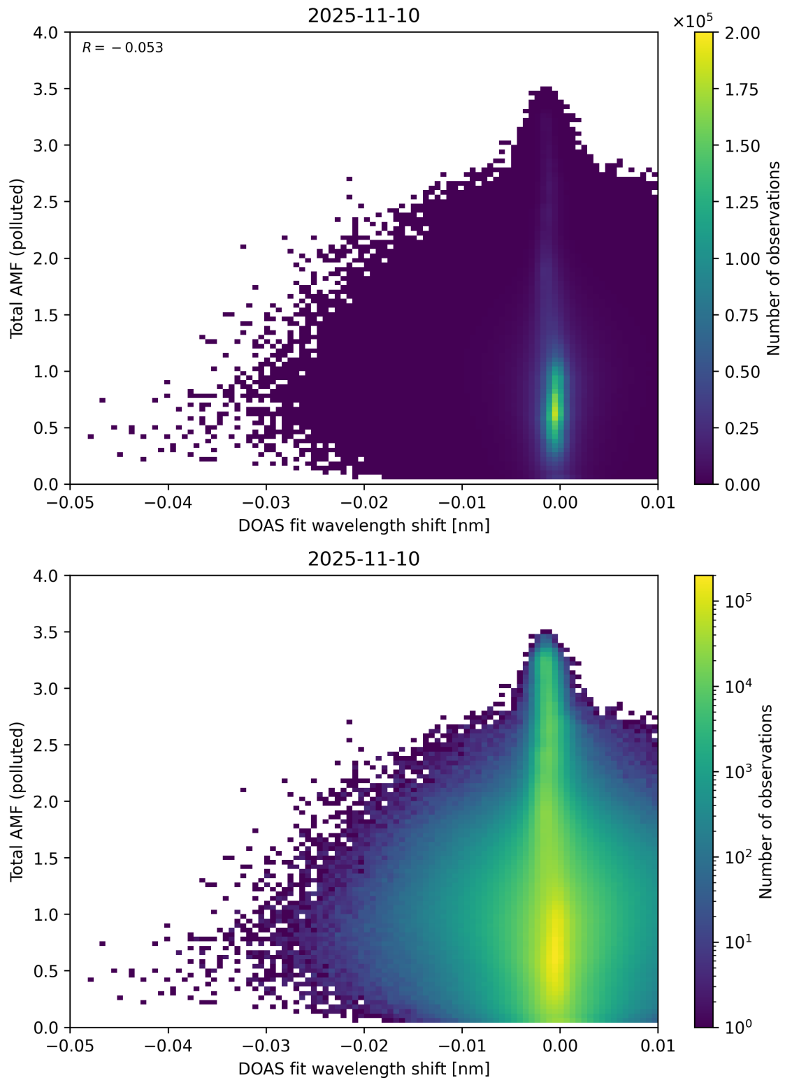
Figure 141: Scatter density plot of “DOAS fit wavelength shift” against “Total AMF (polluted)” for 2025-11-09 to 2025-11-11.
