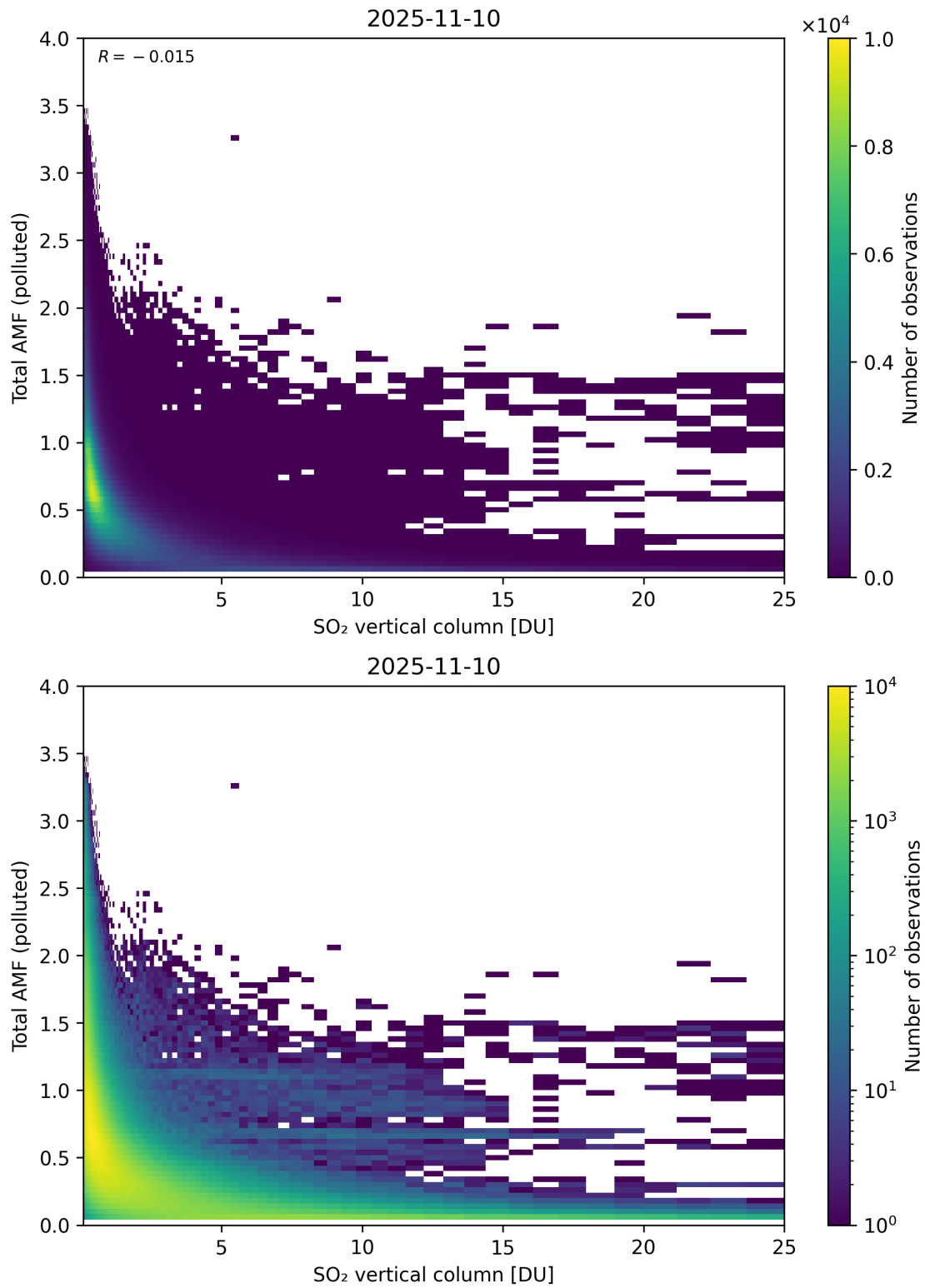
Figure 359: Scatter density plot of “SO 2 vertical column” against “Total AMF (polluted)” for 2025-11-09 to 2025-11-11.
