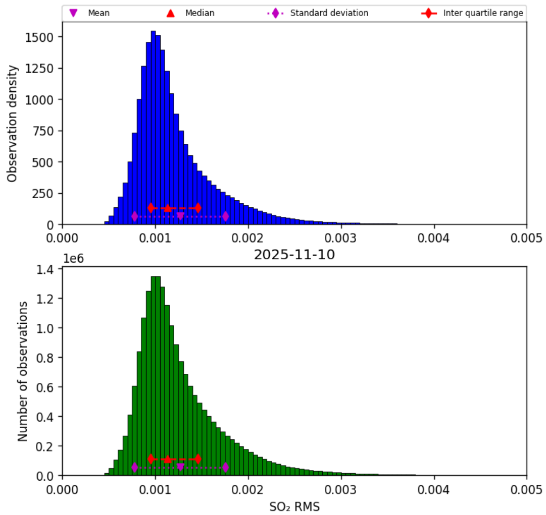
Figure 78: Histogram of “SO 2 RMS” for 2025-11-09 to 2025-11-11
