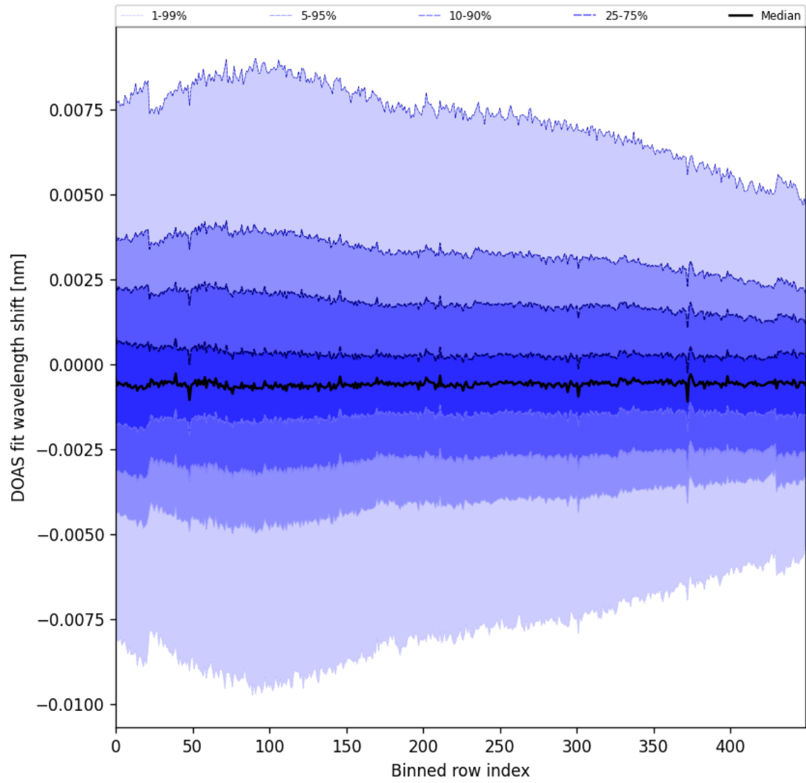
Figure 102: Along track statistics of “DOAS fit wavelength shift” for 2025-11-09 to 2025-11-11
