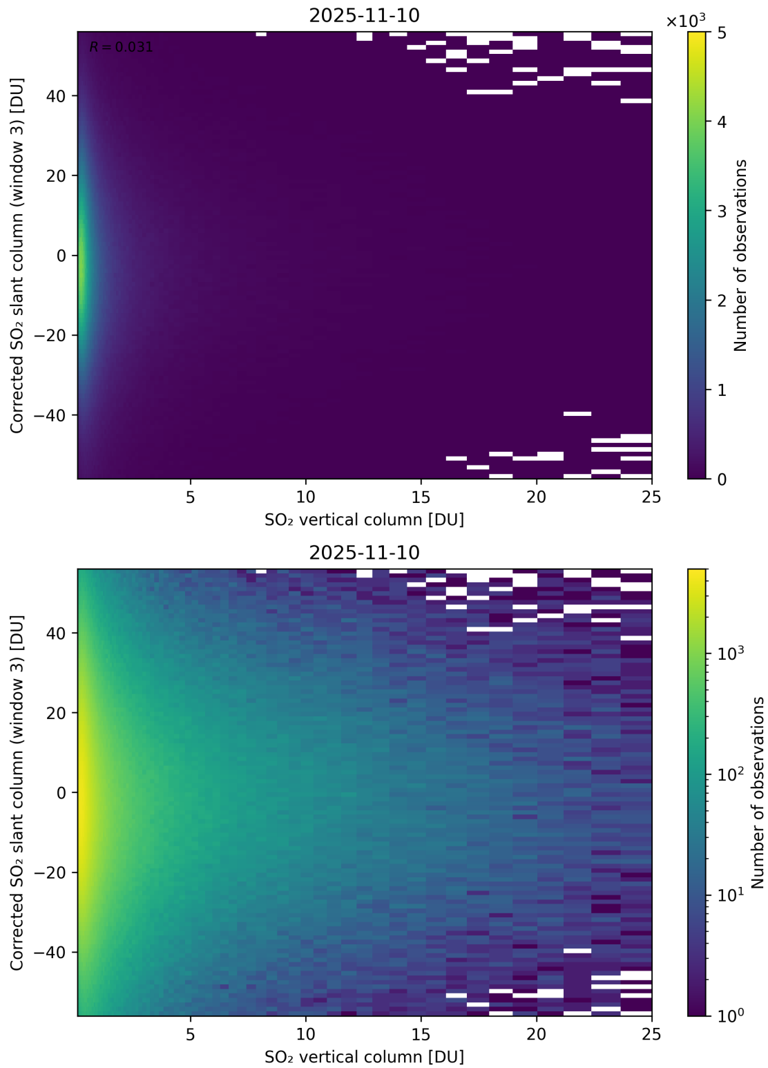
Figure 353: Scatter density plot of “SO 2 vertical column” against “Corrected SO 2 slant column (window 3)” for 2025-11-09 to 2025-11-11.
