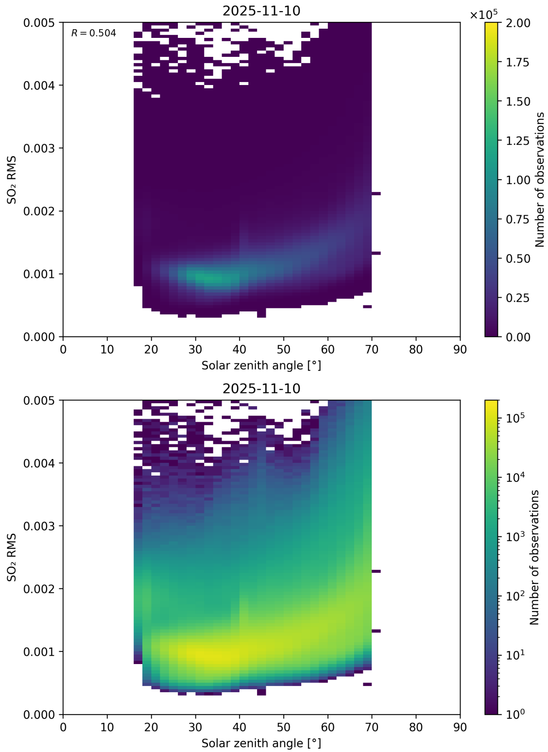
Figure 176: Scatter density plot of “Solar zenith angle” against “SO 2 RMS” for 2025-11-09 to 2025-11-11.
