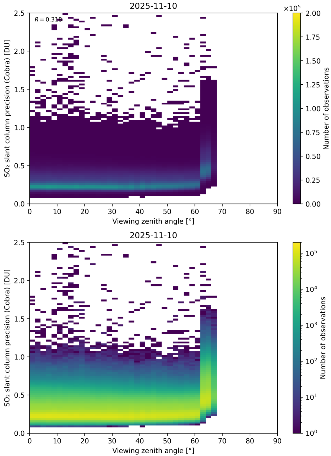
Figure 372: Scatter density plot of “Viewing zenith angle” against “SO 2 slant column precision (Cobra)” for 2025-11-09 to 2025-11-11.
