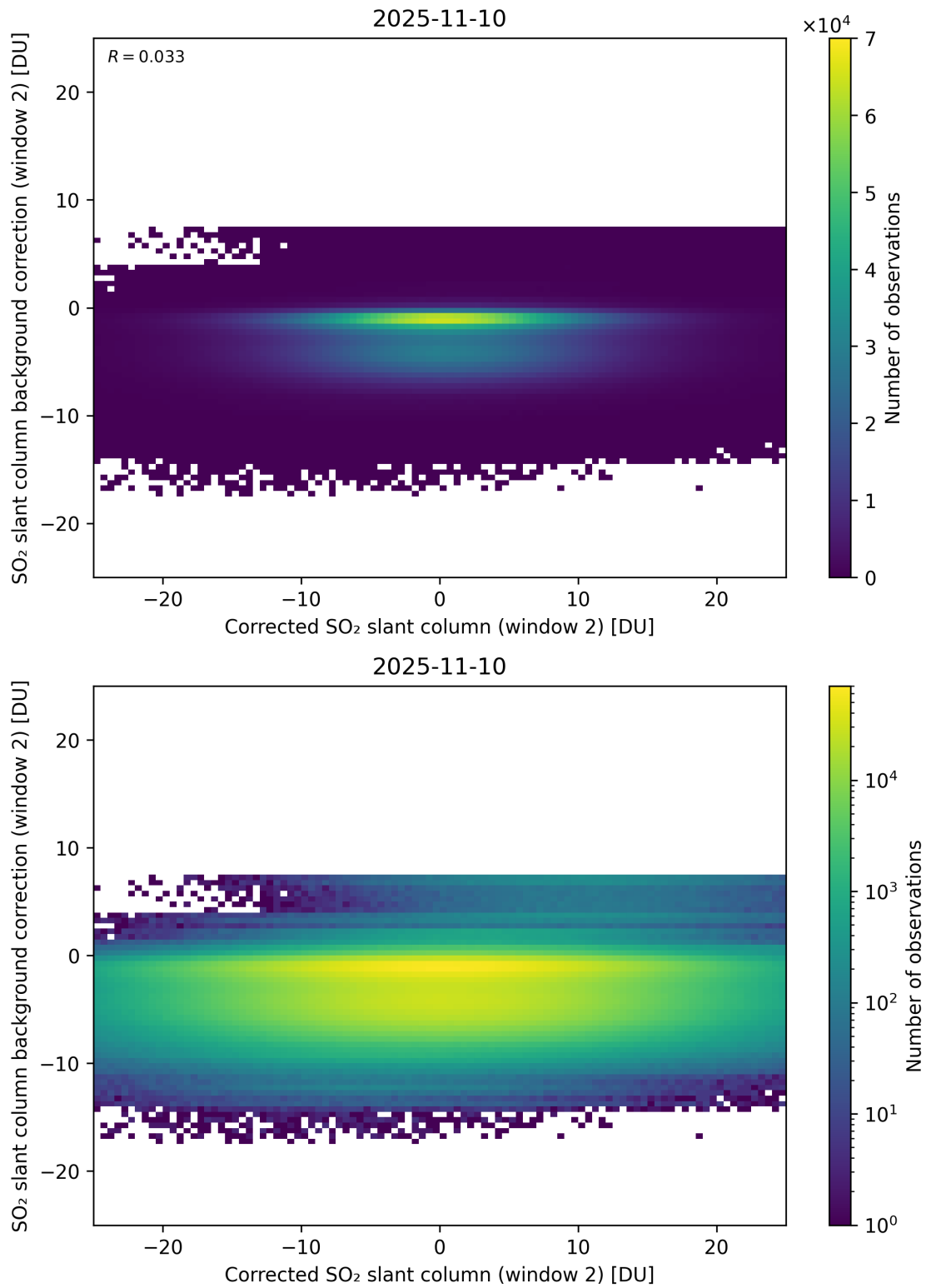
Figure 244: Scatter density plot of “Corrected SO 2 slant column (window 2)” against “SO 2 slant column background correction (window 2)” for 2025-11-09 to 2025-11-11.
