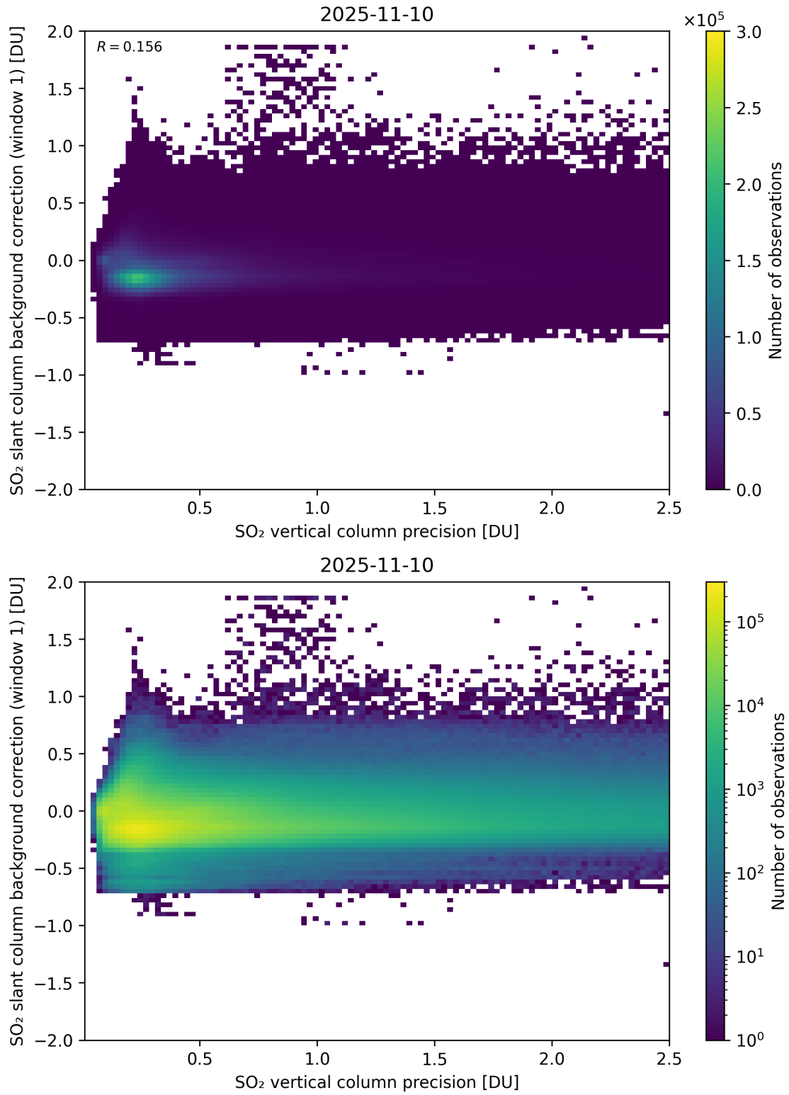
Figure 329: Scatter density plot of “SO 2 vertical column precision” against “SO 2 slant column background correction (window 1)” for 2025-11-09 to 2025-11-11.
