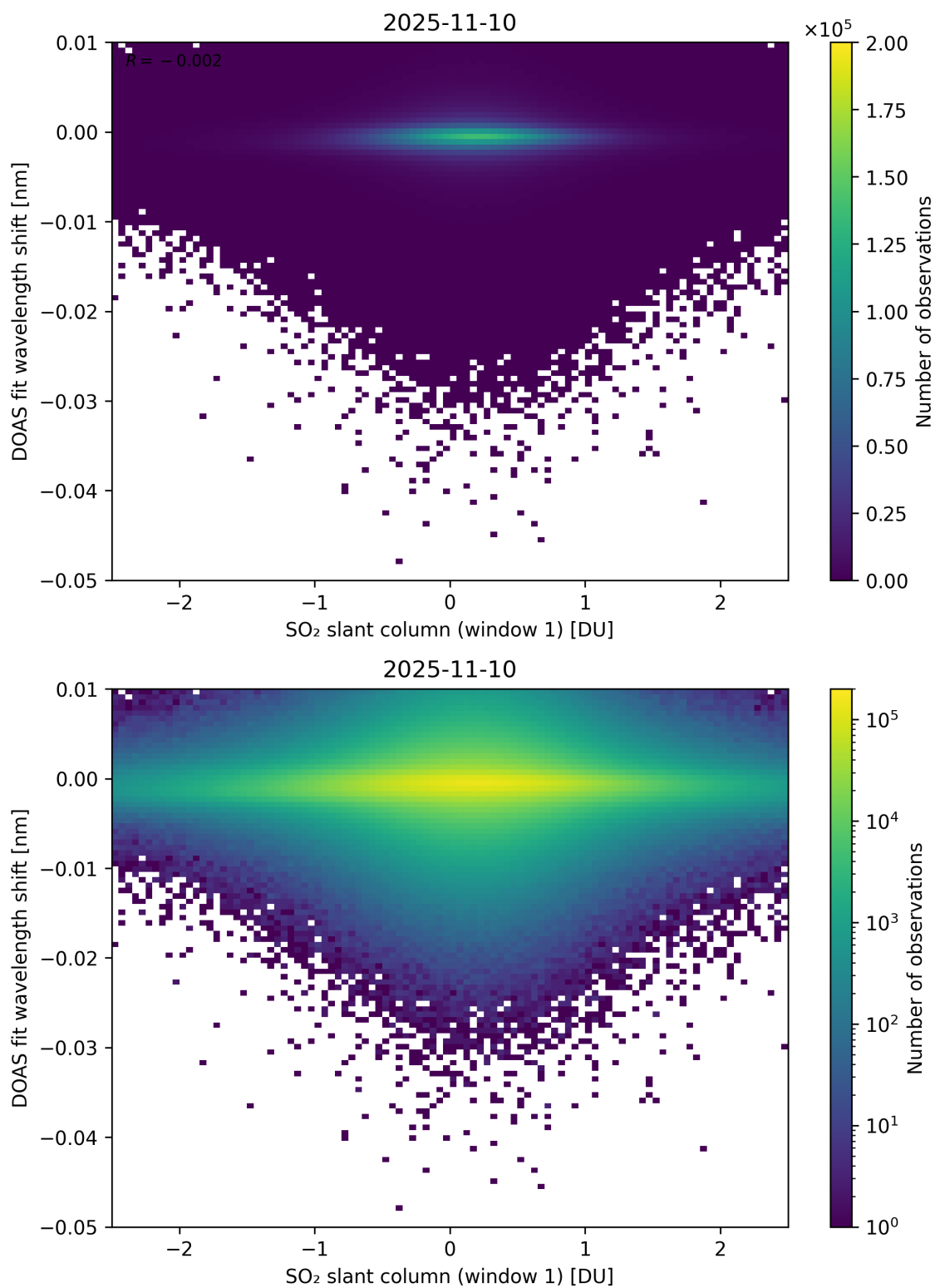
Figure 265: Scatter density plot of “SO 2 slant column (window 1)” against “DOAS fit wavelength shift” for 2025-11-09 to 2025-11-11.
