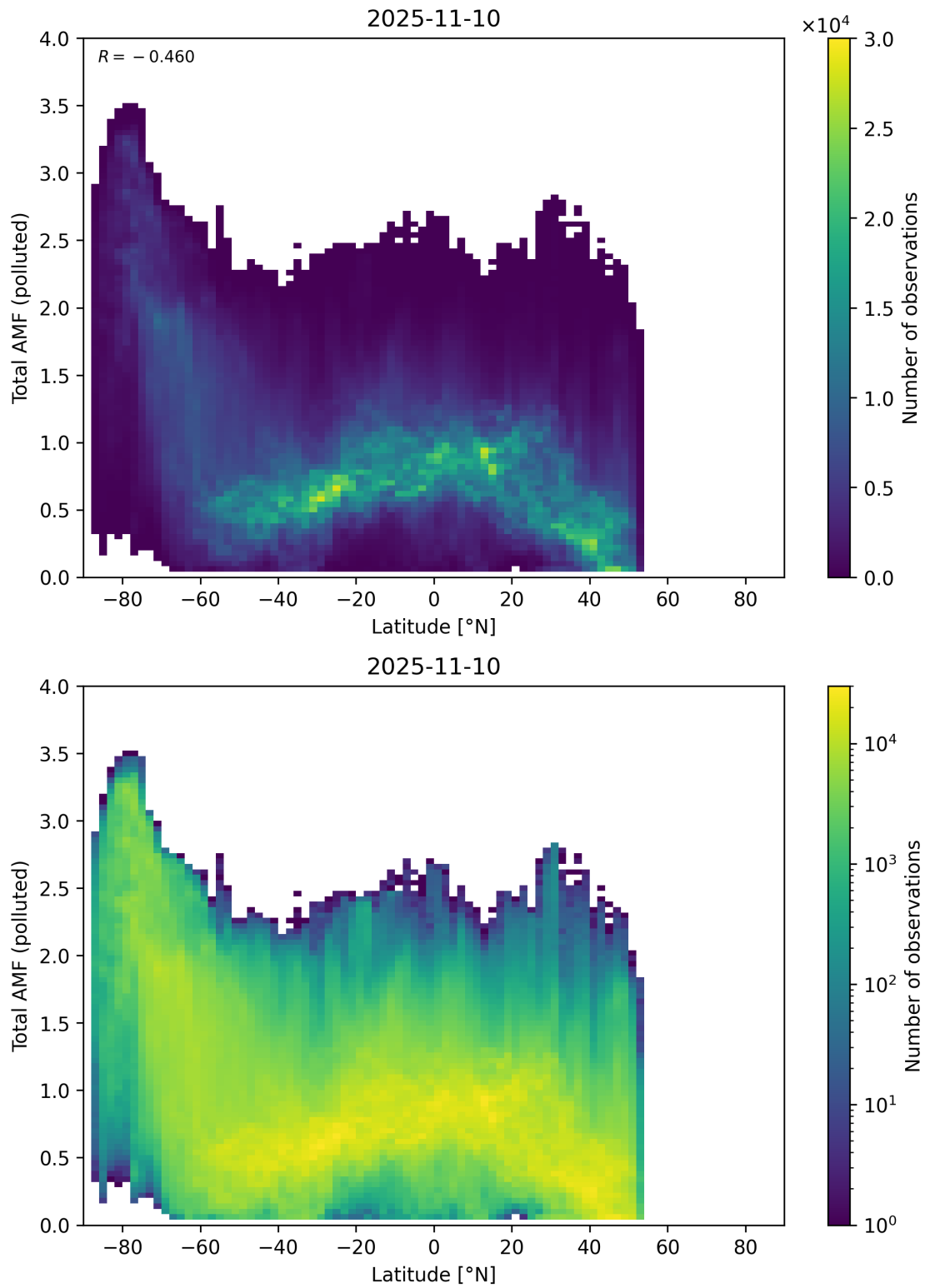
Figure 167: Scatter density plot of “Latitude” against “Total AMF (polluted)” for 2025-11-09 to 2025-11-11.
