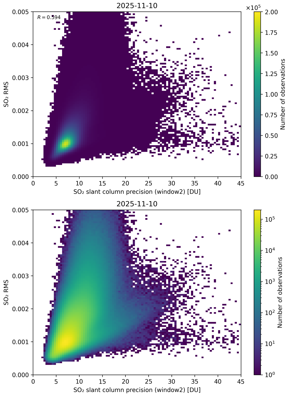
Figure 295: Scatter density plot of “SO 2 slant column precision (window2)” against “SO 2 RMS” for 2025-11-09 to 2025-11-11.
