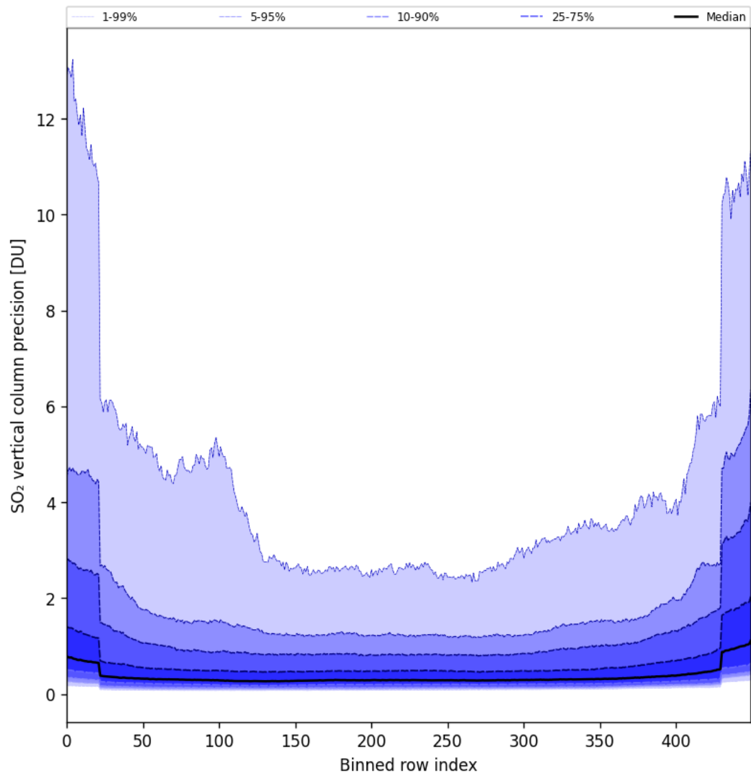
Figure 85: Along track statistics of “SO 2 vertical column precision” for 2025-11-09 to 2025-11-11
