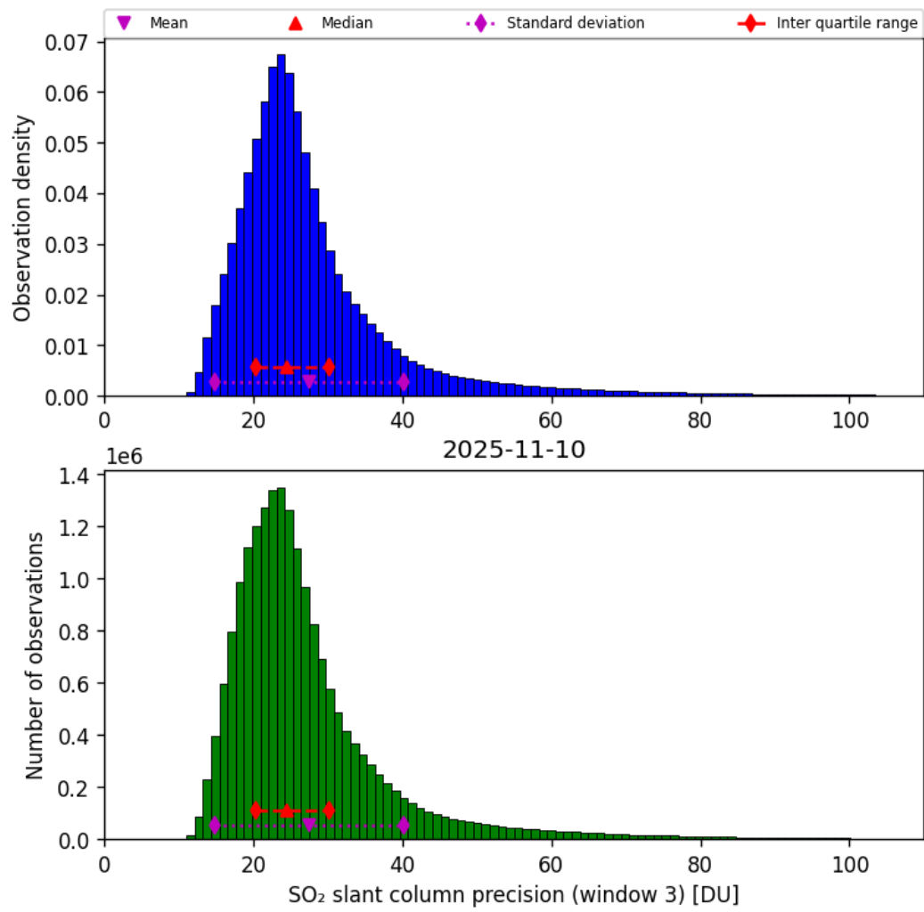
Figure 72: Histogram of “SO 2 slant column precision (window 3)” for 2025-11-09 to 2025-11-11
