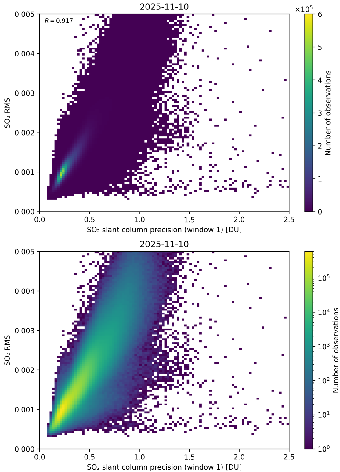
Figure 273: Scatter density plot of “SO 2 slant column precision (window 1)” against “SO 2 RMS” for 2025-11-09 to 2025-11-11.
