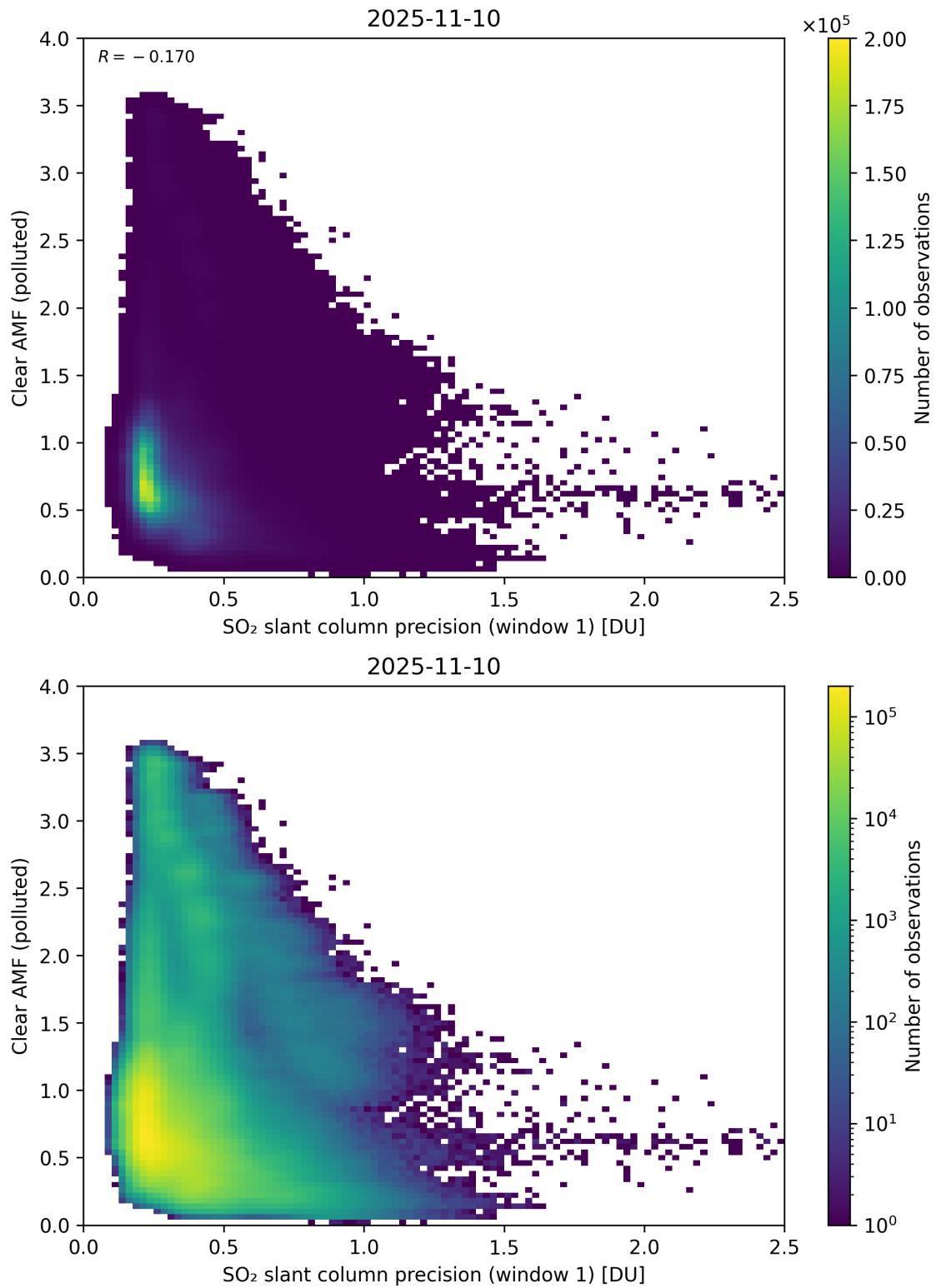
Figure 274: Scatter density plot of “SO 2 slant column precision (window 1)” against “Clear AMF (polluted)” for 2025-11-09 to 2025-11-11.
