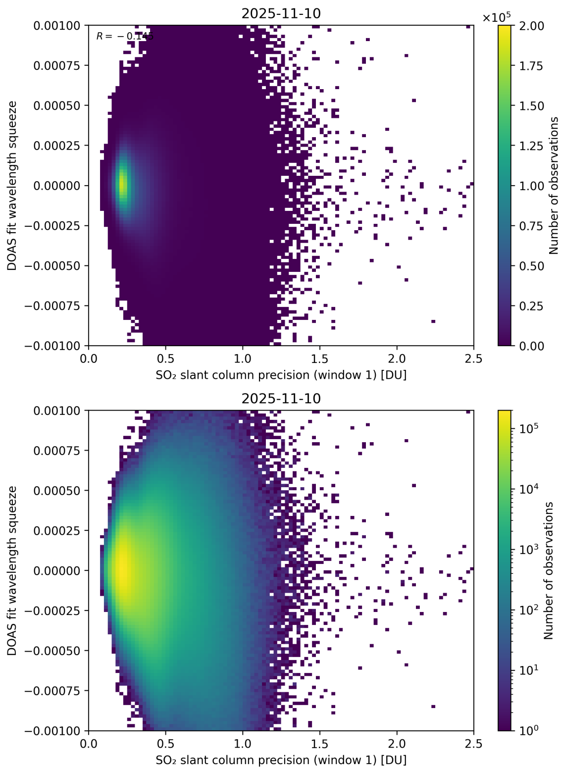
Figure 272: Scatter density plot of “SO 2 slant column precision (window 1)” against “DOAS fit wavelength squeeze” for 2025-11-09 to 2025-11-11.
