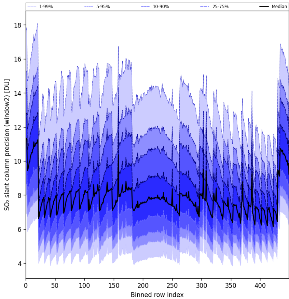
Figure 94: Along track statistics of “SO 2 slant column precision (window2)” for 2025-11-09 to 2025-11-11
