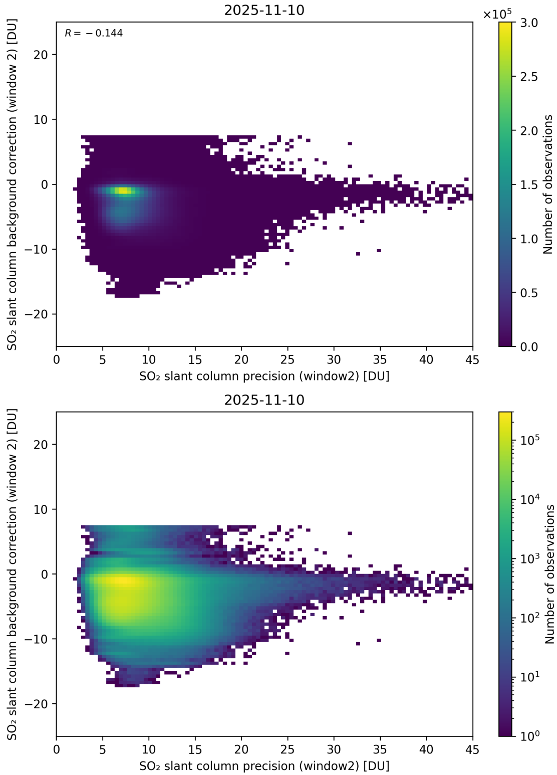
Figure 291: Scatter density plot of “SO 2 slant column precision (window2)” against “SO 2 slant column background correction (window 2)” for 2025-11-09 to 2025-11-11.
