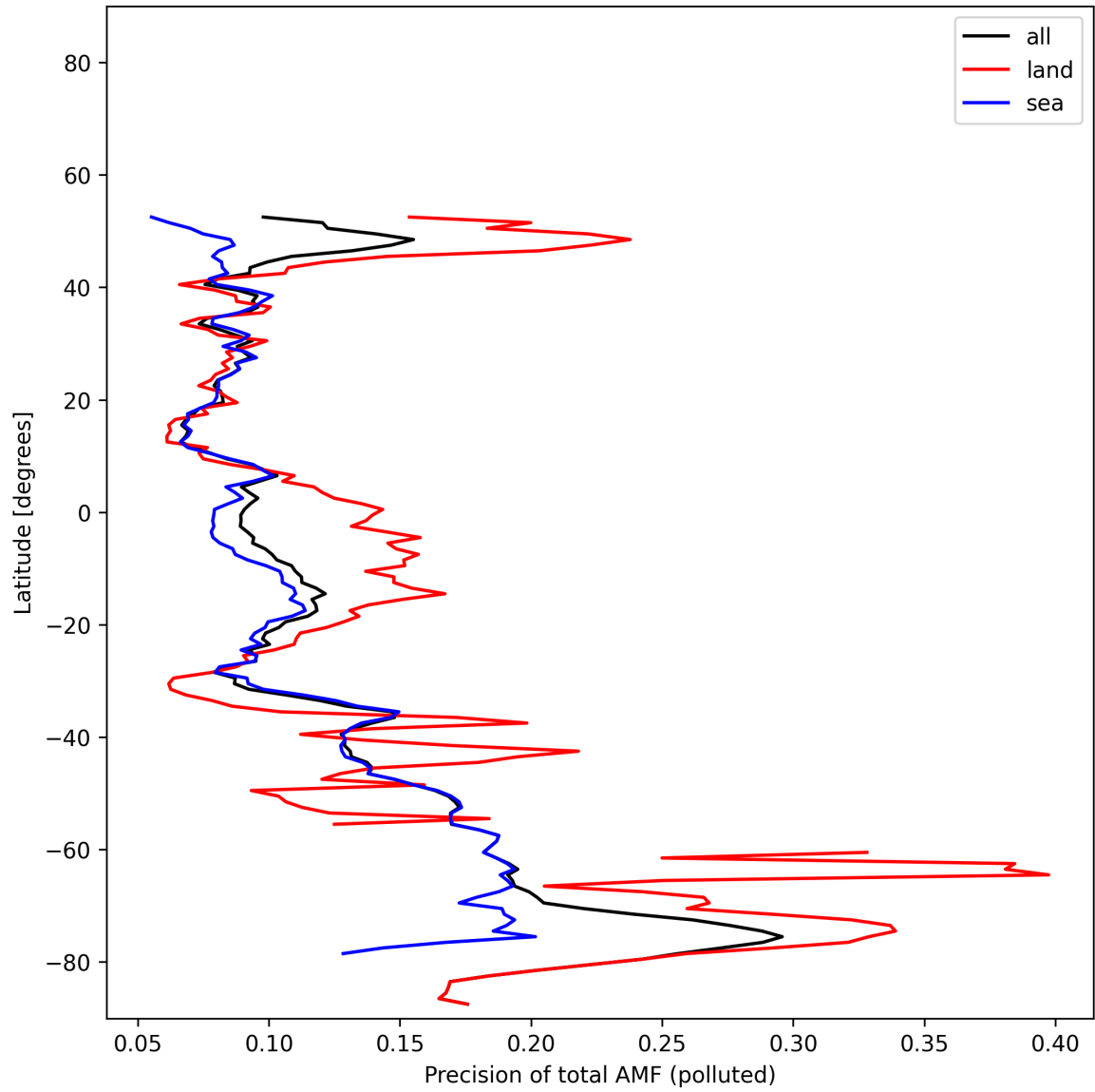
Figure 54: Zonal average of “Precision of total AMF (polluted)” for 2025-11-09 to 2025-11-11.
