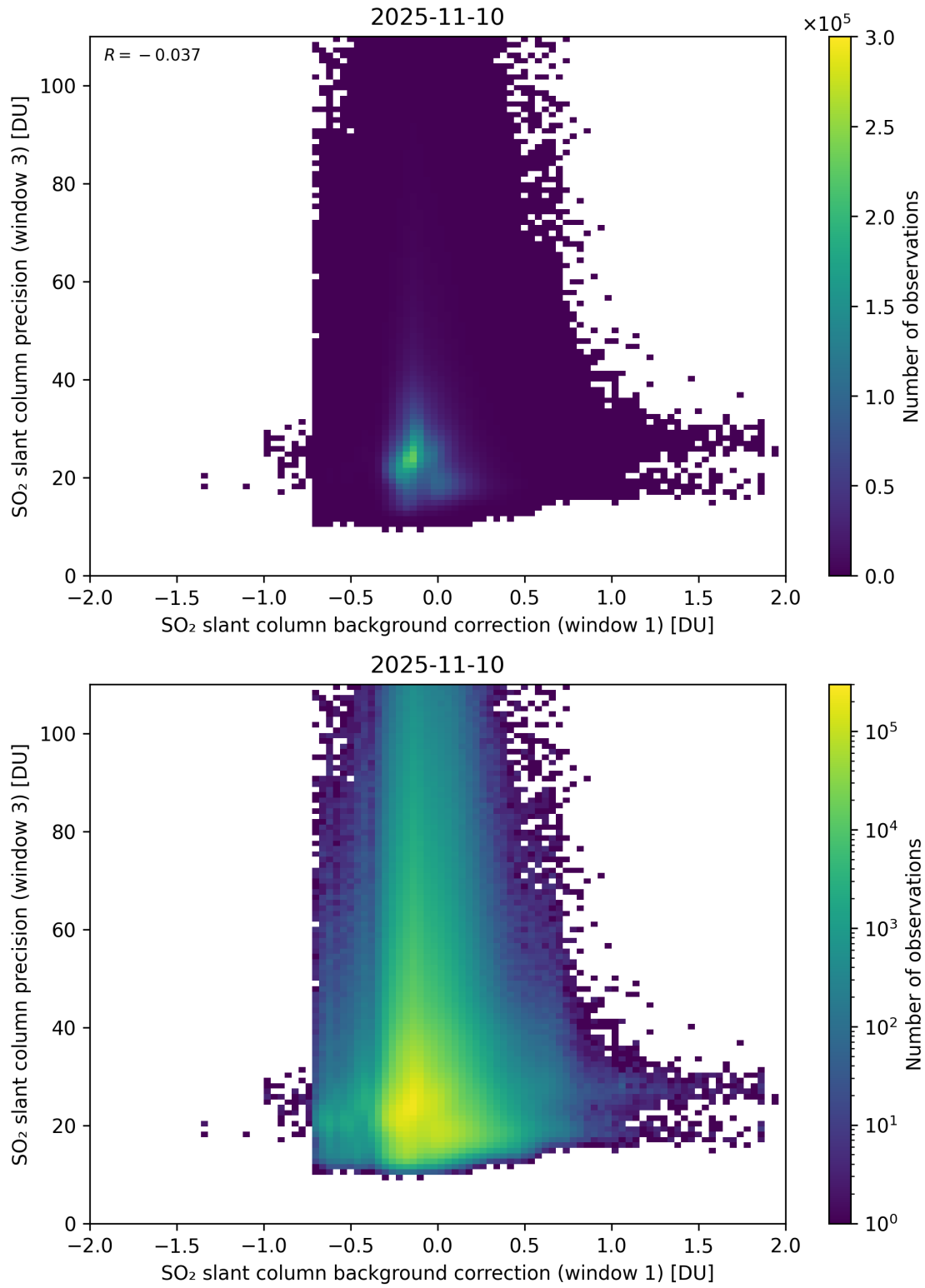
Figure 119: Scatter density plot of “SO 2 slant column background correction (window 1)” against “SO 2 slant column precision (window 3)” for 2025-11-09 to 2025-11-11.
