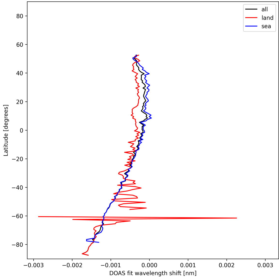
Figure 50: Zonal average of "DOAS fit wavelength shift" for 2025-11-09 to 2025-11-11.
