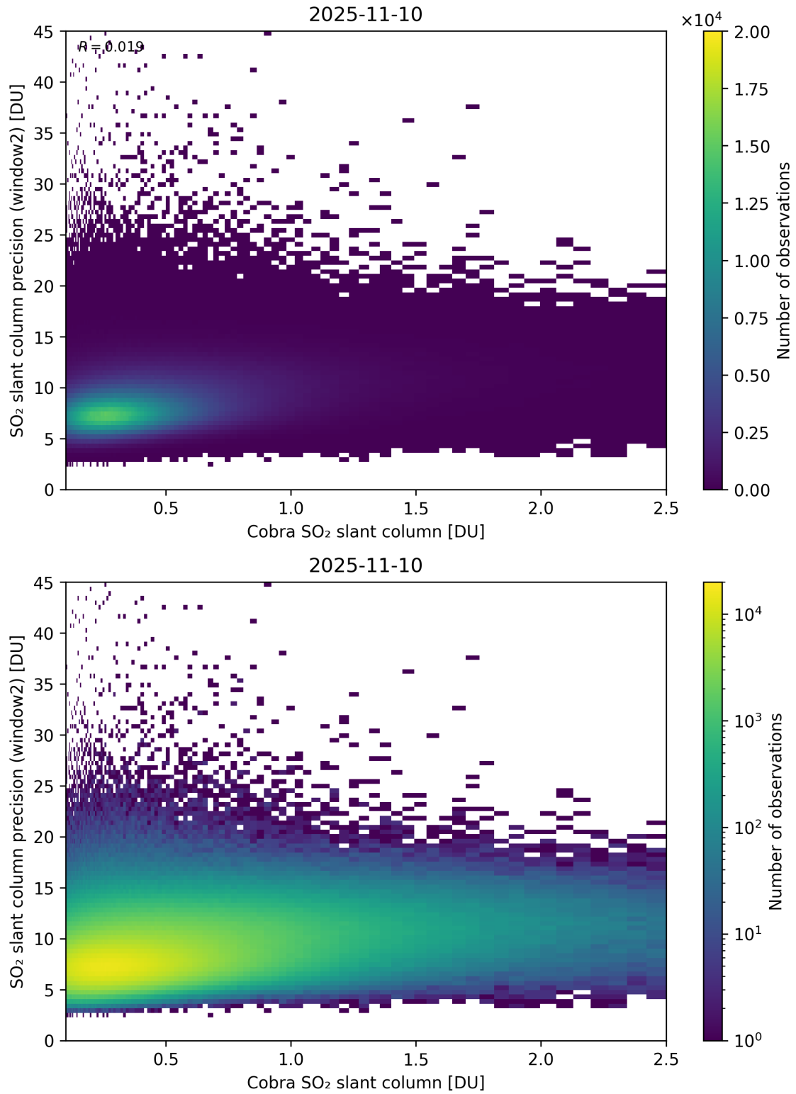
Figure 221: Scatter density plot of “Cobra SO 2 slant column” against “SO 2 slant column precision (window2)” for 2025-11-09 to 2025-11-11.
