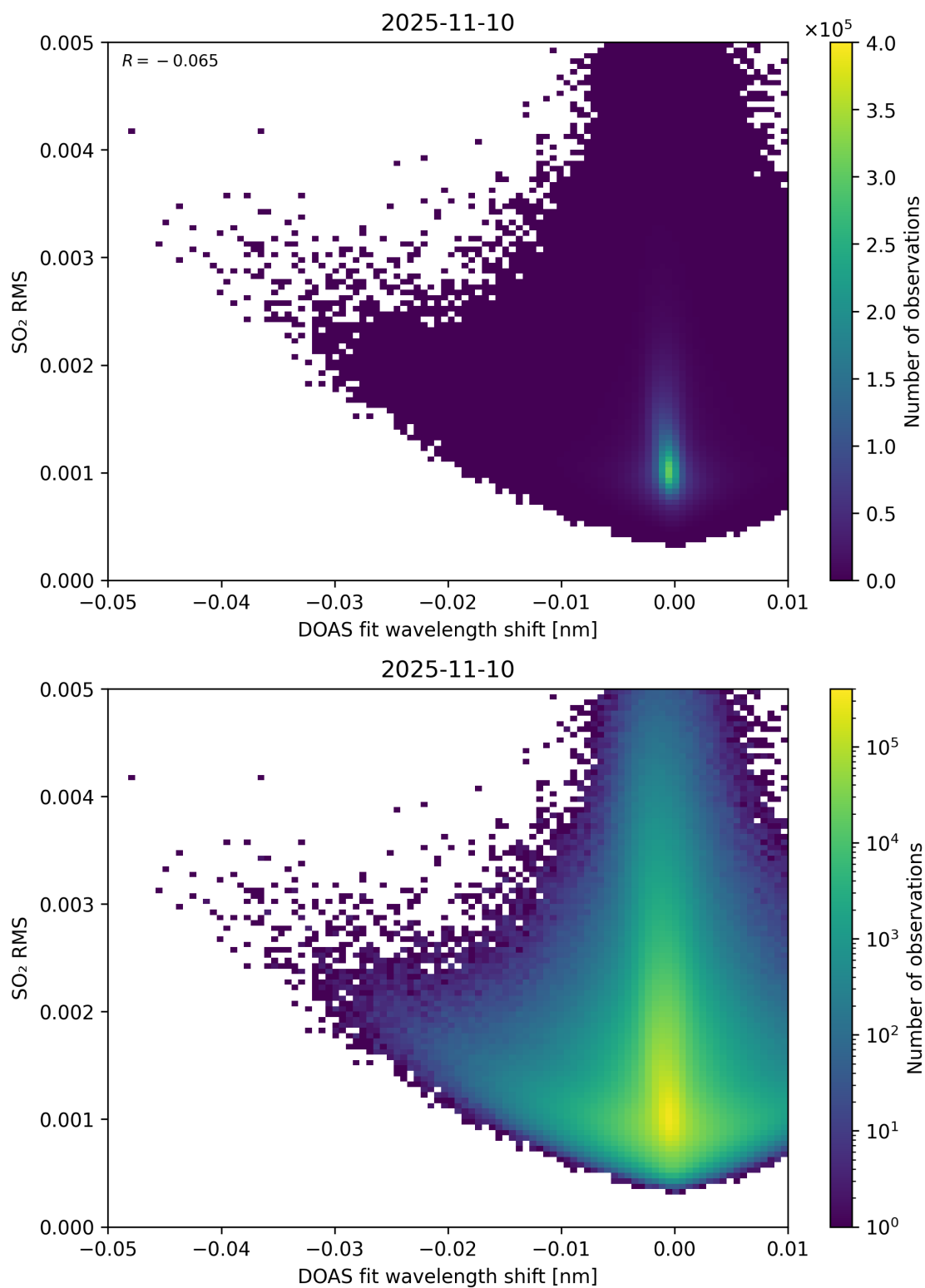
Figure 139: Scatter density plot of “DOAS fit wavelength shift” against “SO 2 RMS” for 2025-11-09 to 2025-11-11.
