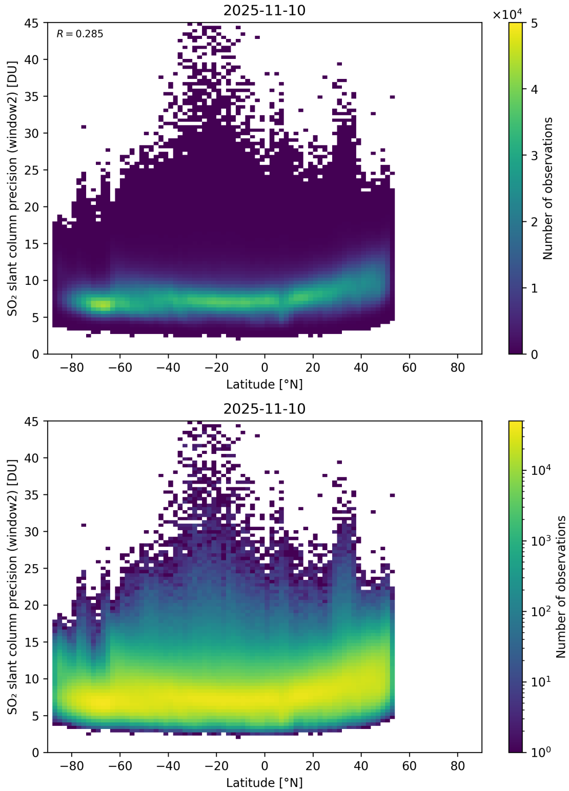
Figure 164: Scatter density plot of “Latitude” against “SO 2 slant column precision (window2)” for 2025-11-09 to 2025-11-11.
