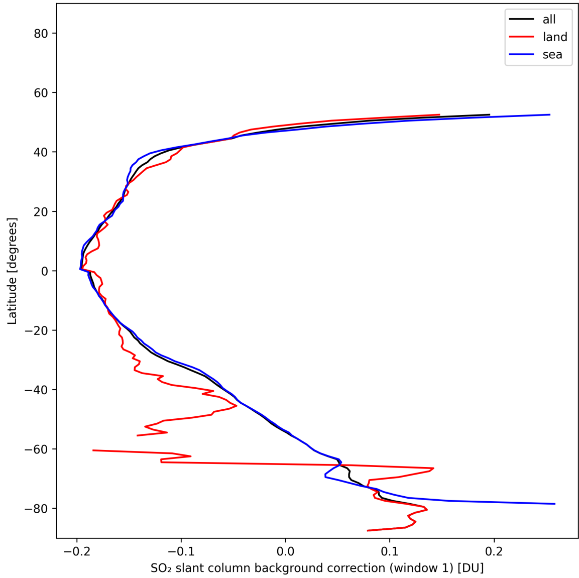
Figure 40: Zonal average of “SO 2 slant column background correction (window 1)” for 2025-11-09 to 2025-11-11.
