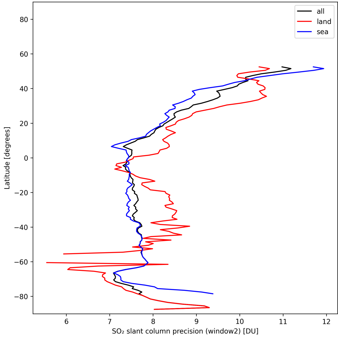
Figure 42: Zonal average of “SO 2 slant column precision (window2)” for 2025-11-09 to 2025-11-11.
