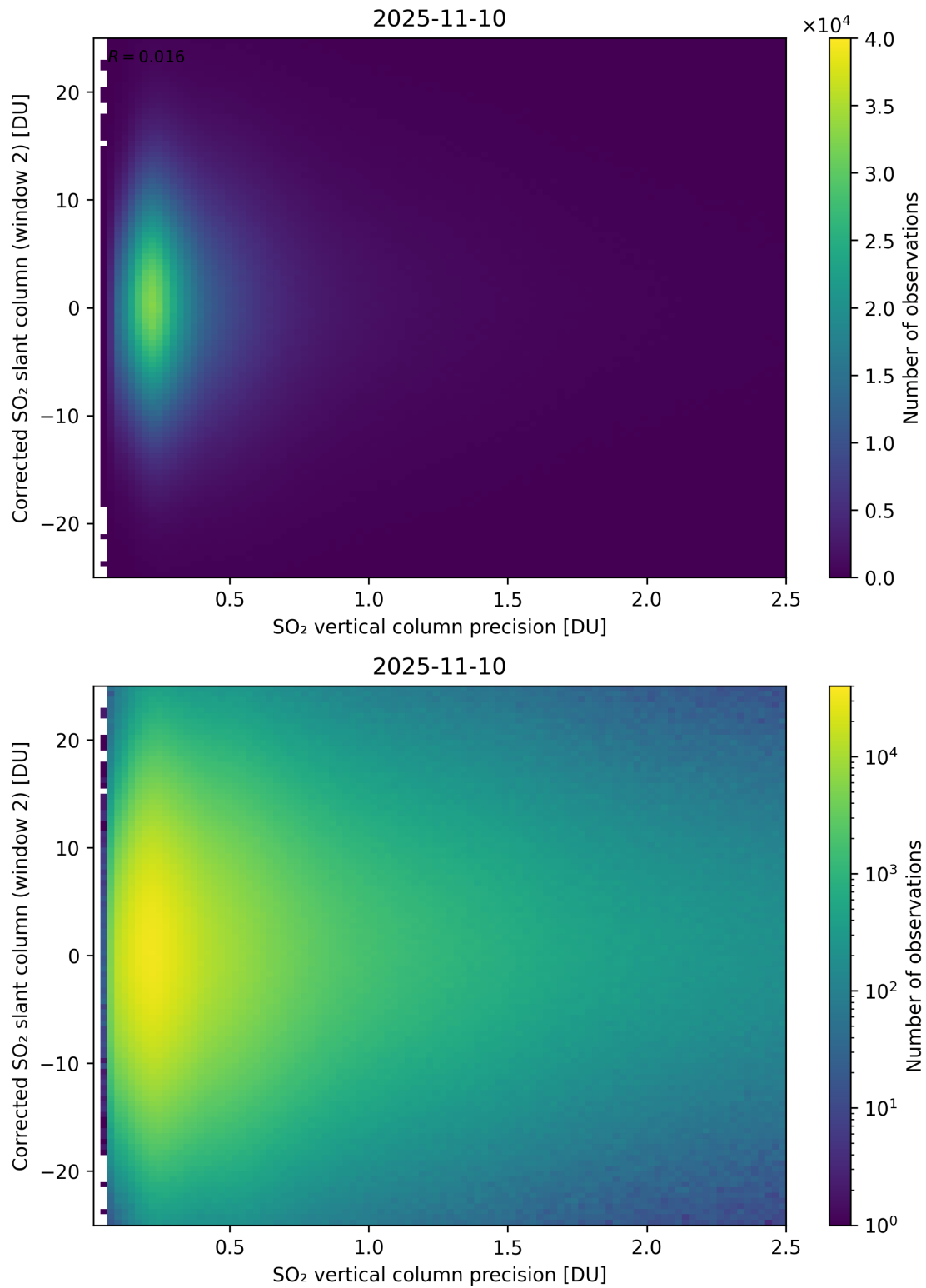
Figure 339: Scatter density plot of “SO 2 vertical column precision” against “Corrected SO 2 slant column (window 2)” for 2025-11-09 to 2025-11-11.
