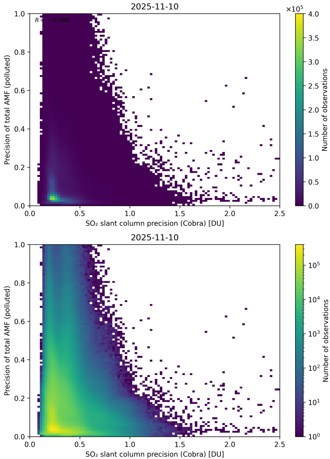
Figure 214: Scatter density plot of “SO 2 slant column precision (Cobra)” against “Precision of total AMF (polluted)” for 2025-11-09 to 2025-11-11.
