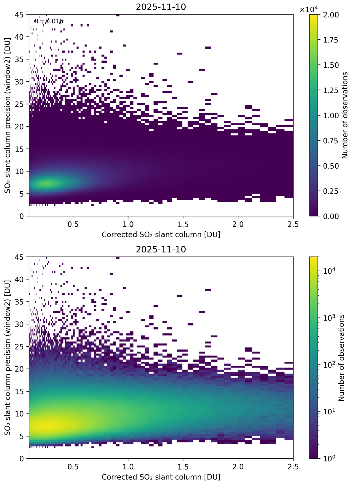
Figure 239: Scatter density plot of “Corrected SO 2 slant column” against “SO 2 slant column precision (window2)” for 2025-11-09 to 2025-11-11.
