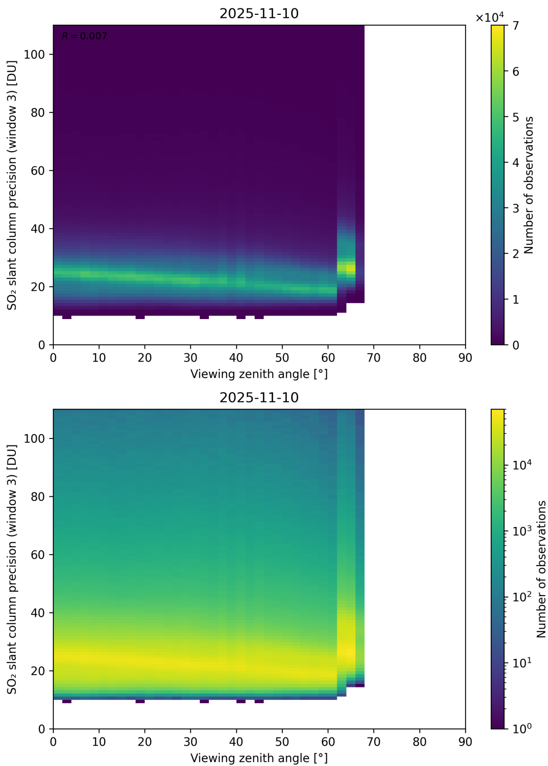
Figure 380: Scatter density plot of “Viewing zenith angle” against “SO 2 slant column precision (window 3)” for 2025-11-09 to 2025-11-11.
