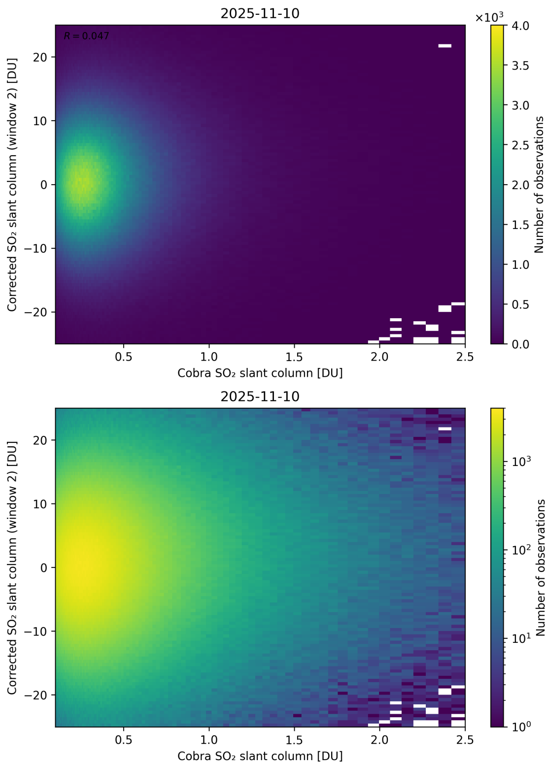
Figure 217: Scatter density plot of “Cobra SO 2 slant column” against “Corrected SO 2 slant column (window 2)” for 2025-11-09 to 2025-11-11.
