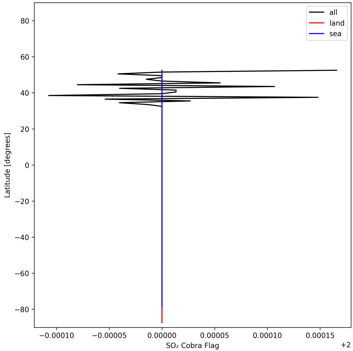
Figure 49: Zonal average of “SO 2 Cobra Flag” for 2025-11-09 to 2025-11-11.
