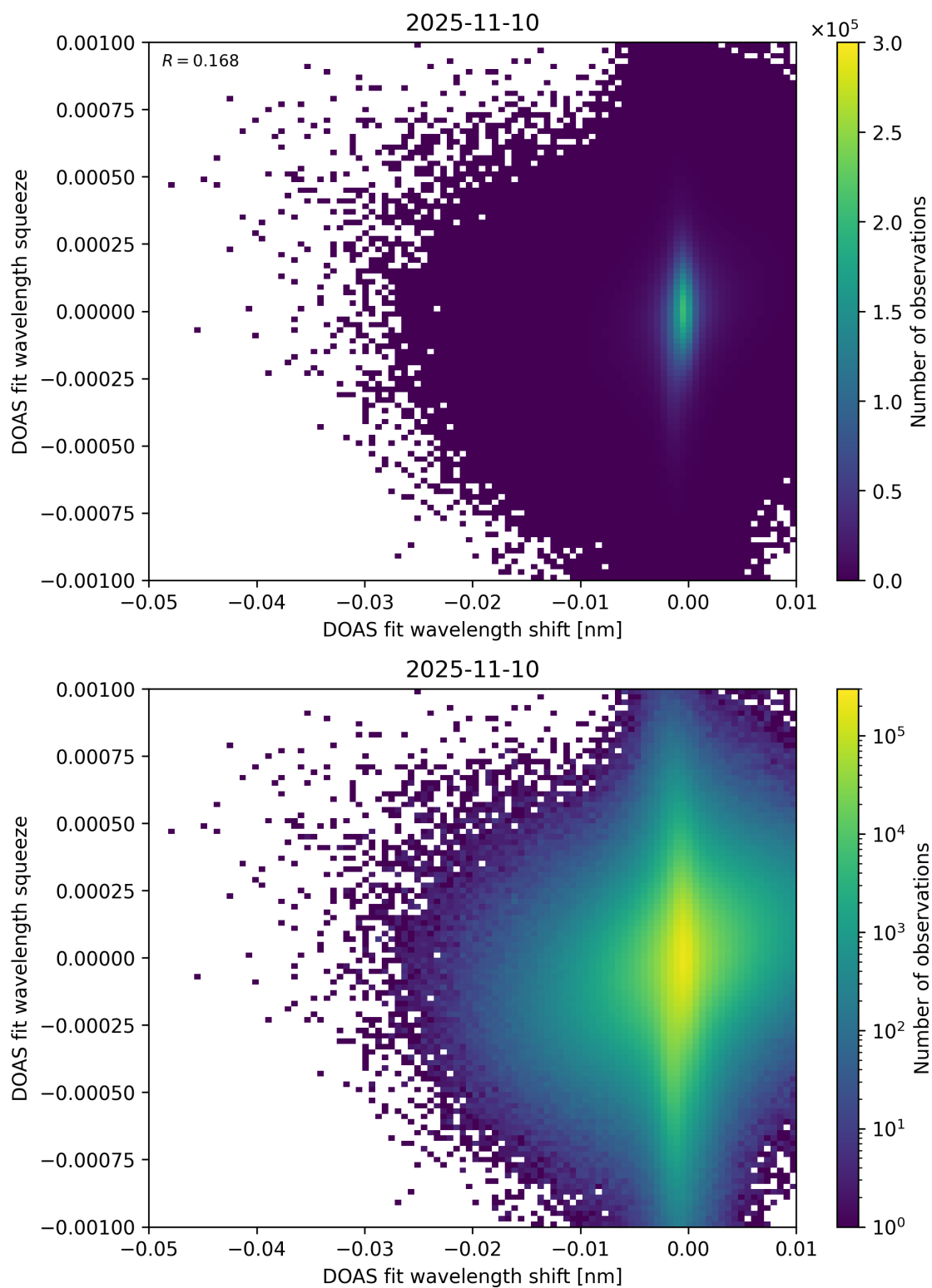
Figure 138: Scatter density plot of “DOAS fit wavelength shift” against “DOAS fit wavelength squeeze” for 2025-11-09 to 2025-11-11.
