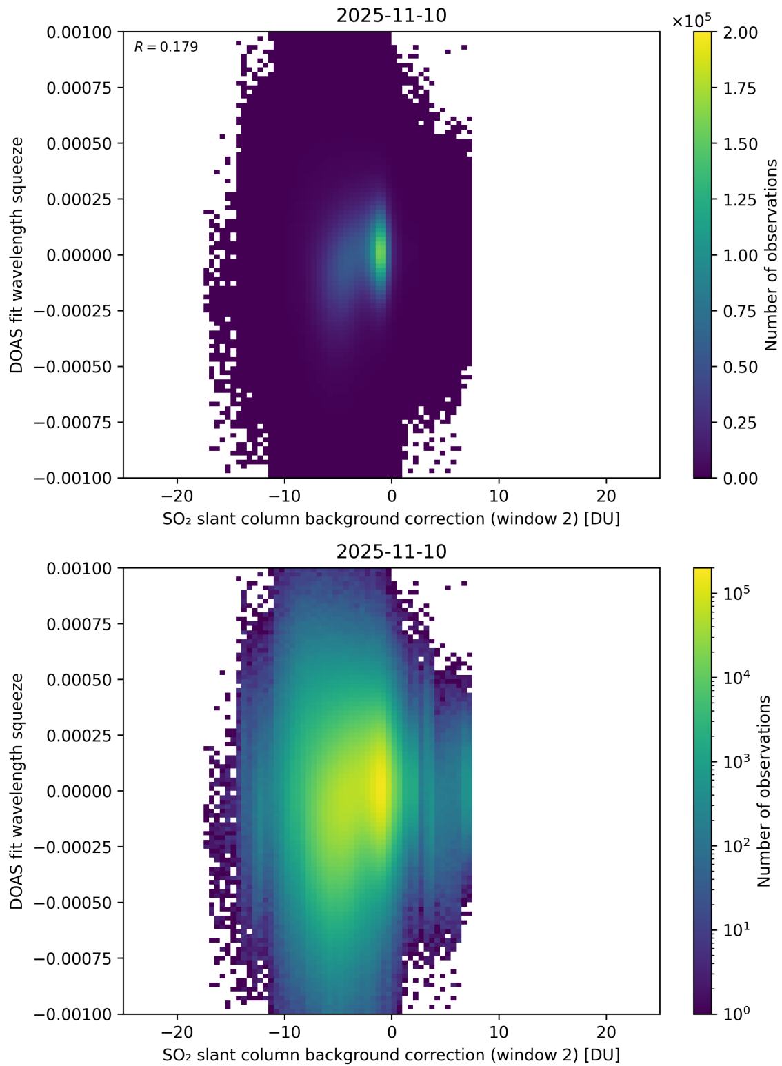
Figure 124: Scatter density plot of “SO 2 slant column background correction (window 2)” against “DOAS fit wavelength squeeze” for 2025-11-09 to 2025-11-11.
