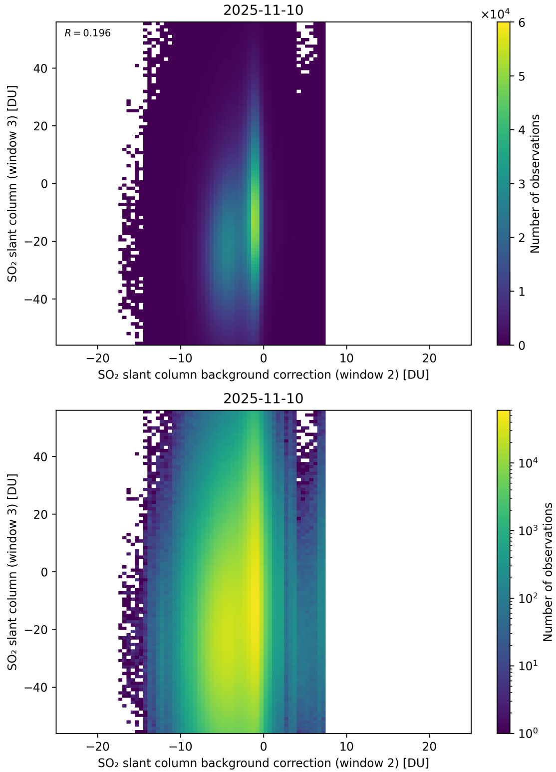
Figure 128: Scatter density plot of “SO 2 slant column background correction (window 2)” against “SO 2 slant column (window 3)” for 2025-11-09 to 2025-11-11.
