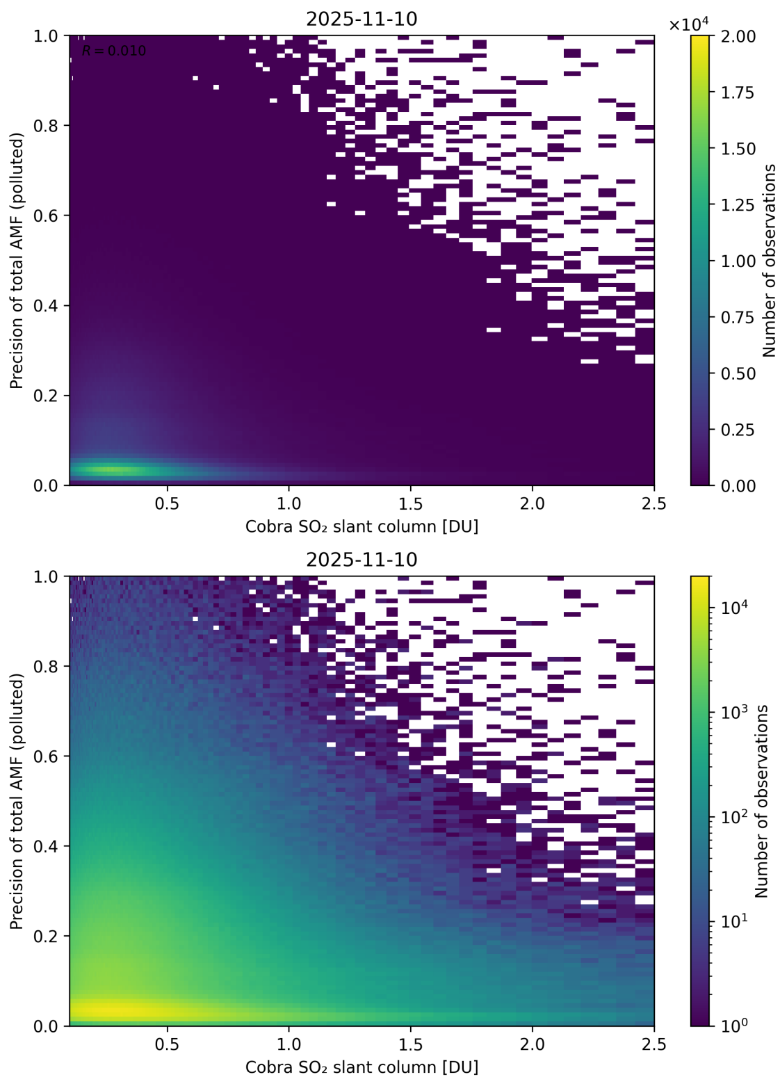
Figure 225: Scatter density plot of “Cobra SO 2 slant column” against “Precision of total AMF (polluted)” for 2025-11-09 to 2025-11-11.
