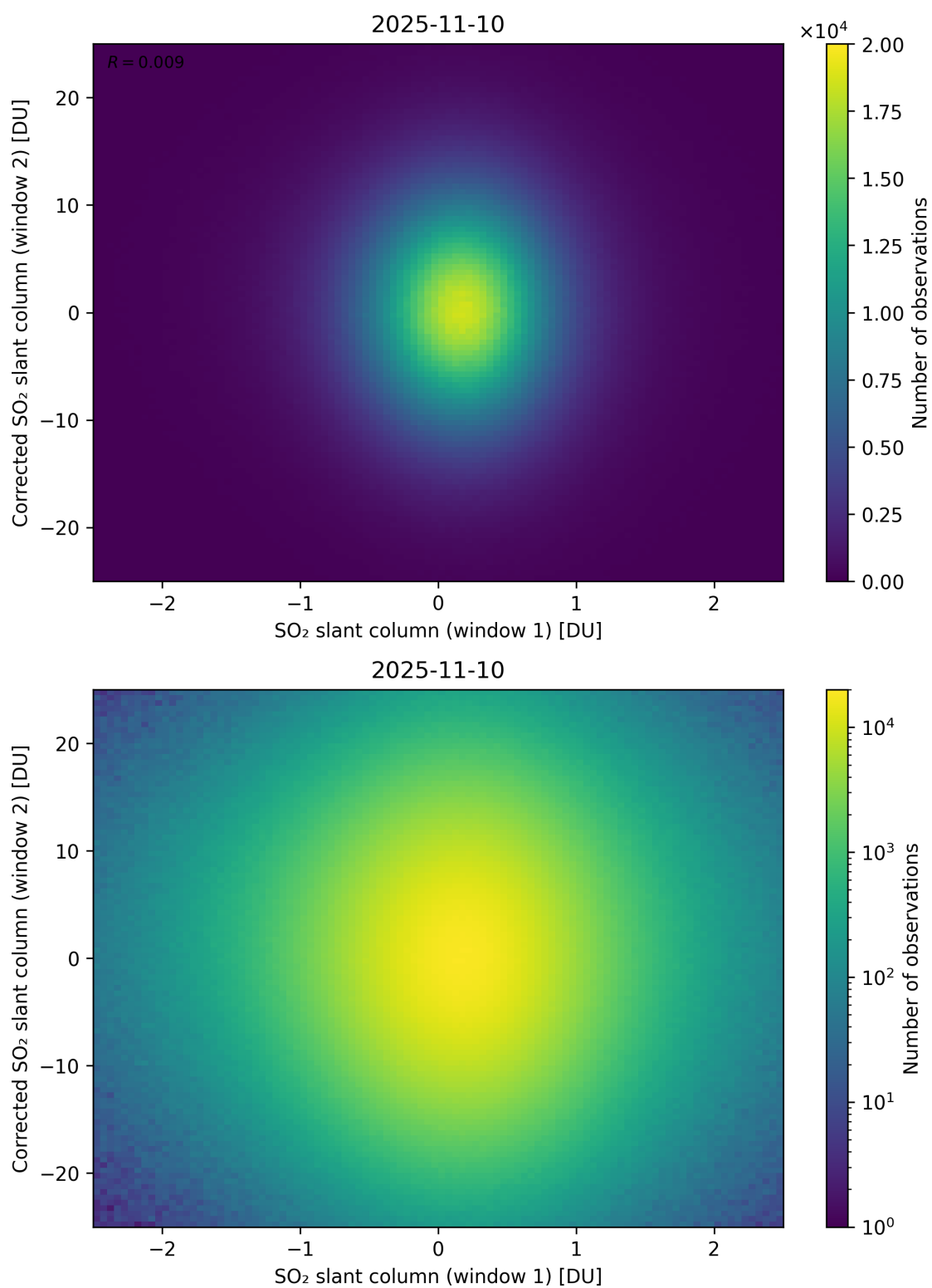
Figure 283: Scatter density plot of “SO 2 slant column (window 1)” against “Corrected SO 2 slant column (window 2)” for 2025-11-09 to 2025-11-11.
