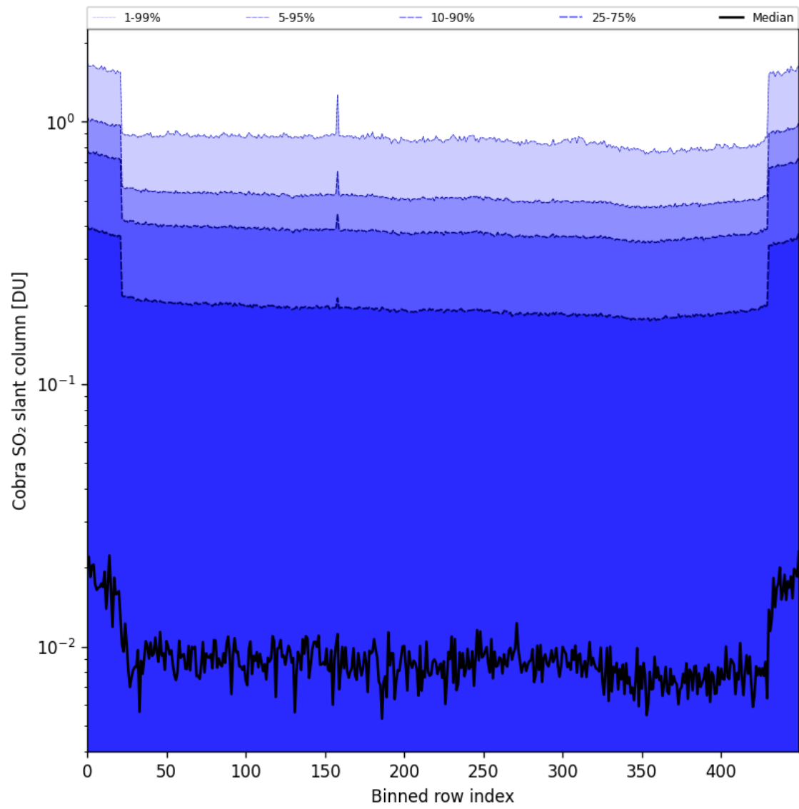
Figure 87: Along track statistics of “Cobra SO 2 slant column” for 2025-11-09 to 2025-11-11
