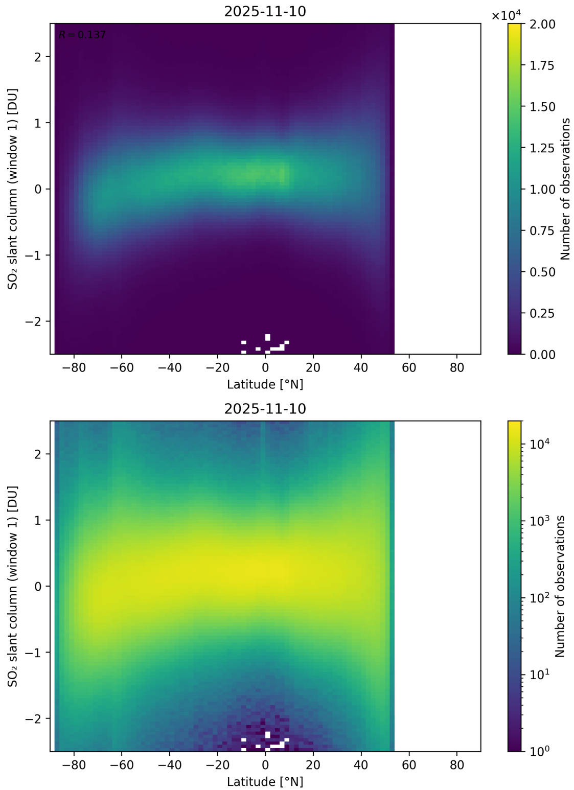
Figure 162: Scatter density plot of “Latitude” against “SO 2 slant column (window 1)” for 2025-11-09 to 2025-11-11.
