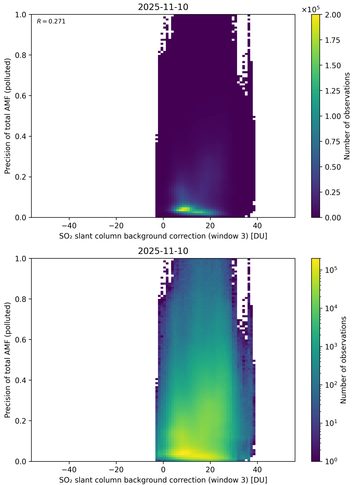
Figure 137: Scatter density plot of “SO 2 slant column background correction (window 3)” against “Precision of total AMF (polluted)” for 2025-11-09 to 2025-11-11.
