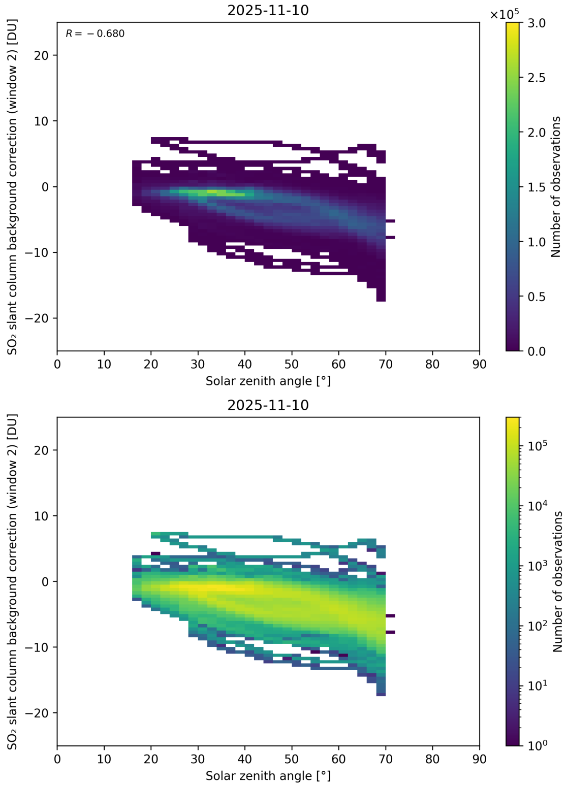
Figure 172: Scatter density plot of “Solar zenith angle” against “SO 2 slant column background correction (window 2)” for 2025-11-09 to 2025-11-11.
