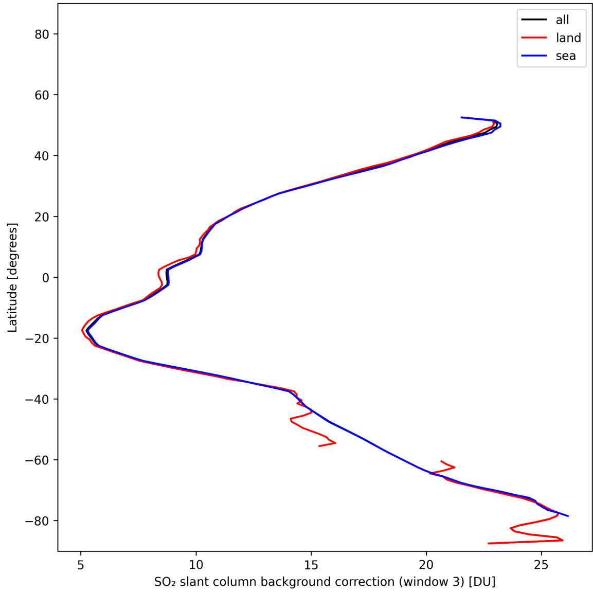
Figure 48: Zonal average of “SO 2 slant column background correction (window 3)” for 2025-11-09 to 2025-11-11.
