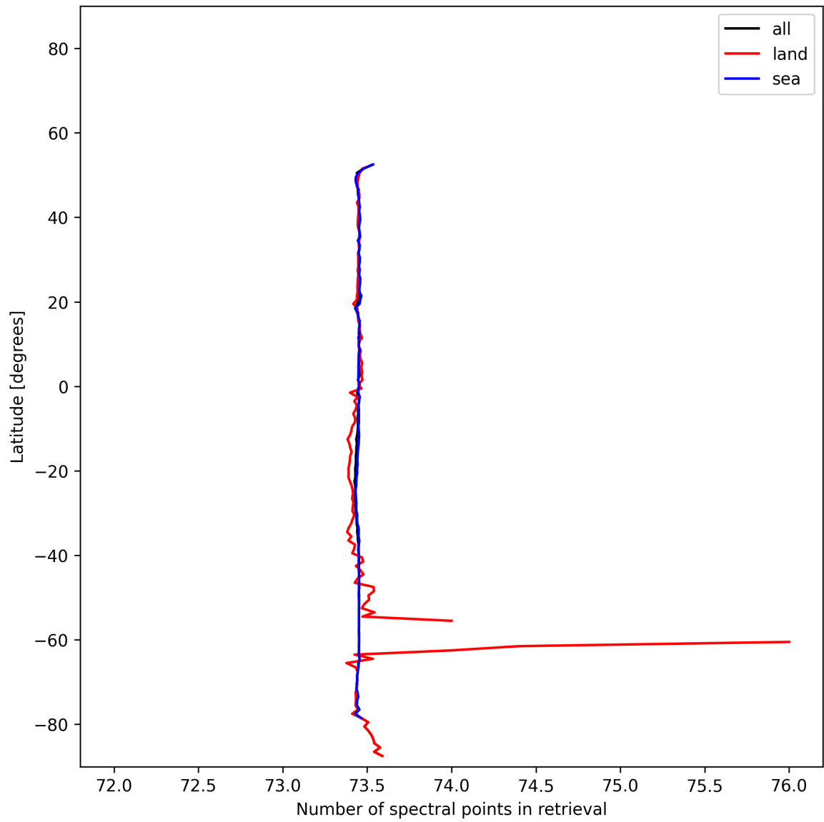
Figure 56: Zonal average of “Number of spectral points in retrieval” for 2025-11-09 to 2025-11-11.
