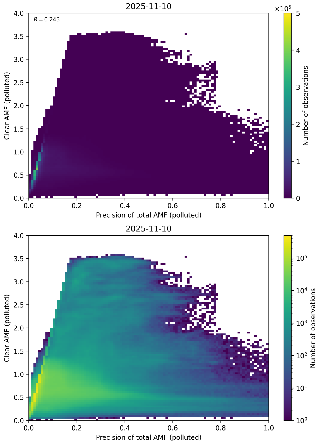
Figure 320: Scatter density plot of “Precision of total AMF (polluted)” against “Clear AMF (polluted)” for 2025-11-09 to 2025-11-11.
