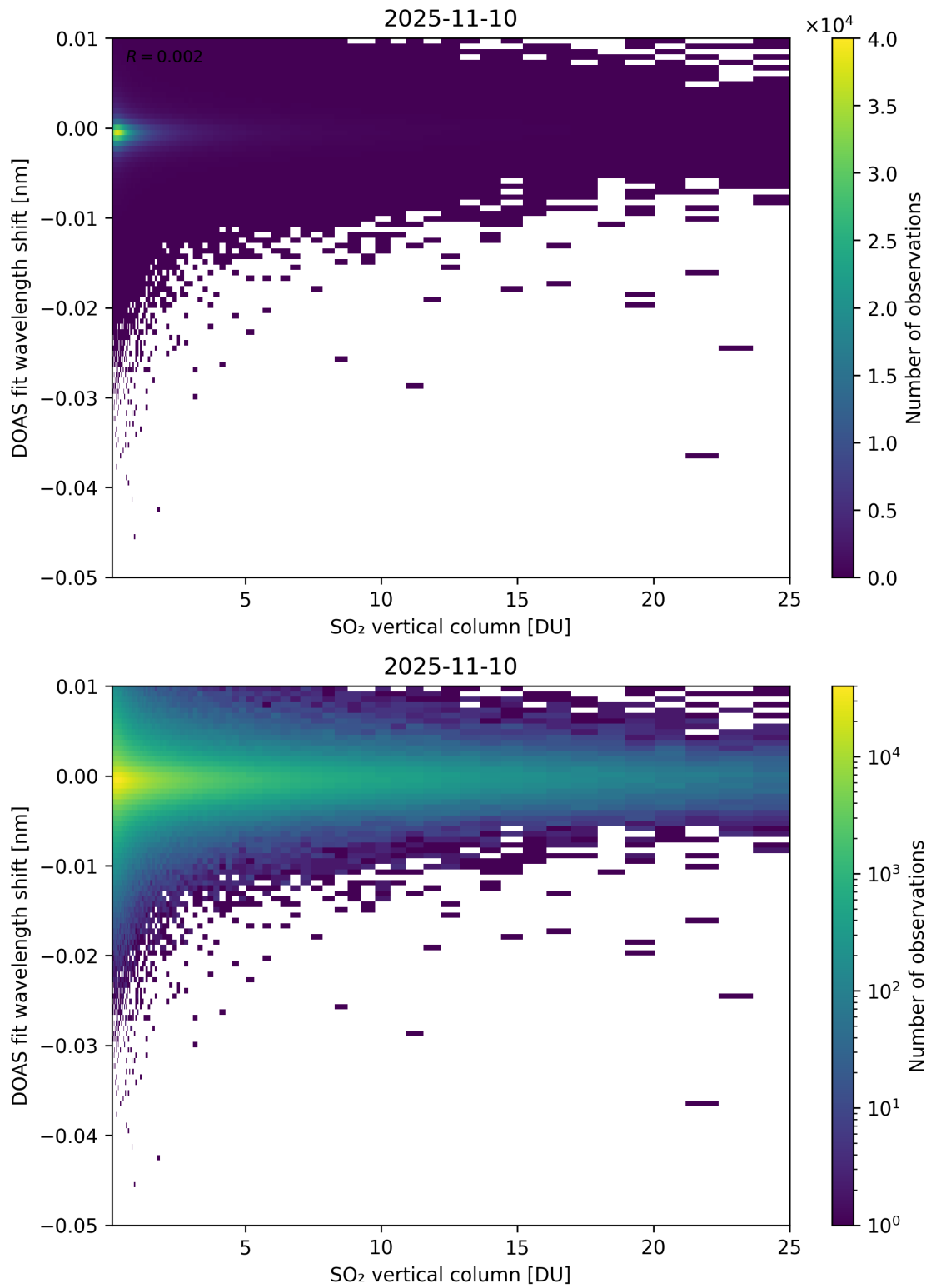
Figure 326: Scatter density plot of “SO 2 vertical column” against “DOAS fit wavelength shift” for 2025-11-09 to 2025-11-11.
