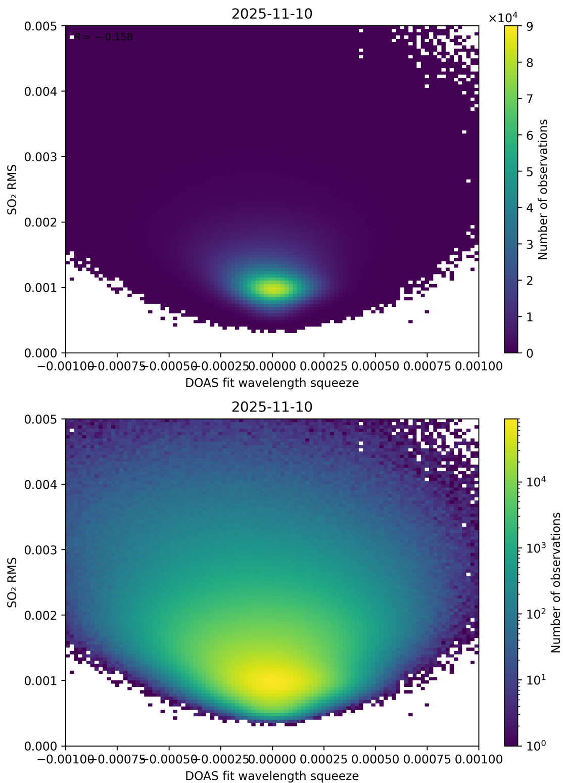
Figure 143: Scatter density plot of “DOAS fit wavelength squeeze” against “SO 2 RMS” for 2025-11-09 to 2025-11-11.
