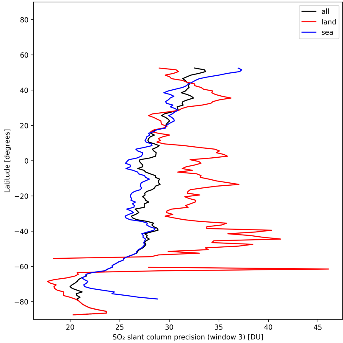
Figure 46: Zonal average of “SO 2 slant column precision (window 3)” for 2025-11-09 to 2025-11-11.
