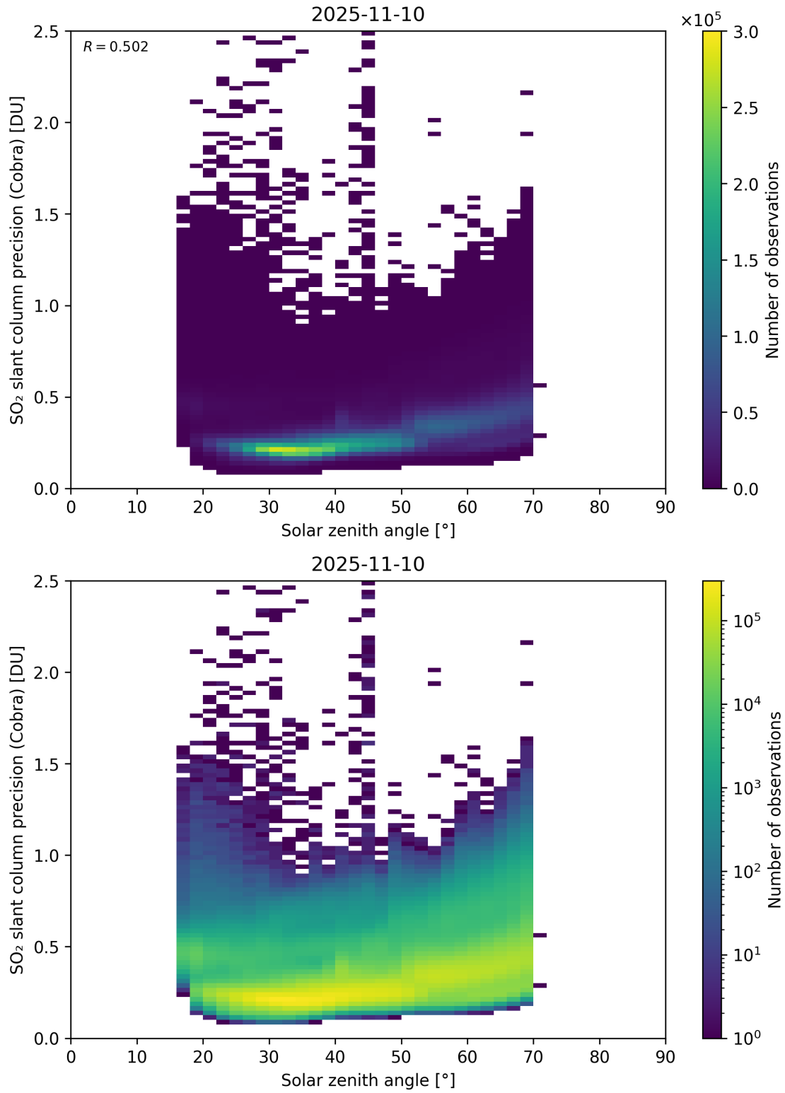
Figure 180: Scatter density plot of “Solar zenith angle” against “SO 2 slant column precision (Cobra)” for 2025-11-09 to 2025-11-11.
