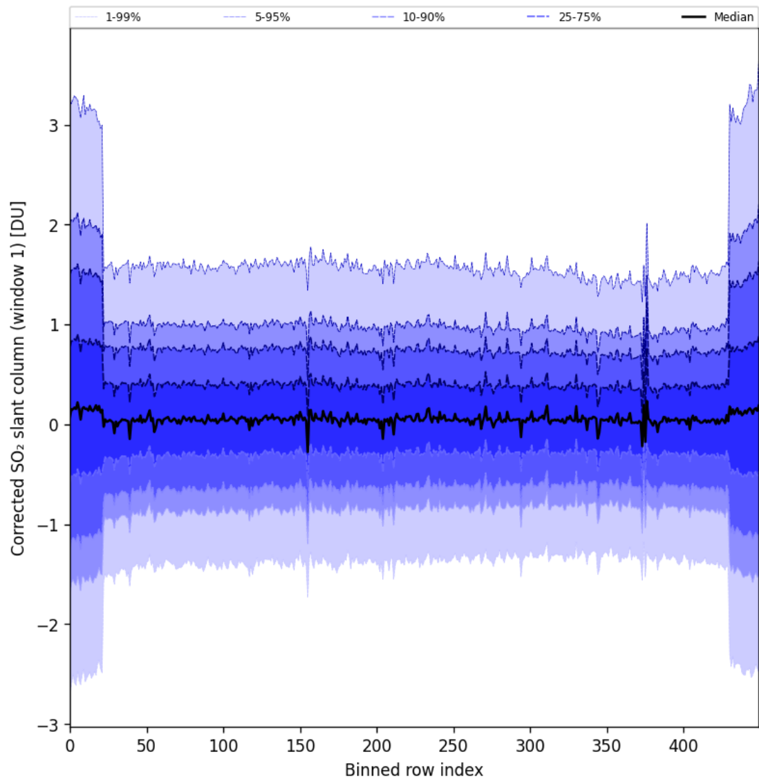
Figure 91: Along track statistics of “Corrected SO 2 slant column (window 1)” for 2025-11-09 to 2025-11-11
