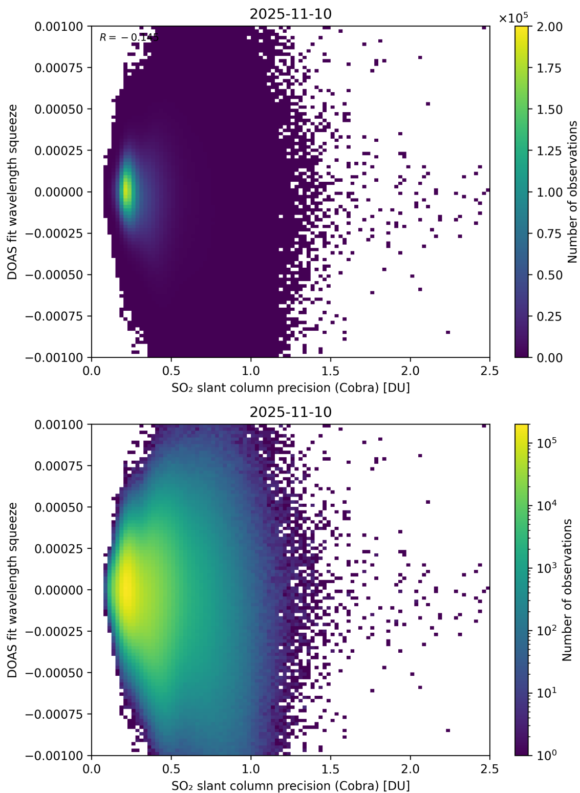
Figure 203: Scatter density plot of “SO 2 slant column precision (Cobra)” against “DOAS fit wavelength squeeze” for 2025-11-09 to 2025-11-11.
