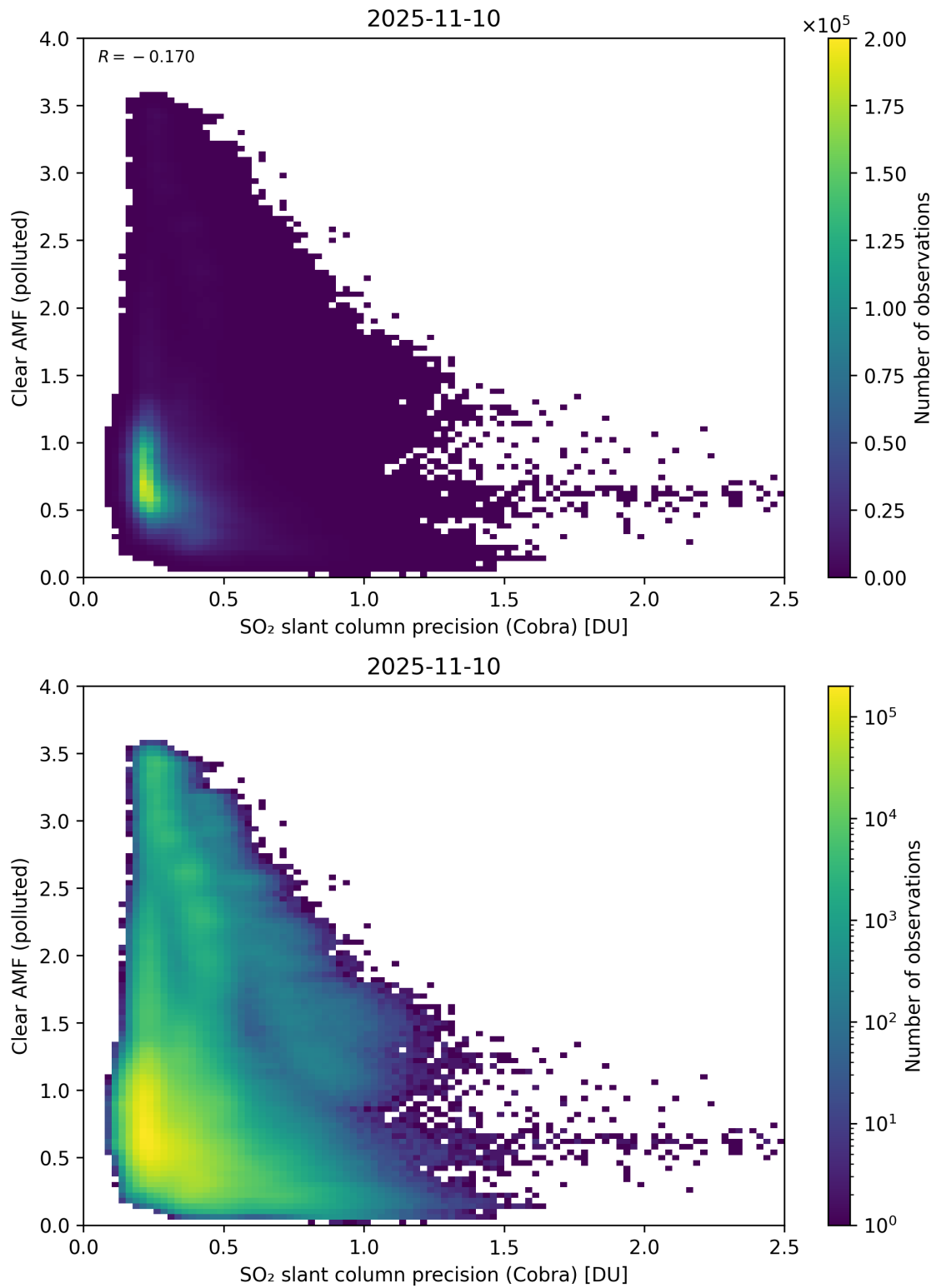
Figure 205: Scatter density plot of “SO 2 slant column precision (Cobra)” against “Clear AMF (polluted)” for 2025-11-09 to 2025-11-11.
