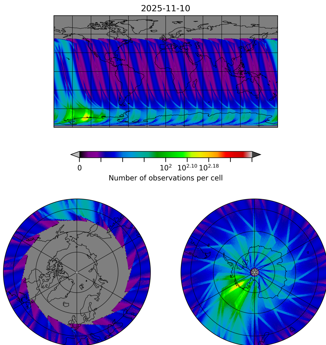
Figure 30: Map of the number of observations for 2025-11-09 to 2025-11-11
