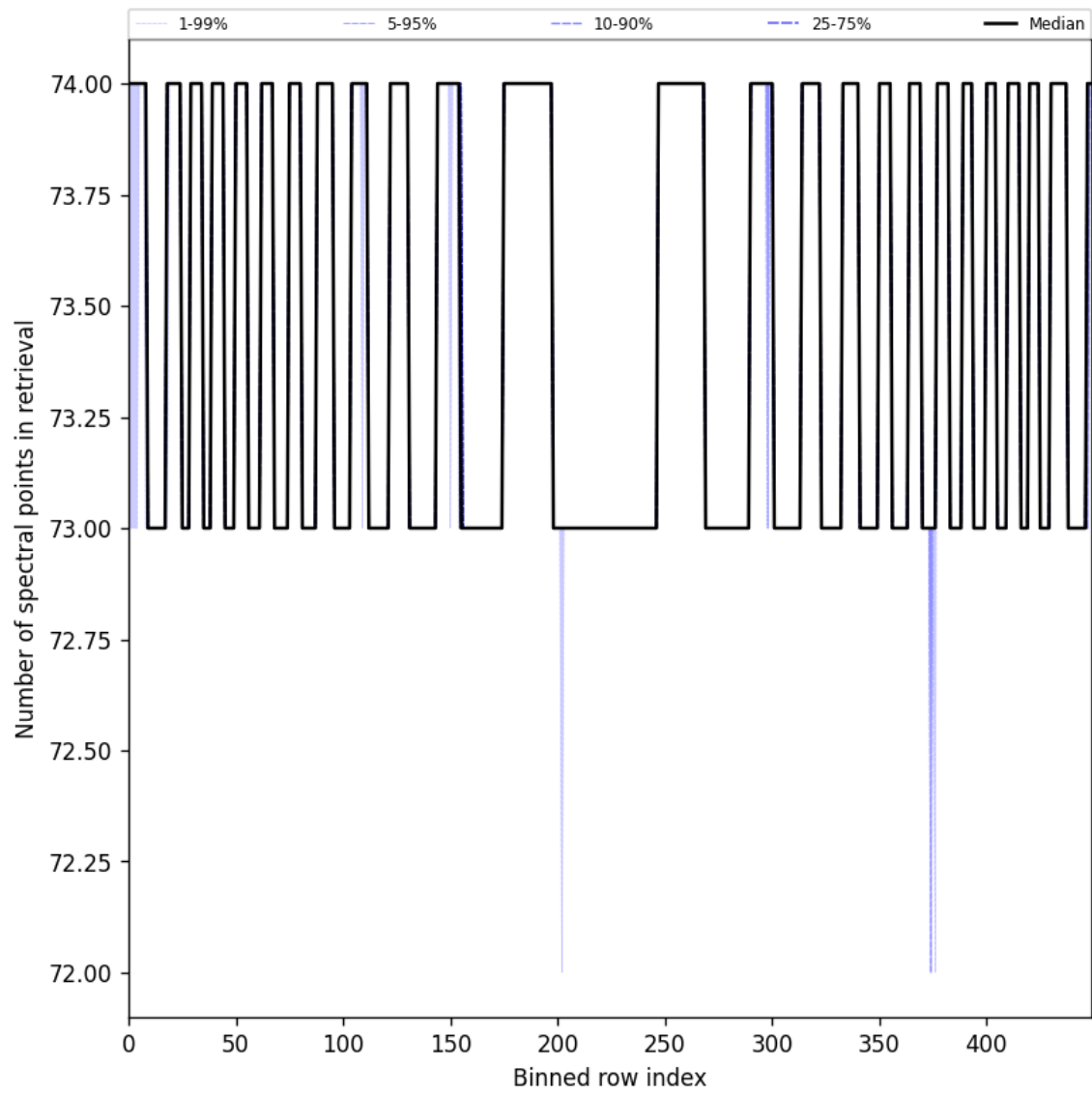
Figure 108: Along track statistics of “Number of spectral points in retrieval” for 2025-11-12 to 2025-11-13
