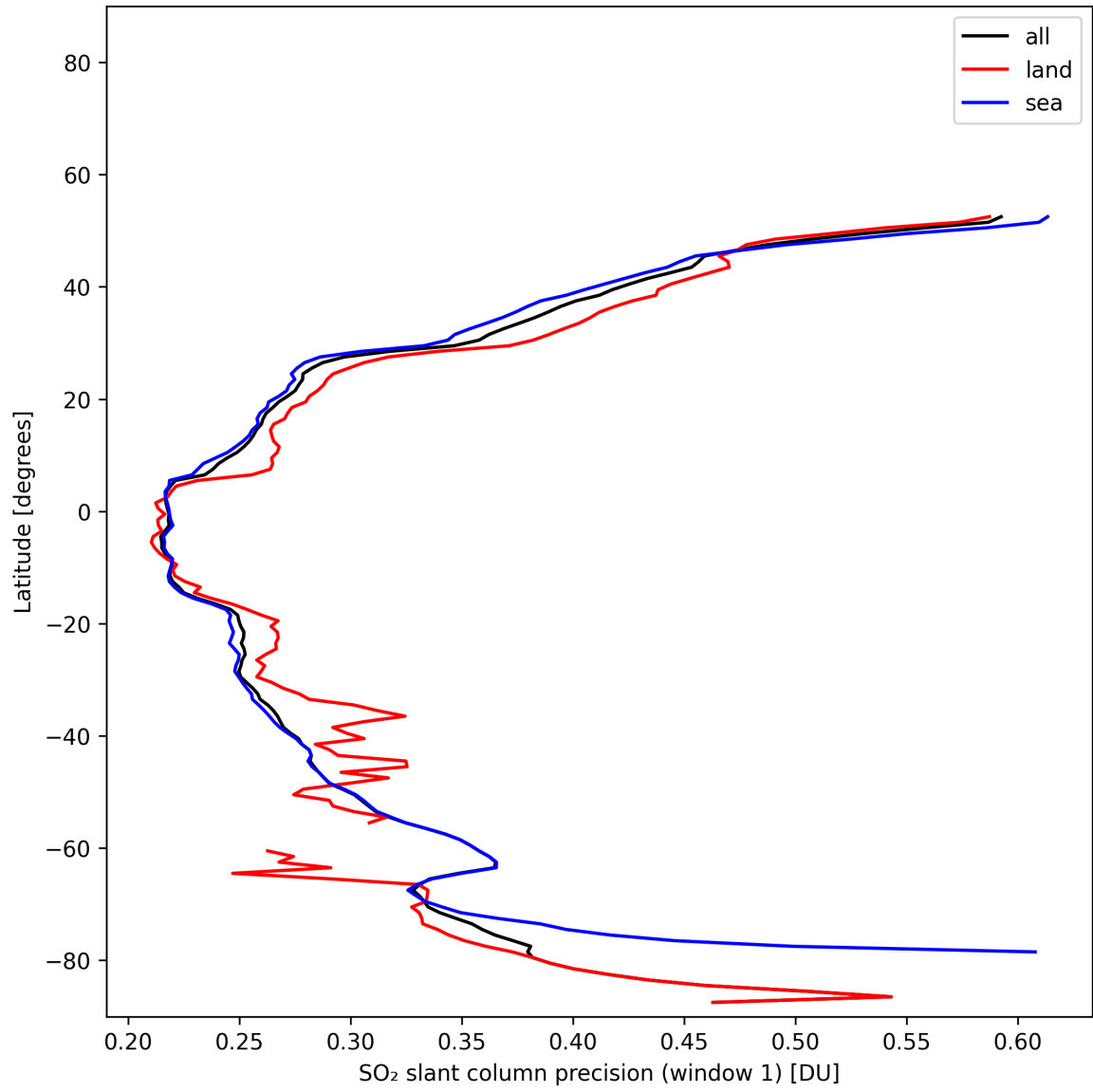
Figure 38: Zonal average of “SO 2 slant column precision (window 1)” for 2025-11-12 to 2025-11-13.
