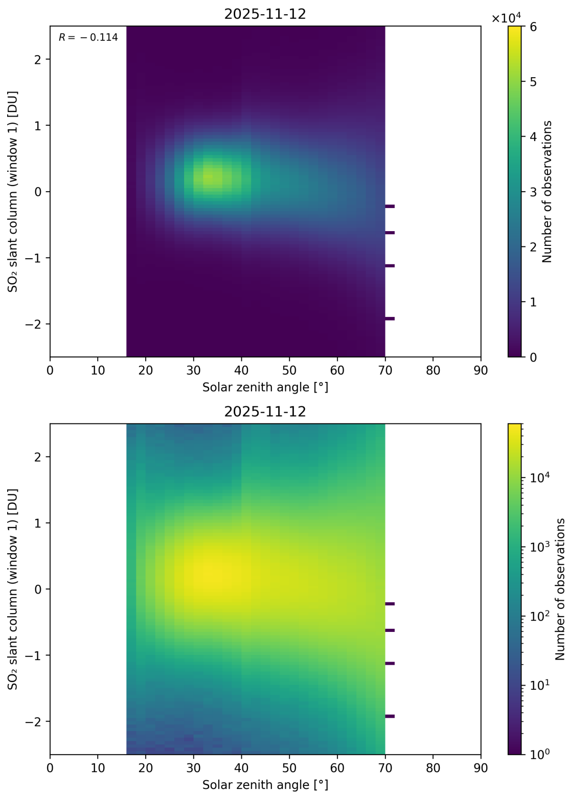
Figure 184: Scatter density plot of “Solar zenith angle” against “SO 2 slant column (window 1)” for 2025-11-12 to 2025-11-13.
