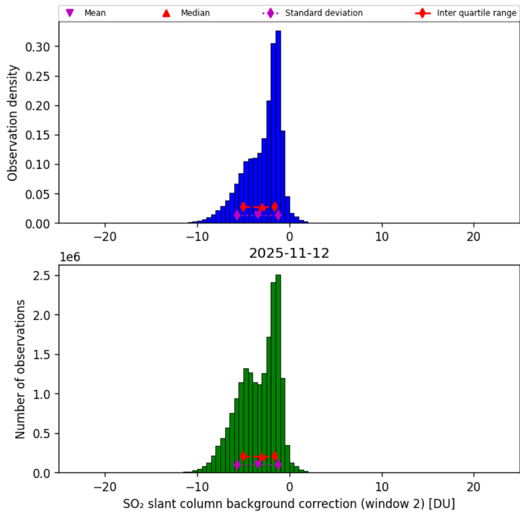
Figure 70: Histogram of “SO 2 slant column background correction (window 2)” for 2025-11-12 to 2025-11-13
