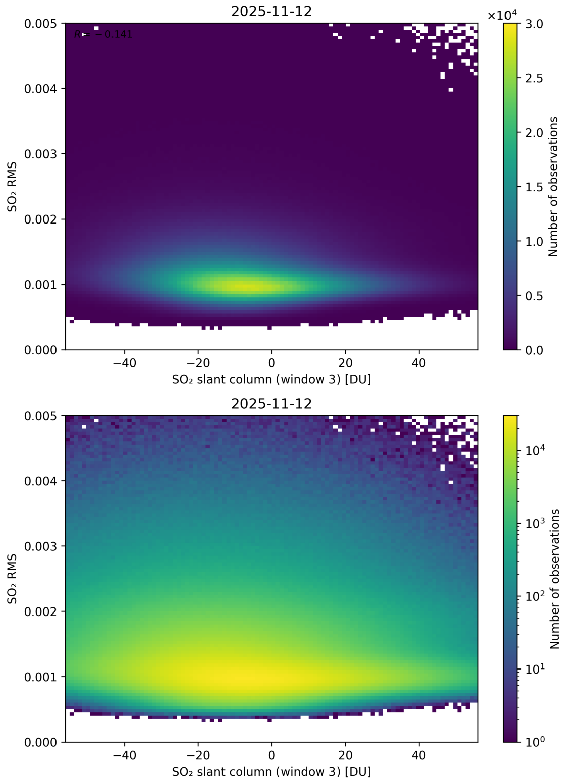
Figure 306: Scatter density plot of “SO 2 slant column (window 3)” against “SO 2 RMS” for 2025-11-12 to 2025-11-13.
