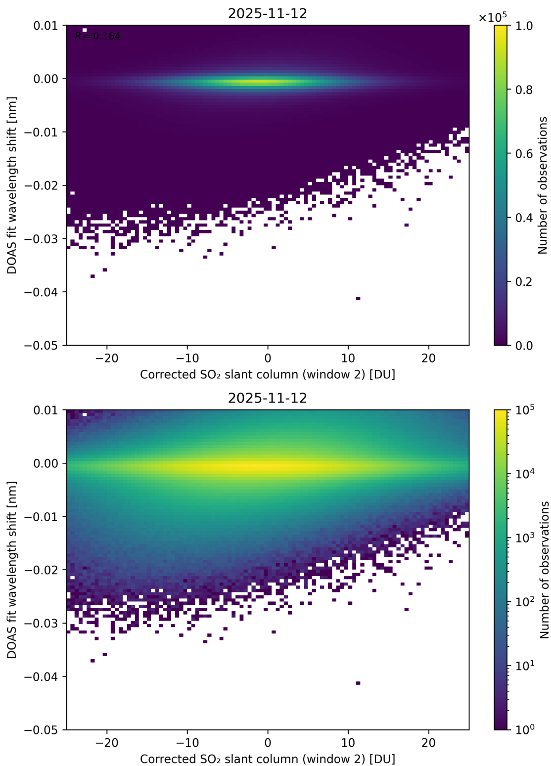
Figure 246: Scatter density plot of “Corrected SO 2 slant column (window 2)” against “DOAS fit wavelength shift” for 2025-11-12 to 2025-11-13.
