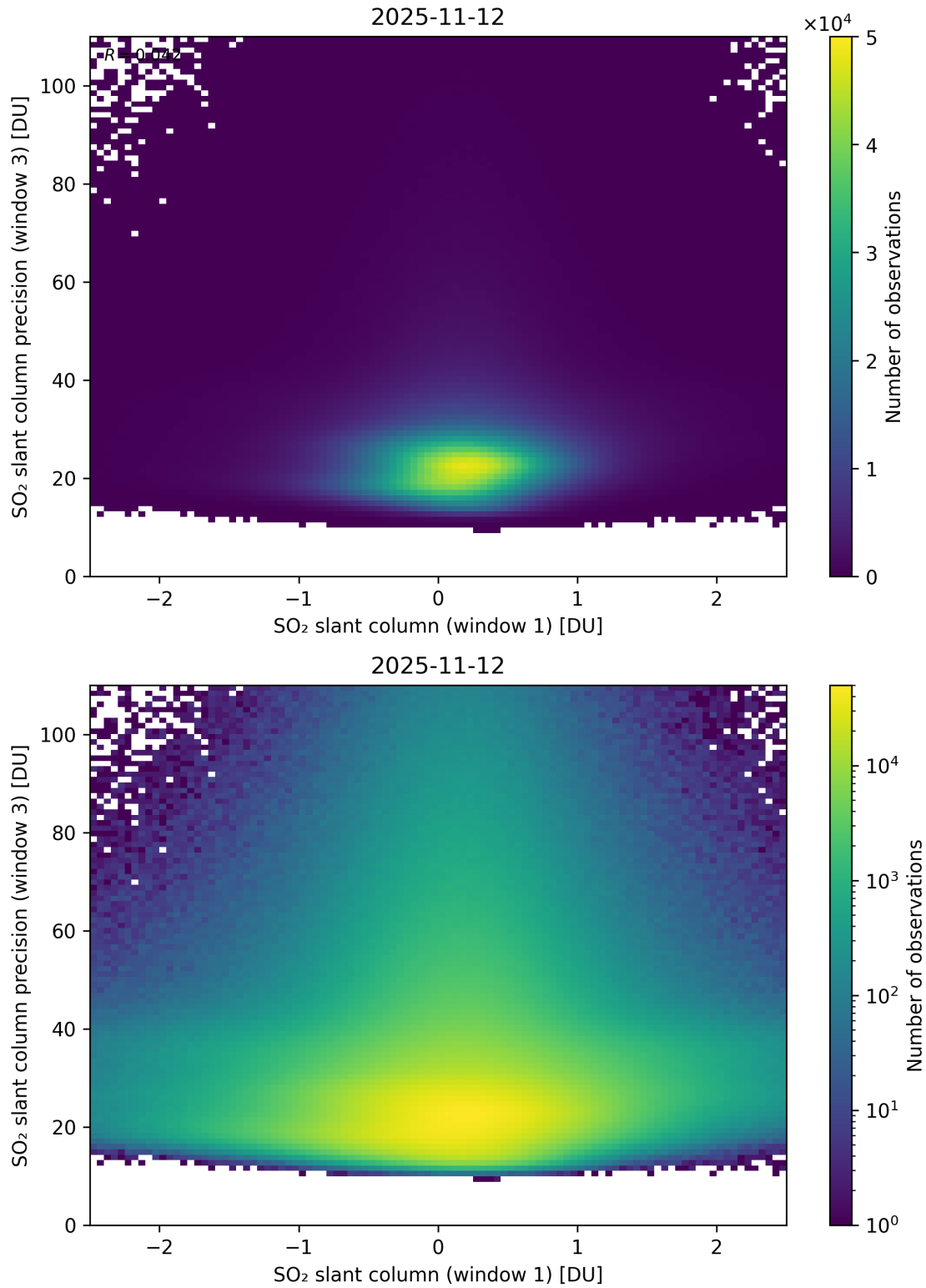
Figure 288: Scatter density plot of “SO 2 slant column (window 1)” against “SO 2 slant column precision (window 3)” for 2025-11-12 to 2025-11-13.
