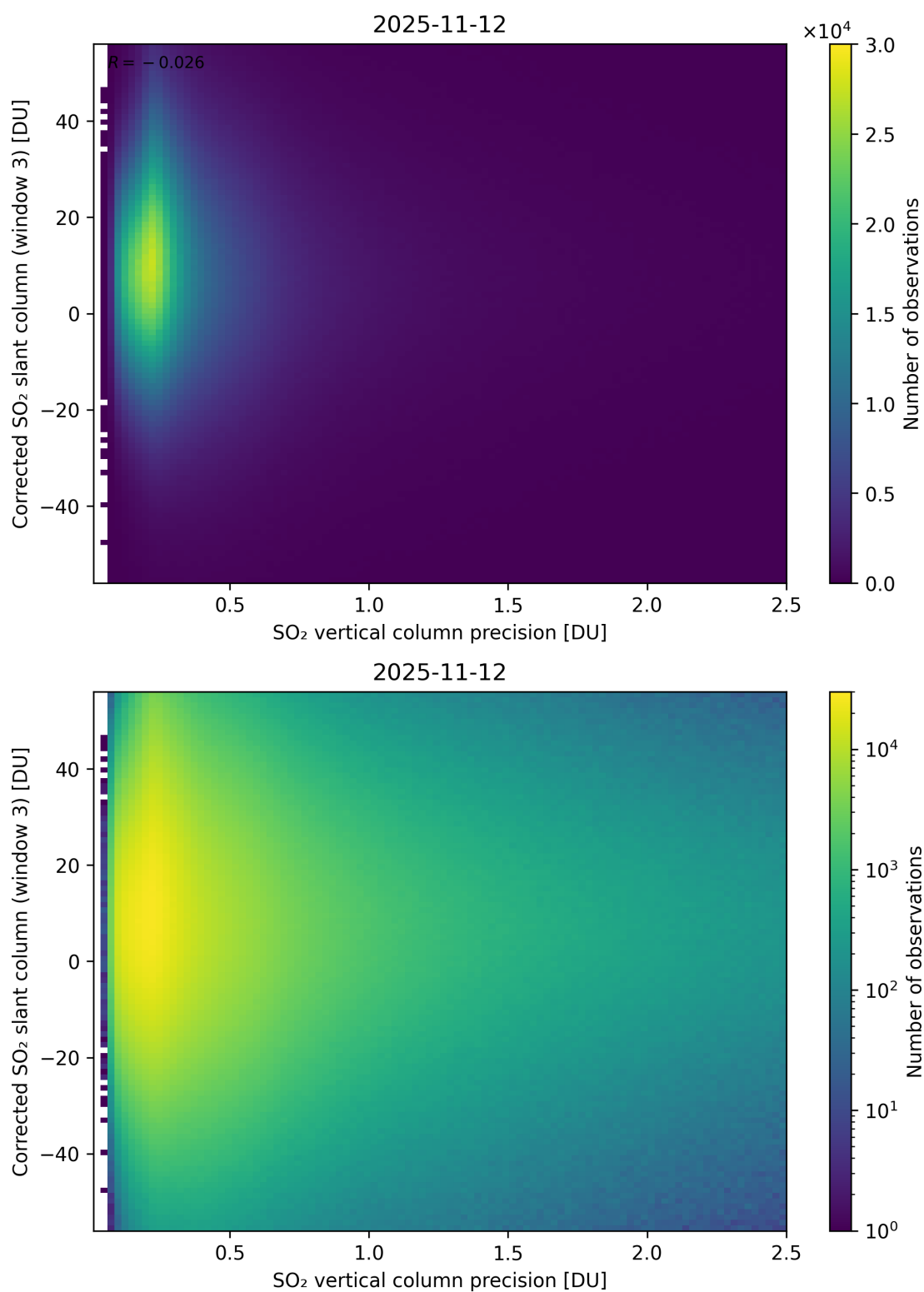
Figure 340: Scatter density plot of “SO 2 vertical column precision” against “Corrected SO 2 slant column (window 3)” for 2025-11-12 to 2025-11-13.
