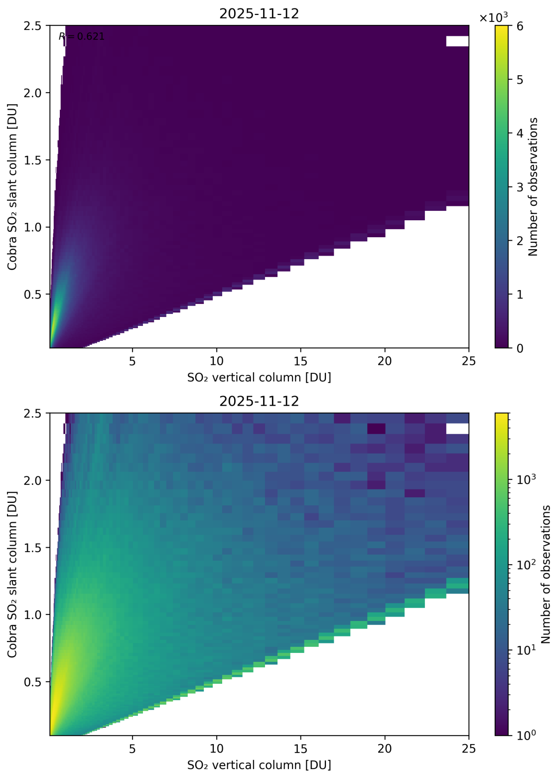
Figure 349: Scatter density plot of “SO 2 vertical column” against “Cobra SO 2 slant column” for 2025-11-12 to 2025-11-13.
