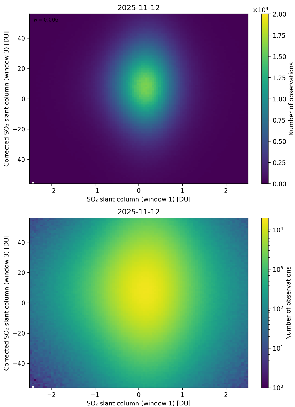
Figure 284: Scatter density plot of “SO 2 slant column (window 1)” against “Corrected SO 2 slant column (window 3)” for 2025-11-12 to 2025-11-13.
