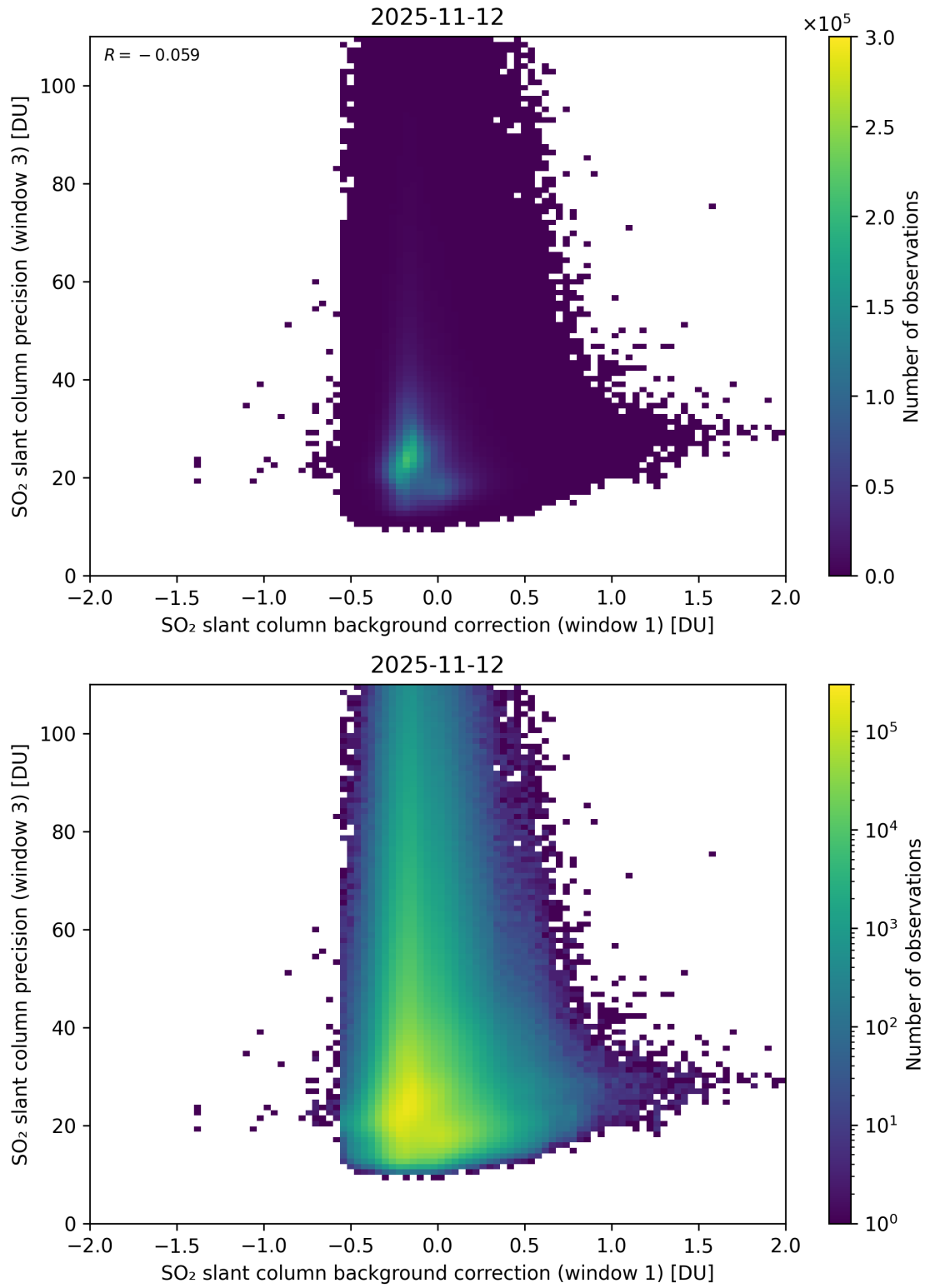
Figure 119: Scatter density plot of “SO 2 slant column background correction (window 1)” against “SO 2 slant column precision (window 3)” for 2025-11-12 to 2025-11-13.
