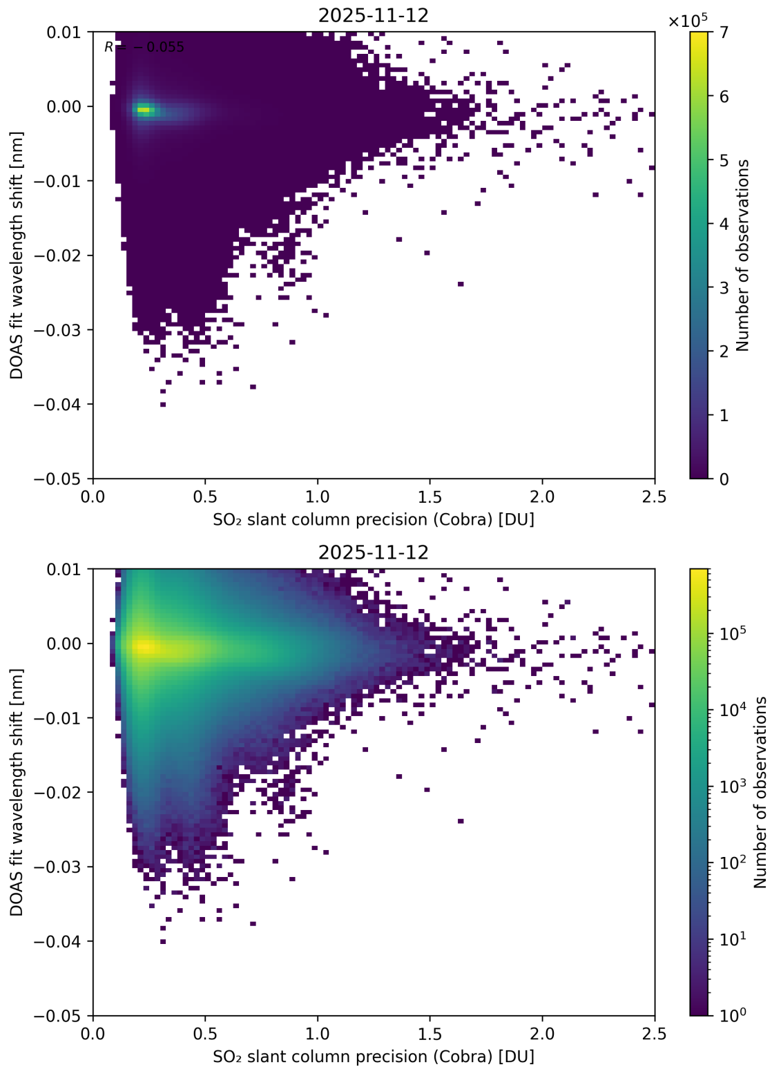
Figure 202: Scatter density plot of “SO 2 slant column precision (Cobra)” against “DOAS fit wavelength shift” for 2025-11-12 to 2025-11-13.
