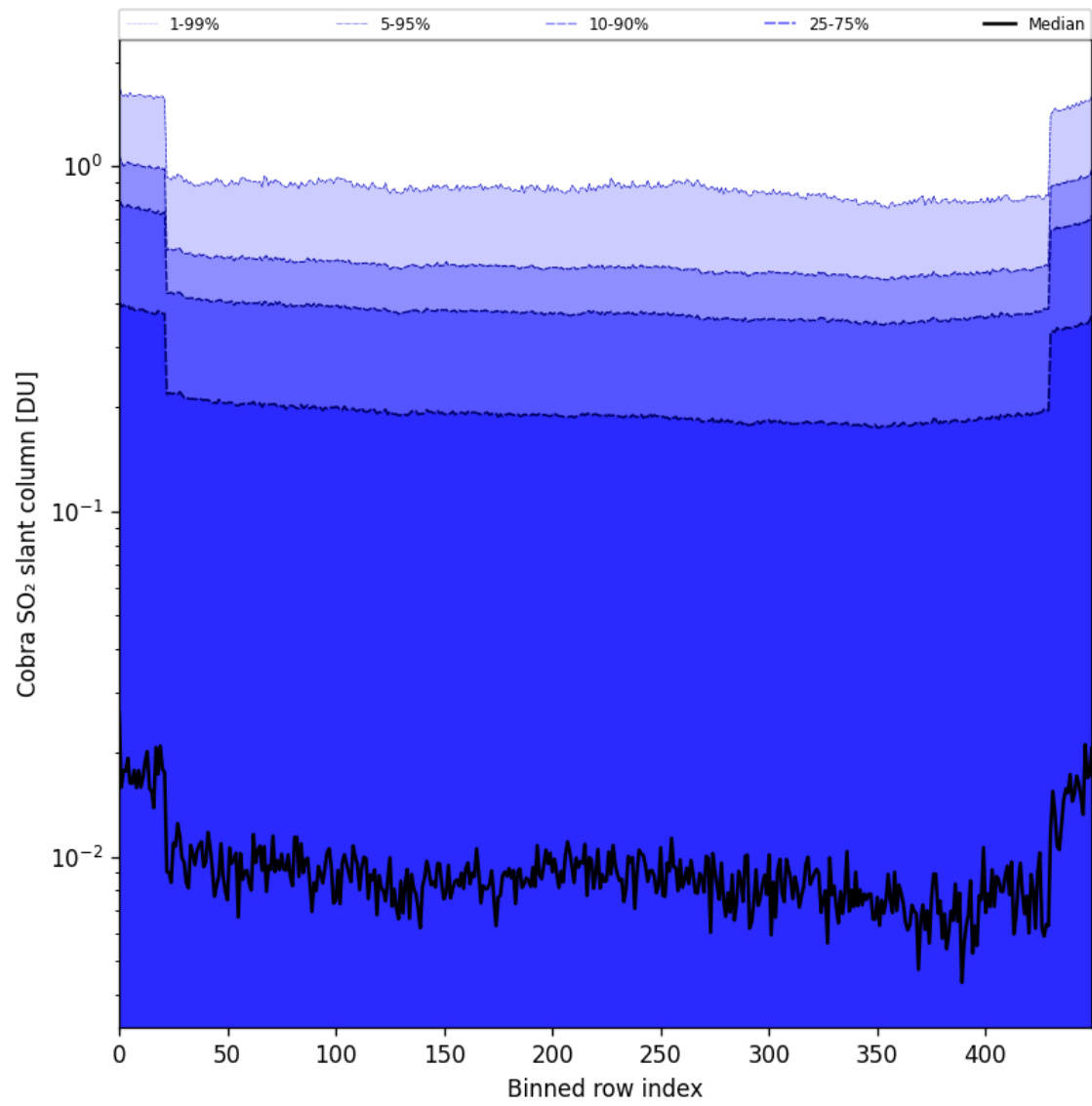
Figure 87: Along track statistics of “Cobra SO 2 slant column” for 2025-11-12 to 2025-11-13
