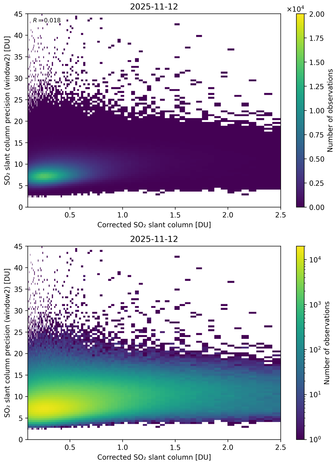
Figure 239: Scatter density plot of “Corrected SO 2 slant column” against “SO 2 slant column precision (window2)” for 2025-11-12 to 2025-11-13.
