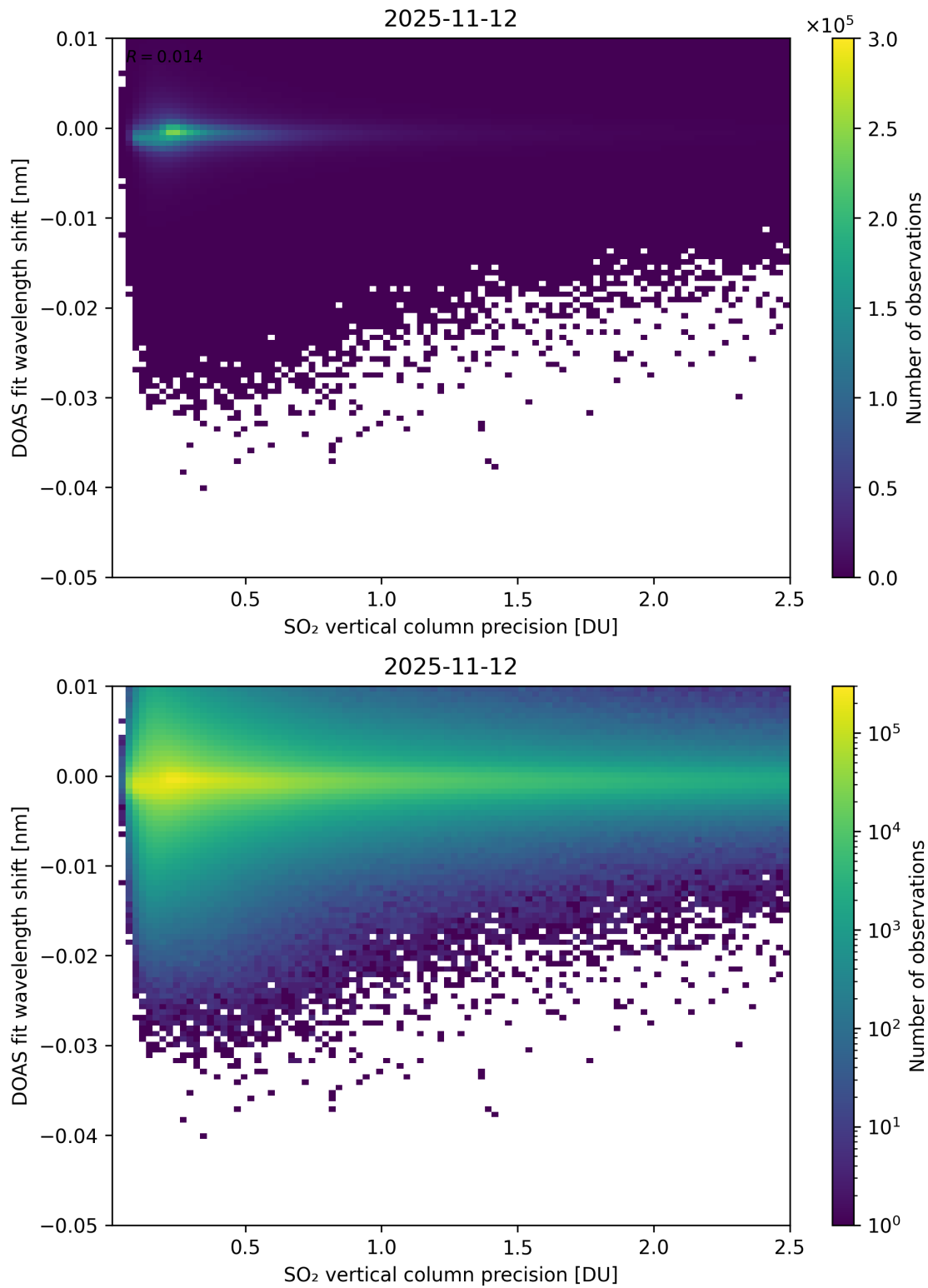
Figure 332: Scatter density plot of “SO 2 vertical column precision” against “DOAS fit wavelength shift” for 2025-11-12 to 2025-11-13.
