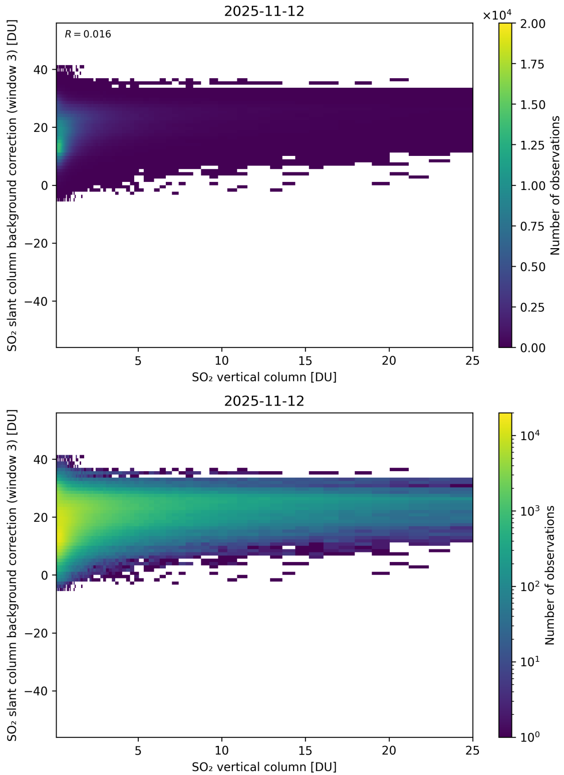
Figure 325: Scatter density plot of “SO 2 vertical column” against “SO 2 slant column background correction (window 3)” for 2025-11-12 to 2025-11-13.
