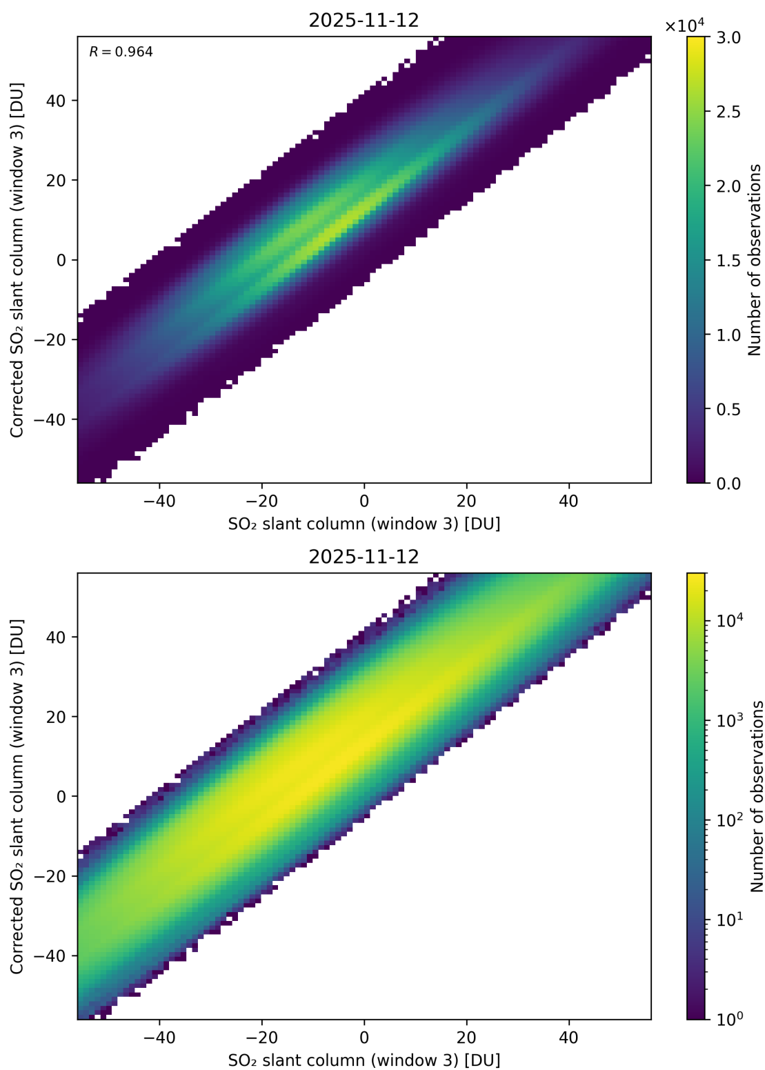
Figure 316: Scatter density plot of “SO 2 slant column (window 3)” against “Corrected SO 2 slant column (window 3)” for 2025-11-12 to 2025-11-13.
