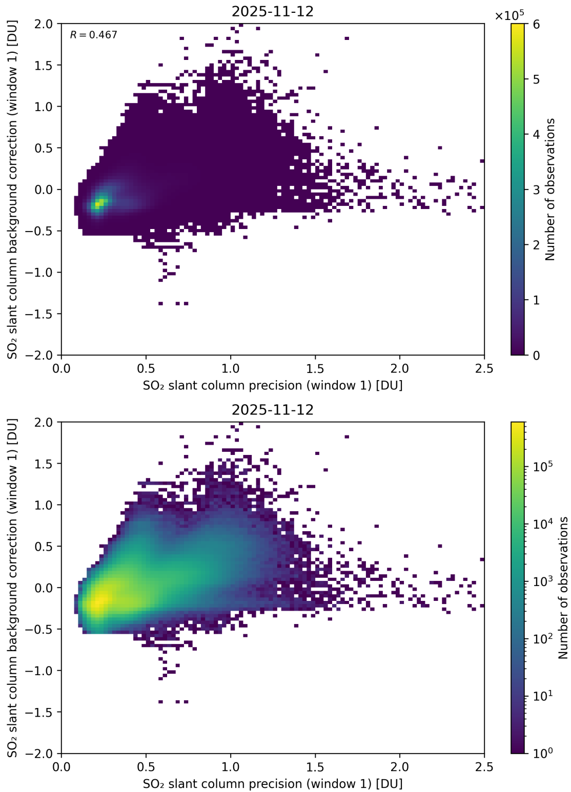
Figure 268: Scatter density plot of “SO 2 slant column precision (window 1)” against “SO 2 slant column background correction (window 1)” for 2025-11-12 to 2025-11-13.
