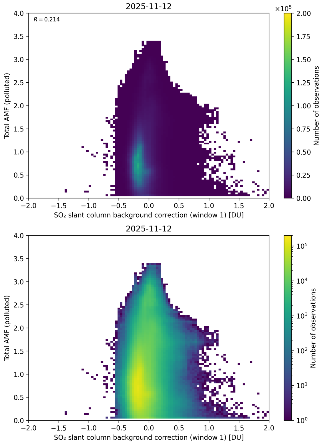
Figure 120: Scatter density plot of “SO 2 slant column background correction (window 1)” against “Total AMF (polluted)” for 2025-11-12 to 2025-11-13.
