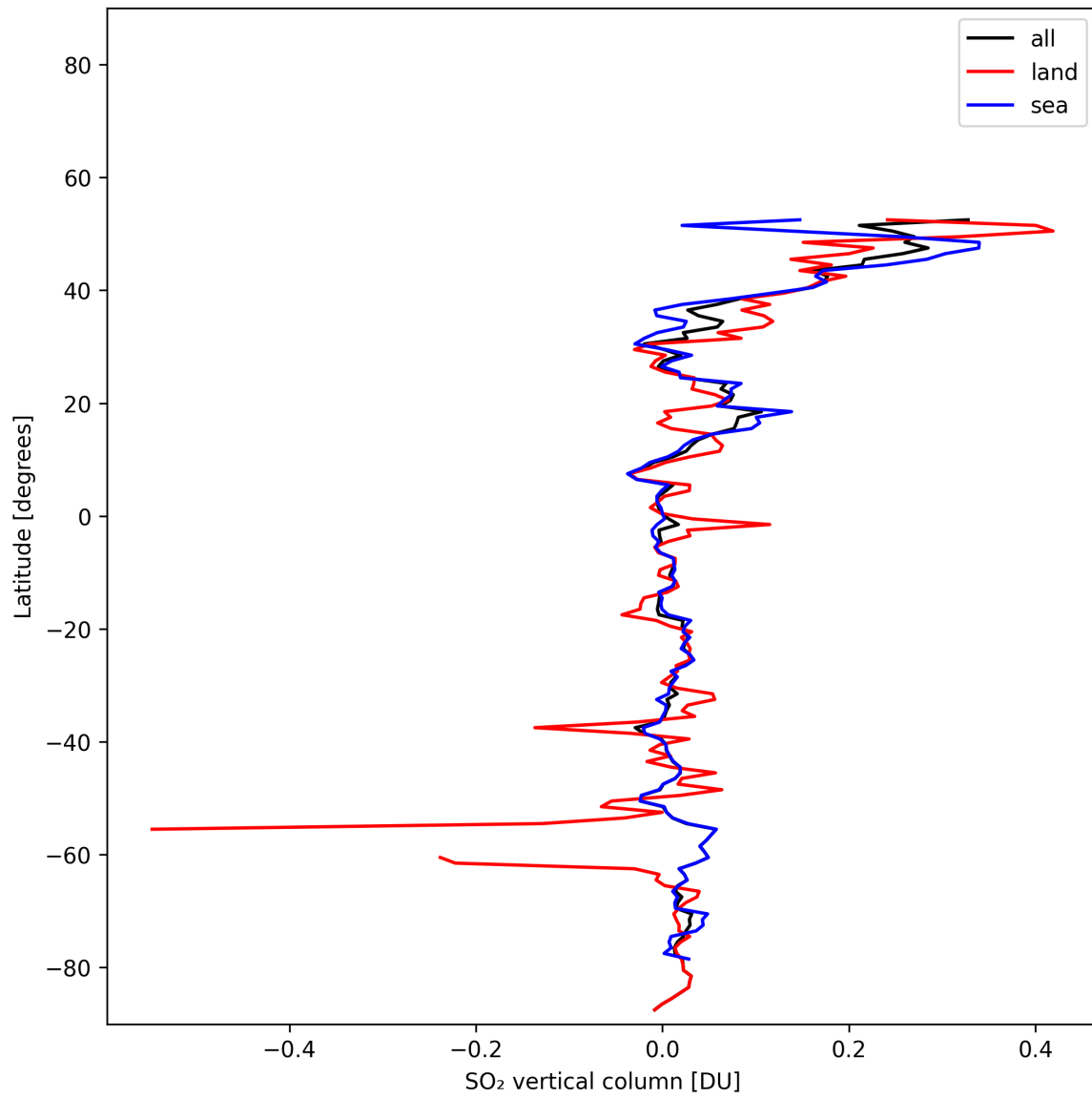
Figure 32: Zonal average of “SO 2 vertical column” for 2025-11-12 to 2025-11-13.
