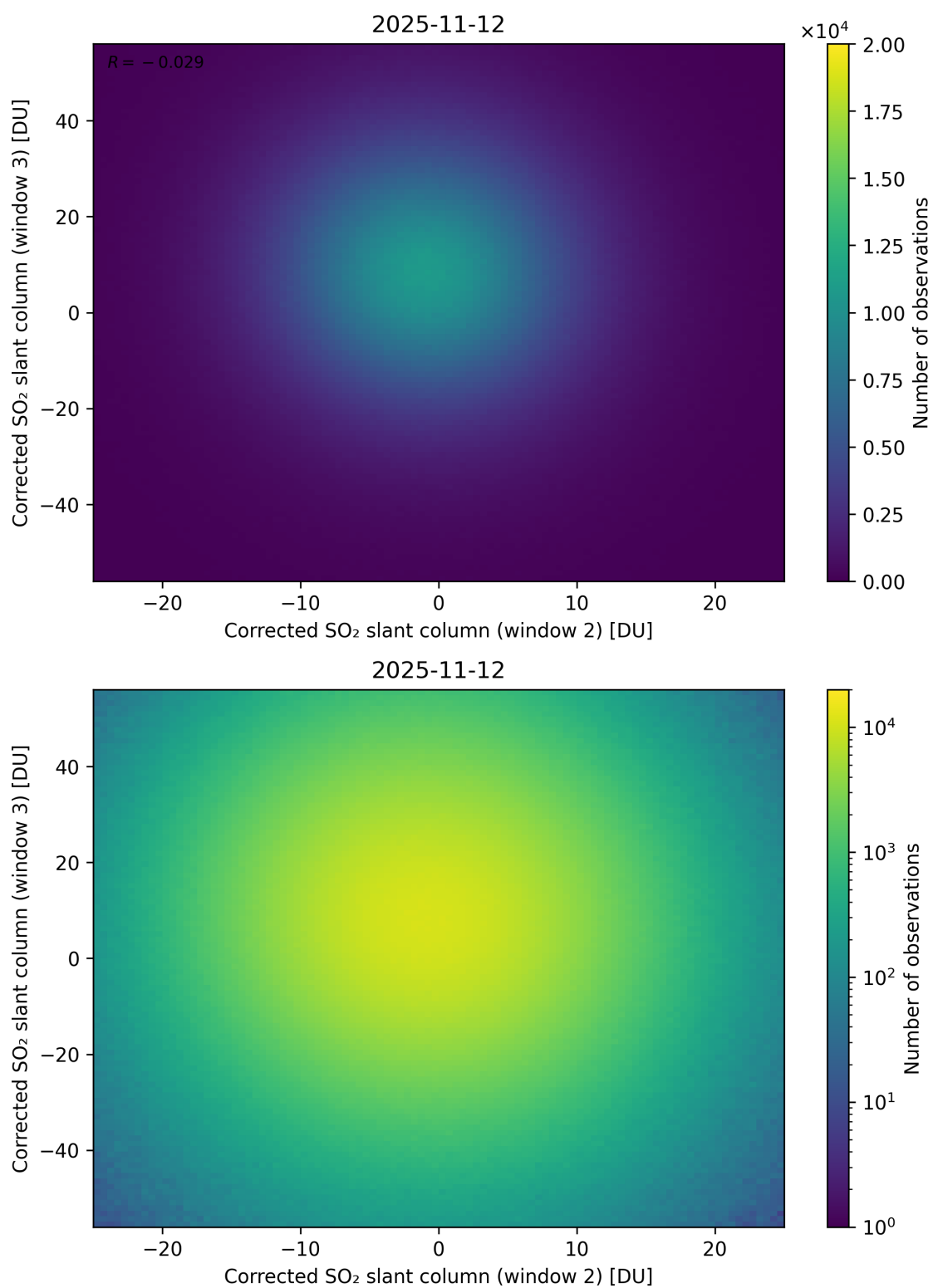
Figure 250: Scatter density plot of “Corrected SO 2 slant column (window 2)” against “Corrected SO 2 slant column (window 3)” for 2025-11-12 to 2025-11-13.
