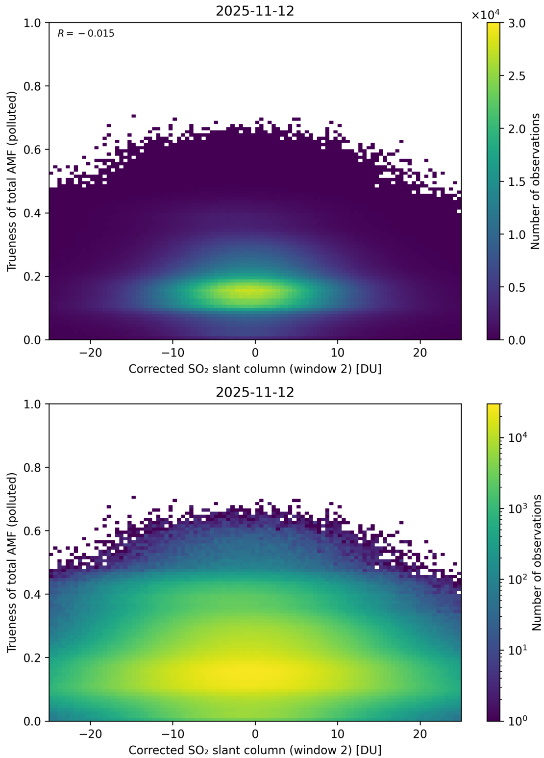
Figure 254: Scatter density plot of “Corrected SO 2 slant column (window 2)” against “Trueness of total AMF (polluted)” for 2025-11-12 to 2025-11-13.
