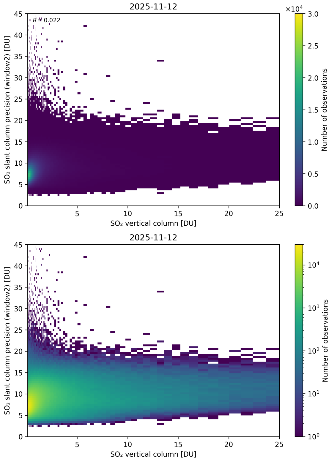
Figure 356: Scatter density plot of “SO 2 vertical column” against “SO 2 slant column precision (window2)” for 2025-11-12 to 2025-11-13.
