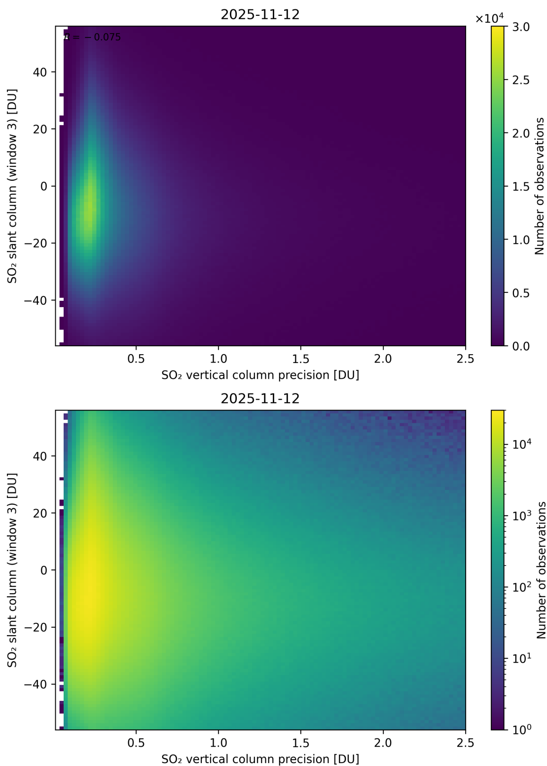
Figure 344: Scatter density plot of “SO 2 vertical column precision” against “SO 2 slant column (window 3)” for 2025-11-12 to 2025-11-13.
