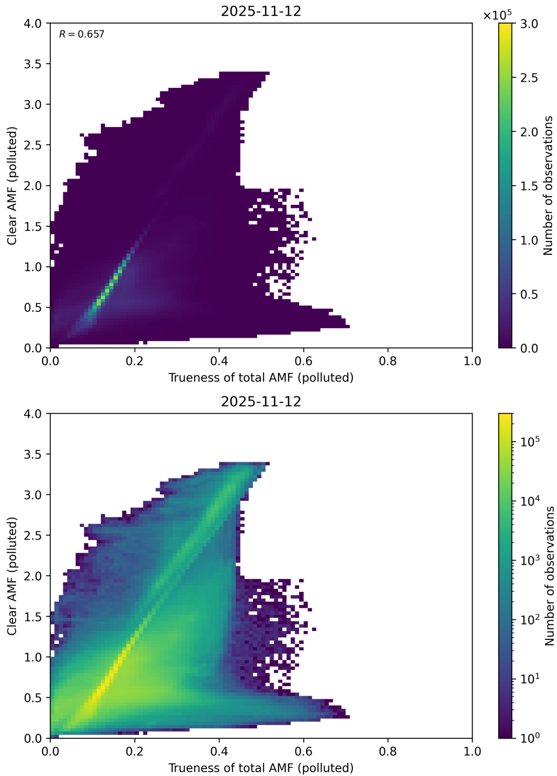
Figure 322: Scatter density plot of “Trueness of total AMF (polluted)” against “Clear AMF (polluted)” for 2025-11-12 to 2025-11-13.
