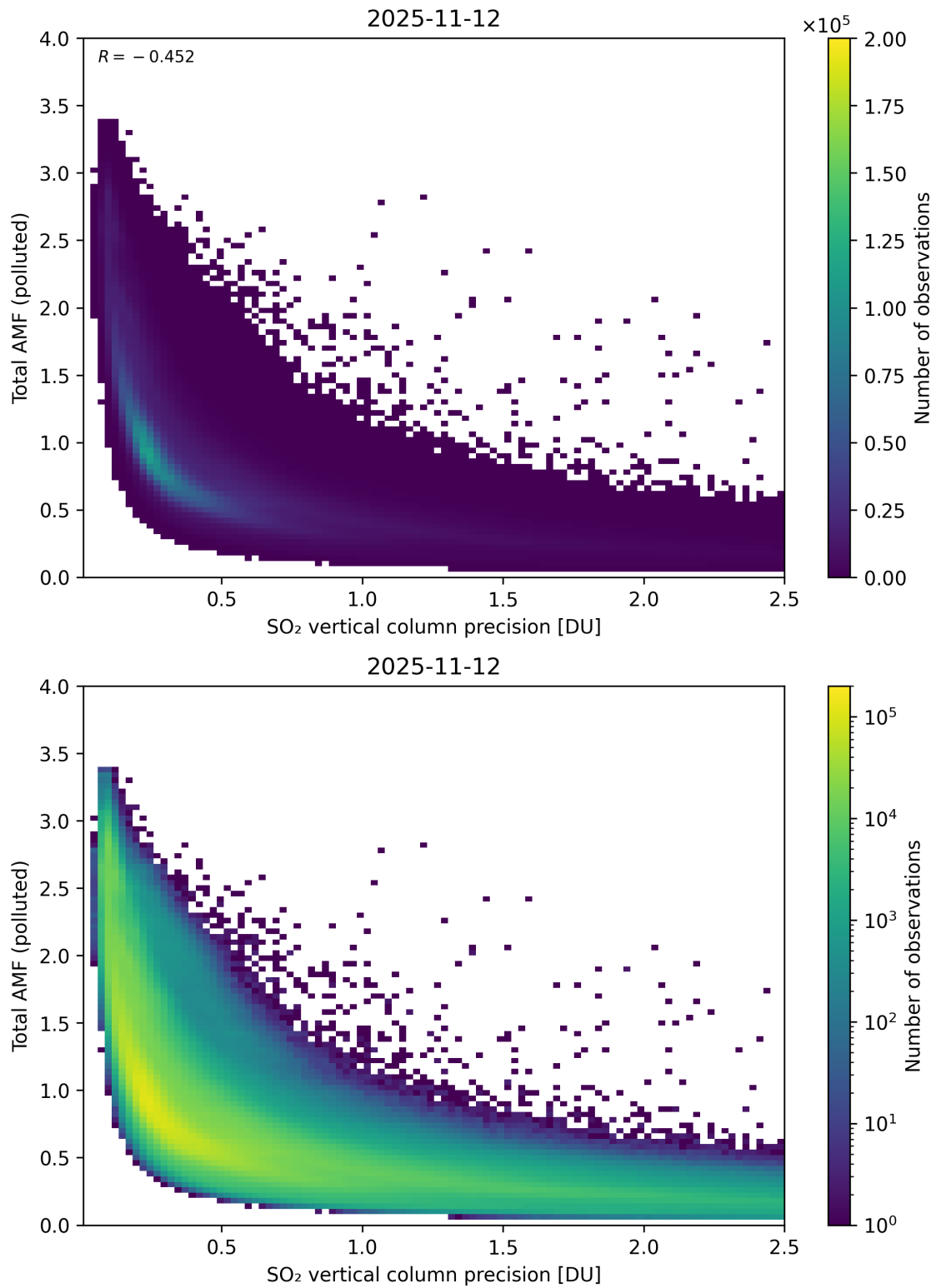
Figure 346: Scatter density plot of “SO 2 vertical column precision” against “Total AMF (polluted)” for 2025-11-12 to 2025-11-13.
