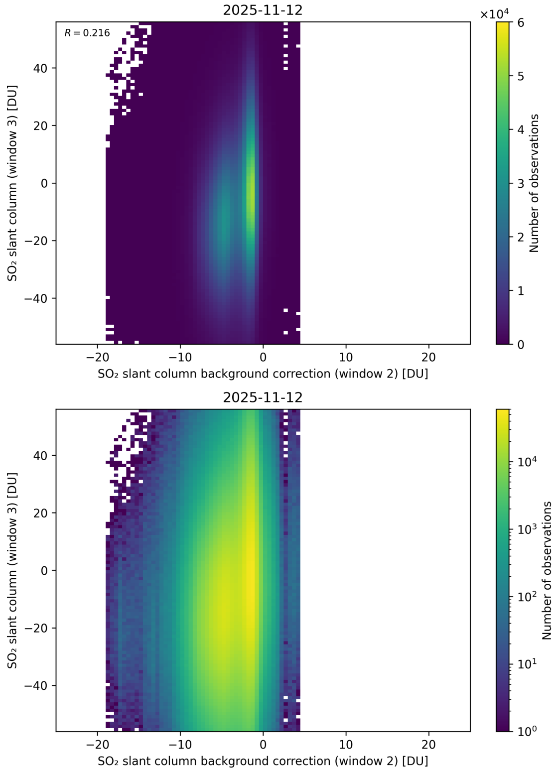
Figure 128: Scatter density plot of “SO 2 slant column background correction (window 2)” against “SO 2 slant column (window 3)” for 2025-11-12 to 2025-11-13.
