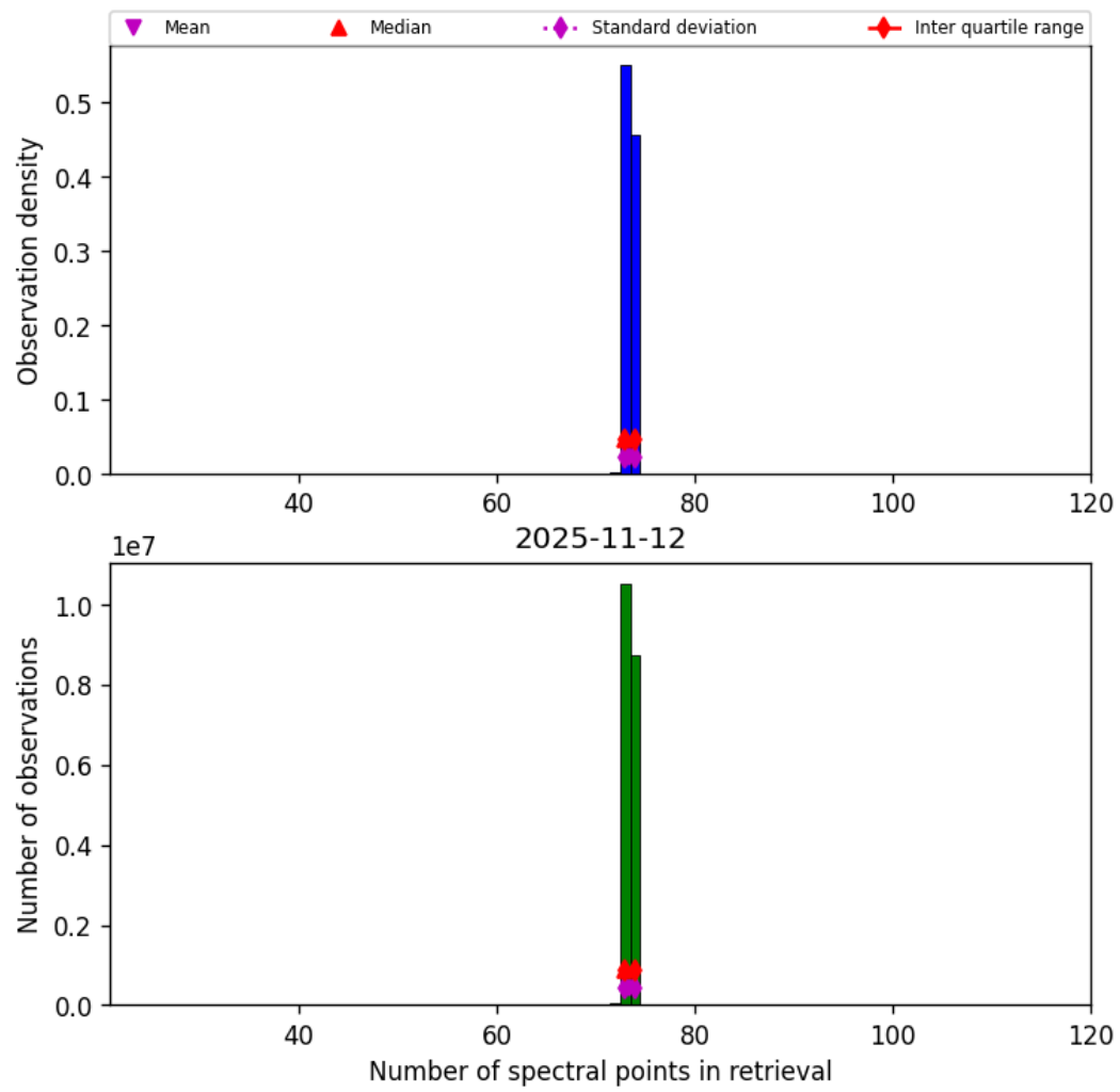
Figure 82: Histogram of “Number of spectral points in retrieval” for 2025-11-12 to 2025-11-13
