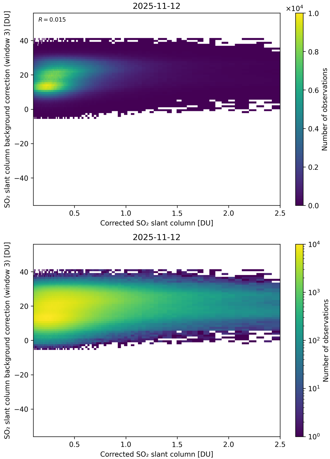
Figure 228: Scatter density plot of “Corrected SO 2 slant column” against “SO 2 slant column background correction (window 3)” for 2025-11-12 to 2025-11-13.
