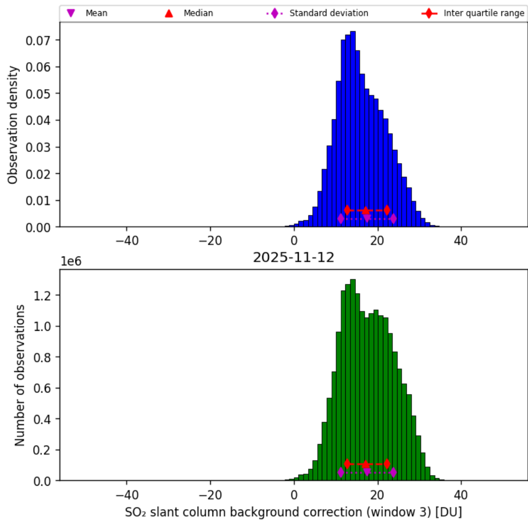
Figure 74: Histogram of “SO 2 slant column background correction (window 3)” for 2025-11-12 to 2025-11-13
