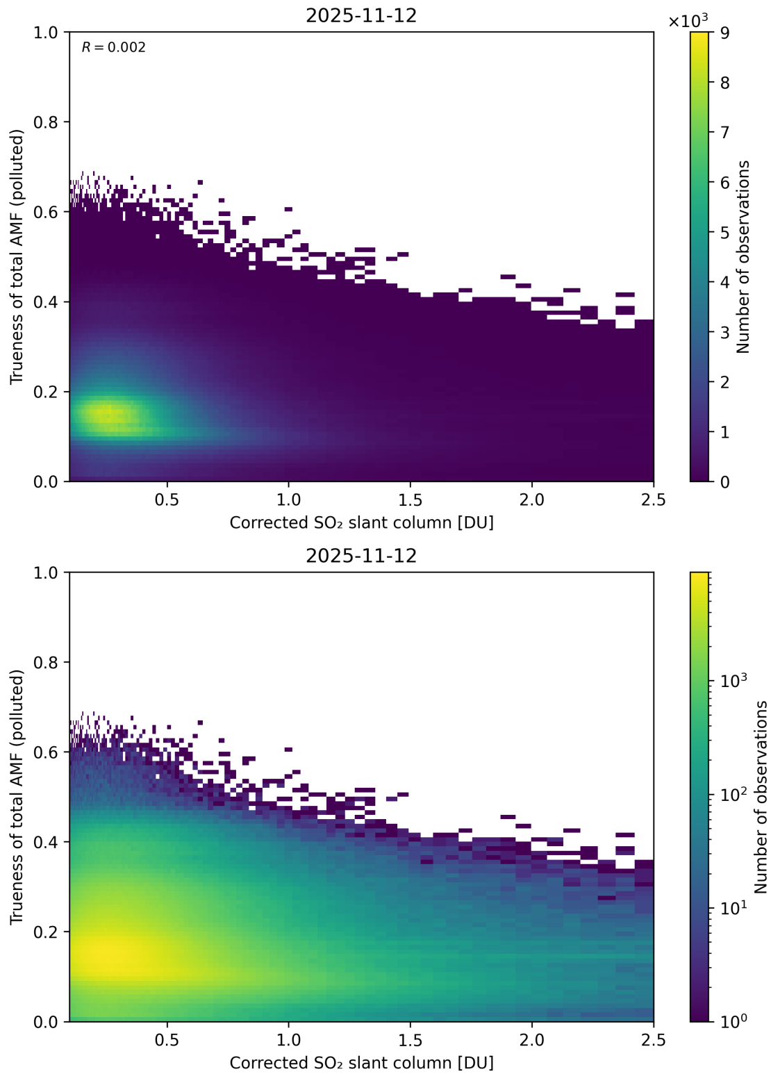
Figure 243: Scatter density plot of “Corrected SO 2 slant column” against “Trueness of total AMF (polluted)” for 2025-11-12 to 2025-11-13.
