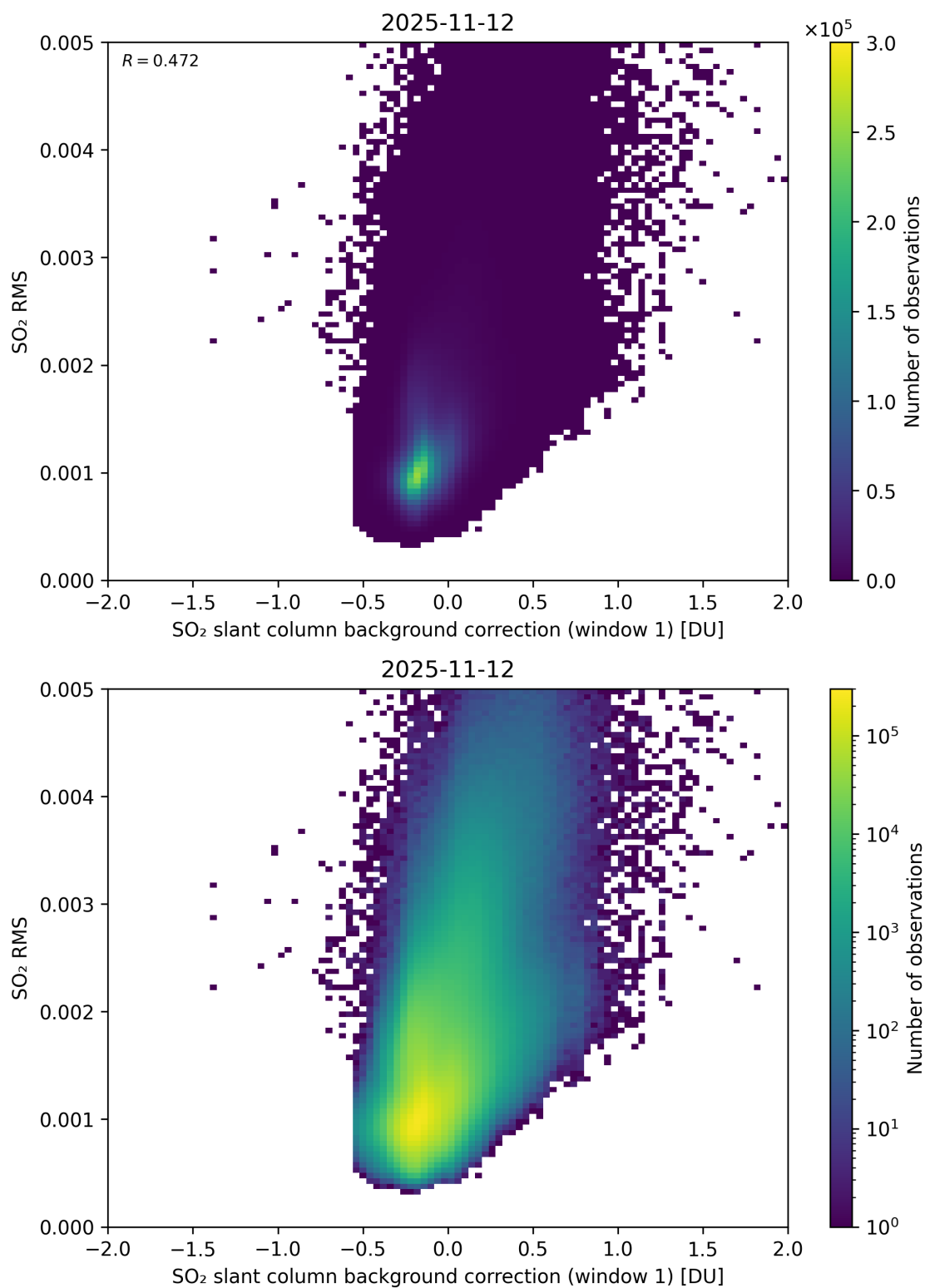
Figure 113: Scatter density plot of “SO 2 slant column background correction (window 1)” against “SO 2 RMS” for 2025-11-12 to 2025-11-13.
