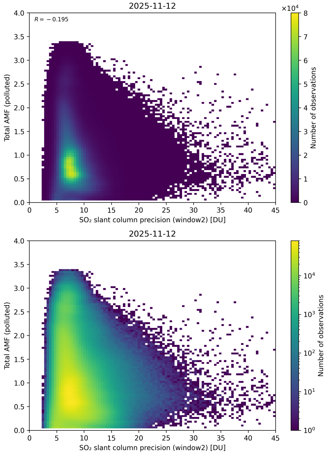
Figure 301: Scatter density plot of “SO 2 slant column precision (window2)” against “Total AMF (polluted)” for 2025-11-12 to 2025-11-13.
