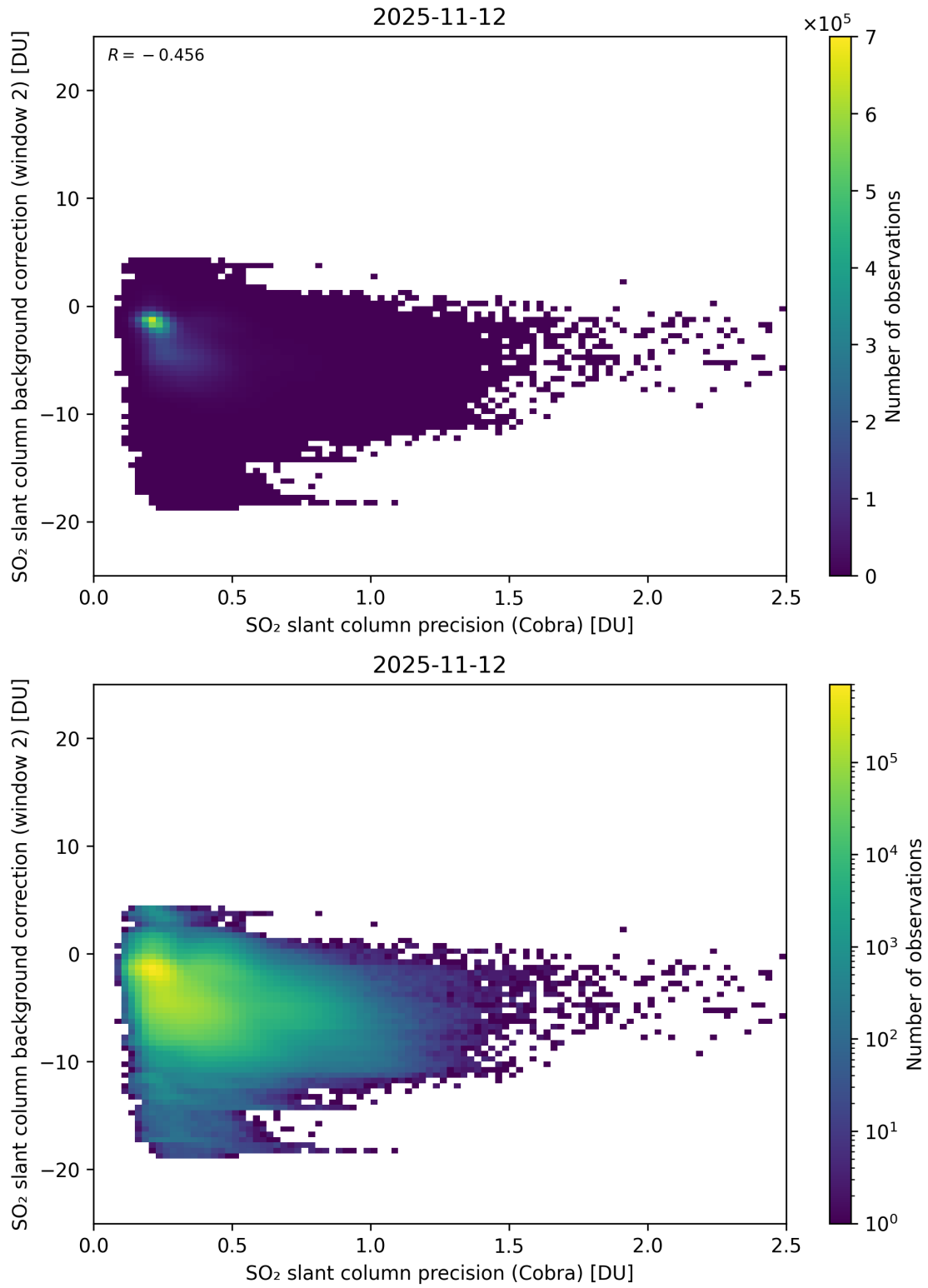
Figure 200: Scatter density plot of “SO 2 slant column precision (Cobra)” against “SO 2 slant column background correction (window 2)” for 2025-11-12 to 2025-11-13.
