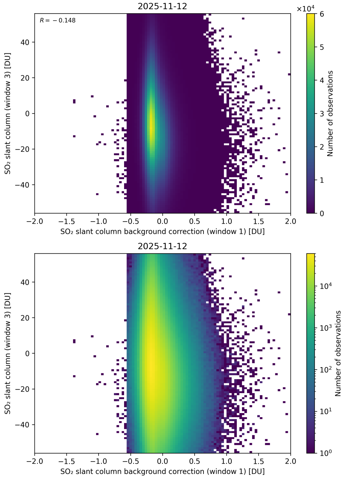
Figure 118: Scatter density plot of “SO 2 slant column background correction (window 1)” against “SO 2 slant column (window 3)” for 2025-11-12 to 2025-11-13.
