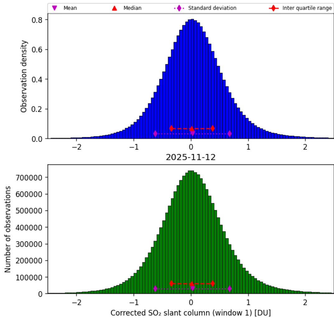
Figure 65: Histogram of “Corrected SO 2 slant column (window 1)” for 2025-11-12 to 2025-11-13
