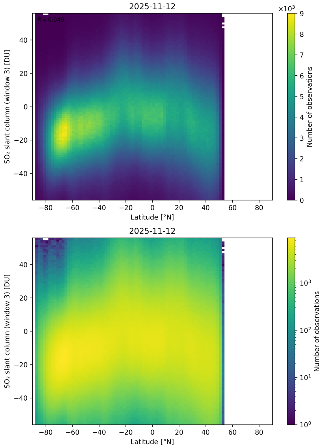
Figure 165: Scatter density plot of “Latitude” against “SO 2 slant column (window 3)” for 2025-11-12 to 2025-11-13.
