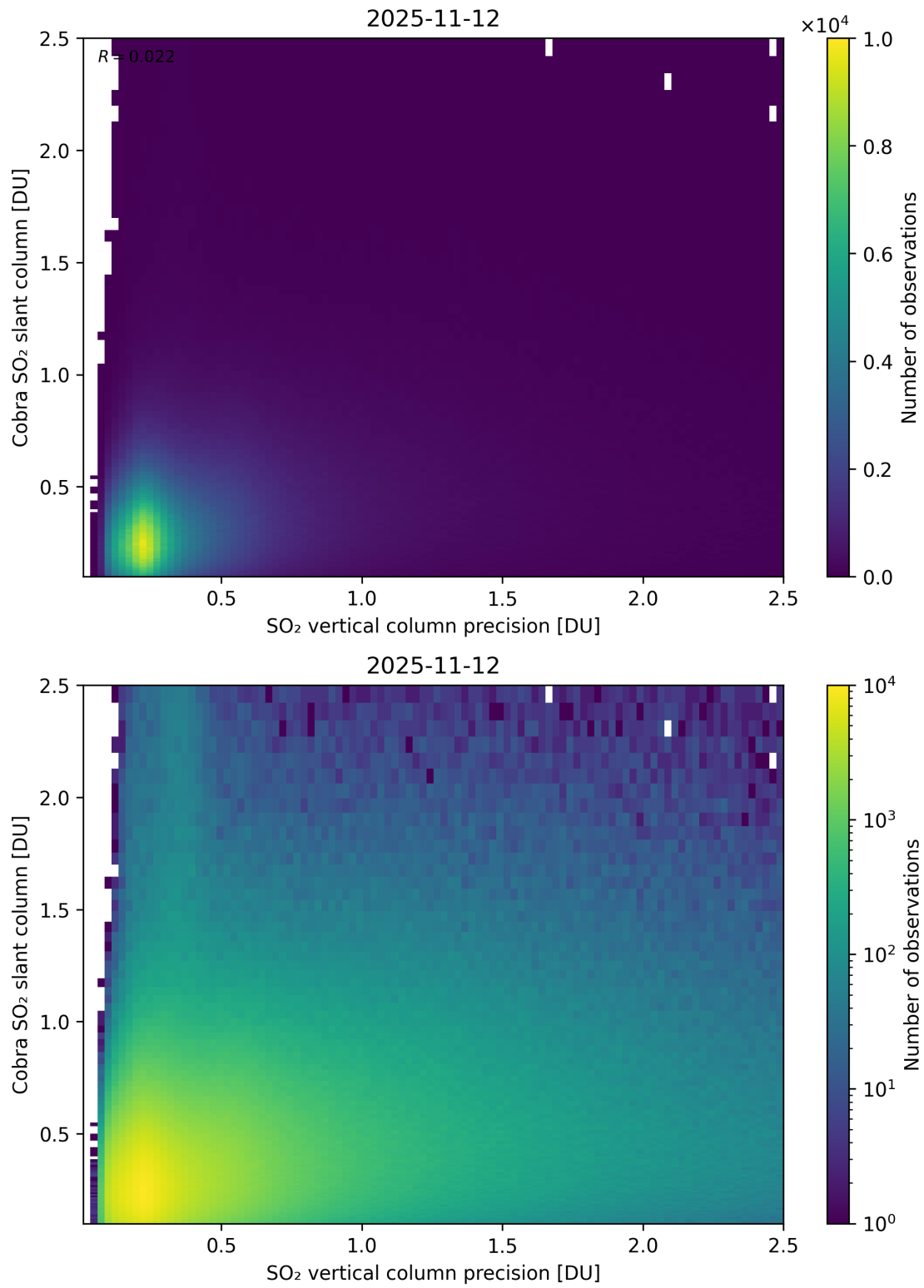
Figure 336: Scatter density plot of “SO 2 vertical column precision” against “Cobra SO 2 slant column” for 2025-11-12 to 2025-11-13.
