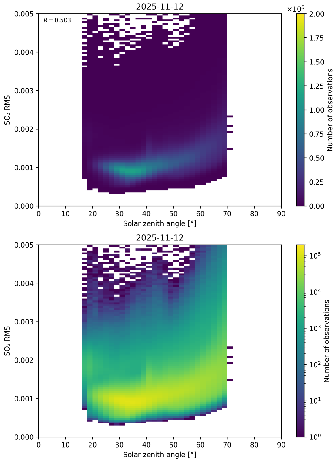
Figure 176: Scatter density plot of “Solar zenith angle” against “SO 2 RMS” for 2025-11-12 to 2025-11-13.
