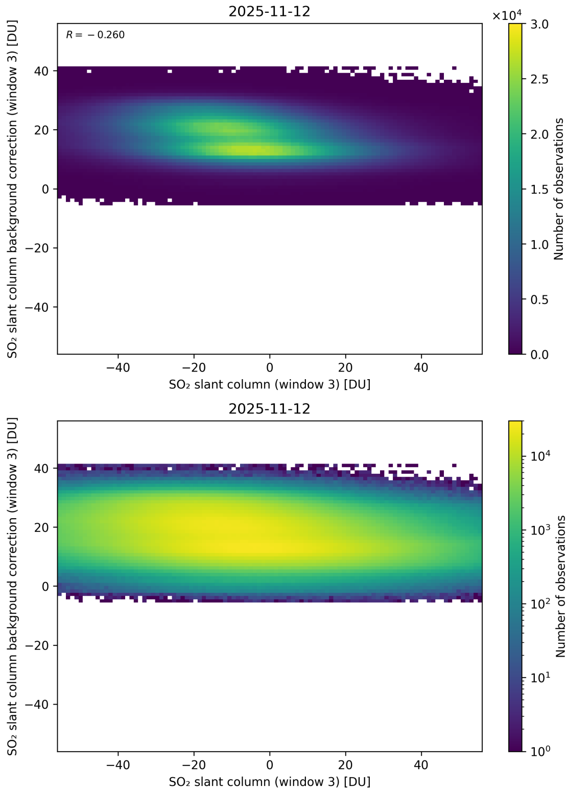
Figure 303: Scatter density plot of “SO 2 slant column (window 3)” against “SO 2 slant column background correction (window 3)” for 2025-11-12 to 2025-11-13.
