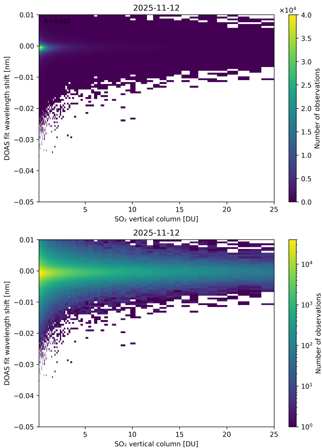
Figure 326: Scatter density plot of “SO 2 vertical column” against “DOAS fit wavelength shift” for 2025-11-12 to 2025-11-13.
