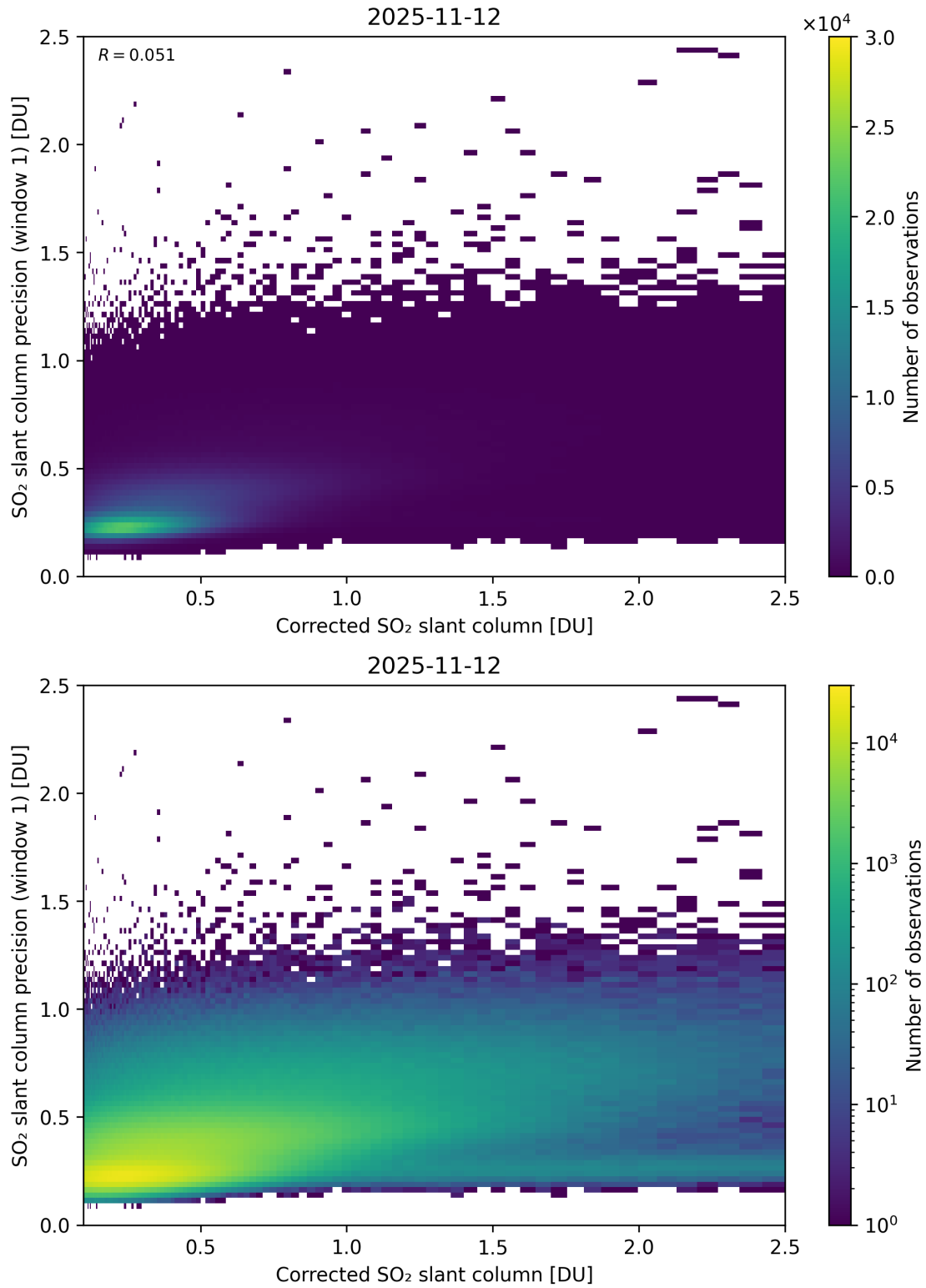
Figure 238: Scatter density plot of “Corrected SO 2 slant column” against “SO 2 slant column precision (window 1)” for 2025-11-12 to 2025-11-13.
