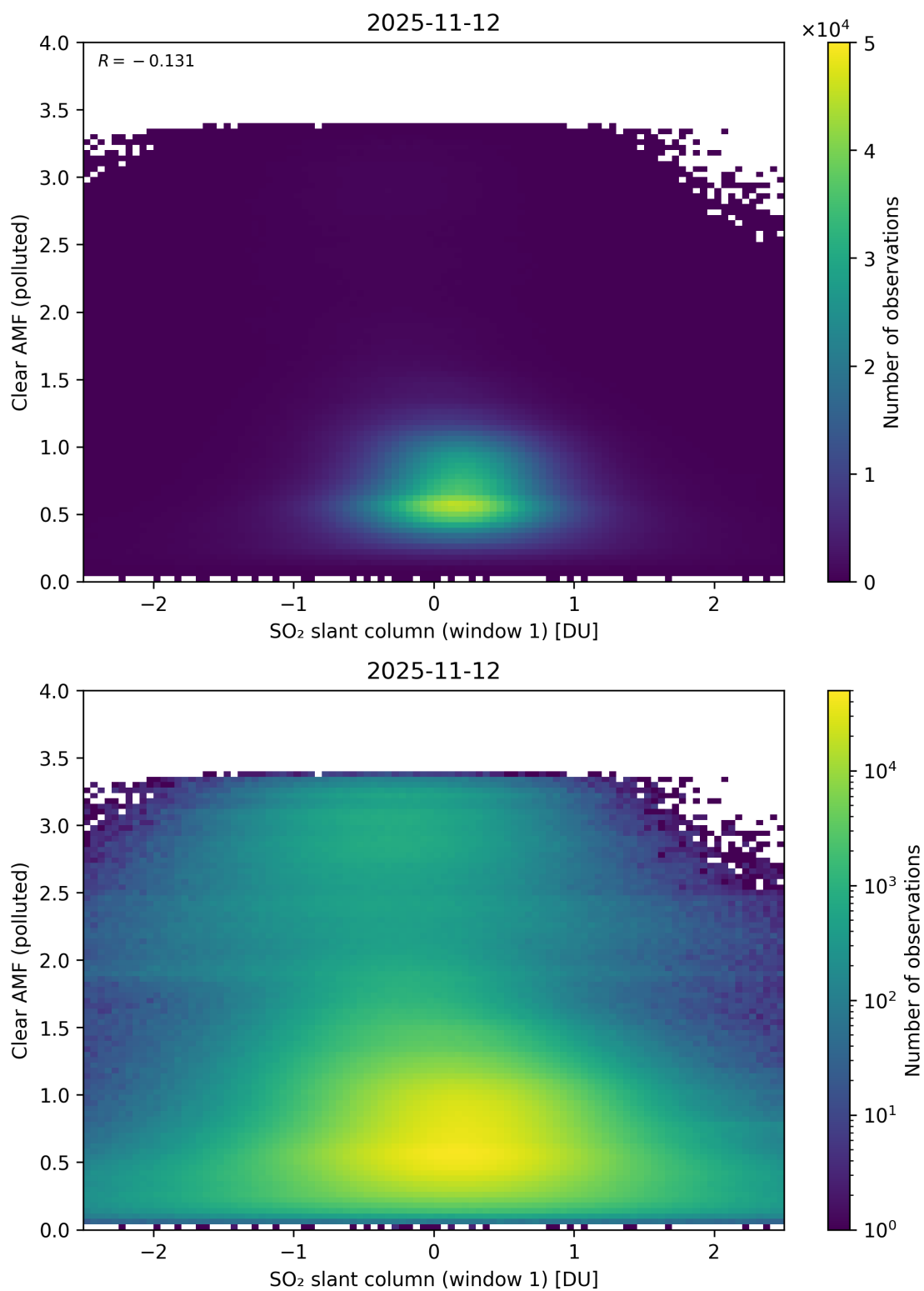
Figure 282: Scatter density plot of “SO 2 slant column (window 1)” against “Clear AMF (polluted)” for 2025-11-12 to 2025-11-13.
