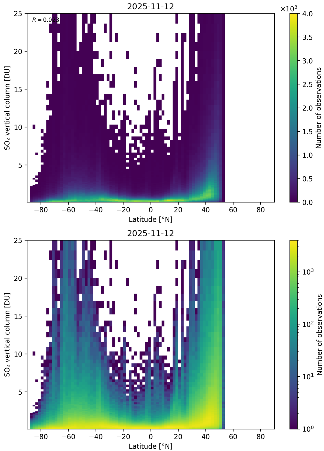
Figure 169: Scatter density plot of “Latitude” against “SO 2 vertical column” for 2025-11-12 to 2025-11-13.
