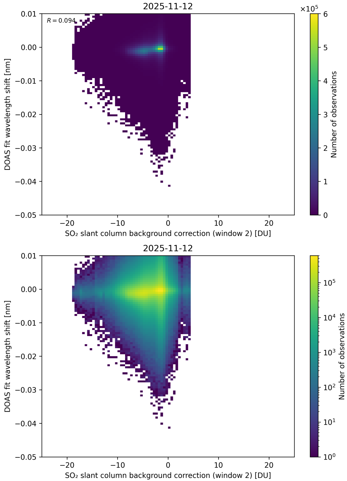
Figure 123: Scatter density plot of “SO 2 slant column background correction (window 2)” against “DOAS fit wavelength shift” for 2025-11-12 to 2025-11-13.
