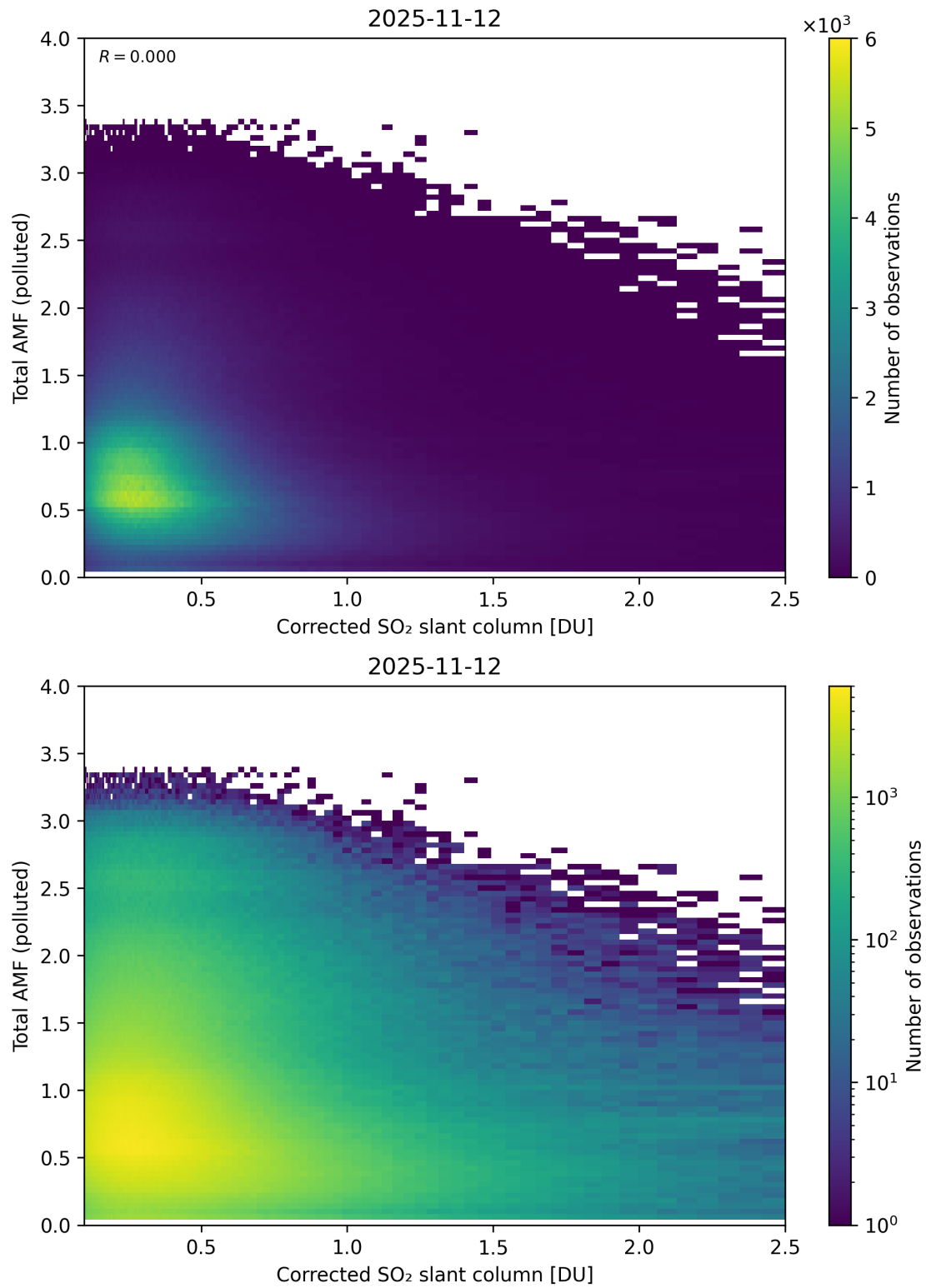
Figure 242: Scatter density plot of “Corrected SO 2 slant column” against “Total AMF (polluted)” for 2025-11-12 to 2025-11-13.
