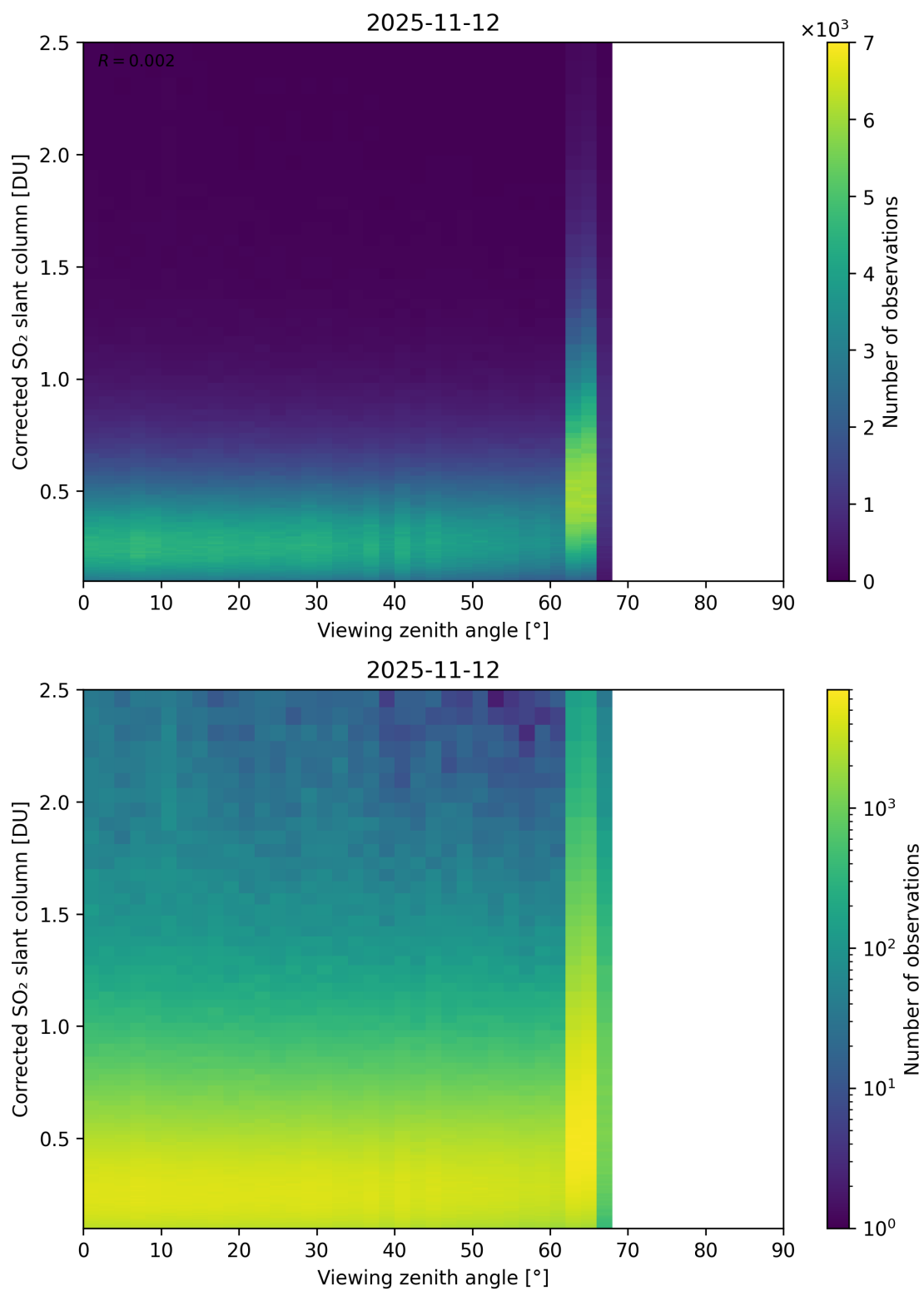
Figure 373: Scatter density plot of “Viewing zenith angle” against “Corrected SO 2 slant column” for 2025-11-12 to 2025-11-13.
