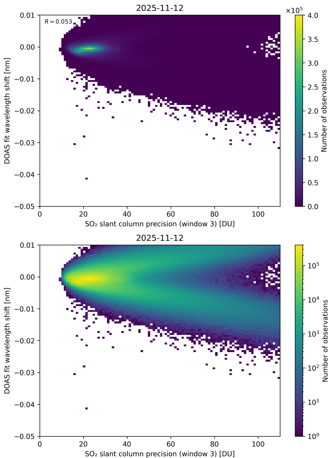
Figure 308: Scatter density plot of “SO 2 slant column precision (window 3)” against “DOAS fit wavelength shift” for 2025-11-12 to 2025-11-13.
