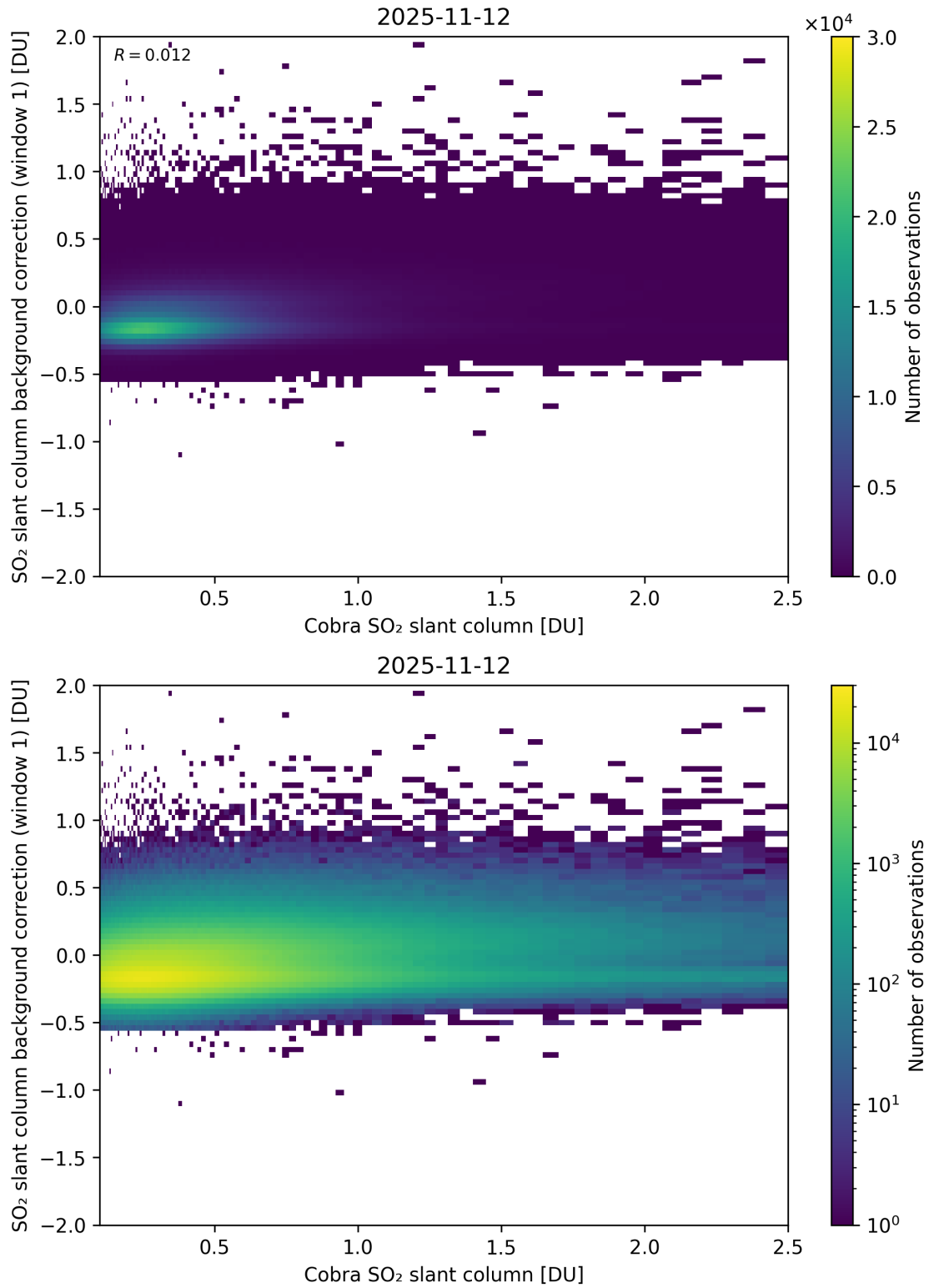
Figure 193: Scatter density plot of “Cobra SO 2 slant column” against “SO 2 slant column background correction (window 1)” for 2025-11-12 to 2025-11-13.
