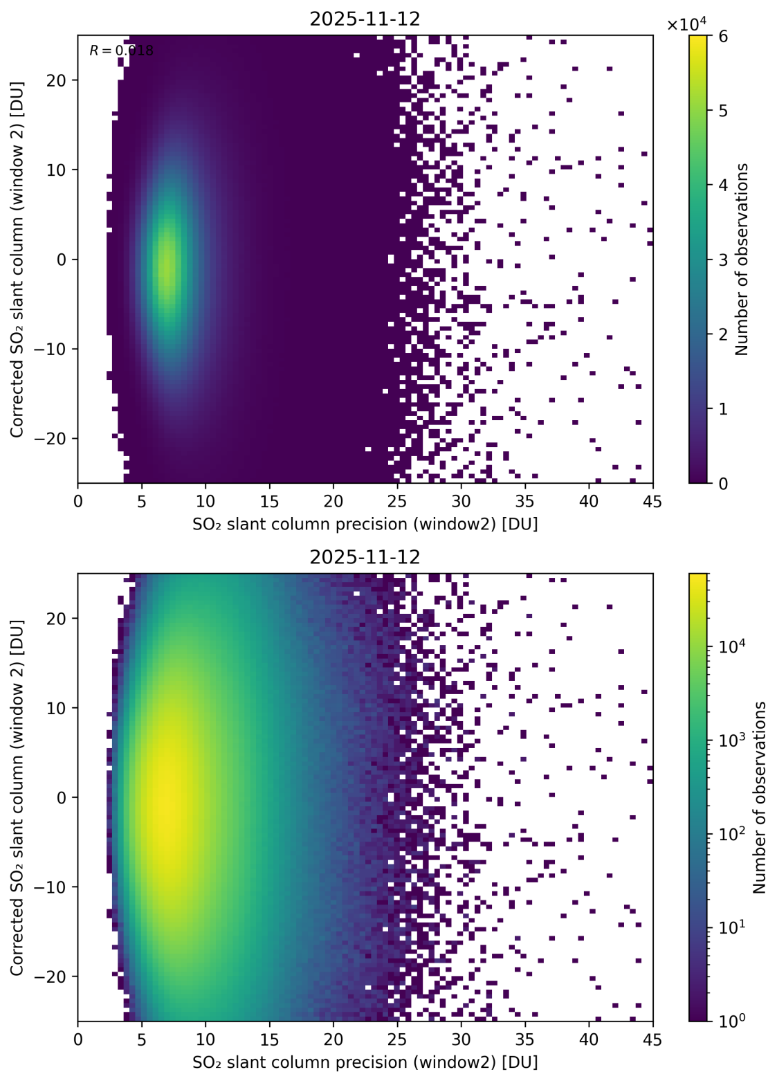
Figure 297: Scatter density plot of “SO 2 slant column precision (window2)” against “Corrected SO 2 slant column (window 2)” for 2025-11-12 to 2025-11-13.
