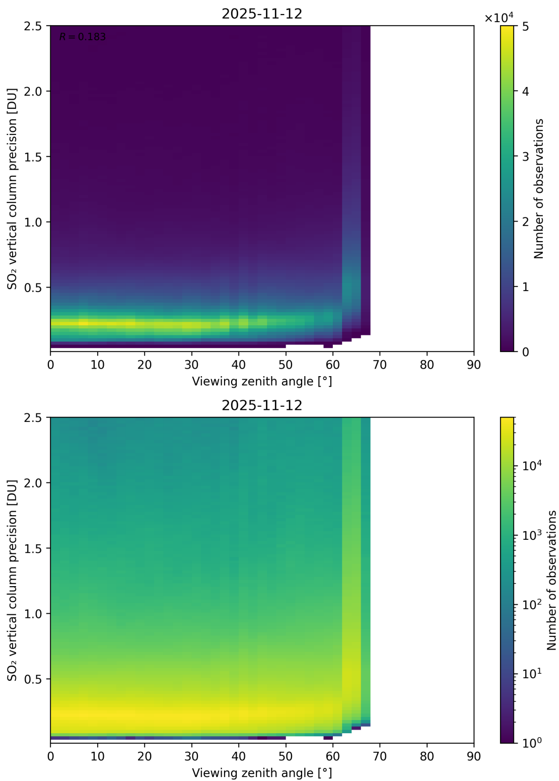
Figure 384: Scatter density plot of “Viewing zenith angle” against “SO 2 vertical column precision” for 2025-11-12 to 2025-11-13.
