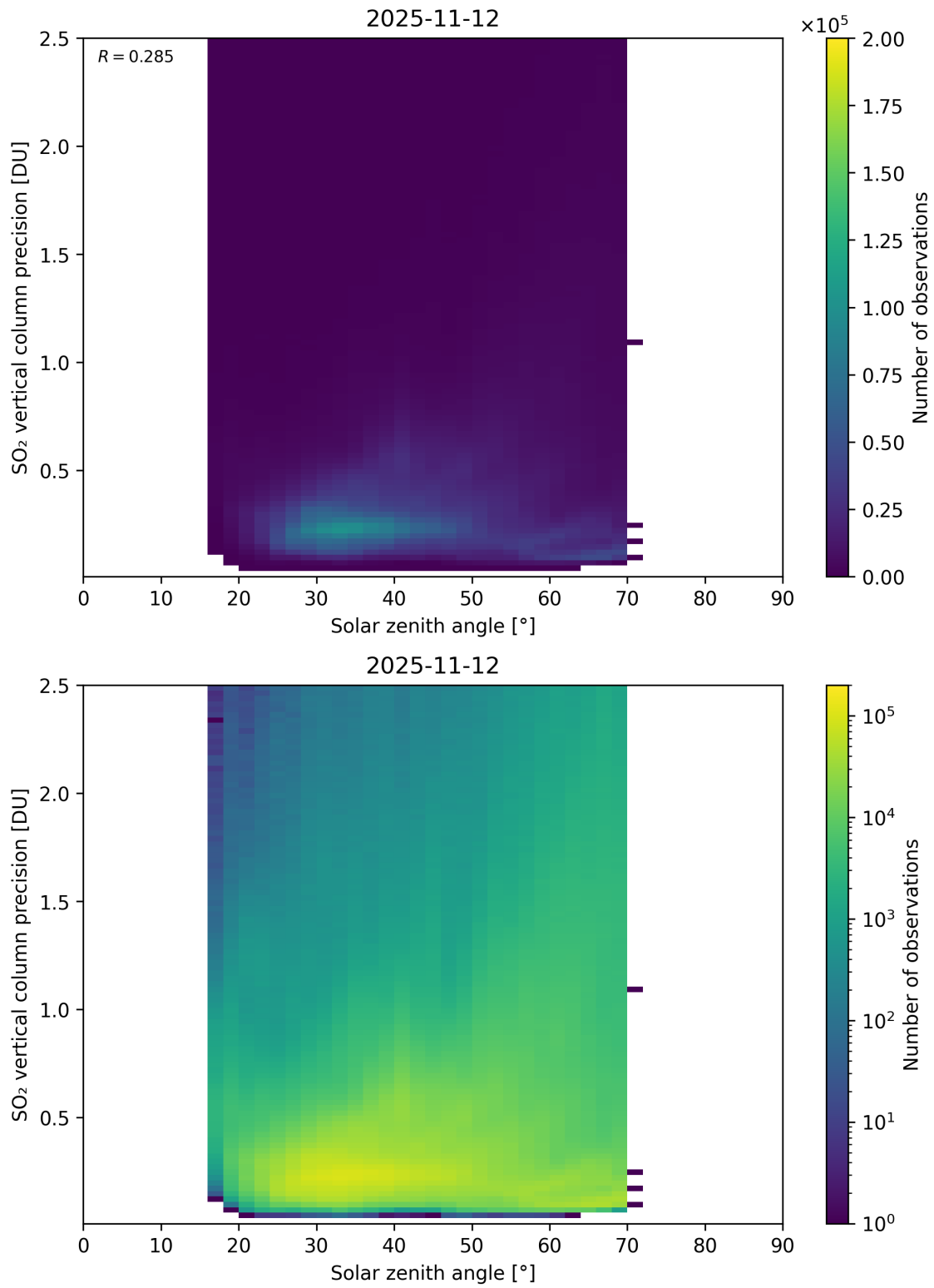
Figure 192: Scatter density plot of “Solar zenith angle” against “SO 2 vertical column precision” for 2025-11-12 to 2025-11-13.
