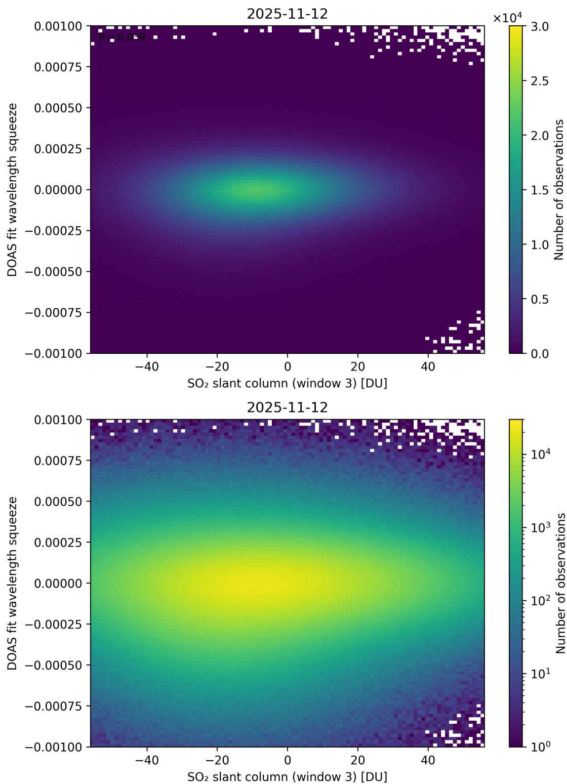
Figure 305: Scatter density plot of “SO 2 slant column (window 3)” against “DOAS fit wavelength squeeze” for 2025-11-12 to 2025-11-13.
