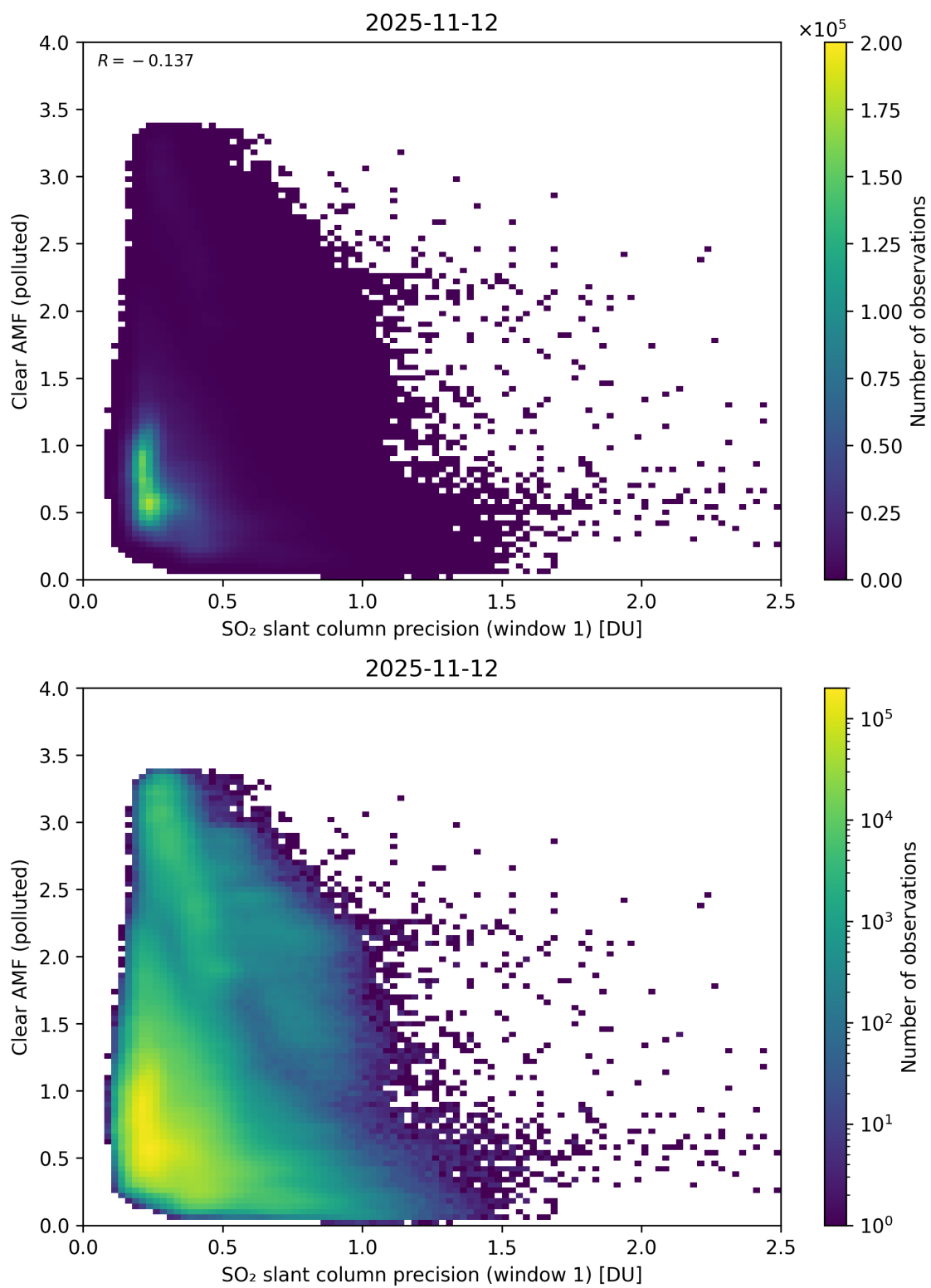
Figure 274: Scatter density plot of “SO 2 slant column precision (window 1)” against “Clear AMF (polluted)” for 2025-11-12 to 2025-11-13.
