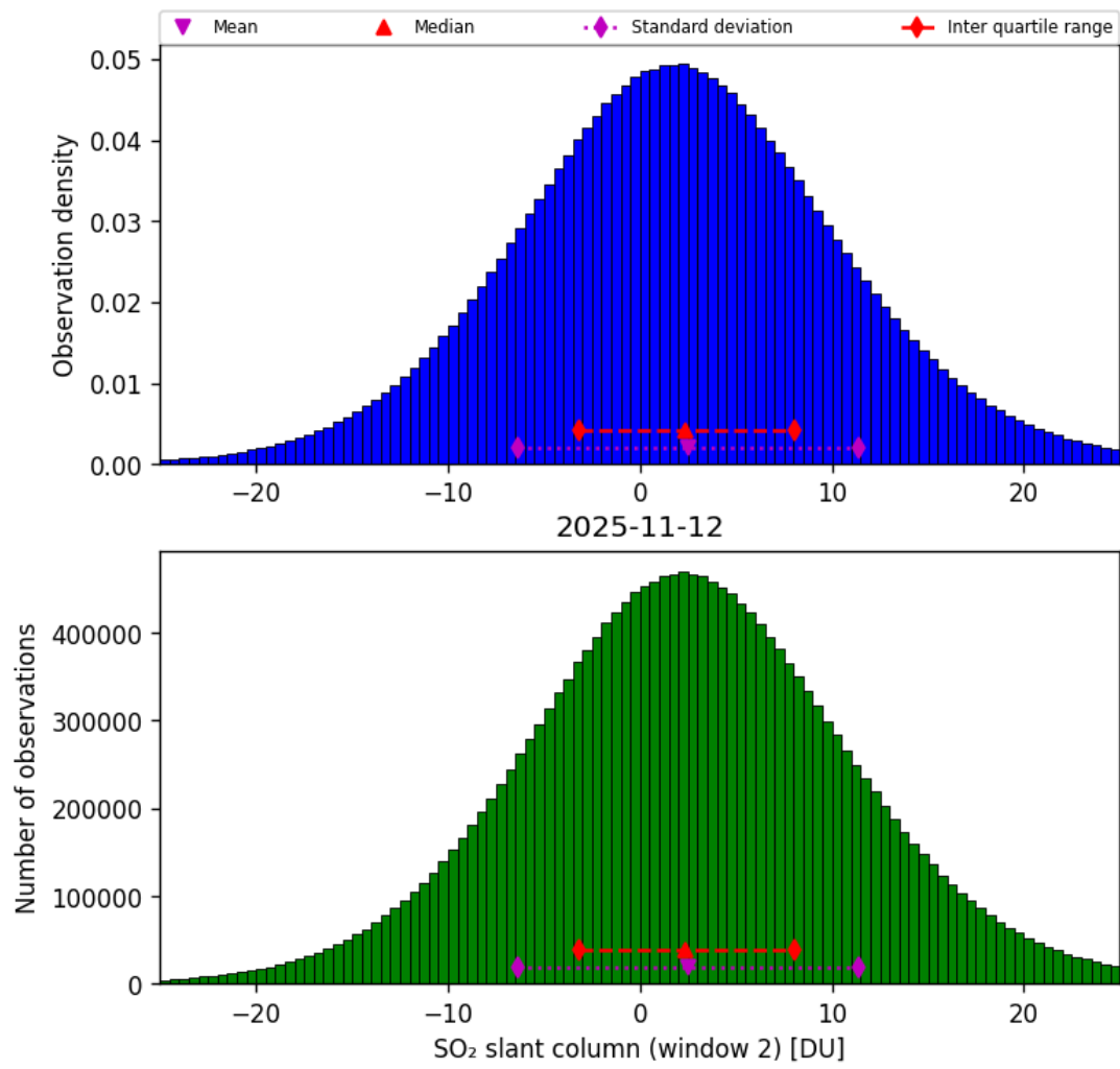
Figure 67: Histogram of “SO 2 slant column (window 2)” for 2025-11-12 to 2025-11-13
