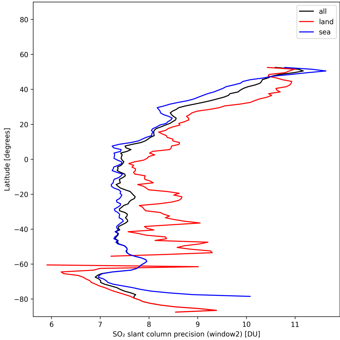
Figure 42: Zonal average of “SO 2 slant column precision (window2)” for 2025-11-12 to 2025-11-13.
