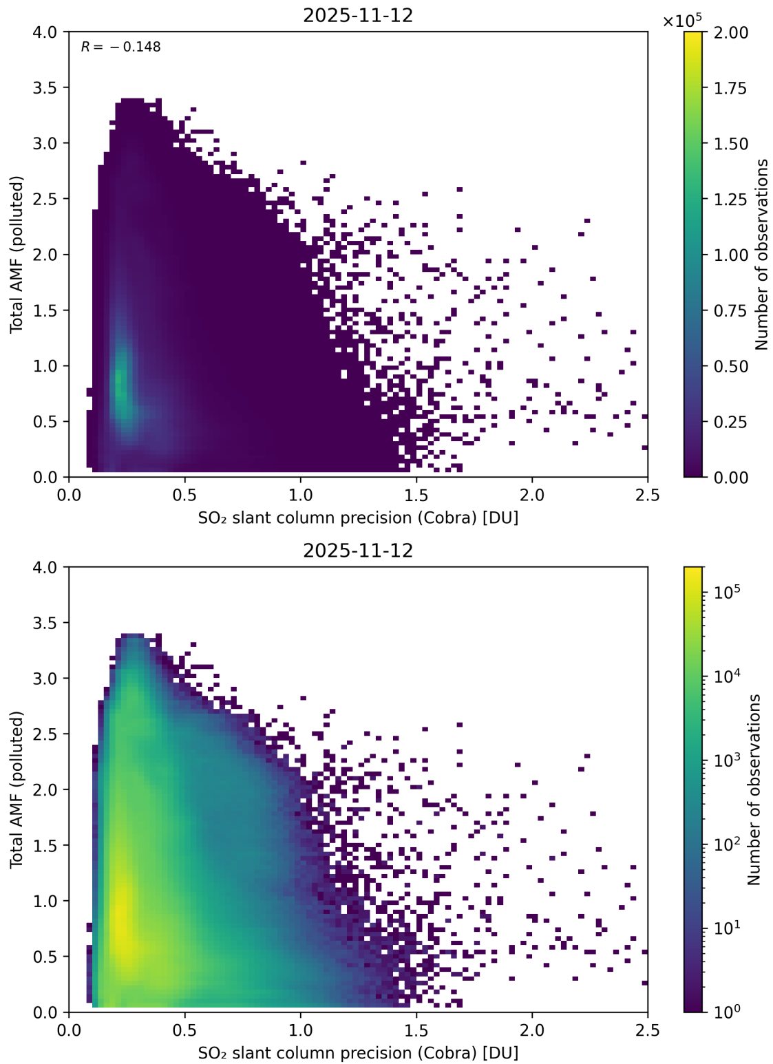
Figure 213: Scatter density plot of “SO 2 slant column precision (Cobra)” against “Total AMF (polluted)” for 2025-11-12 to 2025-11-13.
