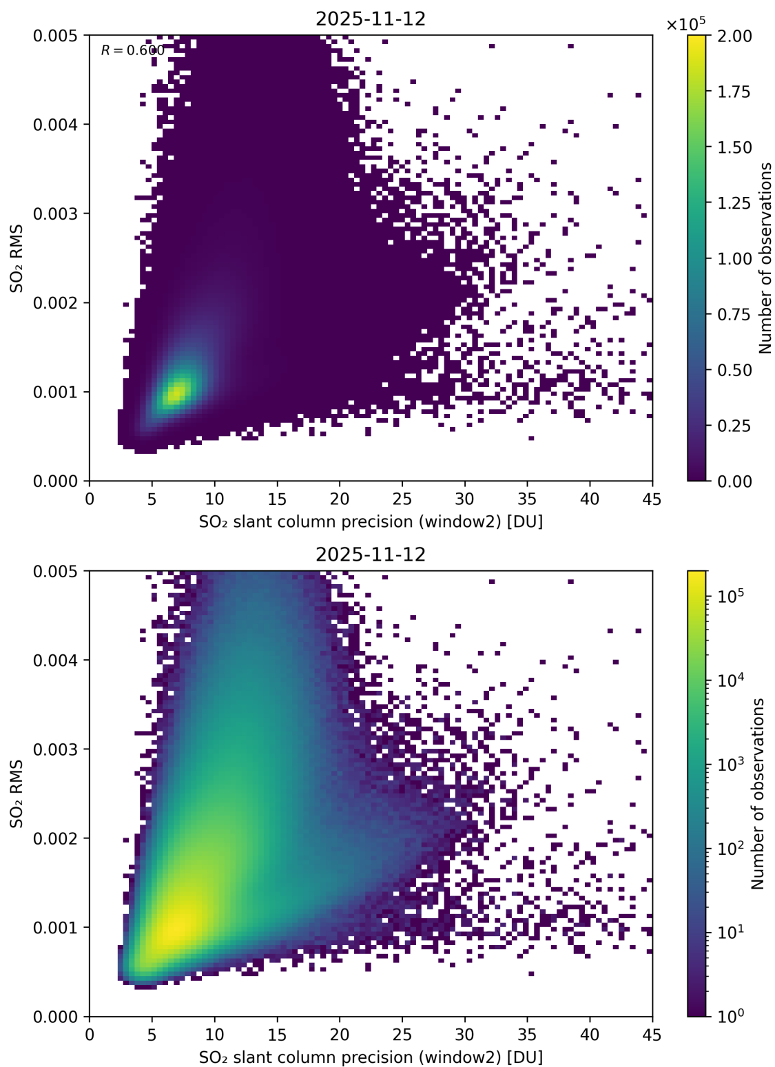
Figure 295: Scatter density plot of “SO 2 slant column precision (window2)” against “SO 2 RMS” for 2025-11-12 to 2025-11-13.
