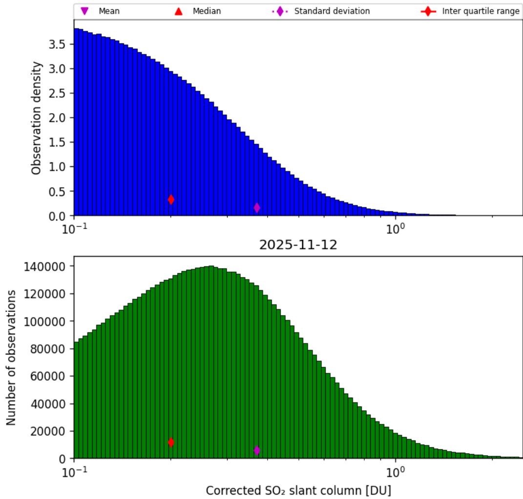
Figure 60: Histogram of “Corrected SO 2 slant column” for 2025-11-12 to 2025-11-13
