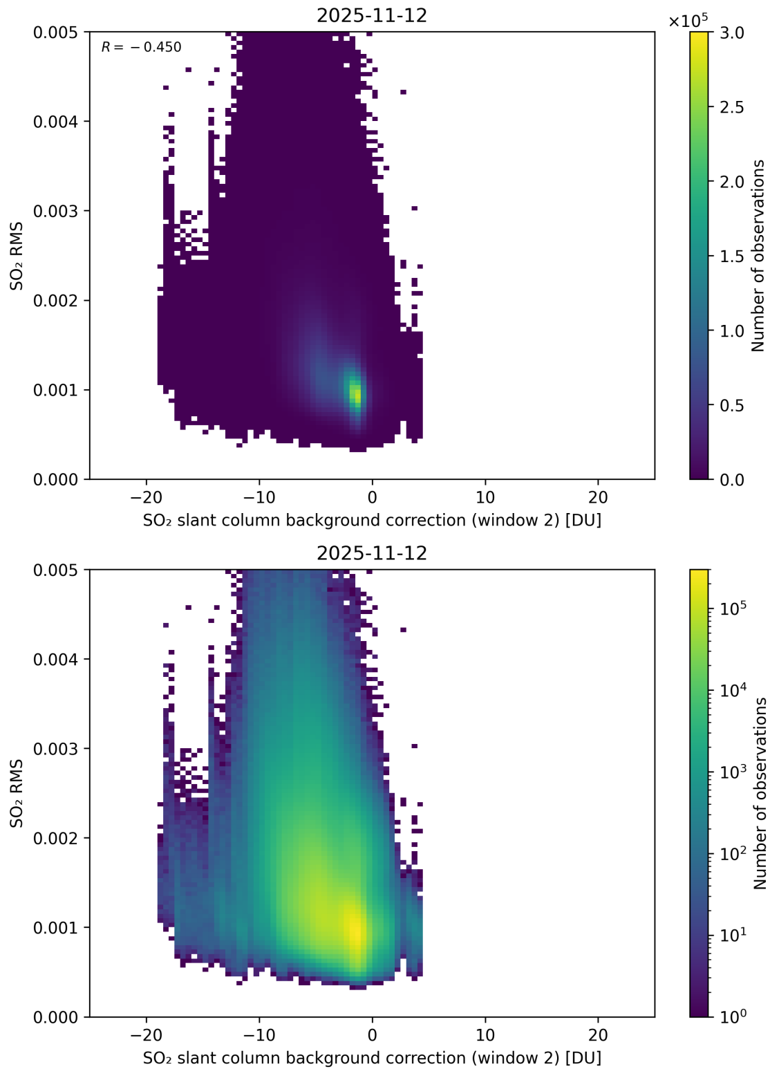
Figure 125: Scatter density plot of “SO 2 slant column background correction (window 2)” against “SO 2 RMS” for 2025-11-12 to 2025-11-13.
