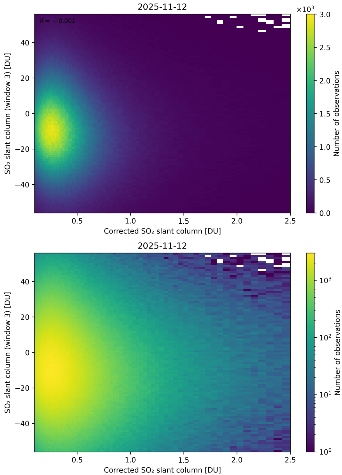
Figure 240: Scatter density plot of “Corrected SO 2 slant column” against “SO 2 slant column (window 3)” for 2025-11-12 to 2025-11-13.
