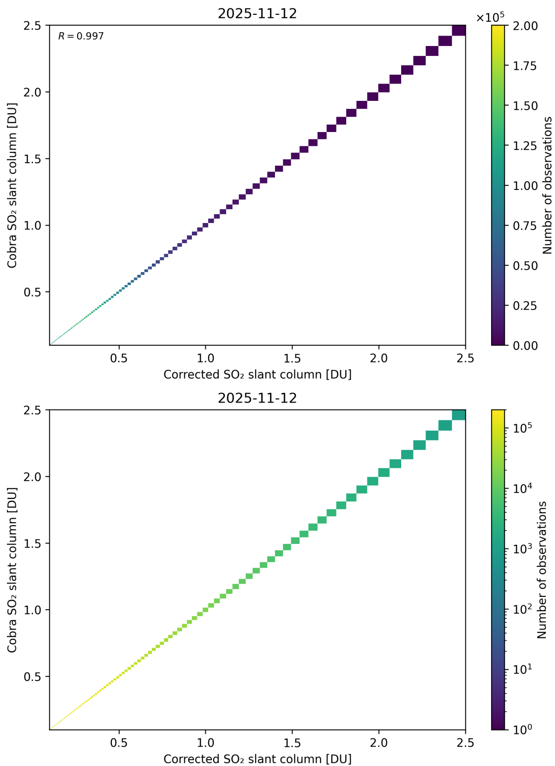
Figure 233: Scatter density plot of “Corrected SO 2 slant column” against “Cobra SO 2 slant column” for 2025-11-12 to 2025-11-13.
