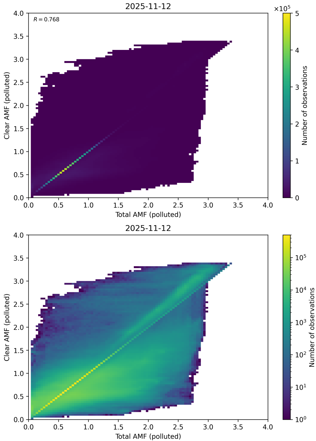
Figure 320: Scatter density plot of “Total AMF (polluted)” against “Clear AMF (polluted)” for 2025-11-12 to 2025-11-13.
