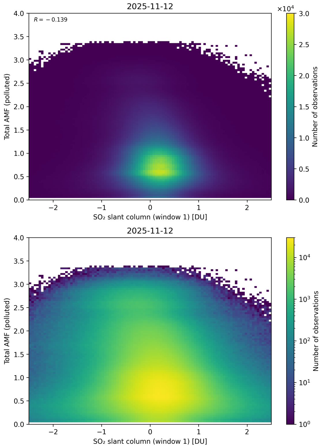
Figure 289: Scatter density plot of “SO 2 slant column (window 1)” against “Total AMF (polluted)” for 2025-11-12 to 2025-11-13.
