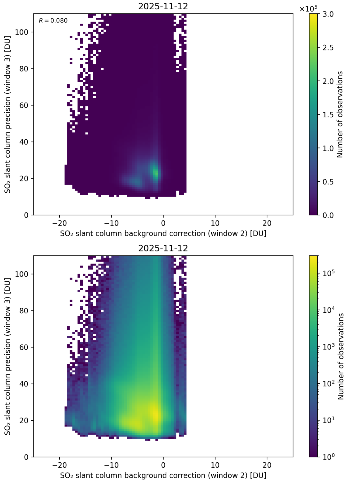
Figure 129: Scatter density plot of “SO 2 slant column background correction (window 2)” against “SO 2 slant column precision (window 3)” for 2025-11-12 to 2025-11-13.
