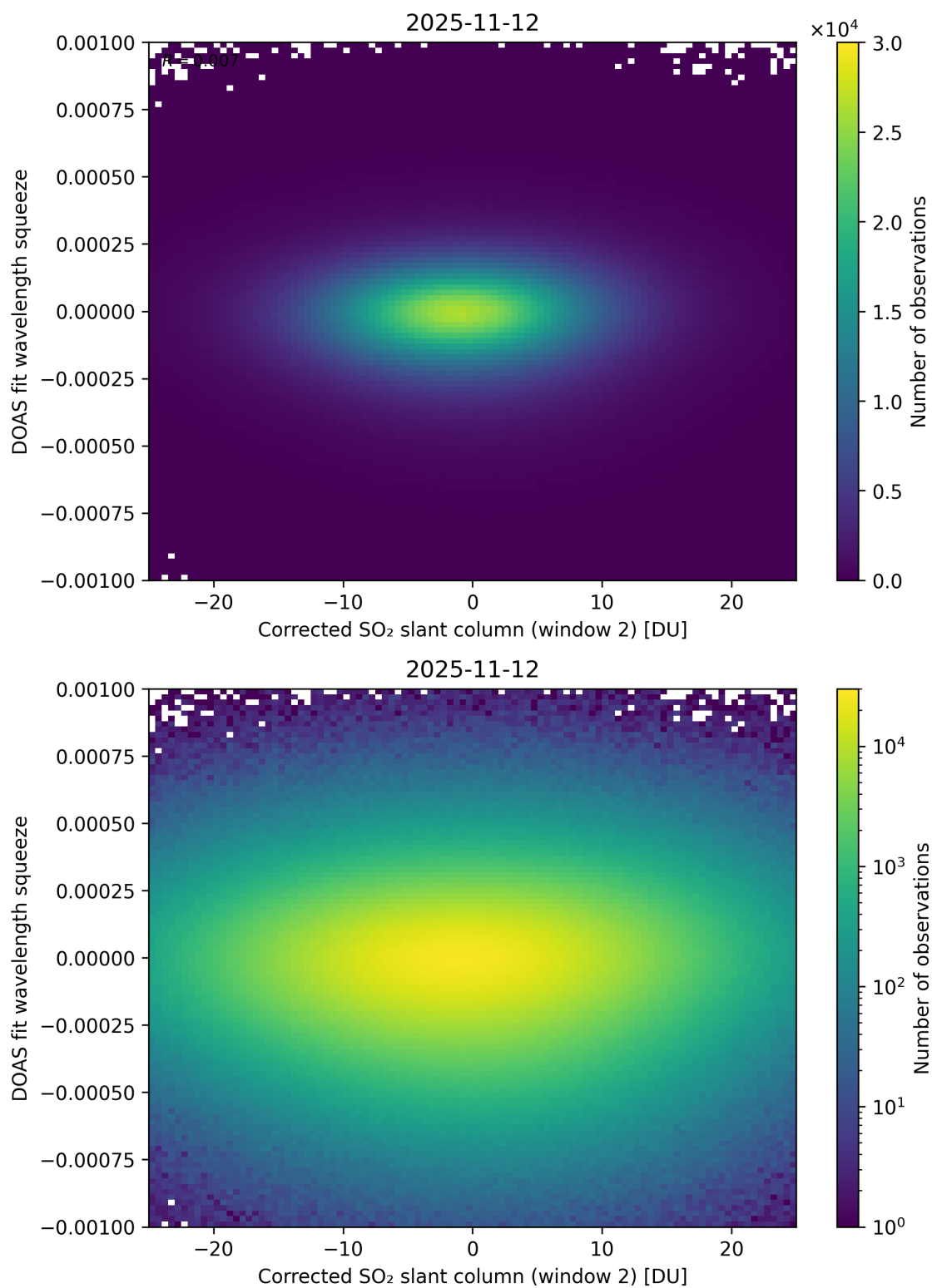
Figure 247: Scatter density plot of “Corrected SO 2 slant column (window 2)” against “DOAS fit wavelength squeeze” for 2025-11-12 to 2025-11-13.
