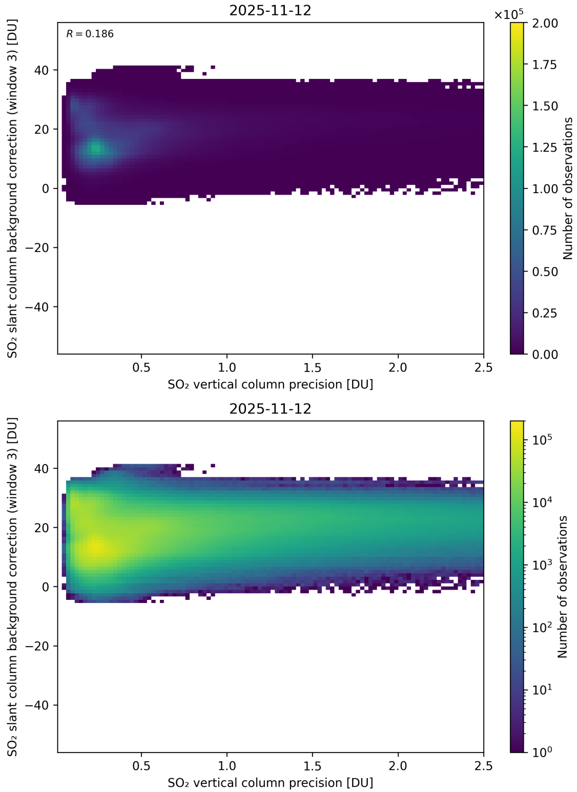
Figure 331: Scatter density plot of “SO 2 vertical column precision” against “SO 2 slant column background correction (window 3)” for 2025-11-12 to 2025-11-13.
