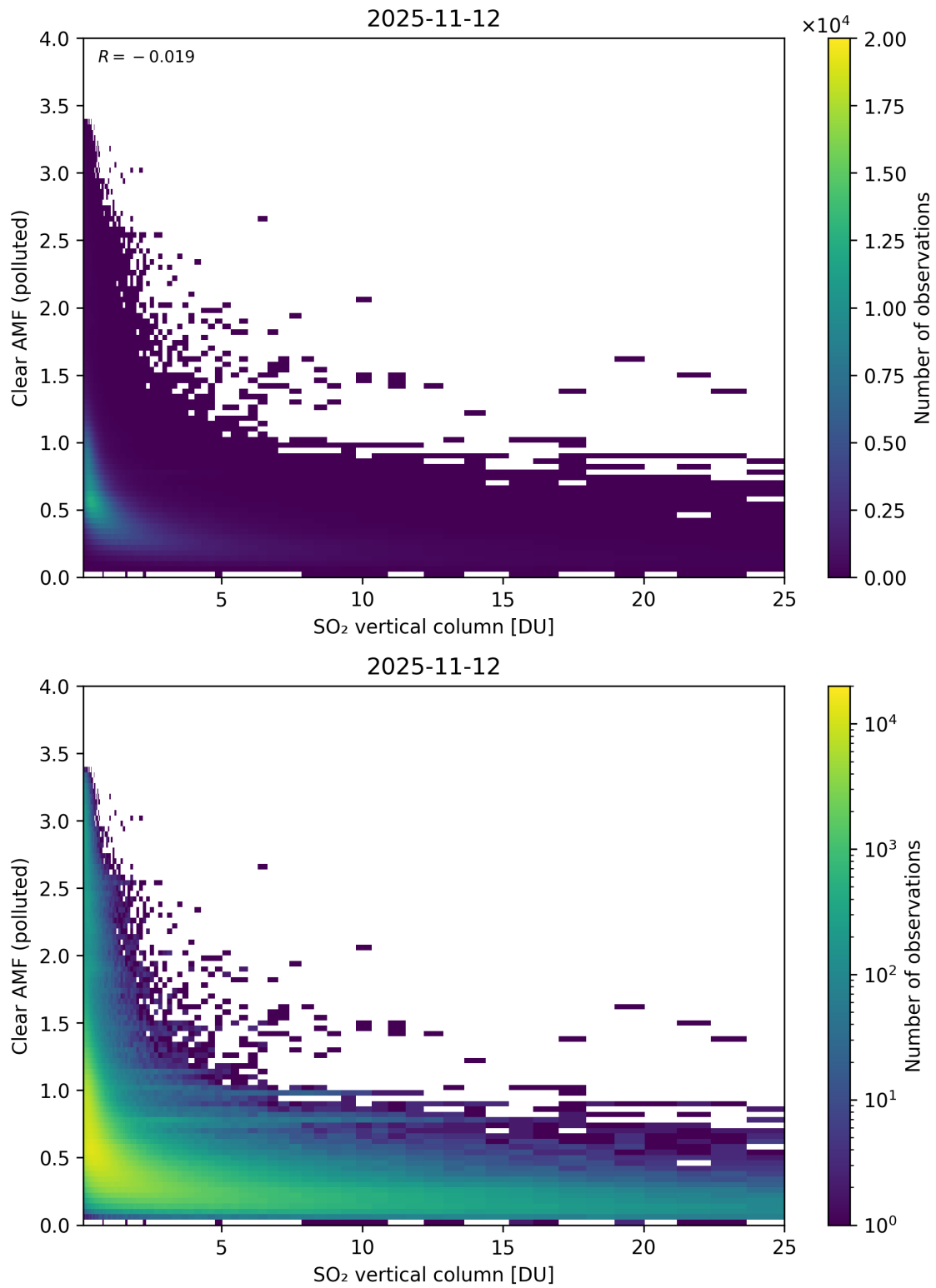
Figure 348: Scatter density plot of “SO 2 vertical column” against “Clear AMF (polluted)” for 2025-11-12 to 2025-11-13.
