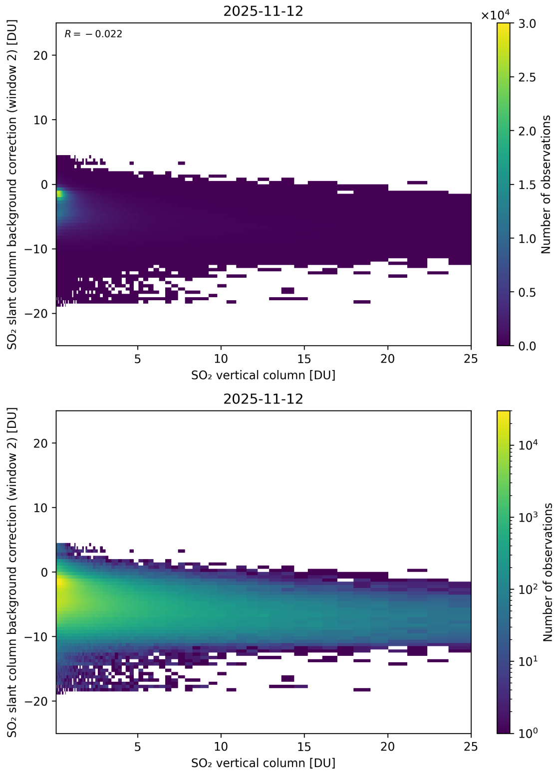
Figure 324: Scatter density plot of “SO 2 vertical column” against “SO 2 slant column background correction (window 2)” for 2025-11-12 to 2025-11-13.
