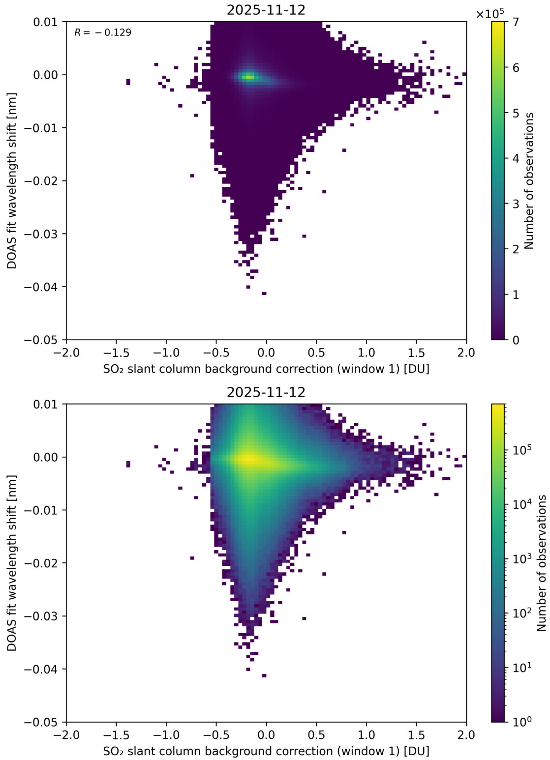
Figure 111: Scatter density plot of “SO 2 slant column background correction (window 1)” against “DOAS fit wavelength shift” for 2025-11-12 to 2025-11-13.
