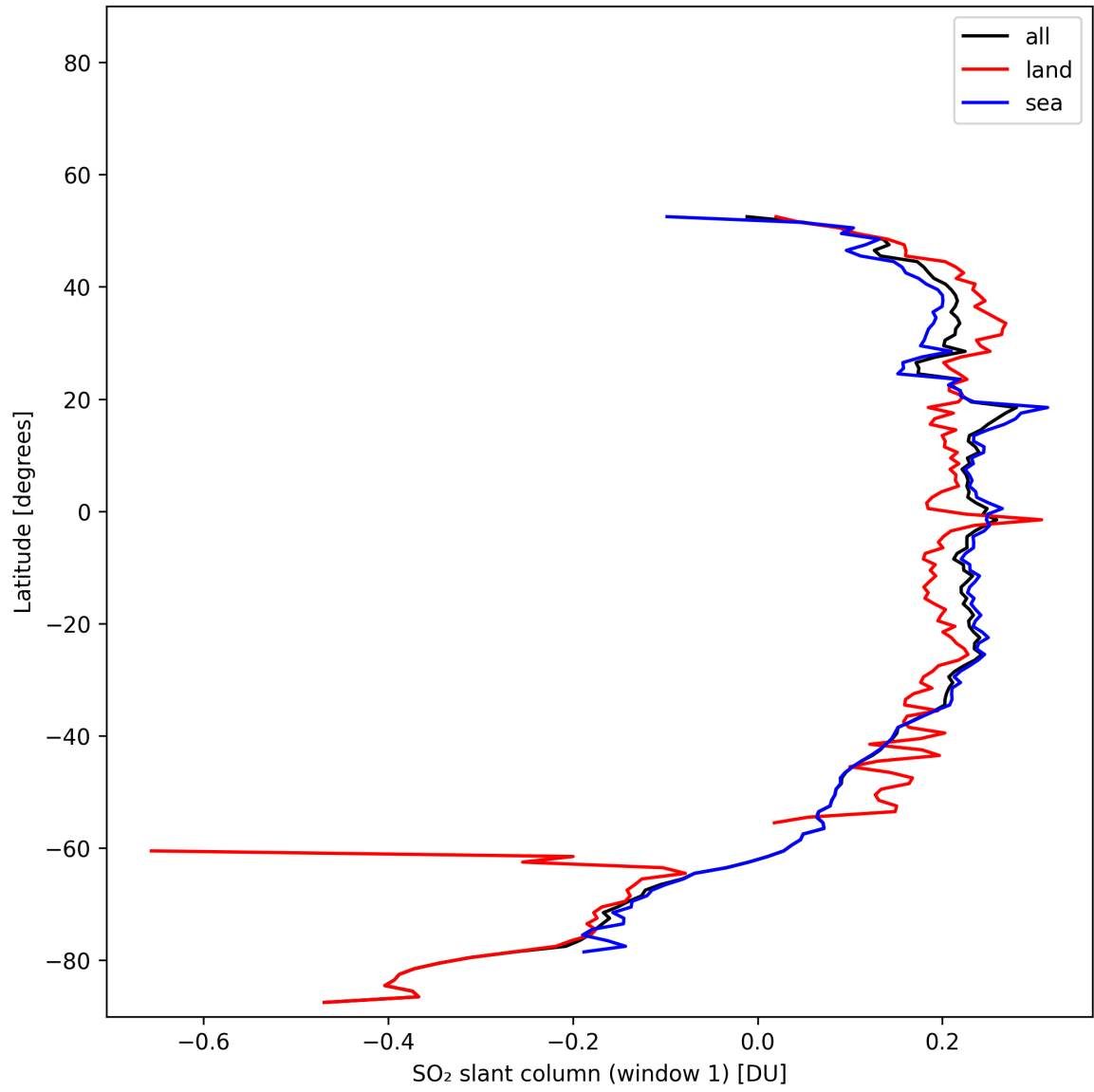
Figure 37: Zonal average of “SO 2 slant column (window 1)” for 2025-11-12 to 2025-11-13.
