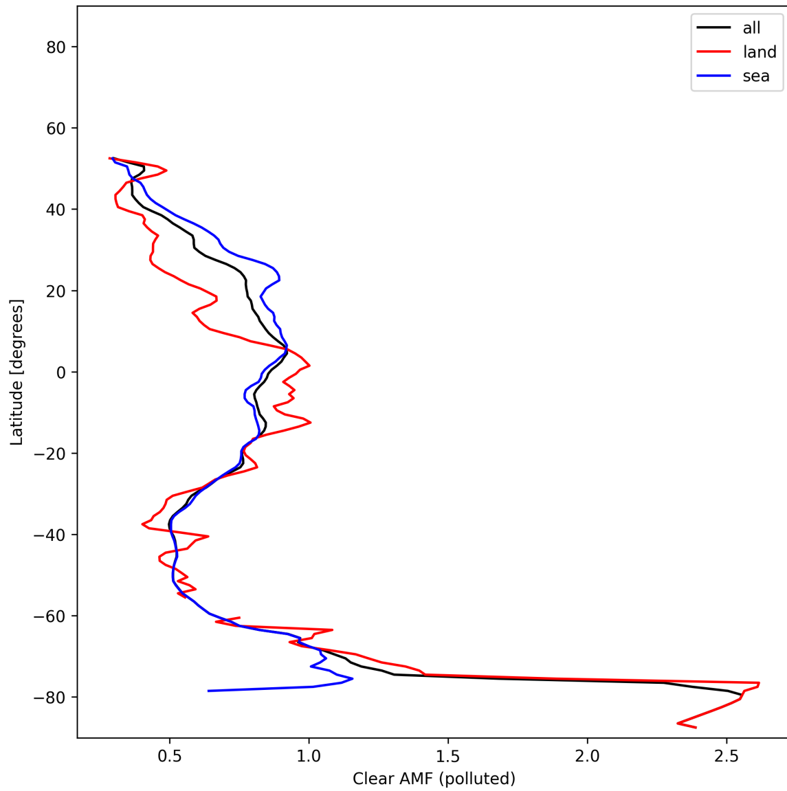
Figure 55: Zonal average of “Clear AMF (polluted)” for 2025-11-12 to 2025-11-13.
