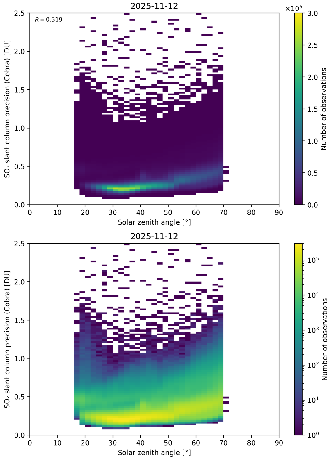
Figure 180: Scatter density plot of “Solar zenith angle” against “SO 2 slant column precision (Cobra)” for 2025-11-12 to 2025-11-13.
