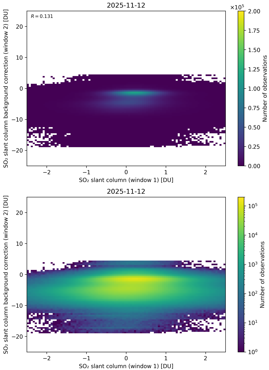
Figure 263: Scatter density plot of “SO 2 slant column (window 1)” against “SO 2 slant column background correction (window 2)” for 2025-11-12 to 2025-11-13.
