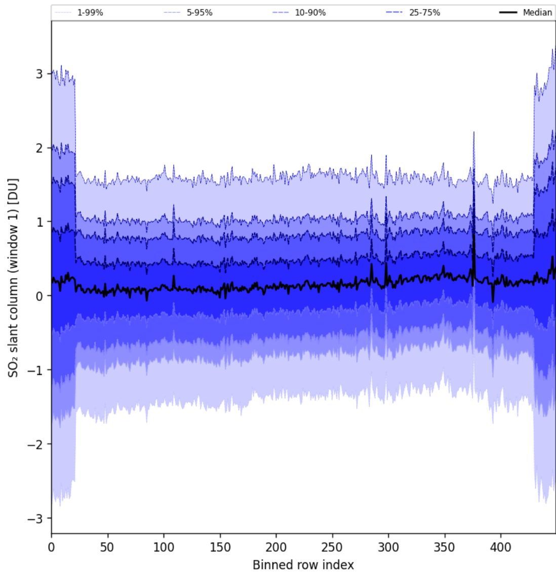
Figure 89: Along track statistics of “SO 2 slant column (window 1)” for 2025-11-12 to 2025-11-13
