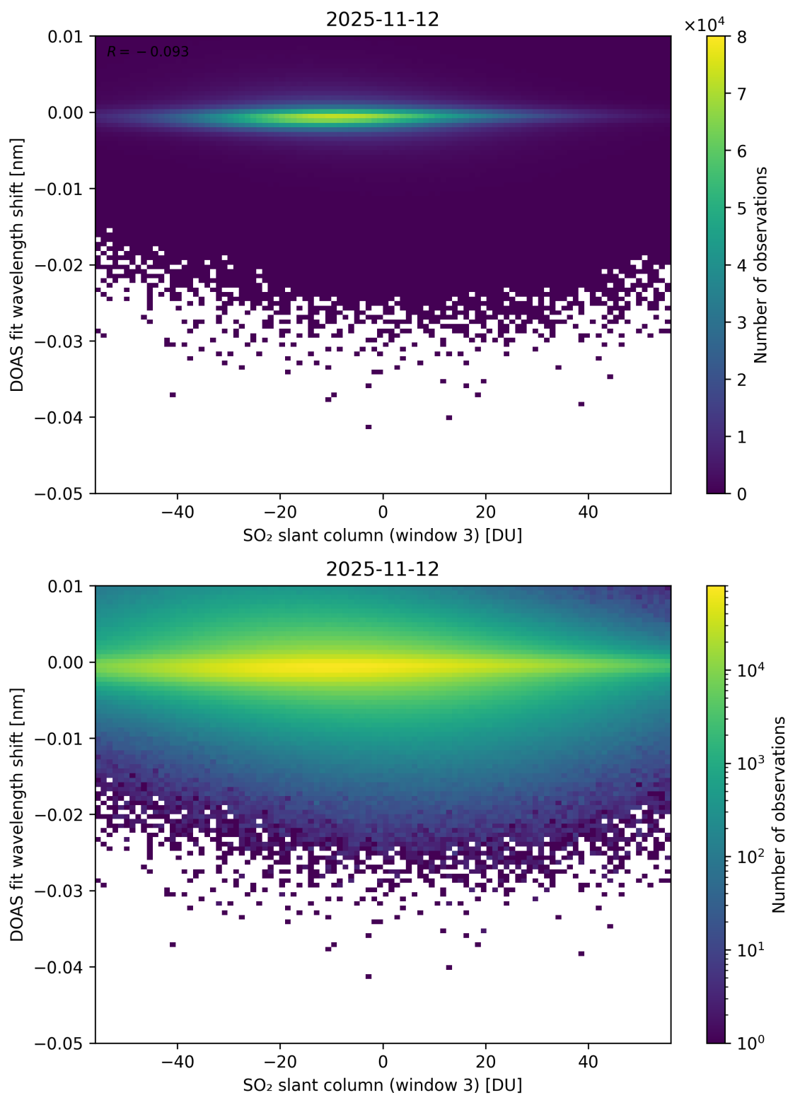
Figure 304: Scatter density plot of “SO 2 slant column (window 3)” against “DOAS fit wavelength shift” for 2025-11-12 to 2025-11-13.
