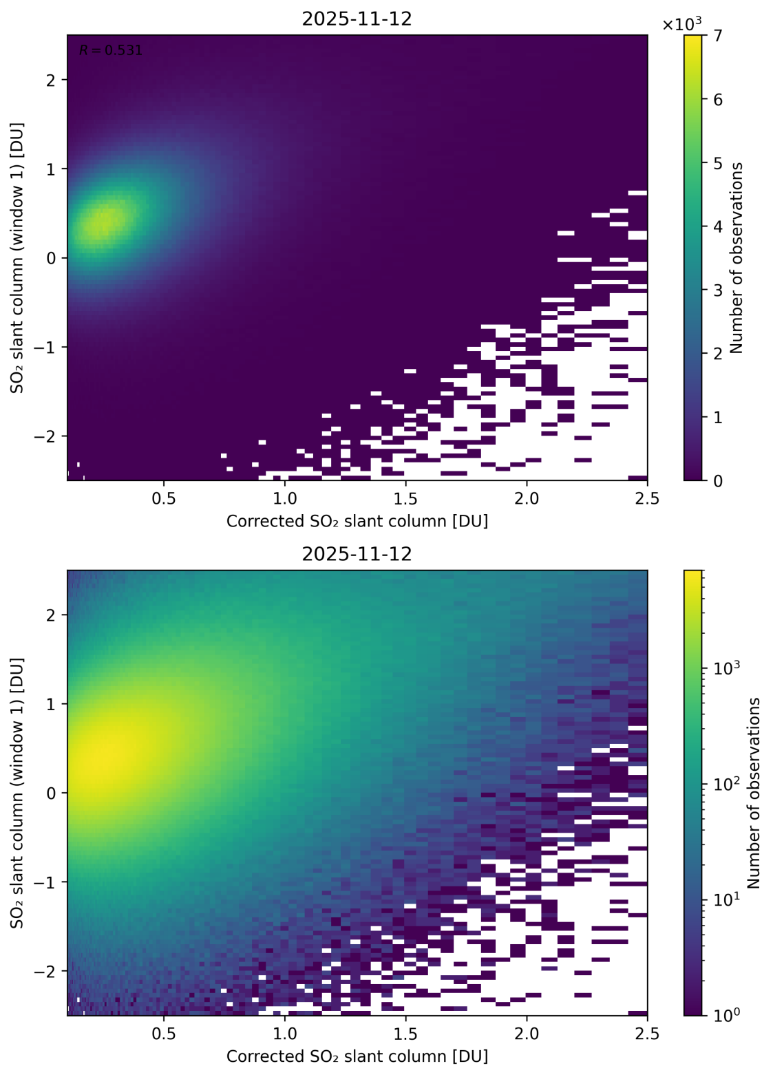
Figure 237: Scatter density plot of “Corrected SO 2 slant column” against “SO 2 slant column (window 1)” for 2025-11-12 to 2025-11-13.
