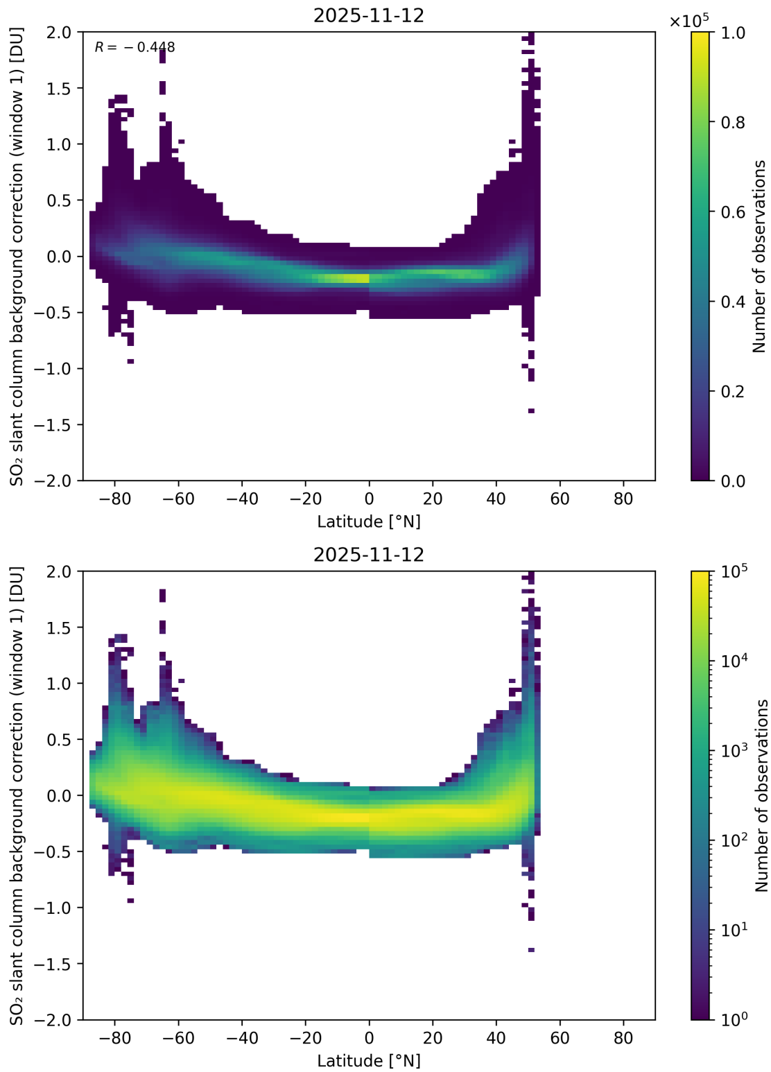
Figure 150: Scatter density plot of “Latitude” against “SO 2 slant column background correction (window 1)” for 2025-11-12 to 2025-11-13.
