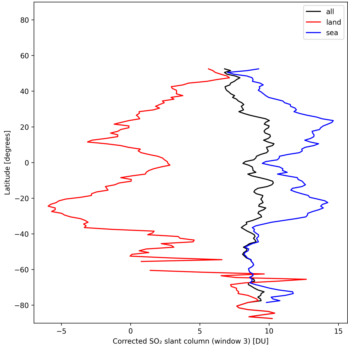
Figure 47: Zonal average of “Corrected SO 2 slant column (window 3)” for 2025-11-12 to 2025-11-13.
