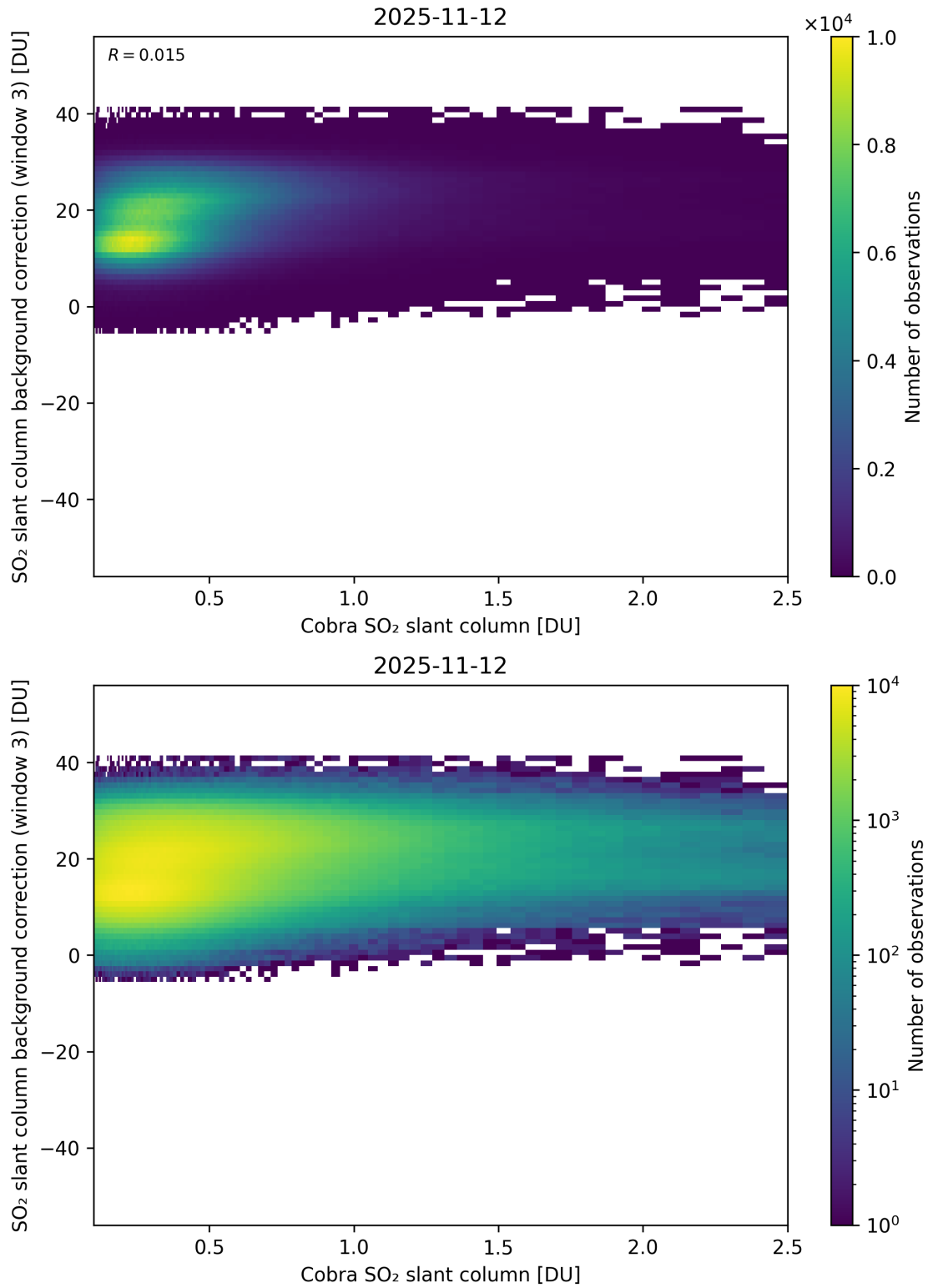
Figure 195: Scatter density plot of “Cobra SO 2 slant column” against “SO 2 slant column background correction (window 3)” for 2025-11-12 to 2025-11-13.
