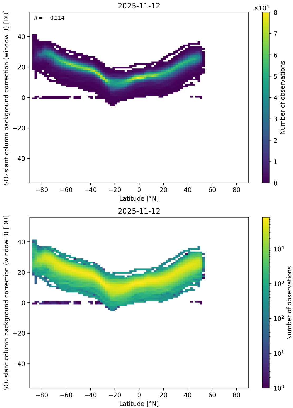
Figure 152: Scatter density plot of “Latitude” against “SO 2 slant column background correction (window 3)” for 2025-11-12 to 2025-11-13.
