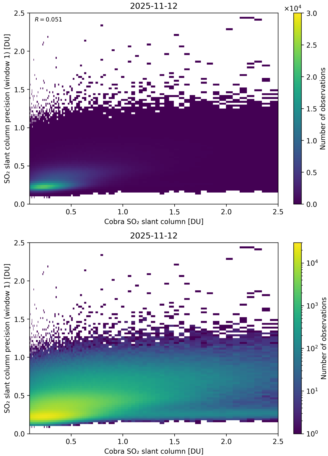
Figure 220: Scatter density plot of “Cobra SO 2 slant column” against “SO 2 slant column precision (window 1)” for 2025-11-12 to 2025-11-13.
