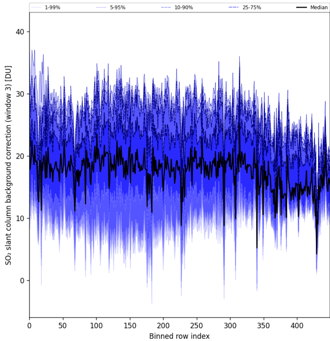
Figure 100: Along track statistics of “SO 2 slant column background correction (window 3)” for 2025-11-12 to 2025-11-13
