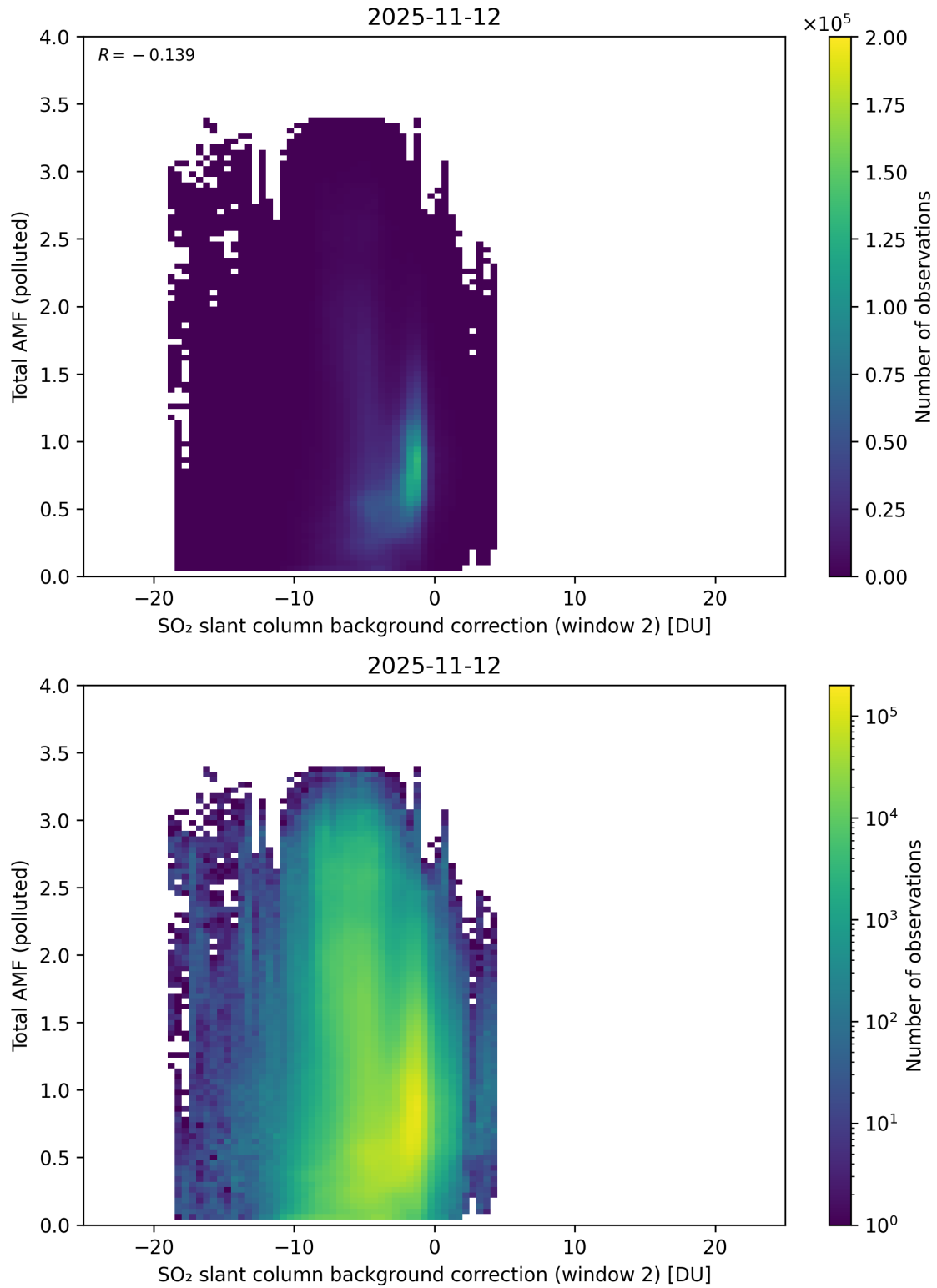
Figure 130: Scatter density plot of “SO 2 slant column background correction (window 2)” against “Total AMF (polluted)” for 2025-11-12 to 2025-11-13.
