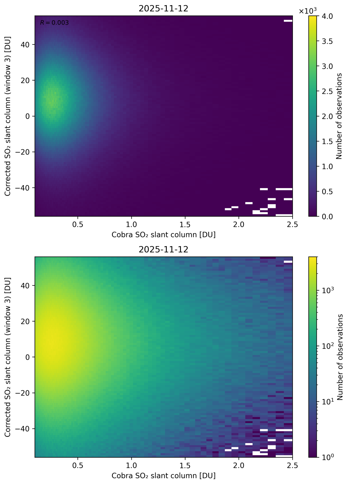
Figure 218: Scatter density plot of “Cobra SO 2 slant column” against “Corrected SO 2 slant column (window 3)” for 2025-11-12 to 2025-11-13.
