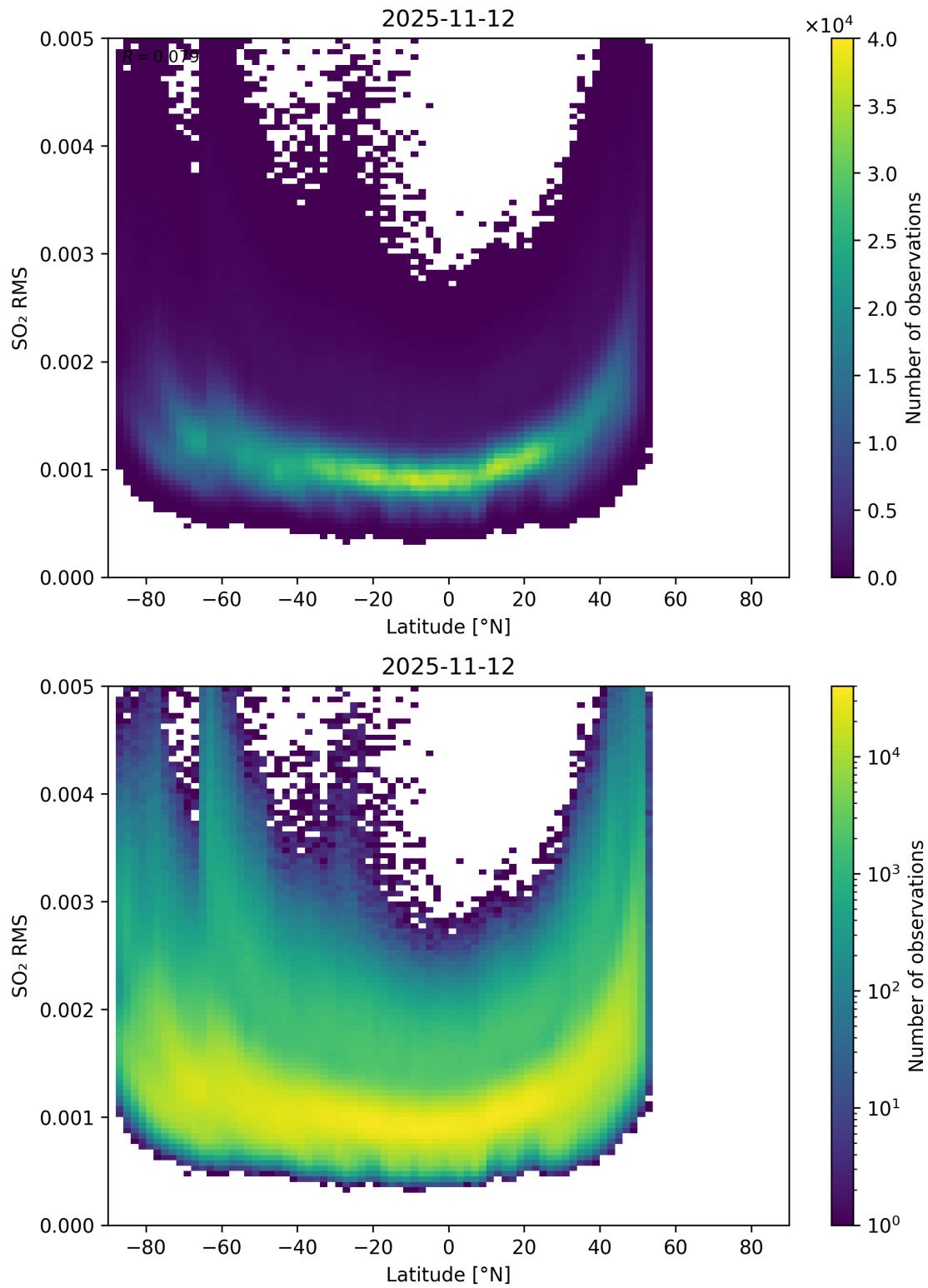
Figure 155: Scatter density plot of “Latitude” against “SO 2 RMS” for 2025-11-12 to 2025-11-13.
