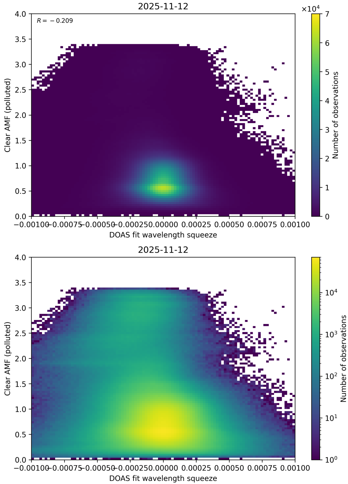
Figure 144: Scatter density plot of “DOAS fit wavelength squeeze” against “Clear AMF (polluted)” for 2025-11-12 to 2025-11-13.
