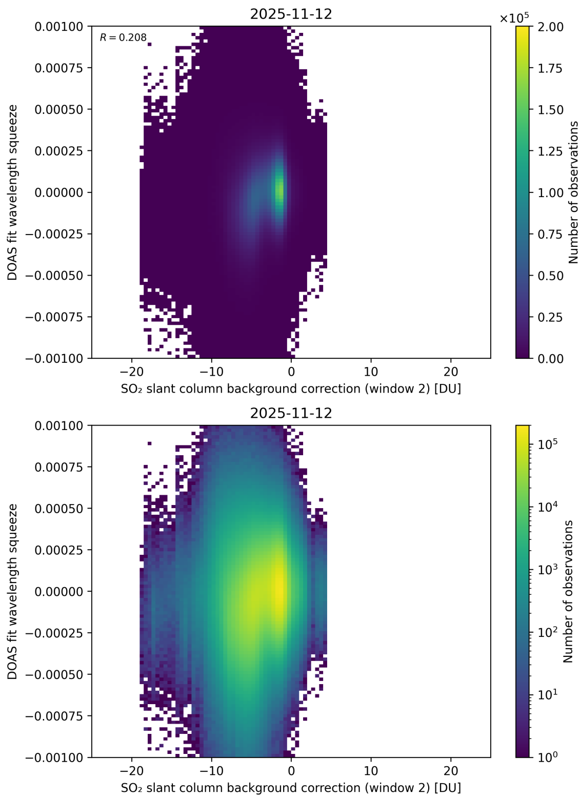
Figure 124: Scatter density plot of “SO 2 slant column background correction (window 2)” against “DOAS fit wavelength squeeze” for 2025-11-12 to 2025-11-13.
