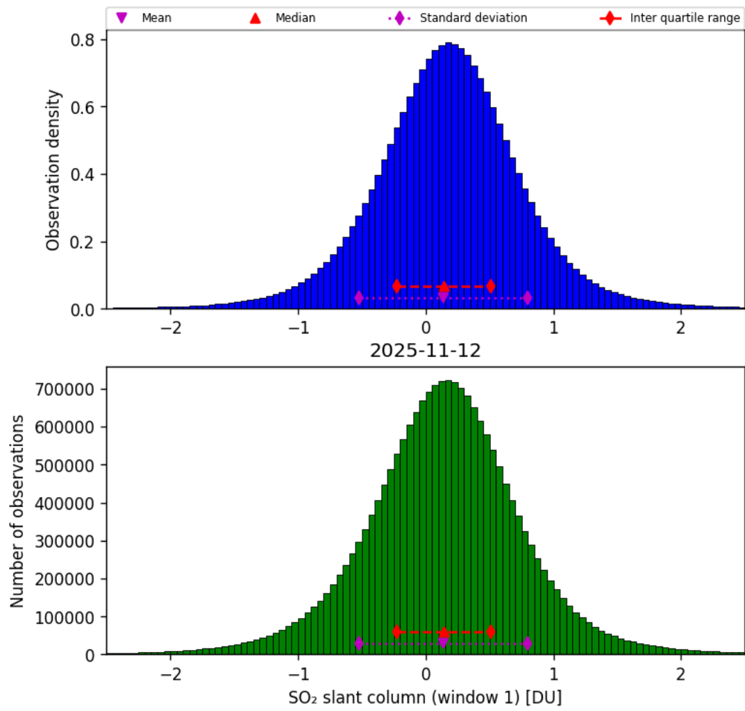
Figure 63: Histogram of “SO 2 slant column (window 1)” for 2025-11-12 to 2025-11-13
