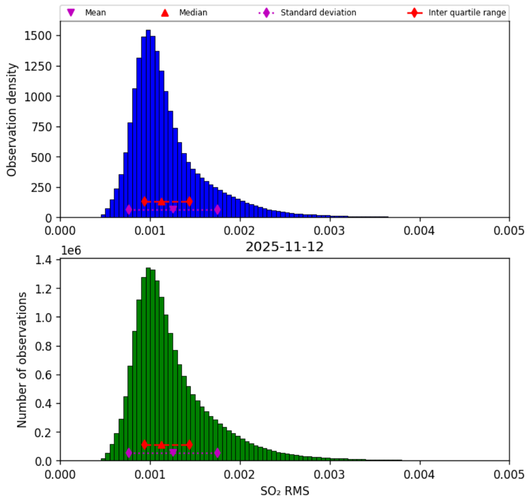
Figure 78: Histogram of “SO 2 RMS” for 2025-11-12 to 2025-11-13
