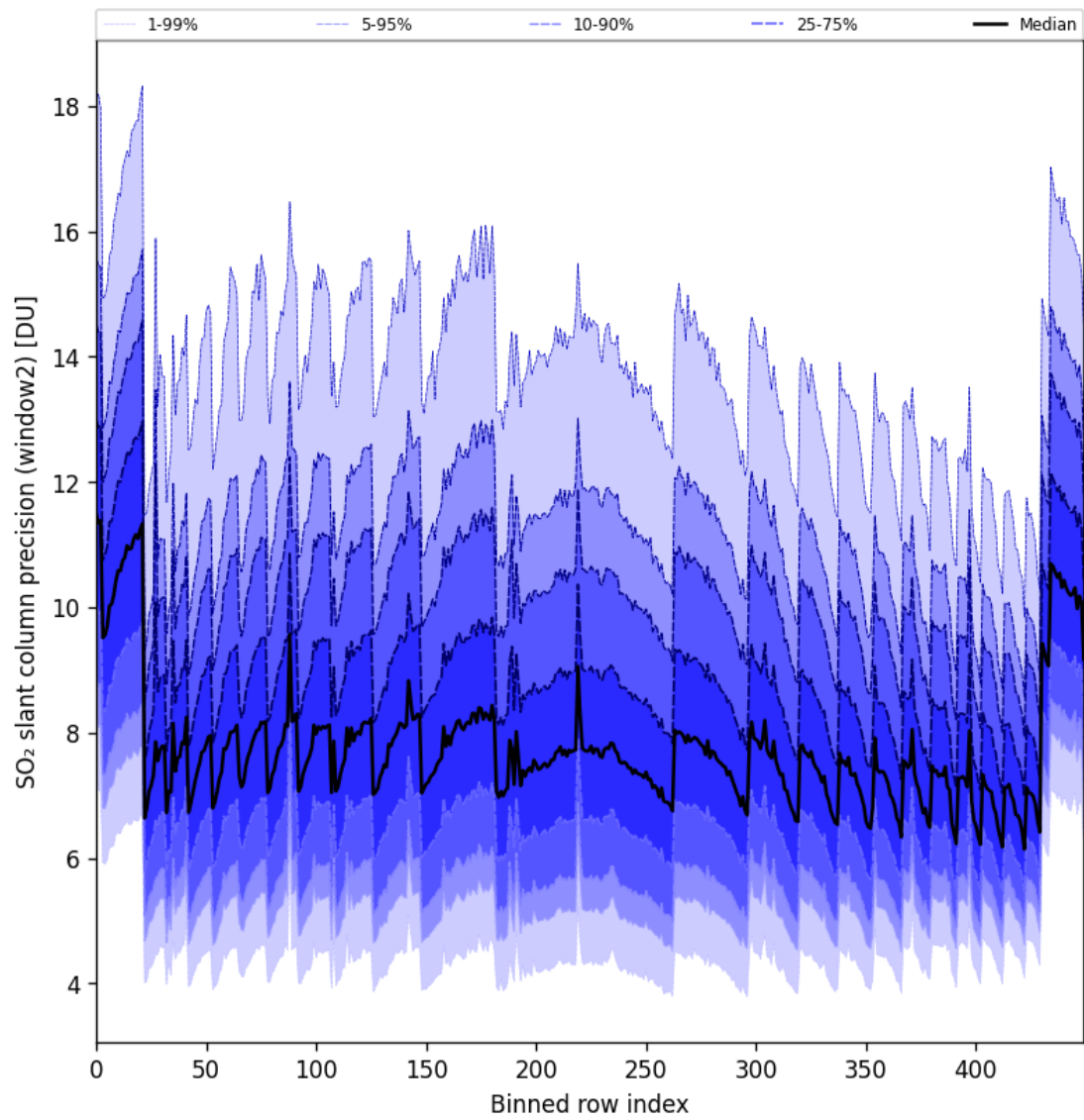
Figure 94: Along track statistics of “SO 2 slant column precision (window2)” for 2025-11-12 to 2025-11-13
