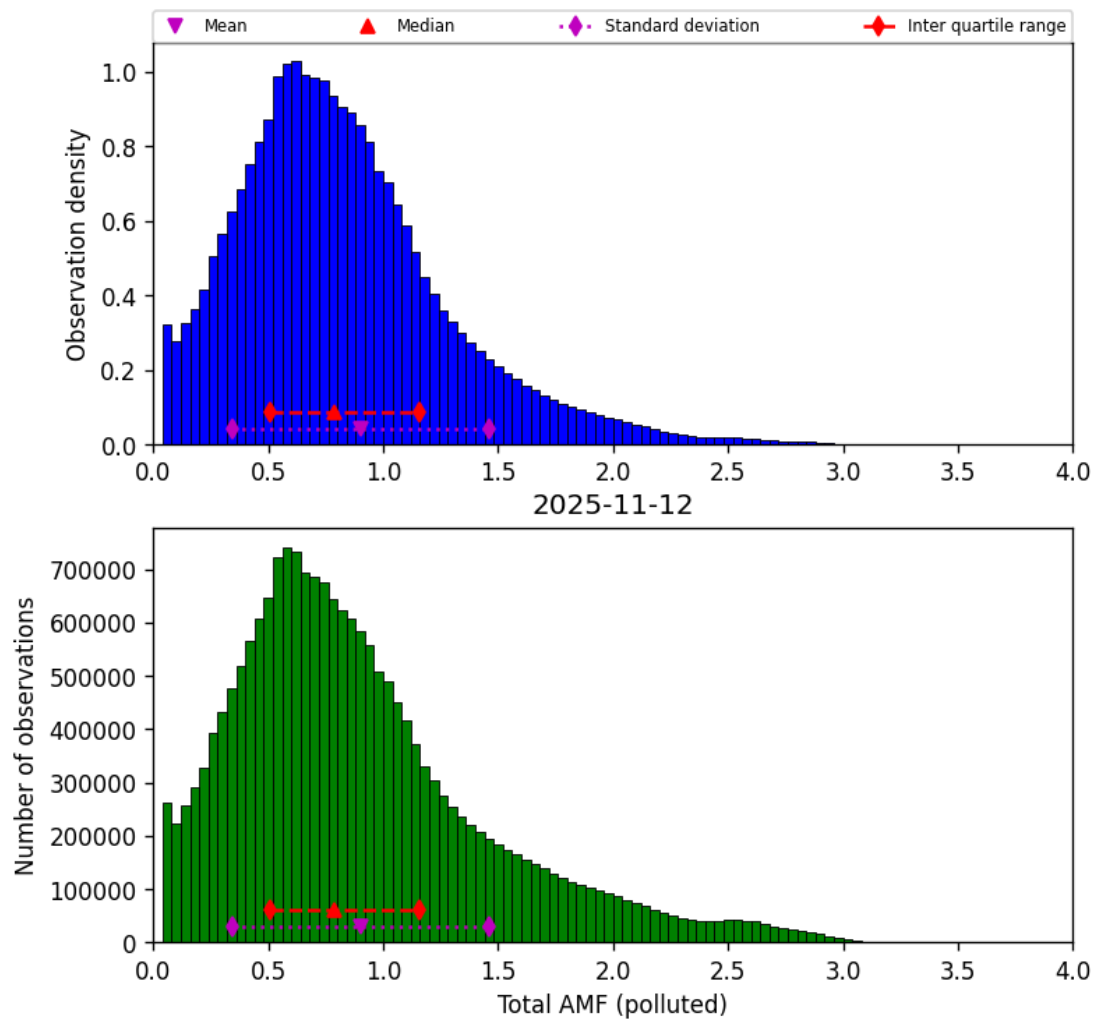
Figure 79: Histogram of “Total AMF (polluted)” for 2025-11-12 to 2025-11-13
