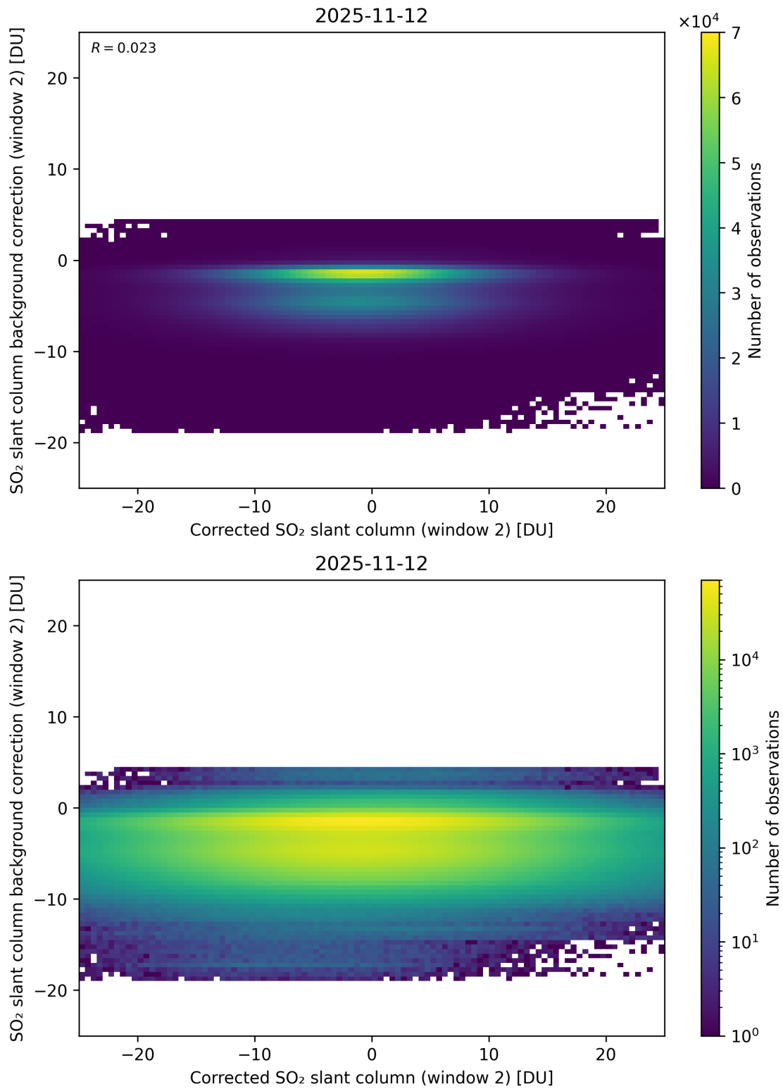
Figure 244: Scatter density plot of “Corrected SO 2 slant column (window 2)” against “SO 2 slant column background correction (window 2)” for 2025-11-12 to 2025-11-13.
