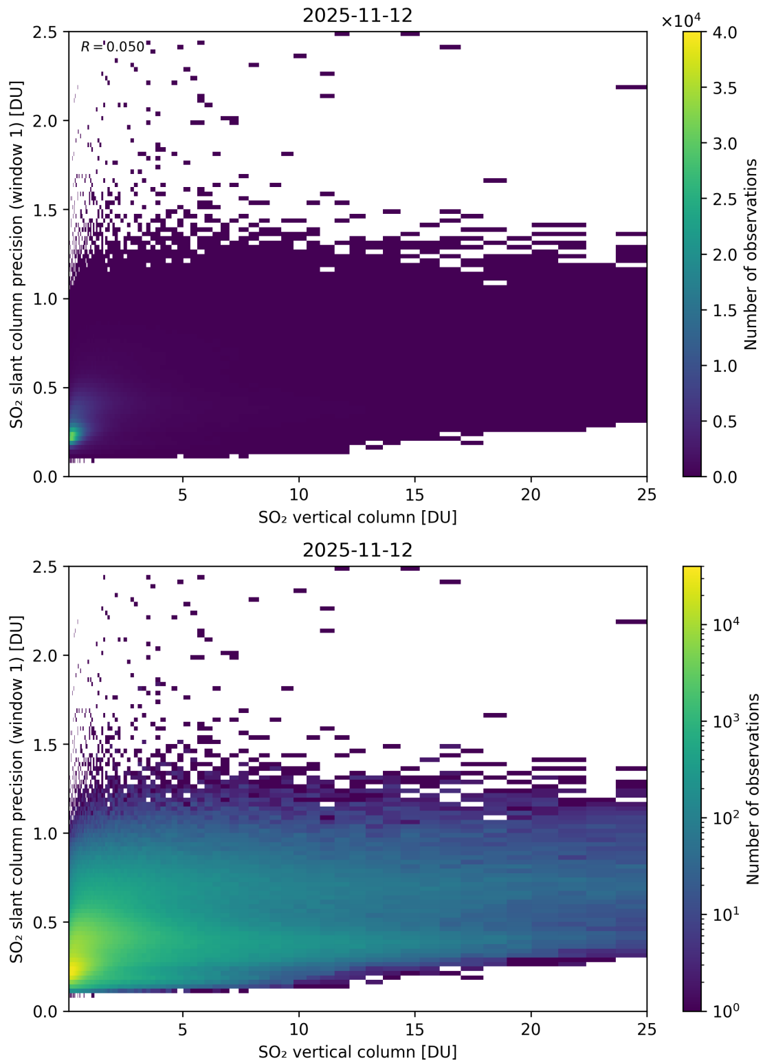
Figure 355: Scatter density plot of “SO 2 vertical column” against “SO 2 slant column precision (window 1)” for 2025-11-12 to 2025-11-13.
