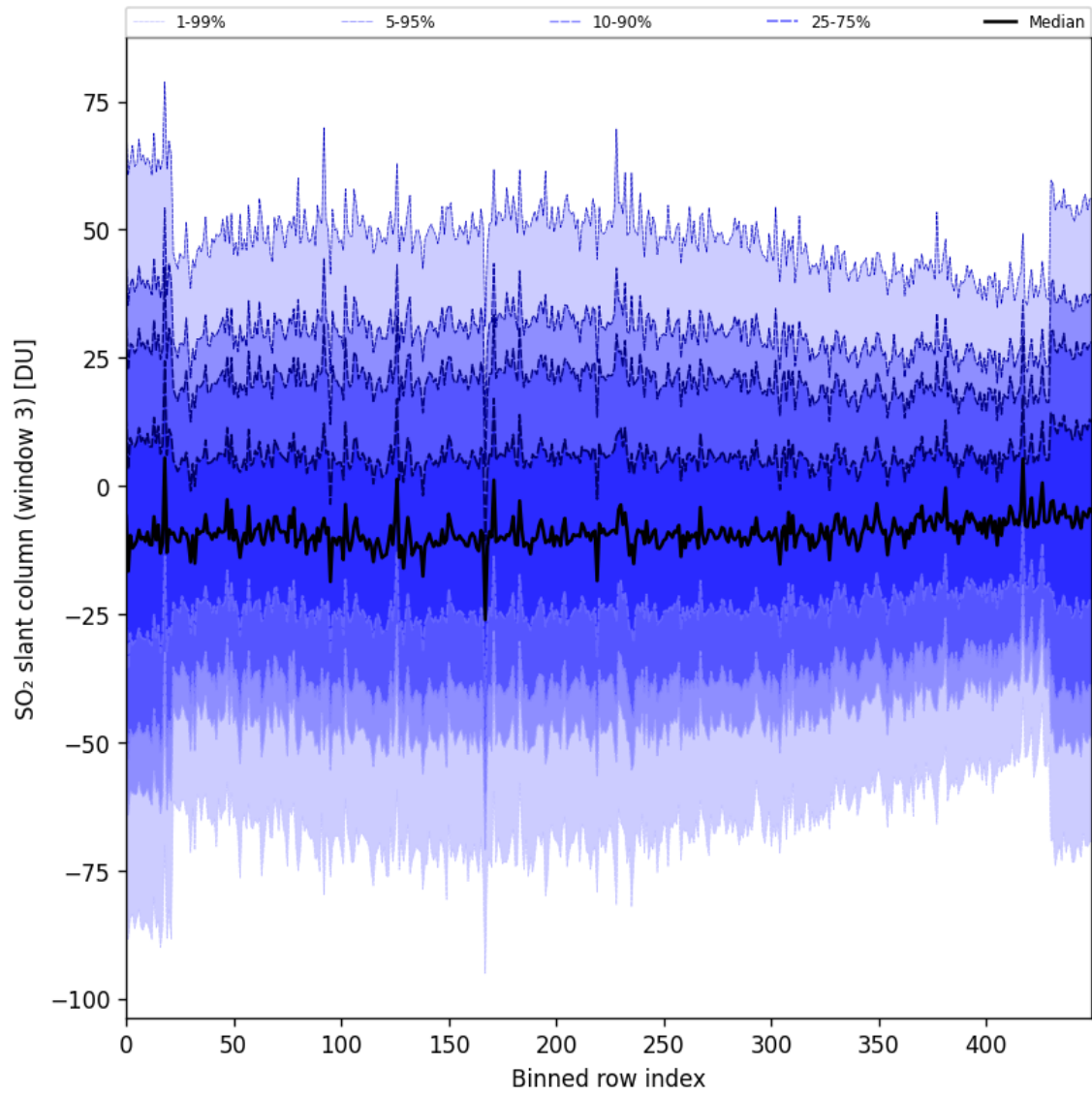
Figure 97: Along track statistics of “SO 2 slant column (window 3)” for 2025-11-12 to 2025-11-13
