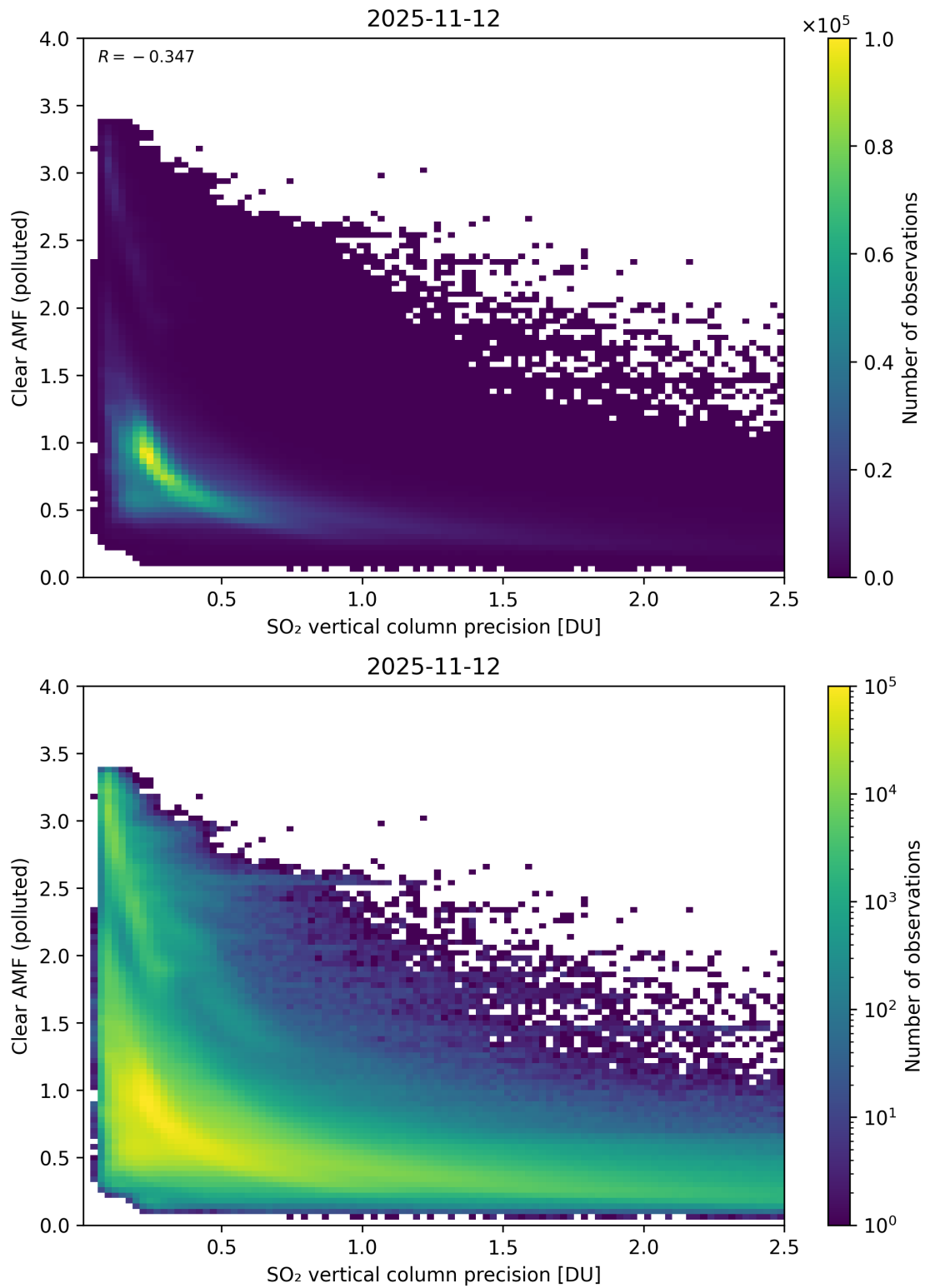
Figure 335: Scatter density plot of “SO 2 vertical column precision” against “Clear AMF (polluted)” for 2025-11-12 to 2025-11-13.
