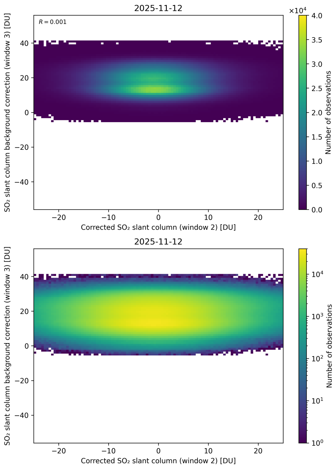
Figure 245: Scatter density plot of “Corrected SO 2 slant column (window 2)” against “SO 2 slant column background correction (window 3)” for 2025-11-12 to 2025-11-13.
