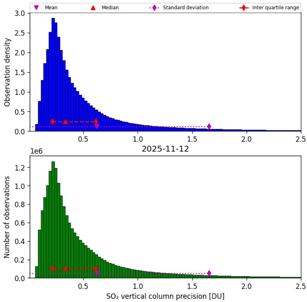
Figure 59: Histogram of “SO 2 vertical column precision” for 2025-11-12 to 2025-11-13
