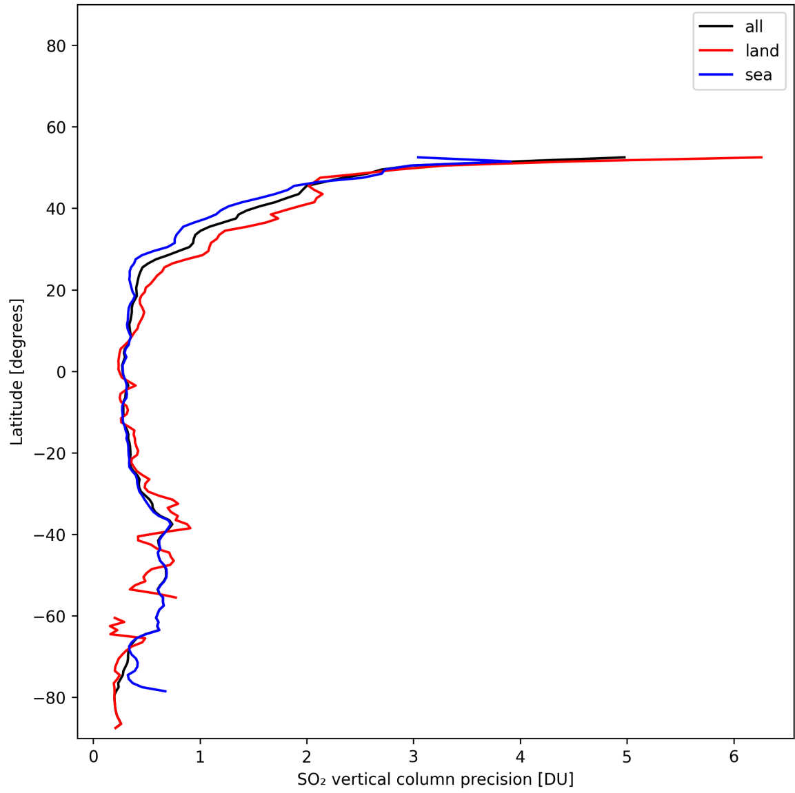
Figure 33: Zonal average of “SO 2 vertical column precision” for 2025-11-12 to 2025-11-13.
