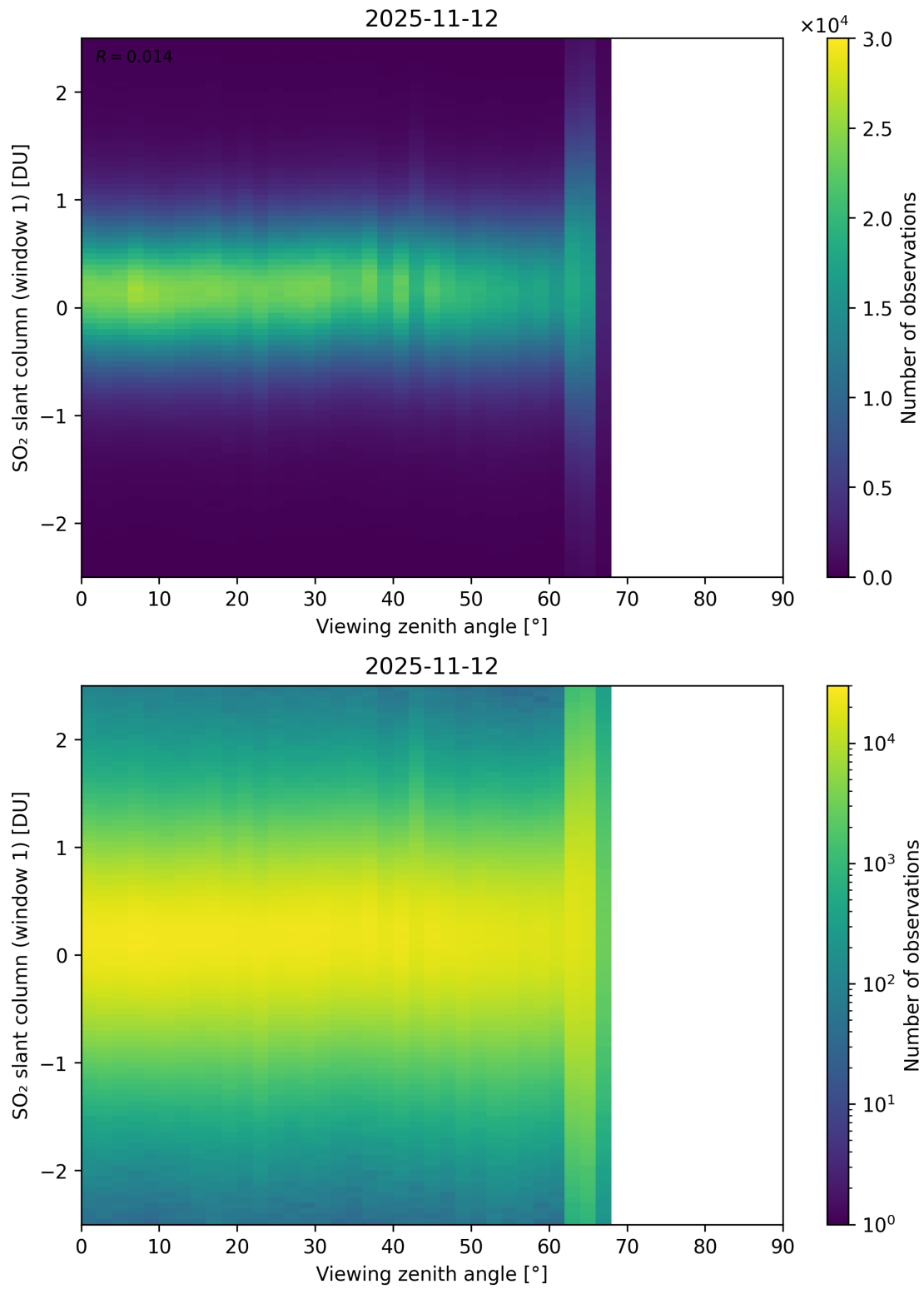
Figure 376: Scatter density plot of “Viewing zenith angle” against “SO 2 slant column (window 1)” for 2025-11-12 to 2025-11-13.
