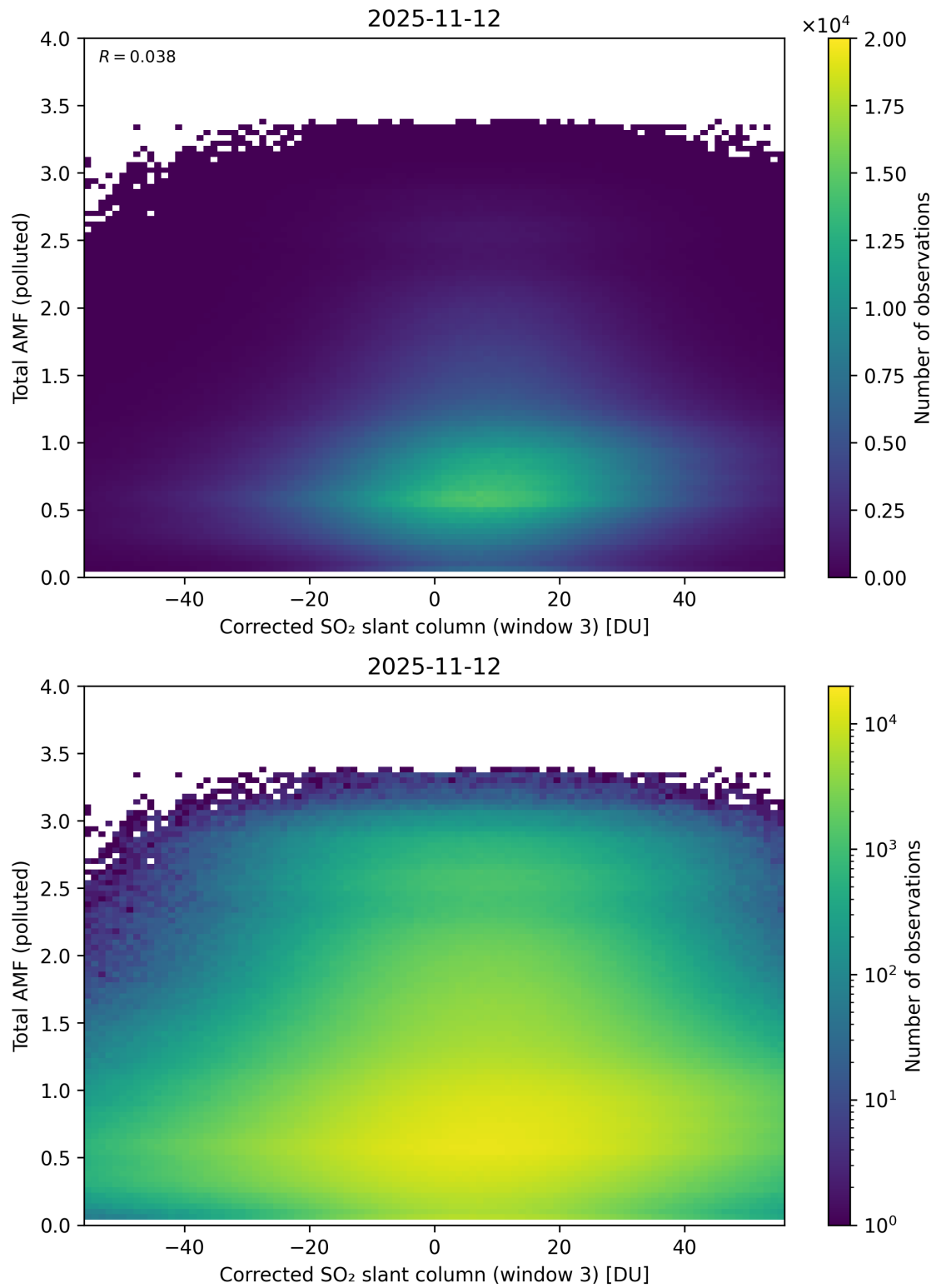
Figure 260: Scatter density plot of “Corrected SO 2 slant column (window 3)” against “Total AMF (polluted)” for 2025-11-12 to 2025-11-13.
