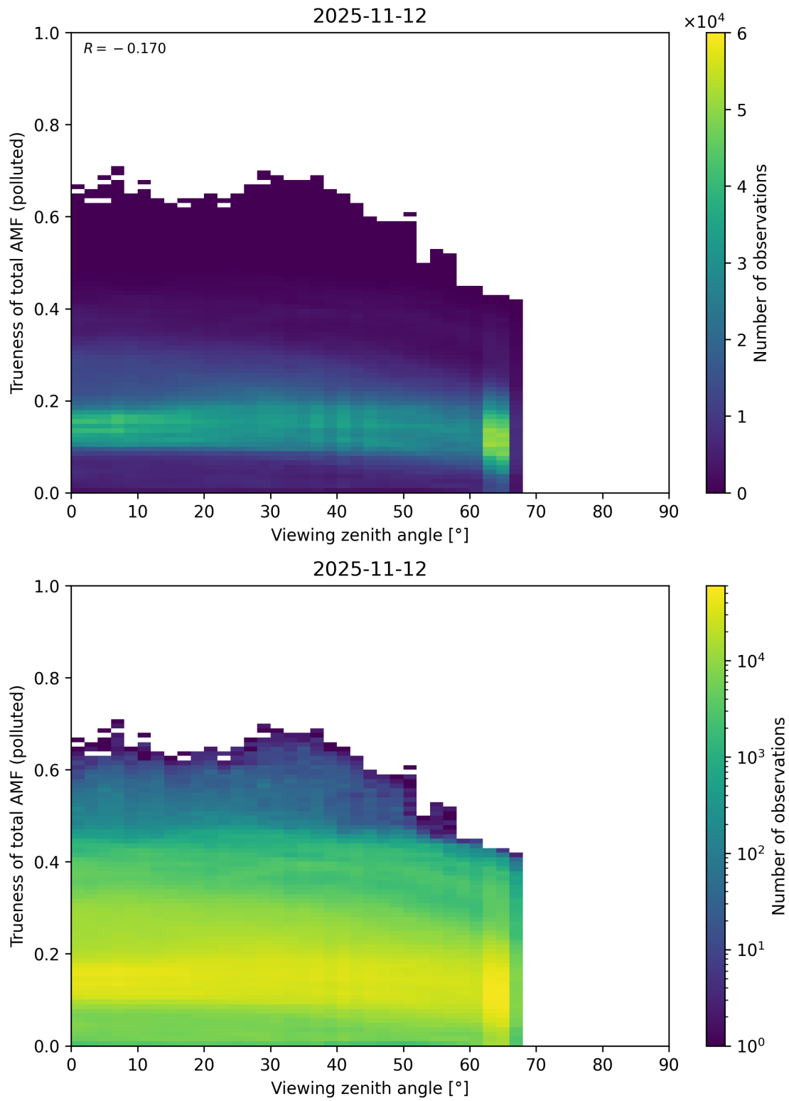
Figure 382: Scatter density plot of “Viewing zenith angle” against “Trueness of total AMF (polluted)” for 2025-11-12 to 2025-11-13.
