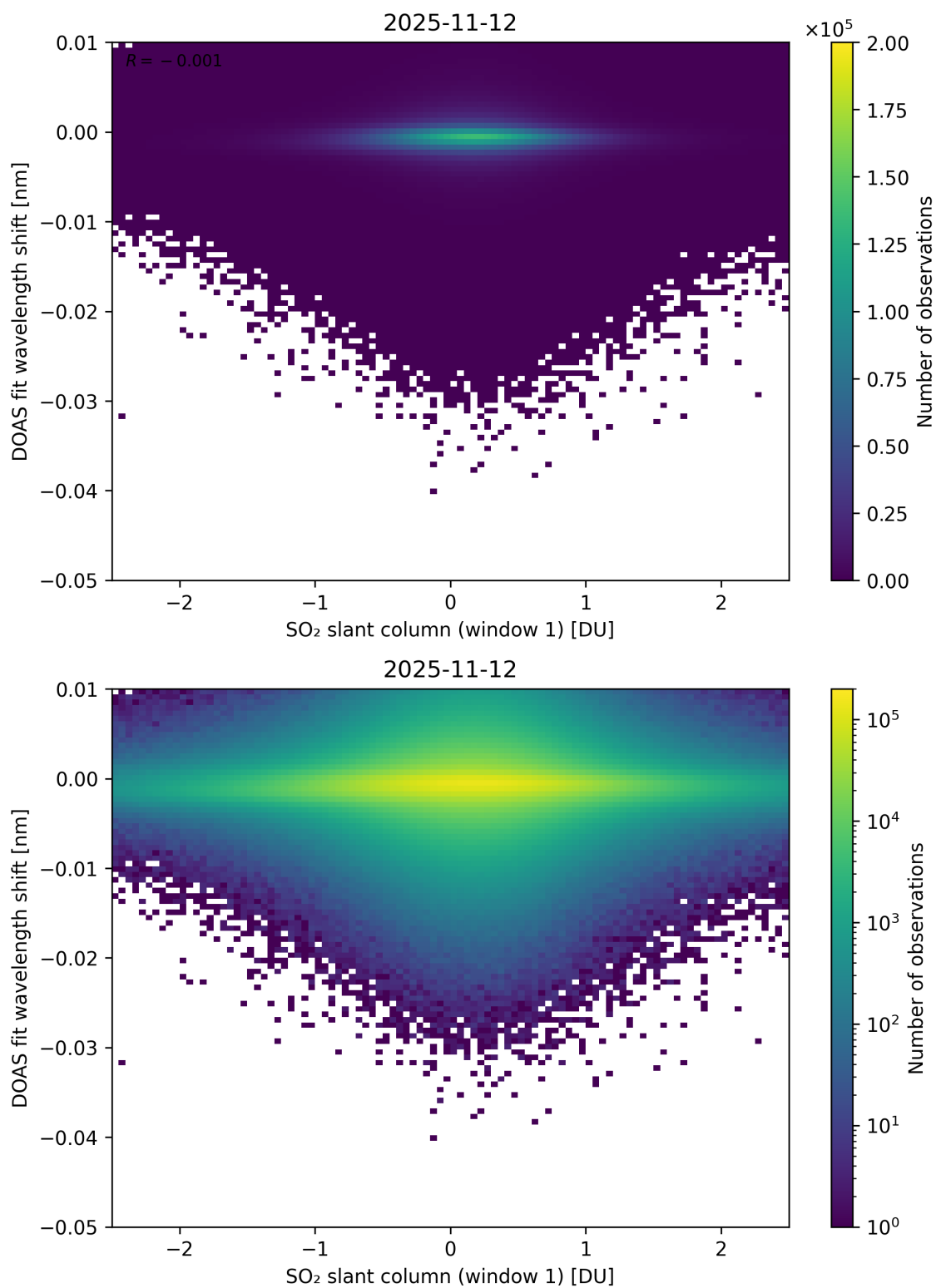
Figure 265: Scatter density plot of “SO 2 slant column (window 1)” against “DOAS fit wavelength shift” for 2025-11-12 to 2025-11-13.
