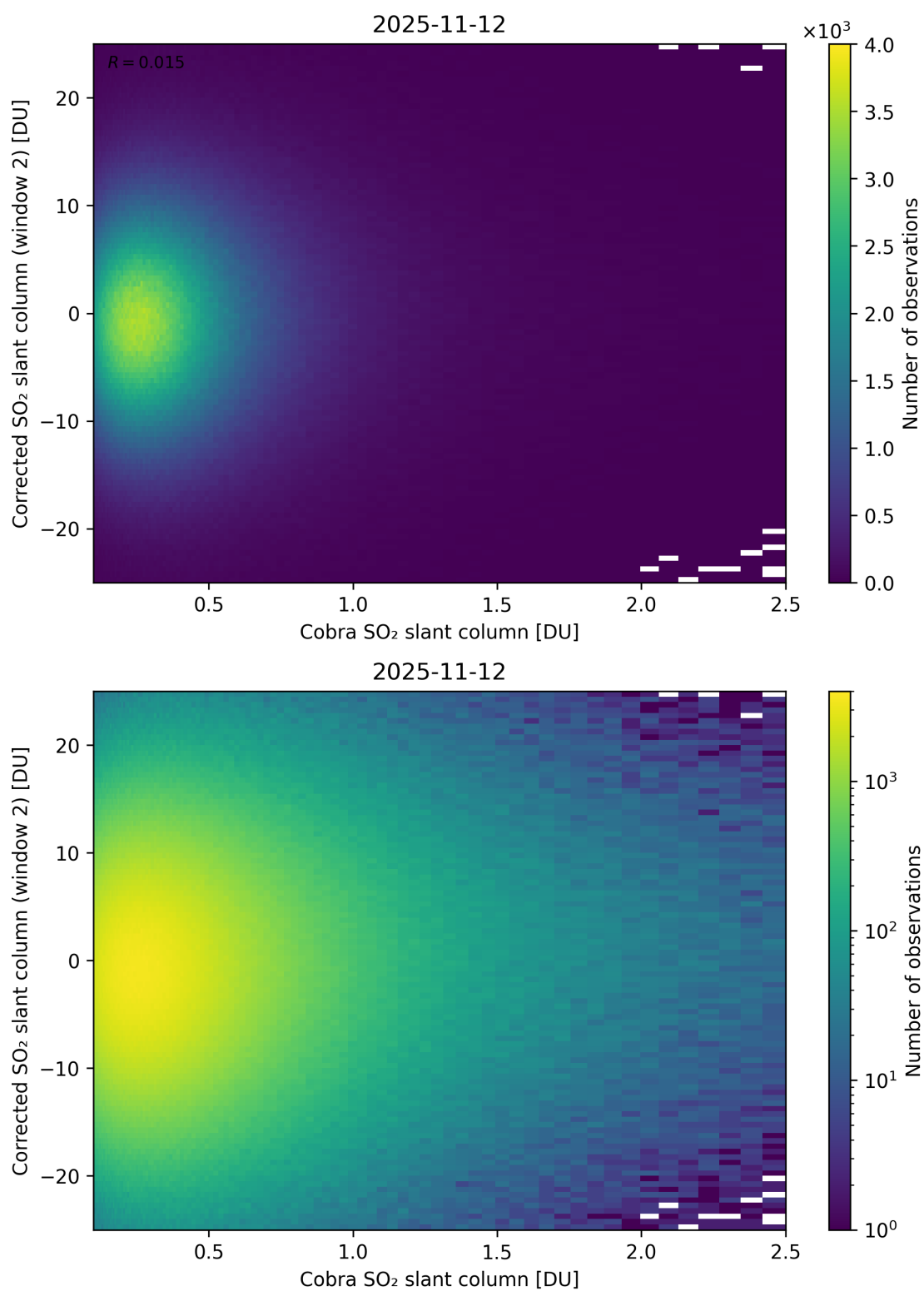
Figure 217: Scatter density plot of “Cobra SO 2 slant column” against “Corrected SO 2 slant column (window 2)” for 2025-11-12 to 2025-11-13.
