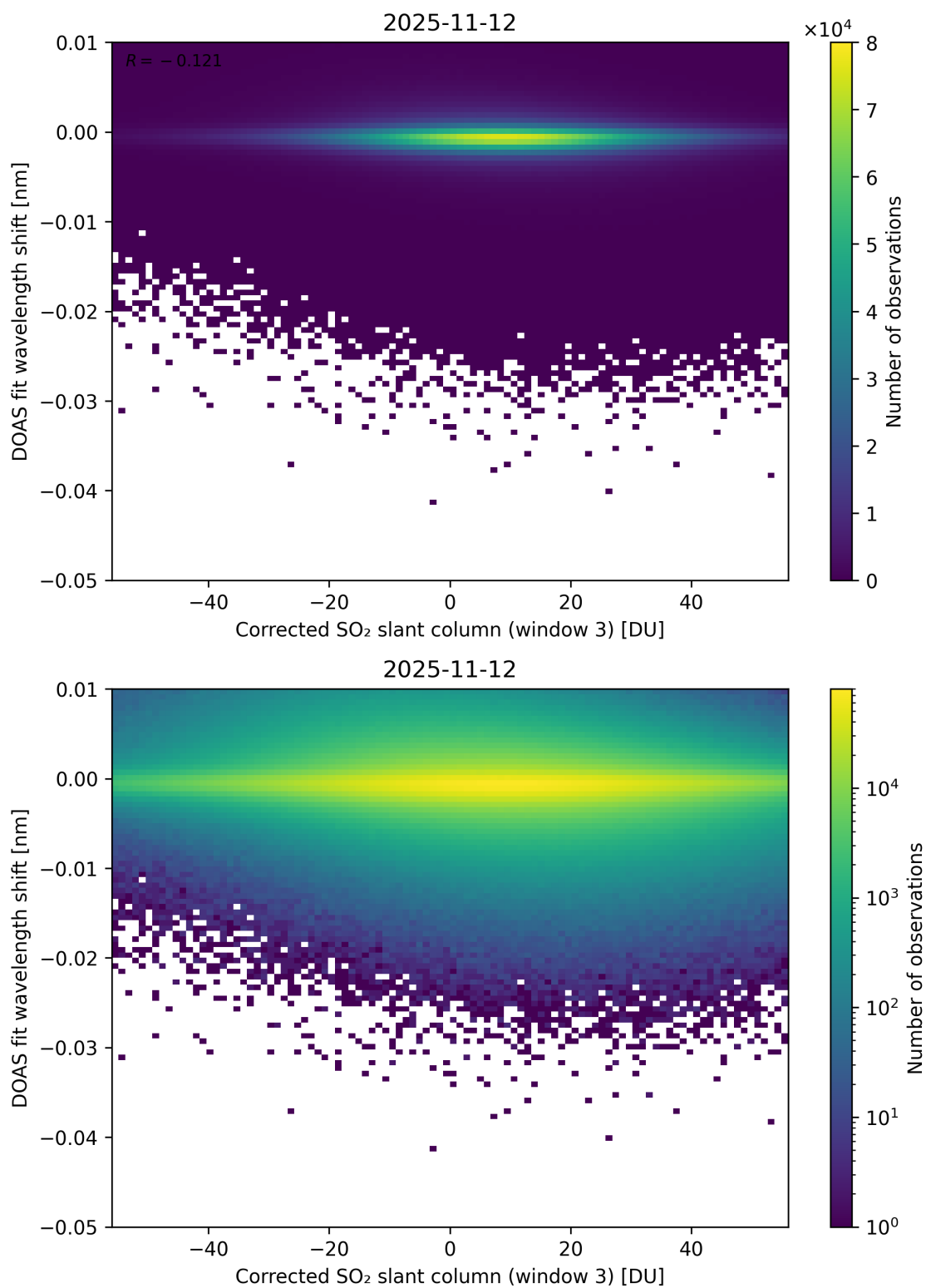
Figure 256: Scatter density plot of “Corrected SO 2 slant column (window 3)” against “DOAS fit wavelength shift” for 2025-11-12 to 2025-11-13.
