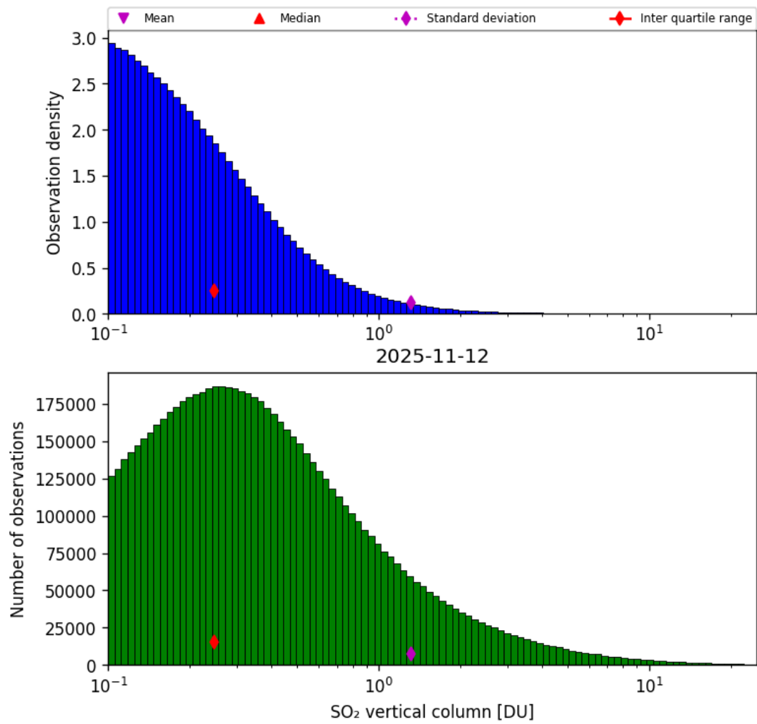
Figure 58: Histogram of “SO 2 vertical column” for 2025-11-12 to 2025-11-13
