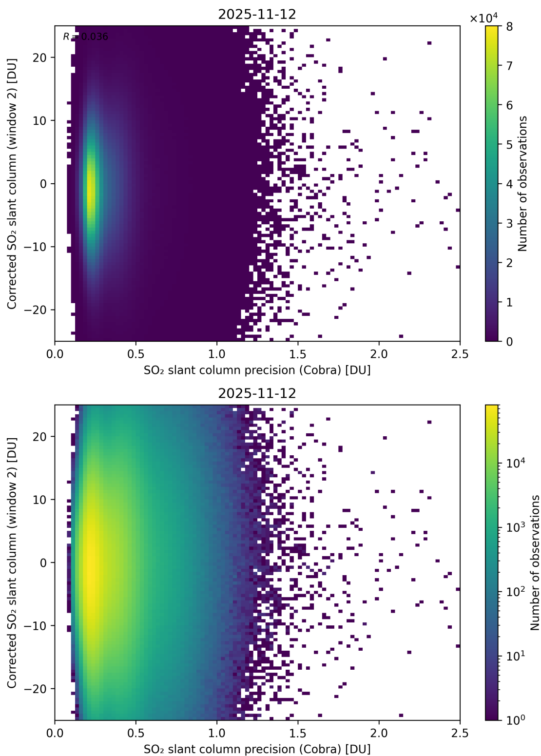
Figure 206: Scatter density plot of “SO 2 slant column precision (Cobra)” against “Corrected SO 2 slant column (window 2)” for 2025-11-12 to 2025-11-13.
