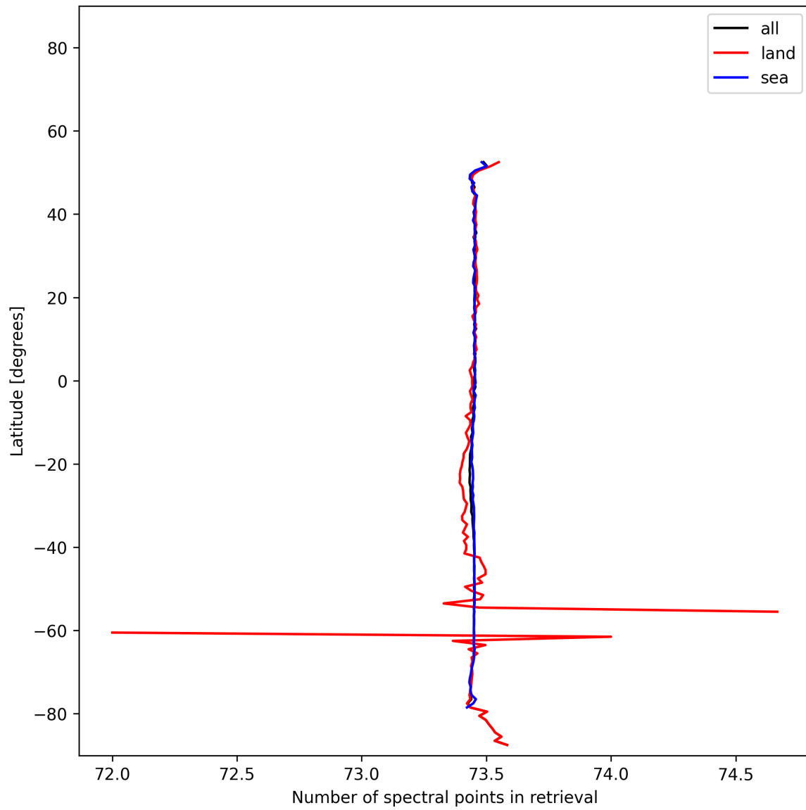
Figure 56: Zonal average of “Number of spectral points in retrieval” for 2025-11-12 to 2025-11-13.
