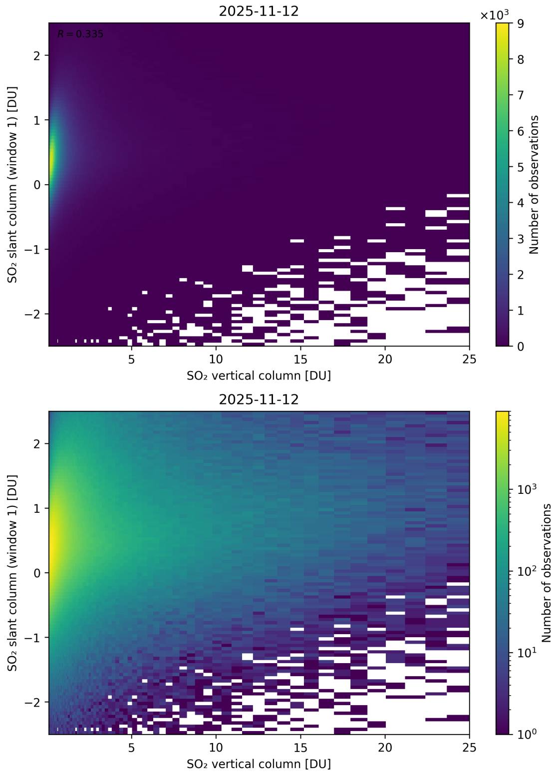
Figure 354: Scatter density plot of “SO 2 vertical column” against “SO 2 slant column (window 1)” for 2025-11-12 to 2025-11-13.
