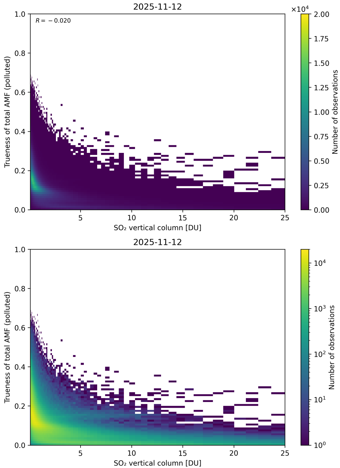
Figure 360: Scatter density plot of “SO 2 vertical column” against “Trueness of total AMF (polluted)” for 2025-11-12 to 2025-11-13.
