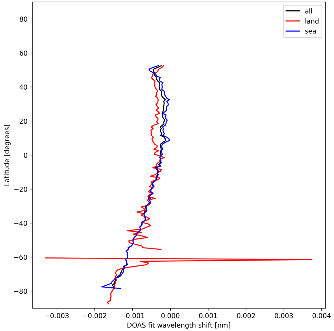
Figure 50: Zonal average of “DOAS fit wavelength shift” for 2025-11-12 to 2025-11-13.
