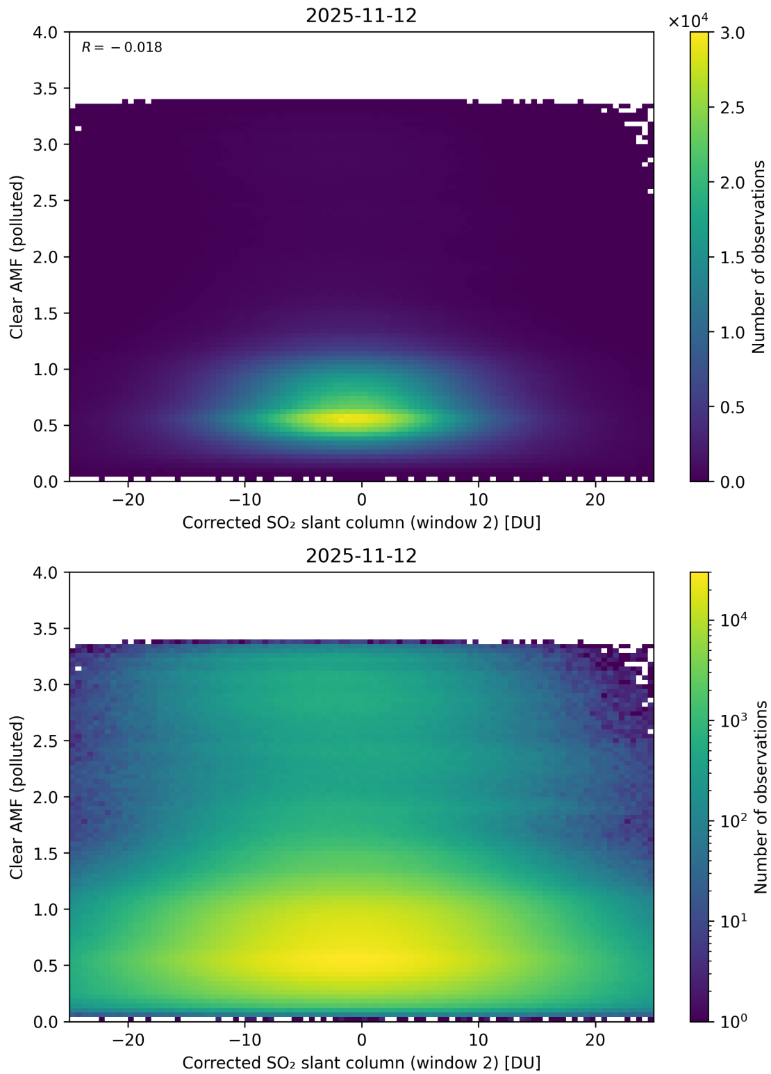
Figure 249: Scatter density plot of “Corrected SO 2 slant column (window 2)” against “Clear AMF (polluted)” for 2025-11-12 to 2025-11-13.
