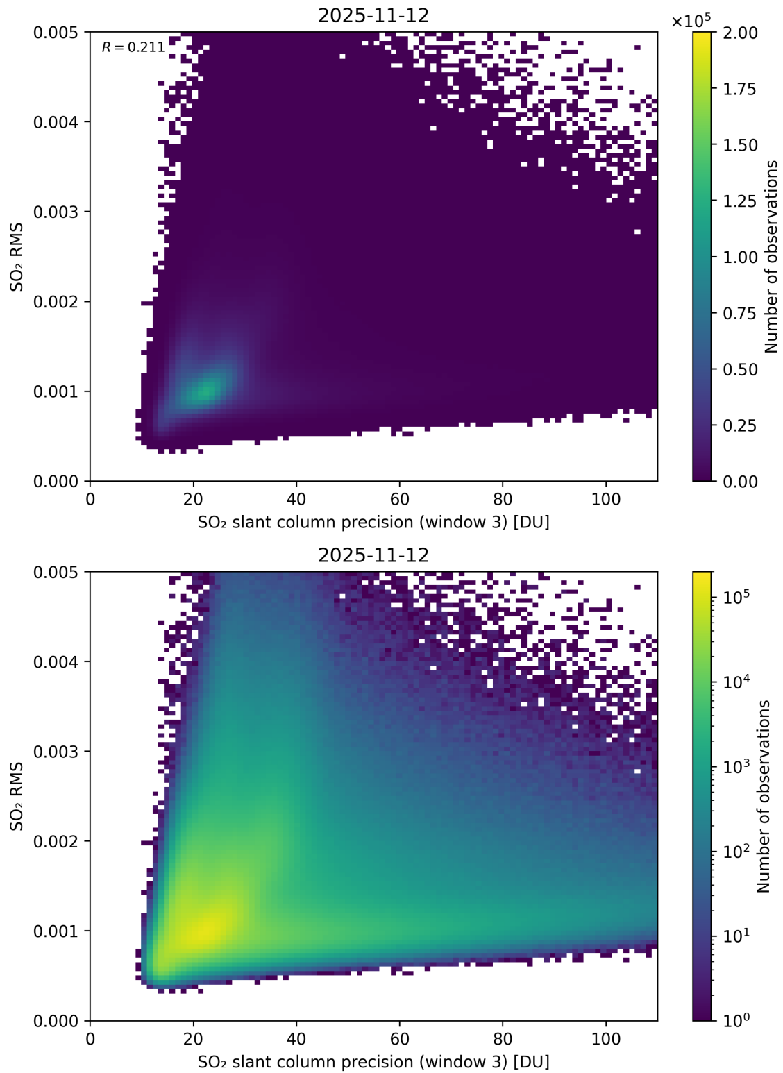
Figure 310: Scatter density plot of “SO 2 slant column precision (window 3)” against “SO 2 RMS” for 2025-11-12 to 2025-11-13.
