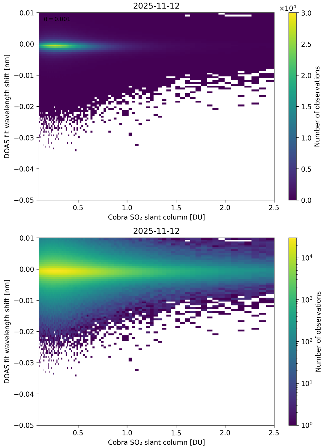
Figure 196: Scatter density plot of “Cobra SO 2 slant column” against “DOAS fit wavelength shift” for 2025-11-12 to 2025-11-13.
