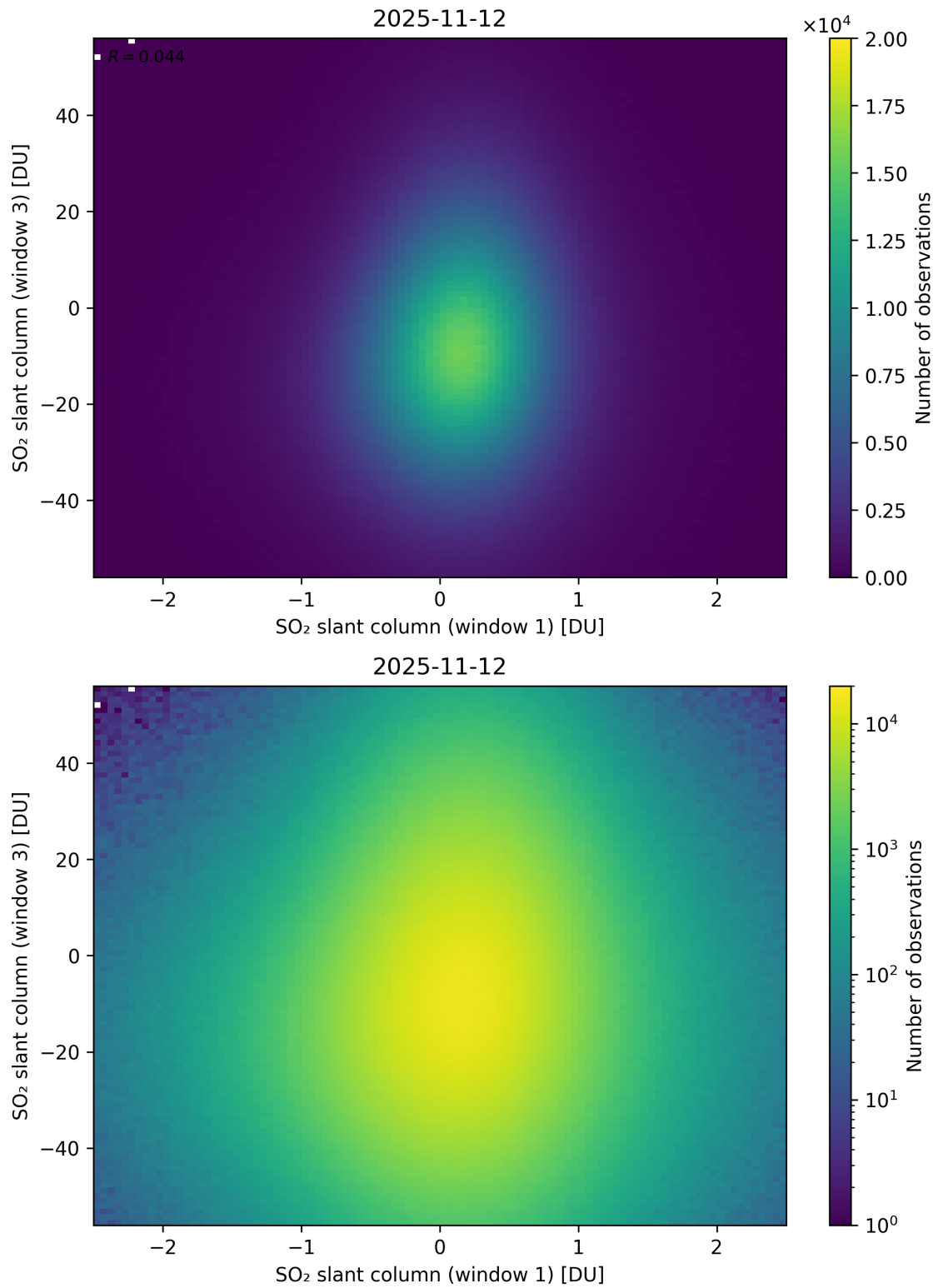
Figure 287: Scatter density plot of “SO 2 slant column (window 1)” against “SO 2 slant column (window 3)” for 2025-11-12 to 2025-11-13.
