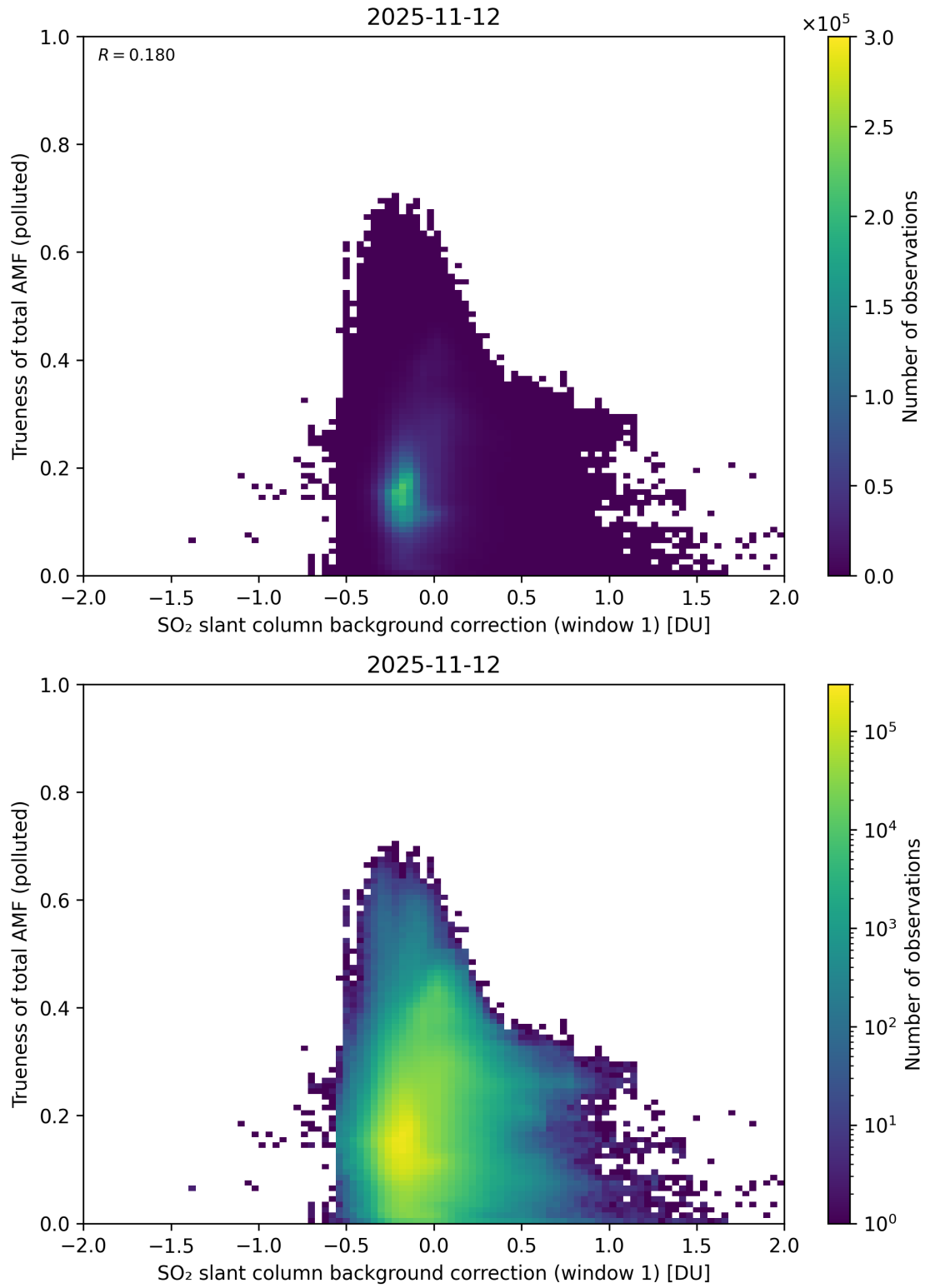
Figure 121: Scatter density plot of “SO 2 slant column background correction (window 1)” against “Trueness of total AMF (polluted)” for 2025-11-12 to 2025-11-13.
