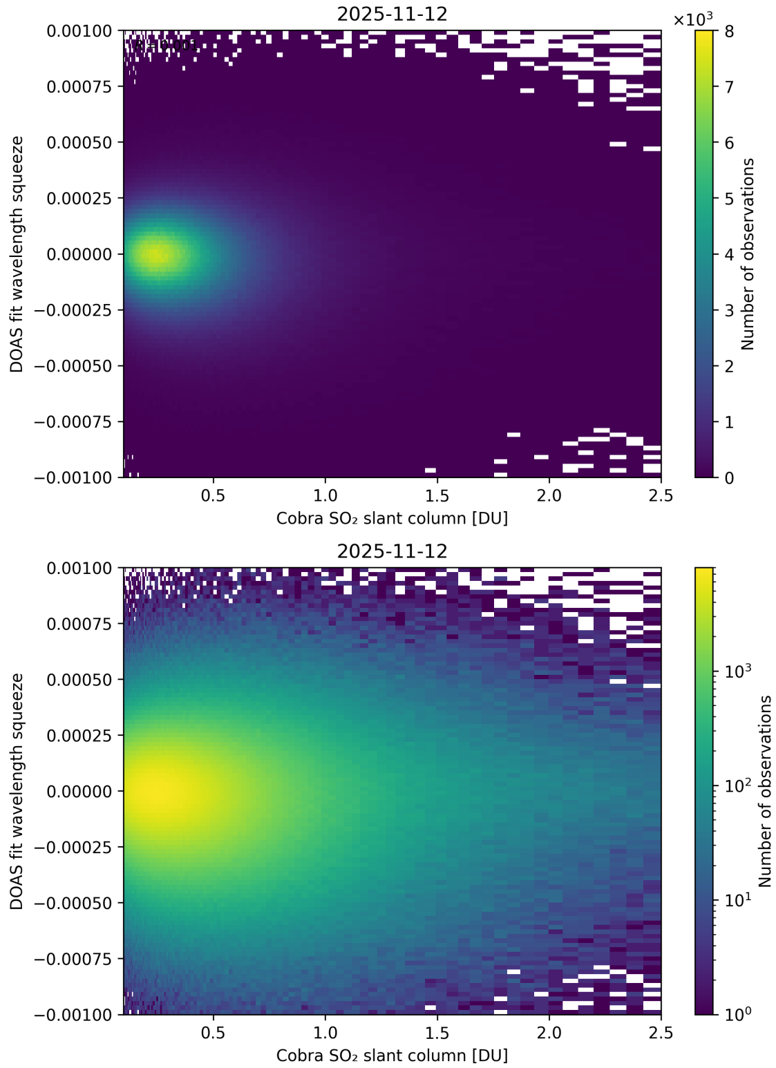
Figure 197: Scatter density plot of “Cobra SO 2 slant column” against “DOAS fit wavelength squeeze” for 2025-11-12 to 2025-11-13.
