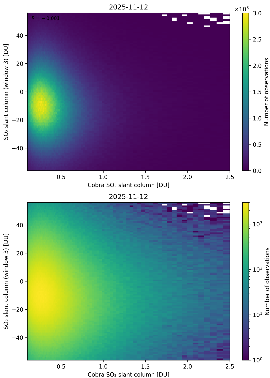
Figure 222: Scatter density plot of “Cobra SO 2 slant column” against “SO 2 slant column (window 3)” for 2025-11-12 to 2025-11-13.
