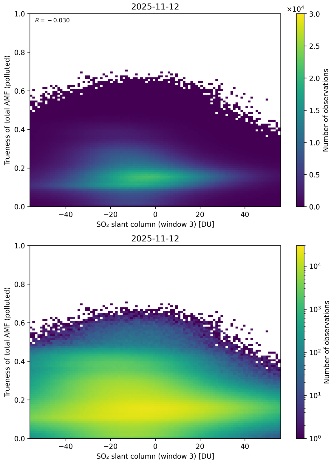
Figure 319: Scatter density plot of “SO 2 slant column (window 3)” against “Trueness of total AMF (polluted)” for 2025-11-12 to 2025-11-13.
