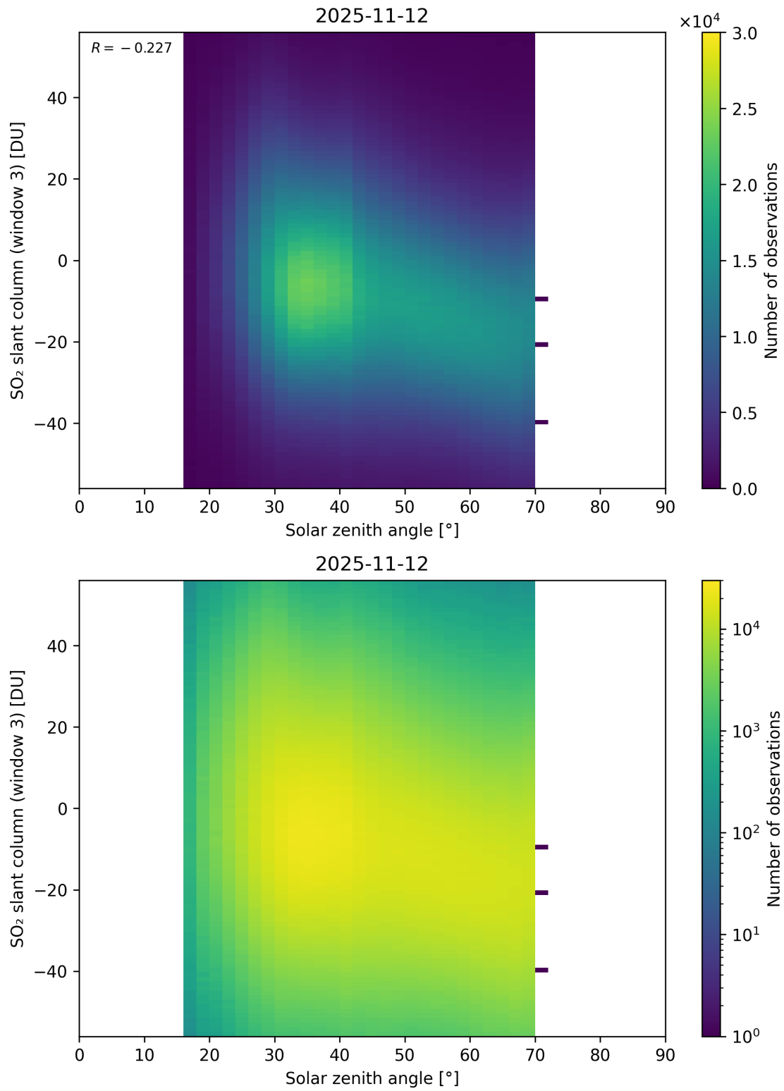
Figure 187: Scatter density plot of “Solar zenith angle” against “SO 2 slant column (window 3)” for 2025-11-12 to 2025-11-13.
