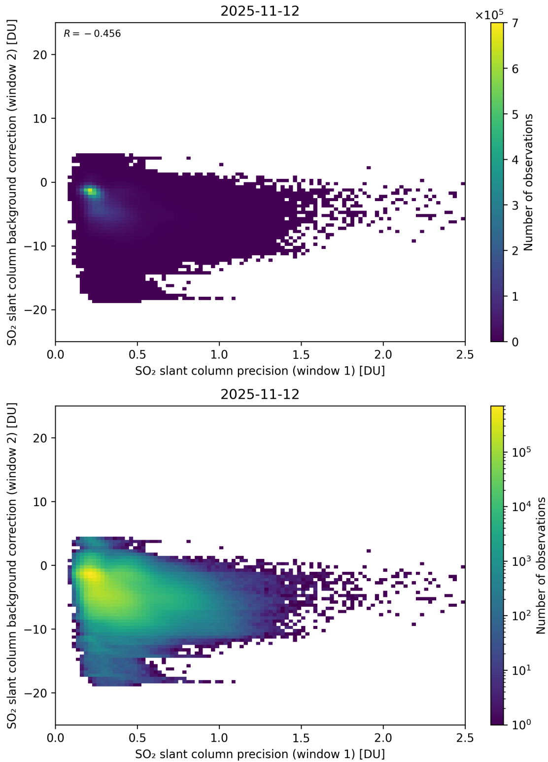
Figure 269: Scatter density plot of “SO 2 slant column precision (window 1)” against “SO 2 slant column background correction (window 2)” for 2025-11-12 to 2025-11-13.
