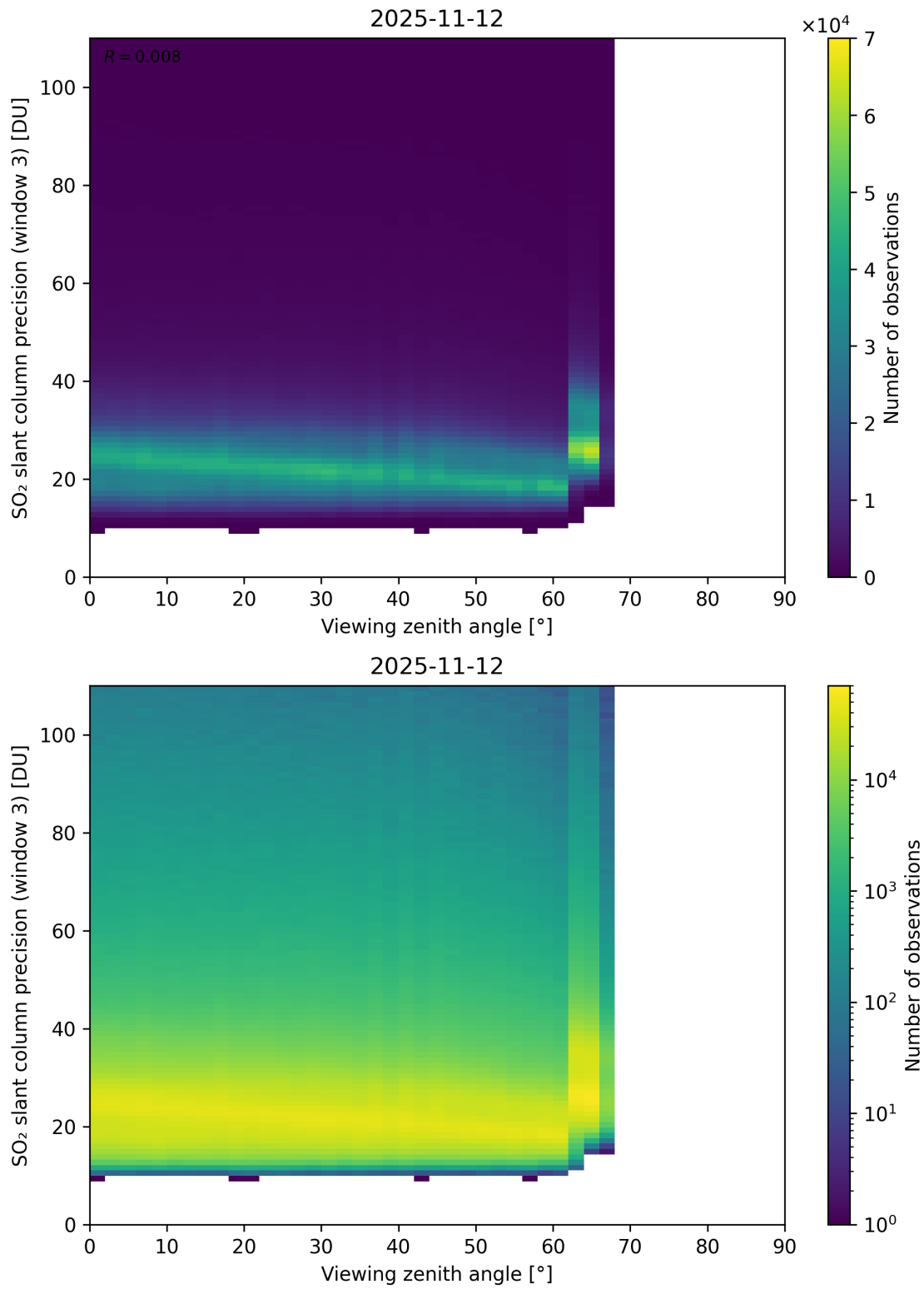
Figure 380: Scatter density plot of “Viewing zenith angle” against “SO 2 slant column precision (window 3)” for 2025-11-12 to 2025-11-13.
