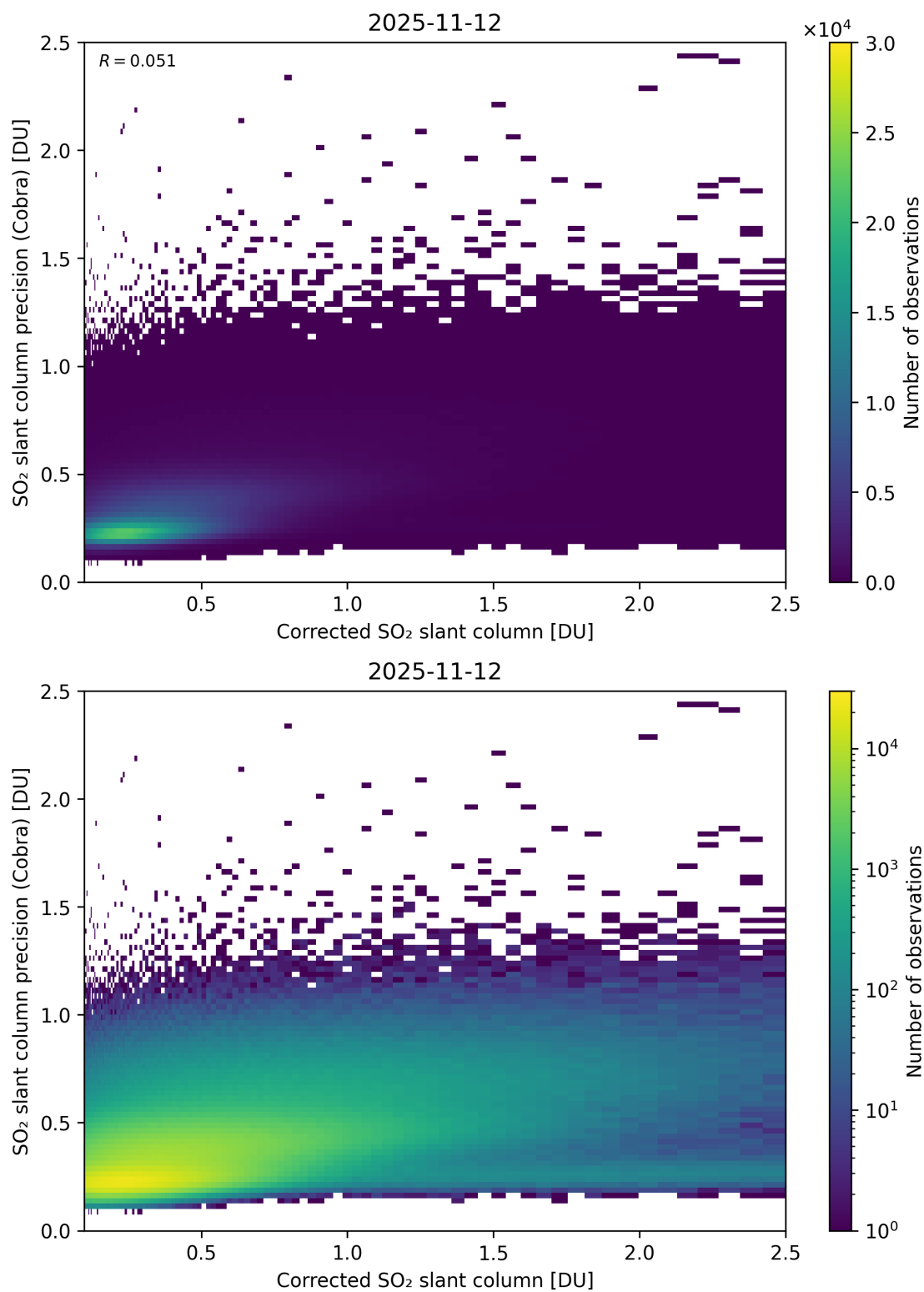
Figure 234: Scatter density plot of “Corrected SO 2 slant column” against “SO 2 slant column precision (Cobra)” for 2025-11-12 to 2025-11-13.
