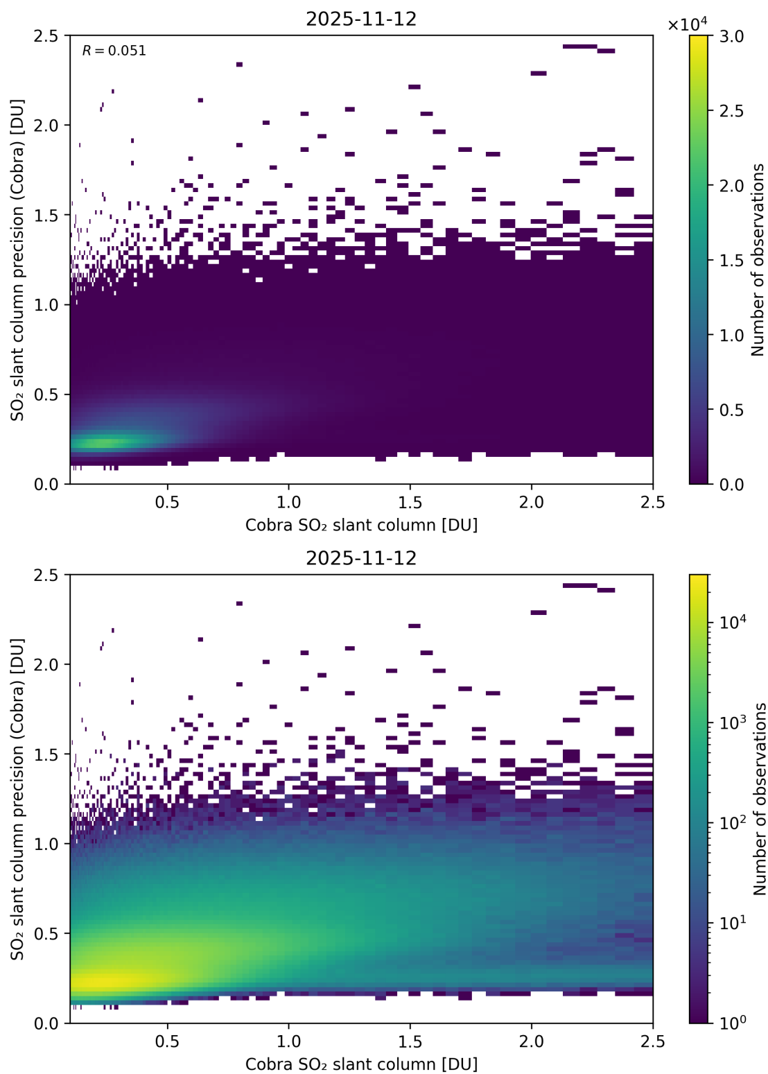
Figure 216: Scatter density plot of “Cobra SO 2 slant column” against “SO 2 slant column precision (Cobra)” for 2025-11-12 to 2025-11-13.
