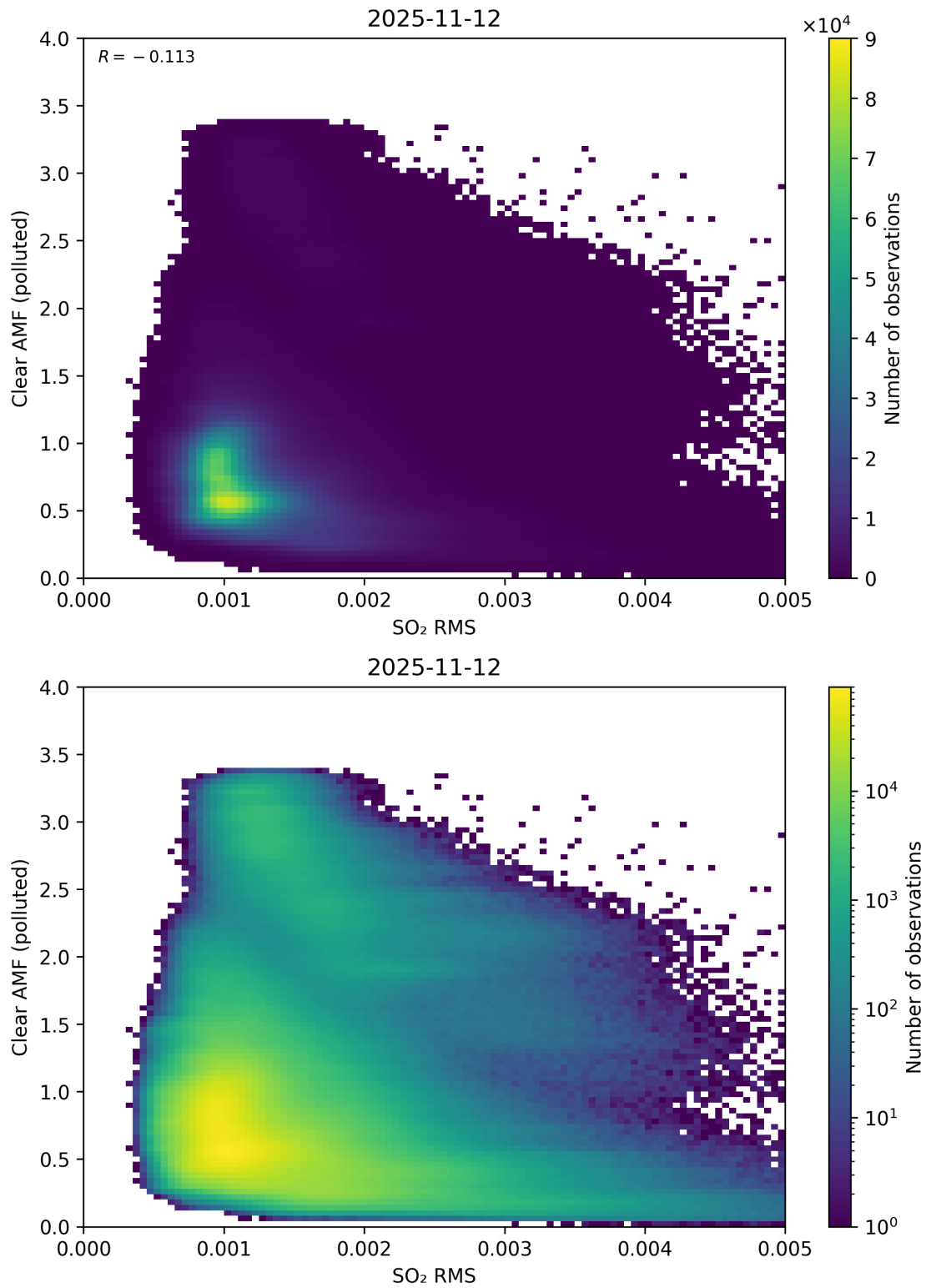
Figure 147: Scatter density plot of “SO 2 RMS” against “Clear AMF (polluted)” for 2025-11-12 to 2025-11-13.
