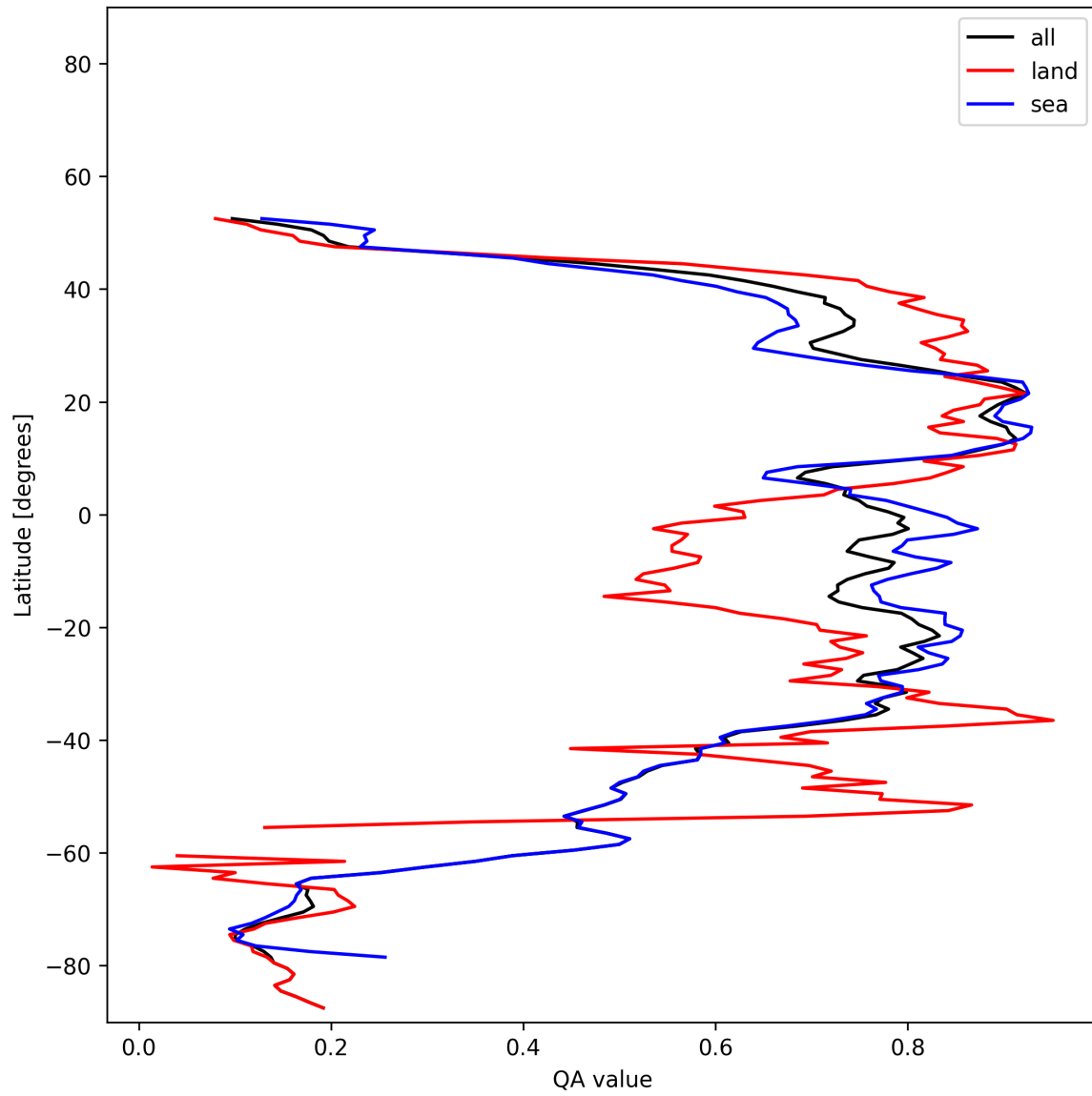
Figure 31: Zonal average of “QA value” for 2025-11-12 to 2025-11-13.
