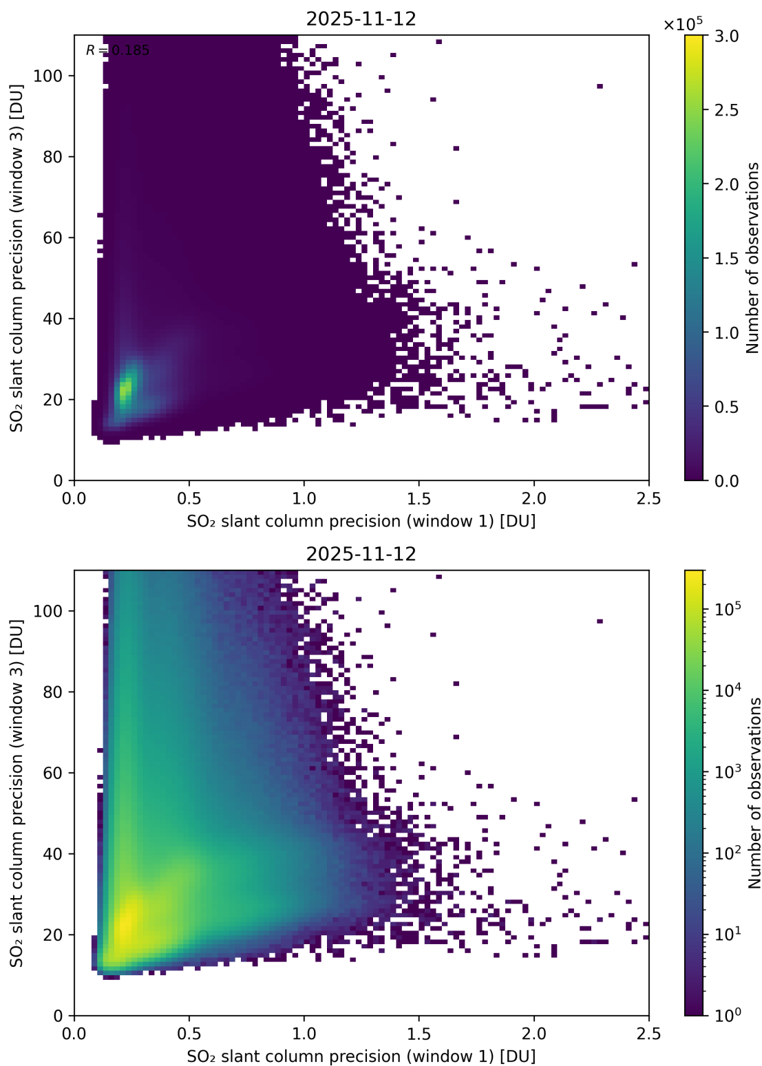
Figure 279: Scatter density plot of “SO 2 slant column precision (window 1)” against “SO 2 slant column precision (window 3)” for 2025-11-12 to 2025-11-13.
