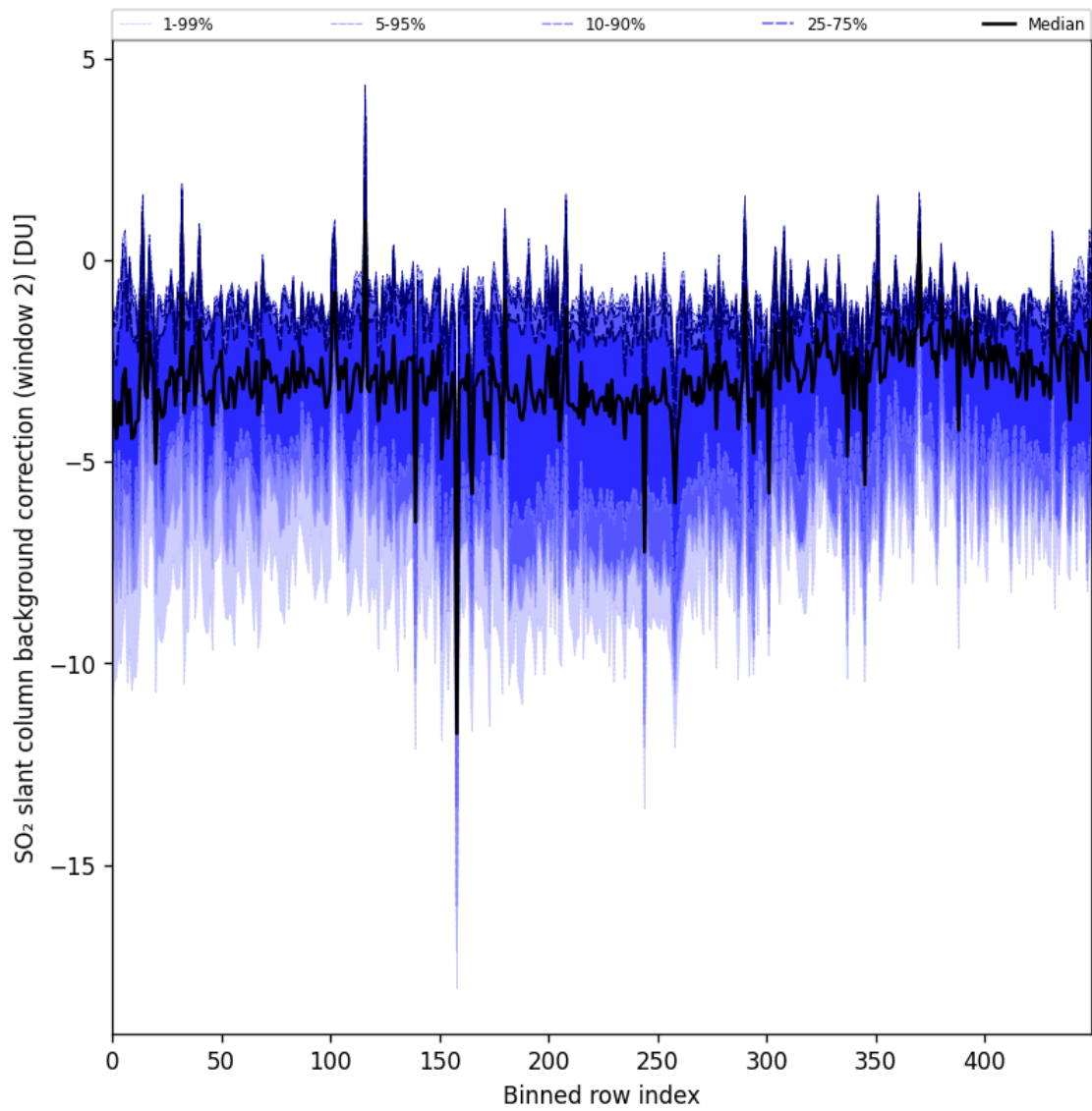
Figure 96: Along track statistics of “SO 2 slant column background correction (window 2)” for 2025-11-12 to 2025-11-13
