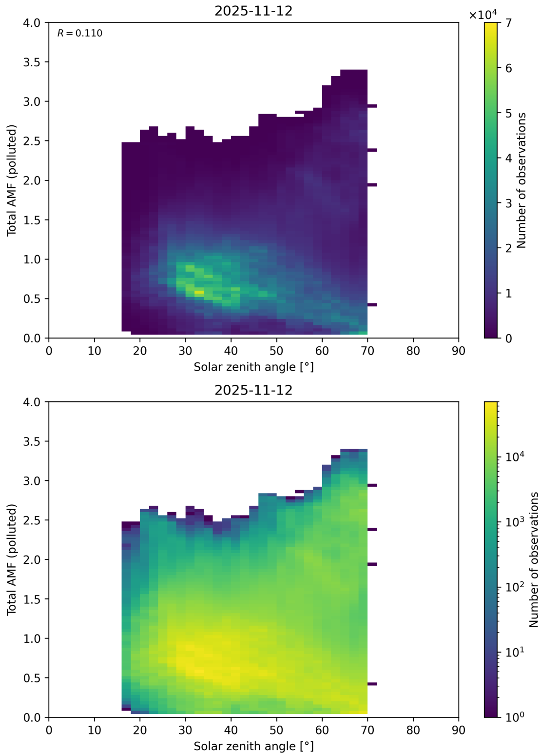
Figure 189: Scatter density plot of “Solar zenith angle” against “Total AMF (polluted)” for 2025-11-12 to 2025-11-13.
