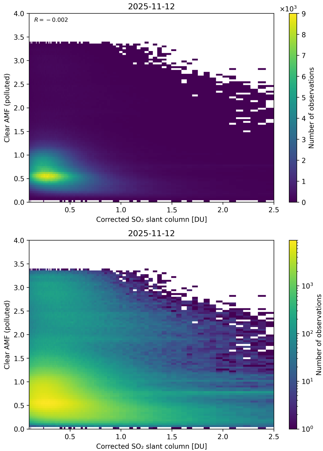
Figure 232: Scatter density plot of “Corrected SO 2 slant column” against “Clear AMF (polluted)” for 2025-11-12 to 2025-11-13.
