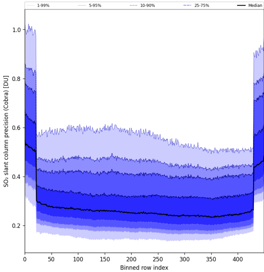
Figure 88: Along track statistics of “SO 2 slant column precision (Cobra)” for 2025-11-12 to 2025-11-13
