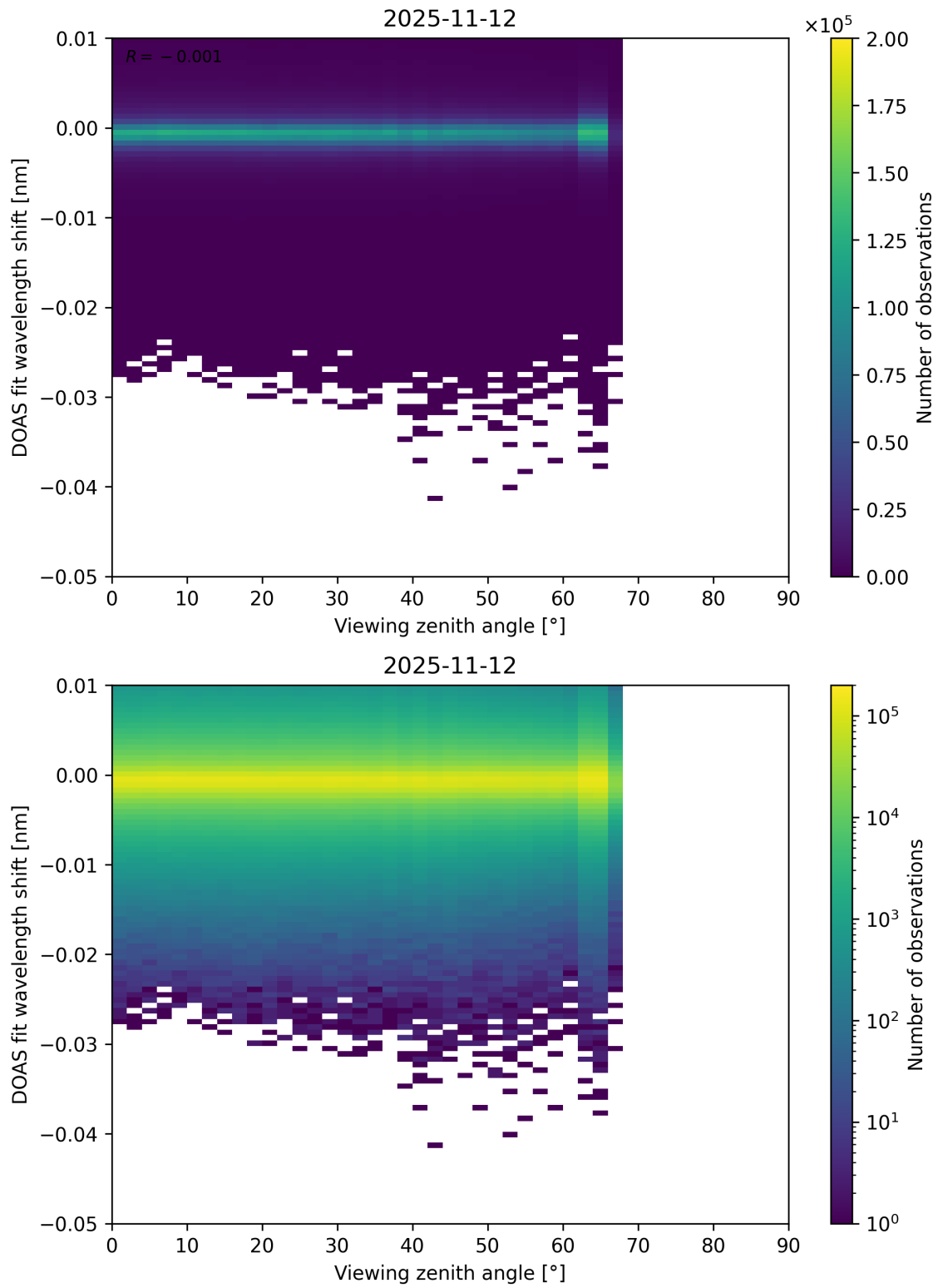
Figure 365: Scatter density plot of “Viewing zenith angle” against “DOAS fit wavelength shift” for 2025-11-12 to 2025-11-13.
