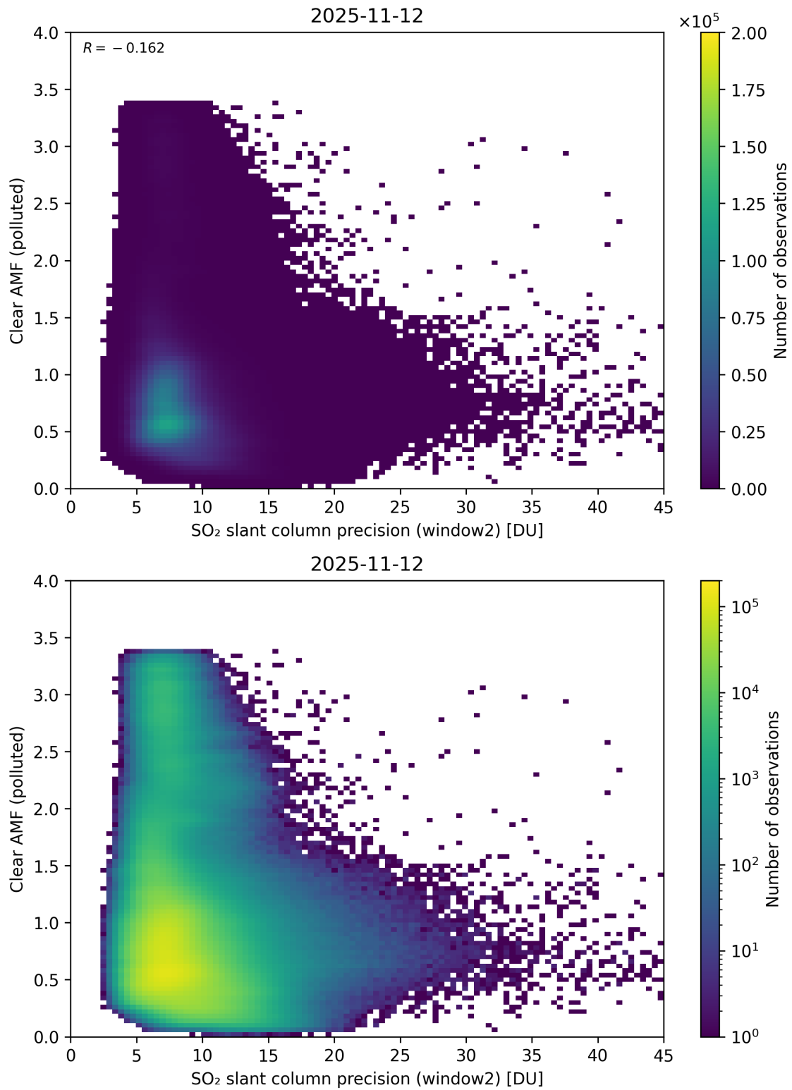
Figure 296: Scatter density plot of “SO 2 slant column precision (window2)” against “Clear AMF (polluted)” for 2025-11-12 to 2025-11-13.
