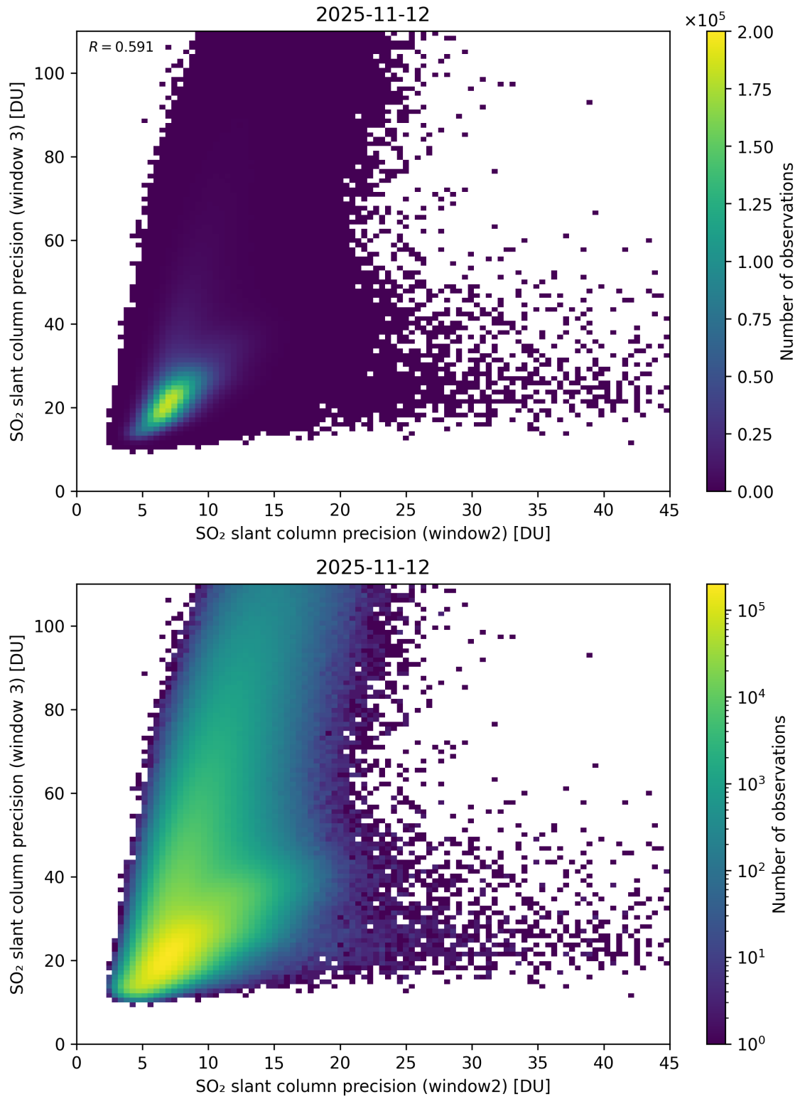
Figure 300: Scatter density plot of “SO 2 slant column precision (window2)” against “SO 2 slant column precision (window 3)” for 2025-11-12 to 2025-11-13.
