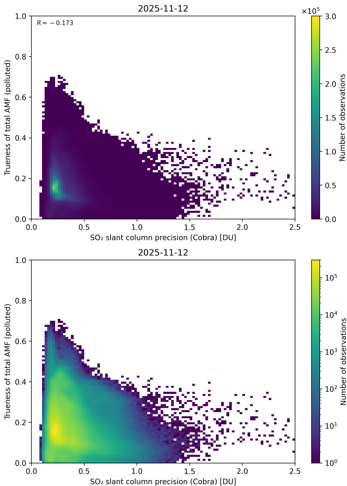
Figure 214: Scatter density plot of “SO 2 slant column precision (Cobra)” against “Trueness of total AMF (polluted)” for 2025-11-12 to 2025-11-13.
