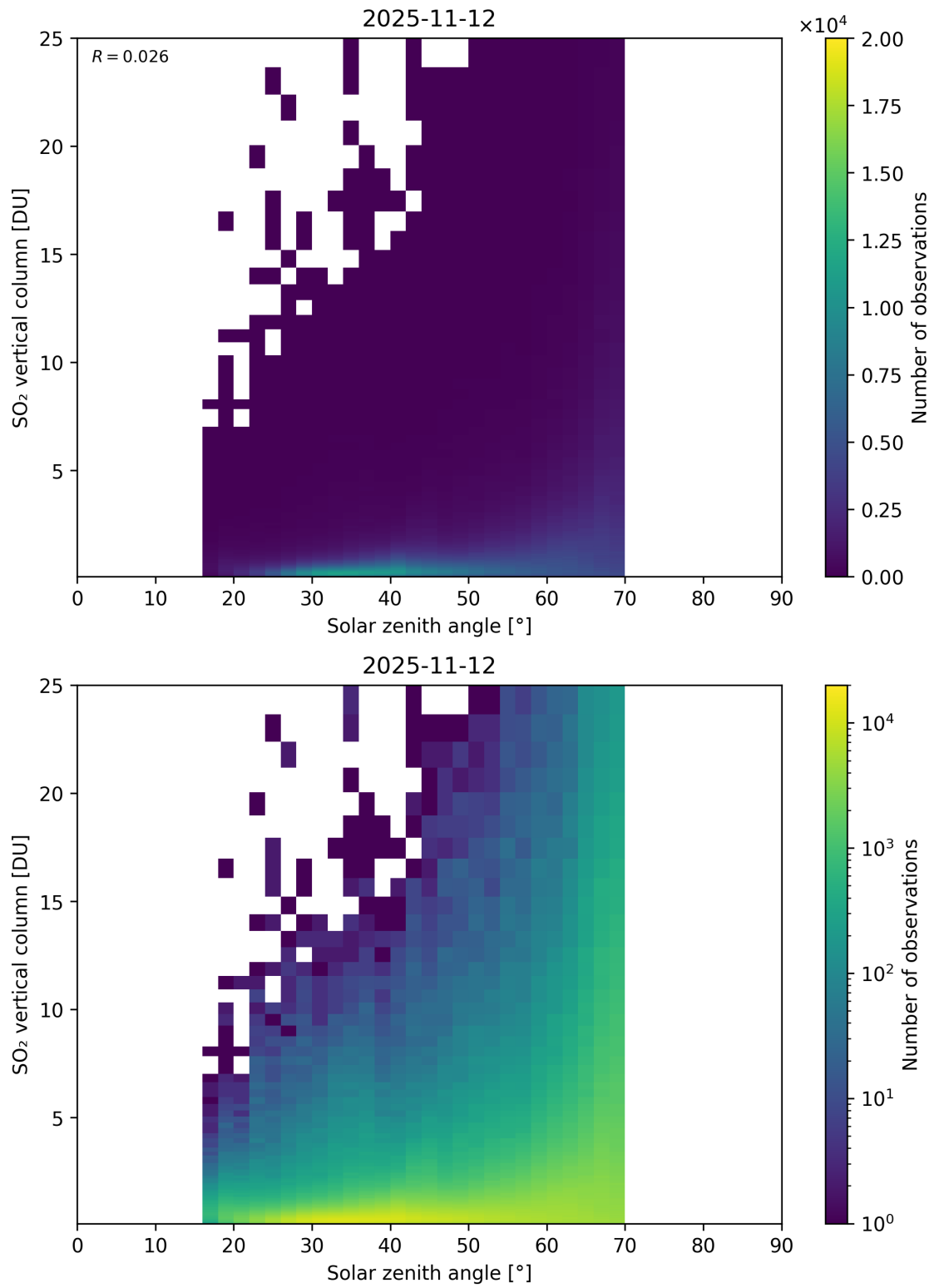
Figure 191: Scatter density plot of “Solar zenith angle” against “SO 2 vertical column” for 2025-11-12 to 2025-11-13.
