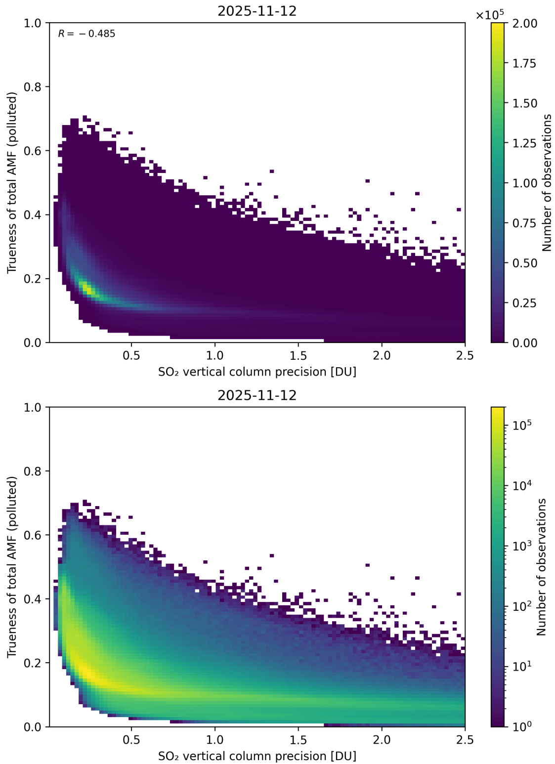
Figure 347: Scatter density plot of “SO 2 vertical column precision” against “Trueness of total AMF (polluted)” for 2025-11-12 to 2025-11-13.
