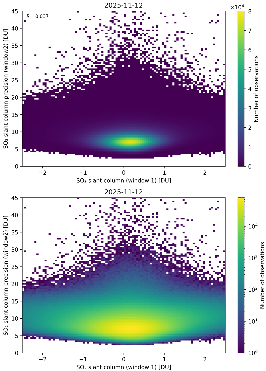
Figure 286: Scatter density plot of “SO 2 slant column (window 1)” against “SO 2 slant column precision (window2)” for 2025-11-12 to 2025-11-13.
