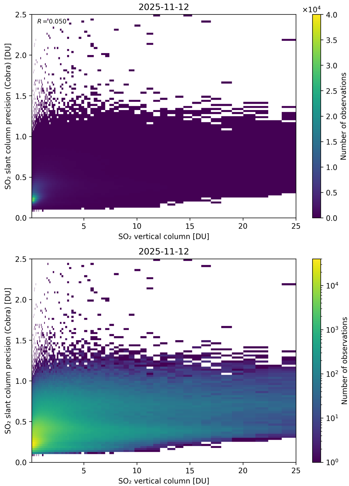
Figure 350: Scatter density plot of “SO 2 vertical column” against “SO 2 slant column precision (Cobra)” for 2025-11-12 to 2025-11-13.
