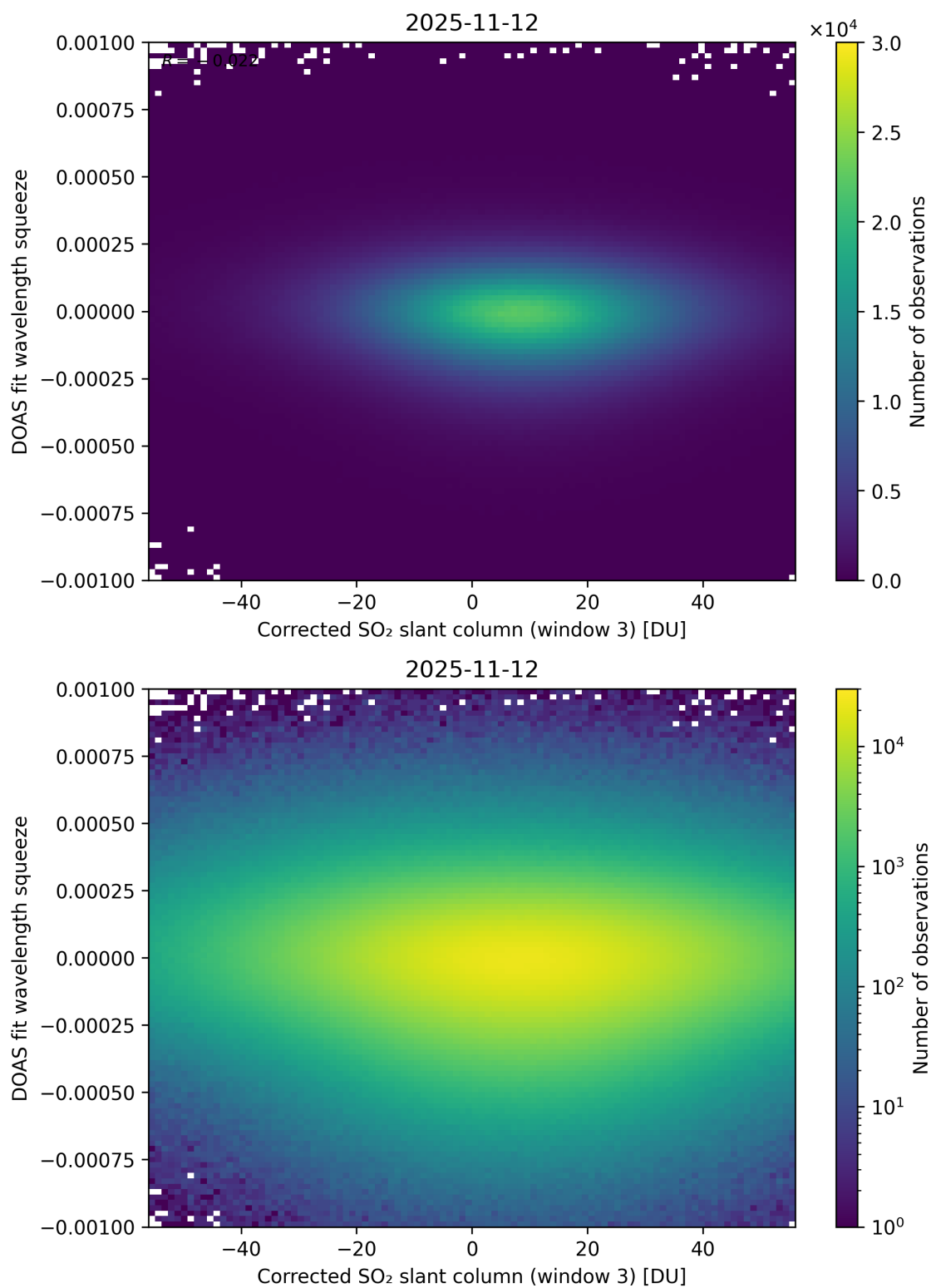
Figure 257: Scatter density plot of “Corrected SO 2 slant column (window 3)” against “DOAS fit wavelength squeeze” for 2025-11-12 to 2025-11-13.
