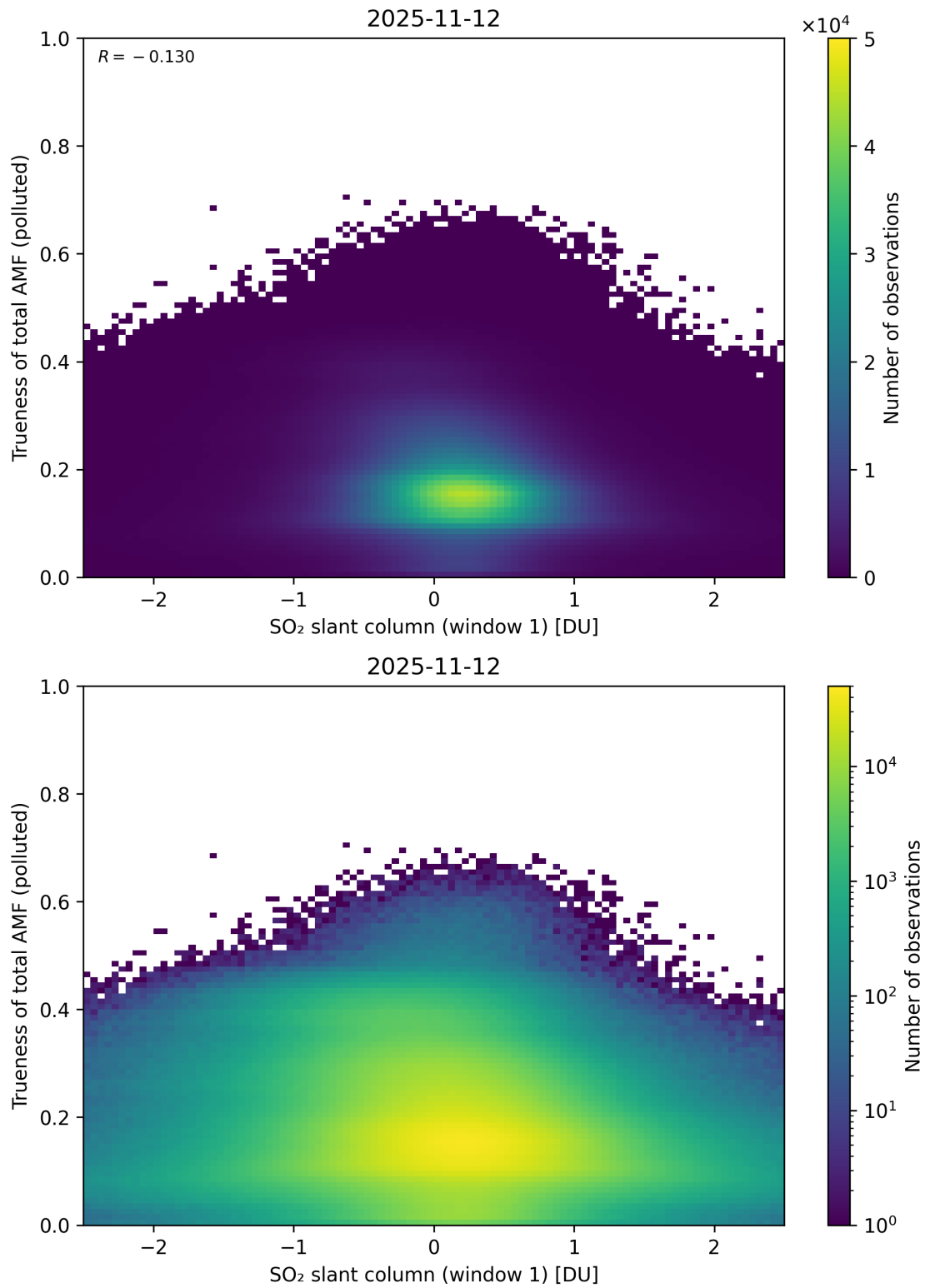
Figure 290: Scatter density plot of “SO 2 slant column (window 1)” against “Trueness of total AMF (polluted)” for 2025-11-12 to 2025-11-13.
