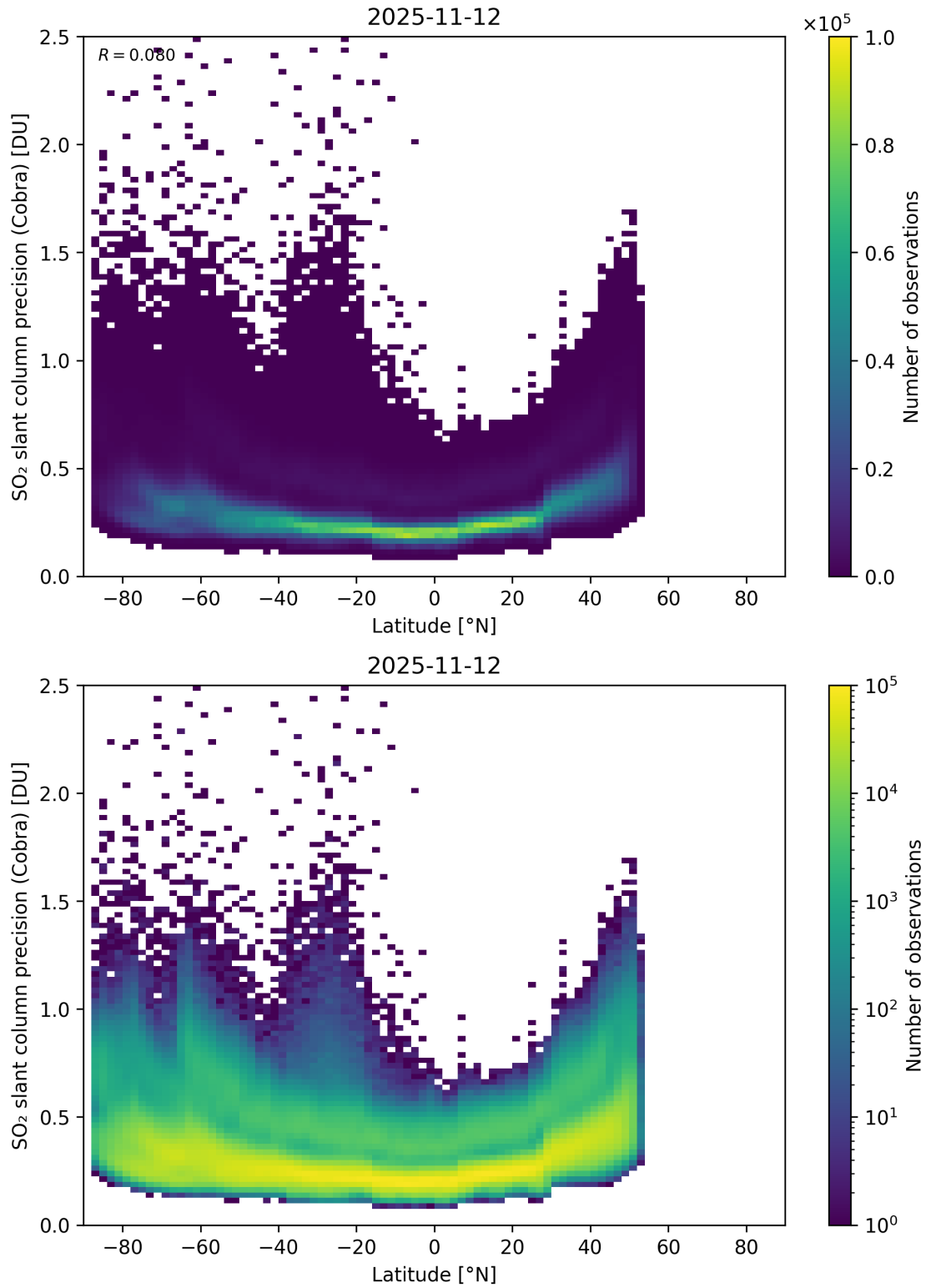
Figure 158: Scatter density plot of “Latitude” against “SO 2 slant column precision (Cobra)” for 2025-11-12 to 2025-11-13.
