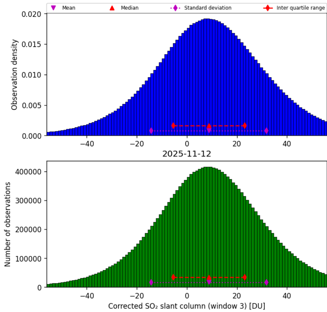
Figure 73: Histogram of “Corrected SO 2 slant column (window 3)” for 2025-11-12 to 2025-11-13
