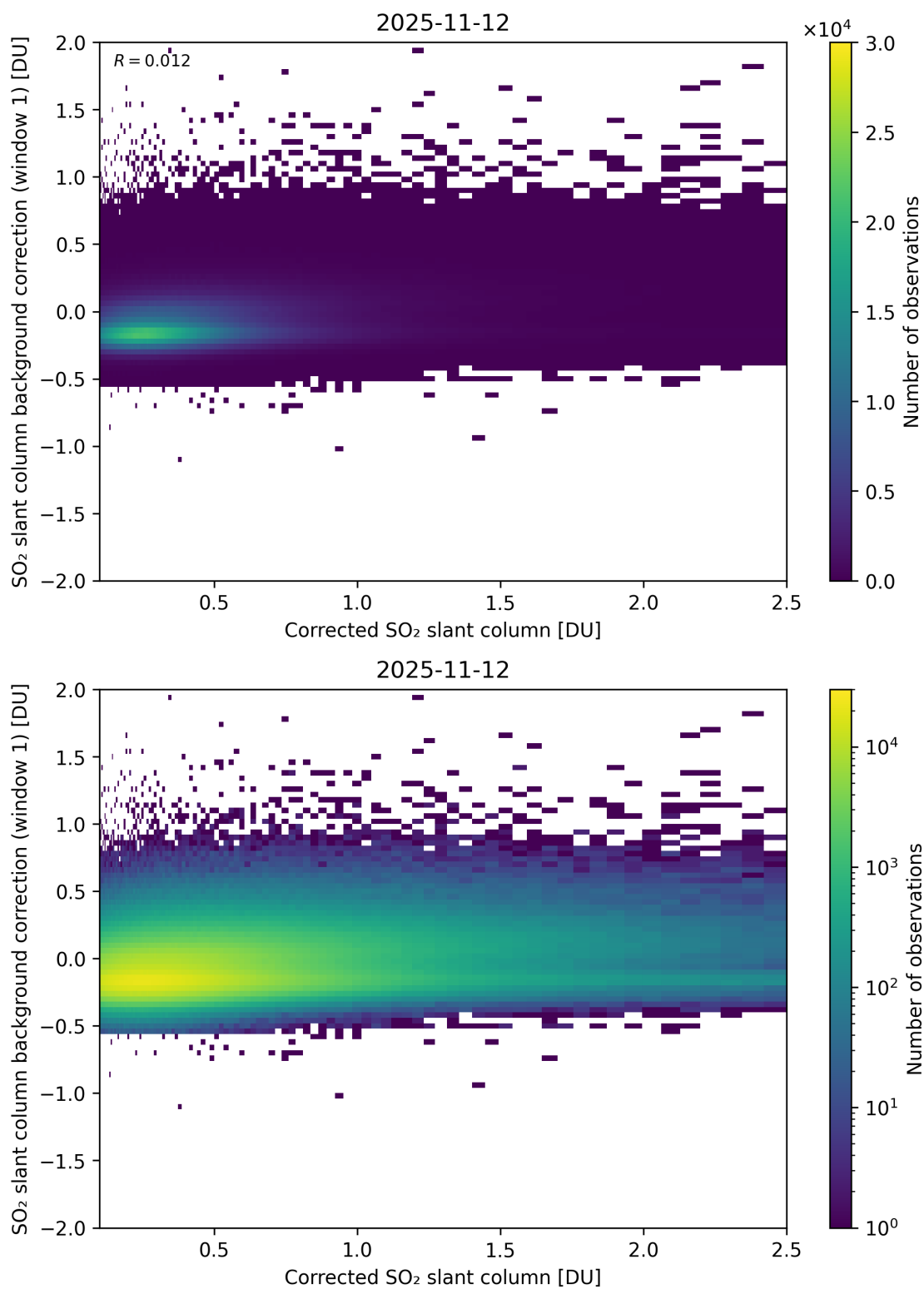
Figure 226: Scatter density plot of “Corrected SO 2 slant column” against “SO 2 slant column background correction (window 1)” for 2025-11-12 to 2025-11-13.
