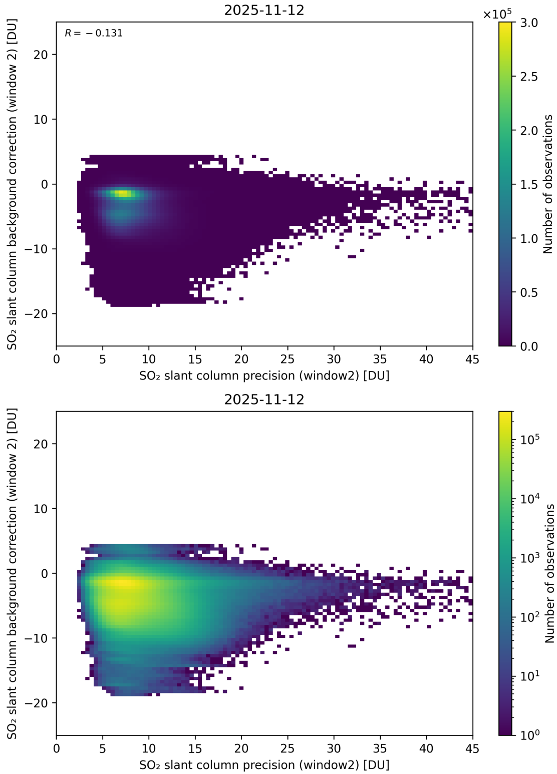
Figure 291: Scatter density plot of “SO 2 slant column precision (window2)” against “SO 2 slant column background correction (window 2)” for 2025-11-12 to 2025-11-13.
