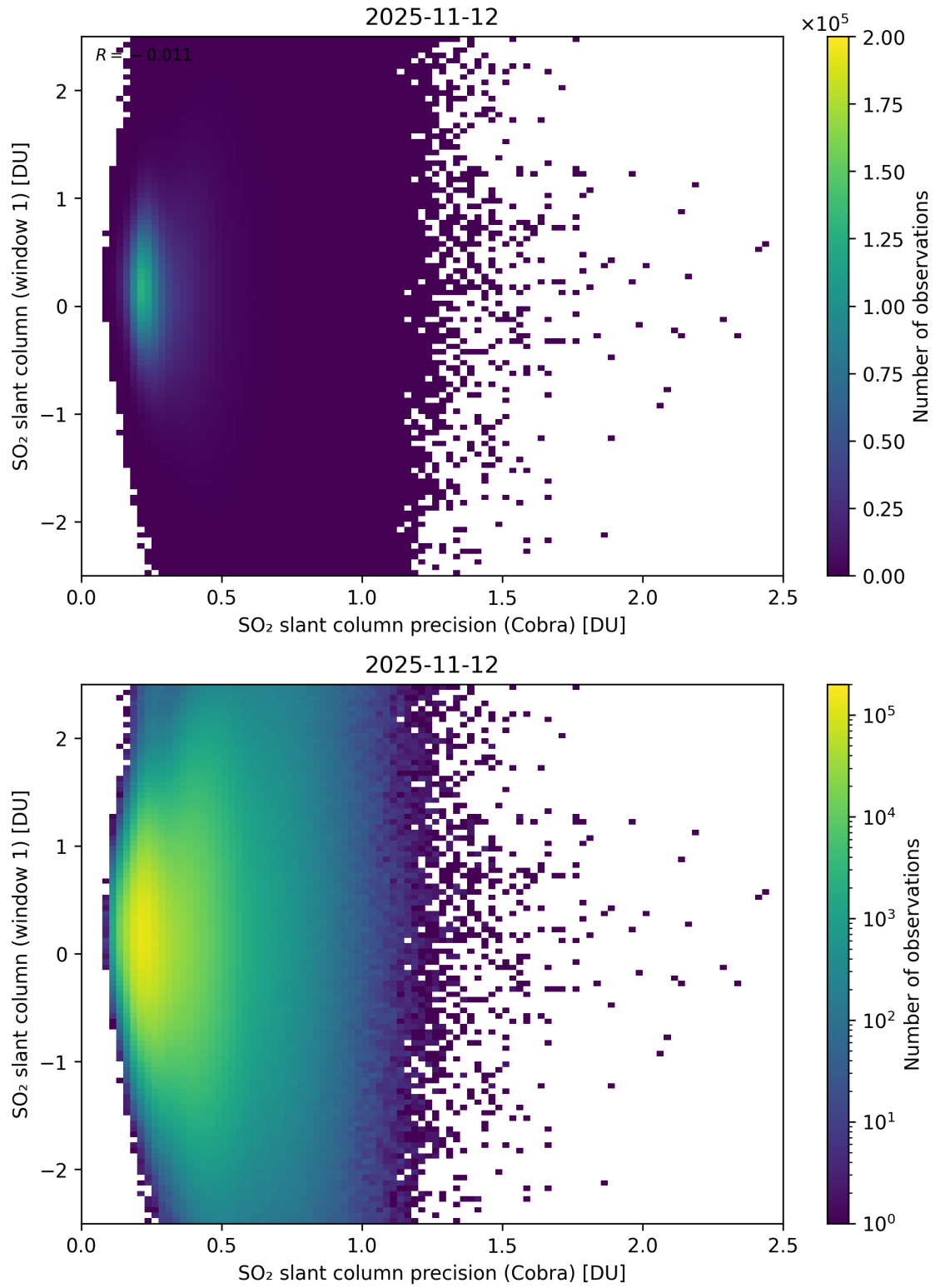
Figure 208: Scatter density plot of “SO 2 slant column precision (Cobra)” against “SO 2 slant column (window 1)” for 2025-11-12 to 2025-11-13.
