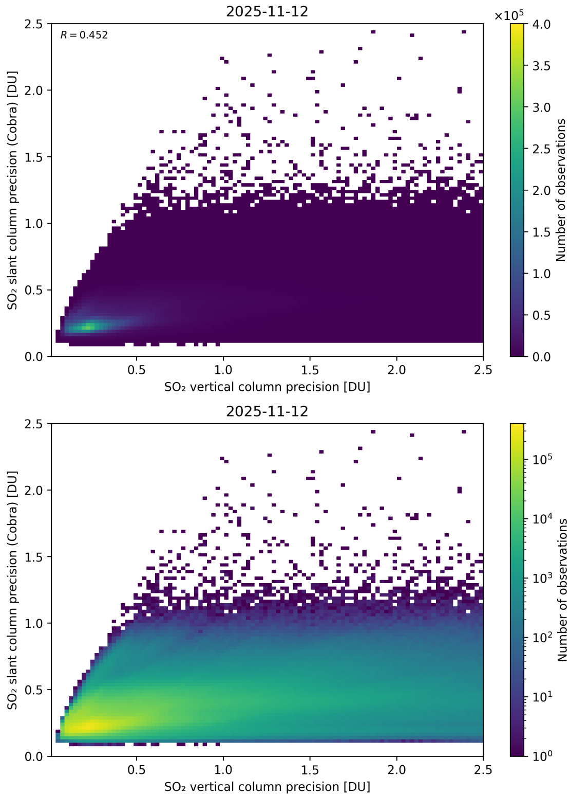
Figure 337: Scatter density plot of “SO 2 vertical column precision” against “SO 2 slant column precision (Cobra)” for 2025-11-12 to 2025-11-13.
