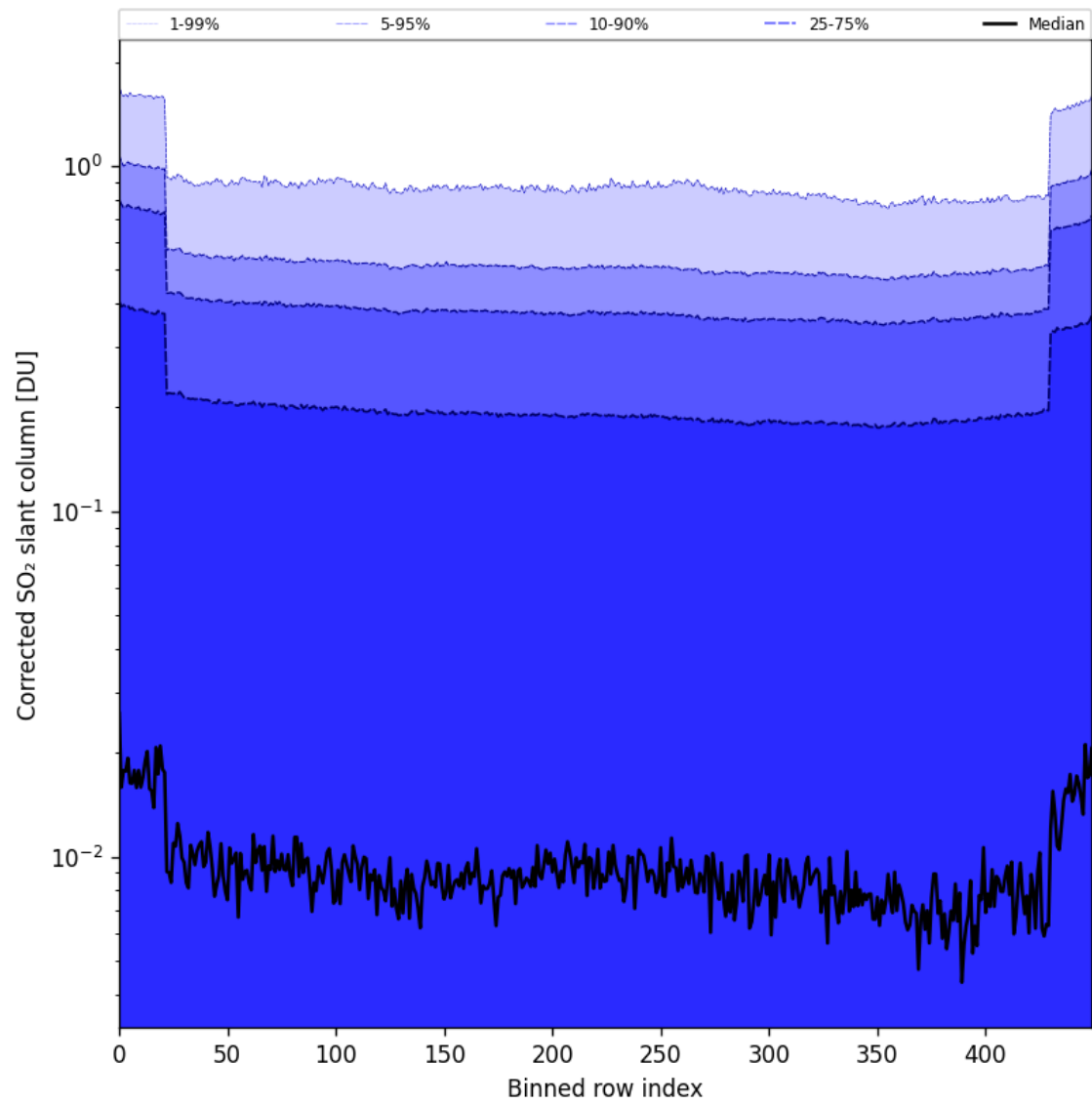
Figure 86: Along track statistics of “Corrected SO 2 slant column” for 2025-11-12 to 2025-11-13
