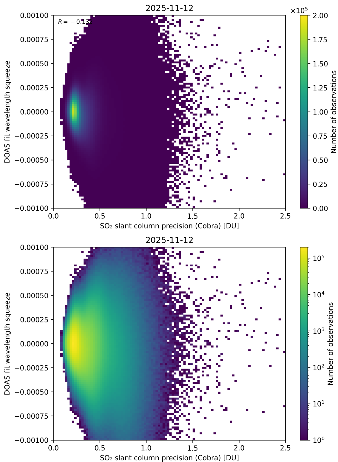
Figure 203: Scatter density plot of “SO 2 slant column precision (Cobra)” against “DOAS fit wavelength squeeze” for 2025-11-12 to 2025-11-13.
