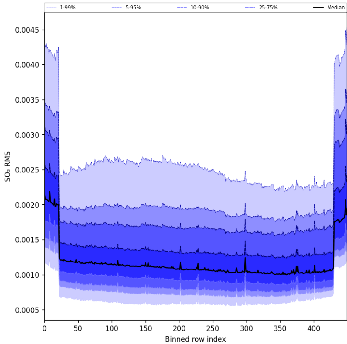
Figure 104: Along track statistics of “SO 2 RMS” for 2025-11-12 to 2025-11-13
