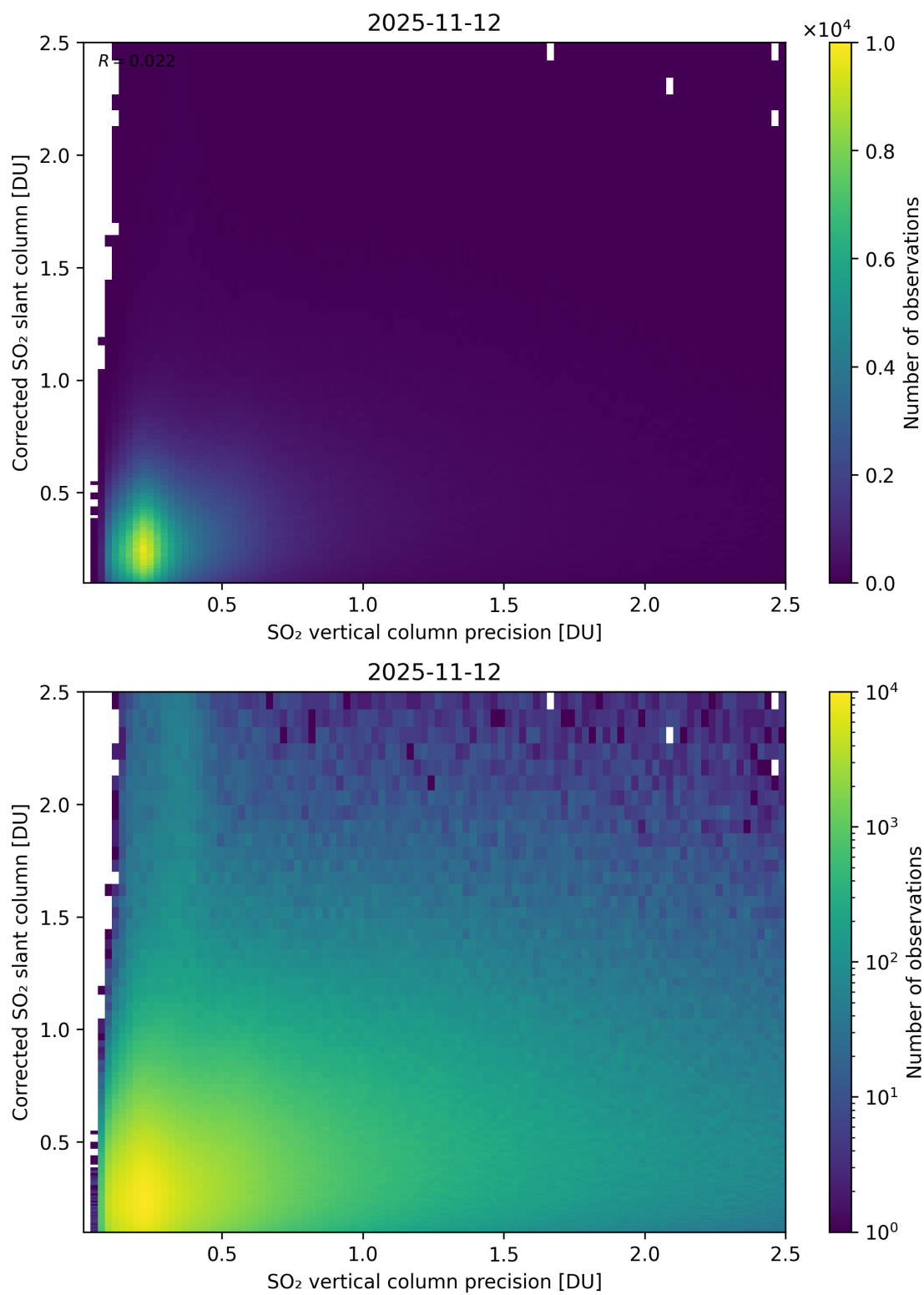
Figure 338: Scatter density plot of “SO 2 vertical column precision” against “Corrected SO 2 slant column” for 2025-11-12 to 2025-11-13.
