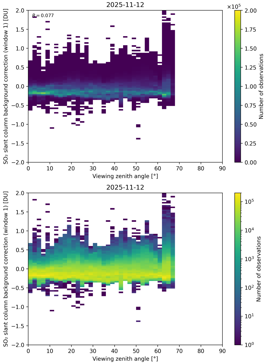
Figure 362: Scatter density plot of “Viewing zenith angle” against “SO 2 slant column background correction (window 1)” for 2025-11-12 to 2025-11-13.
