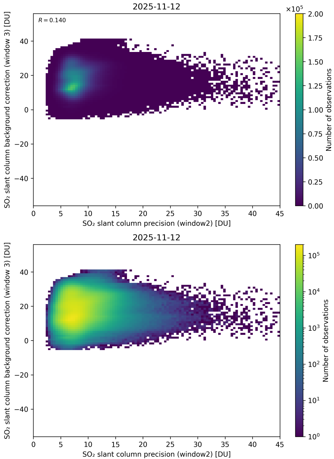
Figure 292: Scatter density plot of “SO 2 slant column precision (window2)” against “SO 2 slant column background correction (window 3)” for 2025-11-12 to 2025-11-13.
