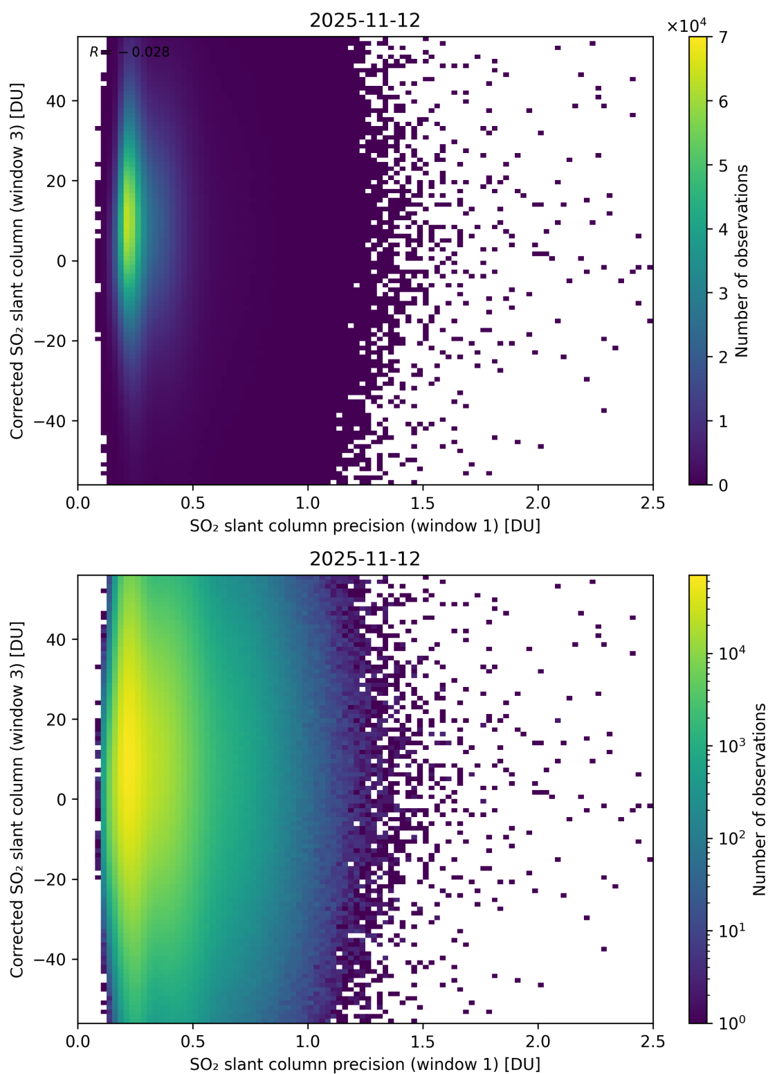
Figure 276: Scatter density plot of “SO 2 slant column precision (window 1)” against “Corrected SO 2 slant column (window 3)” for 2025-11-12 to 2025-11-13.
