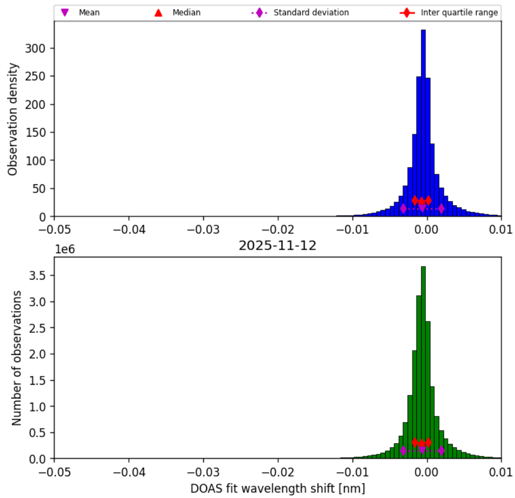
Figure 76: Histogram of “DOAS fit wavelength shift” for 2025-11-12 to 2025-11-13
