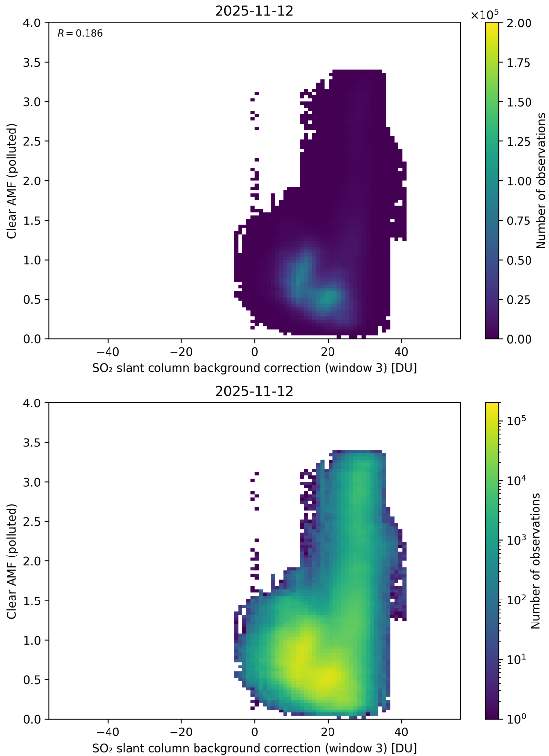
Figure 135: Scatter density plot of “SO 2 slant column background correction (window 3)” against “Clear AMF (polluted)” for 2025-11-12 to 2025-11-13.
