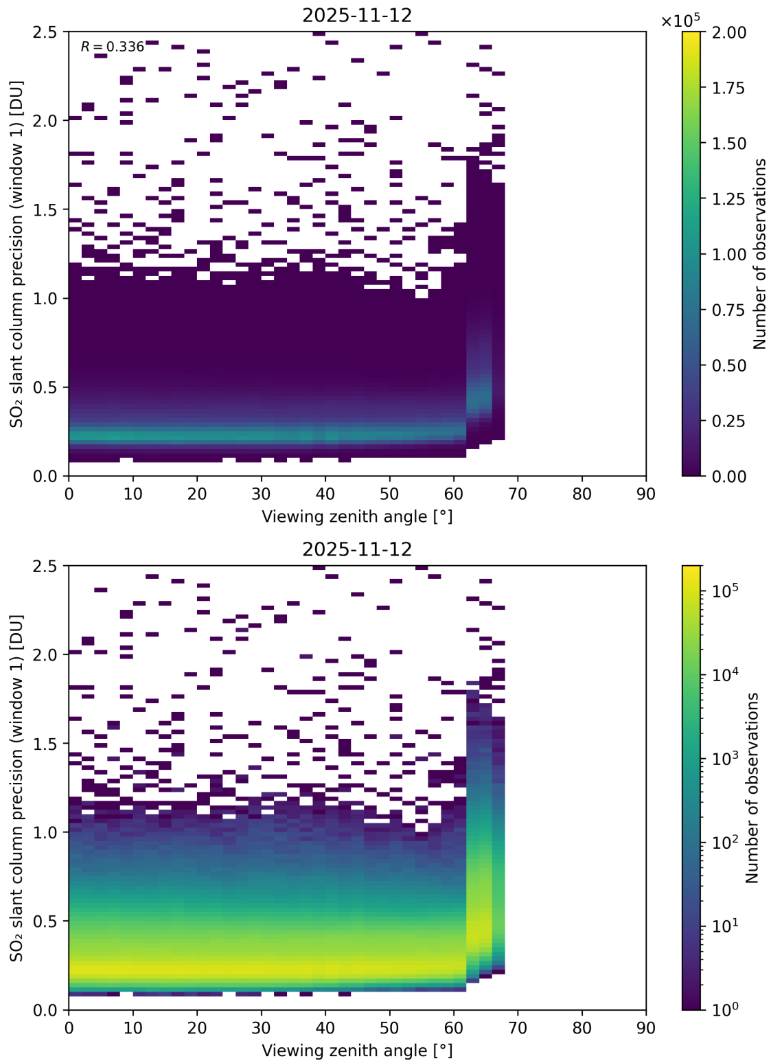
Figure 377: Scatter density plot of “Viewing zenith angle” against “SO 2 slant column precision (window 1)” for 2025-11-12 to 2025-11-13.
