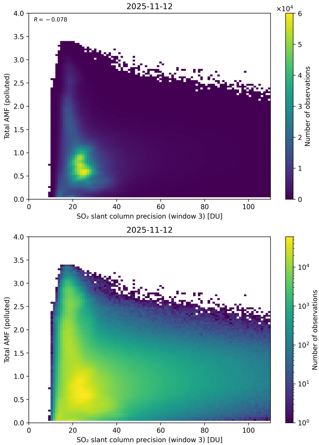
Figure 313: Scatter density plot of “SO 2 slant column precision (window 3)” against “Total AMF (polluted)” for 2025-11-12 to 2025-11-13.
