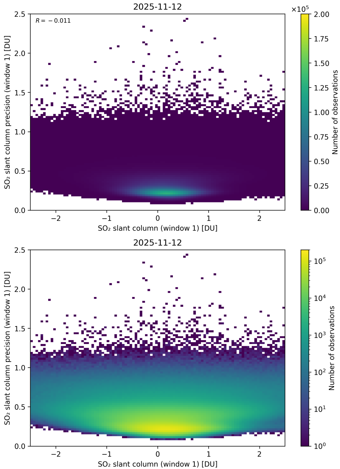
Figure 285: Scatter density plot of “SO 2 slant column (window 1)” against “SO 2 slant column precision (window 1)” for 2025-11-12 to 2025-11-13.
