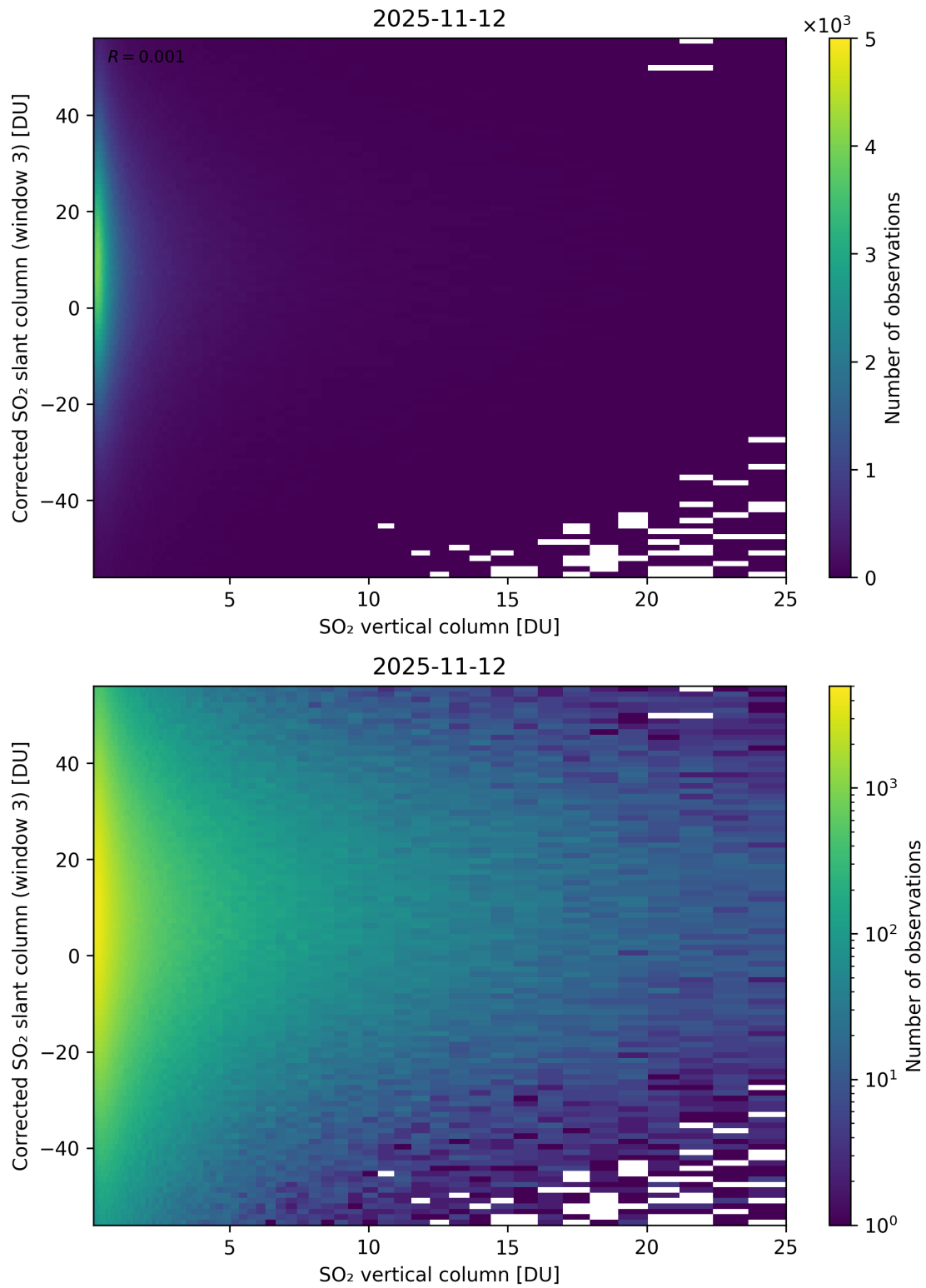
Figure 353: Scatter density plot of “SO 2 vertical column” against “Corrected SO 2 slant column (window 3)” for 2025-11-12 to 2025-11-13.
