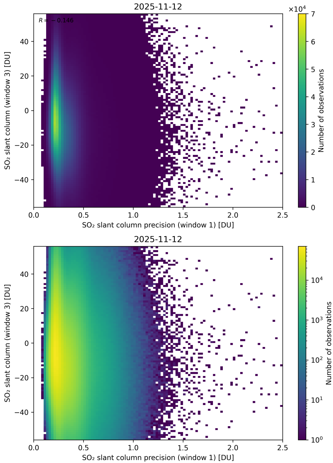
Figure 278: Scatter density plot of “SO 2 slant column precision (window 1)” against “SO 2 slant column (window 3)” for 2025-11-12 to 2025-11-13.
