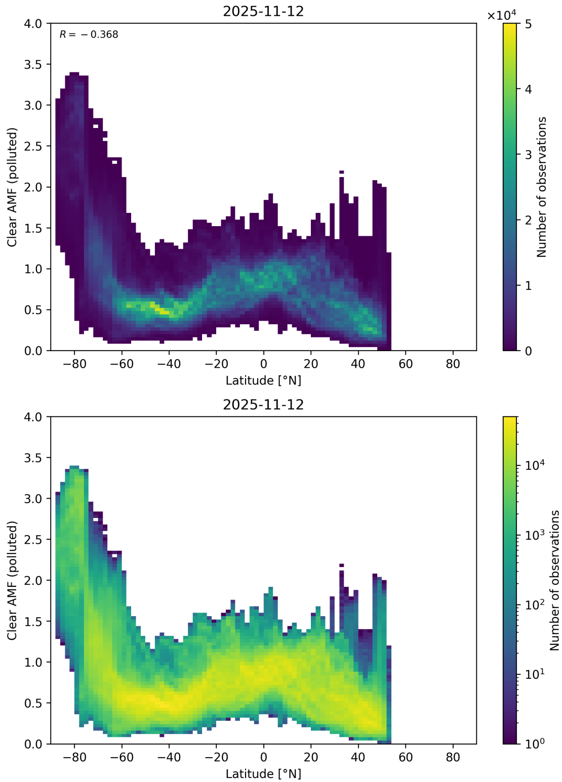
Figure 156: Scatter density plot of “Latitude” against “Clear AMF (polluted)” for 2025-11-12 to 2025-11-13.
