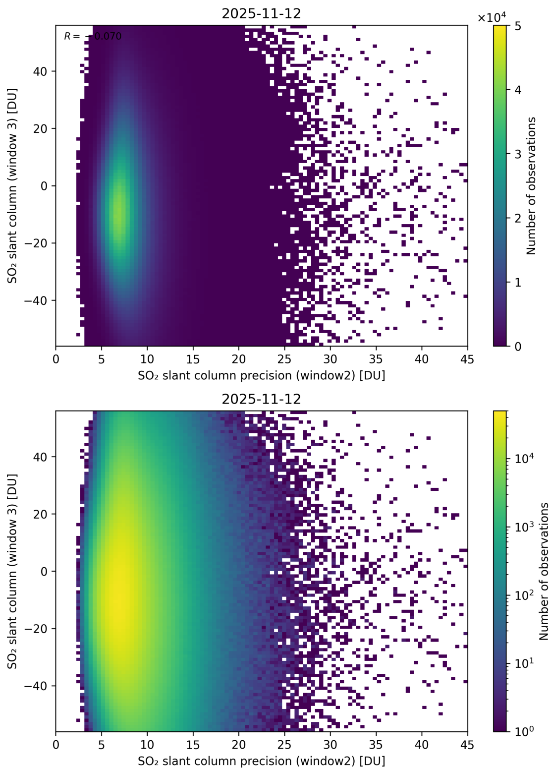
Figure 299: Scatter density plot of “SO 2 slant column precision (window2)” against “SO 2 slant column (window 3)” for 2025-11-12 to 2025-11-13.
