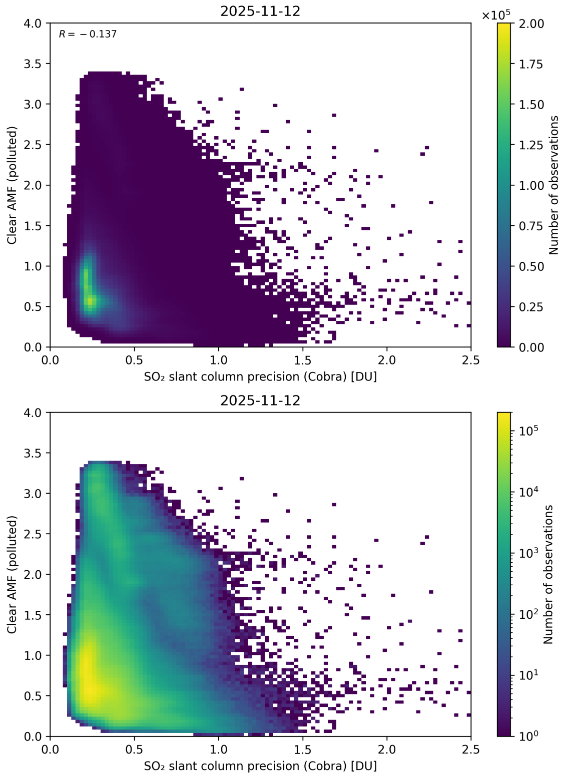
Figure 205: Scatter density plot of “SO 2 slant column precision (Cobra)” against “Clear AMF (polluted)” for 2025-11-12 to 2025-11-13.
