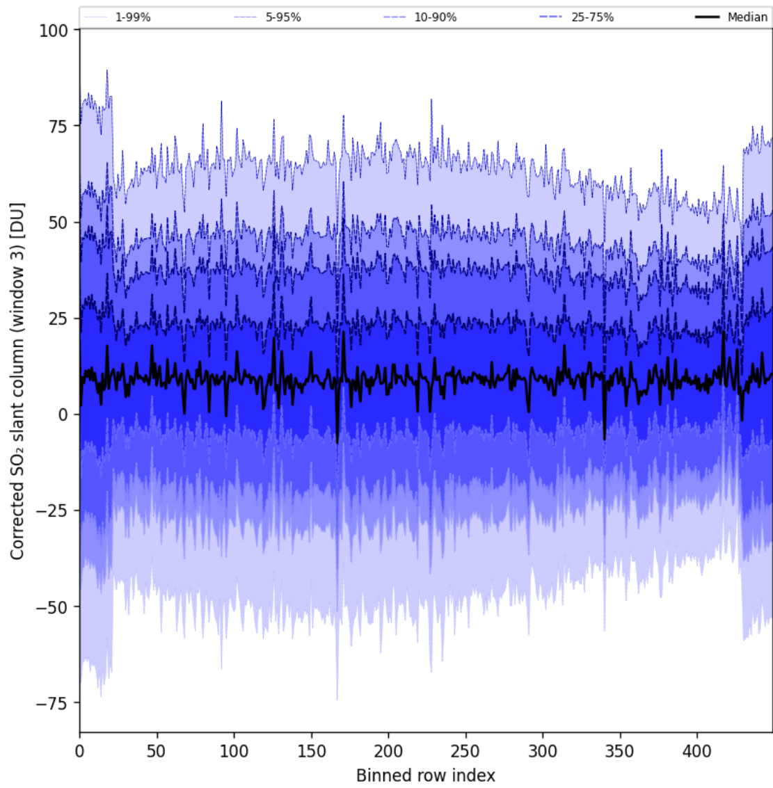
Figure 99: Along track statistics of “Corrected SO 2 slant column (window 3)” for 2025-11-12 to 2025-11-13
