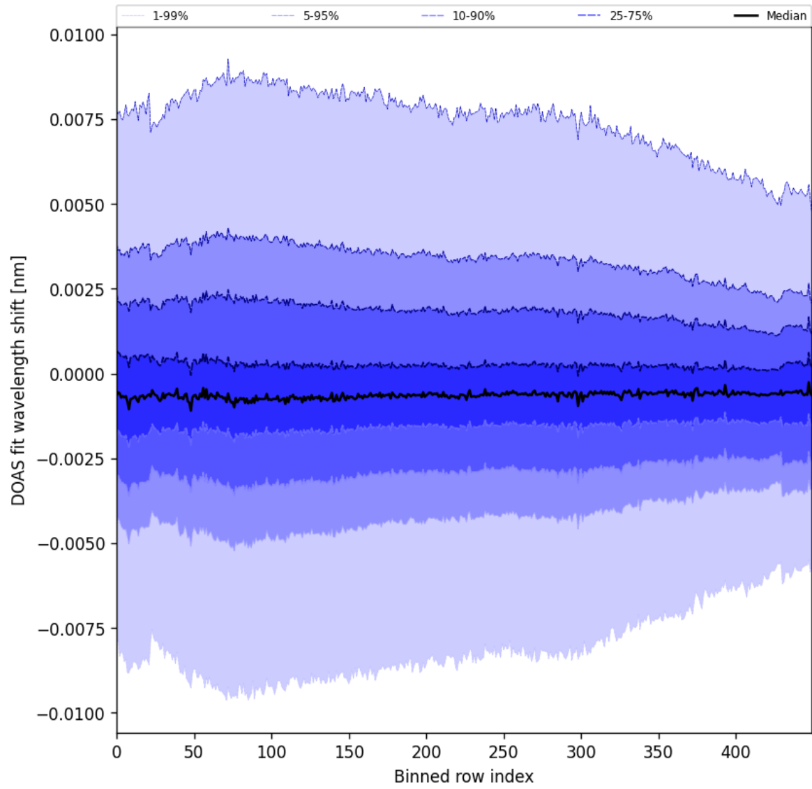
Figure 102: Along track statistics of “DOAS fit wavelength shift” for 2025-11-12 to 2025-11-13
