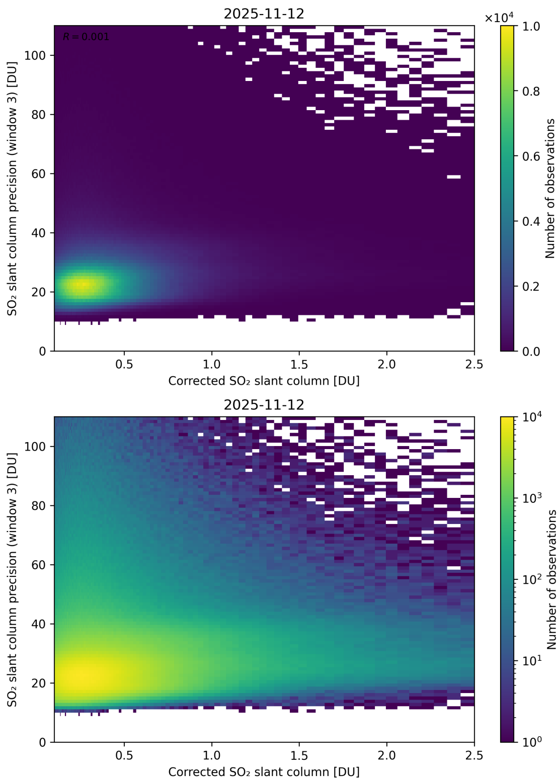
Figure 241: Scatter density plot of “Corrected SO 2 slant column” against “SO 2 slant column precision (window 3)” for 2025-11-12 to 2025-11-13.
