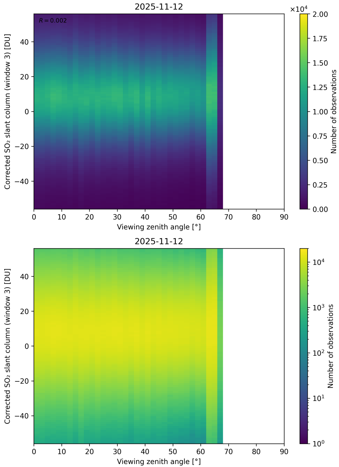
Figure 375: Scatter density plot of “Viewing zenith angle” against “Corrected SO 2 slant column (window 3)” for 2025-11-12 to 2025-11-13.
