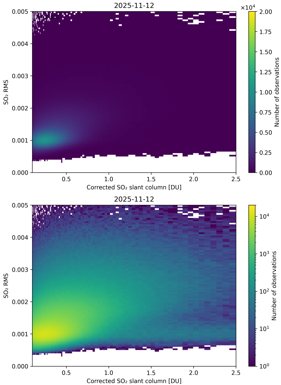
Figure 231: Scatter density plot of “Corrected SO 2 slant column” against “SO 2 RMS” for 2025-11-12 to 2025-11-13.
