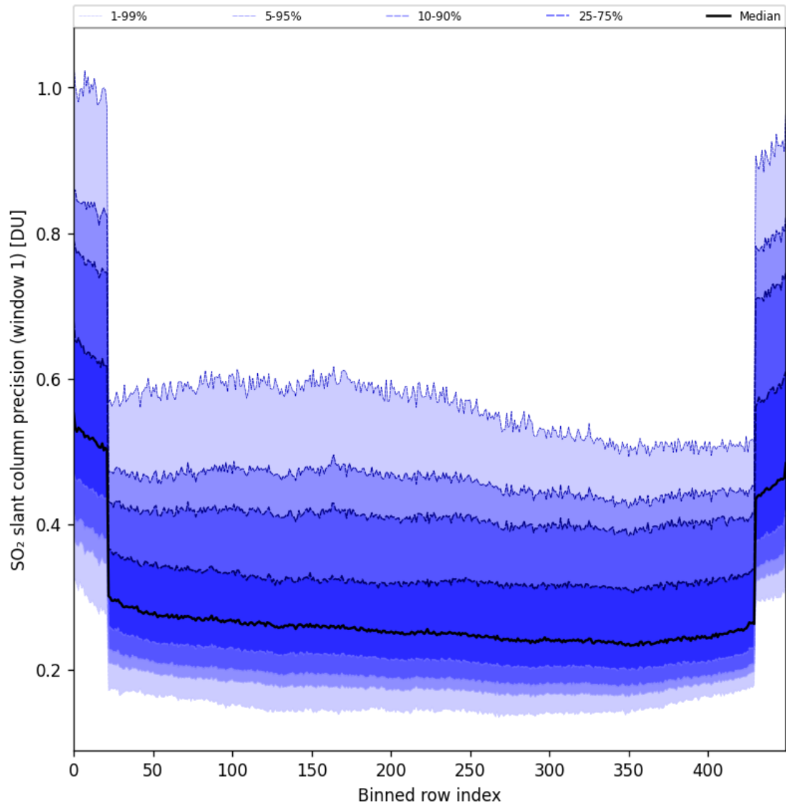
Figure 90: Along track statistics of “SO 2 slant column precision (window 1)” for 2025-11-12 to 2025-11-13
