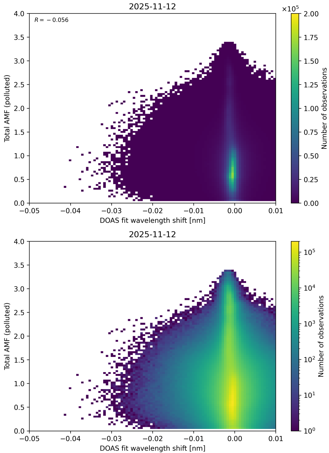
Figure 141: Scatter density plot of “DOAS fit wavelength shift” against “Total AMF (polluted)” for 2025-11-12 to 2025-11-13.
