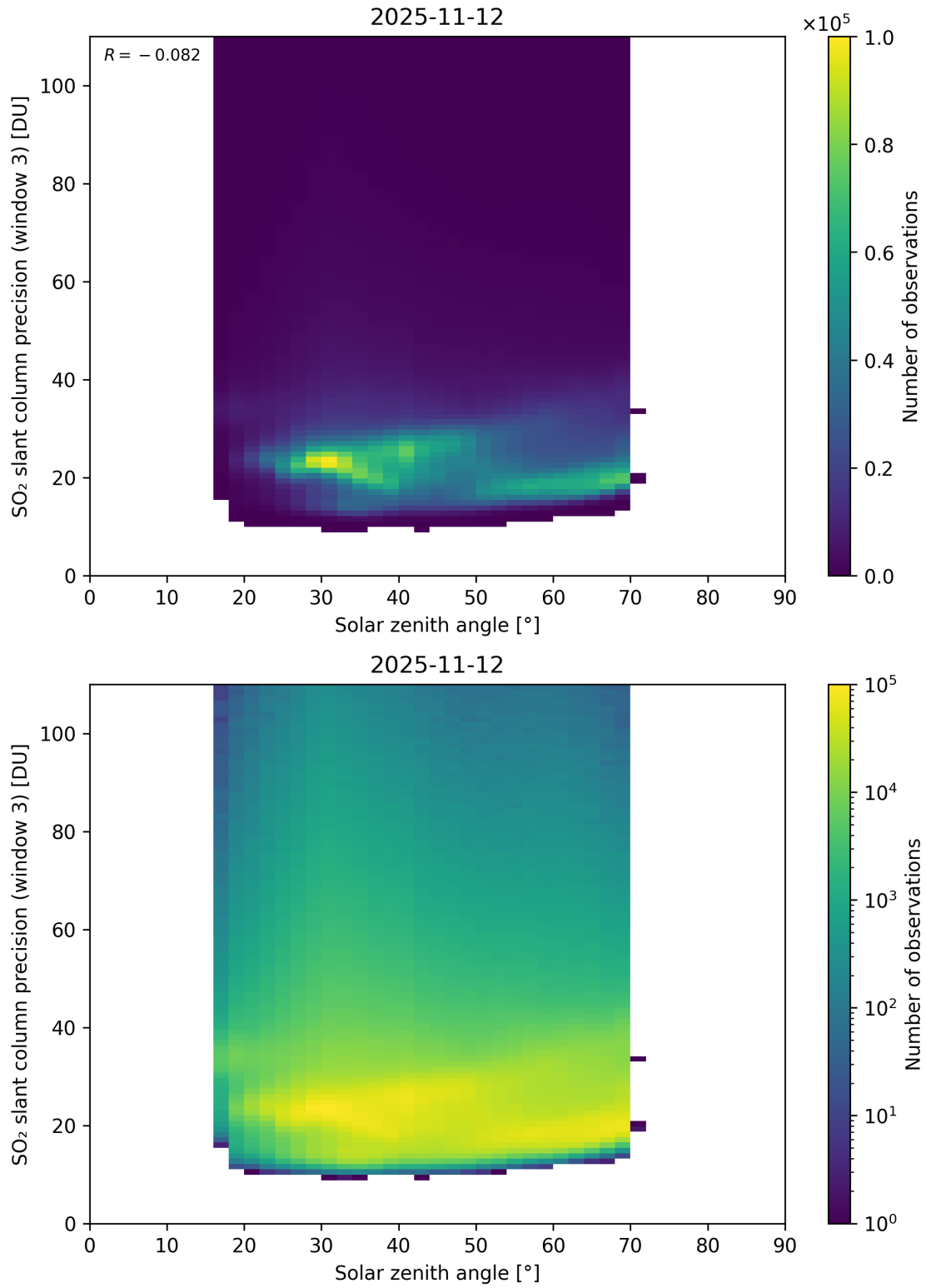
Figure 188: Scatter density plot of “Solar zenith angle” against “SO 2 slant column precision (window 3)” for 2025-11-12 to 2025-11-13.
