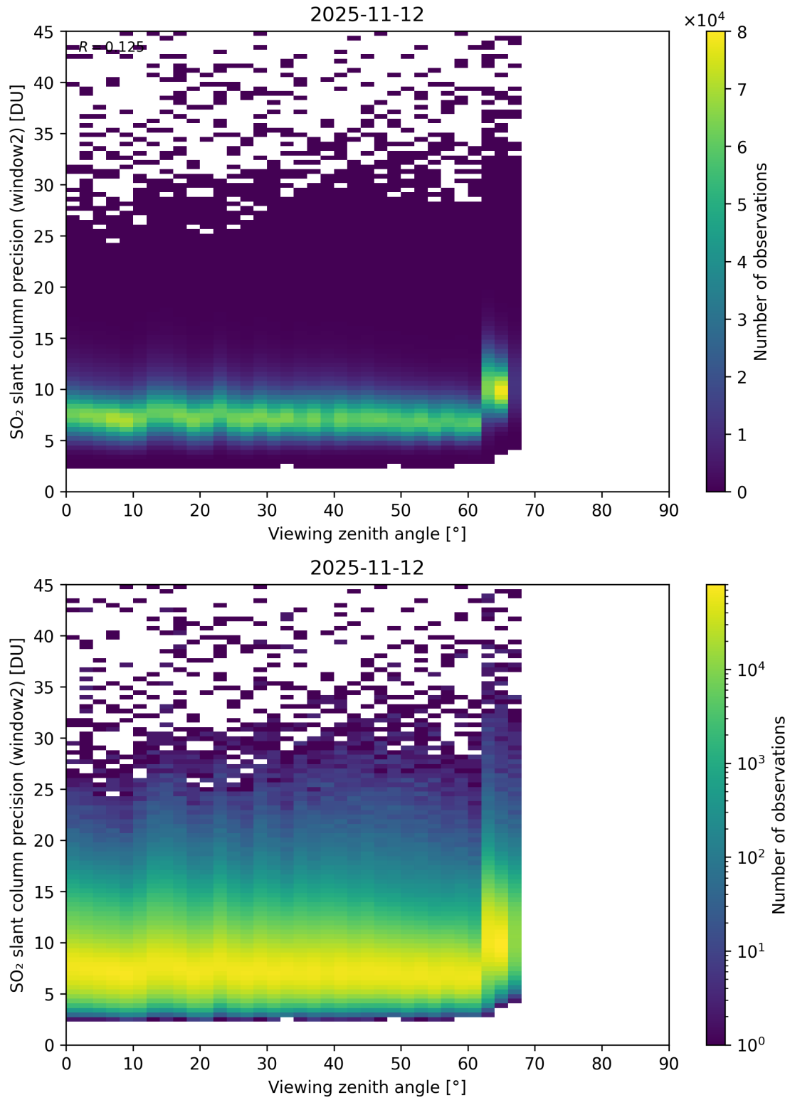
Figure 378: Scatter density plot of “Viewing zenith angle” against “SO 2 slant column precision (window2)” for 2025-11-12 to 2025-11-13.
