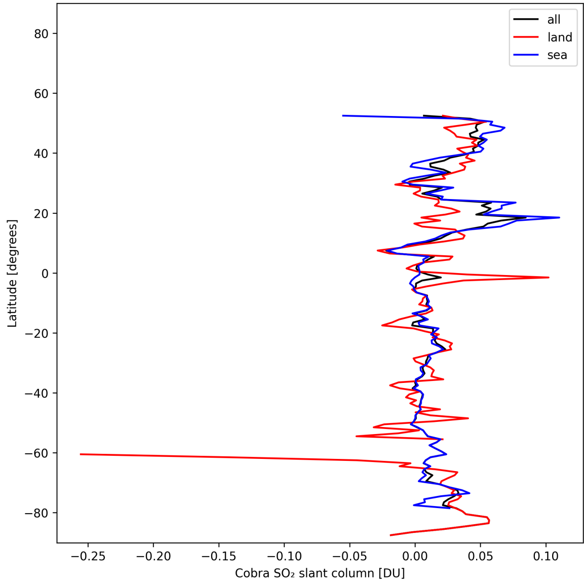
Figure 35: Zonal average of “Cobra SO 2 slant column” for 2025-11-12 to 2025-11-13.
