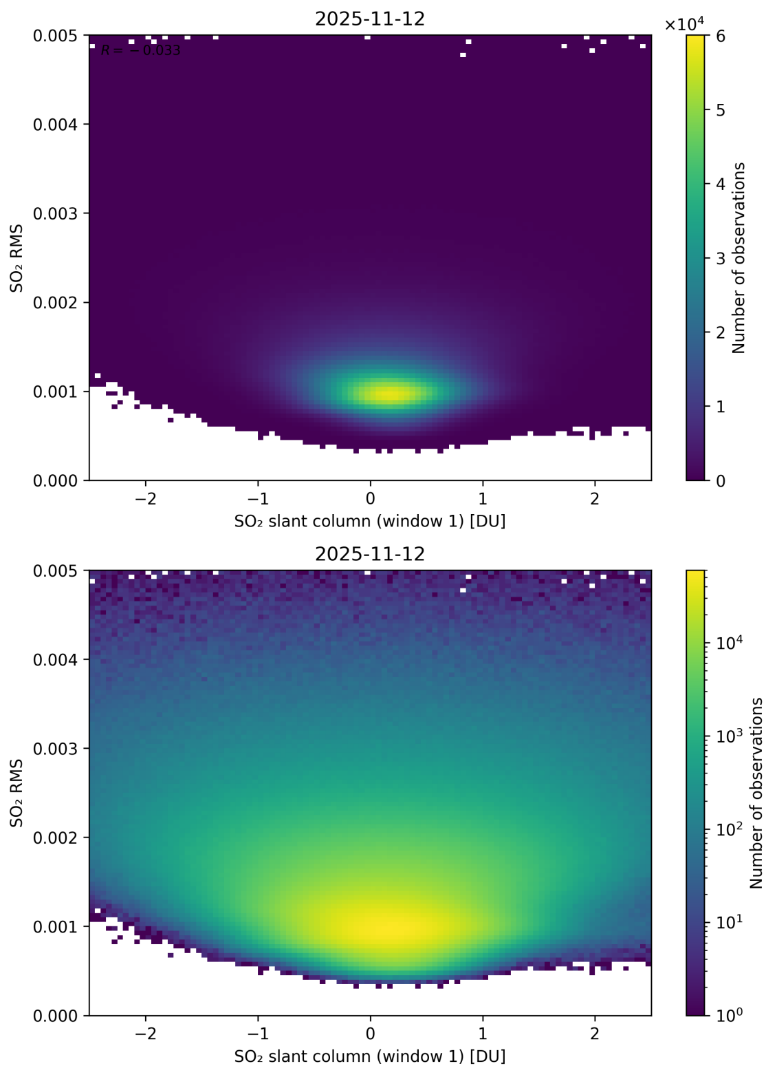
Figure 267: Scatter density plot of “SO 2 slant column (window 1)” against “SO 2 RMS” for 2025-11-12 to 2025-11-13.
