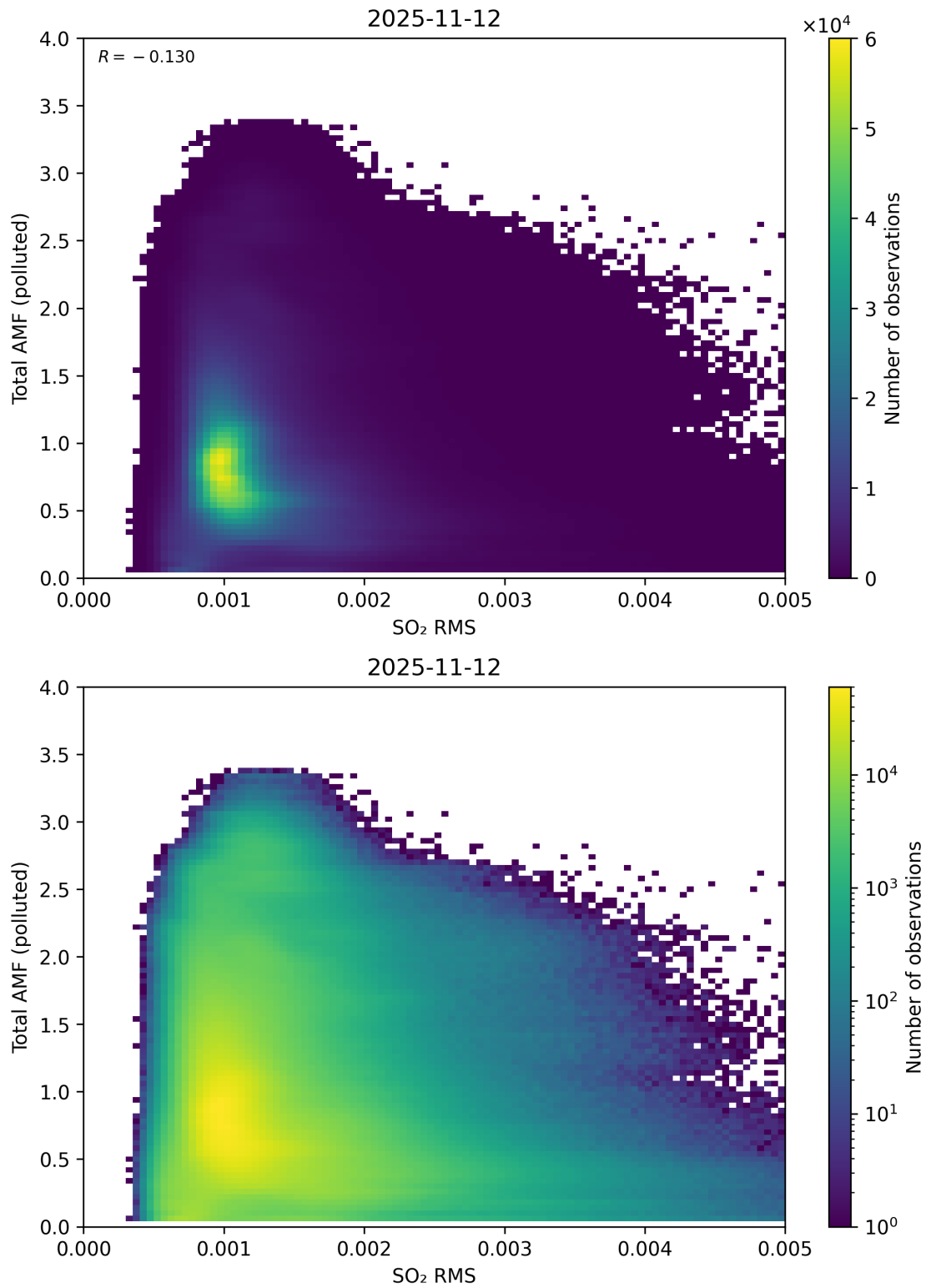
Figure 148: Scatter density plot of “SO 2 RMS” against “Total AMF (polluted)” for 2025-11-12 to 2025-11-13.
