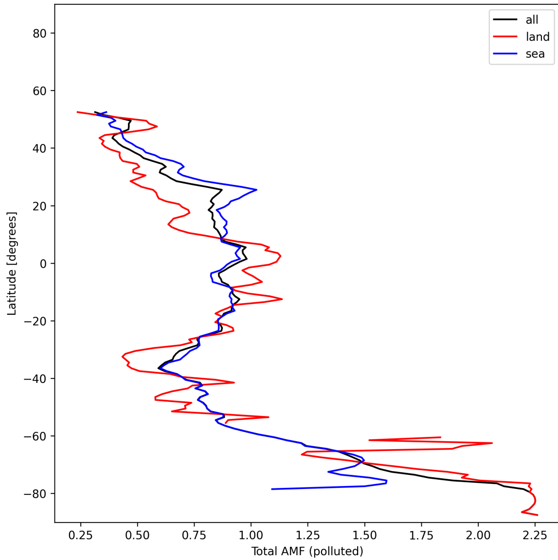
Figure 53: Zonal average of “Total AMF (polluted)” for 2025-11-12 to 2025-11-13.
