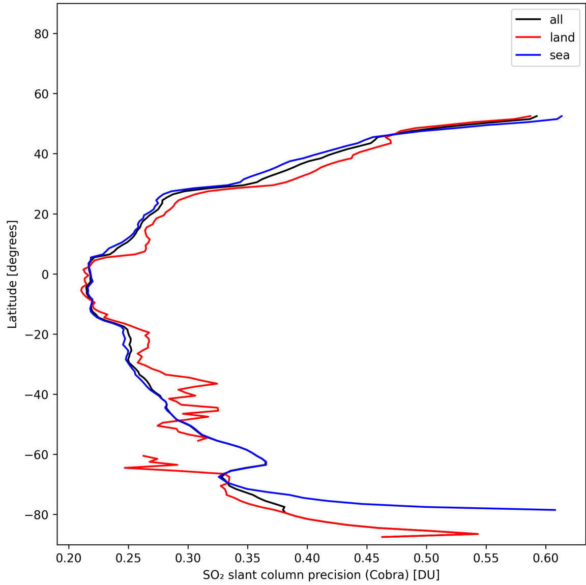
Figure 36: Zonal average of “SO 2 slant column precision (Cobra)” for 2025-11-12 to 2025-11-13.
