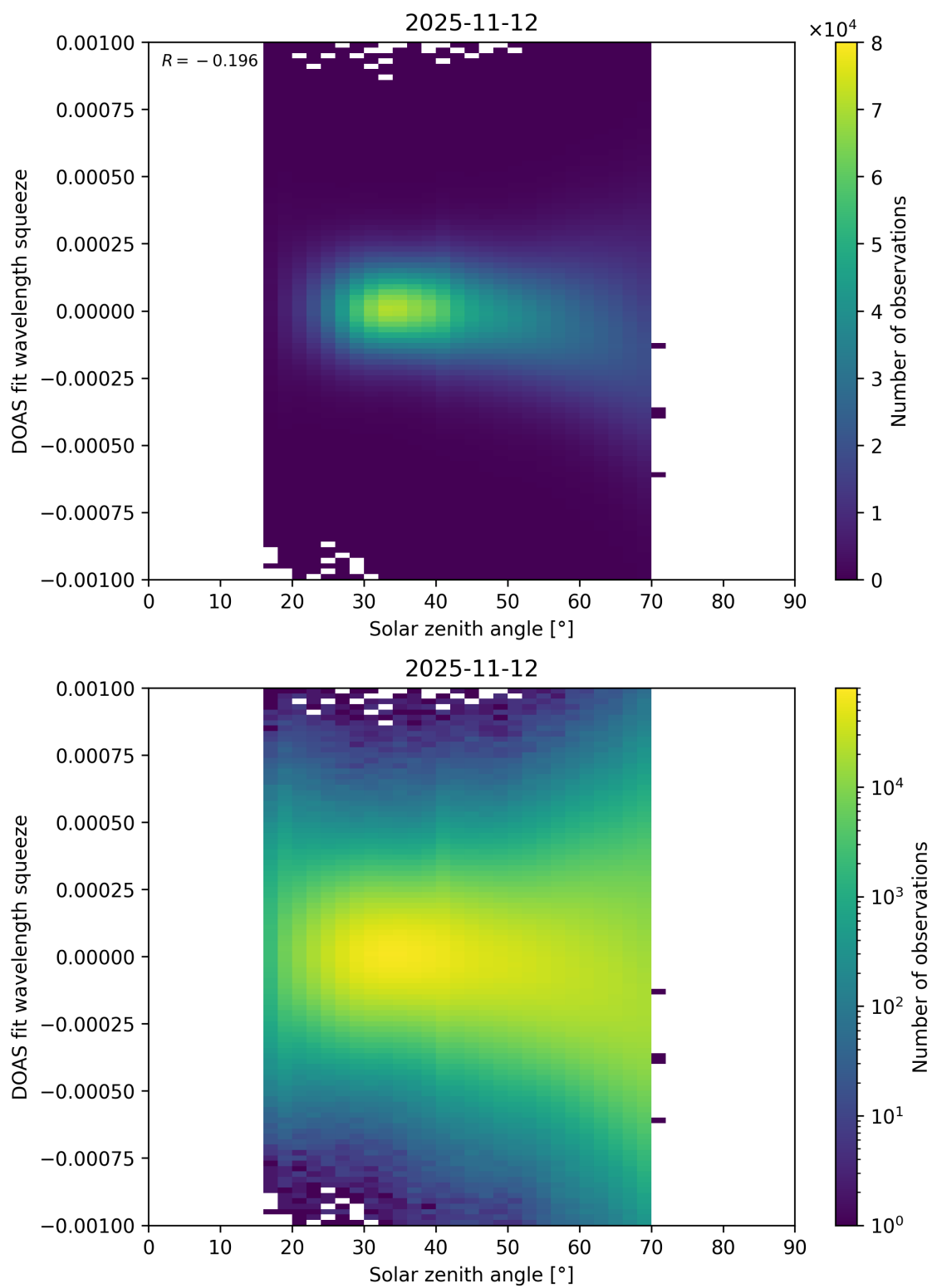
Figure 175: Scatter density plot of “Solar zenith angle” against “DOAS fit wavelength squeeze” for 2025-11-12 to 2025-11-13.
