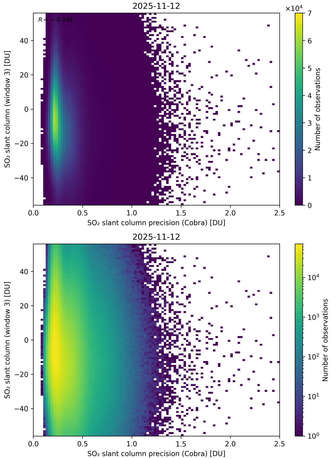
Figure 211: Scatter density plot of “SO 2 slant column precision (Cobra)” against “SO 2 slant column (window 3)” for 2025-11-12 to 2025-11-13.
