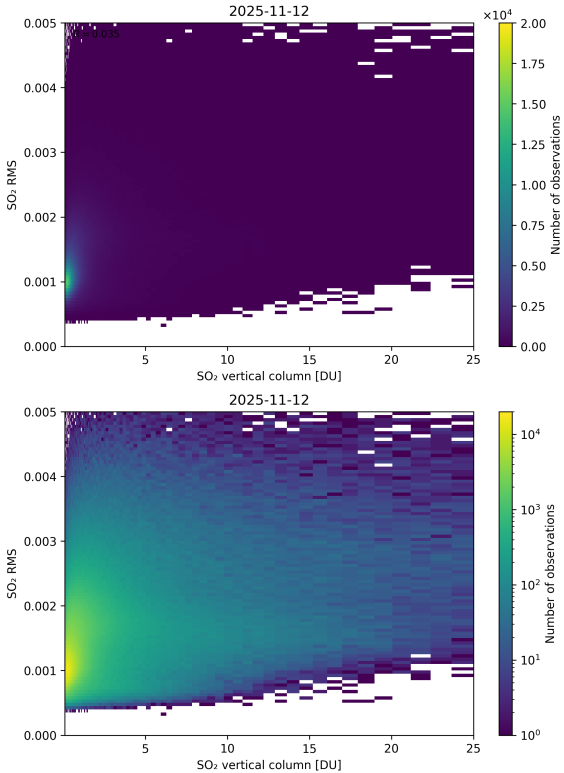
Figure 328: Scatter density plot of “SO 2 vertical column” against “SO 2 RMS” for 2025-11-12 to 2025-11-13.
