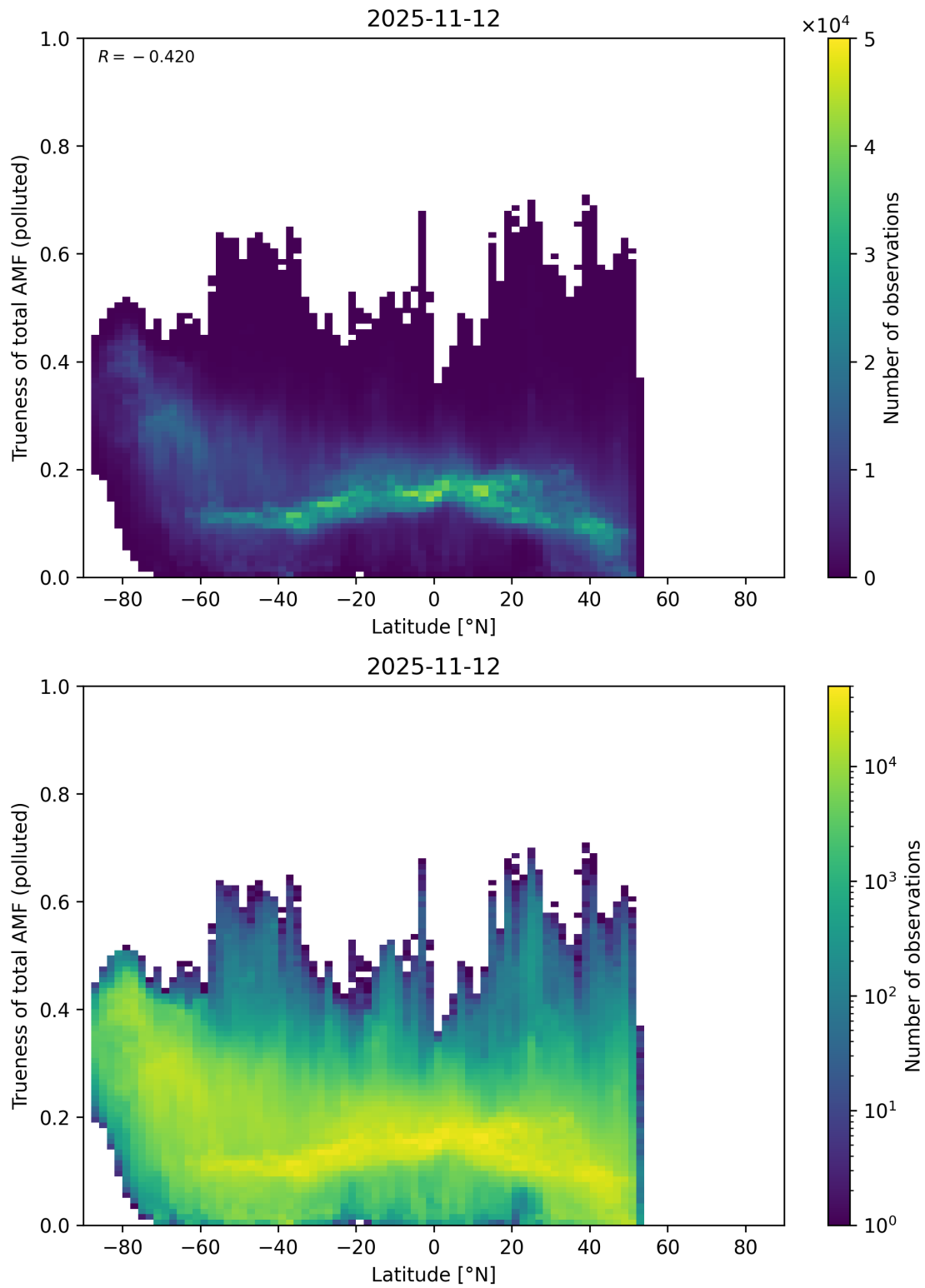
Figure 168: Scatter density plot of “Latitude” against “Trueness of total AMF (polluted)” for 2025-11-12 to 2025-11-13.
