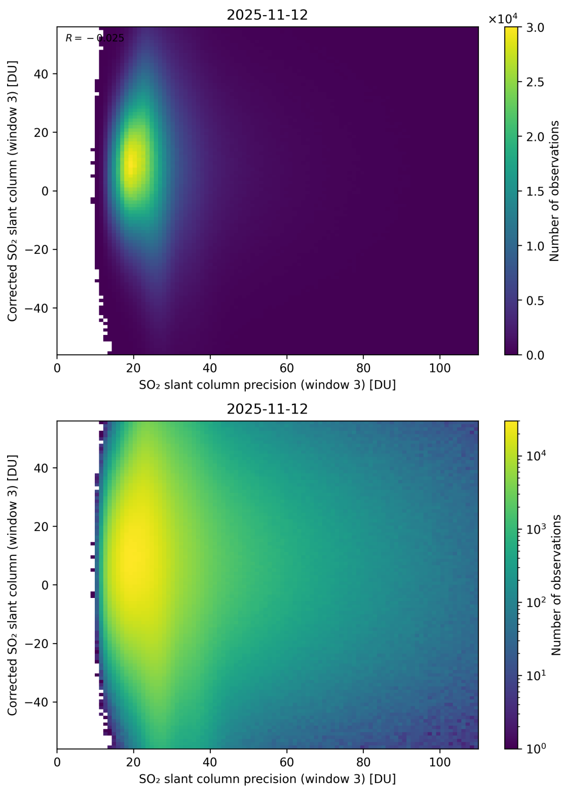
Figure 312: Scatter density plot of “SO 2 slant column precision (window 3)” against “Corrected SO 2 slant column (window 3)” for 2025-11-12 to 2025-11-13.
