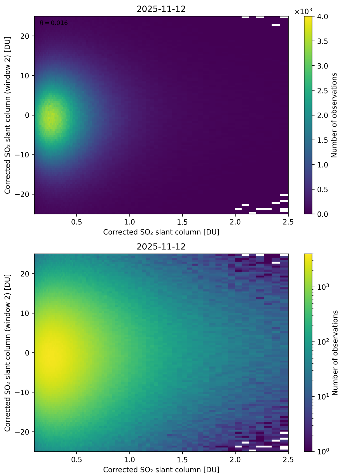
Figure 235: Scatter density plot of “Corrected SO 2 slant column” against “Corrected SO 2 slant column (window 2)” for 2025-11-12 to 2025-11-13.
