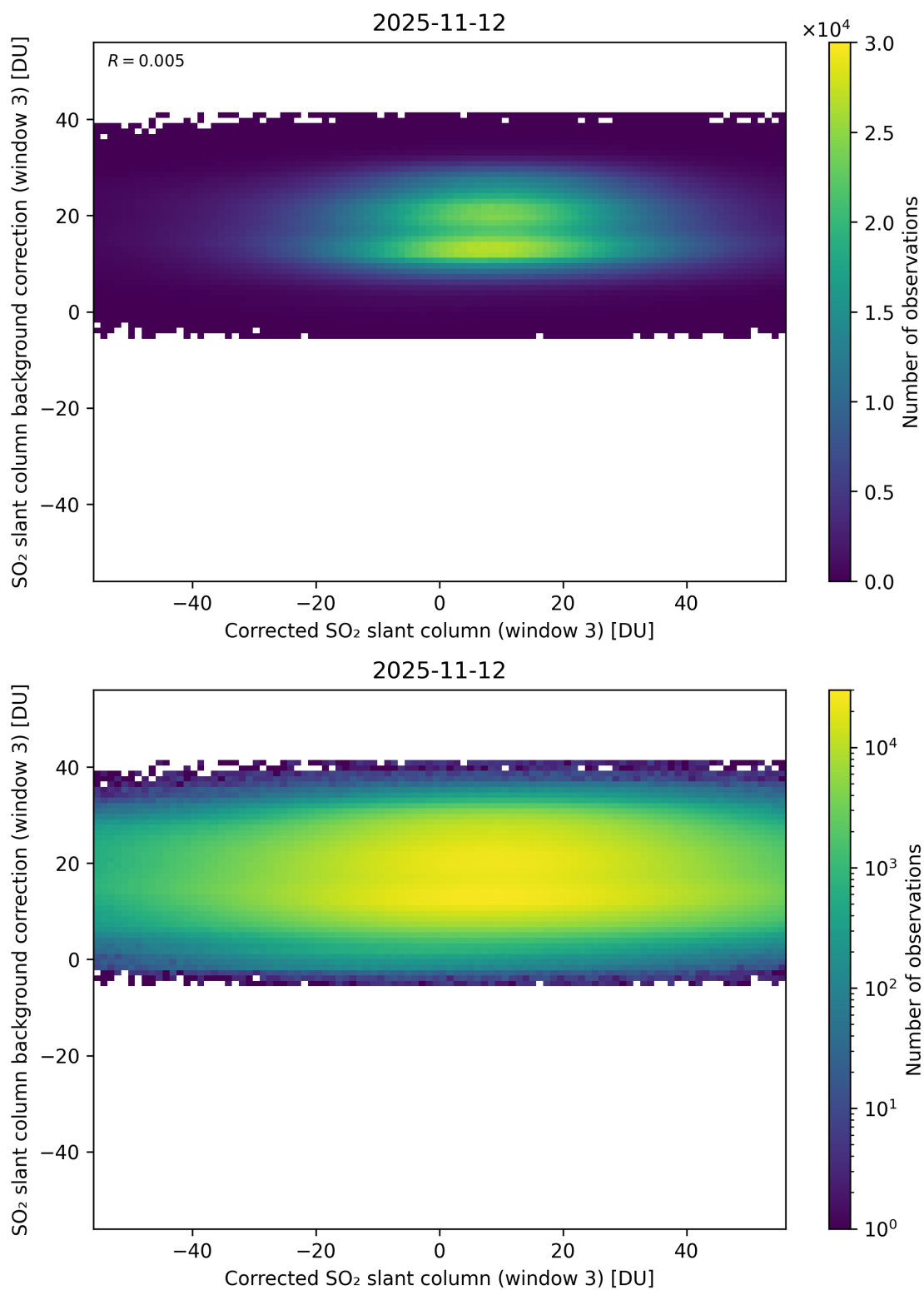
Figure 255: Scatter density plot of “Corrected SO 2 slant column (window 3)” against “SO 2 slant column background correction (window 3)” for 2025-11-12 to 2025-11-13.
