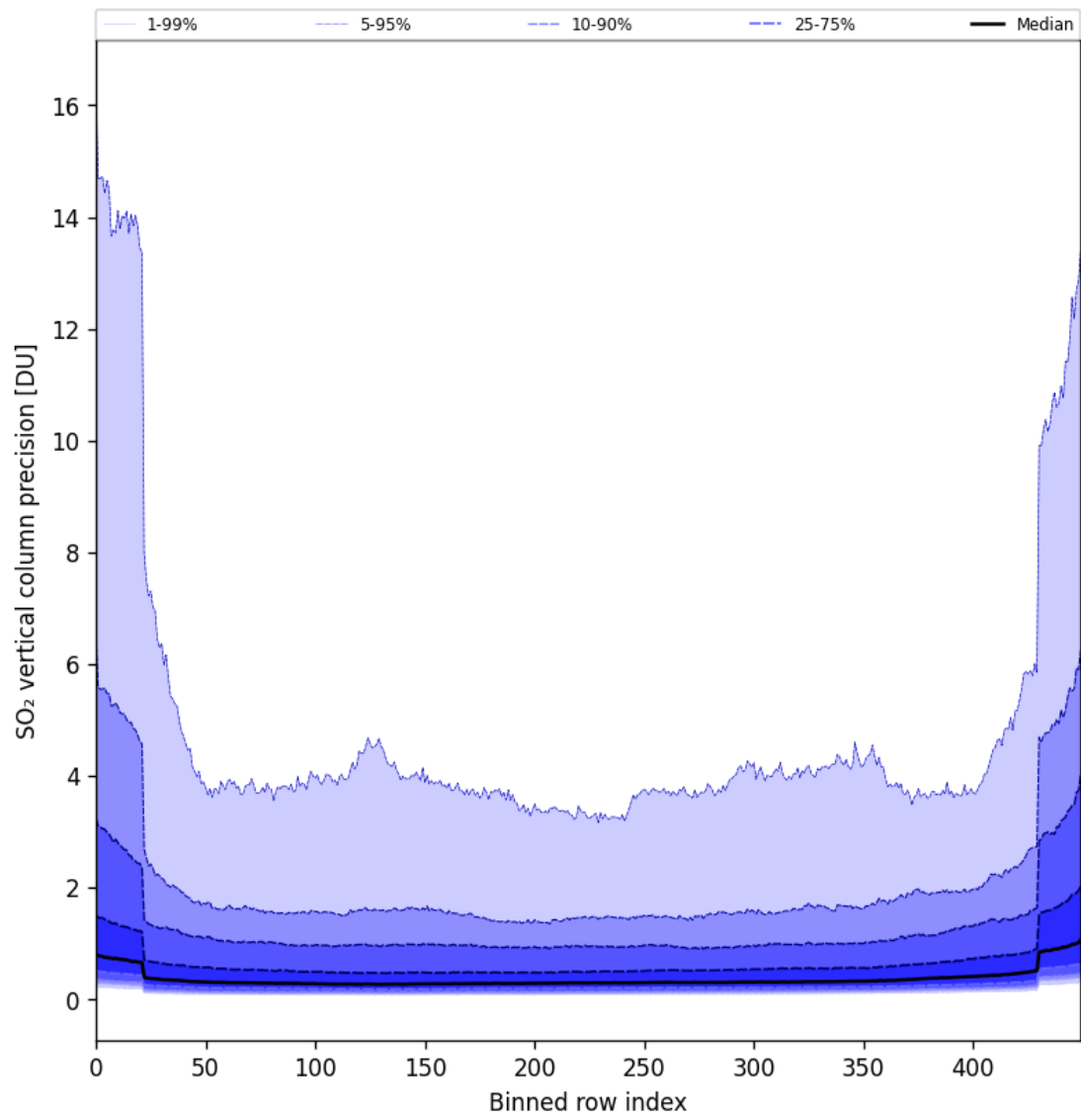
Figure 85: Along track statistics of “SO 2 vertical column precision” for 2025-11-12 to 2025-11-13
