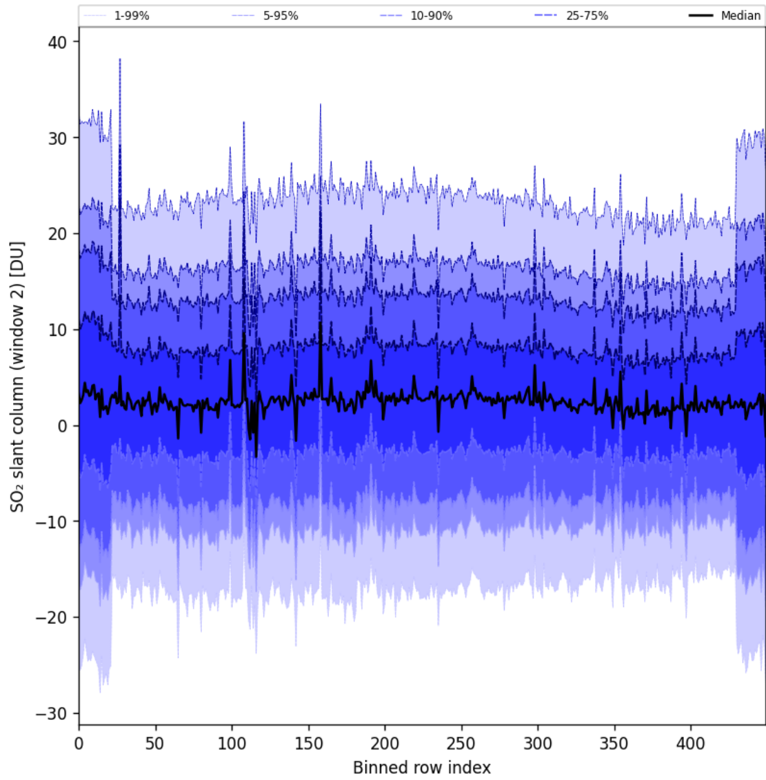
Figure 93: Along track statistics of “SO 2 slant column (window 2)” for 2025-11-12 to 2025-11-13
