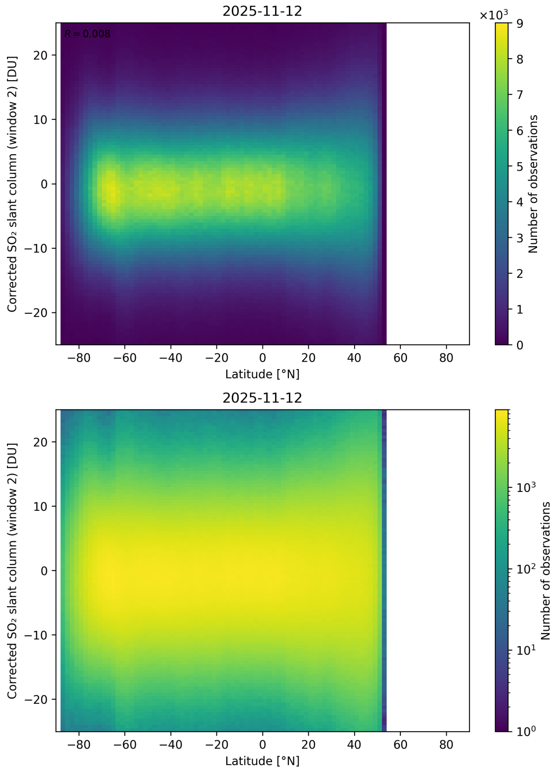
Figure 160: Scatter density plot of “Latitude” against “Corrected SO 2 slant column (window 2)” for 2025-11-12 to 2025-11-13.
