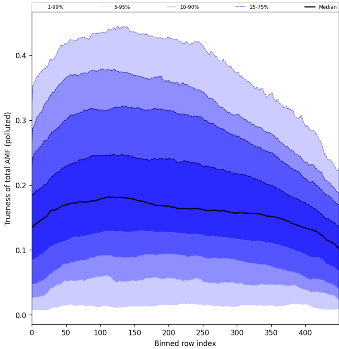
Figure 106: Along track statistics of “Trueness of total AMF (polluted)” for 2025-11-12 to 2025-11-13
