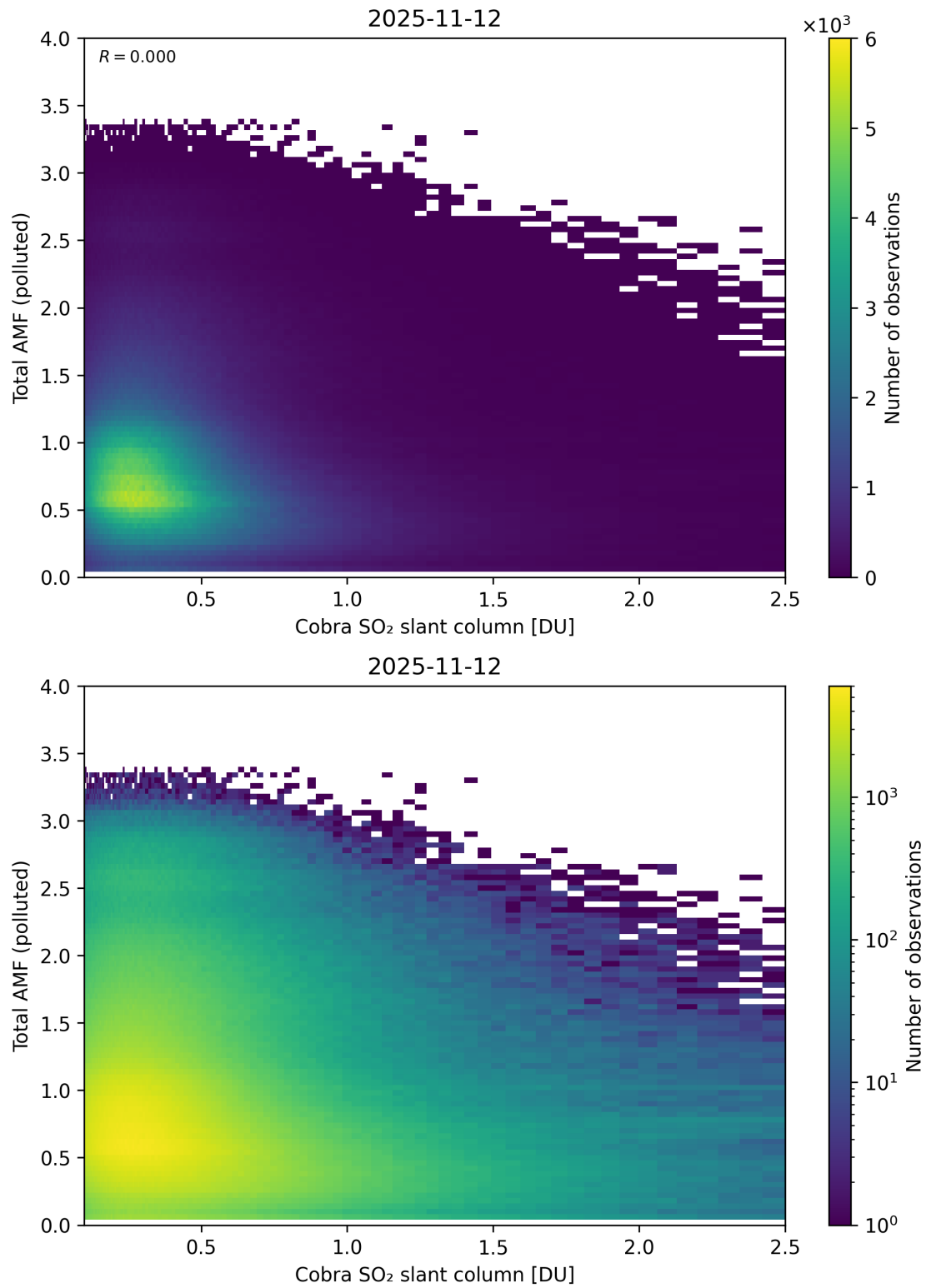
Figure 224: Scatter density plot of “Cobra SO 2 slant column” against “Total AMF (polluted)” for 2025-11-12 to 2025-11-13.
