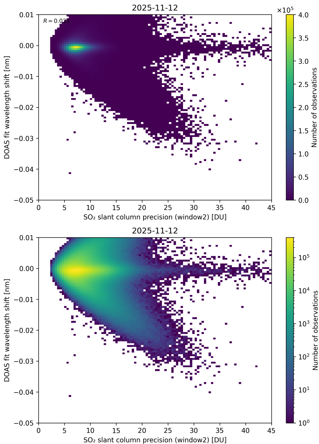
Figure 293: Scatter density plot of “SO 2 slant column precision (window2)” against “DOAS fit wavelength shift” for 2025-11-12 to 2025-11-13.
