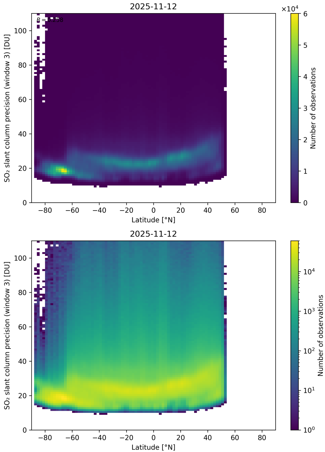
Figure 166: Scatter density plot of “Latitude” against “SO 2 slant column precision (window 3)” for 2025-11-12 to 2025-11-13.
