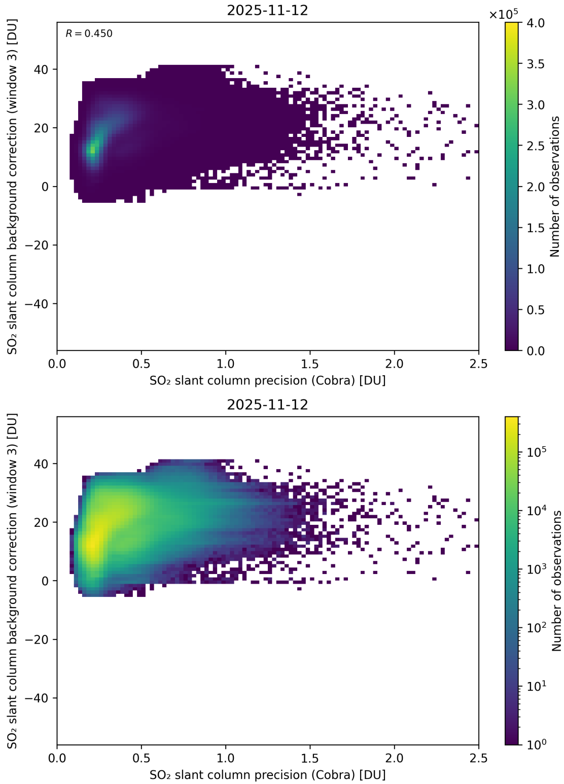
Figure 201: Scatter density plot of “SO 2 slant column precision (Cobra)” against “SO 2 slant column background correction (window 3)” for 2025-11-12 to 2025-11-13.
