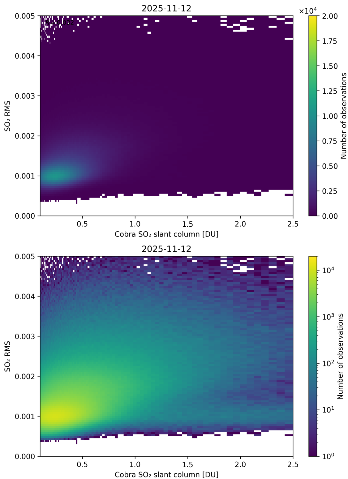
Figure 198: Scatter density plot of “Cobra SO 2 slant column” against “SO 2 RMS” for 2025-11-12 to 2025-11-13.
