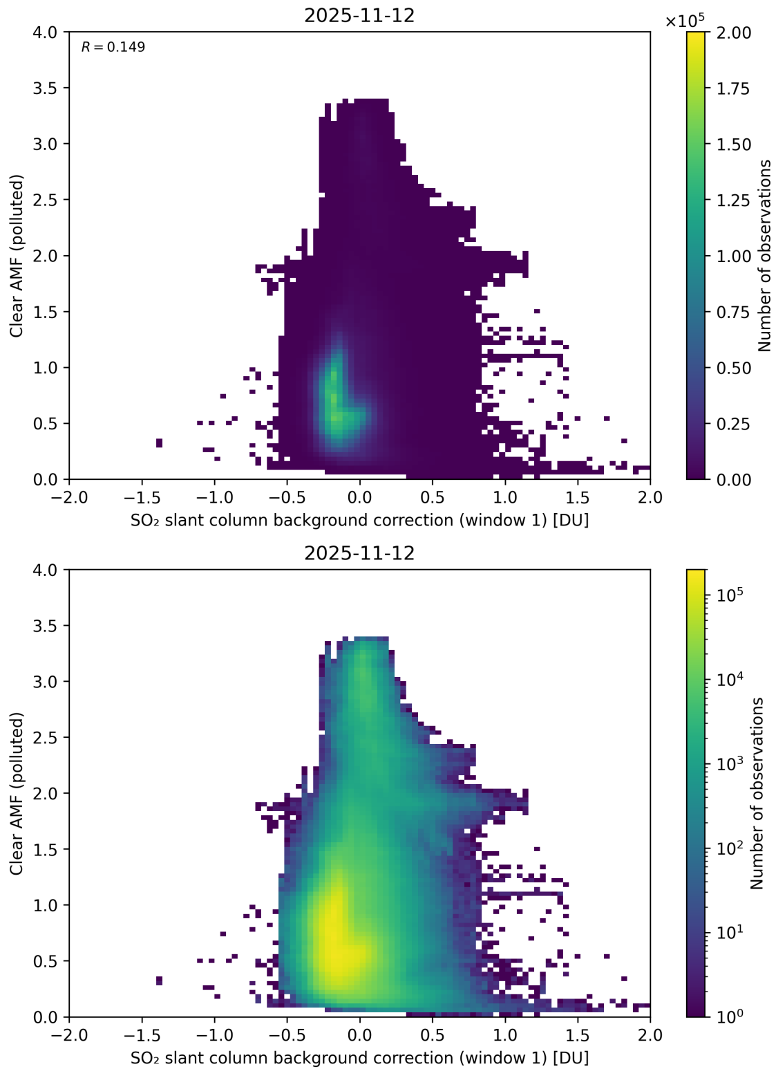
Figure 114: Scatter density plot of “SO 2 slant column background correction (window 1)” against “Clear AMF (polluted)” for 2025-11-12 to 2025-11-13.
