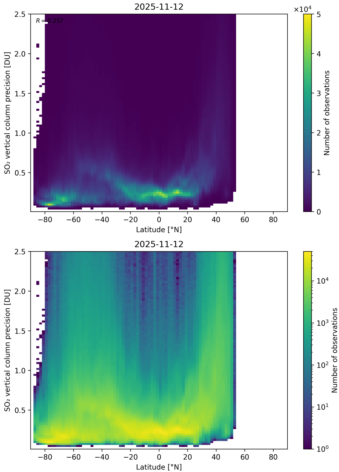
Figure 170: Scatter density plot of “Latitude” against “SO 2 vertical column precision” for 2025-11-12 to 2025-11-13.
