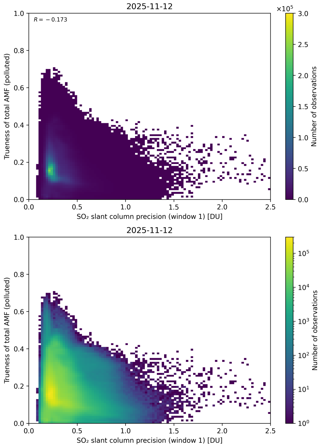
Figure 281: Scatter density plot of “SO 2 slant column precision (window 1)” against “Trueness of total AMF (polluted)” for 2025-11-12 to 2025-11-13.
