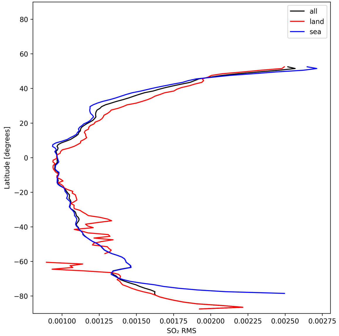
Figure 52: Zonal average of “SO 2 RMS” for 2025-11-12 to 2025-11-13.
