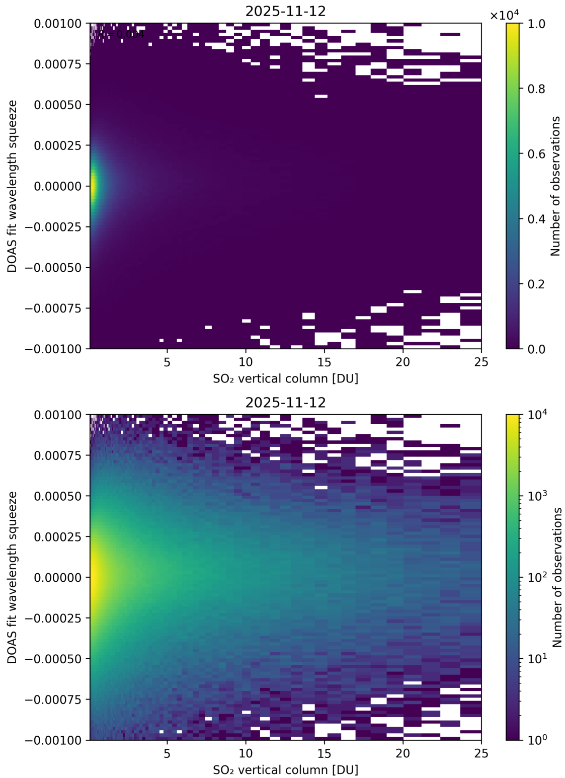
Figure 327: Scatter density plot of “SO 2 vertical column” against “DOAS fit wavelength squeeze” for 2025-11-12 to 2025-11-13.
