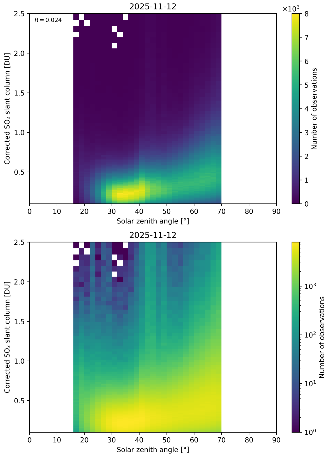
Figure 181: Scatter density plot of “Solar zenith angle” against “Corrected SO 2 slant column” for 2025-11-12 to 2025-11-13.
