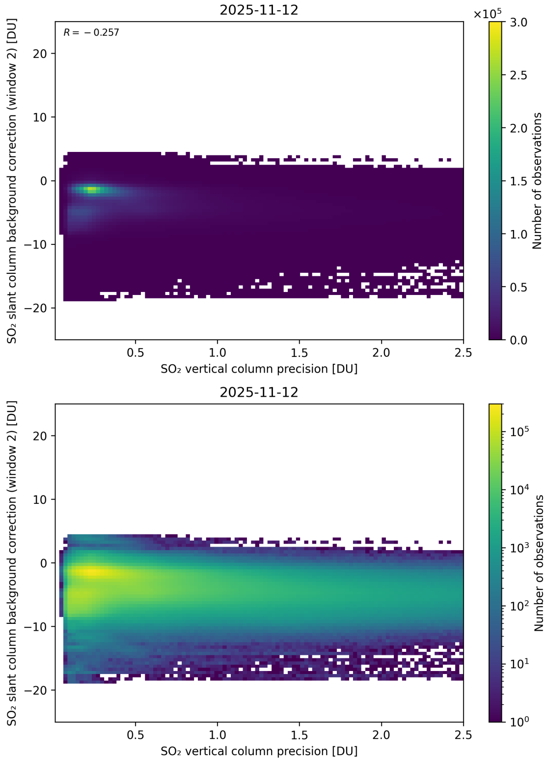
Figure 330: Scatter density plot of “SO 2 vertical column precision” against “SO 2 slant column background correction (window 2)” for 2025-11-12 to 2025-11-13.
