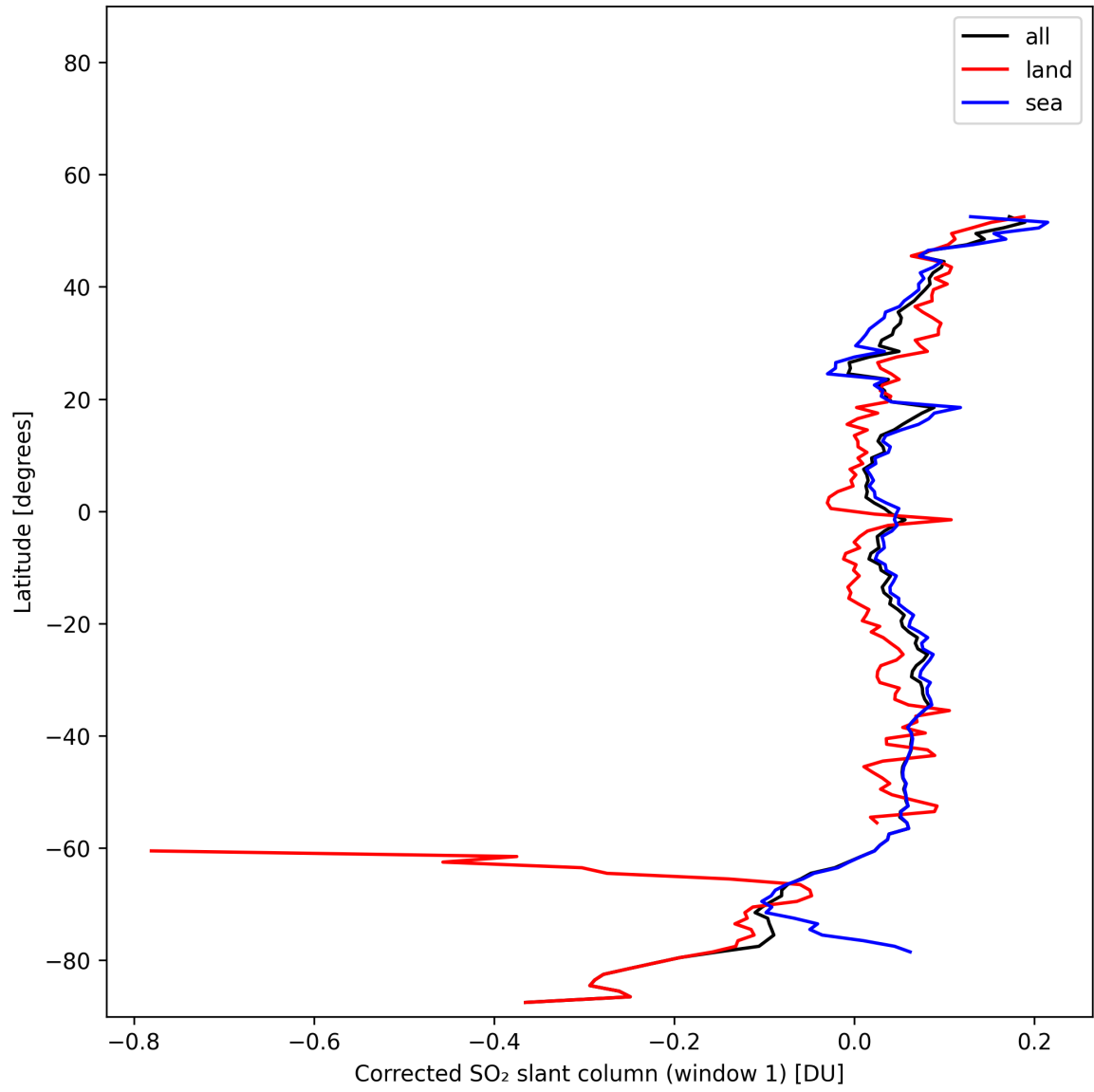
Figure 39: Zonal average of “Corrected SO 2 slant column (window 1)” for 2025-11-12 to 2025-11-13.
