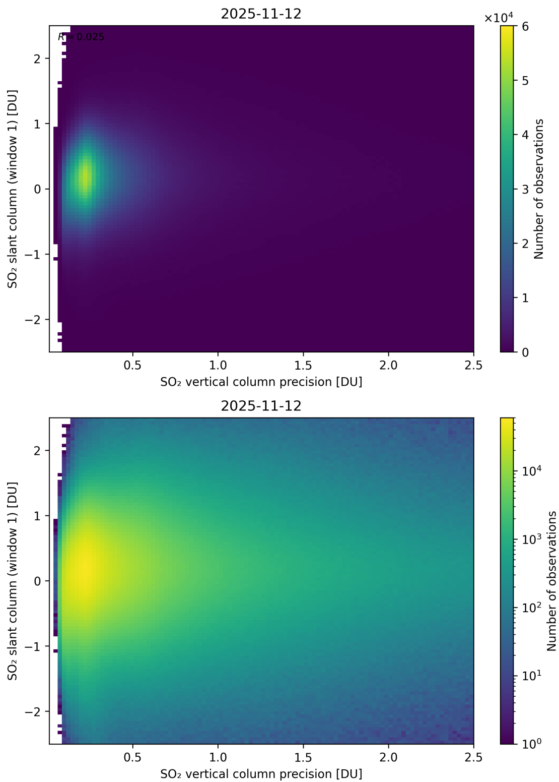
Figure 341: Scatter density plot of “SO 2 vertical column precision” against “SO 2 slant column (window 1)” for 2025-11-12 to 2025-11-13.
