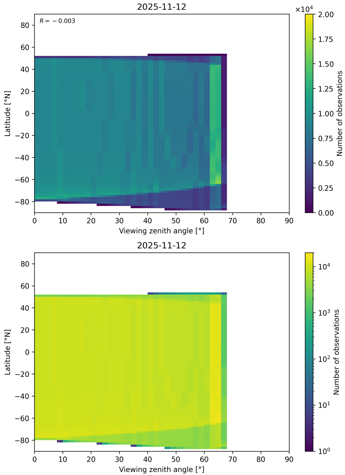
Figure 368: Scatter density plot of “Viewing zenith angle” against “Latitude” for 2025-11-12 to 2025-11-13.
