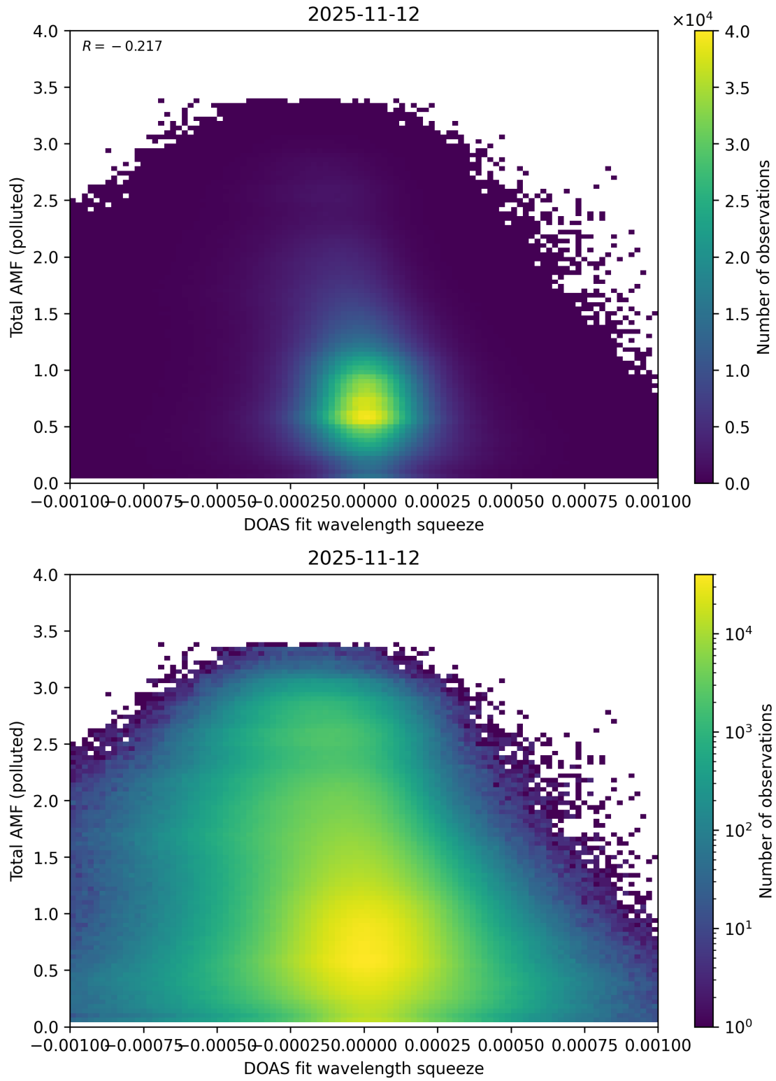
Figure 145: Scatter density plot of “DOAS fit wavelength squeeze” against “Total AMF (polluted)” for 2025-11-12 to 2025-11-13.
