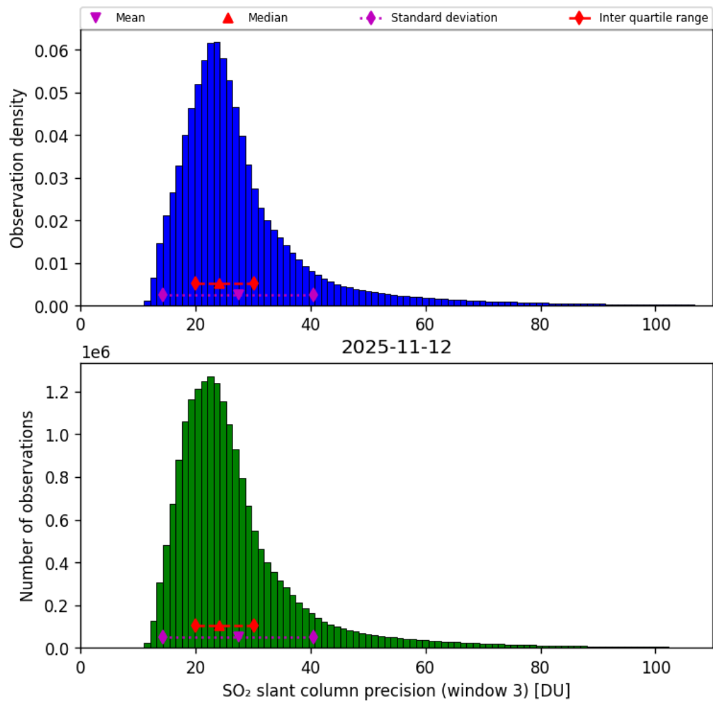
Figure 72: Histogram of “SO 2 slant column precision (window 3)” for 2025-11-12 to 2025-11-13
