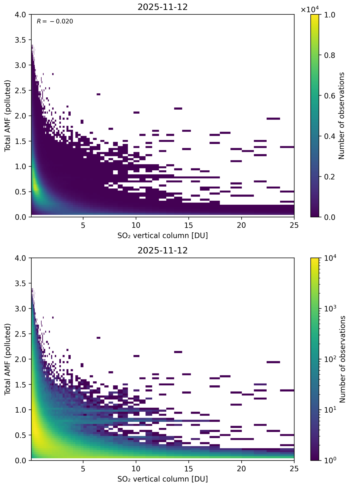
Figure 359: Scatter density plot of “SO 2 vertical column” against “Total AMF (polluted)” for 2025-11-12 to 2025-11-13.
