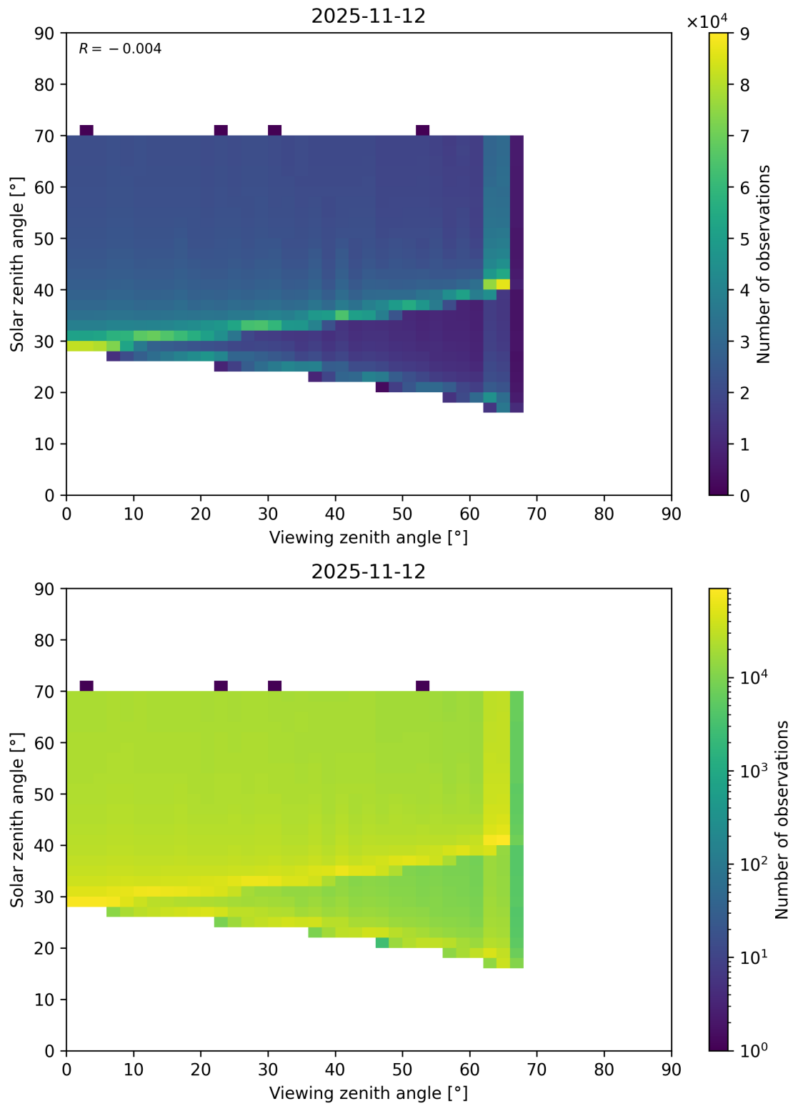
Figure 369: Scatter density plot of “Viewing zenith angle” against “Solar zenith angle” for 2025-11-12 to 2025-11-13.
