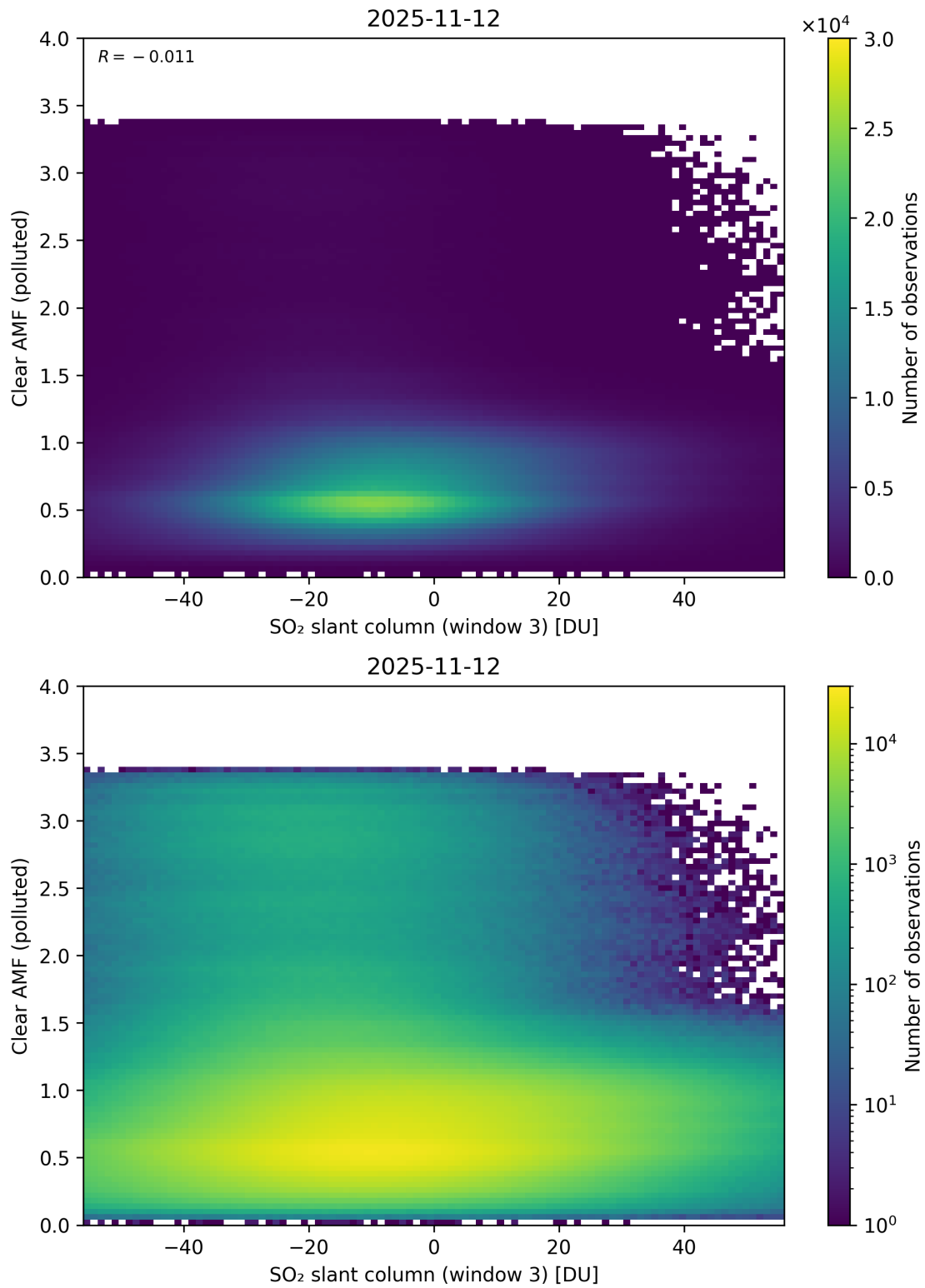
Figure 315: Scatter density plot of “SO 2 slant column (window 3)” against “Clear AMF (polluted)” for 2025-11-12 to 2025-11-13.
