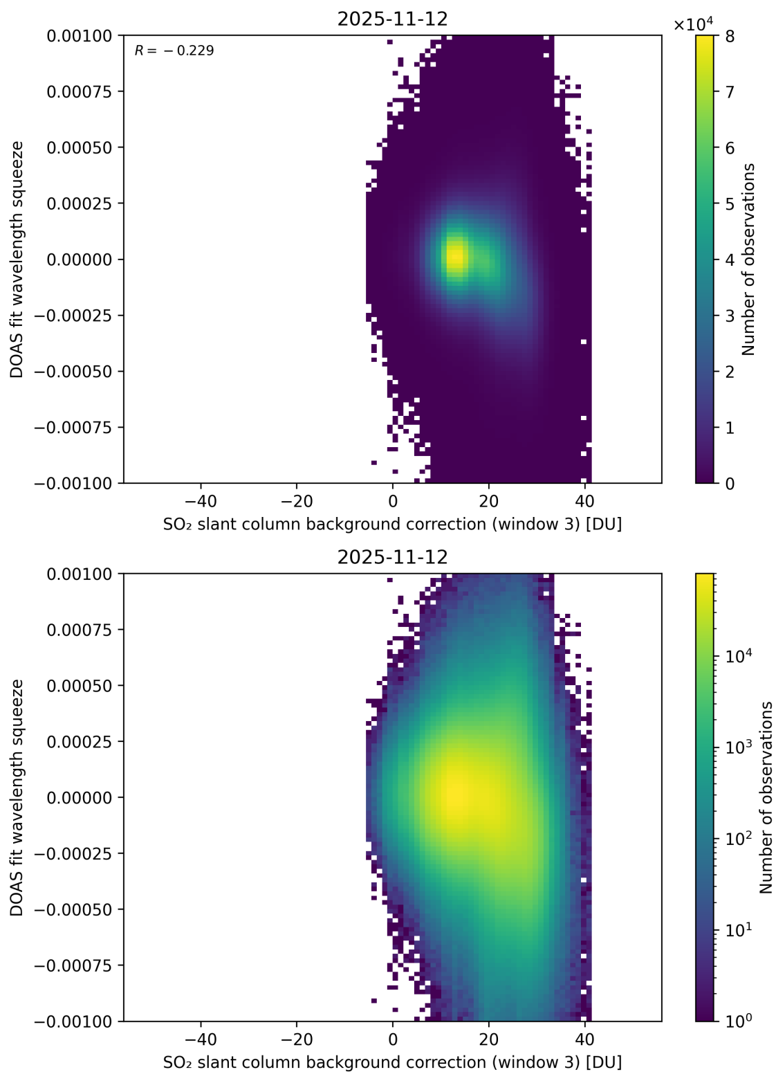
Figure 133: Scatter density plot of “SO 2 slant column background correction (window 3)” against “DOAS fit wavelength squeeze” for 2025-11-12 to 2025-11-13.
