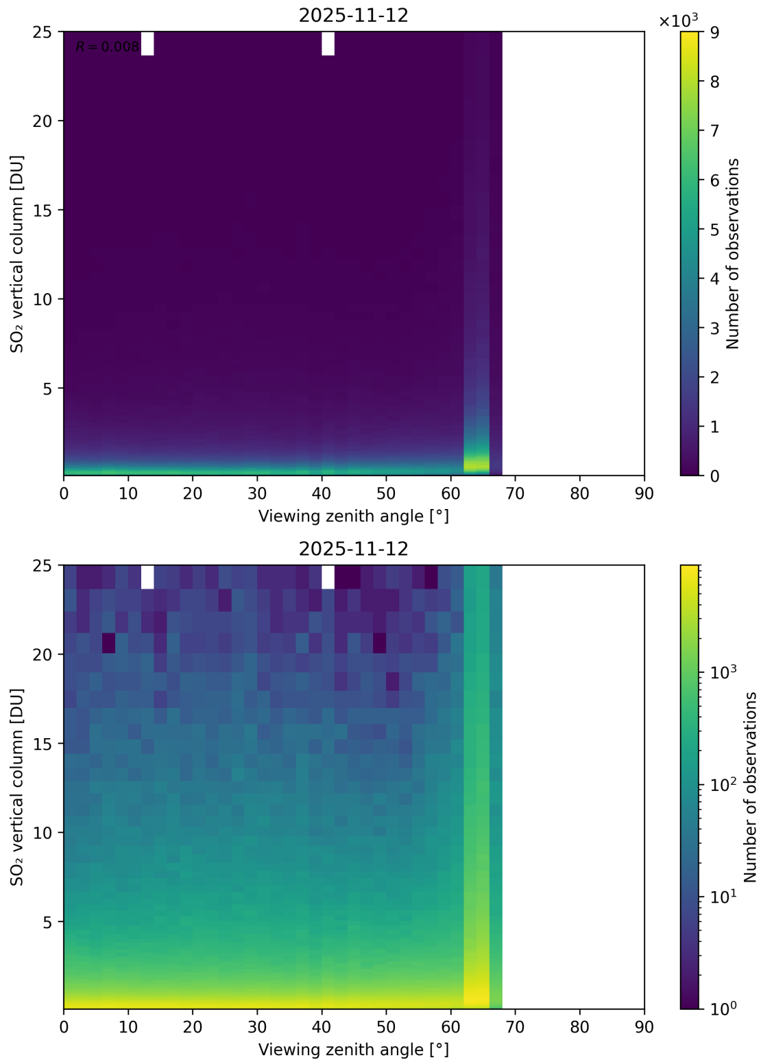
Figure 383: Scatter density plot of “Viewing zenith angle” against “SO 2 vertical column” for 2025-11-12 to 2025-11-13.
