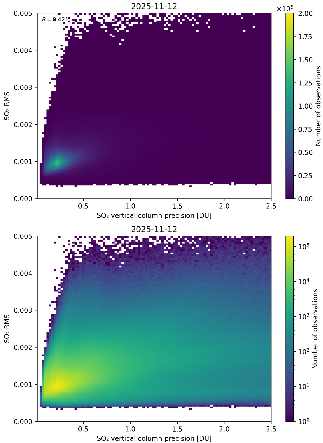
Figure 334: Scatter density plot of “SO 2 vertical column precision” against “SO 2 RMS” for 2025-11-12 to 2025-11-13.
