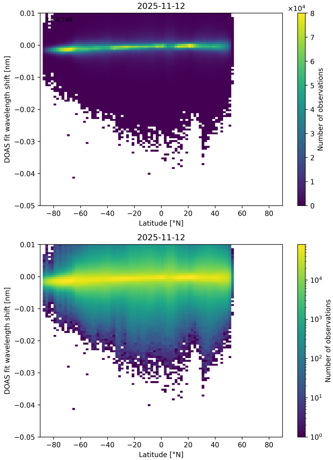
Figure 153: Scatter density plot of “Latitude” against “DOAS fit wavelength shift” for 2025-11-12 to 2025-11-13.
