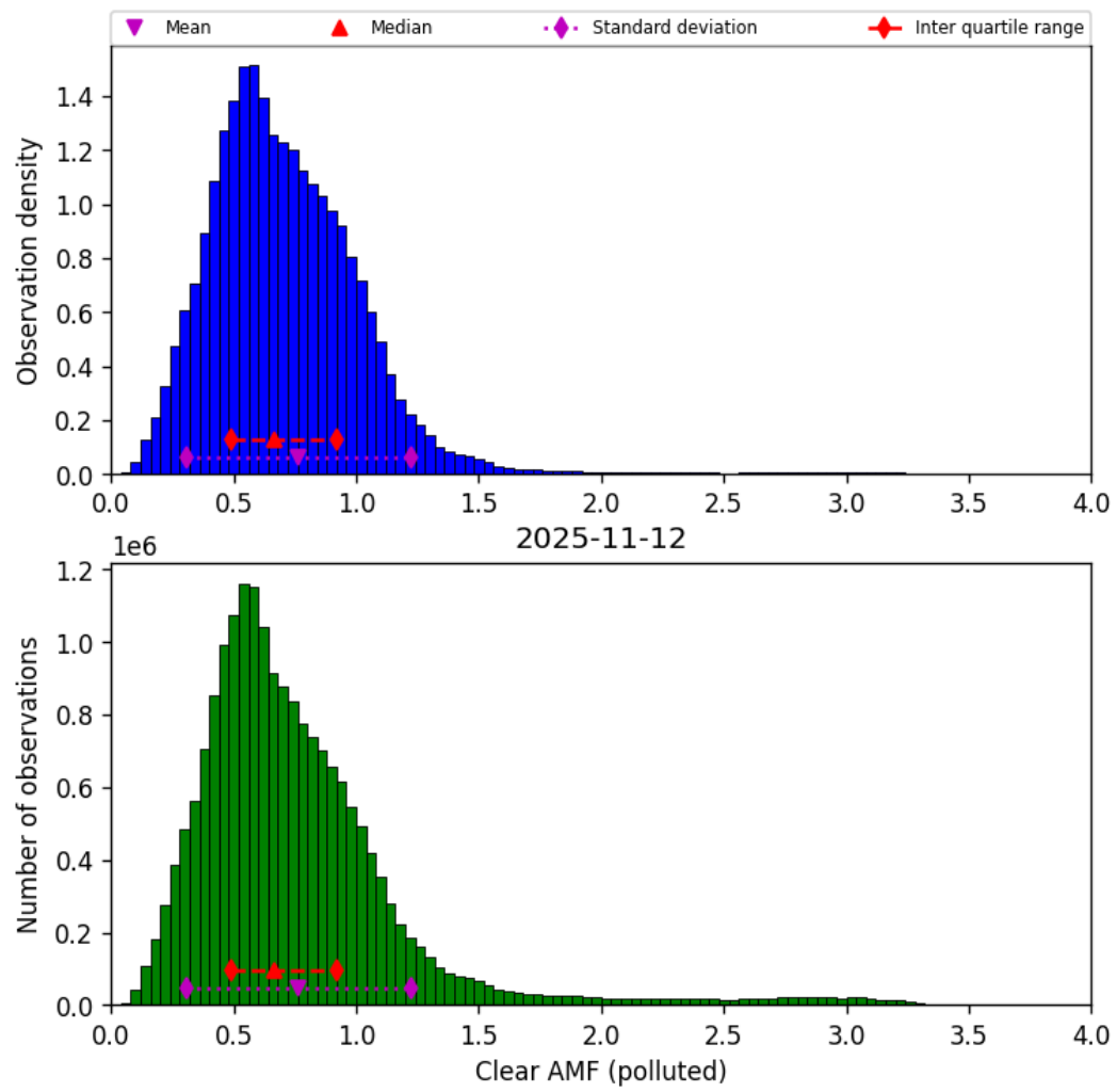
Figure 81: Histogram of “Clear AMF (polluted)” for 2025-11-12 to 2025-11-13
