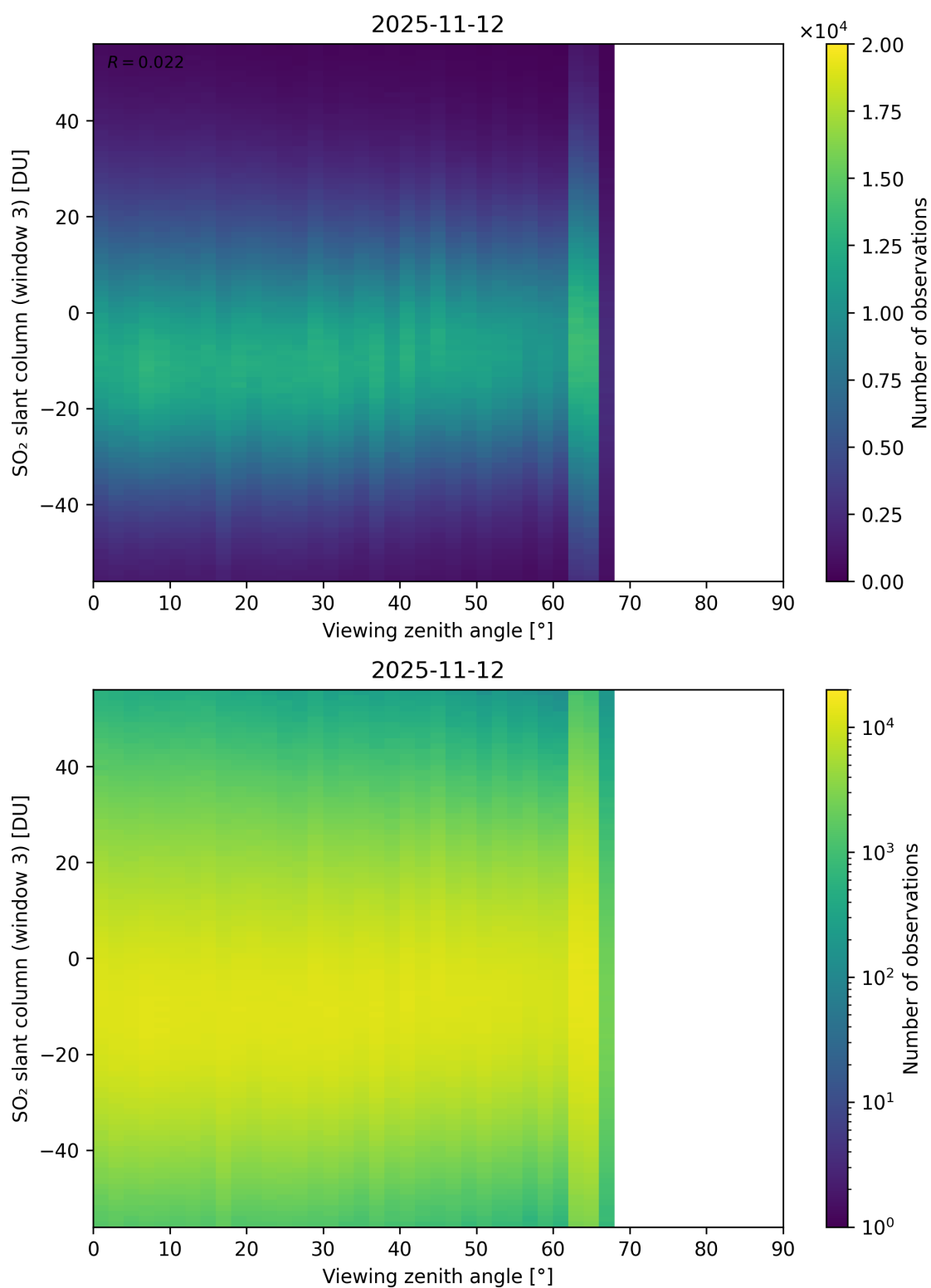
Figure 379: Scatter density plot of “Viewing zenith angle” against “SO 2 slant column (window 3)” for 2025-11-12 to 2025-11-13.
