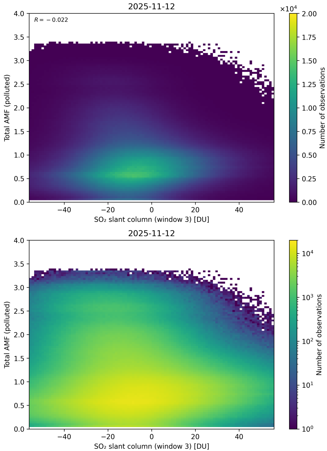
Figure 318: Scatter density plot of “SO 2 slant column (window 3)” against “Total AMF (polluted)” for 2025-11-12 to 2025-11-13.
