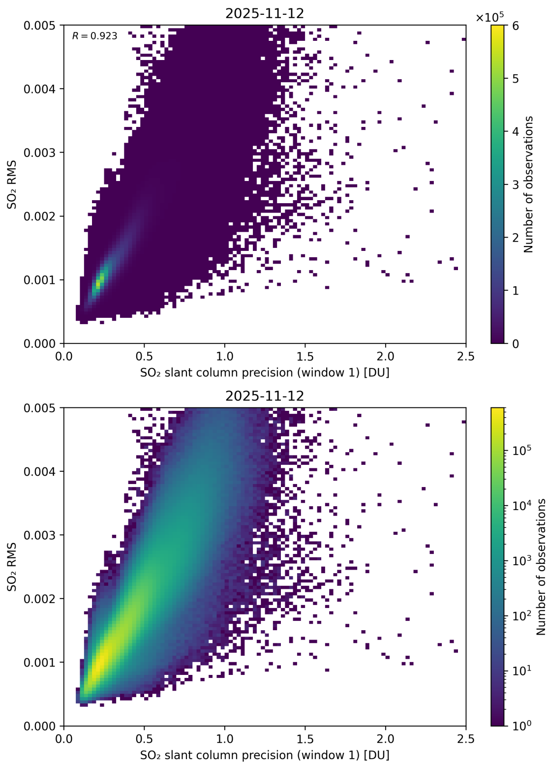
Figure 273: Scatter density plot of “SO 2 slant column precision (window 1)” against “SO 2 RMS” for 2025-11-12 to 2025-11-13.
