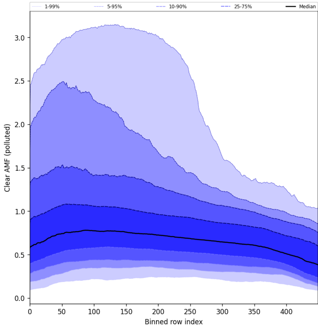
Figure 107: Along track statistics of “Clear AMF (polluted)” for 2025-11-12 to 2025-11-13
