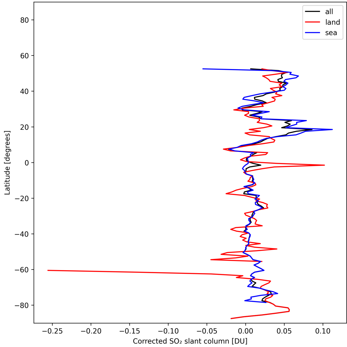
Figure 34: Zonal average of “Corrected SO 2 slant column” for 2025-11-12 to 2025-11-13.
