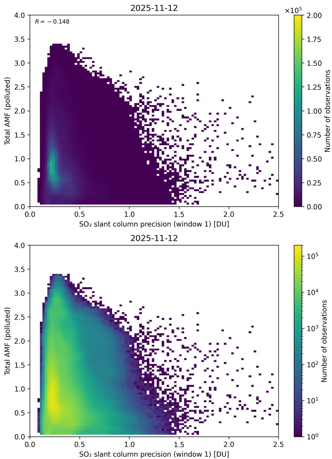
Figure 280: Scatter density plot of “SO 2 slant column precision (window 1)” against “Total AMF (polluted)” for 2025-11-12 to 2025-11-13.
