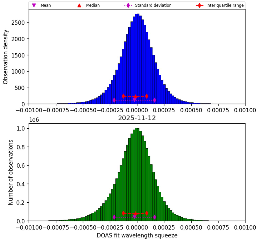
Figure 77: Histogram of “DOAS fit wavelength squeeze” for 2025-11-12 to 2025-11-13
