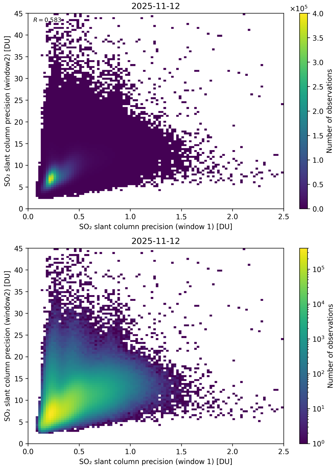
Figure 277: Scatter density plot of “SO 2 slant column precision (window 1)” against “SO 2 slant column precision (window2)” for 2025-11-12 to 2025-11-13.
