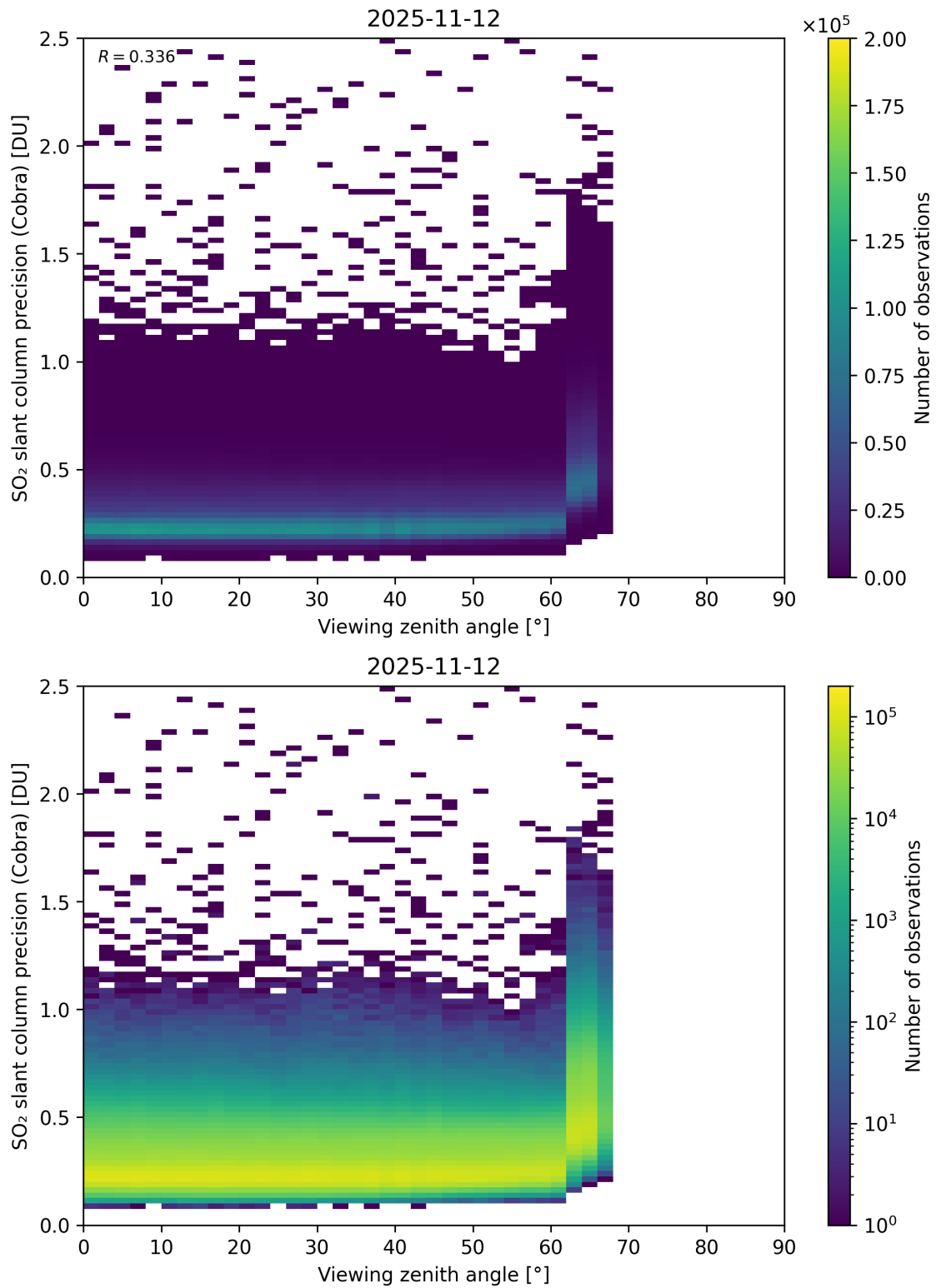
Figure 372: Scatter density plot of “Viewing zenith angle” against “SO 2 slant column precision (Cobra)” for 2025-11-12 to 2025-11-13.
