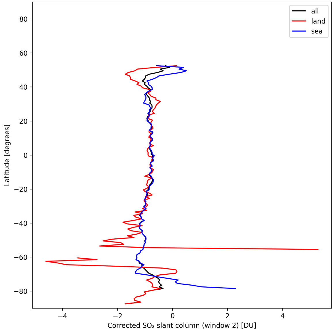
Figure 43: Zonal average of “Corrected SO 2 slant column (window 2)” for 2025-11-12 to 2025-11-13.
