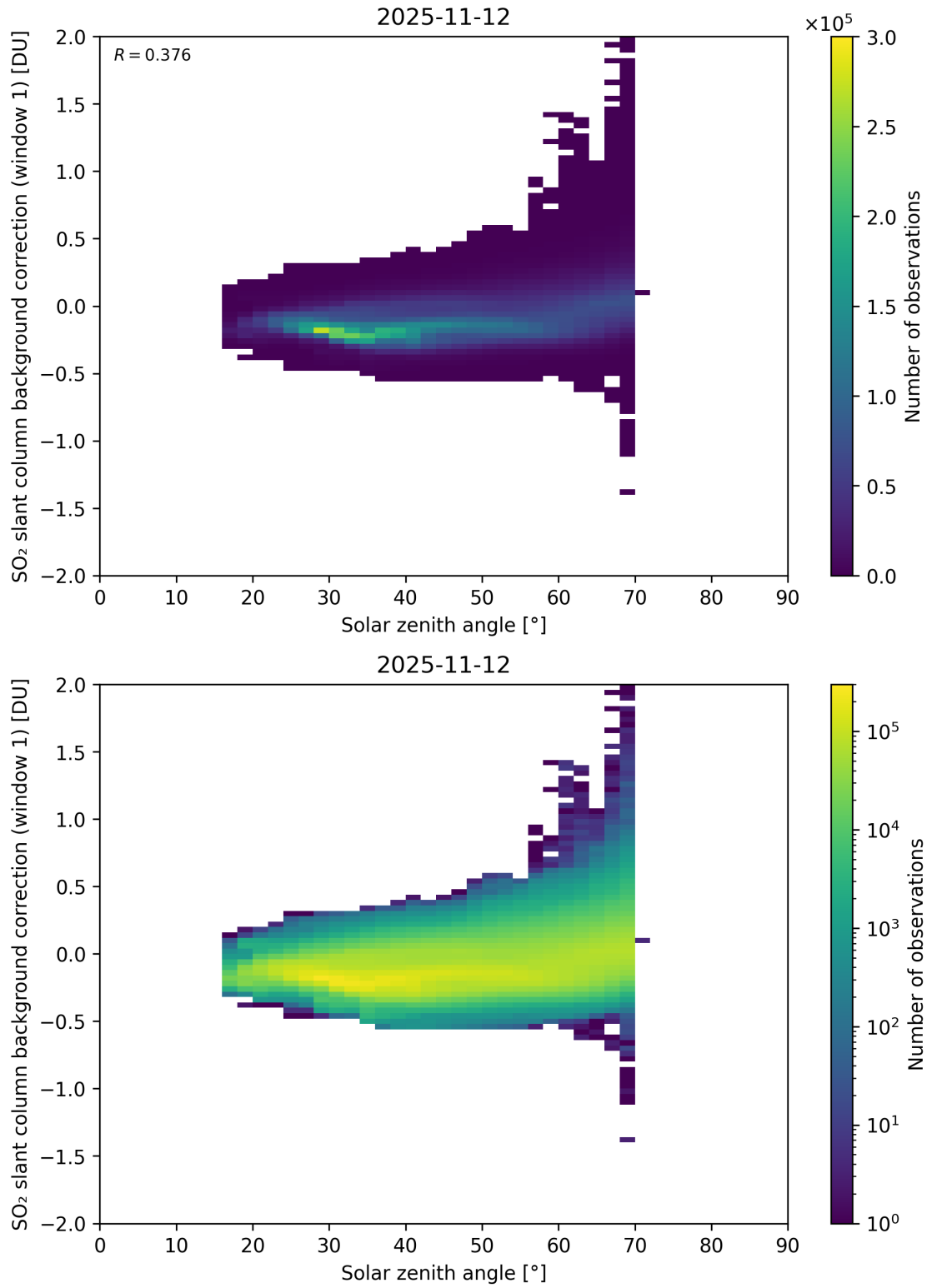
Figure 171: Scatter density plot of “Solar zenith angle” against “SO 2 slant column background correction (window 1)” for 2025-11-12 to 2025-11-13.
