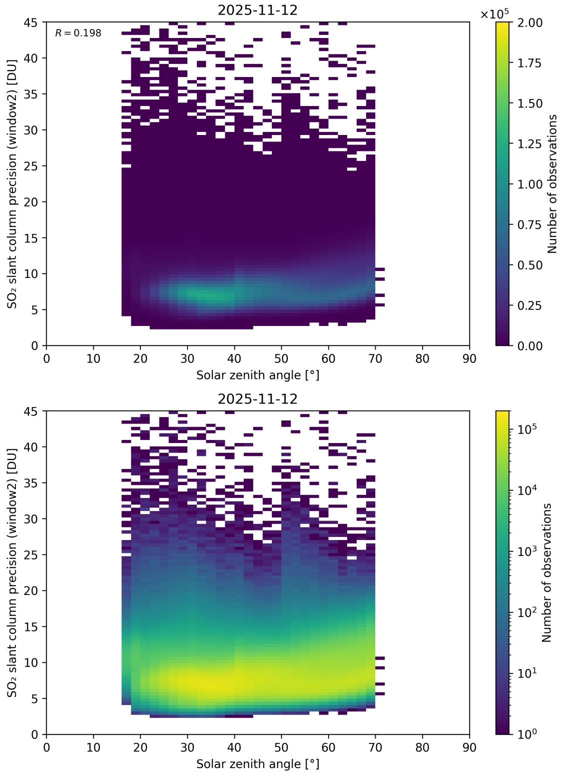
Figure 186: Scatter density plot of “Solar zenith angle” against “SO 2 slant column precision (window2)” for 2025-11-12 to 2025-11-13.
