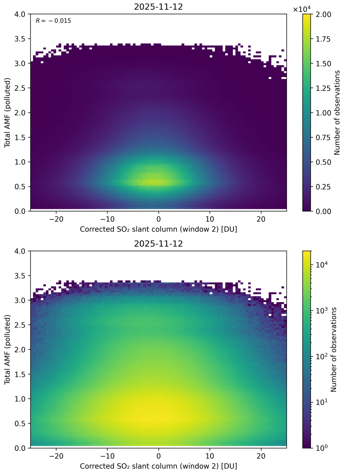
Figure 253: Scatter density plot of “Corrected SO 2 slant column (window 2)” against “Total AMF (polluted)” for 2025-11-12 to 2025-11-13.
