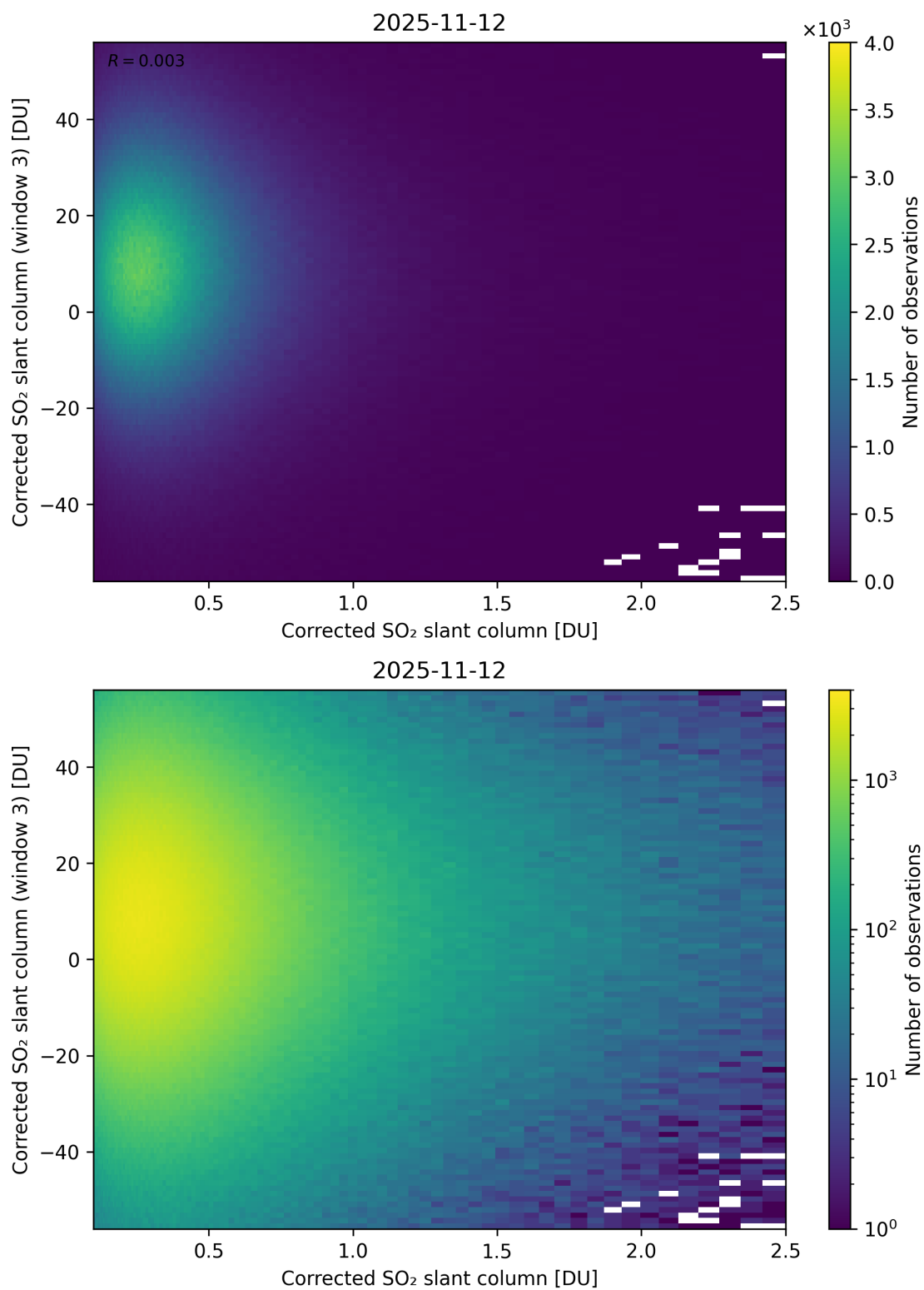
Figure 236: Scatter density plot of “Corrected SO 2 slant column” against “Corrected SO 2 slant column (window 3)” for 2025-11-12 to 2025-11-13.
