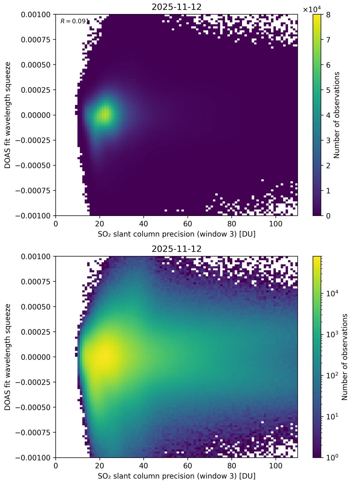
Figure 309: Scatter density plot of “SO 2 slant column precision (window 3)” against “DOAS fit wavelength squeeze” for 2025-11-12 to 2025-11-13.
