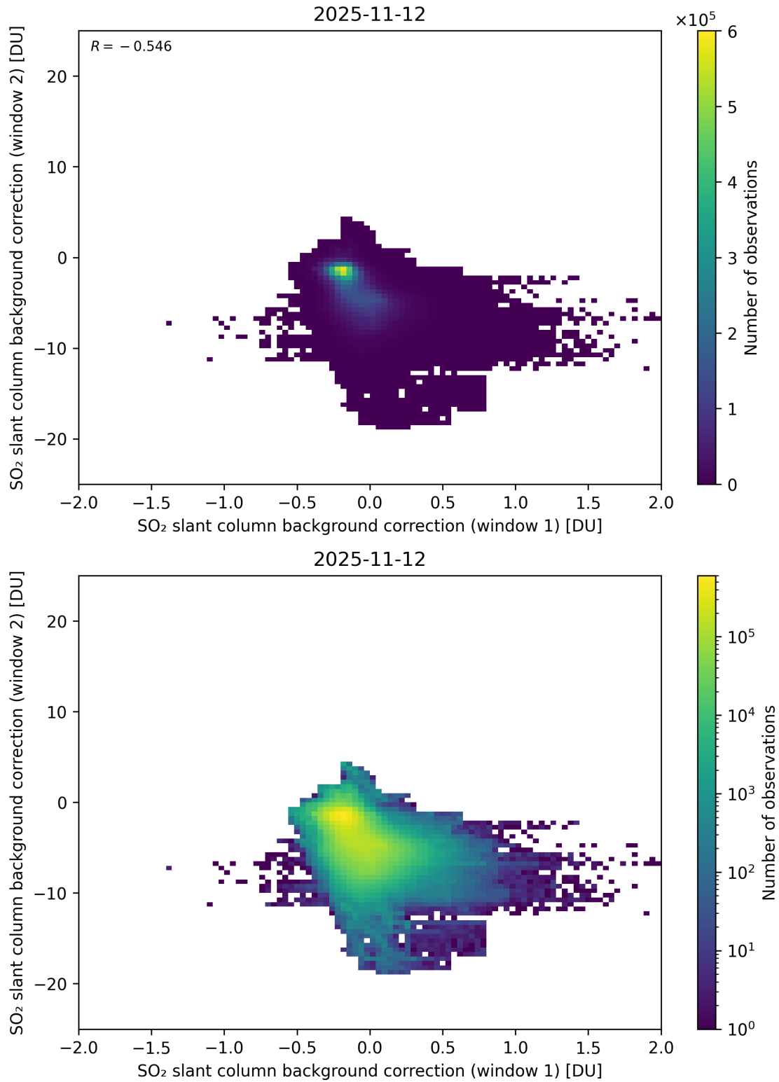
Figure 109: Scatter density plot of “SO 2 slant column background correction (window 1)” against “SO 2 slant column background correction (window 2)” for 2025-11-12 to 2025-11-13.
