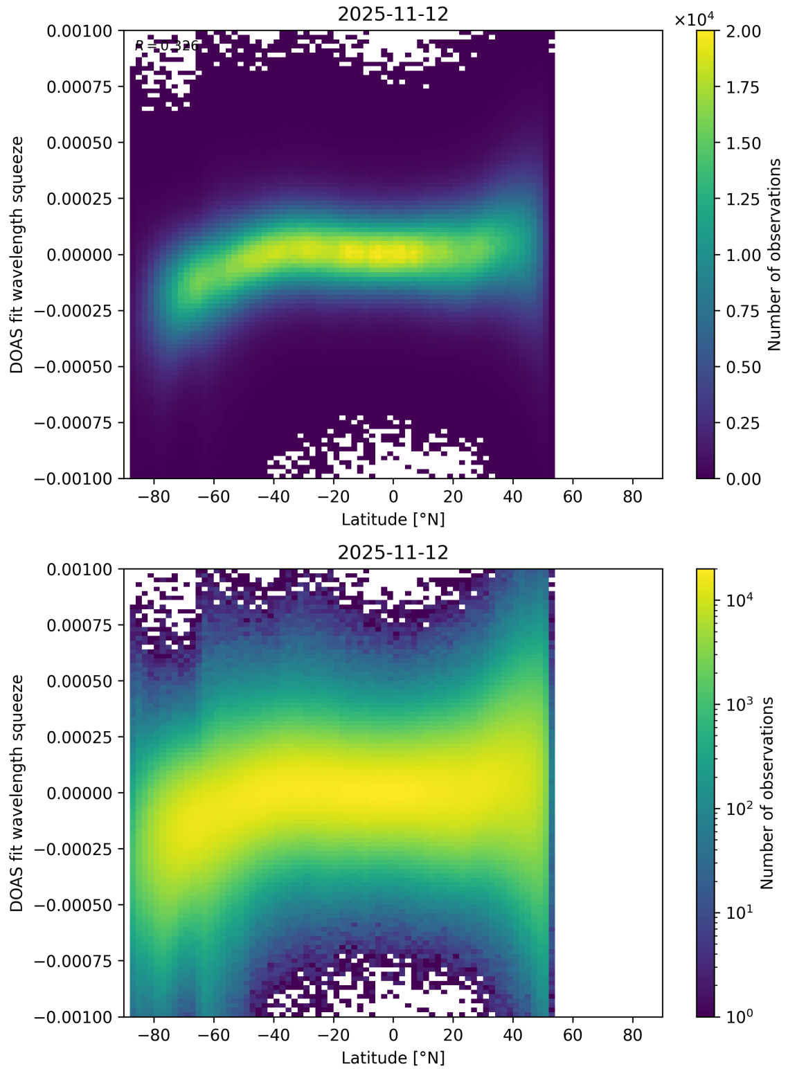
Figure 154: Scatter density plot of “Latitude” against “DOAS fit wavelength squeeze” for 2025-11-12 to 2025-11-13.
