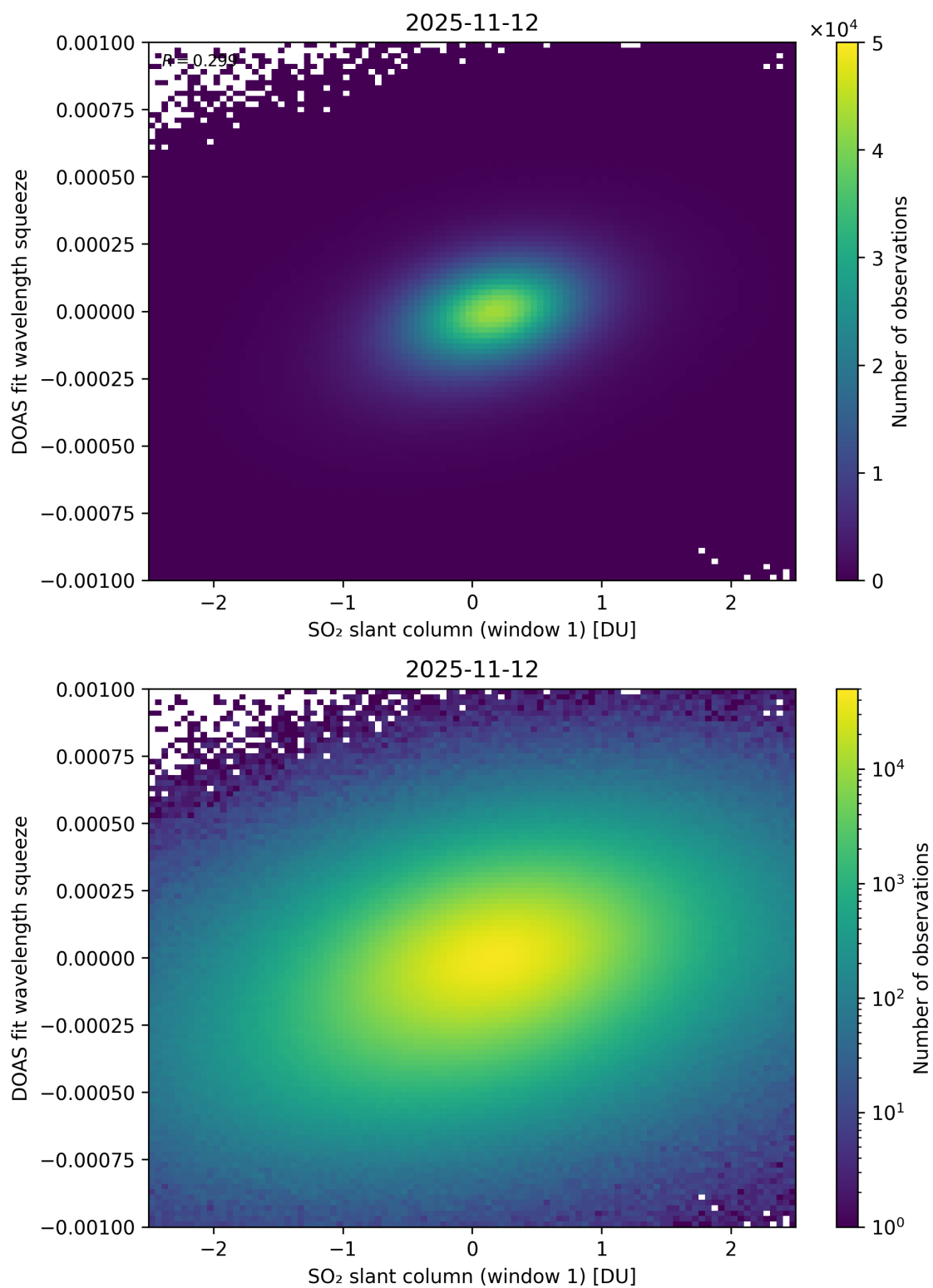
Figure 266: Scatter density plot of “SO 2 slant column (window 1)” against “DOAS fit wavelength squeeze” for 2025-11-12 to 2025-11-13.
