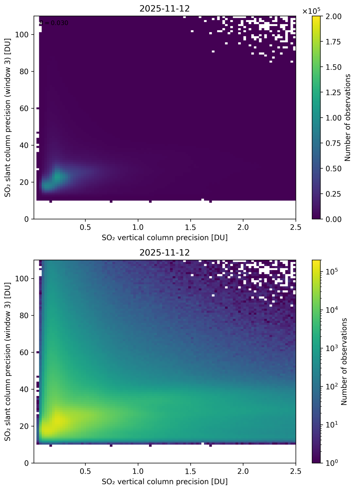
Figure 345: Scatter density plot of “SO 2 vertical column precision” against “SO 2 slant column precision (window 3)” for 2025-11-12 to 2025-11-13.
