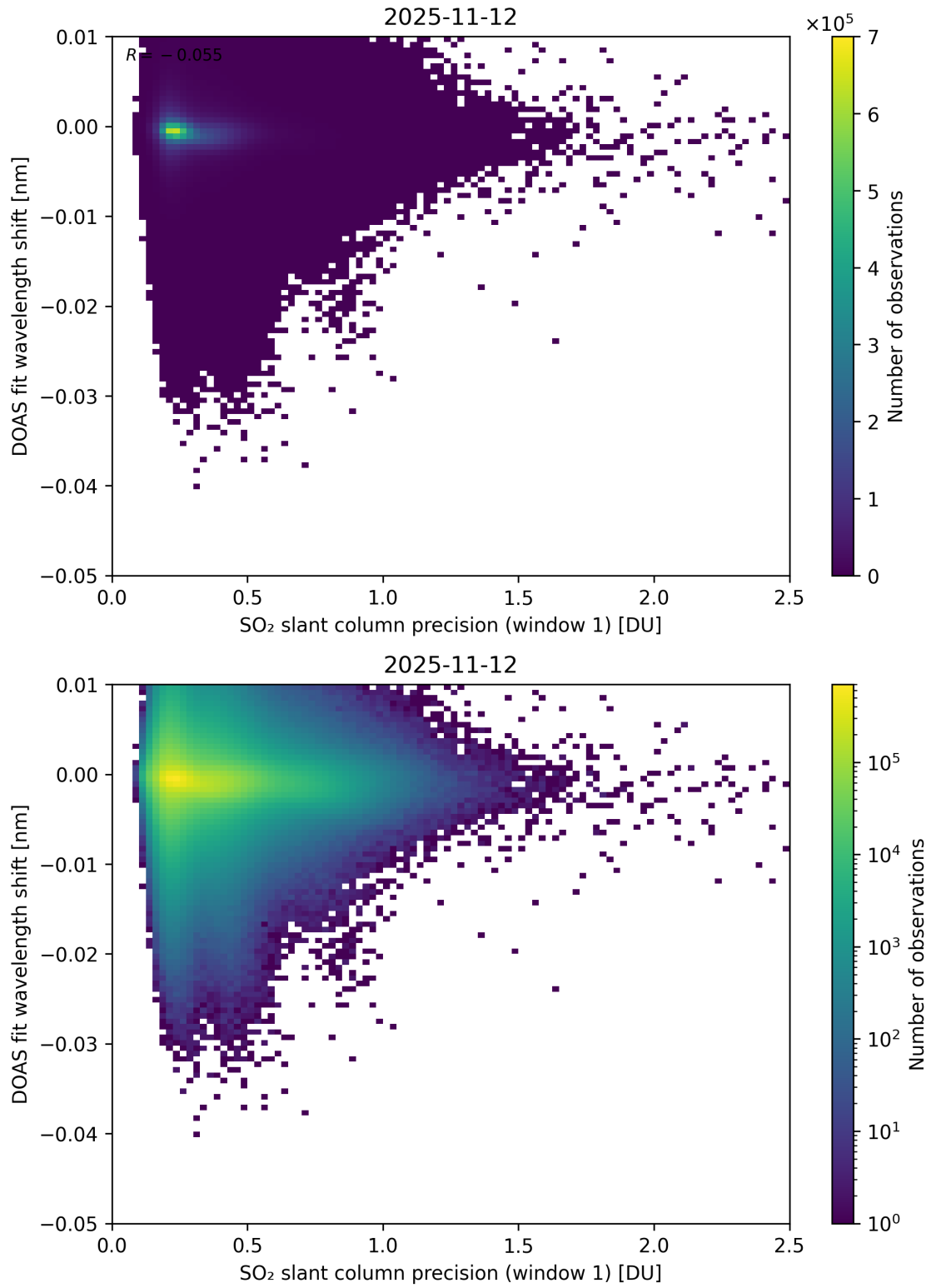
Figure 271: Scatter density plot of “SO 2 slant column precision (window 1)” against “DOAS fit wavelength shift” for 2025-11-12 to 2025-11-13.
