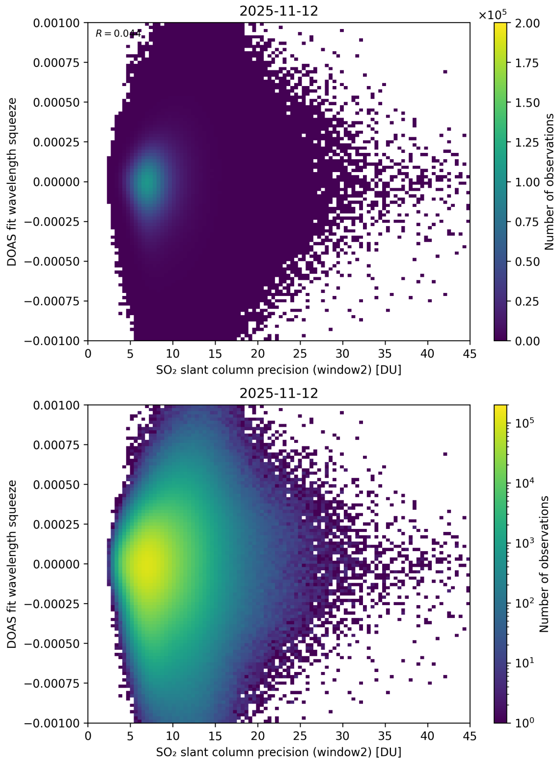
Figure 294: Scatter density plot of “SO 2 slant column precision (window2)” against “DOAS fit wavelength squeeze” for 2025-11-12 to 2025-11-13.
