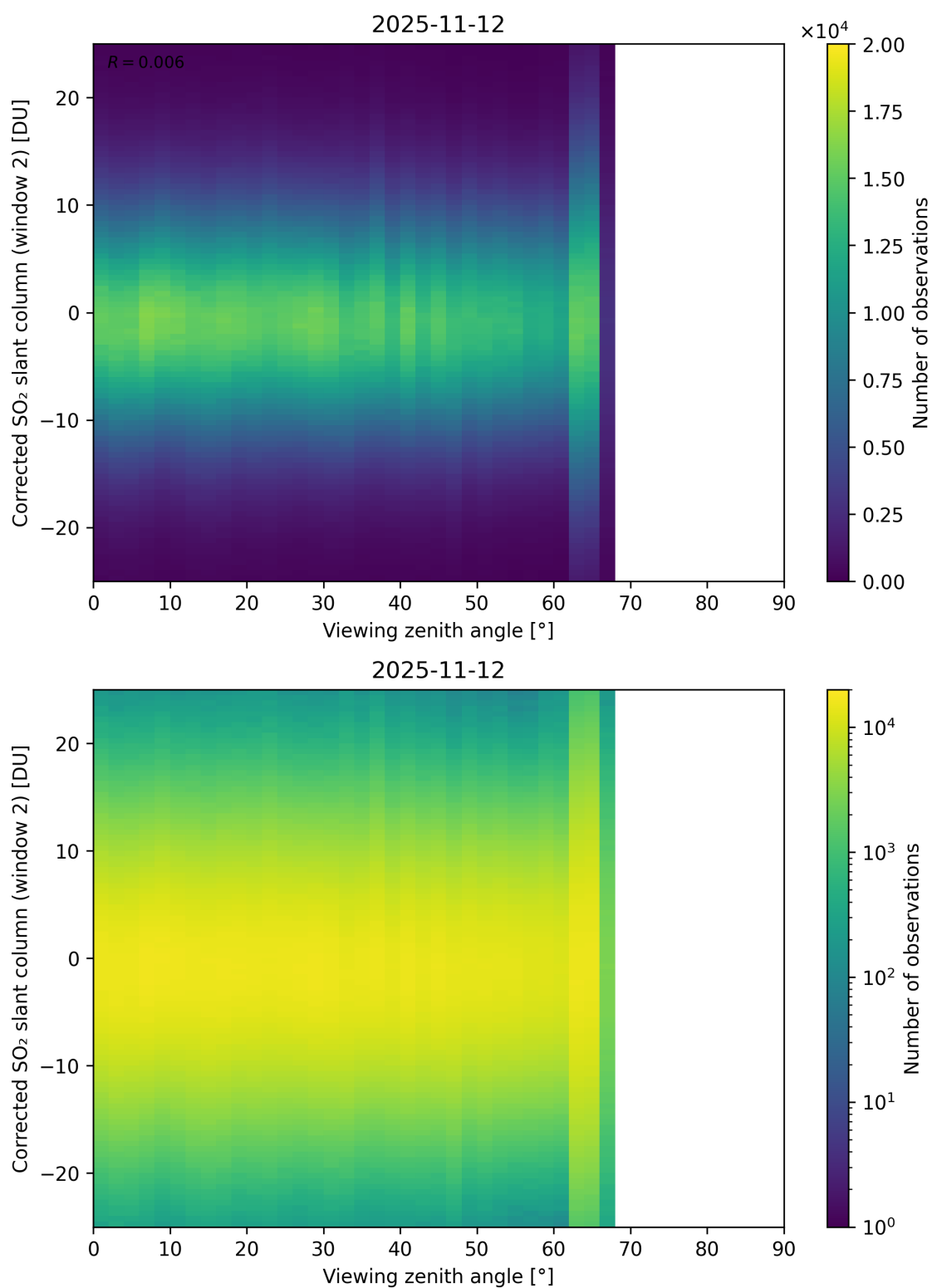
Figure 374: Scatter density plot of “Viewing zenith angle” against “Corrected SO 2 slant column (window 2)” for 2025-11-12 to 2025-11-13.
