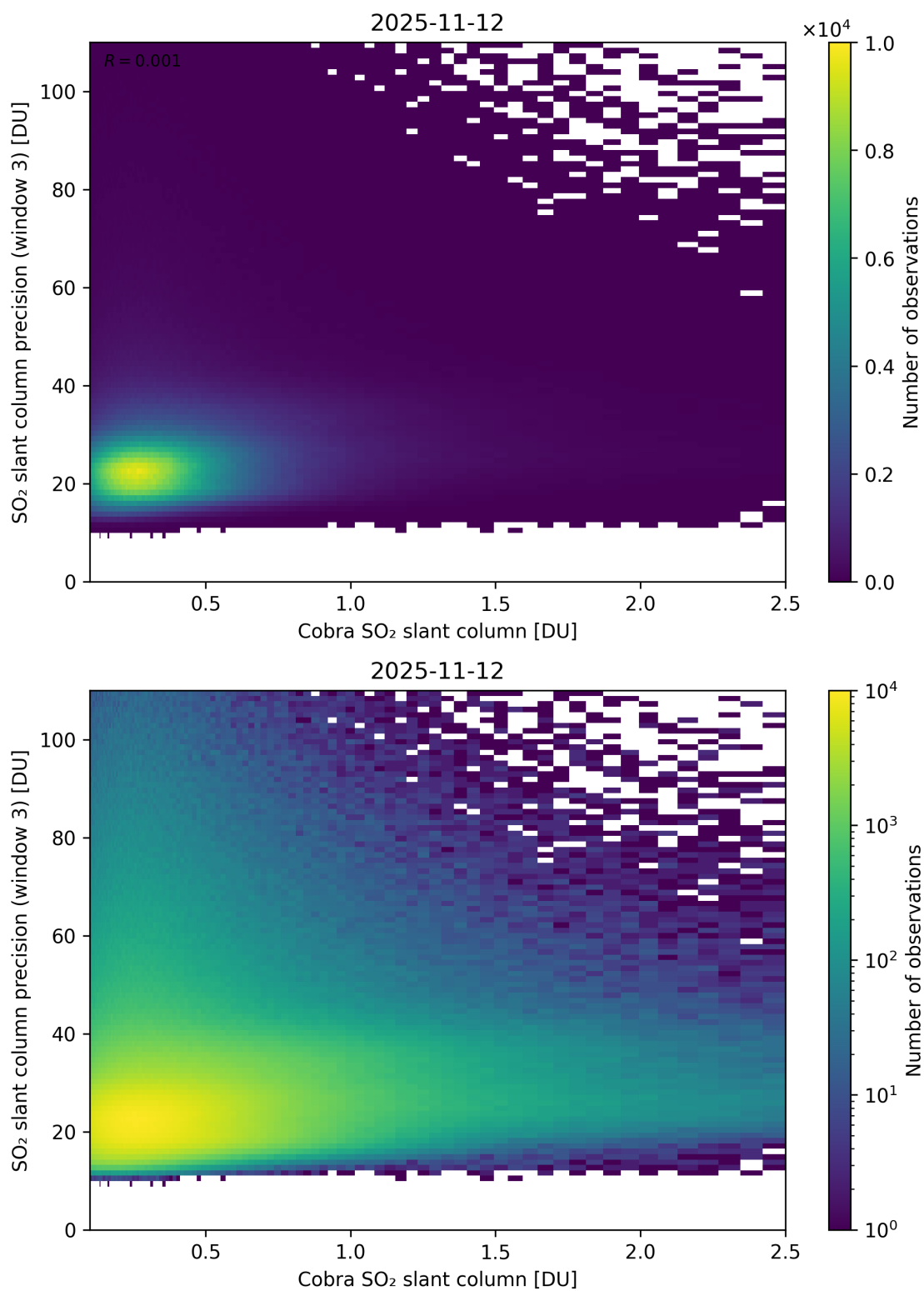
Figure 223: Scatter density plot of “Cobra SO 2 slant column” against “SO 2 slant column precision (window 3)” for 2025-11-12 to 2025-11-13.
