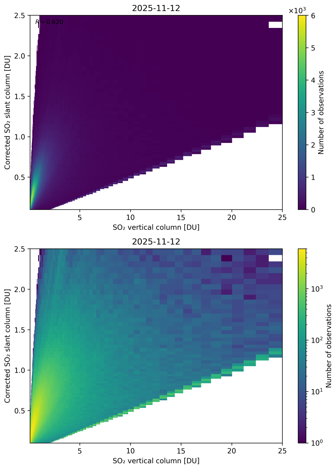
Figure 351: Scatter density plot of “SO 2 vertical column” against “Corrected SO 2 slant column” for 2025-11-12 to 2025-11-13.
