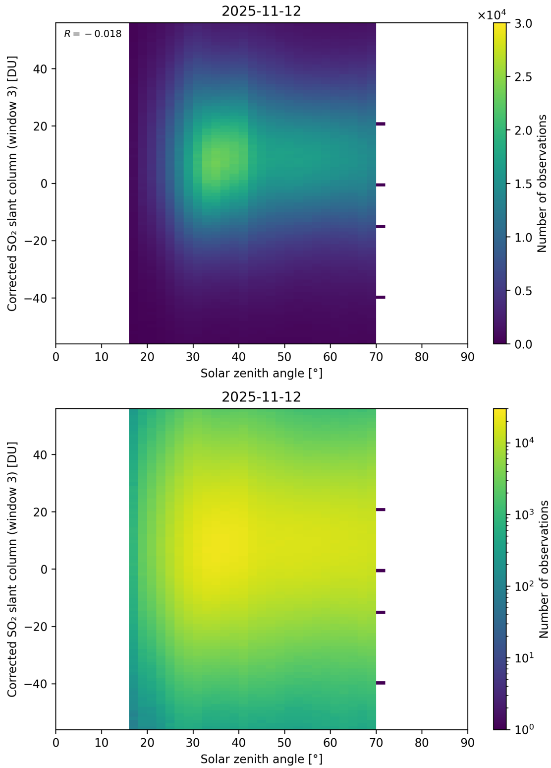
Figure 183: Scatter density plot of “Solar zenith angle” against “Corrected SO 2 slant column (window 3)” for 2025-11-12 to 2025-11-13.
