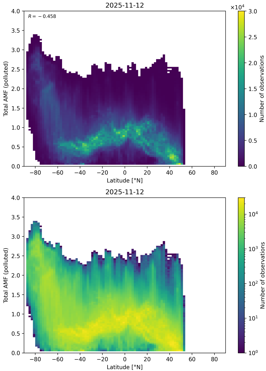
Figure 167: Scatter density plot of “Latitude” against “Total AMF (polluted)” for 2025-11-12 to 2025-11-13.
