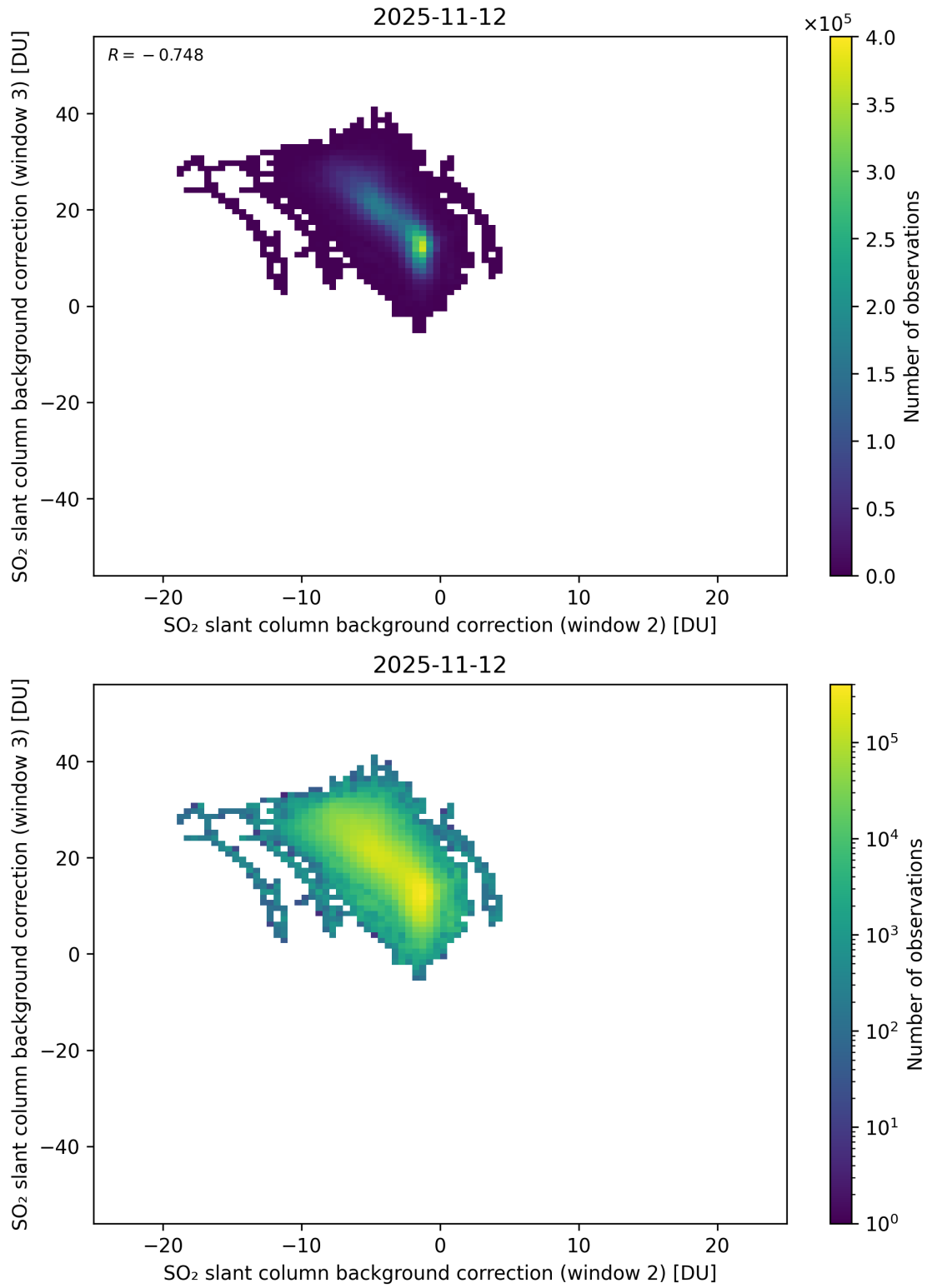
Figure 122: Scatter density plot of “SO 2 slant column background correction (window 2)” against “SO 2 slant column background correction (window 3)” for 2025-11-12 to 2025-11-13.
