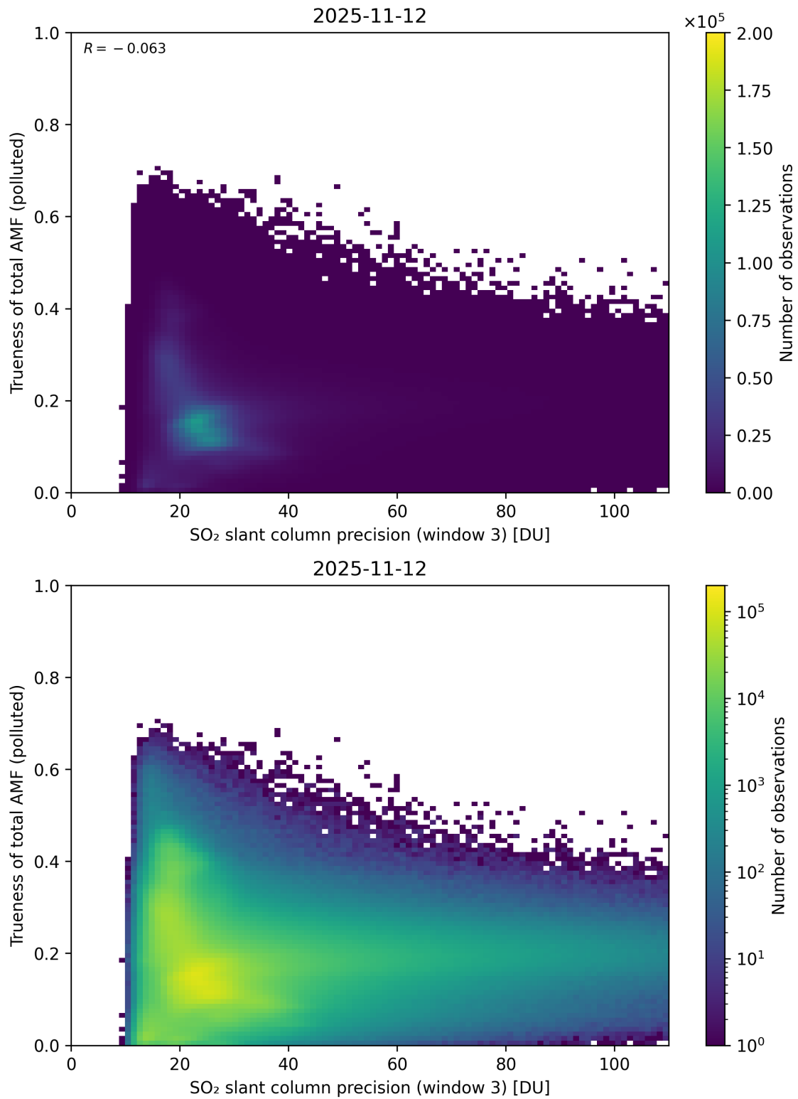
Figure 314: Scatter density plot of “SO 2 slant column precision (window 3)” against “Trueness of total AMF (polluted)” for 2025-11-12 to 2025-11-13.
