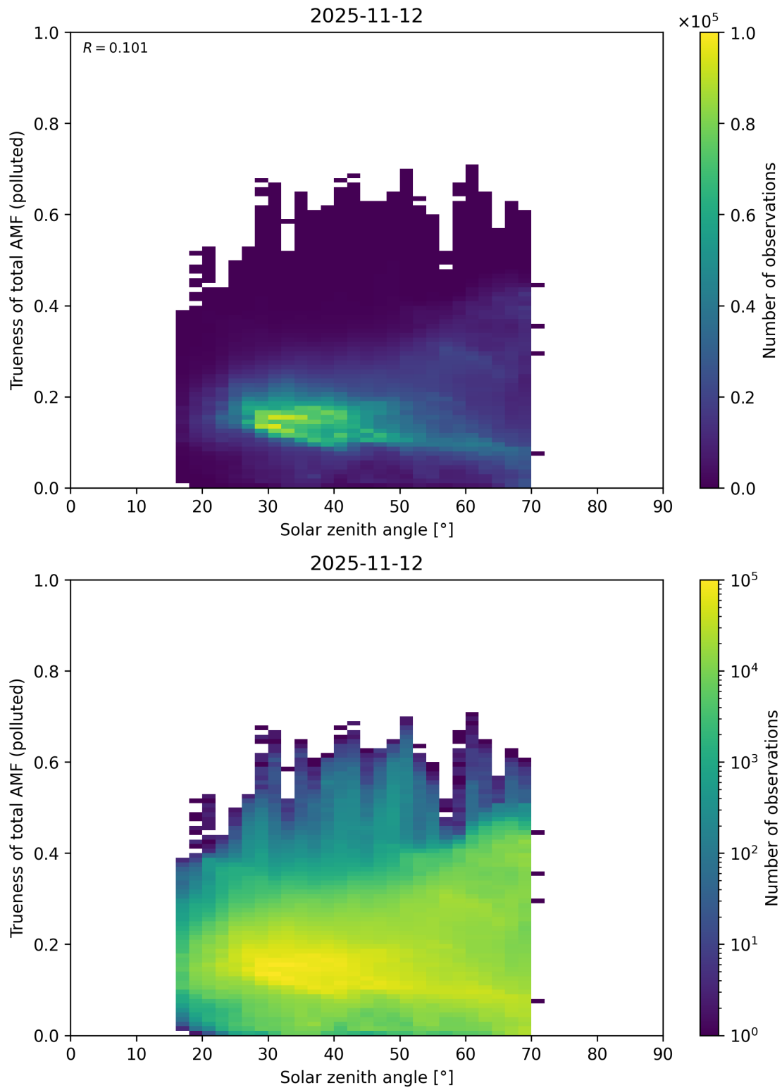
Figure 190: Scatter density plot of “Solar zenith angle” against “Trueness of total AMF (polluted)” for 2025-11-12 to 2025-11-13.
