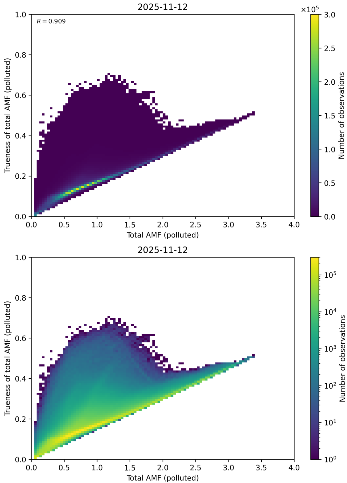
Figure 321: Scatter density plot of “Total AMF (polluted)” against “Trueness of total AMF (polluted)” for 2025-11-12 to 2025-11-13.
