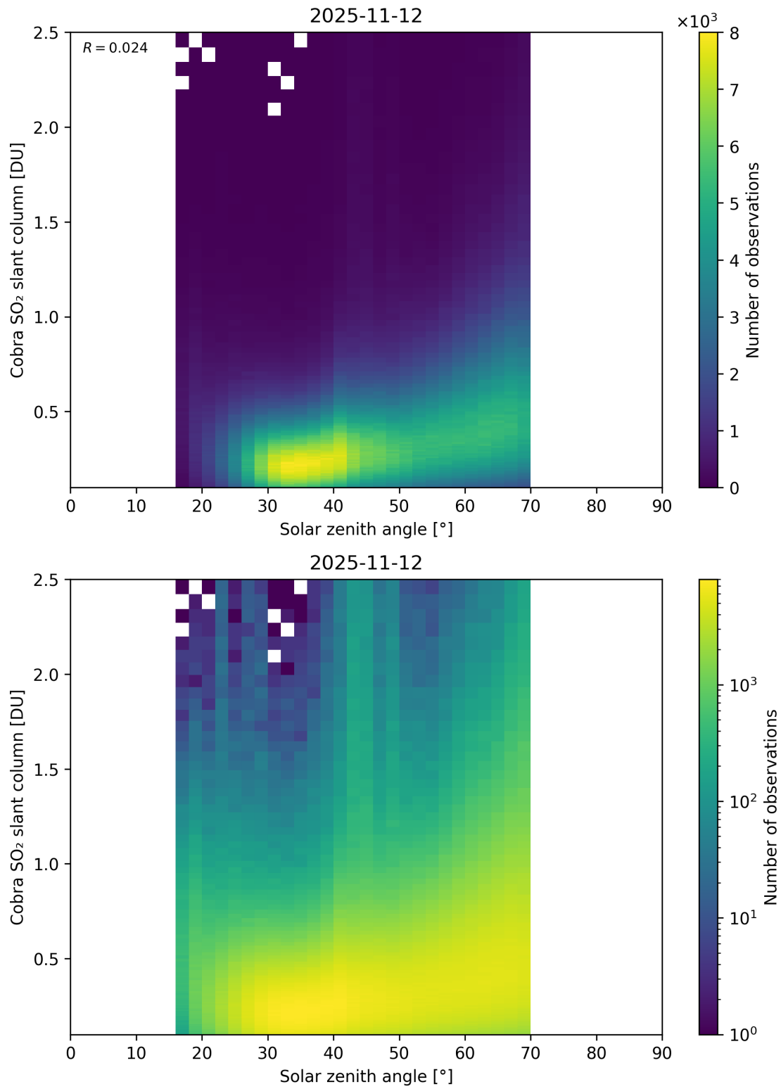
Figure 179: Scatter density plot of “Solar zenith angle” against “Cobra SO 2 slant column” for 2025-11-12 to 2025-11-13.
