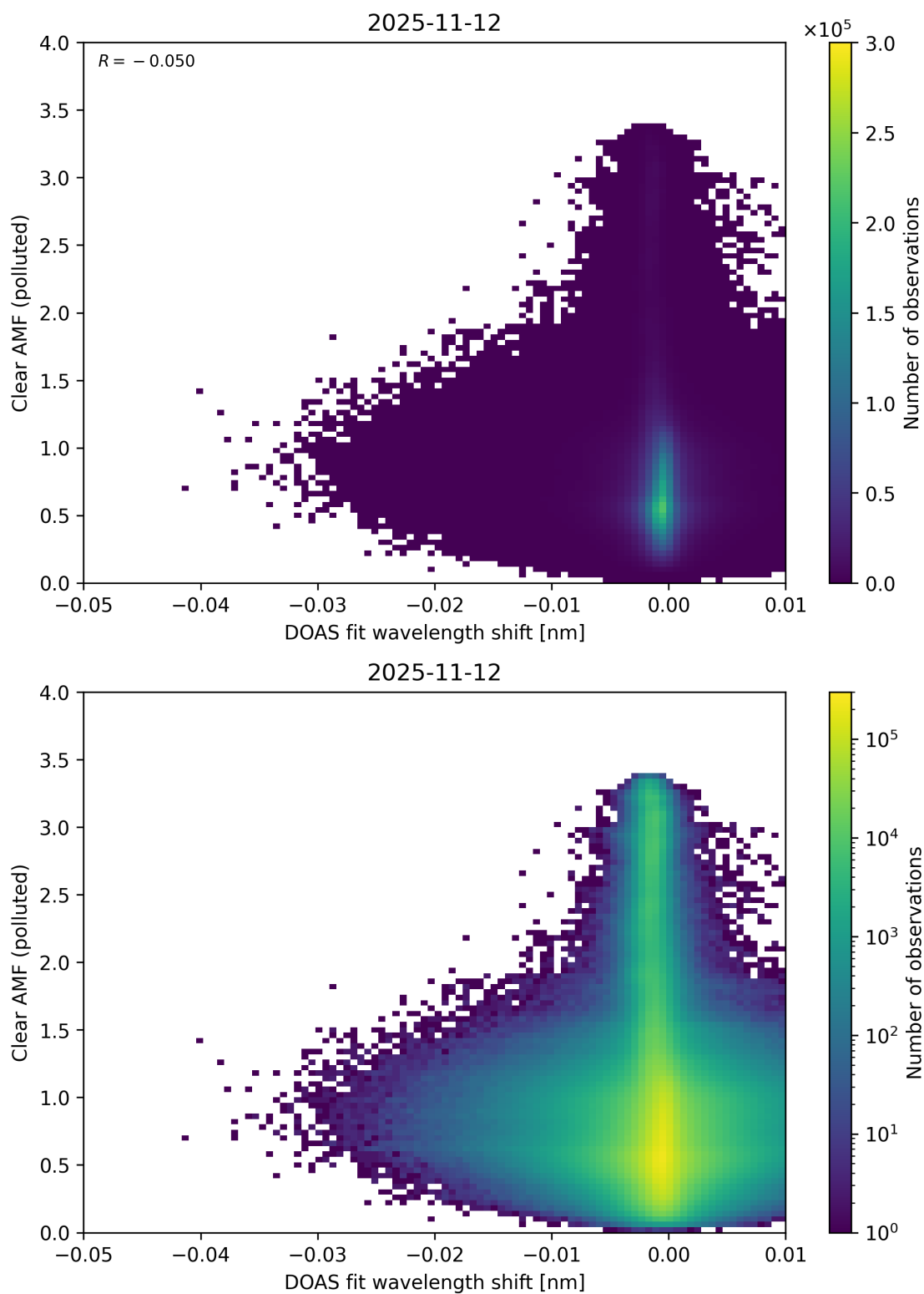
Figure 140: Scatter density plot of “DOAS fit wavelength shift” against “Clear AMF (polluted)” for 2025-11-12 to 2025-11-13.
