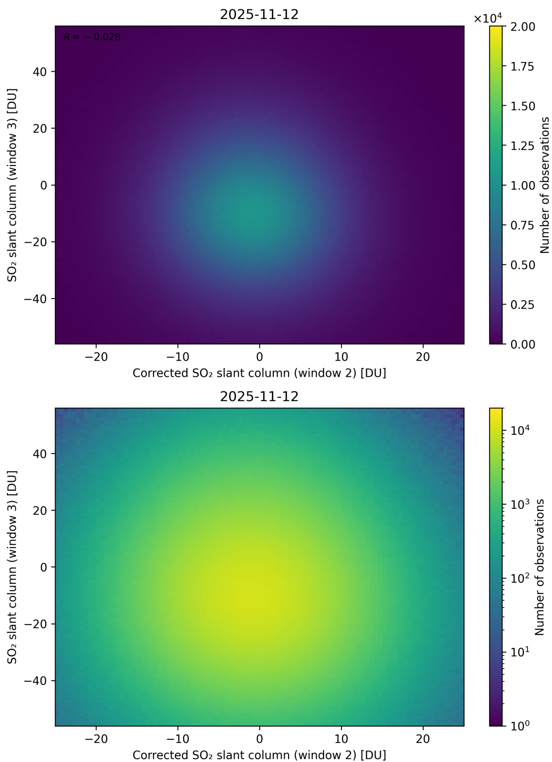
Figure 251: Scatter density plot of “Corrected SO 2 slant column (window 2)” against “SO 2 slant column (window 3)” for 2025-11-12 to 2025-11-13.
