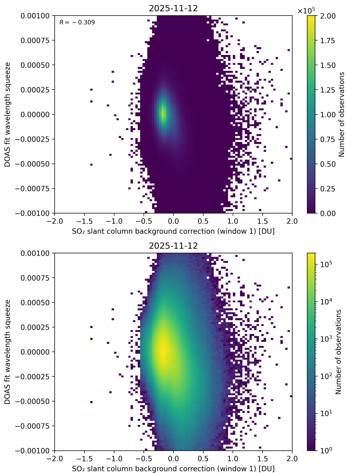
Figure 112: Scatter density plot of “SO 2 slant column background correction (window 1)” against “DOAS fit wavelength squeeze” for 2025-11-12 to 2025-11-13.
