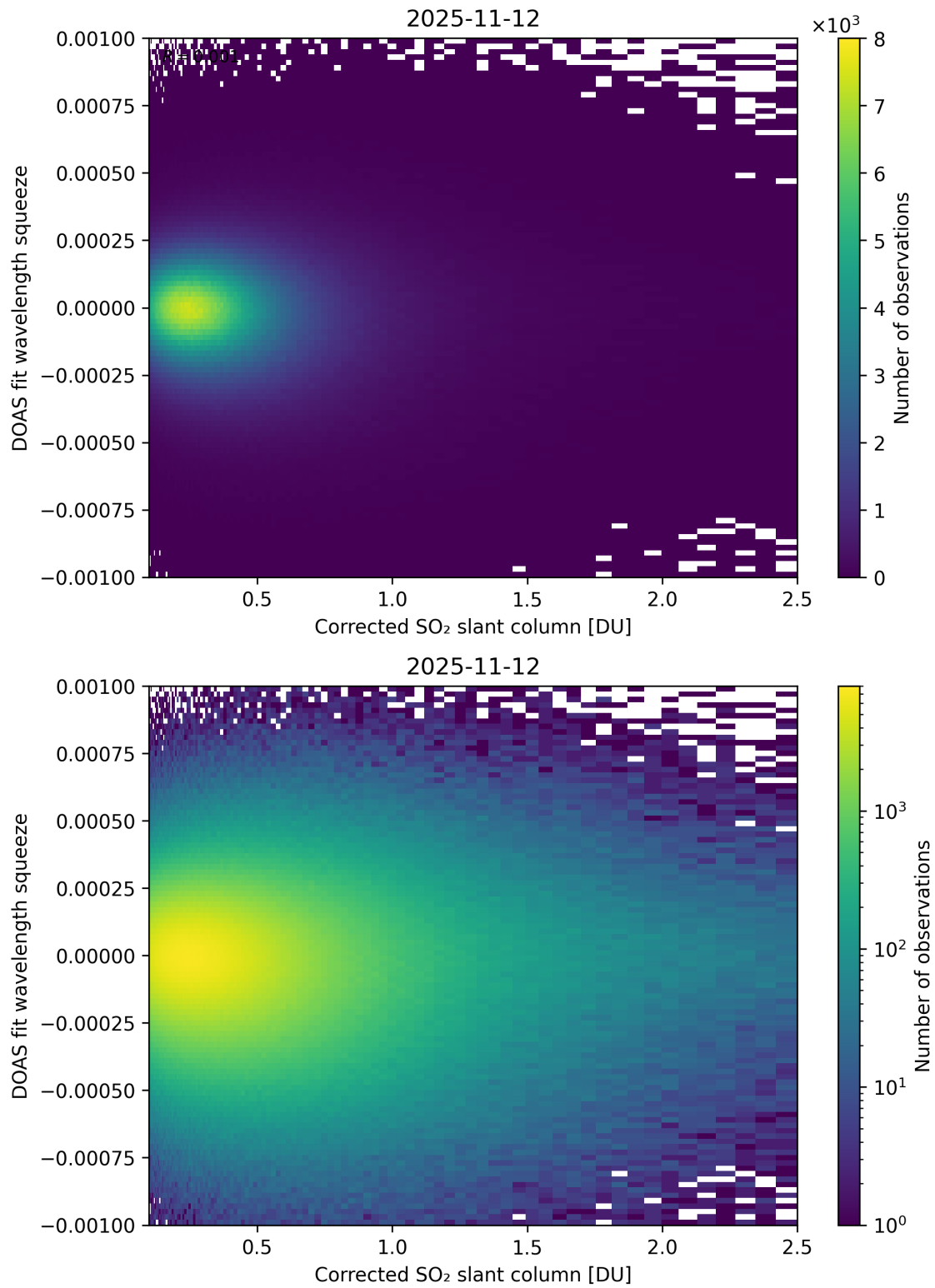
Figure 230: Scatter density plot of "Corrected SO 2 slant column" against "DOAS fit wavelength squeeze" for 2025-11-12 to 2025-11-13.
