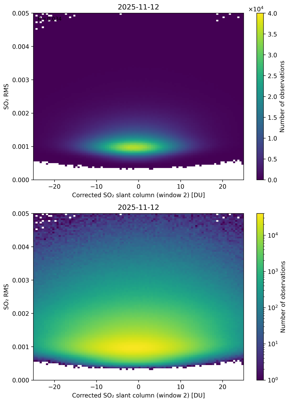
Figure 248: Scatter density plot of “Corrected SO 2 slant column (window 2)” against “SO 2 RMS” for 2025-11-12 to 2025-11-13.
