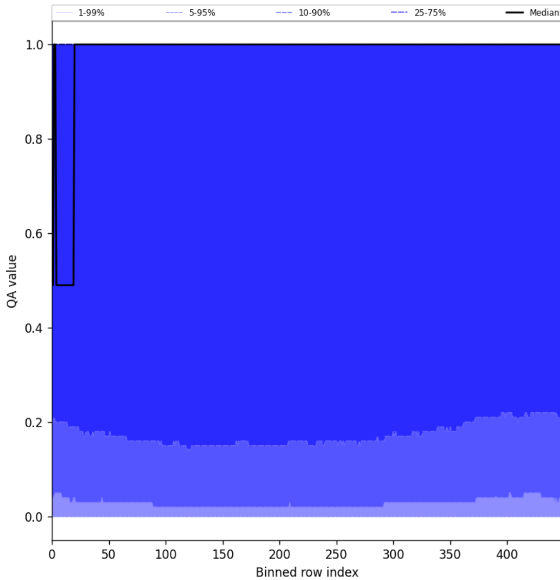
Figure 83: Along track statistics of “QA value” for 2025-11-12 to 2025-11-13
