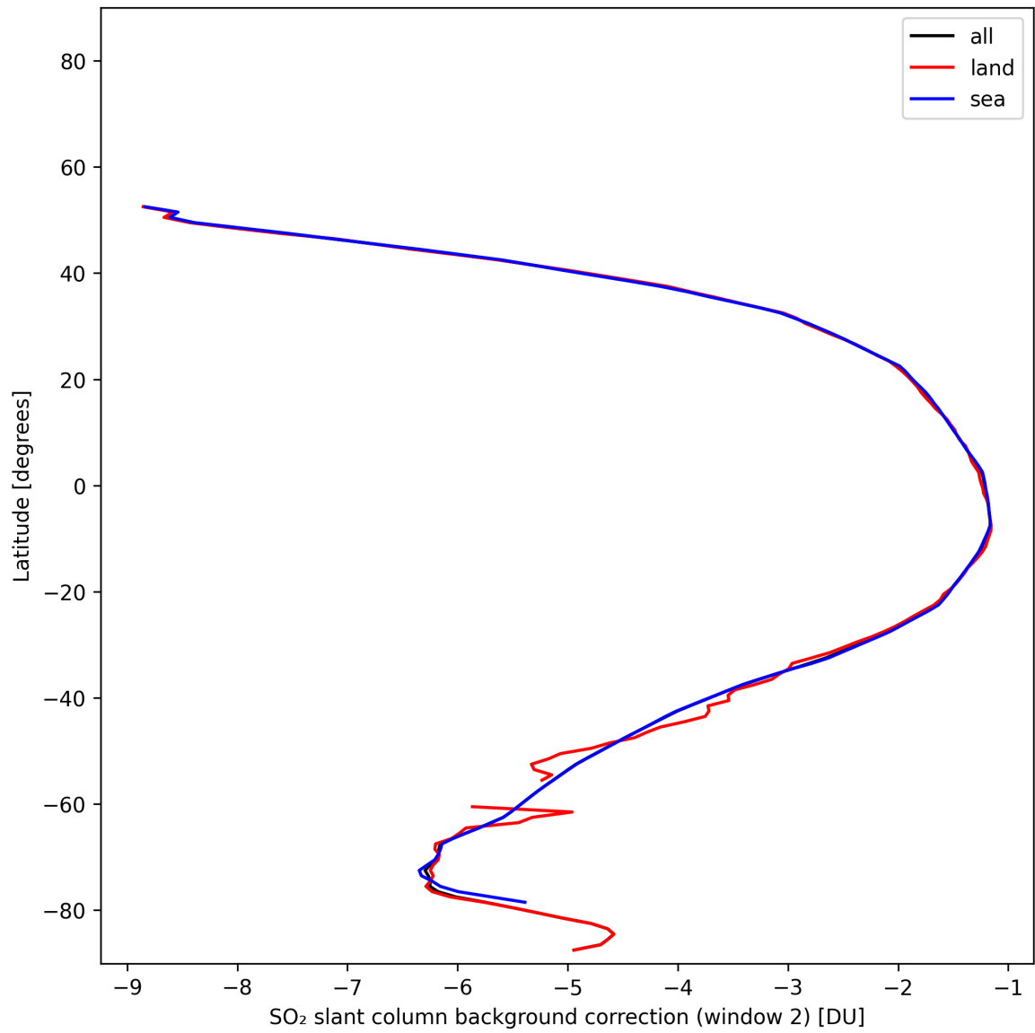
Figure 44: Zonal average of “SO 2 slant column background correction (window 2)” for 2025-11-12 to 2025-11-13.
