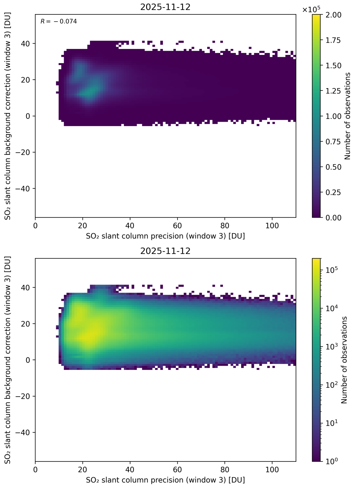
Figure 307: Scatter density plot of “SO 2 slant column precision (window 3)” against “SO 2 slant column background correction (window 3)” for 2025-11-12 to 2025-11-13.
