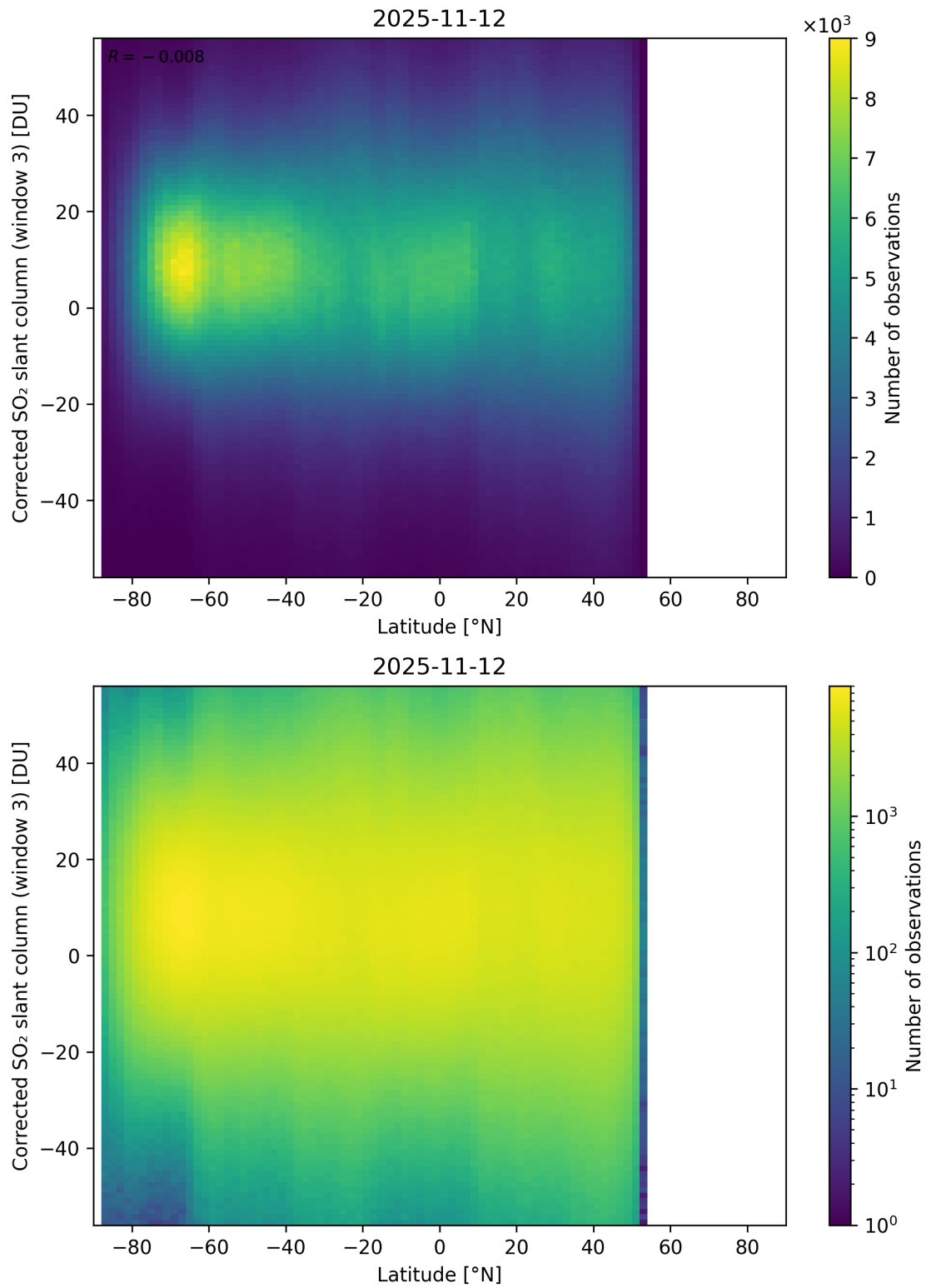
Figure 161: Scatter density plot of “Latitude” against “Corrected SO 2 slant column (window 3)” for 2025-11-12 to 2025-11-13.
