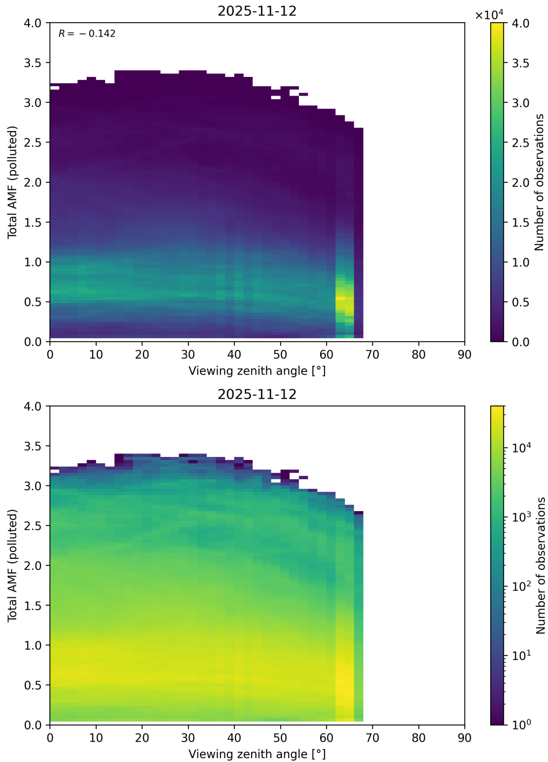
Figure 381: Scatter density plot of “Viewing zenith angle” against “Total AMF (polluted)” for 2025-11-12 to 2025-11-13.
