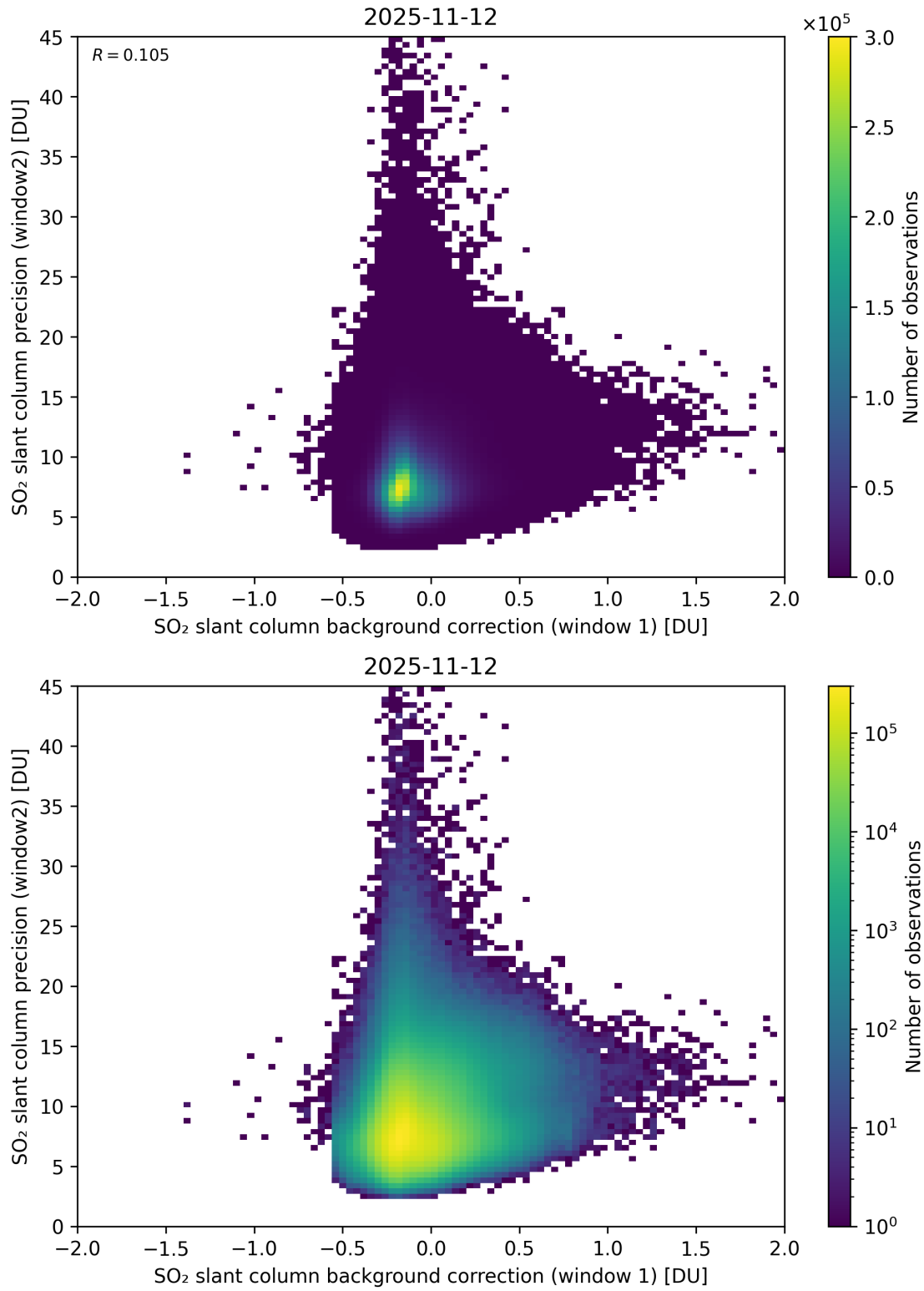
Figure 117: Scatter density plot of “SO 2 slant column background correction (window 1)” against “SO 2 slant column precision (window2)” for 2025-11-12 to 2025-11-13.
