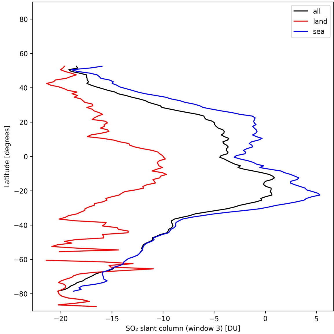
Figure 45: Zonal average of “SO 2 slant column (window 3)” for 2025-11-12 to 2025-11-13.
