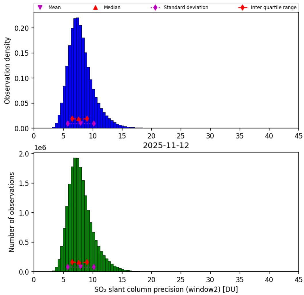
Figure 68: Histogram of “SO 2 slant column precision (window2)” for 2025-11-12 to 2025-11-13
