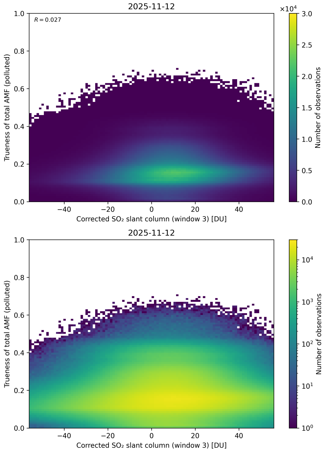
Figure 261: Scatter density plot of “Corrected SO 2 slant column (window 3)” against “Trueness of total AMF (polluted)” for 2025-11-12 to 2025-11-13.
