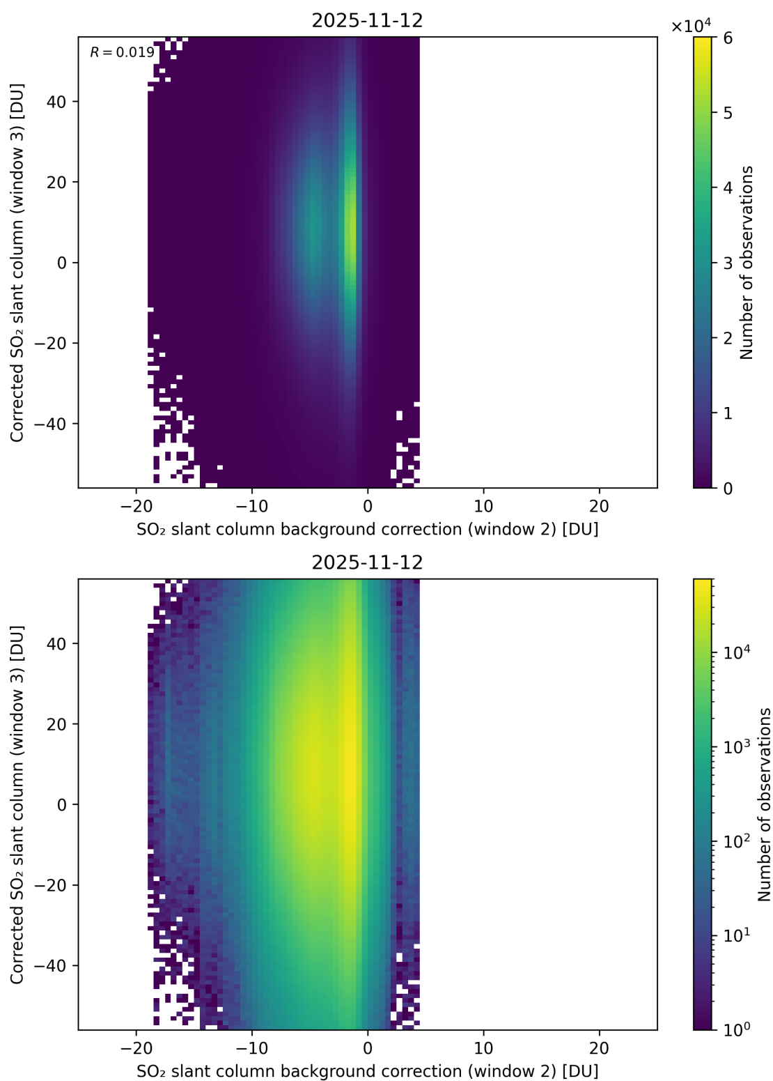
Figure 127: Scatter density plot of “SO 2 slant column background correction (window 2)” against “Corrected SO 2 slant column (window 3)” for 2025-11-12 to 2025-11-13.
