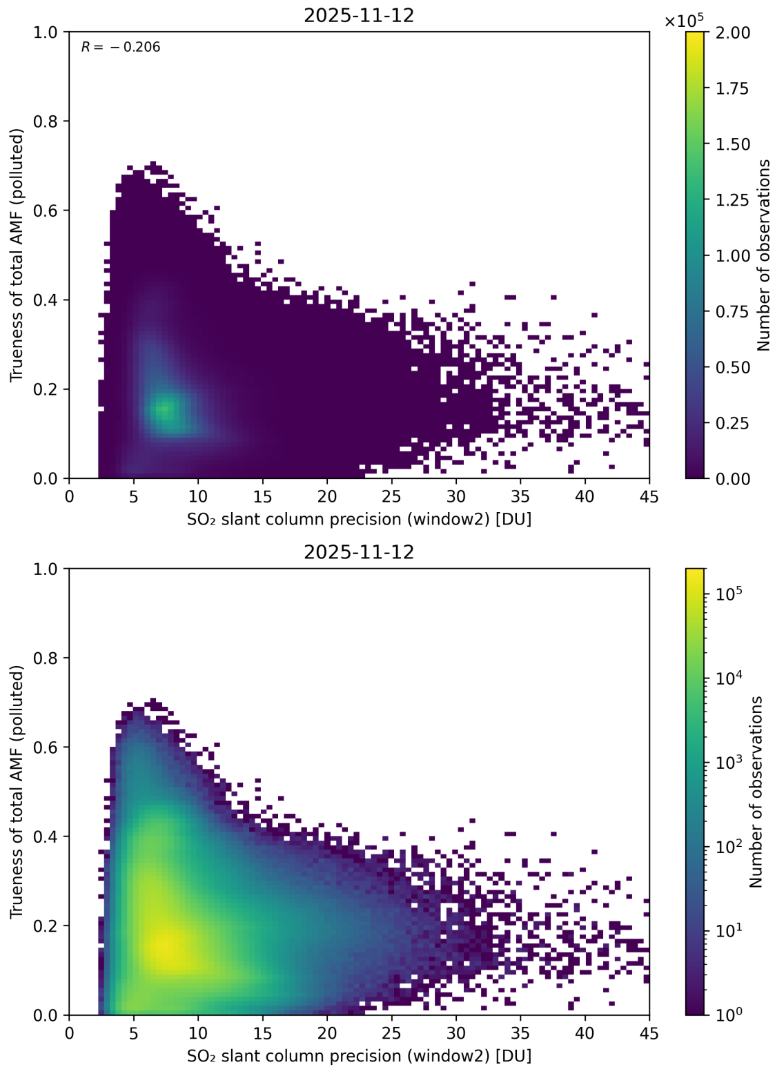
Figure 302: Scatter density plot of “SO 2 slant column precision (window2)” against “Trueness of total AMF (polluted)” for 2025-11-12 to 2025-11-13.
