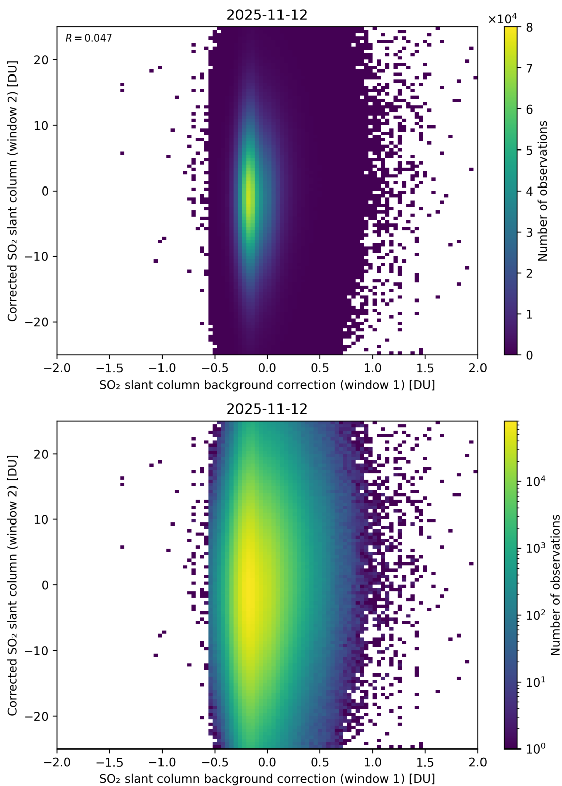
Figure 115: Scatter density plot of “SO 2 slant column background correction (window 1)” against “Corrected SO 2 slant column (window 2)” for 2025-11-12 to 2025-11-13.
