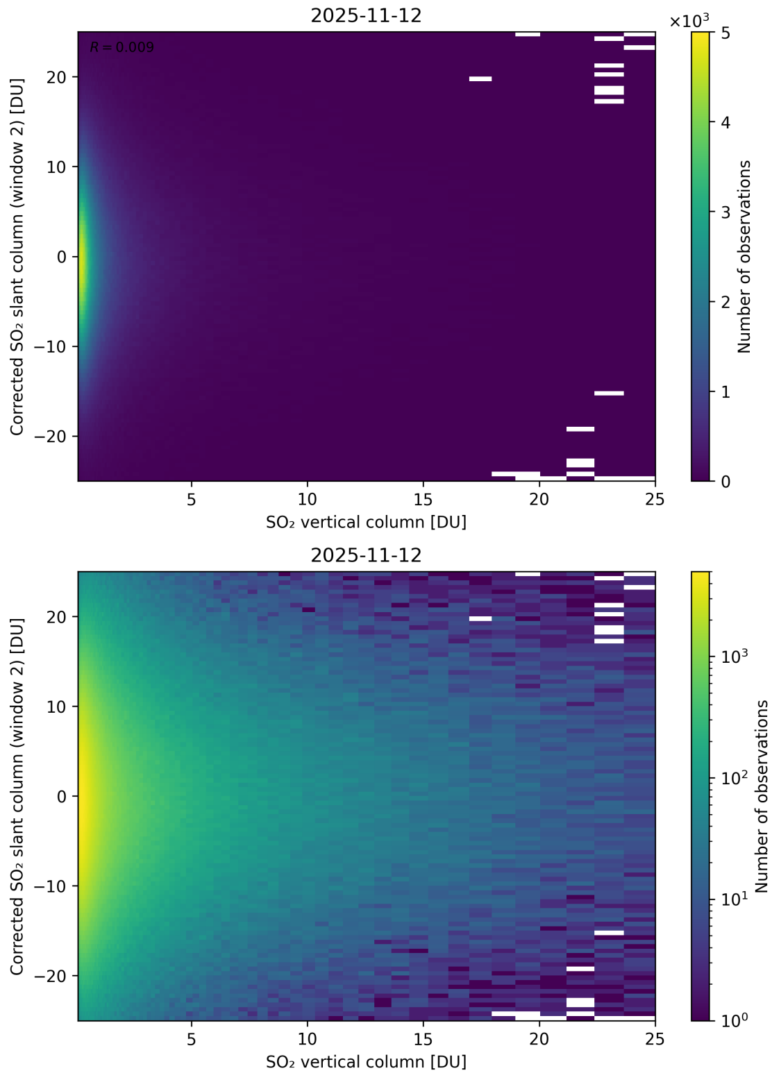
Figure 352: Scatter density plot of “SO 2 vertical column” against “Corrected SO 2 slant column (window 2)” for 2025-11-12 to 2025-11-13.
