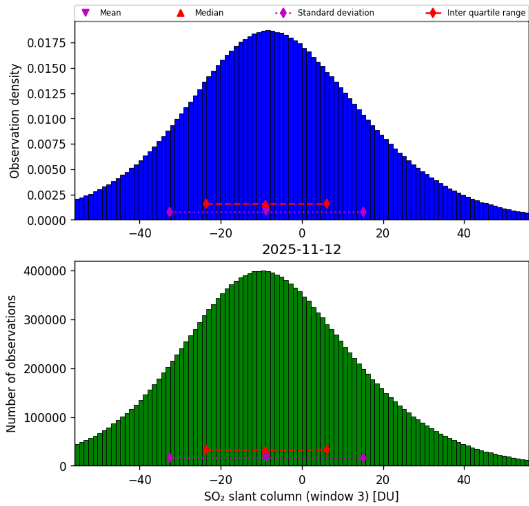
Figure 71: Histogram of “SO 2 slant column (window 3)” for 2025-11-12 to 2025-11-13
