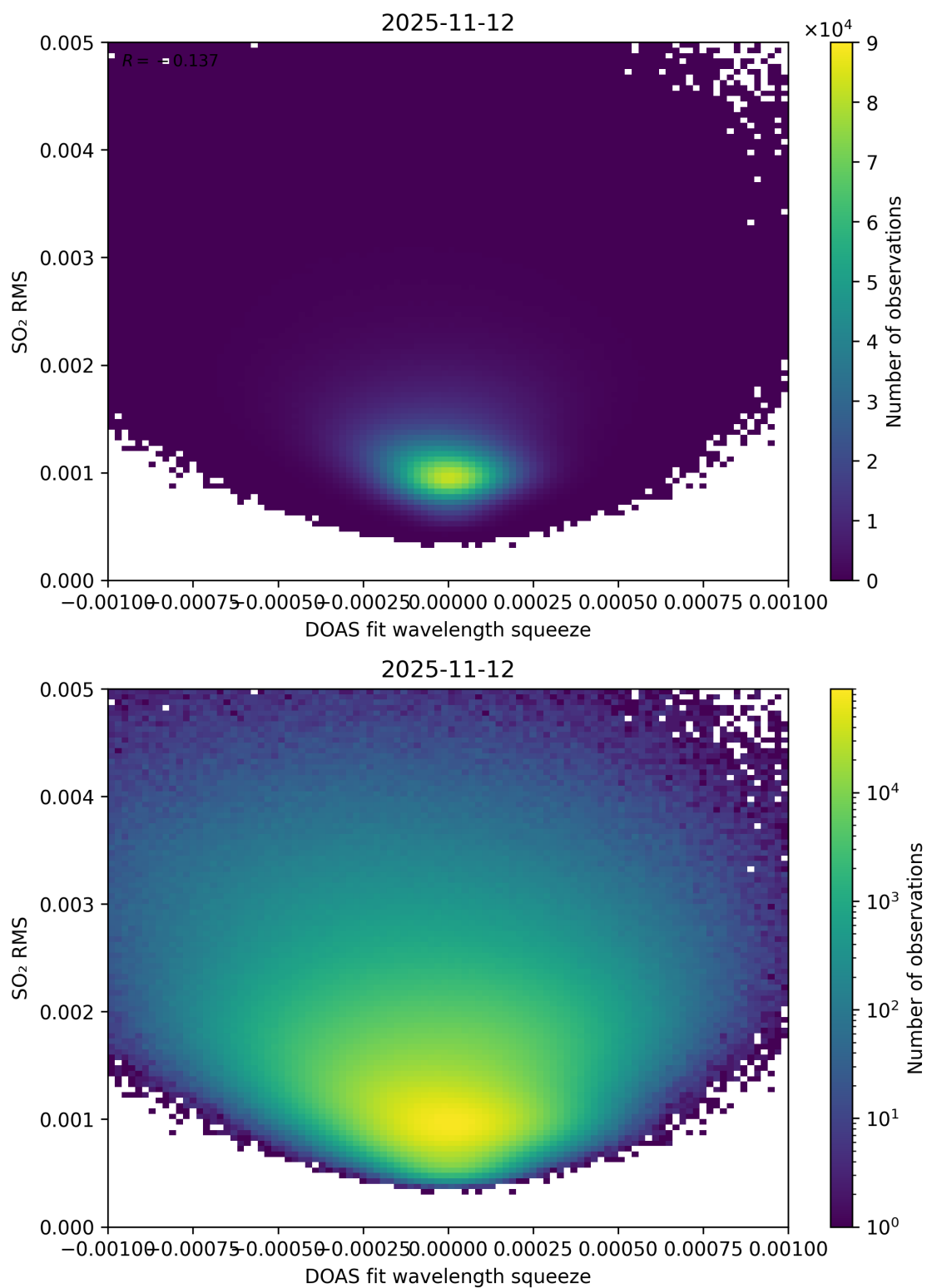
Figure 143: Scatter density plot of “DOAS fit wavelength squeeze” against “SO 2 RMS” for 2025-11-12 to 2025-11-13.
