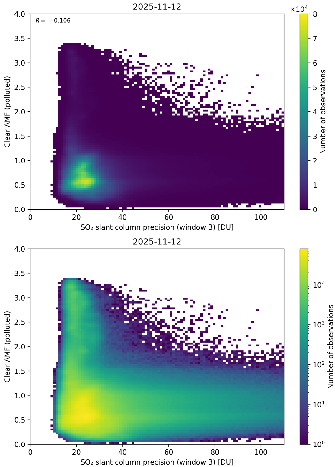
Figure 311: Scatter density plot of “SO 2 slant column precision (window 3)” against “Clear AMF (polluted)” for 2025-11-12 to 2025-11-13.
