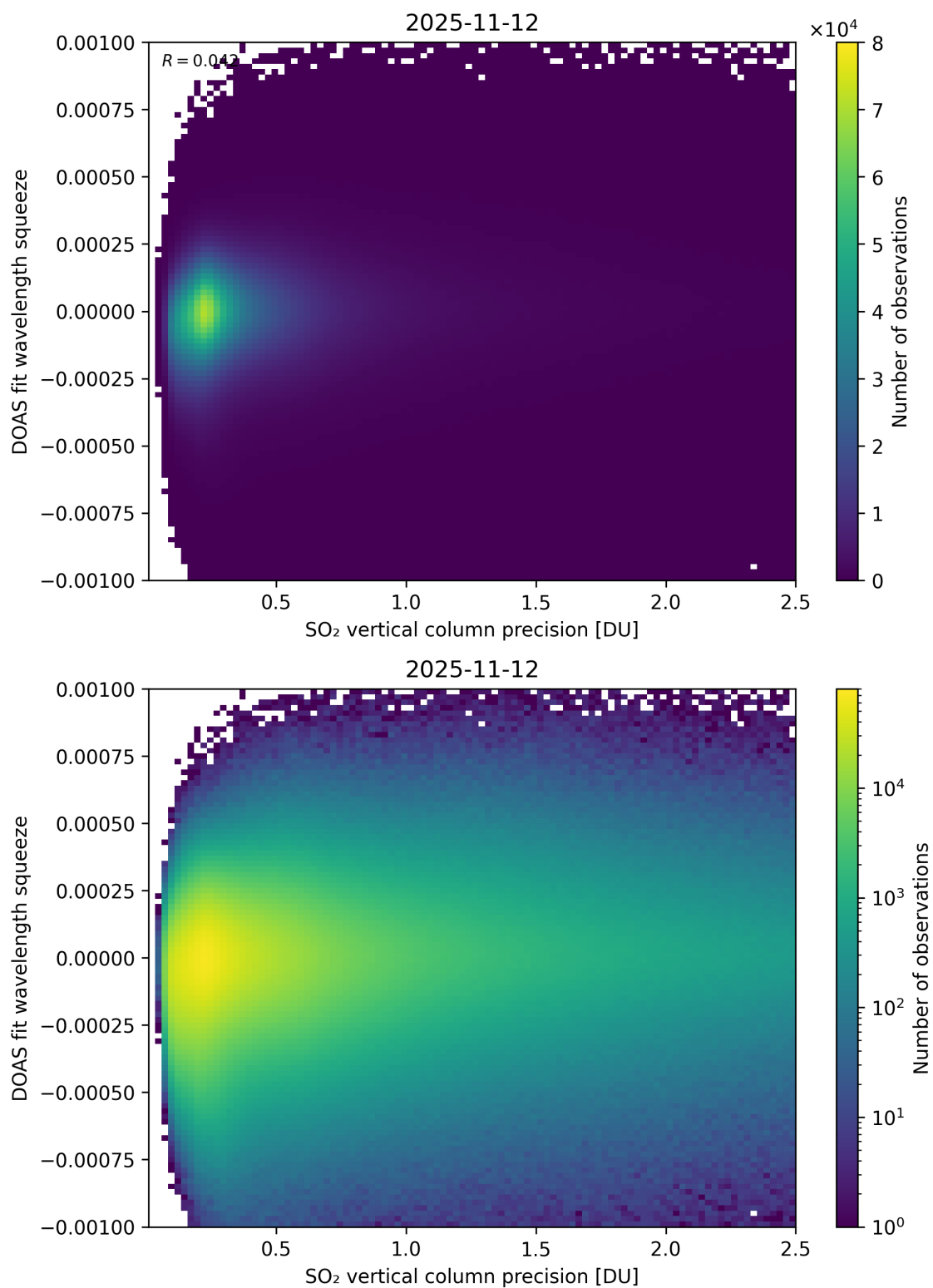
Figure 333: Scatter density plot of “SO 2 vertical column precision” against “DOAS fit wavelength squeeze” for 2025-11-12 to 2025-11-13.
