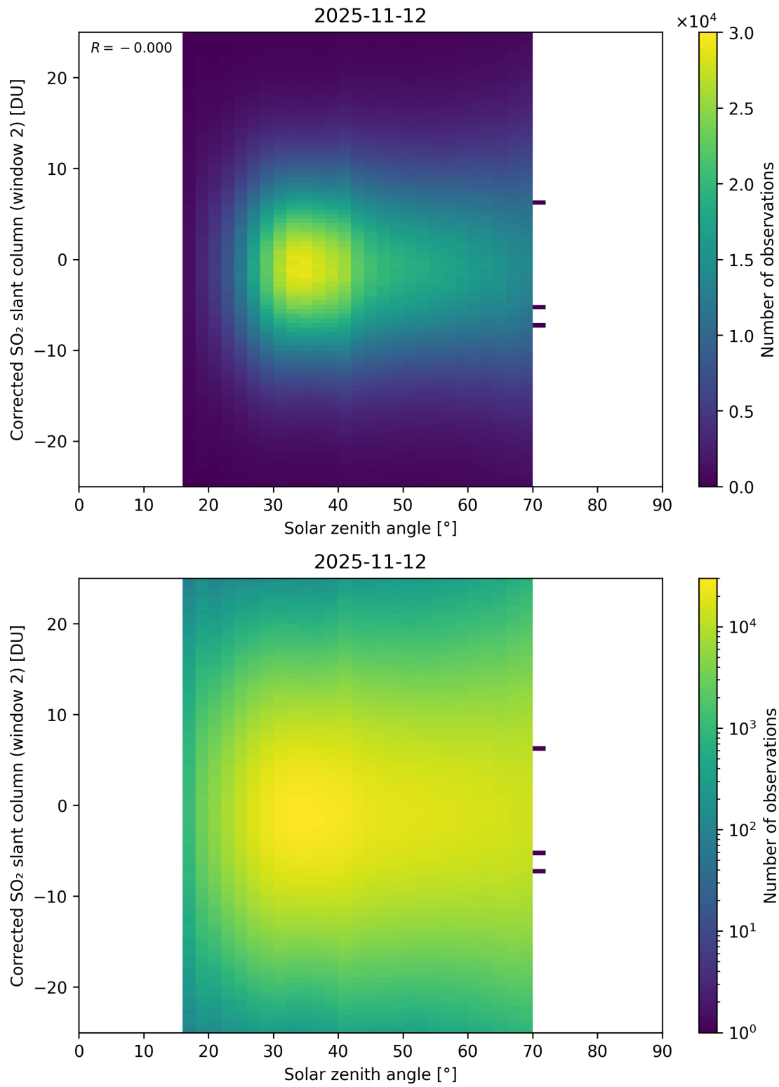
Figure 182: Scatter density plot of “Solar zenith angle” against “Corrected SO 2 slant column (window 2)” for 2025-11-12 to 2025-11-13.
