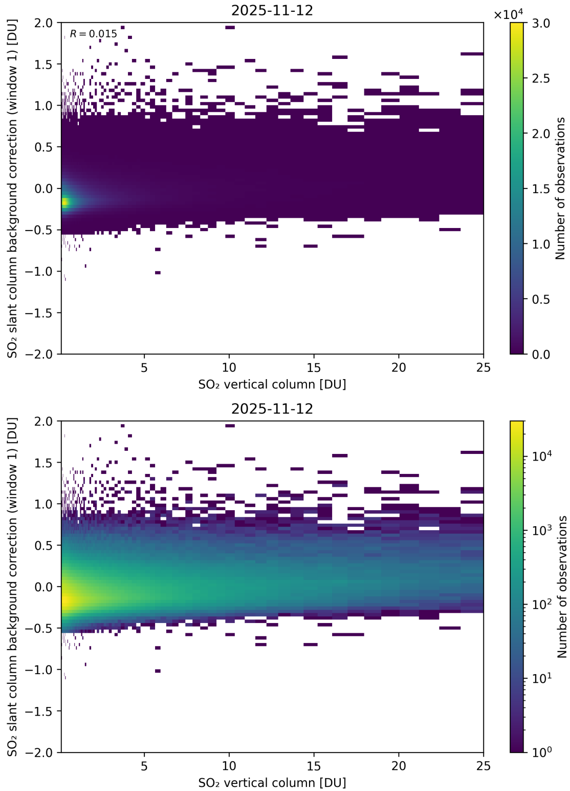
Figure 323: Scatter density plot of “SO 2 vertical column” against “SO 2 slant column background correction (window 1)” for 2025-11-12 to 2025-11-13.
