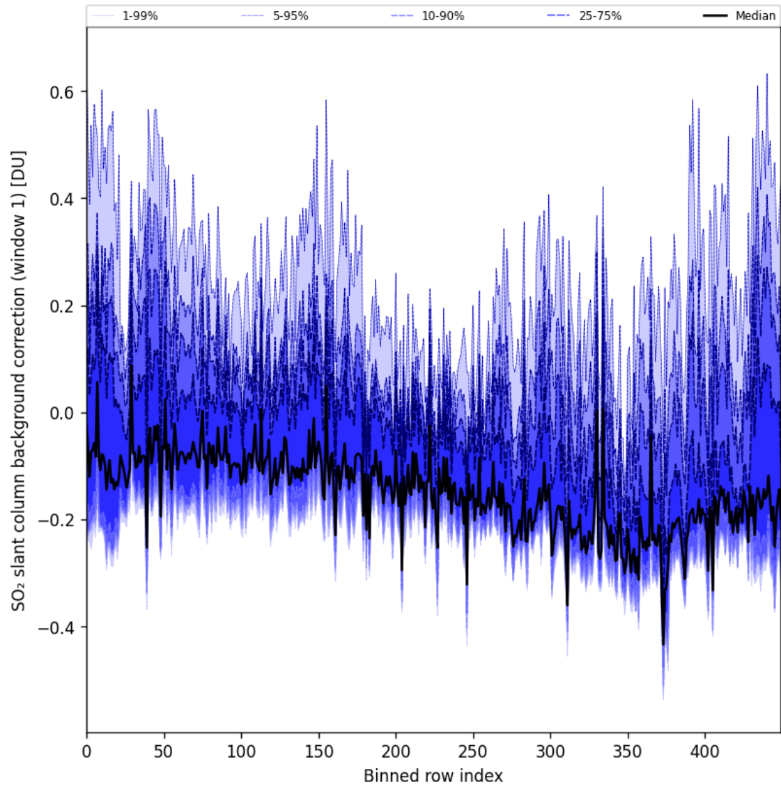
Figure 92: Along track statistics of “SO 2 slant column background correction (window 1)” for 2025-11-12 to 2025-11-13
