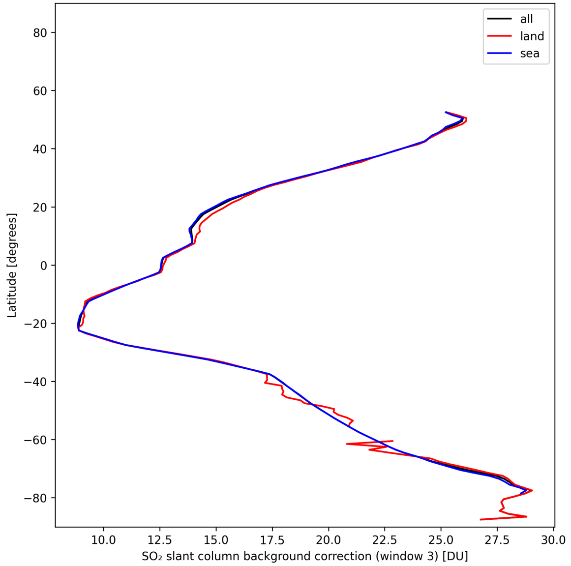
Figure 48: Zonal average of “SO 2 slant column background correction (window 3)” for 2025-11-12 to 2025-11-13.
