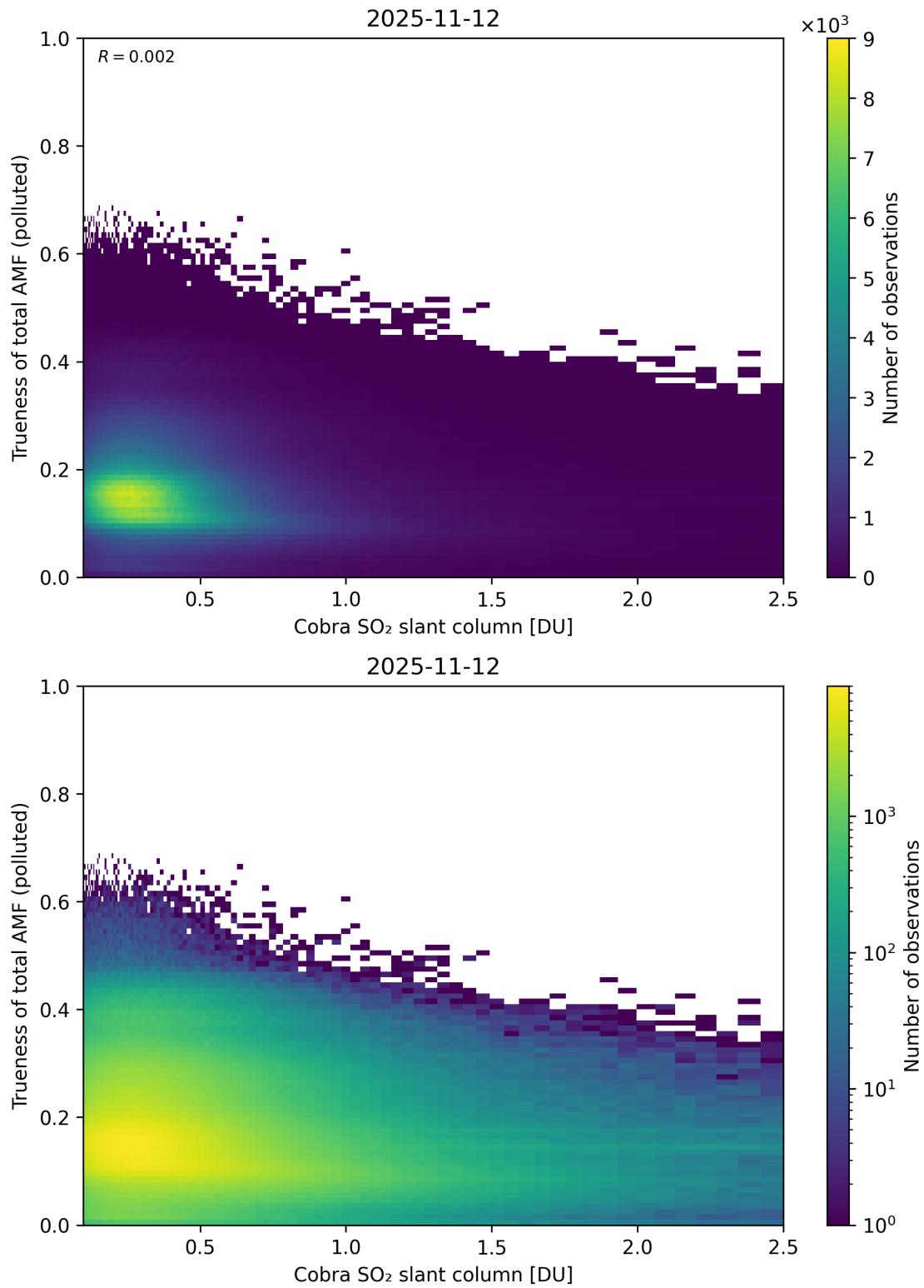
Figure 225: Scatter density plot of “Cobra SO 2 slant column” against “Trueness of total AMF (polluted)” for 2025-11-12 to 2025-11-13.
