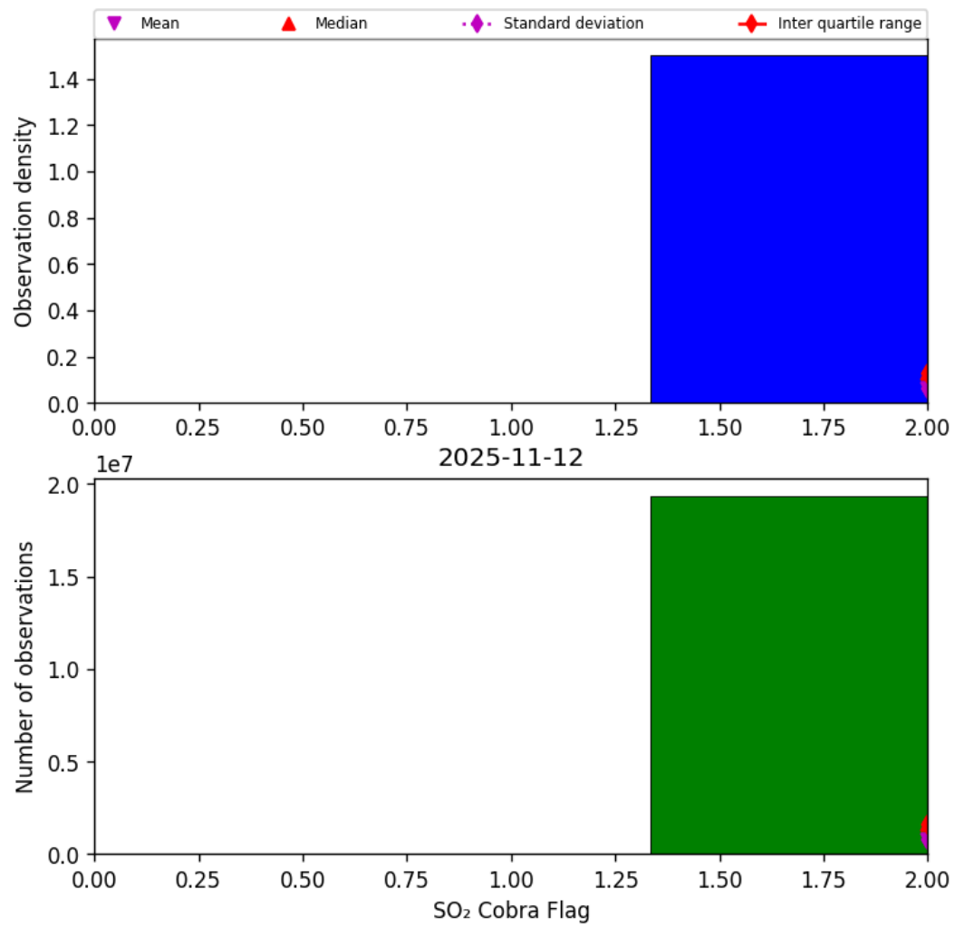
Figure 75: Histogram of “SO 2 Cobra Flag” for 2025-11-12 to 2025-11-13
