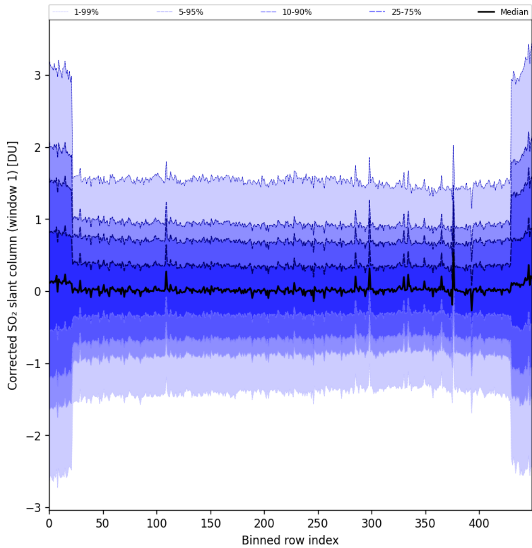
Figure 91: Along track statistics of “Corrected SO 2 slant column (window 1)” for 2025-11-12 to 2025-11-13
