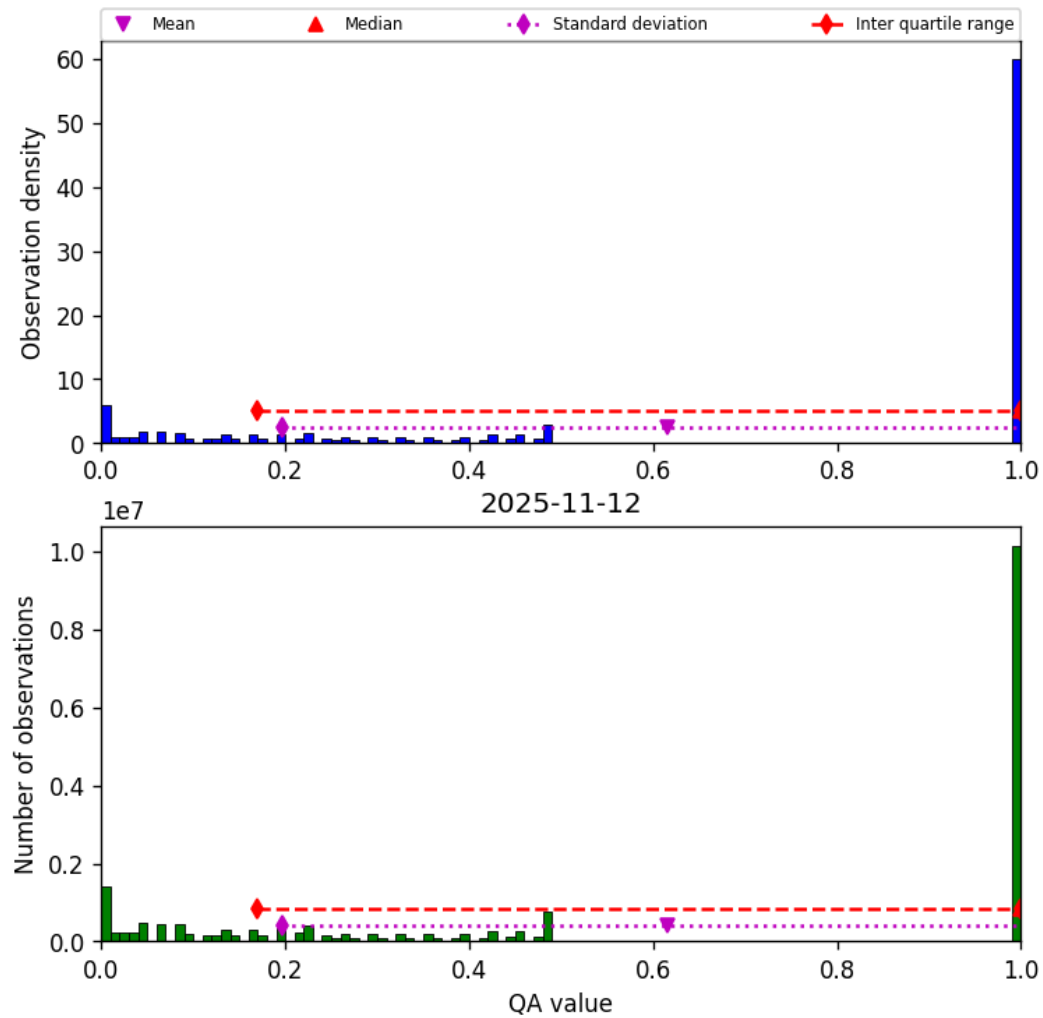
Figure 57: Histogram of “QA value” for 2025-11-12 to 2025-11-13
