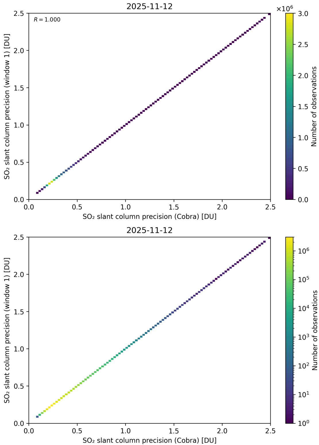
Figure 209: Scatter density plot of “SO 2 slant column precision (Cobra)” against “SO 2 slant column precision (window 1)” for 2025-11-12 to 2025-11-13.
