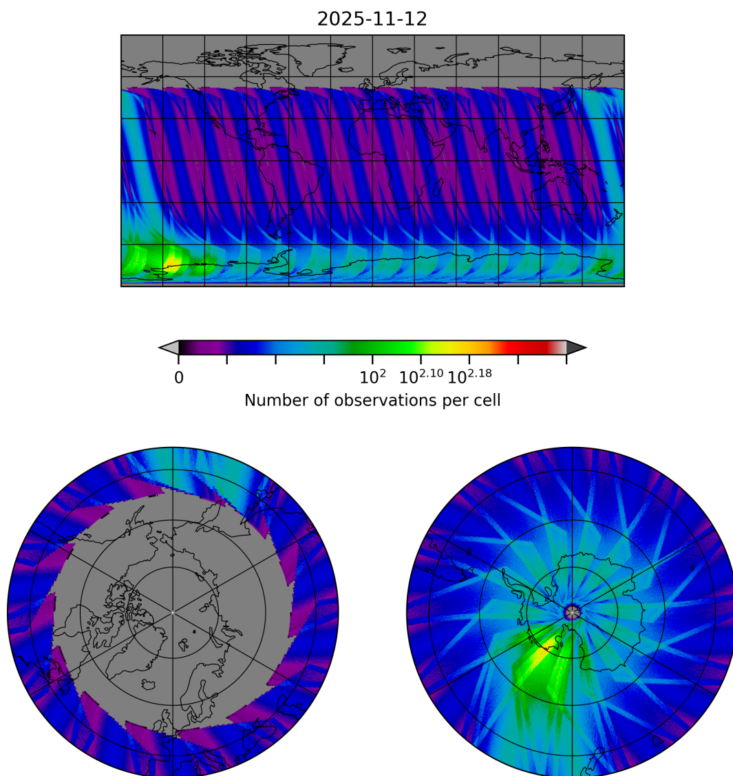
Figure 30: Map of the number of observations for 2025-11-12 to 2025-11-13
