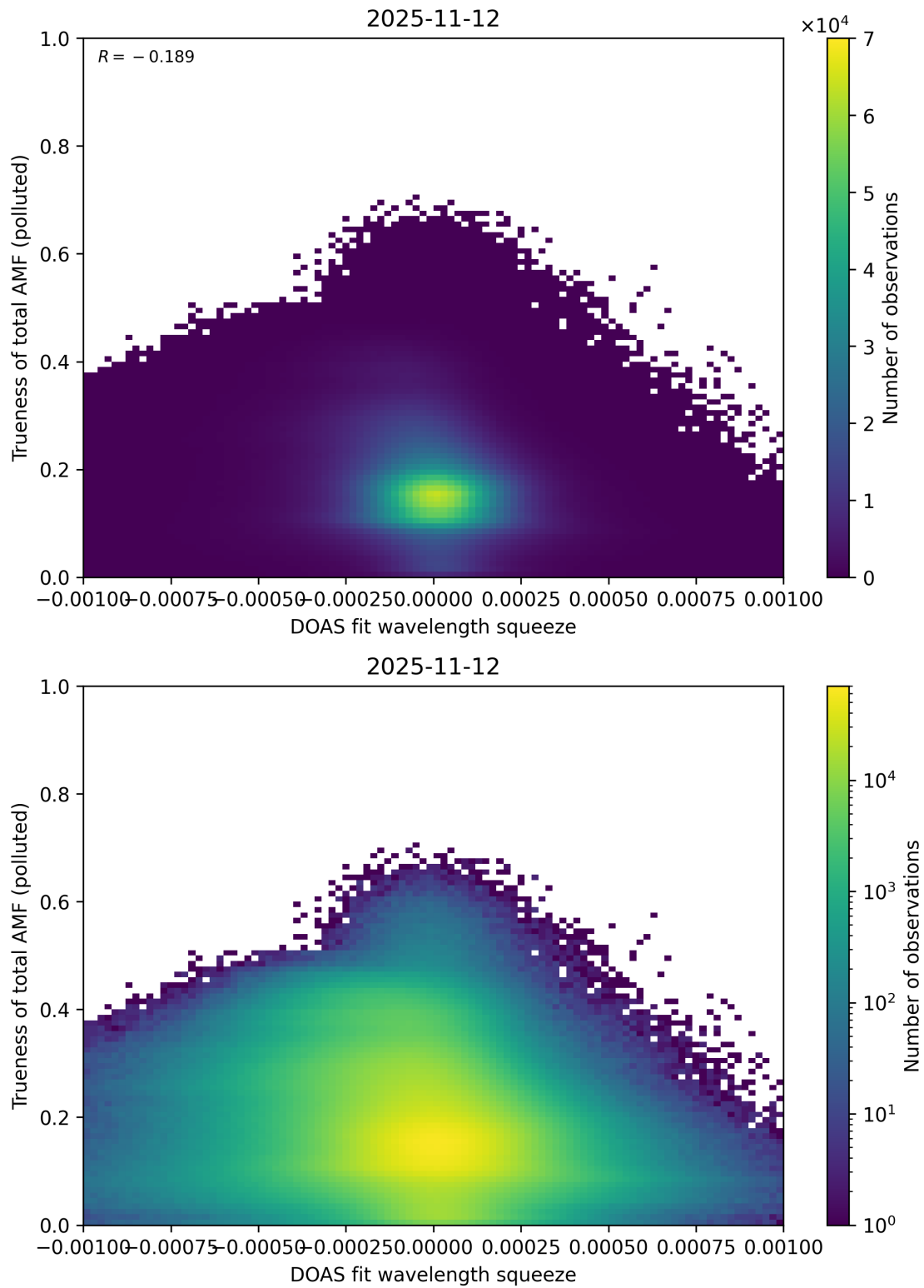
Figure 146: Scatter density plot of “DOAS fit wavelength squeeze” against “Trueness of total AMF (polluted)” for 2025-11-12 to 2025-11-13.
