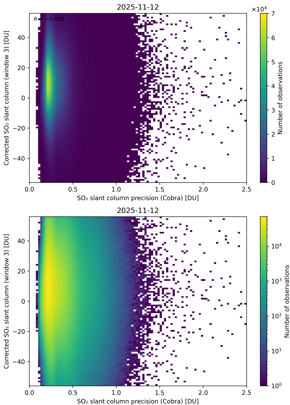
Figure 207: Scatter density plot of “SO 2 slant column precision (Cobra)” against “Corrected SO 2 slant column (window 3)” for 2025-11-12 to 2025-11-13.
