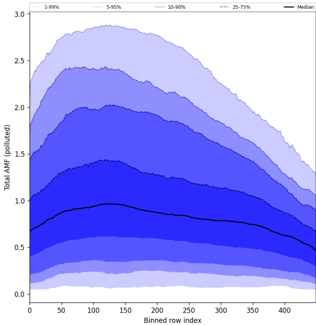
Figure 105: Along track statistics of “Total AMF (polluted)” for 2025-11-12 to 2025-11-13
