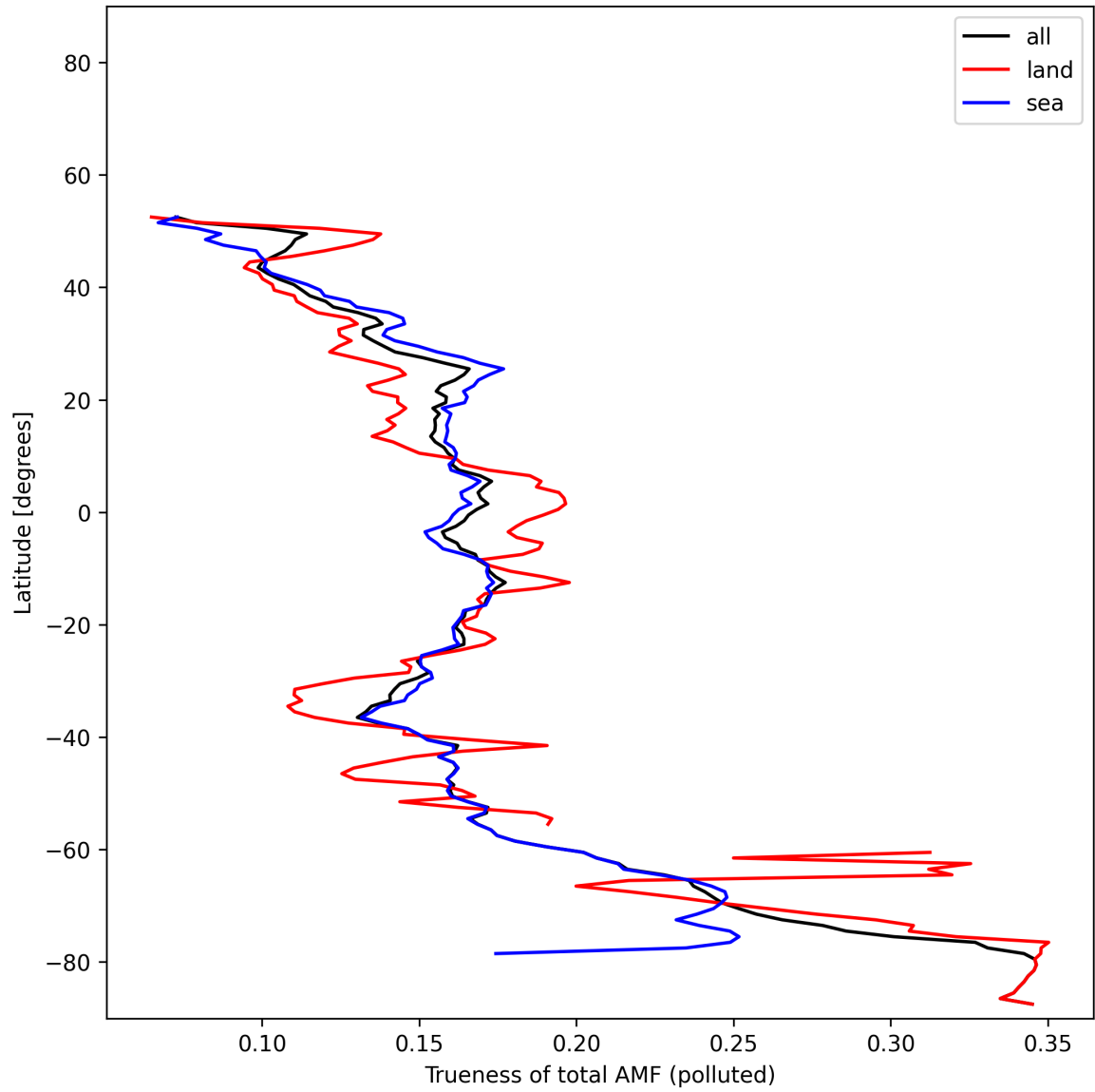
Figure 54: Zonal average of “Trueness of total AMF (polluted)” for 2025-11-12 to 2025-11-13.
