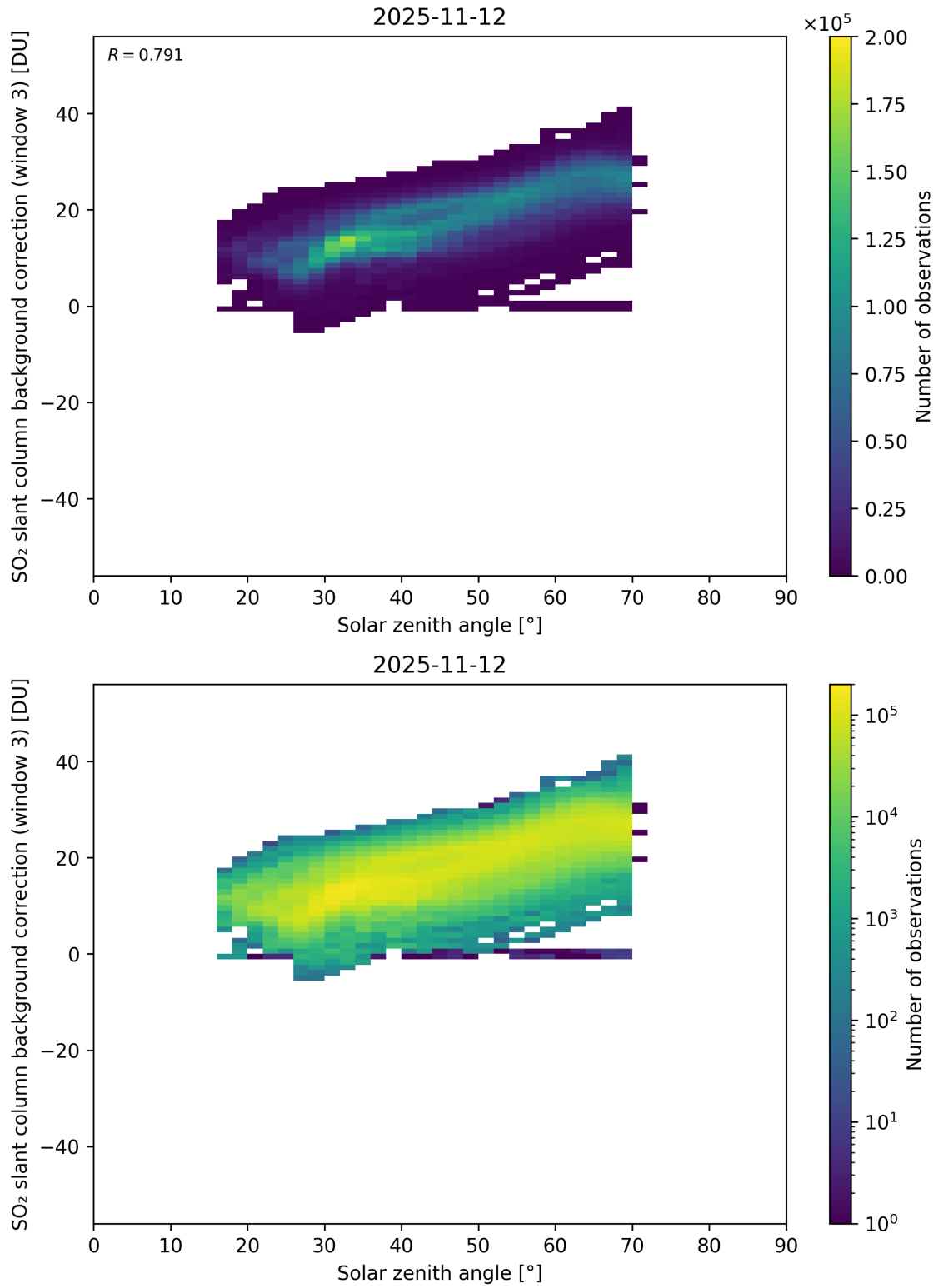
Figure 173: Scatter density plot of “Solar zenith angle” against “SO 2 slant column background correction (window 3)” for 2025-11-12 to 2025-11-13.
