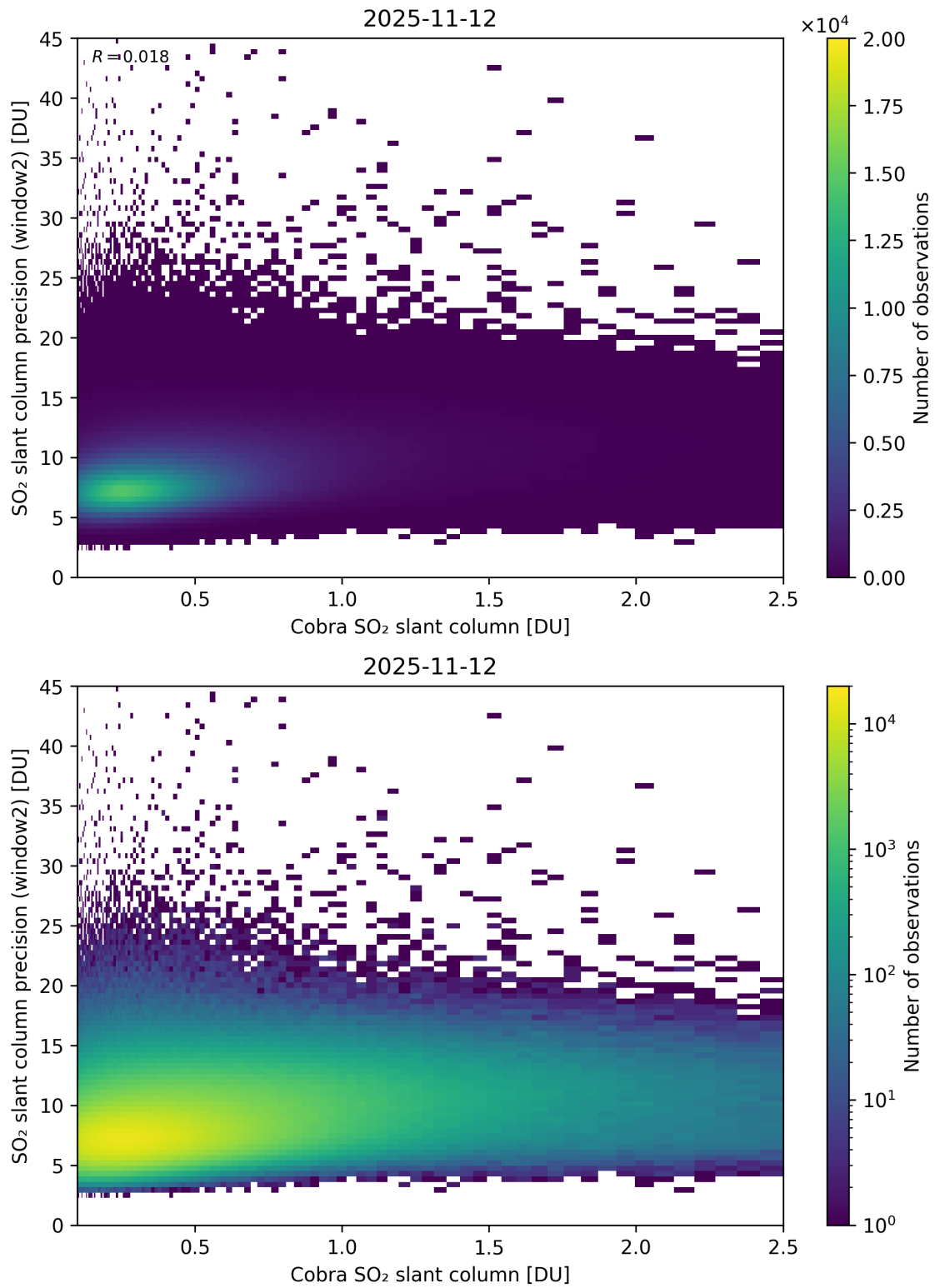
Figure 221: Scatter density plot of “Cobra SO 2 slant column” against “SO 2 slant column precision (window2)” for 2025-11-12 to 2025-11-13.
