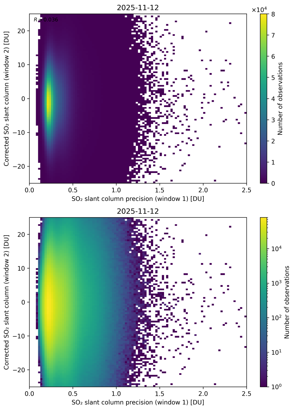
Figure 275: Scatter density plot of “SO 2 slant column precision (window 1)” against “Corrected SO 2 slant column (window 2)” for 2025-11-12 to 2025-11-13.
