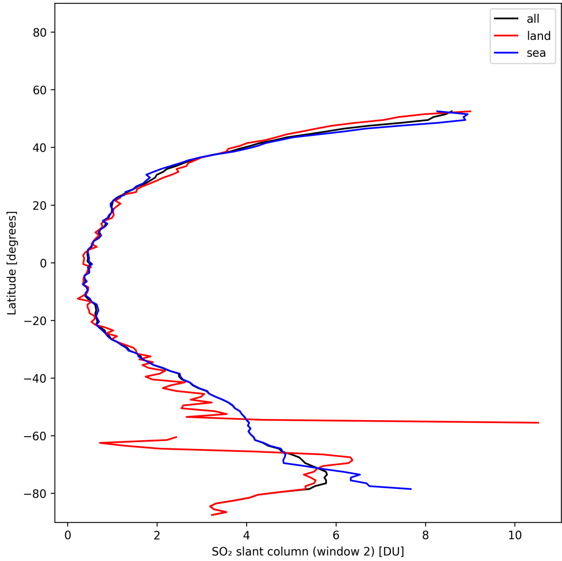
Figure 41: Zonal average of “SO 2 slant column (window 2)” for 2025-11-12 to 2025-11-13.
