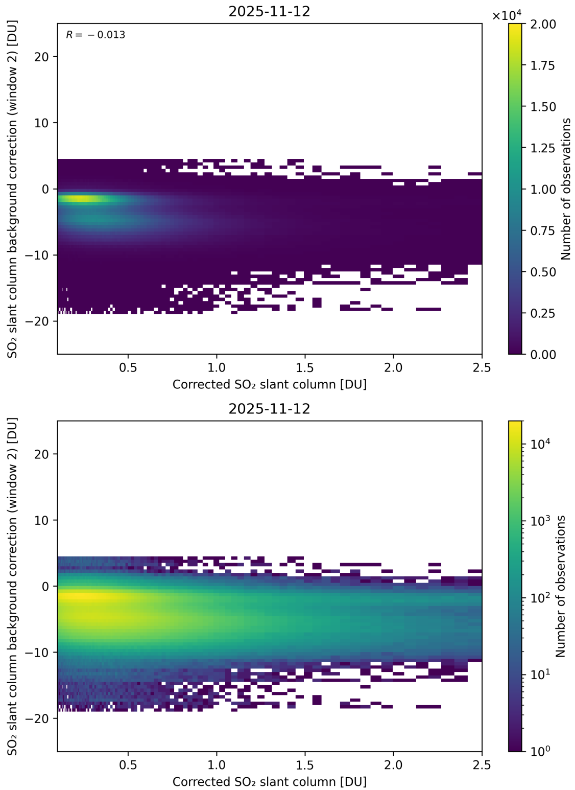
Figure 227: Scatter density plot of “Corrected SO 2 slant column” against “SO 2 slant column background correction (window 2)” for 2025-11-12 to 2025-11-13.
