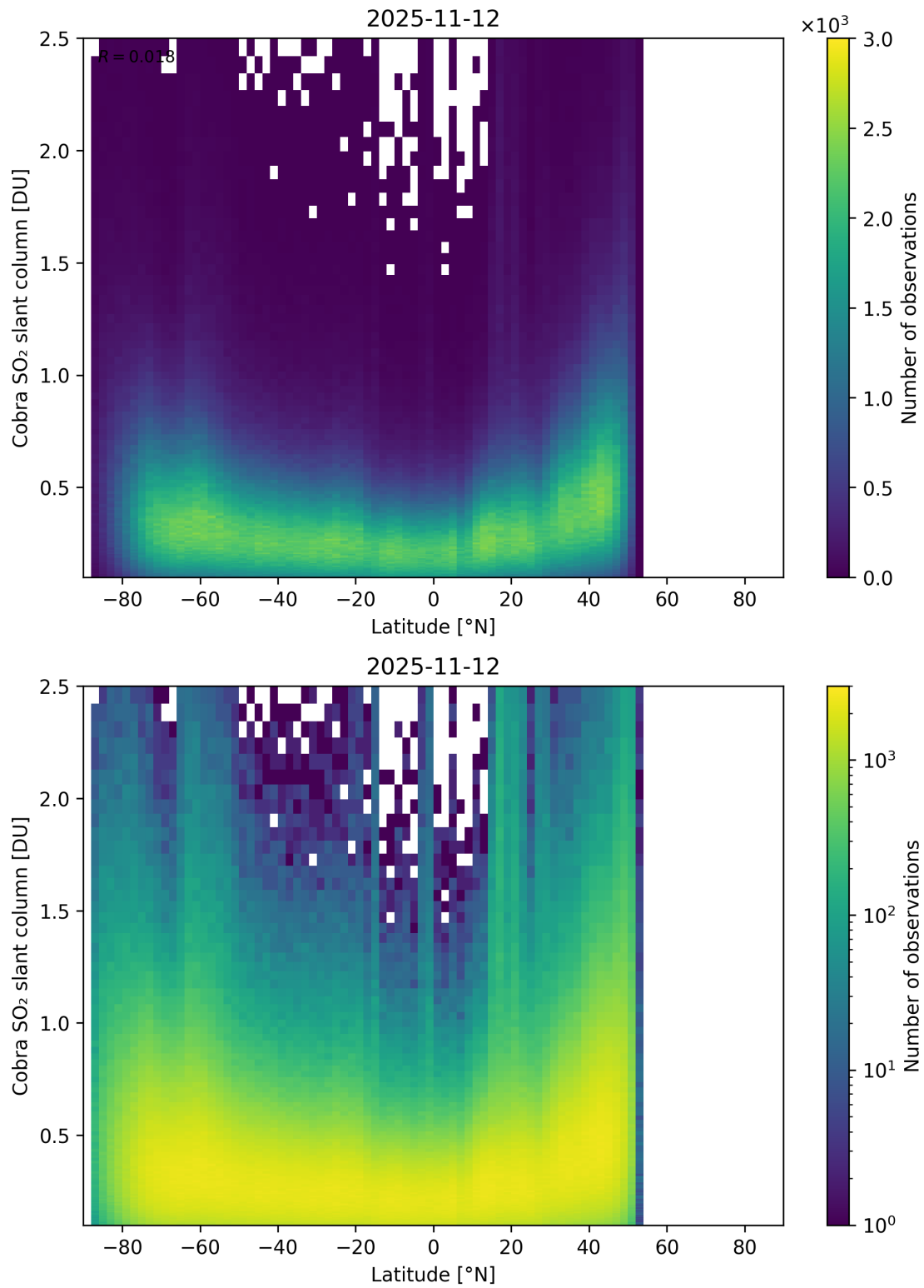
Figure 157: Scatter density plot of “Latitude” against “Cobra SO 2 slant column” for 2025-11-12 to 2025-11-13.
