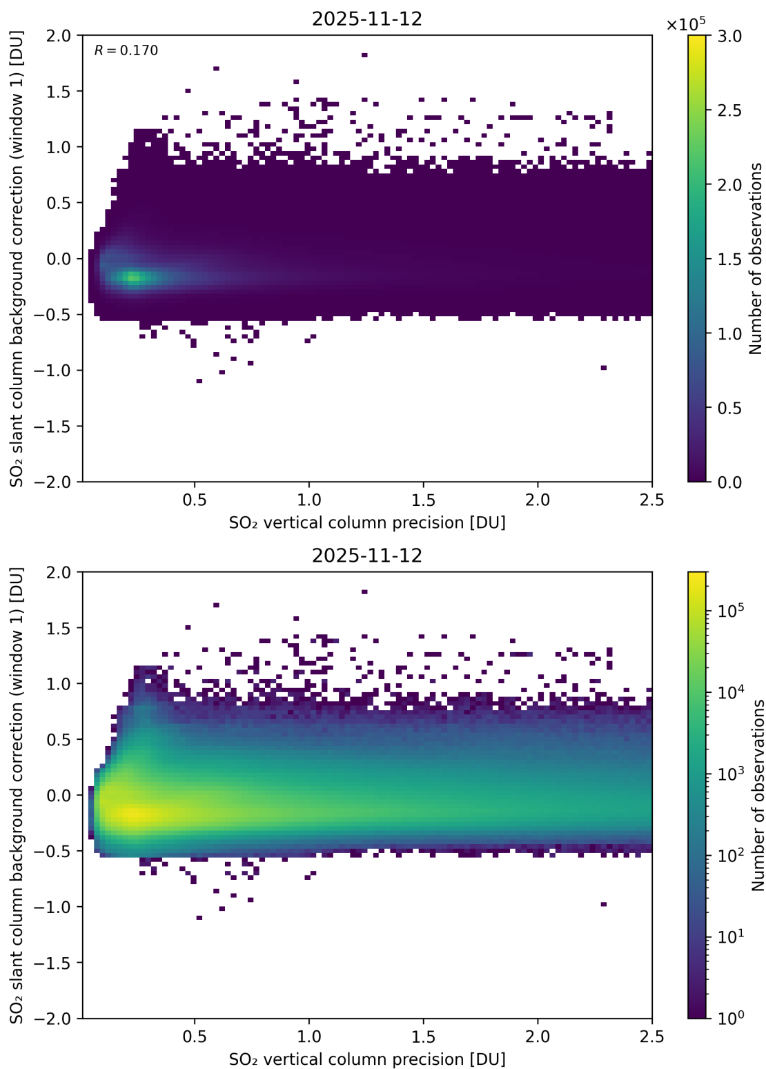
Figure 329: Scatter density plot of “SO 2 vertical column precision” against “SO 2 slant column background correction (window 1)” for 2025-11-12 to 2025-11-13.
