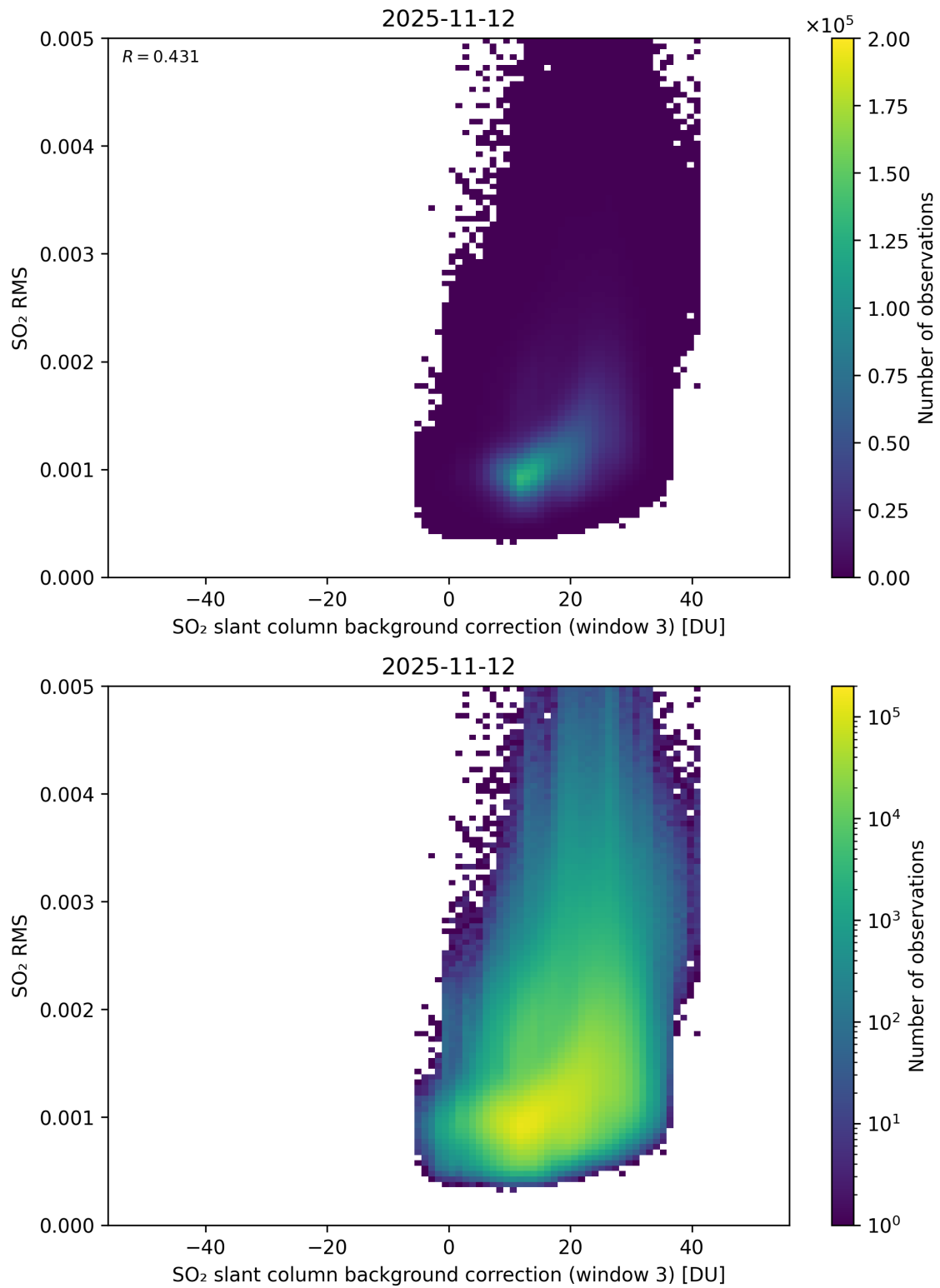
Figure 134: Scatter density plot of “SO 2 slant column background correction (window 3)” against “SO 2 RMS” for 2025-11-12 to 2025-11-13.
