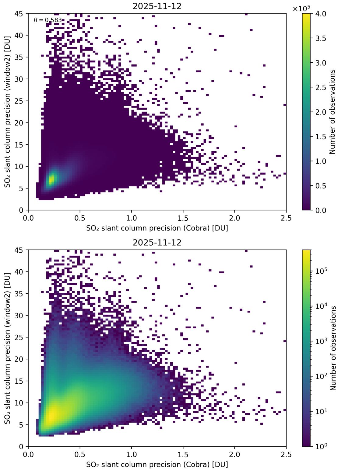
Figure 210: Scatter density plot of “SO 2 slant column precision (Cobra)” against “SO 2 slant column precision (window2)” for 2025-11-12 to 2025-11-13.
