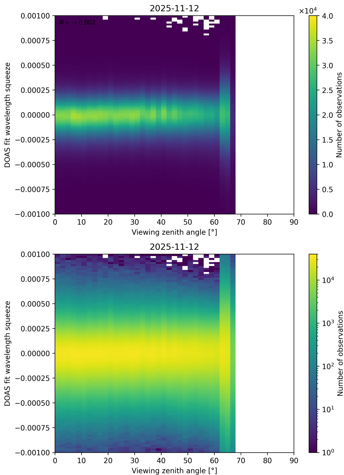
Figure 366: Scatter density plot of “Viewing zenith angle” against “DOAS fit wavelength squeeze” for 2025-11-12 to 2025-11-13.
