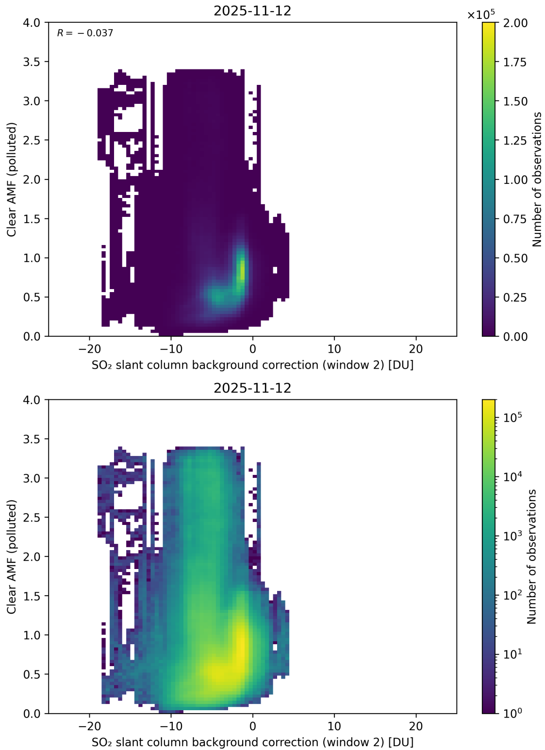
Figure 126: Scatter density plot of “SO 2 slant column background correction (window 2)” against “Clear AMF (polluted)” for 2025-11-12 to 2025-11-13.
