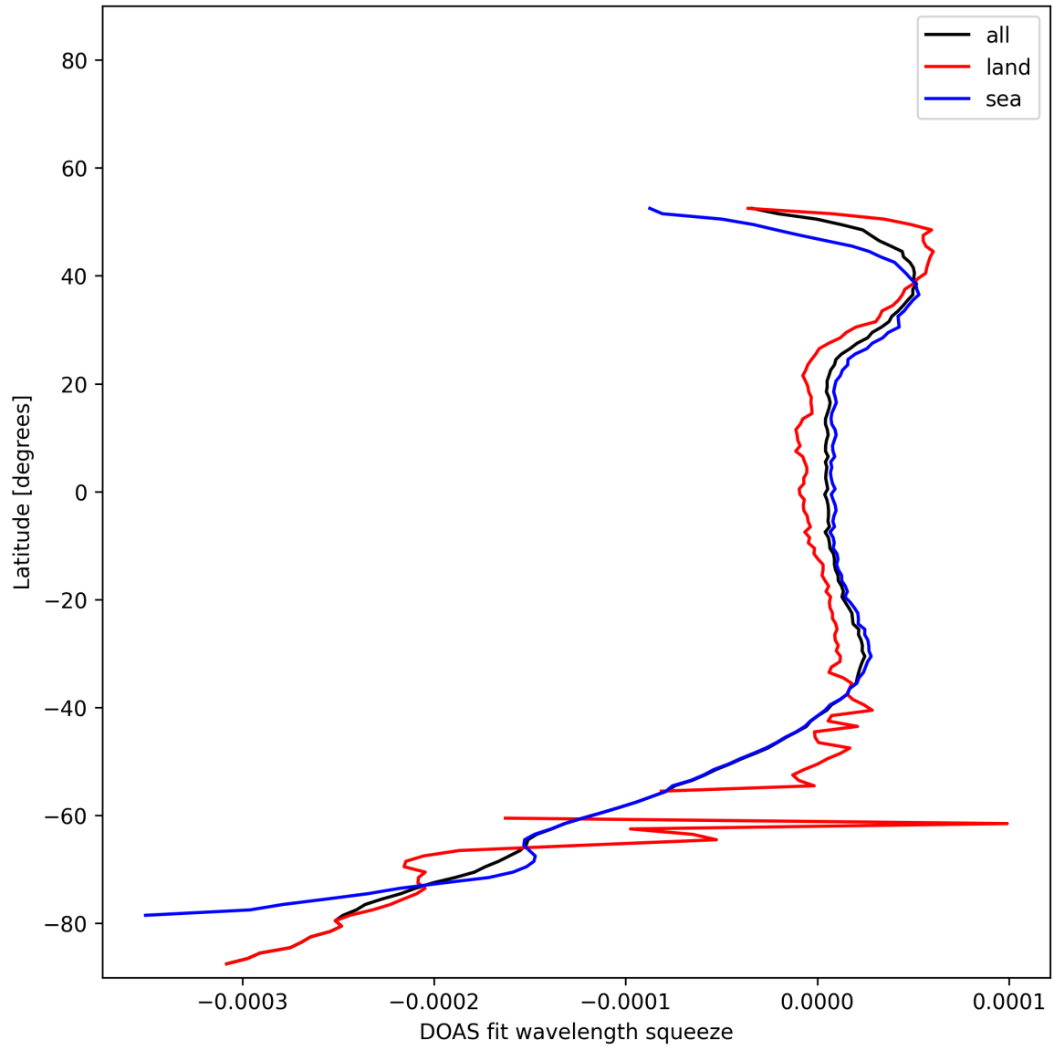
Figure 51: Zonal average of “DOAS fit wavelength squeeze” for 2025-11-12 to 2025-11-13.
