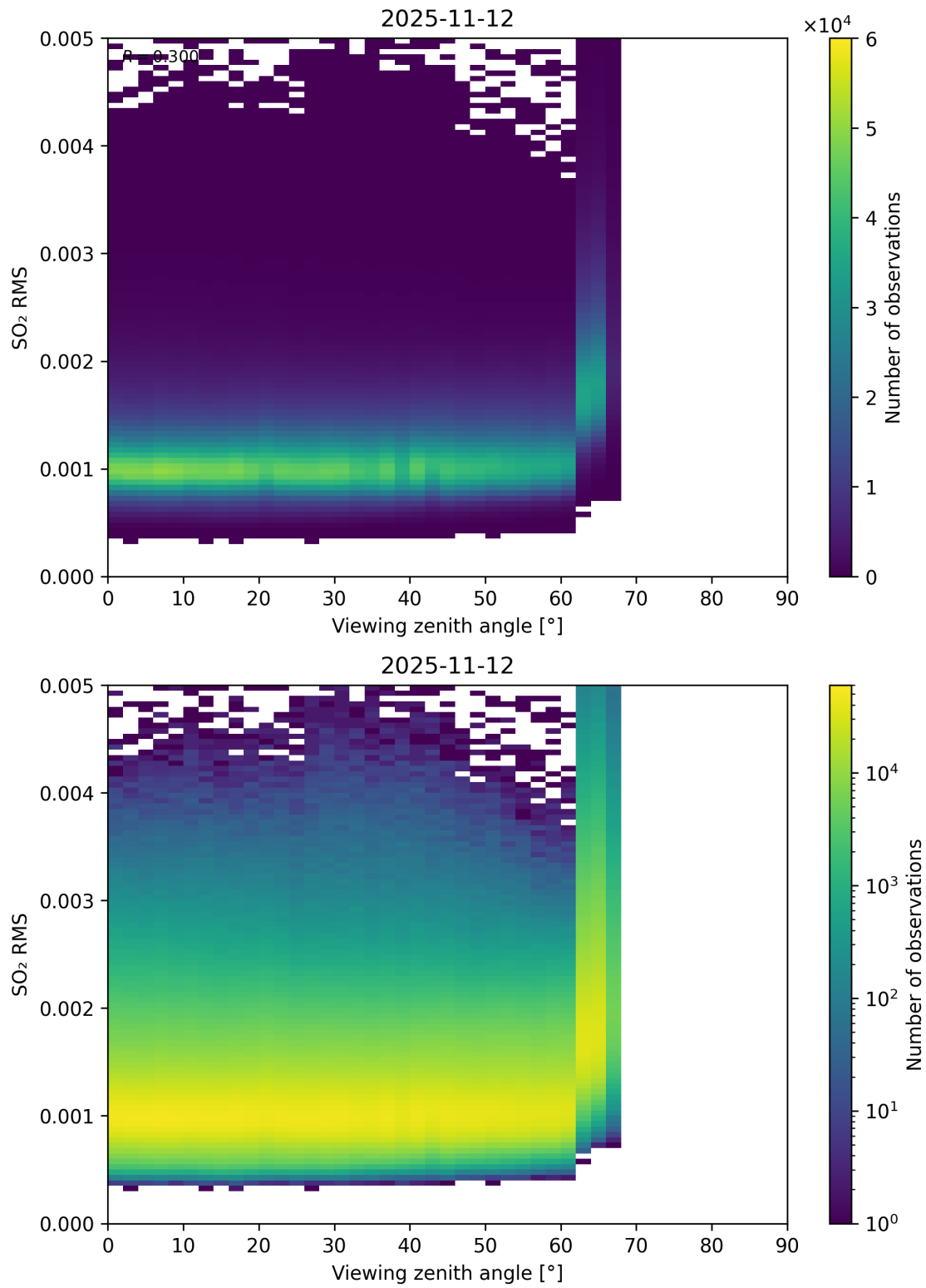
Figure 367: Scatter density plot of “Viewing zenith angle” against “SO 2 RMS” for 2025-11-12 to 2025-11-13.
