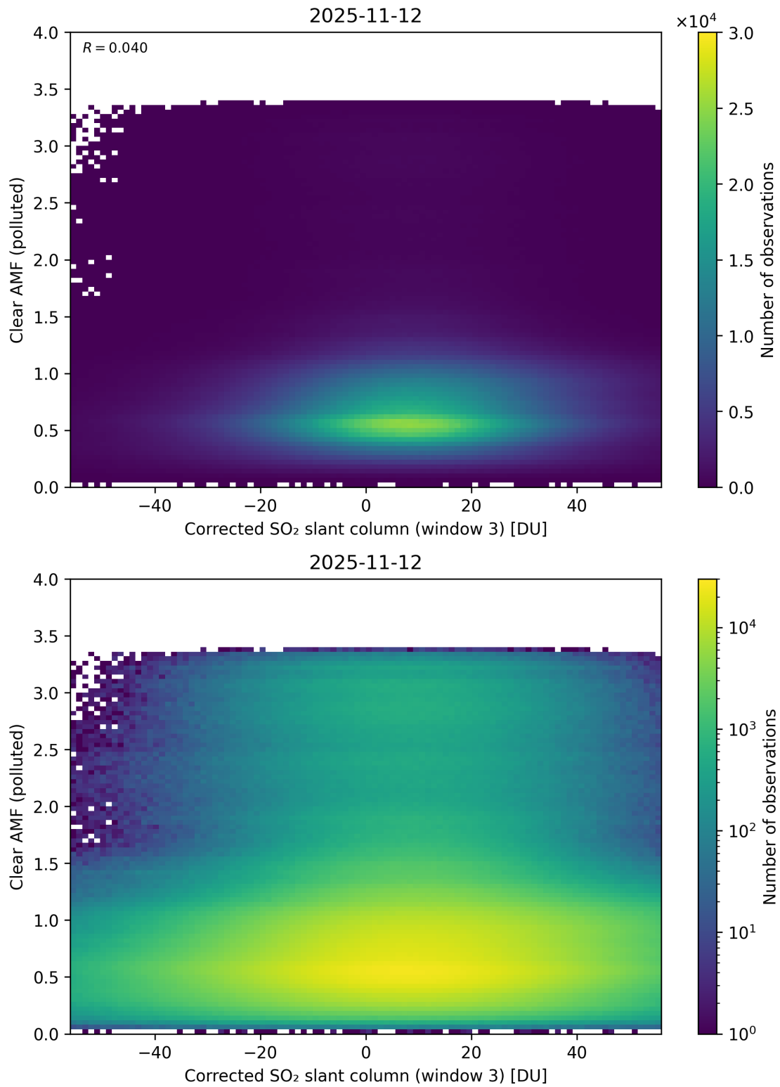
Figure 259: Scatter density plot of “Corrected SO 2 slant column (window 3)” against “Clear AMF (polluted)” for 2025-11-12 to 2025-11-13.
