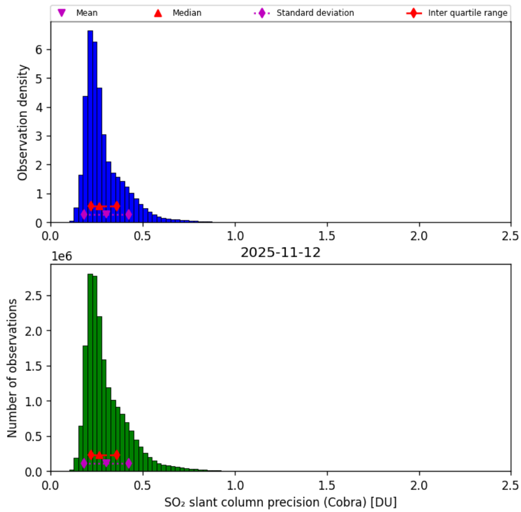
Figure 62: Histogram of “SO 2 slant column precision (Cobra)” for 2025-11-12 to 2025-11-13
