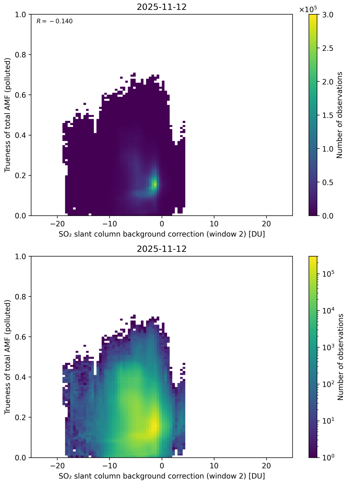
Figure 131: Scatter density plot of “SO 2 slant column background correction (window 2)” against “Trueness of total AMF (polluted)” for 2025-11-12 to 2025-11-13.
