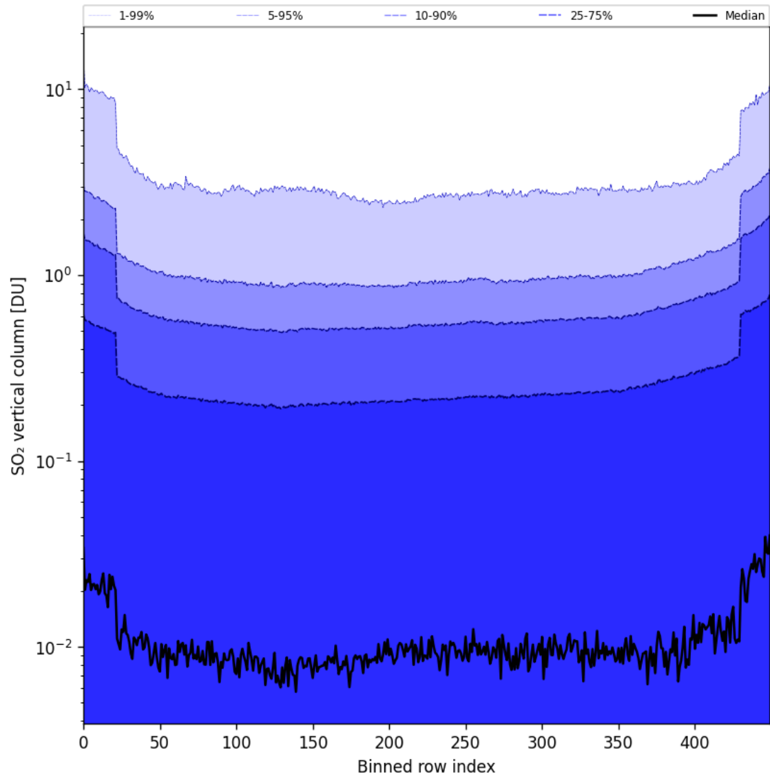
Figure 84: Along track statistics of “SO 2 vertical column” for 2025-11-12 to 2025-11-13
