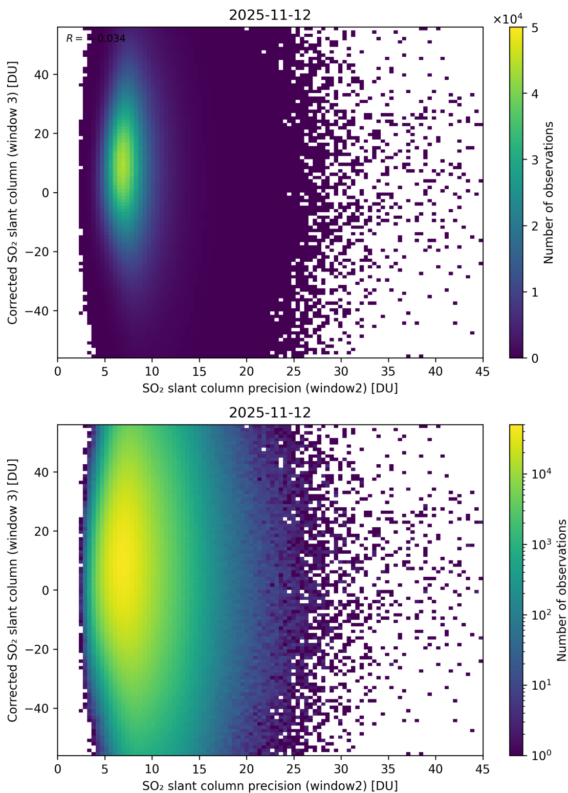
Figure 298: Scatter density plot of “SO 2 slant column precision (window2)” against “Corrected SO 2 slant column (window 3)” for 2025-11-12 to 2025-11-13.
