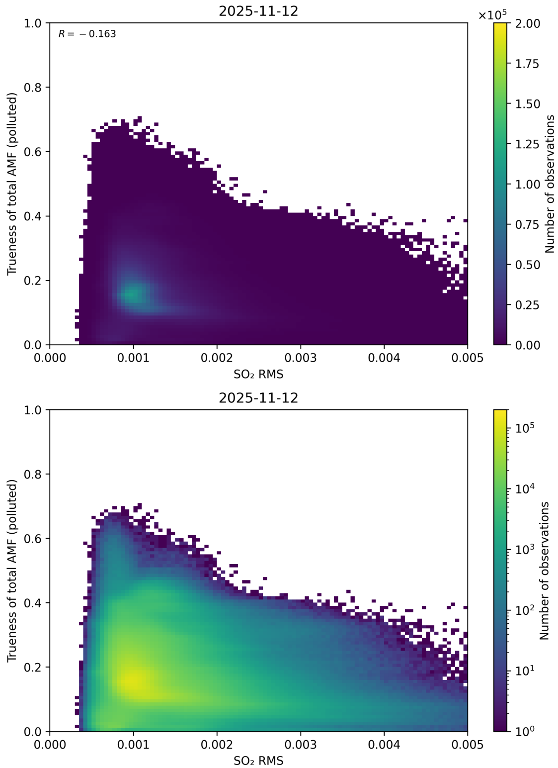
Figure 149: Scatter density plot of “SO 2 RMS” against “Trueness of total AMF (polluted)” for 2025-11-12 to 2025-11-13.
