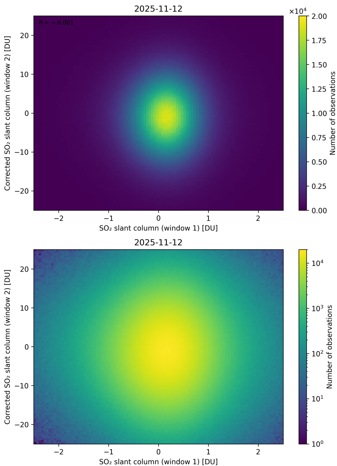
Figure 283: Scatter density plot of “SO 2 slant column (window 1)” against “Corrected SO 2 slant column (window 2)” for 2025-11-12 to 2025-11-13.
