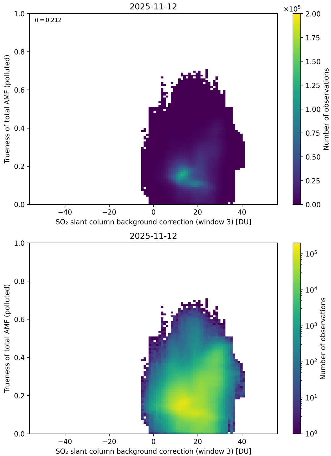
Figure 137: Scatter density plot of “SO 2 slant column background correction (window 3)” against “Trueness of total AMF (polluted)” for 2025-11-12 to 2025-11-13.
