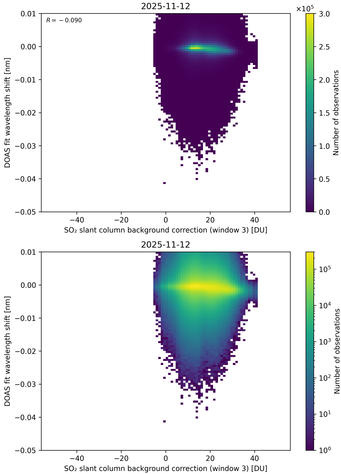
Figure 132: Scatter density plot of “SO 2 slant column background correction (window 3)” against “DOAS fit wavelength shift” for 2025-11-12 to 2025-11-13.
