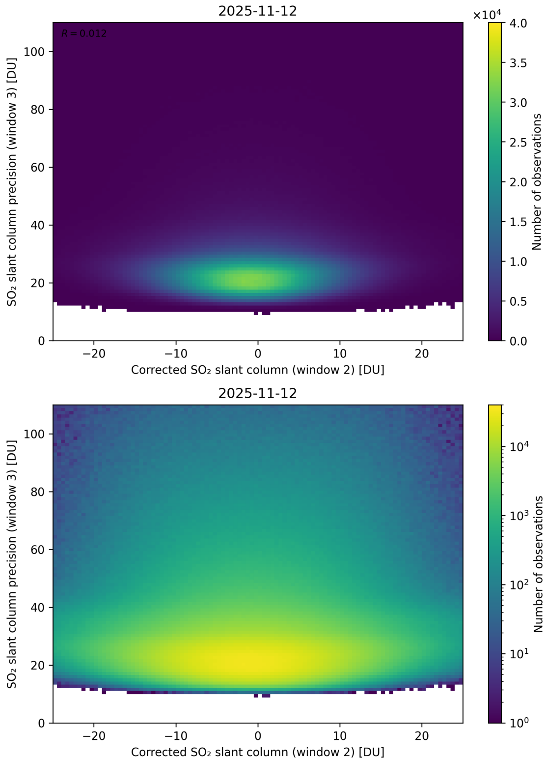
Figure 252: Scatter density plot of “Corrected SO 2 slant column (window 2)” against “SO 2 slant column precision (window 3)” for 2025-11-12 to 2025-11-13.
