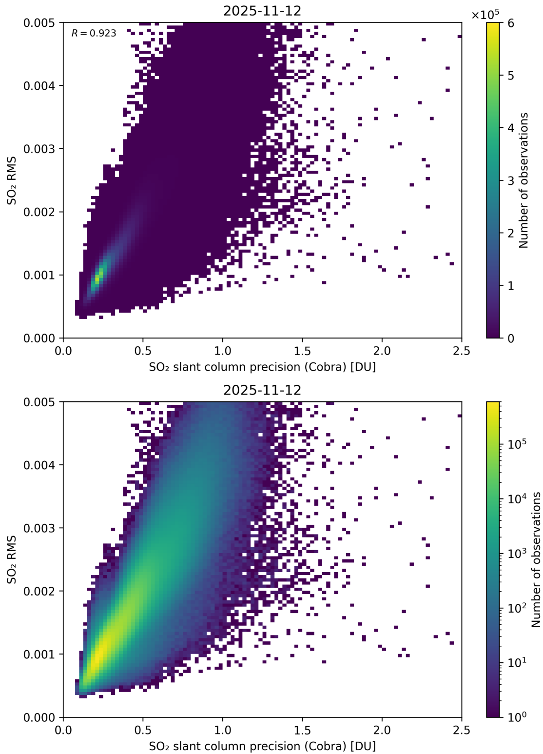
Figure 204: Scatter density plot of “SO 2 slant column precision (Cobra)” against “SO 2 RMS” for 2025-11-12 to 2025-11-13.
