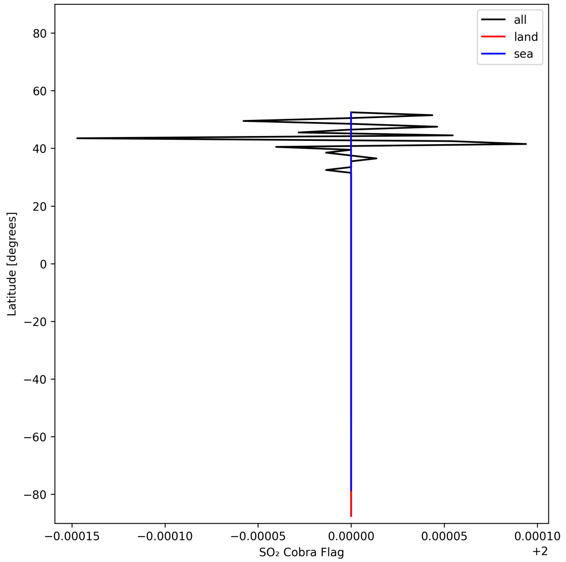
Figure 49: Zonal average of “SO 2 Cobra Flag” for 2025-11-12 to 2025-11-13.
