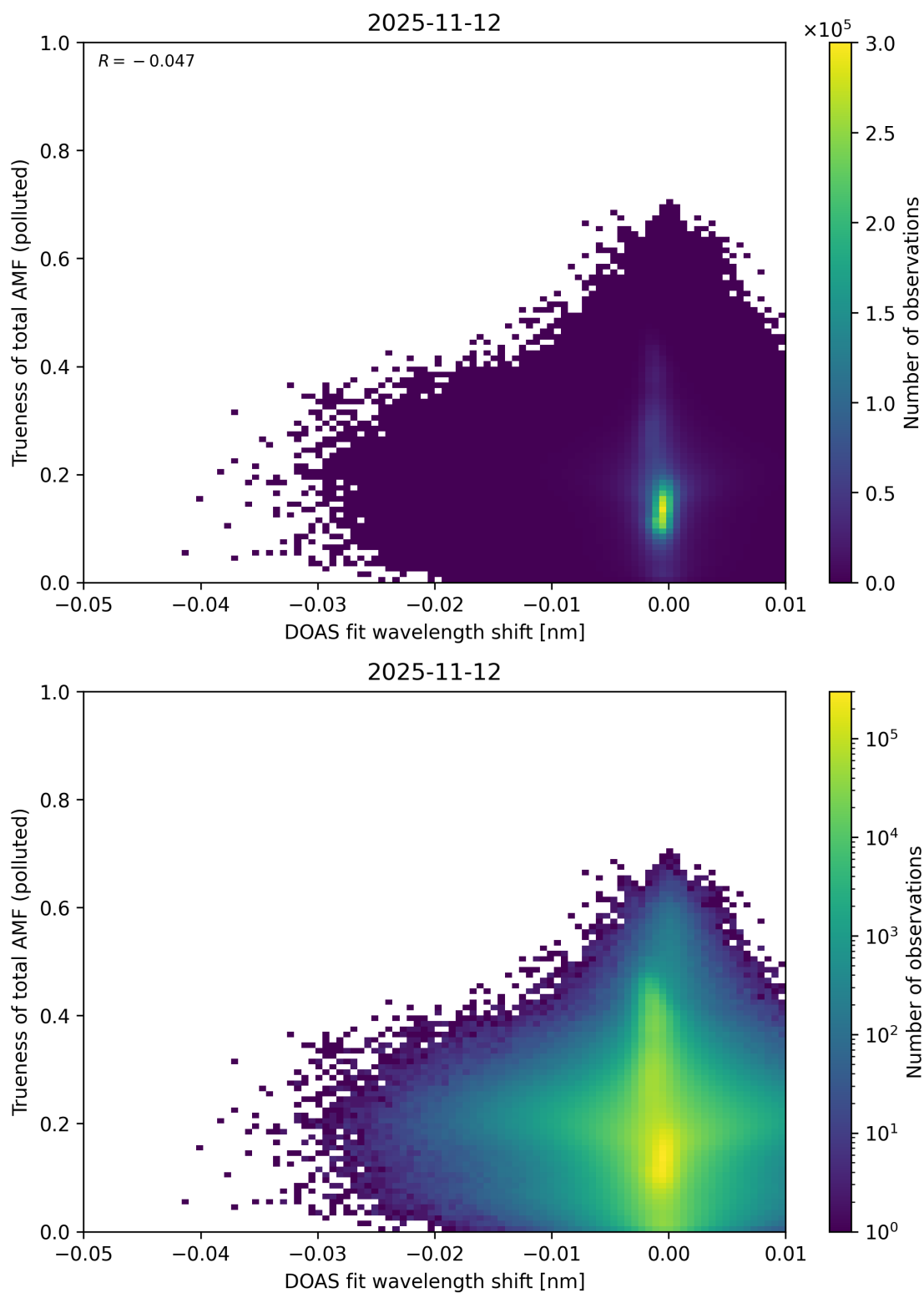
Figure 142: Scatter density plot of “DOAS fit wavelength shift” against “Trueness of total AMF (polluted)” for 2025-11-12 to 2025-11-13.
