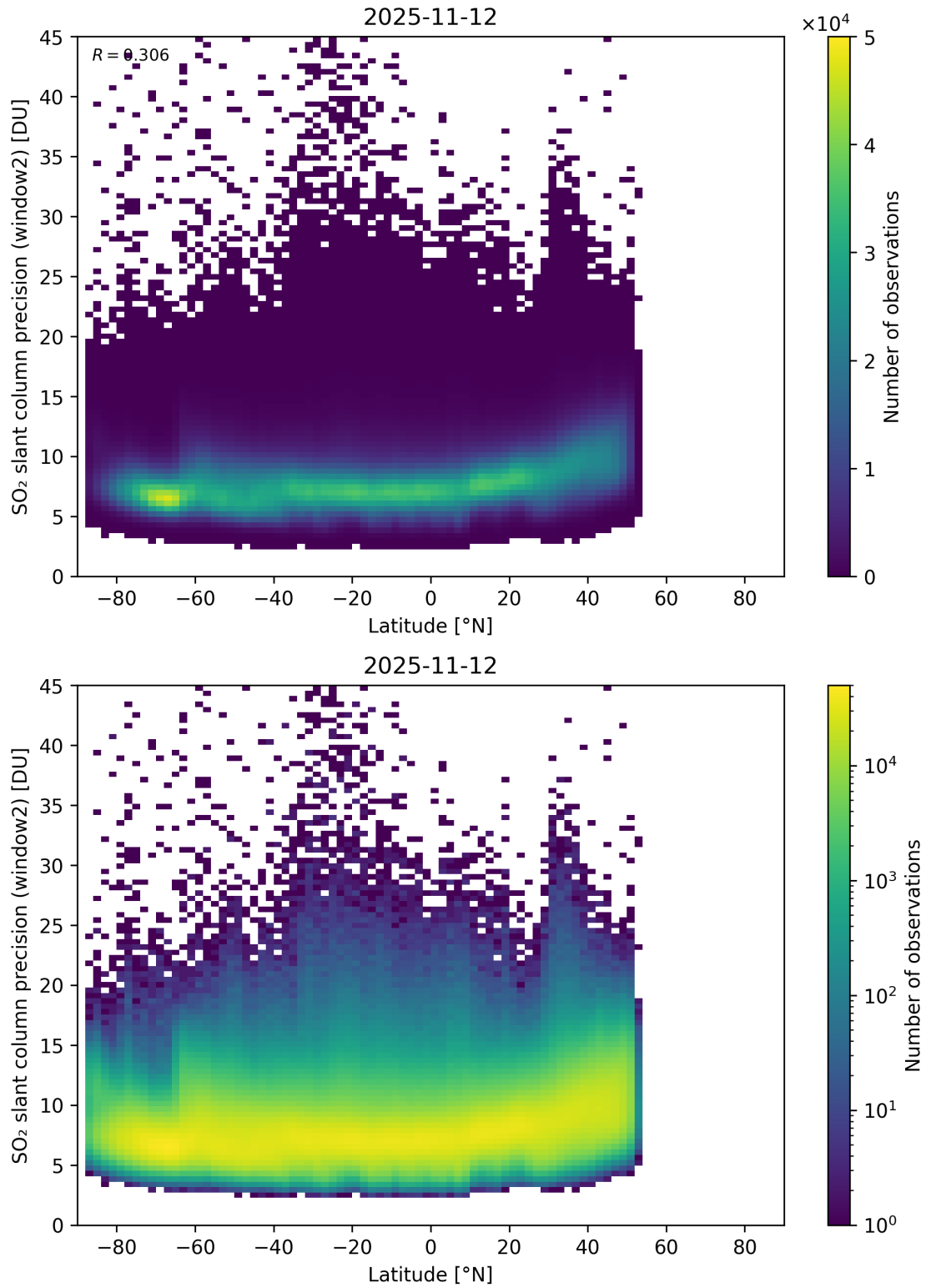
Figure 164: Scatter density plot of “Latitude” against “SO 2 slant column precision (window2)” for 2025-11-12 to 2025-11-13.
