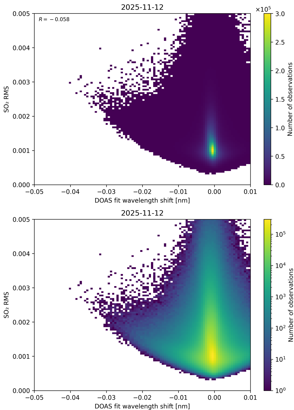
Figure 139: Scatter density plot of “DOAS fit wavelength shift” against “SO 2 RMS” for 2025-11-12 to 2025-11-13.
