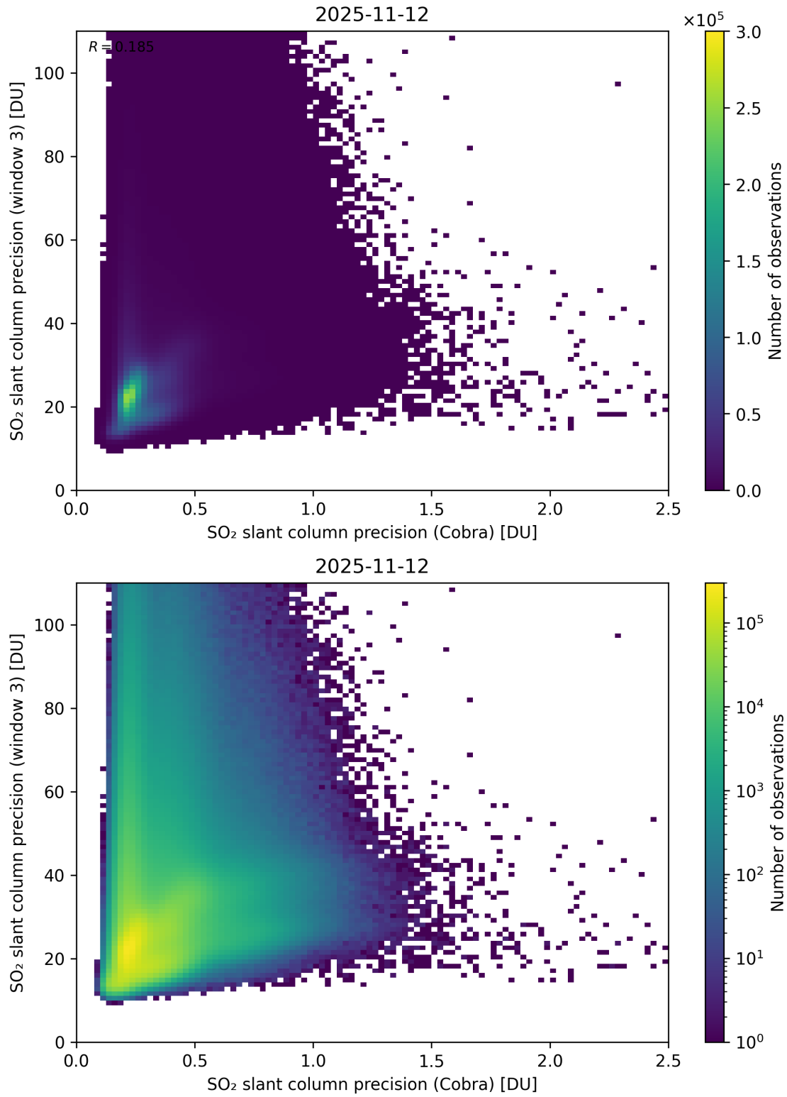
Figure 212: Scatter density plot of “SO 2 slant column precision (Cobra)” against “SO 2 slant column precision (window 3)” for 2025-11-12 to 2025-11-13.
