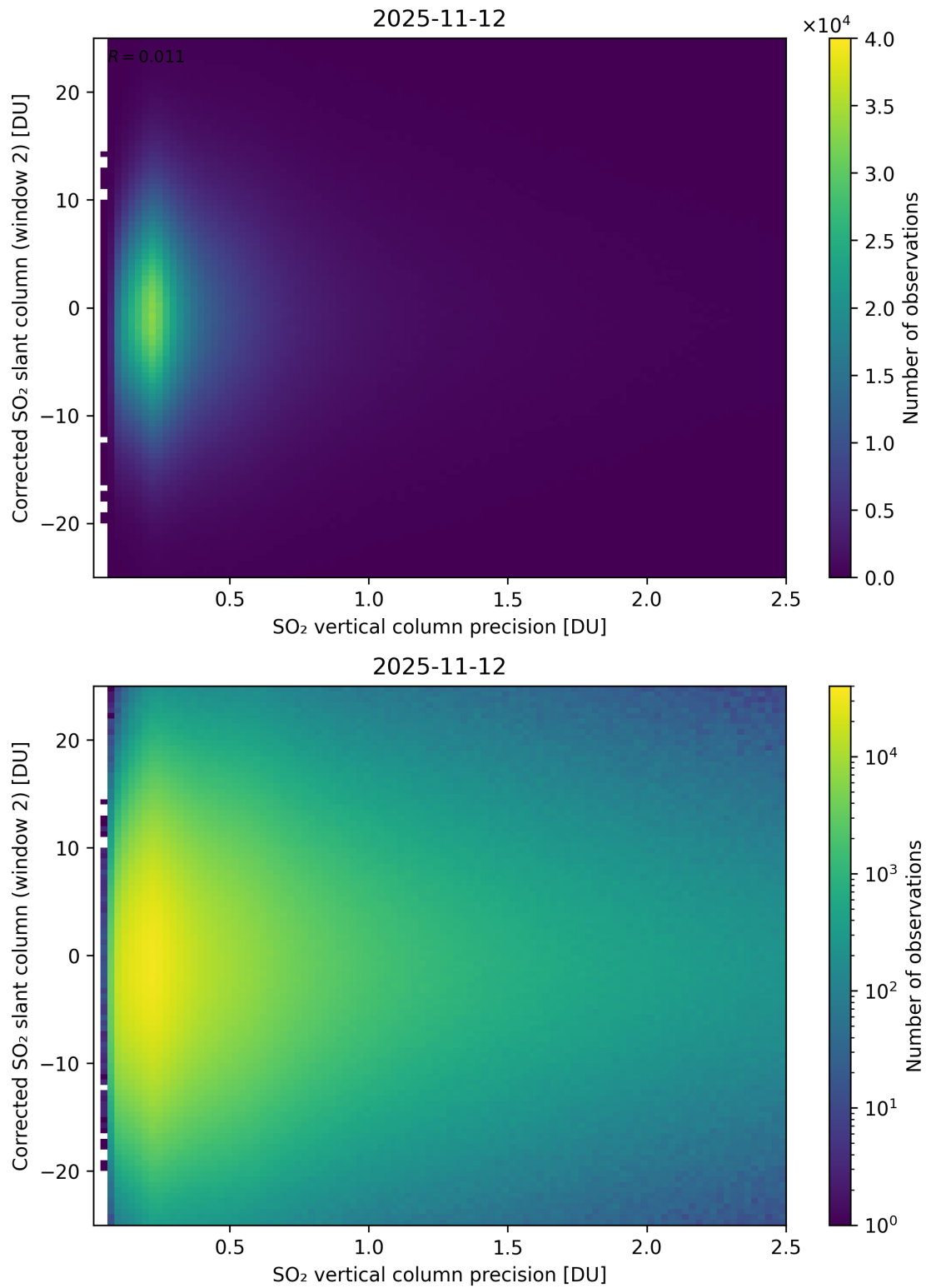
Figure 339: Scatter density plot of “SO 2 vertical column precision” against “Corrected SO 2 slant column (window 2)” for 2025-11-12 to 2025-11-13.
