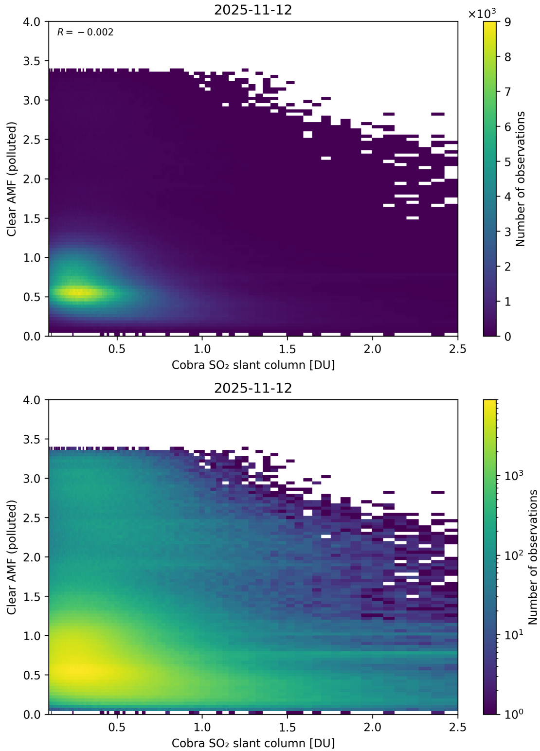
Figure 215: Scatter density plot of “Cobra SO 2 slant column” against “Clear AMF (polluted)” for 2025-11-12 to 2025-11-13.
