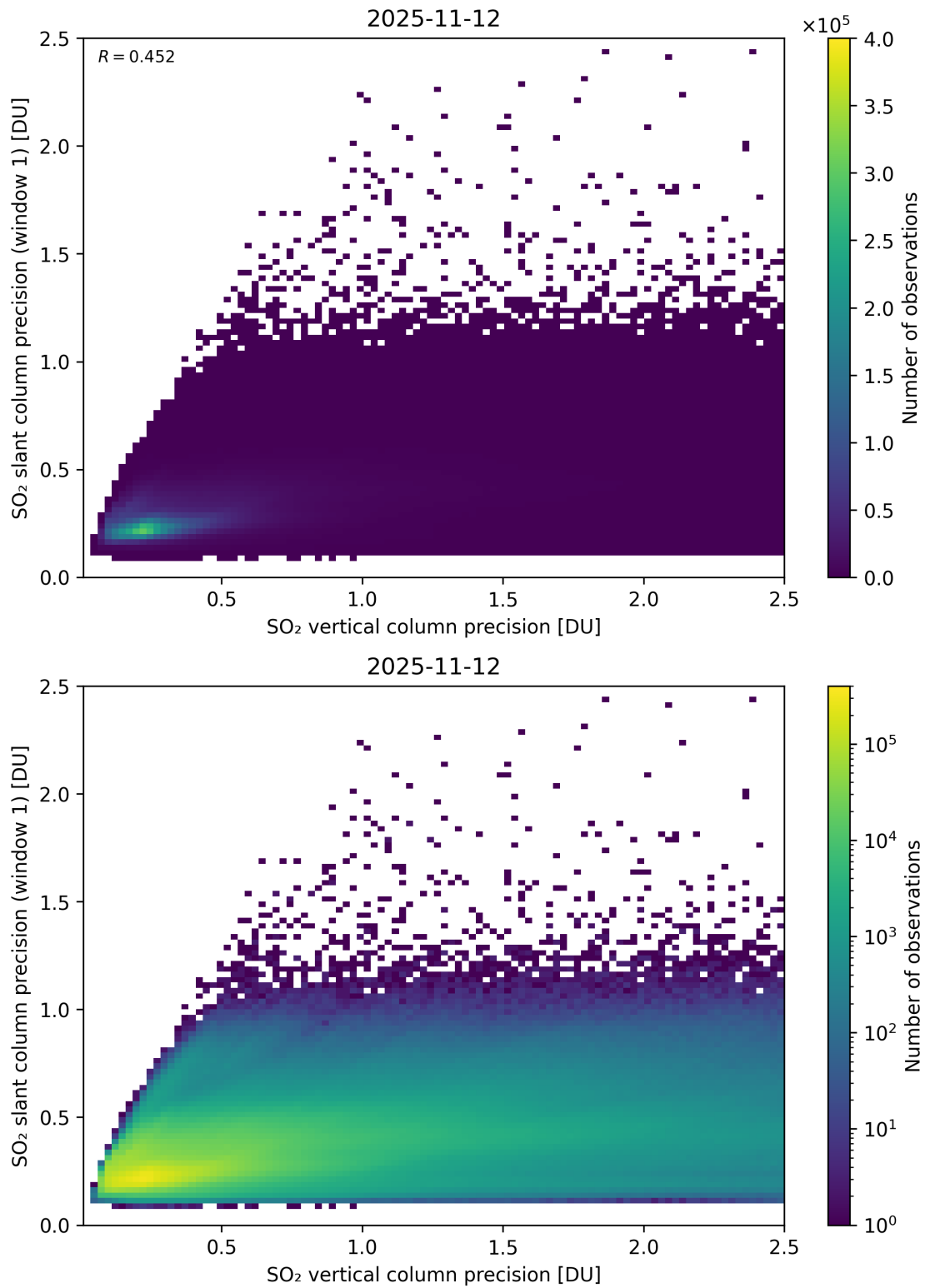
Figure 342: Scatter density plot of “SO 2 vertical column precision” against “SO 2 slant column precision (window 1)” for 2025-11-12 to 2025-11-13.
