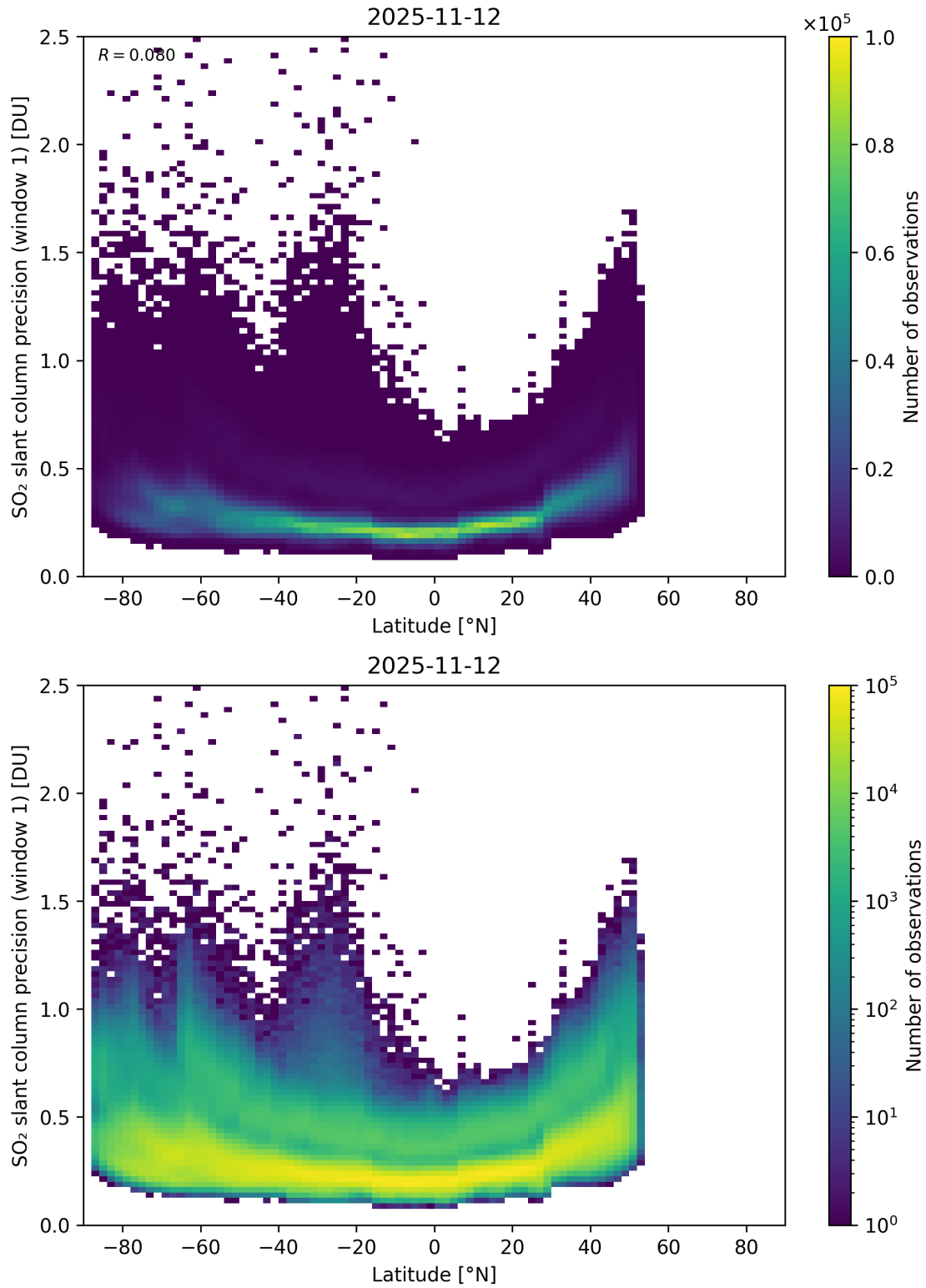
Figure 163: Scatter density plot of “Latitude” against “SO 2 slant column precision (window 1)” for 2025-11-12 to 2025-11-13.
