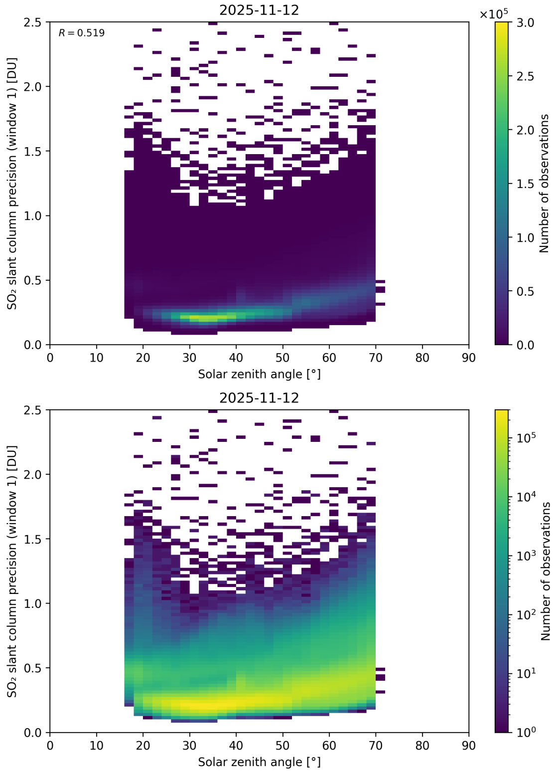
Figure 185: Scatter density plot of “Solar zenith angle” against “SO 2 slant column precision (window 1)” for 2025-11-12 to 2025-11-13.
