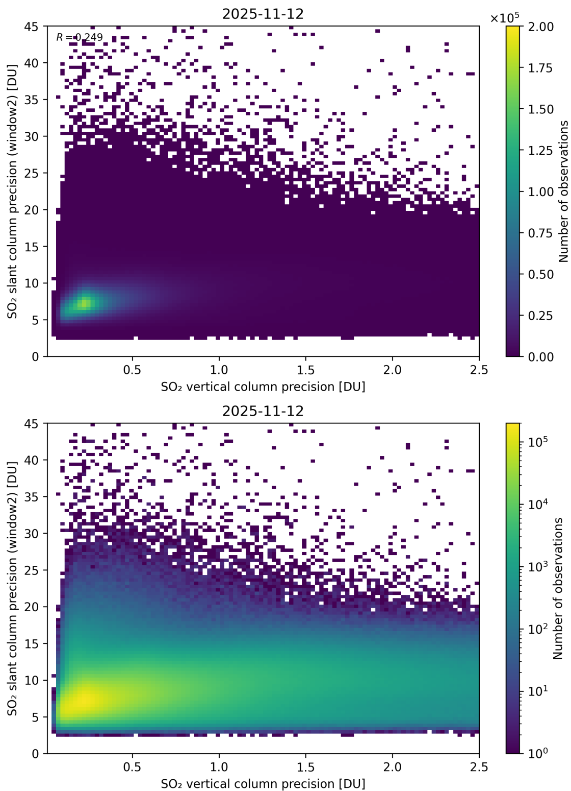
Figure 343: Scatter density plot of “SO 2 vertical column precision” against “SO 2 slant column precision (window2)” for 2025-11-12 to 2025-11-13.
