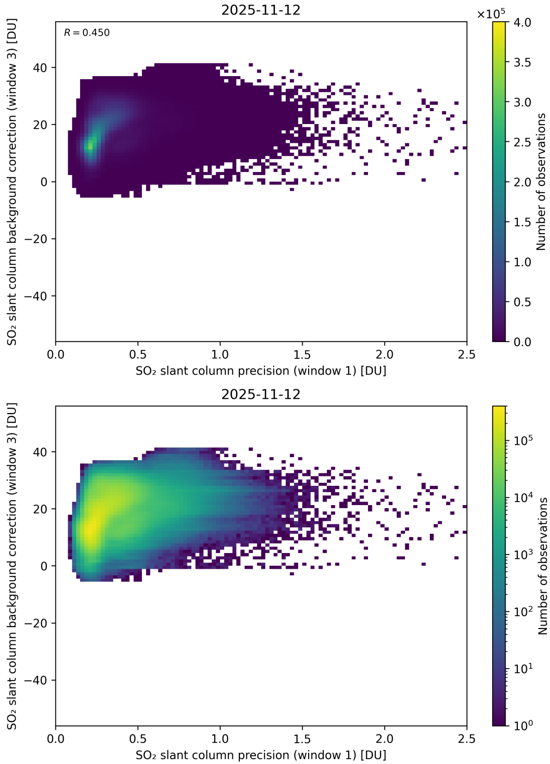
Figure 270: Scatter density plot of “SO 2 slant column precision (window 1)” against “SO 2 slant column background correction (window 3)” for 2025-11-12 to 2025-11-13.
