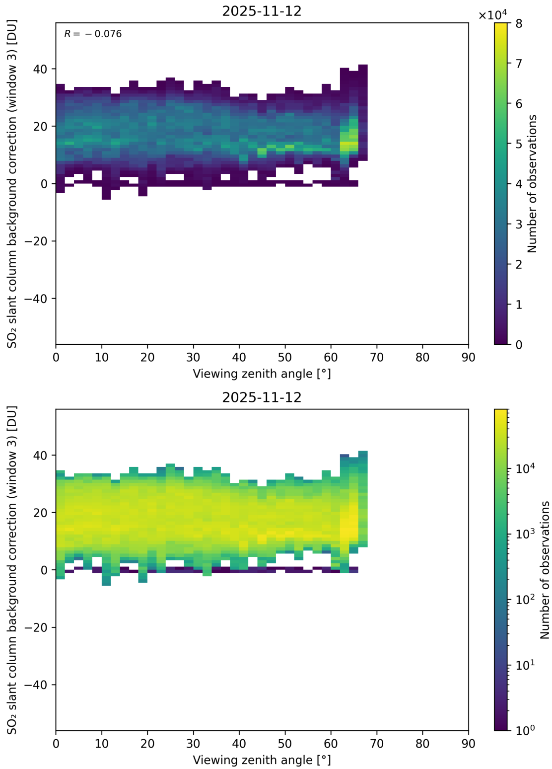
Figure 364: Scatter density plot of “Viewing zenith angle” against “SO 2 slant column background correction (window 3)” for 2025-11-12 to 2025-11-13.
