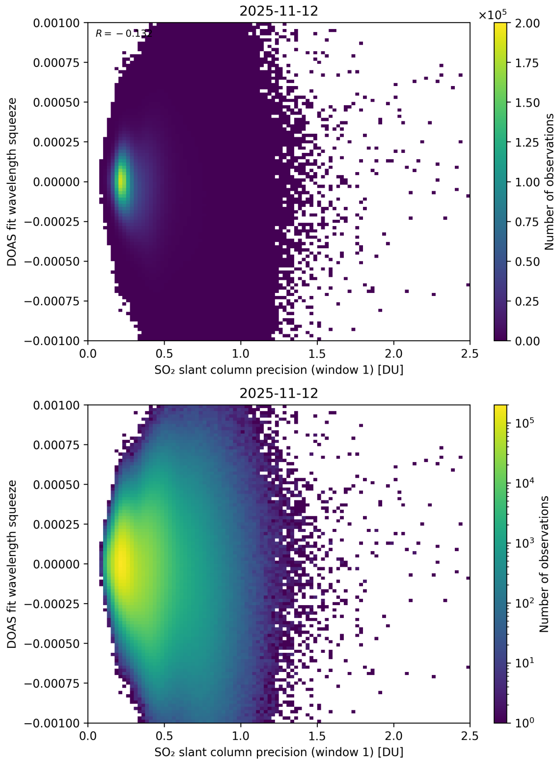
Figure 272: Scatter density plot of “SO 2 slant column precision (window 1)” against “DOAS fit wavelength squeeze” for 2025-11-12 to 2025-11-13.
