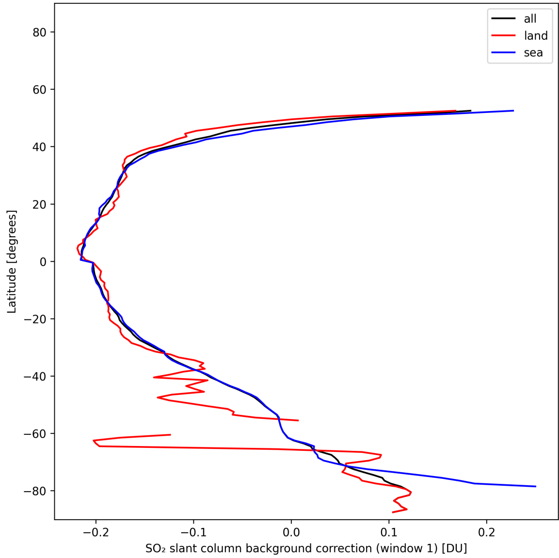
Figure 40: Zonal average of “SO 2 slant column background correction (window 1)” for 2025-11-12 to 2025-11-13.
