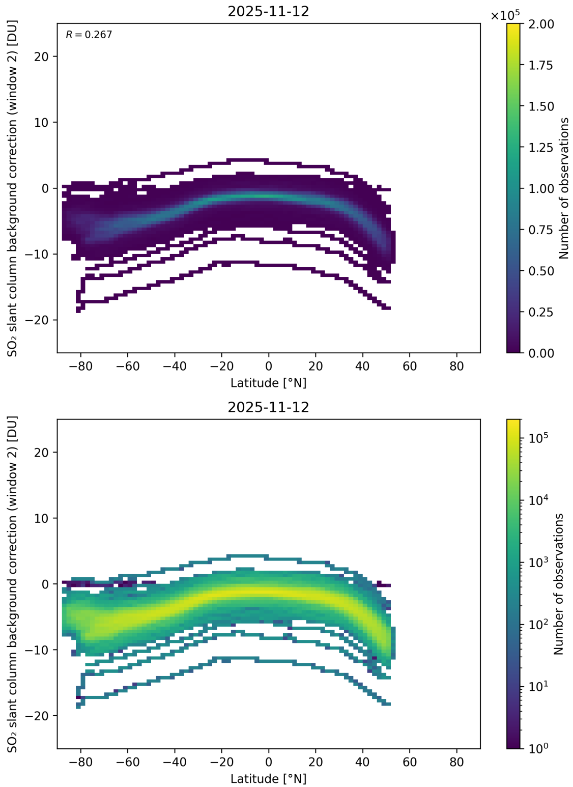
Figure 151: Scatter density plot of “Latitude” against “SO 2 slant column background correction (window 2)” for 2025-11-12 to 2025-11-13.
