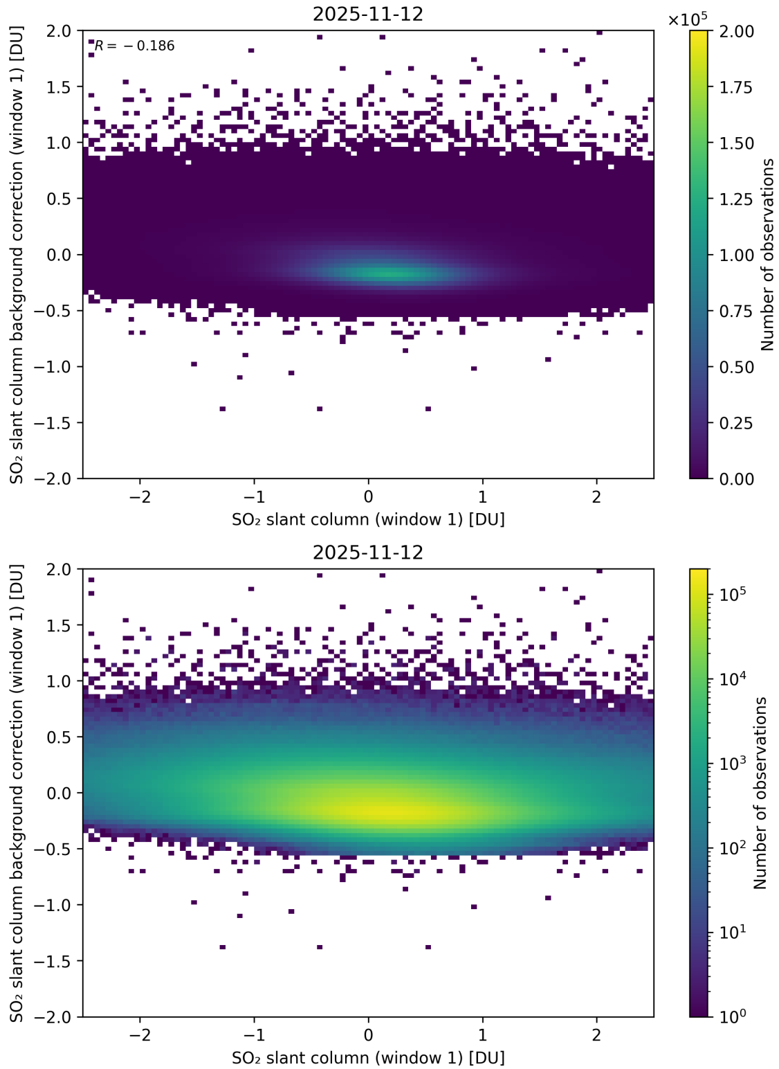
Figure 262: Scatter density plot of “SO 2 slant column (window 1)” against “SO 2 slant column background correction (window 1)” for 2025-11-12 to 2025-11-13.
