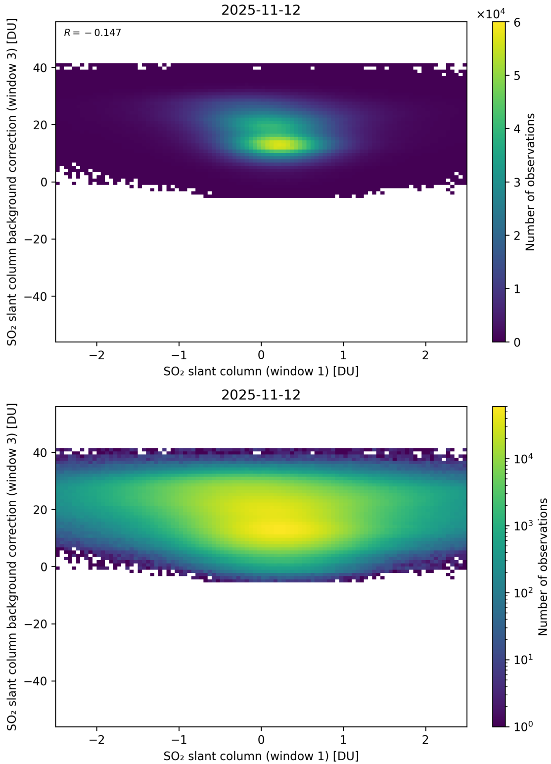
Figure 264: Scatter density plot of “SO 2 slant column (window 1)” against “SO 2 slant column background correction (window 3)” for 2025-11-12 to 2025-11-13.
