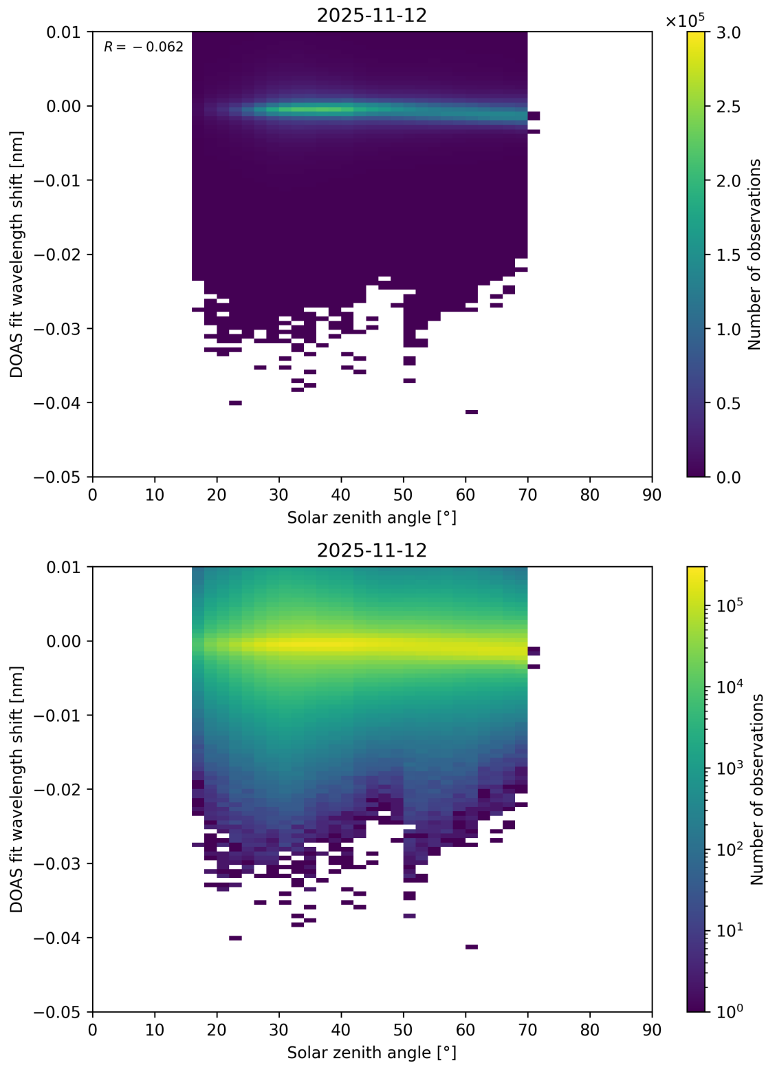
Figure 174: Scatter density plot of “Solar zenith angle” against “DOAS fit wavelength shift” for 2025-11-12 to 2025-11-13.
