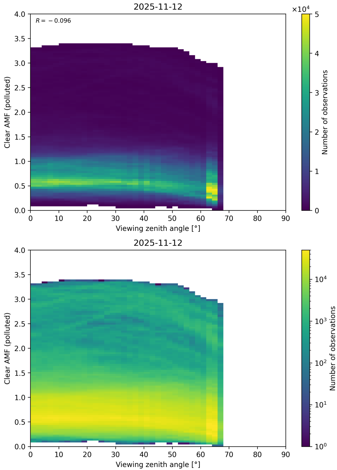
Figure 370: Scatter density plot of “Viewing zenith angle” against “Clear AMF (polluted)” for 2025-11-12 to 2025-11-13.
