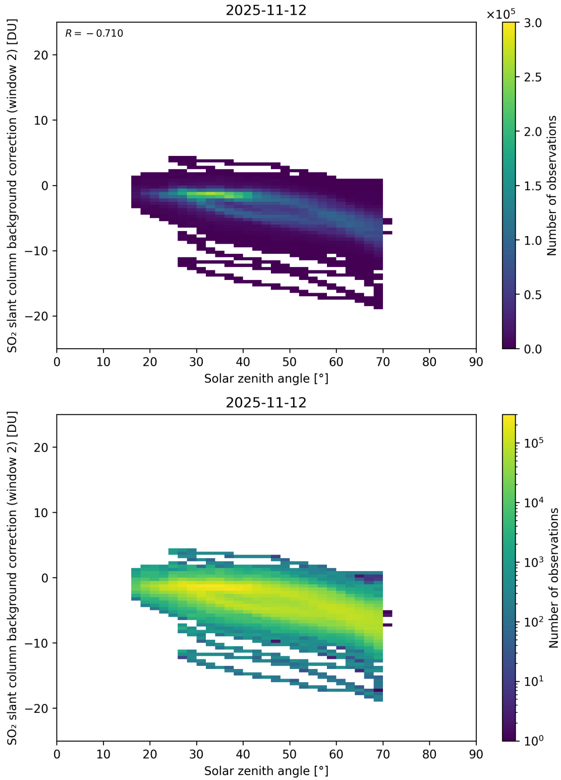
Figure 172: Scatter density plot of “Solar zenith angle” against “SO 2 slant column background correction (window 2)” for 2025-11-12 to 2025-11-13.
