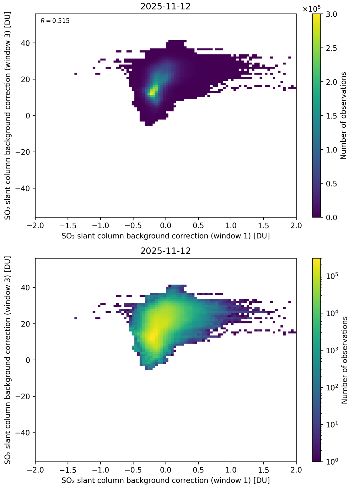
Figure 110: Scatter density plot of “SO 2 slant column background correction (window 1)” against “SO 2 slant column background correction (window 3)” for 2025-11-12 to 2025-11-13.
