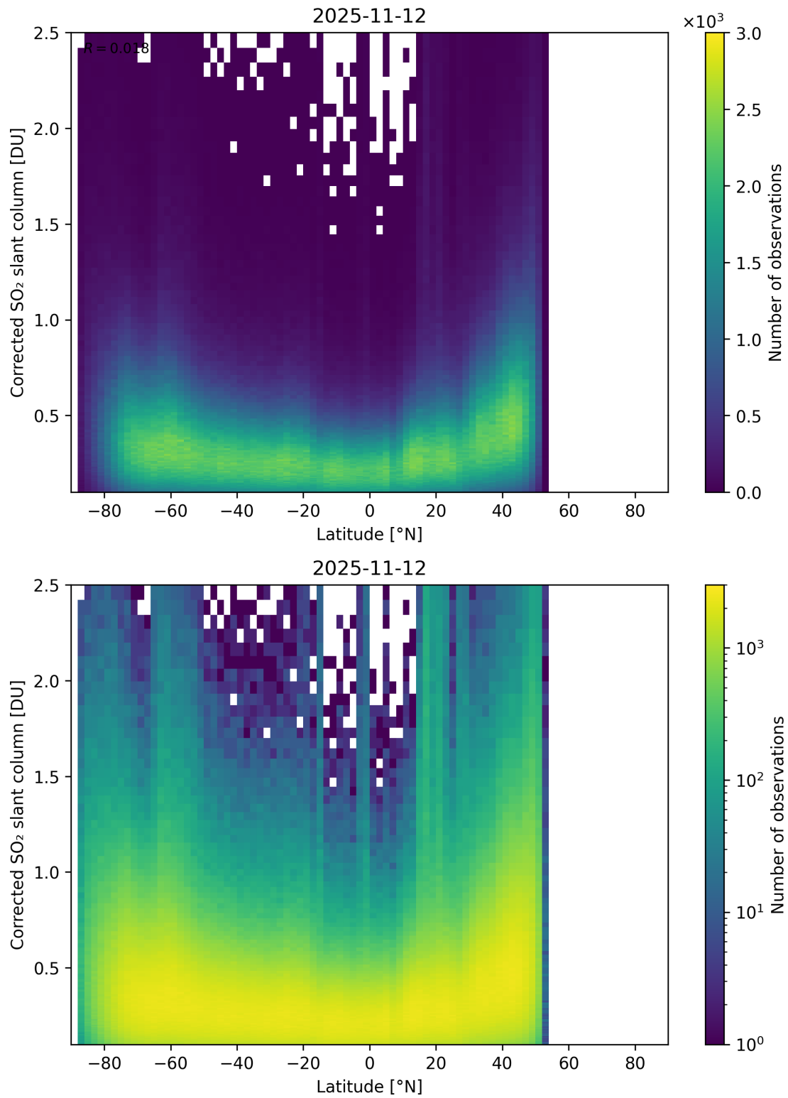
Figure 159: Scatter density plot of “Latitude” against “Corrected SO 2 slant column” for 2025-11-12 to 2025-11-13.
