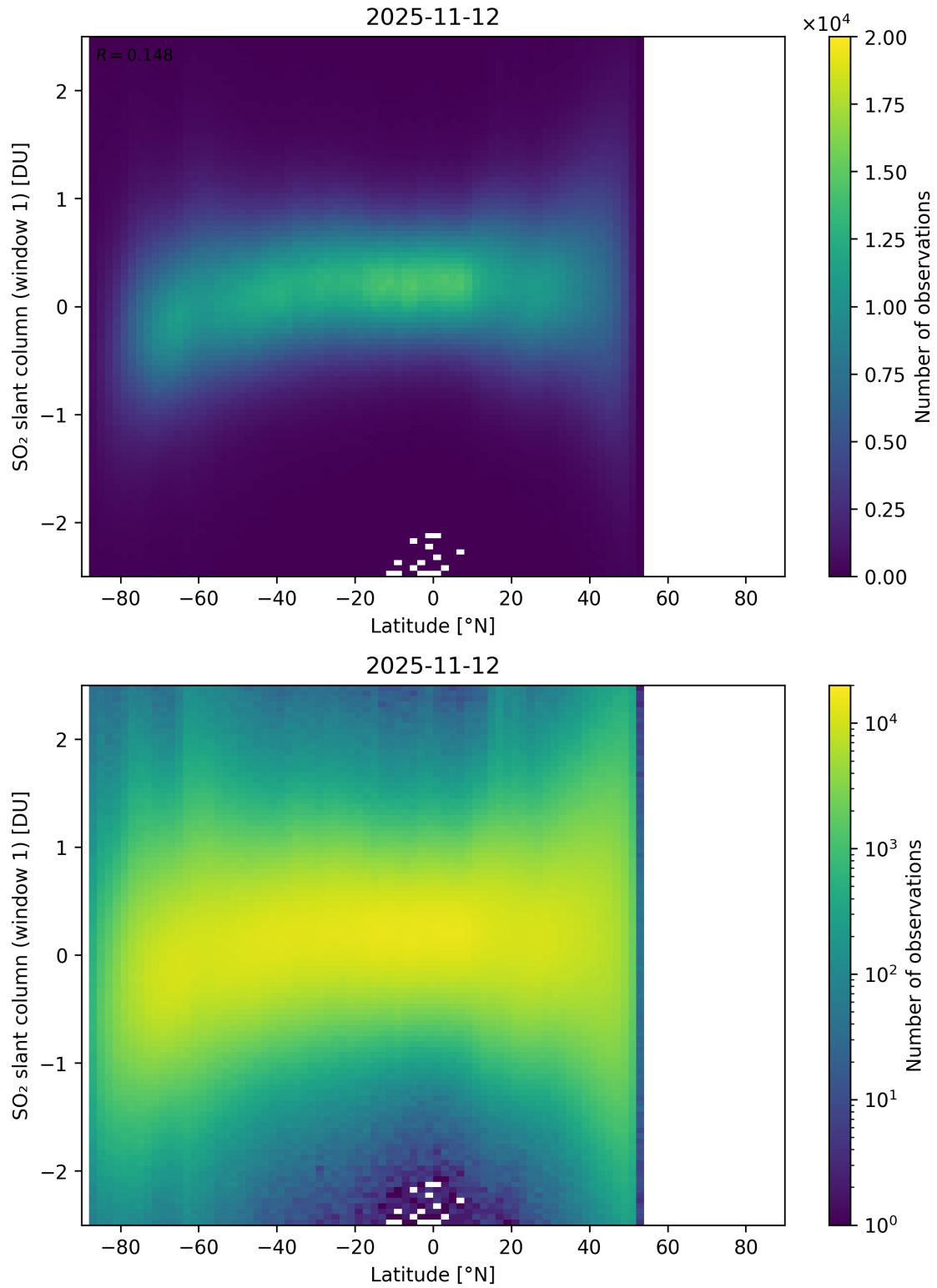
Figure 162: Scatter density plot of “Latitude” against “SO 2 slant column (window 1)” for 2025-11-12 to 2025-11-13.
