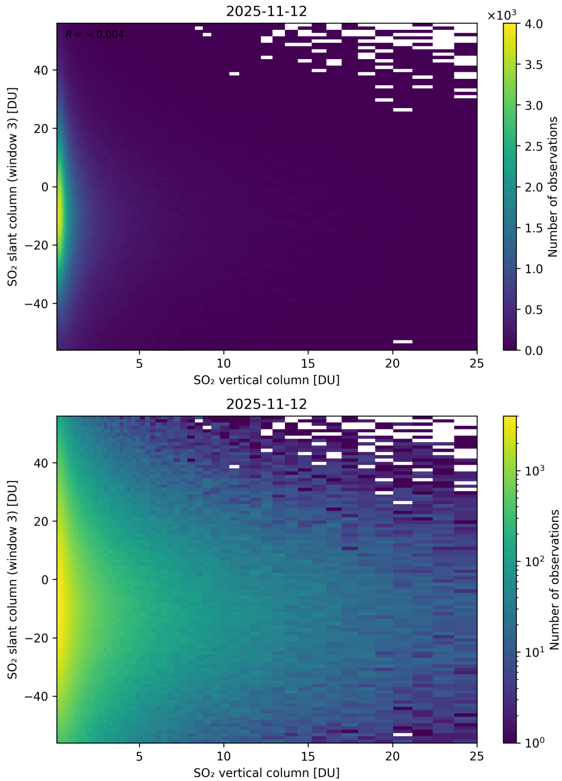
Figure 357: Scatter density plot of “SO 2 vertical column” against “SO 2 slant column (window 3)” for 2025-11-12 to 2025-11-13.
