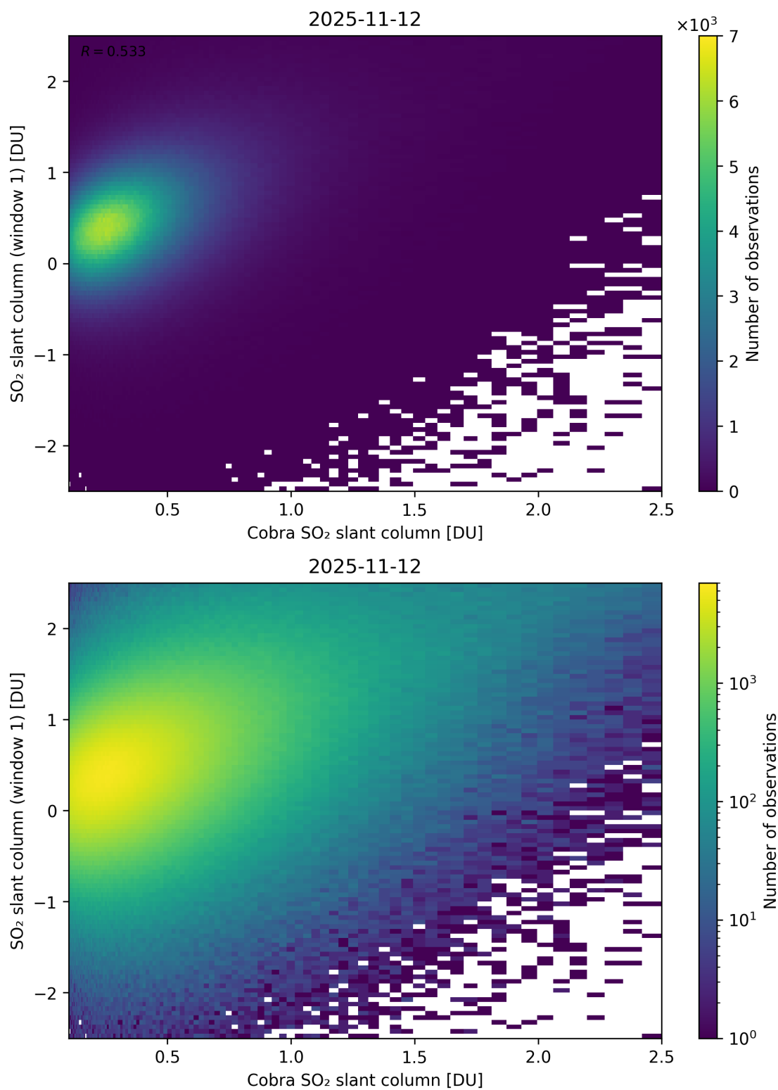
Figure 219: Scatter density plot of “Cobra SO 2 slant column” against “SO 2 slant column (window 1)” for 2025-11-12 to 2025-11-13.
