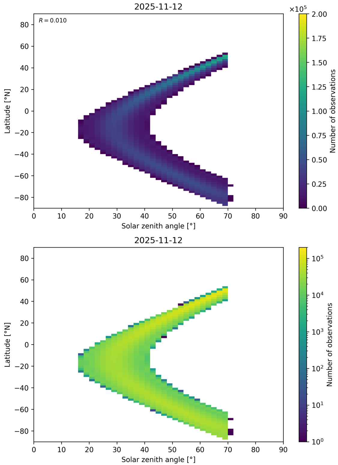
Figure 177: Scatter density plot of “Solar zenith angle” against “Latitude” for 2025-11-12 to 2025-11-13.
