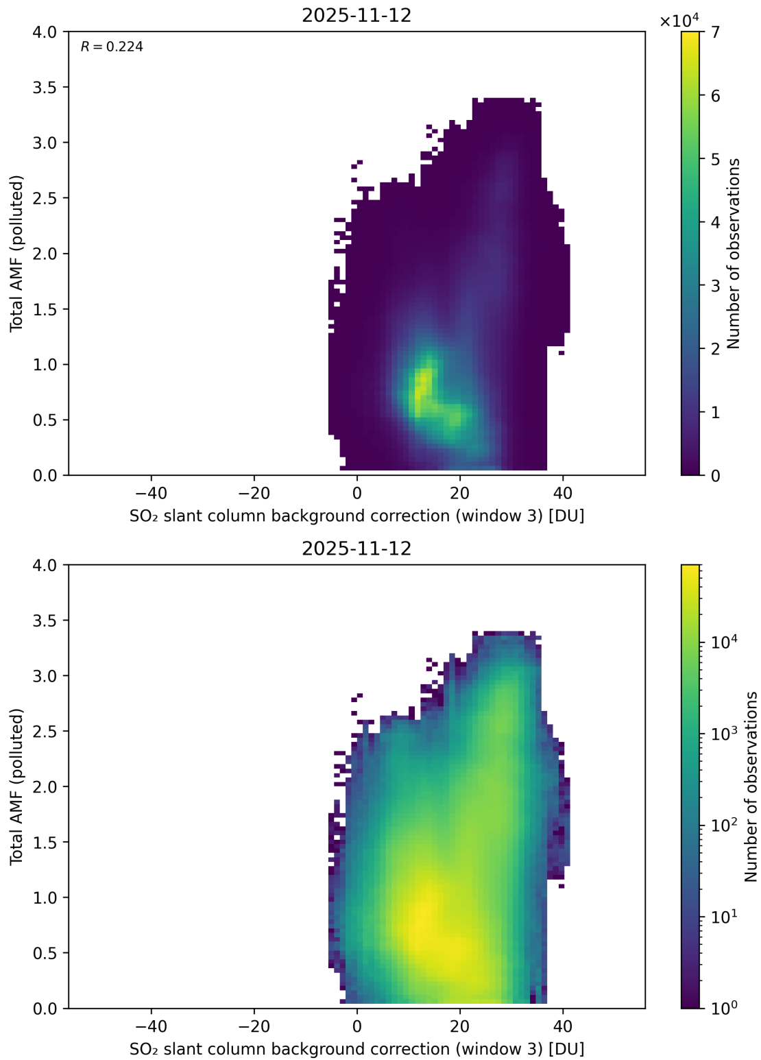
Figure 136: Scatter density plot of “SO 2 slant column background correction (window 3)” against “Total AMF (polluted)” for 2025-11-12 to 2025-11-13.
