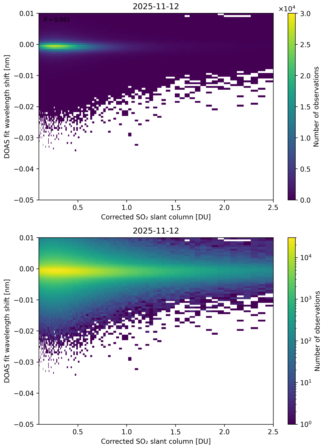
Figure 229: Scatter density plot of “Corrected SO 2 slant column” against “DOAS fit wavelength shift” for 2025-11-12 to 2025-11-13.
