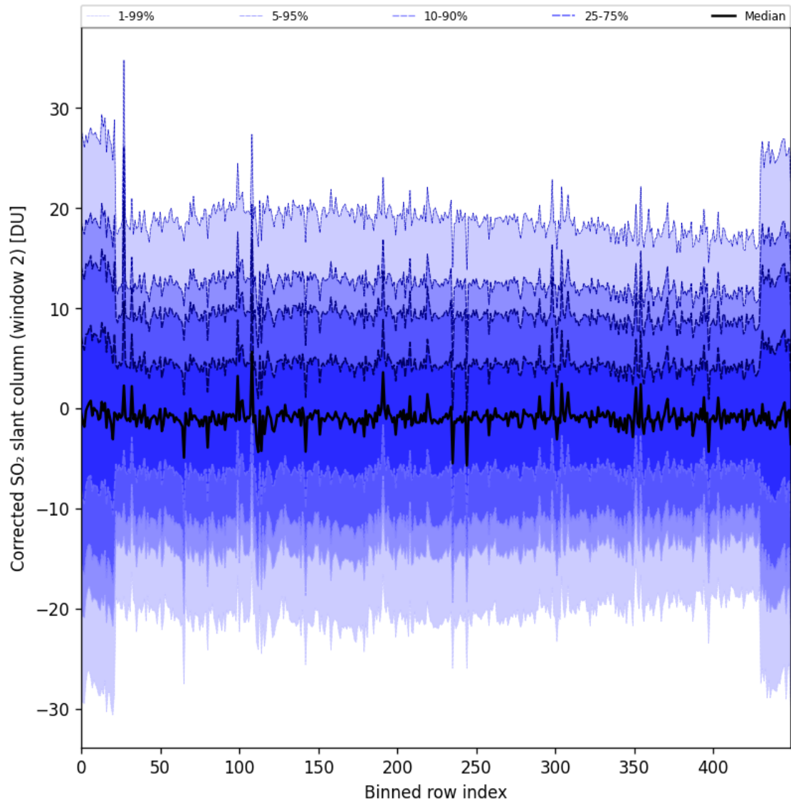
Figure 95: Along track statistics of “Corrected SO 2 slant column (window 2)” for 2025-11-12 to 2025-11-13
