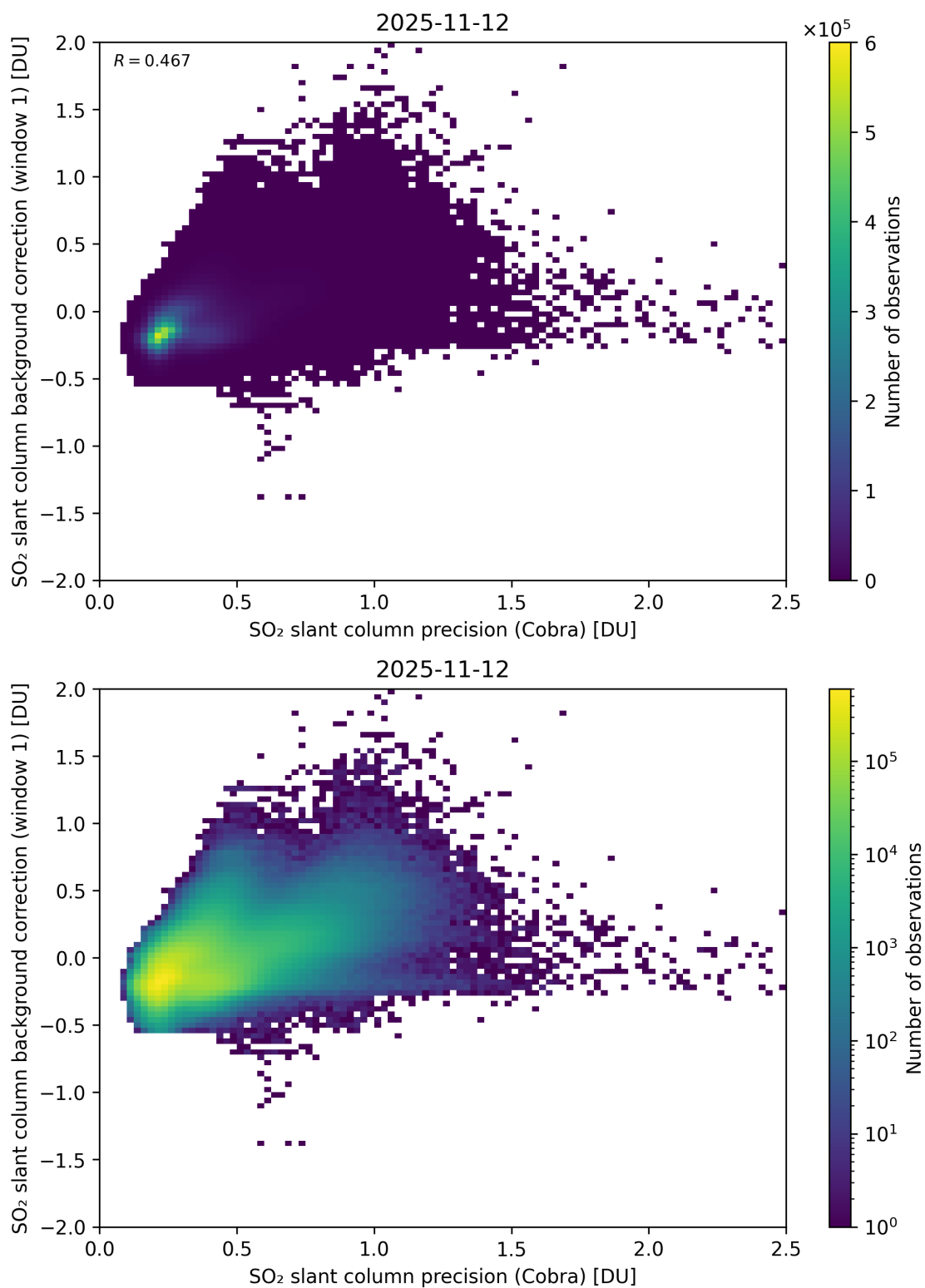
Figure 199: Scatter density plot of “SO 2 slant column precision (Cobra)” against “SO 2 slant column background correction (window 1)” for 2025-11-12 to 2025-11-13.
