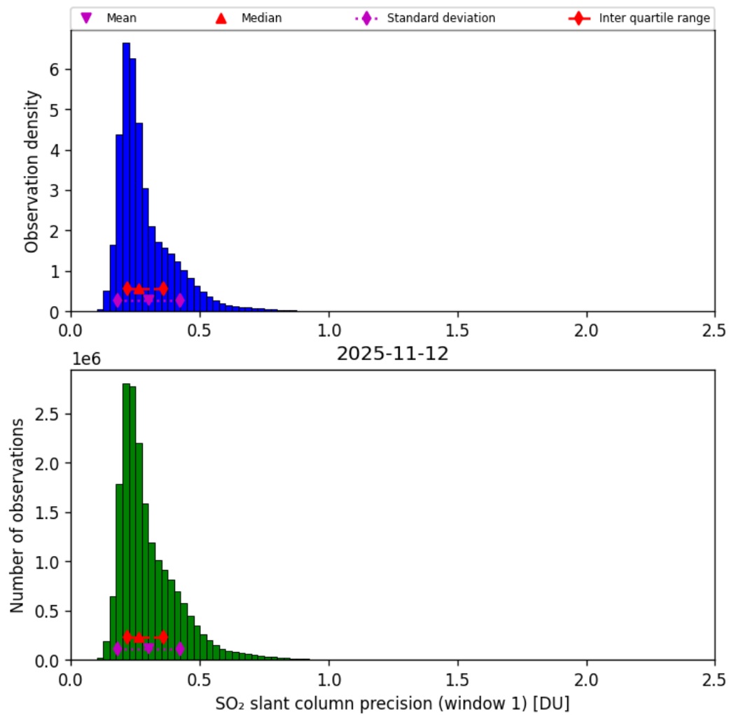
Figure 64: Histogram of “SO 2 slant column precision (window 1)” for 2025-11-12 to 2025-11-13
