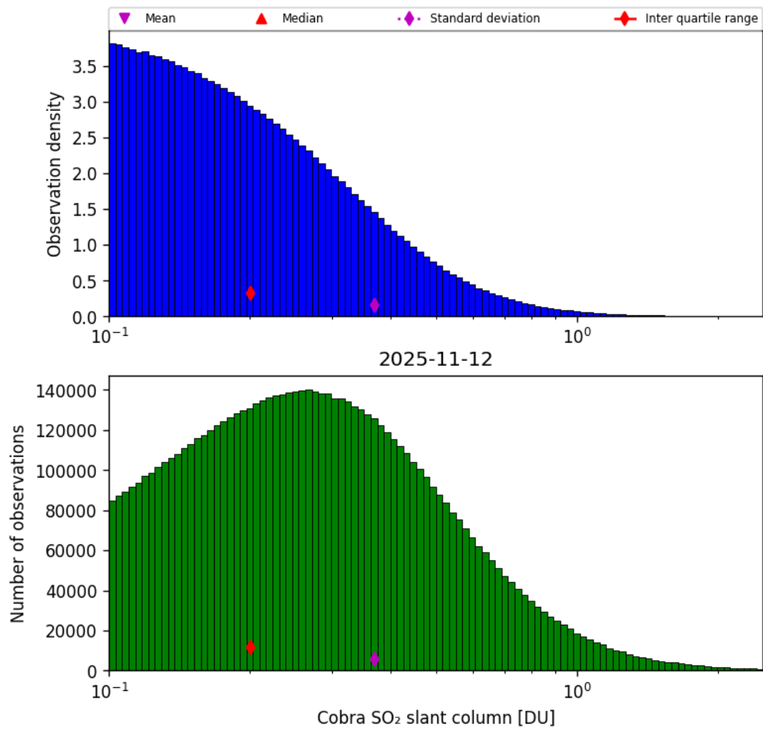
Figure 61: Histogram of “Cobra SO 2 slant column” for 2025-11-12 to 2025-11-13
