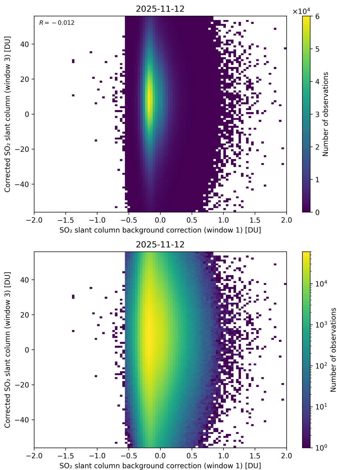
Figure 116: Scatter density plot of “SO 2 slant column background correction (window 1)” against “Corrected SO 2 slant column (window 3)” for 2025-11-12 to 2025-11-13.
