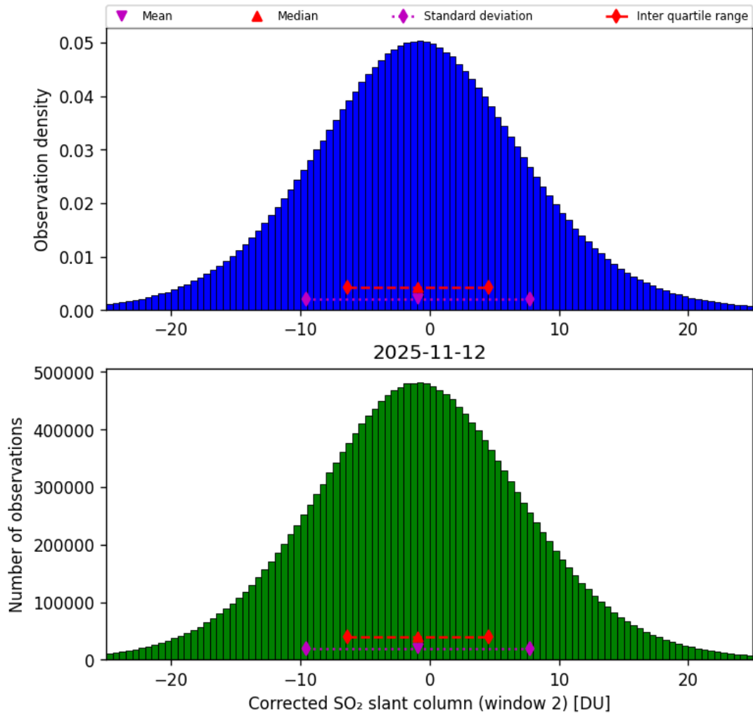
Figure 69: Histogram of “Corrected SO 2 slant column (window 2)” for 2025-11-12 to 2025-11-13
