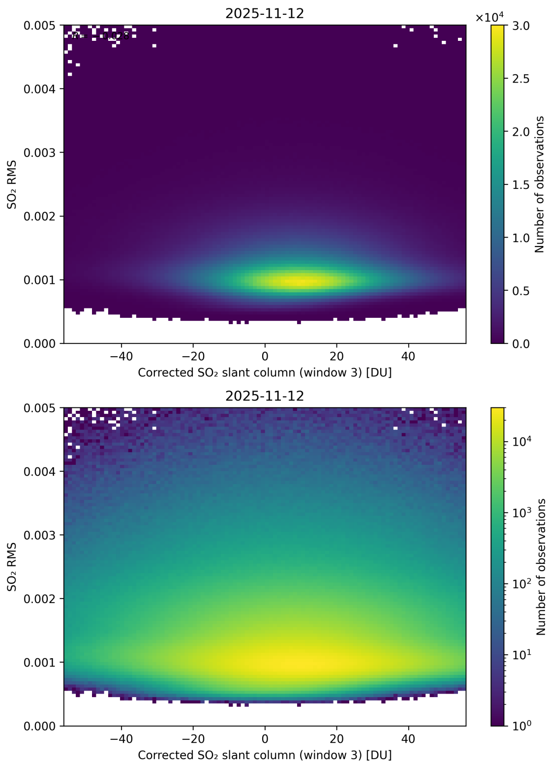
Figure 258: Scatter density plot of “Corrected SO 2 slant column (window 3)” against “SO 2 RMS” for 2025-11-12 to 2025-11-13.
