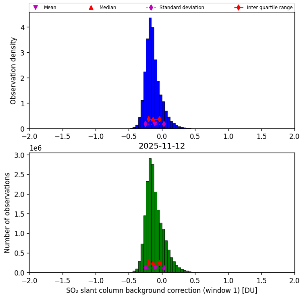
Figure 66: Histogram of “SO 2 slant column background correction (window 1)” for 2025-11-12 to 2025-11-13
