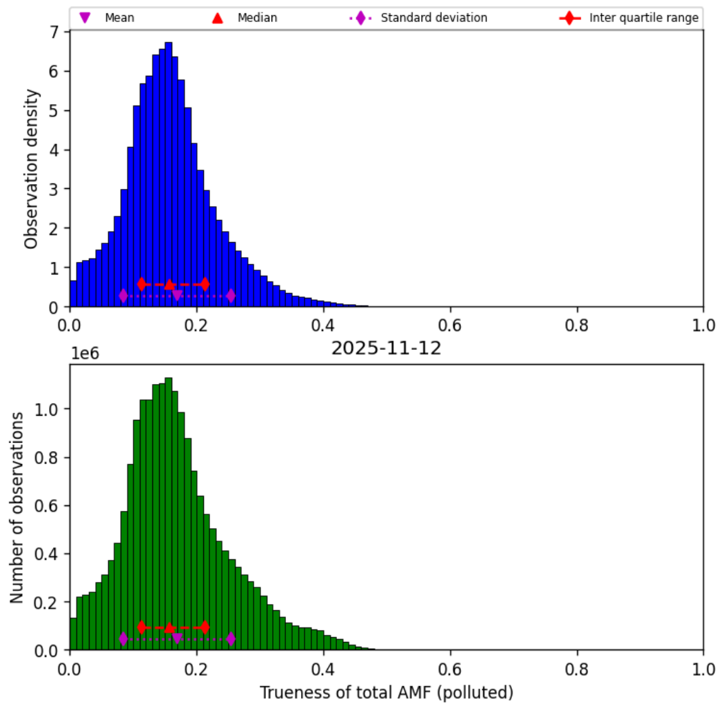
Figure 80: Histogram of “Trueness of total AMF (polluted)” for 2025-11-12 to 2025-11-13
