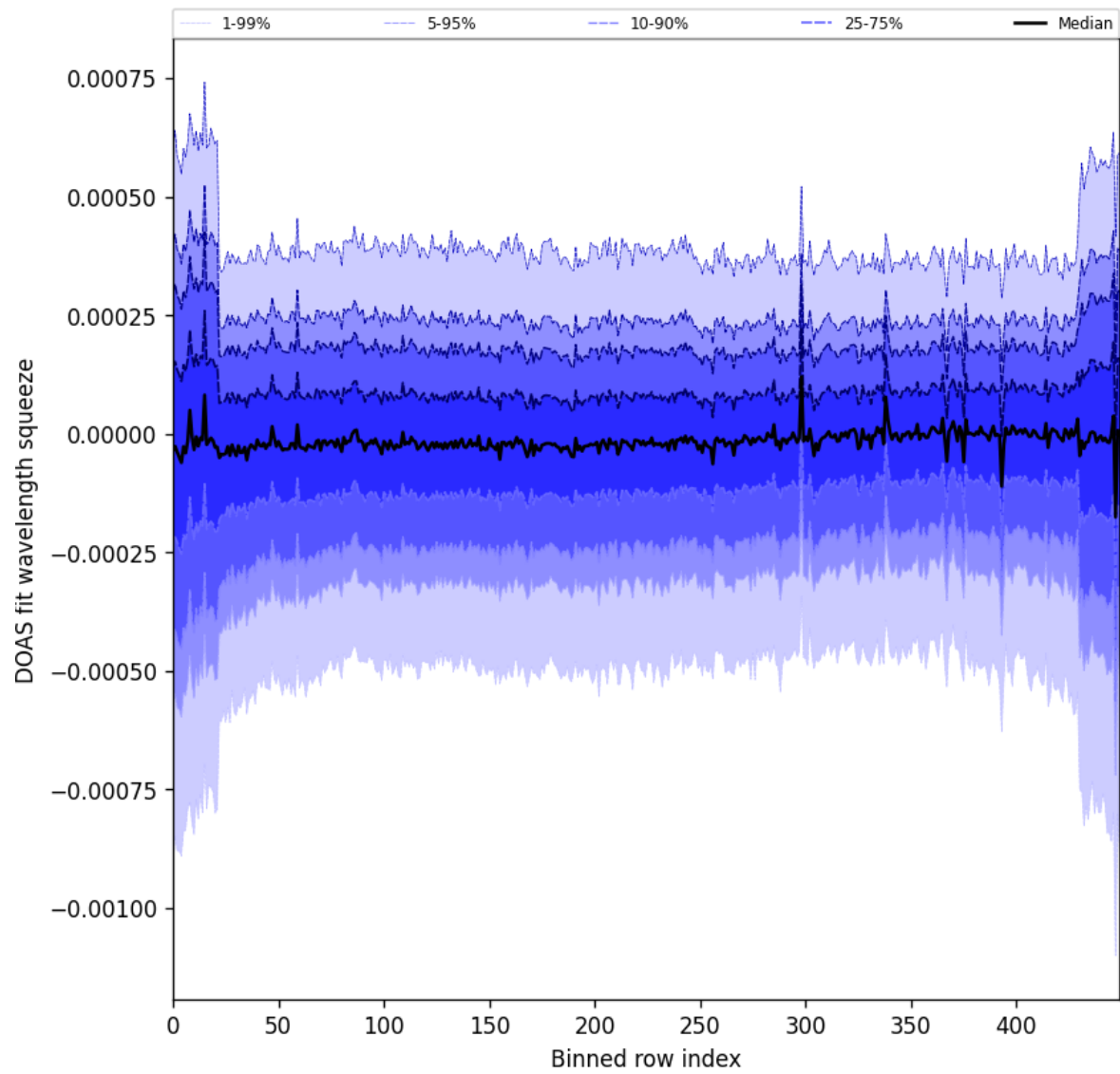
Figure 103: Along track statistics of “DOAS fit wavelength squeeze” for 2025-11-12 to 2025-11-13
