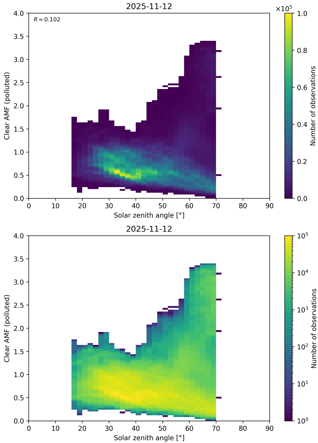
Figure 178: Scatter density plot of “Solar zenith angle” against “Clear AMF (polluted)” for 2025-11-12 to 2025-11-13.
