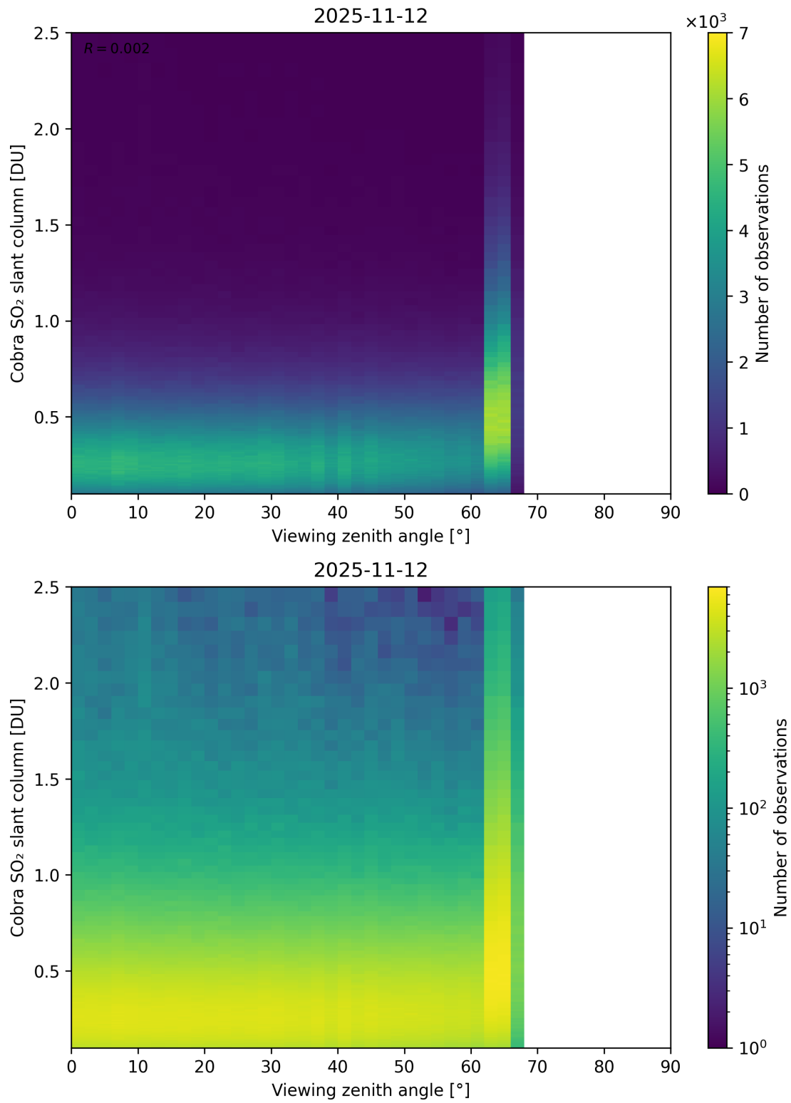
Figure 371: Scatter density plot of “Viewing zenith angle” against “Cobra SO 2 slant column” for 2025-11-12 to 2025-11-13.
