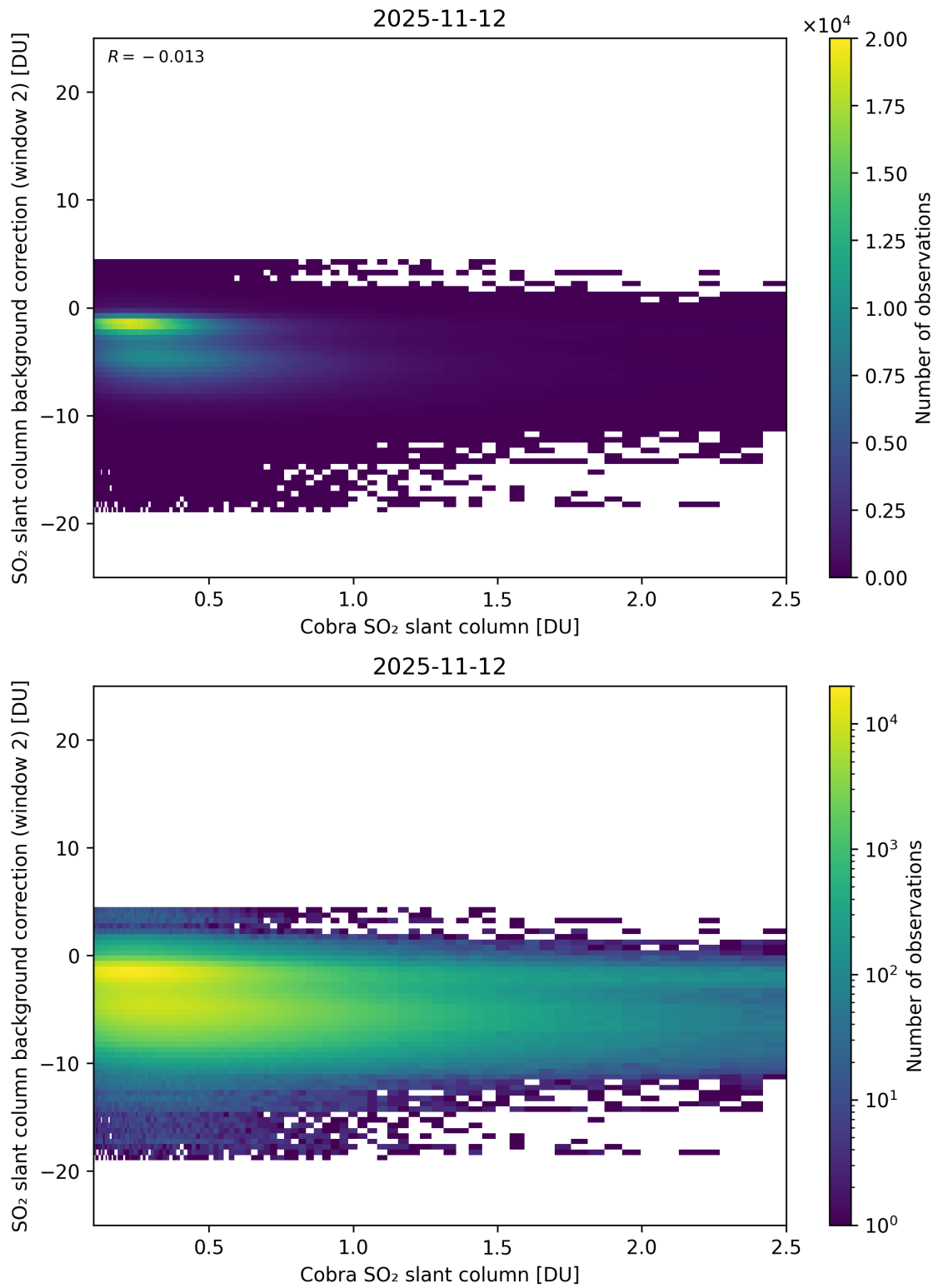
Figure 194: Scatter density plot of “Cobra SO 2 slant column” against “SO 2 slant column background correction (window 2)” for 2025-11-12 to 2025-11-13.
