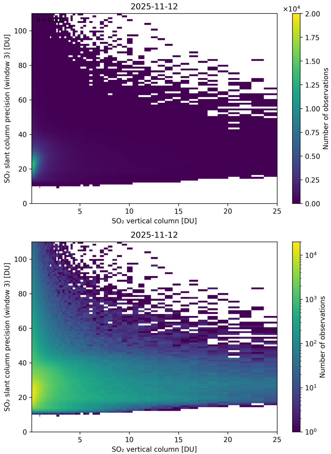
Figure 358: Scatter density plot of “SO 2 vertical column” against “SO 2 slant column precision (window 3)” for 2025-11-12 to 2025-11-13.
