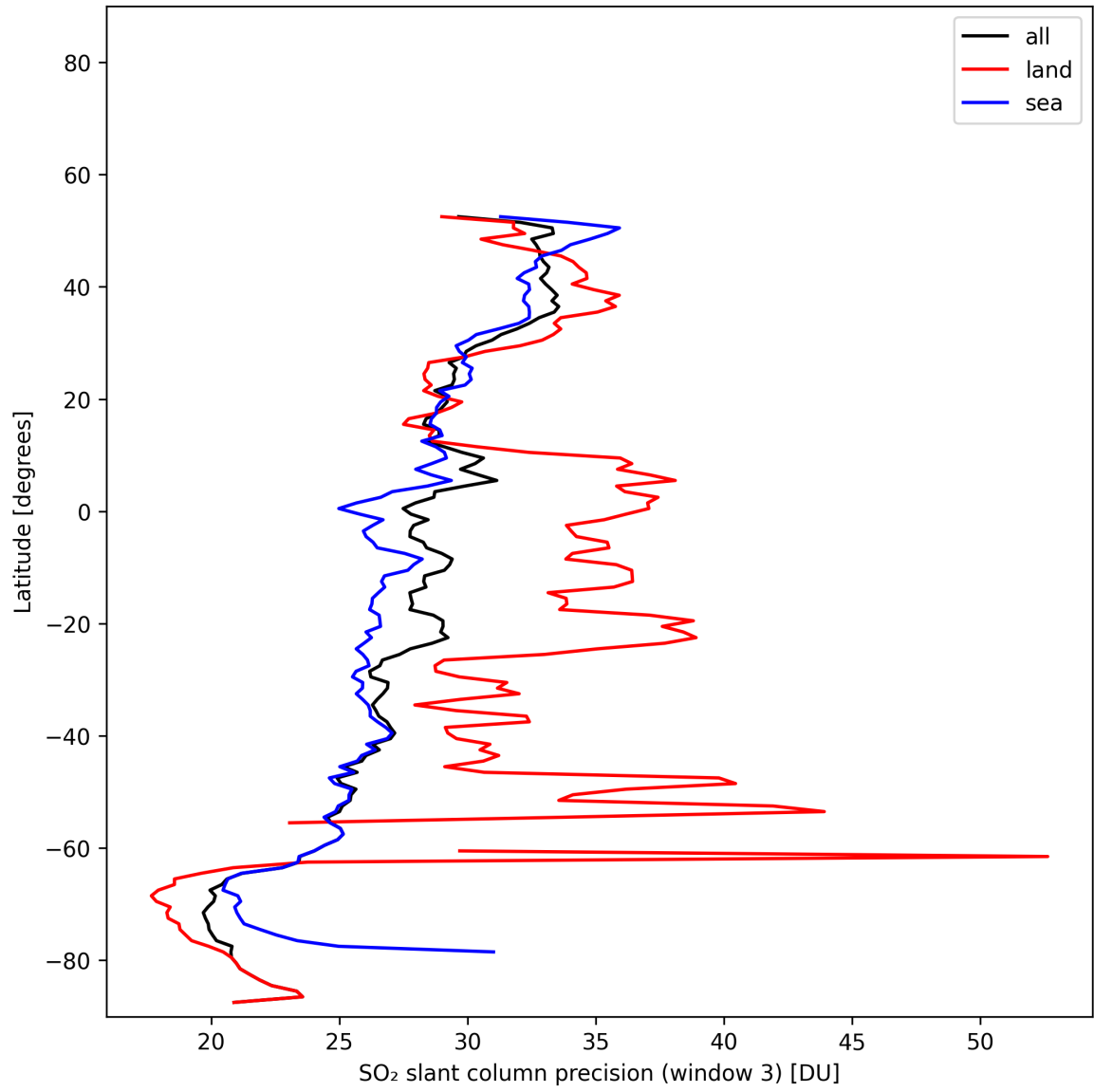
Figure 46: Zonal average of “SO 2 slant column precision (window 3)” for 2025-11-12 to 2025-11-13.
