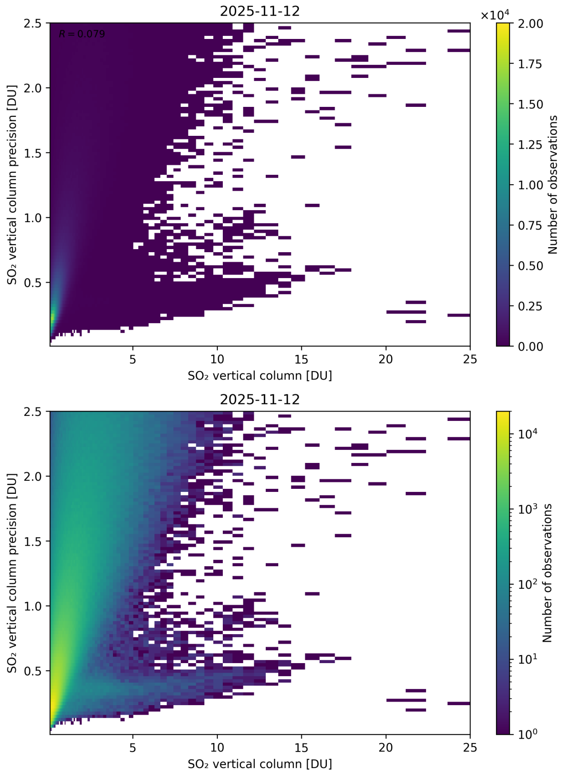
Figure 361: Scatter density plot of “SO 2 vertical column” against “SO 2 vertical column precision” for 2025-11-12 to 2025-11-13.
