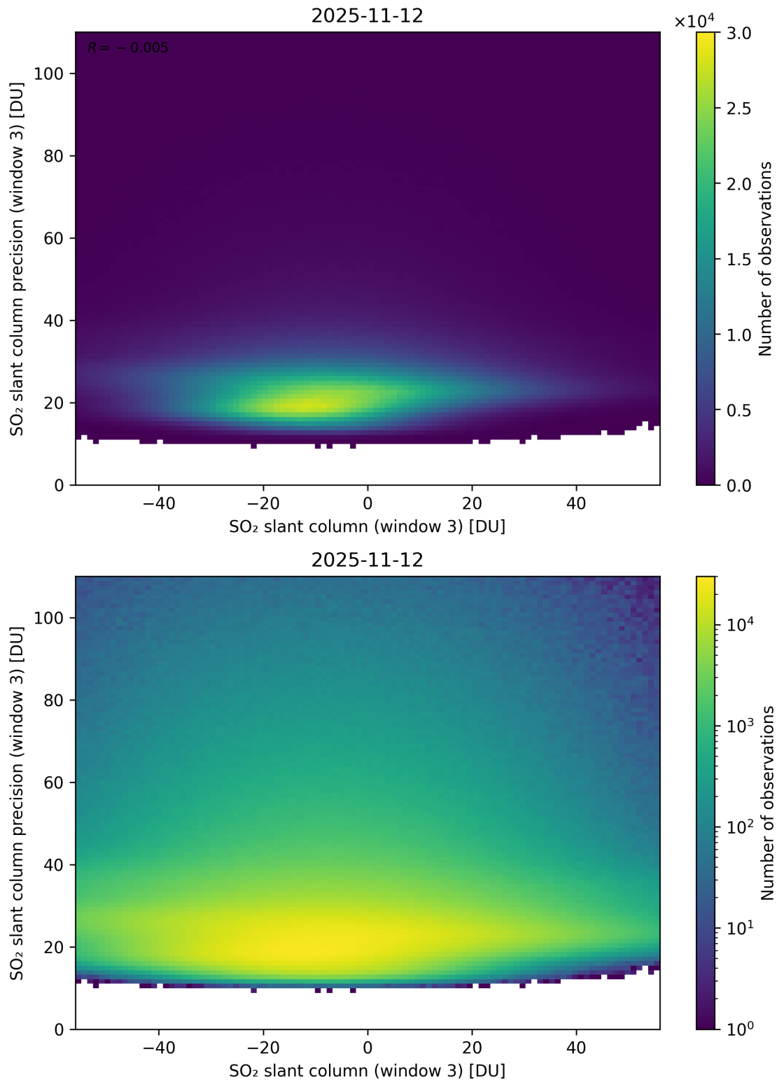
Figure 317: Scatter density plot of “SO 2 slant column (window 3)” against “SO 2 slant column precision (window 3)” for 2025-11-12 to 2025-11-13.
