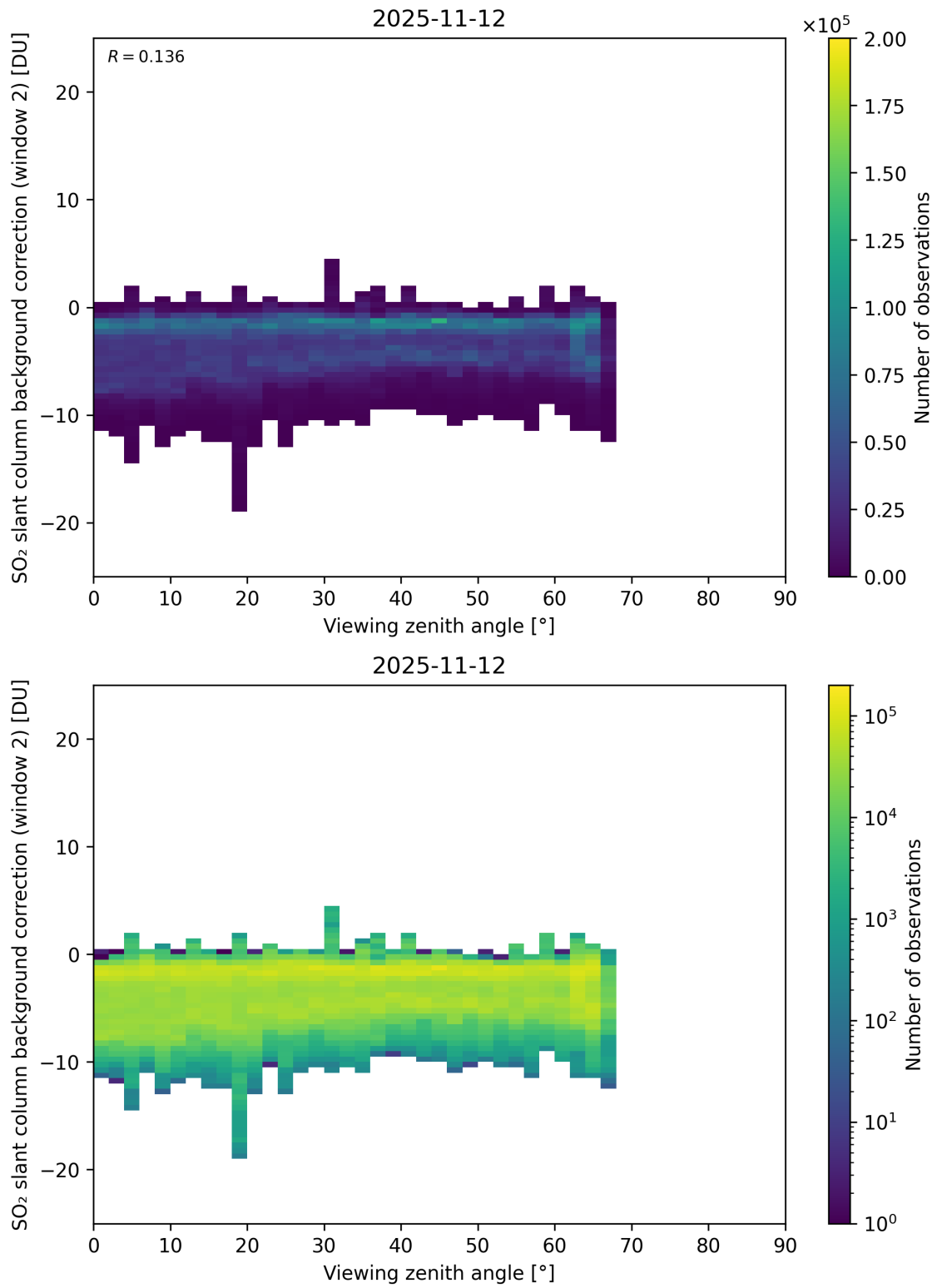
Figure 363: Scatter density plot of “Viewing zenith angle” against “SO 2 slant column background correction (window 2)” for 2025-11-12 to 2025-11-13.
