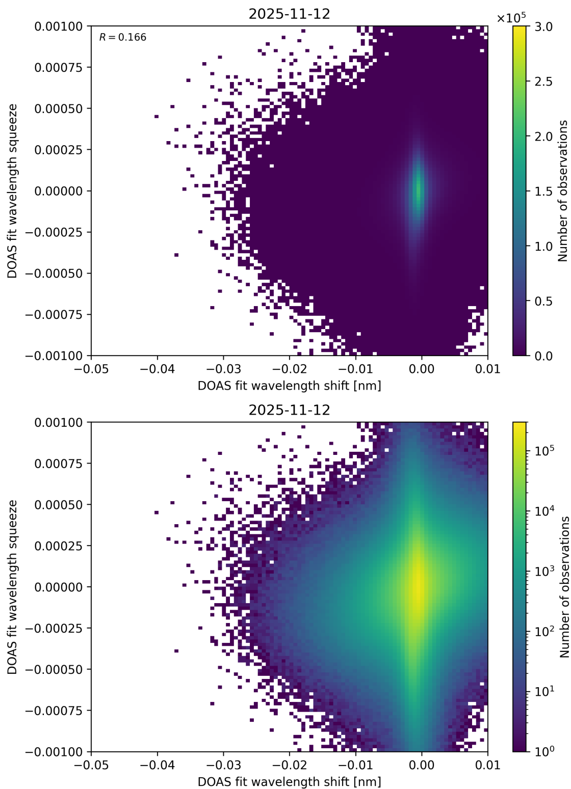
Figure 138: Scatter density plot of “DOAS fit wavelength shift” against “DOAS fit wavelength squeeze” for 2025-11-12 to 2025-11-13.
