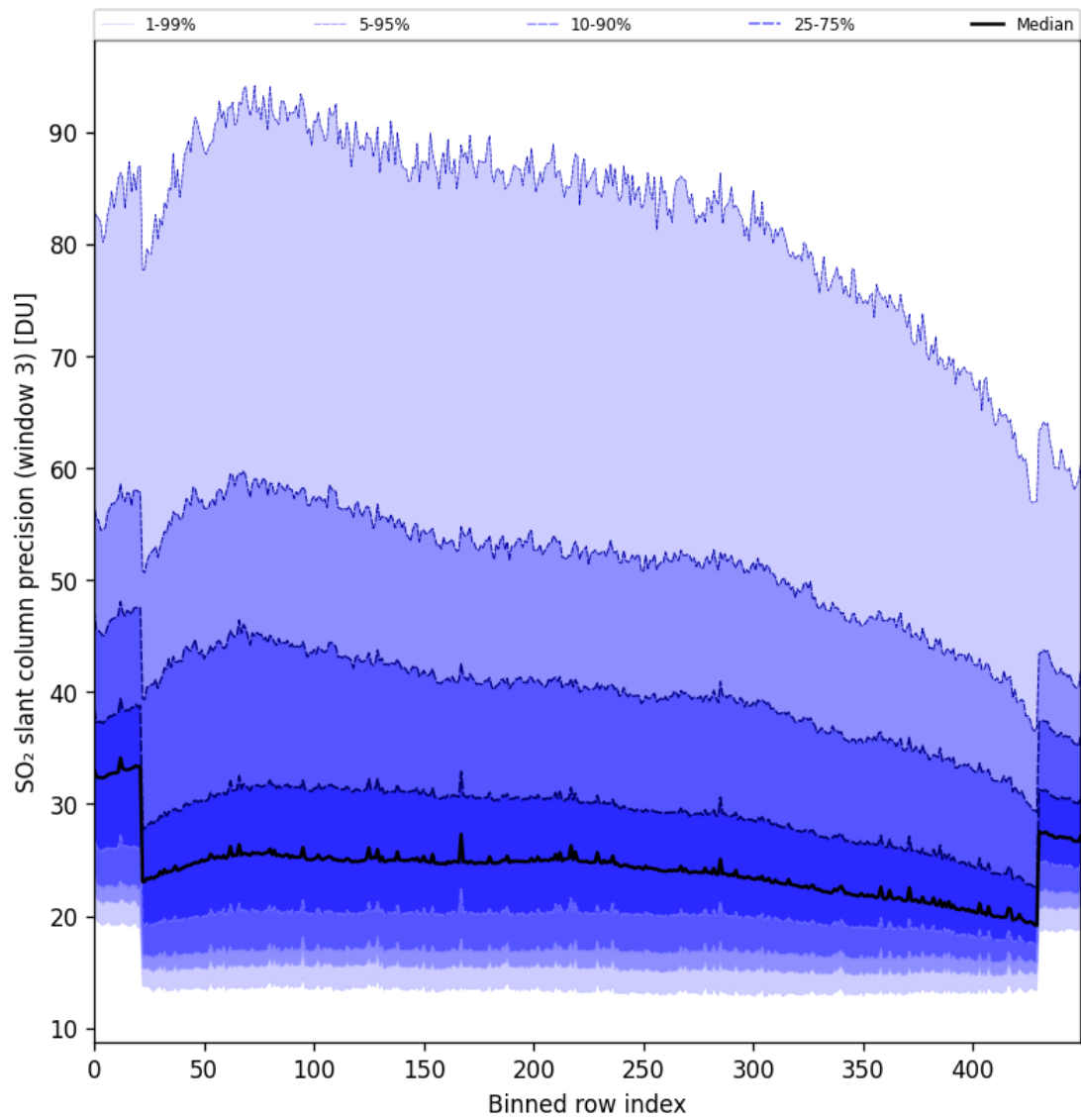
Figure 98: Along track statistics of “SO 2 slant column precision (window 3)” for 2025-11-12 to 2025-11-13
