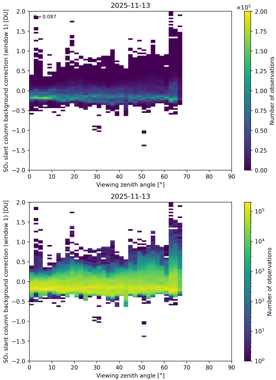
Figure 362: Scatter density plot of “Viewing zenith angle” against “SO 2 slant column background correction (window 1)” for 2025-11-12 to 2025-11-14.
