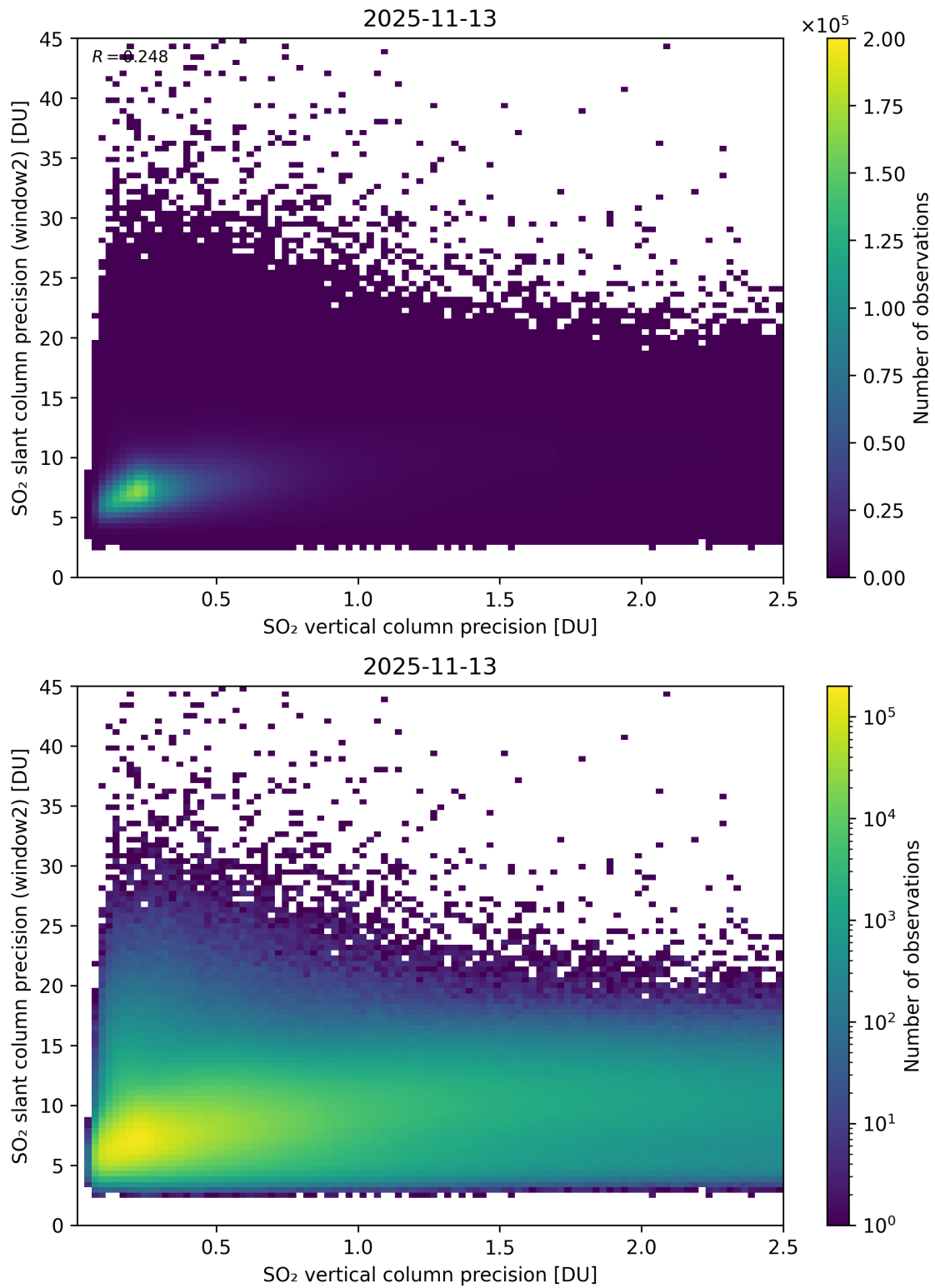
Figure 343: Scatter density plot of “SO 2 vertical column precision” against “SO 2 slant column precision (window2)” for 2025-11-12 to 2025-11-14.
