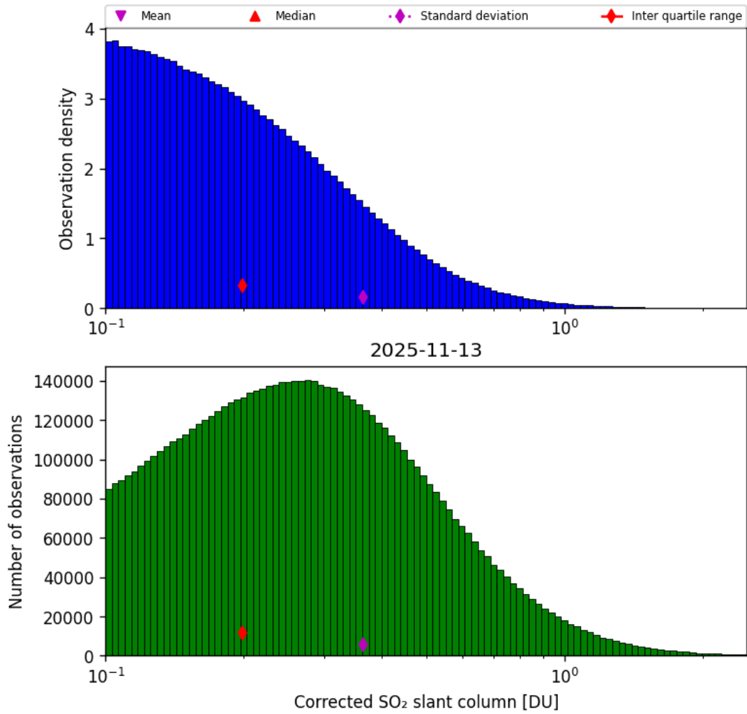
Figure 60: Histogram of “Corrected SO 2 slant column” for 2025-11-12 to 2025-11-14
