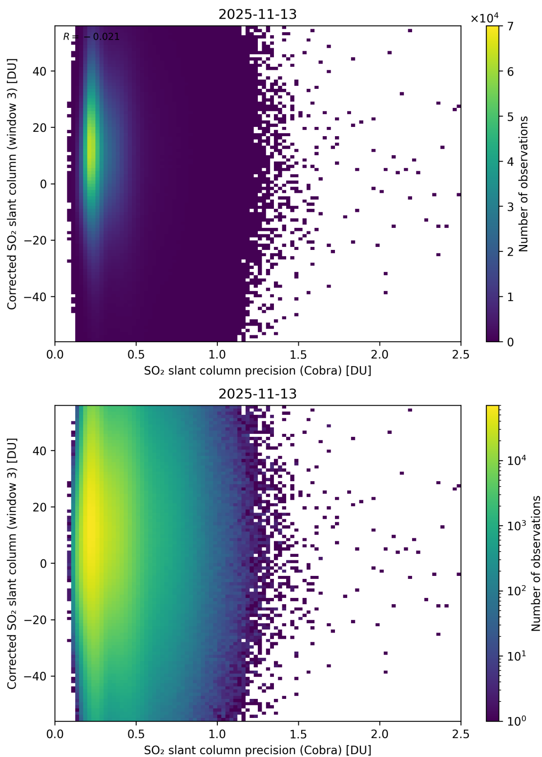
Figure 207: Scatter density plot of “SO 2 slant column precision (Cobra)” against “Corrected SO 2 slant column (window 3)” for 2025-11-12 to 2025-11-14.
