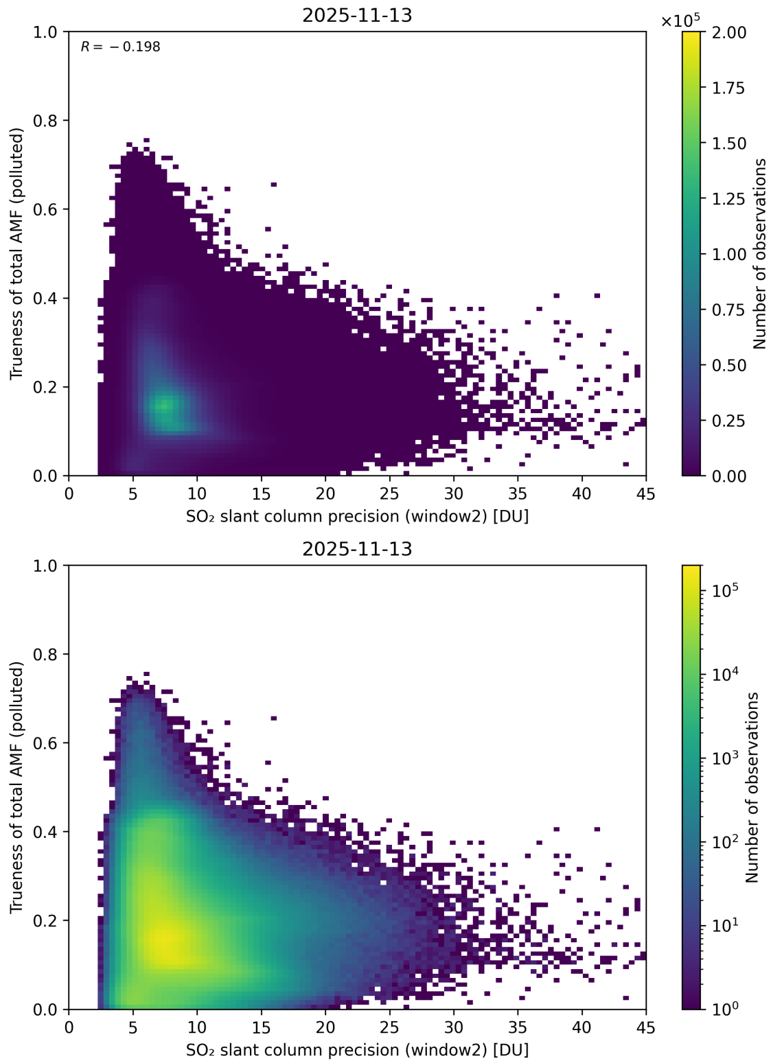
Figure 302: Scatter density plot of “SO 2 slant column precision (window2)” against “Trueness of total AMF (polluted)” for 2025-11-12 to 2025-11-14.
