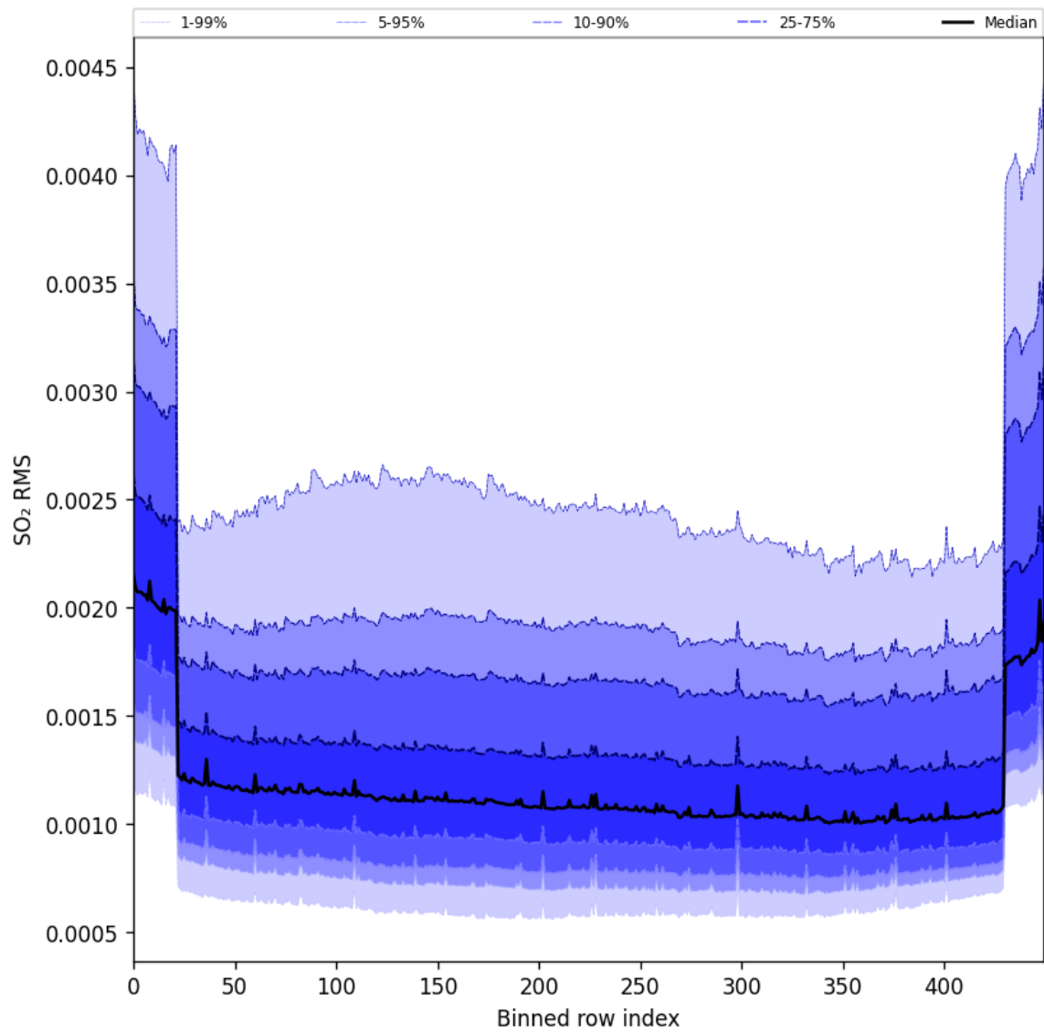
Figure 104: Along track statistics of “SO 2 RMS” for 2025-11-12 to 2025-11-14
