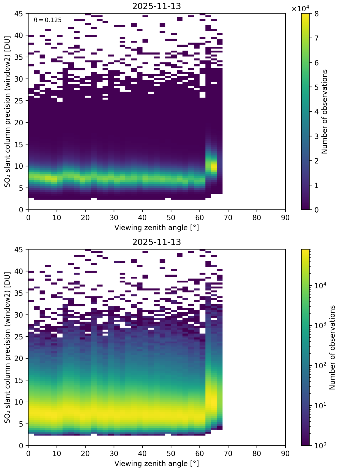
Figure 378: Scatter density plot of “Viewing zenith angle” against “SO 2 slant column precision (window2)” for 2025-11-12 to 2025-11-14.
