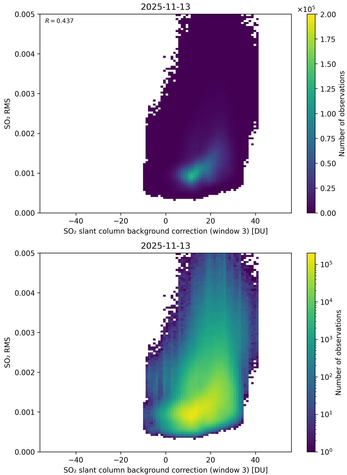
Figure 134: Scatter density plot of “SO 2 slant column background correction (window 3)” against “SO 2 RMS” for 2025-11-12 to 2025-11-14.
