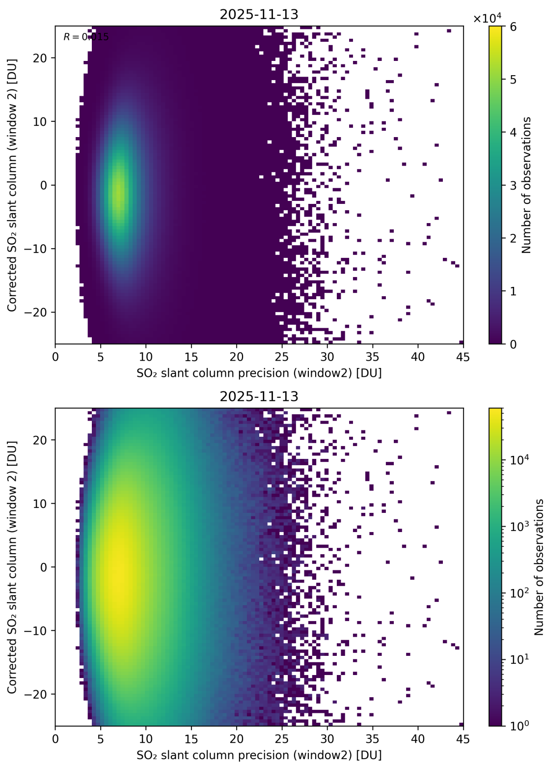
Figure 297: Scatter density plot of “SO 2 slant column precision (window2)” against “Corrected SO 2 slant column (window 2)” for 2025-11-12 to 2025-11-14.
