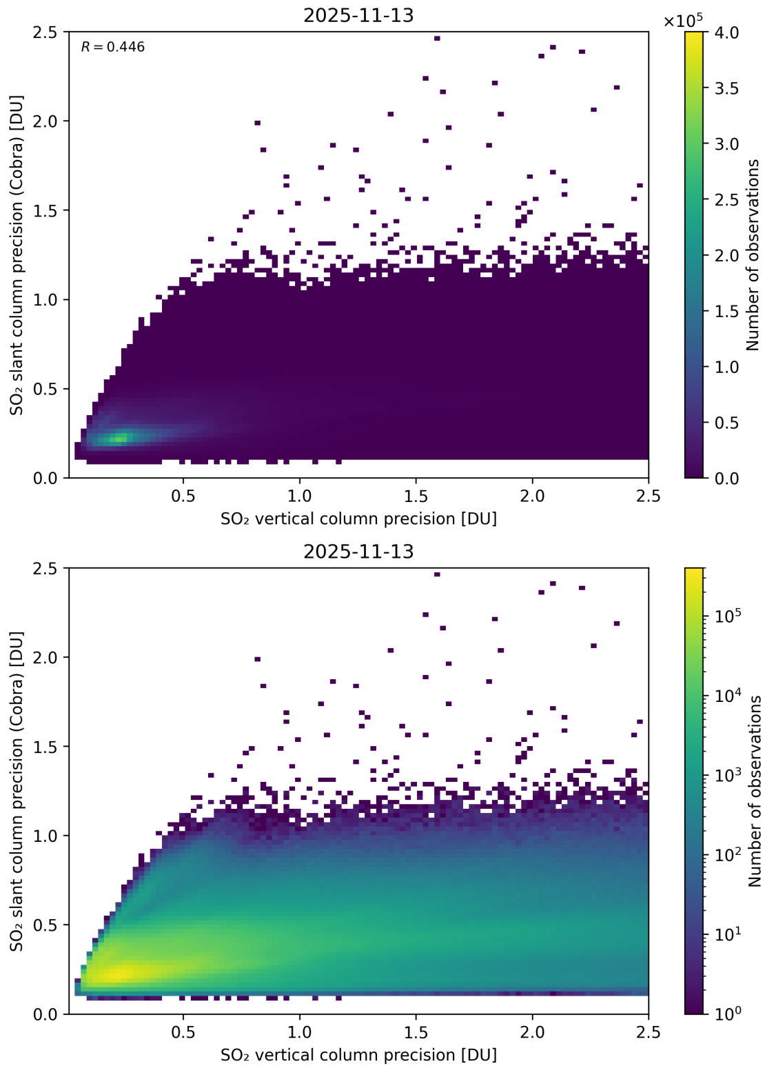
Figure 337: Scatter density plot of “SO 2 vertical column precision” against “SO 2 slant column precision (Cobra)” for 2025-11-12 to 2025-11-14.
