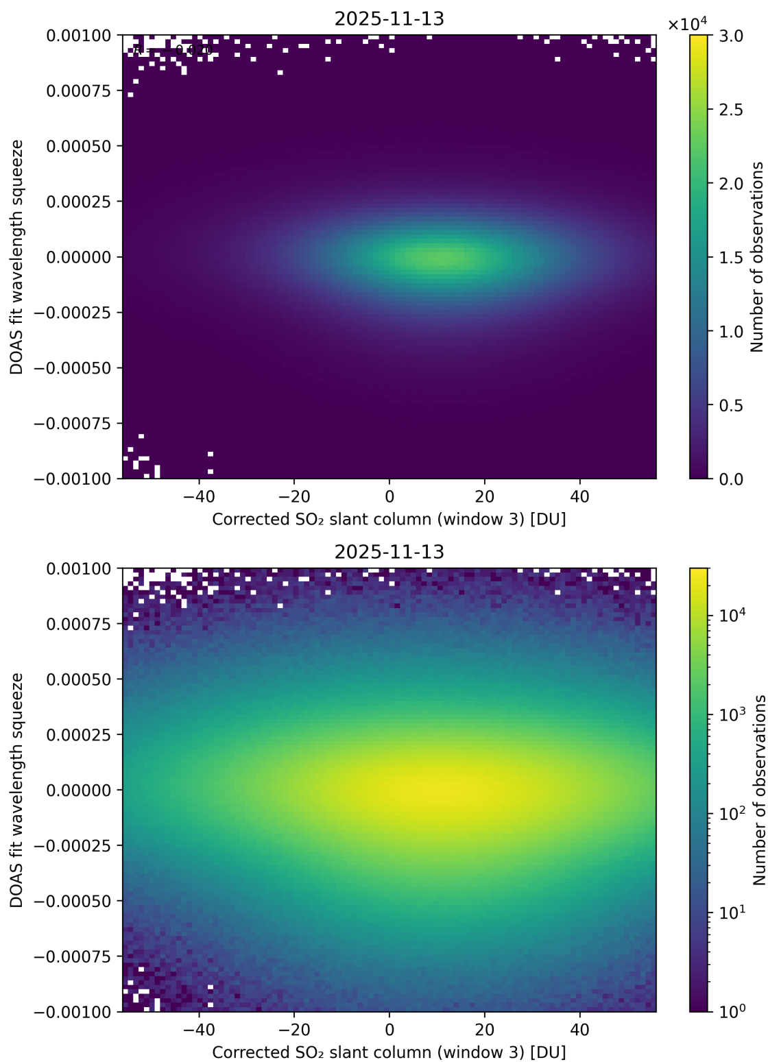
Figure 257: Scatter density plot of “Corrected SO 2 slant column (window 3)” against “DOAS fit wavelength squeeze” for 2025-11-12 to 2025-11-14.
