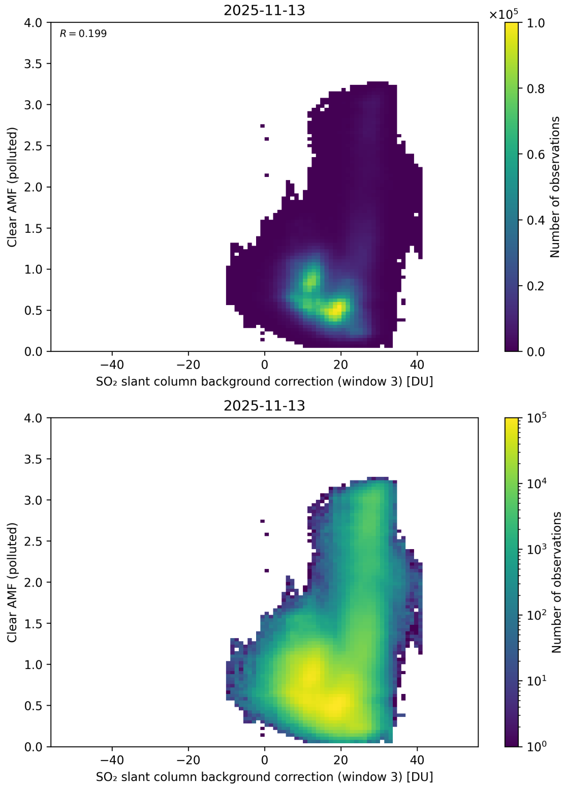
Figure 135: Scatter density plot of “SO 2 slant column background correction (window 3)” against “Clear AMF (polluted)” for 2025-11-12 to 2025-11-14.
