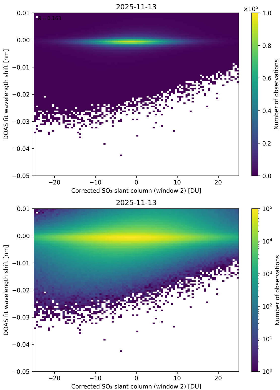
Figure 246: Scatter density plot of “Corrected SO 2 slant column (window 2)” against “DOAS fit wavelength shift” for 2025-11-12 to 2025-11-14.
