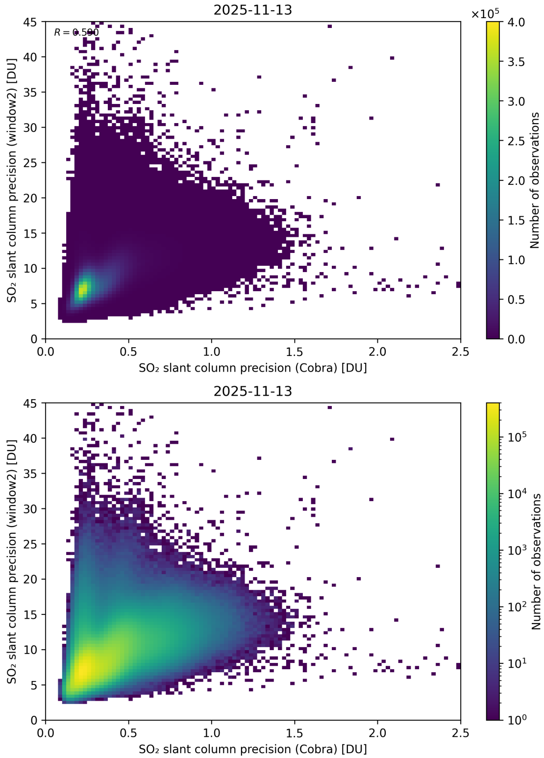
Figure 210: Scatter density plot of “SO 2 slant column precision (Cobra)” against “SO 2 slant column precision (window2)” for 2025-11-12 to 2025-11-14.
