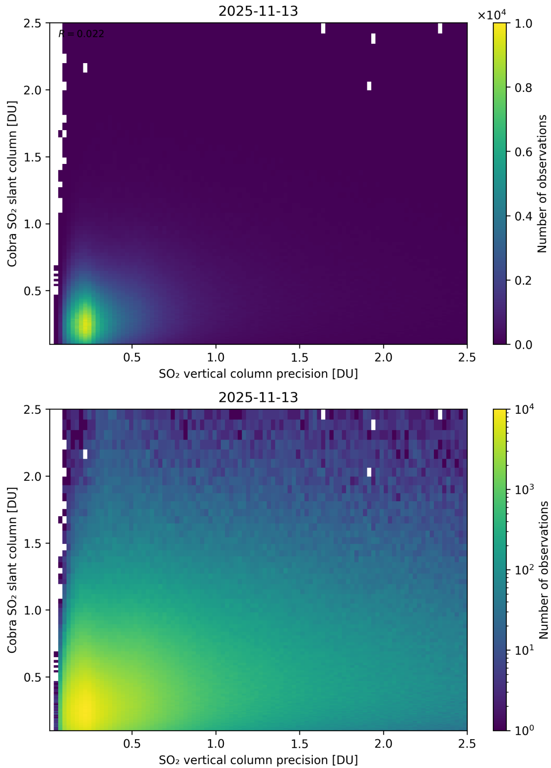
Figure 336: Scatter density plot of “SO 2 vertical column precision” against “Cobra SO 2 slant column” for 2025-11-12 to 2025-11-14.
