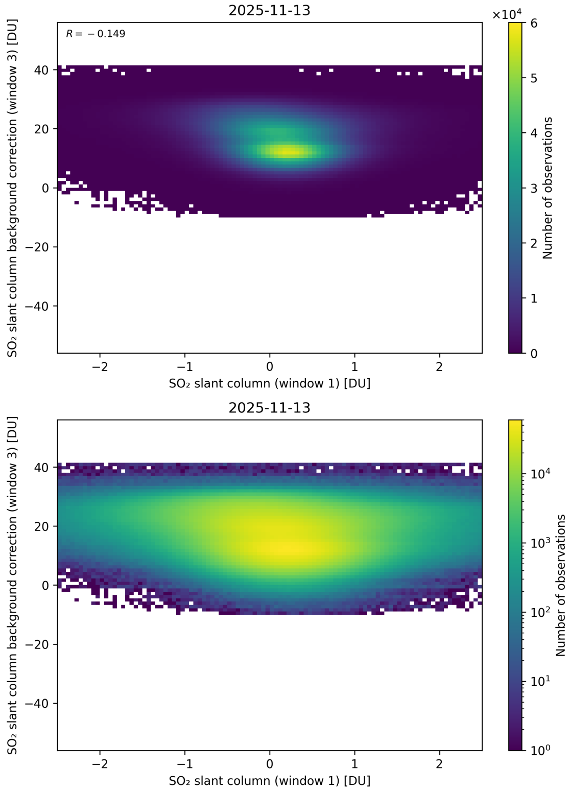
Figure 264: Scatter density plot of “SO 2 slant column (window 1)” against “SO 2 slant column background correction (window 3)” for 2025-11-12 to 2025-11-14.
