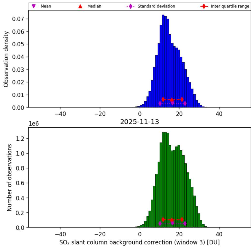
Figure 74: Histogram of “SO 2 slant column background correction (window 3)” for 2025-11-12 to 2025-11-14
