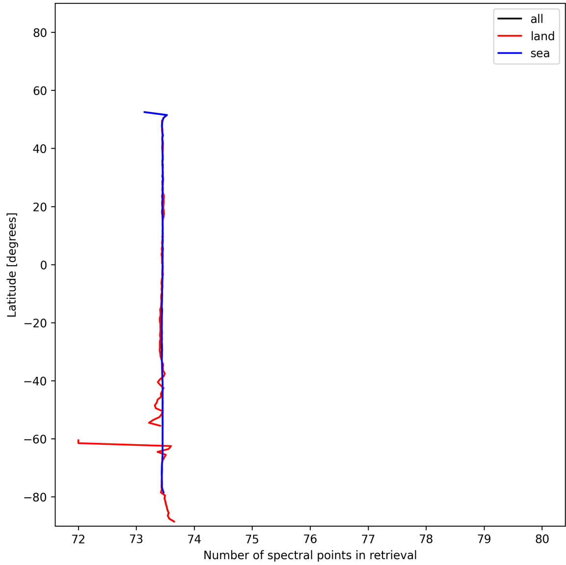
Figure 56: Zonal average of “Number of spectral points in retrieval” for 2025-11-12 to 2025-11-14.
