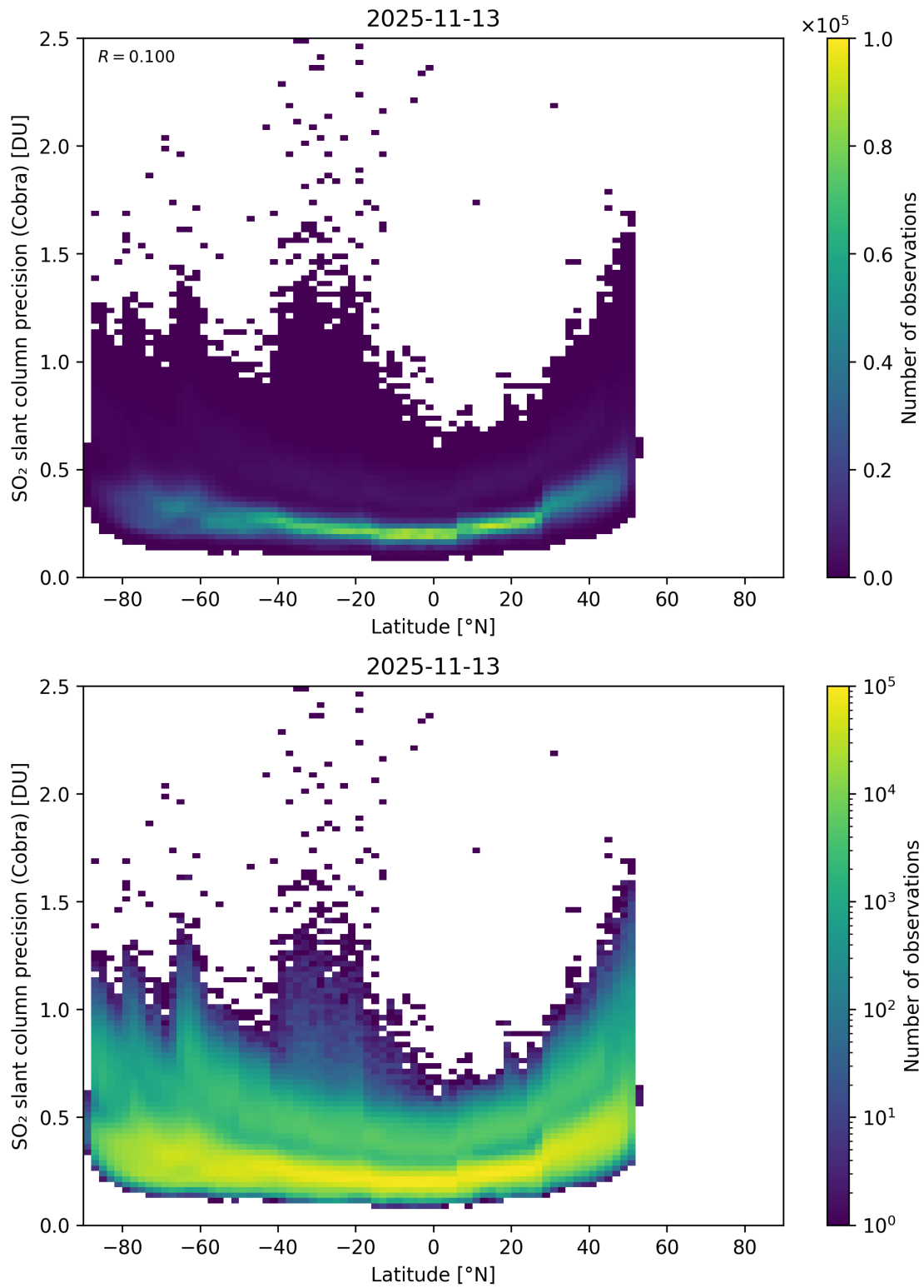
Figure 158: Scatter density plot of “Latitude” against “SO 2 slant column precision (Cobra)” for 2025-11-12 to 2025-11-14.
