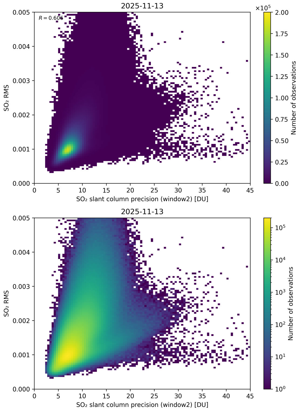
Figure 295: Scatter density plot of “SO 2 slant column precision (window2)” against “SO 2 RMS” for 2025-11-12 to 2025-11-14.
