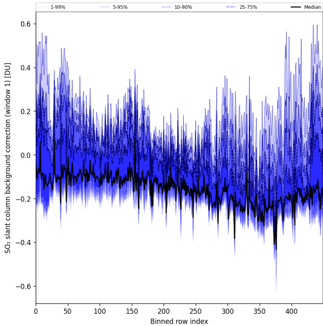
Figure 92: Along track statistics of “SO 2 slant column background correction (window 1)” for 2025-11-12 to 2025-11-14
