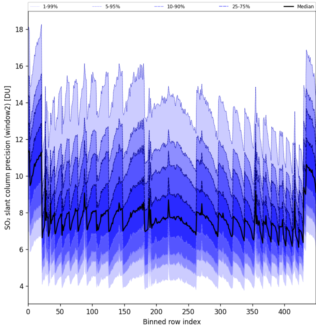
Figure 94: Along track statistics of “SO 2 slant column precision (window2)” for 2025-11-12 to 2025-11-14
