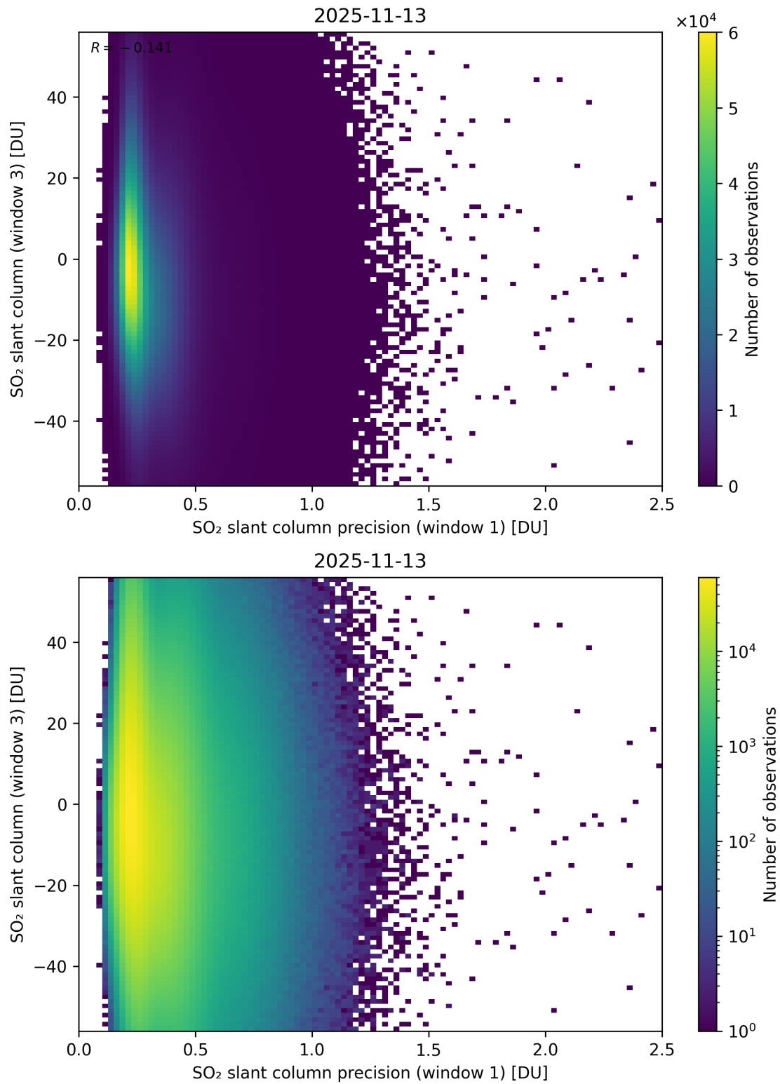
Figure 278: Scatter density plot of “SO 2 slant column precision (window 1)” against “SO 2 slant column (window 3)” for 2025-11-12 to 2025-11-14.
