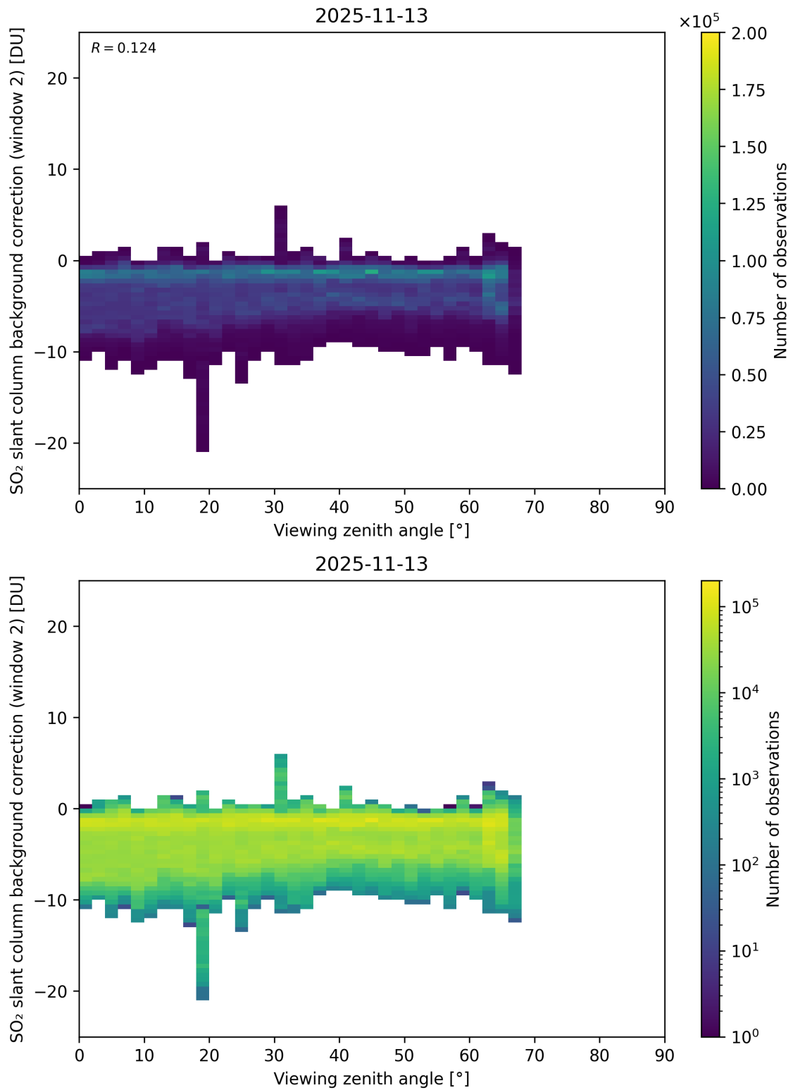
Figure 363: Scatter density plot of “Viewing zenith angle” against “SO 2 slant column background correction (window 2)” for 2025-11-12 to 2025-11-14.
