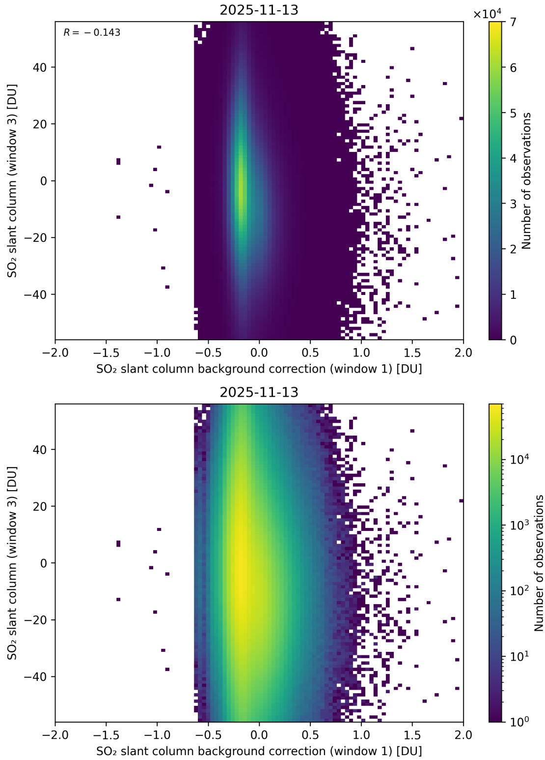
Figure 118: Scatter density plot of “SO 2 slant column background correction (window 1)” against “SO 2 slant column (window 3)” for 2025-11-12 to 2025-11-14.
