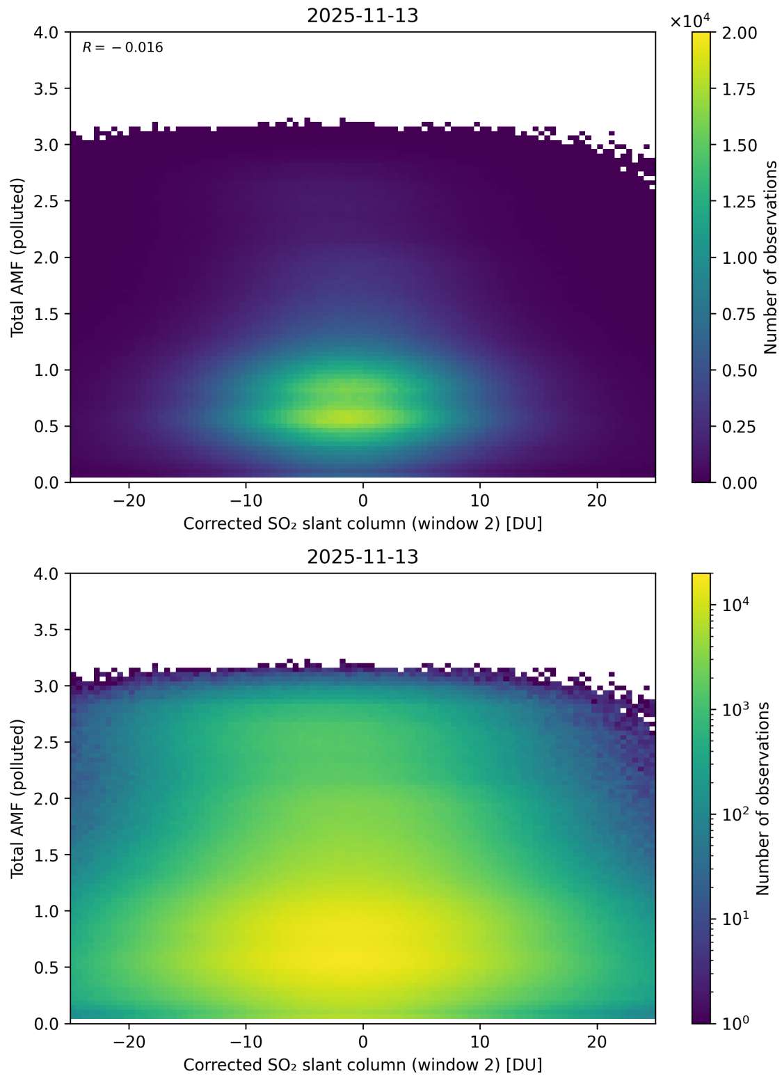
Figure 253: Scatter density plot of “Corrected SO 2 slant column (window 2)” against “Total AMF (polluted)” for 2025-11-12 to 2025-11-14.
