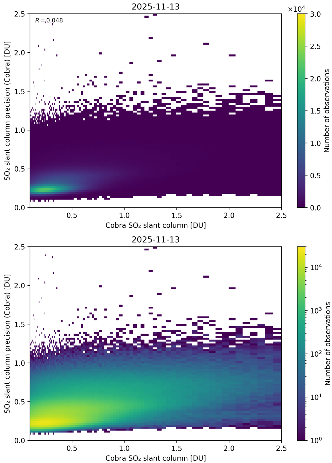
Figure 216: Scatter density plot of “Cobra SO 2 slant column” against “SO 2 slant column precision (Cobra)” for 2025-11-12 to 2025-11-14.
