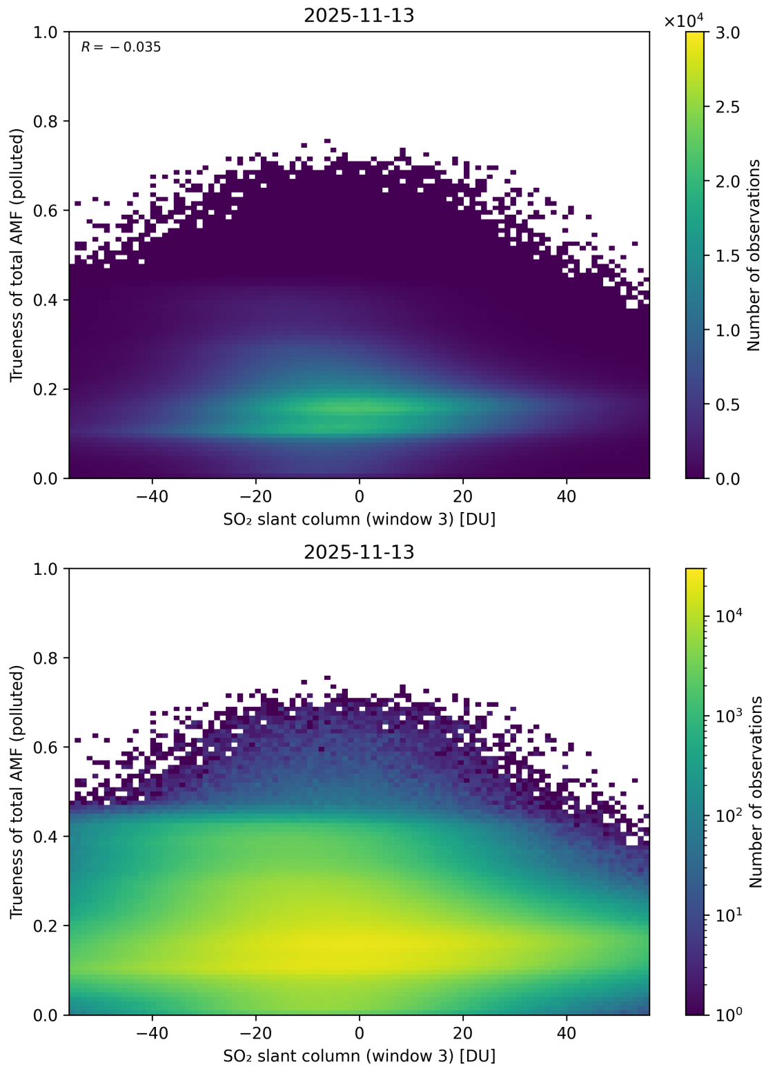
Figure 319: Scatter density plot of “SO 2 slant column (window 3)” against “Trueness of total AMF (polluted)” for 2025-11-12 to 2025-11-14.
