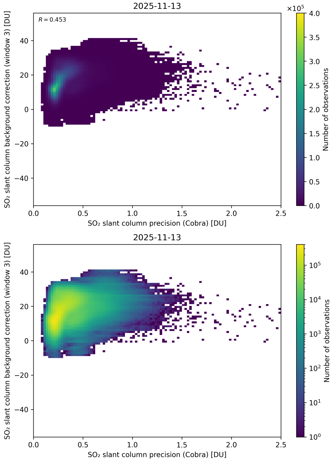
Figure 201: Scatter density plot of “SO 2 slant column precision (Cobra)” against “SO 2 slant column background correction (window 3)” for 2025-11-12 to 2025-11-14.
