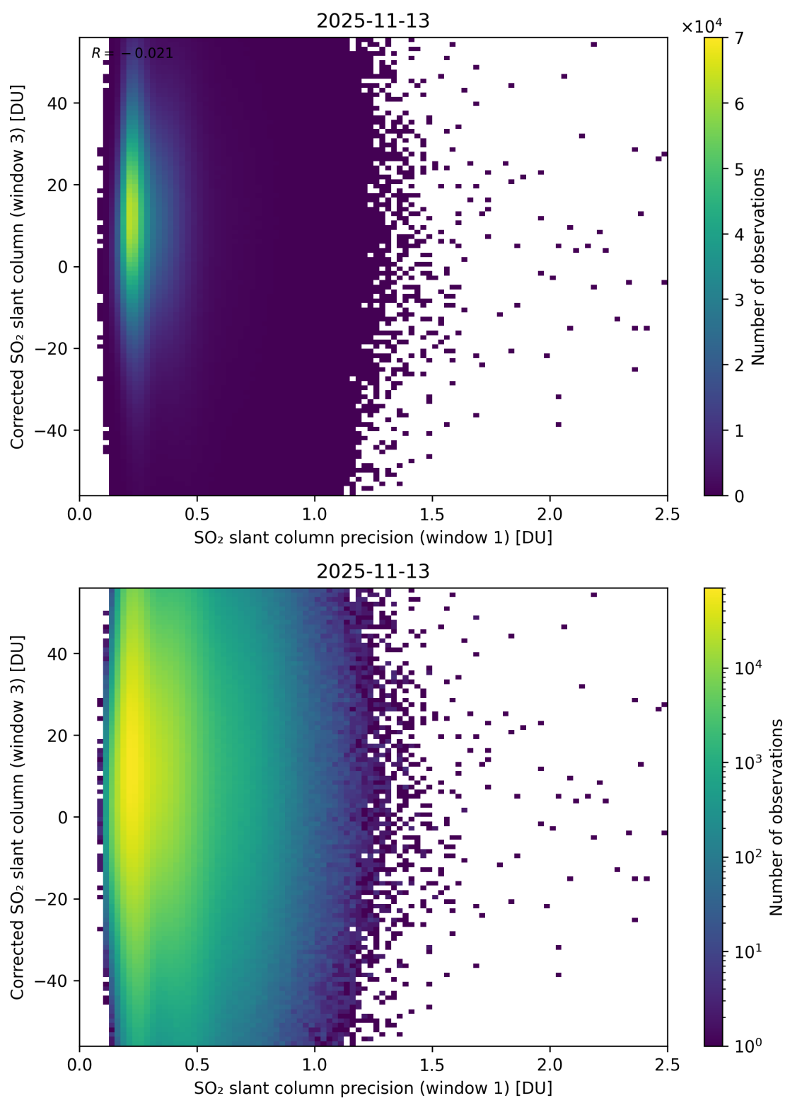
Figure 276: Scatter density plot of “SO 2 slant column precision (window 1)” against “Corrected SO 2 slant column (window 3)” for 2025-11-12 to 2025-11-14.
