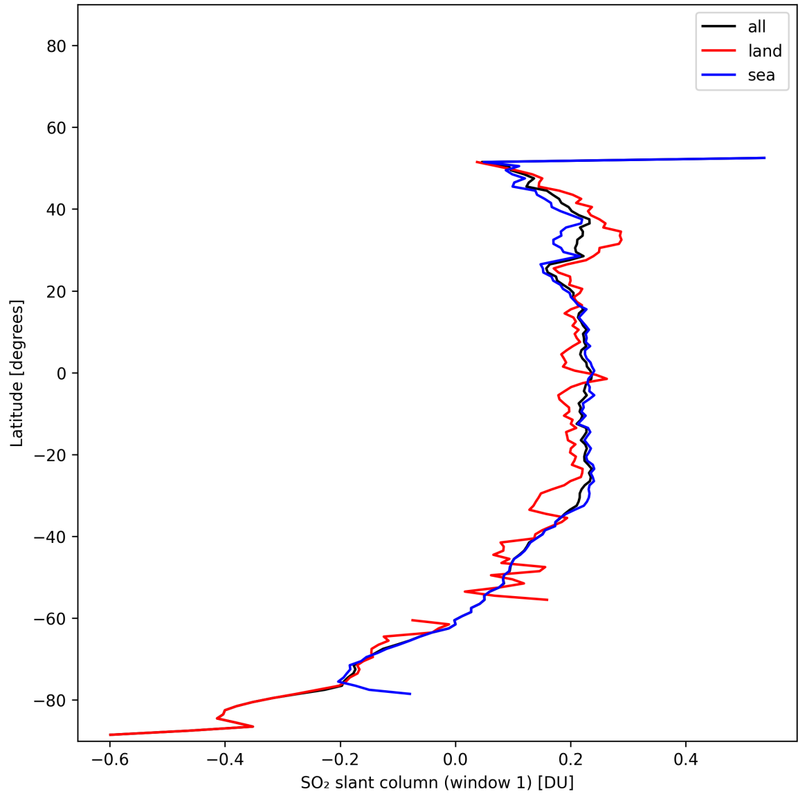
Figure 37: Zonal average of “SO 2 slant column (window 1)” for 2025-11-12 to 2025-11-14.
