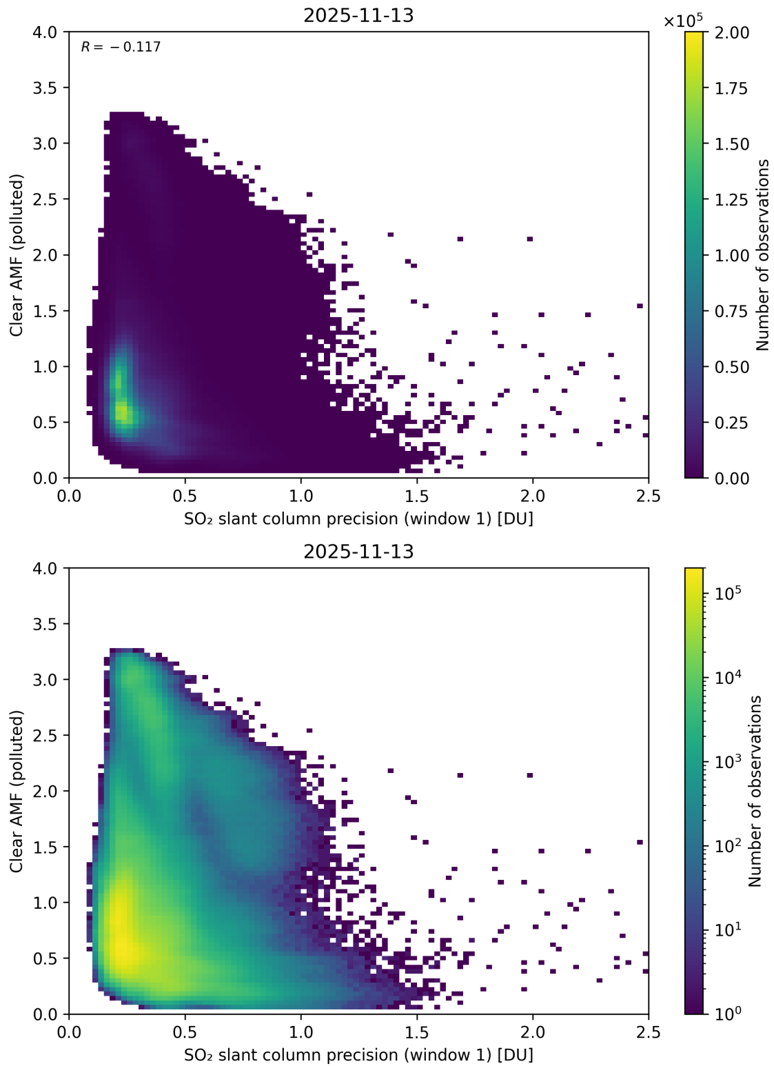
Figure 274: Scatter density plot of “SO 2 slant column precision (window 1)” against “Clear AMF (polluted)” for 2025-11-12 to 2025-11-14.
