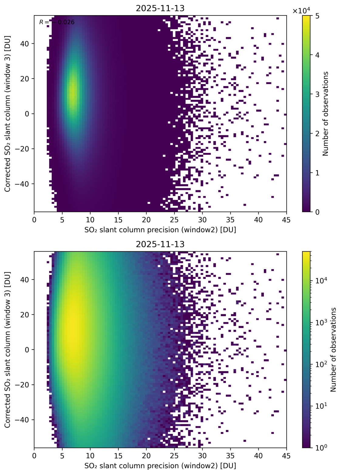
Figure 298: Scatter density plot of “SO 2 slant column precision (window2)” against “Corrected SO 2 slant column (window 3)” for 2025-11-12 to 2025-11-14.
