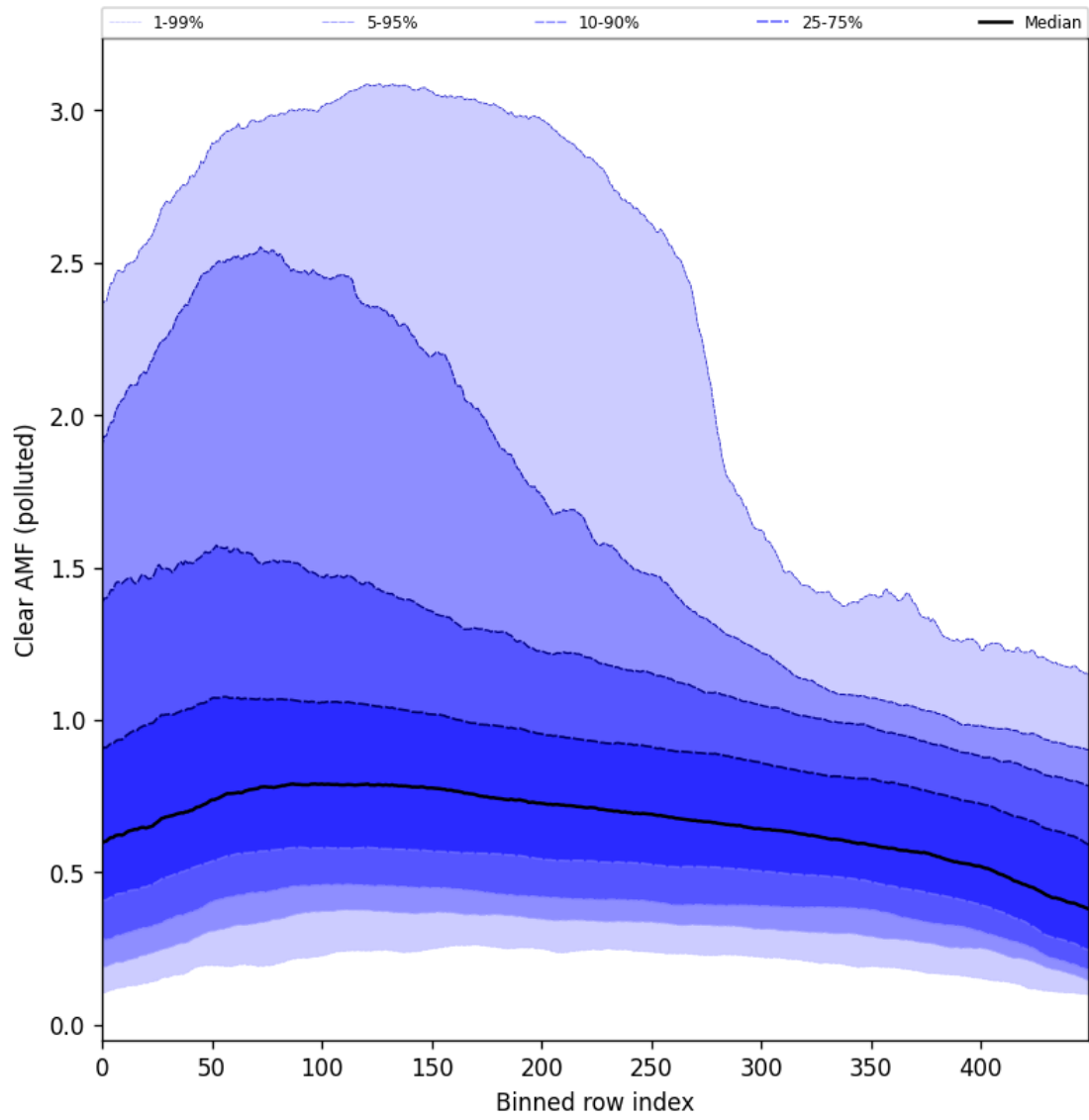
Figure 107: Along track statistics of “Clear AMF (polluted)” for 2025-11-12 to 2025-11-14
