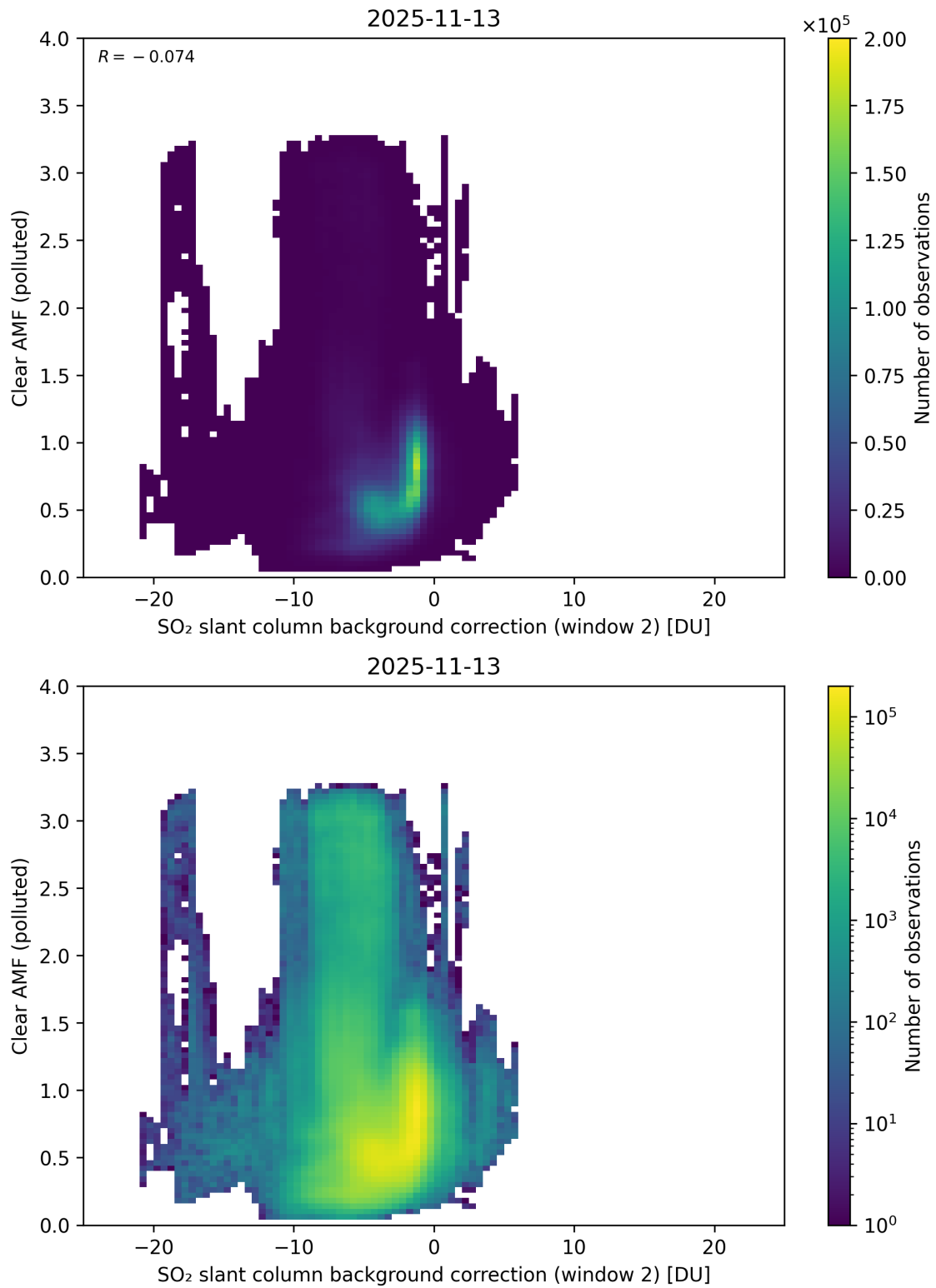
Figure 126: Scatter density plot of “SO 2 slant column background correction (window 2)” against “Clear AMF (polluted)” for 2025-11-12 to 2025-11-14.
