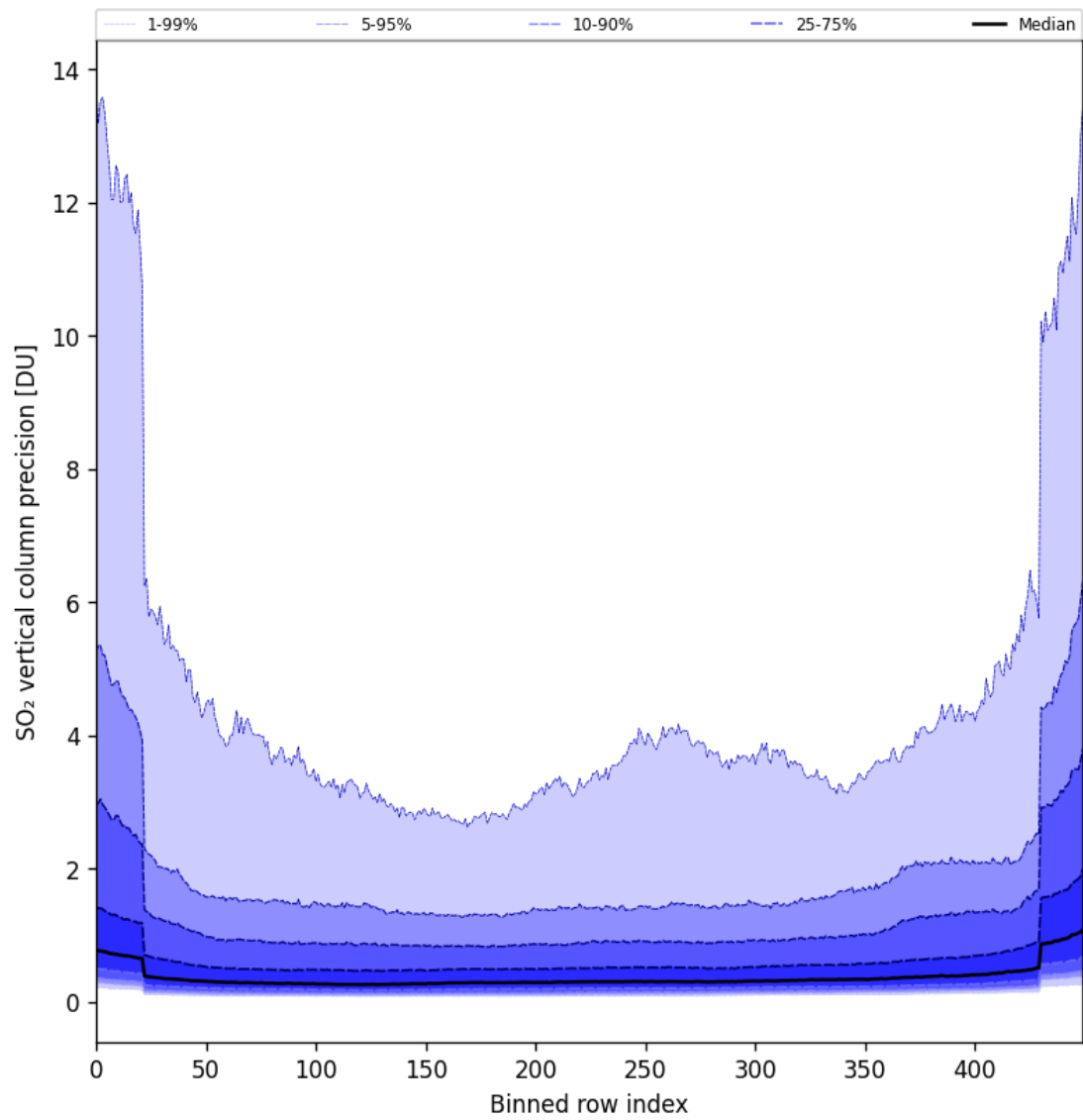
Figure 85: Along track statistics of “SO 2 vertical column precision” for 2025-11-12 to 2025-11-14
