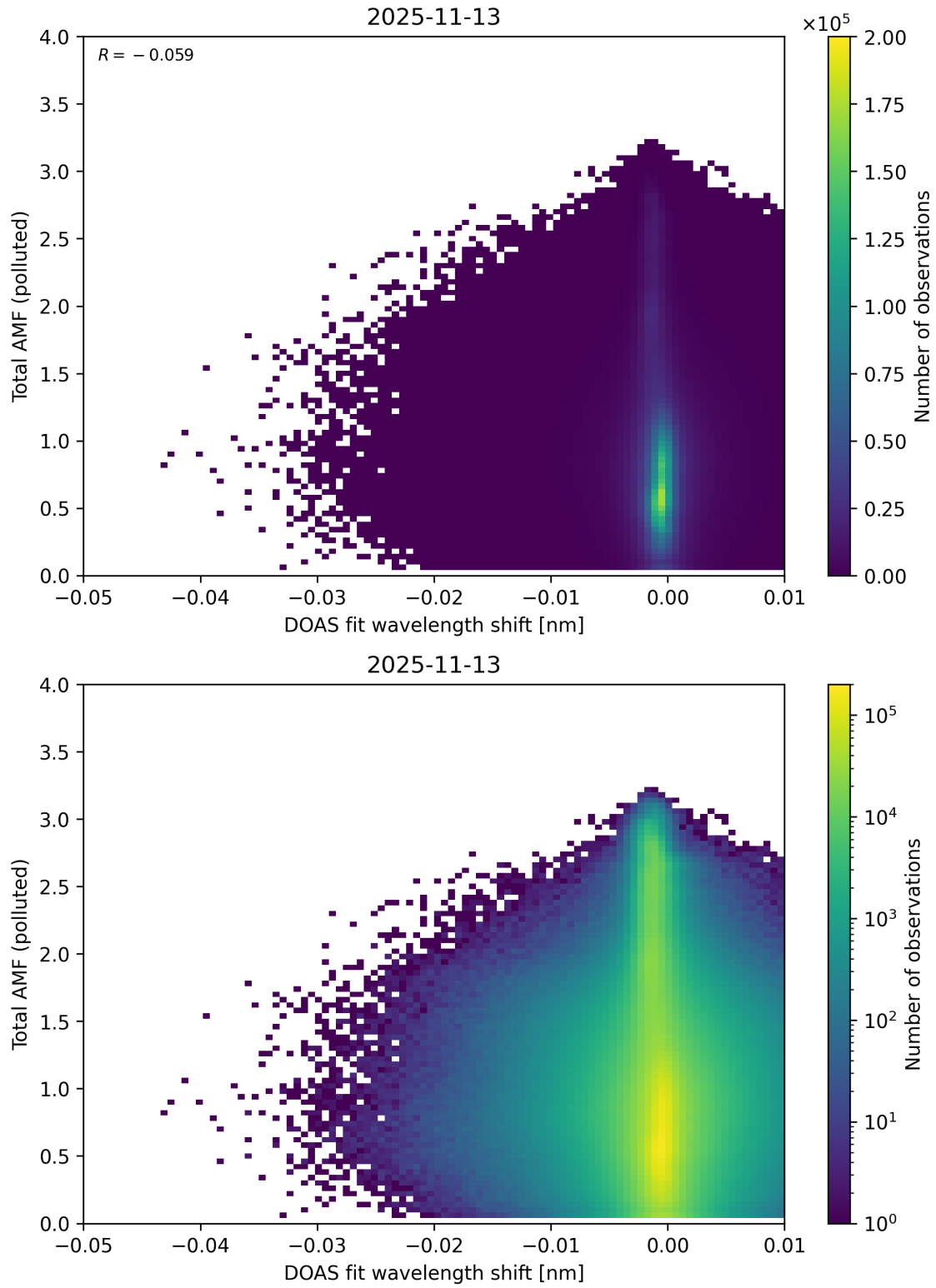
Figure 141: Scatter density plot of “DOAS fit wavelength shift” against “Total AMF (polluted)” for 2025-11-12 to 2025-11-14.
