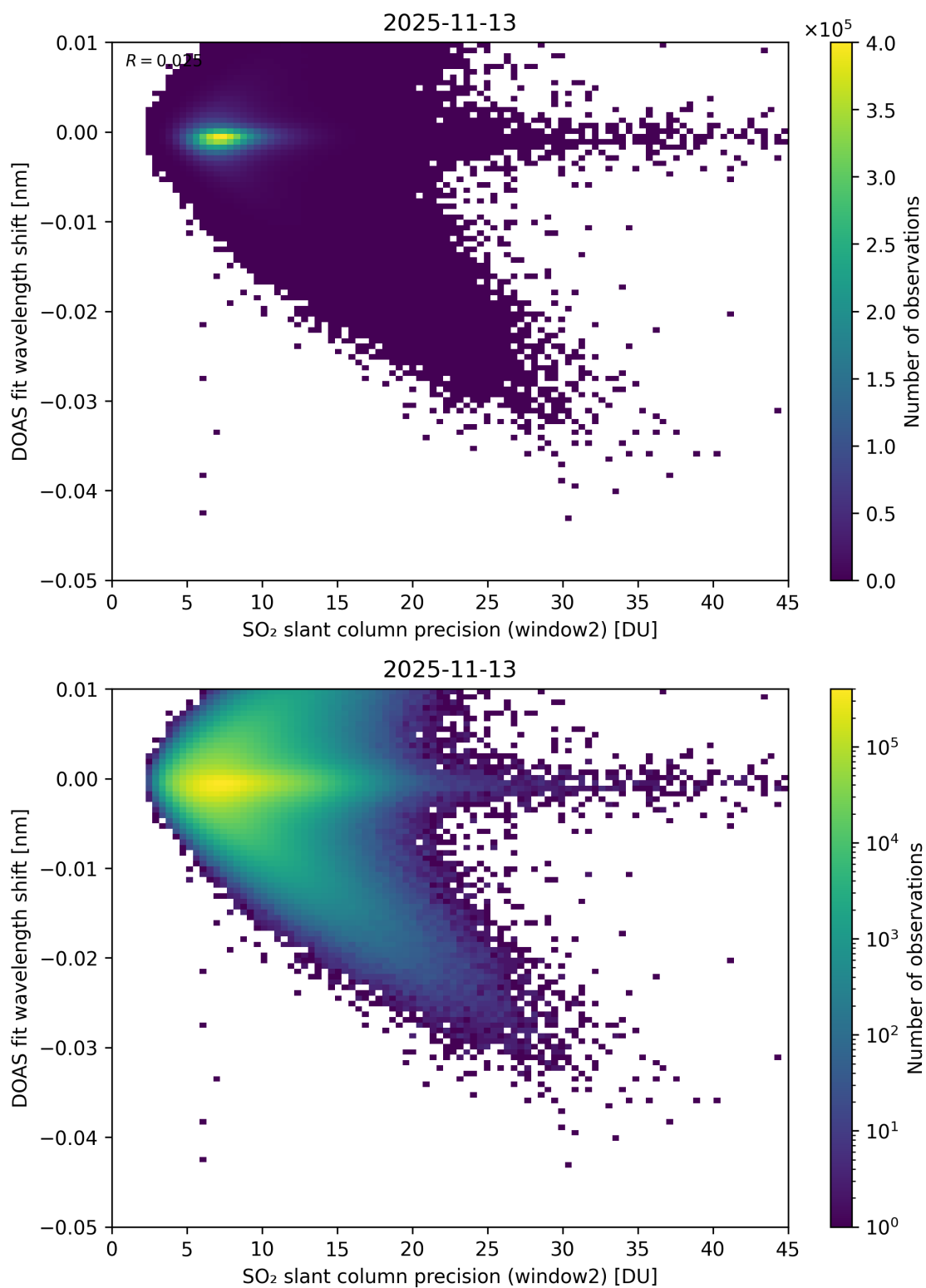
Figure 293: Scatter density plot of “SO 2 slant column precision (window2)” against “DOAS fit wavelength shift” for 2025-11-12 to 2025-11-14.
