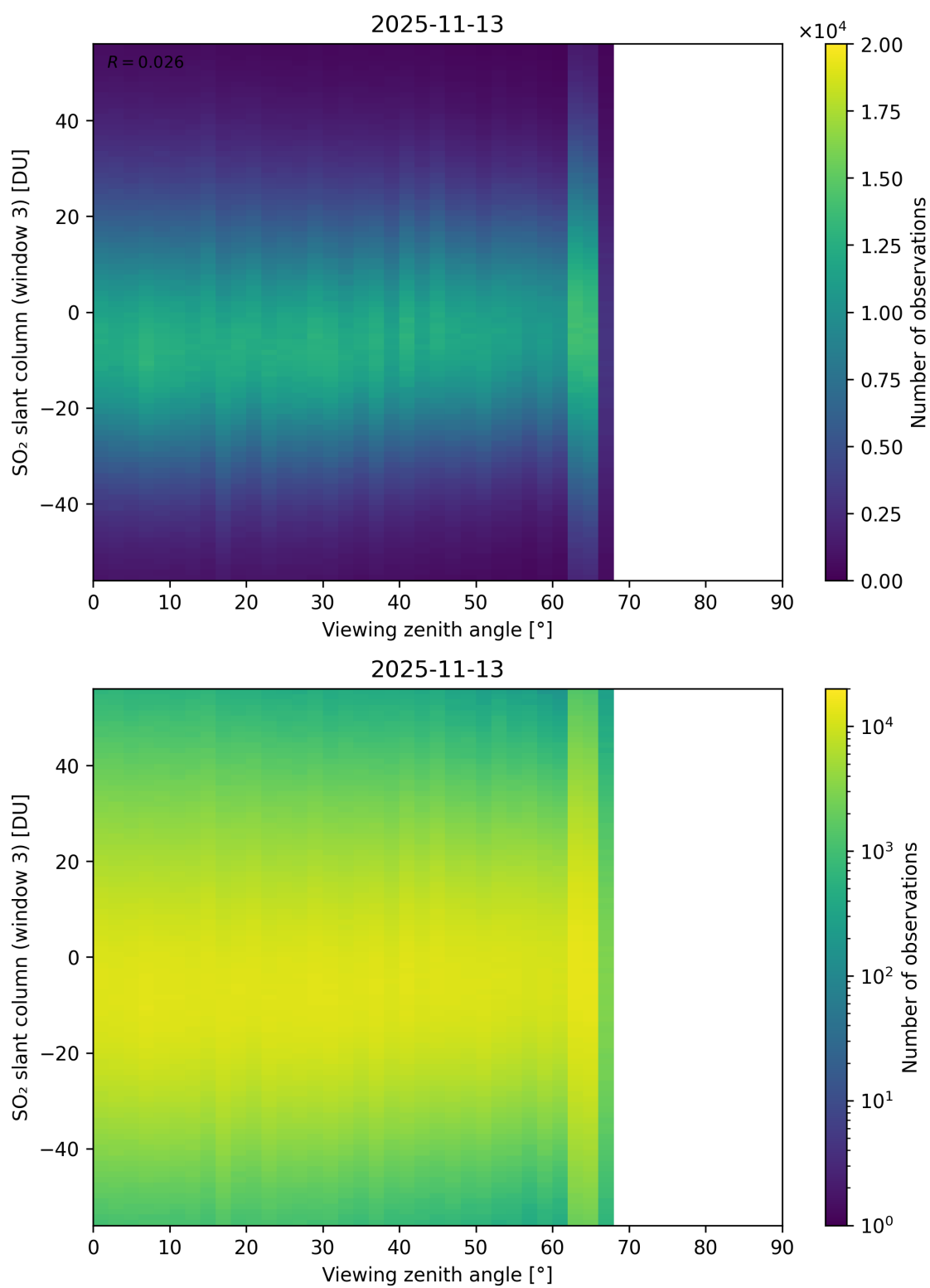
Figure 379: Scatter density plot of “Viewing zenith angle” against “SO 2 slant column (window 3)” for 2025-11-12 to 2025-11-14.
