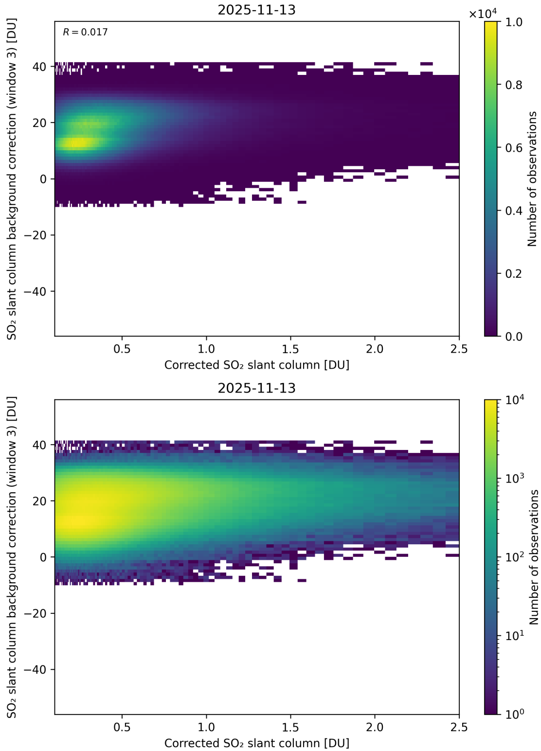
Figure 228: Scatter density plot of “Corrected SO 2 slant column” against “SO 2 slant column background correction (window 3)” for 2025-11-12 to 2025-11-14.
