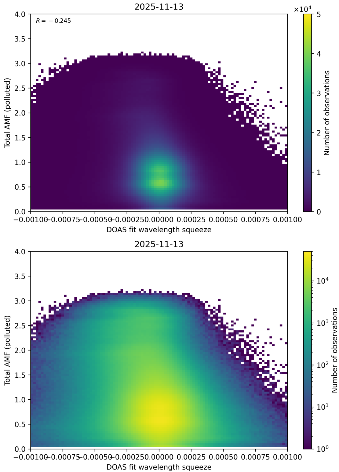
Figure 145: Scatter density plot of “DOAS fit wavelength squeeze” against “Total AMF (polluted)” for 2025-11-12 to 2025-11-14.
