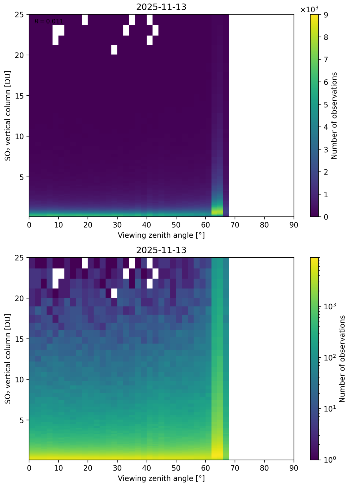
Figure 383: Scatter density plot of “Viewing zenith angle” against “SO 2 vertical column” for 2025-11-12 to 2025-11-14.
