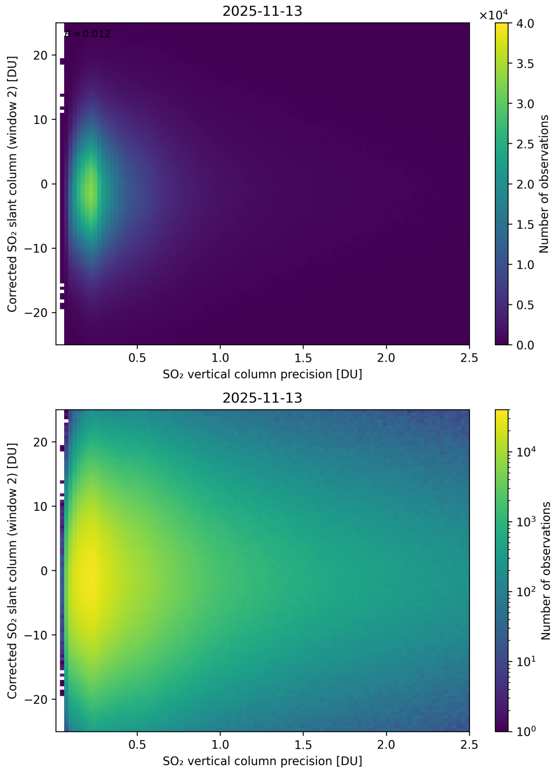
Figure 339: Scatter density plot of “SO 2 vertical column precision” against “Corrected SO 2 slant column (window 2)” for 2025-11-12 to 2025-11-14.
