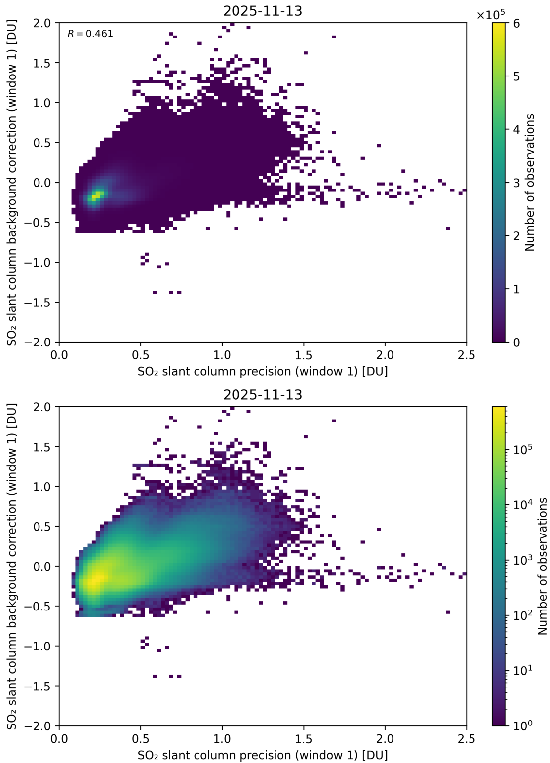
Figure 268: Scatter density plot of “SO 2 slant column precision (window 1)” against “SO 2 slant column background correction (window 1)” for 2025-11-12 to 2025-11-14.
