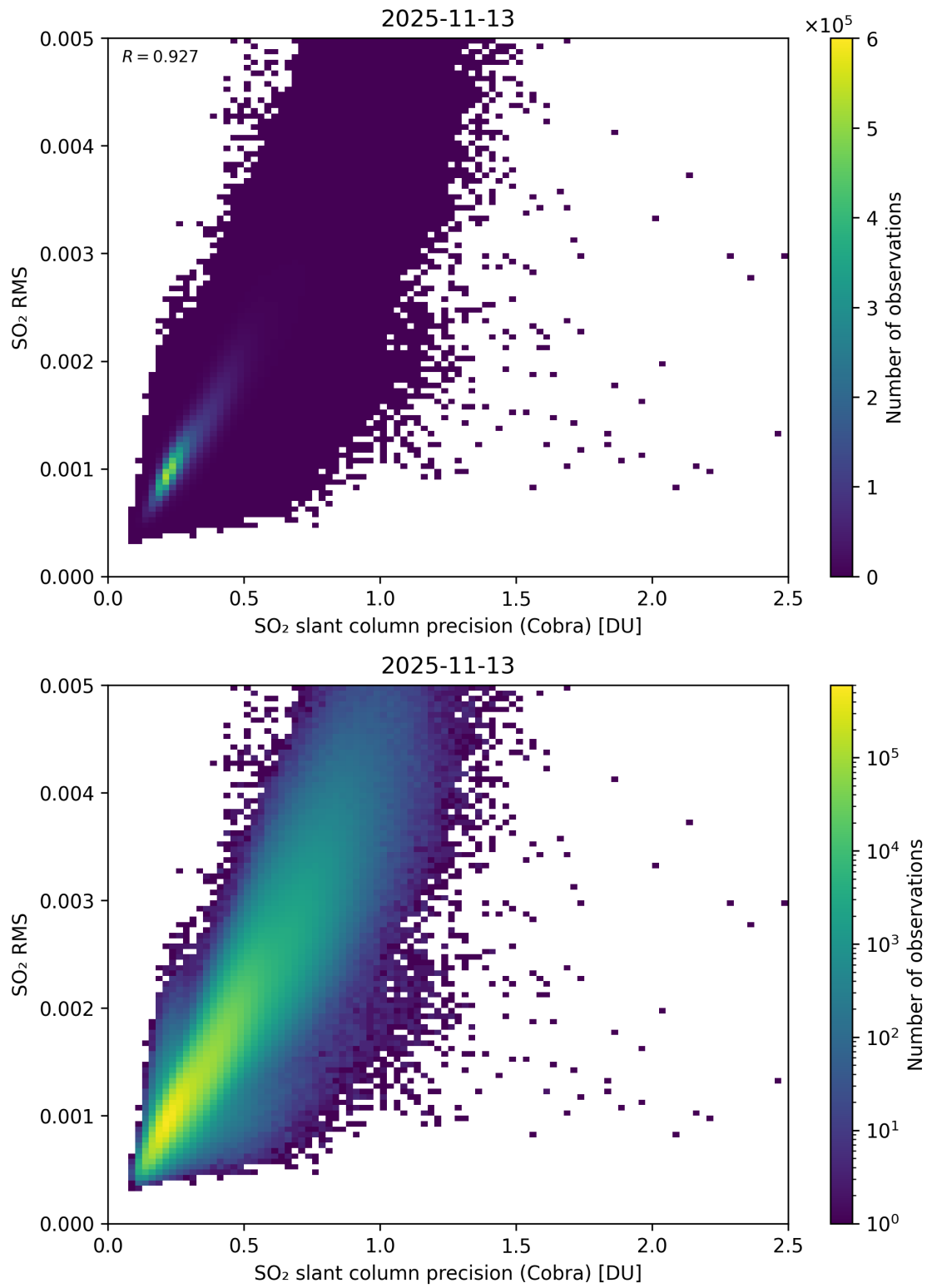
Figure 204: Scatter density plot of “SO 2 slant column precision (Cobra)” against “SO 2 RMS” for 2025-11-12 to 2025-11-14.
