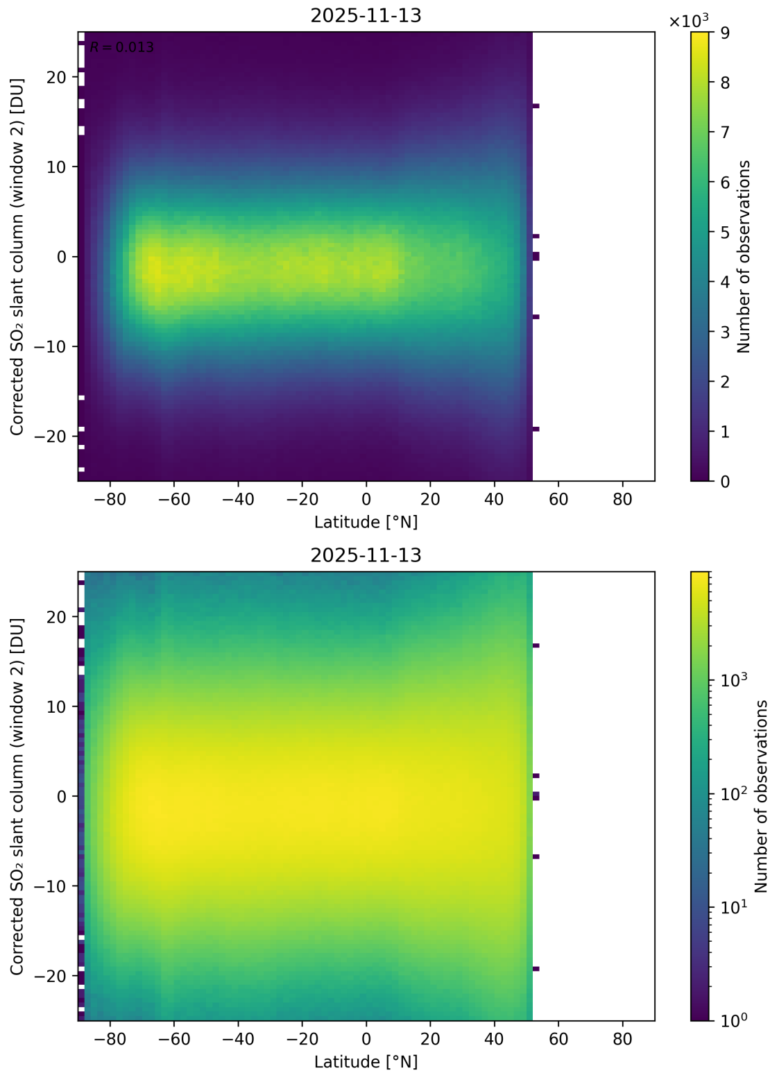
Figure 160: Scatter density plot of “Latitude” against “Corrected SO 2 slant column (window 2)” for 2025-11-12 to 2025-11-14.
