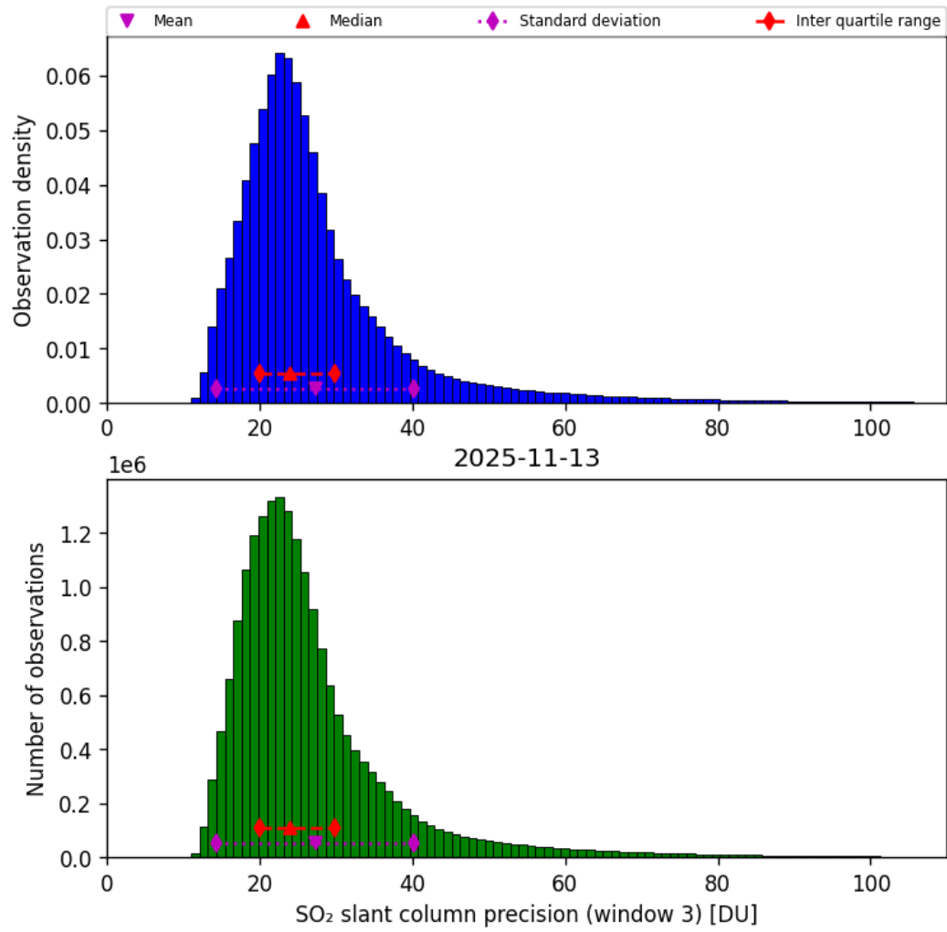
Figure 72: Histogram of “SO 2 slant column precision (window 3)” for 2025-11-12 to 2025-11-14
