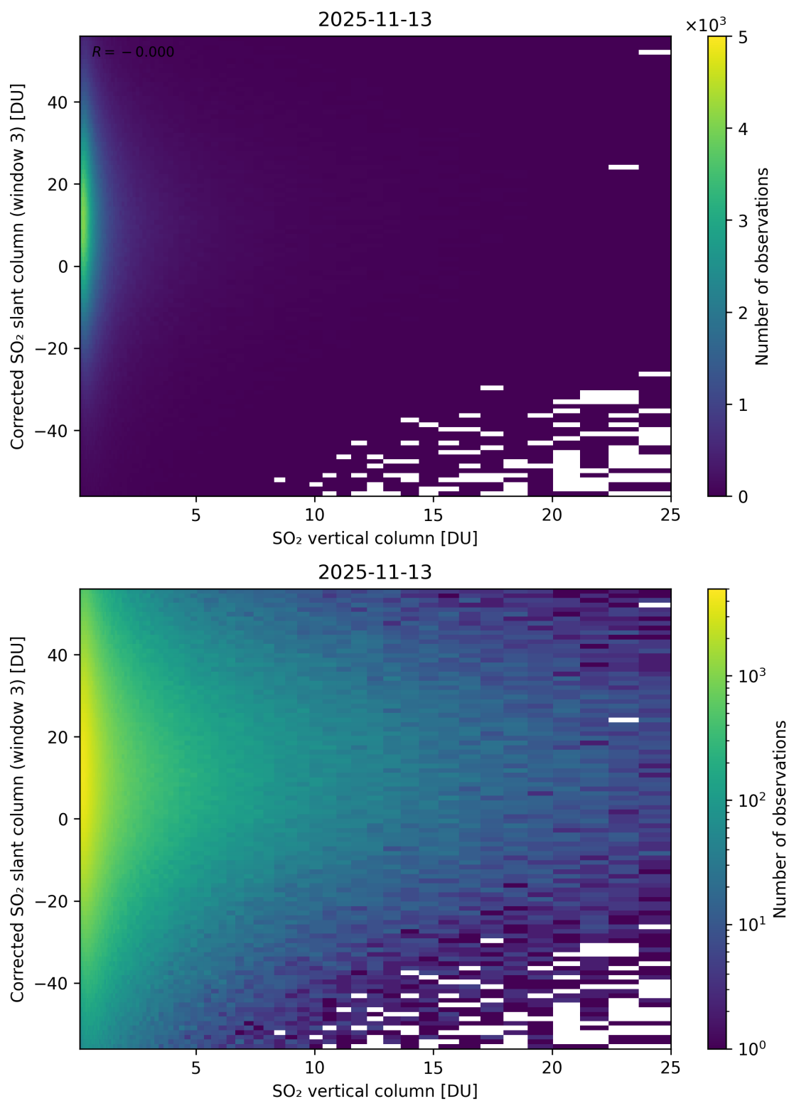
Figure 353: Scatter density plot of “SO 2 vertical column” against “Corrected SO 2 slant column (window 3)” for 2025-11-12 to 2025-11-14.
