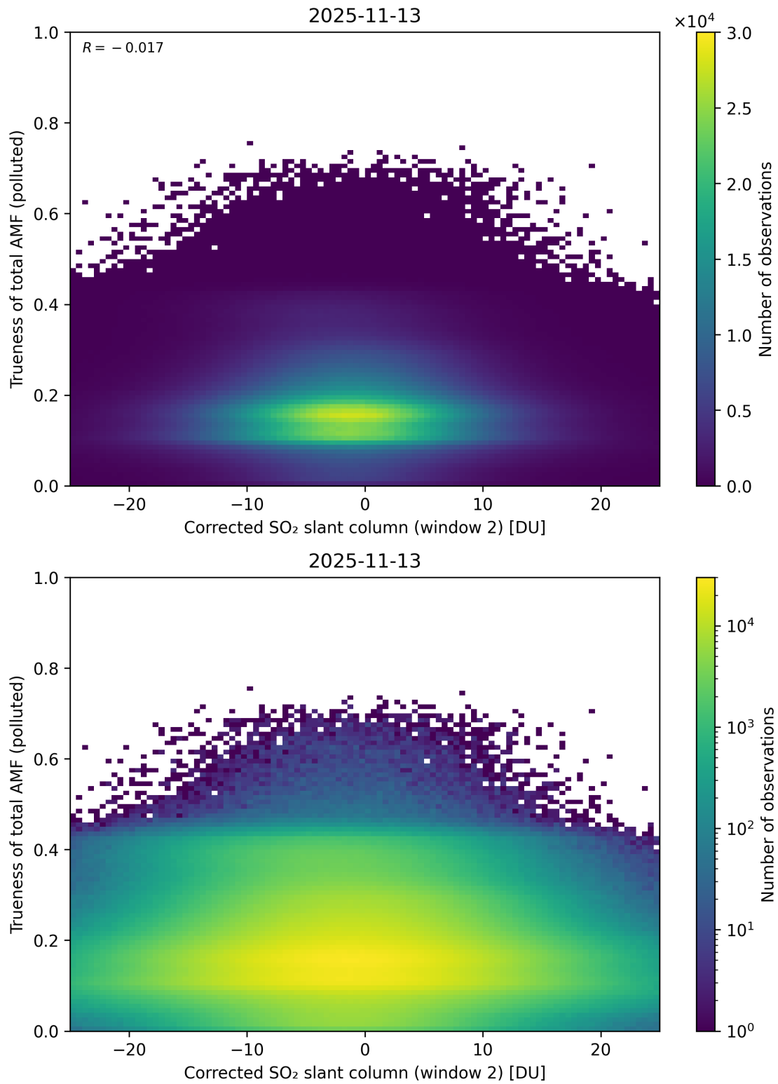
Figure 254: Scatter density plot of “Corrected SO 2 slant column (window 2)” against “Trueness of total AMF (polluted)” for 2025-11-12 to 2025-11-14.
