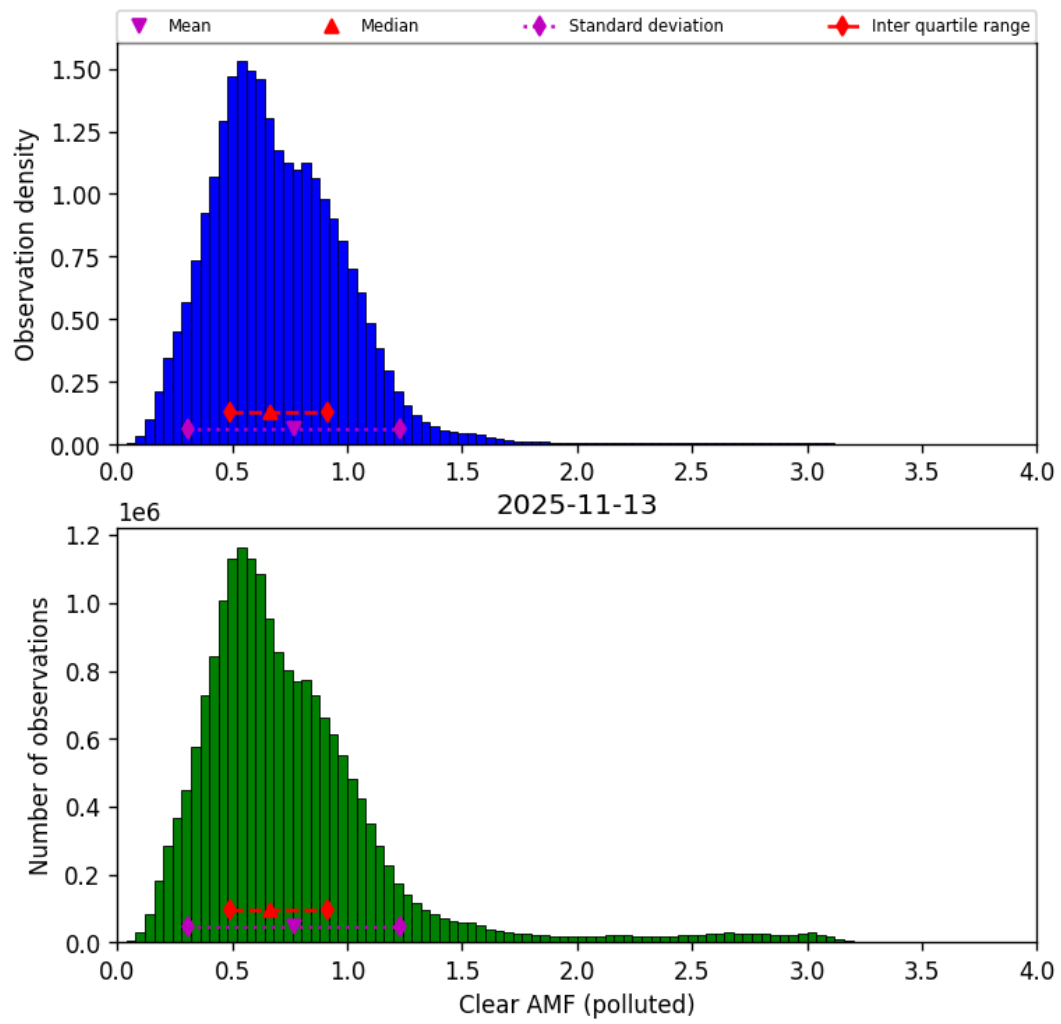
Figure 81: Histogram of “Clear AMF (polluted)” for 2025-11-12 to 2025-11-14
