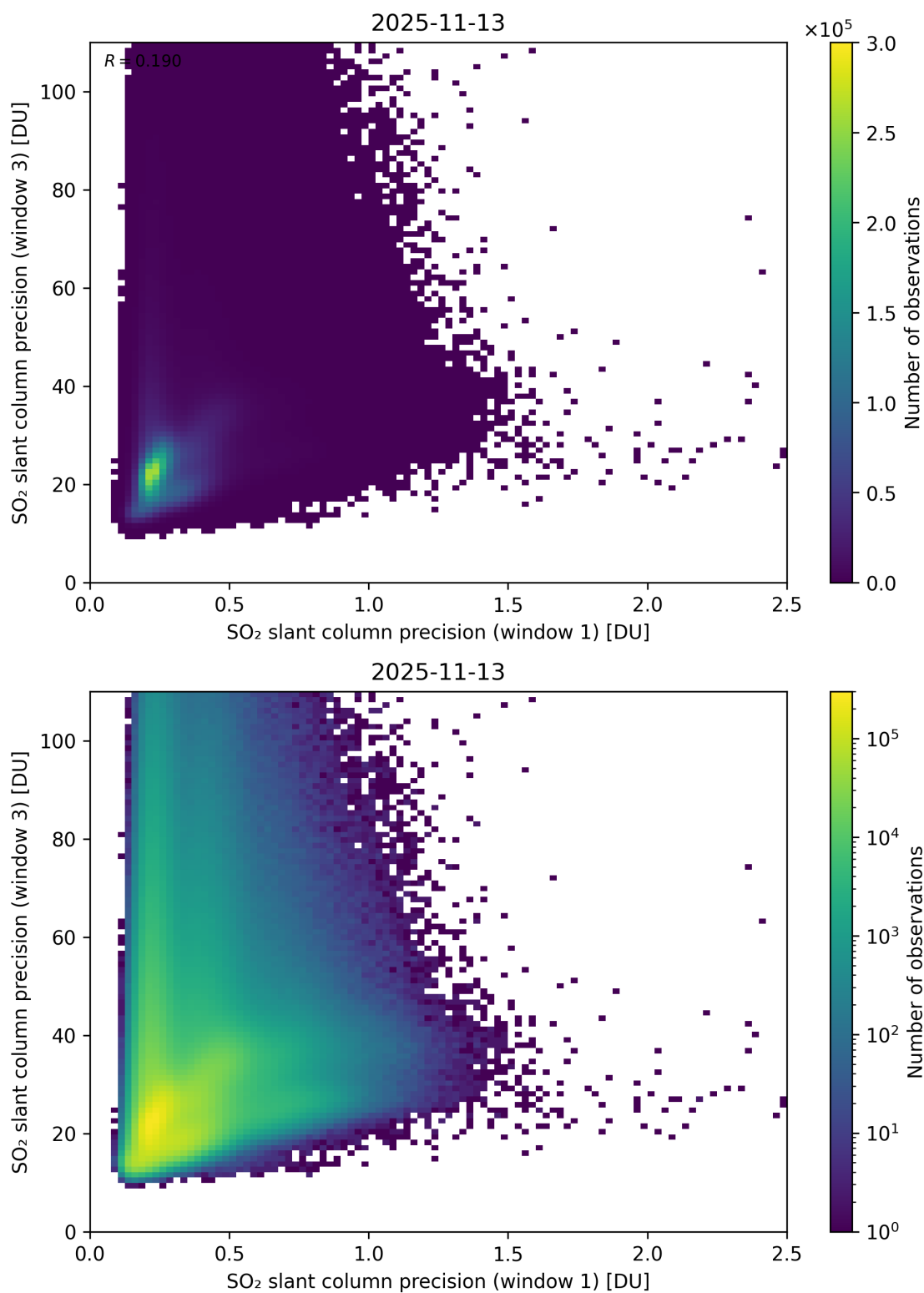
Figure 279: Scatter density plot of “SO 2 slant column precision (window 1)” against “SO 2 slant column precision (window 3)” for 2025-11-12 to 2025-11-14.
