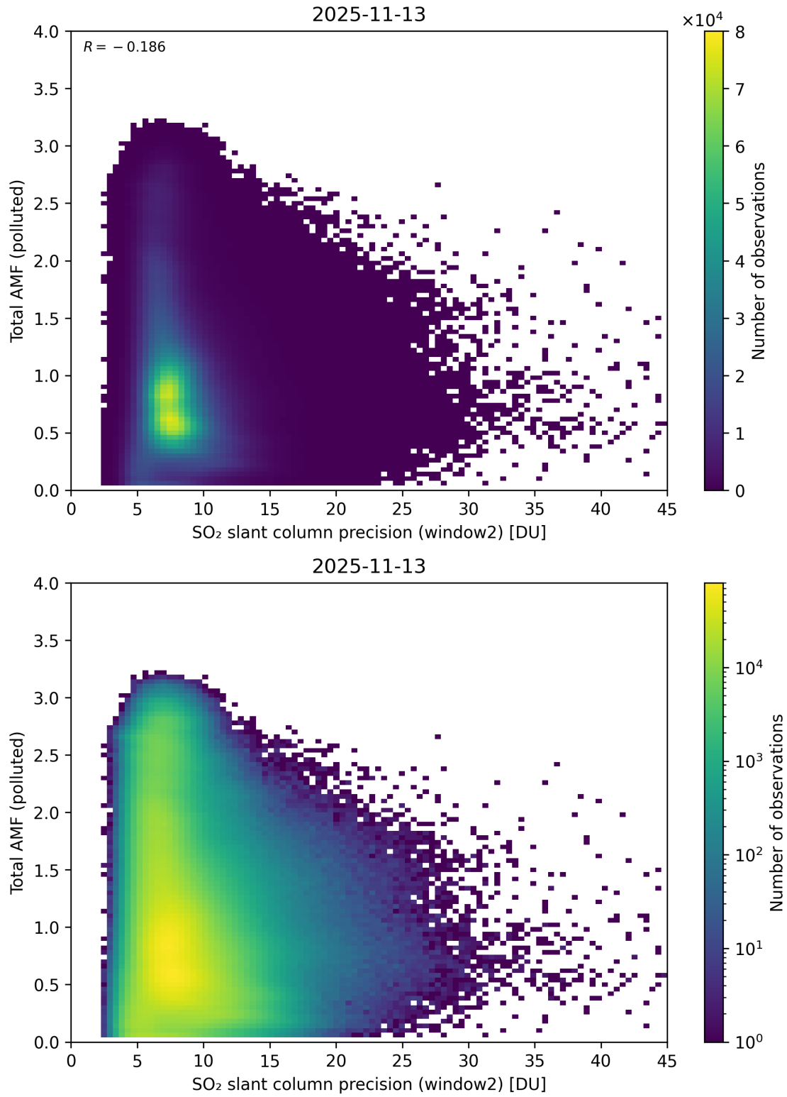
Figure 301: Scatter density plot of “SO 2 slant column precision (window2)” against “Total AMF (polluted)” for 2025-11-12 to 2025-11-14.
