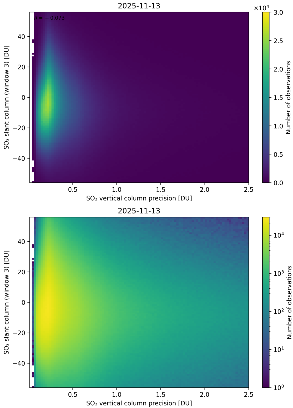
Figure 344: Scatter density plot of “SO 2 vertical column precision” against “SO 2 slant column (window 3)” for 2025-11-12 to 2025-11-14.
