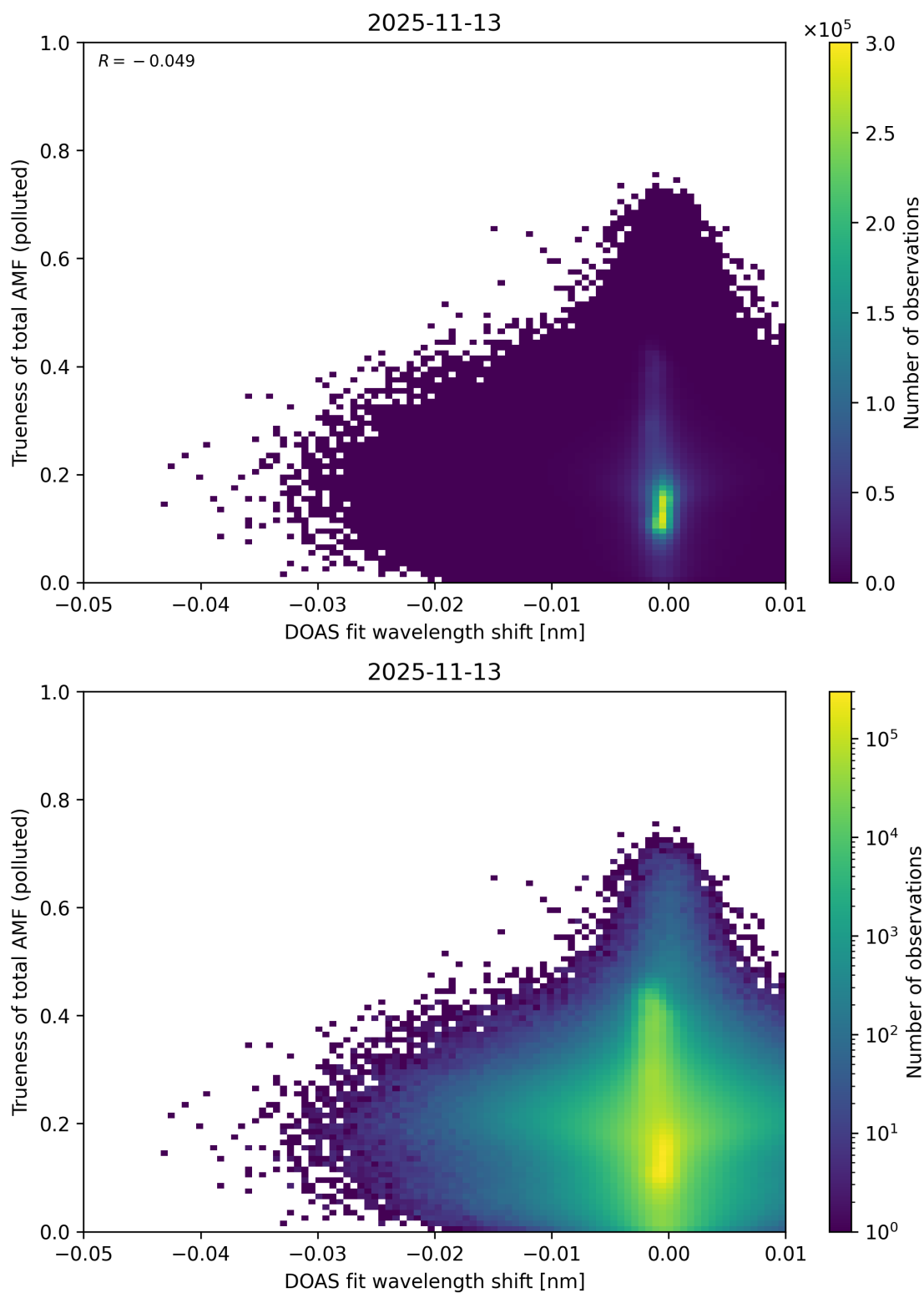
Figure 142: Scatter density plot of “DOAS fit wavelength shift” against “Trueness of total AMF (polluted)” for 2025-11-12 to 2025-11-14.
