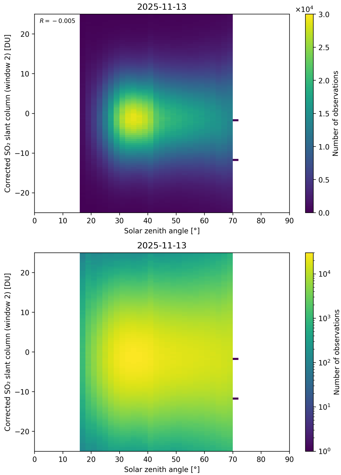
Figure 182: Scatter density plot of “Solar zenith angle” against “Corrected SO 2 slant column (window 2)” for 2025-11-12 to 2025-11-14.
