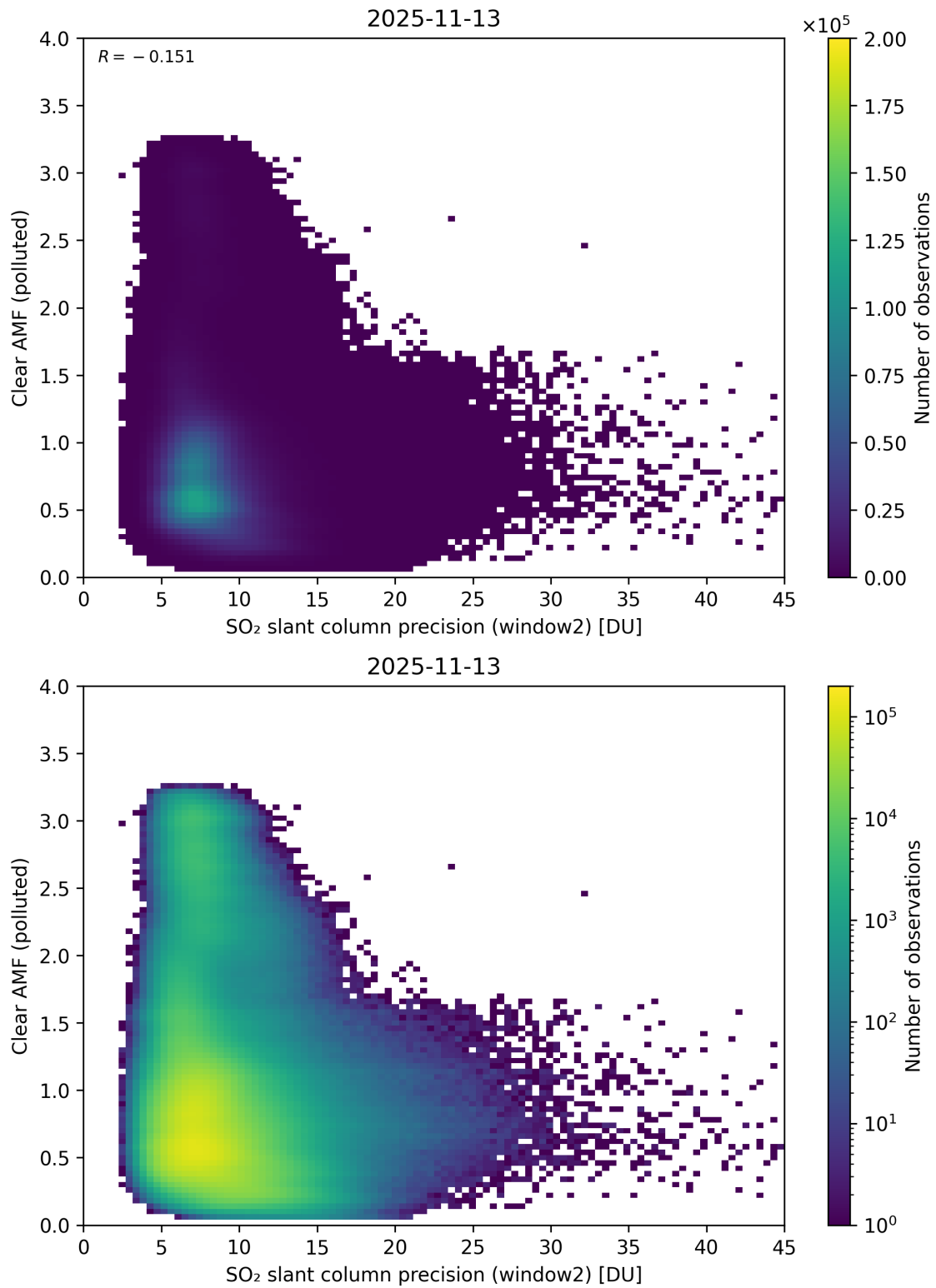
Figure 296: Scatter density plot of “SO 2 slant column precision (window2)” against “Clear AMF (polluted)” for 2025-11-12 to 2025-11-14.
