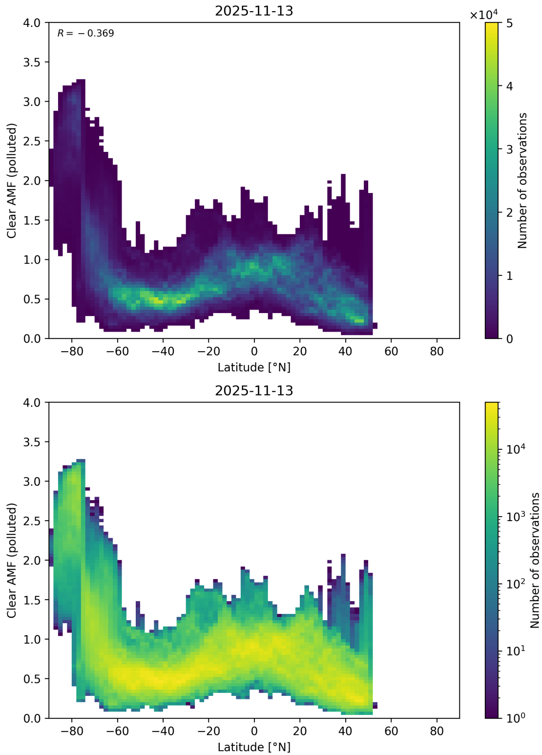
Figure 156: Scatter density plot of “Latitude” against “Clear AMF (polluted)” for 2025-11-12 to 2025-11-14.
