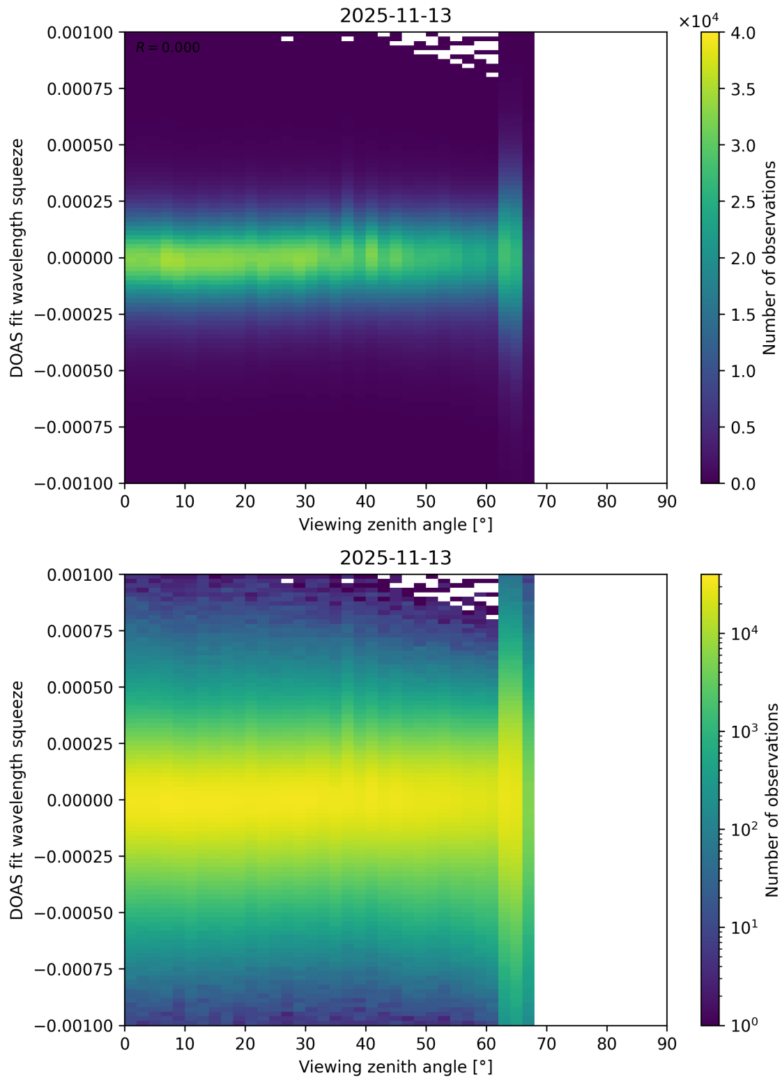
Figure 366: Scatter density plot of “Viewing zenith angle” against “DOAS fit wavelength squeeze” for 2025-11-12 to 2025-11-14.
