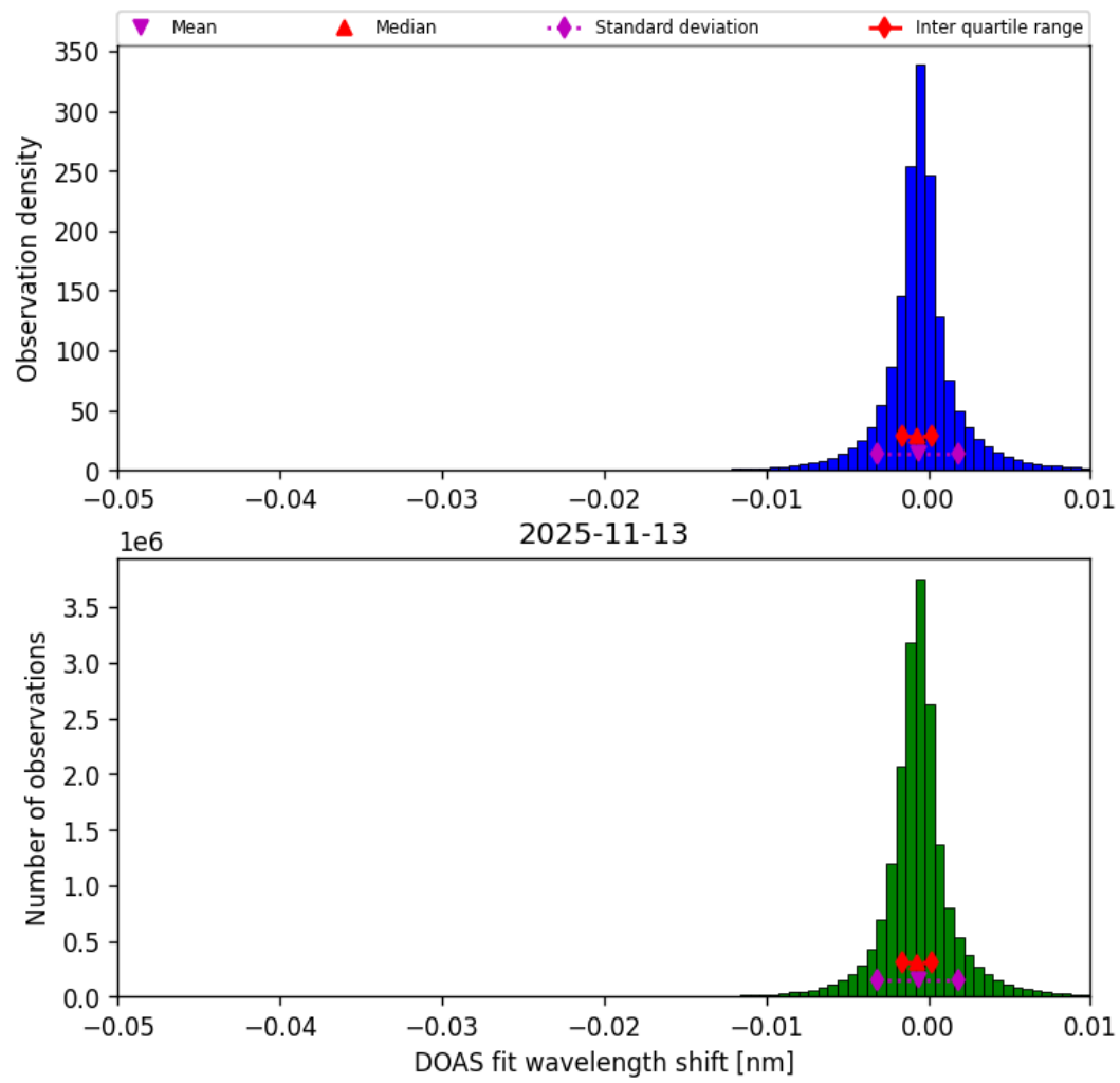
Figure 76: Histogram of “DOAS fit wavelength shift” for 2025-11-12 to 2025-11-14
