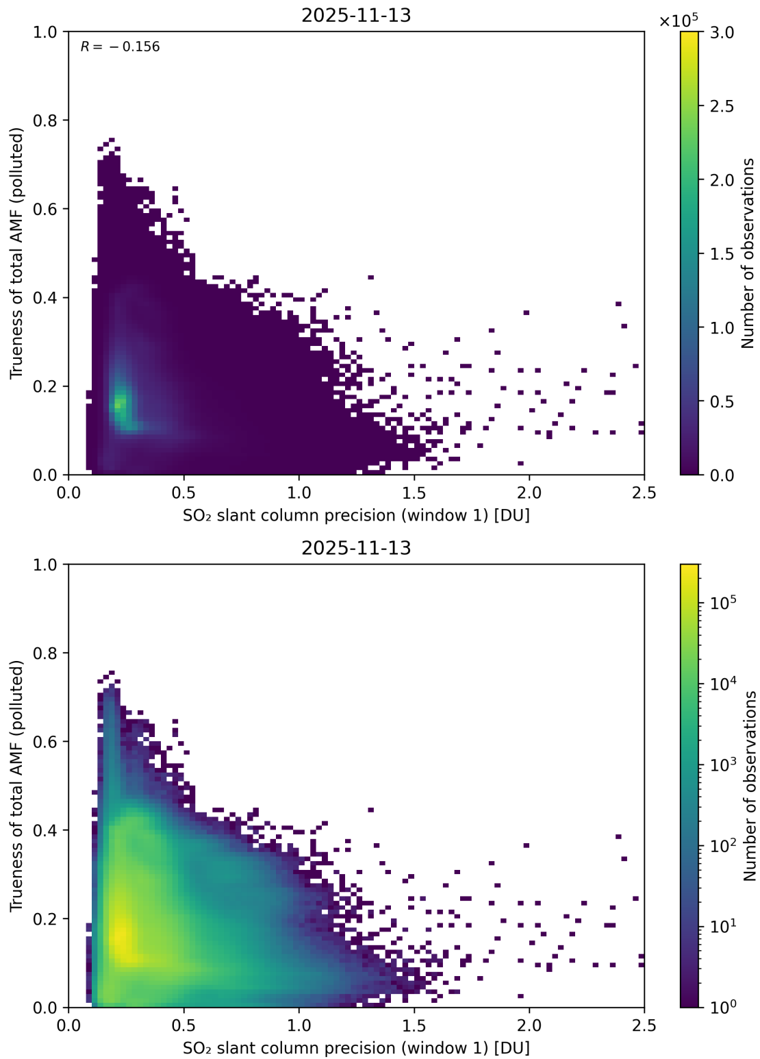
Figure 281: Scatter density plot of “SO 2 slant column precision (window 1)” against “Trueness of total AMF (polluted)” for 2025-11-12 to 2025-11-14.
