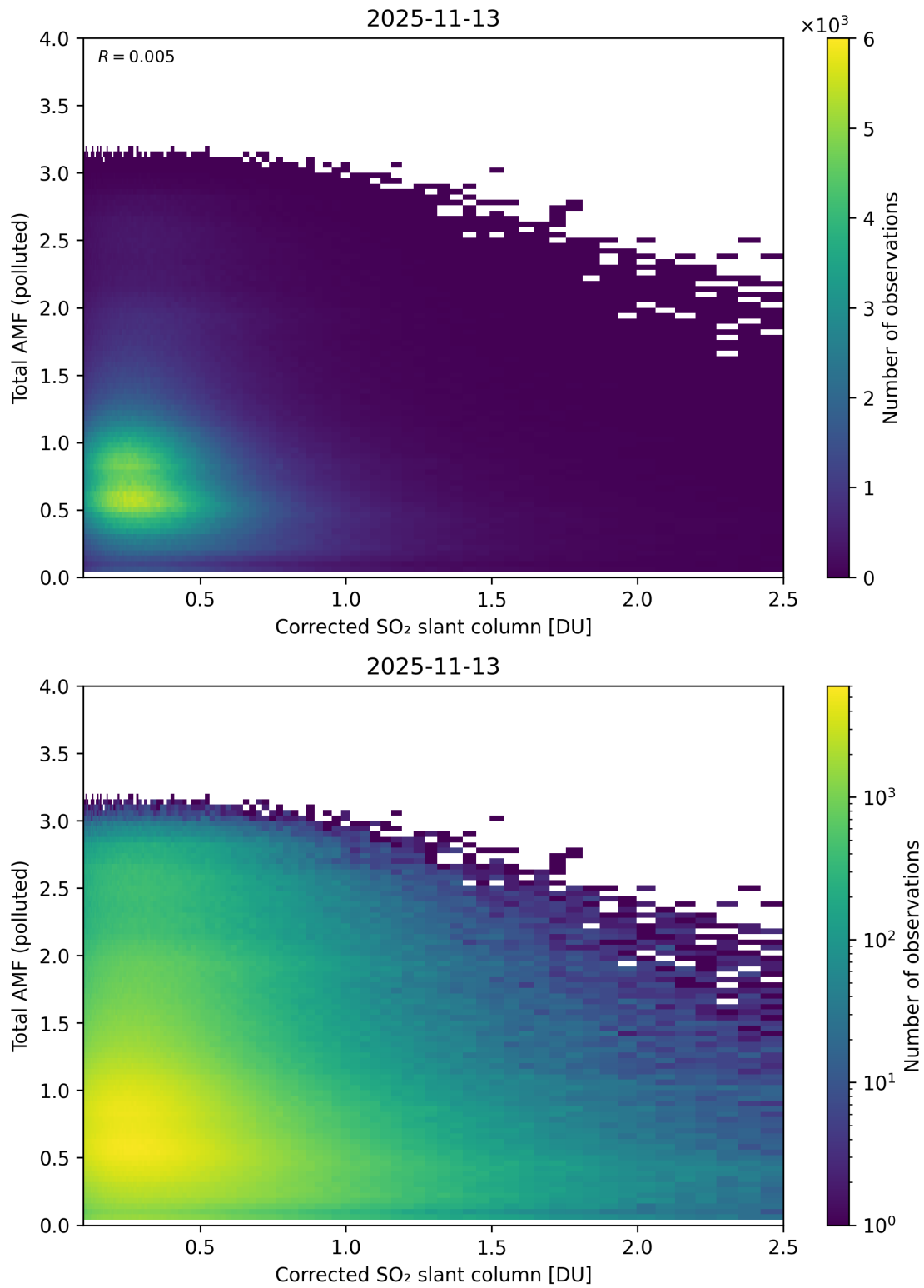
Figure 242: Scatter density plot of “Corrected SO 2 slant column” against “Total AMF (polluted)” for 2025-11-12 to 2025-11-14.
