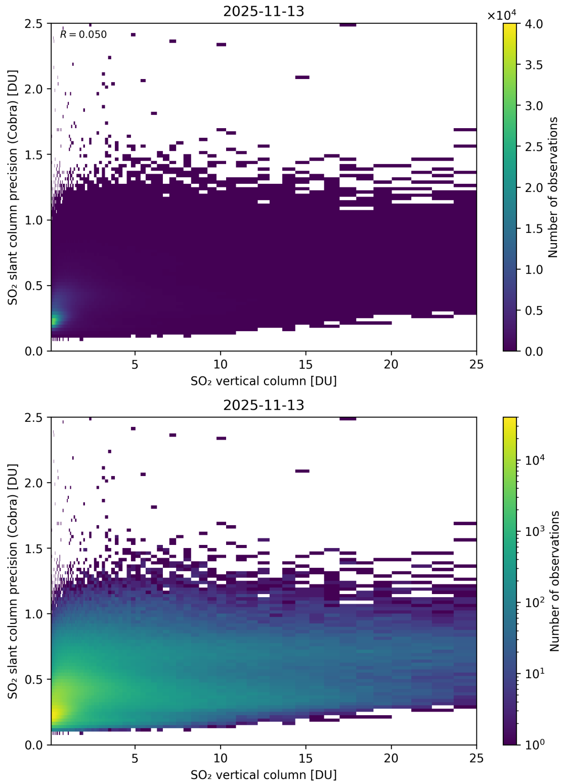
Figure 350: Scatter density plot of “SO 2 vertical column” against “SO 2 slant column precision (Cobra)” for 2025-11-12 to 2025-11-14.
