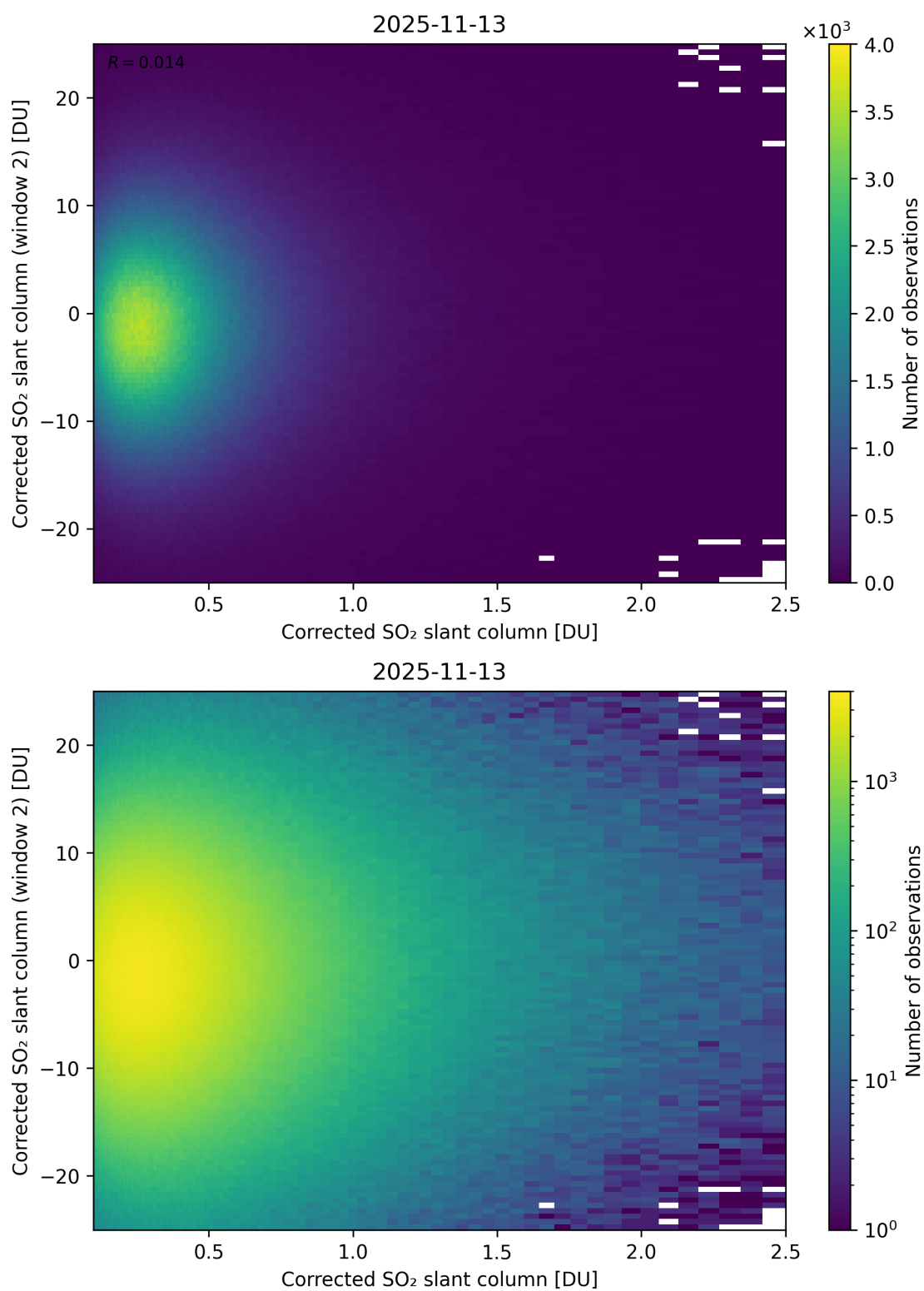
Figure 235: Scatter density plot of “Corrected SO 2 slant column” against “Corrected SO 2 slant column (window 2)” for 2025-11-12 to 2025-11-14.
