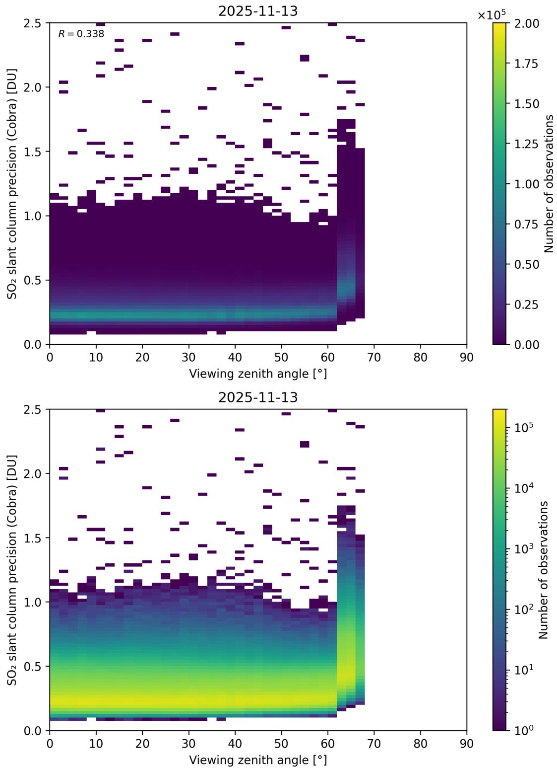
Figure 372: Scatter density plot of “Viewing zenith angle” against “SO 2 slant column precision (Cobra)” for 2025-11-12 to 2025-11-14.
