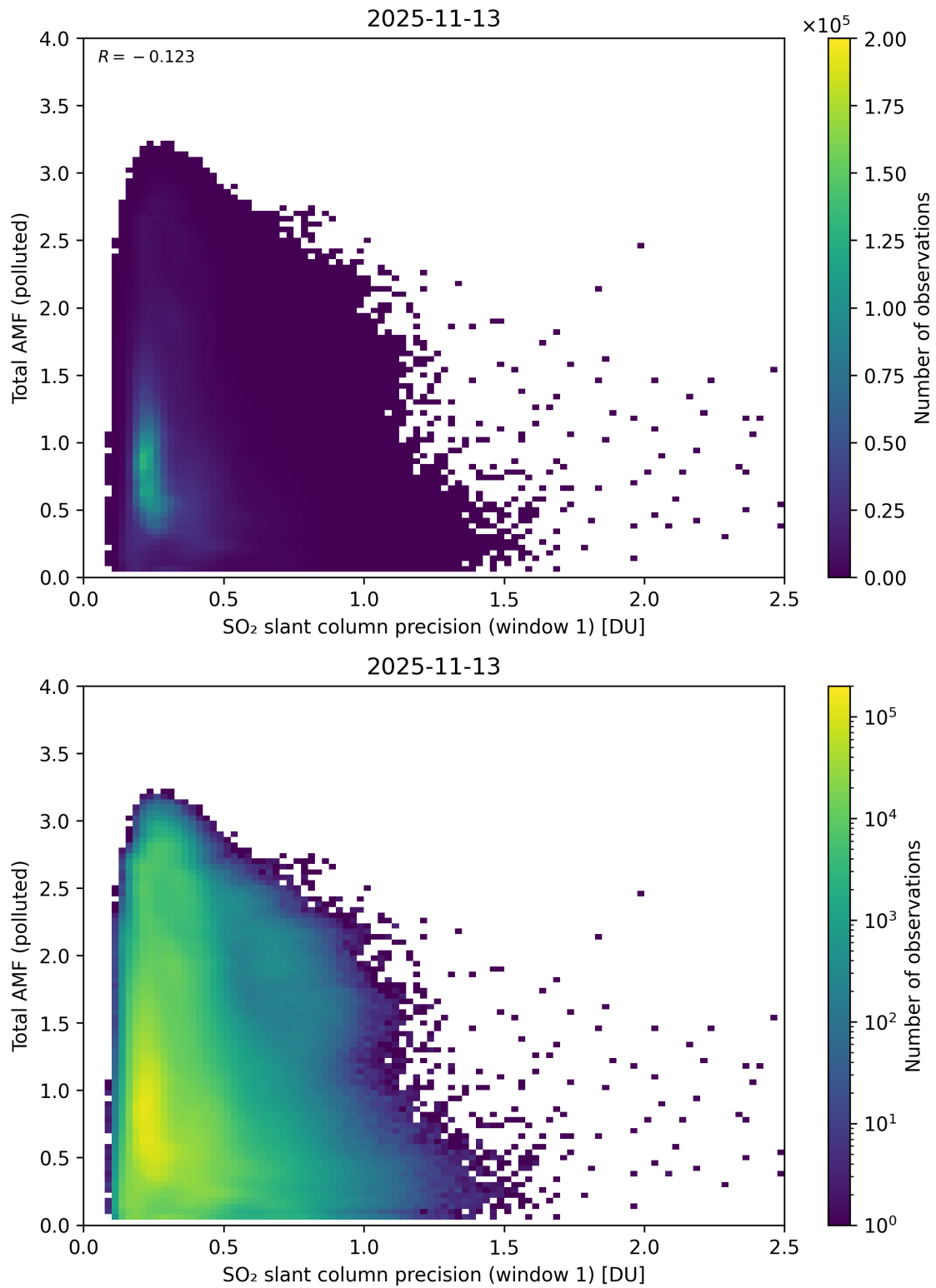
Figure 280: Scatter density plot of “SO 2 slant column precision (window 1)” against “Total AMF (polluted)” for 2025-11-12 to 2025-11-14.
