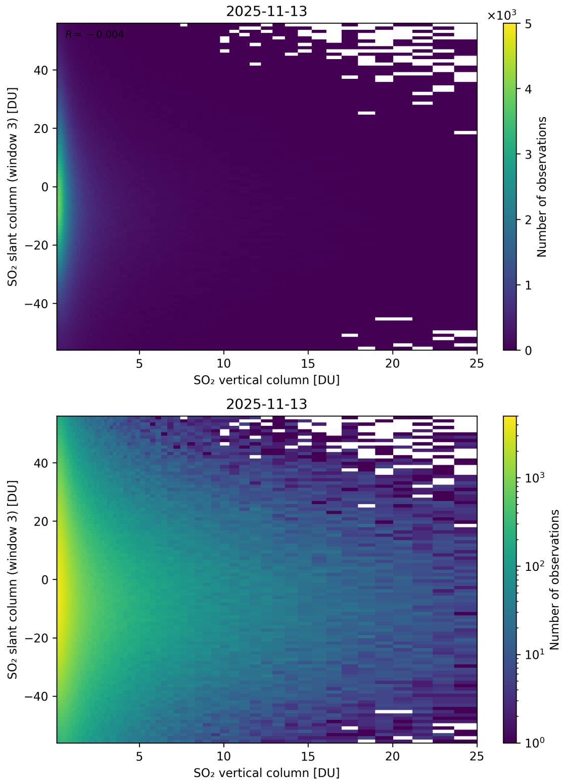
Figure 357: Scatter density plot of “SO 2 vertical column” against “SO 2 slant column (window 3)” for 2025-11-12 to 2025-11-14.
