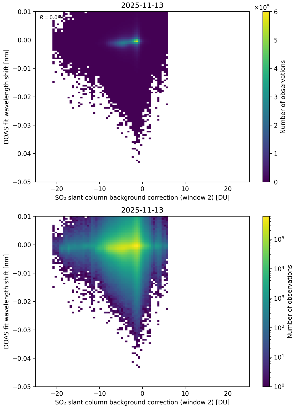
Figure 123: Scatter density plot of “SO 2 slant column background correction (window 2)” against “DOAS fit wavelength shift” for 2025-11-12 to 2025-11-14.
