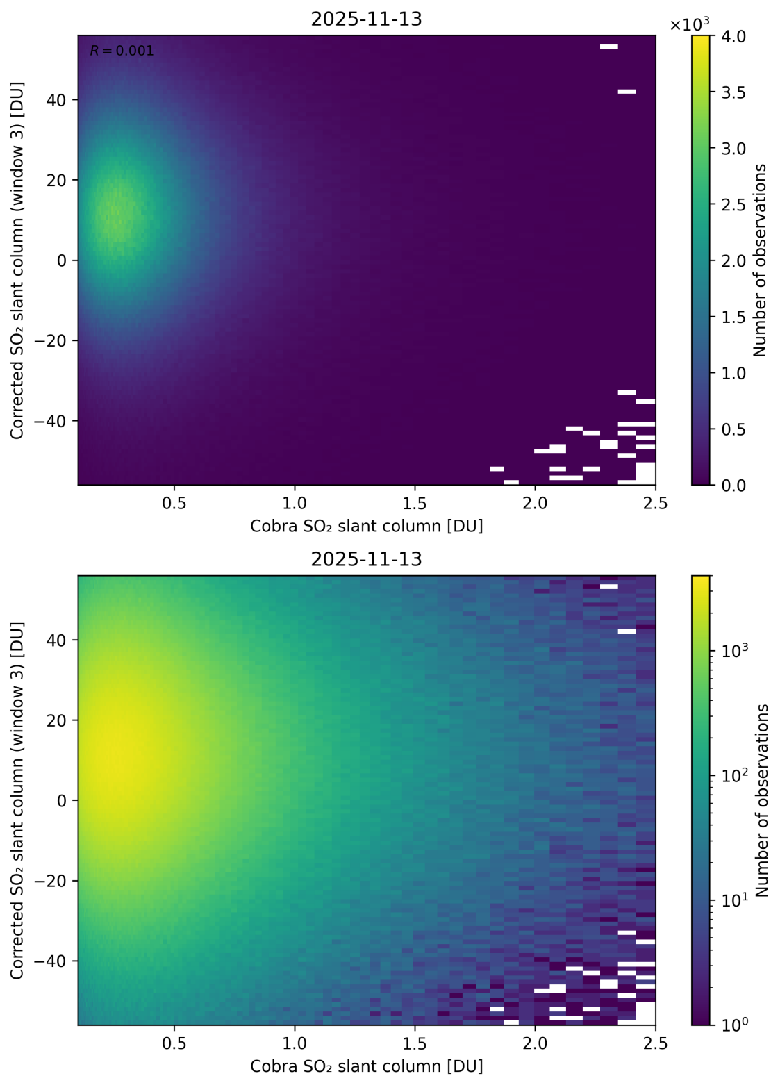
Figure 218: Scatter density plot of “Cobra SO 2 slant column” against “Corrected SO 2 slant column (window 3)” for 2025-11-12 to 2025-11-14.
