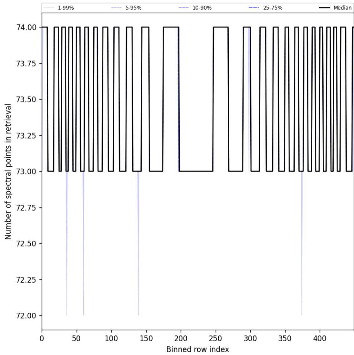
Figure 108: Along track statistics of “Number of spectral points in retrieval” for 2025-11-12 to 2025-11-14
