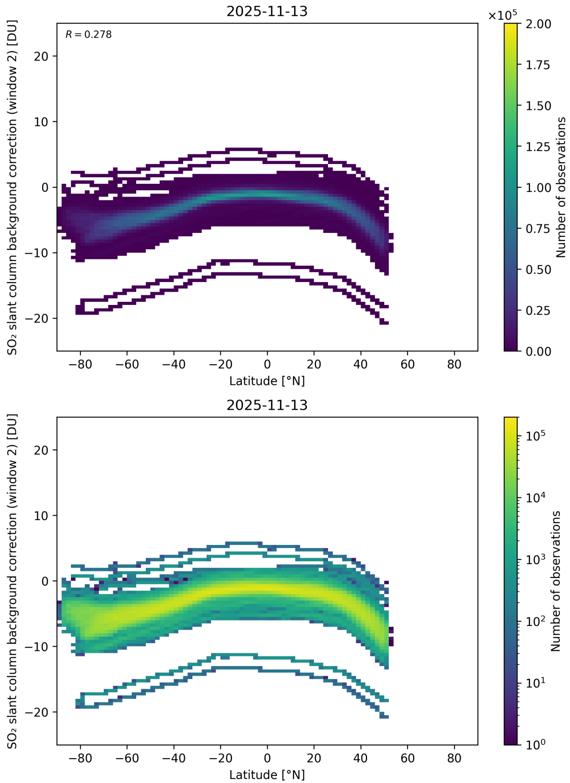
Figure 151: Scatter density plot of “Latitude” against “SO 2 slant column background correction (window 2)” for 2025-11-12 to 2025-11-14.
