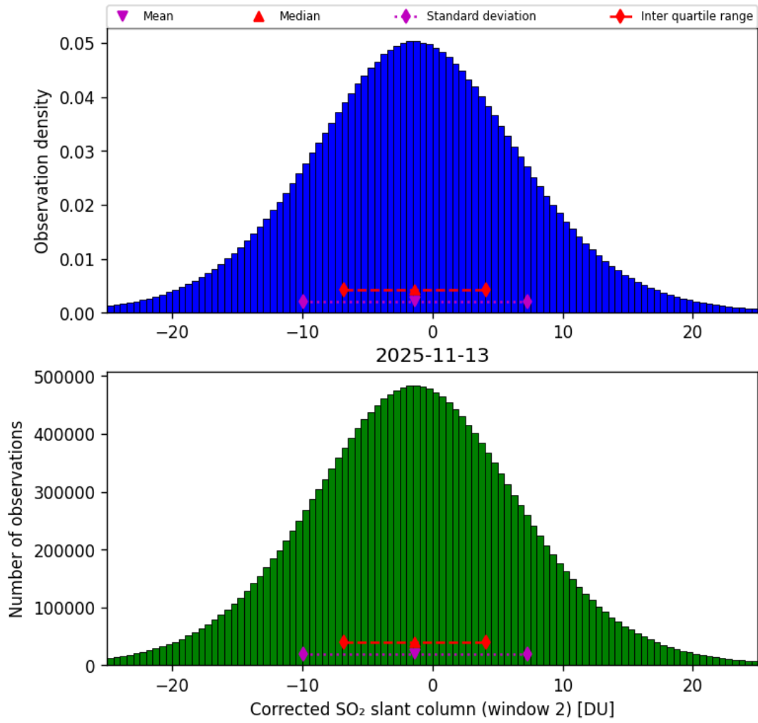
Figure 69: Histogram of “Corrected SO 2 slant column (window 2)” for 2025-11-12 to 2025-11-14
