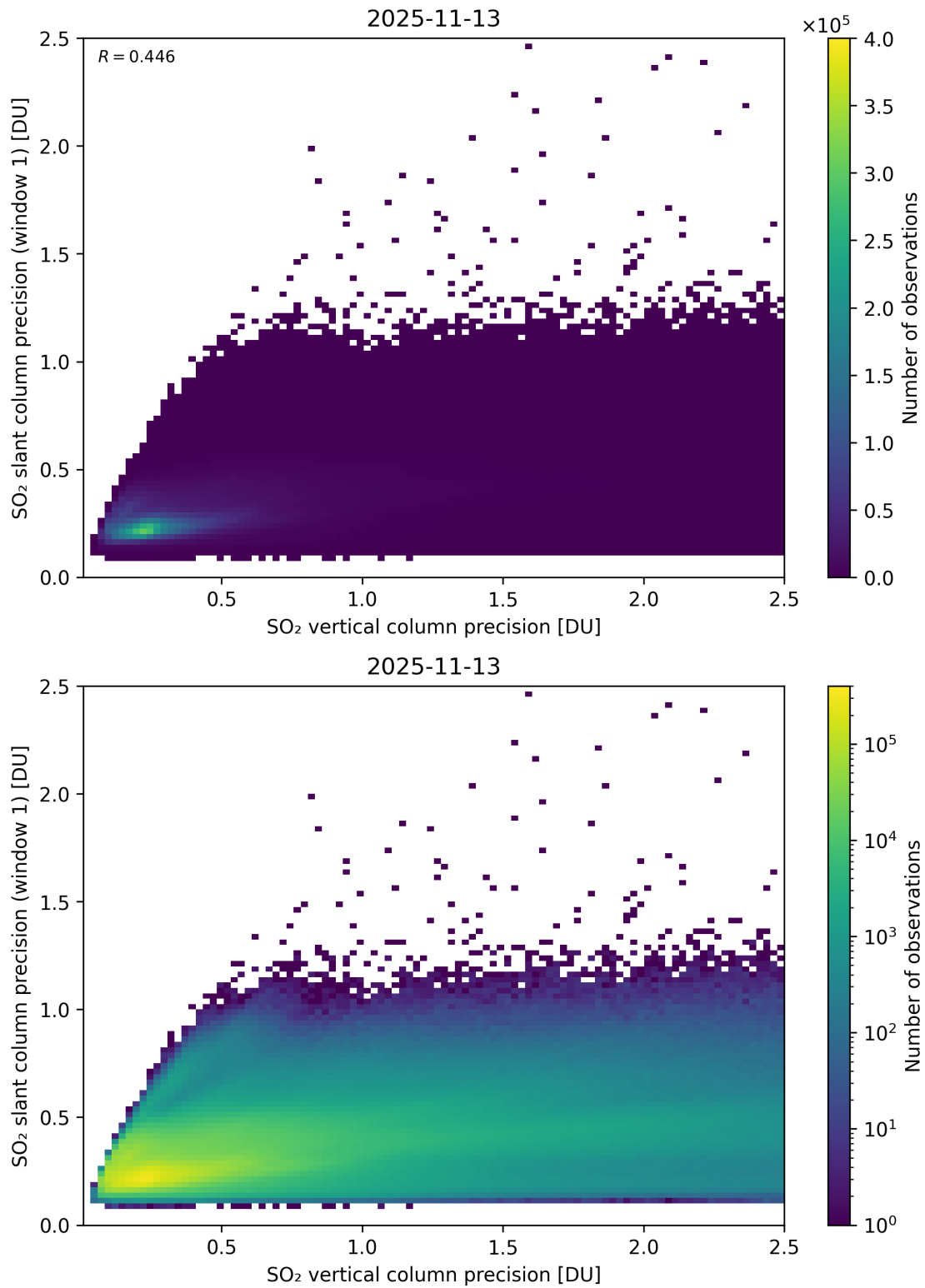
Figure 342: Scatter density plot of “SO 2 vertical column precision” against “SO 2 slant column precision (window 1)” for 2025-11-12 to 2025-11-14.
