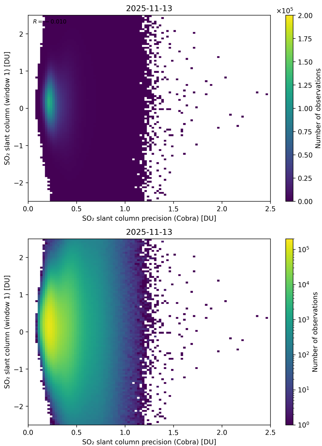
Figure 208: Scatter density plot of “SO 2 slant column precision (Cobra)” against “SO 2 slant column (window 1)” for 2025-11-12 to 2025-11-14.
