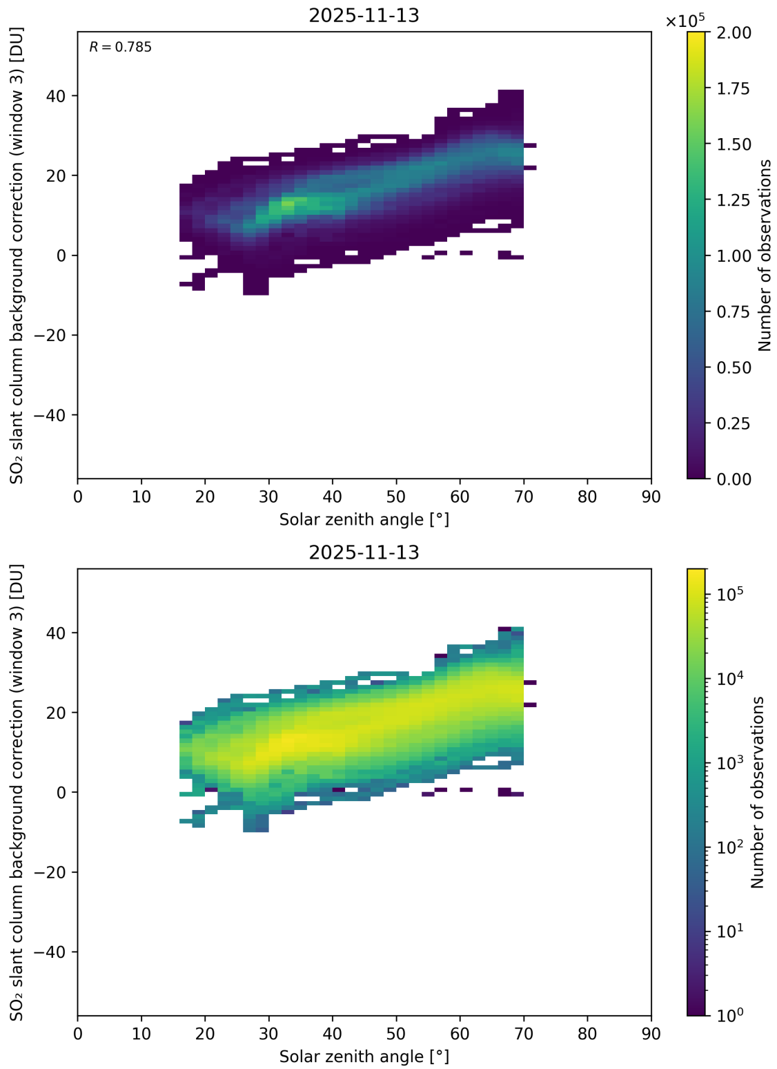
Figure 173: Scatter density plot of “Solar zenith angle” against “SO 2 slant column background correction (window 3)” for 2025-11-12 to 2025-11-14.
