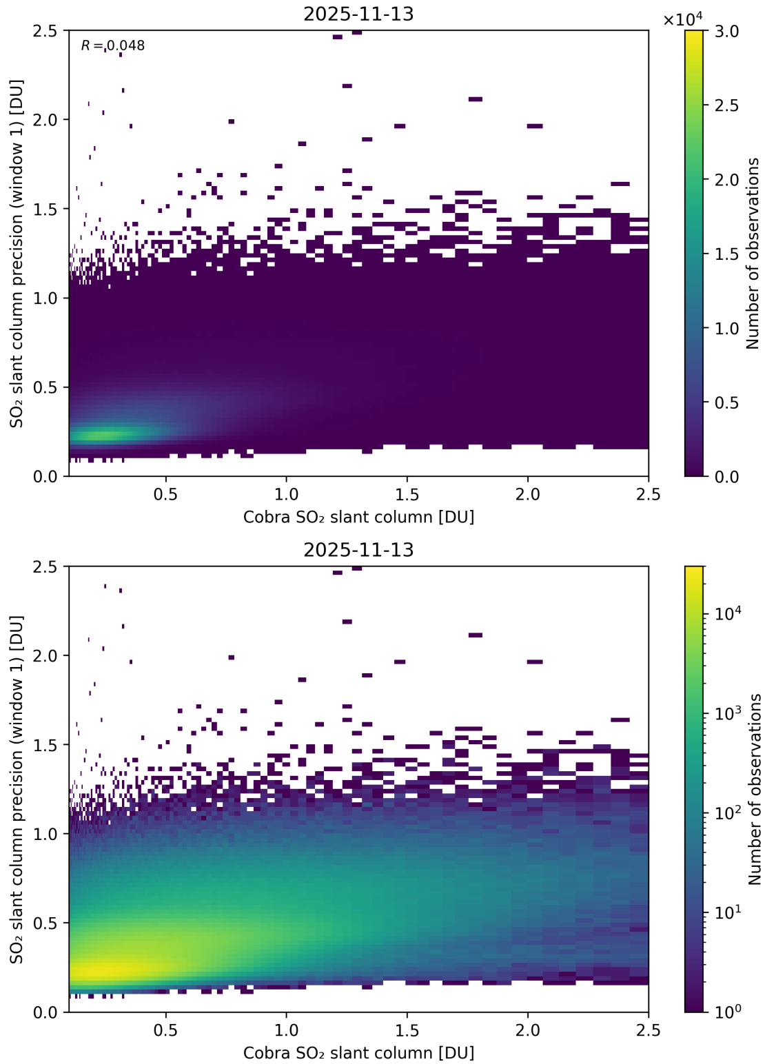
Figure 220: Scatter density plot of “Cobra SO 2 slant column” against “SO 2 slant column precision (window 1)” for 2025-11-12 to 2025-11-14.
