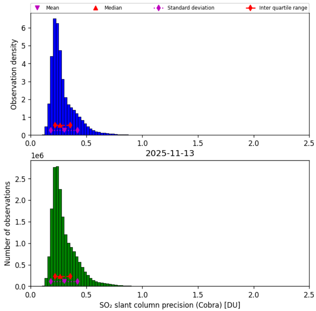
Figure 62: Histogram of “SO 2 slant column precision (Cobra)” for 2025-11-12 to 2025-11-14
