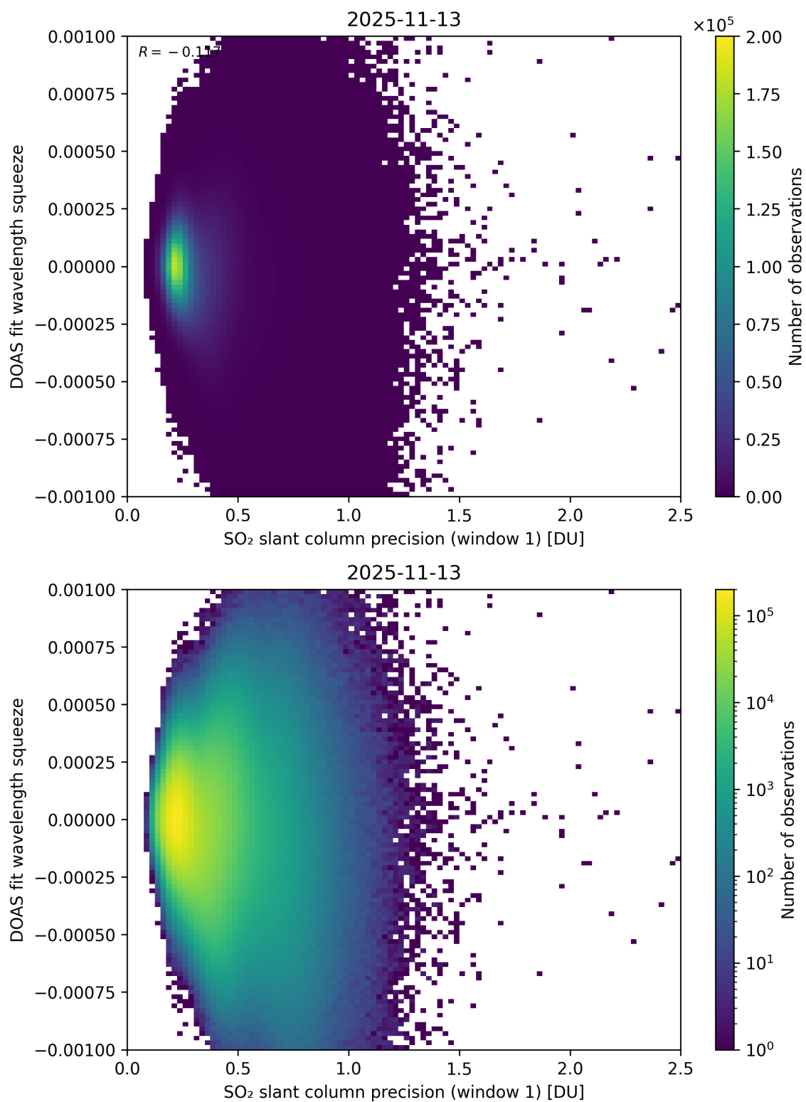
Figure 272: Scatter density plot of “SO 2 slant column precision (window 1)” against “DOAS fit wavelength squeeze” for 2025-11-12 to 2025-11-14.
