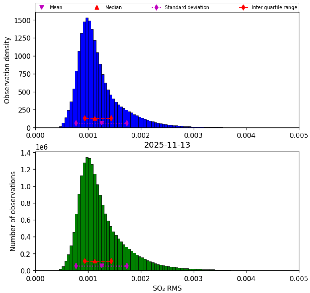
Figure 78: Histogram of “SO 2 RMS” for 2025-11-12 to 2025-11-14
