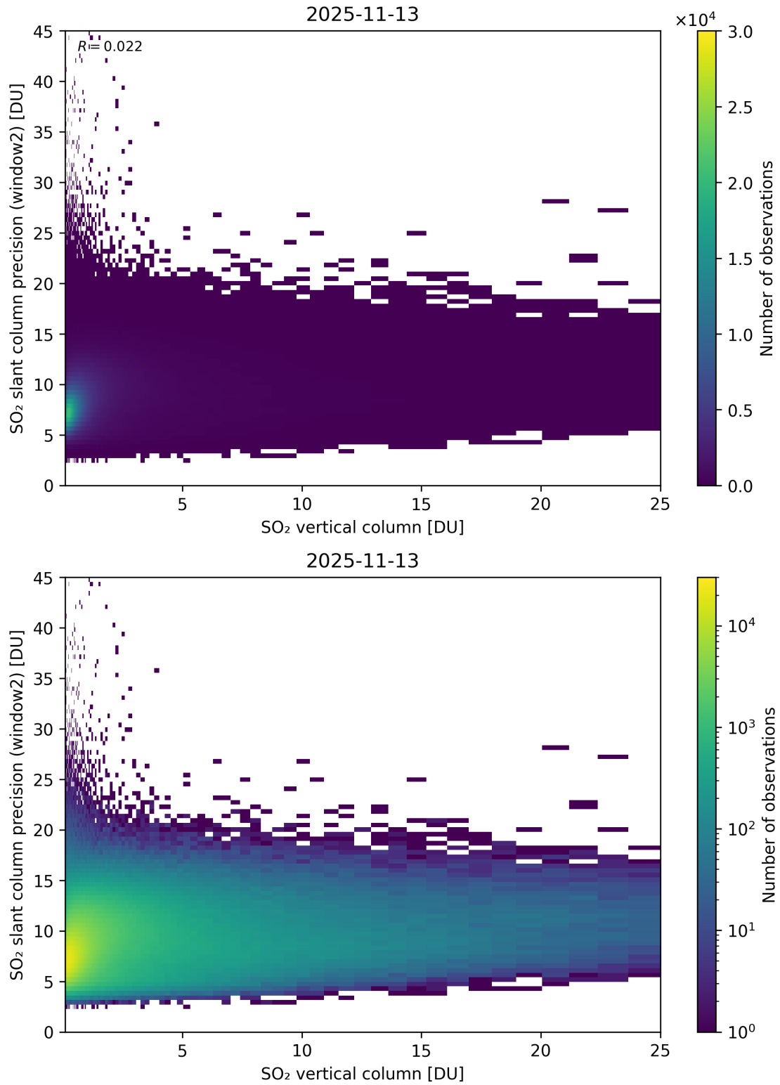
Figure 356: Scatter density plot of “SO 2 vertical column” against “SO 2 slant column precision (window2)” for 2025-11-12 to 2025-11-14.
