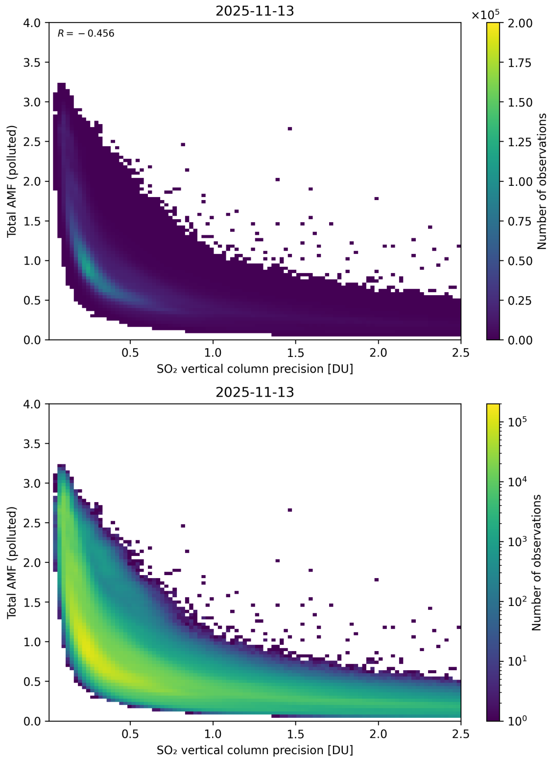
Figure 346: Scatter density plot of “SO 2 vertical column precision” against “Total AMF (polluted)” for 2025-11-12 to 2025-11-14.
