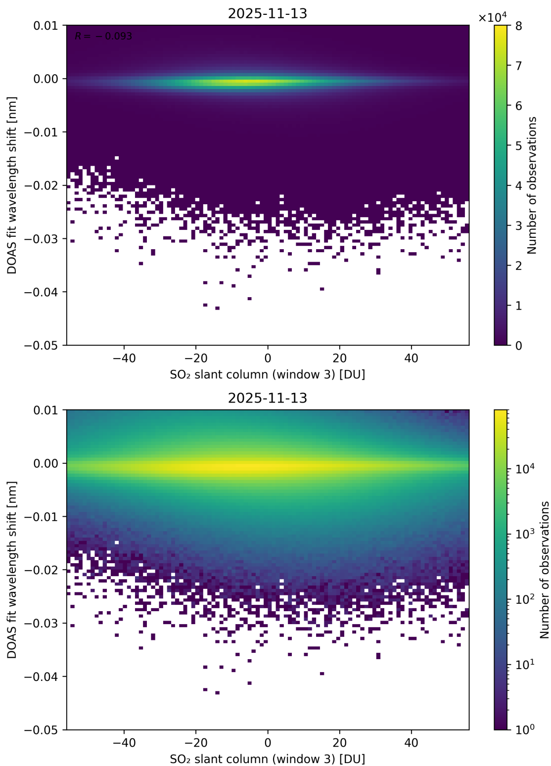
Figure 304: Scatter density plot of “SO 2 slant column (window 3)” against “DOAS fit wavelength shift” for 2025-11-12 to 2025-11-14.
