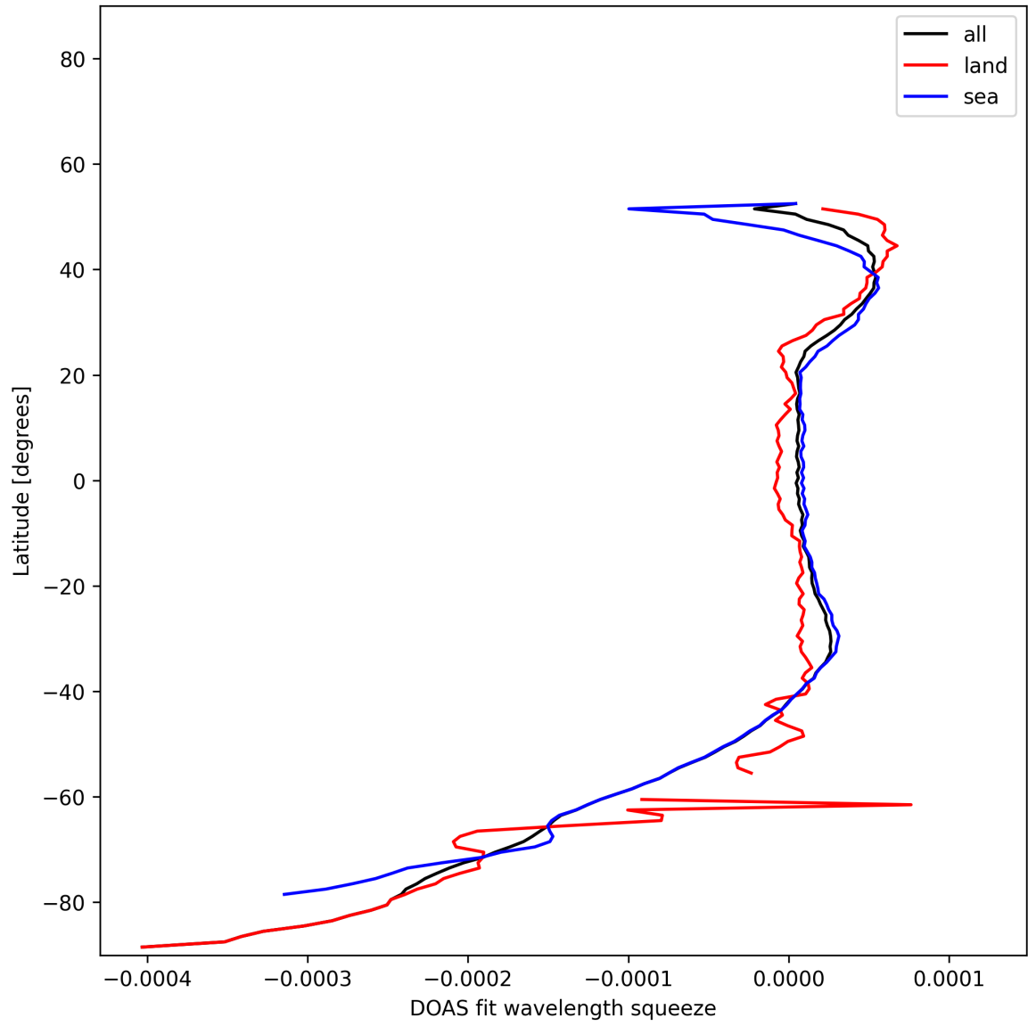
Figure 51: Zonal average of “DOAS fit wavelength squeeze” for 2025-11-12 to 2025-11-14.
