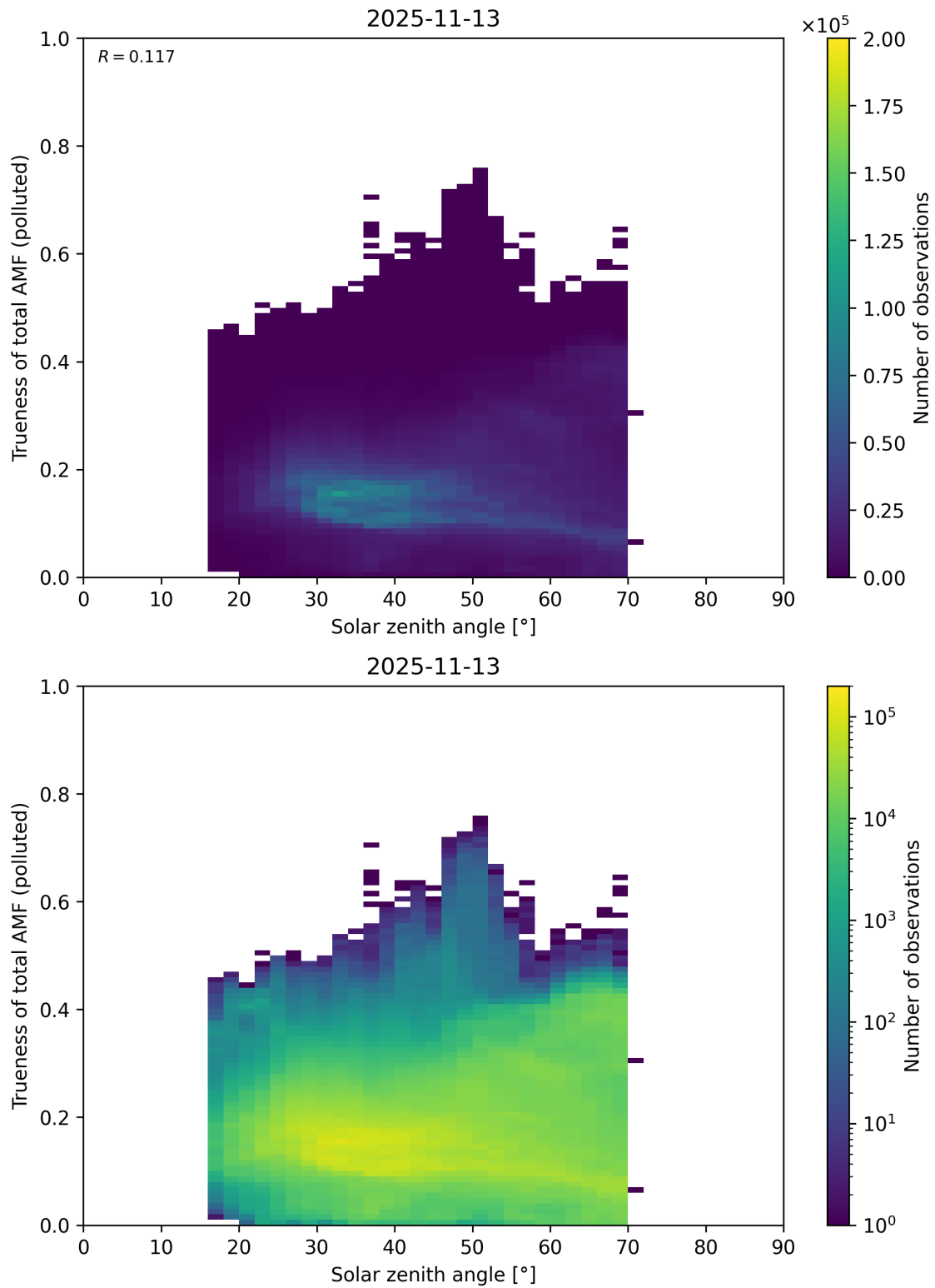
Figure 190: Scatter density plot of “Solar zenith angle” against “Trueness of total AMF (polluted)” for 2025-11-12 to 2025-11-14.
