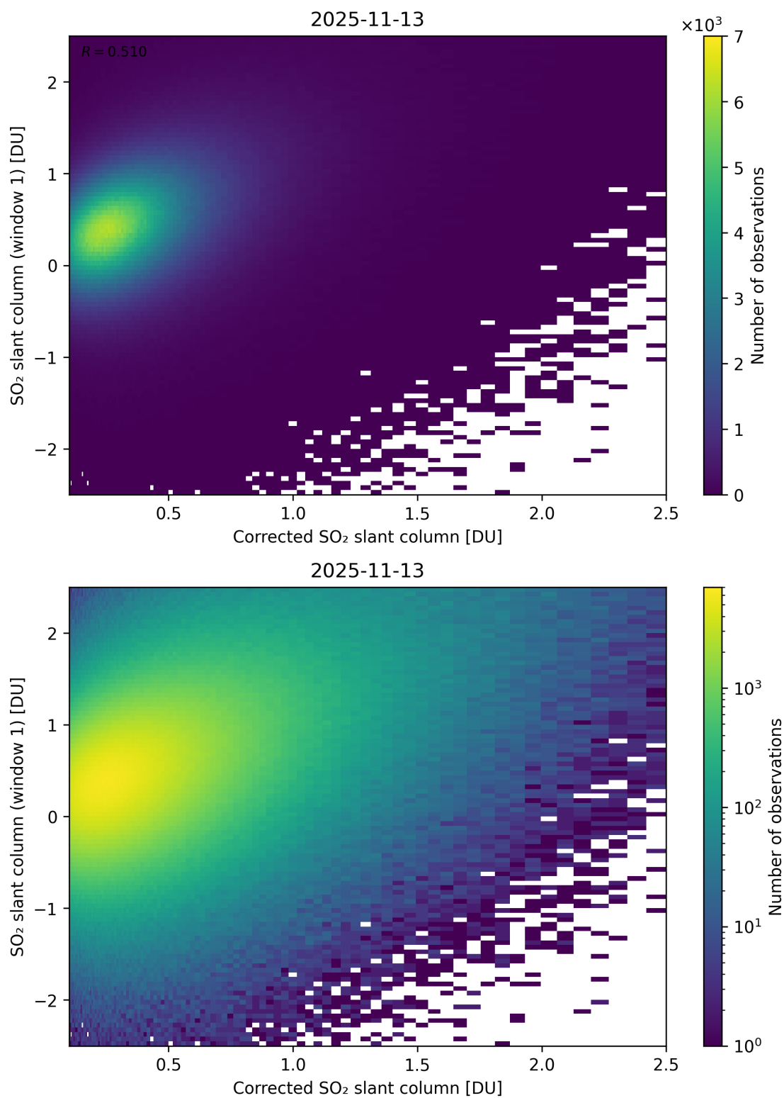
Figure 237: Scatter density plot of “Corrected SO 2 slant column” against “SO 2 slant column (window 1)” for 2025-11-12 to 2025-11-14.
