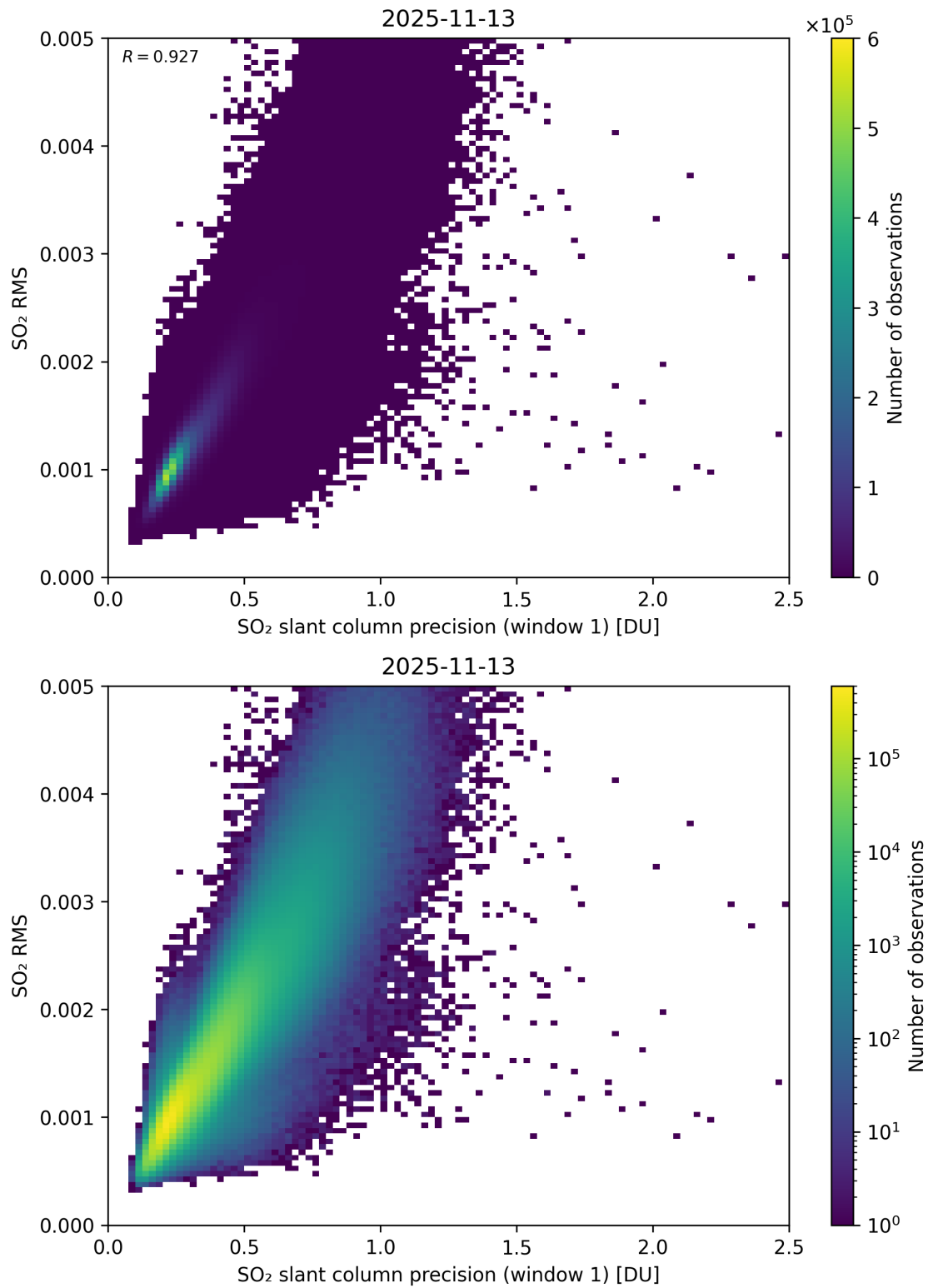
Figure 273: Scatter density plot of “SO 2 slant column precision (window 1)” against “SO 2 RMS” for 2025-11-12 to 2025-11-14.
