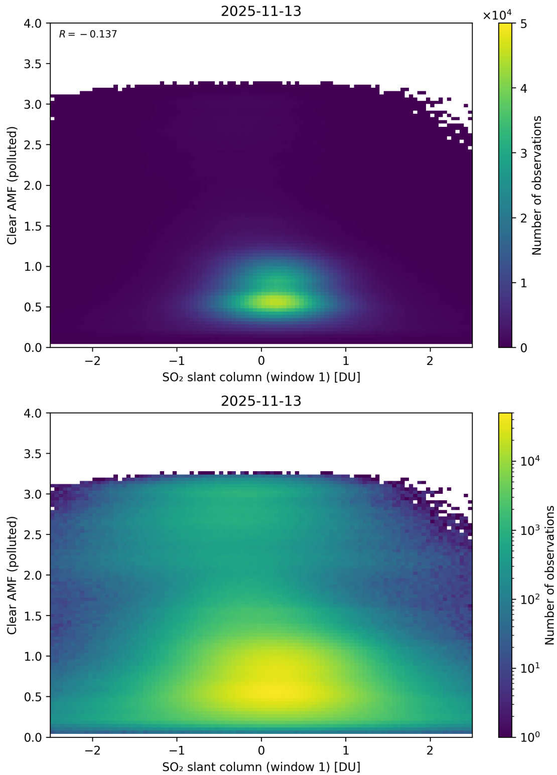
Figure 282: Scatter density plot of “SO 2 slant column (window 1)” against “Clear AMF (polluted)” for 2025-11-12 to 2025-11-14.
