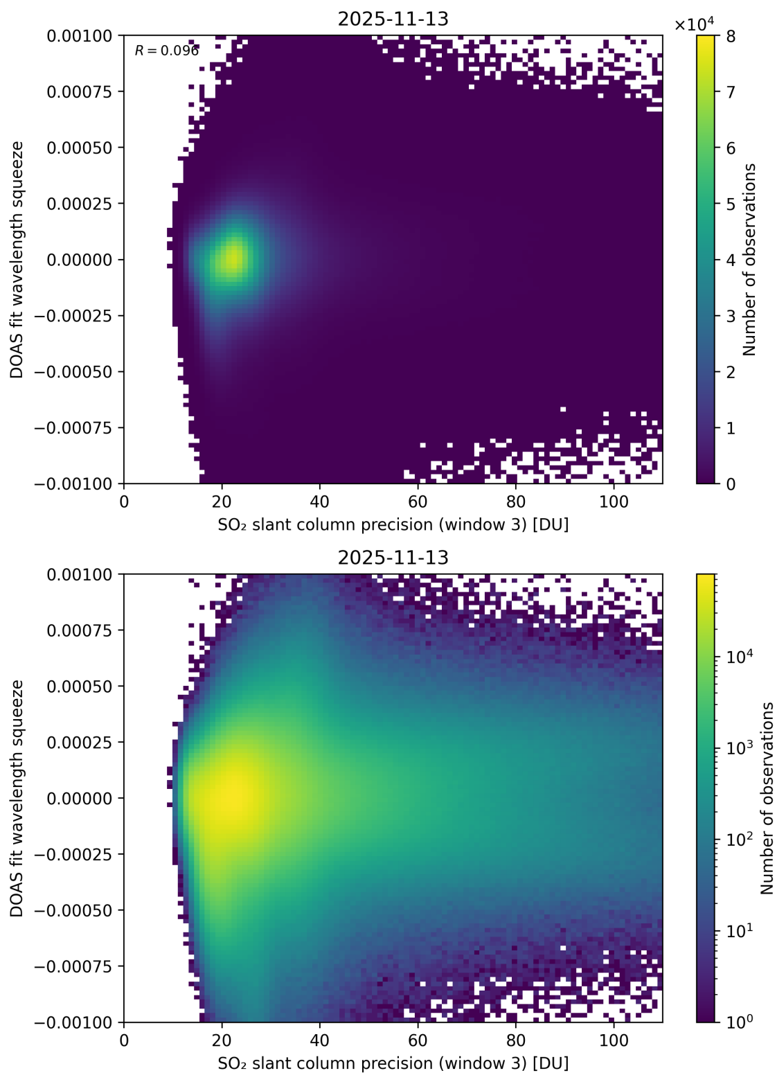
Figure 309: Scatter density plot of “SO 2 slant column precision (window 3)” against “DOAS fit wavelength squeeze” for 2025-11-12 to 2025-11-14.
