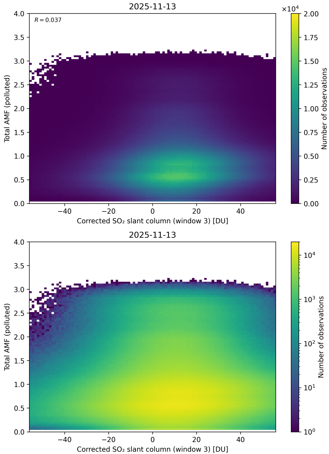
Figure 260: Scatter density plot of “Corrected SO 2 slant column (window 3)” against “Total AMF (polluted)” for 2025-11-12 to 2025-11-14.
