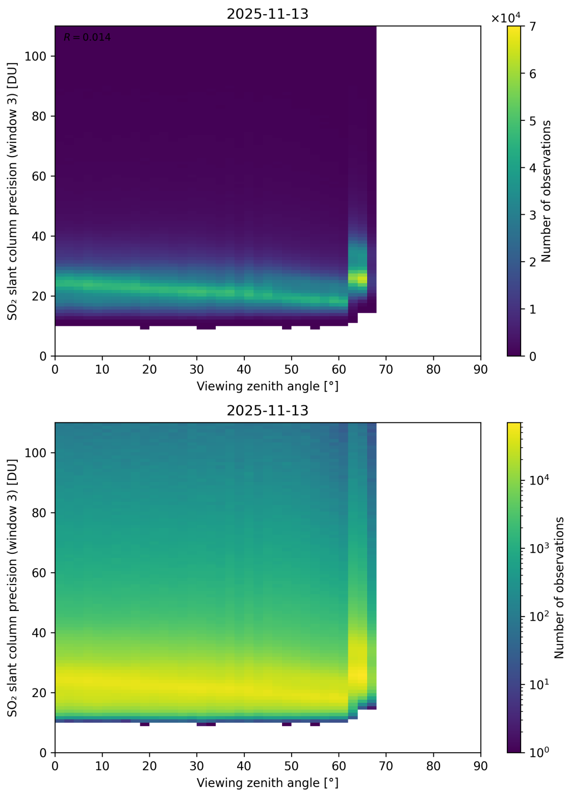
Figure 380: Scatter density plot of “Viewing zenith angle” against “SO 2 slant column precision (window 3)” for 2025-11-12 to 2025-11-14.
