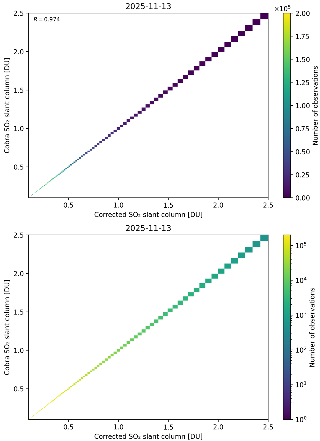
Figure 233: Scatter density plot of “Corrected SO 2 slant column” against “Cobra SO 2 slant column” for 2025-11-12 to 2025-11-14.
