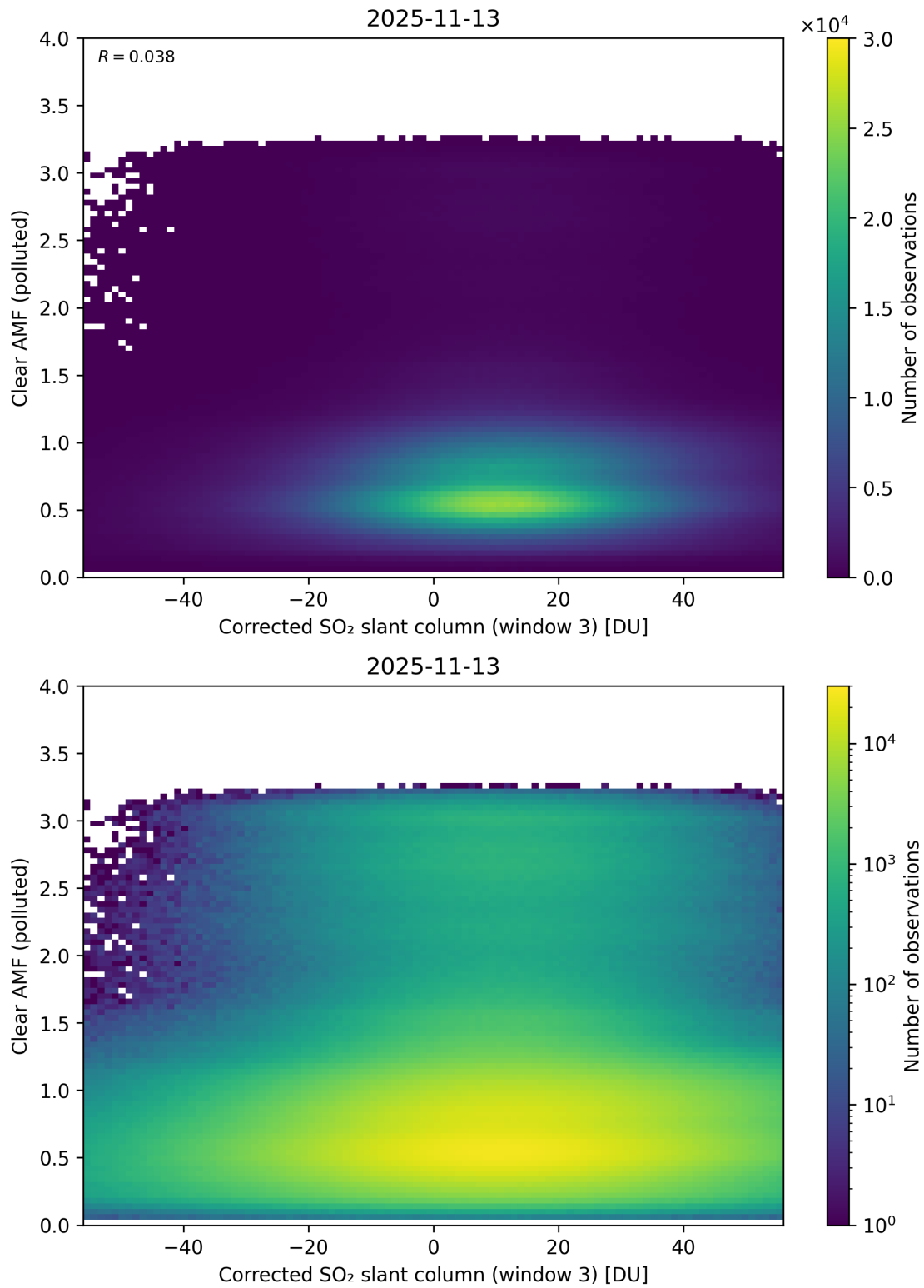
Figure 259: Scatter density plot of “Corrected SO 2 slant column (window 3)” against “Clear AMF (polluted)” for 2025-11-12 to 2025-11-14.
