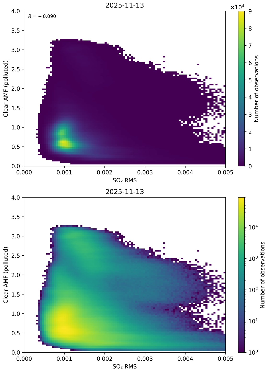
Figure 147: Scatter density plot of “SO 2 RMS” against “Clear AMF (polluted)” for 2025-11-12 to 2025-11-14.
