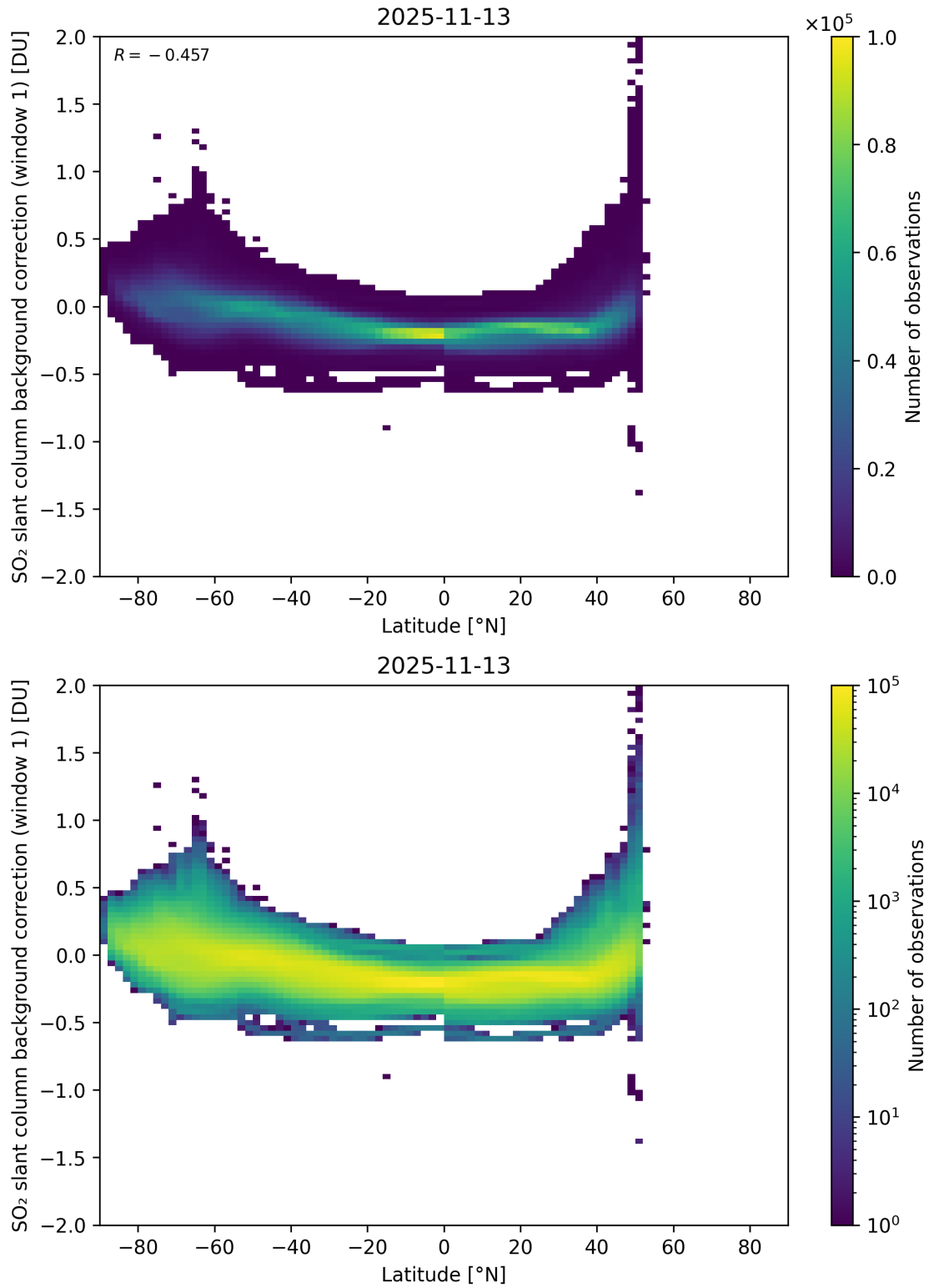
Figure 150: Scatter density plot of “Latitude” against “SO 2 slant column background correction (window 1)” for 2025-11-12 to 2025-11-14.
