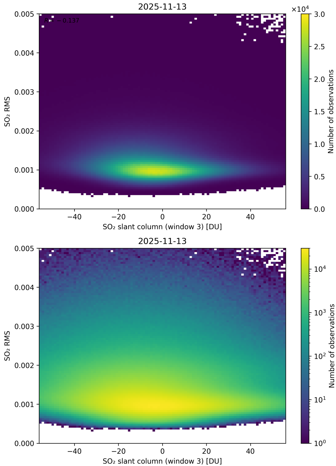
Figure 306: Scatter density plot of “SO 2 slant column (window 3)” against “SO 2 RMS” for 2025-11-12 to 2025-11-14.
