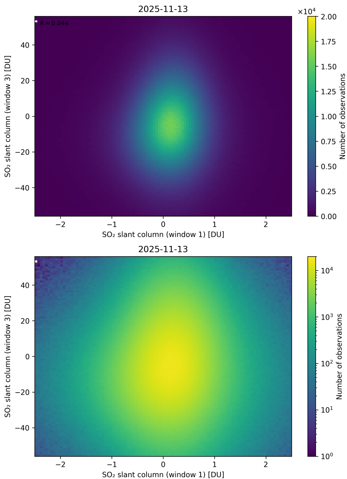
Figure 287: Scatter density plot of “SO 2 slant column (window 1)” against “SO 2 slant column (window 3)” for 2025-11-12 to 2025-11-14.
