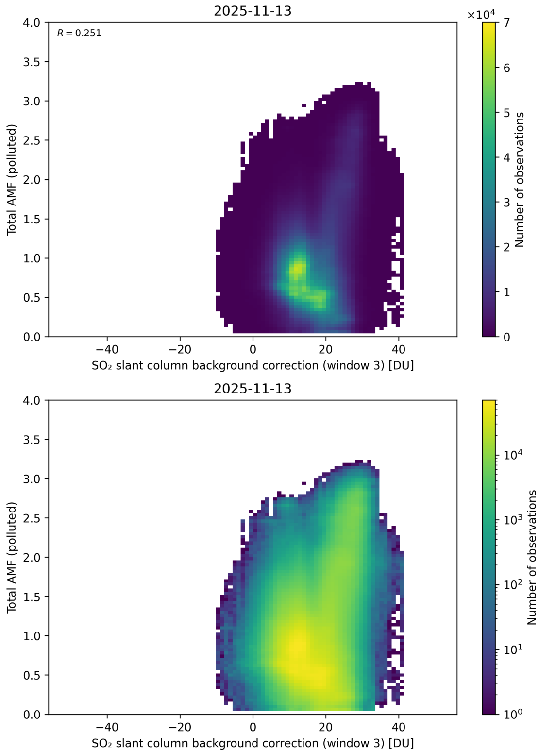
Figure 136: Scatter density plot of “SO 2 slant column background correction (window 3)” against “Total AMF (polluted)” for 2025-11-12 to 2025-11-14.
