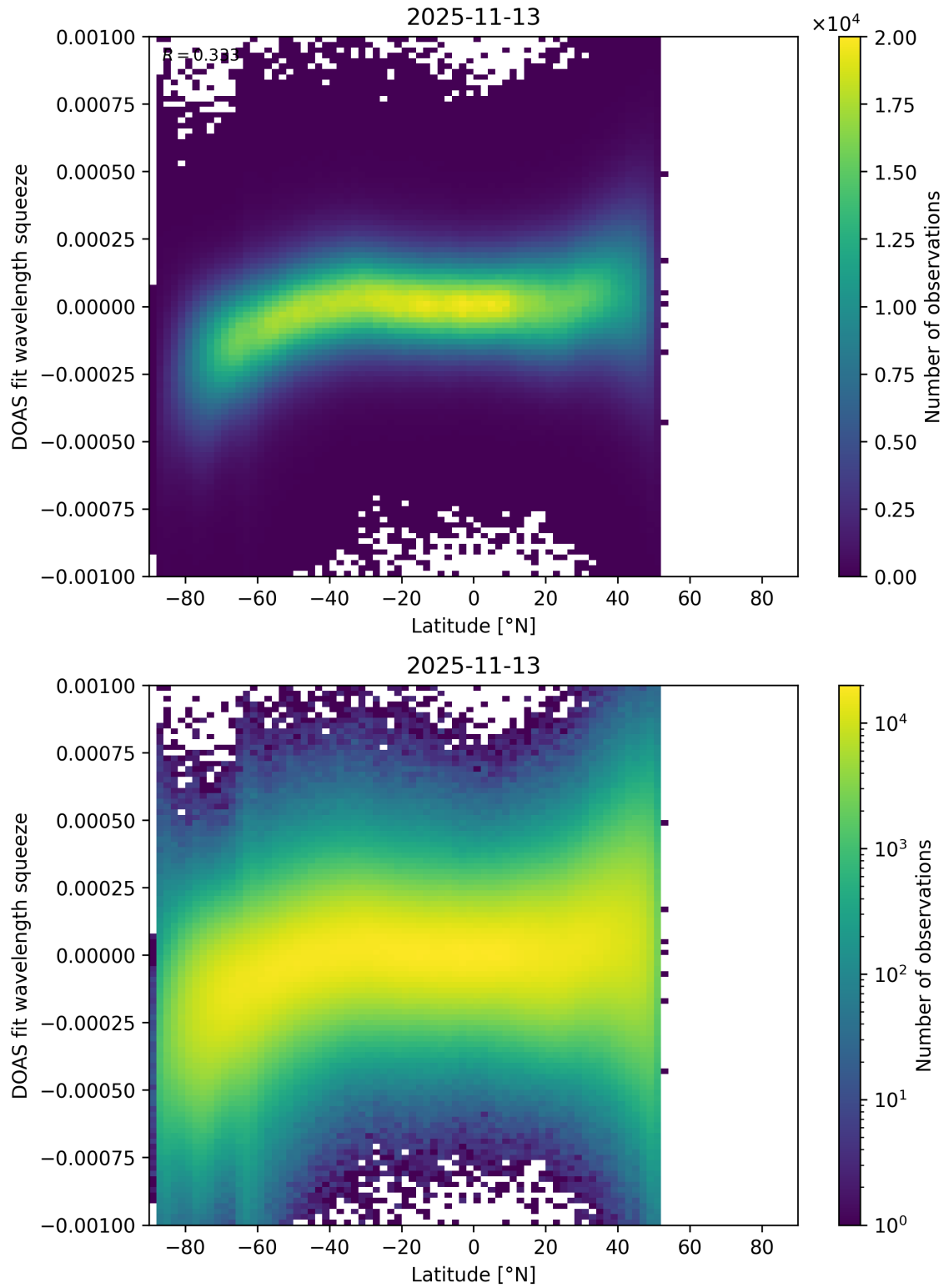
Figure 154: Scatter density plot of "Latitude" against "DOAS fit wavelength squeeze" for 2025-11-12 to 2025-11-14.
