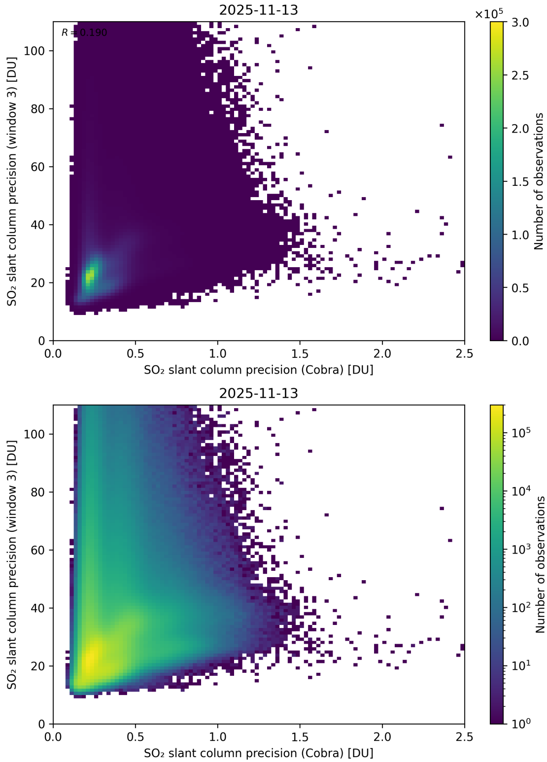
Figure 212: Scatter density plot of “SO 2 slant column precision (Cobra)” against “SO 2 slant column precision (window 3)” for 2025-11-12 to 2025-11-14.
