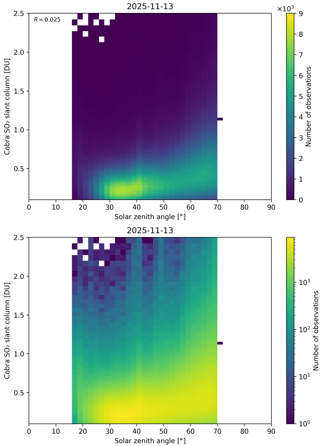
Figure 179: Scatter density plot of “Solar zenith angle” against “Cobra SO 2 slant column” for 2025-11-12 to 2025-11-14.
