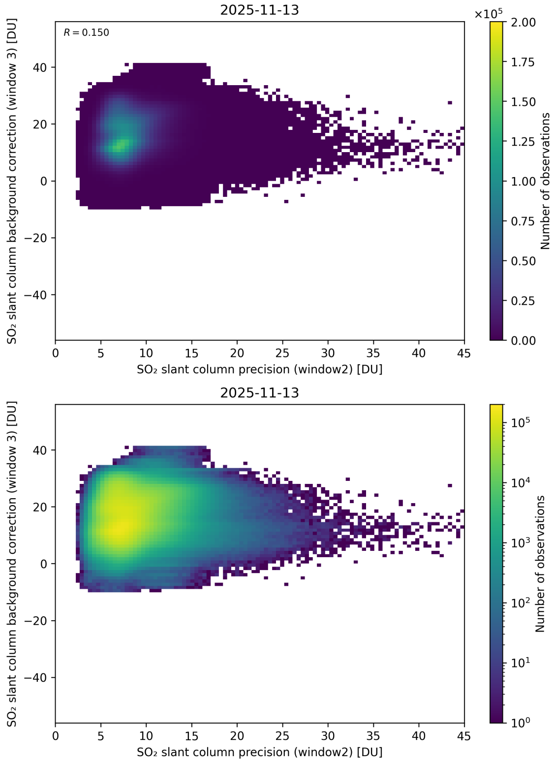
Figure 292: Scatter density plot of “SO 2 slant column precision (window2)” against “SO 2 slant column background correction (window 3)” for 2025-11-12 to 2025-11-14.
