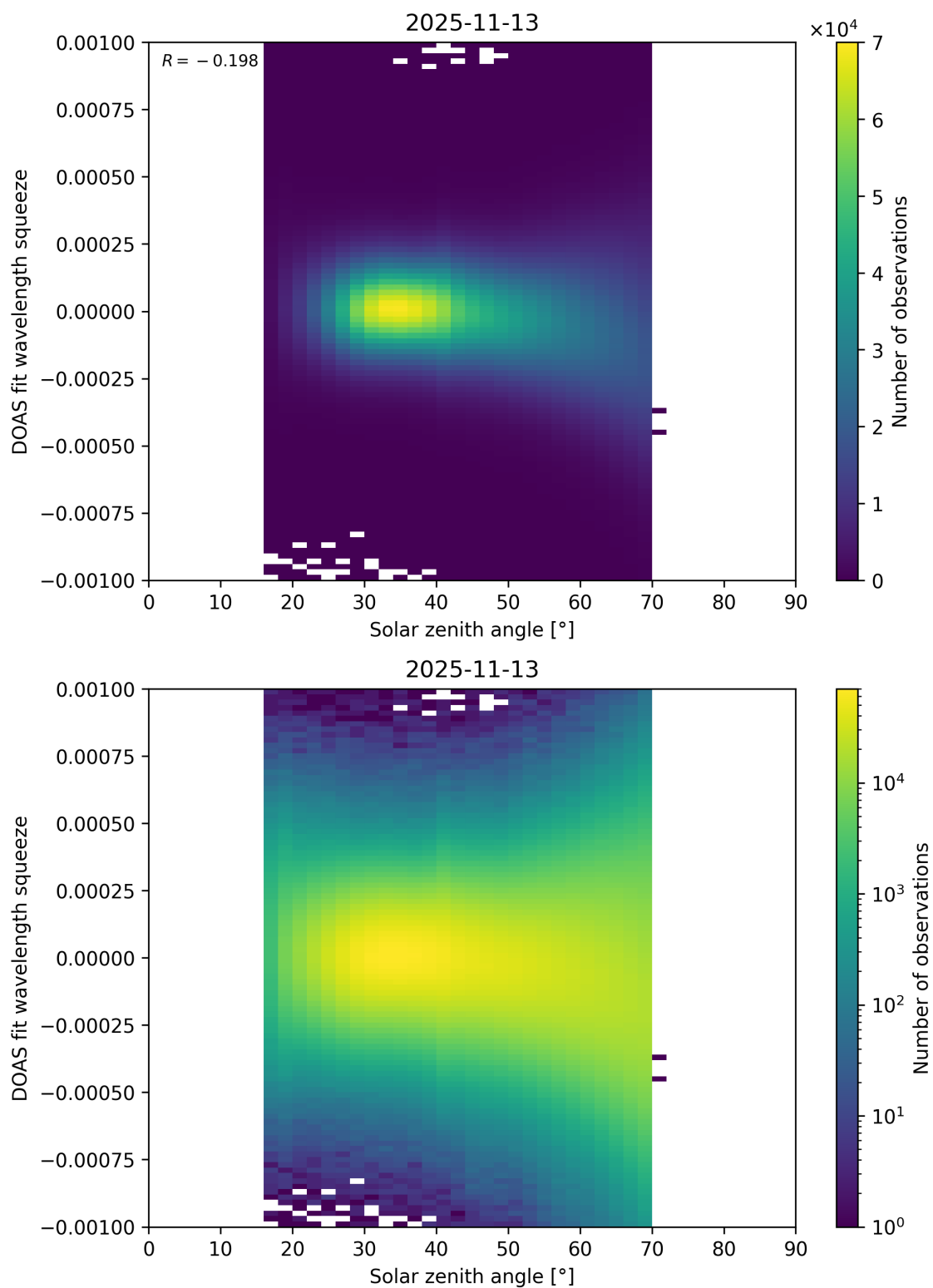
Figure 175: Scatter density plot of “Solar zenith angle” against “DOAS fit wavelength squeeze” for 2025-11-12 to 2025-11-14.
