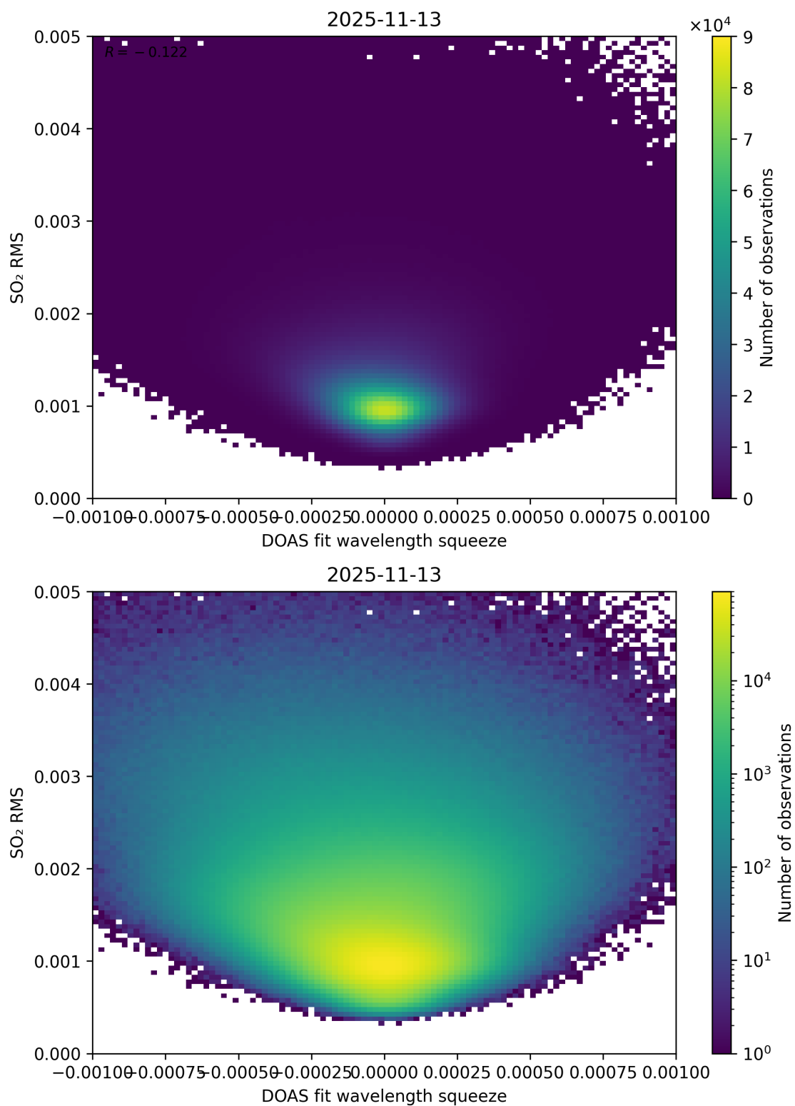
Figure 143: Scatter density plot of “DOAS fit wavelength squeeze” against “SO 2 RMS” for 2025-11-12 to 2025-11-14.
