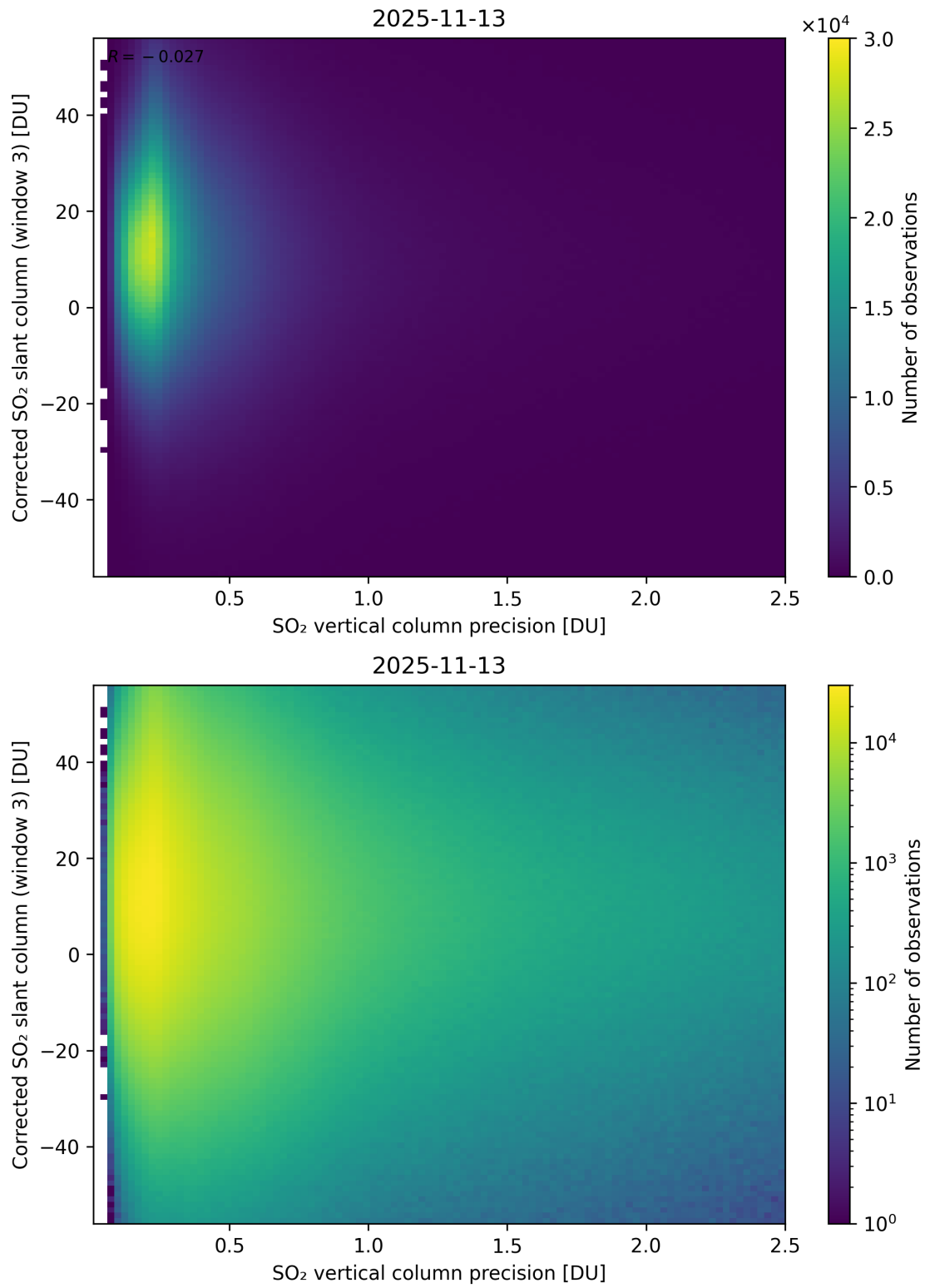
Figure 340: Scatter density plot of “SO 2 vertical column precision” against “Corrected SO 2 slant column (window 3)” for 2025-11-12 to 2025-11-14.
