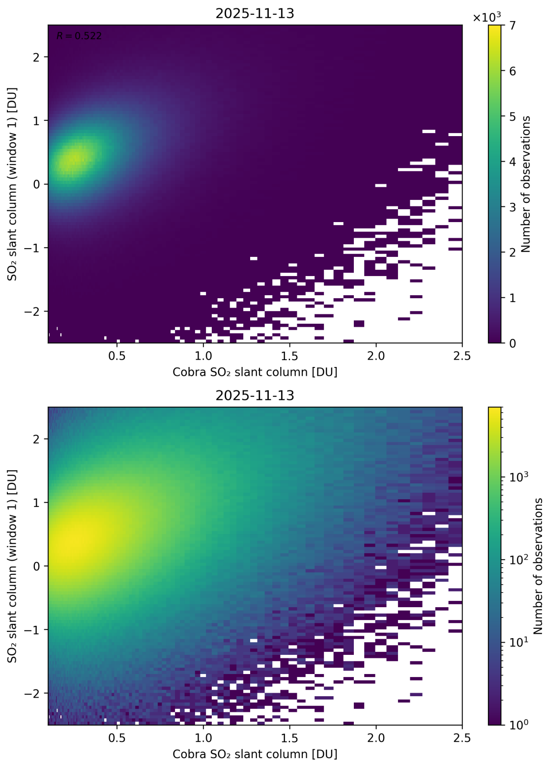
Figure 219: Scatter density plot of “Cobra SO 2 slant column” against “SO 2 slant column (window 1)” for 2025-11-12 to 2025-11-14.
