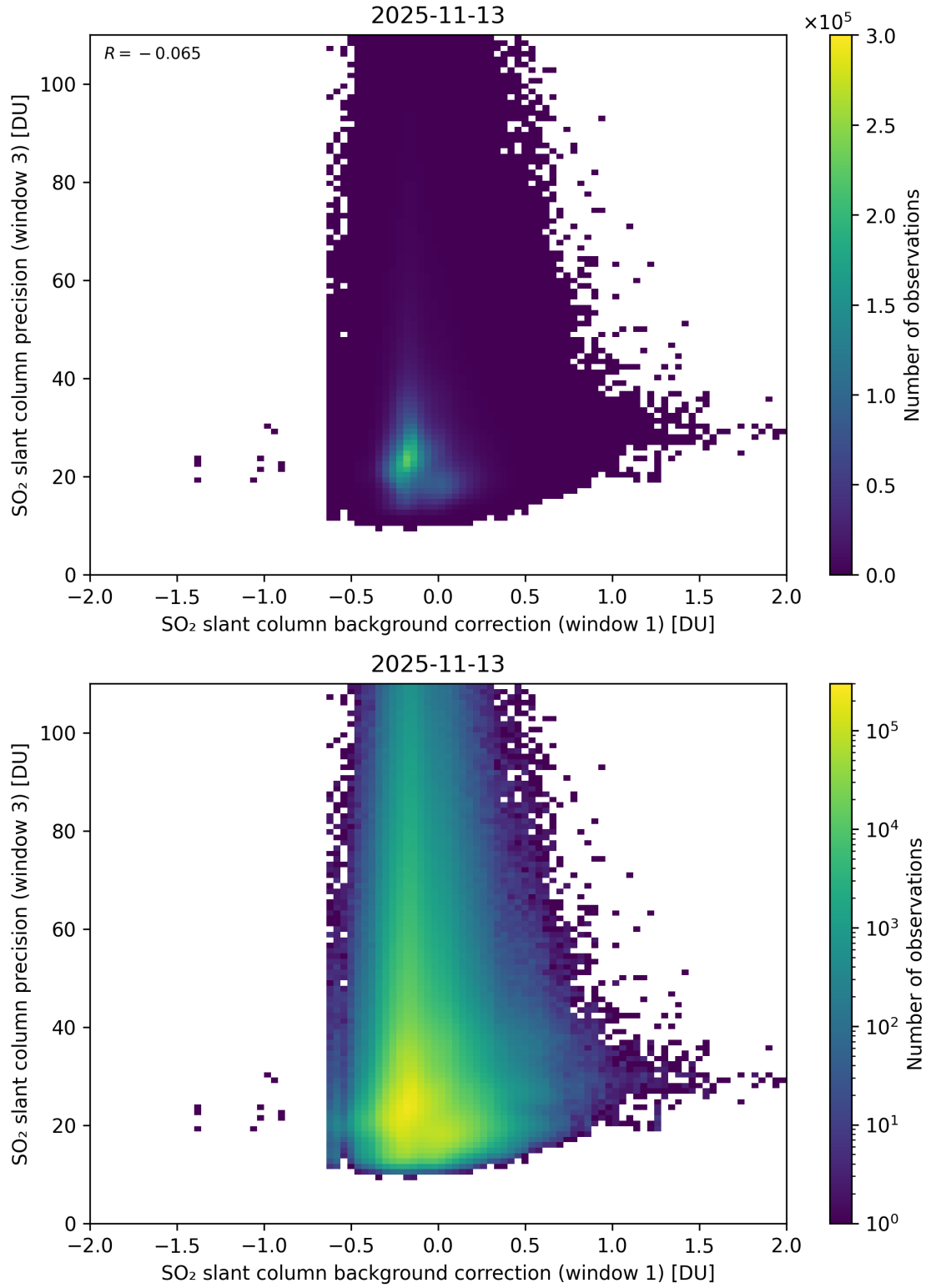
Figure 119: Scatter density plot of “SO 2 slant column background correction (window 1)” against “SO 2 slant column precision (window 3)” for 2025-11-12 to 2025-11-14.
