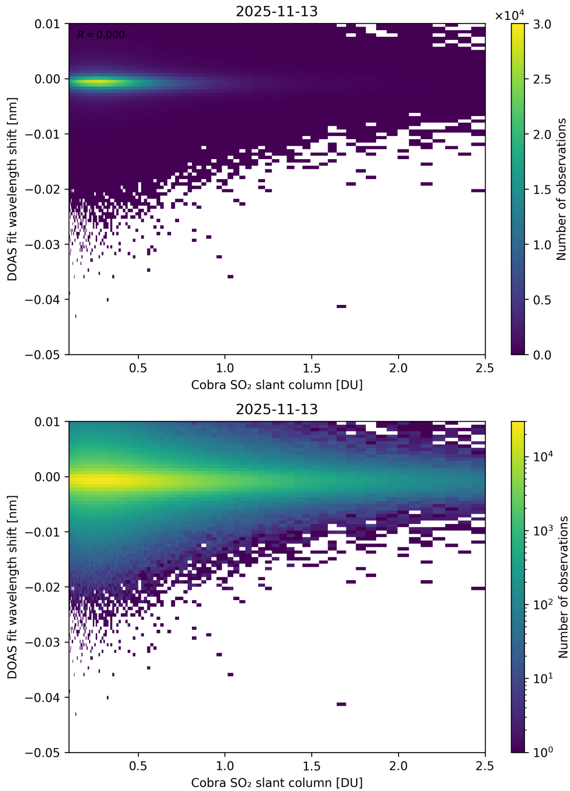
Figure 196: Scatter density plot of “Cobra SO 2 slant column” against “DOAS fit wavelength shift” for 2025-11-12 to 2025-11-14.
