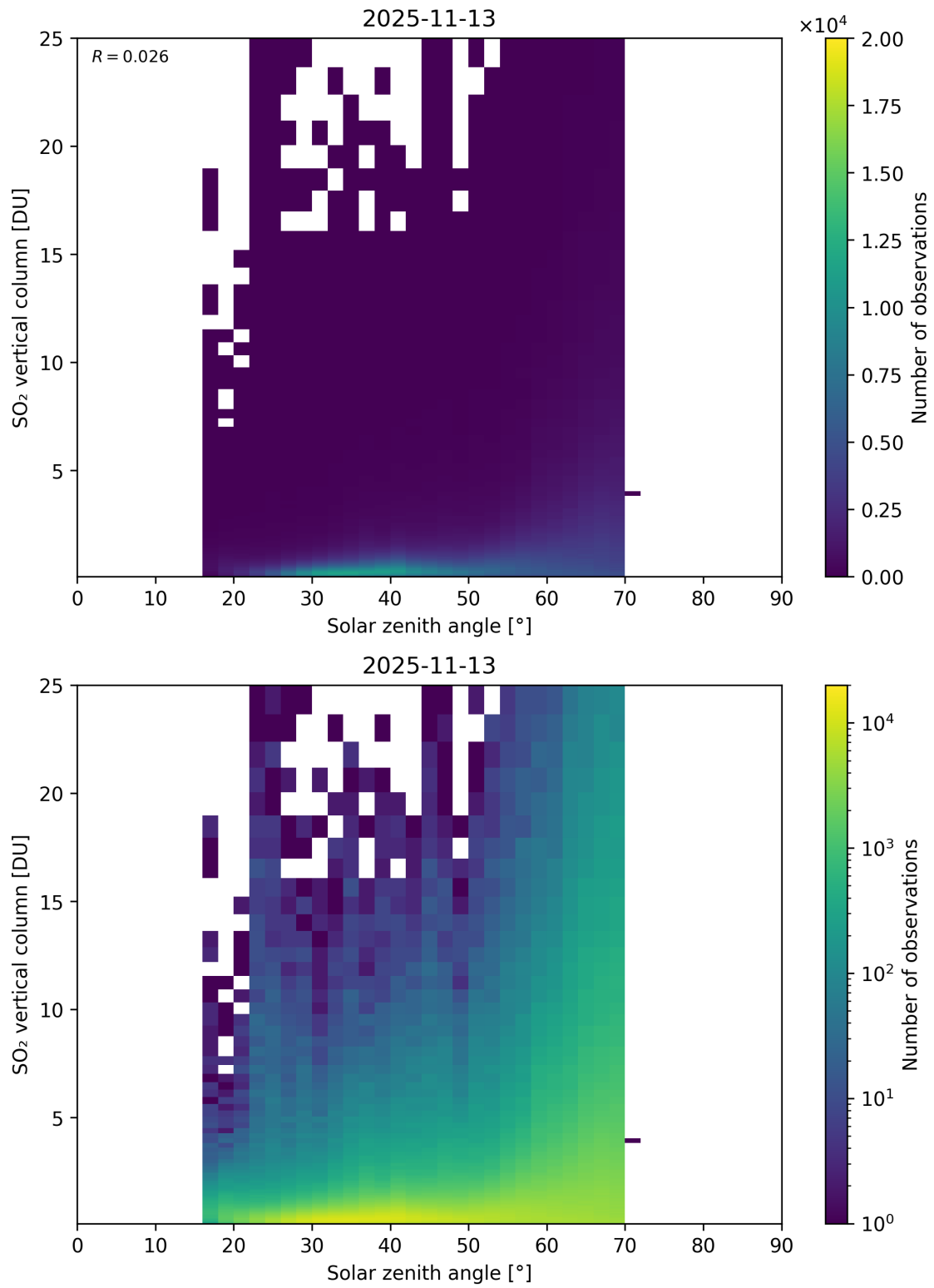
Figure 191: Scatter density plot of “Solar zenith angle” against “SO 2 vertical column” for 2025-11-12 to 2025-11-14.
