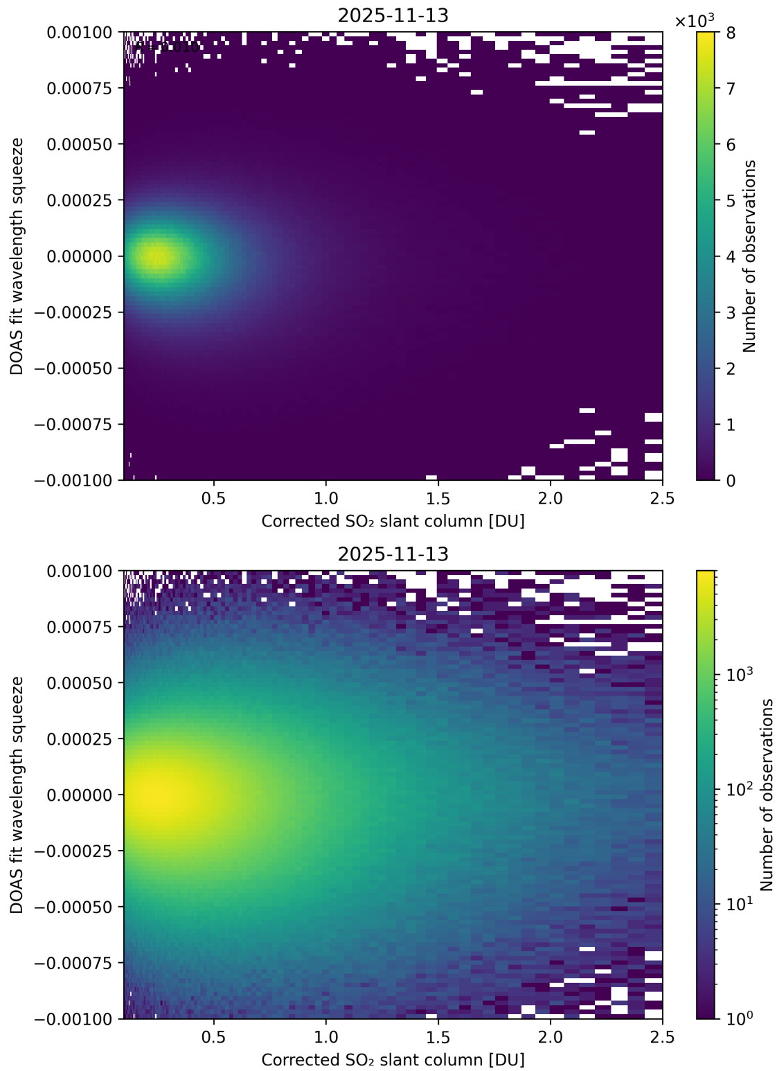
Figure 230: Scatter density plot of “Corrected SO 2 slant column” against “DOAS fit wavelength squeeze” for 2025-11-12 to 2025-11-14.
