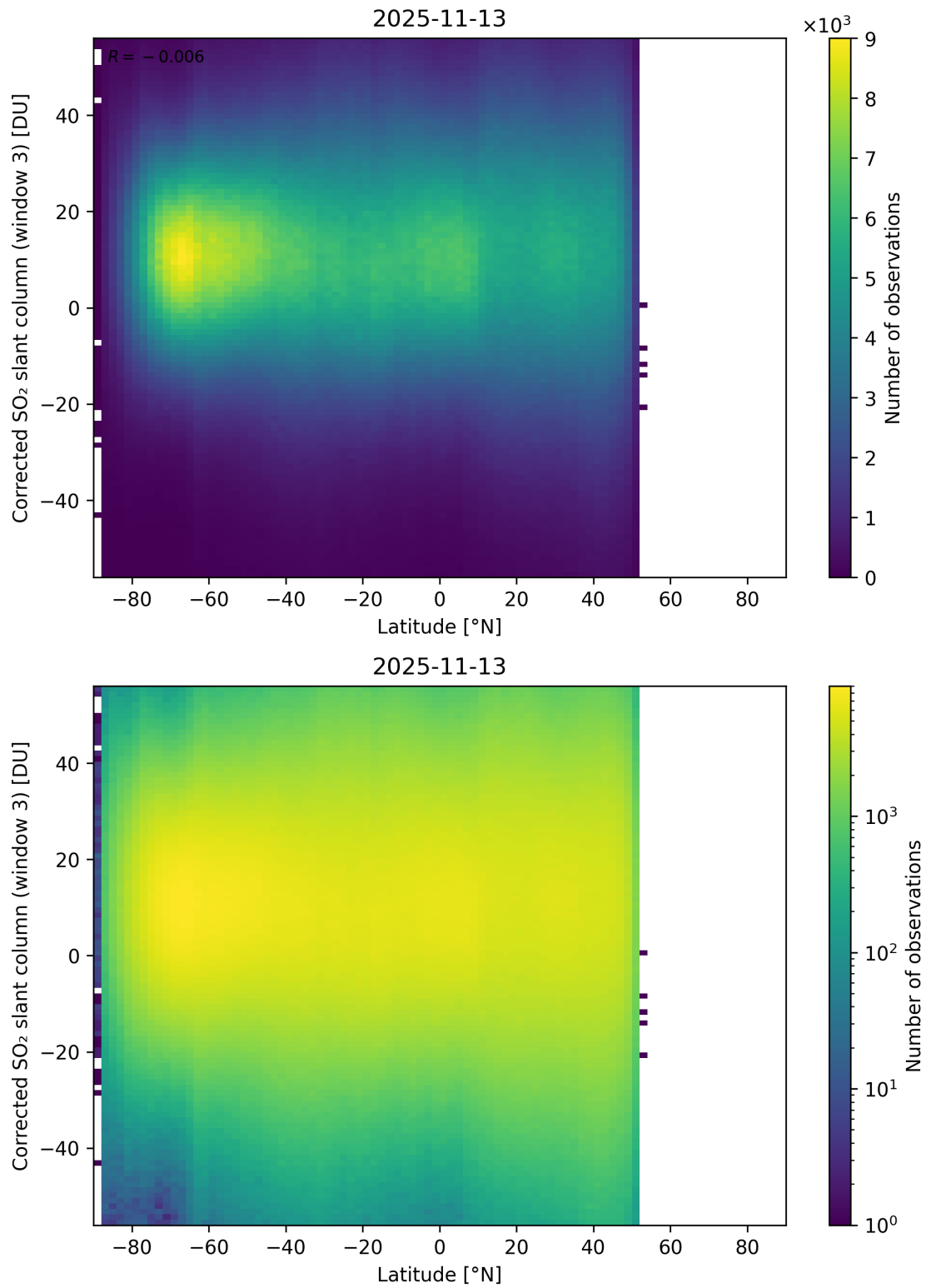
Figure 161: Scatter density plot of “Latitude” against “Corrected SO 2 slant column (window 3)” for 2025-11-12 to 2025-11-14.
