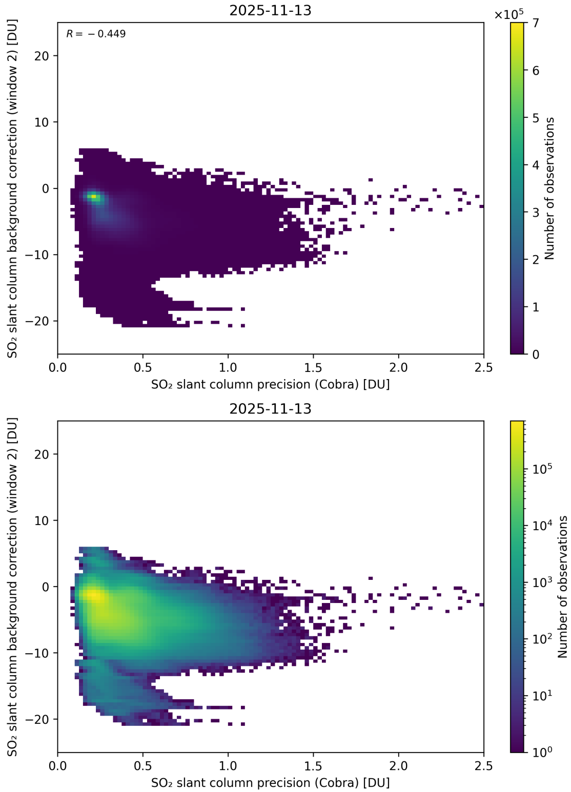
Figure 200: Scatter density plot of “SO 2 slant column precision (Cobra)” against “SO 2 slant column background correction (window 2)” for 2025-11-12 to 2025-11-14.
