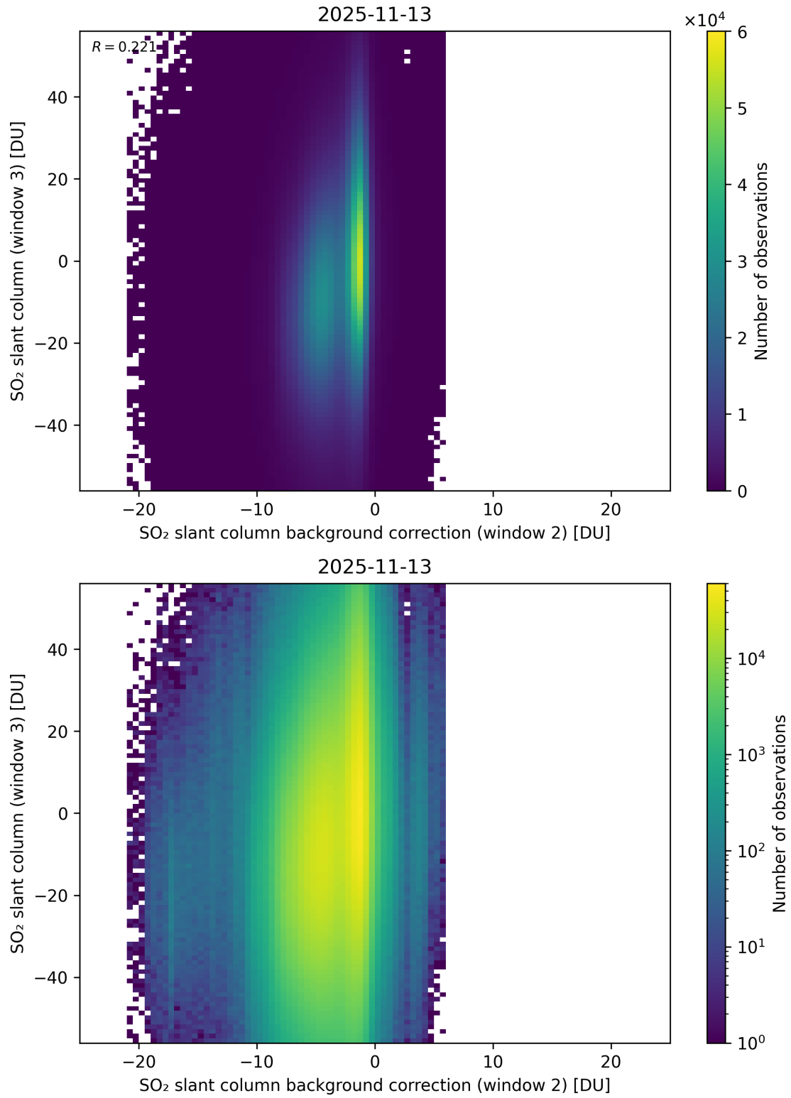
Figure 128: Scatter density plot of “SO 2 slant column background correction (window 2)” against “SO 2 slant column (window 3)” for 2025-11-12 to 2025-11-14.
