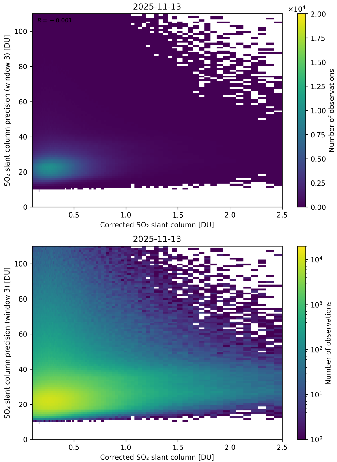
Figure 241: Scatter density plot of “Corrected SO 2 slant column” against “SO 2 slant column precision (window 3)” for 2025-11-12 to 2025-11-14.
