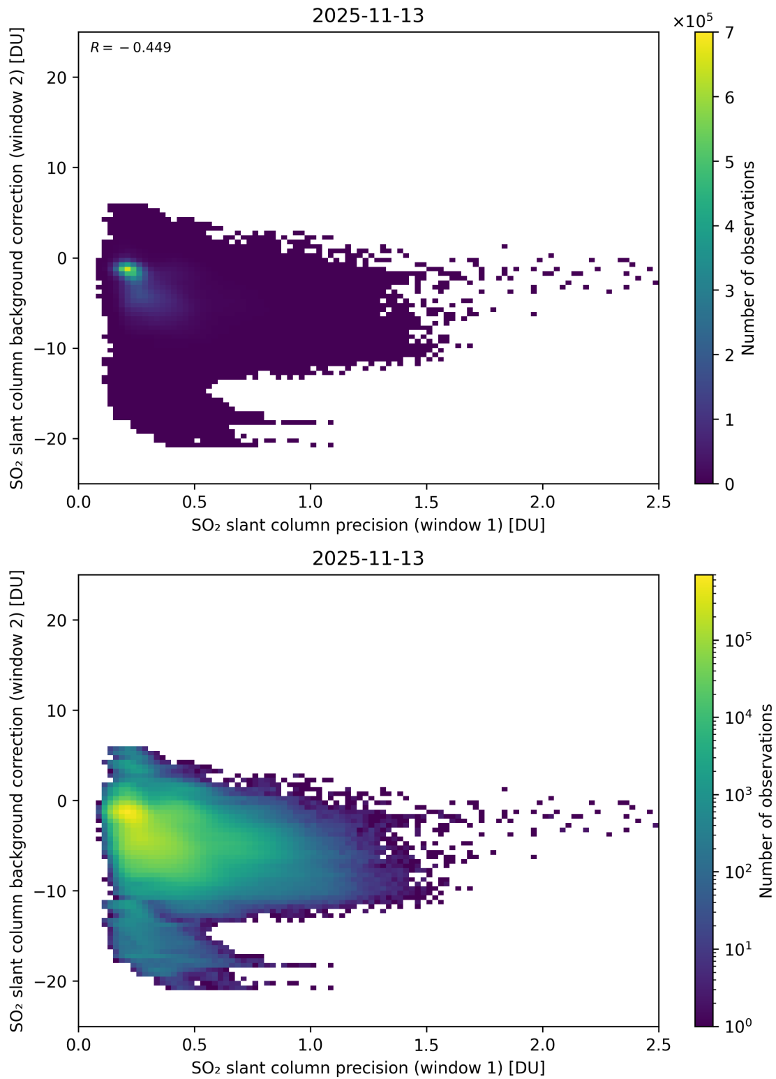
Figure 269: Scatter density plot of “SO 2 slant column precision (window 1)” against “SO 2 slant column background correction (window 2)” for 2025-11-12 to 2025-11-14.
