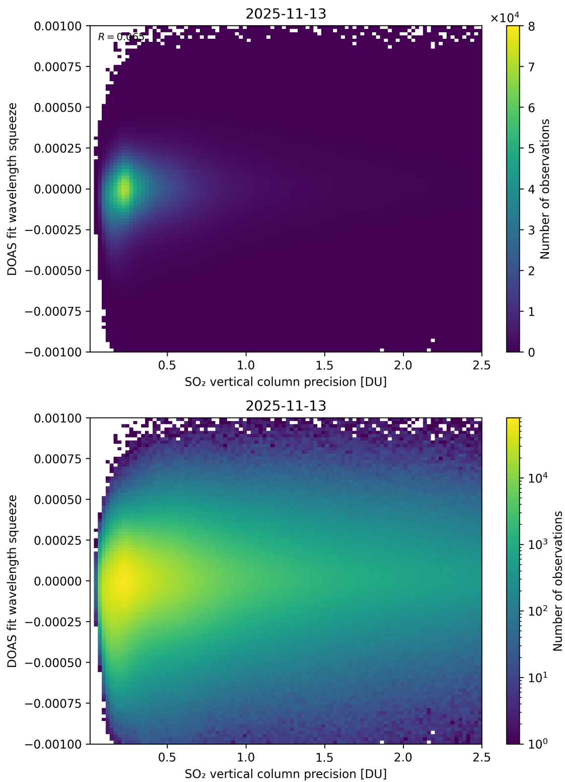
Figure 333: Scatter density plot of “SO 2 vertical column precision” against “DOAS fit wavelength squeeze” for 2025-11-12 to 2025-11-14.
