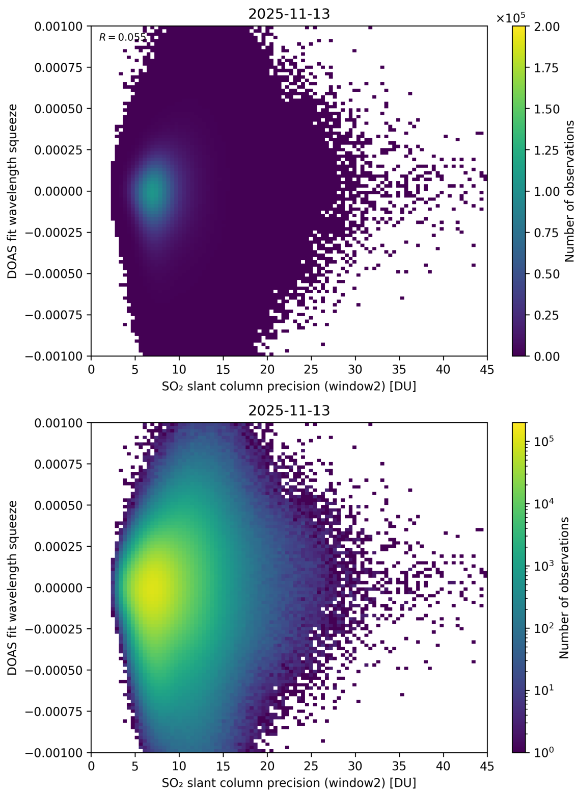
Figure 294: Scatter density plot of “SO 2 slant column precision (window2)” against “DOAS fit wavelength squeeze” for 2025-11-12 to 2025-11-14.
