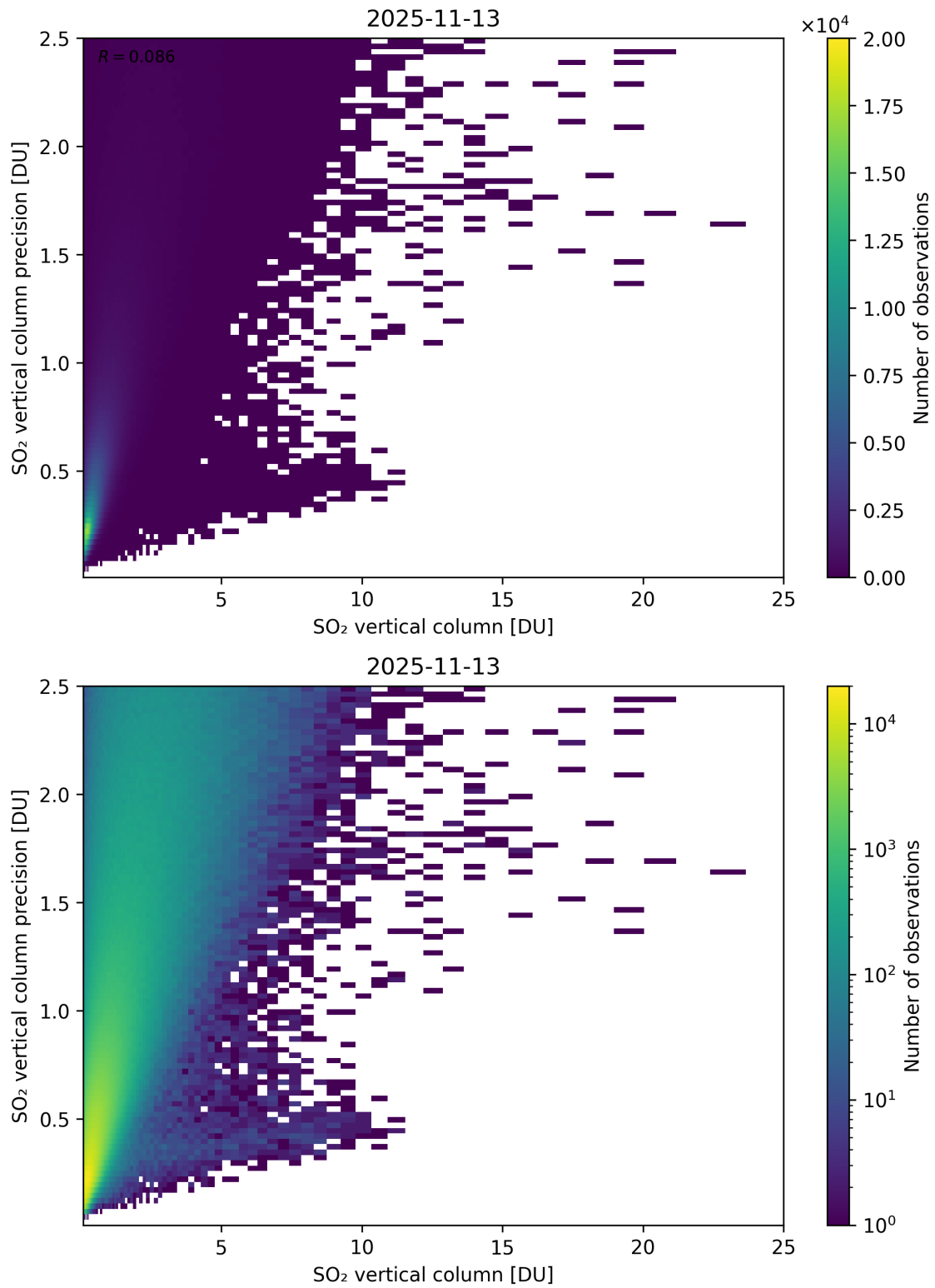
Figure 361: Scatter density plot of “SO 2 vertical column” against “SO 2 vertical column precision” for 2025-11-12 to 2025-11-14.
