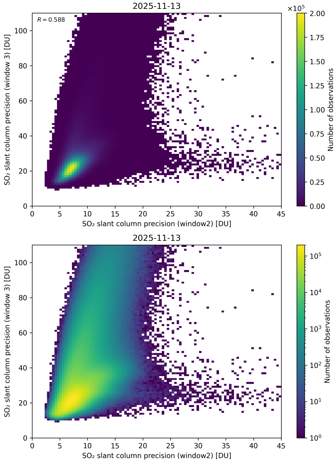
Figure 300: Scatter density plot of “SO 2 slant column precision (window2)” against “SO 2 slant column precision (window 3)” for 2025-11-12 to 2025-11-14.
