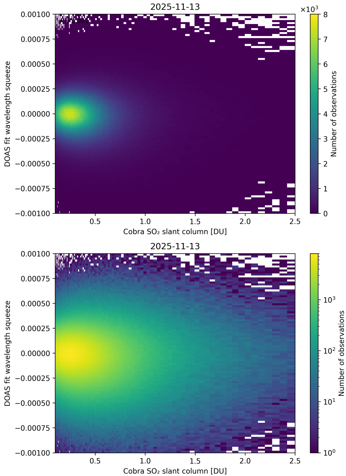
Figure 197: Scatter density plot of “Cobra SO 2 slant column” against “DOAS fit wavelength squeeze” for 2025-11-12 to 2025-11-14.
