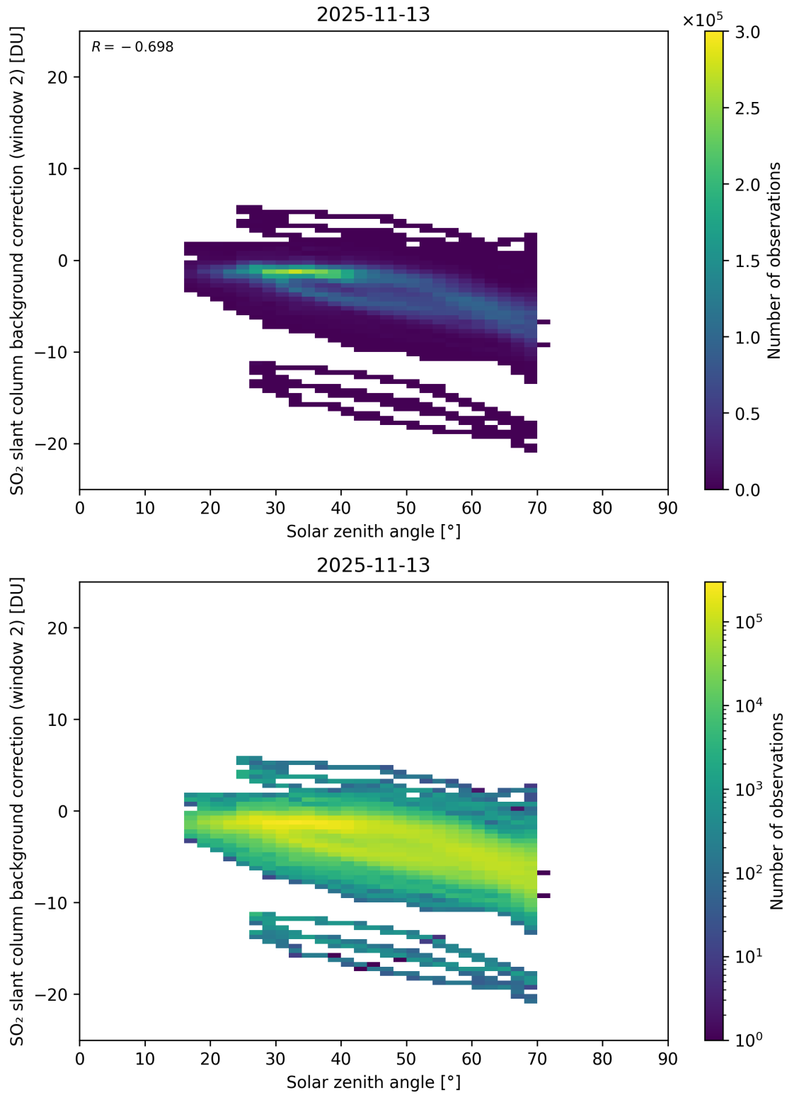
Figure 172: Scatter density plot of “Solar zenith angle” against “SO 2 slant column background correction (window 2)” for 2025-11-12 to 2025-11-14.
