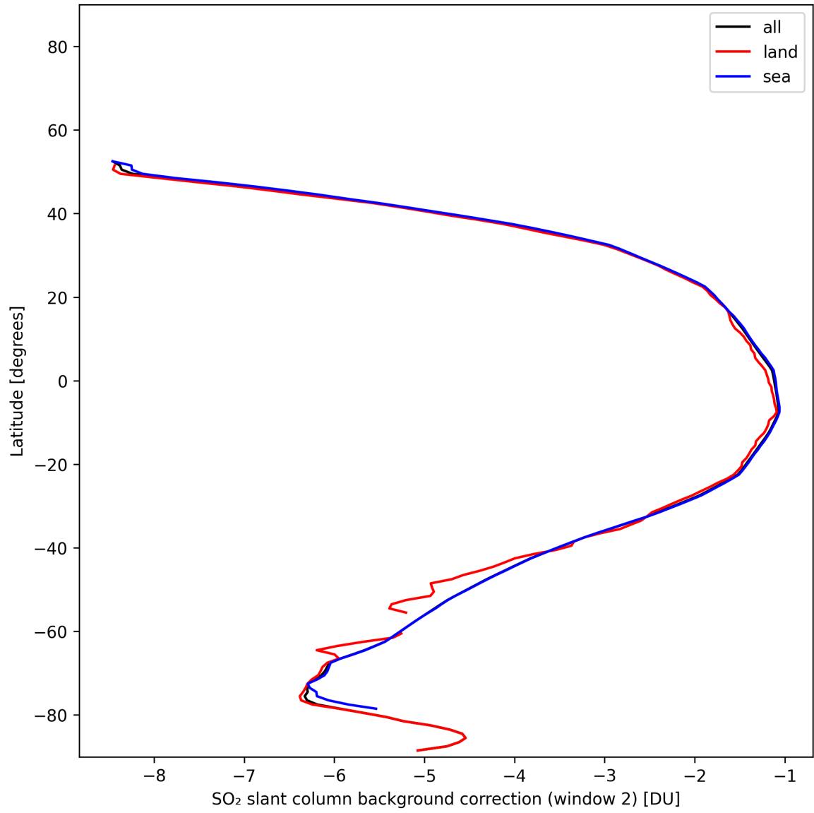
Figure 44: Zonal average of “SO 2 slant column background correction (window 2)” for 2025-11-12 to 2025-11-14.
