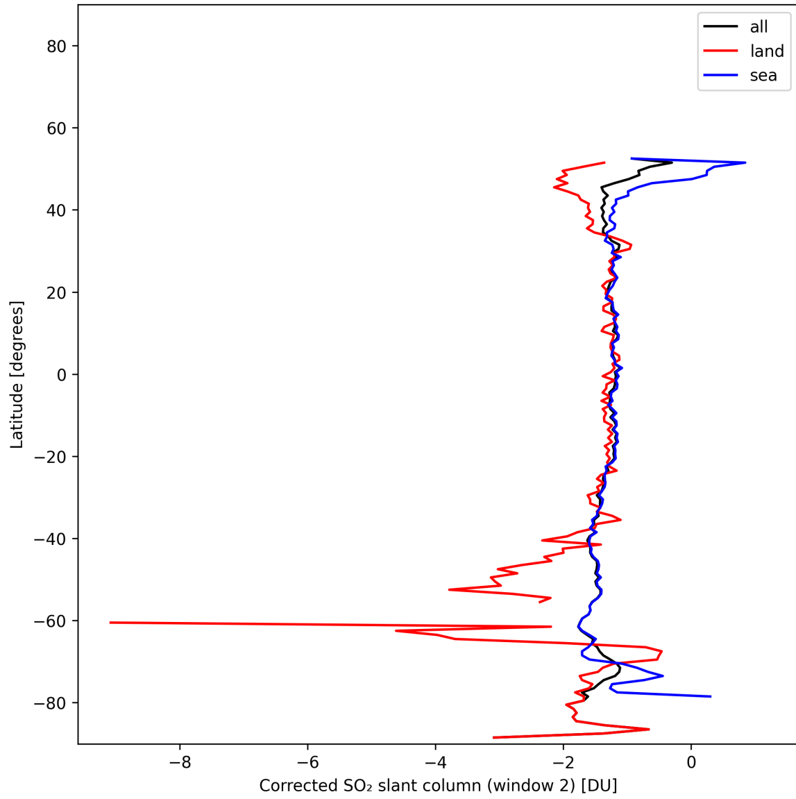
Figure 43: Zonal average of “Corrected SO 2 slant column (window 2)” for 2025-11-12 to 2025-11-14.
