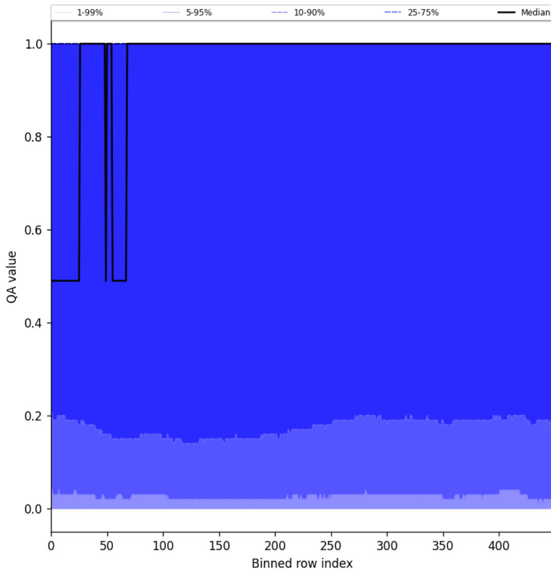
Figure 83: Along track statistics of “QA value” for 2025-11-12 to 2025-11-14
