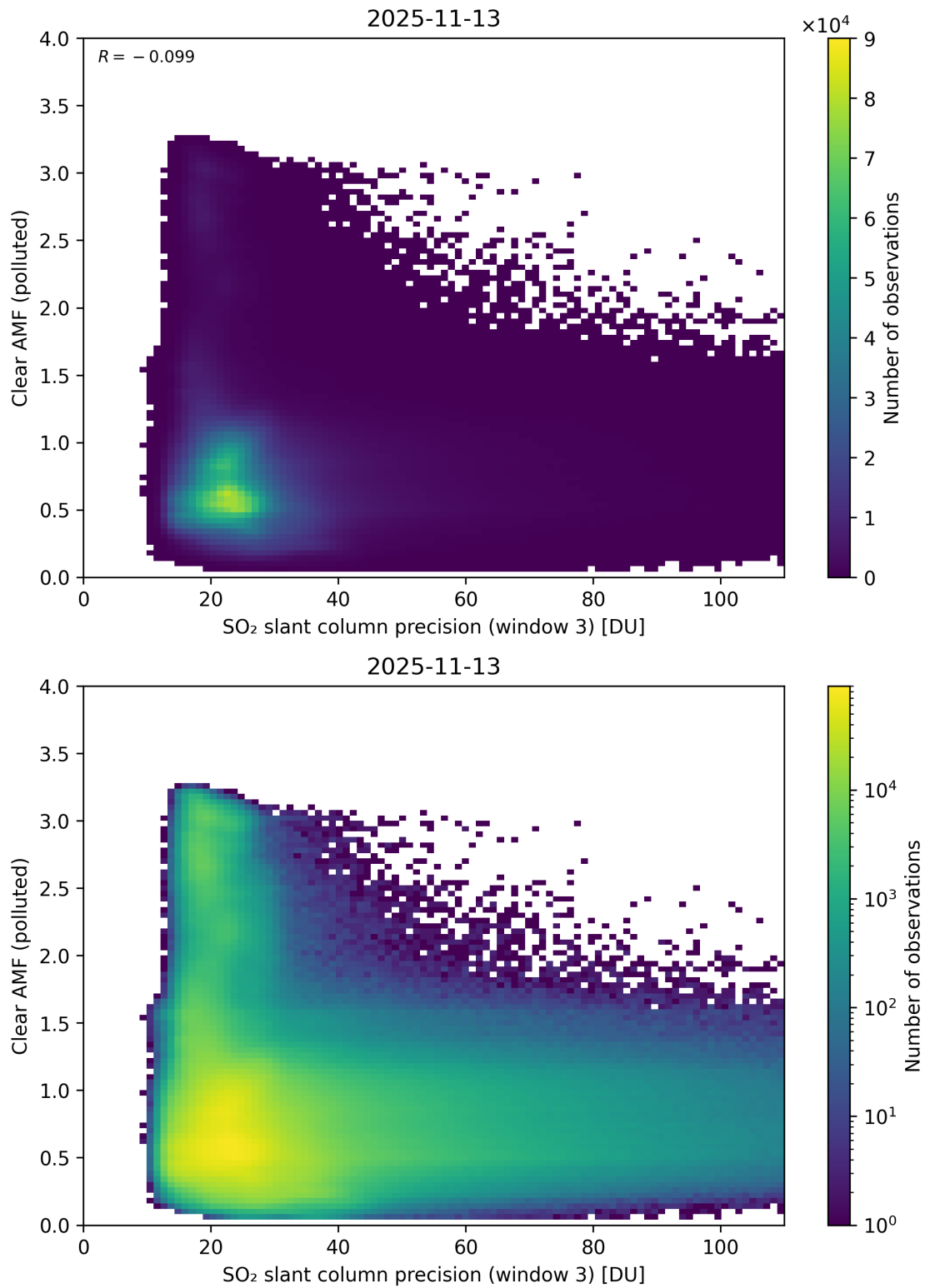
Figure 311: Scatter density plot of “SO 2 slant column precision (window 3)” against “Clear AMF (polluted)” for 2025-11-12 to 2025-11-14.
