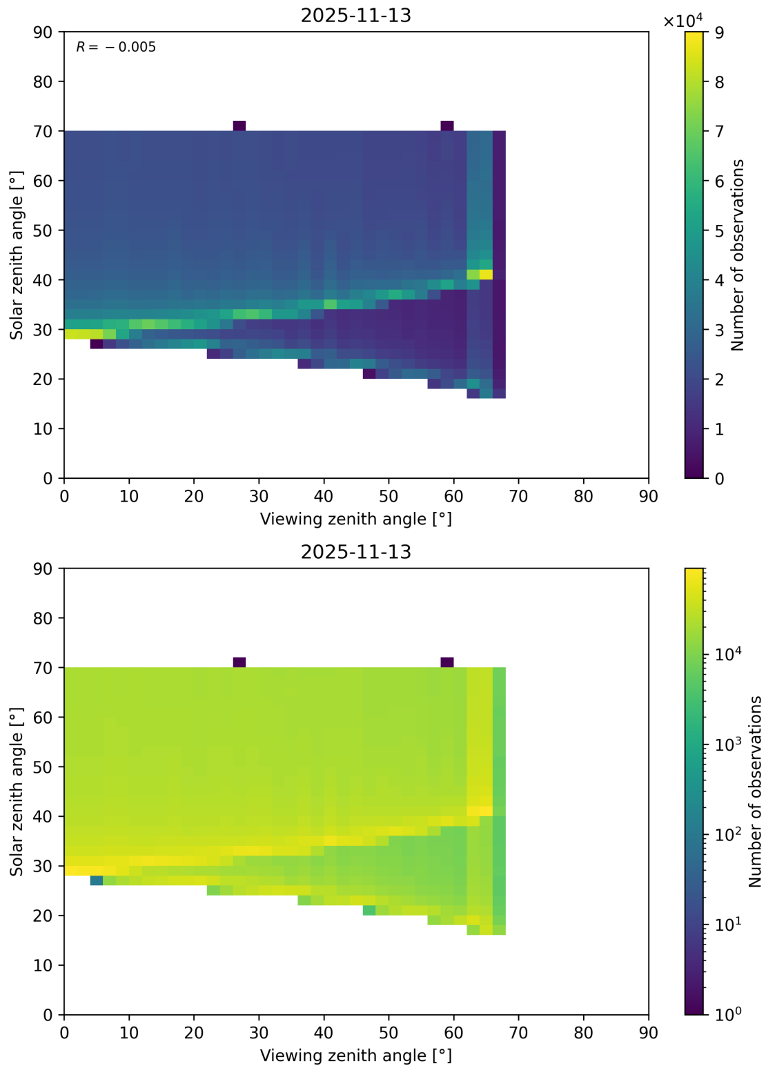
Figure 369: Scatter density plot of “Viewing zenith angle” against “Solar zenith angle” for 2025-11-12 to 2025-11-14.
