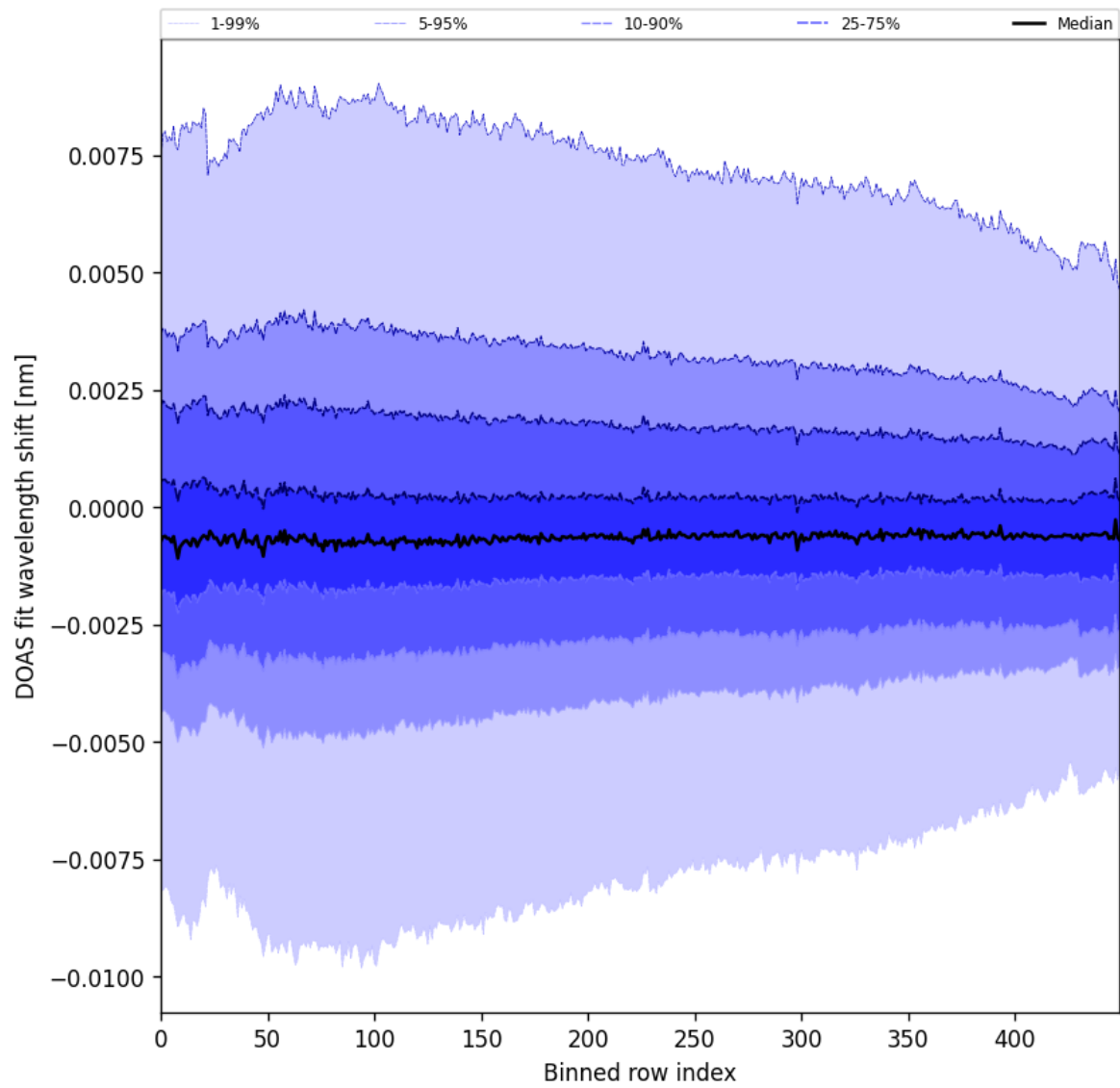
Figure 102: Along track statistics of “DOAS fit wavelength shift” for 2025-11-12 to 2025-11-14
