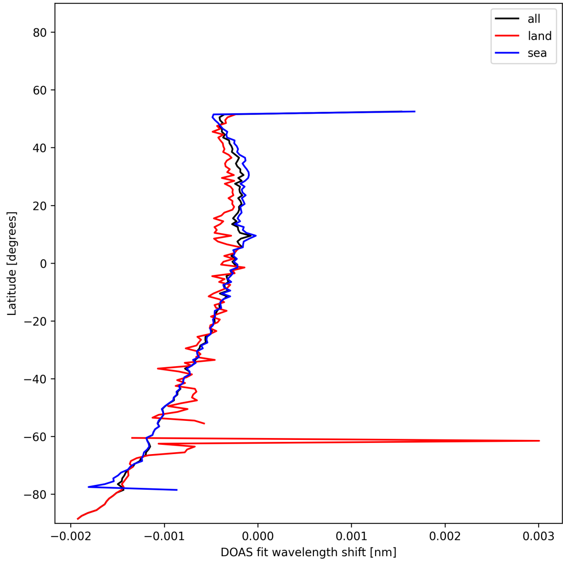
Figure 50: Zonal average of "DOAS fit wavelength shift" for 2025-11-12 to 2025-11-14.
