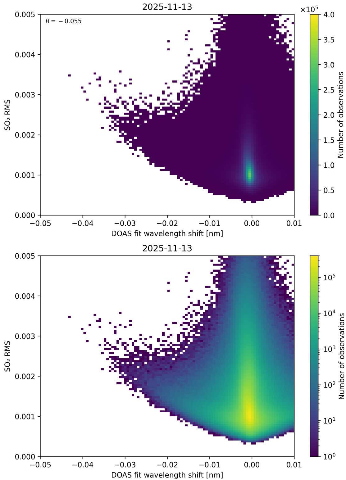
Figure 139: Scatter density plot of “DOAS fit wavelength shift” against “SO 2 RMS” for 2025-11-12 to 2025-11-14.
