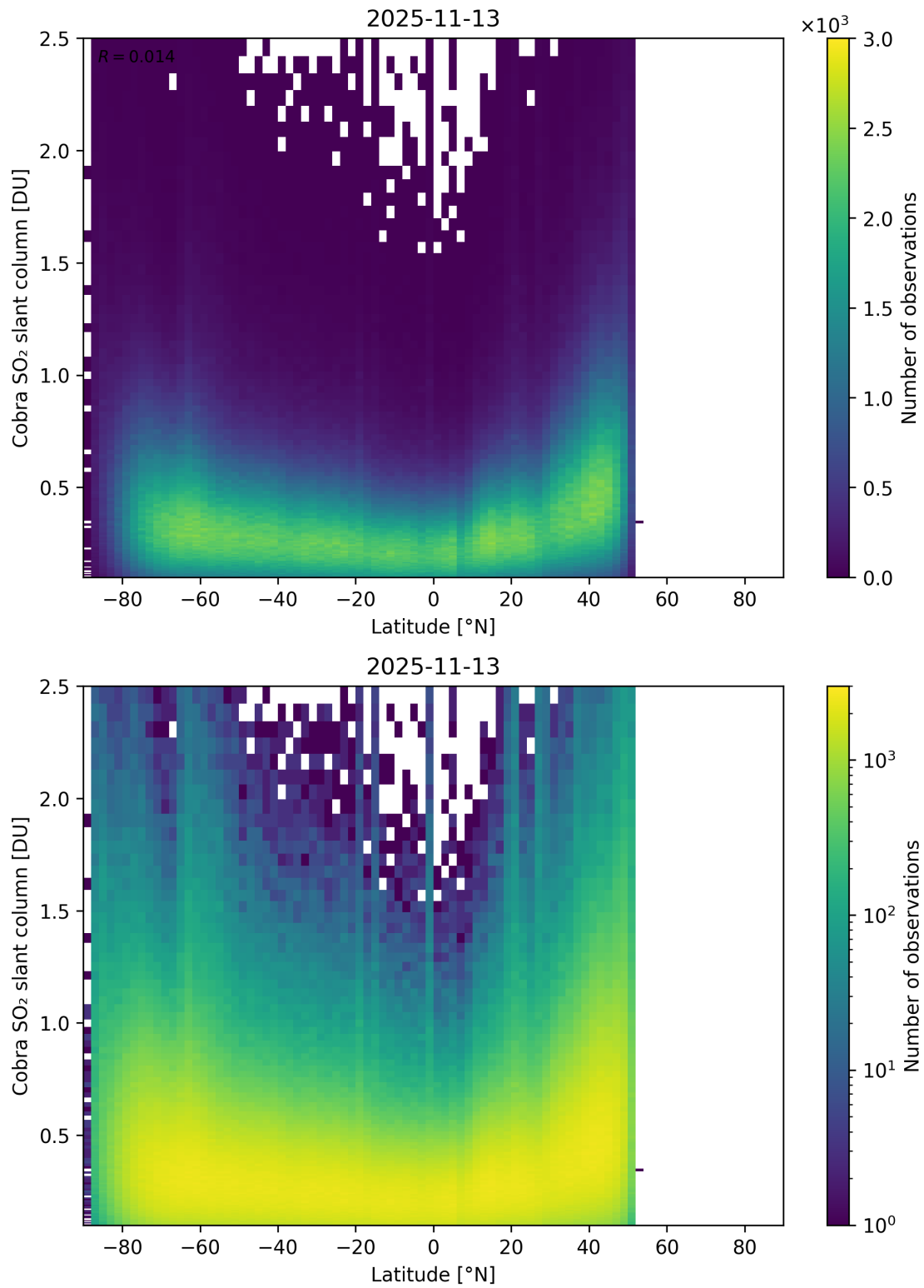
Figure 157: Scatter density plot of “Latitude” against “Cobra SO 2 slant column” for 2025-11-12 to 2025-11-14.
