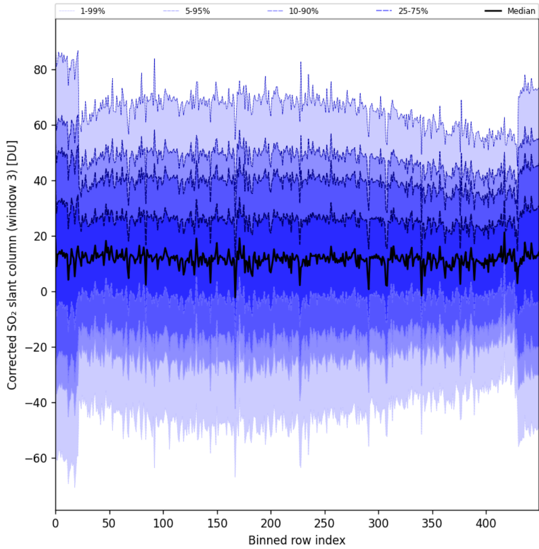
Figure 99: Along track statistics of “Corrected SO 2 slant column (window 3)” for 2025-11-12 to 2025-11-14
