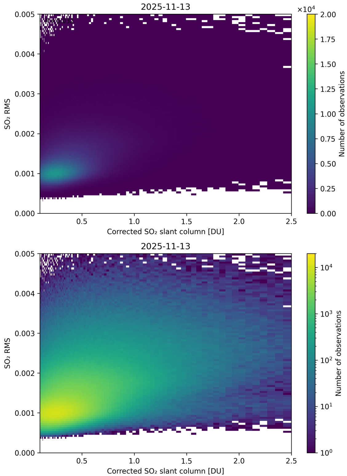
Figure 231: Scatter density plot of “Corrected SO 2 slant column” against “SO 2 RMS” for 2025-11-12 to 2025-11-14.
