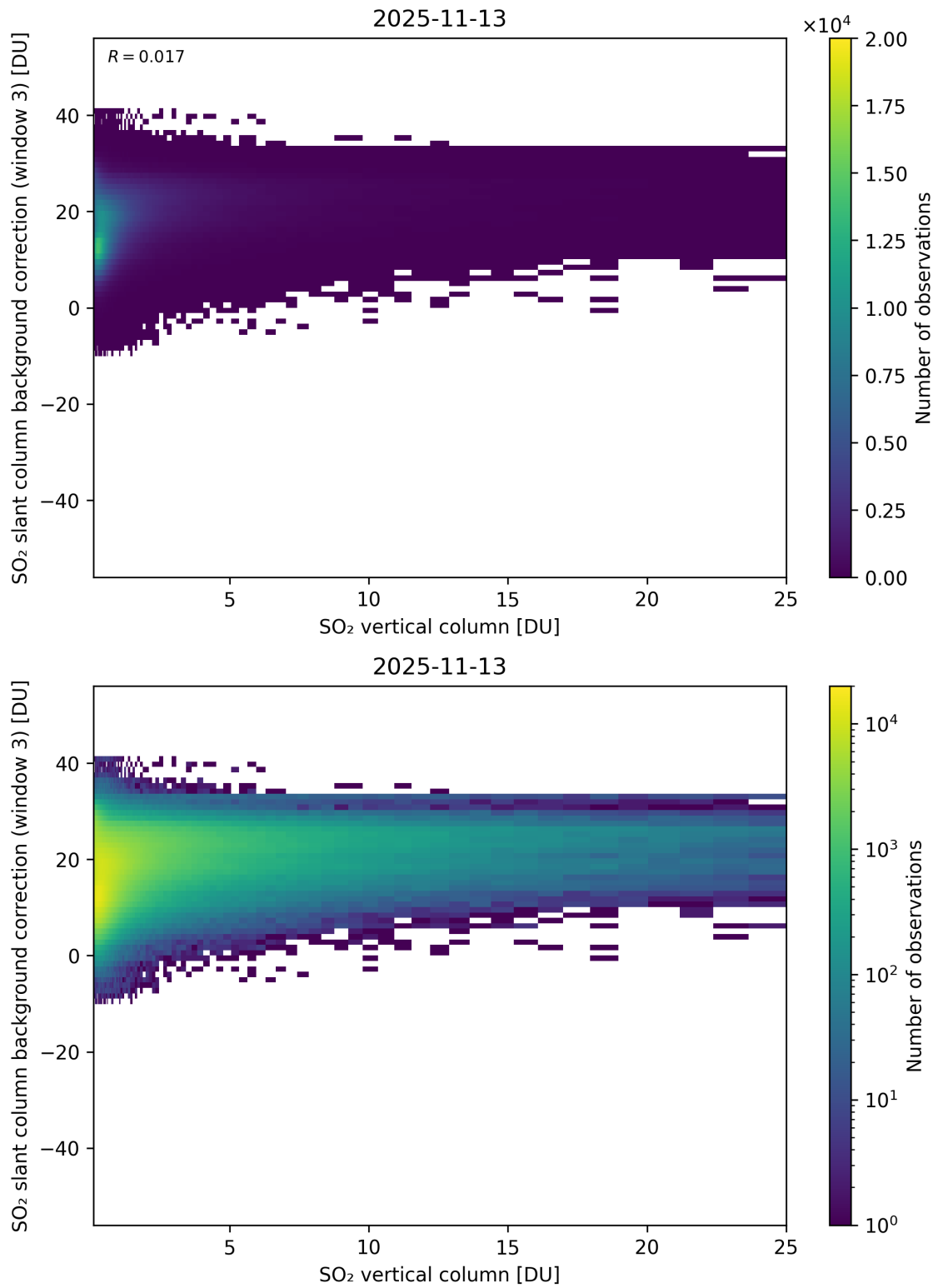
Figure 325: Scatter density plot of “SO 2 vertical column” against “SO 2 slant column background correction (window 3)” for 2025-11-12 to 2025-11-14.
