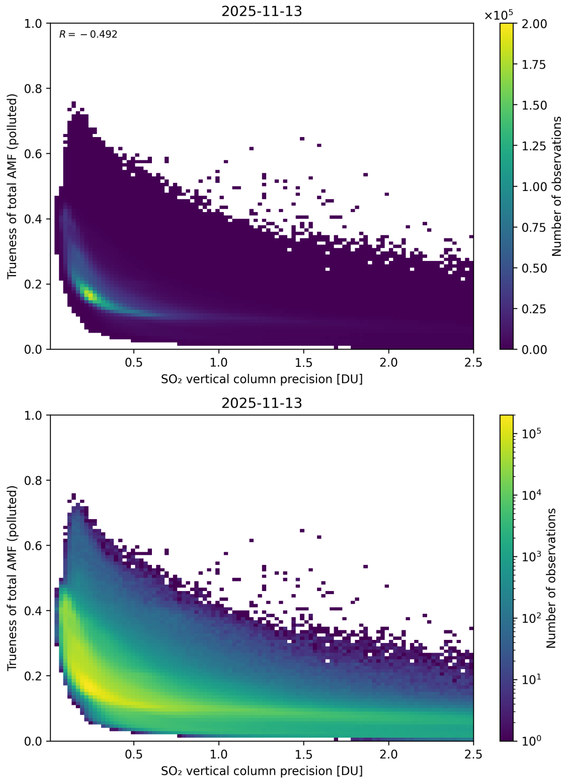
Figure 347: Scatter density plot of “SO 2 vertical column precision” against “Trueness of total AMF (polluted)” for 2025-11-12 to 2025-11-14.
