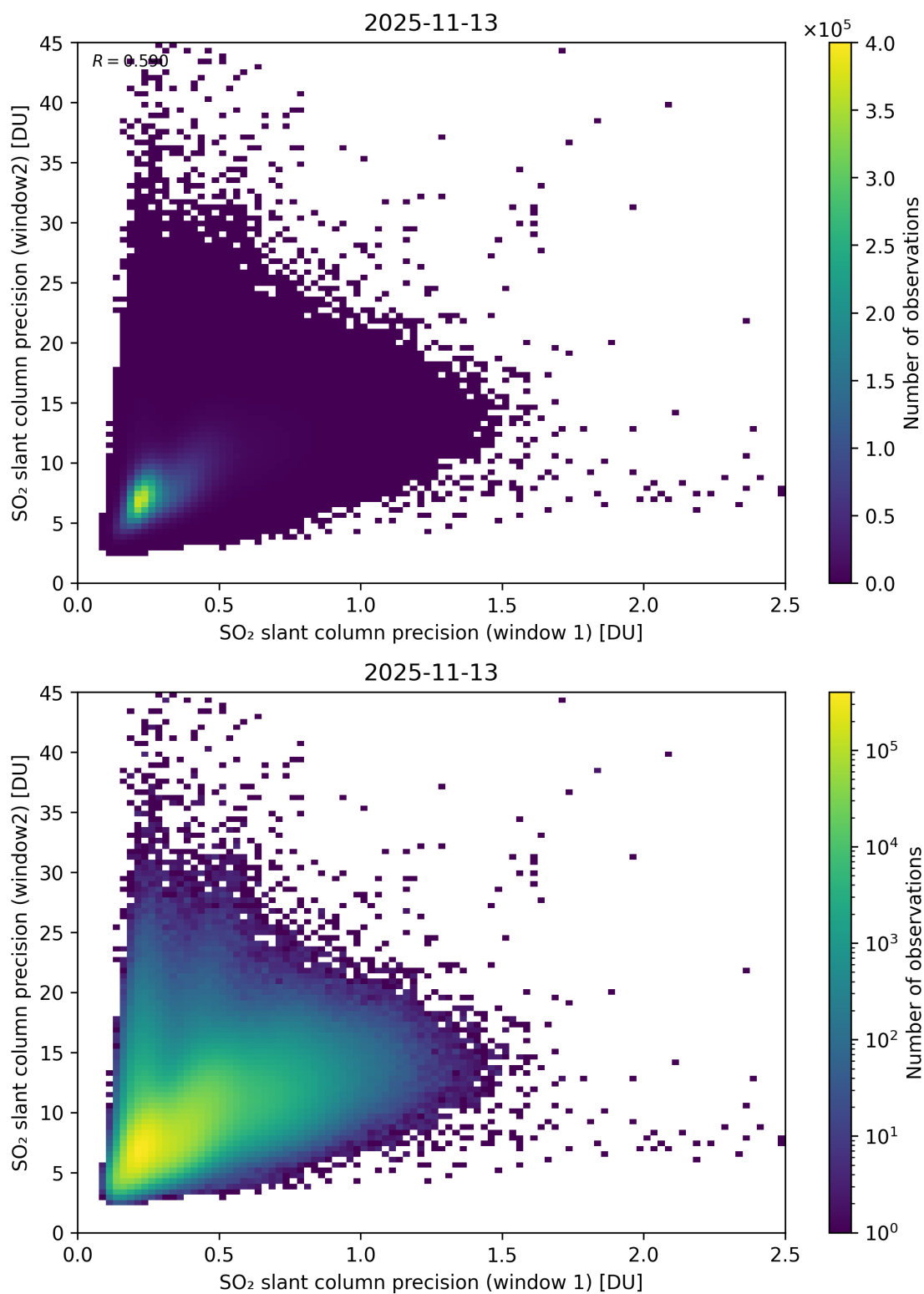
Figure 277: Scatter density plot of “SO 2 slant column precision (window 1)” against “SO 2 slant column precision (window2)” for 2025-11-12 to 2025-11-14.
