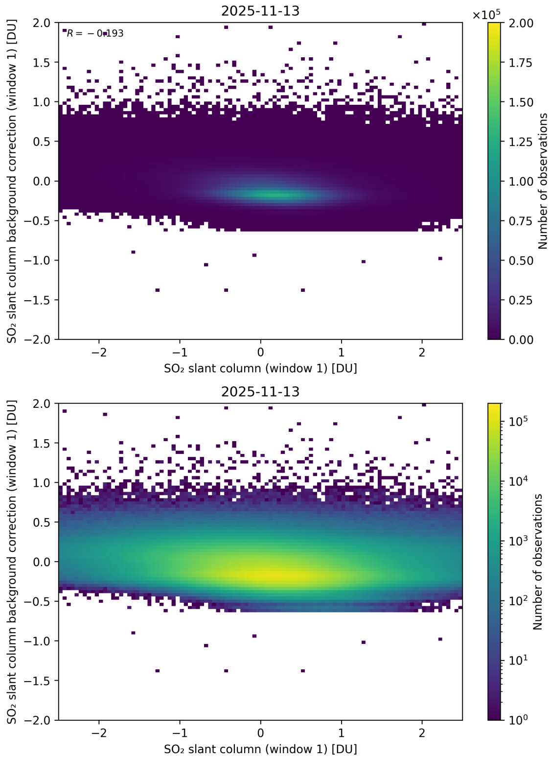
Figure 262: Scatter density plot of “SO 2 slant column (window 1)” against “SO 2 slant column background correction (window 1)” for 2025-11-12 to 2025-11-14.
