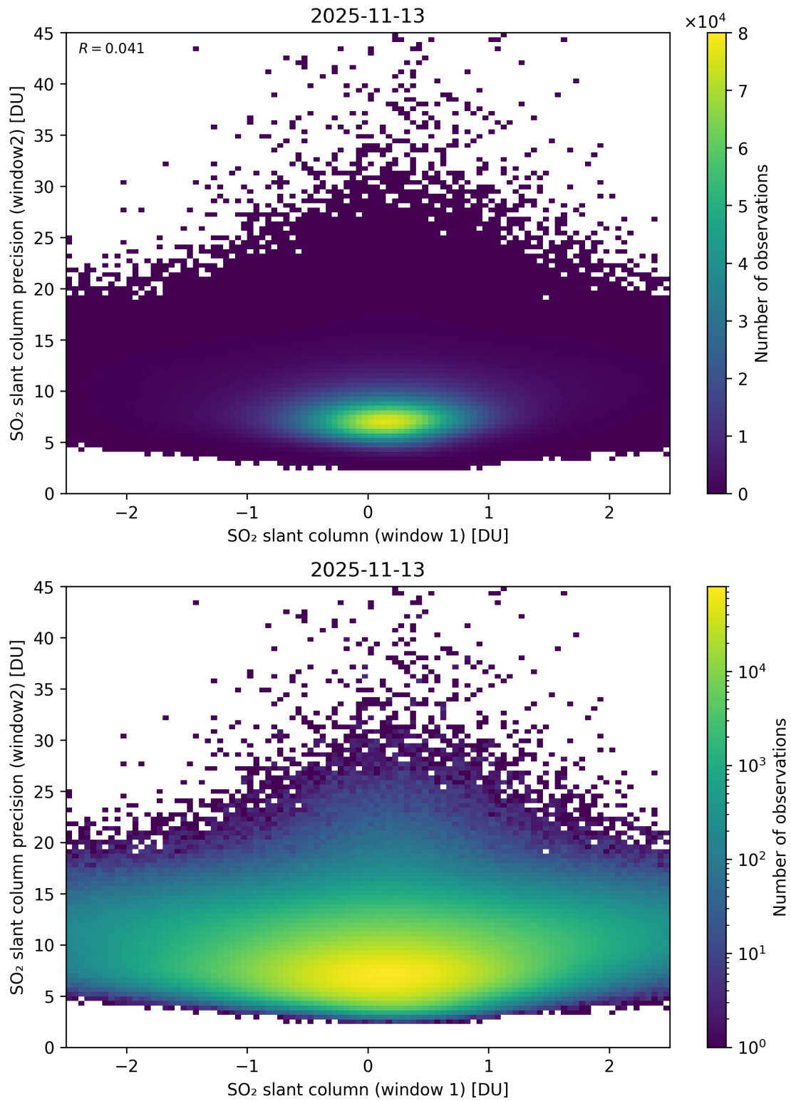
Figure 286: Scatter density plot of “SO 2 slant column (window 1)” against “SO 2 slant column precision (window2)” for 2025-11-12 to 2025-11-14.
