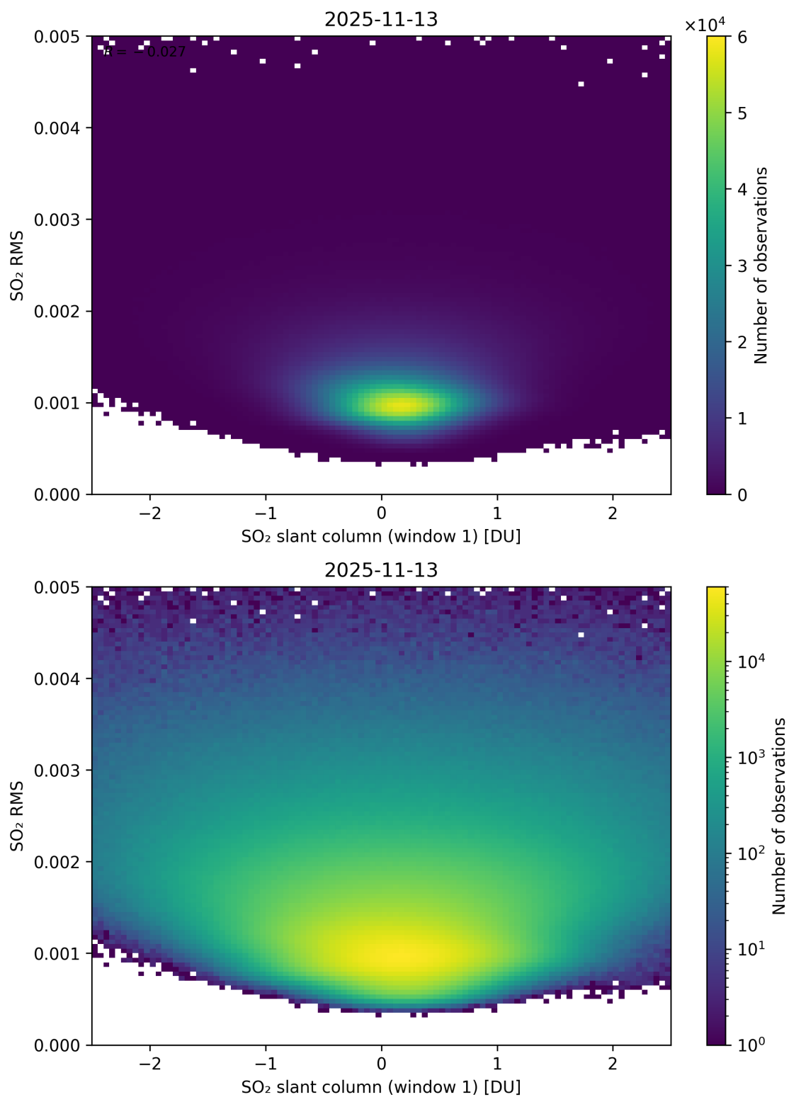
Figure 267: Scatter density plot of “SO 2 slant column (window 1)” against “SO 2 RMS” for 2025-11-12 to 2025-11-14.
