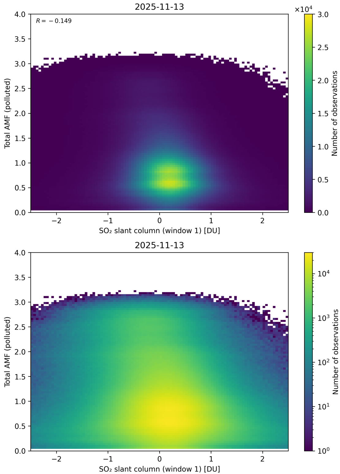
Figure 289: Scatter density plot of “SO 2 slant column (window 1)” against “Total AMF (polluted)” for 2025-11-12 to 2025-11-14.
