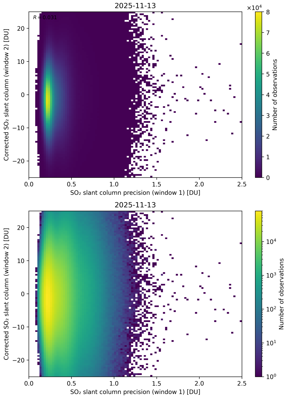
Figure 275: Scatter density plot of “SO 2 slant column precision (window 1)” against “Corrected SO 2 slant column (window 2)” for 2025-11-12 to 2025-11-14.
