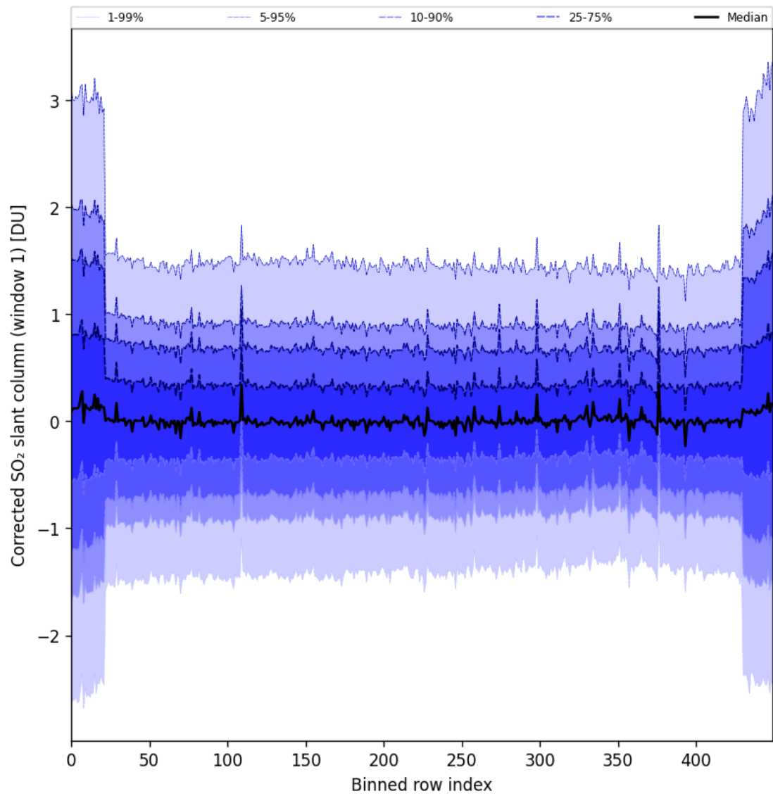
Figure 91: Along track statistics of “Corrected SO 2 slant column (window 1)” for 2025-11-12 to 2025-11-14
