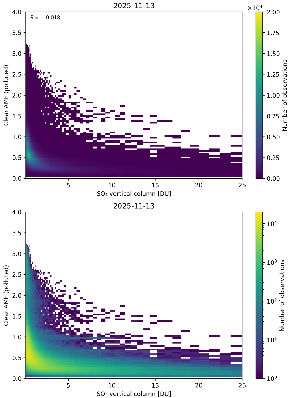
Figure 348: Scatter density plot of “SO 2 vertical column” against “Clear AMF (polluted)” for 2025-11-12 to 2025-11-14.
