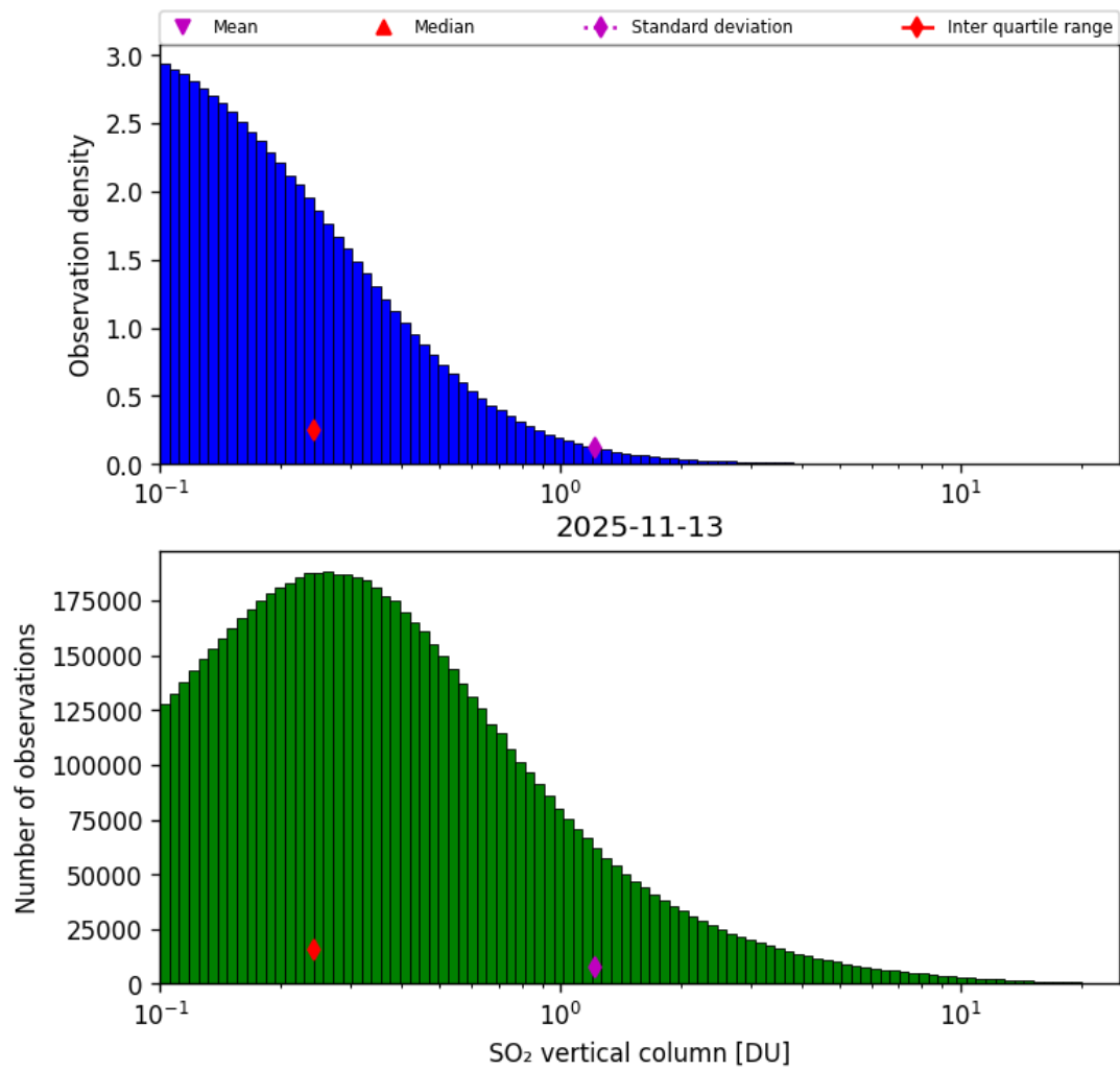
Figure 58: Histogram of “SO 2 vertical column” for 2025-11-12 to 2025-11-14
