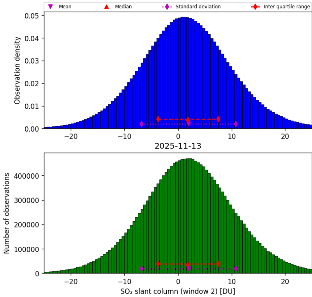
Figure 67: Histogram of “SO 2 slant column (window 2)” for 2025-11-12 to 2025-11-14
