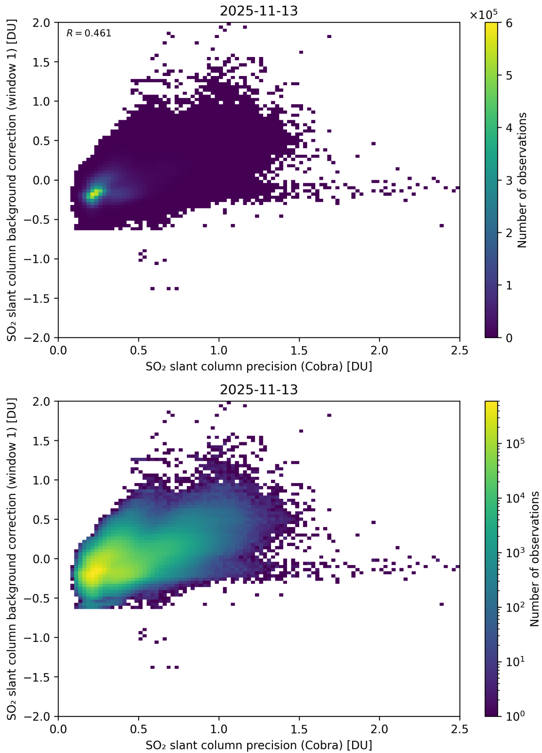
Figure 199: Scatter density plot of “SO 2 slant column precision (Cobra)” against “SO 2 slant column background correction (window 1)” for 2025-11-12 to 2025-11-14.
