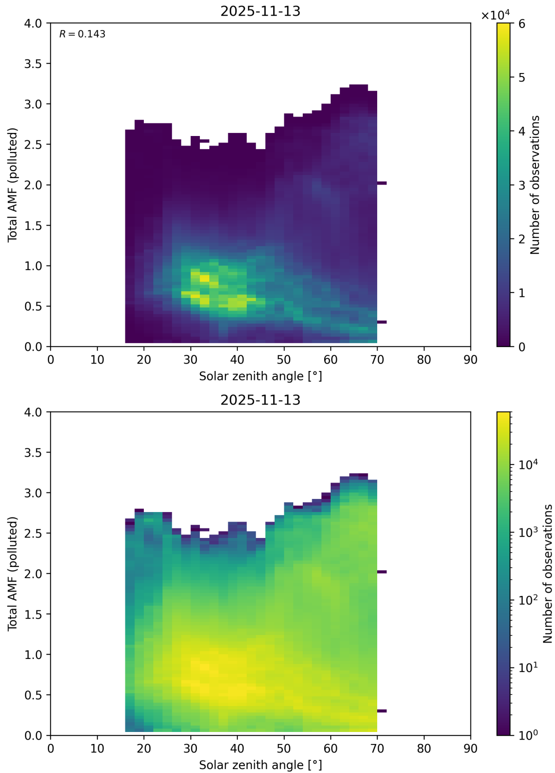
Figure 189: Scatter density plot of “Solar zenith angle” against “Total AMF (polluted)” for 2025-11-12 to 2025-11-14.
