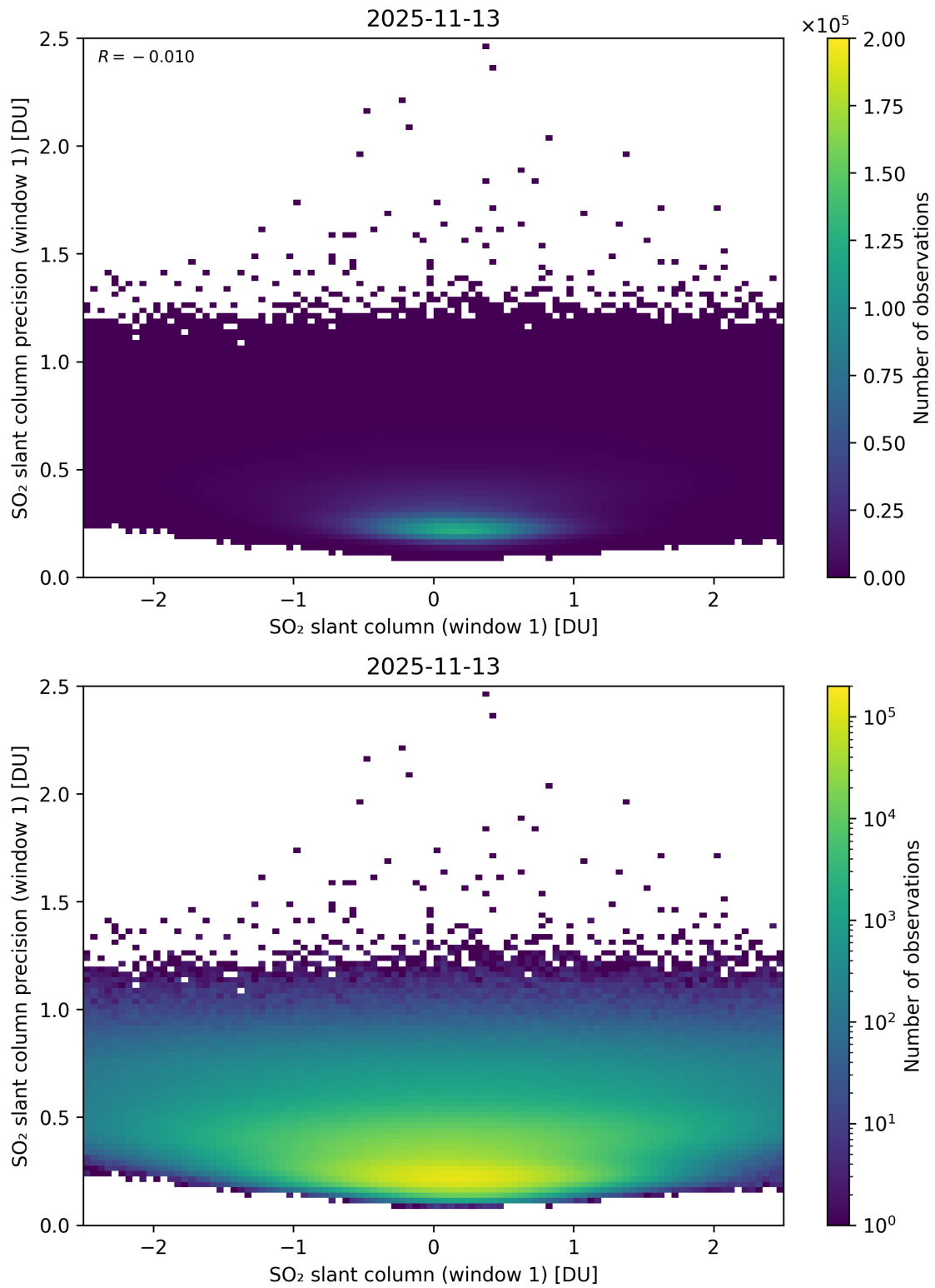
Figure 285: Scatter density plot of “SO 2 slant column (window 1)” against “SO 2 slant column precision (window 1)” for 2025-11-12 to 2025-11-14.
