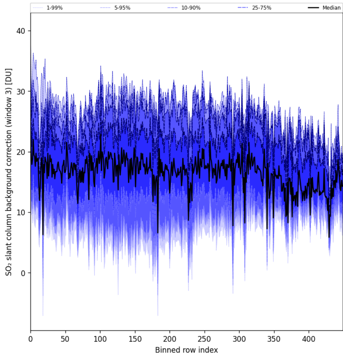
Figure 100: Along track statistics of “SO 2 slant column background correction (window 3)” for 2025-11-12 to 2025-11-14
