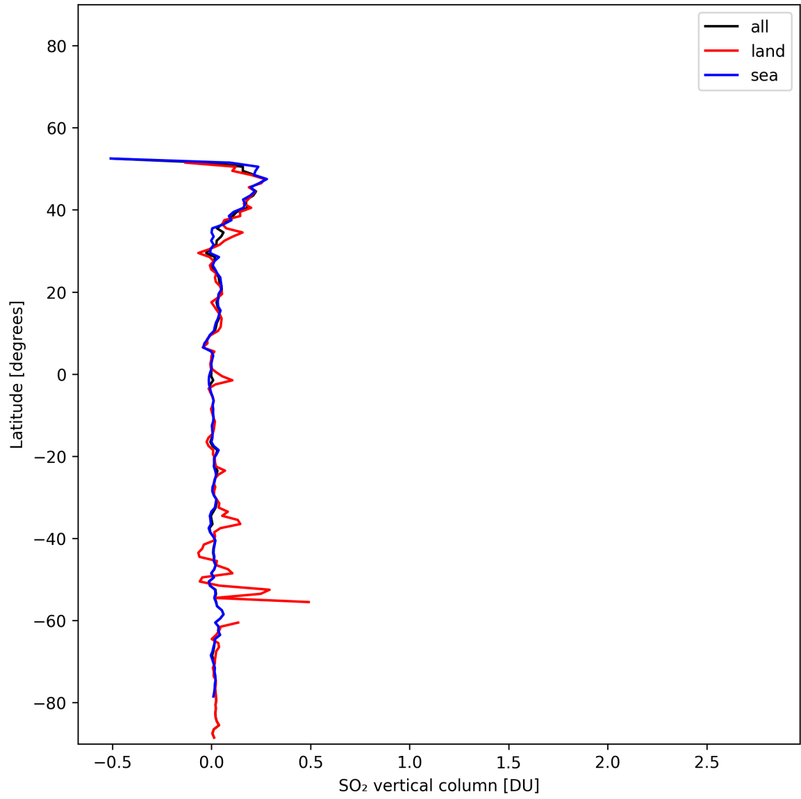
Figure 32: Zonal average of “SO 2 vertical column” for 2025-11-12 to 2025-11-14.
