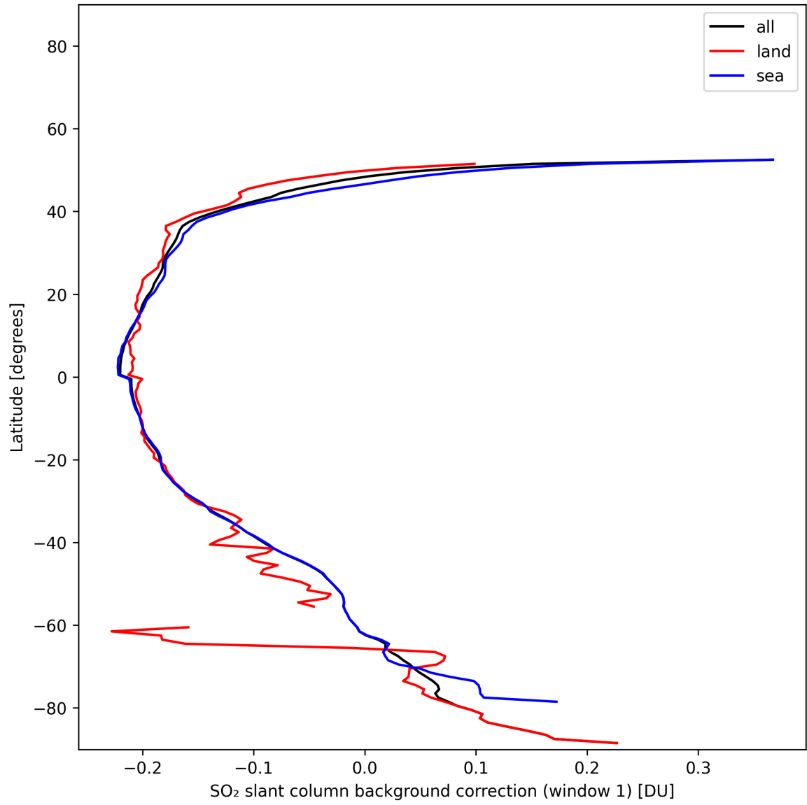
Figure 40: Zonal average of “SO 2 slant column background correction (window 1)” for 2025-11-12 to 2025-11-14.
