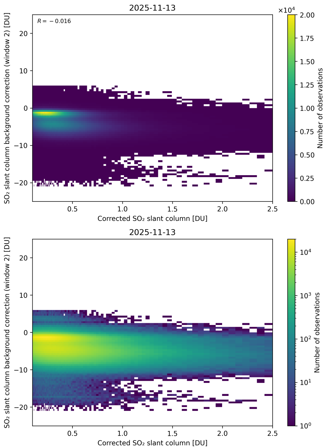
Figure 227: Scatter density plot of “Corrected SO 2 slant column” against “SO 2 slant column background correction (window 2)” for 2025-11-12 to 2025-11-14.
