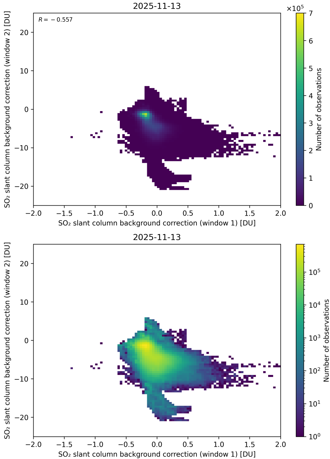
Figure 109: Scatter density plot of “SO 2 slant column background correction (window 1)” against “SO 2 slant column background correction (window 2)” for 2025-11-12 to 2025-11-14.
