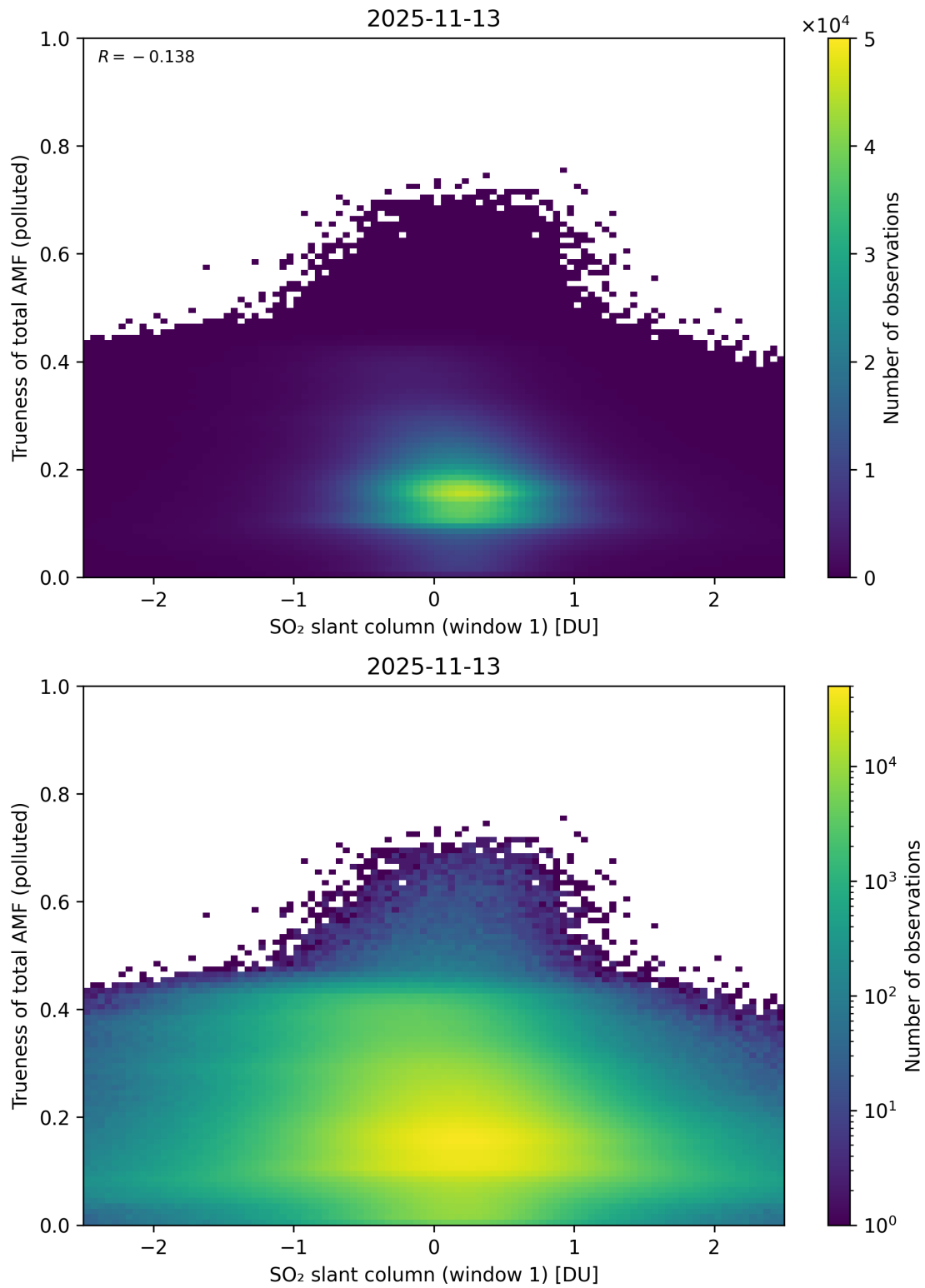
Figure 290: Scatter density plot of “SO 2 slant column (window 1)” against “Trueness of total AMF (polluted)” for 2025-11-12 to 2025-11-14.
