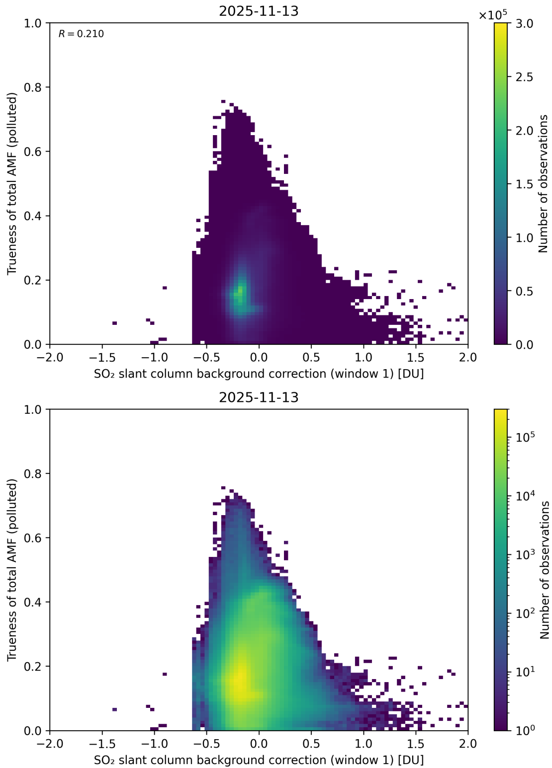
Figure 121: Scatter density plot of “SO 2 slant column background correction (window 1)” against “Trueness of total AMF (polluted)” for 2025-11-12 to 2025-11-14.
