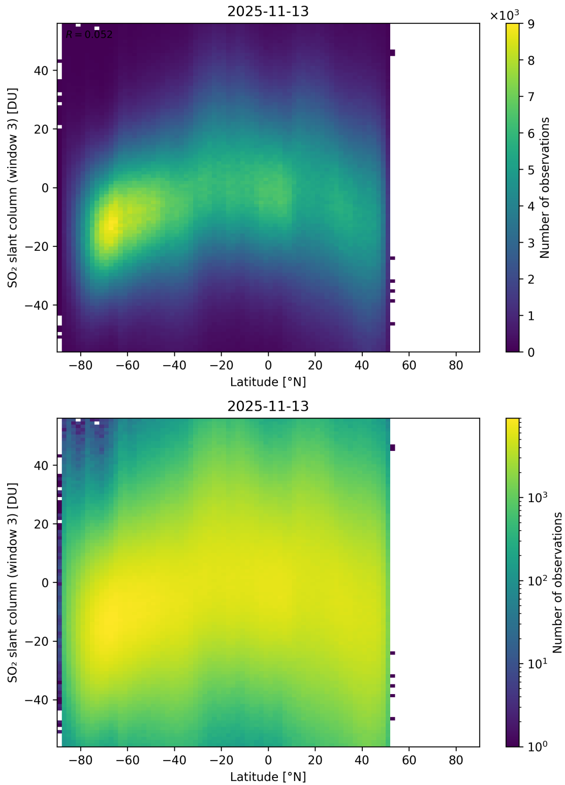
Figure 165: Scatter density plot of “Latitude” against “SO 2 slant column (window 3)” for 2025-11-12 to 2025-11-14.
