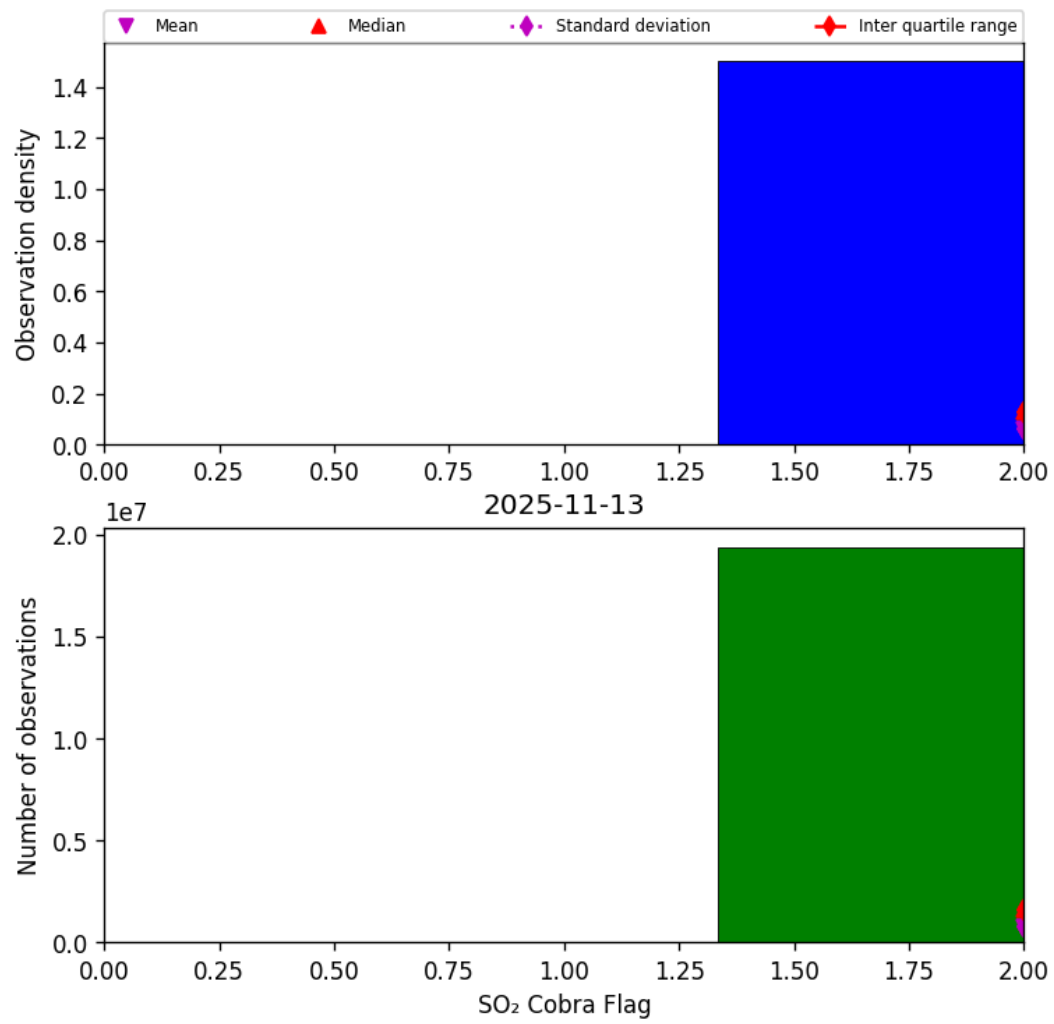
Figure 75: Histogram of “SO 2 Cobra Flag” for 2025-11-12 to 2025-11-14
