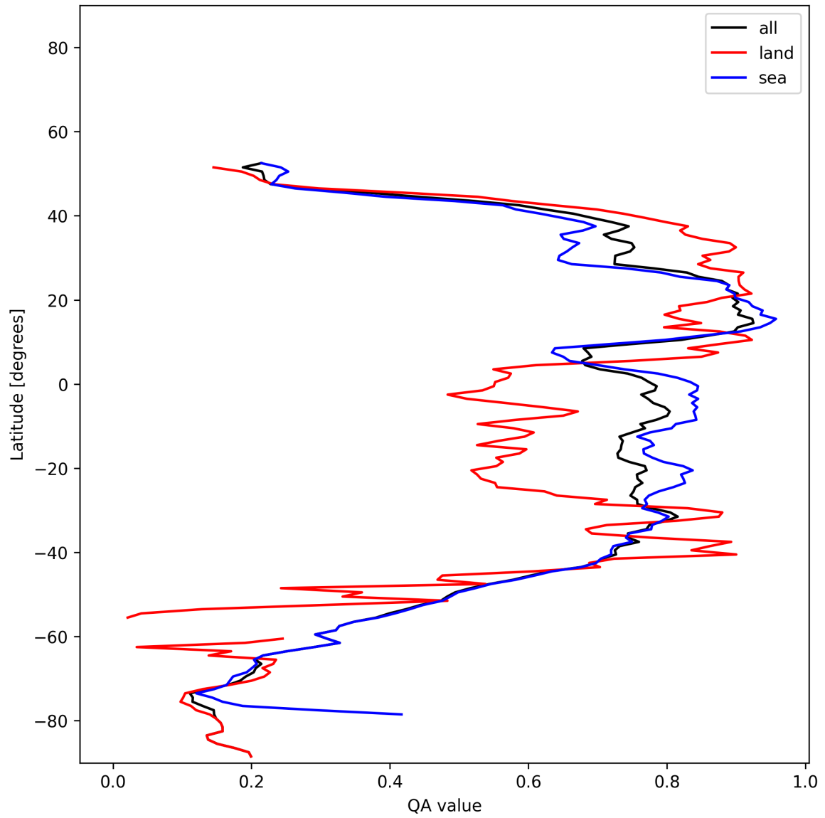
Figure 31: Zonal average of “QA value” for 2025-11-12 to 2025-11-14.
