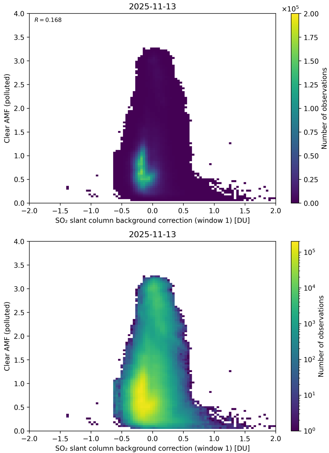
Figure 114: Scatter density plot of “SO 2 slant column background correction (window 1)” against “Clear AMF (polluted)” for 2025-11-12 to 2025-11-14.
