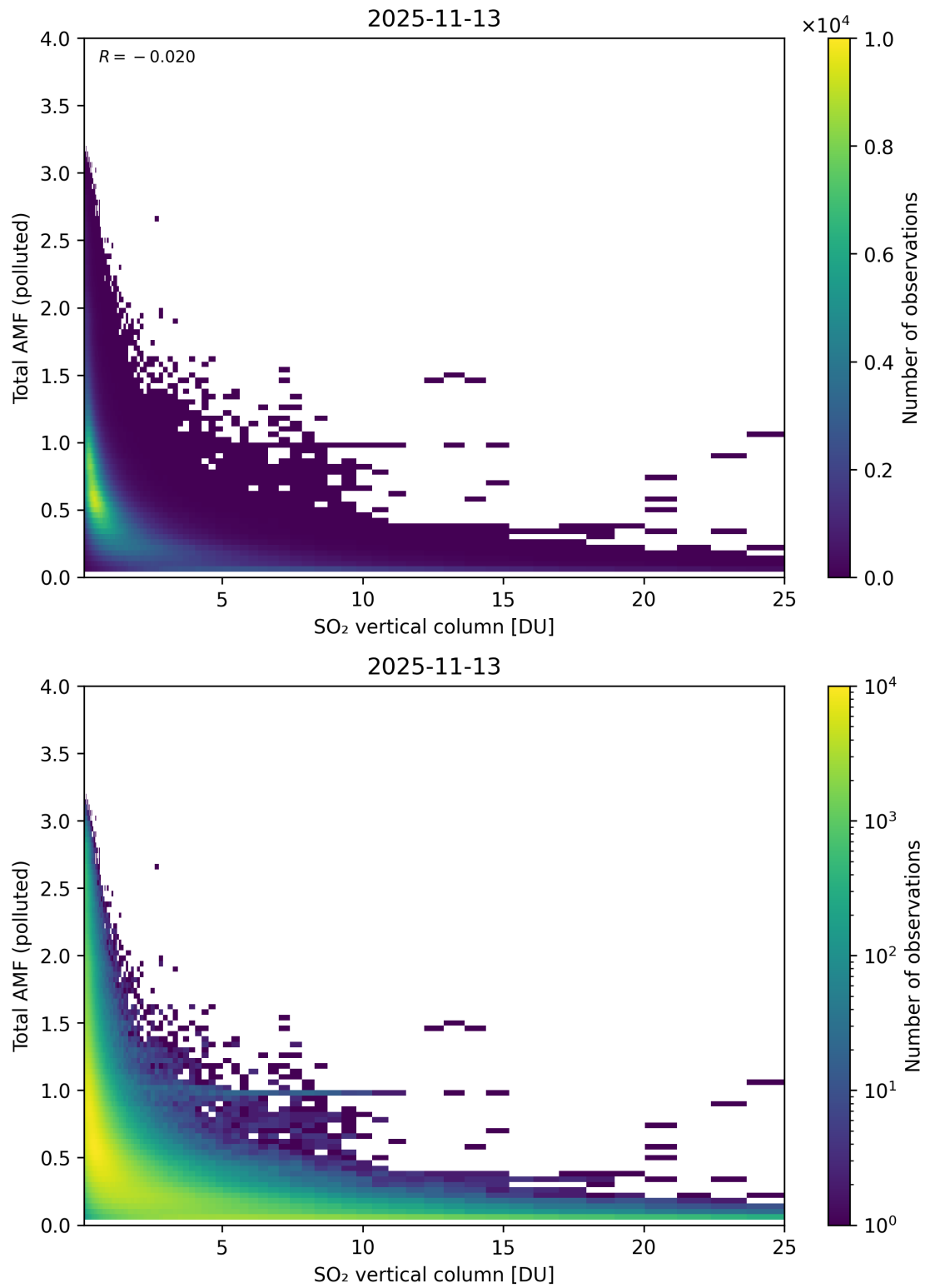
Figure 359: Scatter density plot of “SO 2 vertical column” against “Total AMF (polluted)” for 2025-11-12 to 2025-11-14.
