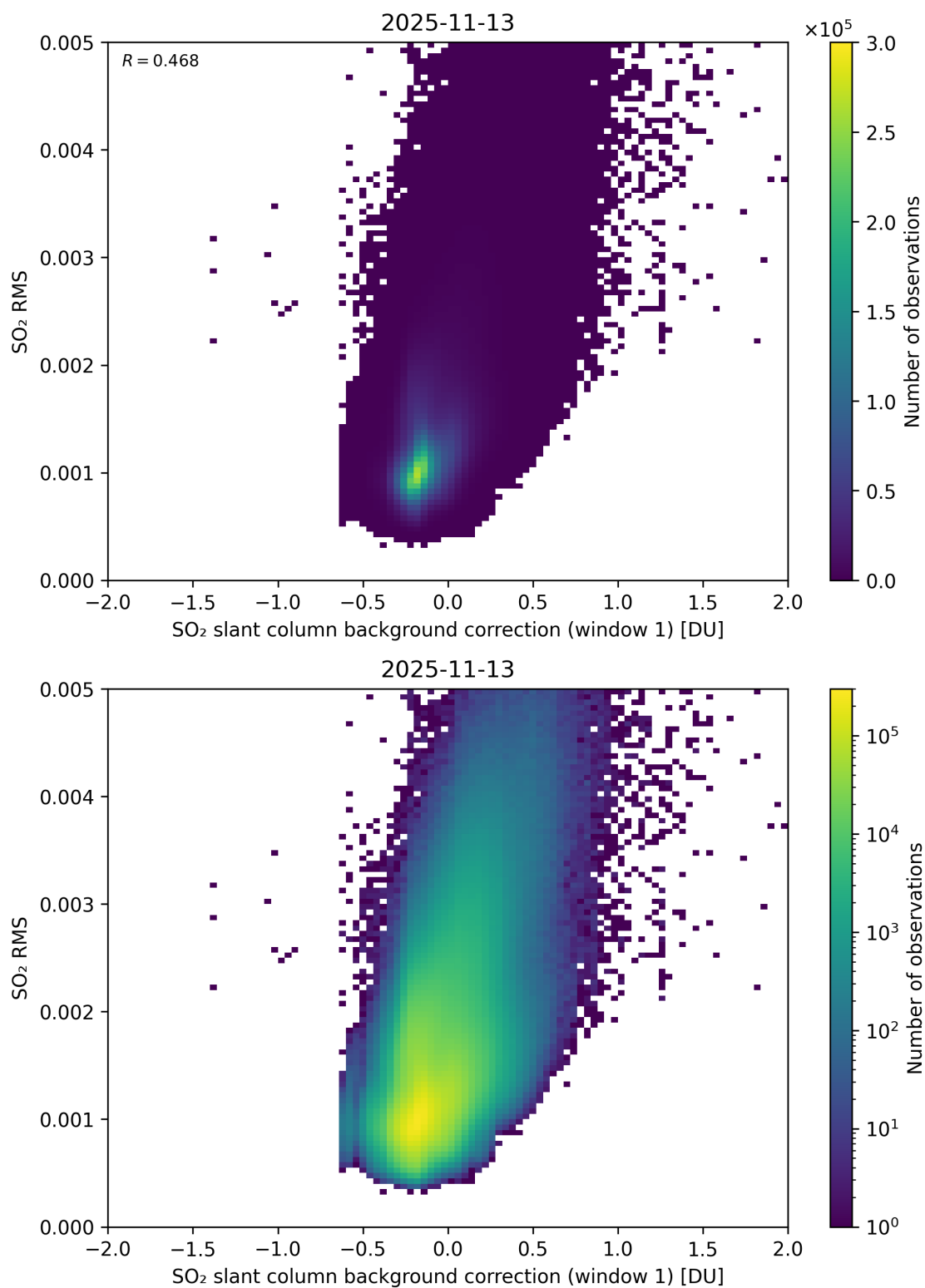
Figure 113: Scatter density plot of “SO 2 slant column background correction (window 1)” against “SO 2 RMS” for 2025-11-12 to 2025-11-14.
