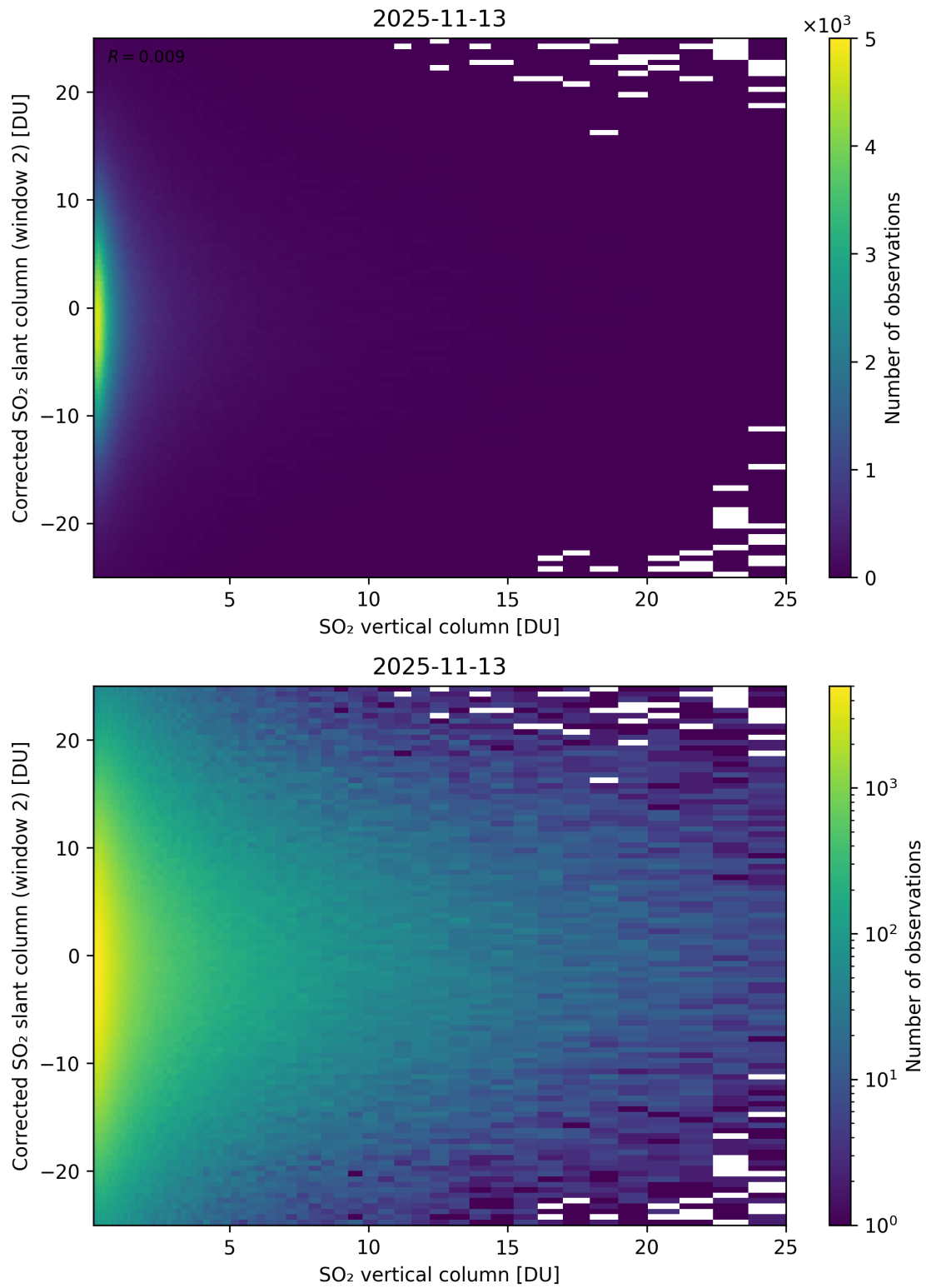
Figure 352: Scatter density plot of “SO 2 vertical column” against “Corrected SO 2 slant column (window 2)” for 2025-11-12 to 2025-11-14.
