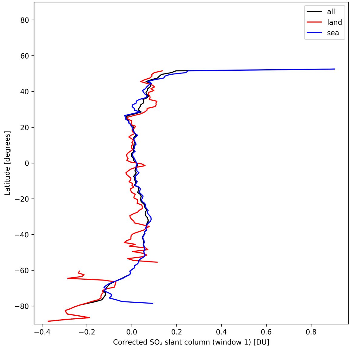
Figure 39: Zonal average of “Corrected SO 2 slant column (window 1)” for 2025-11-12 to 2025-11-14.
