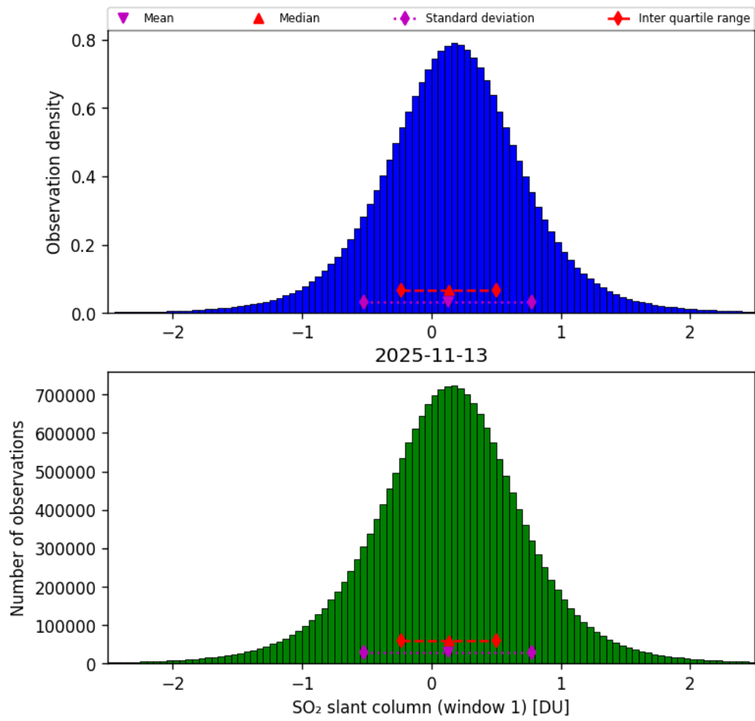
Figure 63: Histogram of “SO 2 slant column (window 1)” for 2025-11-12 to 2025-11-14
