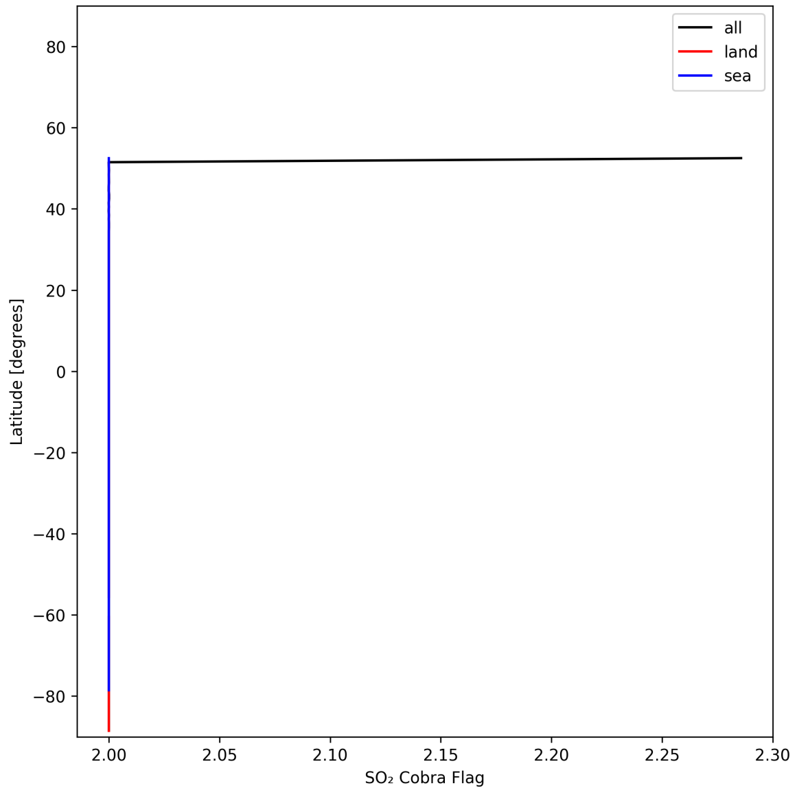
Figure 49: Zonal average of “SO 2 Cobra Flag” for 2025-11-12 to 2025-11-14.
