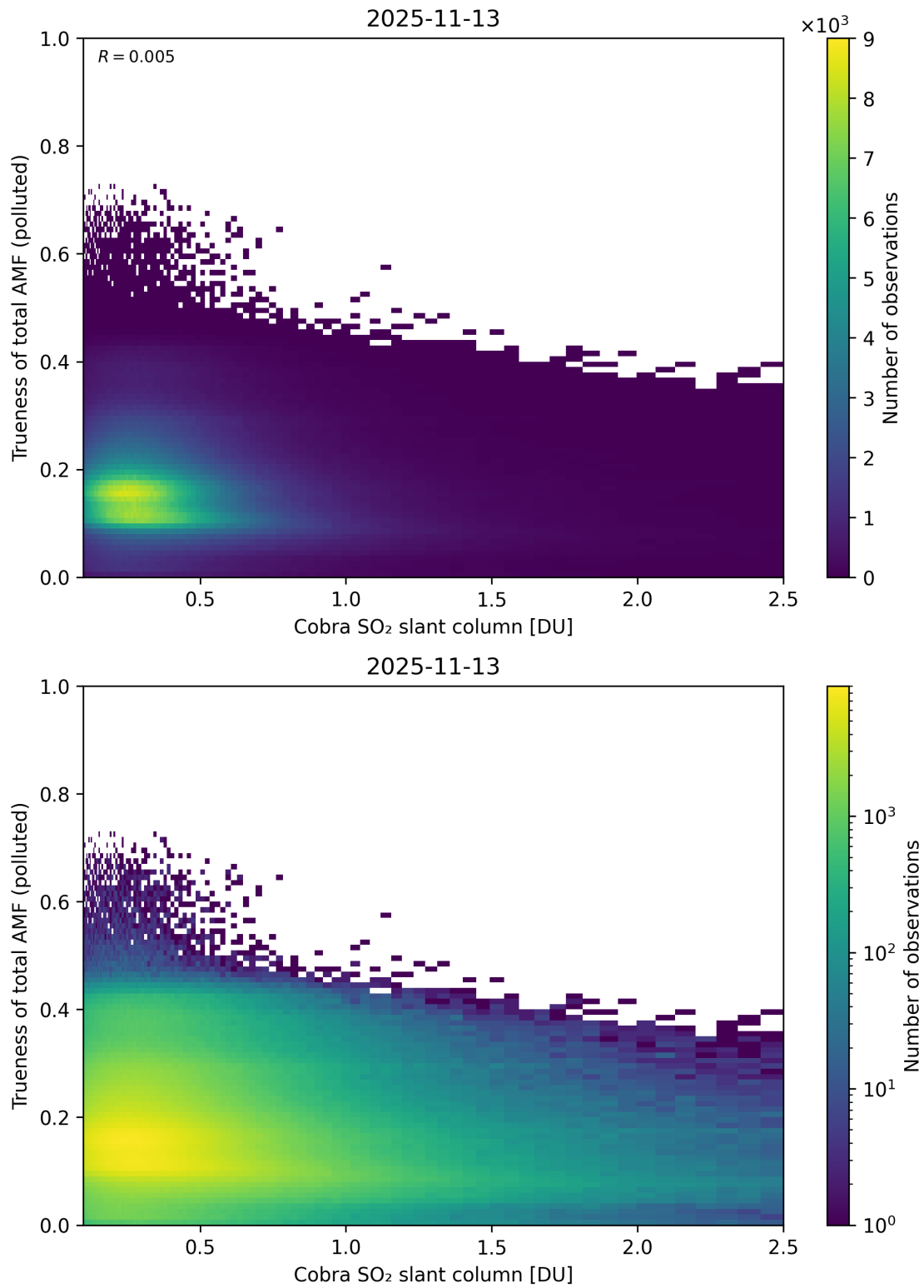
Figure 225: Scatter density plot of “Cobra SO 2 slant column” against “Trueness of total AMF (polluted)” for 2025-11-12 to 2025-11-14.
