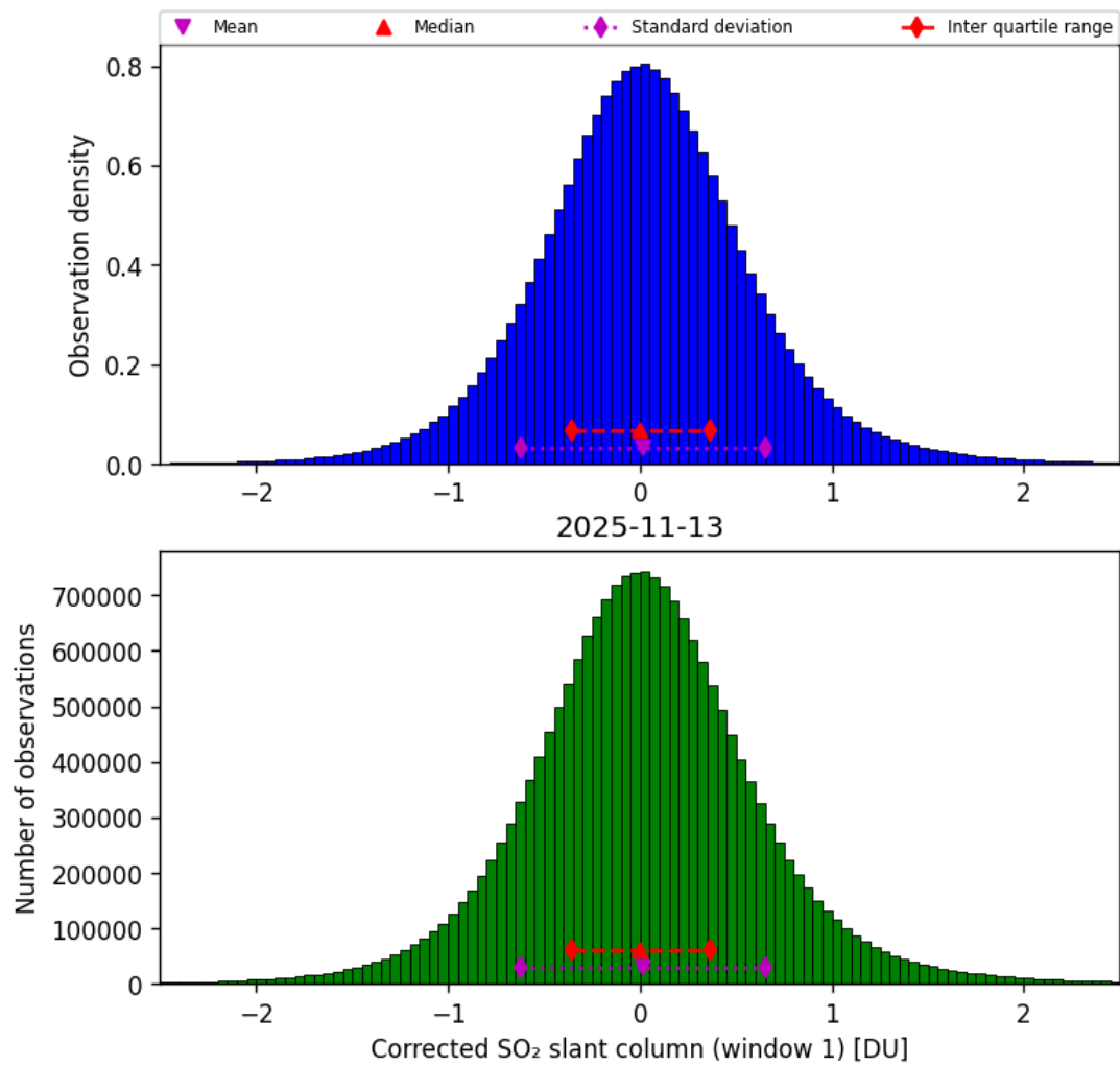
Figure 65: Histogram of “Corrected SO 2 slant column (window 1)” for 2025-11-12 to 2025-11-14
