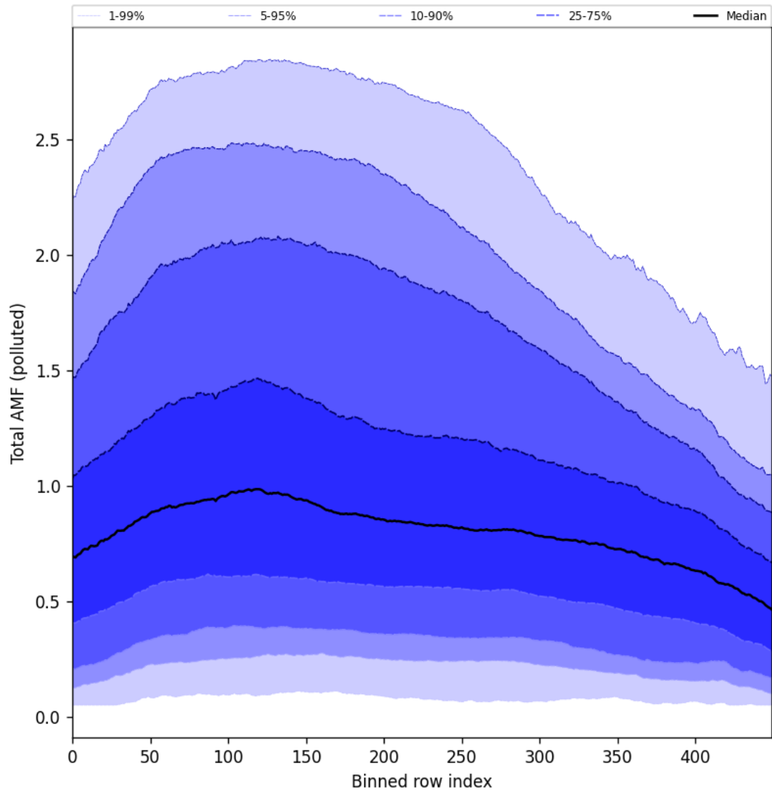
Figure 105: Along track statistics of “Total AMF (polluted)” for 2025-11-12 to 2025-11-14
