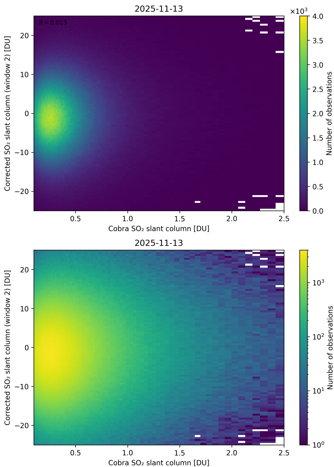
Figure 217: Scatter density plot of “Cobra SO 2 slant column” against “Corrected SO 2 slant column (window 2)” for 2025-11-12 to 2025-11-14.
