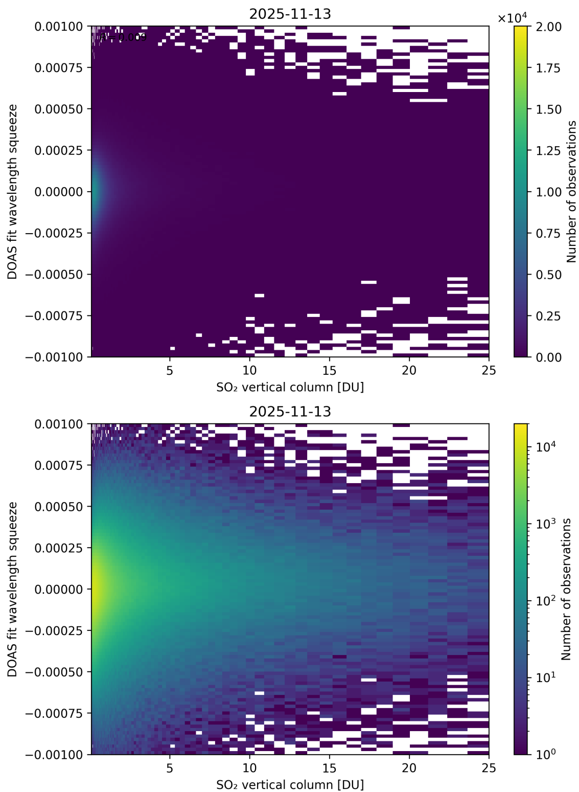
Figure 327: Scatter density plot of “SO 2 vertical column” against “DOAS fit wavelength squeeze” for 2025-11-12 to 2025-11-14.
