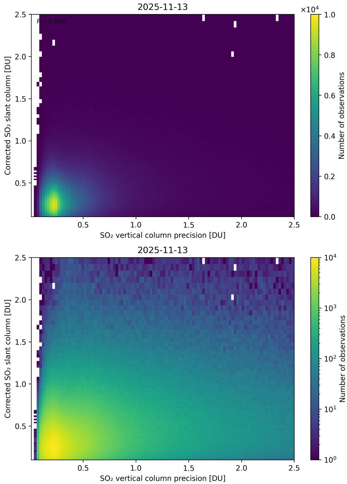
Figure 338: Scatter density plot of “SO 2 vertical column precision” against “Corrected SO 2 slant column” for 2025-11-12 to 2025-11-14.
