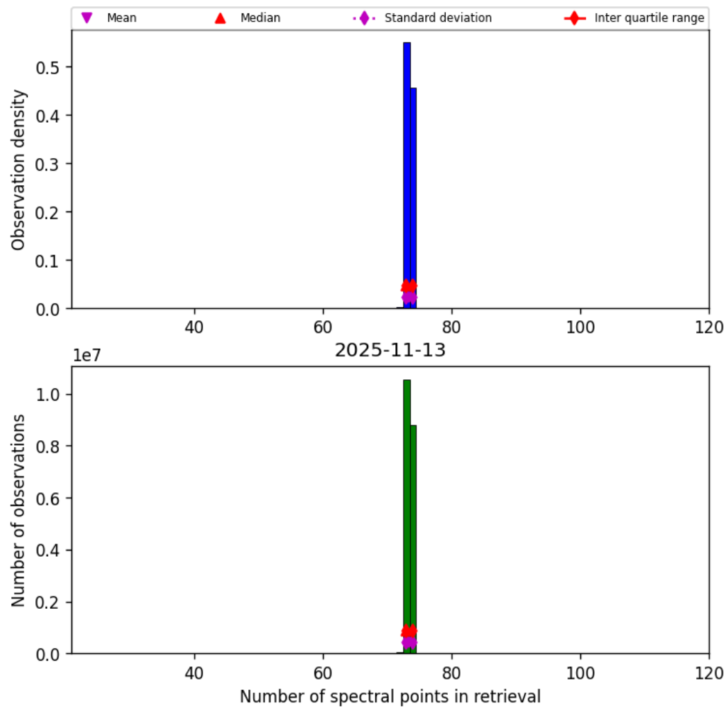
Figure 82: Histogram of “Number of spectral points in retrieval” for 2025-11-12 to 2025-11-14
