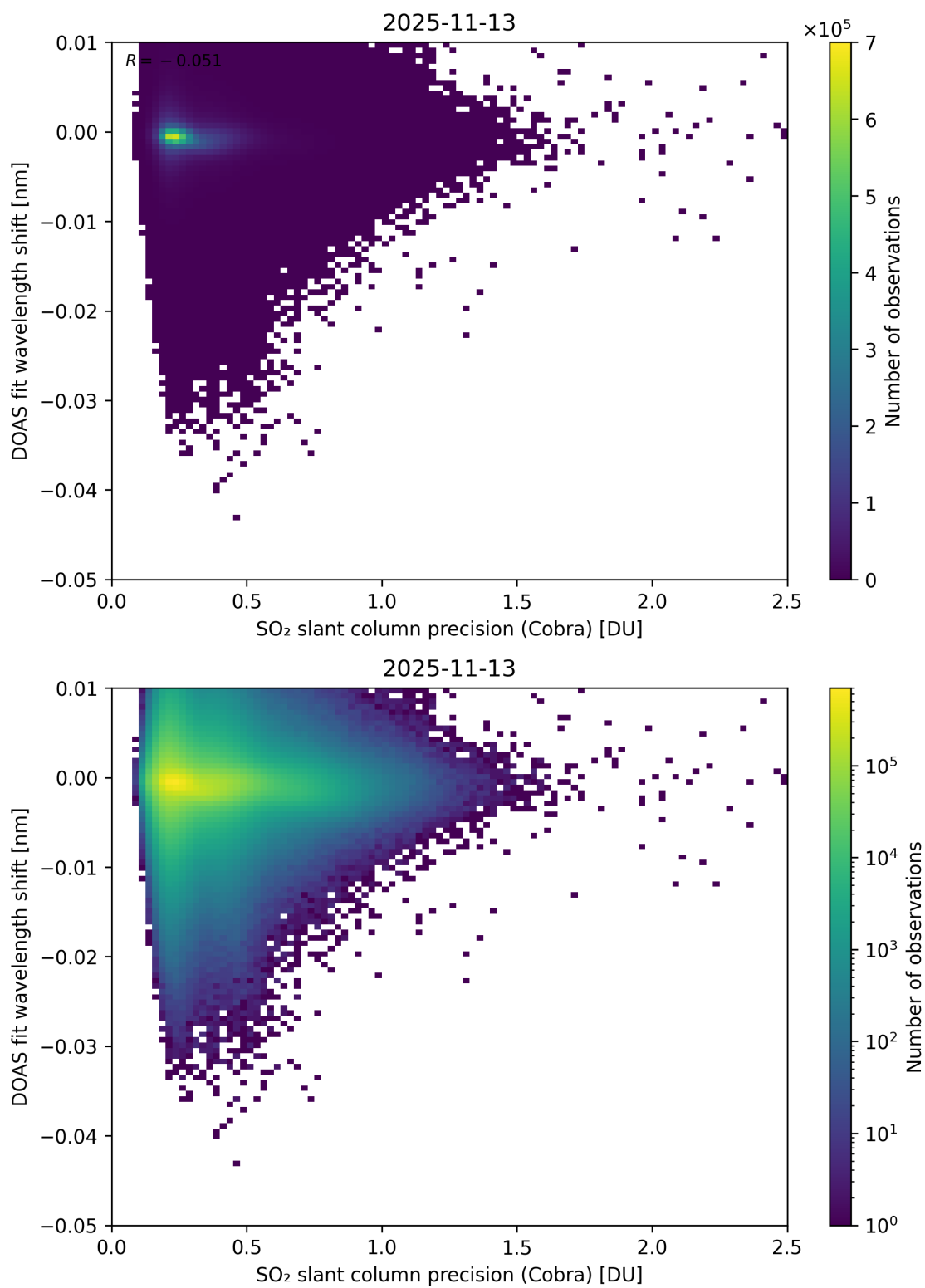
Figure 202: Scatter density plot of “SO 2 slant column precision (Cobra)” against “DOAS fit wavelength shift” for 2025-11-12 to 2025-11-14.
