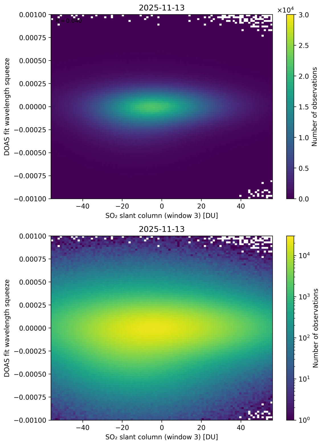
Figure 305: Scatter density plot of “SO 2 slant column (window 3)” against “DOAS fit wavelength squeeze” for 2025-11-12 to 2025-11-14.
