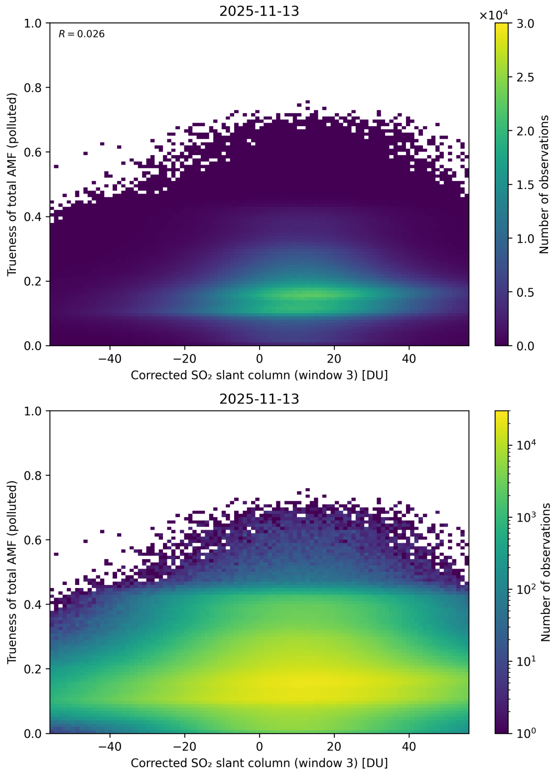
Figure 261: Scatter density plot of “Corrected SO 2 slant column (window 3)” against “Trueness of total AMF (polluted)” for 2025-11-12 to 2025-11-14.
