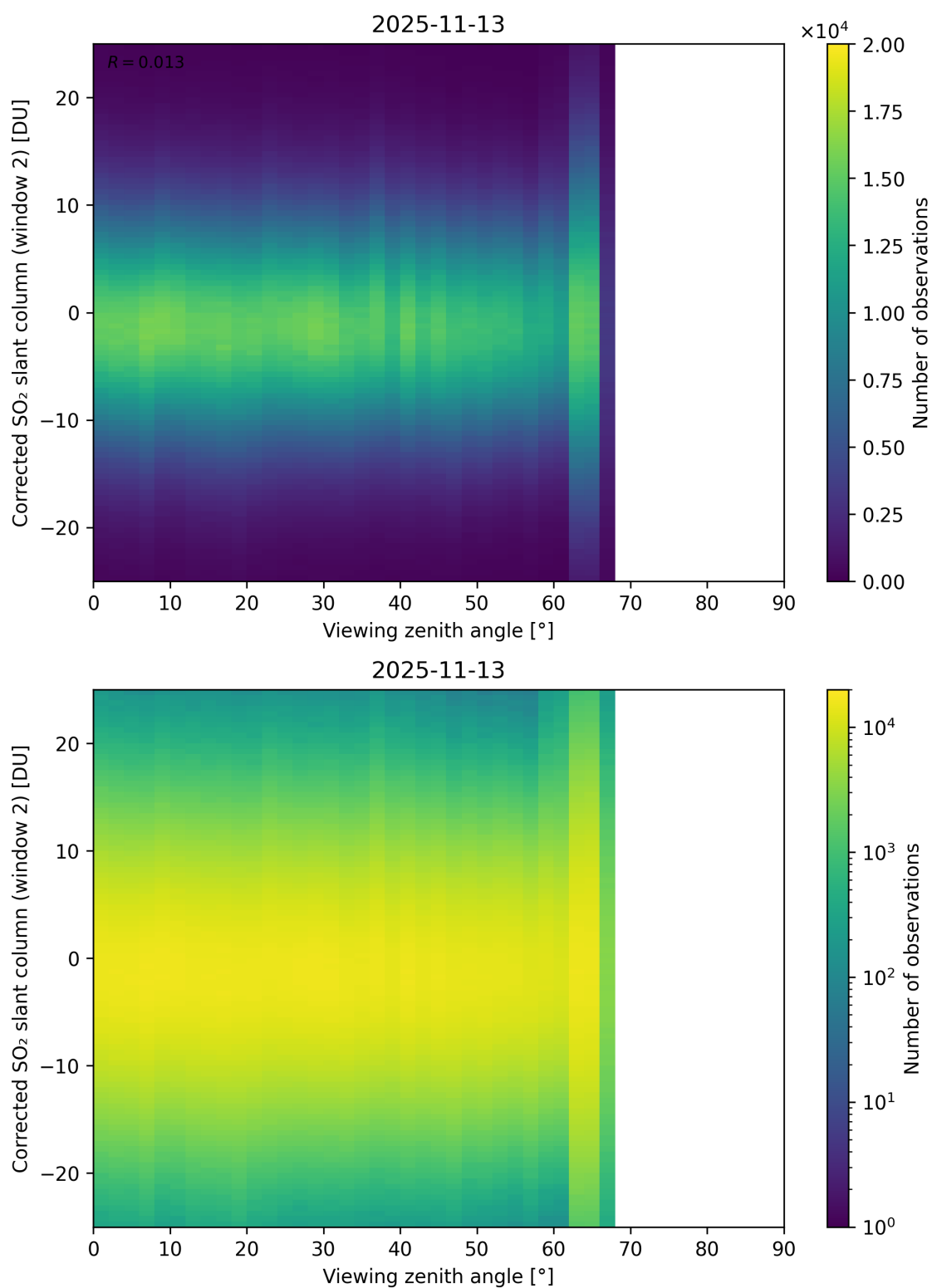
Figure 374: Scatter density plot of “Viewing zenith angle” against “Corrected SO 2 slant column (window 2)” for 2025-11-12 to 2025-11-14.
