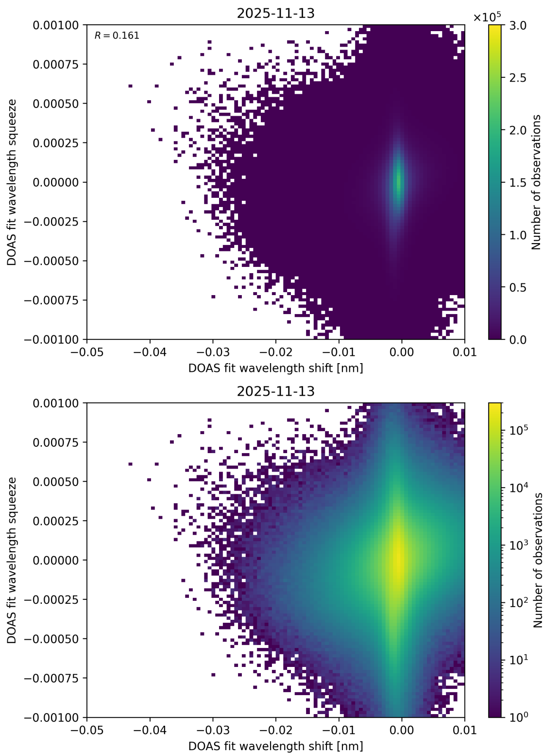
Figure 138: Scatter density plot of “DOAS fit wavelength shift” against “DOAS fit wavelength squeeze” for 2025-11-12 to 2025-11-14.
