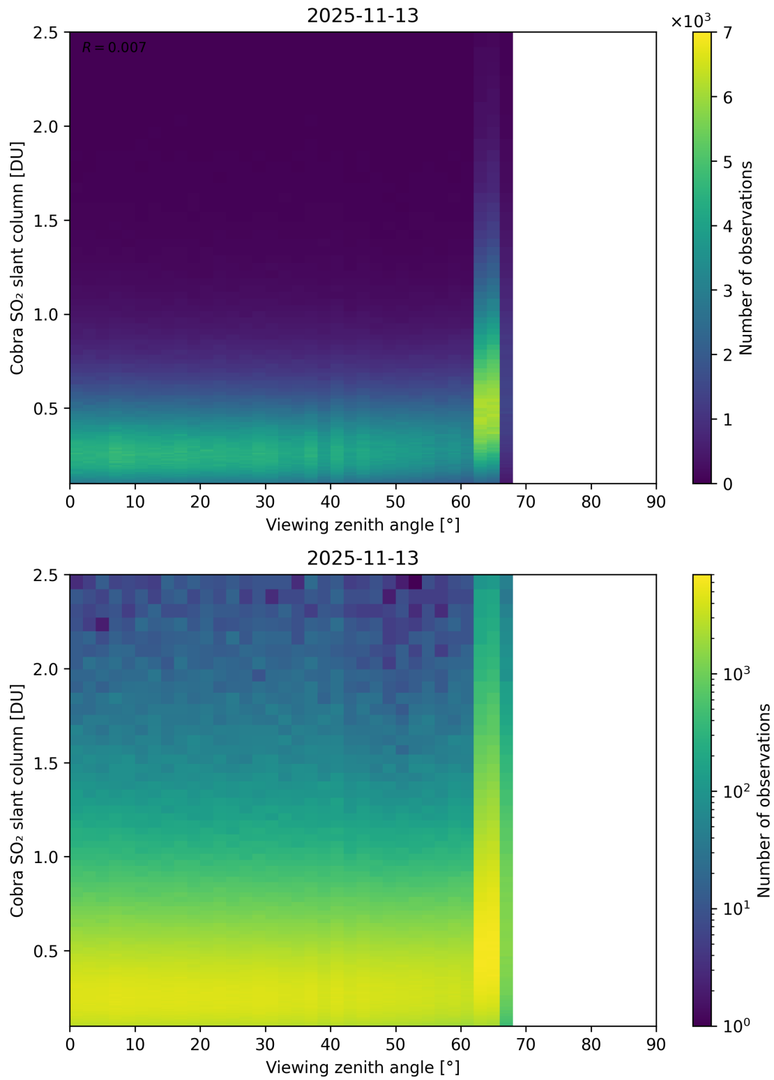
Figure 371: Scatter density plot of “Viewing zenith angle” against “Cobra SO 2 slant column” for 2025-11-12 to 2025-11-14.
