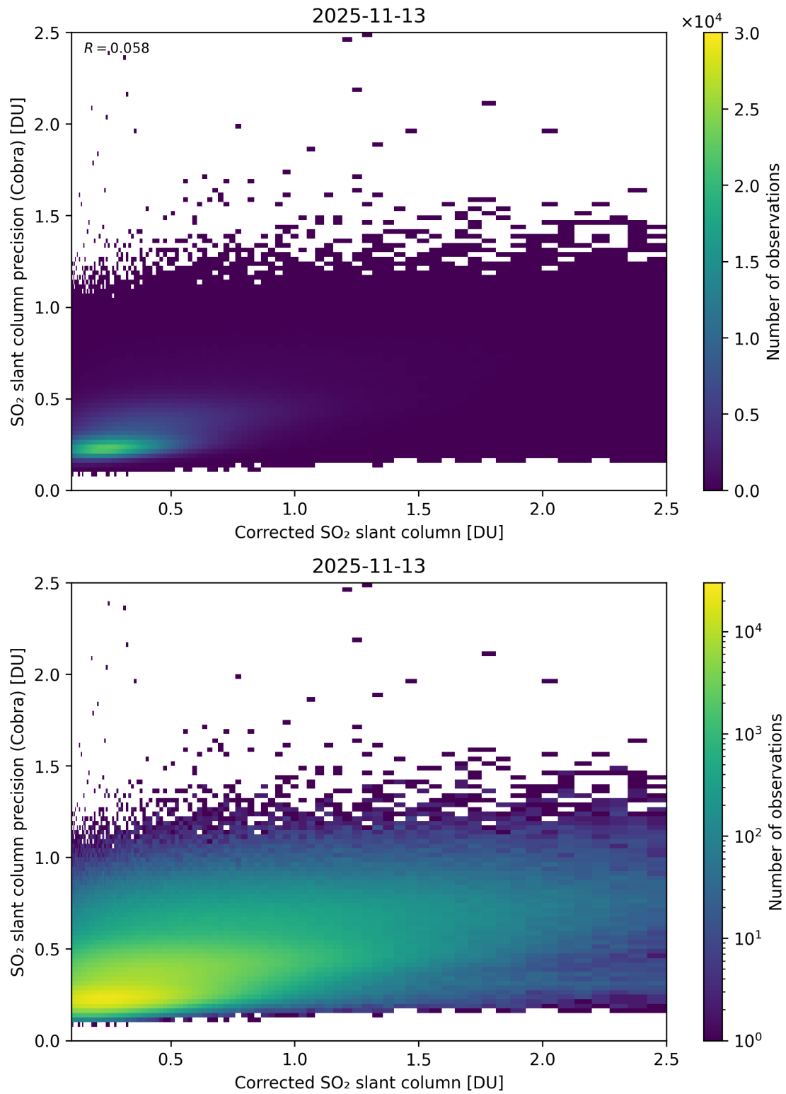
Figure 234: Scatter density plot of “Corrected SO 2 slant column” against “SO 2 slant column precision (Cobra)” for 2025-11-12 to 2025-11-14.
