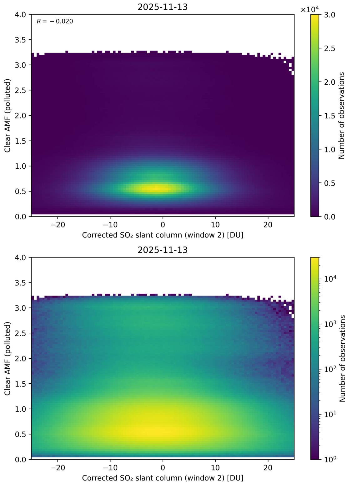
Figure 249: Scatter density plot of “Corrected SO 2 slant column (window 2)” against “Clear AMF (polluted)” for 2025-11-12 to 2025-11-14.
