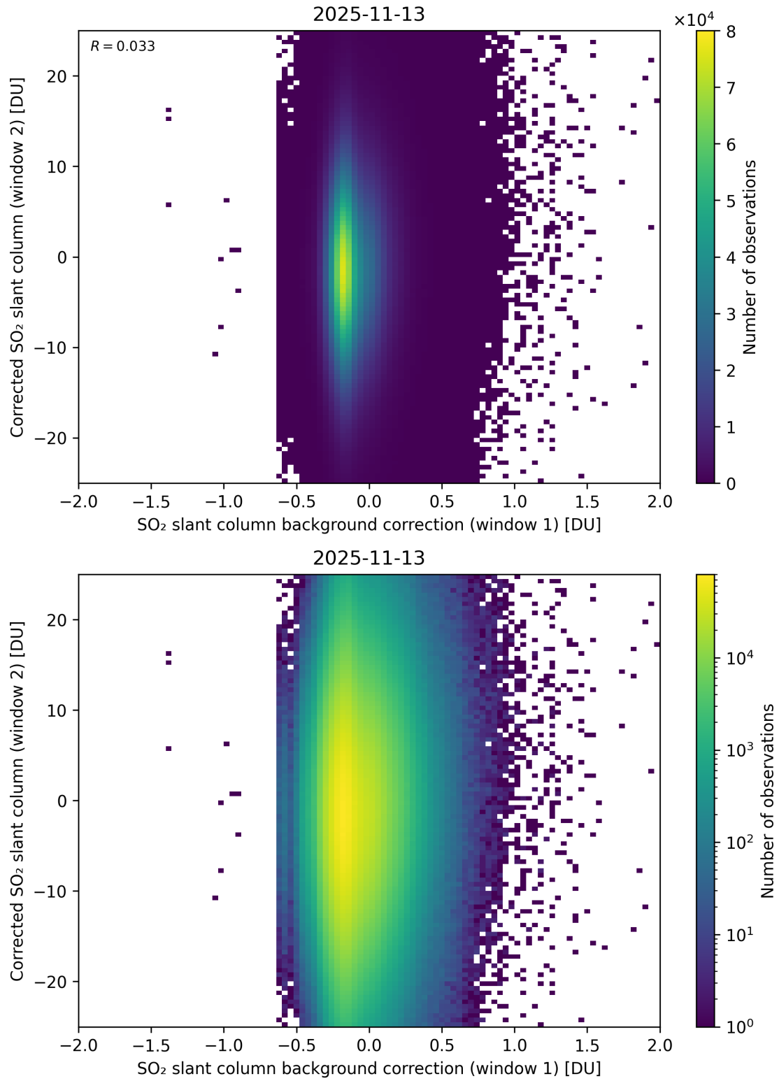
Figure 115: Scatter density plot of “SO 2 slant column background correction (window 1)” against “Corrected SO 2 slant column (window 2)” for 2025-11-12 to 2025-11-14.
