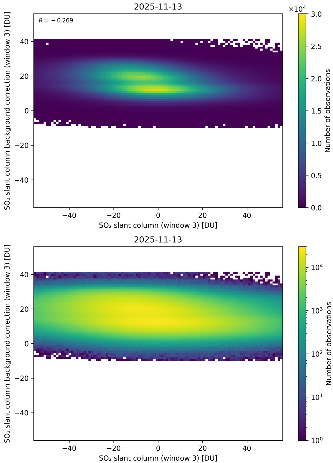
Figure 303: Scatter density plot of “SO 2 slant column (window 3)” against “SO 2 slant column background correction (window 3)” for 2025-11-12 to 2025-11-14.
