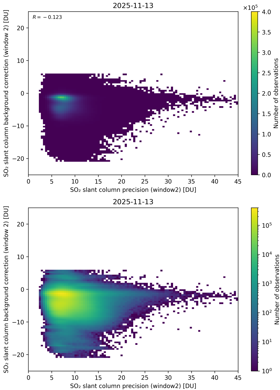
Figure 291: Scatter density plot of “SO 2 slant column precision (window2)” against “SO 2 slant column background correction (window 2)” for 2025-11-12 to 2025-11-14.
