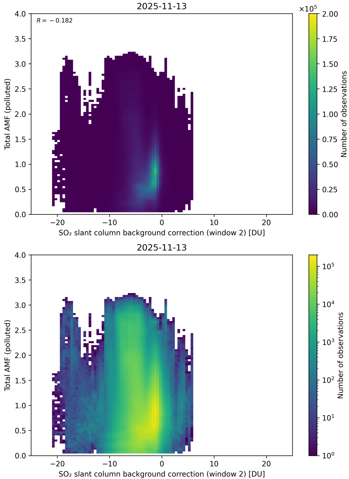
Figure 130: Scatter density plot of “SO 2 slant column background correction (window 2)” against “Total AMF (polluted)” for 2025-11-12 to 2025-11-14.
