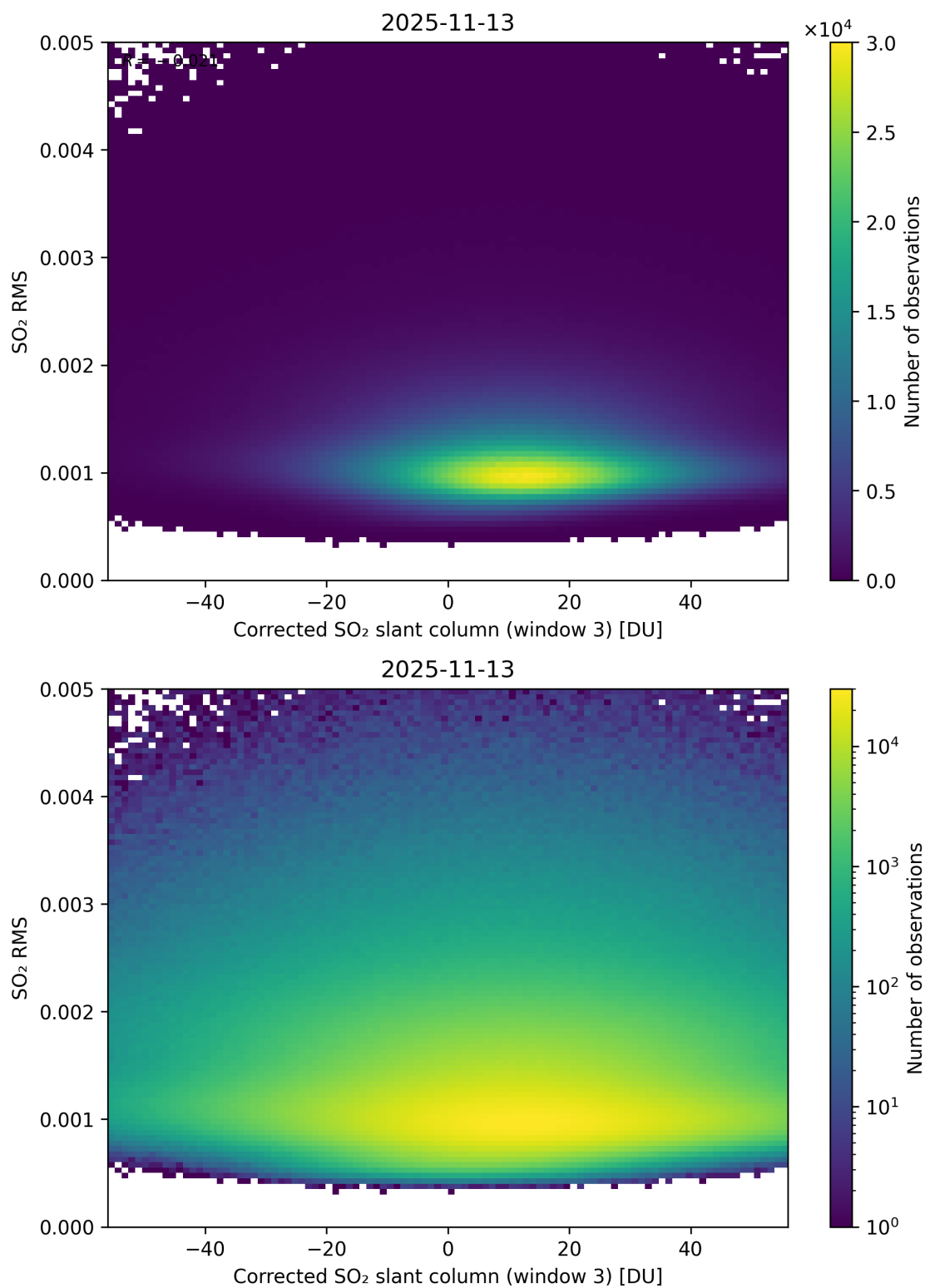
Figure 258: Scatter density plot of “Corrected SO 2 slant column (window 3)” against “SO 2 RMS” for 2025-11-12 to 2025-11-14.
