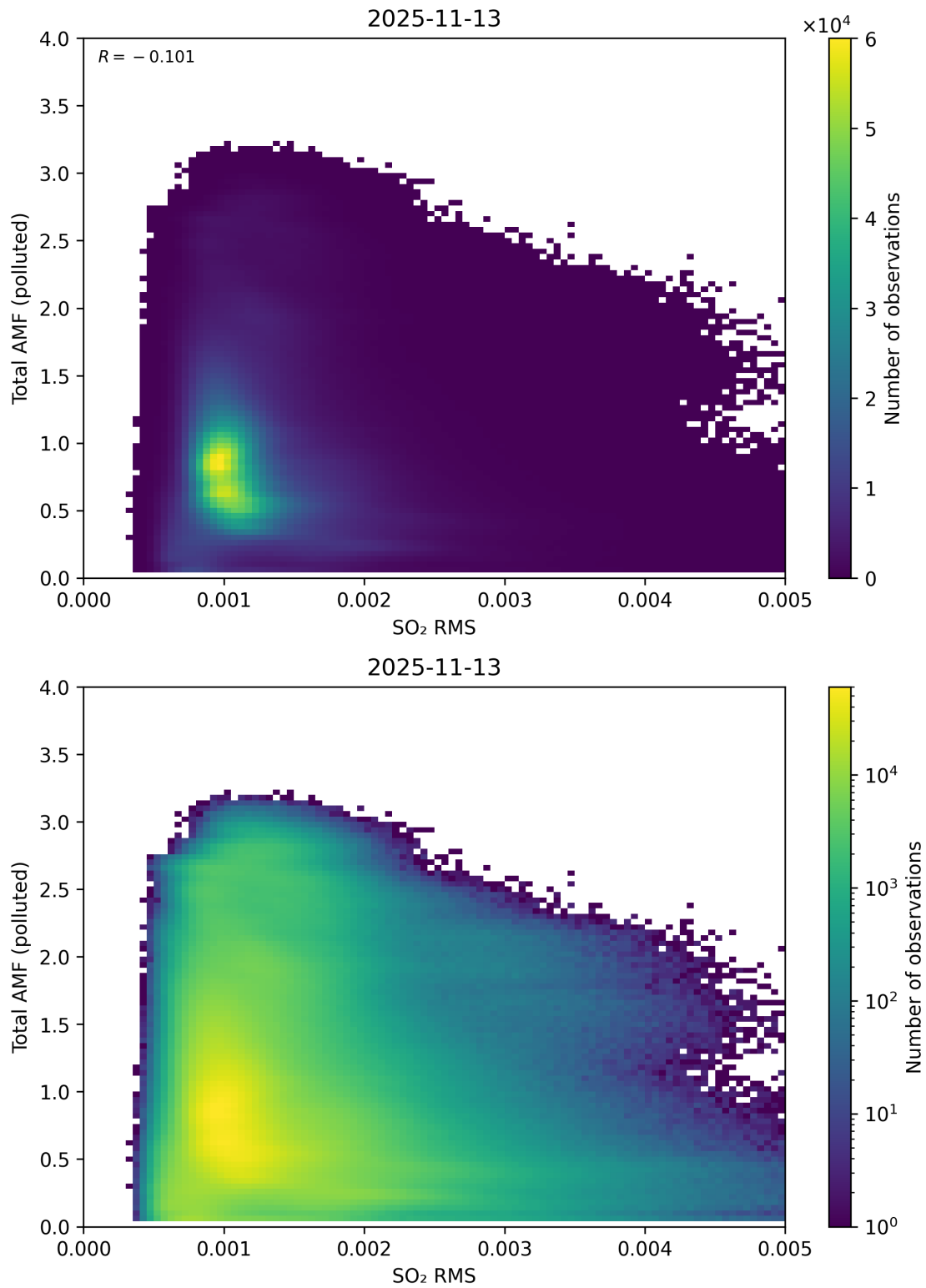
Figure 148: Scatter density plot of “SO 2 RMS” against “Total AMF (polluted)” for 2025-11-12 to 2025-11-14.
