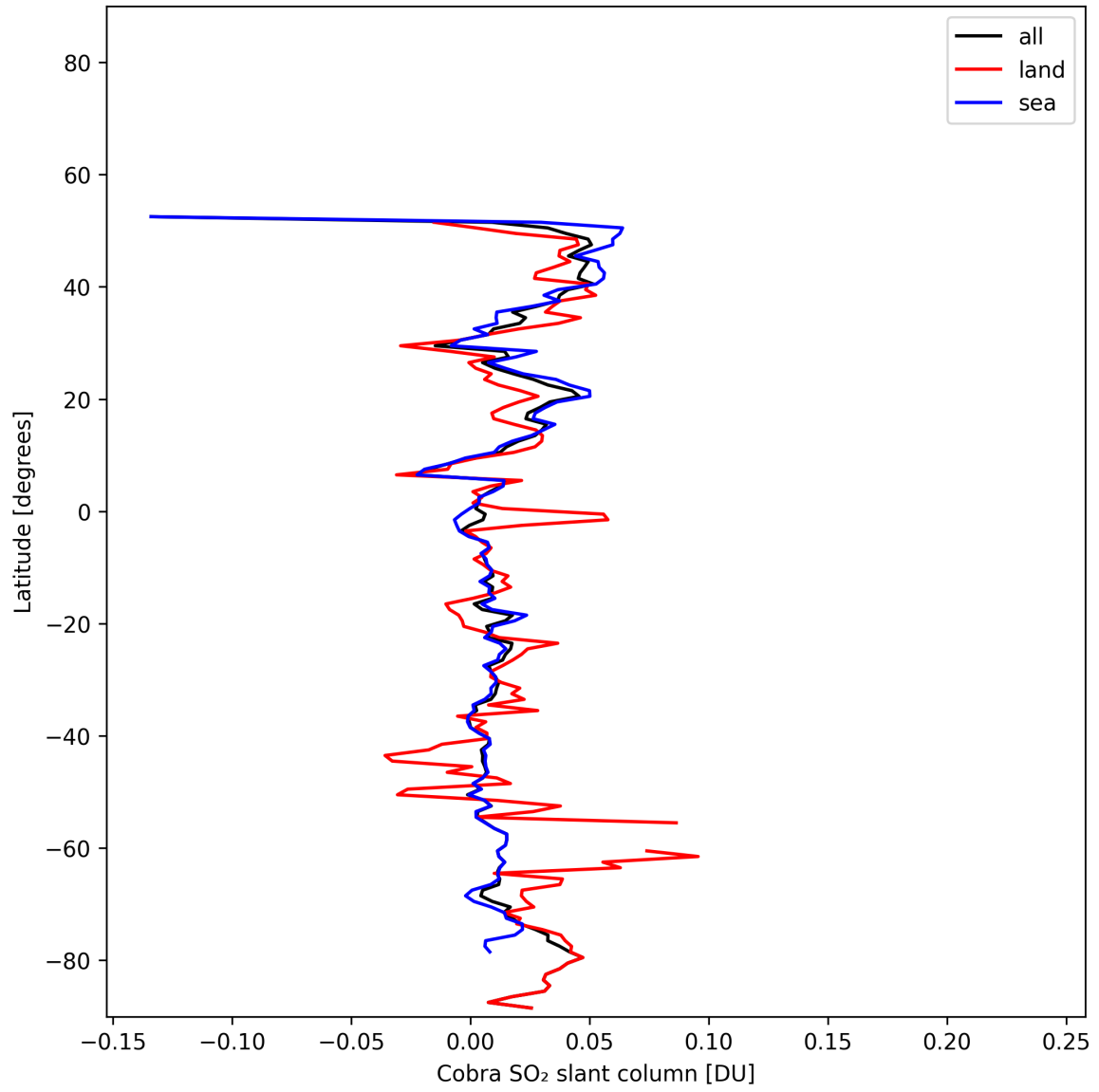
Figure 35: Zonal average of “Cobra SO 2 slant column” for 2025-11-12 to 2025-11-14.
