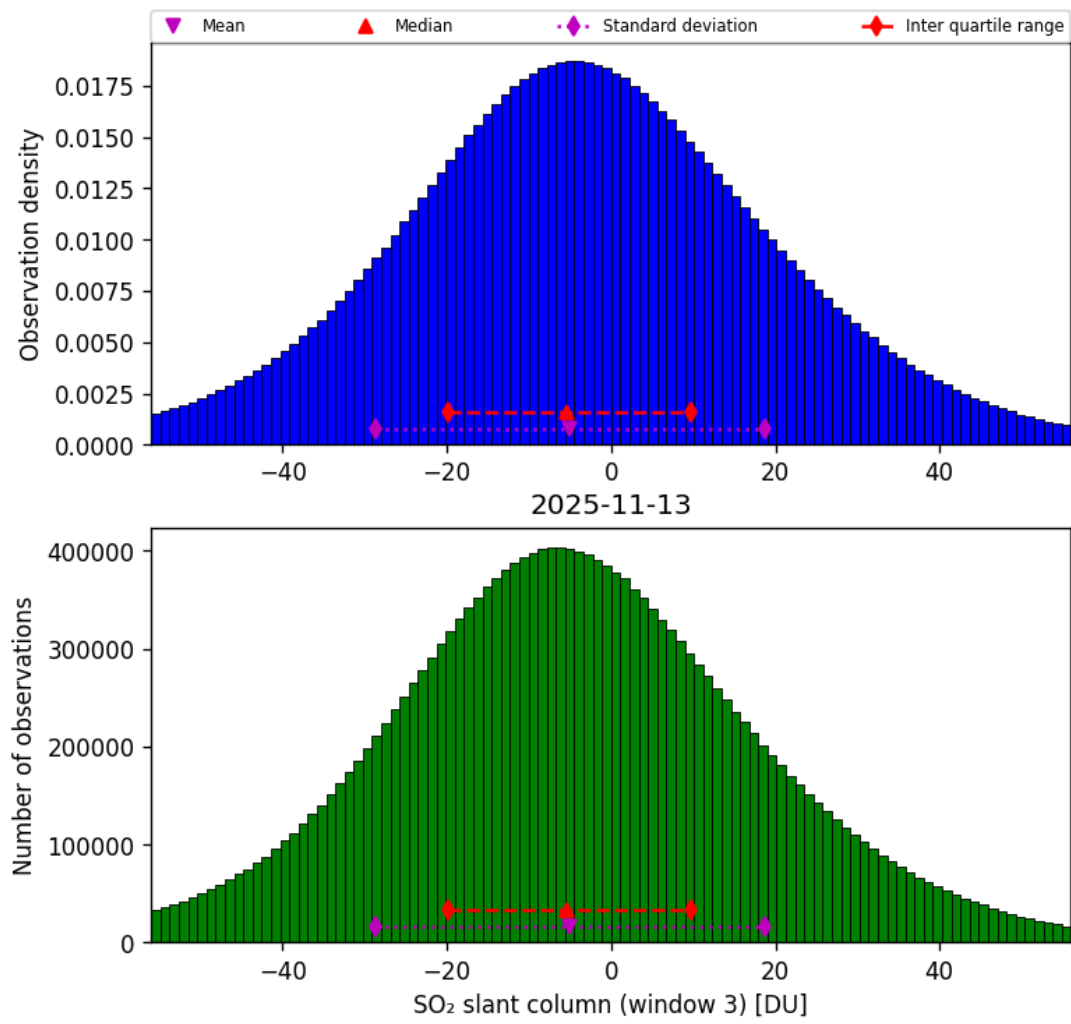
Figure 71: Histogram of “SO 2 slant column (window 3)” for 2025-11-12 to 2025-11-14
