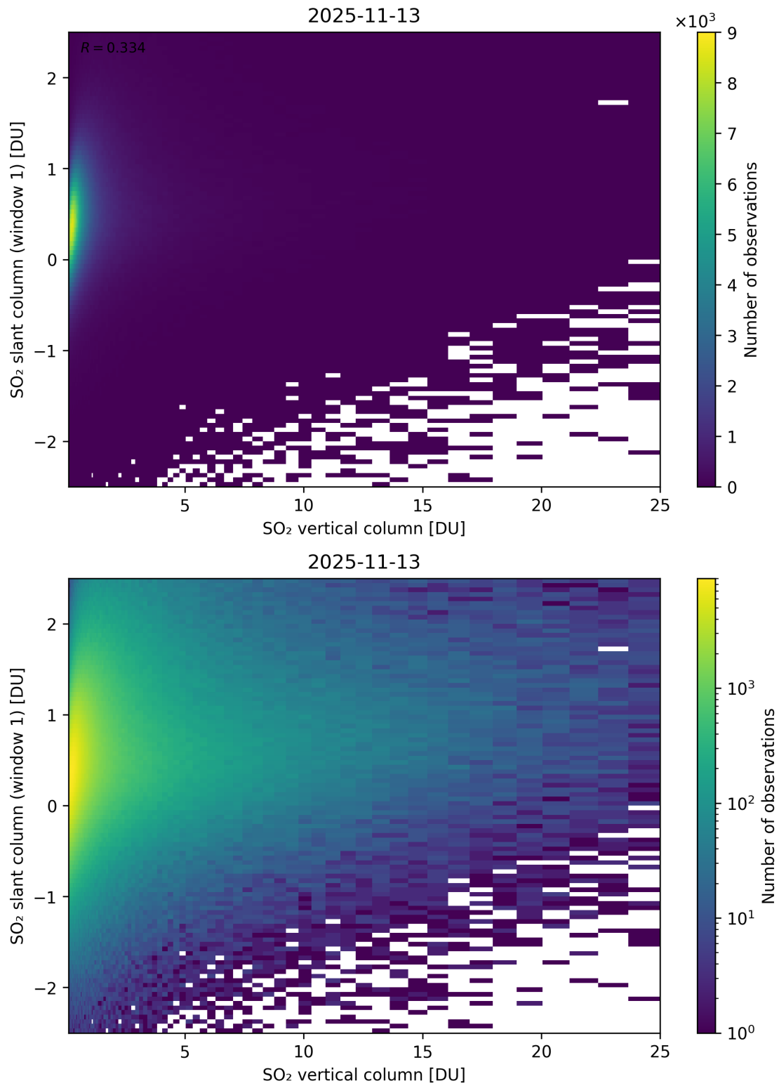
Figure 354: Scatter density plot of “SO 2 vertical column” against “SO 2 slant column (window 1)” for 2025-11-12 to 2025-11-14.
