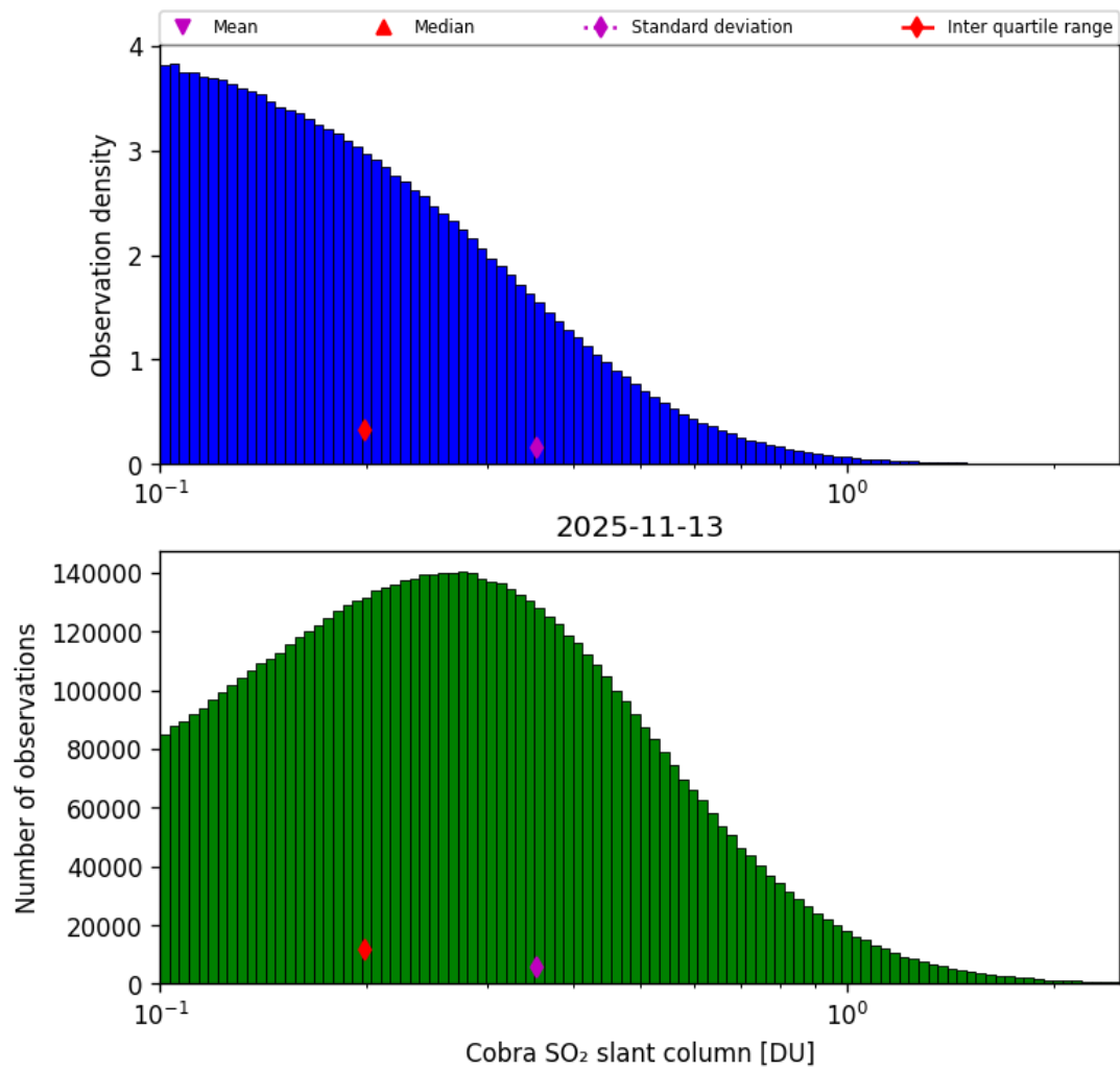
Figure 61: Histogram of “Cobra SO 2 slant column” for 2025-11-12 to 2025-11-14
