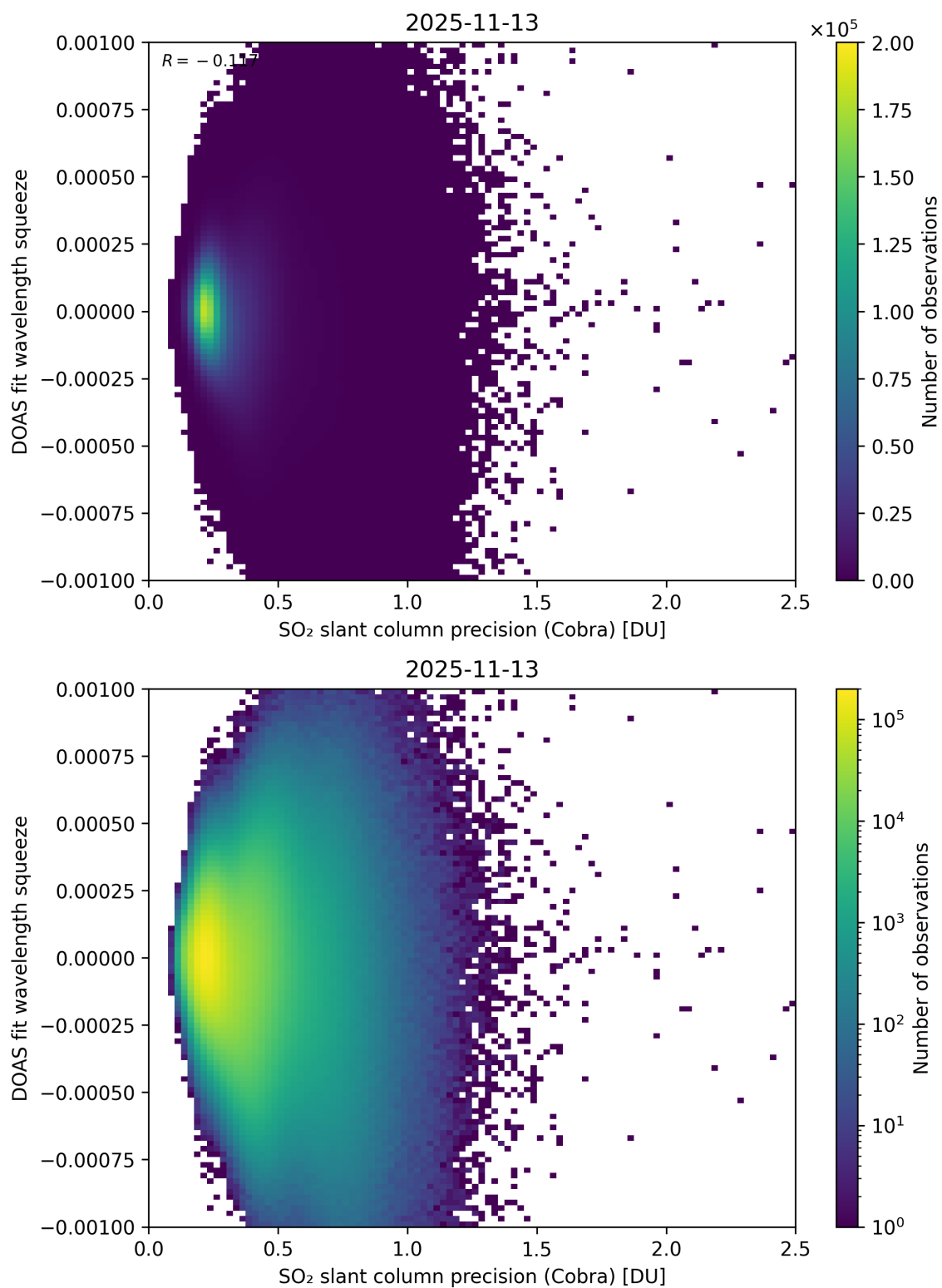
Figure 203: Scatter density plot of “SO 2 slant column precision (Cobra)” against “DOAS fit wavelength squeeze” for 2025-11-12 to 2025-11-14.
