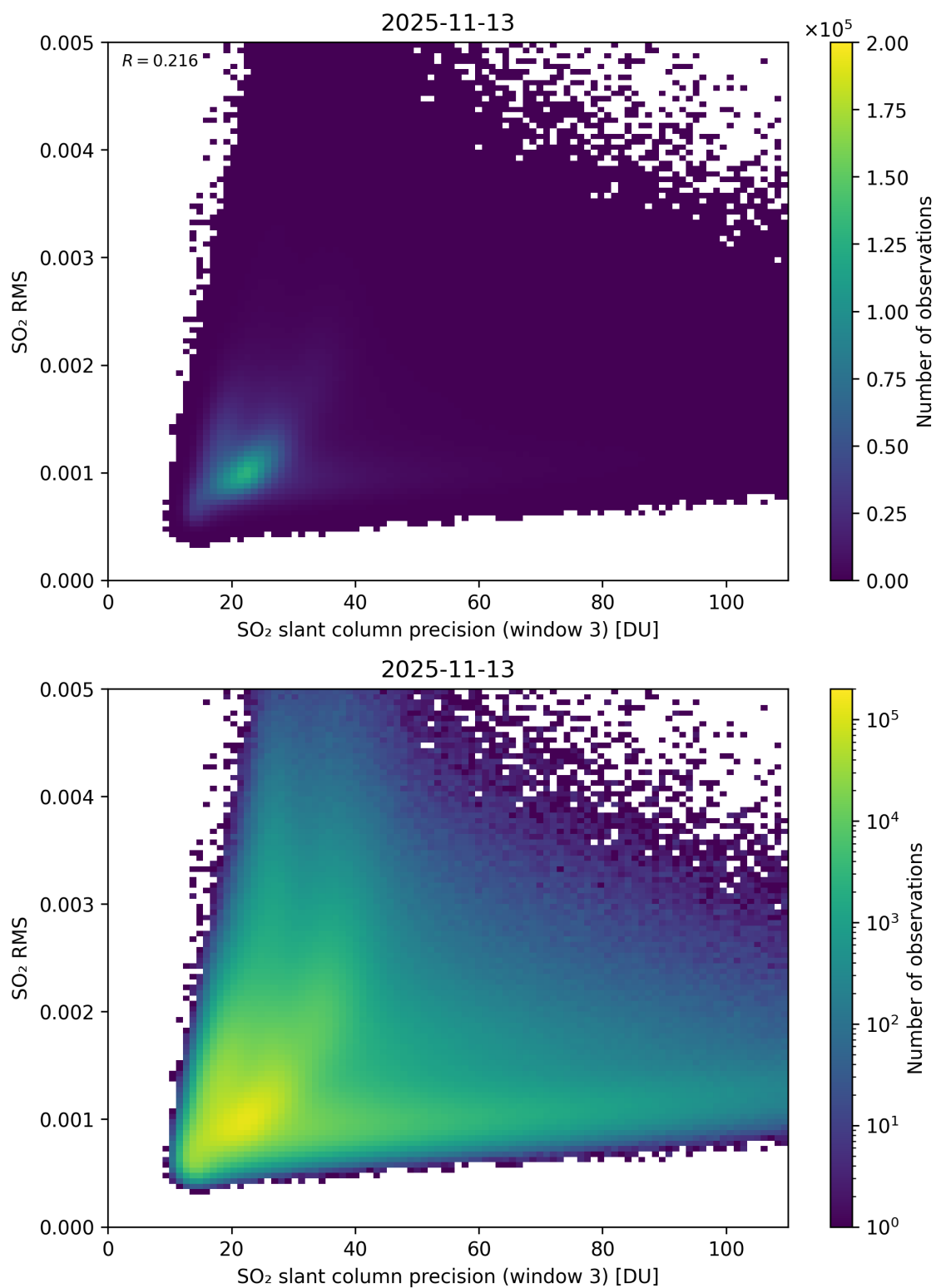
Figure 310: Scatter density plot of “SO 2 slant column precision (window 3)” against “SO 2 RMS” for 2025-11-12 to 2025-11-14.
