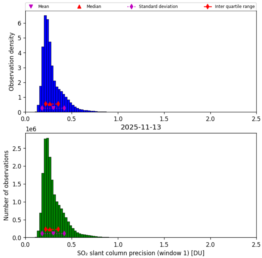
Figure 64: Histogram of “SO 2 slant column precision (window 1)” for 2025-11-12 to 2025-11-14
