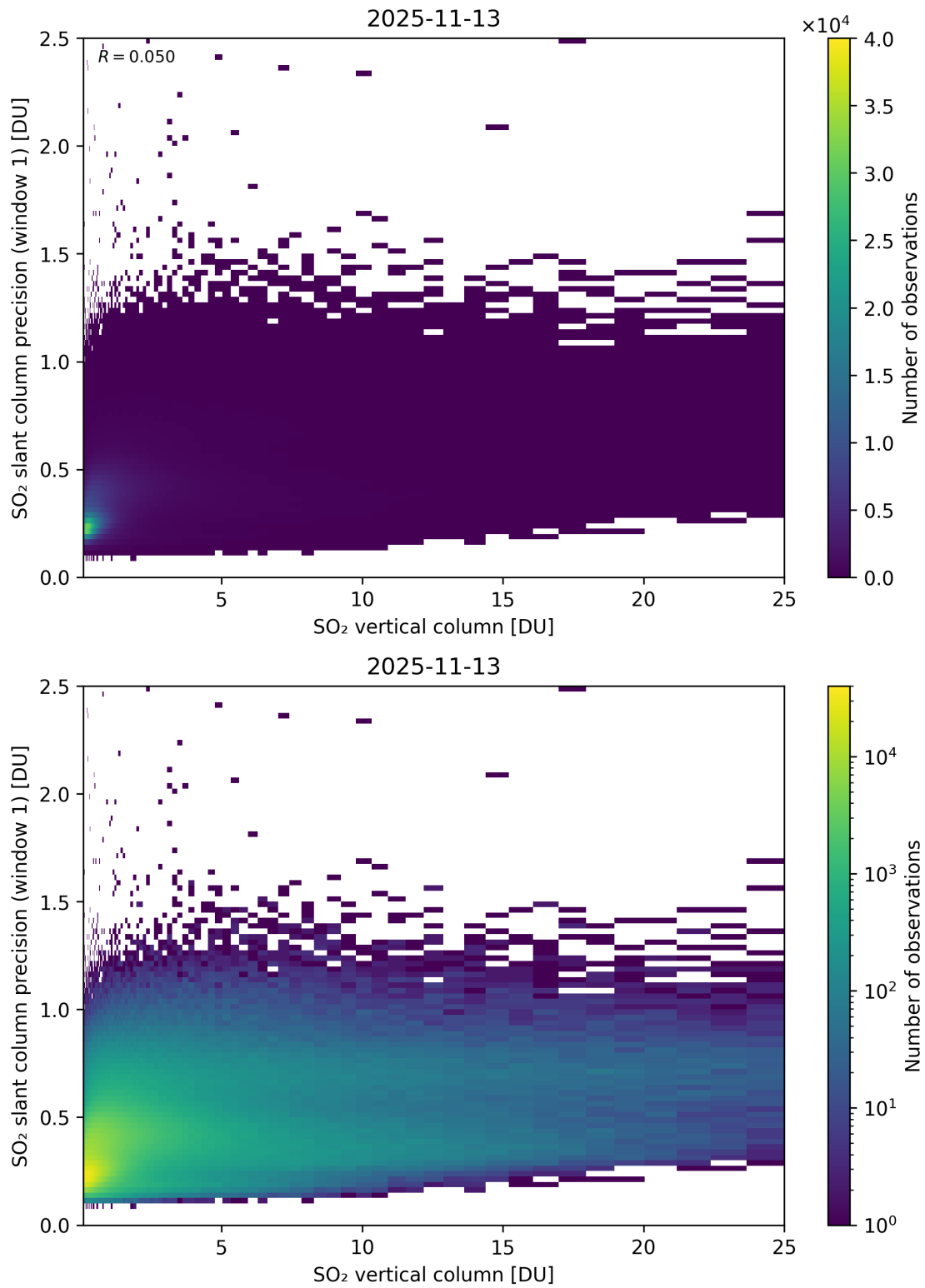
Figure 355: Scatter density plot of “SO 2 vertical column” against “SO 2 slant column precision (window 1)” for 2025-11-12 to 2025-11-14.
