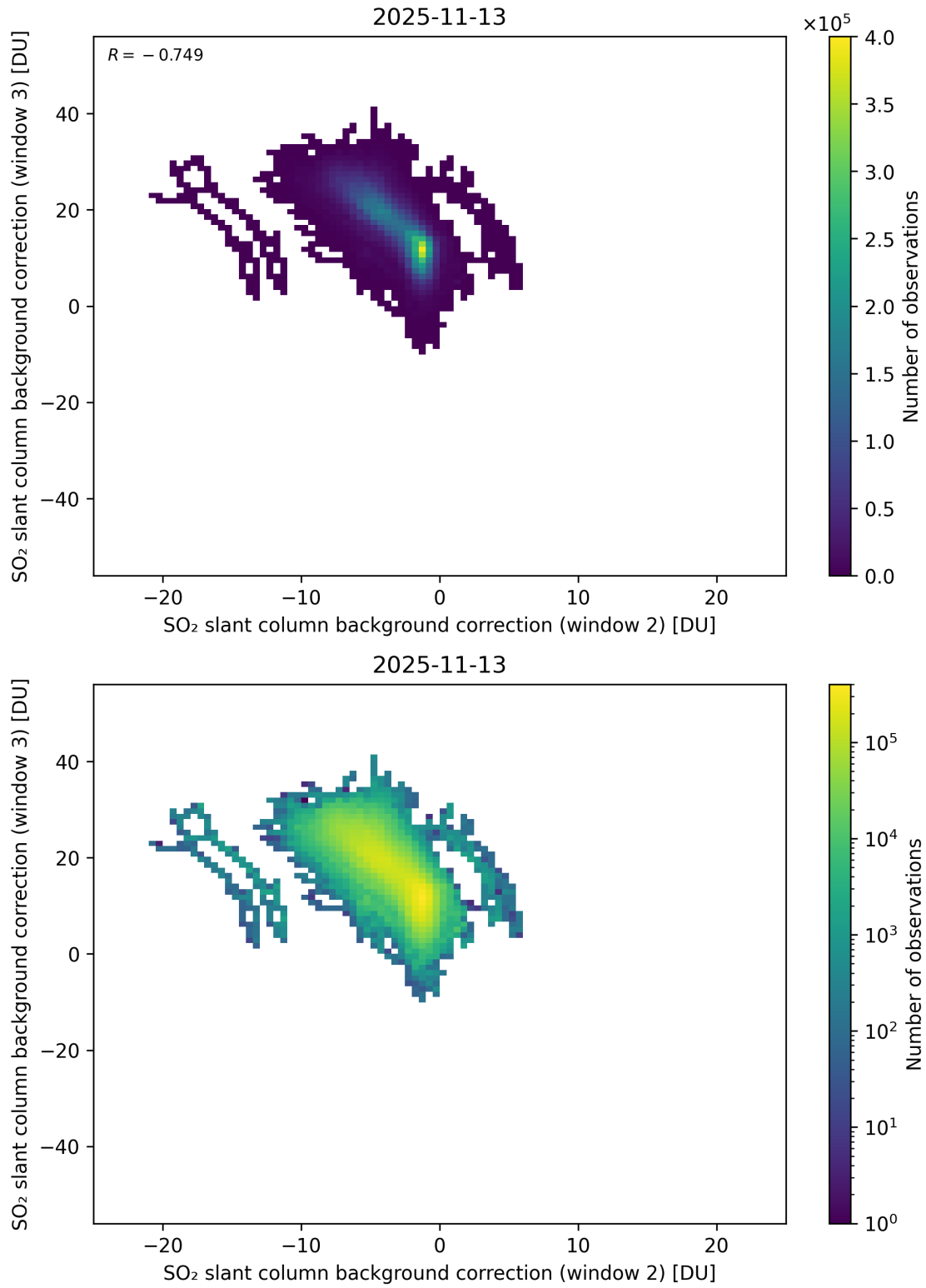
Figure 122: Scatter density plot of “SO 2 slant column background correction (window 2)” against “SO 2 slant column background correction (window 3)” for 2025-11-12 to 2025-11-14.
