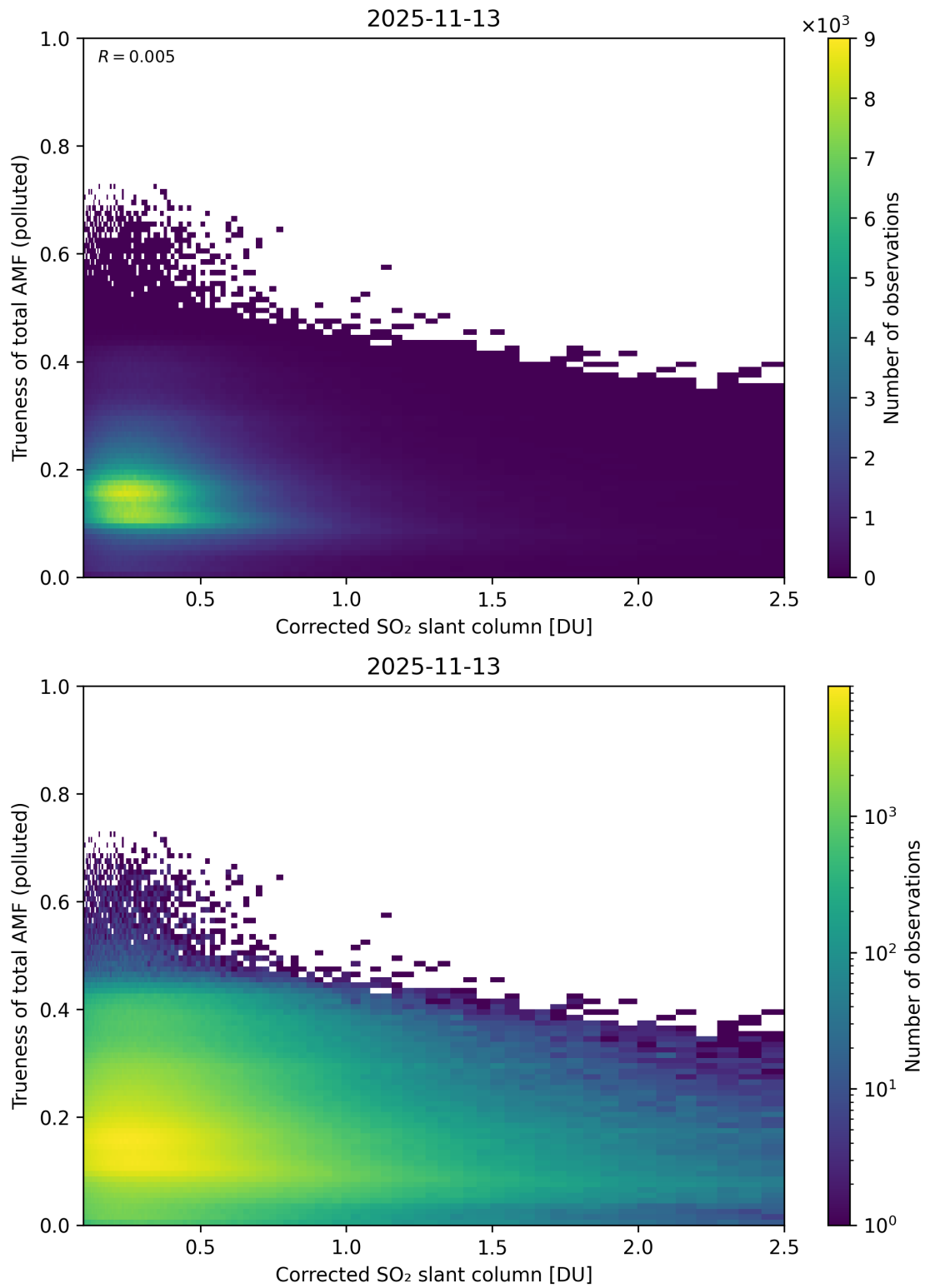
Figure 243: Scatter density plot of “Corrected SO 2 slant column” against “Trueness of total AMF (polluted)” for 2025-11-12 to 2025-11-14.
