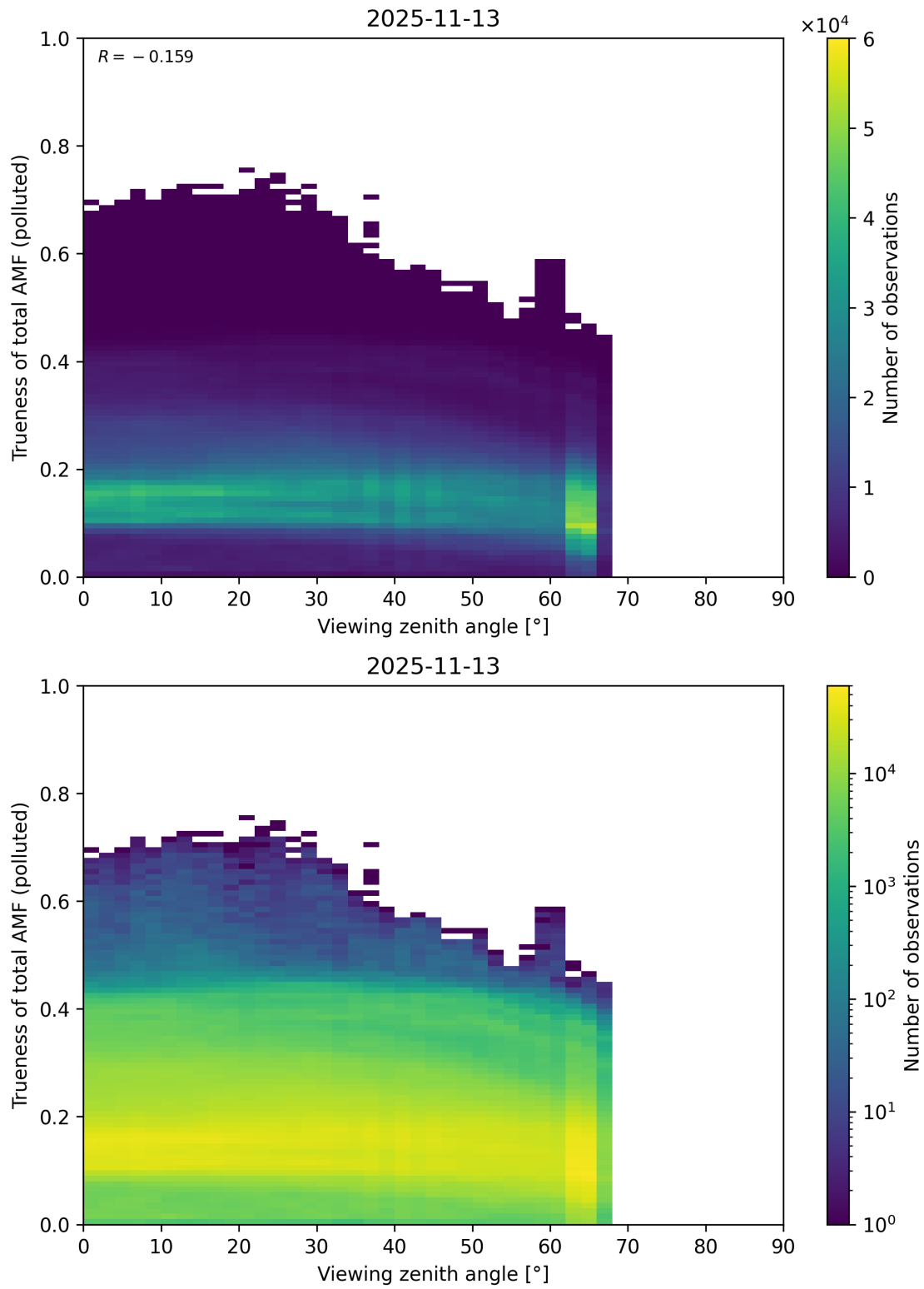
Figure 382: Scatter density plot of “Viewing zenith angle” against “Trueness of total AMF (polluted)” for 2025-11-12 to 2025-11-14.
