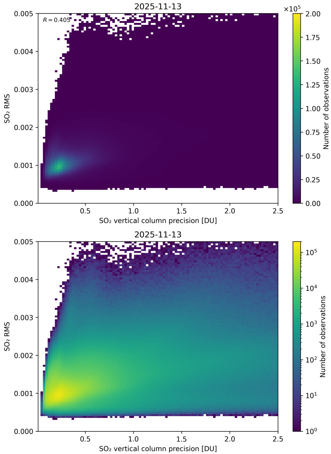
Figure 334: Scatter density plot of “SO 2 vertical column precision” against “SO 2 RMS” for 2025-11-12 to 2025-11-14.
