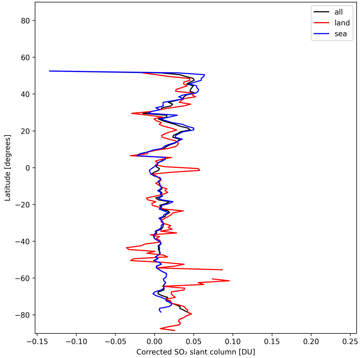
Figure 34: Zonal average of “Corrected SO 2 slant column” for 2025-11-12 to 2025-11-14.
