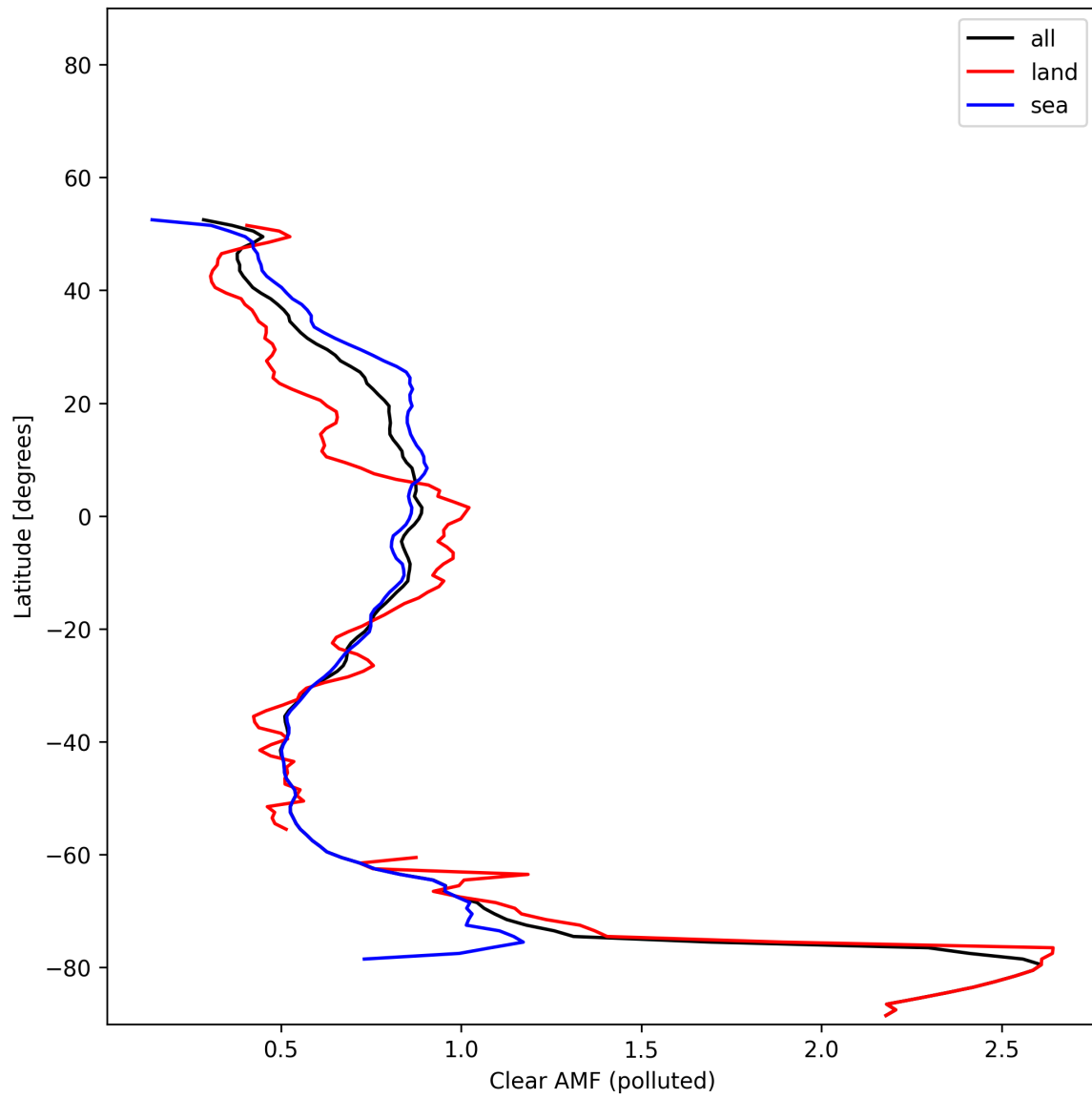
Figure 55: Zonal average of “Clear AMF (polluted)” for 2025-11-12 to 2025-11-14.
