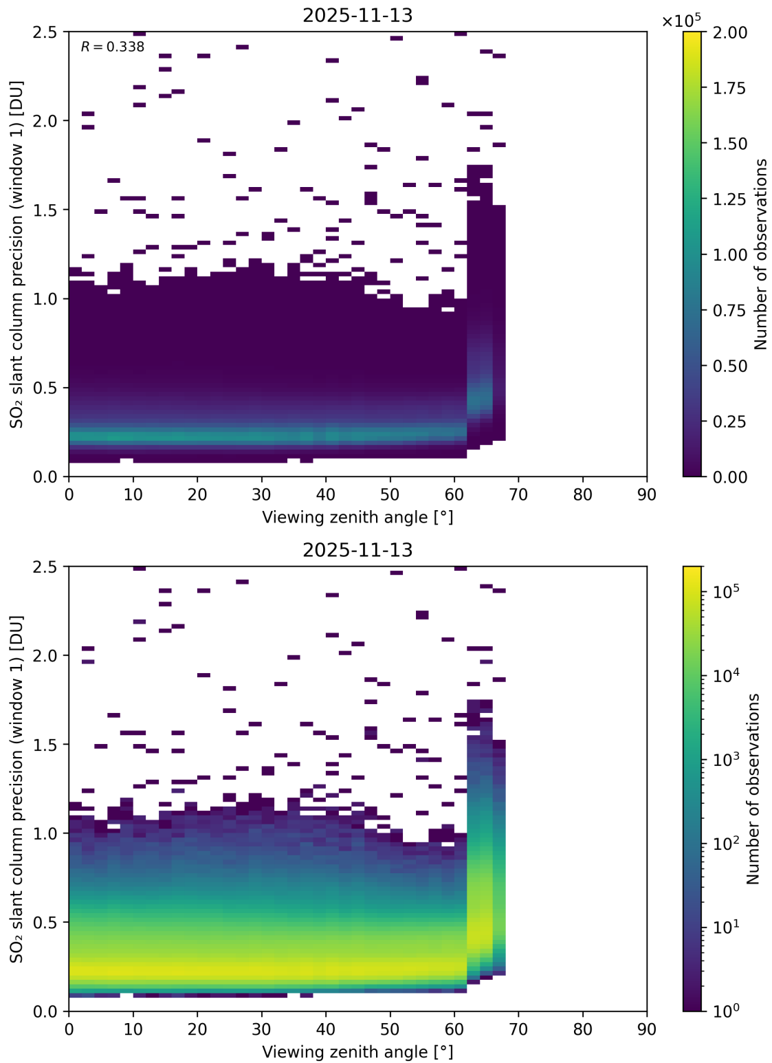
Figure 377: Scatter density plot of “Viewing zenith angle” against “SO 2 slant column precision (window 1)” for 2025-11-12 to 2025-11-14.
