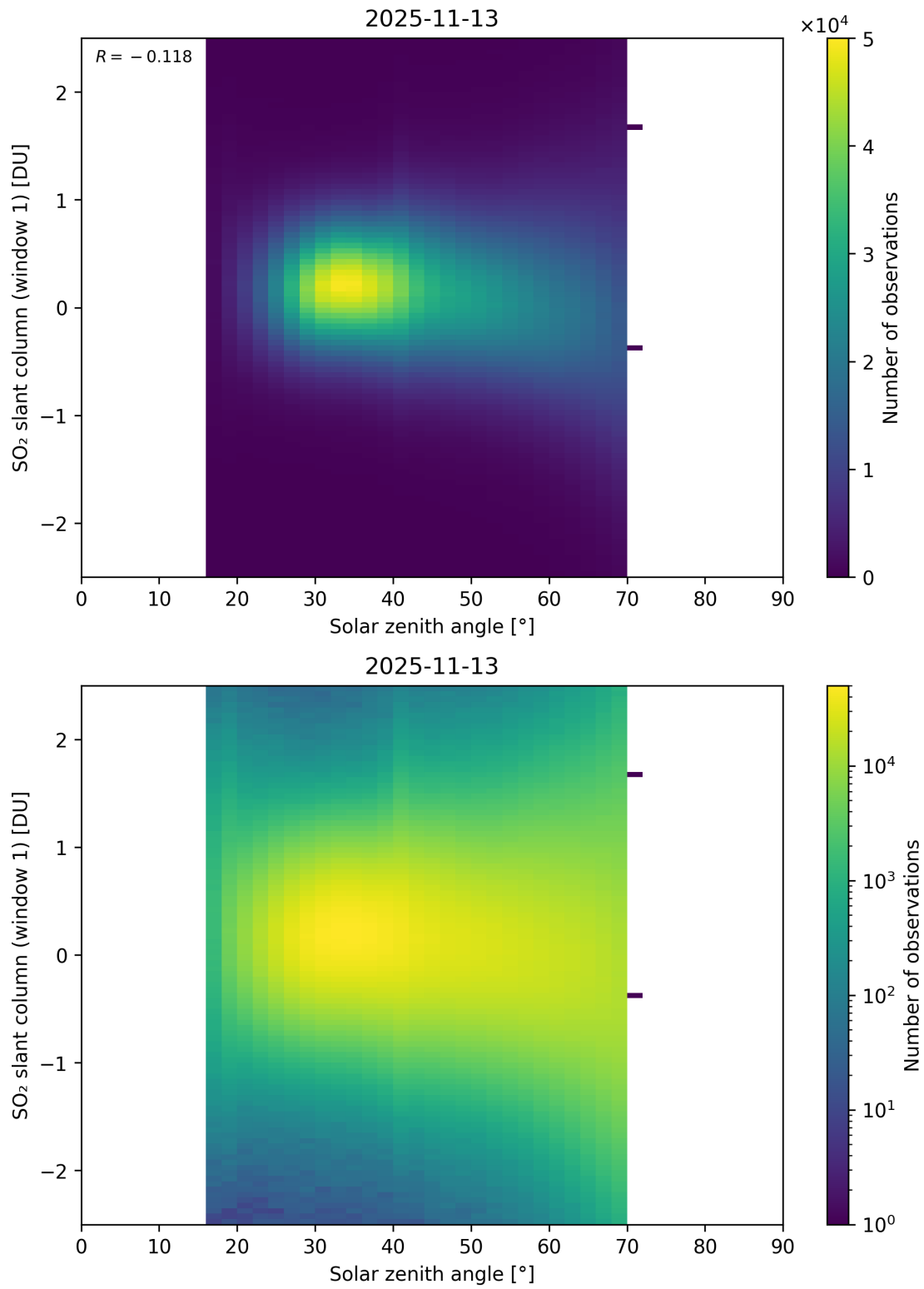
Figure 184: Scatter density plot of “Solar zenith angle” against “SO 2 slant column (window 1)” for 2025-11-12 to 2025-11-14.
