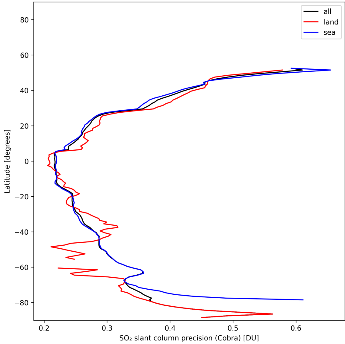
Figure 36: Zonal average of “SO 2 slant column precision (Cobra)” for 2025-11-12 to 2025-11-14.
