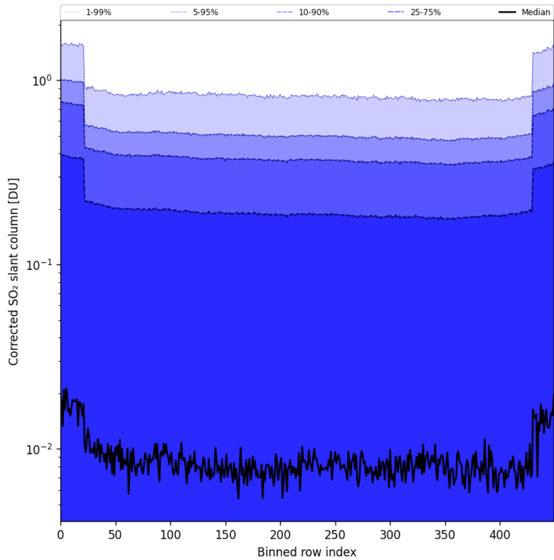
Figure 86: Along track statistics of “Corrected SO 2 slant column” for 2025-11-12 to 2025-11-14
