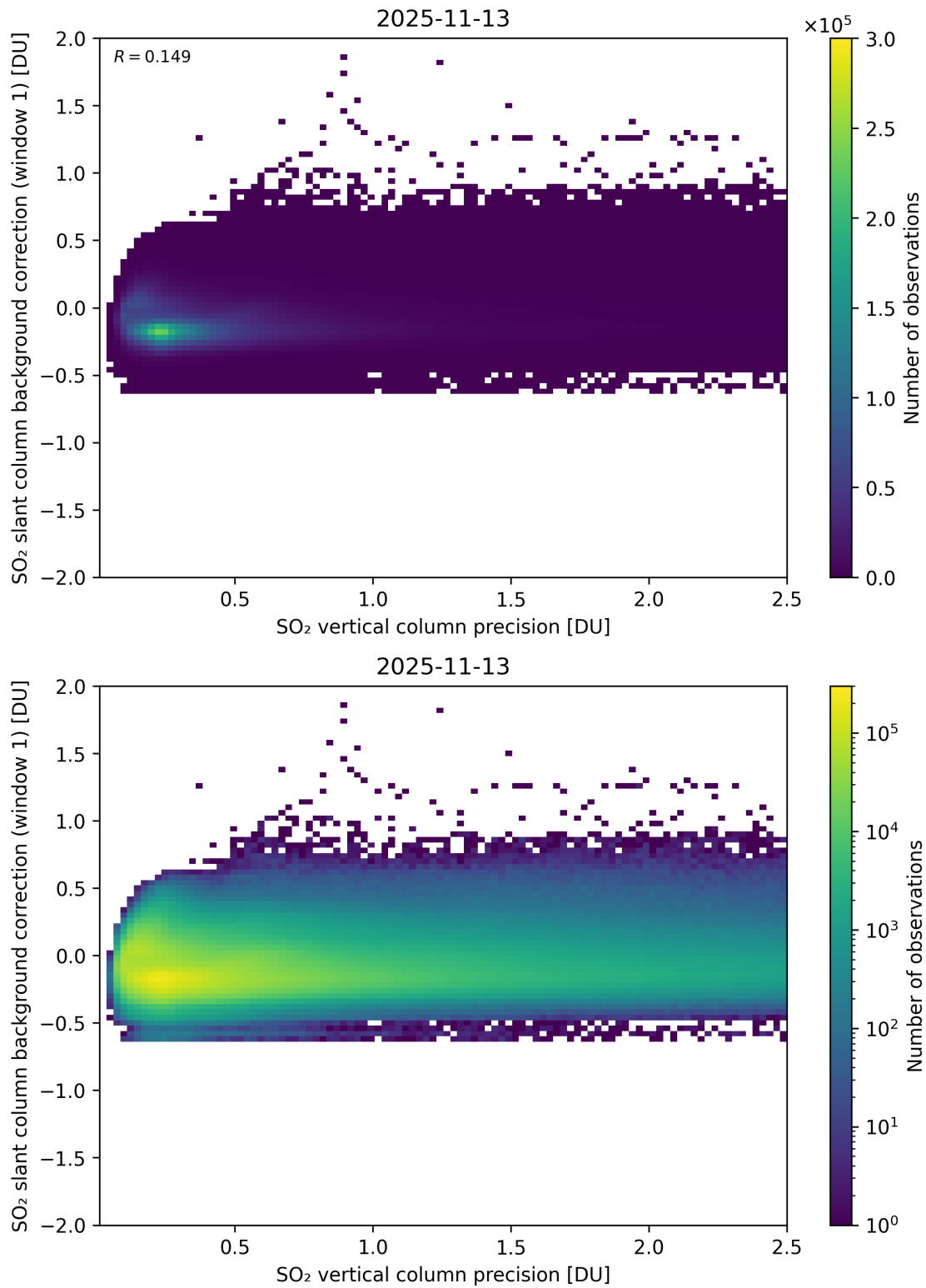
Figure 329: Scatter density plot of “SO 2 vertical column precision” against “SO 2 slant column background correction (window 1)” for 2025-11-12 to 2025-11-14.
