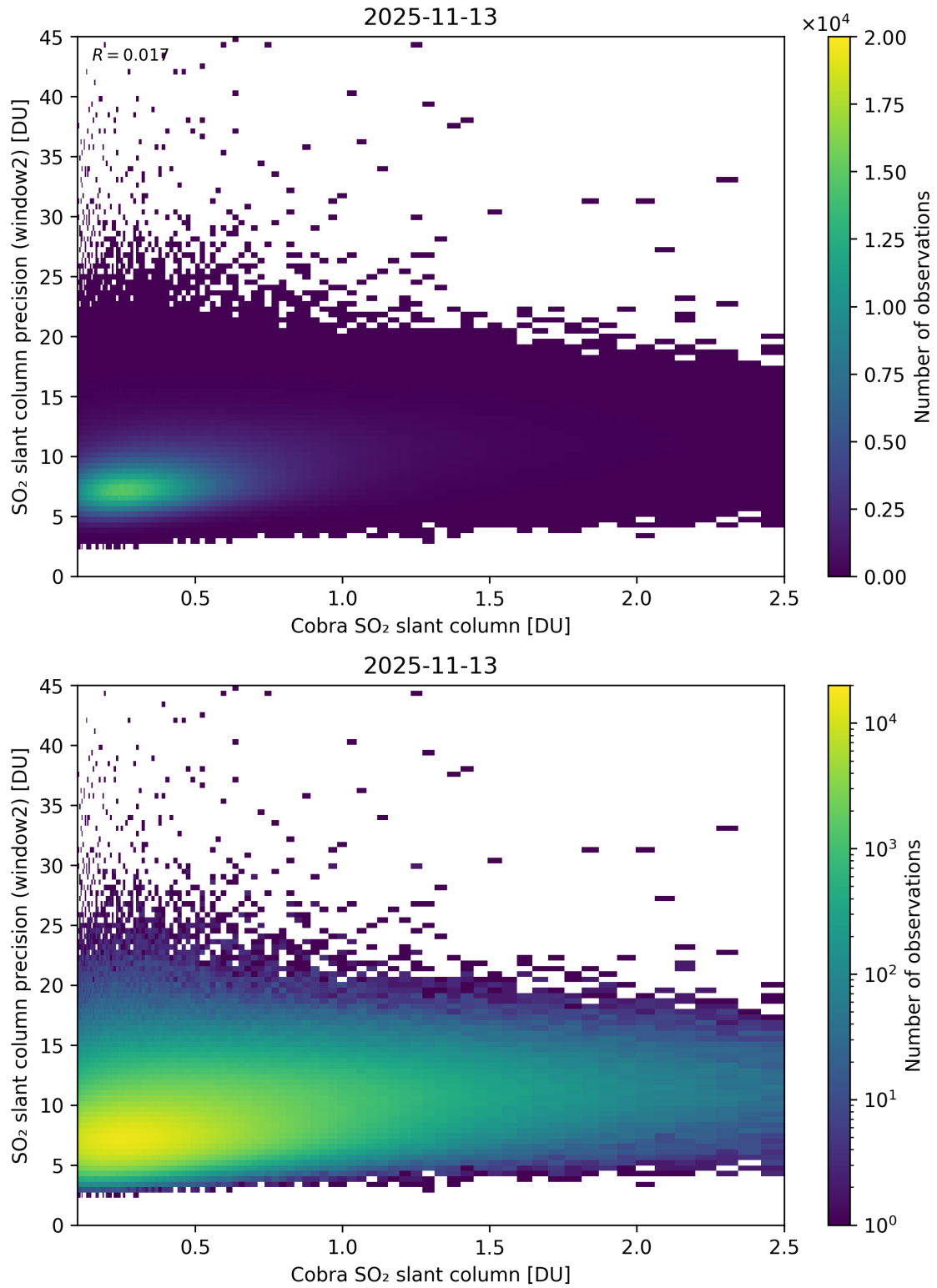
Figure 221: Scatter density plot of “Cobra SO 2 slant column” against “SO 2 slant column precision (window2)” for 2025-11-12 to 2025-11-14.
