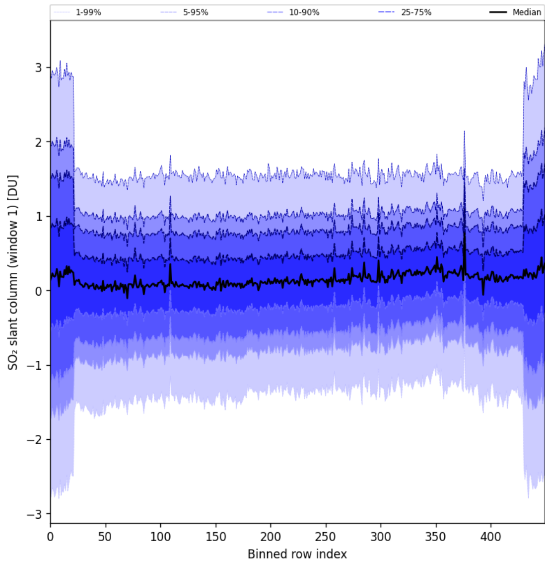
Figure 89: Along track statistics of “SO 2 slant column (window 1)” for 2025-11-12 to 2025-11-14
