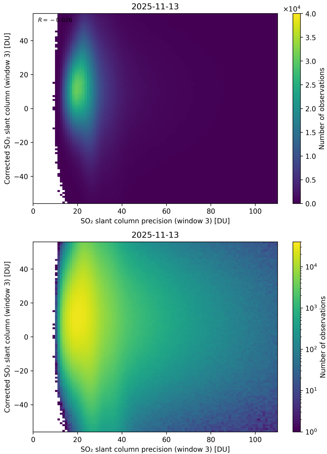
Figure 312: Scatter density plot of “SO 2 slant column precision (window 3)” against “Corrected SO 2 slant column (window 3)” for 2025-11-12 to 2025-11-14.
