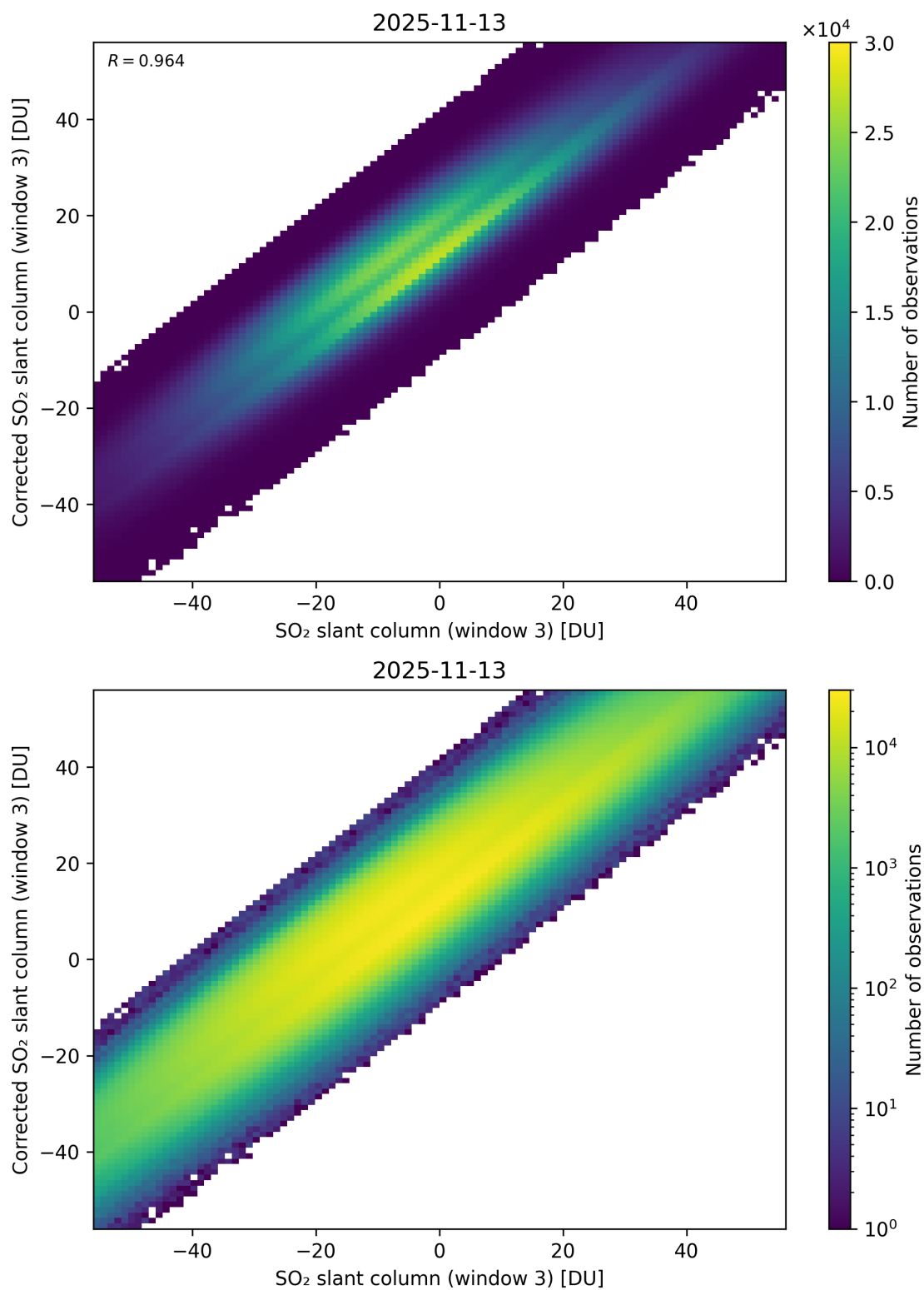
Figure 316: Scatter density plot of “SO 2 slant column (window 3)” against “Corrected SO 2 slant column (window 3)” for 2025-11-12 to 2025-11-14.
