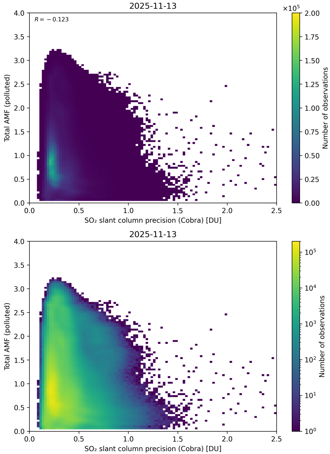
Figure 213: Scatter density plot of “SO 2 slant column precision (Cobra)” against “Total AMF (polluted)” for 2025-11-12 to 2025-11-14.
