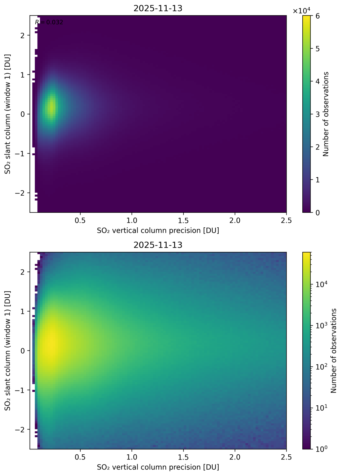
Figure 341: Scatter density plot of “SO 2 vertical column precision” against “SO 2 slant column (window 1)” for 2025-11-12 to 2025-11-14.
