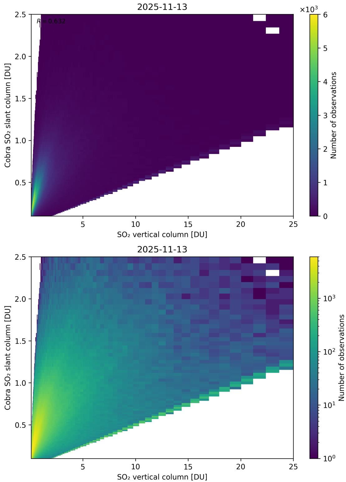
Figure 349: Scatter density plot of “SO 2 vertical column” against “Cobra SO 2 slant column” for 2025-11-12 to 2025-11-14.
