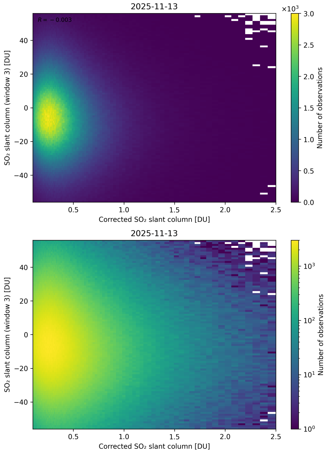
Figure 240: Scatter density plot of “Corrected SO 2 slant column” against “SO 2 slant column (window 3)” for 2025-11-12 to 2025-11-14.
