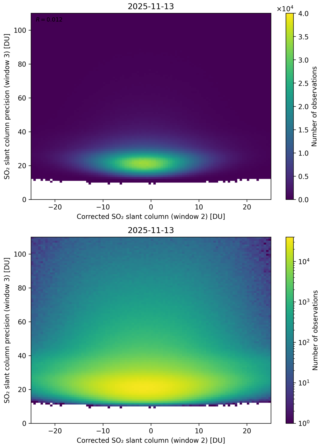
Figure 252: Scatter density plot of “Corrected SO 2 slant column (window 2)” against “SO 2 slant column precision (window 3)” for 2025-11-12 to 2025-11-14.
