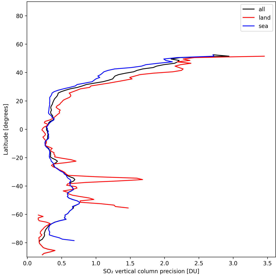
Figure 33: Zonal average of “SO 2 vertical column precision” for 2025-11-12 to 2025-11-14.
