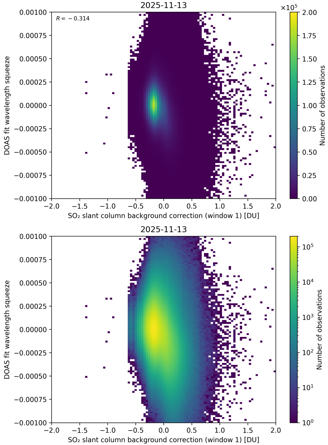
Figure 112: Scatter density plot of “SO 2 slant column background correction (window 1)” against “DOAS fit wavelength squeeze” for 2025-11-12 to 2025-11-14.
