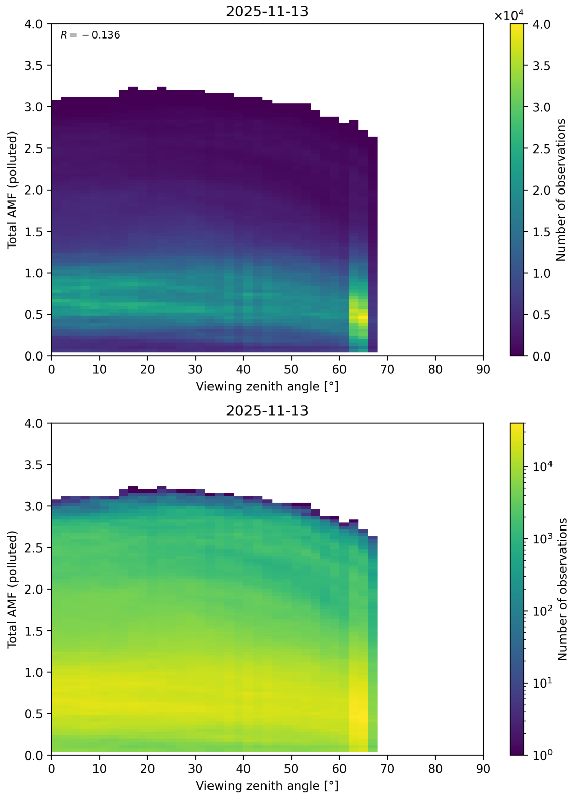
Figure 381: Scatter density plot of “Viewing zenith angle” against “Total AMF (polluted)” for 2025-11-12 to 2025-11-14.
