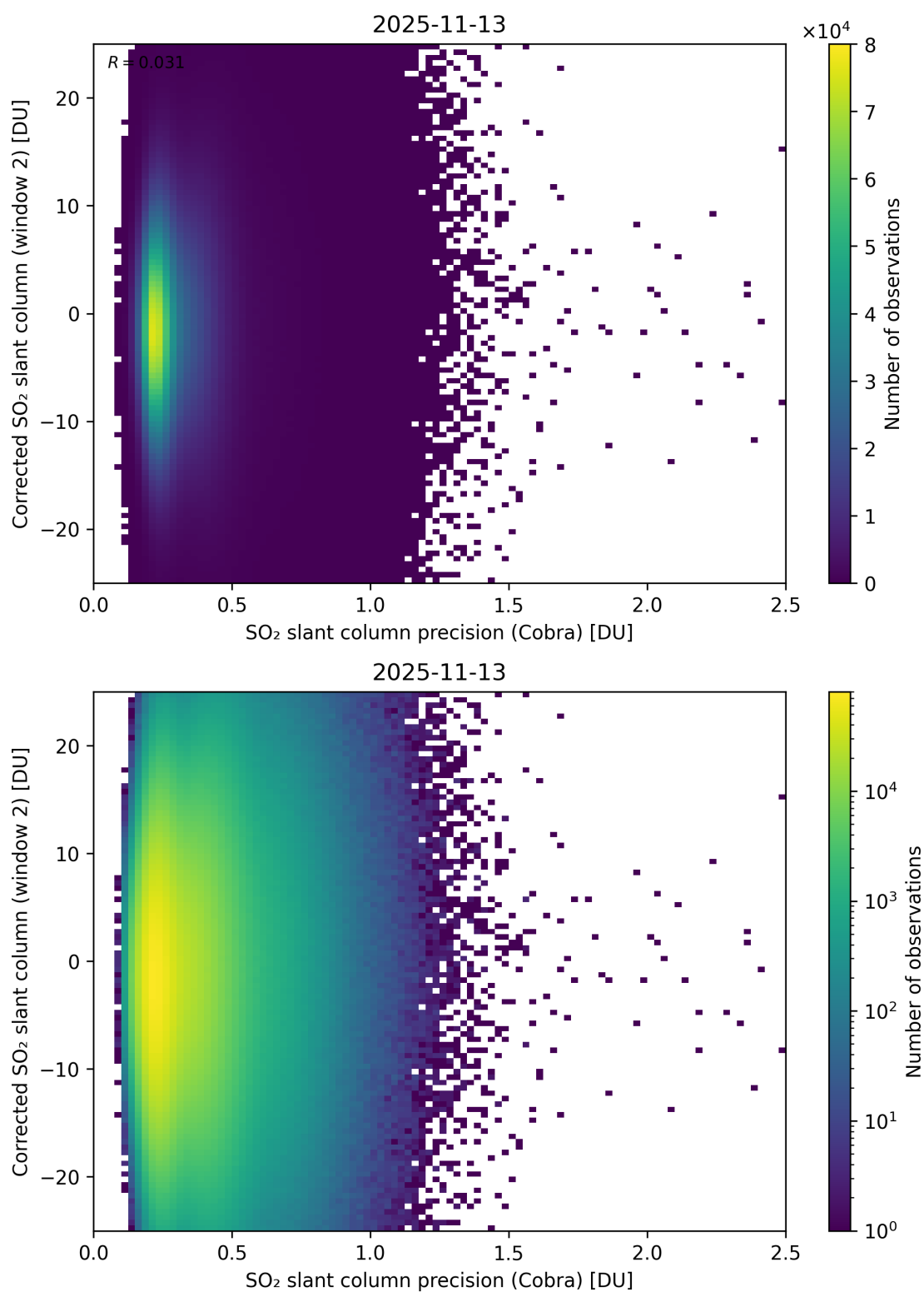
Figure 206: Scatter density plot of “SO 2 slant column precision (Cobra)” against “Corrected SO 2 slant column (window 2)” for 2025-11-12 to 2025-11-14.
