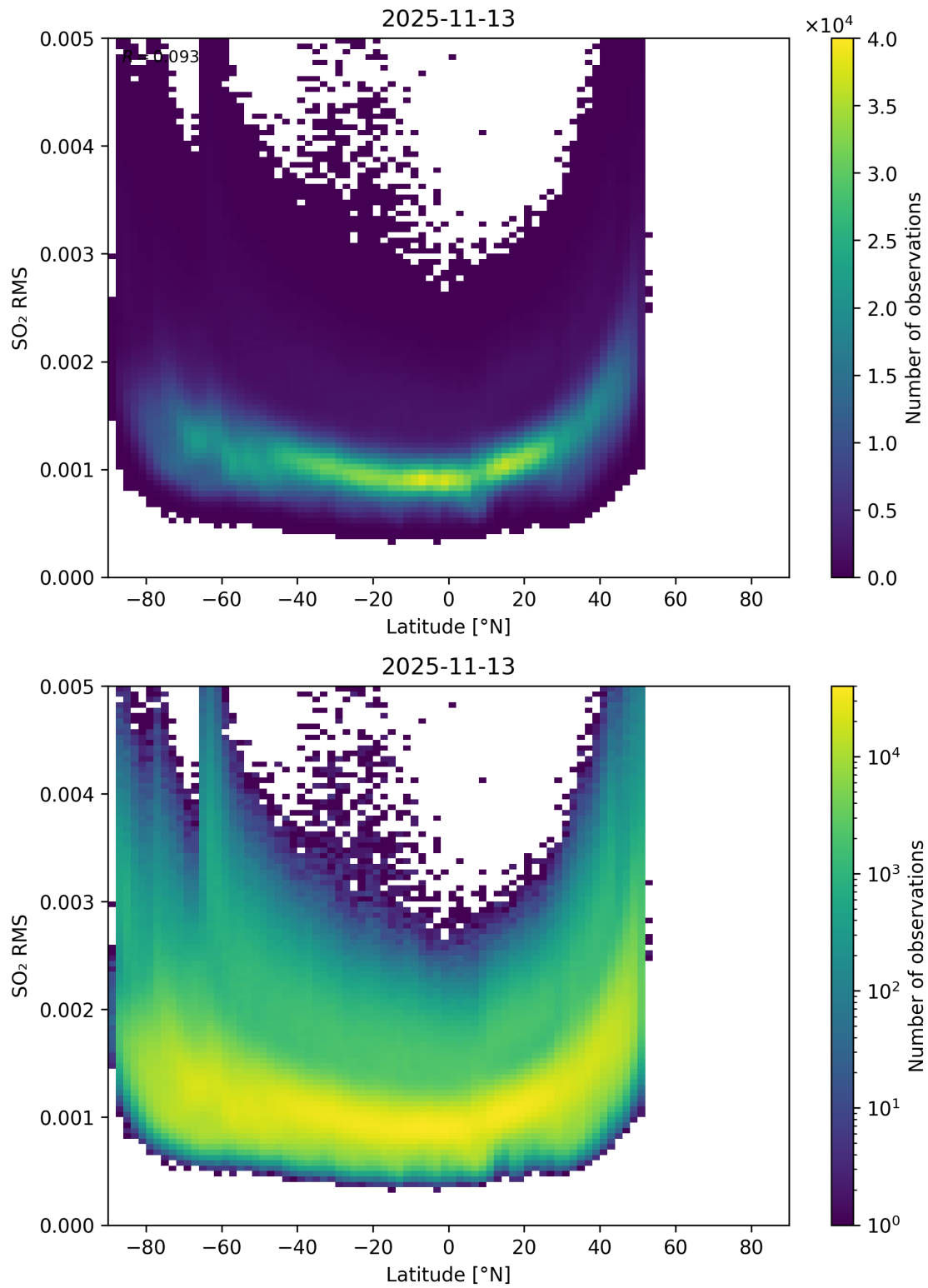
Figure 155: Scatter density plot of “Latitude” against “SO 2 RMS” for 2025-11-12 to 2025-11-14.
