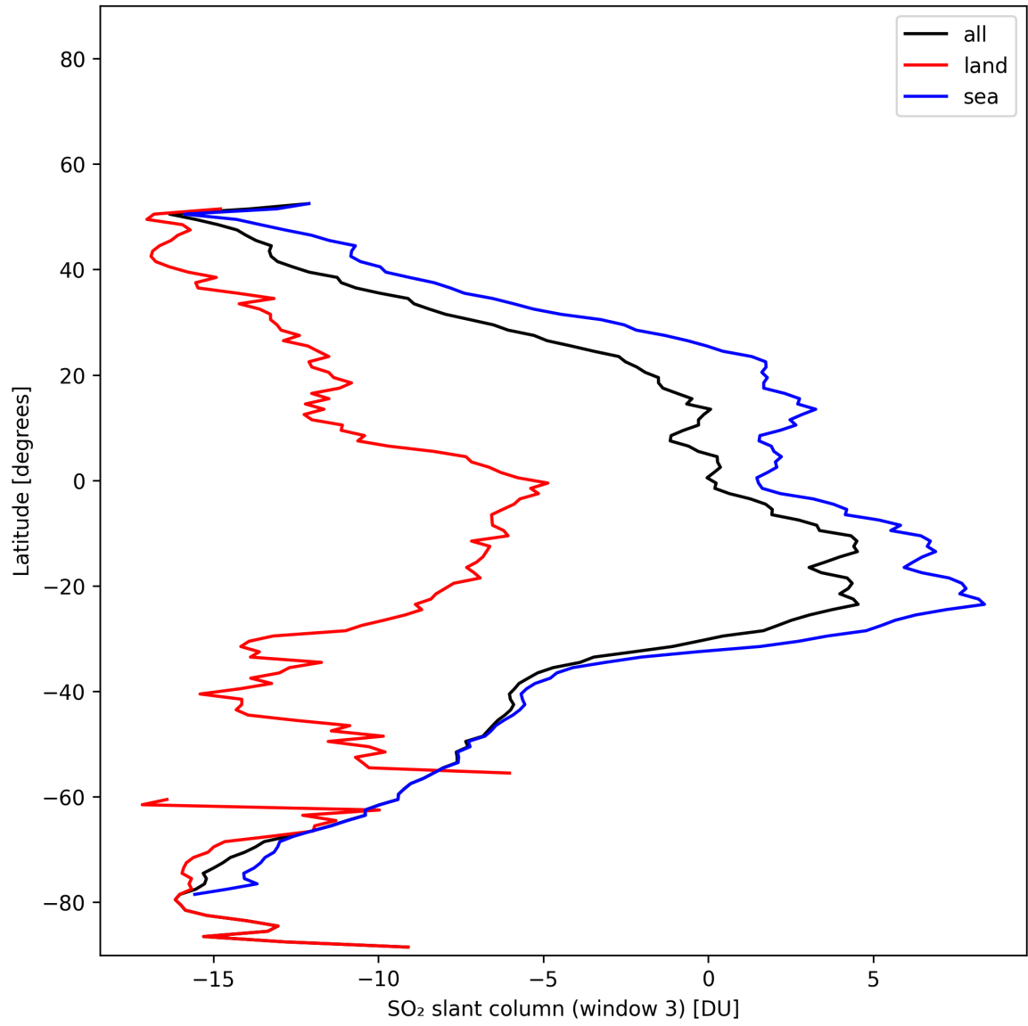
Figure 45: Zonal average of “SO 2 slant column (window 3)” for 2025-11-12 to 2025-11-14.
