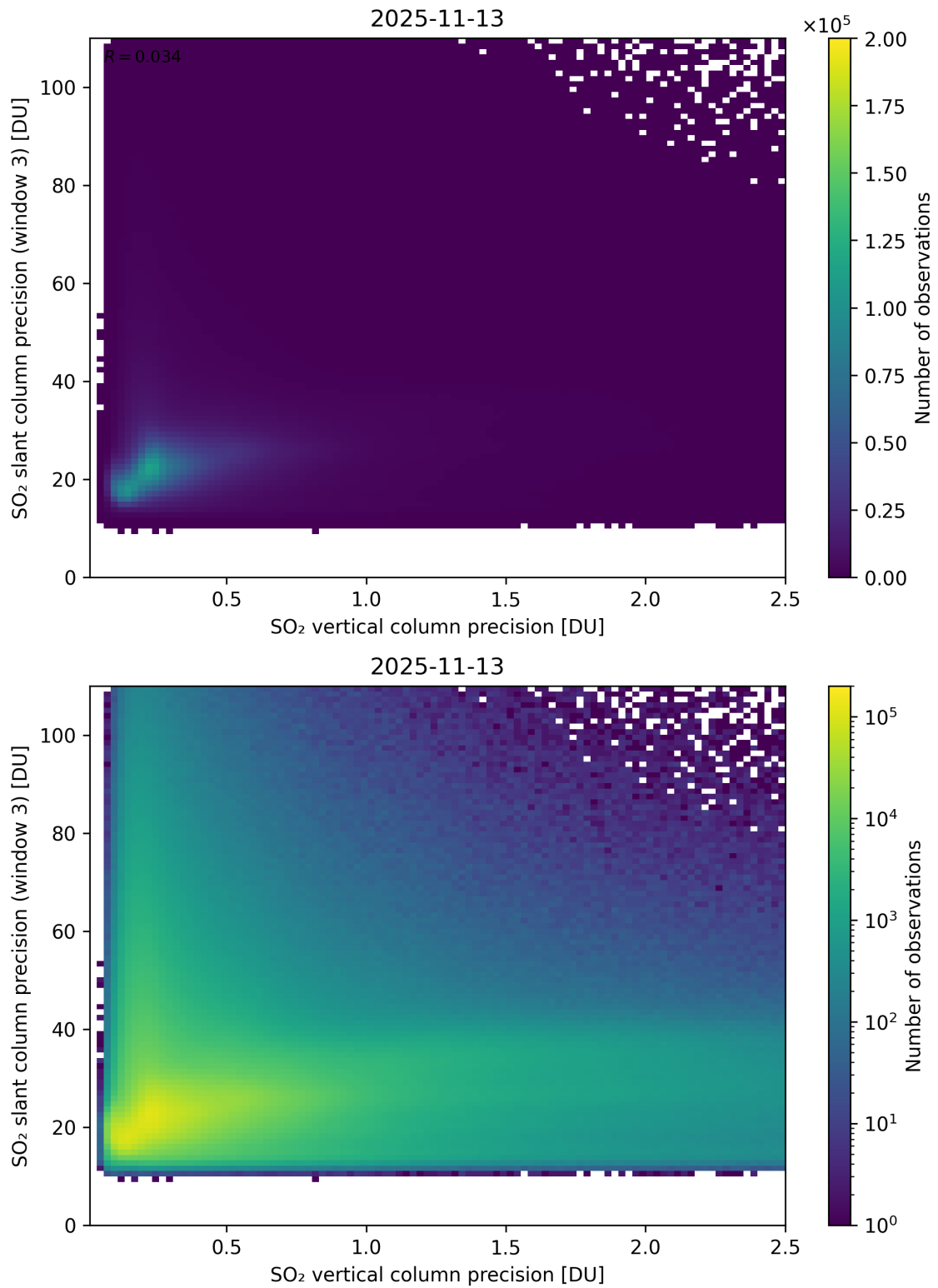
Figure 345: Scatter density plot of “SO 2 vertical column precision” against “SO 2 slant column precision (window 3)” for 2025-11-12 to 2025-11-14.
