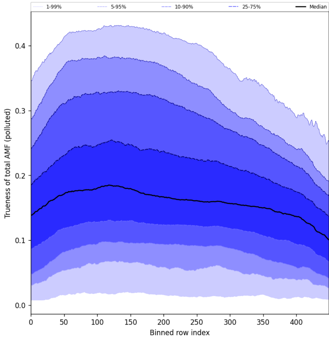
Figure 106: Along track statistics of “Trueness of total AMF (polluted)” for 2025-11-12 to 2025-11-14
