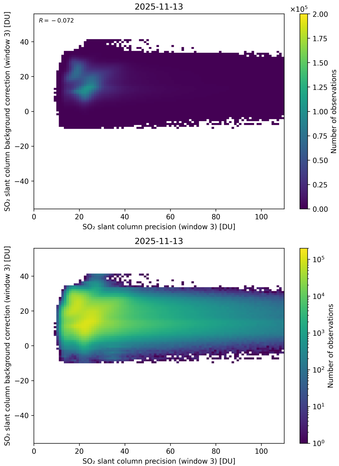
Figure 307: Scatter density plot of “SO 2 slant column precision (window 3)” against “SO 2 slant column background correction (window 3)” for 2025-11-12 to 2025-11-14.
