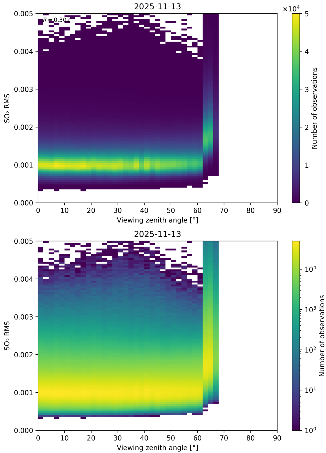
Figure 367: Scatter density plot of “Viewing zenith angle” against “SO 2 RMS” for 2025-11-12 to 2025-11-14.
