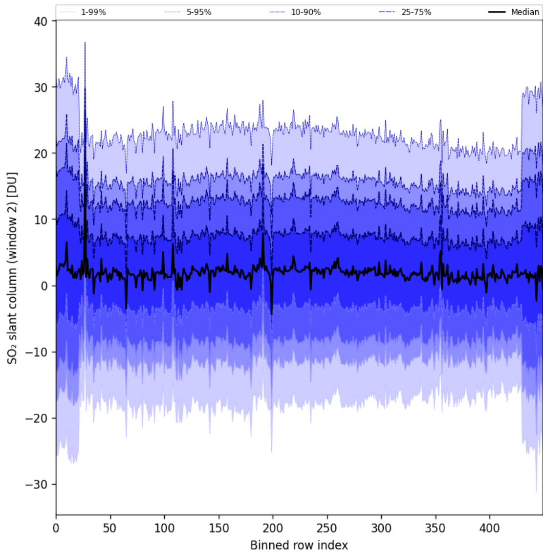
Figure 93: Along track statistics of “SO 2 slant column (window 2)” for 2025-11-12 to 2025-11-14
