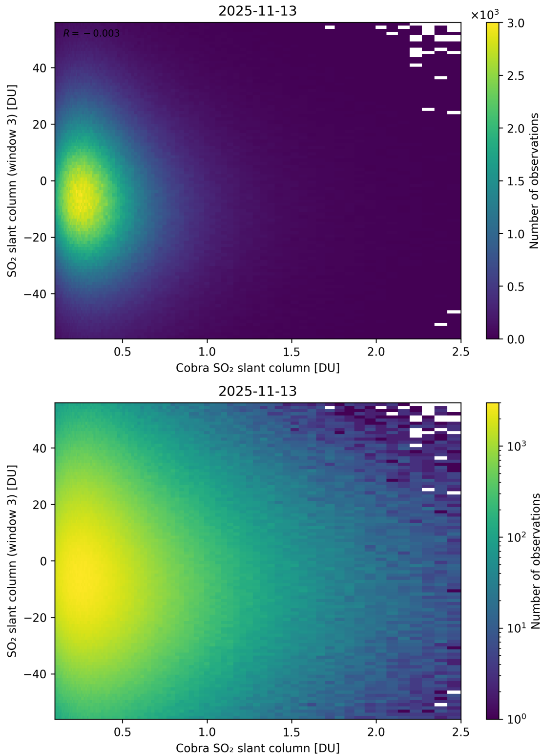
Figure 222: Scatter density plot of “Cobra SO 2 slant column” against “SO 2 slant column (window 3)” for 2025-11-12 to 2025-11-14.
