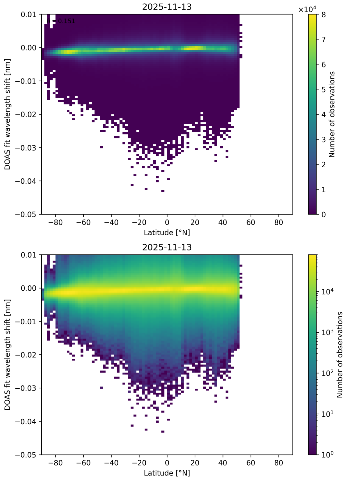
Figure 153: Scatter density plot of “Latitude” against “DOAS fit wavelength shift” for 2025-11-12 to 2025-11-14.
