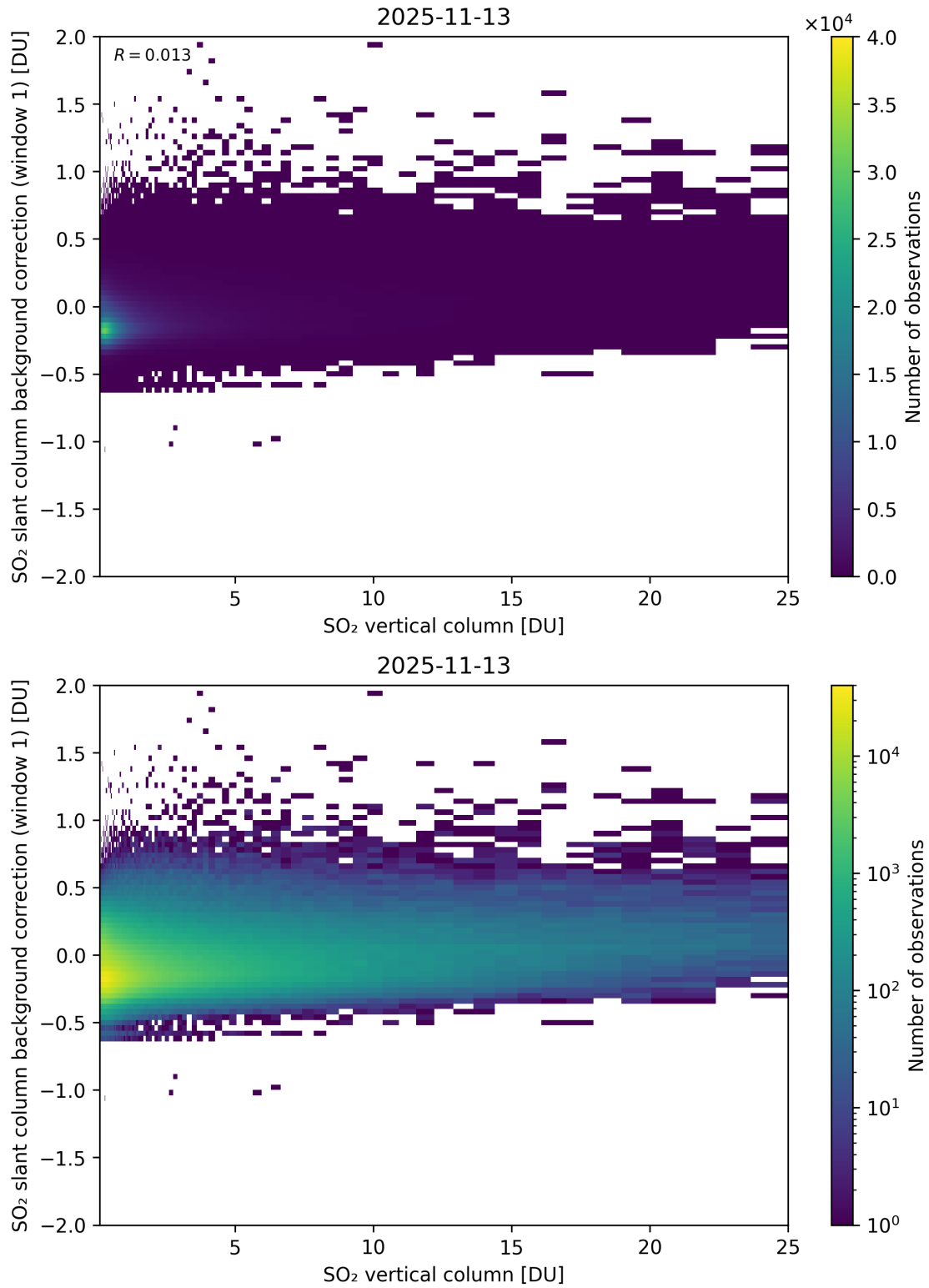
Figure 323: Scatter density plot of “SO 2 vertical column” against “SO 2 slant column background correction (window 1)” for 2025-11-12 to 2025-11-14.
