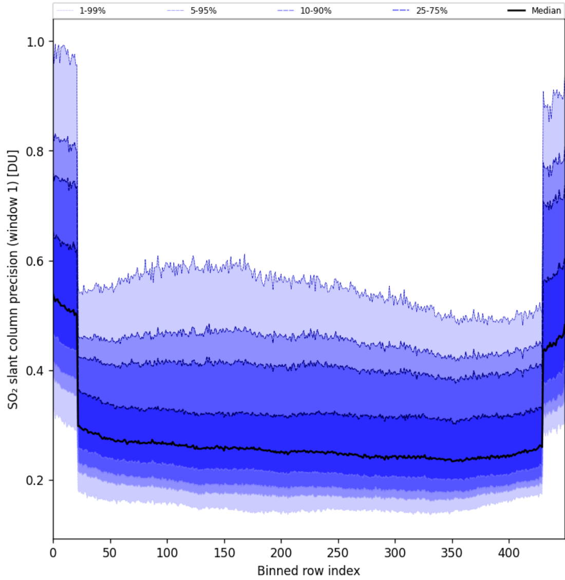
Figure 90: Along track statistics of “SO 2 slant column precision (window 1)” for 2025-11-12 to 2025-11-14
