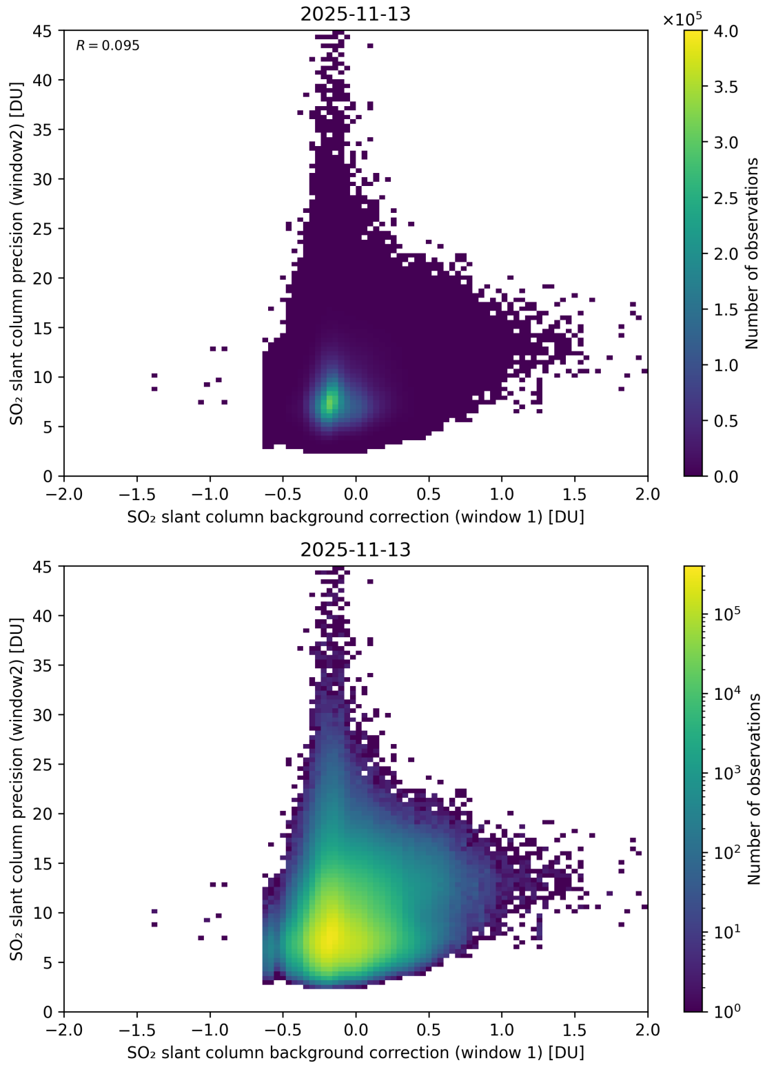
Figure 117: Scatter density plot of “SO 2 slant column background correction (window 1)” against “SO 2 slant column precision (window2)” for 2025-11-12 to 2025-11-14.
