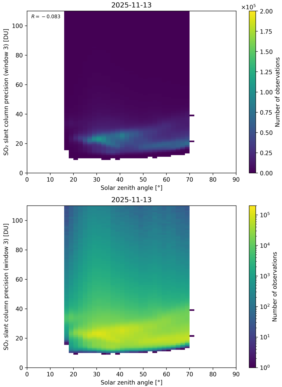
Figure 188: Scatter density plot of “Solar zenith angle” against “SO 2 slant column precision (window 3)” for 2025-11-12 to 2025-11-14.
