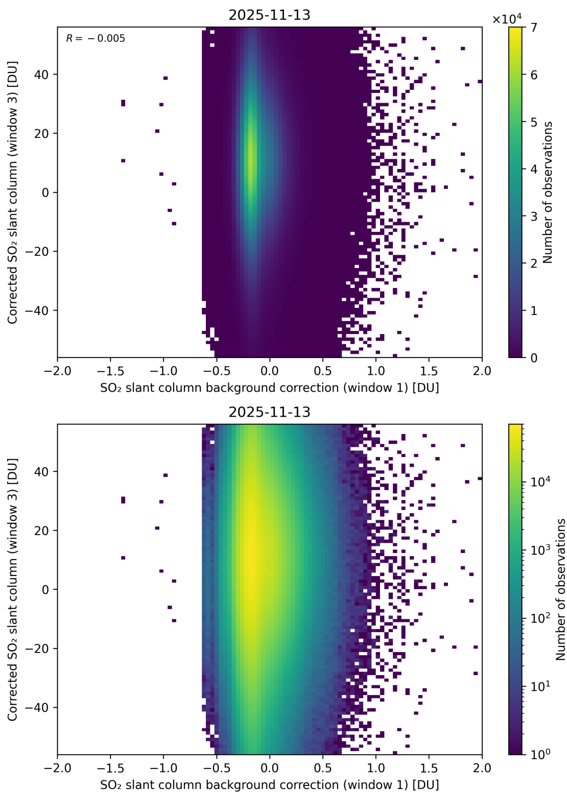
Figure 116: Scatter density plot of “SO 2 slant column background correction (window 1)” against “Corrected SO 2 slant column (window 3)” for 2025-11-12 to 2025-11-14.
