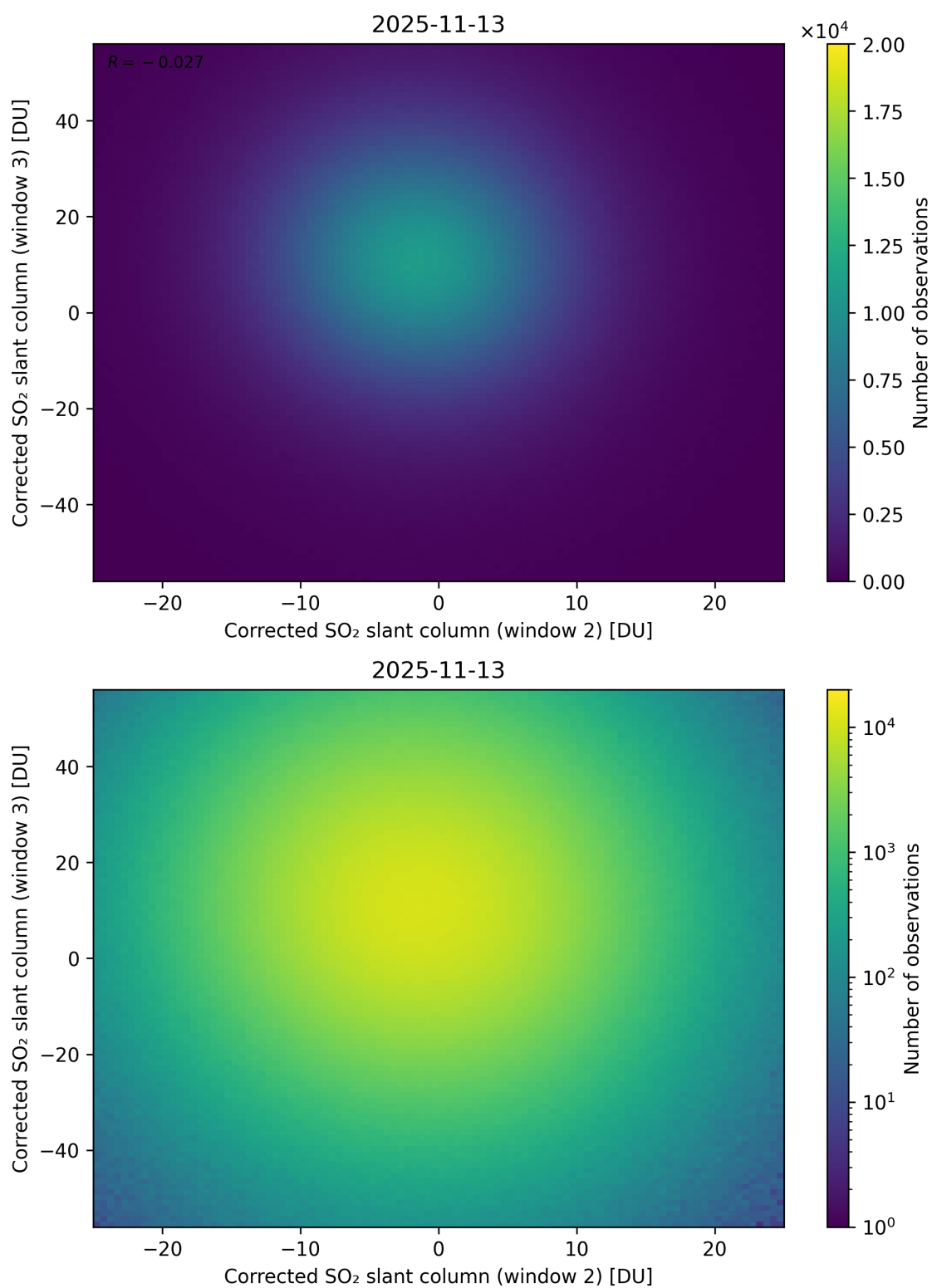
Figure 250: Scatter density plot of “Corrected SO 2 slant column (window 2)” against “Corrected SO 2 slant column (window 3)” for 2025-11-12 to 2025-11-14.
