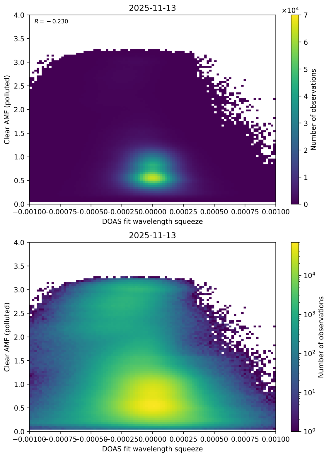
Figure 144: Scatter density plot of “DOAS fit wavelength squeeze” against “Clear AMF (polluted)” for 2025-11-12 to 2025-11-14.
