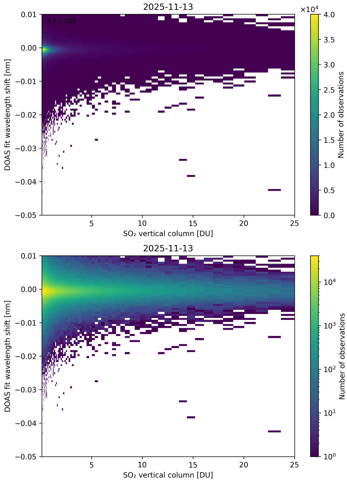
Figure 326: Scatter density plot of “SO 2 vertical column” against “DOAS fit wavelength shift” for 2025-11-12 to 2025-11-14.
