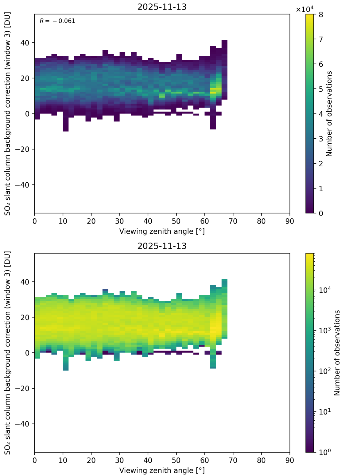
Figure 364: Scatter density plot of “Viewing zenith angle” against “SO 2 slant column background correction (window 3)” for 2025-11-12 to 2025-11-14.
