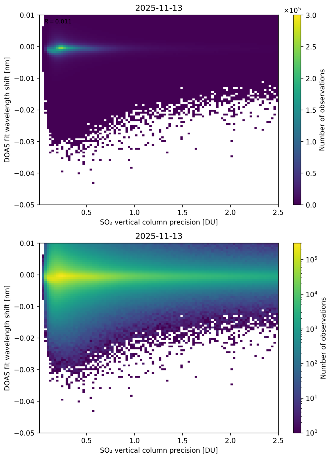
Figure 332: Scatter density plot of “SO 2 vertical column precision” against “DOAS fit wavelength shift” for 2025-11-12 to 2025-11-14.
