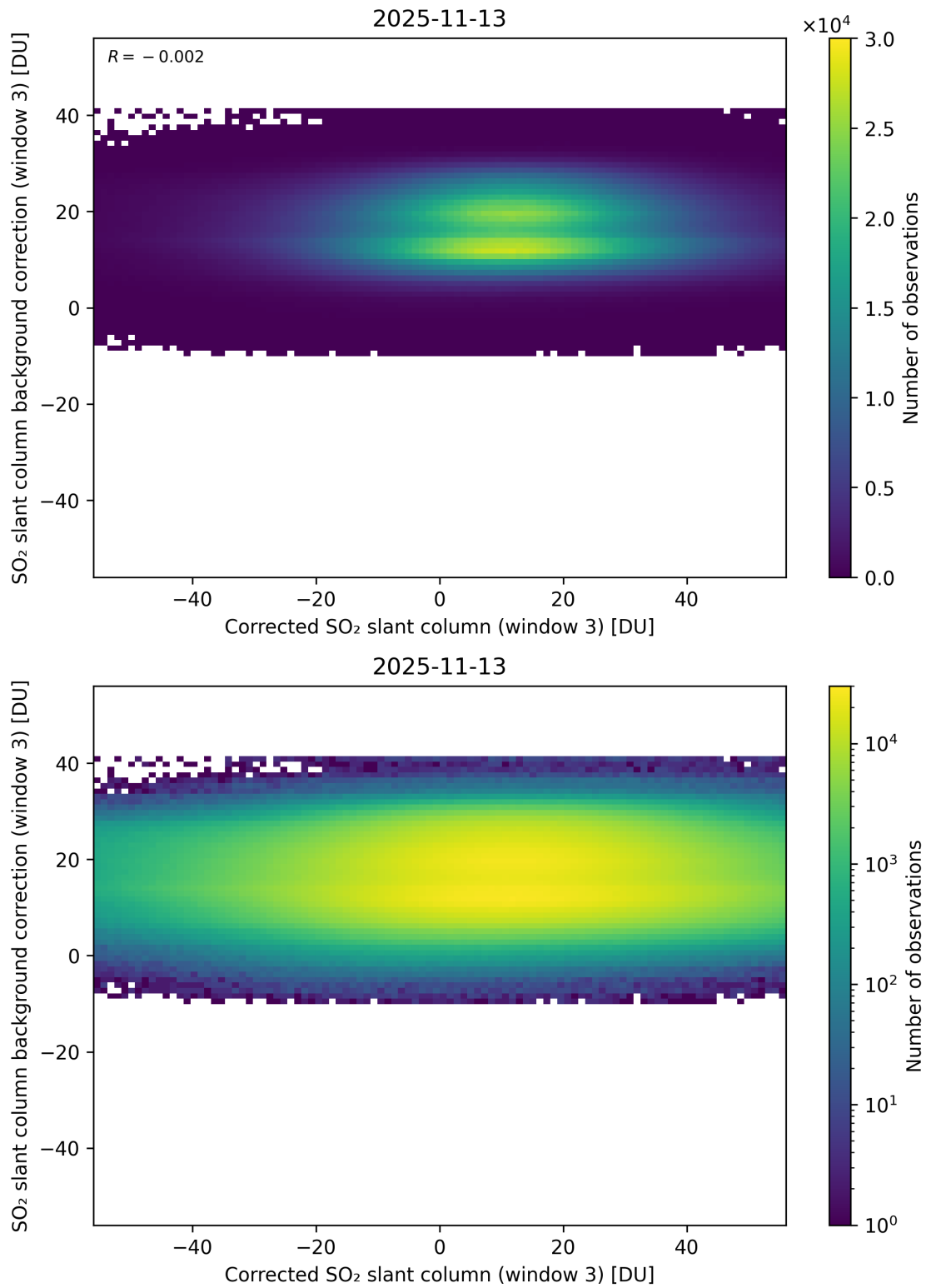
Figure 255: Scatter density plot of “Corrected SO 2 slant column (window 3)” against “SO 2 slant column background correction (window 3)” for 2025-11-12 to 2025-11-14.
