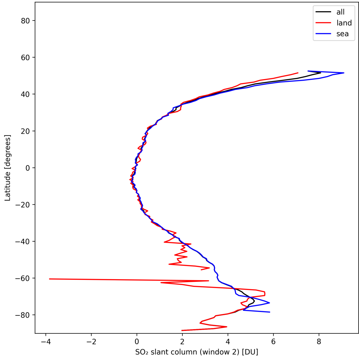
Figure 41: Zonal average of “SO 2 slant column (window 2)” for 2025-11-12 to 2025-11-14.
