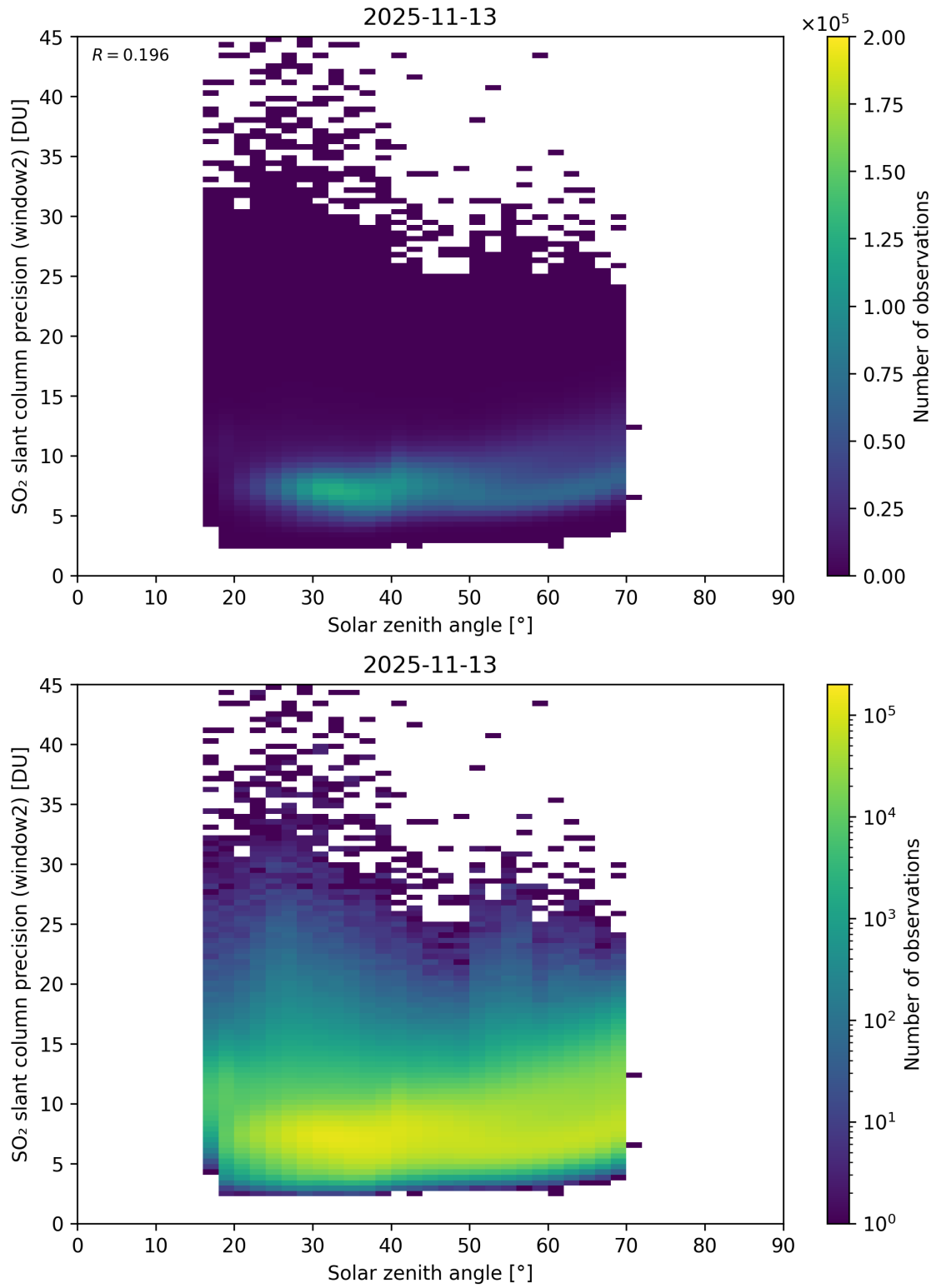
Figure 186: Scatter density plot of “Solar zenith angle” against “SO 2 slant column precision (window2)” for 2025-11-12 to 2025-11-14.
