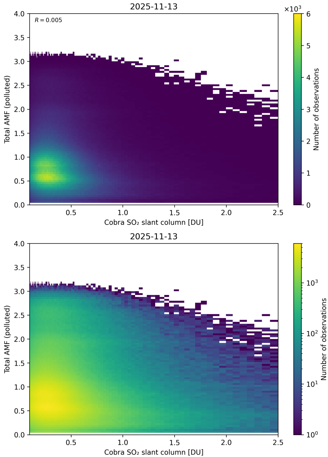
Figure 224: Scatter density plot of “Cobra SO 2 slant column” against “Total AMF (polluted)” for 2025-11-12 to 2025-11-14.
