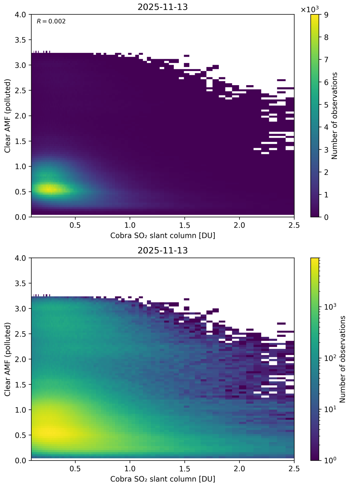
Figure 215: Scatter density plot of “Cobra SO 2 slant column” against “Clear AMF (polluted)” for 2025-11-12 to 2025-11-14.
