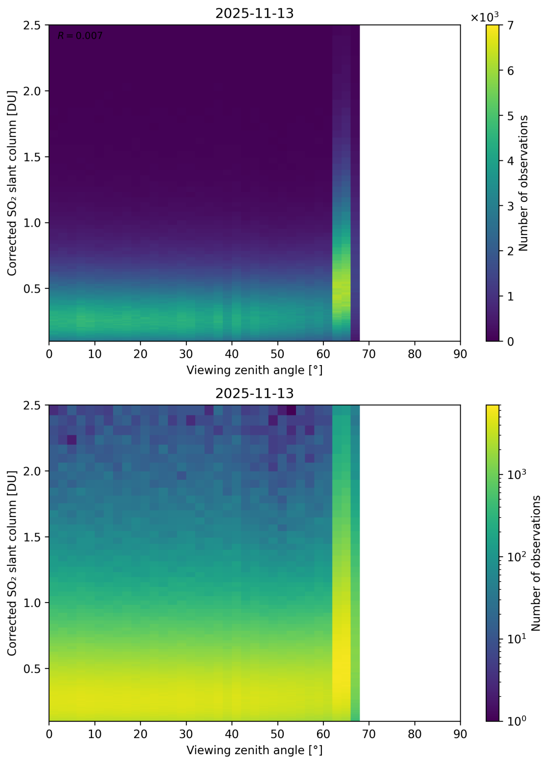
Figure 373: Scatter density plot of “Viewing zenith angle” against “Corrected SO 2 slant column” for 2025-11-12 to 2025-11-14.
