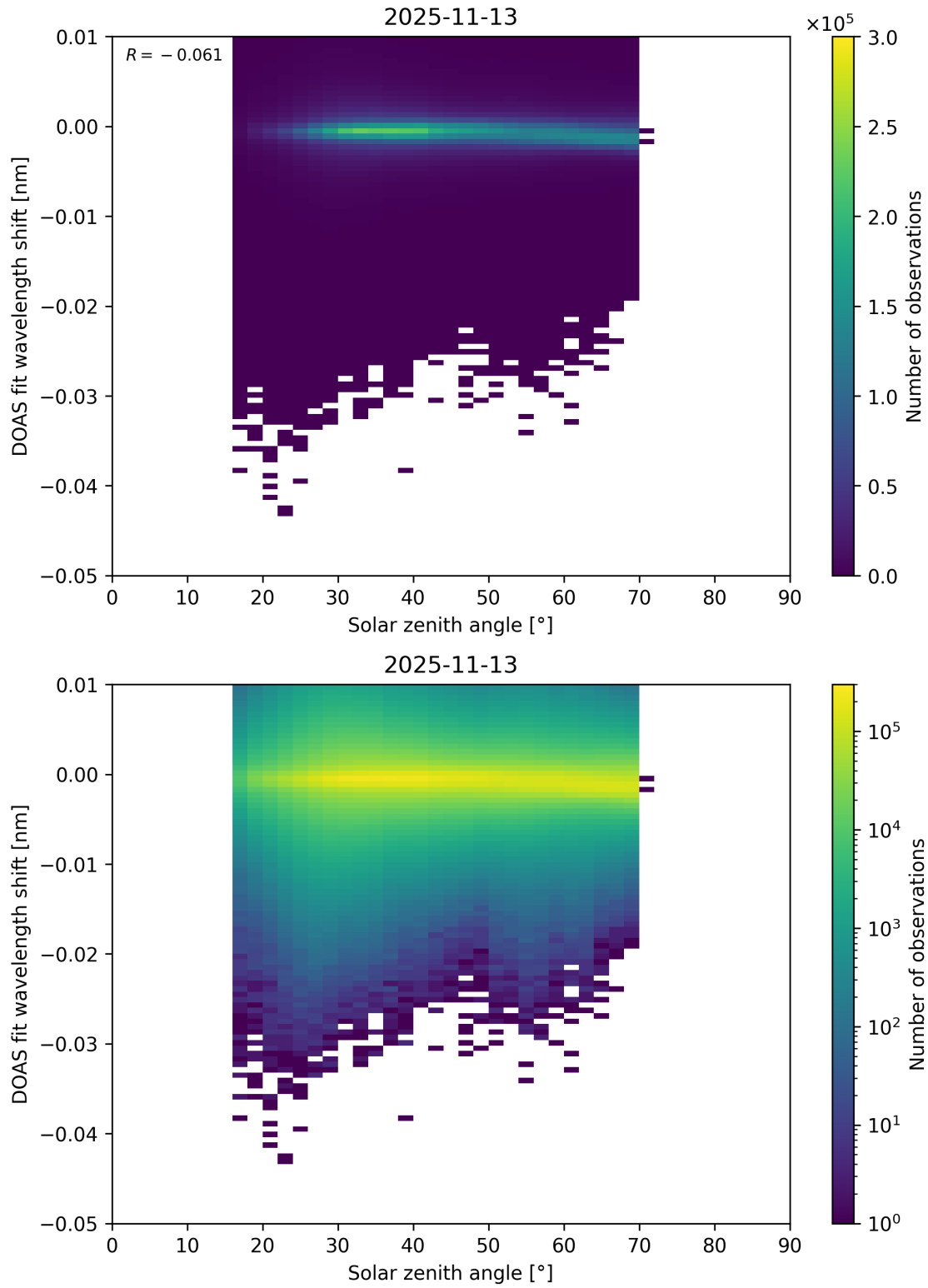
Figure 174: Scatter density plot of “Solar zenith angle” against “DOAS fit wavelength shift” for 2025-11-12 to 2025-11-14.
