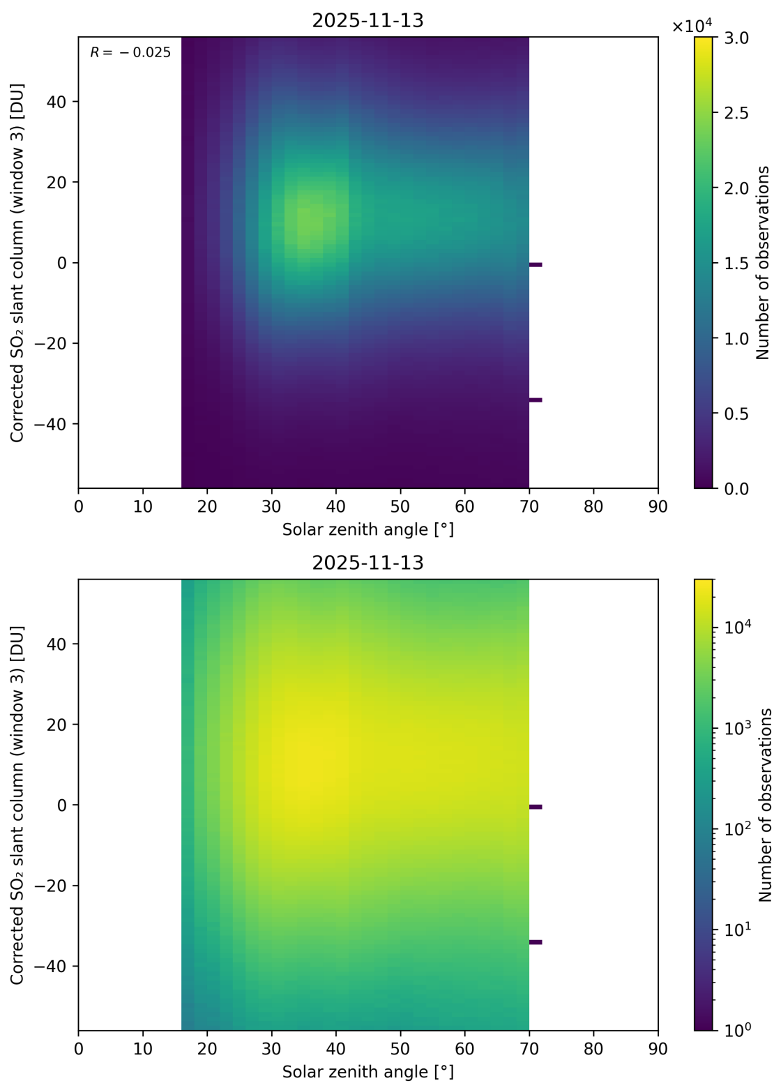
Figure 183: Scatter density plot of “Solar zenith angle” against “Corrected SO 2 slant column (window 3)” for 2025-11-12 to 2025-11-14.
