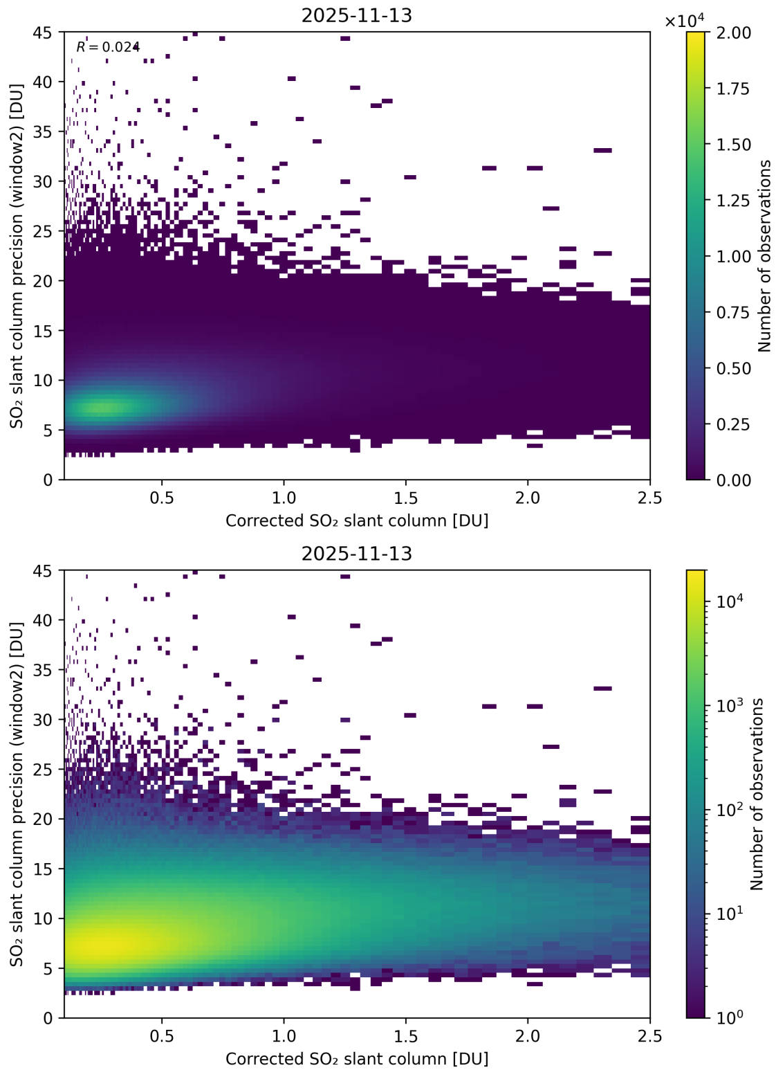
Figure 239: Scatter density plot of “Corrected SO 2 slant column” against “SO 2 slant column precision (window2)” for 2025-11-12 to 2025-11-14.
