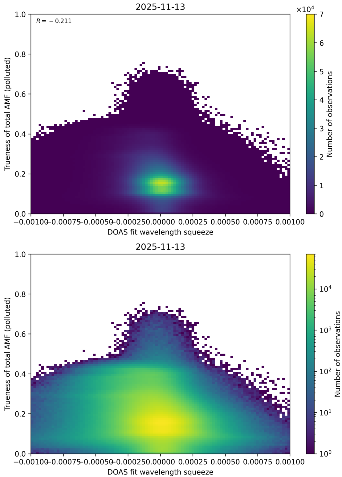
Figure 146: Scatter density plot of “DOAS fit wavelength squeeze” against “Trueness of total AMF (polluted)” for 2025-11-12 to 2025-11-14.
