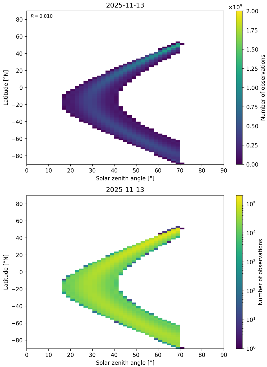
Figure 177: Scatter density plot of “Solar zenith angle” against “Latitude” for 2025-11-12 to 2025-11-14.
