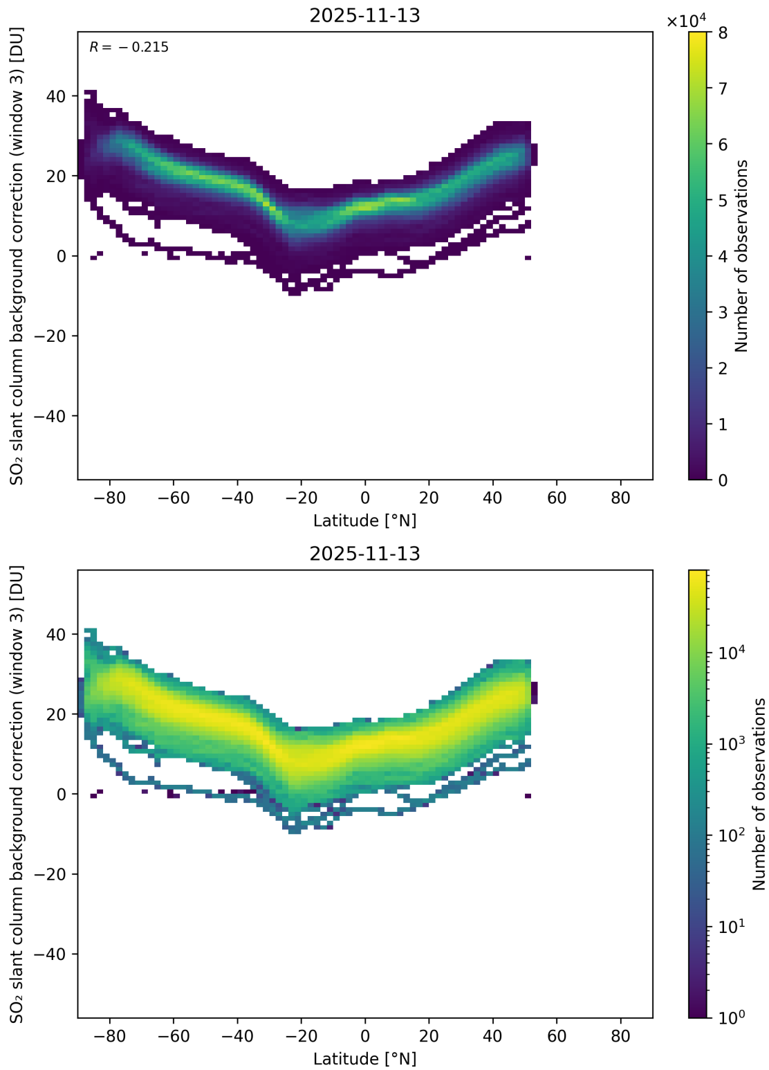
Figure 152: Scatter density plot of “Latitude” against “SO 2 slant column background correction (window 3)” for 2025-11-12 to 2025-11-14.
