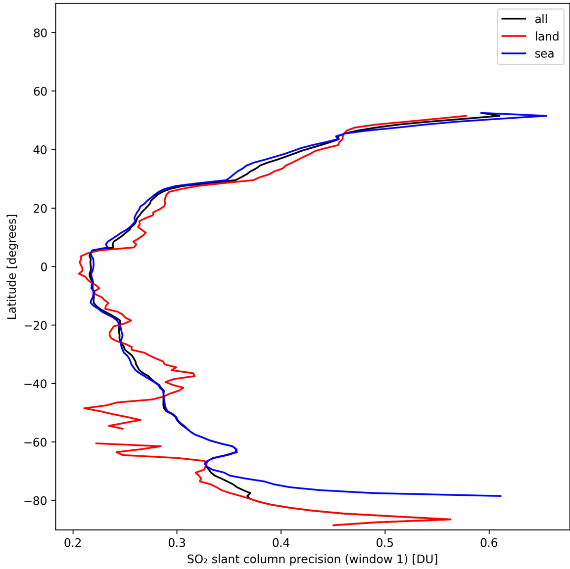
Figure 38: Zonal average of “SO 2 slant column precision (window 1)” for 2025-11-12 to 2025-11-14.
