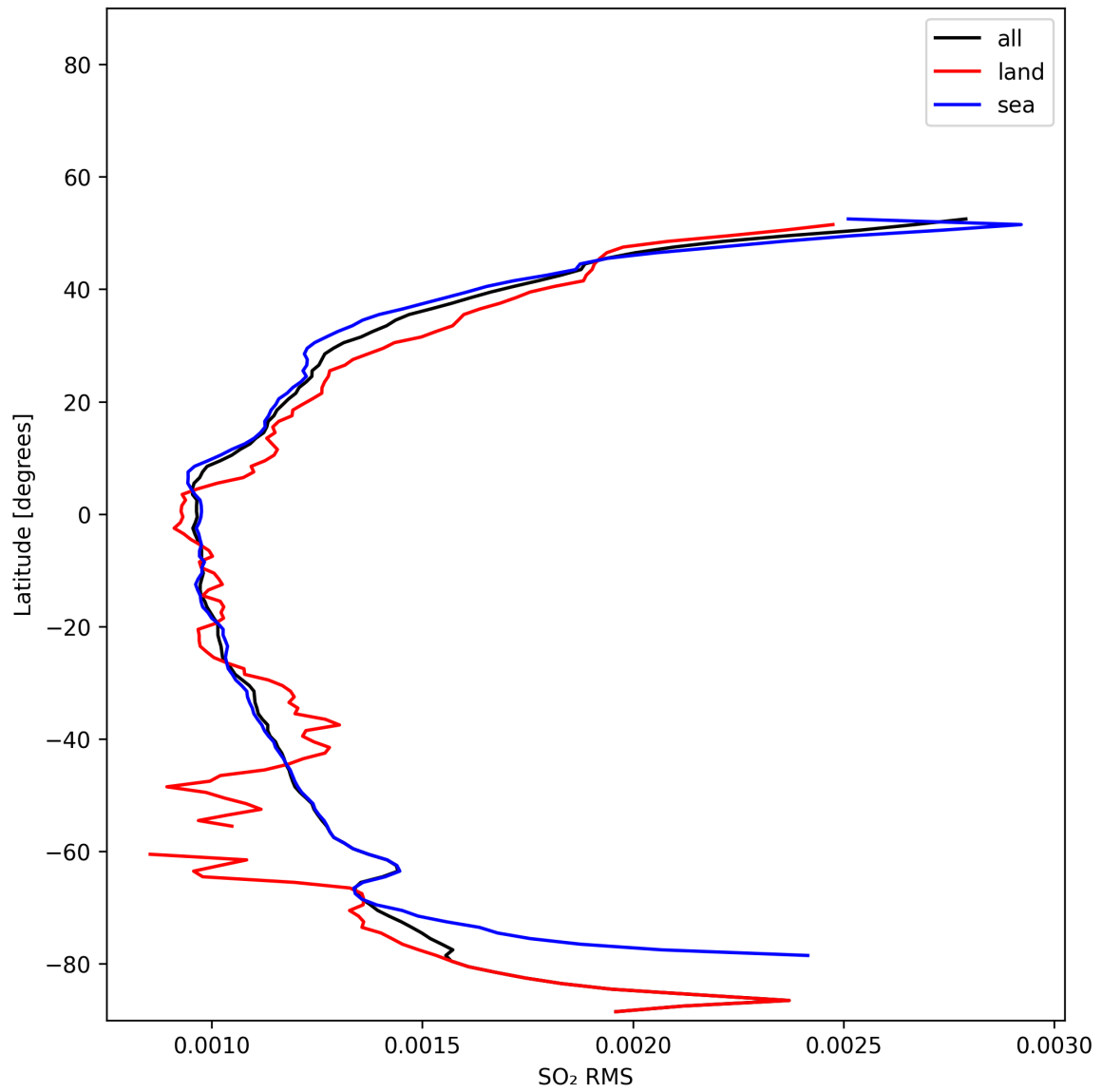
Figure 52: Zonal average of “SO 2 RMS” for 2025-11-12 to 2025-11-14.
