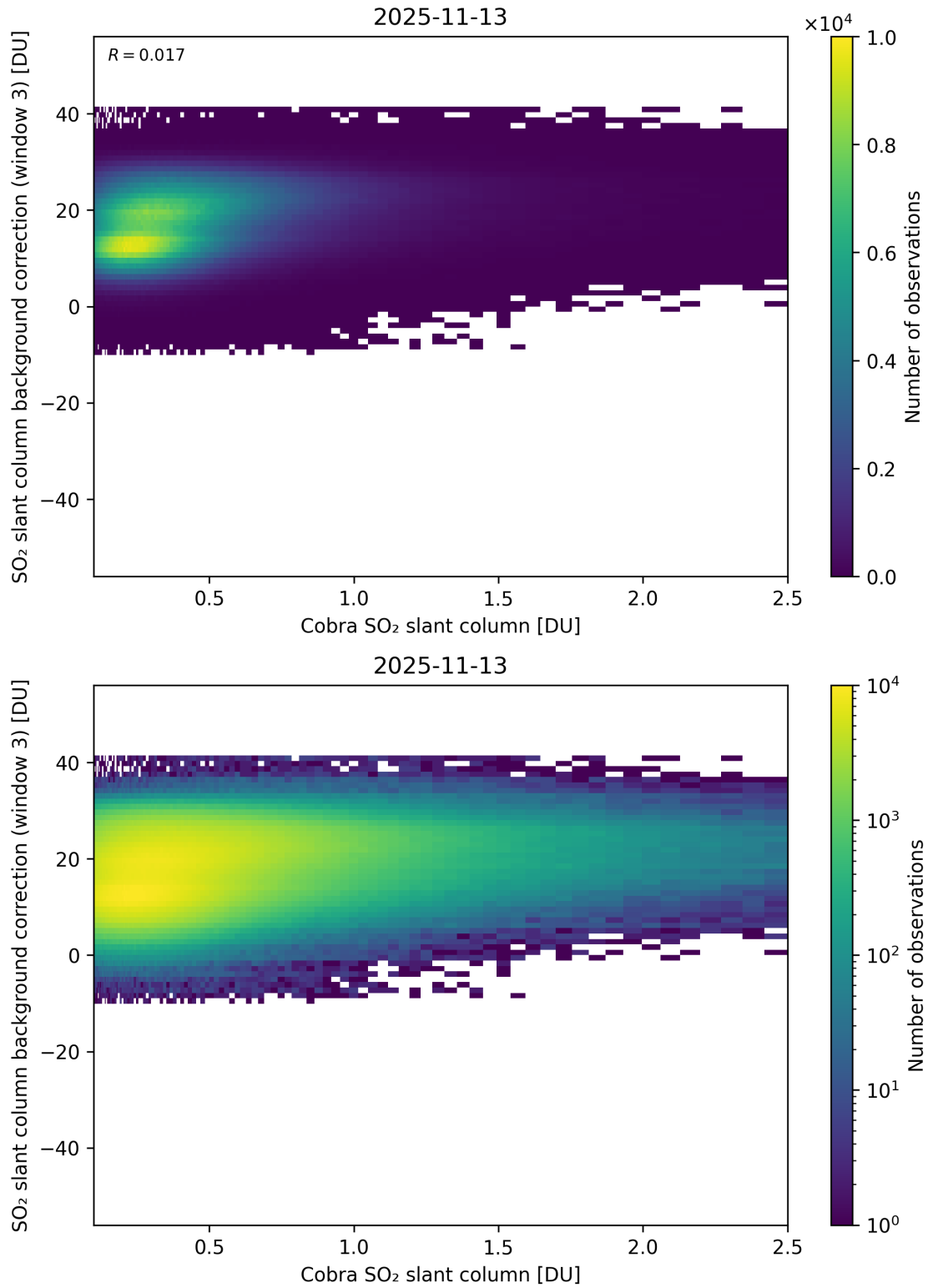
Figure 195: Scatter density plot of “Cobra SO 2 slant column” against “SO 2 slant column background correction (window 3)” for 2025-11-12 to 2025-11-14.
