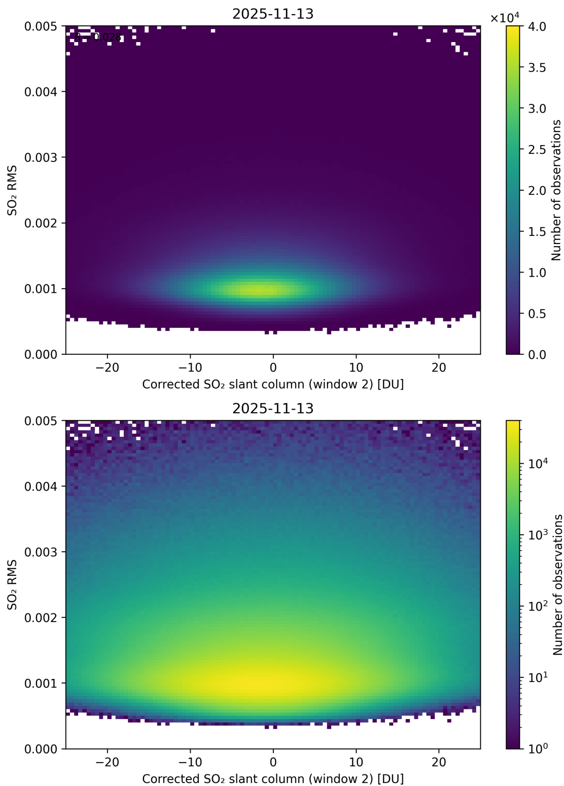
Figure 248: Scatter density plot of “Corrected SO 2 slant column (window 2)” against “SO 2 RMS” for 2025-11-12 to 2025-11-14.
