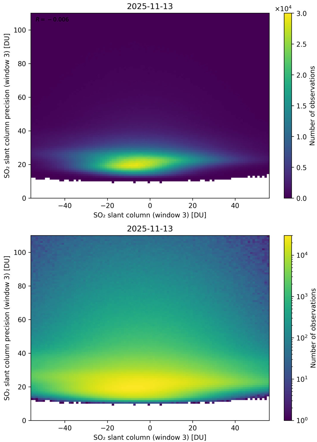
Figure 317: Scatter density plot of “SO 2 slant column (window 3)” against “SO 2 slant column precision (window 3)” for 2025-11-12 to 2025-11-14.
