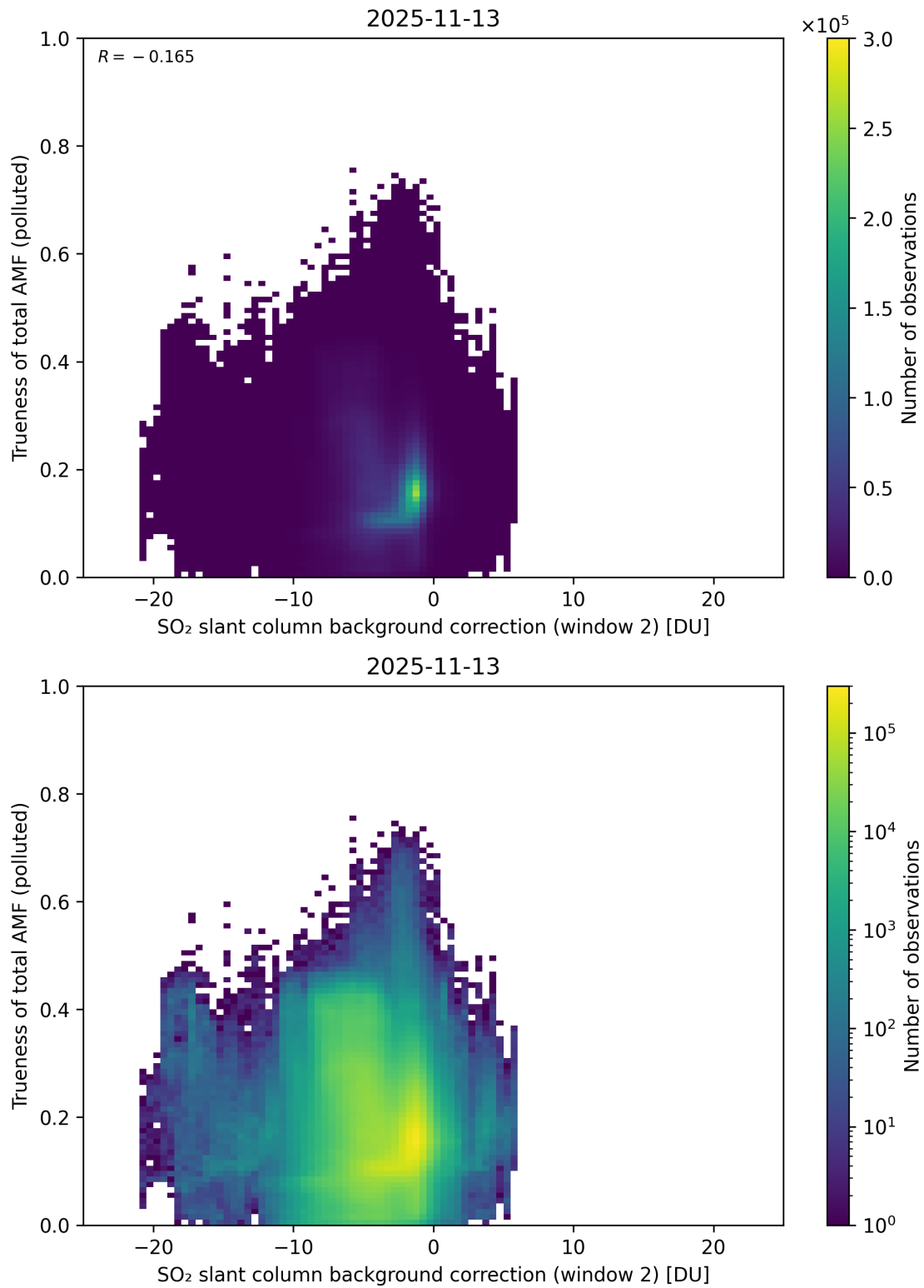
Figure 131: Scatter density plot of “SO 2 slant column background correction (window 2)” against “Trueness of total AMF (polluted)” for 2025-11-12 to 2025-11-14.
