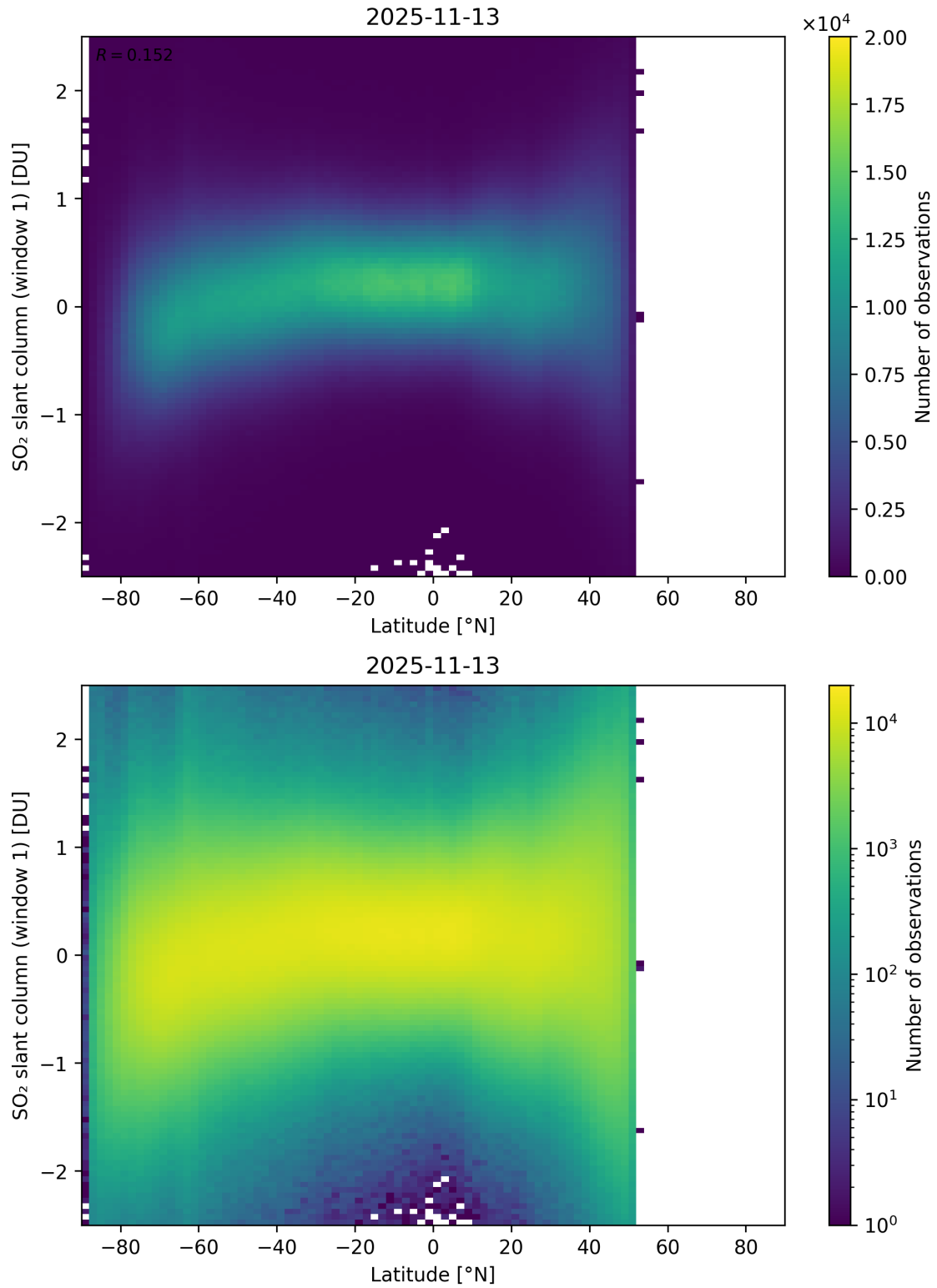
Figure 162: Scatter density plot of “Latitude” against “SO 2 slant column (window 1)” for 2025-11-12 to 2025-11-14.
