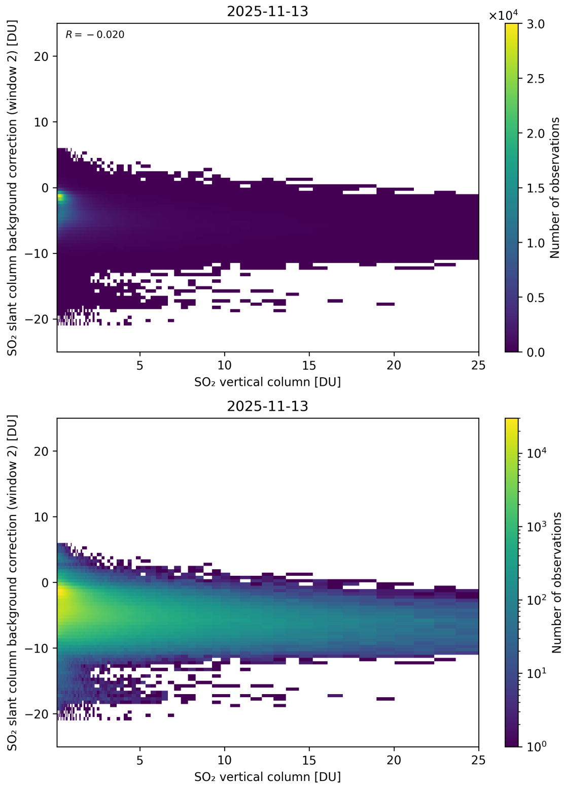
Figure 324: Scatter density plot of “SO 2 vertical column” against “SO 2 slant column background correction (window 2)” for 2025-11-12 to 2025-11-14.
