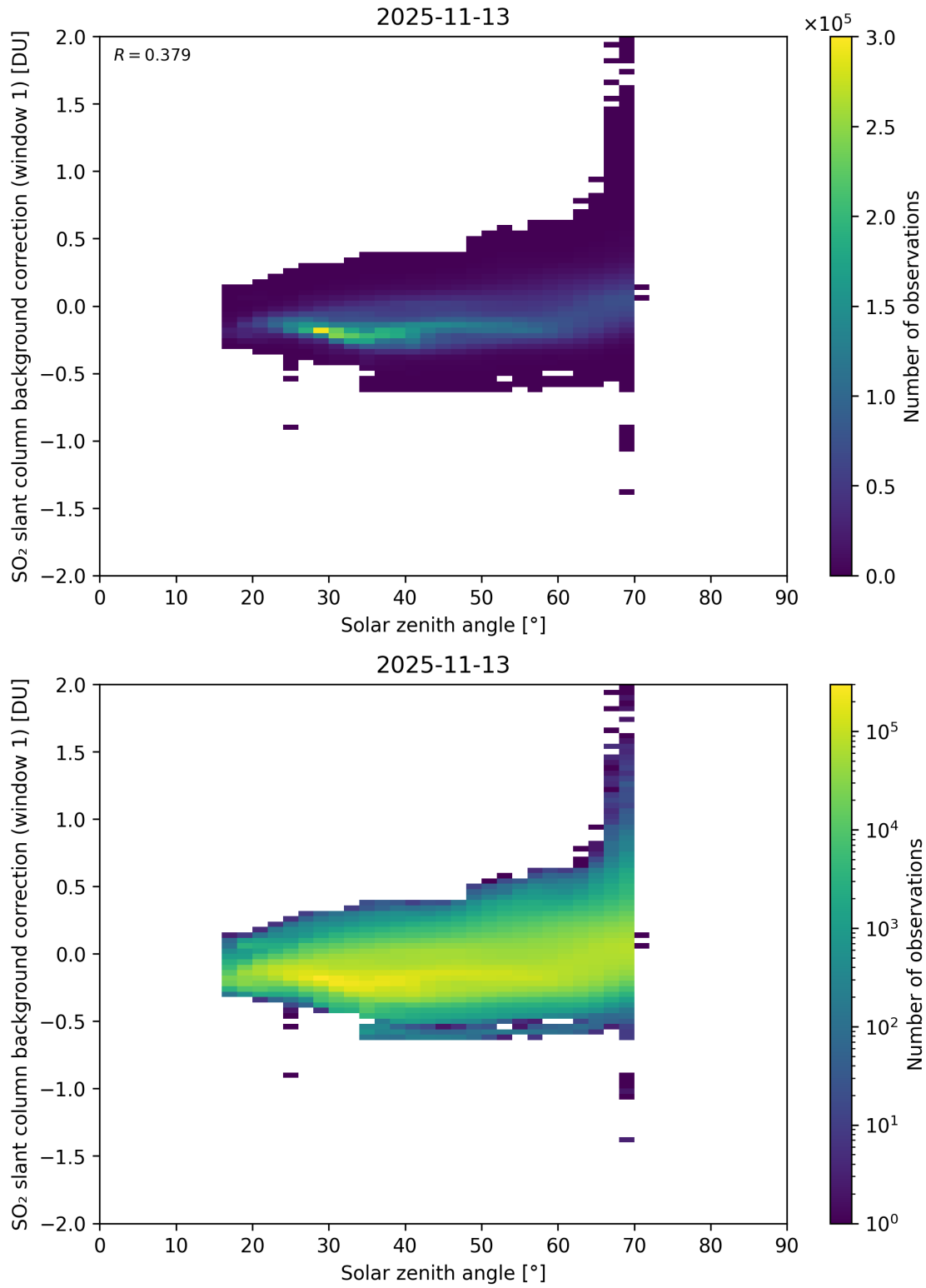
Figure 171: Scatter density plot of “Solar zenith angle” against “SO 2 slant column background correction (window 1)” for 2025-11-12 to 2025-11-14.
