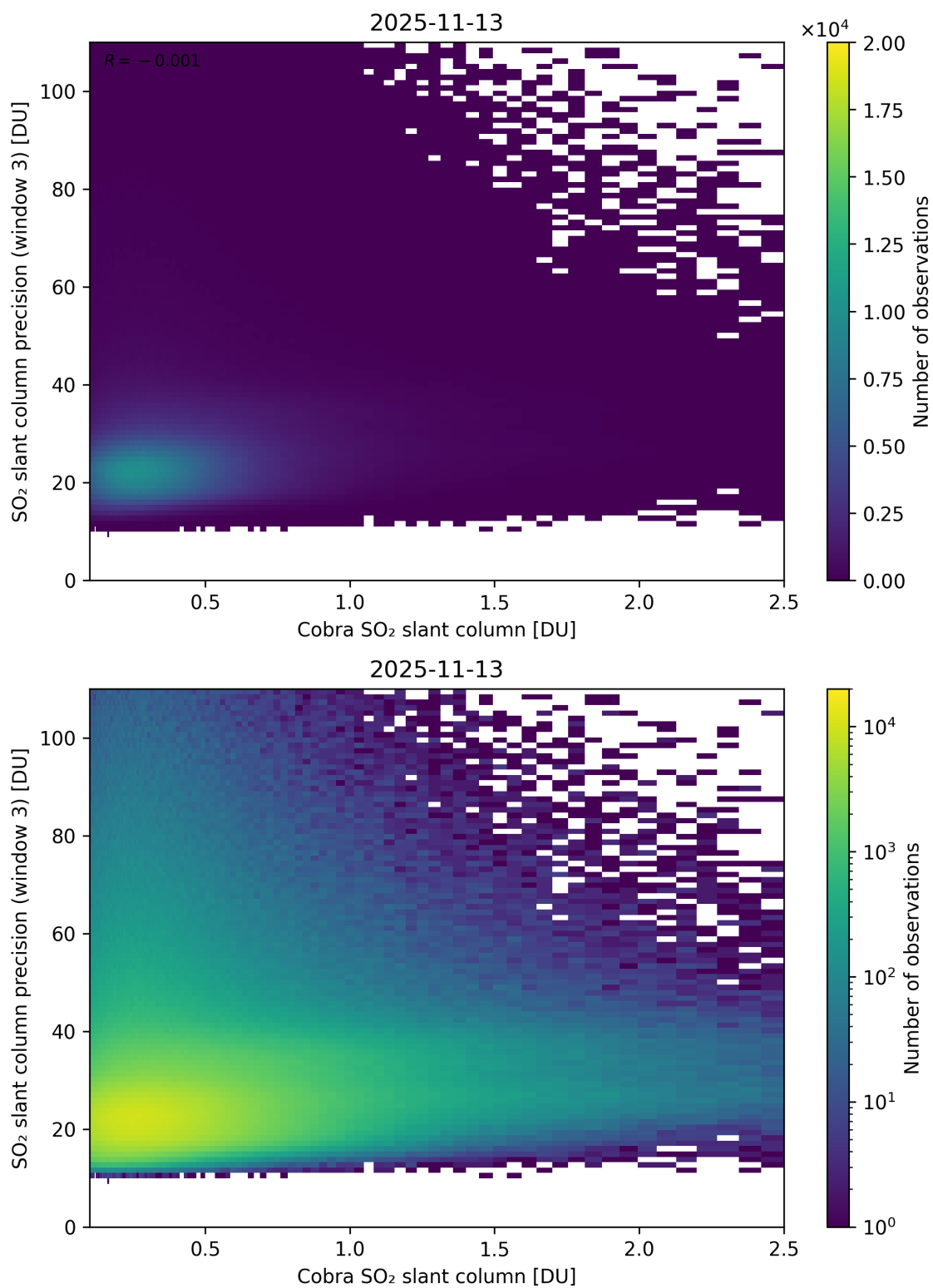
Figure 223: Scatter density plot of “Cobra SO 2 slant column” against “SO 2 slant column precision (window 3)” for 2025-11-12 to 2025-11-14.
