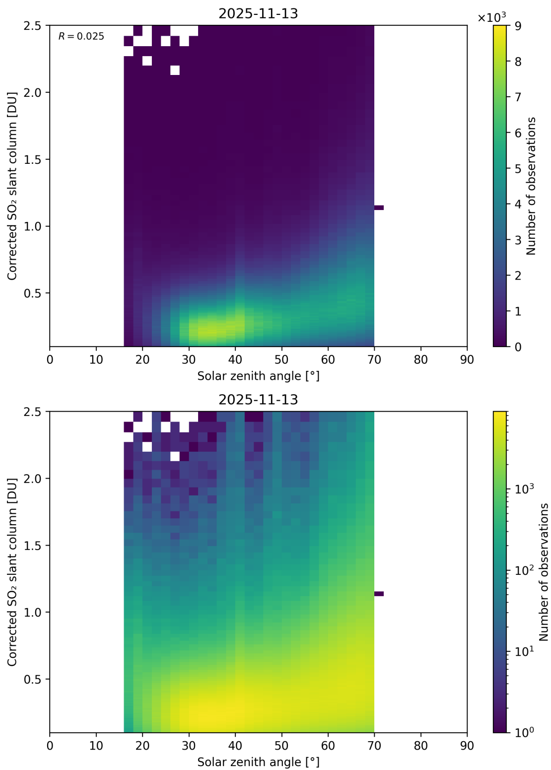
Figure 181: Scatter density plot of “Solar zenith angle” against “Corrected SO 2 slant column” for 2025-11-12 to 2025-11-14.
