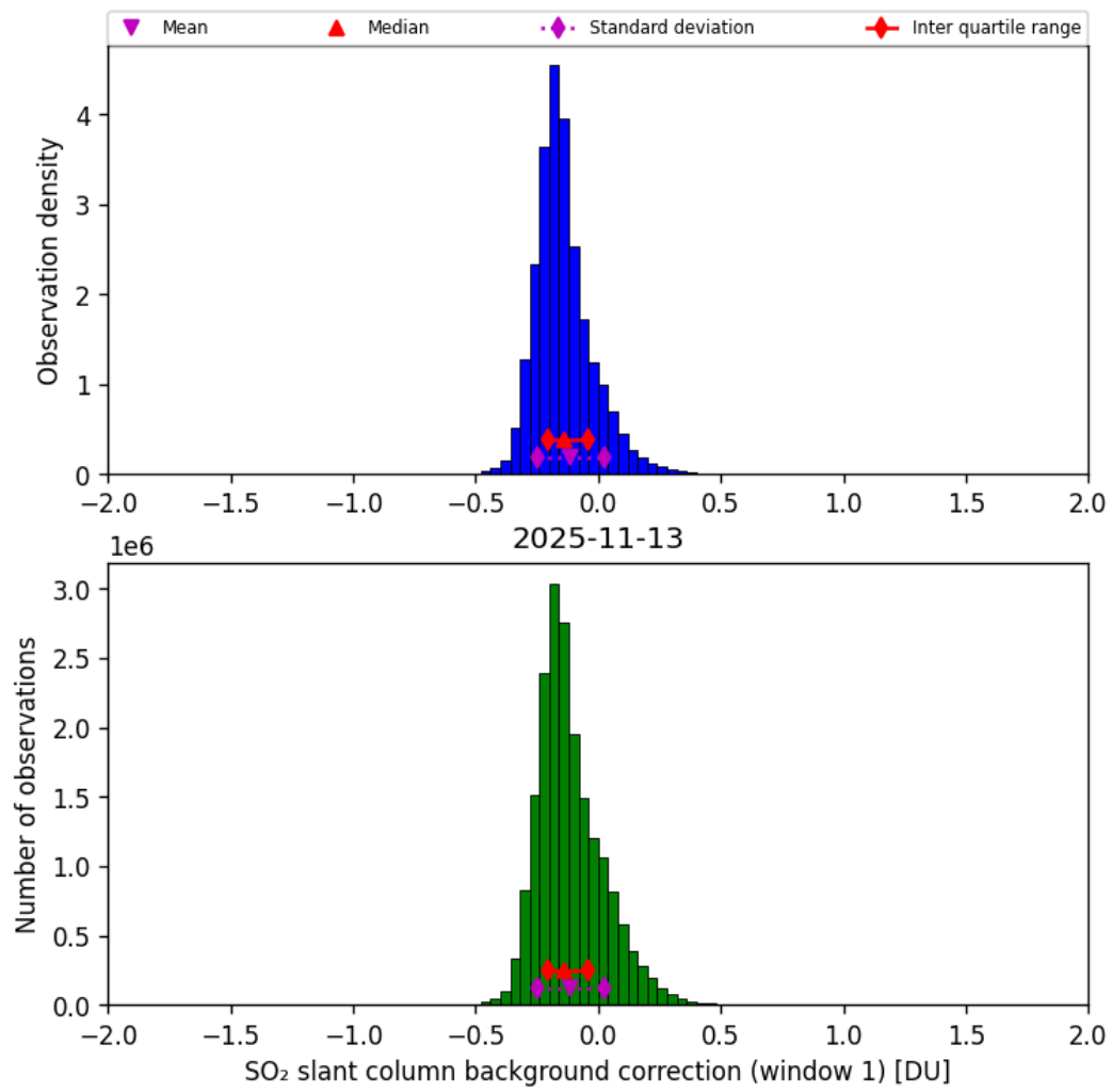
Figure 66: Histogram of “SO 2 slant column background correction (window 1)” for 2025-11-12 to 2025-11-14
