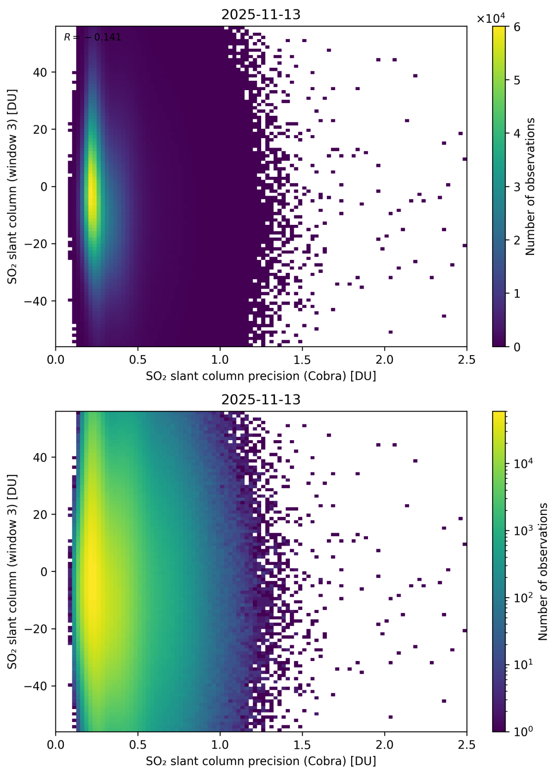
Figure 211: Scatter density plot of “SO 2 slant column precision (Cobra)” against “SO 2 slant column (window 3)” for 2025-11-12 to 2025-11-14.
