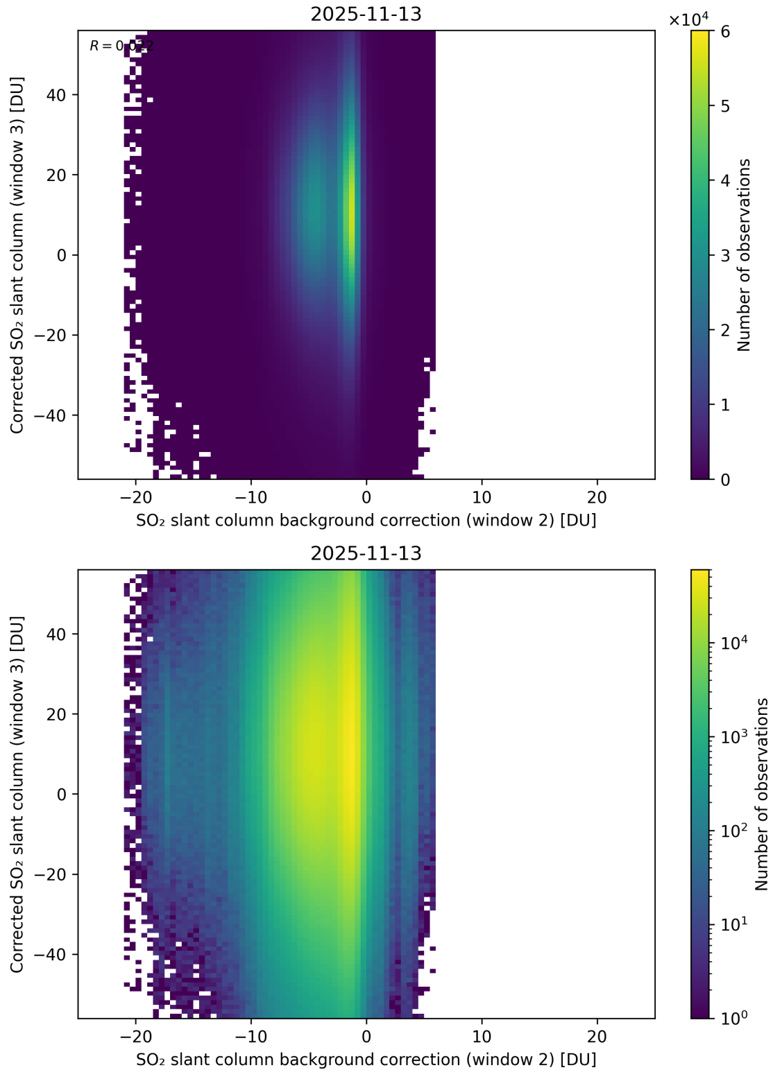
Figure 127: Scatter density plot of “SO 2 slant column background correction (window 2)” against “Corrected SO 2 slant column (window 3)” for 2025-11-12 to 2025-11-14.
