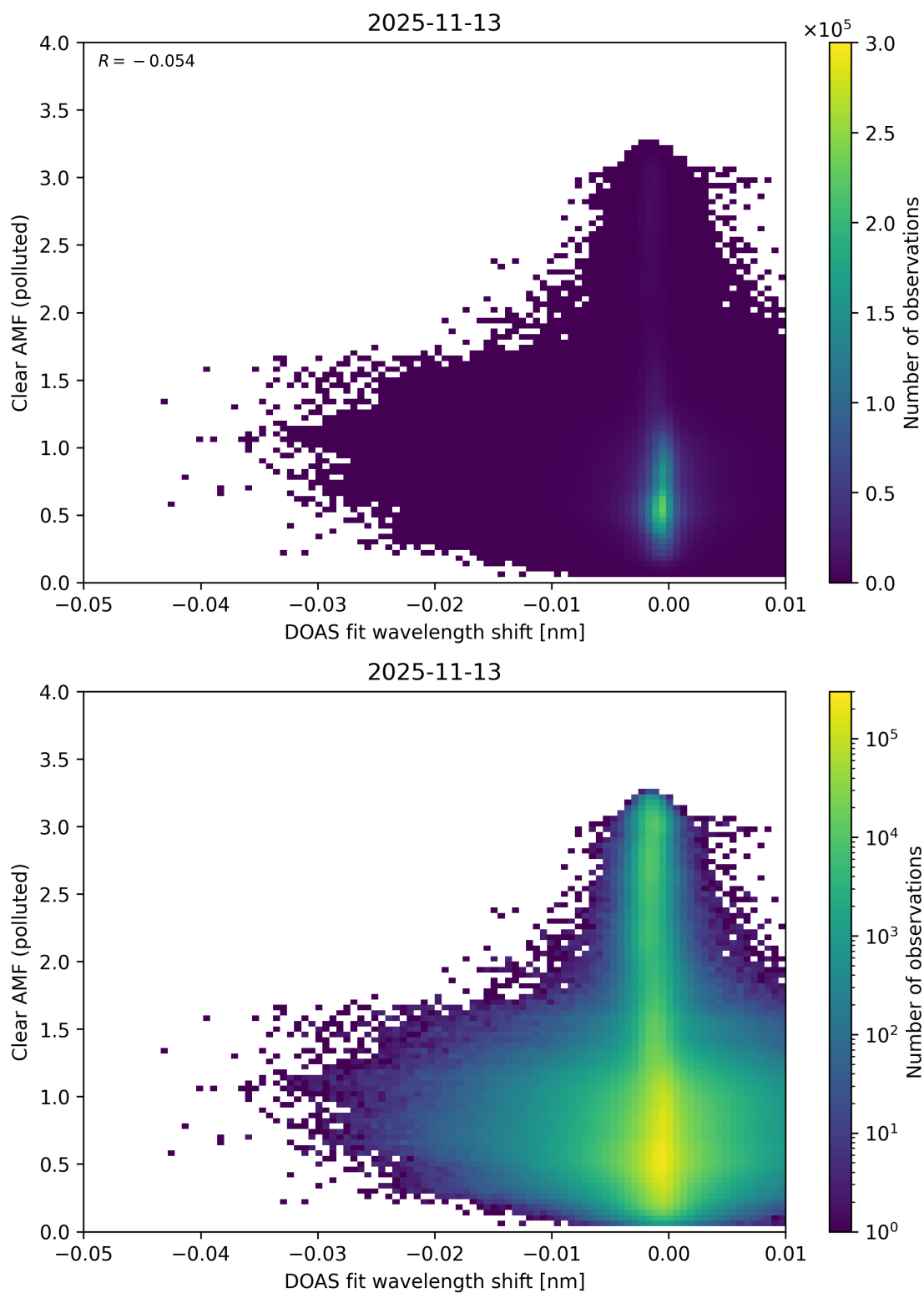
Figure 140: Scatter density plot of “DOAS fit wavelength shift” against “Clear AMF (polluted)” for 2025-11-12 to 2025-11-14.
