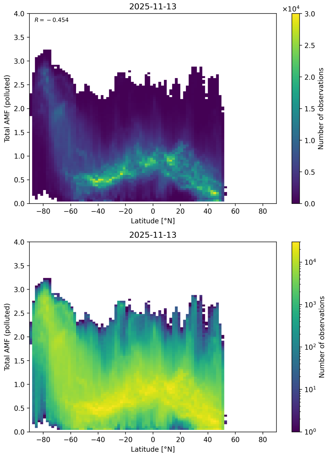
Figure 167: Scatter density plot of “Latitude” against “Total AMF (polluted)” for 2025-11-12 to 2025-11-14.
