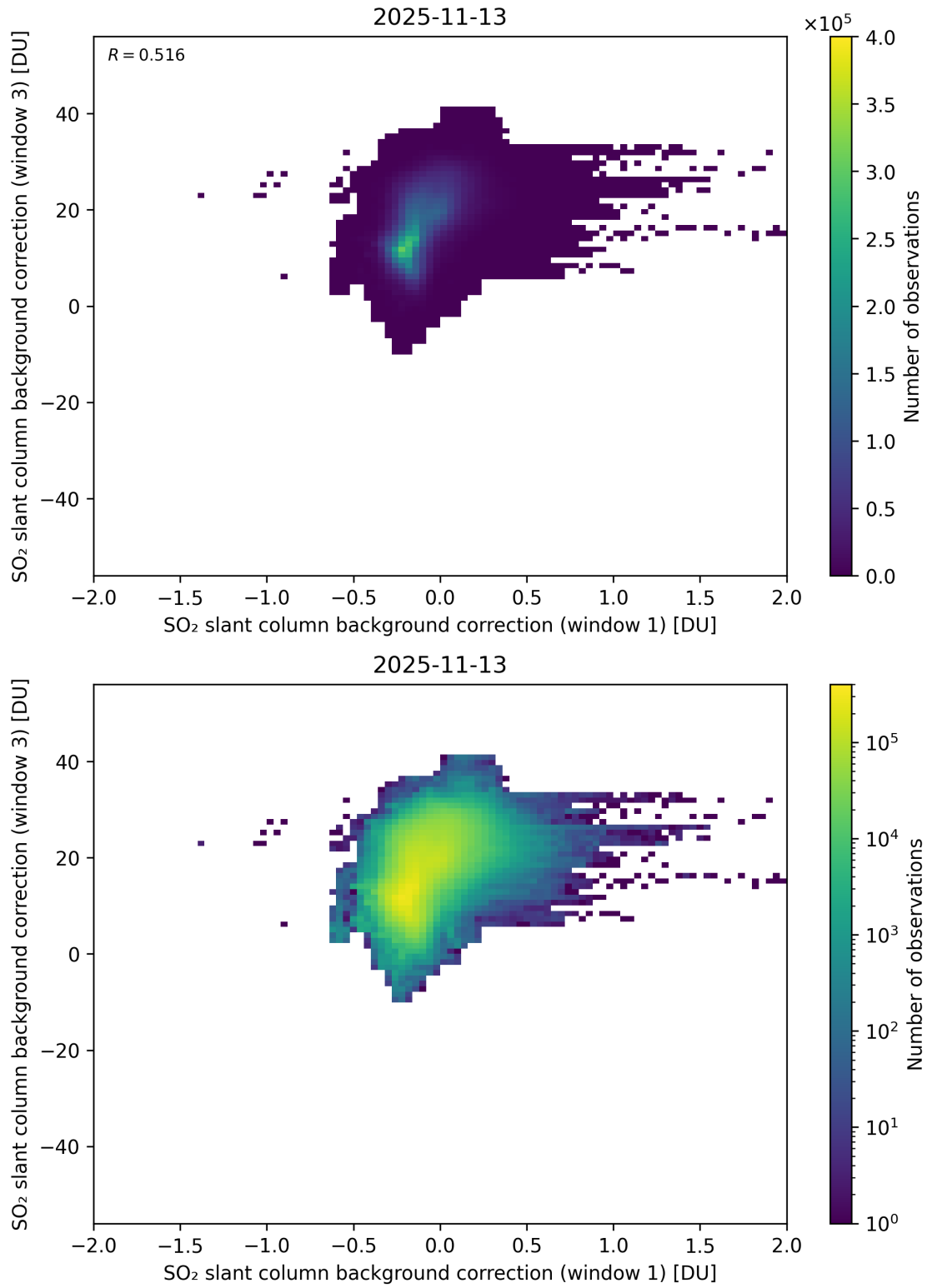
Figure 110: Scatter density plot of “SO 2 slant column background correction (window 1)” against “SO 2 slant column background correction (window 3)” for 2025-11-12 to 2025-11-14.
