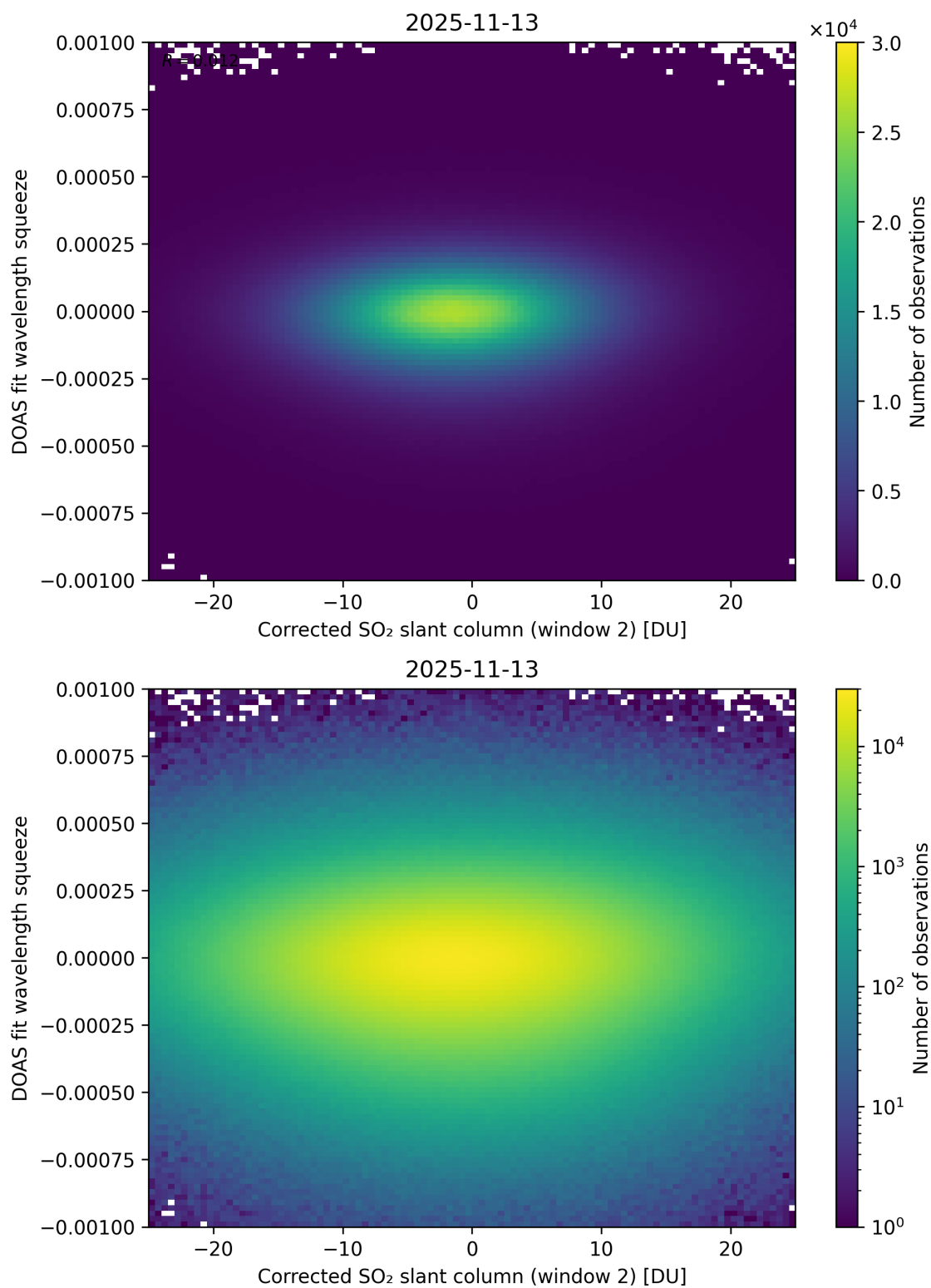
Figure 247: Scatter density plot of “Corrected SO 2 slant column (window 2)” against “DOAS fit wavelength squeeze” for 2025-11-12 to 2025-11-14.
