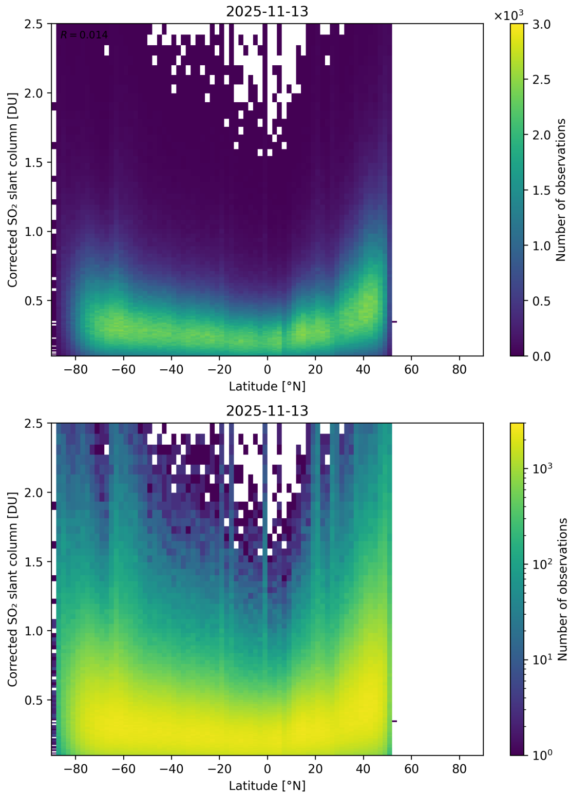
Figure 159: Scatter density plot of “Latitude” against “Corrected SO 2 slant column” for 2025-11-12 to 2025-11-14.
