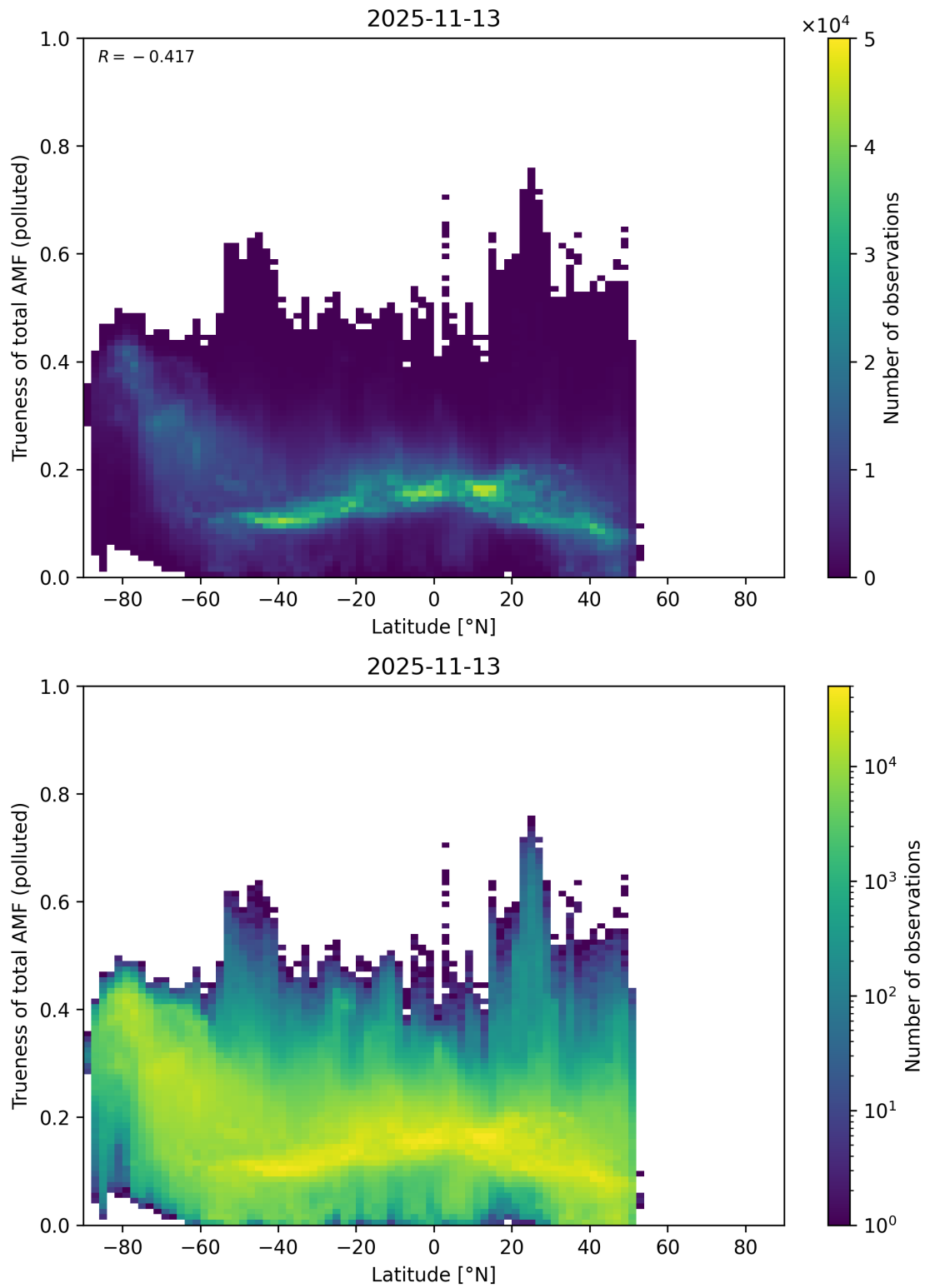
Figure 168: Scatter density plot of “Latitude” against “Trueness of total AMF (polluted)” for 2025-11-12 to 2025-11-14.
