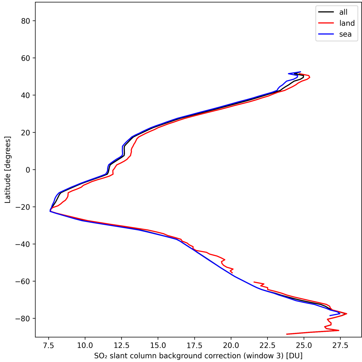
Figure 48: Zonal average of “SO 2 slant column background correction (window 3)” for 2025-11-12 to 2025-11-14.
