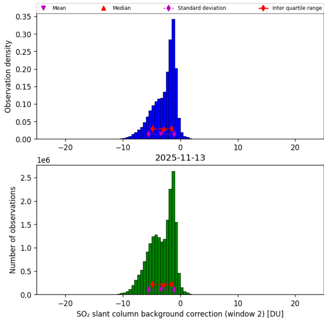
Figure 70: Histogram of “SO 2 slant column background correction (window 2)” for 2025-11-12 to 2025-11-14
