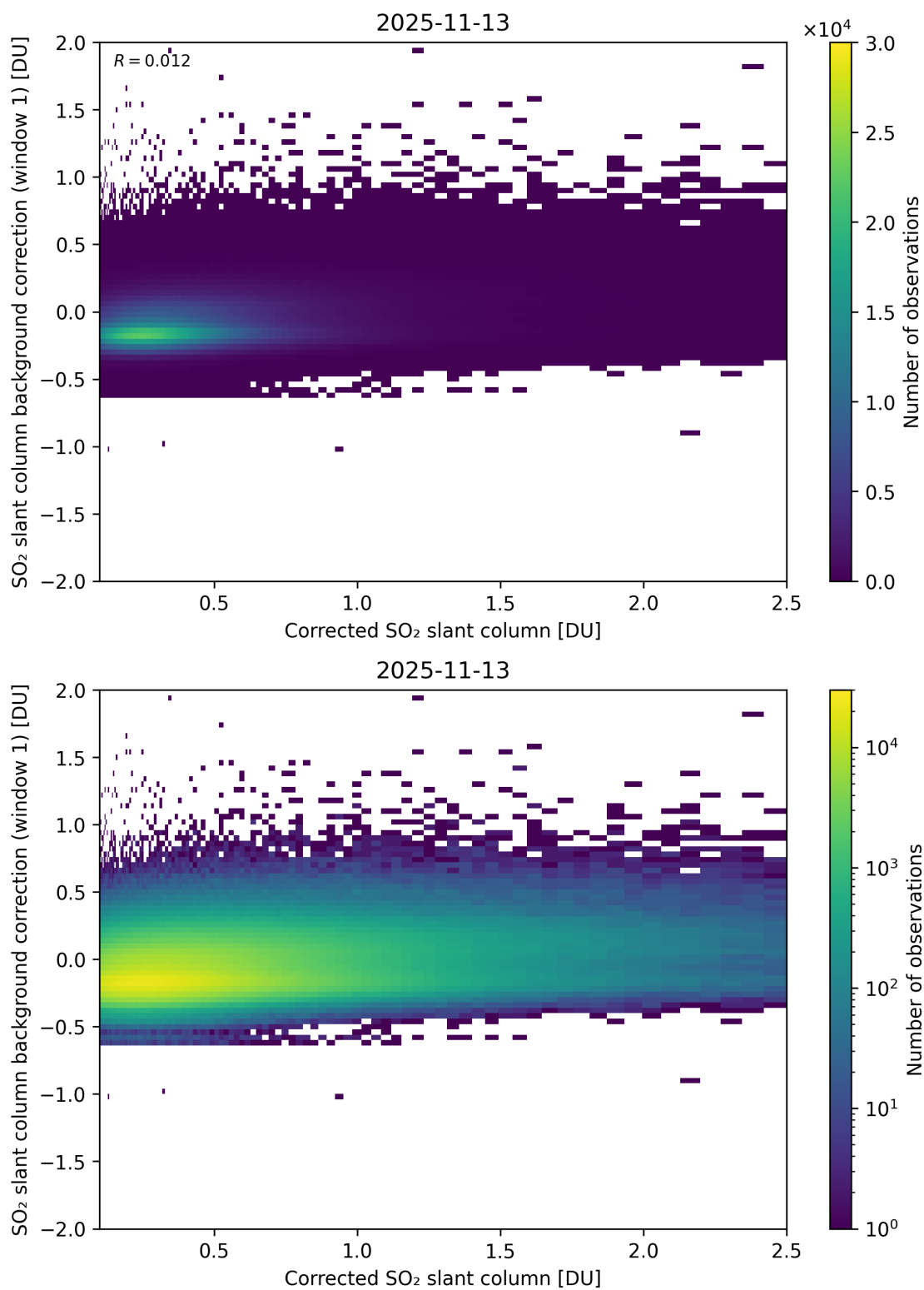
Figure 226: Scatter density plot of “Corrected SO 2 slant column” against “SO 2 slant column background correction (window 1)” for 2025-11-12 to 2025-11-14.
