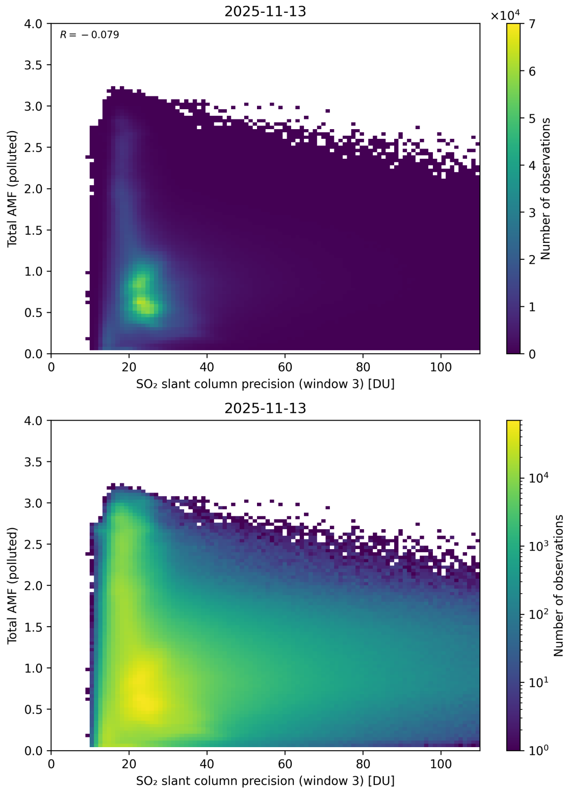
Figure 313: Scatter density plot of “SO 2 slant column precision (window 3)” against “Total AMF (polluted)” for 2025-11-12 to 2025-11-14.
