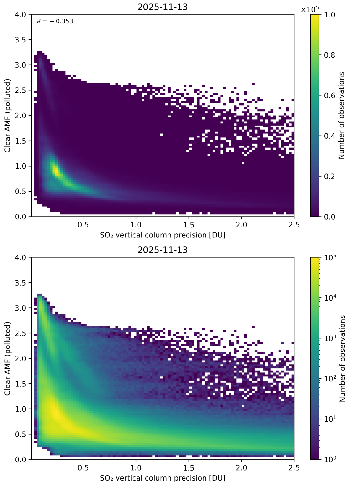
Figure 335: Scatter density plot of “SO 2 vertical column precision” against “Clear AMF (polluted)” for 2025-11-12 to 2025-11-14.
