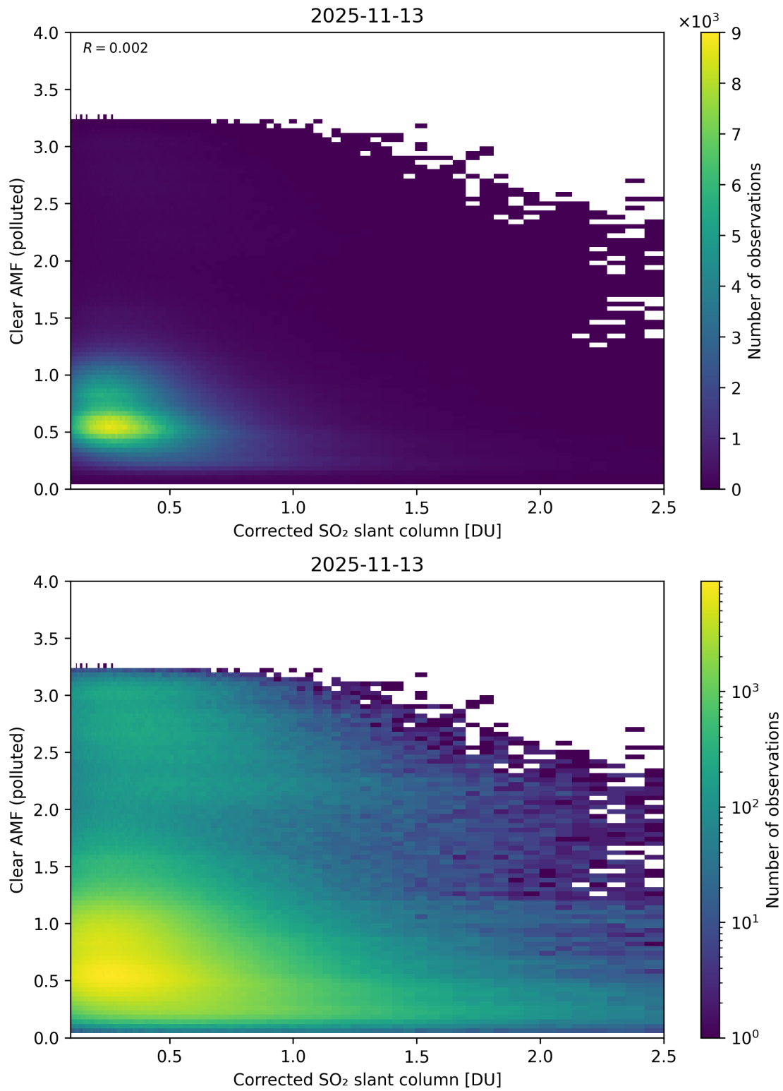
Figure 232: Scatter density plot of “Corrected SO 2 slant column” against “Clear AMF (polluted)” for 2025-11-12 to 2025-11-14.
