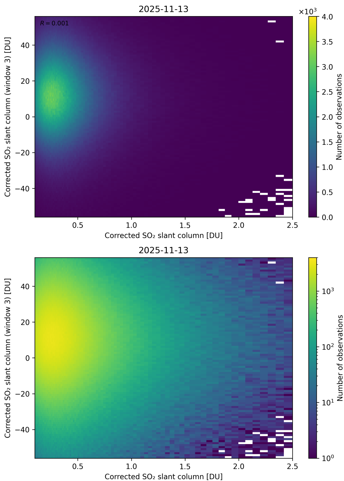
Figure 236: Scatter density plot of “Corrected SO 2 slant column” against “Corrected SO 2 slant column (window 3)” for 2025-11-12 to 2025-11-14.
