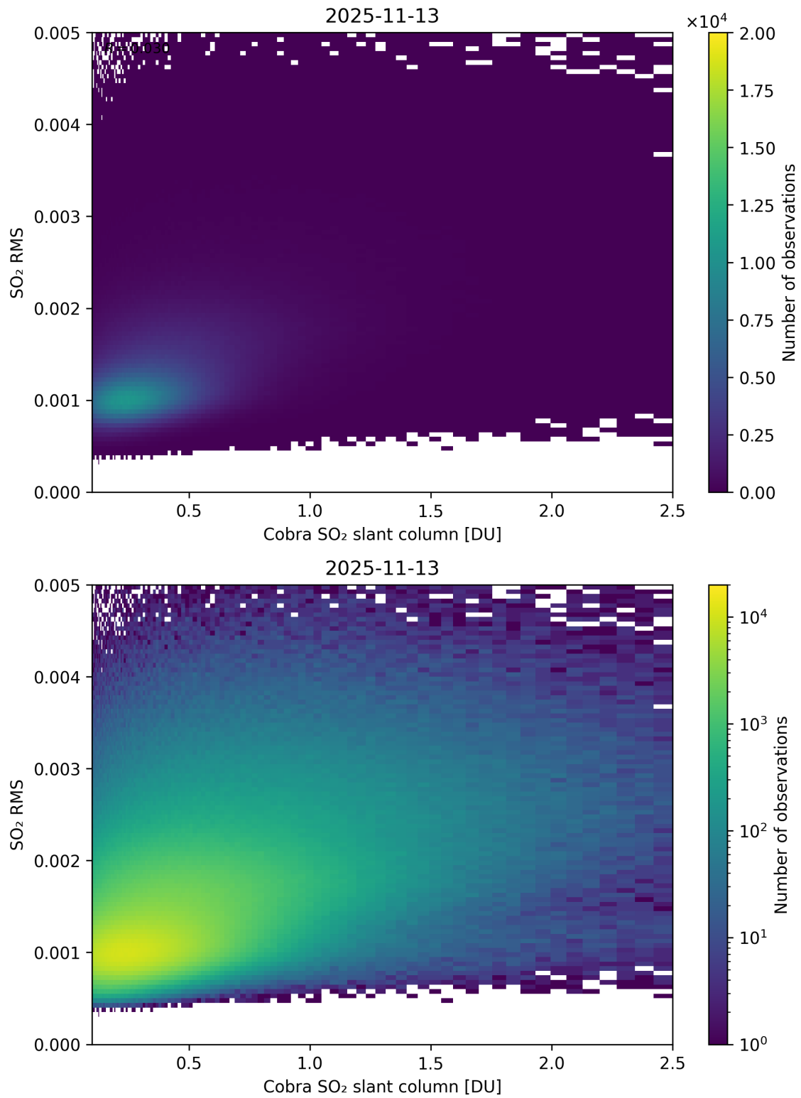
Figure 198: Scatter density plot of “Cobra SO 2 slant column” against “SO 2 RMS” for 2025-11-12 to 2025-11-14.
