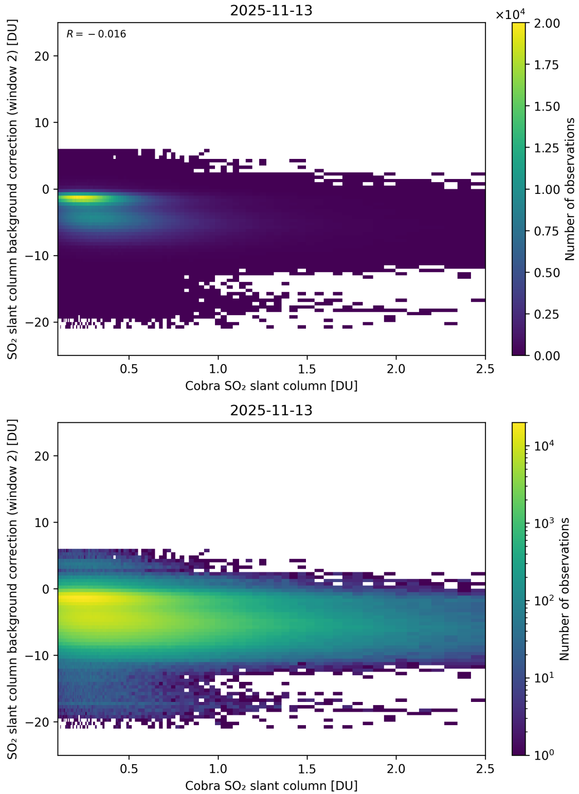
Figure 194: Scatter density plot of “Cobra SO 2 slant column” against “SO 2 slant column background correction (window 2)” for 2025-11-12 to 2025-11-14.
