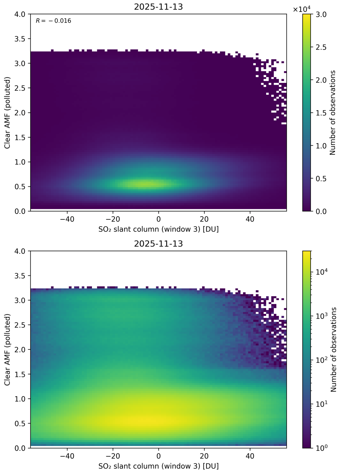
Figure 315: Scatter density plot of “SO 2 slant column (window 3)” against “Clear AMF (polluted)” for 2025-11-12 to 2025-11-14.
