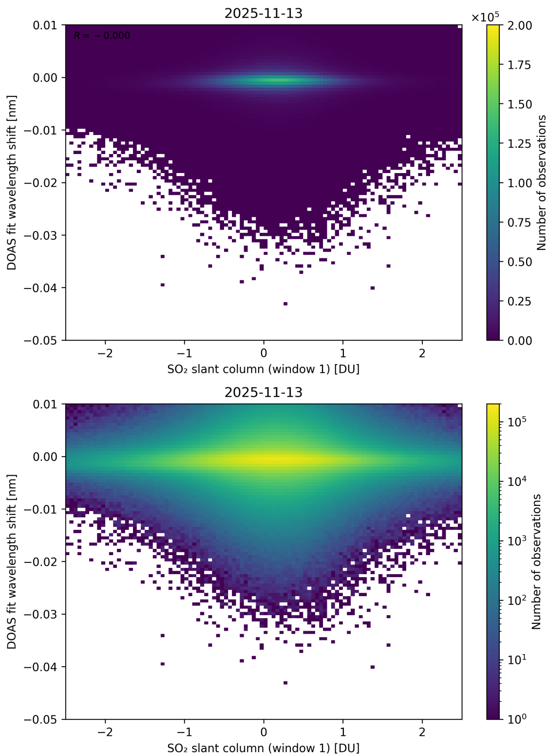
Figure 265: Scatter density plot of “SO 2 slant column (window 1)” against “DOAS fit wavelength shift” for 2025-11-12 to 2025-11-14.
