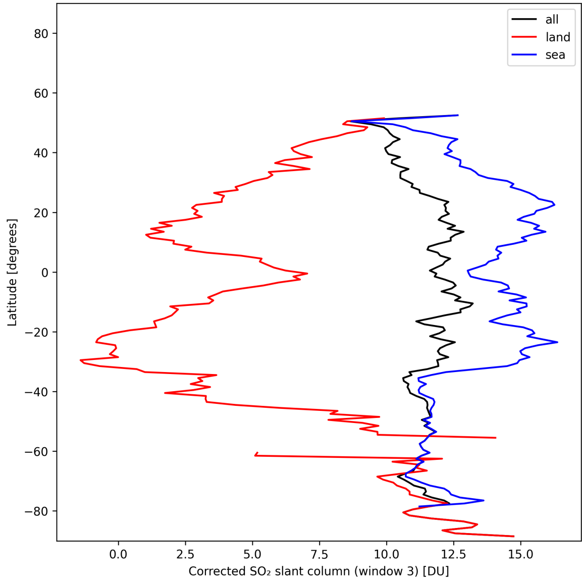
Figure 47: Zonal average of “Corrected SO 2 slant column (window 3)” for 2025-11-12 to 2025-11-14.
