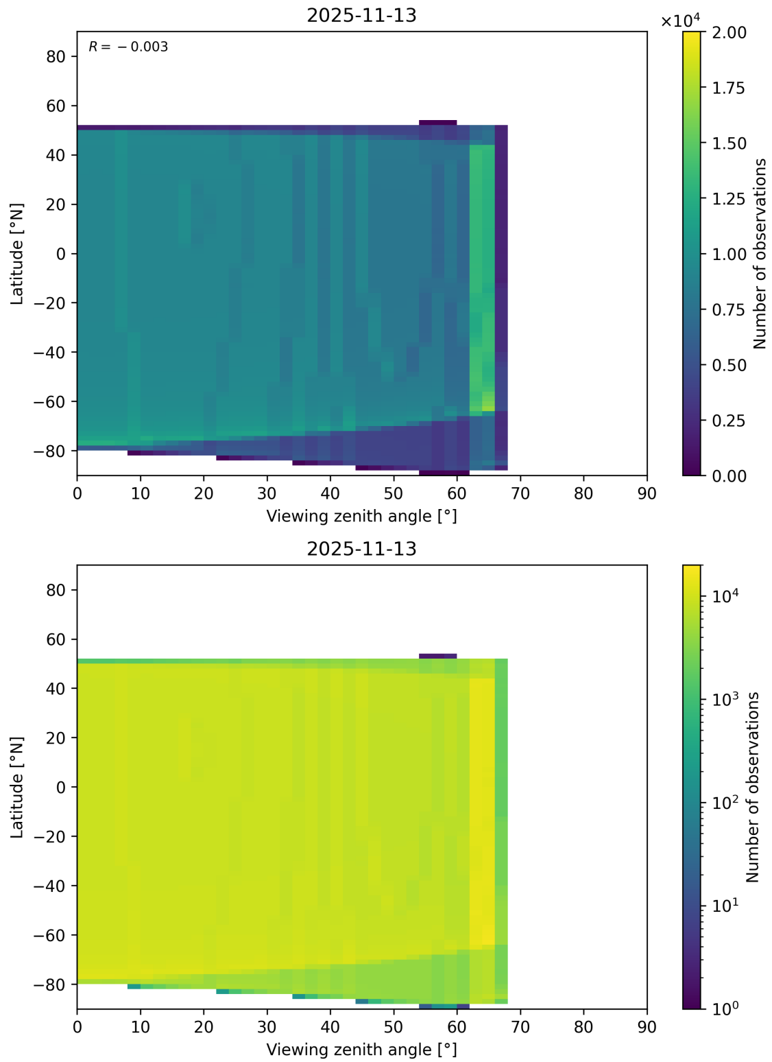
Figure 368: Scatter density plot of “Viewing zenith angle” against “Latitude” for 2025-11-12 to 2025-11-14.
