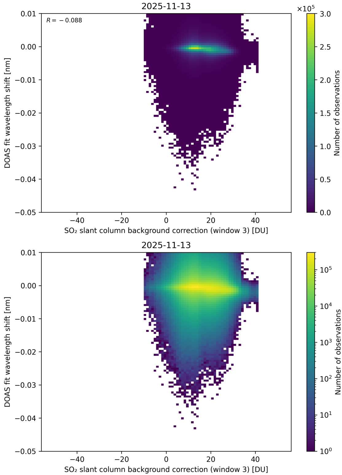
Figure 132: Scatter density plot of “SO 2 slant column background correction (window 3)” against “DOAS fit wavelength shift” for 2025-11-12 to 2025-11-14.
