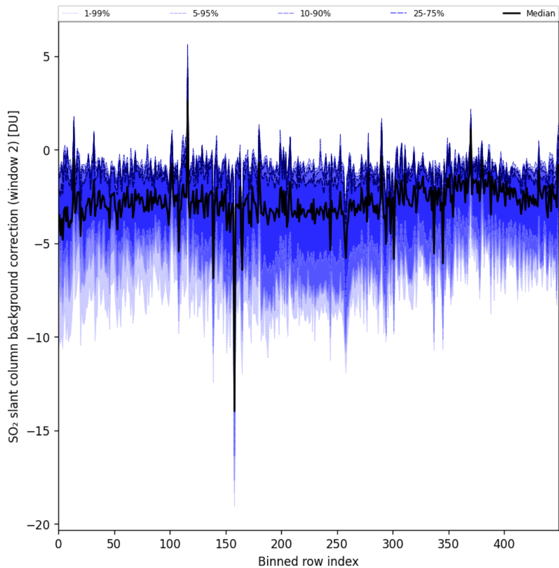
Figure 96: Along track statistics of “SO 2 slant column background correction (window 2)” for 2025-11-12 to 2025-11-14
