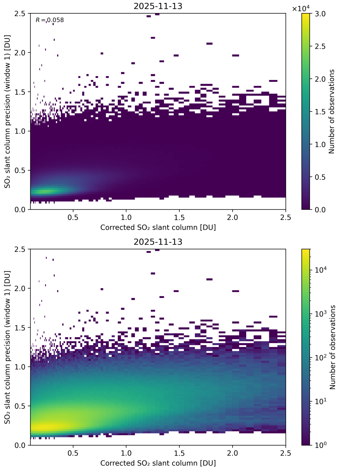
Figure 238: Scatter density plot of “Corrected SO 2 slant column” against “SO 2 slant column precision (window 1)” for 2025-11-12 to 2025-11-14.
