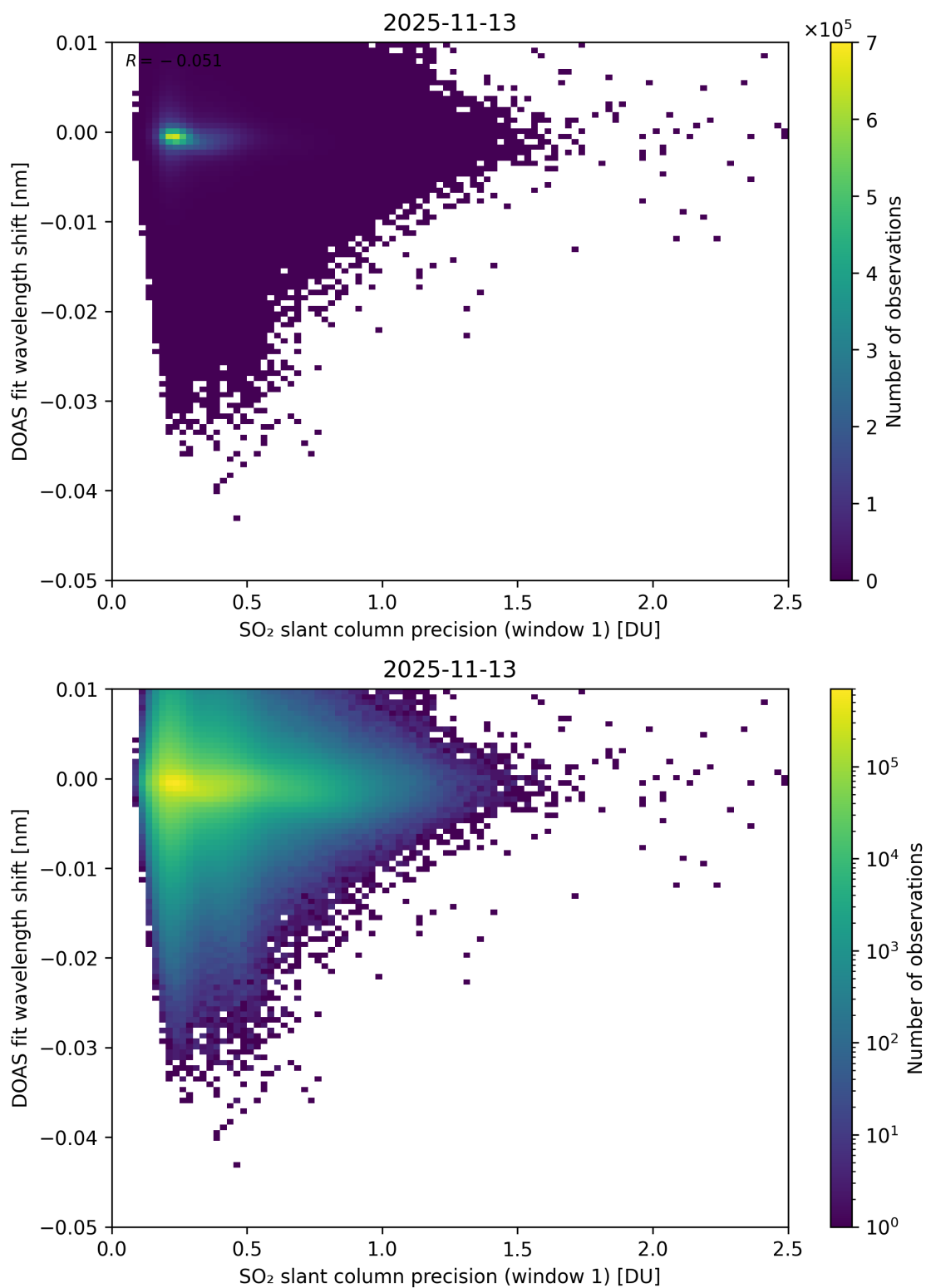
Figure 271: Scatter density plot of “SO 2 slant column precision (window 1)” against “DOAS fit wavelength shift” for 2025-11-12 to 2025-11-14.
