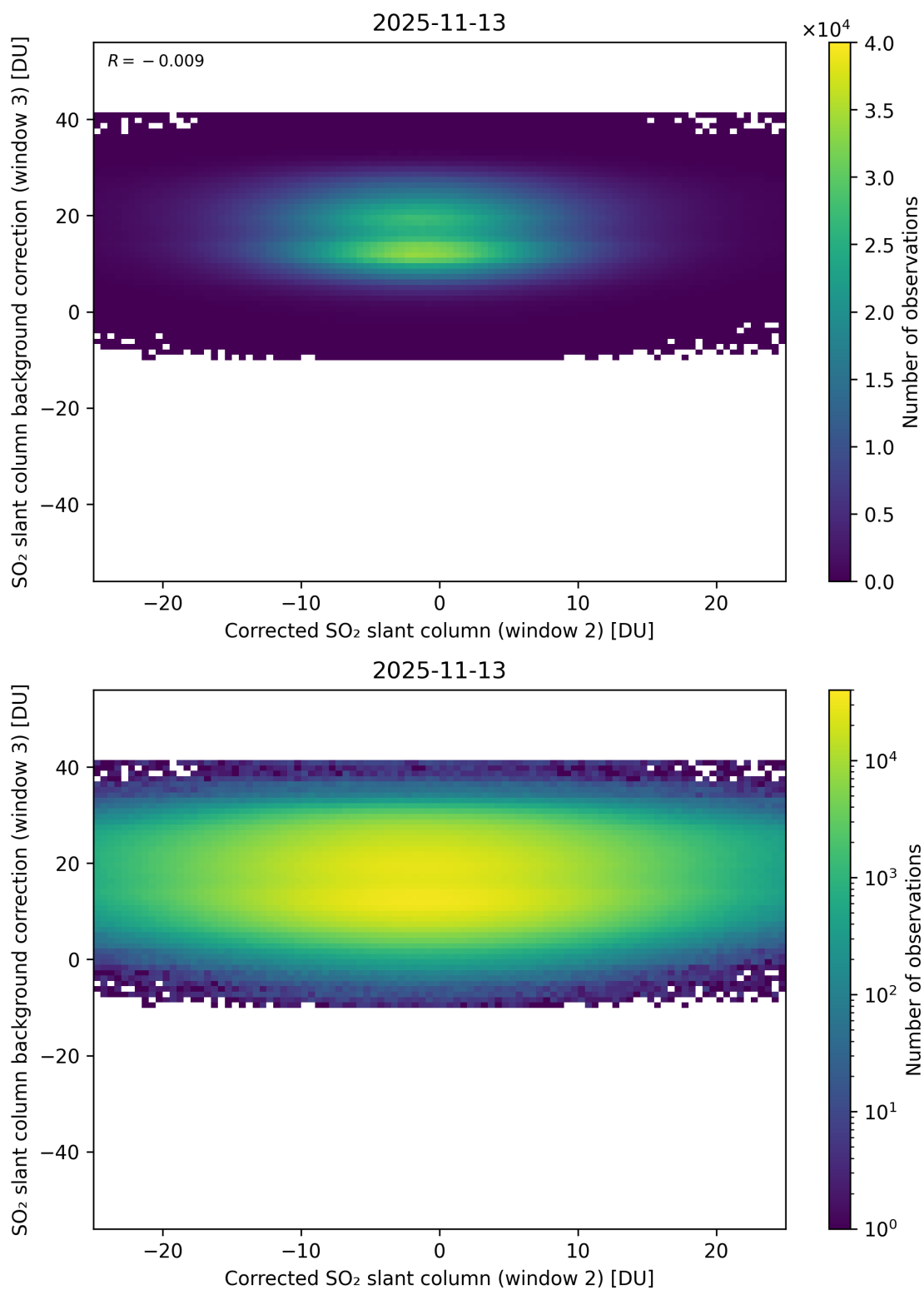
Figure 245: Scatter density plot of “Corrected SO 2 slant column (window 2)” against “SO 2 slant column background correction (window 3)” for 2025-11-12 to 2025-11-14.
