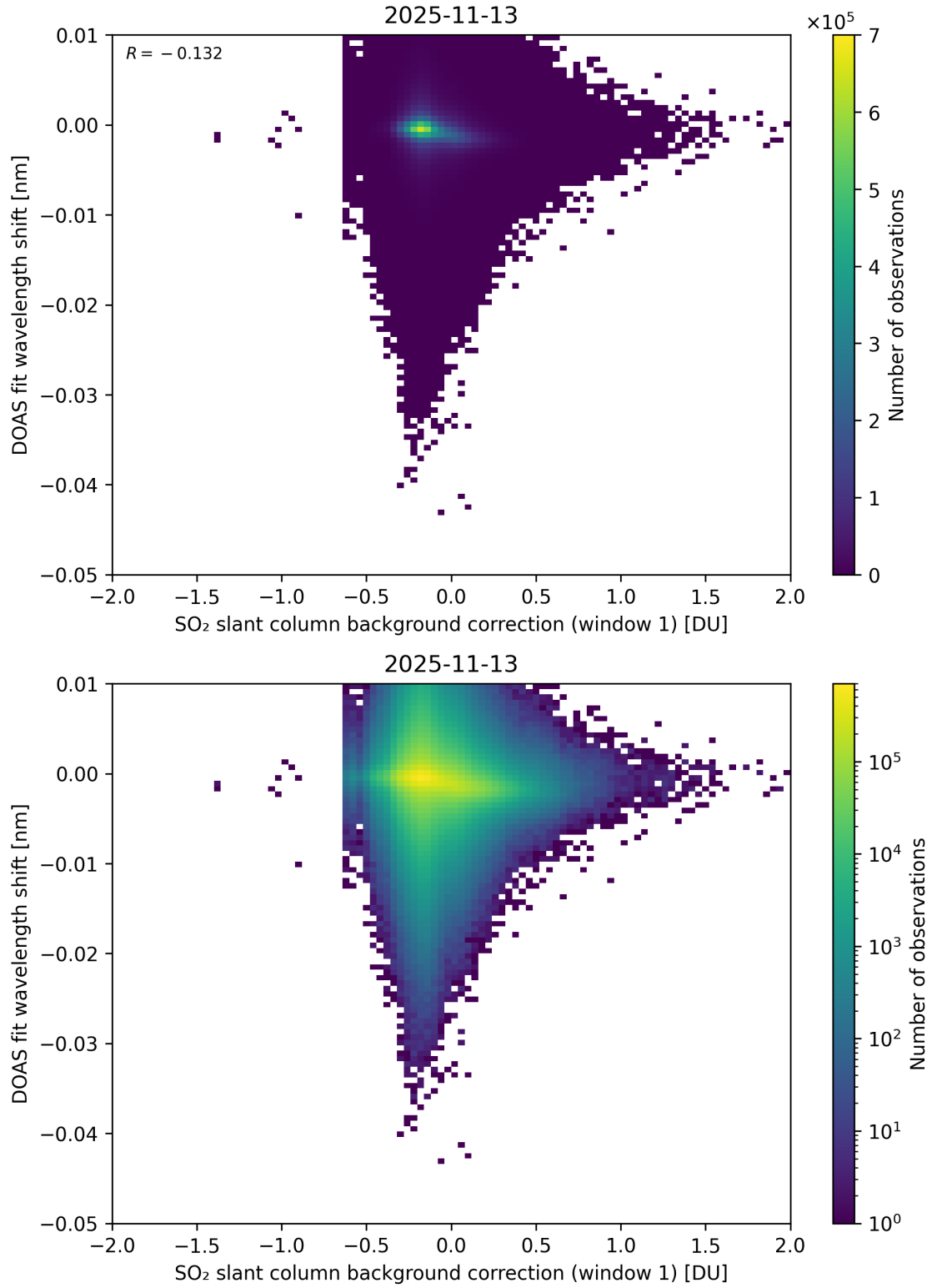
Figure 111: Scatter density plot of “SO 2 slant column background correction (window 1)” against “DOAS fit wavelength shift” for 2025-11-12 to 2025-11-14.
