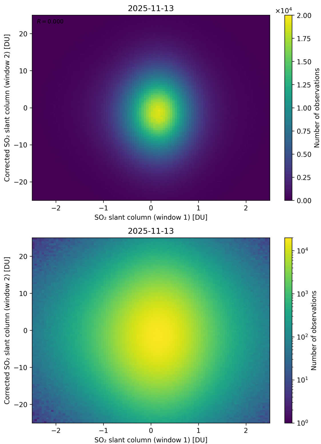
Figure 283: Scatter density plot of “SO 2 slant column (window 1)” against “Corrected SO 2 slant column (window 2)” for 2025-11-12 to 2025-11-14.
