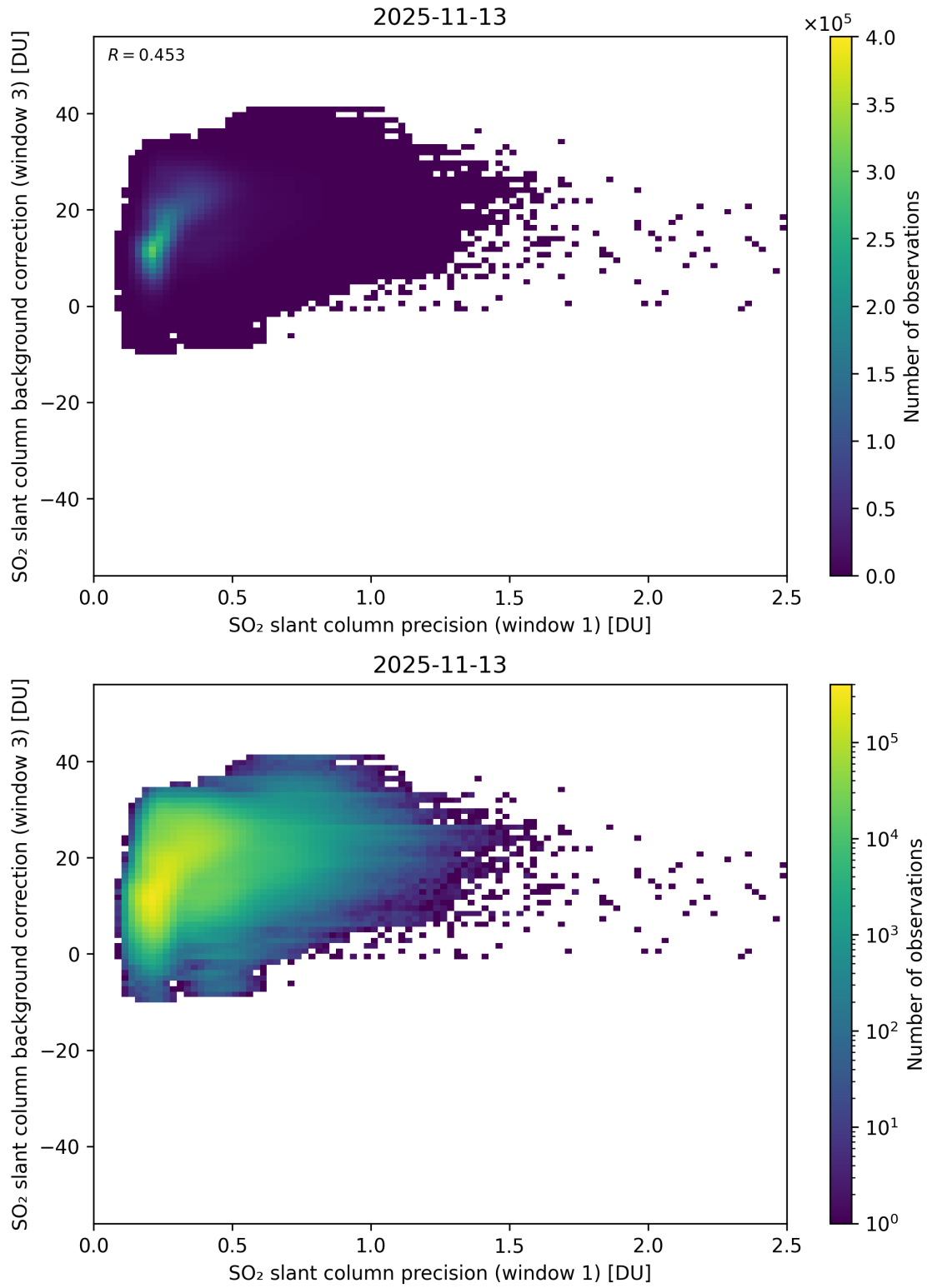
Figure 270: Scatter density plot of “SO 2 slant column precision (window 1)” against “SO 2 slant column background correction (window 3)” for 2025-11-12 to 2025-11-14.
