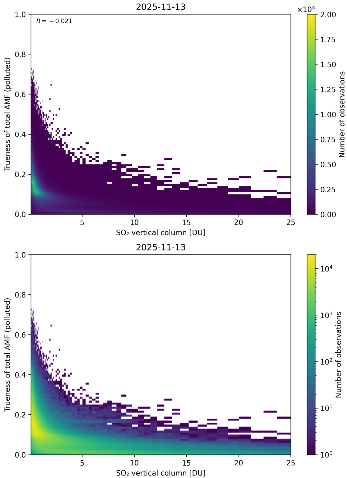
Figure 360: Scatter density plot of “SO 2 vertical column” against “Trueness of total AMF (polluted)” for 2025-11-12 to 2025-11-14.
