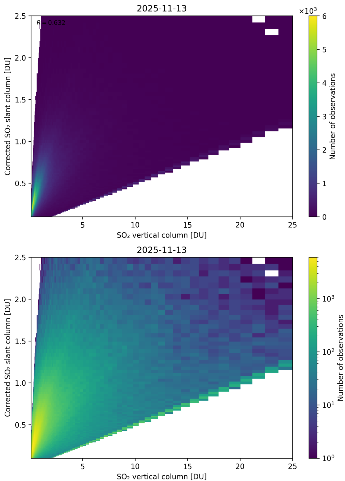
Figure 351: Scatter density plot of “SO 2 vertical column” against “Corrected SO 2 slant column” for 2025-11-12 to 2025-11-14.
