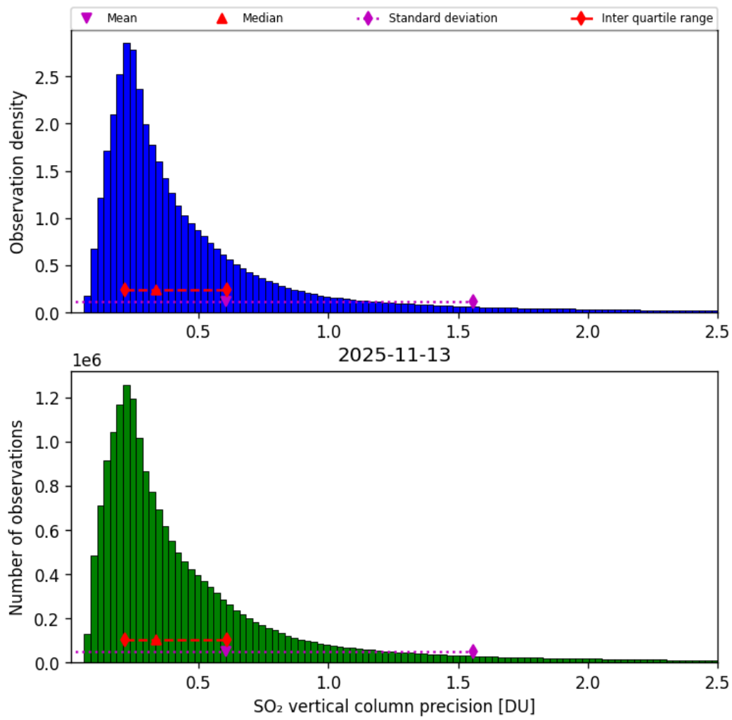
Figure 59: Histogram of “SO 2 vertical column precision” for 2025-11-12 to 2025-11-14
