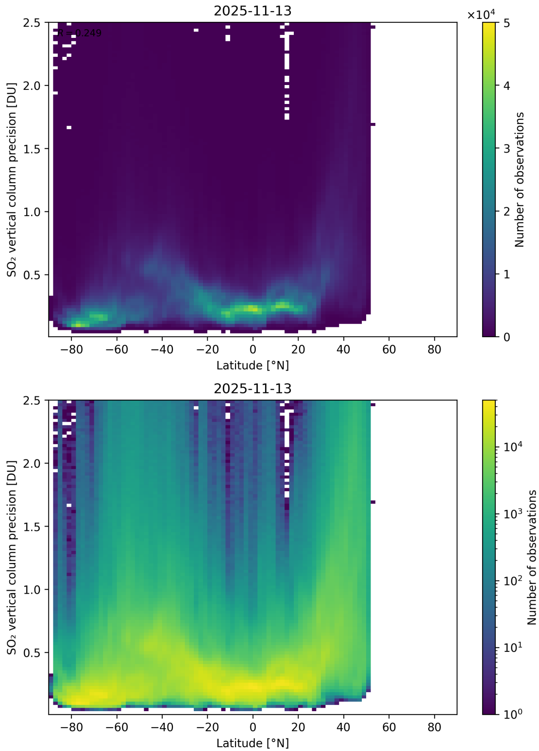
Figure 170: Scatter density plot of “Latitude” against “SO 2 vertical column precision” for 2025-11-12 to 2025-11-14.
