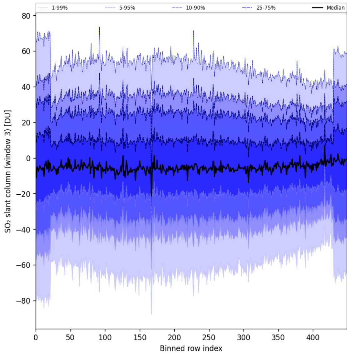
Figure 97: Along track statistics of “SO 2 slant column (window 3)” for 2025-11-12 to 2025-11-14
