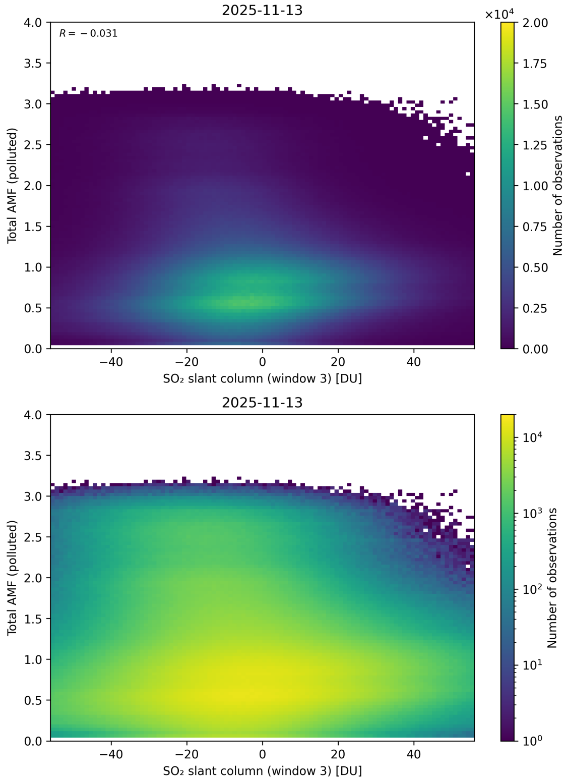
Figure 318: Scatter density plot of “SO 2 slant column (window 3)” against “Total AMF (polluted)” for 2025-11-12 to 2025-11-14.
