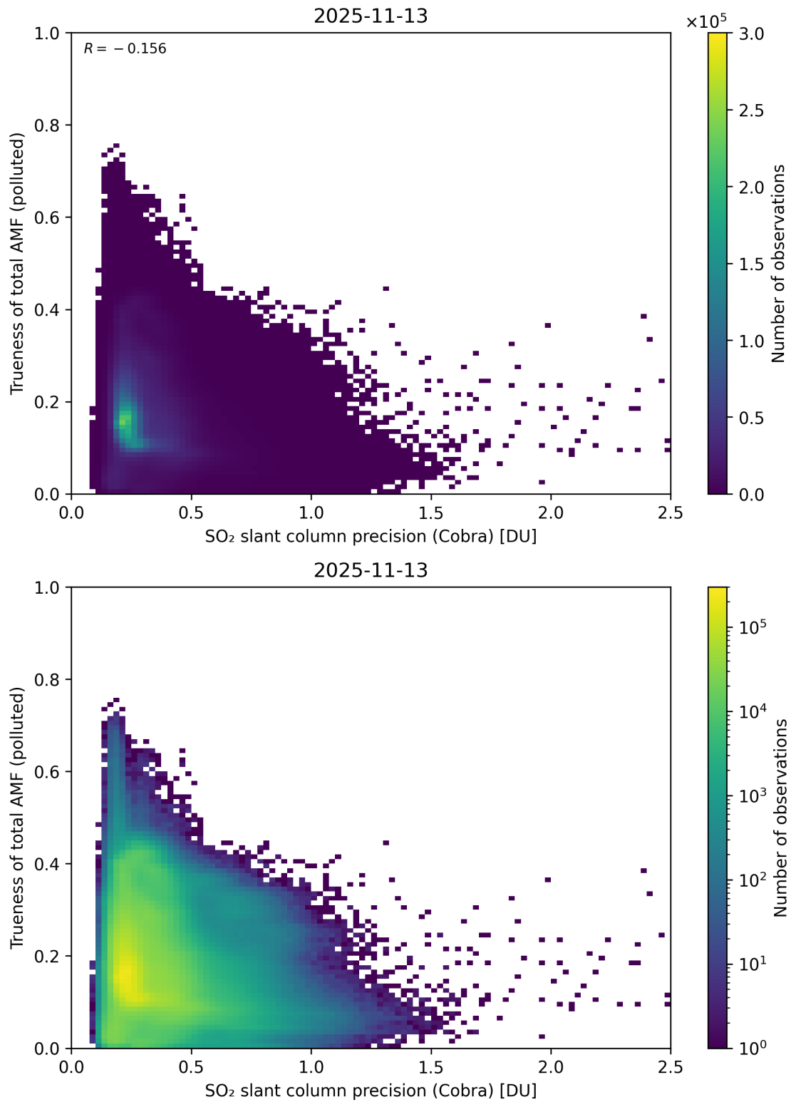
Figure 214: Scatter density plot of “SO 2 slant column precision (Cobra)” against “Trueness of total AMF (polluted)” for 2025-11-12 to 2025-11-14.
