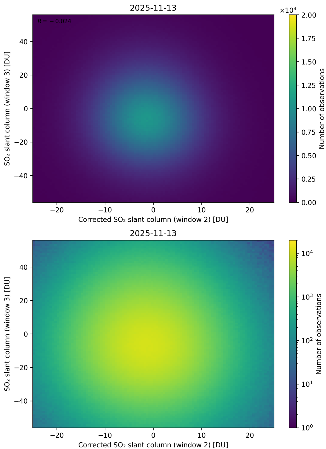
Figure 251: Scatter density plot of “Corrected SO 2 slant column (window 2)” against “SO 2 slant column (window 3)” for 2025-11-12 to 2025-11-14.
