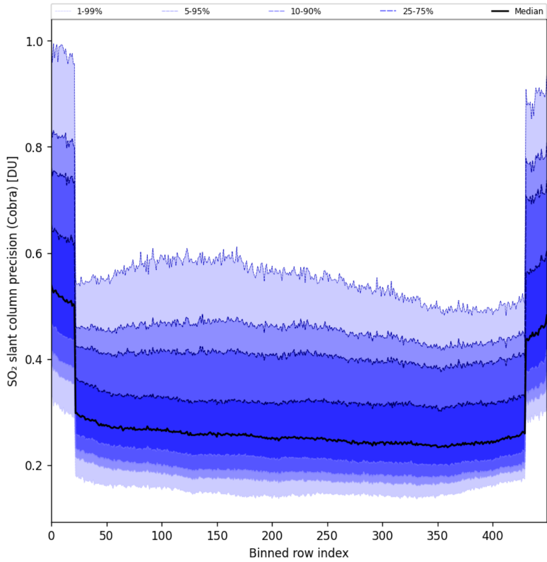
Figure 88: Along track statistics of “SO 2 slant column precision (Cobra)” for 2025-11-12 to 2025-11-14
