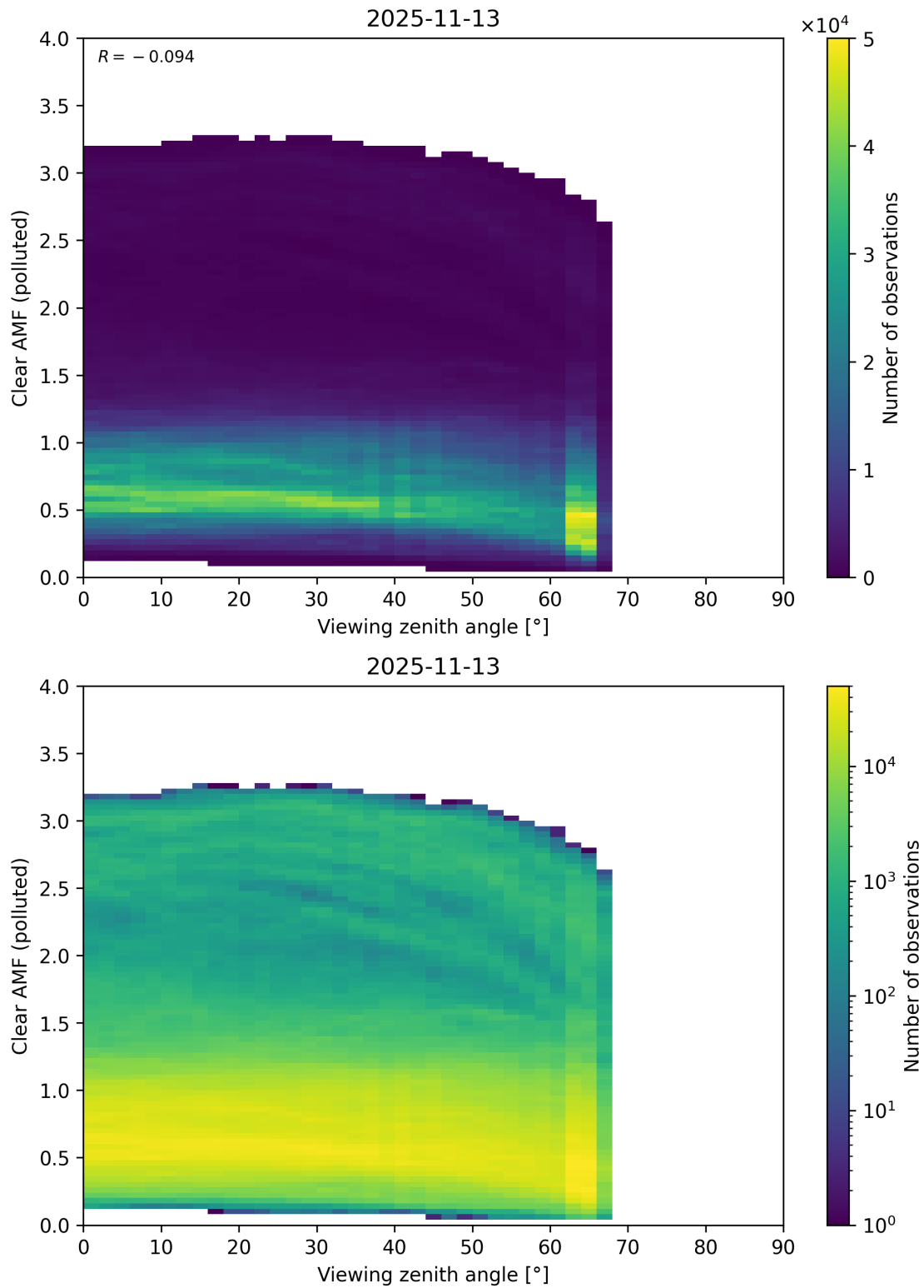
Figure 370: Scatter density plot of “Viewing zenith angle” against “Clear AMF (polluted)” for 2025-11-12 to 2025-11-14.
