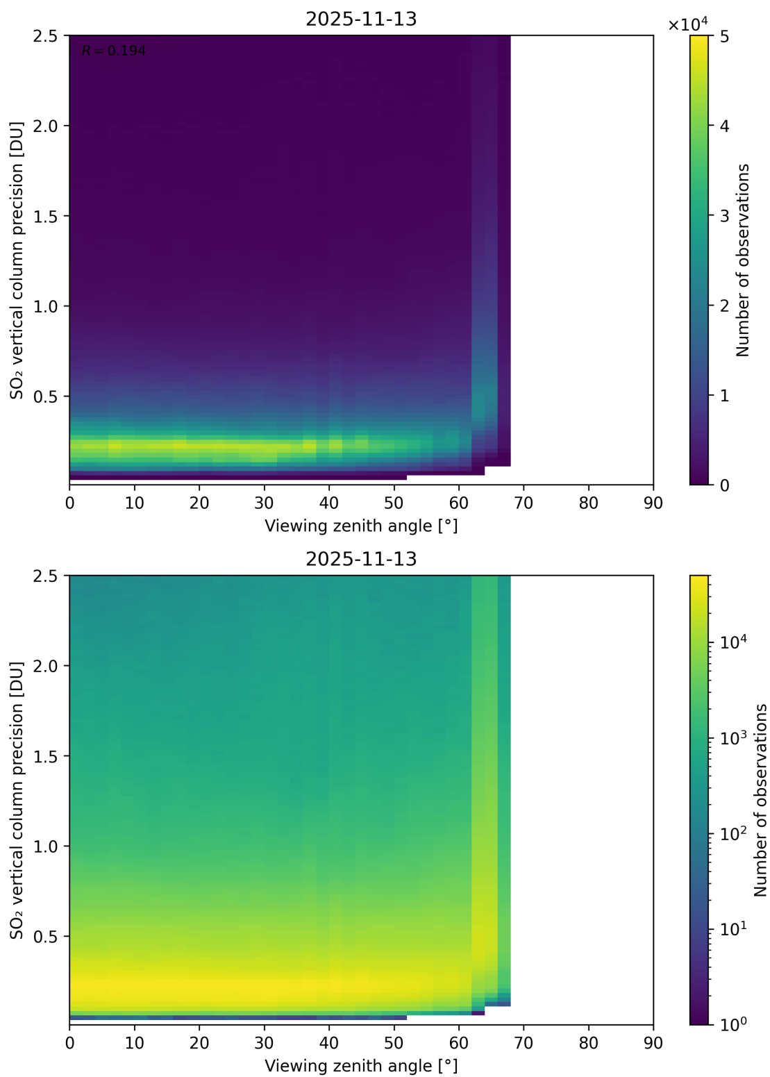
Figure 384: Scatter density plot of “Viewing zenith angle” against “SO 2 vertical column precision” for 2025-11-12 to 2025-11-14.
