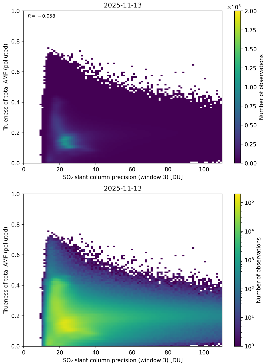
Figure 314: Scatter density plot of “SO 2 slant column precision (window 3)” against “Trueness of total AMF (polluted)” for 2025-11-12 to 2025-11-14.
