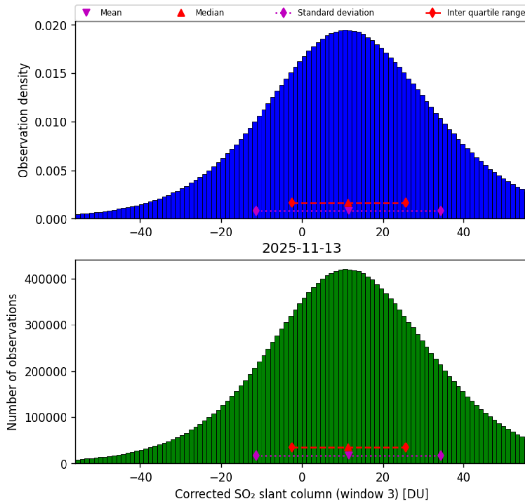
Figure 73: Histogram of “Corrected SO 2 slant column (window 3)” for 2025-11-12 to 2025-11-14
