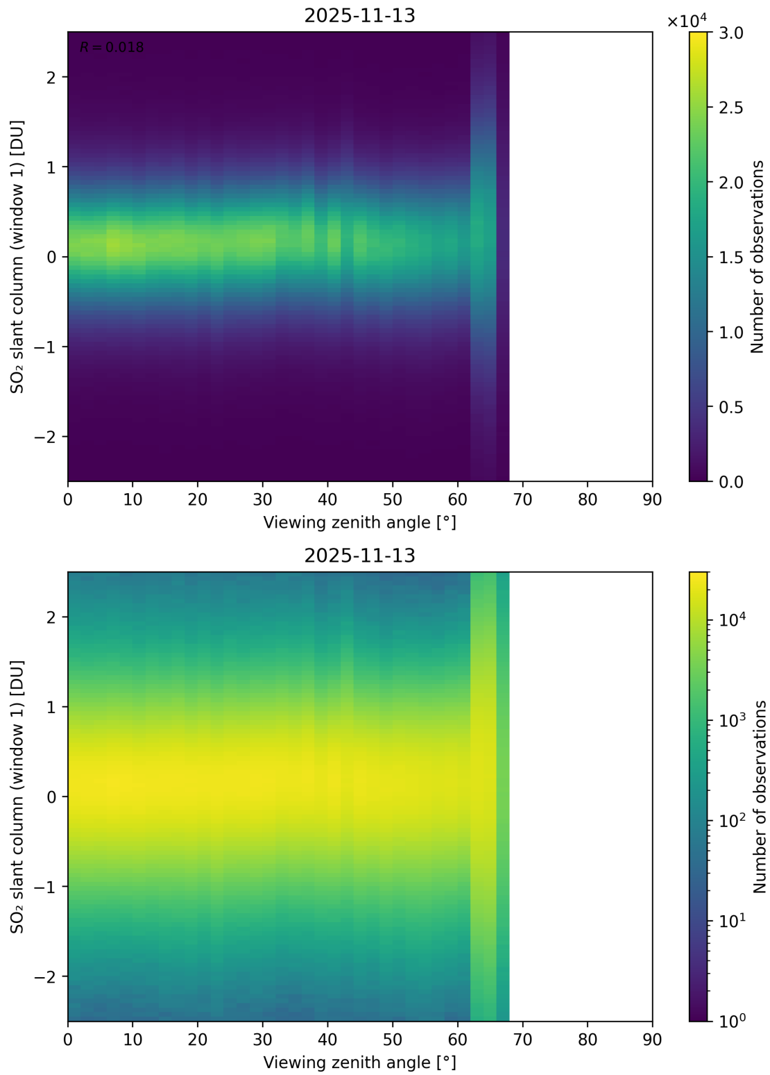
Figure 376: Scatter density plot of “Viewing zenith angle” against “SO 2 slant column (window 1)” for 2025-11-12 to 2025-11-14.
