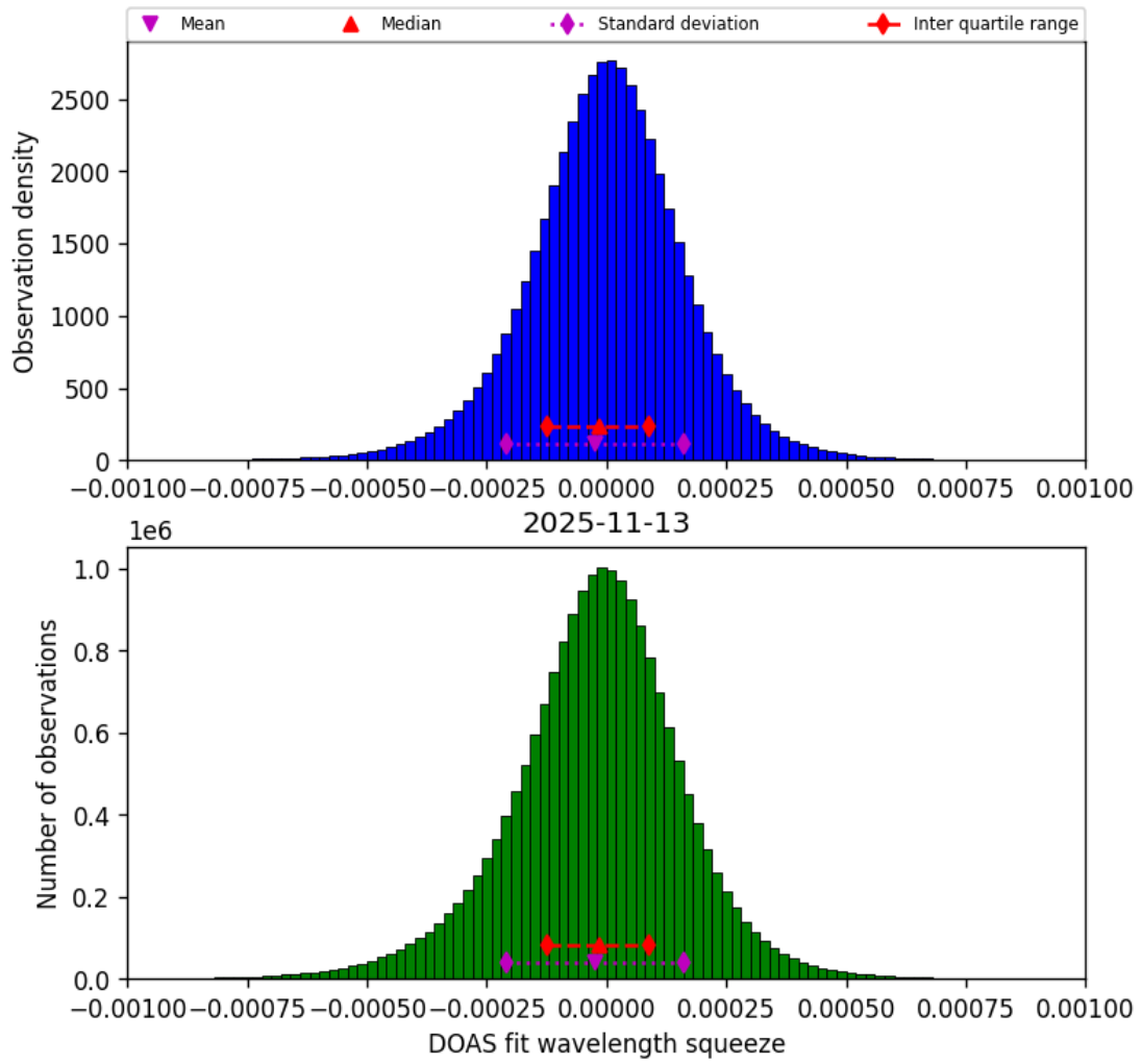
Figure 77: Histogram of “DOAS fit wavelength squeeze” for 2025-11-12 to 2025-11-14
