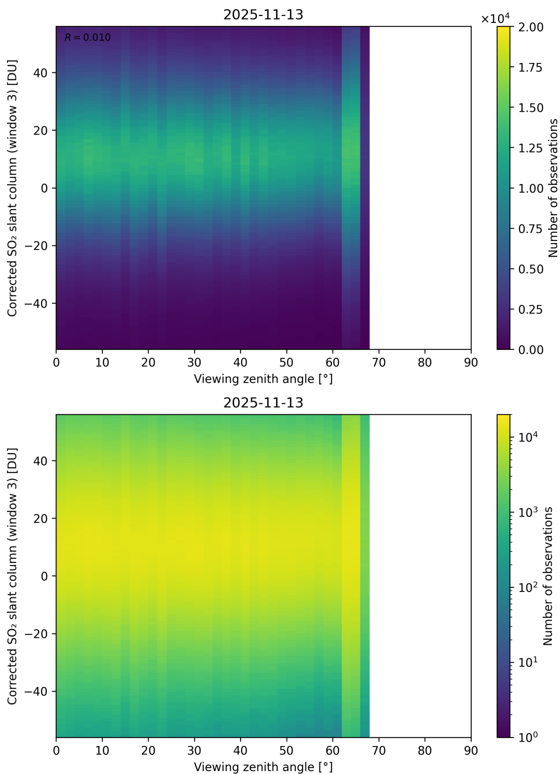
Figure 375: Scatter density plot of “Viewing zenith angle” against “Corrected SO 2 slant column (window 3)” for 2025-11-12 to 2025-11-14.
