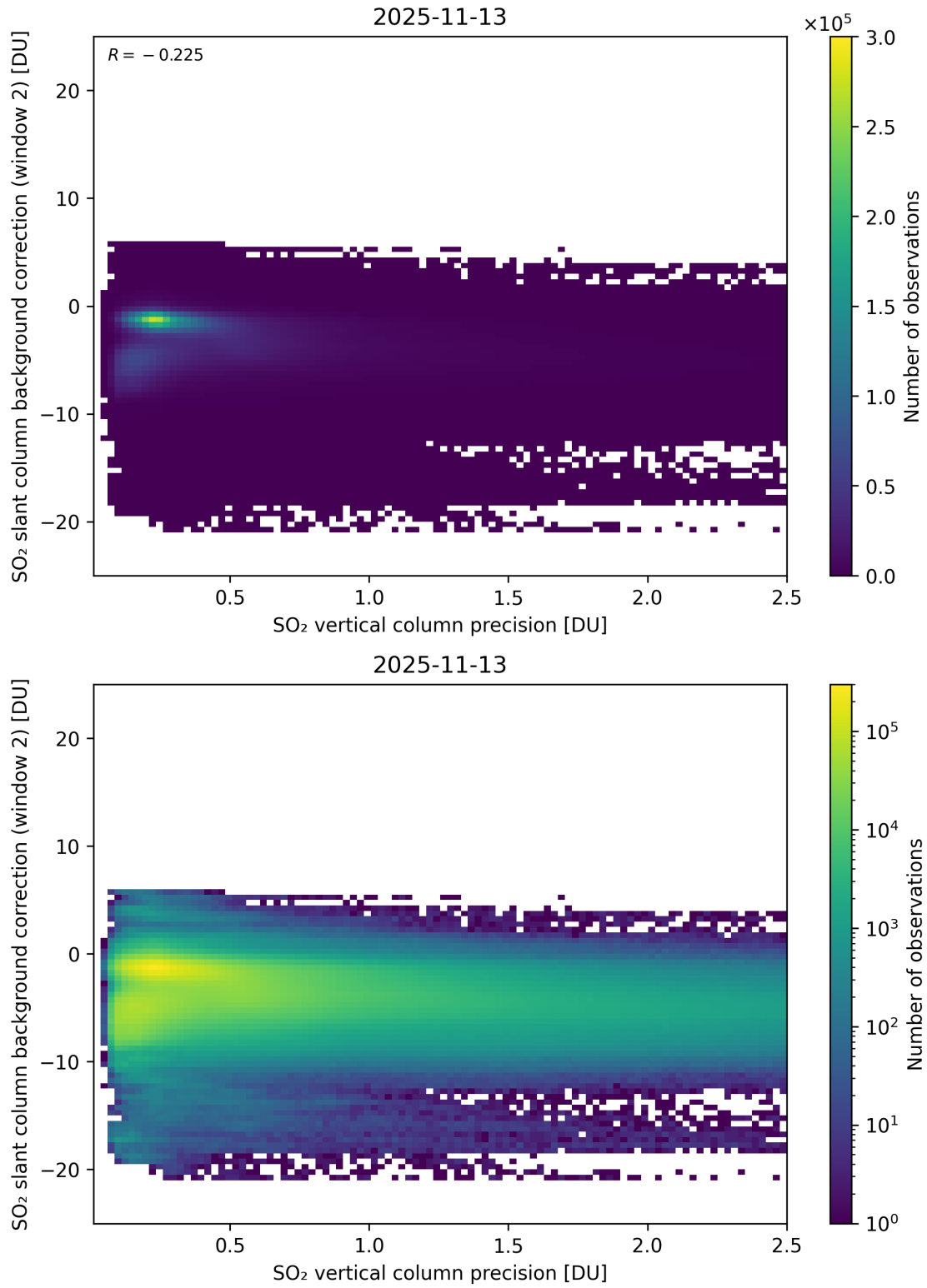
Figure 330: Scatter density plot of “SO 2 vertical column precision” against “SO 2 slant column background correction (window 2)” for 2025-11-12 to 2025-11-14.
