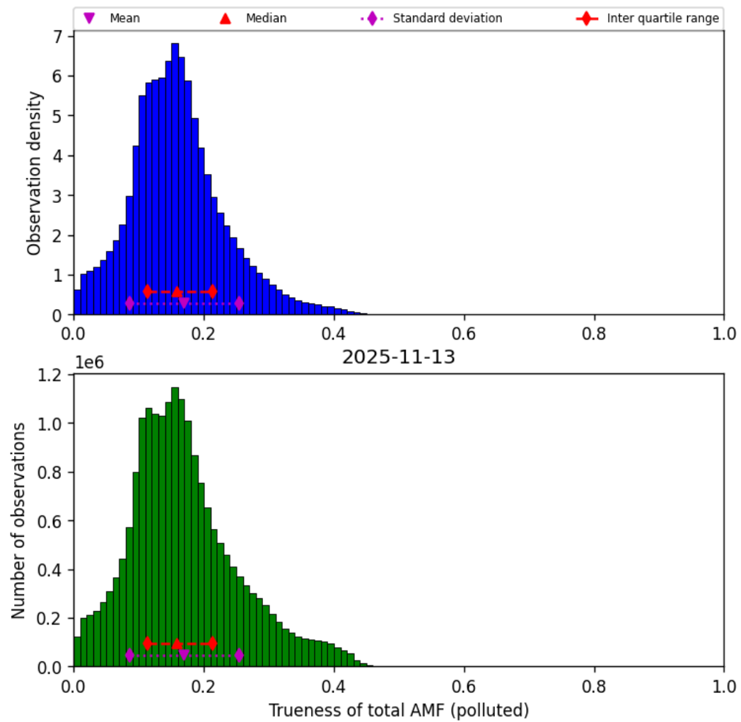
Figure 80: Histogram of “Trueness of total AMF (polluted)” for 2025-11-12 to 2025-11-14
