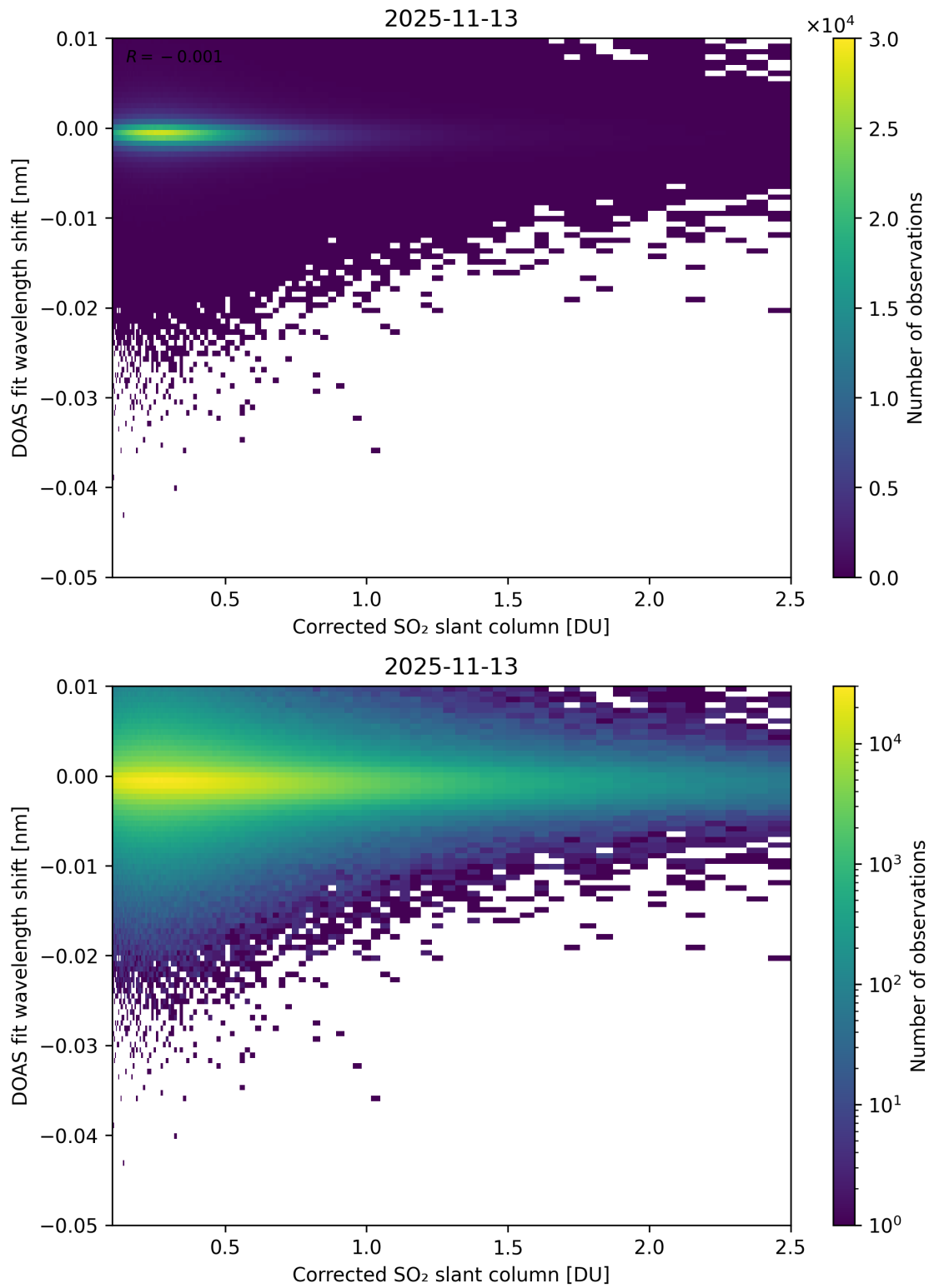
Figure 229: Scatter density plot of “Corrected SO 2 slant column” against “DOAS fit wavelength shift” for 2025-11-12 to 2025-11-14.
