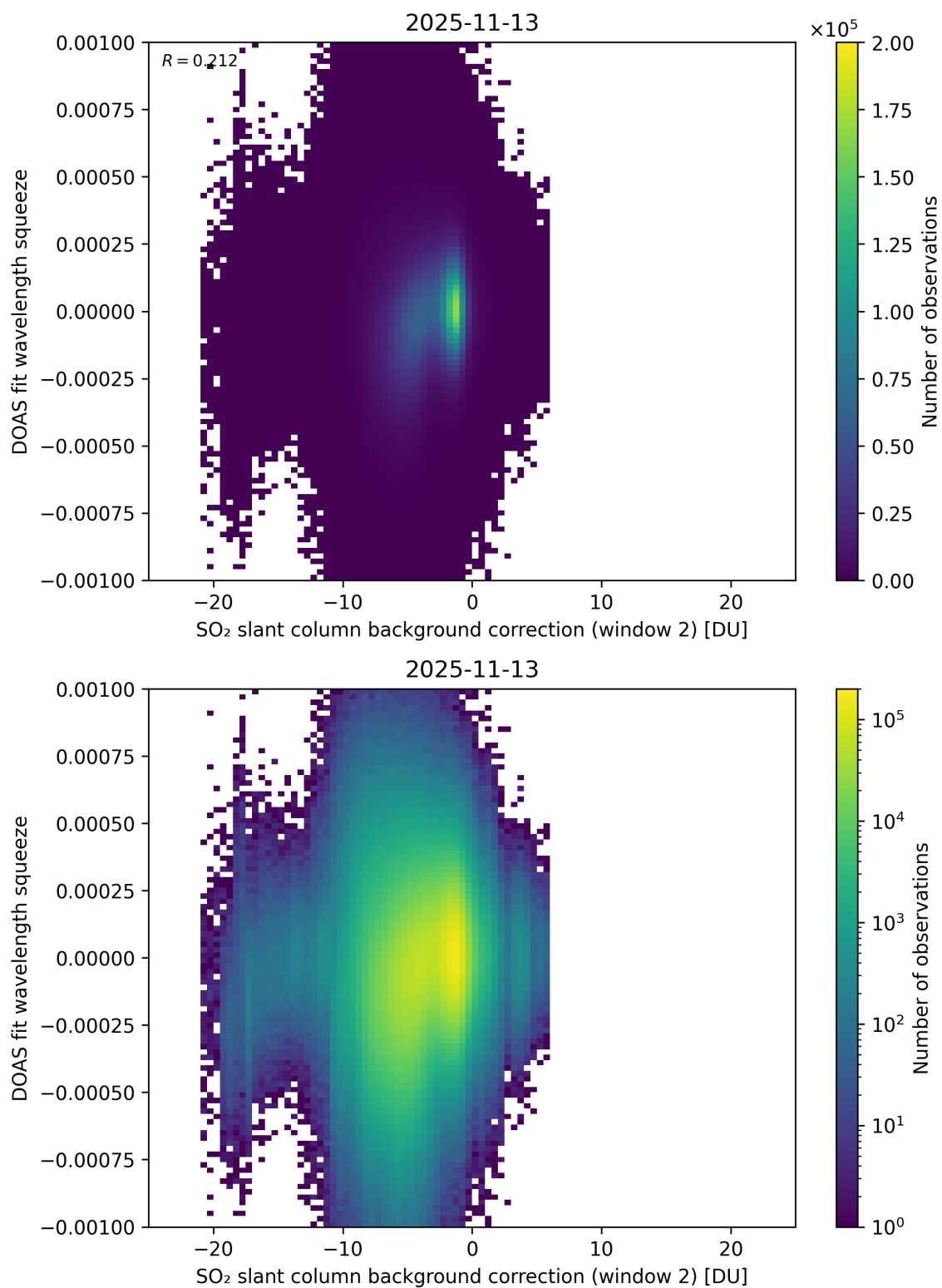
Figure 124: Scatter density plot of “SO 2 slant column background correction (window 2)” against “DOAS fit wavelength squeeze” for 2025-11-12 to 2025-11-14.
