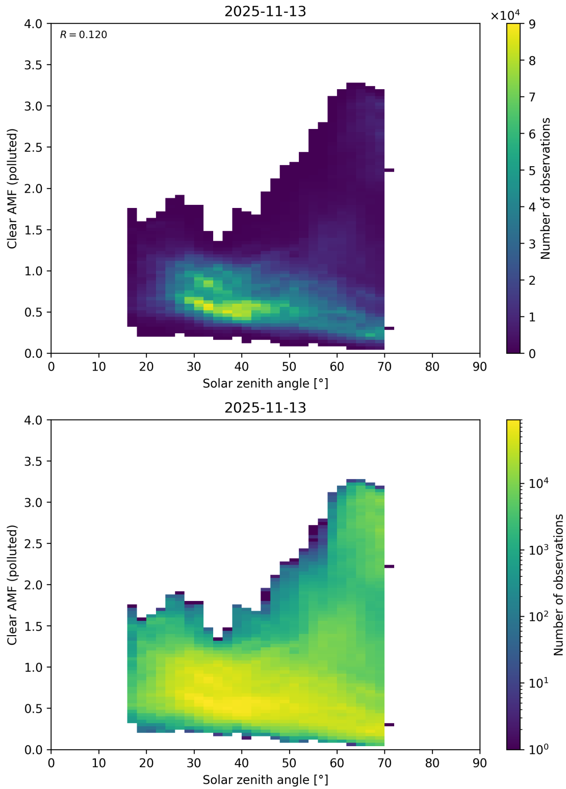
Figure 178: Scatter density plot of “Solar zenith angle” against “Clear AMF (polluted)” for 2025-11-12 to 2025-11-14.
