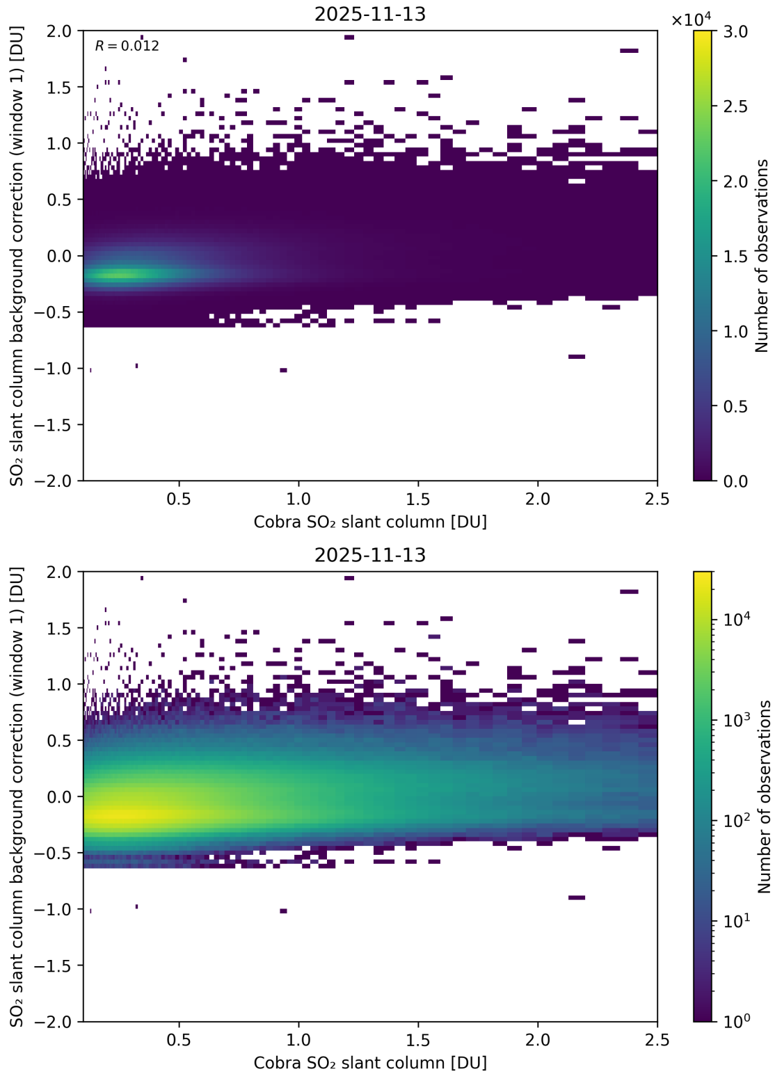
Figure 193: Scatter density plot of “Cobra SO 2 slant column” against “SO 2 slant column background correction (window 1)” for 2025-11-12 to 2025-11-14.
