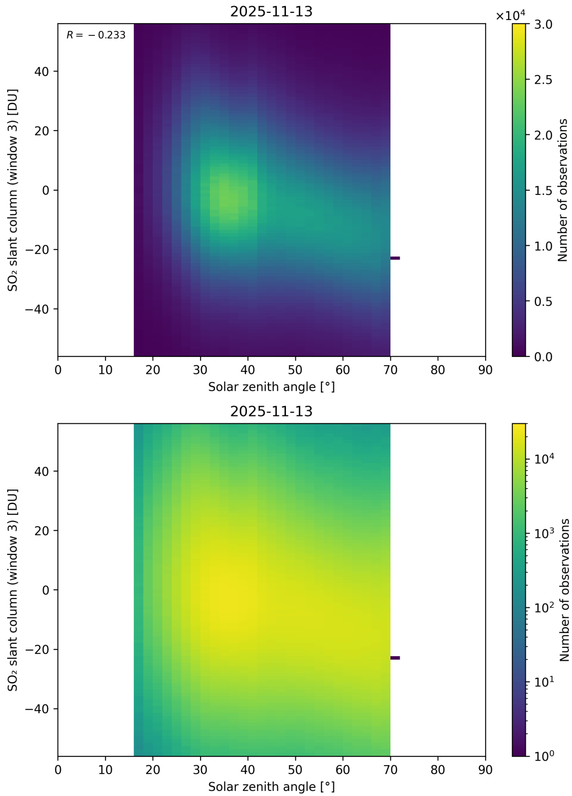
Figure 187: Scatter density plot of “Solar zenith angle” against “SO 2 slant column (window 3)” for 2025-11-12 to 2025-11-14.
