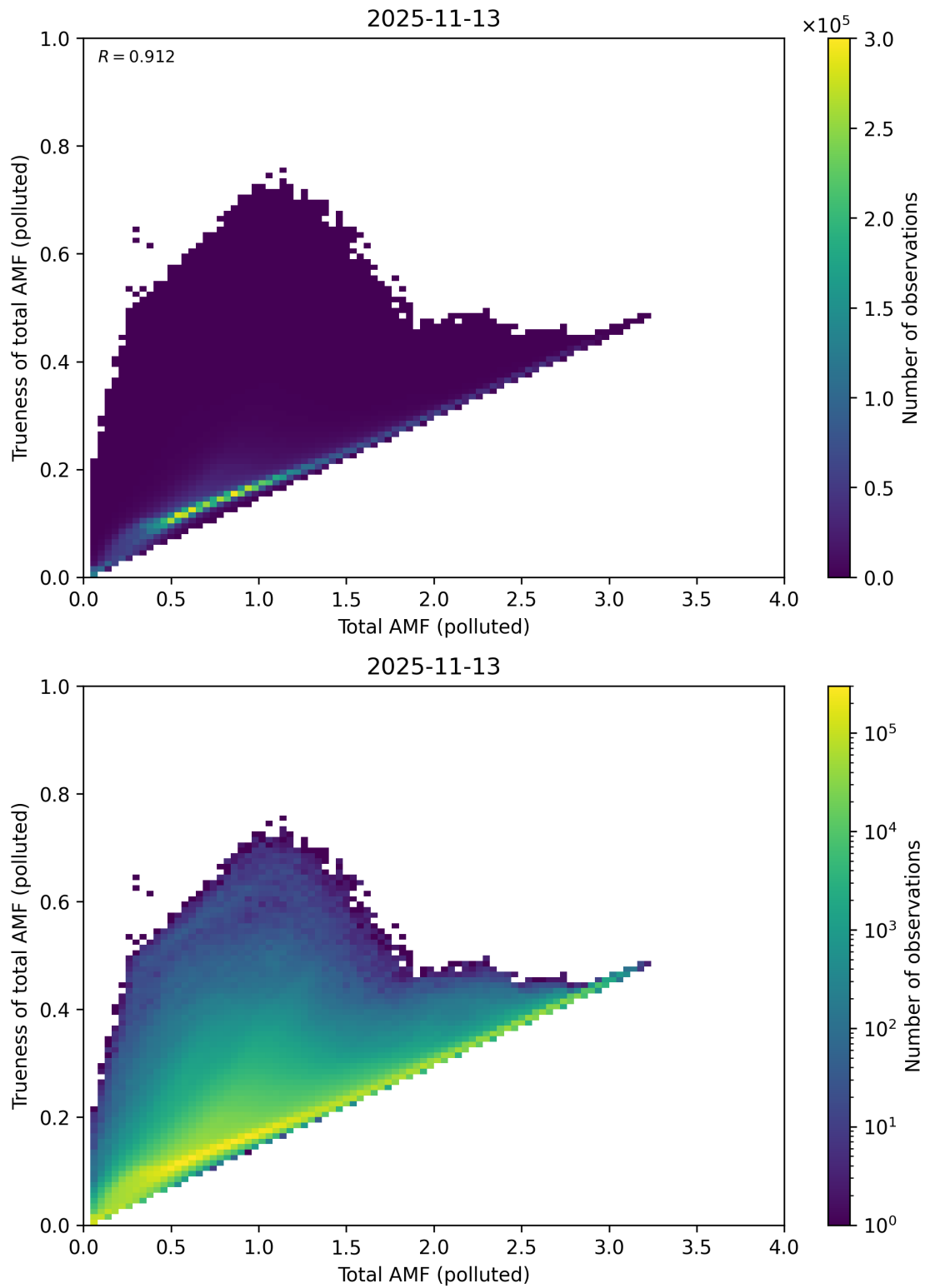
Figure 321: Scatter density plot of “Total AMF (polluted)” against “Trueness of total AMF (polluted)” for 2025-11-12 to 2025-11-14.
