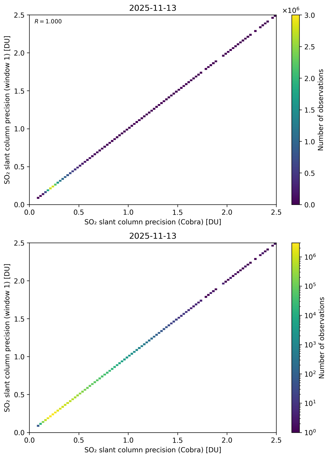
Figure 209: Scatter density plot of “SO 2 slant column precision (Cobra)” against “SO 2 slant column precision (window 1)” for 2025-11-12 to 2025-11-14.
