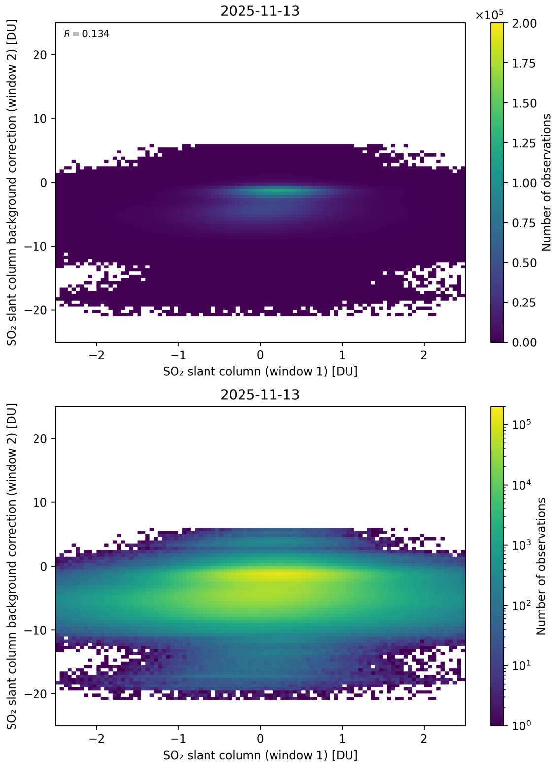
Figure 263: Scatter density plot of “SO 2 slant column (window 1)” against “SO 2 slant column background correction (window 2)” for 2025-11-12 to 2025-11-14.
