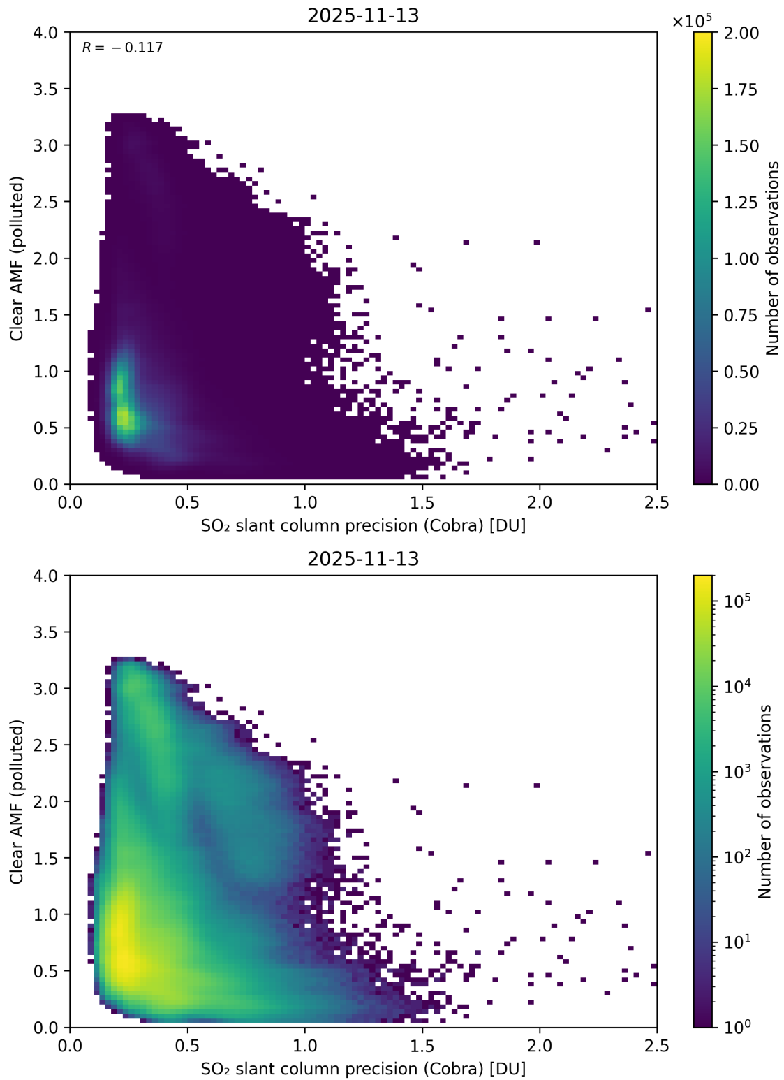
Figure 205: Scatter density plot of “SO 2 slant column precision (Cobra)” against “Clear AMF (polluted)” for 2025-11-12 to 2025-11-14.
