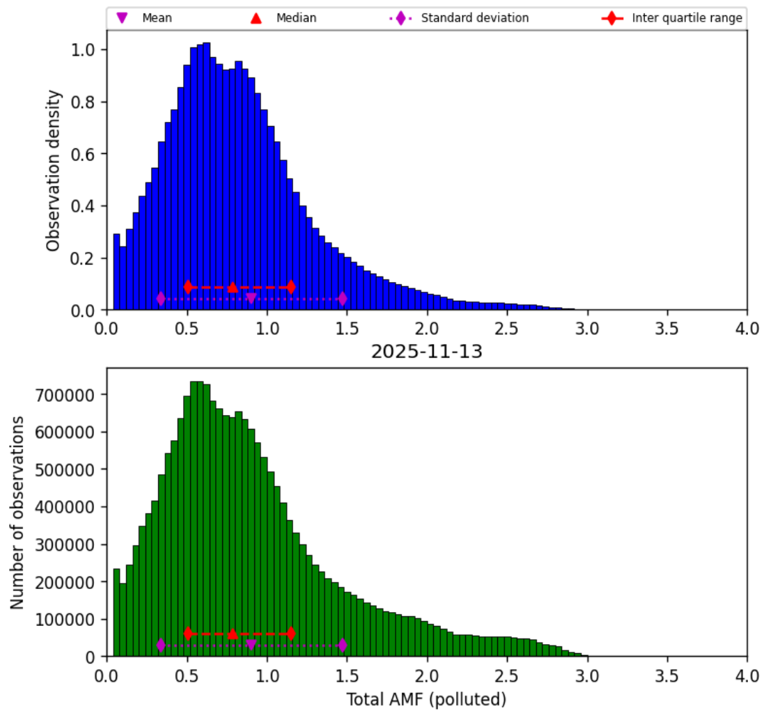
Figure 79: Histogram of “Total AMF (polluted)” for 2025-11-12 to 2025-11-14
