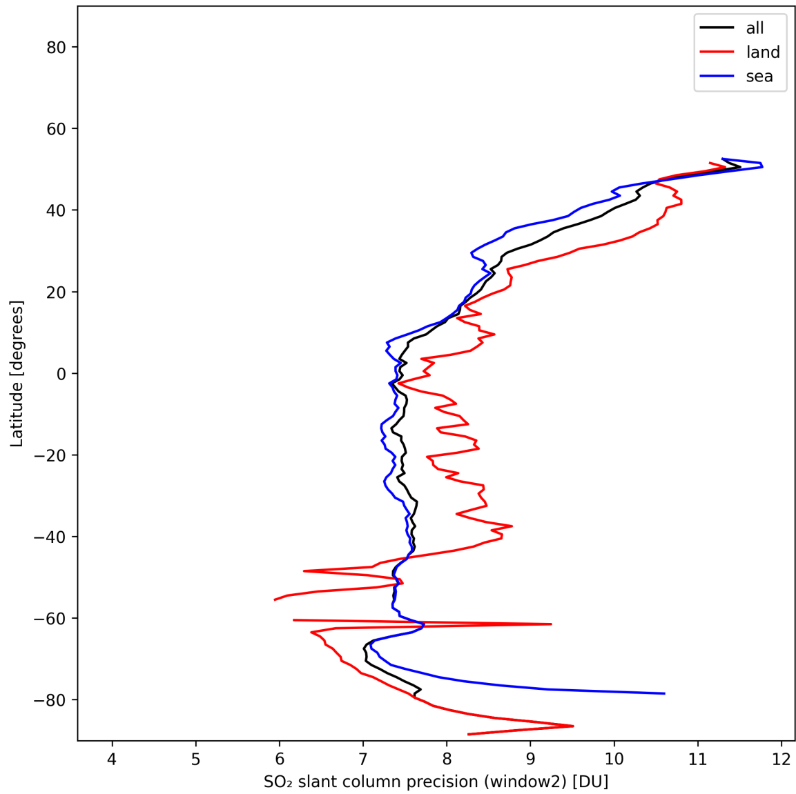
Figure 42: Zonal average of “SO 2 slant column precision (window2)” for 2025-11-12 to 2025-11-14.
