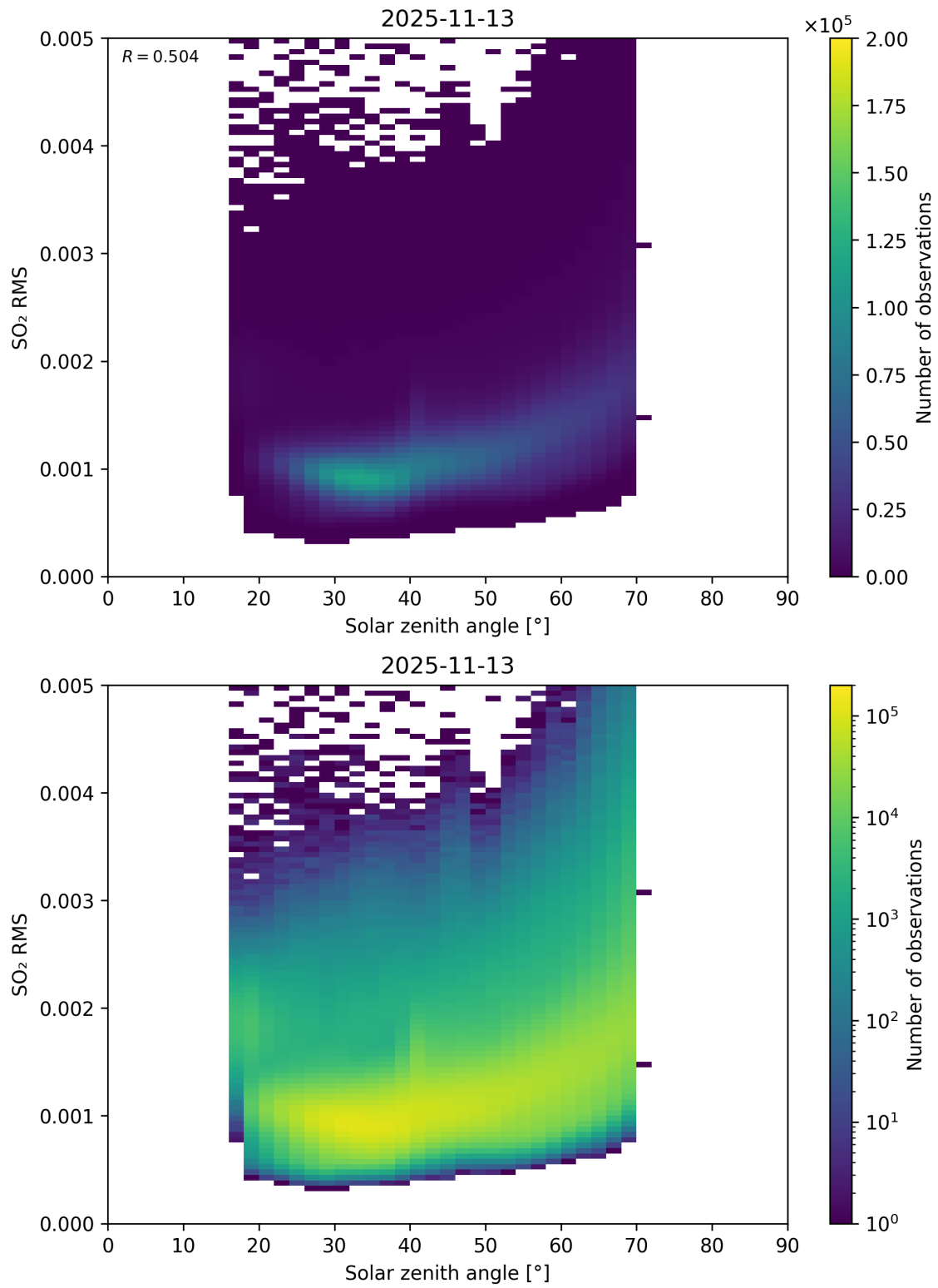
Figure 176: Scatter density plot of “Solar zenith angle” against “SO 2 RMS” for 2025-11-12 to 2025-11-14.
