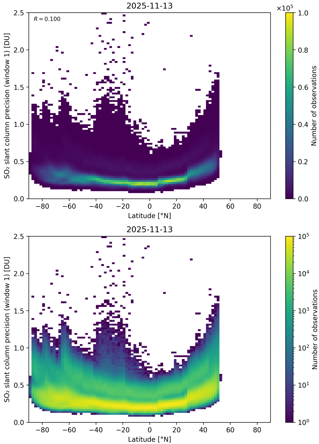
Figure 163: Scatter density plot of “Latitude” against “SO 2 slant column precision (window 1)” for 2025-11-12 to 2025-11-14.
