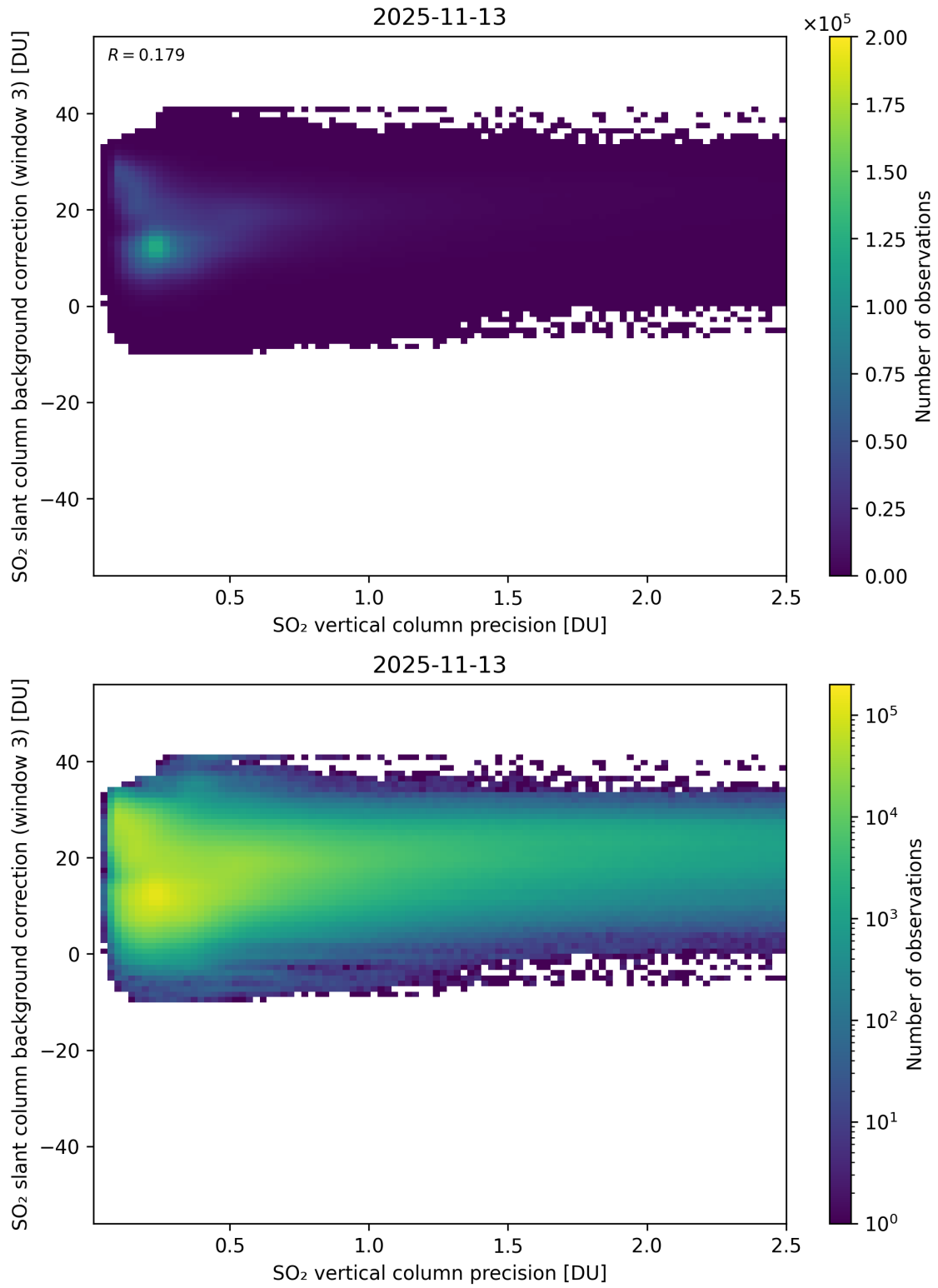
Figure 331: Scatter density plot of “SO 2 vertical column precision” against “SO 2 slant column background correction (window 3)” for 2025-11-12 to 2025-11-14.
