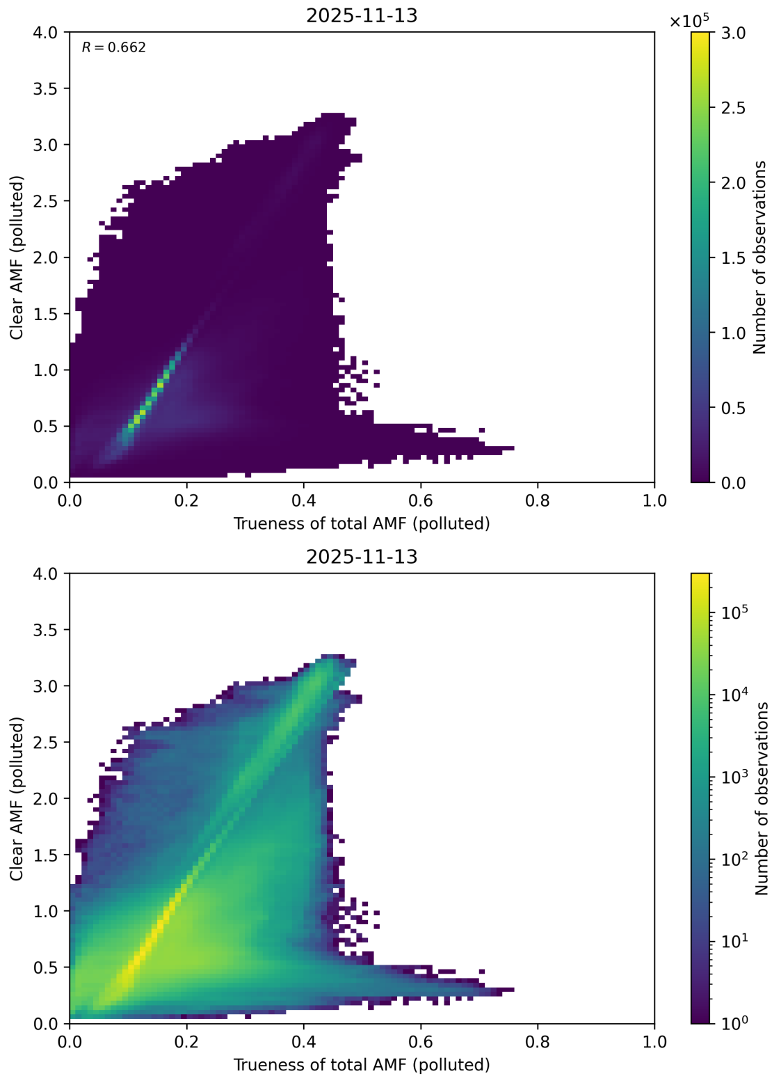
Figure 322: Scatter density plot of “Trueness of total AMF (polluted)” against “Clear AMF (polluted)” for 2025-11-12 to 2025-11-14.
