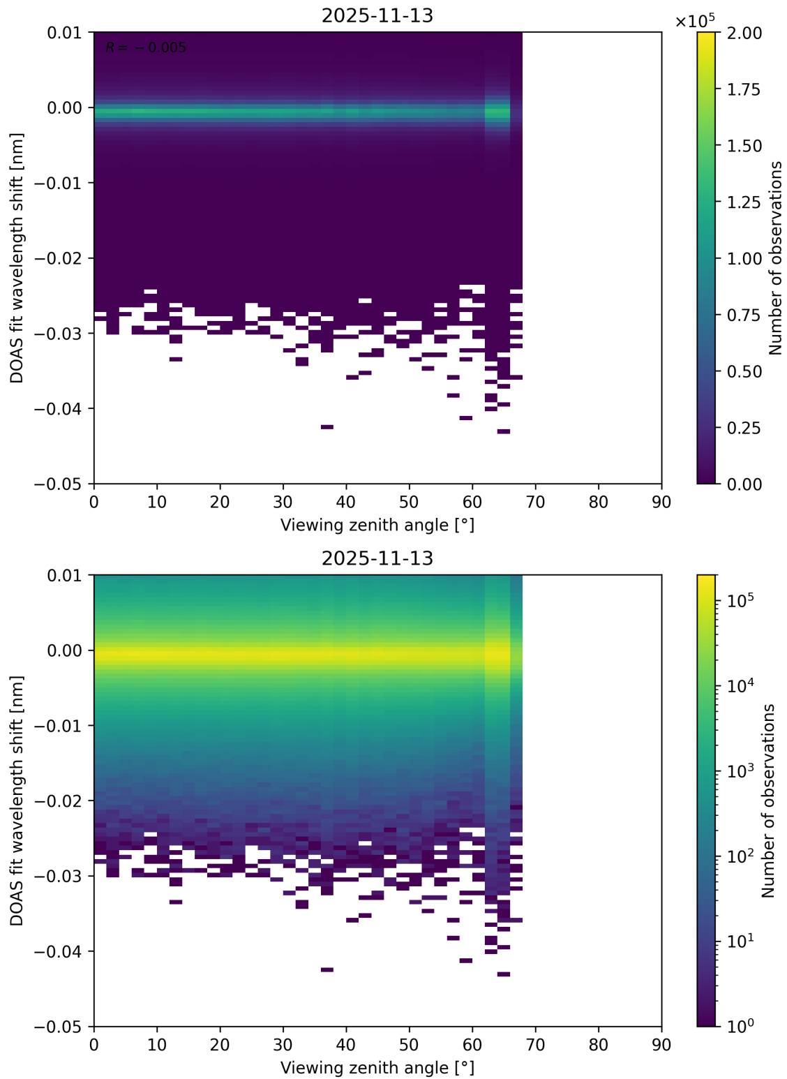
Figure 365: Scatter density plot of “Viewing zenith angle” against “DOAS fit wavelength shift” for 2025-11-12 to 2025-11-14.
