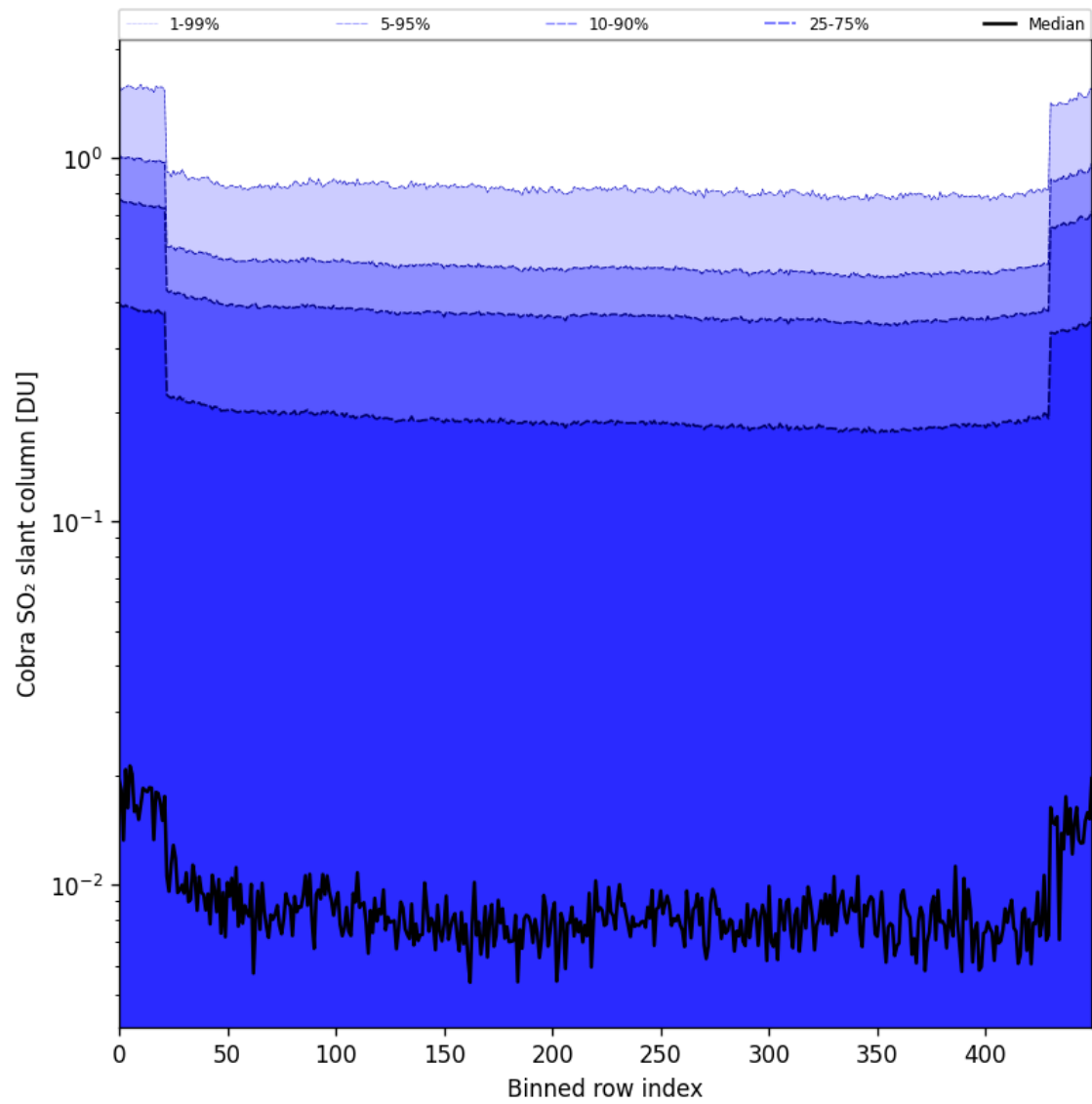
Figure 87: Along track statistics of “Cobra SO 2 slant column” for 2025-11-12 to 2025-11-14
