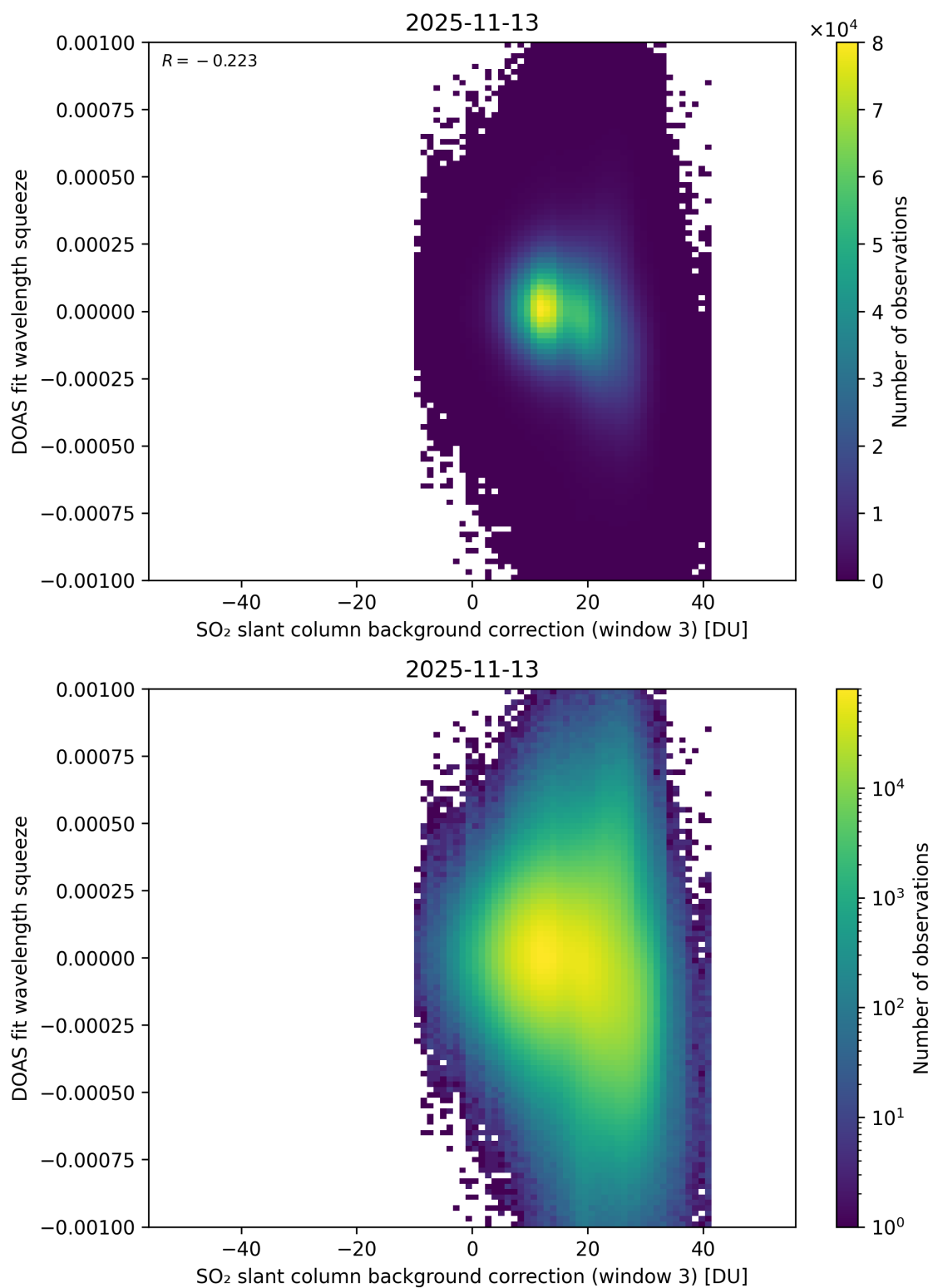
Figure 133: Scatter density plot of “SO 2 slant column background correction (window 3)” against “DOAS fit wavelength squeeze” for 2025-11-12 to 2025-11-14.
