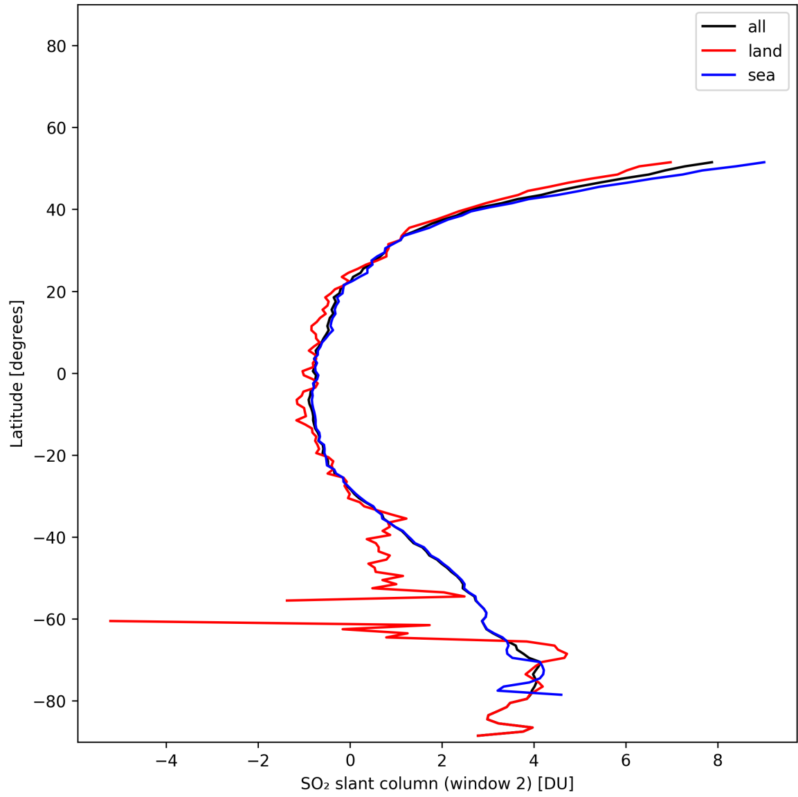
Figure 41: Zonal average of “SO 2 slant column (window 2)” for 2025-11-13 to 2025-11-15.
