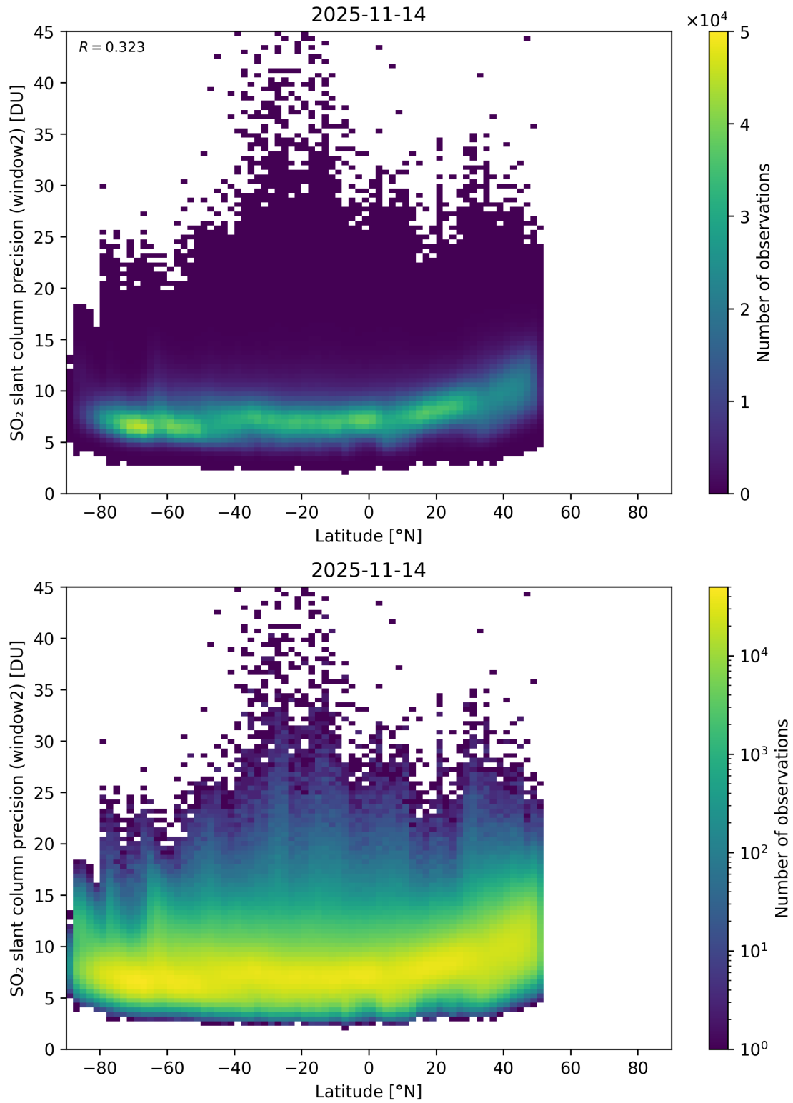
Figure 164: Scatter density plot of “Latitude” against “SO 2 slant column precision (window2)” for 2025-11-13 to 2025-11-15.
