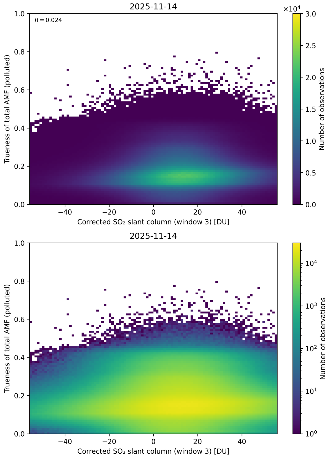
Figure 261: Scatter density plot of “Corrected SO 2 slant column (window 3)” against “Trueness of total AMF (polluted)” for 2025-11-13 to 2025-11-15.
