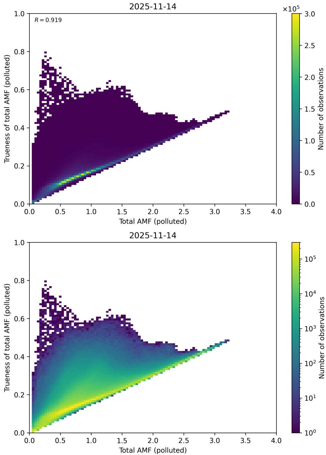
Figure 321: Scatter density plot of “Total AMF (polluted)” against “Trueness of total AMF (polluted)” for 2025-11-13 to 2025-11-15.
