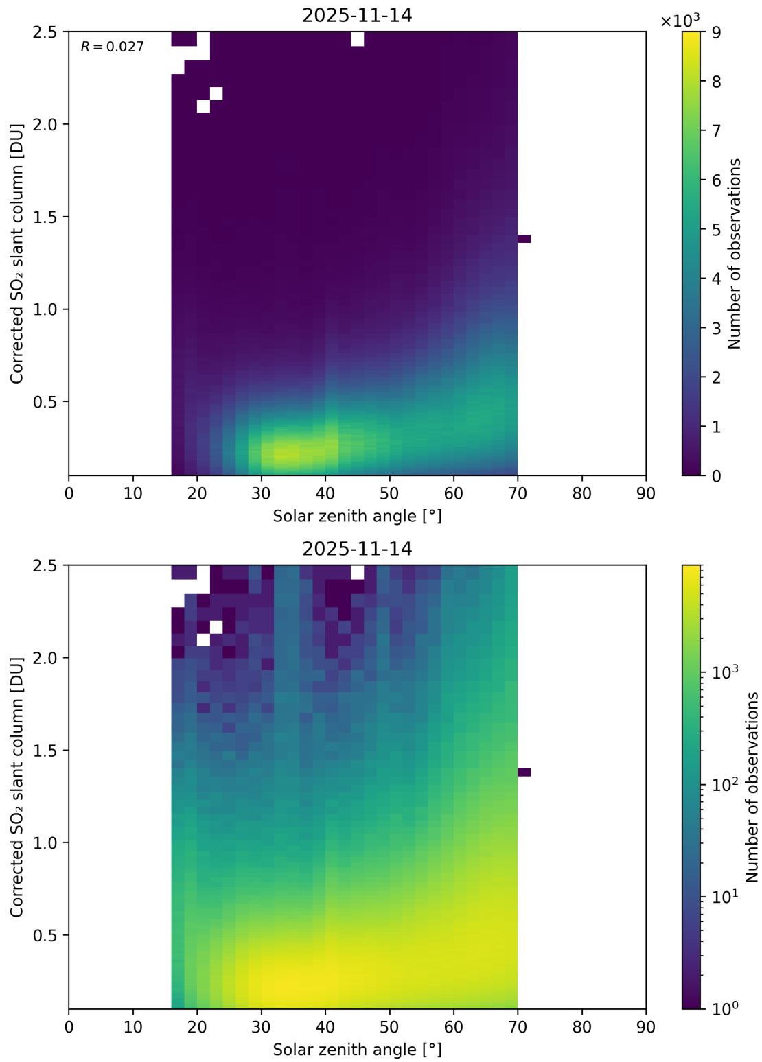
Figure 181: Scatter density plot of “Solar zenith angle” against “Corrected SO 2 slant column” for 2025-11-13 to 2025-11-15.
