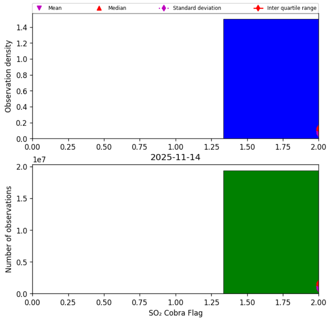
Figure 75: Histogram of “SO 2 Cobra Flag” for 2025-11-13 to 2025-11-15
