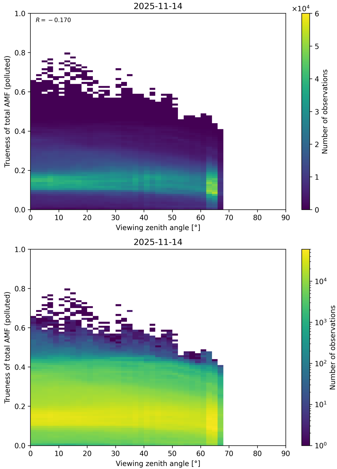
Figure 382: Scatter density plot of “Viewing zenith angle” against “Trueness of total AMF (polluted)” for 2025-11-13 to 2025-11-15.
