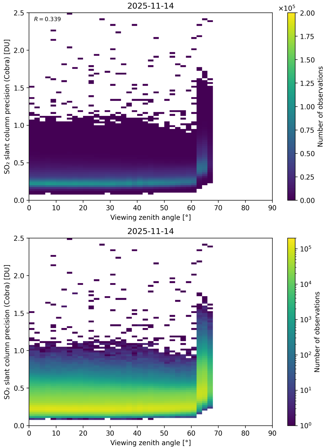
Figure 372: Scatter density plot of “Viewing zenith angle” against “SO 2 slant column precision (Cobra)” for 2025-11-13 to 2025-11-15.
