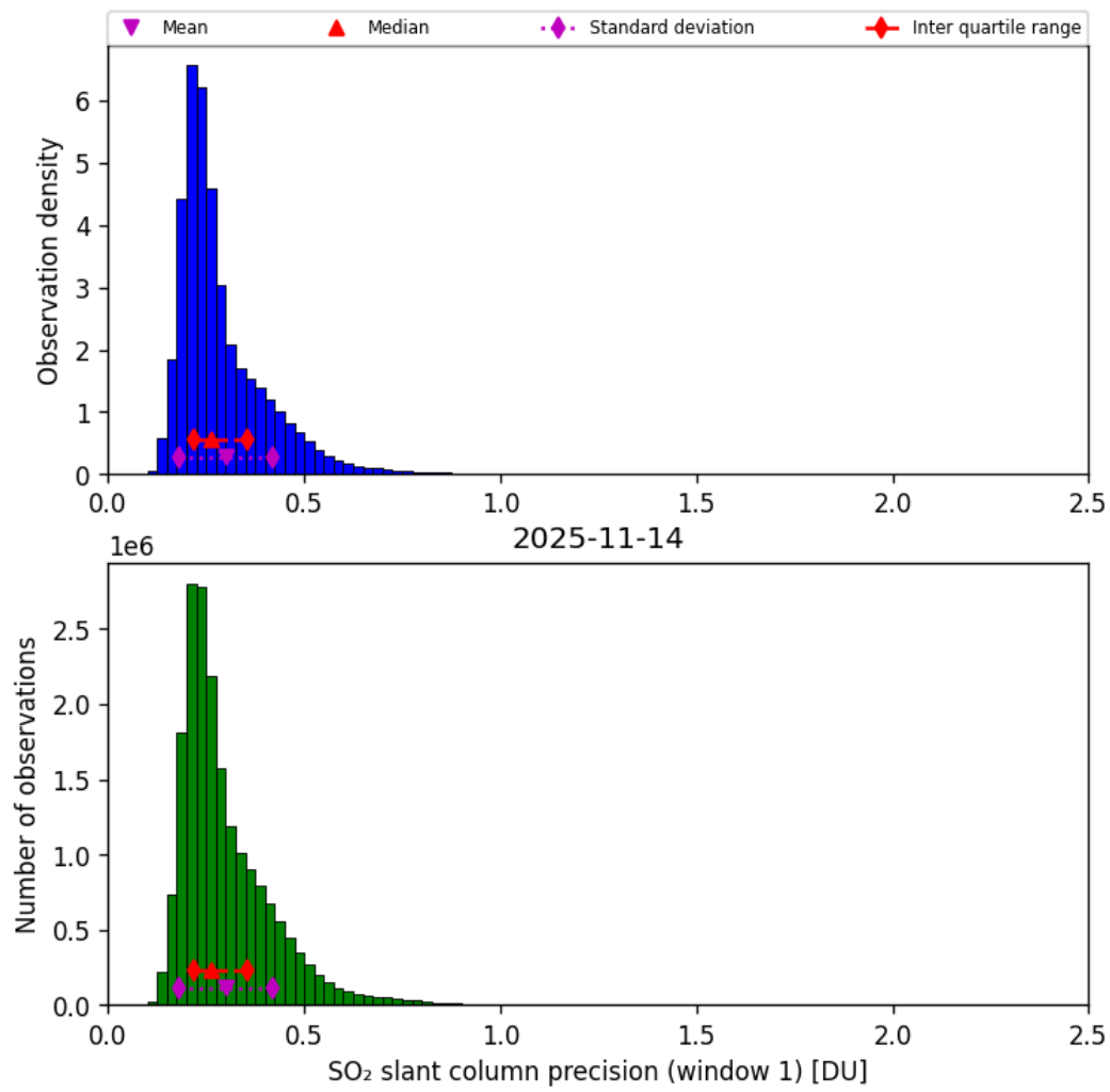
Figure 64: Histogram of “SO 2 slant column precision (window 1)” for 2025-11-13 to 2025-11-15
