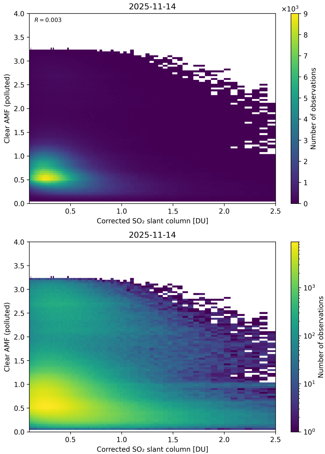
Figure 232: Scatter density plot of “Corrected SO 2 slant column” against “Clear AMF (polluted)” for 2025-11-13 to 2025-11-15.
