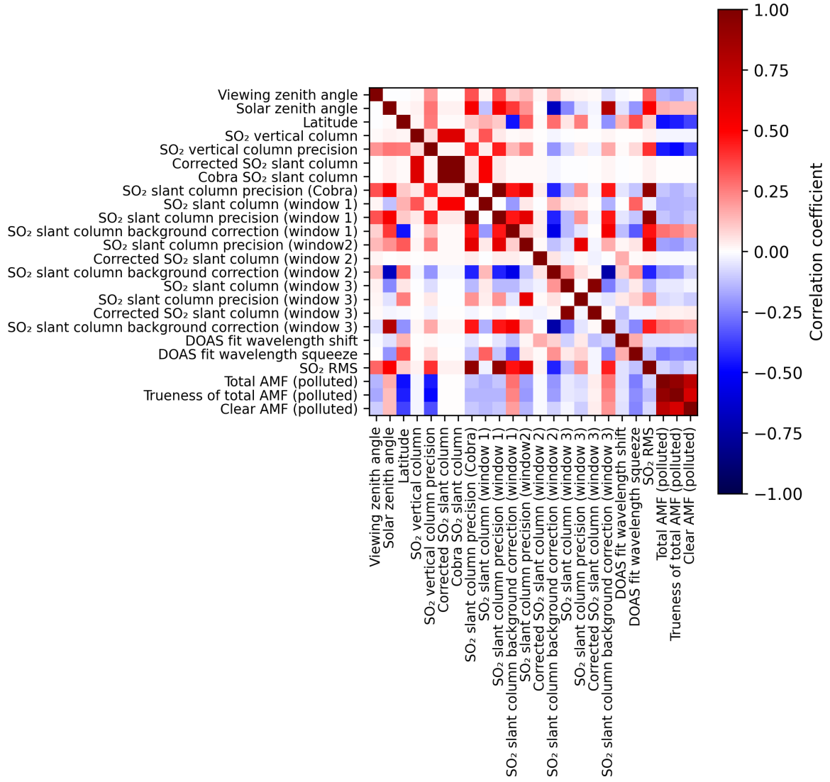
Figure 2: Map of correlation matrix for 2025-11-13 to 2025-11-15.
