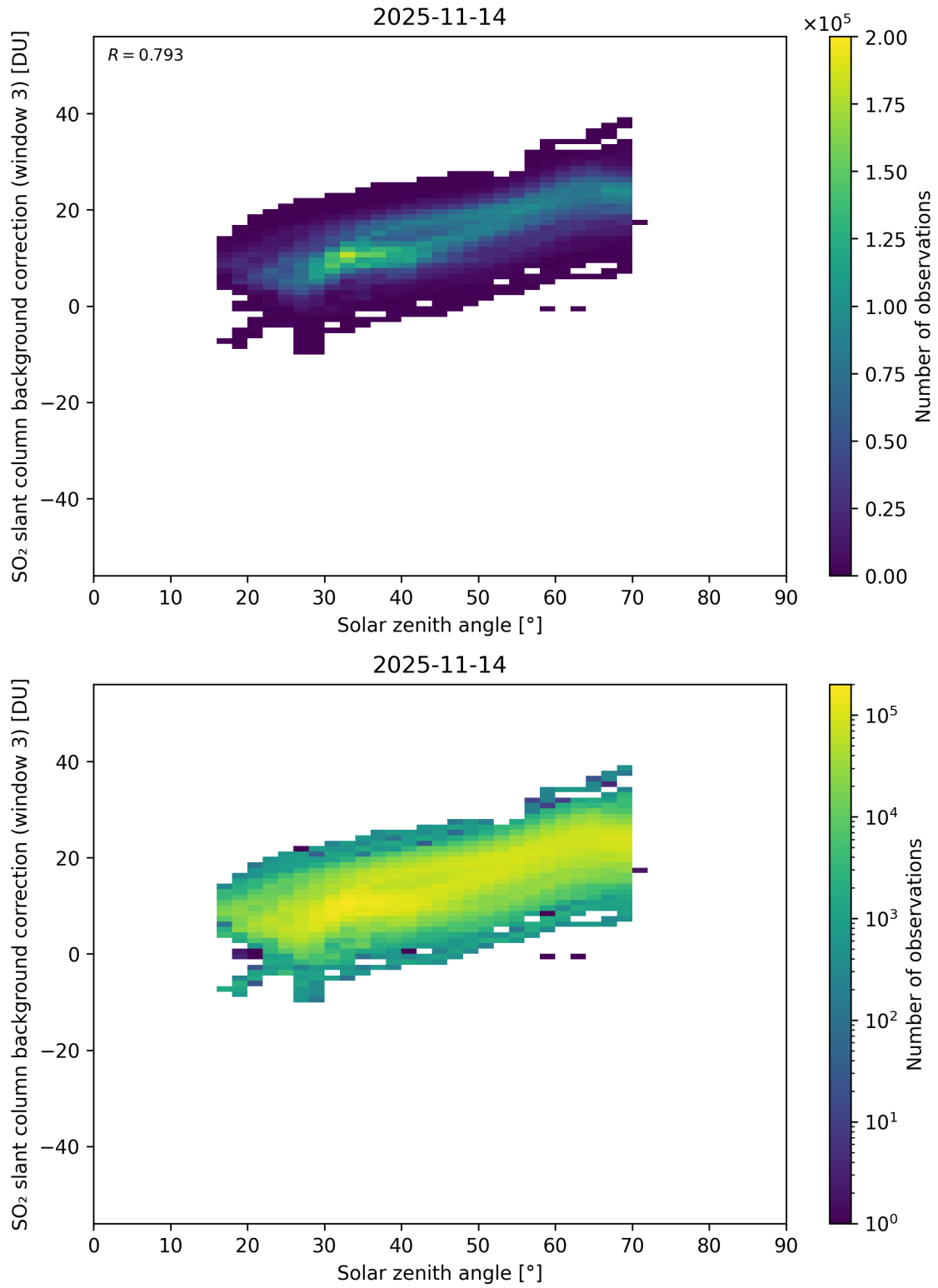
Figure 173: Scatter density plot of “Solar zenith angle” against “SO 2 slant column background correction (window 3)” for 2025-11-13 to 2025-11-15.
