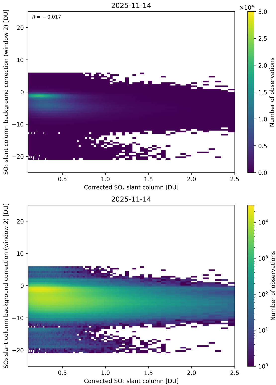
Figure 227: Scatter density plot of “Corrected SO 2 slant column” against “SO 2 slant column background correction (window 2)” for 2025-11-13 to 2025-11-15.
