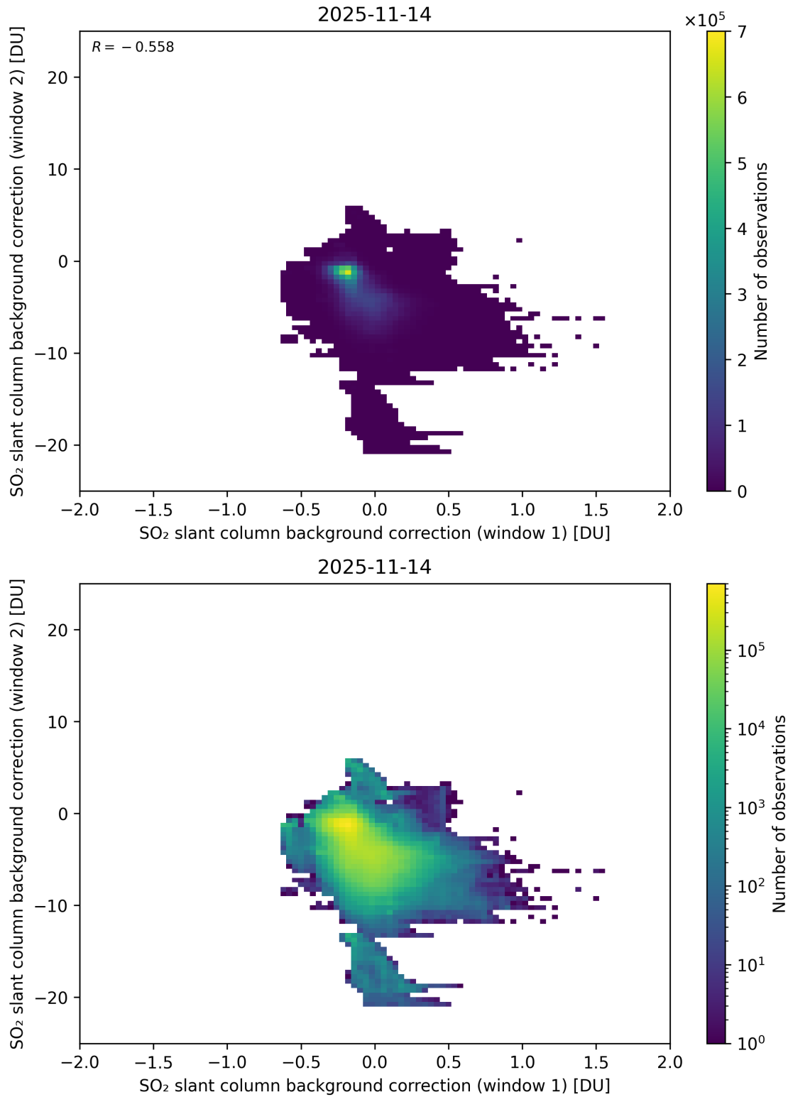
Figure 109: Scatter density plot of “SO 2 slant column background correction (window 1)” against “SO 2 slant column background correction (window 2)” for 2025-11-13 to 2025-11-15.
