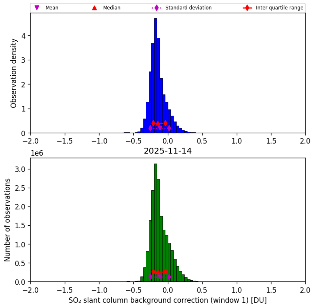
Figure 66: Histogram of “SO 2 slant column background correction (window 1)” for 2025-11-13 to 2025-11-15
