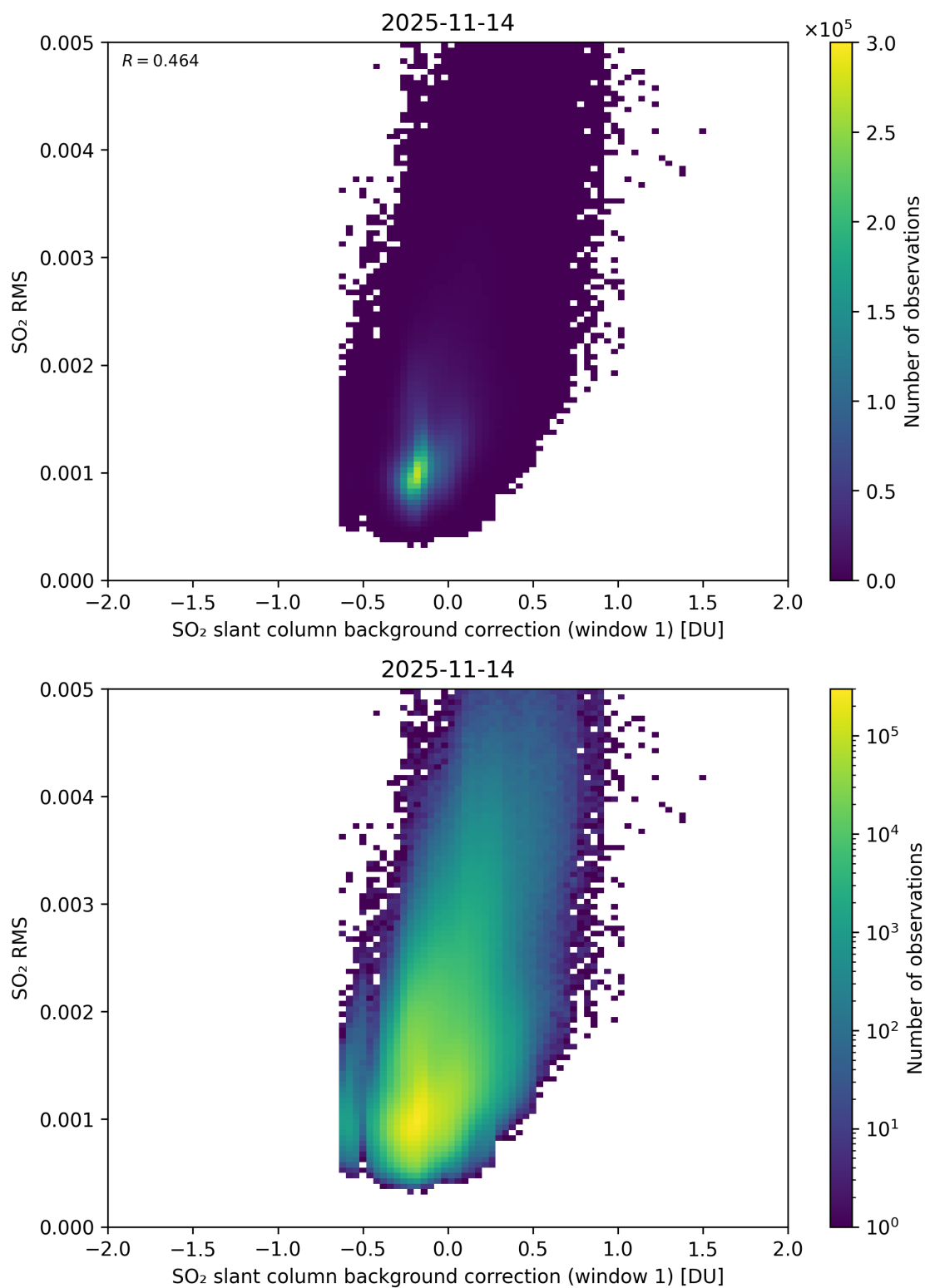
Figure 113: Scatter density plot of “SO 2 slant column background correction (window 1)” against “SO 2 RMS” for 2025-11-13 to 2025-11-15.
