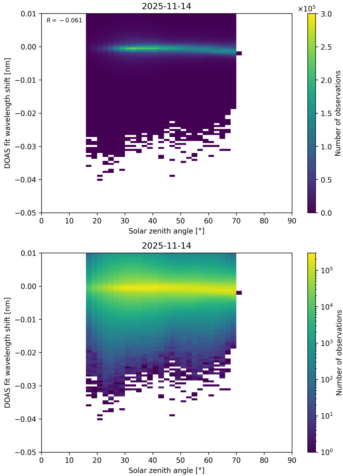
Figure 174: Scatter density plot of “Solar zenith angle” against “DOAS fit wavelength shift” for 2025-11-13 to 2025-11-15.
