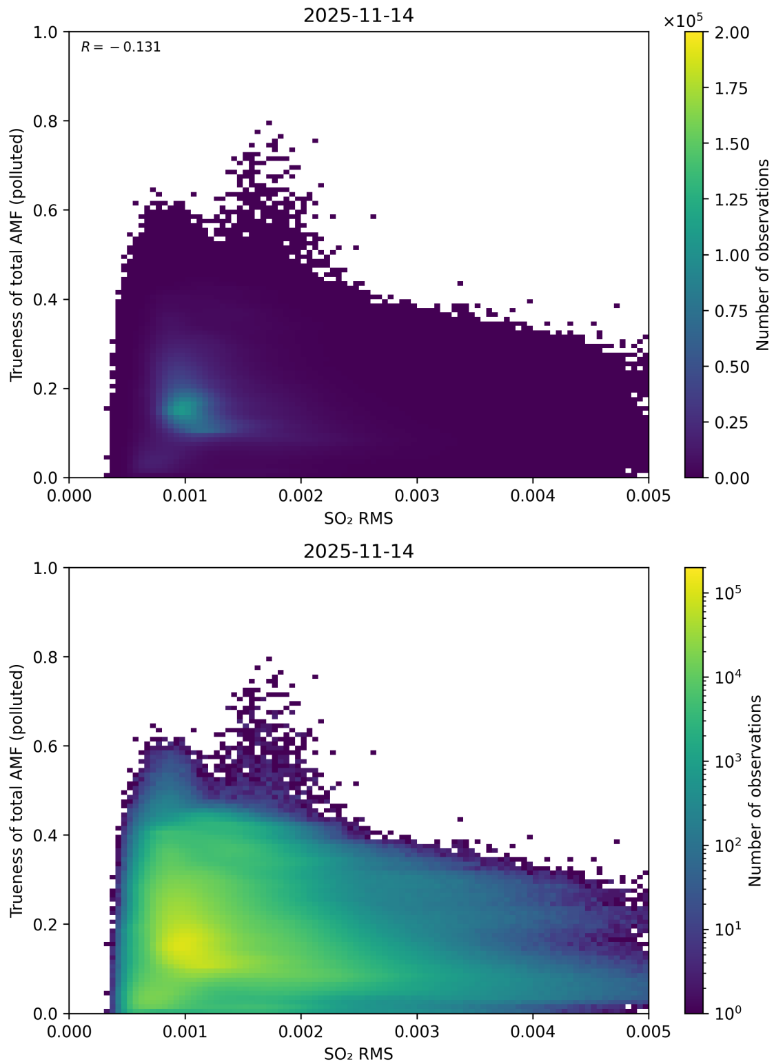
Figure 149: Scatter density plot of “SO 2 RMS” against “Trueness of total AMF (polluted)” for 2025-11-13 to 2025-11-15.
