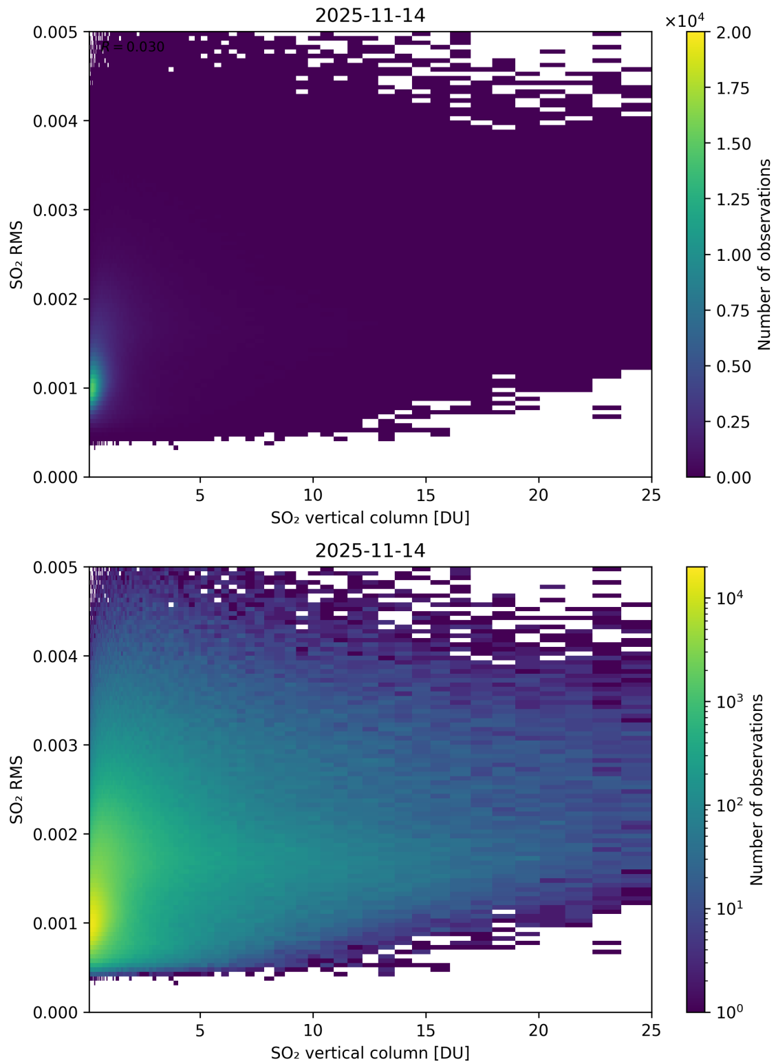
Figure 328: Scatter density plot of “SO 2 vertical column” against “SO 2 RMS” for 2025-11-13 to 2025-11-15.
