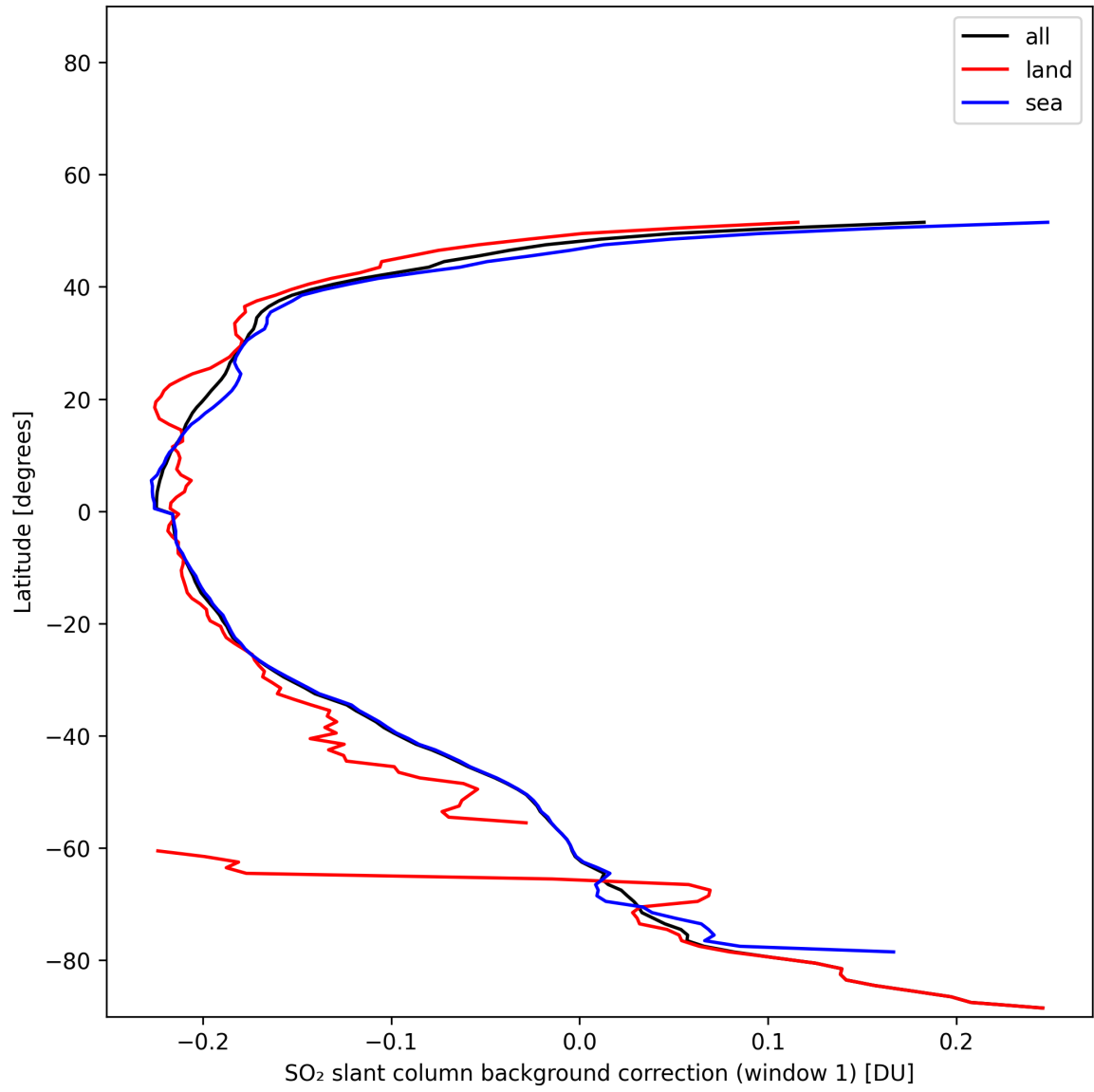
Figure 40: Zonal average of “SO 2 slant column background correction (window 1)” for 2025-11-13 to 2025-11-15.
