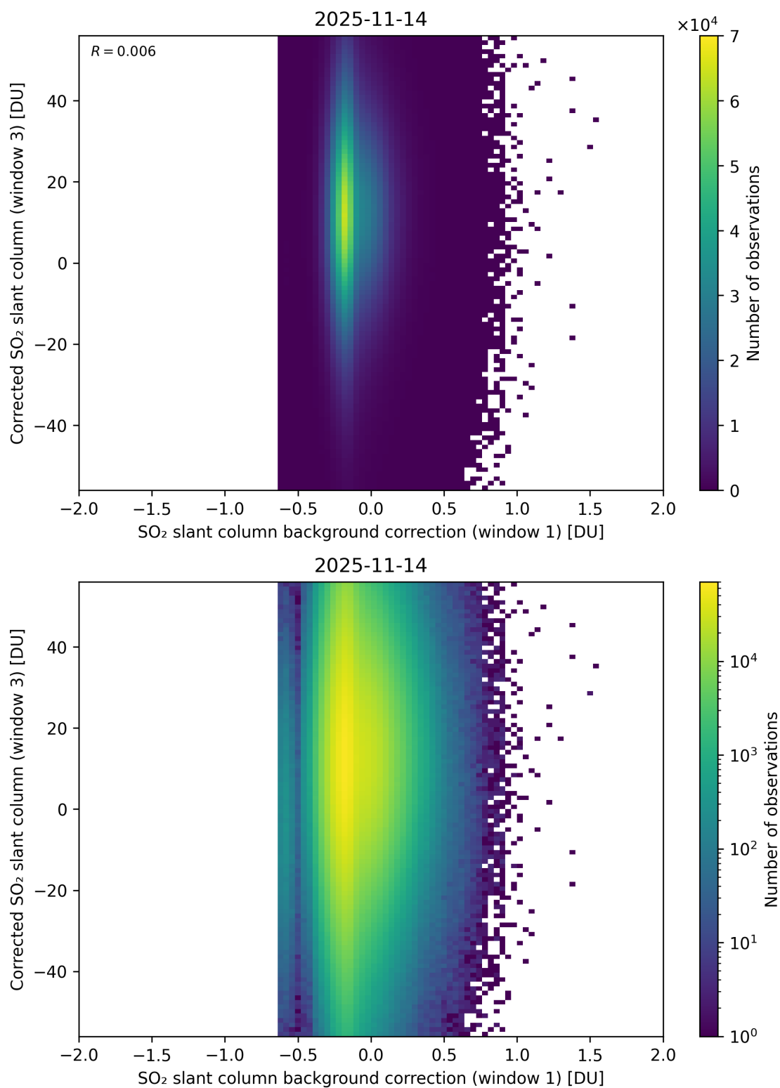
Figure 116: Scatter density plot of “SO 2 slant column background correction (window 1)” against “Corrected SO 2 slant column (window 3)” for 2025-11-13 to 2025-11-15.
