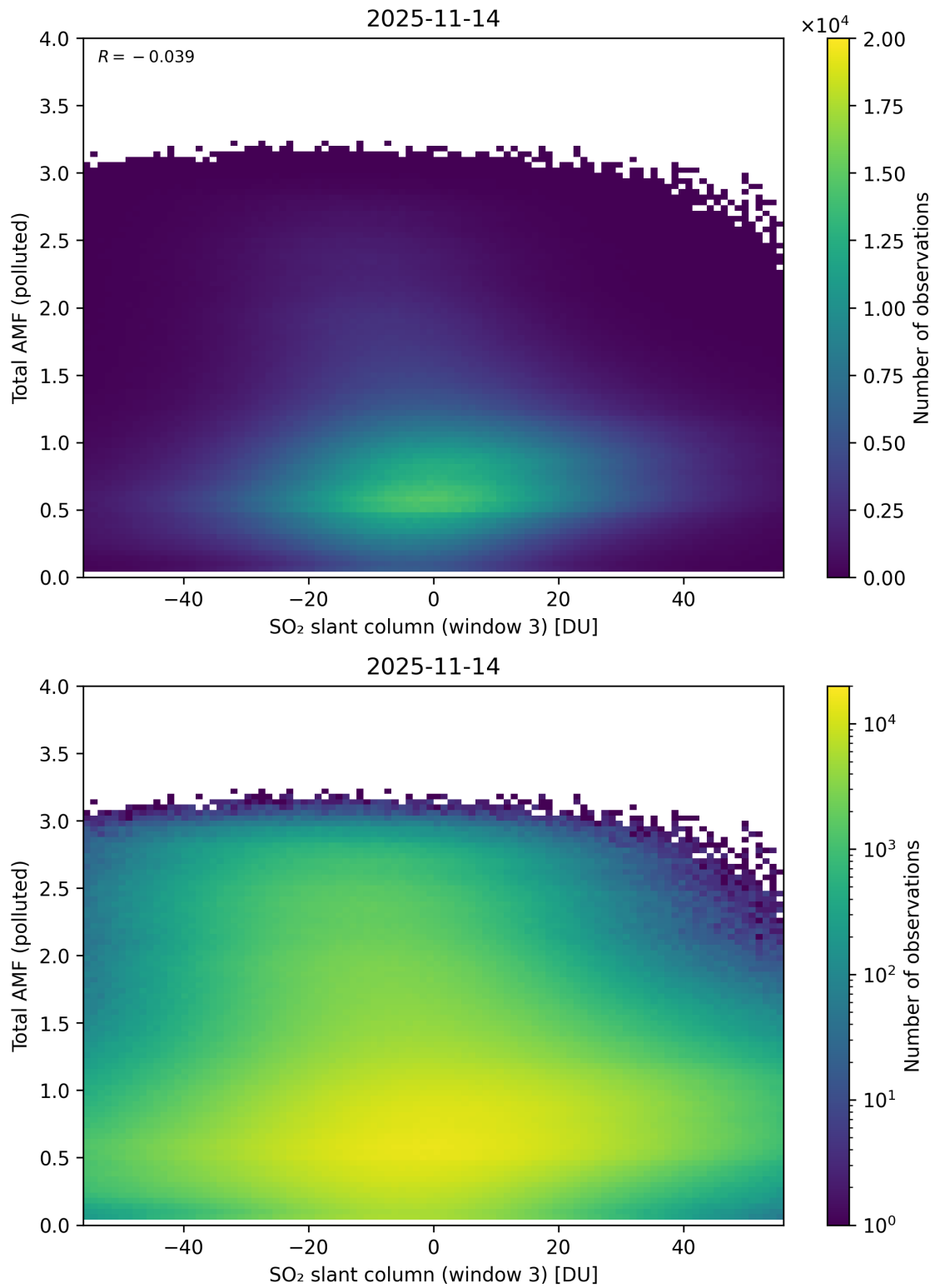
Figure 318: Scatter density plot of “SO 2 slant column (window 3)” against “Total AMF (polluted)” for 2025-11-13 to 2025-11-15.
