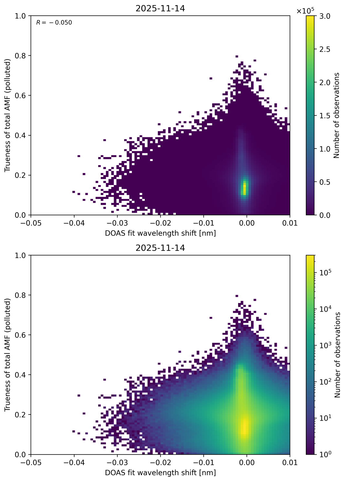
Figure 142: Scatter density plot of “DOAS fit wavelength shift” against “Trueness of total AMF (polluted)” for 2025-11-13 to 2025-11-15.
