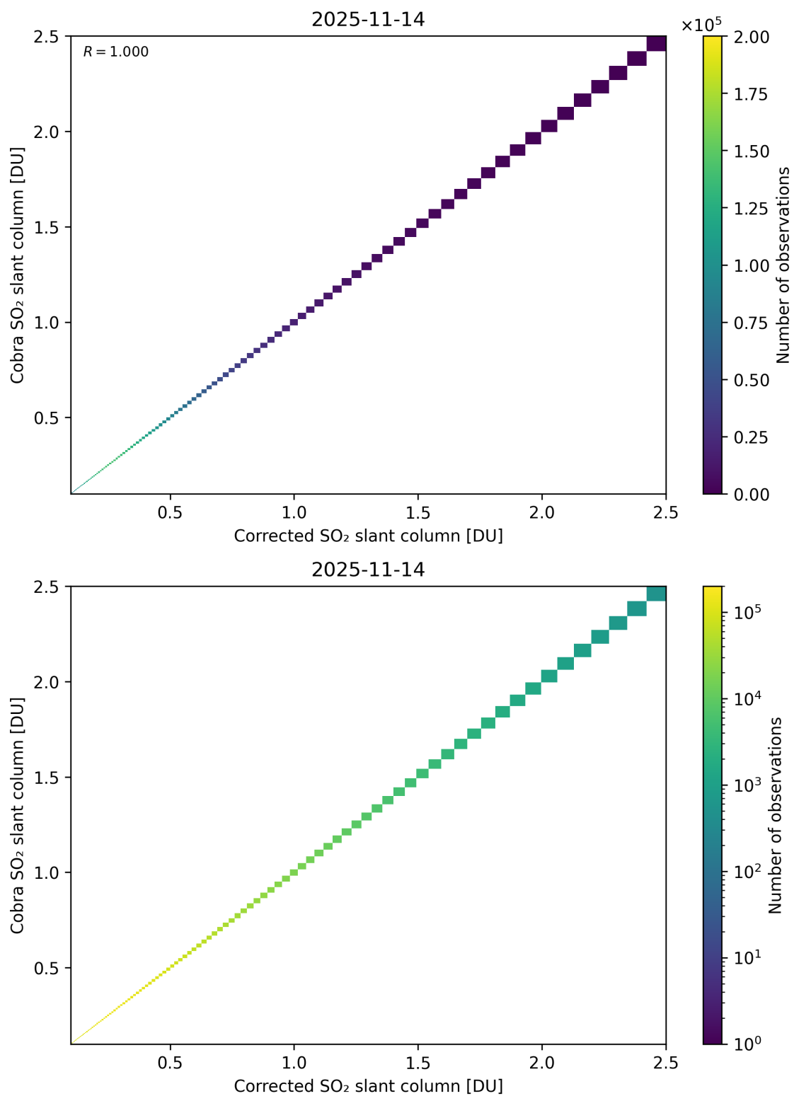
Figure 233: Scatter density plot of “Corrected SO 2 slant column” against “Cobra SO 2 slant column” for 2025-11-13 to 2025-11-15.
