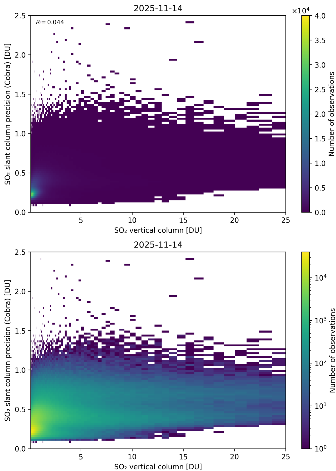
Figure 350: Scatter density plot of “SO 2 vertical column” against “SO 2 slant column precision (Cobra)” for 2025-11-13 to 2025-11-15.
