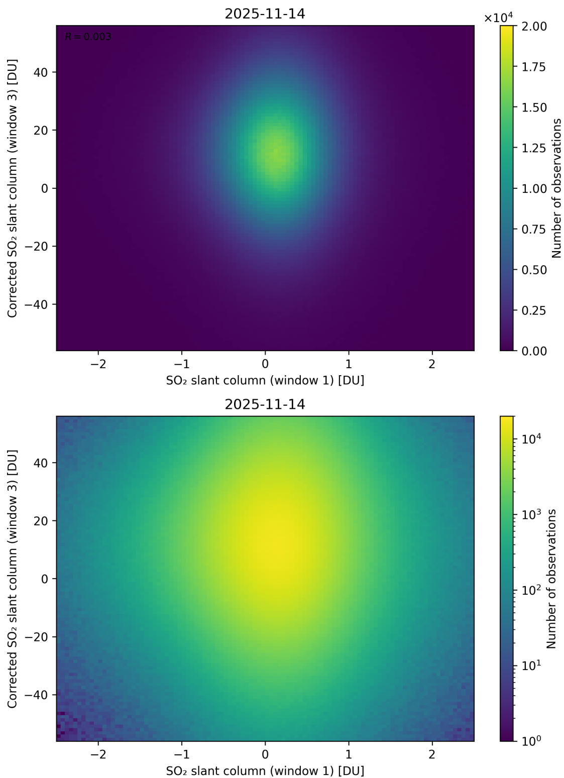
Figure 284: Scatter density plot of “SO 2 slant column (window 1)” against “Corrected SO 2 slant column (window 3)” for 2025-11-13 to 2025-11-15.
