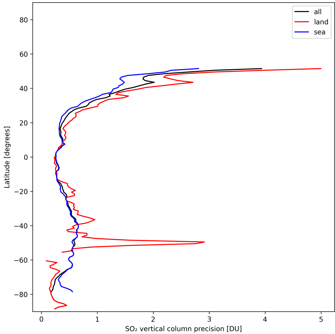
Figure 33: Zonal average of “SO 2 vertical column precision” for 2025-11-13 to 2025-11-15.
