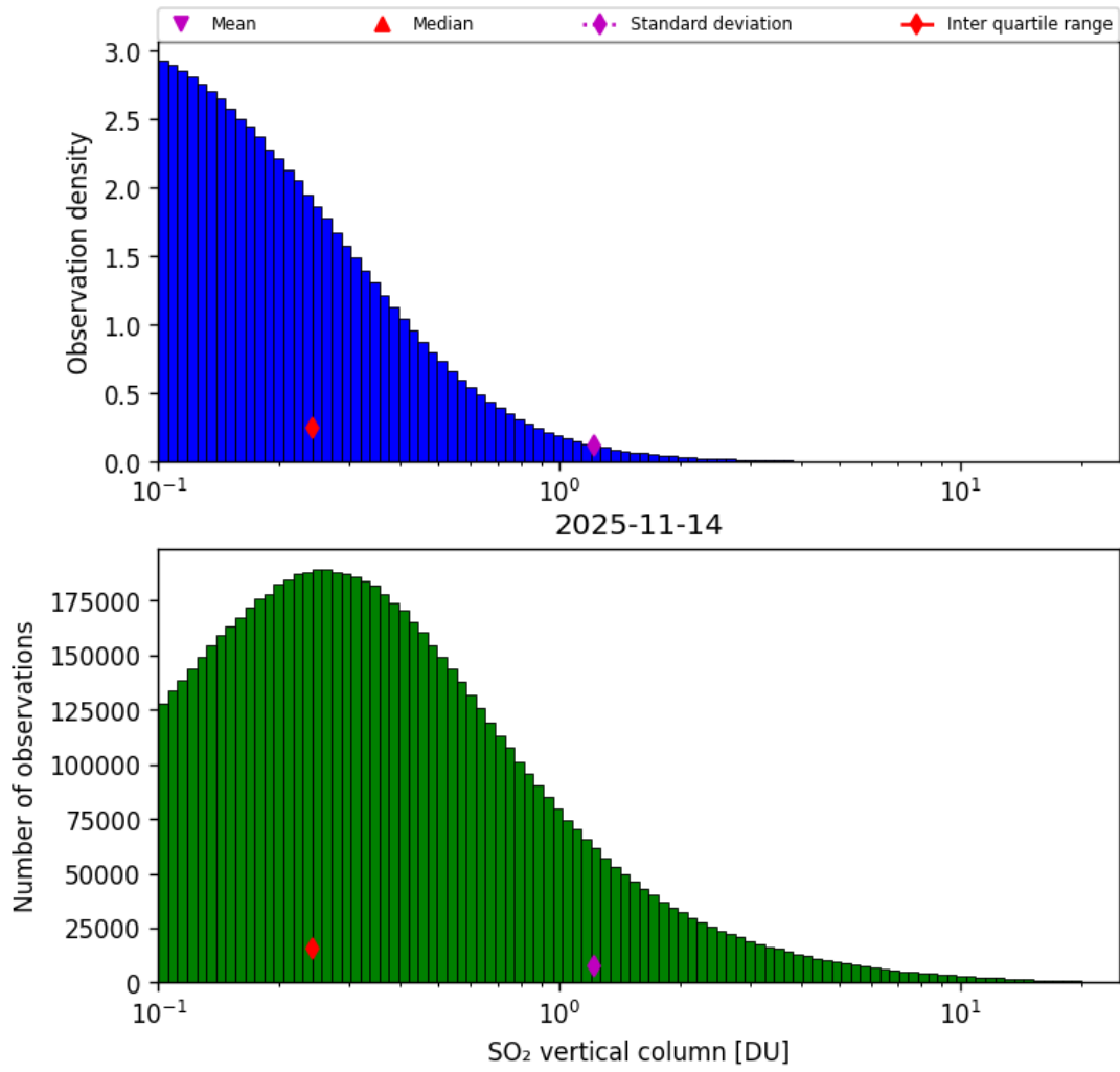
Figure 58: Histogram of “SO 2 vertical column” for 2025-11-13 to 2025-11-15
