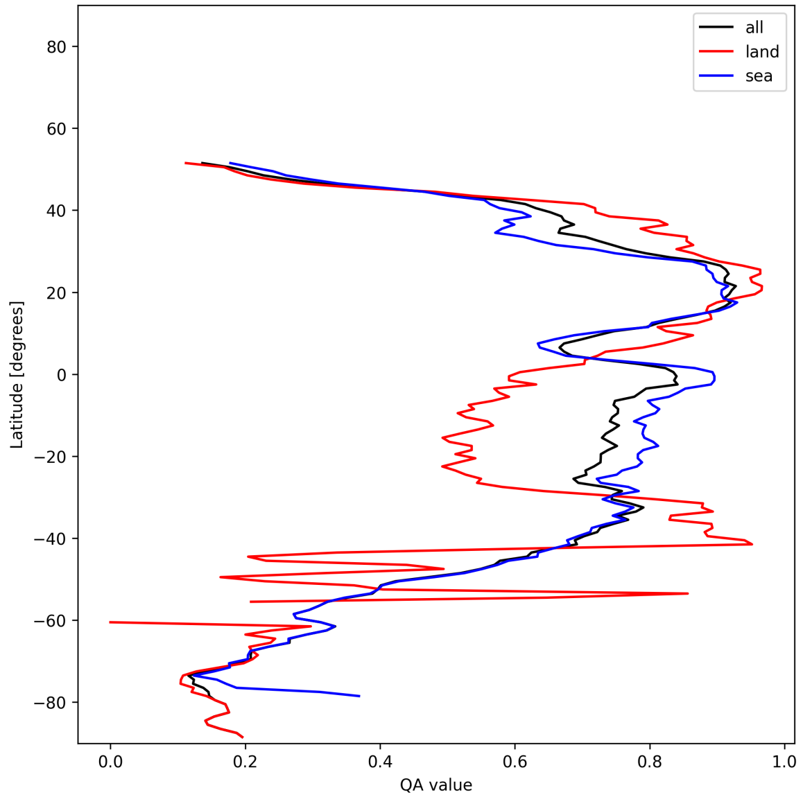
Figure 31: Zonal average of “QA value” for 2025-11-13 to 2025-11-15.
