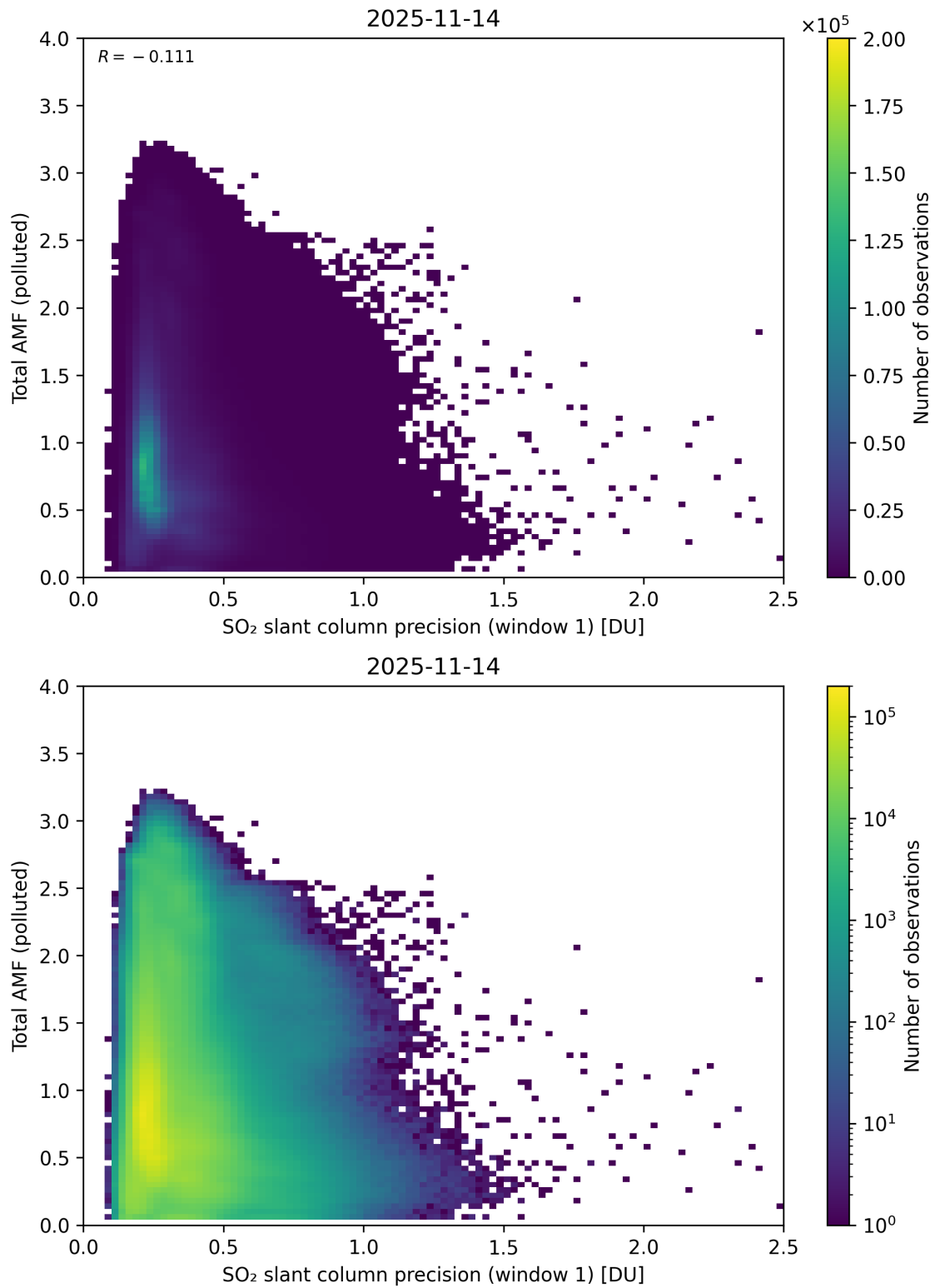
Figure 280: Scatter density plot of “SO 2 slant column precision (window 1)” against “Total AMF (polluted)” for 2025-11-13 to 2025-11-15.
