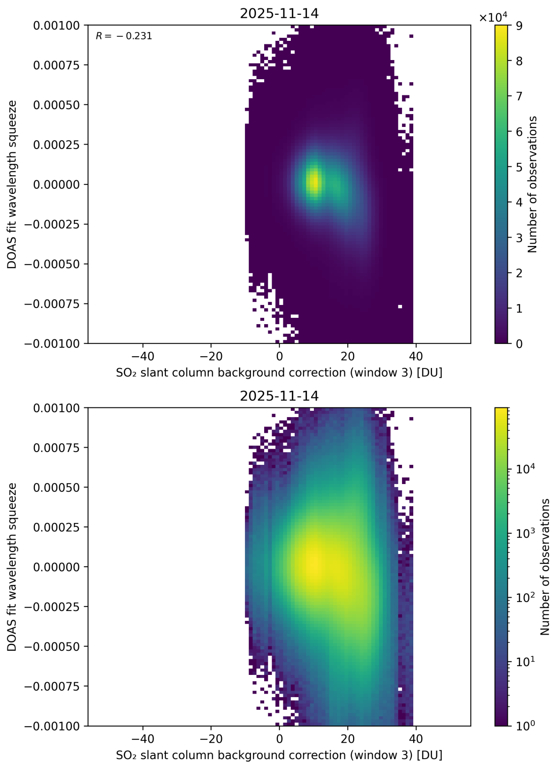
Figure 133: Scatter density plot of “SO 2 slant column background correction (window 3)” against “DOAS fit wavelength squeeze” for 2025-11-13 to 2025-11-15.
