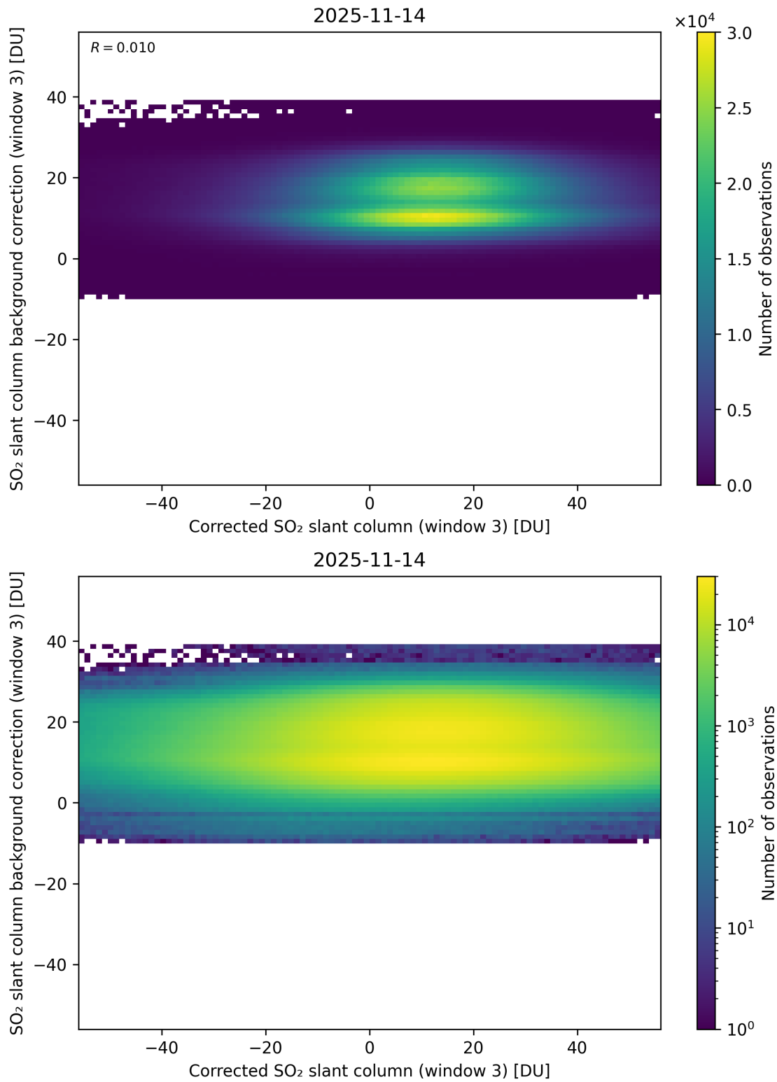
Figure 255: Scatter density plot of “Corrected SO 2 slant column (window 3)” against “SO 2 slant column background correction (window 3)” for 2025-11-13 to 2025-11-15.
