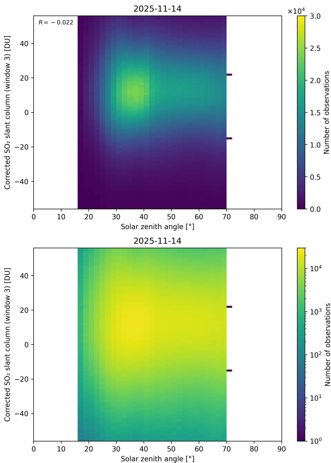
Figure 183: Scatter density plot of “Solar zenith angle” against “Corrected SO 2 slant column (window 3)” for 2025-11-13 to 2025-11-15.
