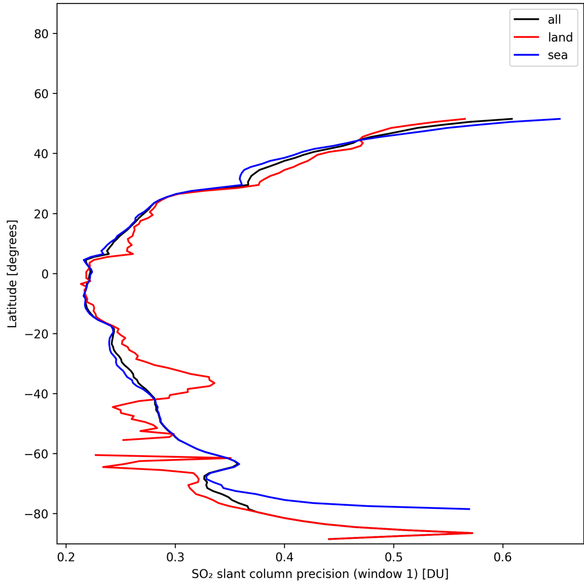
Figure 38: Zonal average of “SO 2 slant column precision (window 1)” for 2025-11-13 to 2025-11-15.
