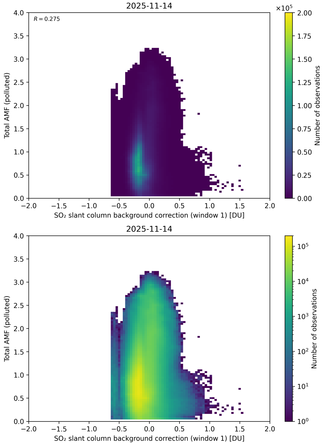
Figure 120: Scatter density plot of “SO 2 slant column background correction (window 1)” against “Total AMF (polluted)” for 2025-11-13 to 2025-11-15.
