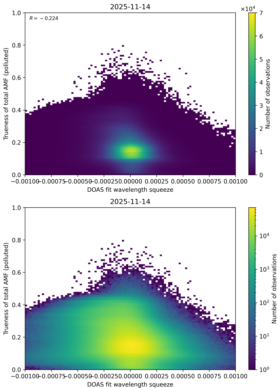
Figure 146: Scatter density plot of “DOAS fit wavelength squeeze” against “Trueness of total AMF (polluted)” for 2025-11-13 to 2025-11-15.
