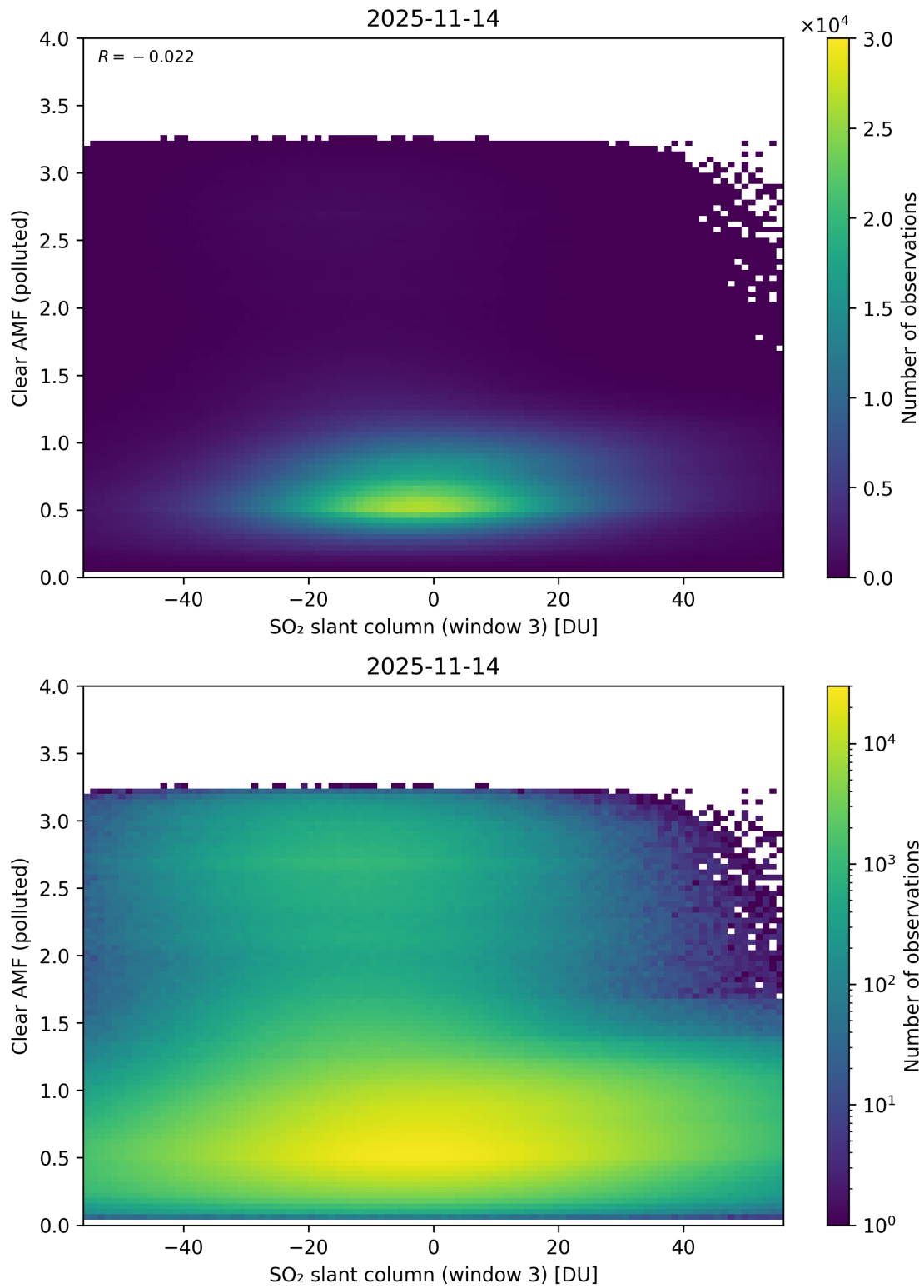
Figure 315: Scatter density plot of “SO 2 slant column (window 3)” against “Clear AMF (polluted)” for 2025-11-13 to 2025-11-15.
