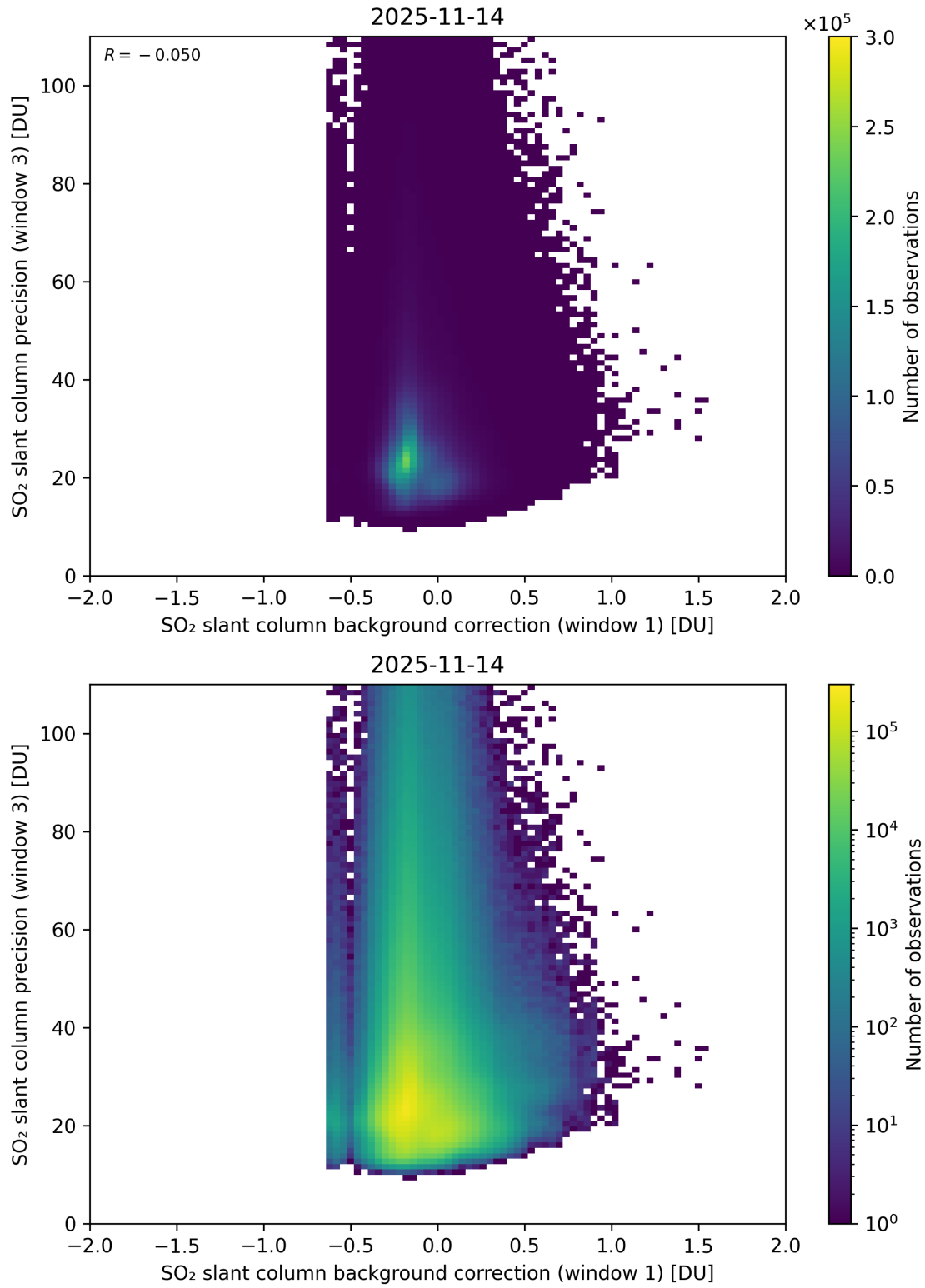
Figure 119: Scatter density plot of “SO 2 slant column background correction (window 1)” against “SO 2 slant column precision (window 3)” for 2025-11-13 to 2025-11-15.
