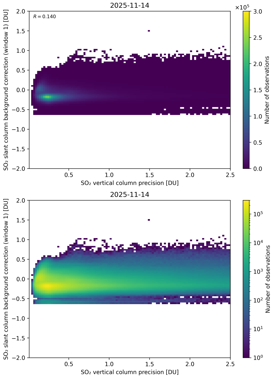
Figure 329: Scatter density plot of “SO 2 vertical column precision” against “SO 2 slant column background correction (window 1)” for 2025-11-13 to 2025-11-15.
