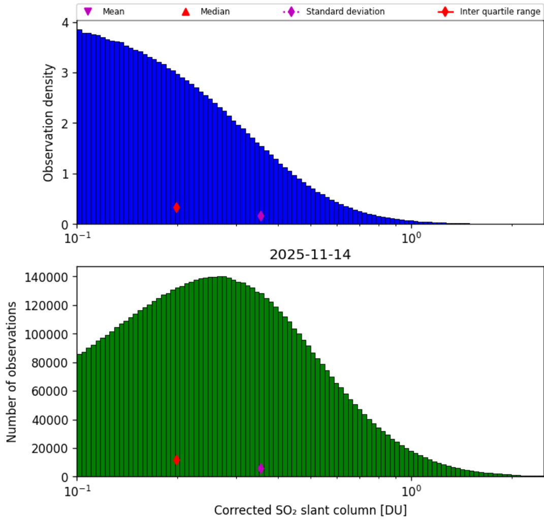
Figure 60: Histogram of “Corrected SO 2 slant column” for 2025-11-13 to 2025-11-15
