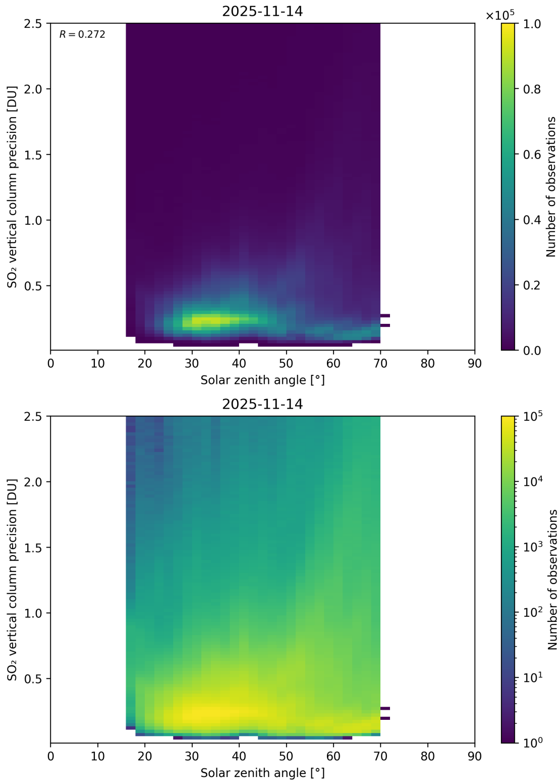
Figure 192: Scatter density plot of “Solar zenith angle” against “SO 2 vertical column precision” for 2025-11-13 to 2025-11-15.
