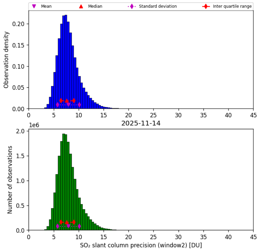
Figure 68: Histogram of “SO 2 slant column precision (window2)” for 2025-11-13 to 2025-11-15
