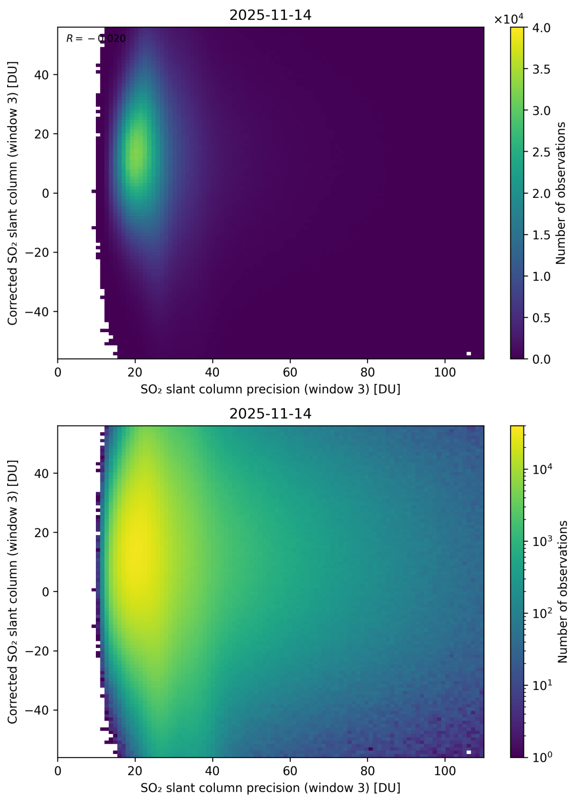
Figure 312: Scatter density plot of “SO 2 slant column precision (window 3)” against “Corrected SO 2 slant column (window 3)” for 2025-11-13 to 2025-11-15.
