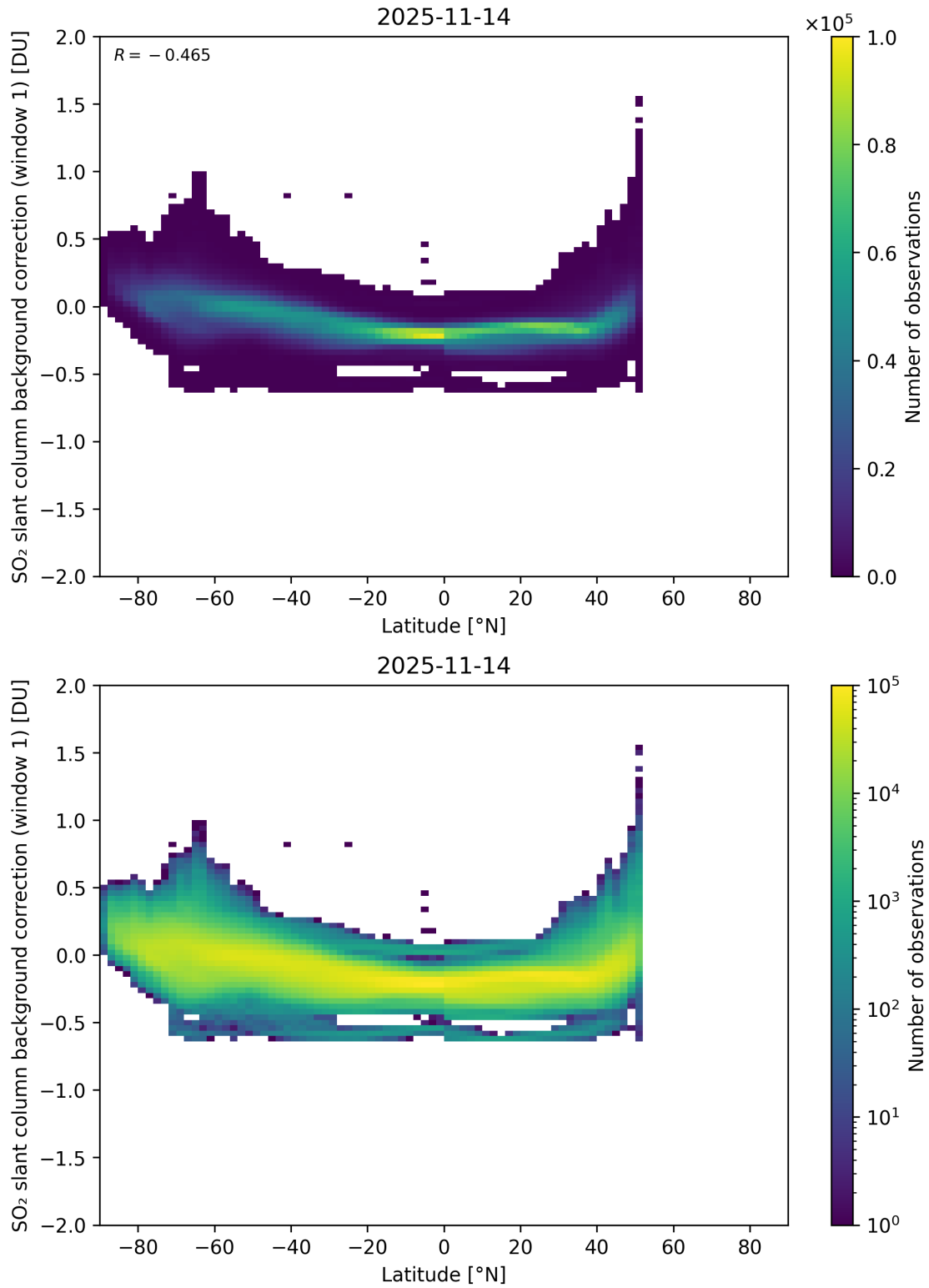
Figure 150: Scatter density plot of “Latitude” against “SO 2 slant column background correction (window 1)” for 2025-11-13 to 2025-11-15.
