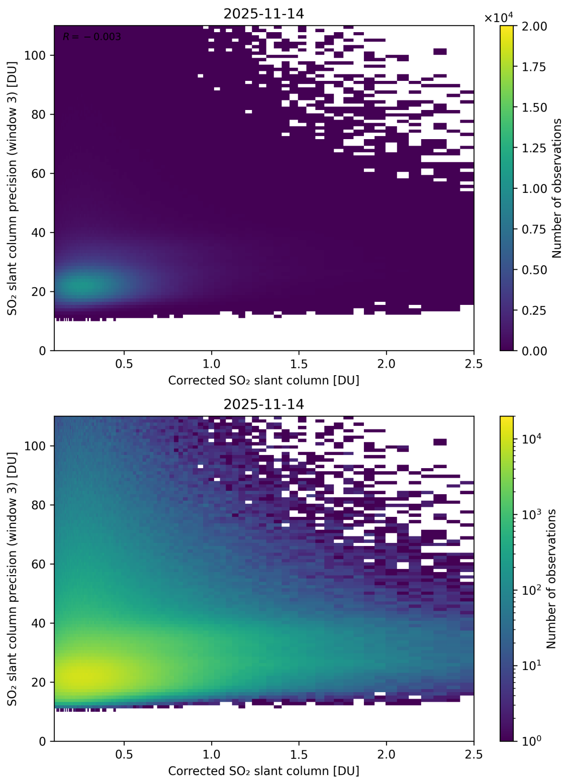
Figure 241: Scatter density plot of “Corrected SO 2 slant column” against “SO 2 slant column precision (window 3)” for 2025-11-13 to 2025-11-15.
