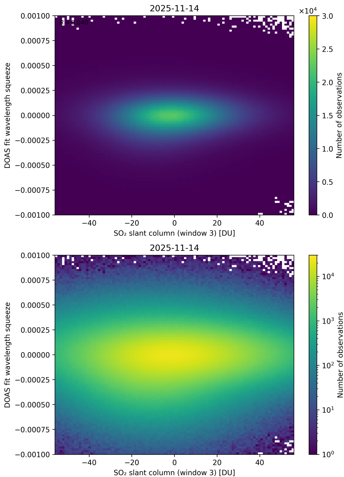
Figure 305: Scatter density plot of “SO 2 slant column (window 3)” against “DOAS fit wavelength squeeze” for 2025-11-13 to 2025-11-15.
