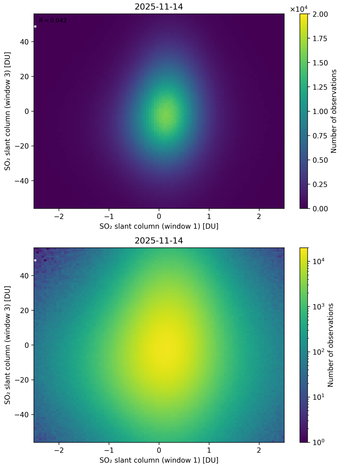
Figure 287: Scatter density plot of “SO 2 slant column (window 1)” against “SO 2 slant column (window 3)” for 2025-11-13 to 2025-11-15.
