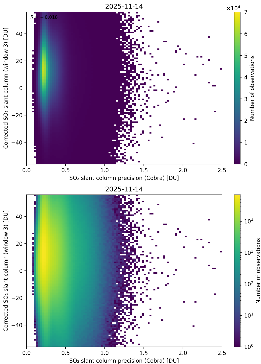
Figure 207: Scatter density plot of “SO 2 slant column precision (Cobra)” against “Corrected SO 2 slant column (window 3)” for 2025-11-13 to 2025-11-15.
