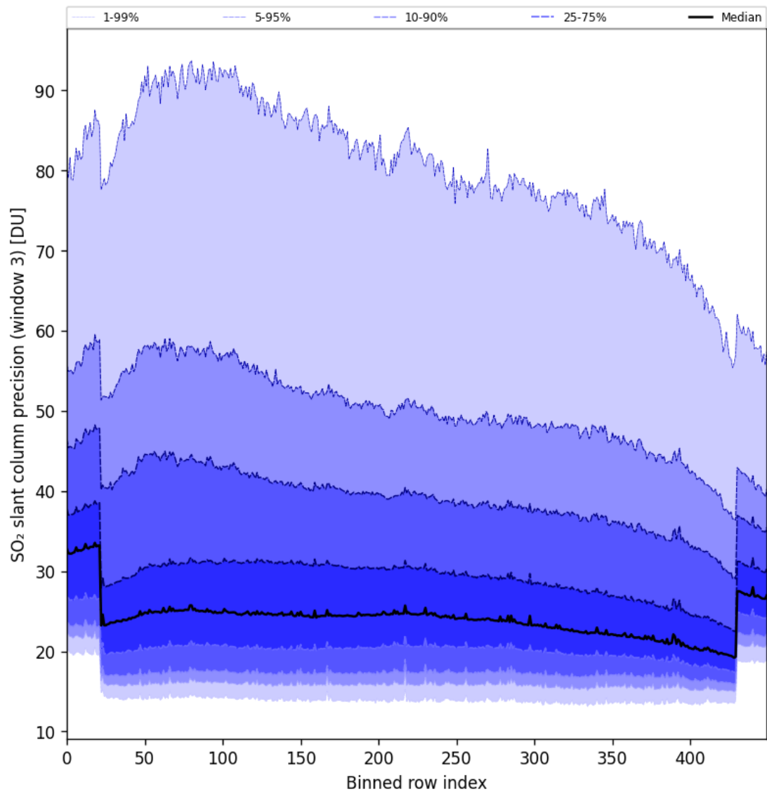
Figure 98: Along track statistics of “SO 2 slant column precision (window 3)” for 2025-11-13 to 2025-11-15
