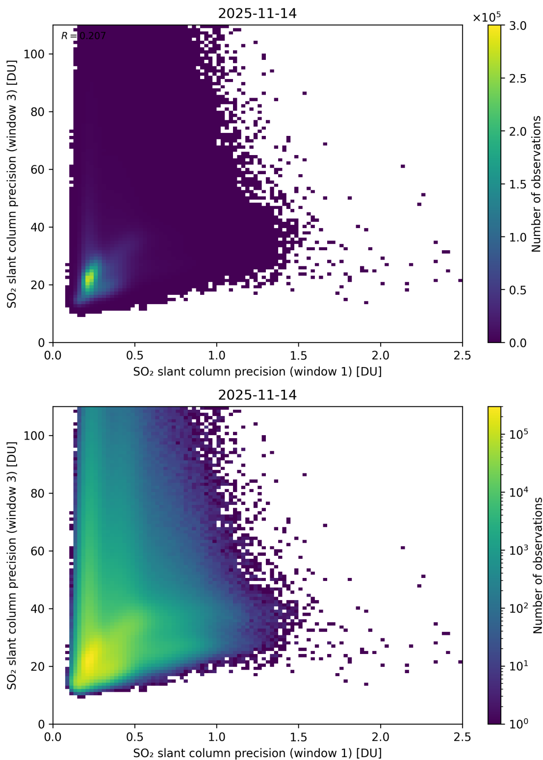
Figure 279: Scatter density plot of “SO 2 slant column precision (window 1)” against “SO 2 slant column precision (window 3)” for 2025-11-13 to 2025-11-15.
