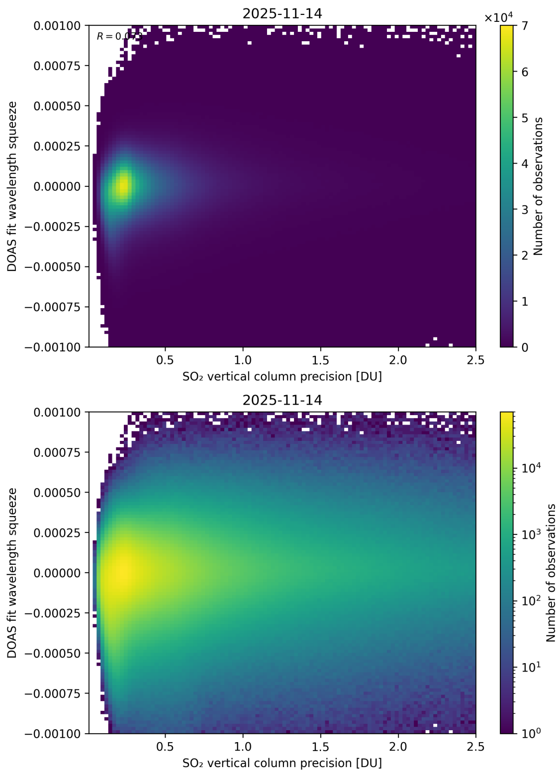
Figure 333: Scatter density plot of “SO 2 vertical column precision” against “DOAS fit wavelength squeeze” for 2025-11-13 to 2025-11-15.
