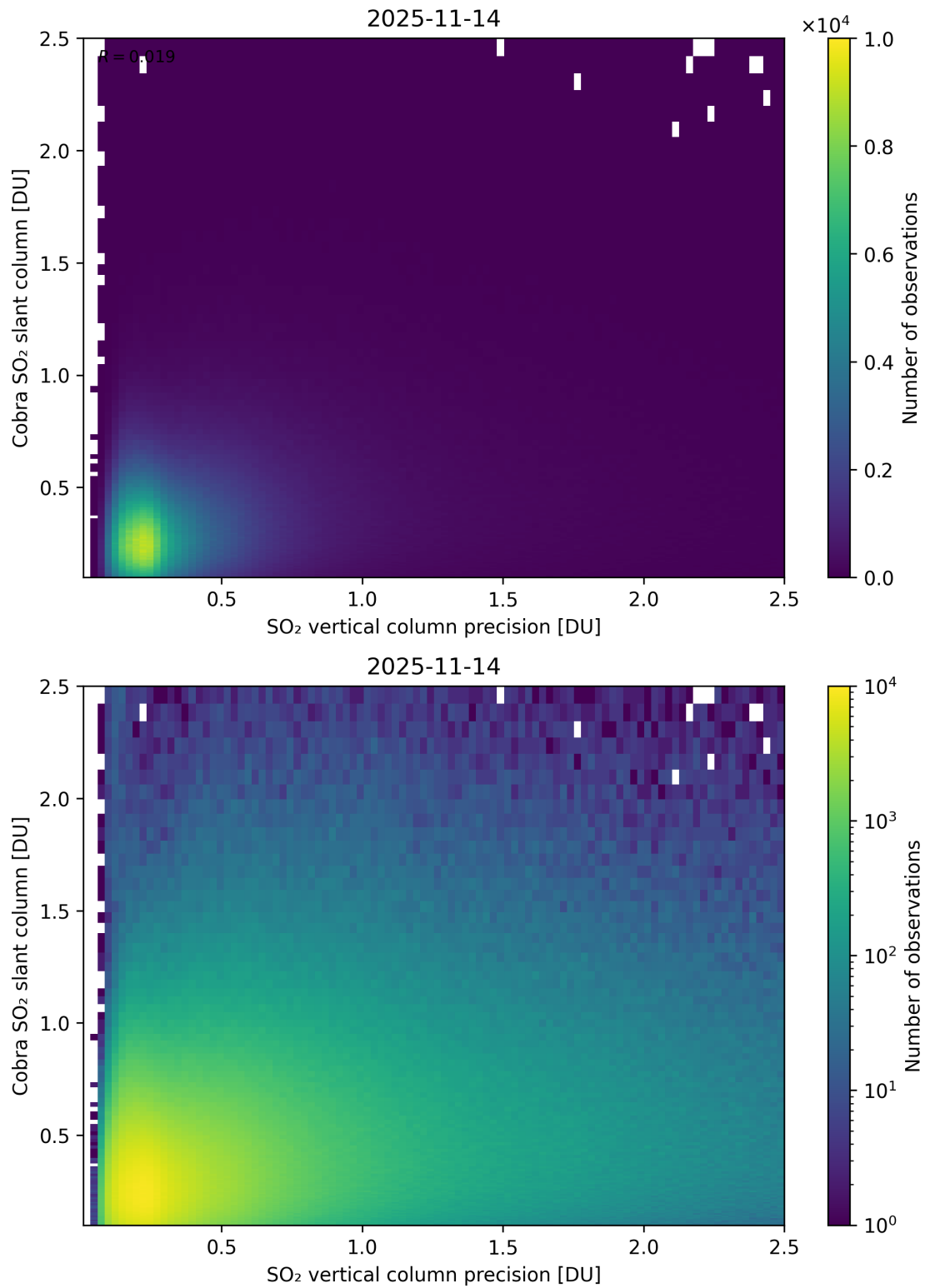
Figure 336: Scatter density plot of “SO 2 vertical column precision” against “Cobra SO 2 slant column” for 2025-11-13 to 2025-11-15.
