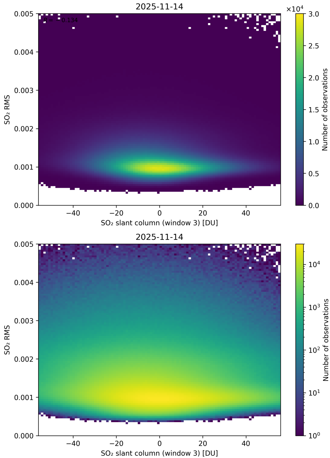
Figure 306: Scatter density plot of “SO 2 slant column (window 3)” against “SO 2 RMS” for 2025-11-13 to 2025-11-15.
