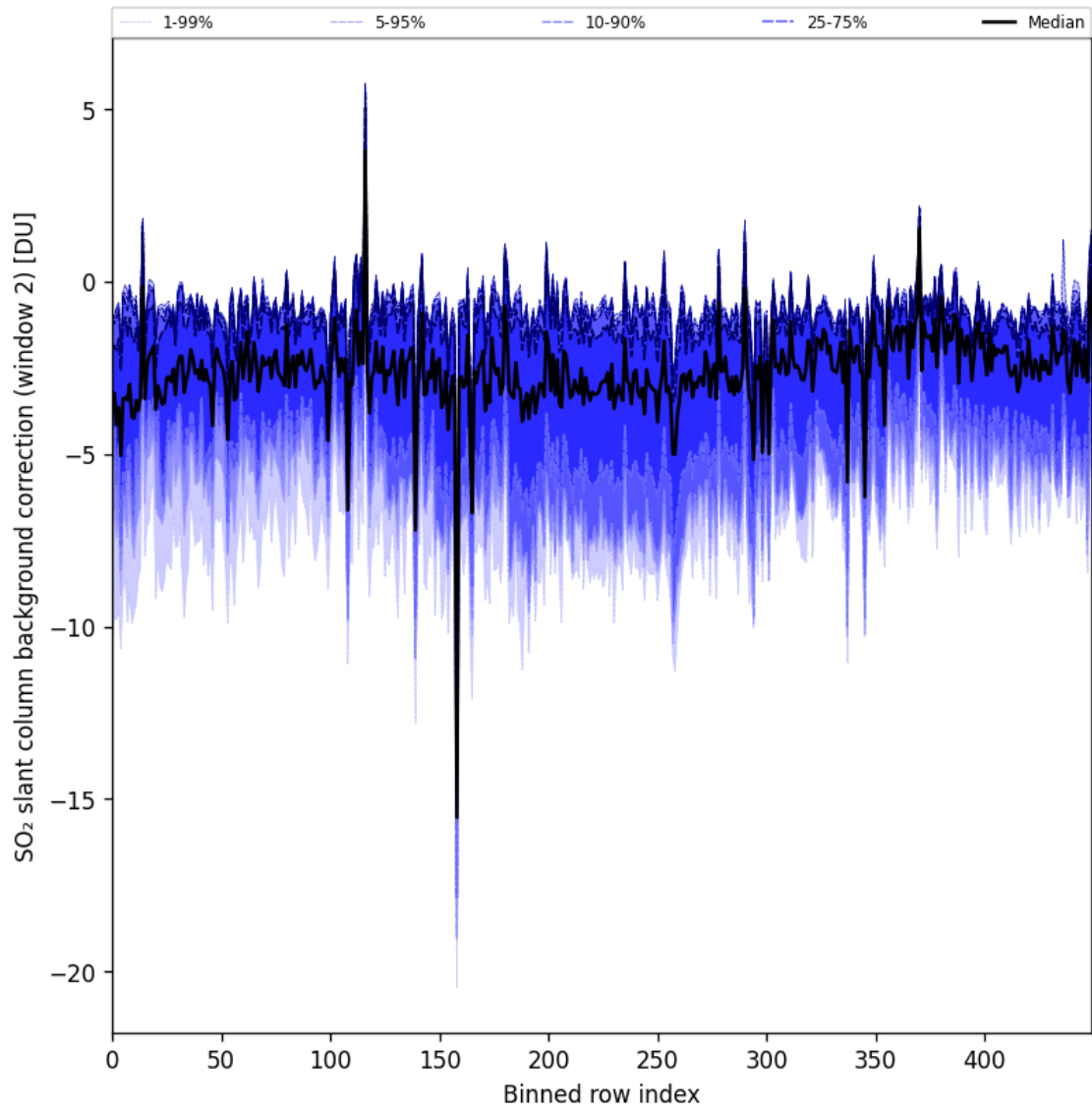
Figure 96: Along track statistics of “SO 2 slant column background correction (window 2)” for 2025-11-13 to 2025-11-15
