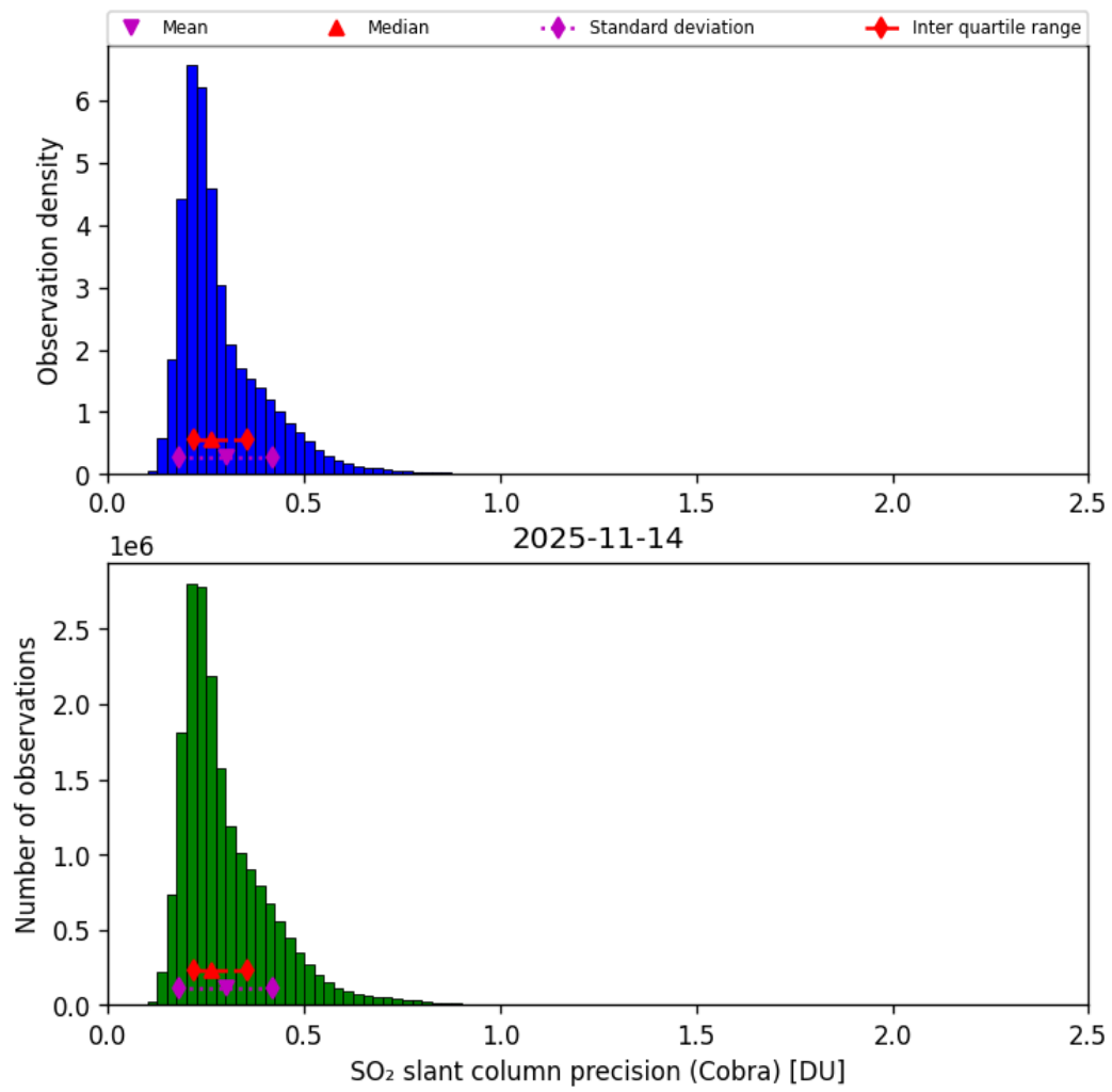
Figure 62: Histogram of “SO 2 slant column precision (Cobra)” for 2025-11-13 to 2025-11-15
