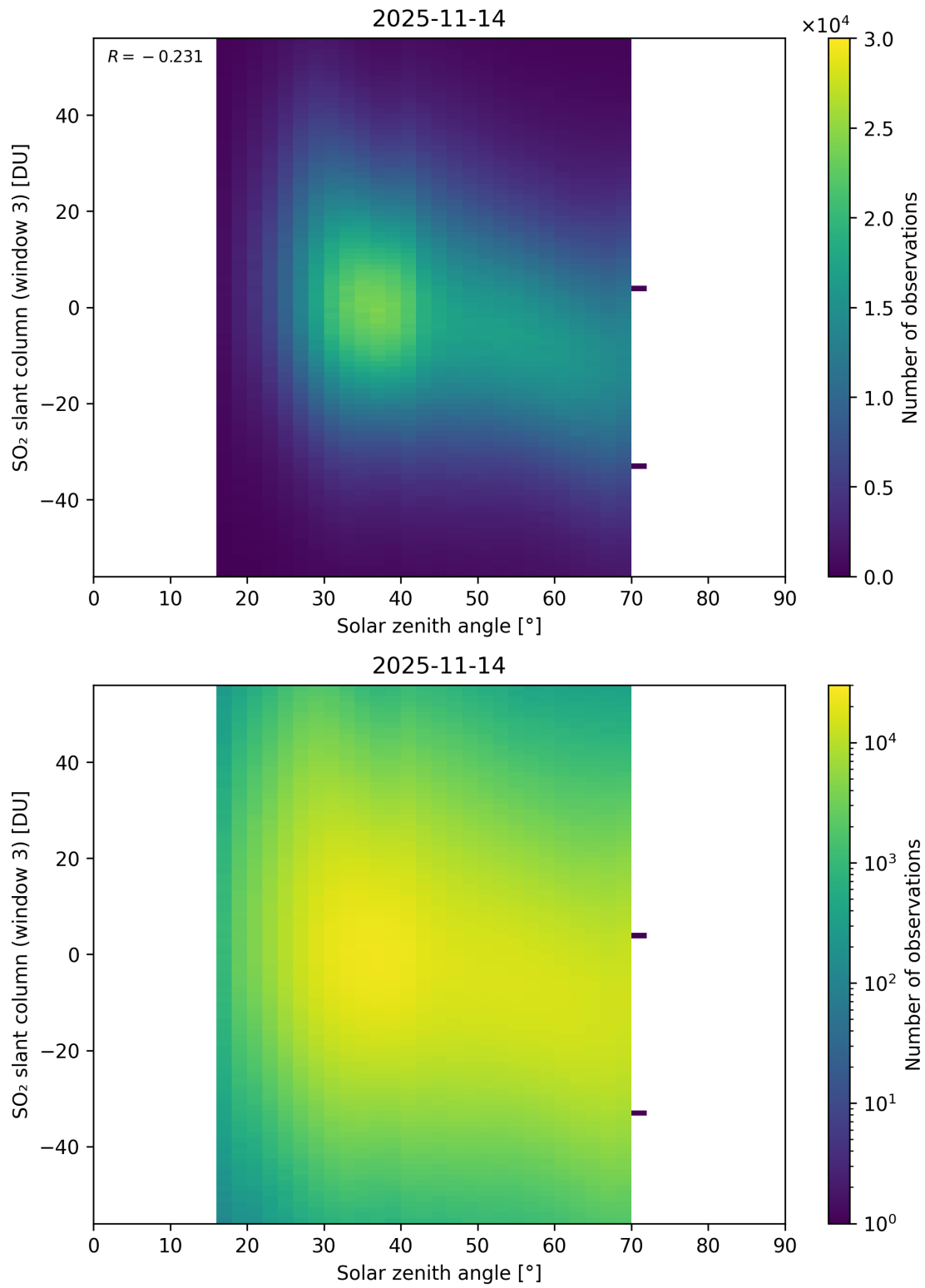
Figure 187: Scatter density plot of “Solar zenith angle” against “SO 2 slant column (window 3)” for 2025-11-13 to 2025-11-15.
