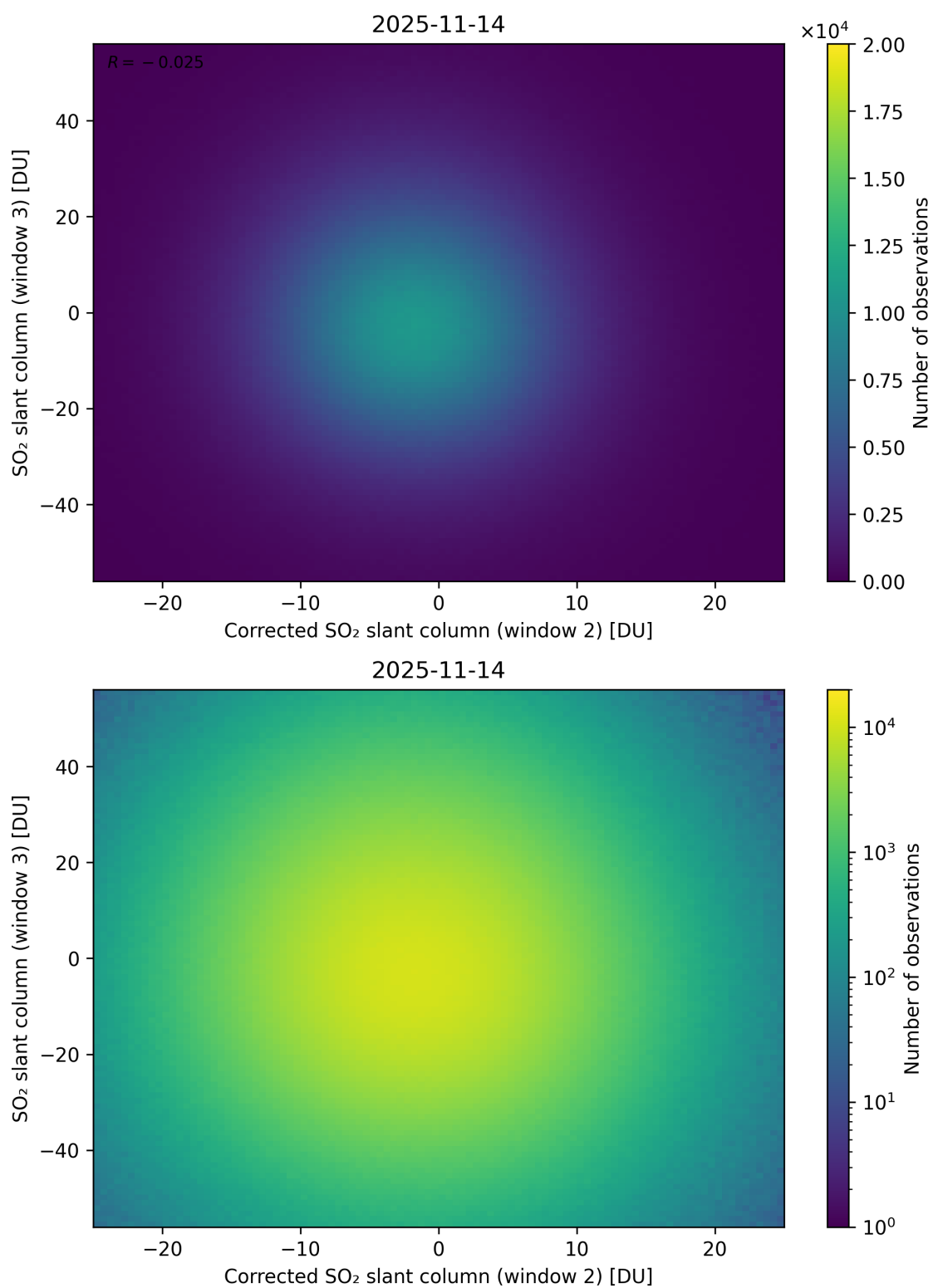
Figure 251: Scatter density plot of “Corrected SO 2 slant column (window 2)” against “SO 2 slant column (window 3)” for 2025-11-13 to 2025-11-15.
