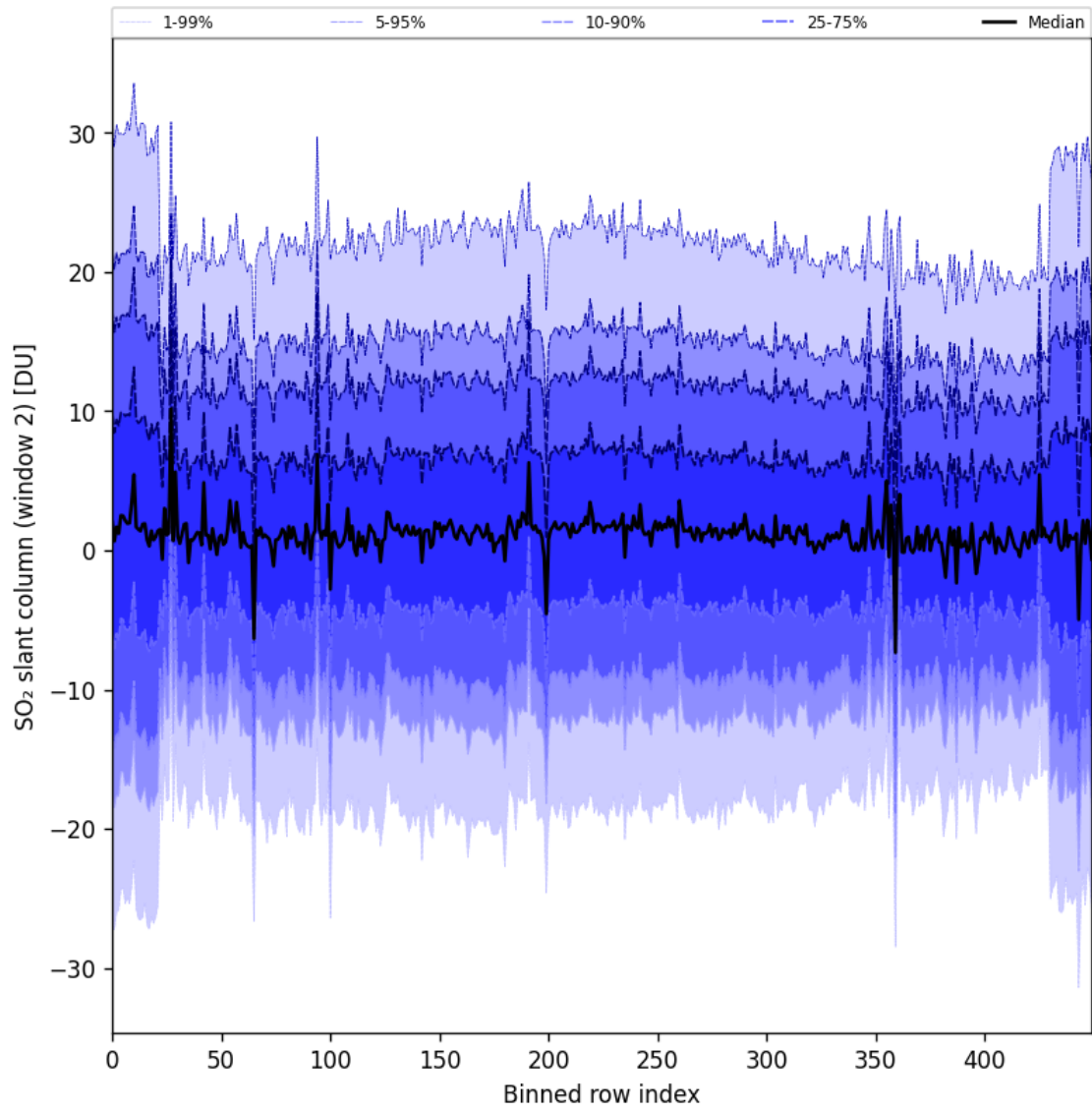
Figure 93: Along track statistics of “SO 2 slant column (window 2)” for 2025-11-13 to 2025-11-15
