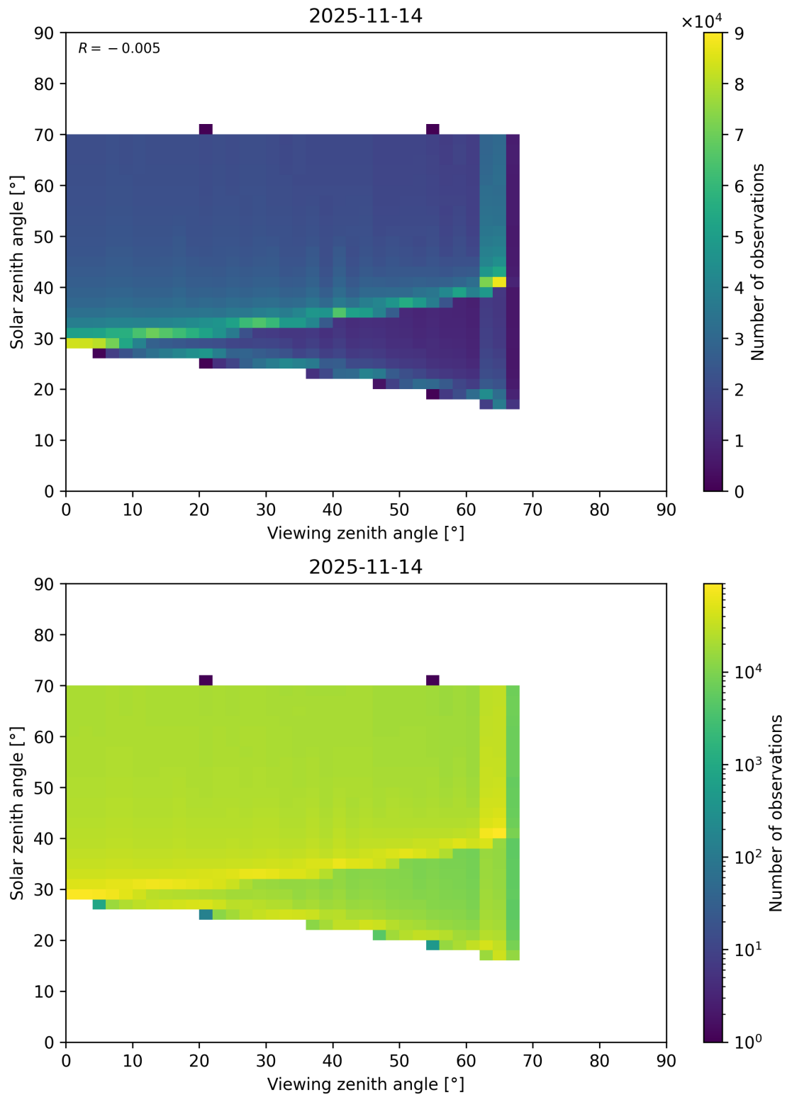
Figure 369: Scatter density plot of “Viewing zenith angle” against “Solar zenith angle” for 2025-11-13 to 2025-11-15.
