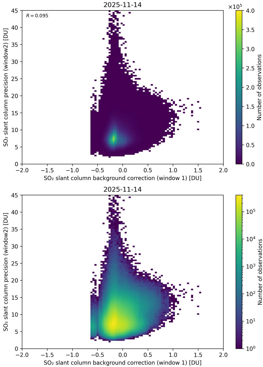
Figure 117: Scatter density plot of “SO 2 slant column background correction (window 1)” against “SO 2 slant column precision (window2)” for 2025-11-13 to 2025-11-15.
