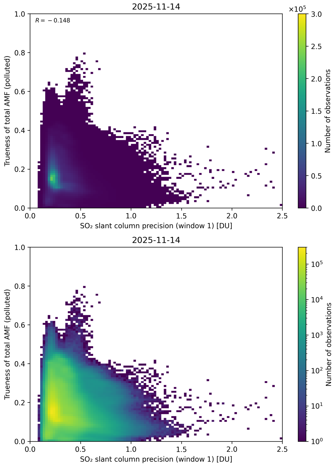
Figure 281: Scatter density plot of “SO 2 slant column precision (window 1)” against “Trueness of total AMF (polluted)” for 2025-11-13 to 2025-11-15.
