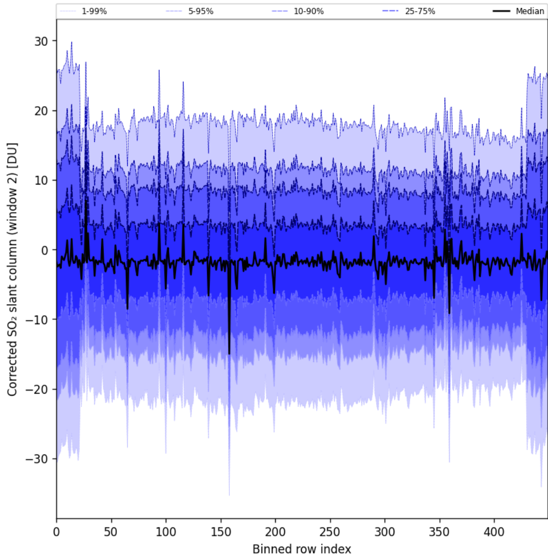
Figure 95: Along track statistics of “Corrected SO 2 slant column (window 2)” for 2025-11-13 to 2025-11-15
