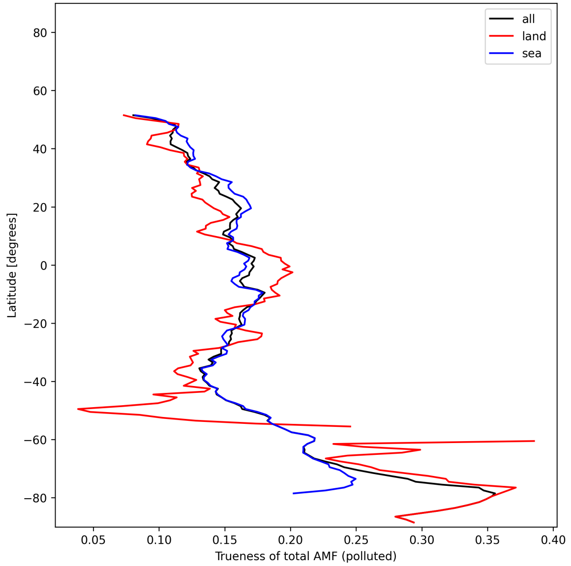
Figure 54: Zonal average of “Trueness of total AMF (polluted)” for 2025-11-13 to 2025-11-15.
