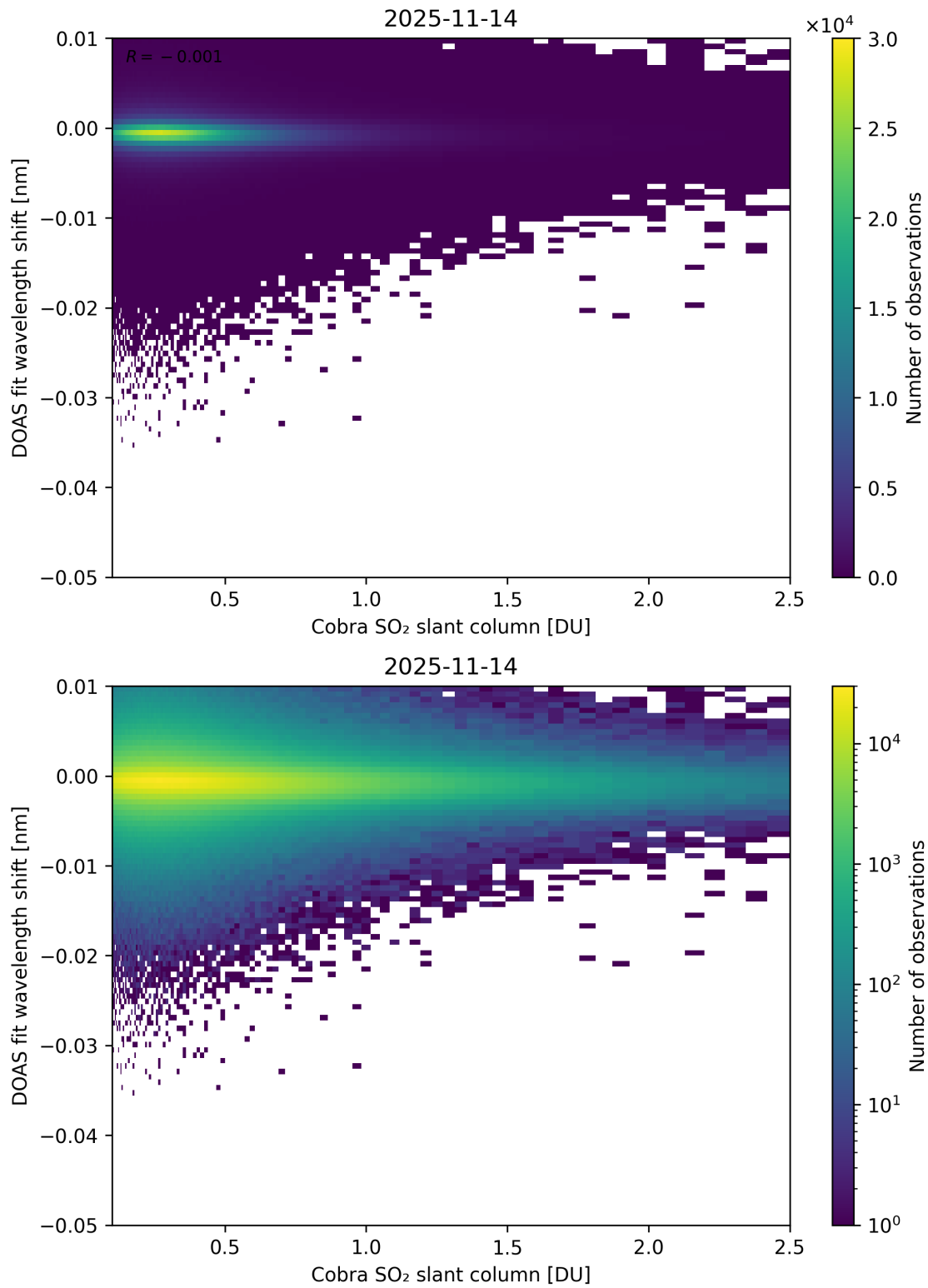
Figure 196: Scatter density plot of “Cobra SO 2 slant column” against “DOAS fit wavelength shift” for 2025-11-13 to 2025-11-15.
