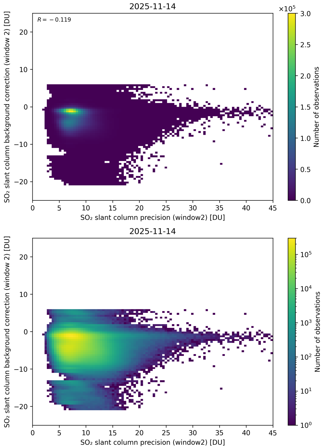
Figure 291: Scatter density plot of “SO 2 slant column precision (window2)” against “SO 2 slant column background correction (window 2)” for 2025-11-13 to 2025-11-15.
