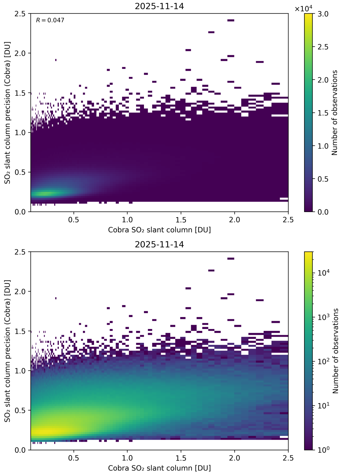
Figure 216: Scatter density plot of “Cobra SO 2 slant column” against “SO 2 slant column precision (Cobra)” for 2025-11-13 to 2025-11-15.
