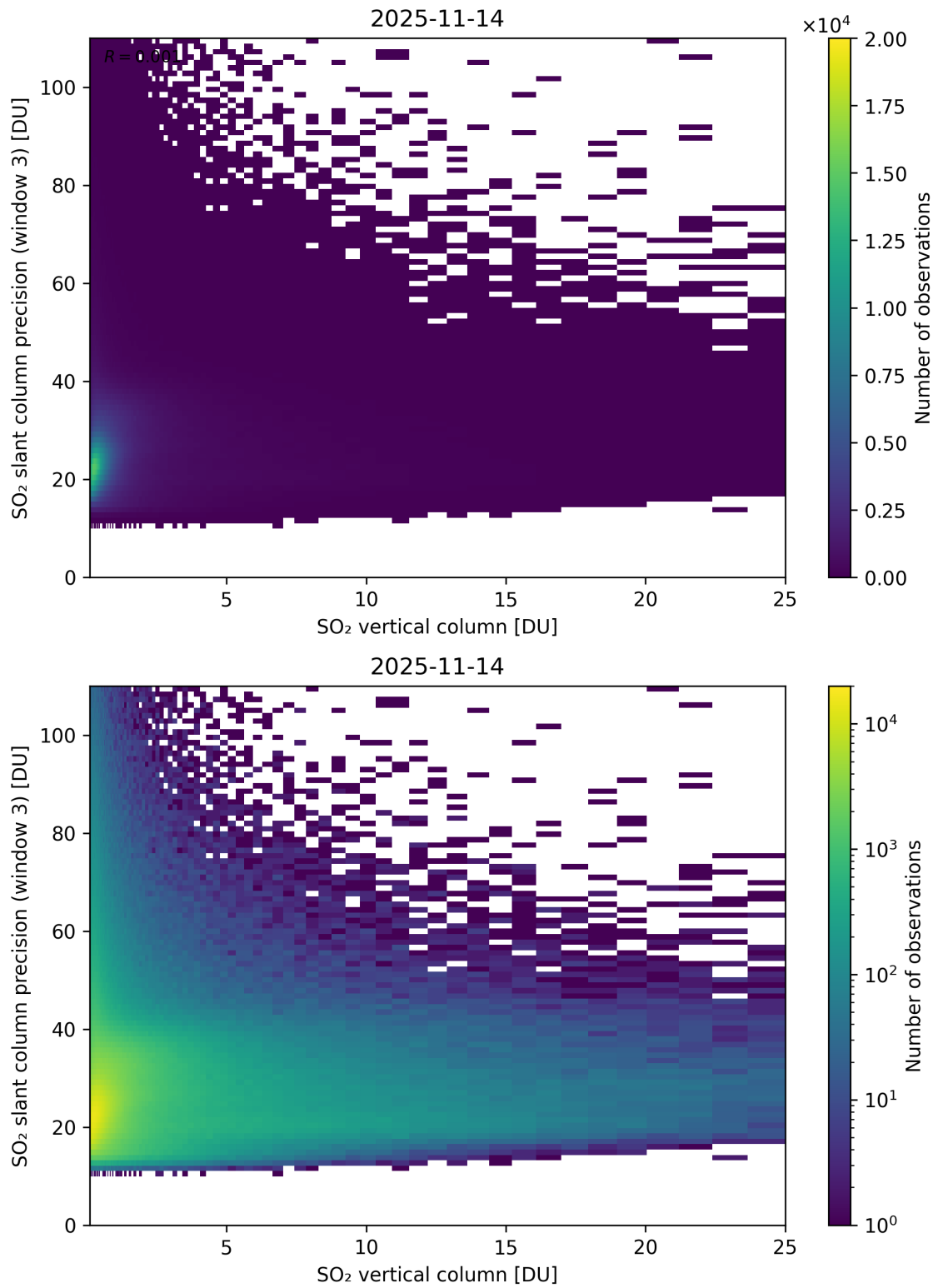
Figure 358: Scatter density plot of “SO 2 vertical column” against “SO 2 slant column precision (window 3)” for 2025-11-13 to 2025-11-15.
