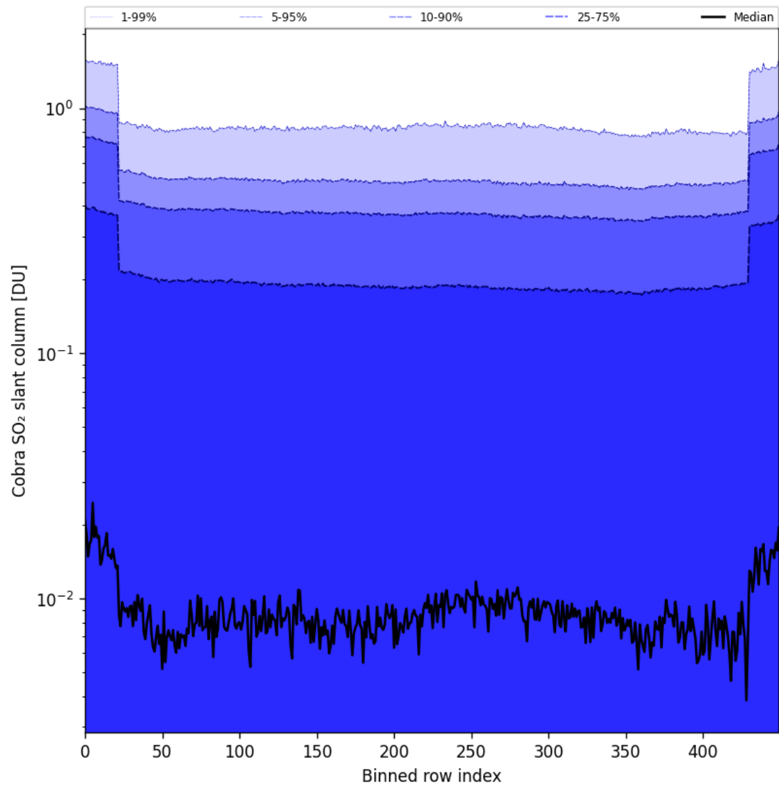
Figure 87: Along track statistics of “Cobra SO 2 slant column” for 2025-11-13 to 2025-11-15
