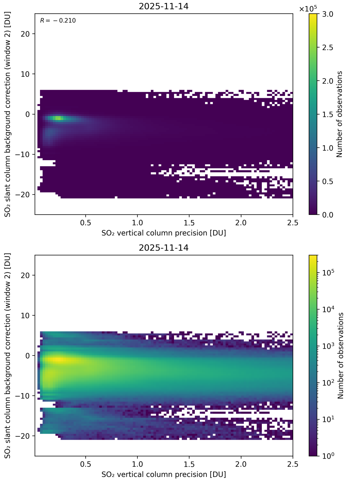
Figure 330: Scatter density plot of “SO 2 vertical column precision” against “SO 2 slant column background correction (window 2)” for 2025-11-13 to 2025-11-15.
