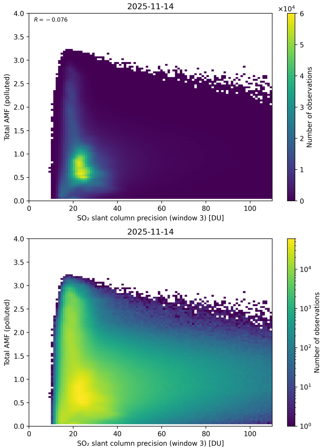
Figure 313: Scatter density plot of “SO 2 slant column precision (window 3)” against “Total AMF (polluted)” for 2025-11-13 to 2025-11-15.
