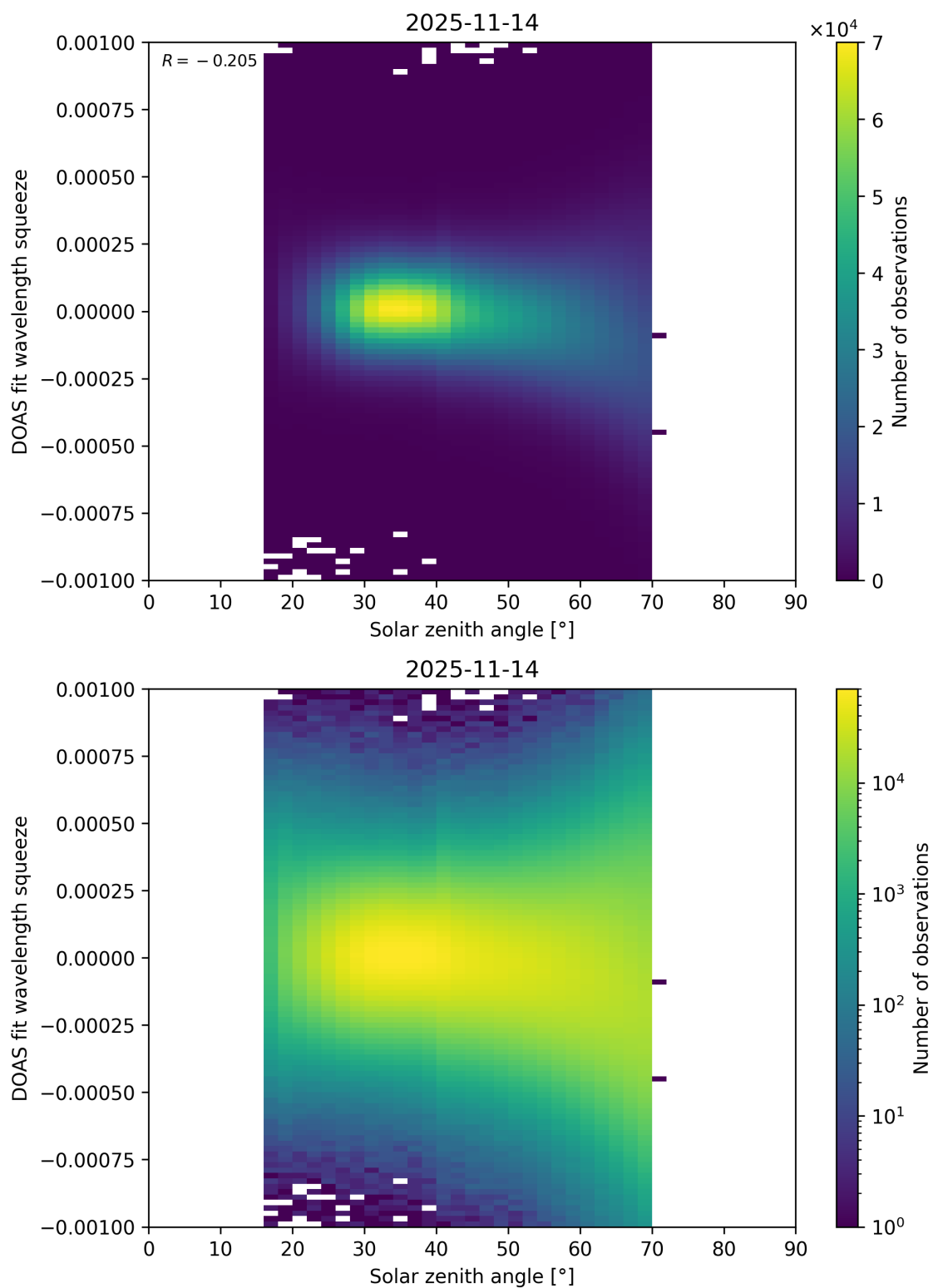
Figure 175: Scatter density plot of “Solar zenith angle” against “DOAS fit wavelength squeeze” for 2025-11-13 to 2025-11-15.
