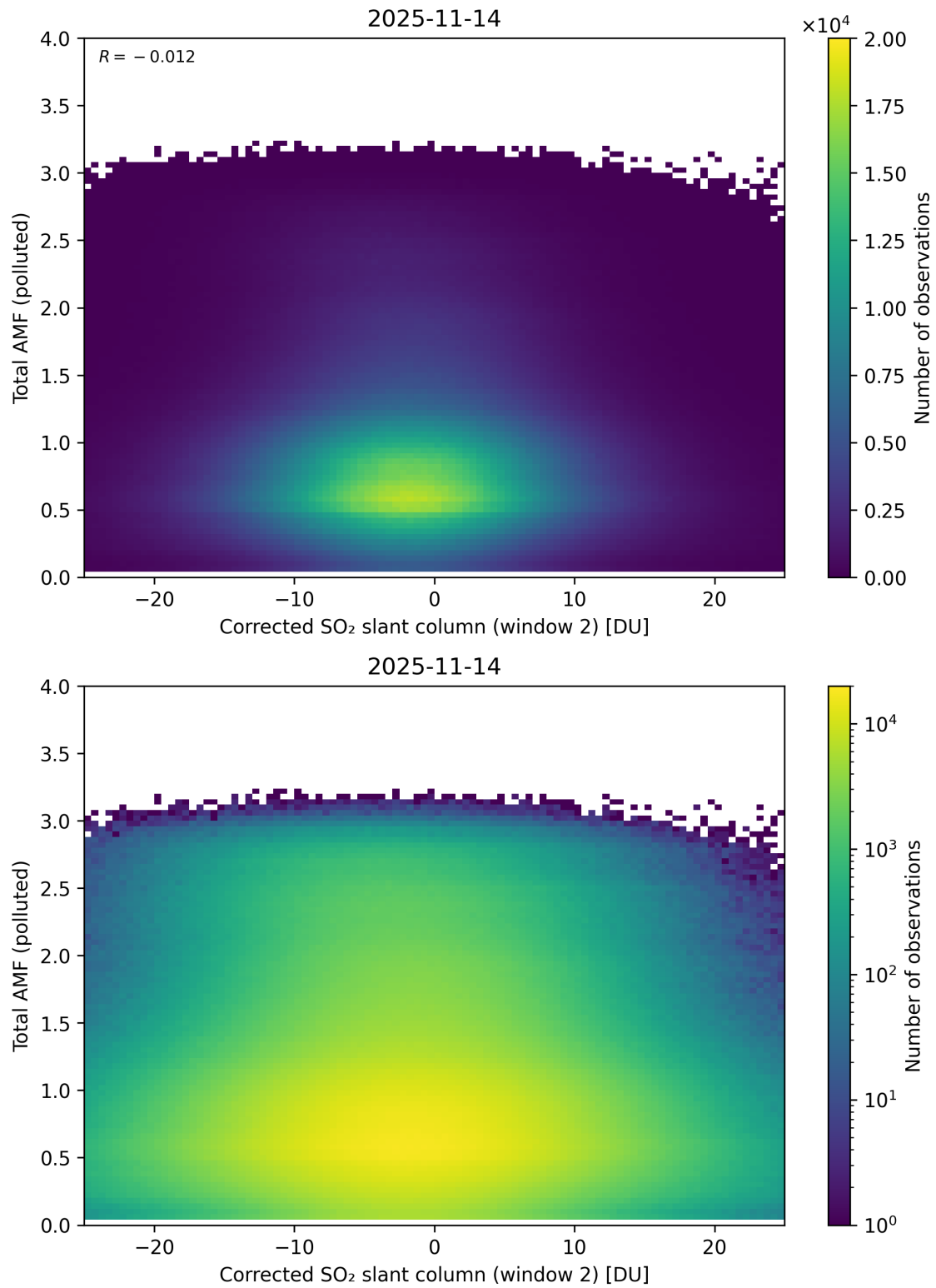
Figure 253: Scatter density plot of “Corrected SO 2 slant column (window 2)” against “Total AMF (polluted)” for 2025-11-13 to 2025-11-15.
