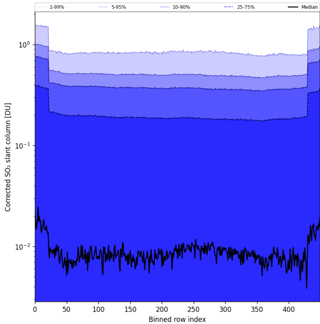
Figure 86: Along track statistics of “Corrected SO 2 slant column” for 2025-11-13 to 2025-11-15
