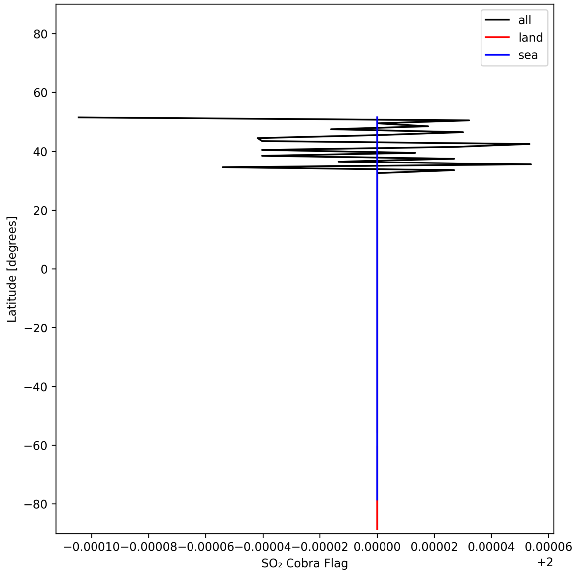
Figure 49: Zonal average of "SO 2 Cobra Flag" for 2025-11-13 to 2025-11-15.
