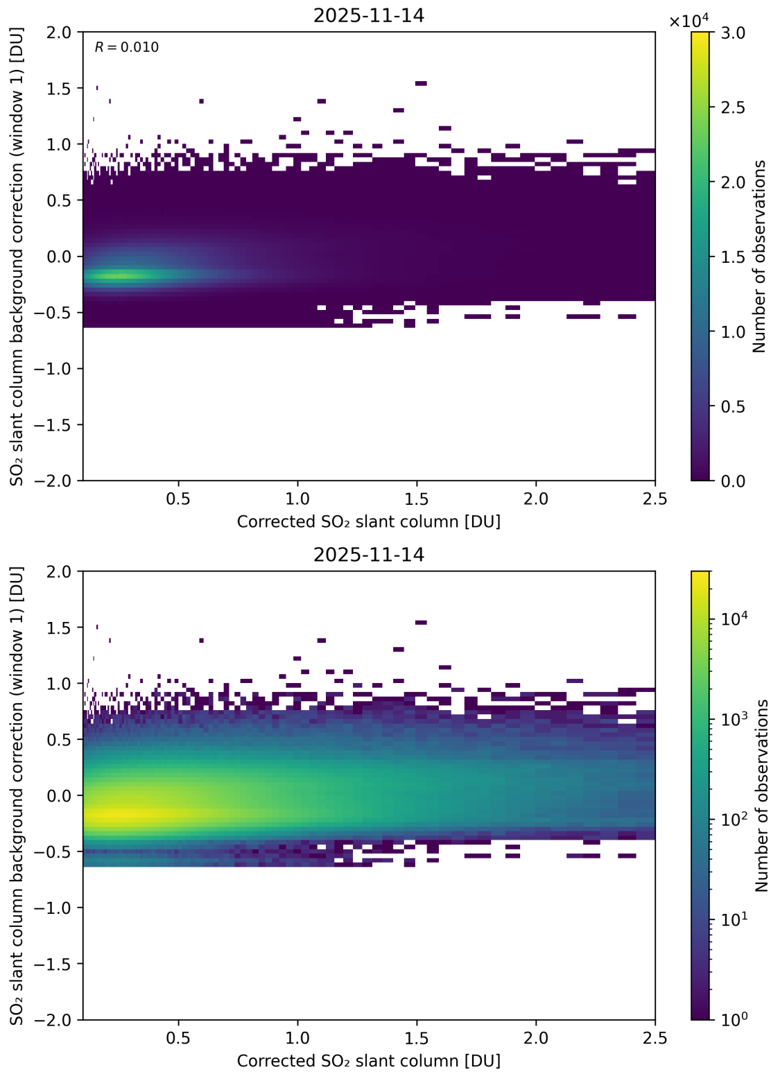
Figure 226: Scatter density plot of “Corrected SO 2 slant column” against “SO 2 slant column background correction (window 1)” for 2025-11-13 to 2025-11-15.
