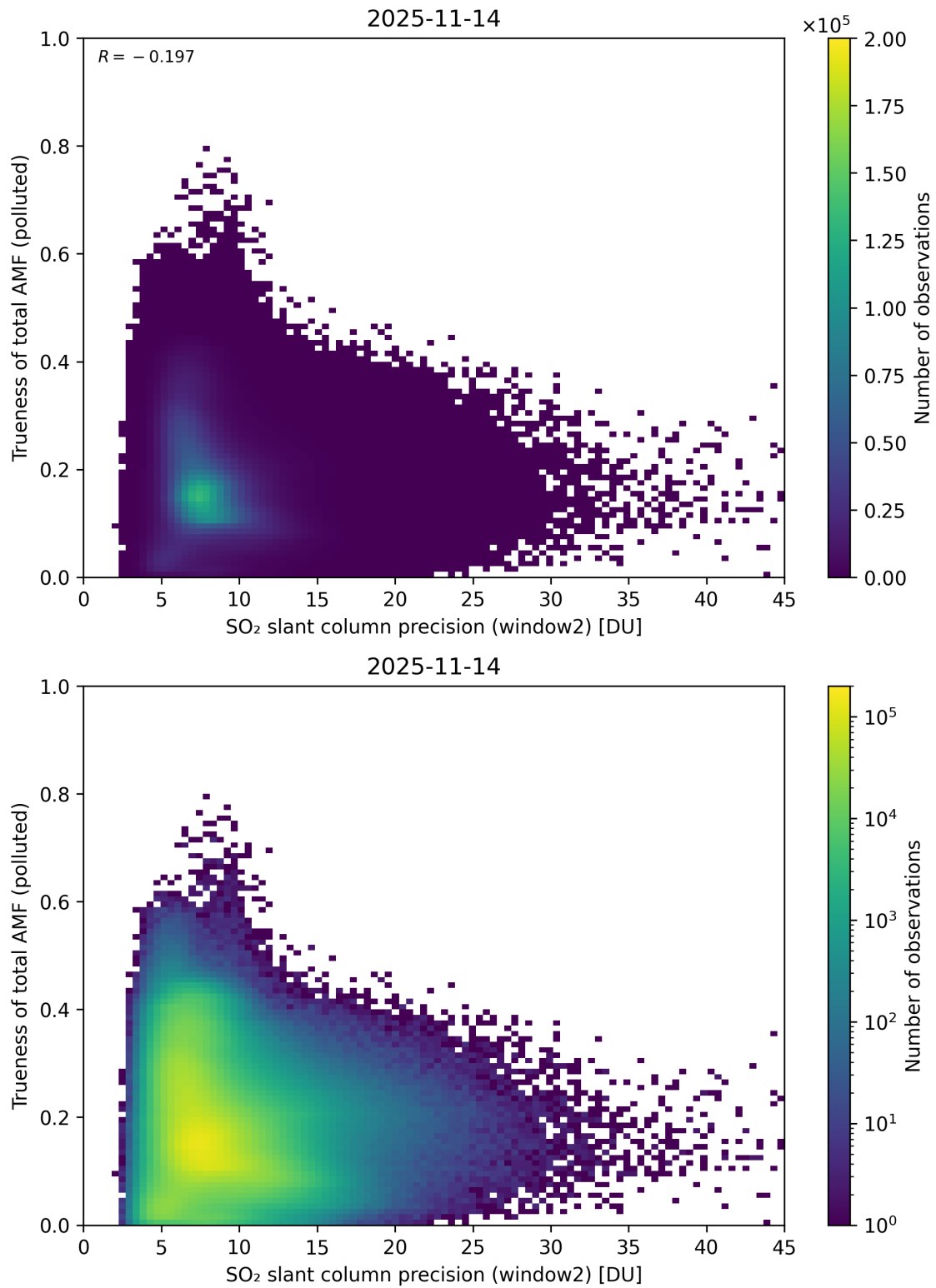
Figure 302: Scatter density plot of “SO 2 slant column precision (window2)” against “Trueness of total AMF (polluted)” for 2025-11-13 to 2025-11-15.
