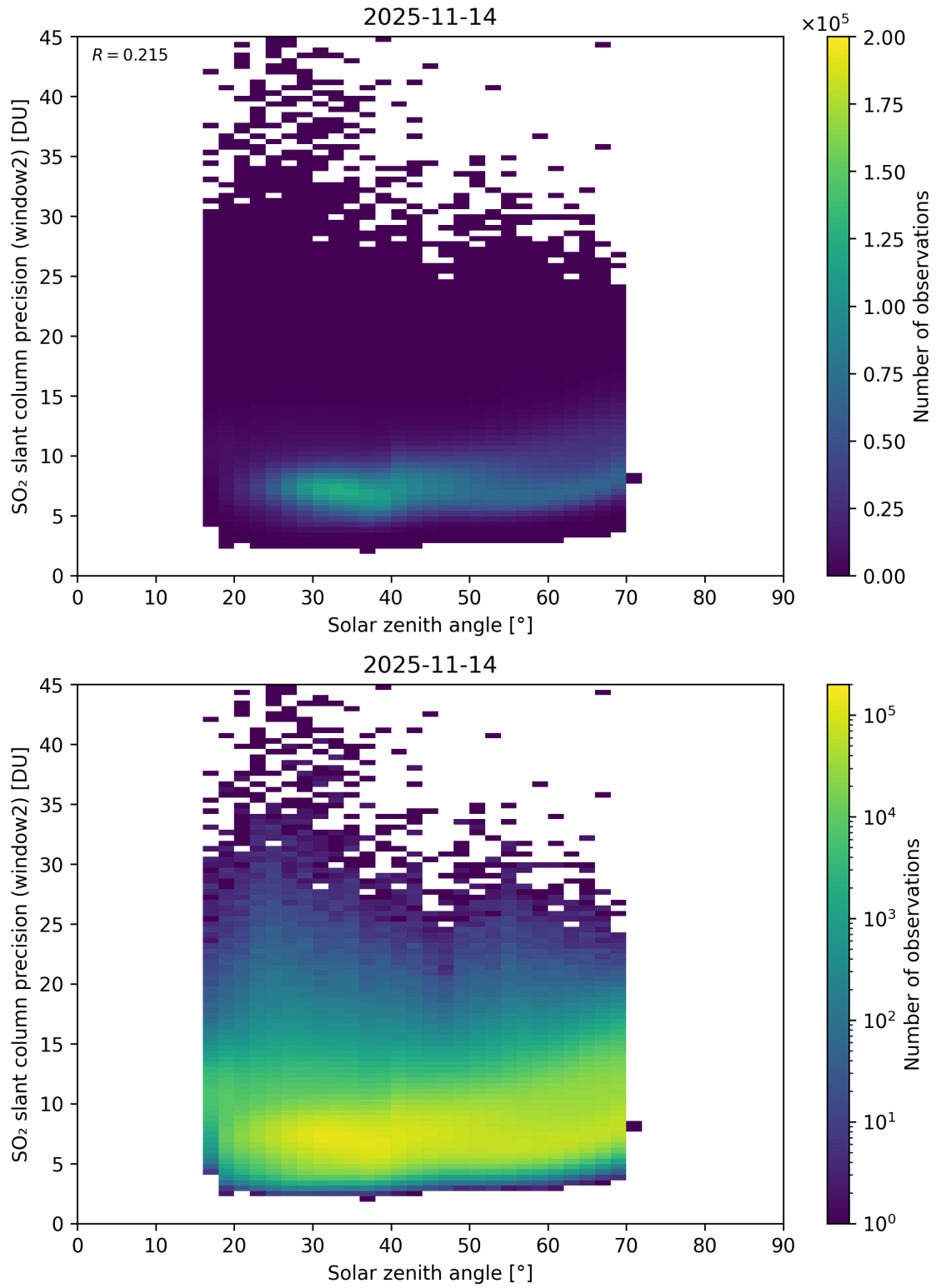
Figure 186: Scatter density plot of “Solar zenith angle” against “SO 2 slant column precision (window2)” for 2025-11-13 to 2025-11-15.
