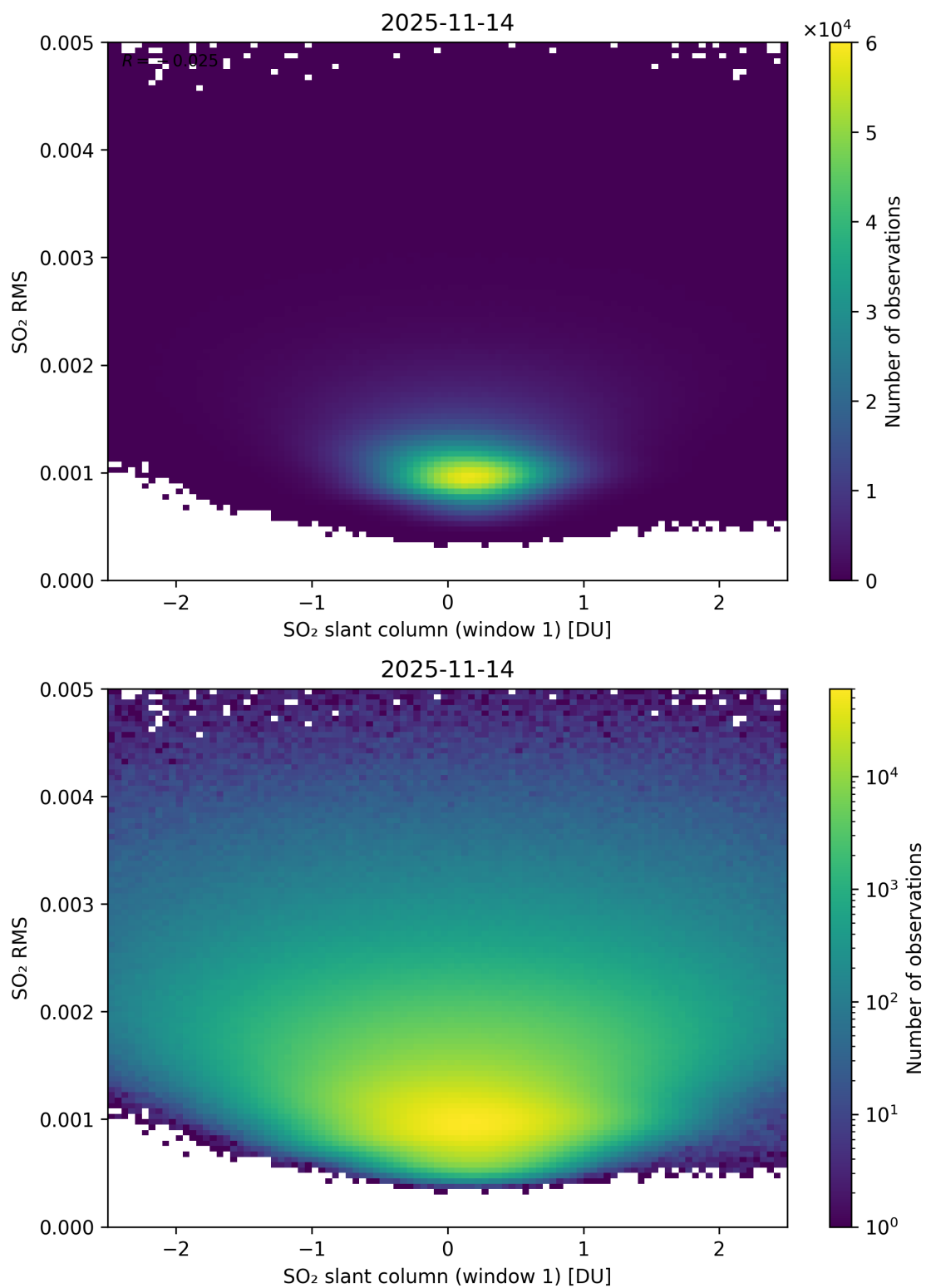
Figure 267: Scatter density plot of “SO 2 slant column (window 1)” against “SO 2 RMS” for 2025-11-13 to 2025-11-15.
