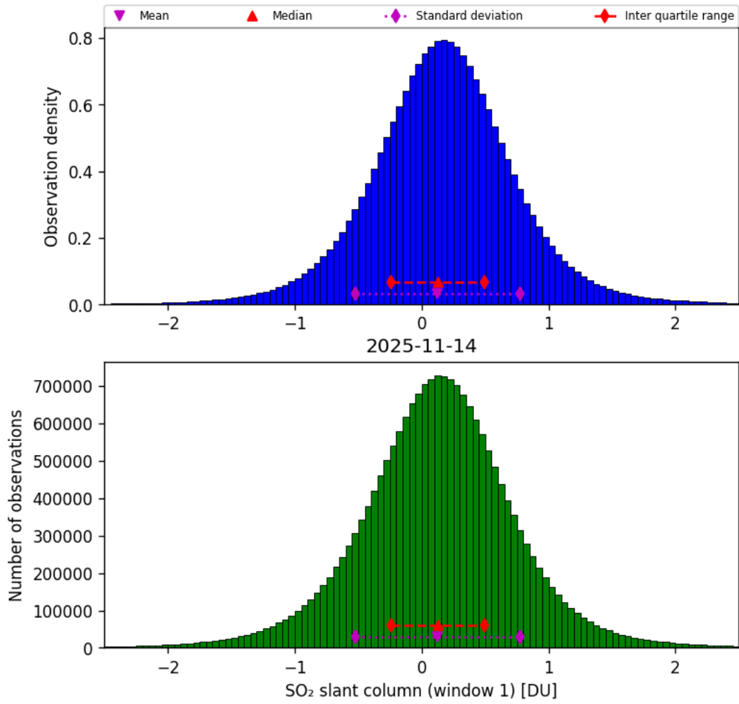
Figure 63: Histogram of “SO 2 slant column (window 1)” for 2025-11-13 to 2025-11-15
