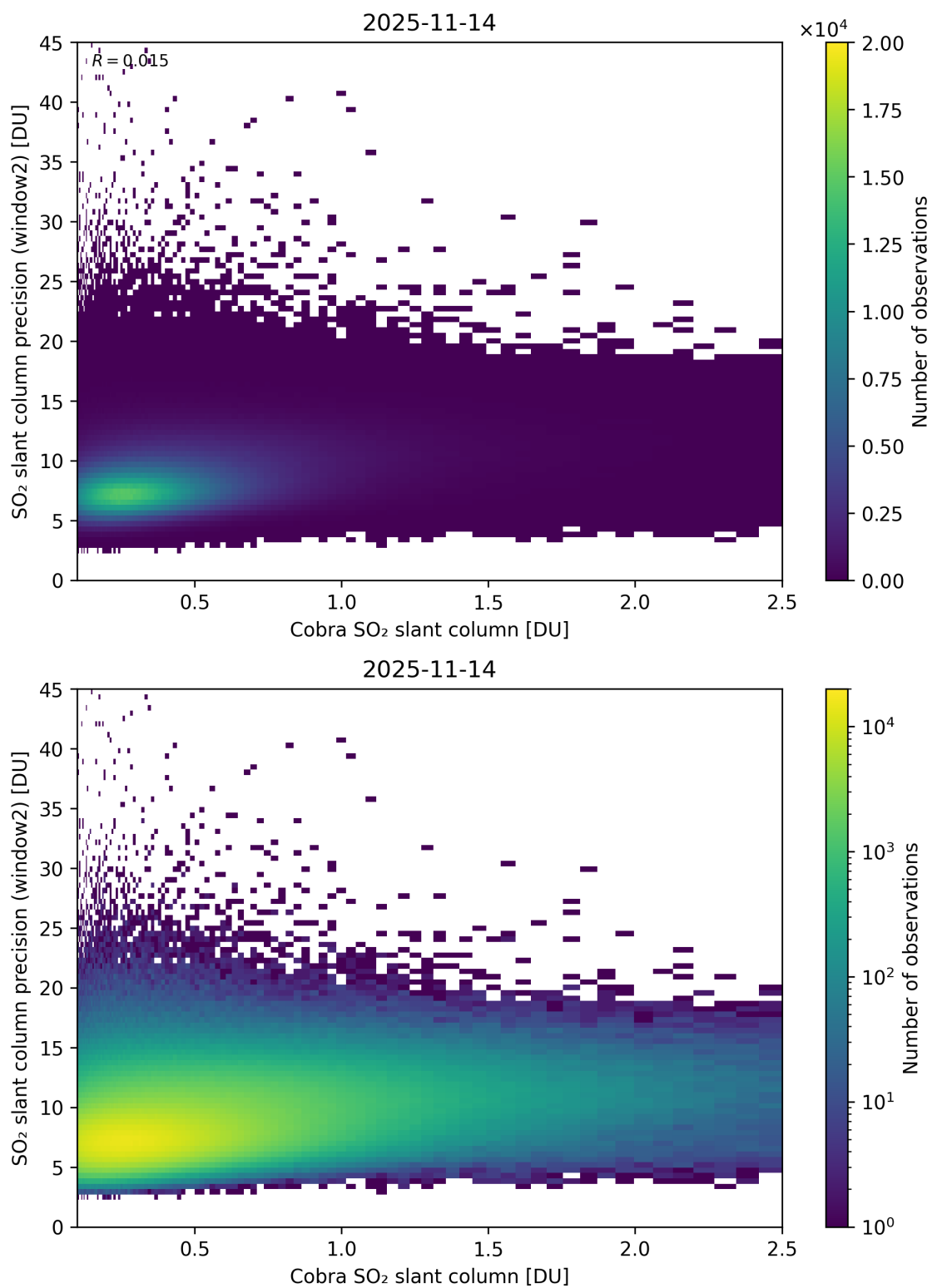
Figure 221: Scatter density plot of “Cobra SO 2 slant column” against “SO 2 slant column precision (window2)” for 2025-11-13 to 2025-11-15.
