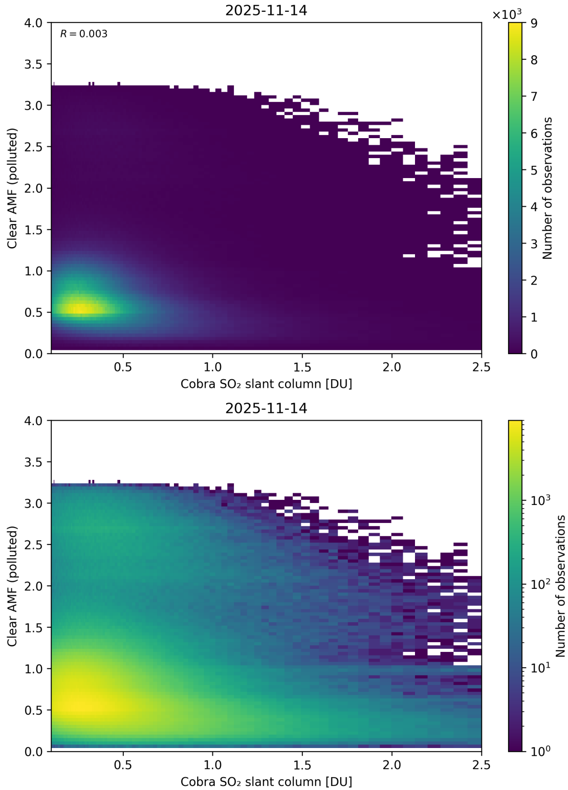
Figure 215: Scatter density plot of “Cobra SO 2 slant column” against “Clear AMF (polluted)” for 2025-11-13 to 2025-11-15.
