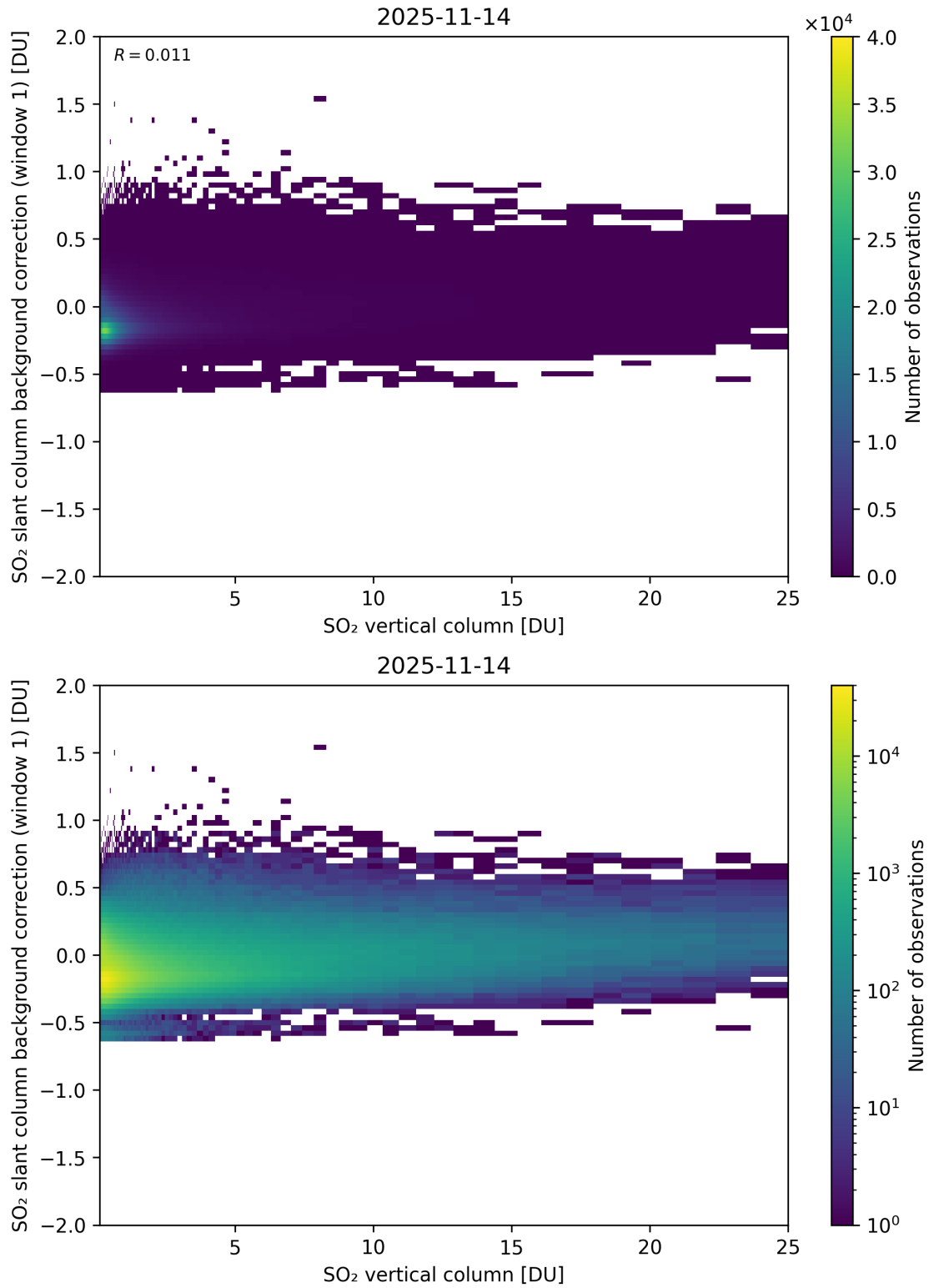
Figure 323: Scatter density plot of “SO 2 vertical column” against “SO 2 slant column background correction (window 1)” for 2025-11-13 to 2025-11-15.
