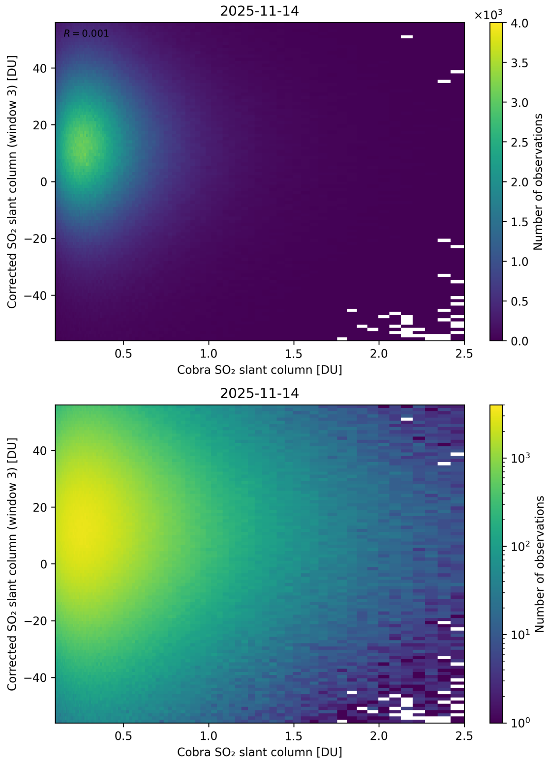
Figure 218: Scatter density plot of “Cobra SO 2 slant column” against “Corrected SO 2 slant column (window 3)” for 2025-11-13 to 2025-11-15.
