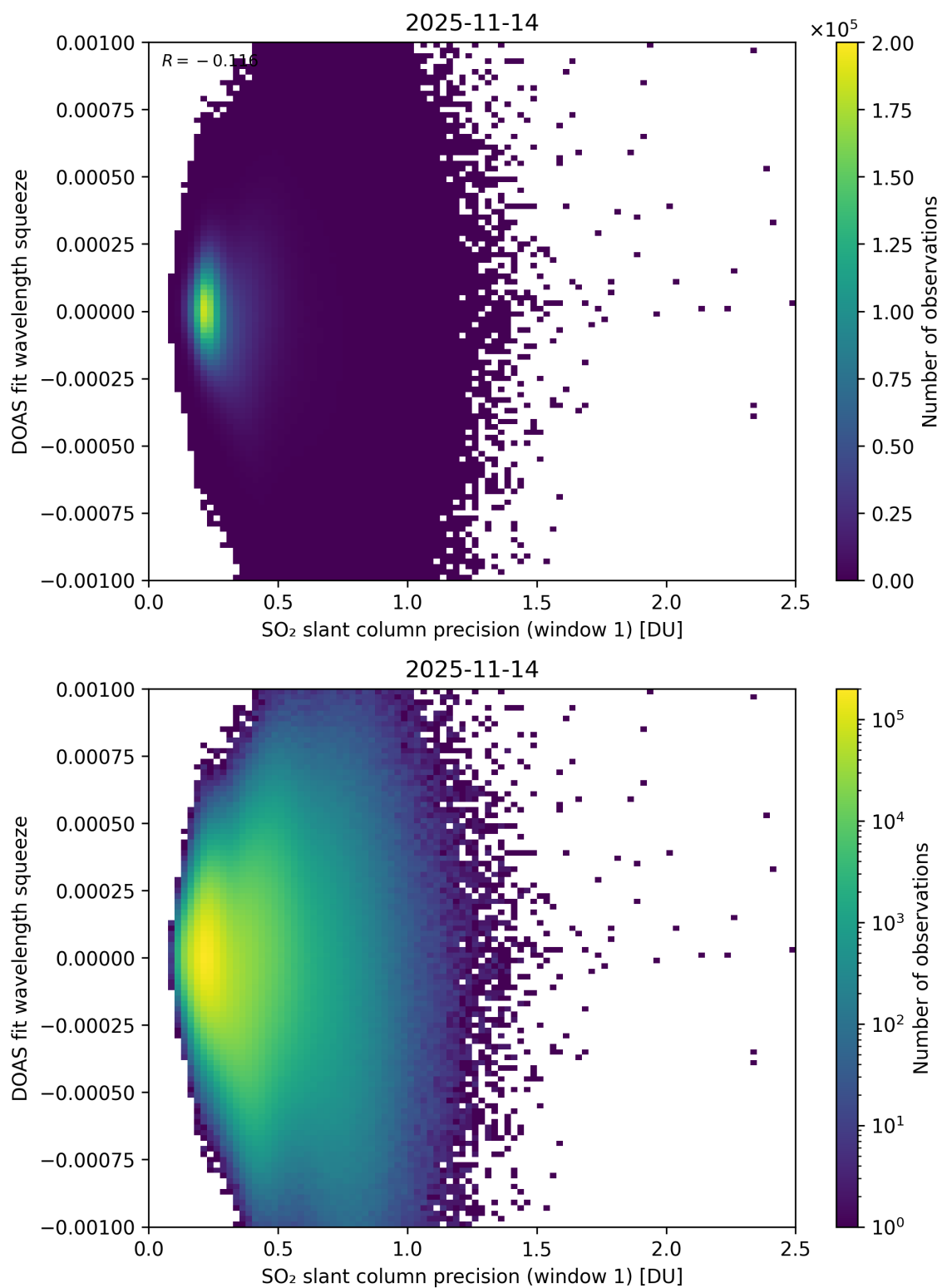
Figure 272: Scatter density plot of “SO 2 slant column precision (window 1)” against “DOAS fit wavelength squeeze” for 2025-11-13 to 2025-11-15.
