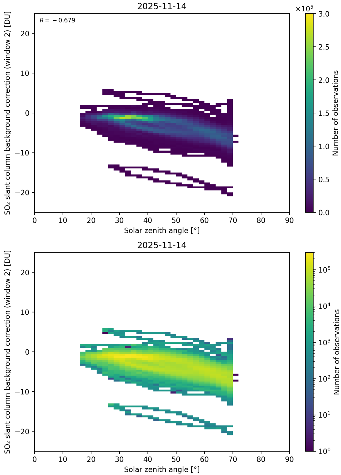
Figure 172: Scatter density plot of “Solar zenith angle” against “SO 2 slant column background correction (window 2)” for 2025-11-13 to 2025-11-15.
