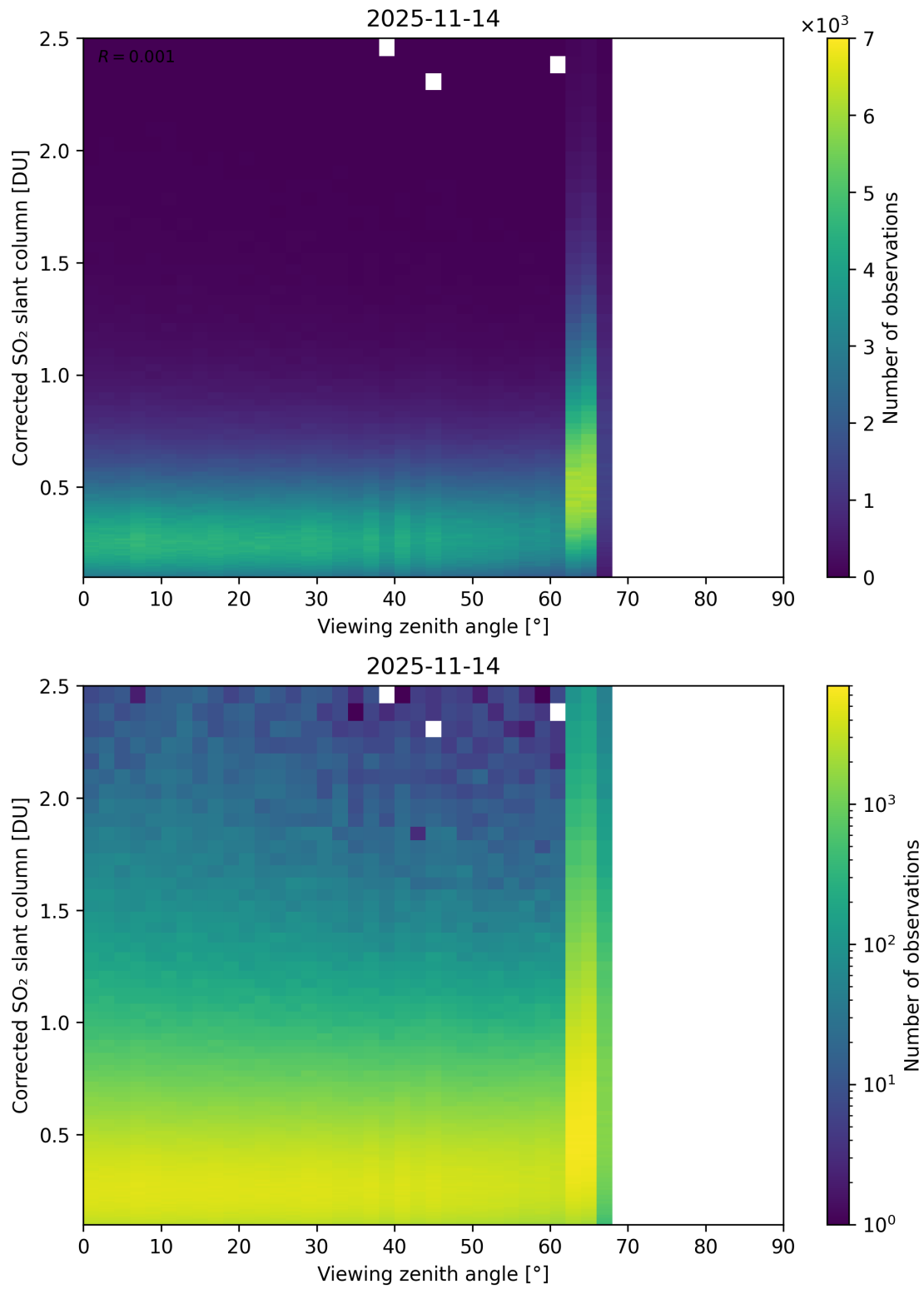
Figure 373: Scatter density plot of “Viewing zenith angle” against “Corrected SO 2 slant column” for 2025-11-13 to 2025-11-15.
