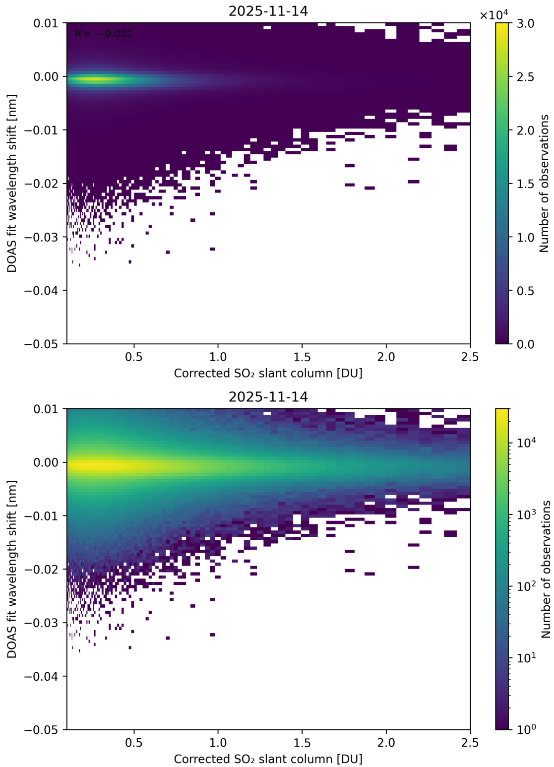
Figure 229: Scatter density plot of “Corrected SO 2 slant column” against “DOAS fit wavelength shift” for 2025-11-13 to 2025-11-15.
