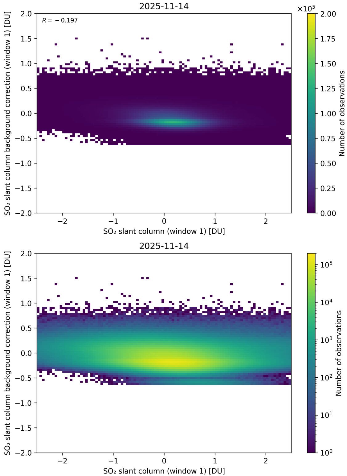
Figure 262: Scatter density plot of “SO 2 slant column (window 1)” against “SO 2 slant column background correction (window 1)” for 2025-11-13 to 2025-11-15.
