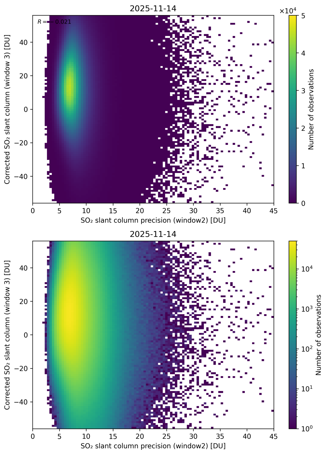
Figure 298: Scatter density plot of “SO 2 slant column precision (window2)” against “Corrected SO 2 slant column (window 3)” for 2025-11-13 to 2025-11-15.
