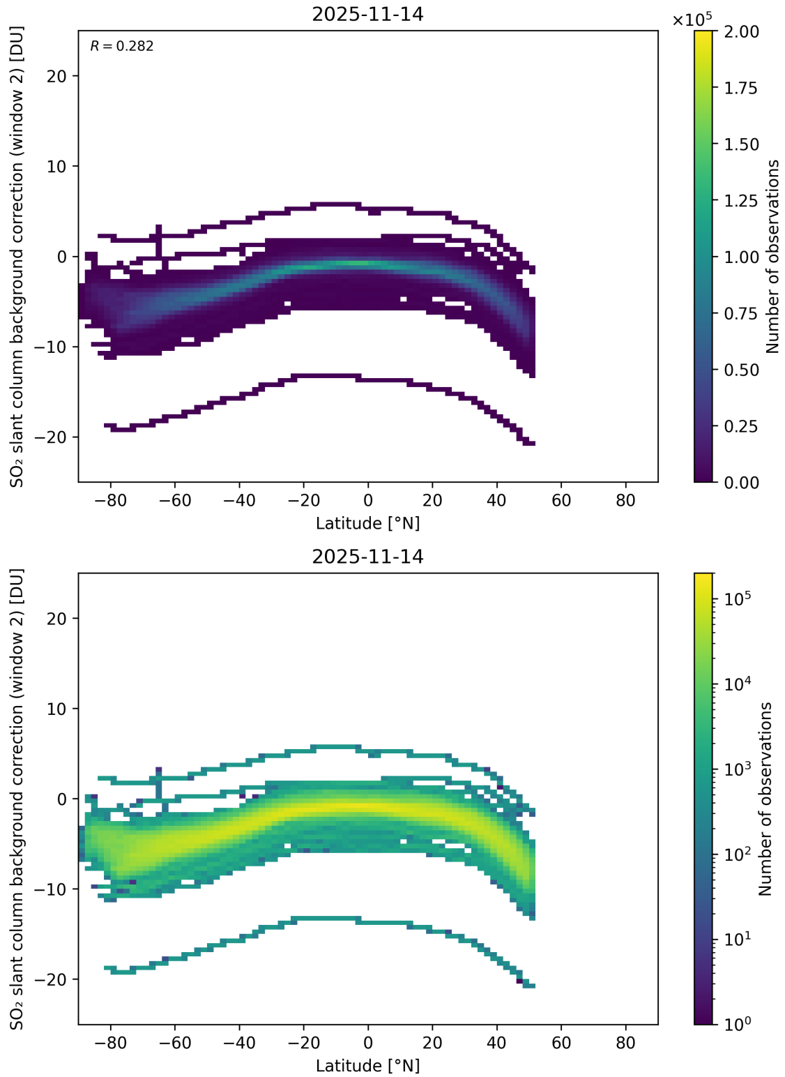
Figure 151: Scatter density plot of “Latitude” against “SO 2 slant column background correction (window 2)” for 2025-11-13 to 2025-11-15.
