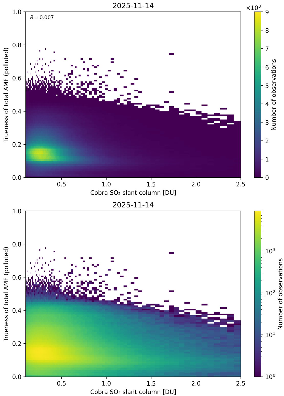
Figure 225: Scatter density plot of “Cobra SO 2 slant column” against “Trueness of total AMF (polluted)” for 2025-11-13 to 2025-11-15.
