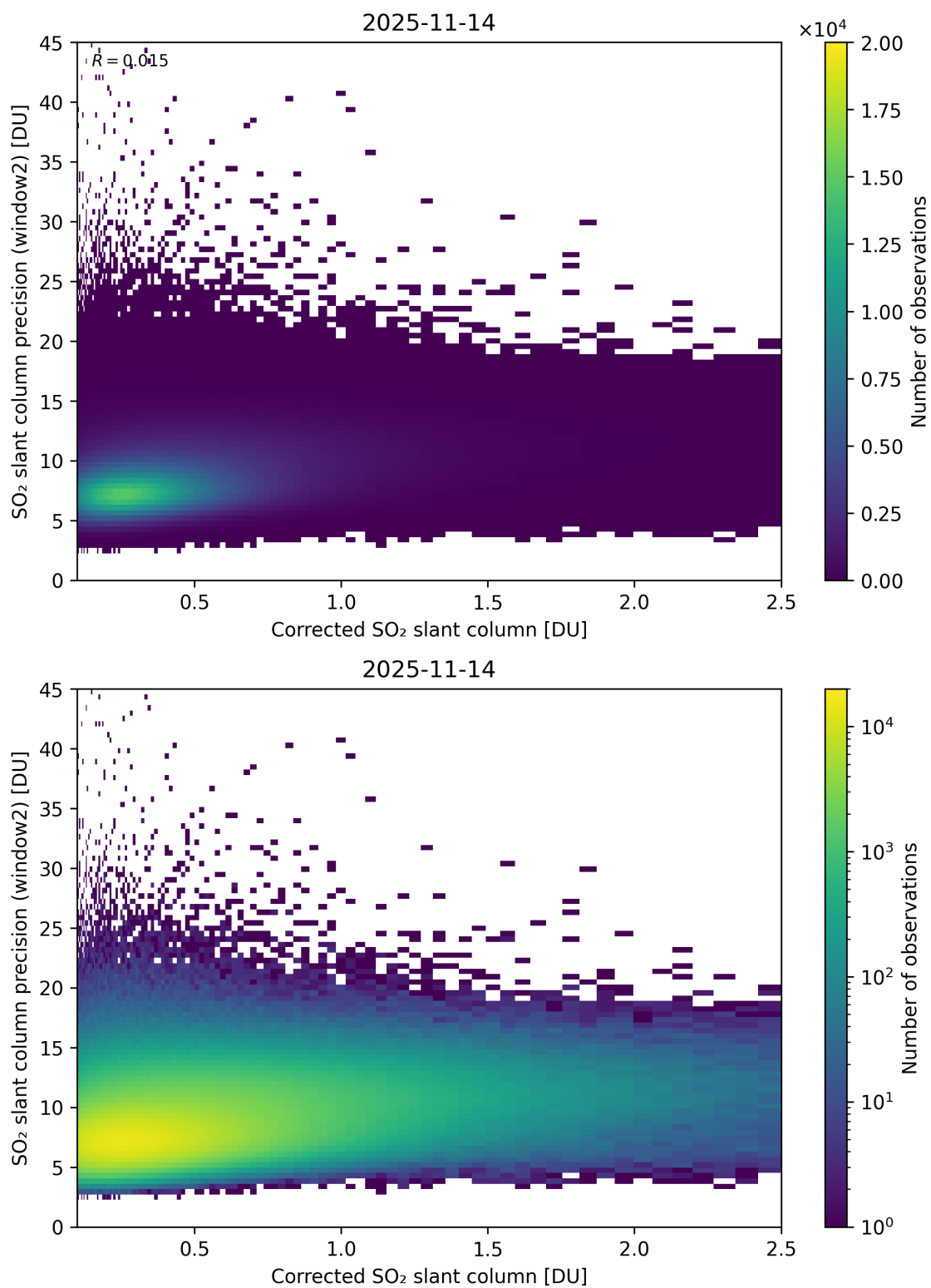
Figure 239: Scatter density plot of “Corrected SO 2 slant column” against “SO 2 slant column precision (window2)” for 2025-11-13 to 2025-11-15.
