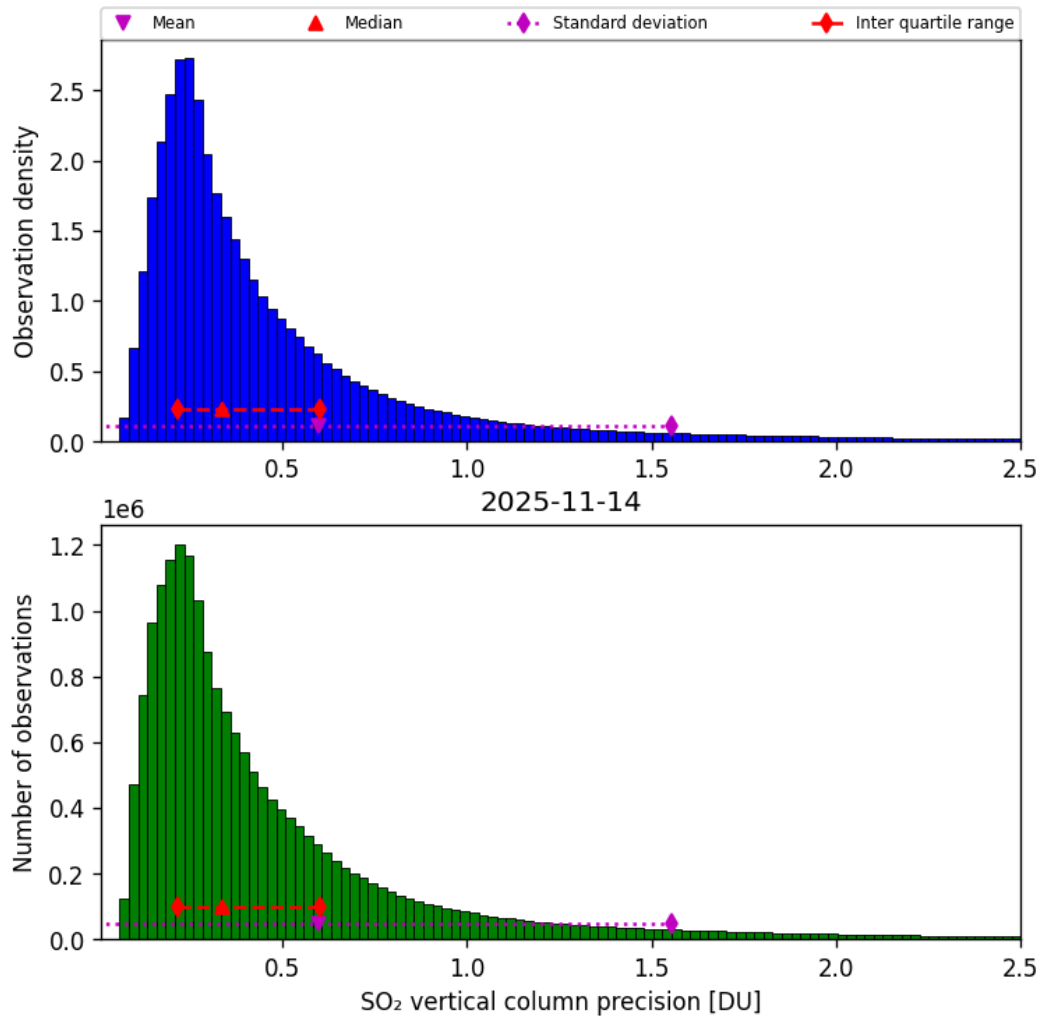
Figure 59: Histogram of “SO 2 vertical column precision” for 2025-11-13 to 2025-11-15
