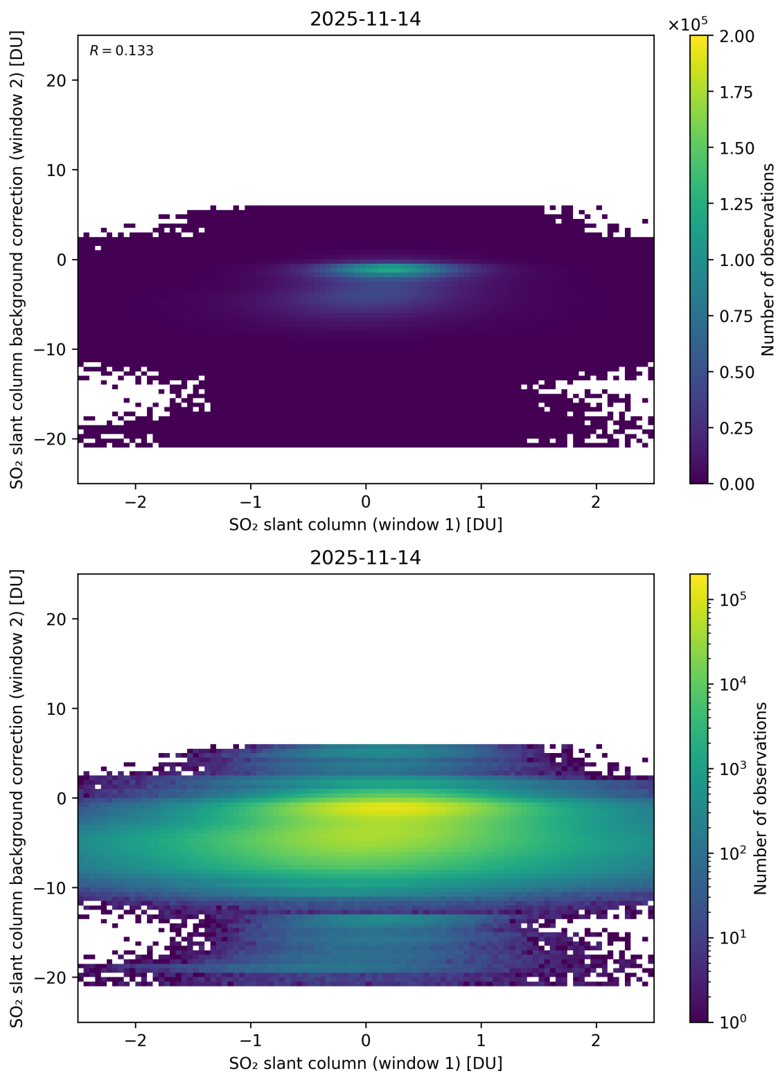
Figure 263: Scatter density plot of “SO 2 slant column (window 1)” against “SO 2 slant column background correction (window 2)” for 2025-11-13 to 2025-11-15.
