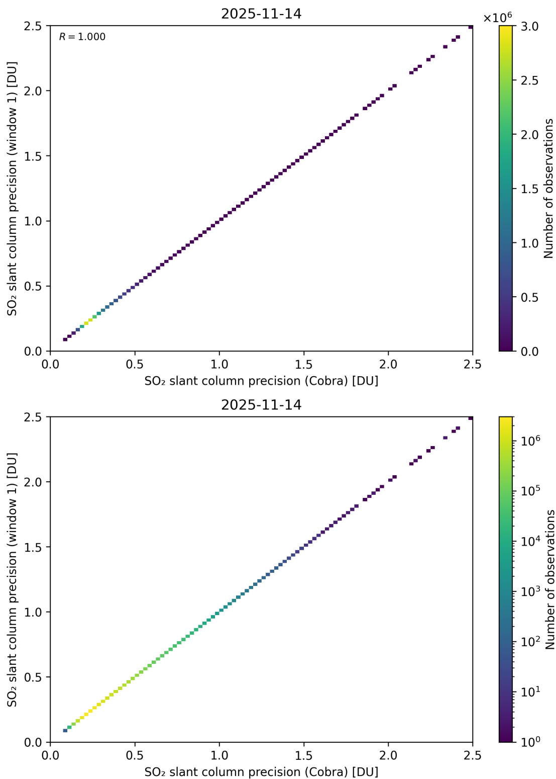
Figure 209: Scatter density plot of “SO 2 slant column precision (Cobra)” against “SO 2 slant column precision (window 1)” for 2025-11-13 to 2025-11-15.
