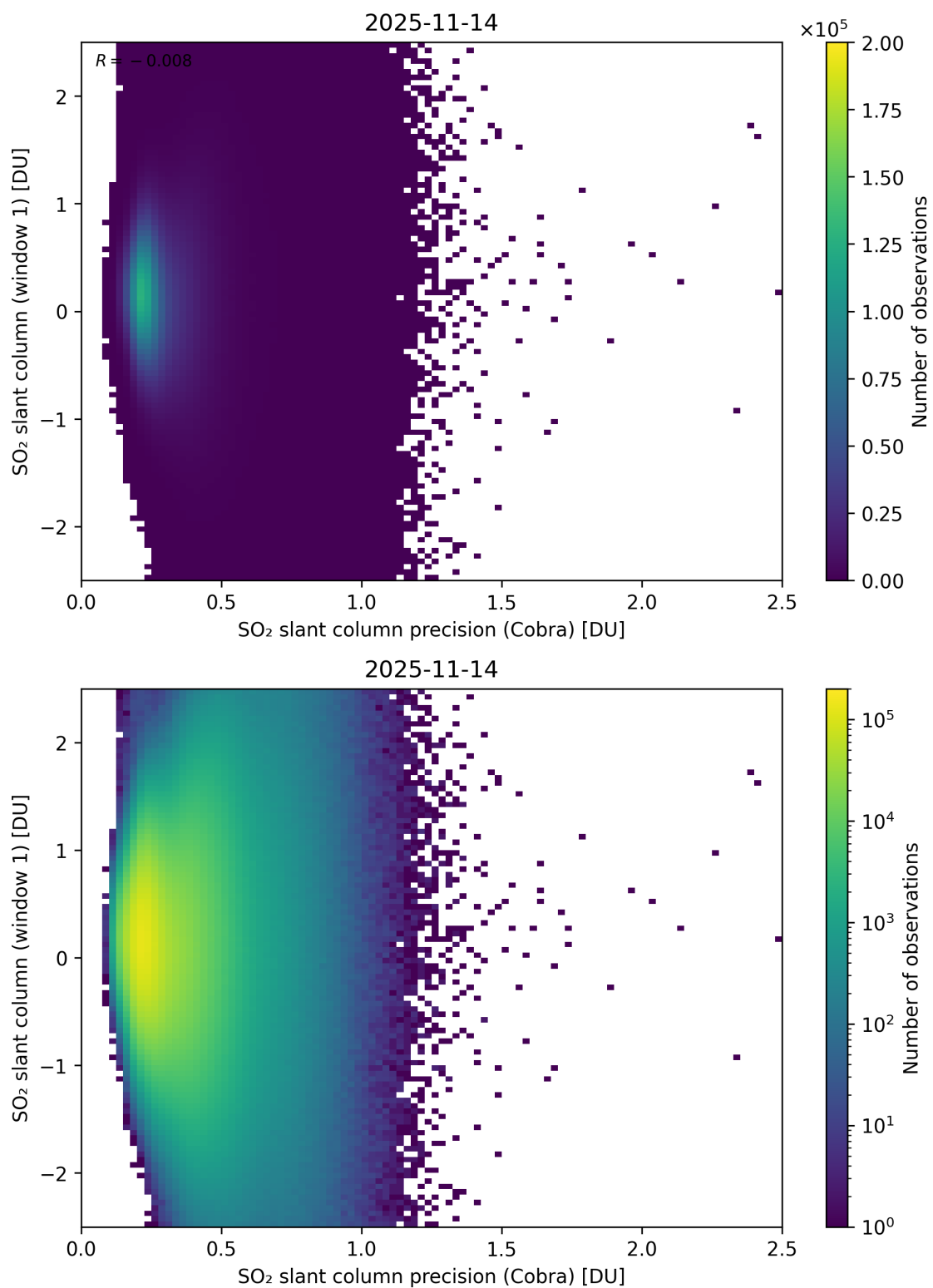
Figure 208: Scatter density plot of “SO 2 slant column precision (Cobra)” against “SO 2 slant column (window 1)” for 2025-11-13 to 2025-11-15.
