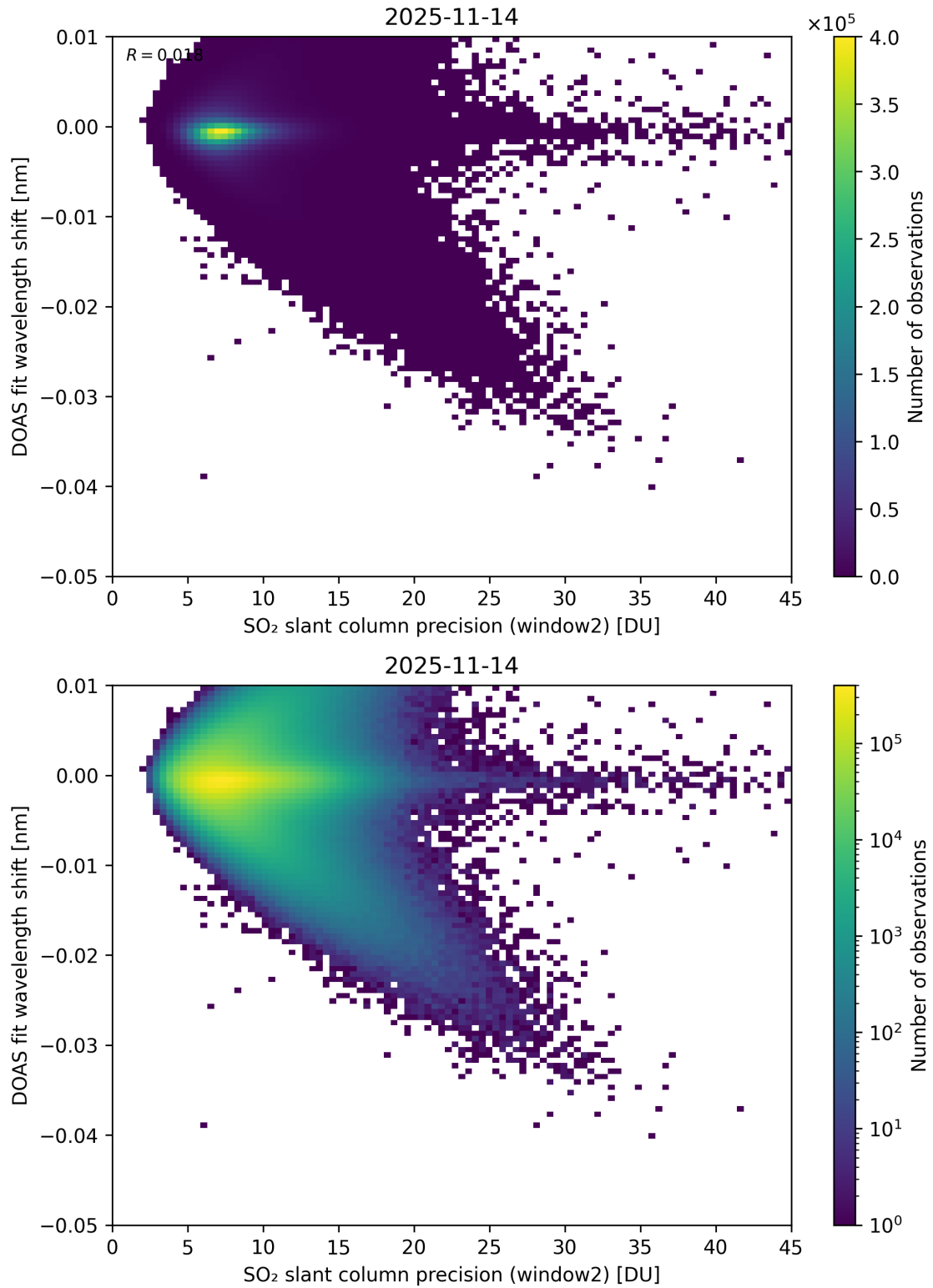
Figure 293: Scatter density plot of “SO 2 slant column precision (window2)” against “DOAS fit wavelength shift” for 2025-11-13 to 2025-11-15.
