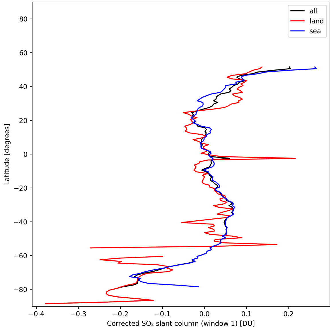
Figure 39: Zonal average of “Corrected SO 2 slant column (window 1)” for 2025-11-13 to 2025-11-15.
