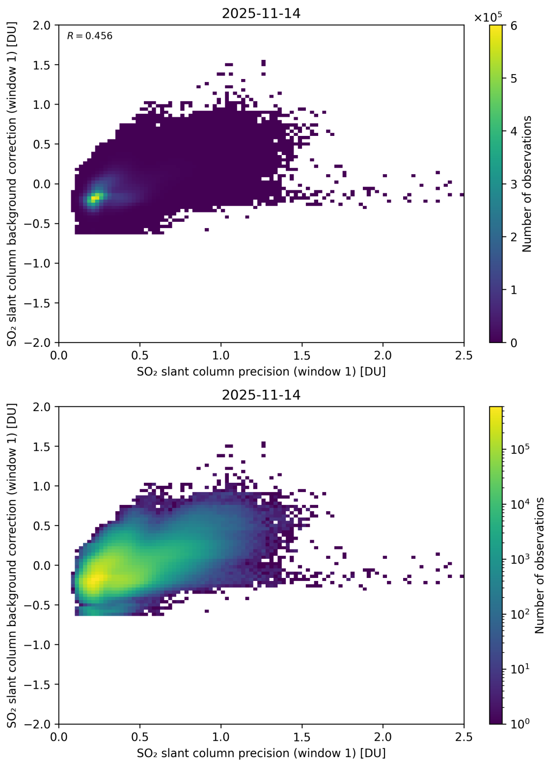
Figure 268: Scatter density plot of “SO 2 slant column precision (window 1)” against “SO 2 slant column background correction (window 1)” for 2025-11-13 to 2025-11-15.
