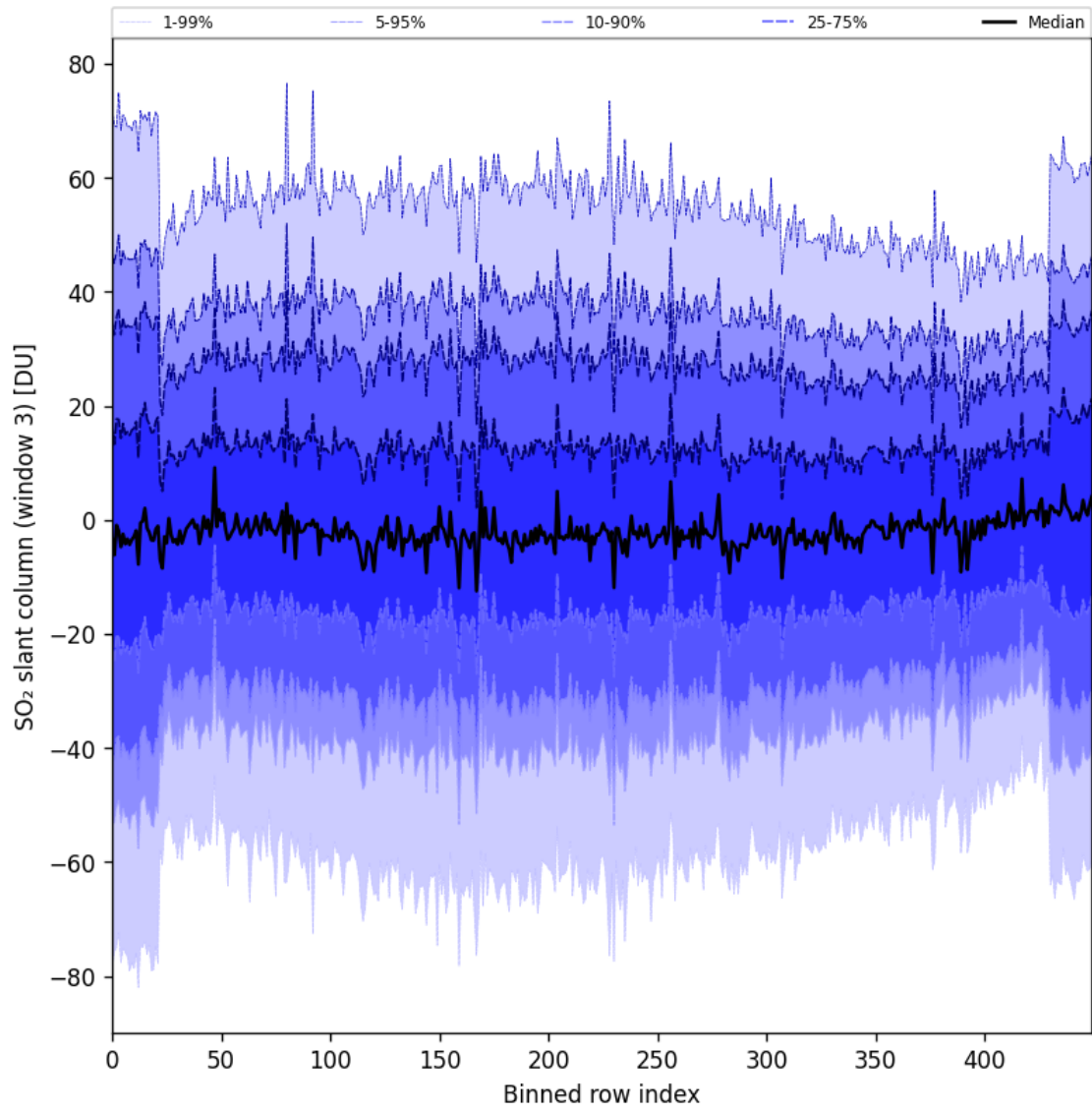
Figure 97: Along track statistics of “SO 2 slant column (window 3)” for 2025-11-13 to 2025-11-15
