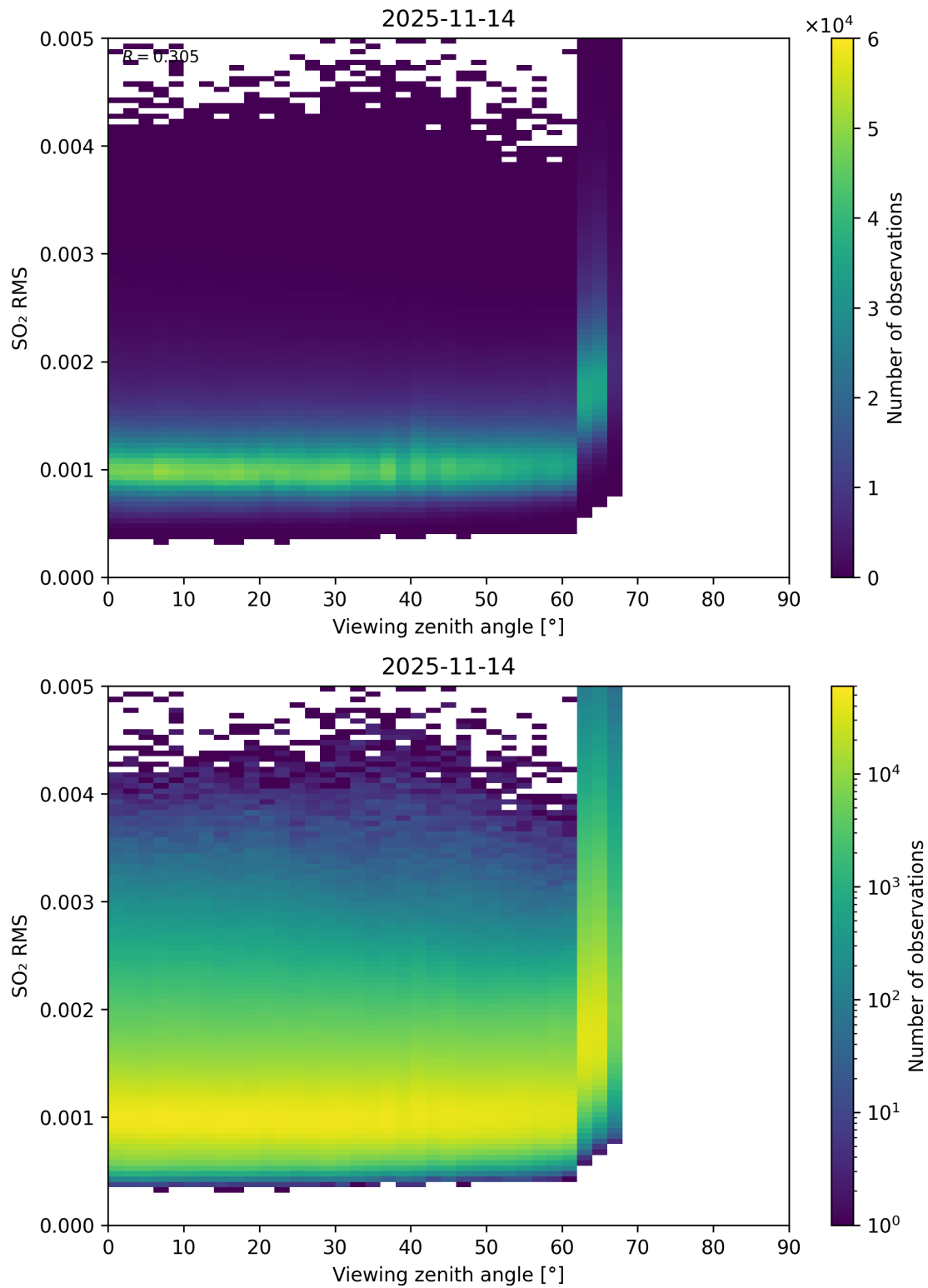
Figure 367: Scatter density plot of “Viewing zenith angle” against “SO 2 RMS” for 2025-11-13 to 2025-11-15.
