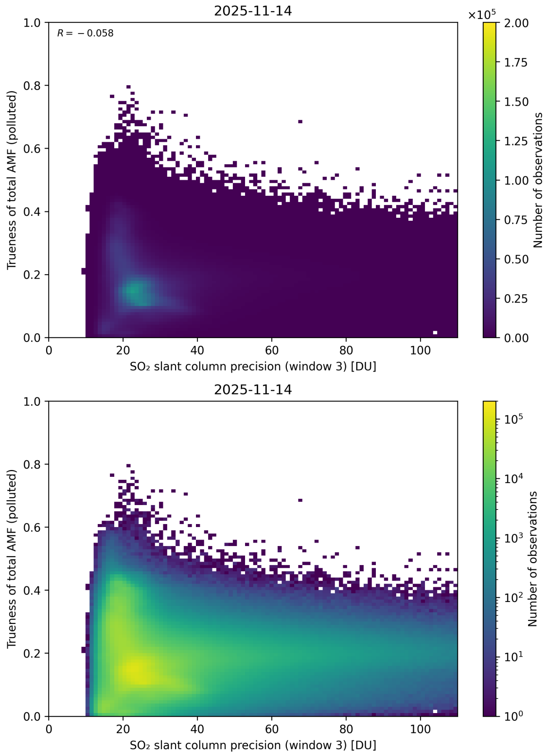
Figure 314: Scatter density plot of “SO 2 slant column precision (window 3)” against “Trueness of total AMF (polluted)” for 2025-11-13 to 2025-11-15.
