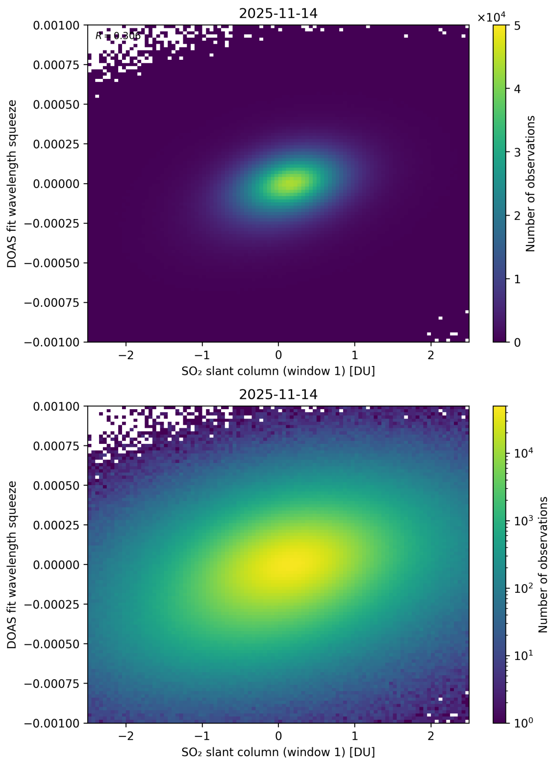
Figure 266: Scatter density plot of “SO 2 slant column (window 1)” against “DOAS fit wavelength squeeze” for 2025-11-13 to 2025-11-15.
