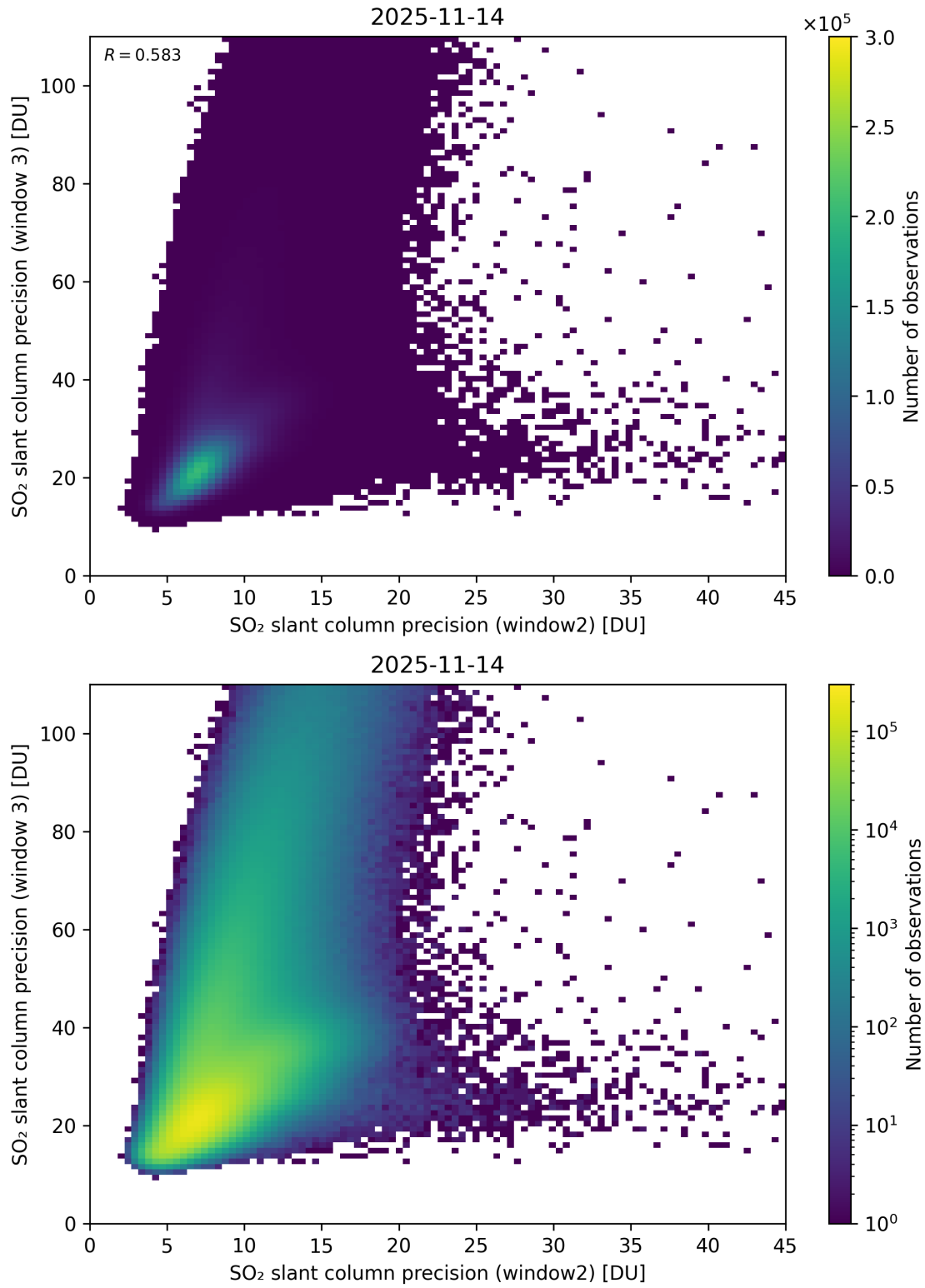
Figure 300: Scatter density plot of “SO 2 slant column precision (window2)” against “SO 2 slant column precision (window 3)” for 2025-11-13 to 2025-11-15.
