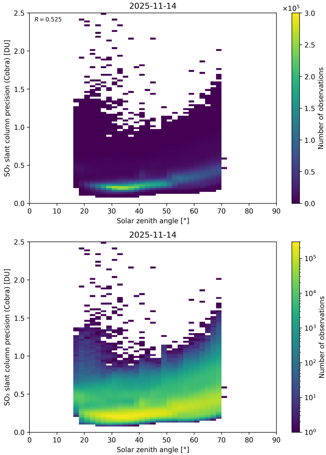
Figure 180: Scatter density plot of “Solar zenith angle” against “SO 2 slant column precision (Cobra)” for 2025-11-13 to 2025-11-15.
