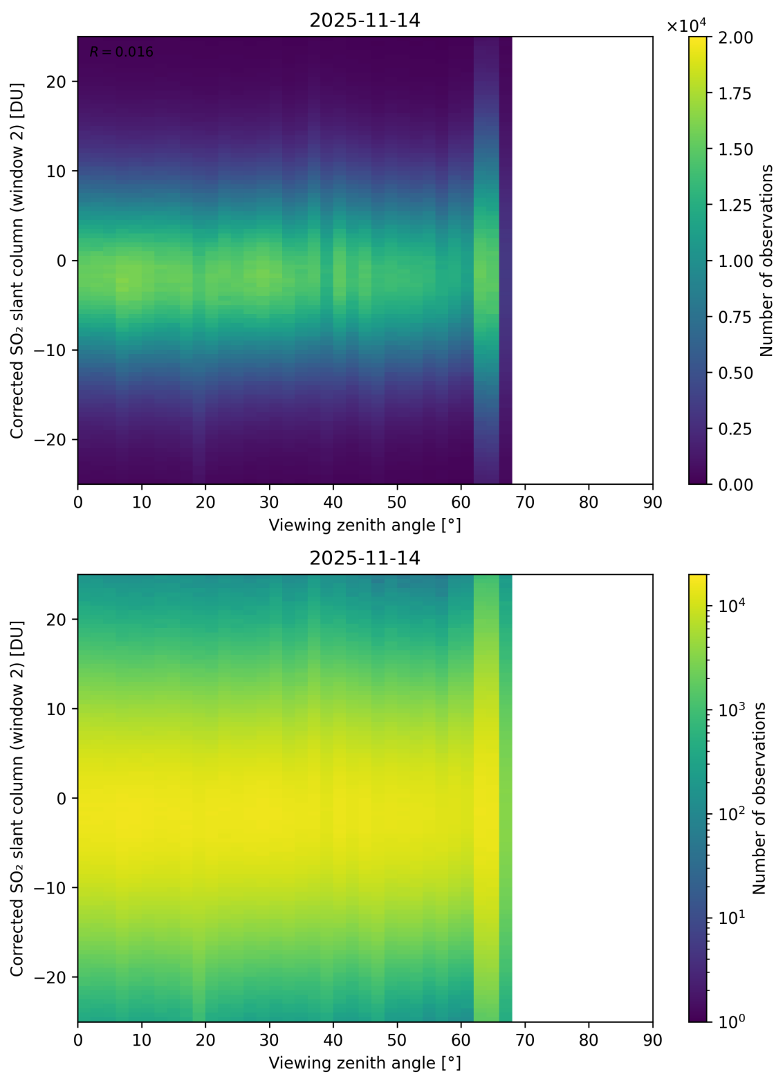
Figure 374: Scatter density plot of “Viewing zenith angle” against “Corrected SO 2 slant column (window 2)” for 2025-11-13 to 2025-11-15.
