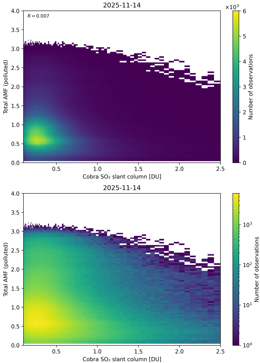
Figure 224: Scatter density plot of “Cobra SO 2 slant column” against “Total AMF (polluted)” for 2025-11-13 to 2025-11-15.
