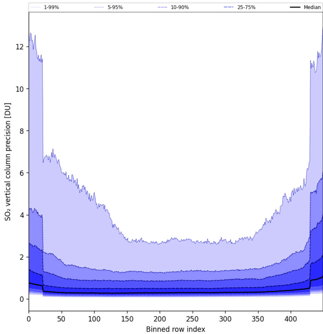
Figure 85: Along track statistics of "SO 2 vertical column precision" for 2025-11-13 to 2025-11-15
