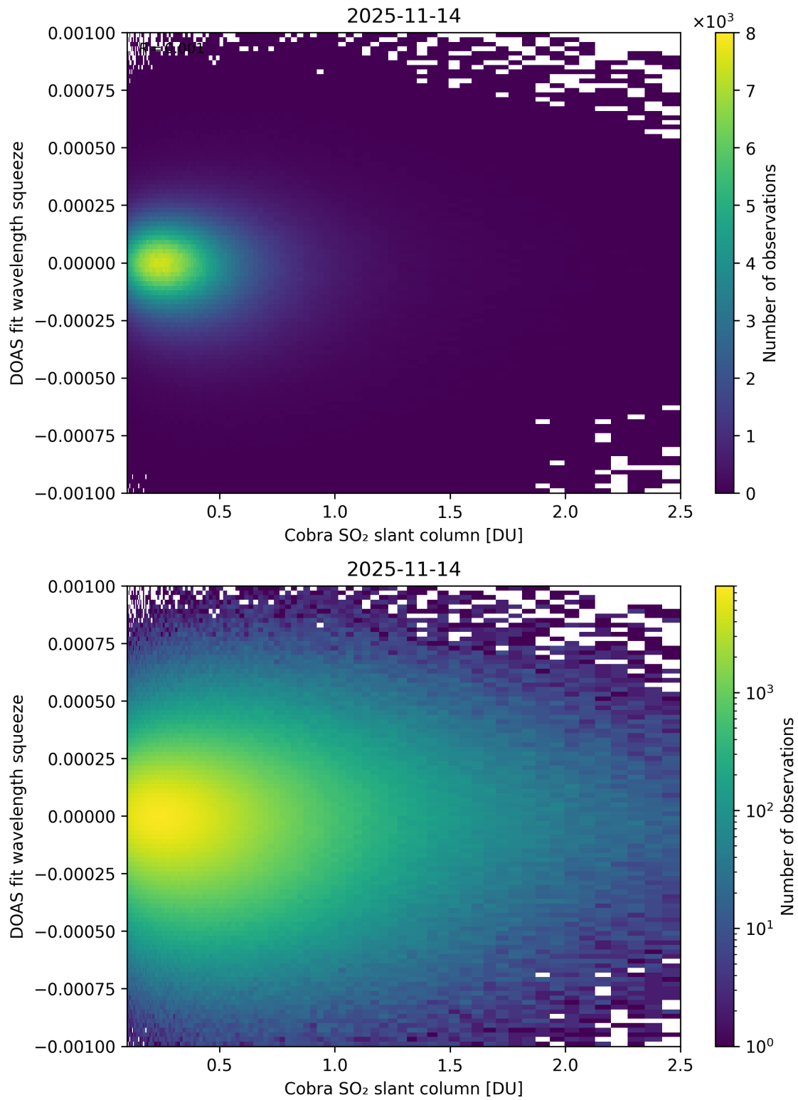
Figure 197: Scatter density plot of “Cobra SO 2 slant column” against “DOAS fit wavelength squeeze” for 2025-11-13 to 2025-11-15.
