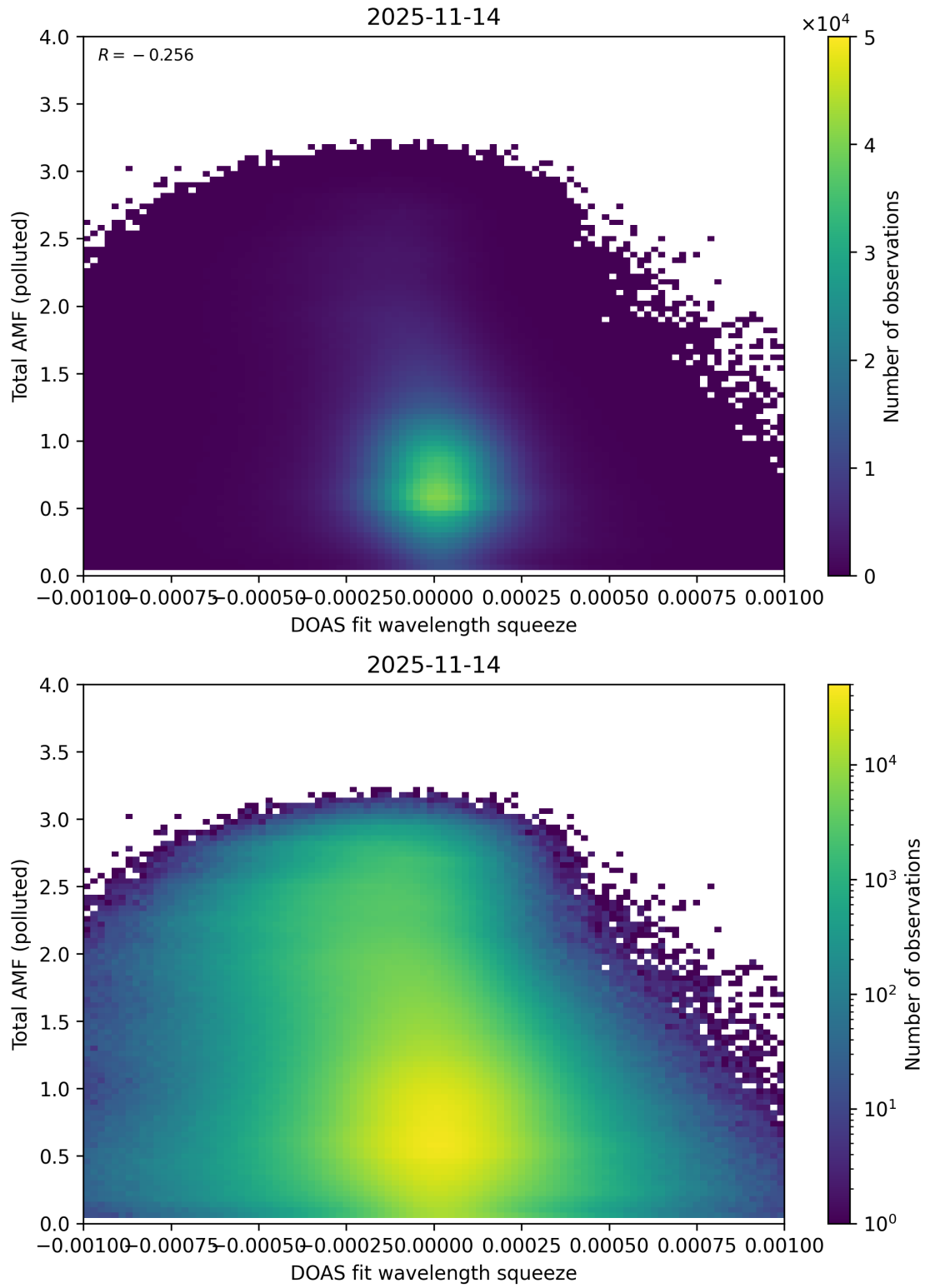
Figure 145: Scatter density plot of “DOAS fit wavelength squeeze” against “Total AMF (polluted)” for 2025-11-13 to 2025-11-15.
