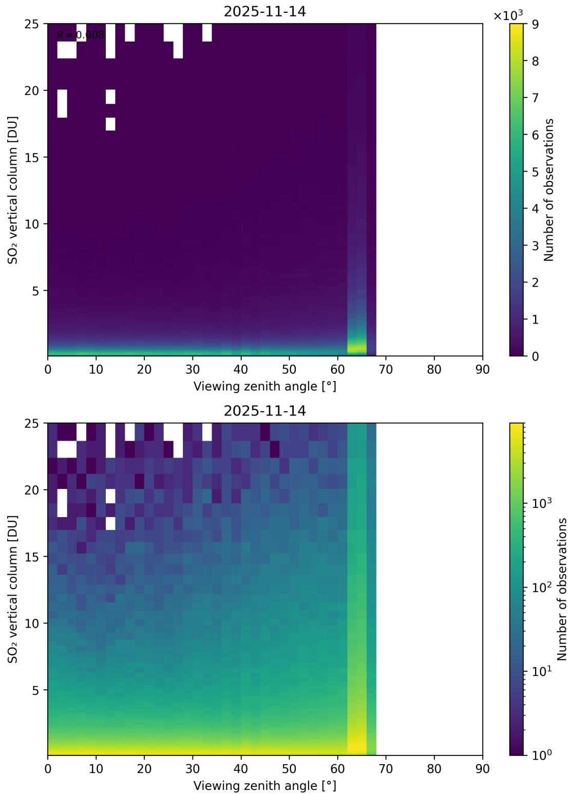
Figure 383: Scatter density plot of “Viewing zenith angle” against “SO 2 vertical column” for 2025-11-13 to 2025-11-15.
