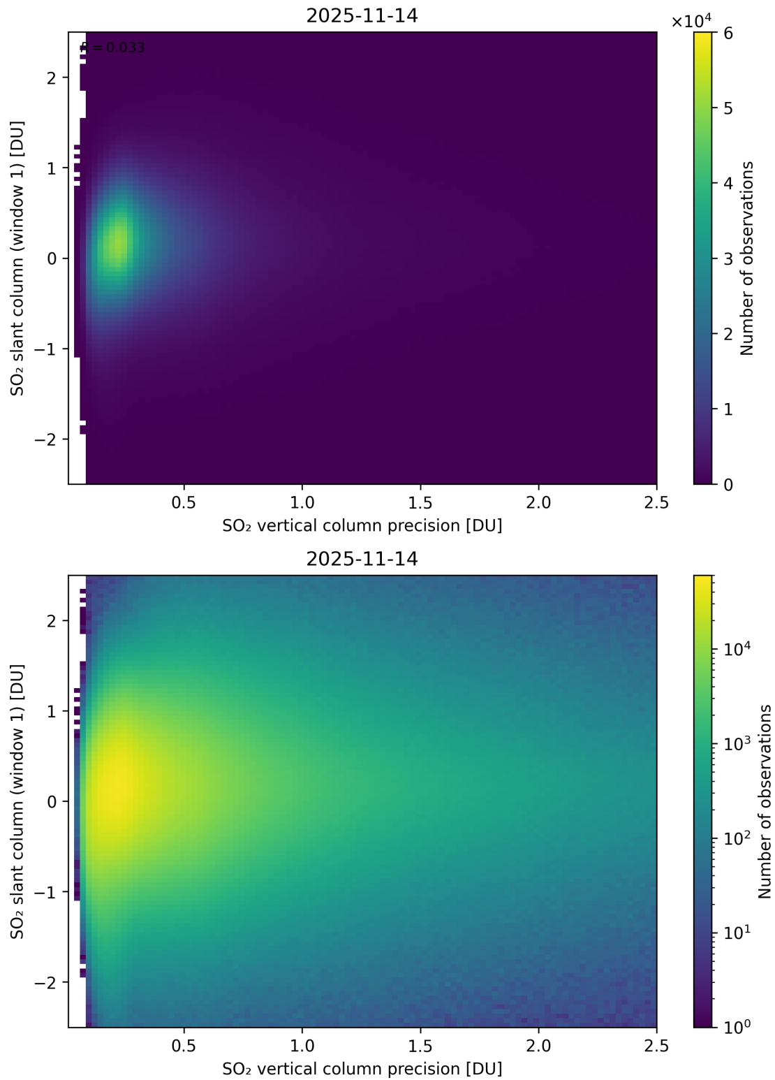
Figure 341: Scatter density plot of “SO 2 vertical column precision” against “SO 2 slant column (window 1)” for 2025-11-13 to 2025-11-15.
