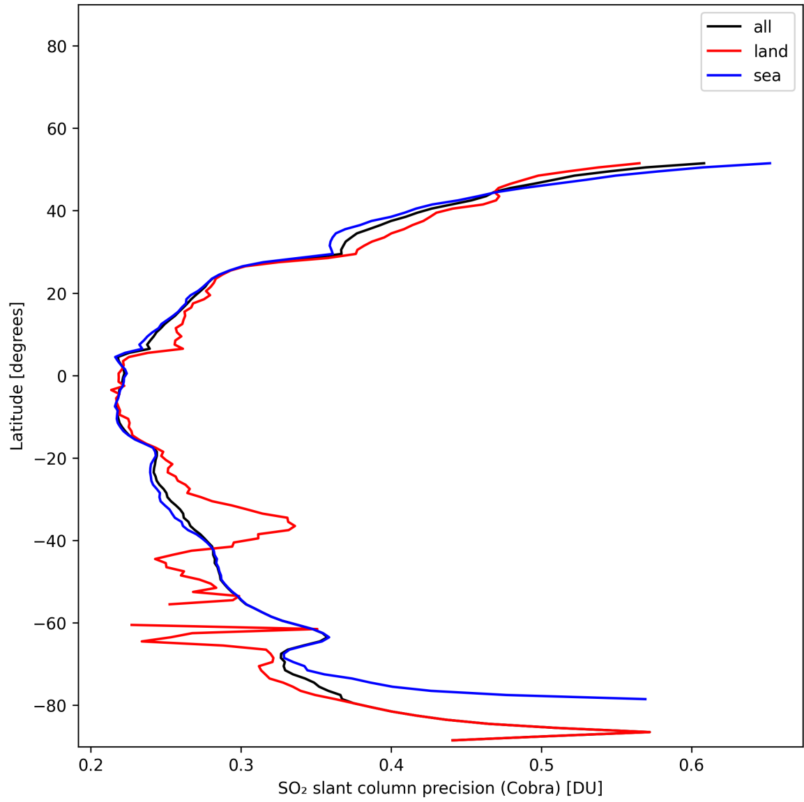
Figure 36: Zonal average of “SO 2 slant column precision (Cobra)” for 2025-11-13 to 2025-11-15.
