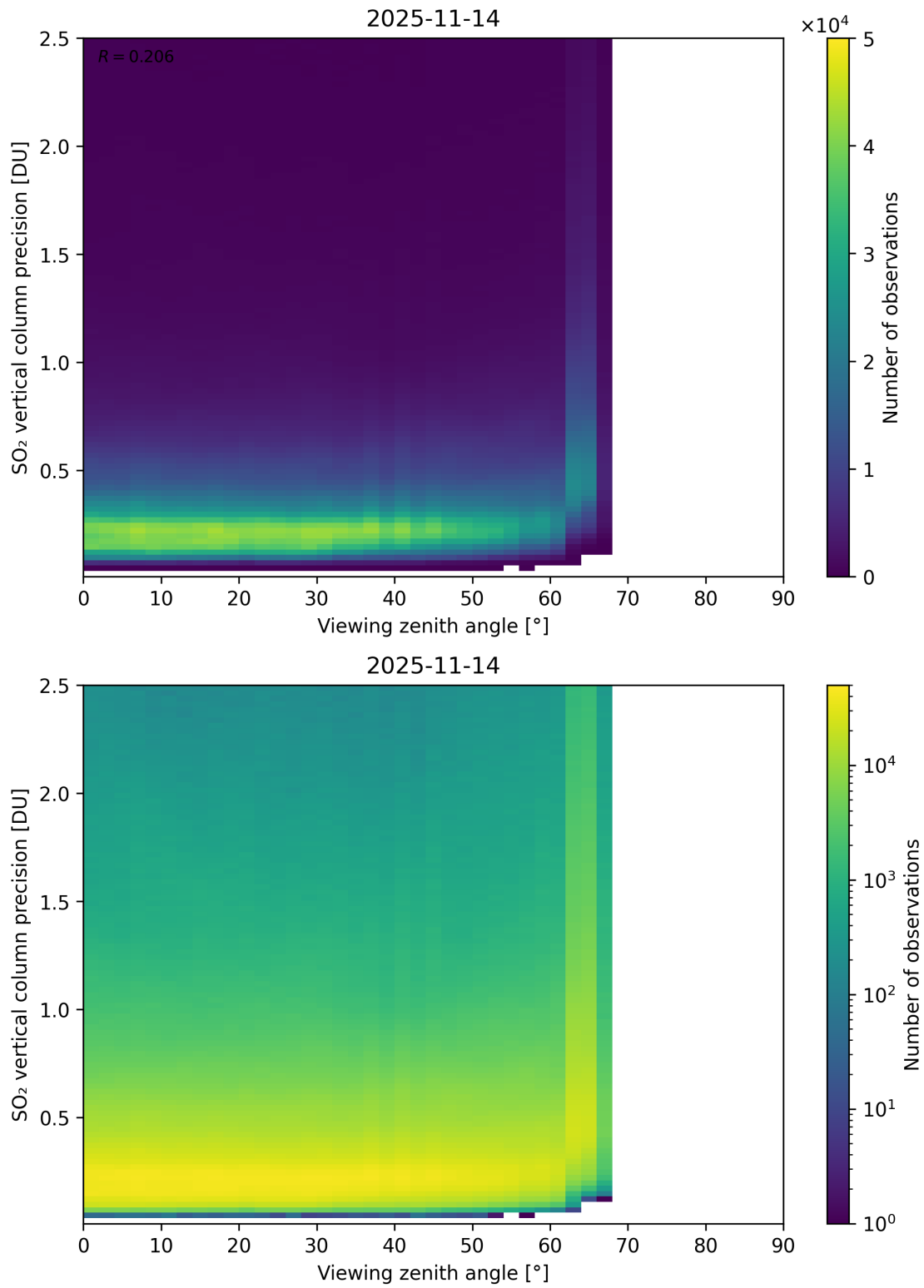
Figure 384: Scatter density plot of “Viewing zenith angle” against “SO 2 vertical column precision” for 2025-11-13 to 2025-11-15.
