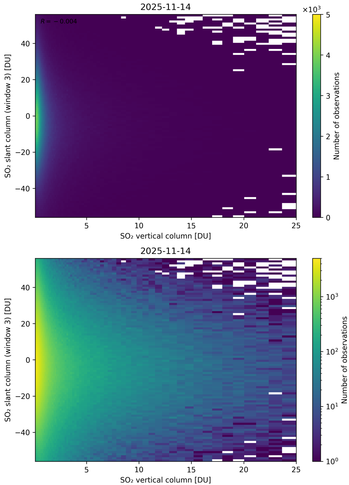
Figure 357: Scatter density plot of “SO 2 vertical column” against “SO 2 slant column (window 3)” for 2025-11-13 to 2025-11-15.
