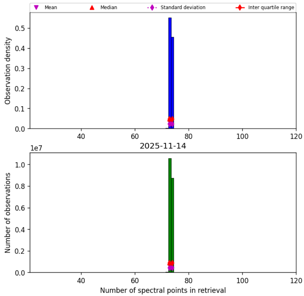
Figure 82: Histogram of “Number of spectral points in retrieval” for 2025-11-13 to 2025-11-15
