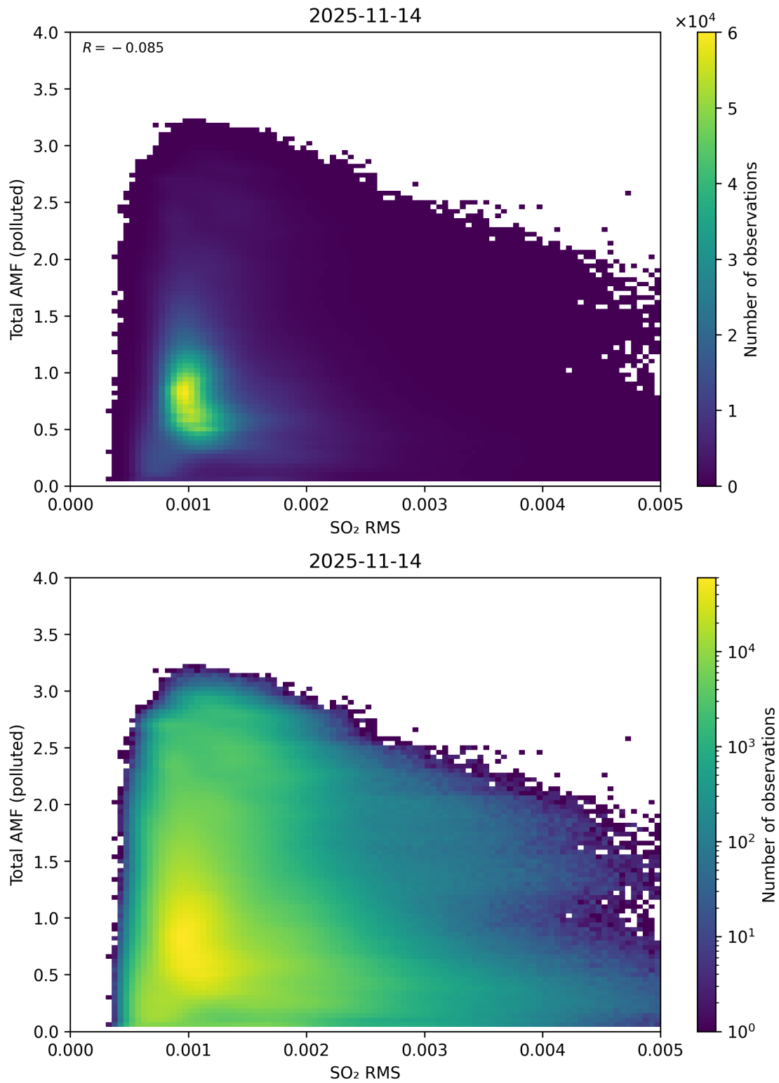
Figure 148: Scatter density plot of “SO 2 RMS” against “Total AMF (polluted)” for 2025-11-13 to 2025-11-15.
