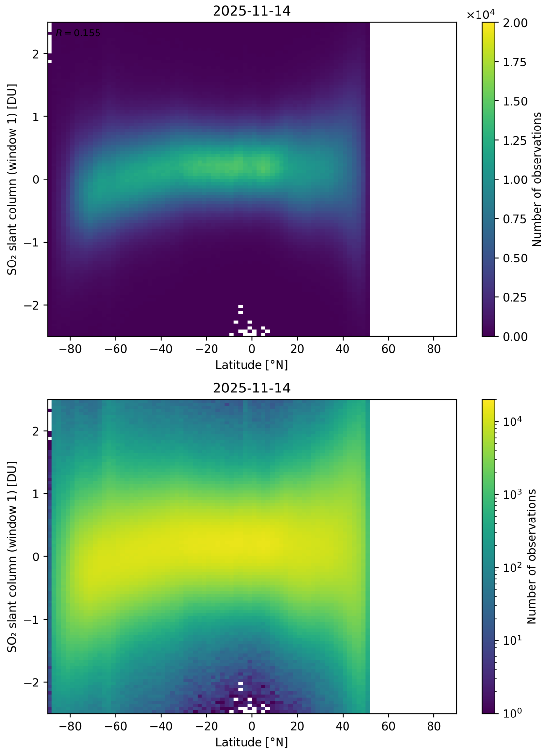
Figure 162: Scatter density plot of “Latitude” against “SO 2 slant column (window 1)” for 2025-11-13 to 2025-11-15.
