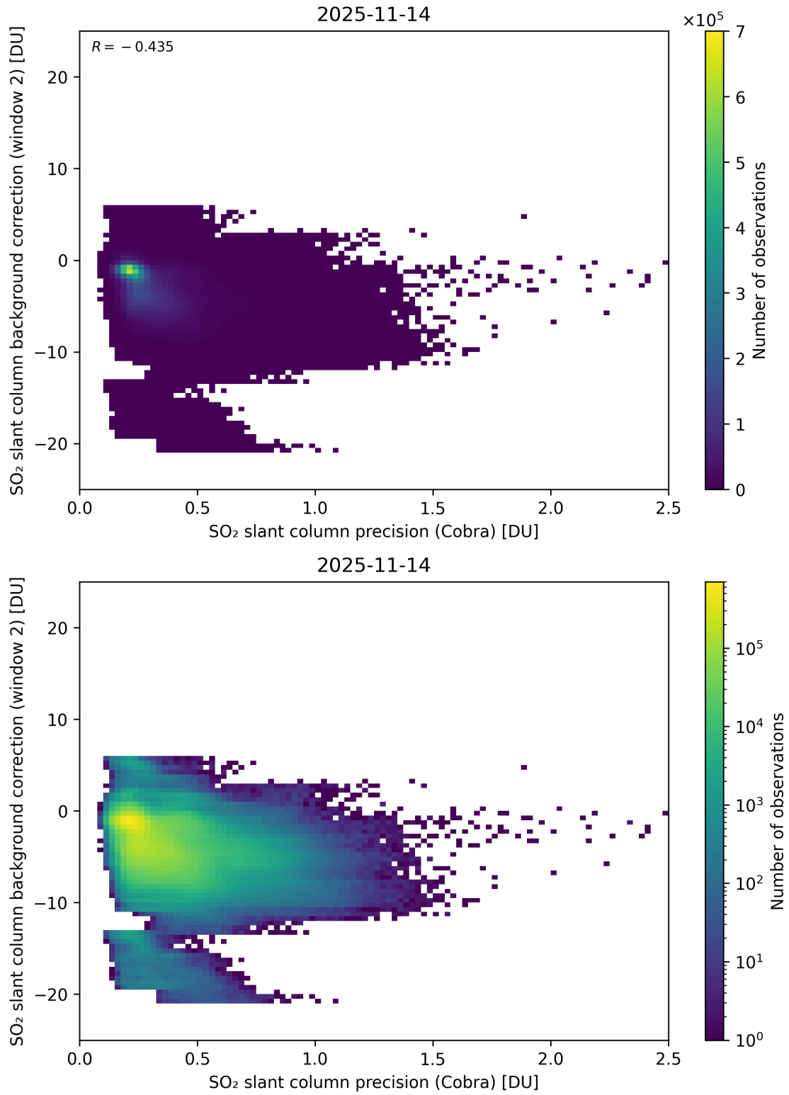
Figure 200: Scatter density plot of “SO 2 slant column precision (Cobra)” against “SO 2 slant column background correction (window 2)” for 2025-11-13 to 2025-11-15.
