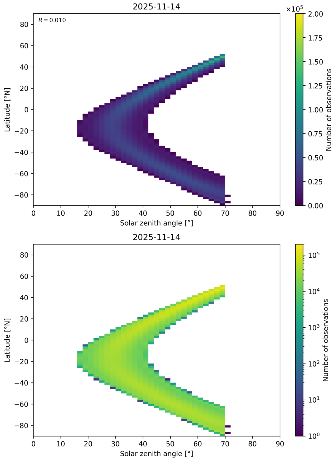
Figure 177: Scatter density plot of “Solar zenith angle” against “Latitude” for 2025-11-13 to 2025-11-15.
