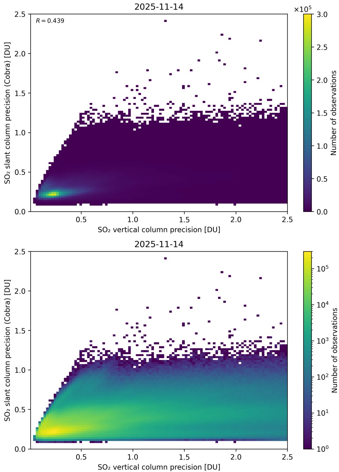
Figure 337: Scatter density plot of “SO 2 vertical column precision” against “SO 2 slant column precision (Cobra)” for 2025-11-13 to 2025-11-15.
