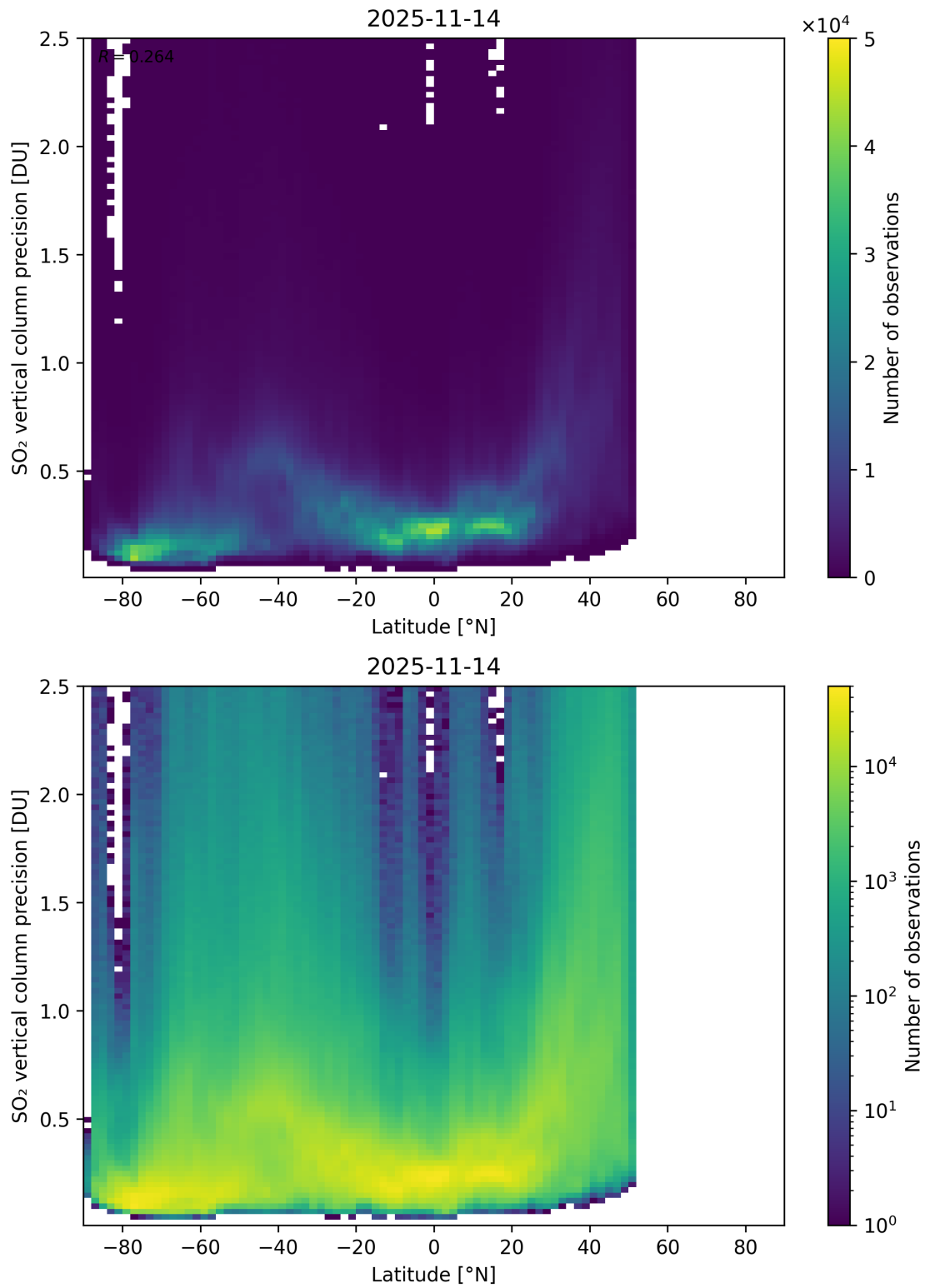
Figure 170: Scatter density plot of “Latitude” against “SO 2 vertical column precision” for 2025-11-13 to 2025-11-15.
