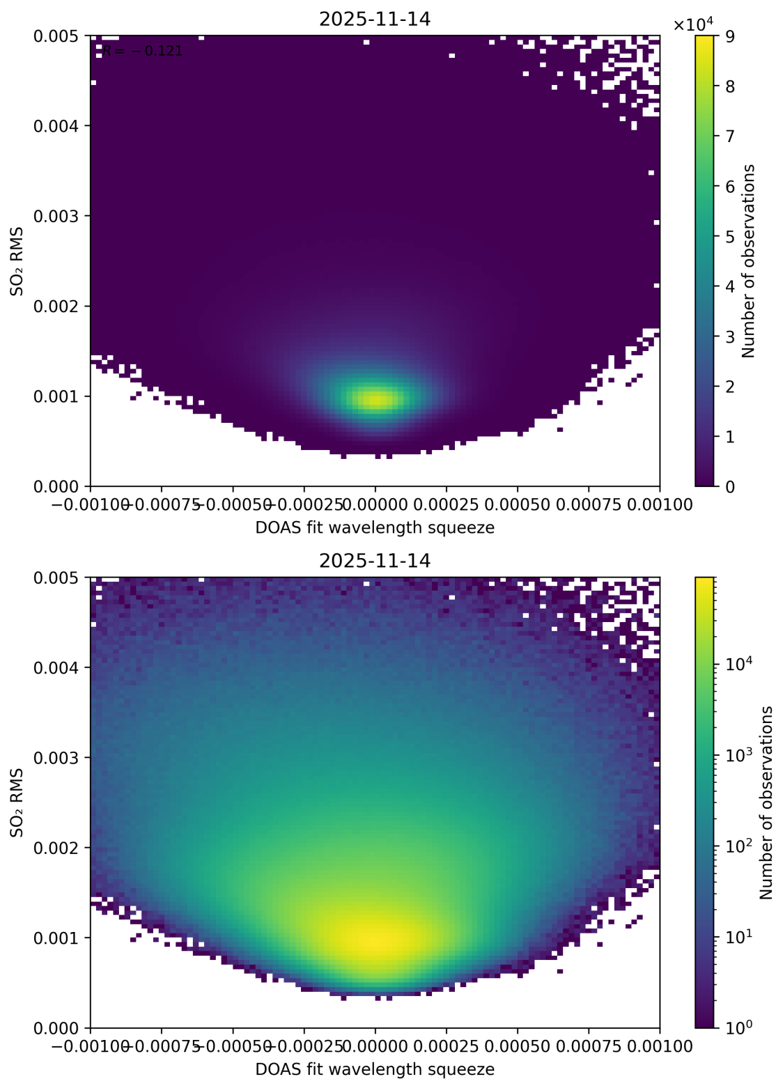
Figure 143: Scatter density plot of “DOAS fit wavelength squeeze” against “SO 2 RMS” for 2025-11-13 to 2025-11-15.
