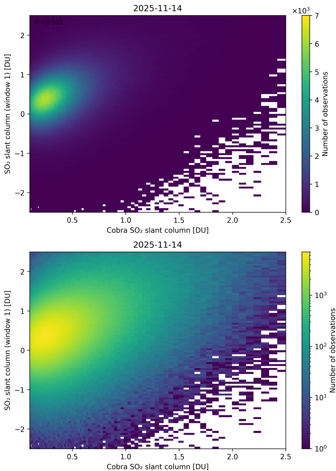
Figure 219: Scatter density plot of “Cobra SO 2 slant column” against “SO 2 slant column (window 1)” for 2025-11-13 to 2025-11-15.
