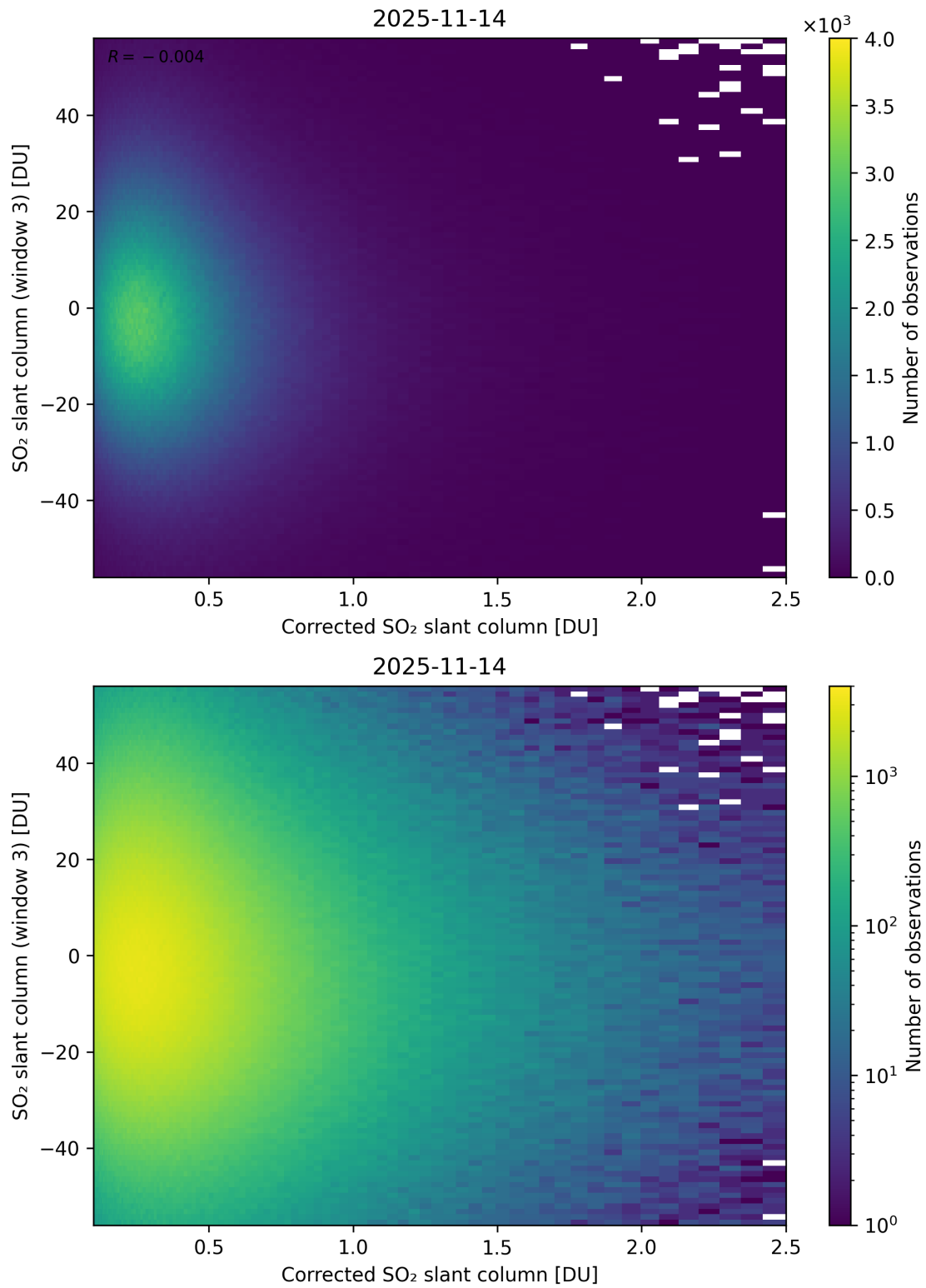
Figure 240: Scatter density plot of “Corrected SO 2 slant column” against “SO 2 slant column (window 3)” for 2025-11-13 to 2025-11-15.
