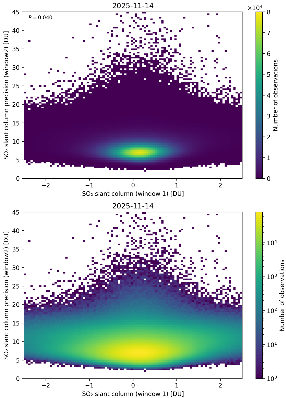
Figure 286: Scatter density plot of “SO 2 slant column (window 1)” against “SO 2 slant column precision (window2)” for 2025-11-13 to 2025-11-15.
