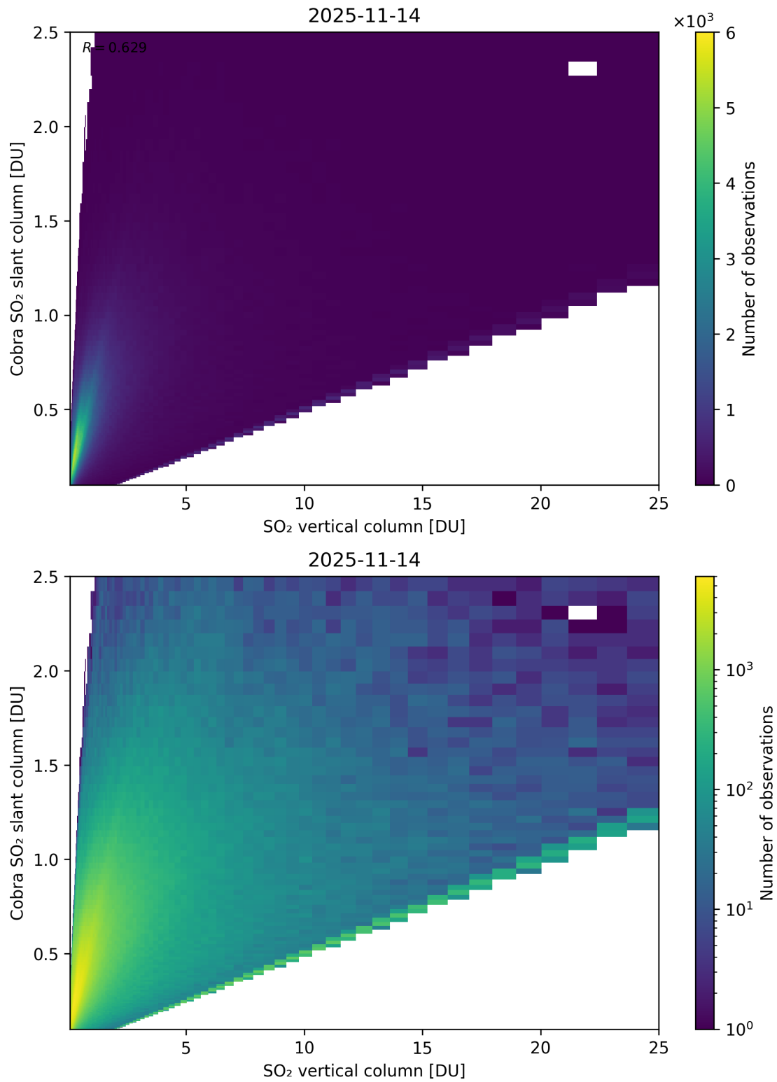
Figure 349: Scatter density plot of “SO 2 vertical column” against “Cobra SO 2 slant column” for 2025-11-13 to 2025-11-15.
