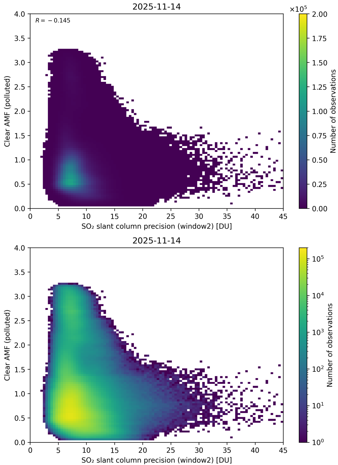
Figure 296: Scatter density plot of “SO 2 slant column precision (window2)” against “Clear AMF (polluted)” for 2025-11-13 to 2025-11-15.
