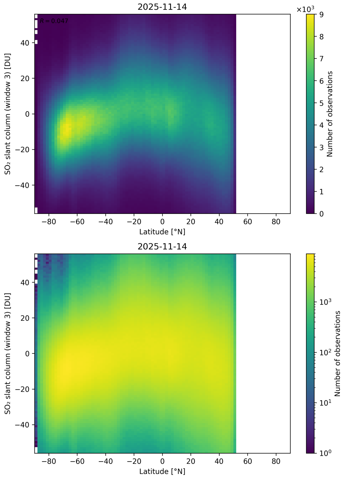
Figure 165: Scatter density plot of “Latitude” against “SO 2 slant column (window 3)” for 2025-11-13 to 2025-11-15.
