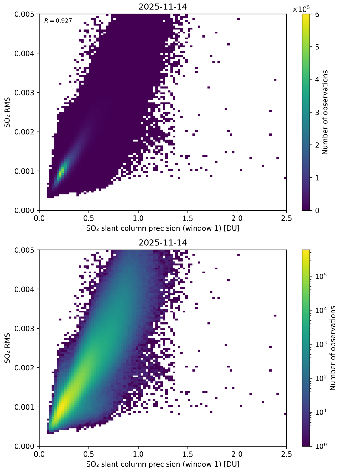
Figure 273: Scatter density plot of “SO 2 slant column precision (window 1)” against “SO 2 RMS” for 2025-11-13 to 2025-11-15.
