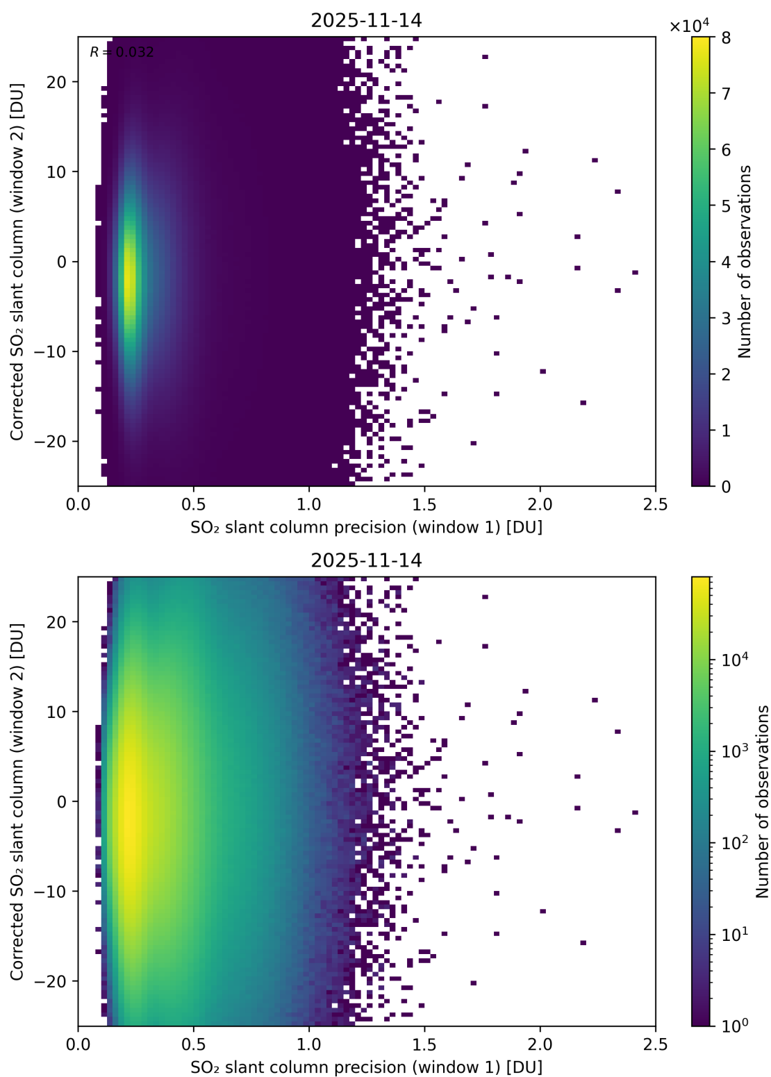
Figure 275: Scatter density plot of “SO 2 slant column precision (window 1)” against “Corrected SO 2 slant column (window 2)” for 2025-11-13 to 2025-11-15.
