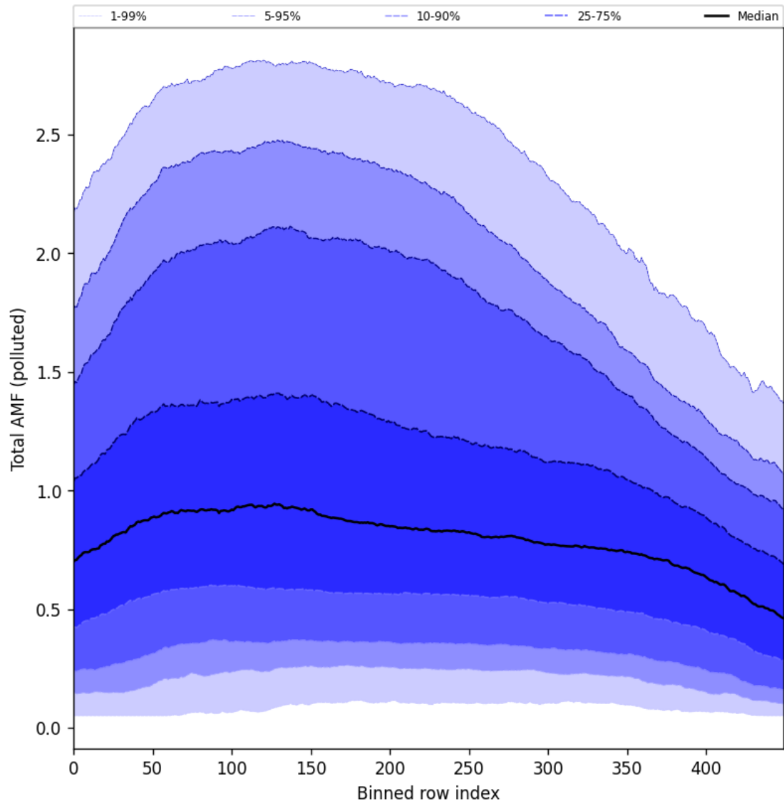
Figure 105: Along track statistics of “Total AMF (polluted)” for 2025-11-13 to 2025-11-15
