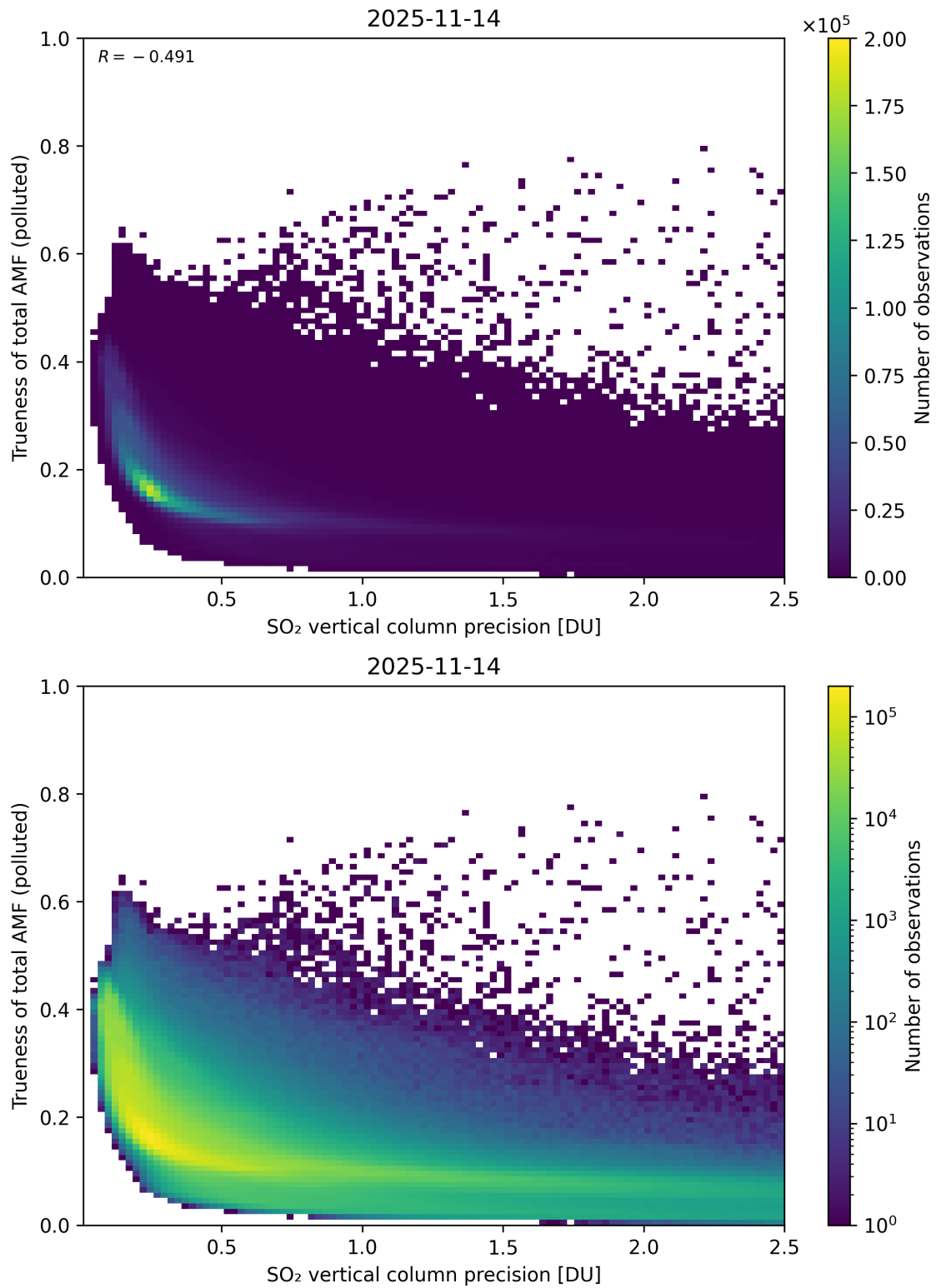
Figure 347: Scatter density plot of “SO 2 vertical column precision” against “Trueness of total AMF (polluted)” for 2025-11-13 to 2025-11-15.
