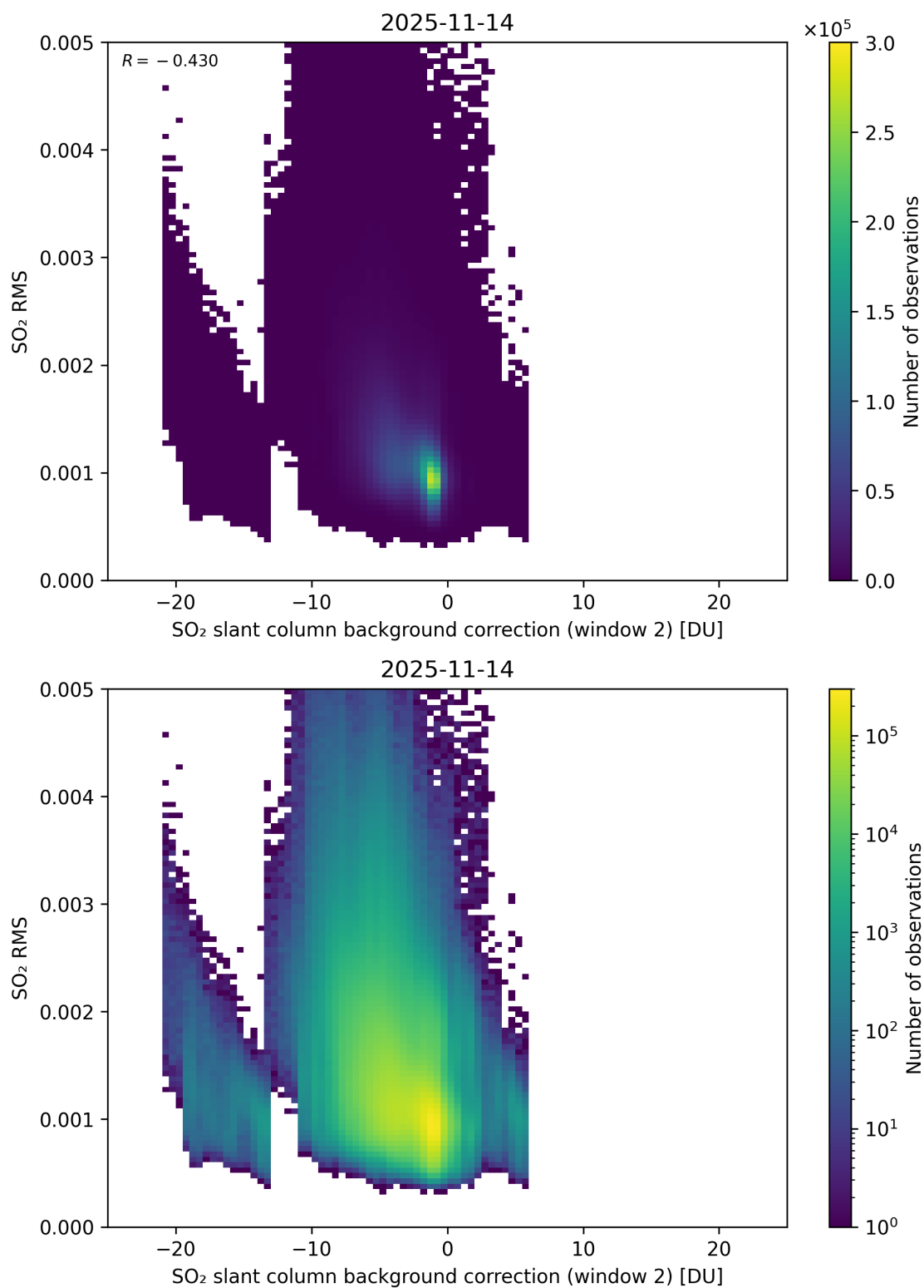
Figure 125: Scatter density plot of “SO 2 slant column background correction (window 2)” against “SO 2 RMS” for 2025-11-13 to 2025-11-15.
