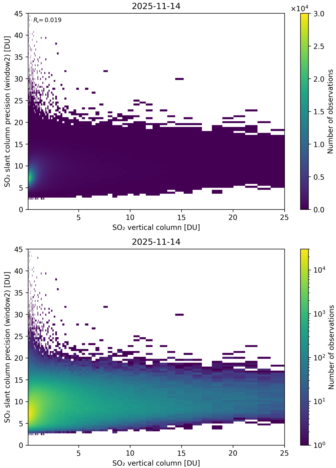
Figure 356: Scatter density plot of “SO 2 vertical column” against “SO 2 slant column precision (window2)” for 2025-11-13 to 2025-11-15.
