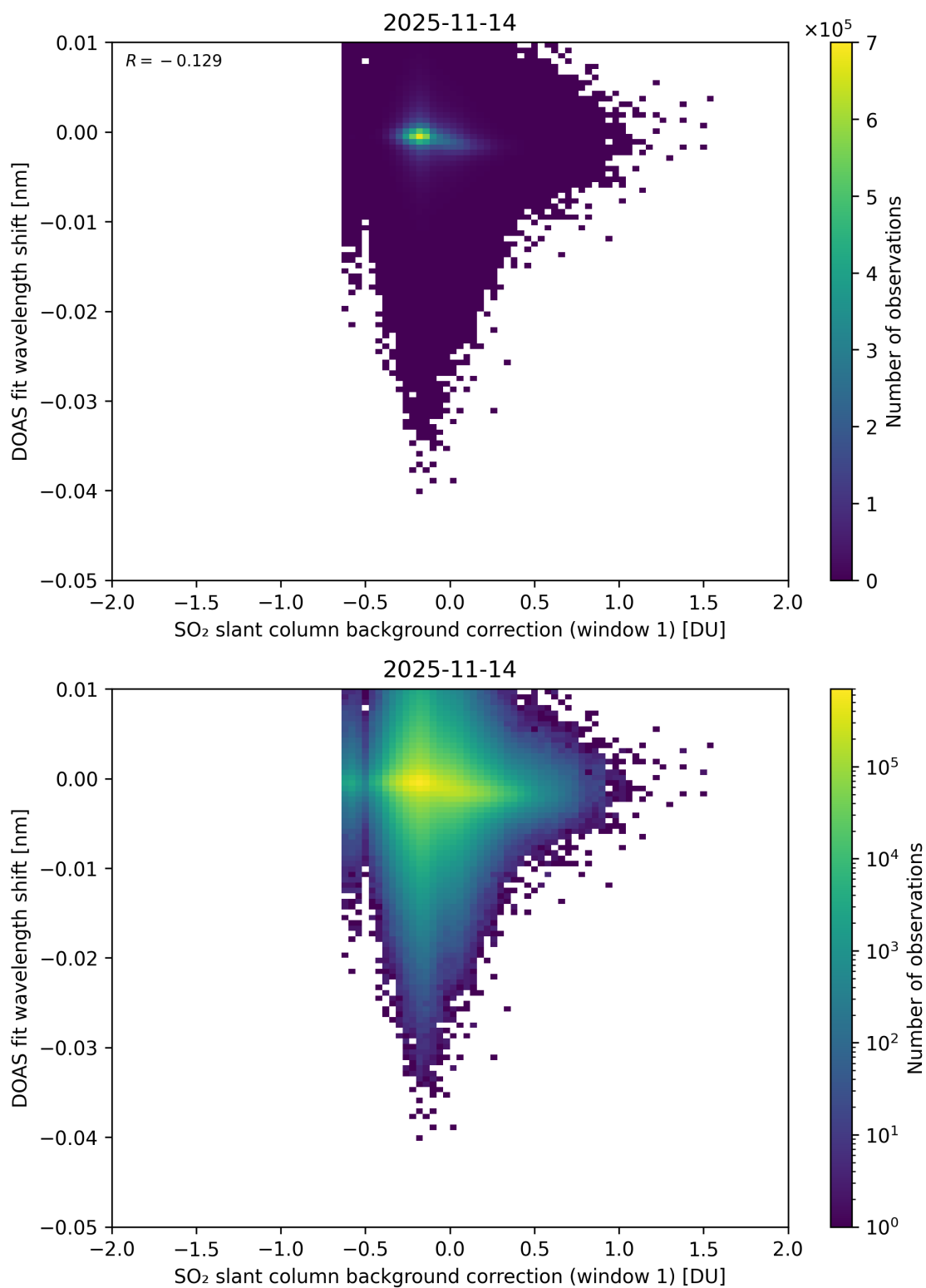
Figure 111: Scatter density plot of “SO 2 slant column background correction (window 1)” against “DOAS fit wavelength shift” for 2025-11-13 to 2025-11-15.
