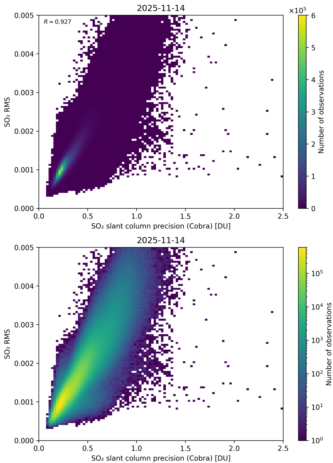
Figure 204: Scatter density plot of “SO 2 slant column precision (Cobra)” against “SO 2 RMS” for 2025-11-13 to 2025-11-15.
