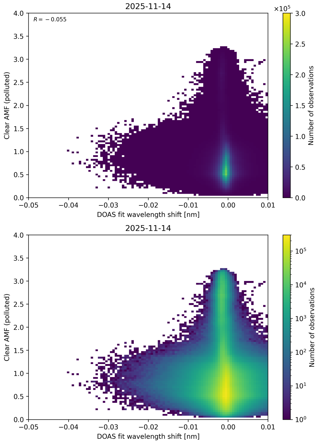
Figure 140: Scatter density plot of “DOAS fit wavelength shift” against “Clear AMF (polluted)” for 2025-11-13 to 2025-11-15.
