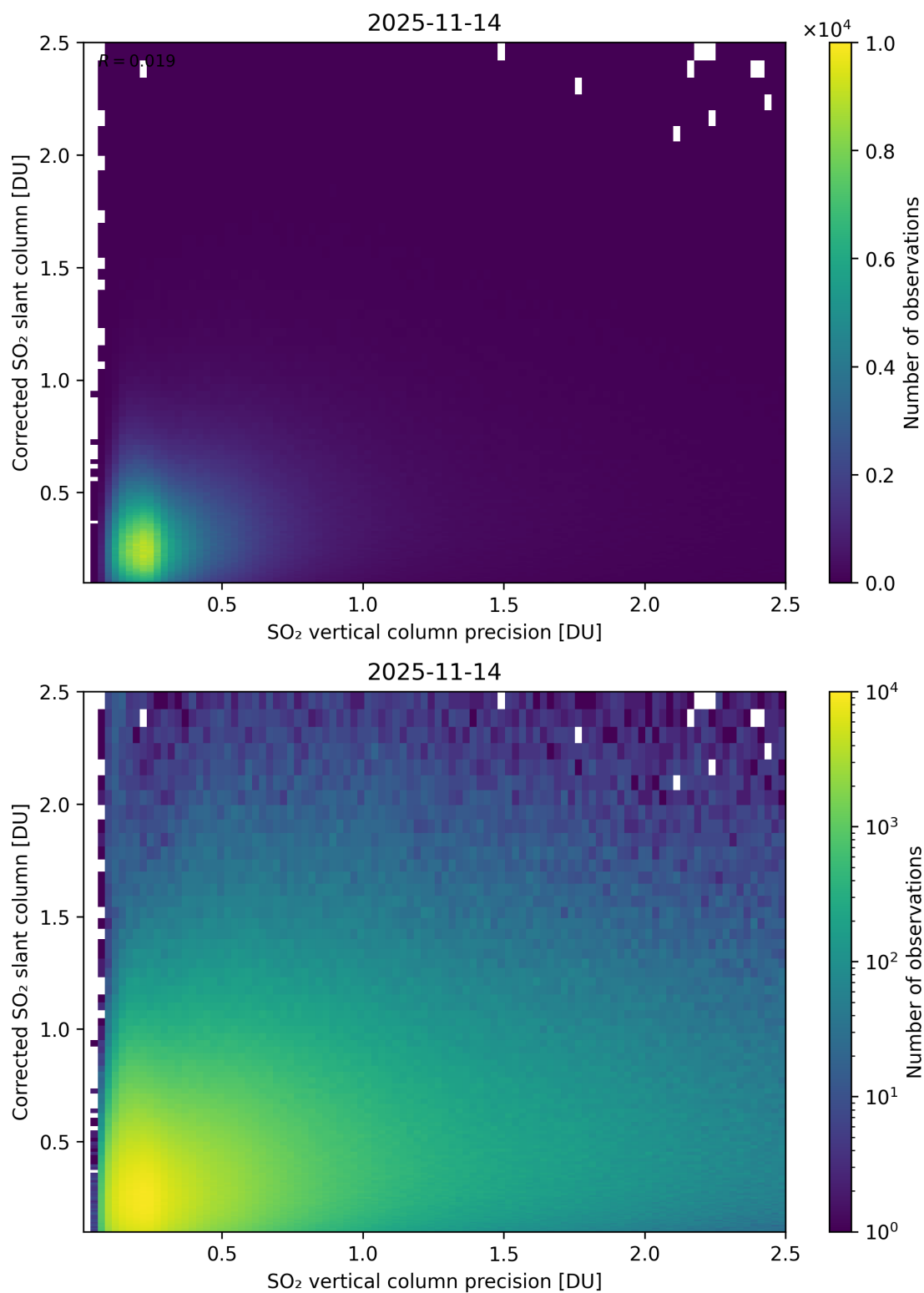
Figure 338: Scatter density plot of “SO 2 vertical column precision” against “Corrected SO 2 slant column” for 2025-11-13 to 2025-11-15.
