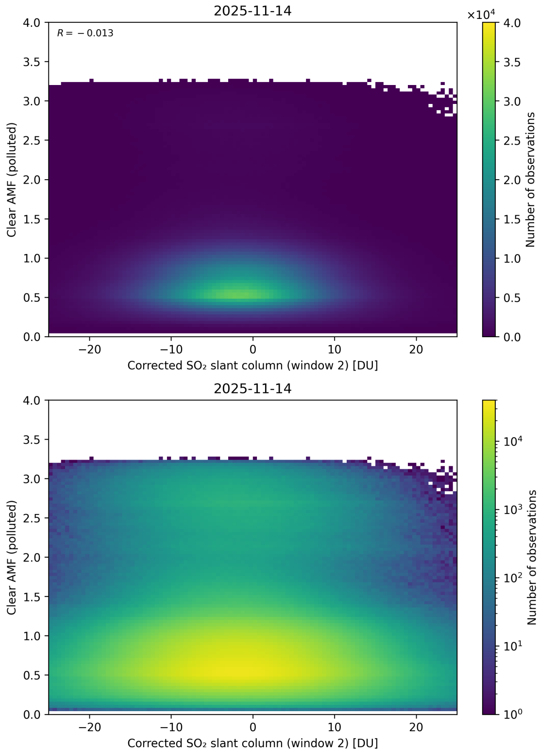
Figure 249: Scatter density plot of “Corrected SO 2 slant column (window 2)” against “Clear AMF (polluted)” for 2025-11-13 to 2025-11-15.
