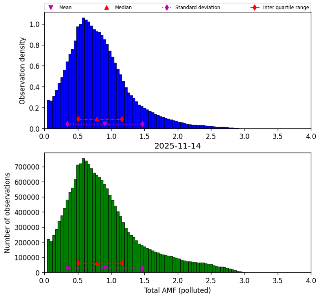
Figure 79: Histogram of “Total AMF (polluted)” for 2025-11-13 to 2025-11-15
