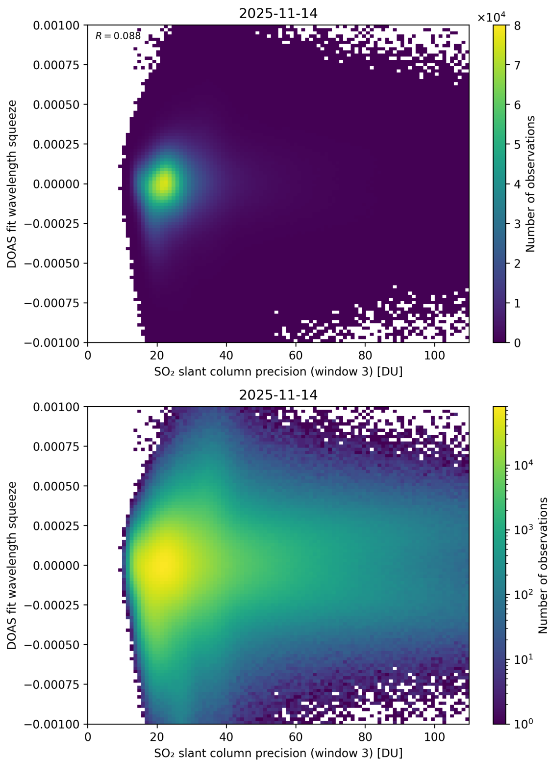
Figure 309: Scatter density plot of “SO 2 slant column precision (window 3)” against “DOAS fit wavelength squeeze” for 2025-11-13 to 2025-11-15.
