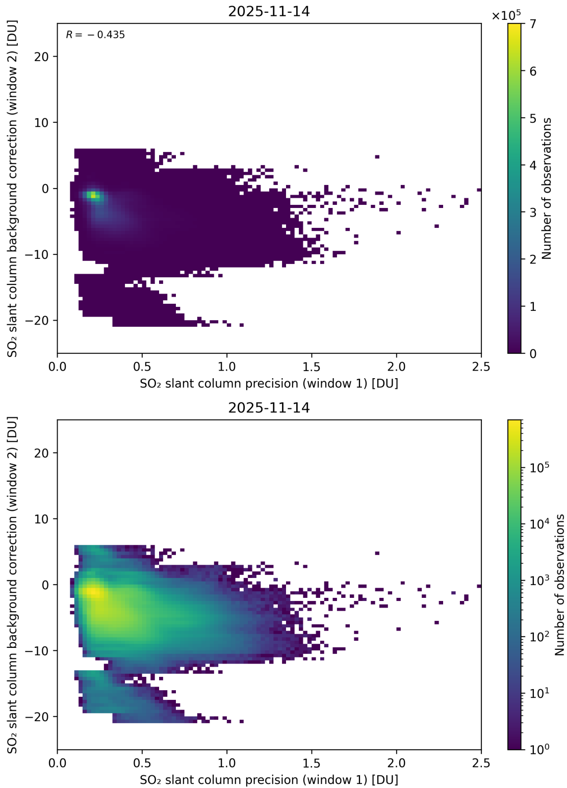
Figure 269: Scatter density plot of “SO 2 slant column precision (window 1)” against “SO 2 slant column background correction (window 2)” for 2025-11-13 to 2025-11-15.
