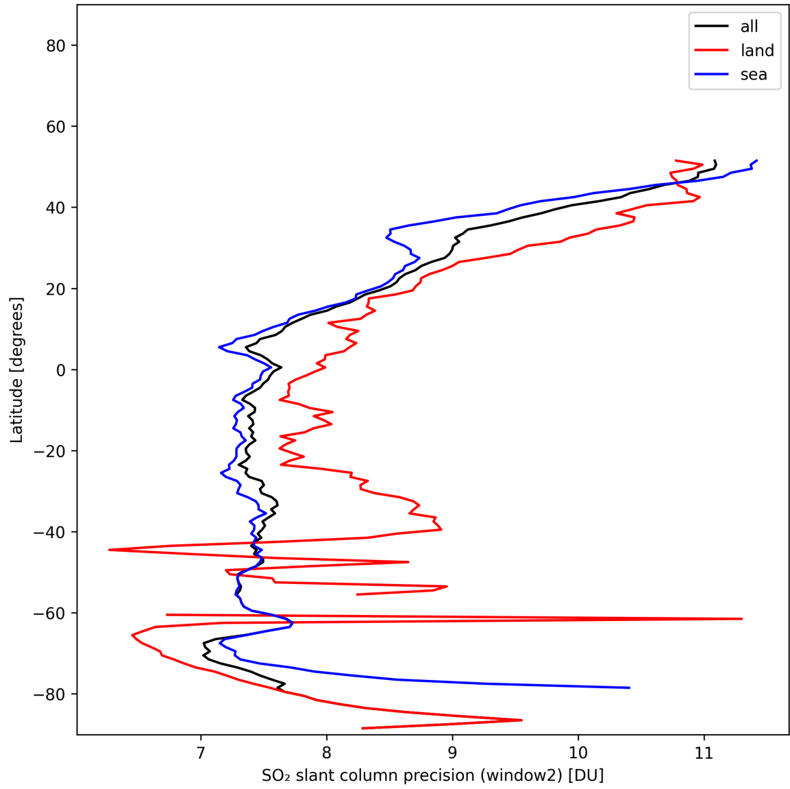
Figure 42: Zonal average of “SO 2 slant column precision (window2)” for 2025-11-13 to 2025-11-15.
