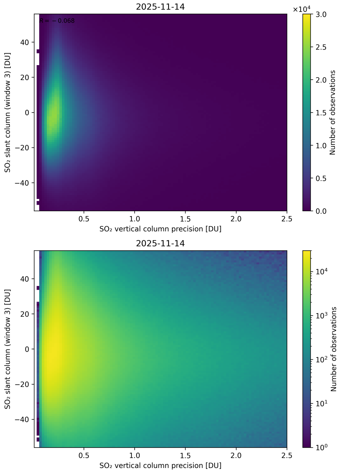
Figure 344: Scatter density plot of “SO 2 vertical column precision” against “SO 2 slant column (window 3)” for 2025-11-13 to 2025-11-15.
