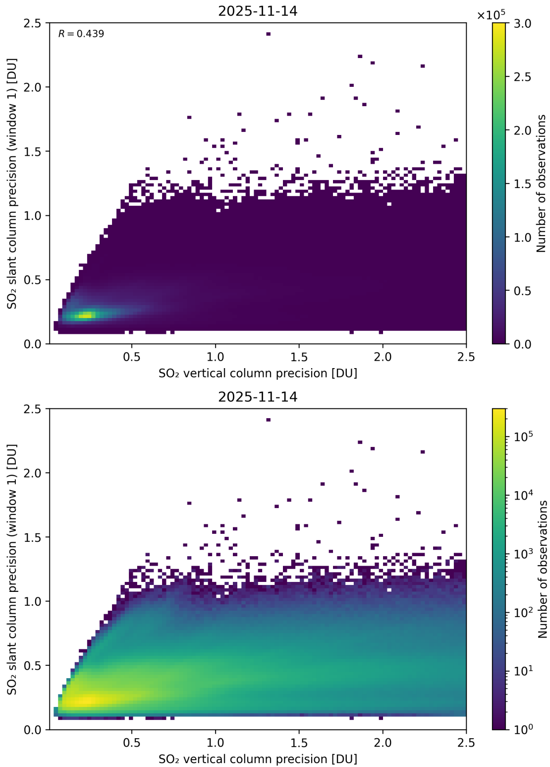
Figure 342: Scatter density plot of “SO 2 vertical column precision” against “SO 2 slant column precision (window 1)” for 2025-11-13 to 2025-11-15.
