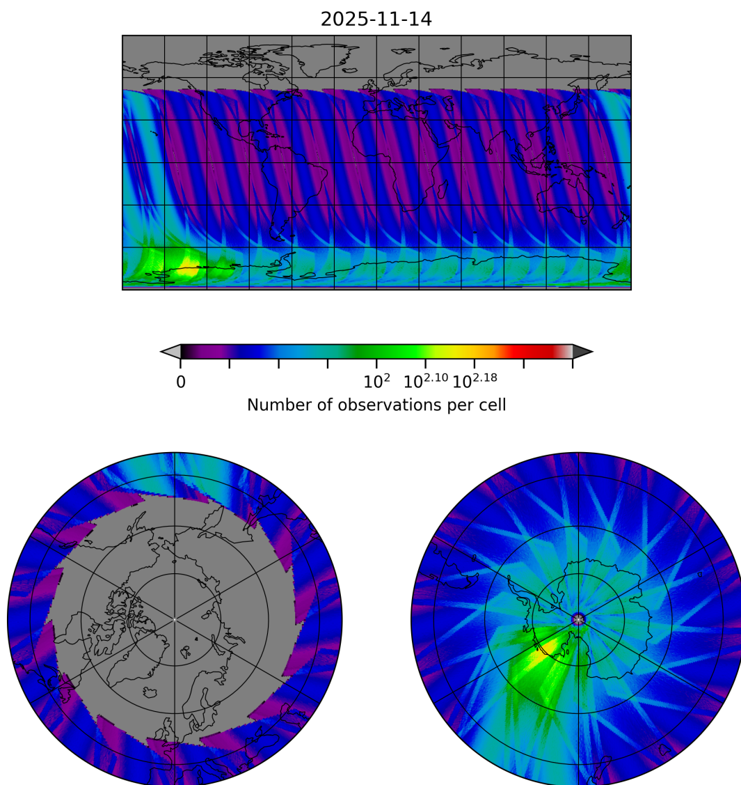
Figure 30: Map of the number of observations for 2025-11-13 to 2025-11-15
