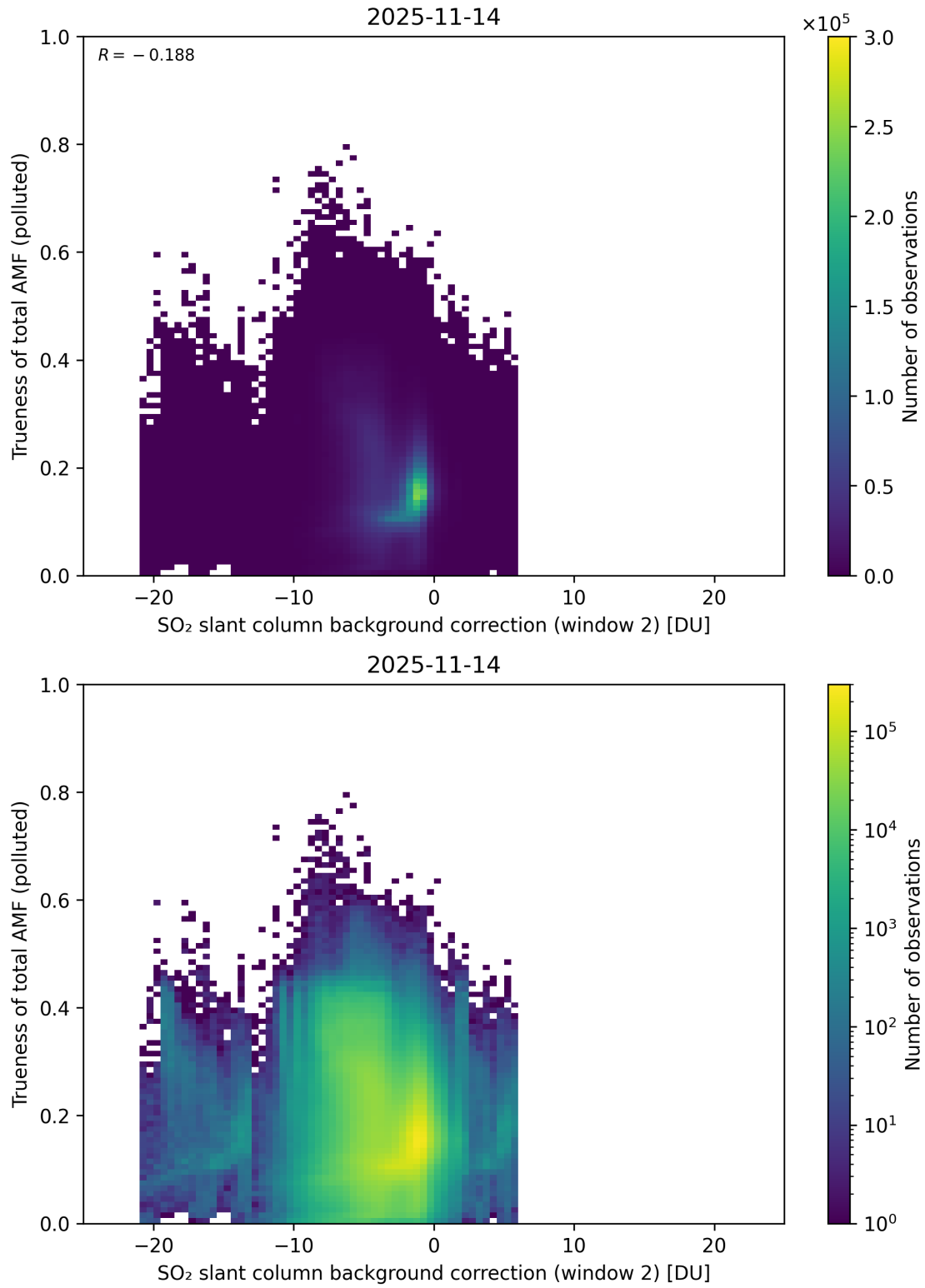
Figure 131: Scatter density plot of “SO 2 slant column background correction (window 2)” against “Trueness of total AMF (polluted)” for 2025-11-13 to 2025-11-15.
