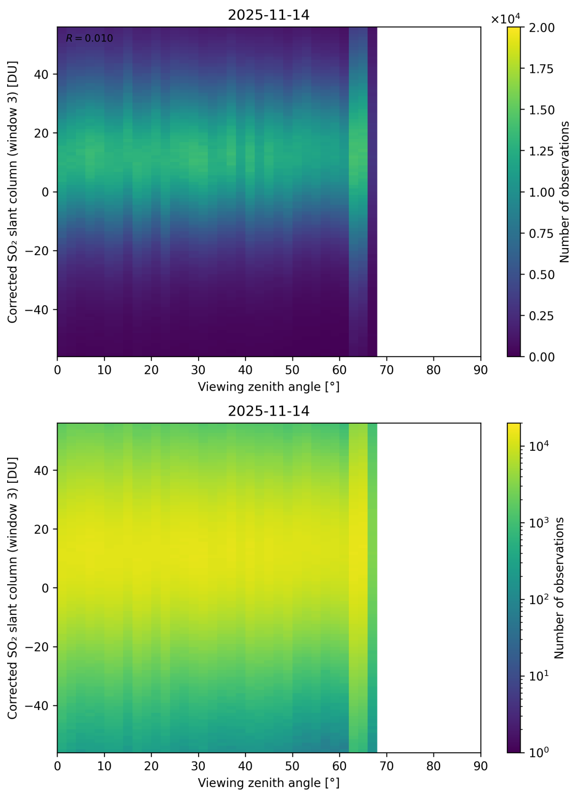
Figure 375: Scatter density plot of “Viewing zenith angle” against “Corrected SO 2 slant column (window 3)” for 2025-11-13 to 2025-11-15.
