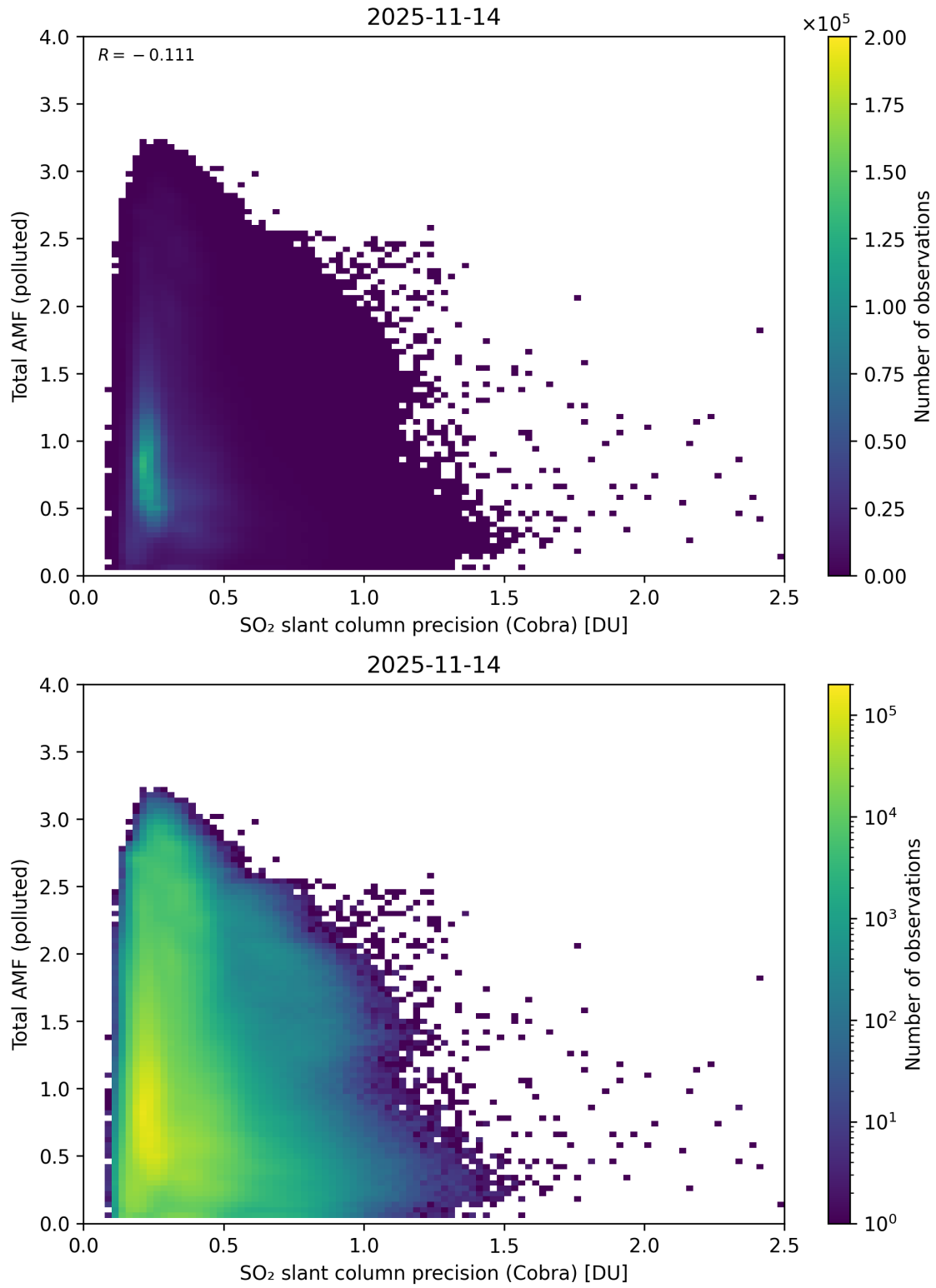
Figure 213: Scatter density plot of “SO 2 slant column precision (Cobra)” against “Total AMF (polluted)” for 2025-11-13 to 2025-11-15.
