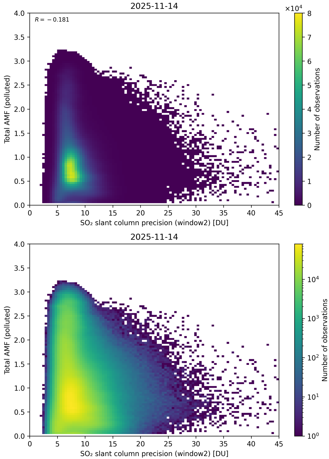
Figure 301: Scatter density plot of “SO 2 slant column precision (window2)” against “Total AMF (polluted)” for 2025-11-13 to 2025-11-15.
