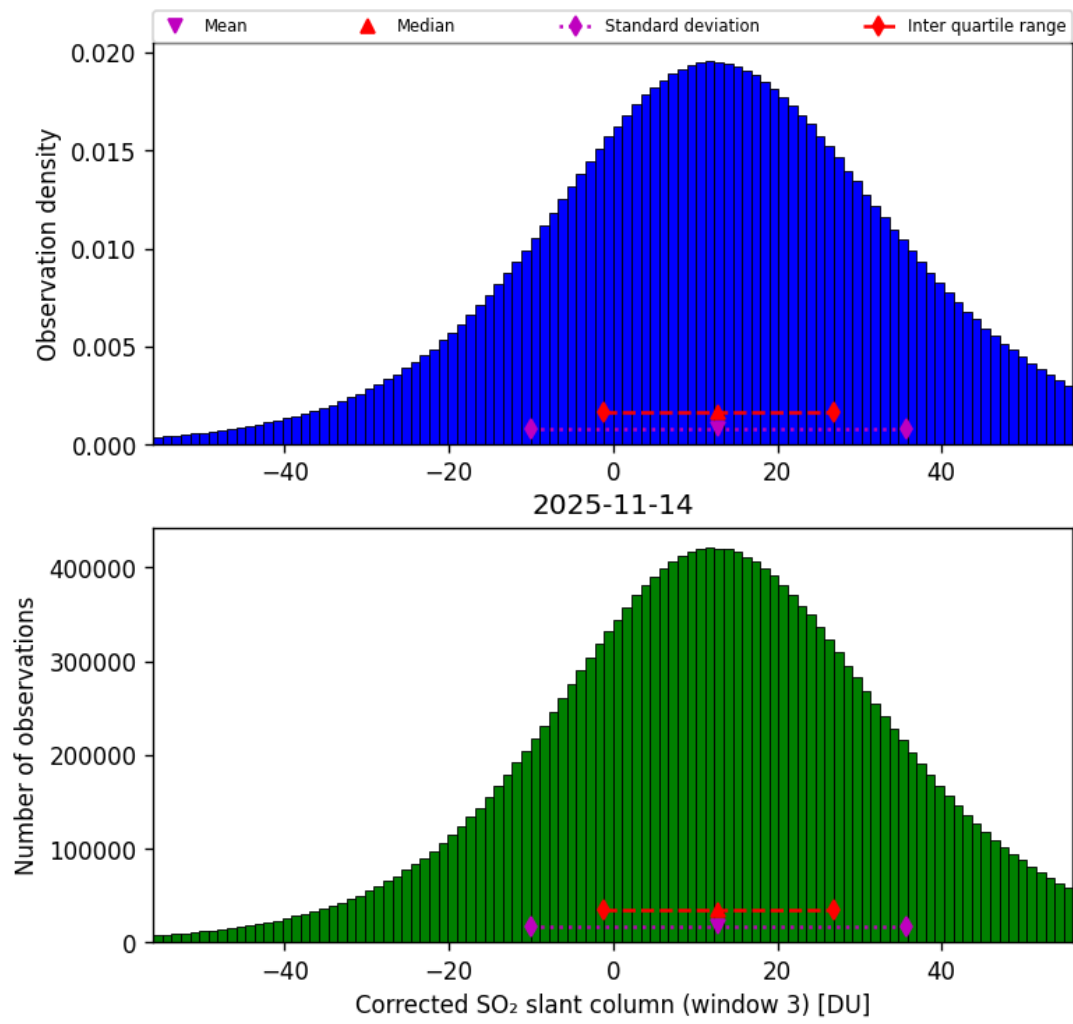
Figure 73: Histogram of “Corrected SO 2 slant column (window 3)” for 2025-11-13 to 2025-11-15
