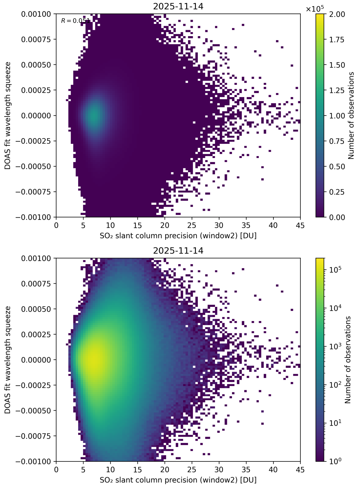
Figure 294: Scatter density plot of “SO 2 slant column precision (window2)” against “DOAS fit wavelength squeeze” for 2025-11-13 to 2025-11-15.
