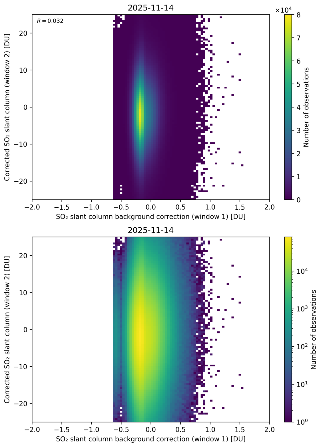
Figure 115: Scatter density plot of “SO 2 slant column background correction (window 1)” against “Corrected SO 2 slant column (window 2)” for 2025-11-13 to 2025-11-15.
