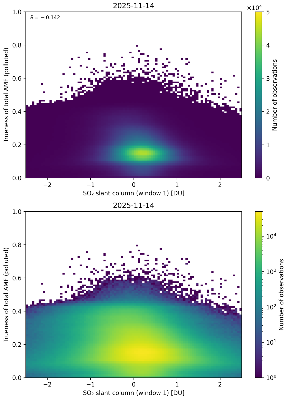
Figure 290: Scatter density plot of “SO 2 slant column (window 1)” against “Trueness of total AMF (polluted)” for 2025-11-13 to 2025-11-15.
