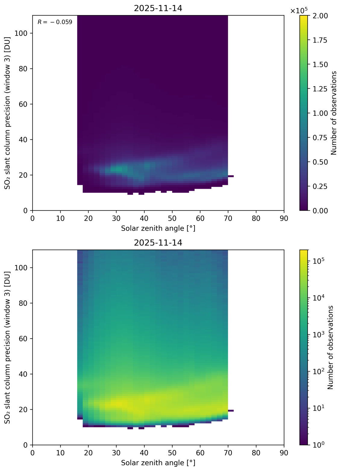
Figure 188: Scatter density plot of “Solar zenith angle” against “SO 2 slant column precision (window 3)” for 2025-11-13 to 2025-11-15.
