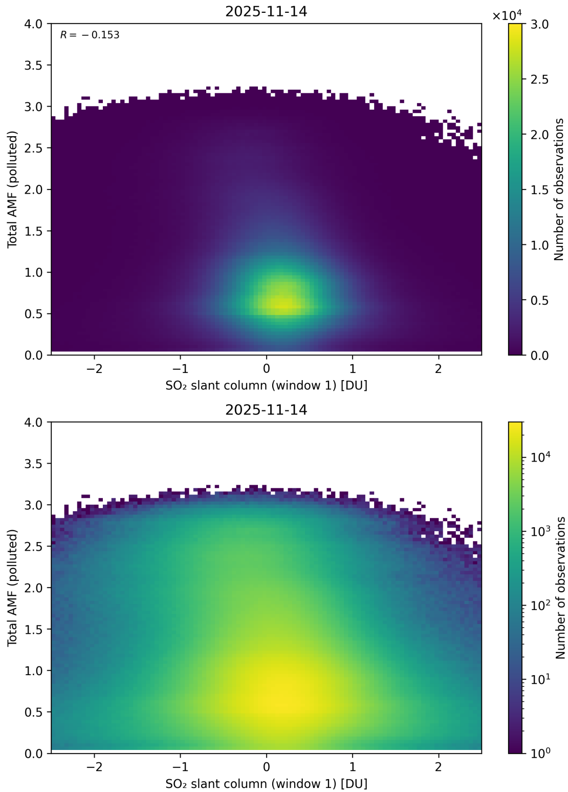
Figure 289: Scatter density plot of “SO 2 slant column (window 1)” against “Total AMF (polluted)” for 2025-11-13 to 2025-11-15.
