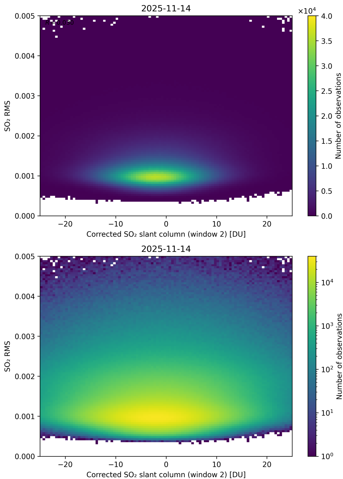
Figure 248: Scatter density plot of “Corrected SO 2 slant column (window 2)” against “SO 2 RMS” for 2025-11-13 to 2025-11-15.
