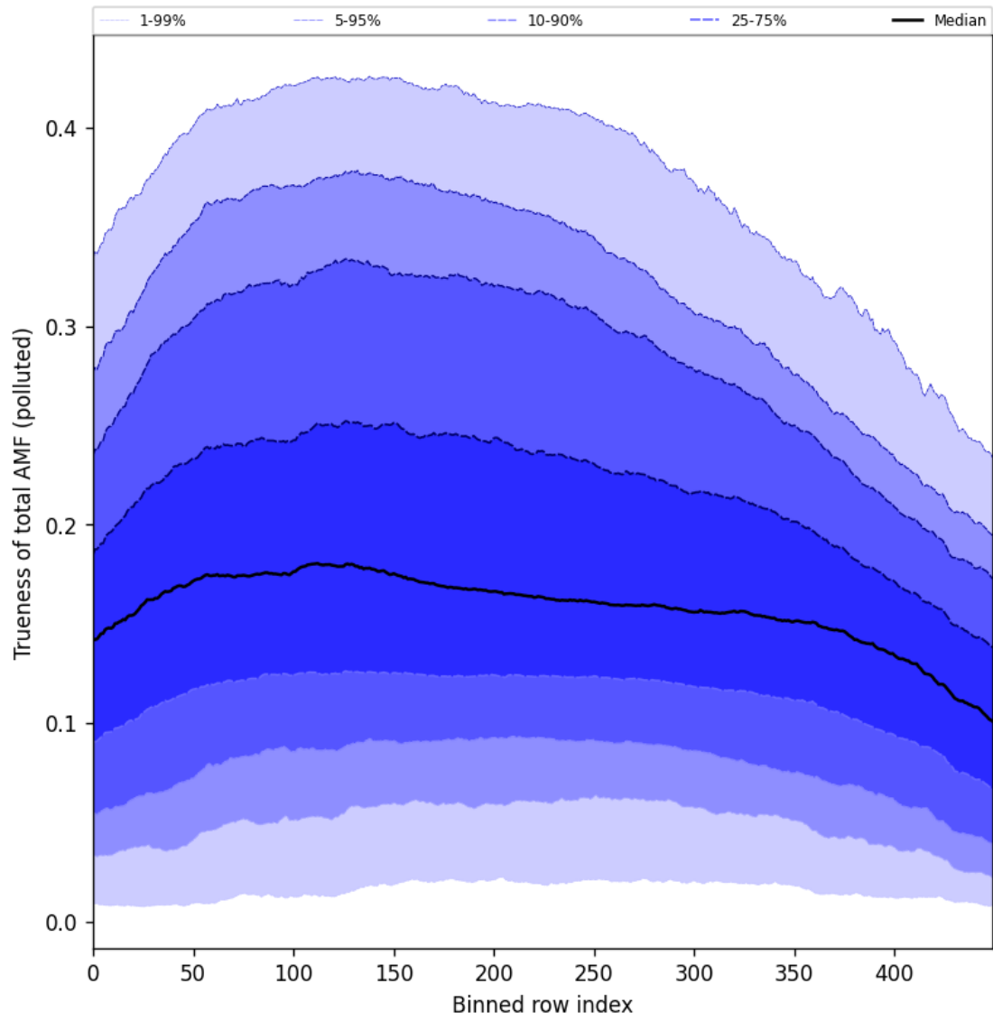
Figure 106: Along track statistics of “Trueness of total AMF (polluted)” for 2025-11-13 to 2025-11-15
