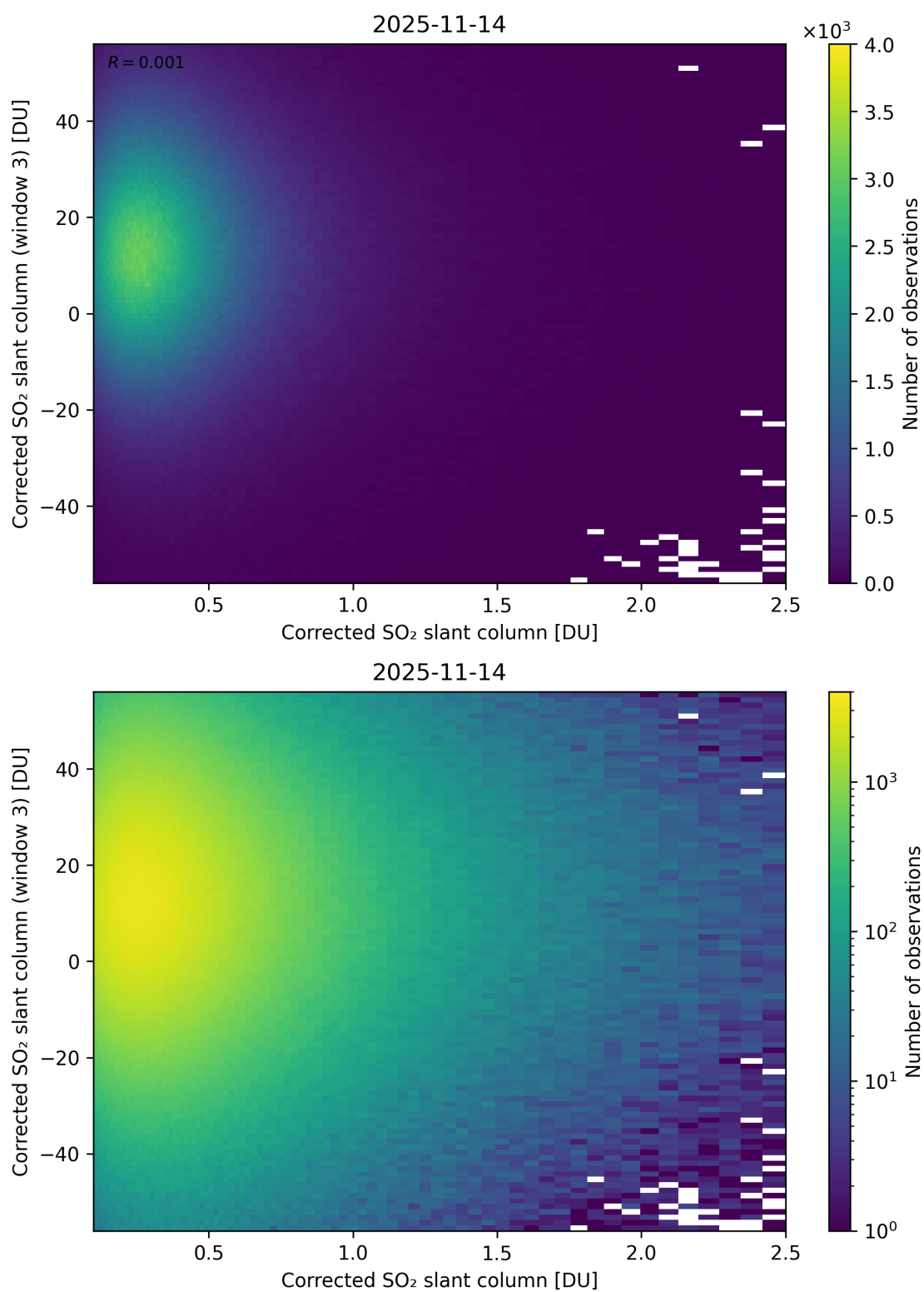
Figure 236: Scatter density plot of “Corrected SO 2 slant column” against “Corrected SO 2 slant column (window 3)” for 2025-11-13 to 2025-11-15.
