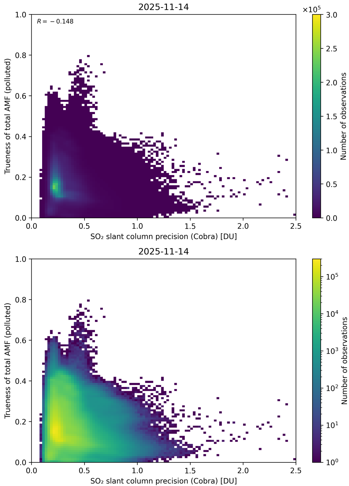
Figure 214: Scatter density plot of “SO 2 slant column precision (Cobra)” against “Trueness of total AMF (polluted)” for 2025-11-13 to 2025-11-15.
