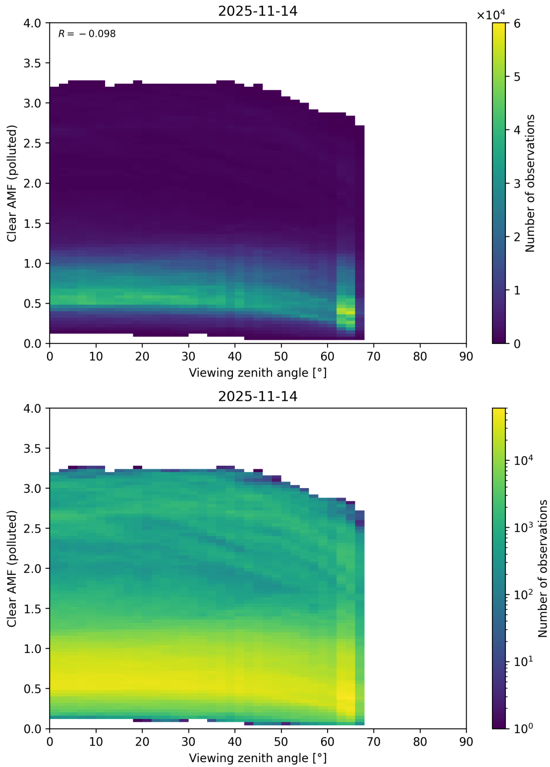
Figure 370: Scatter density plot of “Viewing zenith angle” against “Clear AMF (polluted)” for 2025-11-13 to 2025-11-15.
