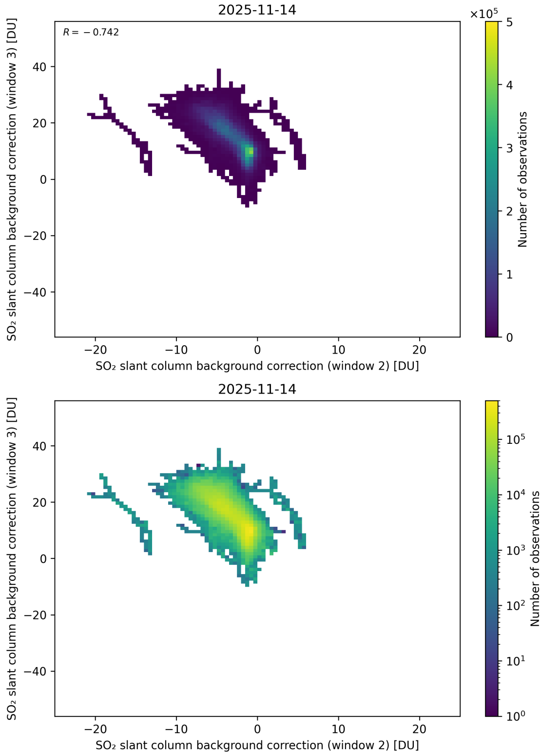
Figure 122: Scatter density plot of “SO 2 slant column background correction (window 2)” against “SO 2 slant column background correction (window 3)” for 2025-11-13 to 2025-11-15.
