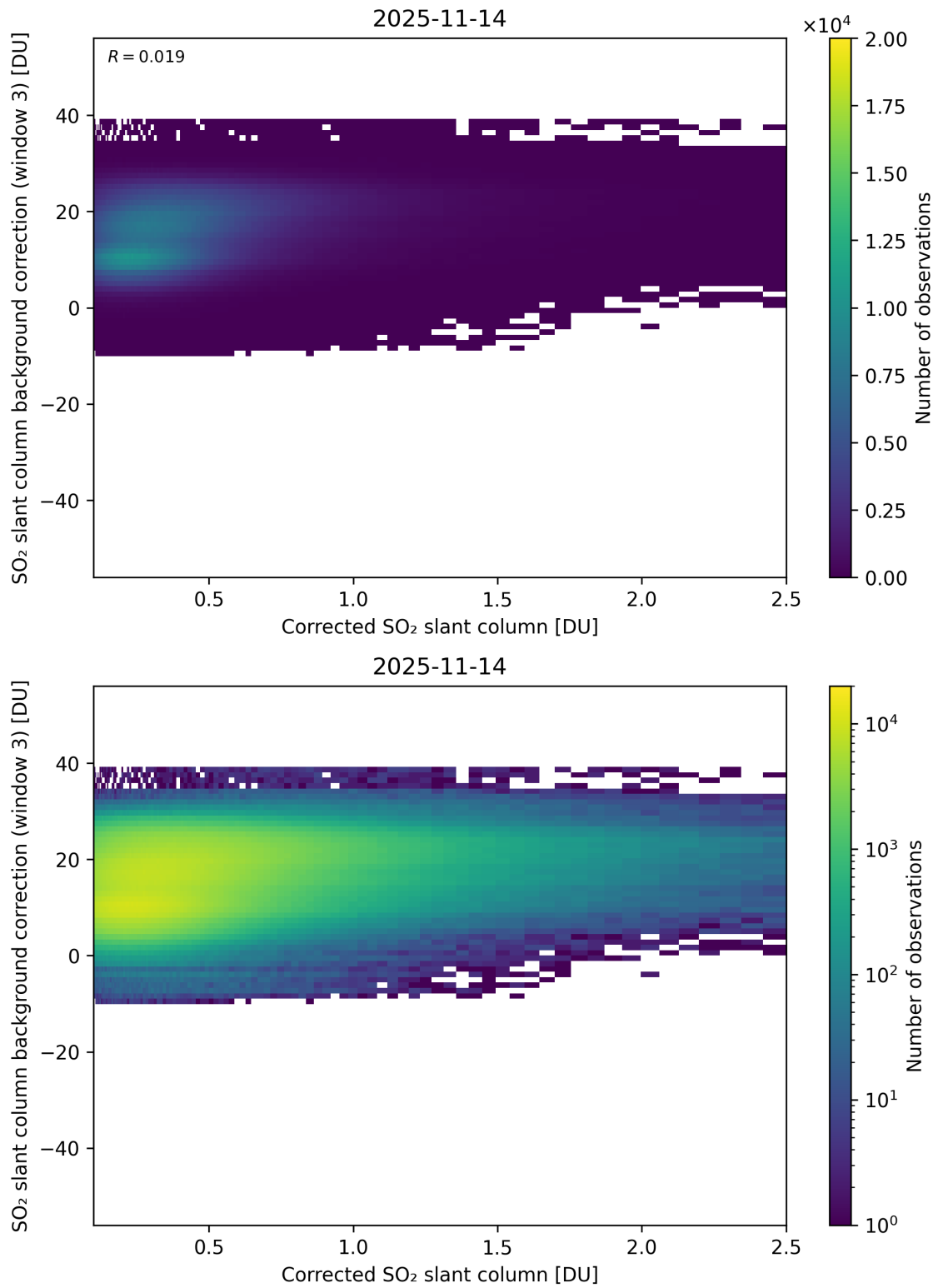
Figure 228: Scatter density plot of “Corrected SO 2 slant column” against “SO 2 slant column background correction (window 3)” for 2025-11-13 to 2025-11-15.
