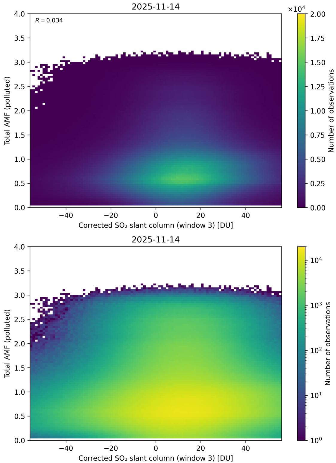
Figure 260: Scatter density plot of “Corrected SO 2 slant column (window 3)” against “Total AMF (polluted)” for 2025-11-13 to 2025-11-15.
