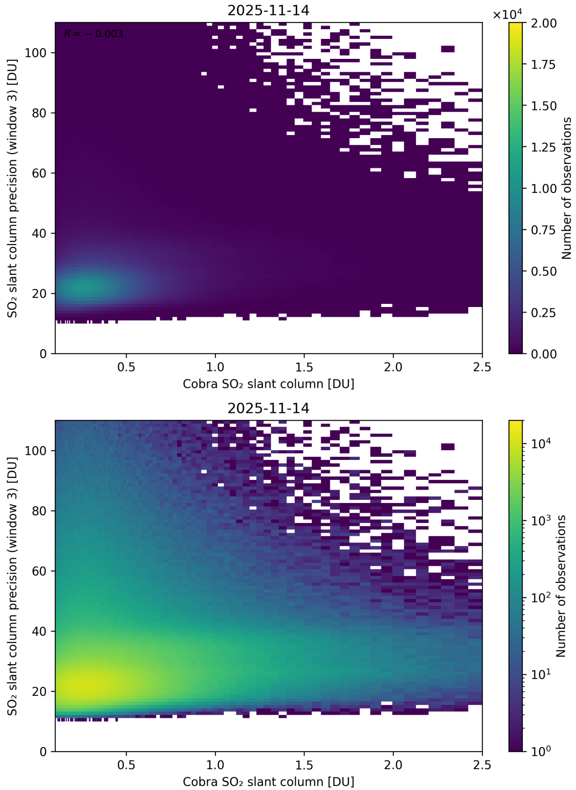
Figure 223: Scatter density plot of “Cobra SO 2 slant column” against “SO 2 slant column precision (window 3)” for 2025-11-13 to 2025-11-15.
