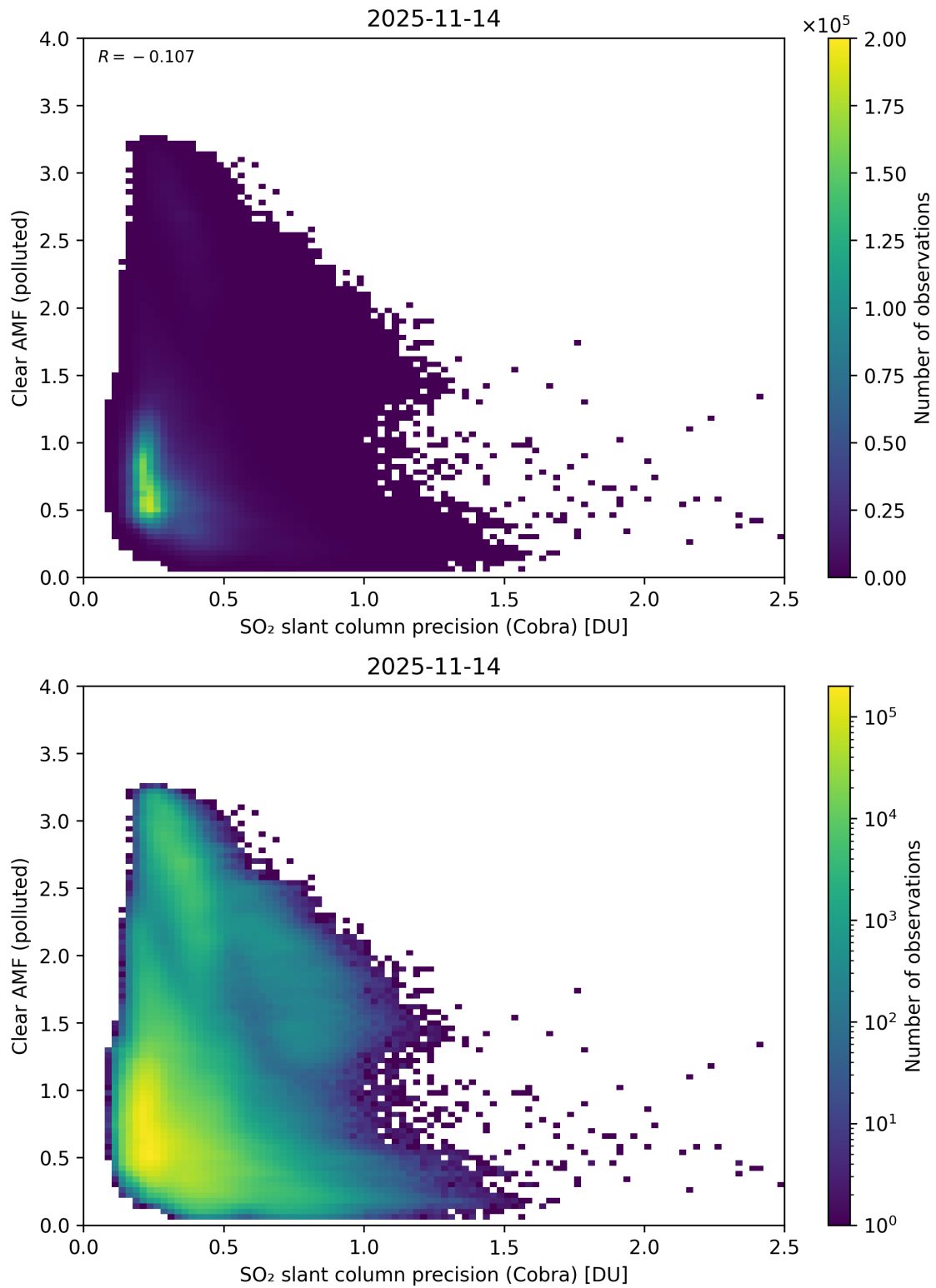
Figure 205: Scatter density plot of “SO 2 slant column precision (Cobra)” against “Clear AMF (polluted)” for 2025-11-13 to 2025-11-15.
