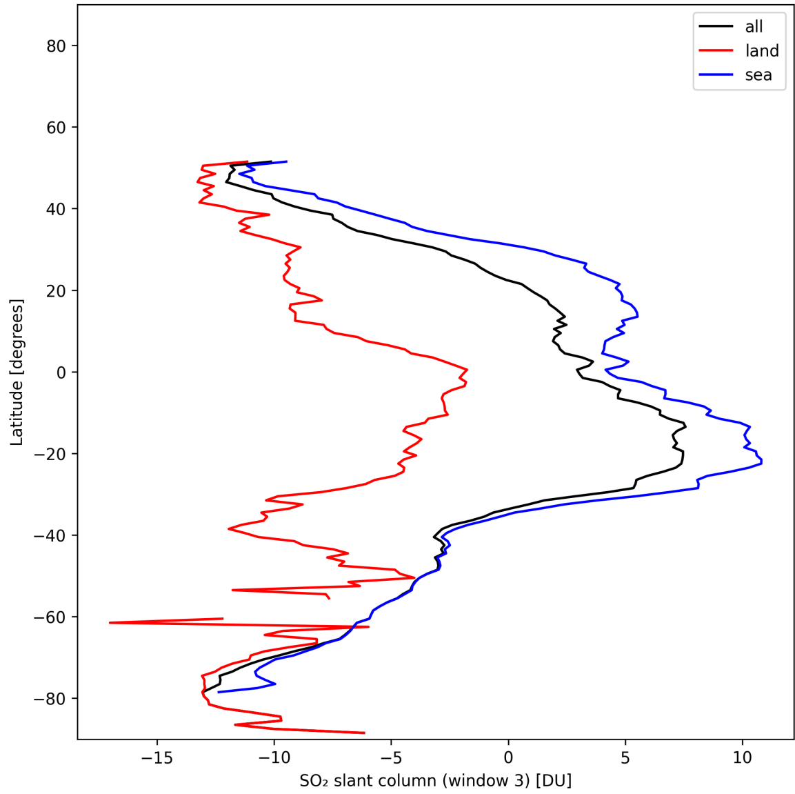
Figure 45: Zonal average of “SO 2 slant column (window 3)” for 2025-11-13 to 2025-11-15.
