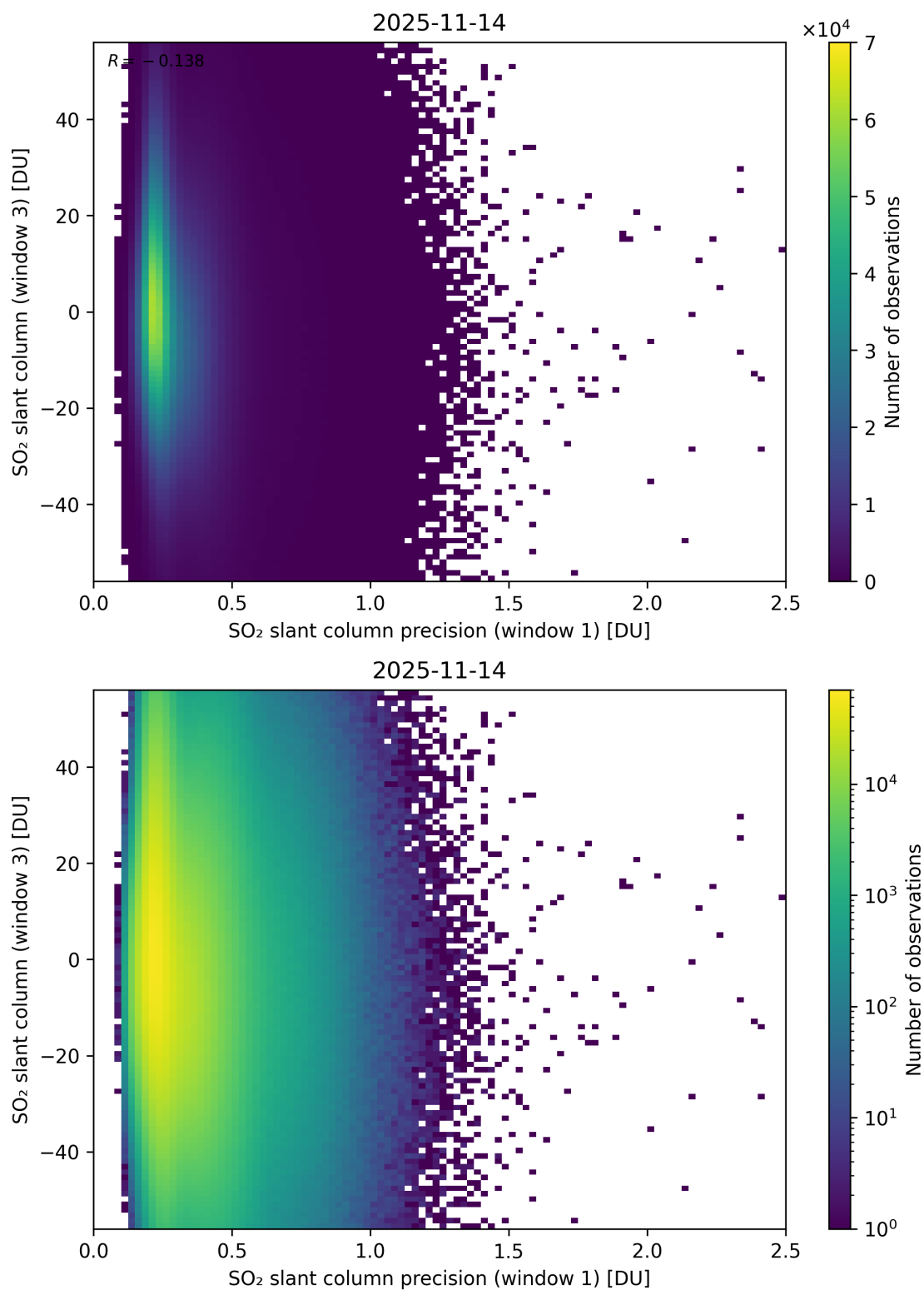
Figure 278: Scatter density plot of “SO 2 slant column precision (window 1)” against “SO 2 slant column (window 3)” for 2025-11-13 to 2025-11-15.
