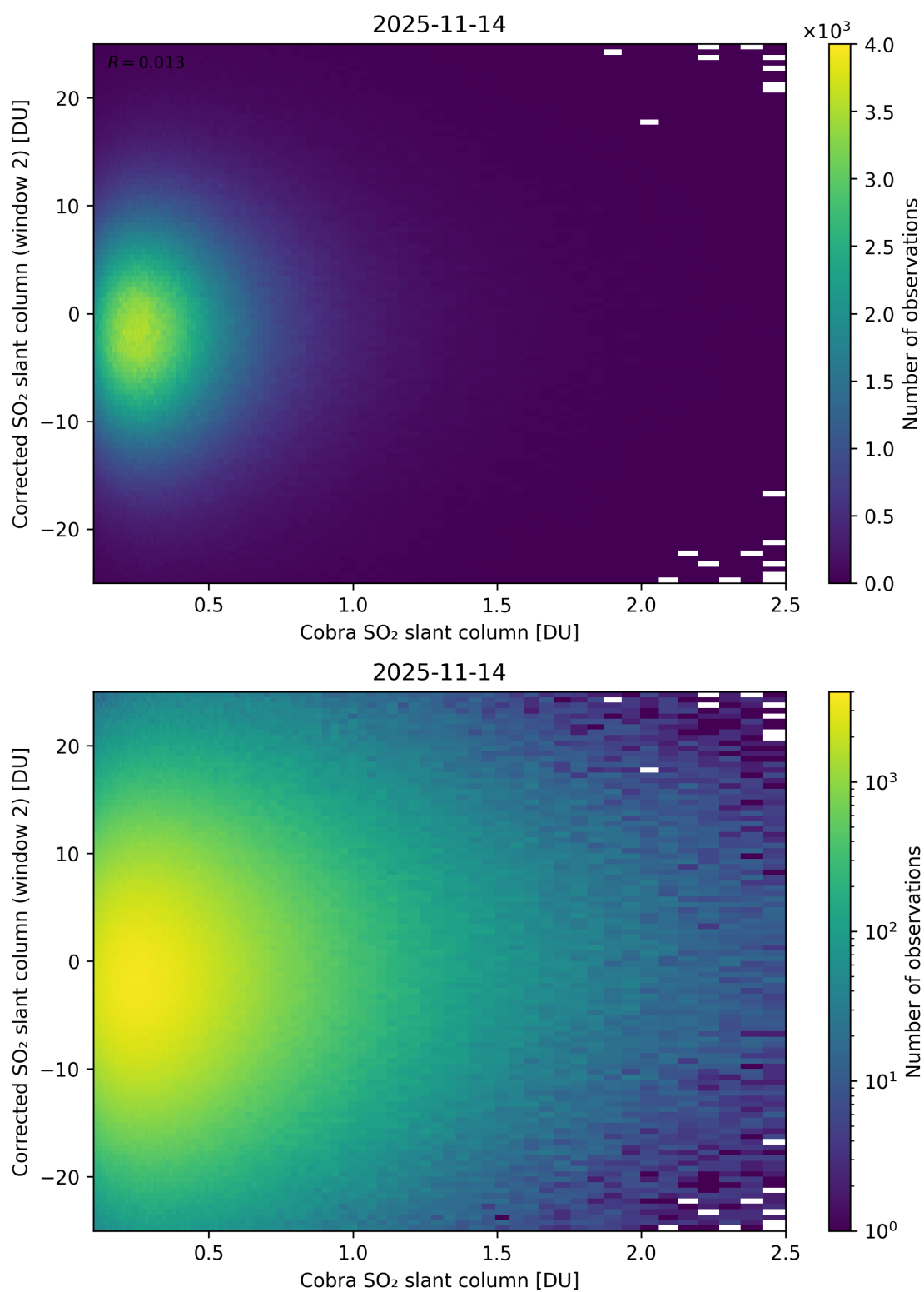
Figure 217: Scatter density plot of “Cobra SO 2 slant column” against “Corrected SO 2 slant column (window 2)” for 2025-11-13 to 2025-11-15.
