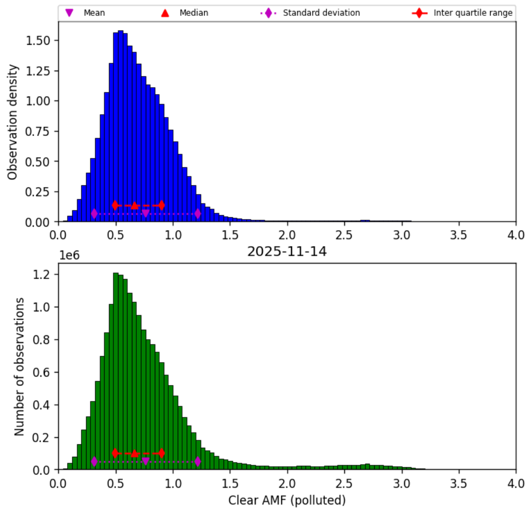
Figure 81: Histogram of “Clear AMF (polluted)” for 2025-11-13 to 2025-11-15
