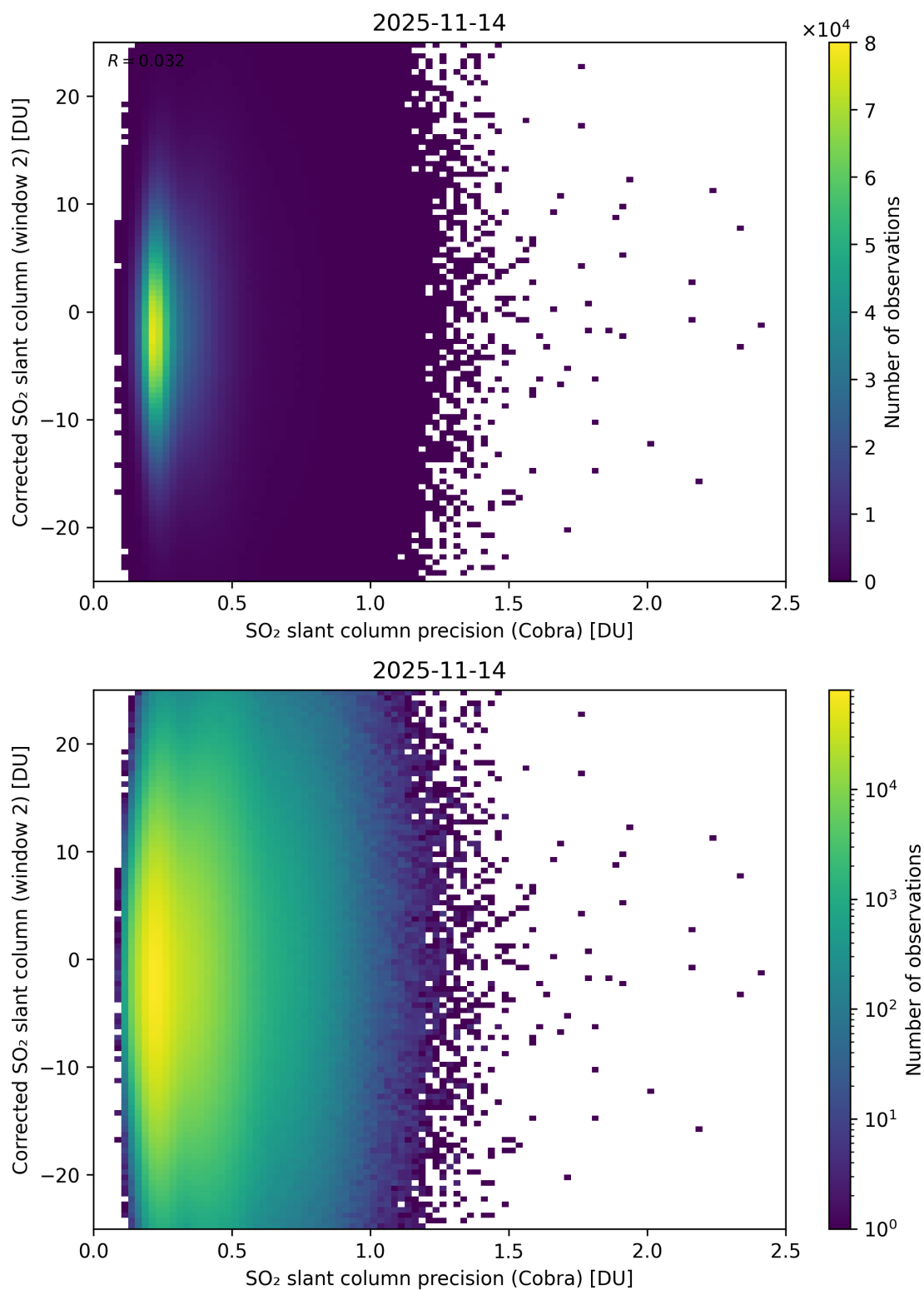
Figure 206: Scatter density plot of “SO 2 slant column precision (Cobra)” against “Corrected SO 2 slant column (window 2)” for 2025-11-13 to 2025-11-15.
