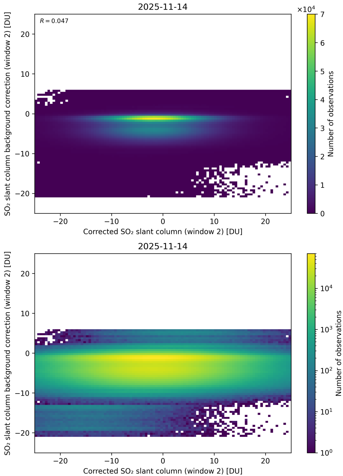
Figure 244: Scatter density plot of “Corrected SO 2 slant column (window 2)” against “SO 2 slant column background correction (window 2)” for 2025-11-13 to 2025-11-15.
