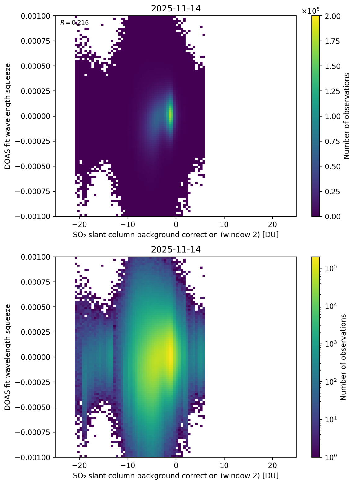
Figure 124: Scatter density plot of “SO 2 slant column background correction (window 2)” against “DOAS fit wavelength squeeze” for 2025-11-13 to 2025-11-15.
