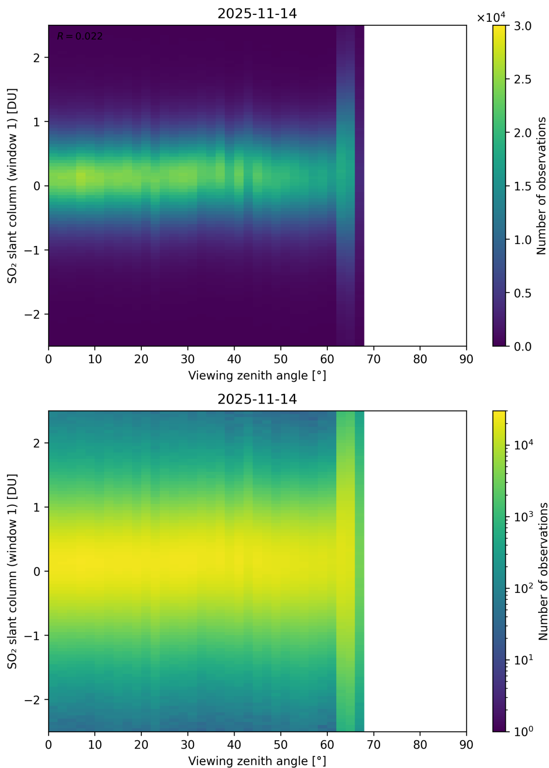
Figure 376: Scatter density plot of “Viewing zenith angle” against “SO 2 slant column (window 1)” for 2025-11-13 to 2025-11-15.
