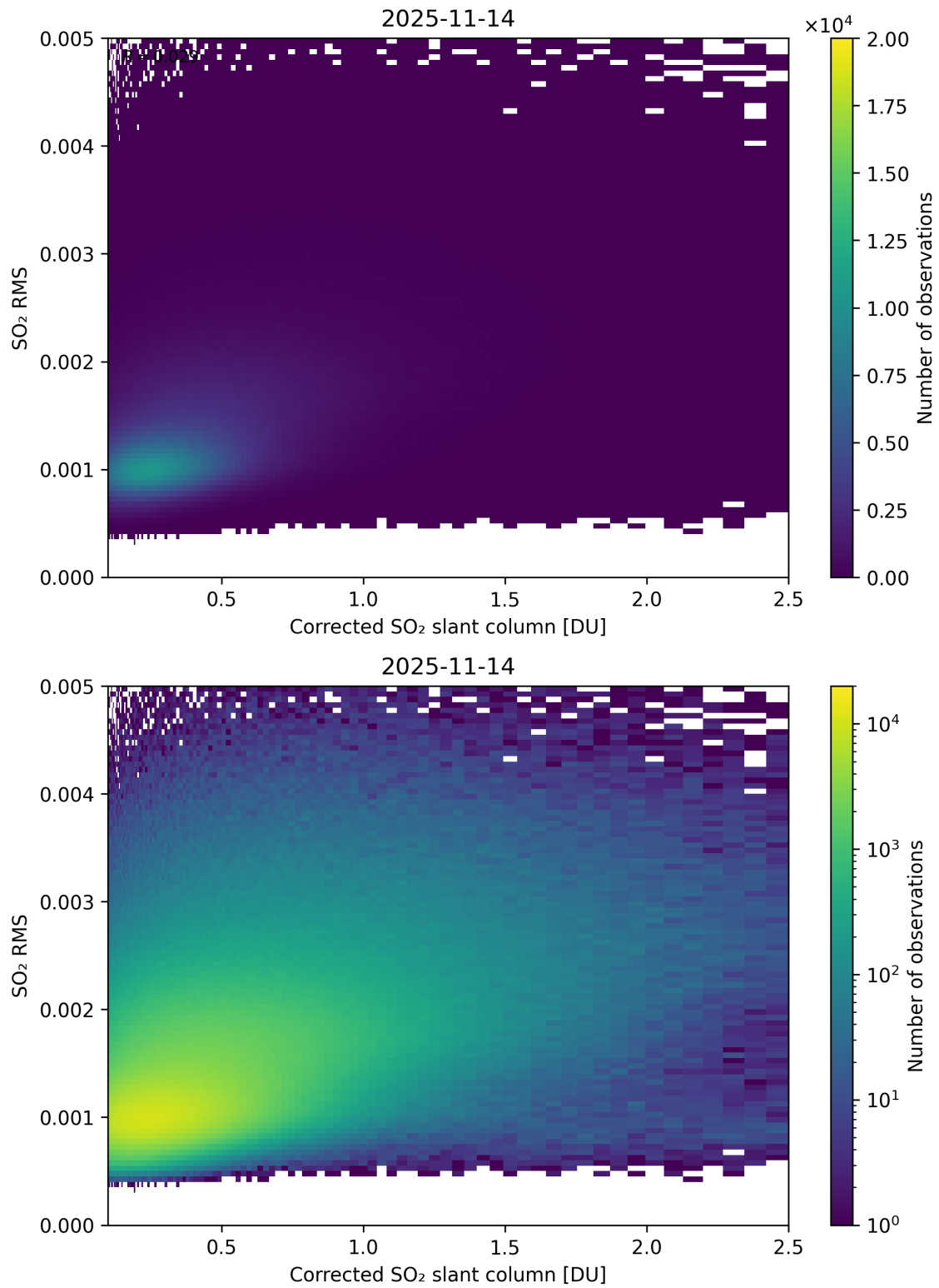
Figure 231: Scatter density plot of “Corrected SO 2 slant column” against “SO 2 RMS” for 2025-11-13 to 2025-11-15.
