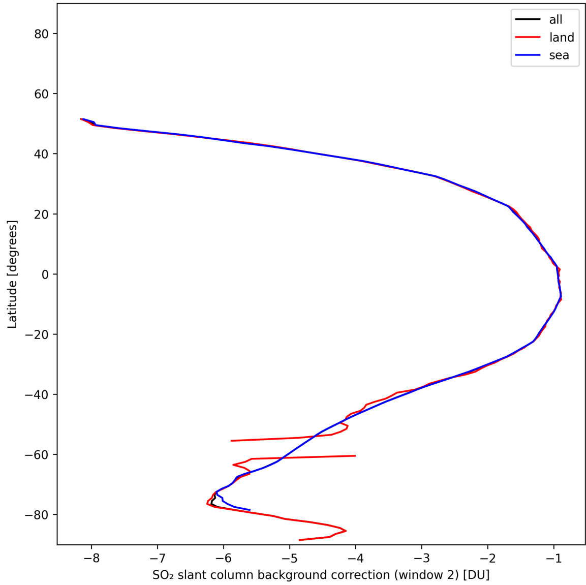
Figure 44: Zonal average of “SO 2 slant column background correction (window 2)” for 2025-11-13 to 2025-11-15.
