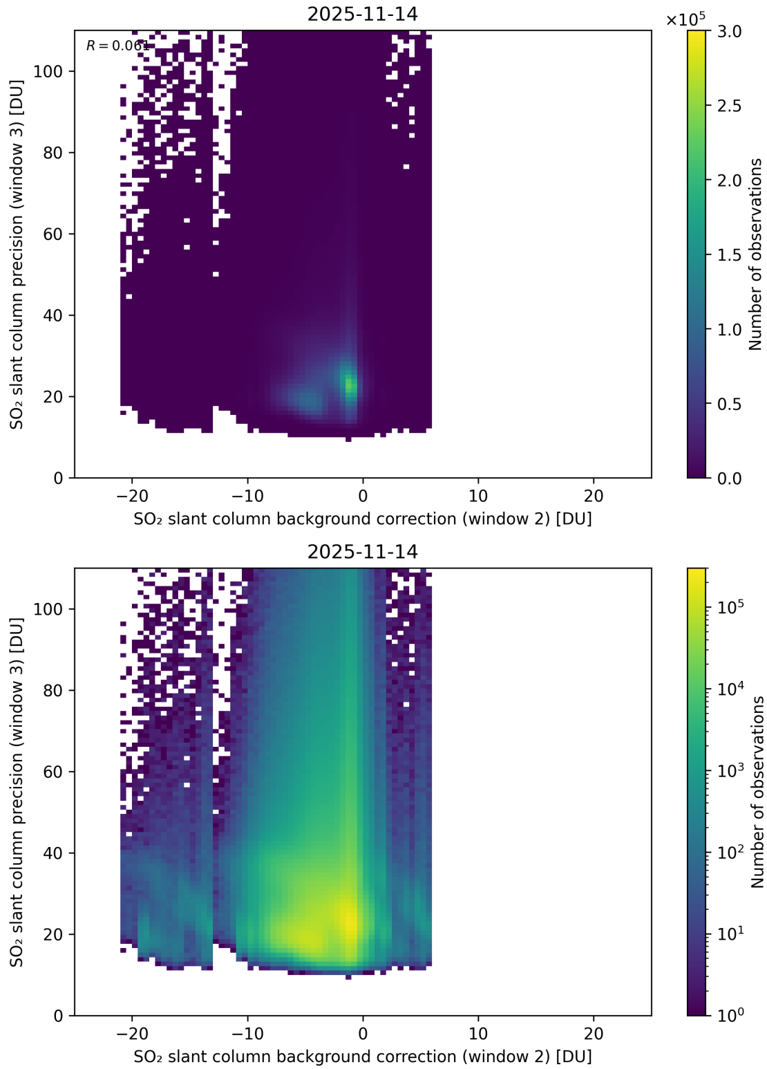
Figure 129: Scatter density plot of “SO 2 slant column background correction (window 2)” against “SO 2 slant column precision (window 3)” for 2025-11-13 to 2025-11-15.
