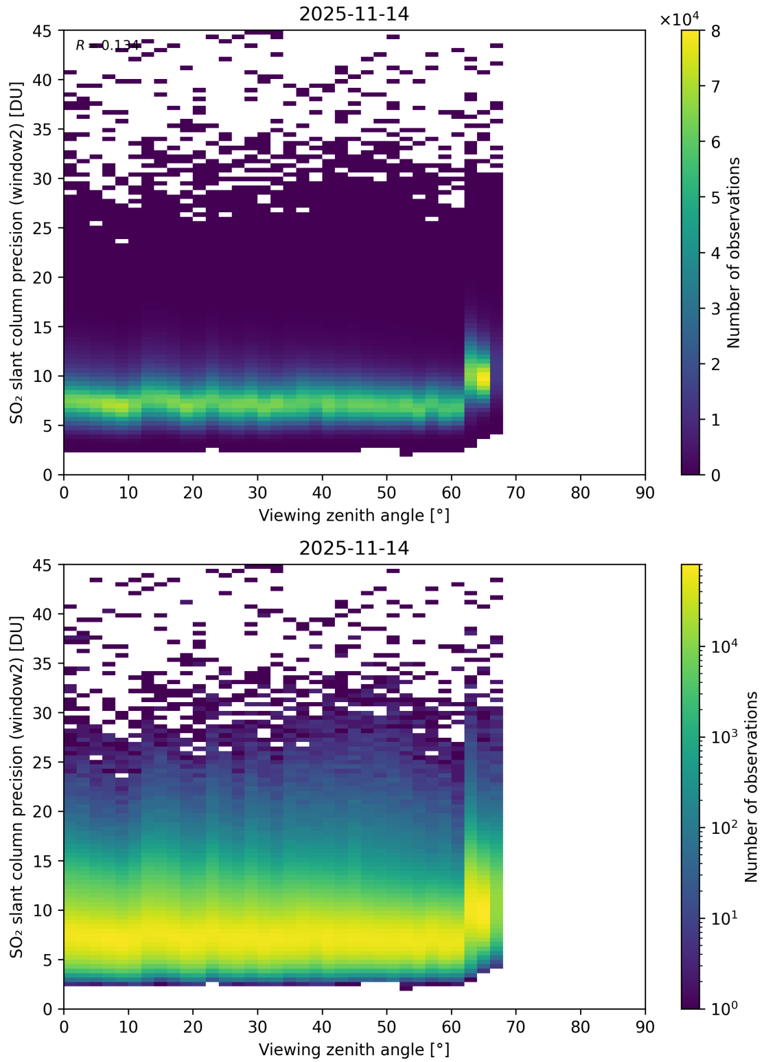
Figure 378: Scatter density plot of “Viewing zenith angle” against “SO 2 slant column precision (window2)” for 2025-11-13 to 2025-11-15.
