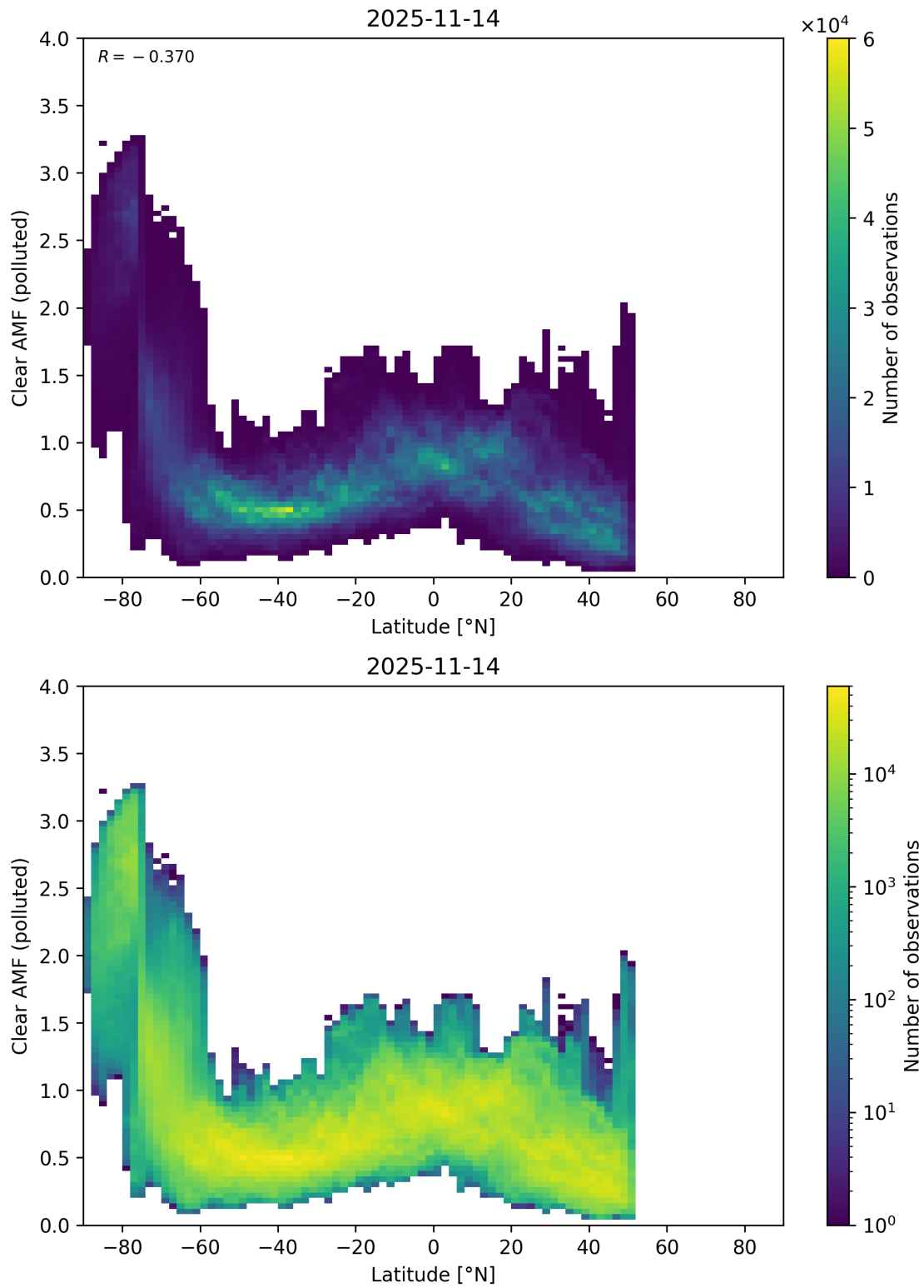
Figure 156: Scatter density plot of “Latitude” against “Clear AMF (polluted)” for 2025-11-13 to 2025-11-15.
