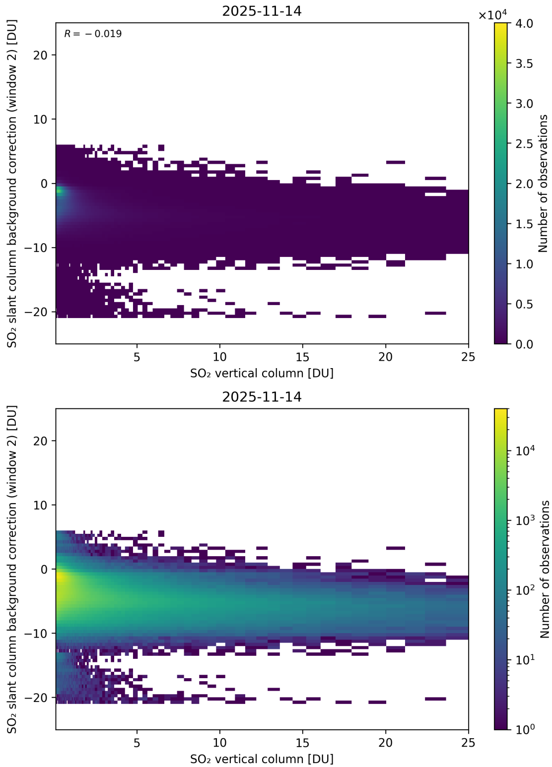
Figure 324: Scatter density plot of “SO 2 vertical column” against “SO 2 slant column background correction (window 2)” for 2025-11-13 to 2025-11-15.
