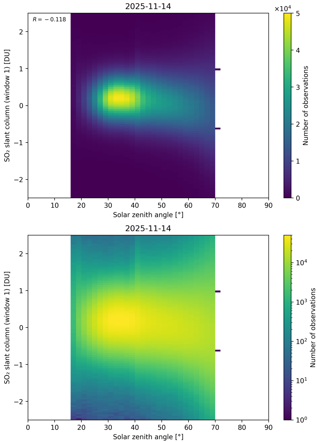
Figure 184: Scatter density plot of “Solar zenith angle” against “SO 2 slant column (window 1)” for 2025-11-13 to 2025-11-15.
