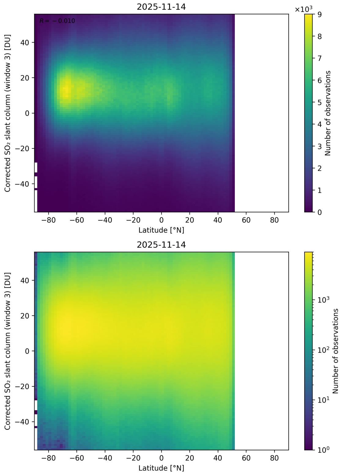
Figure 161: Scatter density plot of “Latitude” against “Corrected SO 2 slant column (window 3)” for 2025-11-13 to 2025-11-15.
