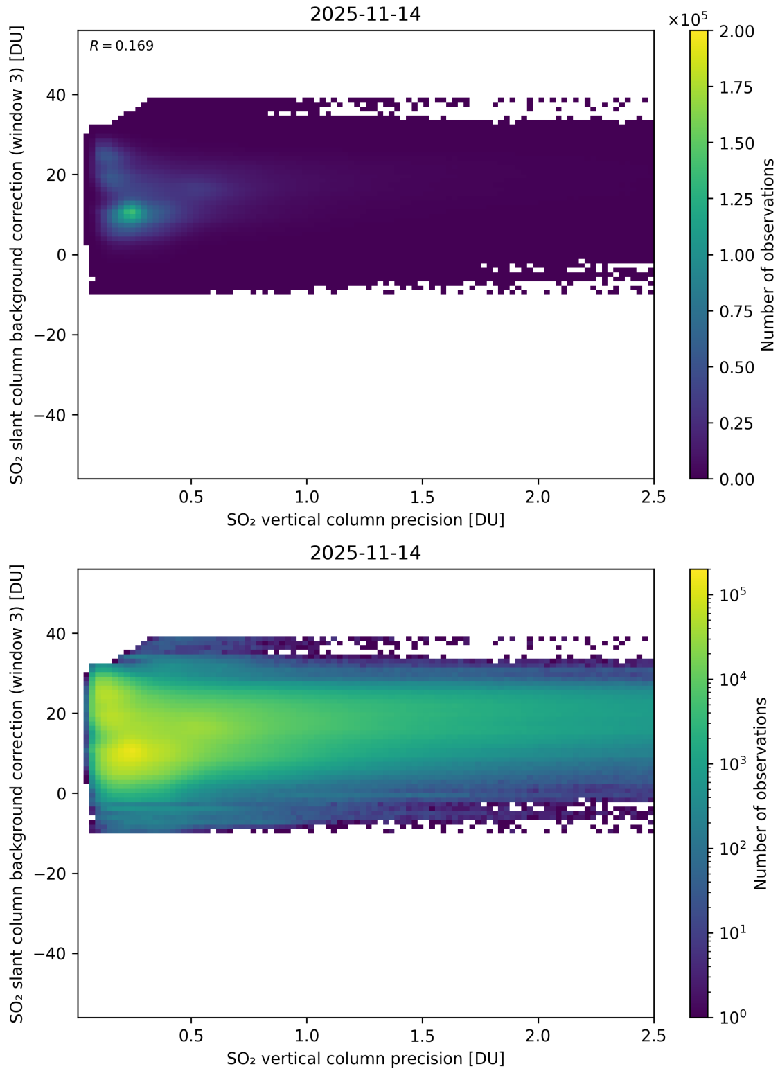
Figure 331: Scatter density plot of “SO 2 vertical column precision” against “SO 2 slant column background correction (window 3)” for 2025-11-13 to 2025-11-15.
