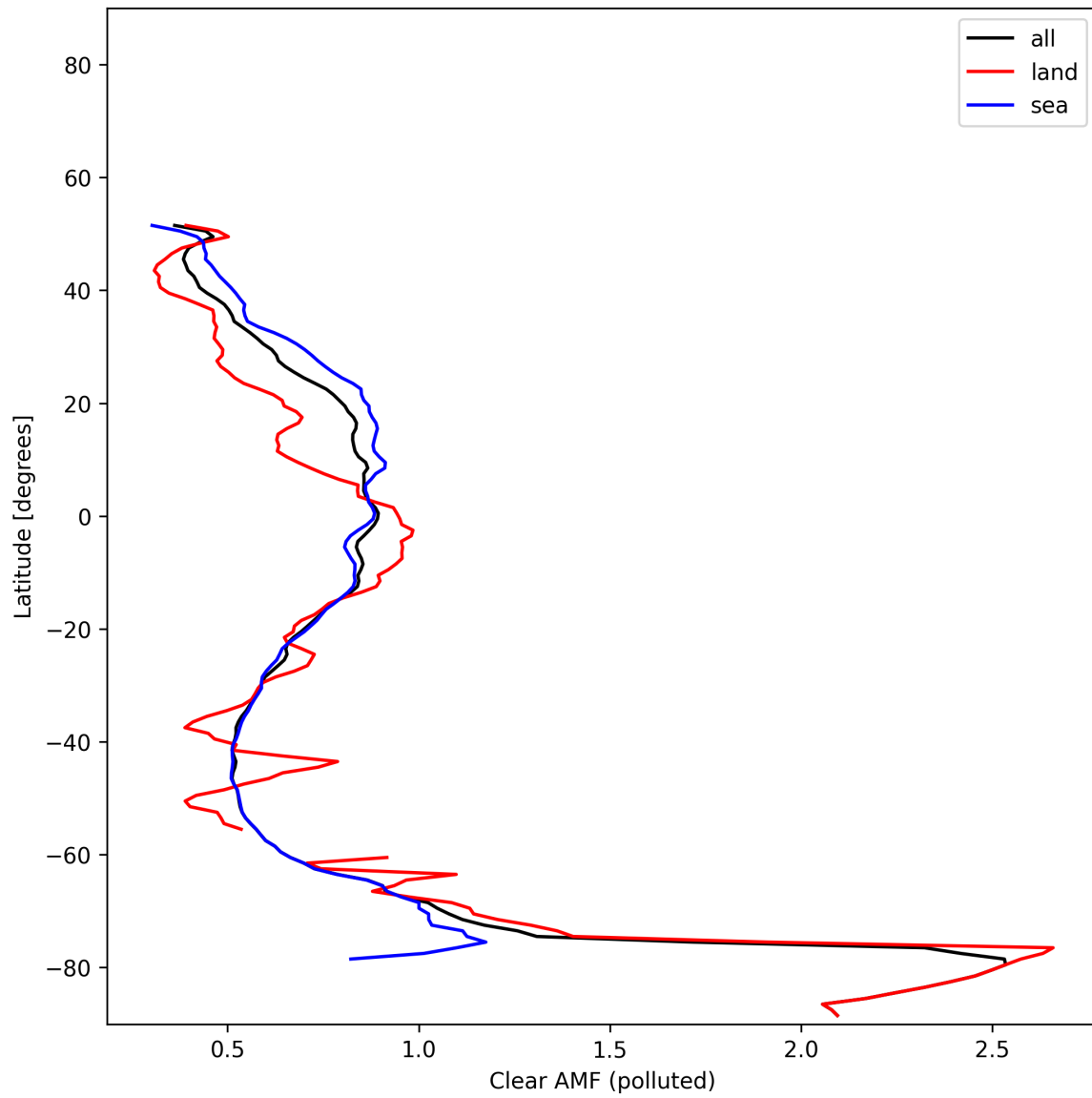
Figure 55: Zonal average of “Clear AMF (polluted)” for 2025-11-13 to 2025-11-15.
