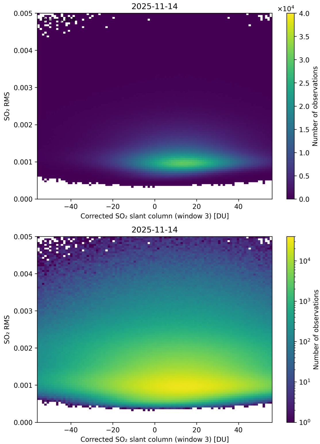
Figure 258: Scatter density plot of “Corrected SO 2 slant column (window 3)” against “SO 2 RMS” for 2025-11-13 to 2025-11-15.
