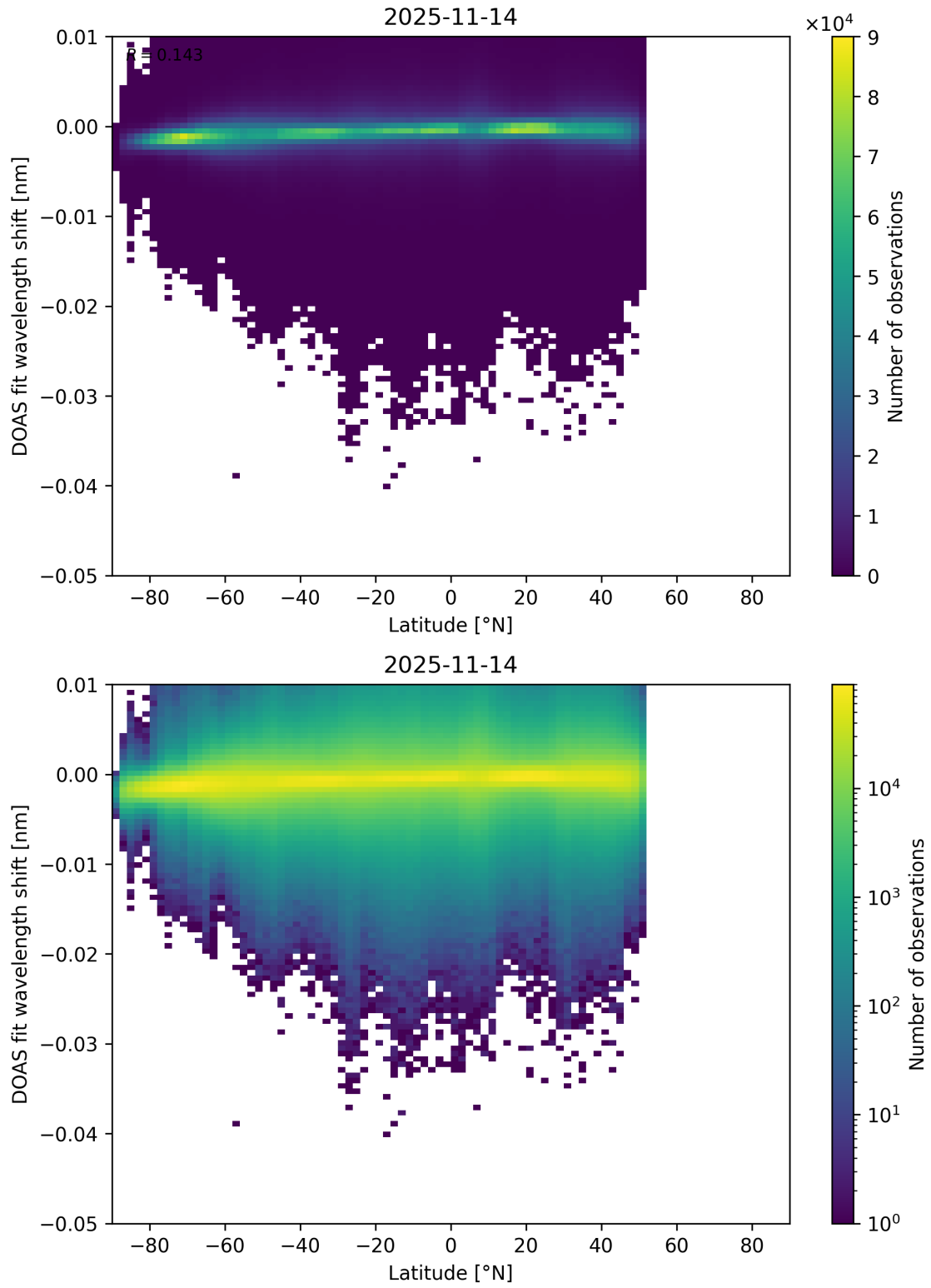
Figure 153: Scatter density plot of “Latitude” against “DOAS fit wavelength shift” for 2025-11-13 to 2025-11-15.
