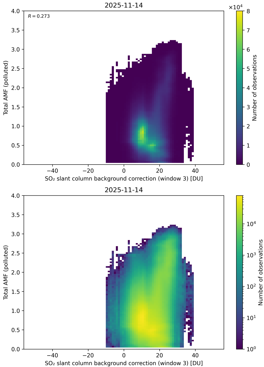
Figure 136: Scatter density plot of “SO 2 slant column background correction (window 3)” against “Total AMF (polluted)” for 2025-11-13 to 2025-11-15.
