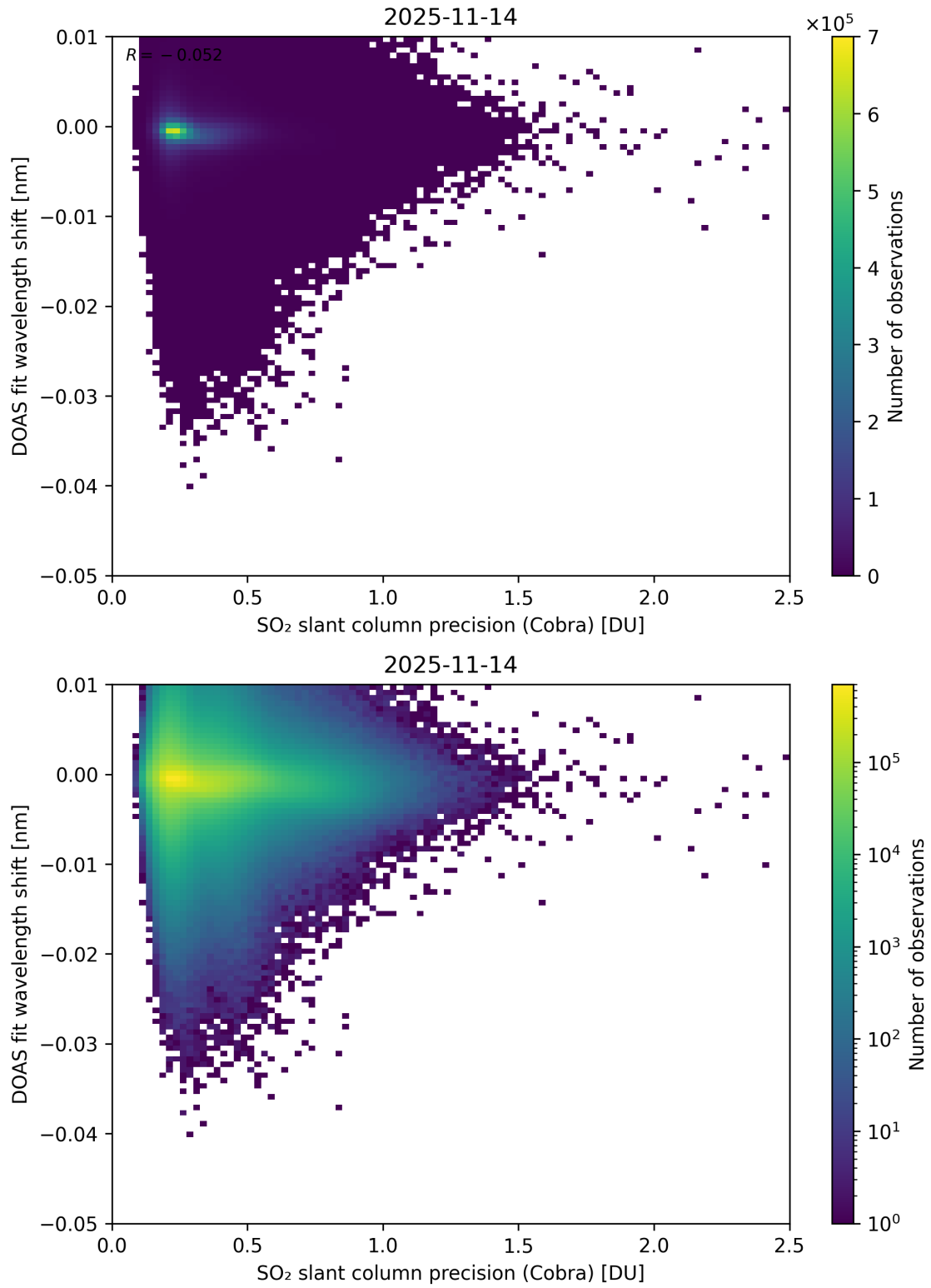
Figure 202: Scatter density plot of “SO 2 slant column precision (Cobra)” against “DOAS fit wavelength shift” for 2025-11-13 to 2025-11-15.
