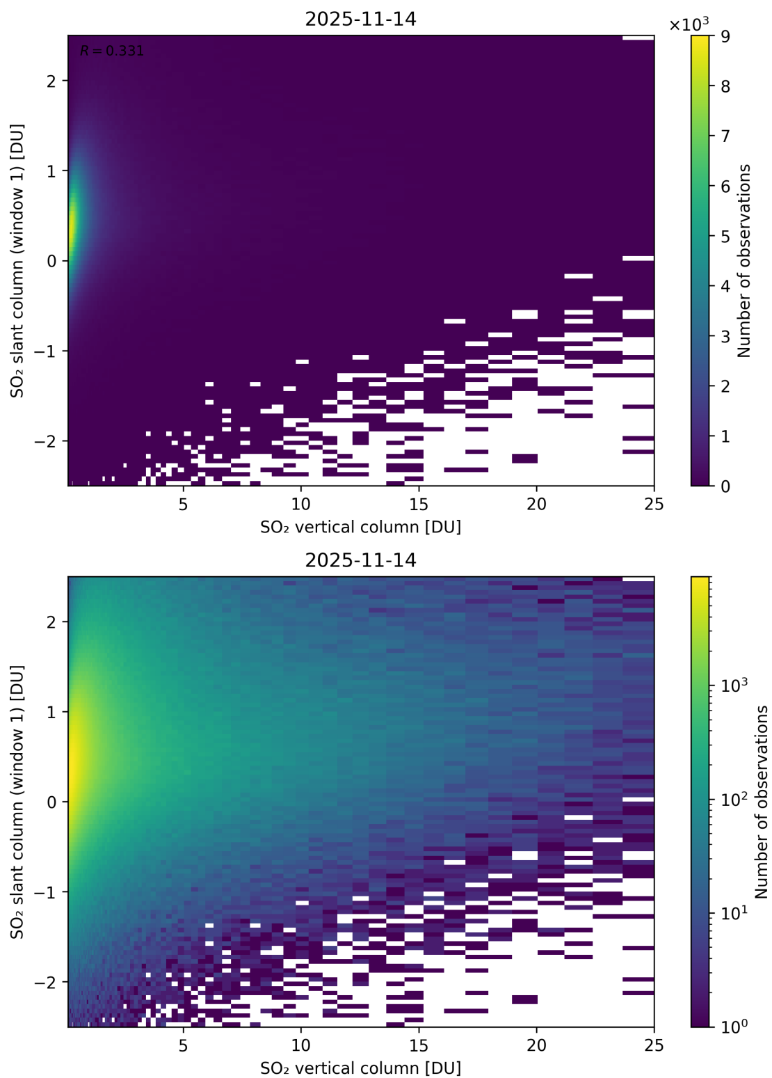
Figure 354: Scatter density plot of “SO 2 vertical column” against “SO 2 slant column (window 1)” for 2025-11-13 to 2025-11-15.
