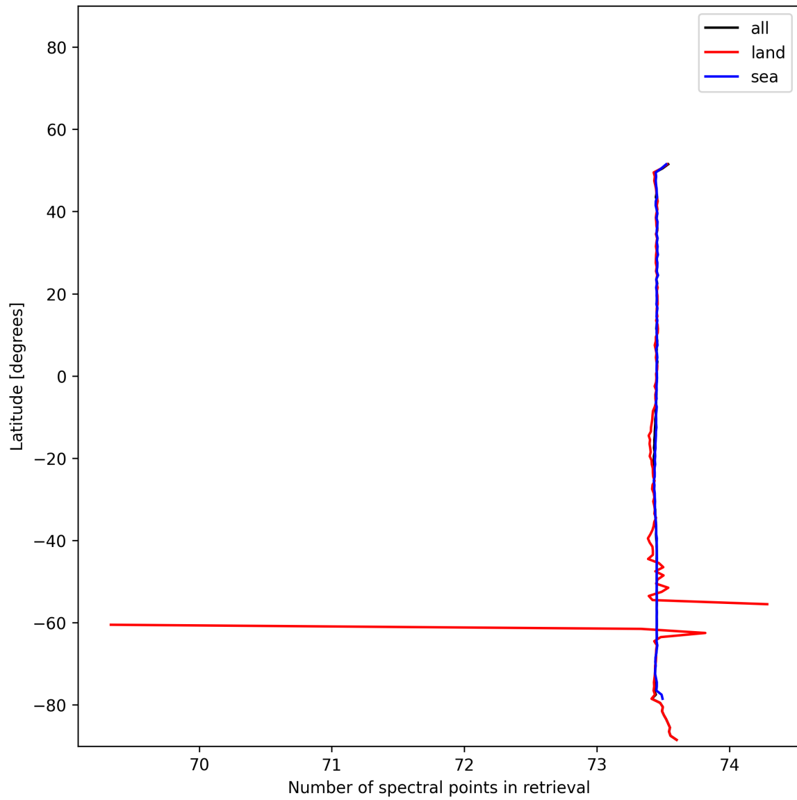
Figure 56: Zonal average of “Number of spectral points in retrieval” for 2025-11-13 to 2025-11-15.
