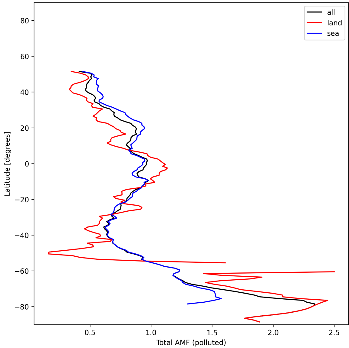
Figure 53: Zonal average of “Total AMF (polluted)” for 2025-11-13 to 2025-11-15.
