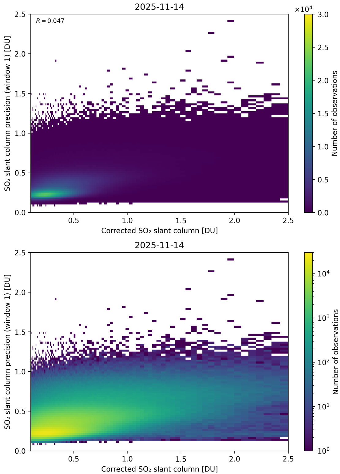
Figure 238: Scatter density plot of “Corrected SO 2 slant column” against “SO 2 slant column precision (window 1)” for 2025-11-13 to 2025-11-15.
