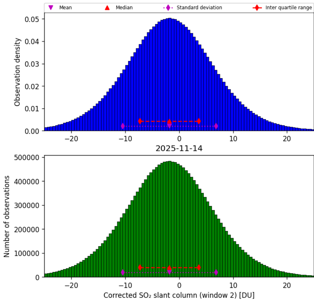
Figure 69: Histogram of “Corrected SO 2 slant column (window 2)” for 2025-11-13 to 2025-11-15
