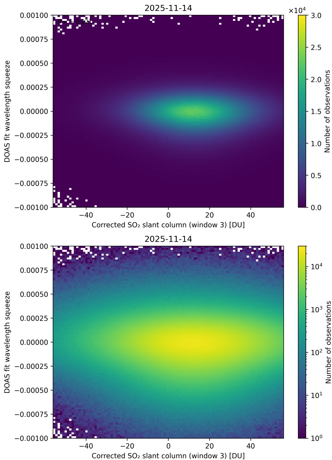
Figure 257: Scatter density plot of “Corrected SO 2 slant column (window 3)” against “DOAS fit wavelength squeeze” for 2025-11-13 to 2025-11-15.
