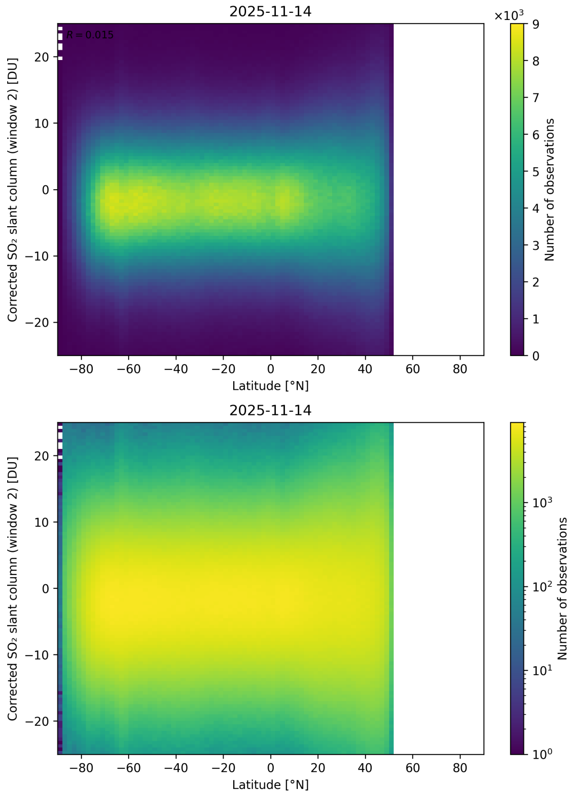
Figure 160: Scatter density plot of “Latitude” against “Corrected SO 2 slant column (window 2)” for 2025-11-13 to 2025-11-15.
