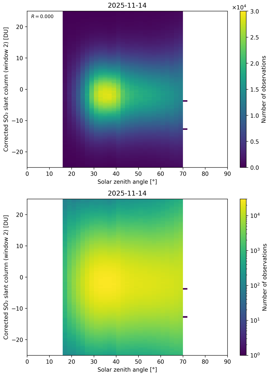
Figure 182: Scatter density plot of “Solar zenith angle” against “Corrected SO 2 slant column (window 2)” for 2025-11-13 to 2025-11-15.
