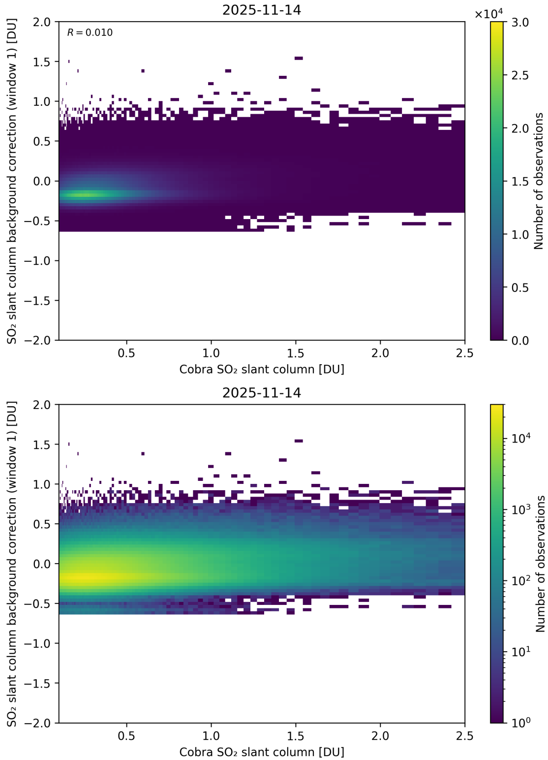
Figure 193: Scatter density plot of “Cobra SO 2 slant column” against “SO 2 slant column background correction (window 1)” for 2025-11-13 to 2025-11-15.
