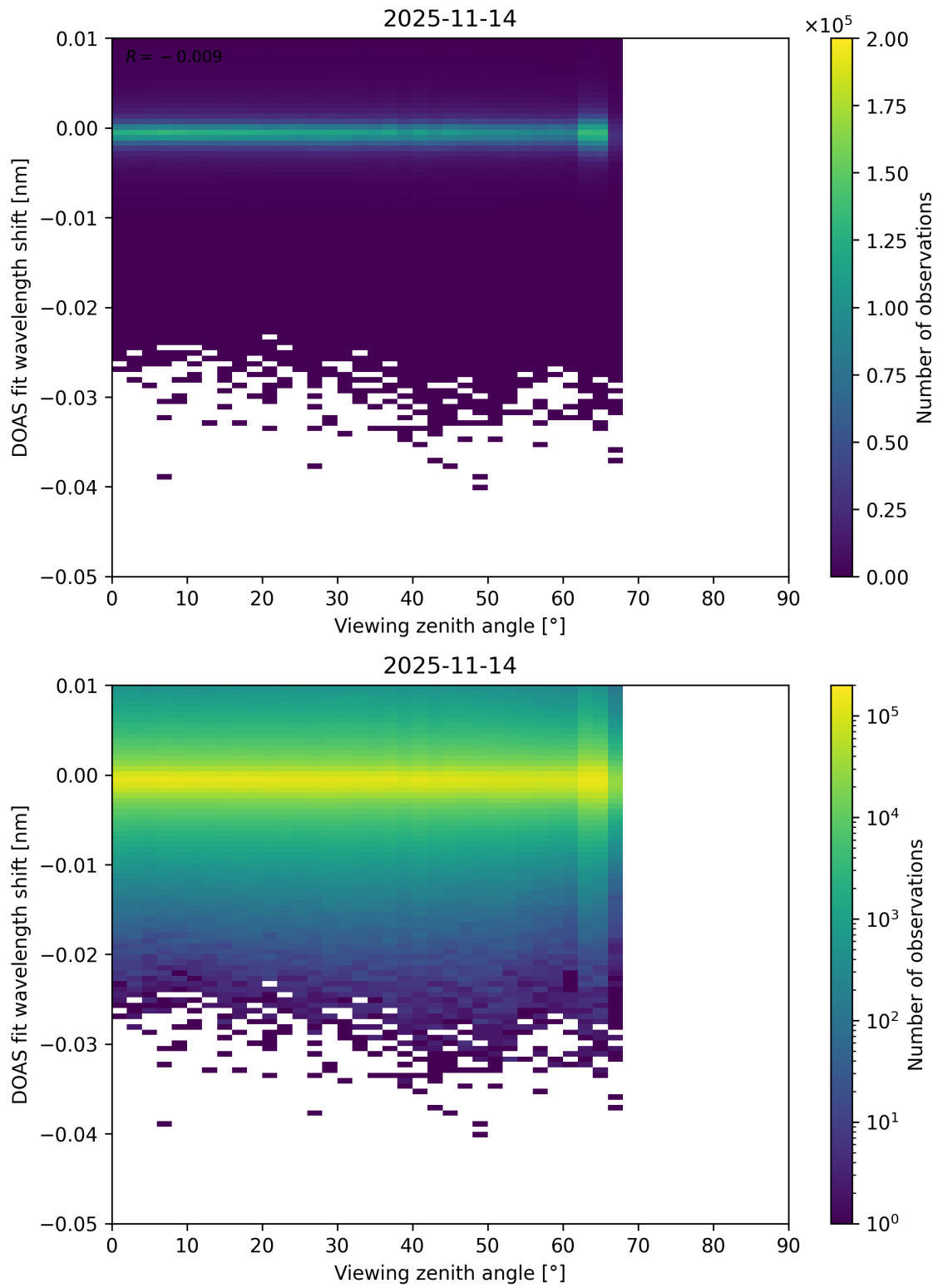
Figure 365: Scatter density plot of “Viewing zenith angle” against “DOAS fit wavelength shift” for 2025-11-13 to 2025-11-15.
