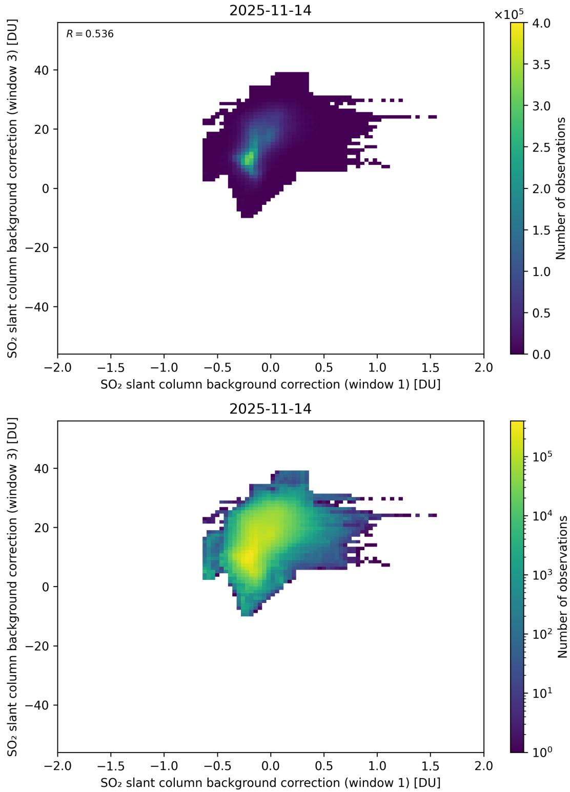
Figure 110: Scatter density plot of “SO 2 slant column background correction (window 1)” against “SO 2 slant column background correction (window 3)” for 2025-11-13 to 2025-11-15.
