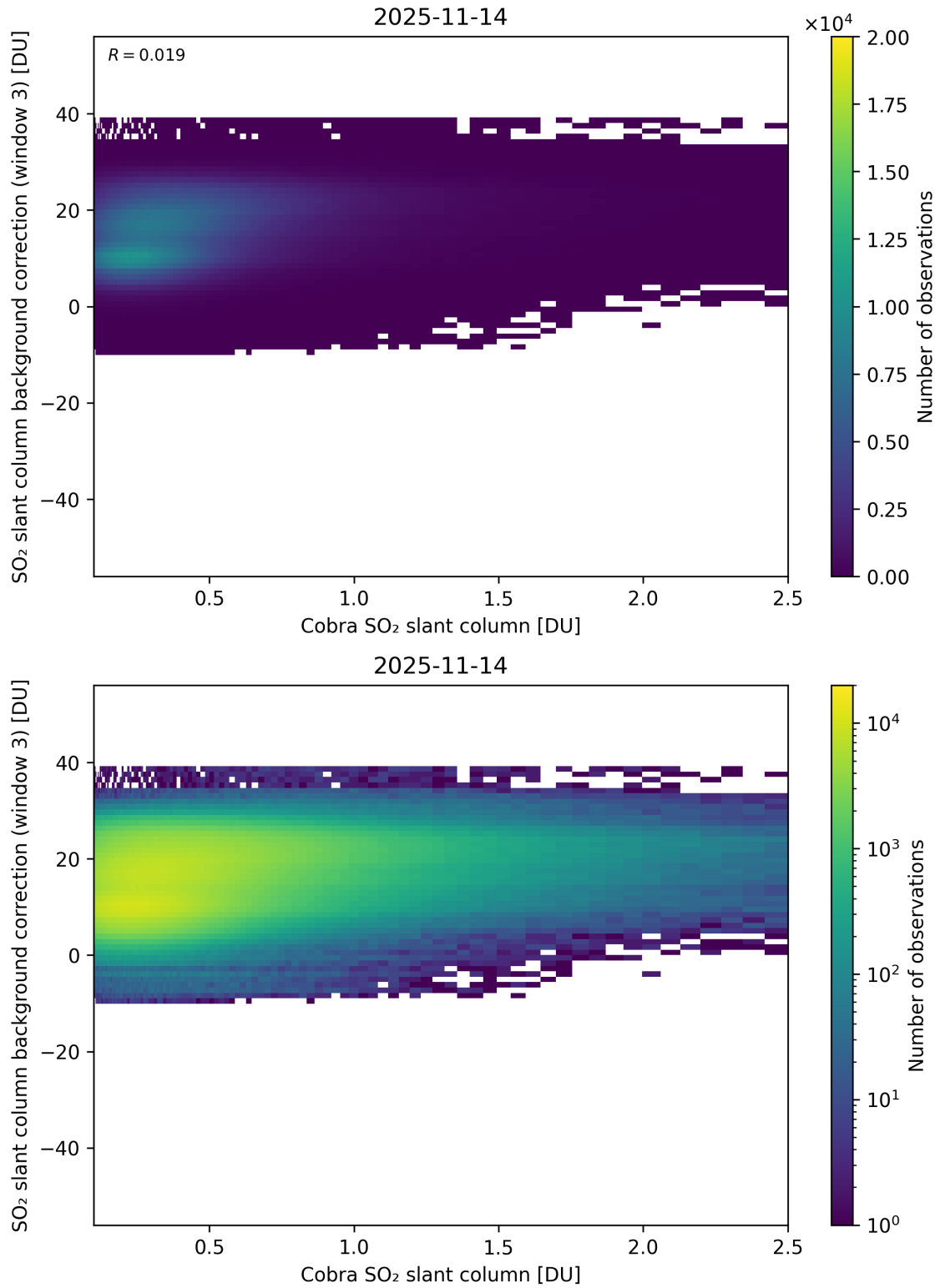
Figure 195: Scatter density plot of “Cobra SO 2 slant column” against “SO 2 slant column background correction (window 3)” for 2025-11-13 to 2025-11-15.
