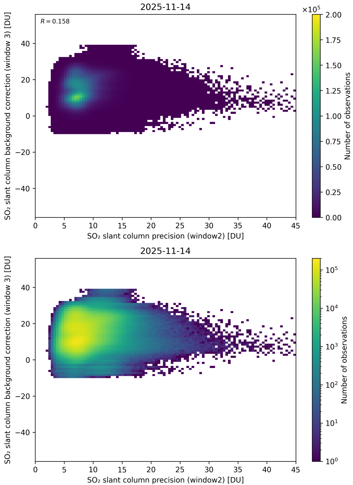
Figure 292: Scatter density plot of “SO 2 slant column precision (window2)” against “SO 2 slant column background correction (window 3)” for 2025-11-13 to 2025-11-15.
