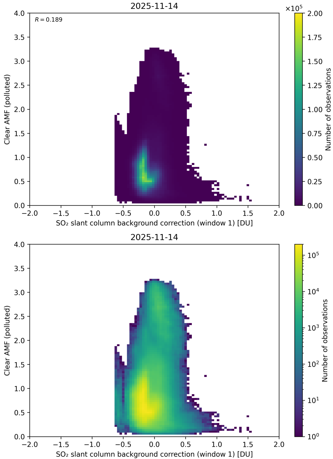
Figure 114: Scatter density plot of “SO 2 slant column background correction (window 1)” against “Clear AMF (polluted)” for 2025-11-13 to 2025-11-15.
