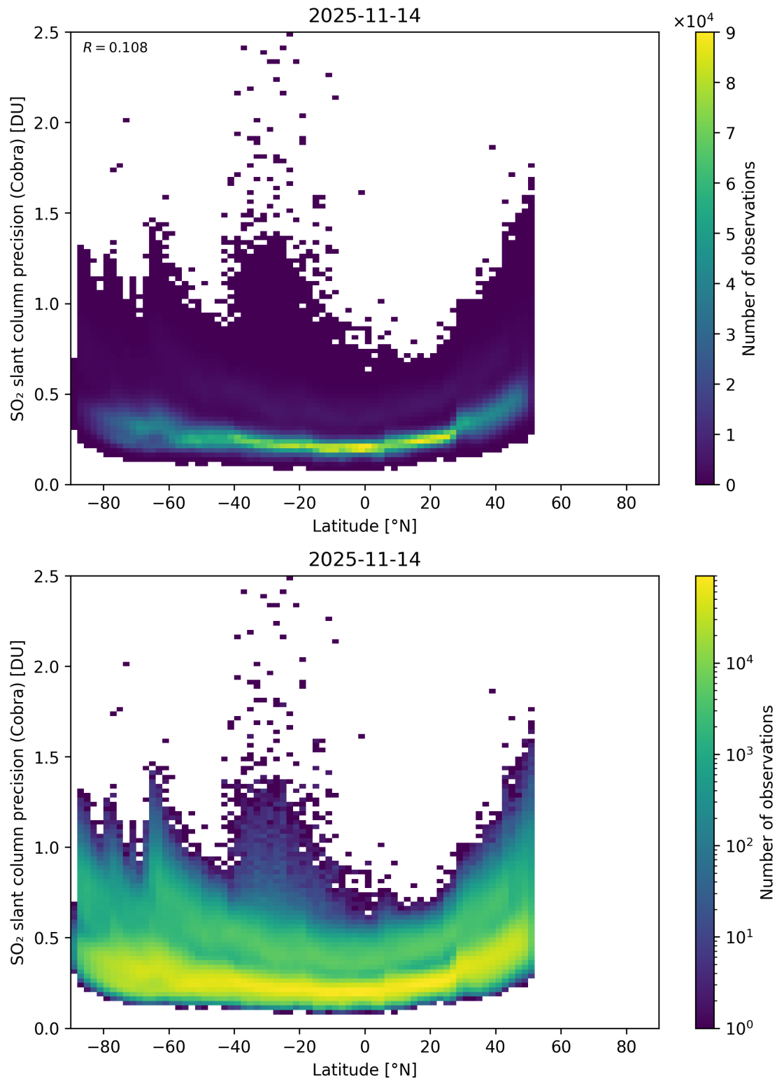
Figure 158: Scatter density plot of “Latitude” against “SO 2 slant column precision (Cobra)” for 2025-11-13 to 2025-11-15.
