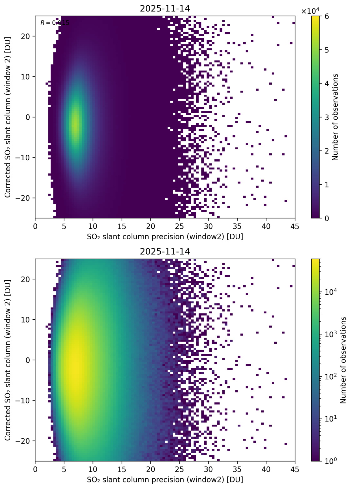
Figure 297: Scatter density plot of “SO 2 slant column precision (window2)” against “Corrected SO 2 slant column (window 2)” for 2025-11-13 to 2025-11-15.
