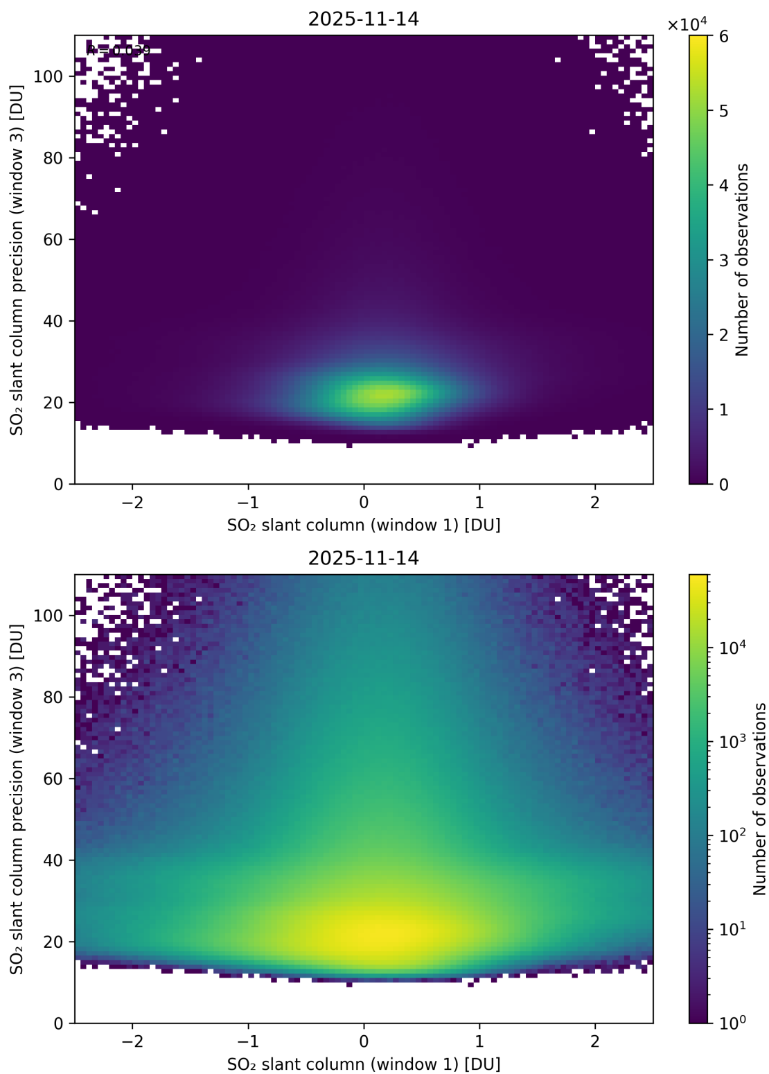
Figure 288: Scatter density plot of “SO 2 slant column (window 1)” against “SO 2 slant column precision (window 3)” for 2025-11-13 to 2025-11-15.
