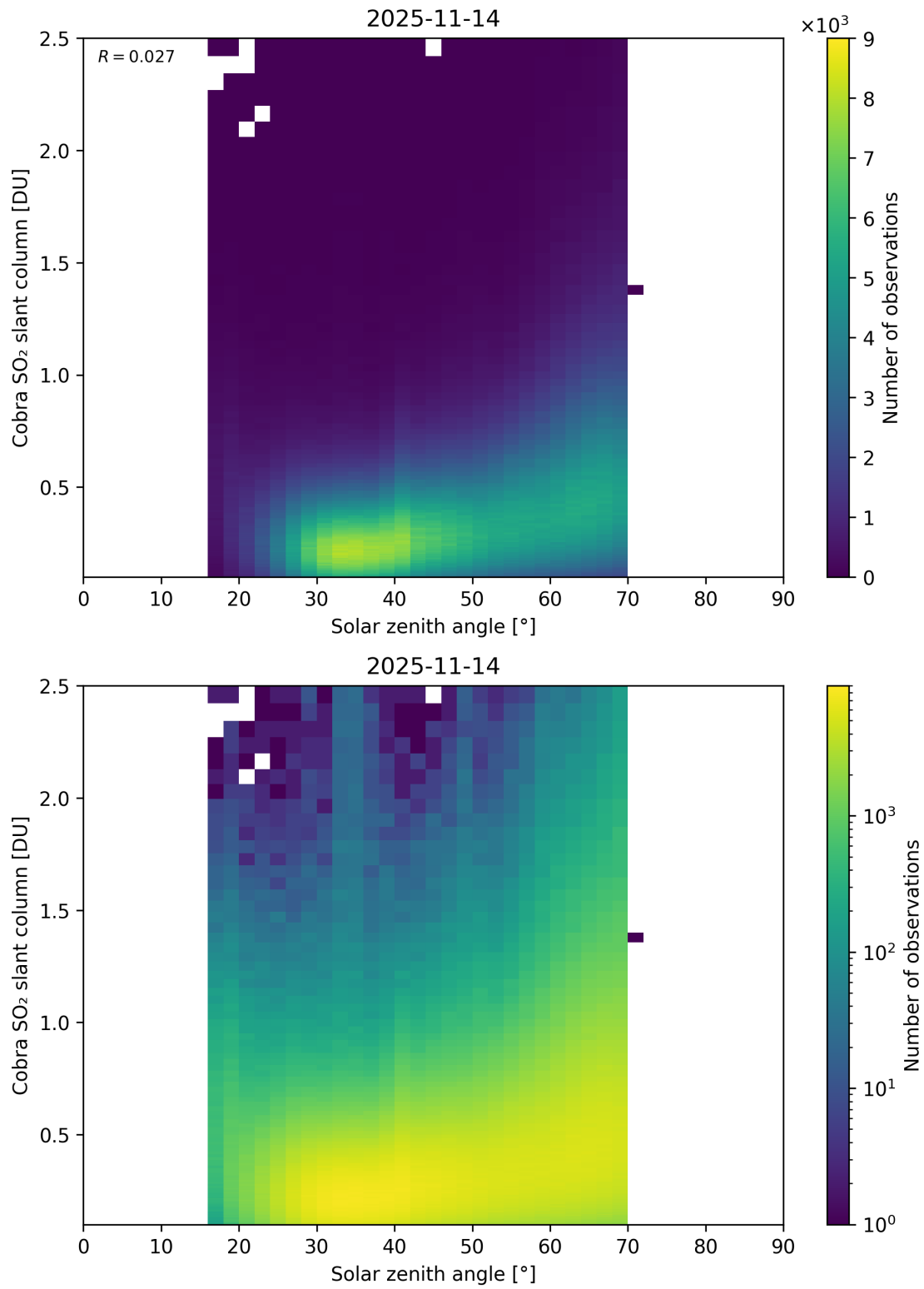
Figure 179: Scatter density plot of “Solar zenith angle” against “Cobra SO 2 slant column” for 2025-11-13 to 2025-11-15.
