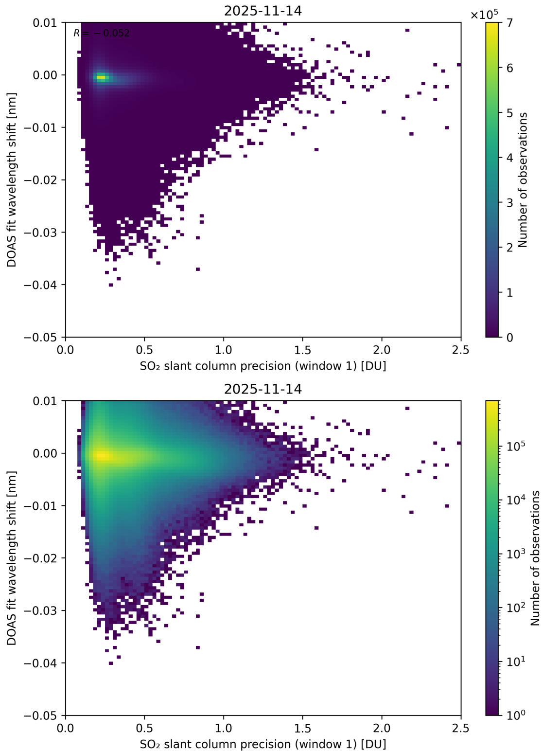
Figure 271: Scatter density plot of “SO 2 slant column precision (window 1)” against “DOAS fit wavelength shift” for 2025-11-13 to 2025-11-15.
