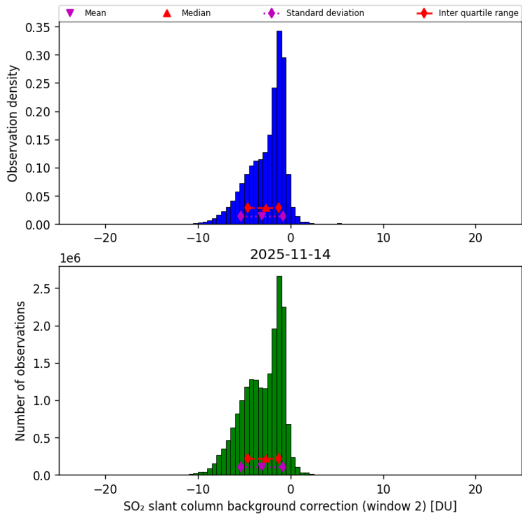
Figure 70: Histogram of “SO 2 slant column background correction (window 2)” for 2025-11-13 to 2025-11-15
