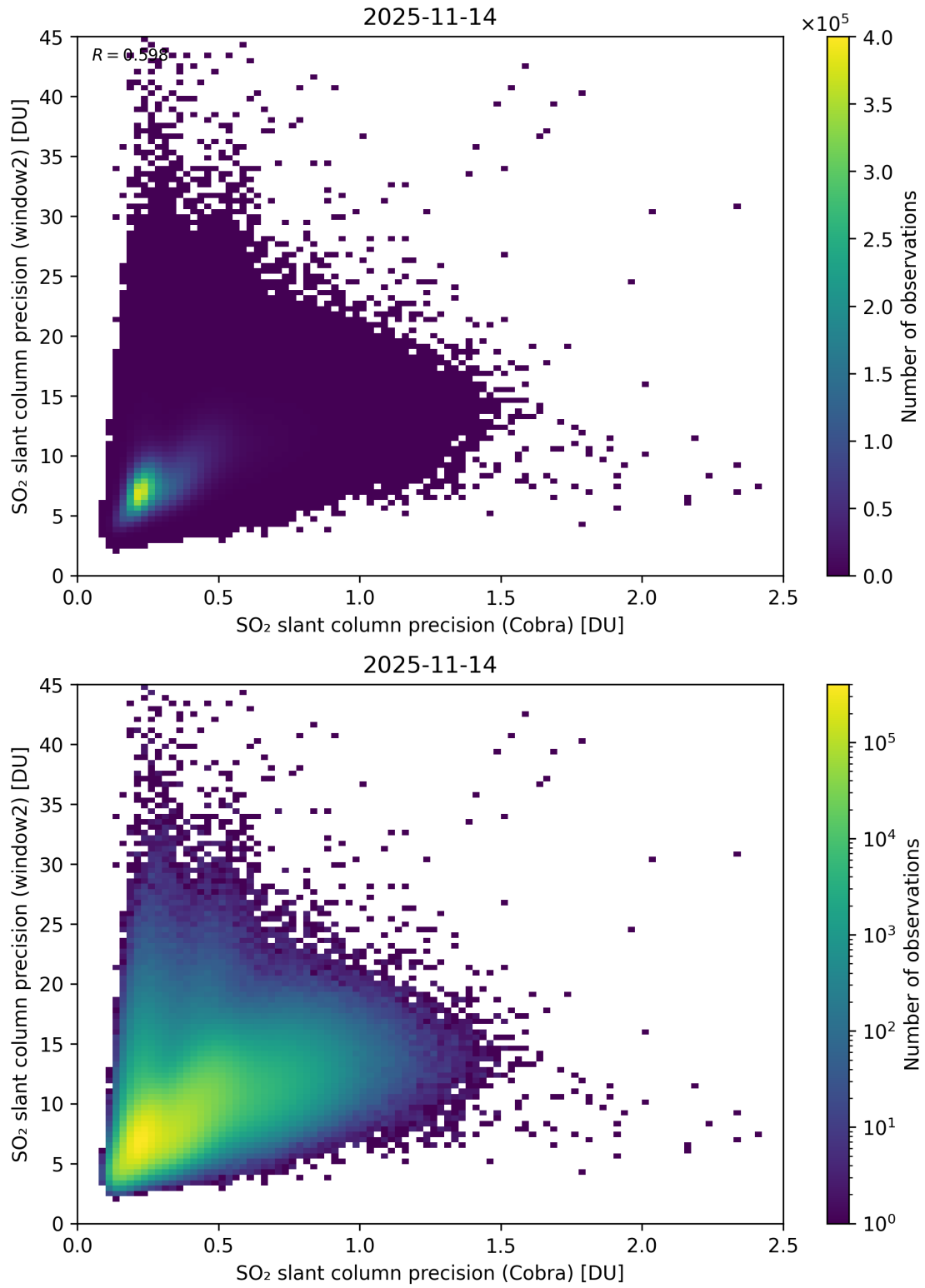
Figure 210: Scatter density plot of “SO 2 slant column precision (Cobra)” against “SO 2 slant column precision (window2)” for 2025-11-13 to 2025-11-15.
