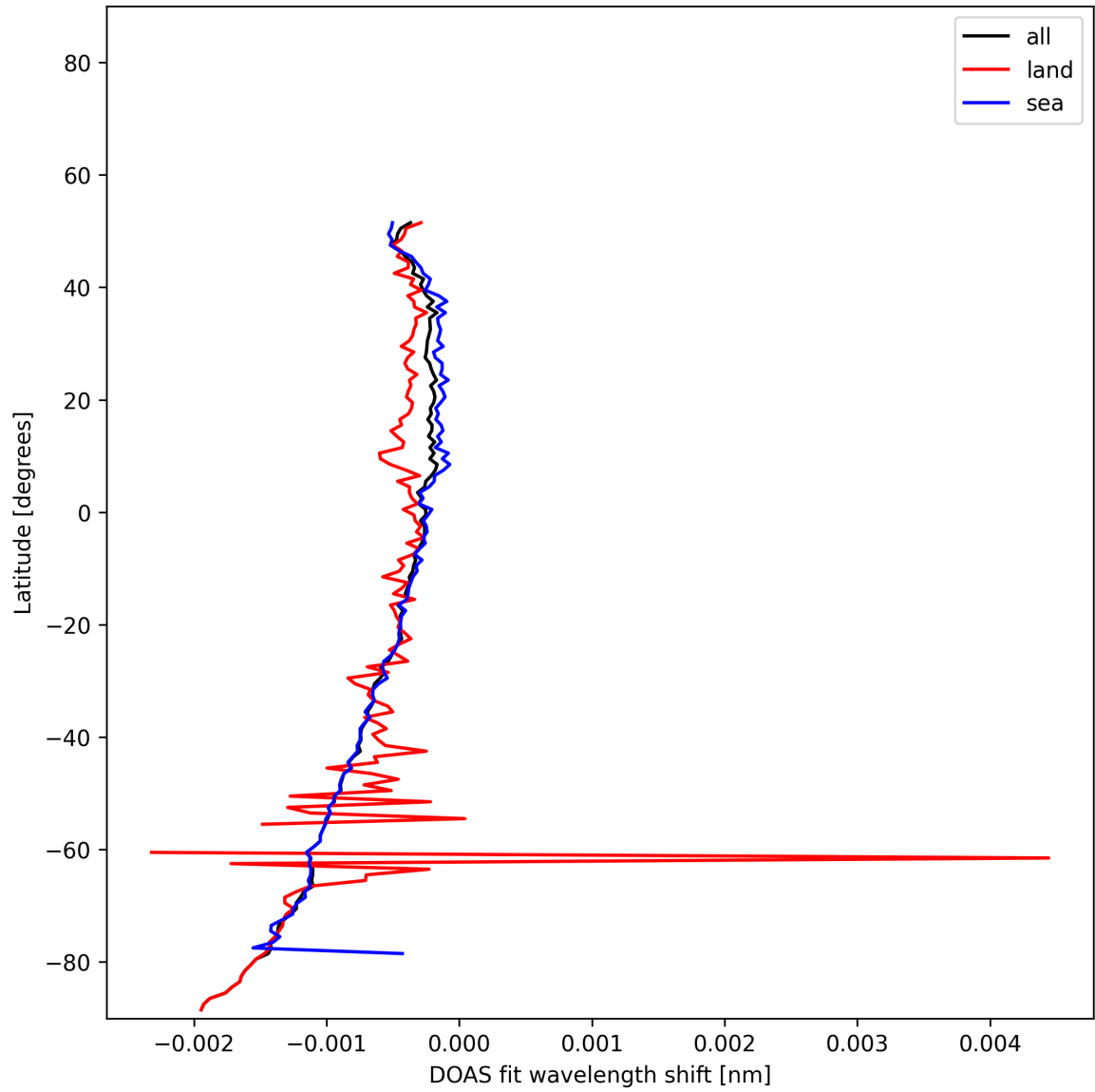
Figure 50: Zonal average of "DOAS fit wavelength shift" for 2025-11-13 to 2025-11-15.
