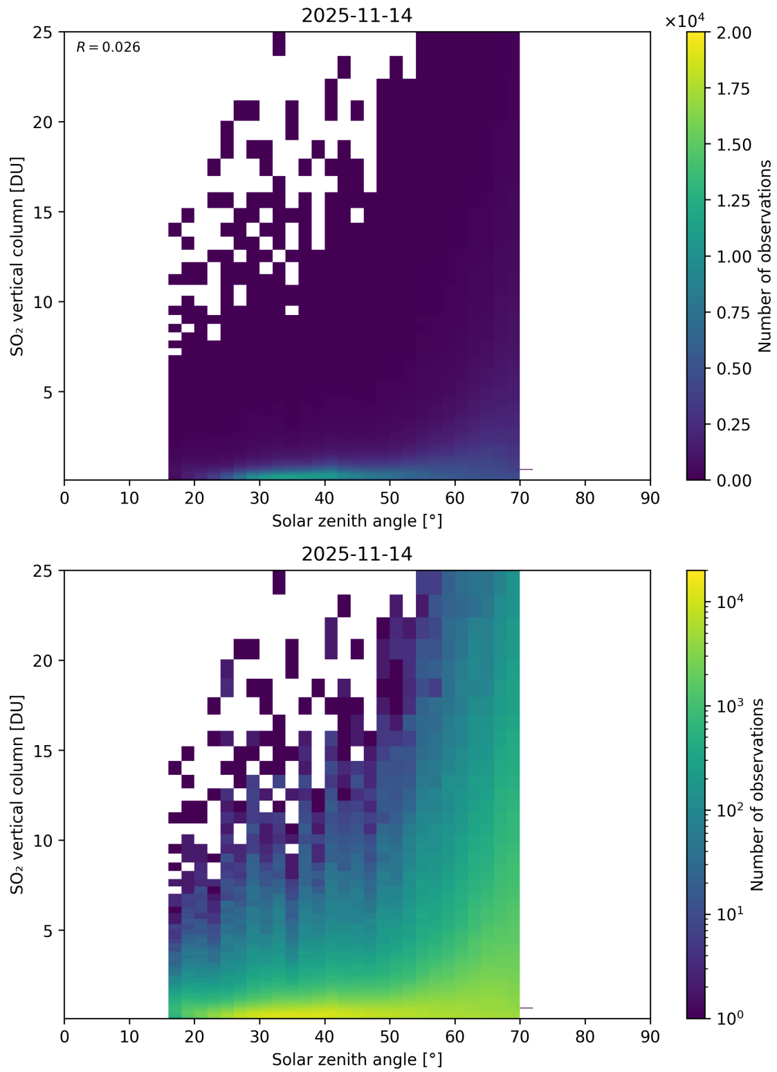
Figure 191: Scatter density plot of “Solar zenith angle” against “SO 2 vertical column” for 2025-11-13 to 2025-11-15.
