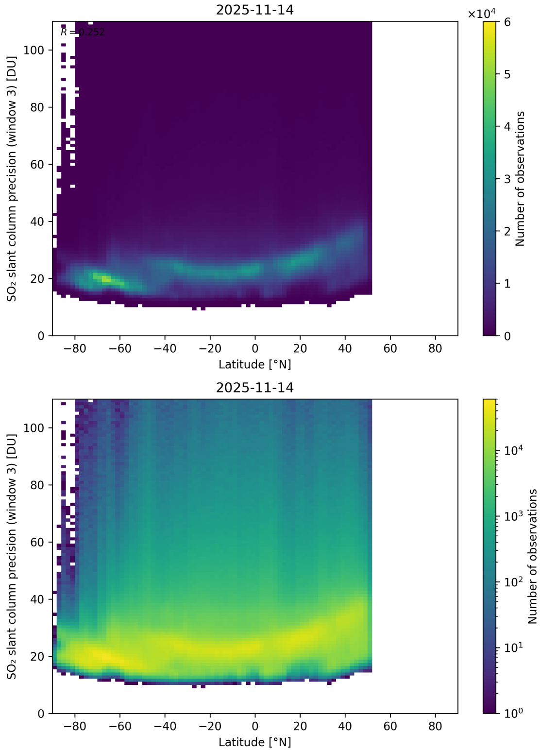
Figure 166: Scatter density plot of “Latitude” against “SO 2 slant column precision (window 3)” for 2025-11-13 to 2025-11-15.
