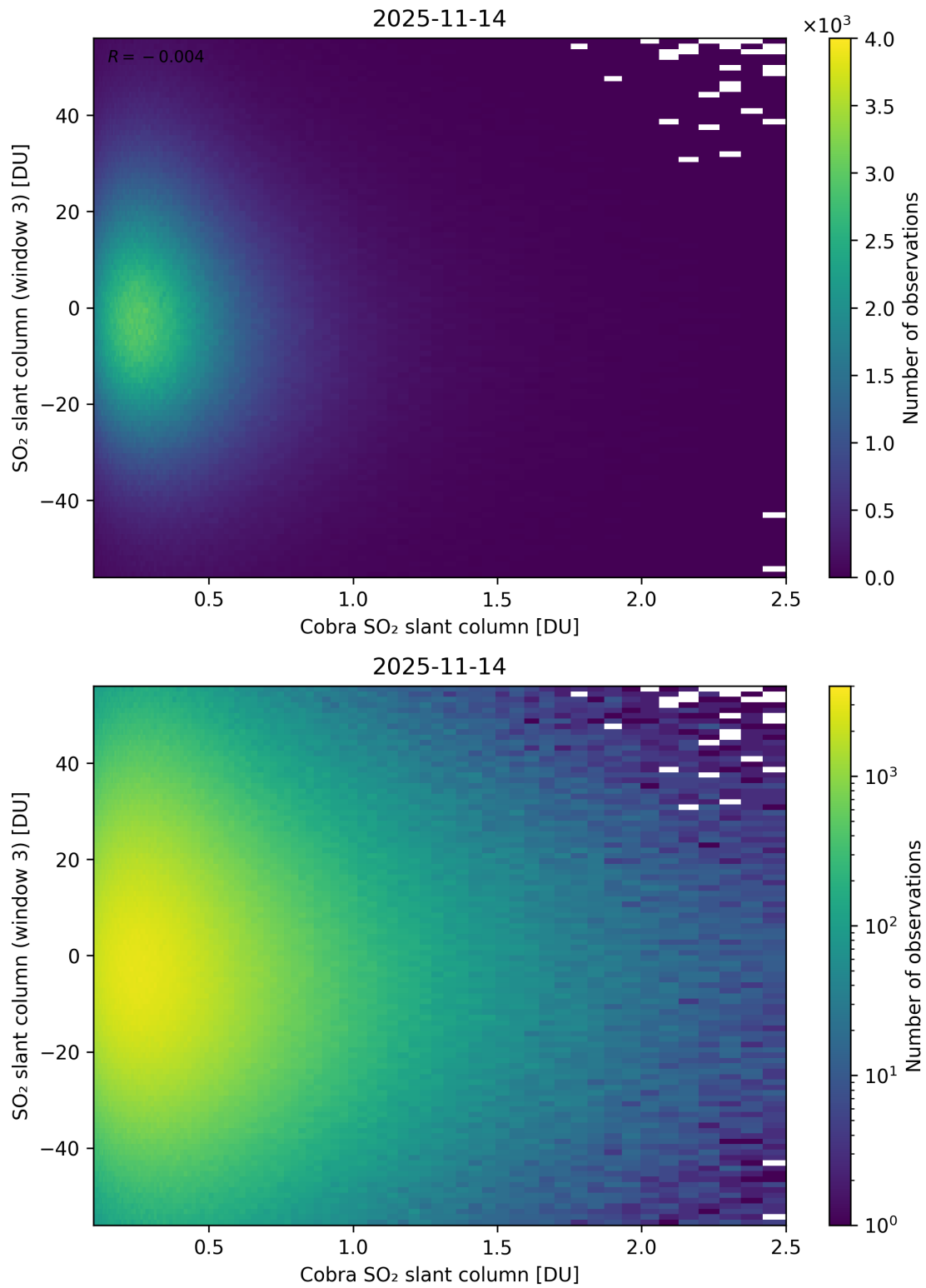
Figure 222: Scatter density plot of “Cobra SO 2 slant column” against “SO 2 slant column (window 3)” for 2025-11-13 to 2025-11-15.
