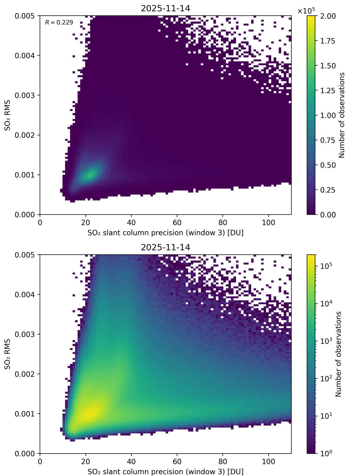
Figure 310: Scatter density plot of “SO 2 slant column precision (window 3)” against “SO 2 RMS” for 2025-11-13 to 2025-11-15.
