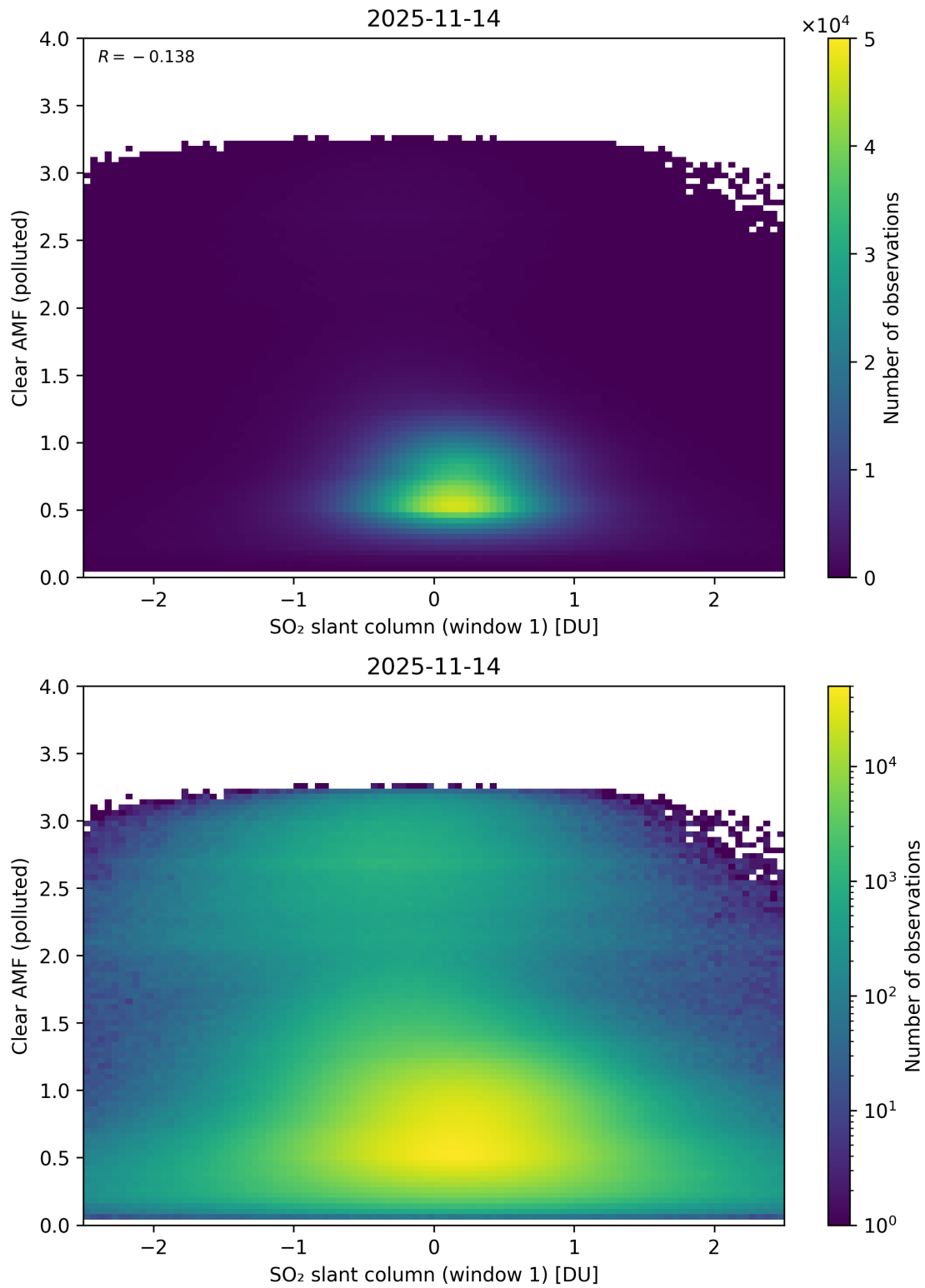
Figure 282: Scatter density plot of “SO 2 slant column (window 1)” against “Clear AMF (polluted)” for 2025-11-13 to 2025-11-15.
