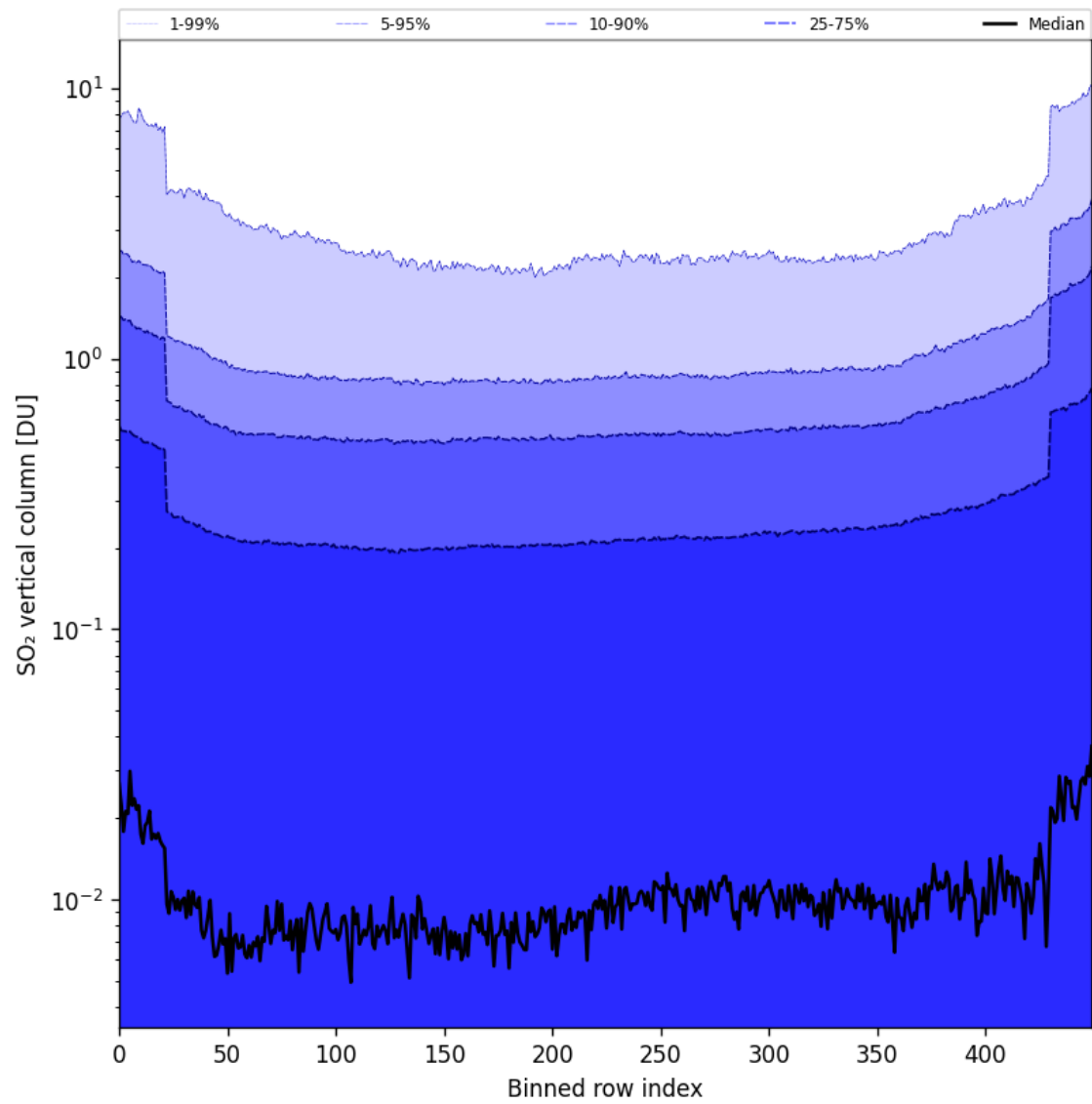
Figure 84: Along track statistics of “SO 2 vertical column” for 2025-11-13 to 2025-11-15
