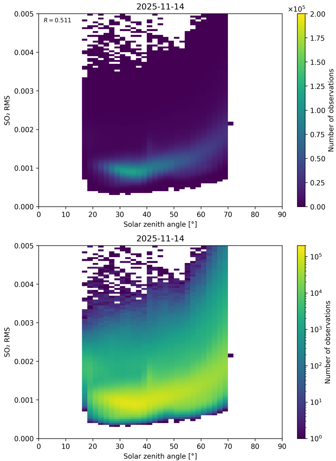
Figure 176: Scatter density plot of “Solar zenith angle” against “SO 2 RMS” for 2025-11-13 to 2025-11-15.
