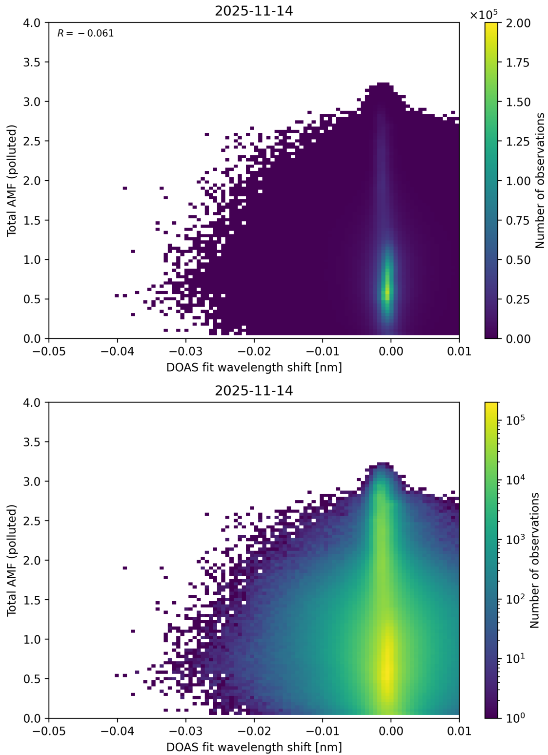
Figure 141: Scatter density plot of “DOAS fit wavelength shift” against “Total AMF (polluted)” for 2025-11-13 to 2025-11-15.
