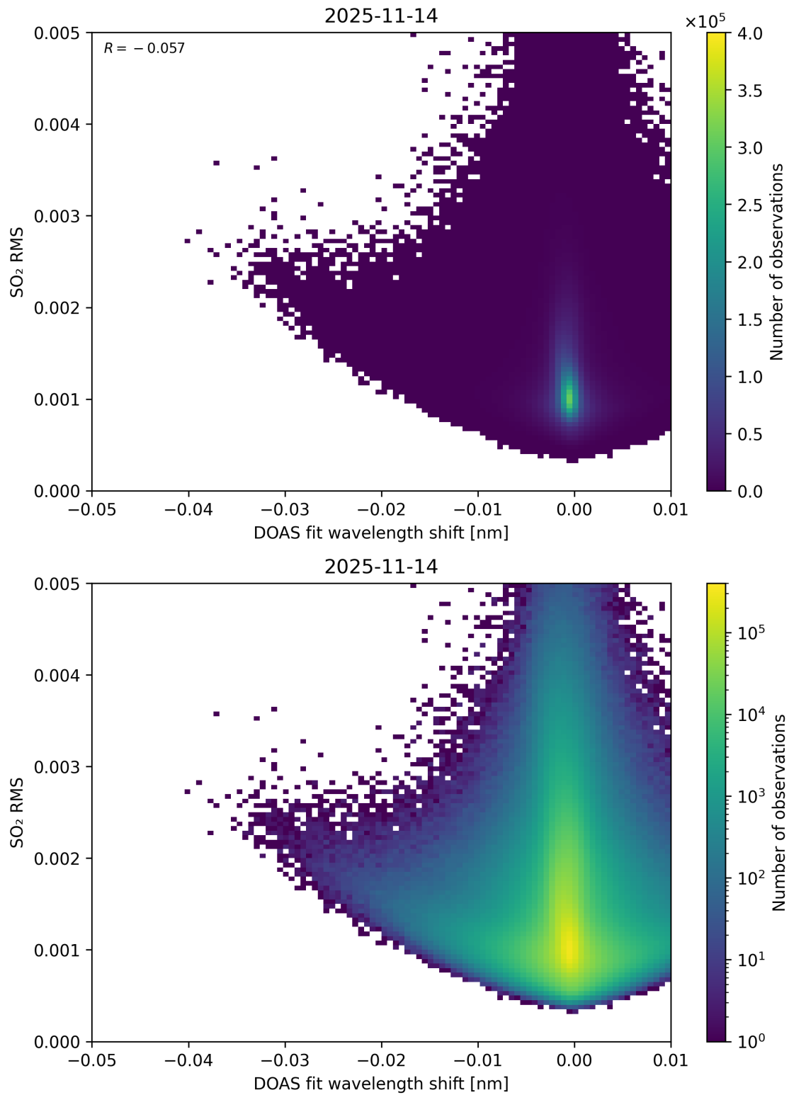
Figure 139: Scatter density plot of “DOAS fit wavelength shift” against “SO 2 RMS” for 2025-11-13 to 2025-11-15.
