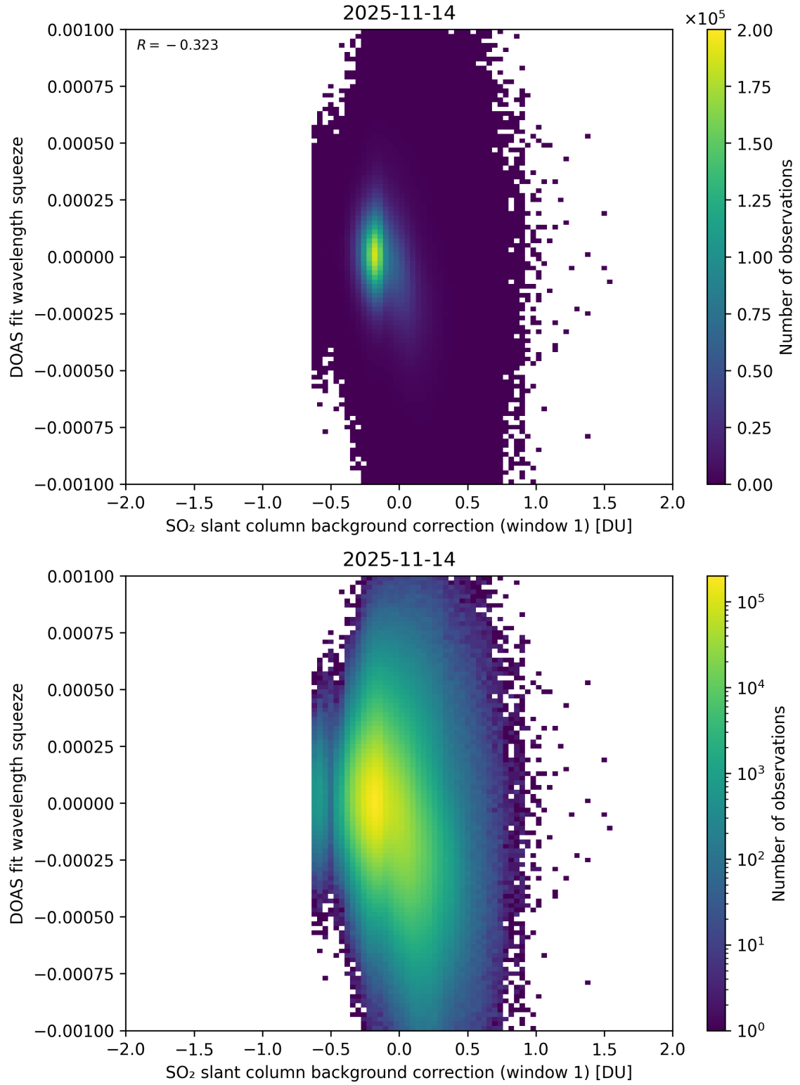
Figure 112: Scatter density plot of “SO 2 slant column background correction (window 1)” against “DOAS fit wavelength squeeze” for 2025-11-13 to 2025-11-15.
