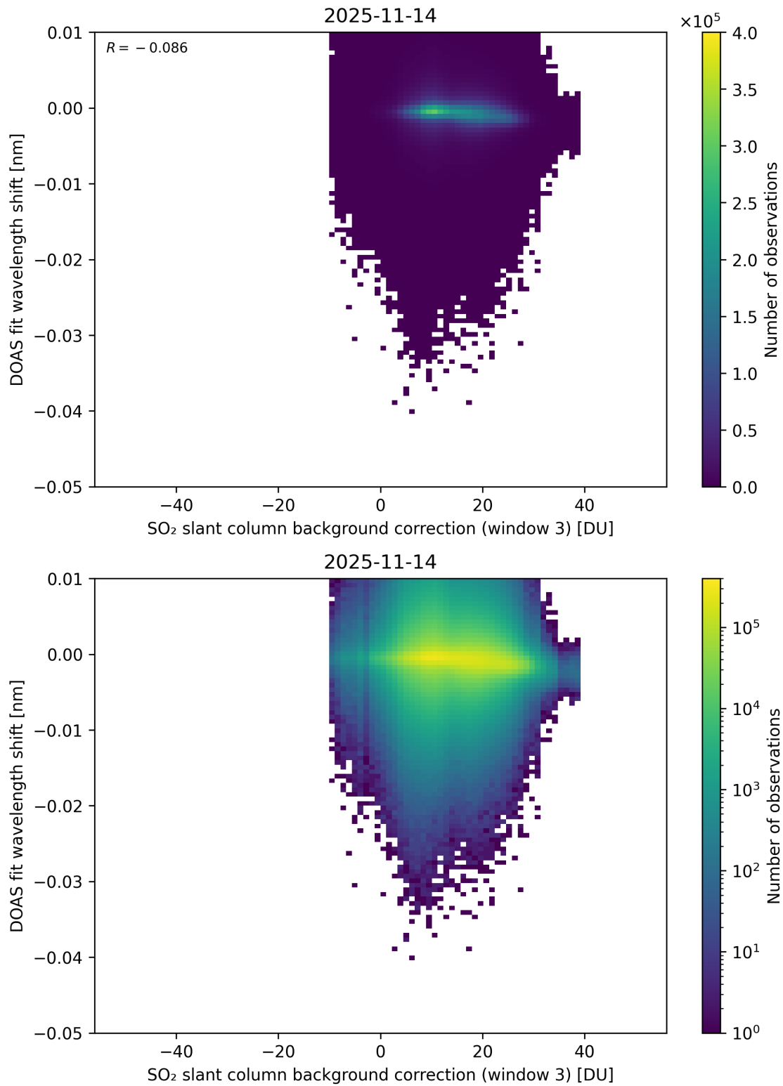
Figure 132: Scatter density plot of “SO 2 slant column background correction (window 3)” against “DOAS fit wavelength shift” for 2025-11-13 to 2025-11-15.
