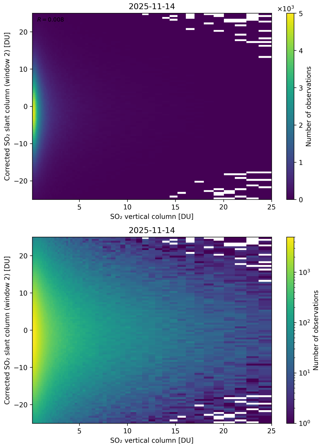
Figure 352: Scatter density plot of “SO 2 vertical column” against “Corrected SO 2 slant column (window 2)” for 2025-11-13 to 2025-11-15.
