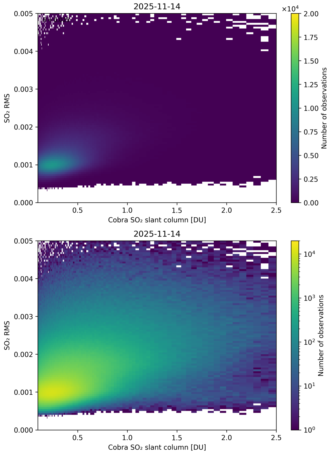
Figure 198: Scatter density plot of “Cobra SO 2 slant column” against “SO 2 RMS” for 2025-11-13 to 2025-11-15.
