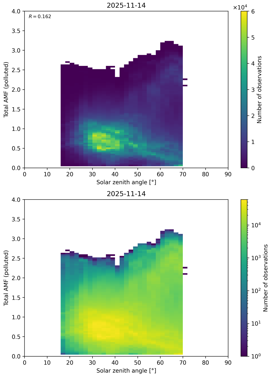
Figure 189: Scatter density plot of “Solar zenith angle” against “Total AMF (polluted)” for 2025-11-13 to 2025-11-15.
