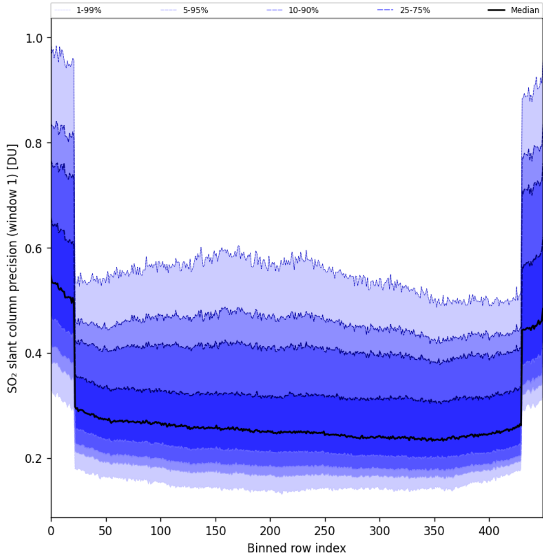
Figure 90: Along track statistics of “SO 2 slant column precision (window 1)” for 2025-11-13 to 2025-11-15
