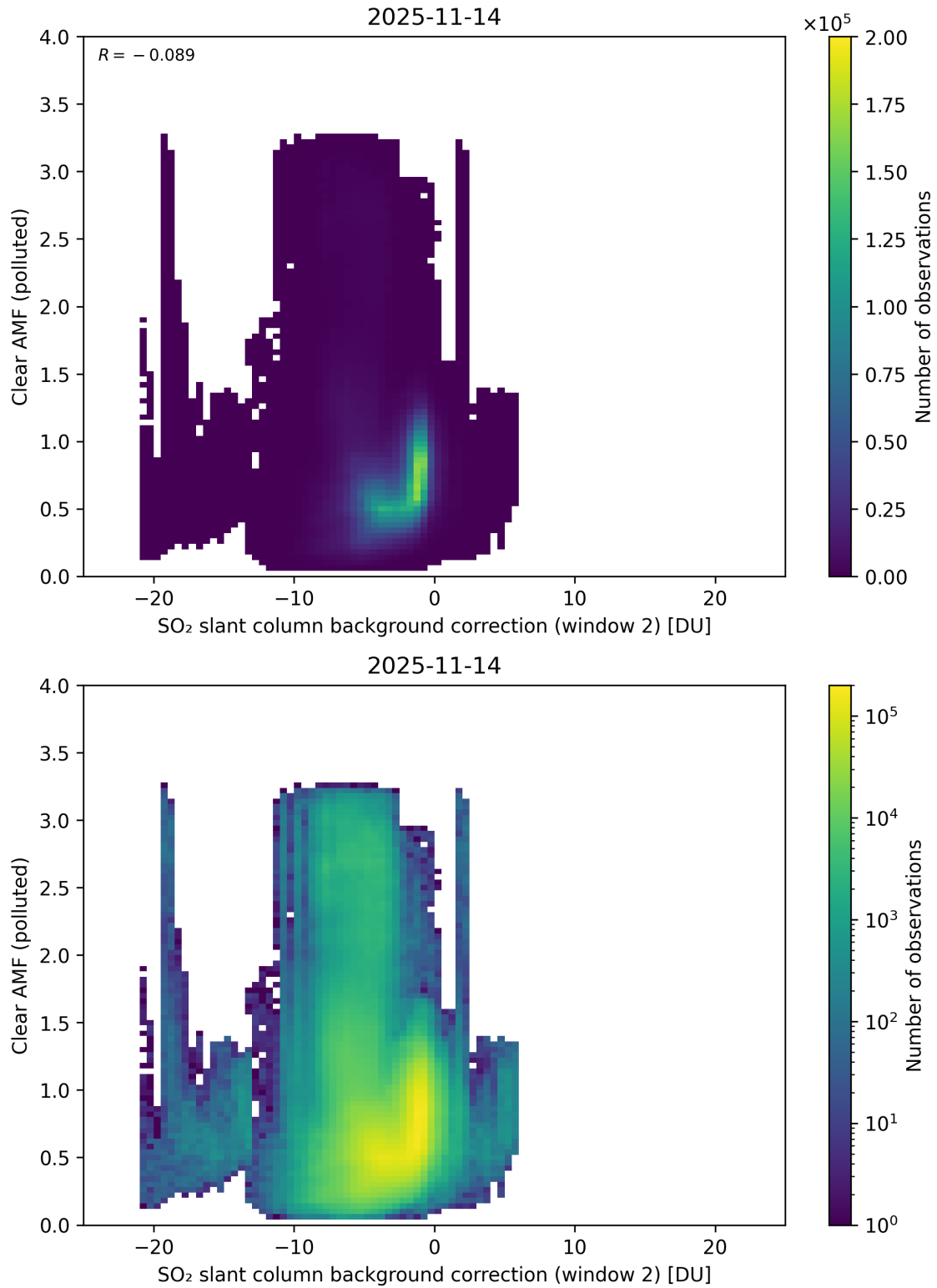
Figure 126: Scatter density plot of “SO 2 slant column background correction (window 2)” against “Clear AMF (polluted)” for 2025-11-13 to 2025-11-15.
