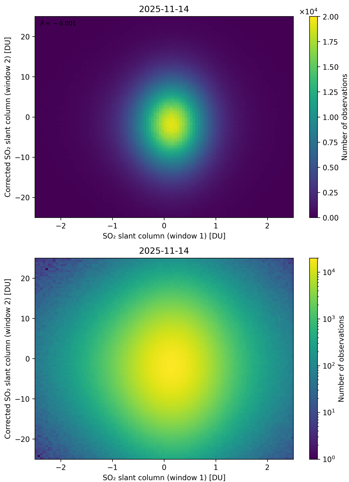
Figure 283: Scatter density plot of “SO 2 slant column (window 1)” against “Corrected SO 2 slant column (window 2)” for 2025-11-13 to 2025-11-15.
