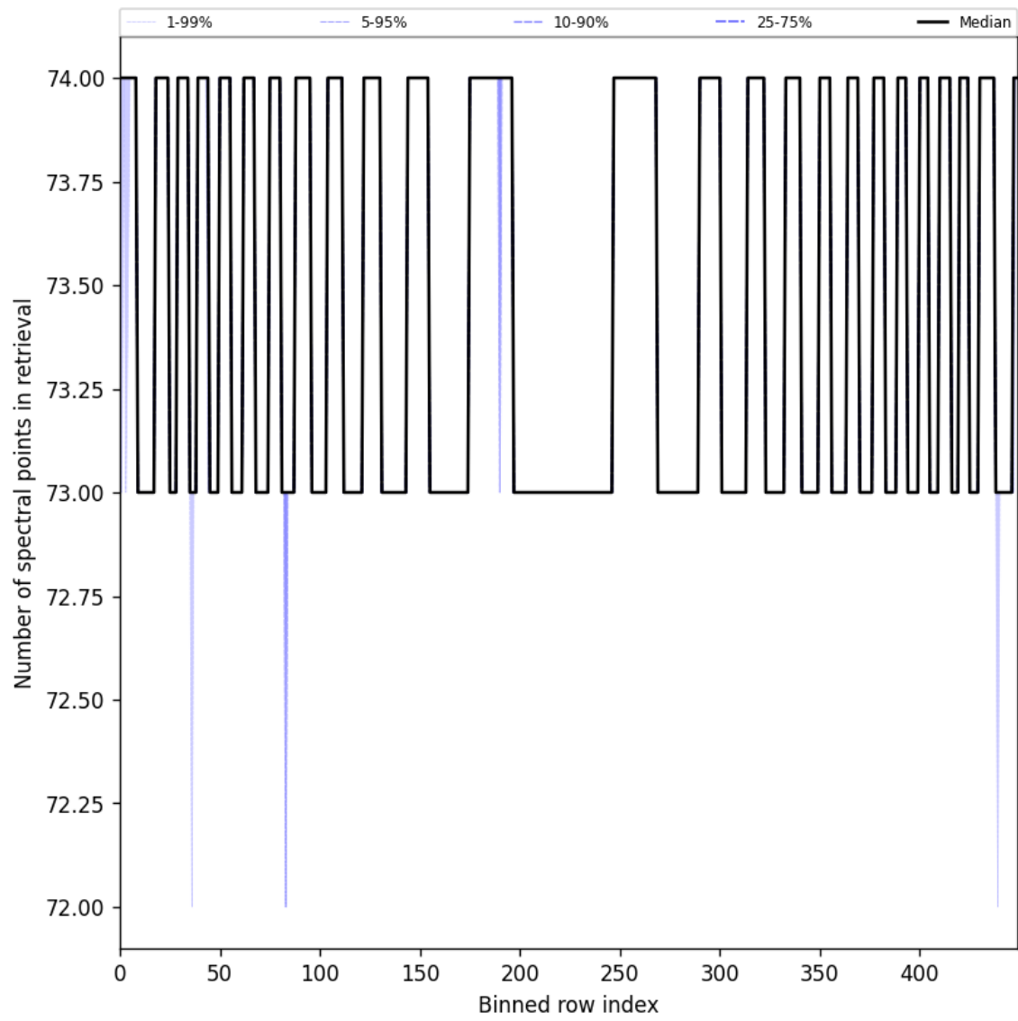
Figure 108: Along track statistics of “Number of spectral points in retrieval” for 2025-11-13 to 2025-11-15
