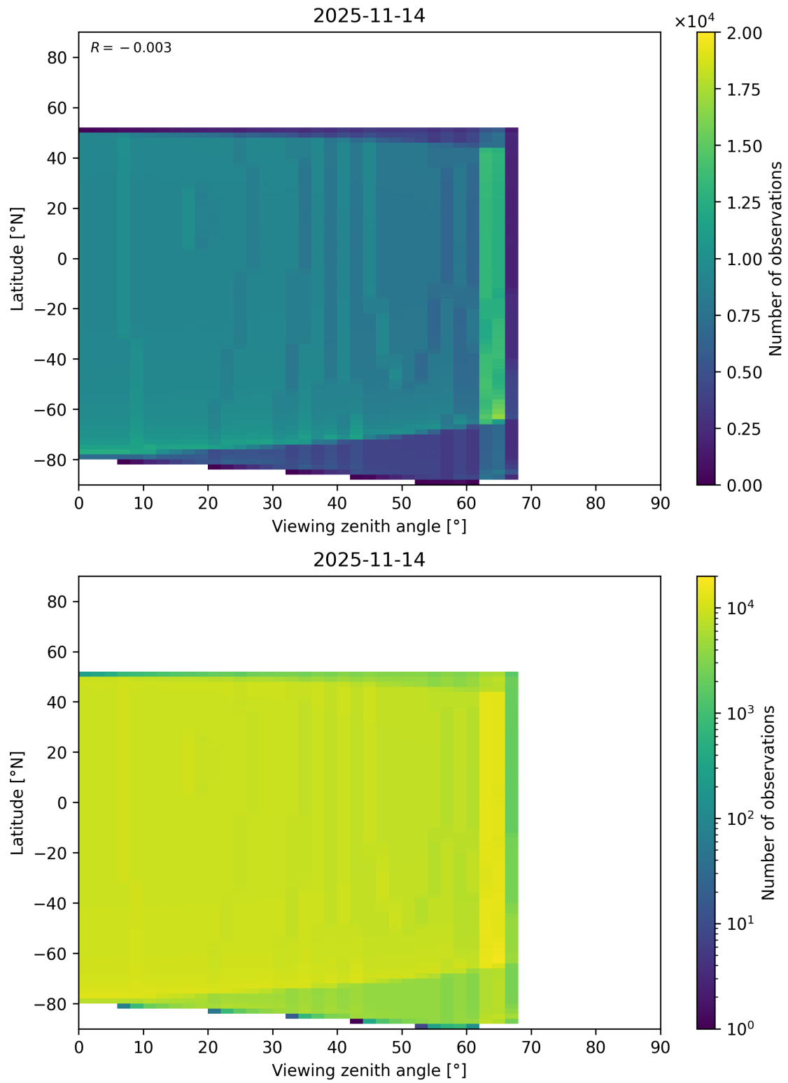
Figure 368: Scatter density plot of “Viewing zenith angle” against “Latitude” for 2025-11-13 to 2025-11-15.
