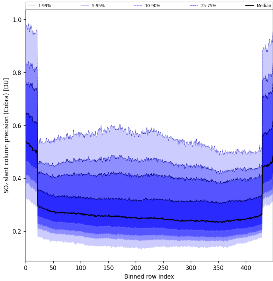
Figure 88: Along track statistics of “SO 2 slant column precision (Cobra)” for 2025-11-13 to 2025-11-15
