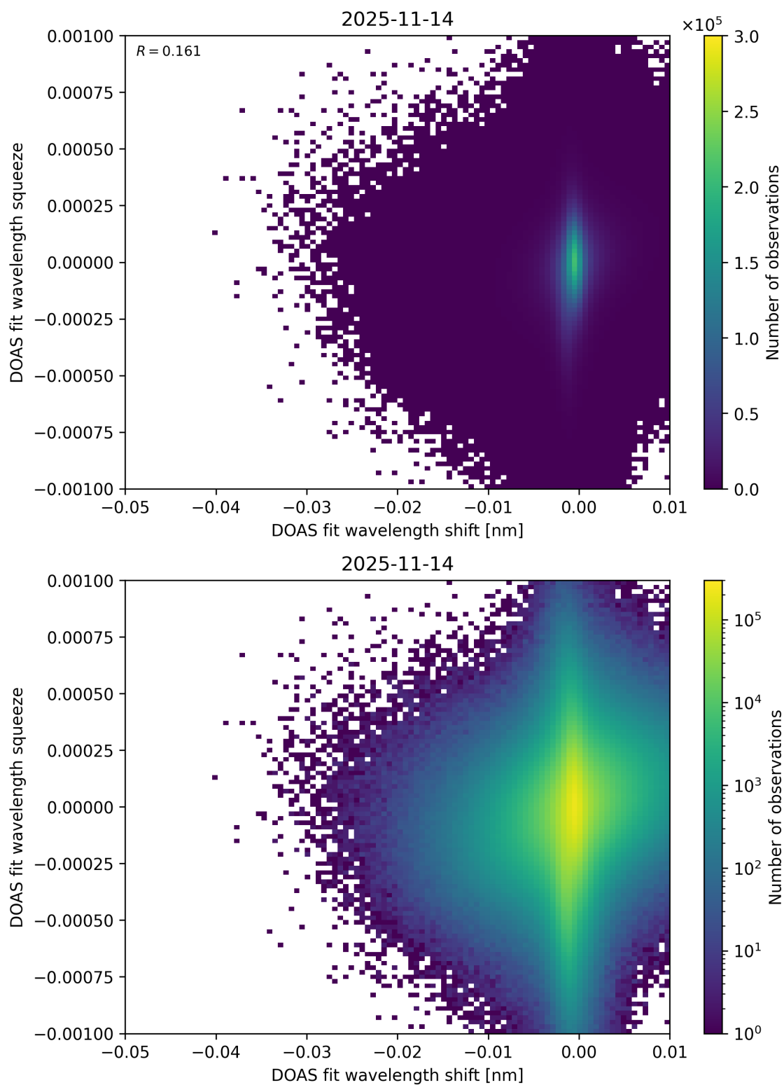
Figure 138: Scatter density plot of “DOAS fit wavelength shift” against “DOAS fit wavelength squeeze” for 2025-11-13 to 2025-11-15.
