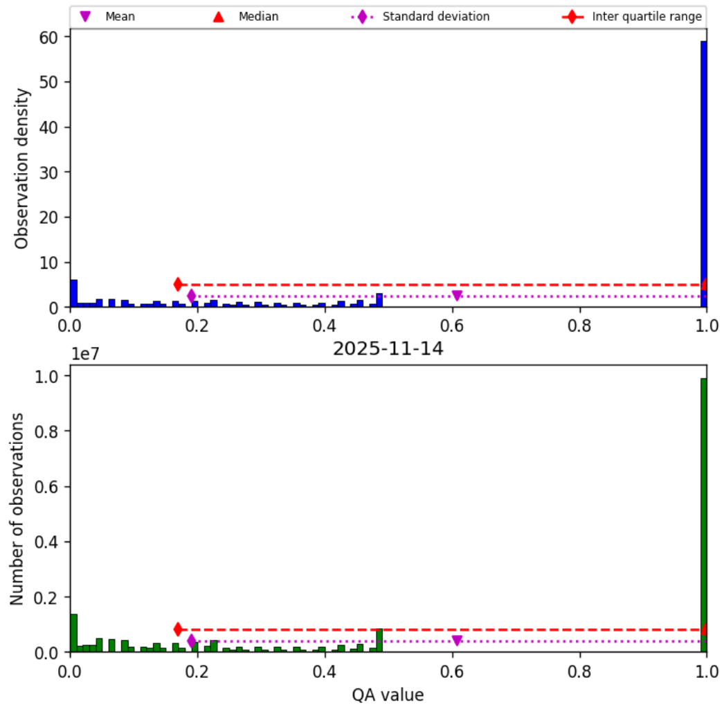
Figure 57: Histogram of “QA value” for 2025-11-13 to 2025-11-15
