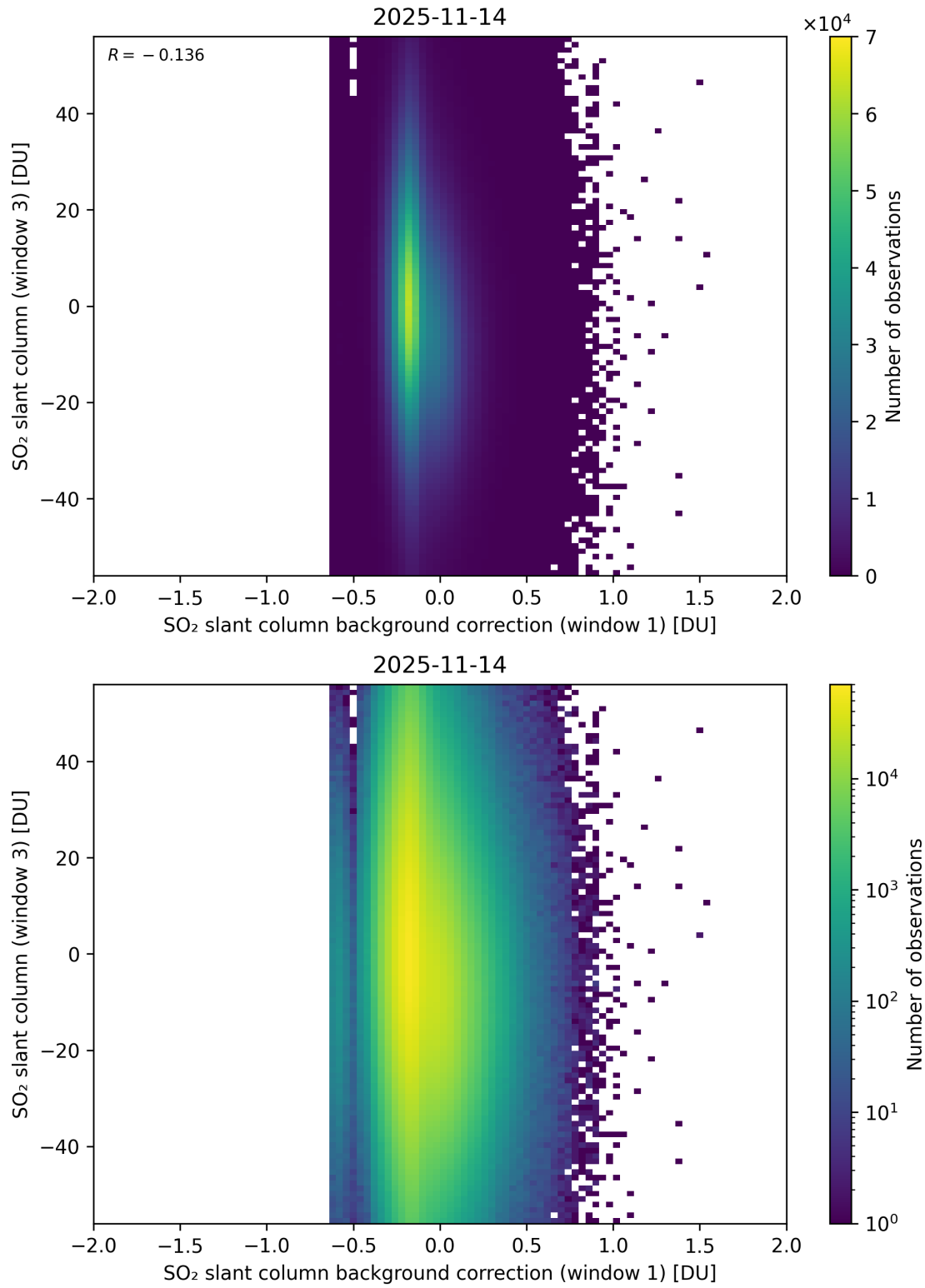
Figure 118: Scatter density plot of “SO 2 slant column background correction (window 1)” against “SO 2 slant column (window 3)” for 2025-11-13 to 2025-11-15.
