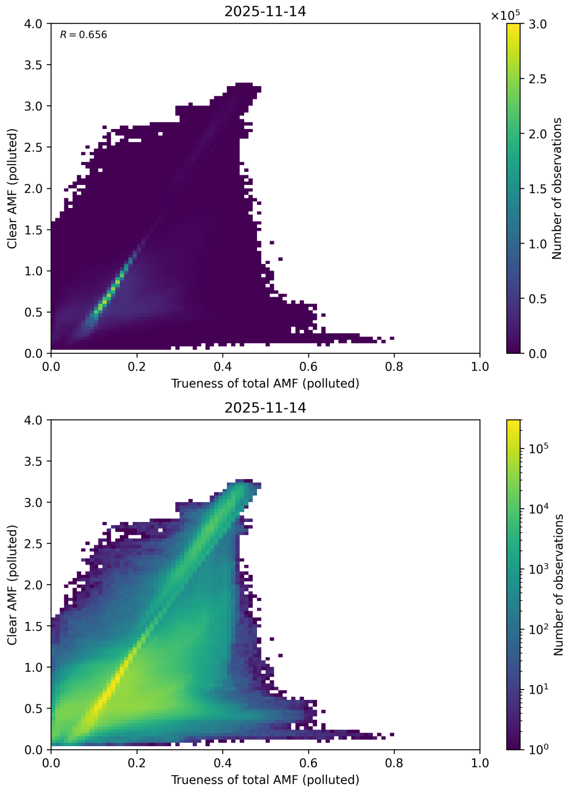
Figure 322: Scatter density plot of “Trueness of total AMF (polluted)” against “Clear AMF (polluted)” for 2025-11-13 to 2025-11-15.
