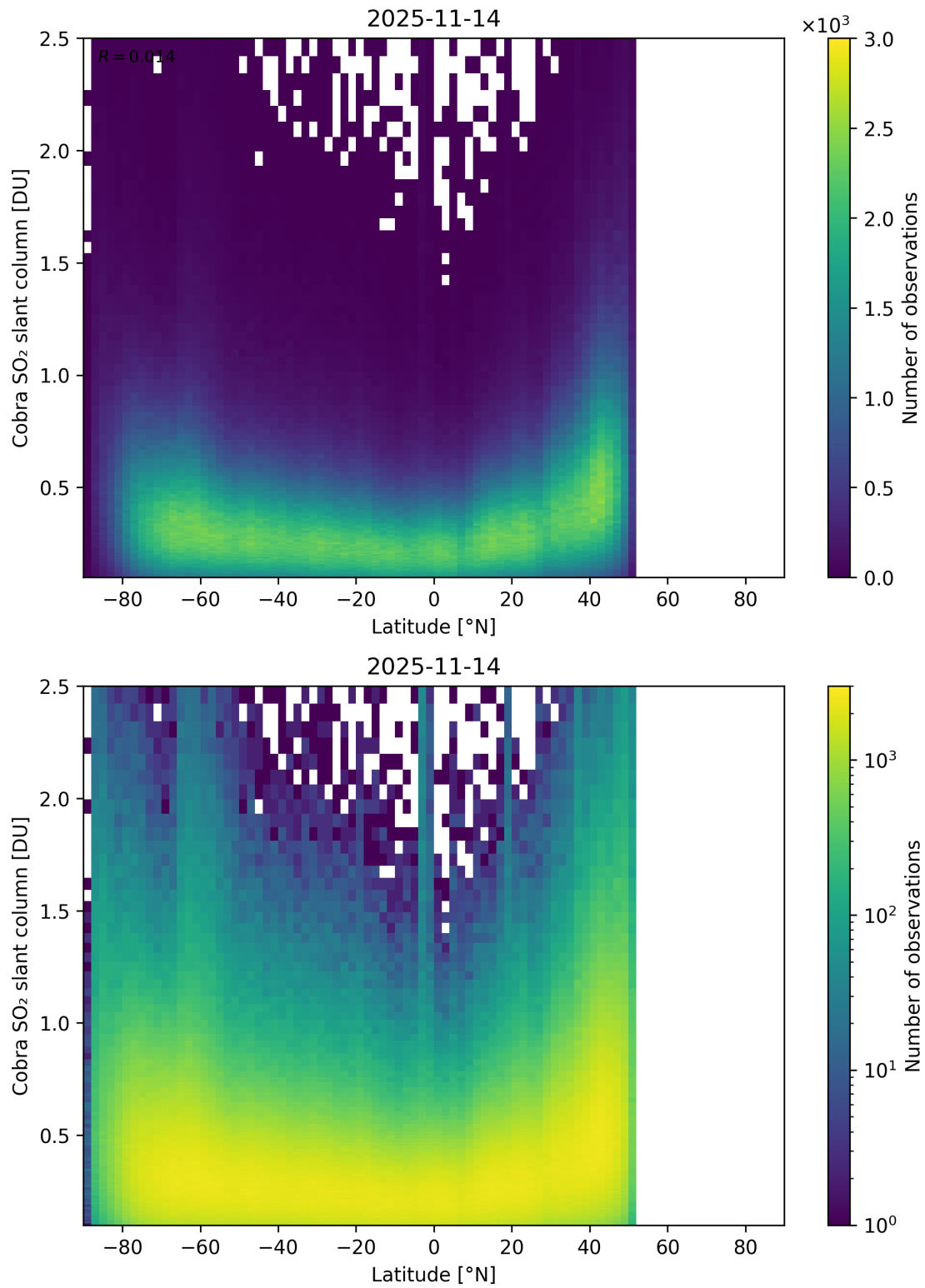
Figure 157: Scatter density plot of “Latitude” against “Cobra SO 2 slant column” for 2025-11-13 to 2025-11-15.
