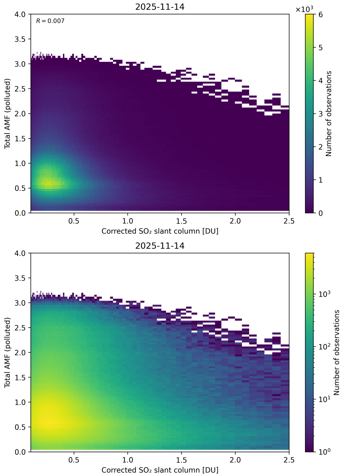
Figure 242: Scatter density plot of “Corrected SO 2 slant column” against “Total AMF (polluted)” for 2025-11-13 to 2025-11-15.
