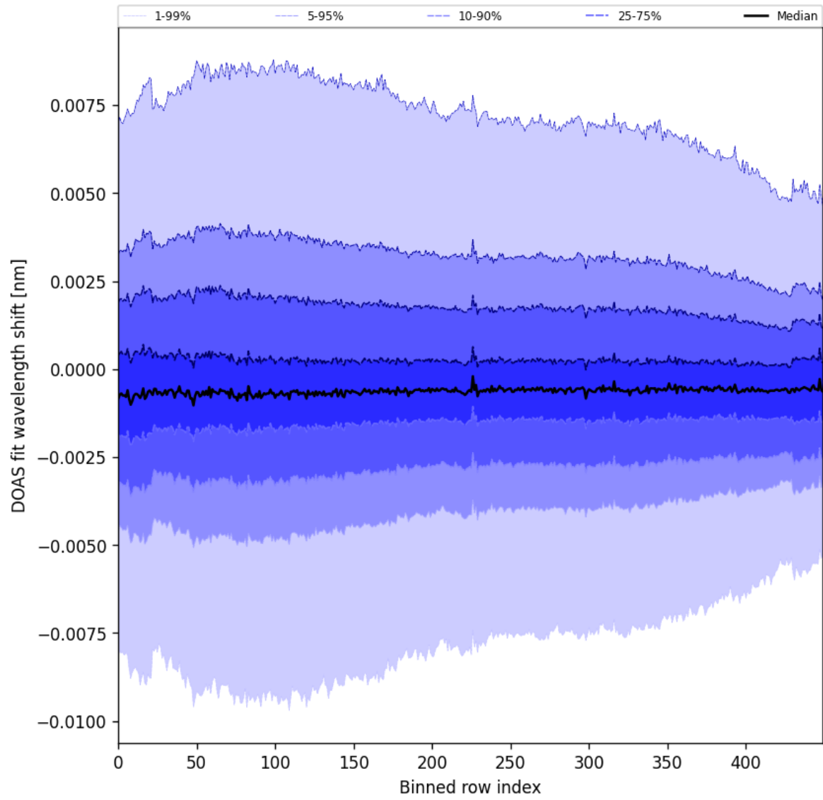
Figure 102: Along track statistics of “DOAS fit wavelength shift” for 2025-11-13 to 2025-11-15
