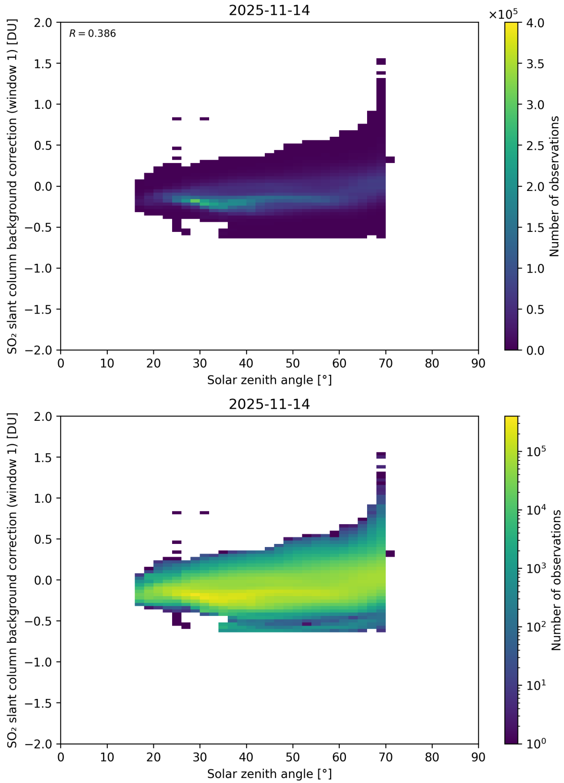
Figure 171: Scatter density plot of “Solar zenith angle” against “SO 2 slant column background correction (window 1)” for 2025-11-13 to 2025-11-15.
