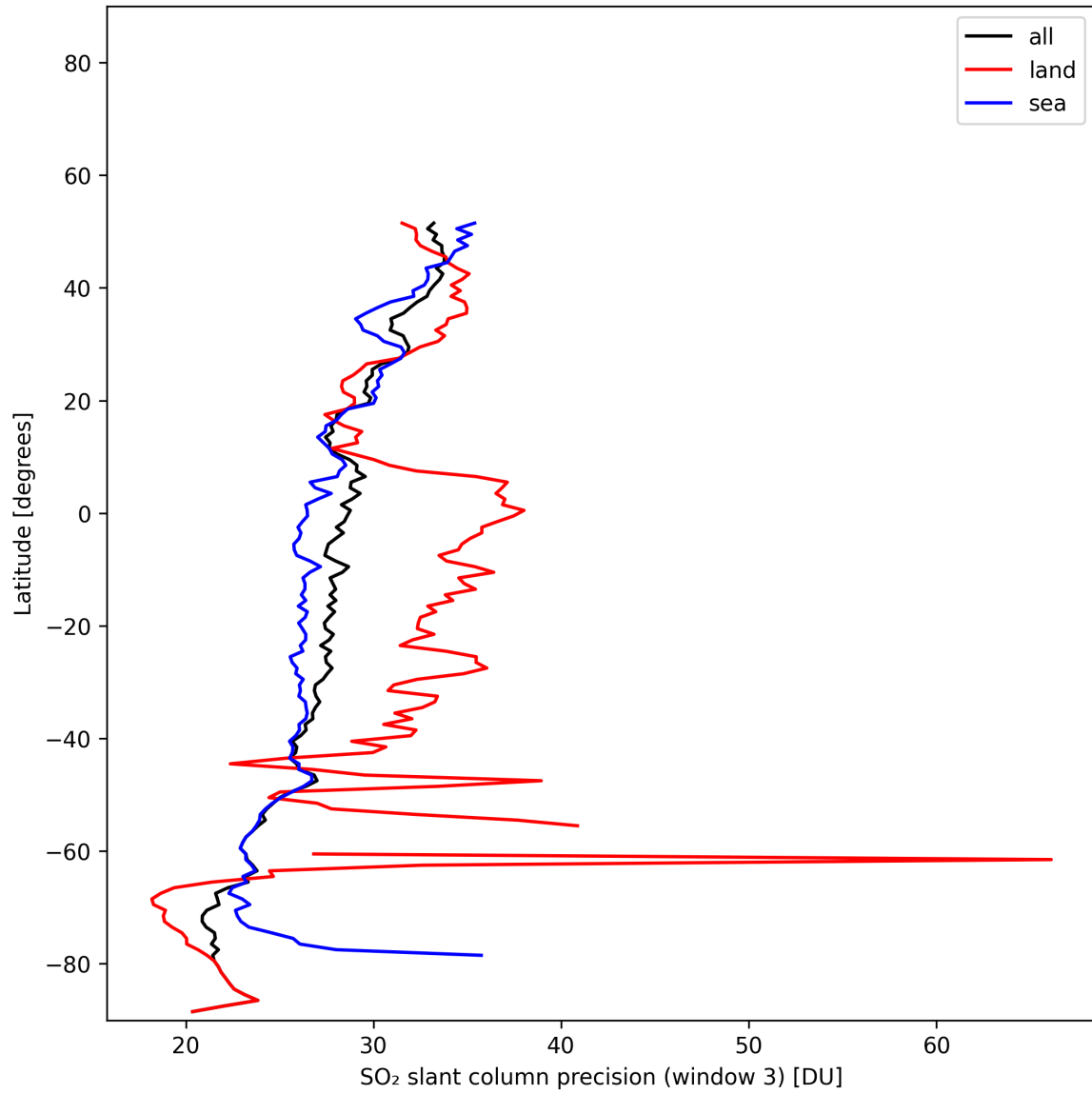
Figure 46: Zonal average of “SO 2 slant column precision (window 3)” for 2025-11-13 to 2025-11-15.
