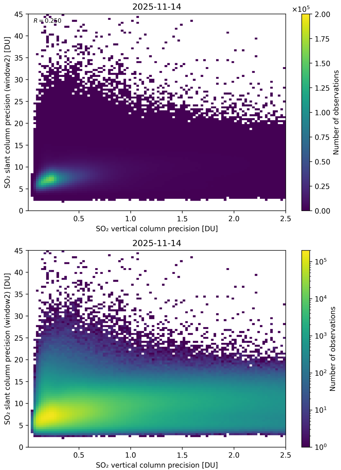
Figure 343: Scatter density plot of “SO 2 vertical column precision” against “SO 2 slant column precision (window2)” for 2025-11-13 to 2025-11-15.
