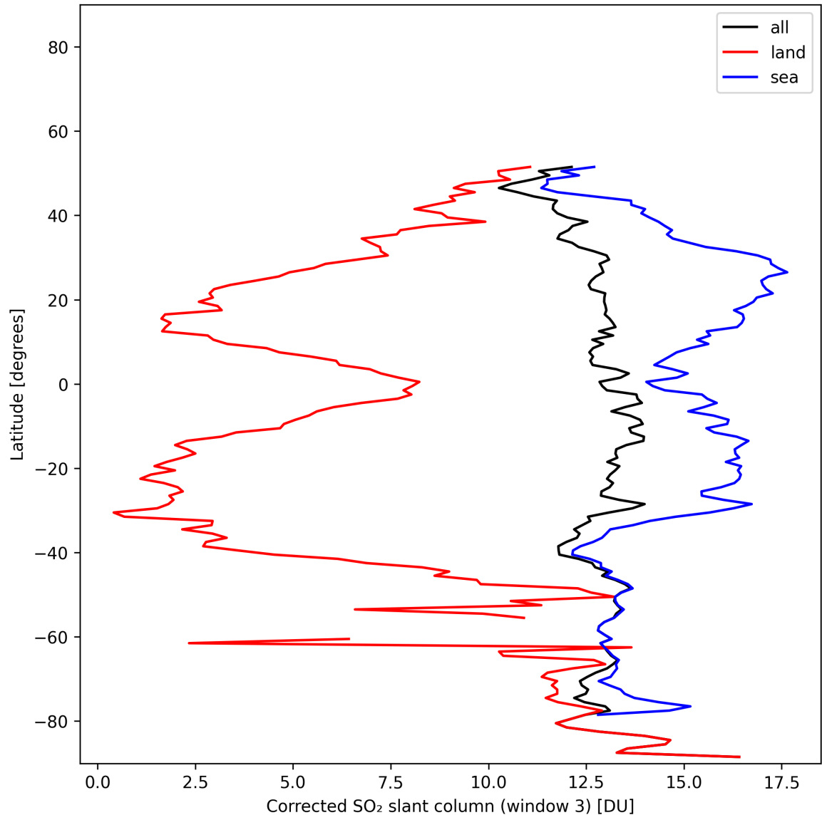
Figure 47: Zonal average of “Corrected SO 2 slant column (window 3)” for 2025-11-13 to 2025-11-15.
