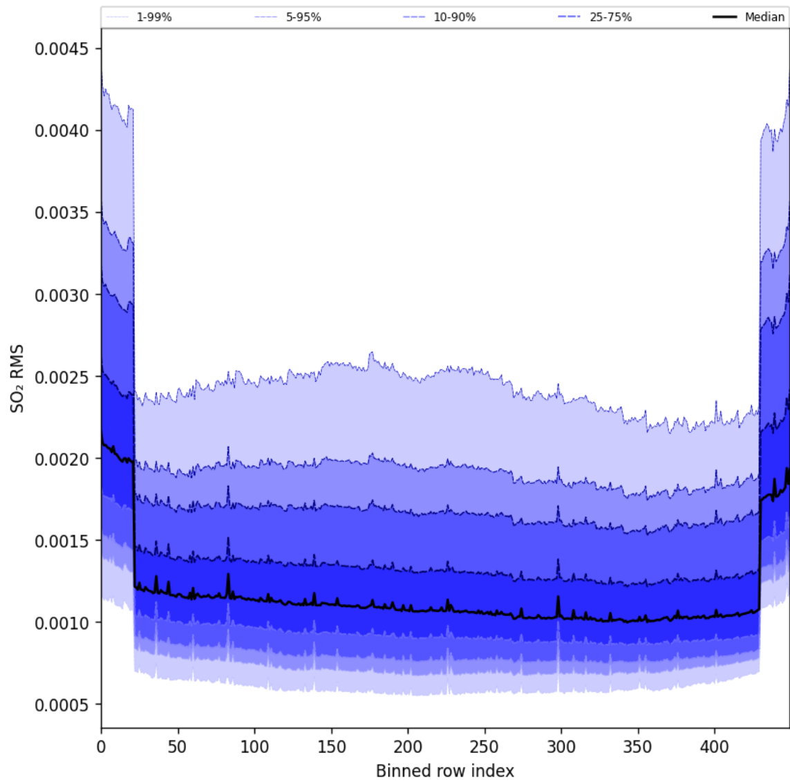
Figure 104: Along track statistics of “SO 2 RMS” for 2025-11-13 to 2025-11-15
