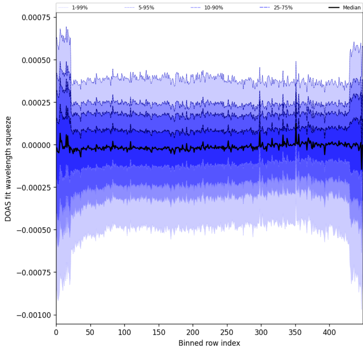
Figure 103: Along track statistics of “DOAS fit wavelength squeeze” for 2025-11-13 to 2025-11-15
