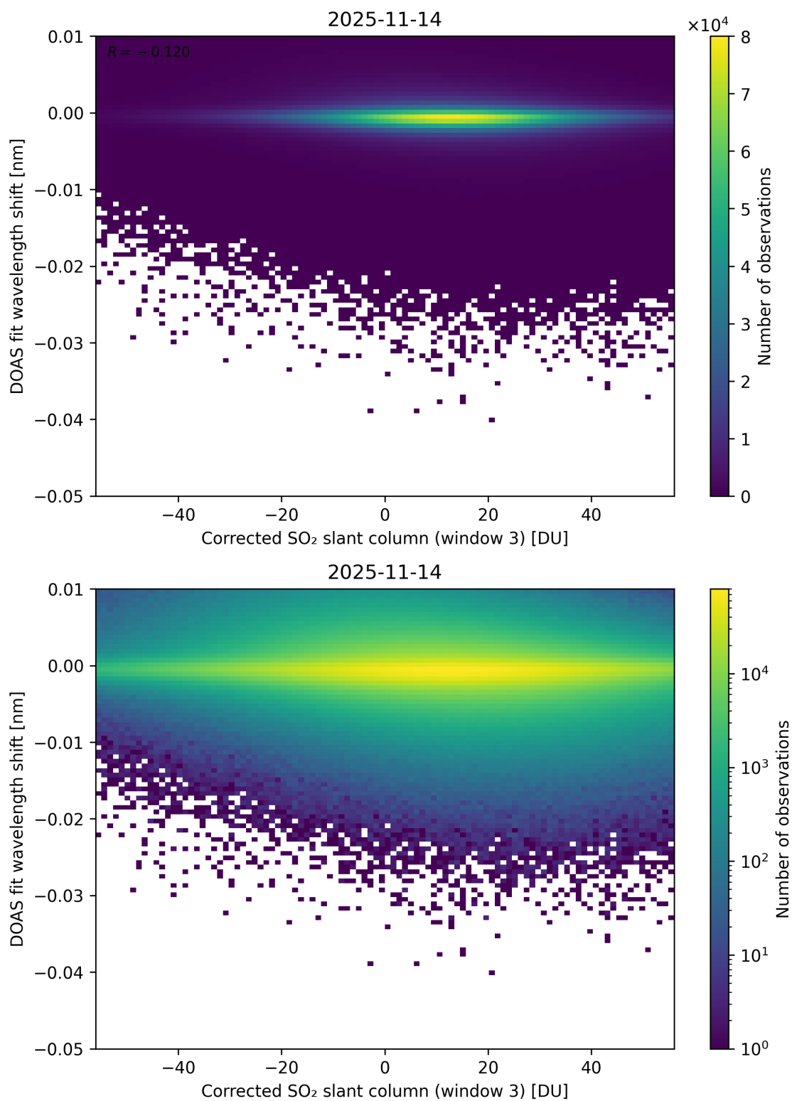
Figure 256: Scatter density plot of “Corrected SO 2 slant column (window 3)” against “DOAS fit wavelength shift” for 2025-11-13 to 2025-11-15.
