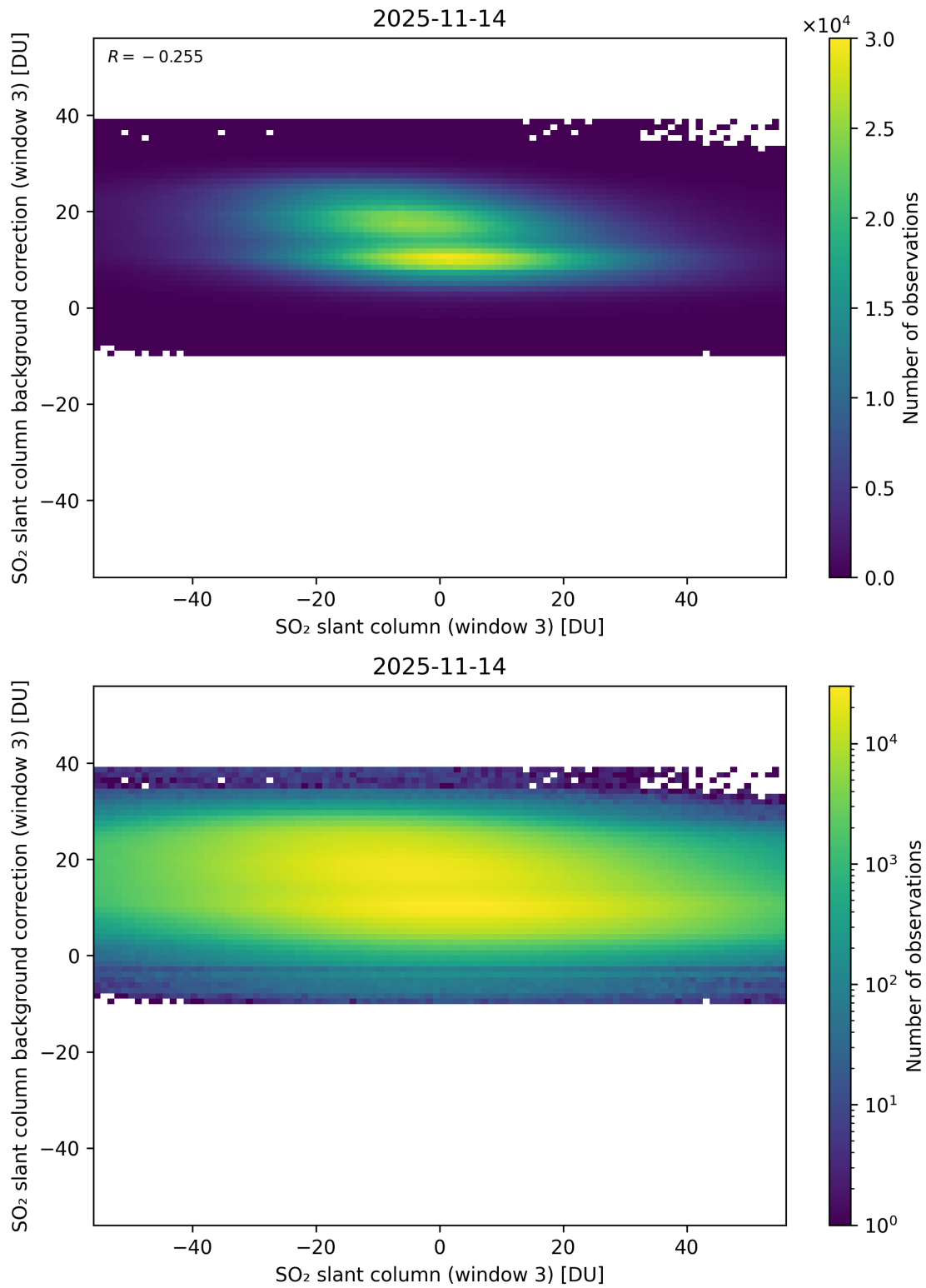
Figure 303: Scatter density plot of “SO 2 slant column (window 3)” against “SO 2 slant column background correction (window 3)” for 2025-11-13 to 2025-11-15.
