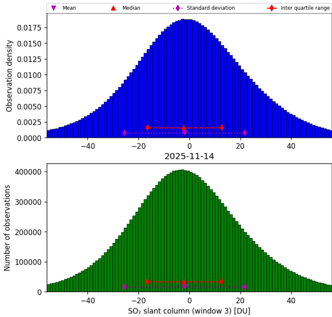
Figure 71: Histogram of “SO 2 slant column (window 3)” for 2025-11-13 to 2025-11-15
