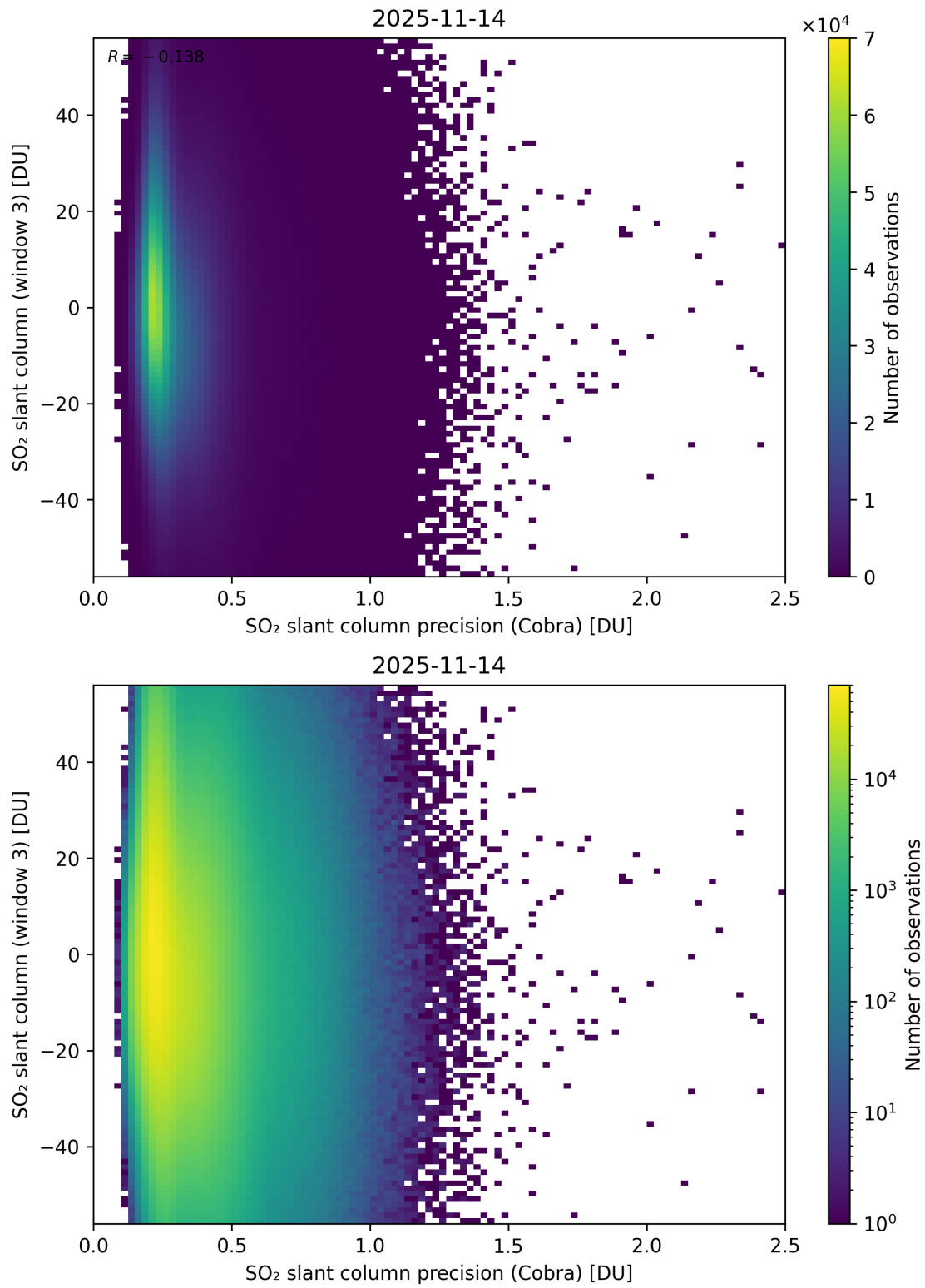
Figure 211: Scatter density plot of “SO 2 slant column precision (Cobra)” against “SO 2 slant column (window 3)” for 2025-11-13 to 2025-11-15.
