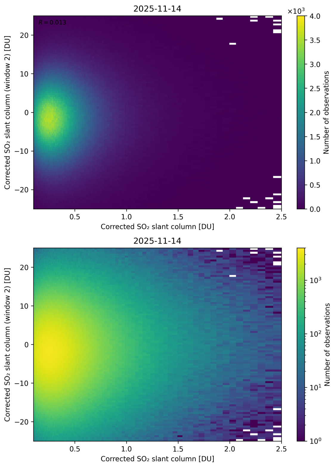
Figure 235: Scatter density plot of “Corrected SO 2 slant column” against “Corrected SO 2 slant column (window 2)” for 2025-11-13 to 2025-11-15.
