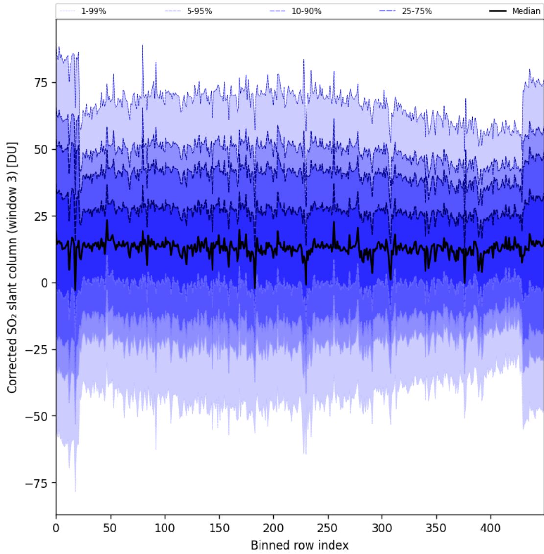
Figure 99: Along track statistics of “Corrected SO 2 slant column (window 3)” for 2025-11-13 to 2025-11-15
