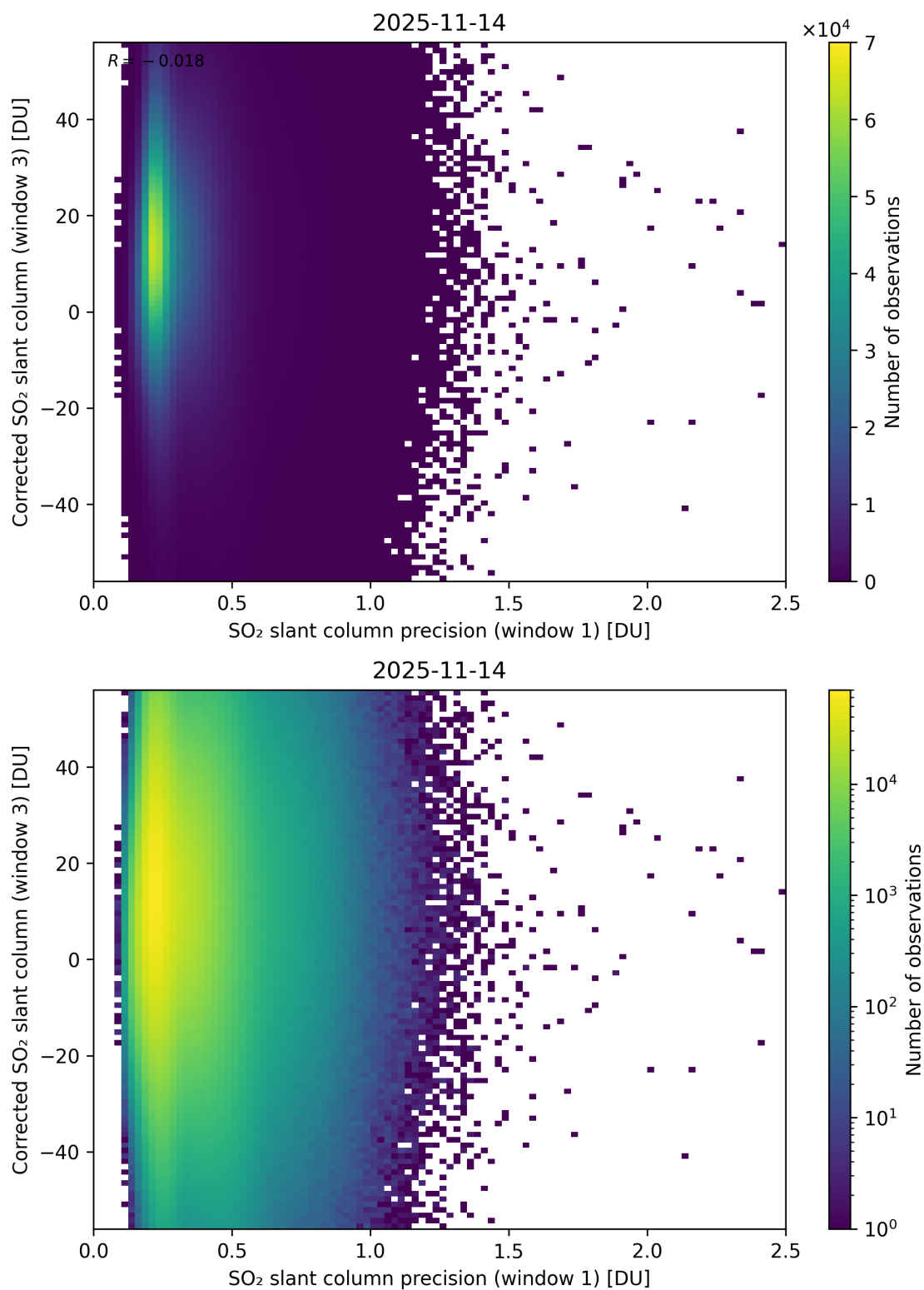
Figure 276: Scatter density plot of “SO 2 slant column precision (window 1)” against “Corrected SO 2 slant column (window 3)” for 2025-11-13 to 2025-11-15.
