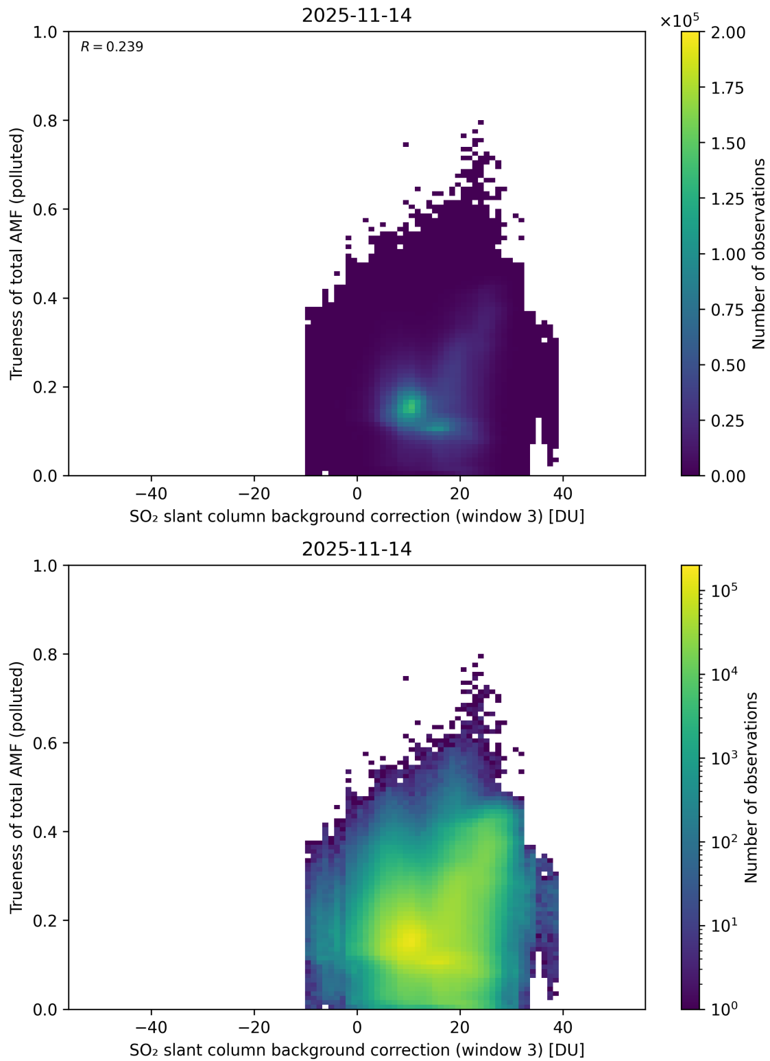
Figure 137: Scatter density plot of “SO 2 slant column background correction (window 3)” against “Trueness of total AMF (polluted)” for 2025-11-13 to 2025-11-15.
