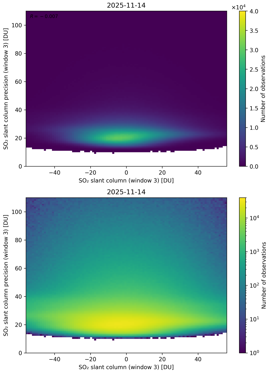
Figure 317: Scatter density plot of “SO 2 slant column (window 3)” against “SO 2 slant column precision (window 3)” for 2025-11-13 to 2025-11-15.
