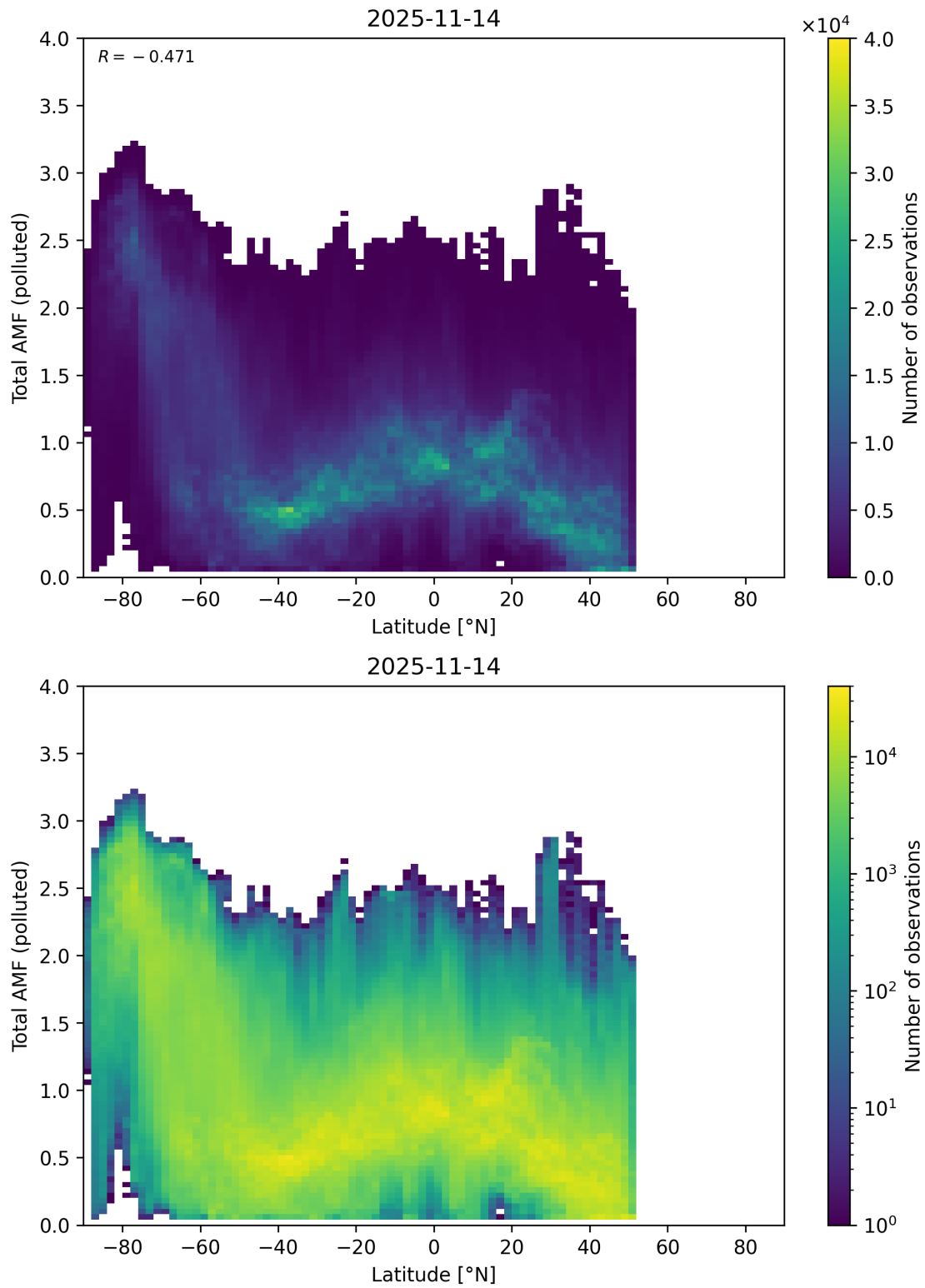
Figure 167: Scatter density plot of “Latitude” against “Total AMF (polluted)” for 2025-11-13 to 2025-11-15.
