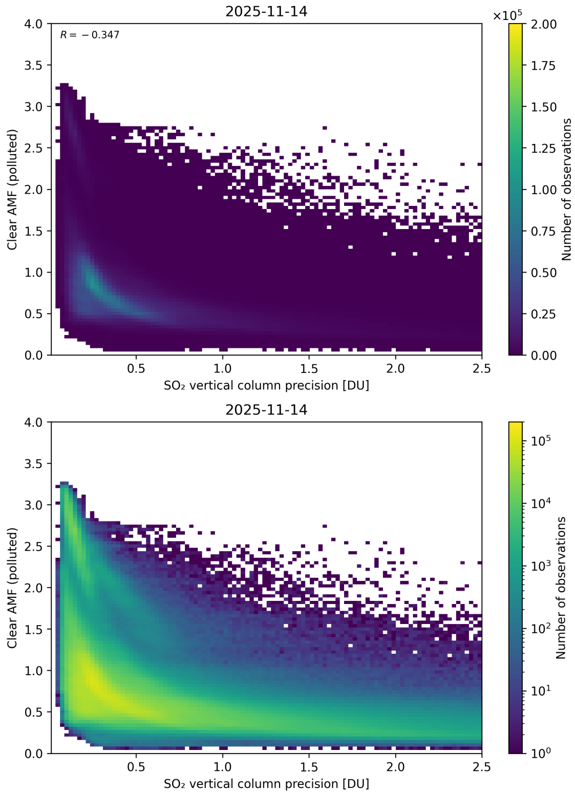
Figure 335: Scatter density plot of “SO 2 vertical column precision” against “Clear AMF (polluted)” for 2025-11-13 to 2025-11-15.
