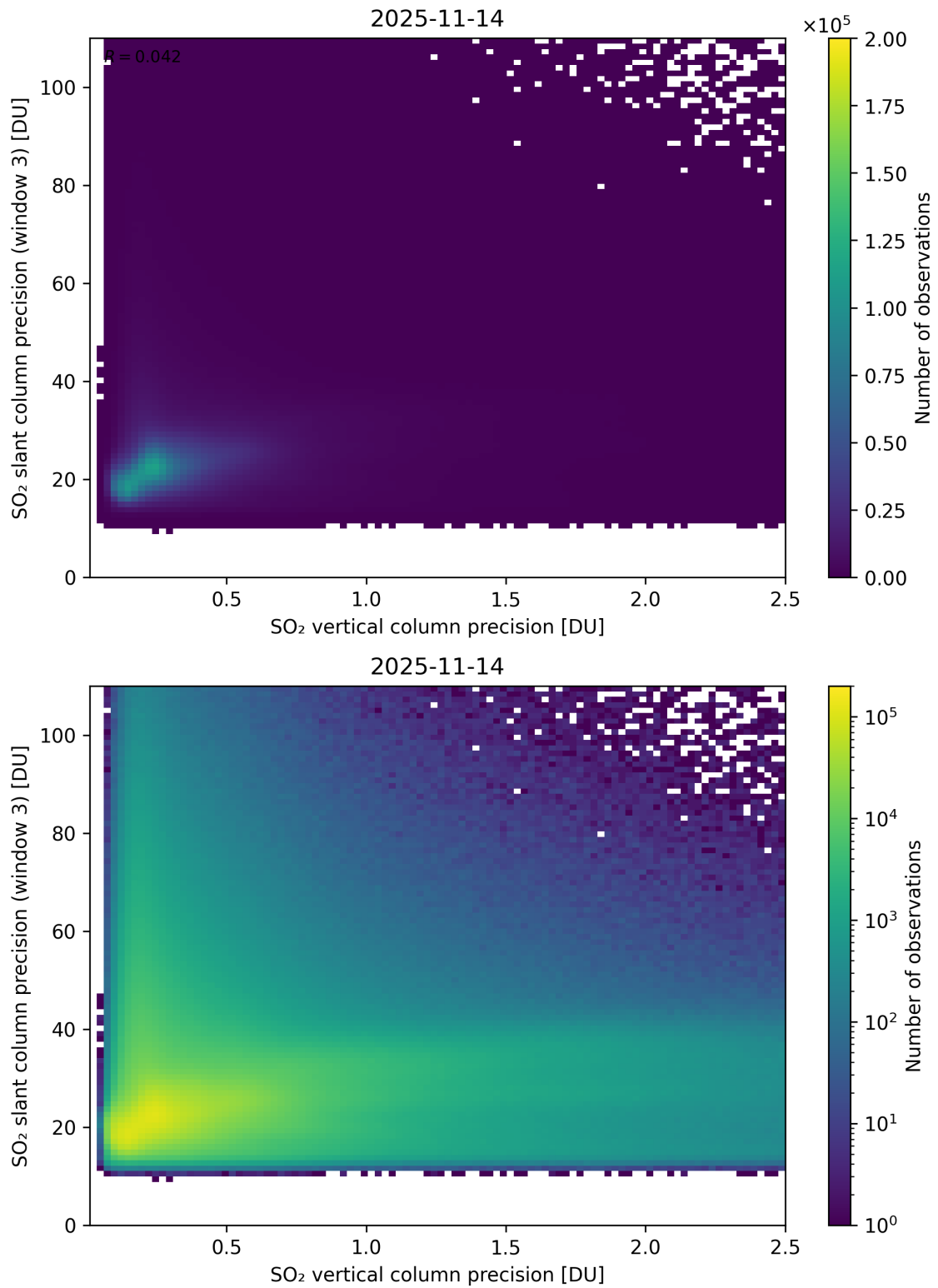
Figure 345: Scatter density plot of “SO 2 vertical column precision” against “SO 2 slant column precision (window 3)” for 2025-11-13 to 2025-11-15.
