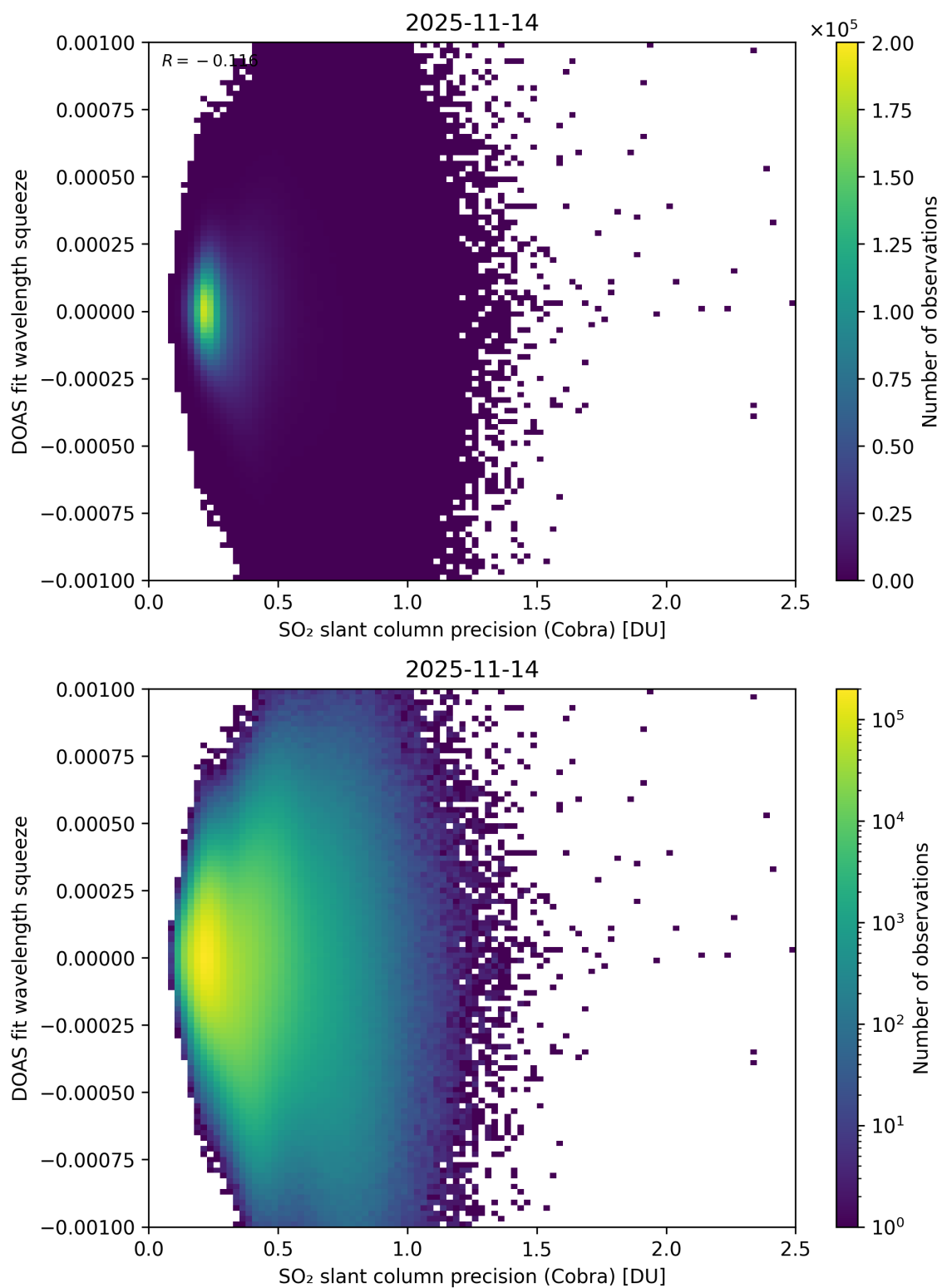
Figure 203: Scatter density plot of “SO 2 slant column precision (Cobra)” against “DOAS fit wavelength squeeze” for 2025-11-13 to 2025-11-15.
