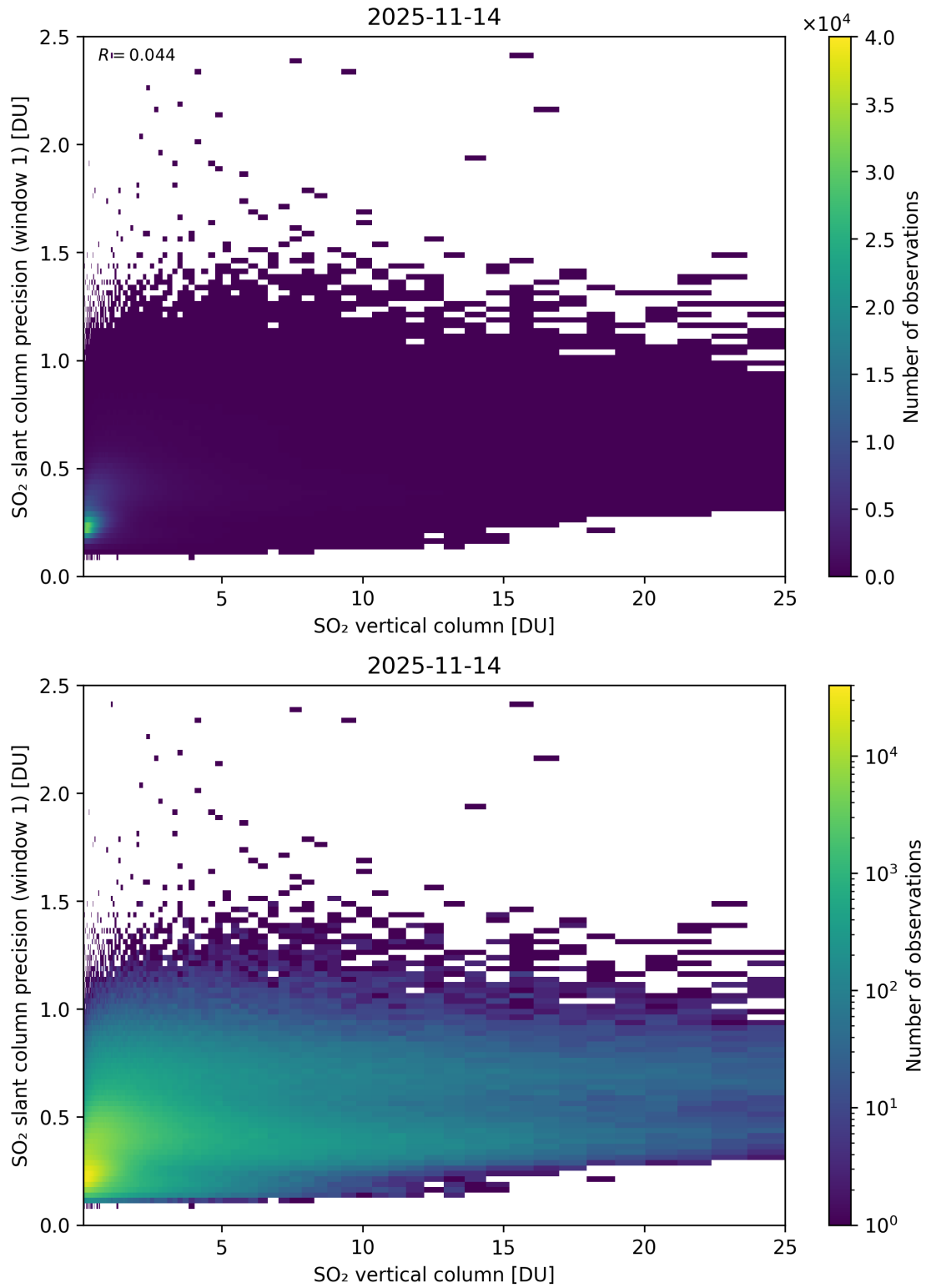
Figure 355: Scatter density plot of “SO 2 vertical column” against “SO 2 slant column precision (window 1)” for 2025-11-13 to 2025-11-15.
