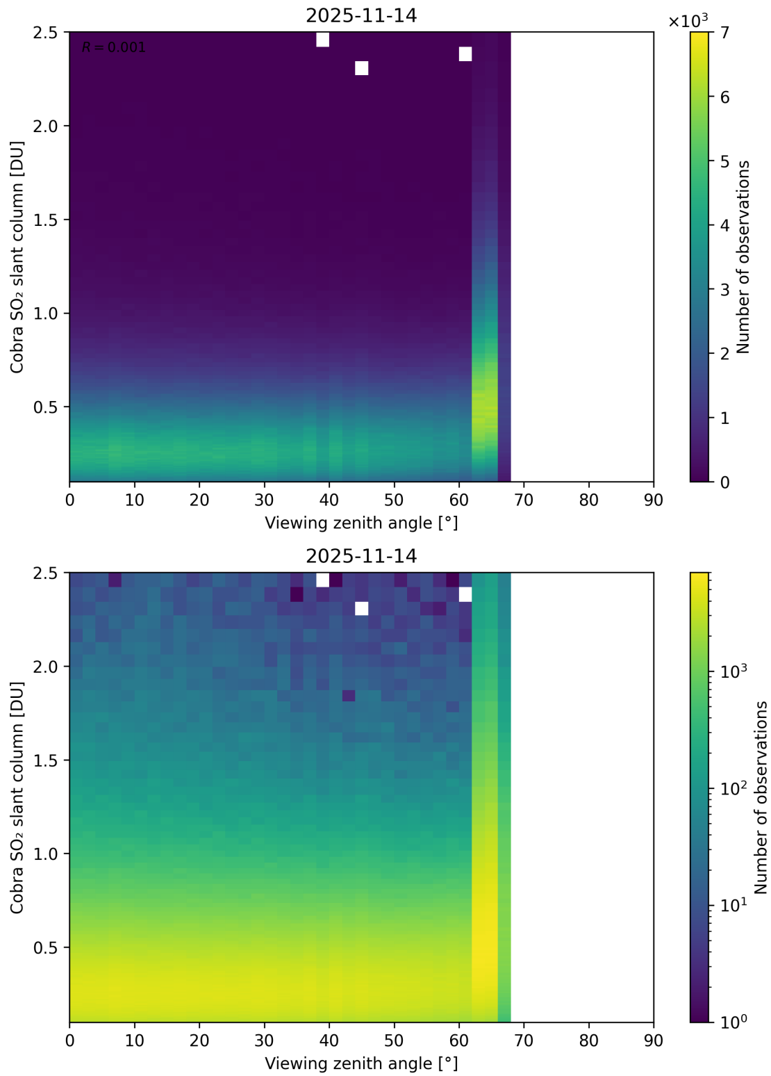
Figure 371: Scatter density plot of “Viewing zenith angle” against “Cobra SO 2 slant column” for 2025-11-13 to 2025-11-15.
