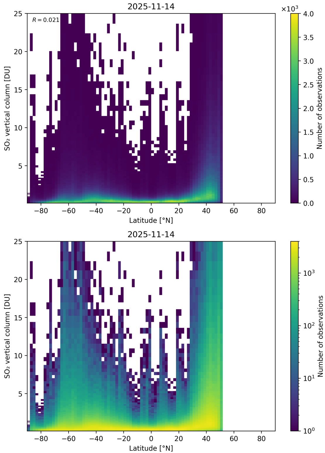
Figure 169: Scatter density plot of “Latitude” against “SO 2 vertical column” for 2025-11-13 to 2025-11-15.
