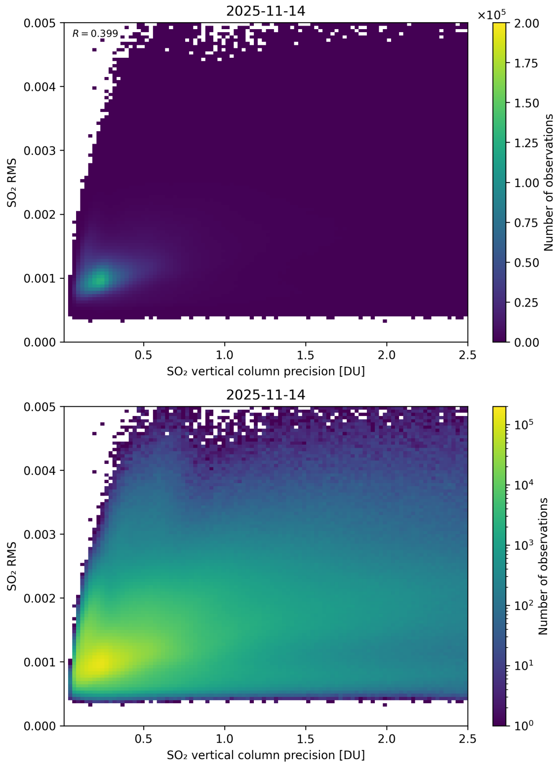
Figure 334: Scatter density plot of “SO 2 vertical column precision” against “SO 2 RMS” for 2025-11-13 to 2025-11-15.
