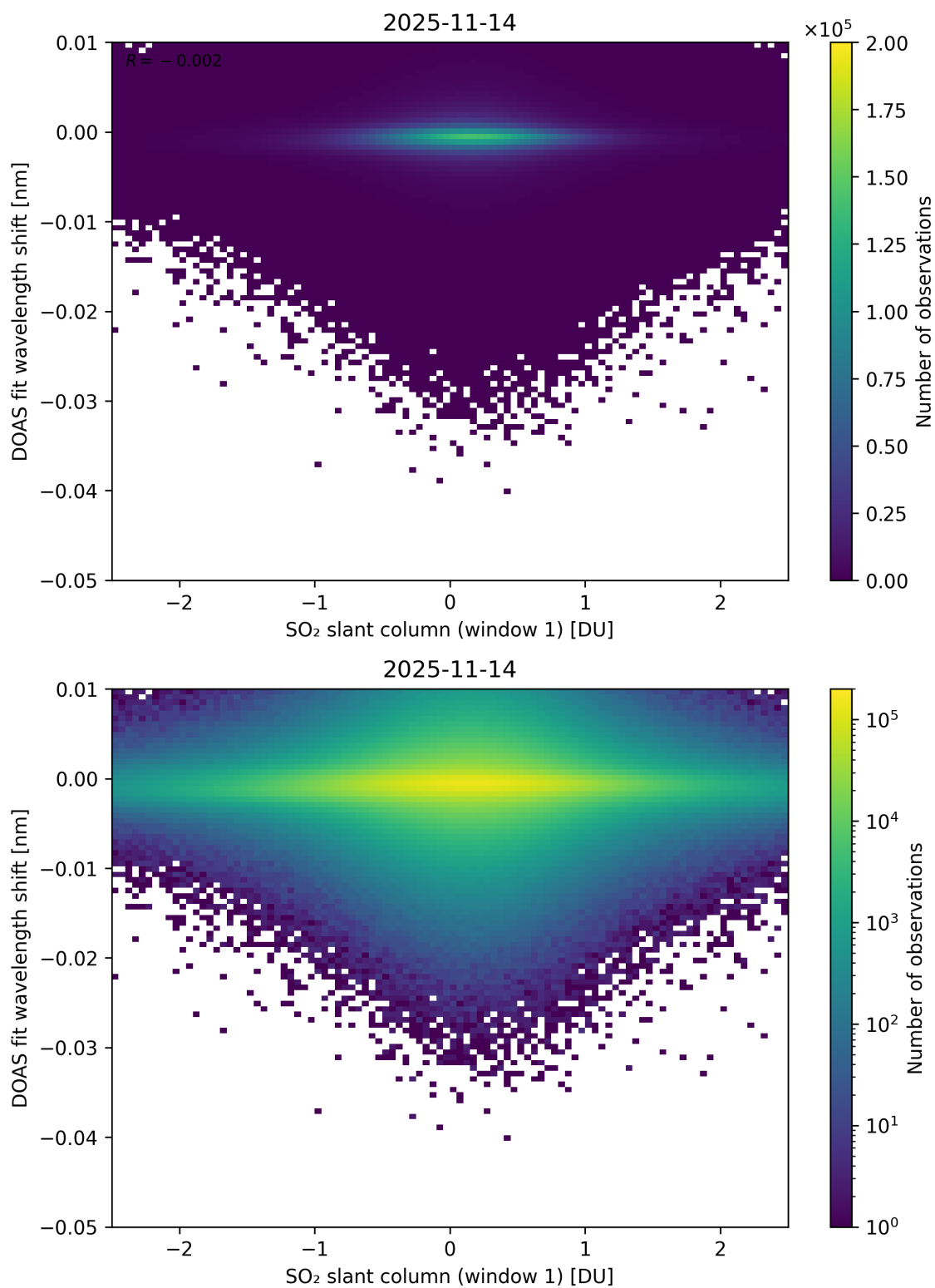
Figure 265: Scatter density plot of “SO 2 slant column (window 1)” against “DOAS fit wavelength shift” for 2025-11-13 to 2025-11-15.
