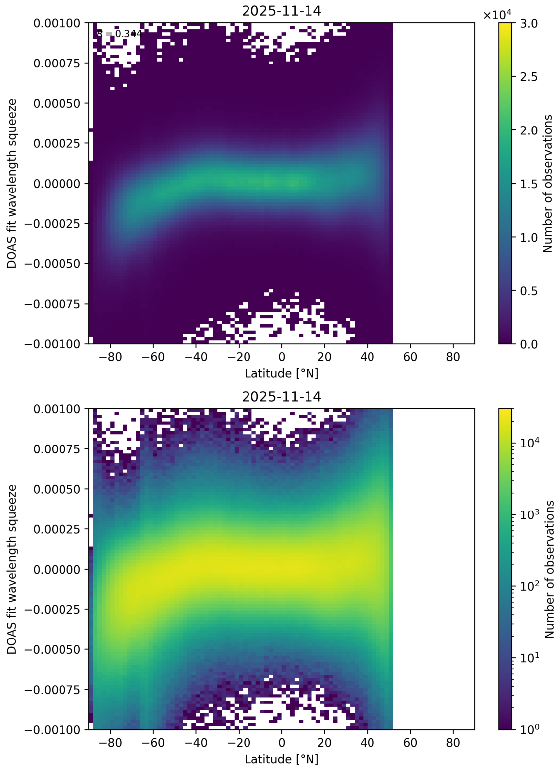
Figure 154: Scatter density plot of “Latitude” against “DOAS fit wavelength squeeze” for 2025-11-13 to 2025-11-15.
