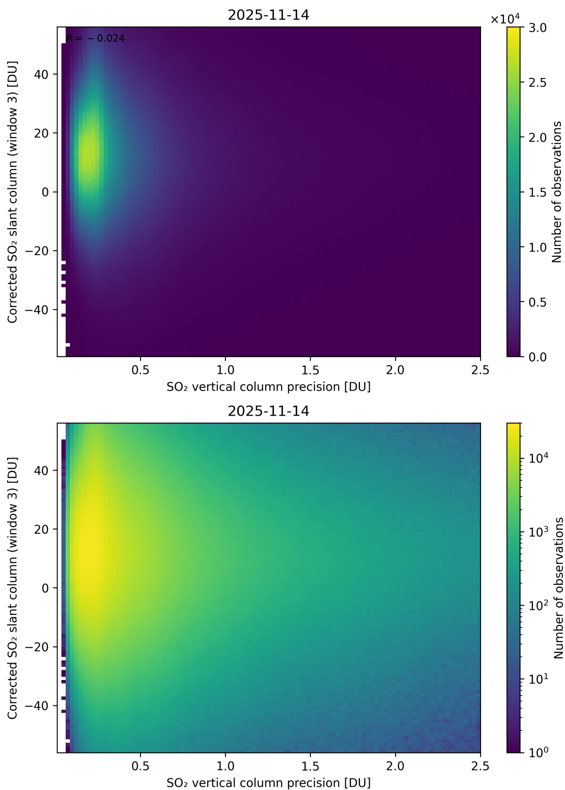
Figure 340: Scatter density plot of “SO 2 vertical column precision” against “Corrected SO 2 slant column (window 3)” for 2025-11-13 to 2025-11-15.
