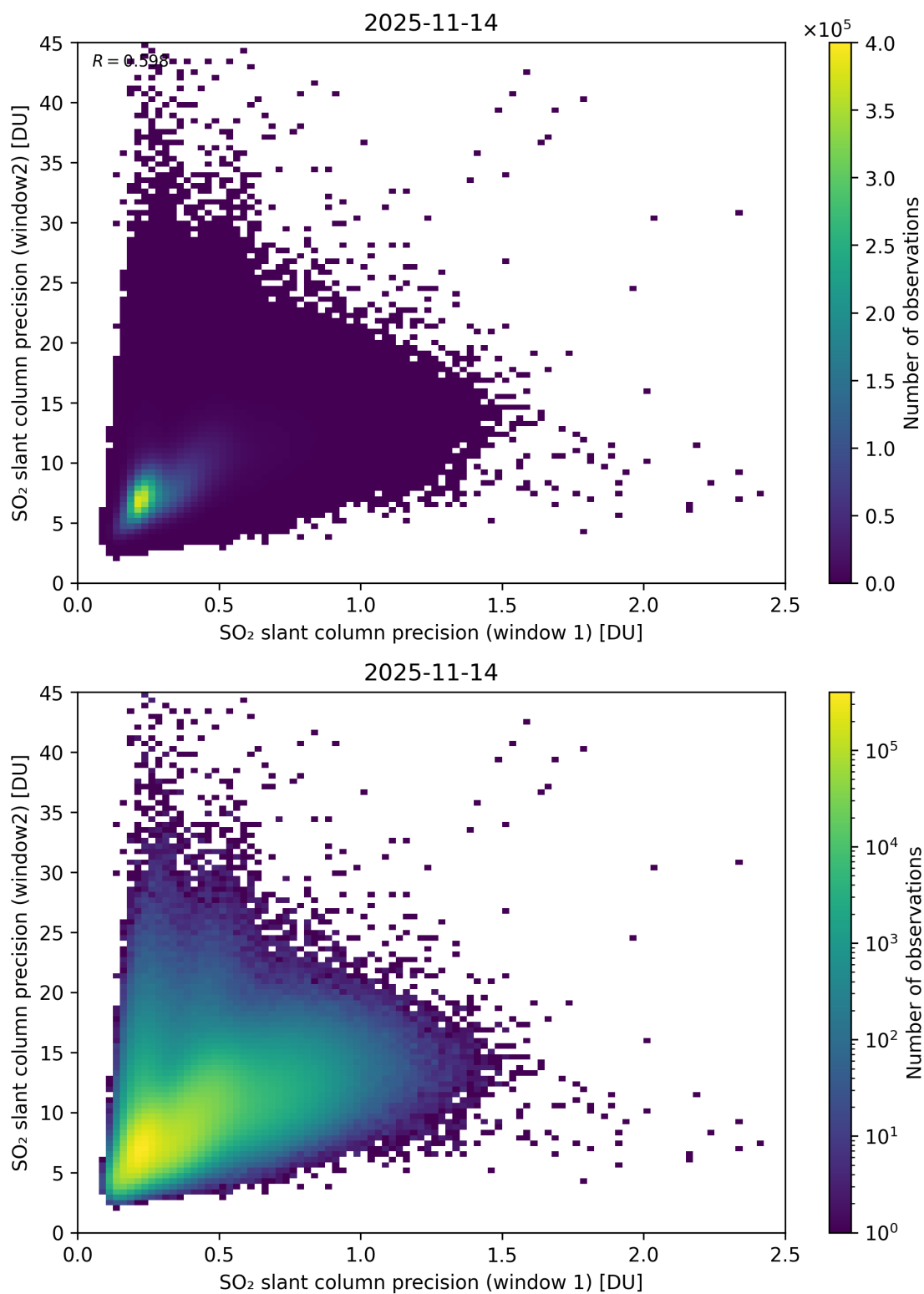
Figure 277: Scatter density plot of “SO 2 slant column precision (window 1)” against “SO 2 slant column precision (window2)” for 2025-11-13 to 2025-11-15.
