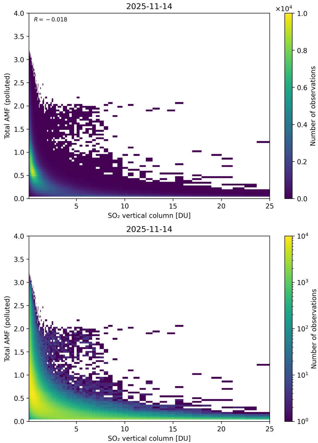
Figure 359: Scatter density plot of “SO 2 vertical column” against “Total AMF (polluted)” for 2025-11-13 to 2025-11-15.
