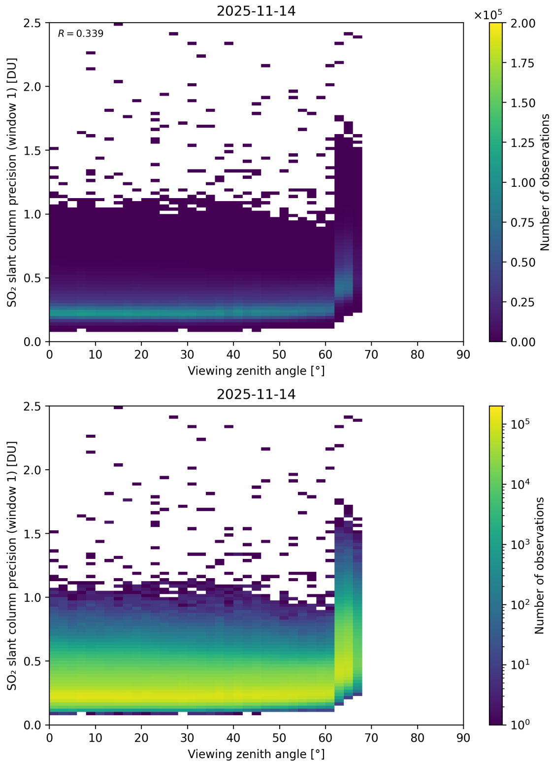
Figure 377: Scatter density plot of “Viewing zenith angle” against “SO 2 slant column precision (window 1)” for 2025-11-13 to 2025-11-15.
