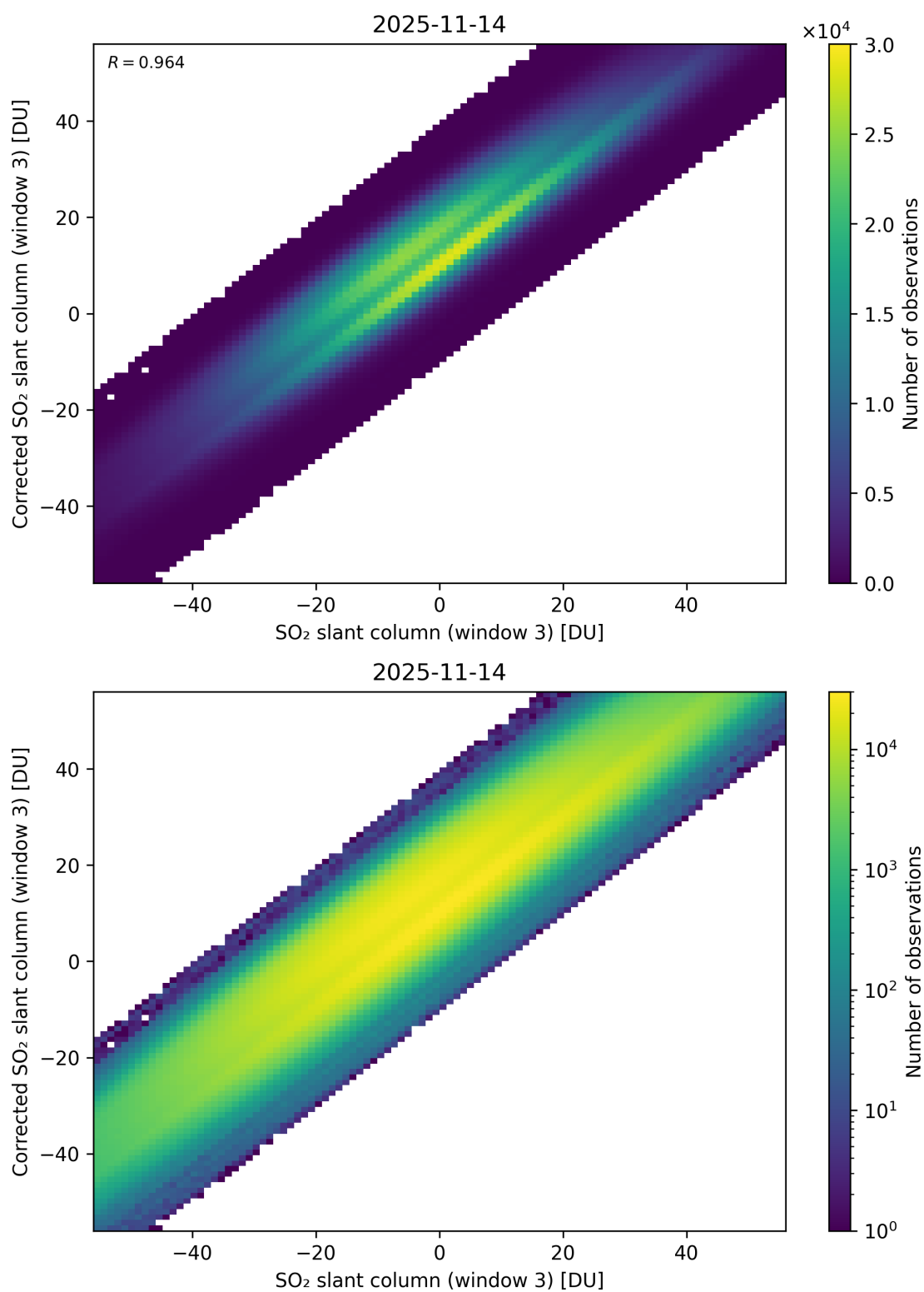
Figure 316: Scatter density plot of “SO 2 slant column (window 3)” against “Corrected SO 2 slant column (window 3)” for 2025-11-13 to 2025-11-15.
