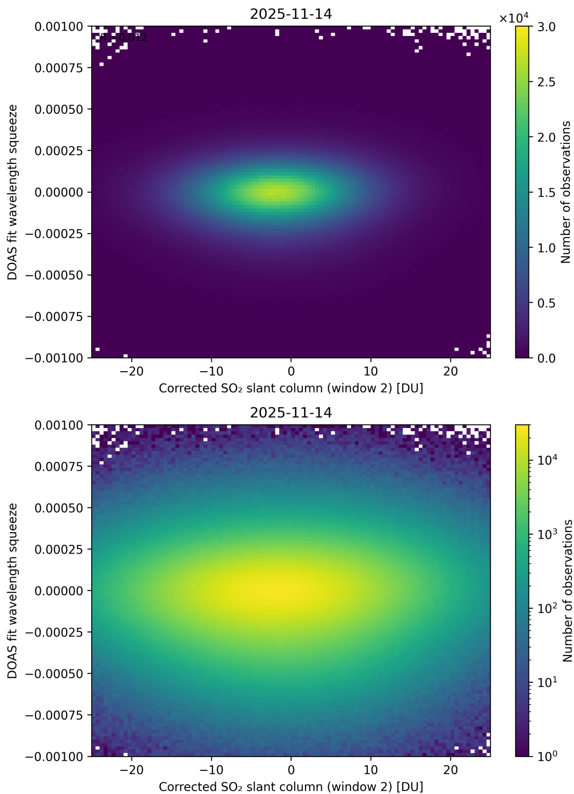
Figure 247: Scatter density plot of “Corrected SO 2 slant column (window 2)” against “DOAS fit wavelength squeeze” for 2025-11-13 to 2025-11-15.
