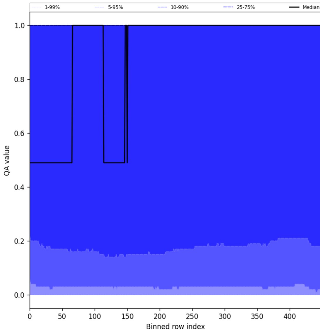
Figure 83: Along track statistics of “QA value” for 2025-11-13 to 2025-11-15
