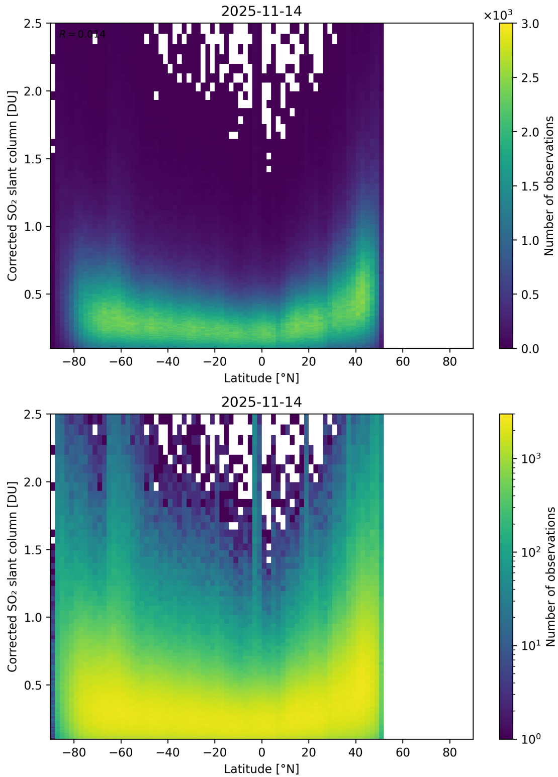
Figure 159: Scatter density plot of “Latitude” against “Corrected SO 2 slant column” for 2025-11-13 to 2025-11-15.
