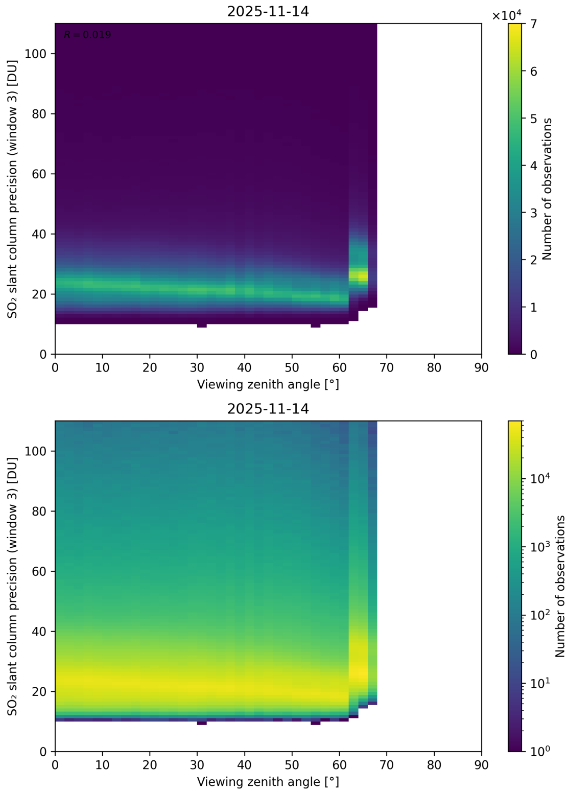
Figure 380: Scatter density plot of “Viewing zenith angle” against “SO 2 slant column precision (window 3)” for 2025-11-13 to 2025-11-15.
