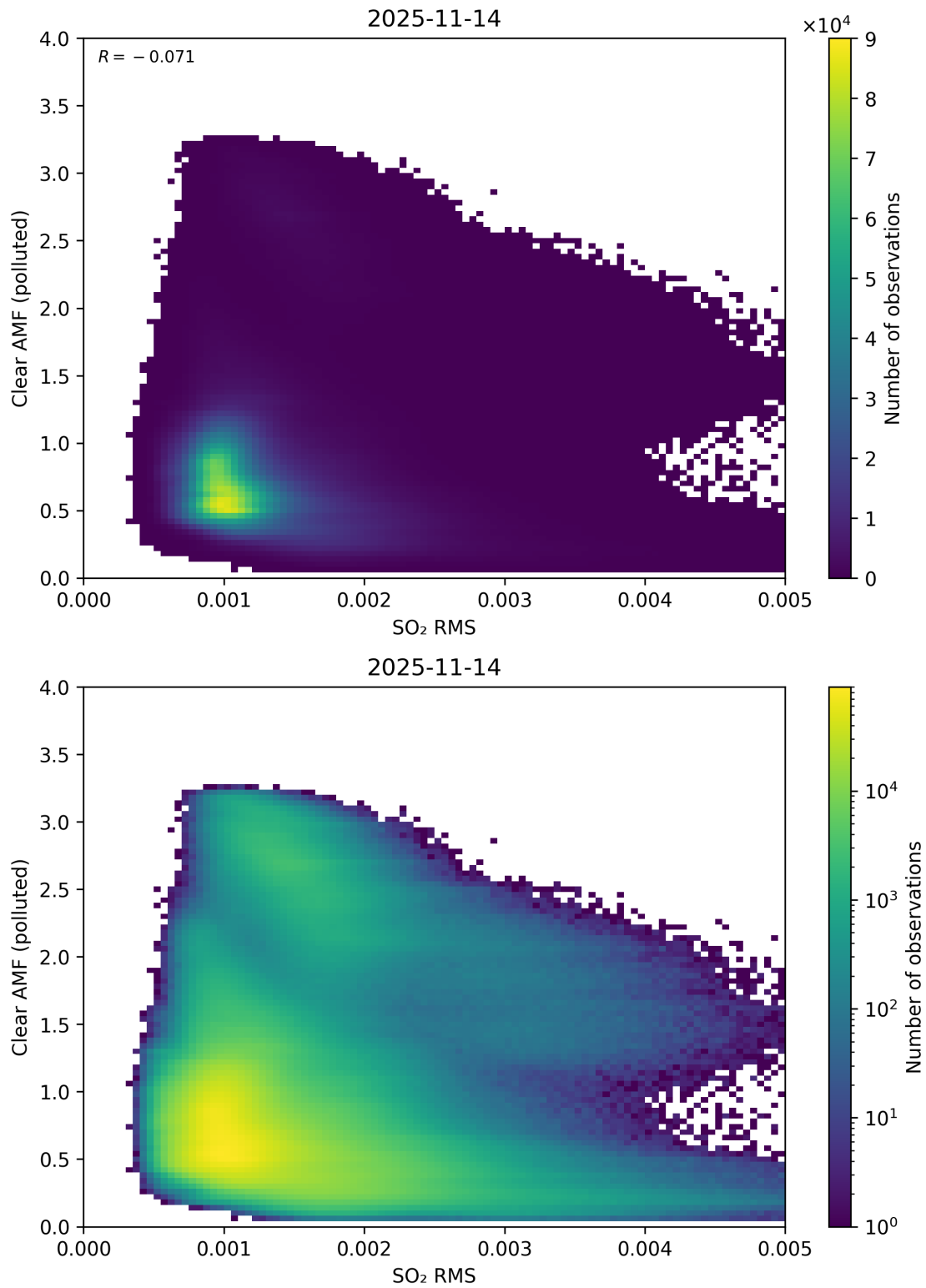
Figure 147: Scatter density plot of “SO 2 RMS” against “Clear AMF (polluted)” for 2025-11-13 to 2025-11-15.
