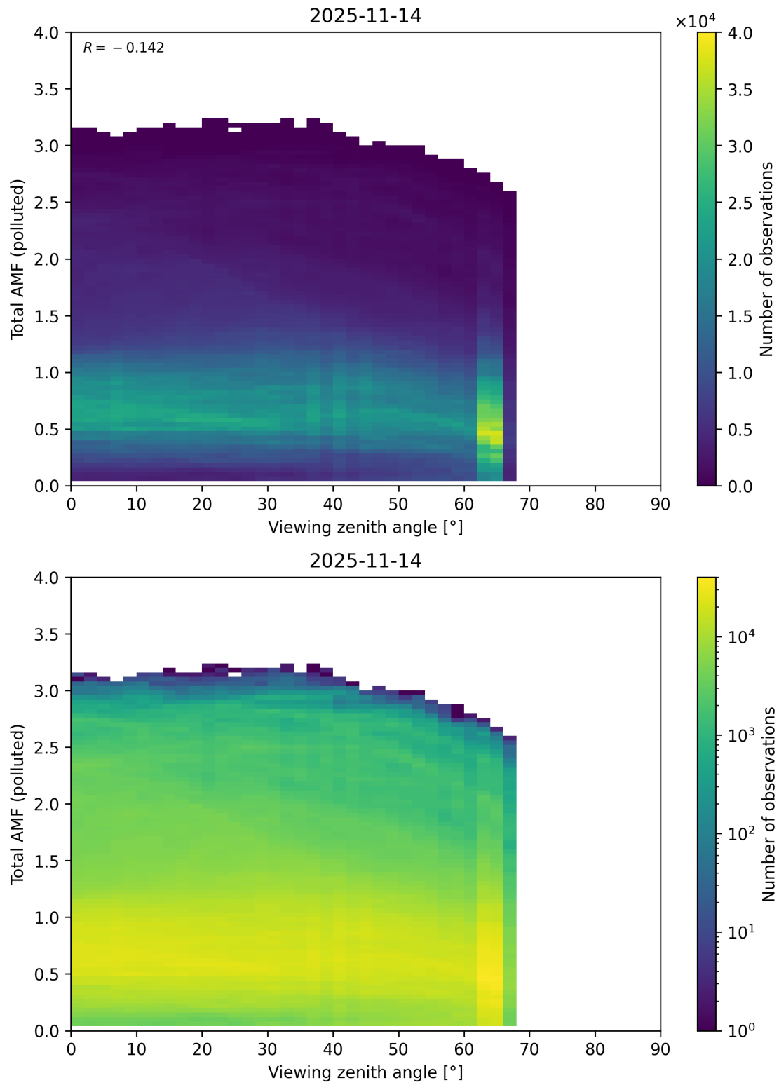
Figure 381: Scatter density plot of “Viewing zenith angle” against “Total AMF (polluted)” for 2025-11-13 to 2025-11-15.
