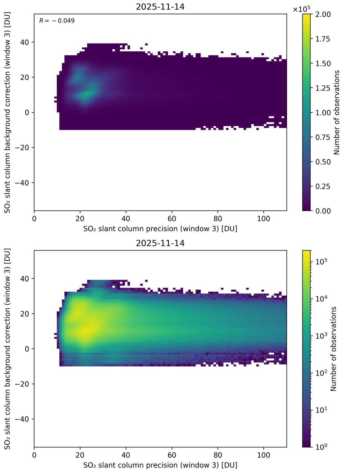
Figure 307: Scatter density plot of “SO 2 slant column precision (window 3)” against “SO 2 slant column background correction (window 3)” for 2025-11-13 to 2025-11-15.
