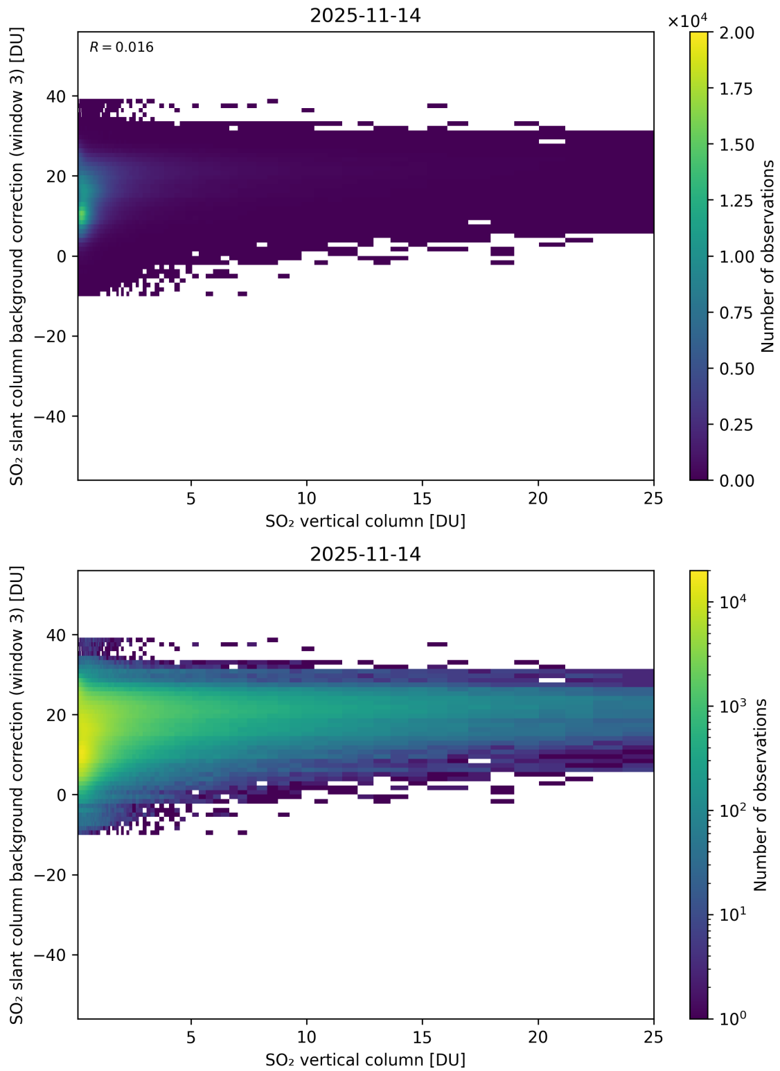
Figure 325: Scatter density plot of “SO 2 vertical column” against “SO 2 slant column background correction (window 3)” for 2025-11-13 to 2025-11-15.
