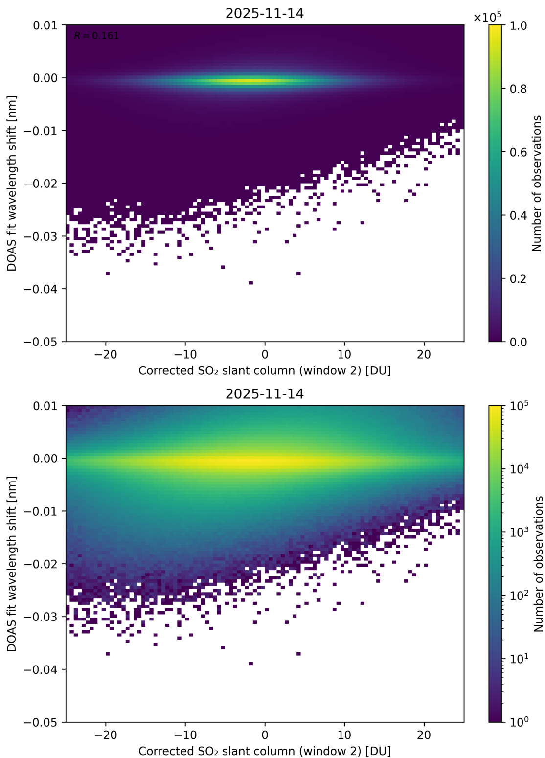
Figure 246: Scatter density plot of “Corrected SO 2 slant column (window 2)” against “DOAS fit wavelength shift” for 2025-11-13 to 2025-11-15.
