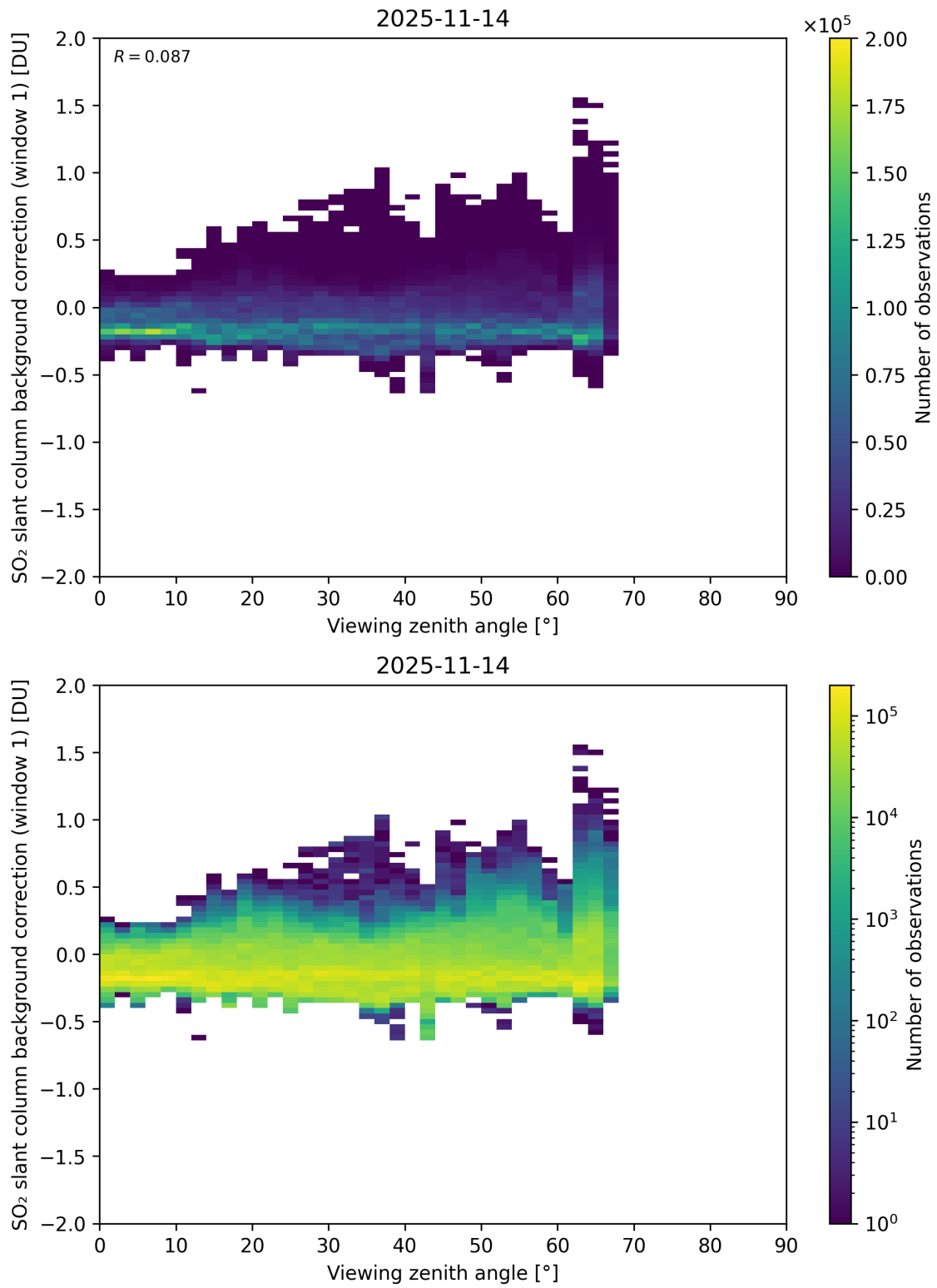
Figure 362: Scatter density plot of “Viewing zenith angle” against “SO 2 slant column background correction (window 1)” for 2025-11-13 to 2025-11-15.
