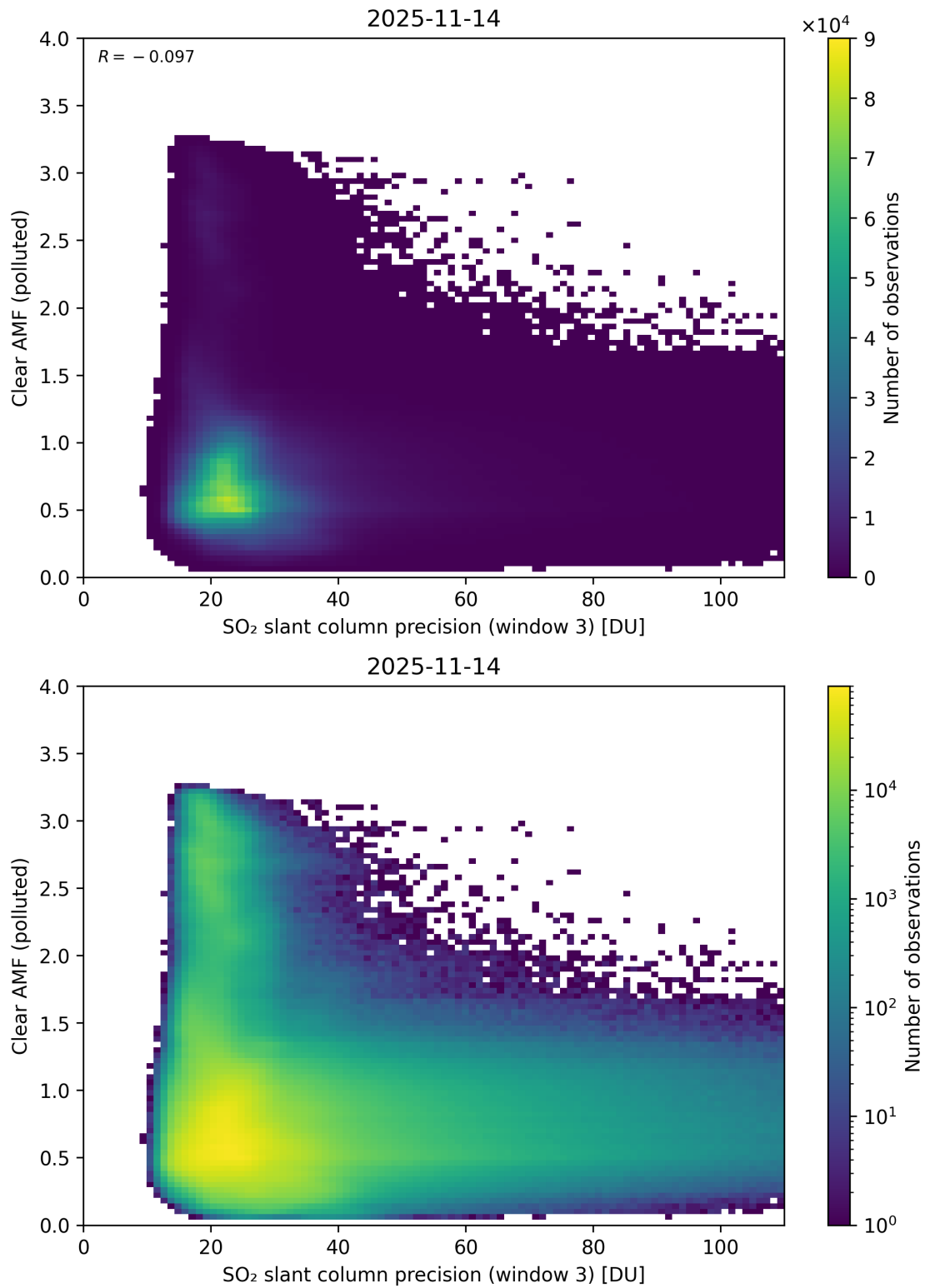
Figure 311: Scatter density plot of “SO 2 slant column precision (window 3)” against “Clear AMF (polluted)” for 2025-11-13 to 2025-11-15.
