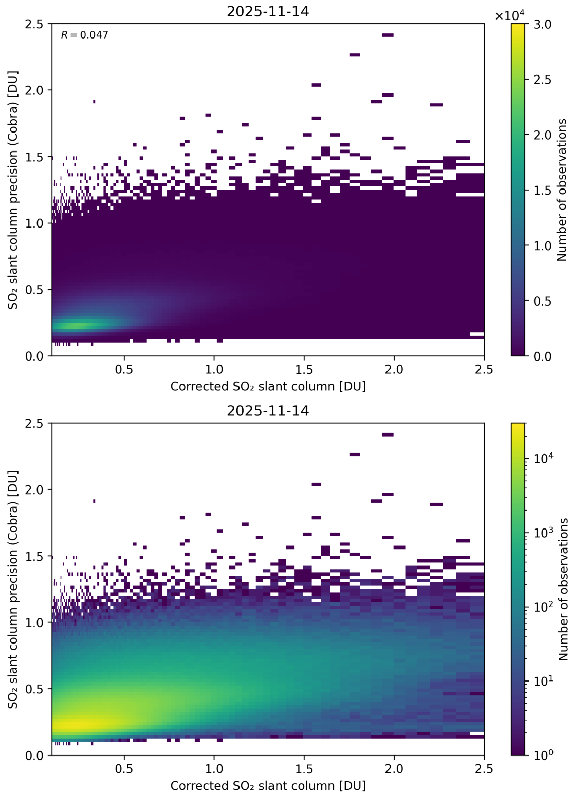
Figure 234: Scatter density plot of “Corrected SO 2 slant column” against “SO 2 slant column precision (Cobra)” for 2025-11-13 to 2025-11-15.
