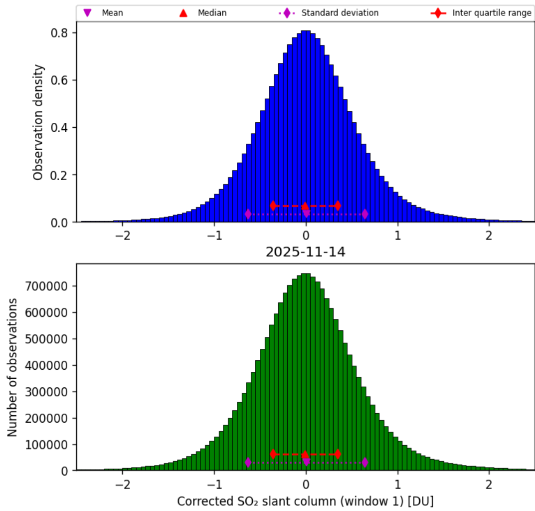
Figure 65: Histogram of “Corrected SO 2 slant column (window 1)” for 2025-11-13 to 2025-11-15
