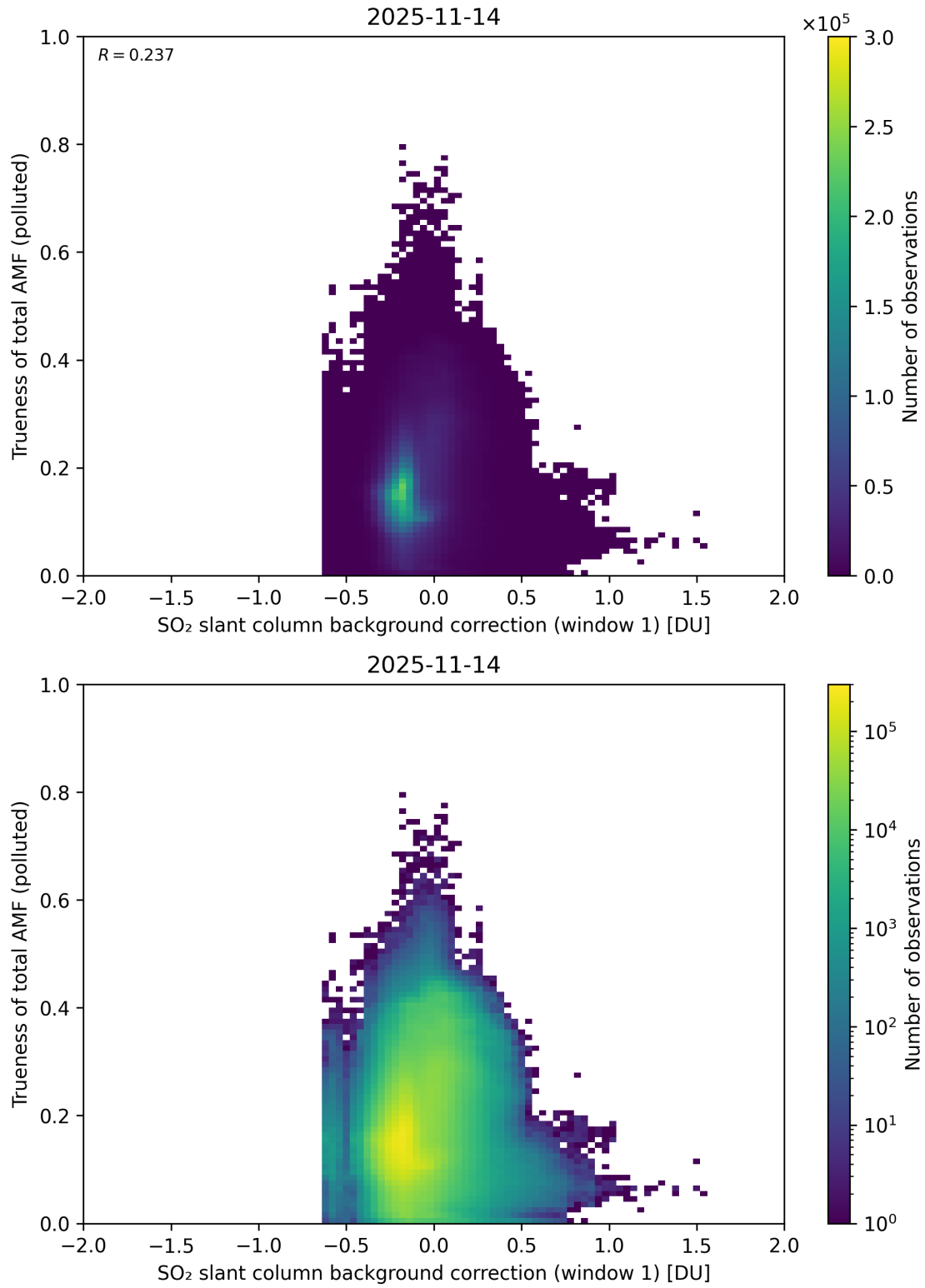
Figure 121: Scatter density plot of “SO 2 slant column background correction (window 1)” against “Trueness of total AMF (polluted)” for 2025-11-13 to 2025-11-15.
