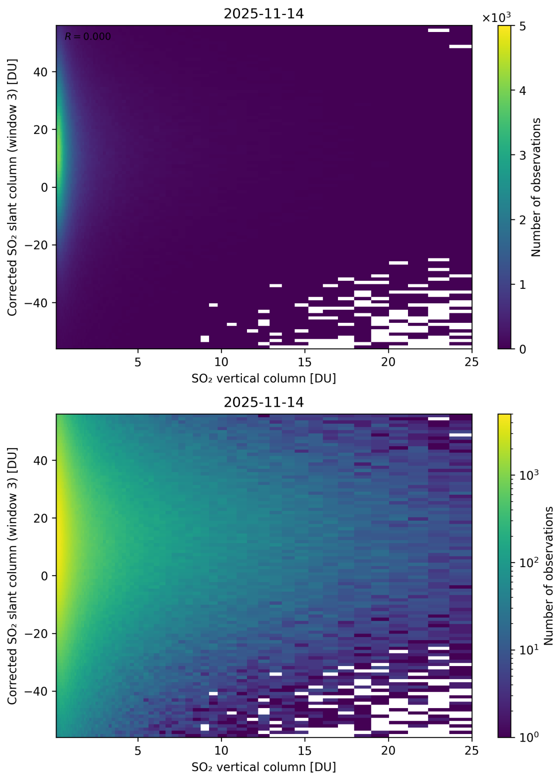
Figure 353: Scatter density plot of “SO 2 vertical column” against “Corrected SO 2 slant column (window 3)” for 2025-11-13 to 2025-11-15.
