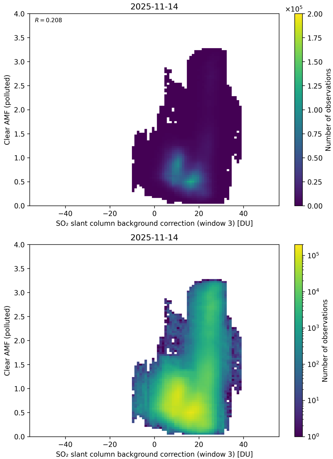
Figure 135: Scatter density plot of “SO 2 slant column background correction (window 3)” against “Clear AMF (polluted)” for 2025-11-13 to 2025-11-15.
