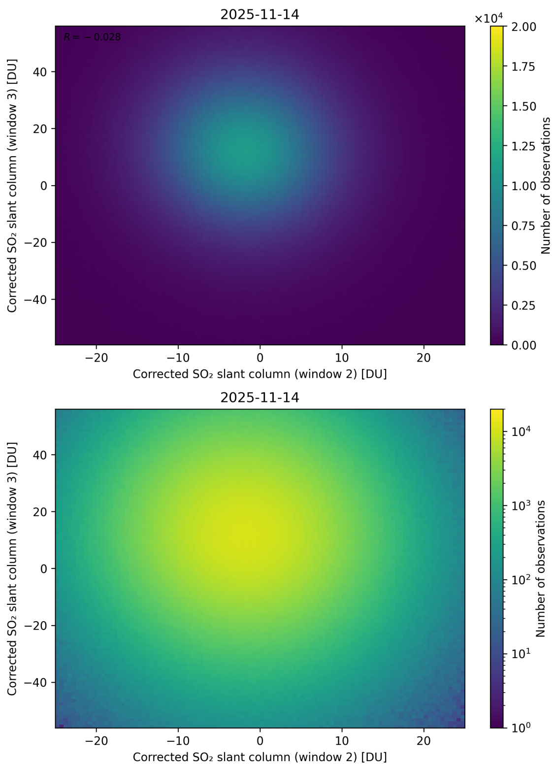
Figure 250: Scatter density plot of “Corrected SO 2 slant column (window 2)” against “Corrected SO 2 slant column (window 3)” for 2025-11-13 to 2025-11-15.
