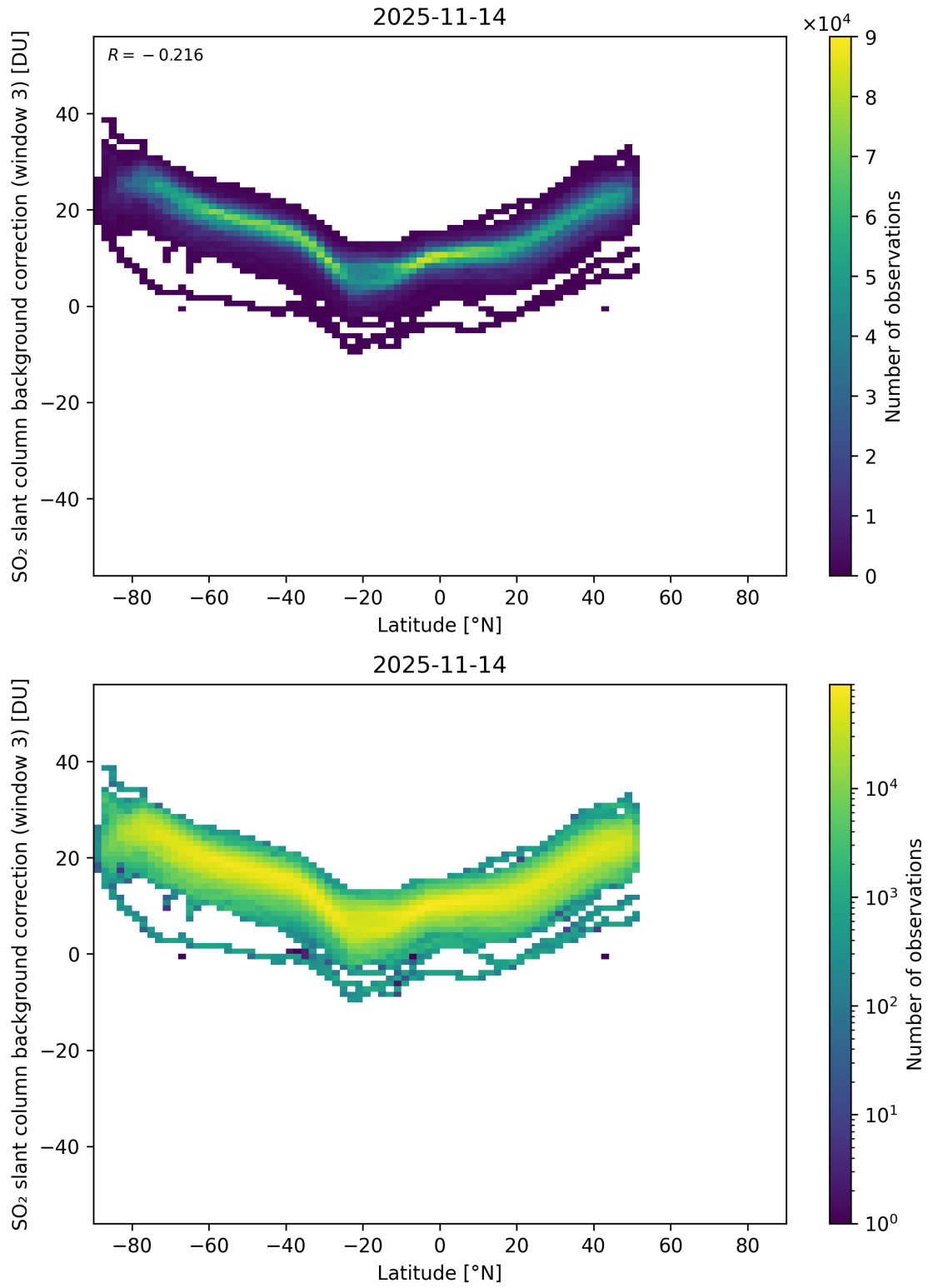
Figure 152: Scatter density plot of “Latitude” against “SO 2 slant column background correction (window 3)” for 2025-11-13 to 2025-11-15.
