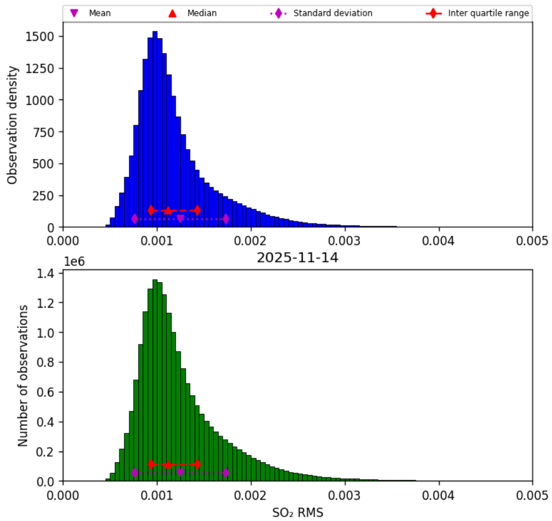
Figure 78: Histogram of “SO 2 RMS” for 2025-11-13 to 2025-11-15
