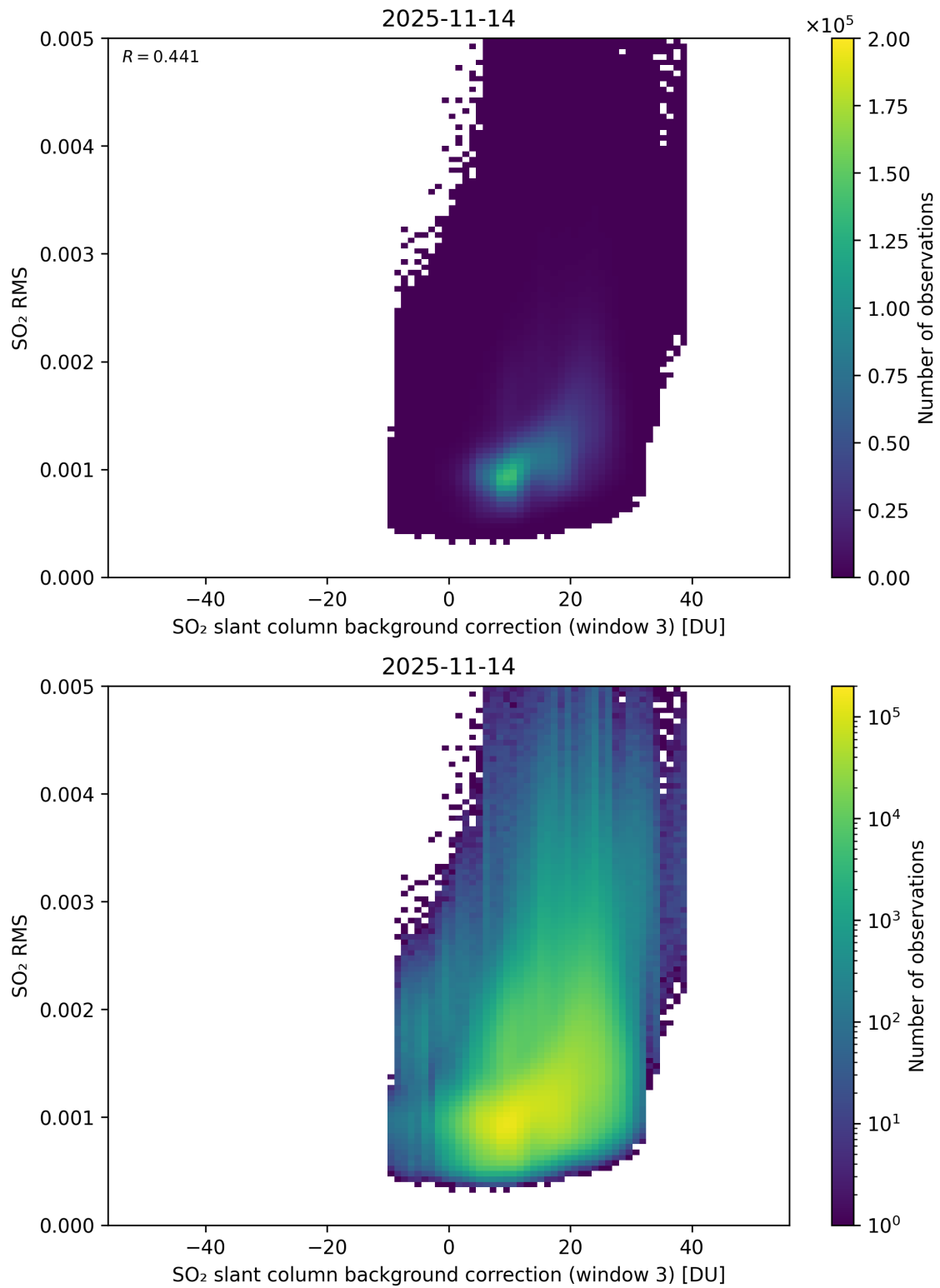
Figure 134: Scatter density plot of “SO 2 slant column background correction (window 3)” against “SO 2 RMS” for 2025-11-13 to 2025-11-15.
