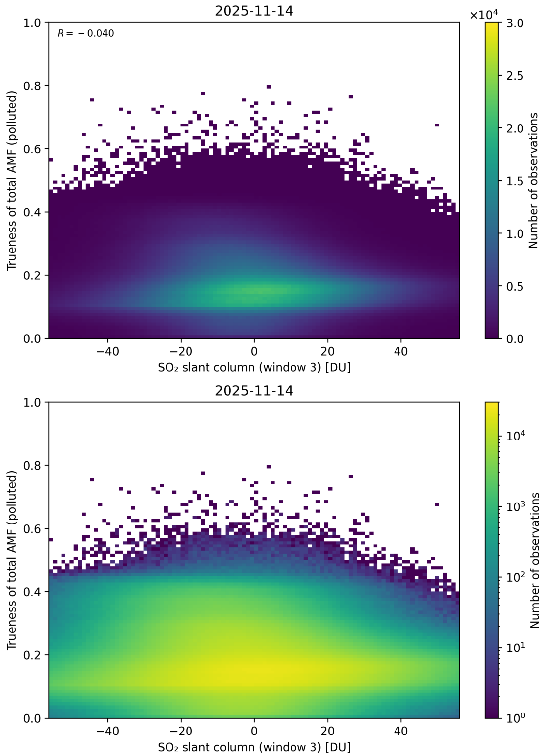
Figure 319: Scatter density plot of “SO 2 slant column (window 3)” against “Trueness of total AMF (polluted)” for 2025-11-13 to 2025-11-15.
