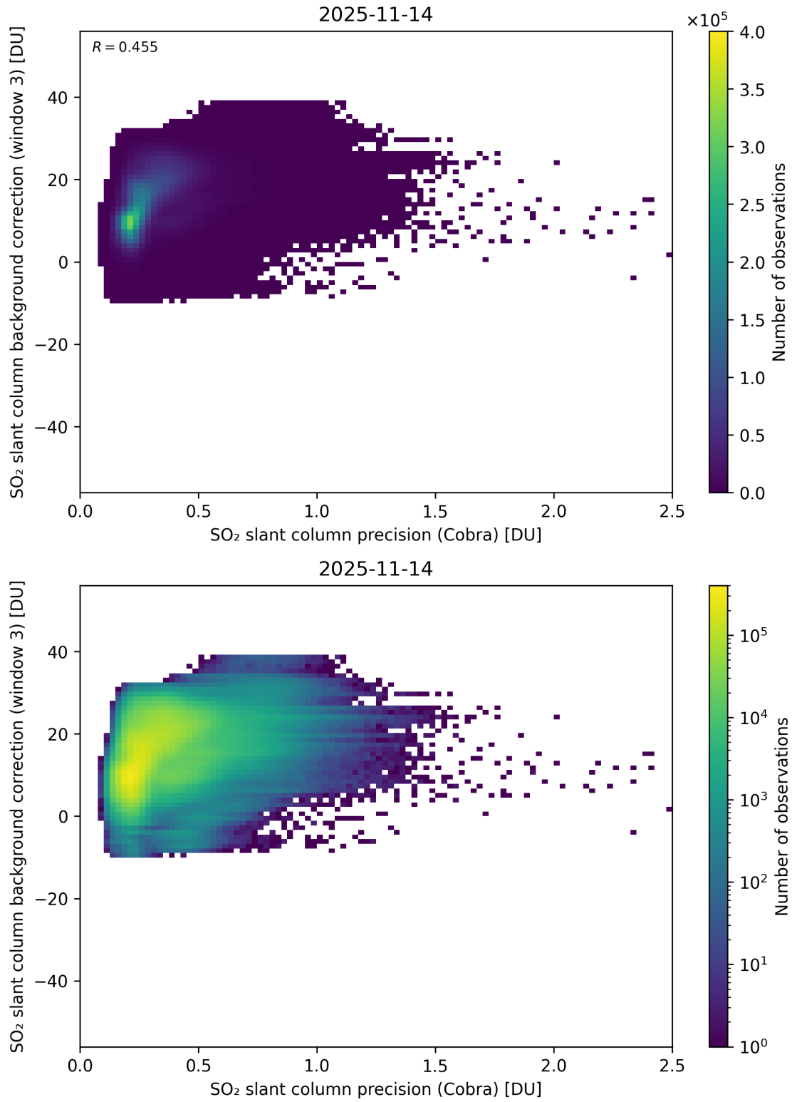
Figure 201: Scatter density plot of “SO 2 slant column precision (Cobra)” against “SO 2 slant column background correction (window 3)” for 2025-11-13 to 2025-11-15.
