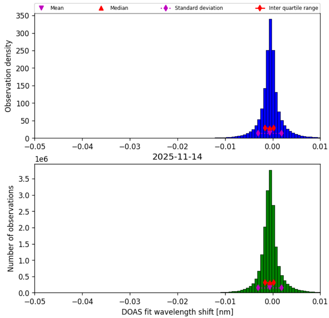
Figure 76: Histogram of “DOAS fit wavelength shift” for 2025-11-13 to 2025-11-15
