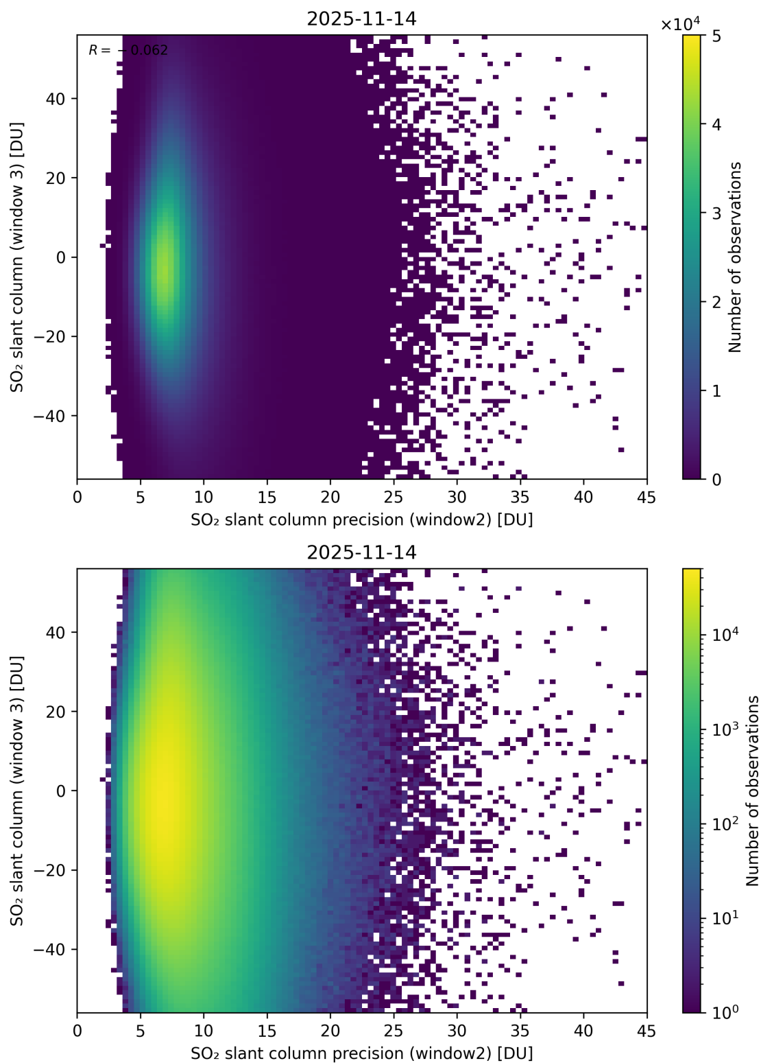
Figure 299: Scatter density plot of “SO 2 slant column precision (window2)” against “SO 2 slant column (window 3)” for 2025-11-13 to 2025-11-15.
