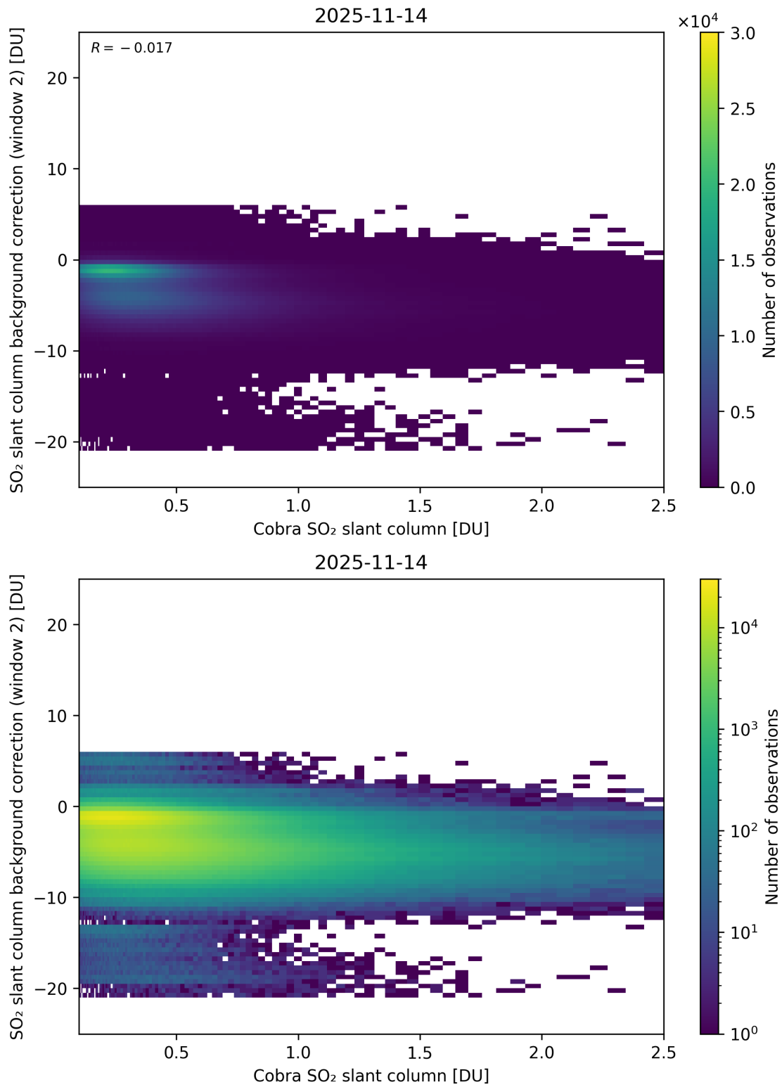
Figure 194: Scatter density plot of “Cobra SO 2 slant column” against “SO 2 slant column background correction (window 2)” for 2025-11-13 to 2025-11-15.
