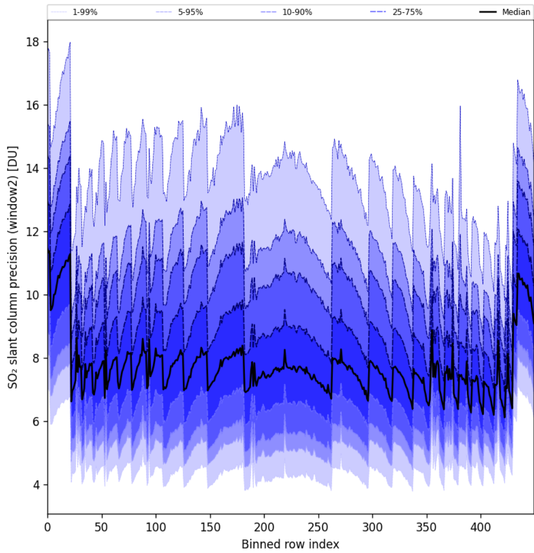
Figure 94: Along track statistics of “SO 2 slant column precision (window2)” for 2025-11-13 to 2025-11-15
