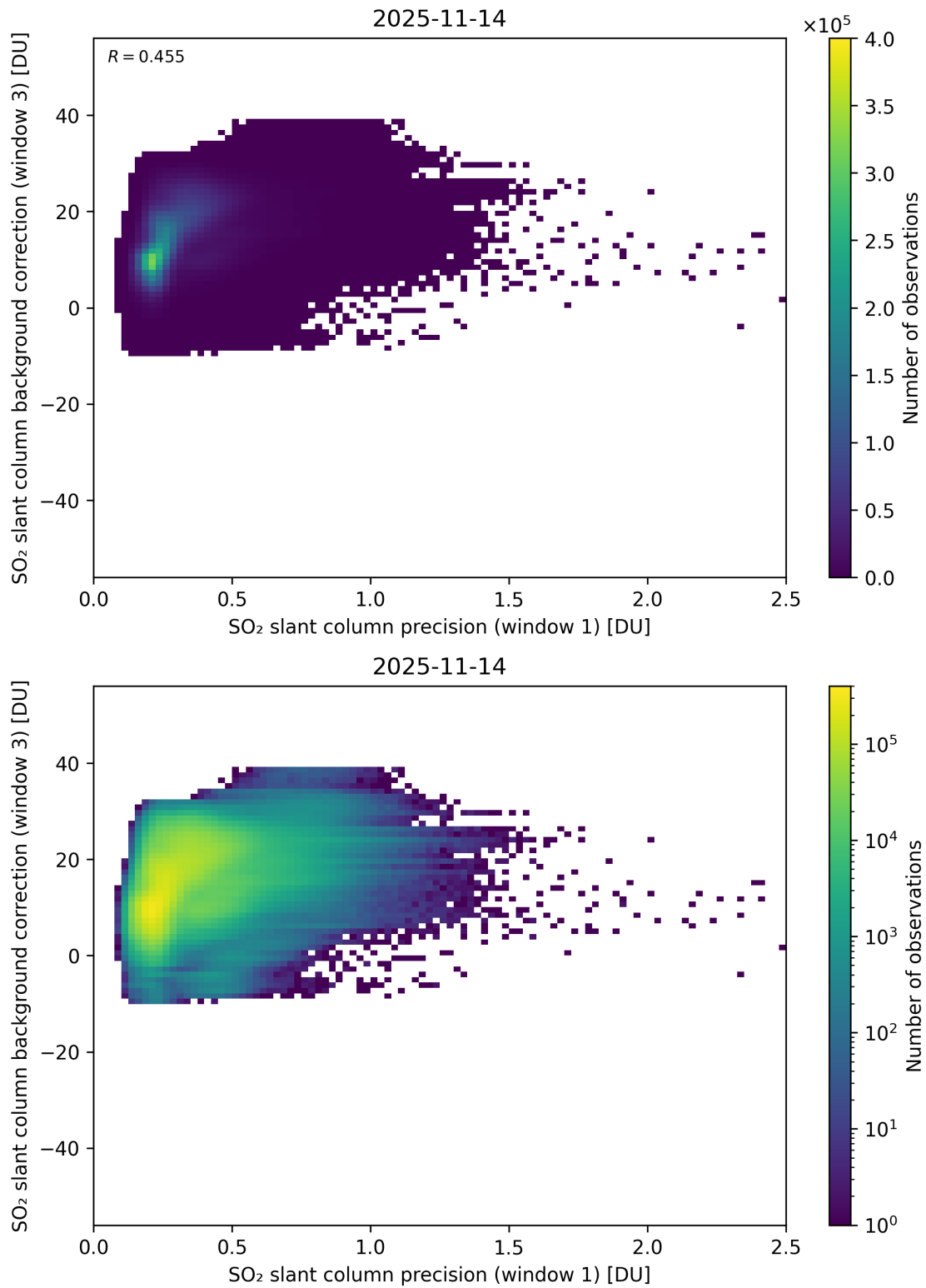
Figure 270: Scatter density plot of “SO 2 slant column precision (window 1)” against “SO 2 slant column background correction (window 3)” for 2025-11-13 to 2025-11-15.
