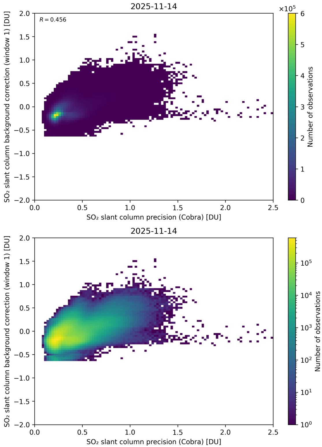
Figure 199: Scatter density plot of “SO 2 slant column precision (Cobra)” against “SO 2 slant column background correction (window 1)” for 2025-11-13 to 2025-11-15.
