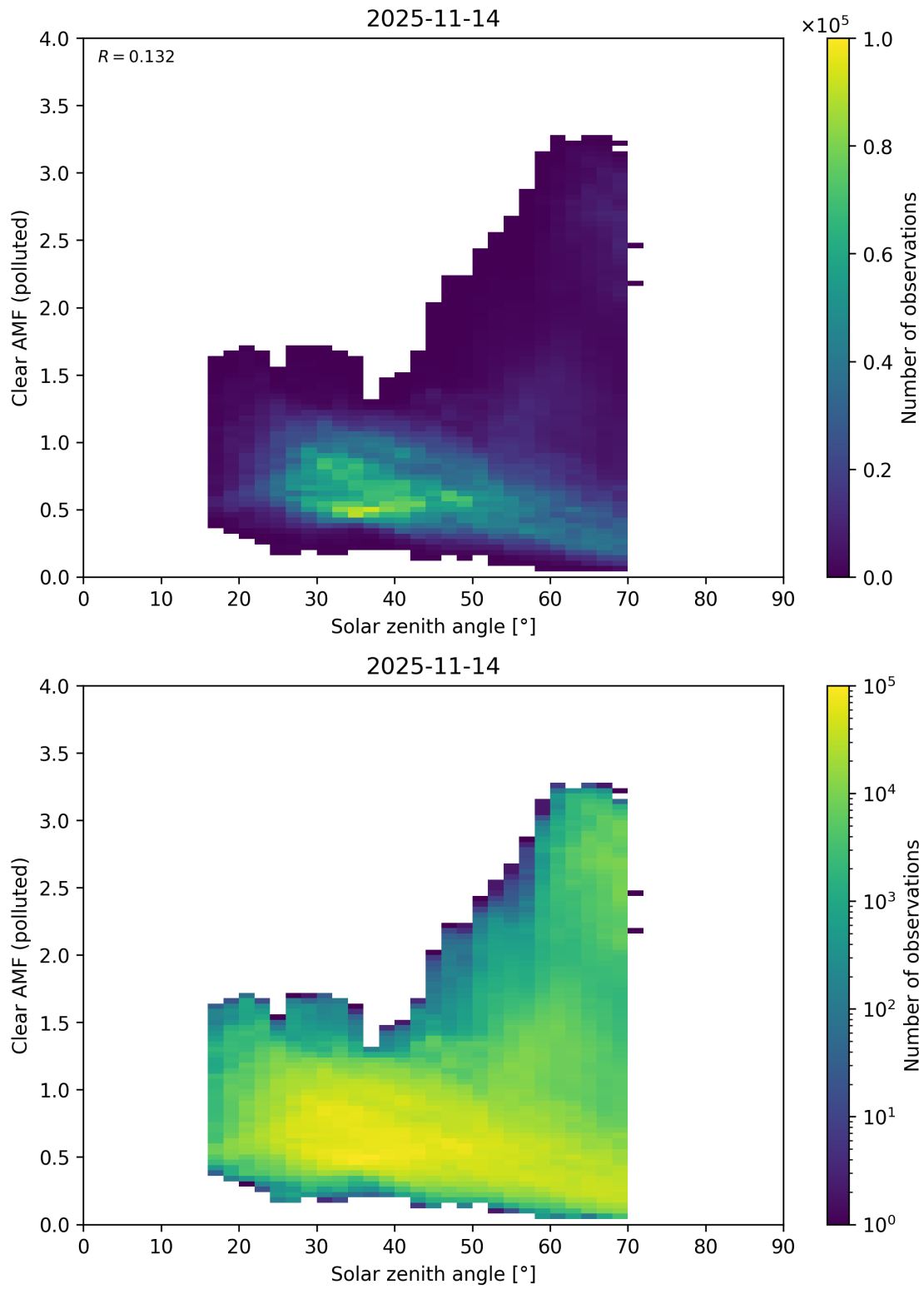
Figure 178: Scatter density plot of “Solar zenith angle” against “Clear AMF (polluted)” for 2025-11-13 to 2025-11-15.
