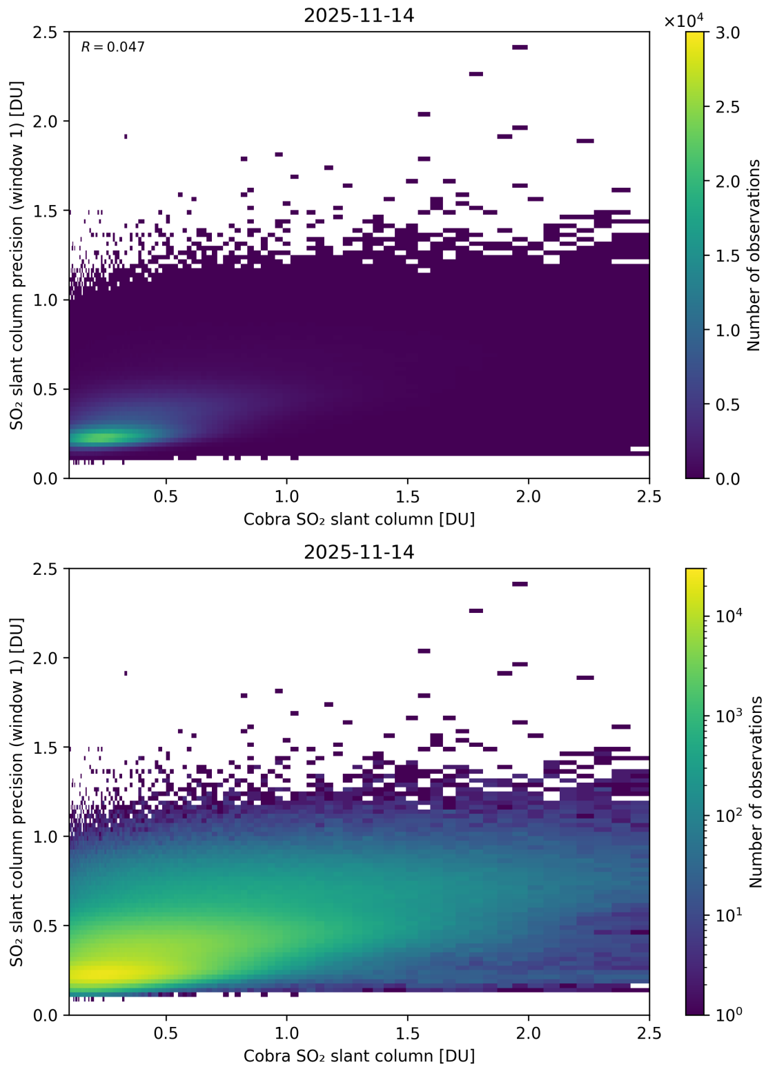
Figure 220: Scatter density plot of “Cobra SO 2 slant column” against “SO 2 slant column precision (window 1)” for 2025-11-13 to 2025-11-15.
