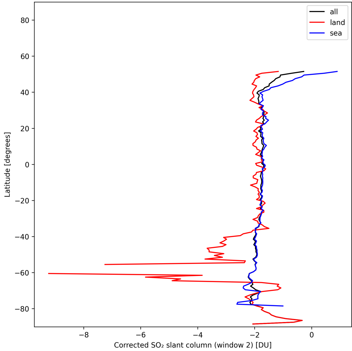
Figure 43: Zonal average of “Corrected SO 2 slant column (window 2)” for 2025-11-13 to 2025-11-15.
