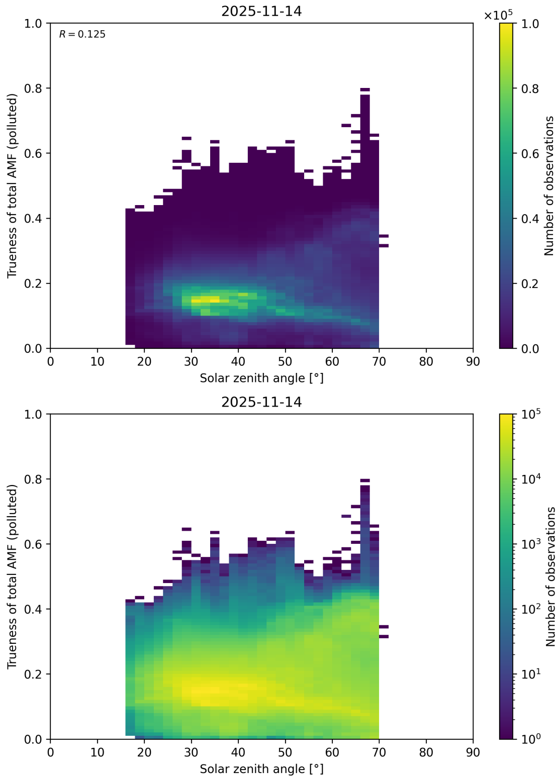
Figure 190: Scatter density plot of “Solar zenith angle” against “Trueness of total AMF (polluted)” for 2025-11-13 to 2025-11-15.
