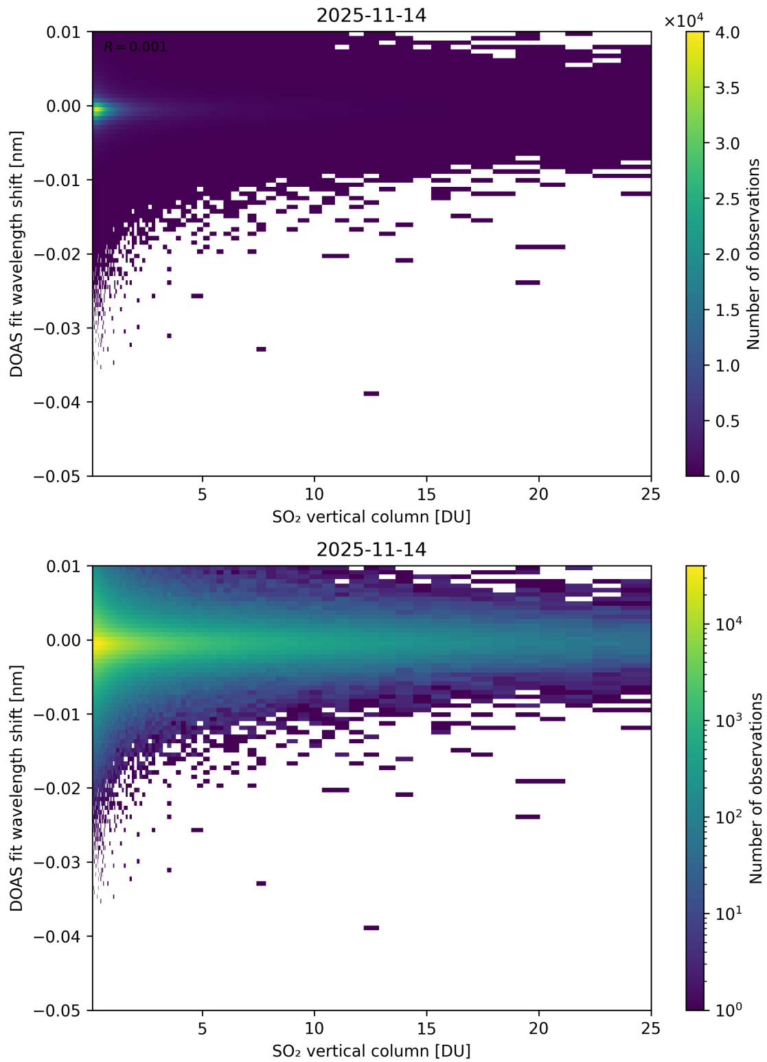
Figure 326: Scatter density plot of “SO 2 vertical column” against “DOAS fit wavelength shift” for 2025-11-13 to 2025-11-15.
