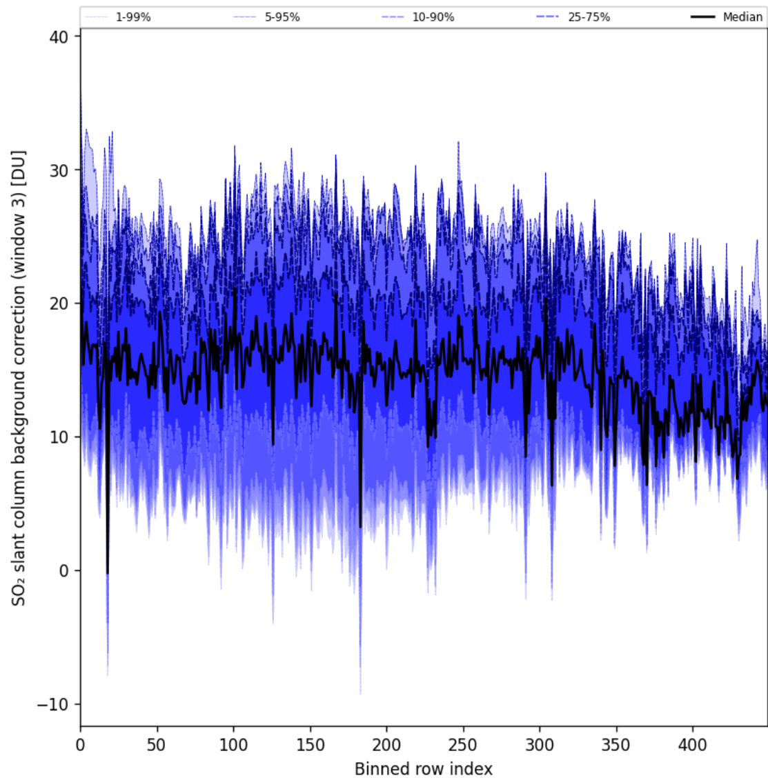
Figure 100: Along track statistics of “SO 2 slant column background correction (window 3)” for 2025-11-13 to 2025-11-15
