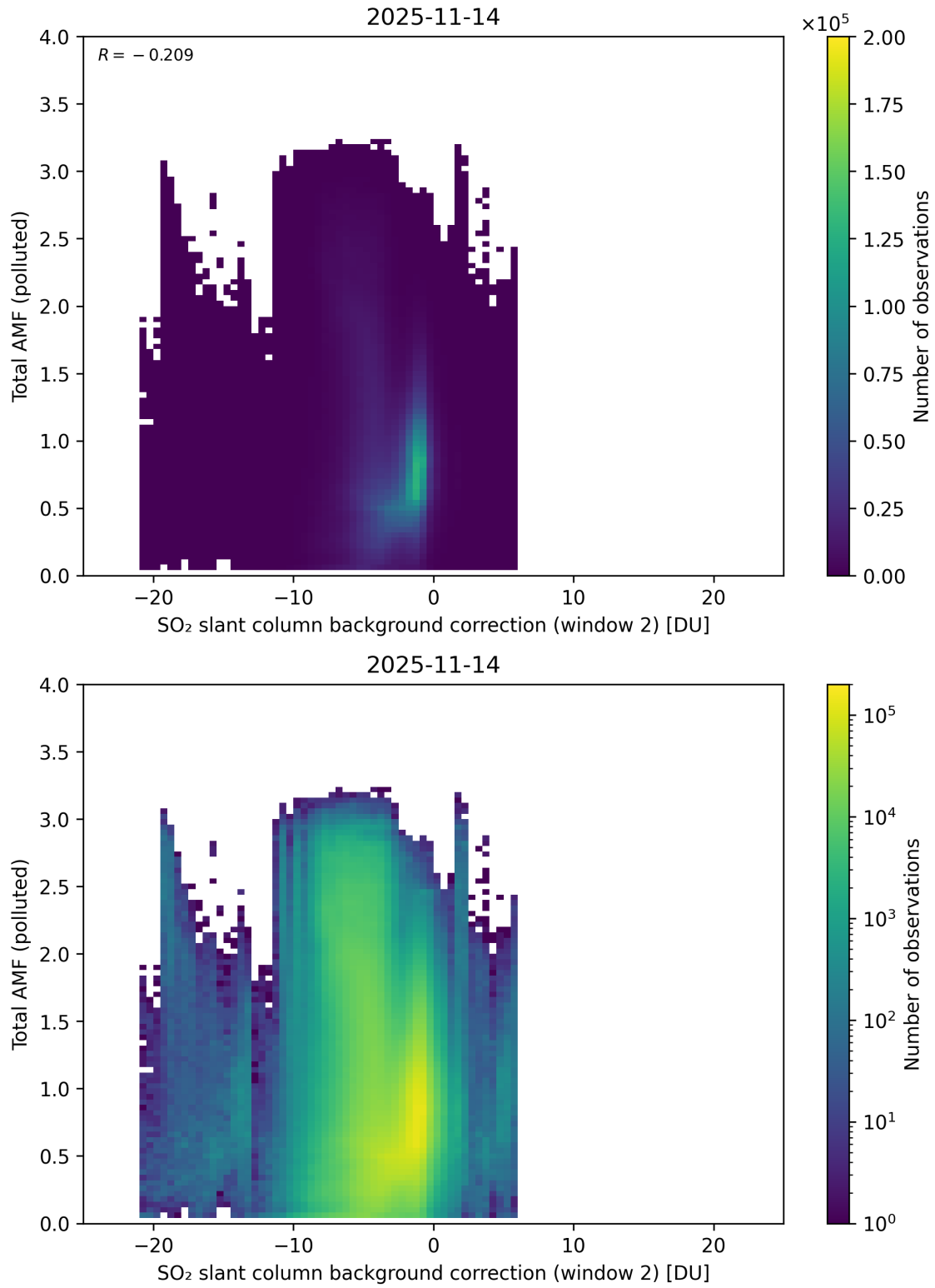
Figure 130: Scatter density plot of “SO 2 slant column background correction (window 2)” against “Total AMF (polluted)” for 2025-11-13 to 2025-11-15.
