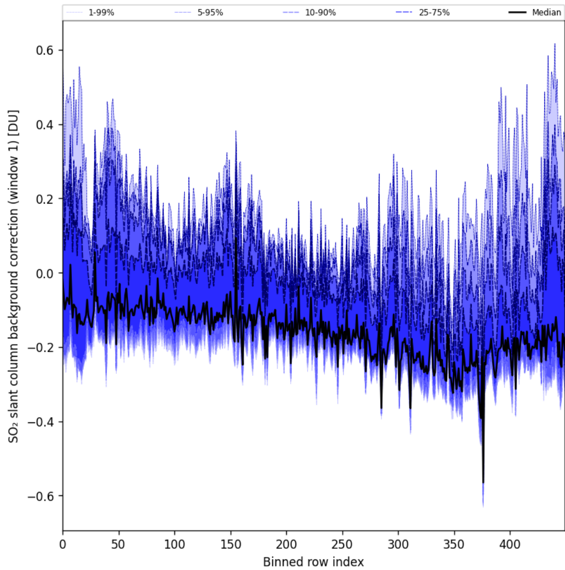
Figure 92: Along track statistics of “SO 2 slant column background correction (window 1)” for 2025-11-13 to 2025-11-15
