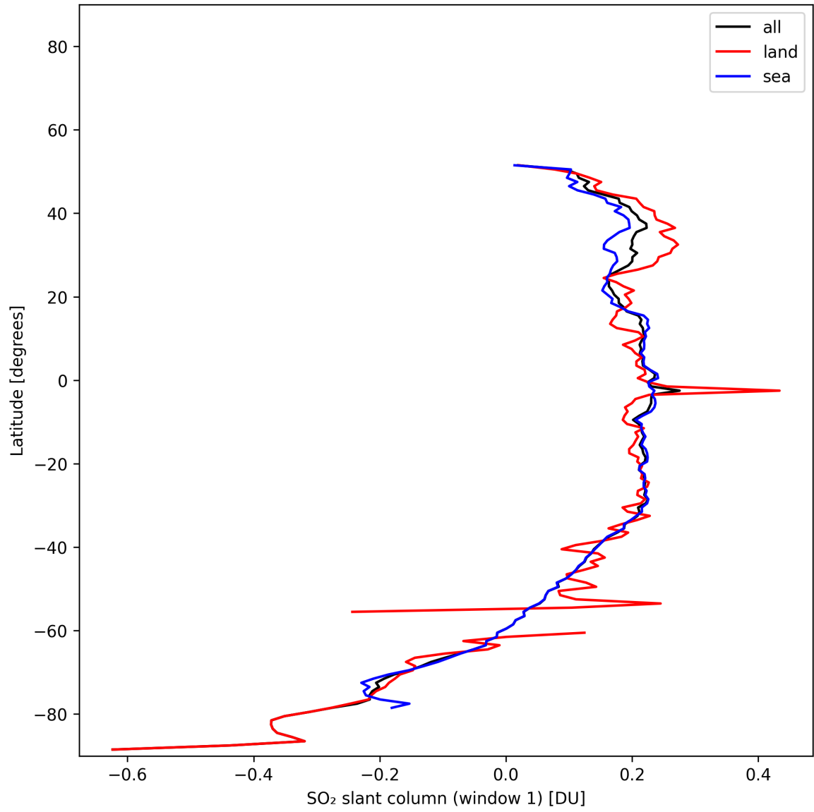
Figure 37: Zonal average of “SO 2 slant column (window 1)” for 2025-11-13 to 2025-11-15.
