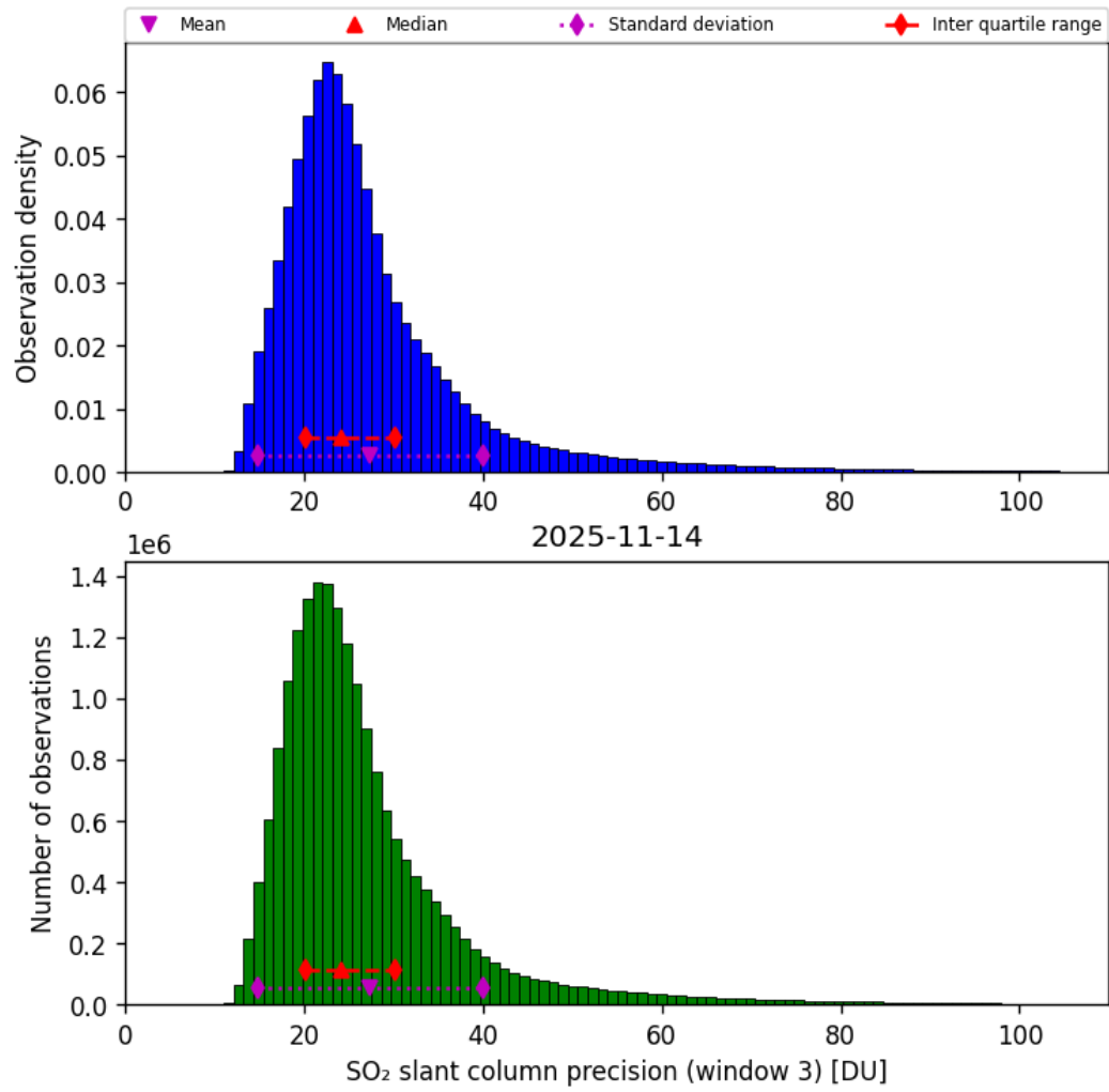
Figure 72: Histogram of “SO 2 slant column precision (window 3)” for 2025-11-13 to 2025-11-15
