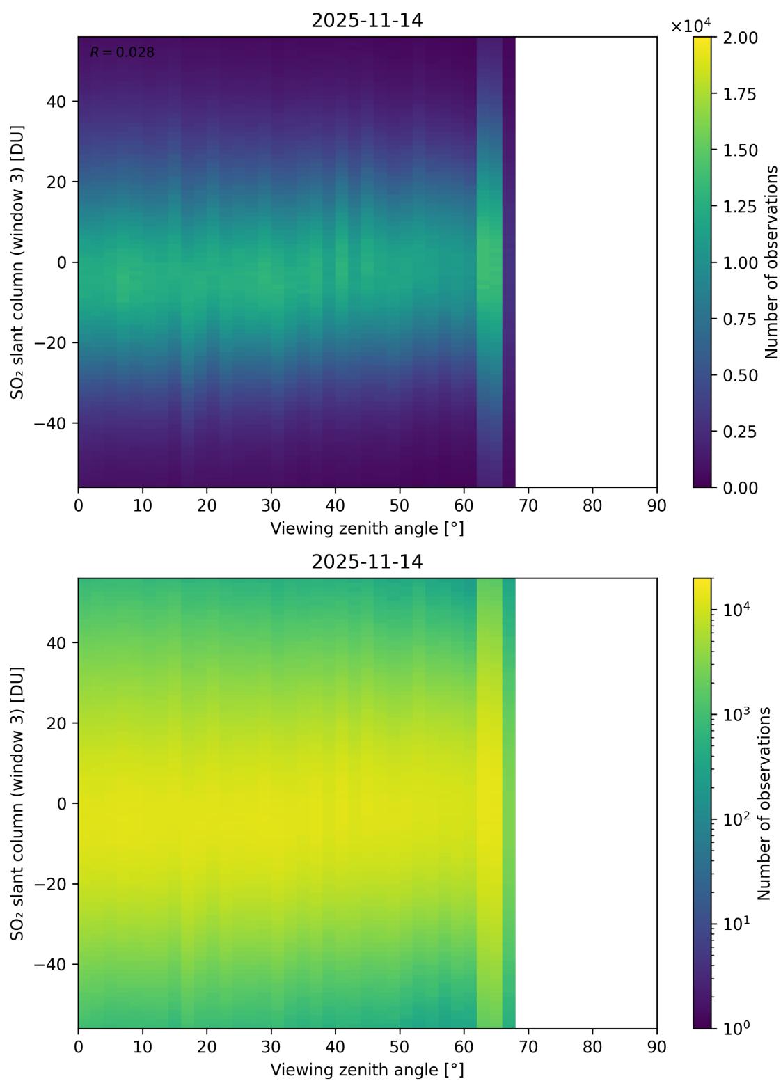
Figure 379: Scatter density plot of “Viewing zenith angle” against “SO 2 slant column (window 3)” for 2025-11-13 to 2025-11-15.
