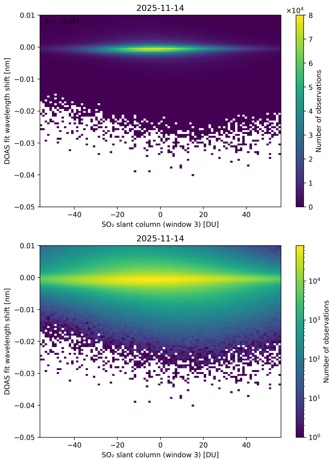
Figure 304: Scatter density plot of “SO 2 slant column (window 3)” against “DOAS fit wavelength shift” for 2025-11-13 to 2025-11-15.
