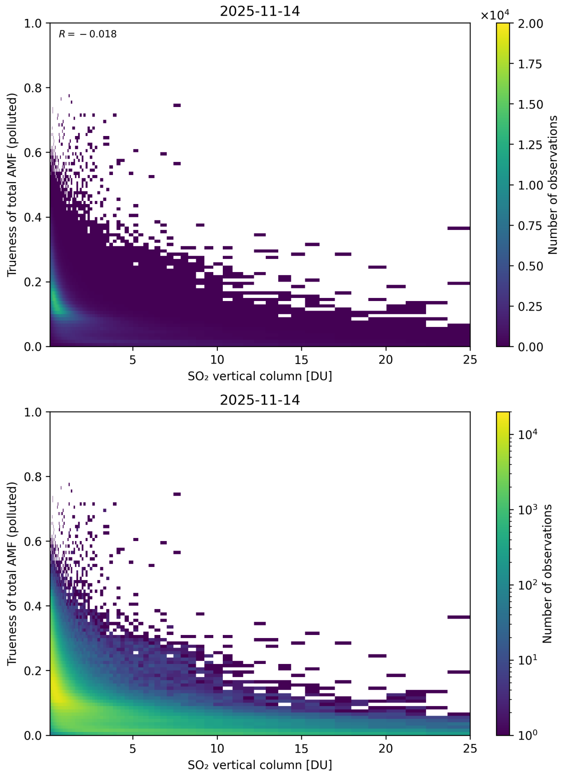
Figure 360: Scatter density plot of “SO 2 vertical column” against “Trueness of total AMF (polluted)” for 2025-11-13 to 2025-11-15.
