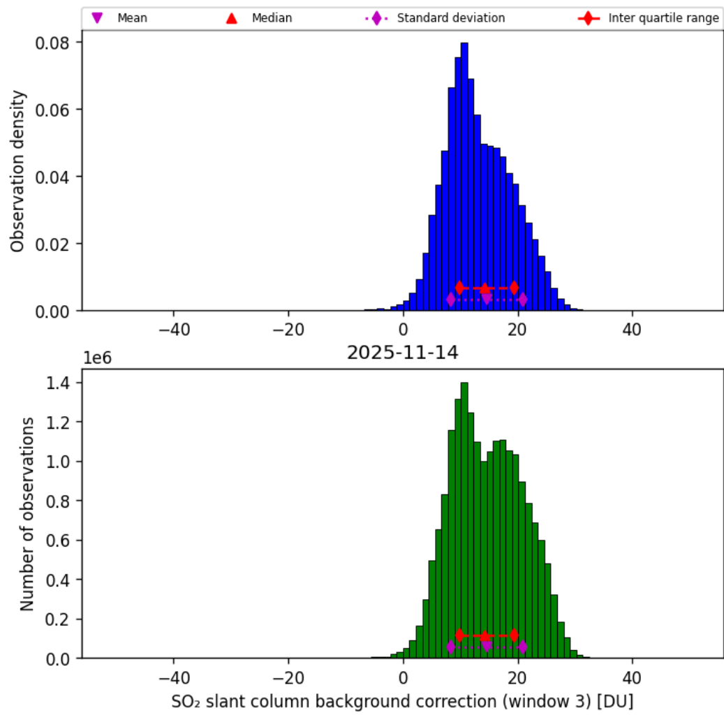
Figure 74: Histogram of “SO 2 slant column background correction (window 3)” for 2025-11-13 to 2025-11-15
