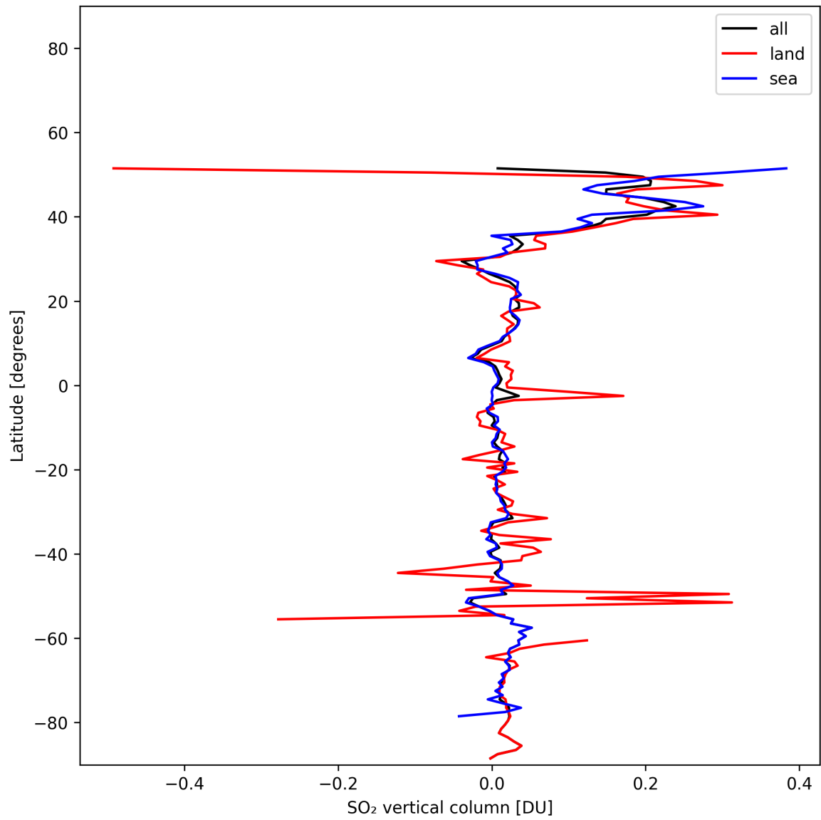
Figure 32: Zonal average of “SO 2 vertical column” for 2025-11-13 to 2025-11-15.
