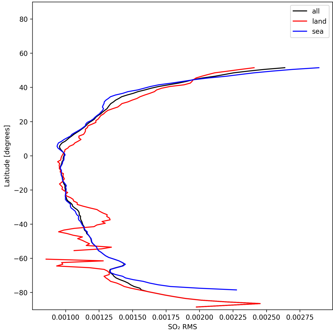
Figure 52: Zonal average of “SO 2 RMS” for 2025-11-13 to 2025-11-15.
