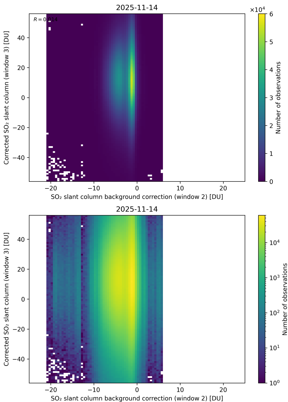
Figure 127: Scatter density plot of “SO 2 slant column background correction (window 2)” against “Corrected SO 2 slant column (window 3)” for 2025-11-13 to 2025-11-15.
