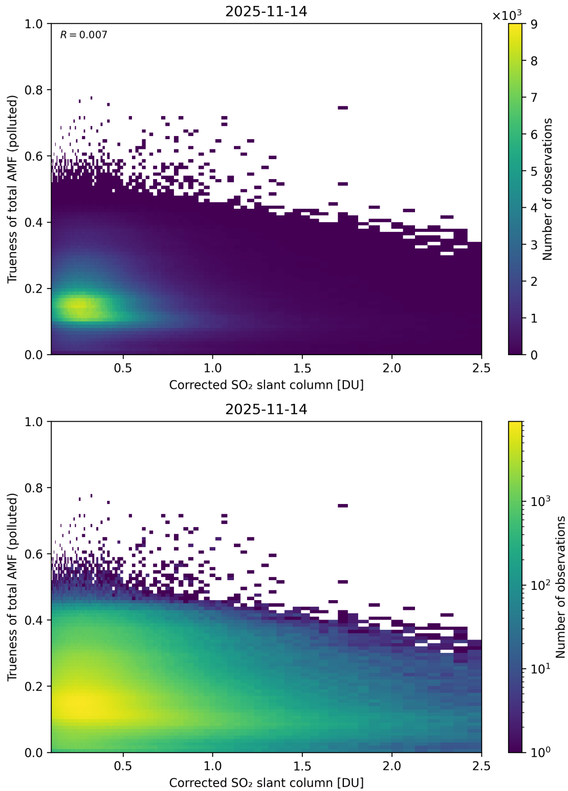
Figure 243: Scatter density plot of “Corrected SO 2 slant column” against “Trueness of total AMF (polluted)” for 2025-11-13 to 2025-11-15.
