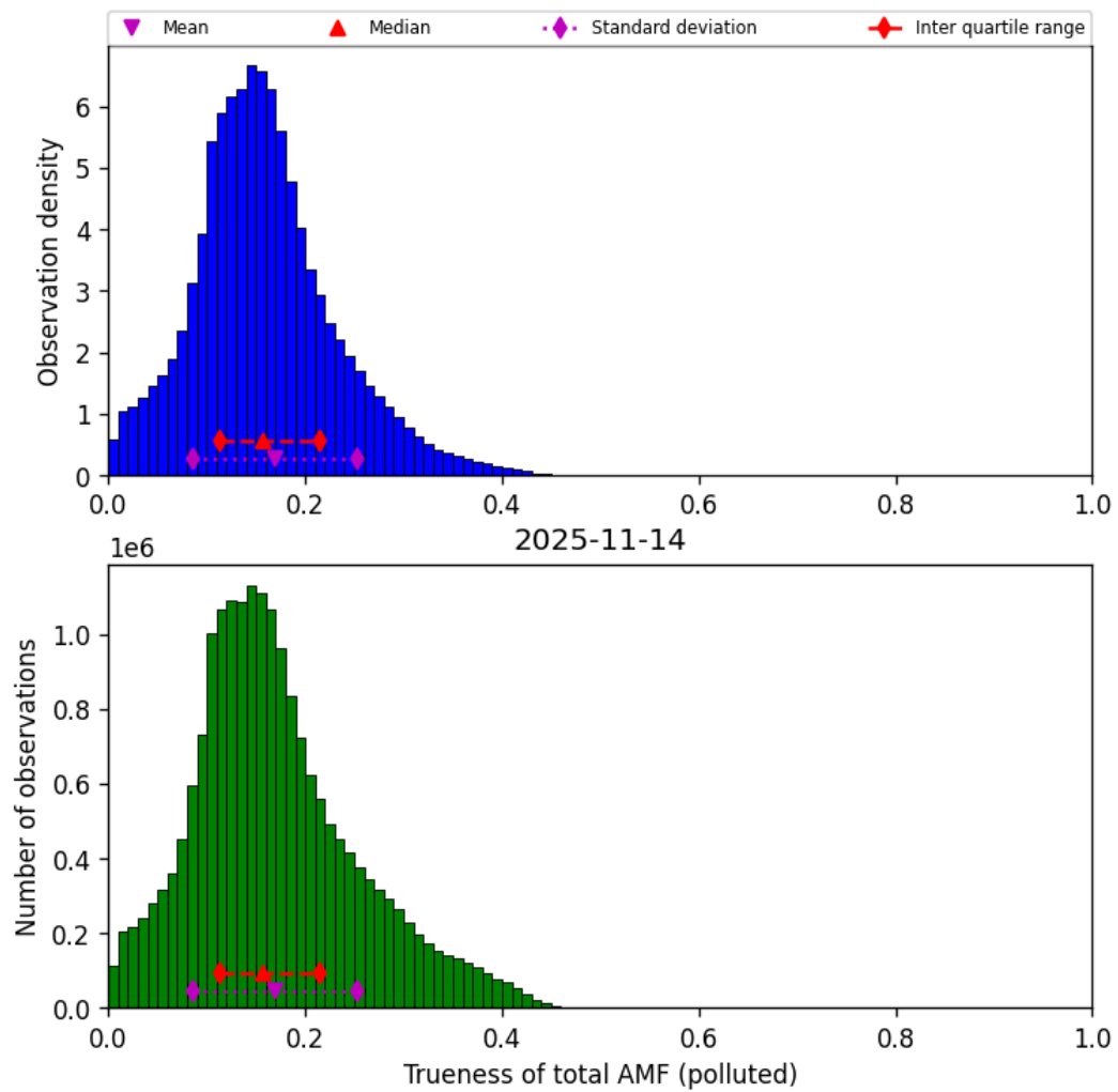
Figure 80: Histogram of “Trueness of total AMF (polluted)” for 2025-11-13 to 2025-11-15
