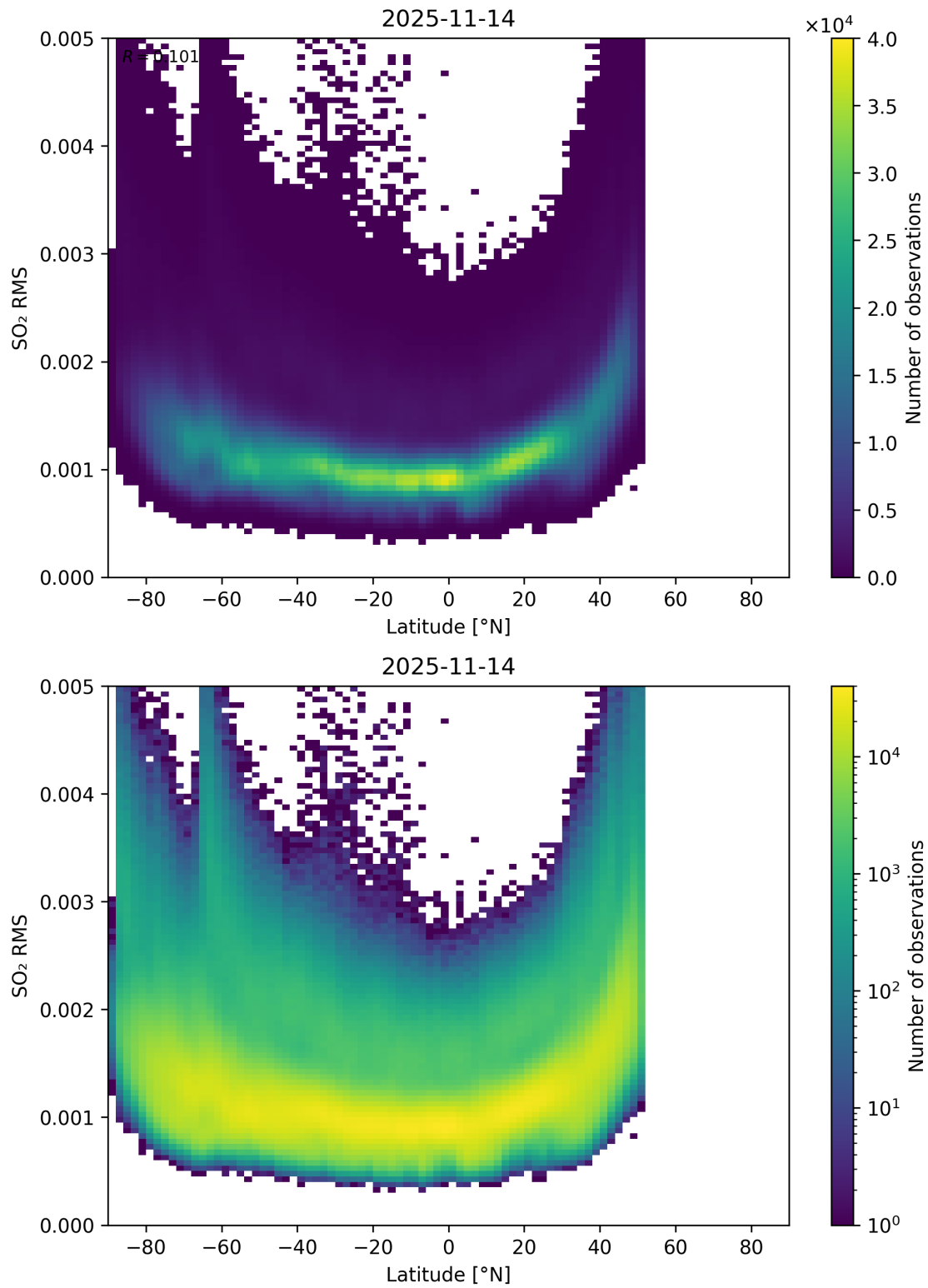
Figure 155: Scatter density plot of “Latitude” against “SO 2 RMS” for 2025-11-13 to 2025-11-15.
