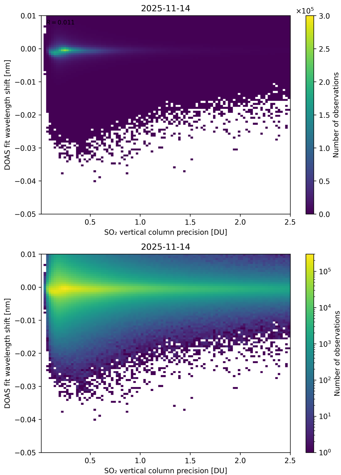
Figure 332: Scatter density plot of “SO 2 vertical column precision” against “DOAS fit wavelength shift” for 2025-11-13 to 2025-11-15.
