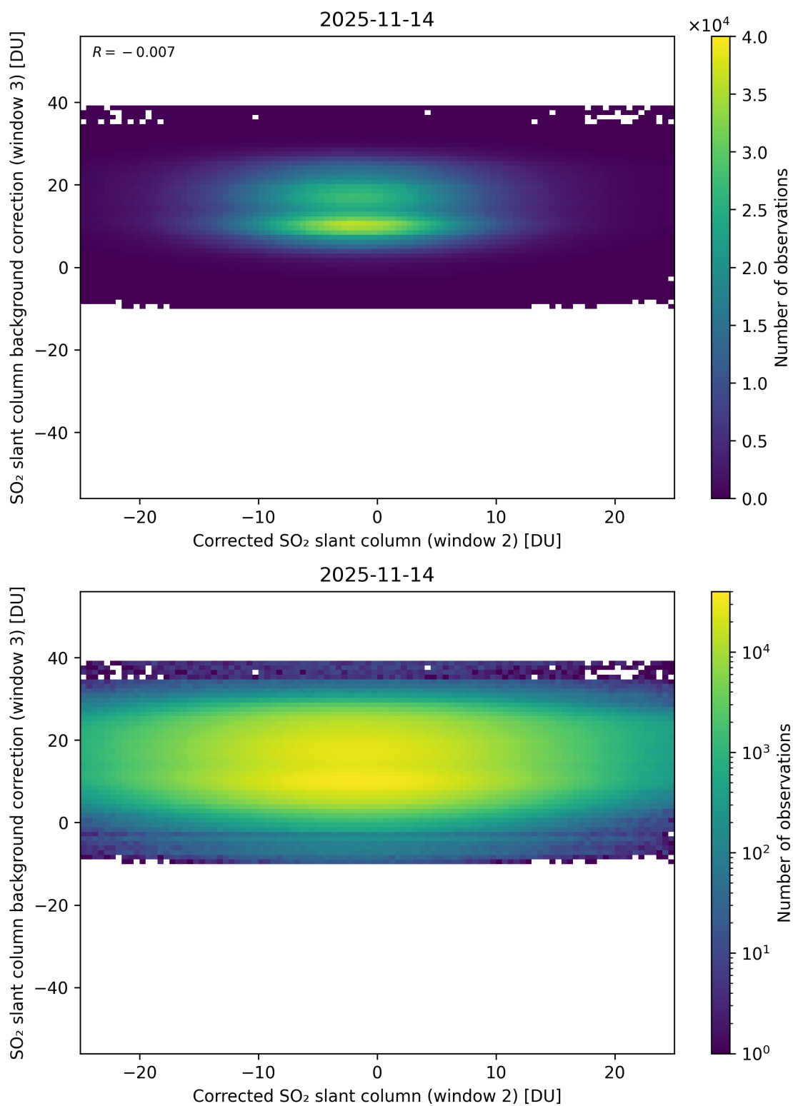
Figure 245: Scatter density plot of “Corrected SO 2 slant column (window 2)” against “SO 2 slant column background correction (window 3)” for 2025-11-13 to 2025-11-15.
