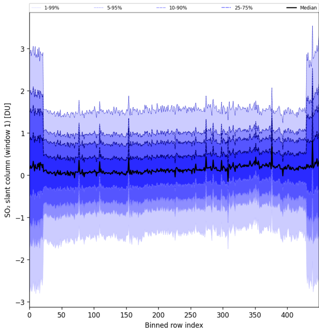
Figure 89: Along track statistics of “SO 2 slant column (window 1)” for 2025-11-13 to 2025-11-15
