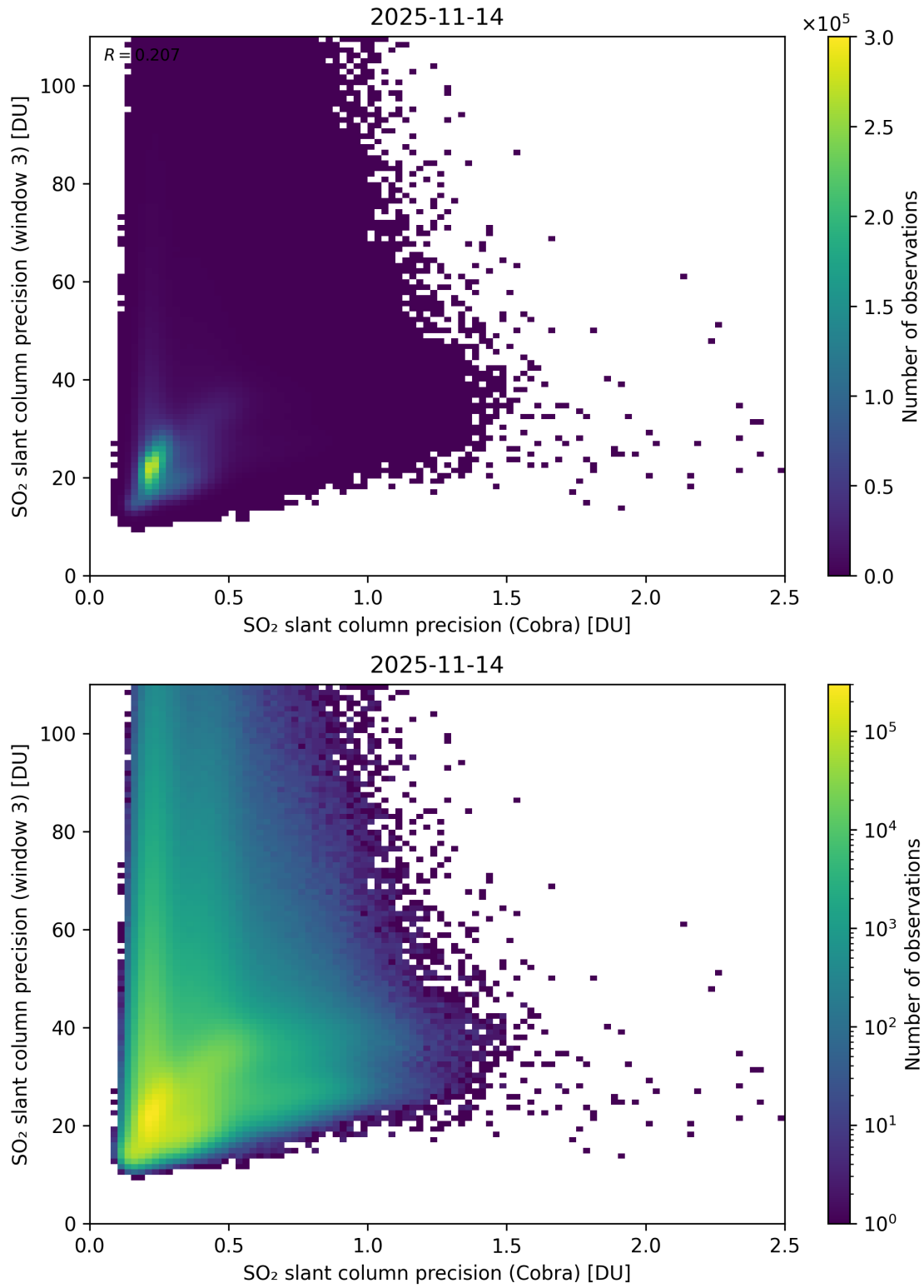
Figure 212: Scatter density plot of “SO 2 slant column precision (Cobra)” against “SO 2 slant column precision (window 3)” for 2025-11-13 to 2025-11-15.
