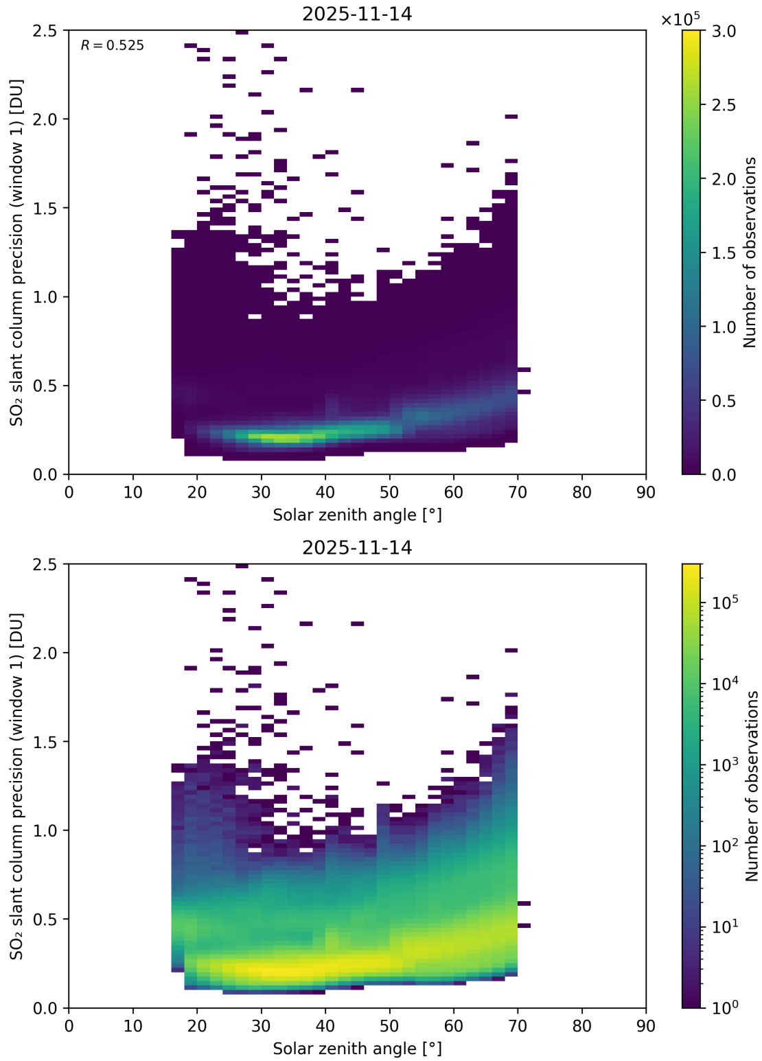
Figure 185: Scatter density plot of “Solar zenith angle” against “SO 2 slant column precision (window 1)” for 2025-11-13 to 2025-11-15.
