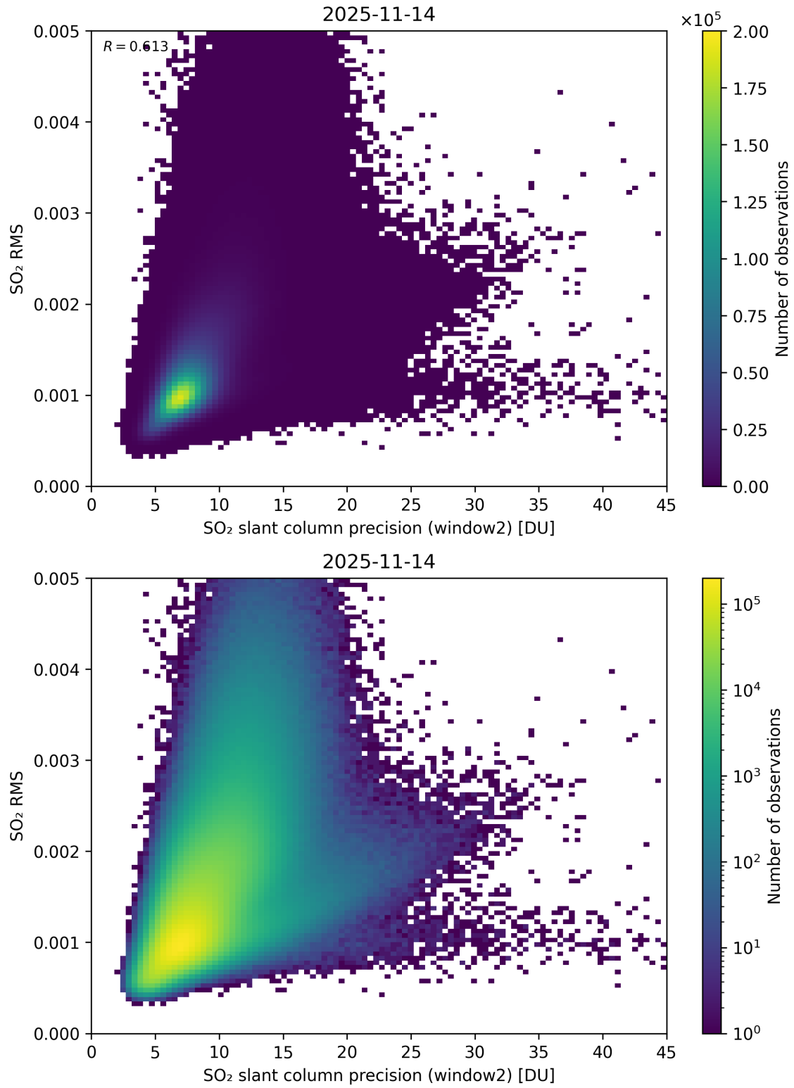
Figure 295: Scatter density plot of “SO 2 slant column precision (window2)” against “SO 2 RMS” for 2025-11-13 to 2025-11-15.
