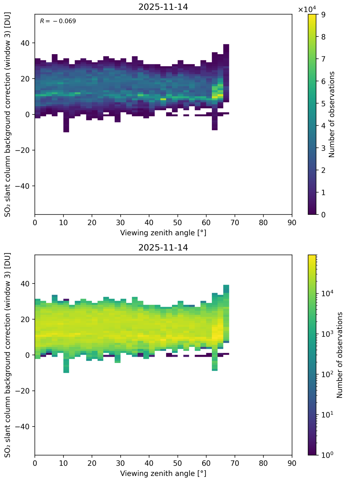
Figure 364: Scatter density plot of “Viewing zenith angle” against “SO 2 slant column background correction (window 3)” for 2025-11-13 to 2025-11-15.
