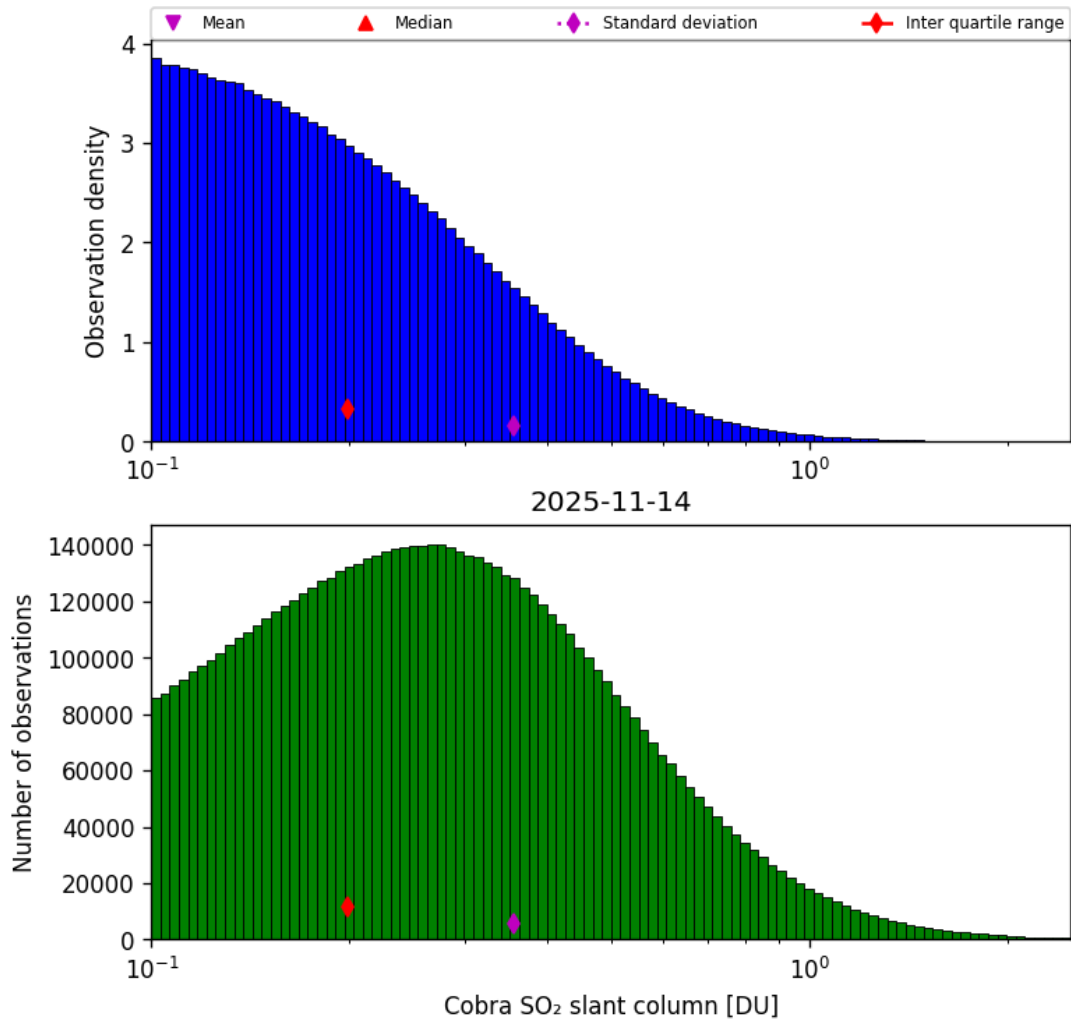
Figure 61: Histogram of “Cobra SO 2 slant column” for 2025-11-13 to 2025-11-15
