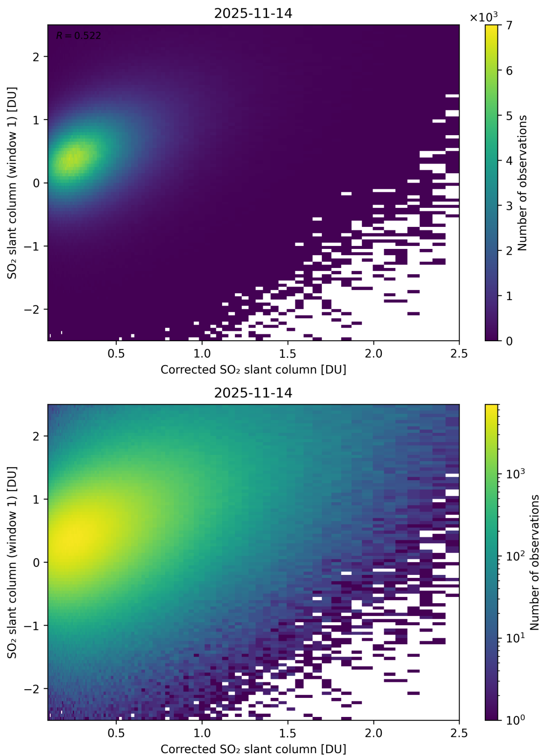
Figure 237: Scatter density plot of “Corrected SO 2 slant column” against “SO 2 slant column (window 1)” for 2025-11-13 to 2025-11-15.
