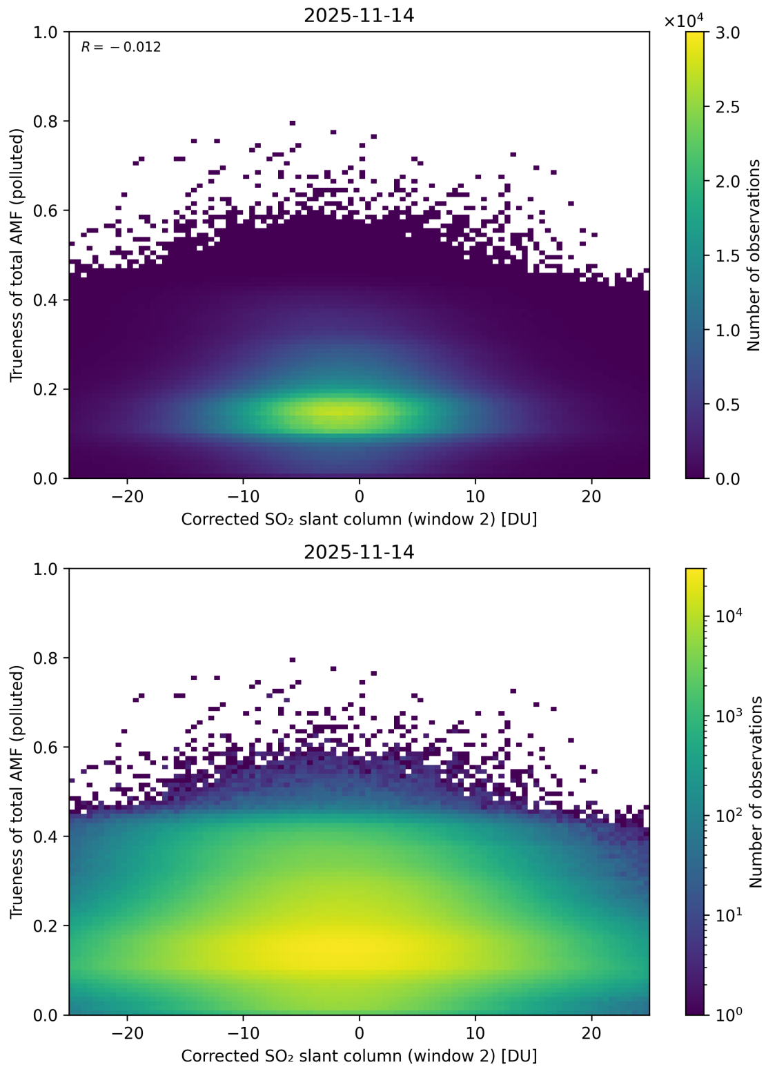
Figure 254: Scatter density plot of “Corrected SO 2 slant column (window 2)” against “Trueness of total AMF (polluted)” for 2025-11-13 to 2025-11-15.
