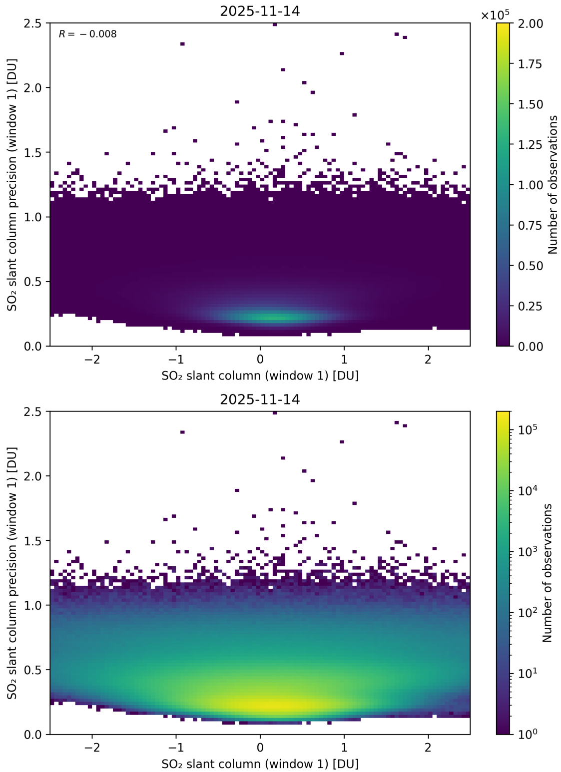
Figure 285: Scatter density plot of “SO 2 slant column (window 1)” against “SO 2 slant column precision (window 1)” for 2025-11-13 to 2025-11-15.
