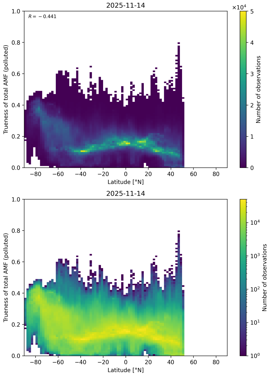
Figure 168: Scatter density plot of “Latitude” against “Trueness of total AMF (polluted)” for 2025-11-13 to 2025-11-15.
