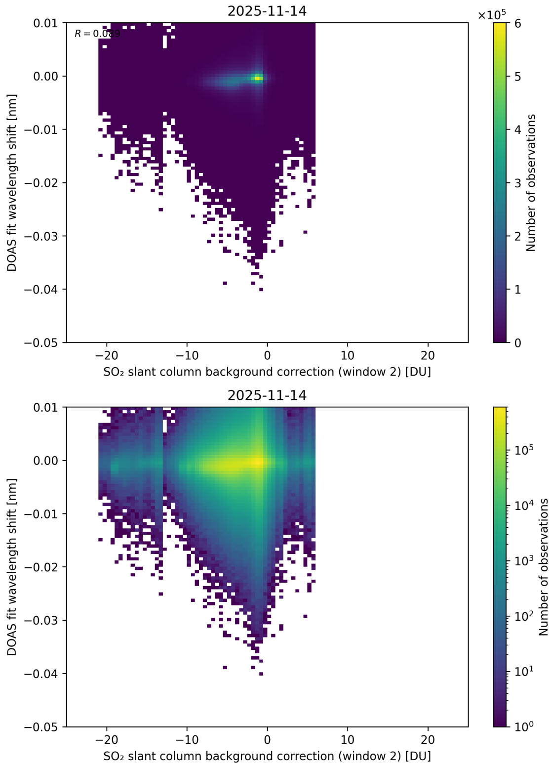
Figure 123: Scatter density plot of “SO 2 slant column background correction (window 2)” against “DOAS fit wavelength shift” for 2025-11-13 to 2025-11-15.
