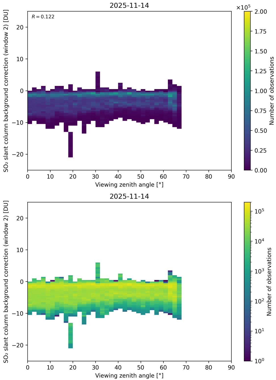
Figure 363: Scatter density plot of “Viewing zenith angle” against “SO 2 slant column background correction (window 2)” for 2025-11-13 to 2025-11-15.
