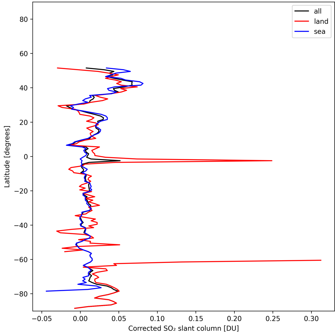
Figure 34: Zonal average of “Corrected SO 2 slant column” for 2025-11-13 to 2025-11-15.
