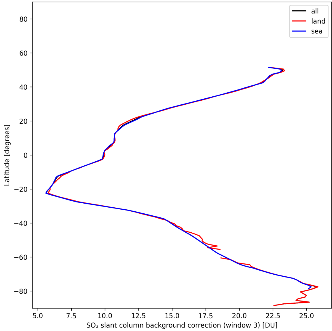
Figure 48: Zonal average of “SO 2 slant column background correction (window 3)” for 2025-11-13 to 2025-11-15.
