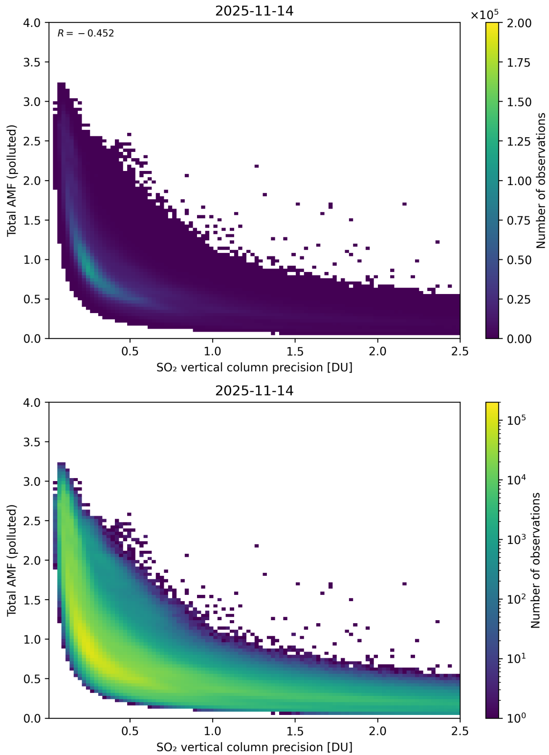
Figure 346: Scatter density plot of “SO 2 vertical column precision” against “Total AMF (polluted)” for 2025-11-13 to 2025-11-15.
