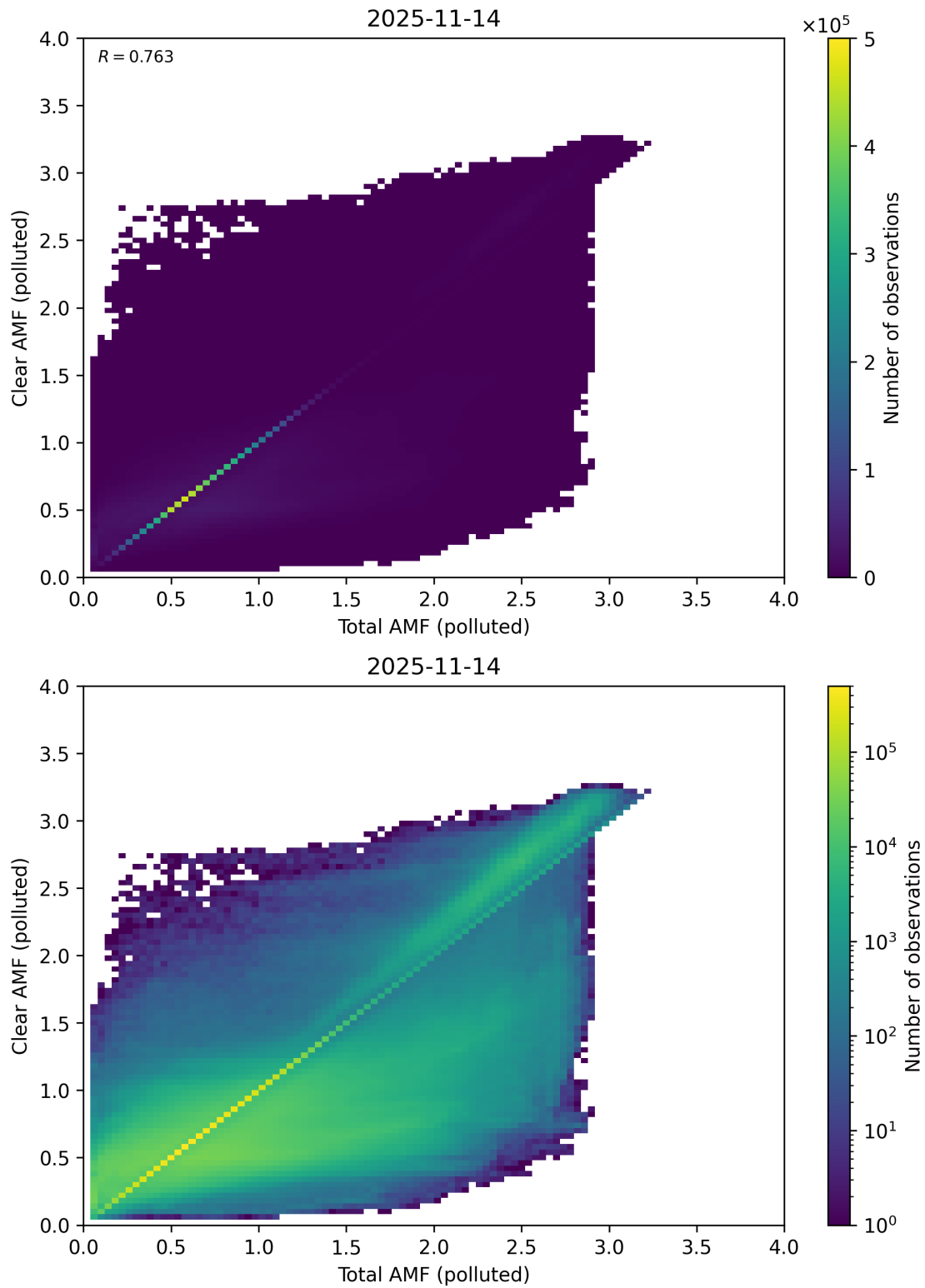
Figure 320: Scatter density plot of “Total AMF (polluted)” against “Clear AMF (polluted)” for 2025-11-13 to 2025-11-15.
