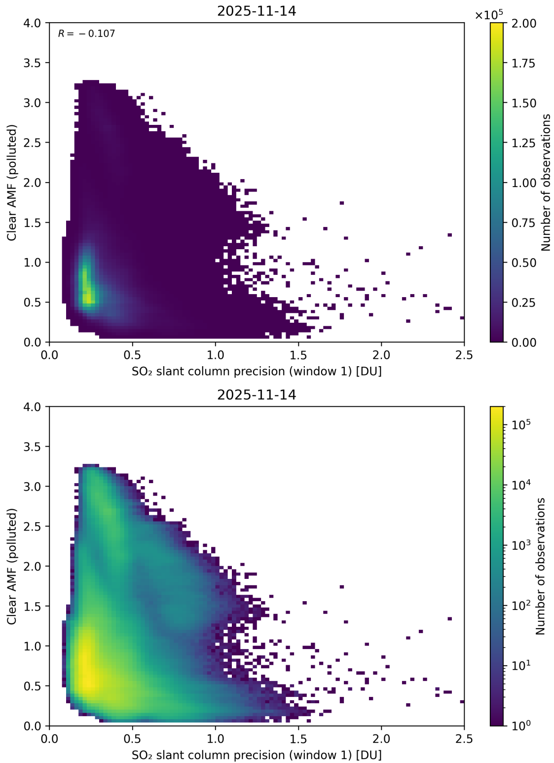
Figure 274: Scatter density plot of “SO 2 slant column precision (window 1)” against “Clear AMF (polluted)” for 2025-11-13 to 2025-11-15.
