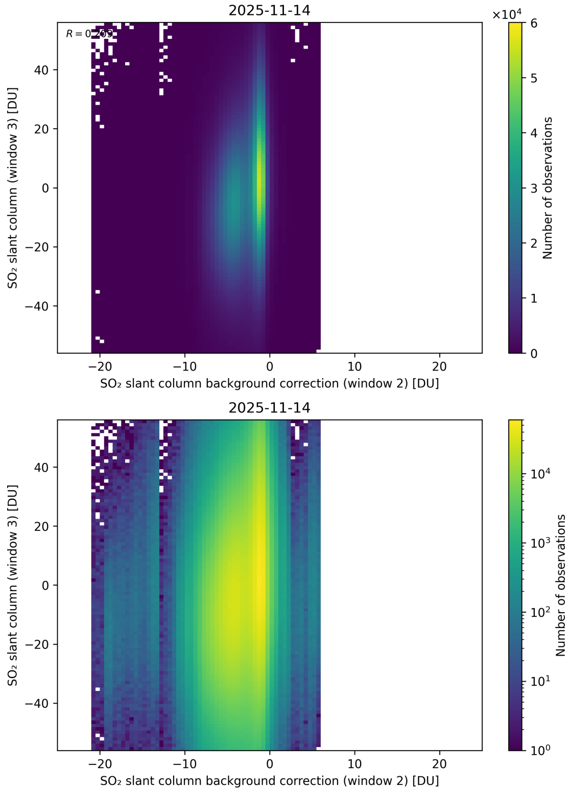
Figure 128: Scatter density plot of “SO 2 slant column background correction (window 2)” against “SO 2 slant column (window 3)” for 2025-11-13 to 2025-11-15.
