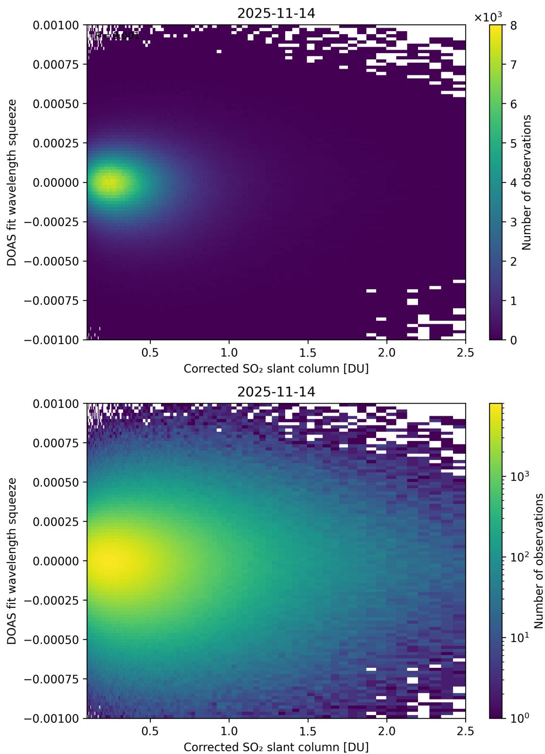
Figure 230: Scatter density plot of "Corrected SO 2 slant column" against "DOAS fit wavelength squeeze" for 2025-11-13 to 2025-11-15.
