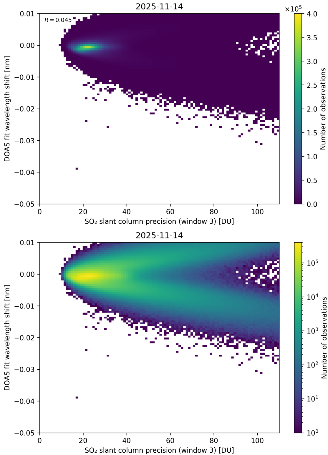
Figure 308: Scatter density plot of “SO 2 slant column precision (window 3)” against “DOAS fit wavelength shift” for 2025-11-13 to 2025-11-15.
