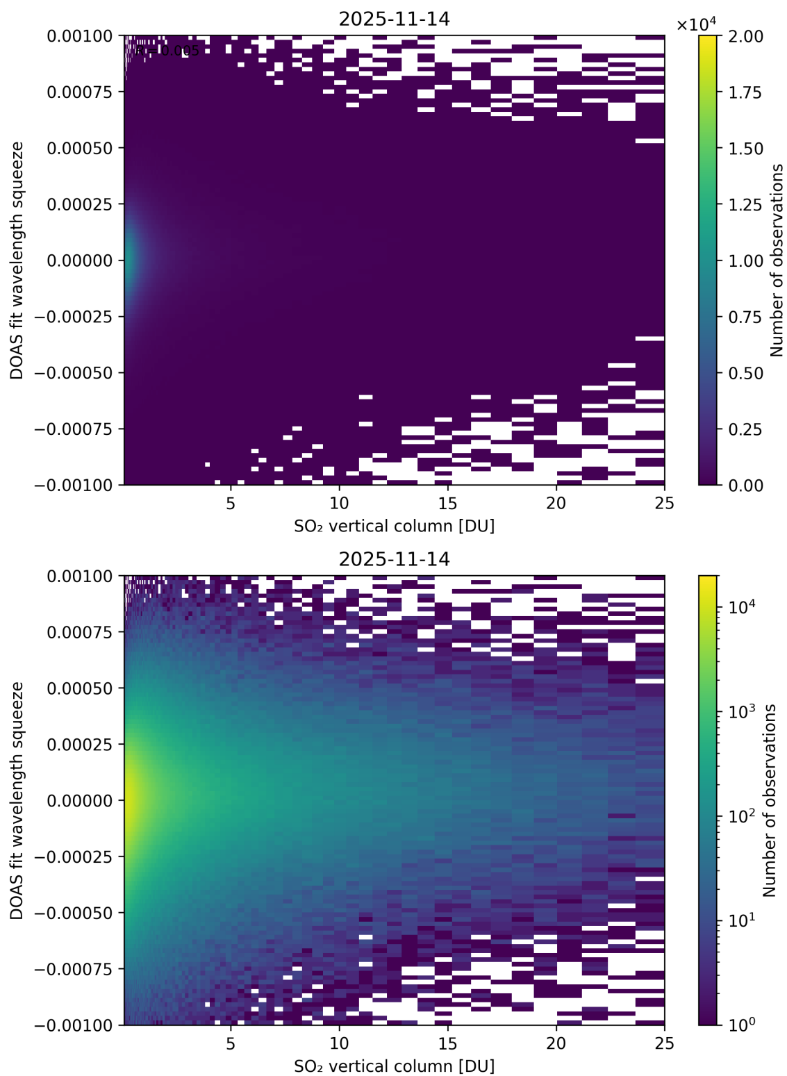
Figure 327: Scatter density plot of “SO 2 vertical column” against “DOAS fit wavelength squeeze” for 2025-11-13 to 2025-11-15.
