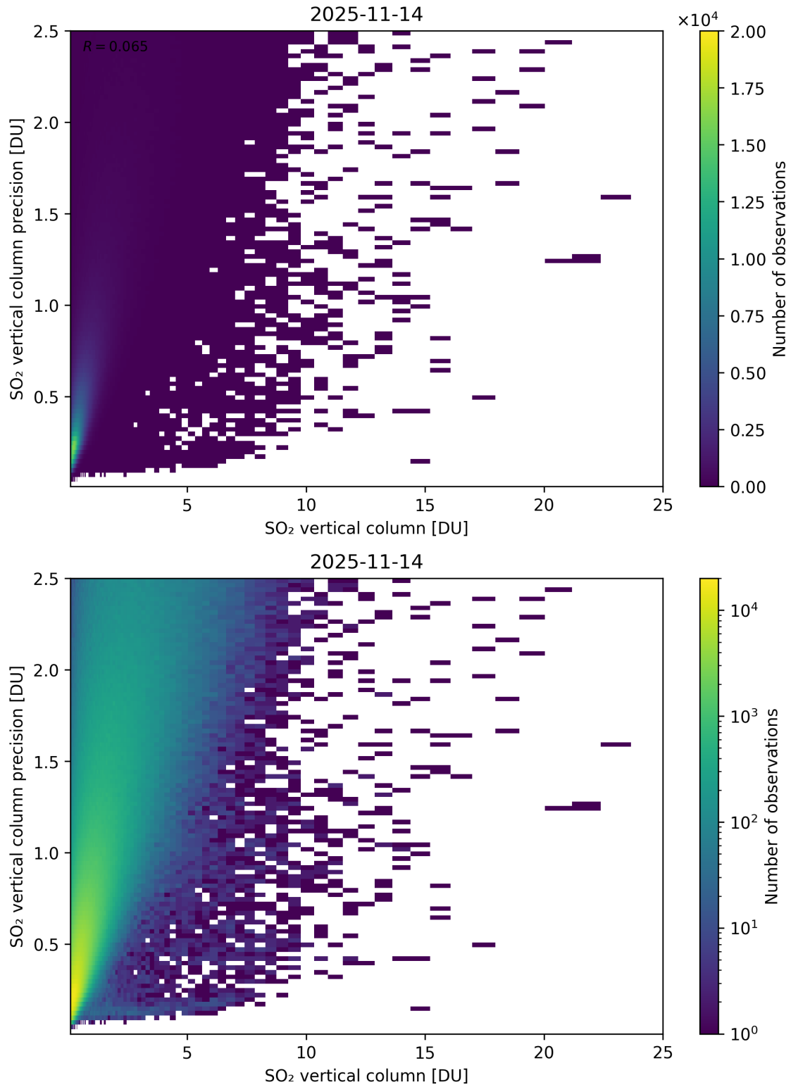
Figure 361: Scatter density plot of “SO 2 vertical column” against “SO 2 vertical column precision” for 2025-11-13 to 2025-11-15.
