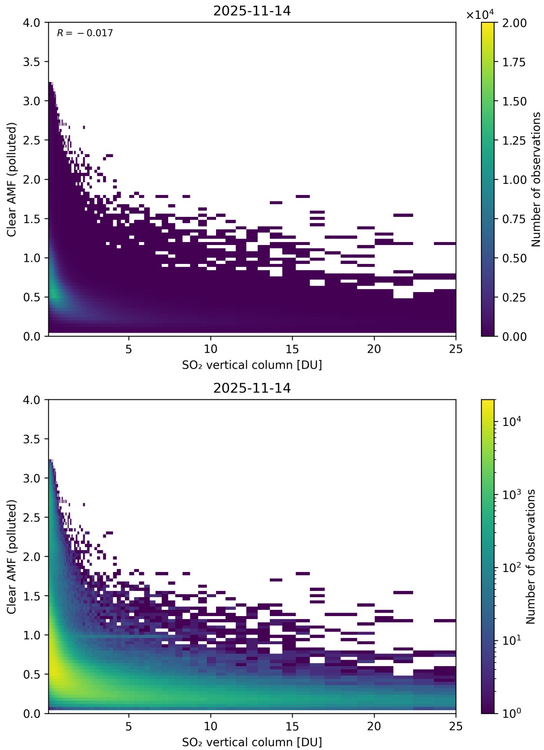
Figure 348: Scatter density plot of “SO 2 vertical column” against “Clear AMF (polluted)” for 2025-11-13 to 2025-11-15.
