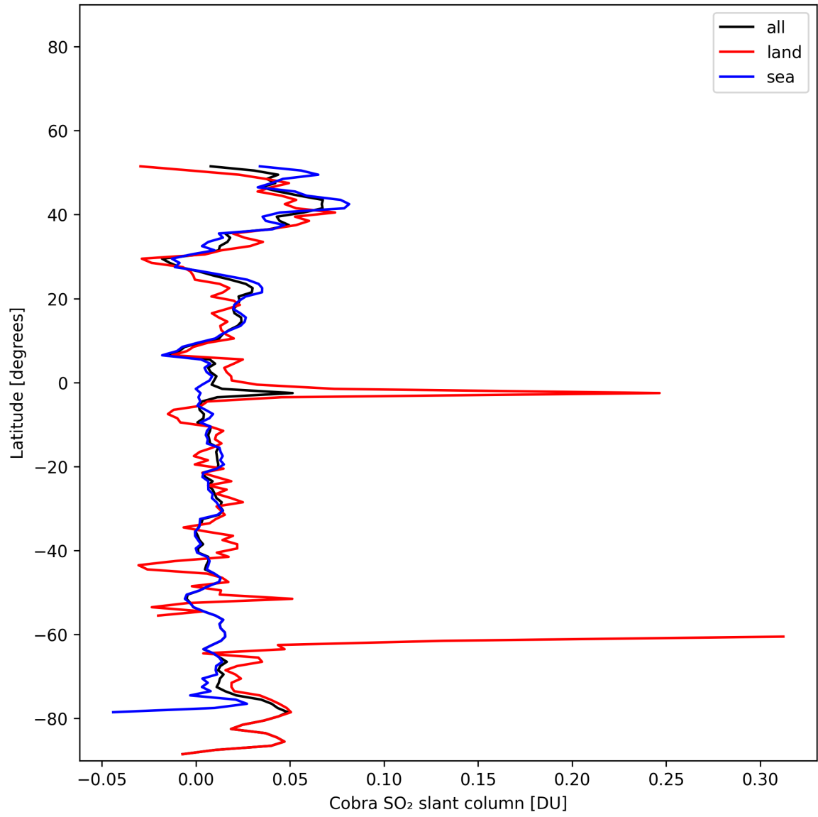
Figure 35: Zonal average of “Cobra SO 2 slant column” for 2025-11-13 to 2025-11-15.
