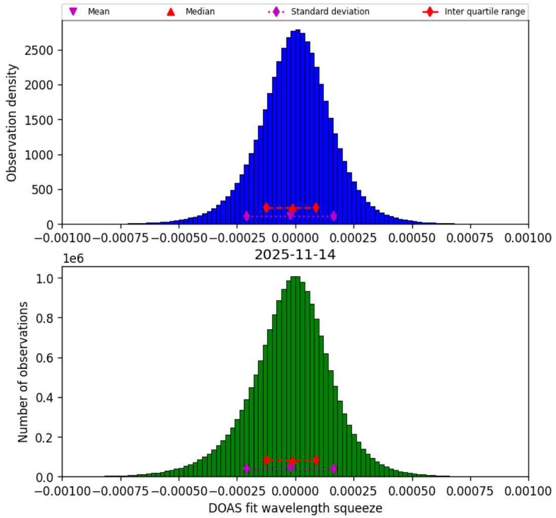
Figure 77: Histogram of “DOAS fit wavelength squeeze” for 2025-11-13 to 2025-11-15
