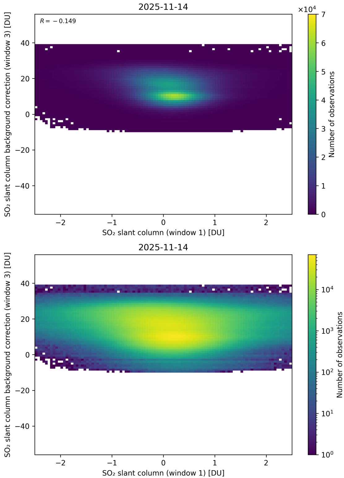
Figure 264: Scatter density plot of “SO 2 slant column (window 1)” against “SO 2 slant column background correction (window 3)” for 2025-11-13 to 2025-11-15.
