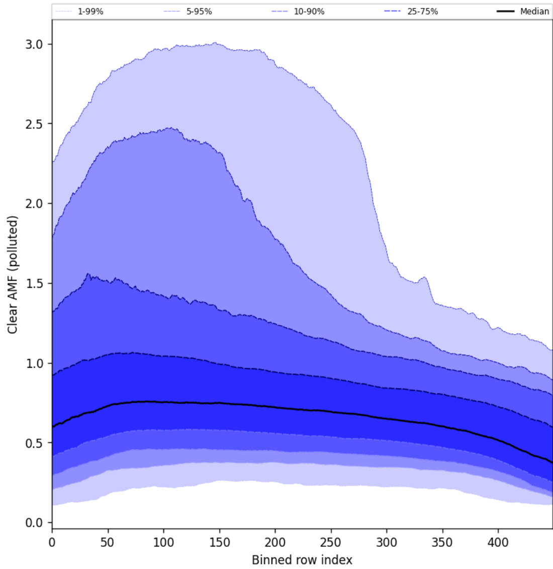
Figure 107: Along track statistics of “Clear AMF (polluted)” for 2025-11-13 to 2025-11-15
