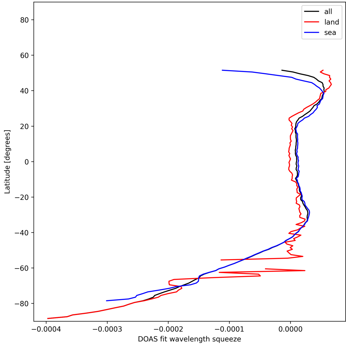
Figure 51: Zonal average of “DOAS fit wavelength squeeze” for 2025-11-13 to 2025-11-15.
