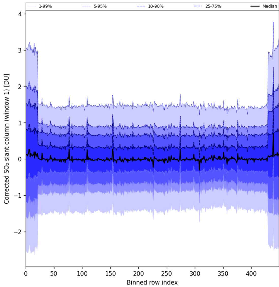
Figure 91: Along track statistics of “Corrected SO 2 slant column (window 1)” for 2025-11-13 to 2025-11-15
