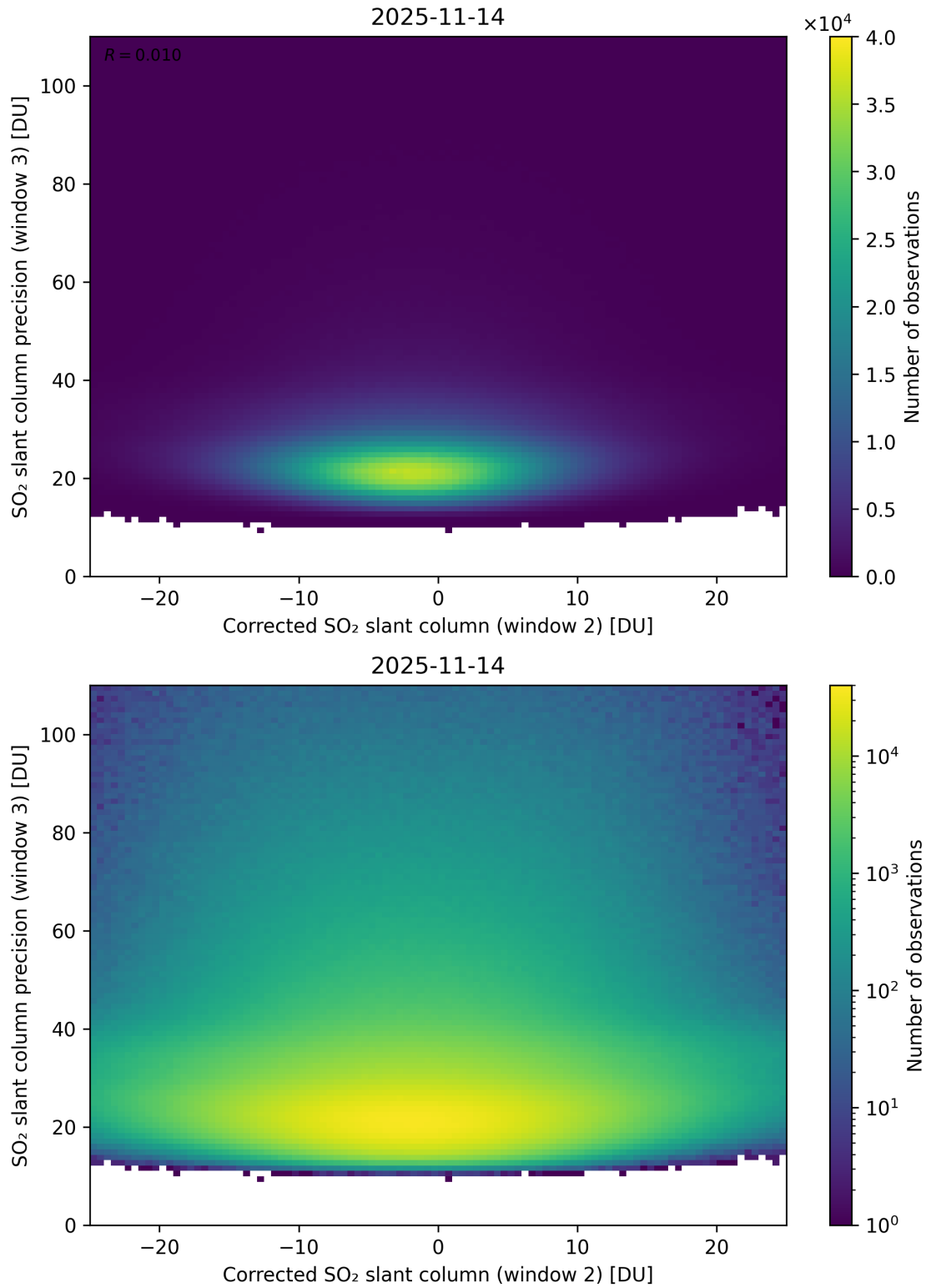
Figure 252: Scatter density plot of “Corrected SO 2 slant column (window 2)” against “SO 2 slant column precision (window 3)” for 2025-11-13 to 2025-11-15.
