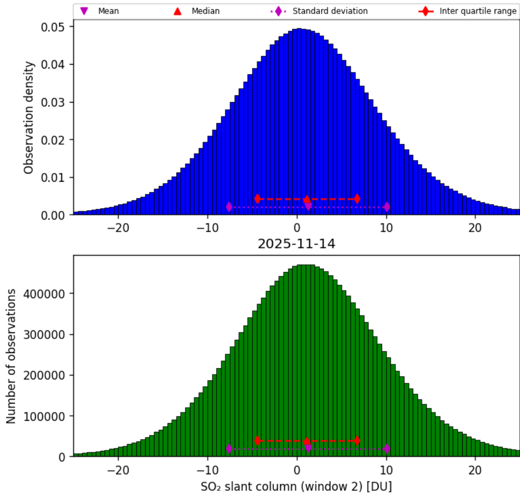
Figure 67: Histogram of “SO 2 slant column (window 2)” for 2025-11-13 to 2025-11-15
