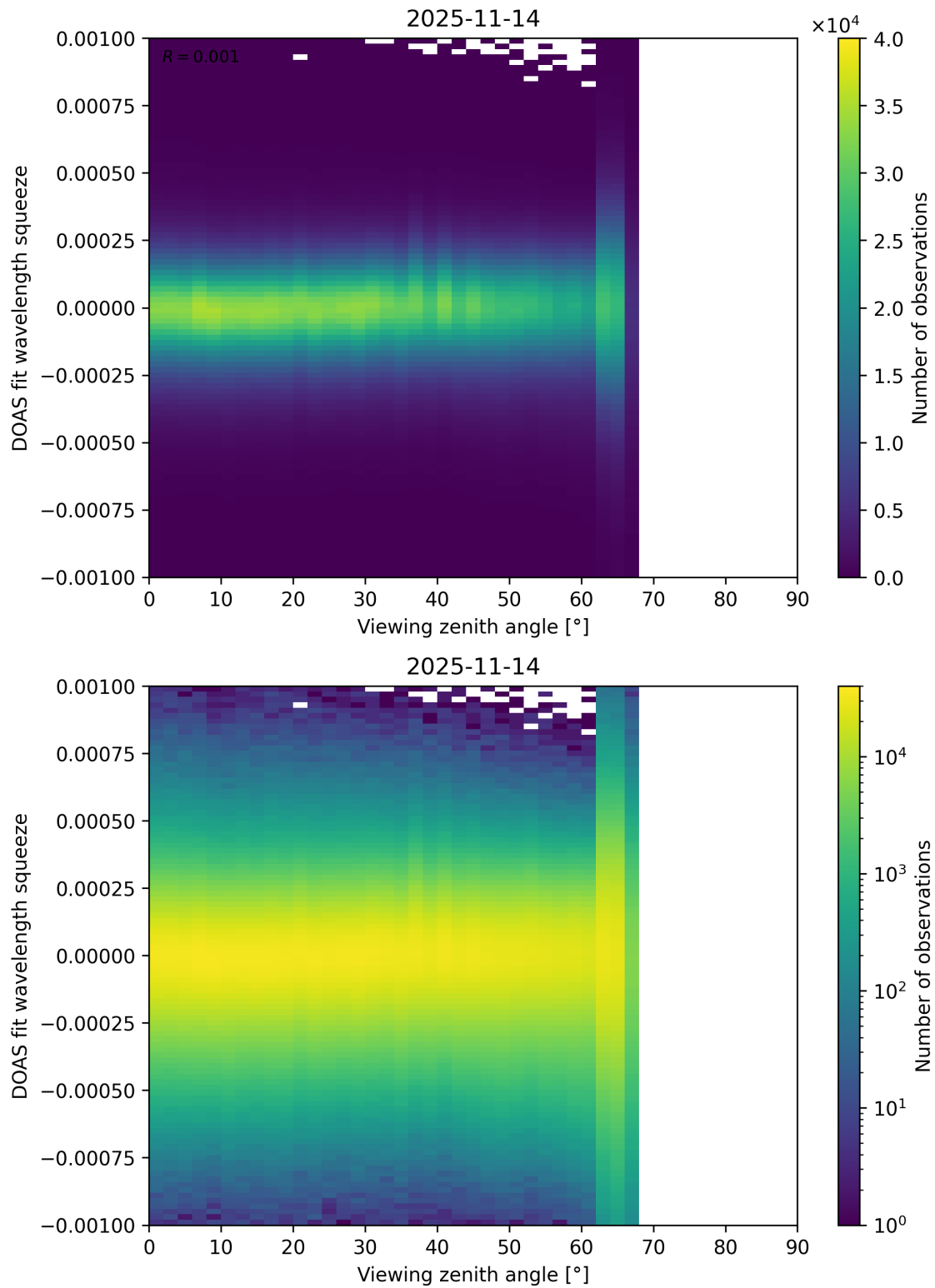
Figure 366: Scatter density plot of “Viewing zenith angle” against “DOAS fit wavelength squeeze” for 2025-11-13 to 2025-11-15.
