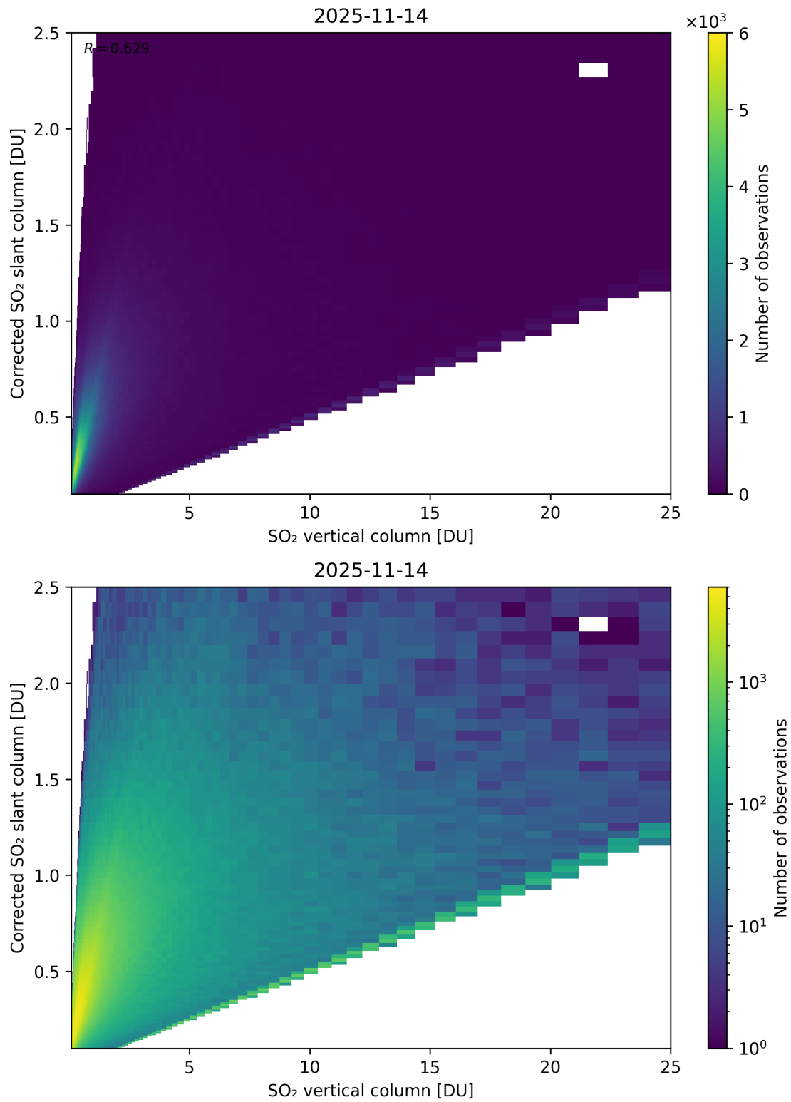
Figure 351: Scatter density plot of “SO 2 vertical column” against “Corrected SO 2 slant column” for 2025-11-13 to 2025-11-15.
