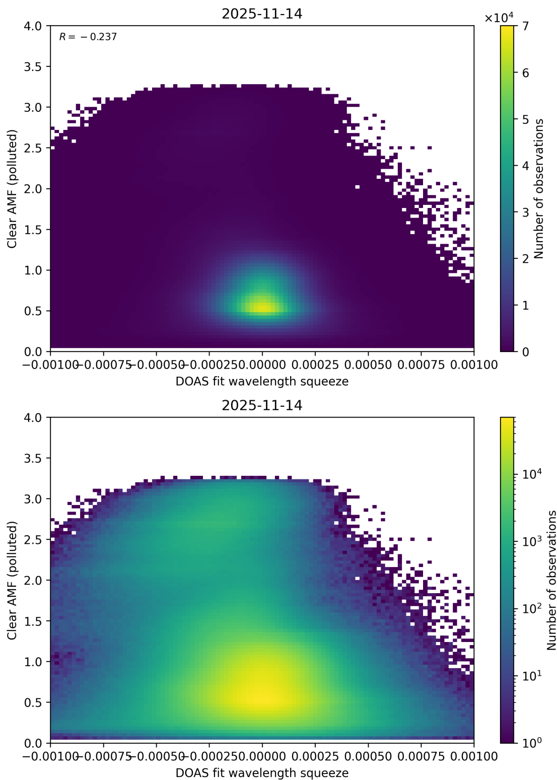
Figure 144: Scatter density plot of “DOAS fit wavelength squeeze” against “Clear AMF (polluted)” for 2025-11-13 to 2025-11-15.
