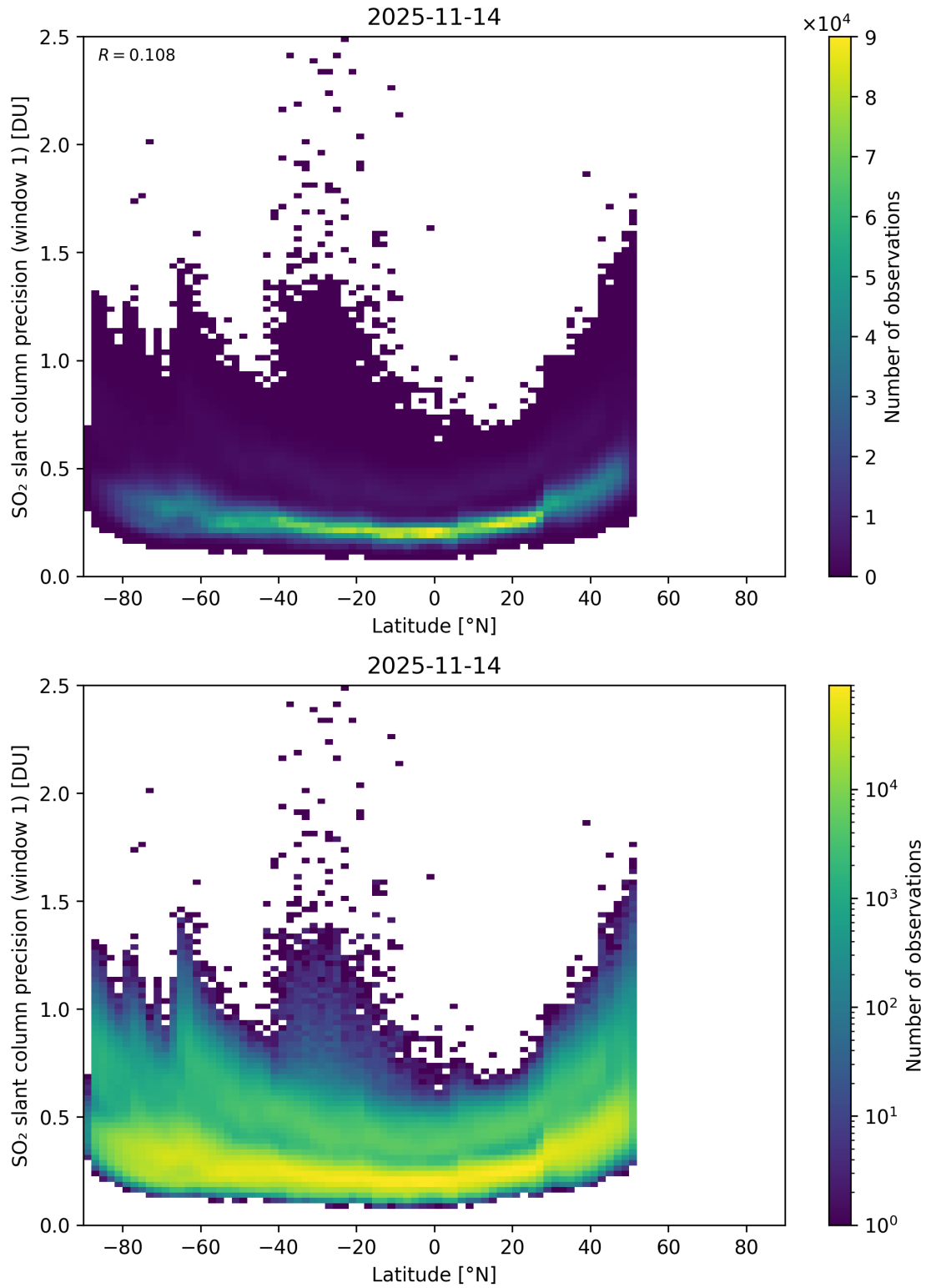
Figure 163: Scatter density plot of “Latitude” against “SO 2 slant column precision (window 1)” for 2025-11-13 to 2025-11-15.
