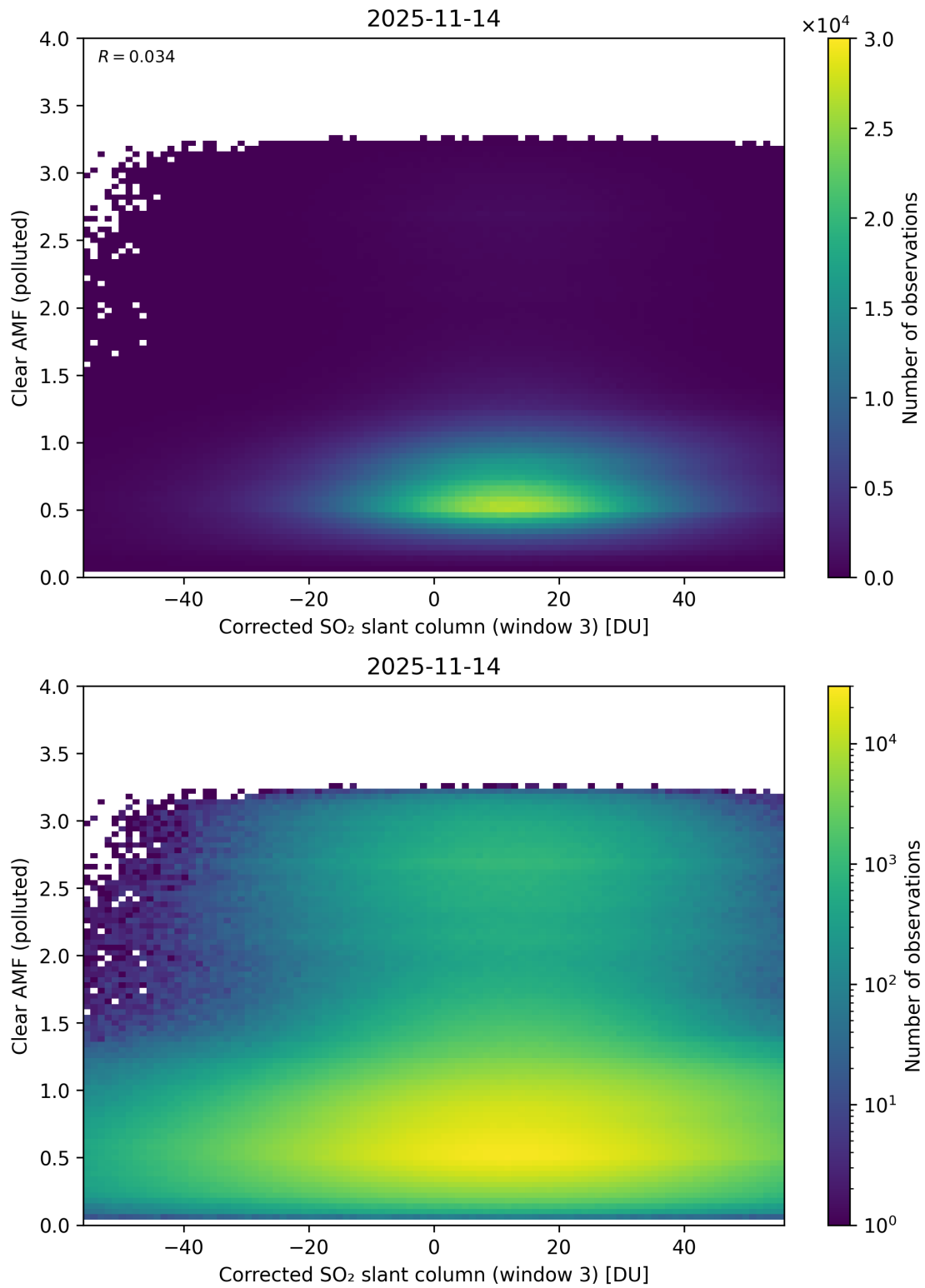
Figure 259: Scatter density plot of “Corrected SO 2 slant column (window 3)” against “Clear AMF (polluted)” for 2025-11-13 to 2025-11-15.
