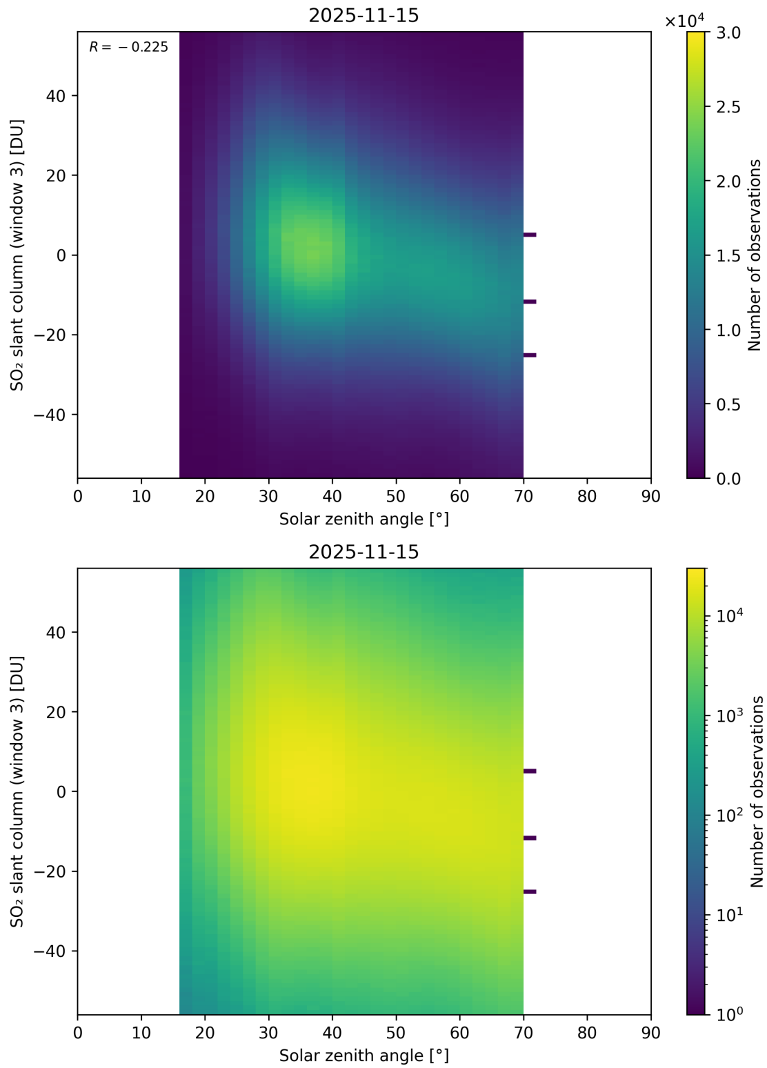
Figure 187: Scatter density plot of “Solar zenith angle” against “SO 2 slant column (window 3)” for 2025-11-14 to 2025-11-16.
