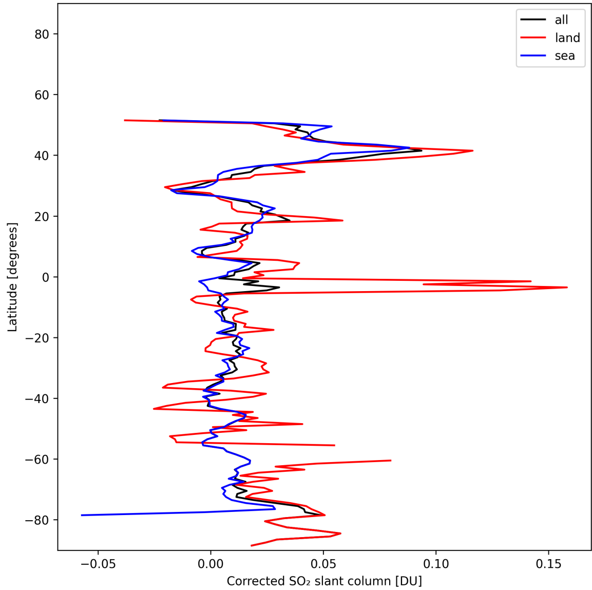
Figure 34: Zonal average of “Corrected SO 2 slant column” for 2025-11-14 to 2025-11-16.
