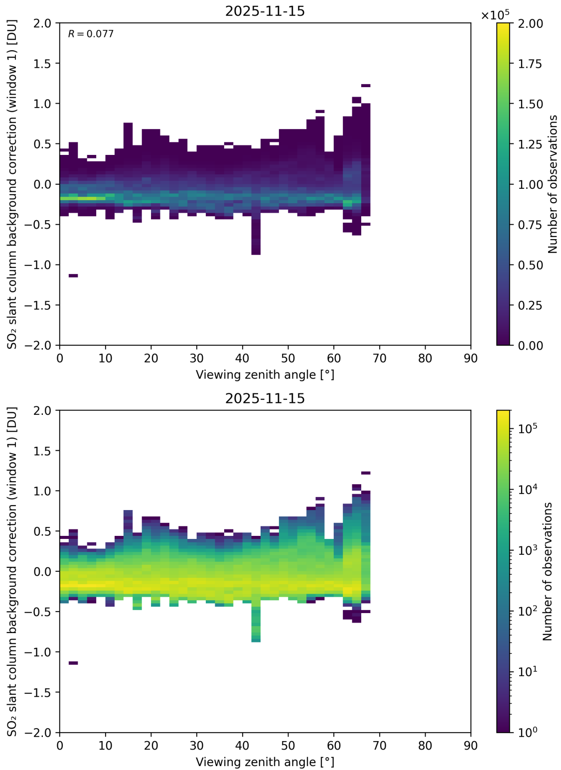
Figure 362: Scatter density plot of “Viewing zenith angle” against “SO 2 slant column background correction (window 1)” for 2025-11-14 to 2025-11-16.
