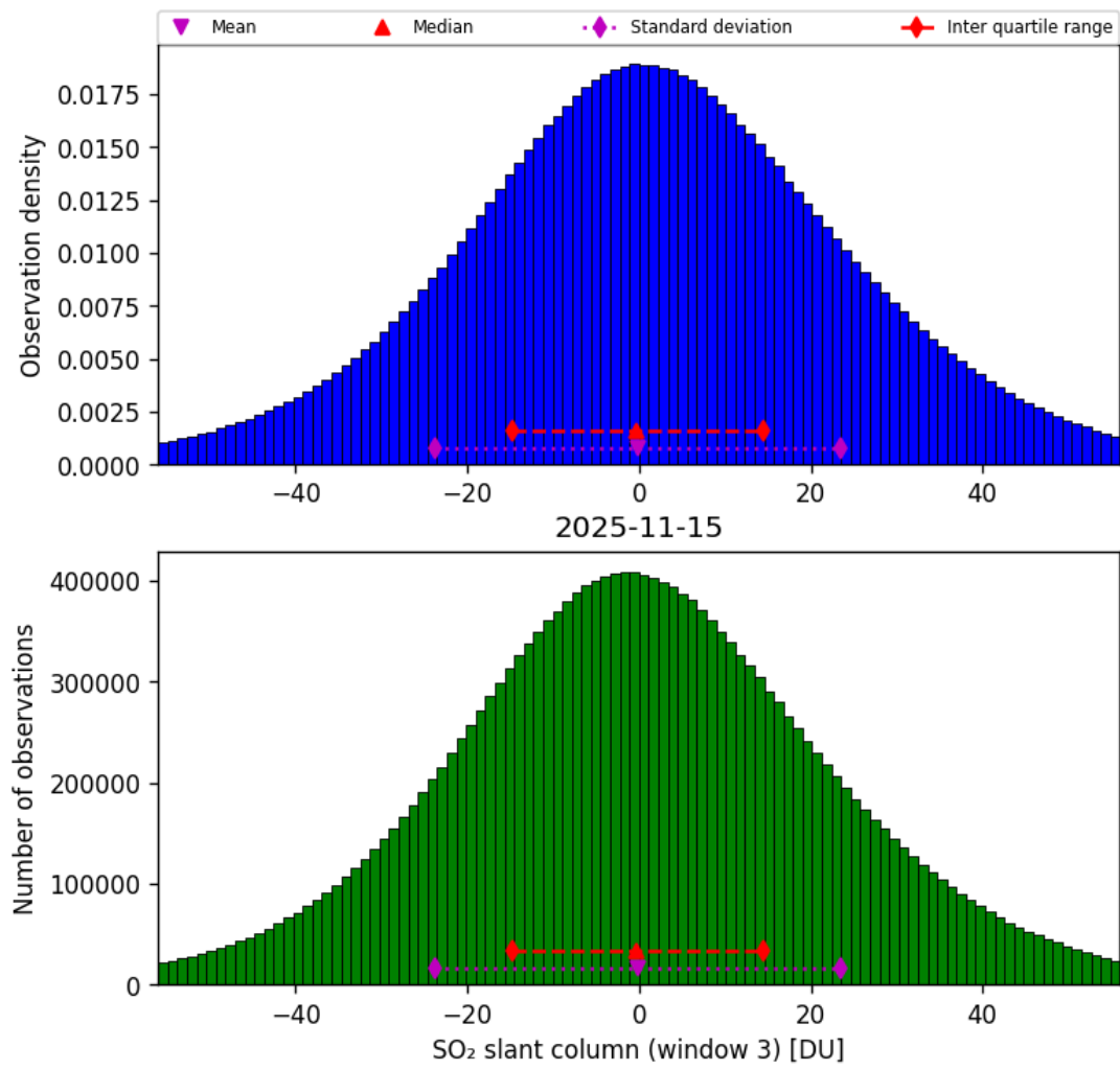
Figure 71: Histogram of “SO 2 slant column (window 3)” for 2025-11-14 to 2025-11-16
