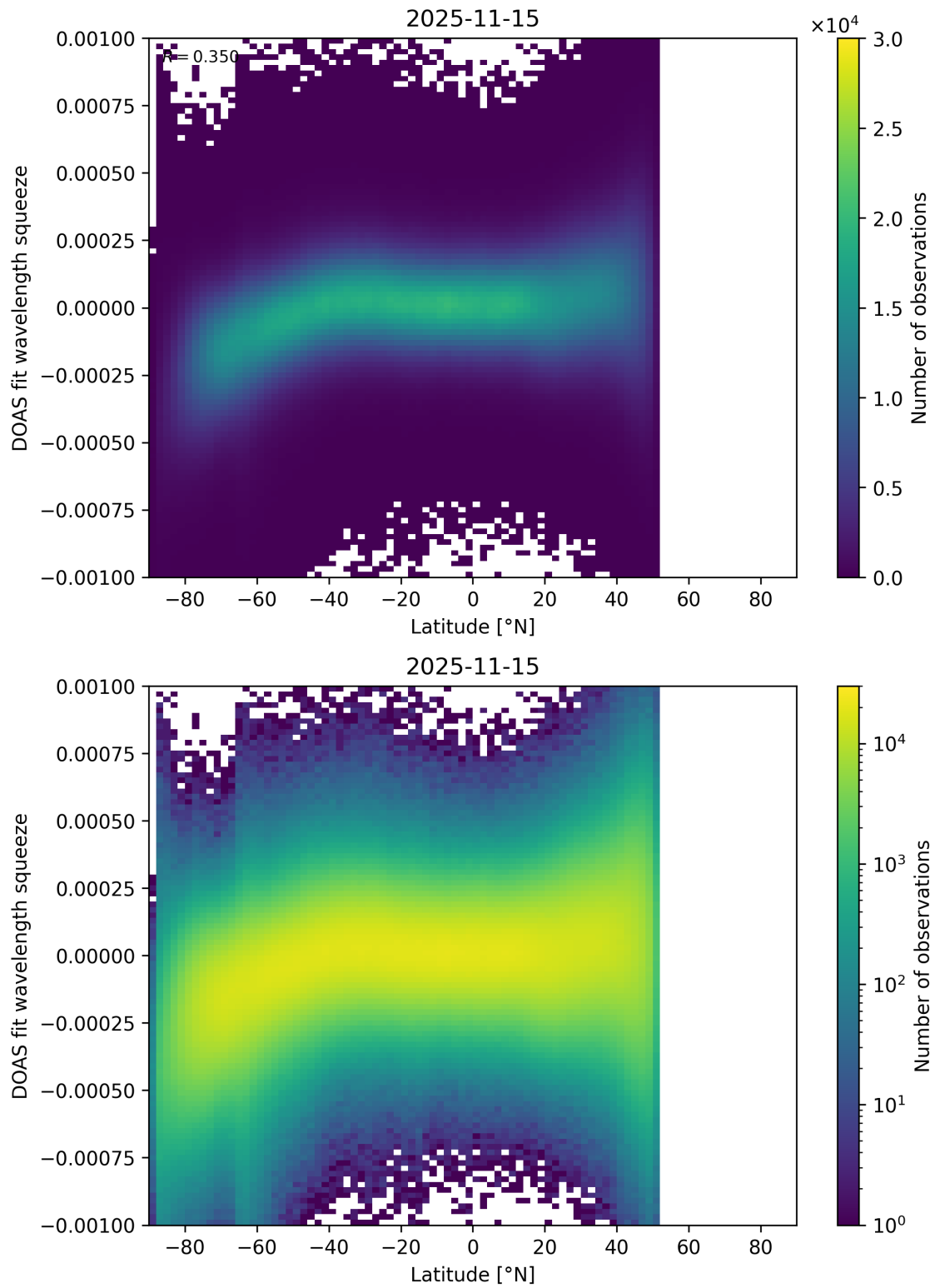
Figure 154: Scatter density plot of "Latitude" against "DOAS fit wavelength squeeze" for 2025-11-14 to 2025-11-16.
