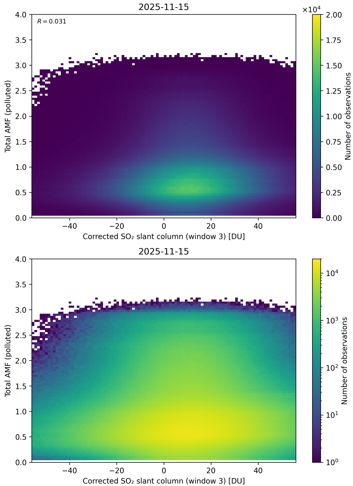
Figure 260: Scatter density plot of “Corrected SO 2 slant column (window 3)” against “Total AMF (polluted)” for 2025-11-14 to 2025-11-16.
