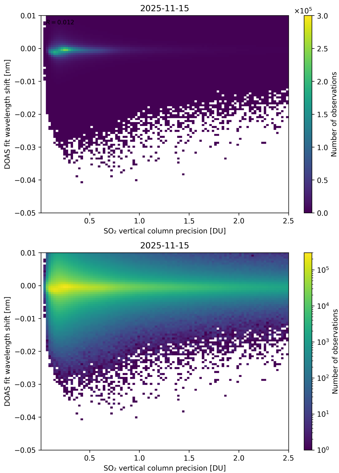
Figure 332: Scatter density plot of “SO 2 vertical column precision” against “DOAS fit wavelength shift” for 2025-11-14 to 2025-11-16.
