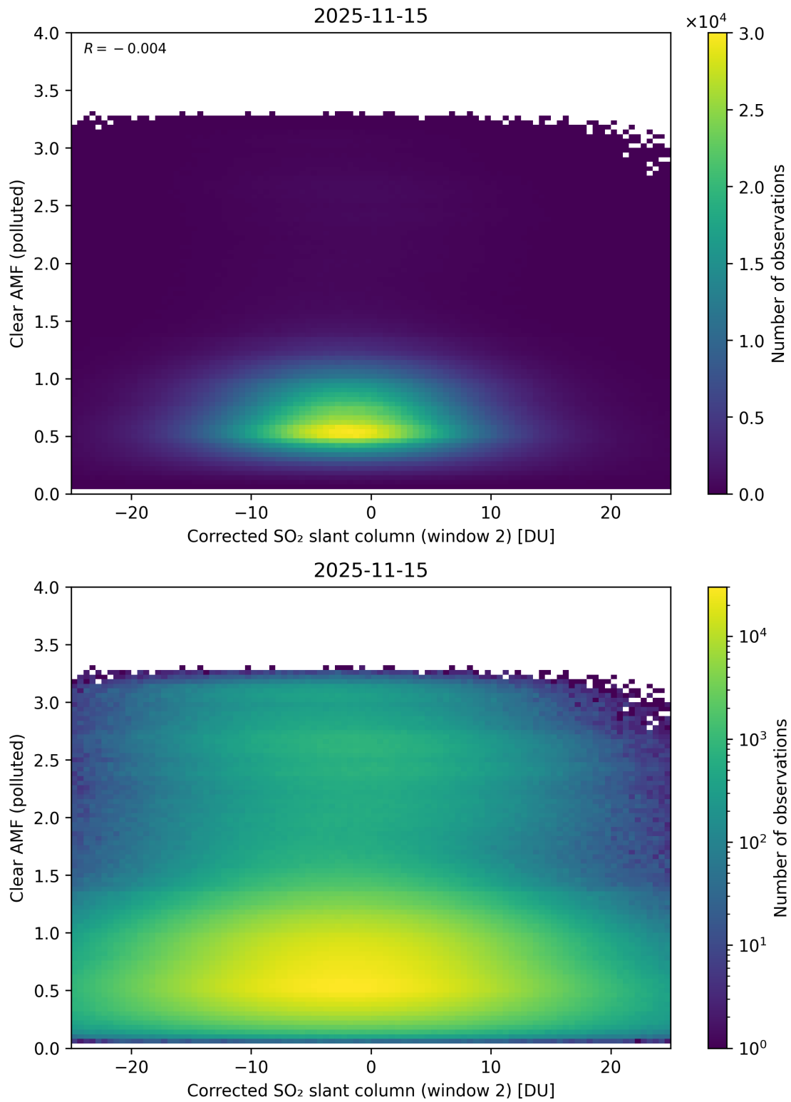
Figure 249: Scatter density plot of “Corrected SO 2 slant column (window 2)” against “Clear AMF (polluted)” for 2025-11-14 to 2025-11-16.
