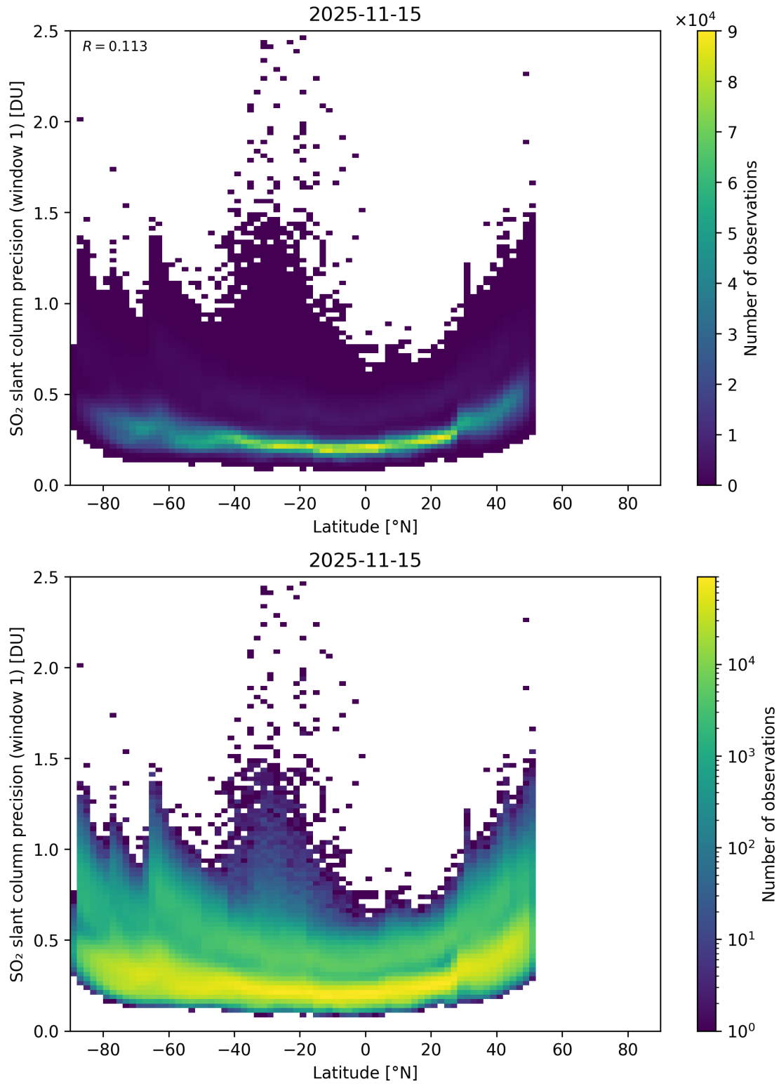
Figure 163: Scatter density plot of “Latitude” against “SO 2 slant column precision (window 1)” for 2025-11-14 to 2025-11-16.
