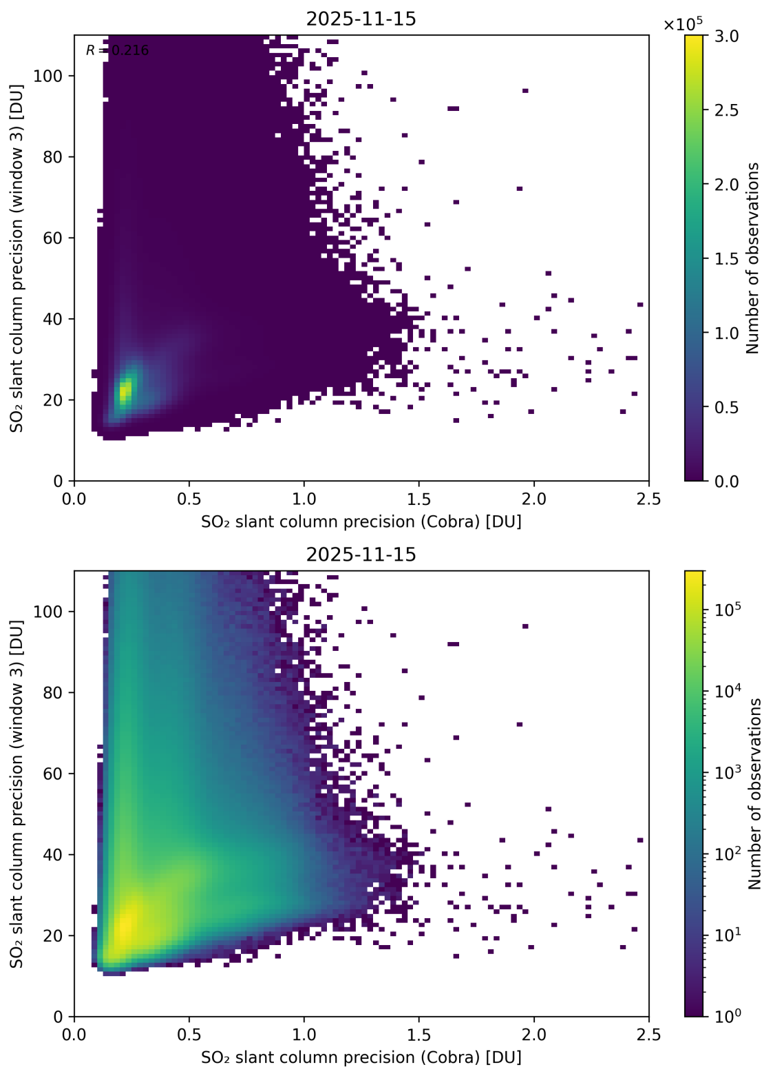
Figure 212: Scatter density plot of “SO 2 slant column precision (Cobra)” against “SO 2 slant column precision (window 3)” for 2025-11-14 to 2025-11-16.
