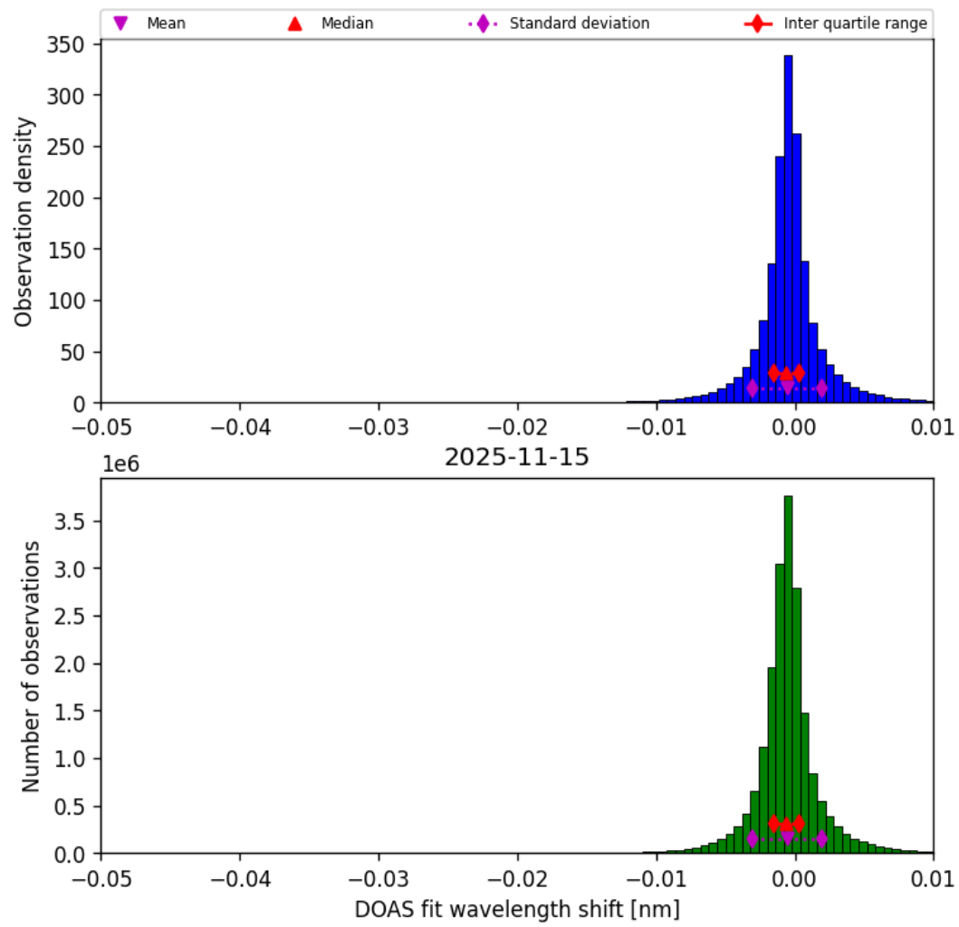
Figure 76: Histogram of “DOAS fit wavelength shift” for 2025-11-14 to 2025-11-16
