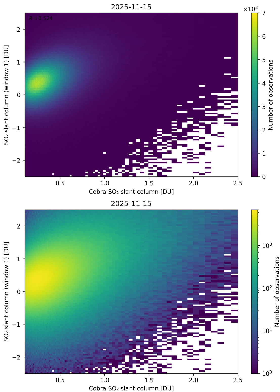
Figure 219: Scatter density plot of “Cobra SO 2 slant column” against “SO 2 slant column (window 1)” for 2025-11-14 to 2025-11-16.
