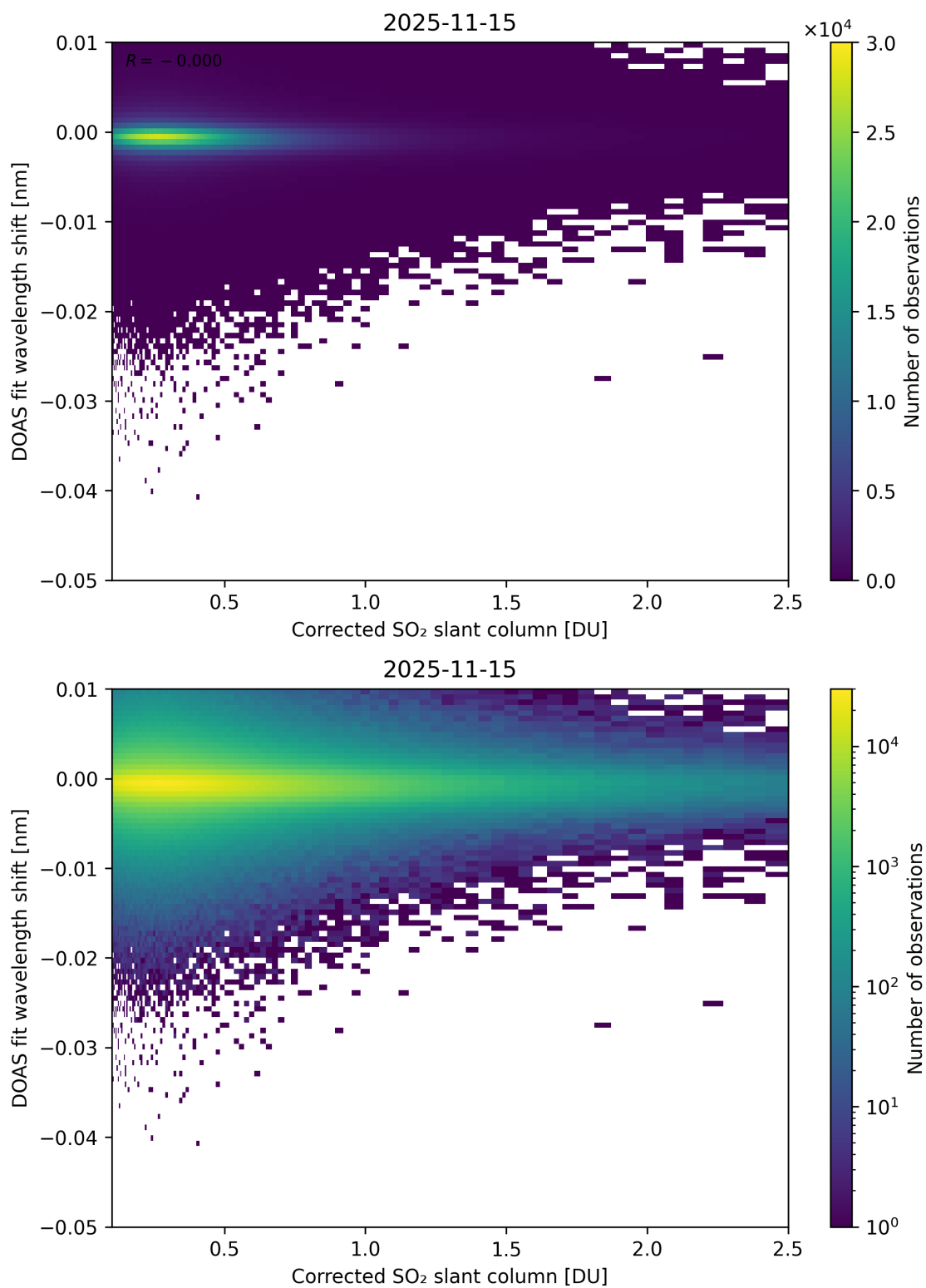
Figure 229: Scatter density plot of “Corrected SO 2 slant column” against “DOAS fit wavelength shift” for 2025-11-14 to 2025-11-16.
