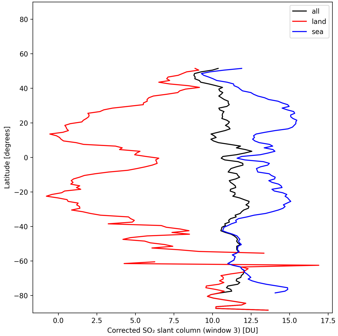
Figure 47: Zonal average of “Corrected SO 2 slant column (window 3)” for 2025-11-14 to 2025-11-16.
