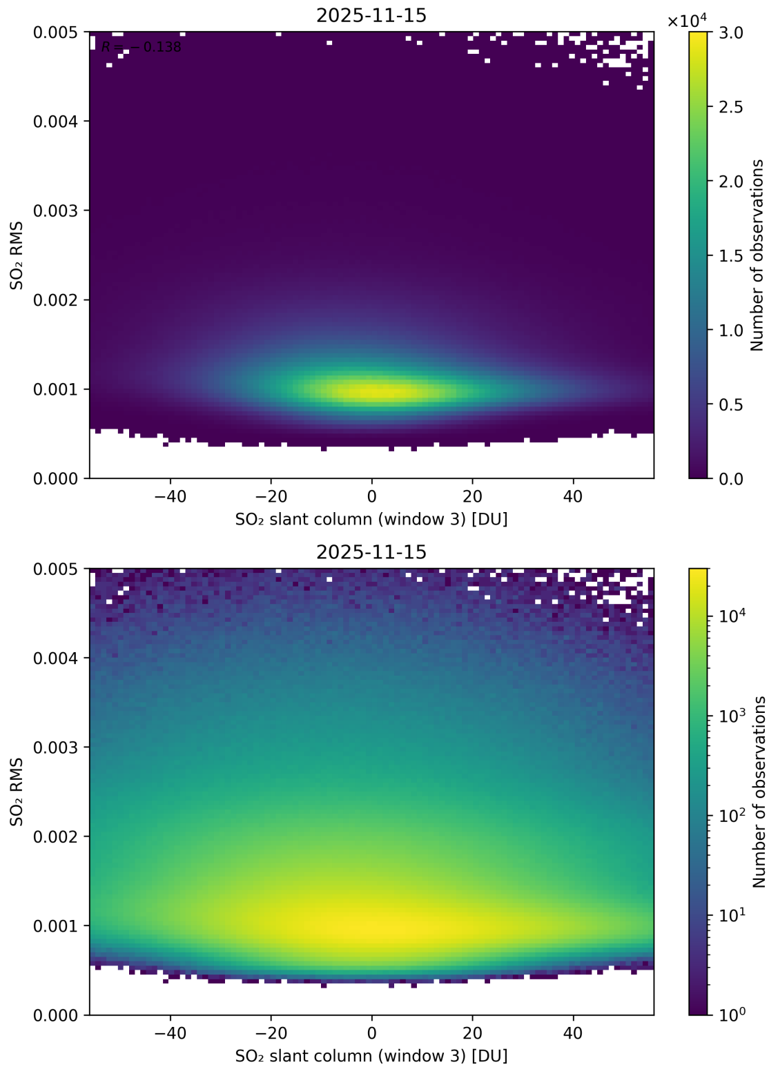
Figure 306: Scatter density plot of “SO 2 slant column (window 3)” against “SO 2 RMS” for 2025-11-14 to 2025-11-16.
