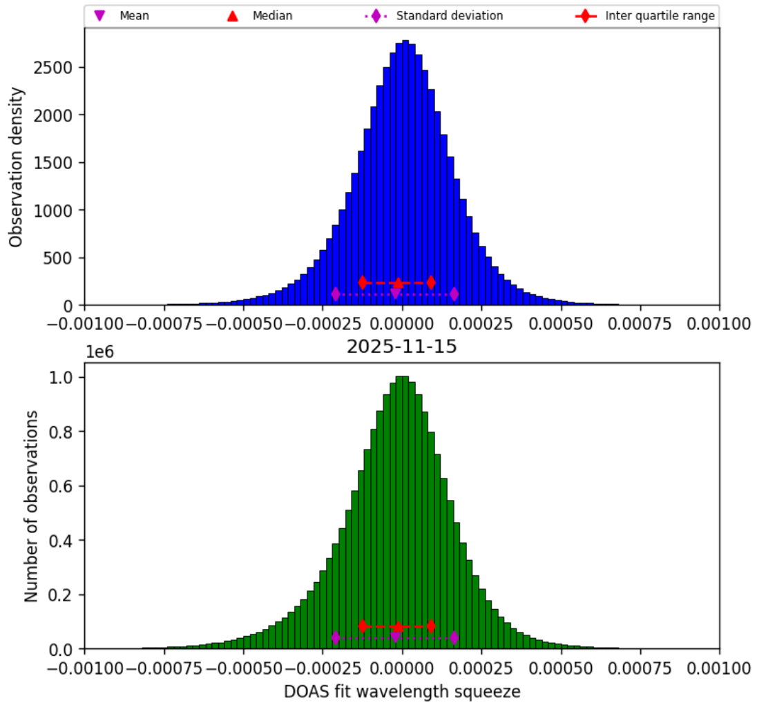
Figure 77: Histogram of “DOAS fit wavelength squeeze” for 2025-11-14 to 2025-11-16
