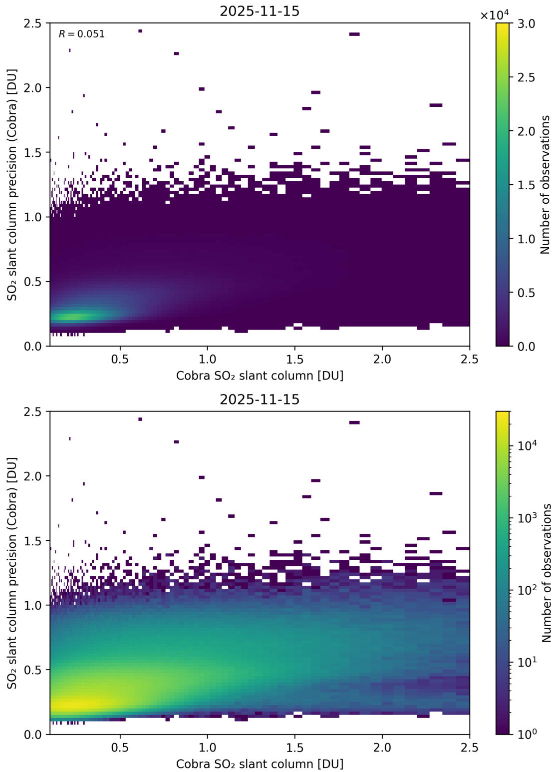
Figure 216: Scatter density plot of “Cobra SO 2 slant column” against “SO 2 slant column precision (Cobra)” for 2025-11-14 to 2025-11-16.
