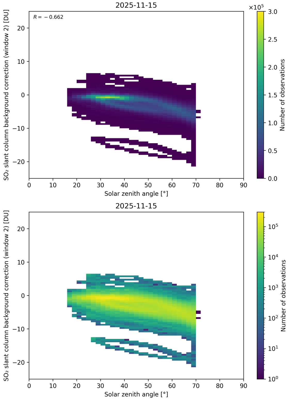
Figure 172: Scatter density plot of “Solar zenith angle” against “SO 2 slant column background correction (window 2)” for 2025-11-14 to 2025-11-16.
