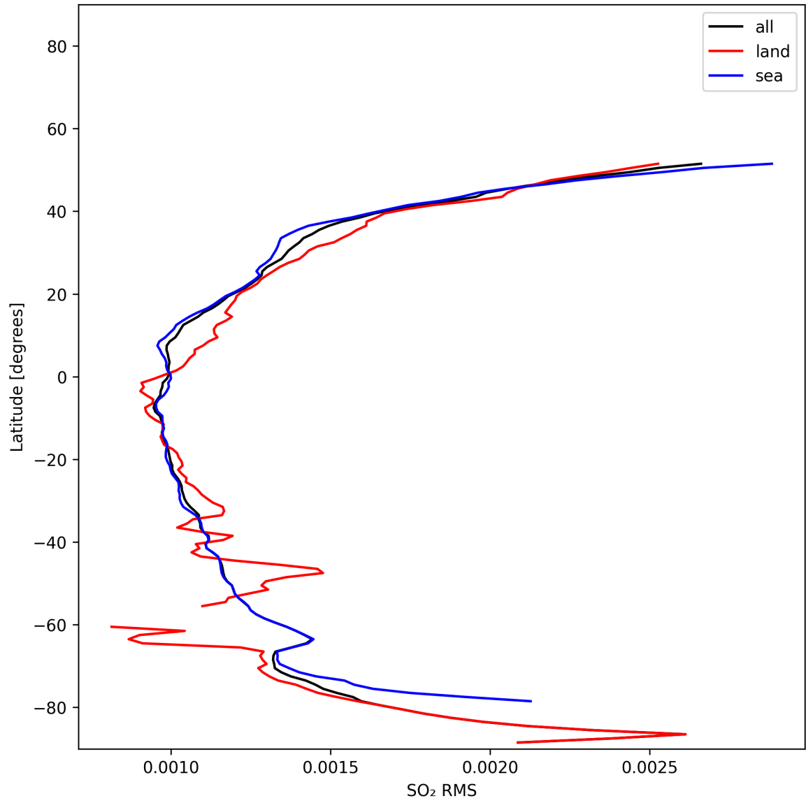
Figure 52: Zonal average of “SO 2 RMS” for 2025-11-14 to 2025-11-16.
