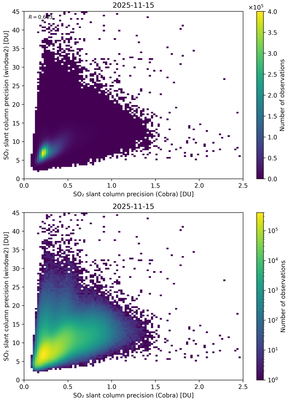
Figure 210: Scatter density plot of “SO 2 slant column precision (Cobra)” against “SO 2 slant column precision (window2)” for 2025-11-14 to 2025-11-16.
