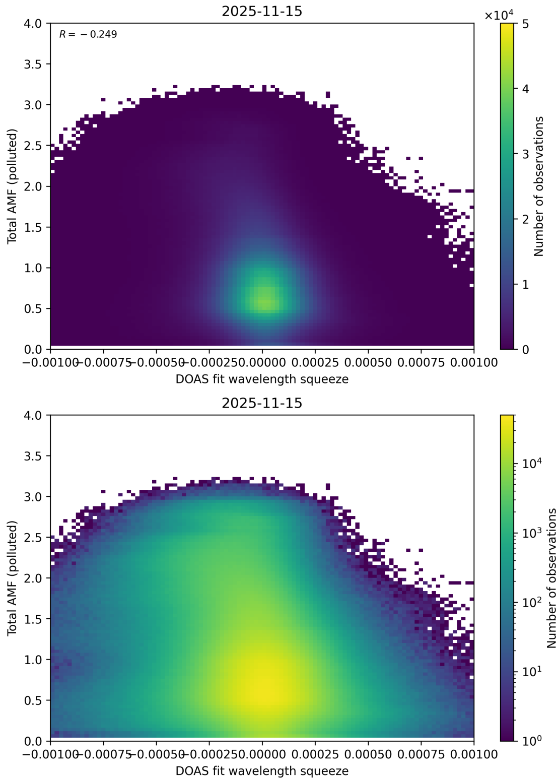
Figure 145: Scatter density plot of “DOAS fit wavelength squeeze” against “Total AMF (polluted)” for 2025-11-14 to 2025-11-16.
