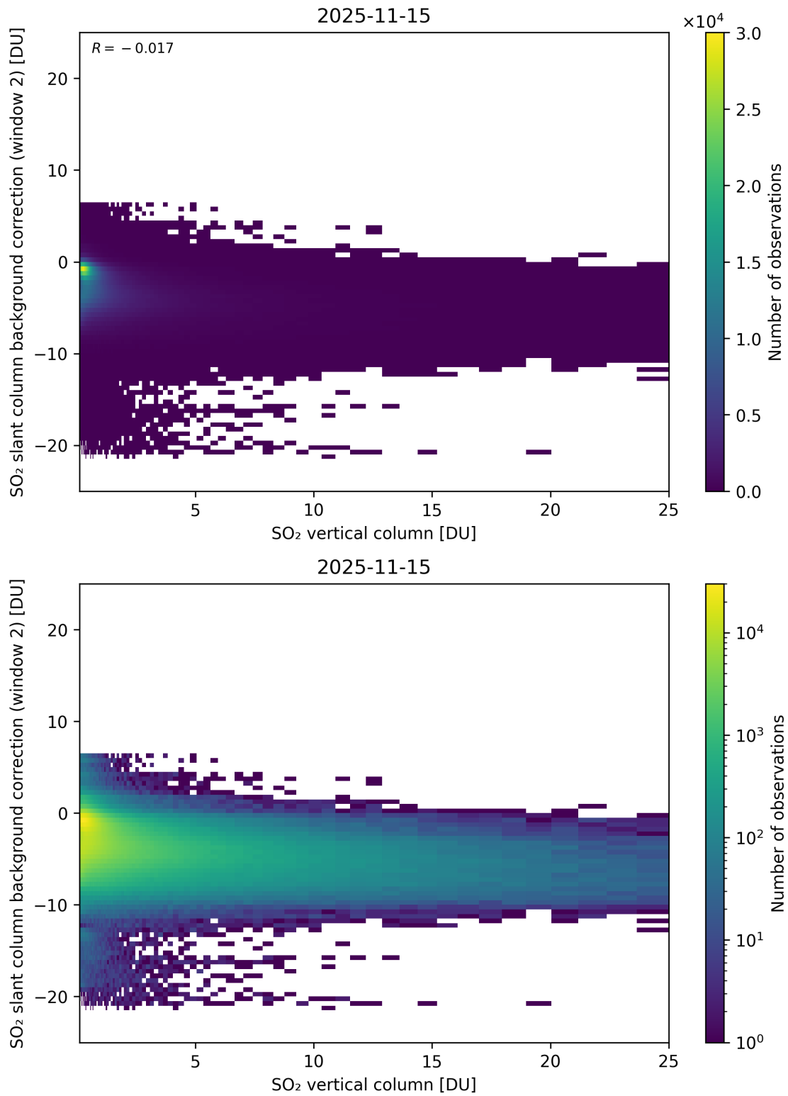
Figure 324: Scatter density plot of “SO 2 vertical column” against “SO 2 slant column background correction (window 2)” for 2025-11-14 to 2025-11-16.
