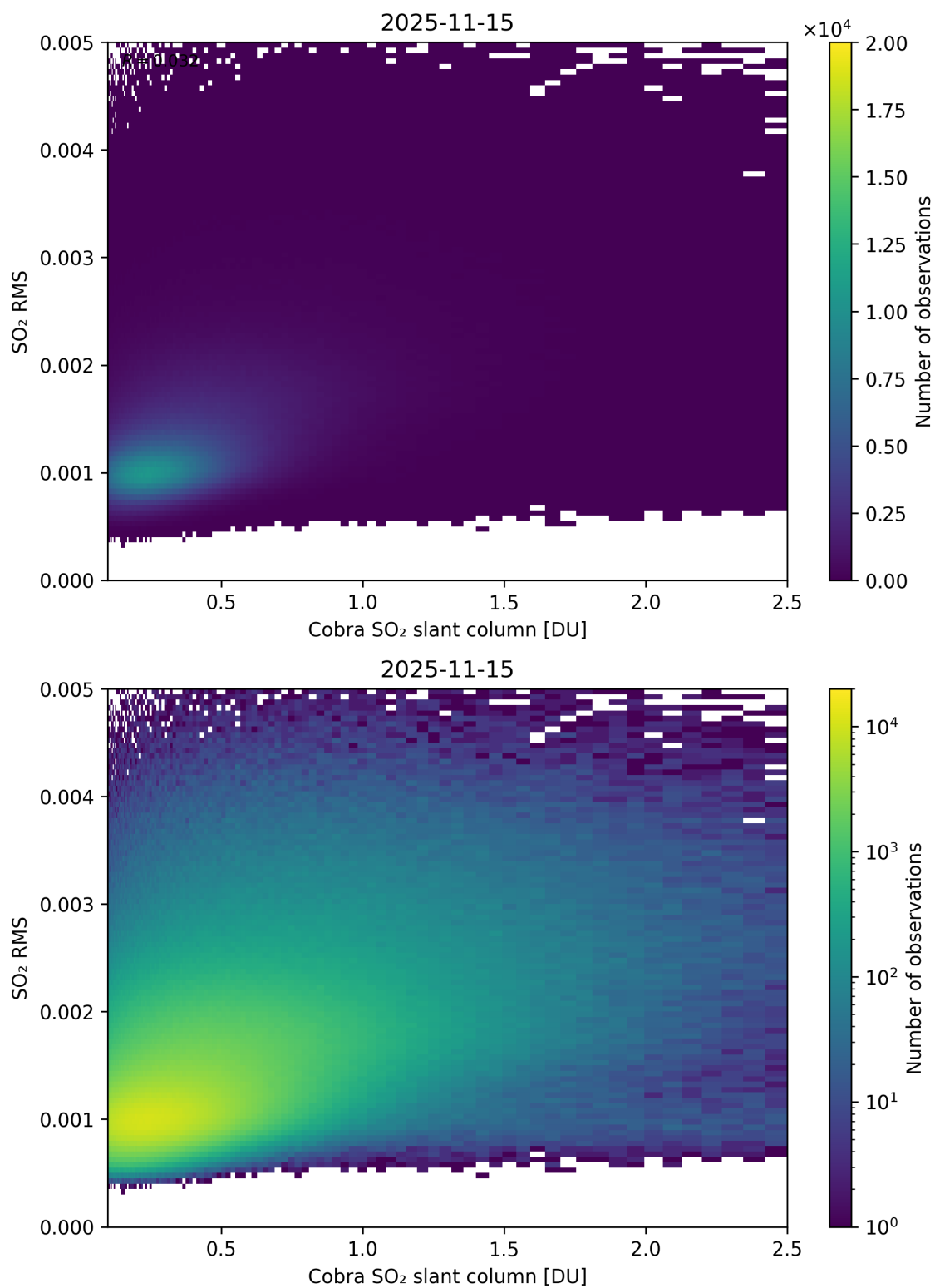
Figure 198: Scatter density plot of “Cobra SO 2 slant column” against “SO 2 RMS” for 2025-11-14 to 2025-11-16.
