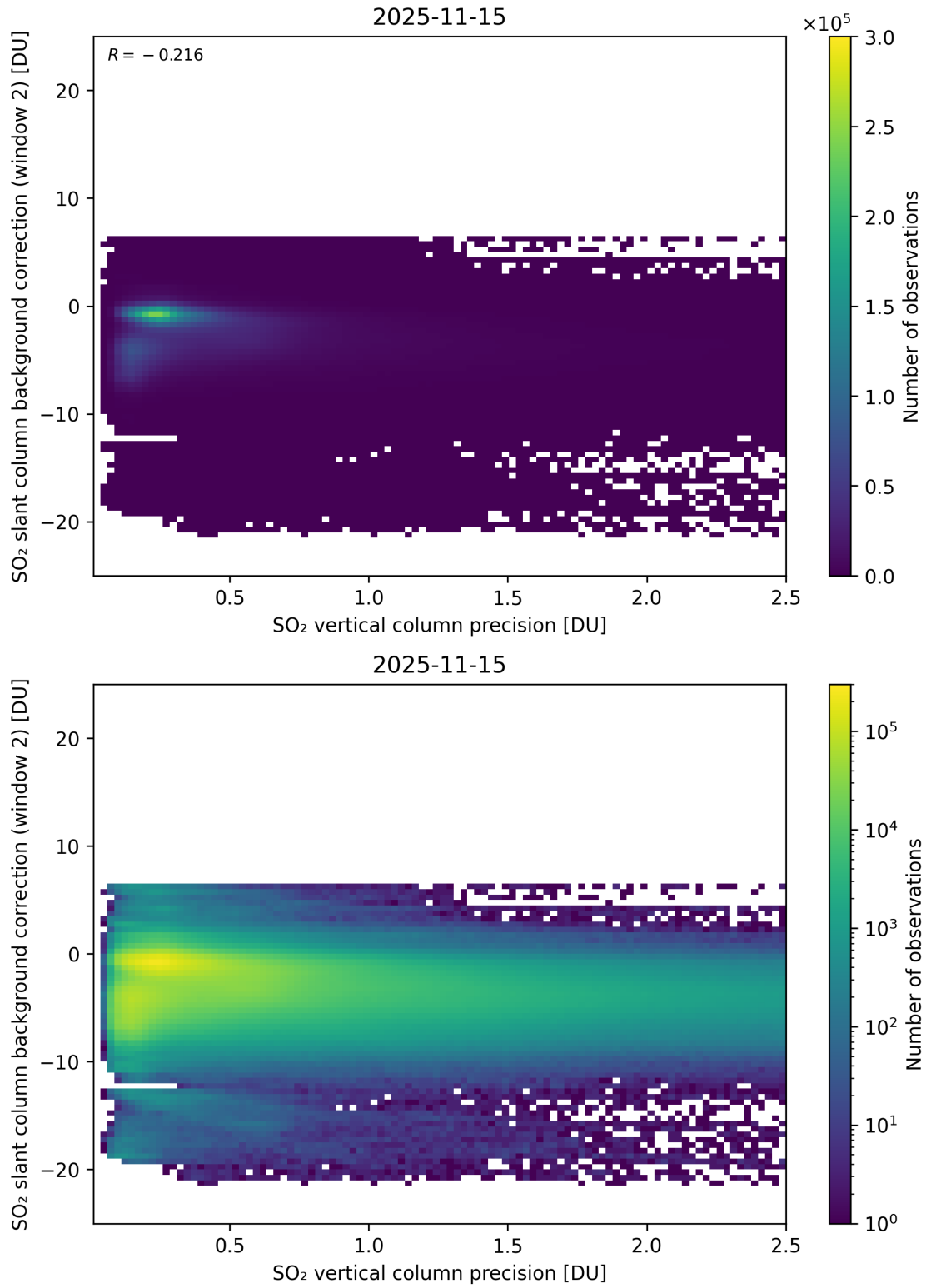
Figure 330: Scatter density plot of “SO 2 vertical column precision” against “SO 2 slant column background correction (window 2)” for 2025-11-14 to 2025-11-16.
