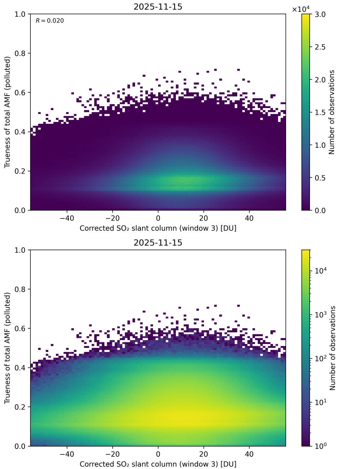
Figure 261: Scatter density plot of “Corrected SO 2 slant column (window 3)” against “Trueness of total AMF (polluted)” for 2025-11-14 to 2025-11-16.
