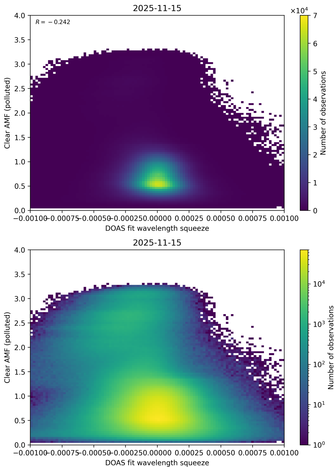
Figure 144: Scatter density plot of “DOAS fit wavelength squeeze” against “Clear AMF (polluted)” for 2025-11-14 to 2025-11-16.
