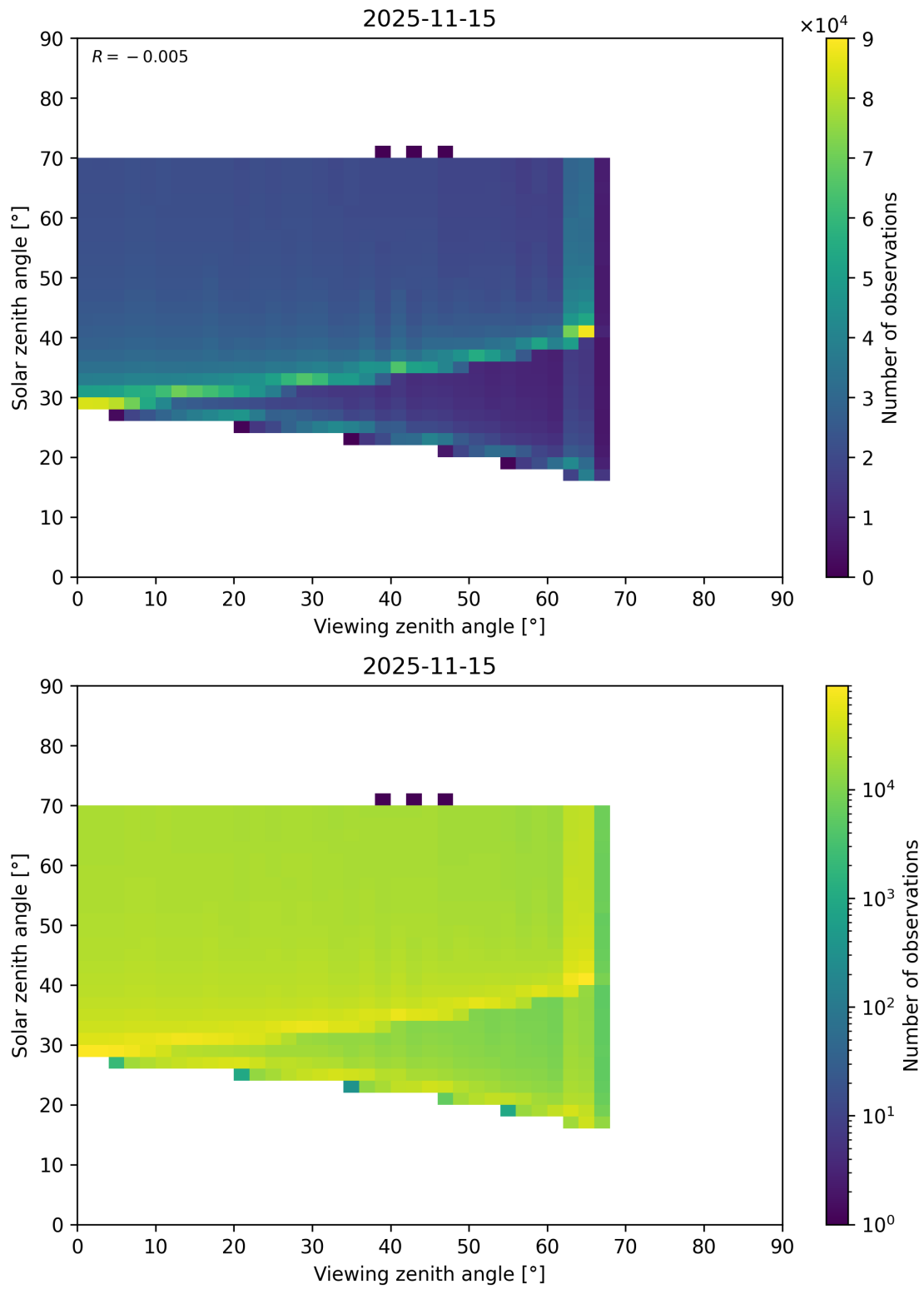
Figure 369: Scatter density plot of “Viewing zenith angle” against “Solar zenith angle” for 2025-11-14 to 2025-11-16.
