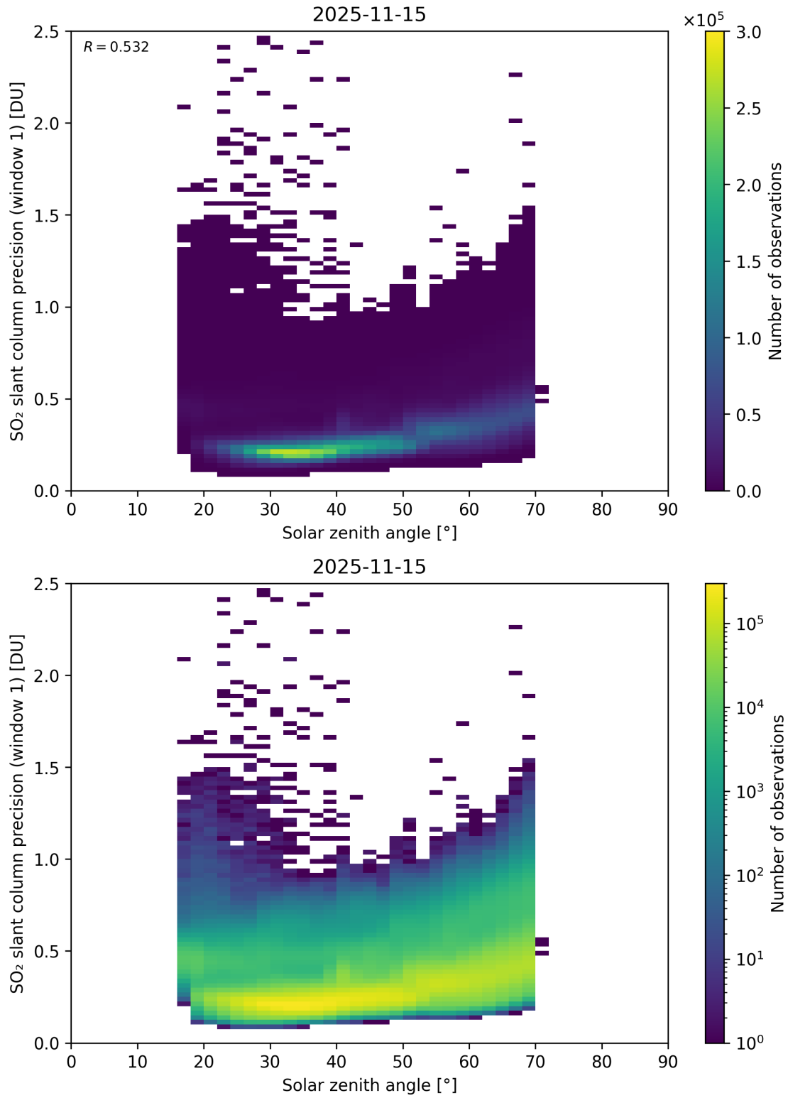
Figure 185: Scatter density plot of “Solar zenith angle” against “SO 2 slant column precision (window 1)” for 2025-11-14 to 2025-11-16.
