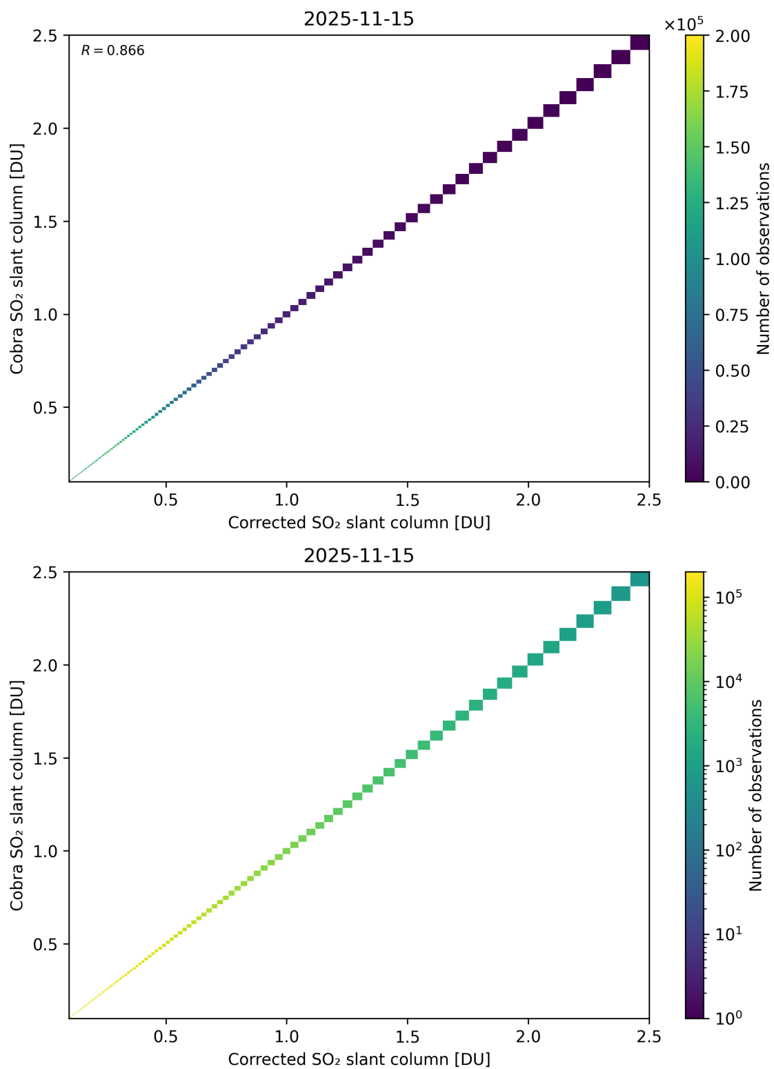
Figure 233: Scatter density plot of “Corrected SO 2 slant column” against “Cobra SO 2 slant column” for 2025-11-14 to 2025-11-16.
