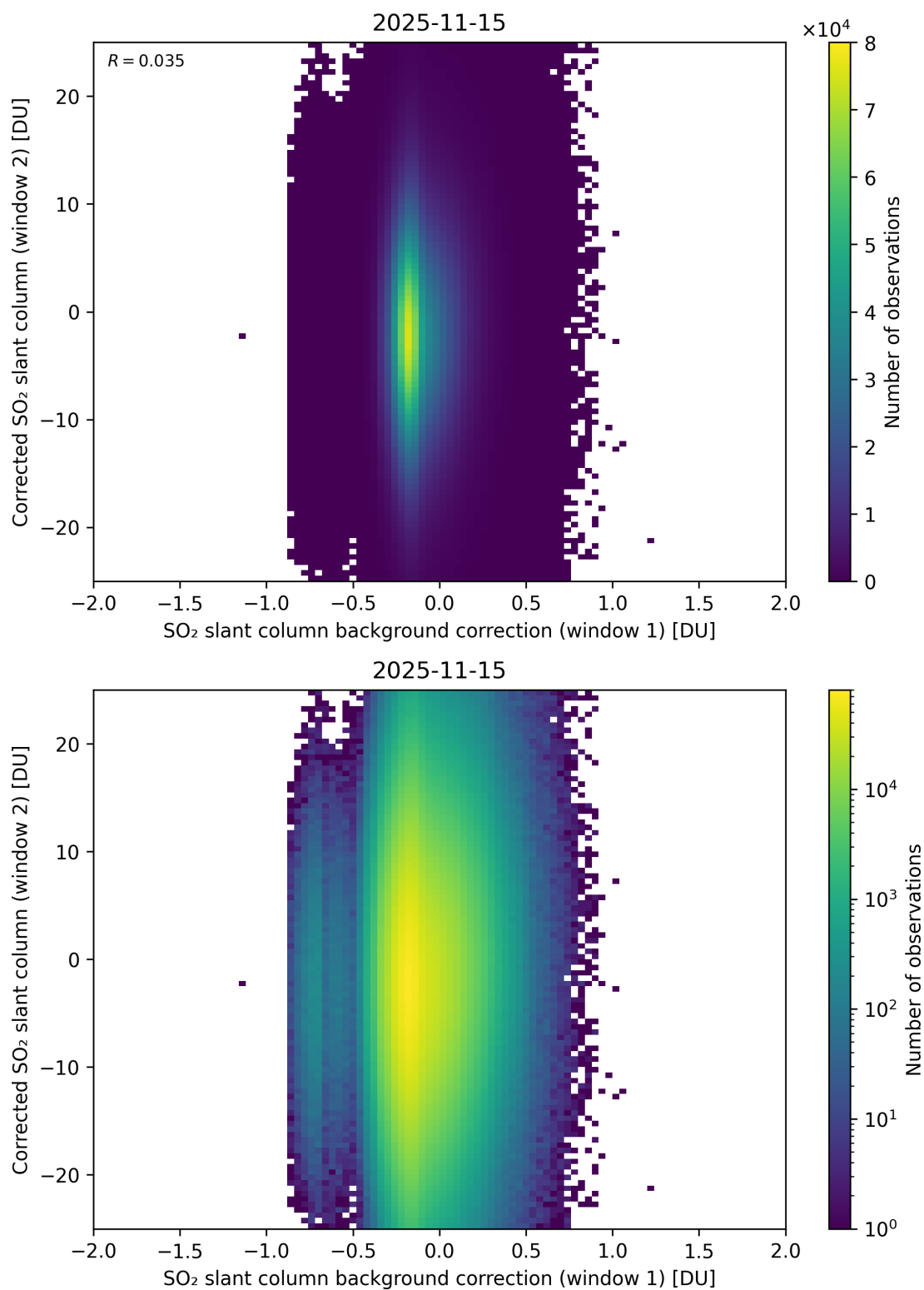
Figure 115: Scatter density plot of “SO 2 slant column background correction (window 1)” against “Corrected SO 2 slant column (window 2)” for 2025-11-14 to 2025-11-16.
