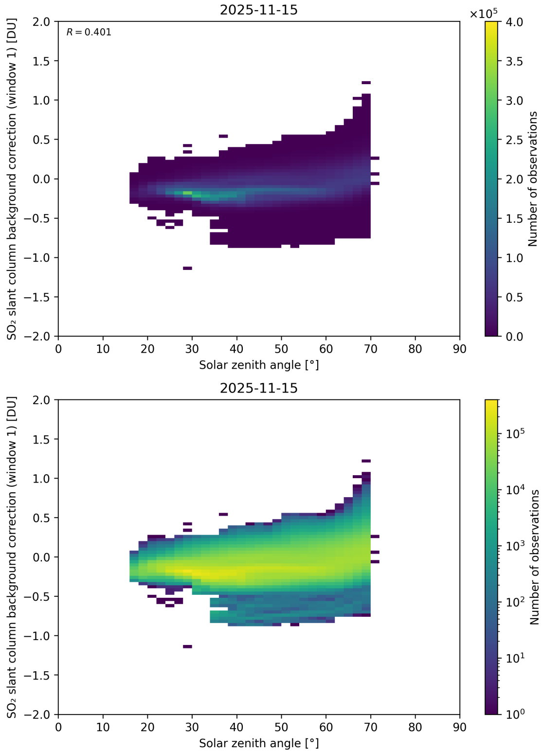
Figure 171: Scatter density plot of “Solar zenith angle” against “SO 2 slant column background correction (window 1)” for 2025-11-14 to 2025-11-16.
