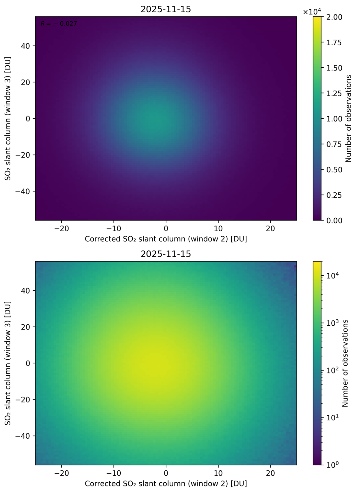
Figure 251: Scatter density plot of “Corrected SO 2 slant column (window 2)” against “SO 2 slant column (window 3)” for 2025-11-14 to 2025-11-16.
