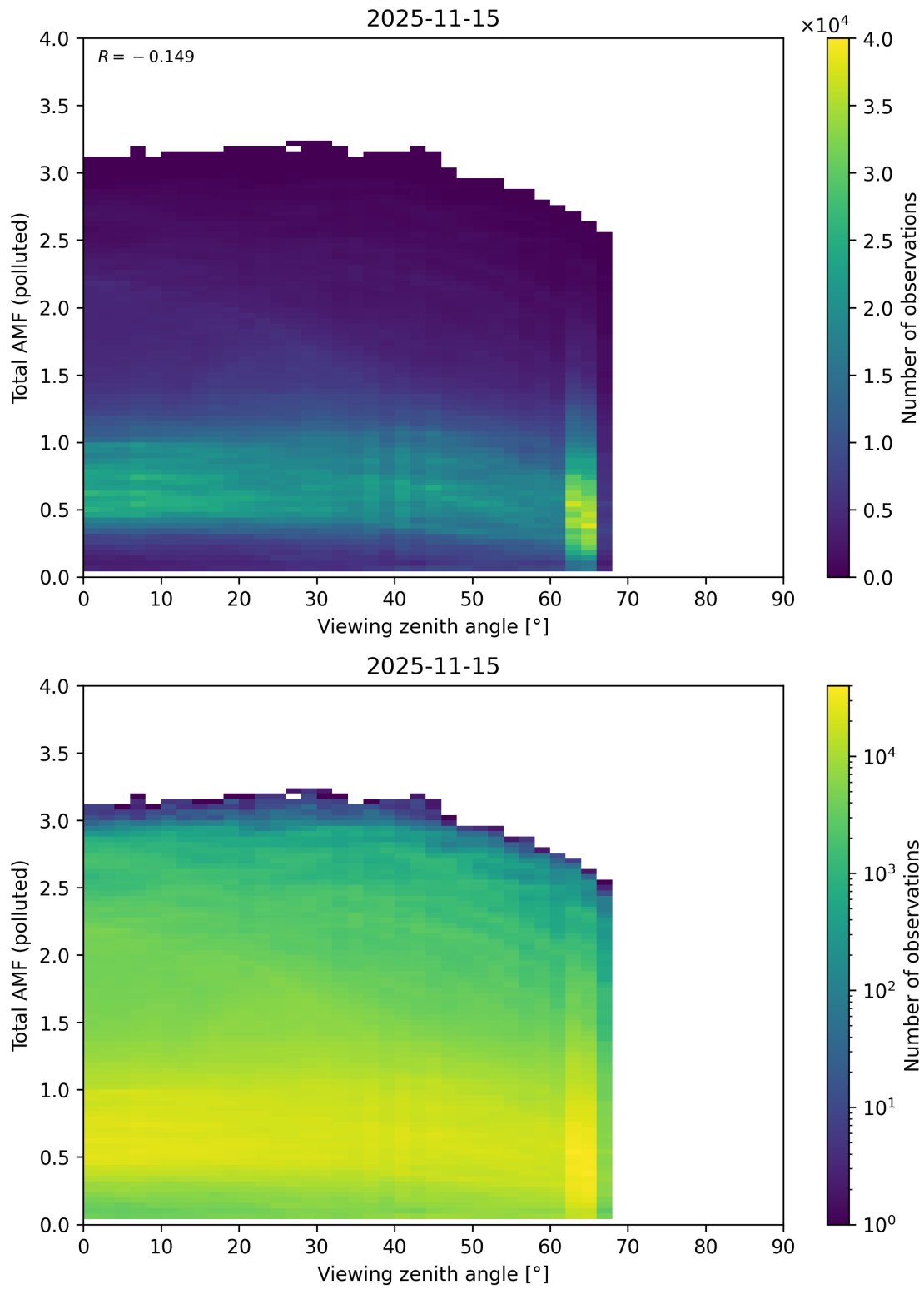
Figure 381: Scatter density plot of “Viewing zenith angle” against “Total AMF (polluted)” for 2025-11-14 to 2025-11-16.
