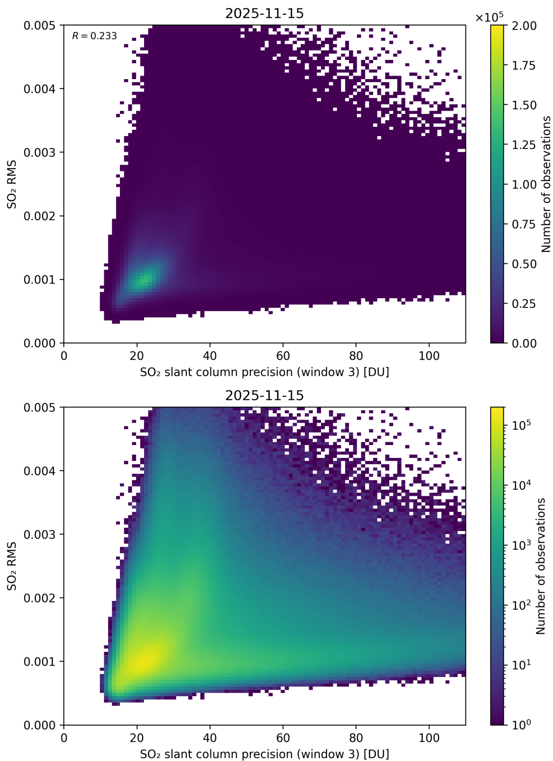
Figure 310: Scatter density plot of “SO 2 slant column precision (window 3)” against “SO 2 RMS” for 2025-11-14 to 2025-11-16.
