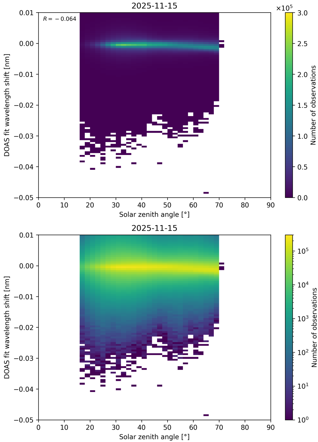
Figure 174: Scatter density plot of “Solar zenith angle” against “DOAS fit wavelength shift” for 2025-11-14 to 2025-11-16.
