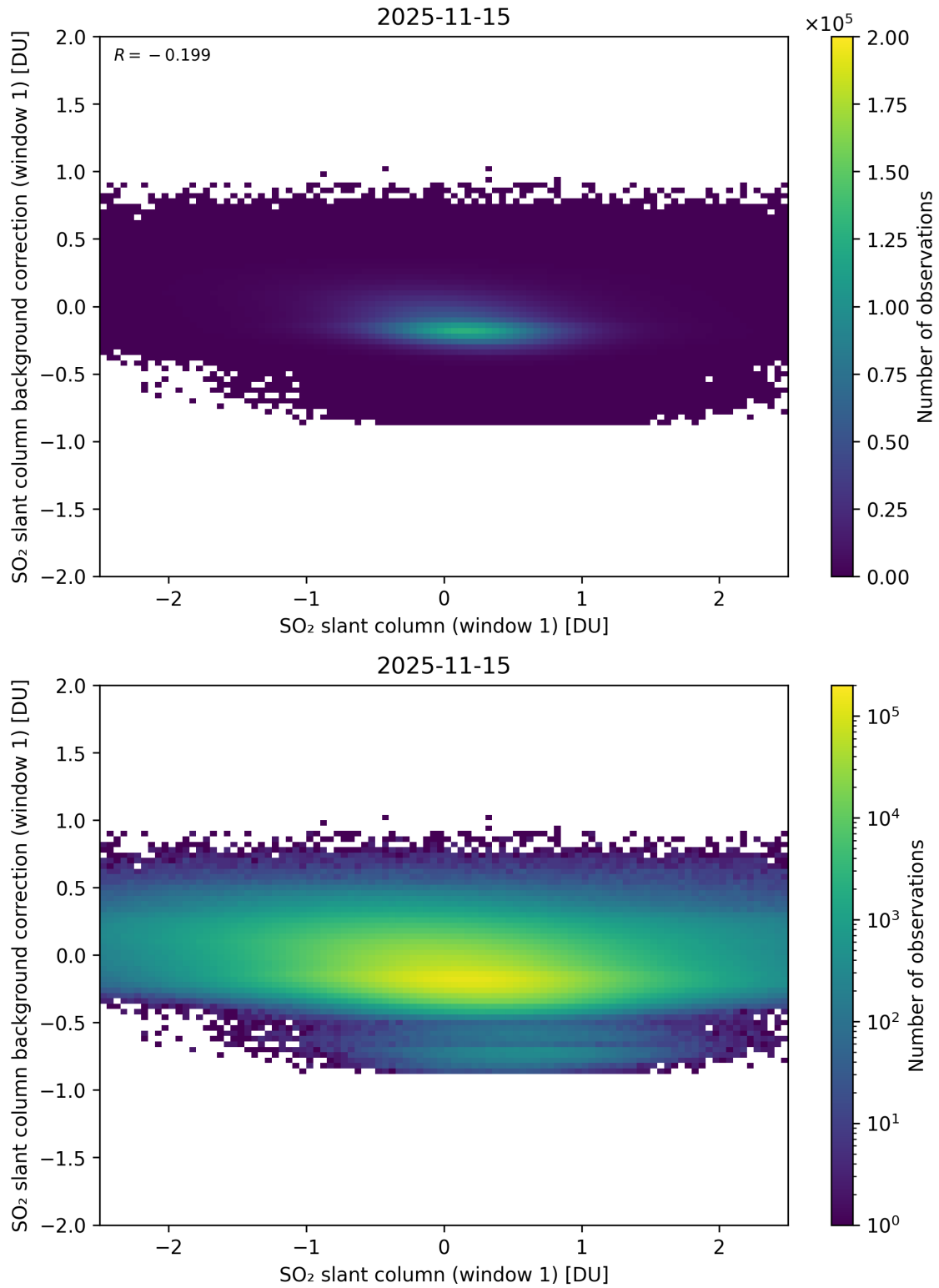
Figure 262: Scatter density plot of “SO 2 slant column (window 1)” against “SO 2 slant column background correction (window 1)” for 2025-11-14 to 2025-11-16.
