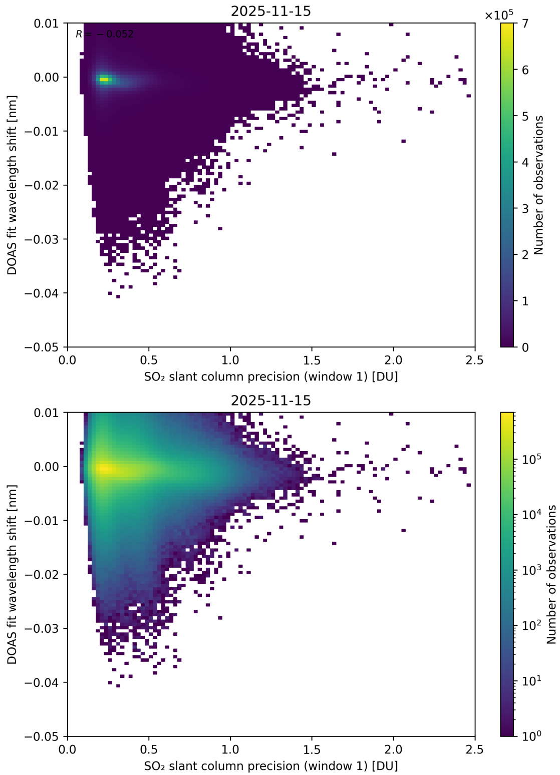
Figure 271: Scatter density plot of “SO 2 slant column precision (window 1)” against “DOAS fit wavelength shift” for 2025-11-14 to 2025-11-16.
