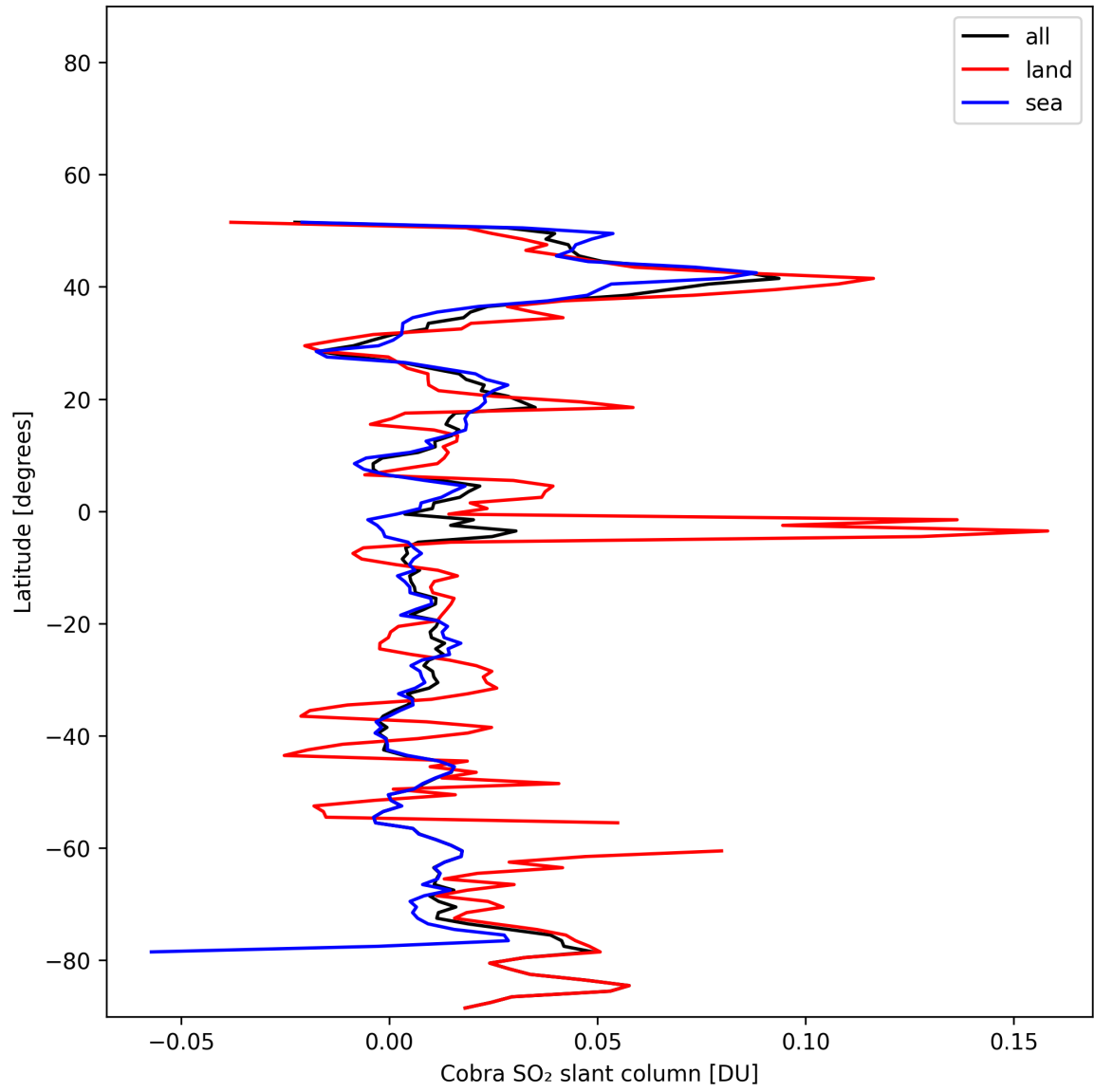
Figure 35: Zonal average of “Cobra SO 2 slant column” for 2025-11-14 to 2025-11-16.
