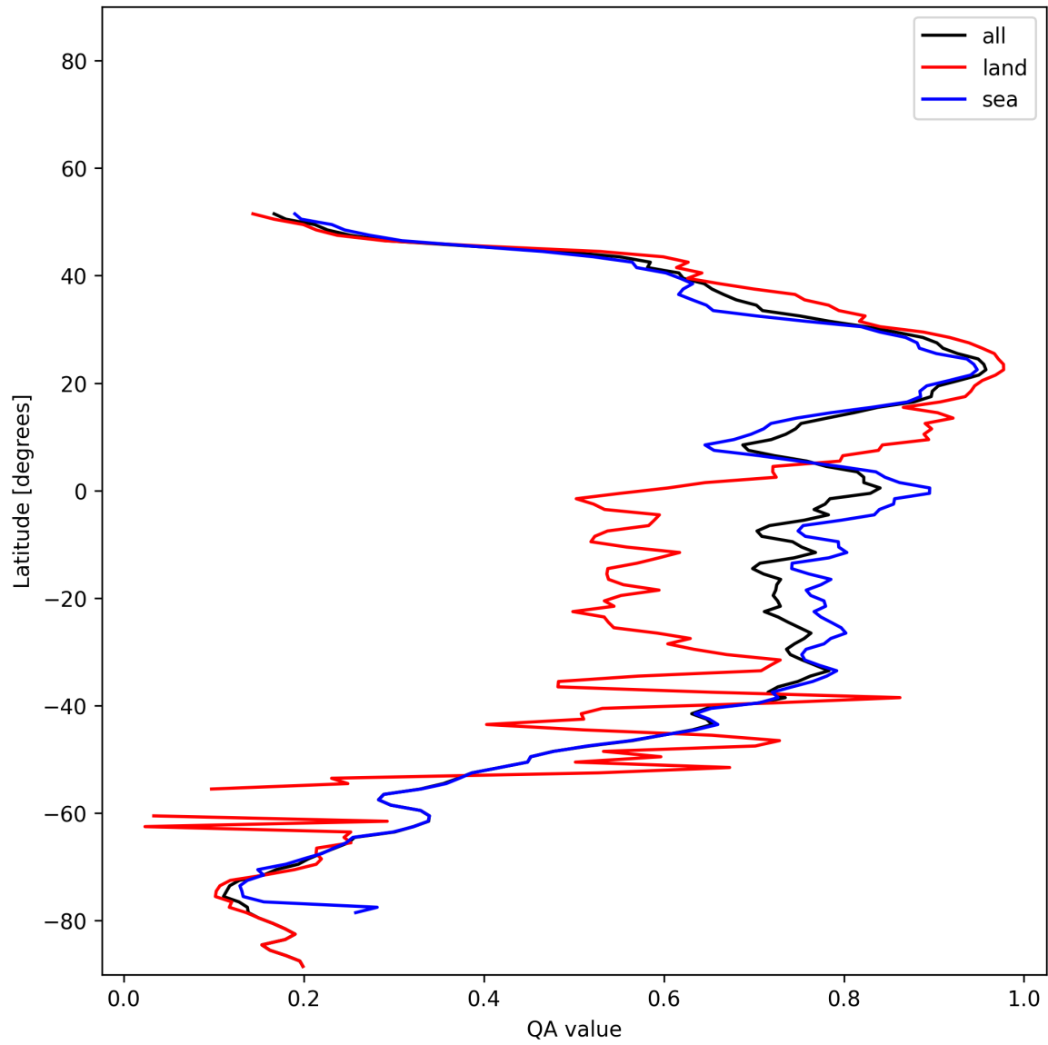
Figure 31: Zonal average of “QA value” for 2025-11-14 to 2025-11-16.
