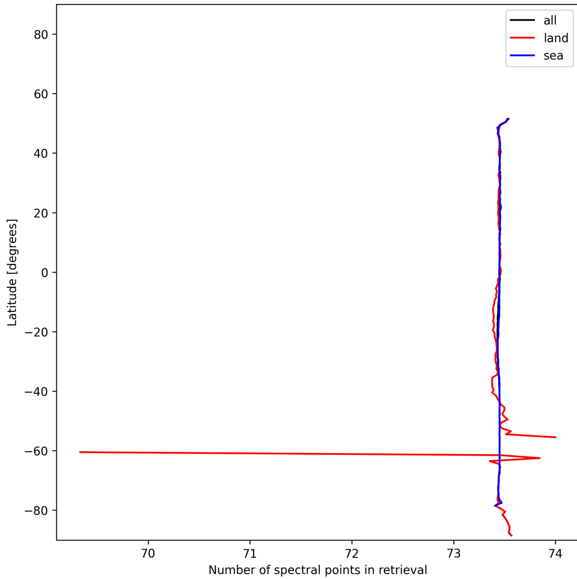
Figure 56: Zonal average of “Number of spectral points in retrieval” for 2025-11-14 to 2025-11-16.
