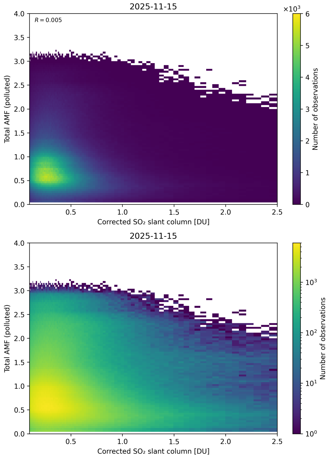
Figure 242: Scatter density plot of “Corrected SO 2 slant column” against “Total AMF (polluted)” for 2025-11-14 to 2025-11-16.
