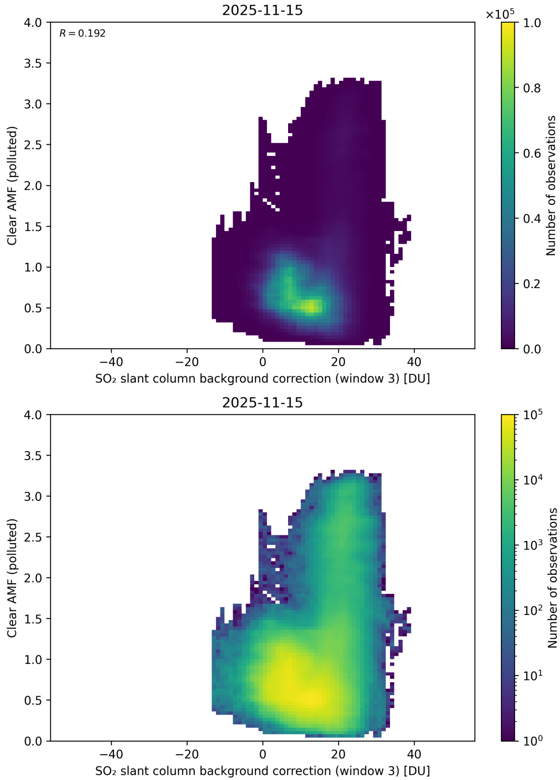
Figure 135: Scatter density plot of “SO 2 slant column background correction (window 3)” against “Clear AMF (polluted)” for 2025-11-14 to 2025-11-16.
