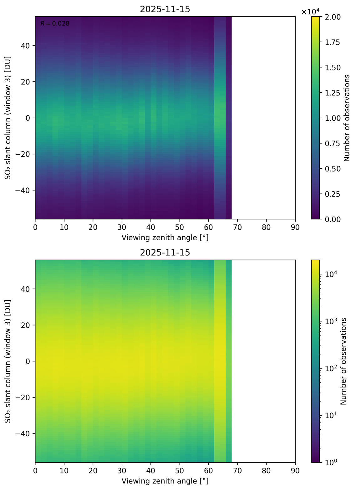
Figure 379: Scatter density plot of “Viewing zenith angle” against “SO 2 slant column (window 3)” for 2025-11-14 to 2025-11-16.
