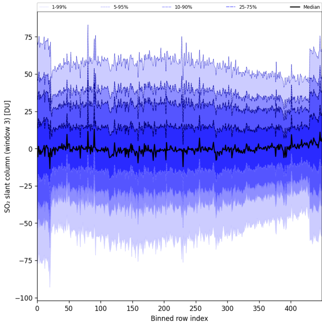
Figure 97: Along track statistics of “SO 2 slant column (window 3)” for 2025-11-14 to 2025-11-16
