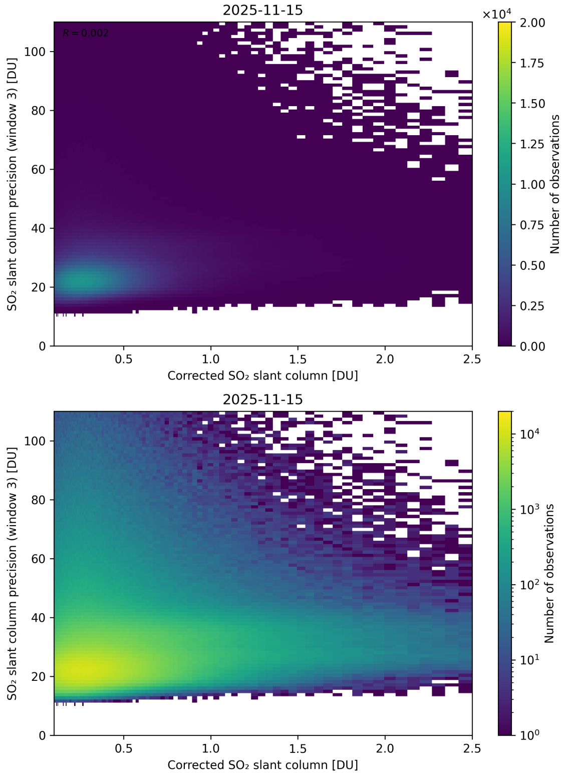
Figure 241: Scatter density plot of “Corrected SO 2 slant column” against “SO 2 slant column precision (window 3)” for 2025-11-14 to 2025-11-16.
