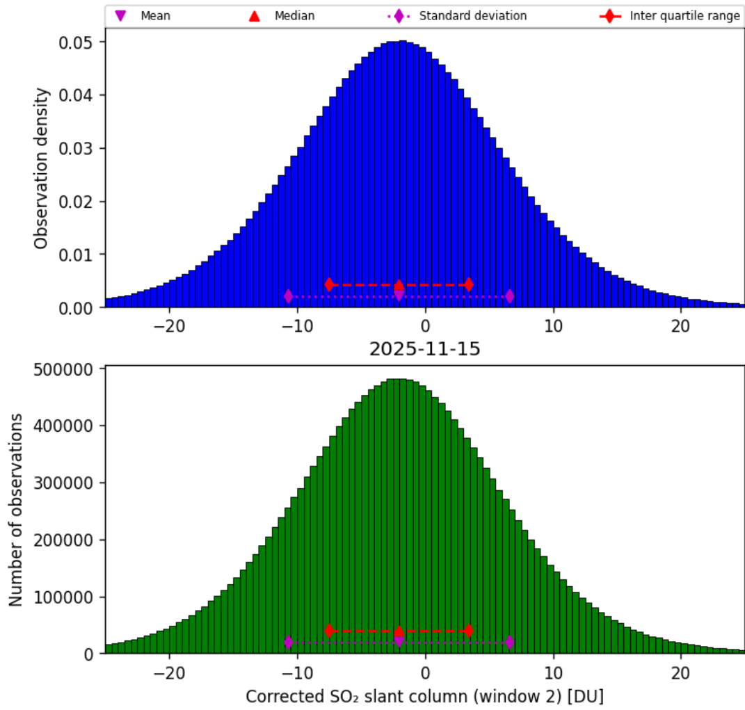
Figure 69: Histogram of “Corrected SO 2 slant column (window 2)” for 2025-11-14 to 2025-11-16
