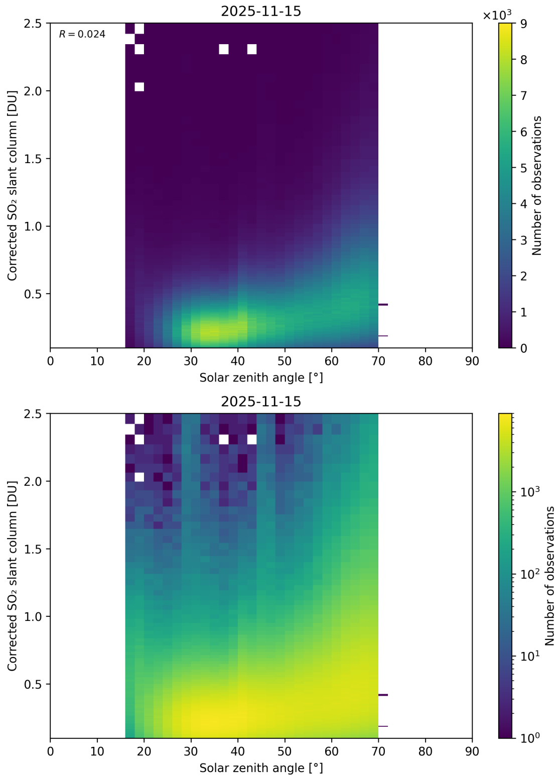
Figure 181: Scatter density plot of “Solar zenith angle” against “Corrected SO 2 slant column” for 2025-11-14 to 2025-11-16.
