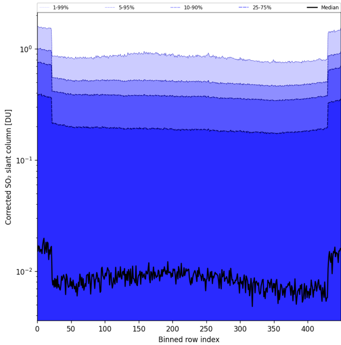
Figure 86: Along track statistics of “Corrected SO 2 slant column” for 2025-11-14 to 2025-11-16
