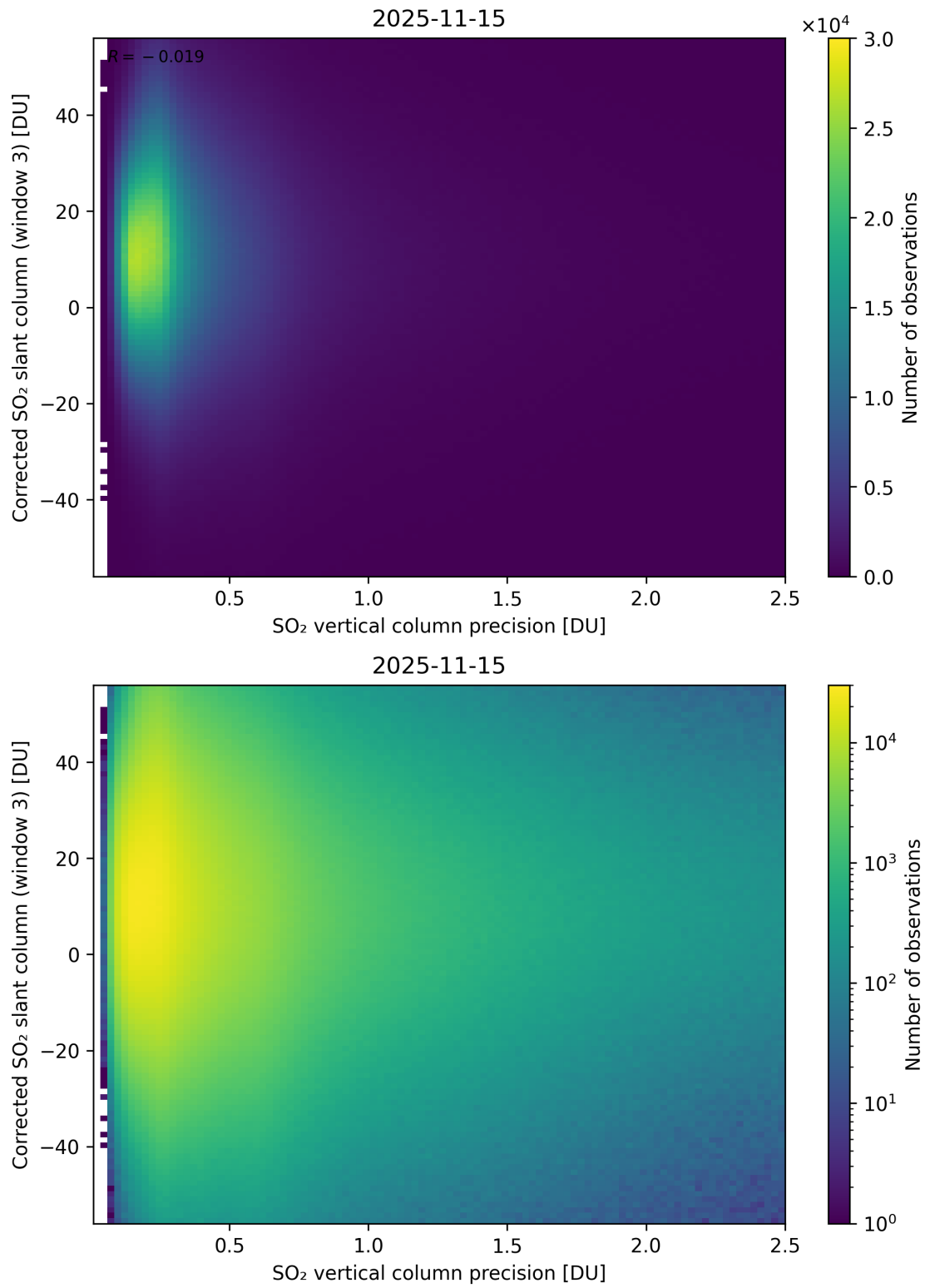
Figure 340: Scatter density plot of “SO 2 vertical column precision” against “Corrected SO 2 slant column (window 3)” for 2025-11-14 to 2025-11-16.
