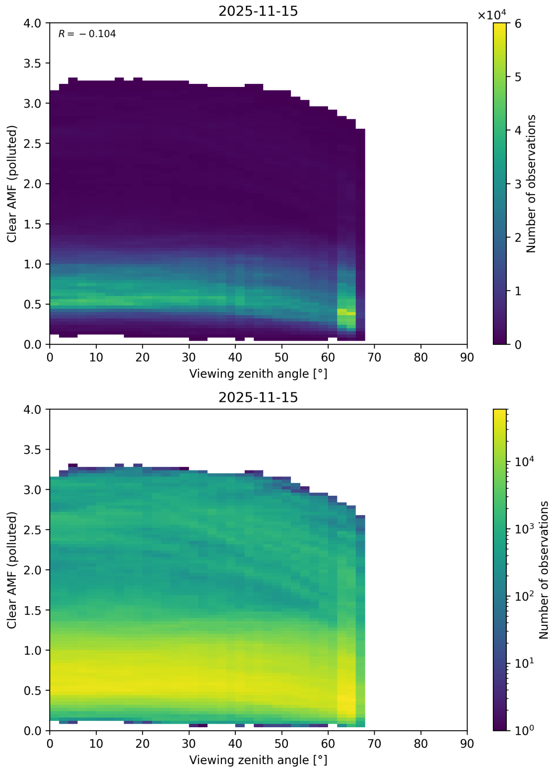
Figure 370: Scatter density plot of “Viewing zenith angle” against “Clear AMF (polluted)” for 2025-11-14 to 2025-11-16.
