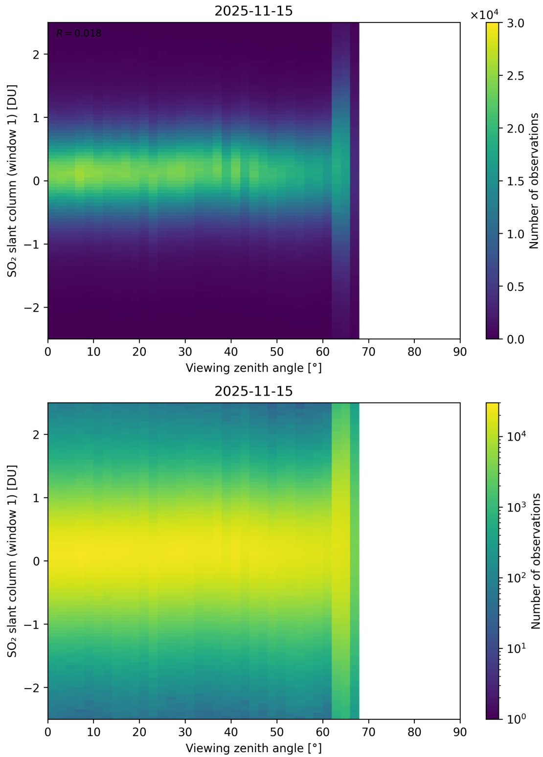
Figure 376: Scatter density plot of “Viewing zenith angle” against “SO 2 slant column (window 1)” for 2025-11-14 to 2025-11-16.
