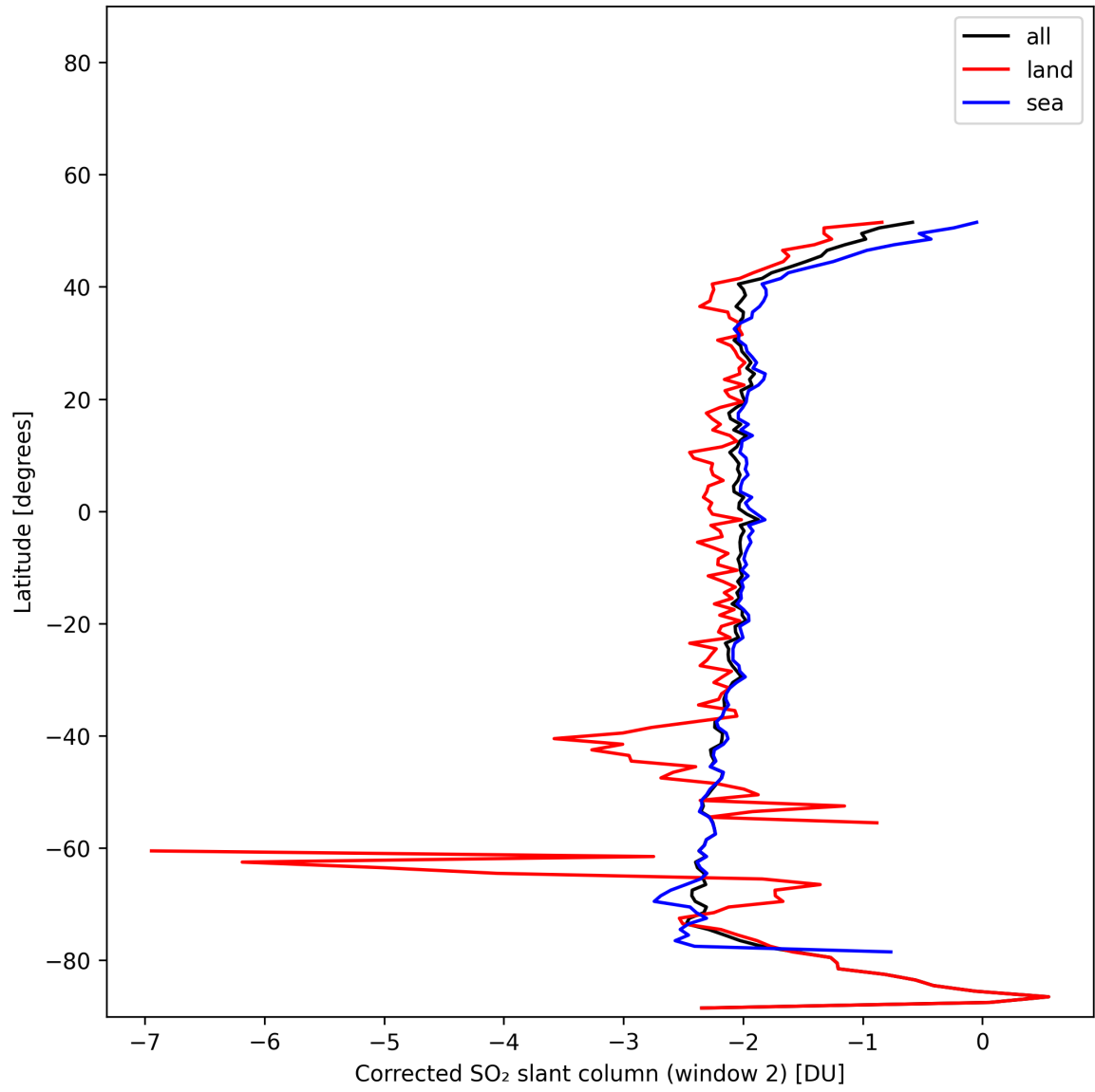
Figure 43: Zonal average of “Corrected SO 2 slant column (window 2)” for 2025-11-14 to 2025-11-16.
