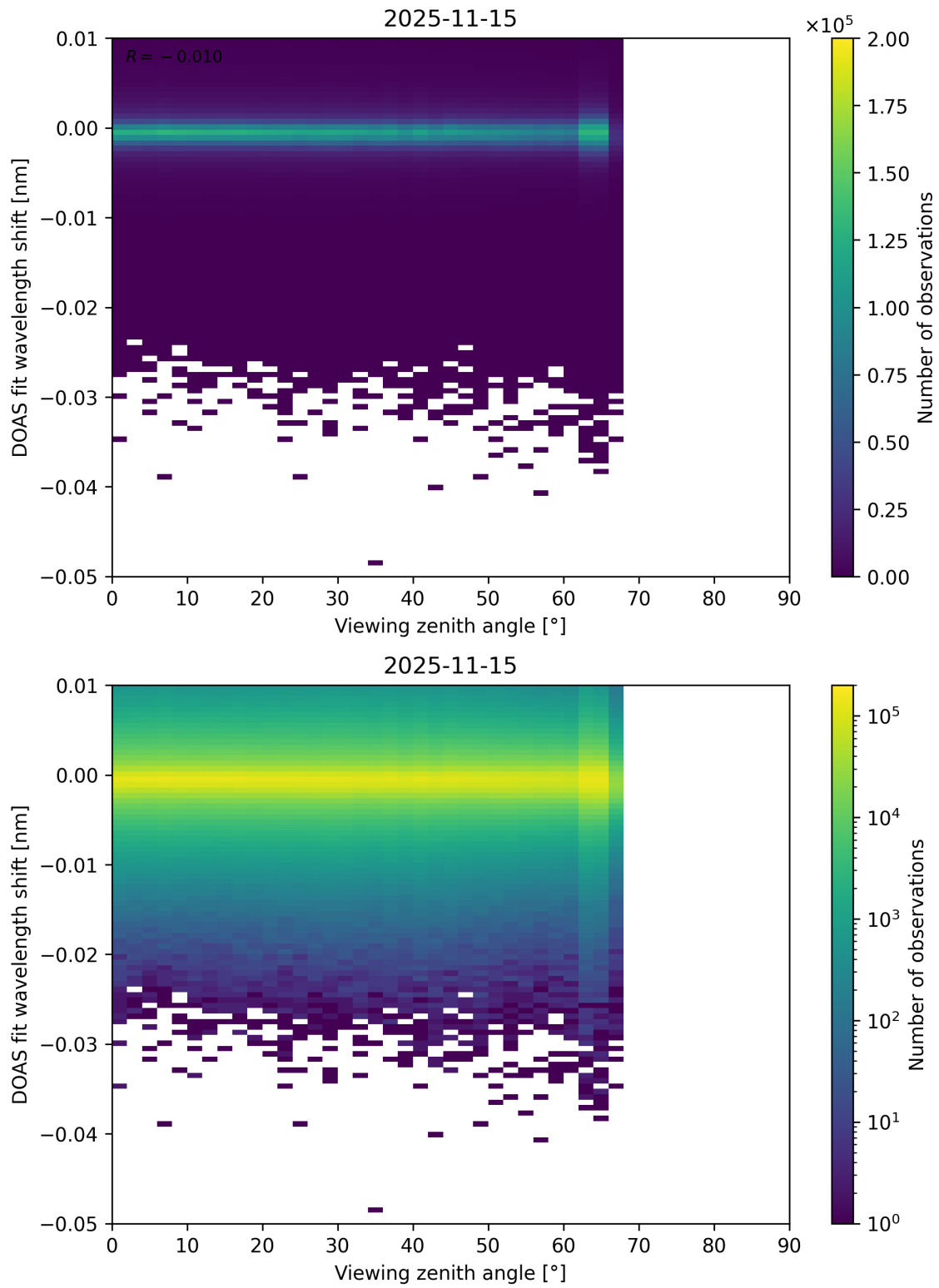
Figure 365: Scatter density plot of “Viewing zenith angle” against “DOAS fit wavelength shift” for 2025-11-14 to 2025-11-16.
