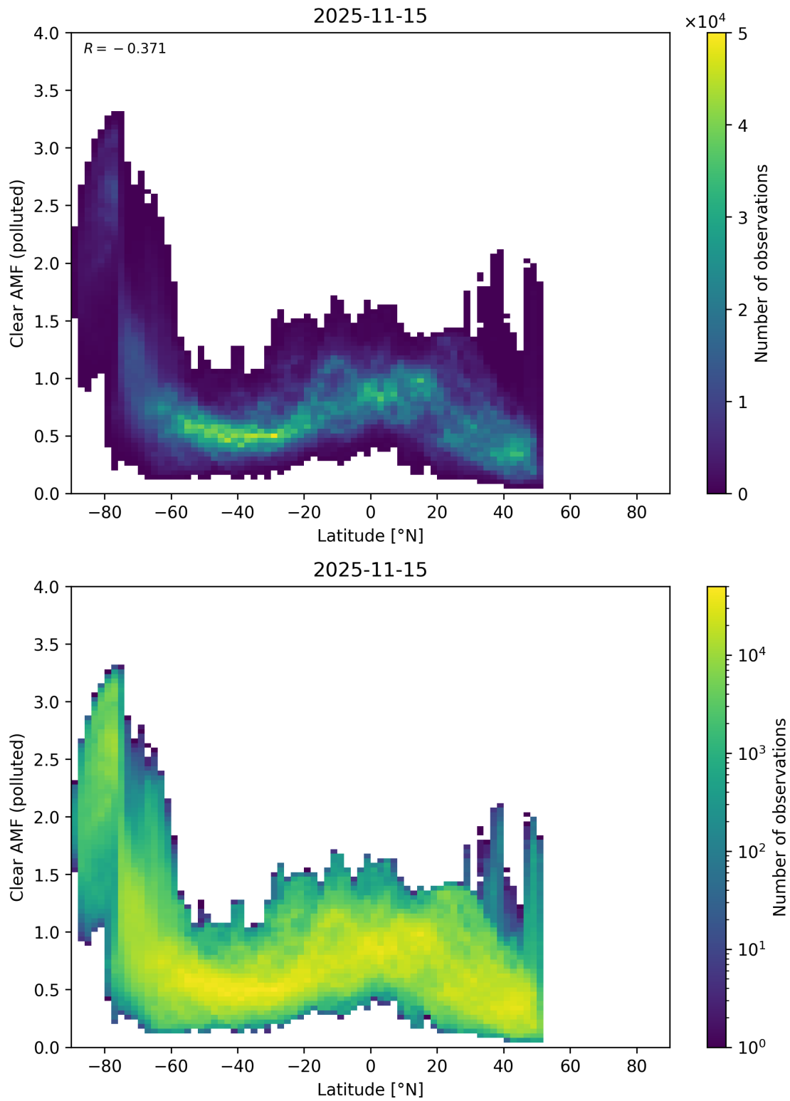
Figure 156: Scatter density plot of “Latitude” against “Clear AMF (polluted)” for 2025-11-14 to 2025-11-16.
