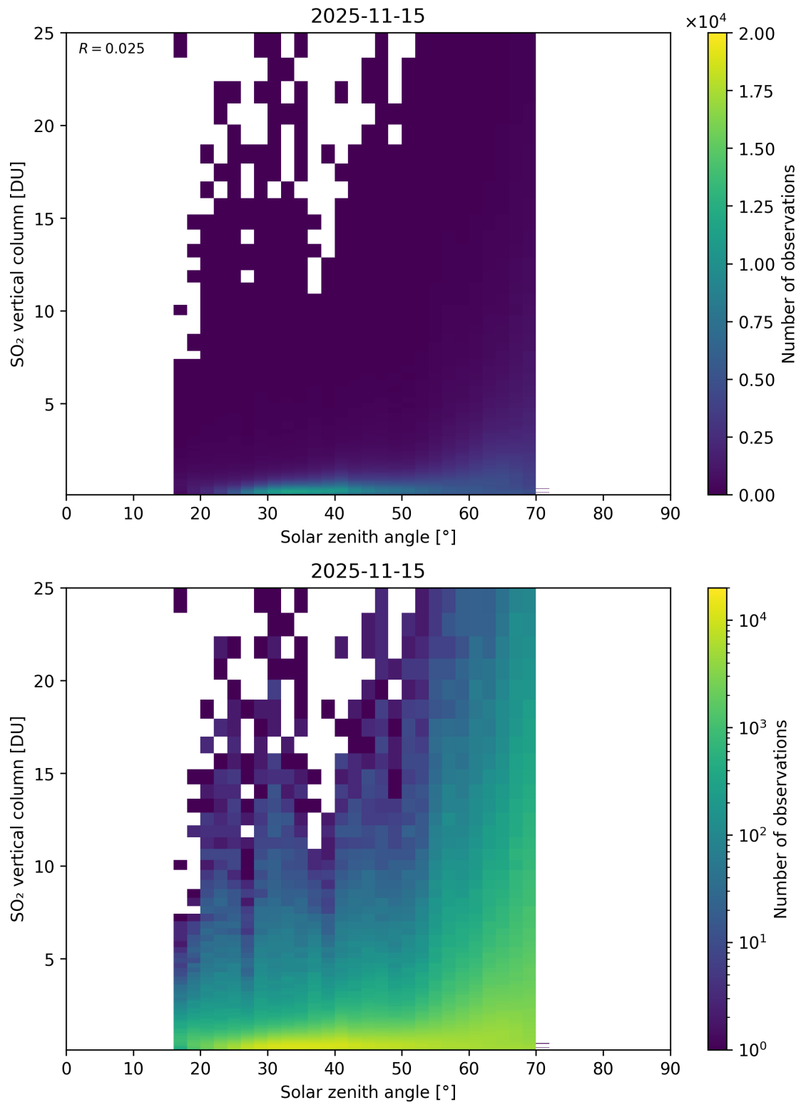
Figure 191: Scatter density plot of “Solar zenith angle” against “SO 2 vertical column” for 2025-11-14 to 2025-11-16.
