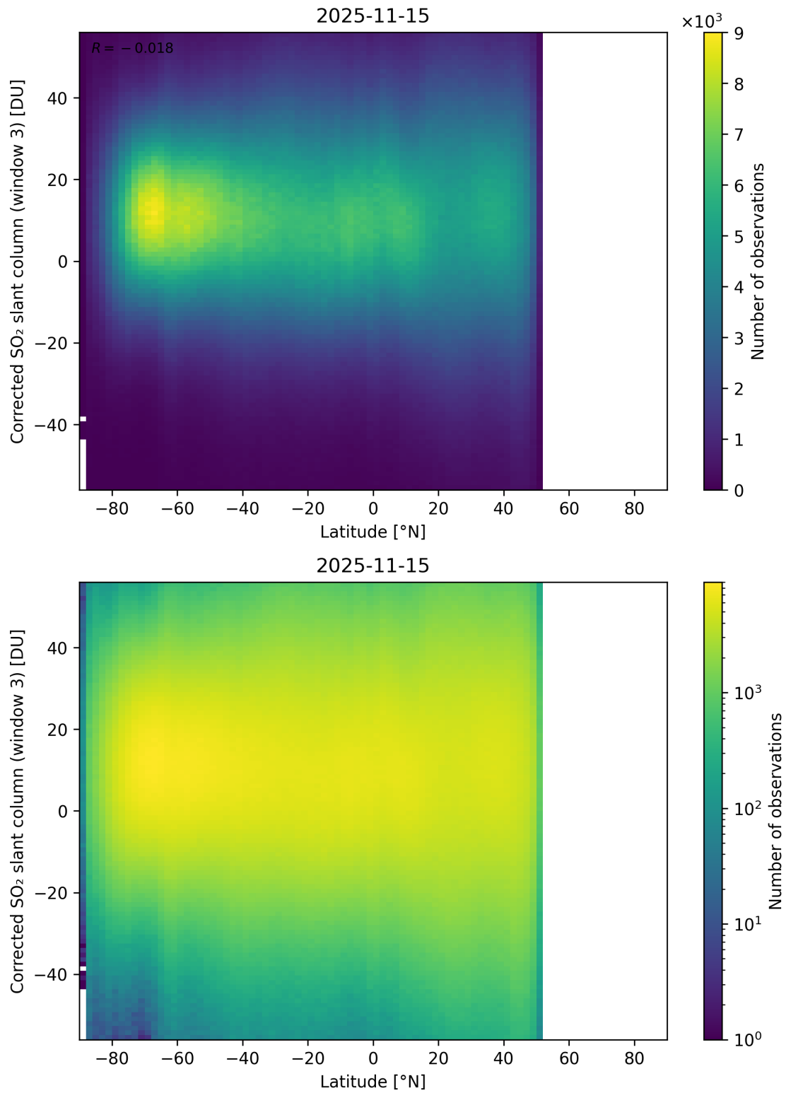
Figure 161: Scatter density plot of “Latitude” against “Corrected SO 2 slant column (window 3)” for 2025-11-14 to 2025-11-16.
