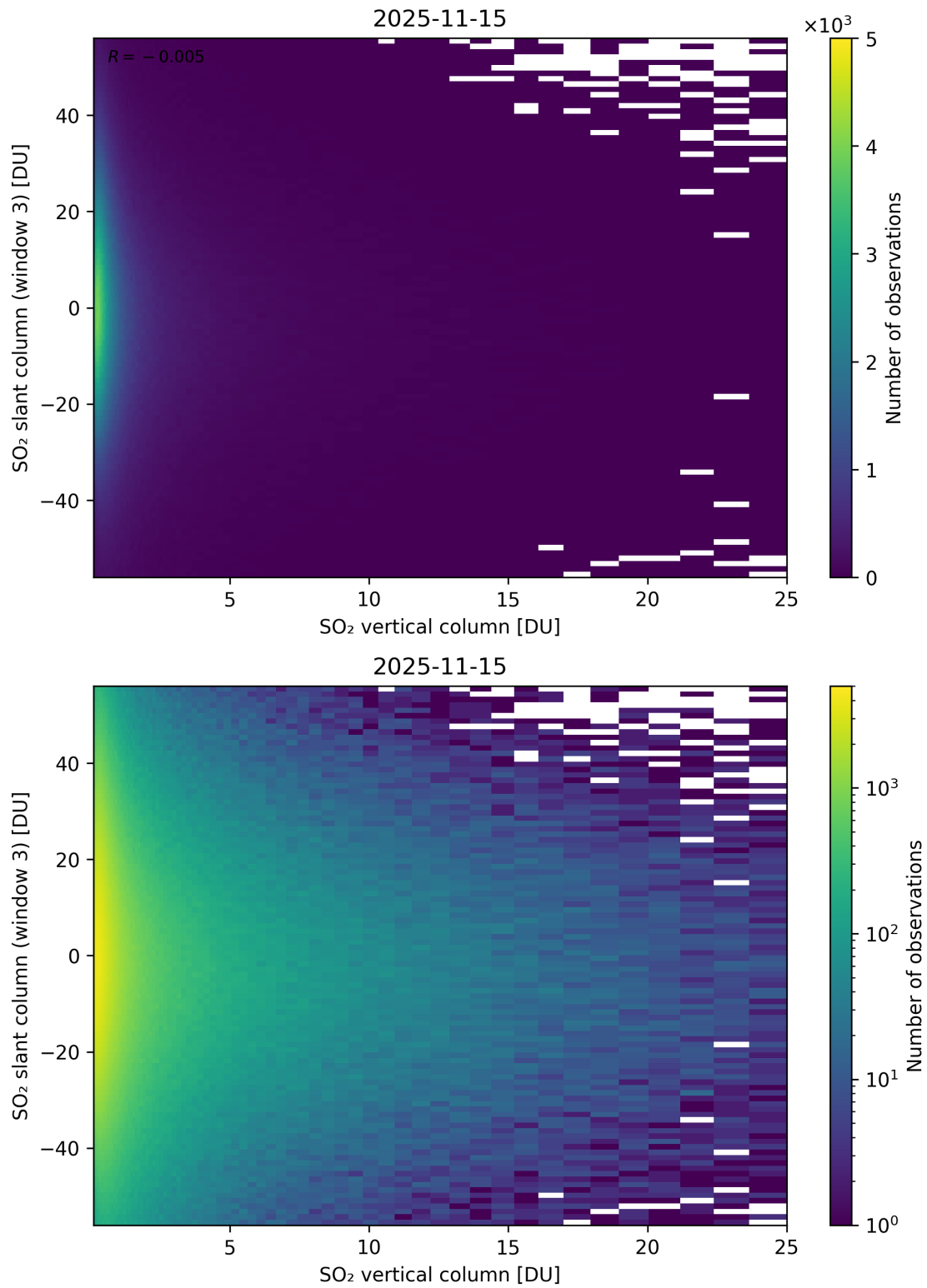
Figure 357: Scatter density plot of “SO 2 vertical column” against “SO 2 slant column (window 3)” for 2025-11-14 to 2025-11-16.
