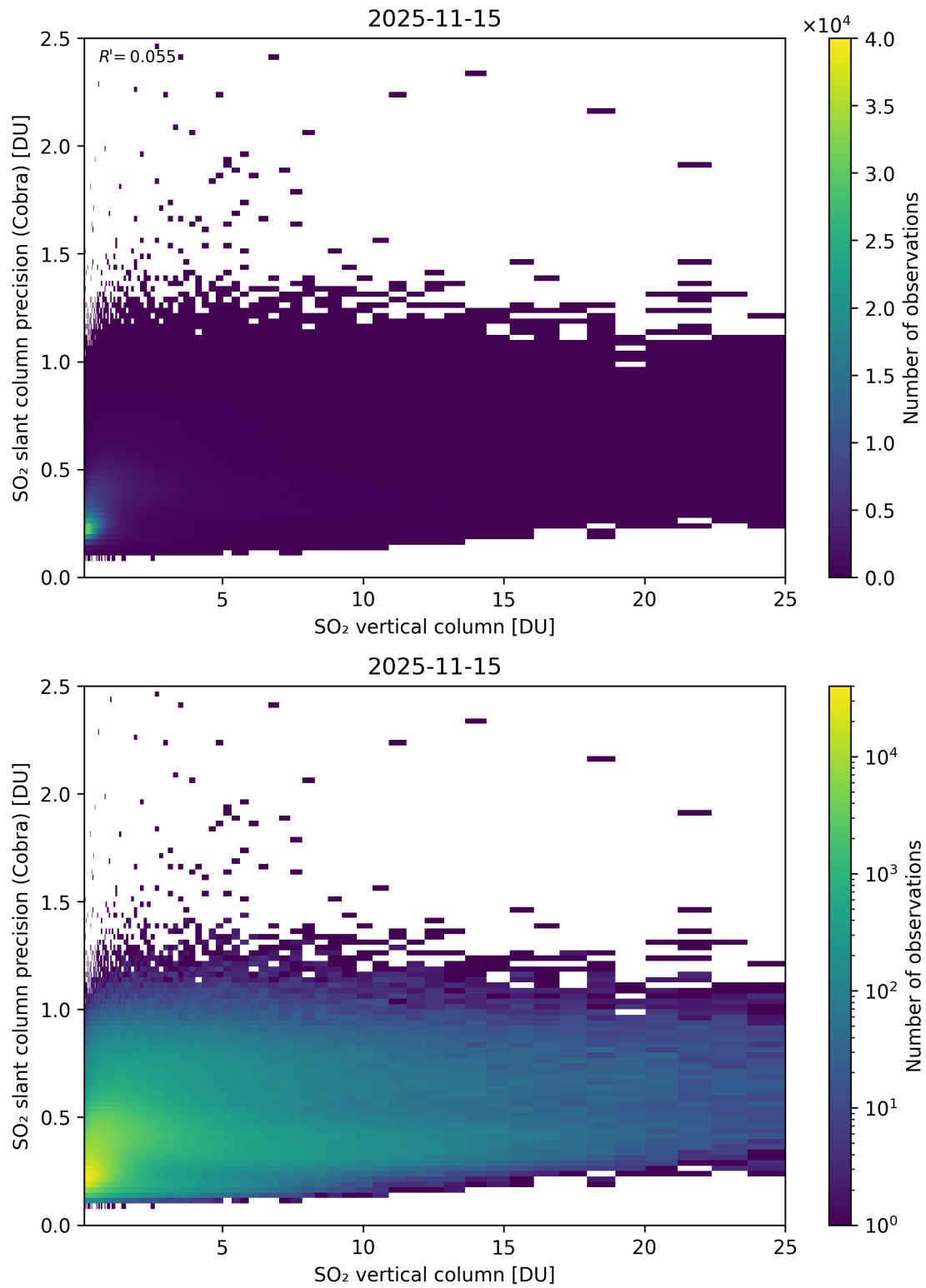
Figure 350: Scatter density plot of “SO 2 vertical column” against “SO 2 slant column precision (Cobra)” for 2025-11-14 to 2025-11-16.
