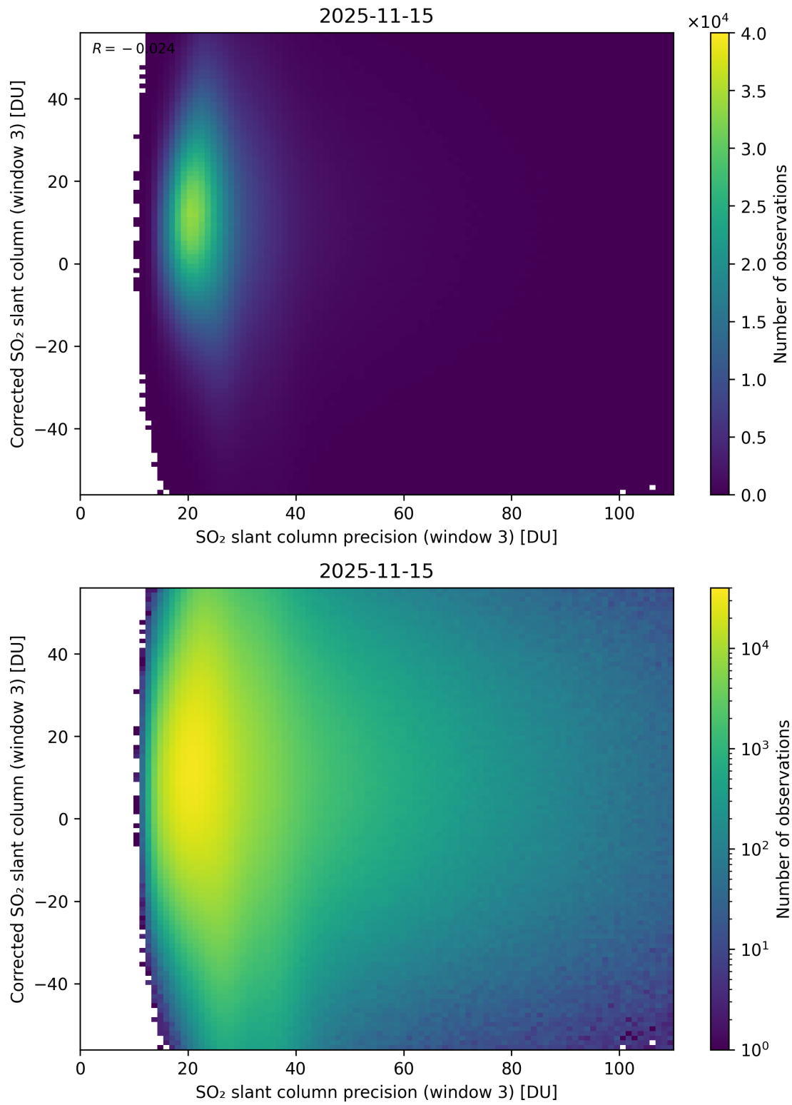
Figure 312: Scatter density plot of “SO 2 slant column precision (window 3)” against “Corrected SO 2 slant column (window 3)” for 2025-11-14 to 2025-11-16.
