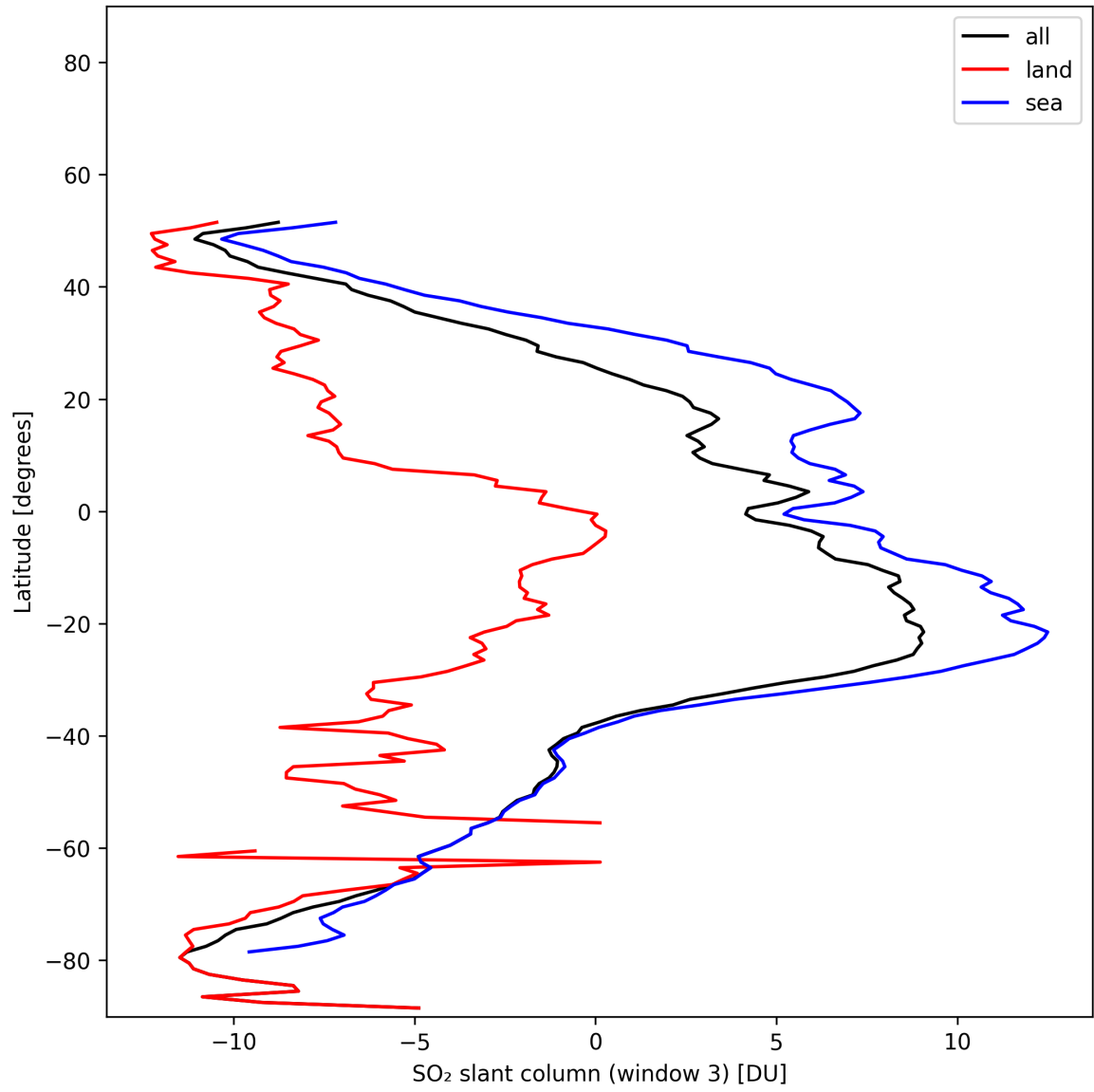
Figure 45: Zonal average of “SO 2 slant column (window 3)” for 2025-11-14 to 2025-11-16.
