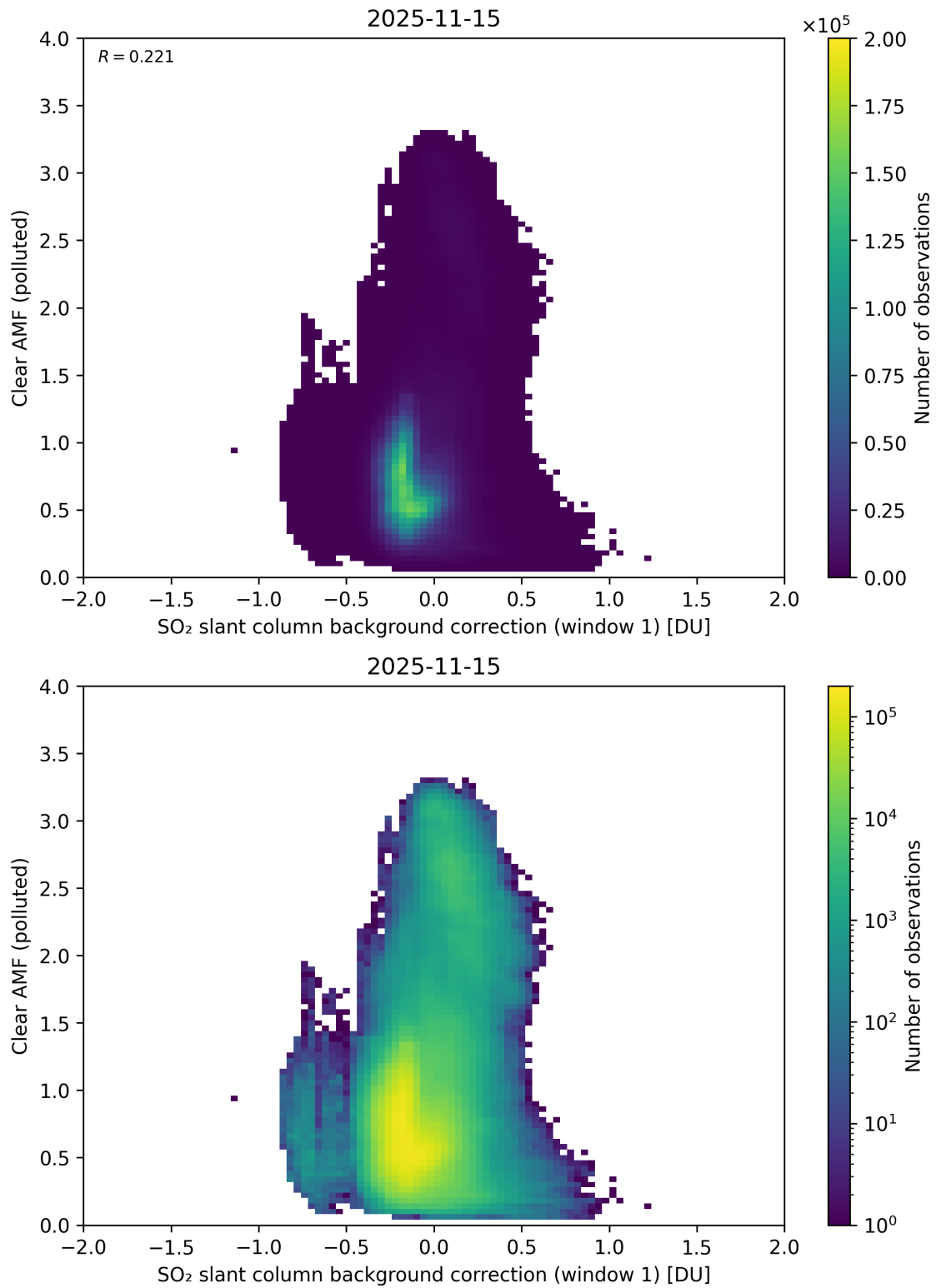
Figure 114: Scatter density plot of “SO 2 slant column background correction (window 1)” against “Clear AMF (polluted)” for 2025-11-14 to 2025-11-16.
