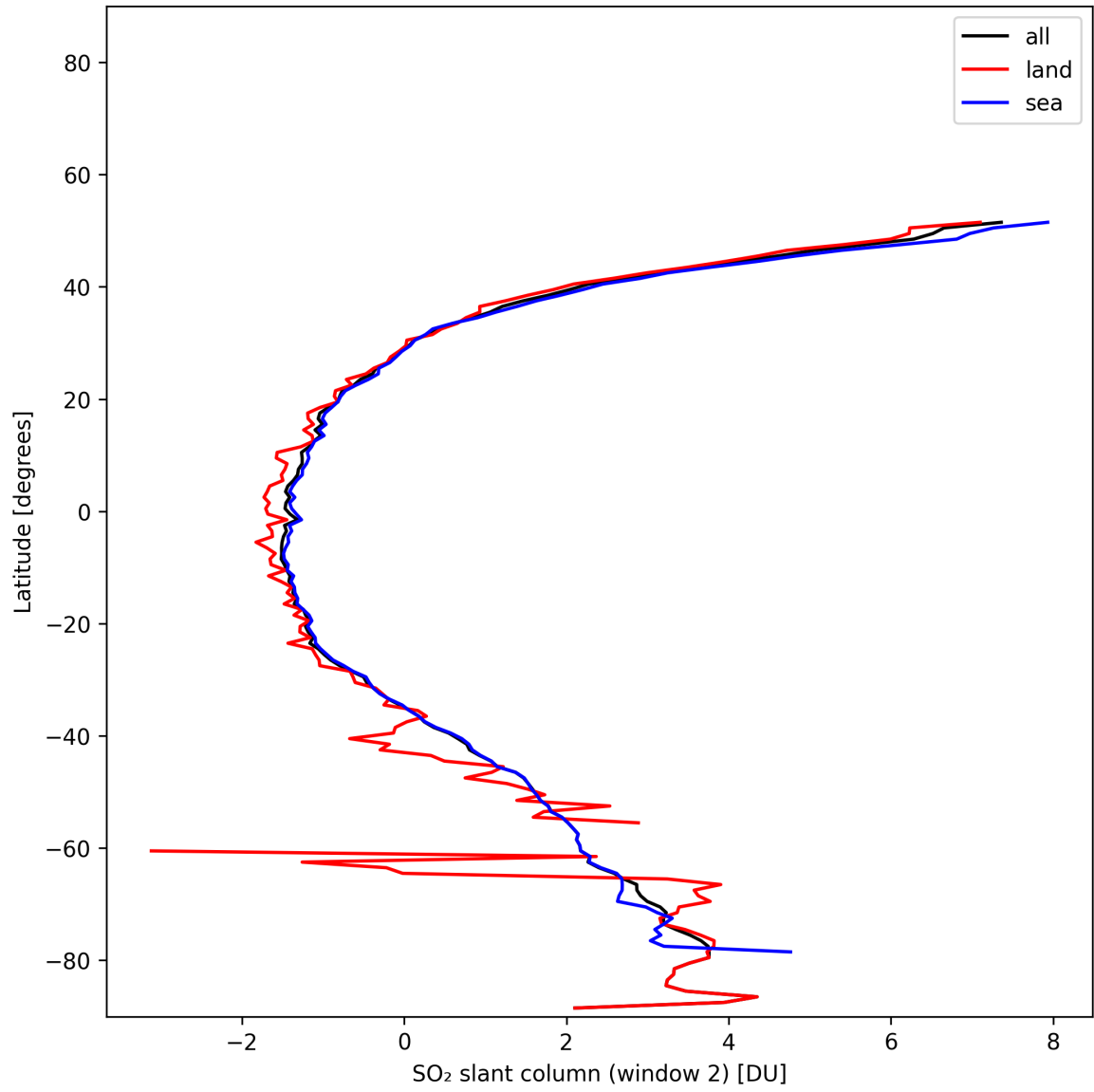
Figure 41: Zonal average of “SO 2 slant column (window 2)” for 2025-11-14 to 2025-11-16.
