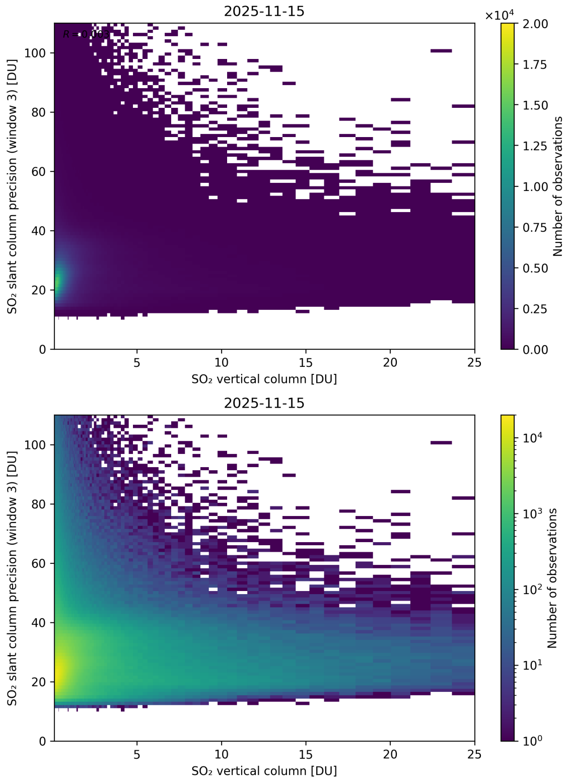
Figure 358: Scatter density plot of “SO 2 vertical column” against “SO 2 slant column precision (window 3)” for 2025-11-14 to 2025-11-16.
