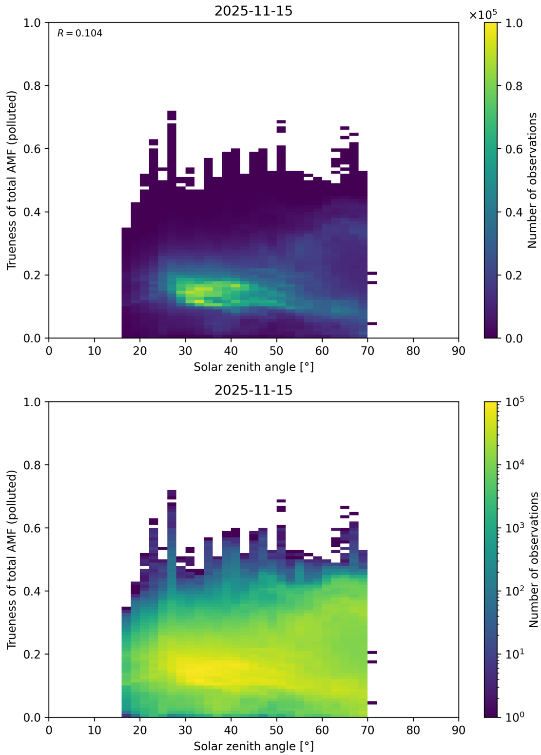
Figure 190: Scatter density plot of “Solar zenith angle” against “Trueness of total AMF (polluted)” for 2025-11-14 to 2025-11-16.
