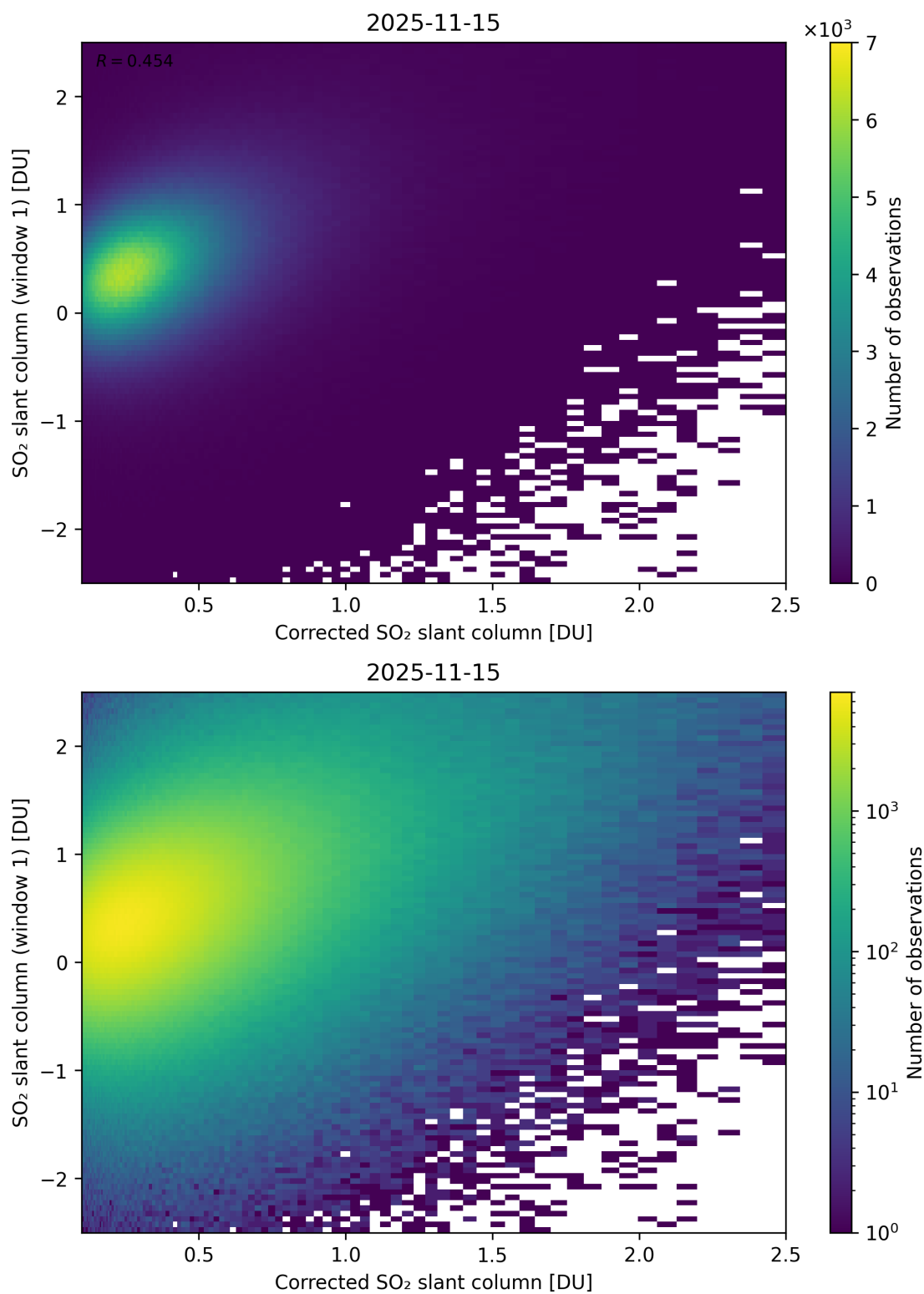
Figure 237: Scatter density plot of “Corrected SO 2 slant column” against “SO 2 slant column (window 1)” for 2025-11-14 to 2025-11-16.
