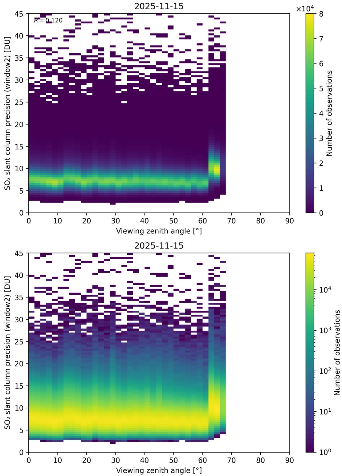
Figure 378: Scatter density plot of “Viewing zenith angle” against “SO 2 slant column precision (window2)” for 2025-11-14 to 2025-11-16.
