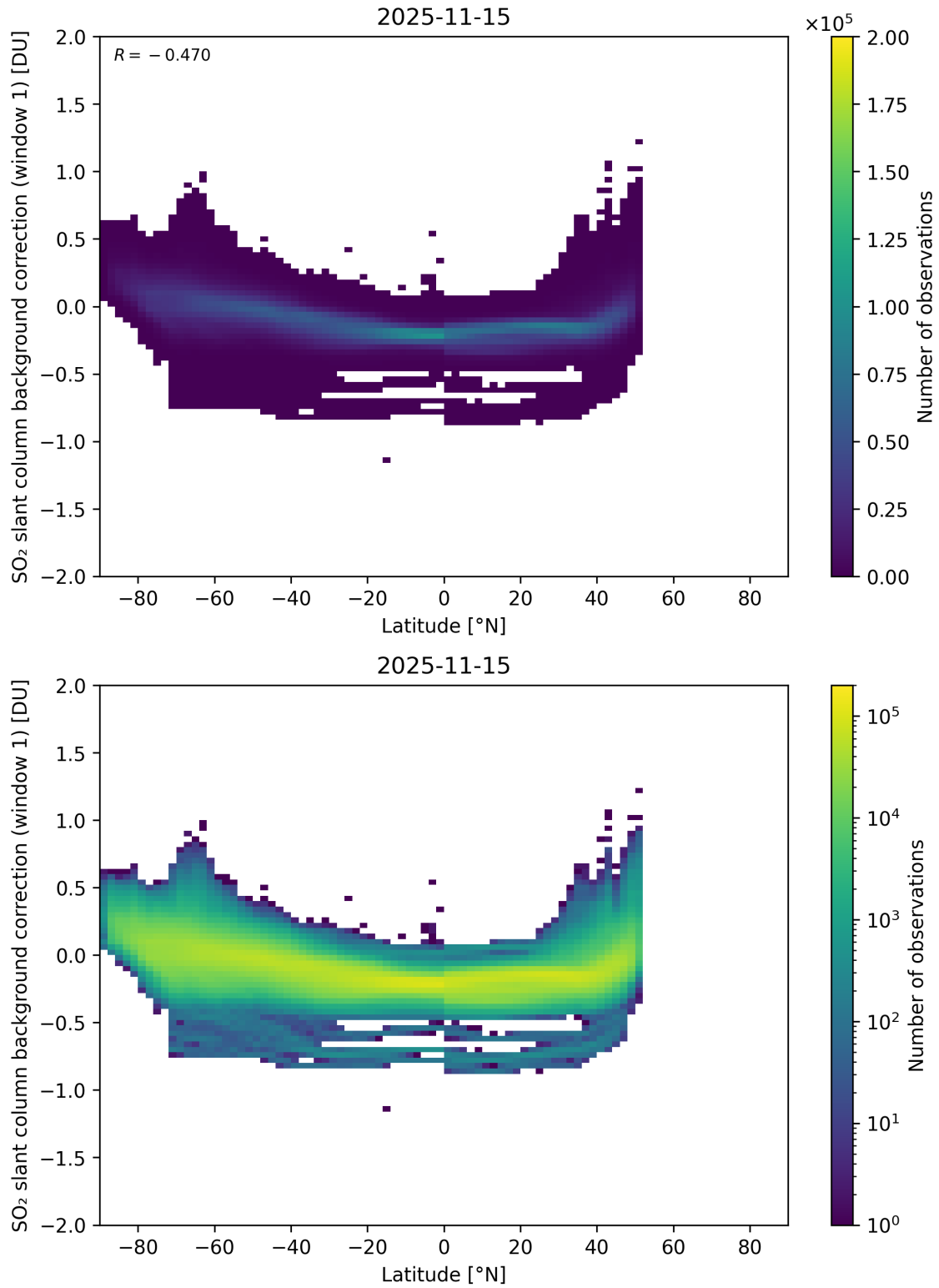
Figure 150: Scatter density plot of “Latitude” against “SO 2 slant column background correction (window 1)” for 2025-11-14 to 2025-11-16.
