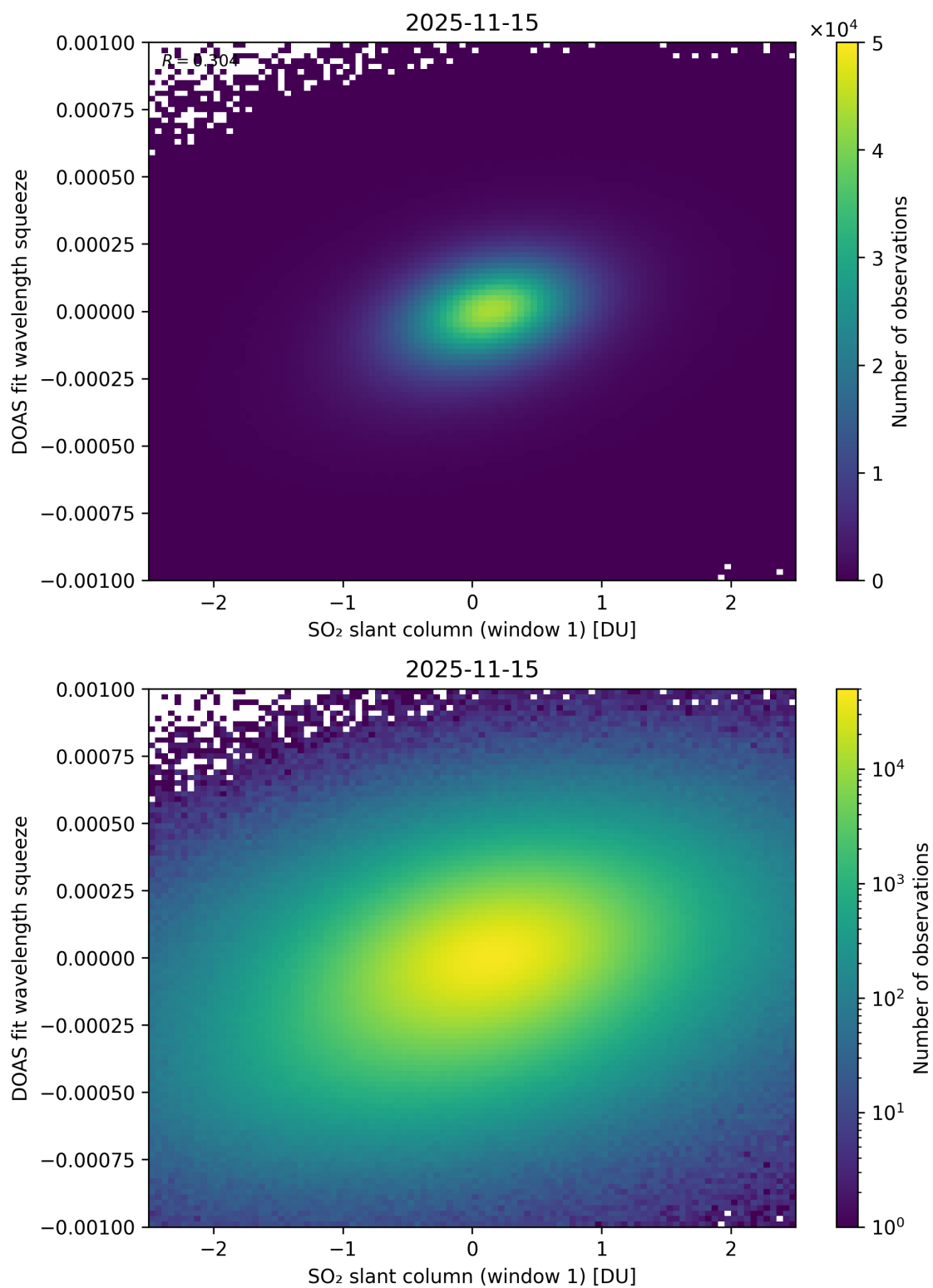
Figure 266: Scatter density plot of “SO 2 slant column (window 1)” against “DOAS fit wavelength squeeze” for 2025-11-14 to 2025-11-16.
