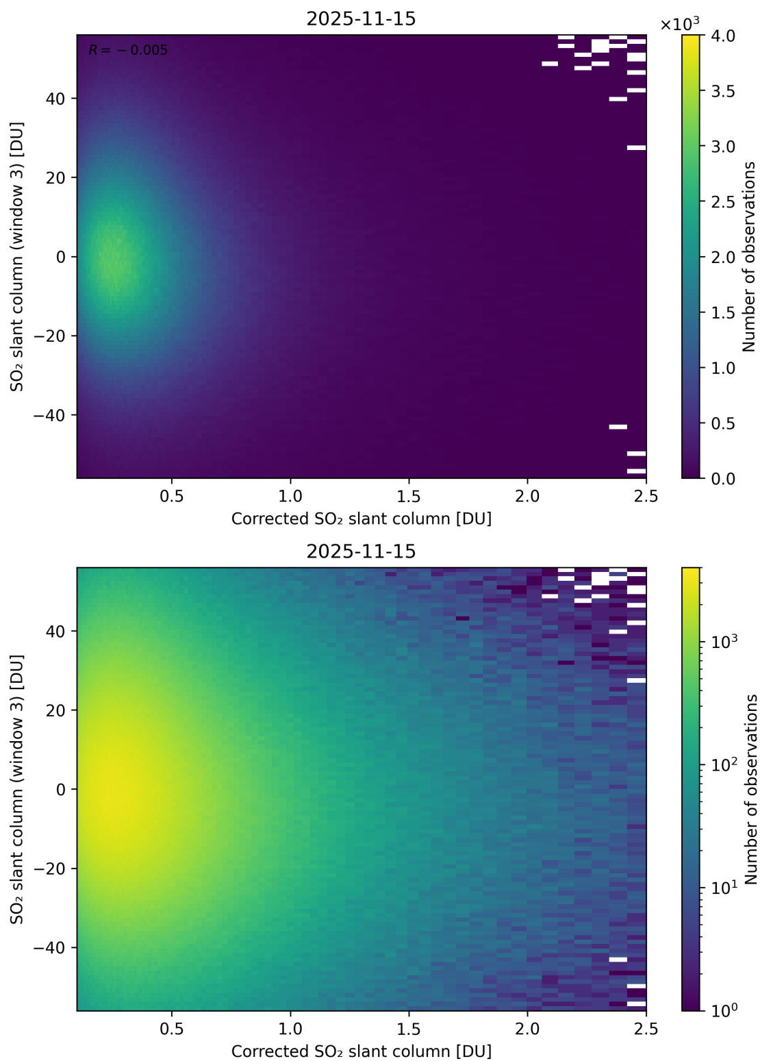
Figure 240: Scatter density plot of “Corrected SO 2 slant column” against “SO 2 slant column (window 3)” for 2025-11-14 to 2025-11-16.
