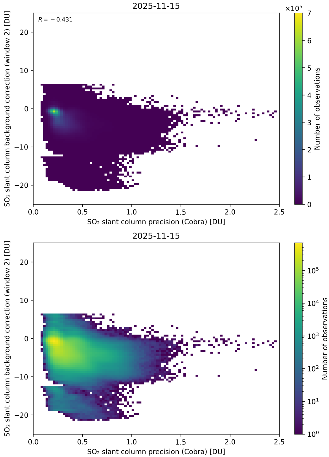
Figure 200: Scatter density plot of “SO 2 slant column precision (Cobra)” against “SO 2 slant column background correction (window 2)” for 2025-11-14 to 2025-11-16.
