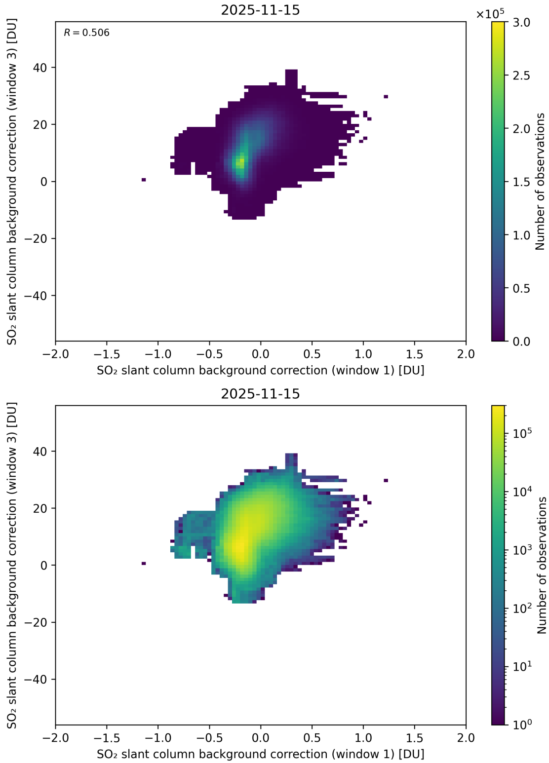
Figure 110: Scatter density plot of “SO 2 slant column background correction (window 1)” against “SO 2 slant column background correction (window 3)” for 2025-11-14 to 2025-11-16.
