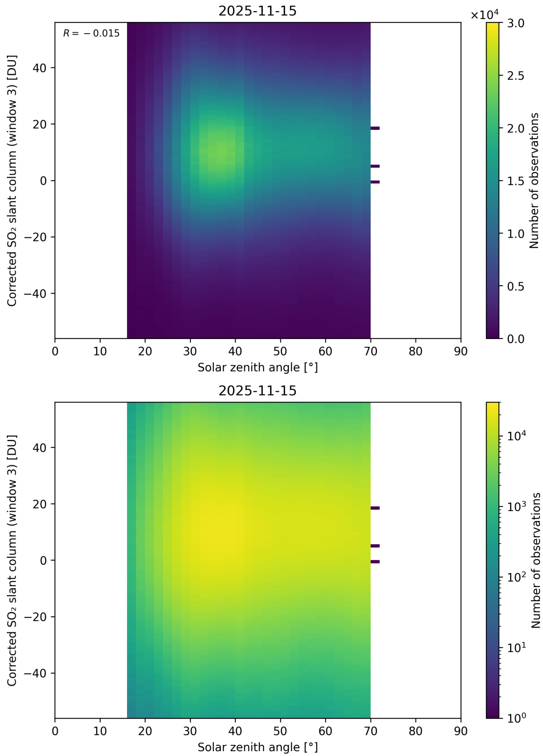
Figure 183: Scatter density plot of “Solar zenith angle” against “Corrected SO 2 slant column (window 3)” for 2025-11-14 to 2025-11-16.
