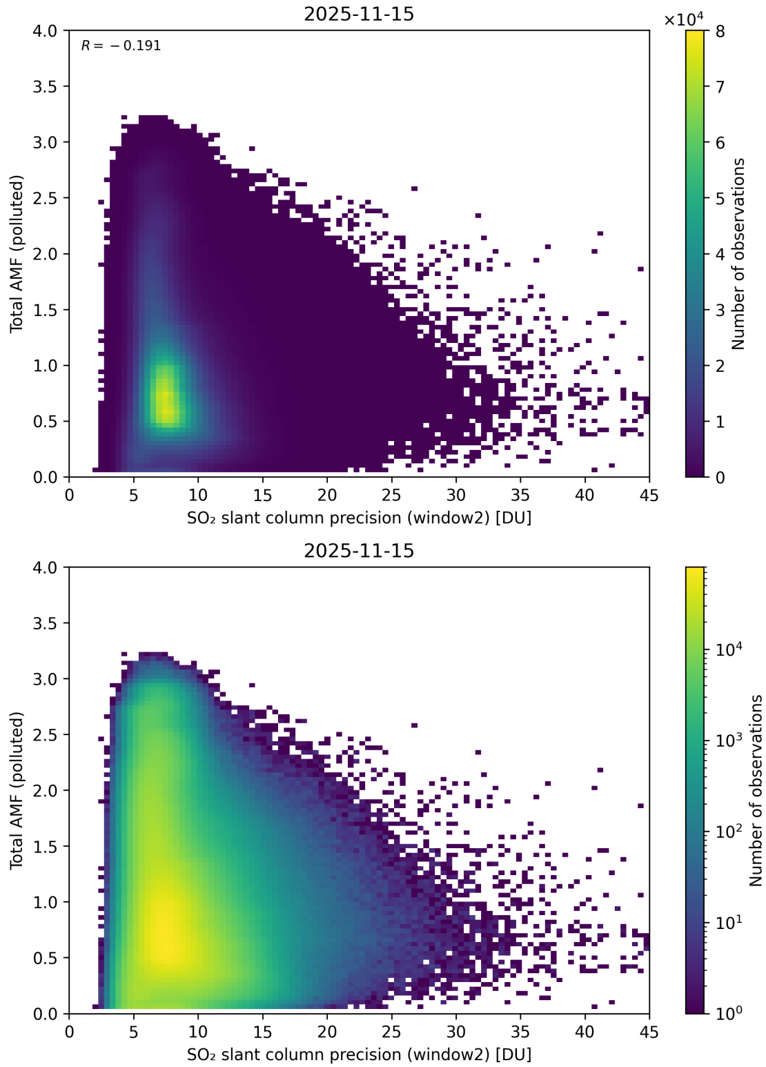
Figure 301: Scatter density plot of “SO 2 slant column precision (window2)” against “Total AMF (polluted)” for 2025-11-14 to 2025-11-16.
