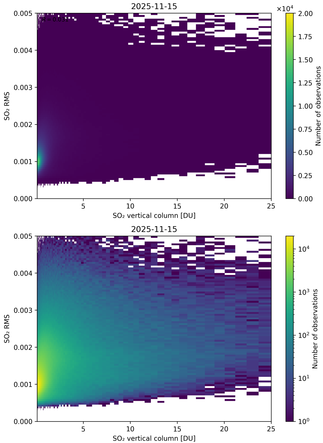
Figure 328: Scatter density plot of “SO 2 vertical column” against “SO 2 RMS” for 2025-11-14 to 2025-11-16.
