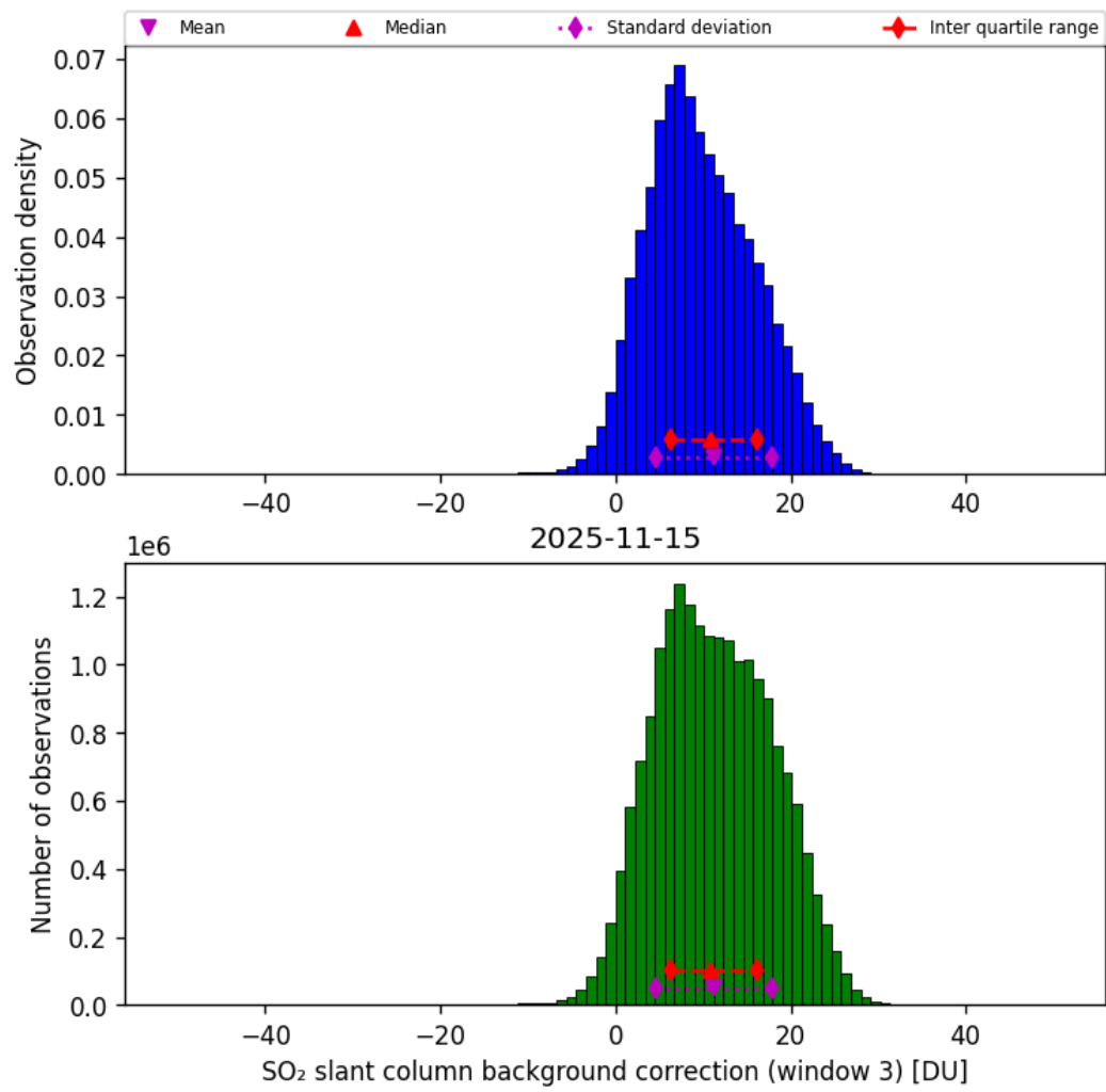
Figure 74: Histogram of “SO 2 slant column background correction (window 3)” for 2025-11-14 to 2025-11-16
