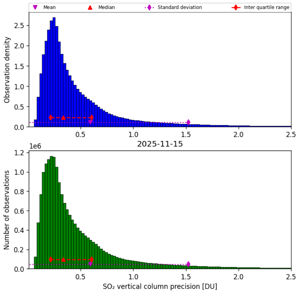
Figure 59: Histogram of “SO 2 vertical column precision” for 2025-11-14 to 2025-11-16
