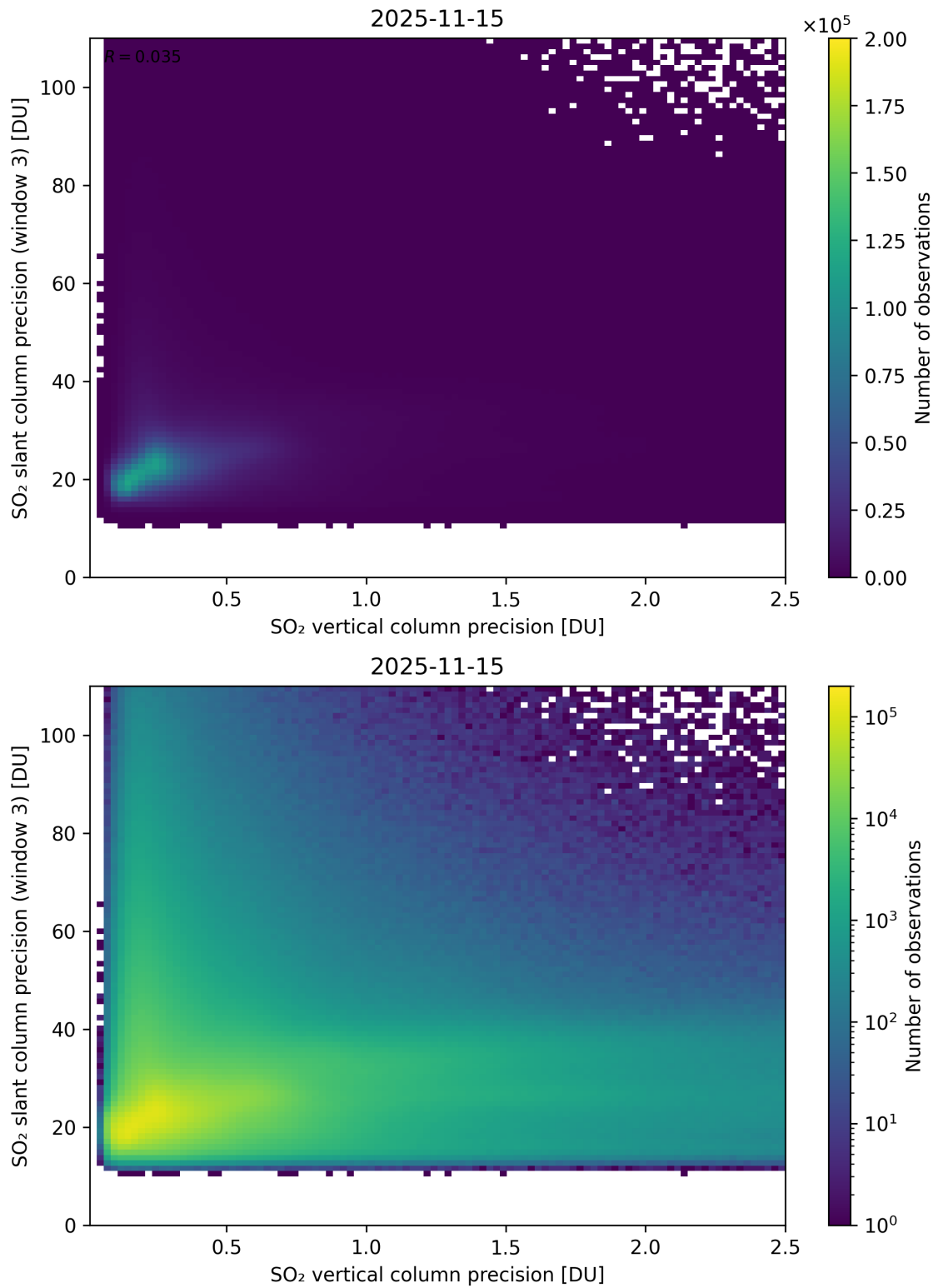
Figure 345: Scatter density plot of “SO 2 vertical column precision” against “SO 2 slant column precision (window 3)” for 2025-11-14 to 2025-11-16.
