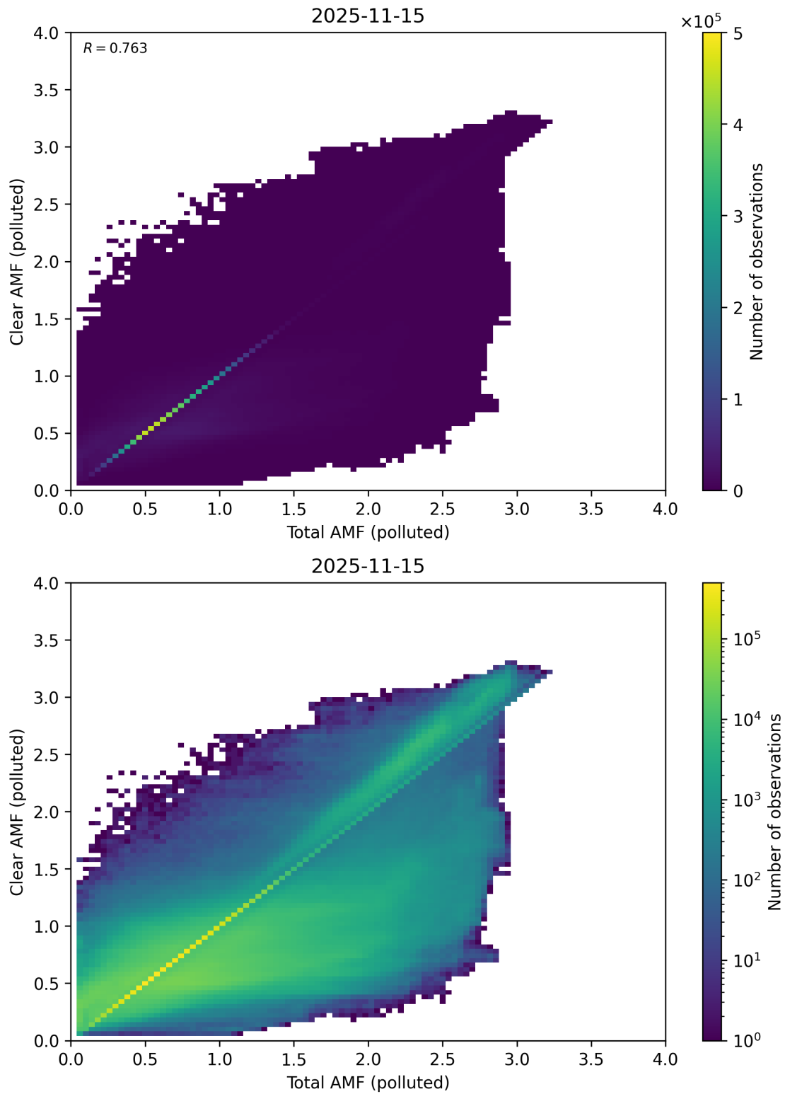
Figure 320: Scatter density plot of “Total AMF (polluted)” against “Clear AMF (polluted)” for 2025-11-14 to 2025-11-16.
