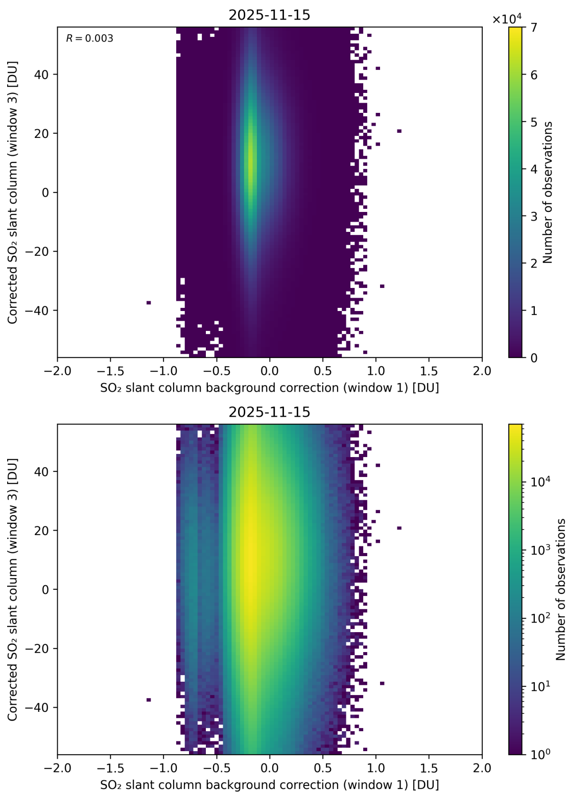
Figure 116: Scatter density plot of “SO 2 slant column background correction (window 1)” against “Corrected SO 2 slant column (window 3)” for 2025-11-14 to 2025-11-16.
