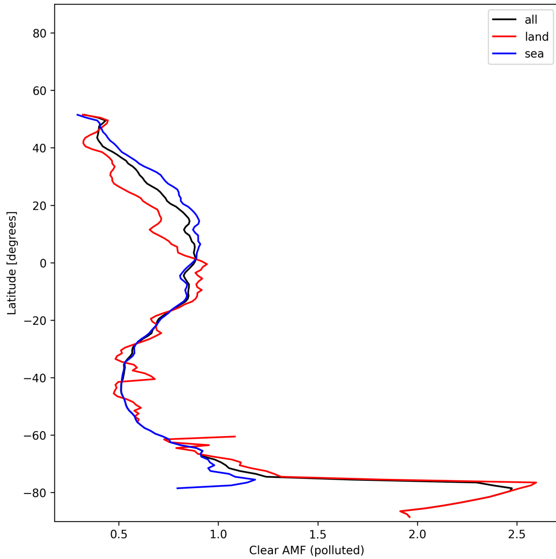
Figure 55: Zonal average of “Clear AMF (polluted)” for 2025-11-14 to 2025-11-16.
