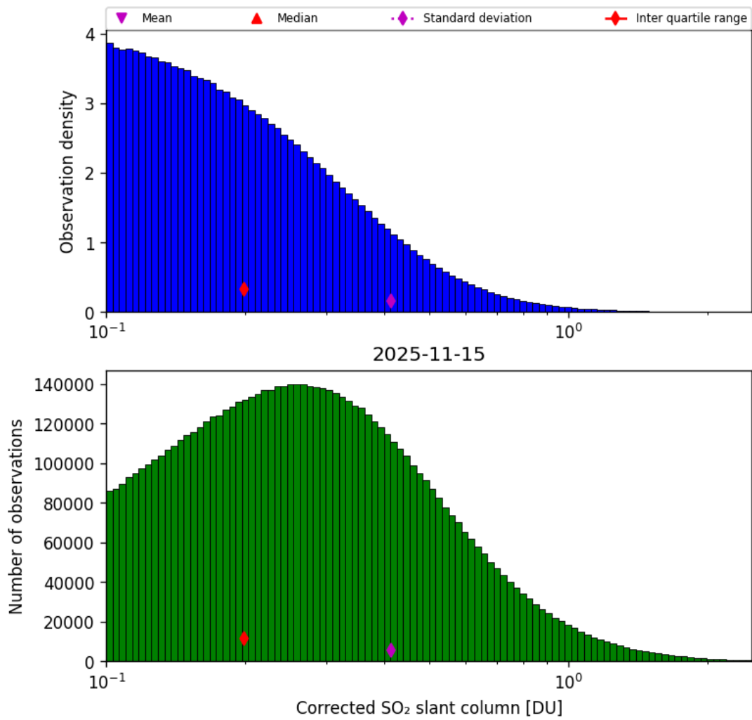
Figure 60: Histogram of “Corrected SO 2 slant column” for 2025-11-14 to 2025-11-16
