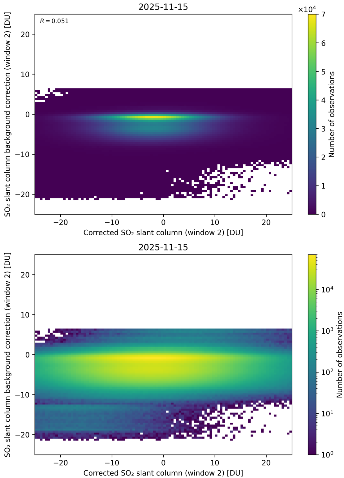
Figure 244: Scatter density plot of “Corrected SO 2 slant column (window 2)” against “SO 2 slant column background correction (window 2)” for 2025-11-14 to 2025-11-16.
