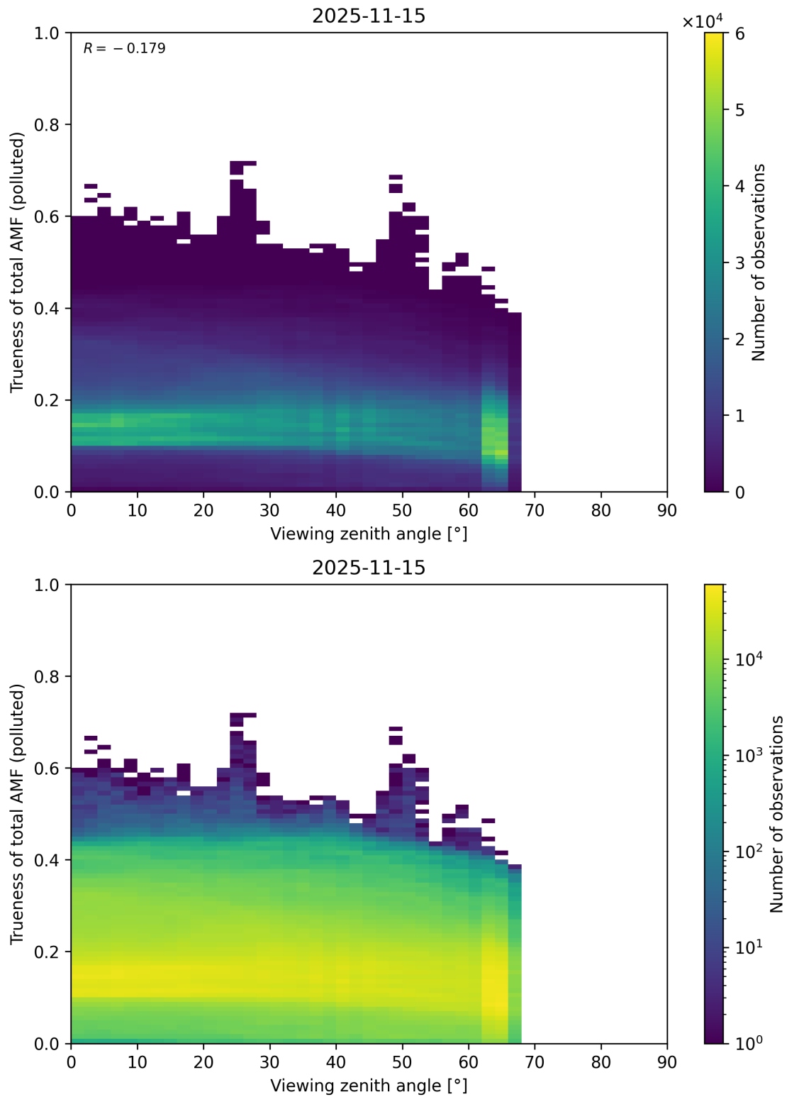
Figure 382: Scatter density plot of “Viewing zenith angle” against “Trueness of total AMF (polluted)” for 2025-11-14 to 2025-11-16.
