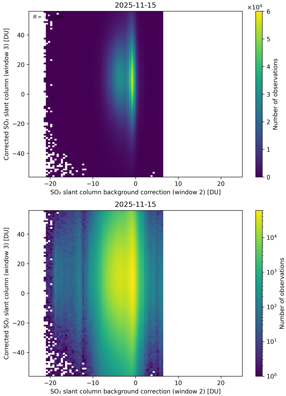
Figure 127: Scatter density plot of “SO 2 slant column background correction (window 2)” against “Corrected SO 2 slant column (window 3)” for 2025-11-14 to 2025-11-16.
