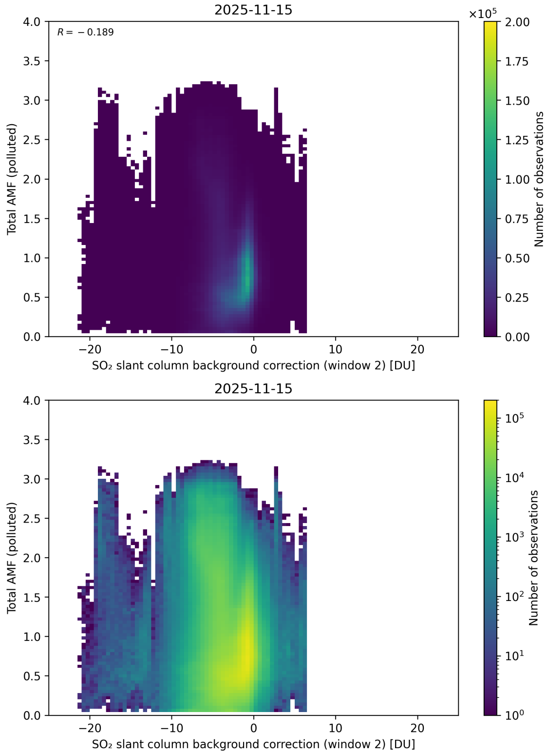
Figure 130: Scatter density plot of “SO 2 slant column background correction (window 2)” against “Total AMF (polluted)” for 2025-11-14 to 2025-11-16.
