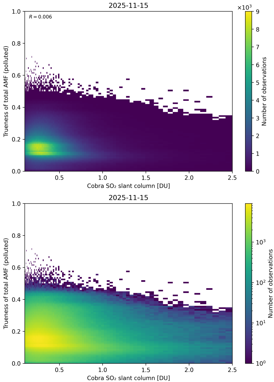
Figure 225: Scatter density plot of “Cobra SO 2 slant column” against “Trueness of total AMF (polluted)” for 2025-11-14 to 2025-11-16.
