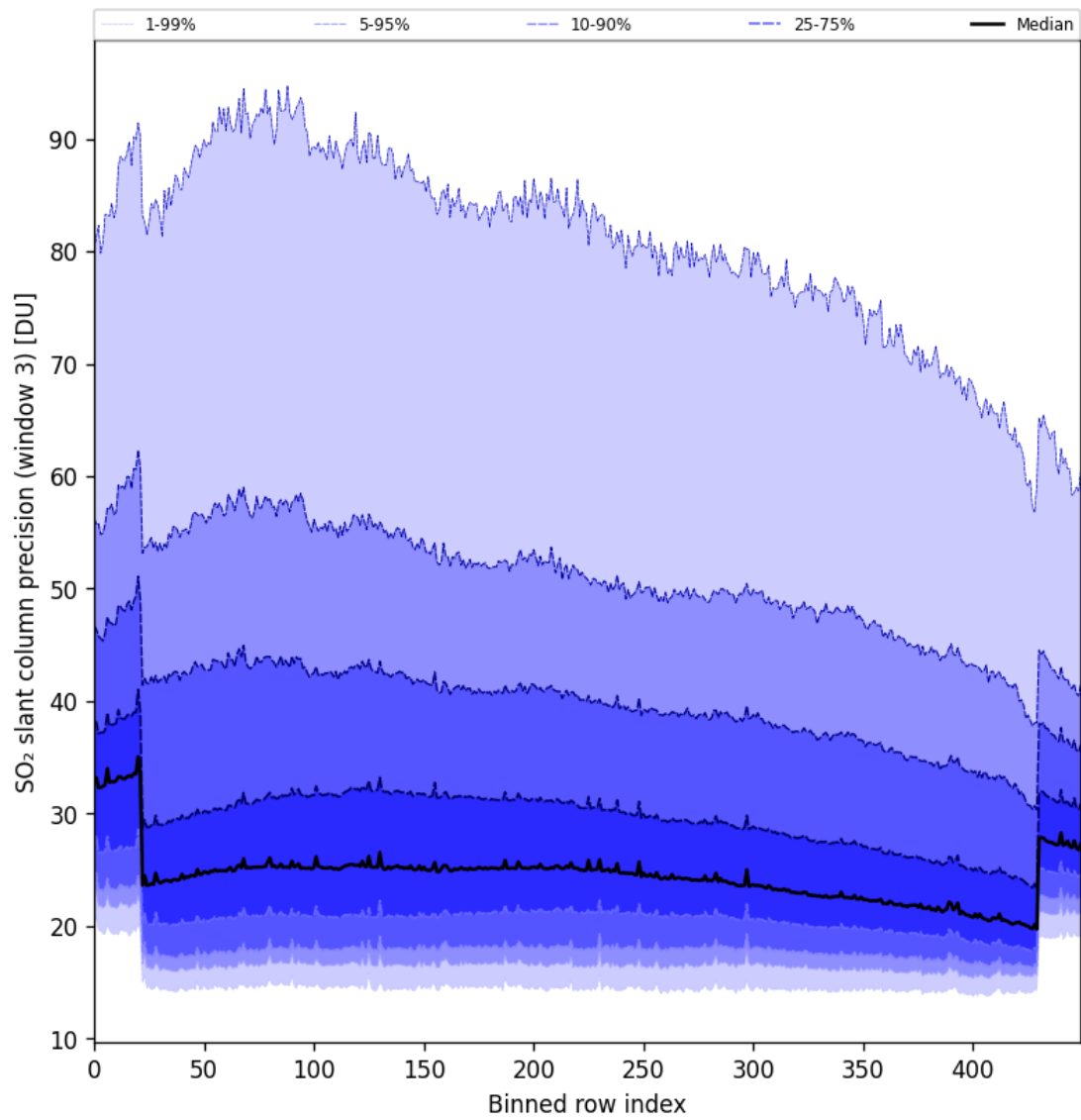
Figure 98: Along track statistics of “SO 2 slant column precision (window 3)” for 2025-11-14 to 2025-11-16
