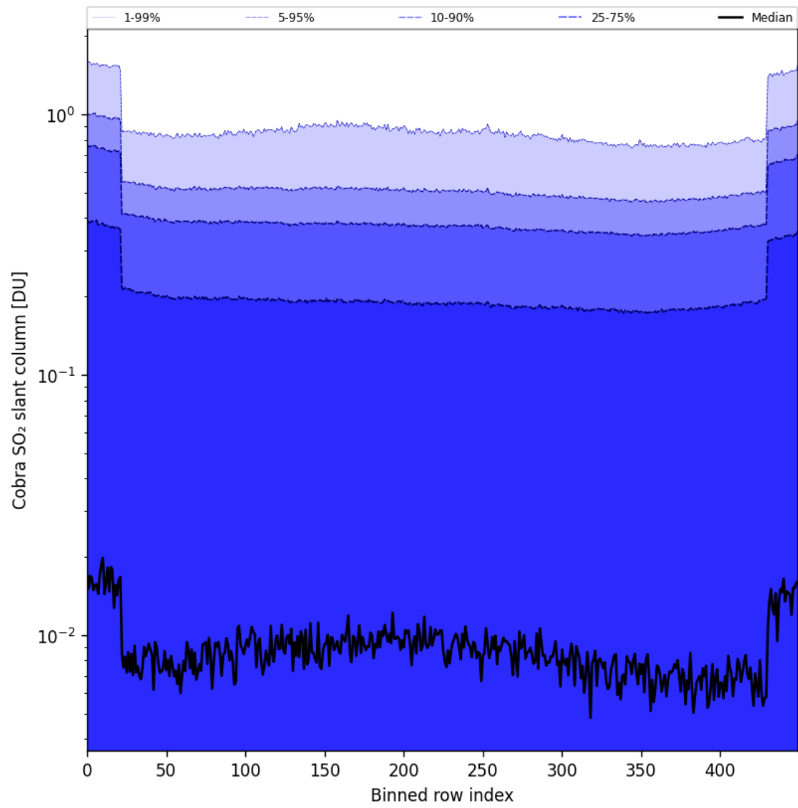
Figure 87: Along track statistics of "Cobra SO 2 slant column" for 2025-11-14 to 2025-11-16
