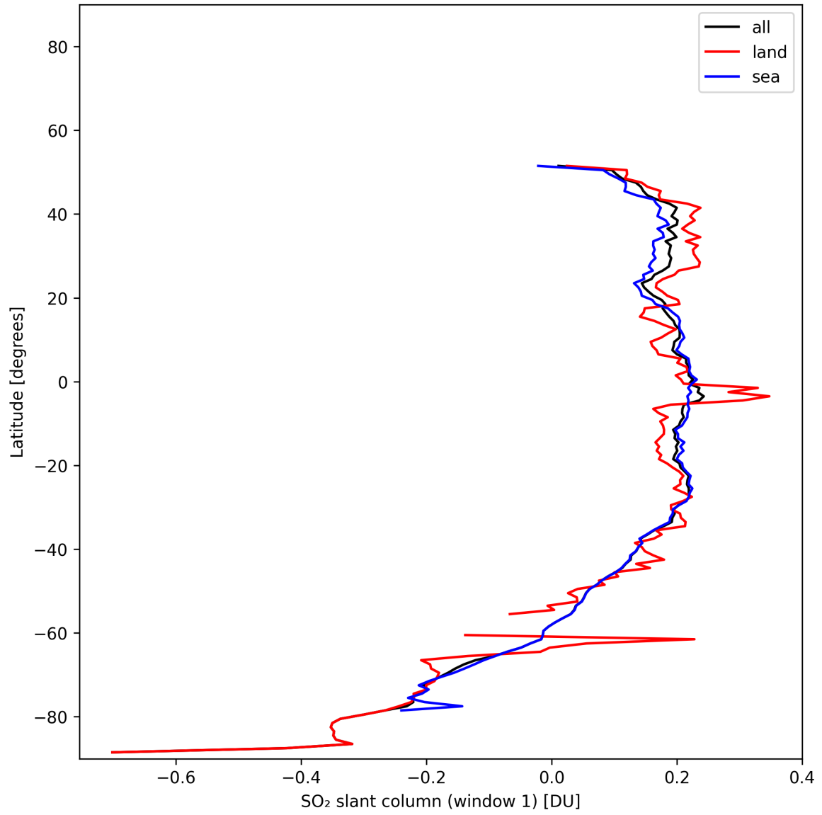
Figure 37: Zonal average of “SO 2 slant column (window 1)” for 2025-11-14 to 2025-11-16.
