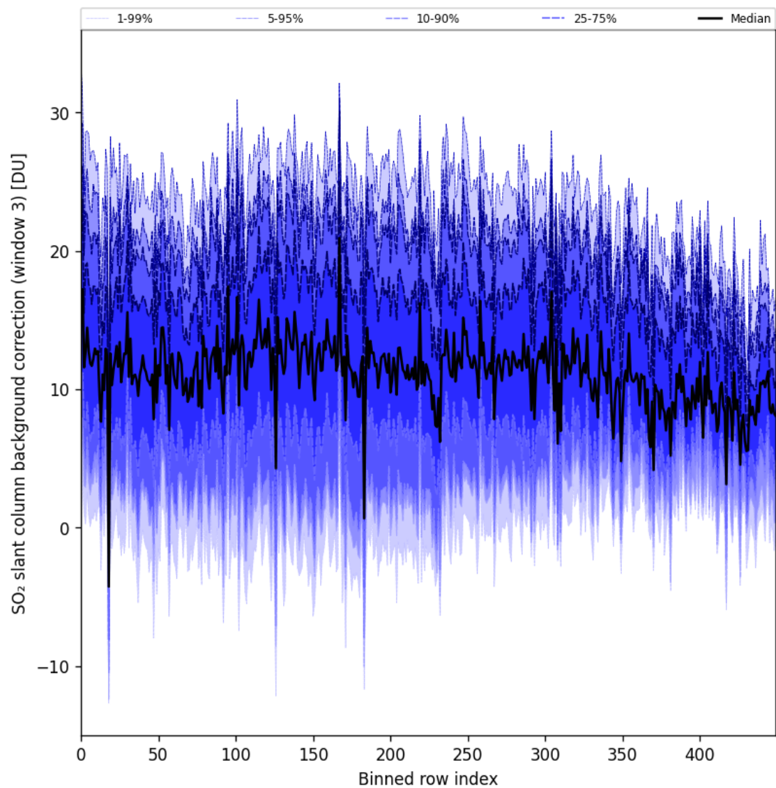
Figure 100: Along track statistics of “SO 2 slant column background correction (window 3)” for 2025-11-14 to 2025-11-16
