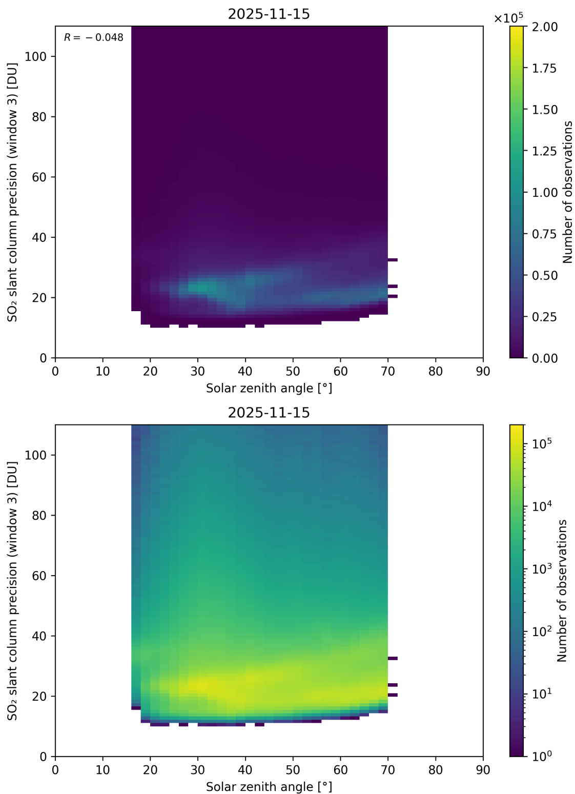
Figure 188: Scatter density plot of “Solar zenith angle” against “SO 2 slant column precision (window 3)” for 2025-11-14 to 2025-11-16.
