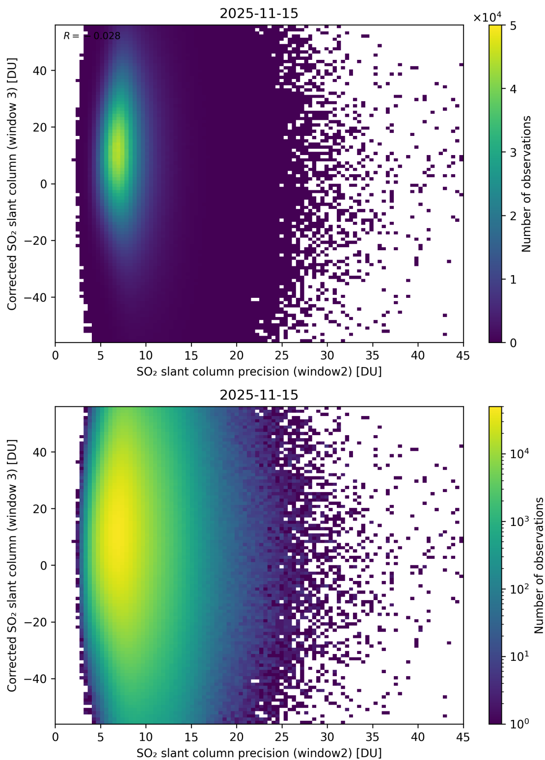
Figure 298: Scatter density plot of “SO 2 slant column precision (window2)” against “Corrected SO 2 slant column (window 3)” for 2025-11-14 to 2025-11-16.
