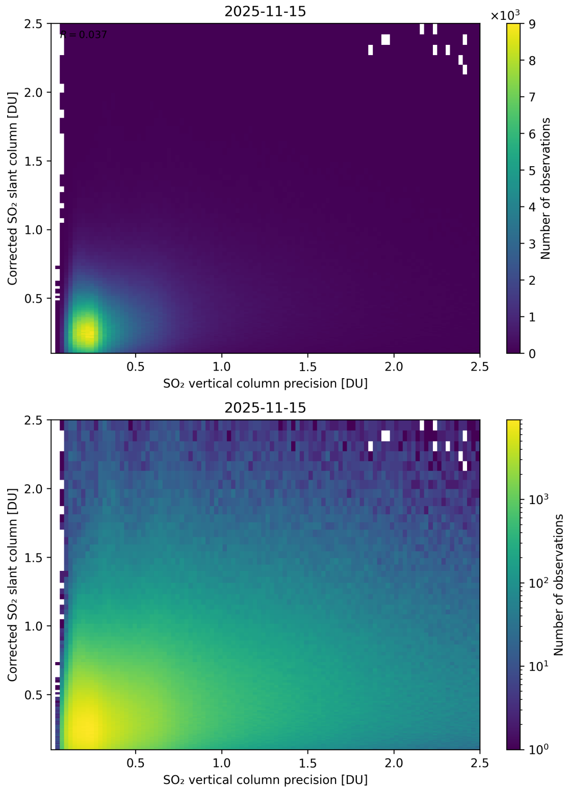
Figure 338: Scatter density plot of “SO 2 vertical column precision” against “Corrected SO 2 slant column” for 2025-11-14 to 2025-11-16.
