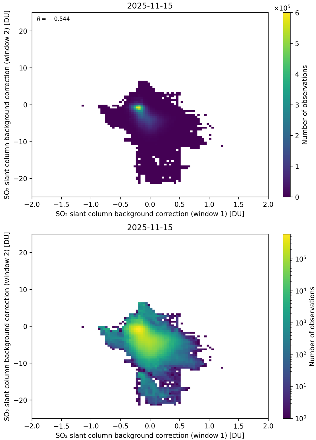
Figure 109: Scatter density plot of “SO 2 slant column background correction (window 1)” against “SO 2 slant column background correction (window 2)” for 2025-11-14 to 2025-11-16.
