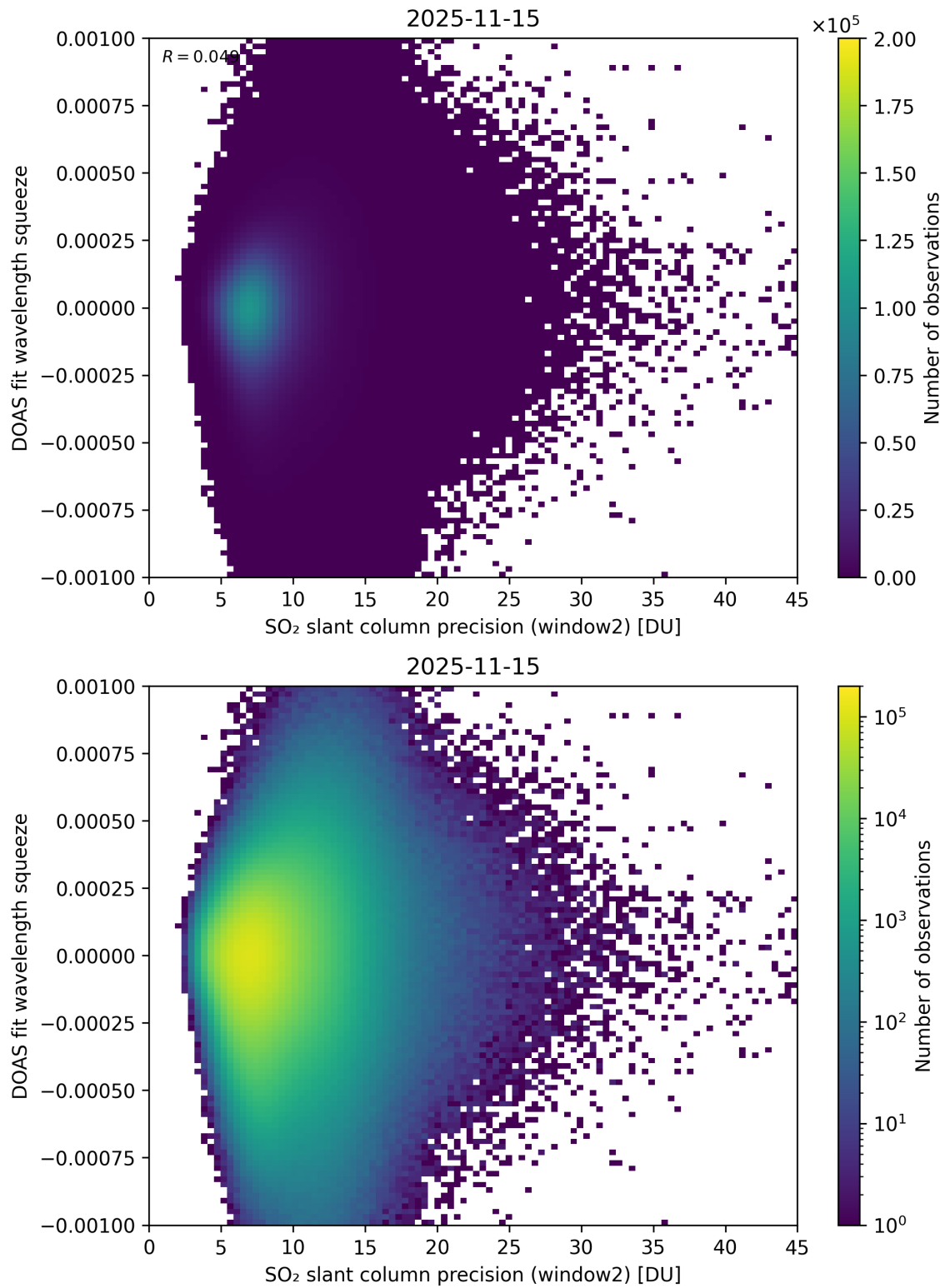
Figure 294: Scatter density plot of “SO 2 slant column precision (window2)” against “DOAS fit wavelength squeeze” for 2025-11-14 to 2025-11-16.
