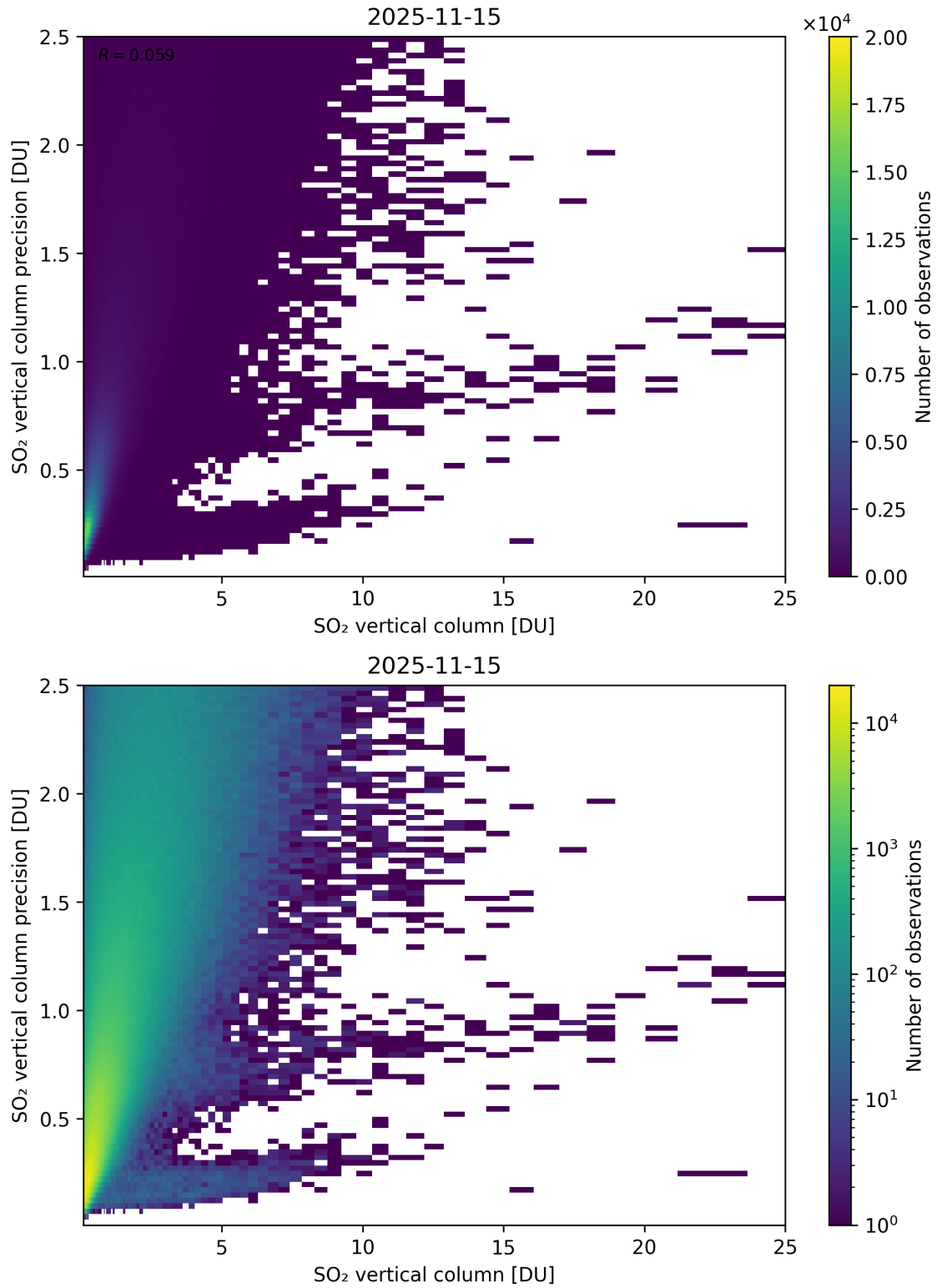
Figure 361: Scatter density plot of “SO 2 vertical column” against “SO 2 vertical column precision” for 2025-11-14 to 2025-11-16.
