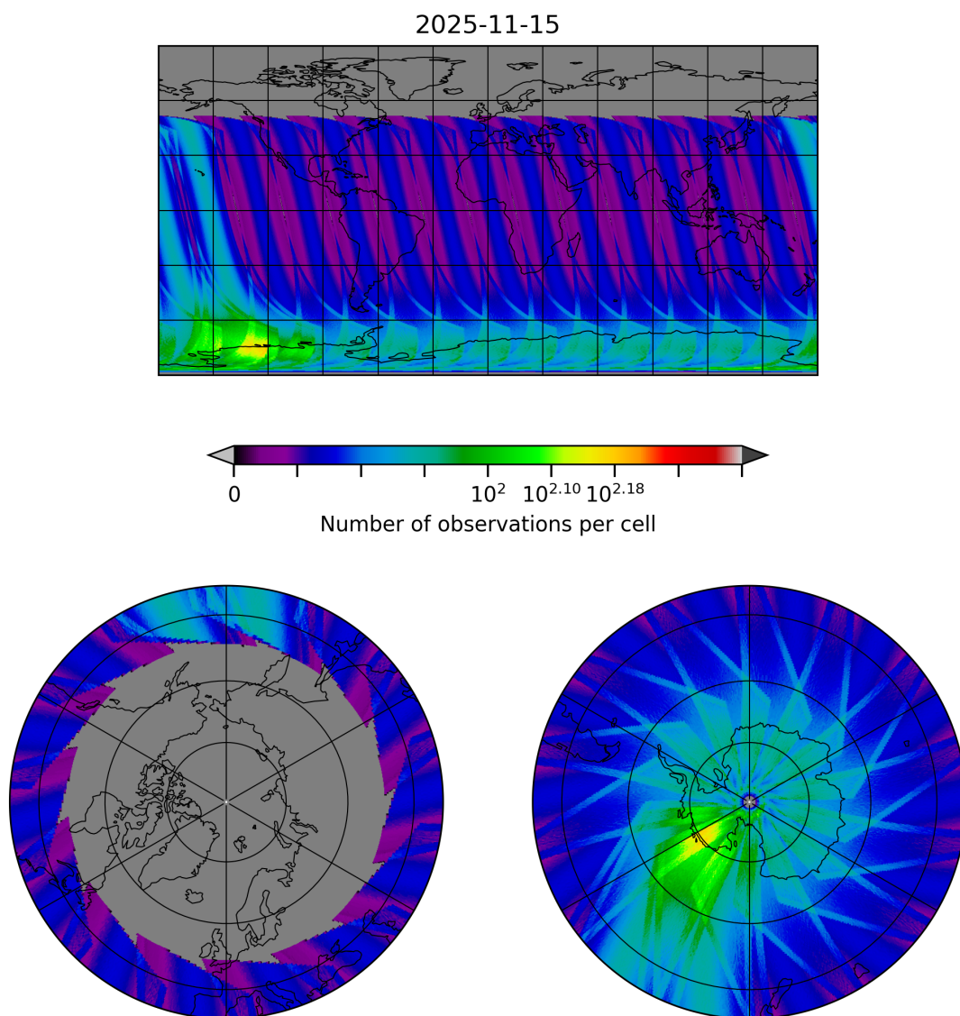
Figure 30: Map of the number of observations for 2025-11-14 to 2025-11-16
