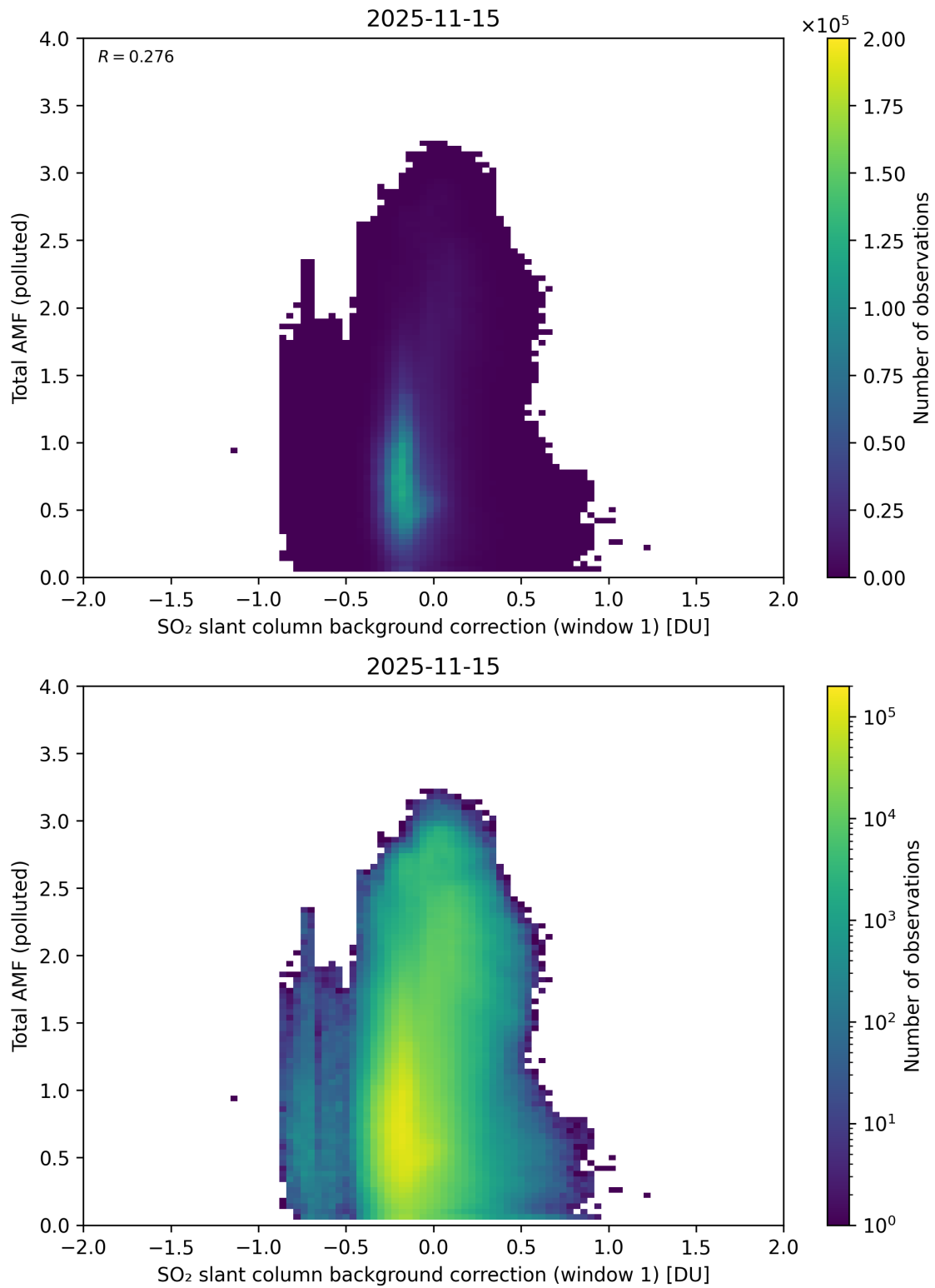
Figure 120: Scatter density plot of “SO 2 slant column background correction (window 1)” against “Total AMF (polluted)” for 2025-11-14 to 2025-11-16.
