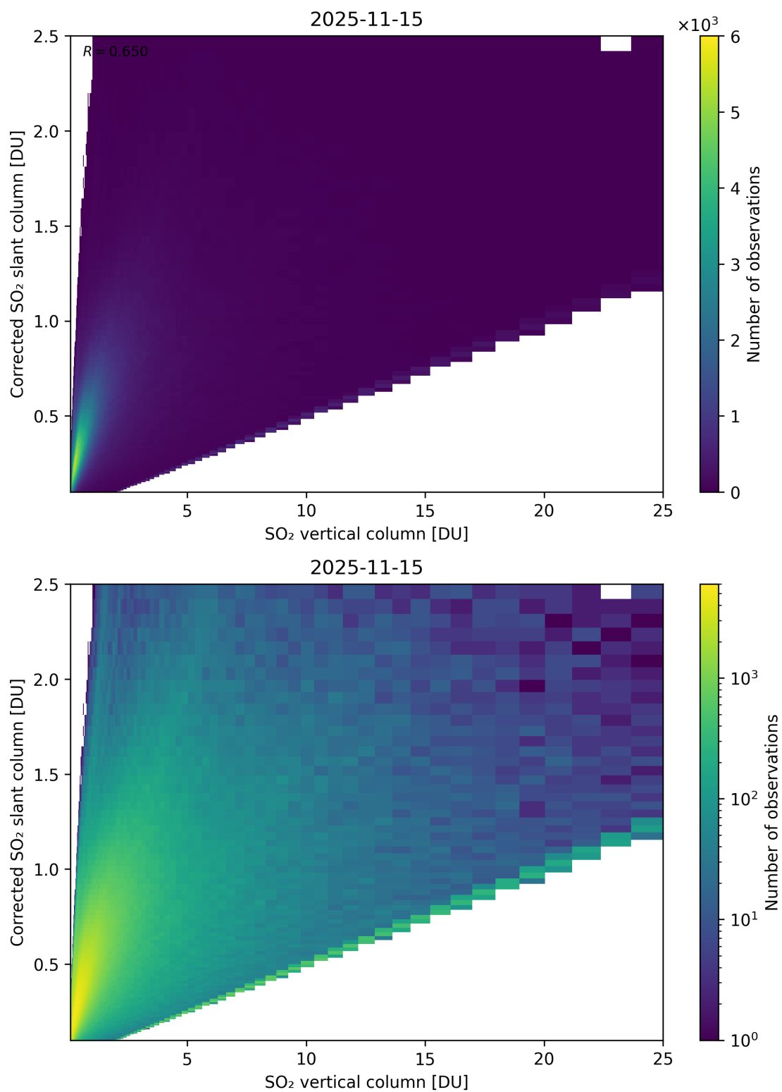
Figure 351: Scatter density plot of “SO 2 vertical column” against “Corrected SO 2 slant column” for 2025-11-14 to 2025-11-16.
