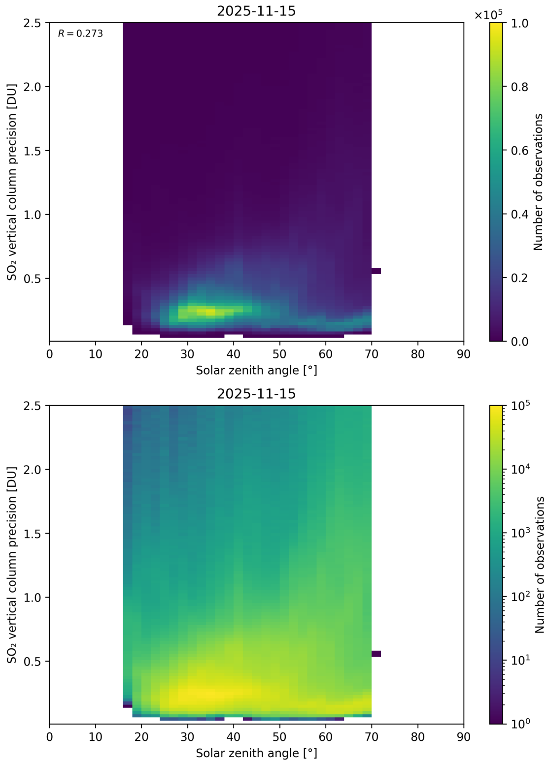
Figure 192: Scatter density plot of “Solar zenith angle” against “SO 2 vertical column precision” for 2025-11-14 to 2025-11-16.
