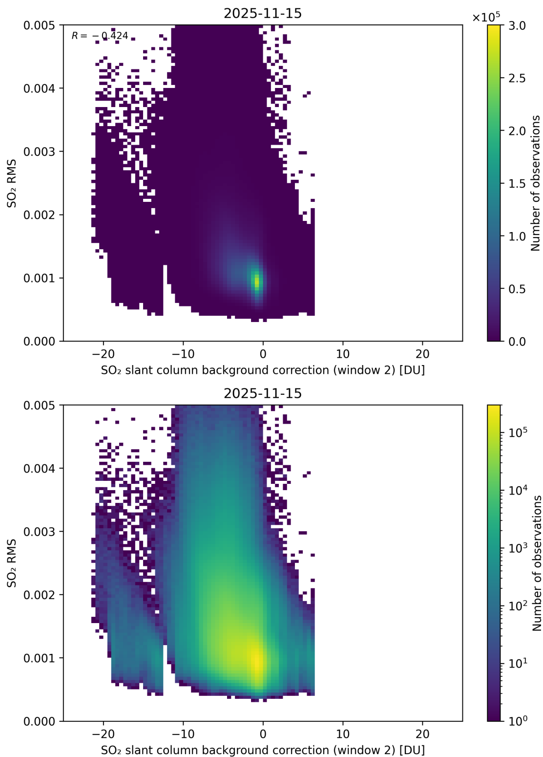
Figure 125: Scatter density plot of “SO 2 slant column background correction (window 2)” against “SO 2 RMS” for 2025-11-14 to 2025-11-16.
