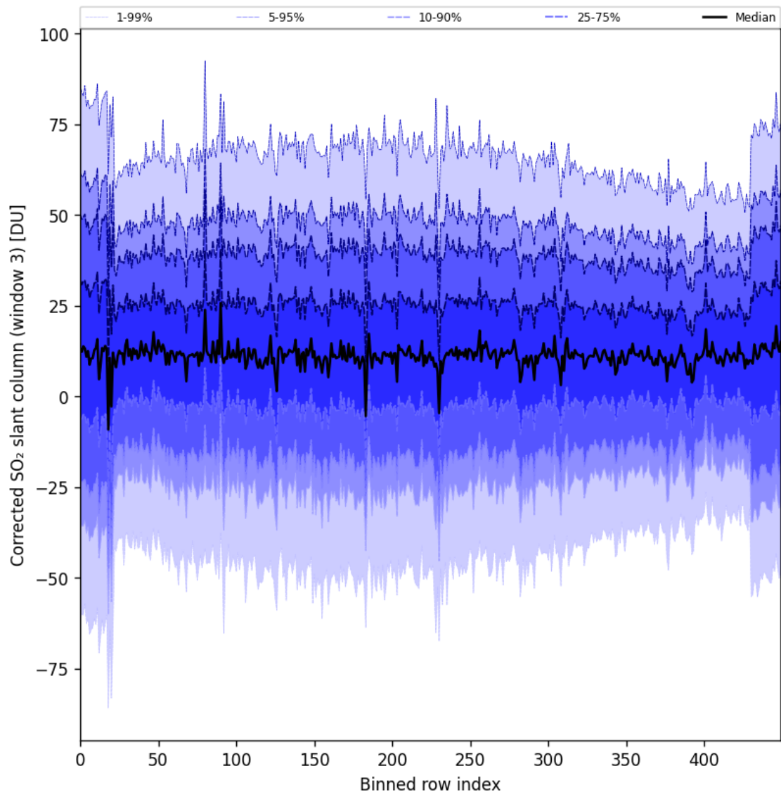
Figure 99: Along track statistics of “Corrected SO 2 slant column (window 3)” for 2025-11-14 to 2025-11-16
