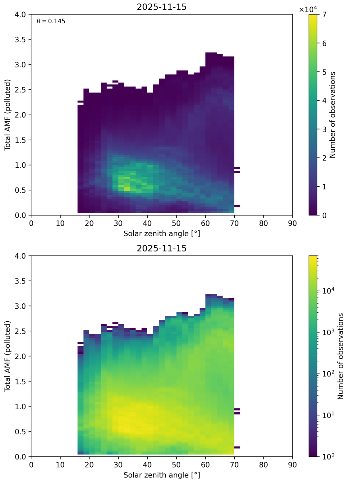
Figure 189: Scatter density plot of “Solar zenith angle” against “Total AMF (polluted)” for 2025-11-14 to 2025-11-16.
