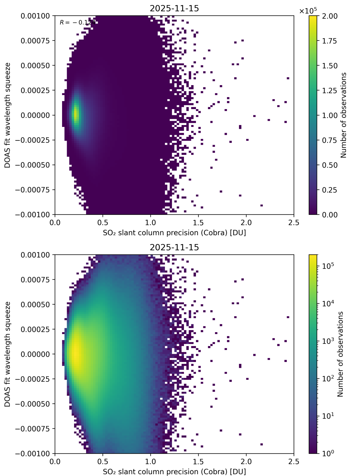
Figure 203: Scatter density plot of “SO 2 slant column precision (Cobra)” against “DOAS fit wavelength squeeze” for 2025-11-14 to 2025-11-16.
