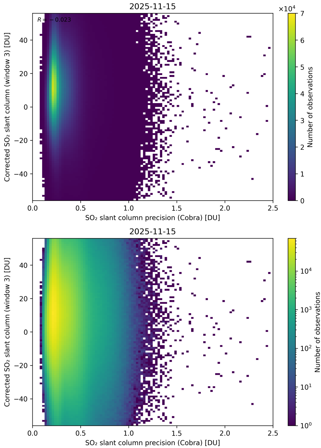
Figure 207: Scatter density plot of “SO 2 slant column precision (Cobra)” against “Corrected SO 2 slant column (window 3)” for 2025-11-14 to 2025-11-16.
