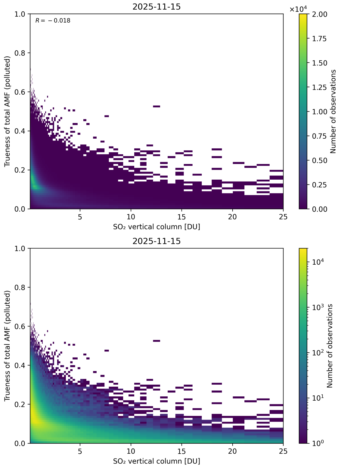
Figure 360: Scatter density plot of “SO 2 vertical column” against “Trueness of total AMF (polluted)” for 2025-11-14 to 2025-11-16.
