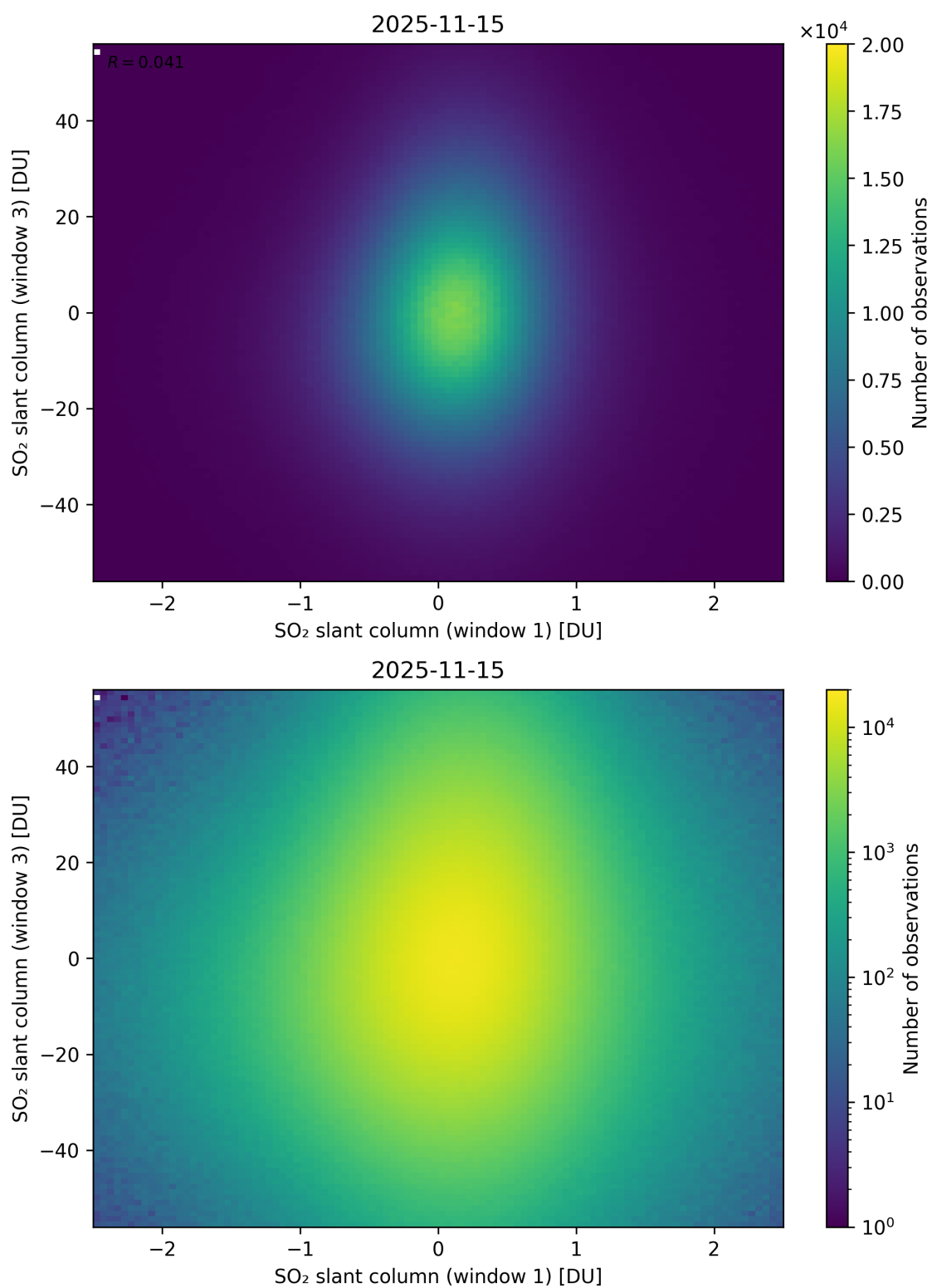
Figure 287: Scatter density plot of “SO 2 slant column (window 1)” against “SO 2 slant column (window 3)” for 2025-11-14 to 2025-11-16.
