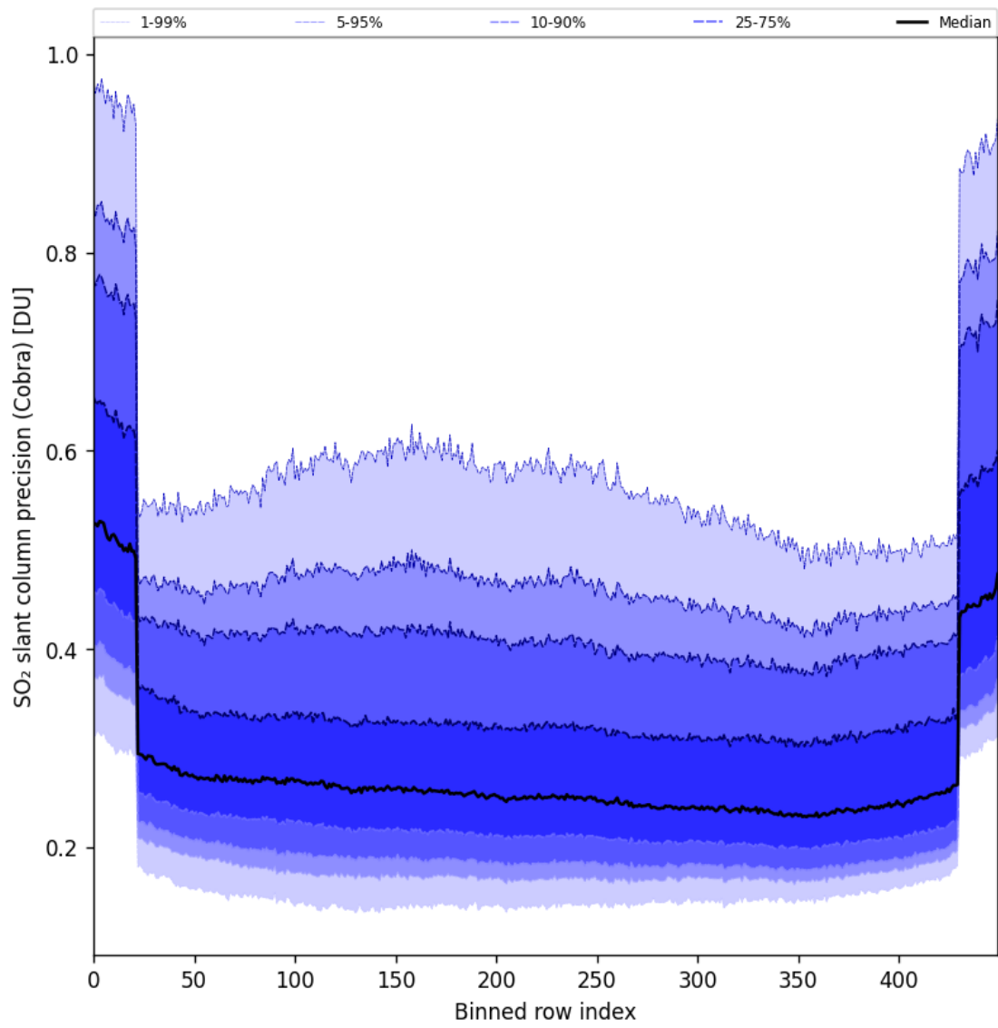
Figure 88: Along track statistics of “SO 2 slant column precision (Cobra)” for 2025-11-14 to 2025-11-16
