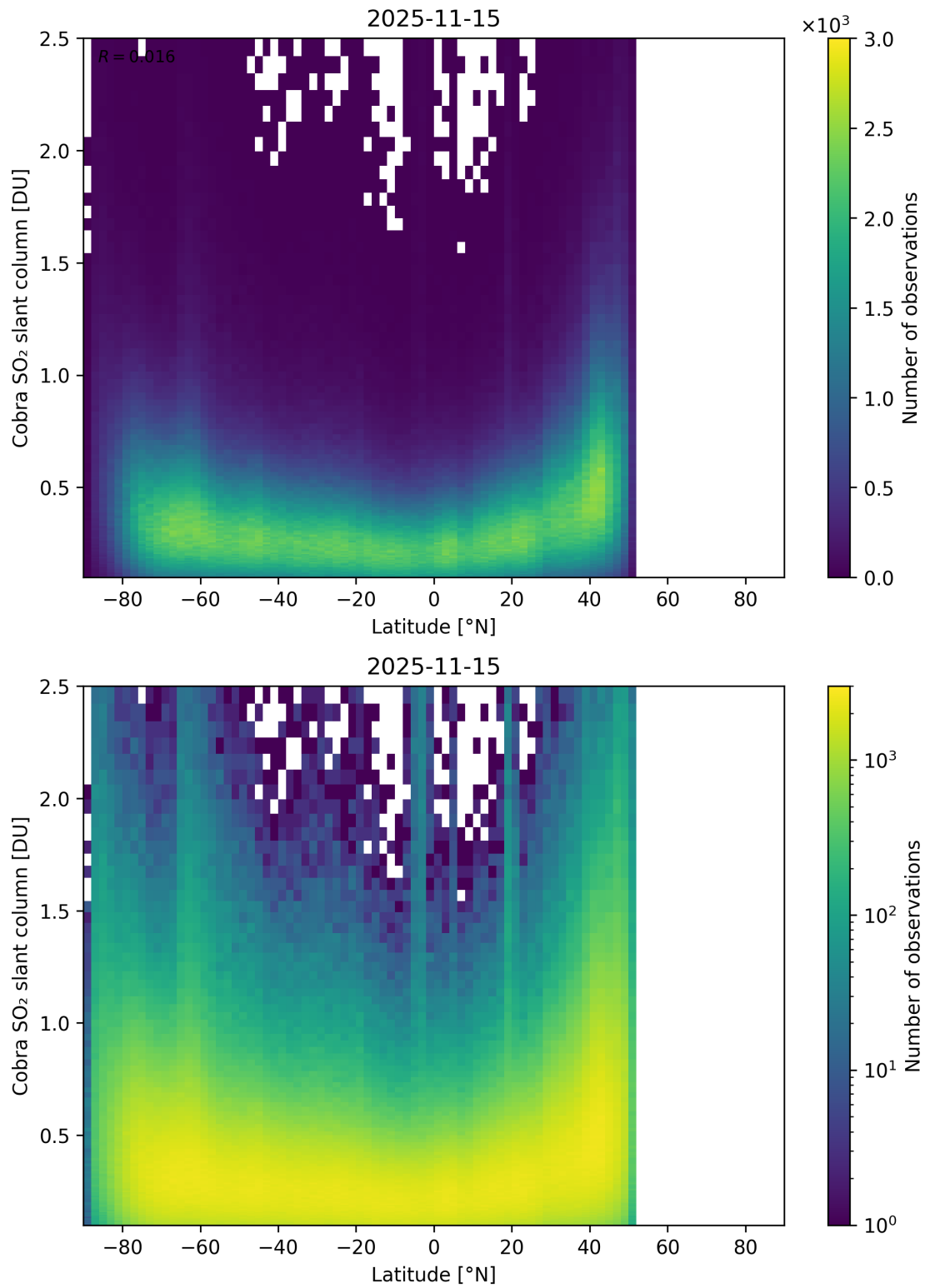
Figure 157: Scatter density plot of “Latitude” against “Cobra SO 2 slant column” for 2025-11-14 to 2025-11-16.
