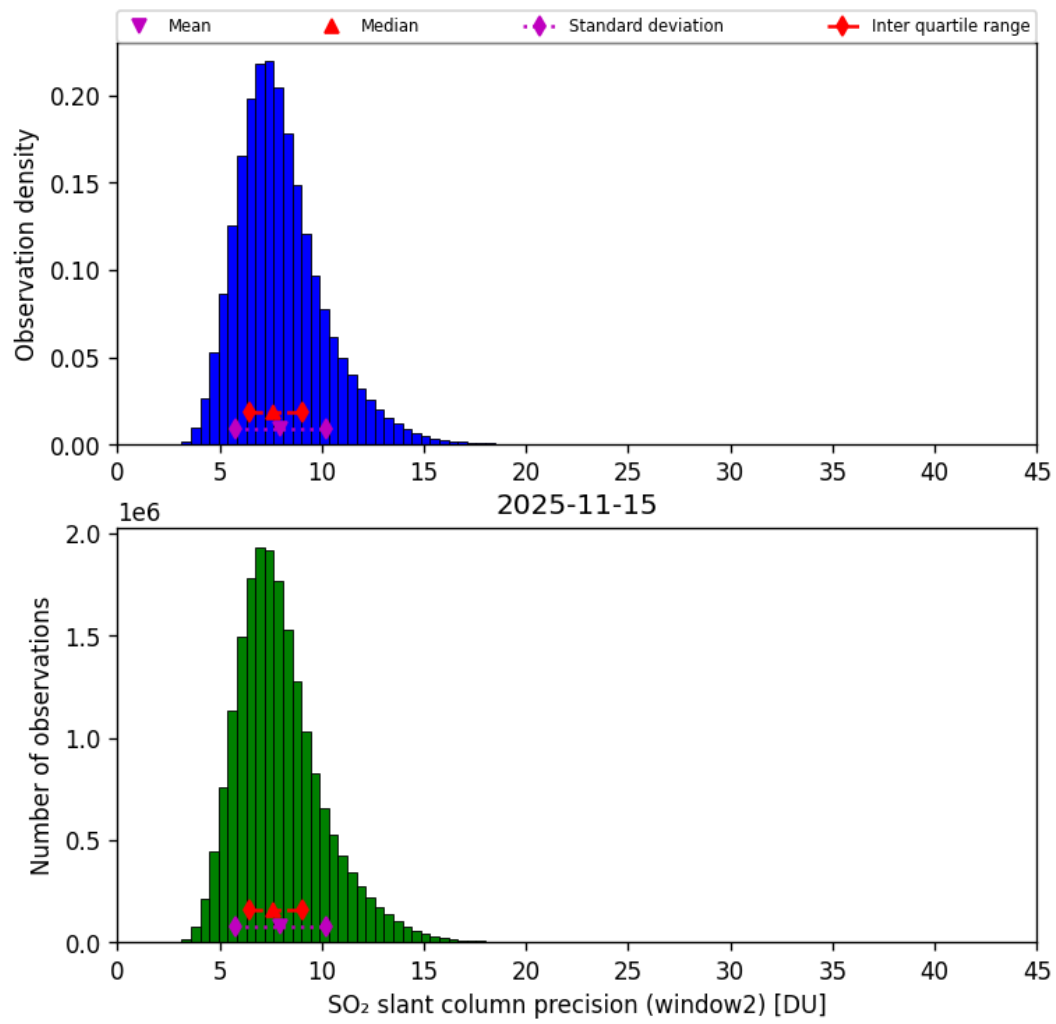
Figure 68: Histogram of “SO 2 slant column precision (window2)” for 2025-11-14 to 2025-11-16
