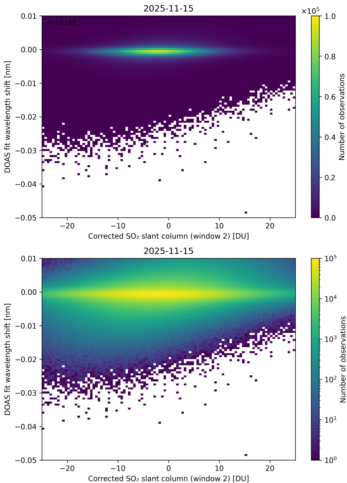
Figure 246: Scatter density plot of “Corrected SO 2 slant column (window 2)” against “DOAS fit wavelength shift” for 2025-11-14 to 2025-11-16.
