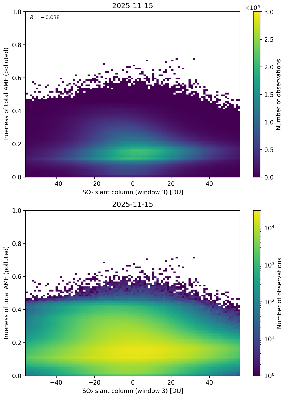
Figure 319: Scatter density plot of “SO 2 slant column (window 3)” against “Trueness of total AMF (polluted)” for 2025-11-14 to 2025-11-16.
