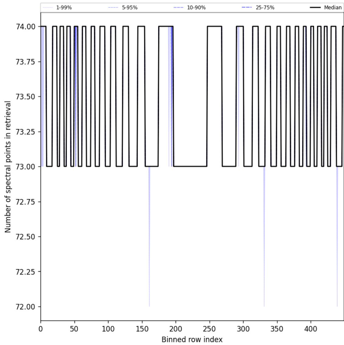
Figure 108: Along track statistics of “Number of spectral points in retrieval” for 2025-11-14 to 2025-11-16
