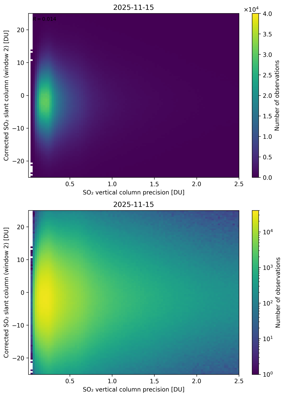
Figure 339: Scatter density plot of “SO 2 vertical column precision” against “Corrected SO 2 slant column (window 2)” for 2025-11-14 to 2025-11-16.
