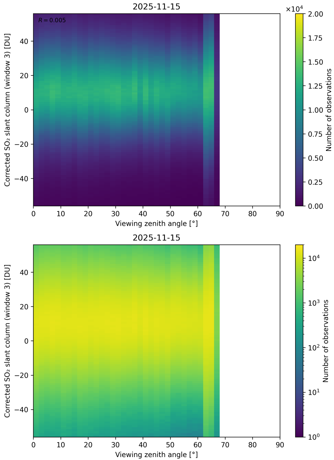
Figure 375: Scatter density plot of “Viewing zenith angle” against “Corrected SO 2 slant column (window 3)” for 2025-11-14 to 2025-11-16.
