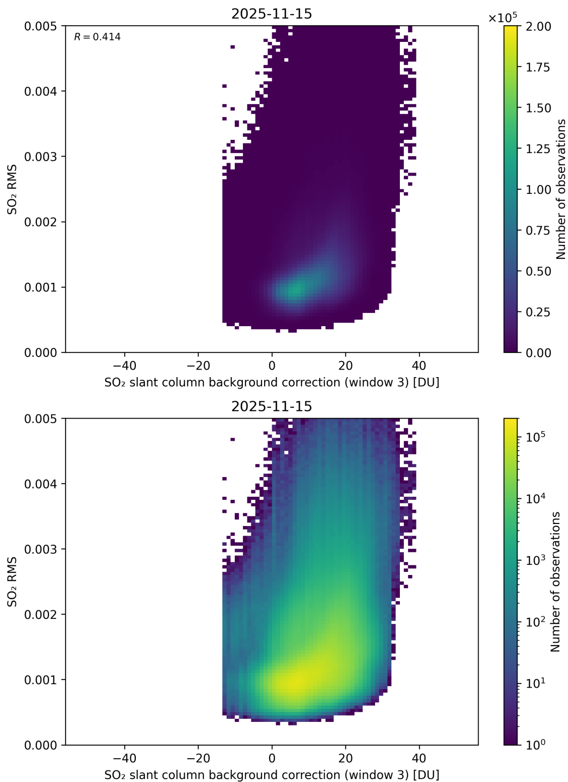
Figure 134: Scatter density plot of “SO 2 slant column background correction (window 3)” against “SO 2 RMS” for 2025-11-14 to 2025-11-16.
