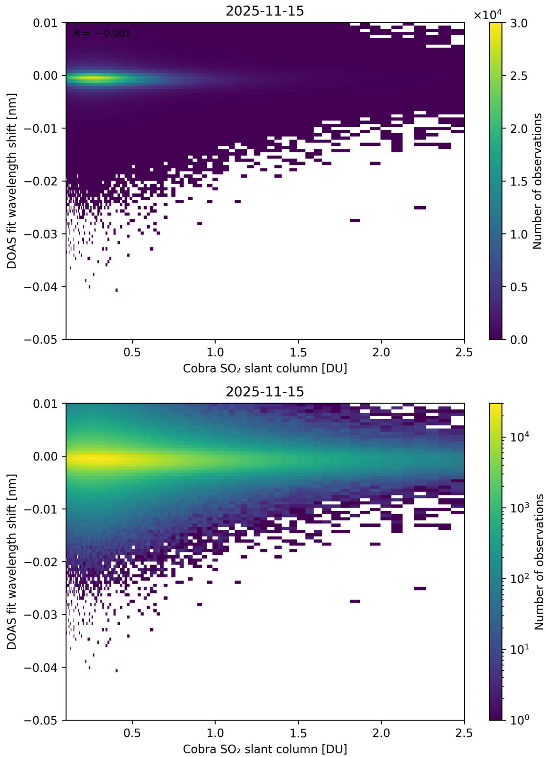
Figure 196: Scatter density plot of “Cobra SO 2 slant column” against “DOAS fit wavelength shift” for 2025-11-14 to 2025-11-16.
