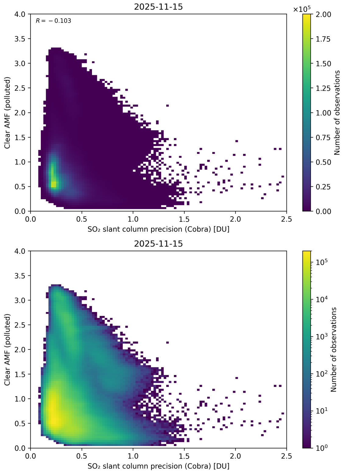
Figure 205: Scatter density plot of “SO 2 slant column precision (Cobra)” against “Clear AMF (polluted)” for 2025-11-14 to 2025-11-16.
