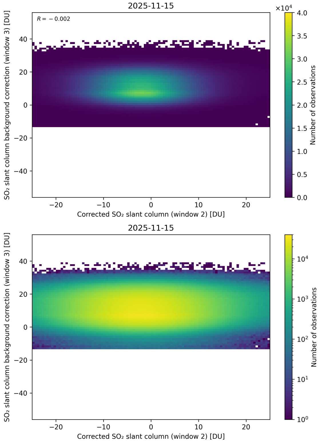
Figure 245: Scatter density plot of “Corrected SO 2 slant column (window 2)” against “SO 2 slant column background correction (window 3)” for 2025-11-14 to 2025-11-16.
