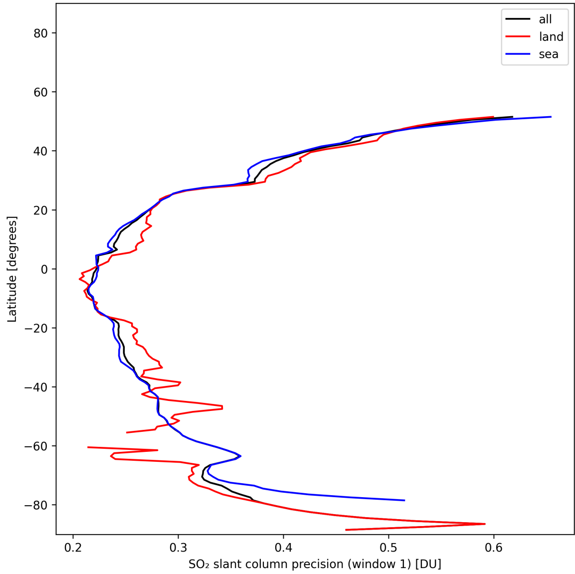
Figure 38: Zonal average of “SO 2 slant column precision (window 1)” for 2025-11-14 to 2025-11-16.
