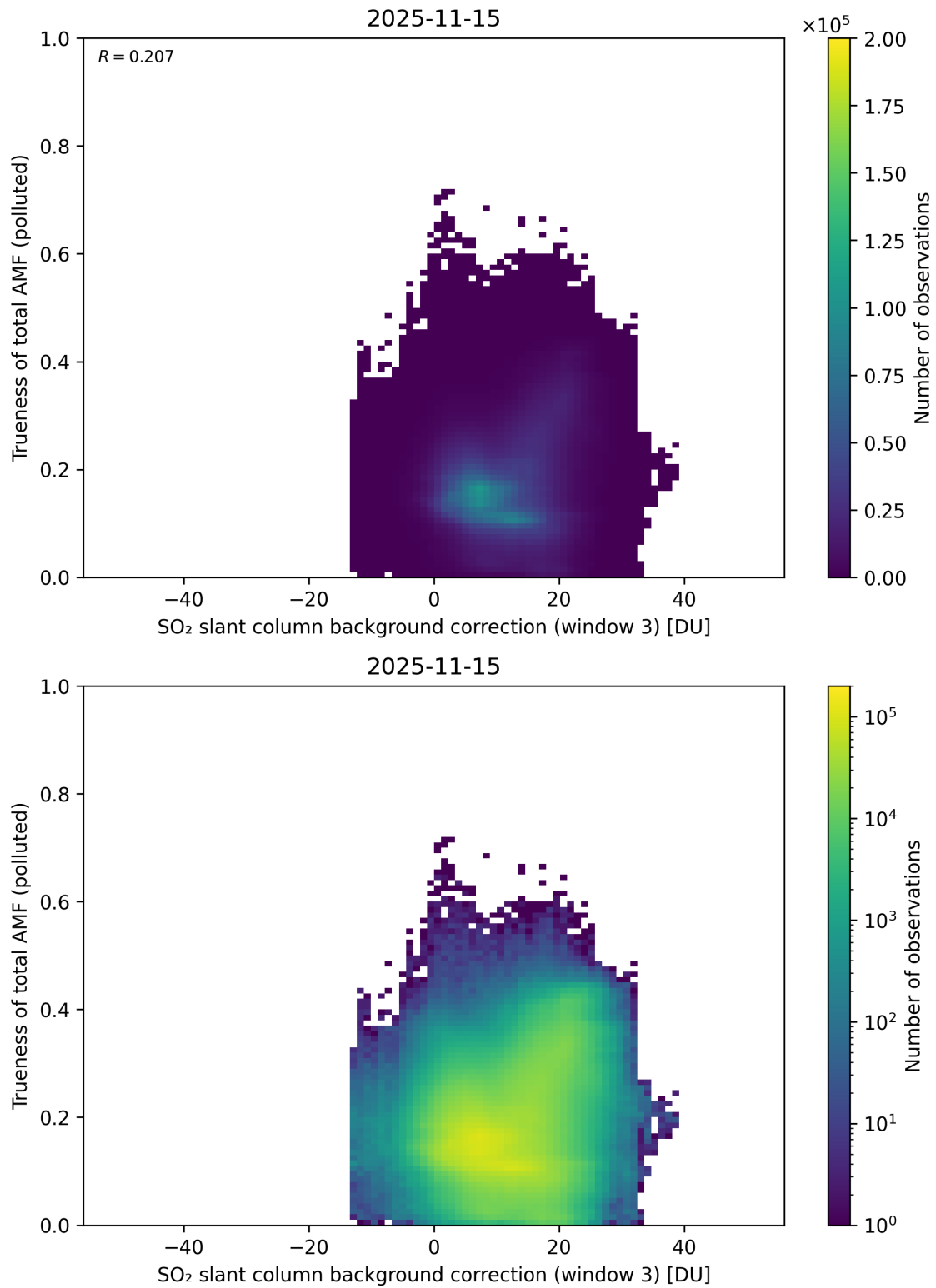
Figure 137: Scatter density plot of “SO 2 slant column background correction (window 3)” against “Trueness of total AMF (polluted)” for 2025-11-14 to 2025-11-16.
