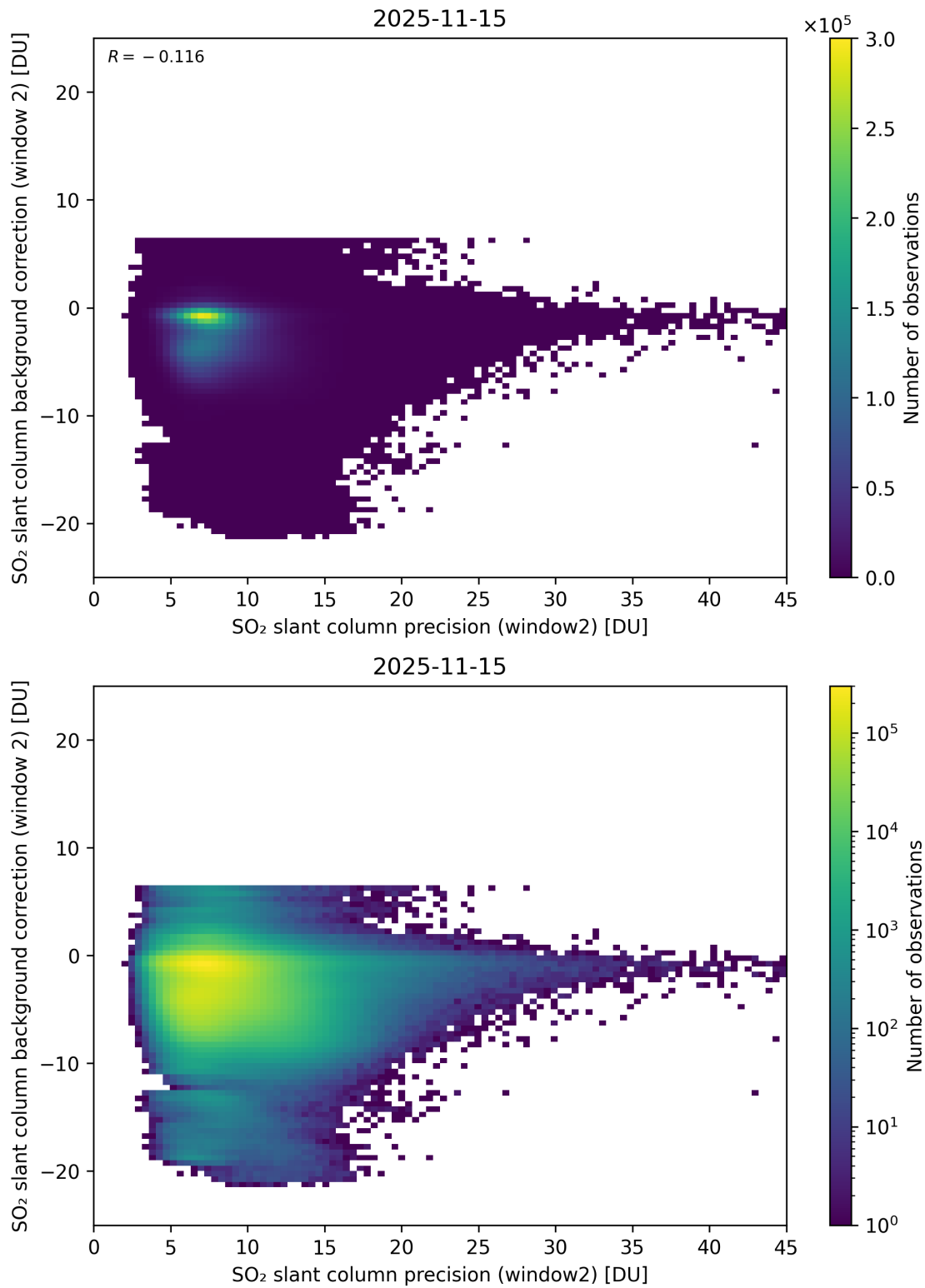
Figure 291: Scatter density plot of “SO 2 slant column precision (window2)” against “SO 2 slant column background correction (window 2)” for 2025-11-14 to 2025-11-16.
