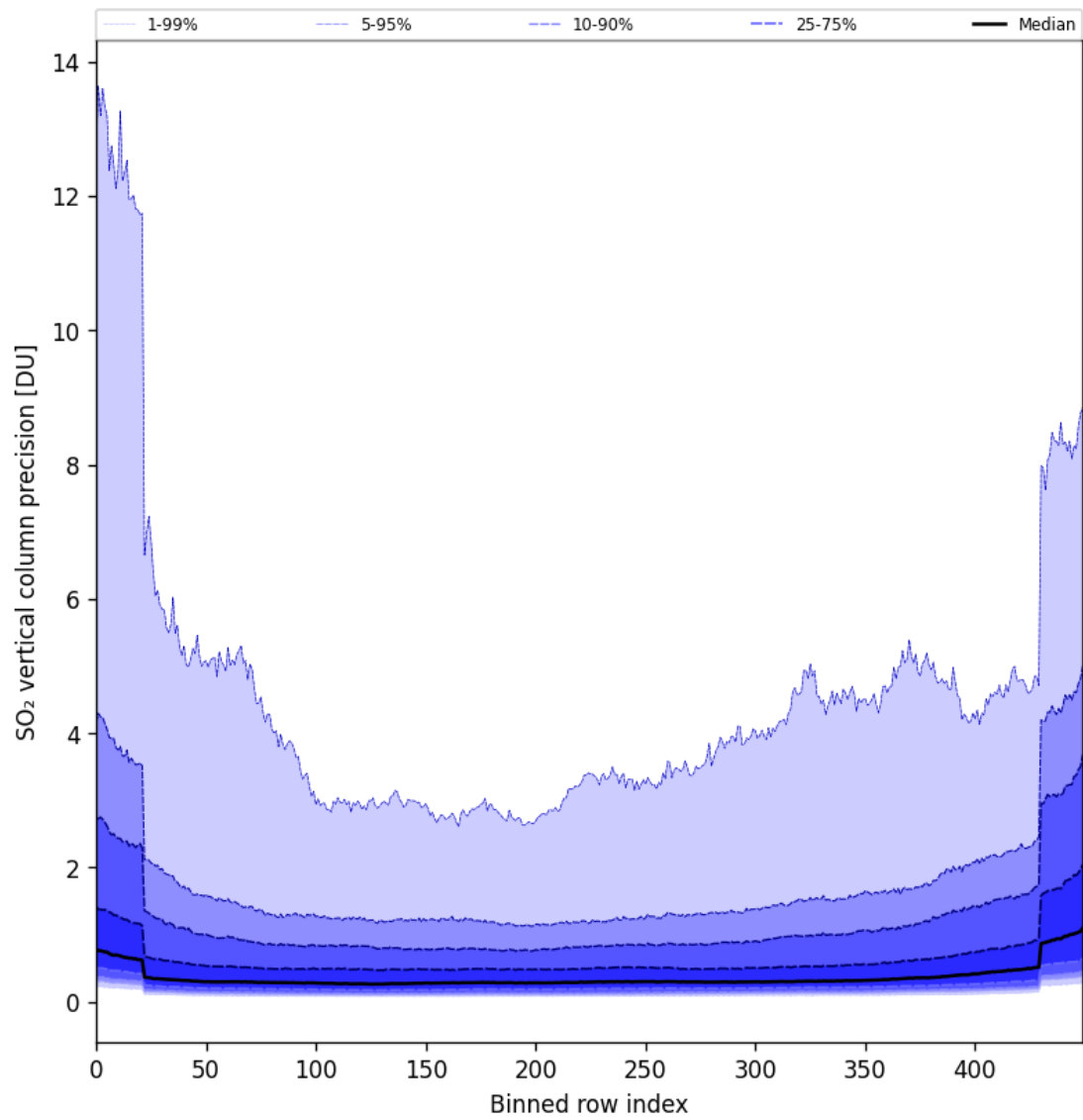
Figure 85: Along track statistics of “SO 2 vertical column precision” for 2025-11-14 to 2025-11-16
