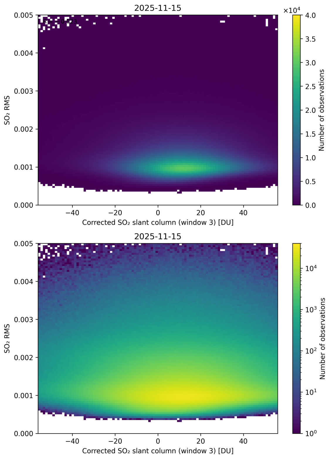
Figure 258: Scatter density plot of “Corrected SO 2 slant column (window 3)” against “SO 2 RMS” for 2025-11-14 to 2025-11-16.
