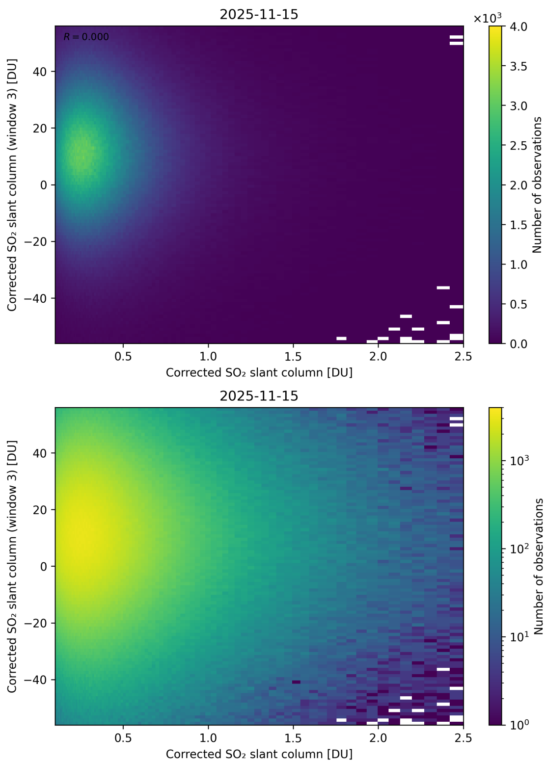
Figure 236: Scatter density plot of “Corrected SO 2 slant column” against “Corrected SO 2 slant column (window 3)” for 2025-11-14 to 2025-11-16.
