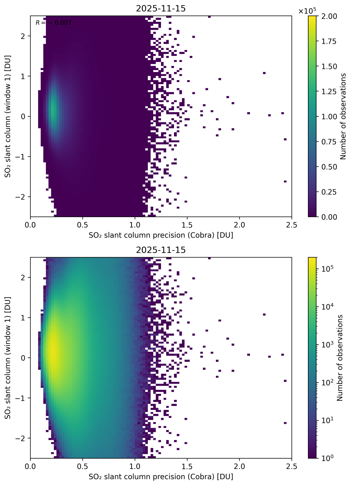
Figure 208: Scatter density plot of “SO 2 slant column precision (Cobra)” against “SO 2 slant column (window 1)” for 2025-11-14 to 2025-11-16.
