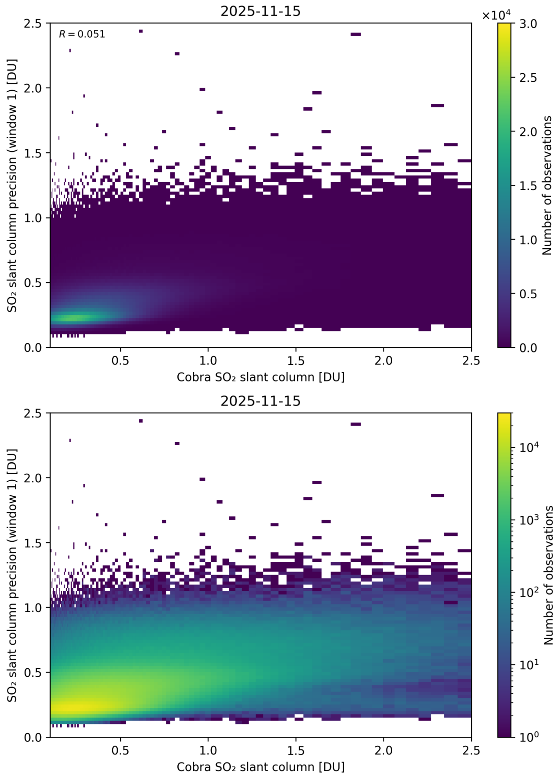
Figure 220: Scatter density plot of “Cobra SO 2 slant column” against “SO 2 slant column precision (window 1)” for 2025-11-14 to 2025-11-16.
