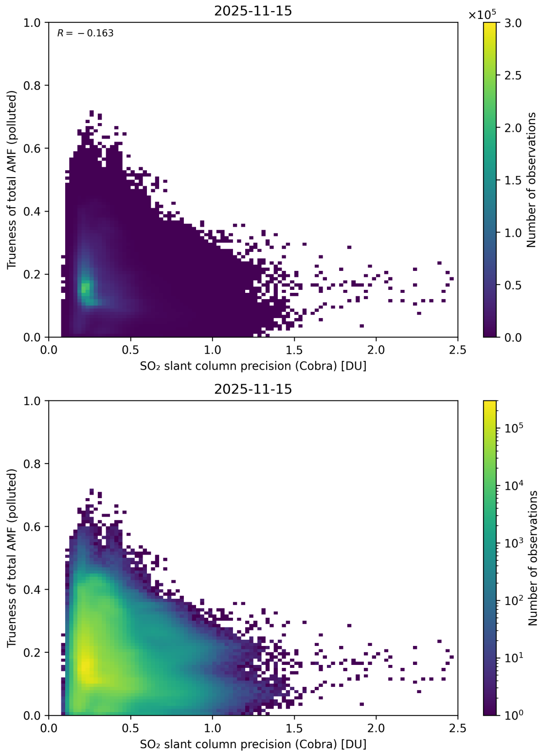
Figure 214: Scatter density plot of “SO 2 slant column precision (Cobra)” against “Trueness of total AMF (polluted)” for 2025-11-14 to 2025-11-16.
