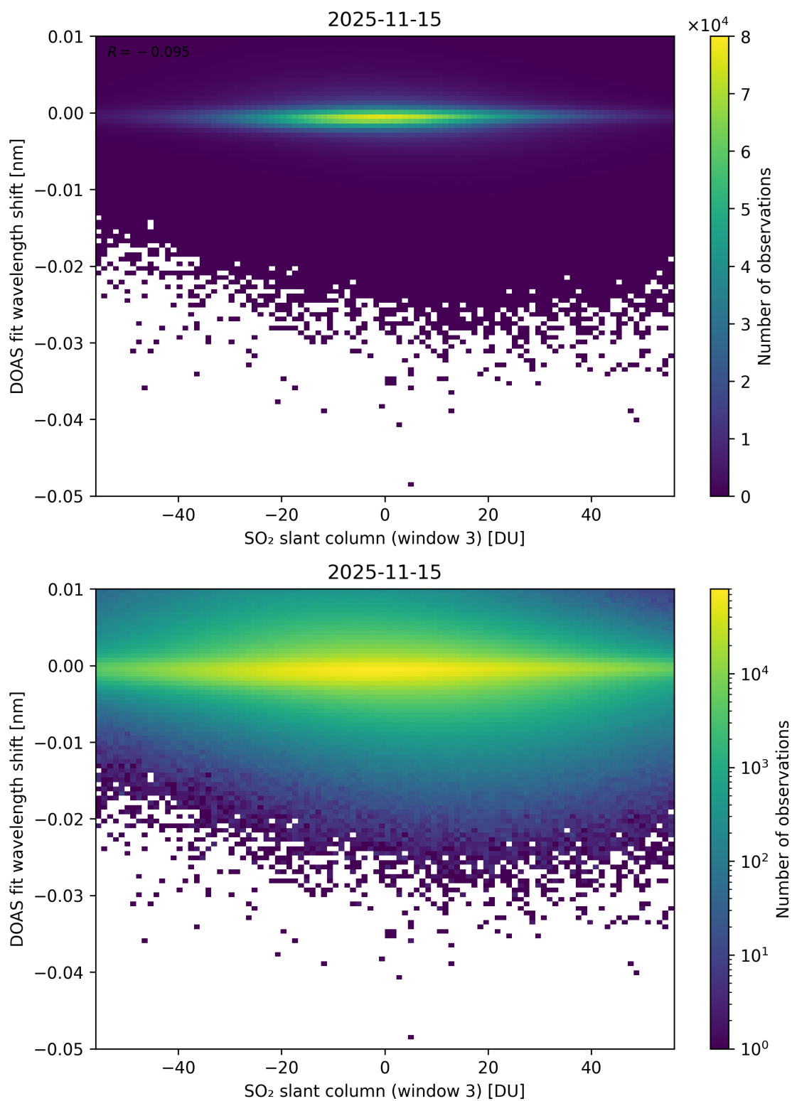
Figure 304: Scatter density plot of “SO 2 slant column (window 3)” against “DOAS fit wavelength shift” for 2025-11-14 to 2025-11-16.
