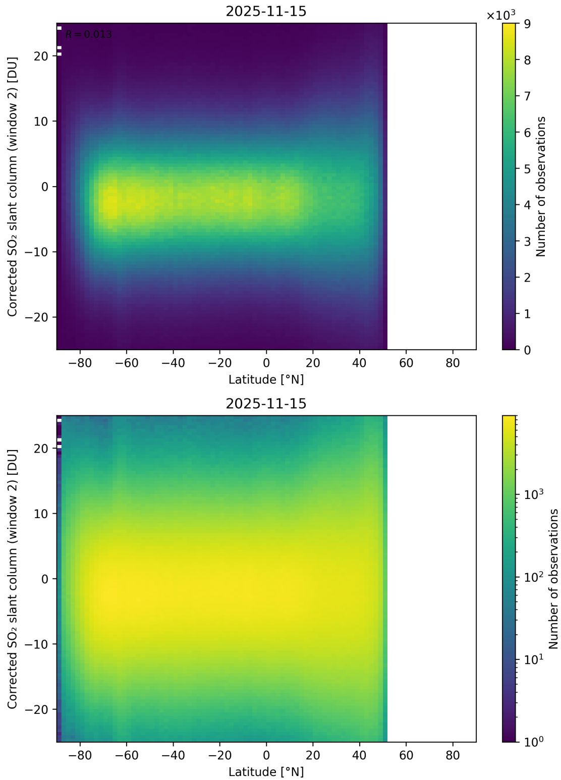
Figure 160: Scatter density plot of “Latitude” against “Corrected SO 2 slant column (window 2)” for 2025-11-14 to 2025-11-16.
