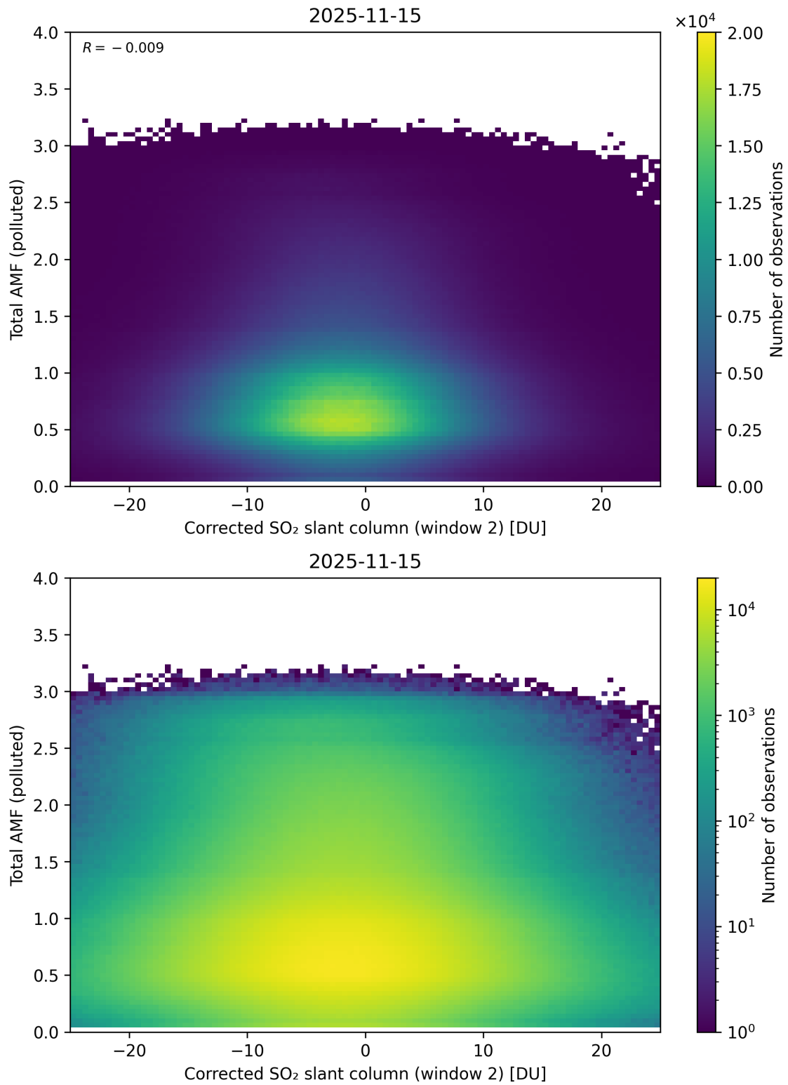
Figure 253: Scatter density plot of “Corrected SO 2 slant column (window 2)” against “Total AMF (polluted)” for 2025-11-14 to 2025-11-16.
