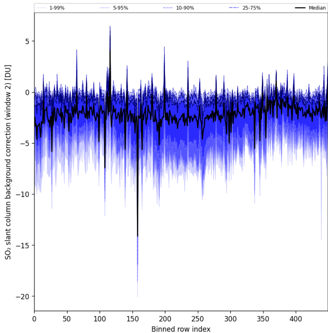
Figure 96: Along track statistics of “SO 2 slant column background correction (window 2)” for 2025-11-14 to 2025-11-16
