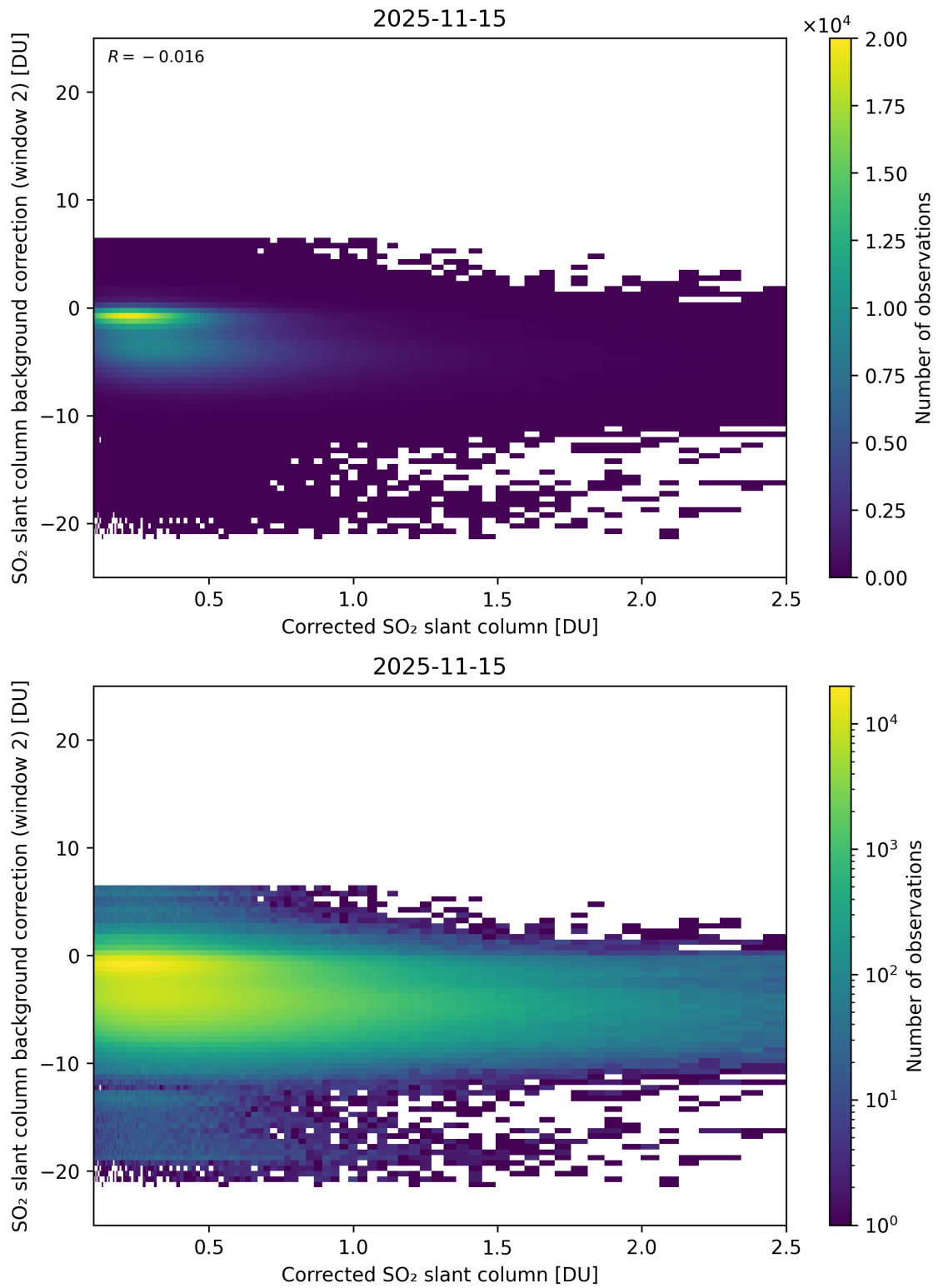
Figure 227: Scatter density plot of “Corrected SO 2 slant column” against “SO 2 slant column background correction (window 2)” for 2025-11-14 to 2025-11-16.
