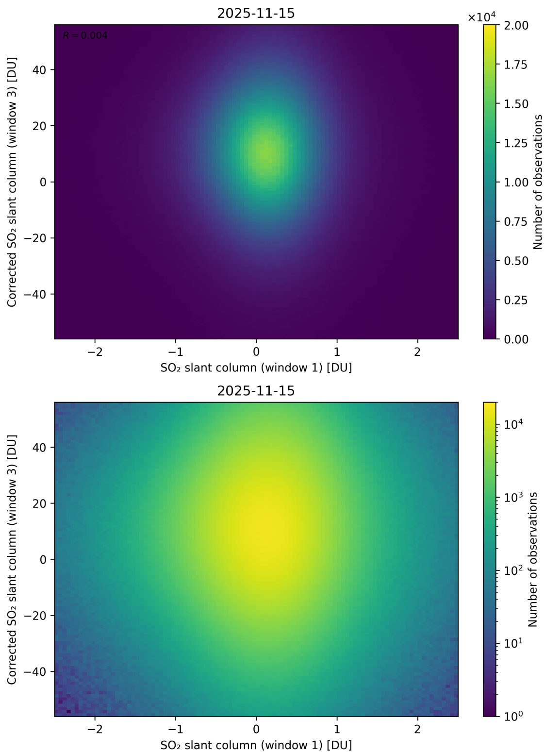
Figure 284: Scatter density plot of “SO 2 slant column (window 1)” against “Corrected SO 2 slant column (window 3)” for 2025-11-14 to 2025-11-16.
