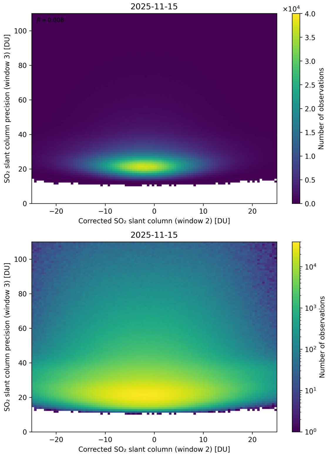
Figure 252: Scatter density plot of “Corrected SO 2 slant column (window 2)” against “SO 2 slant column precision (window 3)” for 2025-11-14 to 2025-11-16.
