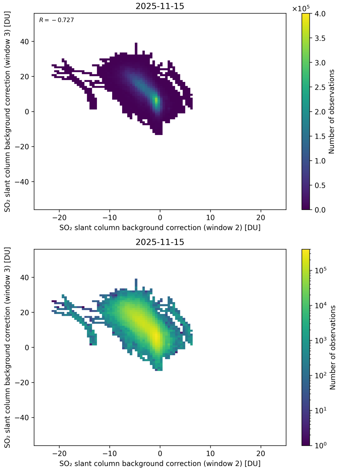
Figure 122: Scatter density plot of “SO 2 slant column background correction (window 2)” against “SO 2 slant column background correction (window 3)” for 2025-11-14 to 2025-11-16.
