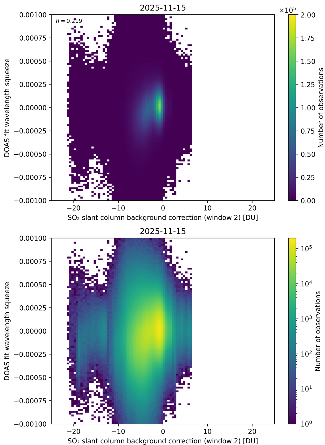
Figure 124: Scatter density plot of “SO 2 slant column background correction (window 2)” against “DOAS fit wavelength squeeze” for 2025-11-14 to 2025-11-16.
