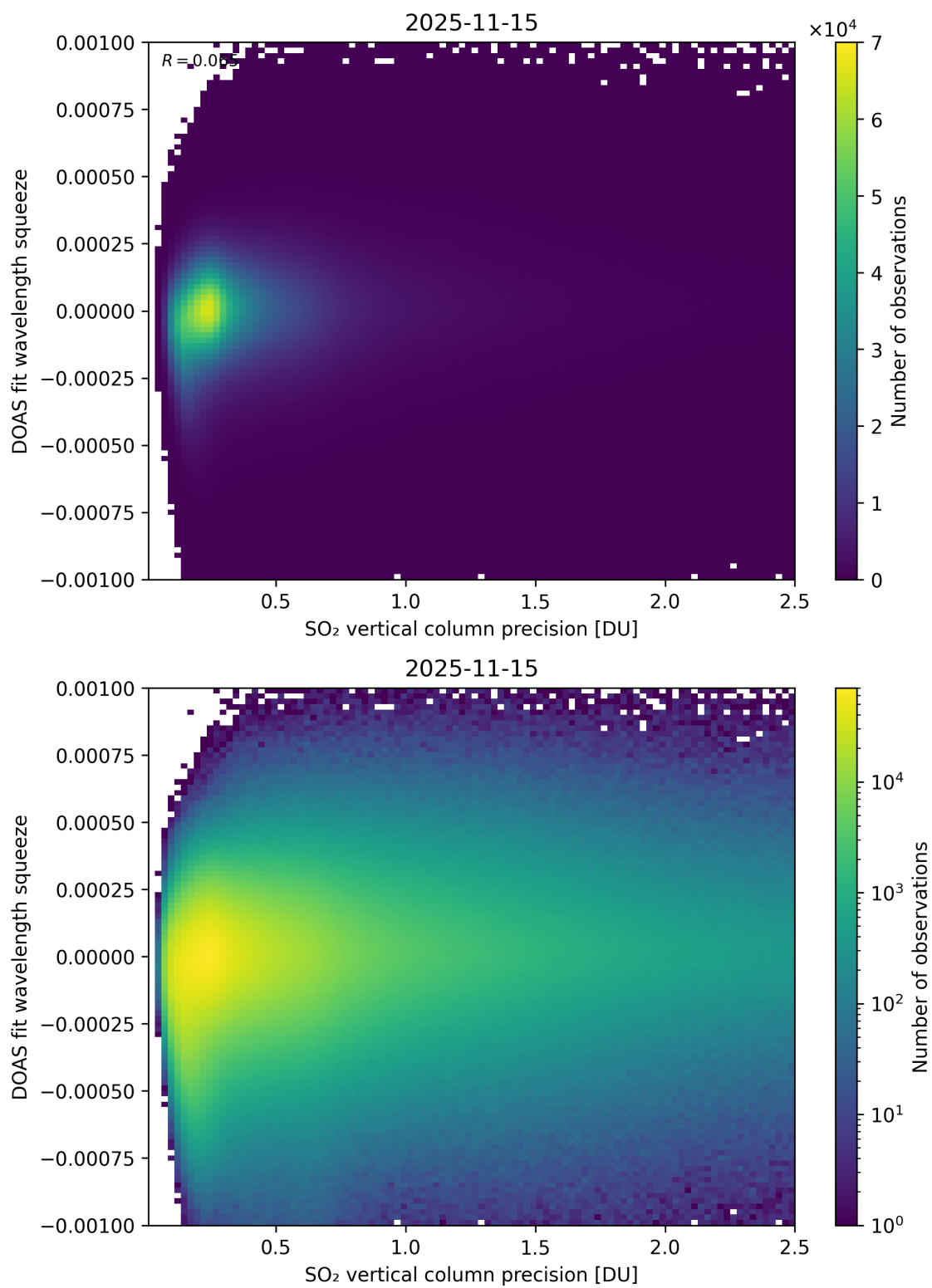
Figure 333: Scatter density plot of “SO 2 vertical column precision” against “DOAS fit wavelength squeeze” for 2025-11-14 to 2025-11-16.
