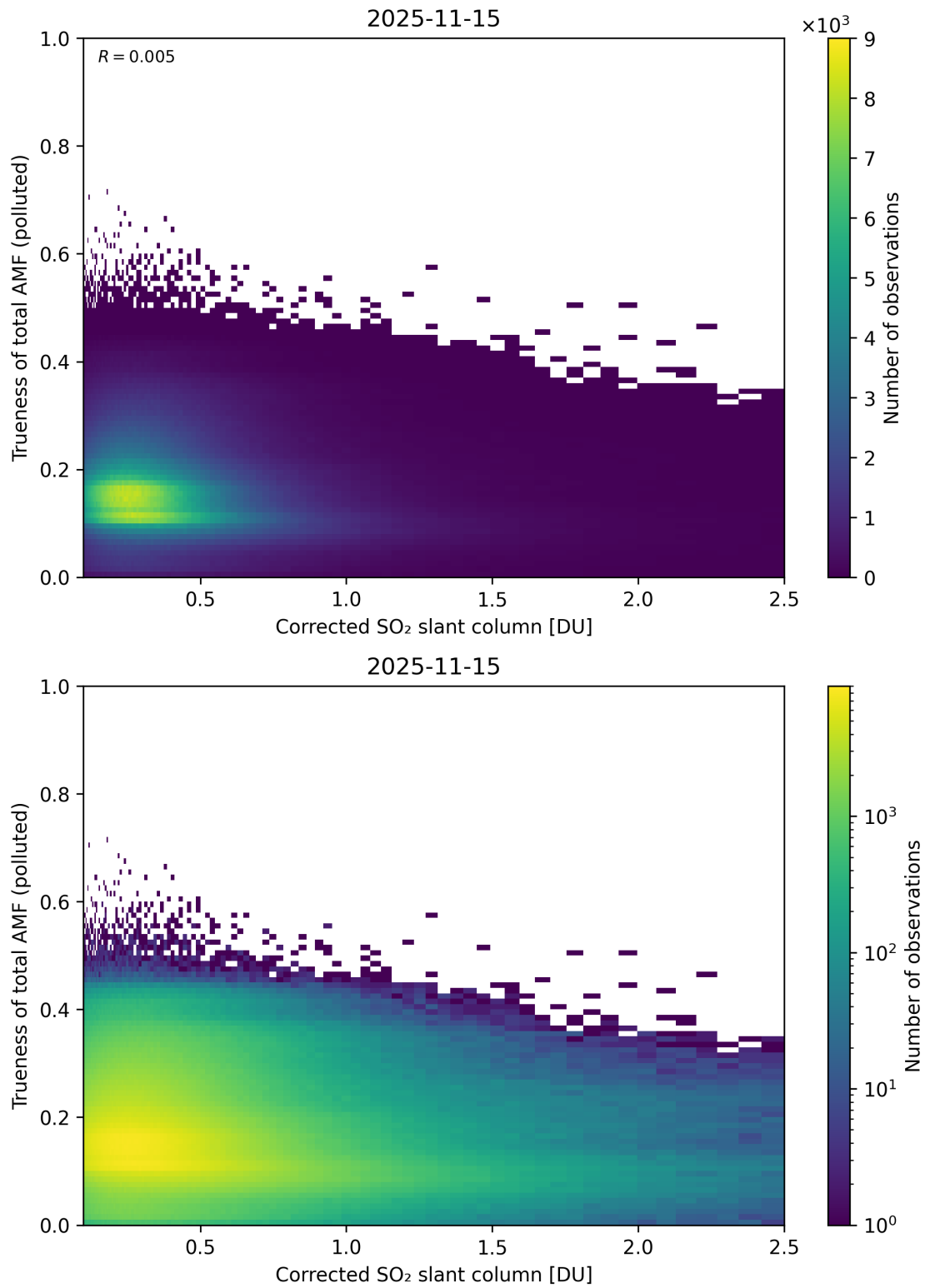
Figure 243: Scatter density plot of “Corrected SO 2 slant column” against “Trueness of total AMF (polluted)” for 2025-11-14 to 2025-11-16.
