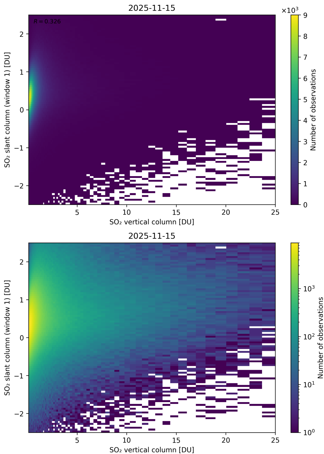
Figure 354: Scatter density plot of “SO 2 vertical column” against “SO 2 slant column (window 1)” for 2025-11-14 to 2025-11-16.
