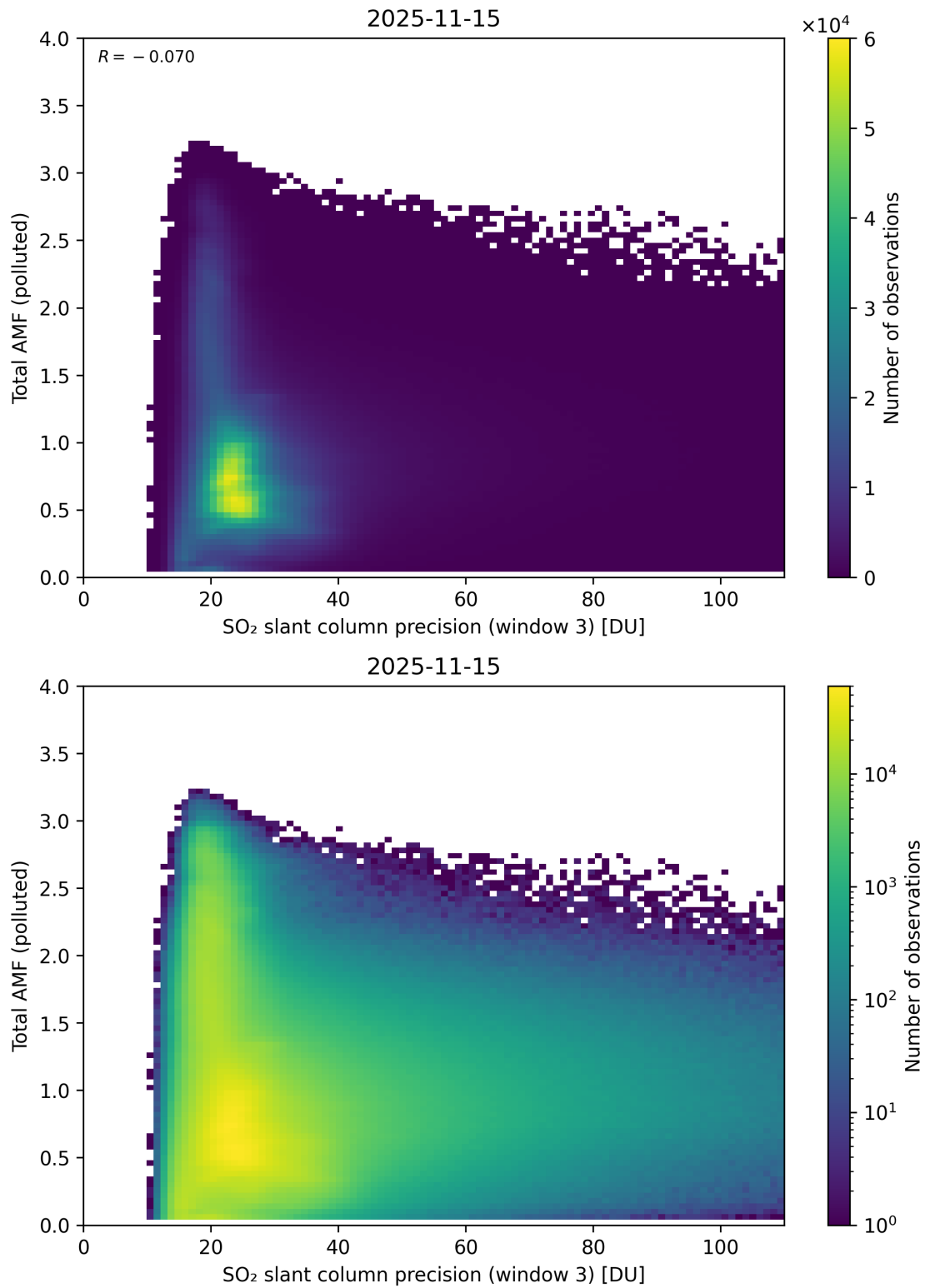
Figure 313: Scatter density plot of “SO 2 slant column precision (window 3)” against “Total AMF (polluted)” for 2025-11-14 to 2025-11-16.
