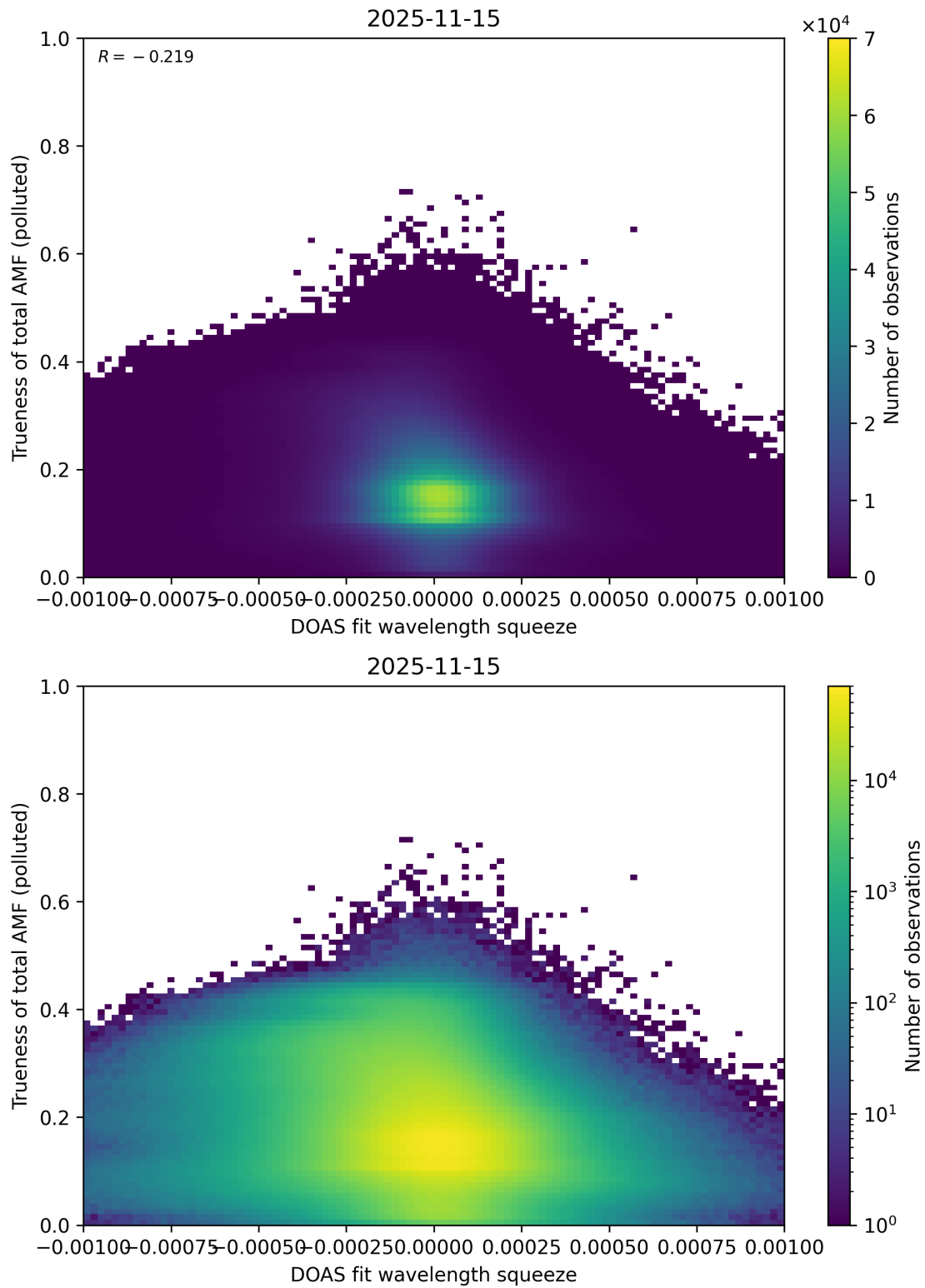
Figure 146: Scatter density plot of “DOAS fit wavelength squeeze” against “Trueness of total AMF (polluted)” for 2025-11-14 to 2025-11-16.
