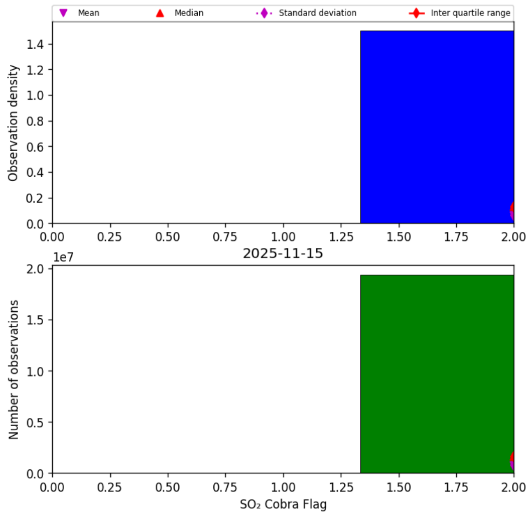
Figure 75: Histogram of “SO 2 Cobra Flag” for 2025-11-14 to 2025-11-16
