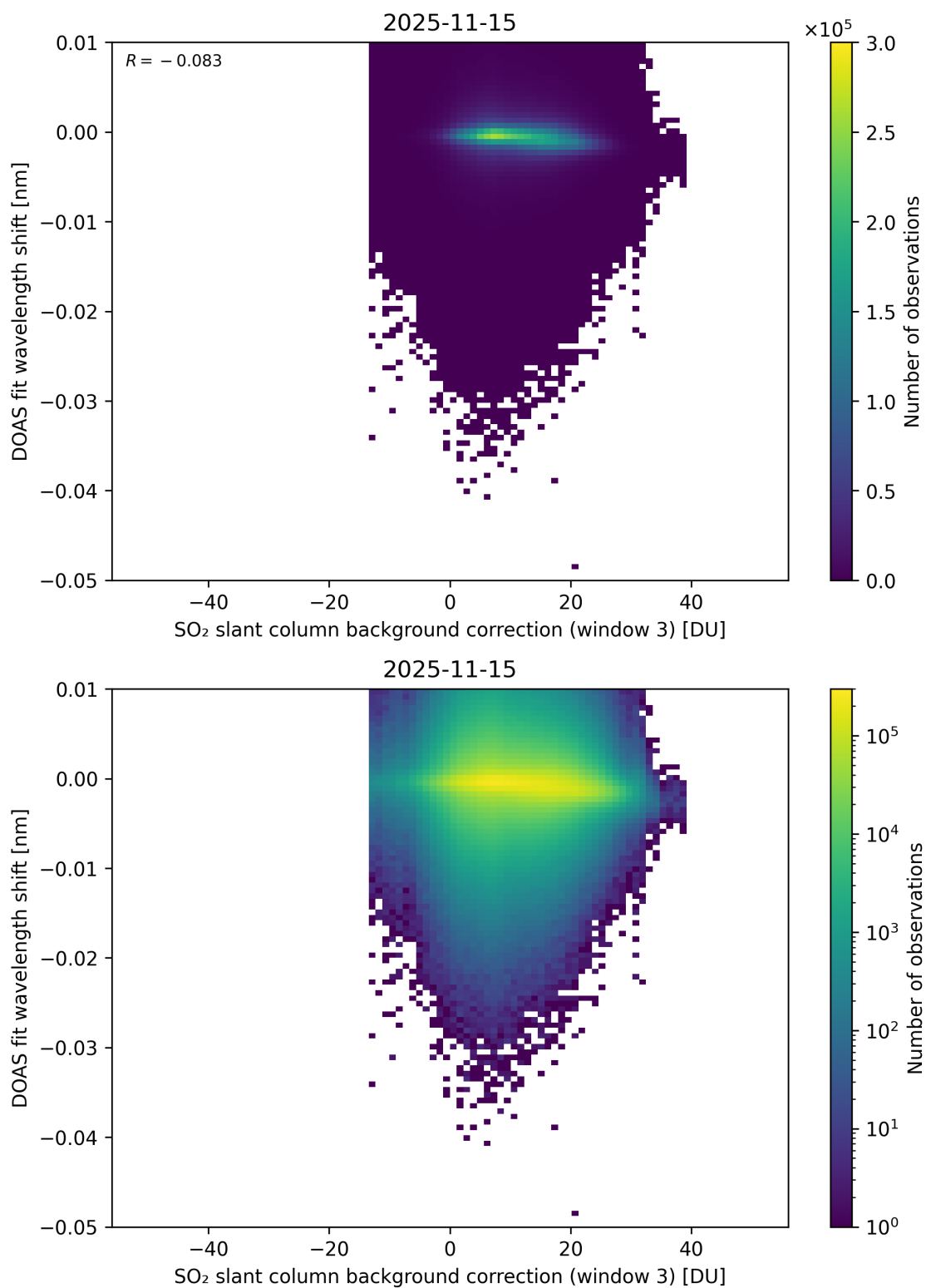
Figure 132: Scatter density plot of “SO 2 slant column background correction (window 3)” against “DOAS fit wavelength shift” for 2025-11-14 to 2025-11-16.
