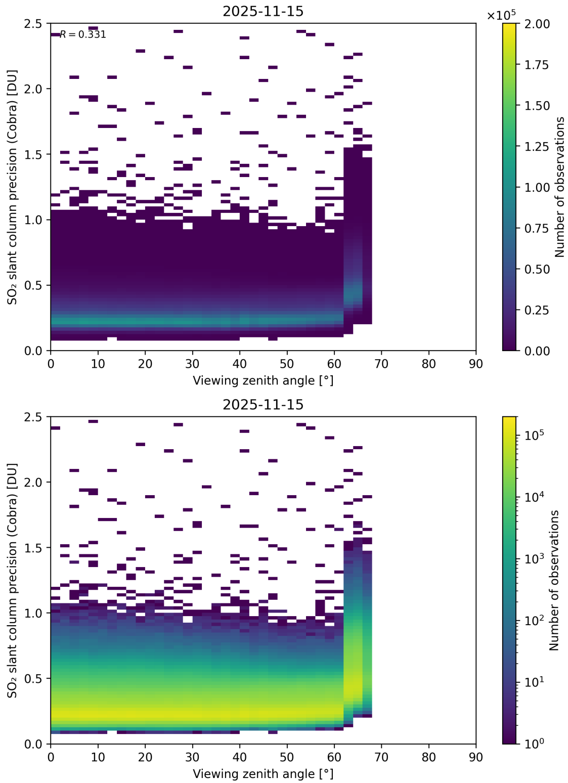
Figure 372: Scatter density plot of “Viewing zenith angle” against “SO 2 slant column precision (Cobra)” for 2025-11-14 to 2025-11-16.
