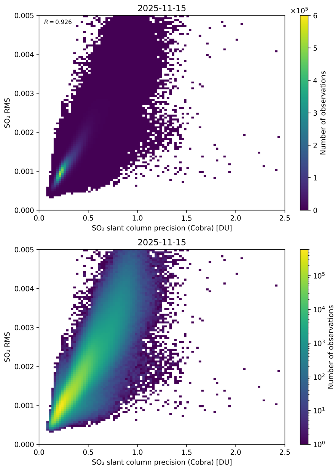
Figure 204: Scatter density plot of “SO 2 slant column precision (Cobra)” against “SO 2 RMS” for 2025-11-14 to 2025-11-16.
