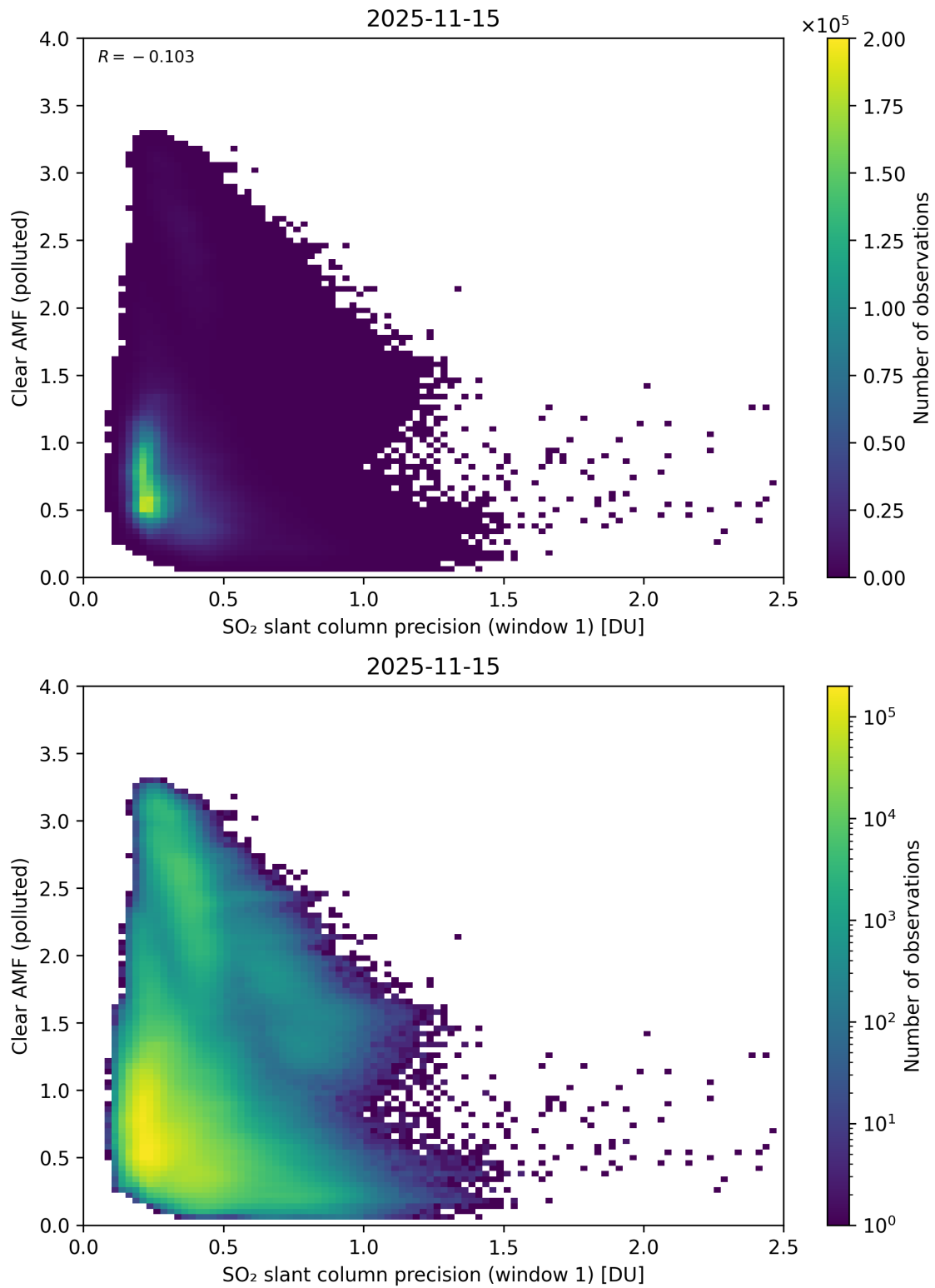
Figure 274: Scatter density plot of “SO 2 slant column precision (window 1)” against “Clear AMF (polluted)” for 2025-11-14 to 2025-11-16.
