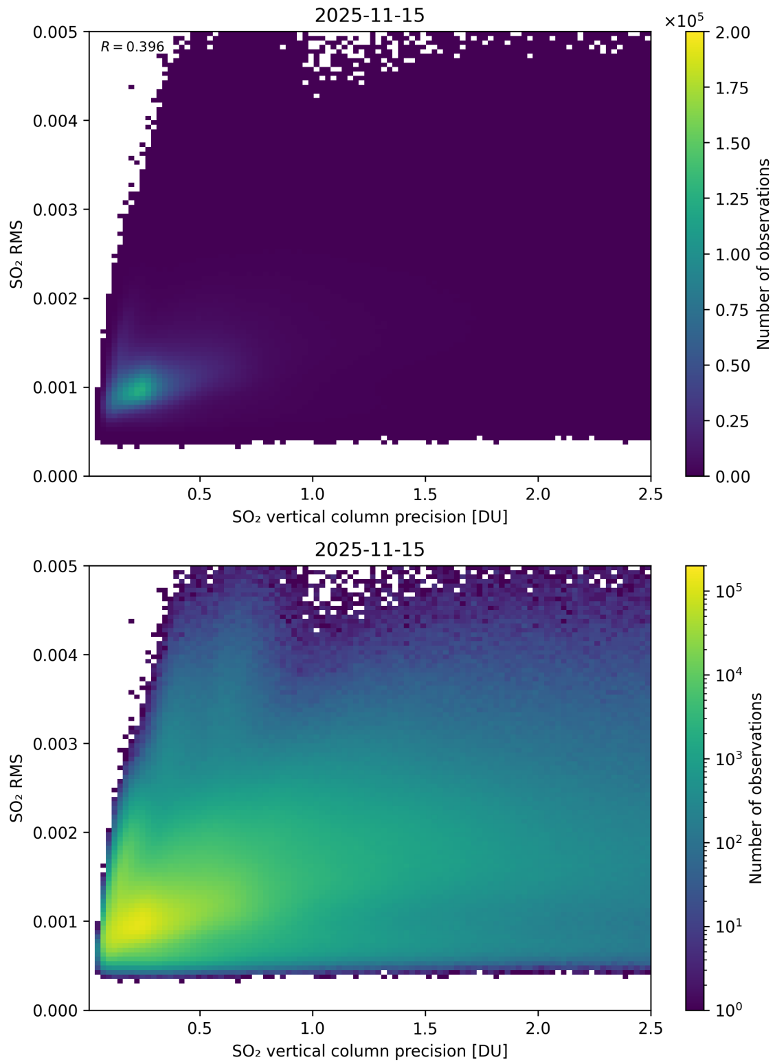
Figure 334: Scatter density plot of “SO 2 vertical column precision” against “SO 2 RMS” for 2025-11-14 to 2025-11-16.
