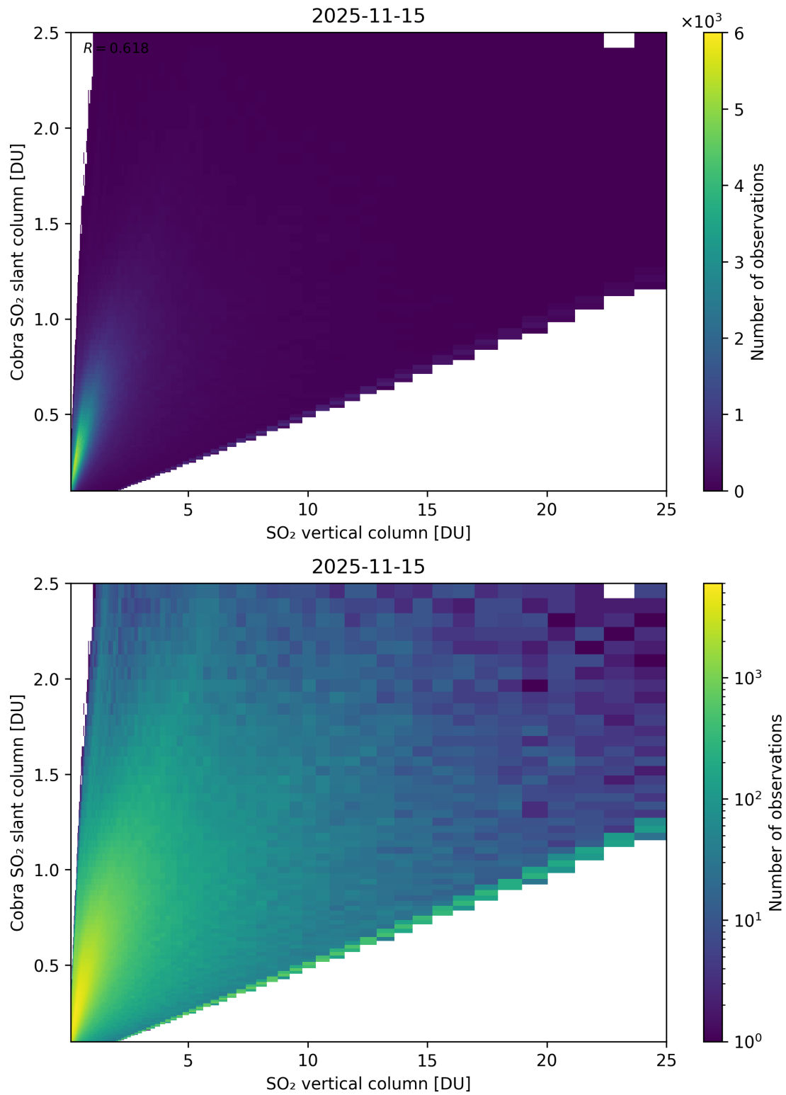
Figure 349: Scatter density plot of “SO 2 vertical column” against “Cobra SO 2 slant column” for 2025-11-14 to 2025-11-16.
