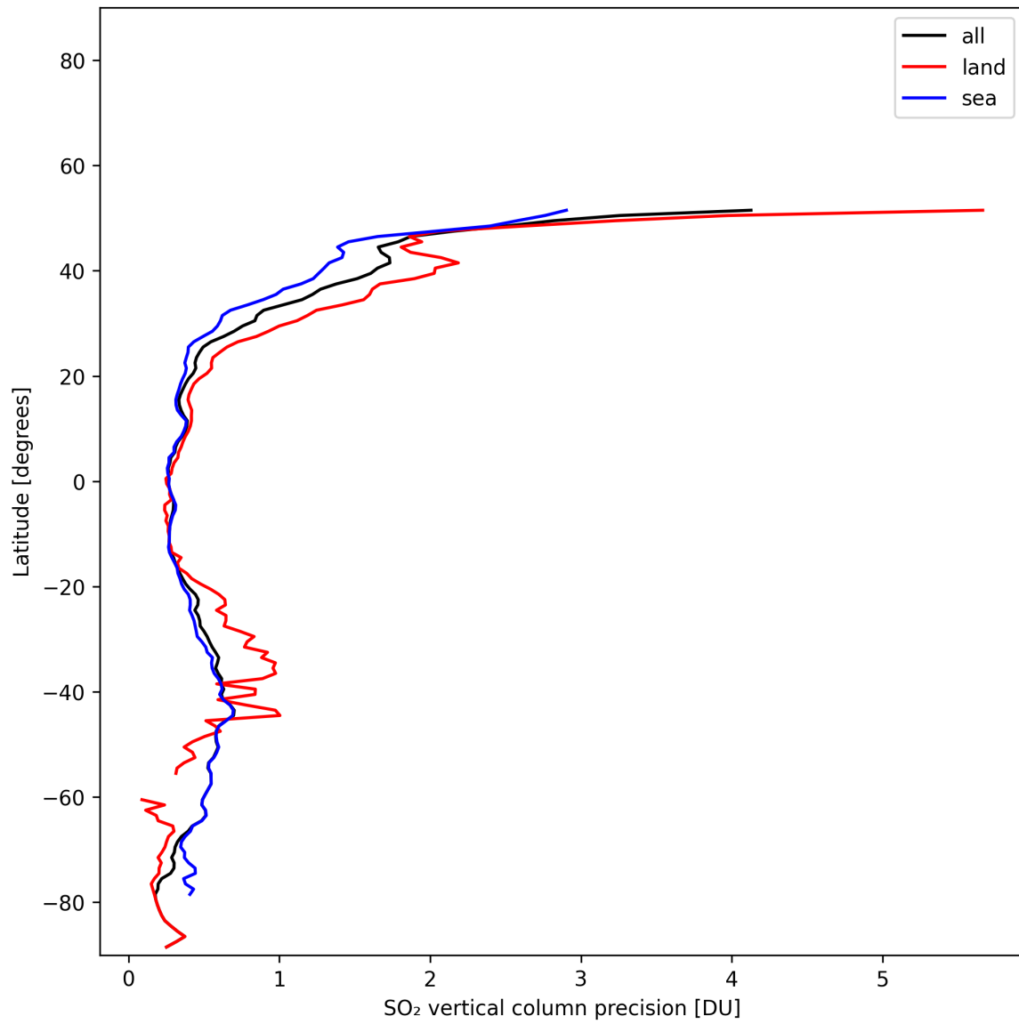
Figure 33: Zonal average of “SO 2 vertical column precision” for 2025-11-14 to 2025-11-16.
