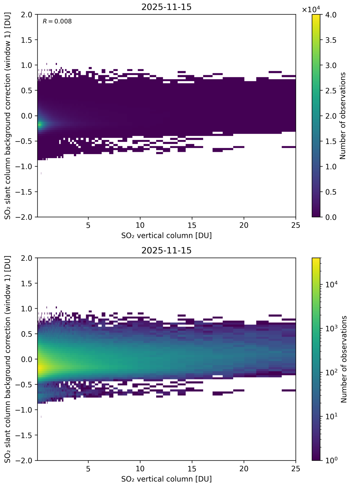
Figure 323: Scatter density plot of “SO 2 vertical column” against “SO 2 slant column background correction (window 1)” for 2025-11-14 to 2025-11-16.
