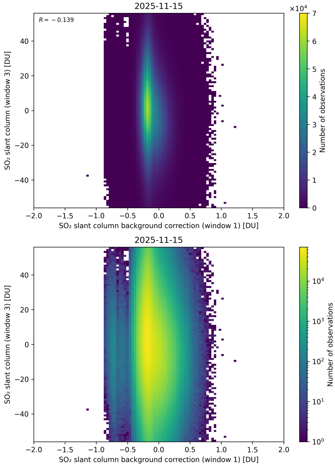
Figure 118: Scatter density plot of “SO 2 slant column background correction (window 1)” against “SO 2 slant column (window 3)” for 2025-11-14 to 2025-11-16.
