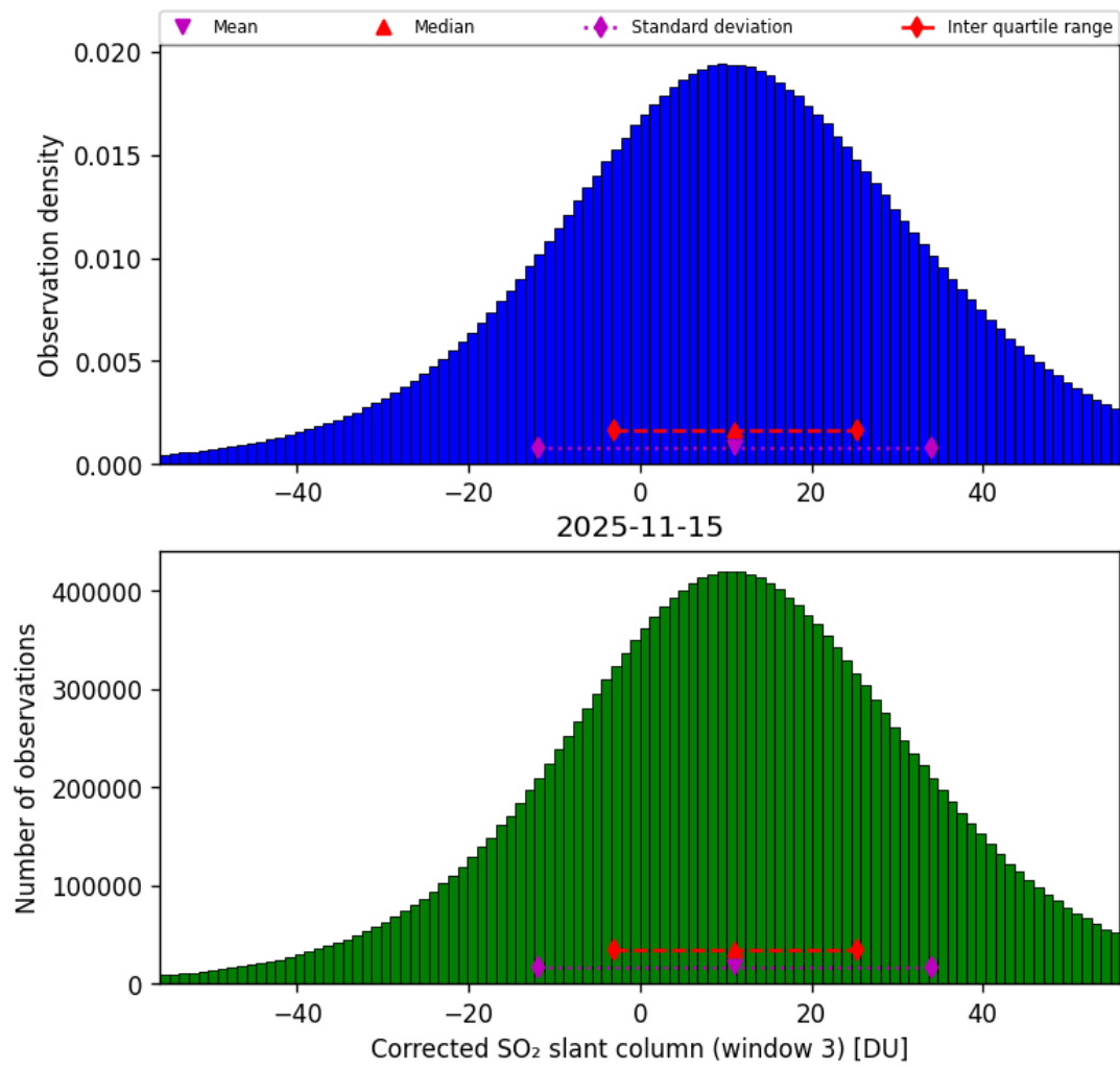
Figure 73: Histogram of “Corrected SO 2 slant column (window 3)” for 2025-11-14 to 2025-11-16
