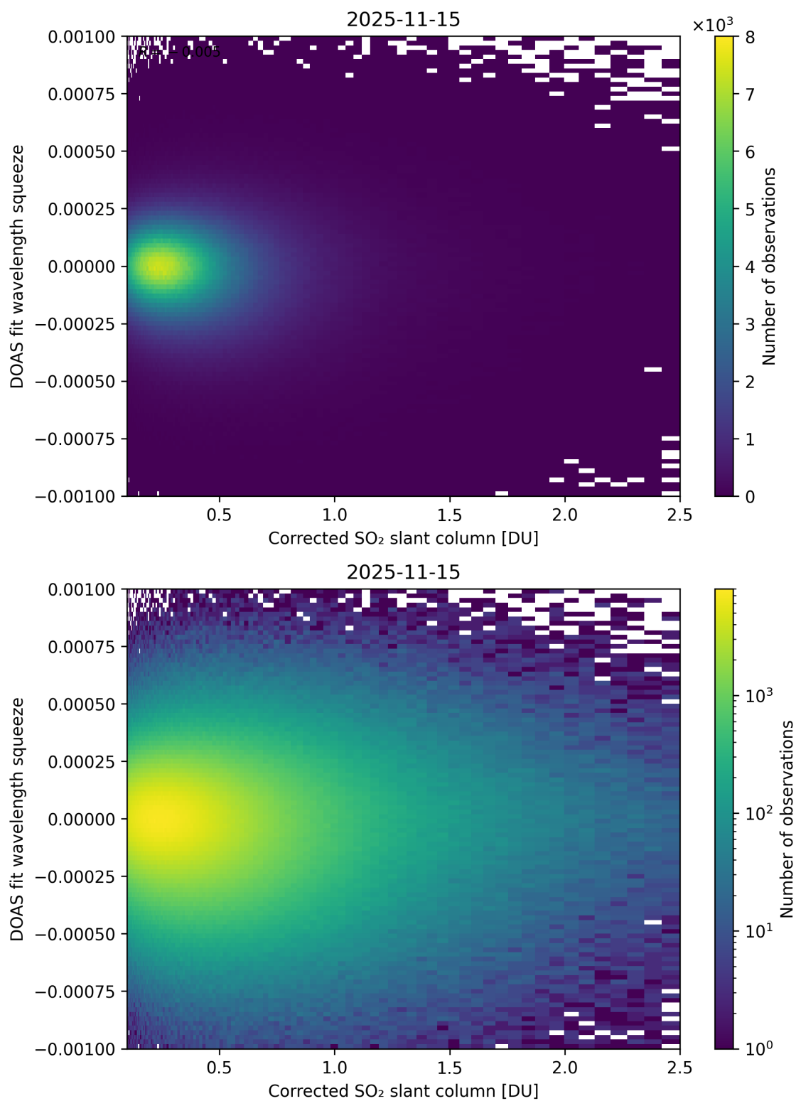
Figure 230: Scatter density plot of “Corrected SO 2 slant column” against “DOAS fit wavelength squeeze” for 2025-11-14 to 2025-11-16.
