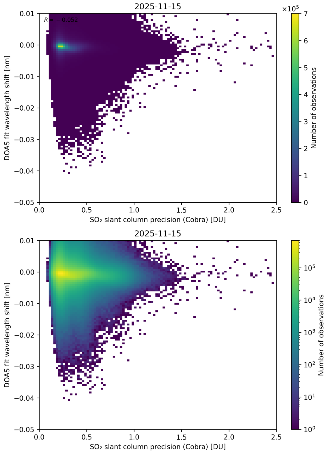
Figure 202: Scatter density plot of “SO 2 slant column precision (Cobra)” against “DOAS fit wavelength shift” for 2025-11-14 to 2025-11-16.
