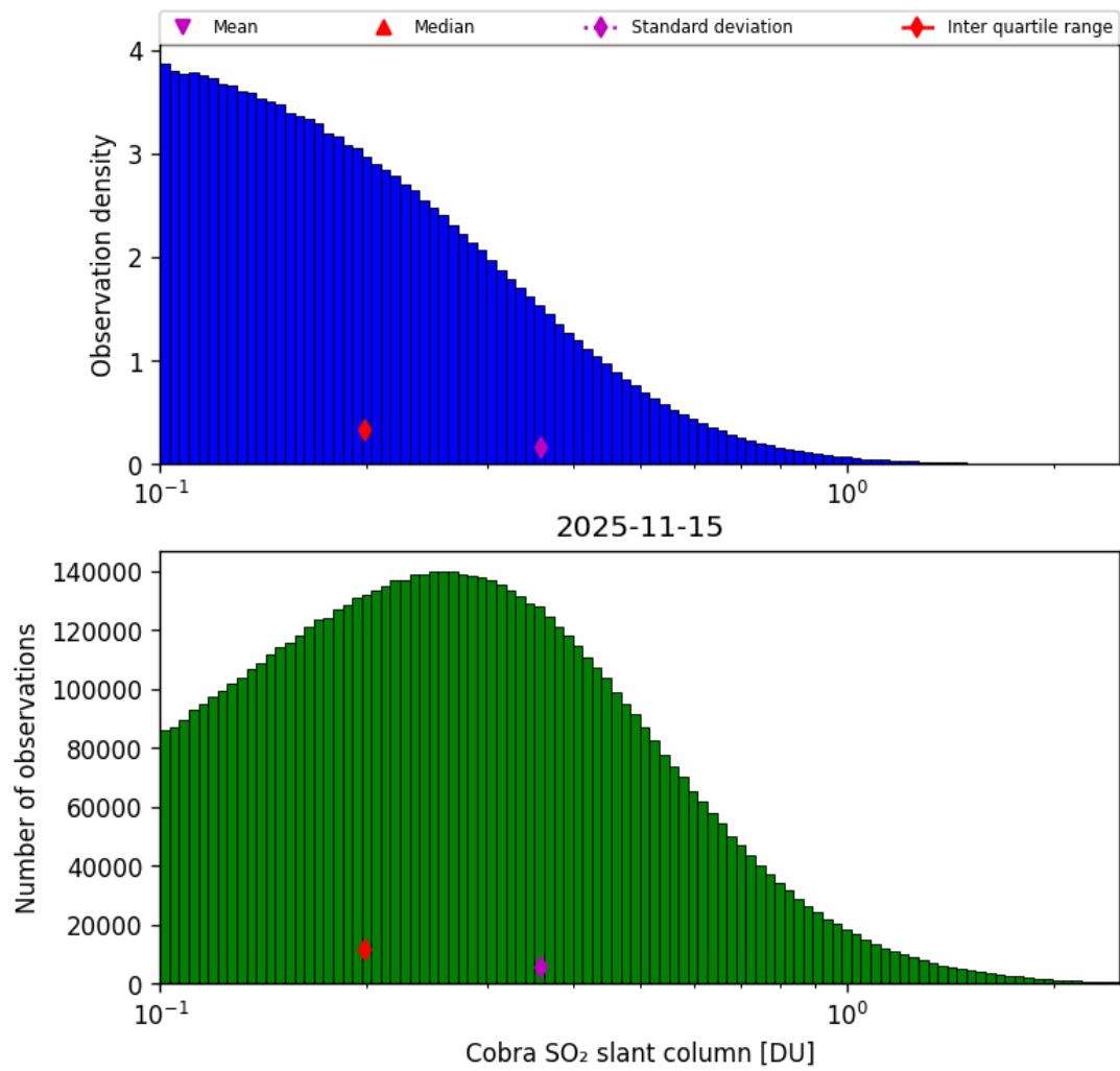
Figure 61: Histogram of “Cobra SO 2 slant column” for 2025-11-14 to 2025-11-16
