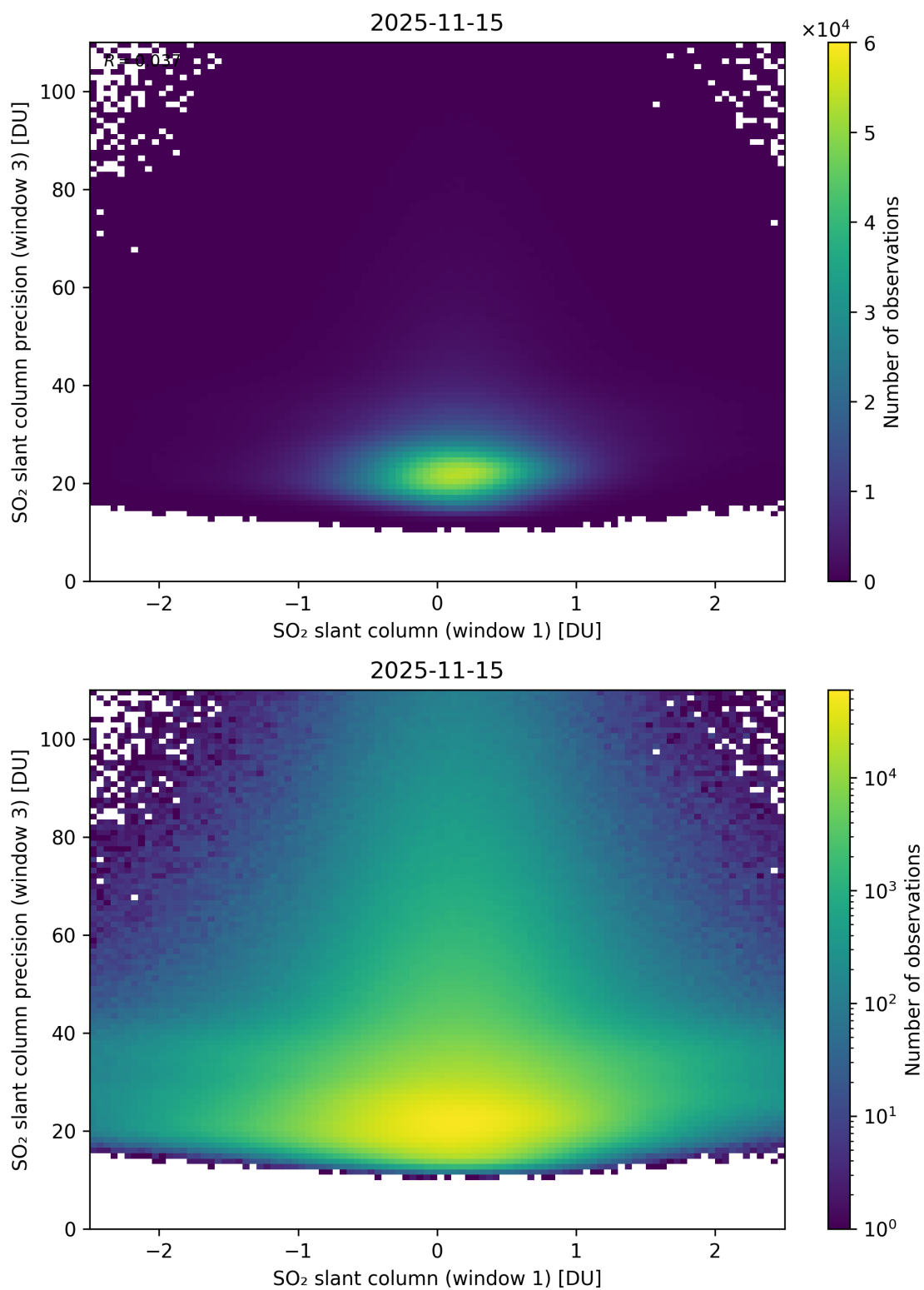
Figure 288: Scatter density plot of “SO 2 slant column (window 1)” against “SO 2 slant column precision (window 3)” for 2025-11-14 to 2025-11-16.
