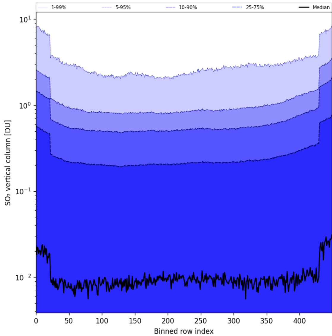
Figure 84: Along track statistics of “SO 2 vertical column” for 2025-11-14 to 2025-11-16
