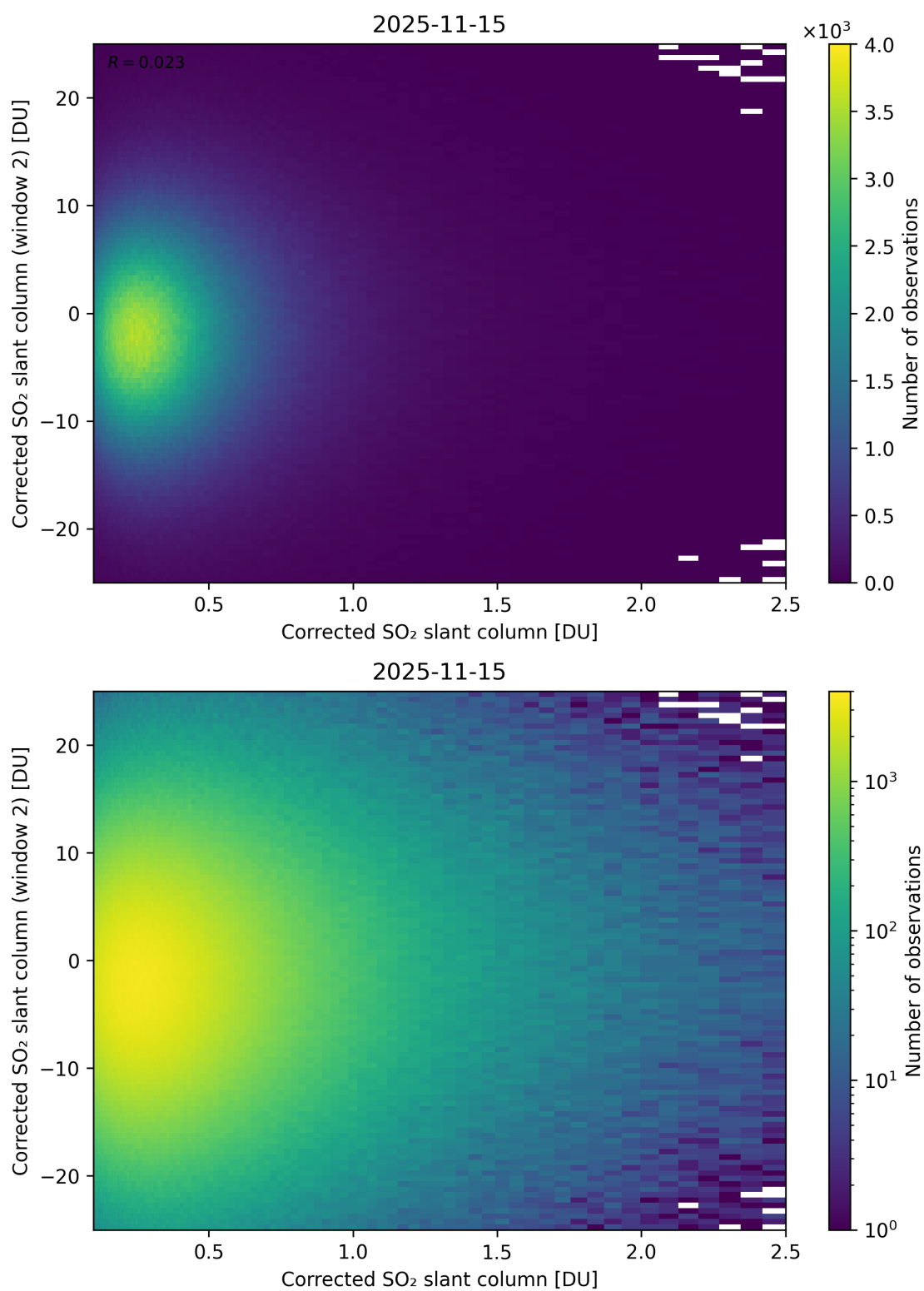
Figure 235: Scatter density plot of “Corrected SO 2 slant column” against “Corrected SO 2 slant column (window 2)” for 2025-11-14 to 2025-11-16.
