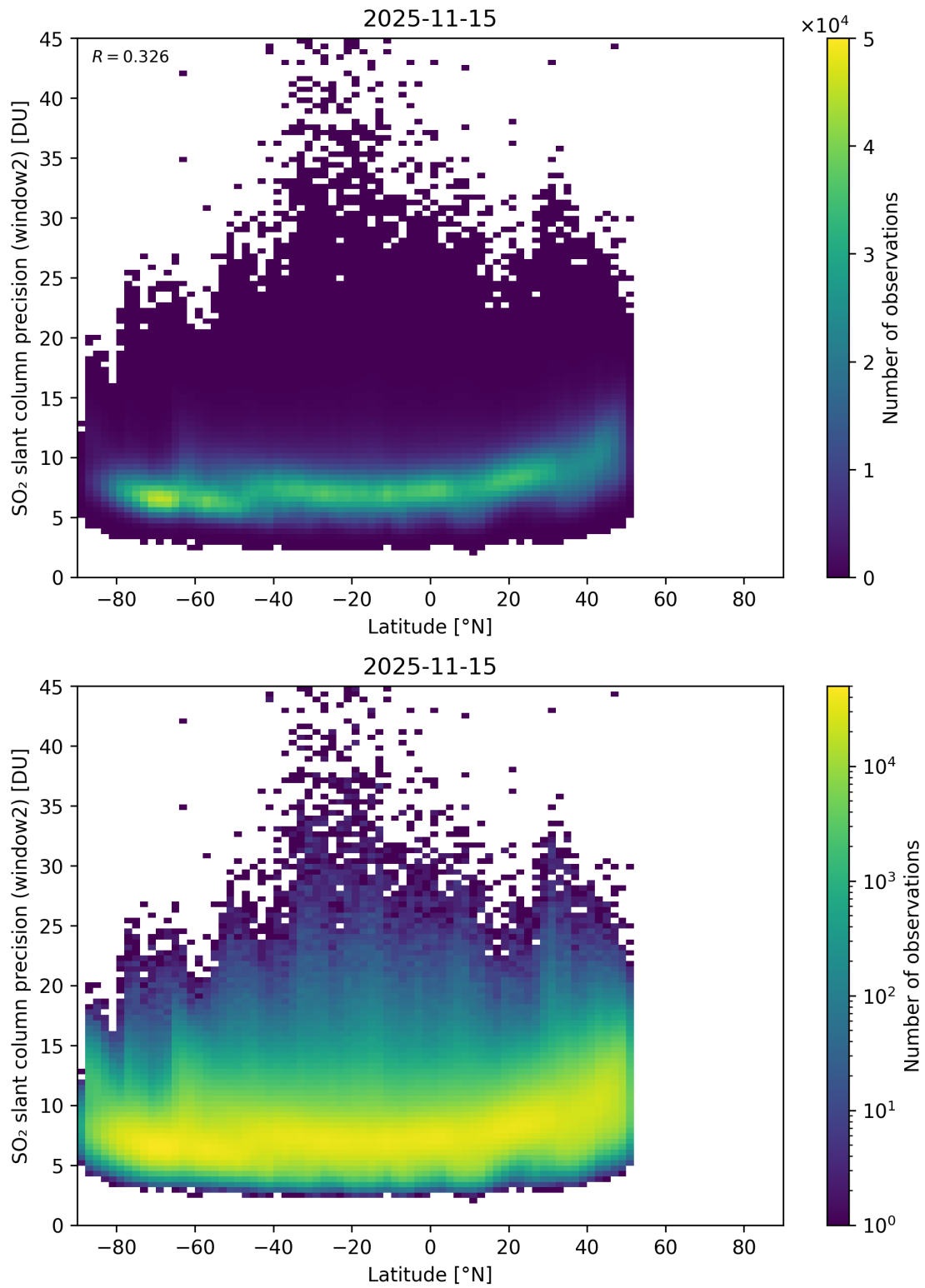
Figure 164: Scatter density plot of “Latitude” against “SO 2 slant column precision (window2)” for 2025-11-14 to 2025-11-16.
