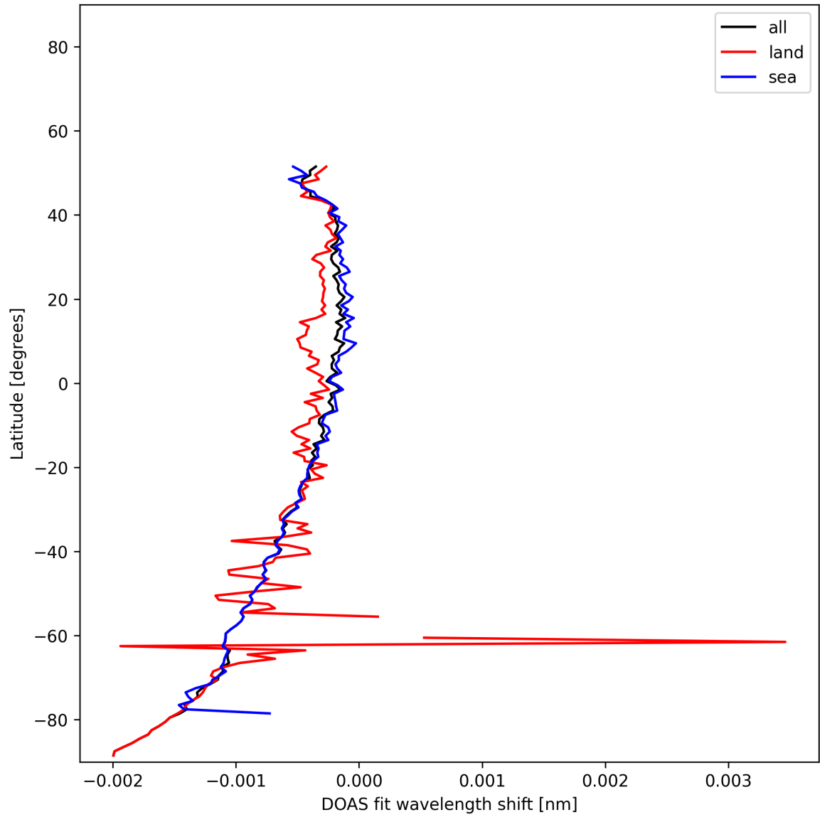
Figure 50: Zonal average of “DOAS fit wavelength shift” for 2025-11-14 to 2025-11-16.
