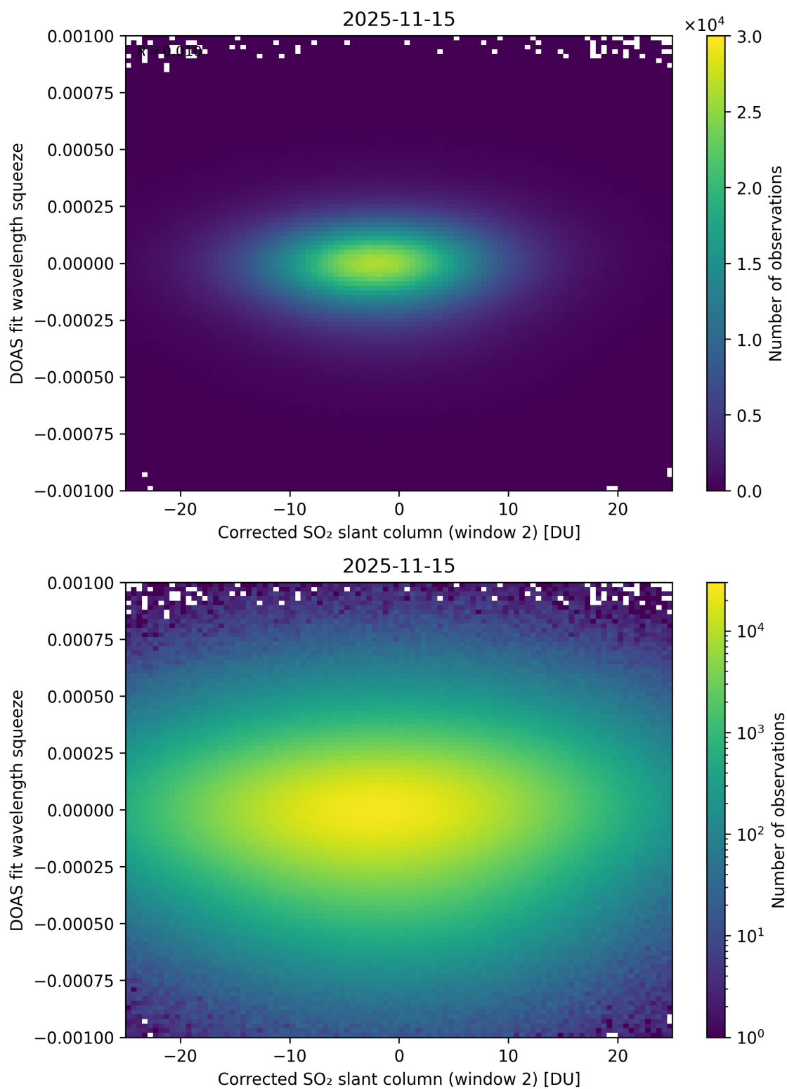
Figure 247: Scatter density plot of “Corrected SO 2 slant column (window 2)” against “DOAS fit wavelength squeeze” for 2025-11-14 to 2025-11-16.
