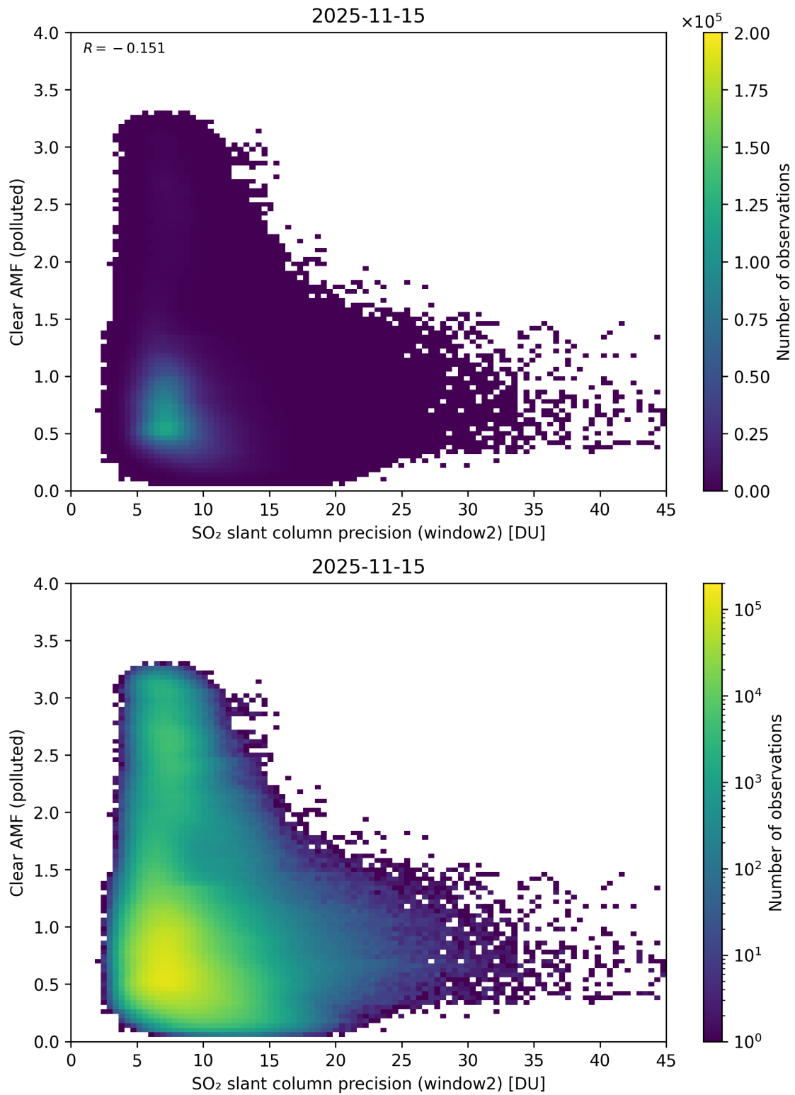
Figure 296: Scatter density plot of “SO 2 slant column precision (window2)” against “Clear AMF (polluted)” for 2025-11-14 to 2025-11-16.
