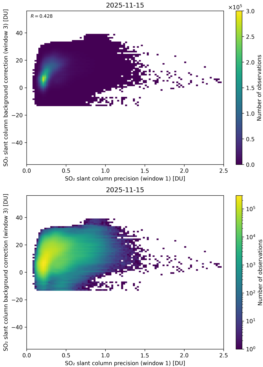
Figure 270: Scatter density plot of “SO 2 slant column precision (window 1)” against “SO 2 slant column background correction (window 3)” for 2025-11-14 to 2025-11-16.
