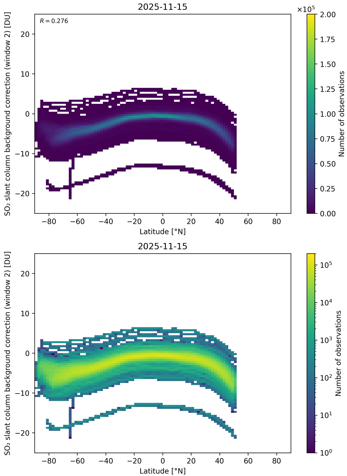
Figure 151: Scatter density plot of “Latitude” against “SO 2 slant column background correction (window 2)” for 2025-11-14 to 2025-11-16.
