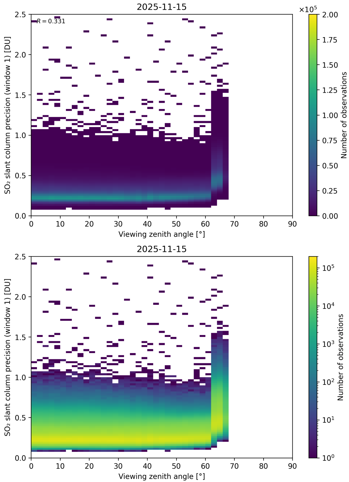
Figure 377: Scatter density plot of “Viewing zenith angle” against “SO 2 slant column precision (window 1)” for 2025-11-14 to 2025-11-16.
