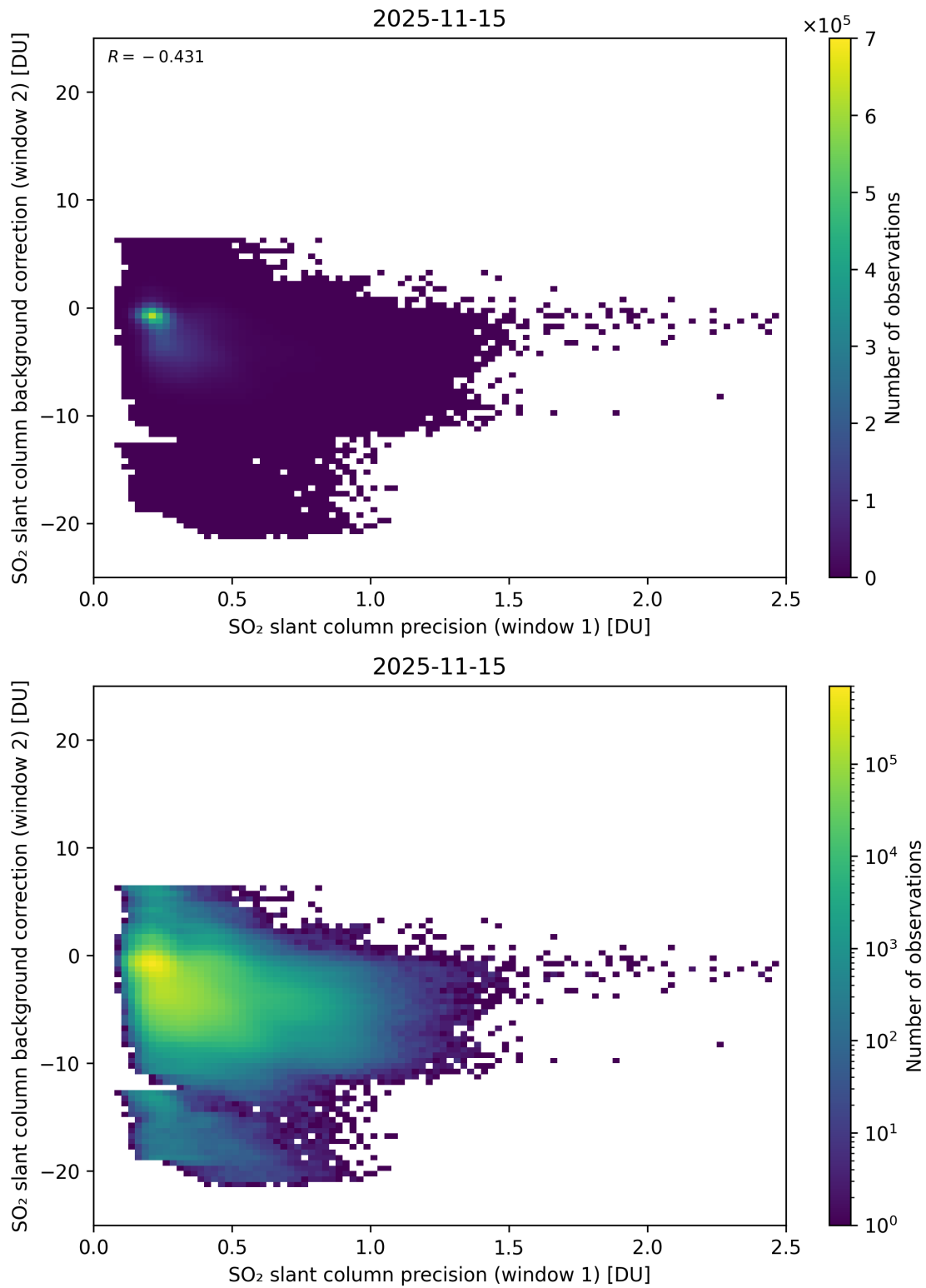
Figure 269: Scatter density plot of “SO 2 slant column precision (window 1)” against “SO 2 slant column background correction (window 2)” for 2025-11-14 to 2025-11-16.
