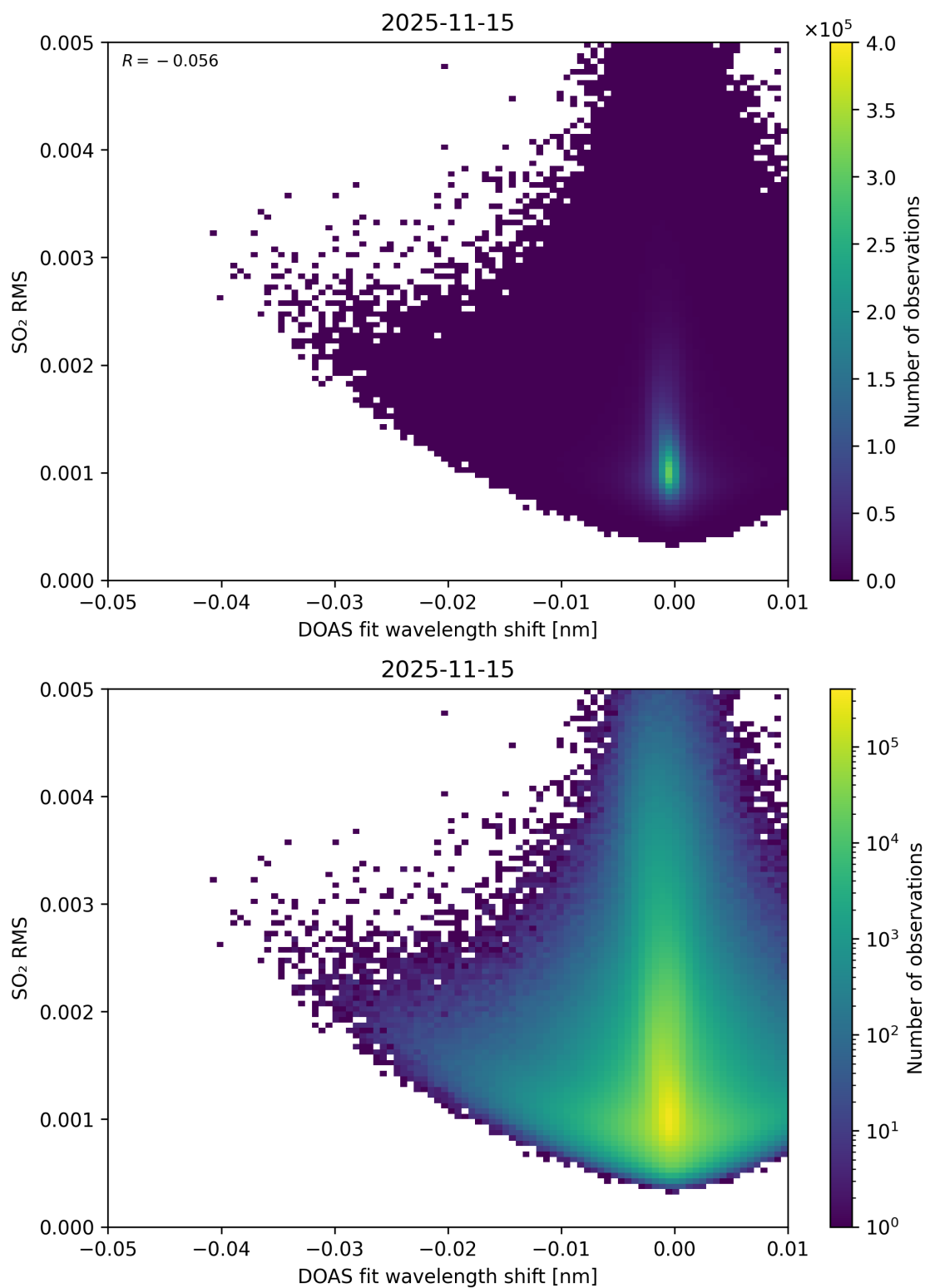
Figure 139: Scatter density plot of “DOAS fit wavelength shift” against “SO 2 RMS” for 2025-11-14 to 2025-11-16.
