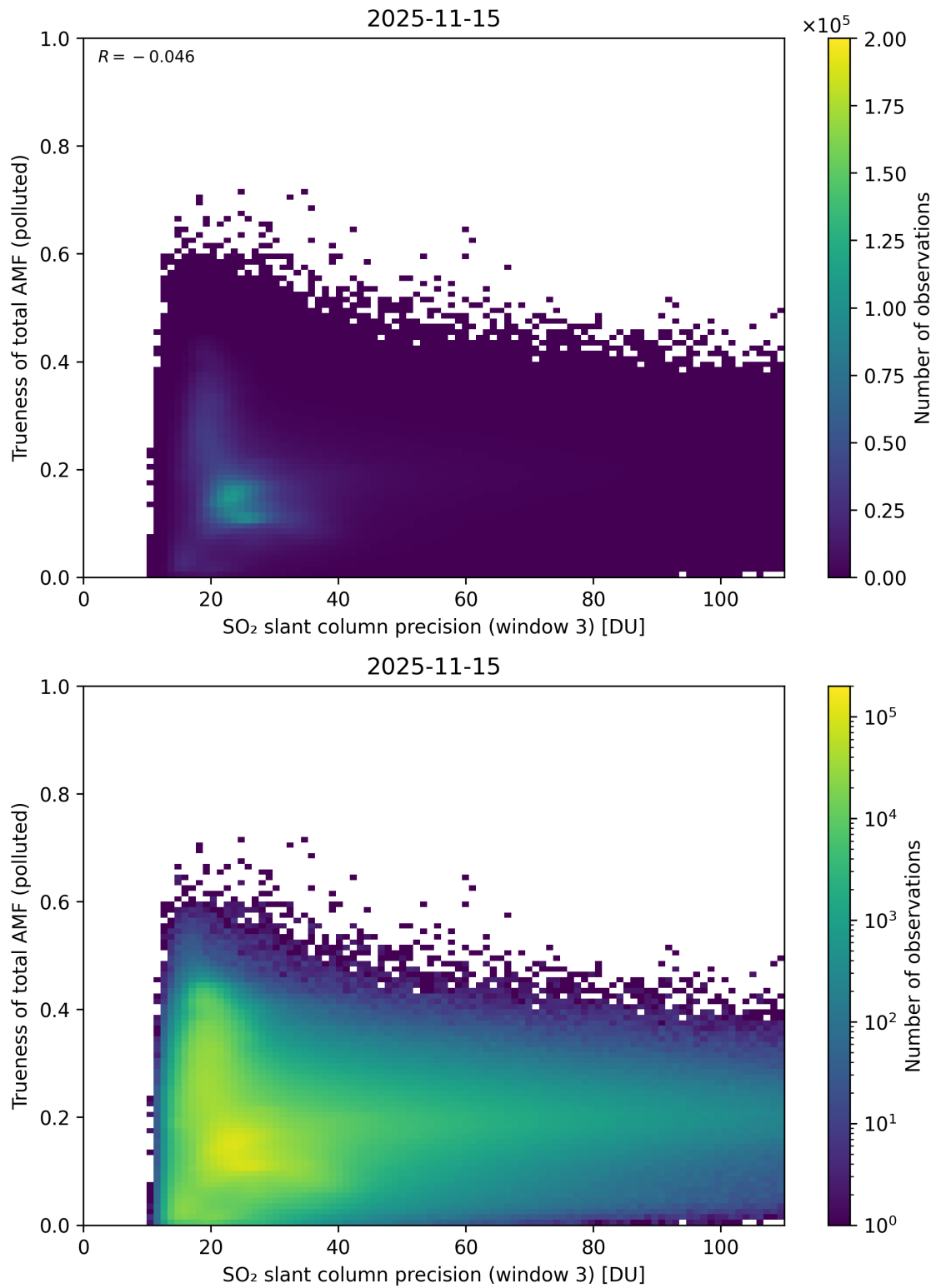
Figure 314: Scatter density plot of “SO 2 slant column precision (window 3)” against “Trueness of total AMF (polluted)” for 2025-11-14 to 2025-11-16.
