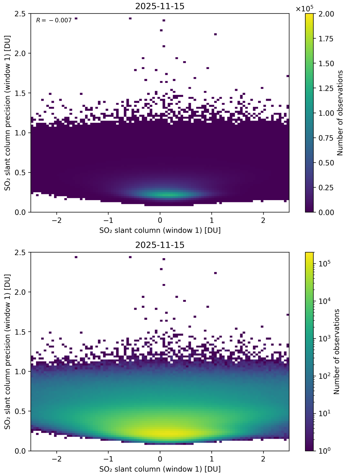
Figure 285: Scatter density plot of “SO 2 slant column (window 1)” against “SO 2 slant column precision (window 1)” for 2025-11-14 to 2025-11-16.
