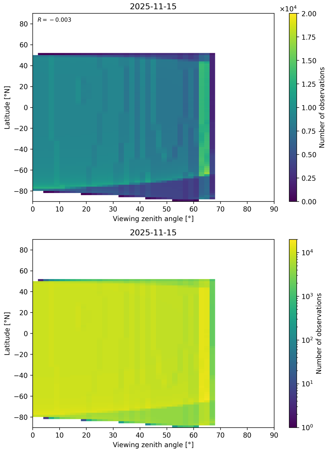
Figure 368: Scatter density plot of “Viewing zenith angle” against “Latitude” for 2025-11-14 to 2025-11-16.
