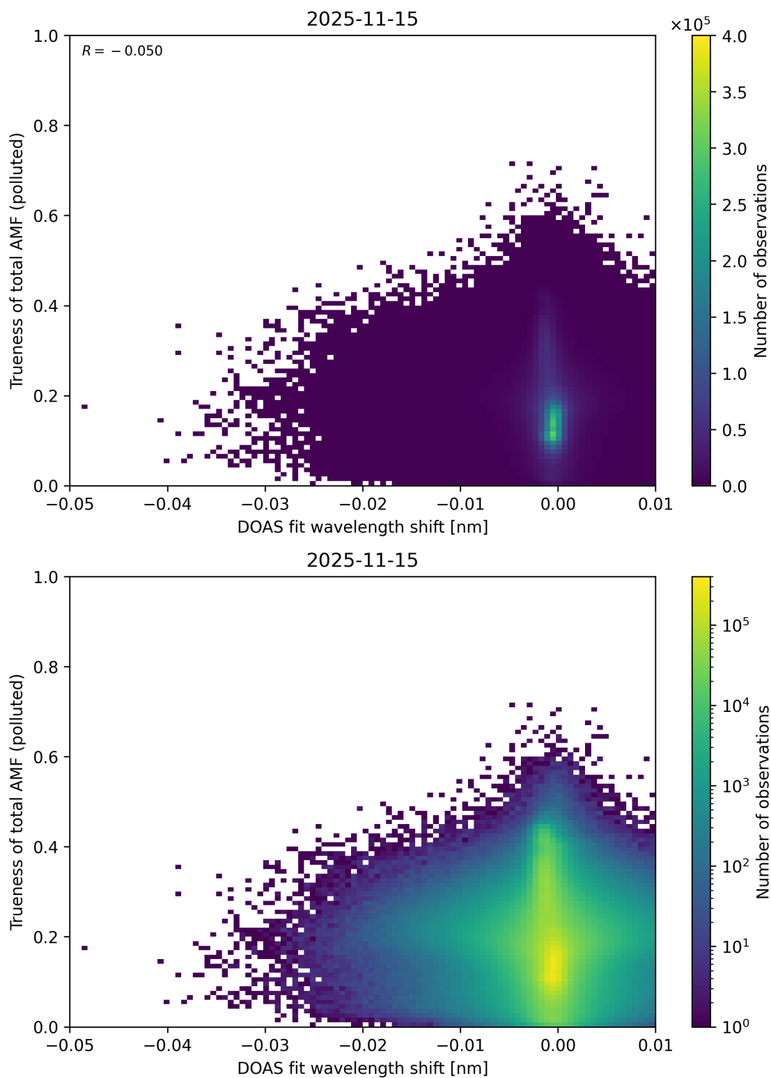
Figure 142: Scatter density plot of “DOAS fit wavelength shift” against “Trueness of total AMF (polluted)” for 2025-11-14 to 2025-11-16.
