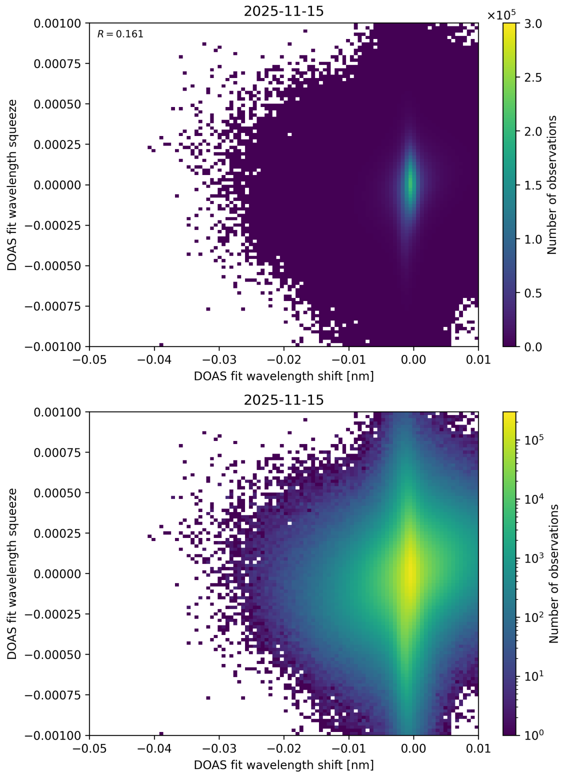
Figure 138: Scatter density plot of “DOAS fit wavelength shift” against “DOAS fit wavelength squeeze” for 2025-11-14 to 2025-11-16.
