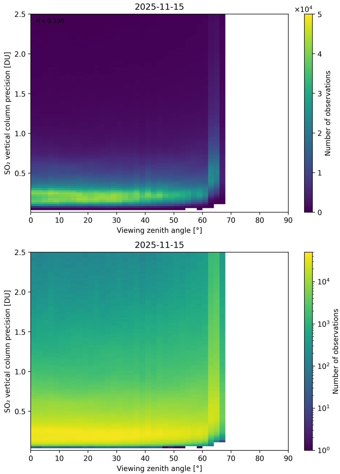
Figure 384: Scatter density plot of “Viewing zenith angle” against “SO 2 vertical column precision” for 2025-11-14 to 2025-11-16.
