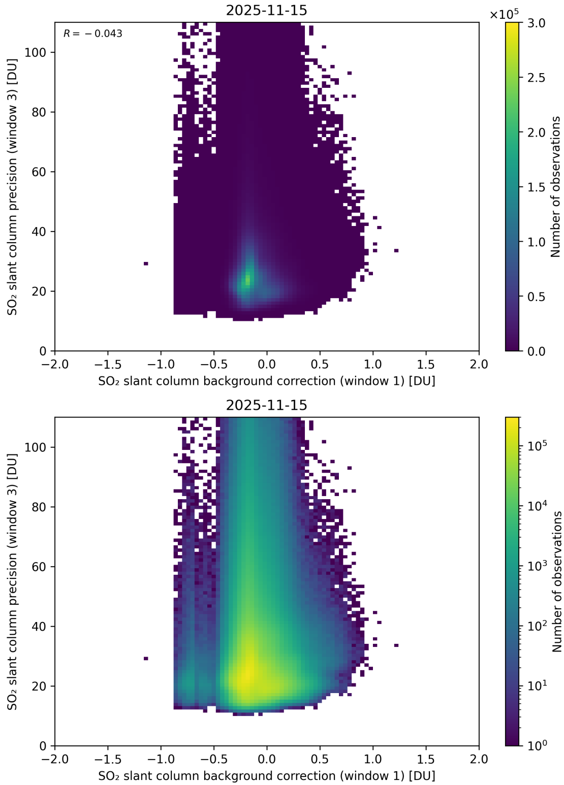
Figure 119: Scatter density plot of “SO 2 slant column background correction (window 1)” against “SO 2 slant column precision (window 3)” for 2025-11-14 to 2025-11-16.
