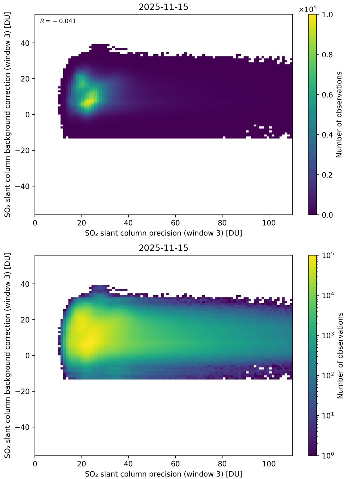
Figure 307: Scatter density plot of “SO 2 slant column precision (window 3)” against “SO 2 slant column background correction (window 3)” for 2025-11-14 to 2025-11-16.
