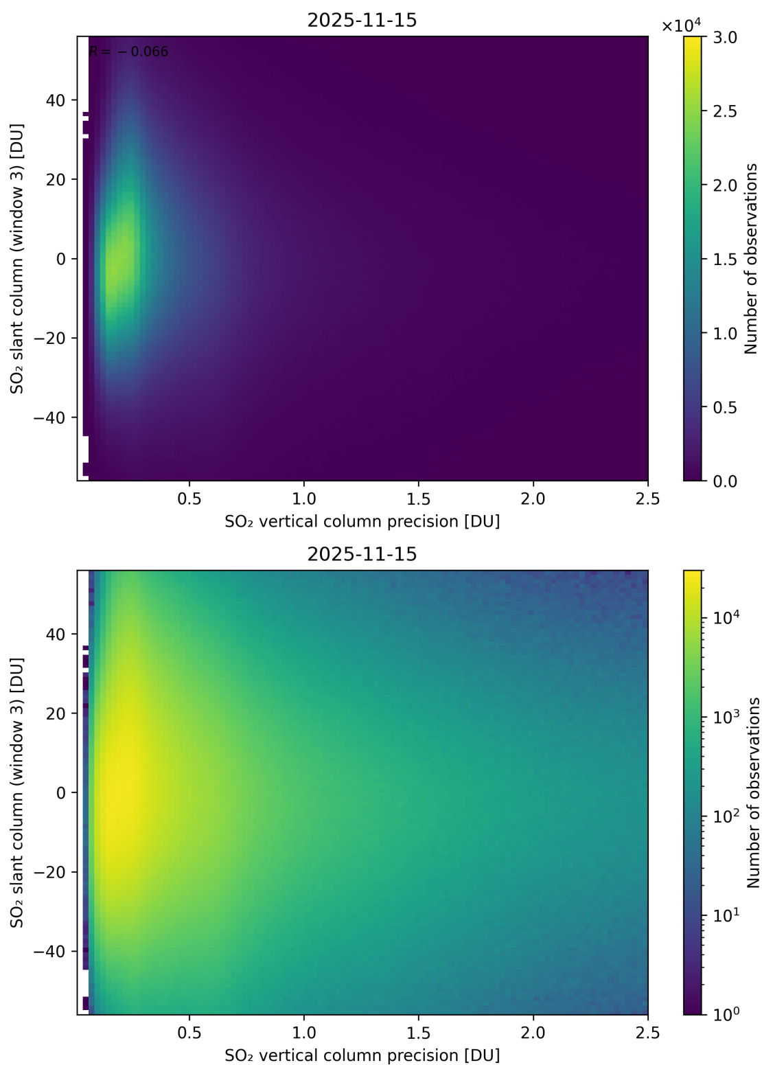
Figure 344: Scatter density plot of “SO 2 vertical column precision” against “SO 2 slant column (window 3)” for 2025-11-14 to 2025-11-16.
