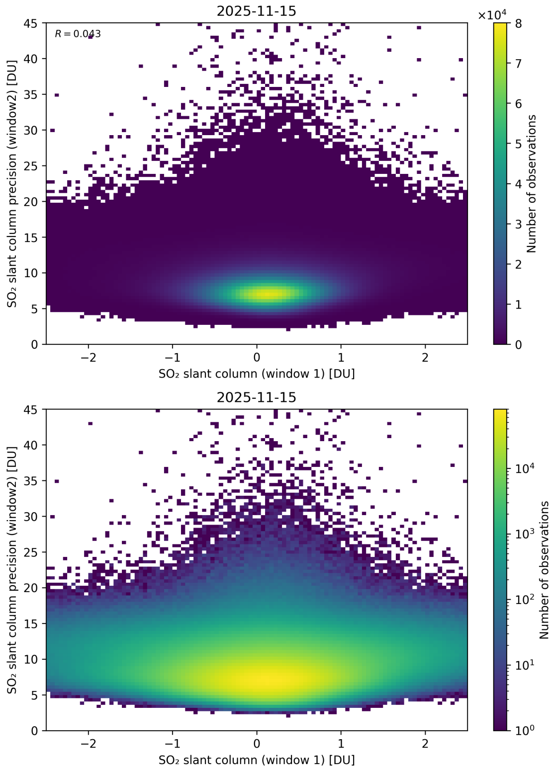
Figure 286: Scatter density plot of “SO 2 slant column (window 1)” against “SO 2 slant column precision (window2)” for 2025-11-14 to 2025-11-16.
