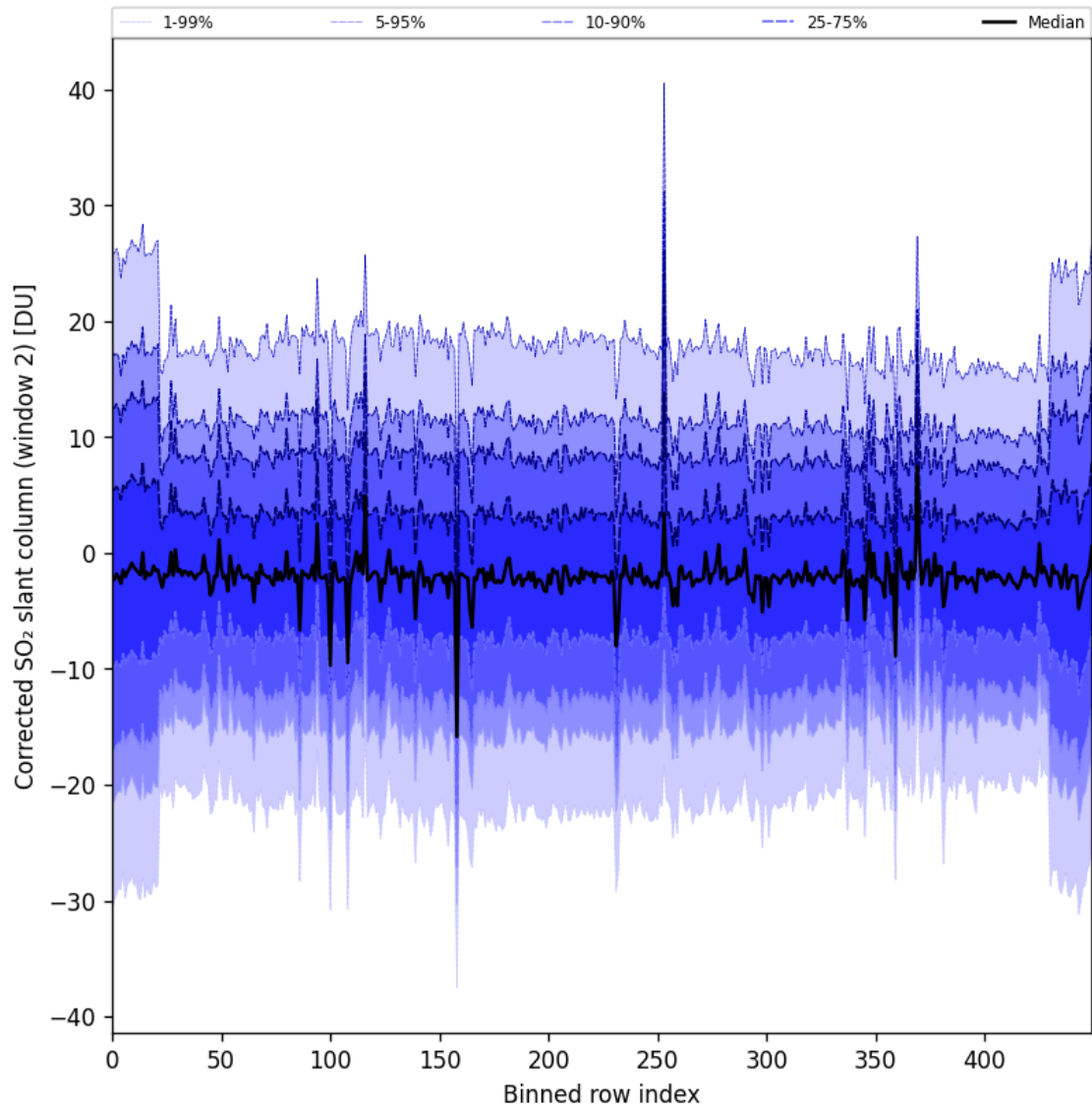
Figure 95: Along track statistics of "Corrected SO 2 slant column (window 2)" for 2025-11-14 to 2025-11-16
