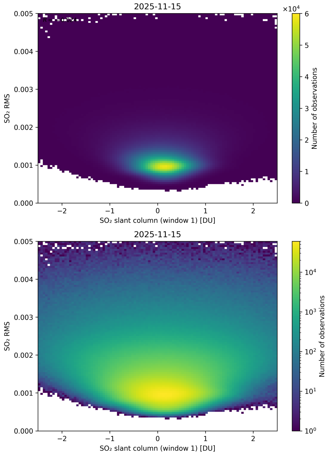
Figure 267: Scatter density plot of “SO 2 slant column (window 1)” against “SO 2 RMS” for 2025-11-14 to 2025-11-16.
