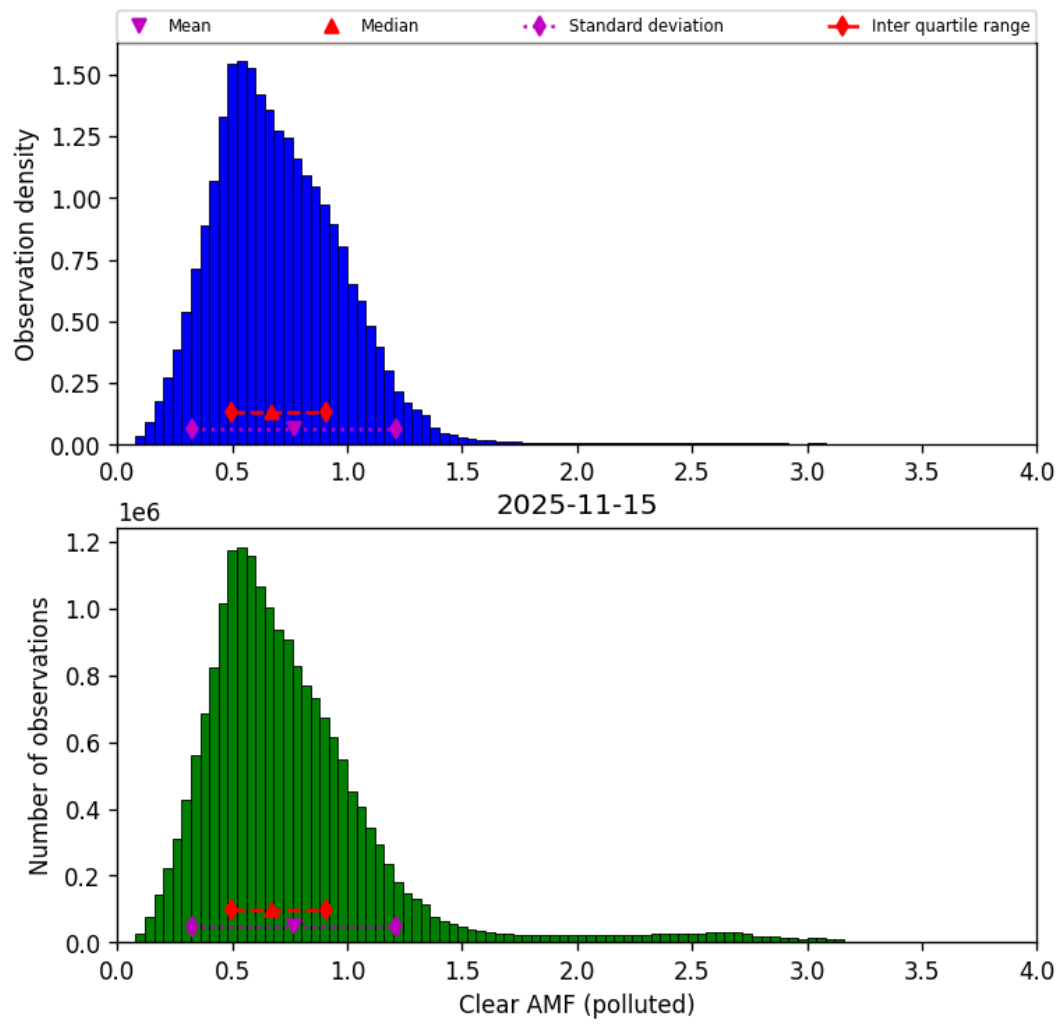
Figure 81: Histogram of “Clear AMF (polluted)” for 2025-11-14 to 2025-11-16
