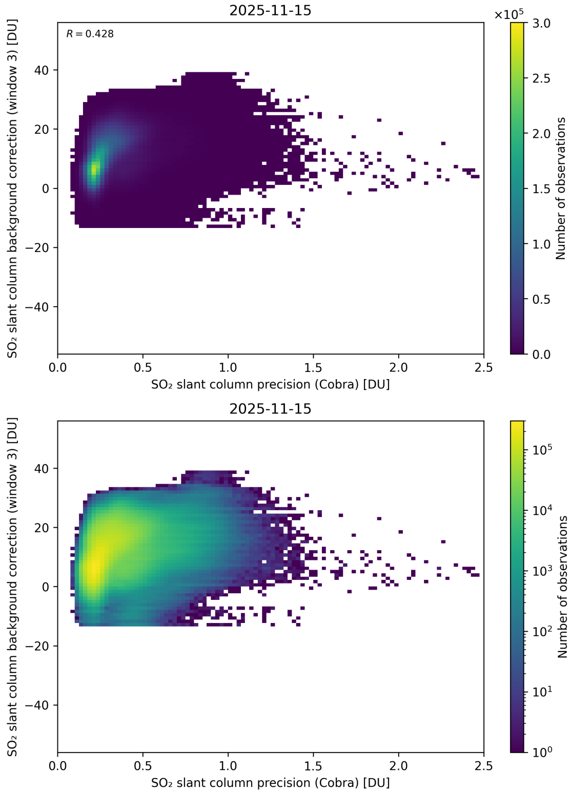
Figure 201: Scatter density plot of “SO 2 slant column precision (Cobra)” against “SO 2 slant column background correction (window 3)” for 2025-11-14 to 2025-11-16.
