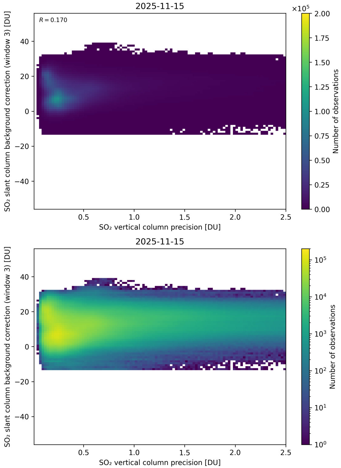
Figure 331: Scatter density plot of “SO 2 vertical column precision” against “SO 2 slant column background correction (window 3)” for 2025-11-14 to 2025-11-16.
