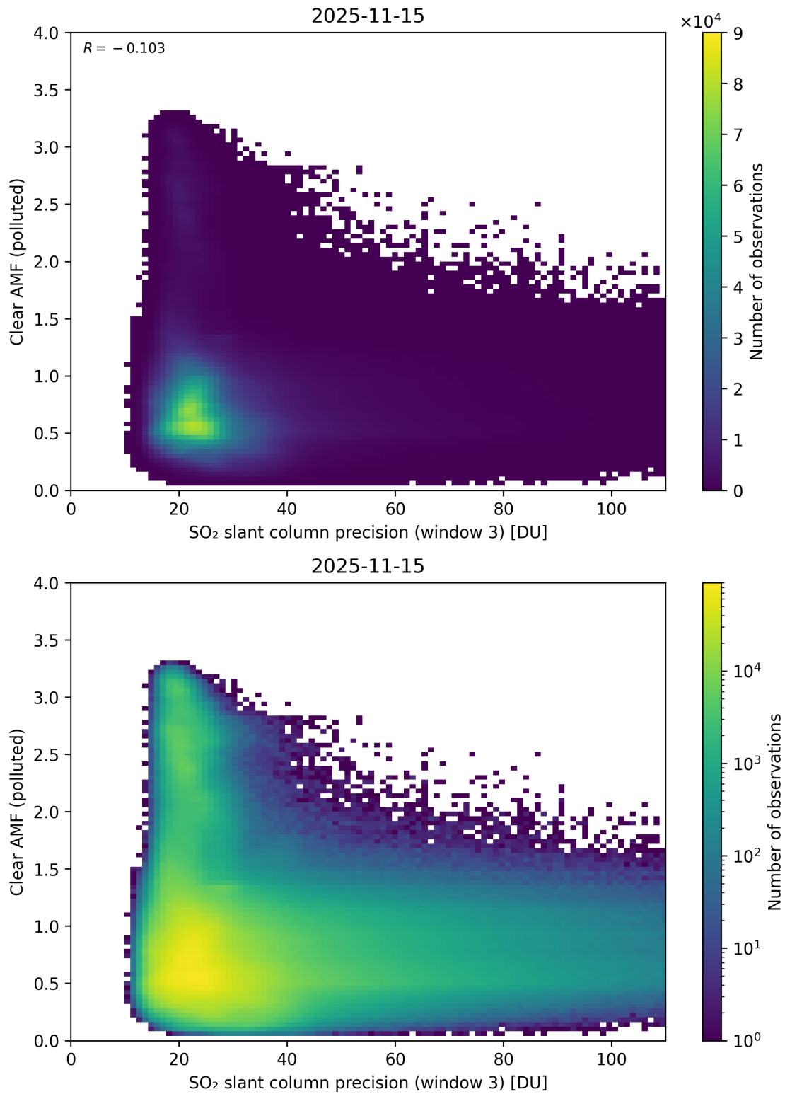
Figure 311: Scatter density plot of “SO 2 slant column precision (window 3)” against “Clear AMF (polluted)” for 2025-11-14 to 2025-11-16.
