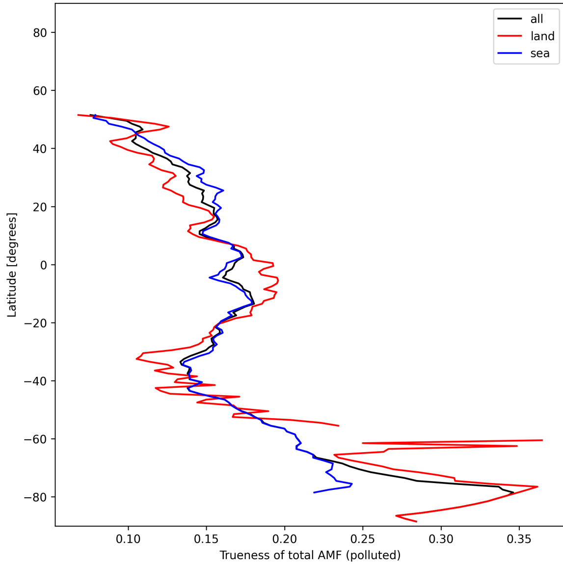
Figure 54: Zonal average of “Trueness of total AMF (polluted)” for 2025-11-14 to 2025-11-16.
