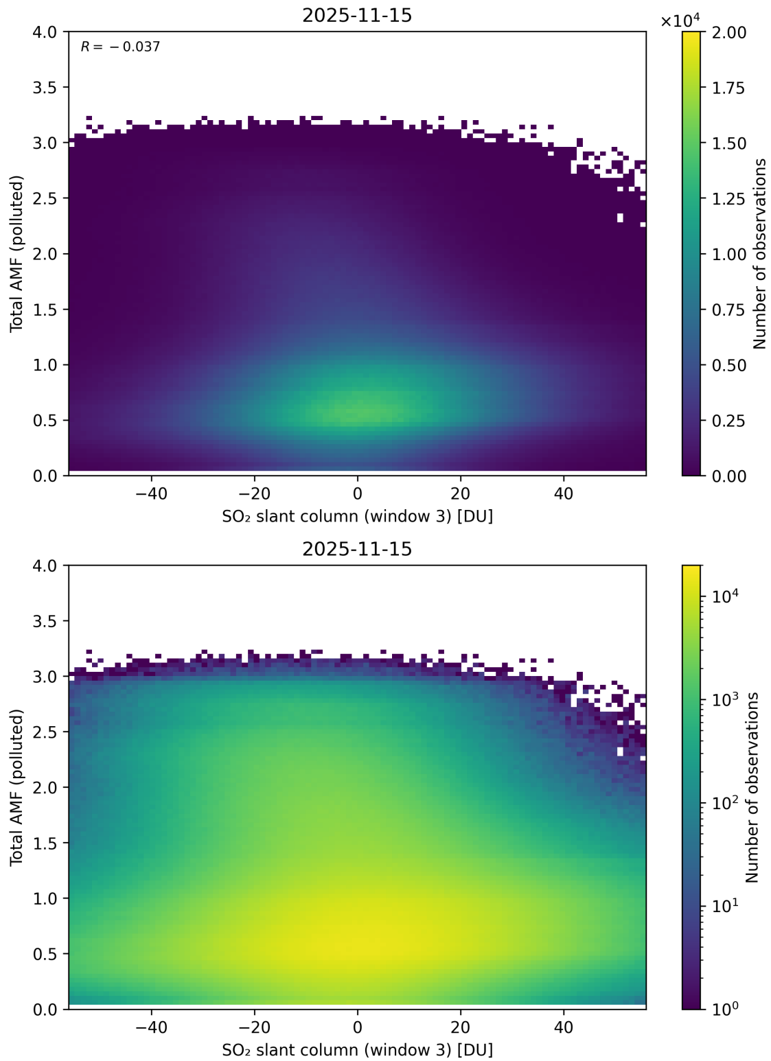
Figure 318: Scatter density plot of “SO 2 slant column (window 3)” against “Total AMF (polluted)” for 2025-11-14 to 2025-11-16.
