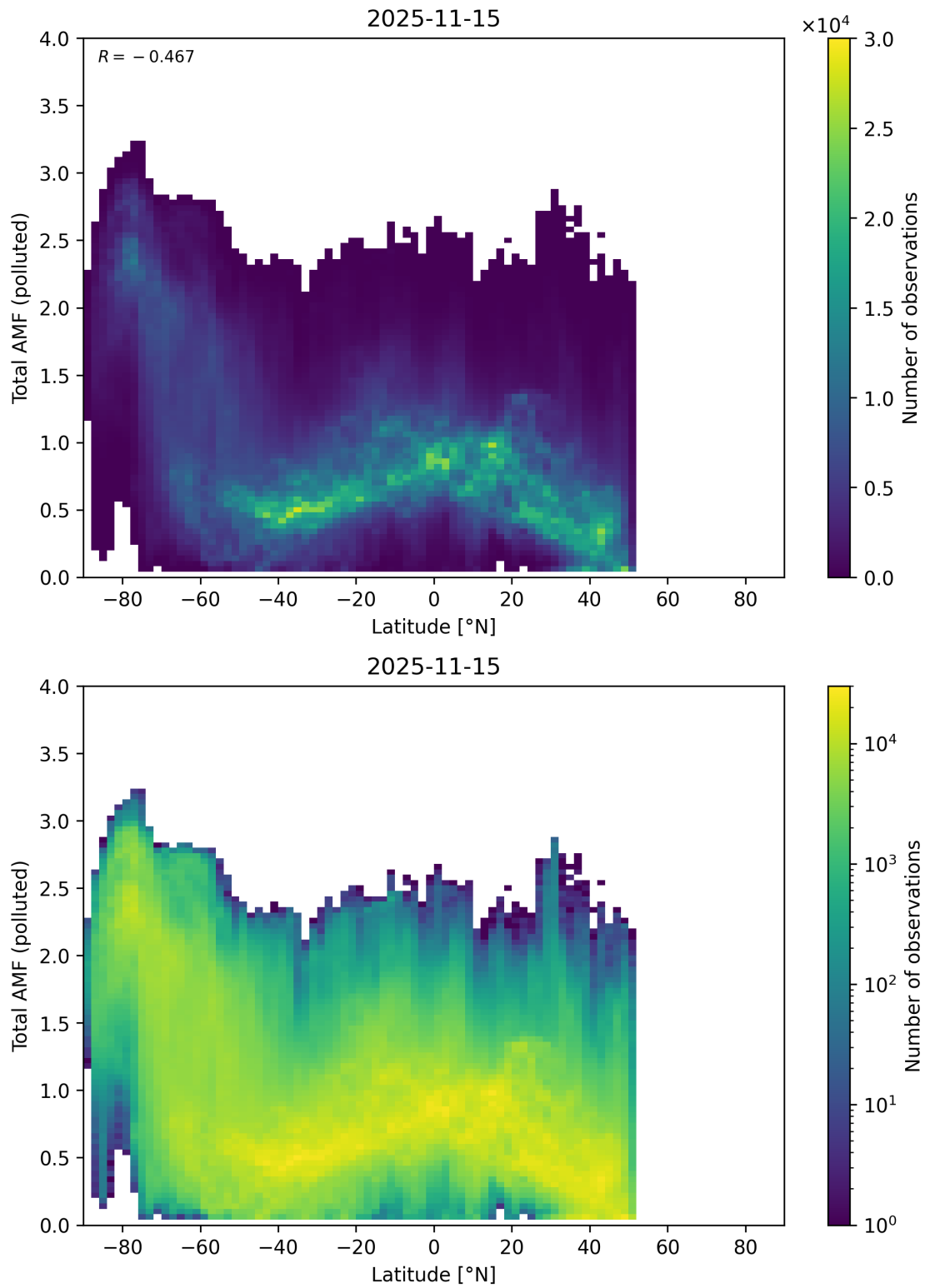
Figure 167: Scatter density plot of “Latitude” against “Total AMF (polluted)” for 2025-11-14 to 2025-11-16.
