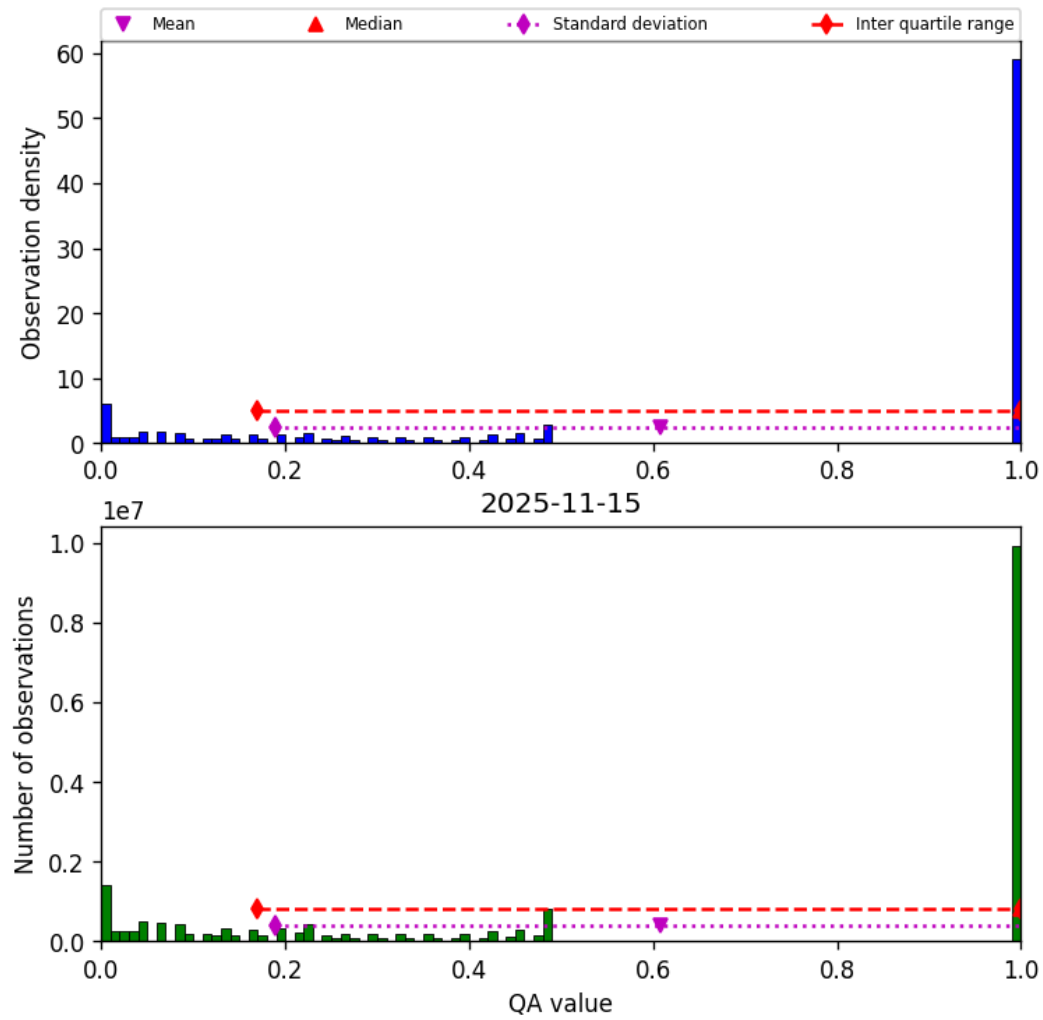
Figure 57: Histogram of “QA value” for 2025-11-14 to 2025-11-16
