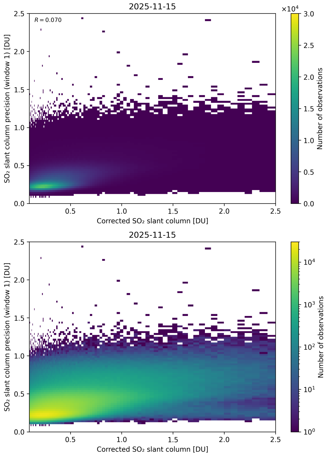
Figure 238: Scatter density plot of “Corrected SO 2 slant column” against “SO 2 slant column precision (window 1)” for 2025-11-14 to 2025-11-16.
