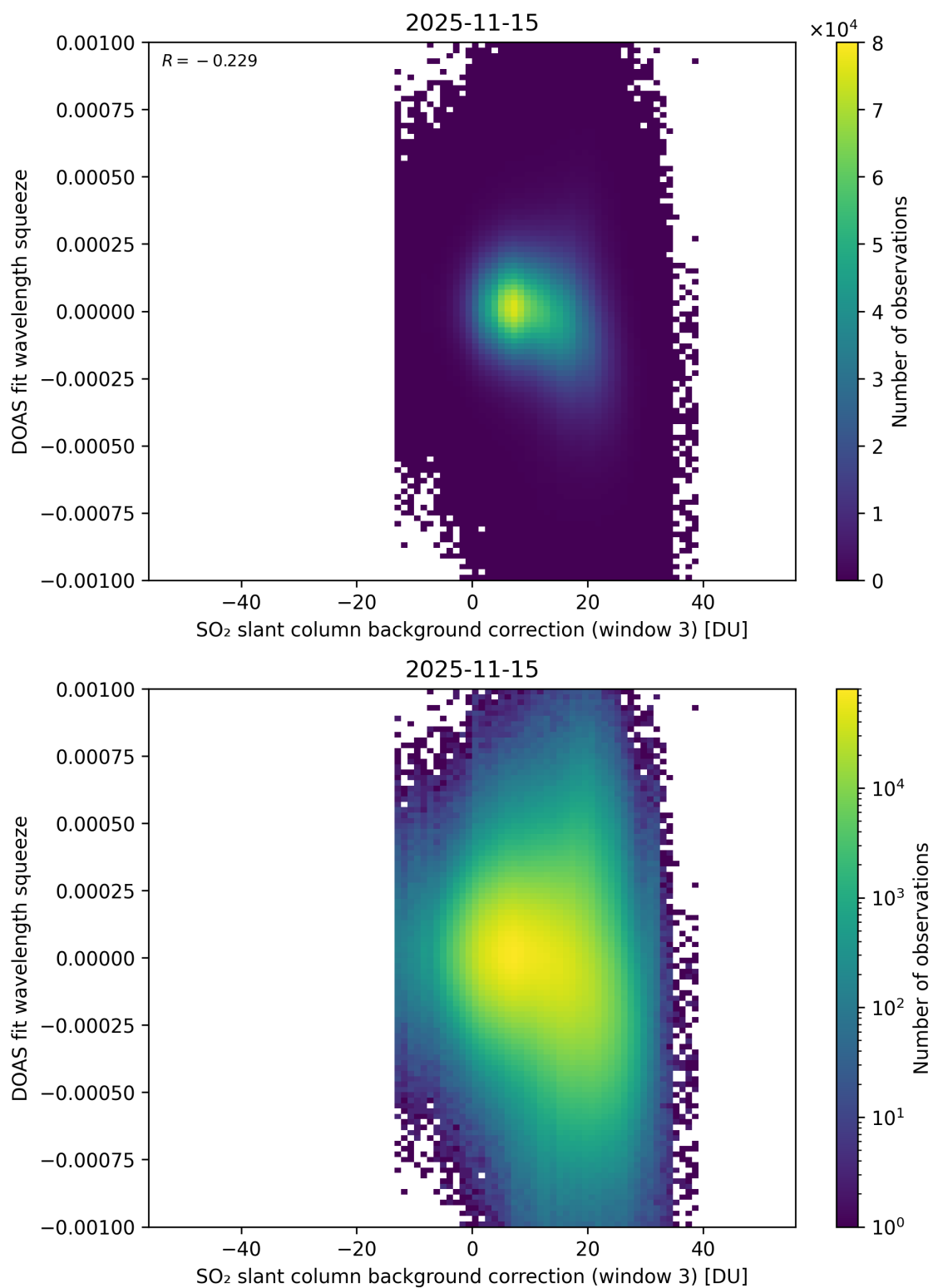
Figure 133: Scatter density plot of “SO 2 slant column background correction (window 3)” against “DOAS fit wavelength squeeze” for 2025-11-14 to 2025-11-16.
