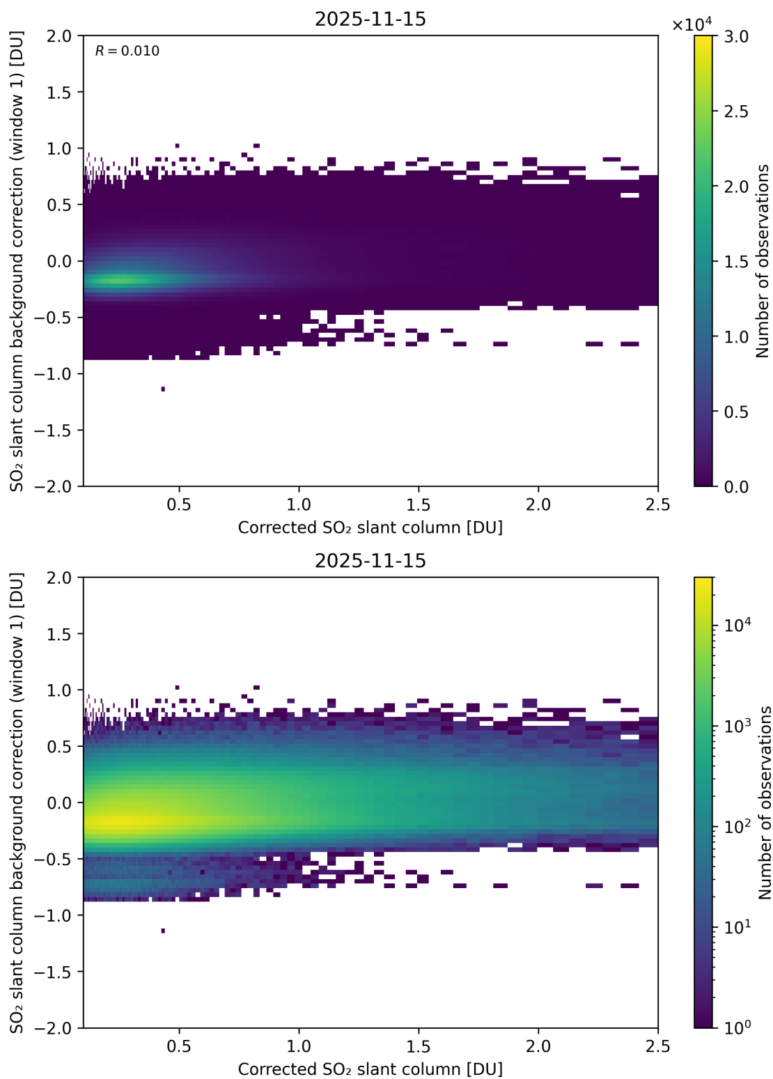
Figure 226: Scatter density plot of “Corrected SO 2 slant column” against “SO 2 slant column background correction (window 1)” for 2025-11-14 to 2025-11-16.
