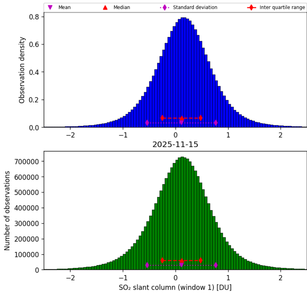
Figure 63: Histogram of “SO 2 slant column (window 1)” for 2025-11-14 to 2025-11-16
