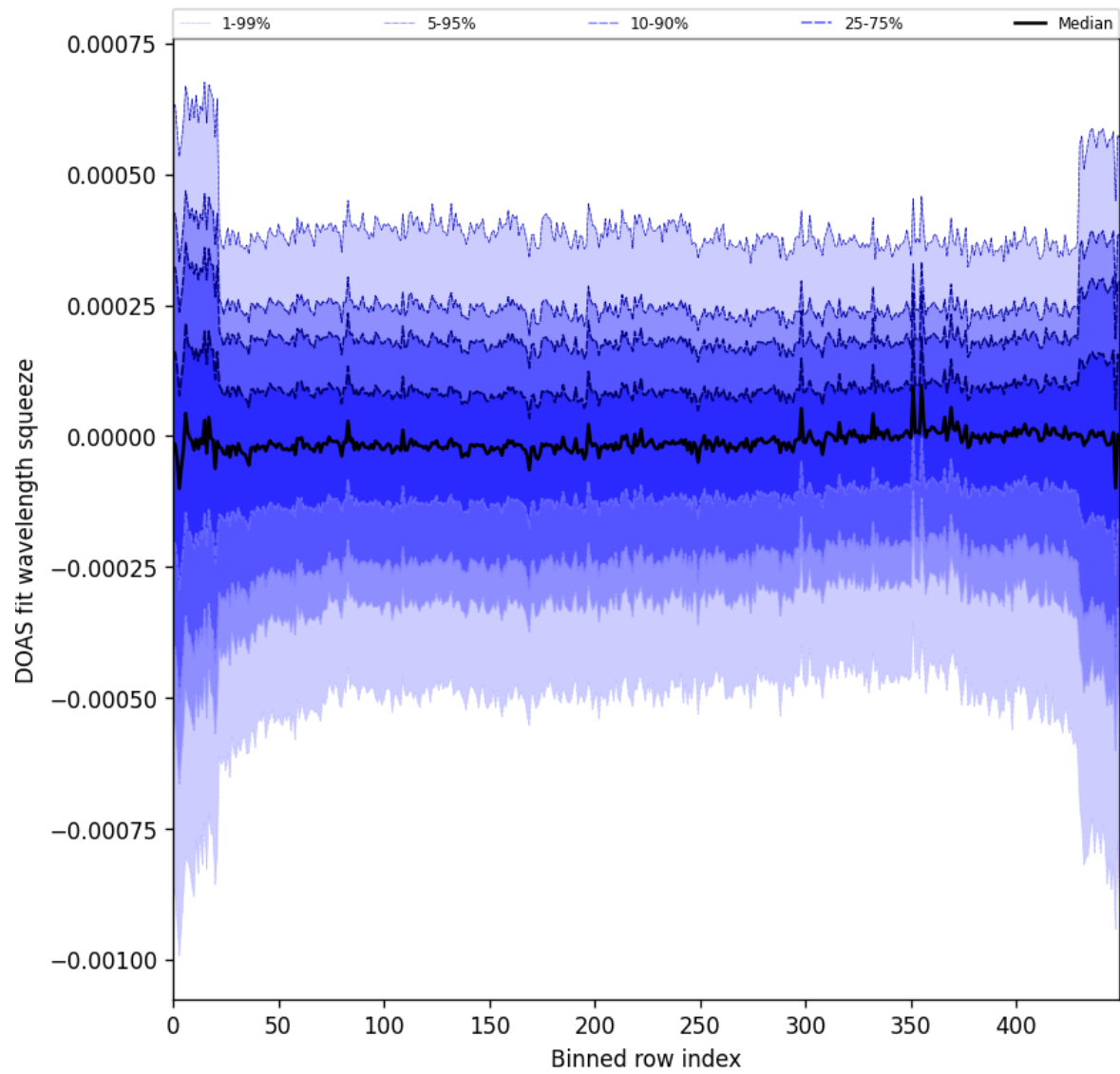
Figure 103: Along track statistics of “DOAS fit wavelength squeeze” for 2025-11-14 to 2025-11-16
