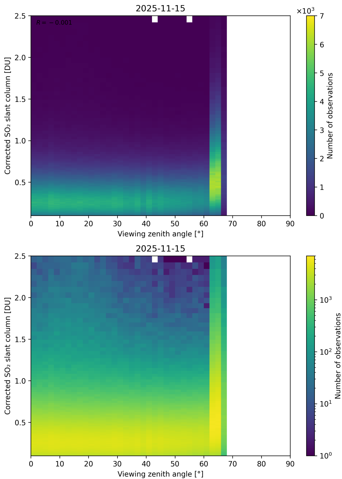
Figure 373: Scatter density plot of “Viewing zenith angle” against “Corrected SO 2 slant column” for 2025-11-14 to 2025-11-16.
