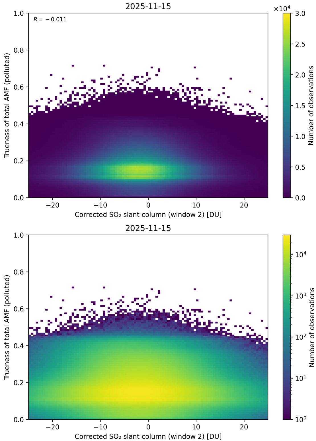
Figure 254: Scatter density plot of “Corrected SO 2 slant column (window 2)” against “Trueness of total AMF (polluted)” for 2025-11-14 to 2025-11-16.
