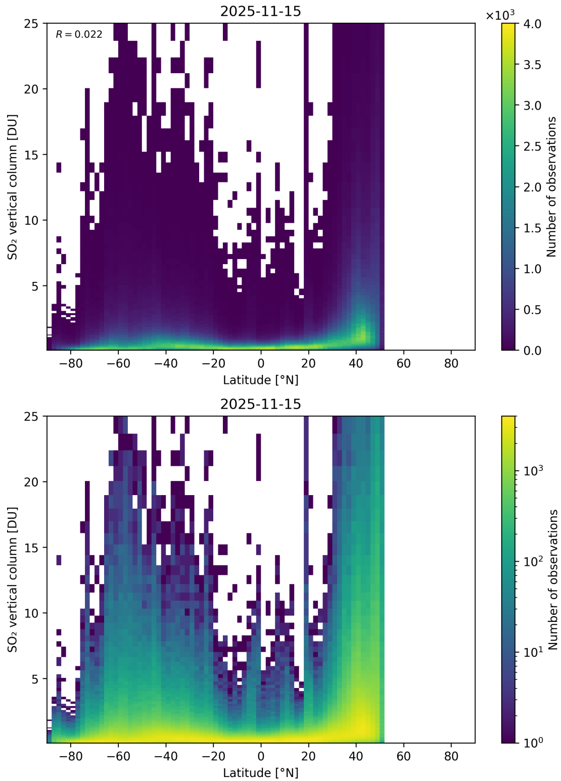
Figure 169: Scatter density plot of “Latitude” against “SO 2 vertical column” for 2025-11-14 to 2025-11-16.
