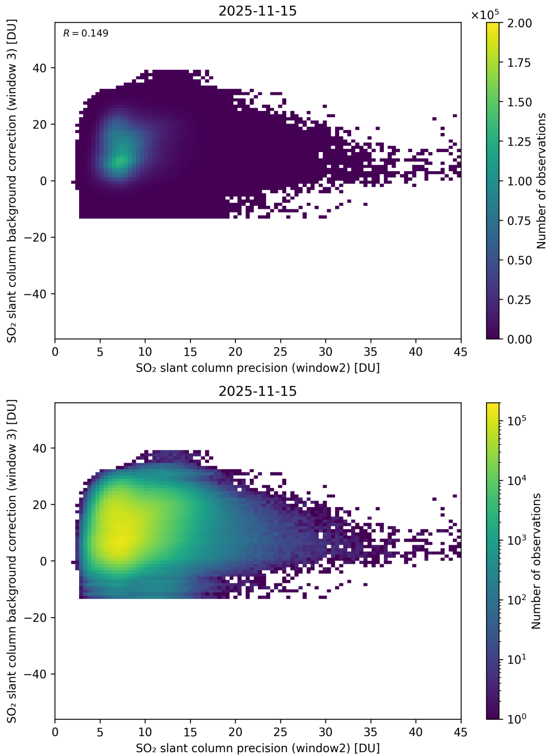
Figure 292: Scatter density plot of “SO 2 slant column precision (window2)” against “SO 2 slant column background correction (window 3)” for 2025-11-14 to 2025-11-16.
