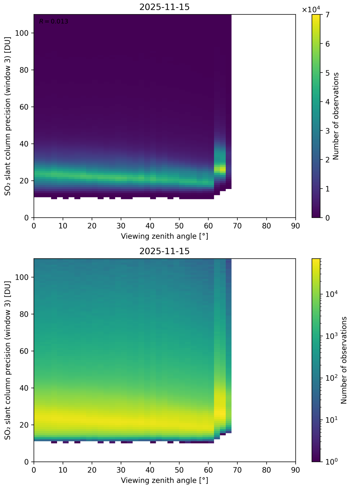
Figure 380: Scatter density plot of “Viewing zenith angle” against “SO 2 slant column precision (window 3)” for 2025-11-14 to 2025-11-16.
