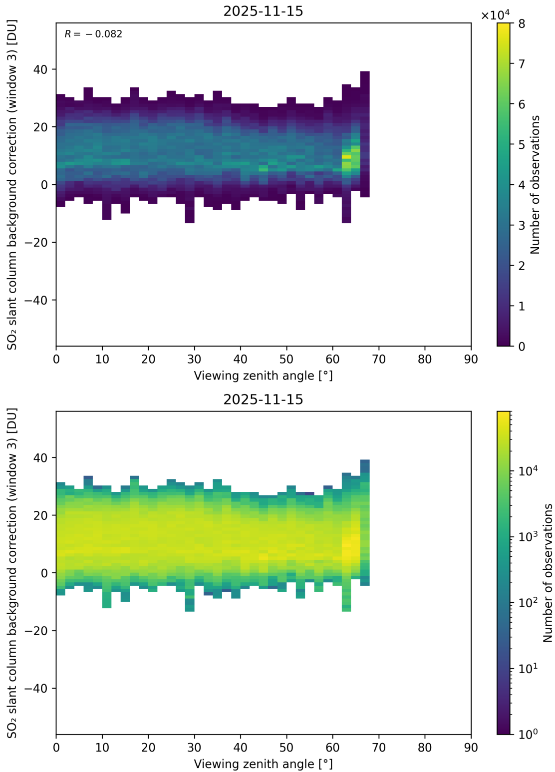
Figure 364: Scatter density plot of “Viewing zenith angle” against “SO 2 slant column background correction (window 3)” for 2025-11-14 to 2025-11-16.
