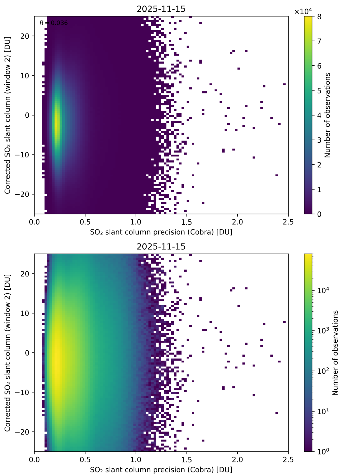
Figure 206: Scatter density plot of “SO 2 slant column precision (Cobra)” against “Corrected SO 2 slant column (window 2)” for 2025-11-14 to 2025-11-16.
