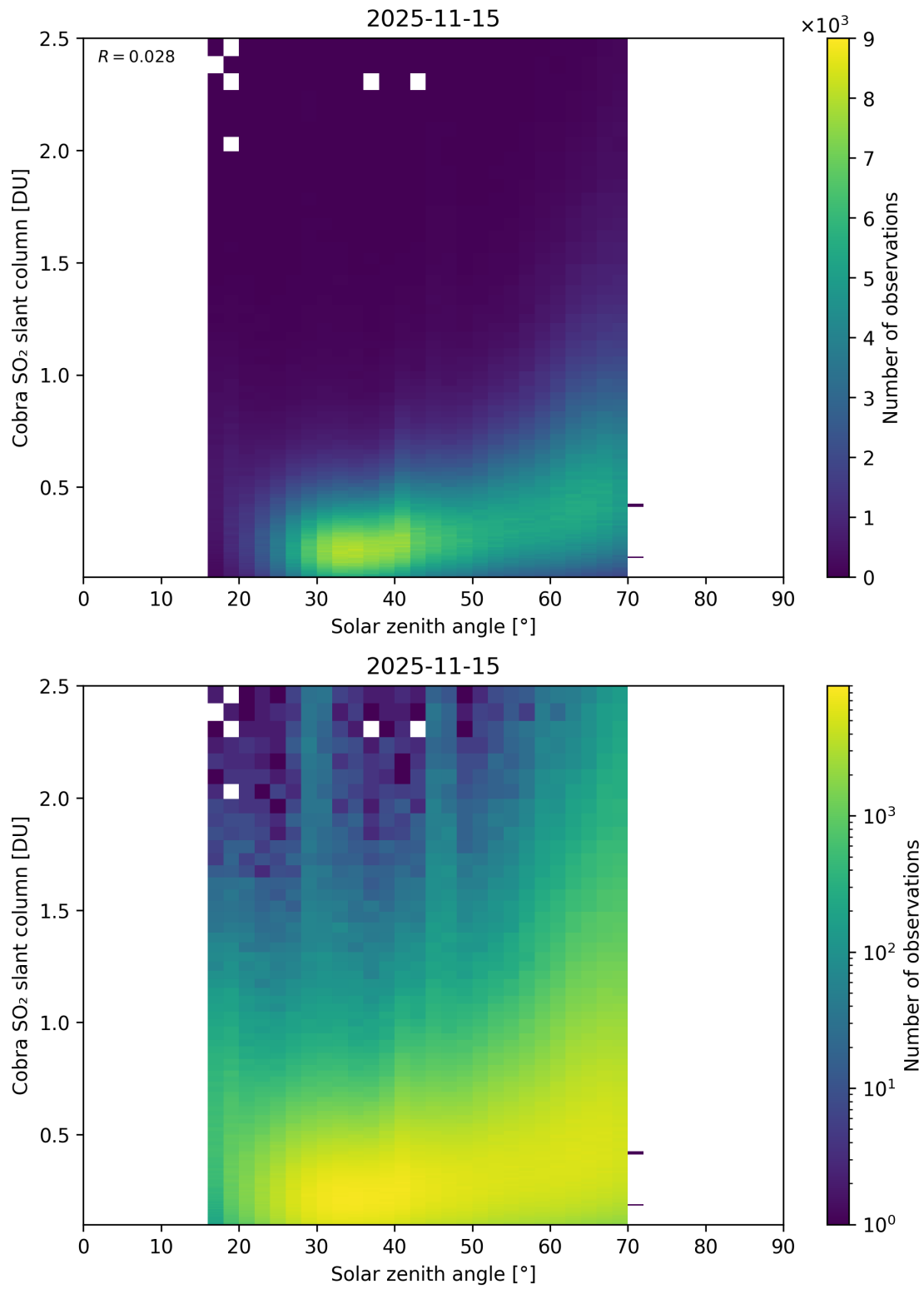
Figure 179: Scatter density plot of “Solar zenith angle” against “Cobra SO 2 slant column” for 2025-11-14 to 2025-11-16.
