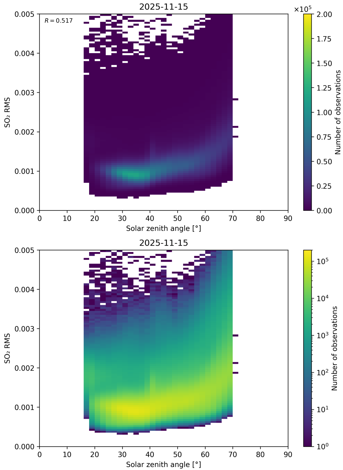
Figure 176: Scatter density plot of “Solar zenith angle” against “SO 2 RMS” for 2025-11-14 to 2025-11-16.
