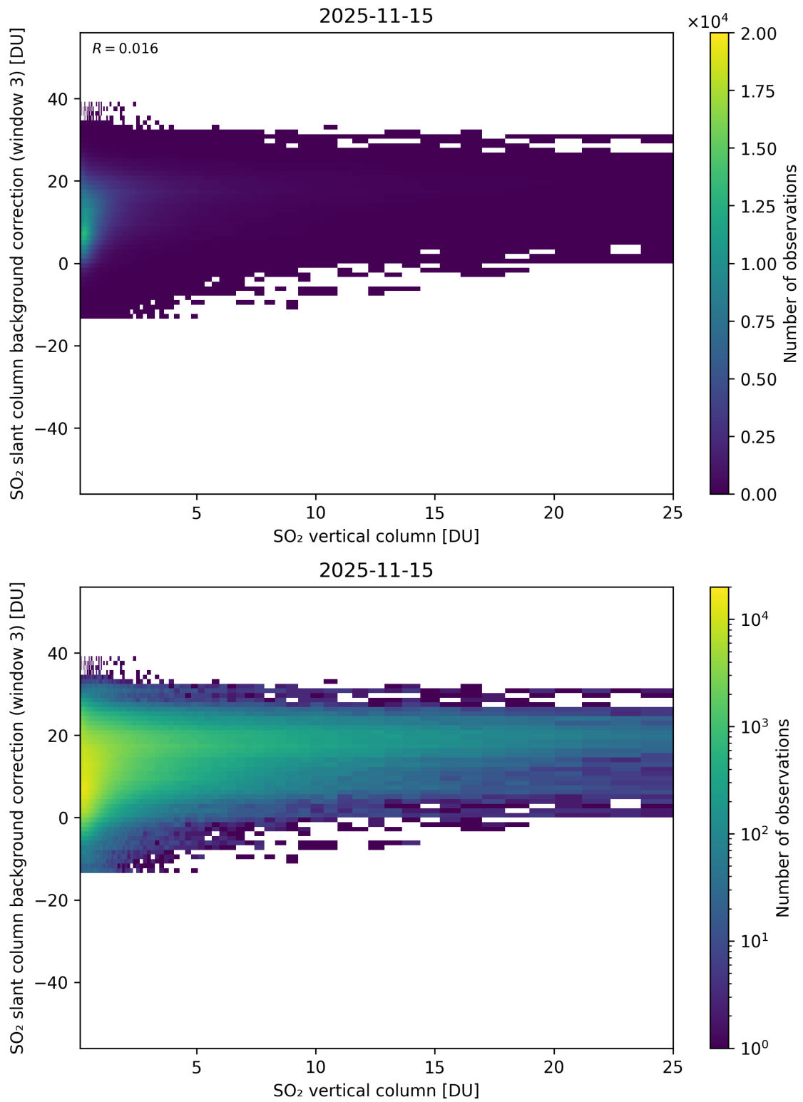
Figure 325: Scatter density plot of “SO 2 vertical column” against “SO 2 slant column background correction (window 3)” for 2025-11-14 to 2025-11-16.
