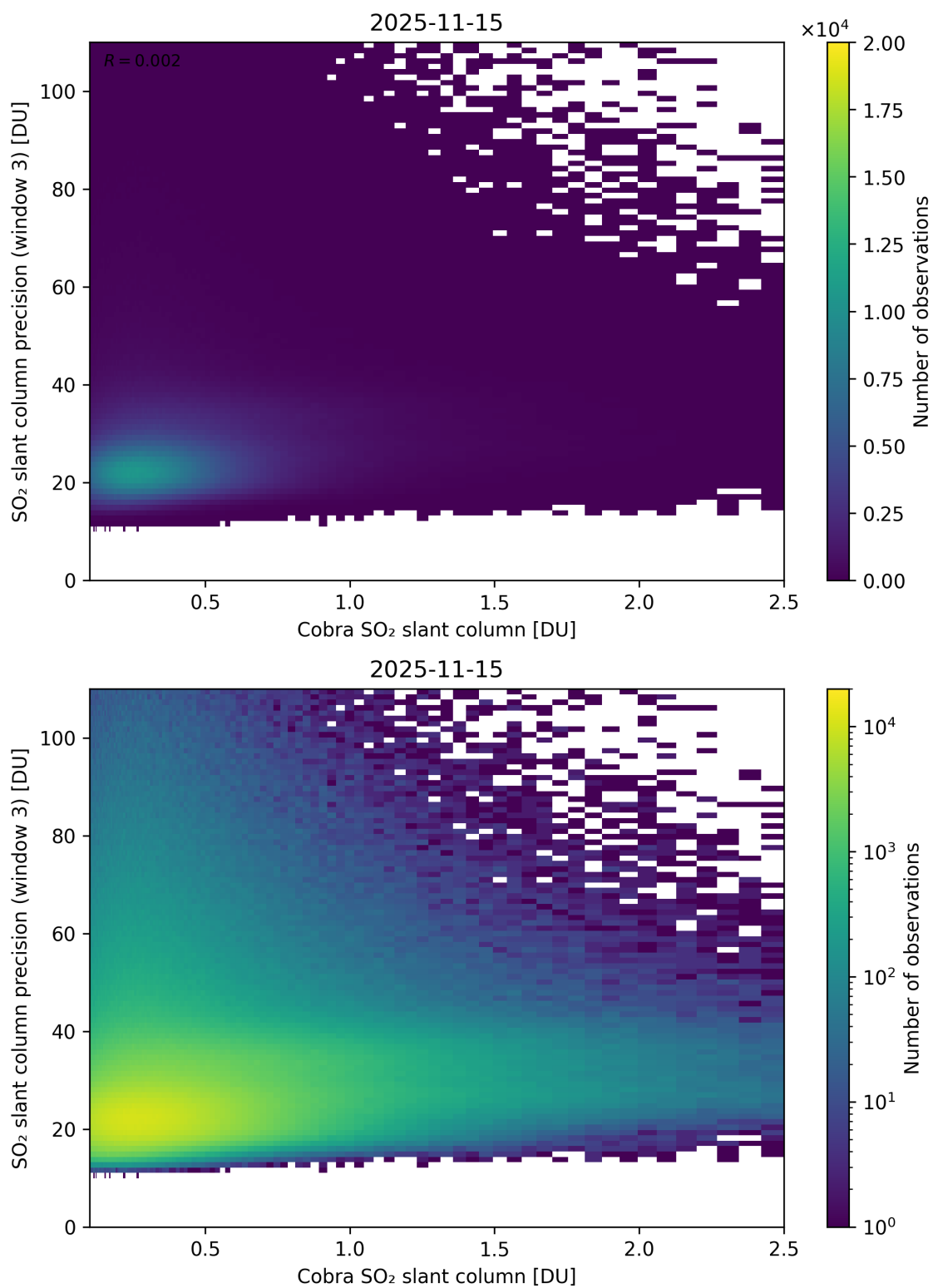
Figure 223: Scatter density plot of “Cobra SO 2 slant column” against “SO 2 slant column precision (window 3)” for 2025-11-14 to 2025-11-16.
