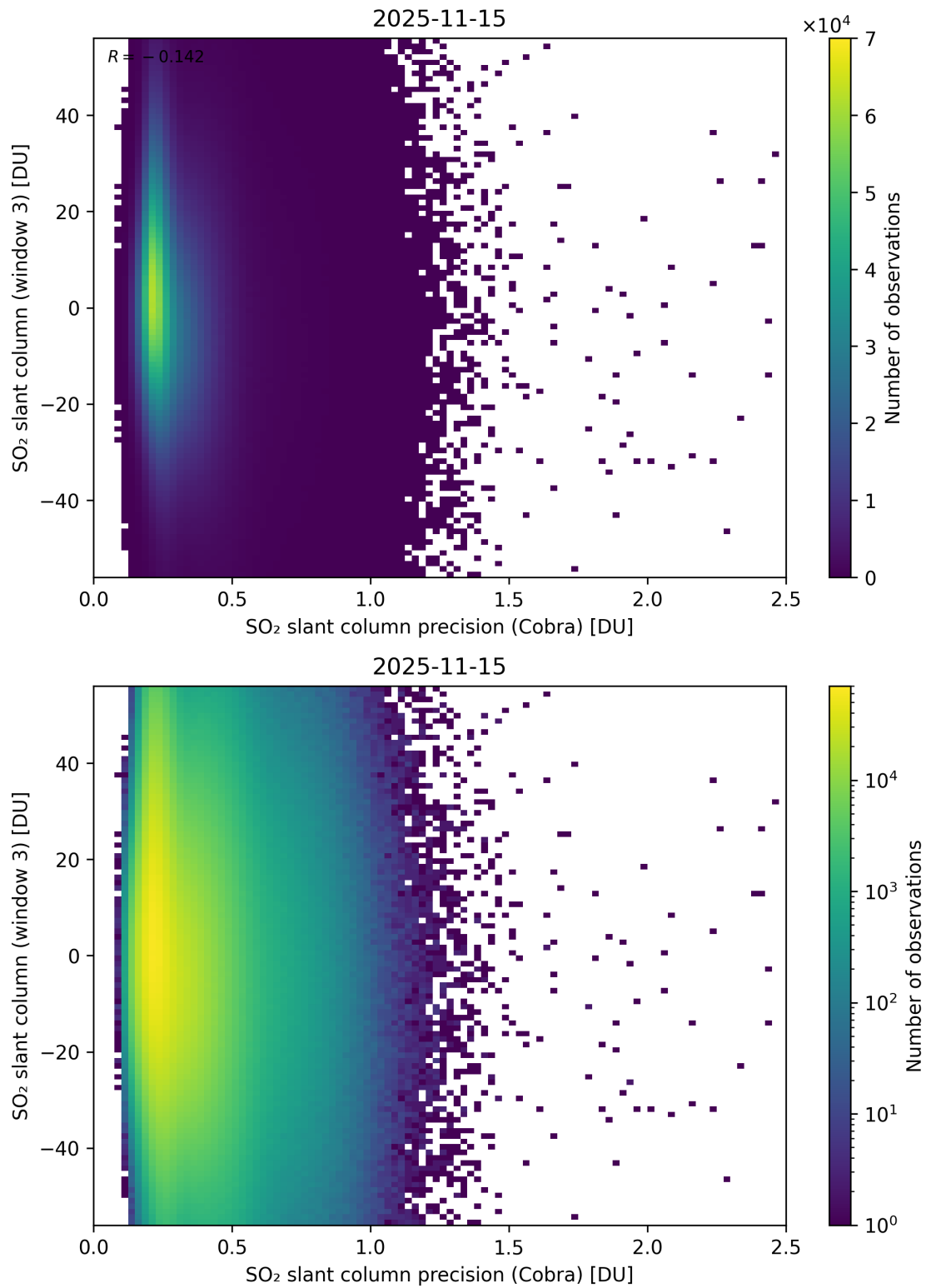
Figure 211: Scatter density plot of “SO 2 slant column precision (Cobra)” against “SO 2 slant column (window 3)” for 2025-11-14 to 2025-11-16.
