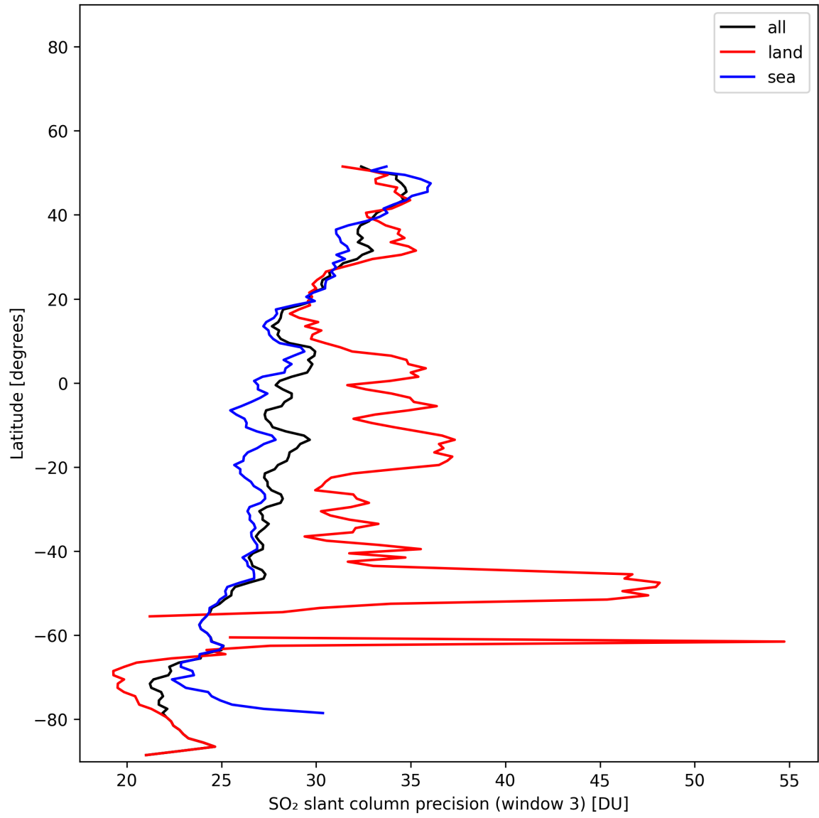
Figure 46: Zonal average of “SO 2 slant column precision (window 3)” for 2025-11-14 to 2025-11-16.
