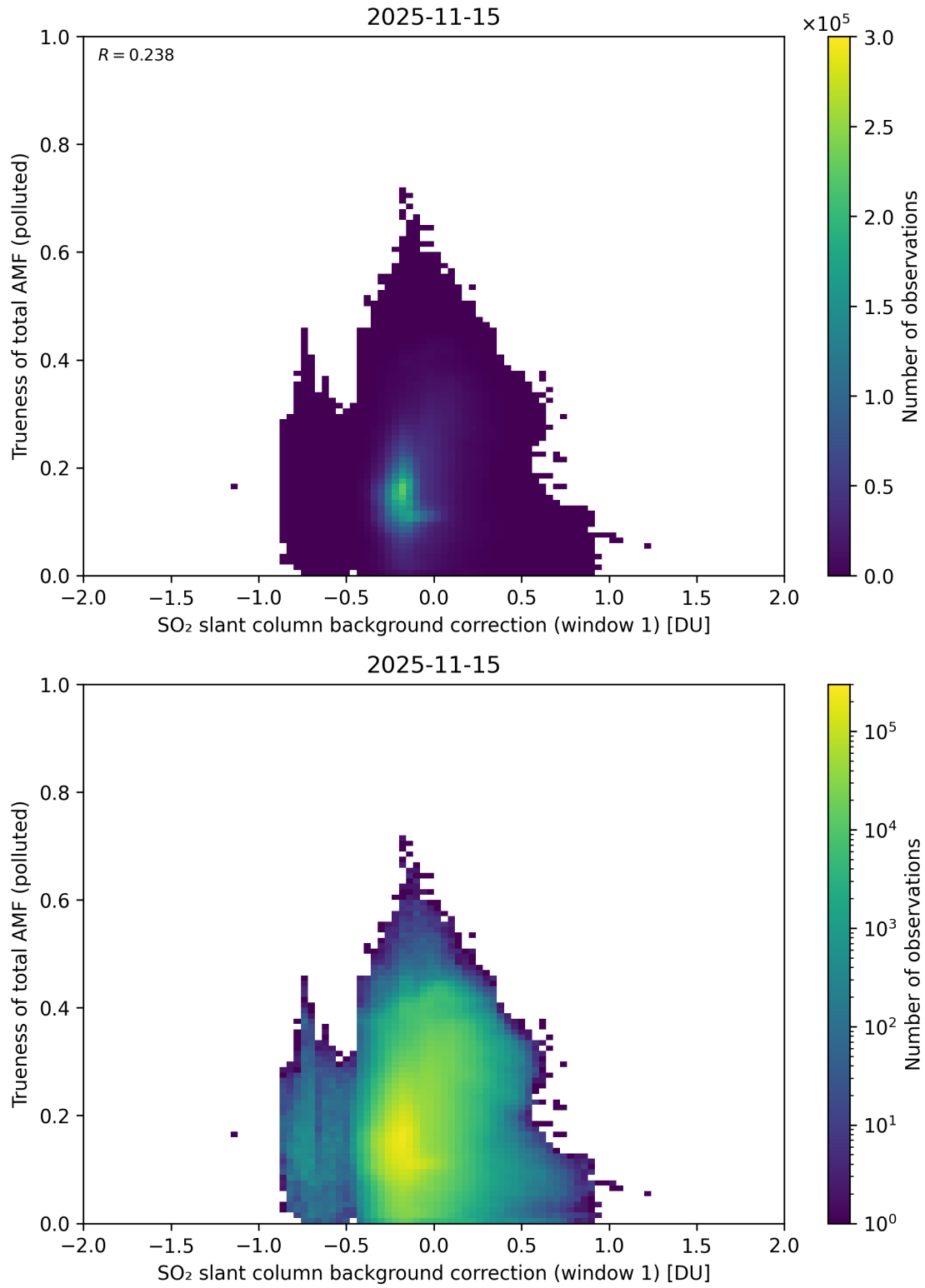
Figure 121: Scatter density plot of “SO 2 slant column background correction (window 1)” against “Trueness of total AMF (polluted)” for 2025-11-14 to 2025-11-16.
