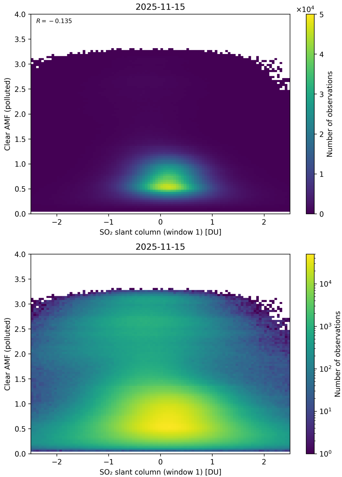
Figure 282: Scatter density plot of “SO 2 slant column (window 1)” against “Clear AMF (polluted)” for 2025-11-14 to 2025-11-16.
