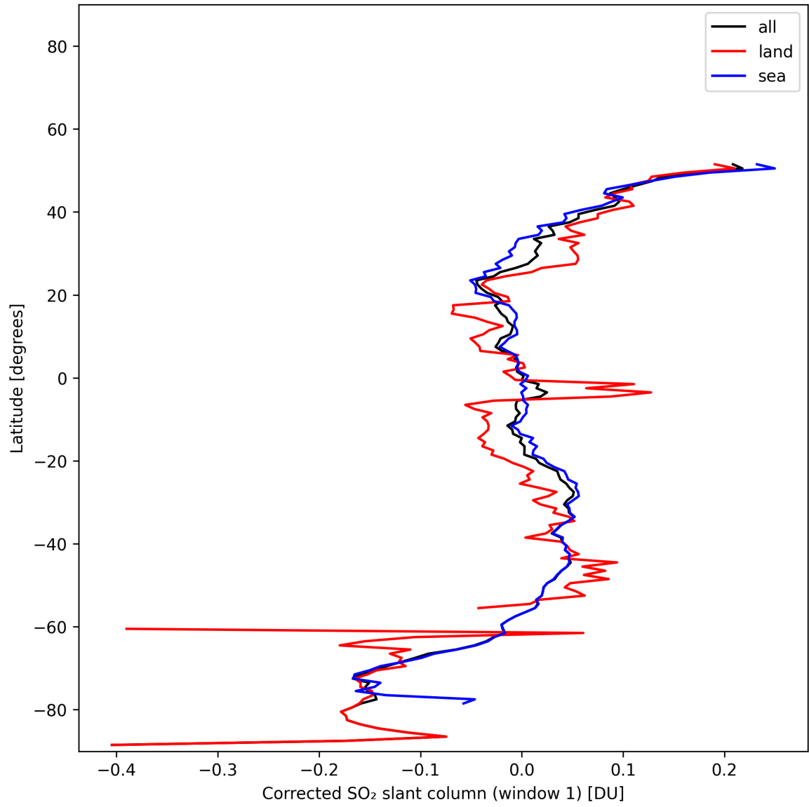
Figure 39: Zonal average of “Corrected SO 2 slant column (window 1)” for 2025-11-14 to 2025-11-16.
