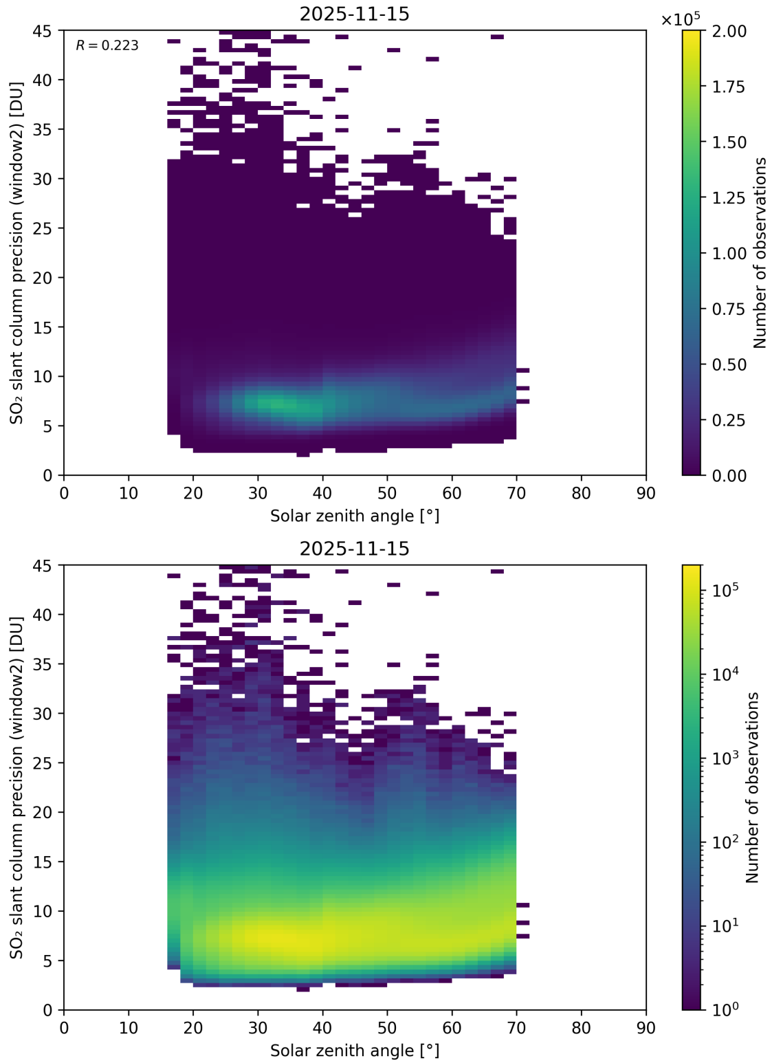
Figure 186: Scatter density plot of “Solar zenith angle” against “SO 2 slant column precision (window2)” for 2025-11-14 to 2025-11-16.
