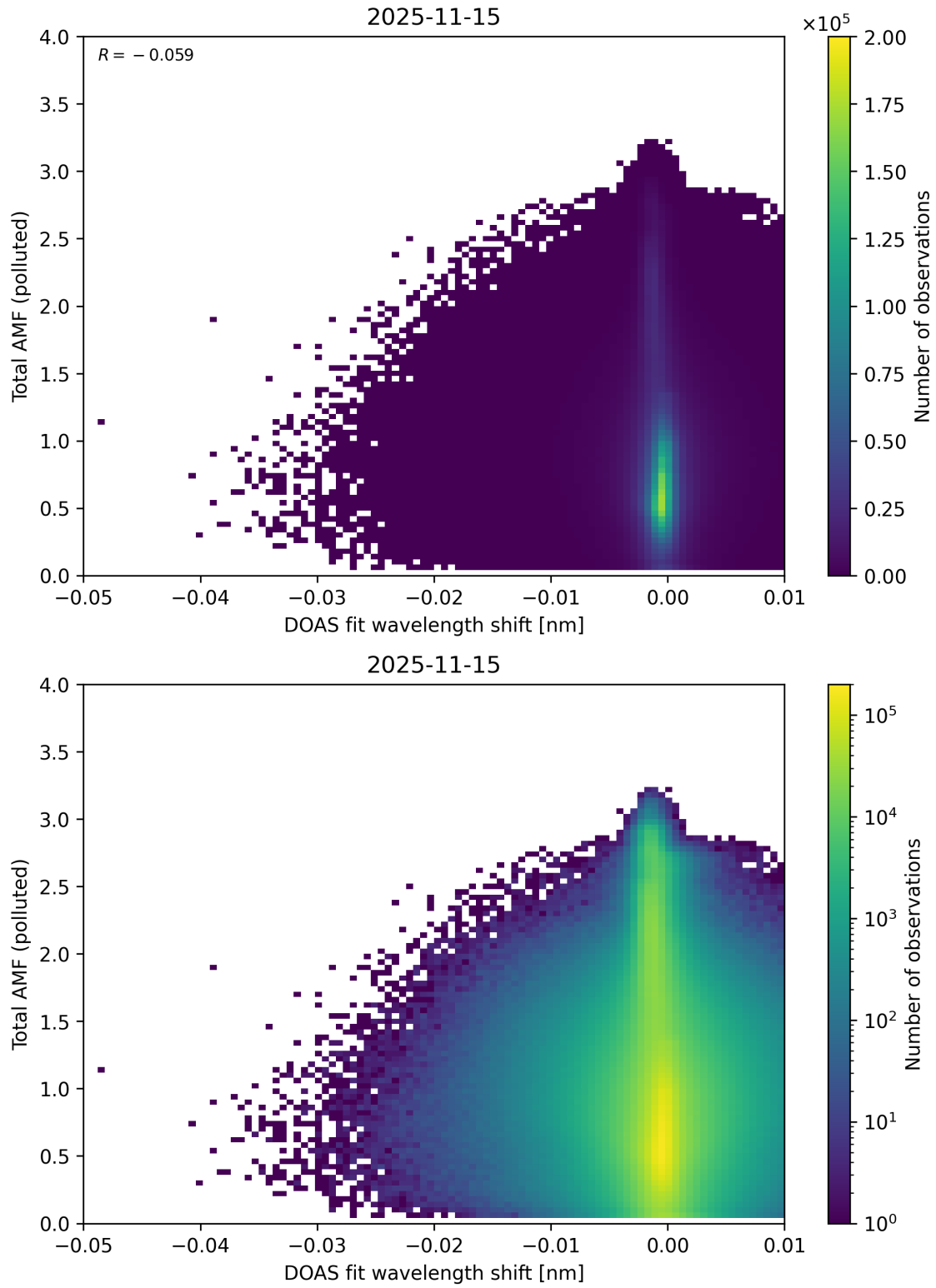
Figure 141: Scatter density plot of “DOAS fit wavelength shift” against “Total AMF (polluted)” for 2025-11-14 to 2025-11-16.
