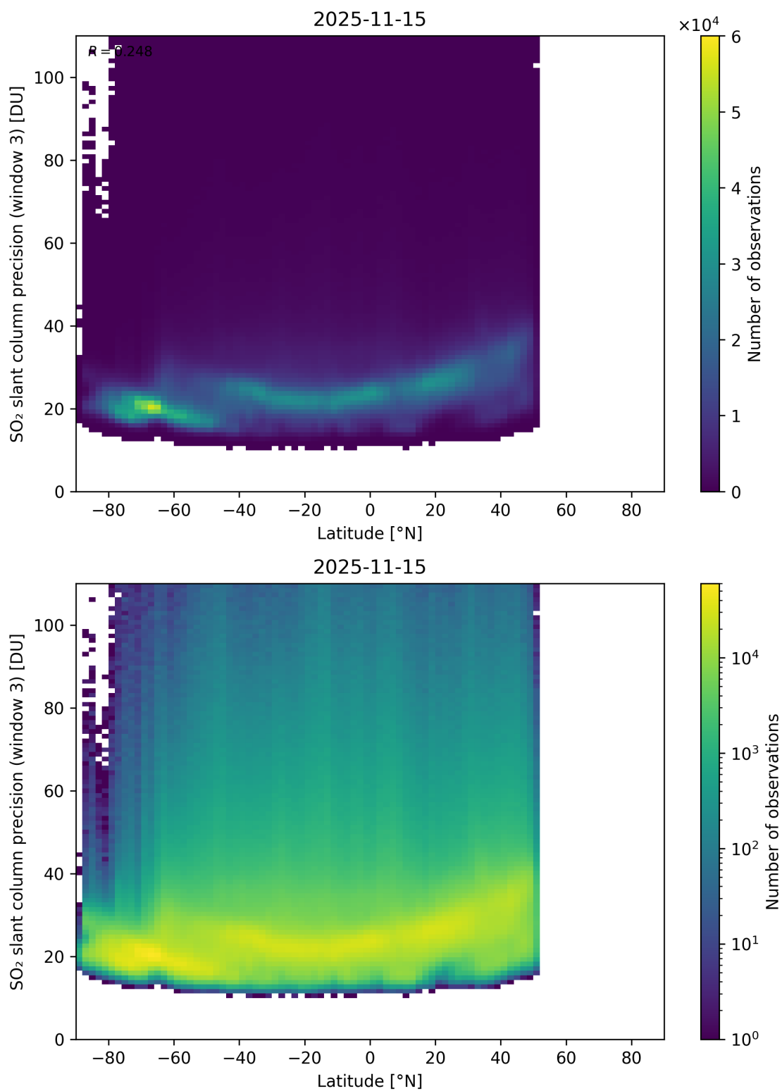
Figure 166: Scatter density plot of “Latitude” against “SO 2 slant column precision (window 3)” for 2025-11-14 to 2025-11-16.
