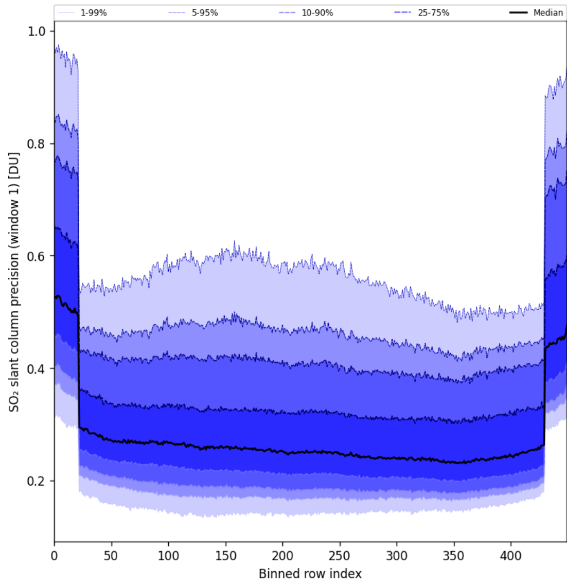
Figure 90: Along track statistics of “SO 2 slant column precision (window 1)” for 2025-11-14 to 2025-11-16
