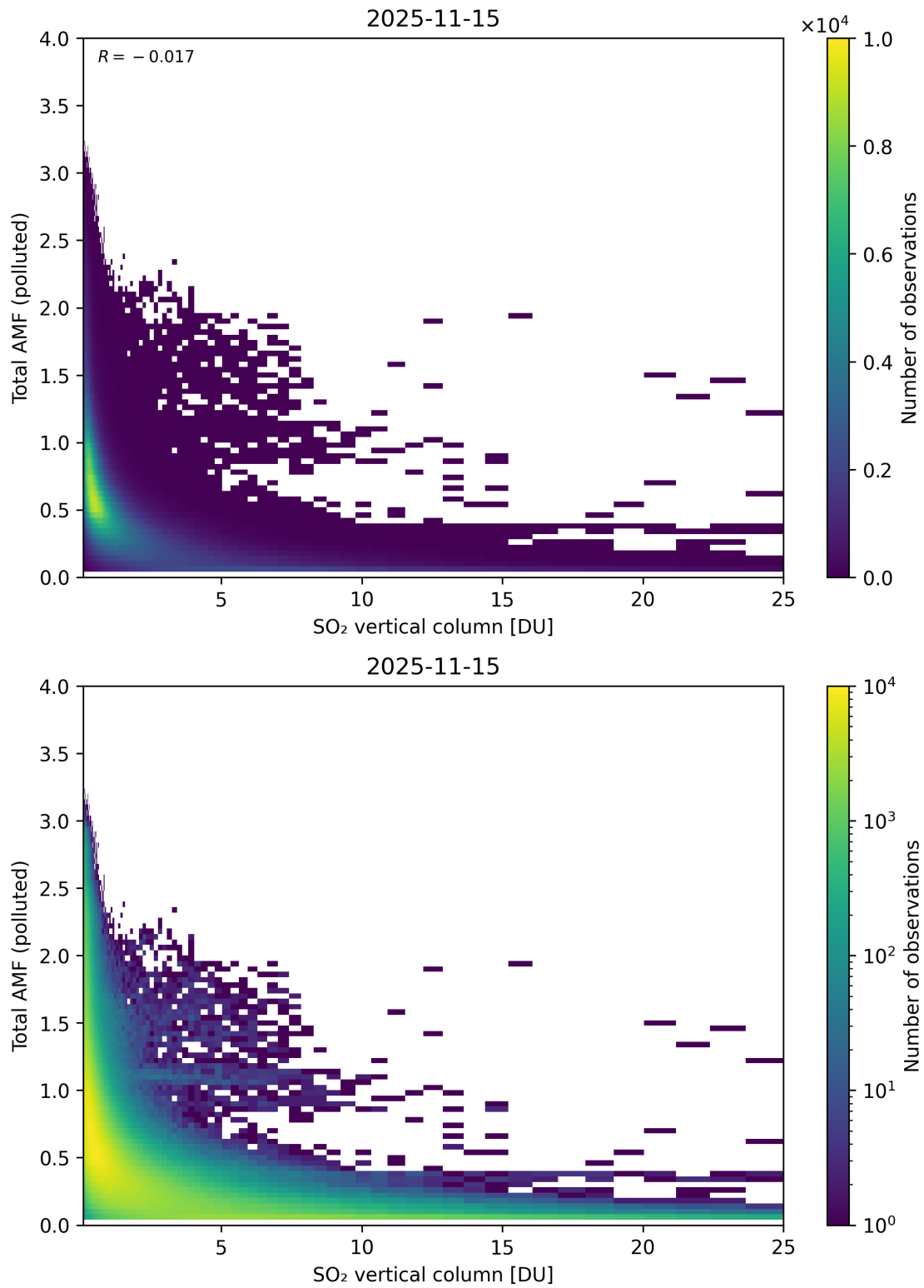
Figure 359: Scatter density plot of “SO 2 vertical column” against “Total AMF (polluted)” for 2025-11-14 to 2025-11-16.
