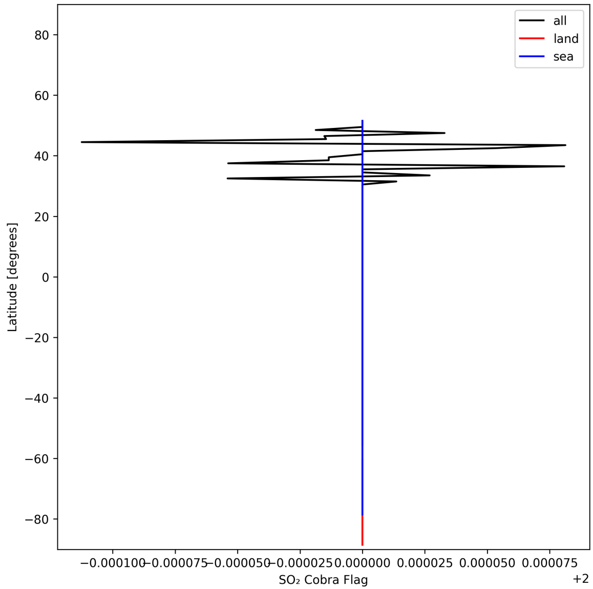
Figure 49: Zonal average of "SO 2 Cobra Flag" for 2025-11-14 to 2025-11-16.
