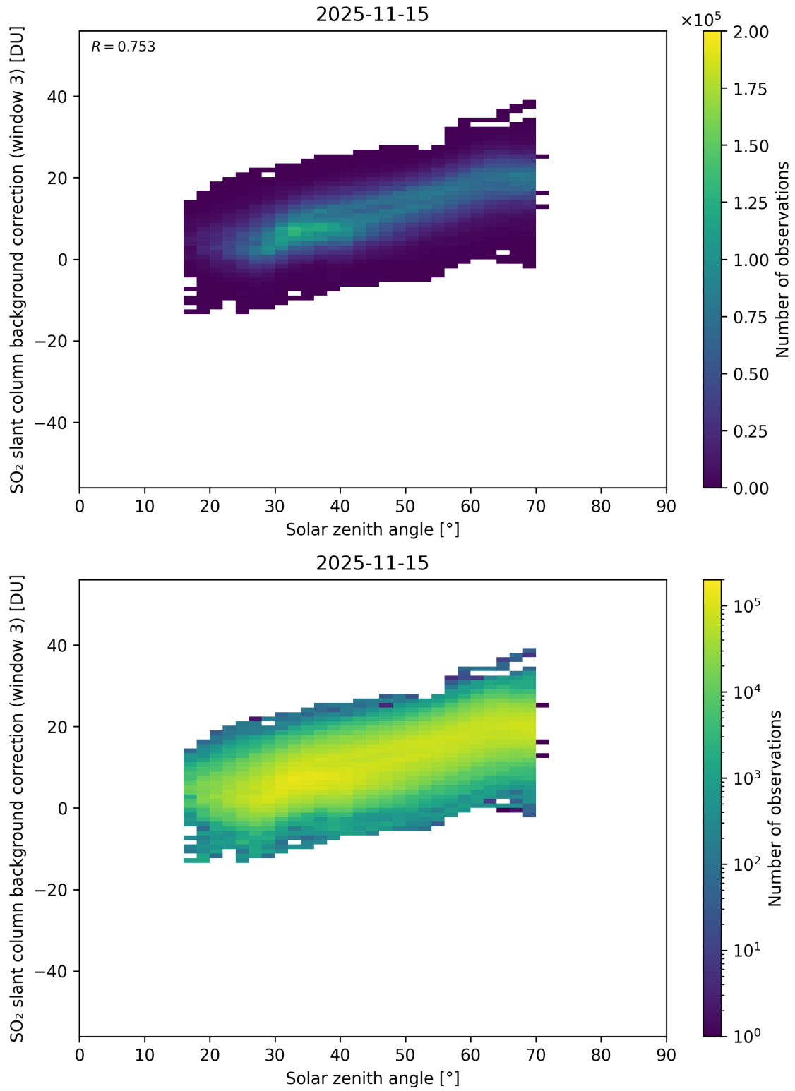
Figure 173: Scatter density plot of “Solar zenith angle” against “SO 2 slant column background correction (window 3)” for 2025-11-14 to 2025-11-16.
