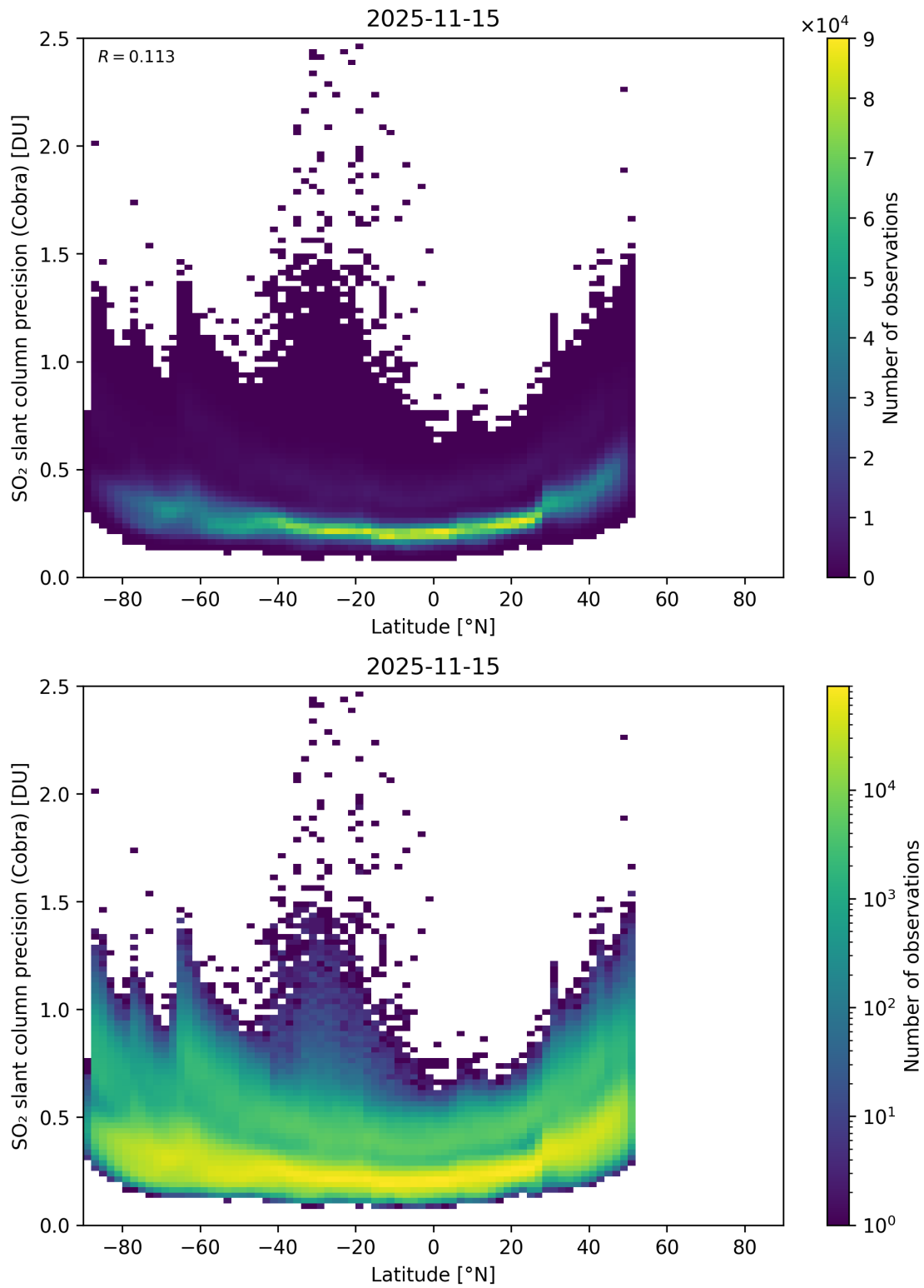
Figure 158: Scatter density plot of “Latitude” against “SO 2 slant column precision (Cobra)” for 2025-11-14 to 2025-11-16.
