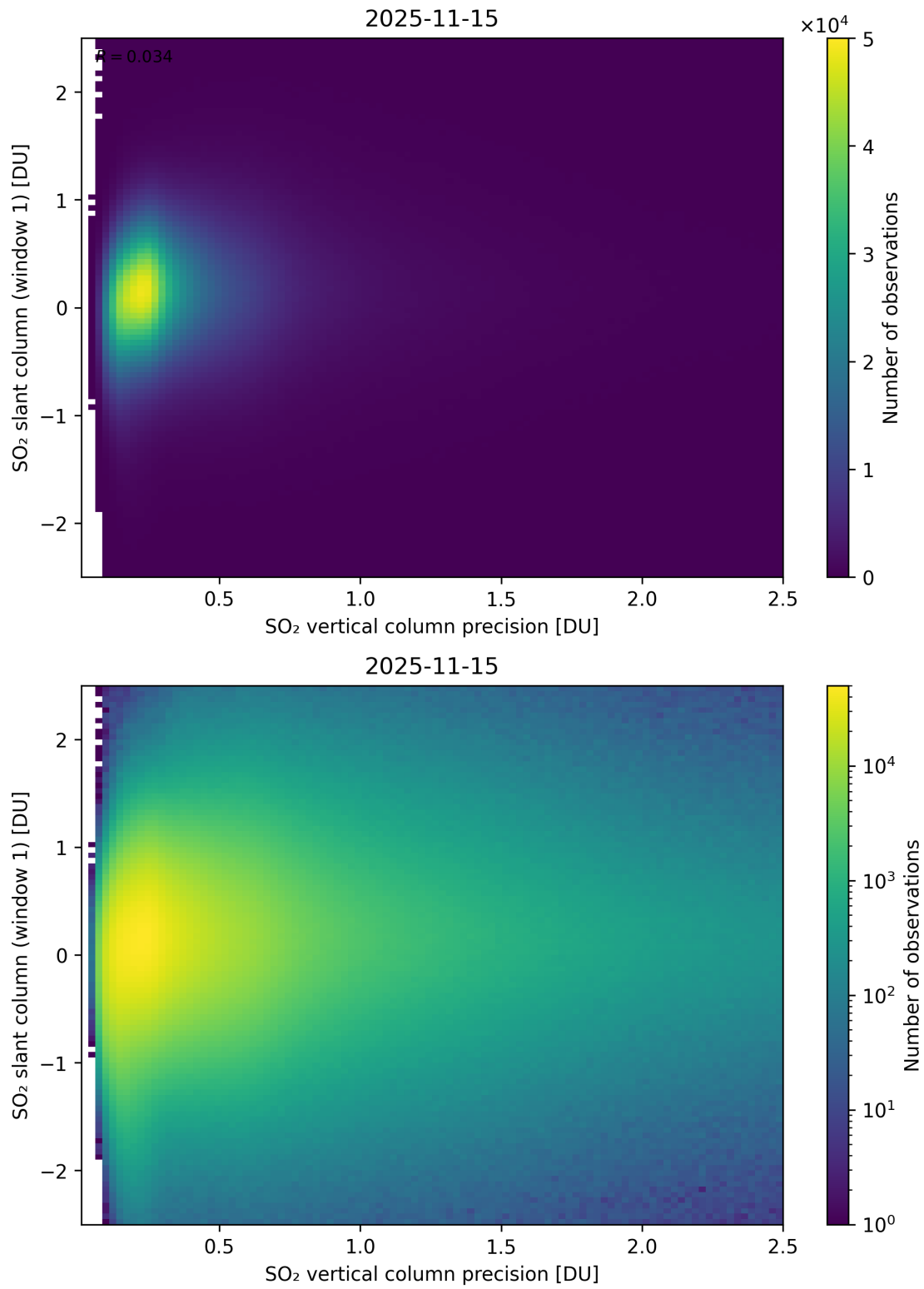
Figure 341: Scatter density plot of “SO 2 vertical column precision” against “SO 2 slant column (window 1)” for 2025-11-14 to 2025-11-16.
