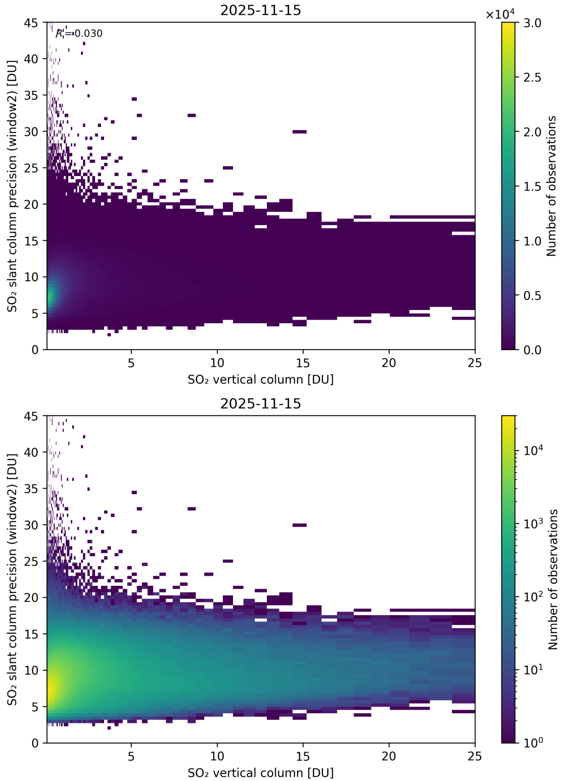
Figure 356: Scatter density plot of “SO 2 vertical column” against “SO 2 slant column precision (window2)” for 2025-11-14 to 2025-11-16.
