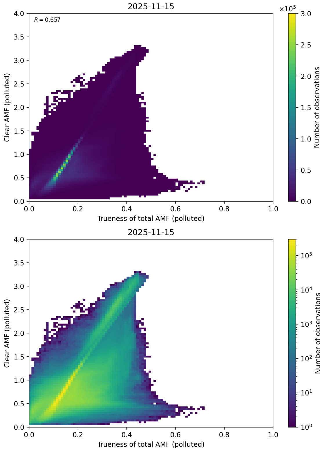
Figure 322: Scatter density plot of “Trueness of total AMF (polluted)” against “Clear AMF (polluted)” for 2025-11-14 to 2025-11-16.
