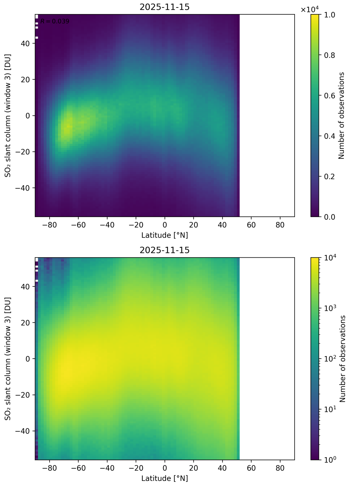
Figure 165: Scatter density plot of “Latitude” against “SO 2 slant column (window 3)” for 2025-11-14 to 2025-11-16.
