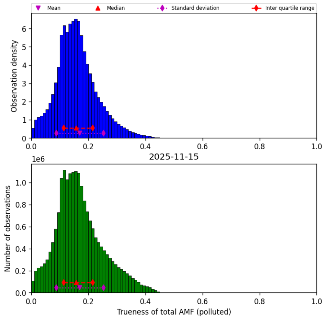
Figure 80: Histogram of “Trueness of total AMF (polluted)” for 2025-11-14 to 2025-11-16
