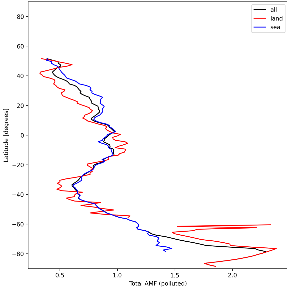
Figure 53: Zonal average of “Total AMF (polluted)” for 2025-11-14 to 2025-11-16.
