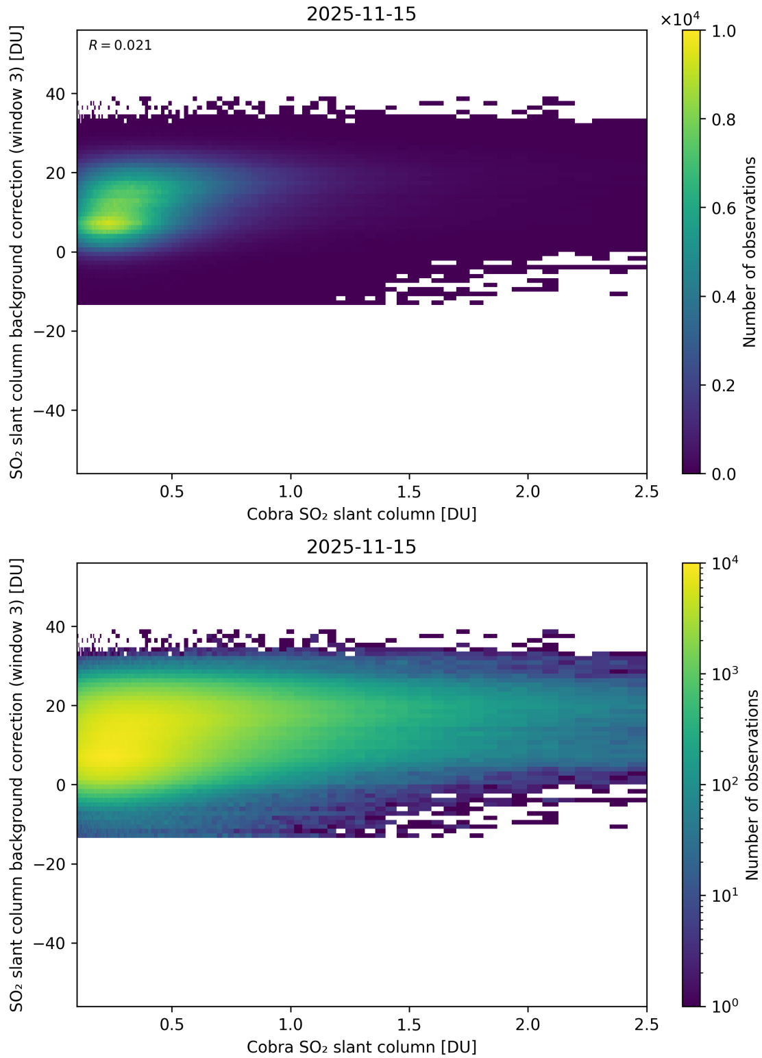
Figure 195: Scatter density plot of “Cobra SO 2 slant column” against “SO 2 slant column background correction (window 3)” for 2025-11-14 to 2025-11-16.
