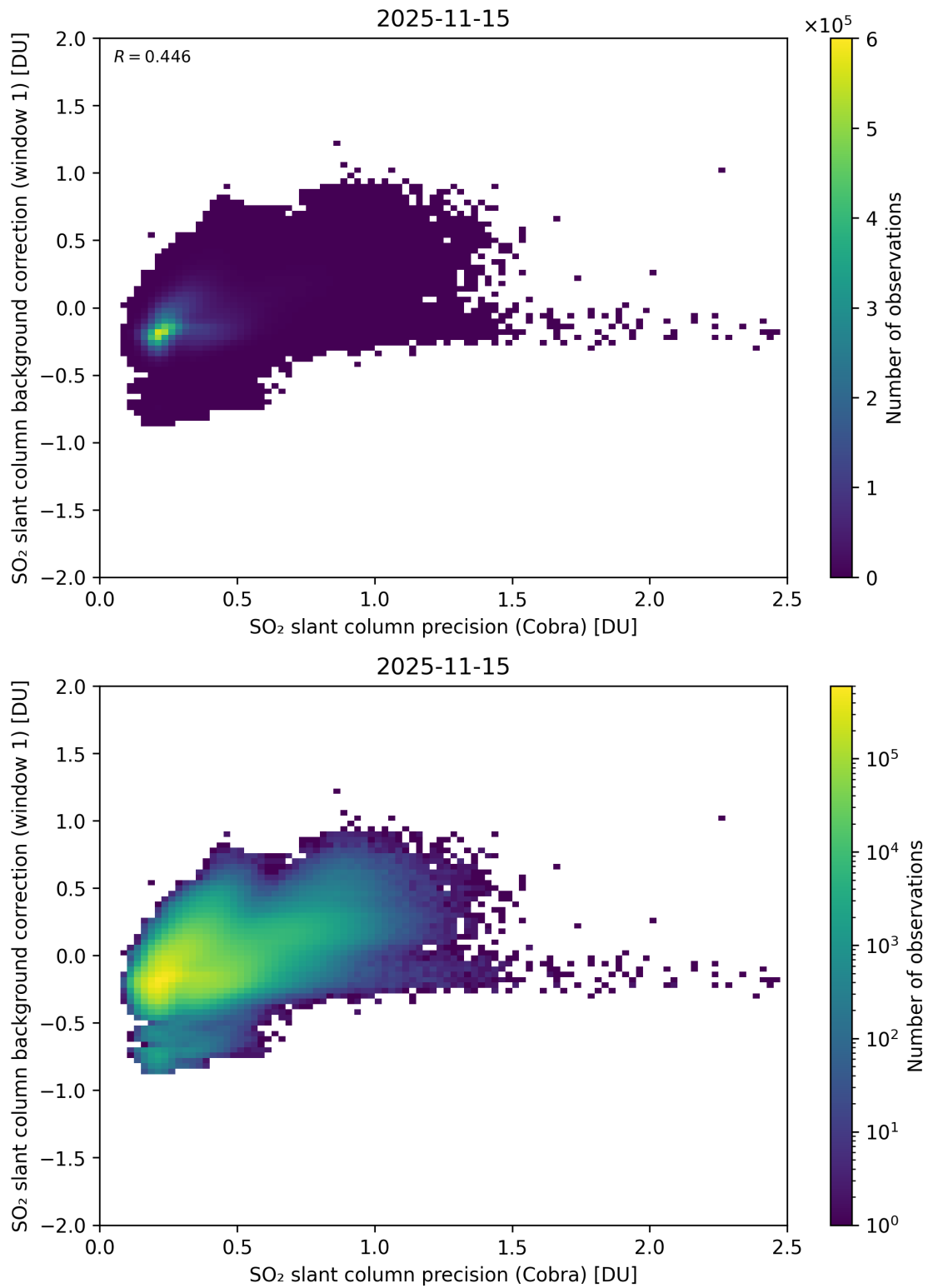
Figure 199: Scatter density plot of “SO 2 slant column precision (Cobra)” against “SO 2 slant column background correction (window 1)” for 2025-11-14 to 2025-11-16.
