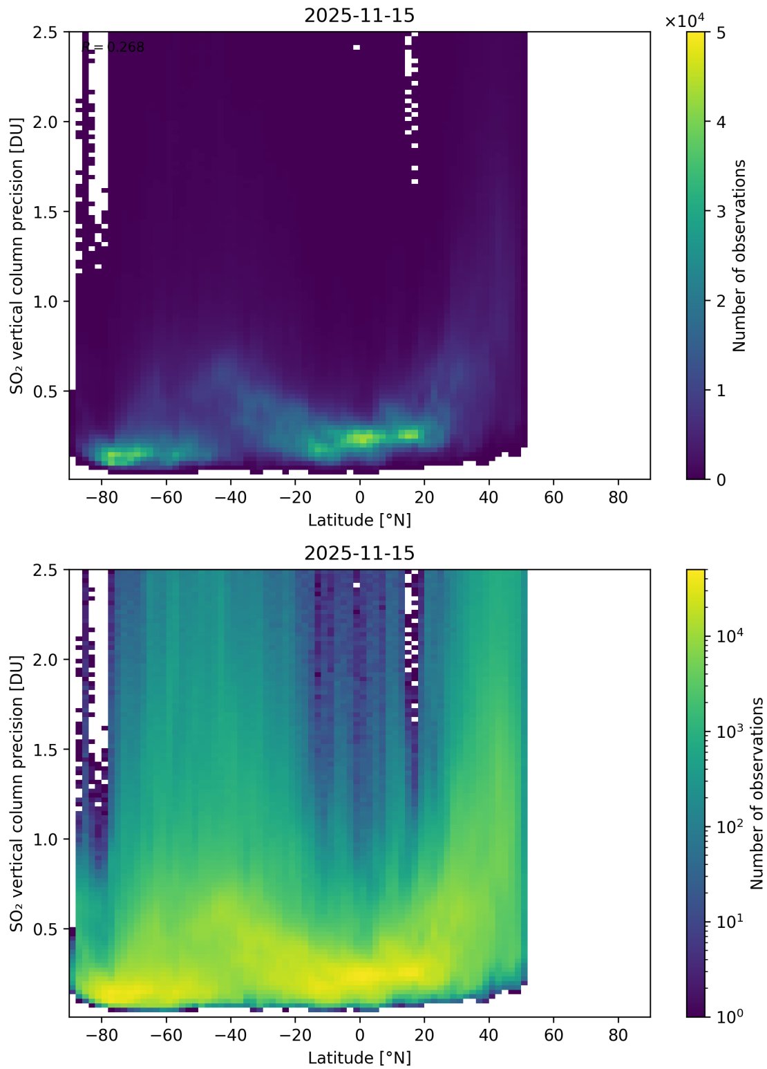
Figure 170: Scatter density plot of “Latitude” against “SO 2 vertical column precision” for 2025-11-14 to 2025-11-16.
