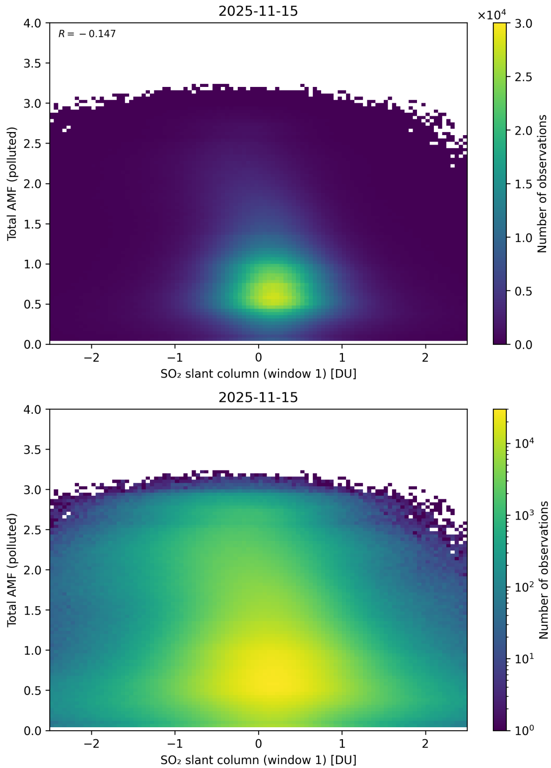
Figure 289: Scatter density plot of “SO 2 slant column (window 1)” against “Total AMF (polluted)” for 2025-11-14 to 2025-11-16.
