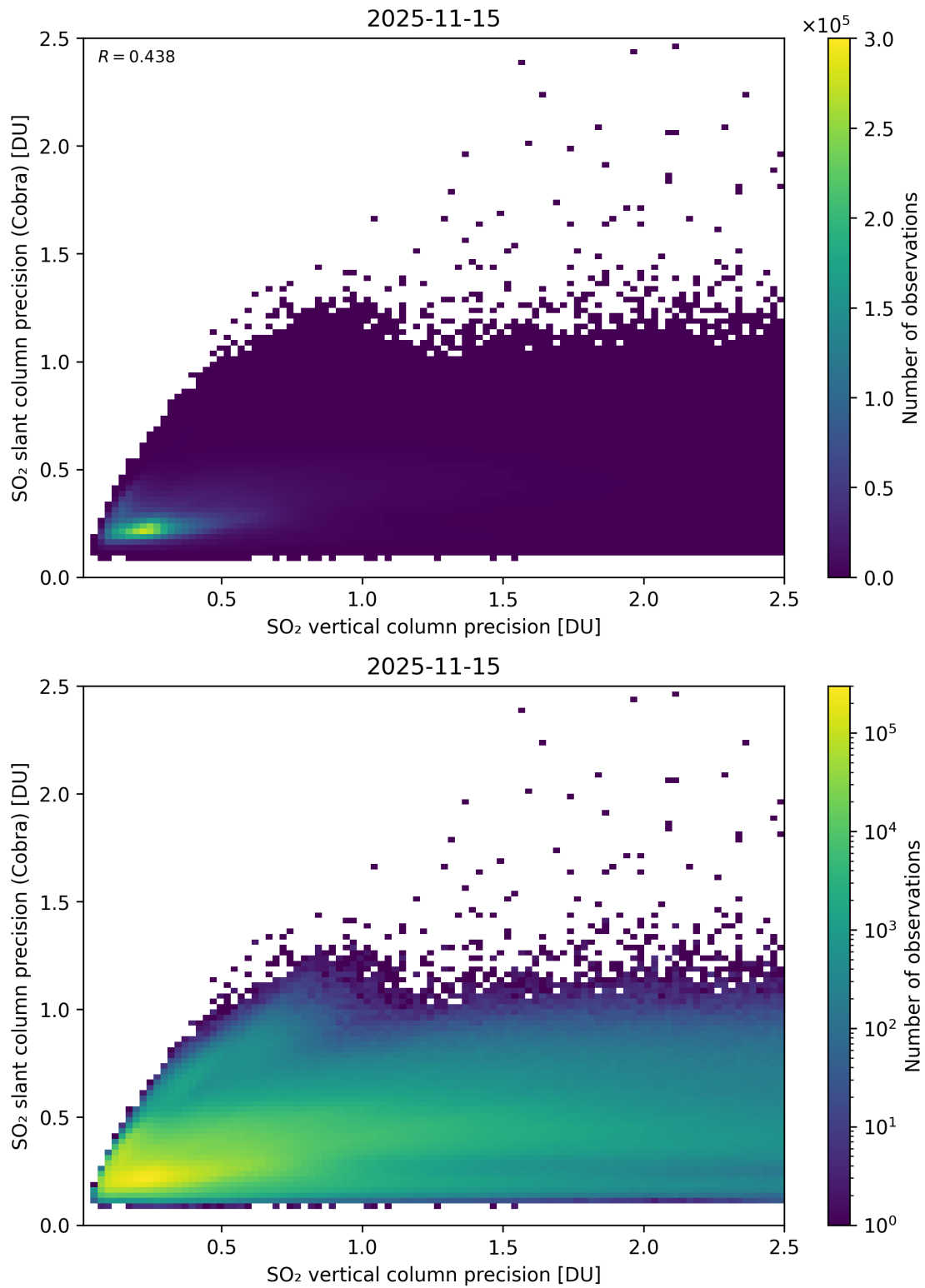
Figure 337: Scatter density plot of “SO 2 vertical column precision” against “SO 2 slant column precision (Cobra)” for 2025-11-14 to 2025-11-16.
