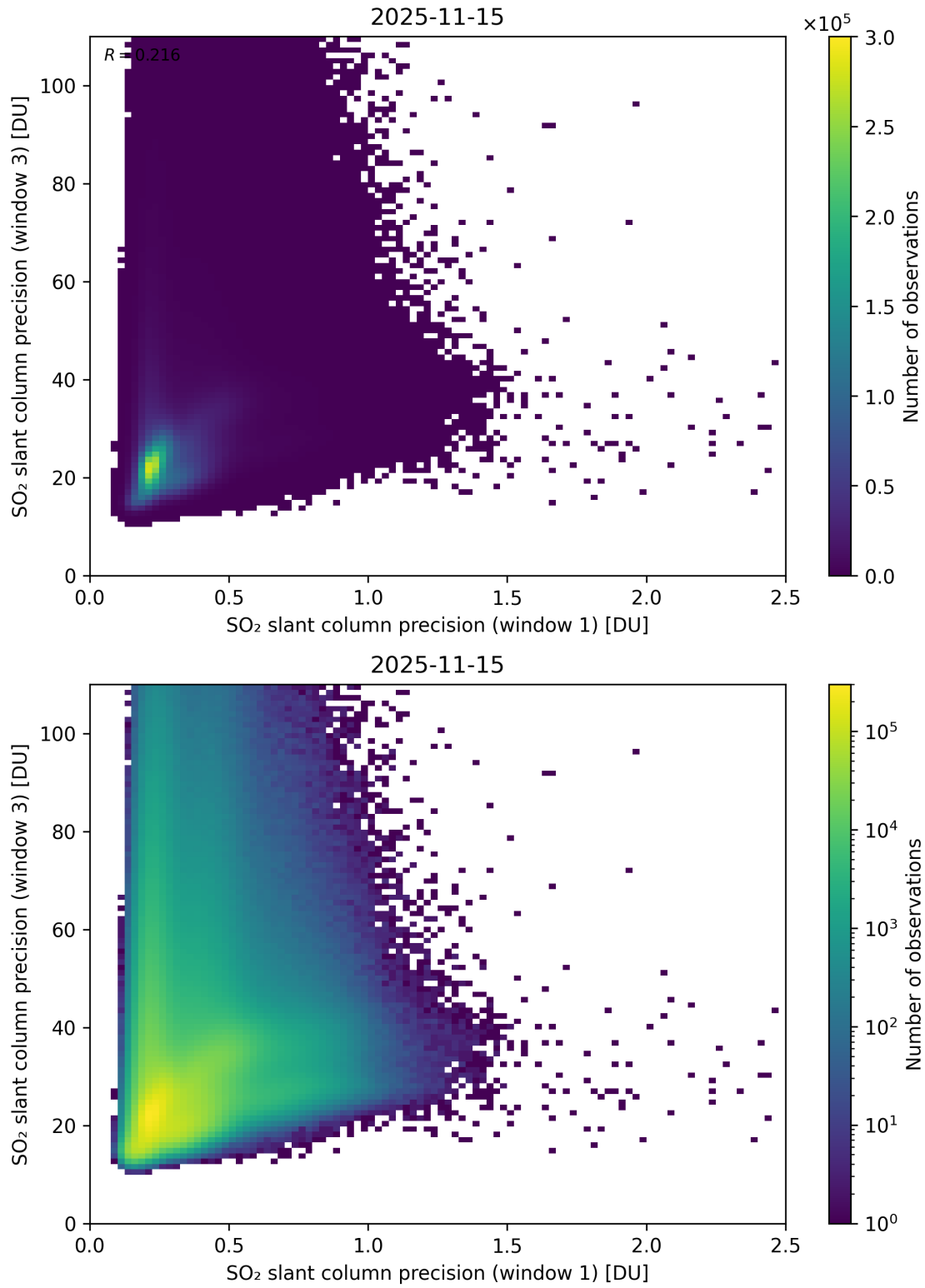
Figure 279: Scatter density plot of “SO 2 slant column precision (window 1)” against “SO 2 slant column precision (window 3)” for 2025-11-14 to 2025-11-16.
