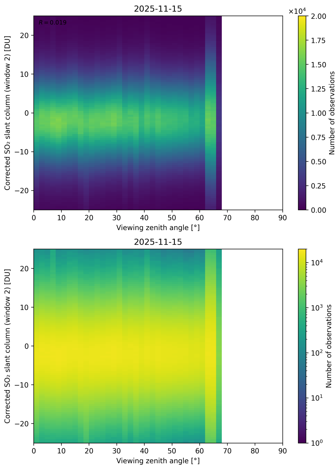
Figure 374: Scatter density plot of “Viewing zenith angle” against “Corrected SO 2 slant column (window 2)” for 2025-11-14 to 2025-11-16.
