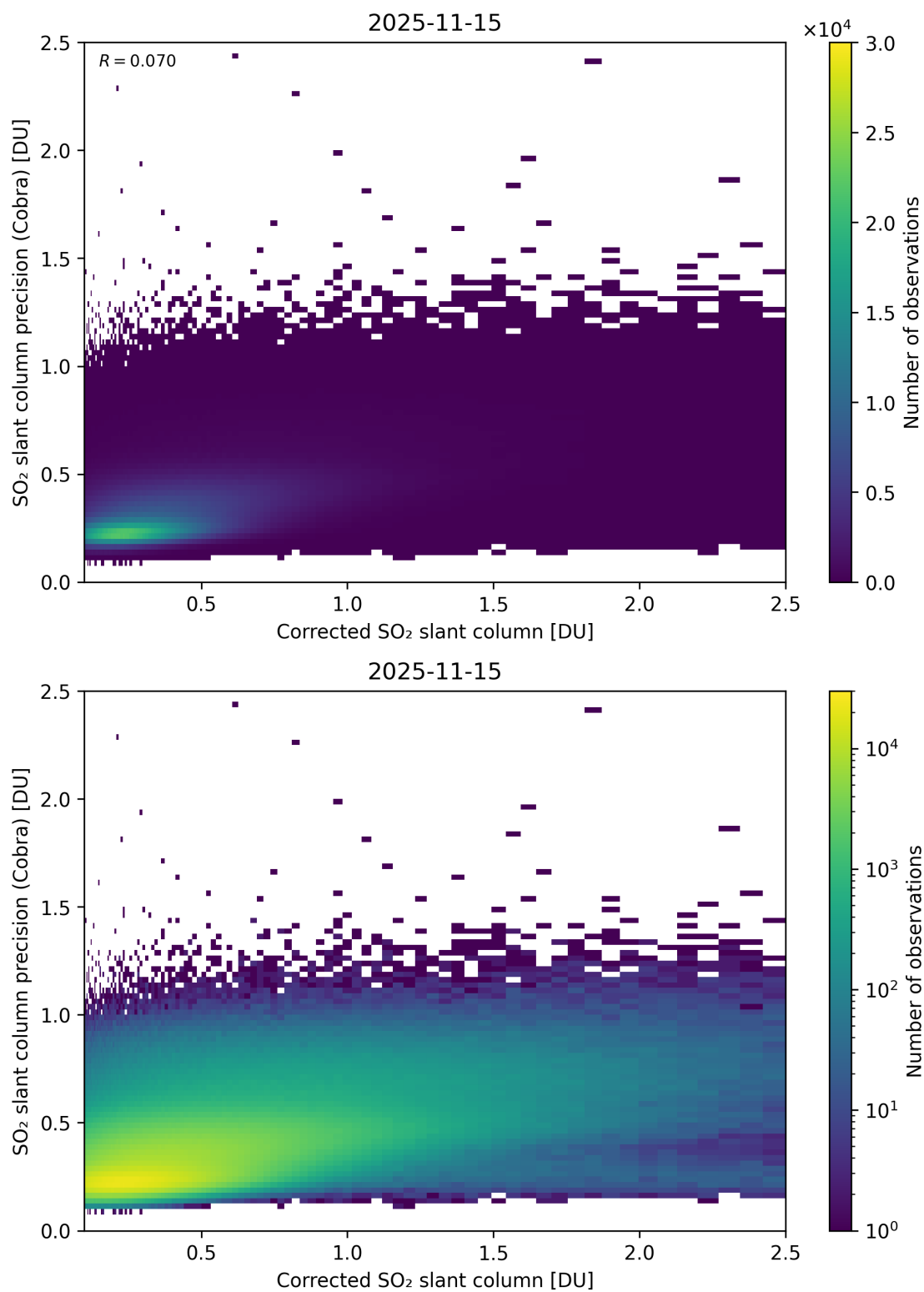
Figure 234: Scatter density plot of “Corrected SO 2 slant column” against “SO 2 slant column precision (Cobra)” for 2025-11-14 to 2025-11-16.
