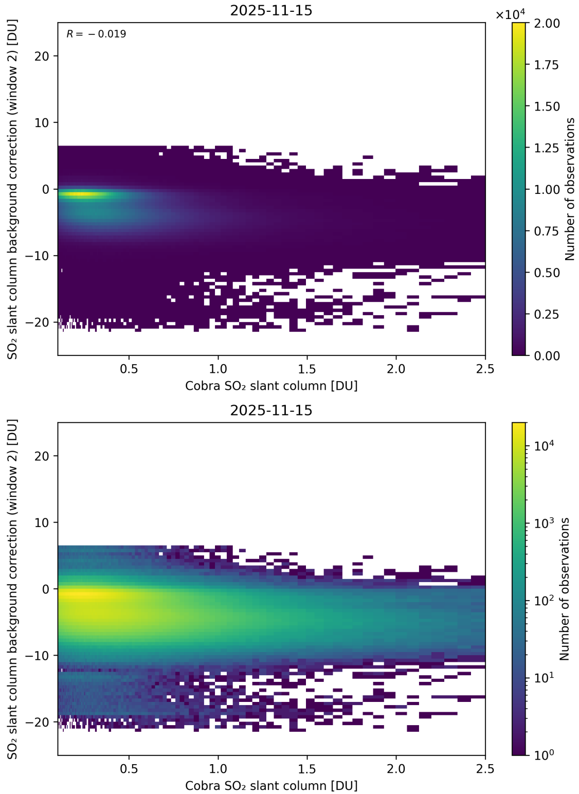
Figure 194: Scatter density plot of “Cobra SO 2 slant column” against “SO 2 slant column background correction (window 2)” for 2025-11-14 to 2025-11-16.
