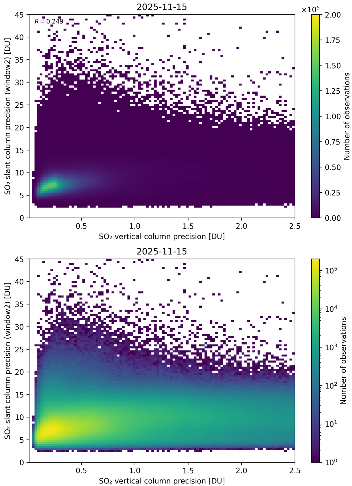
Figure 343: Scatter density plot of “SO 2 vertical column precision” against “SO 2 slant column precision (window2)” for 2025-11-14 to 2025-11-16.
