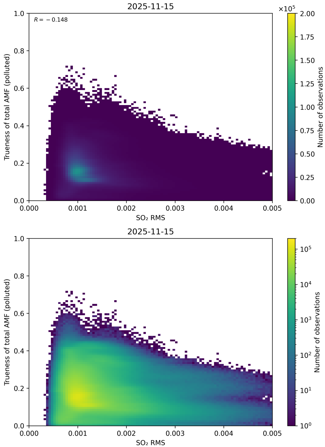
Figure 149: Scatter density plot of “SO 2 RMS” against “Trueness of total AMF (polluted)” for 2025-11-14 to 2025-11-16.
