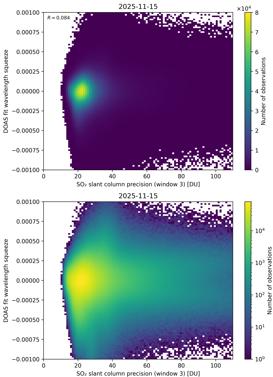
Figure 309: Scatter density plot of “SO 2 slant column precision (window 3)” against “DOAS fit wavelength squeeze” for 2025-11-14 to 2025-11-16.
