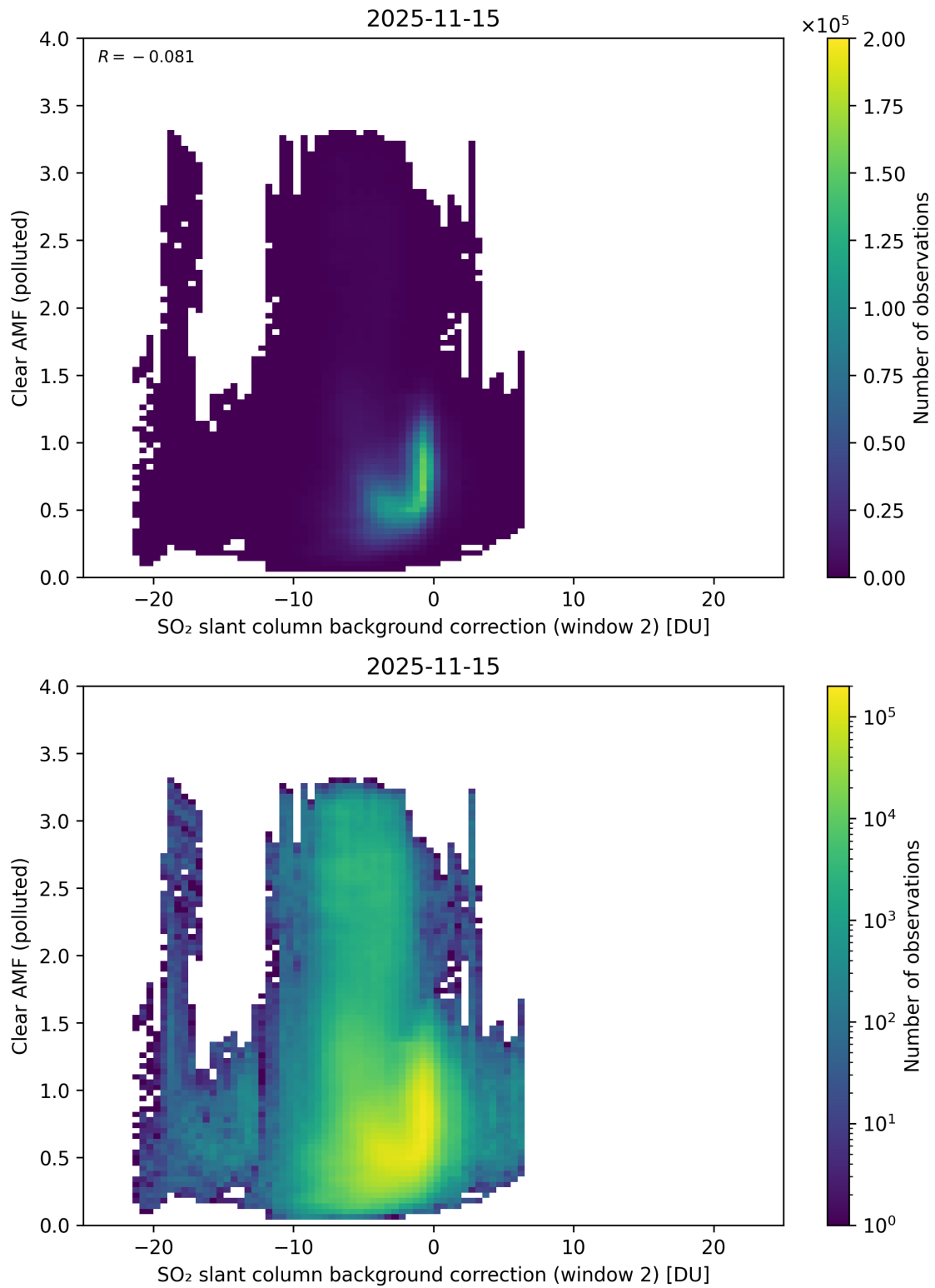
Figure 126: Scatter density plot of “SO 2 slant column background correction (window 2)” against “Clear AMF (polluted)” for 2025-11-14 to 2025-11-16.
