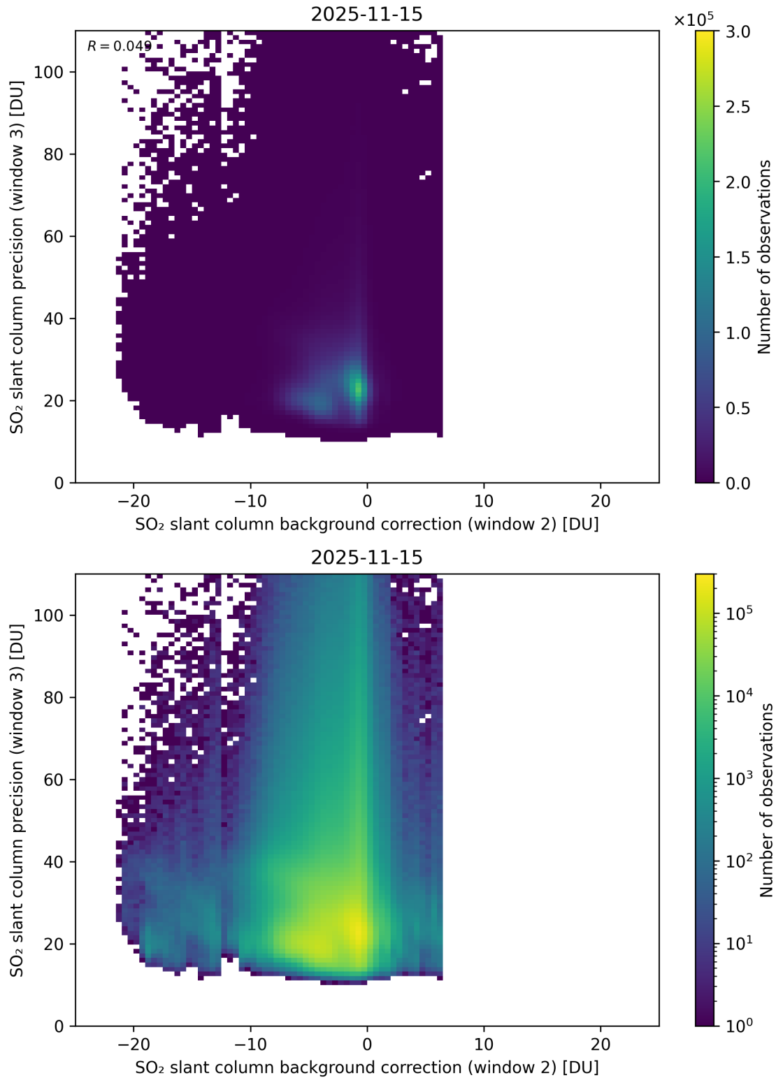
Figure 129: Scatter density plot of “SO 2 slant column background correction (window 2)” against “SO 2 slant column precision (window 3)” for 2025-11-14 to 2025-11-16.
