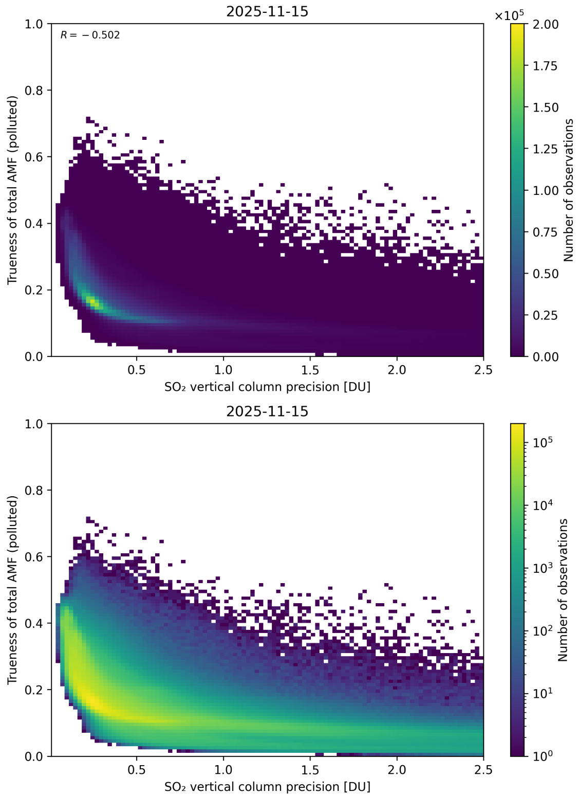
Figure 347: Scatter density plot of “SO 2 vertical column precision” against “Trueness of total AMF (polluted)” for 2025-11-14 to 2025-11-16.
