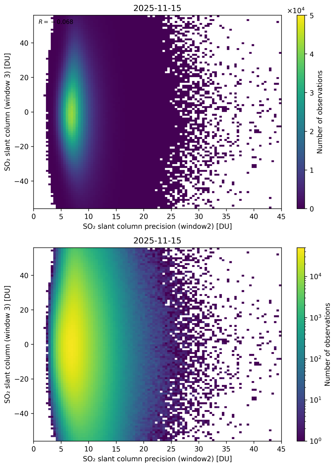
Figure 299: Scatter density plot of “SO 2 slant column precision (window2)” against “SO 2 slant column (window 3)” for 2025-11-14 to 2025-11-16.
