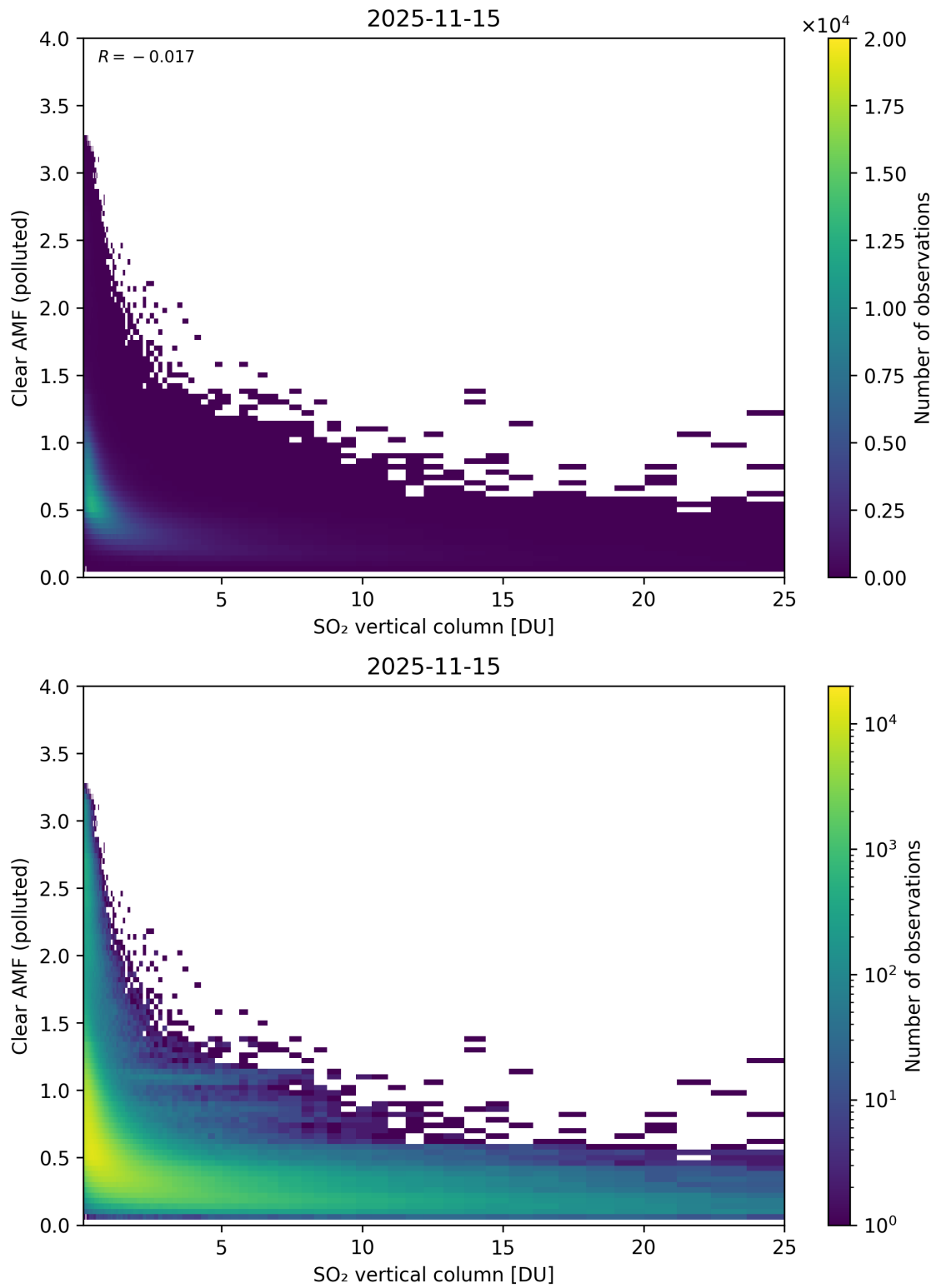
Figure 348: Scatter density plot of “SO 2 vertical column” against “Clear AMF (polluted)” for 2025-11-14 to 2025-11-16.
