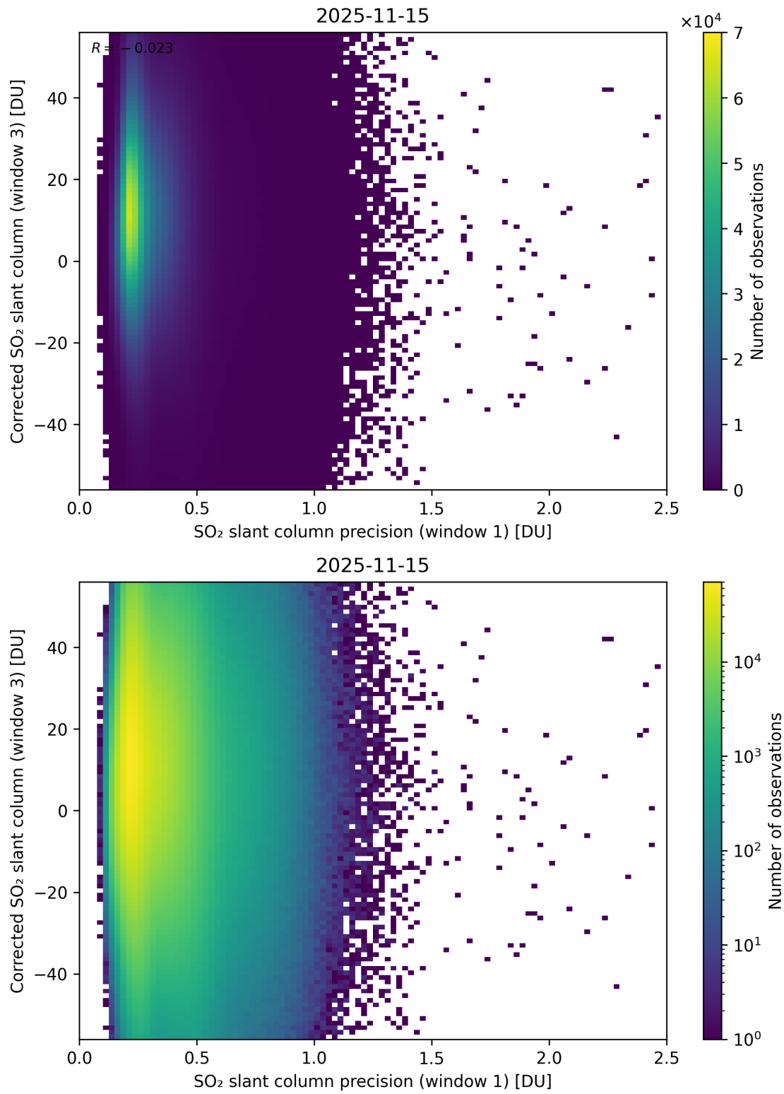
Figure 276: Scatter density plot of “SO 2 slant column precision (window 1)” against “Corrected SO 2 slant column (window 3)” for 2025-11-14 to 2025-11-16.
