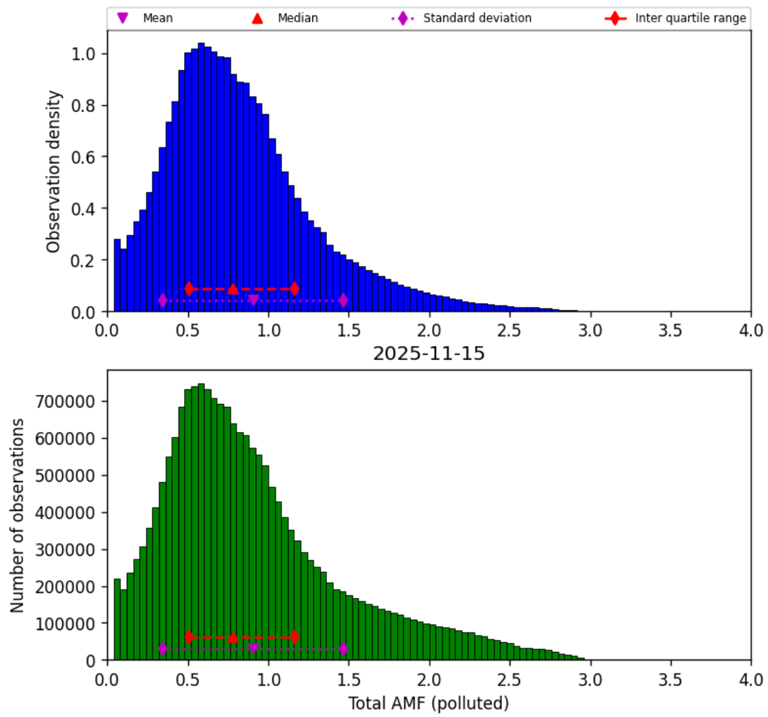
Figure 79: Histogram of “Total AMF (polluted)” for 2025-11-14 to 2025-11-16
