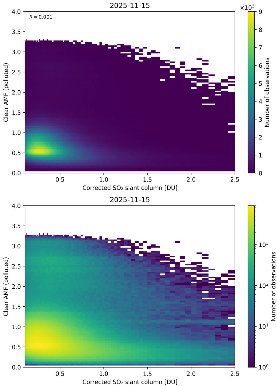
Figure 232: Scatter density plot of “Corrected SO 2 slant column” against “Clear AMF (polluted)” for 2025-11-14 to 2025-11-16.
