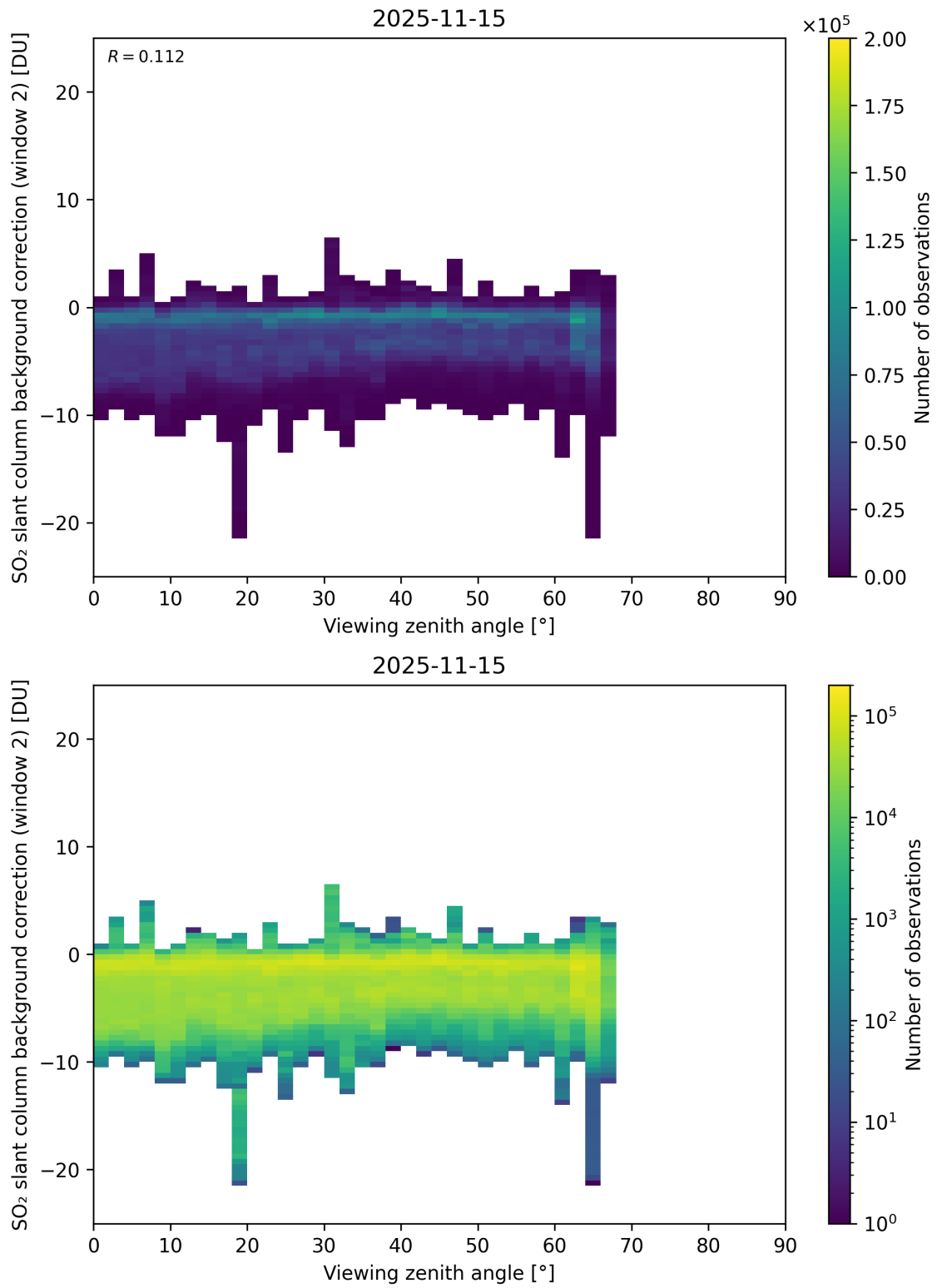
Figure 363: Scatter density plot of “Viewing zenith angle” against “SO 2 slant column background correction (window 2)” for 2025-11-14 to 2025-11-16.
