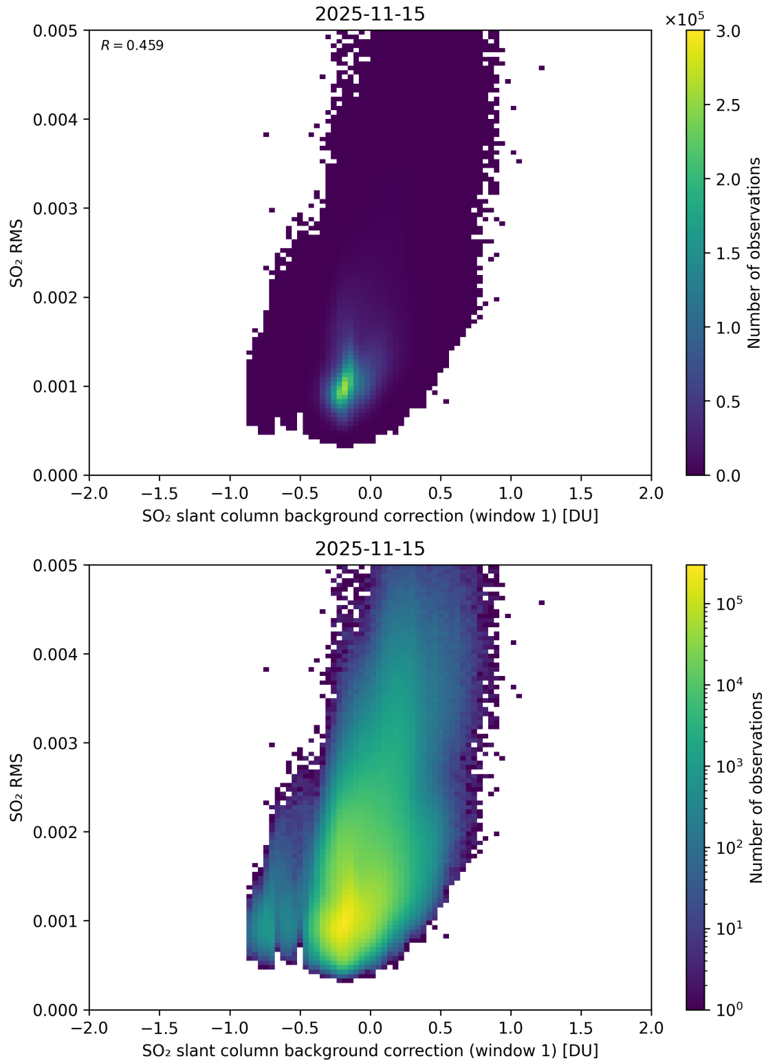
Figure 113: Scatter density plot of “SO 2 slant column background correction (window 1)” against “SO 2 RMS” for 2025-11-14 to 2025-11-16.
