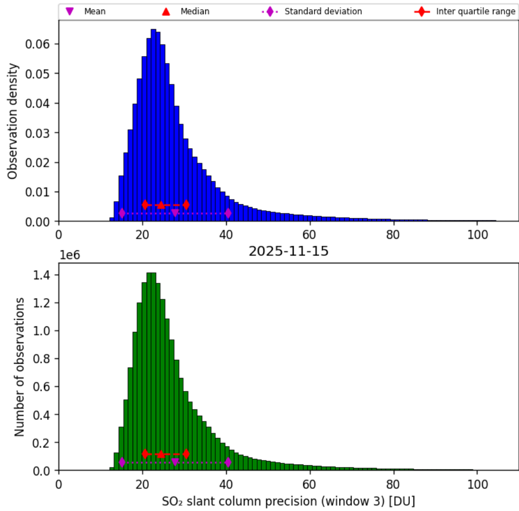
Figure 72: Histogram of “SO 2 slant column precision (window 3)” for 2025-11-14 to 2025-11-16
