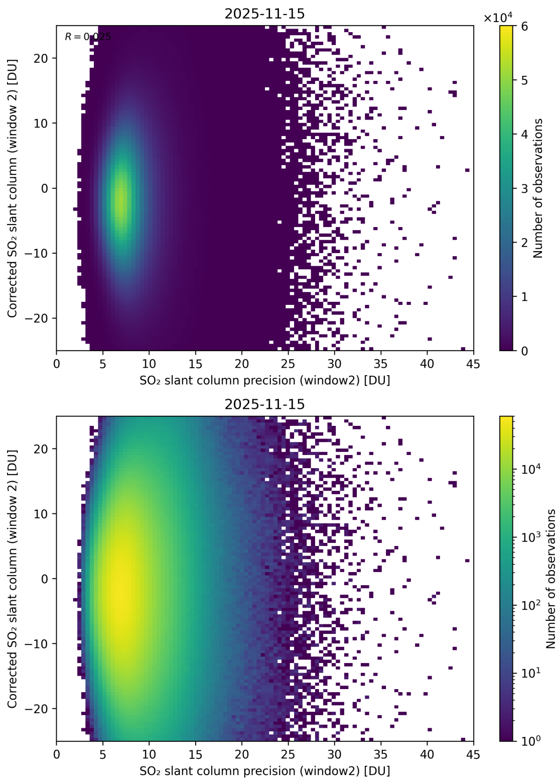
Figure 297: Scatter density plot of “SO 2 slant column precision (window2)” against “Corrected SO 2 slant column (window 2)” for 2025-11-14 to 2025-11-16.
