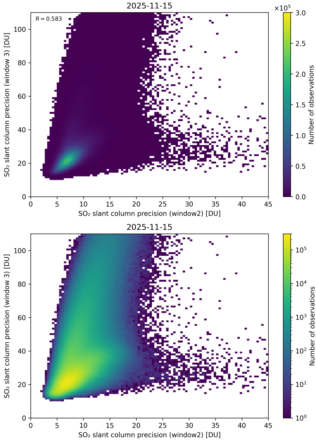
Figure 300: Scatter density plot of “SO 2 slant column precision (window2)” against “SO 2 slant column precision (window 3)” for 2025-11-14 to 2025-11-16.
