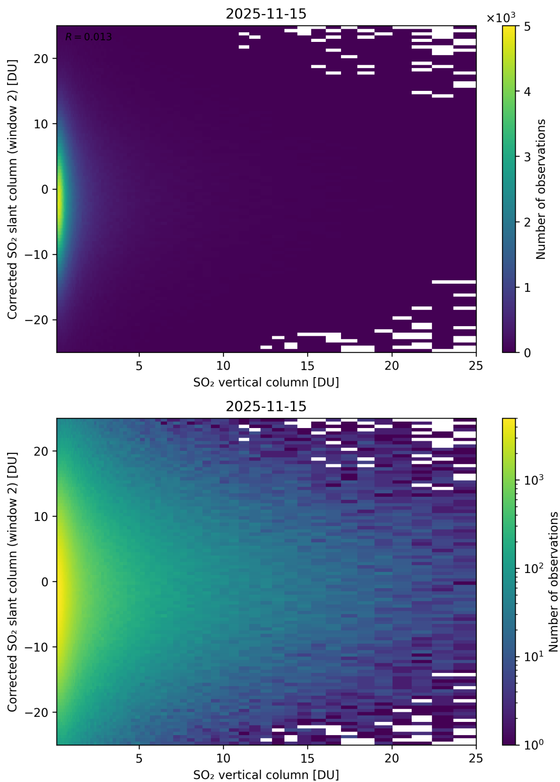
Figure 352: Scatter density plot of “SO 2 vertical column” against “Corrected SO 2 slant column (window 2)” for 2025-11-14 to 2025-11-16.
