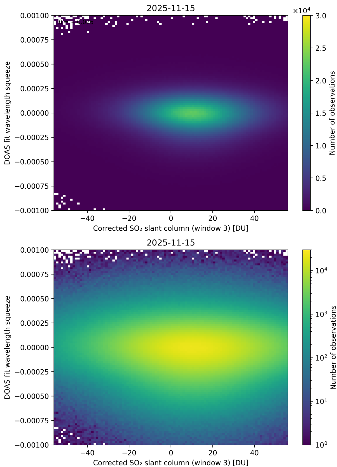
Figure 257: Scatter density plot of “Corrected SO 2 slant column (window 3)” against “DOAS fit wavelength squeeze” for 2025-11-14 to 2025-11-16.
