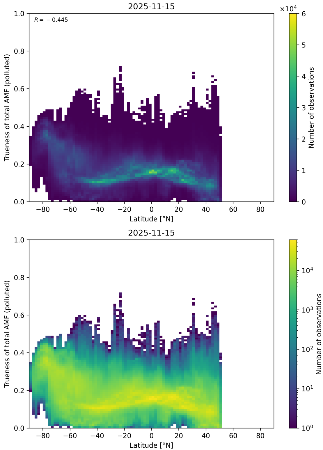
Figure 168: Scatter density plot of “Latitude” against “Trueness of total AMF (polluted)” for 2025-11-14 to 2025-11-16.
