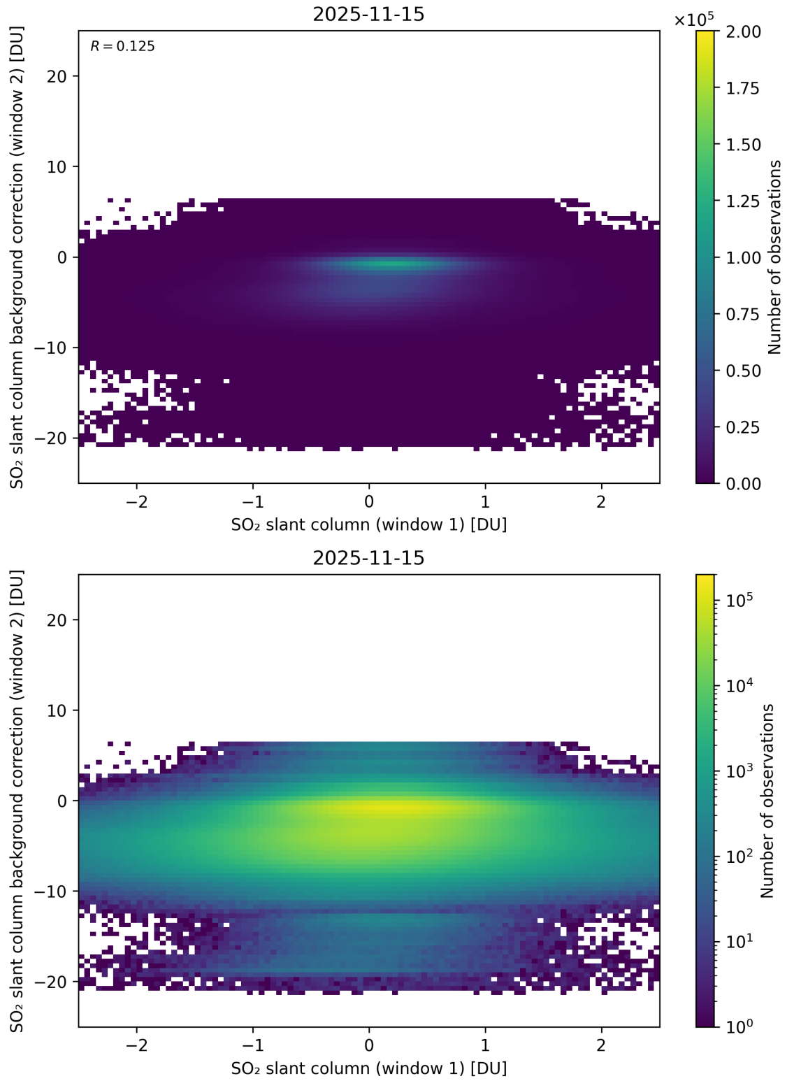
Figure 263: Scatter density plot of “SO 2 slant column (window 1)” against “SO 2 slant column background correction (window 2)” for 2025-11-14 to 2025-11-16.
