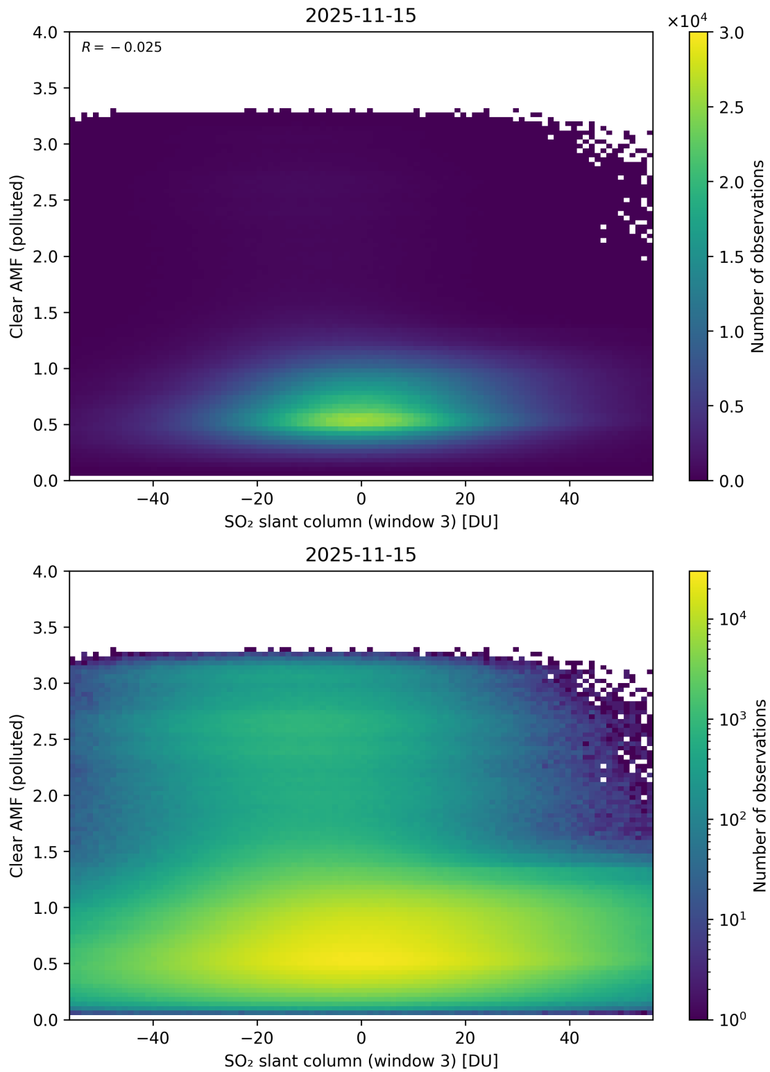
Figure 315: Scatter density plot of “SO 2 slant column (window 3)” against “Clear AMF (polluted)” for 2025-11-14 to 2025-11-16.
