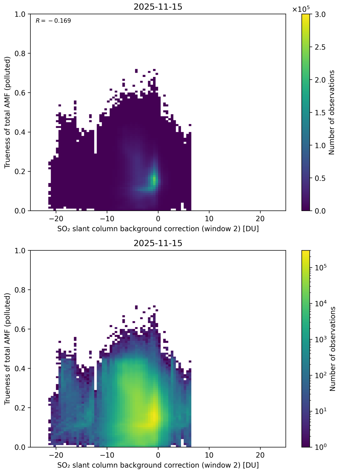
Figure 131: Scatter density plot of “SO 2 slant column background correction (window 2)” against “Trueness of total AMF (polluted)” for 2025-11-14 to 2025-11-16.
