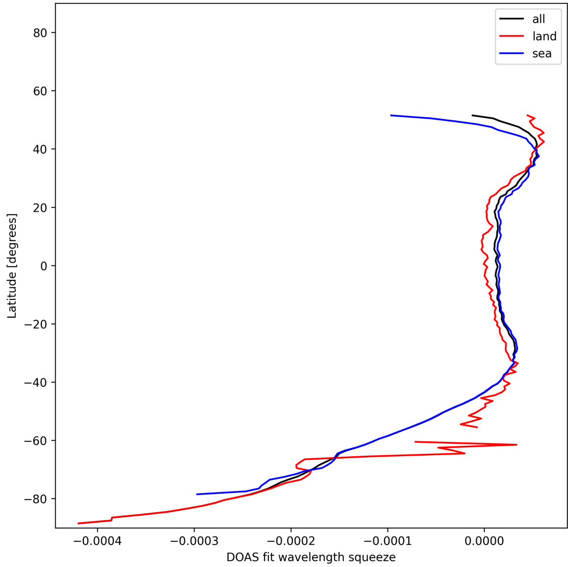
Figure 51: Zonal average of “DOAS fit wavelength squeeze” for 2025-11-14 to 2025-11-16.
