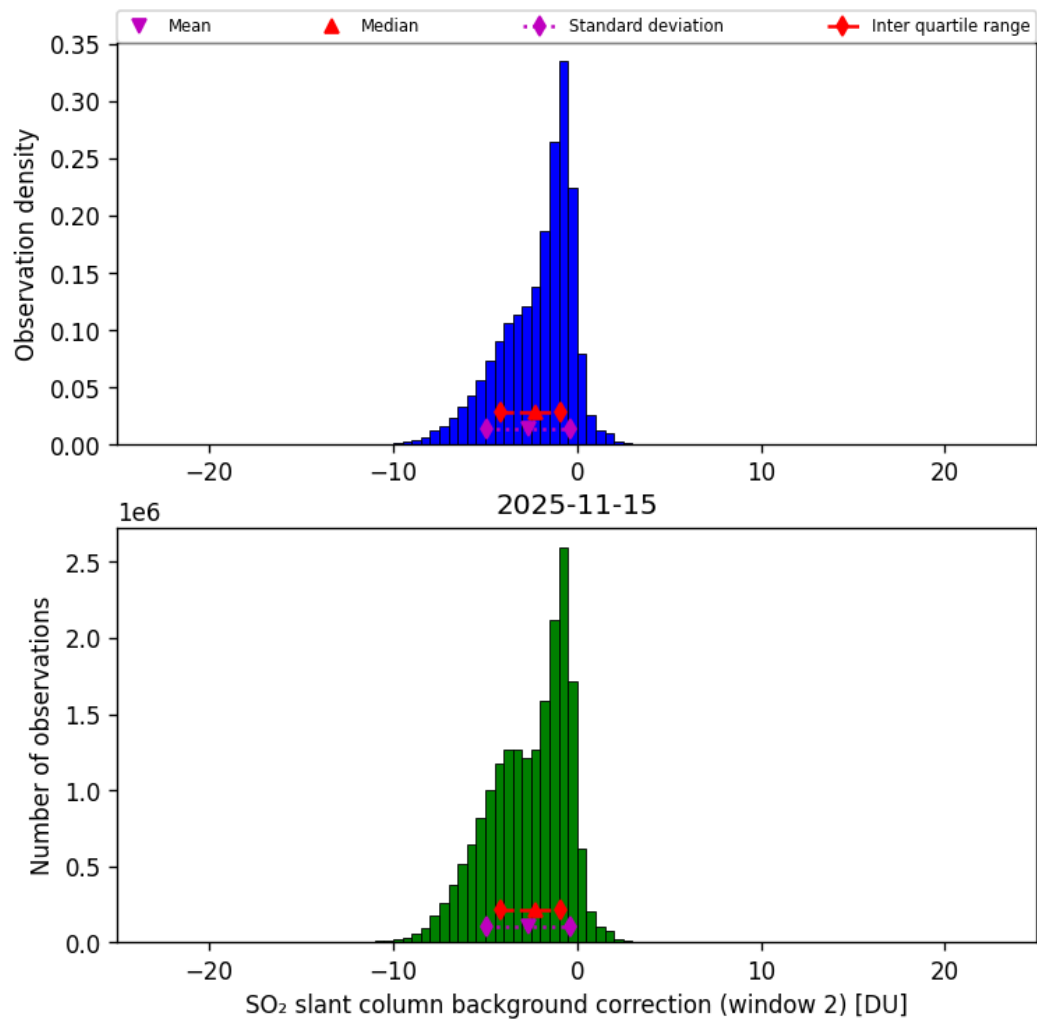
Figure 70: Histogram of “SO 2 slant column background correction (window 2)” for 2025-11-14 to 2025-11-16
