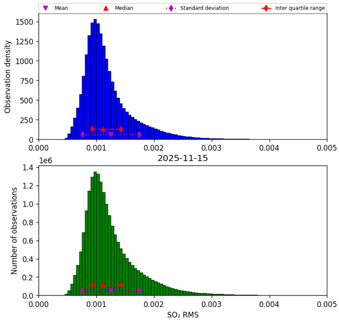
Figure 78: Histogram of “SO 2 RMS” for 2025-11-14 to 2025-11-16
