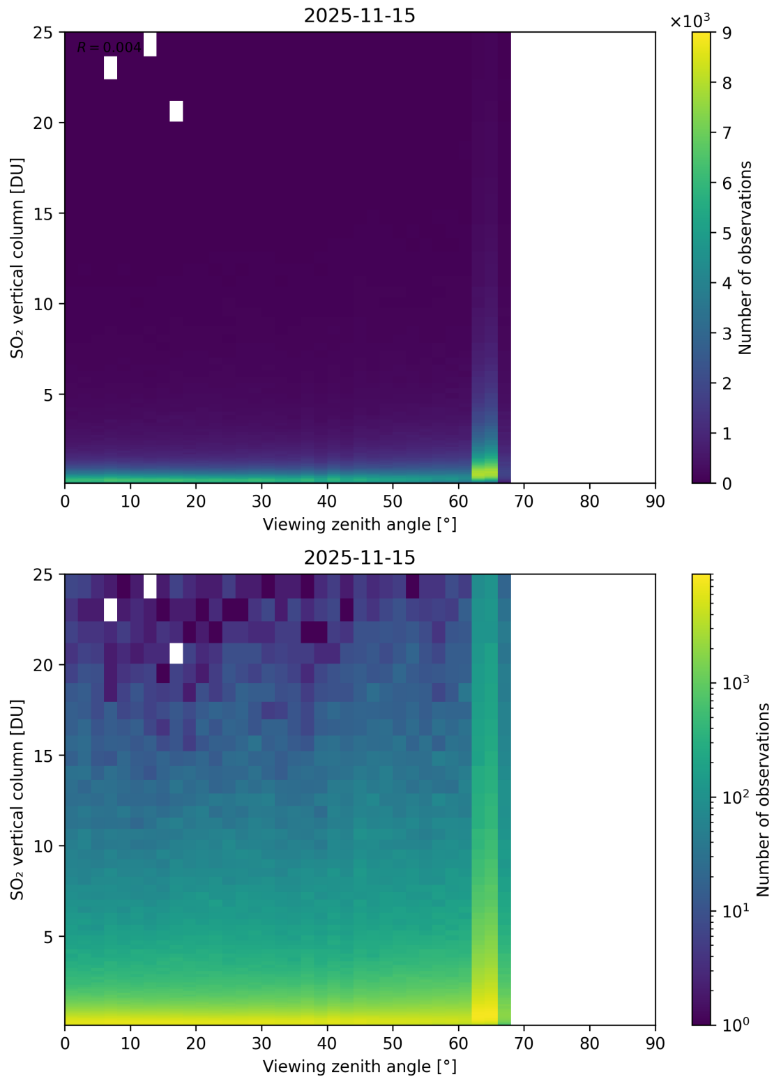
Figure 383: Scatter density plot of “Viewing zenith angle” against “SO 2 vertical column” for 2025-11-14 to 2025-11-16.
