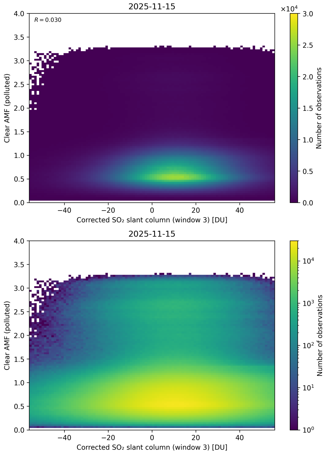
Figure 259: Scatter density plot of “Corrected SO 2 slant column (window 3)” against “Clear AMF (polluted)” for 2025-11-14 to 2025-11-16.
