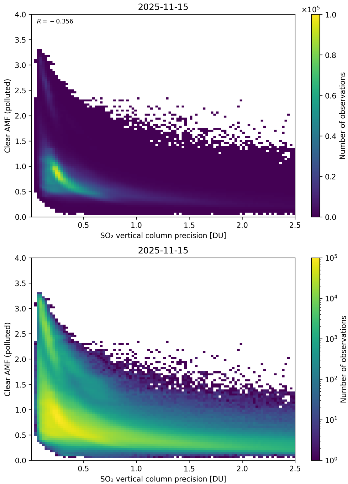
Figure 335: Scatter density plot of “SO 2 vertical column precision” against “Clear AMF (polluted)” for 2025-11-14 to 2025-11-16.
