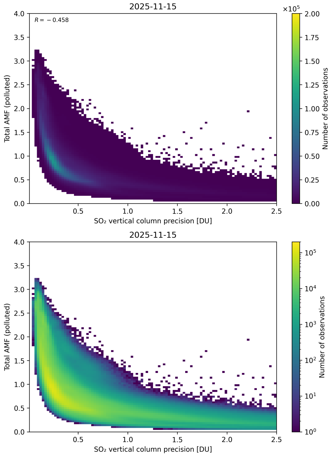
Figure 346: Scatter density plot of “SO 2 vertical column precision” against “Total AMF (polluted)” for 2025-11-14 to 2025-11-16.
