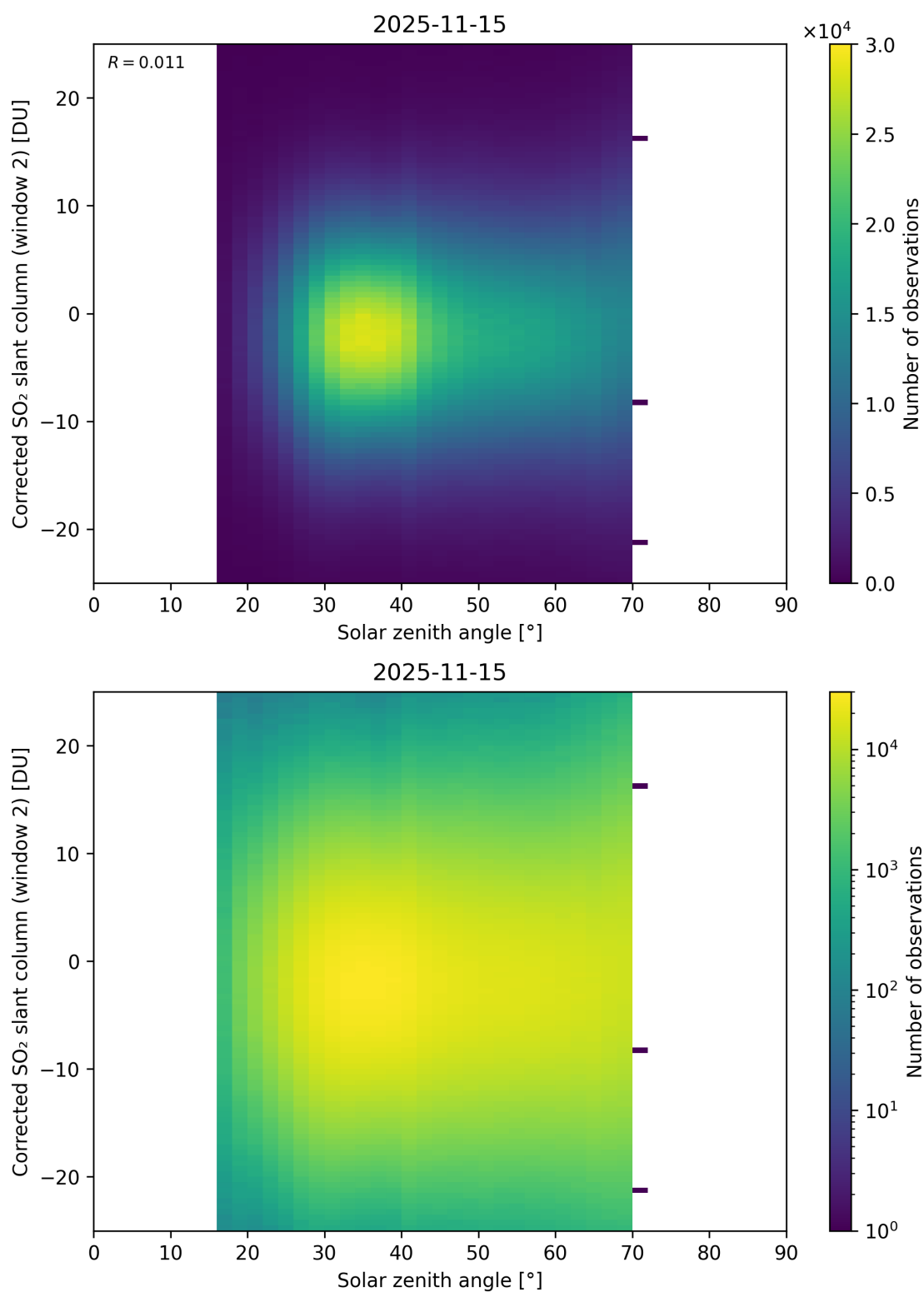
Figure 182: Scatter density plot of “Solar zenith angle” against “Corrected SO 2 slant column (window 2)” for 2025-11-14 to 2025-11-16.
