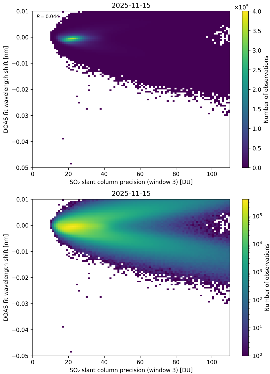
Figure 308: Scatter density plot of “SO 2 slant column precision (window 3)” against “DOAS fit wavelength shift” for 2025-11-14 to 2025-11-16.
