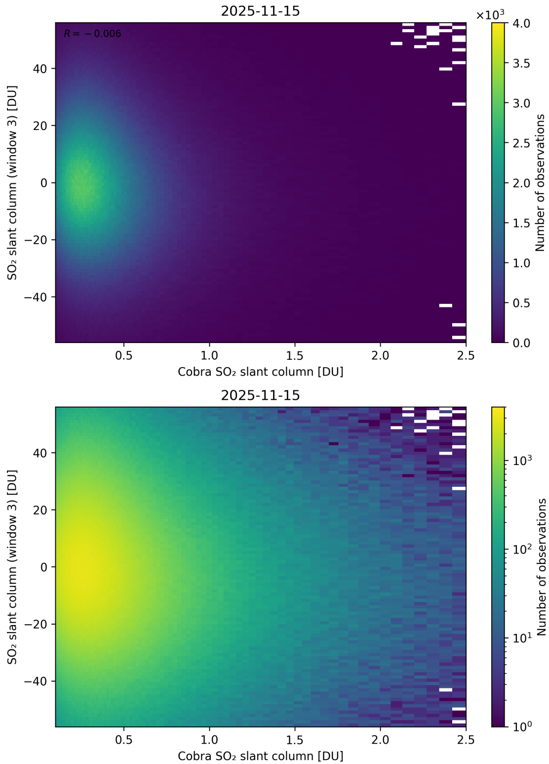
Figure 222: Scatter density plot of “Cobra SO 2 slant column” against “SO 2 slant column (window 3)” for 2025-11-14 to 2025-11-16.
