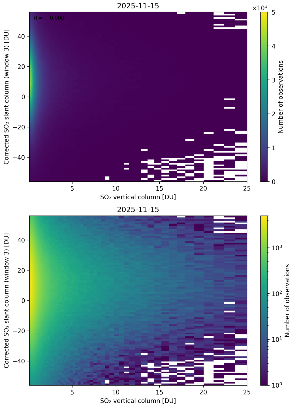
Figure 353: Scatter density plot of “SO 2 vertical column” against “Corrected SO 2 slant column (window 3)” for 2025-11-14 to 2025-11-16.
