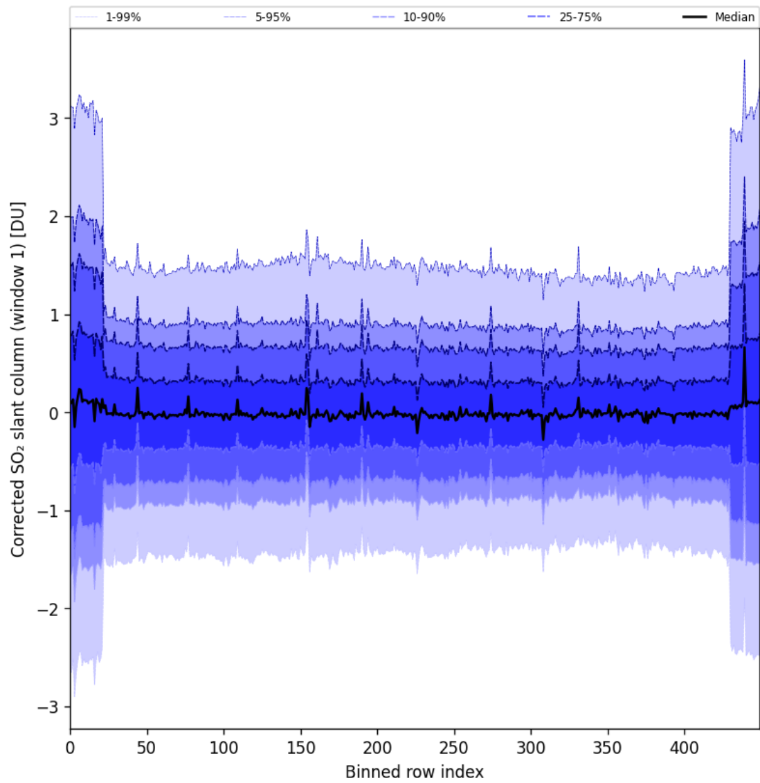
Figure 91: Along track statistics of “Corrected SO 2 slant column (window 1)” for 2025-11-14 to 2025-11-16
