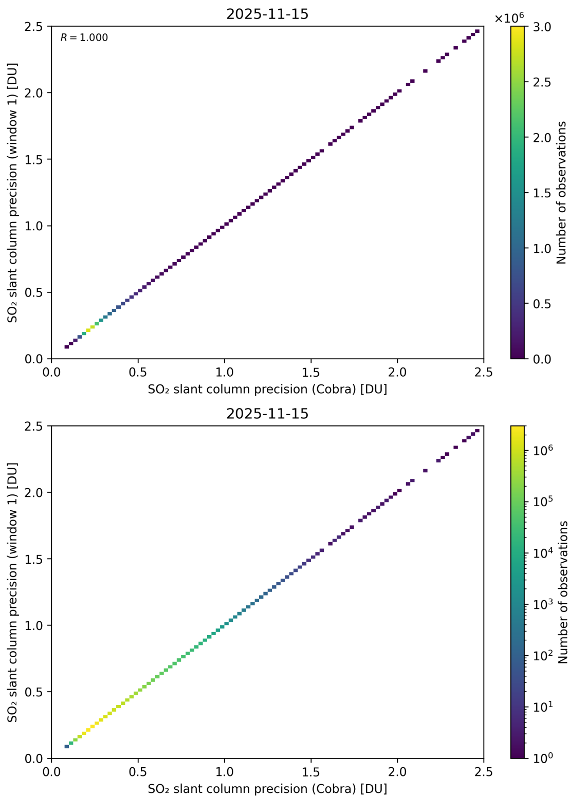
Figure 209: Scatter density plot of “SO 2 slant column precision (Cobra)” against “SO 2 slant column precision (window 1)” for 2025-11-14 to 2025-11-16.
