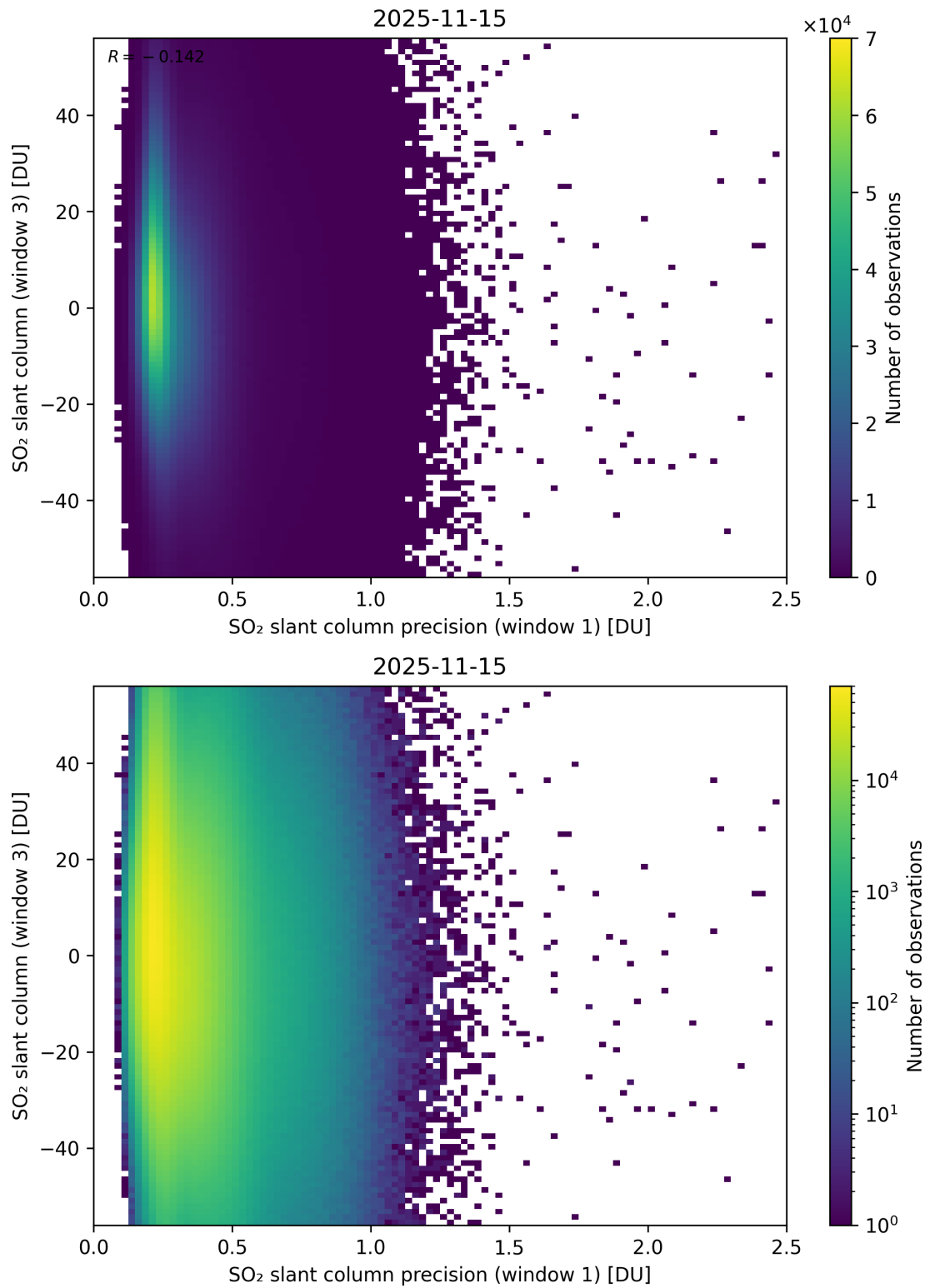
Figure 278: Scatter density plot of “SO 2 slant column precision (window 1)” against “SO 2 slant column (window 3)” for 2025-11-14 to 2025-11-16.
