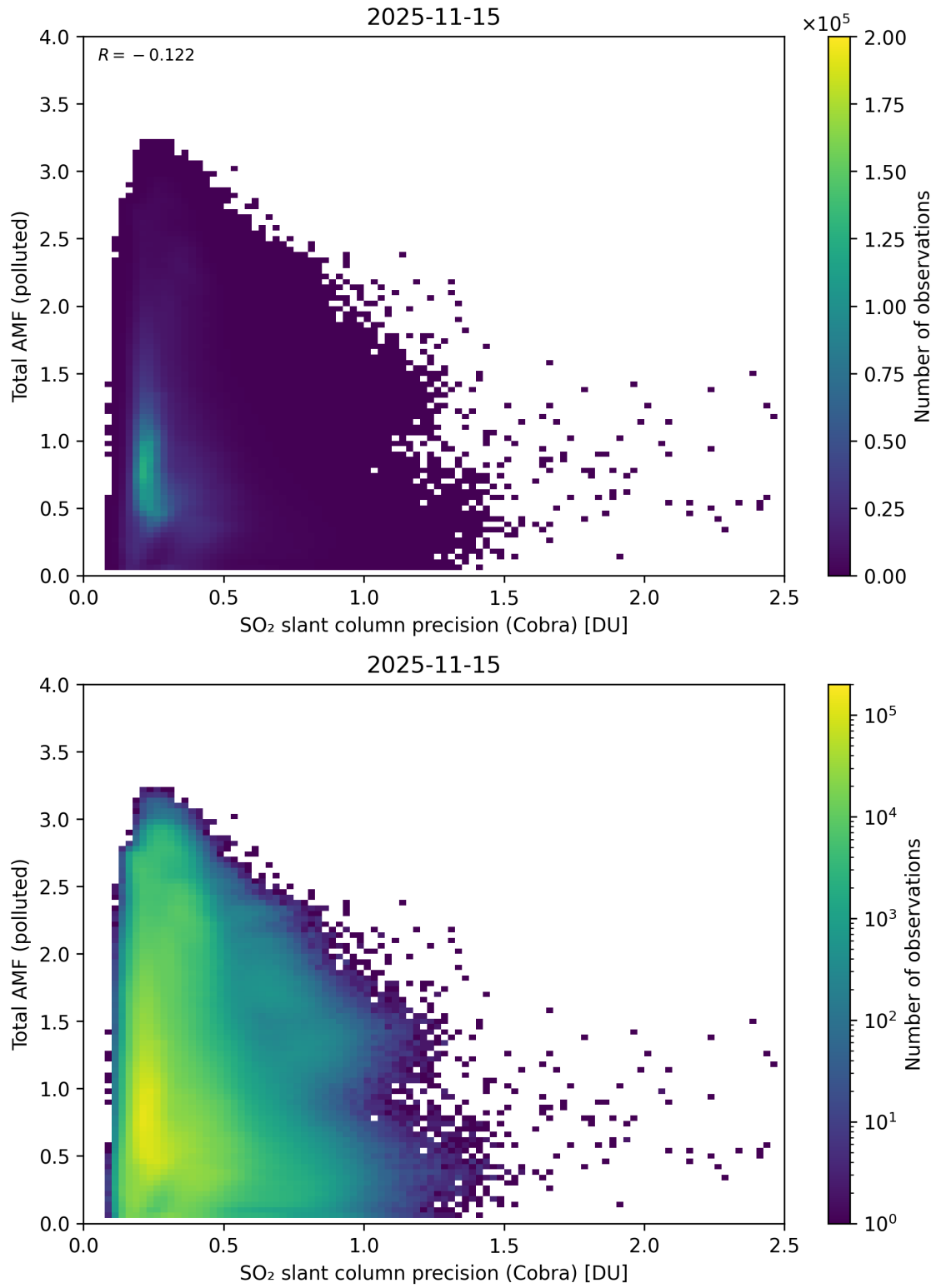
Figure 213: Scatter density plot of “SO 2 slant column precision (Cobra)” against “Total AMF (polluted)” for 2025-11-14 to 2025-11-16.
