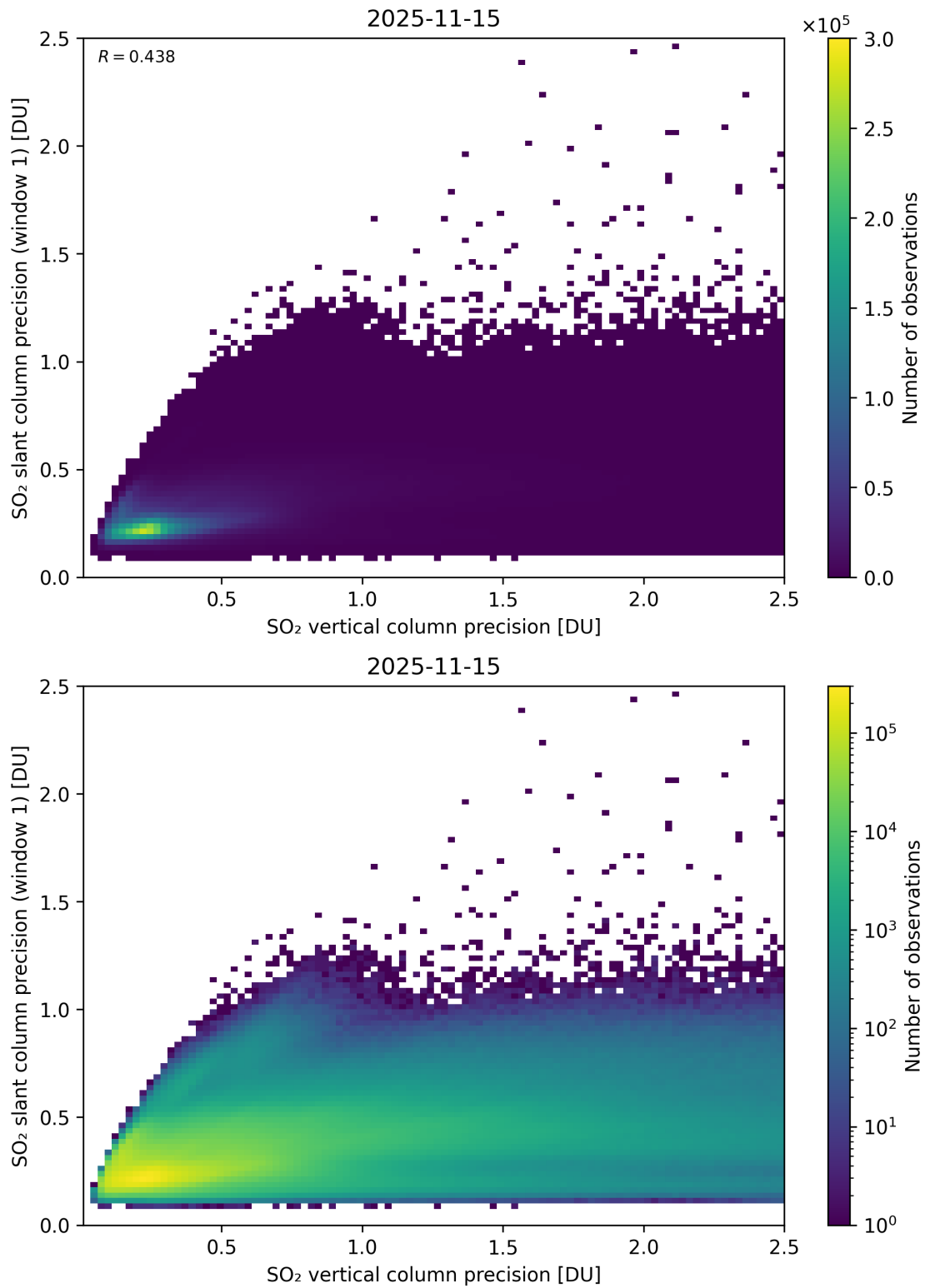
Figure 342: Scatter density plot of “SO 2 vertical column precision” against “SO 2 slant column precision (window 1)” for 2025-11-14 to 2025-11-16.
