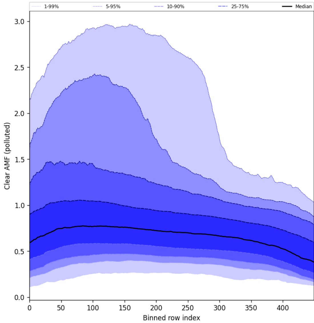
Figure 107: Along track statistics of “Clear AMF (polluted)” for 2025-11-14 to 2025-11-16
