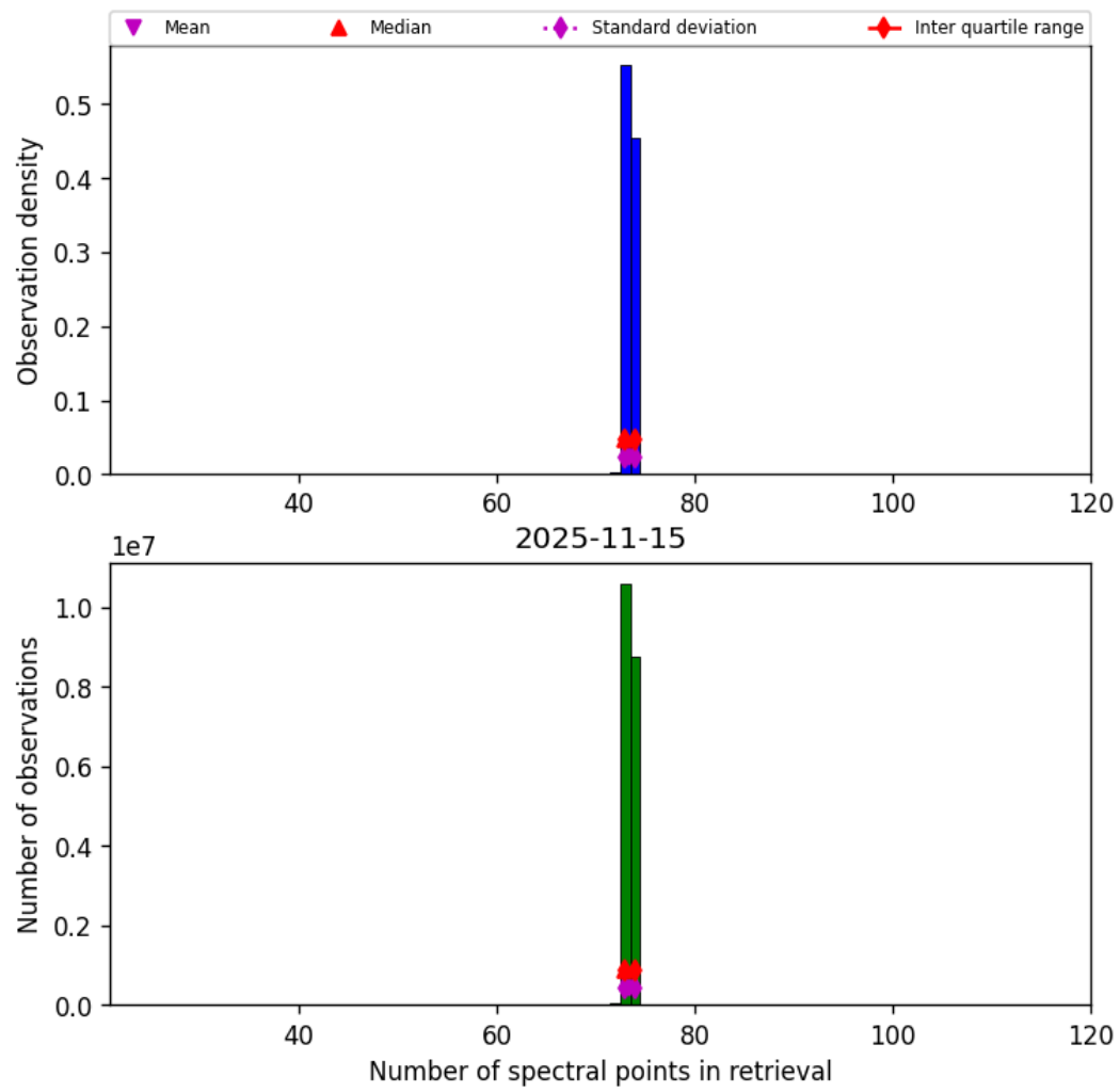
Figure 82: Histogram of “Number of spectral points in retrieval” for 2025-11-14 to 2025-11-16
