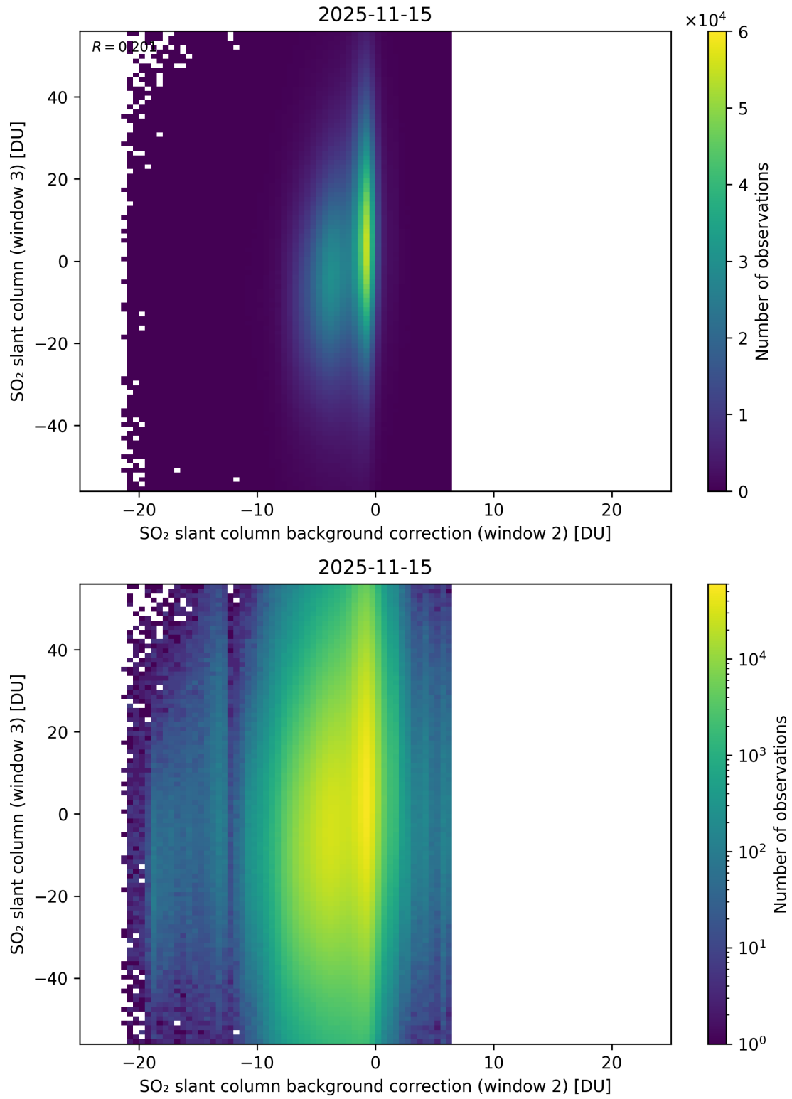
Figure 128: Scatter density plot of “SO 2 slant column background correction (window 2)” against “SO 2 slant column (window 3)” for 2025-11-14 to 2025-11-16.
