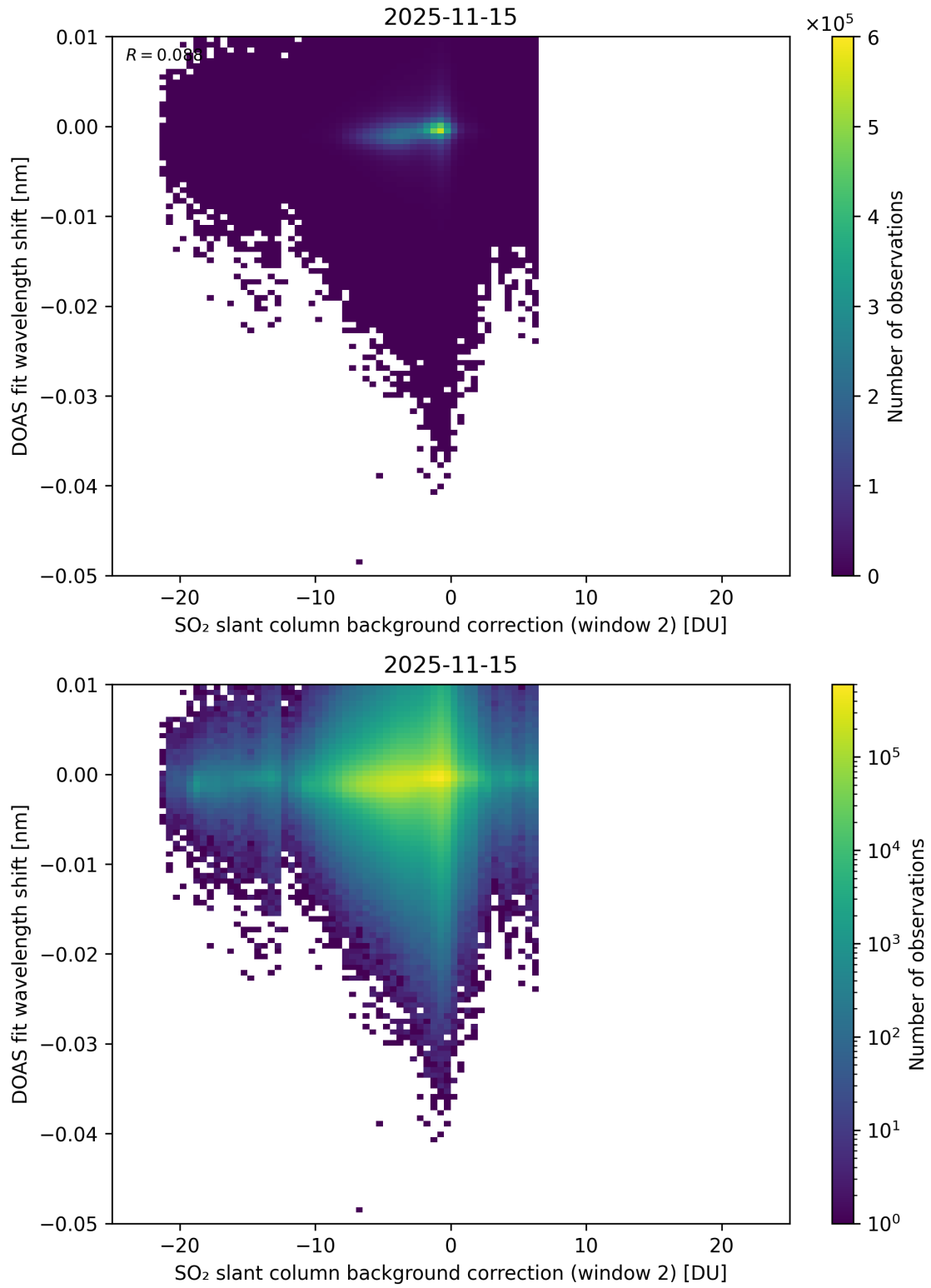
Figure 123: Scatter density plot of “SO 2 slant column background correction (window 2)” against “DOAS fit wavelength shift” for 2025-11-14 to 2025-11-16.
