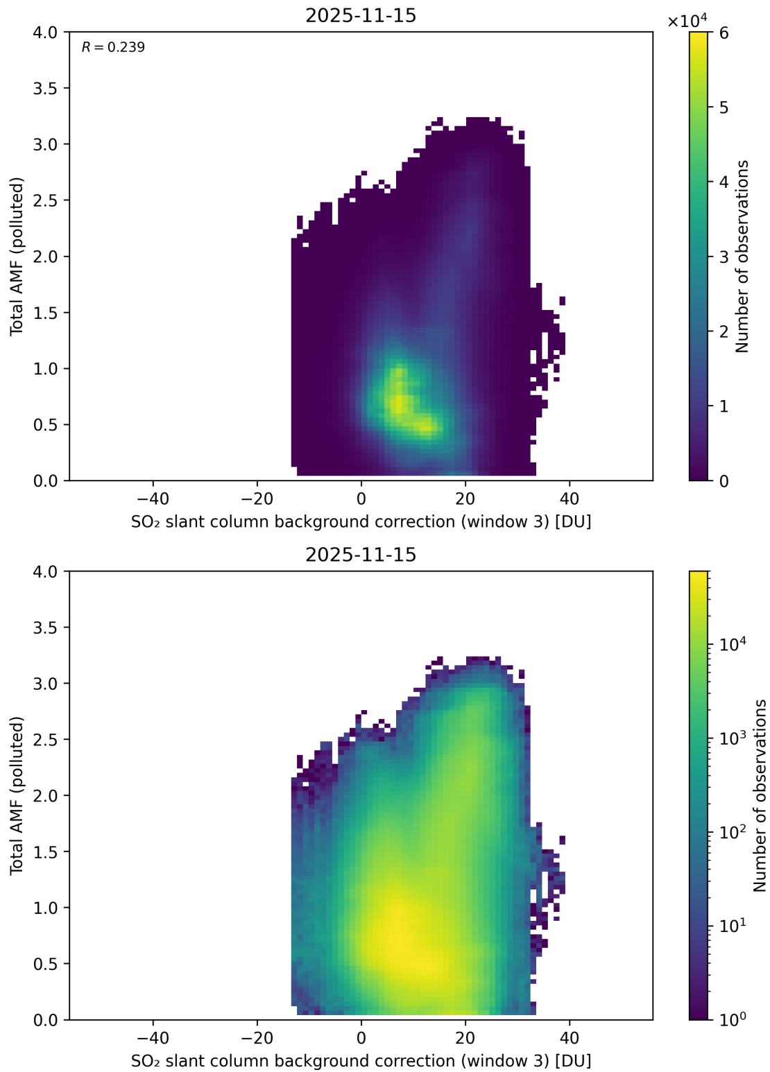
Figure 136: Scatter density plot of “SO 2 slant column background correction (window 3)” against “Total AMF (polluted)” for 2025-11-14 to 2025-11-16.
