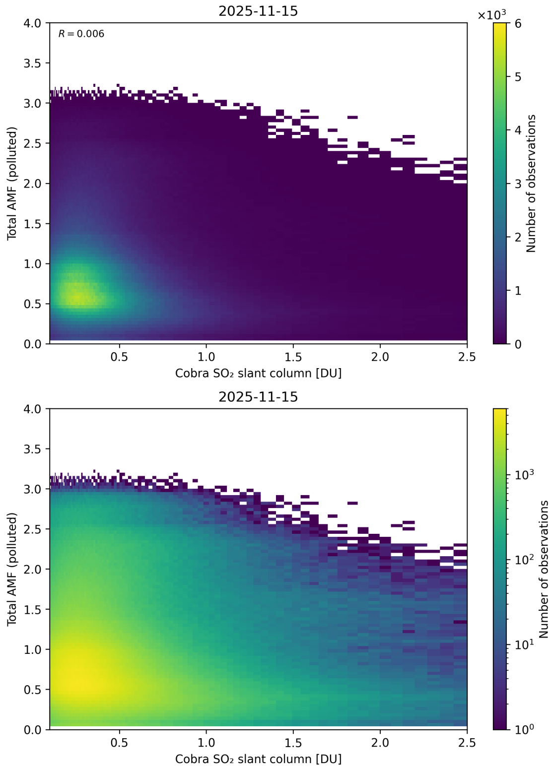
Figure 224: Scatter density plot of “Cobra SO 2 slant column” against “Total AMF (polluted)” for 2025-11-14 to 2025-11-16.
