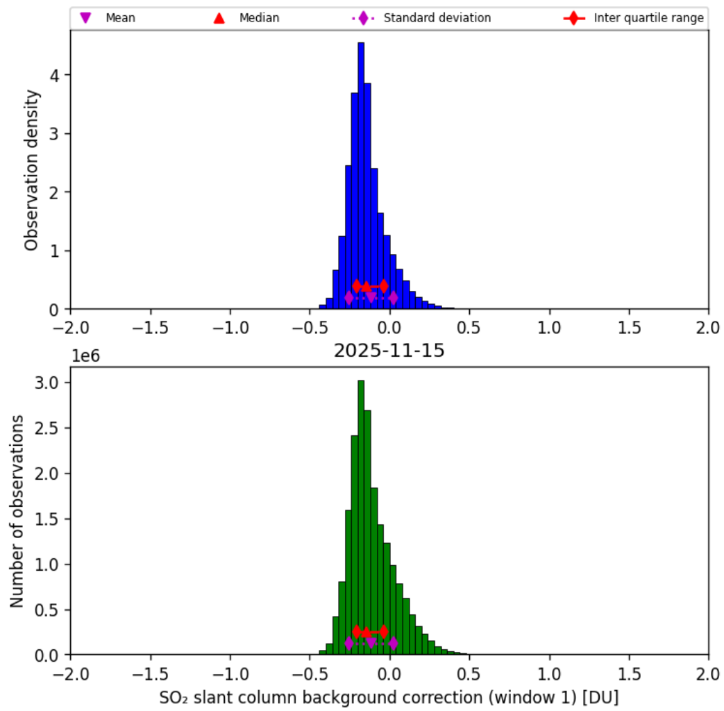
Figure 66: Histogram of “SO 2 slant column background correction (window 1)” for 2025-11-14 to 2025-11-16
