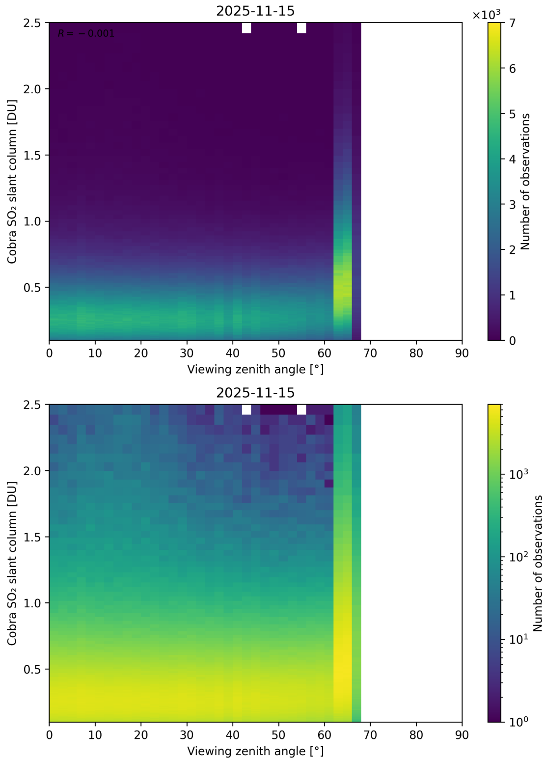
Figure 371: Scatter density plot of “Viewing zenith angle” against “Cobra SO 2 slant column” for 2025-11-14 to 2025-11-16.
