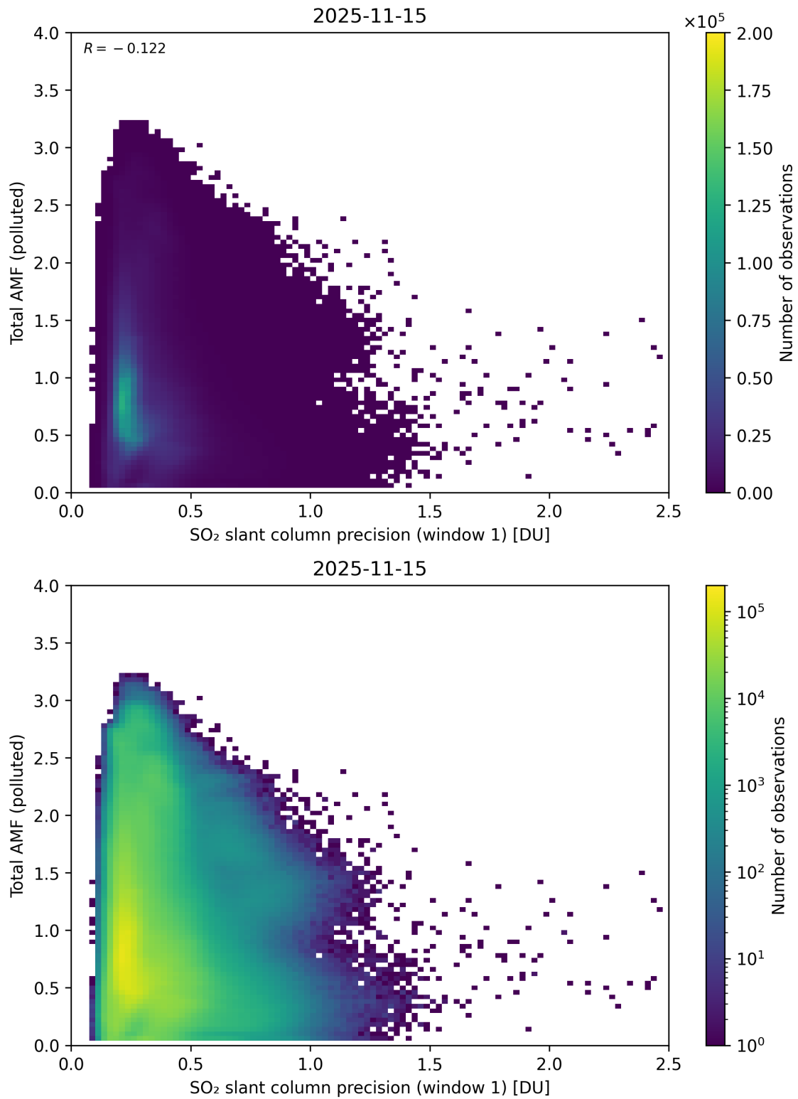
Figure 280: Scatter density plot of “SO 2 slant column precision (window 1)” against “Total AMF (polluted)” for 2025-11-14 to 2025-11-16.
