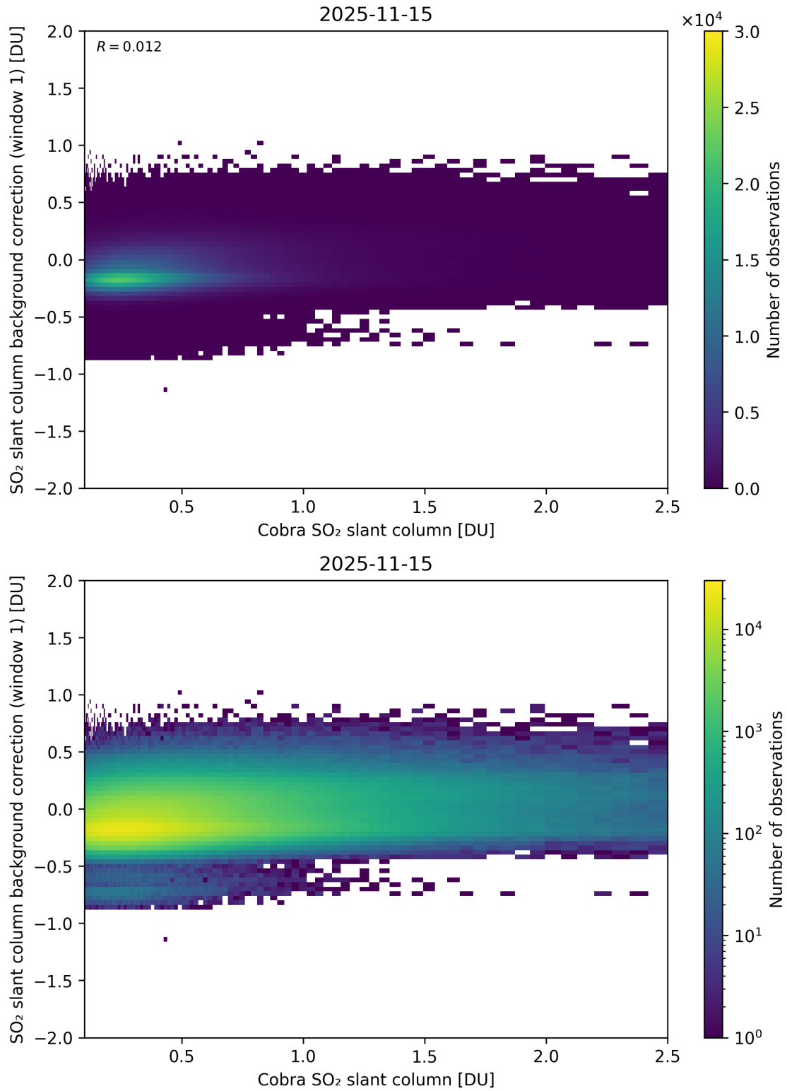
Figure 193: Scatter density plot of “Cobra SO 2 slant column” against “SO 2 slant column background correction (window 1)” for 2025-11-14 to 2025-11-16.
