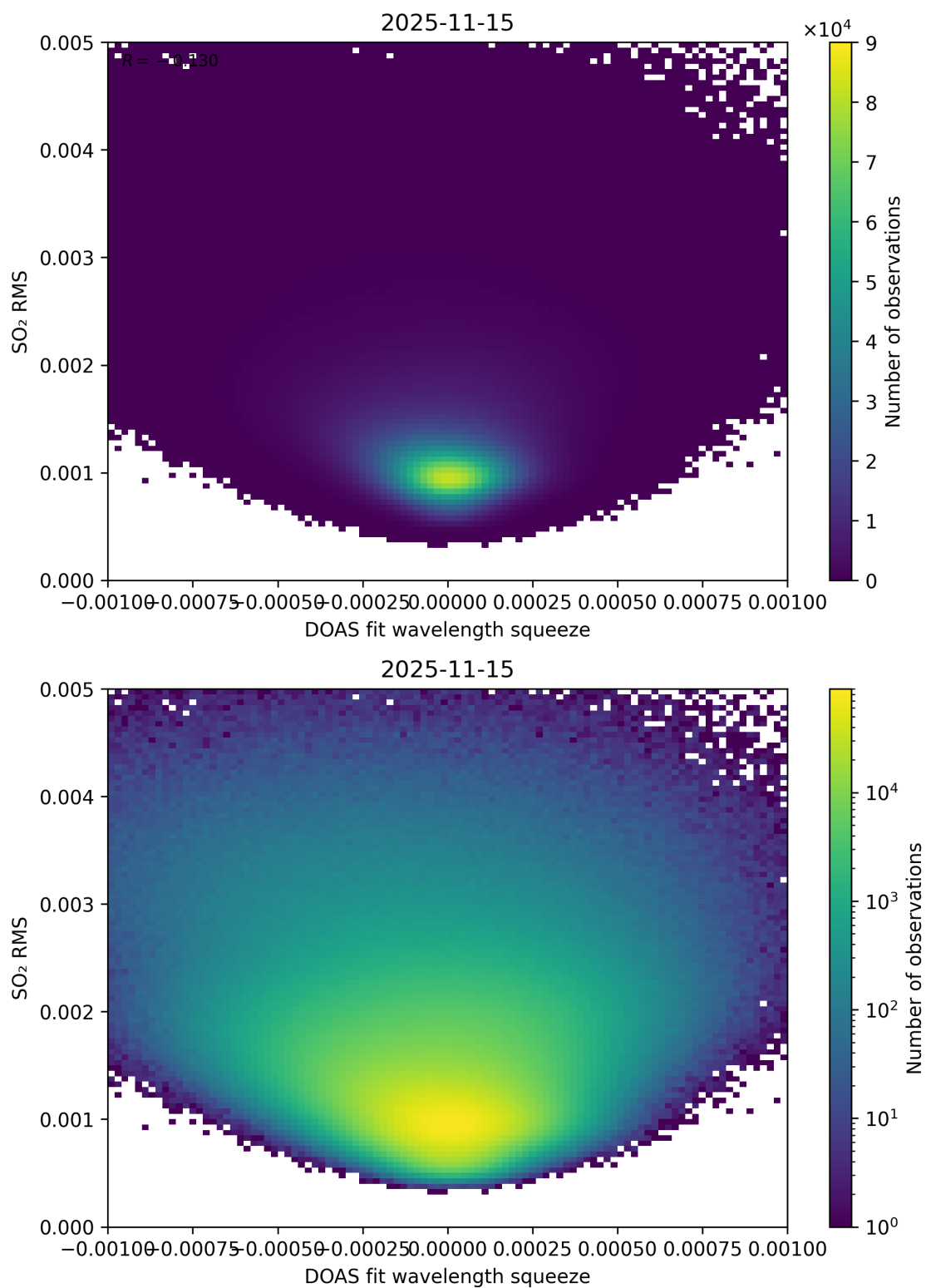
Figure 143: Scatter density plot of “DOAS fit wavelength squeeze” against “SO 2 RMS” for 2025-11-14 to 2025-11-16.
