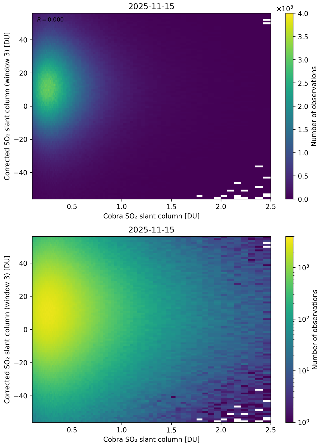
Figure 218: Scatter density plot of “Cobra SO 2 slant column” against “Corrected SO 2 slant column (window 3)” for 2025-11-14 to 2025-11-16.
