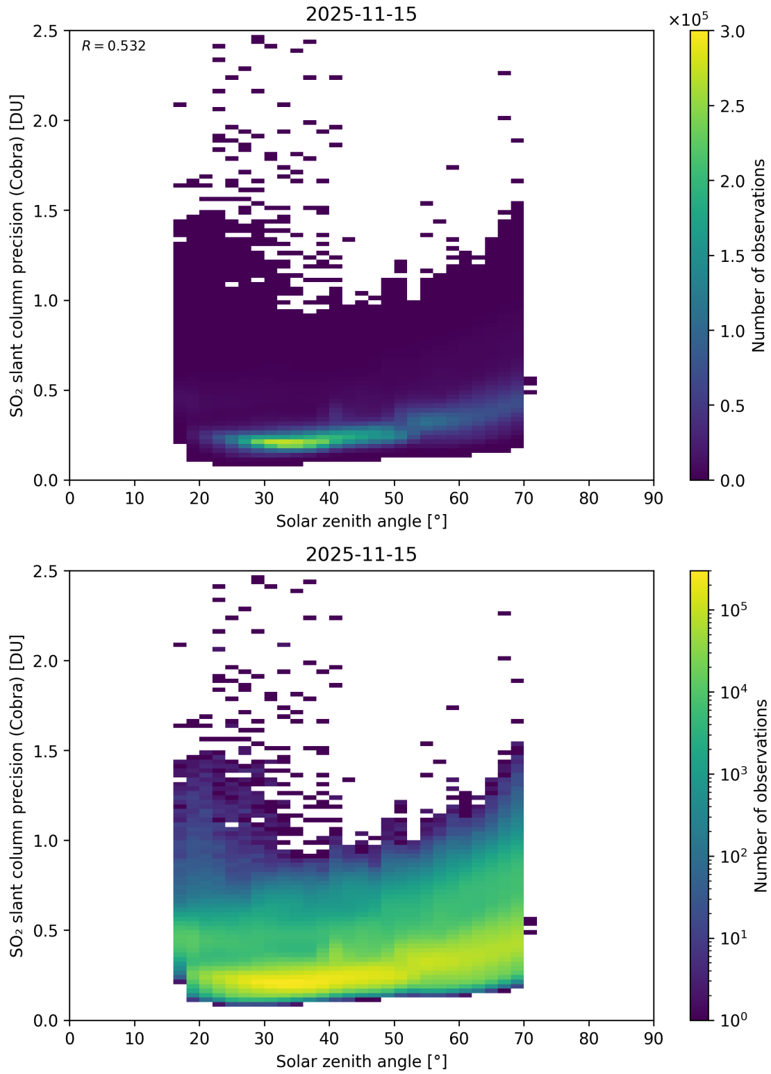
Figure 180: Scatter density plot of “Solar zenith angle” against “SO 2 slant column precision (Cobra)” for 2025-11-14 to 2025-11-16.
