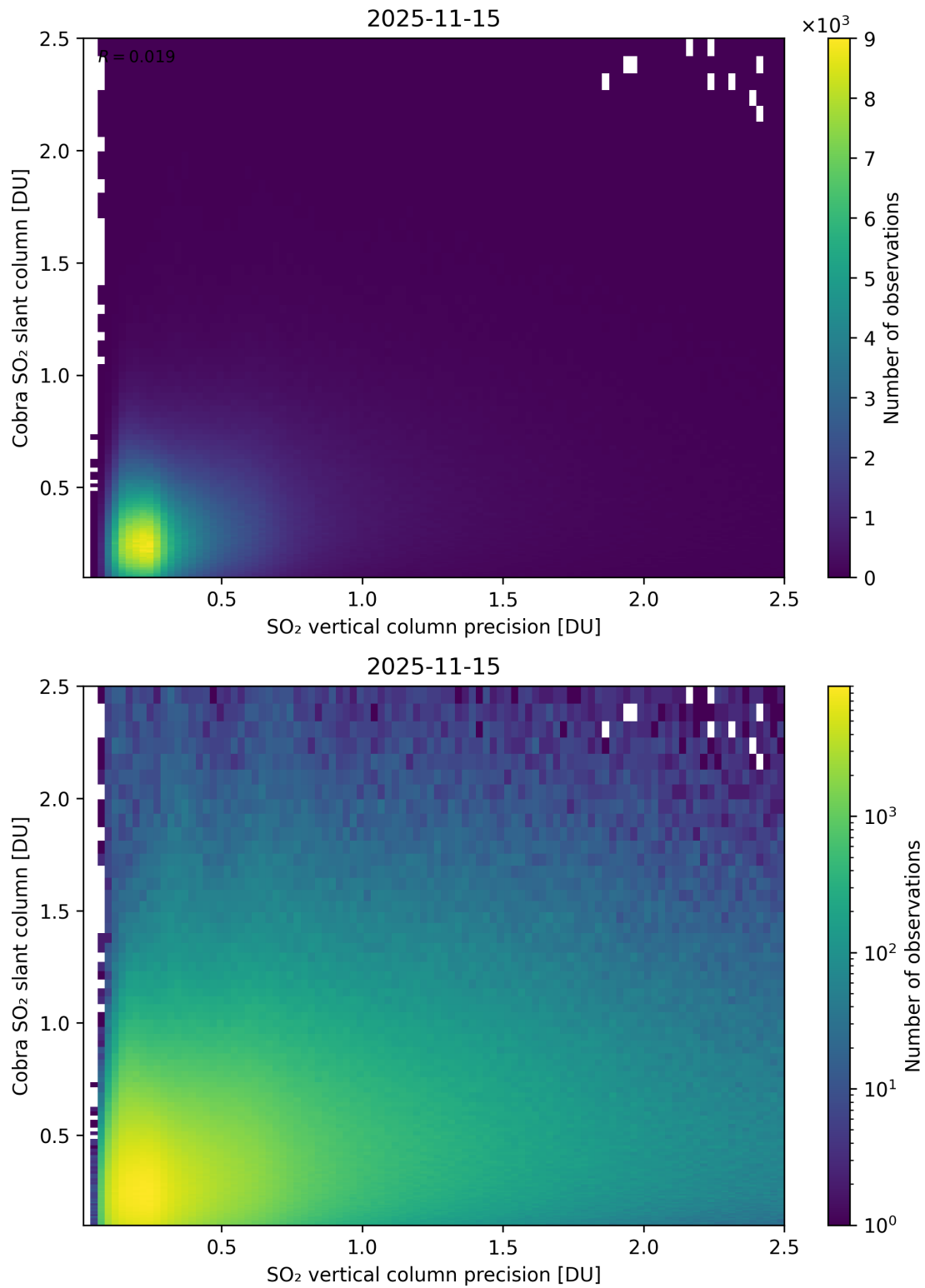
Figure 336: Scatter density plot of “SO 2 vertical column precision” against “Cobra SO 2 slant column” for 2025-11-14 to 2025-11-16.
