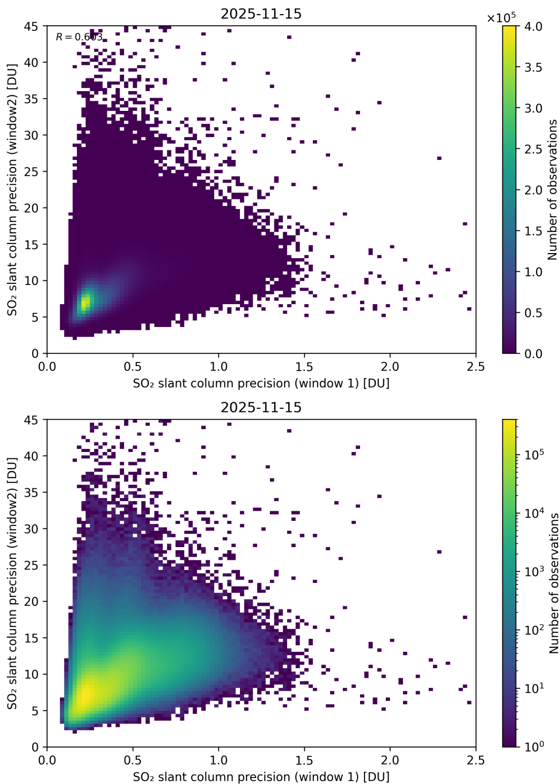
Figure 277: Scatter density plot of “SO 2 slant column precision (window 1)” against “SO 2 slant column precision (window2)” for 2025-11-14 to 2025-11-16.
