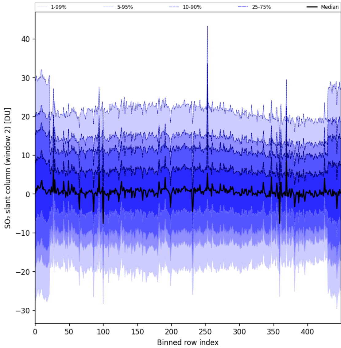
Figure 93: Along track statistics of “SO 2 slant column (window 2)” for 2025-11-14 to 2025-11-16
