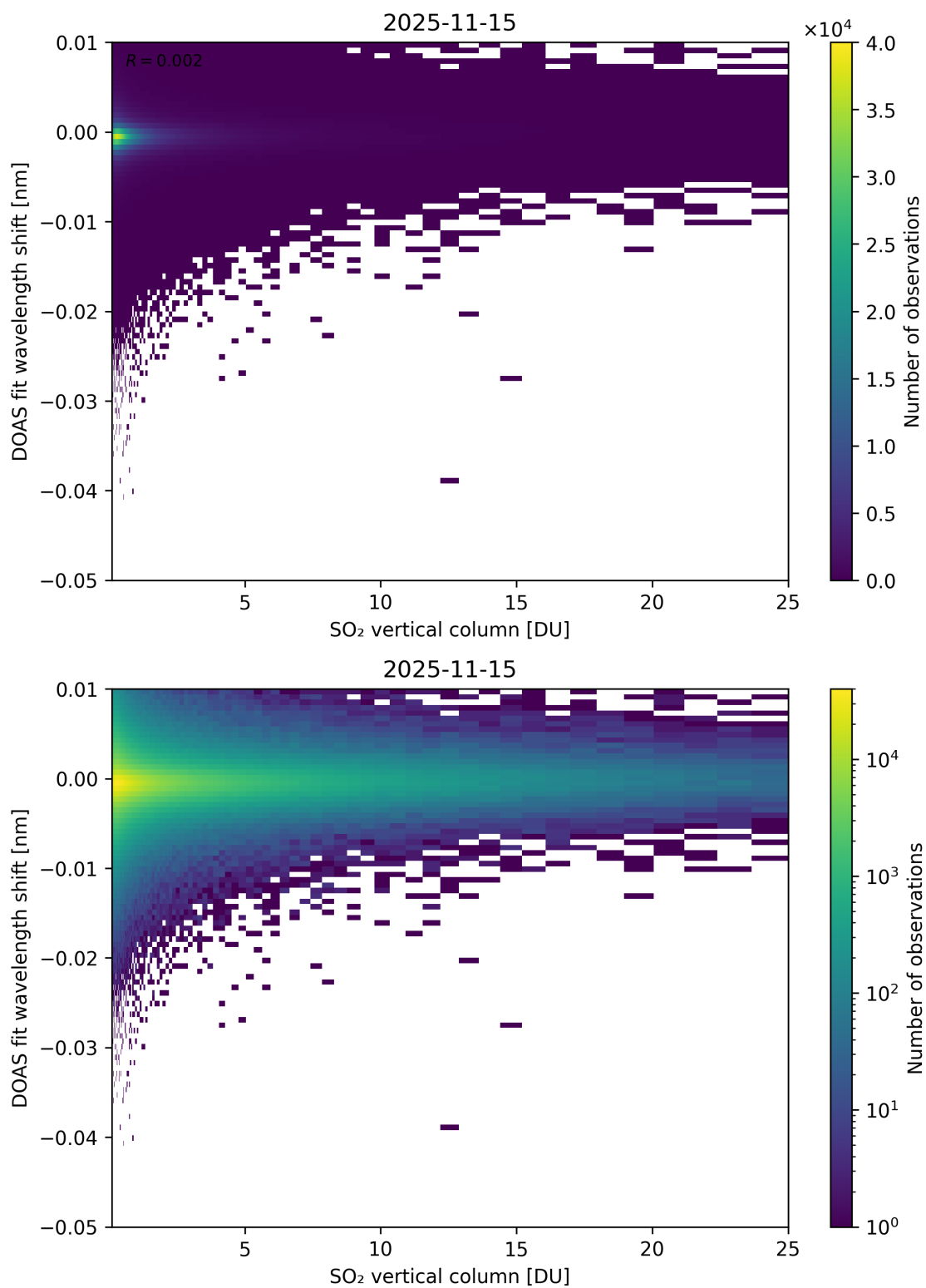
Figure 326: Scatter density plot of “SO 2 vertical column” against “DOAS fit wavelength shift” for 2025-11-14 to 2025-11-16.
