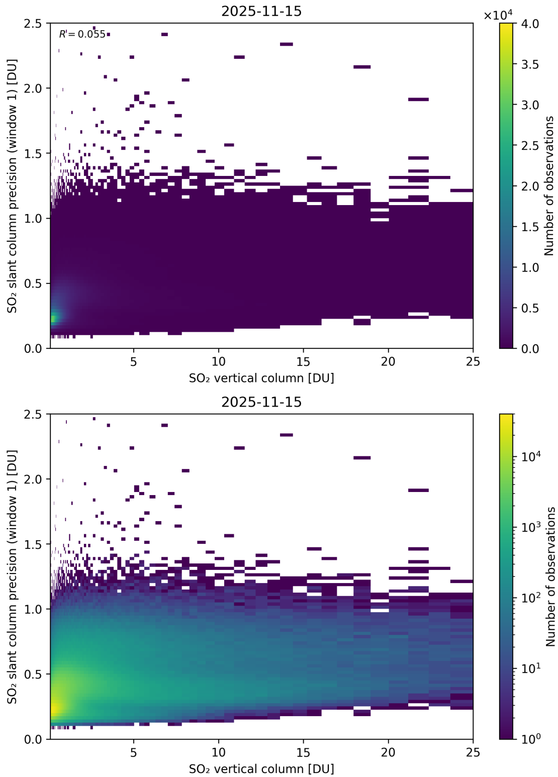
Figure 355: Scatter density plot of “SO 2 vertical column” against “SO 2 slant column precision (window 1)” for 2025-11-14 to 2025-11-16.
