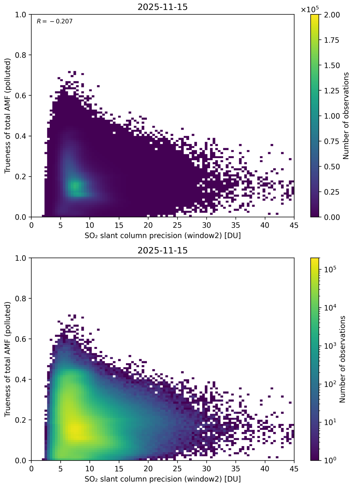
Figure 302: Scatter density plot of “SO 2 slant column precision (window2)” against “Trueness of total AMF (polluted)” for 2025-11-14 to 2025-11-16.
