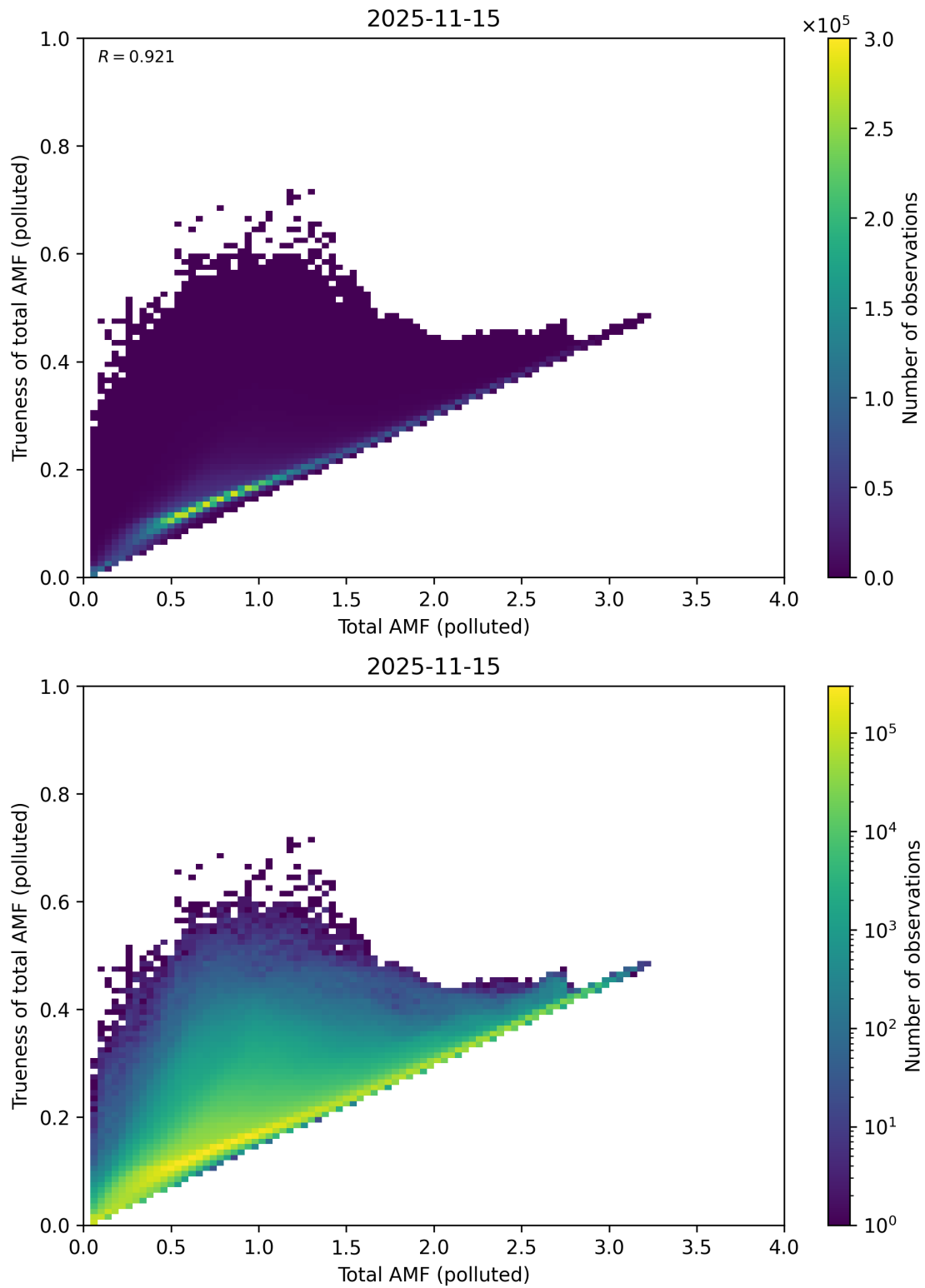
Figure 321: Scatter density plot of “Total AMF (polluted)” against “Trueness of total AMF (polluted)” for 2025-11-14 to 2025-11-16.
