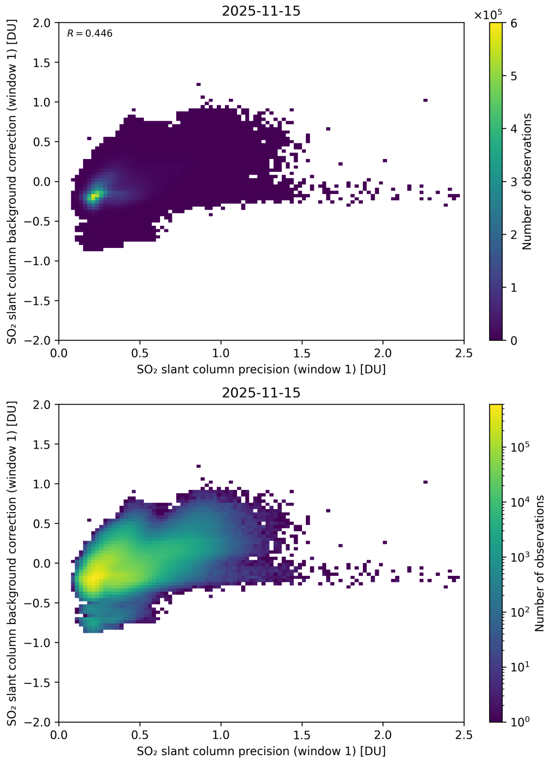
Figure 268: Scatter density plot of “SO 2 slant column precision (window 1)” against “SO 2 slant column background correction (window 1)” for 2025-11-14 to 2025-11-16.
