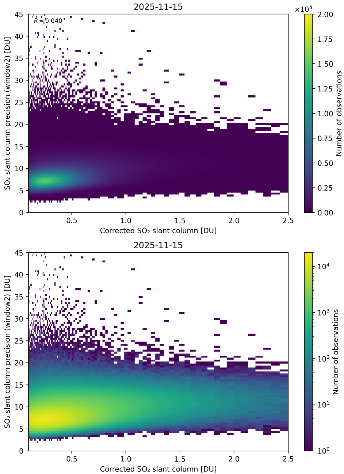
Figure 239: Scatter density plot of “Corrected SO 2 slant column” against “SO 2 slant column precision (window2)” for 2025-11-14 to 2025-11-16.
