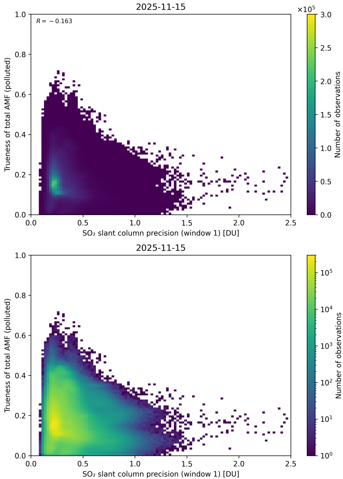
Figure 281: Scatter density plot of “SO 2 slant column precision (window 1)” against “Trueness of total AMF (polluted)” for 2025-11-14 to 2025-11-16.
