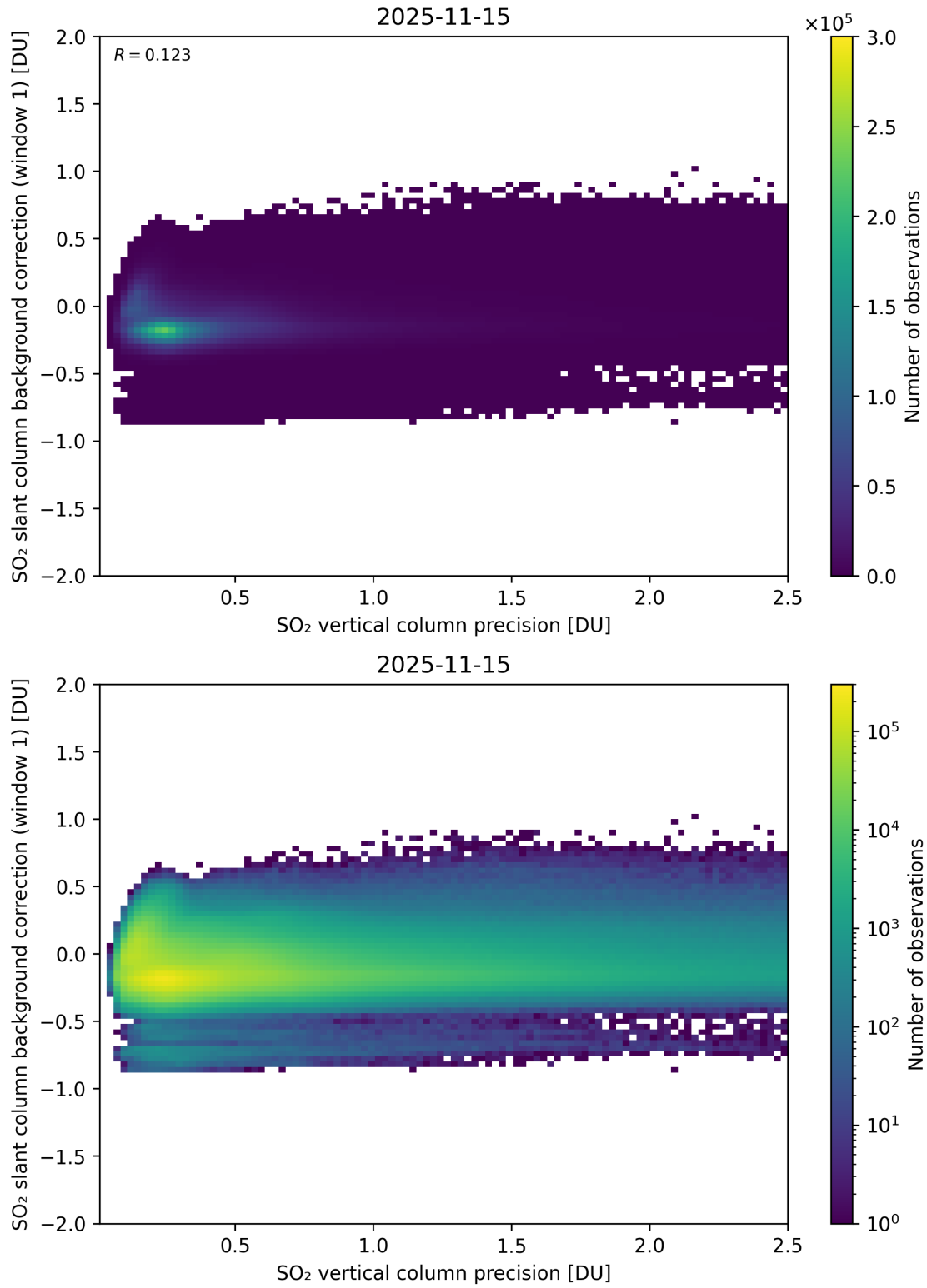
Figure 329: Scatter density plot of “SO 2 vertical column precision” against “SO 2 slant column background correction (window 1)” for 2025-11-14 to 2025-11-16.
