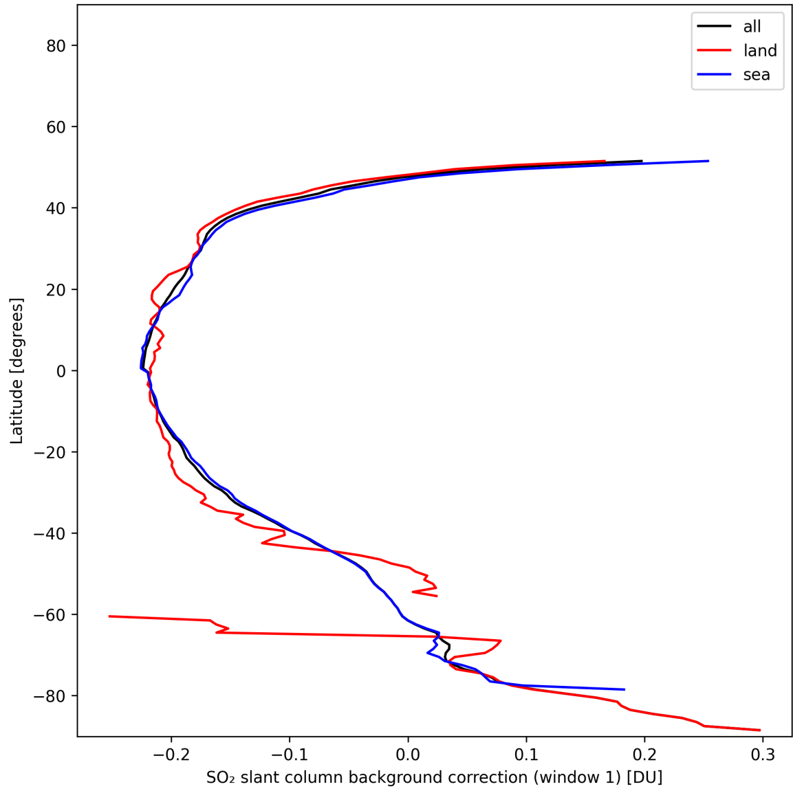
Figure 40: Zonal average of “SO 2 slant column background correction (window 1)” for 2025-11-14 to 2025-11-16.
