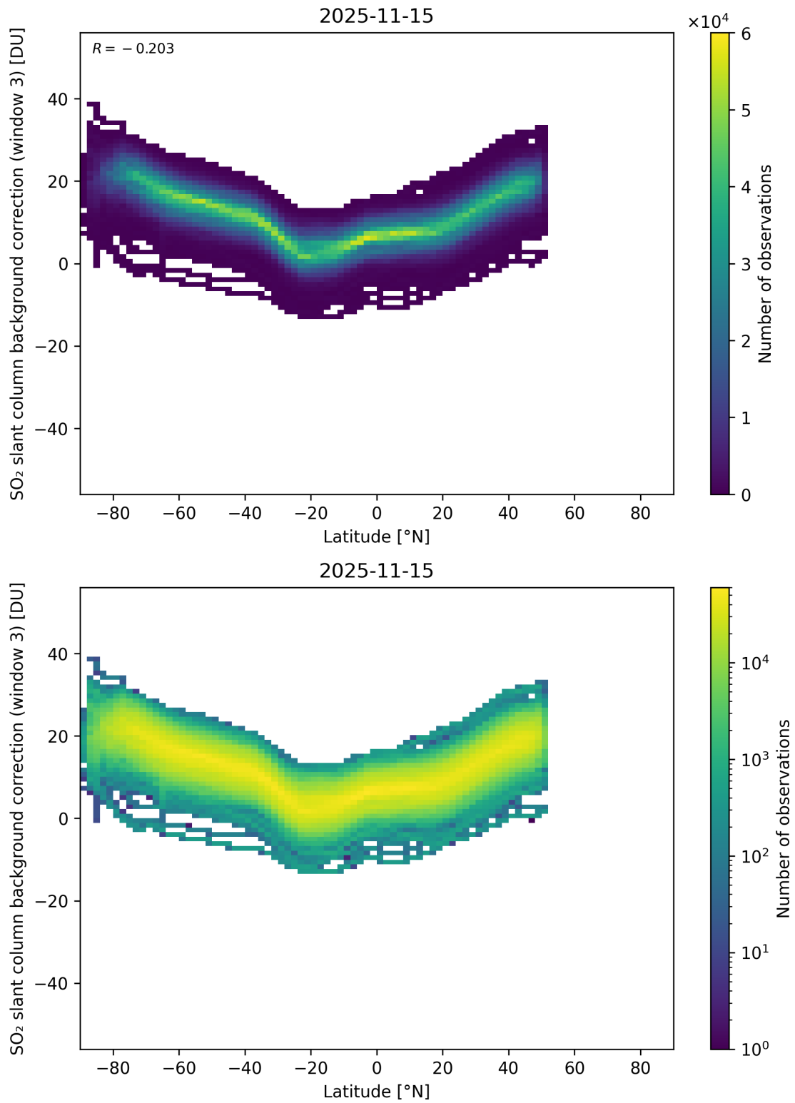
Figure 152: Scatter density plot of “Latitude” against “SO 2 slant column background correction (window 3)” for 2025-11-14 to 2025-11-16.
