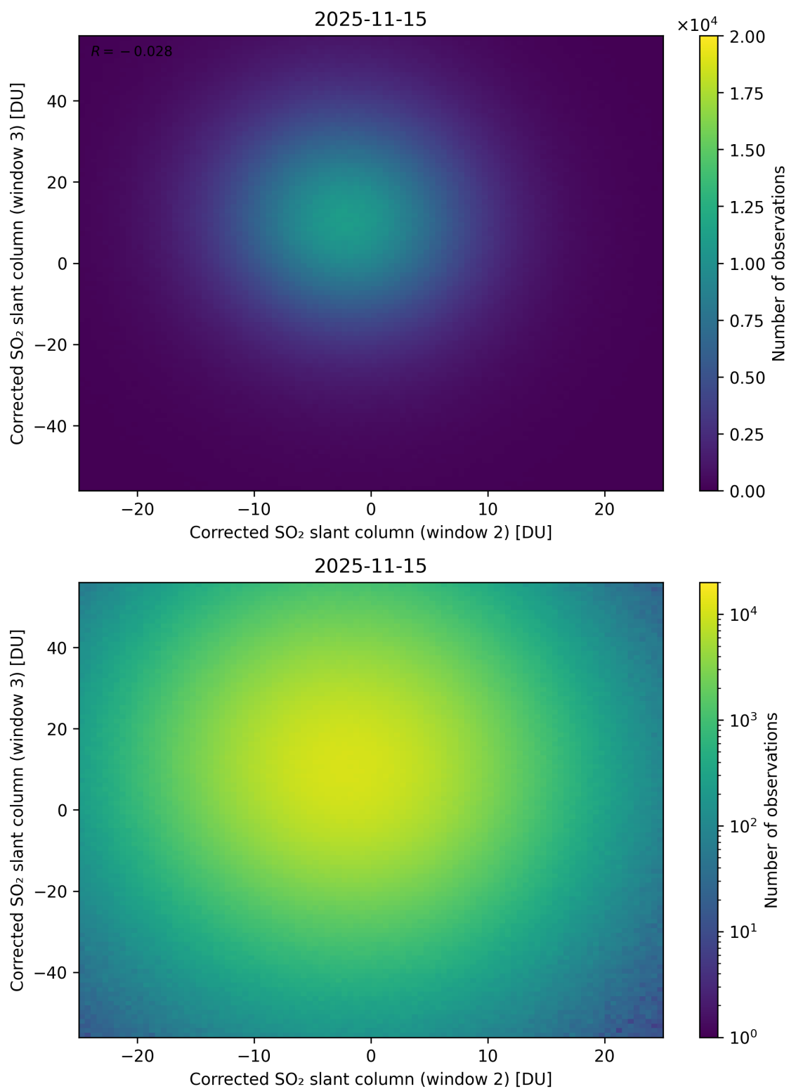
Figure 250: Scatter density plot of “Corrected SO 2 slant column (window 2)” against “Corrected SO 2 slant column (window 3)” for 2025-11-14 to 2025-11-16.
