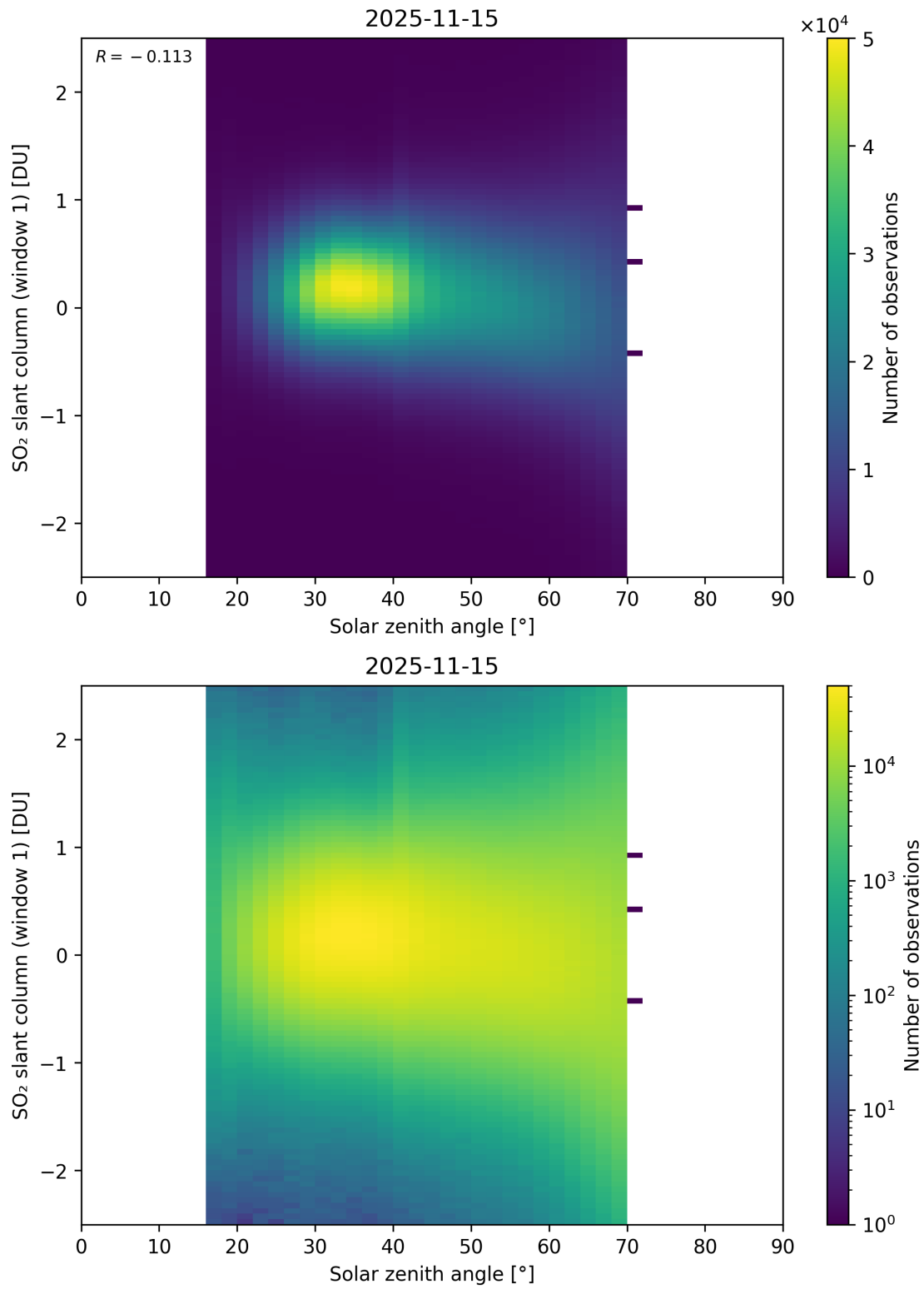
Figure 184: Scatter density plot of “Solar zenith angle” against “SO 2 slant column (window 1)” for 2025-11-14 to 2025-11-16.
