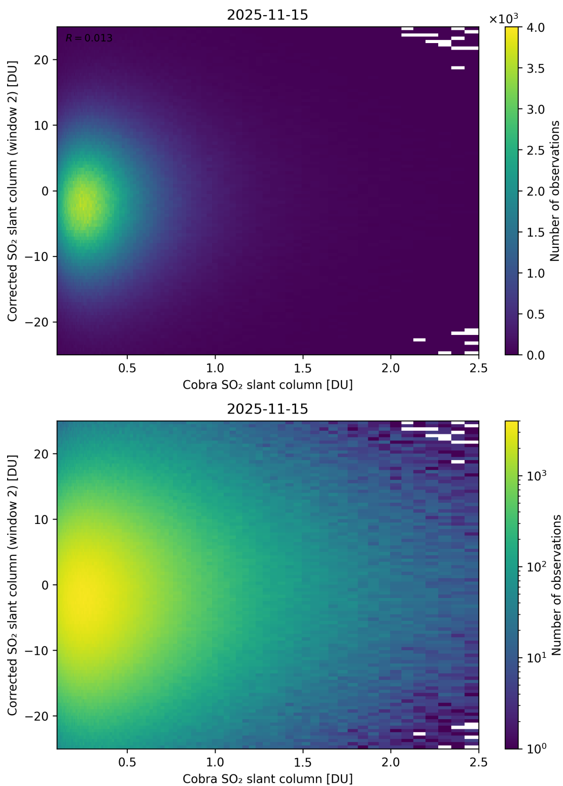
Figure 217: Scatter density plot of “Cobra SO 2 slant column” against “Corrected SO 2 slant column (window 2)” for 2025-11-14 to 2025-11-16.
