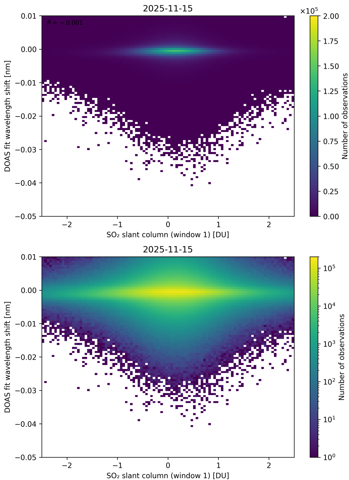
Figure 265: Scatter density plot of “SO 2 slant column (window 1)” against “DOAS fit wavelength shift” for 2025-11-14 to 2025-11-16.
