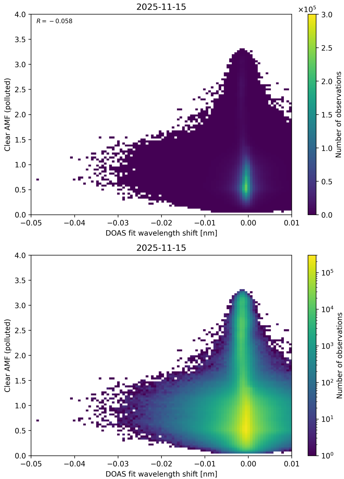
Figure 140: Scatter density plot of “DOAS fit wavelength shift” against “Clear AMF (polluted)” for 2025-11-14 to 2025-11-16.
