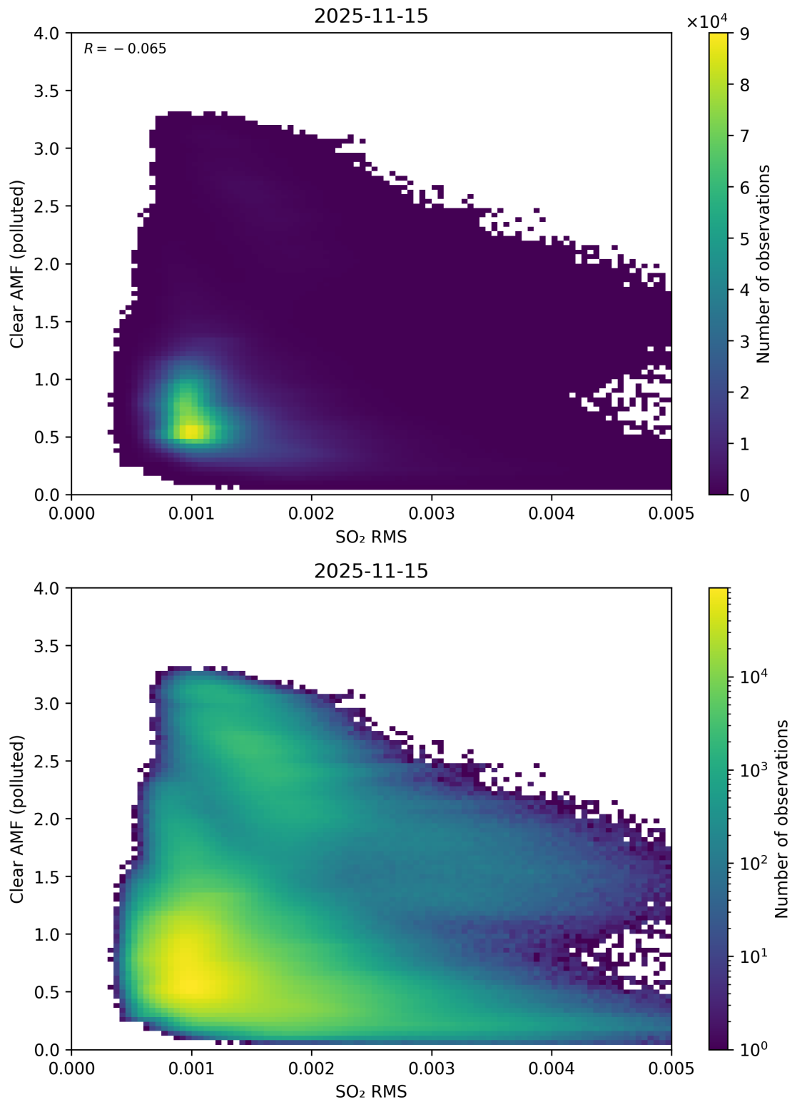
Figure 147: Scatter density plot of “SO 2 RMS” against “Clear AMF (polluted)” for 2025-11-14 to 2025-11-16.
