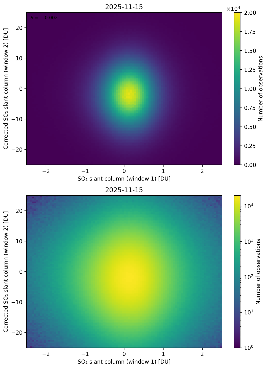
Figure 283: Scatter density plot of “SO 2 slant column (window 1)” against “Corrected SO 2 slant column (window 2)” for 2025-11-14 to 2025-11-16.
