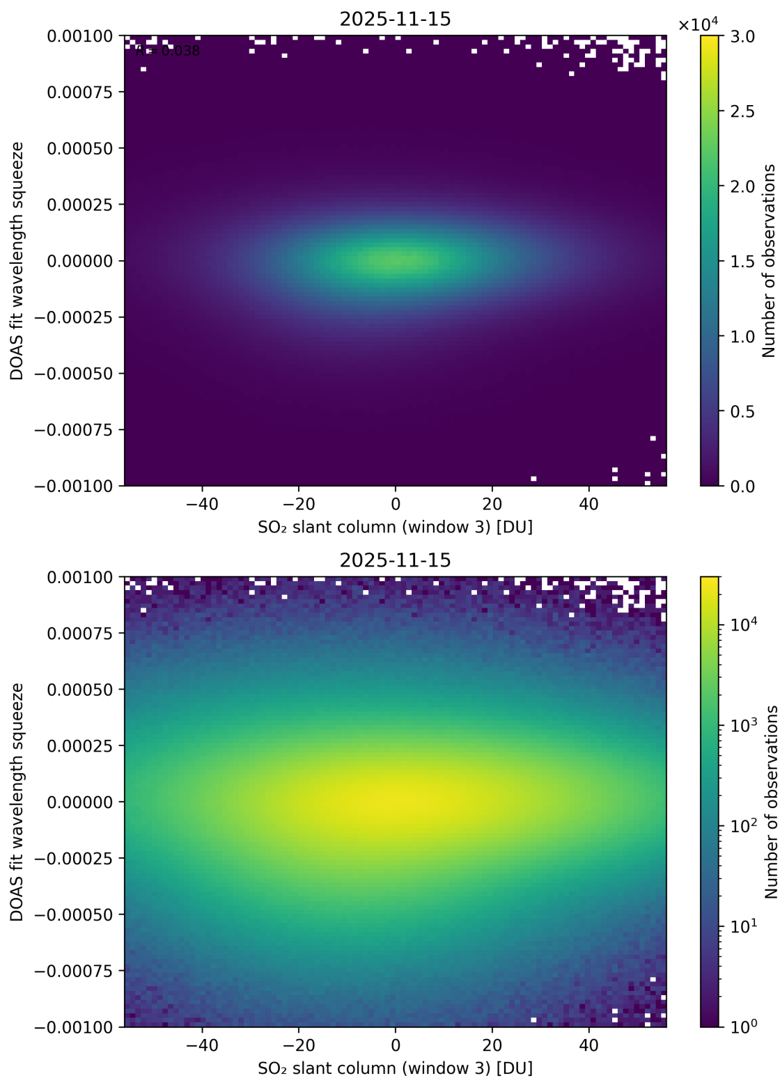
Figure 305: Scatter density plot of “SO 2 slant column (window 3)” against “DOAS fit wavelength squeeze” for 2025-11-14 to 2025-11-16.
