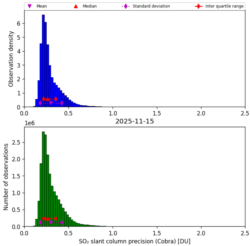
Figure 62: Histogram of “SO 2 slant column precision (Cobra)” for 2025-11-14 to 2025-11-16
