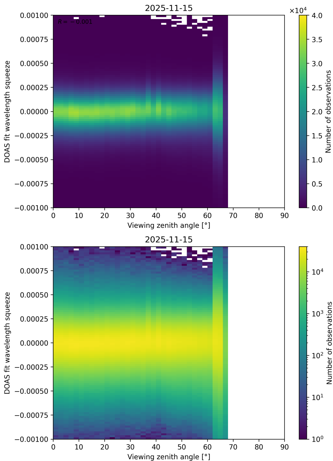
Figure 366: Scatter density plot of “Viewing zenith angle” against “DOAS fit wavelength squeeze” for 2025-11-14 to 2025-11-16.
