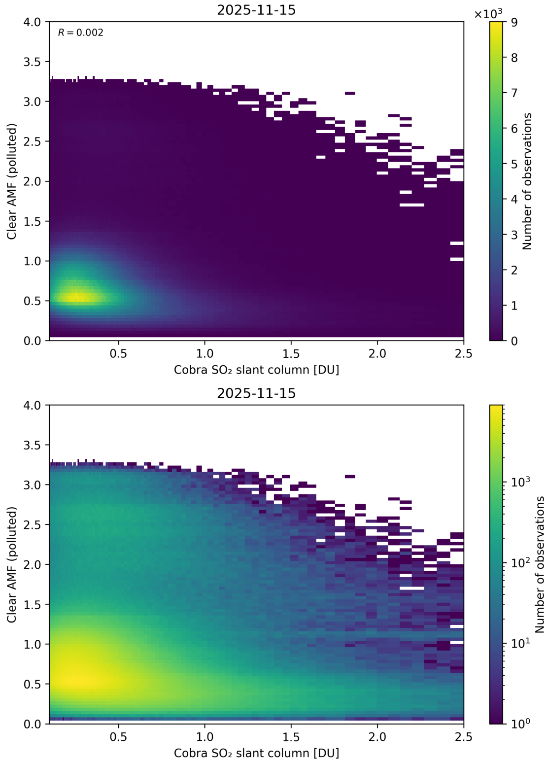
Figure 215: Scatter density plot of “Cobra SO 2 slant column” against “Clear AMF (polluted)” for 2025-11-14 to 2025-11-16.
