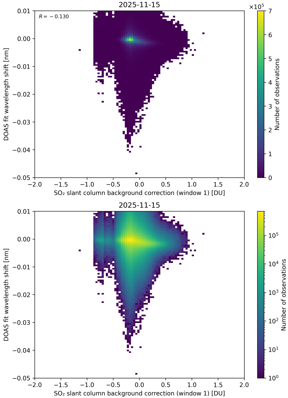
Figure 111: Scatter density plot of “SO 2 slant column background correction (window 1)” against “DOAS fit wavelength shift” for 2025-11-14 to 2025-11-16.
