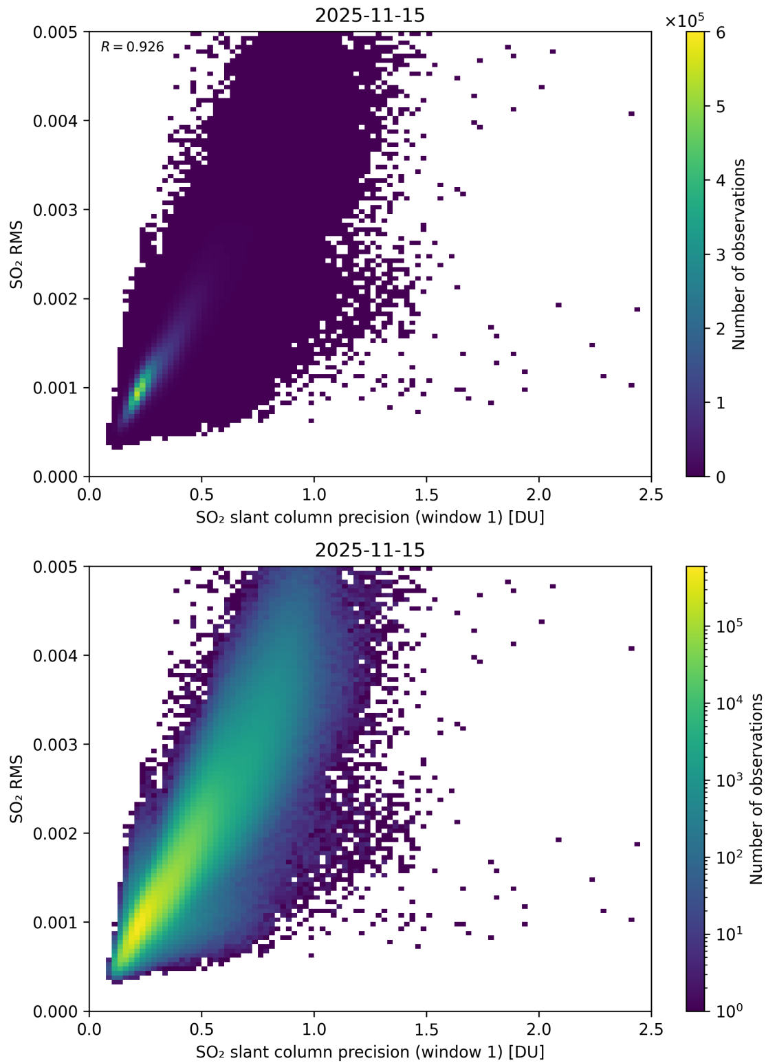
Figure 273: Scatter density plot of “SO 2 slant column precision (window 1)” against “SO 2 RMS” for 2025-11-14 to 2025-11-16.
