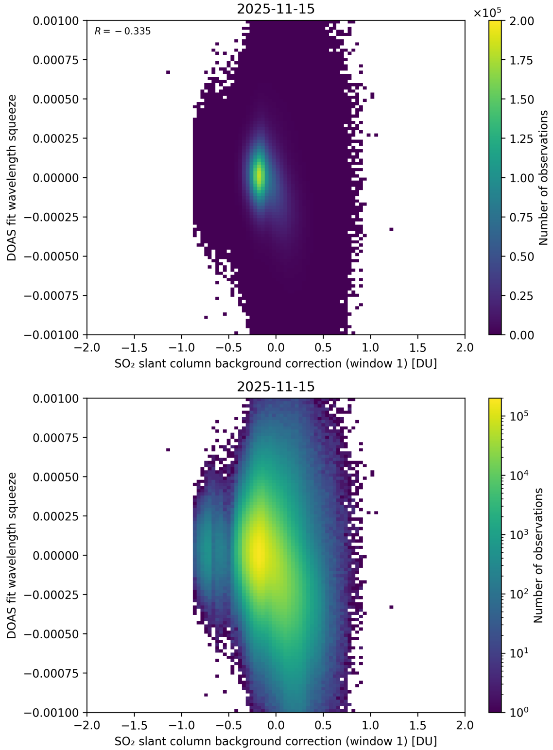
Figure 112: Scatter density plot of “SO 2 slant column background correction (window 1)” against “DOAS fit wavelength squeeze” for 2025-11-14 to 2025-11-16.
