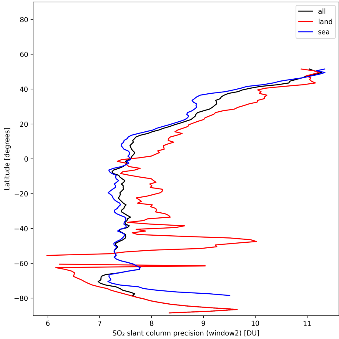
Figure 42: Zonal average of “SO 2 slant column precision (window2)” for 2025-11-14 to 2025-11-16.
