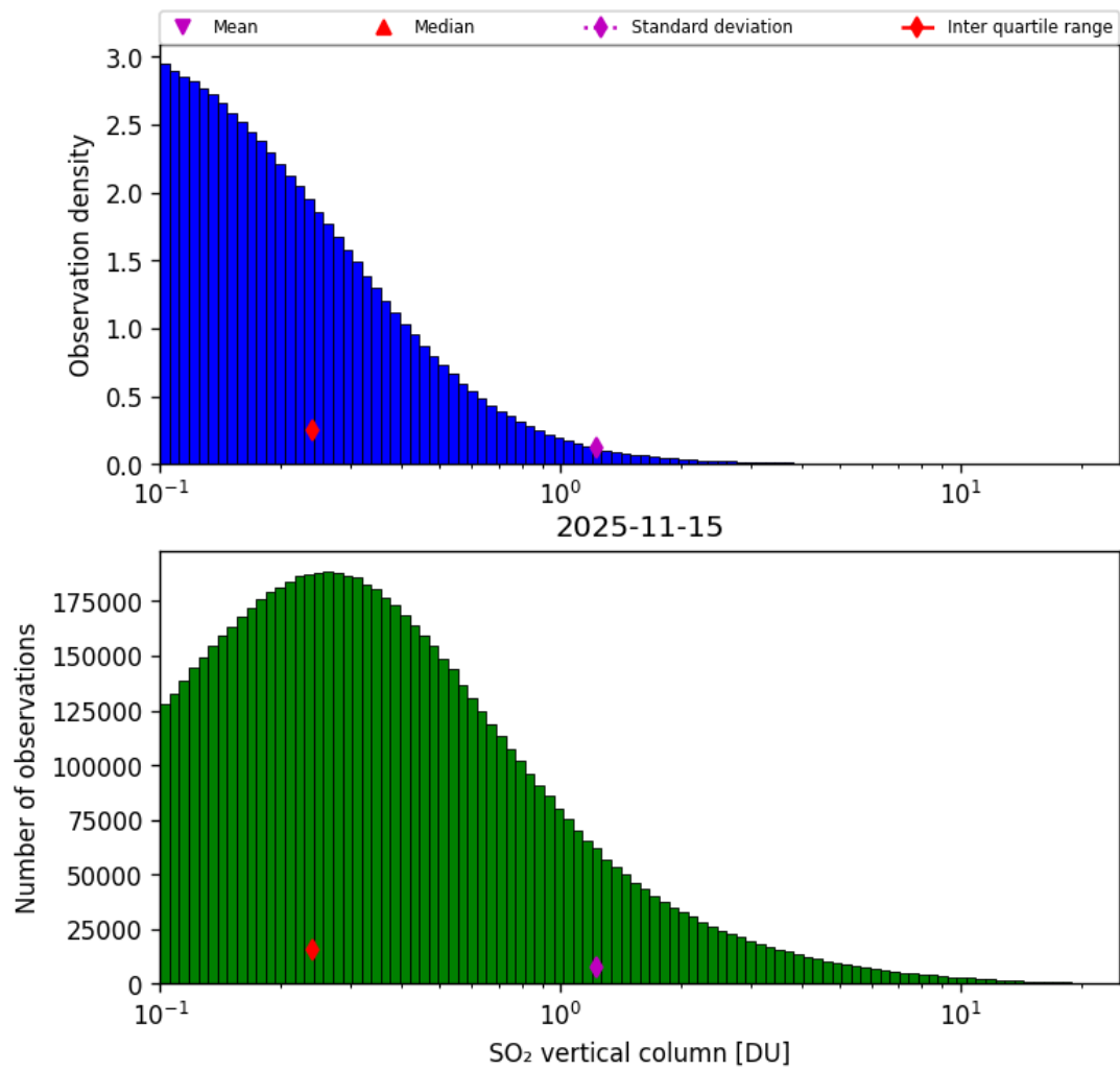
Figure 58: Histogram of “SO 2 vertical column” for 2025-11-14 to 2025-11-16
