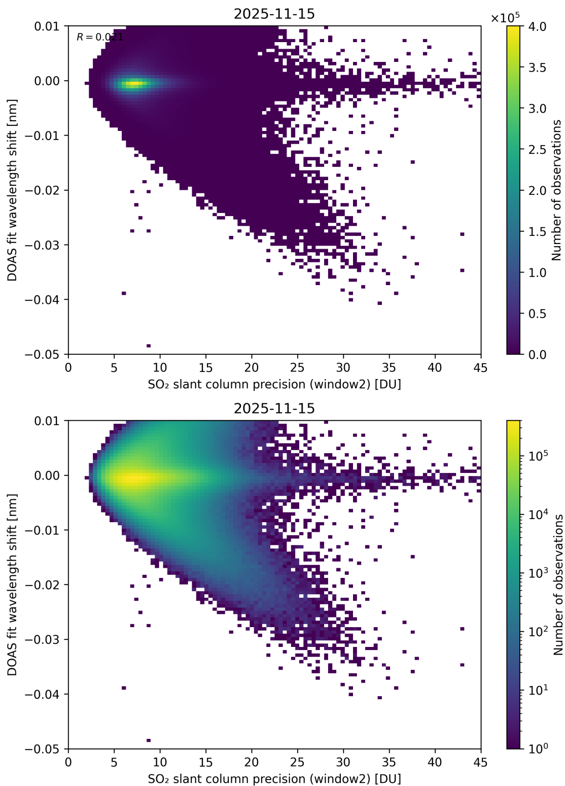
Figure 293: Scatter density plot of “SO 2 slant column precision (window2)” against “DOAS fit wavelength shift” for 2025-11-14 to 2025-11-16.
