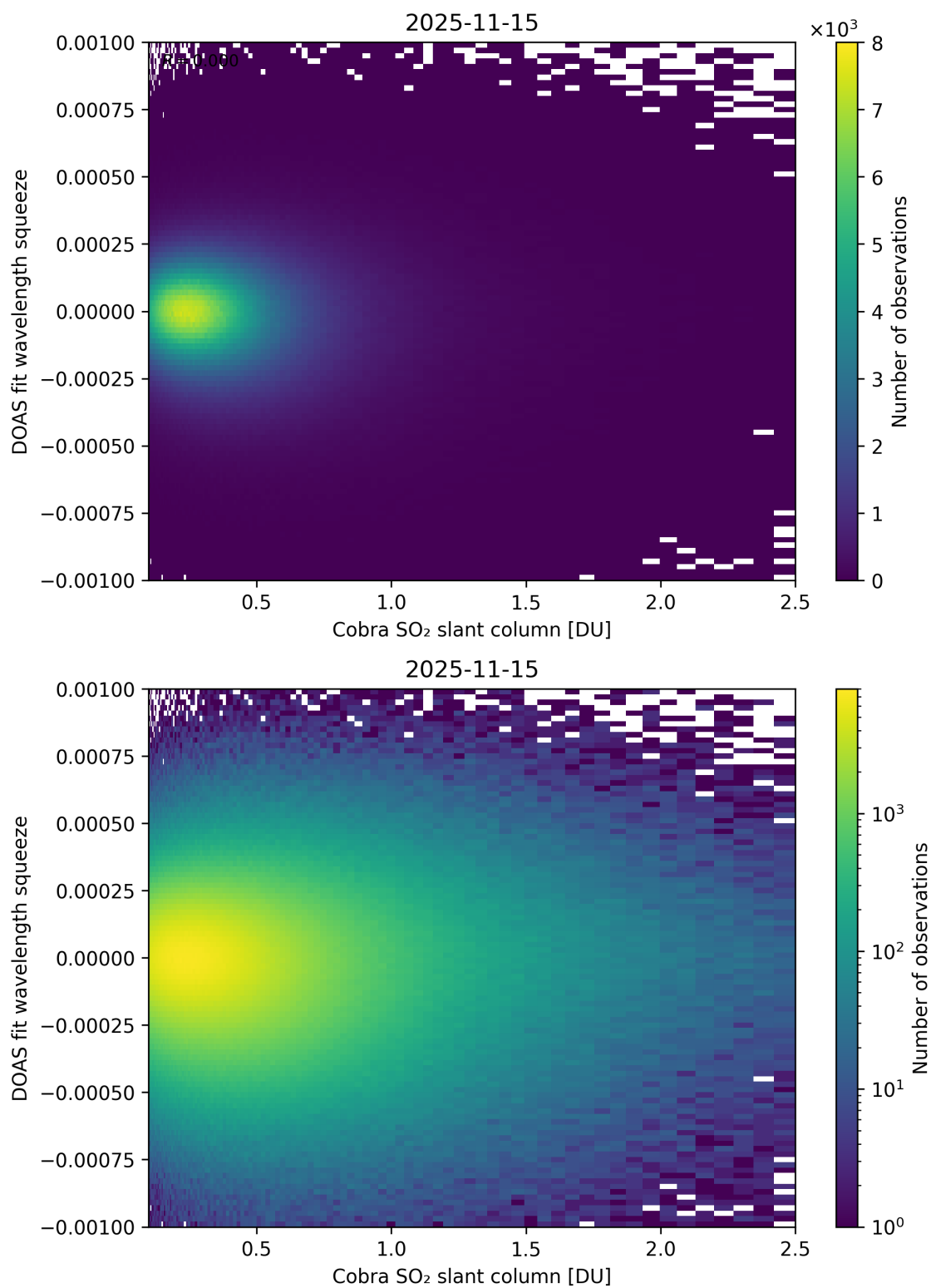
Figure 197: Scatter density plot of “Cobra SO 2 slant column” against “DOAS fit wavelength squeeze” for 2025-11-14 to 2025-11-16.
