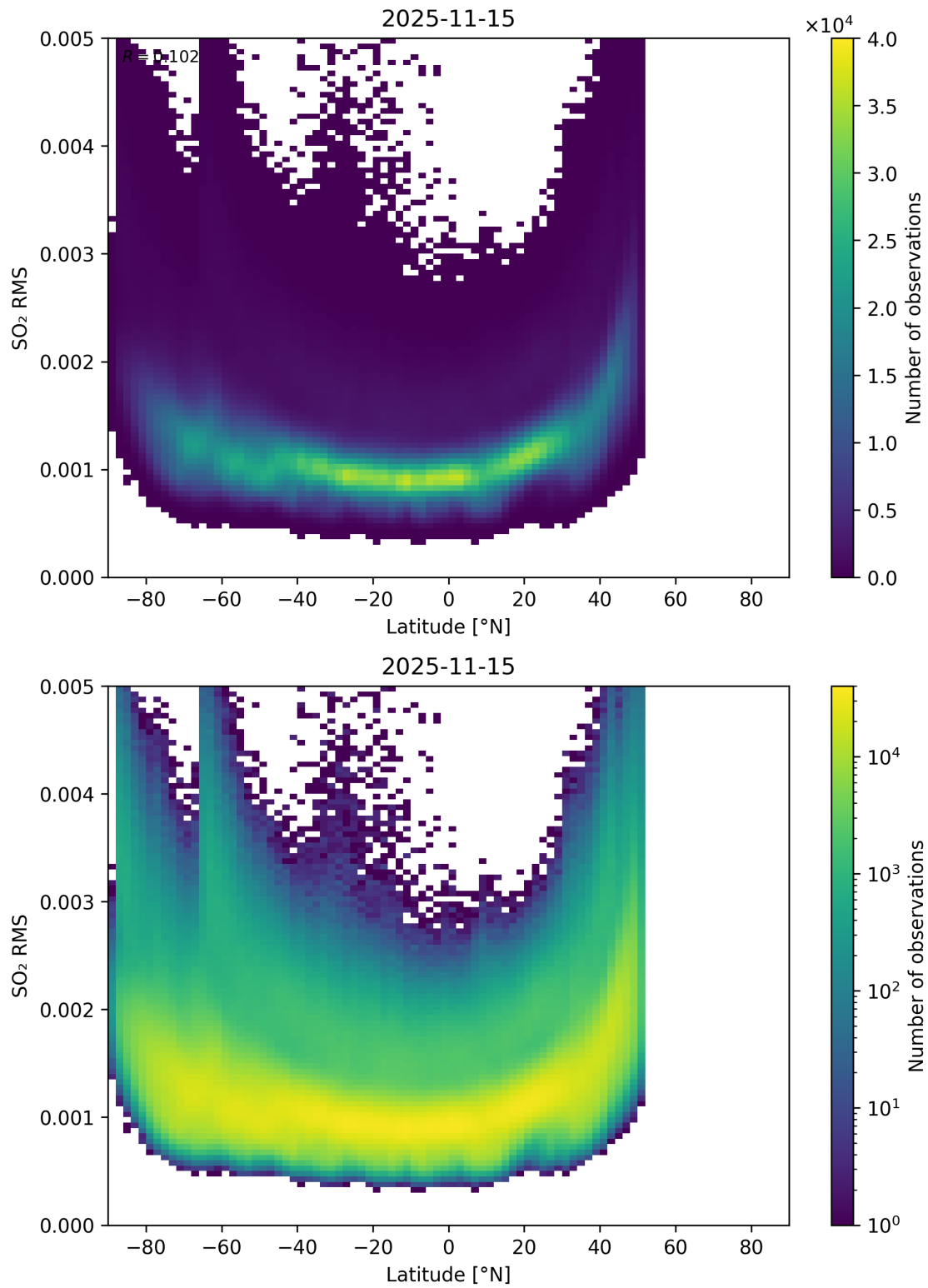
Figure 155: Scatter density plot of “Latitude” against “SO 2 RMS” for 2025-11-14 to 2025-11-16.
