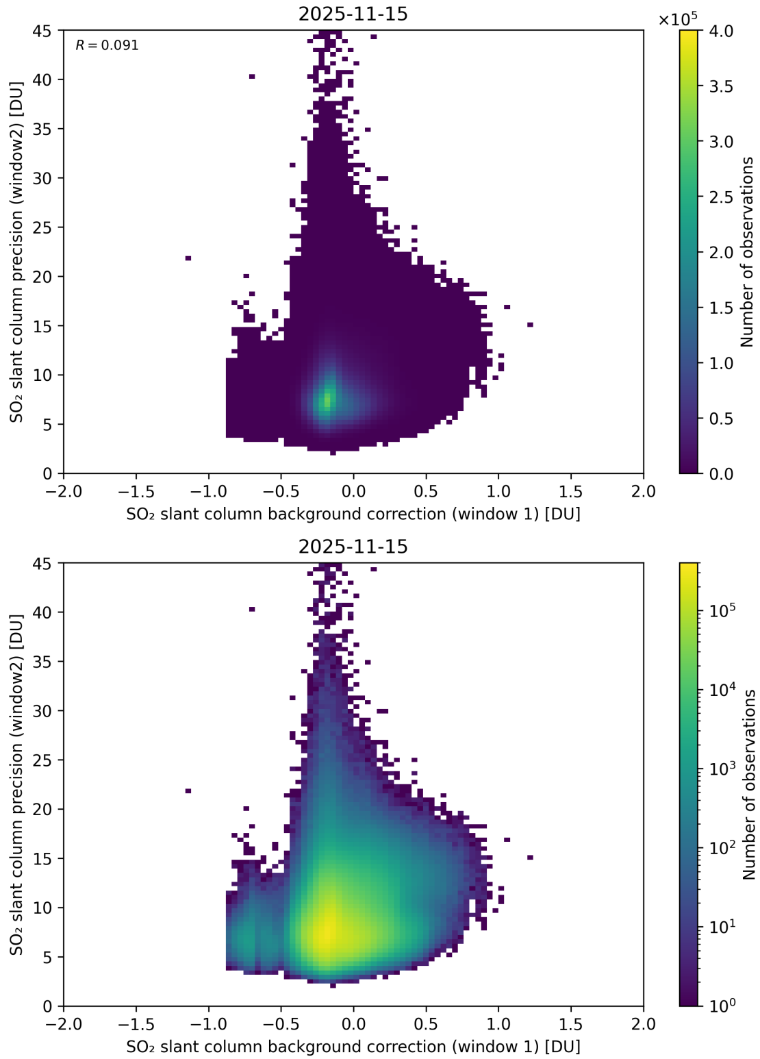
Figure 117: Scatter density plot of “SO 2 slant column background correction (window 1)” against “SO 2 slant column precision (window2)” for 2025-11-14 to 2025-11-16.
