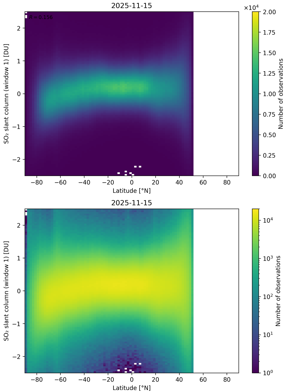
Figure 162: Scatter density plot of “Latitude” against “SO 2 slant column (window 1)” for 2025-11-14 to 2025-11-16.
