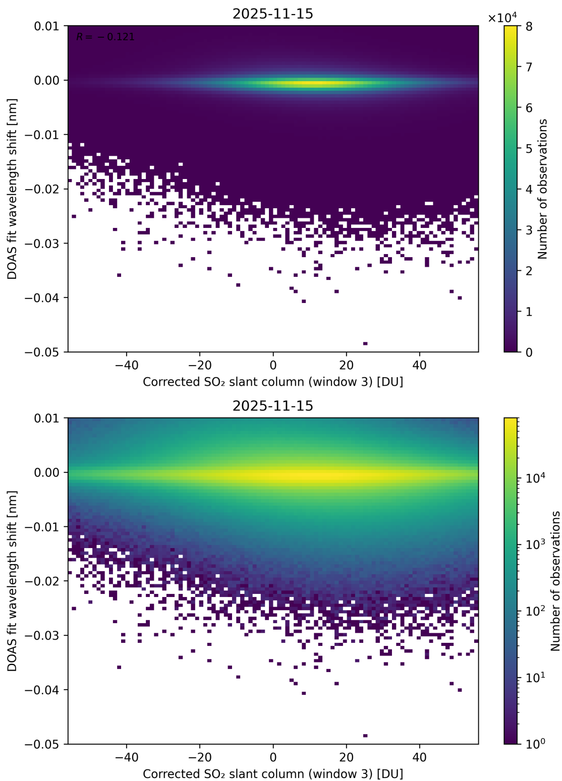
Figure 256: Scatter density plot of “Corrected SO 2 slant column (window 3)” against “DOAS fit wavelength shift” for 2025-11-14 to 2025-11-16.
