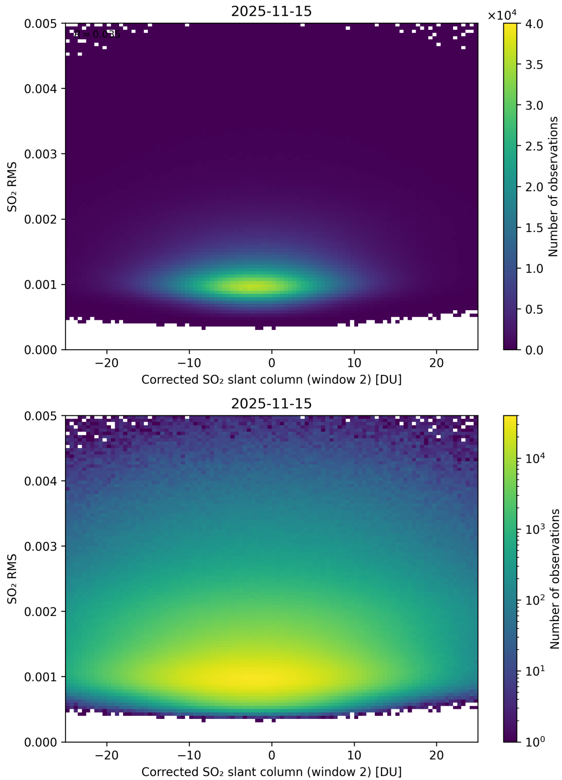
Figure 248: Scatter density plot of “Corrected SO 2 slant column (window 2)” against “SO 2 RMS” for 2025-11-14 to 2025-11-16.
