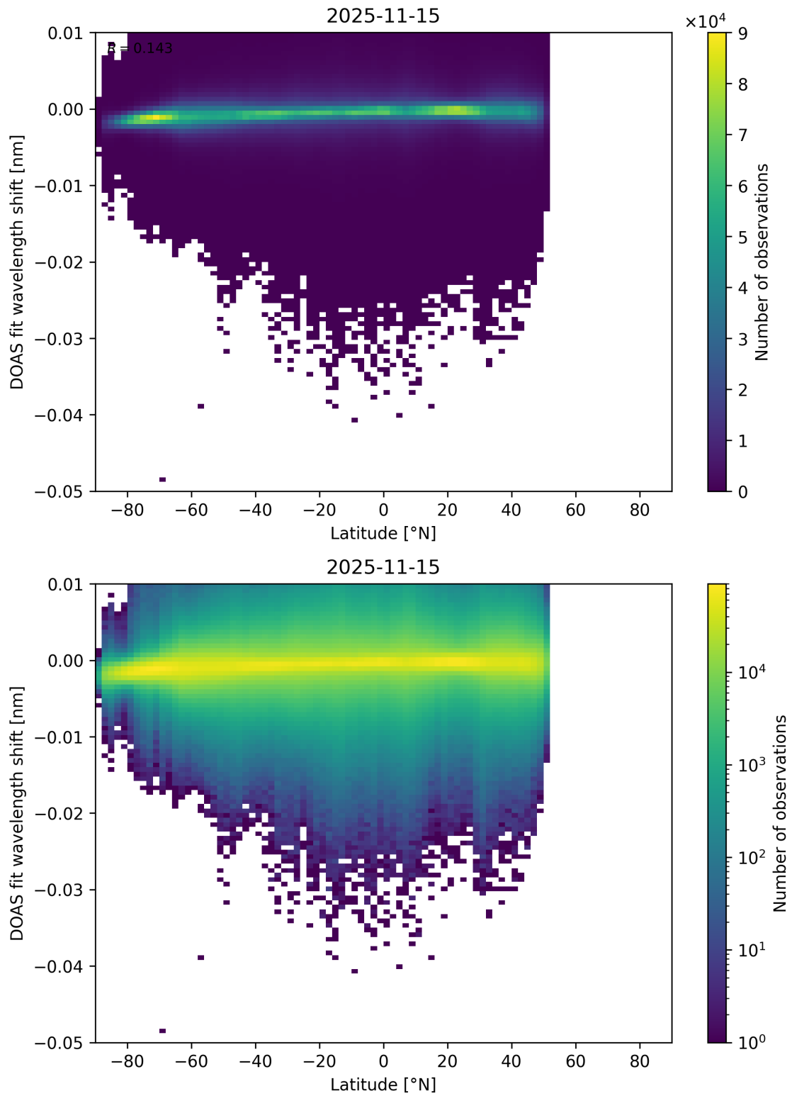
Figure 153: Scatter density plot of “Latitude” against “DOAS fit wavelength shift” for 2025-11-14 to 2025-11-16.
