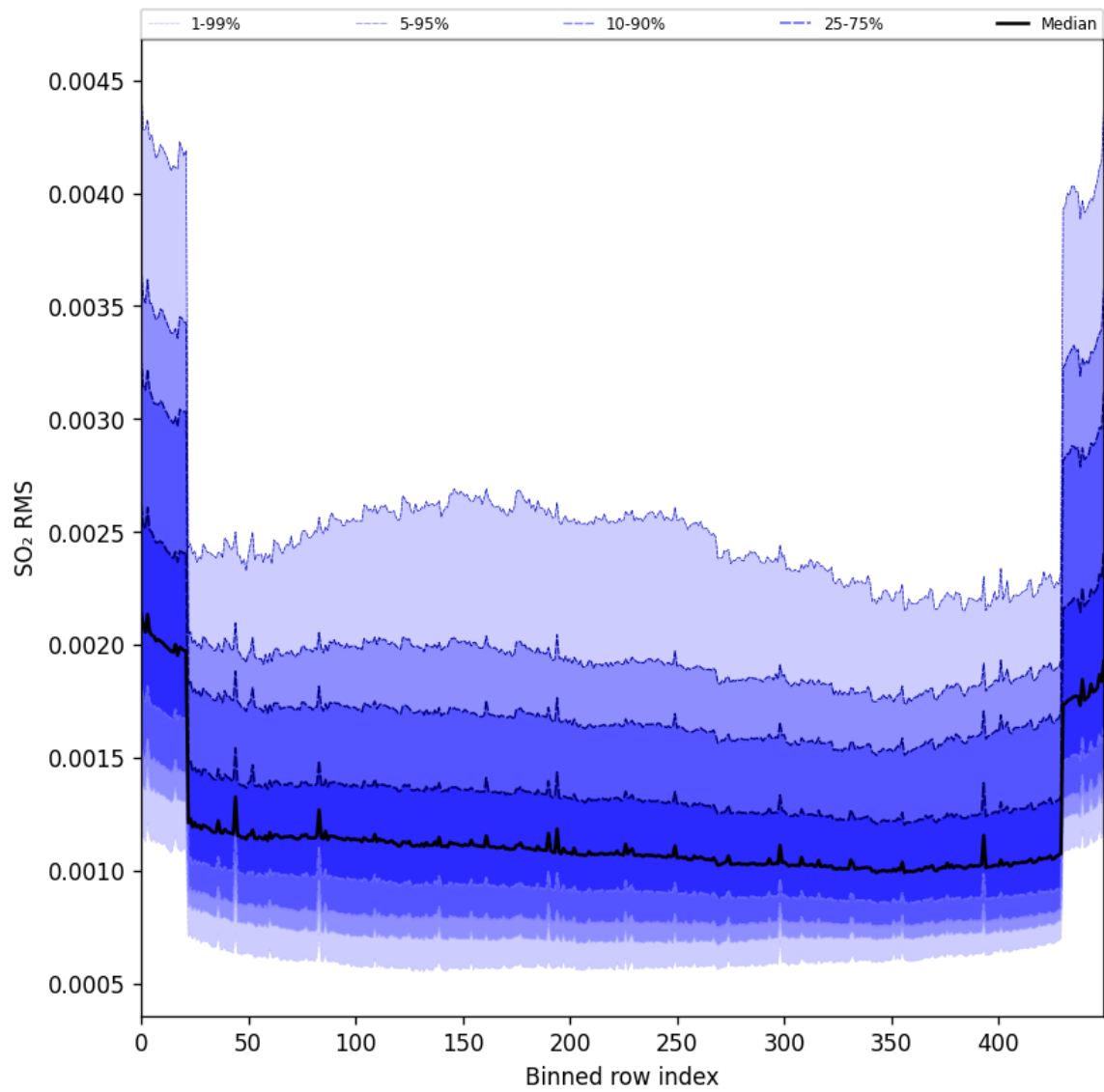
Figure 104: Along track statistics of “SO 2 RMS” for 2025-11-14 to 2025-11-16
