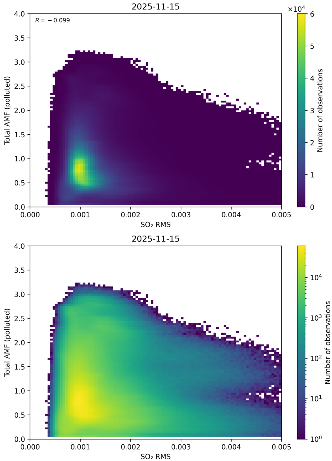
Figure 148: Scatter density plot of “SO 2 RMS” against “Total AMF (polluted)” for 2025-11-14 to 2025-11-16.
