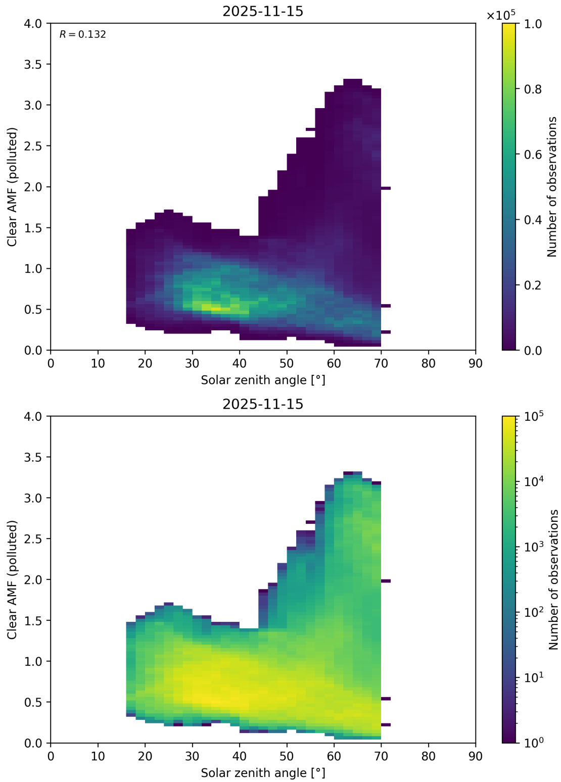
Figure 178: Scatter density plot of “Solar zenith angle” against “Clear AMF (polluted)” for 2025-11-14 to 2025-11-16.
