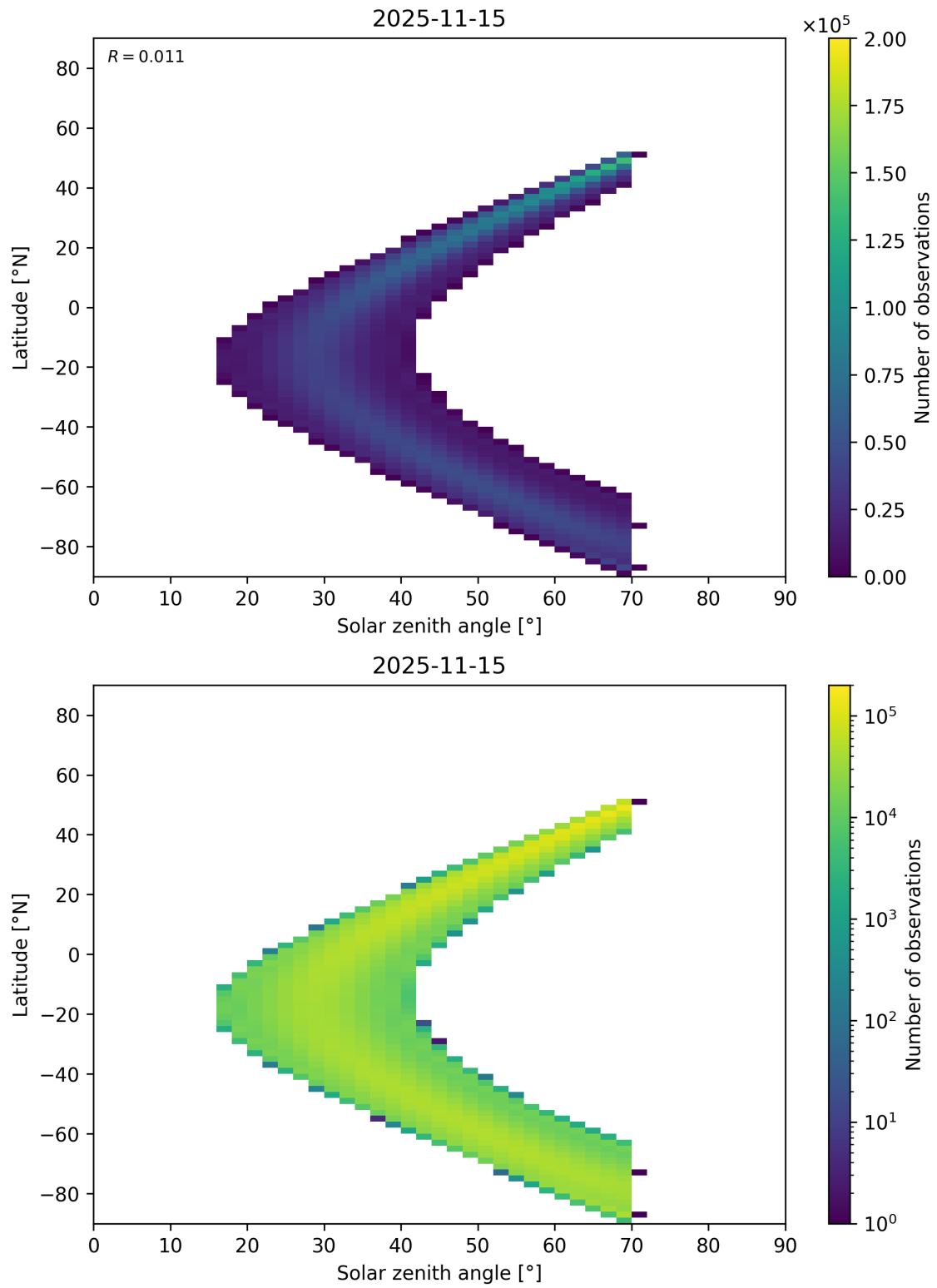
Figure 177: Scatter density plot of “Solar zenith angle” against “Latitude” for 2025-11-14 to 2025-11-16.
