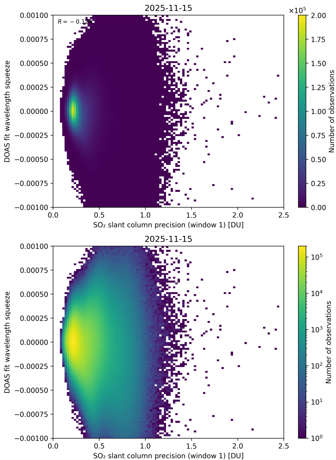
Figure 272: Scatter density plot of “SO 2 slant column precision (window 1)” against “DOAS fit wavelength squeeze” for 2025-11-14 to 2025-11-16.
