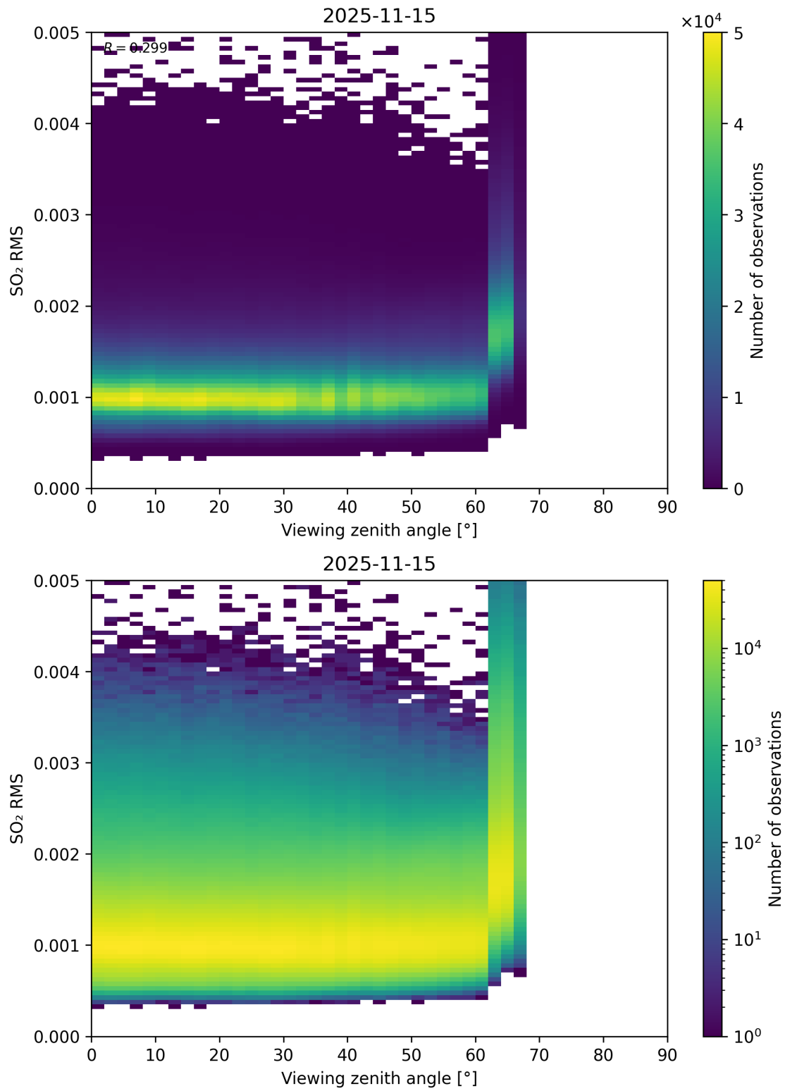
Figure 367: Scatter density plot of “Viewing zenith angle” against “SO 2 RMS” for 2025-11-14 to 2025-11-16.
