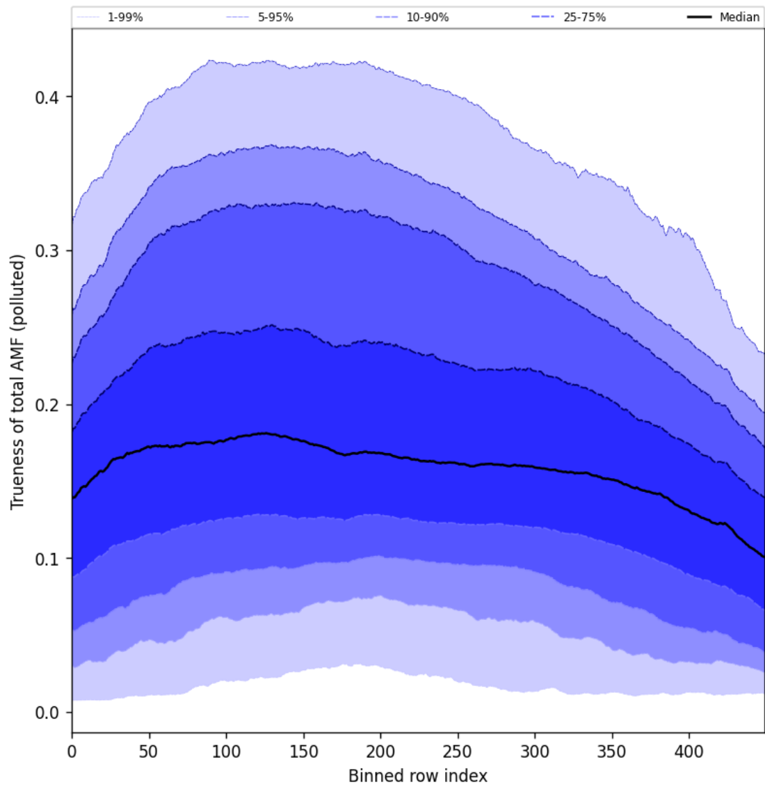
Figure 106: Along track statistics of “Trueness of total AMF (polluted)” for 2025-11-14 to 2025-11-16
