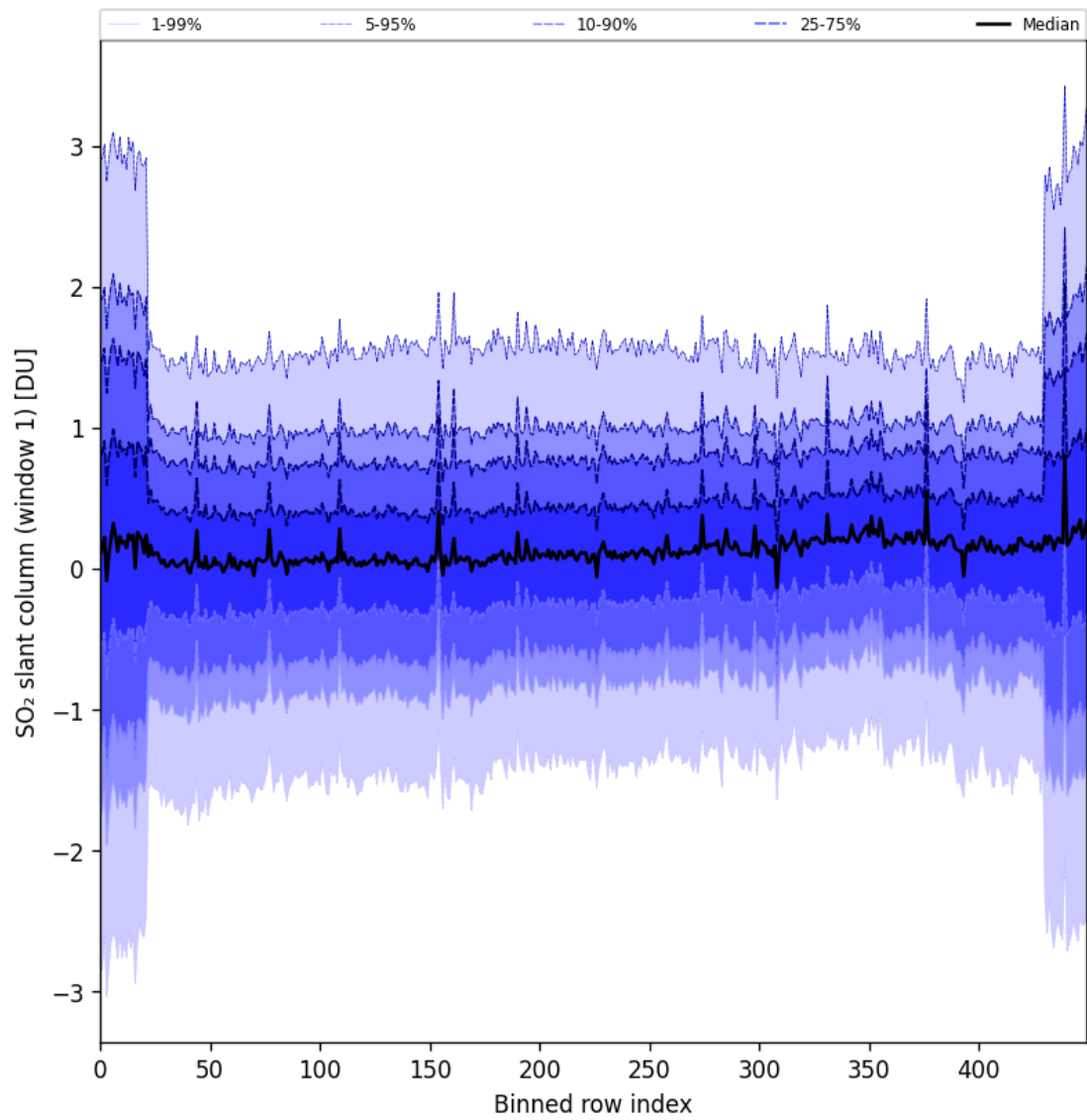
Figure 89: Along track statistics of “SO 2 slant column (window 1)” for 2025-11-14 to 2025-11-16
