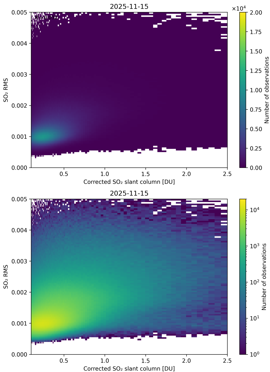
Figure 231: Scatter density plot of “Corrected SO 2 slant column” against “SO 2 RMS” for 2025-11-14 to 2025-11-16.
