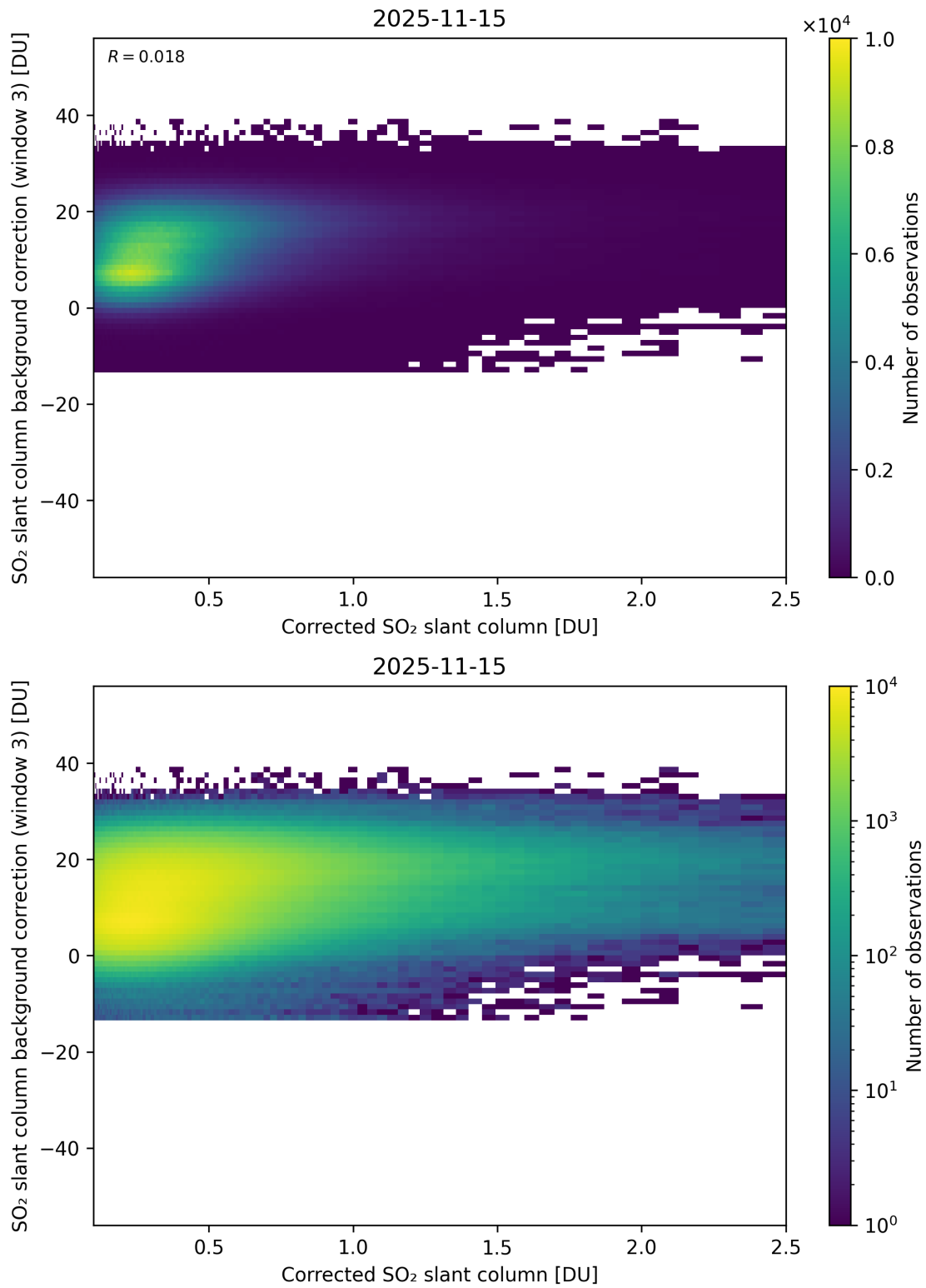
Figure 228: Scatter density plot of “Corrected SO 2 slant column” against “SO 2 slant column background correction (window 3)” for 2025-11-14 to 2025-11-16.
