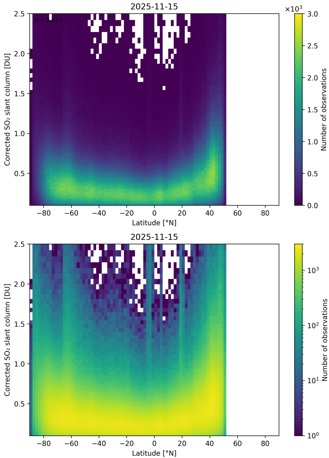
Figure 159: Scatter density plot of “Latitude” against “Corrected SO 2 slant column” for 2025-11-14 to 2025-11-16.
