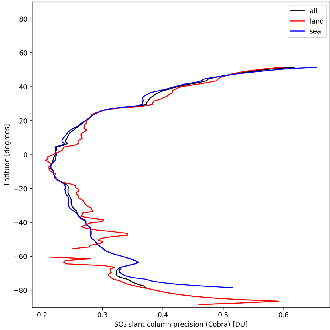
Figure 36: Zonal average of “SO 2 slant column precision (Cobra)” for 2025-11-14 to 2025-11-16.
