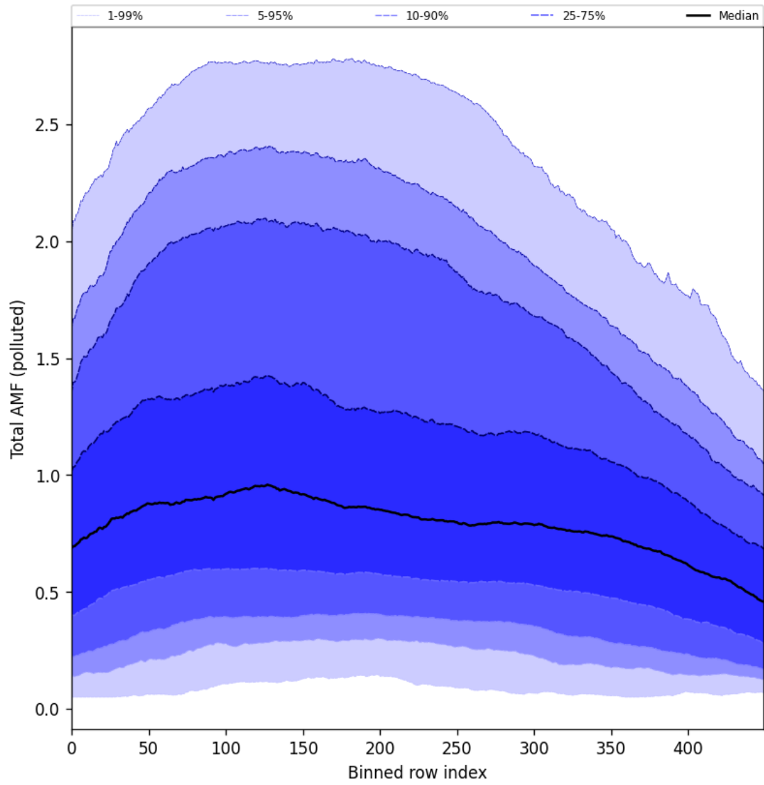
Figure 105: Along track statistics of “Total AMF (polluted)” for 2025-11-14 to 2025-11-16
