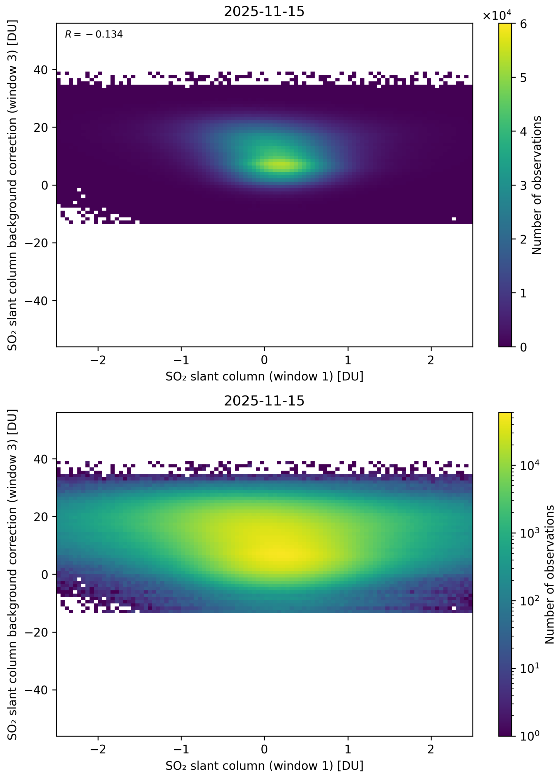
Figure 264: Scatter density plot of “SO 2 slant column (window 1)” against “SO 2 slant column background correction (window 3)” for 2025-11-14 to 2025-11-16.
