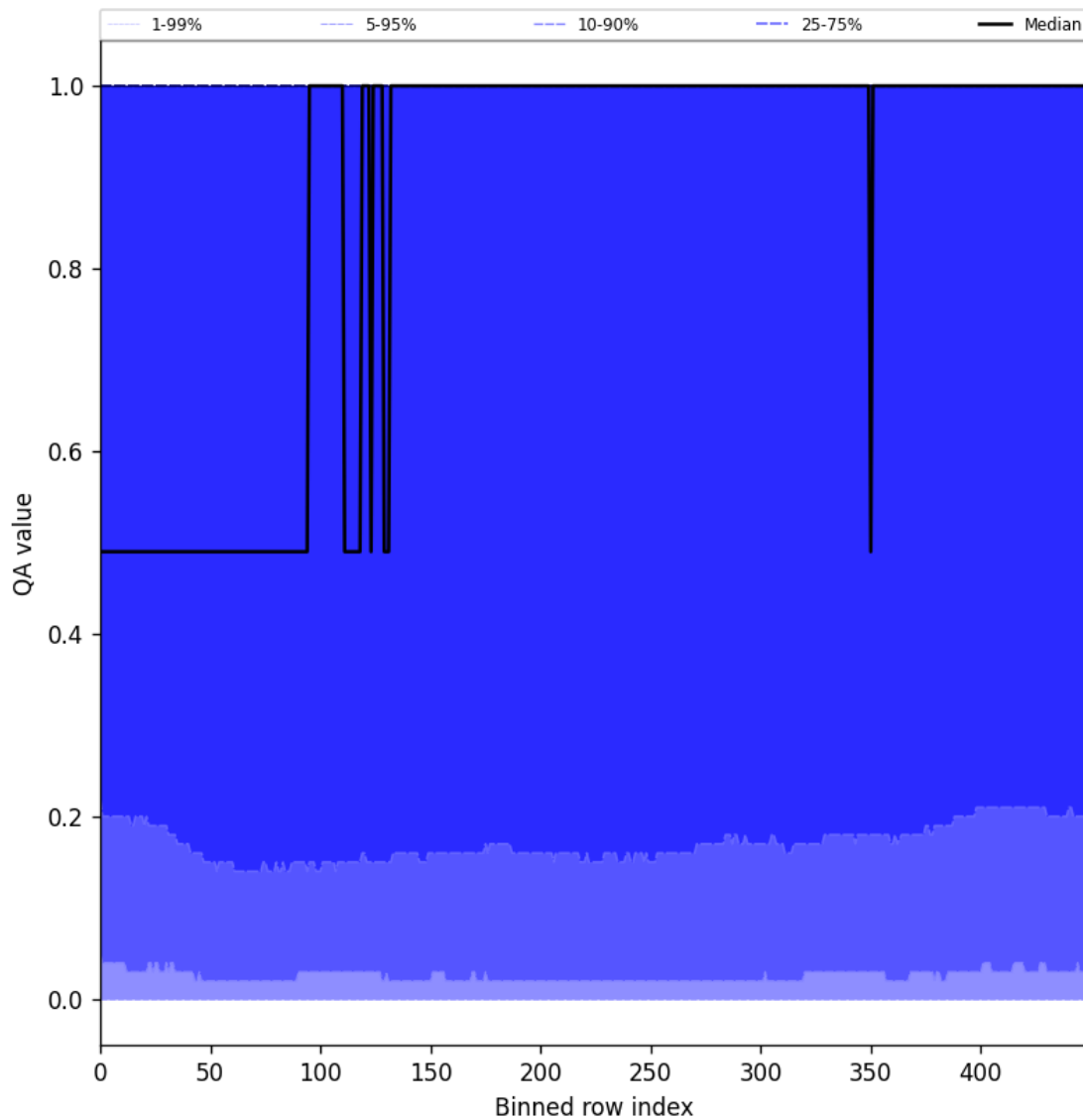
Figure 83: Along track statistics of “QA value” for 2025-11-14 to 2025-11-16
