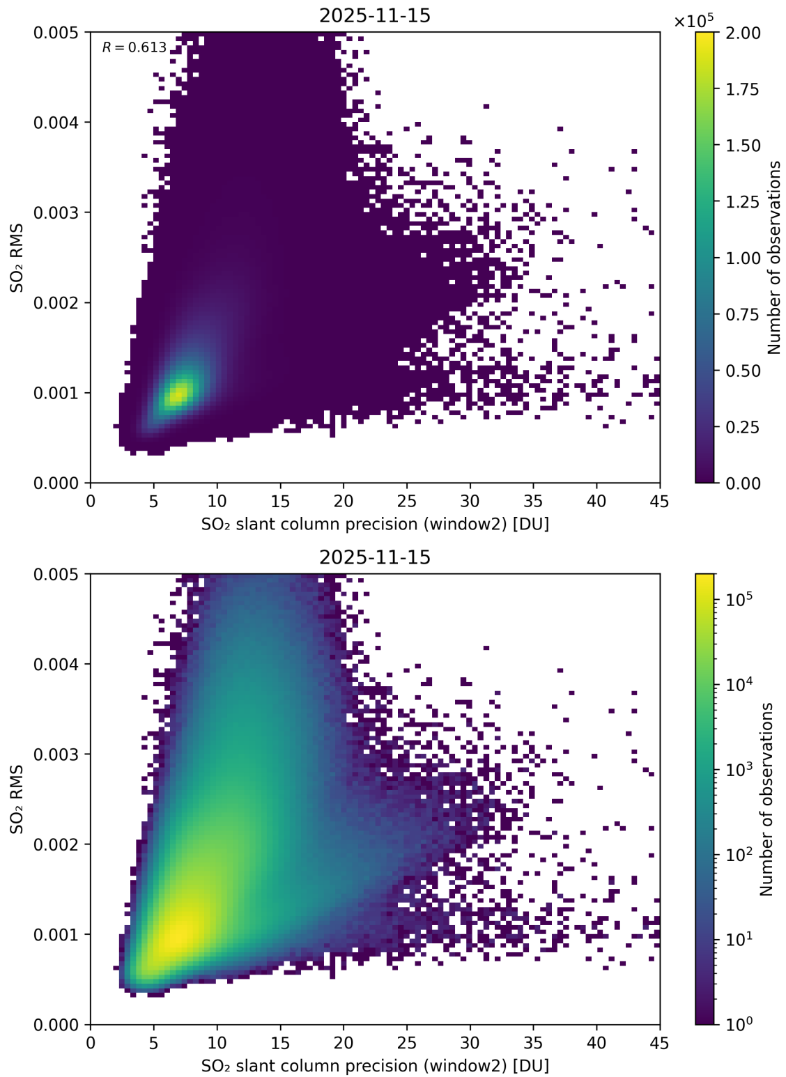
Figure 295: Scatter density plot of “SO 2 slant column precision (window2)” against “SO 2 RMS” for 2025-11-14 to 2025-11-16.
