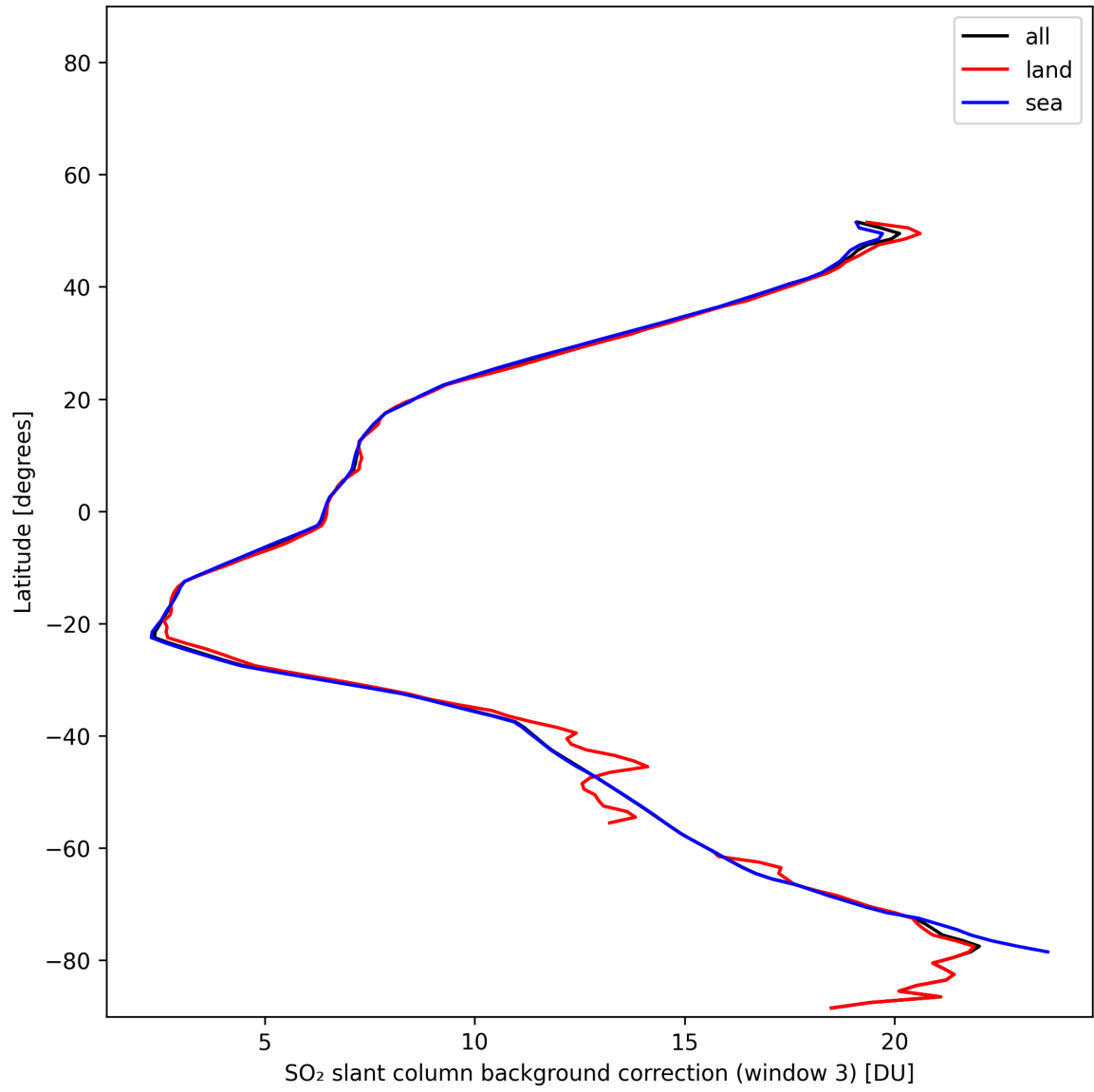
Figure 48: Zonal average of “SO 2 slant column background correction (window 3)” for 2025-11-14 to 2025-11-16.
