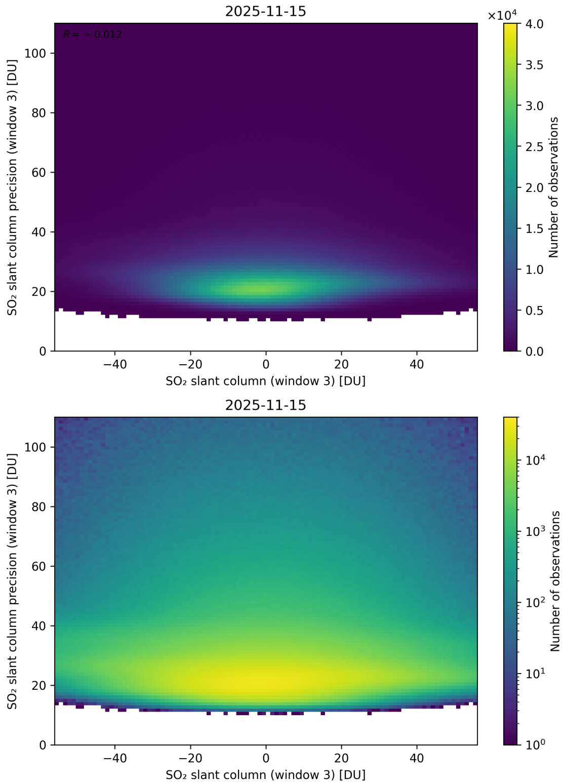
Figure 317: Scatter density plot of “SO 2 slant column (window 3)” against “SO 2 slant column precision (window 3)” for 2025-11-14 to 2025-11-16.
