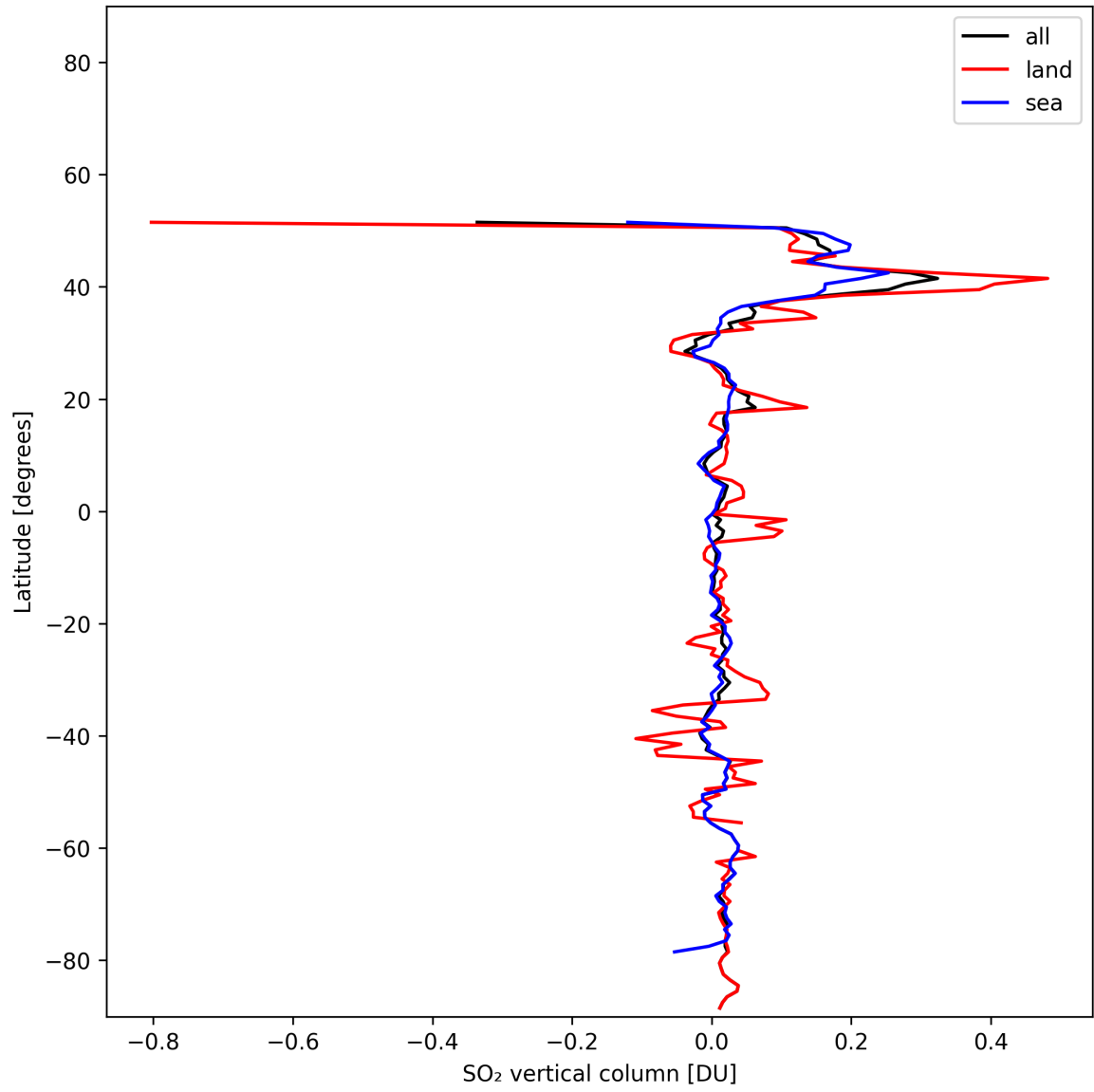
Figure 32: Zonal average of “SO 2 vertical column” for 2025-11-14 to 2025-11-16.
