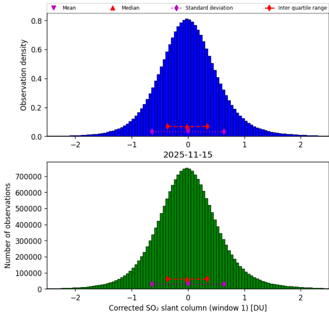
Figure 65: Histogram of “Corrected SO 2 slant column (window 1)” for 2025-11-14 to 2025-11-16
