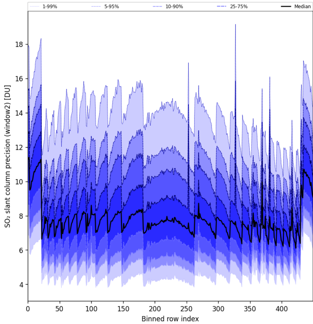
Figure 94: Along track statistics of “SO 2 slant column precision (window2)” for 2025-11-14 to 2025-11-16
