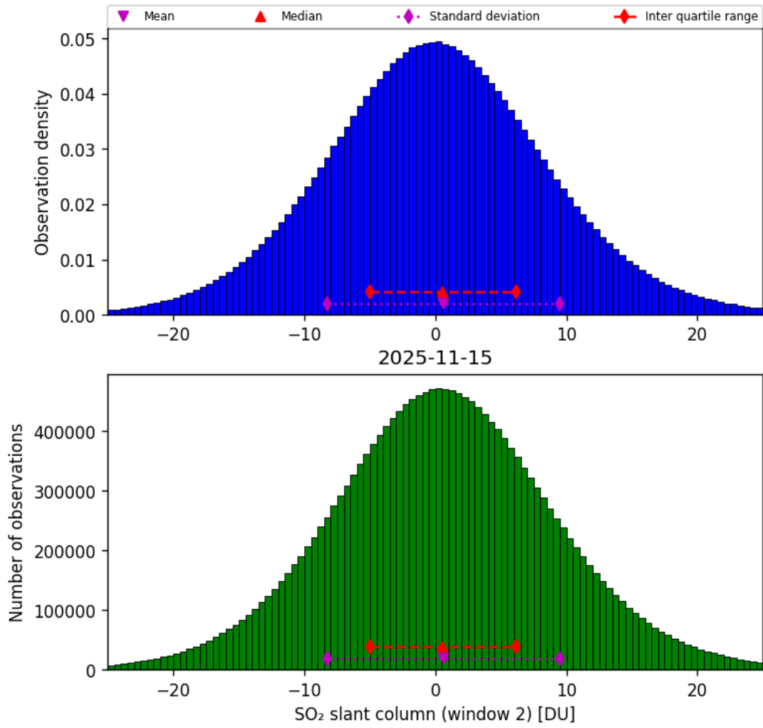
Figure 67: Histogram of “SO 2 slant column (window 2)” for 2025-11-14 to 2025-11-16
