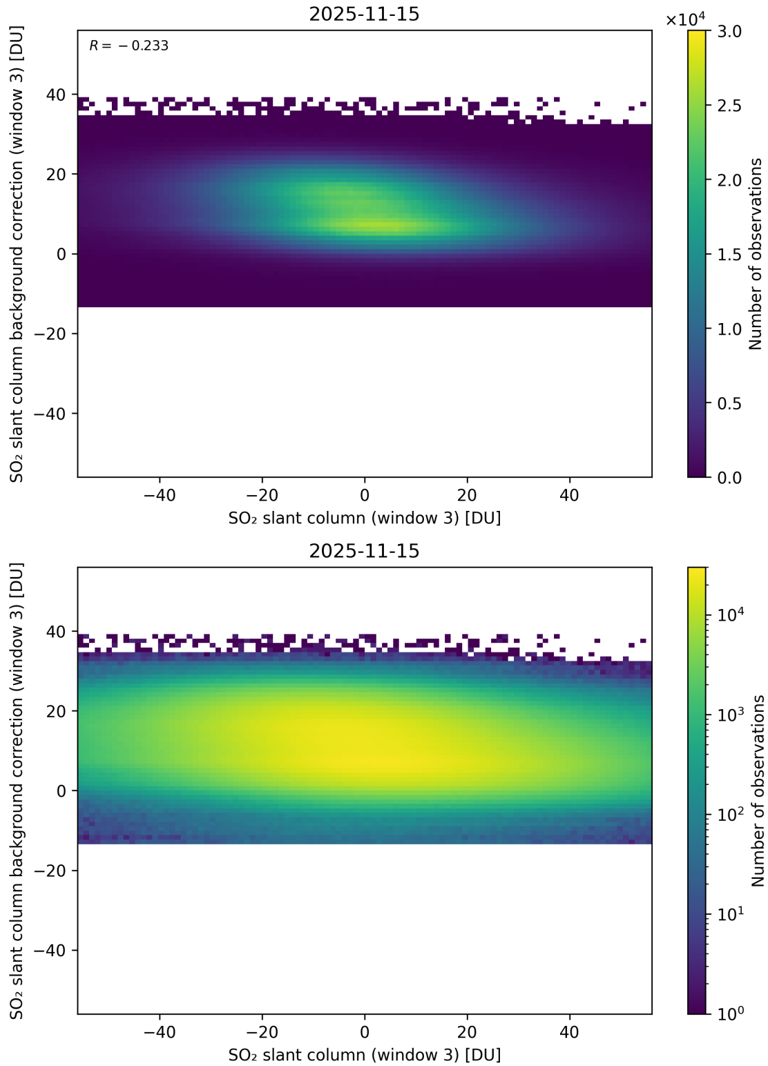
Figure 303: Scatter density plot of “SO 2 slant column (window 3)” against “SO 2 slant column background correction (window 3)” for 2025-11-14 to 2025-11-16.
