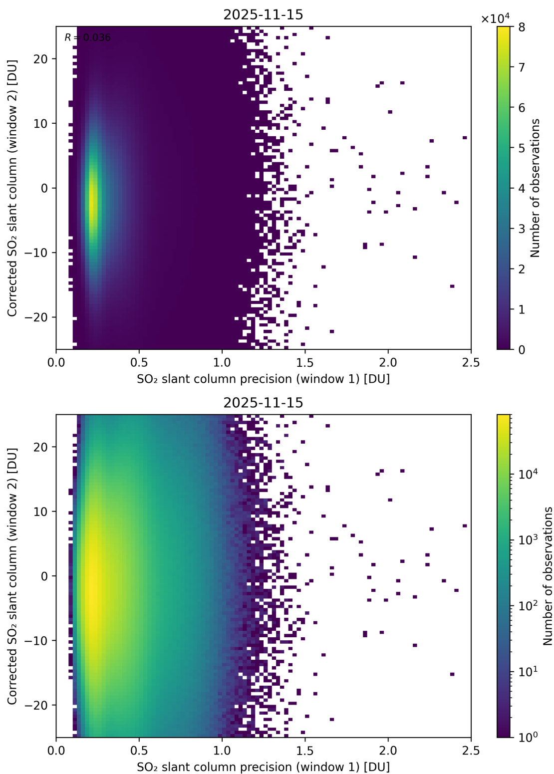
Figure 275: Scatter density plot of “SO 2 slant column precision (window 1)” against “Corrected SO 2 slant column (window 2)” for 2025-11-14 to 2025-11-16.
