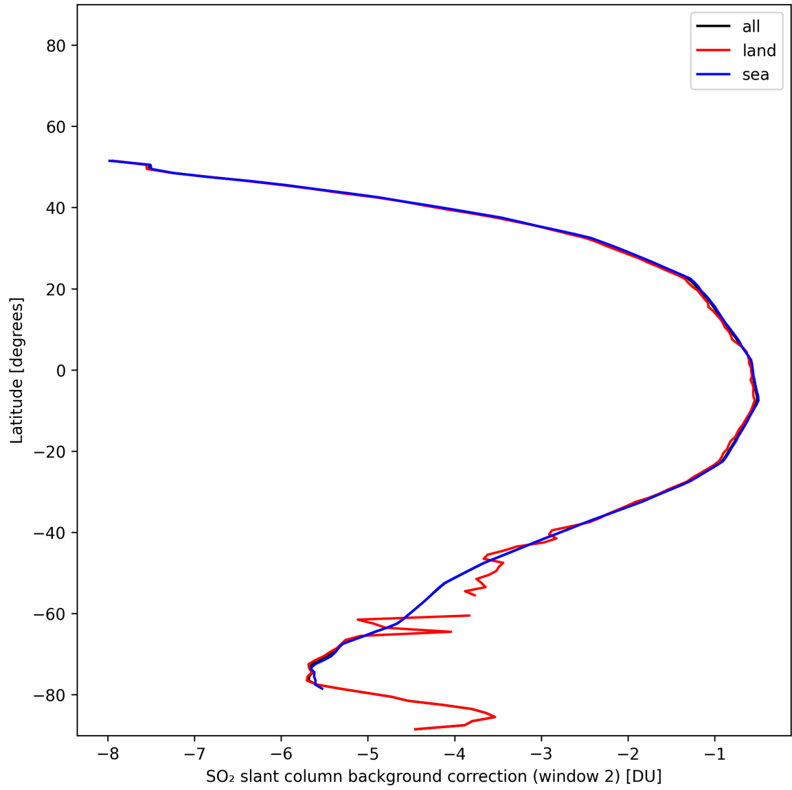
Figure 44: Zonal average of “SO 2 slant column background correction (window 2)” for 2025-11-14 to 2025-11-16.
