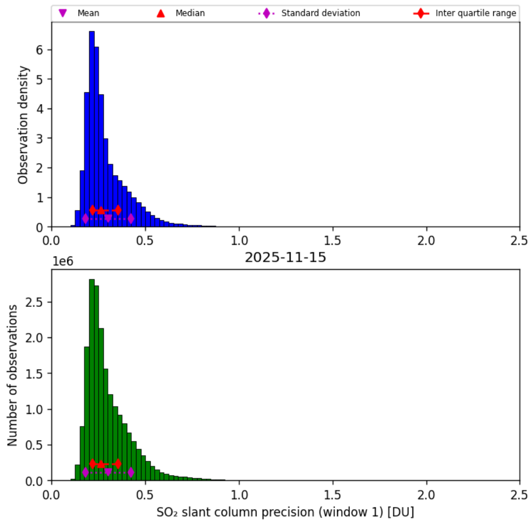
Figure 64: Histogram of “SO 2 slant column precision (window 1)” for 2025-11-14 to 2025-11-16
