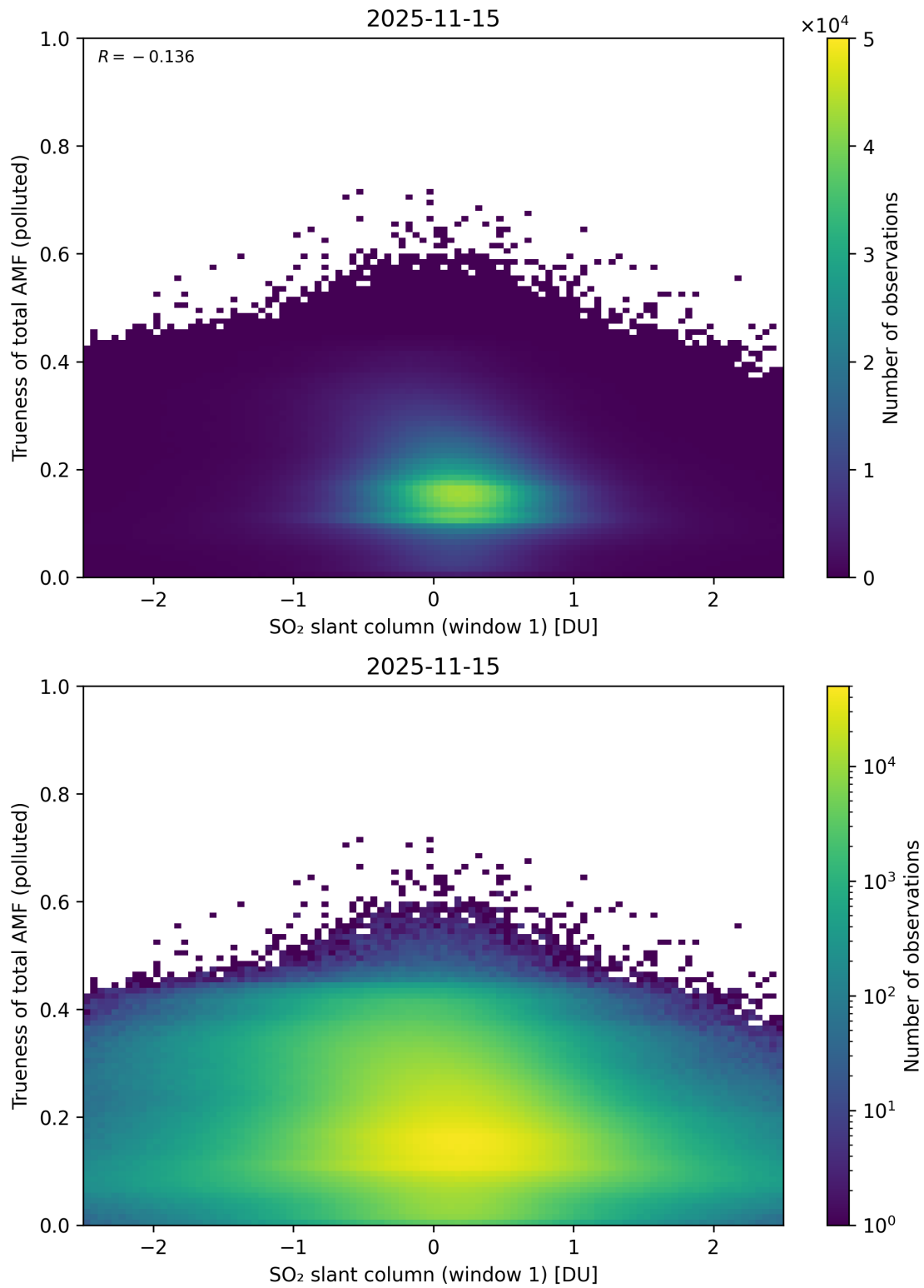
Figure 290: Scatter density plot of “SO 2 slant column (window 1)” against “Trueness of total AMF (polluted)” for 2025-11-14 to 2025-11-16.
