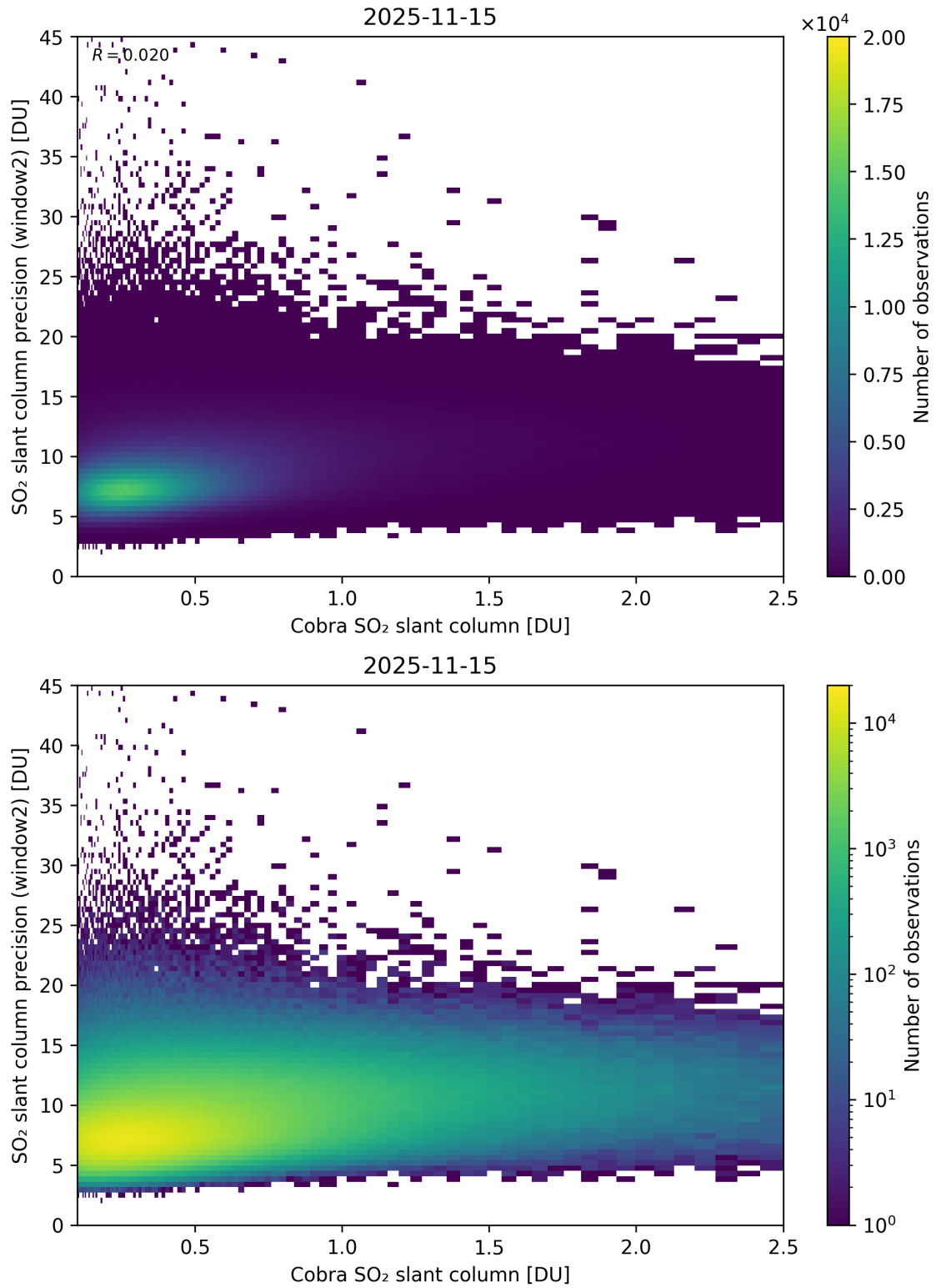
Figure 221: Scatter density plot of “Cobra SO 2 slant column” against “SO 2 slant column precision (window2)” for 2025-11-14 to 2025-11-16.
