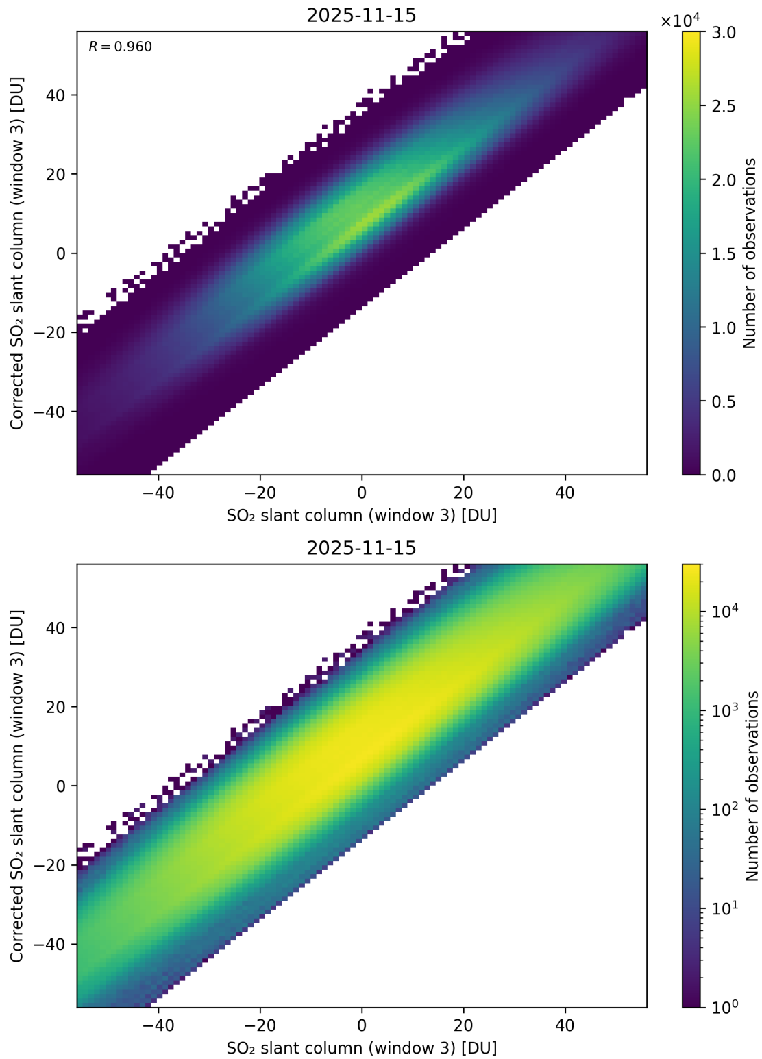
Figure 316: Scatter density plot of “SO 2 slant column (window 3)” against “Corrected SO 2 slant column (window 3)” for 2025-11-14 to 2025-11-16.
