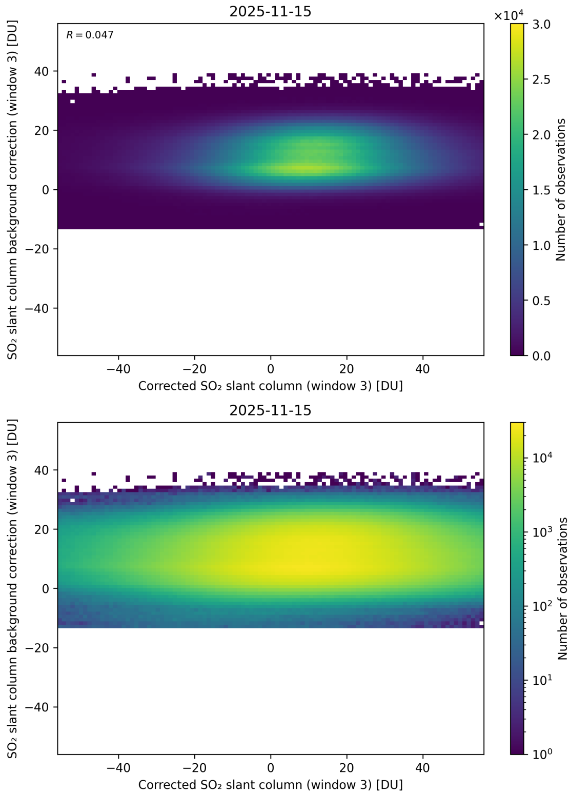
Figure 255: Scatter density plot of “Corrected SO 2 slant column (window 3)” against “SO 2 slant column background correction (window 3)” for 2025-11-14 to 2025-11-16.
