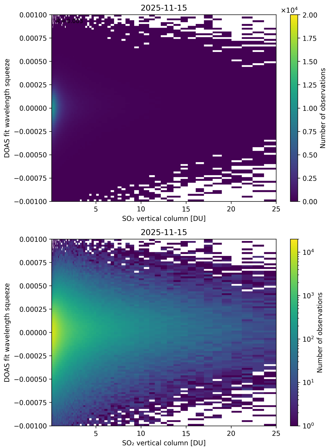
Figure 327: Scatter density plot of “SO 2 vertical column” against “DOAS fit wavelength squeeze” for 2025-11-14 to 2025-11-16.
