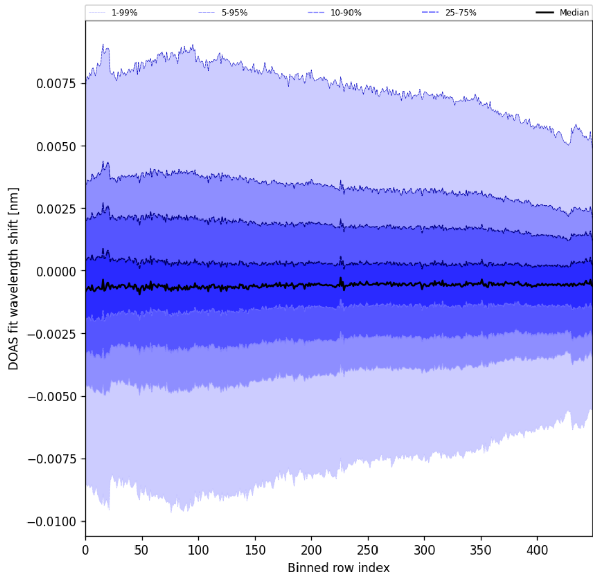
Figure 102: Along track statistics of “DOAS fit wavelength shift” for 2025-11-14 to 2025-11-16
