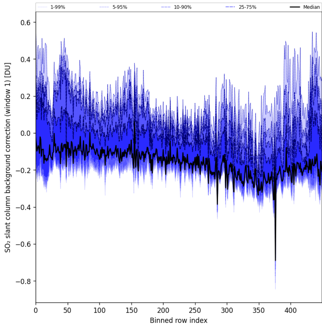
Figure 92: Along track statistics of “SO 2 slant column background correction (window 1)” for 2025-11-14 to 2025-11-16
