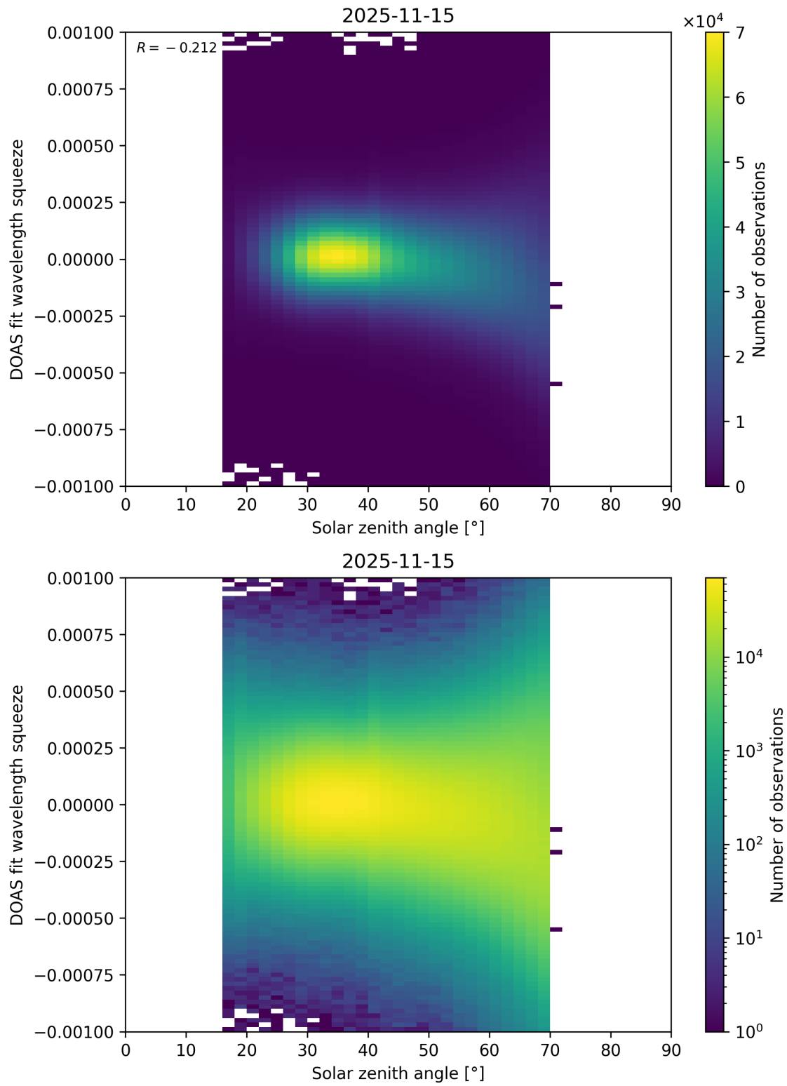
Figure 175: Scatter density plot of “Solar zenith angle” against “DOAS fit wavelength squeeze” for 2025-11-14 to 2025-11-16.
