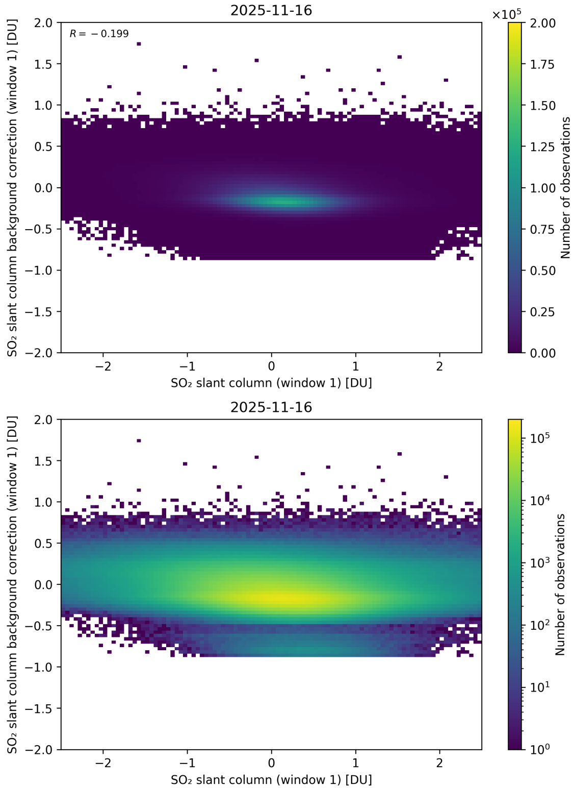
Figure 262: Scatter density plot of “SO 2 slant column (window 1)” against “SO 2 slant column background correction (window 1)” for 2025-11-15 to 2025-11-17.
