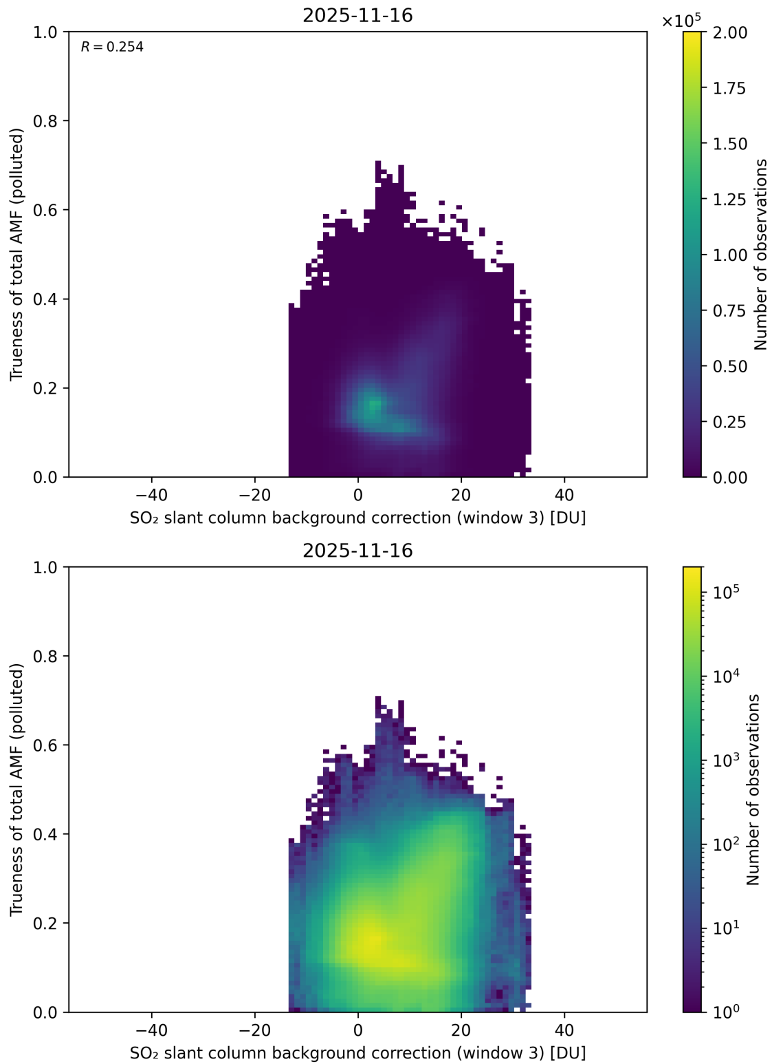
Figure 137: Scatter density plot of “SO 2 slant column background correction (window 3)” against “Trueness of total AMF (polluted)” for 2025-11-15 to 2025-11-17.
