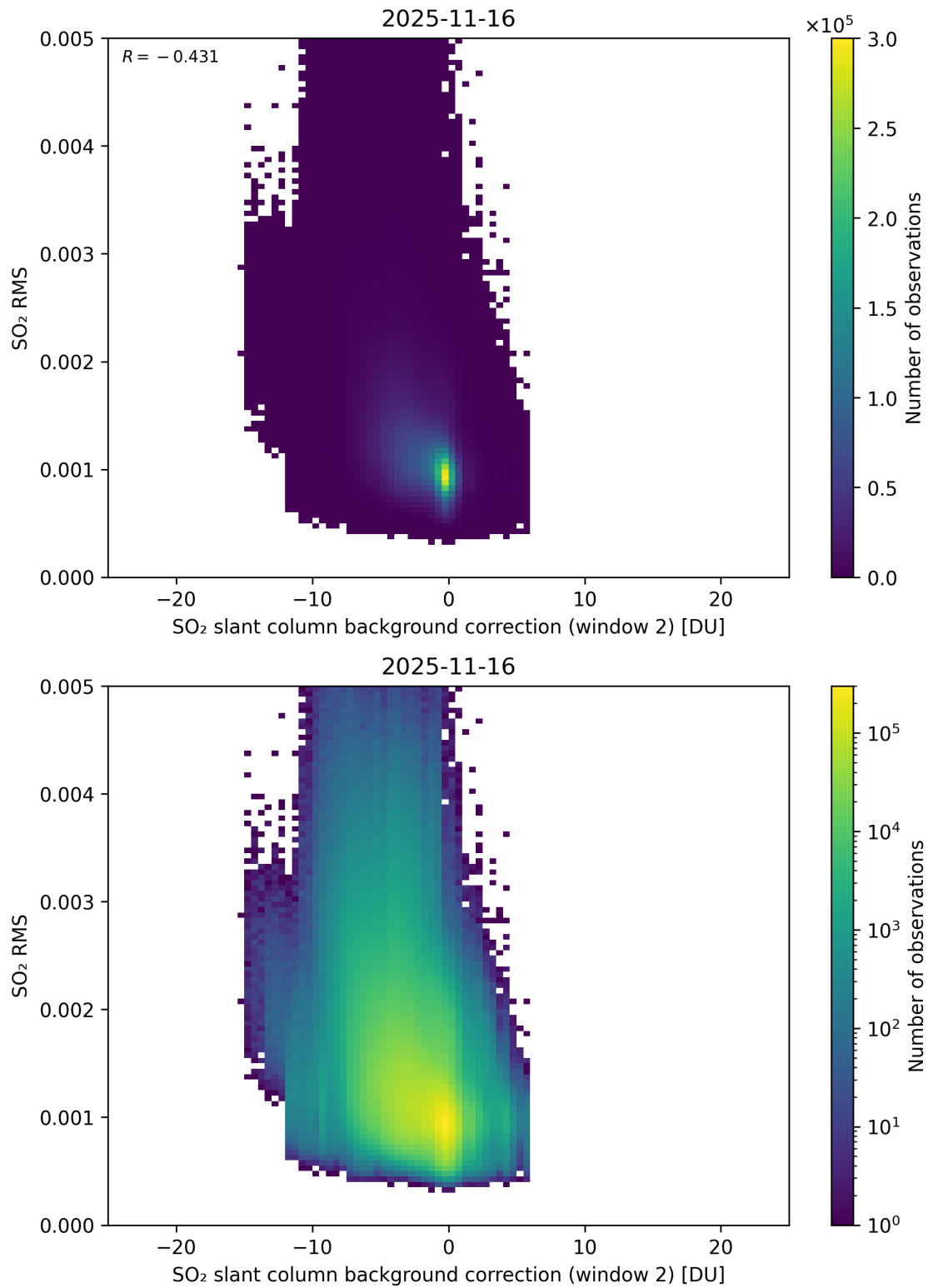
Figure 125: Scatter density plot of “SO 2 slant column background correction (window 2)” against “SO 2 RMS” for 2025-11-15 to 2025-11-17.
