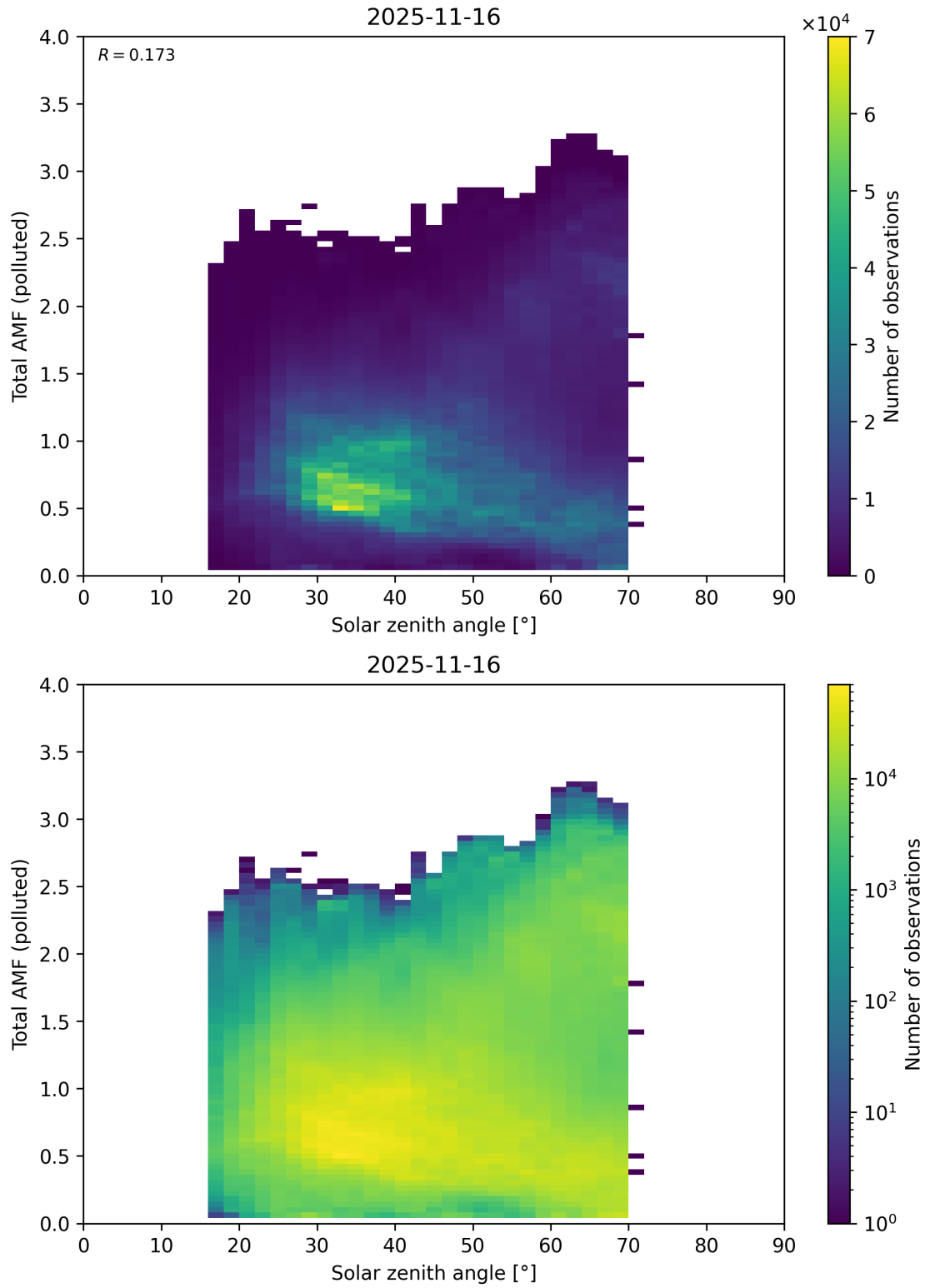
Figure 189: Scatter density plot of “Solar zenith angle” against “Total AMF (polluted)” for 2025-11-15 to 2025-11-17.
