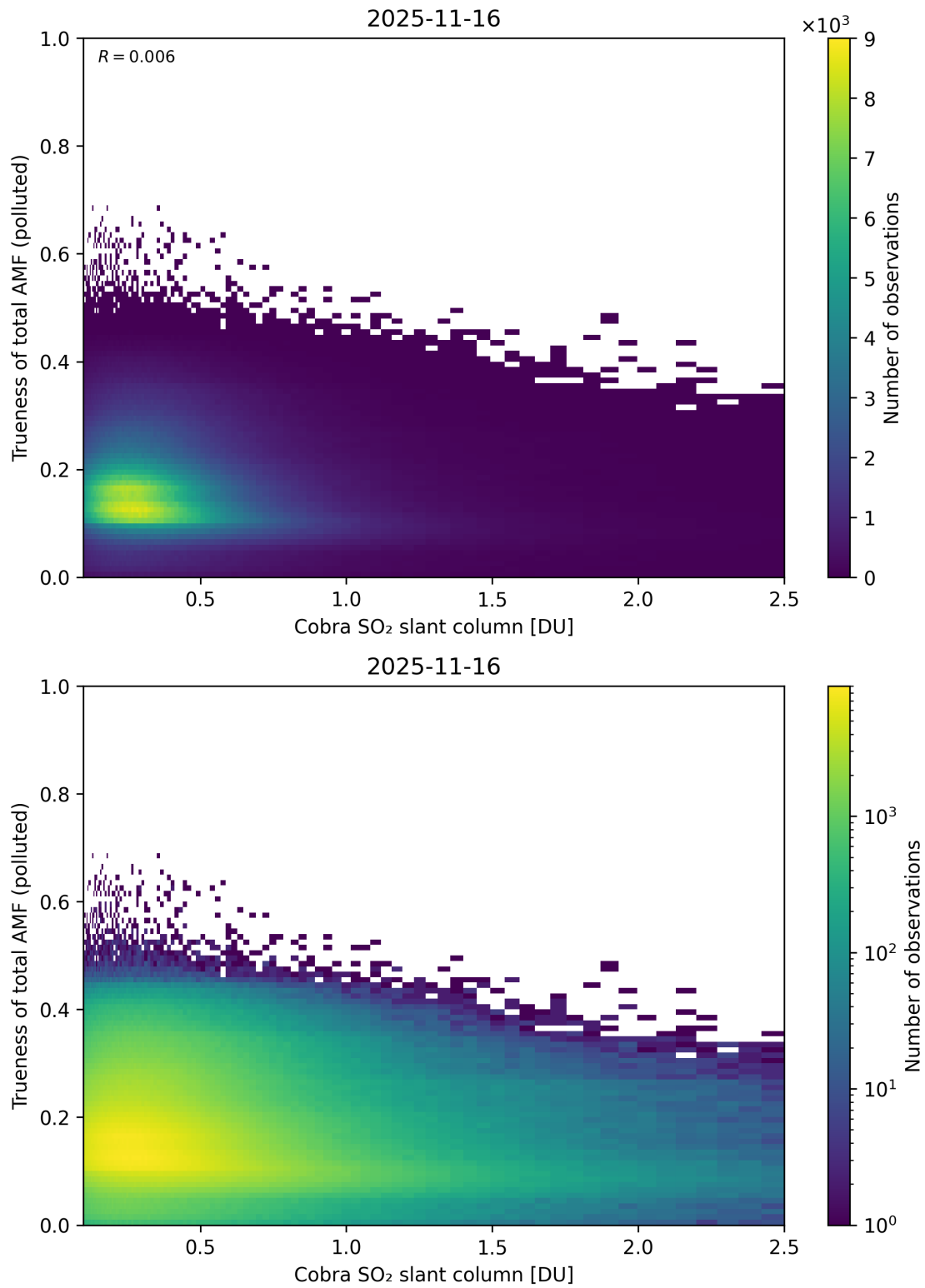
Figure 225: Scatter density plot of “Cobra SO 2 slant column” against “Trueness of total AMF (polluted)” for 2025-11-15 to 2025-11-17.
