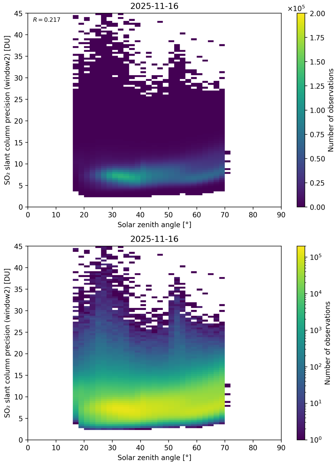
Figure 186: Scatter density plot of “Solar zenith angle” against “SO 2 slant column precision (window2)” for 2025-11-15 to 2025-11-17.
