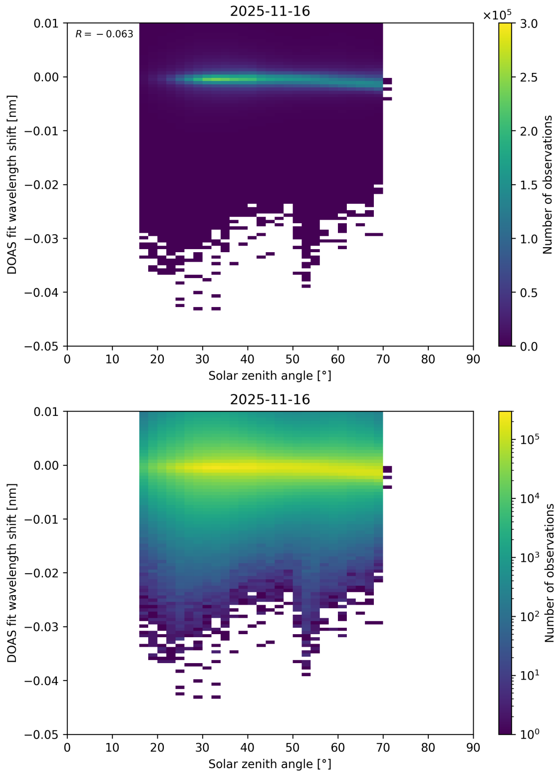
Figure 174: Scatter density plot of “Solar zenith angle” against “DOAS fit wavelength shift” for 2025-11-15 to 2025-11-17.
