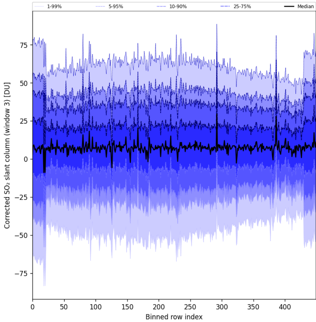
Figure 99: Along track statistics of “Corrected SO 2 slant column (window 3)” for 2025-11-15 to 2025-11-17
