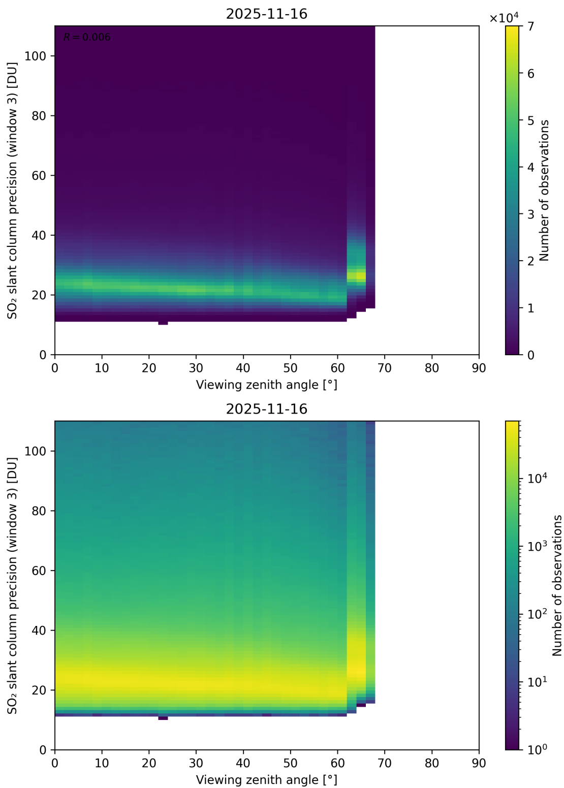
Figure 380: Scatter density plot of “Viewing zenith angle” against “SO 2 slant column precision (window 3)” for 2025-11-15 to 2025-11-17.
