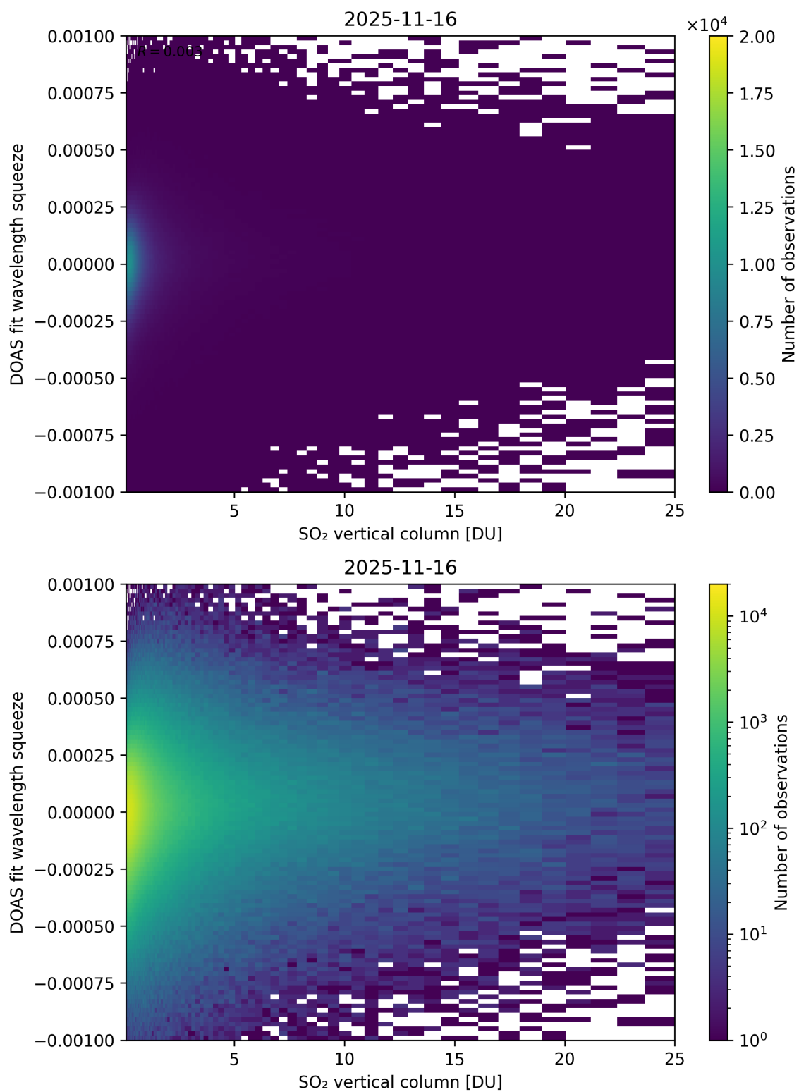
Figure 327: Scatter density plot of “SO 2 vertical column” against “DOAS fit wavelength squeeze” for 2025-11-15 to 2025-11-17.
