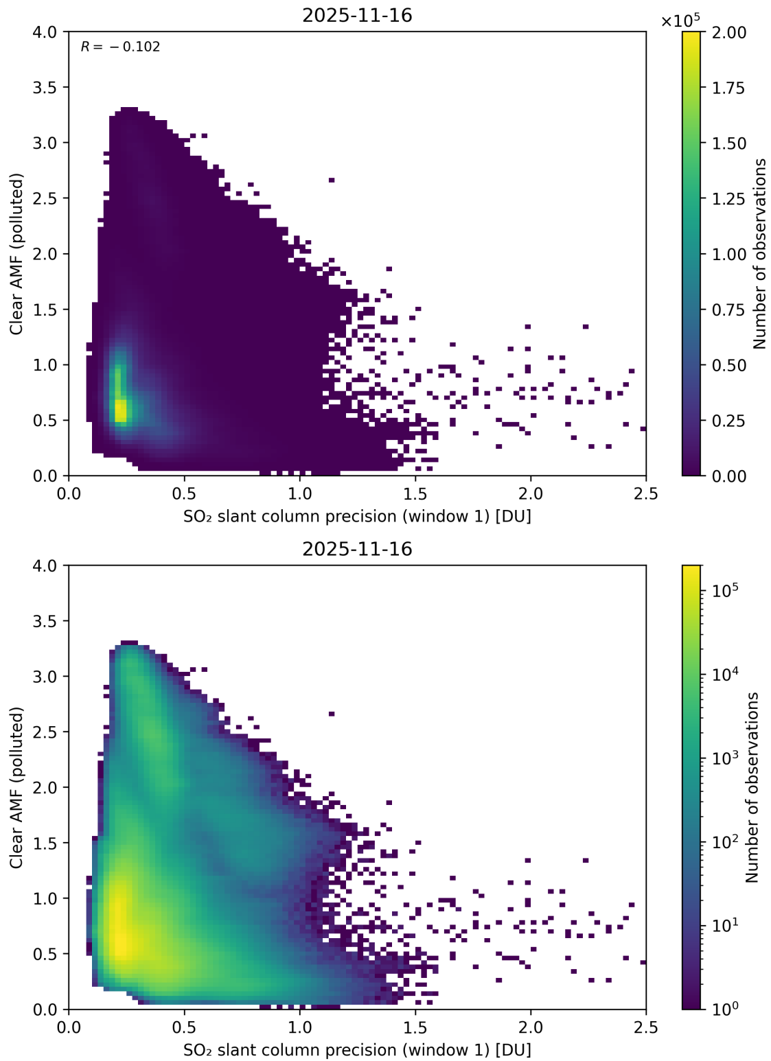
Figure 274: Scatter density plot of “SO 2 slant column precision (window 1)” against “Clear AMF (polluted)” for 2025-11-15 to 2025-11-17.
