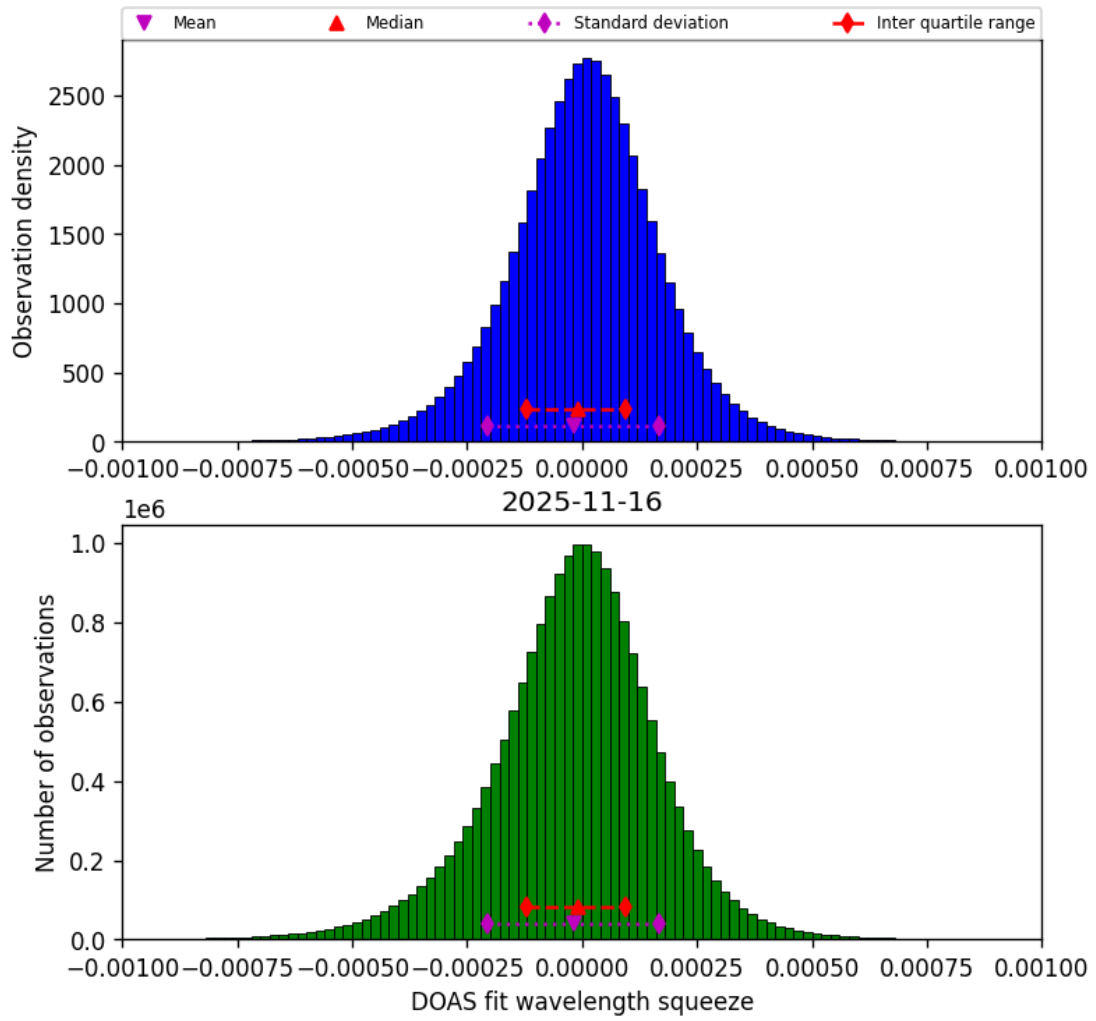
Figure 77: Histogram of “DOAS fit wavelength squeeze” for 2025-11-15 to 2025-11-17
