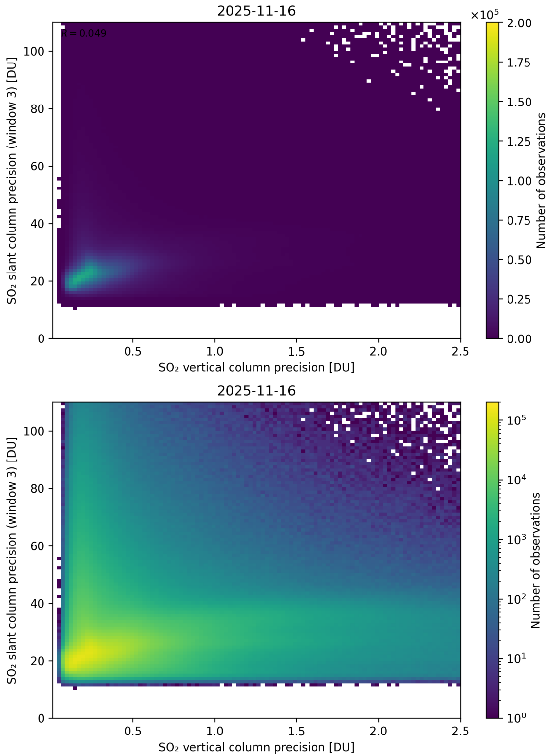
Figure 345: Scatter density plot of “SO 2 vertical column precision” against “SO 2 slant column precision (window 3)” for 2025-11-15 to 2025-11-17.
