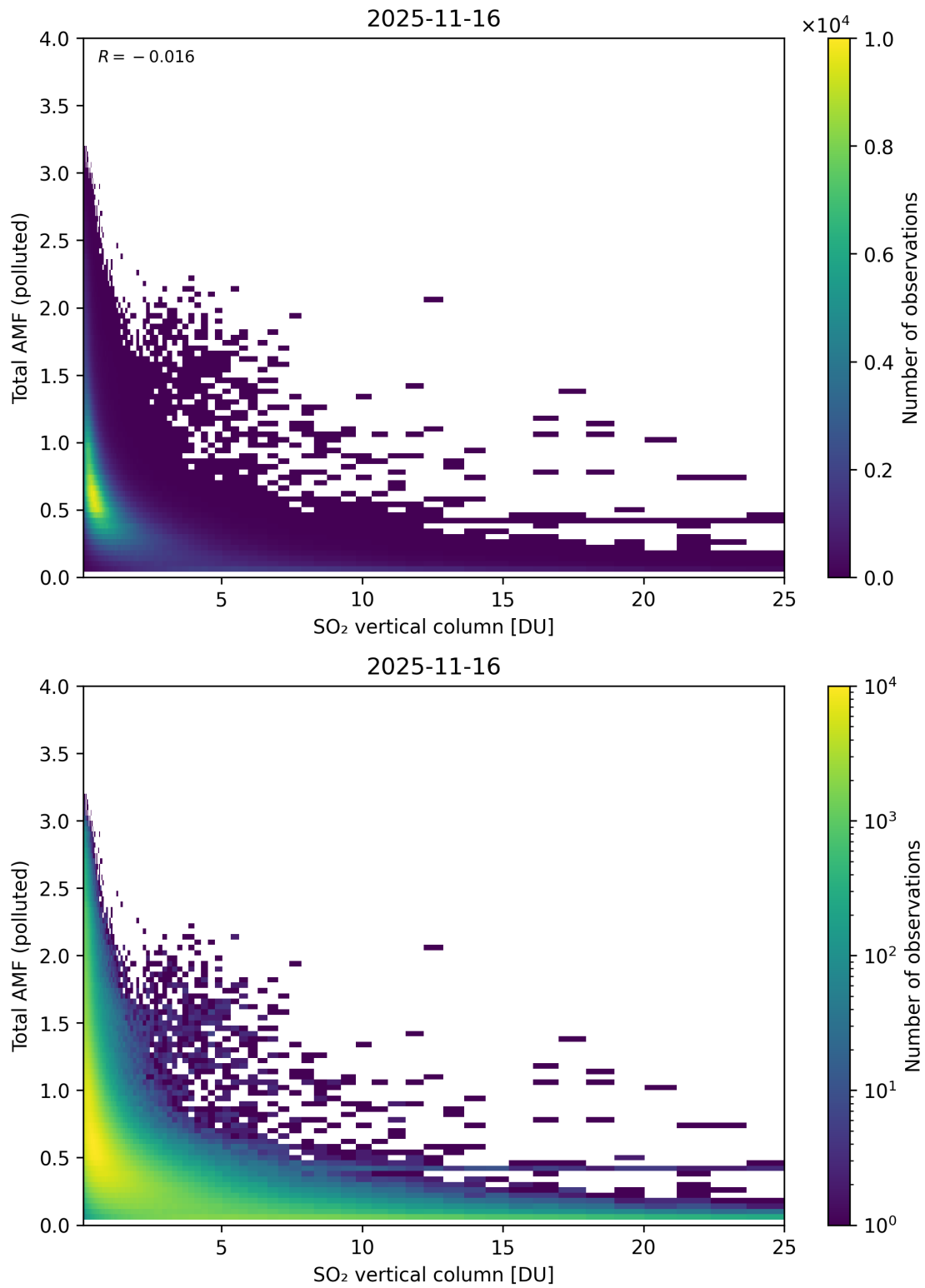
Figure 359: Scatter density plot of “SO 2 vertical column” against “Total AMF (polluted)” for 2025-11-15 to 2025-11-17.
