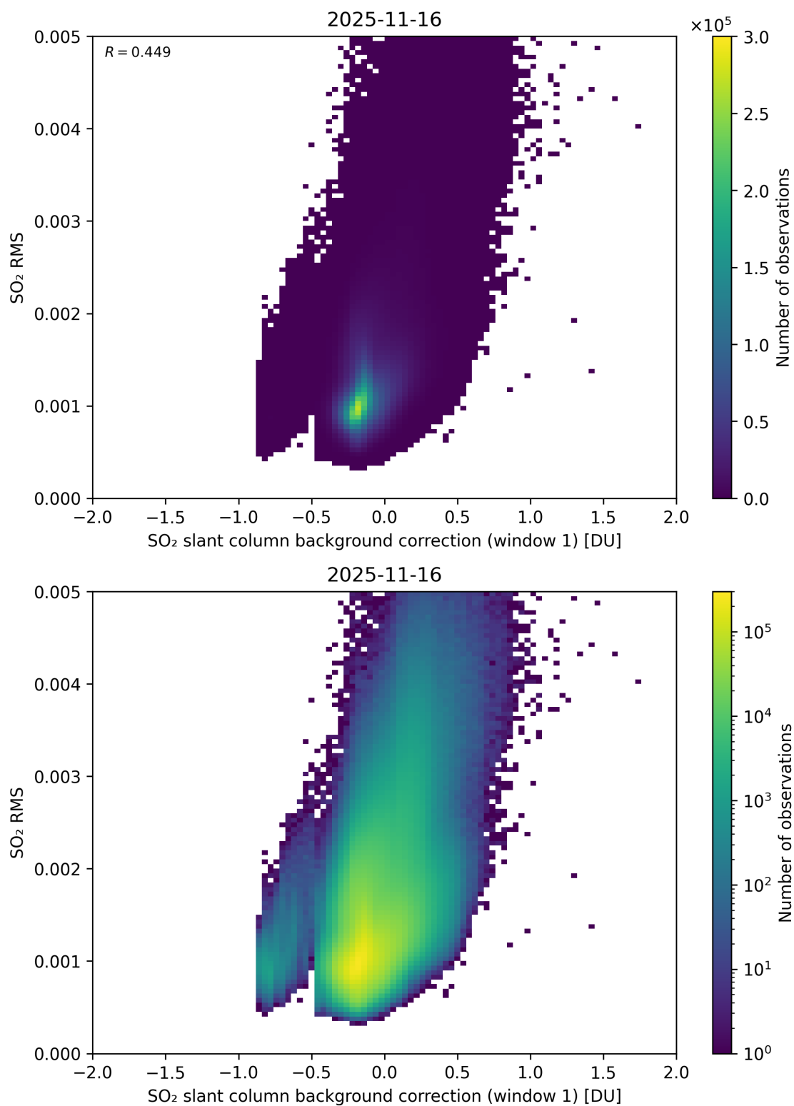
Figure 113: Scatter density plot of “SO 2 slant column background correction (window 1)” against “SO 2 RMS” for 2025-11-15 to 2025-11-17.
