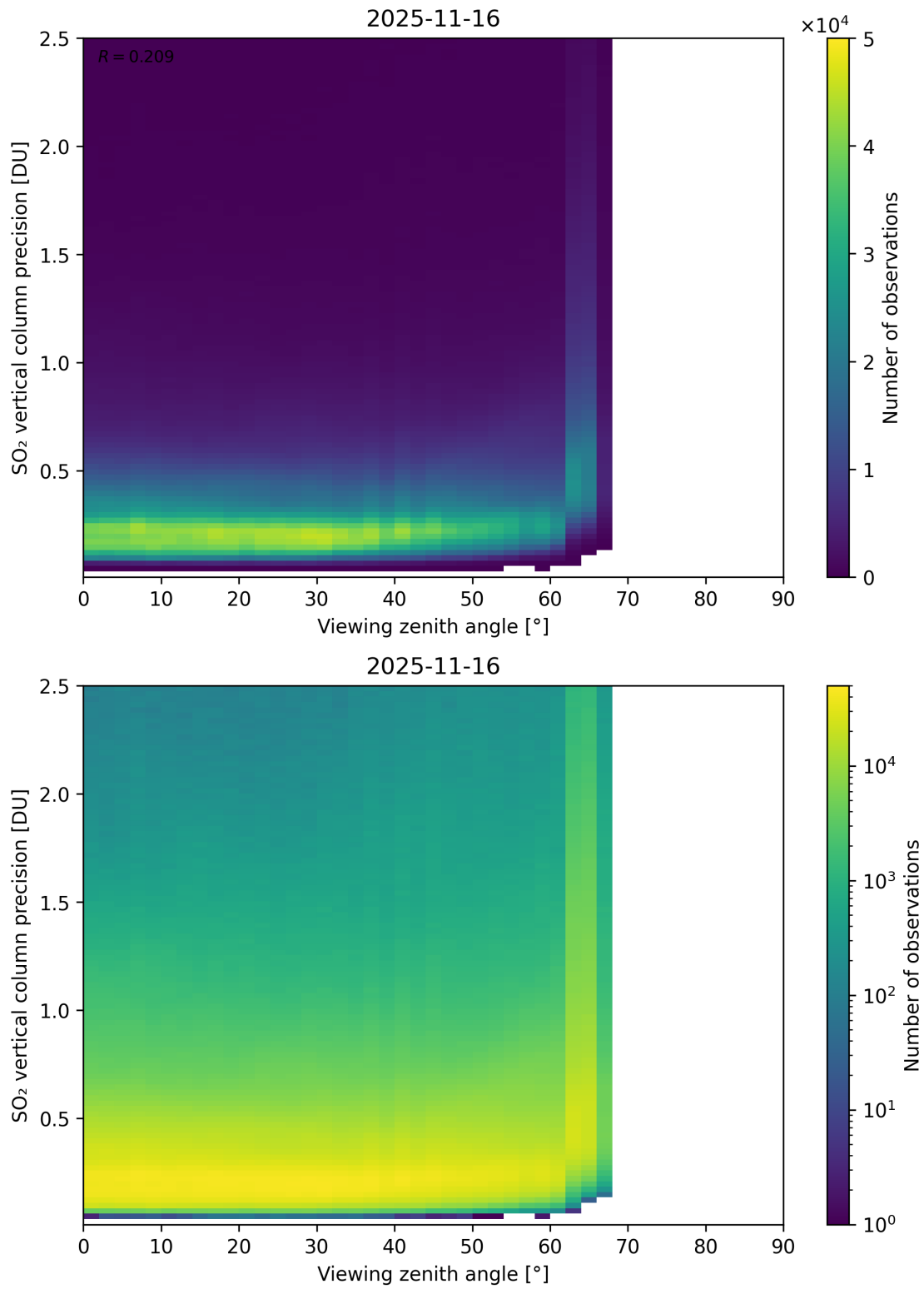
Figure 384: Scatter density plot of “Viewing zenith angle” against “SO 2 vertical column precision” for 2025-11-15 to 2025-11-17.
