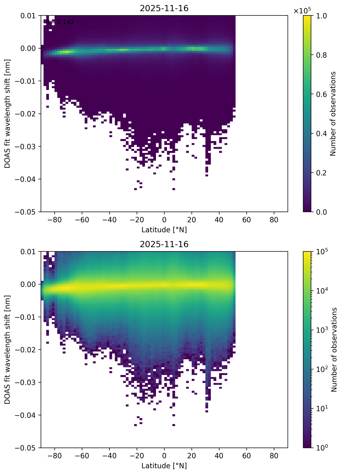
Figure 153: Scatter density plot of “Latitude” against “DOAS fit wavelength shift” for 2025-11-15 to 2025-11-17.
