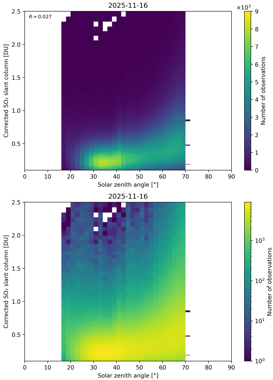
Figure 181: Scatter density plot of “Solar zenith angle” against “Corrected SO 2 slant column” for 2025-11-15 to 2025-11-17.
