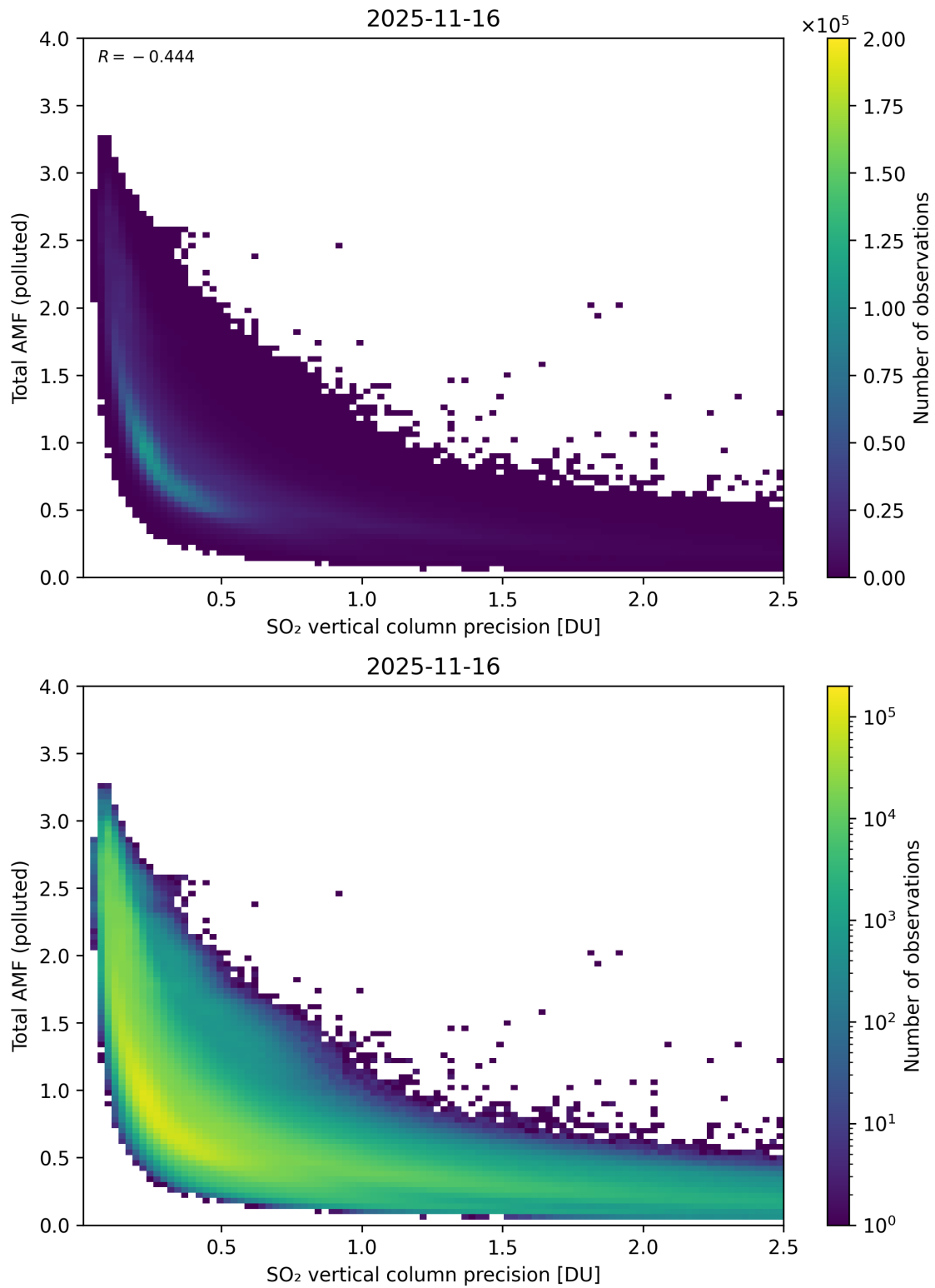
Figure 346: Scatter density plot of “SO 2 vertical column precision” against “Total AMF (polluted)” for 2025-11-15 to 2025-11-17.
