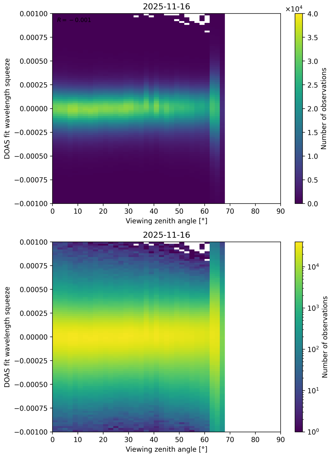
Figure 366: Scatter density plot of “Viewing zenith angle” against “DOAS fit wavelength squeeze” for 2025-11-15 to 2025-11-17.
