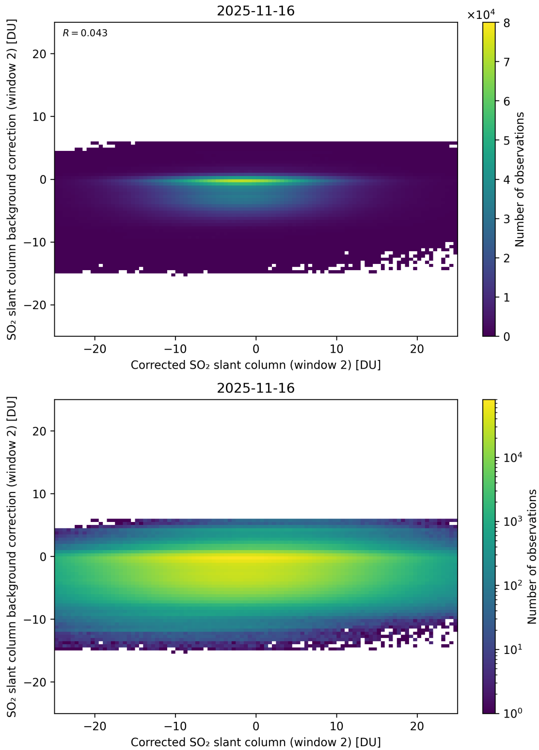
Figure 244: Scatter density plot of “Corrected SO 2 slant column (window 2)” against “SO 2 slant column background correction (window 2)” for 2025-11-15 to 2025-11-17.
