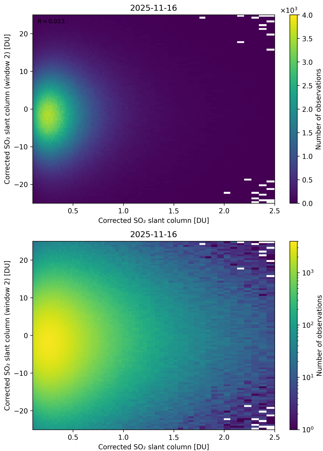
Figure 235: Scatter density plot of “Corrected SO 2 slant column” against “Corrected SO 2 slant column (window 2)” for 2025-11-15 to 2025-11-17.
