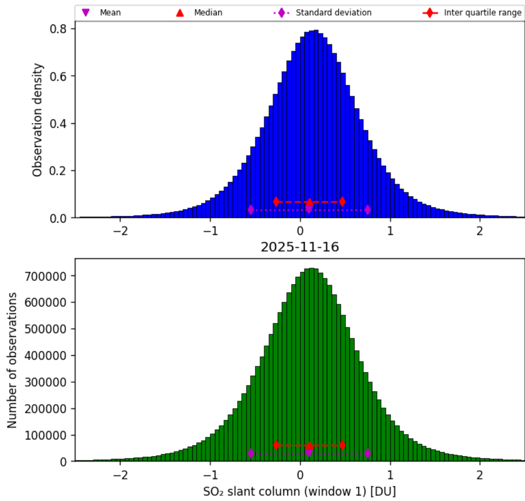
Figure 63: Histogram of “SO 2 slant column (window 1)” for 2025-11-15 to 2025-11-17
