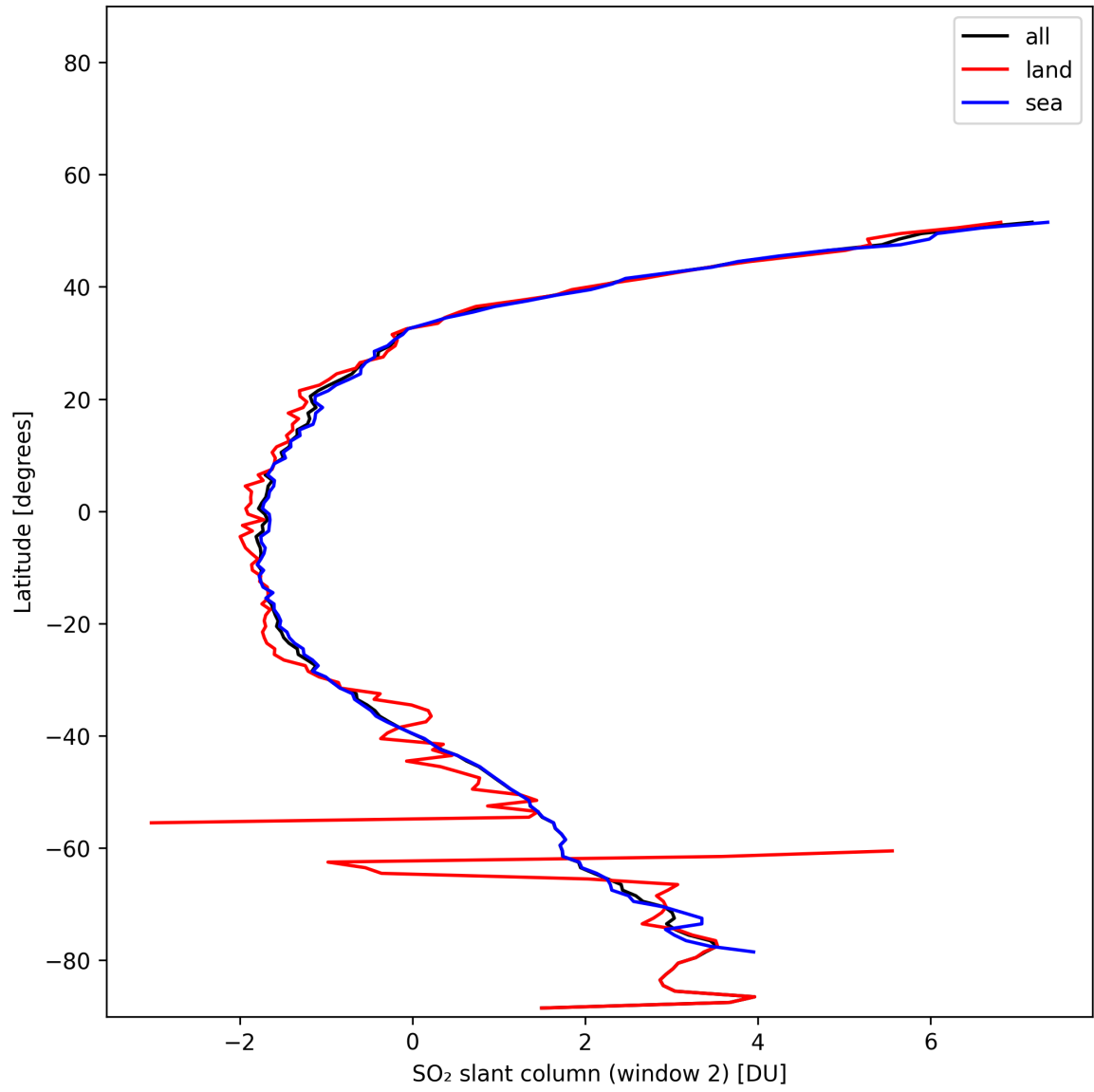
Figure 41: Zonal average of “SO 2 slant column (window 2)” for 2025-11-15 to 2025-11-17.
