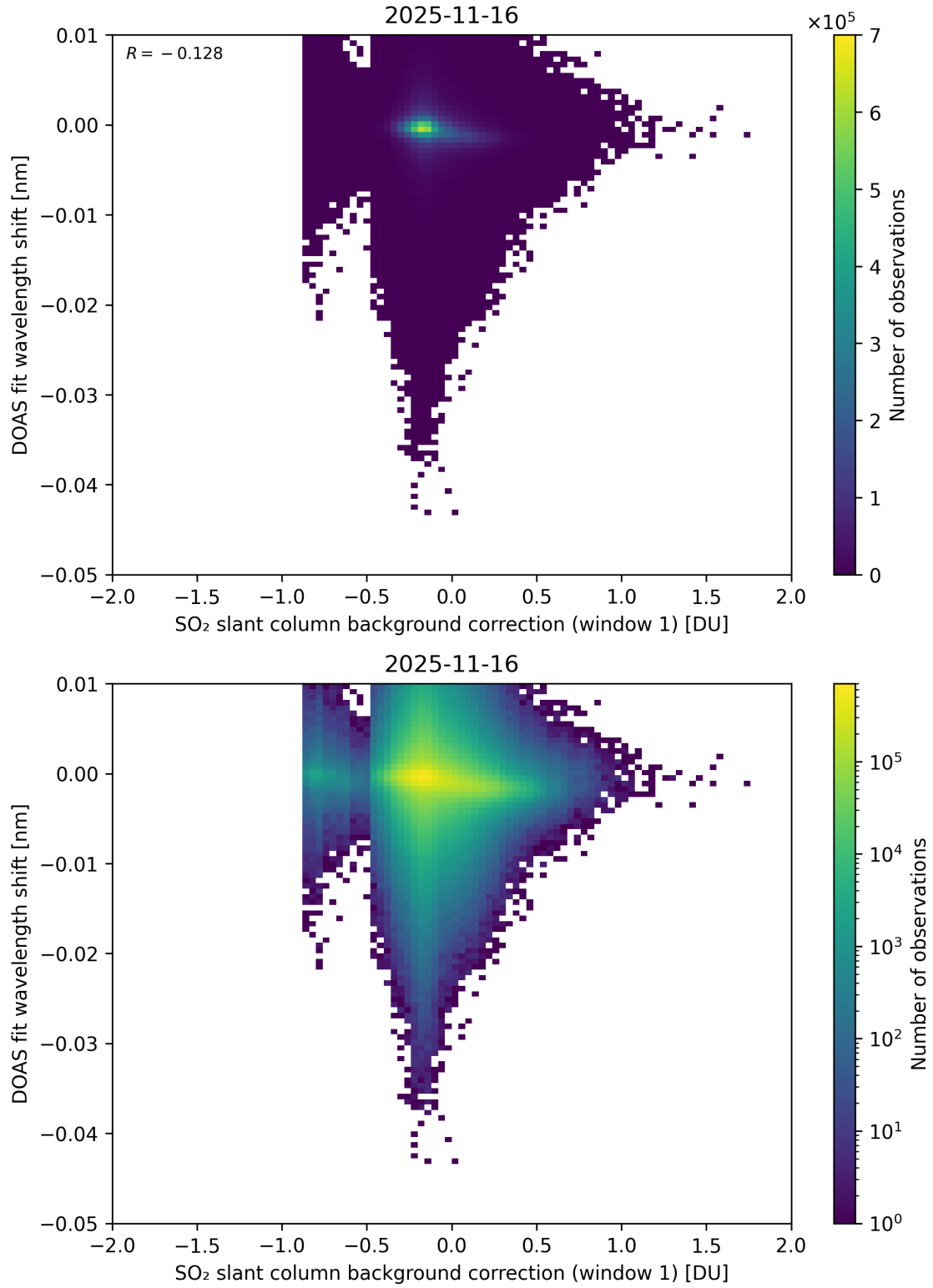
Figure 111: Scatter density plot of “SO 2 slant column background correction (window 1)” against “DOAS fit wavelength shift” for 2025-11-15 to 2025-11-17.
