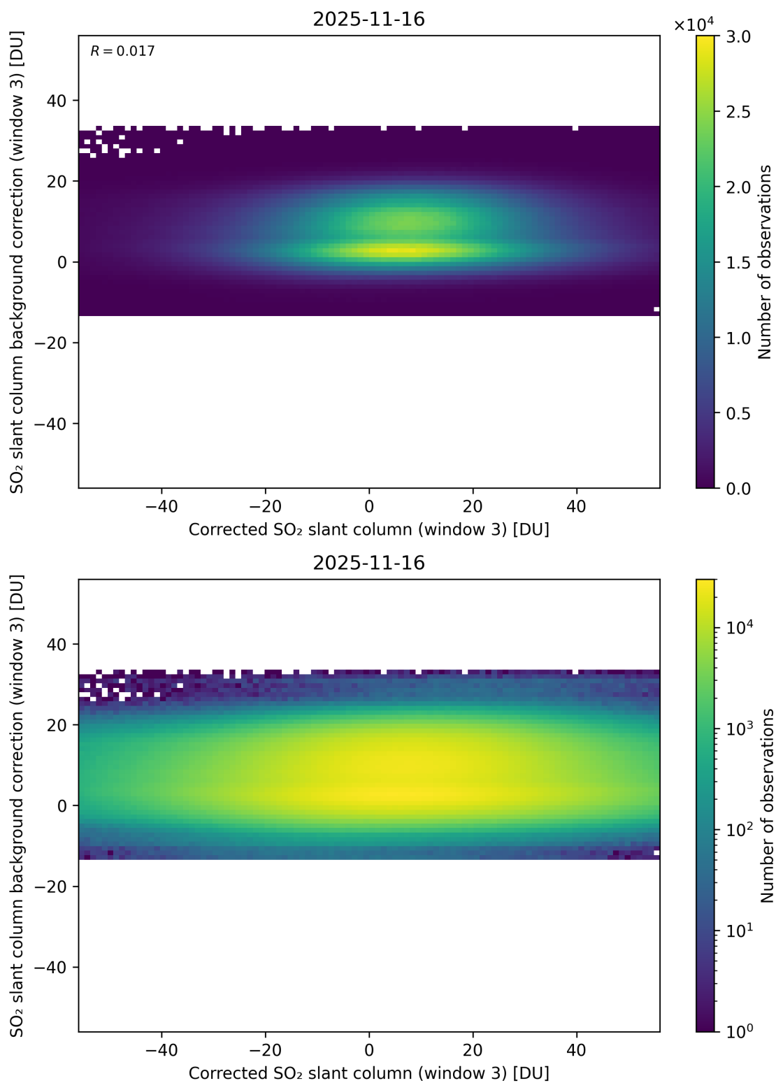
Figure 255: Scatter density plot of “Corrected SO 2 slant column (window 3)” against “SO 2 slant column background correction (window 3)” for 2025-11-15 to 2025-11-17.
