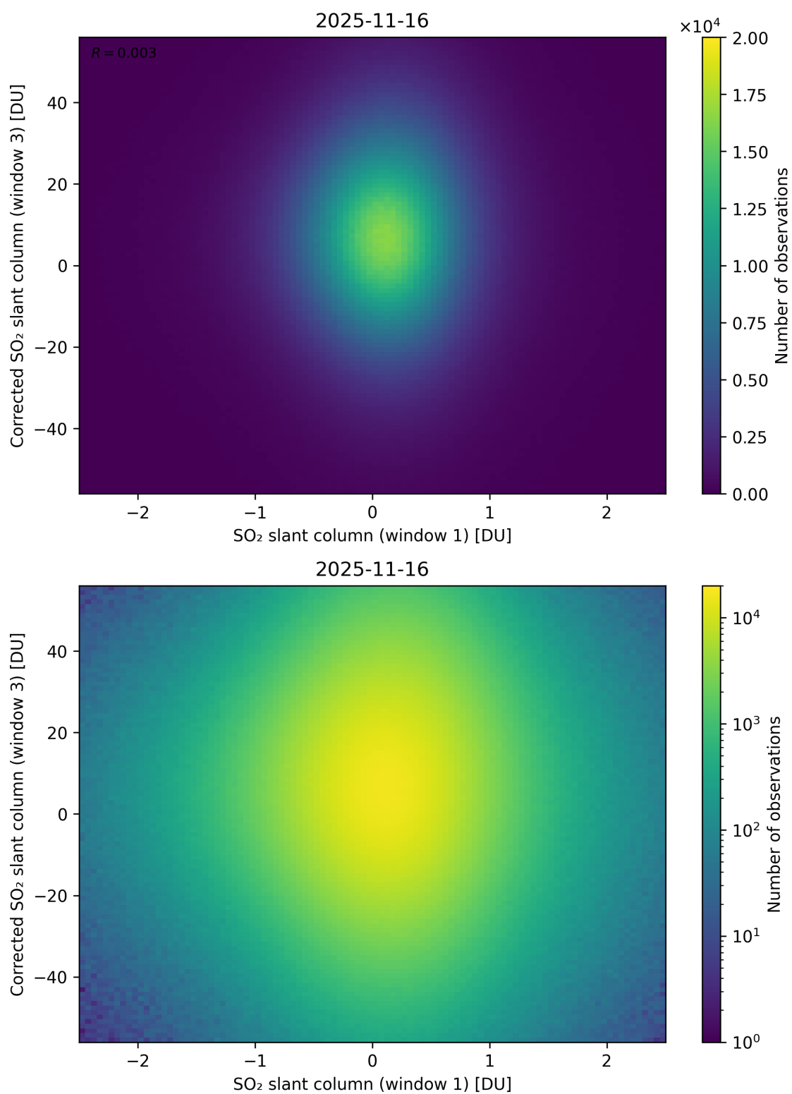
Figure 284: Scatter density plot of “SO 2 slant column (window 1)” against “Corrected SO 2 slant column (window 3)” for 2025-11-15 to 2025-11-17.
