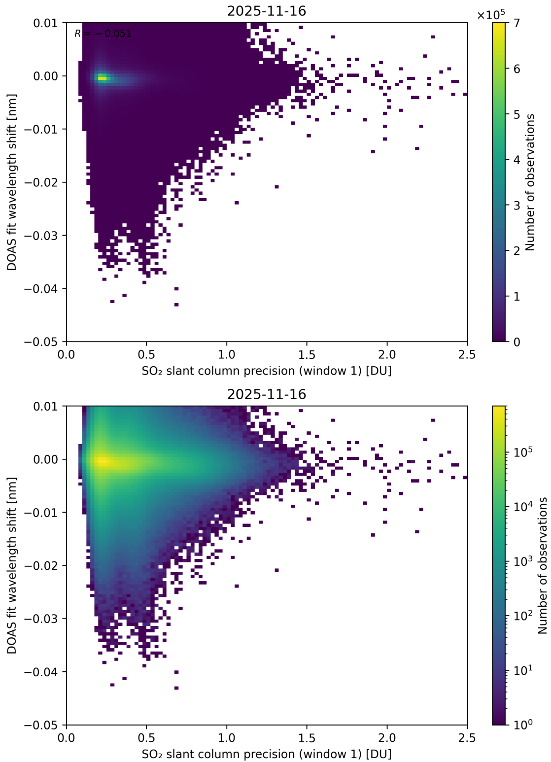
Figure 271: Scatter density plot of “SO 2 slant column precision (window 1)” against “DOAS fit wavelength shift” for 2025-11-15 to 2025-11-17.
