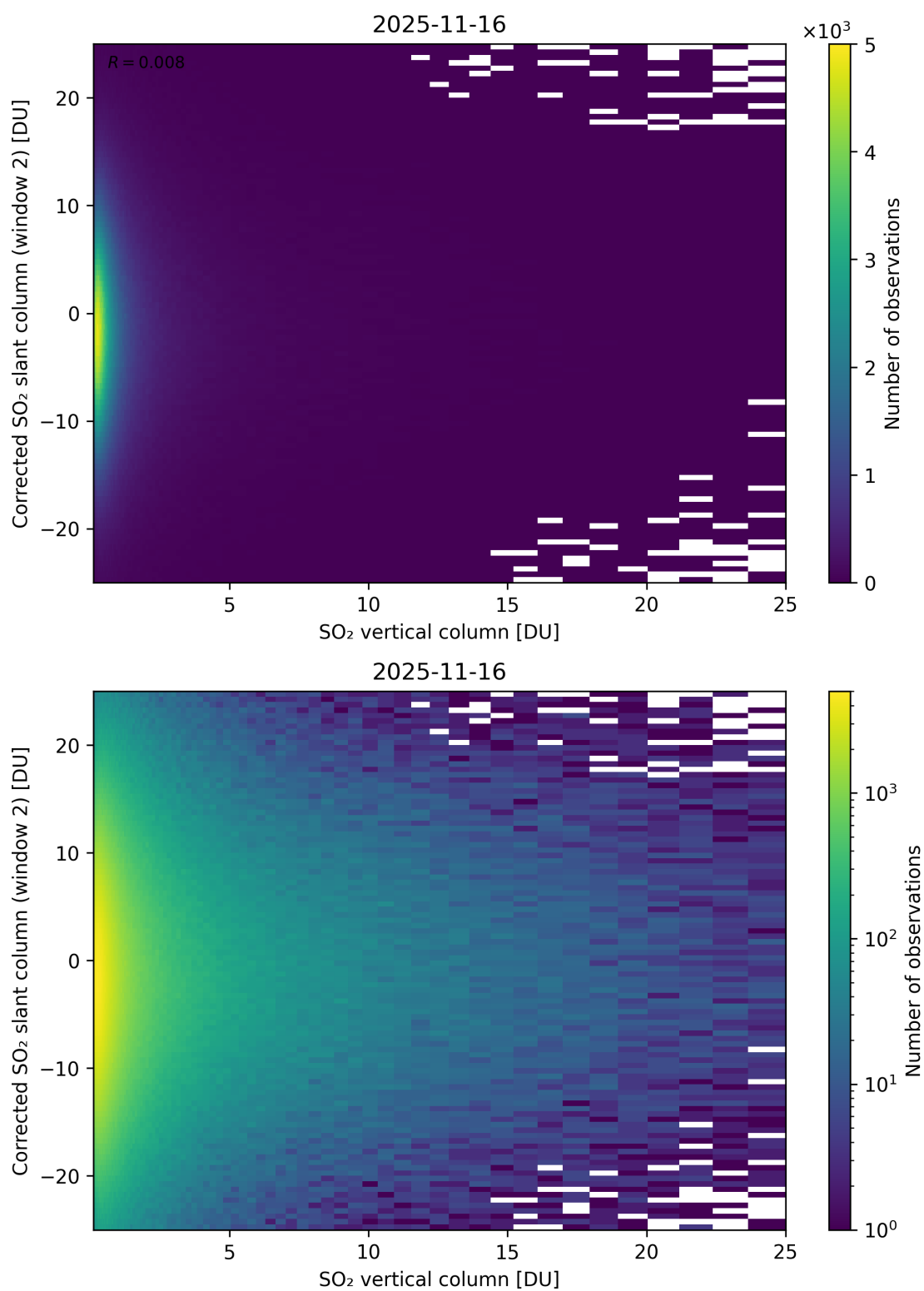
Figure 352: Scatter density plot of “SO 2 vertical column” against “Corrected SO 2 slant column (window 2)” for 2025-11-15 to 2025-11-17.
