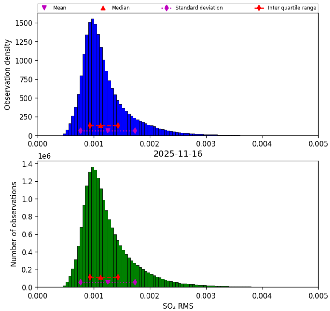
Figure 78: Histogram of “SO 2 RMS” for 2025-11-15 to 2025-11-17
