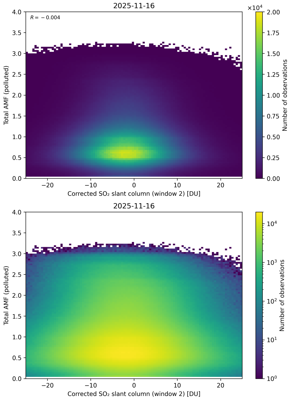
Figure 253: Scatter density plot of “Corrected SO 2 slant column (window 2)” against “Total AMF (polluted)” for 2025-11-15 to 2025-11-17.
