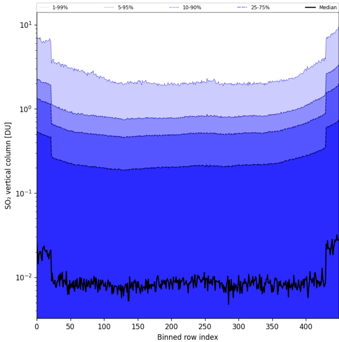
Figure 84: Along track statistics of “SO 2 vertical column” for 2025-11-15 to 2025-11-17
