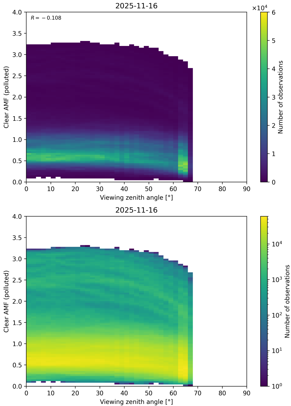
Figure 370: Scatter density plot of “Viewing zenith angle” against “Clear AMF (polluted)” for 2025-11-15 to 2025-11-17.
