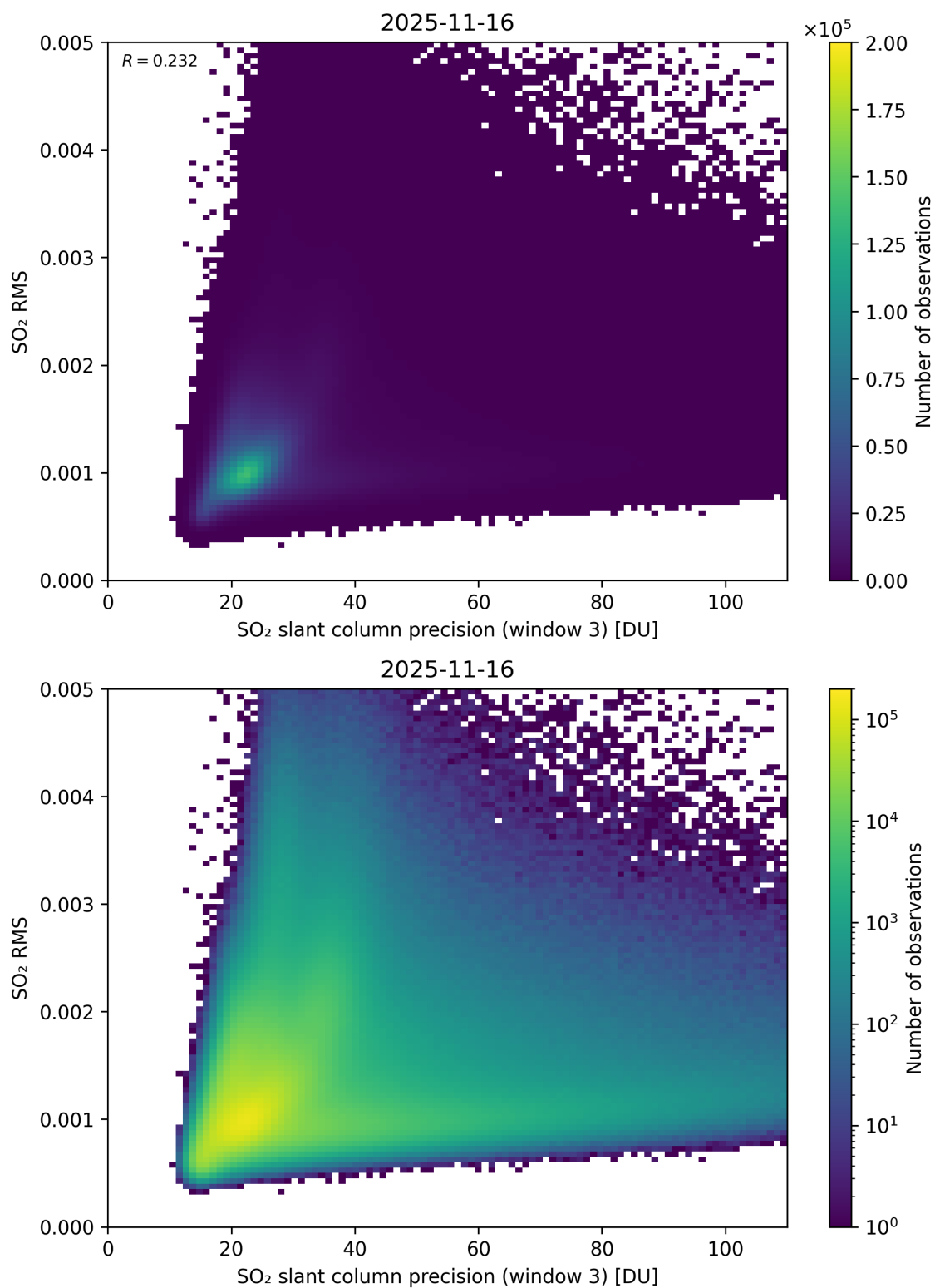
Figure 310: Scatter density plot of “SO 2 slant column precision (window 3)” against “SO 2 RMS” for 2025-11-15 to 2025-11-17.
