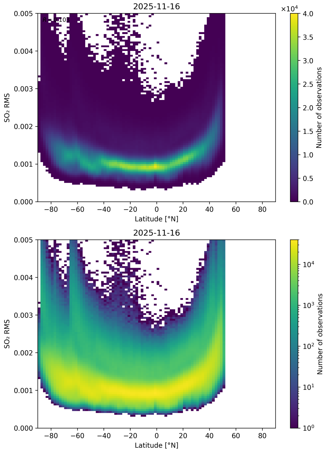
Figure 155: Scatter density plot of “Latitude” against “SO 2 RMS” for 2025-11-15 to 2025-11-17.
