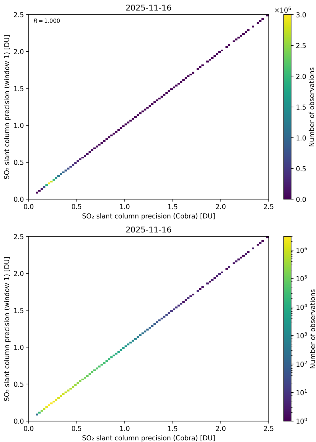
Figure 209: Scatter density plot of “SO 2 slant column precision (Cobra)” against “SO 2 slant column precision (window 1)” for 2025-11-15 to 2025-11-17.
