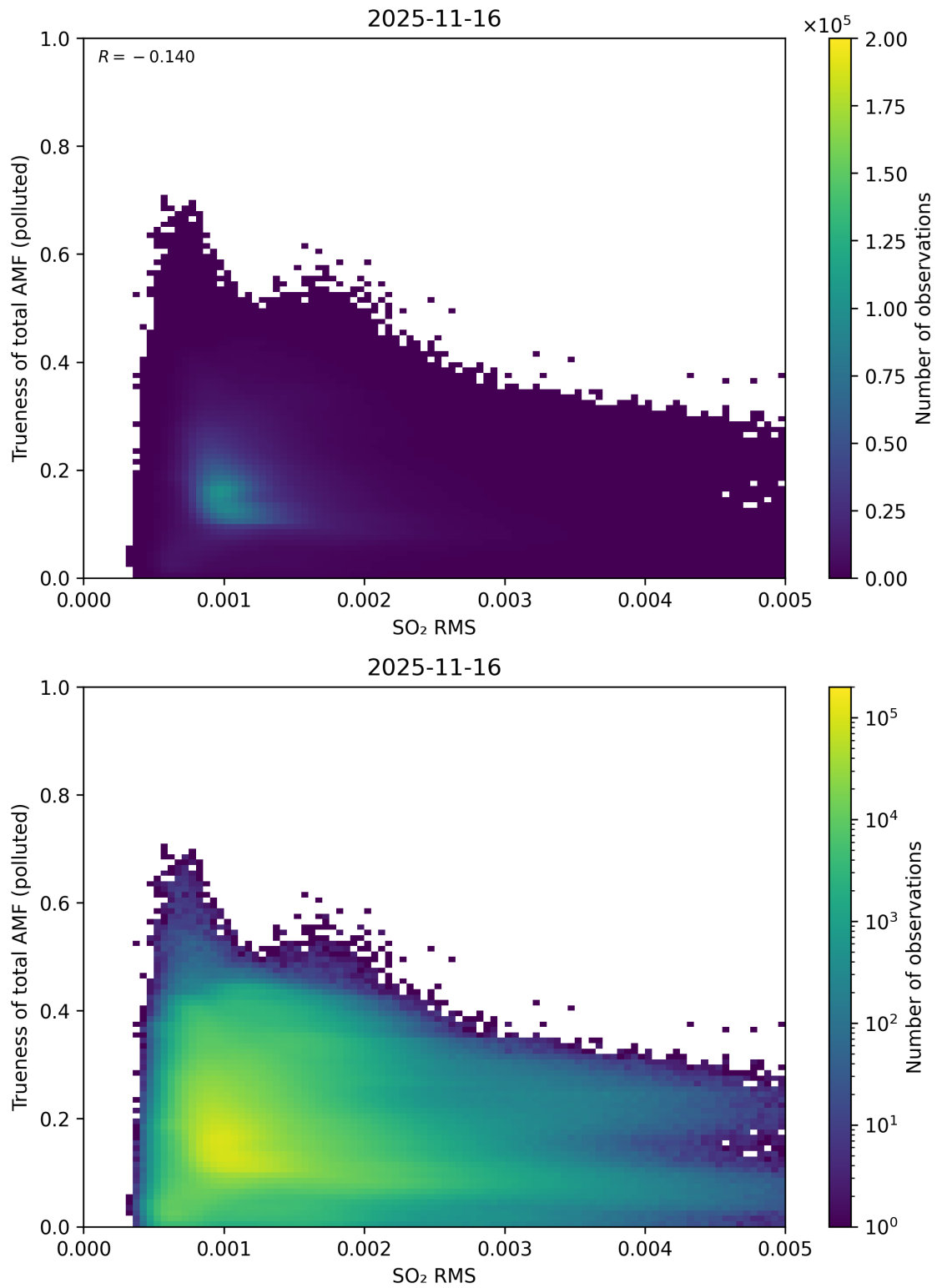
Figure 149: Scatter density plot of “SO 2 RMS” against “Trueness of total AMF (polluted)” for 2025-11-15 to 2025-11-17.
