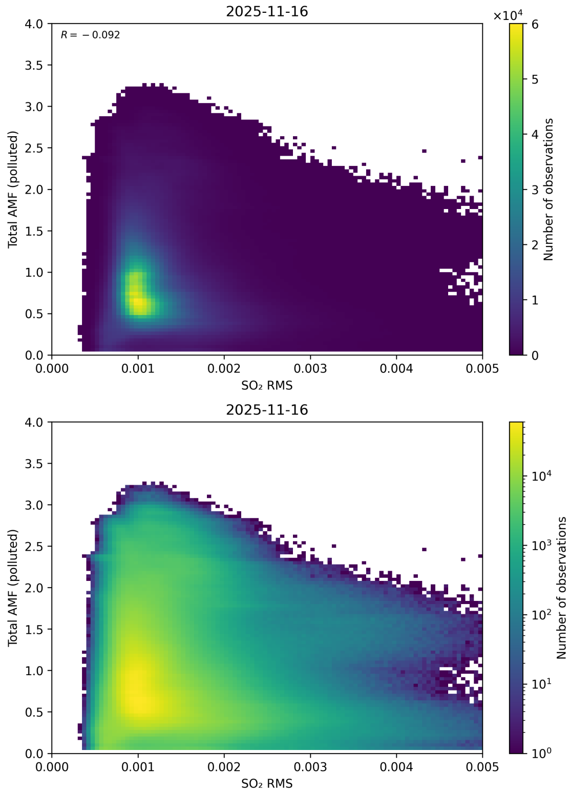
Figure 148: Scatter density plot of “SO 2 RMS” against “Total AMF (polluted)” for 2025-11-15 to 2025-11-17.
