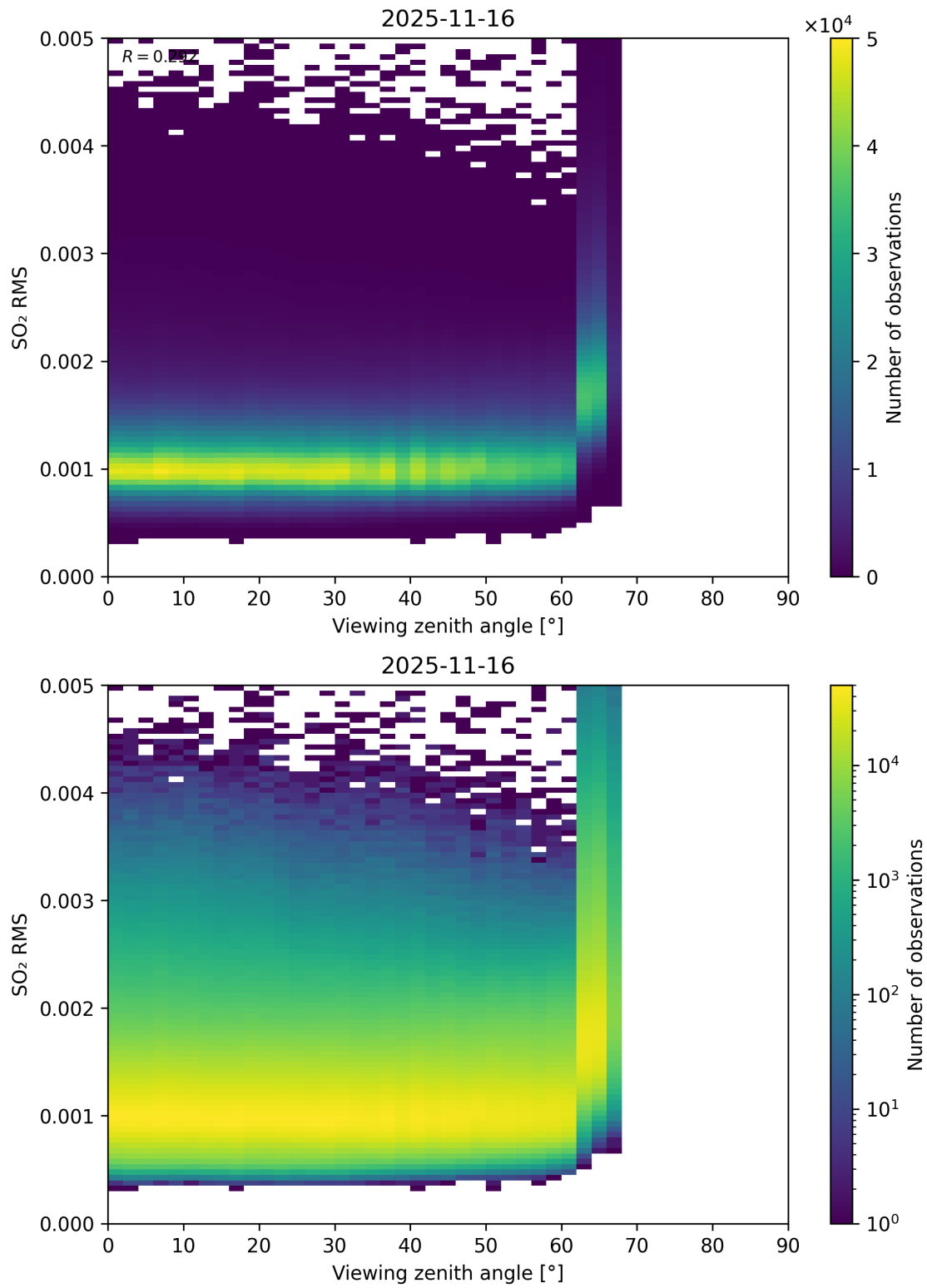
Figure 367: Scatter density plot of “Viewing zenith angle” against “SO 2 RMS” for 2025-11-15 to 2025-11-17.
