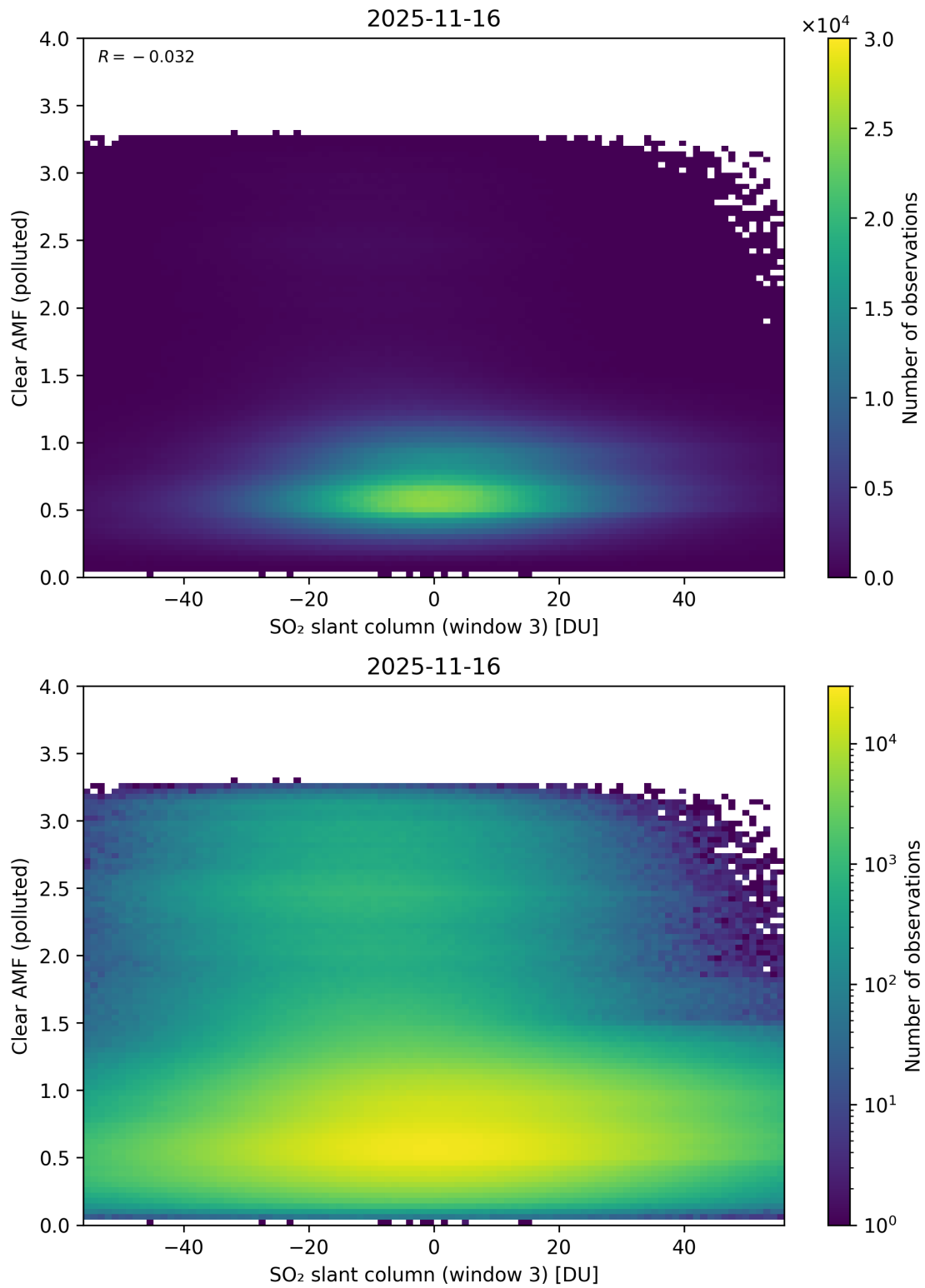
Figure 315: Scatter density plot of “SO 2 slant column (window 3)” against “Clear AMF (polluted)” for 2025-11-15 to 2025-11-17.
