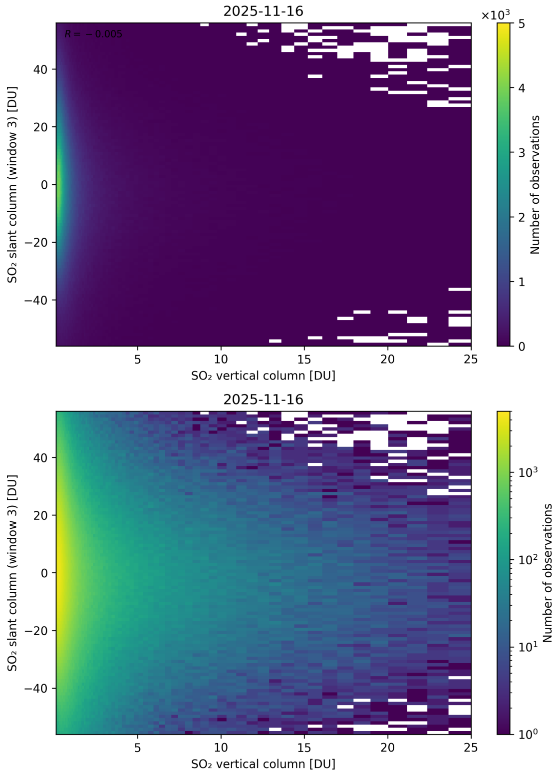
Figure 357: Scatter density plot of “SO 2 vertical column” against “SO 2 slant column (window 3)” for 2025-11-15 to 2025-11-17.
