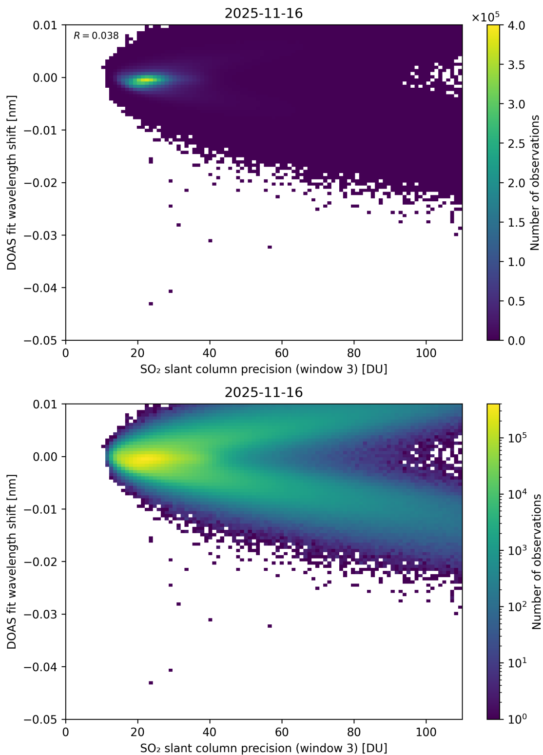
Figure 308: Scatter density plot of “SO 2 slant column precision (window 3)” against “DOAS fit wavelength shift” for 2025-11-15 to 2025-11-17.
