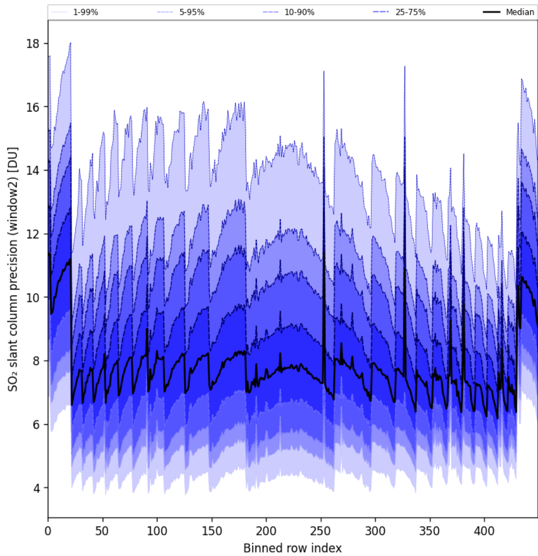
Figure 94: Along track statistics of “SO 2 slant column precision (window2)” for 2025-11-15 to 2025-11-17
