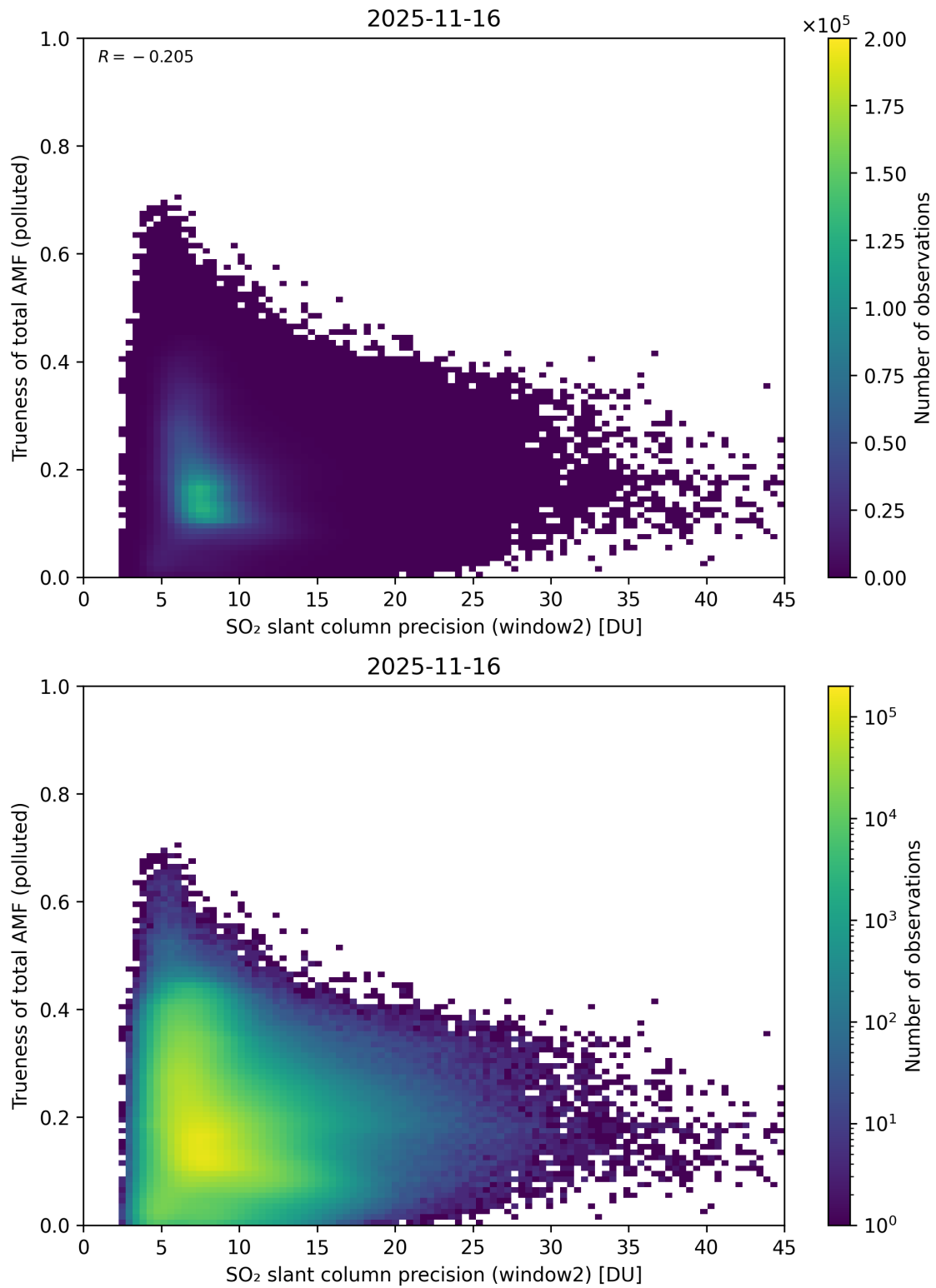
Figure 302: Scatter density plot of “SO 2 slant column precision (window2)” against “Trueness of total AMF (polluted)” for 2025-11-15 to 2025-11-17.
