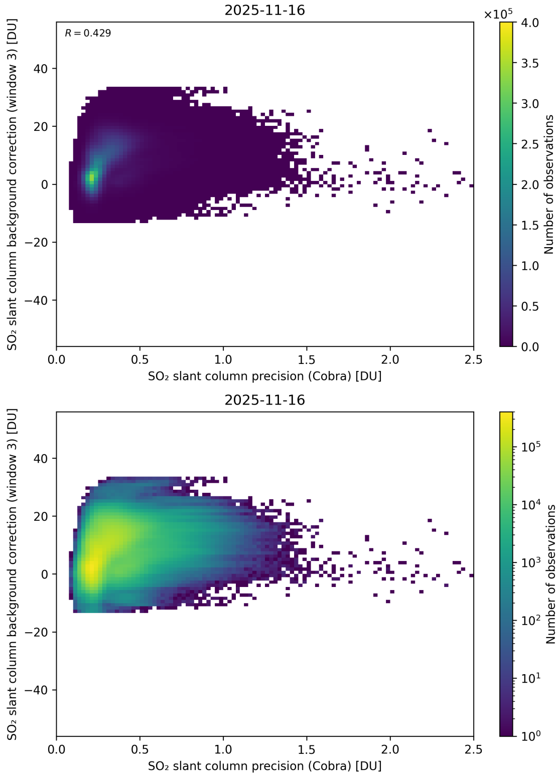
Figure 201: Scatter density plot of “SO 2 slant column precision (Cobra)” against “SO 2 slant column background correction (window 3)” for 2025-11-15 to 2025-11-17.
