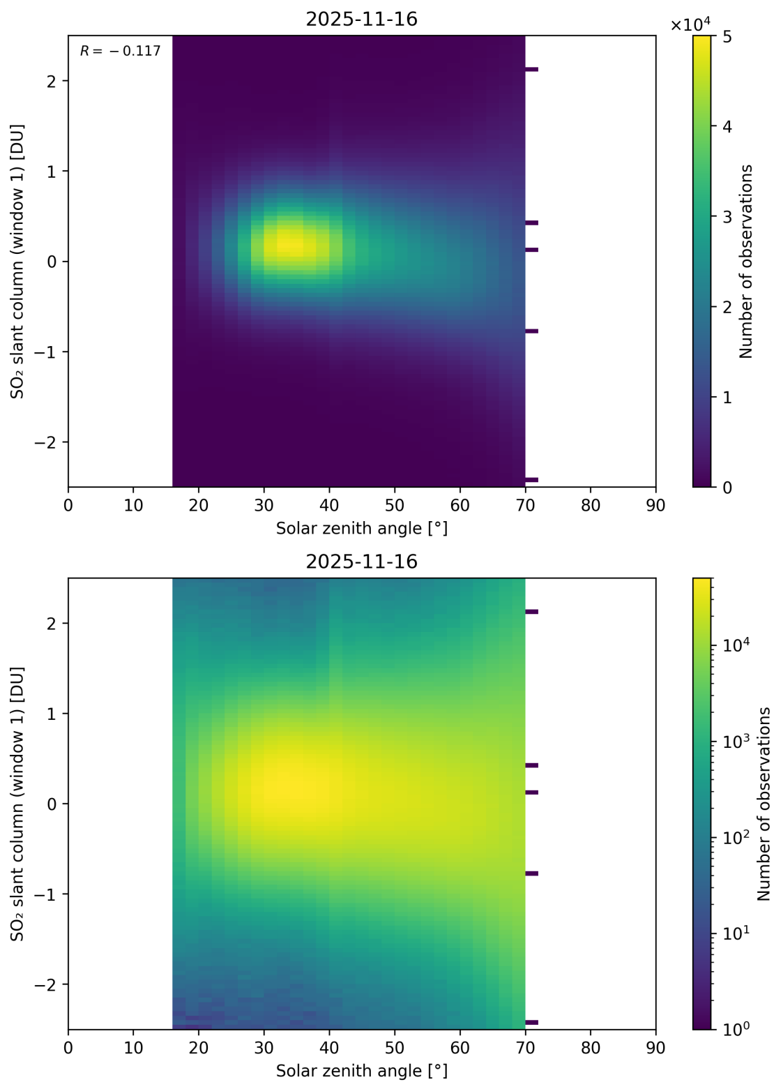
Figure 184: Scatter density plot of “Solar zenith angle” against “SO 2 slant column (window 1)” for 2025-11-15 to 2025-11-17.
