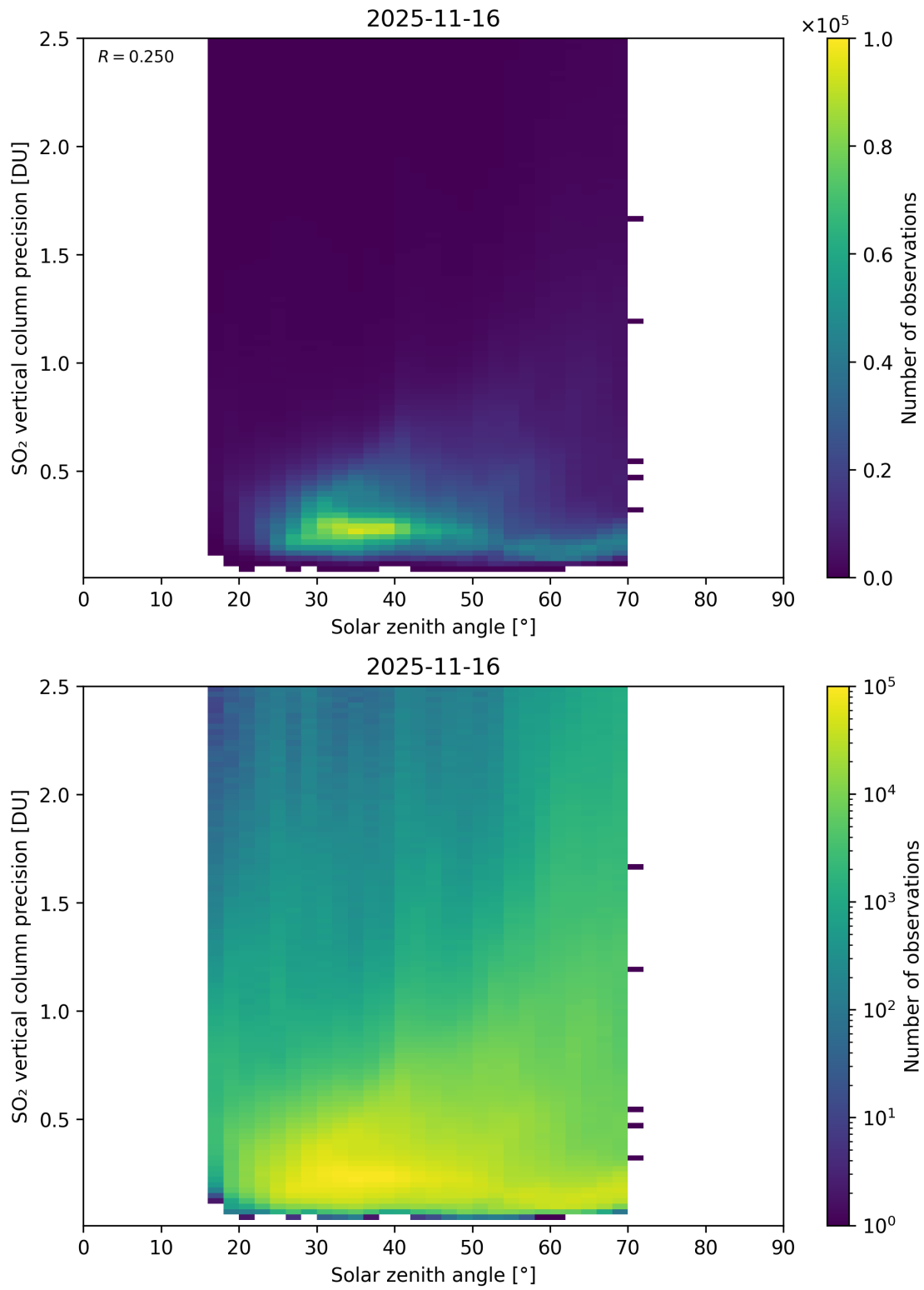
Figure 192: Scatter density plot of “Solar zenith angle” against “SO 2 vertical column precision” for 2025-11-15 to 2025-11-17.
