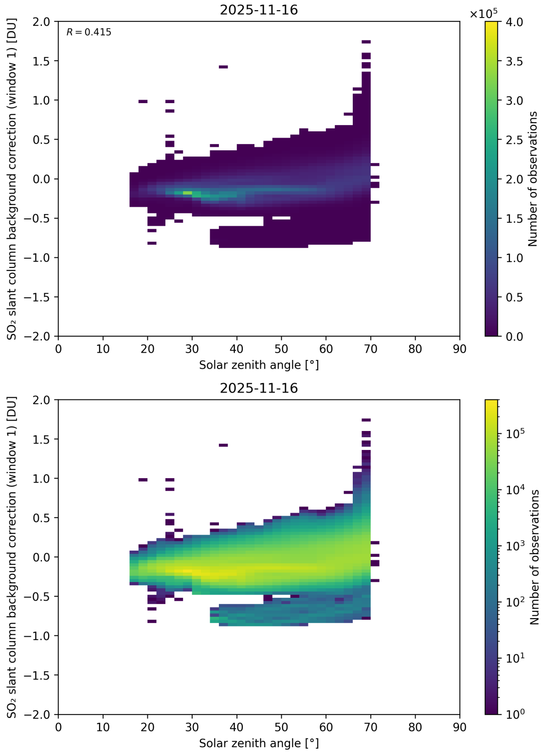
Figure 171: Scatter density plot of “Solar zenith angle” against “SO 2 slant column background correction (window 1)” for 2025-11-15 to 2025-11-17.
