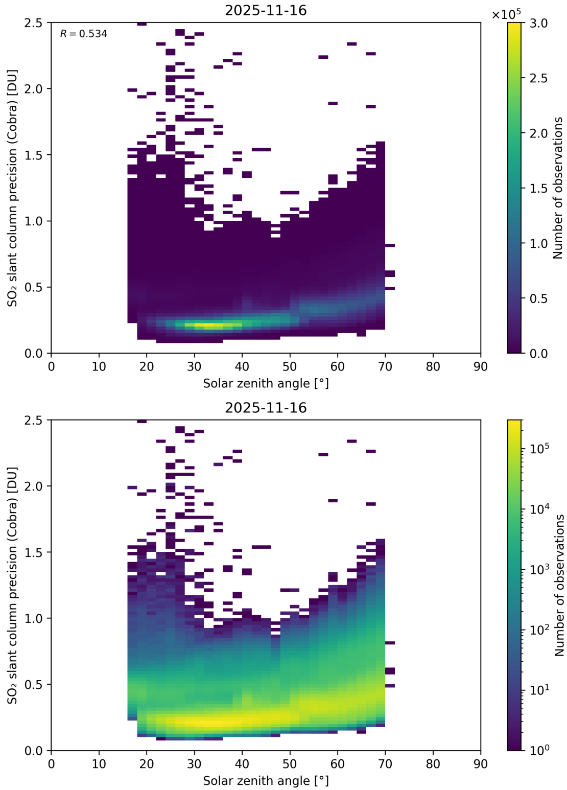
Figure 180: Scatter density plot of “Solar zenith angle” against “SO 2 slant column precision (Cobra)” for 2025-11-15 to 2025-11-17.
