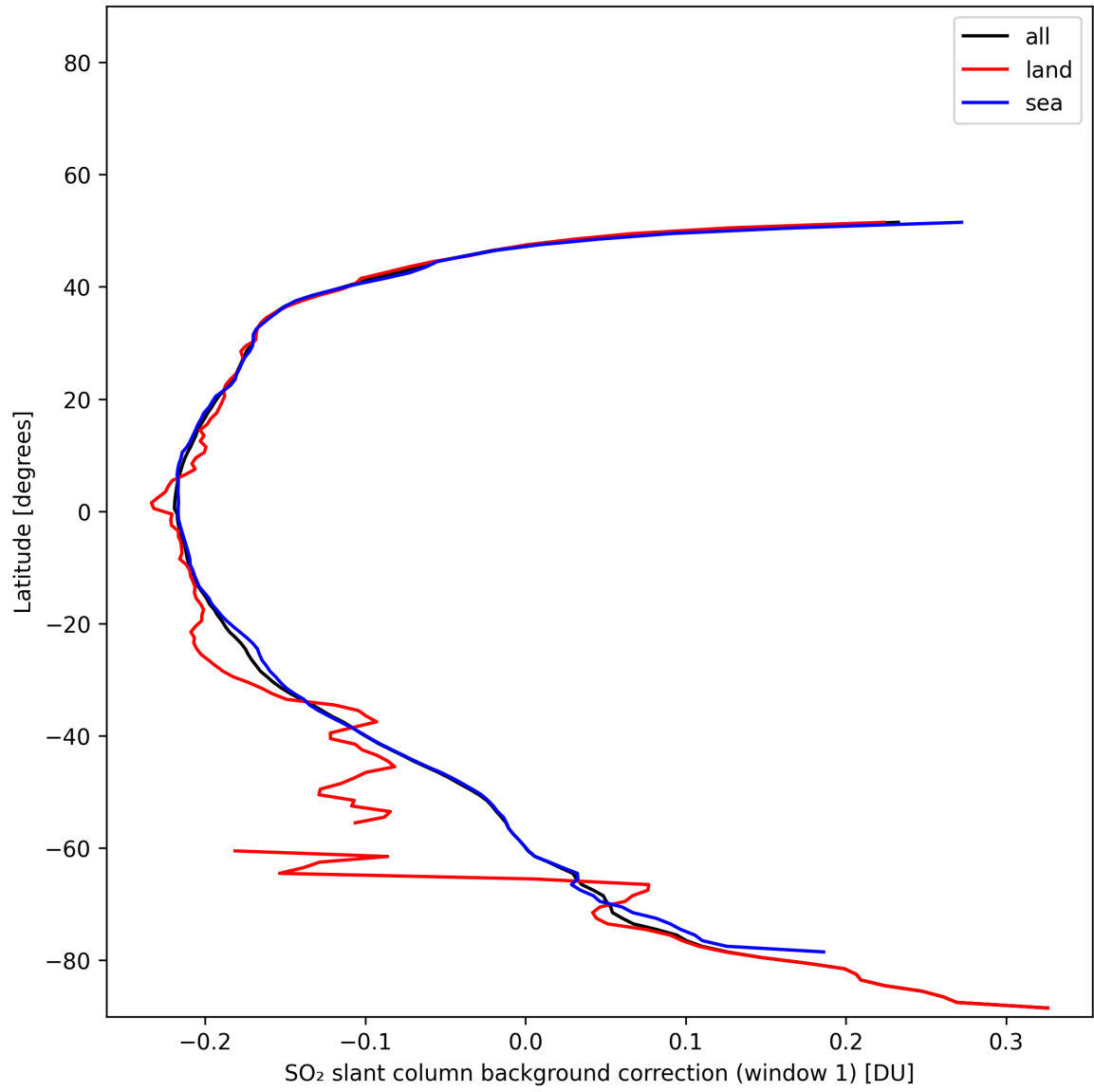
Figure 40: Zonal average of “SO 2 slant column background correction (window 1)” for 2025-11-15 to 2025-11-17.
