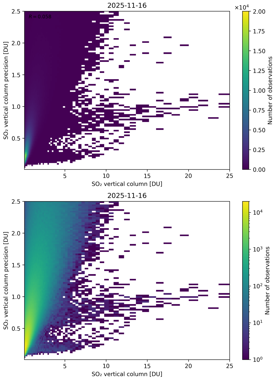
Figure 361: Scatter density plot of “SO 2 vertical column” against “SO 2 vertical column precision” for 2025-11-15 to 2025-11-17.
