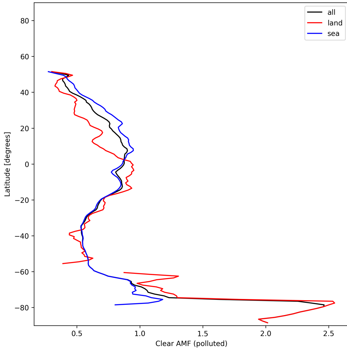
Figure 55: Zonal average of “Clear AMF (polluted)” for 2025-11-15 to 2025-11-17.
