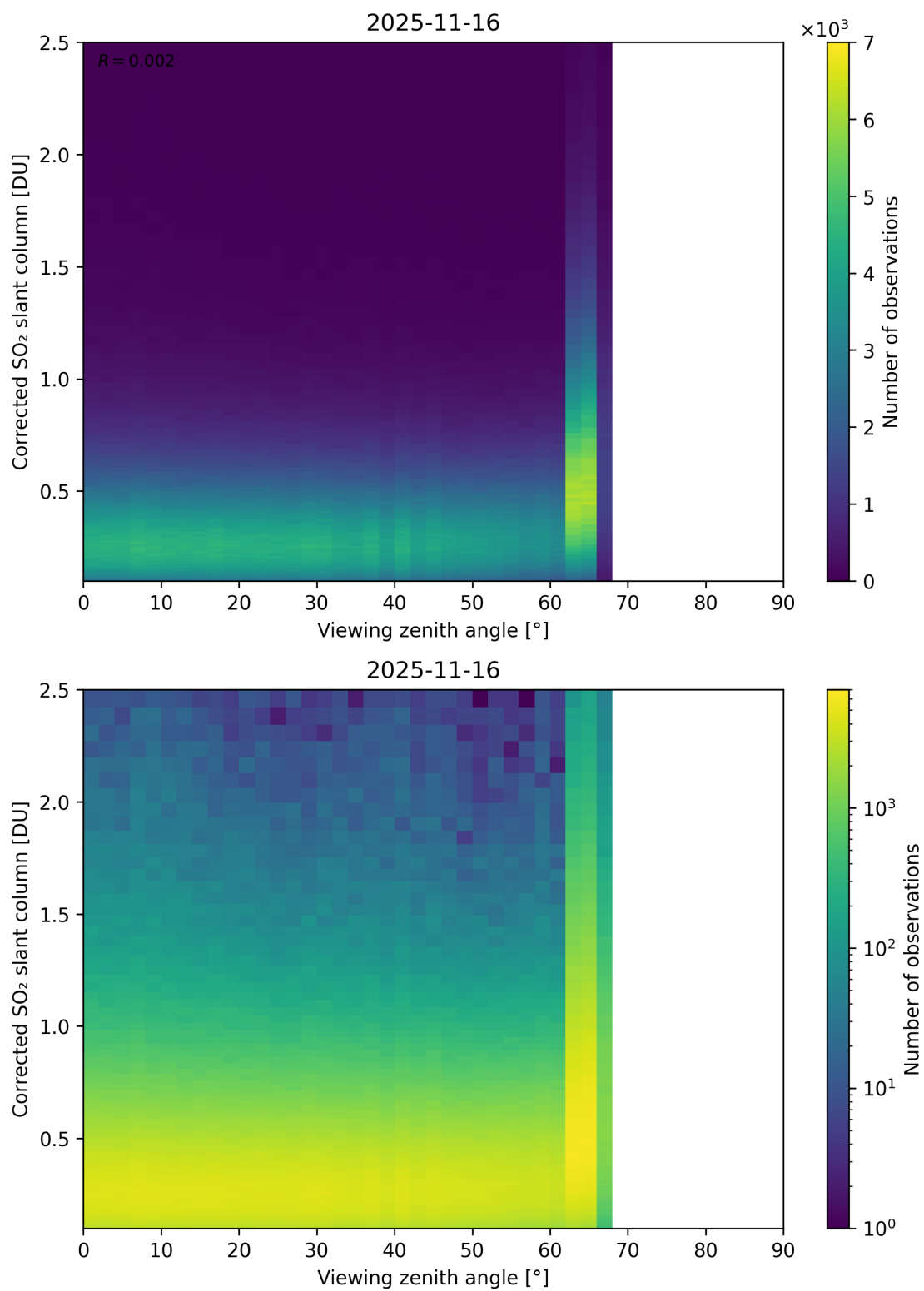
Figure 373: Scatter density plot of “Viewing zenith angle” against “Corrected SO 2 slant column” for 2025-11-15 to 2025-11-17.
