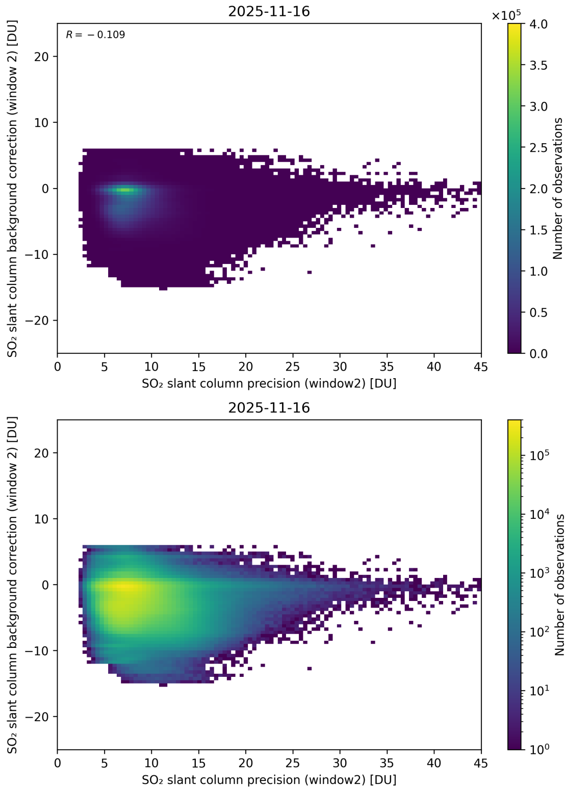
Figure 291: Scatter density plot of “SO 2 slant column precision (window2)” against “SO 2 slant column background correction (window 2)” for 2025-11-15 to 2025-11-17.
