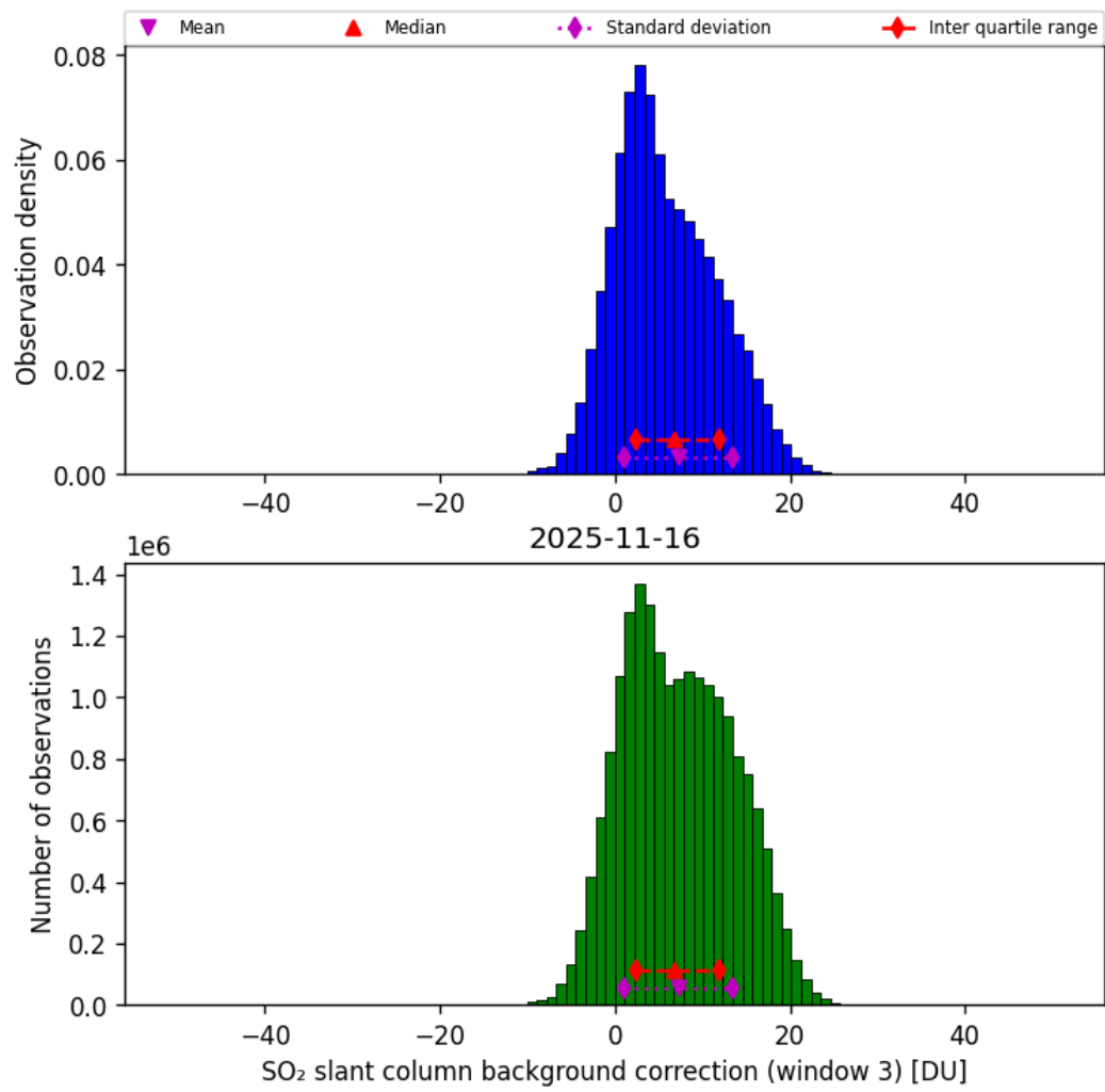
Figure 74: Histogram of “SO 2 slant column background correction (window 3)” for 2025-11-15 to 2025-11-17
