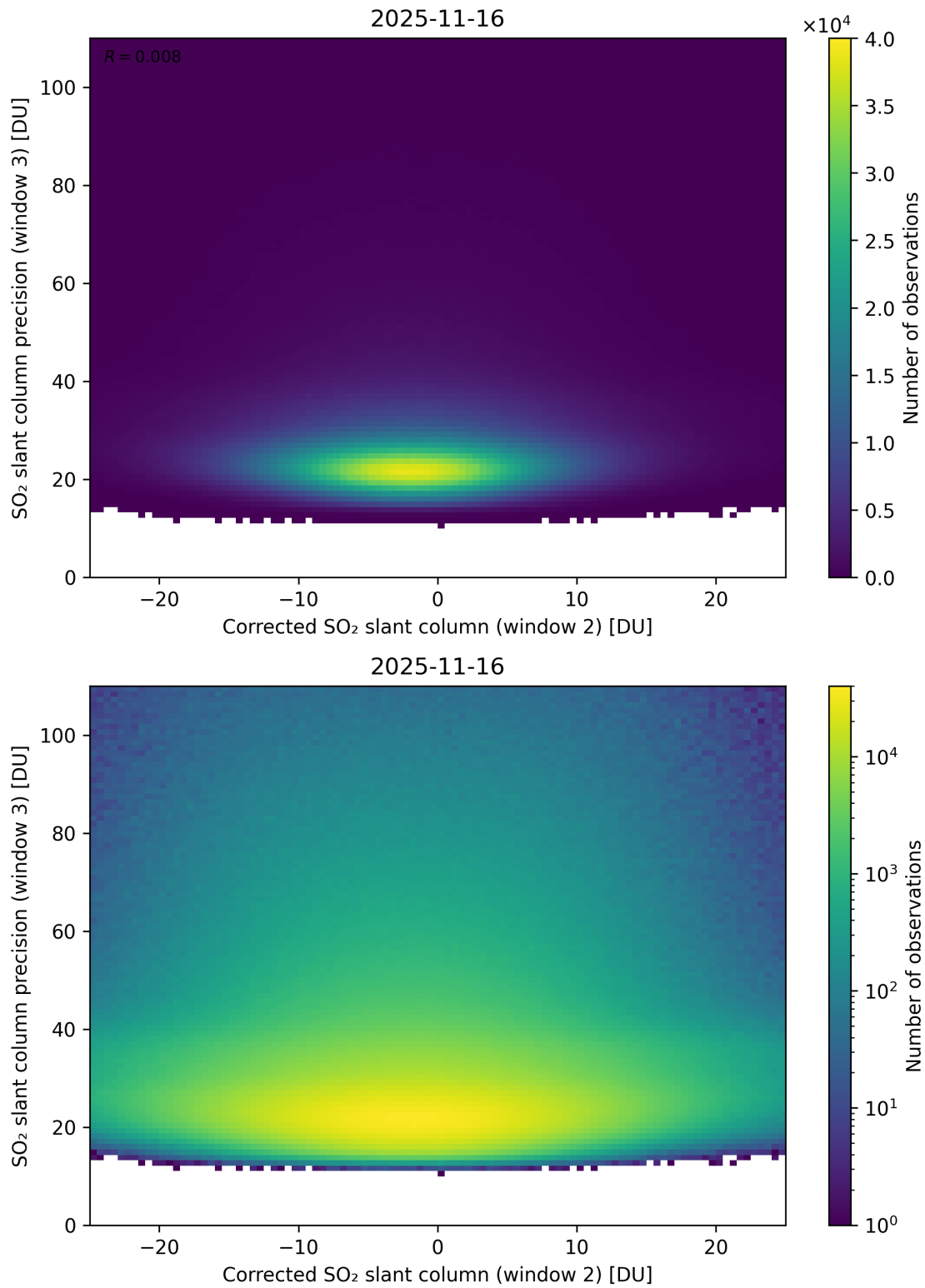
Figure 252: Scatter density plot of “Corrected SO 2 slant column (window 2)” against “SO 2 slant column precision (window 3)” for 2025-11-15 to 2025-11-17.
