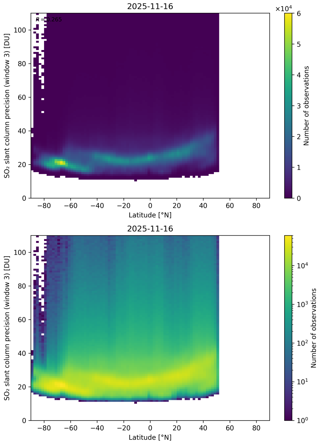
Figure 166: Scatter density plot of “Latitude” against “SO 2 slant column precision (window 3)” for 2025-11-15 to 2025-11-17.
