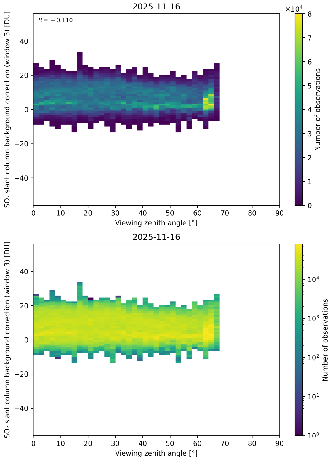
Figure 364: Scatter density plot of “Viewing zenith angle” against “SO 2 slant column background correction (window 3)” for 2025-11-15 to 2025-11-17.
