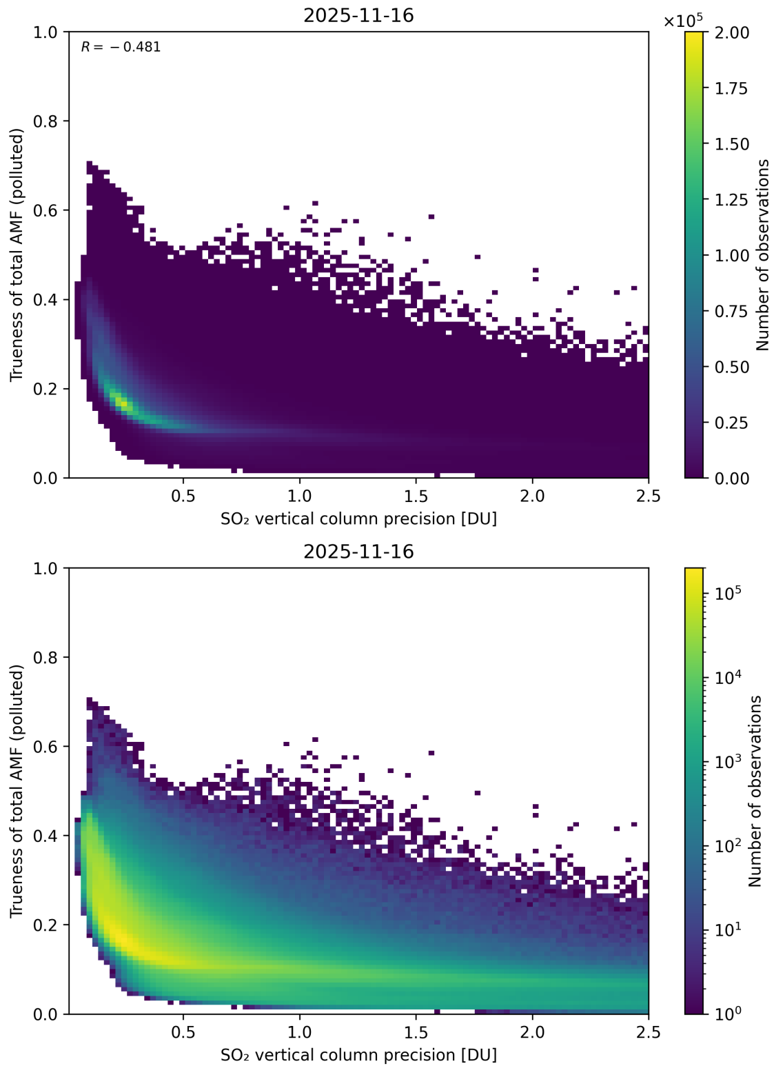
Figure 347: Scatter density plot of “SO 2 vertical column precision” against “Trueness of total AMF (polluted)” for 2025-11-15 to 2025-11-17.
