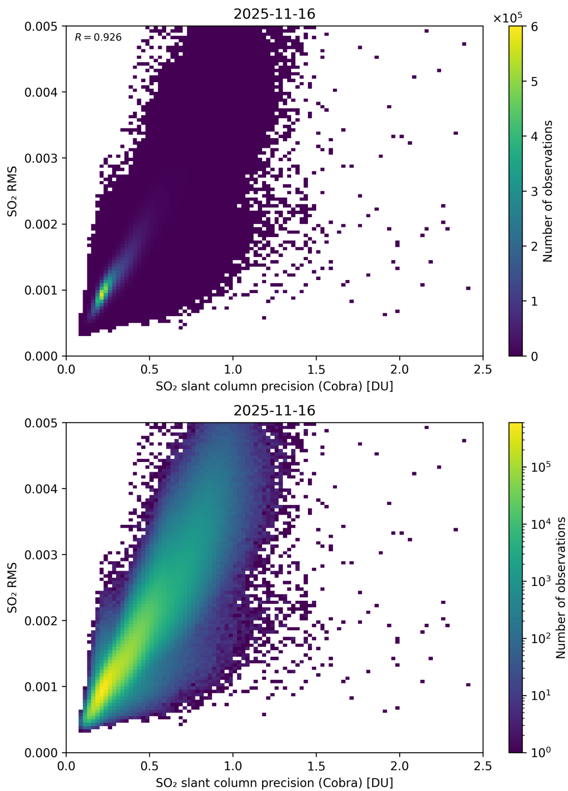
Figure 204: Scatter density plot of “SO 2 slant column precision (Cobra)” against “SO 2 RMS” for 2025-11-15 to 2025-11-17.
