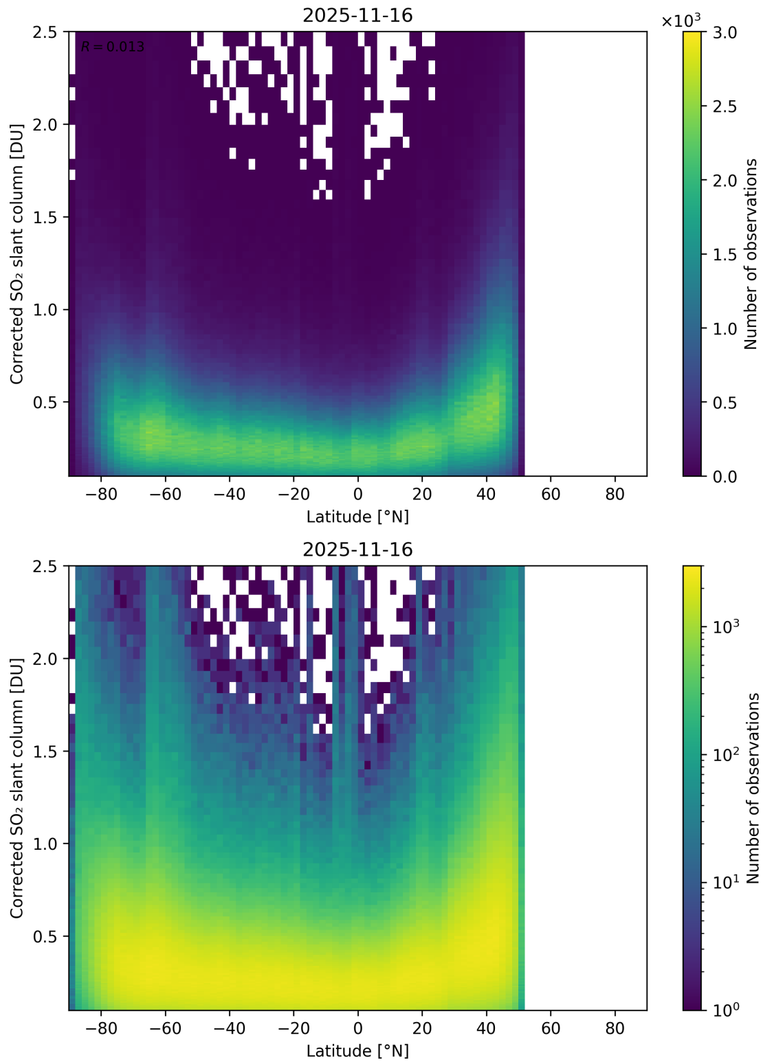
Figure 159: Scatter density plot of “Latitude” against “Corrected SO 2 slant column” for 2025-11-15 to 2025-11-17.
