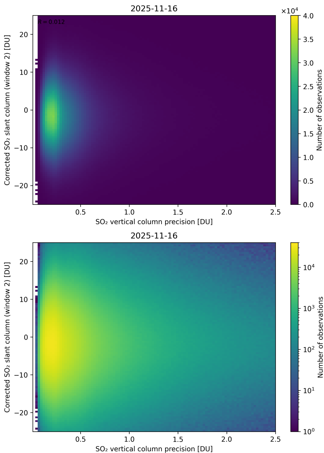
Figure 339: Scatter density plot of “SO 2 vertical column precision” against “Corrected SO 2 slant column (window 2)” for 2025-11-15 to 2025-11-17.
