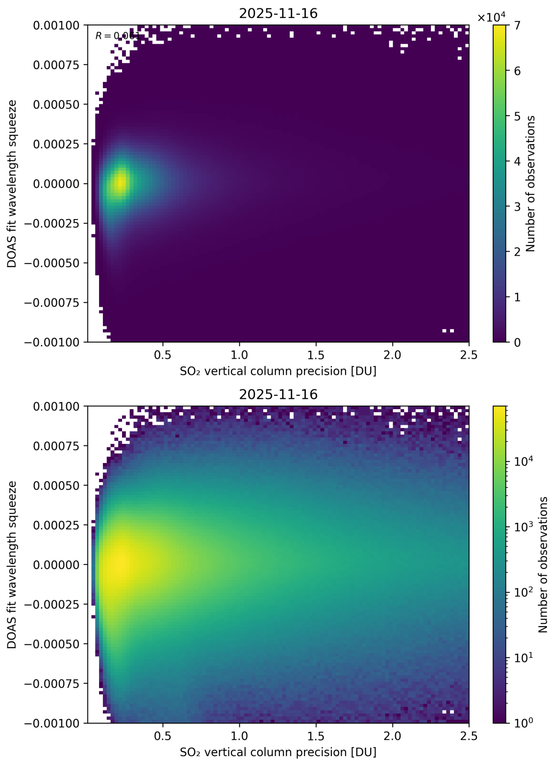
Figure 333: Scatter density plot of “SO 2 vertical column precision” against “DOAS fit wavelength squeeze” for 2025-11-15 to 2025-11-17.
