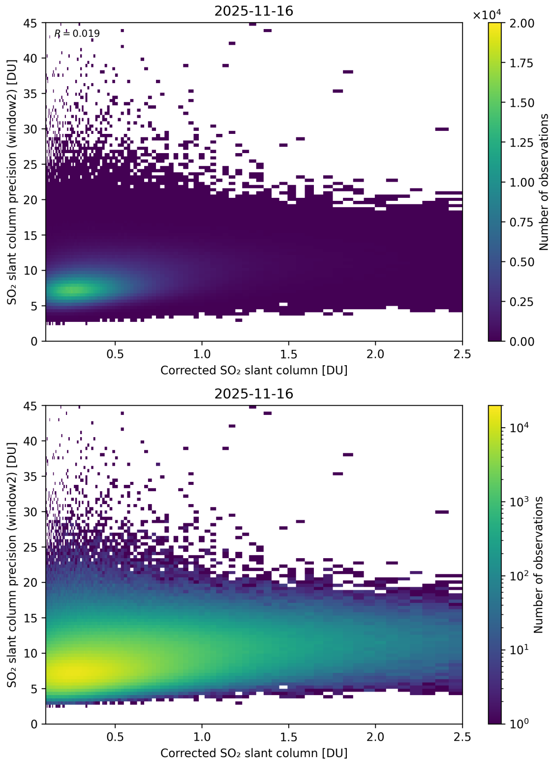
Figure 239: Scatter density plot of “Corrected SO 2 slant column” against “SO 2 slant column precision (window2)” for 2025-11-15 to 2025-11-17.
