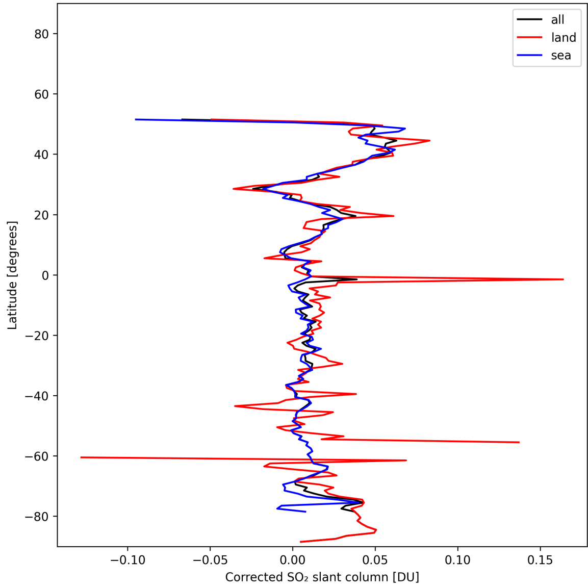
Figure 34: Zonal average of “Corrected SO 2 slant column” for 2025-11-15 to 2025-11-17.
