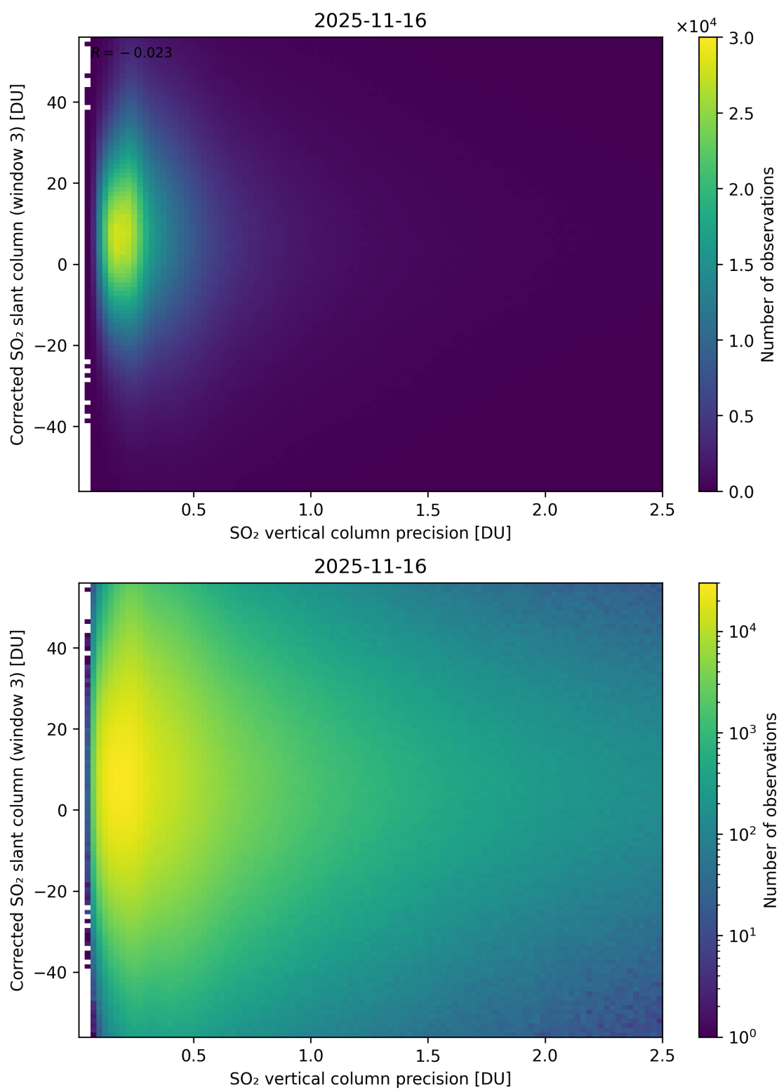
Figure 340: Scatter density plot of “SO 2 vertical column precision” against “Corrected SO 2 slant column (window 3)” for 2025-11-15 to 2025-11-17.
