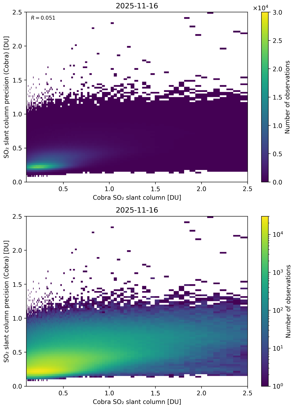
Figure 216: Scatter density plot of “Cobra SO 2 slant column” against “SO 2 slant column precision (Cobra)” for 2025-11-15 to 2025-11-17.
