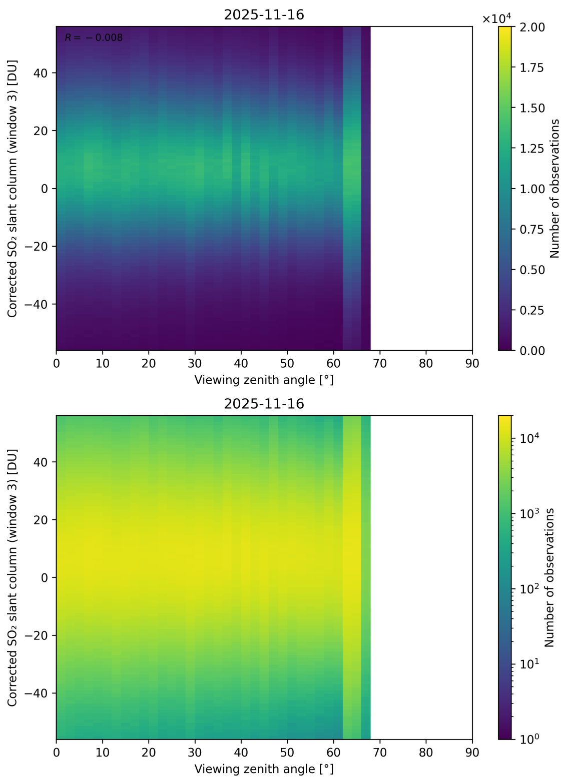
Figure 375: Scatter density plot of “Viewing zenith angle” against “Corrected SO 2 slant column (window 3)” for 2025-11-15 to 2025-11-17.
