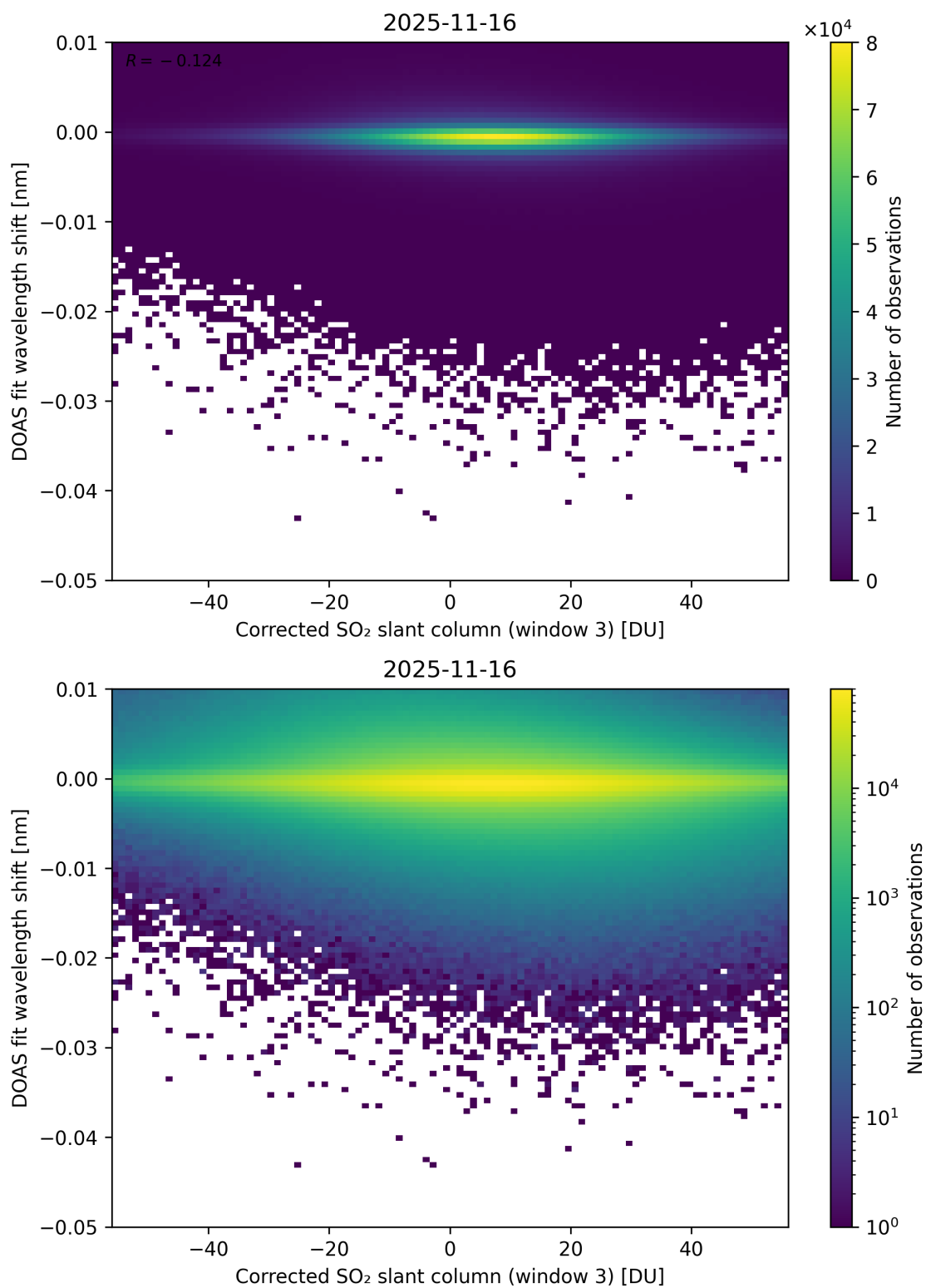
Figure 256: Scatter density plot of “Corrected SO 2 slant column (window 3)” against “DOAS fit wavelength shift” for 2025-11-15 to 2025-11-17.
