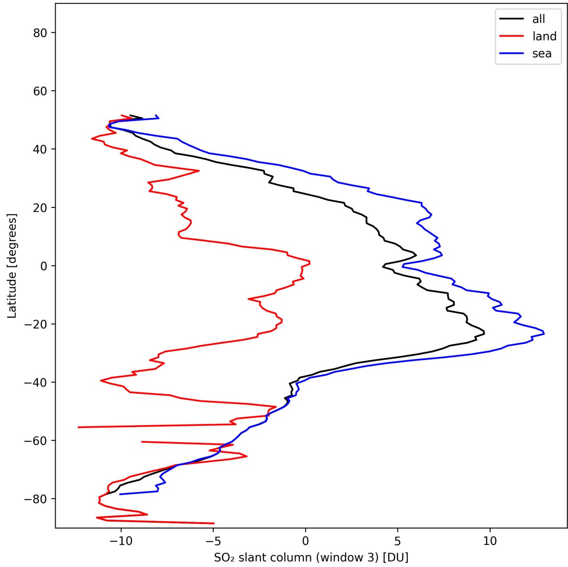
Figure 45: Zonal average of “SO 2 slant column (window 3)” for 2025-11-15 to 2025-11-17.
