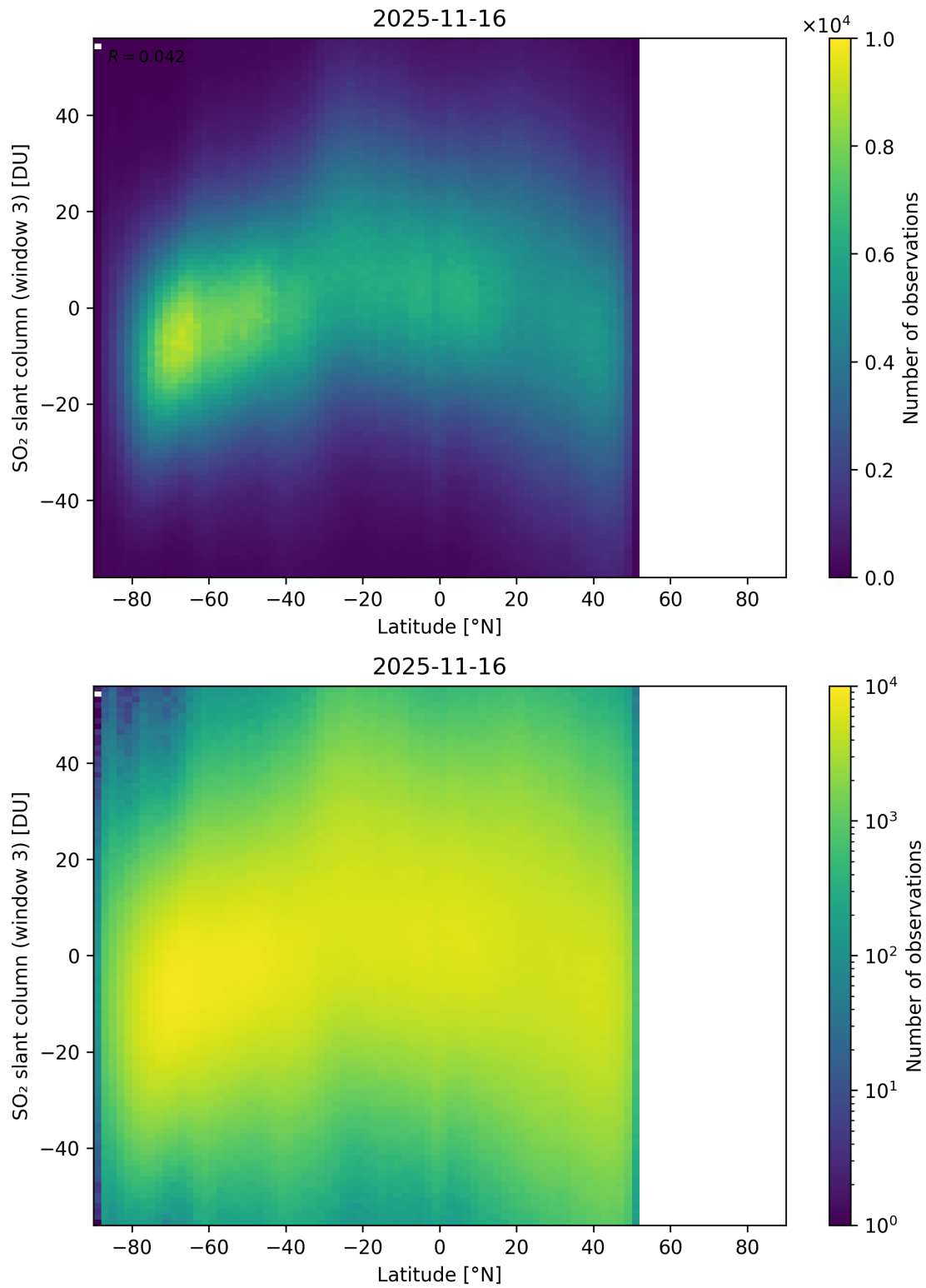
Figure 165: Scatter density plot of “Latitude” against “SO 2 slant column (window 3)” for 2025-11-15 to 2025-11-17.
