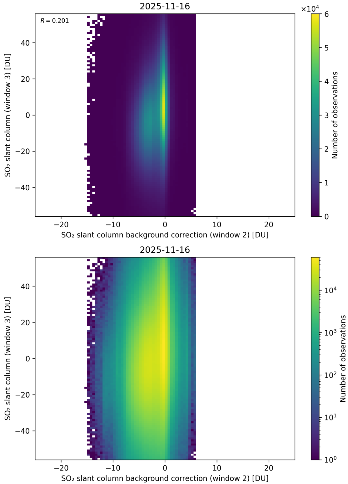
Figure 128: Scatter density plot of “SO 2 slant column background correction (window 2)” against “SO 2 slant column (window 3)” for 2025-11-15 to 2025-11-17.
