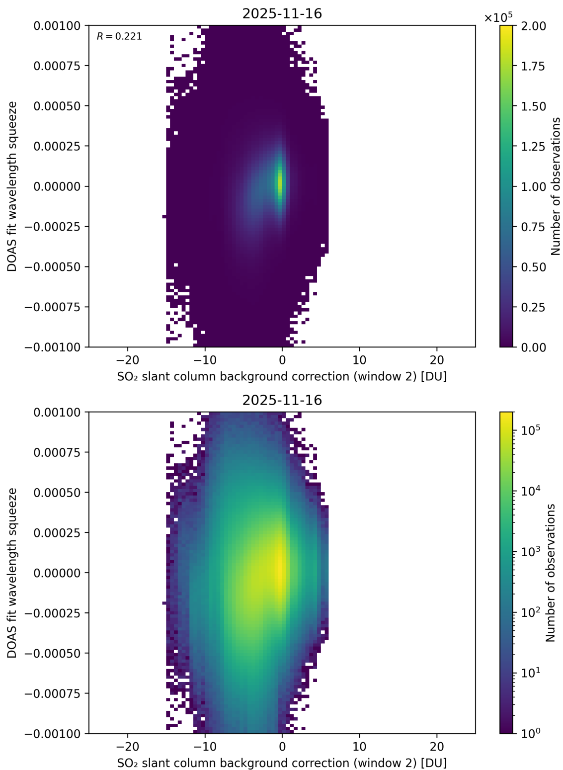
Figure 124: Scatter density plot of “SO 2 slant column background correction (window 2)” against “DOAS fit wavelength squeeze” for 2025-11-15 to 2025-11-17.
