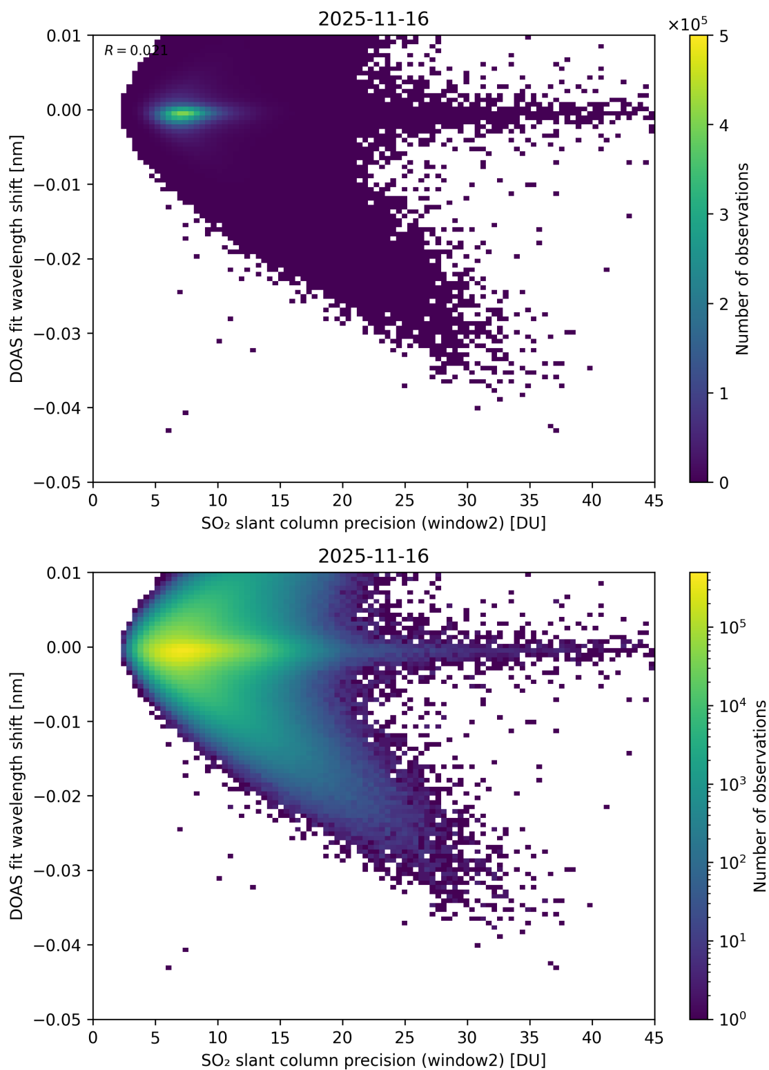
Figure 293: Scatter density plot of “SO 2 slant column precision (window2)” against “DOAS fit wavelength shift” for 2025-11-15 to 2025-11-17.
