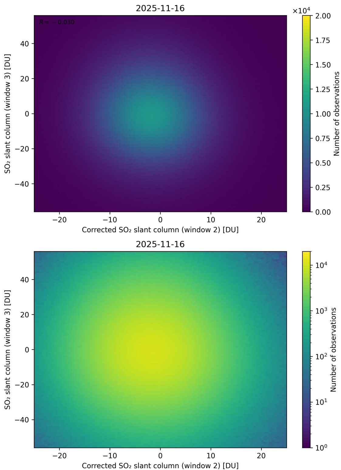
Figure 251: Scatter density plot of “Corrected SO 2 slant column (window 2)” against “SO 2 slant column (window 3)” for 2025-11-15 to 2025-11-17.
