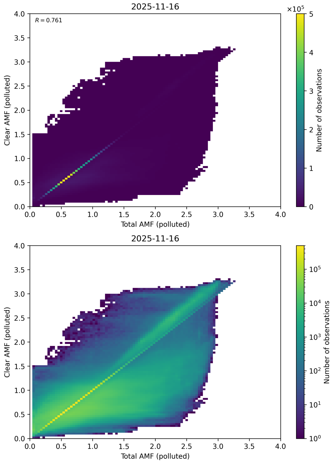
Figure 320: Scatter density plot of “Total AMF (polluted)” against “Clear AMF (polluted)” for 2025-11-15 to 2025-11-17.
