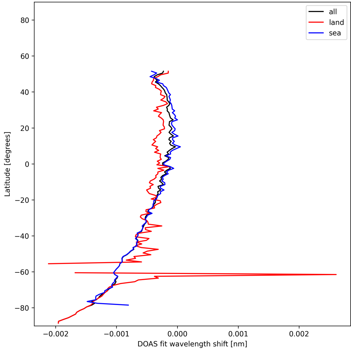
Figure 50: Zonal average of "DOAS fit wavelength shift" for 2025-11-15 to 2025-11-17.
