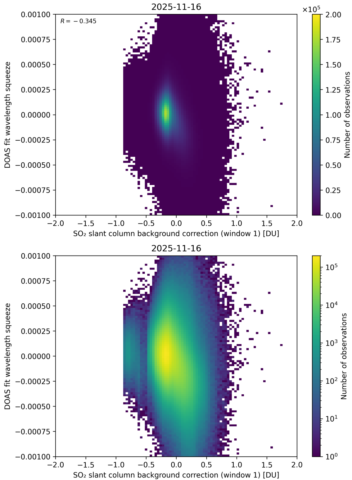
Figure 112: Scatter density plot of “SO 2 slant column background correction (window 1)” against “DOAS fit wavelength squeeze” for 2025-11-15 to 2025-11-17.
