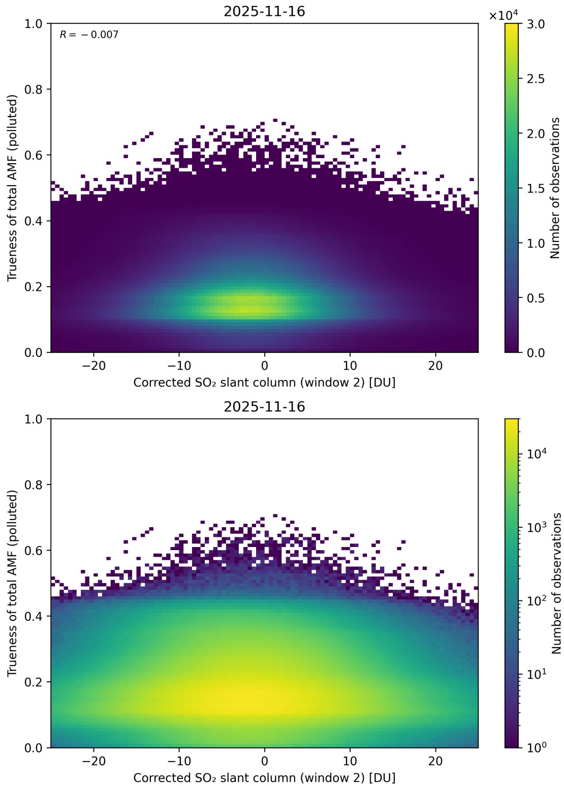
Figure 254: Scatter density plot of “Corrected SO 2 slant column (window 2)” against “Trueness of total AMF (polluted)” for 2025-11-15 to 2025-11-17.
