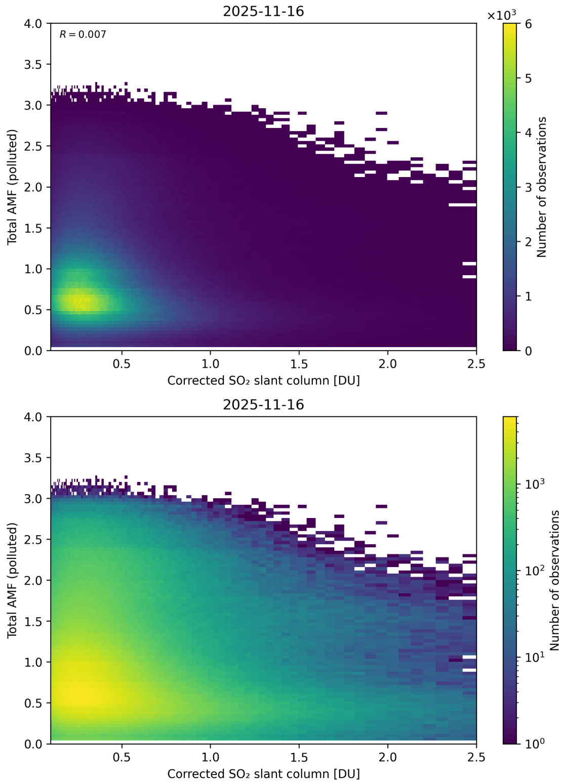
Figure 242: Scatter density plot of “Corrected SO 2 slant column” against “Total AMF (polluted)” for 2025-11-15 to 2025-11-17.
