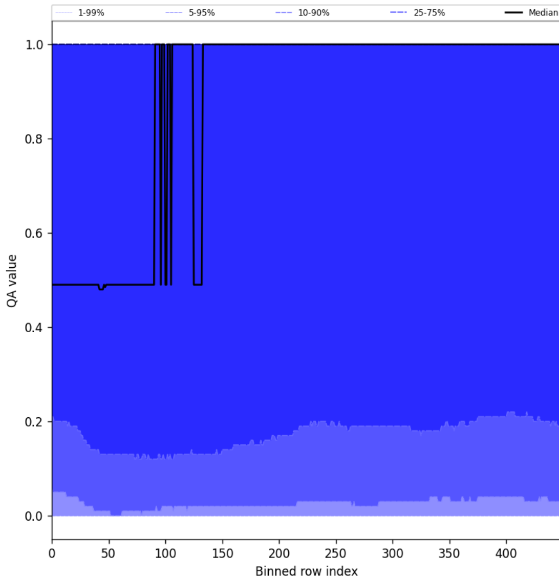
Figure 83: Along track statistics of “QA value” for 2025-11-15 to 2025-11-17
