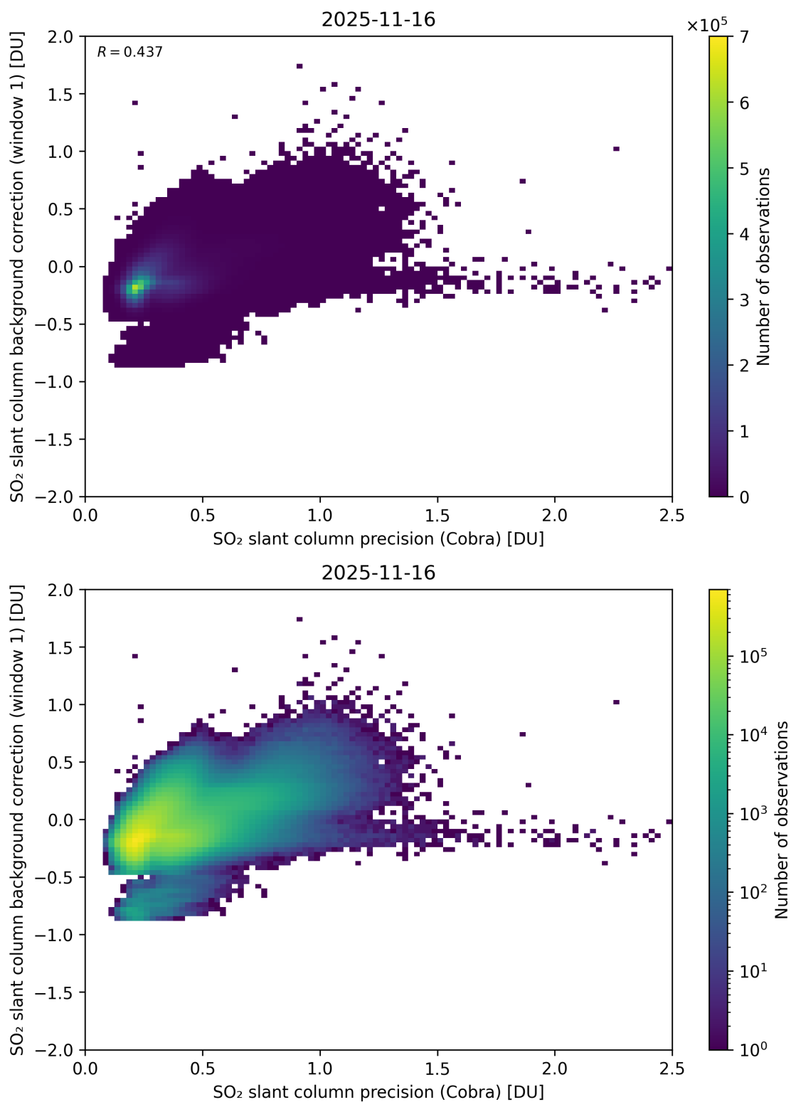
Figure 199: Scatter density plot of “SO 2 slant column precision (Cobra)” against “SO 2 slant column background correction (window 1)” for 2025-11-15 to 2025-11-17.
