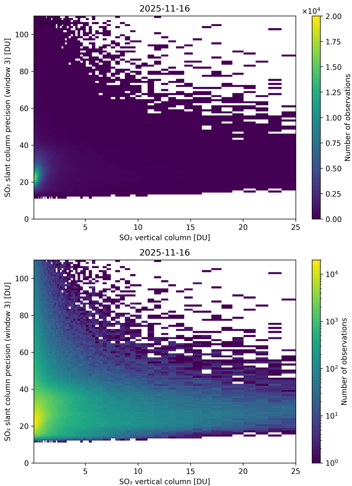
Figure 358: Scatter density plot of “SO 2 vertical column” against “SO 2 slant column precision (window 3)” for 2025-11-15 to 2025-11-17.
