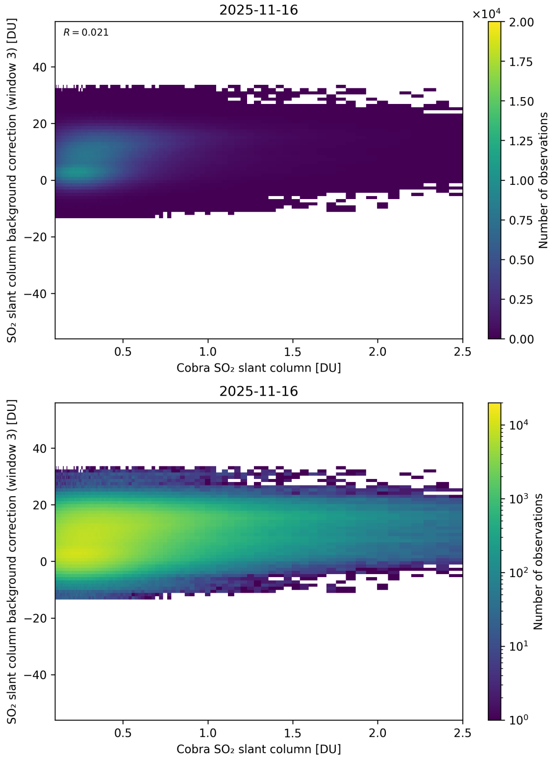
Figure 195: Scatter density plot of “Cobra SO 2 slant column” against “SO 2 slant column background correction (window 3)” for 2025-11-15 to 2025-11-17.
