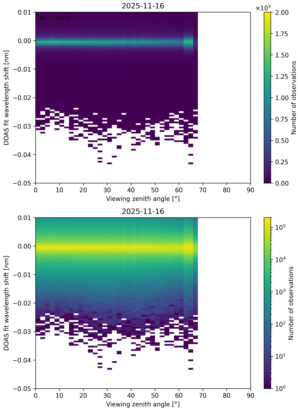
Figure 365: Scatter density plot of “Viewing zenith angle” against “DOAS fit wavelength shift” for 2025-11-15 to 2025-11-17.
