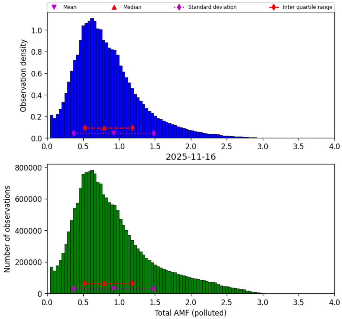
Figure 79: Histogram of “Total AMF (polluted)” for 2025-11-15 to 2025-11-17
