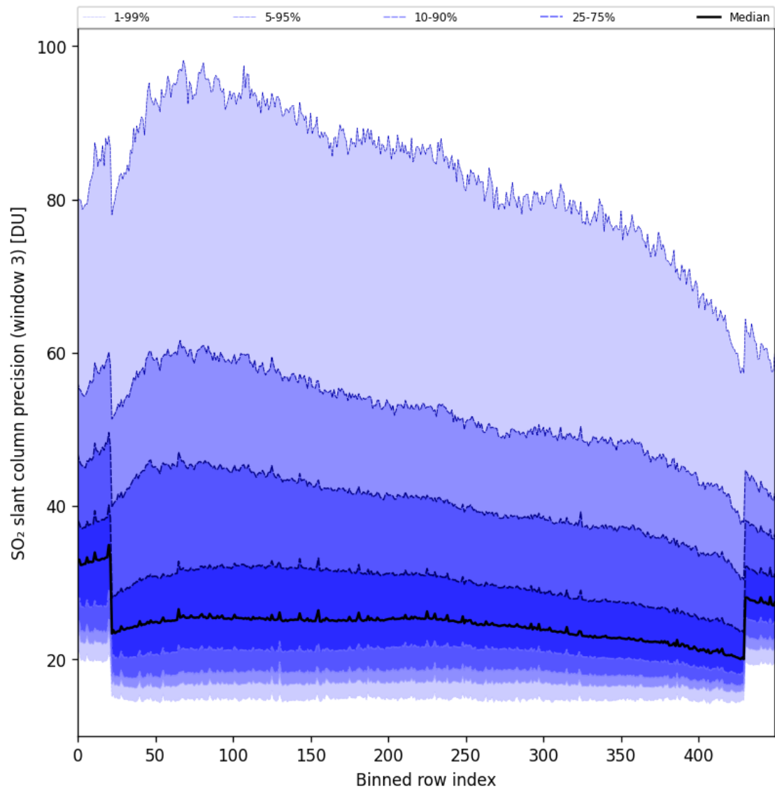
Figure 98: Along track statistics of “SO 2 slant column precision (window 3)” for 2025-11-15 to 2025-11-17
