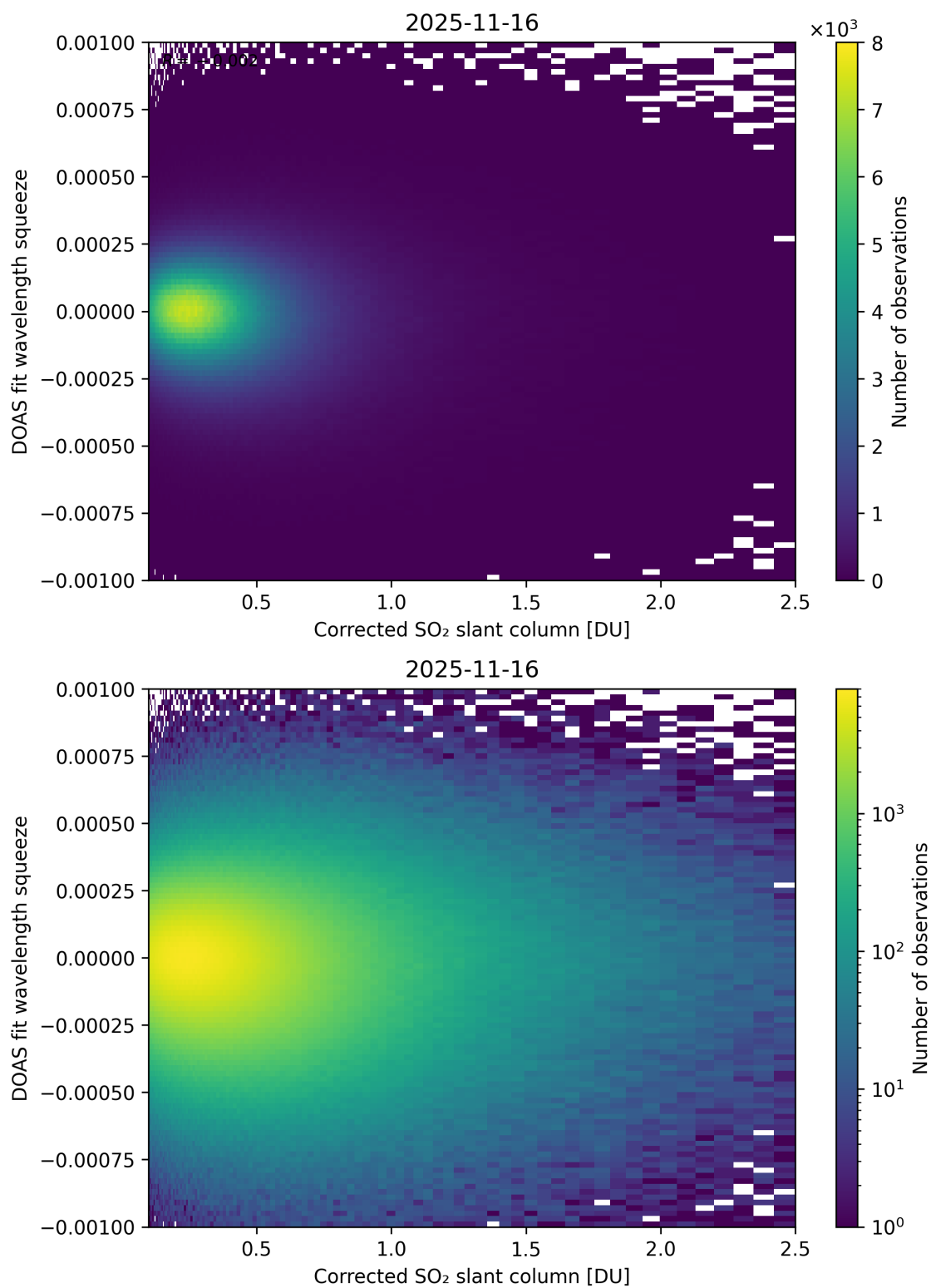
Figure 230: Scatter density plot of “Corrected SO 2 slant column” against “DOAS fit wavelength squeeze” for 2025-11-15 to 2025-11-17.
