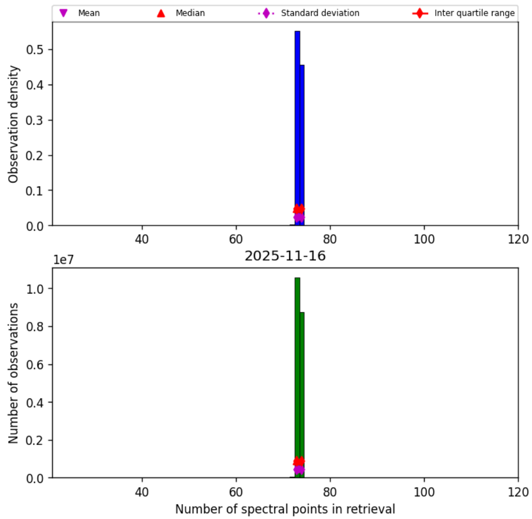
Figure 82: Histogram of "Number of spectral points in retrieval" for 2025-11-15 to 2025-11-17
