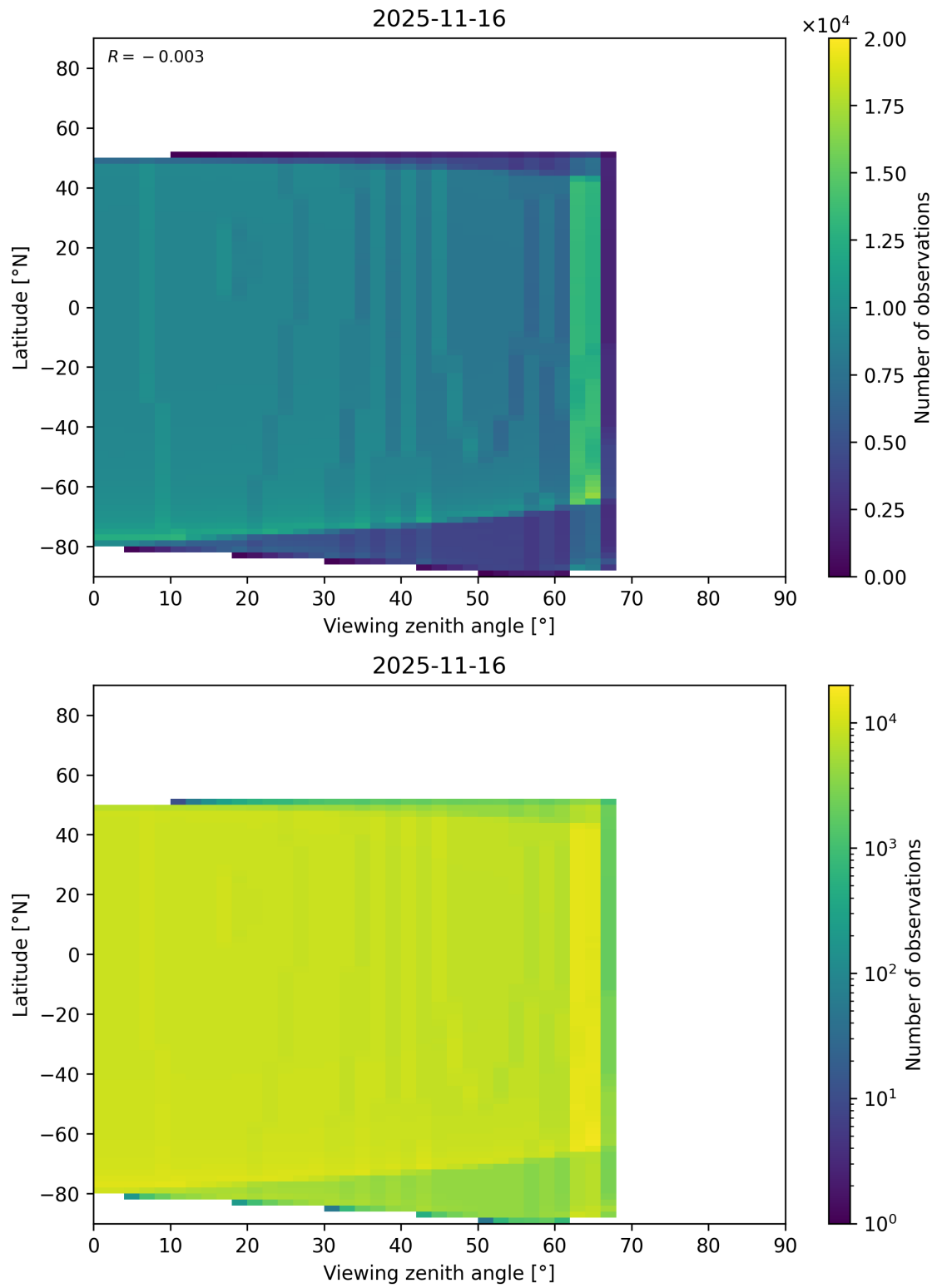
Figure 368: Scatter density plot of “Viewing zenith angle” against “Latitude” for 2025-11-15 to 2025-11-17.
