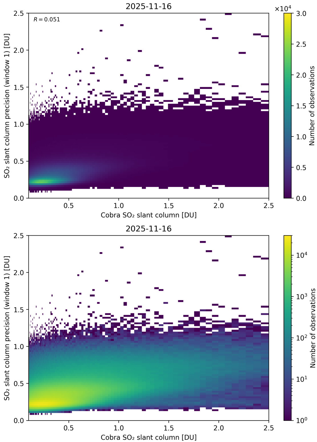
Figure 220: Scatter density plot of “Cobra SO 2 slant column” against “SO 2 slant column precision (window 1)” for 2025-11-15 to 2025-11-17.
