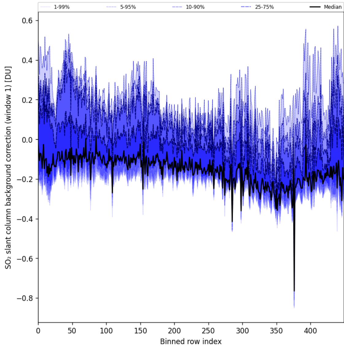
Figure 92: Along track statistics of “SO 2 slant column background correction (window 1)” for 2025-11-15 to 2025-11-17
