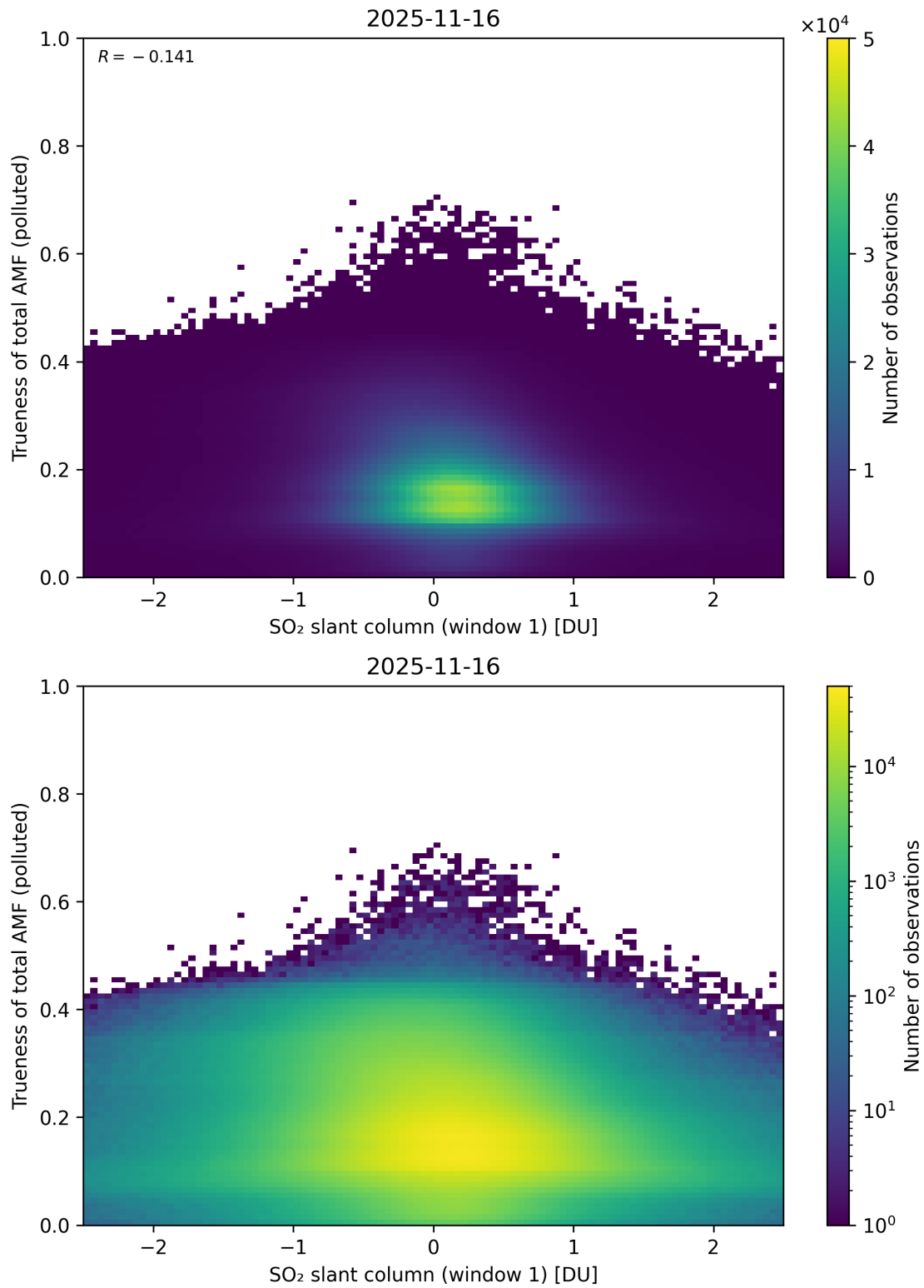
Figure 290: Scatter density plot of “SO 2 slant column (window 1)” against “Trueness of total AMF (polluted)” for 2025-11-15 to 2025-11-17.
