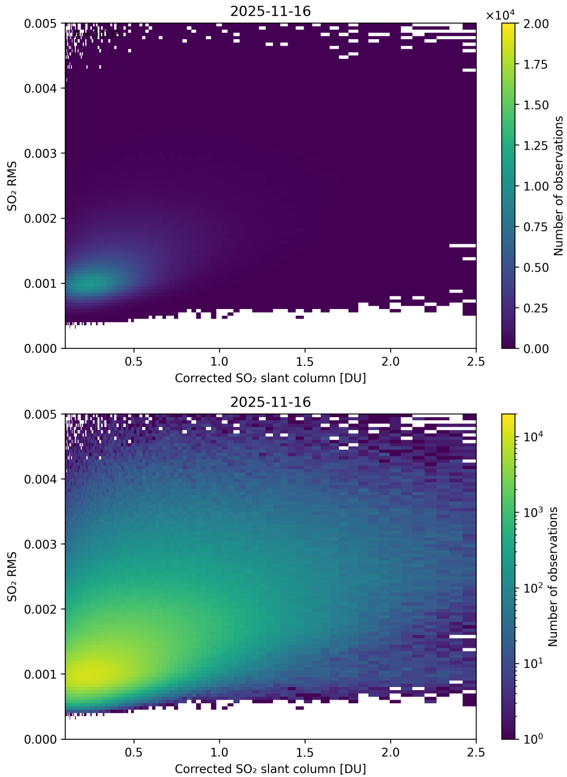
Figure 231: Scatter density plot of “Corrected SO 2 slant column” against “SO 2 RMS” for 2025-11-15 to 2025-11-17.
