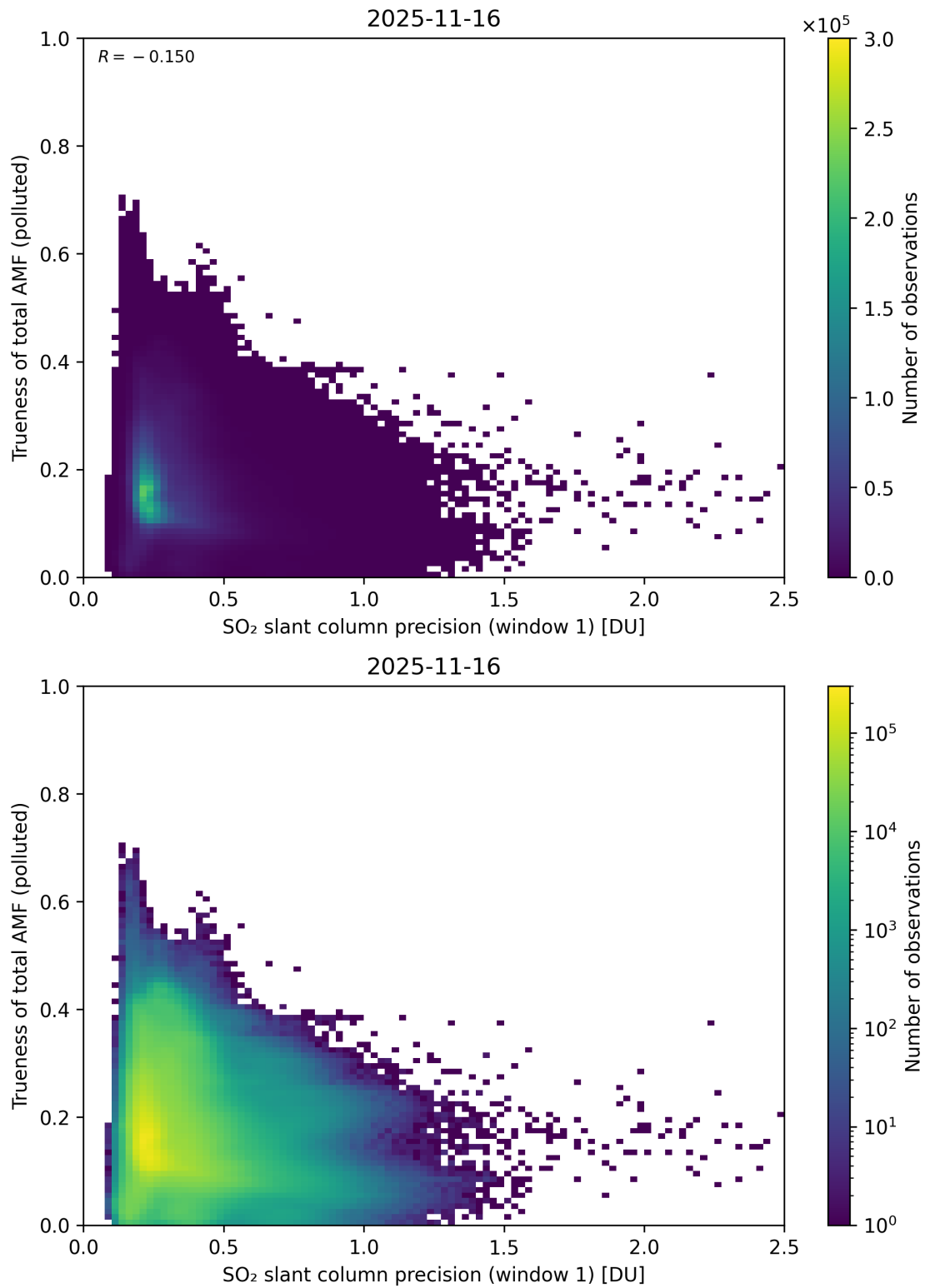
Figure 281: Scatter density plot of “SO 2 slant column precision (window 1)” against “Trueness of total AMF (polluted)” for 2025-11-15 to 2025-11-17.
