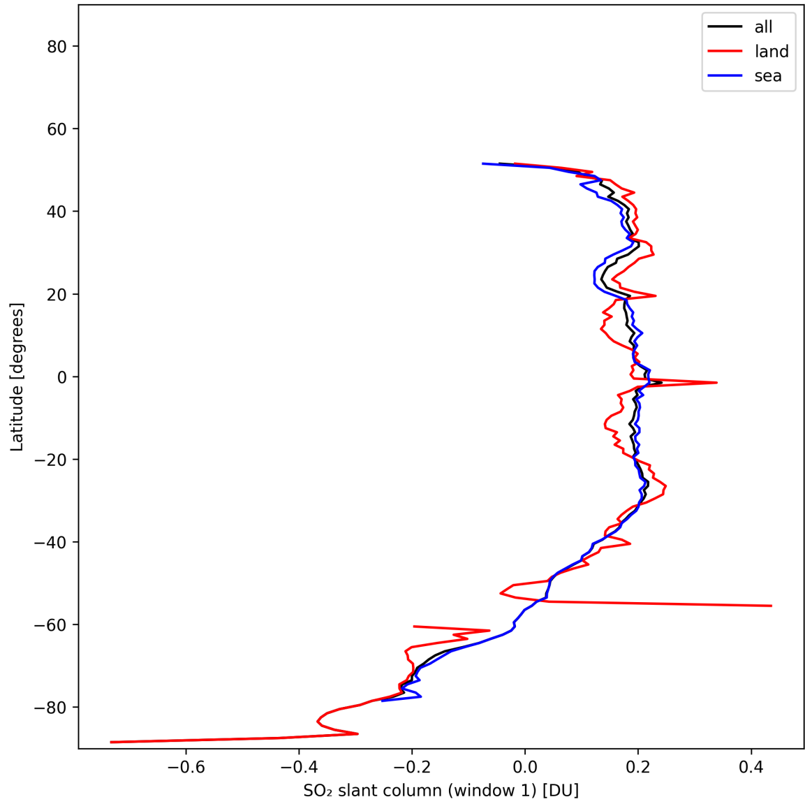
Figure 37: Zonal average of “SO 2 slant column (window 1)” for 2025-11-15 to 2025-11-17.
