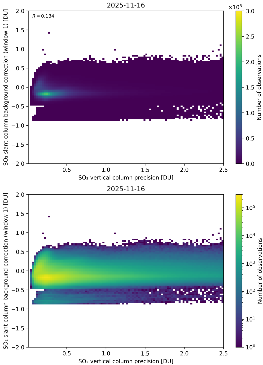
Figure 329: Scatter density plot of “SO 2 vertical column precision” against “SO 2 slant column background correction (window 1)” for 2025-11-15 to 2025-11-17.
