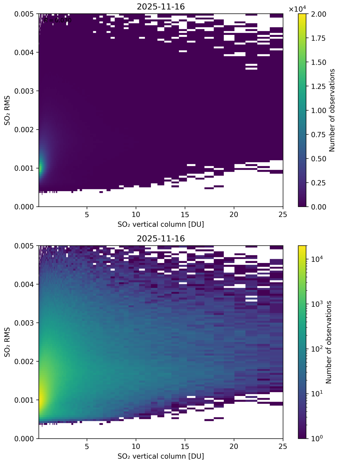
Figure 328: Scatter density plot of “SO 2 vertical column” against “SO 2 RMS” for 2025-11-15 to 2025-11-17.
