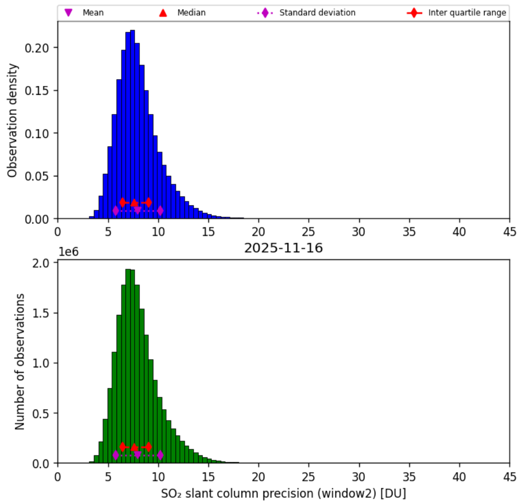
Figure 68: Histogram of “SO 2 slant column precision (window2)” for 2025-11-15 to 2025-11-17
