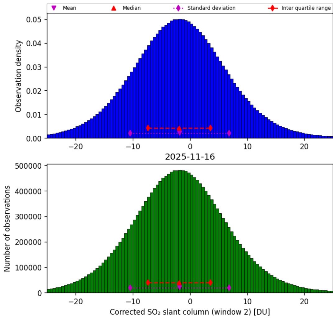
Figure 69: Histogram of “Corrected SO 2 slant column (window 2)” for 2025-11-15 to 2025-11-17
