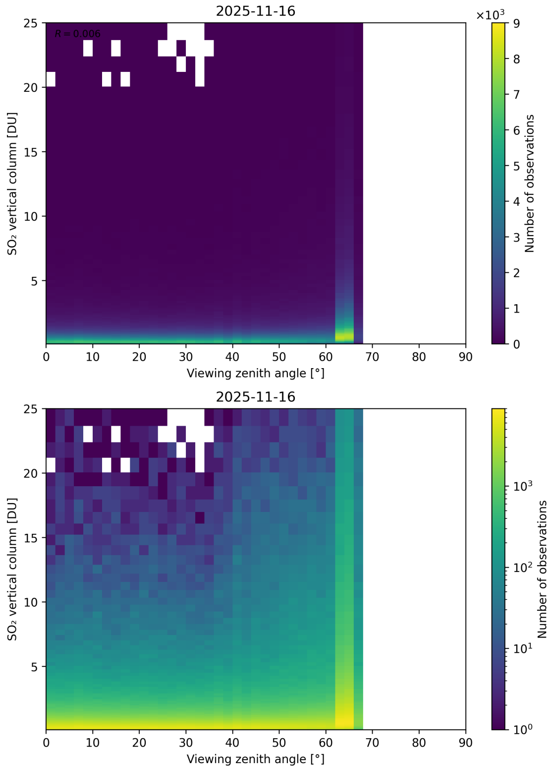
Figure 383: Scatter density plot of “Viewing zenith angle” against “SO 2 vertical column” for 2025-11-15 to 2025-11-17.
