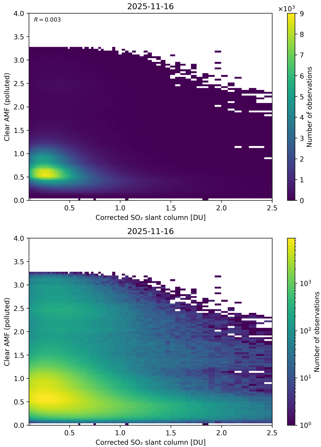
Figure 232: Scatter density plot of “Corrected SO 2 slant column” against “Clear AMF (polluted)” for 2025-11-15 to 2025-11-17.
