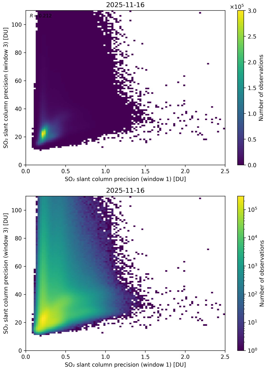
Figure 279: Scatter density plot of “SO 2 slant column precision (window 1)” against “SO 2 slant column precision (window 3)” for 2025-11-15 to 2025-11-17.
