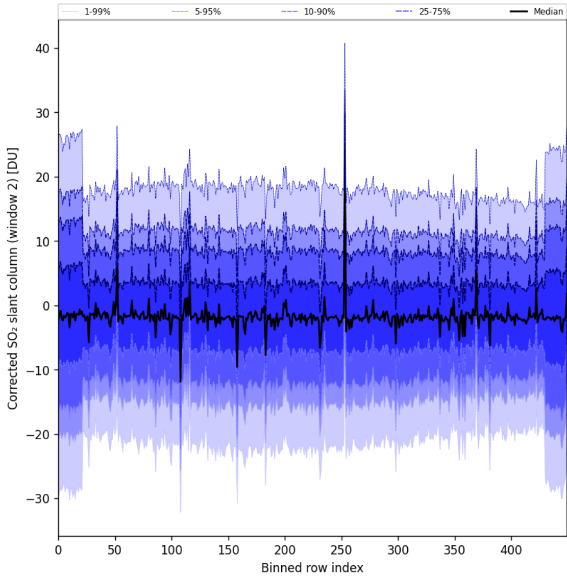
Figure 95: Along track statistics of “Corrected SO 2 slant column (window 2)” for 2025-11-15 to 2025-11-17
