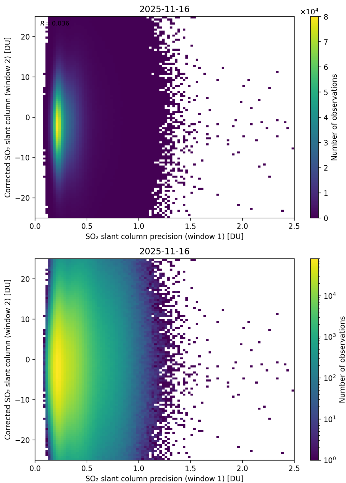
Figure 275: Scatter density plot of “SO 2 slant column precision (window 1)” against “Corrected SO 2 slant column (window 2)” for 2025-11-15 to 2025-11-17.
