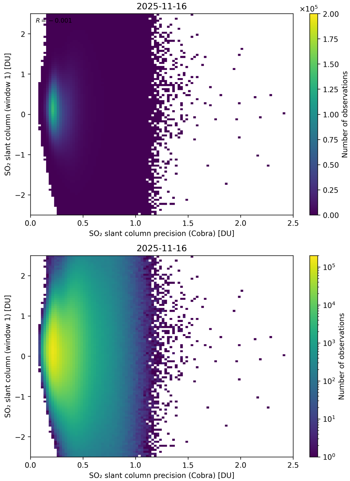
Figure 208: Scatter density plot of “SO 2 slant column precision (Cobra)” against “SO 2 slant column (window 1)” for 2025-11-15 to 2025-11-17.
