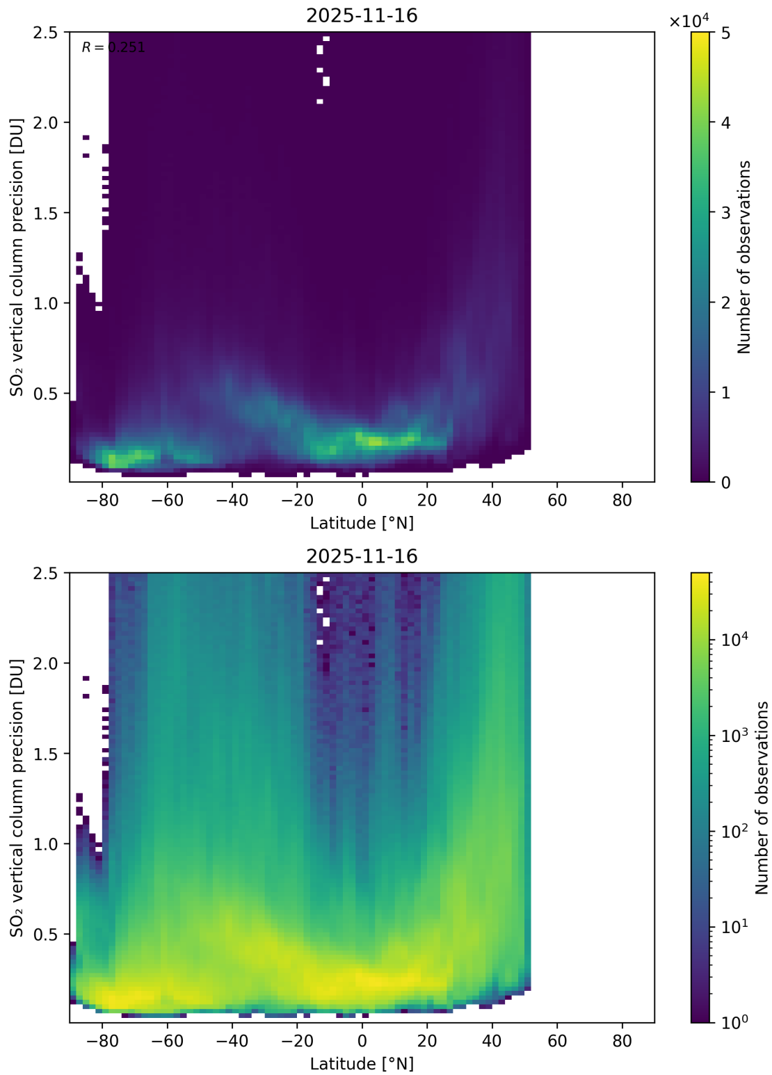
Figure 170: Scatter density plot of “Latitude” against “SO 2 vertical column precision” for 2025-11-15 to 2025-11-17.
