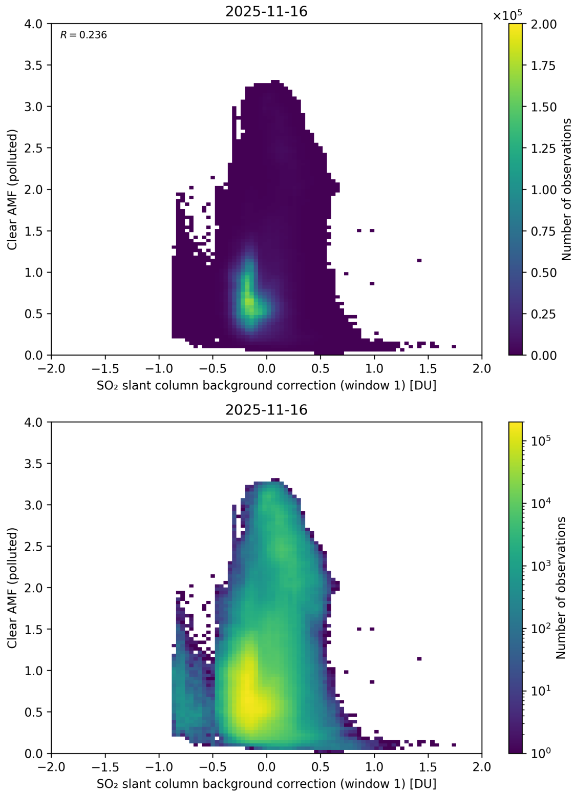
Figure 114: Scatter density plot of “SO 2 slant column background correction (window 1)” against “Clear AMF (polluted)” for 2025-11-15 to 2025-11-17.
