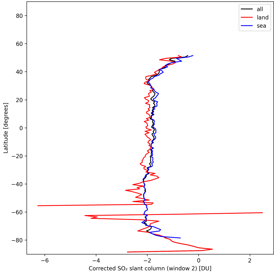
Figure 43: Zonal average of “Corrected SO 2 slant column (window 2)” for 2025-11-15 to 2025-11-17.
