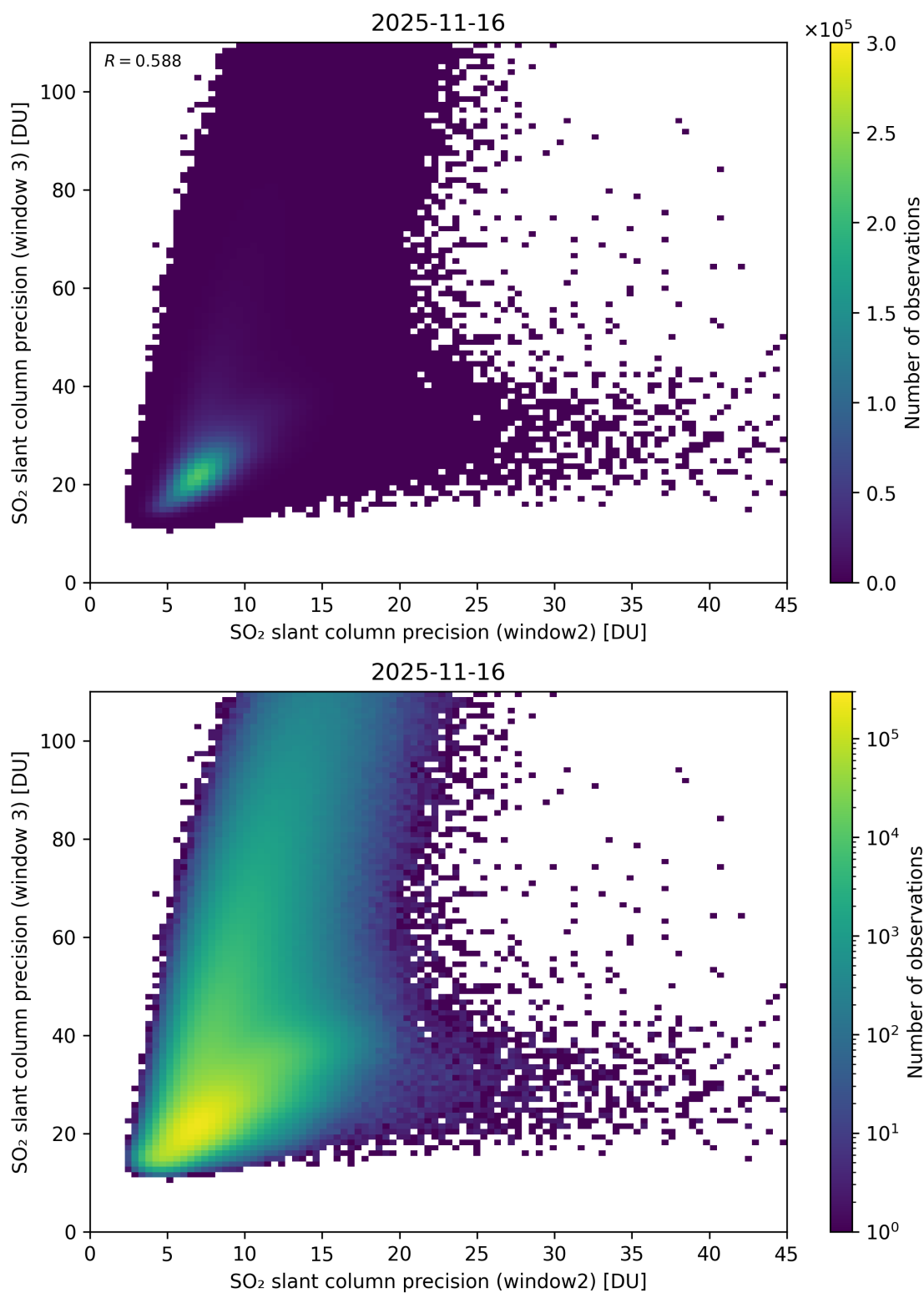
Figure 300: Scatter density plot of “SO 2 slant column precision (window2)” against “SO 2 slant column precision (window 3)” for 2025-11-15 to 2025-11-17.
