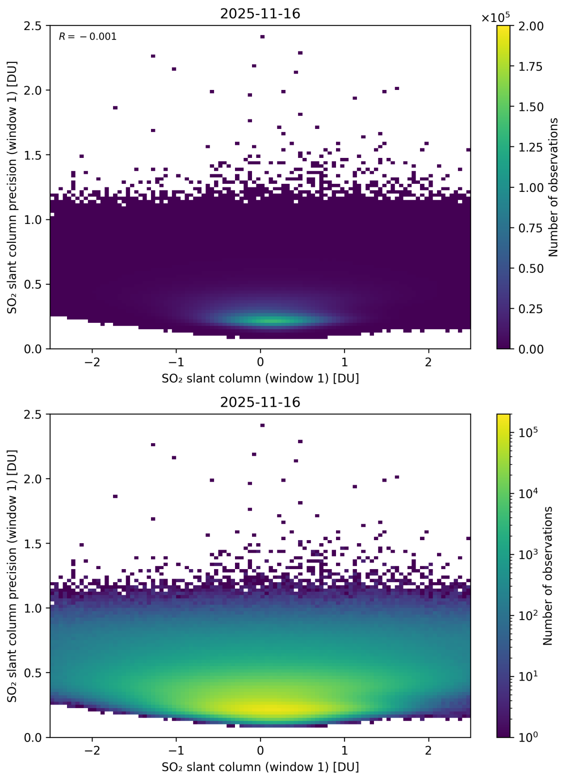
Figure 285: Scatter density plot of “SO 2 slant column (window 1)” against “SO 2 slant column precision (window 1)” for 2025-11-15 to 2025-11-17.
