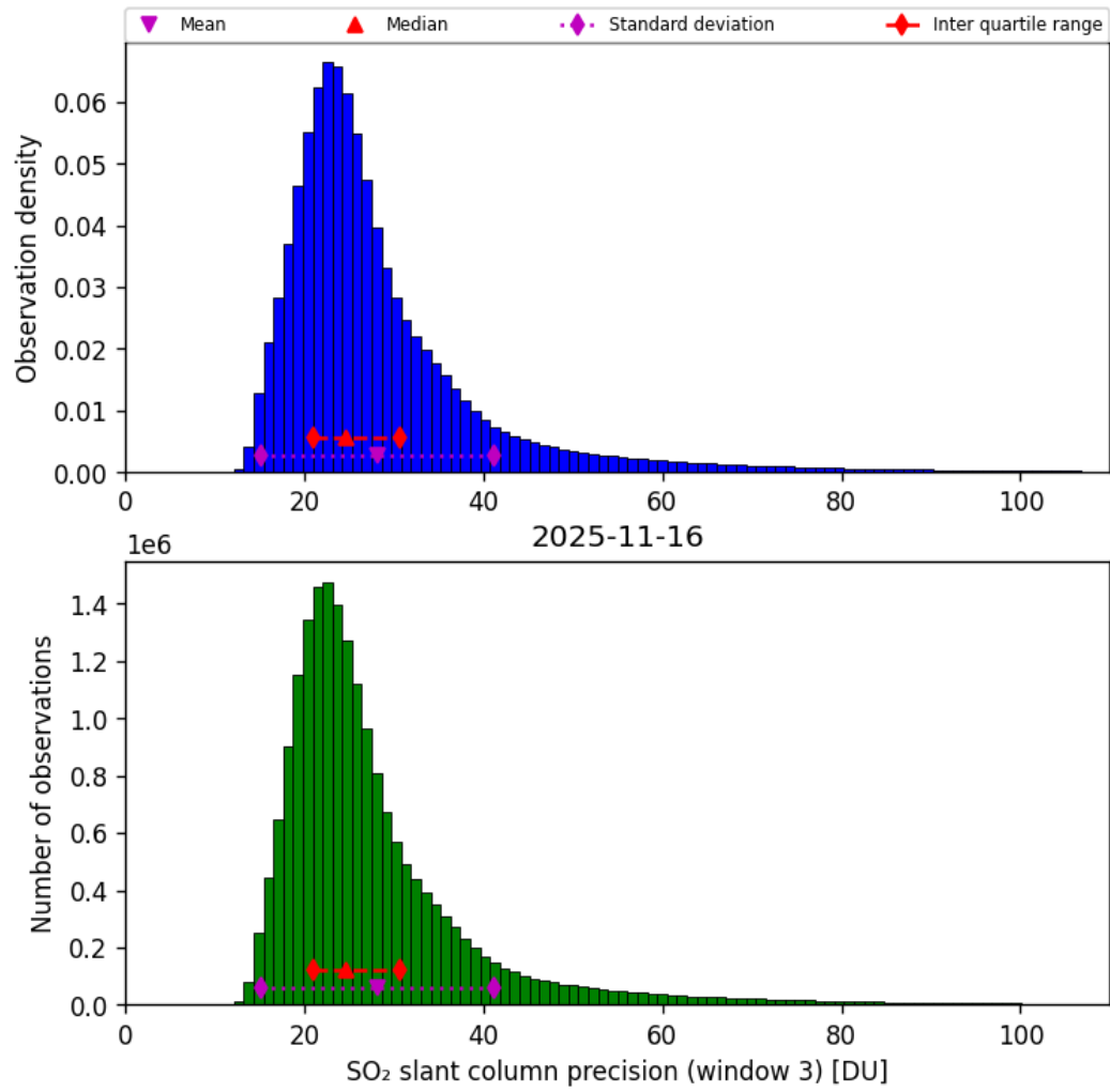
Figure 72: Histogram of “SO 2 slant column precision (window 3)” for 2025-11-15 to 2025-11-17
