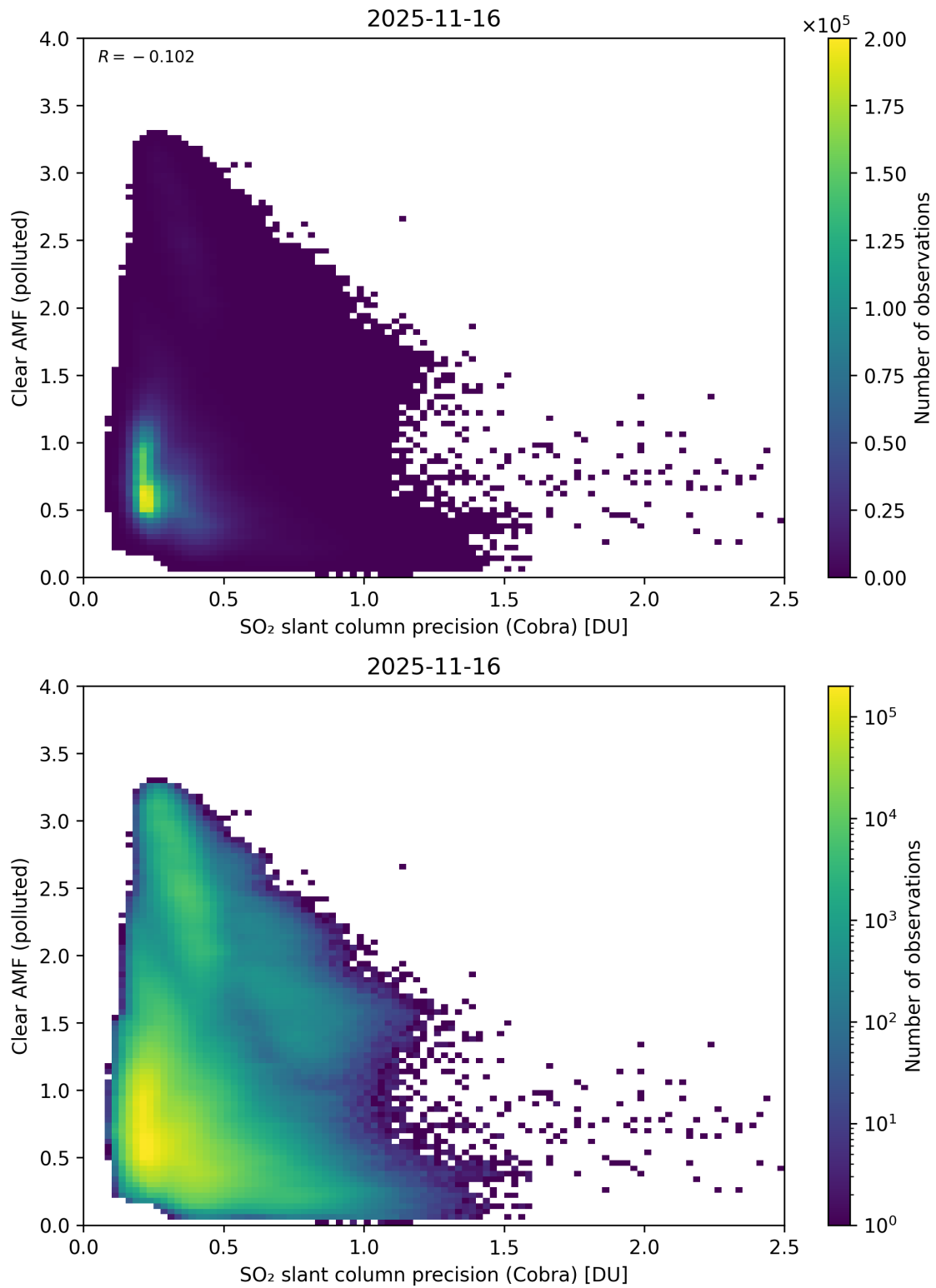
Figure 205: Scatter density plot of “SO 2 slant column precision (Cobra)” against “Clear AMF (polluted)” for 2025-11-15 to 2025-11-17.
