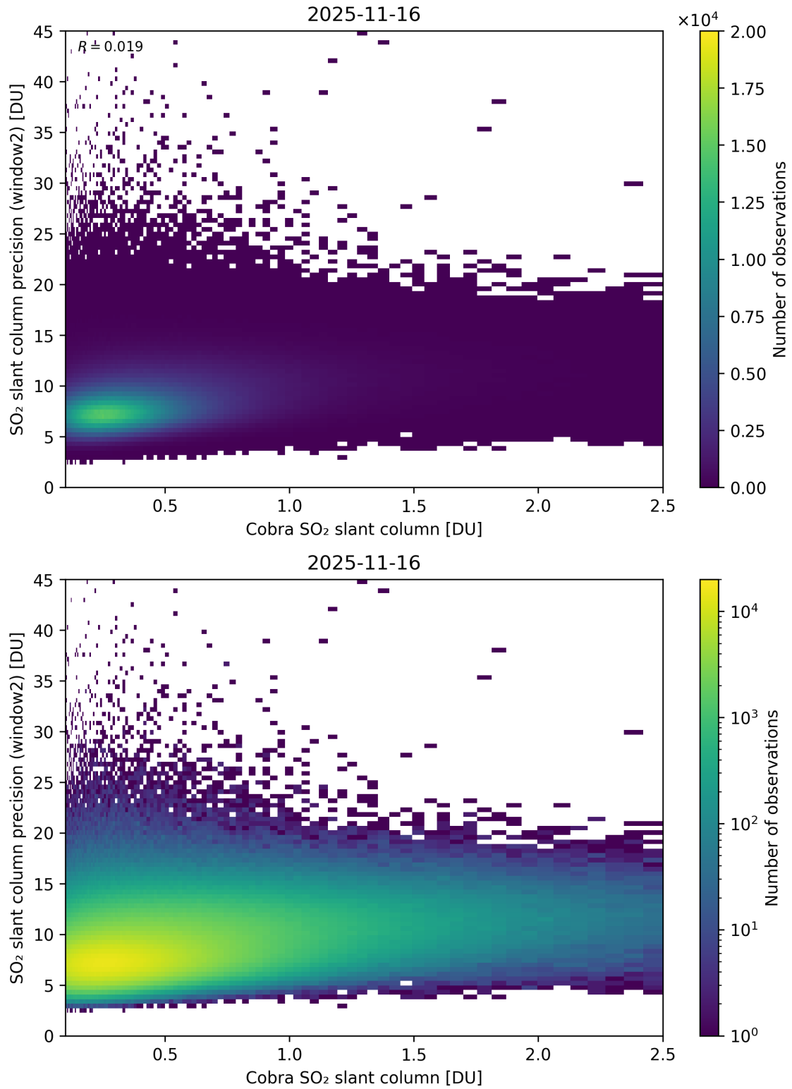
Figure 221: Scatter density plot of “Cobra SO 2 slant column” against “SO 2 slant column precision (window2)” for 2025-11-15 to 2025-11-17.
