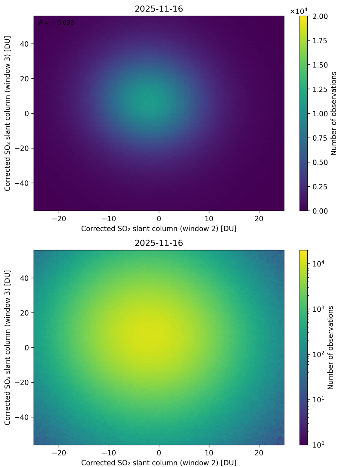
Figure 250: Scatter density plot of “Corrected SO 2 slant column (window 2)” against “Corrected SO 2 slant column (window 3)” for 2025-11-15 to 2025-11-17.
