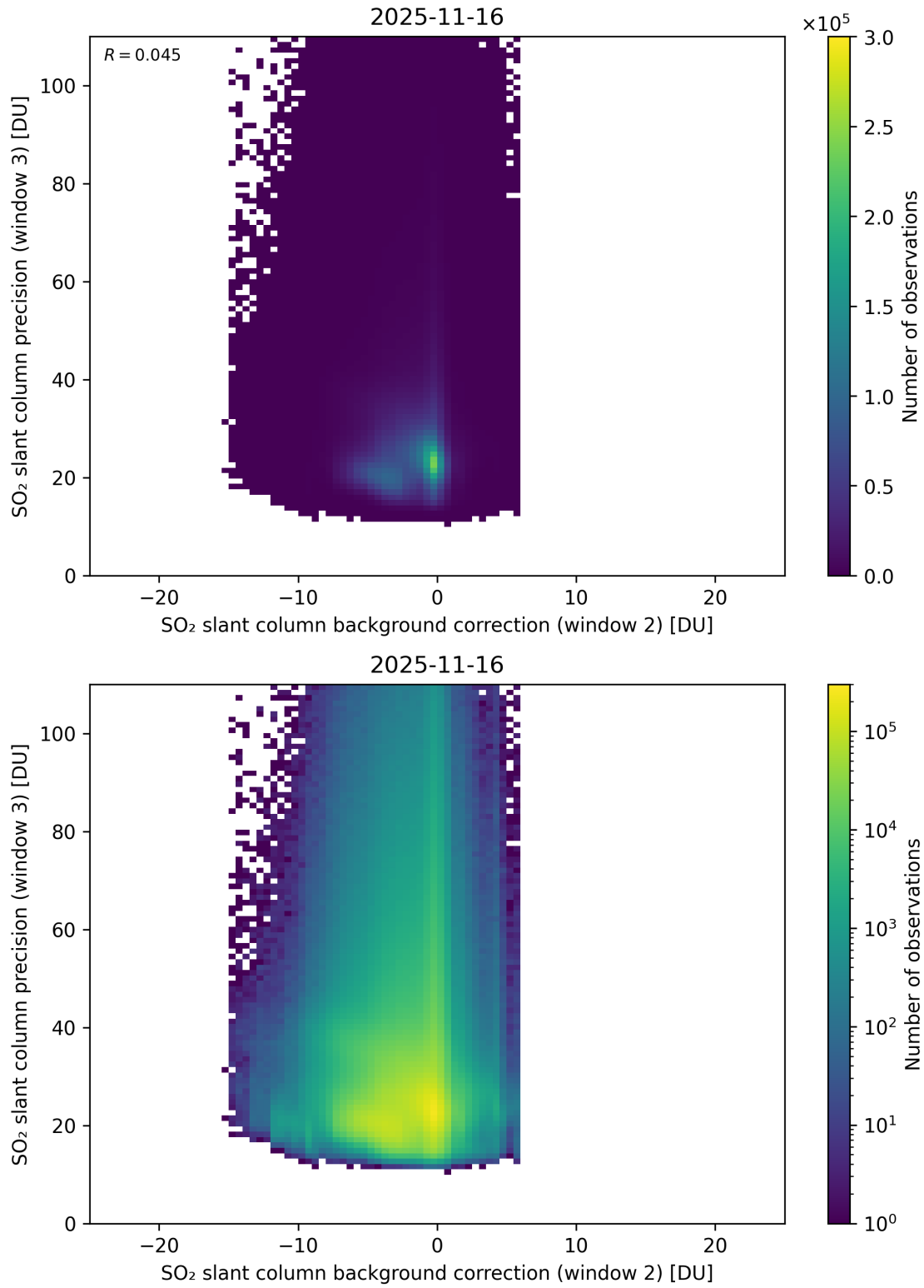
Figure 129: Scatter density plot of “SO 2 slant column background correction (window 2)” against “SO 2 slant column precision (window 3)” for 2025-11-15 to 2025-11-17.
