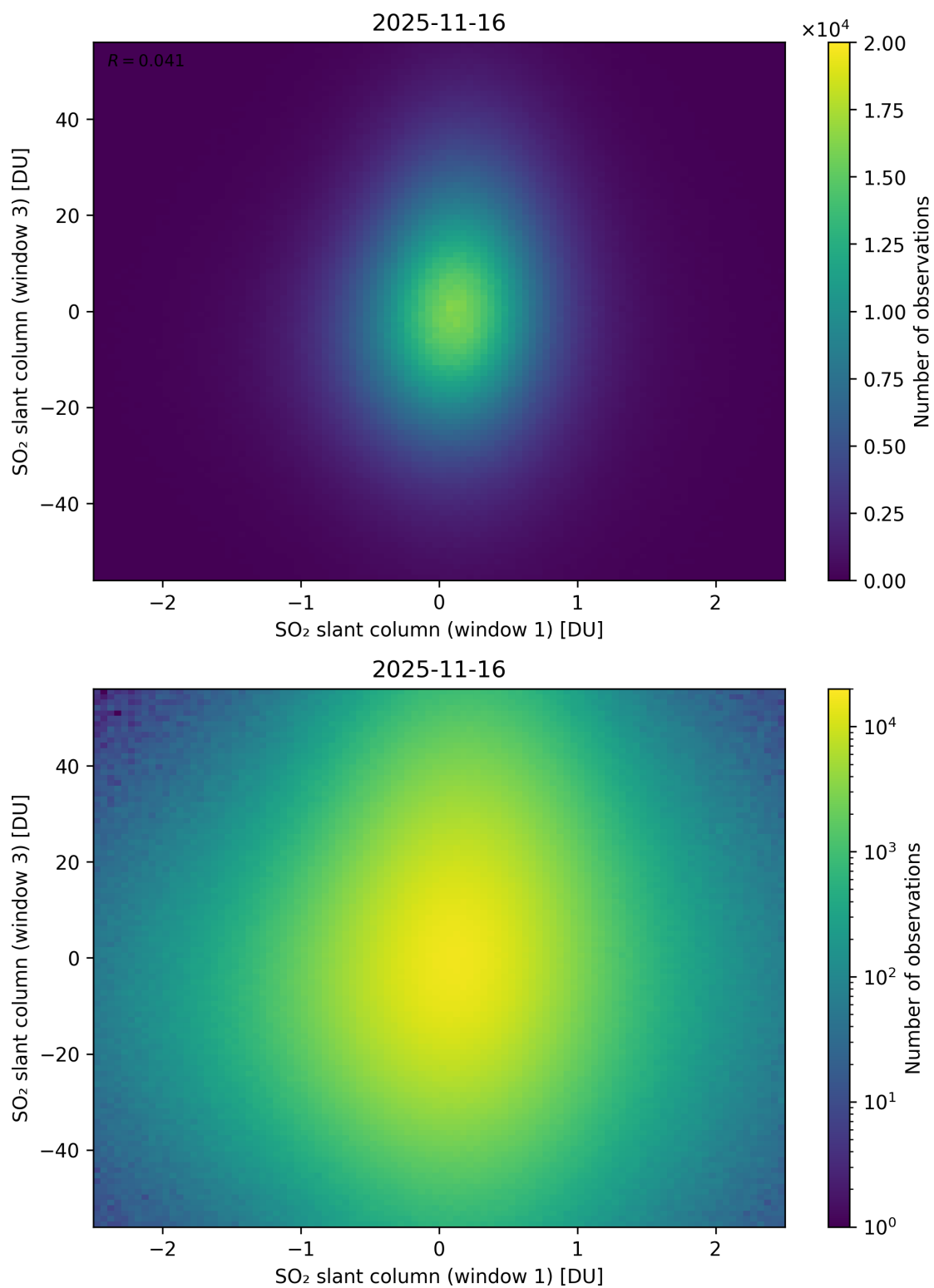
Figure 287: Scatter density plot of “SO 2 slant column (window 1)” against “SO 2 slant column (window 3)” for 2025-11-15 to 2025-11-17.
