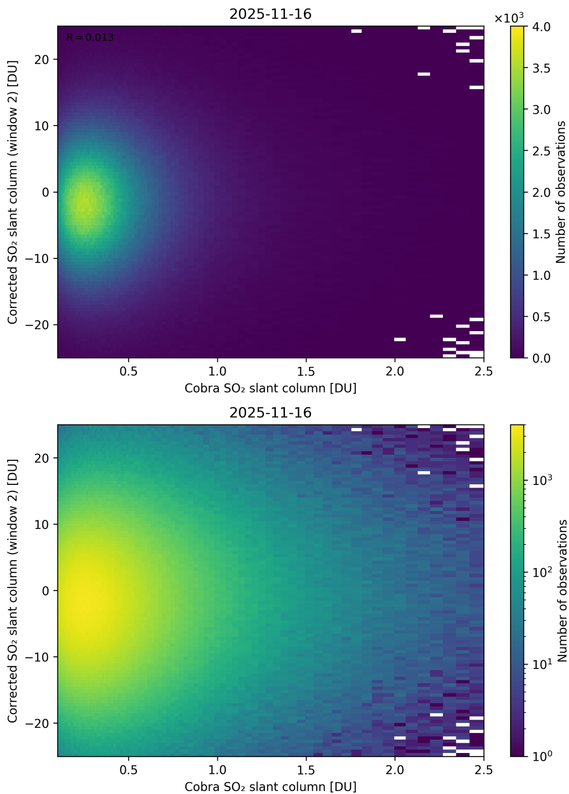
Figure 217: Scatter density plot of “Cobra SO 2 slant column” against “Corrected SO 2 slant column (window 2)” for 2025-11-15 to 2025-11-17.
