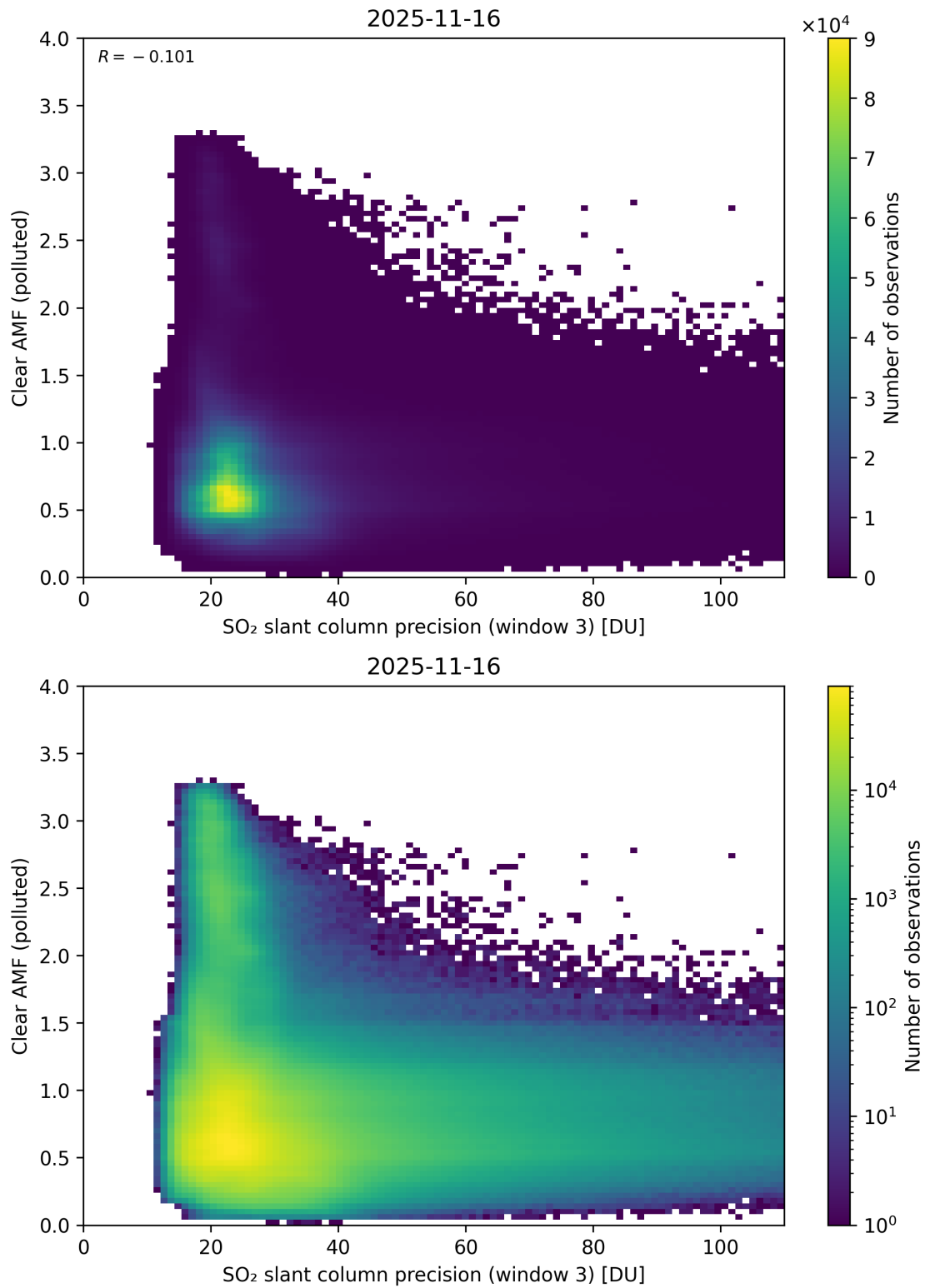
Figure 311: Scatter density plot of “SO 2 slant column precision (window 3)” against “Clear AMF (polluted)” for 2025-11-15 to 2025-11-17.
