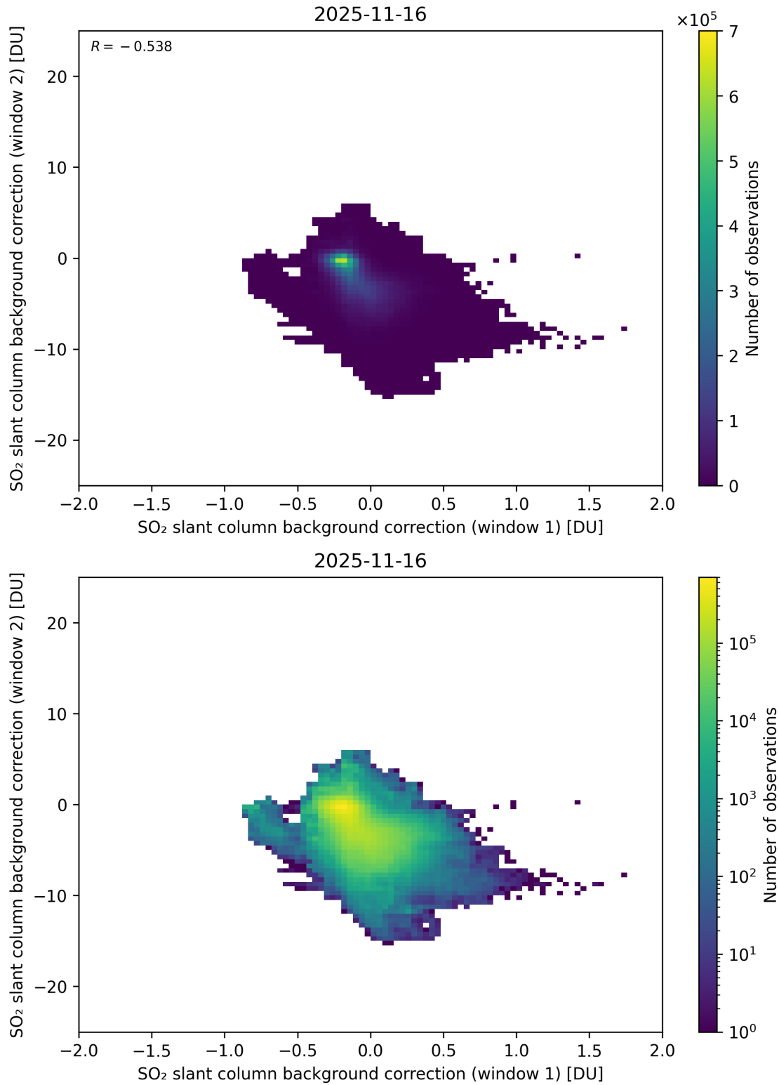
Figure 109: Scatter density plot of “SO 2 slant column background correction (window 1)” against “SO 2 slant column background correction (window 2)” for 2025-11-15 to 2025-11-17.
