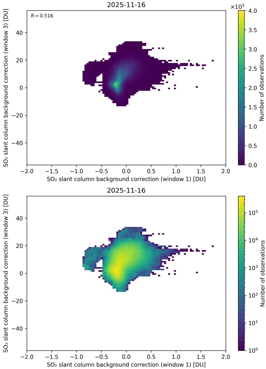
Figure 110: Scatter density plot of “SO 2 slant column background correction (window 1)” against “SO 2 slant column background correction (window 3)” for 2025-11-15 to 2025-11-17.
