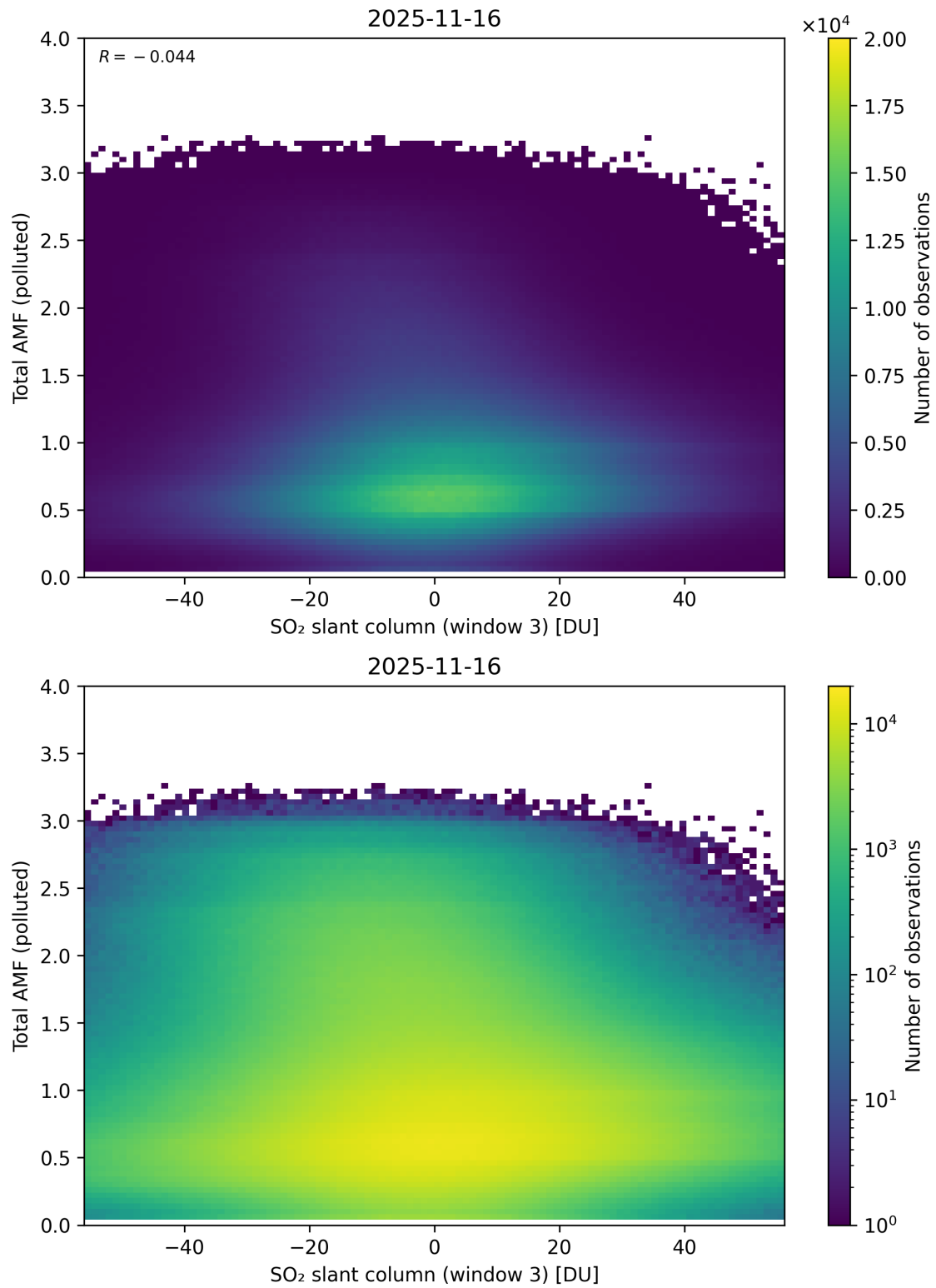
Figure 318: Scatter density plot of “SO 2 slant column (window 3)” against “Total AMF (polluted)” for 2025-11-15 to 2025-11-17.
