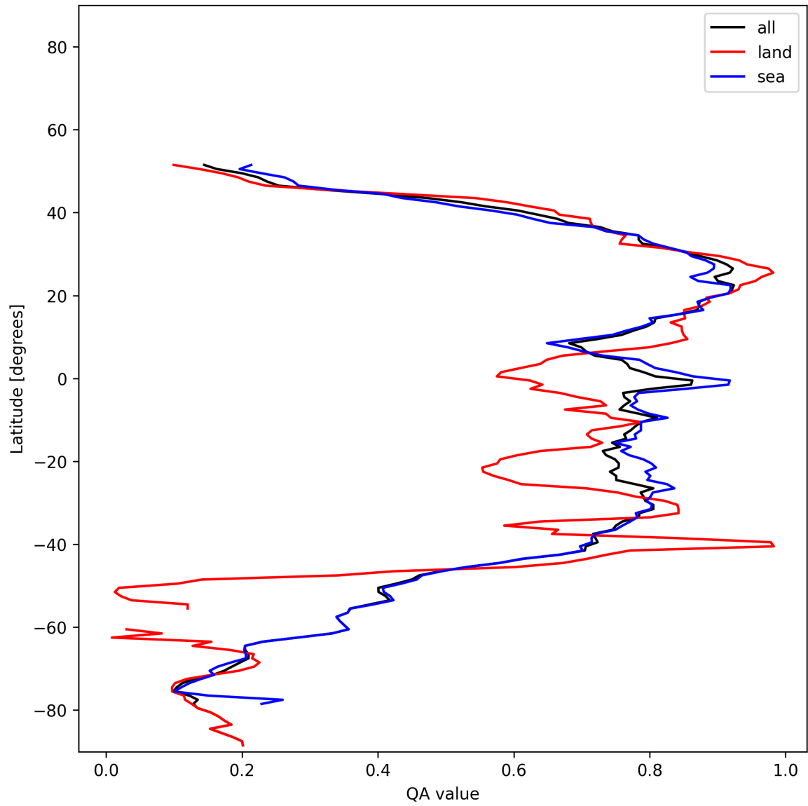
Figure 31: Zonal average of “QA value” for 2025-11-15 to 2025-11-17.
