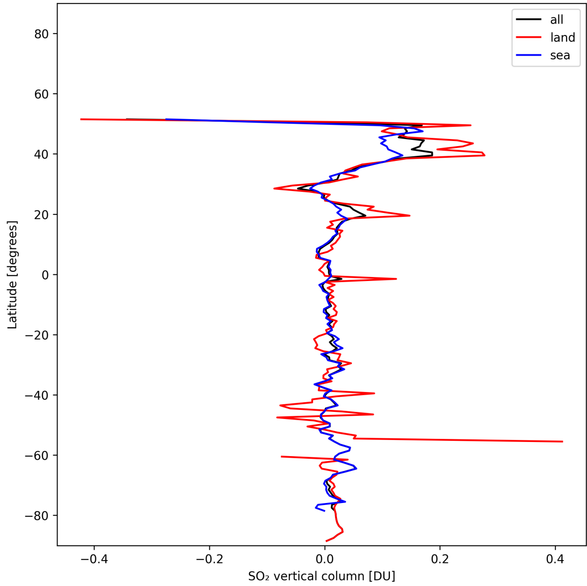
Figure 32: Zonal average of “SO 2 vertical column” for 2025-11-15 to 2025-11-17.
