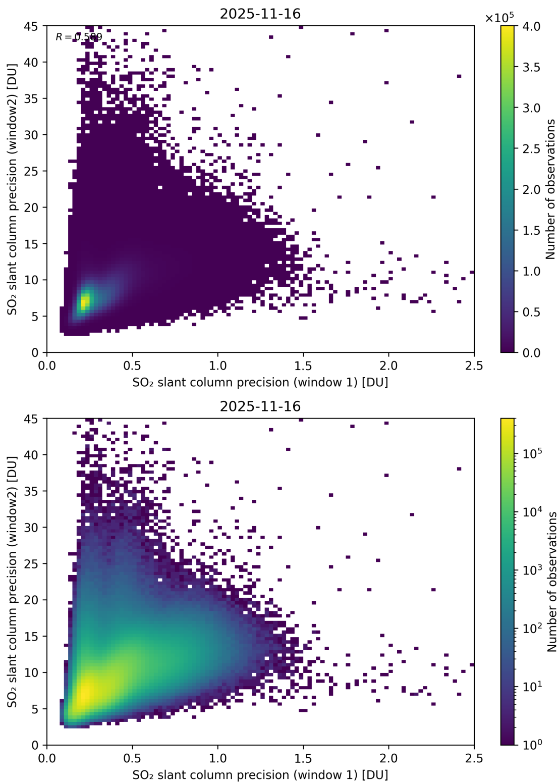
Figure 277: Scatter density plot of “SO 2 slant column precision (window 1)” against “SO 2 slant column precision (window2)” for 2025-11-15 to 2025-11-17.
