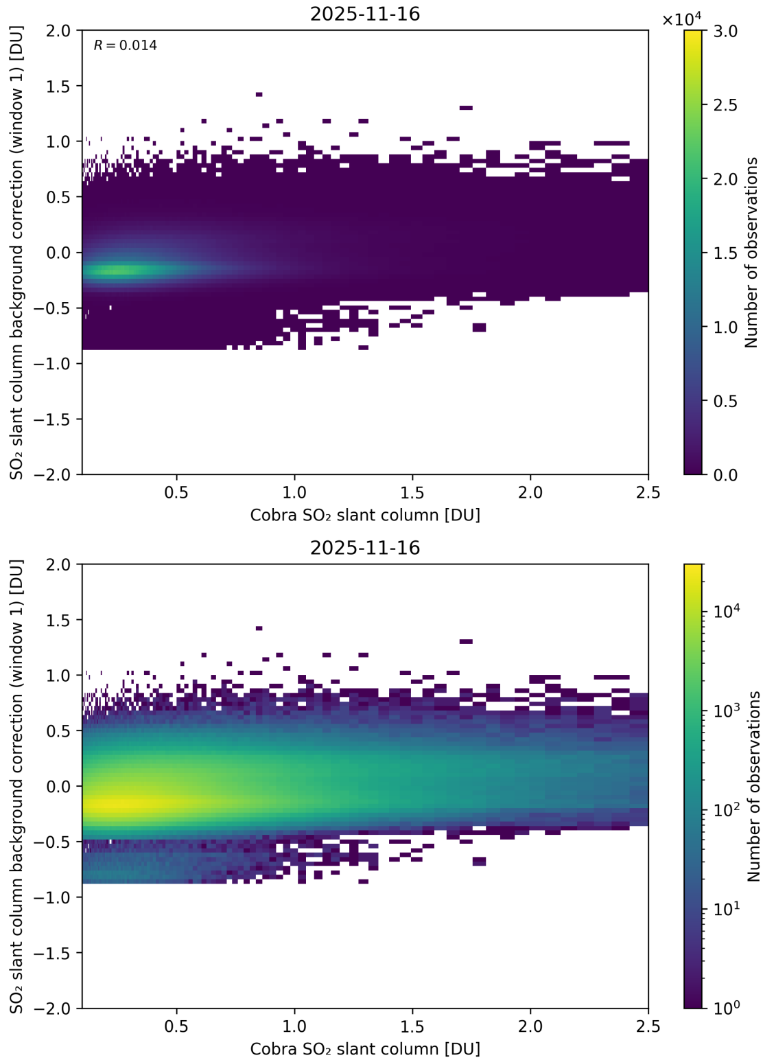
Figure 193: Scatter density plot of “Cobra SO 2 slant column” against “SO 2 slant column background correction (window 1)” for 2025-11-15 to 2025-11-17.
