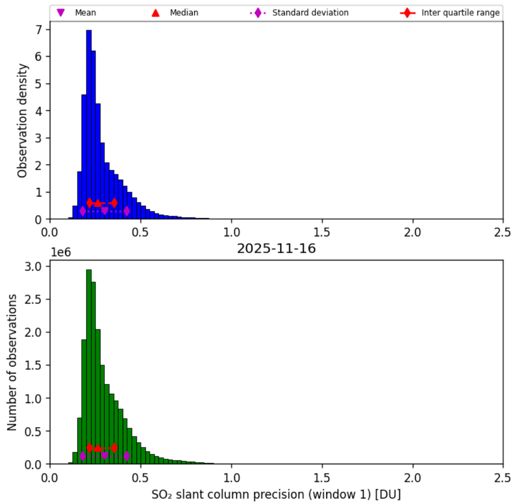
Figure 64: Histogram of “SO 2 slant column precision (window 1)” for 2025-11-15 to 2025-11-17
