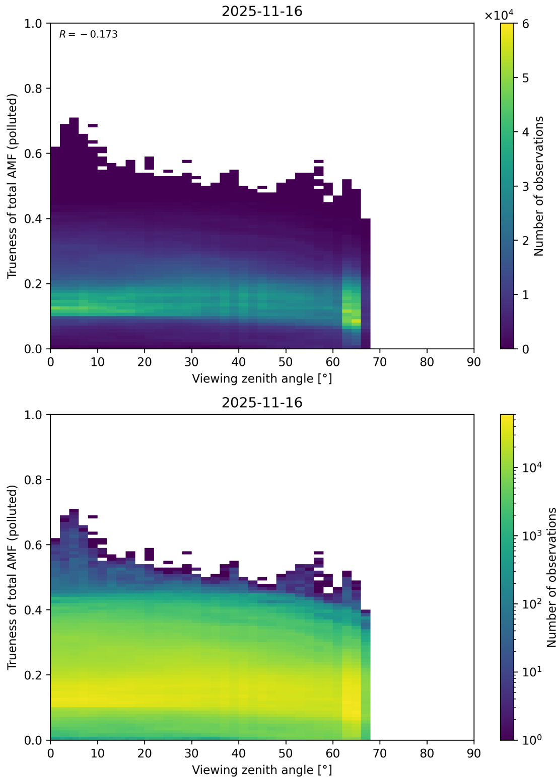
Figure 382: Scatter density plot of “Viewing zenith angle” against “Trueness of total AMF (polluted)” for 2025-11-15 to 2025-11-17.
