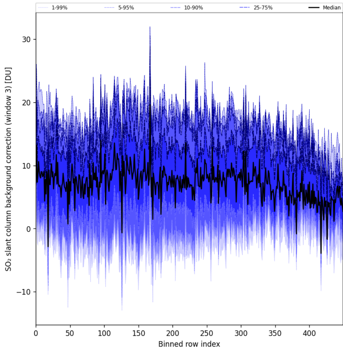
Figure 100: Along track statistics of “SO 2 slant column background correction (window 3)” for 2025-11-15 to 2025-11-17
