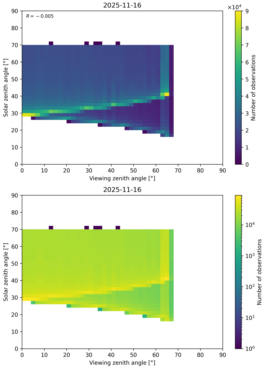
Figure 369: Scatter density plot of “Viewing zenith angle” against “Solar zenith angle” for 2025-11-15 to 2025-11-17.
