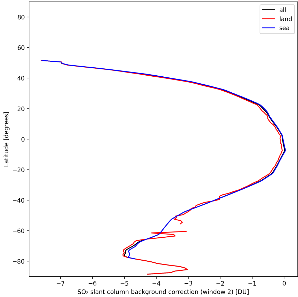
Figure 44: Zonal average of "SO 2 slant column background correction (window 2)" for 2025-11-15 to 2025-11-17.
