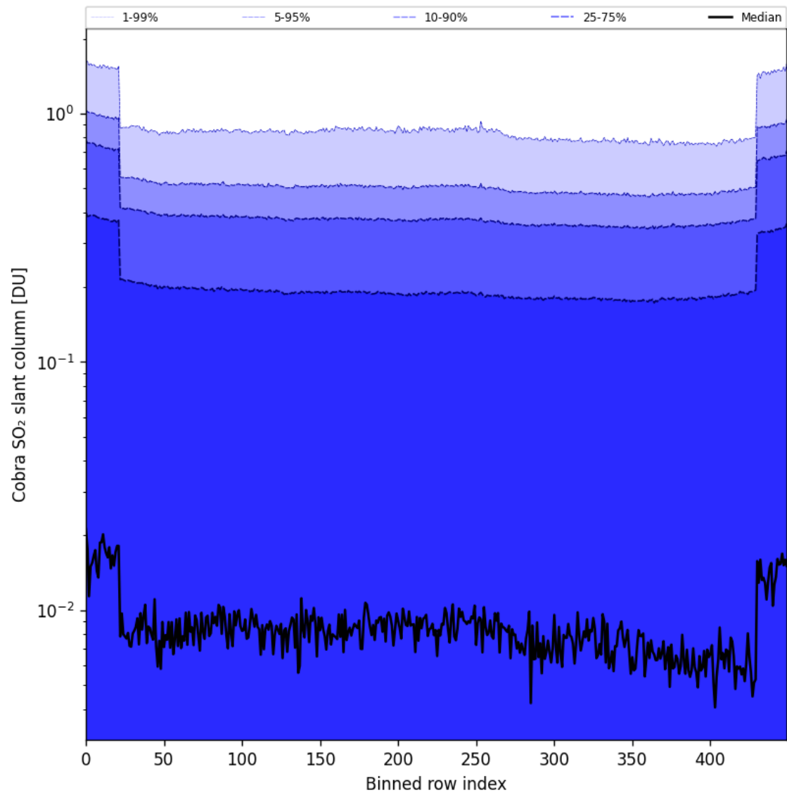
Figure 87: Along track statistics of "Cobra SO 2 slant column" for 2025-11-15 to 2025-11-17
