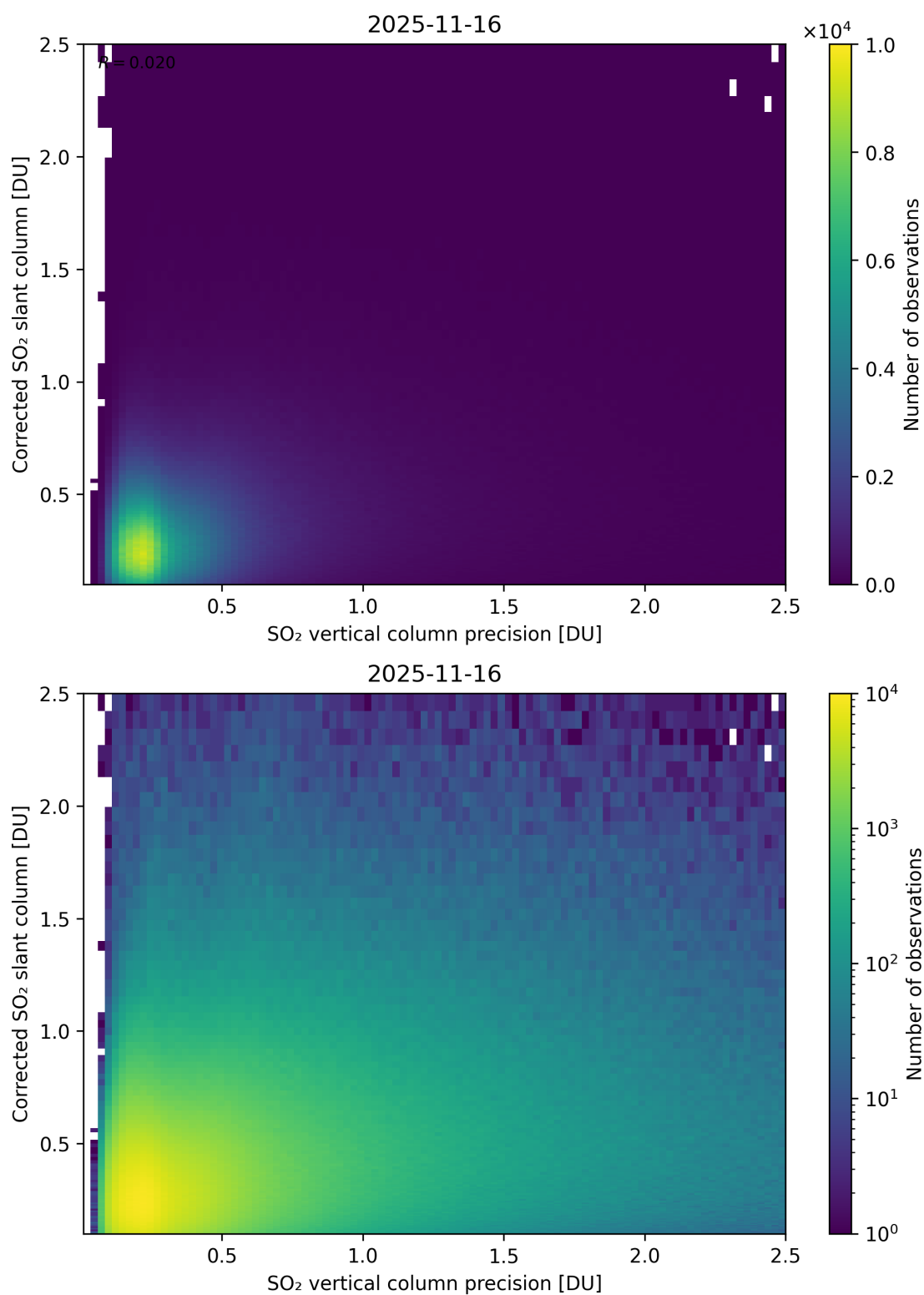
Figure 338: Scatter density plot of “SO 2 vertical column precision” against “Corrected SO 2 slant column” for 2025-11-15 to 2025-11-17.
