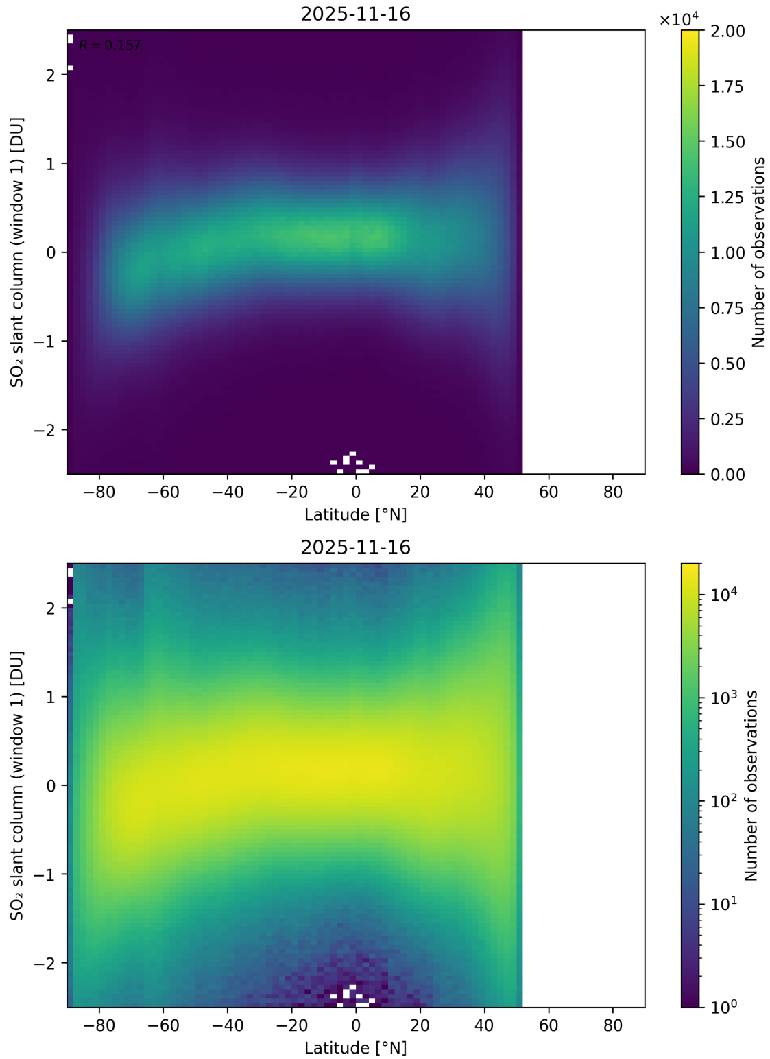
Figure 162: Scatter density plot of “Latitude” against “SO 2 slant column (window 1)” for 2025-11-15 to 2025-11-17.
