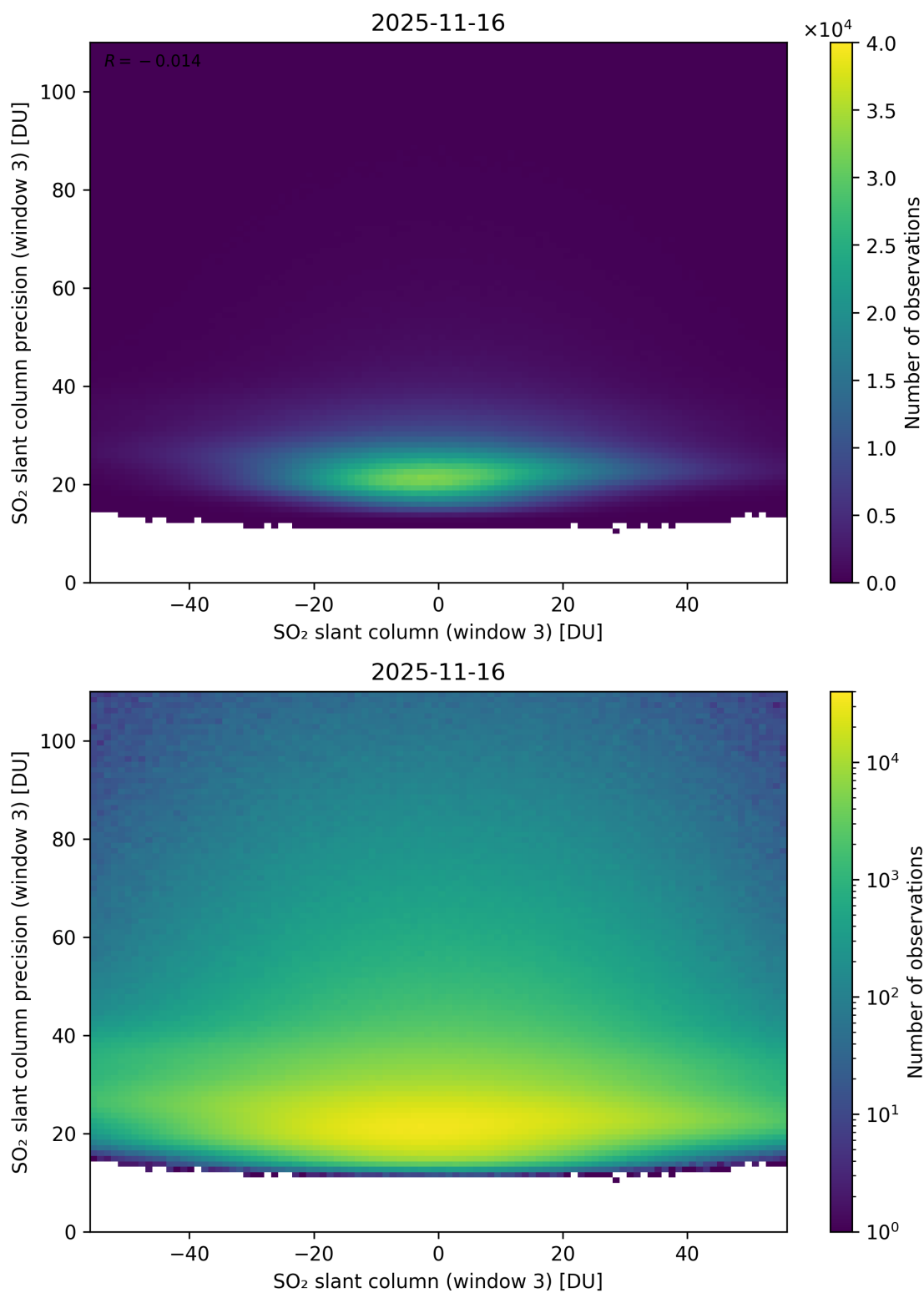
Figure 317: Scatter density plot of “SO 2 slant column (window 3)” against “SO 2 slant column precision (window 3)” for 2025-11-15 to 2025-11-17.
