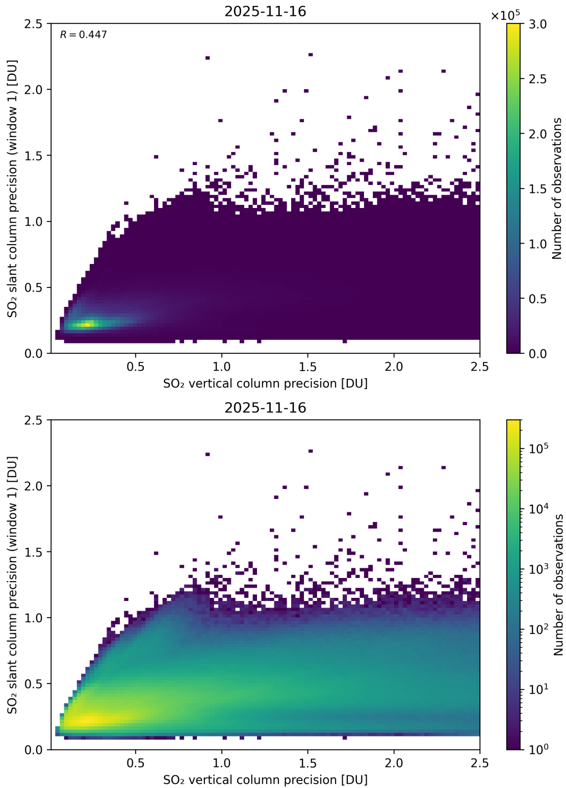
Figure 342: Scatter density plot of “SO 2 vertical column precision” against “SO 2 slant column precision (window 1)” for 2025-11-15 to 2025-11-17.
