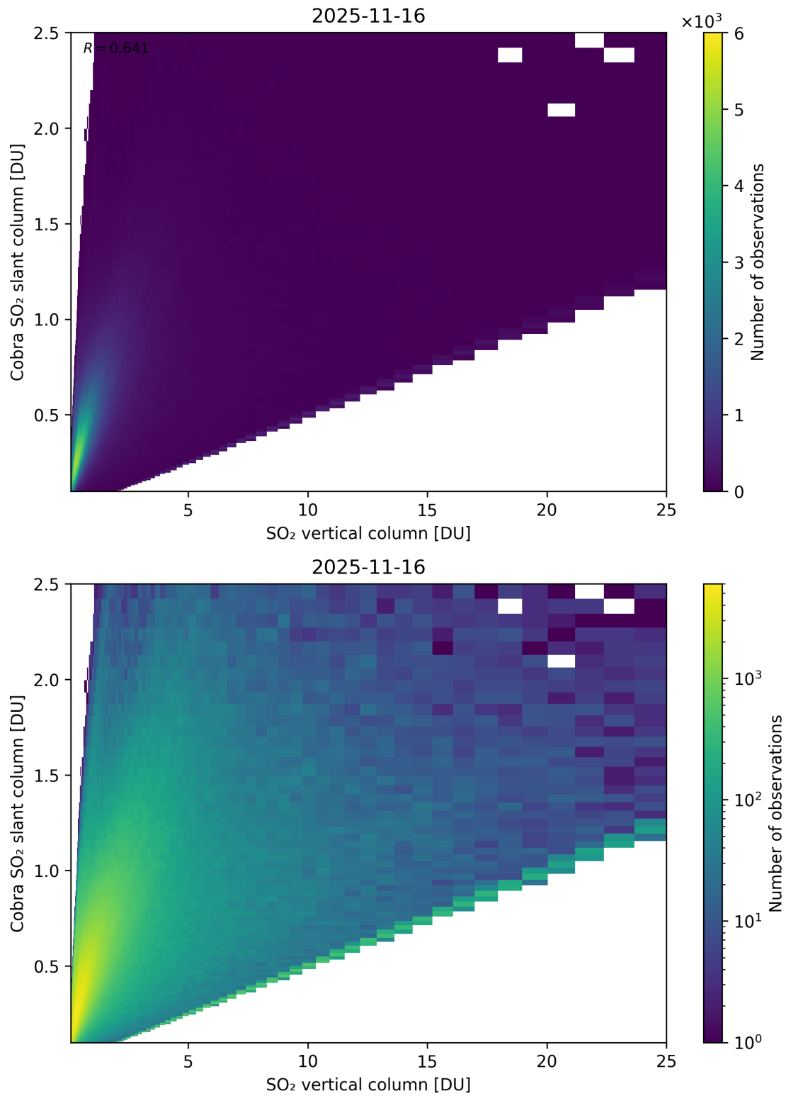
Figure 349: Scatter density plot of “SO 2 vertical column” against “Cobra SO 2 slant column” for 2025-11-15 to 2025-11-17.
