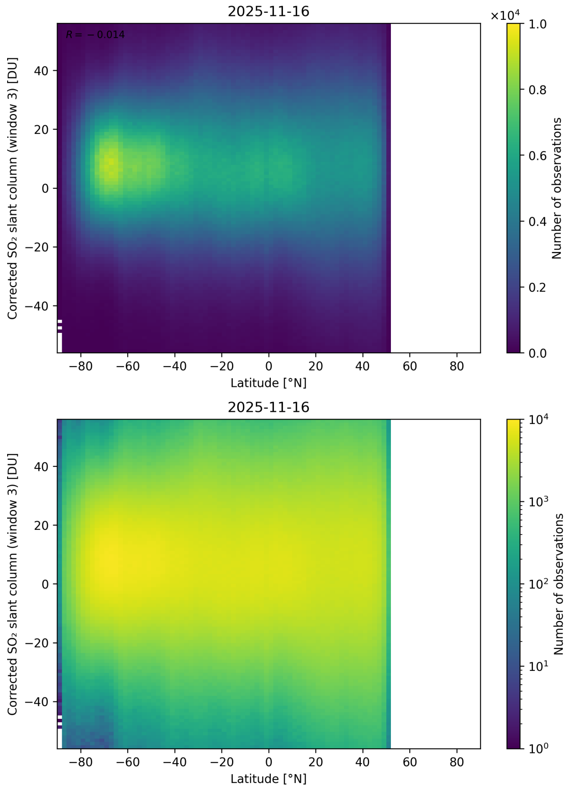
Figure 161: Scatter density plot of “Latitude” against “Corrected SO 2 slant column (window 3)” for 2025-11-15 to 2025-11-17.
