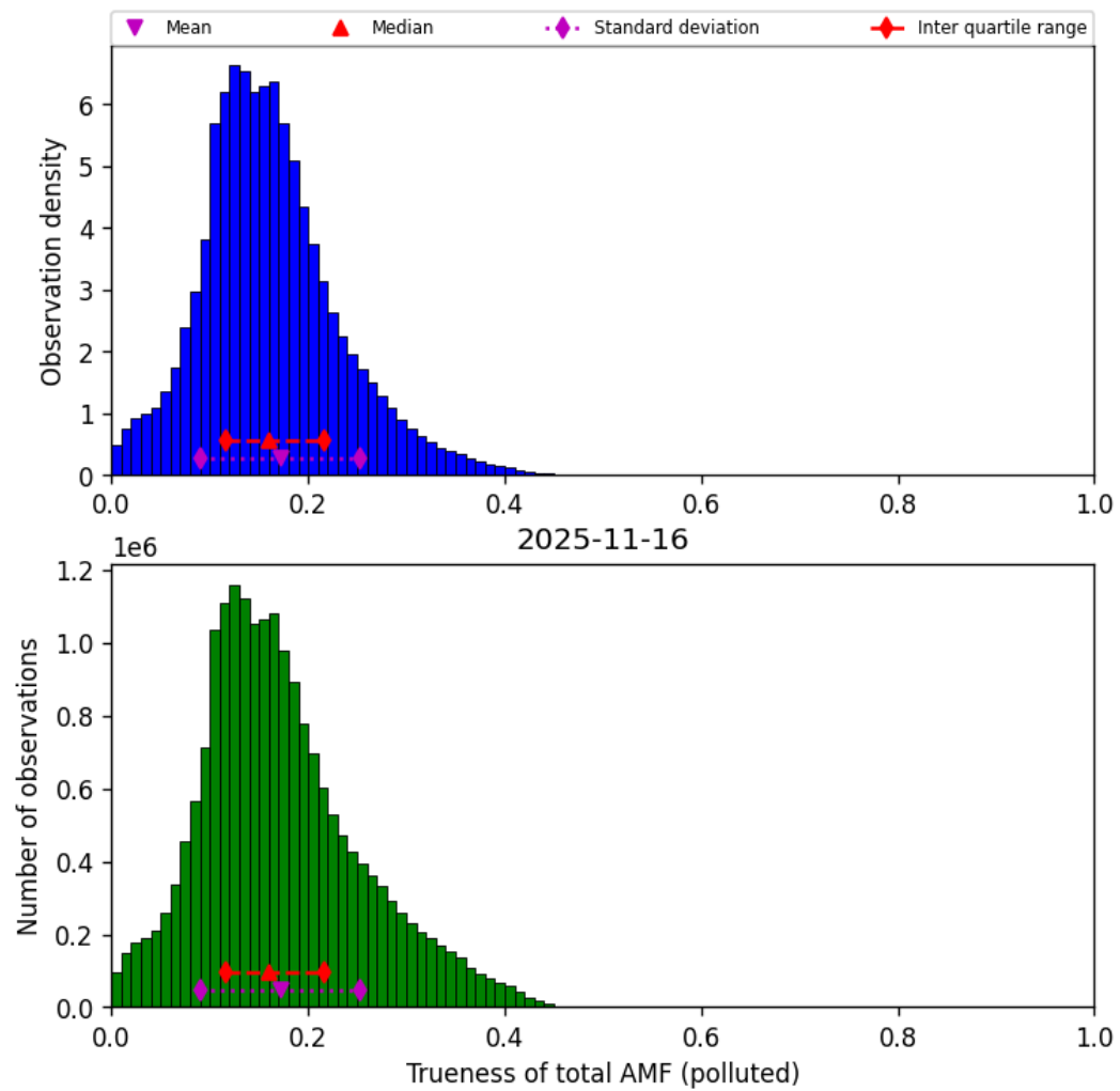
Figure 80: Histogram of “Trueness of total AMF (polluted)” for 2025-11-15 to 2025-11-17
