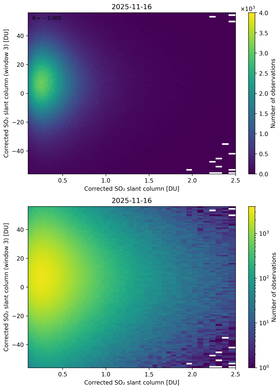
Figure 236: Scatter density plot of “Corrected SO 2 slant column” against “Corrected SO 2 slant column (window 3)” for 2025-11-15 to 2025-11-17.
