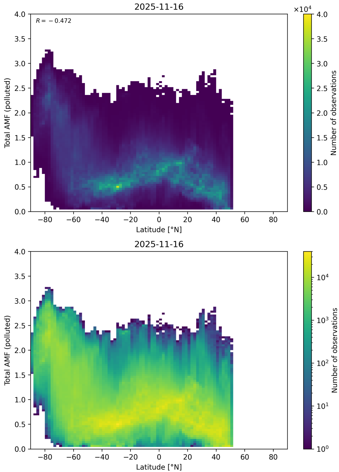
Figure 167: Scatter density plot of “Latitude” against “Total AMF (polluted)” for 2025-11-15 to 2025-11-17.
