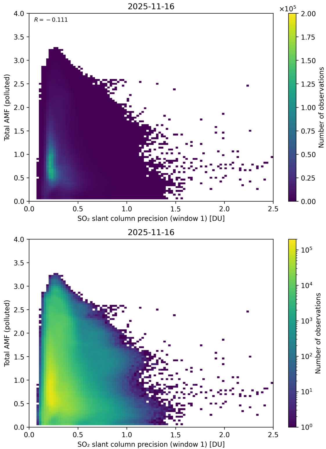
Figure 280: Scatter density plot of “SO 2 slant column precision (window 1)” against “Total AMF (polluted)” for 2025-11-15 to 2025-11-17.
