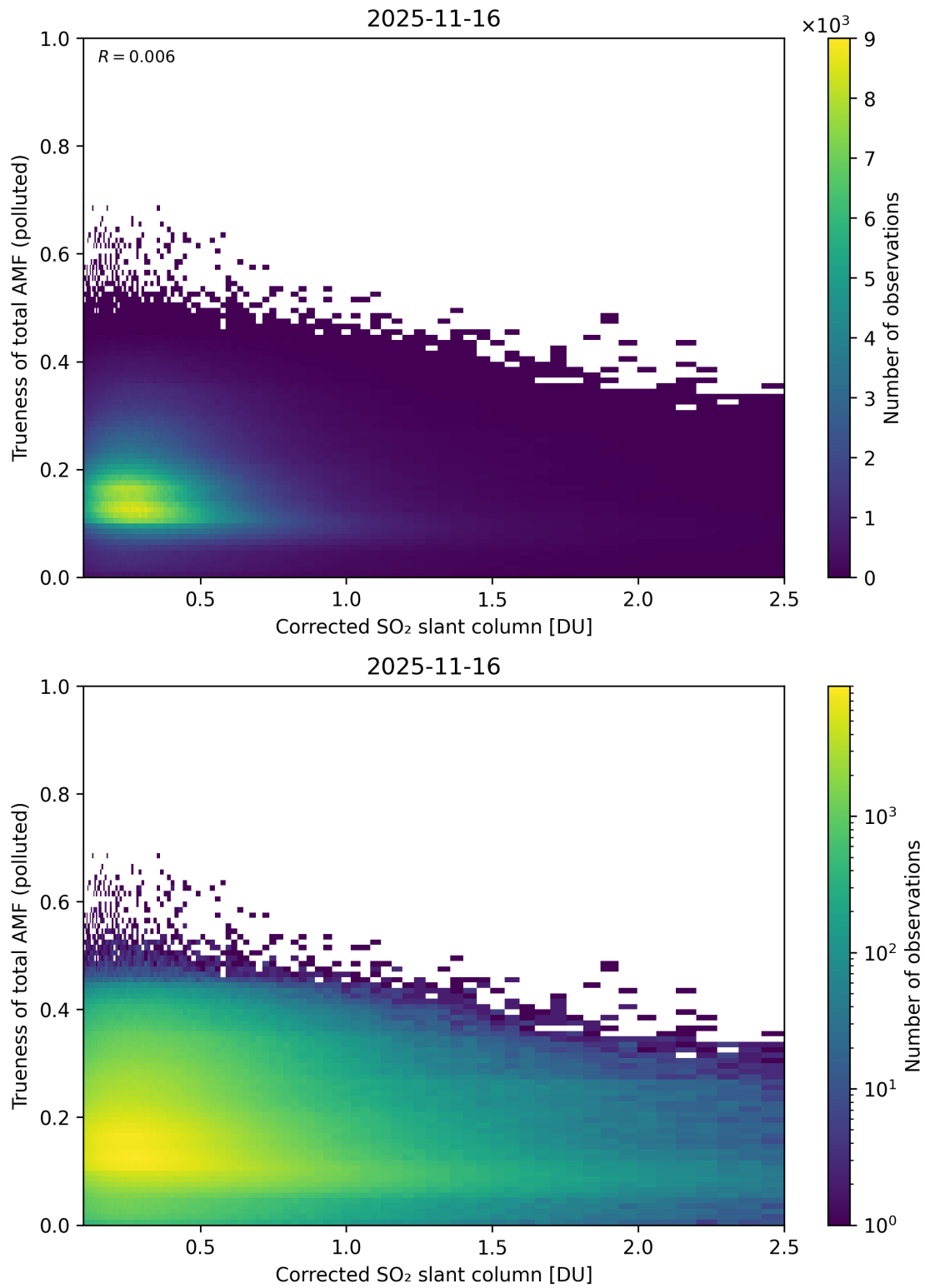
Figure 243: Scatter density plot of “Corrected SO 2 slant column” against “Trueness of total AMF (polluted)” for 2025-11-15 to 2025-11-17.
