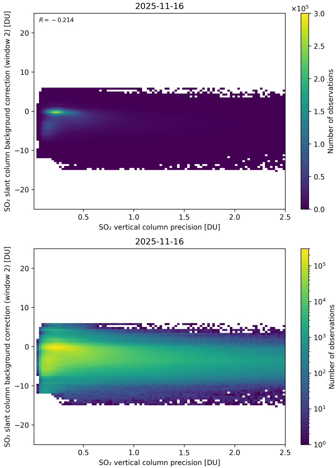
Figure 330: Scatter density plot of “SO 2 vertical column precision” against “SO 2 slant column background correction (window 2)” for 2025-11-15 to 2025-11-17.
