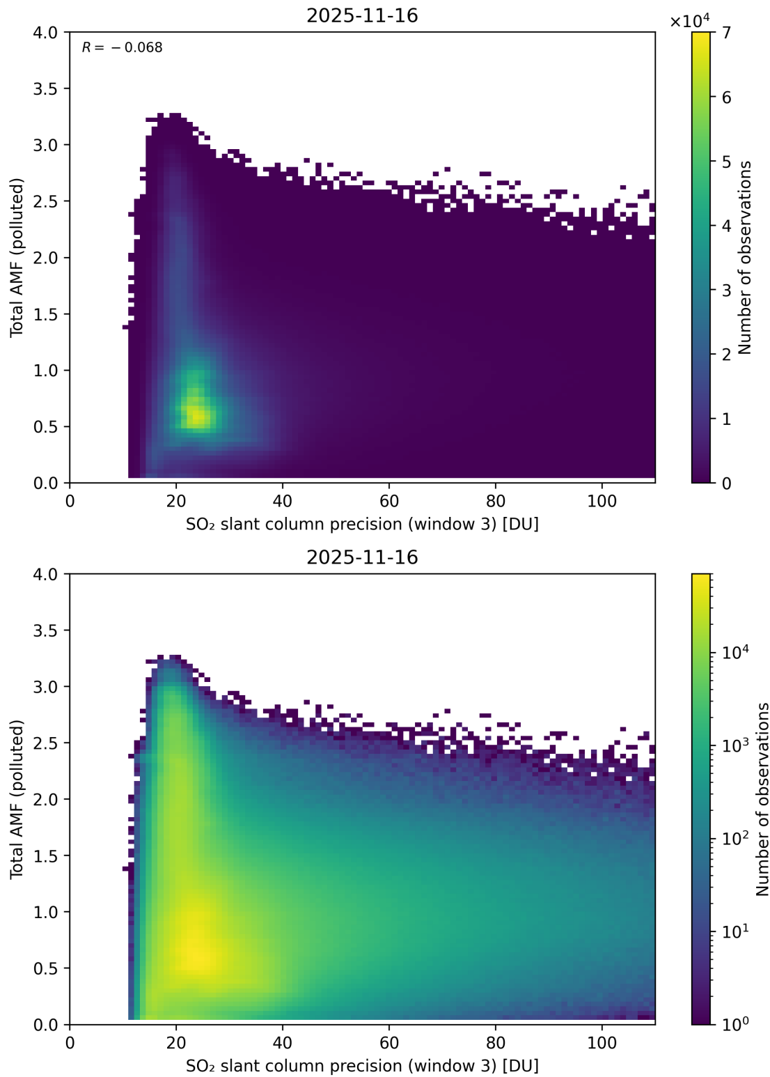
Figure 313: Scatter density plot of “SO 2 slant column precision (window 3)” against “Total AMF (polluted)” for 2025-11-15 to 2025-11-17.
