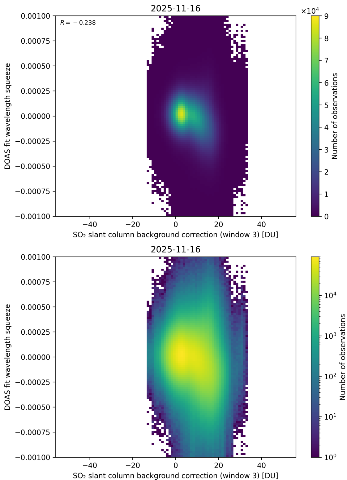
Figure 133: Scatter density plot of “SO 2 slant column background correction (window 3)” against “DOAS fit wavelength squeeze” for 2025-11-15 to 2025-11-17.
