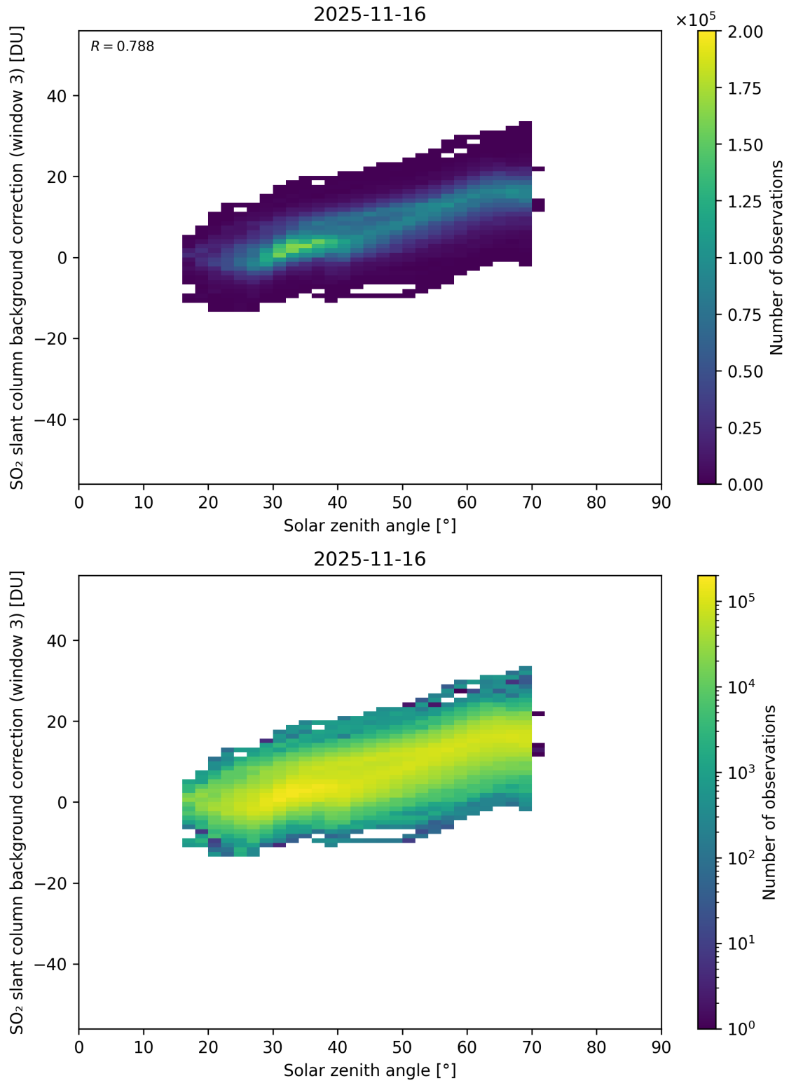
Figure 173: Scatter density plot of “Solar zenith angle” against “SO 2 slant column background correction (window 3)” for 2025-11-15 to 2025-11-17.
