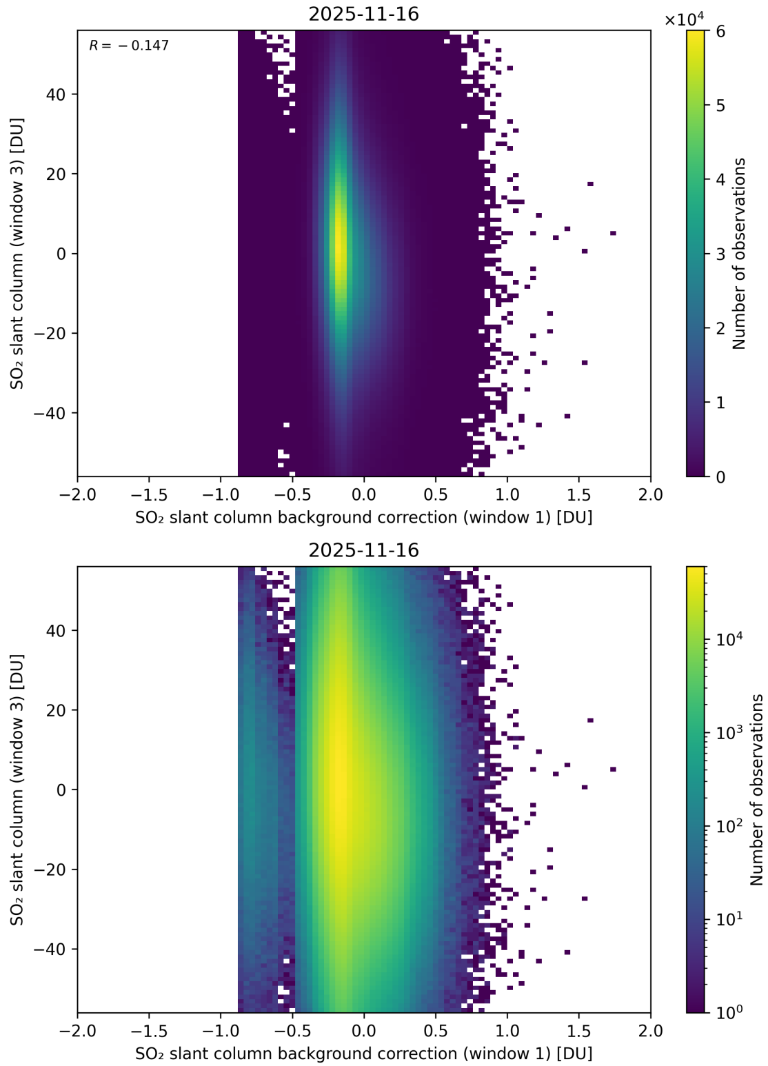
Figure 118: Scatter density plot of “SO 2 slant column background correction (window 1)” against “SO 2 slant column (window 3)” for 2025-11-15 to 2025-11-17.
