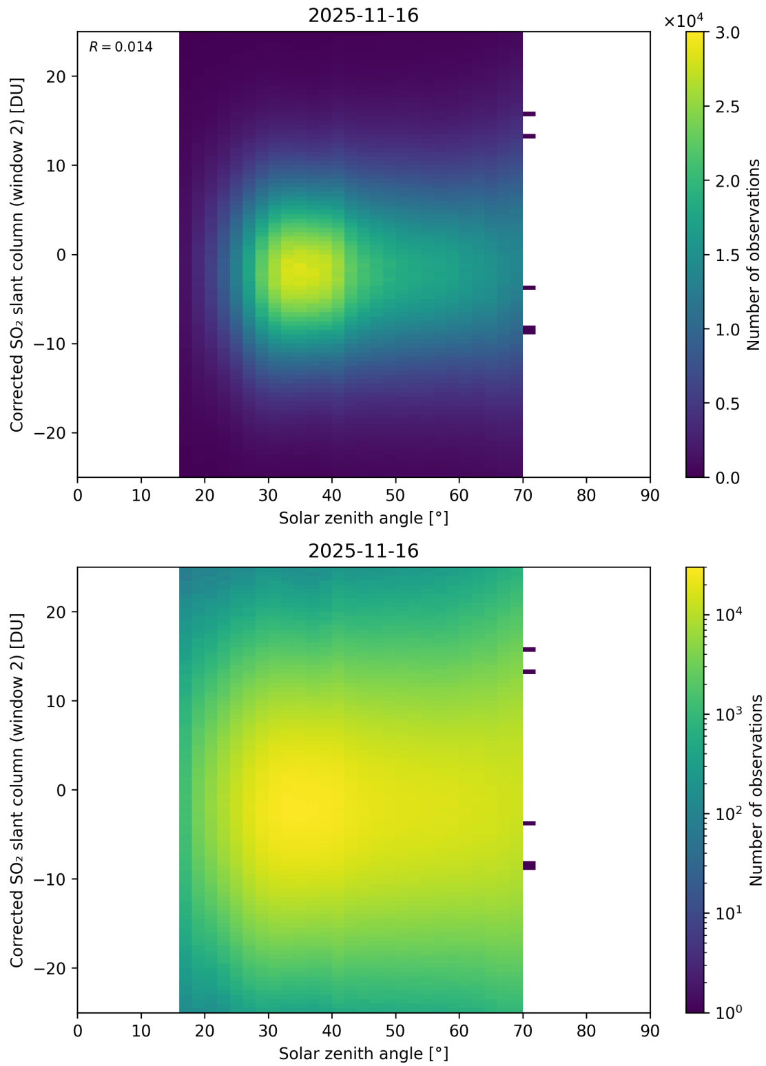
Figure 182: Scatter density plot of “Solar zenith angle” against “Corrected SO 2 slant column (window 2)” for 2025-11-15 to 2025-11-17.
