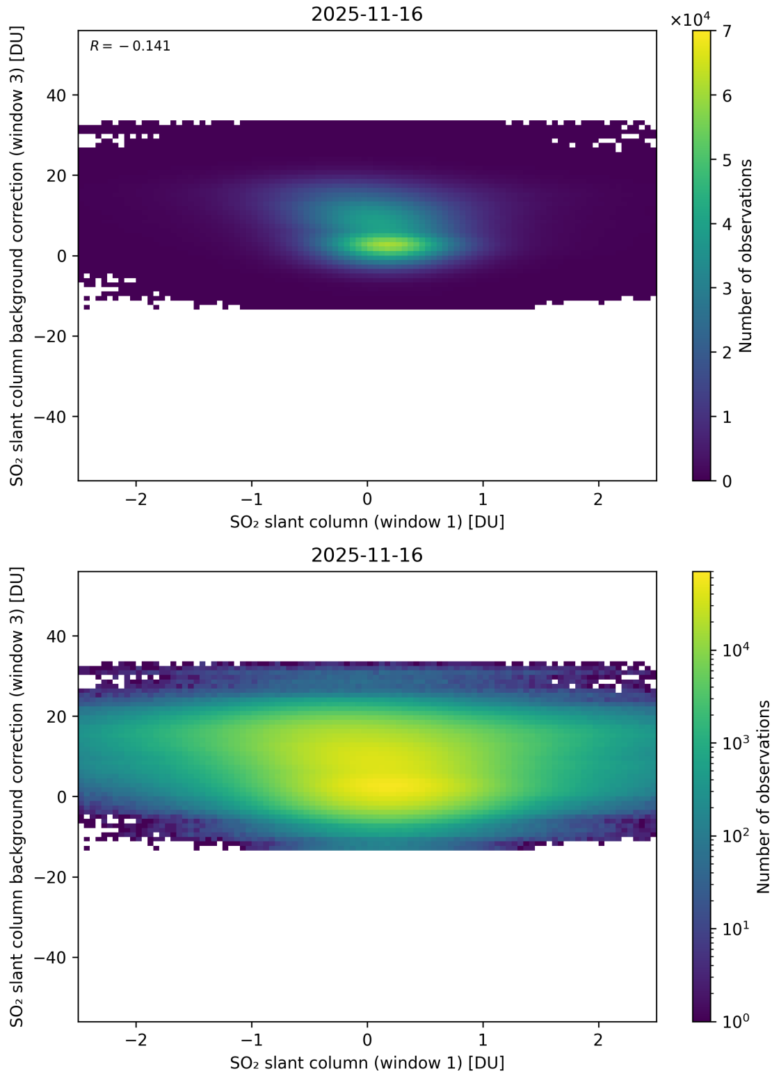
Figure 264: Scatter density plot of “SO 2 slant column (window 1)” against “SO 2 slant column background correction (window 3)” for 2025-11-15 to 2025-11-17.
