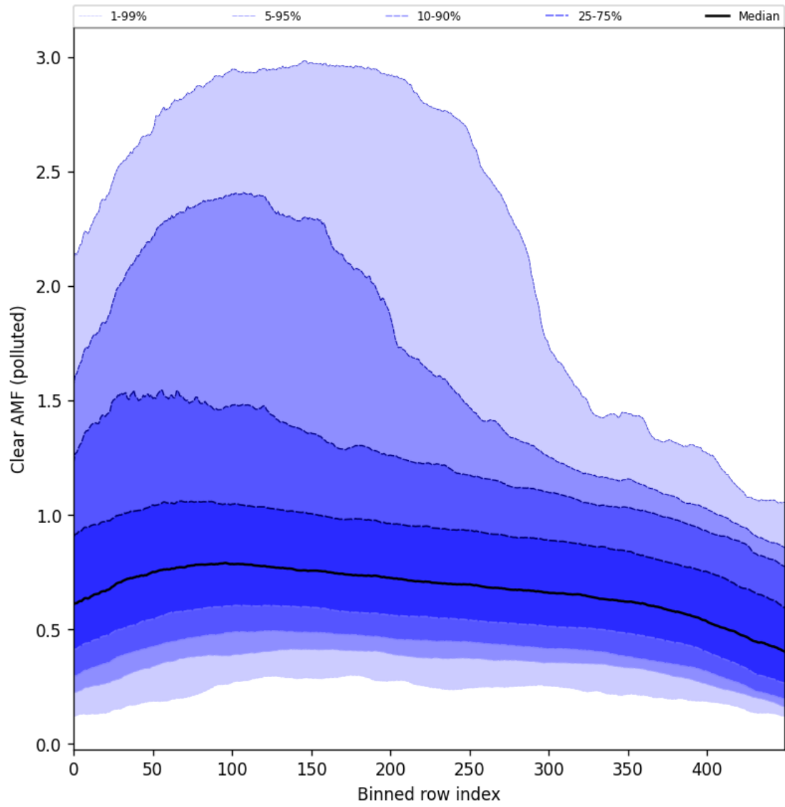
Figure 107: Along track statistics of “Clear AMF (polluted)” for 2025-11-15 to 2025-11-17
