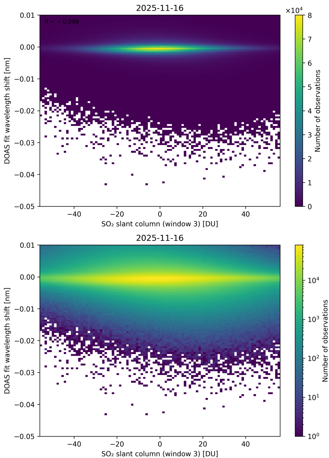
Figure 304: Scatter density plot of “SO 2 slant column (window 3)” against “DOAS fit wavelength shift” for 2025-11-15 to 2025-11-17.
