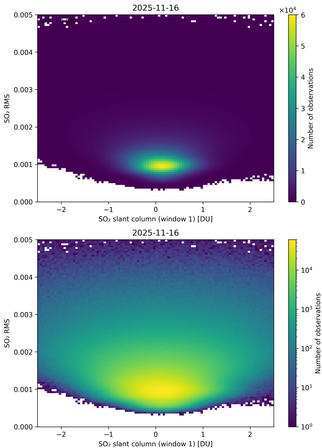
Figure 267: Scatter density plot of “SO 2 slant column (window 1)” against “SO 2 RMS” for 2025-11-15 to 2025-11-17.
