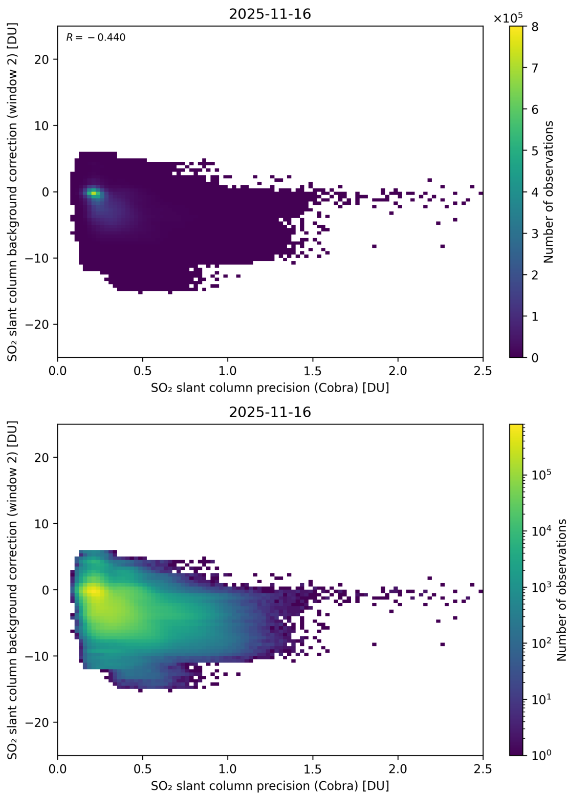
Figure 200: Scatter density plot of “SO 2 slant column precision (Cobra)” against “SO 2 slant column background correction (window 2)” for 2025-11-15 to 2025-11-17.
