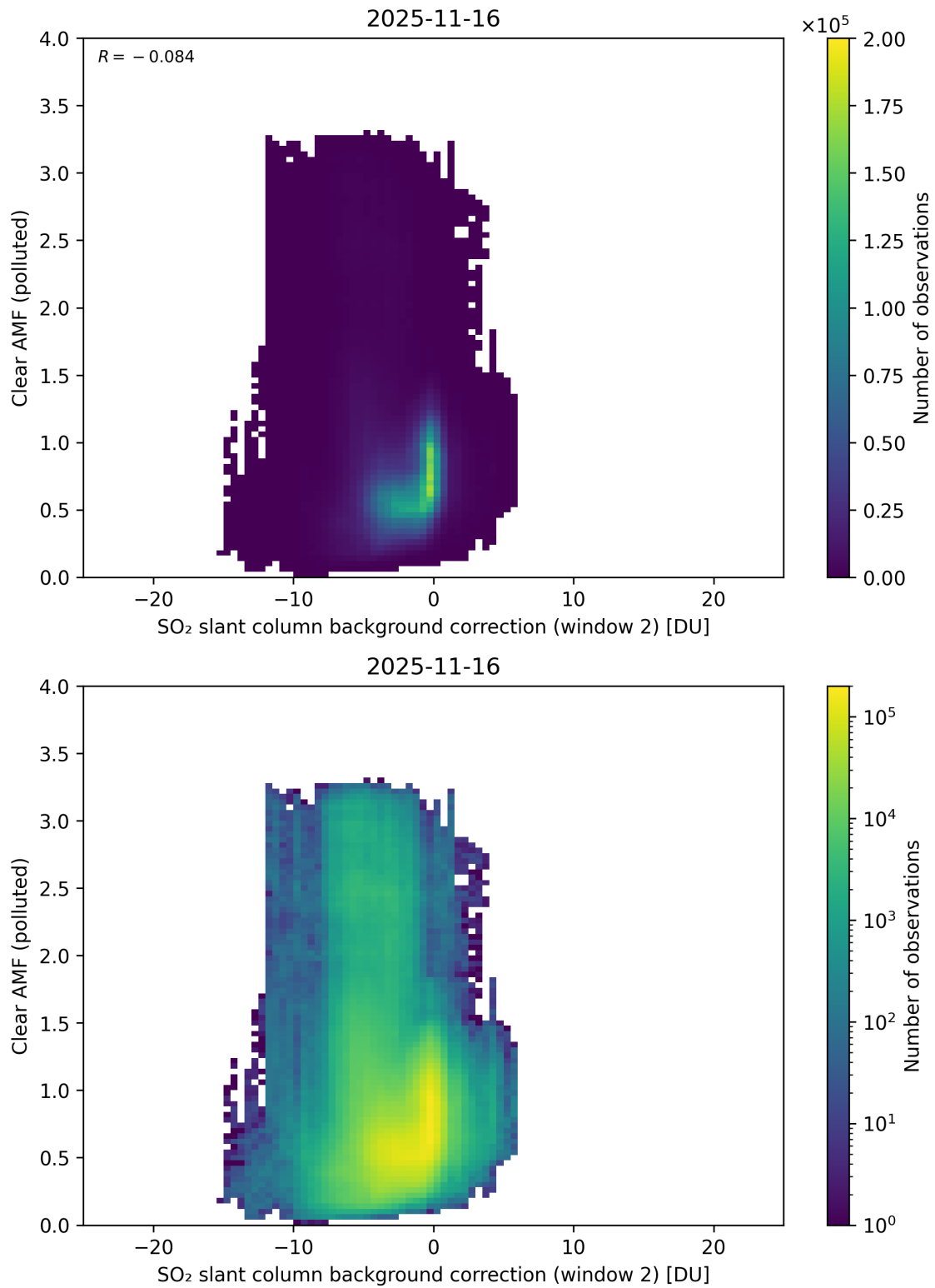
Figure 126: Scatter density plot of “SO 2 slant column background correction (window 2)” against “Clear AMF (polluted)” for 2025-11-15 to 2025-11-17.
