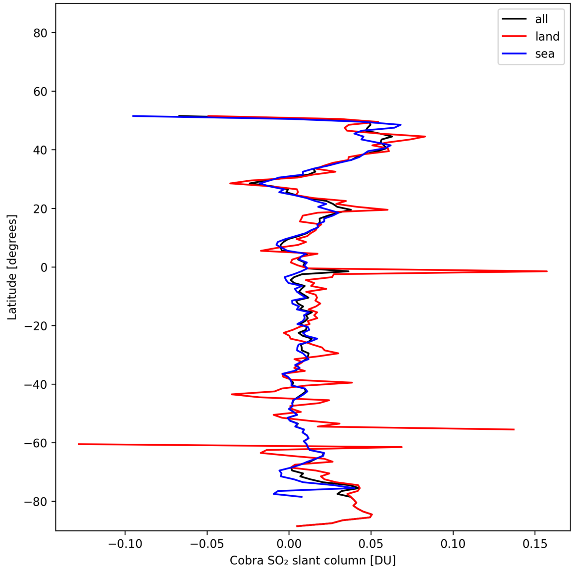
Figure 35: Zonal average of “Cobra SO 2 slant column” for 2025-11-15 to 2025-11-17.
