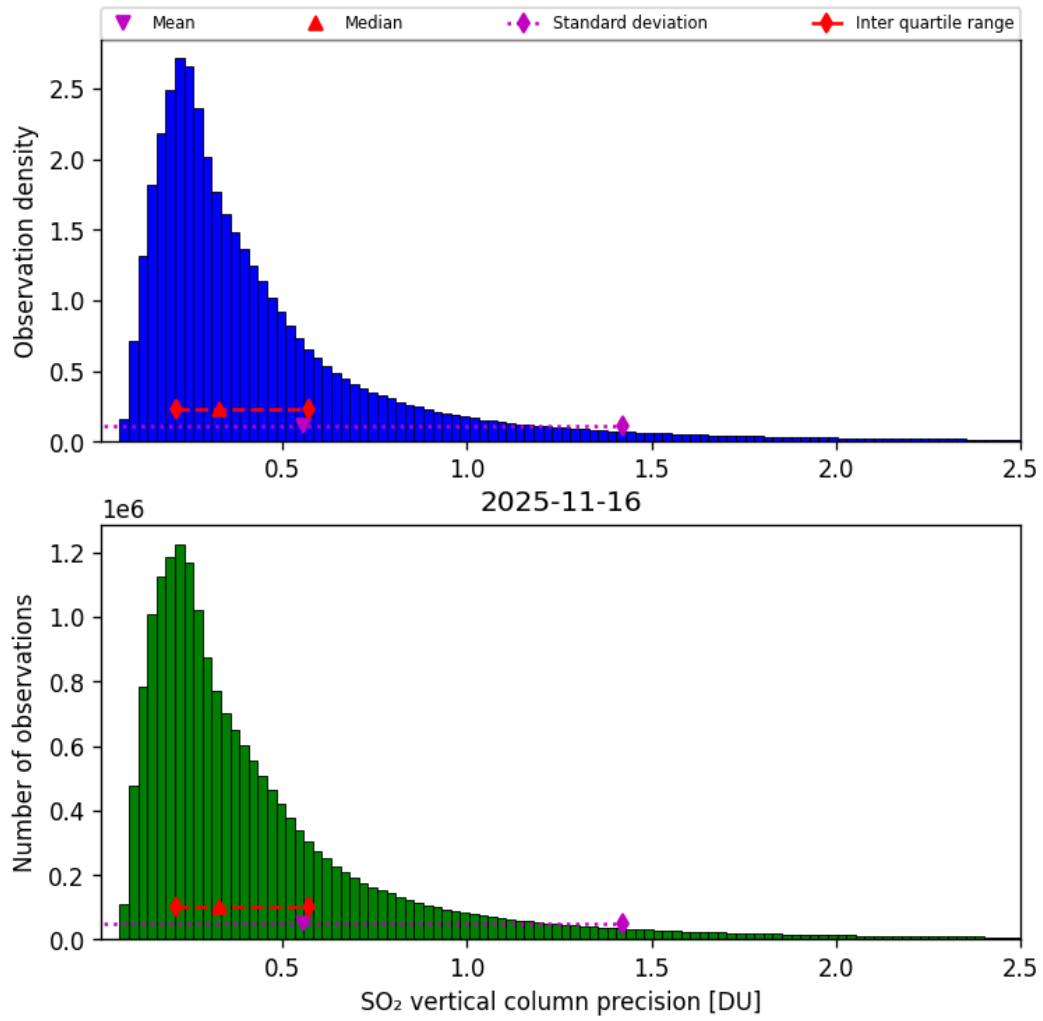
Figure 59: Histogram of “SO 2 vertical column precision” for 2025-11-15 to 2025-11-17
