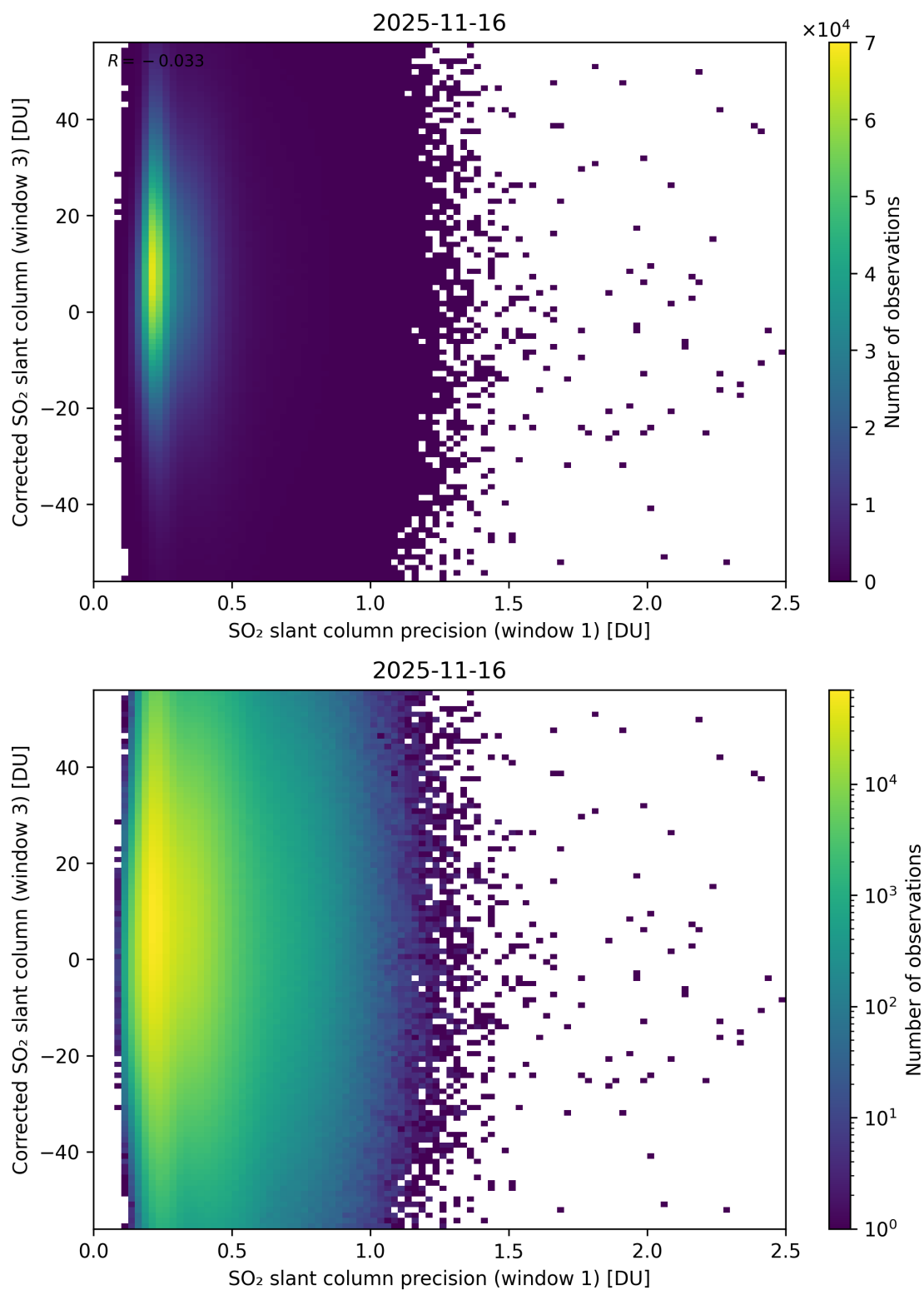
Figure 276: Scatter density plot of “SO 2 slant column precision (window 1)” against “Corrected SO 2 slant column (window 3)” for 2025-11-15 to 2025-11-17.
