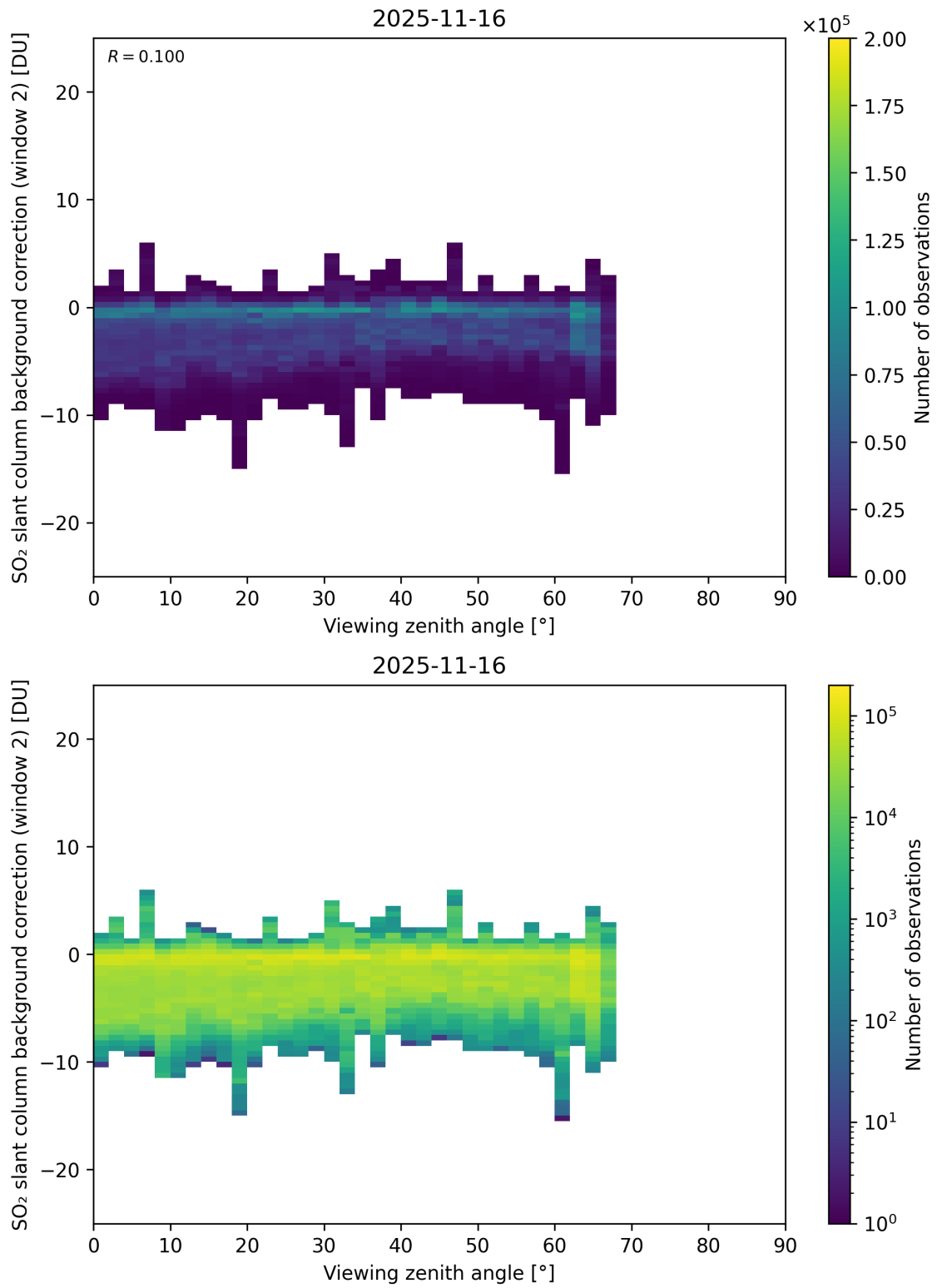
Figure 363: Scatter density plot of “Viewing zenith angle” against “SO 2 slant column background correction (window 2)” for 2025-11-15 to 2025-11-17.
