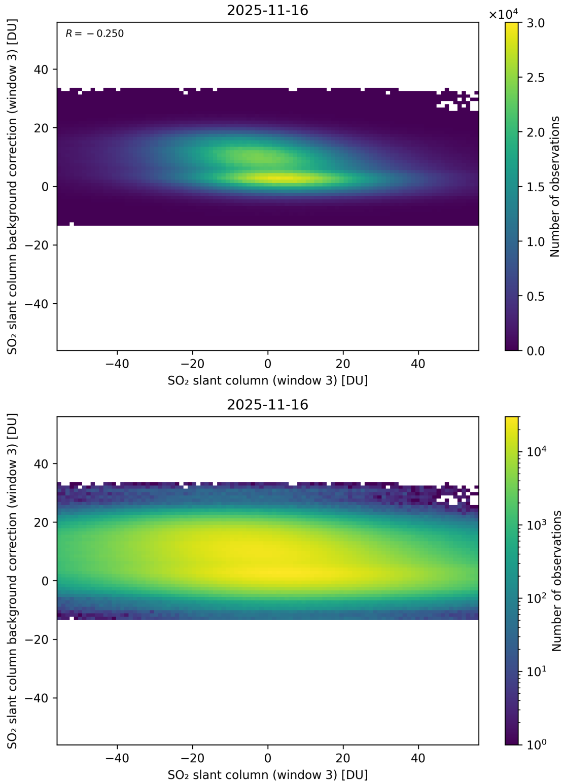
Figure 303: Scatter density plot of “SO 2 slant column (window 3)” against “SO 2 slant column background correction (window 3)” for 2025-11-15 to 2025-11-17.
