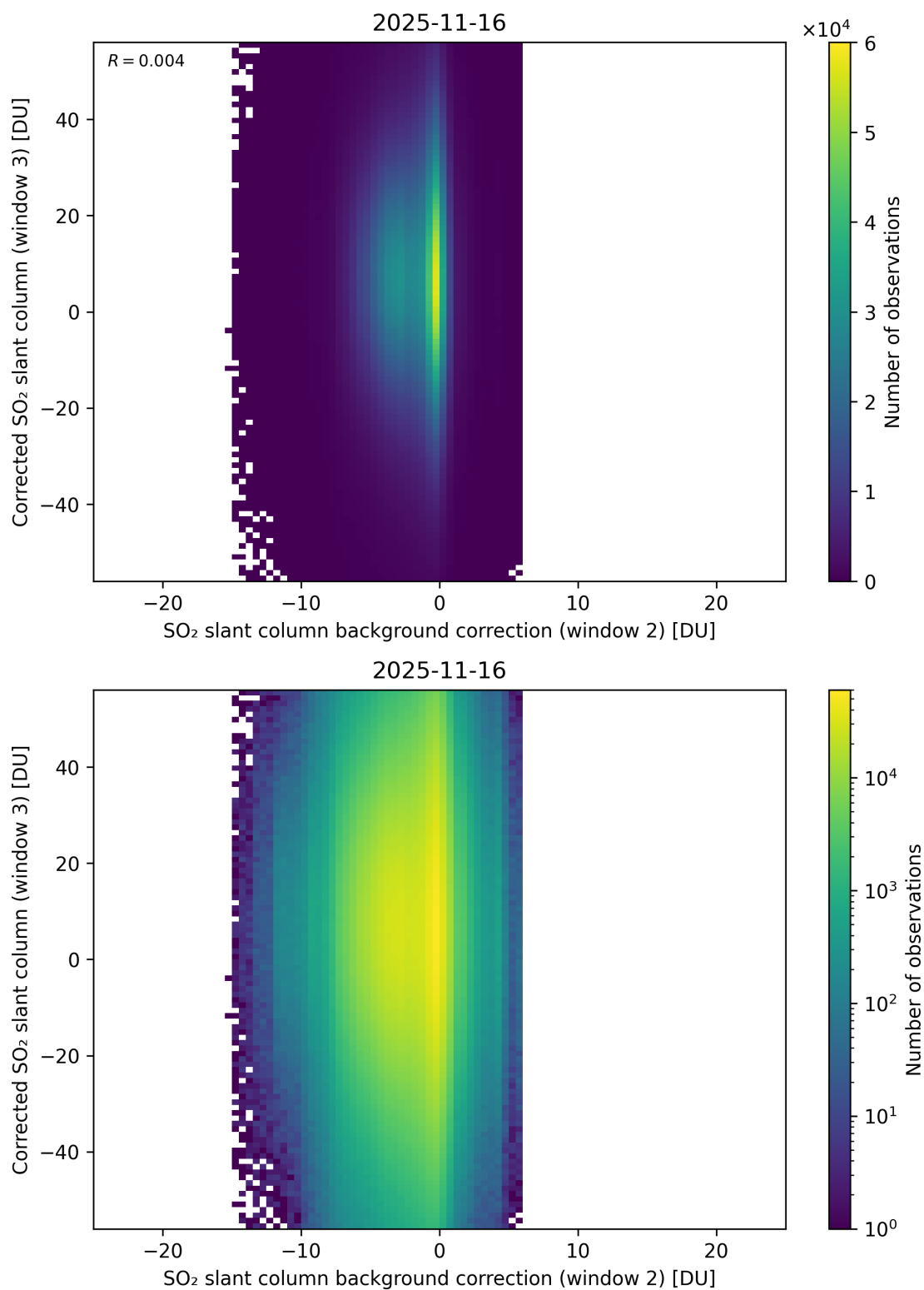
Figure 127: Scatter density plot of “SO 2 slant column background correction (window 2)” against “Corrected SO 2 slant column (window 3)” for 2025-11-15 to 2025-11-17.
