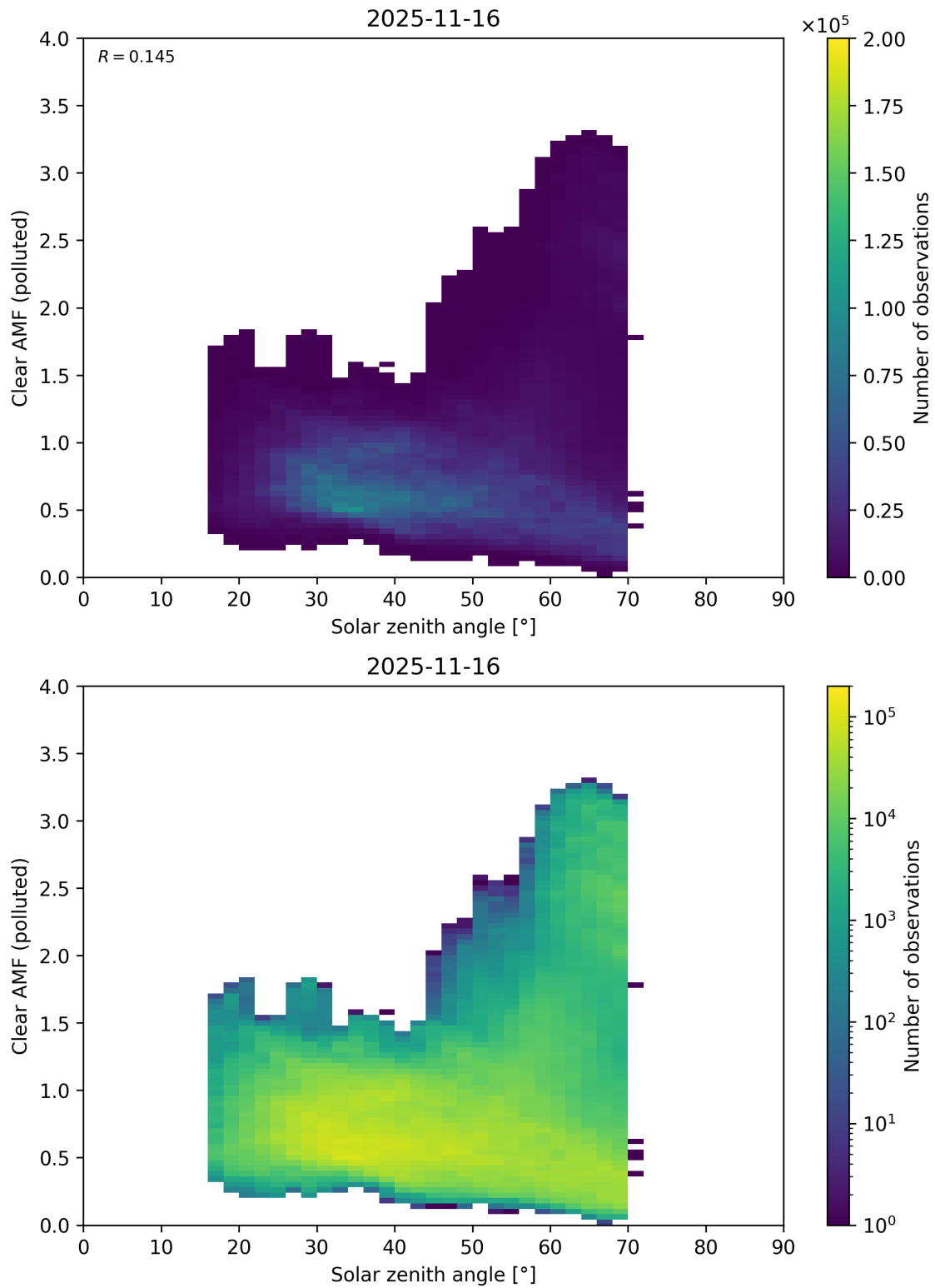
Figure 178: Scatter density plot of “Solar zenith angle” against “Clear AMF (polluted)” for 2025-11-15 to 2025-11-17.
