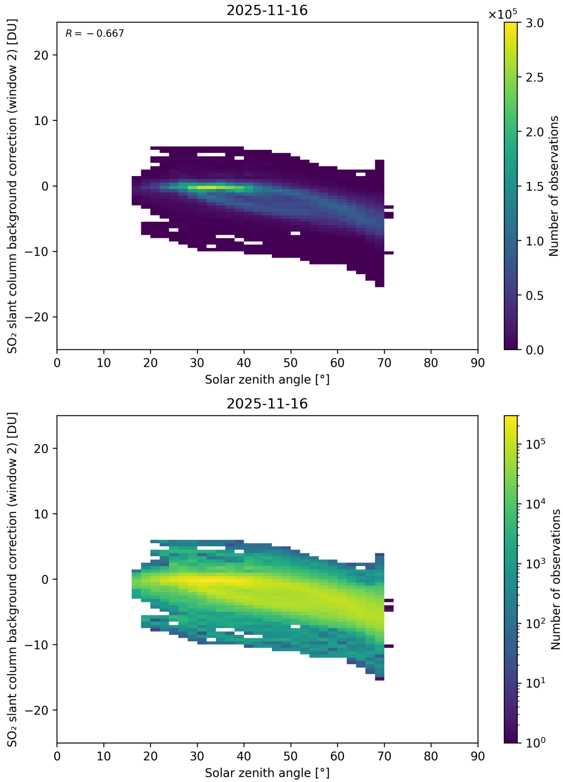
Figure 172: Scatter density plot of “Solar zenith angle” against “SO 2 slant column background correction (window 2)” for 2025-11-15 to 2025-11-17.
