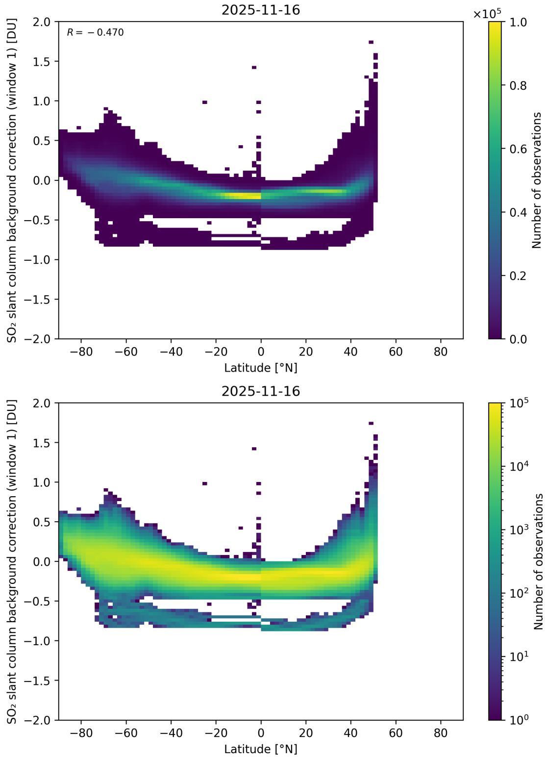
Figure 150: Scatter density plot of “Latitude” against “SO 2 slant column background correction (window 1)” for 2025-11-15 to 2025-11-17.
