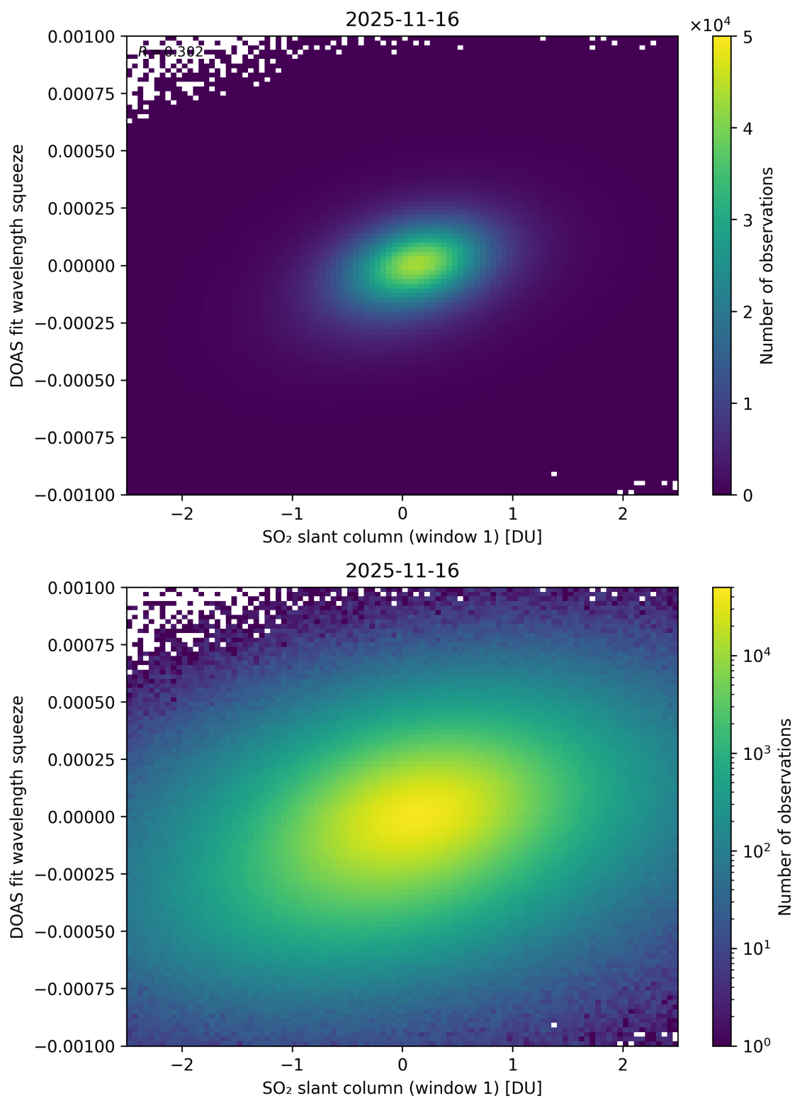
Figure 266: Scatter density plot of “SO 2 slant column (window 1)” against “DOAS fit wavelength squeeze” for 2025-11-15 to 2025-11-17.
