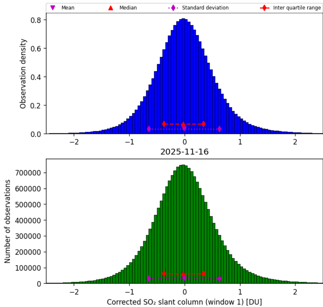
Figure 65: Histogram of “Corrected SO 2 slant column (window 1)” for 2025-11-15 to 2025-11-17
