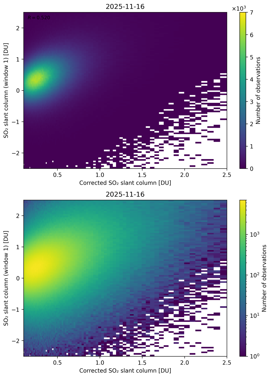
Figure 237: Scatter density plot of “Corrected SO 2 slant column” against “SO 2 slant column (window 1)” for 2025-11-15 to 2025-11-17.
