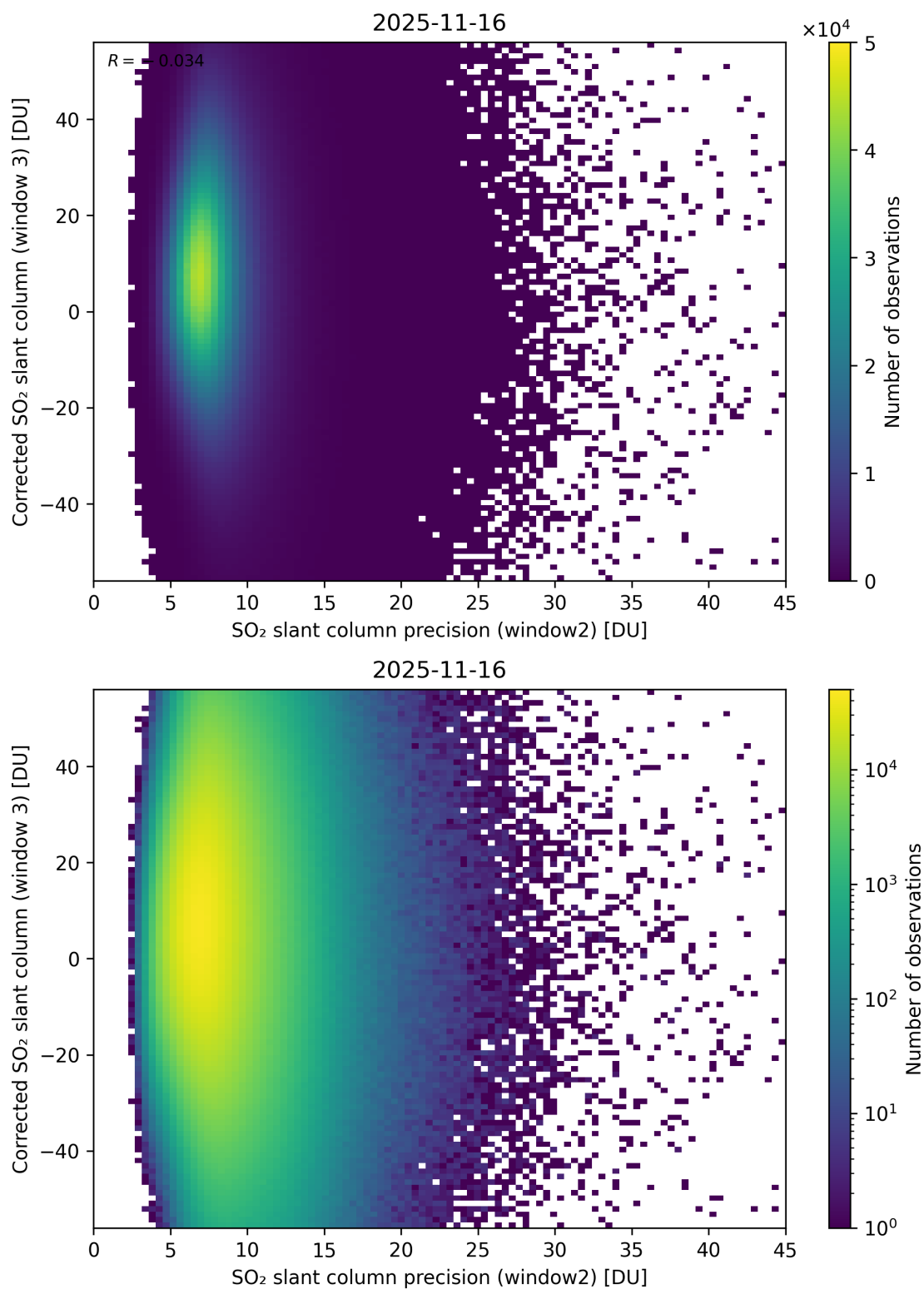
Figure 298: Scatter density plot of “SO 2 slant column precision (window2)” against “Corrected SO 2 slant column (window 3)” for 2025-11-15 to 2025-11-17.
