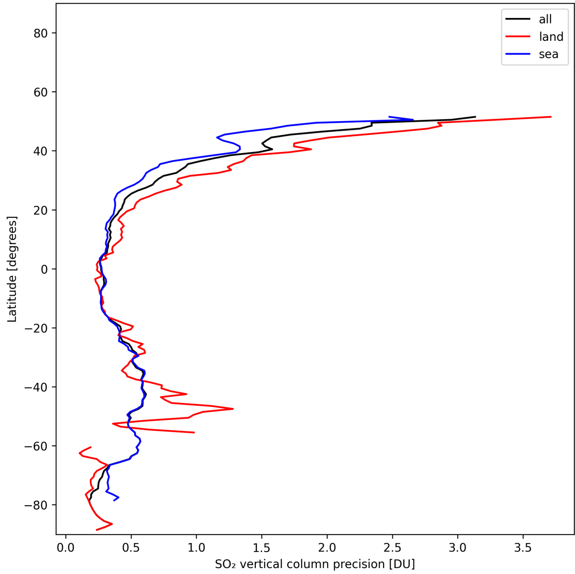
Figure 33: Zonal average of “SO 2 vertical column precision” for 2025-11-15 to 2025-11-17.
