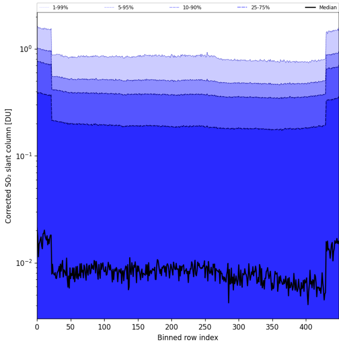
Figure 86: Along track statistics of “Corrected SO 2 slant column” for 2025-11-15 to 2025-11-17
