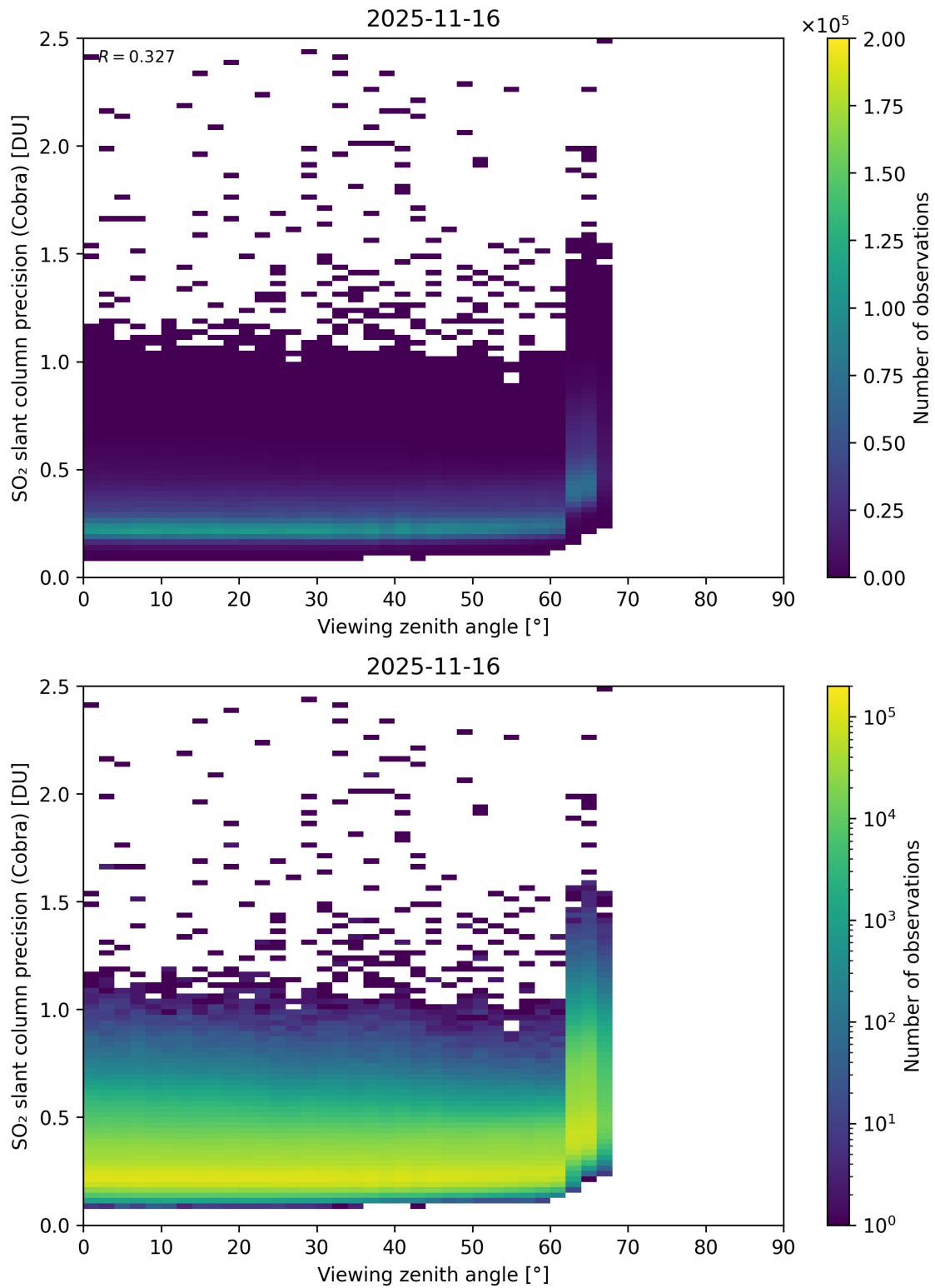
Figure 372: Scatter density plot of “Viewing zenith angle” against “SO 2 slant column precision (Cobra)” for 2025-11-15 to 2025-11-17.
