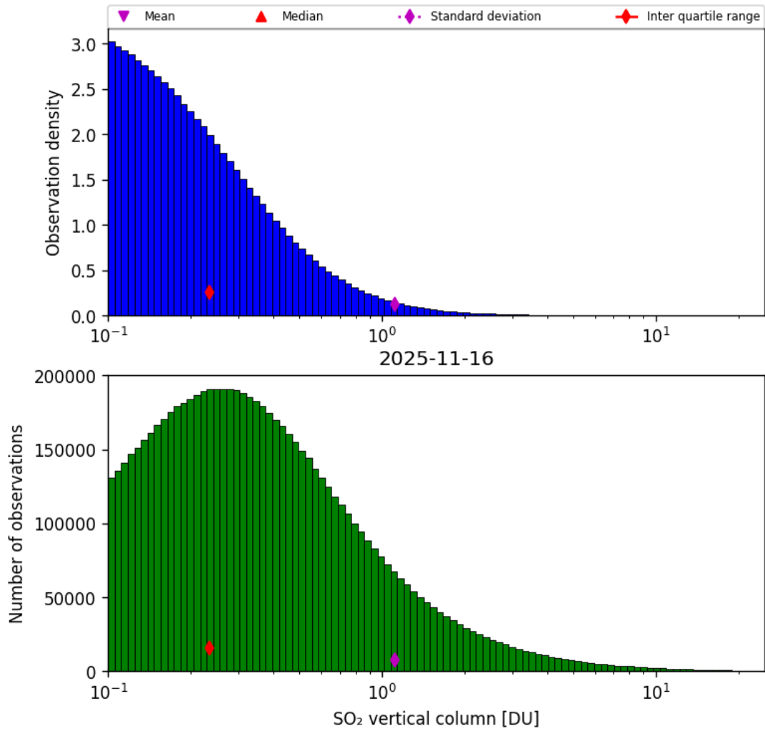
Figure 58: Histogram of “SO 2 vertical column” for 2025-11-15 to 2025-11-17
