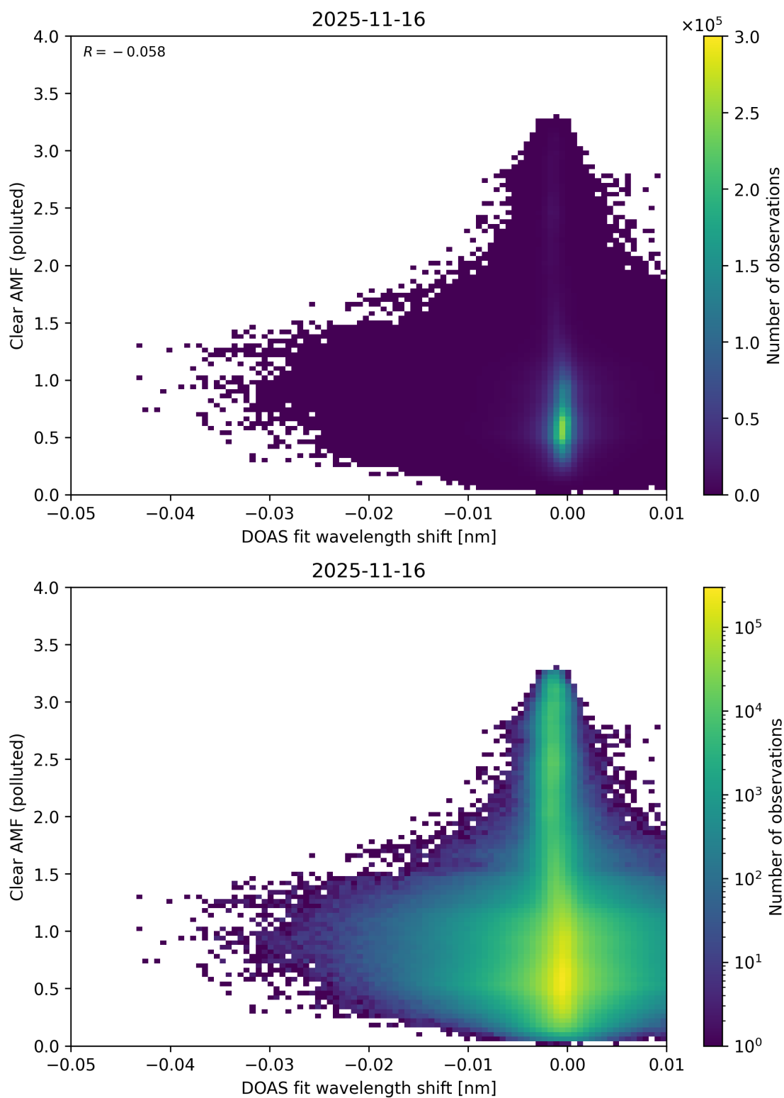
Figure 140: Scatter density plot of “DOAS fit wavelength shift” against “Clear AMF (polluted)” for 2025-11-15 to 2025-11-17.
