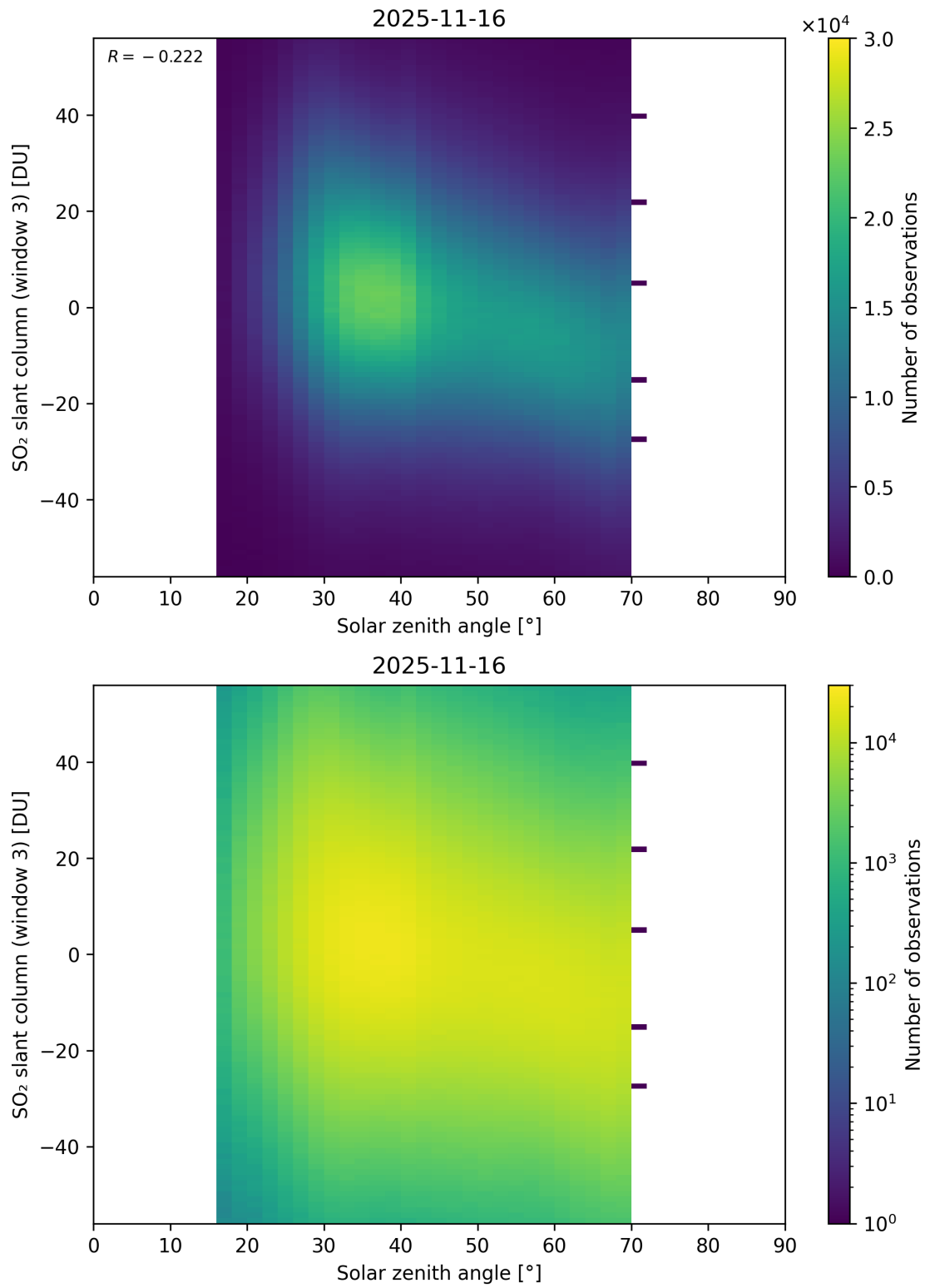
Figure 187: Scatter density plot of “Solar zenith angle” against “SO 2 slant column (window 3)” for 2025-11-15 to 2025-11-17.
