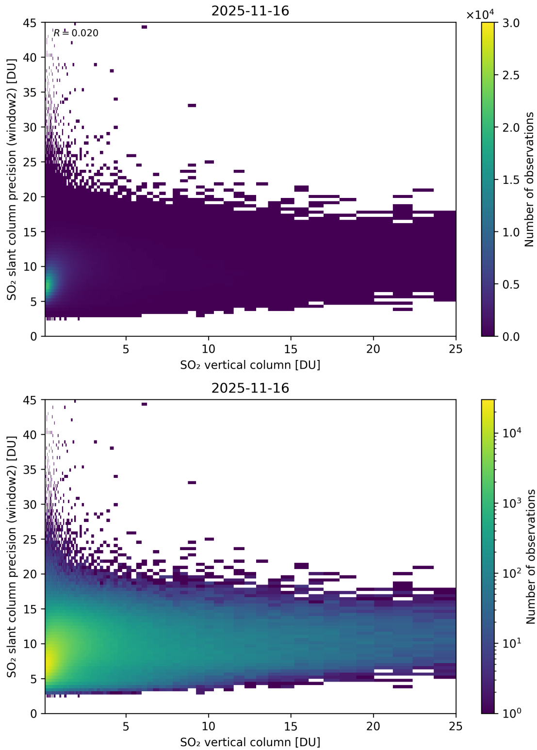
Figure 356: Scatter density plot of “SO 2 vertical column” against “SO 2 slant column precision (window2)” for 2025-11-15 to 2025-11-17.
