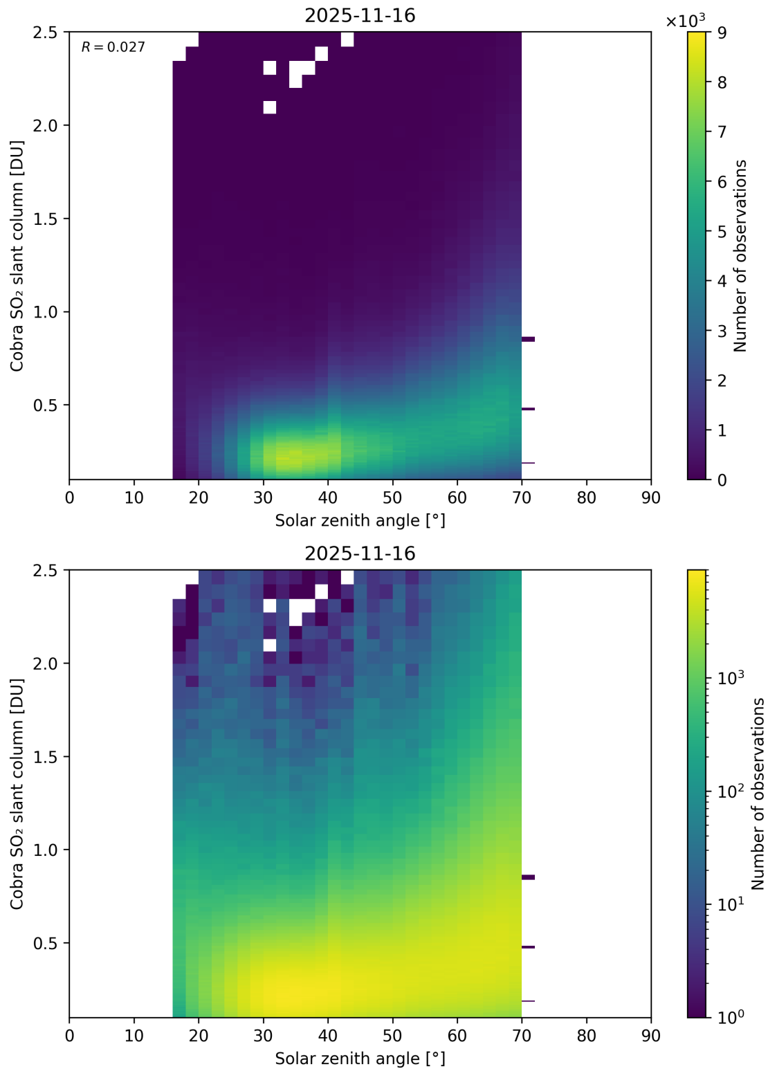
Figure 179: Scatter density plot of “Solar zenith angle” against “Cobra SO 2 slant column” for 2025-11-15 to 2025-11-17.
