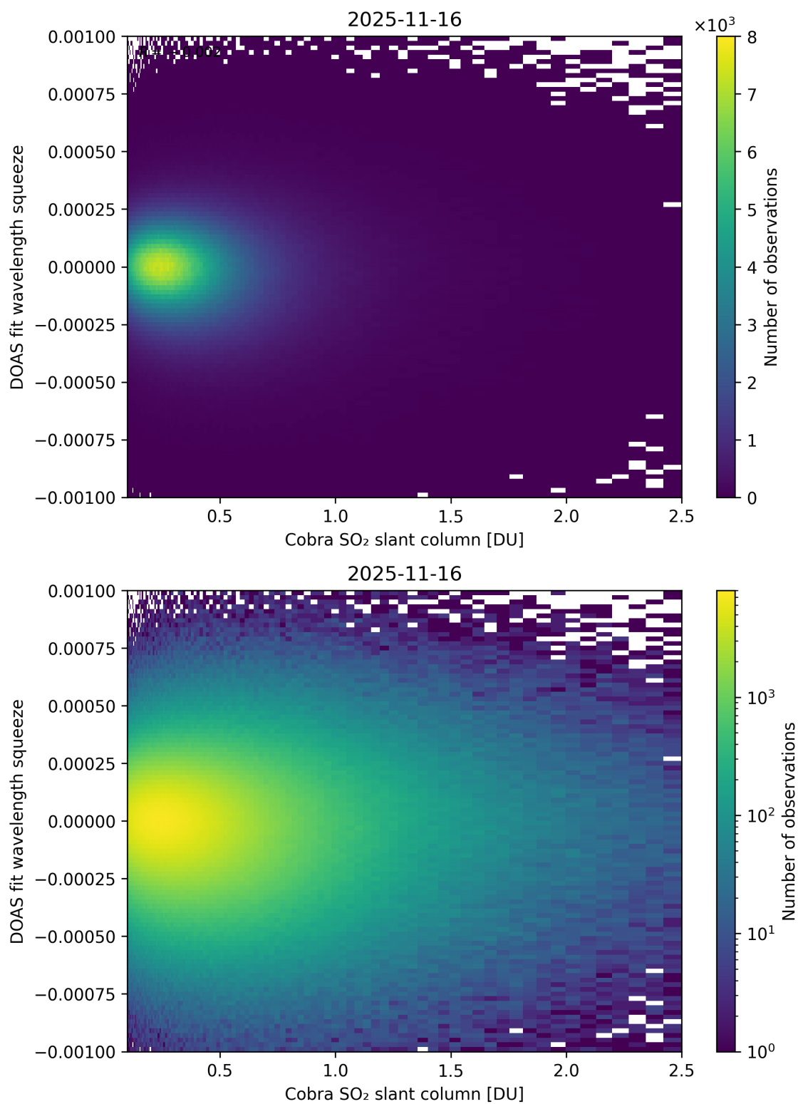
Figure 197: Scatter density plot of “Cobra SO 2 slant column” against “DOAS fit wavelength squeeze” for 2025-11-15 to 2025-11-17.
