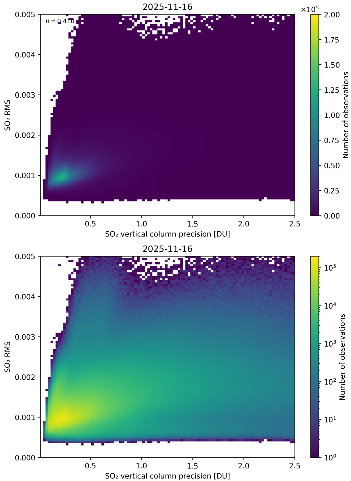
Figure 334: Scatter density plot of “SO 2 vertical column precision” against “SO 2 RMS” for 2025-11-15 to 2025-11-17.
