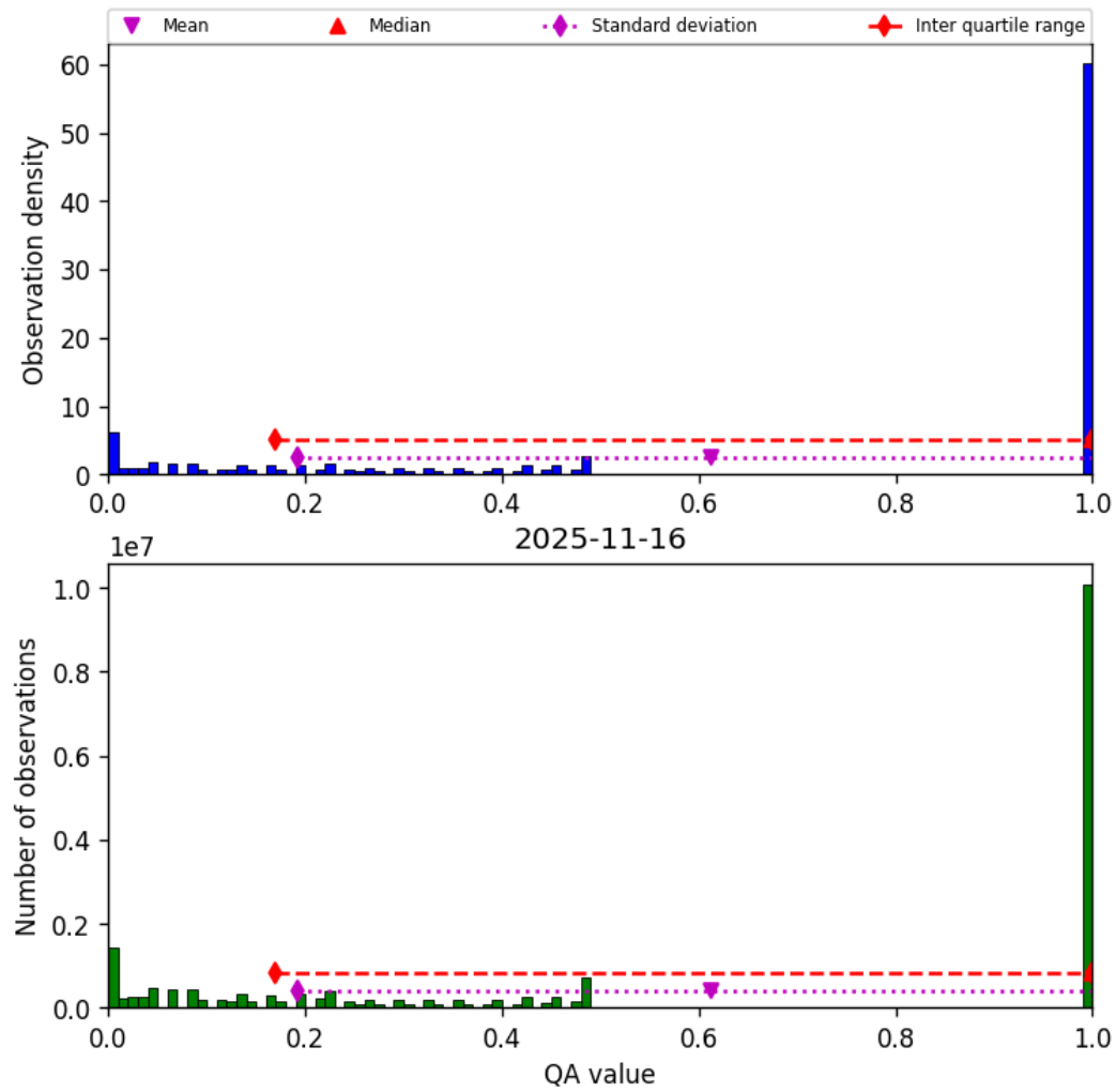
Figure 57: Histogram of “QA value” for 2025-11-15 to 2025-11-17
