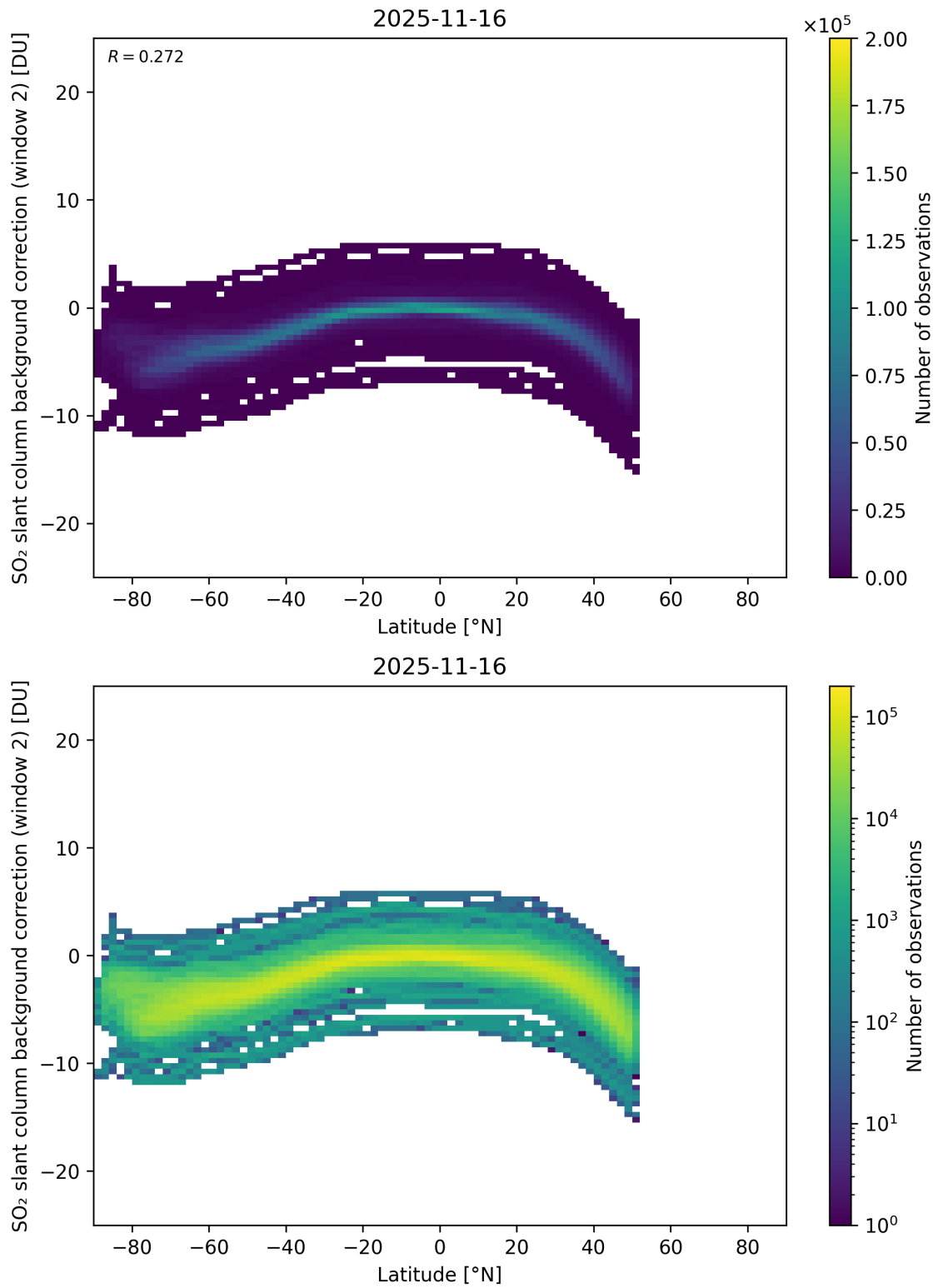
Figure 151: Scatter density plot of “Latitude” against “SO 2 slant column background correction (window 2)” for 2025-11-15 to 2025-11-17.
