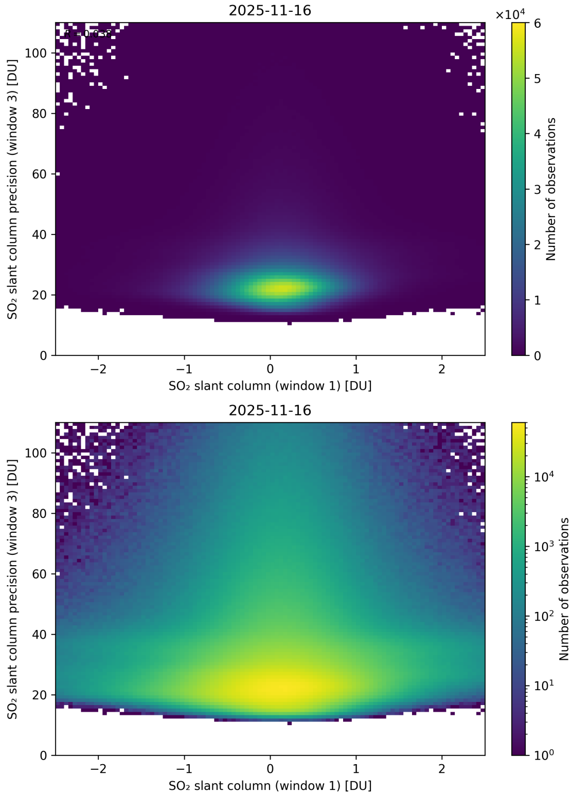
Figure 288: Scatter density plot of “SO 2 slant column (window 1)” against “SO 2 slant column precision (window 3)” for 2025-11-15 to 2025-11-17.
