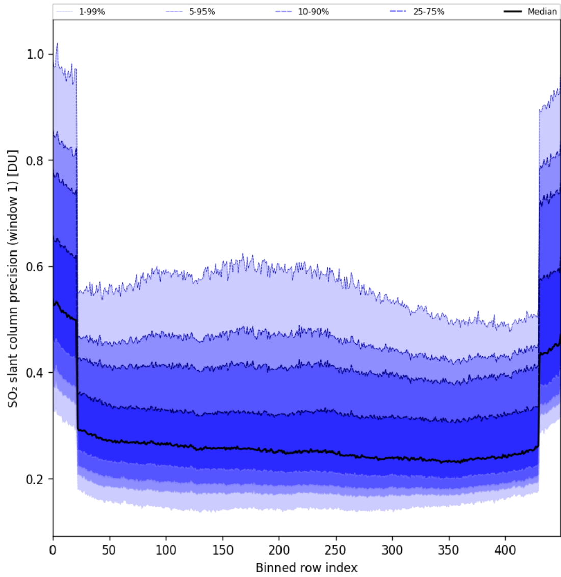
Figure 90: Along track statistics of “SO 2 slant column precision (window 1)” for 2025-11-15 to 2025-11-17
