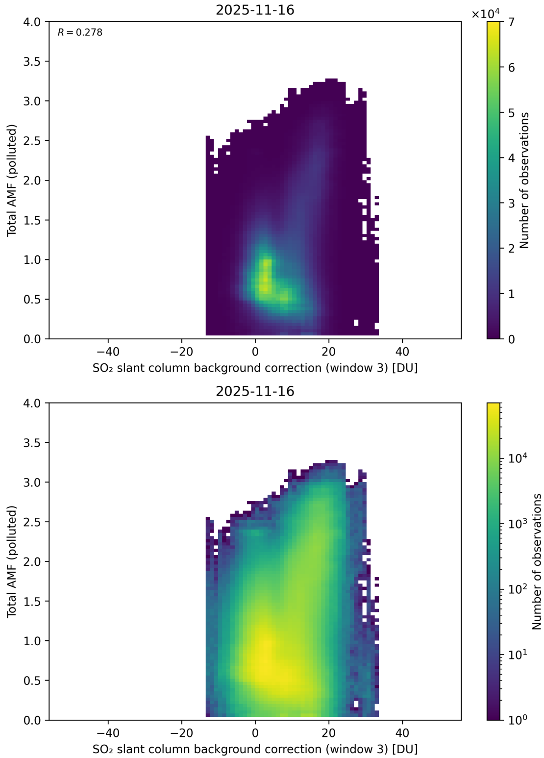
Figure 136: Scatter density plot of “SO 2 slant column background correction (window 3)” against “Total AMF (polluted)” for 2025-11-15 to 2025-11-17.
