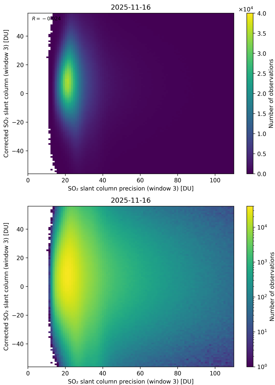
Figure 312: Scatter density plot of “SO 2 slant column precision (window 3)” against “Corrected SO 2 slant column (window 3)” for 2025-11-15 to 2025-11-17.
