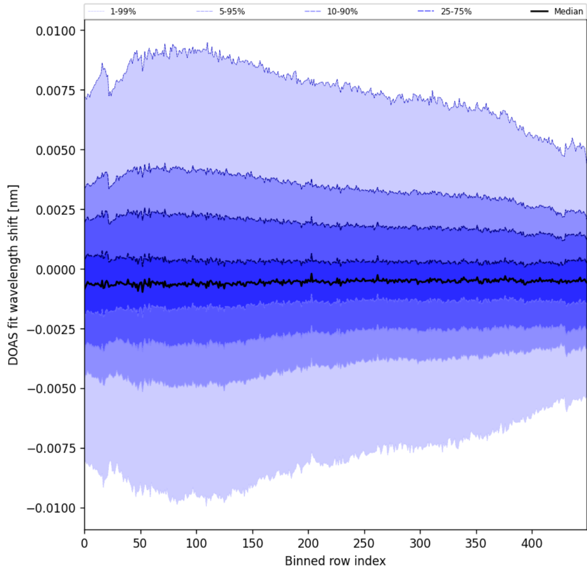
Figure 102: Along track statistics of “DOAS fit wavelength shift” for 2025-11-15 to 2025-11-17
