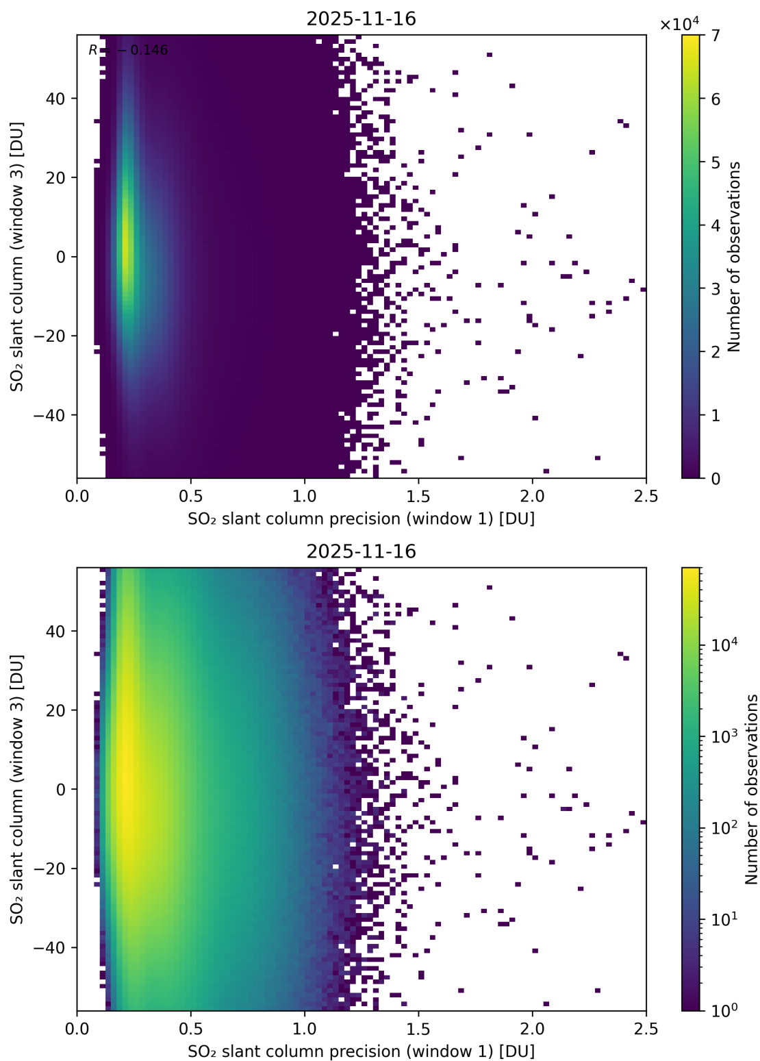
Figure 278: Scatter density plot of “SO 2 slant column precision (window 1)” against “SO 2 slant column (window 3)” for 2025-11-15 to 2025-11-17.
