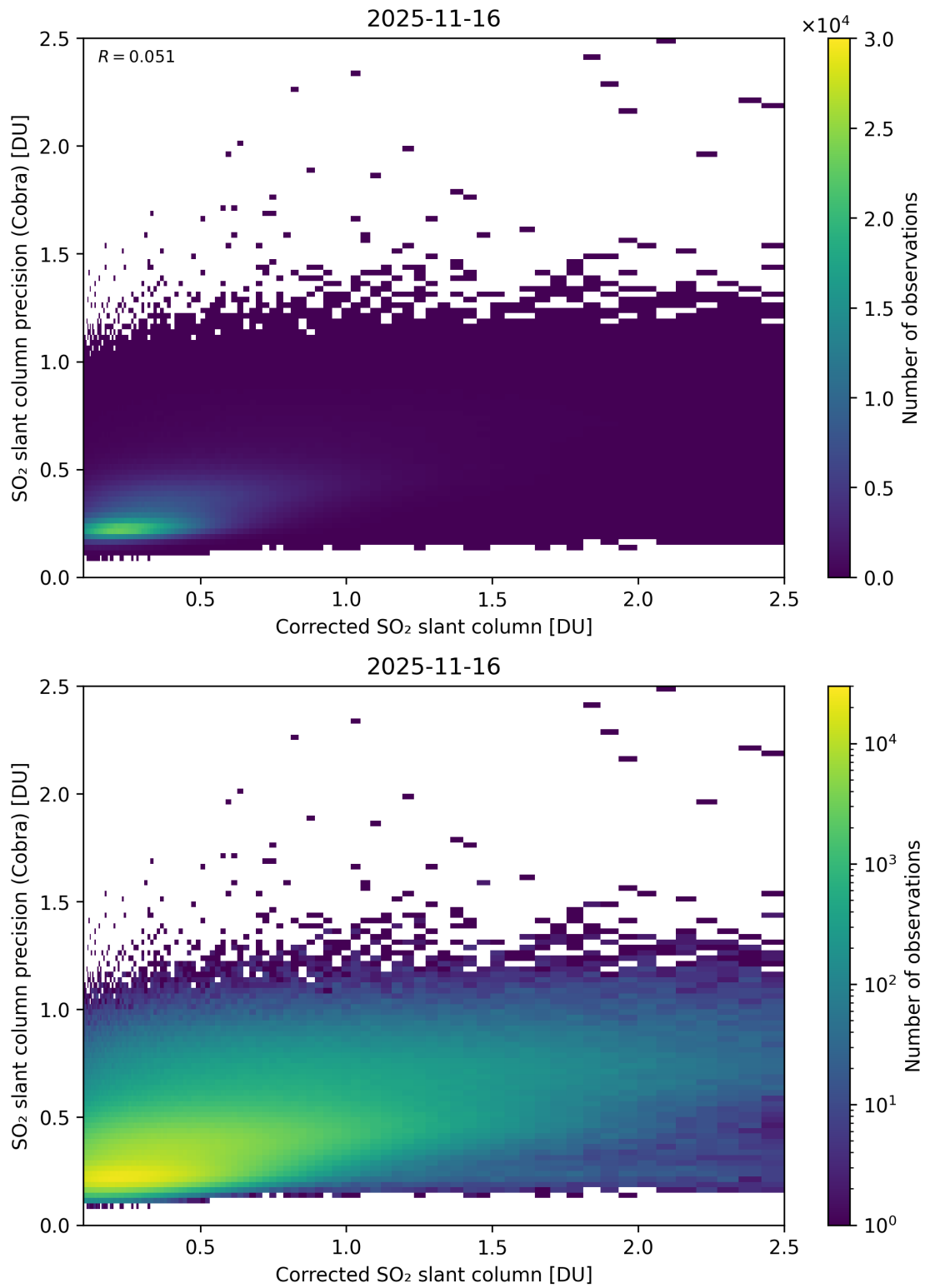
Figure 234: Scatter density plot of “Corrected SO 2 slant column” against “SO 2 slant column precision (Cobra)” for 2025-11-15 to 2025-11-17.
