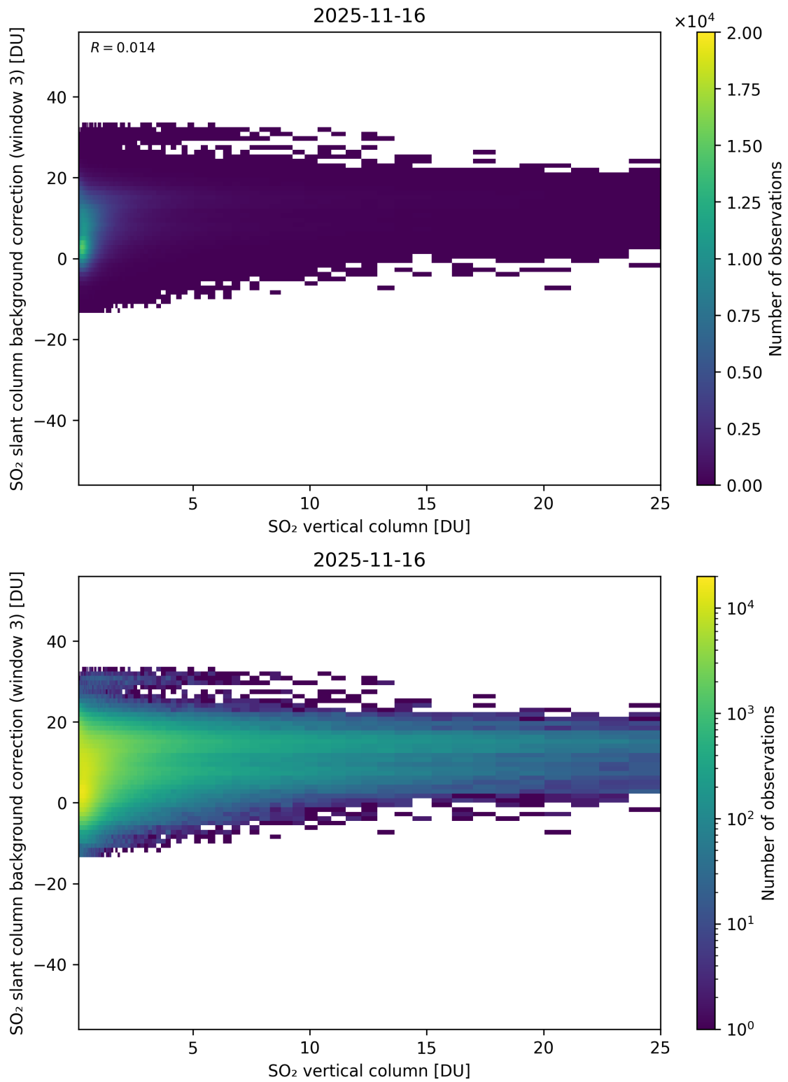
Figure 325: Scatter density plot of “SO 2 vertical column” against “SO 2 slant column background correction (window 3)” for 2025-11-15 to 2025-11-17.
