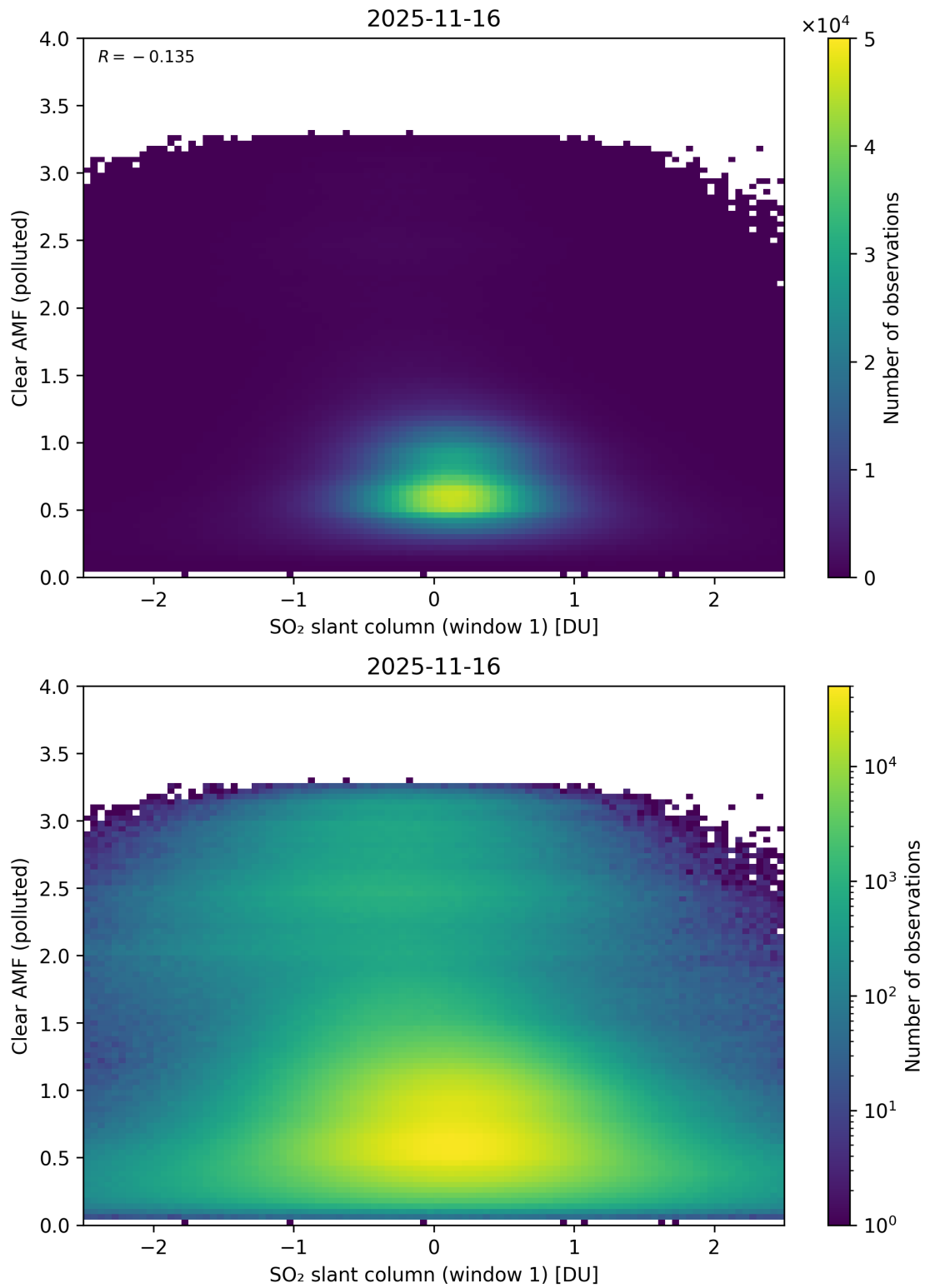
Figure 282: Scatter density plot of “SO 2 slant column (window 1)” against “Clear AMF (polluted)” for 2025-11-15 to 2025-11-17.
