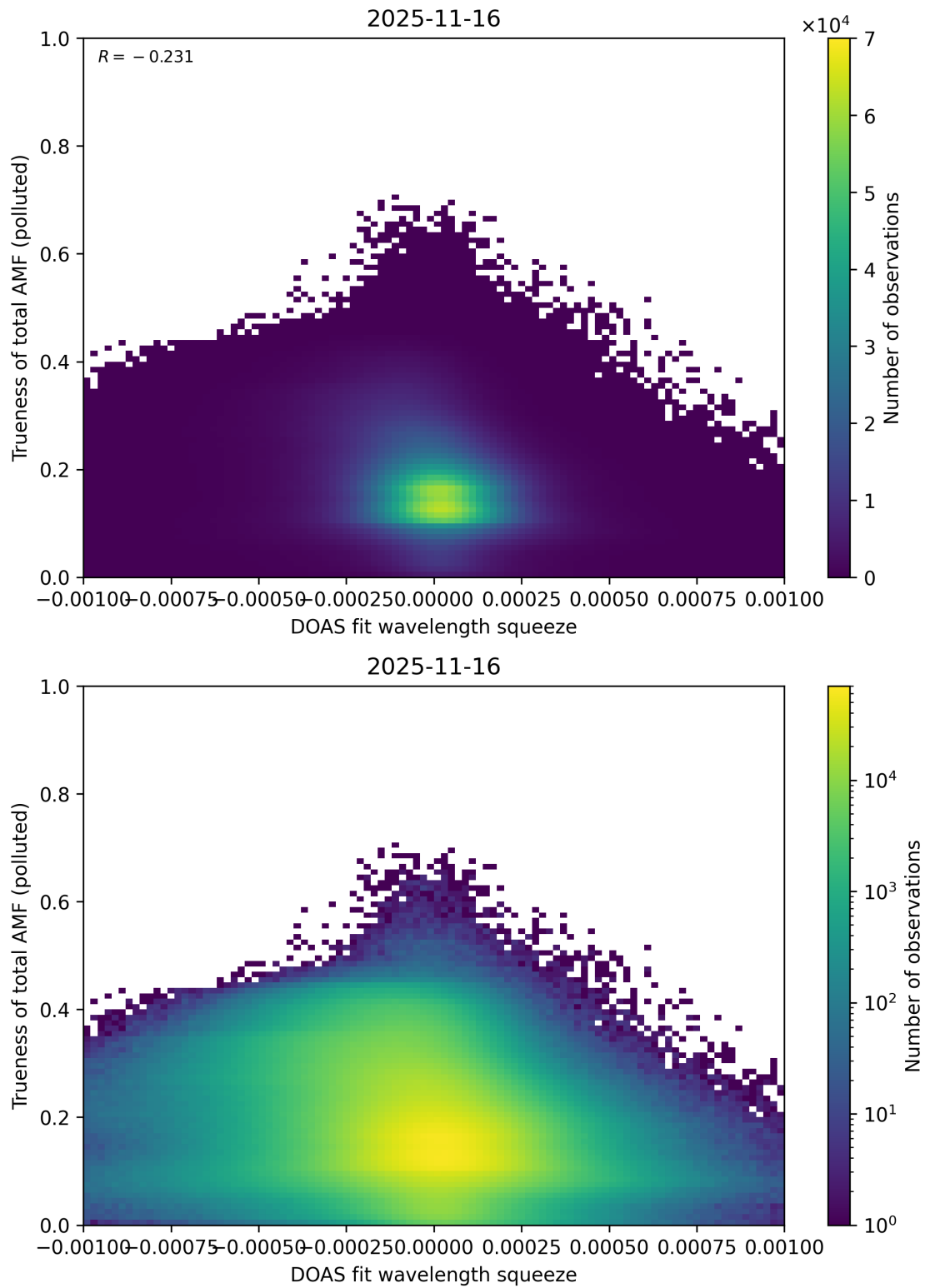
Figure 146: Scatter density plot of “DOAS fit wavelength squeeze” against “Trueness of total AMF (polluted)” for 2025-11-15 to 2025-11-17.
