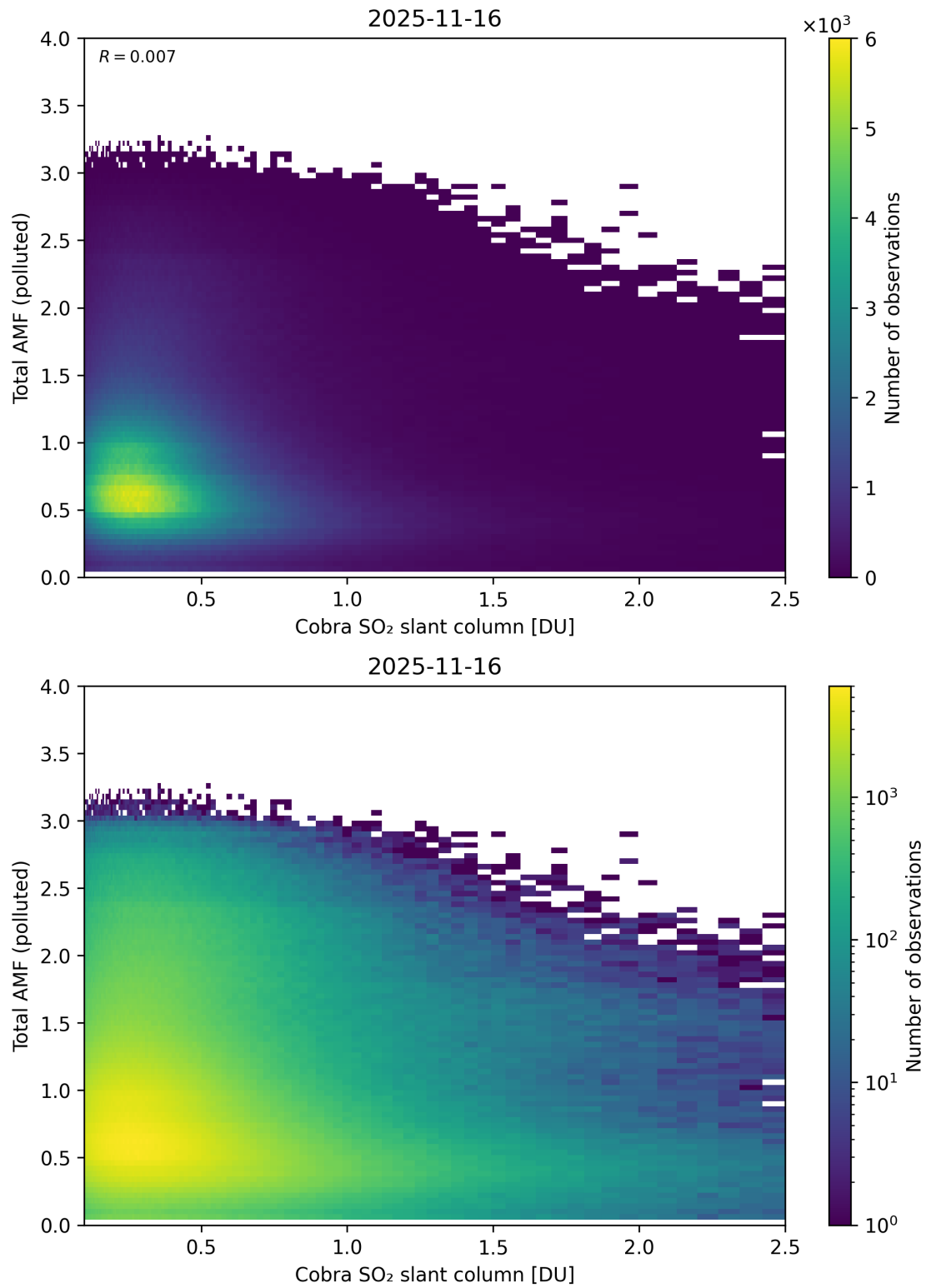
Figure 224: Scatter density plot of “Cobra SO 2 slant column” against “Total AMF (polluted)” for 2025-11-15 to 2025-11-17.
