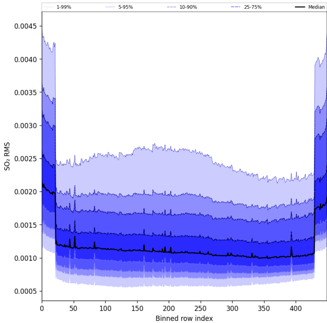
Figure 104: Along track statistics of “SO 2 RMS” for 2025-11-15 to 2025-11-17
