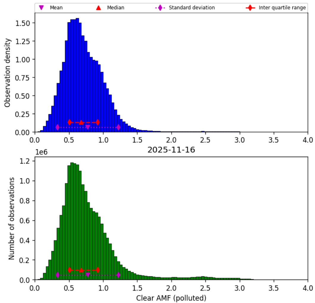
Figure 81: Histogram of “Clear AMF (polluted)” for 2025-11-15 to 2025-11-17
