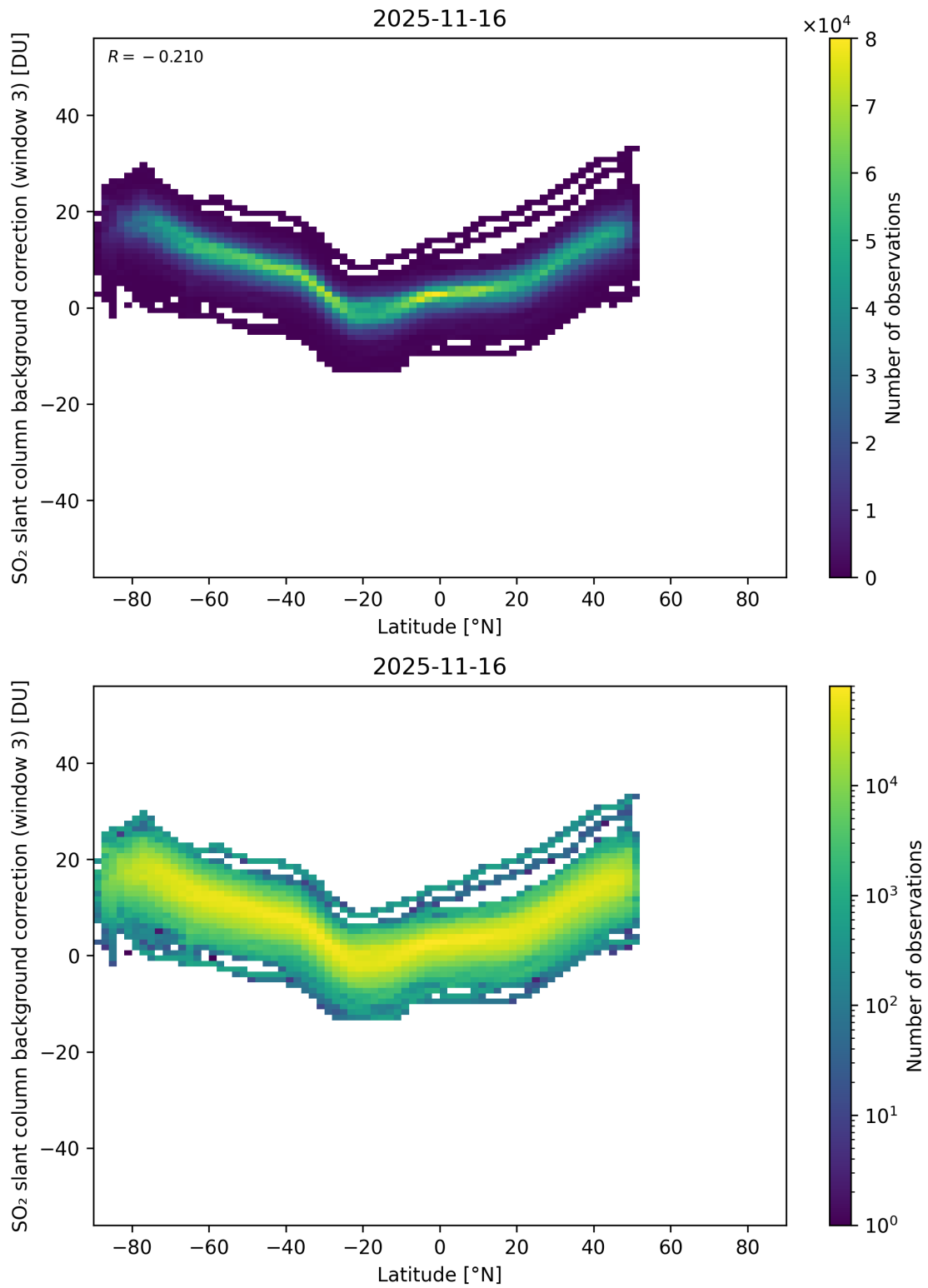
Figure 152: Scatter density plot of “Latitude” against “SO 2 slant column background correction (window 3)” for 2025-11-15 to 2025-11-17.
