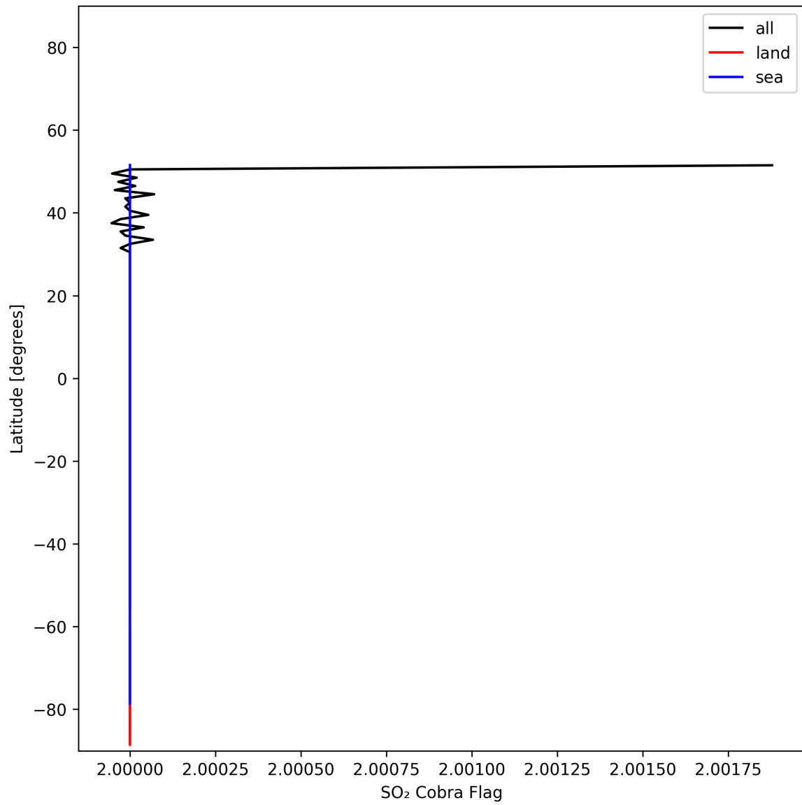
Figure 49: Zonal average of “SO 2 Cobra Flag” for 2025-11-15 to 2025-11-17.
