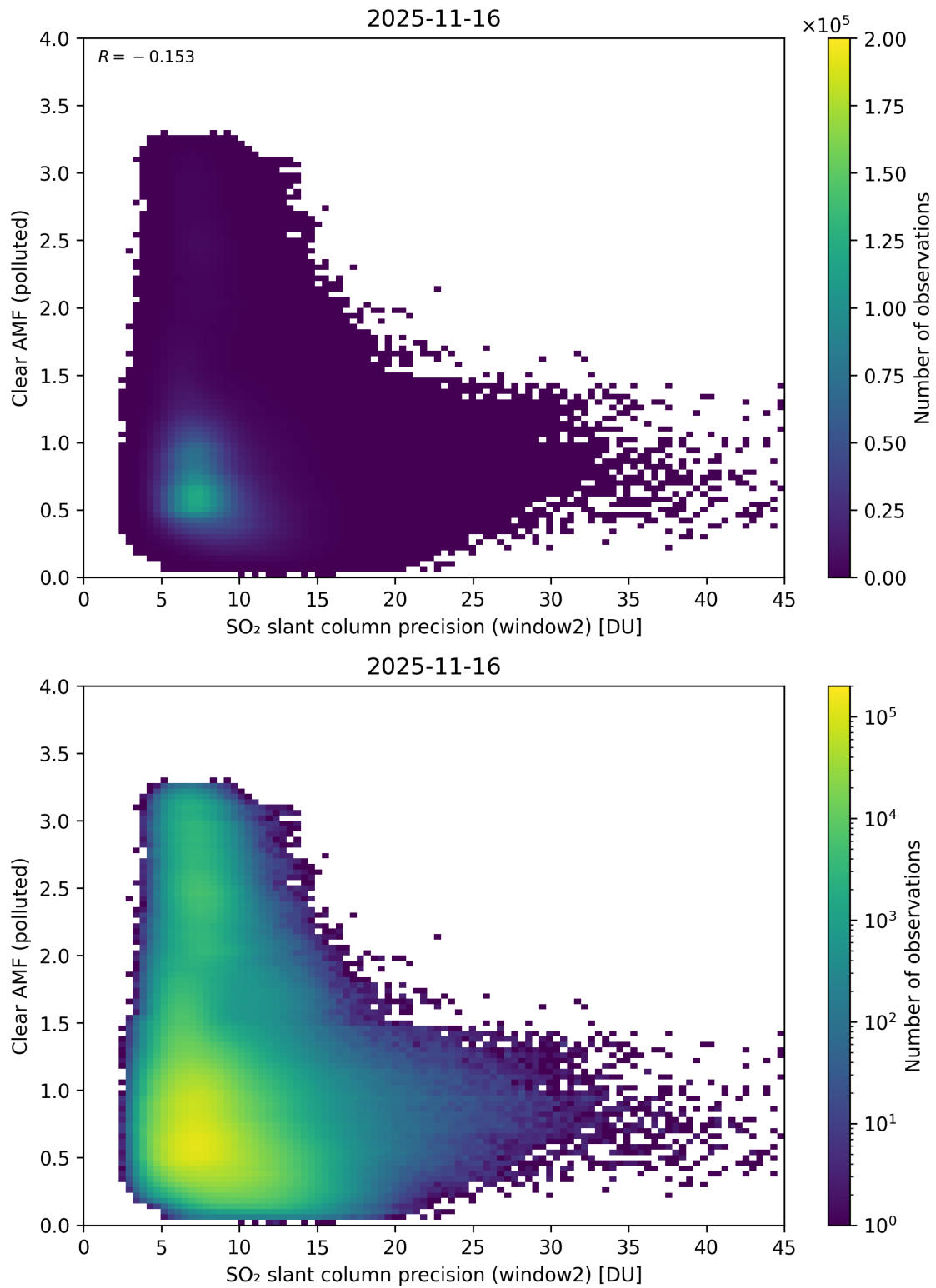
Figure 296: Scatter density plot of “SO 2 slant column precision (window2)” against “Clear AMF (polluted)” for 2025-11-15 to 2025-11-17.
