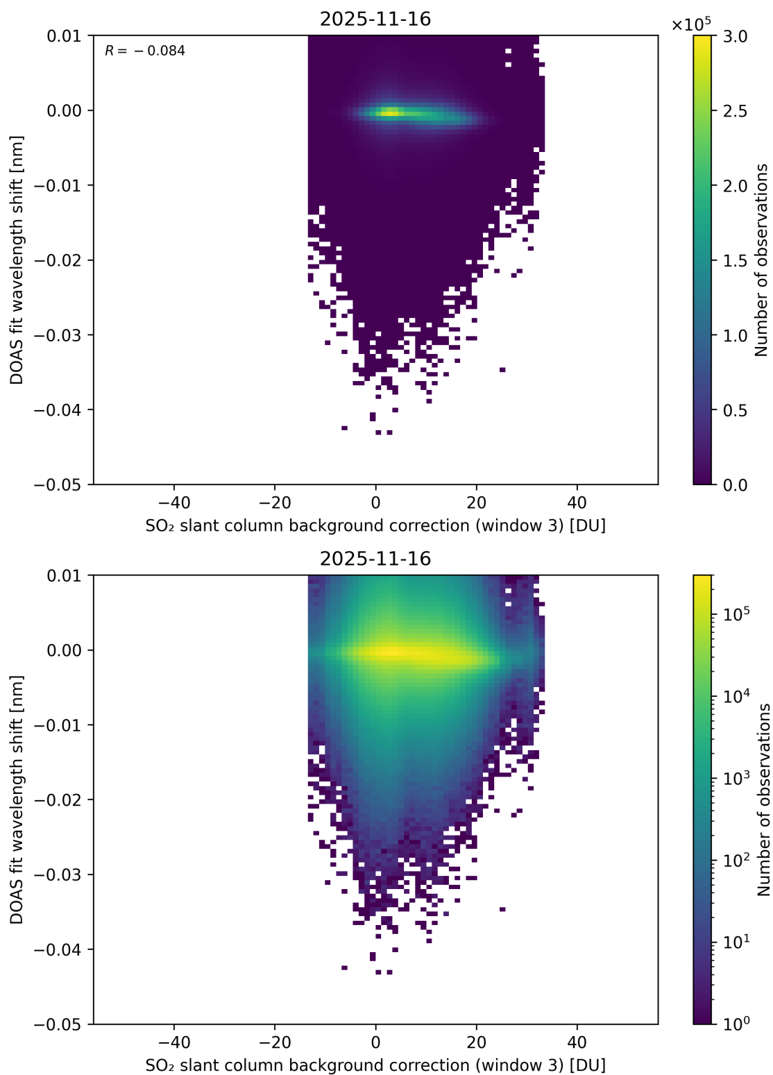
Figure 132: Scatter density plot of “SO 2 slant column background correction (window 3)” against “DOAS fit wavelength shift” for 2025-11-15 to 2025-11-17.
