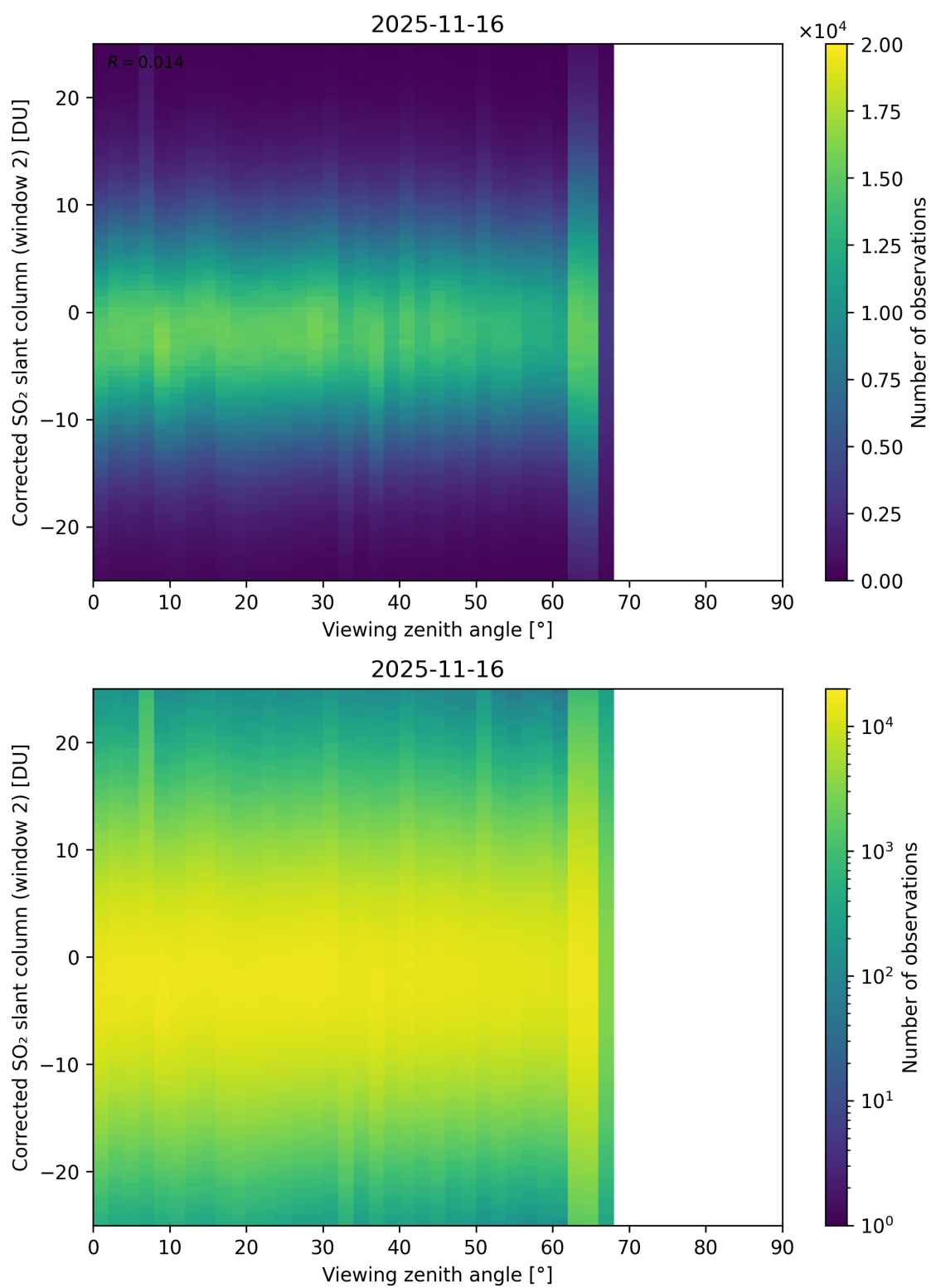
Figure 374: Scatter density plot of “Viewing zenith angle” against “Corrected SO 2 slant column (window 2)” for 2025-11-15 to 2025-11-17.
