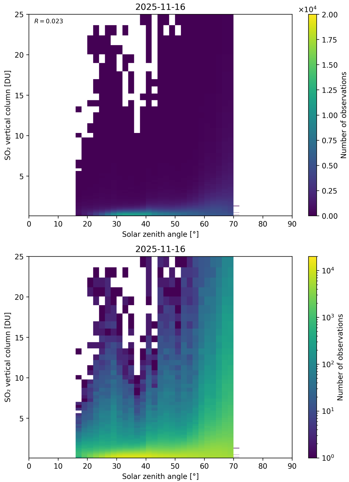
Figure 191: Scatter density plot of “Solar zenith angle” against “SO 2 vertical column” for 2025-11-15 to 2025-11-17.
