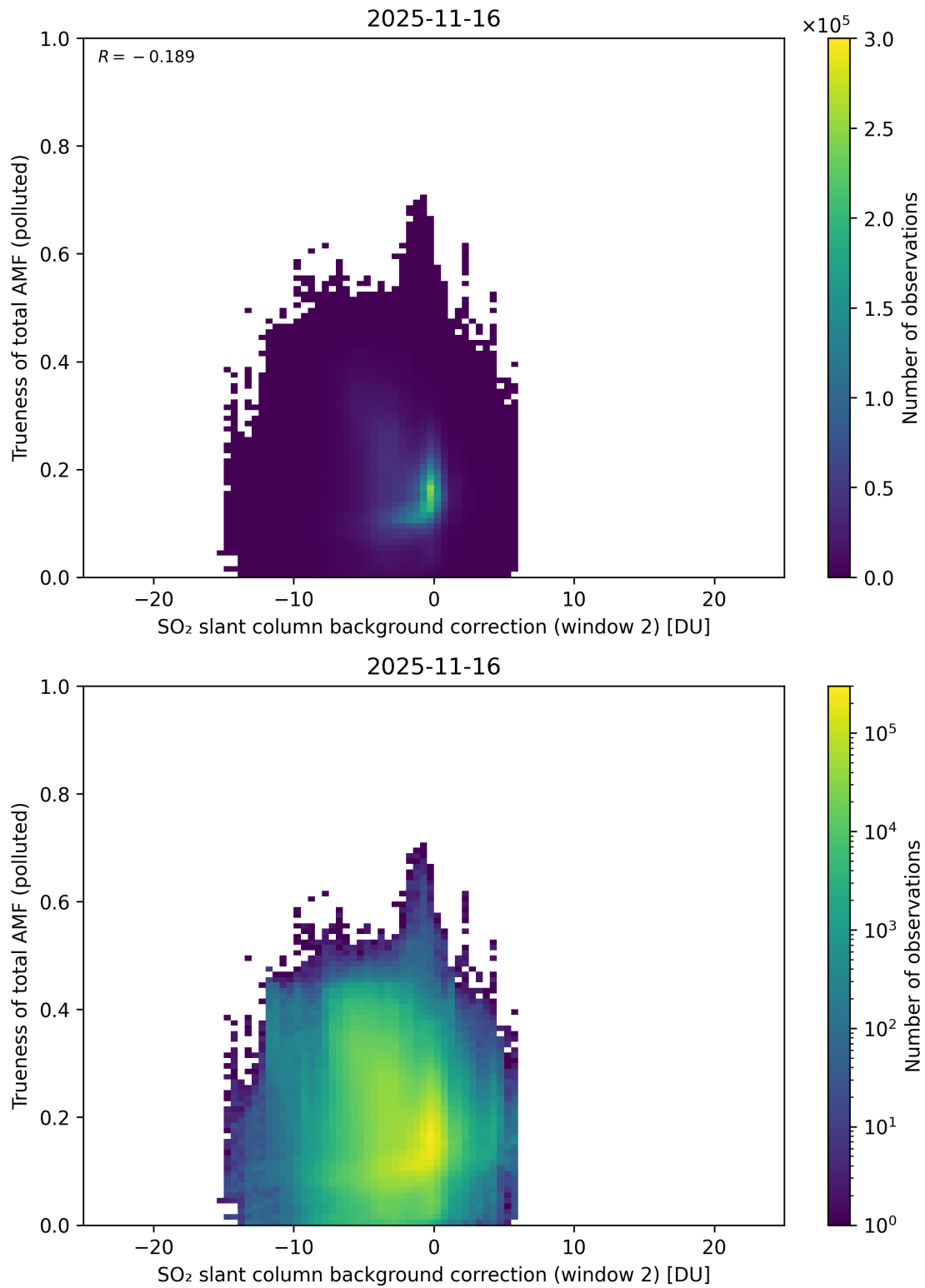
Figure 131: Scatter density plot of “SO 2 slant column background correction (window 2)” against “Trueness of total AMF (polluted)” for 2025-11-15 to 2025-11-17.
