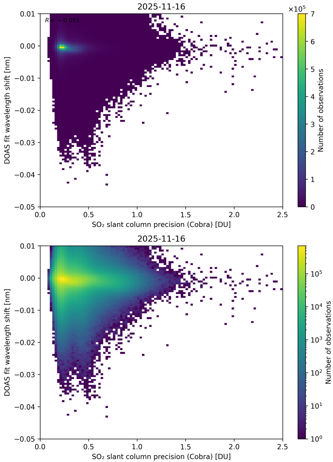
Figure 202: Scatter density plot of “SO 2 slant column precision (Cobra)” against “DOAS fit wavelength shift” for 2025-11-15 to 2025-11-17.
