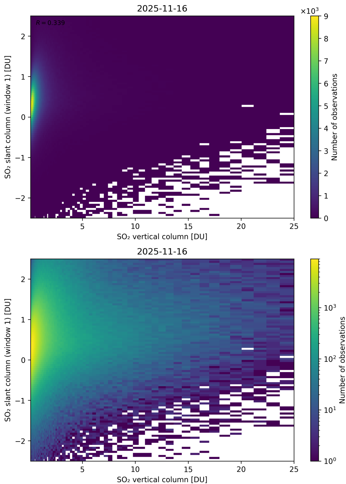
Figure 354: Scatter density plot of “SO 2 vertical column” against “SO 2 slant column (window 1)” for 2025-11-15 to 2025-11-17.
