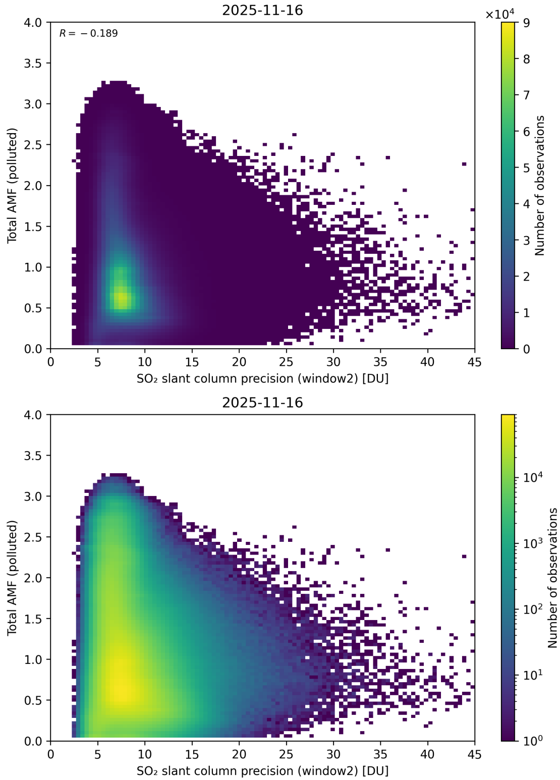
Figure 301: Scatter density plot of “SO 2 slant column precision (window2)” against “Total AMF (polluted)” for 2025-11-15 to 2025-11-17.
