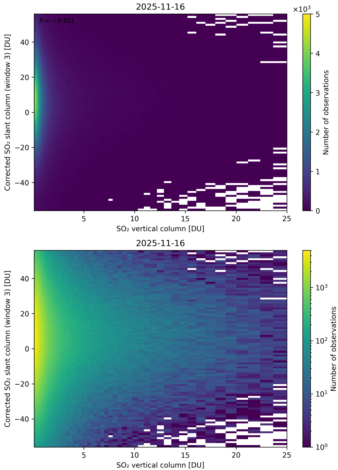
Figure 353: Scatter density plot of “SO 2 vertical column” against “Corrected SO 2 slant column (window 3)” for 2025-11-15 to 2025-11-17.
