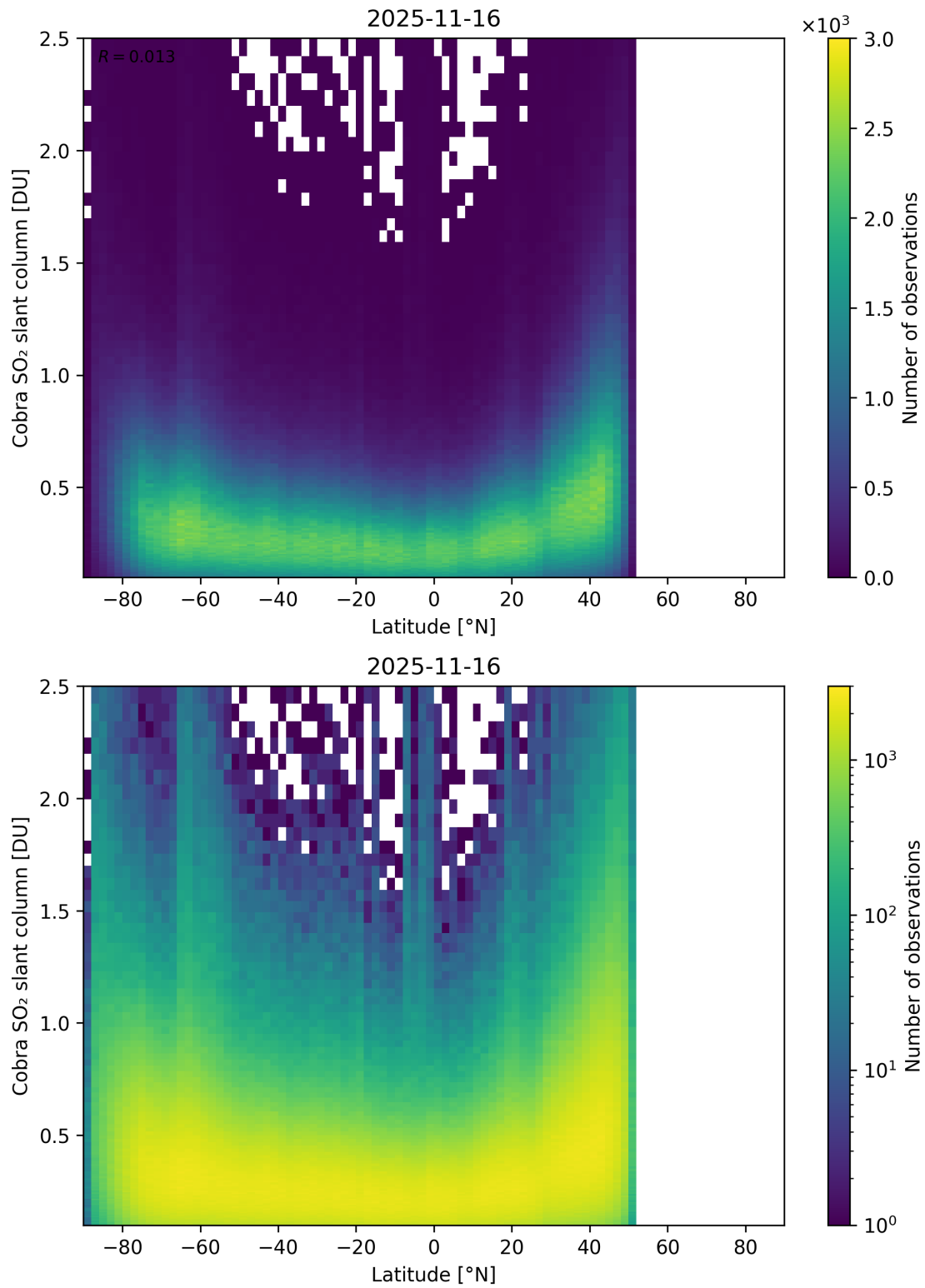
Figure 157: Scatter density plot of “Latitude” against “Cobra SO 2 slant column” for 2025-11-15 to 2025-11-17.
