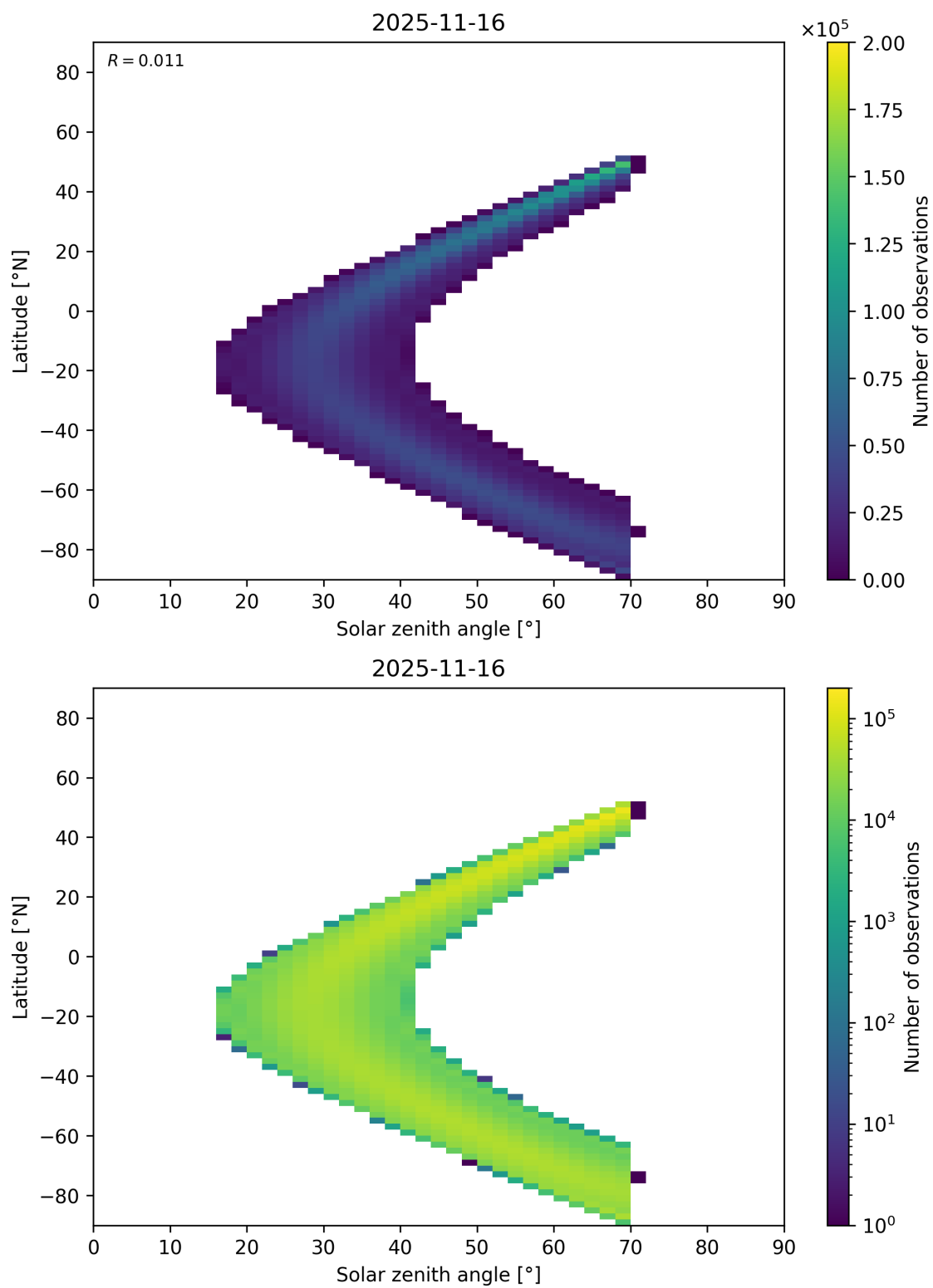
Figure 177: Scatter density plot of “Solar zenith angle” against “Latitude” for 2025-11-15 to 2025-11-17.
