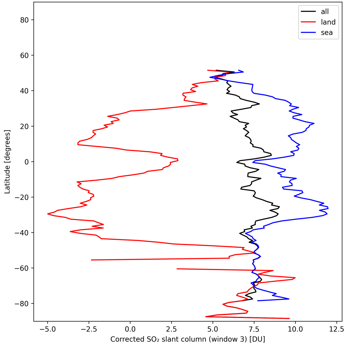
Figure 47: Zonal average of “Corrected SO 2 slant column (window 3)” for 2025-11-15 to 2025-11-17.
