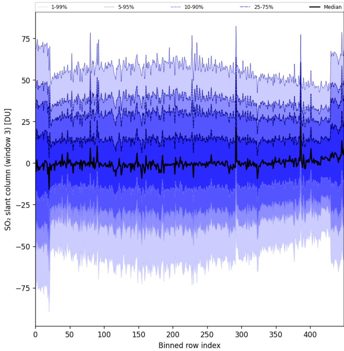
Figure 97: Along track statistics of “SO 2 slant column (window 3)” for 2025-11-15 to 2025-11-17
