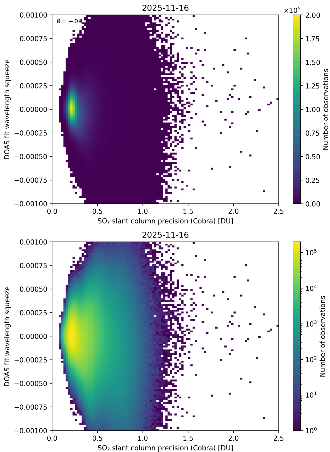
Figure 203: Scatter density plot of “SO 2 slant column precision (Cobra)” against “DOAS fit wavelength squeeze” for 2025-11-15 to 2025-11-17.
