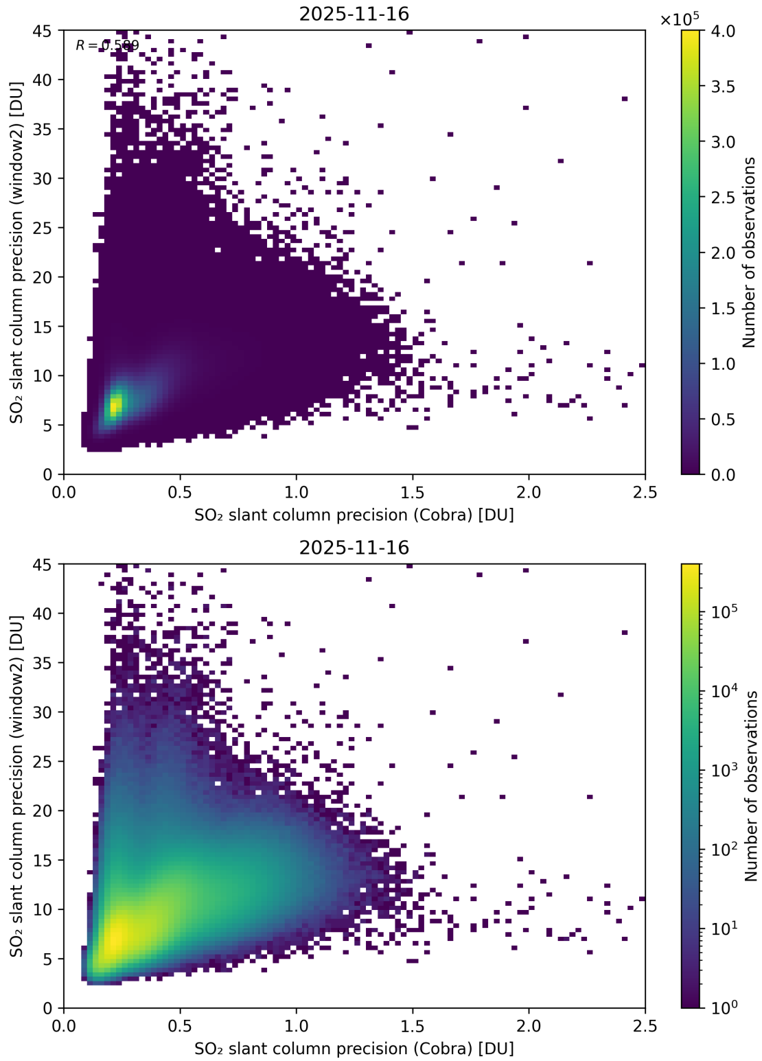
Figure 210: Scatter density plot of “SO 2 slant column precision (Cobra)” against “SO 2 slant column precision (window2)” for 2025-11-15 to 2025-11-17.
