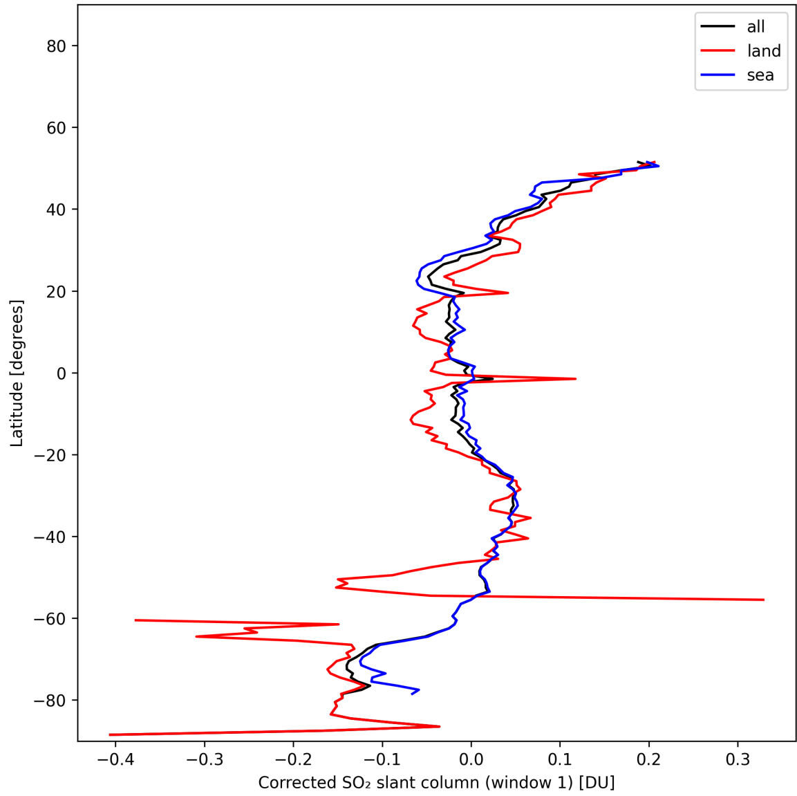
Figure 39: Zonal average of “Corrected SO 2 slant column (window 1)” for 2025-11-15 to 2025-11-17.
