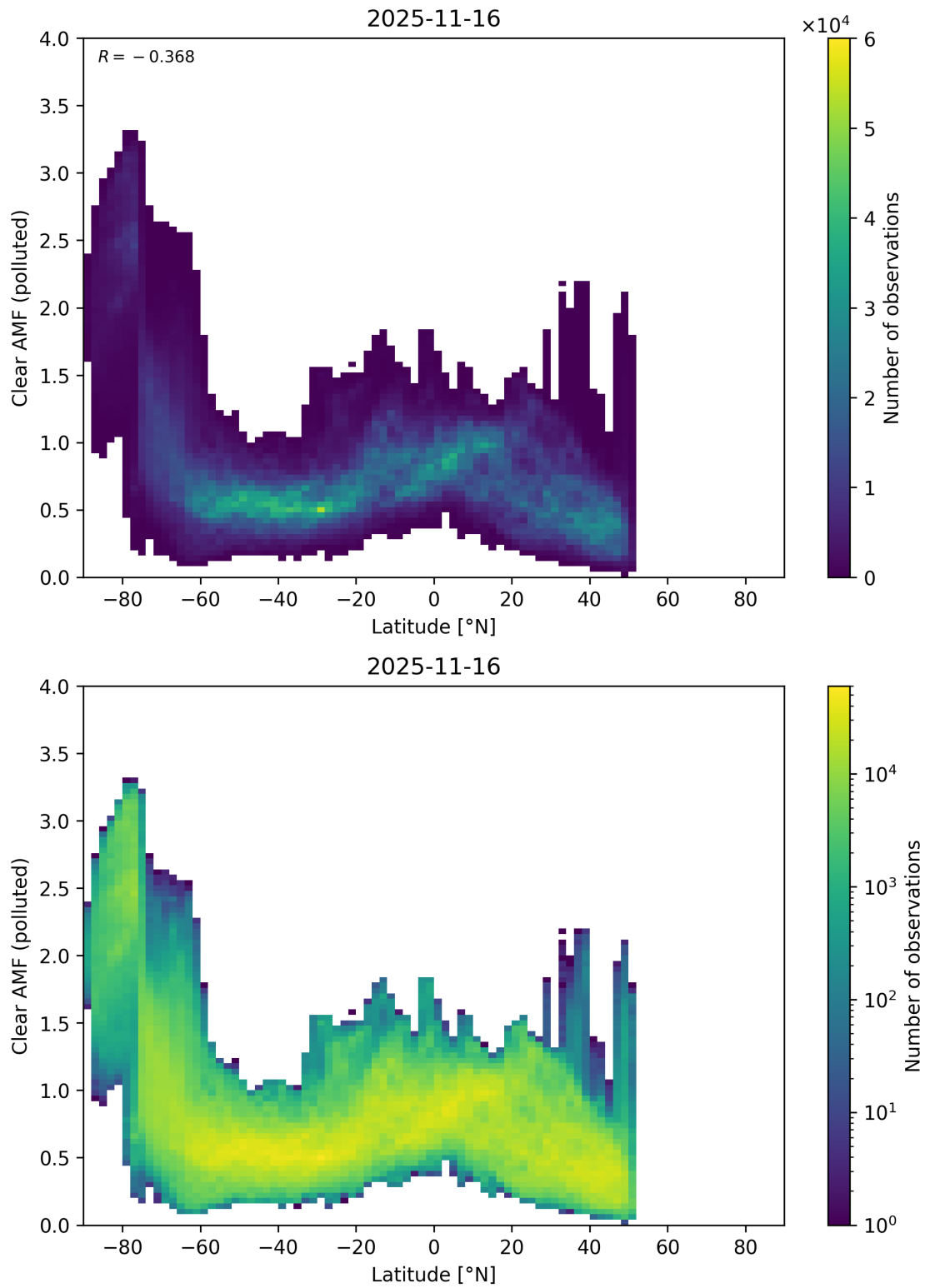
Figure 156: Scatter density plot of “Latitude” against “Clear AMF (polluted)” for 2025-11-15 to 2025-11-17.
