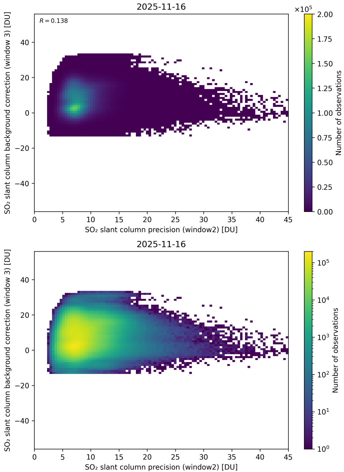
Figure 292: Scatter density plot of “SO 2 slant column precision (window2)” against “SO 2 slant column background correction (window 3)” for 2025-11-15 to 2025-11-17.
