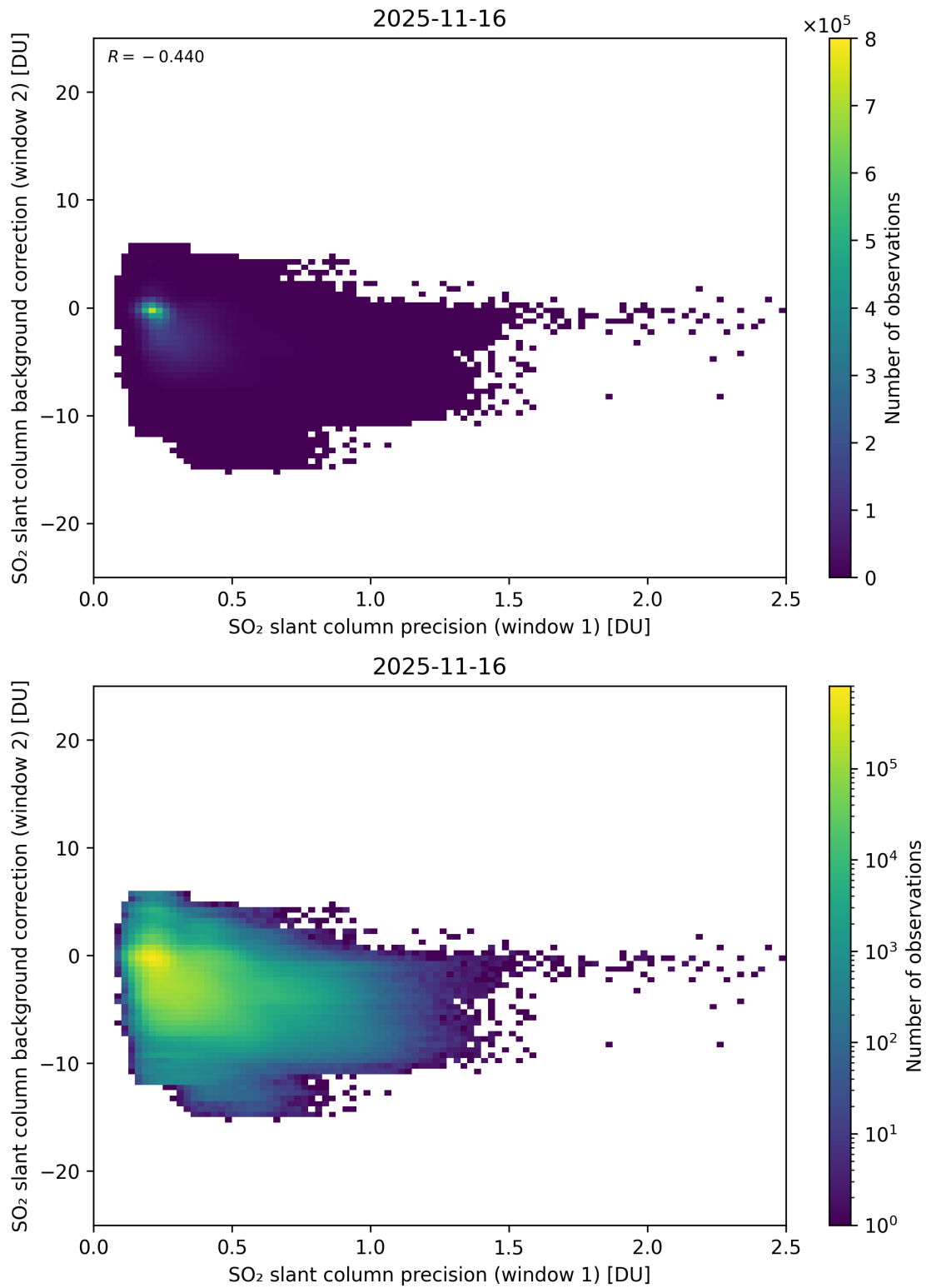
Figure 269: Scatter density plot of “SO 2 slant column precision (window 1)” against “SO 2 slant column background correction (window 2)” for 2025-11-15 to 2025-11-17.
