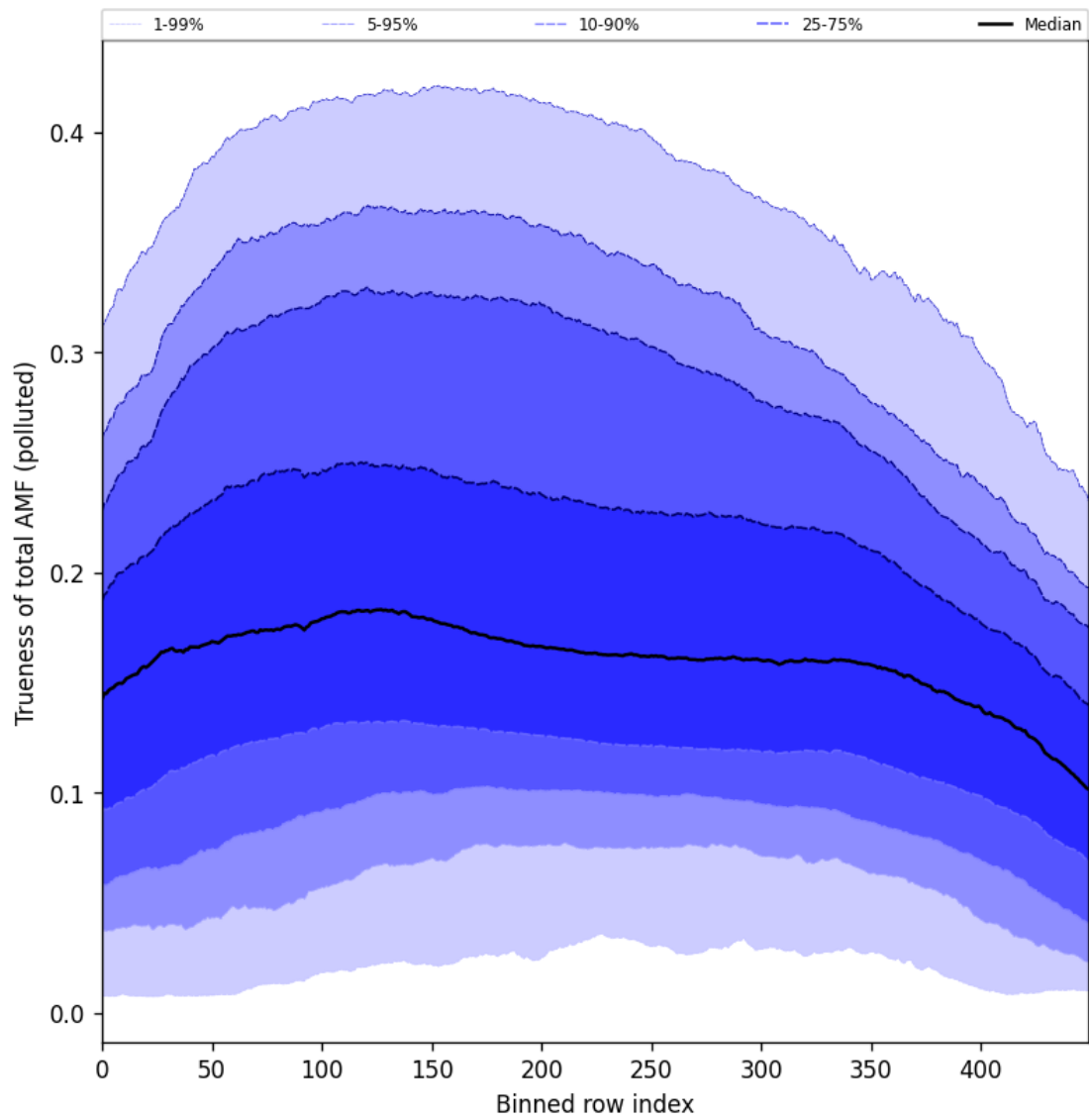
Figure 106: Along track statistics of “Trueness of total AMF (polluted)” for 2025-11-15 to 2025-11-17
