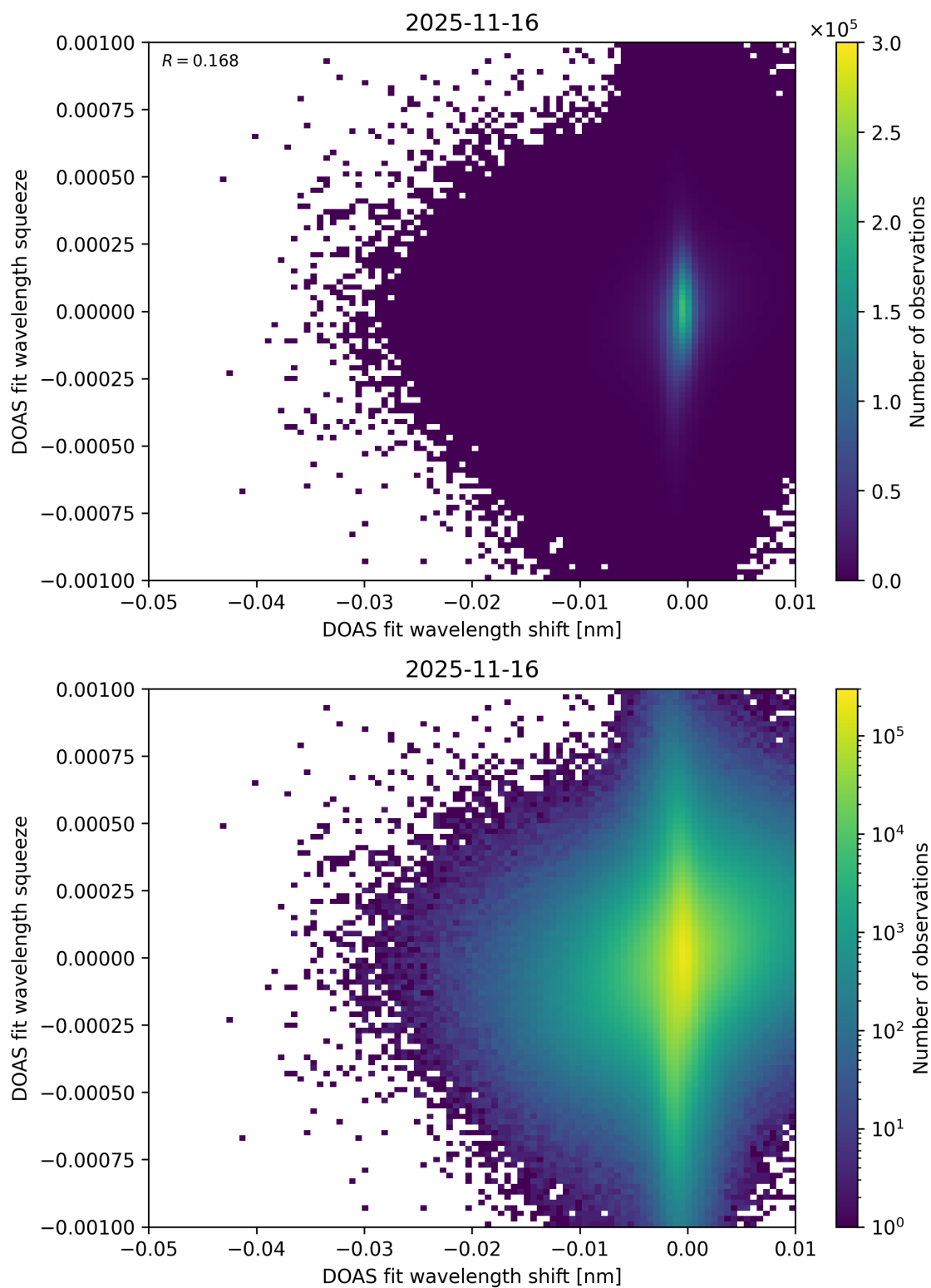
Figure 138: Scatter density plot of “DOAS fit wavelength shift” against “DOAS fit wavelength squeeze” for 2025-11-15 to 2025-11-17.
