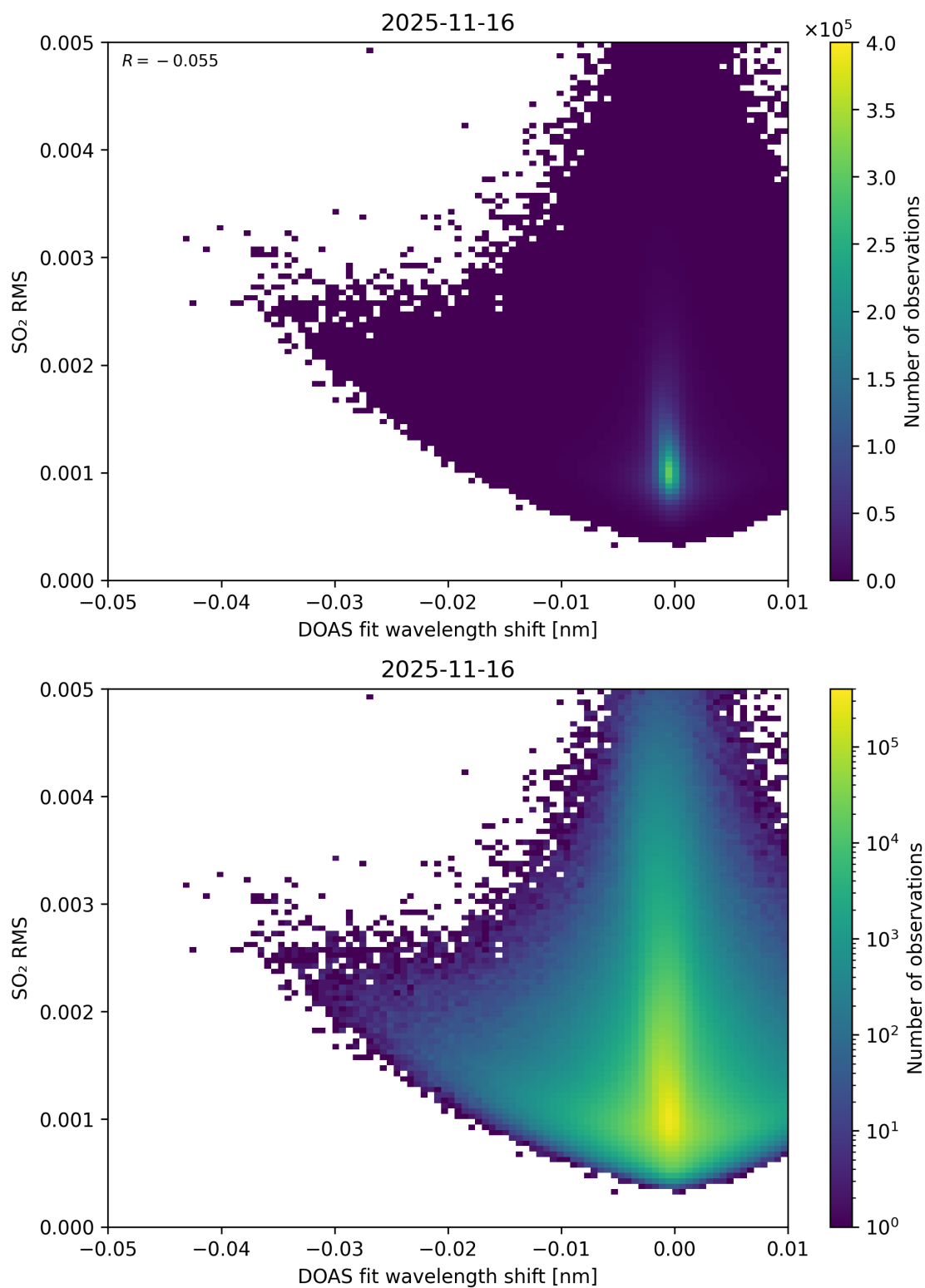
Figure 139: Scatter density plot of “DOAS fit wavelength shift” against “SO 2 RMS” for 2025-11-15 to 2025-11-17.
