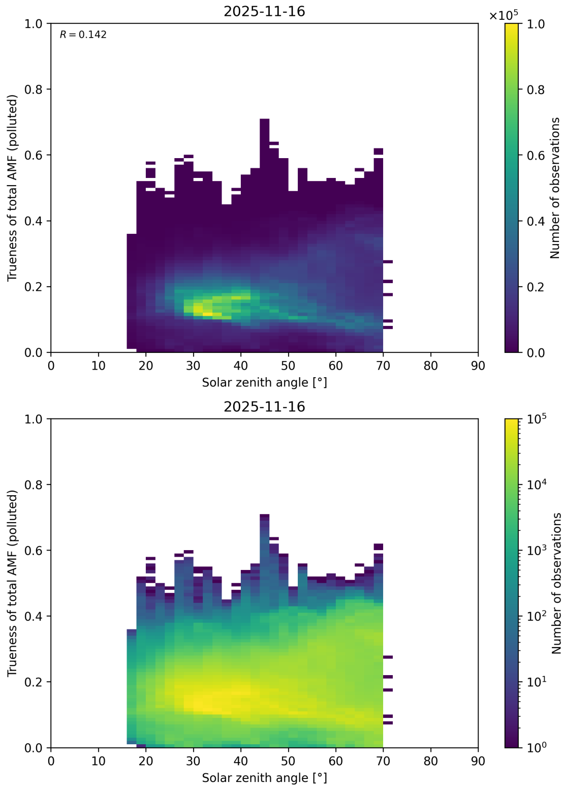
Figure 190: Scatter density plot of “Solar zenith angle” against “Trueness of total AMF (polluted)” for 2025-11-15 to 2025-11-17.
