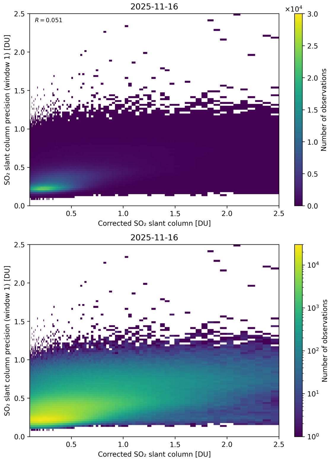
Figure 238: Scatter density plot of “Corrected SO 2 slant column” against “SO 2 slant column precision (window 1)” for 2025-11-15 to 2025-11-17.
