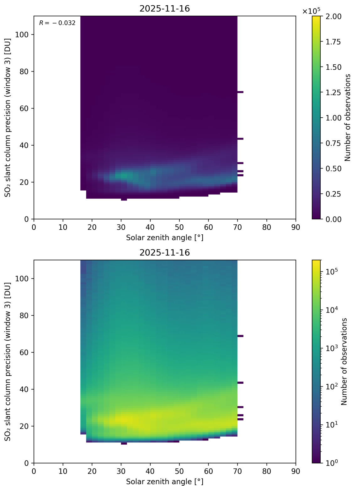
Figure 188: Scatter density plot of “Solar zenith angle” against “SO 2 slant column precision (window 3)” for 2025-11-15 to 2025-11-17.
