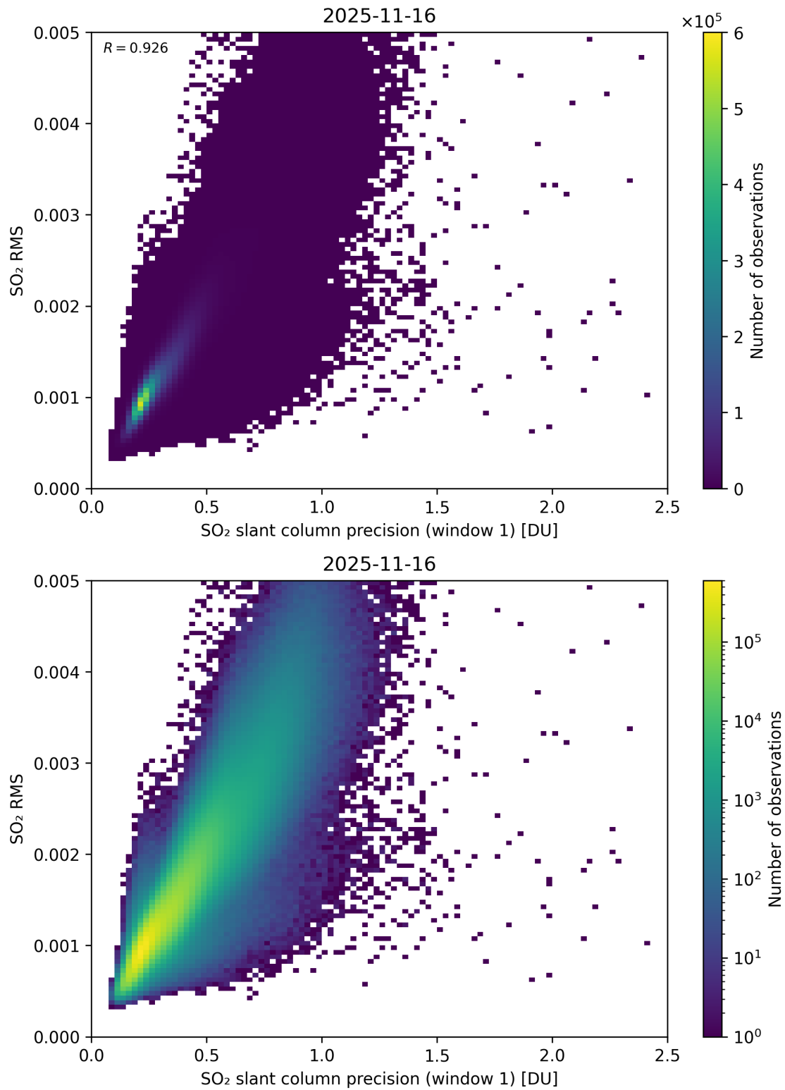
Figure 273: Scatter density plot of “SO 2 slant column precision (window 1)” against “SO 2 RMS” for 2025-11-15 to 2025-11-17.
