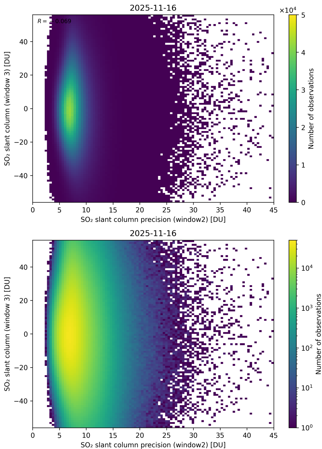
Figure 299: Scatter density plot of “SO 2 slant column precision (window2)” against “SO 2 slant column (window 3)” for 2025-11-15 to 2025-11-17.
