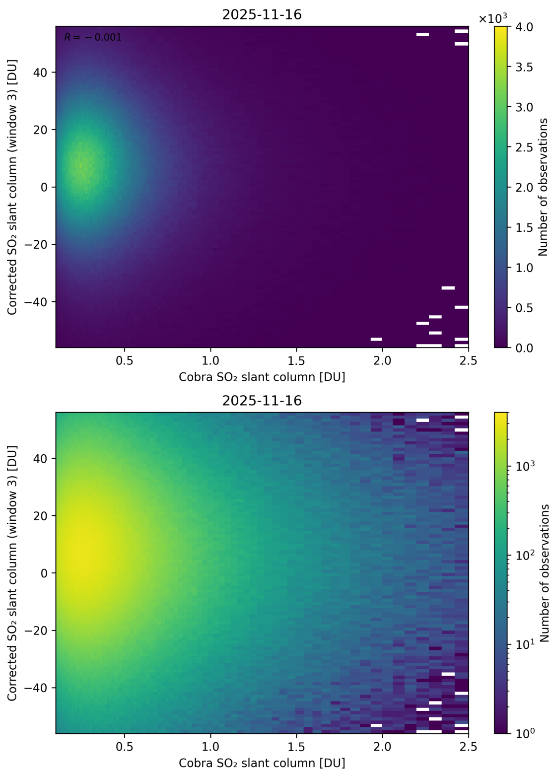
Figure 218: Scatter density plot of “Cobra SO 2 slant column” against “Corrected SO 2 slant column (window 3)” for 2025-11-15 to 2025-11-17.
