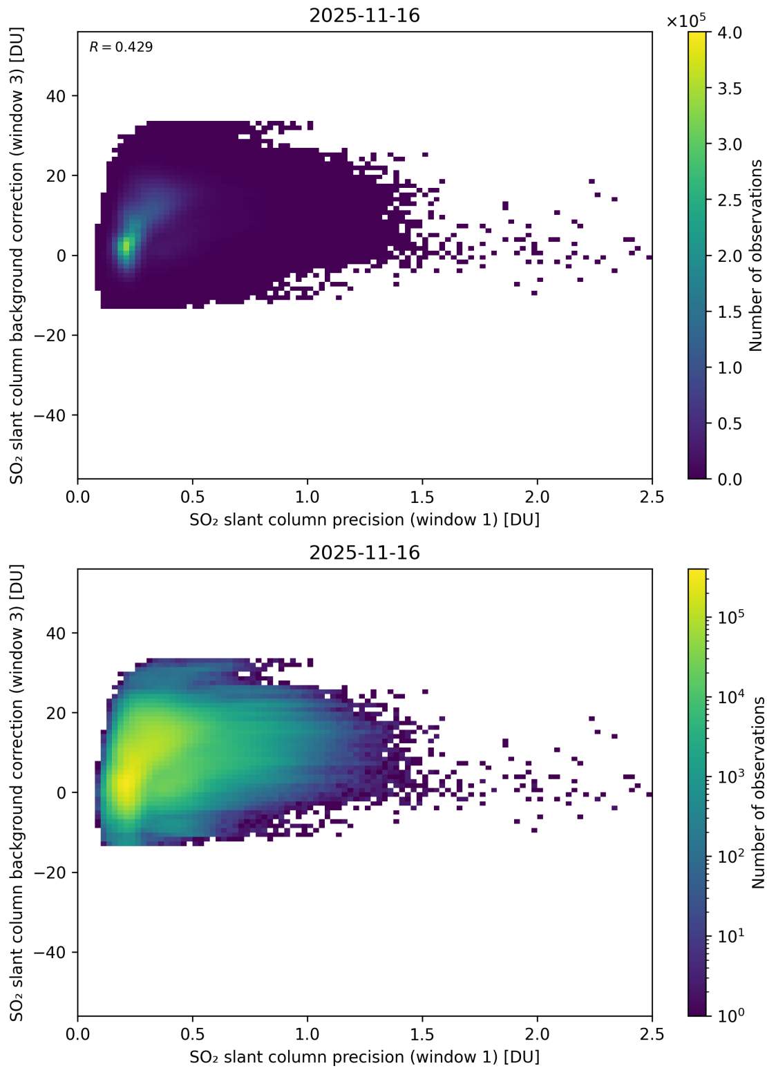
Figure 270: Scatter density plot of “SO 2 slant column precision (window 1)” against “SO 2 slant column background correction (window 3)” for 2025-11-15 to 2025-11-17.
