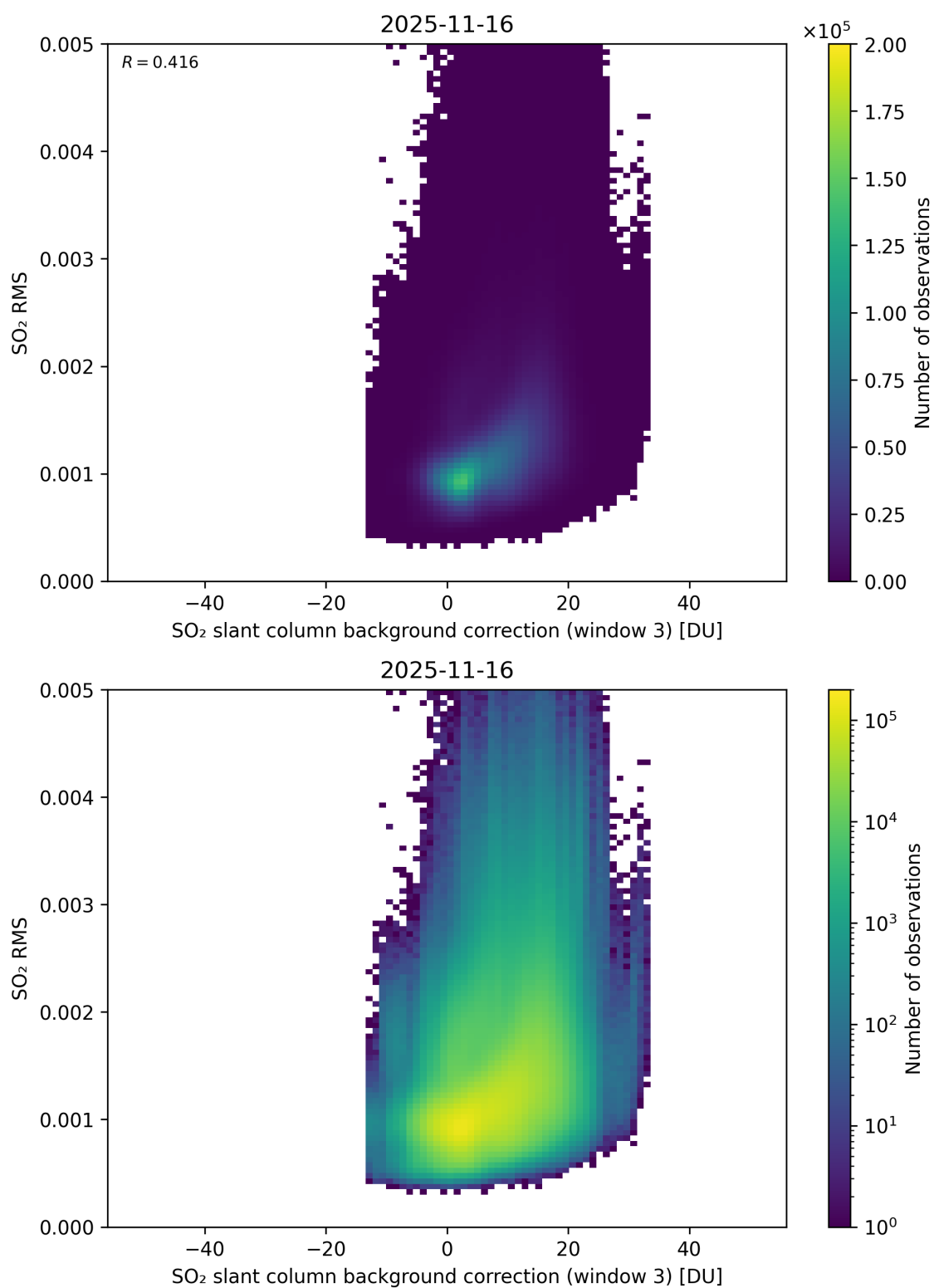
Figure 134: Scatter density plot of “SO 2 slant column background correction (window 3)” against “SO 2 RMS” for 2025-11-15 to 2025-11-17.
