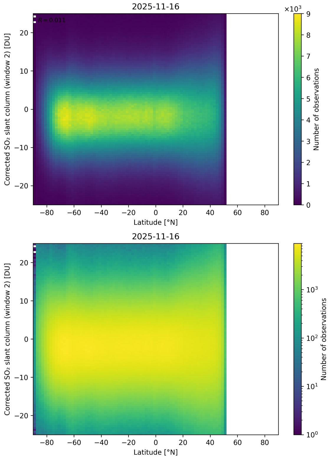
Figure 160: Scatter density plot of “Latitude” against “Corrected SO 2 slant column (window 2)” for 2025-11-15 to 2025-11-17.
