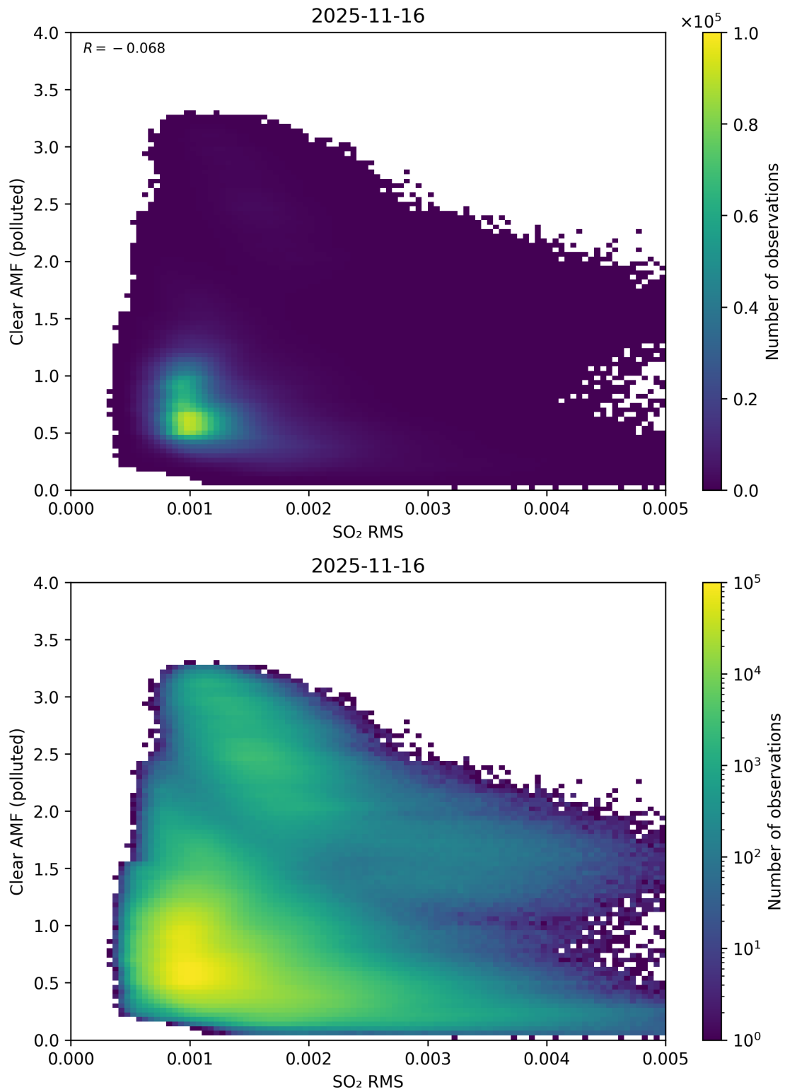
Figure 147: Scatter density plot of “SO 2 RMS” against “Clear AMF (polluted)” for 2025-11-15 to 2025-11-17.
