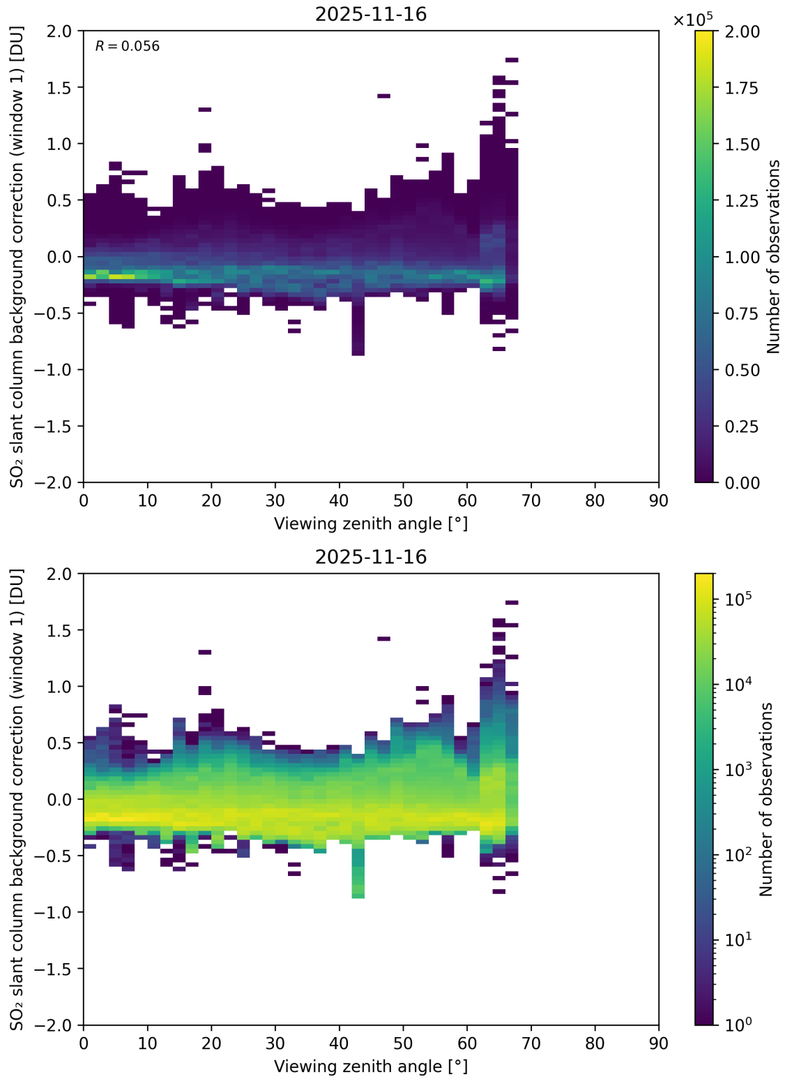
Figure 362: Scatter density plot of “Viewing zenith angle” against “SO 2 slant column background correction (window 1)” for 2025-11-15 to 2025-11-17.
