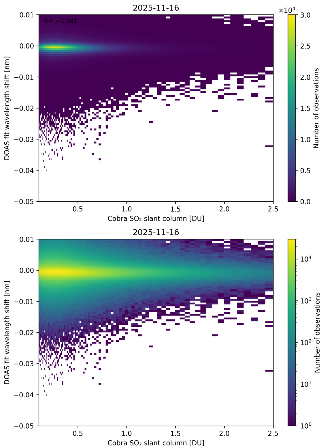
Figure 196: Scatter density plot of “Cobra SO 2 slant column” against “DOAS fit wavelength shift” for 2025-11-15 to 2025-11-17.
