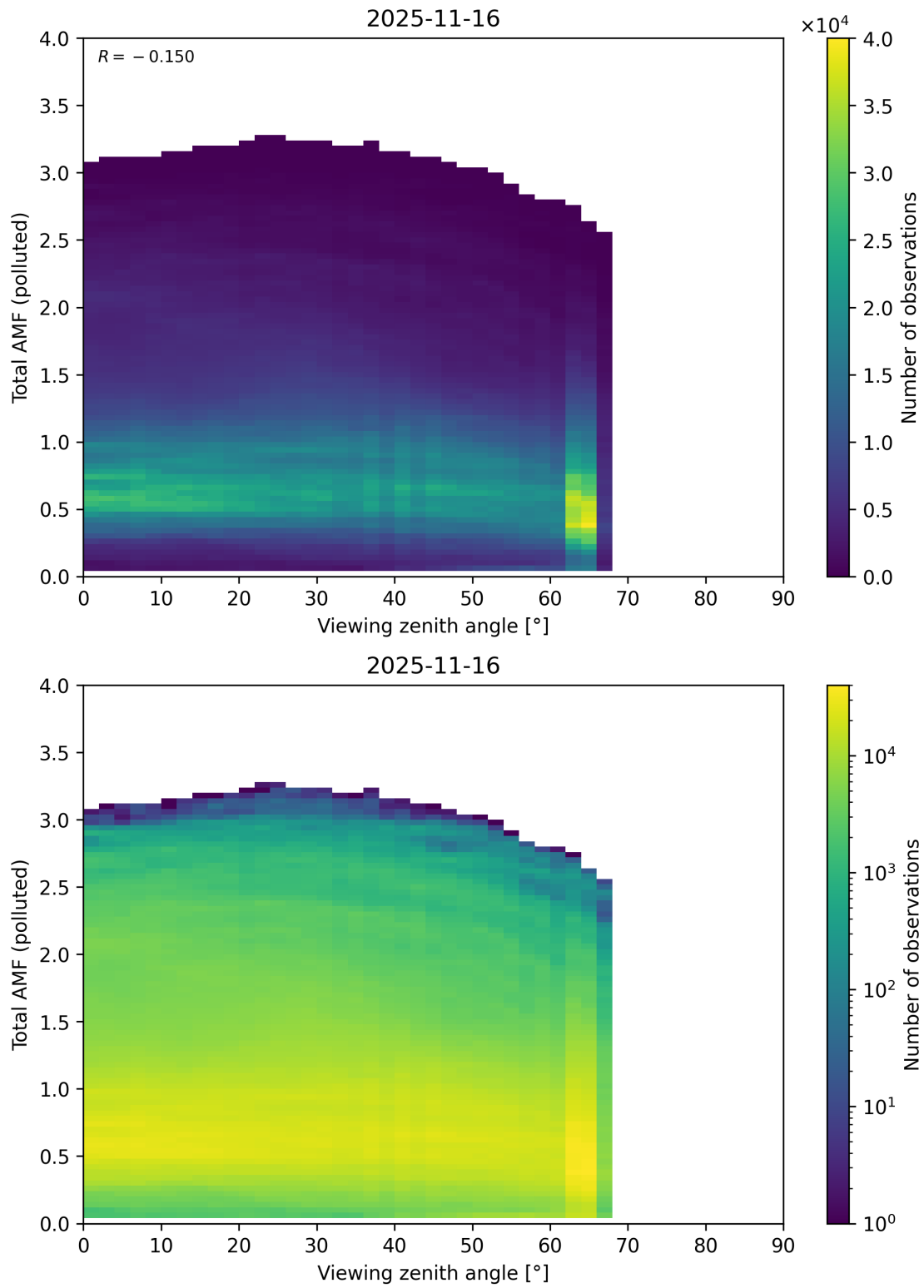
Figure 381: Scatter density plot of “Viewing zenith angle” against “Total AMF (polluted)” for 2025-11-15 to 2025-11-17.
