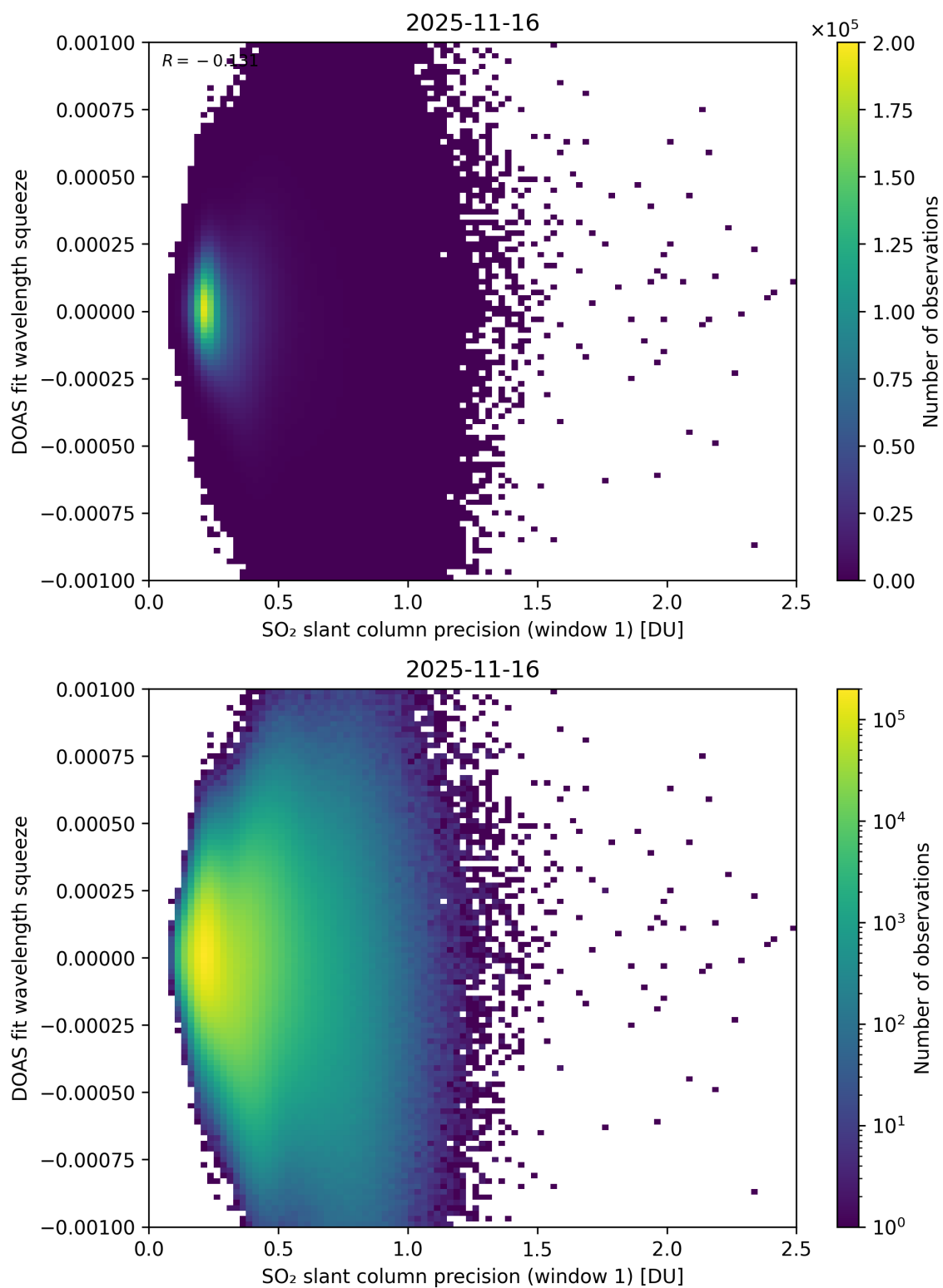
Figure 272: Scatter density plot of “SO 2 slant column precision (window 1)” against “DOAS fit wavelength squeeze” for 2025-11-15 to 2025-11-17.
