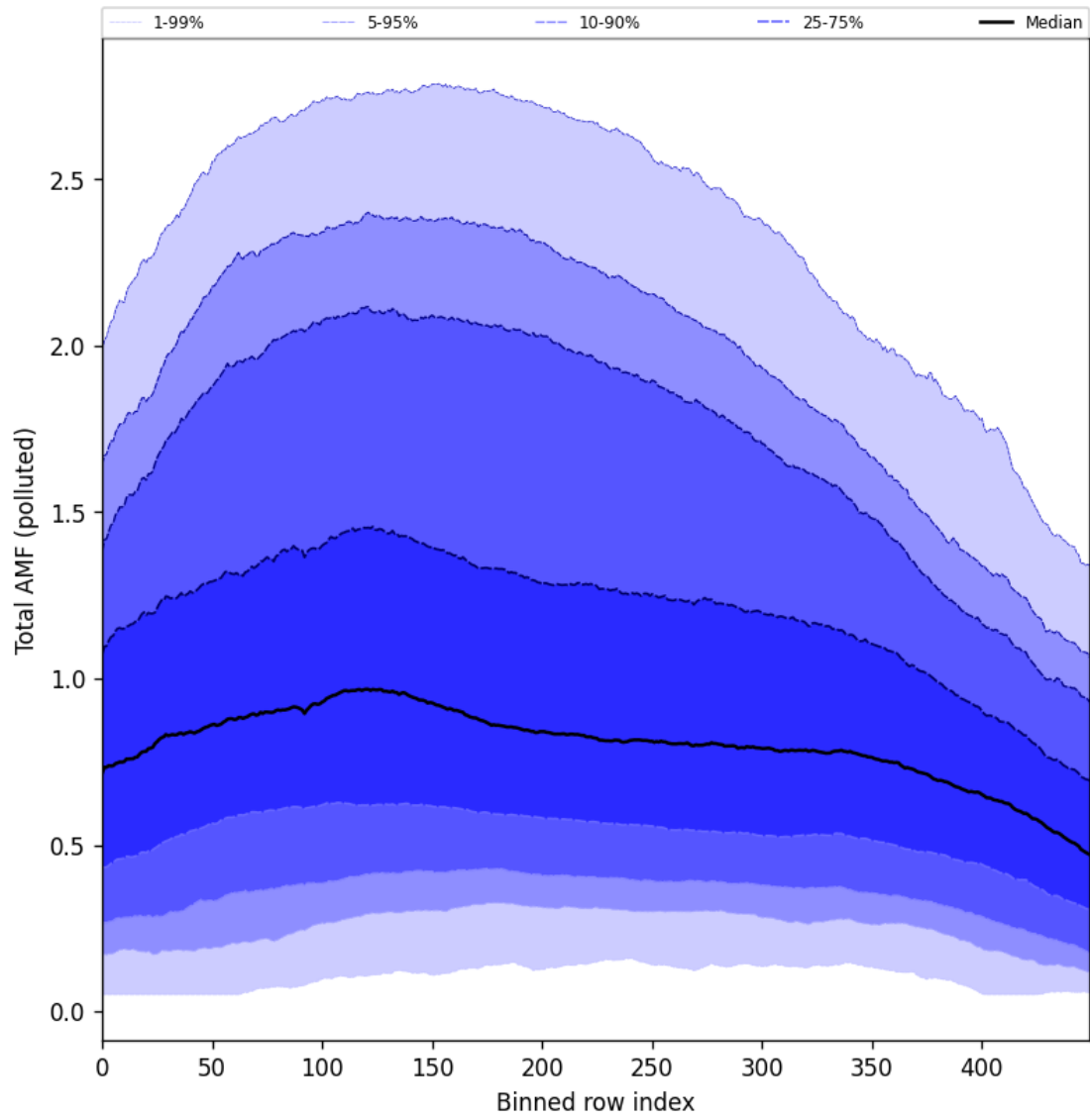
Figure 105: Along track statistics of “Total AMF (polluted)” for 2025-11-15 to 2025-11-17
