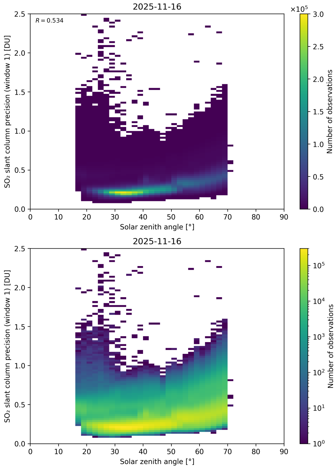
Figure 185: Scatter density plot of “Solar zenith angle” against “SO 2 slant column precision (window 1)” for 2025-11-15 to 2025-11-17.
