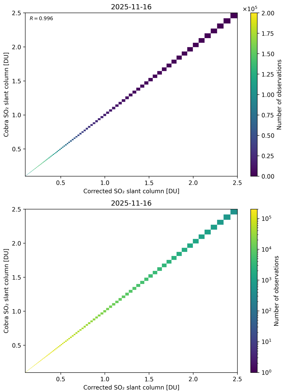
Figure 233: Scatter density plot of “Corrected SO 2 slant column” against “Cobra SO 2 slant column” for 2025-11-15 to 2025-11-17.
