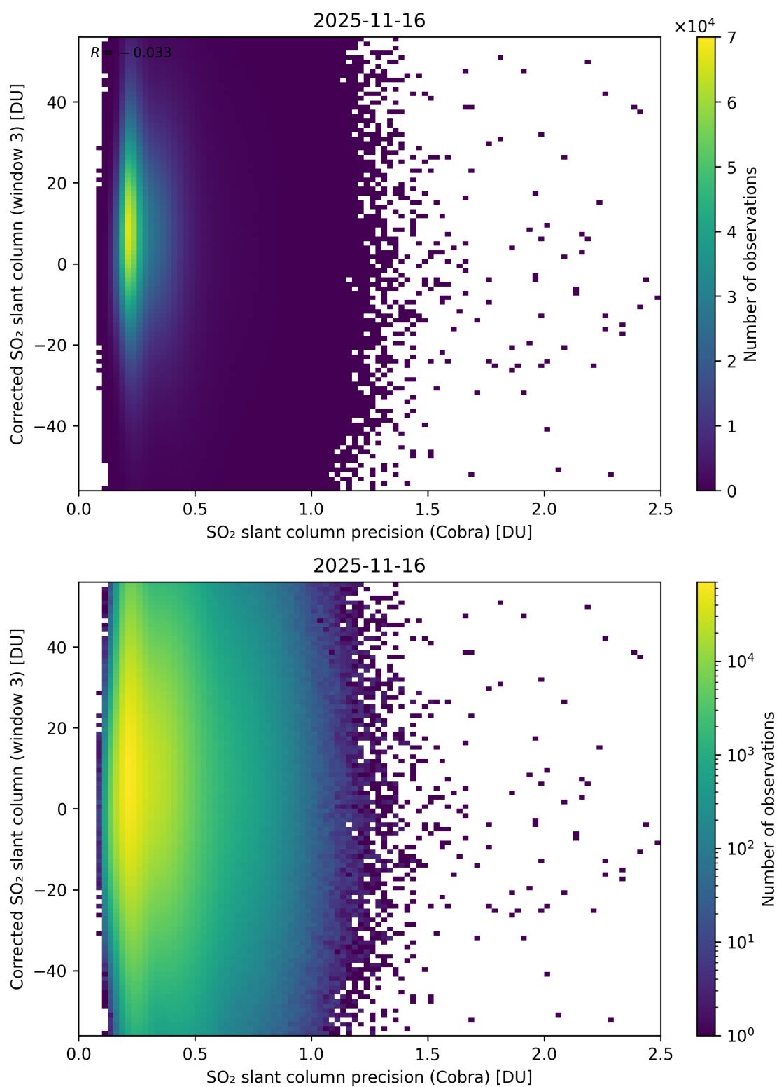
Figure 207: Scatter density plot of “SO 2 slant column precision (Cobra)” against “Corrected SO 2 slant column (window 3)” for 2025-11-15 to 2025-11-17.
