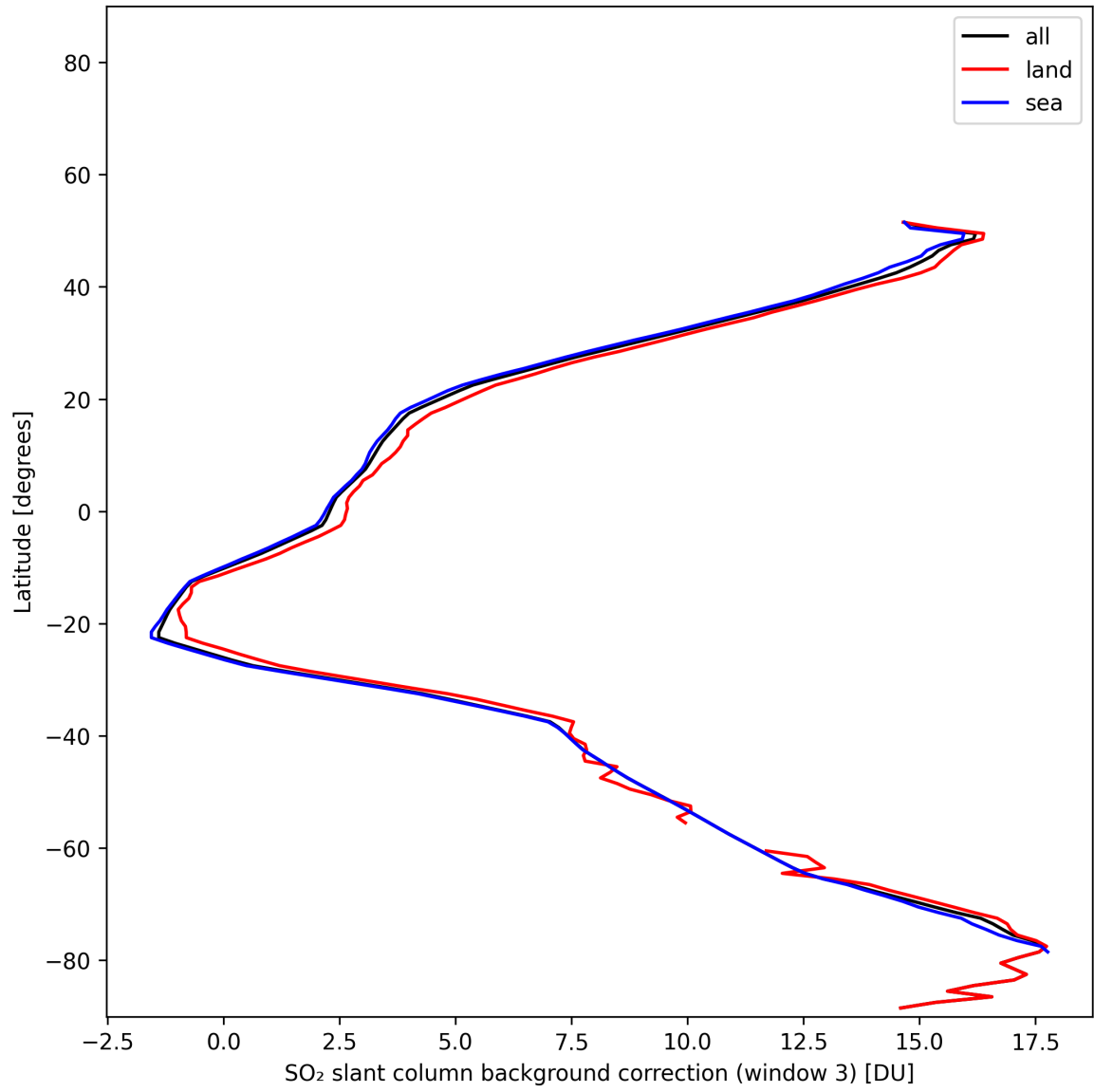
Figure 48: Zonal average of “SO 2 slant column background correction (window 3)” for 2025-11-15 to 2025-11-17.
