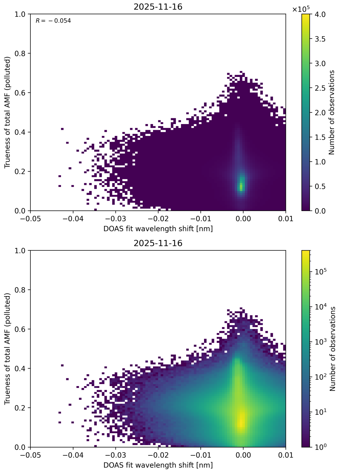
Figure 142: Scatter density plot of “DOAS fit wavelength shift” against “Trueness of total AMF (polluted)” for 2025-11-15 to 2025-11-17.
