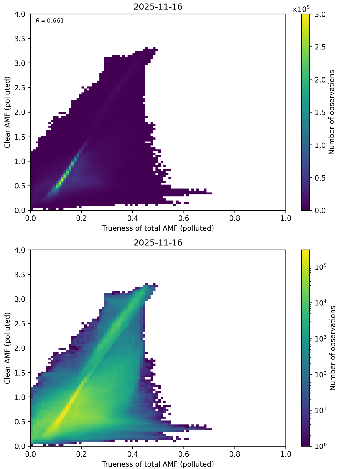
Figure 322: Scatter density plot of “Trueness of total AMF (polluted)” against “Clear AMF (polluted)” for 2025-11-15 to 2025-11-17.
