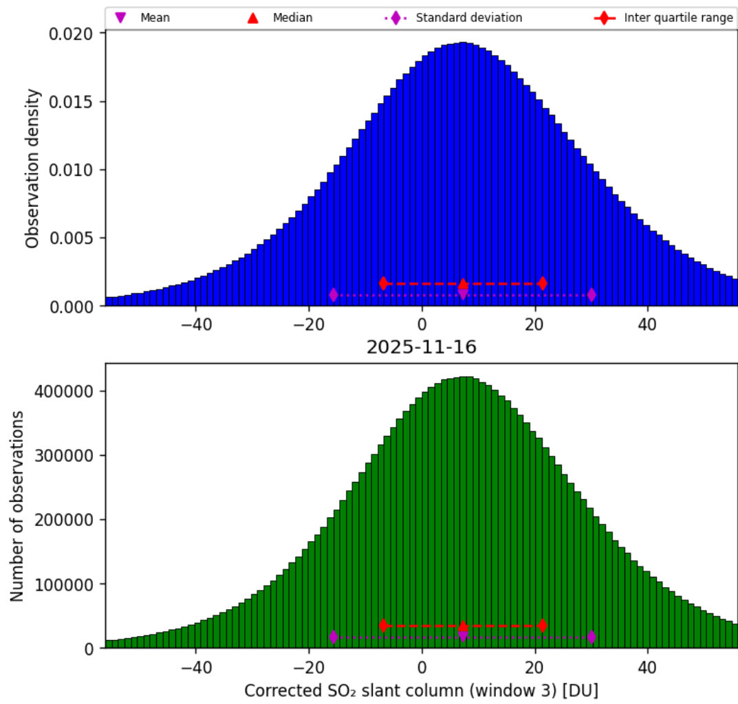
Figure 73: Histogram of “Corrected SO 2 slant column (window 3)” for 2025-11-15 to 2025-11-17
