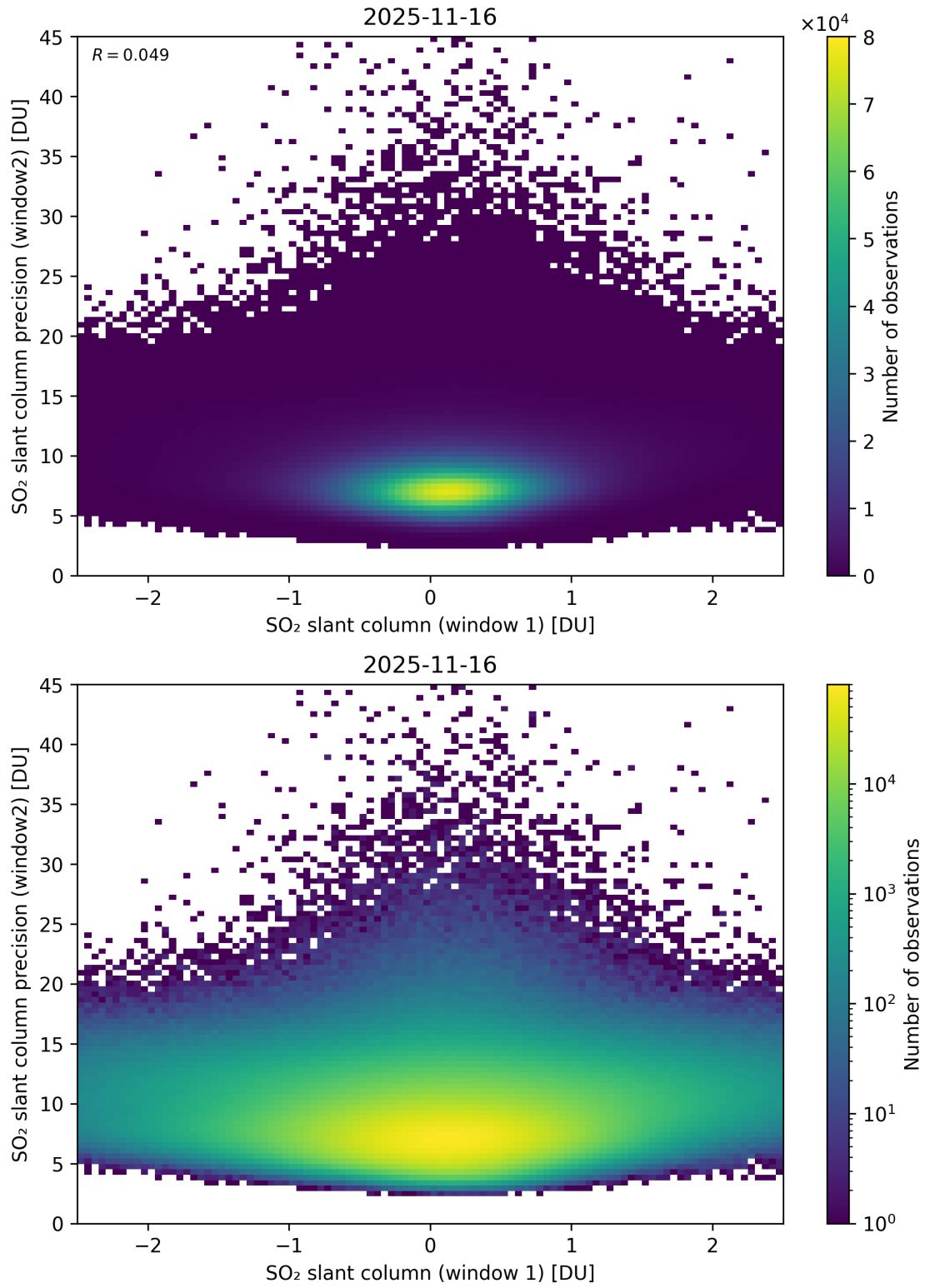
Figure 286: Scatter density plot of “SO 2 slant column (window 1)” against “SO 2 slant column precision (window2)” for 2025-11-15 to 2025-11-17.
