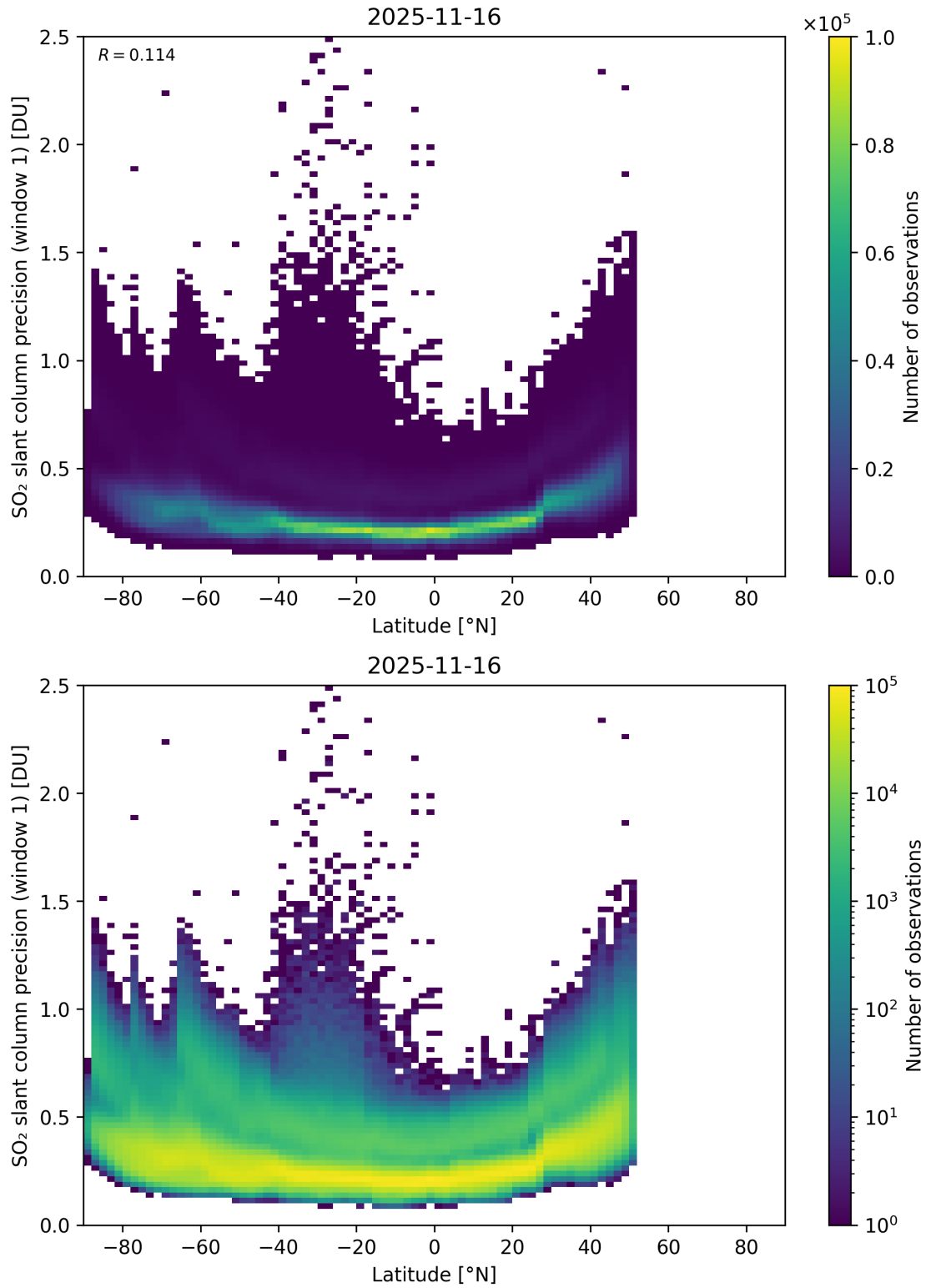
Figure 163: Scatter density plot of “Latitude” against “SO 2 slant column precision (window 1)” for 2025-11-15 to 2025-11-17.
