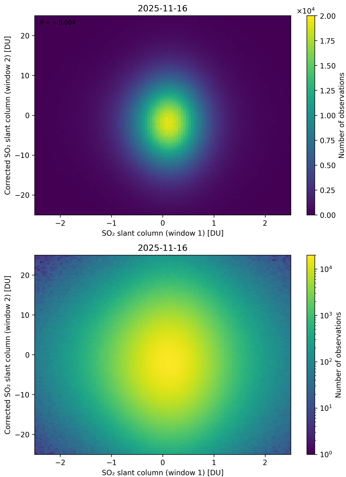
Figure 283: Scatter density plot of “SO 2 slant column (window 1)” against “Corrected SO 2 slant column (window 2)” for 2025-11-15 to 2025-11-17.
