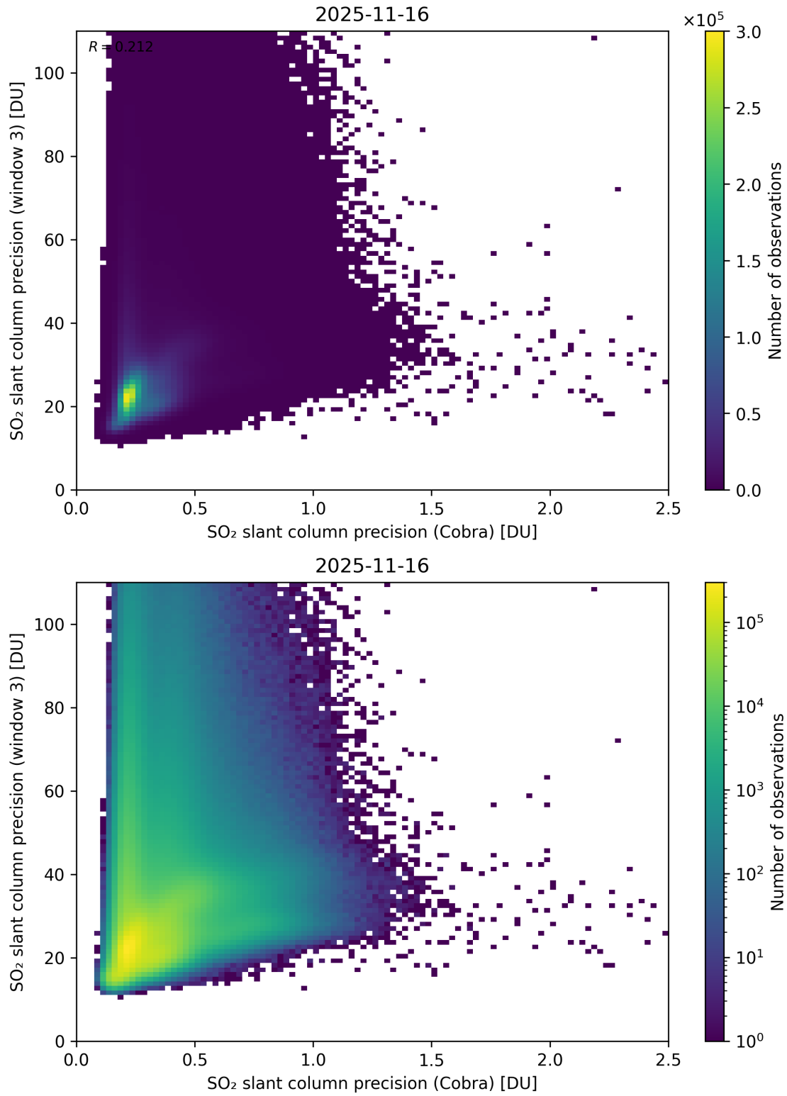
Figure 212: Scatter density plot of “SO 2 slant column precision (Cobra)” against “SO 2 slant column precision (window 3)” for 2025-11-15 to 2025-11-17.
