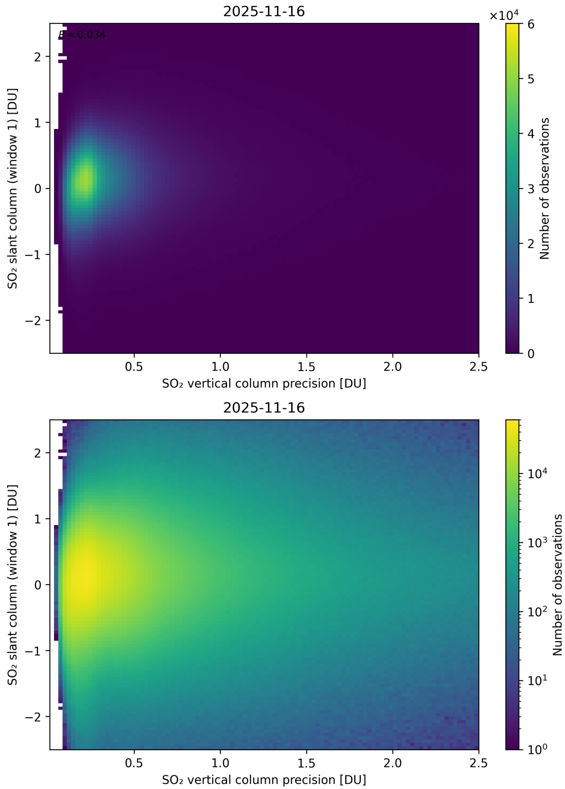
Figure 341: Scatter density plot of “SO 2 vertical column precision” against “SO 2 slant column (window 1)” for 2025-11-15 to 2025-11-17.
