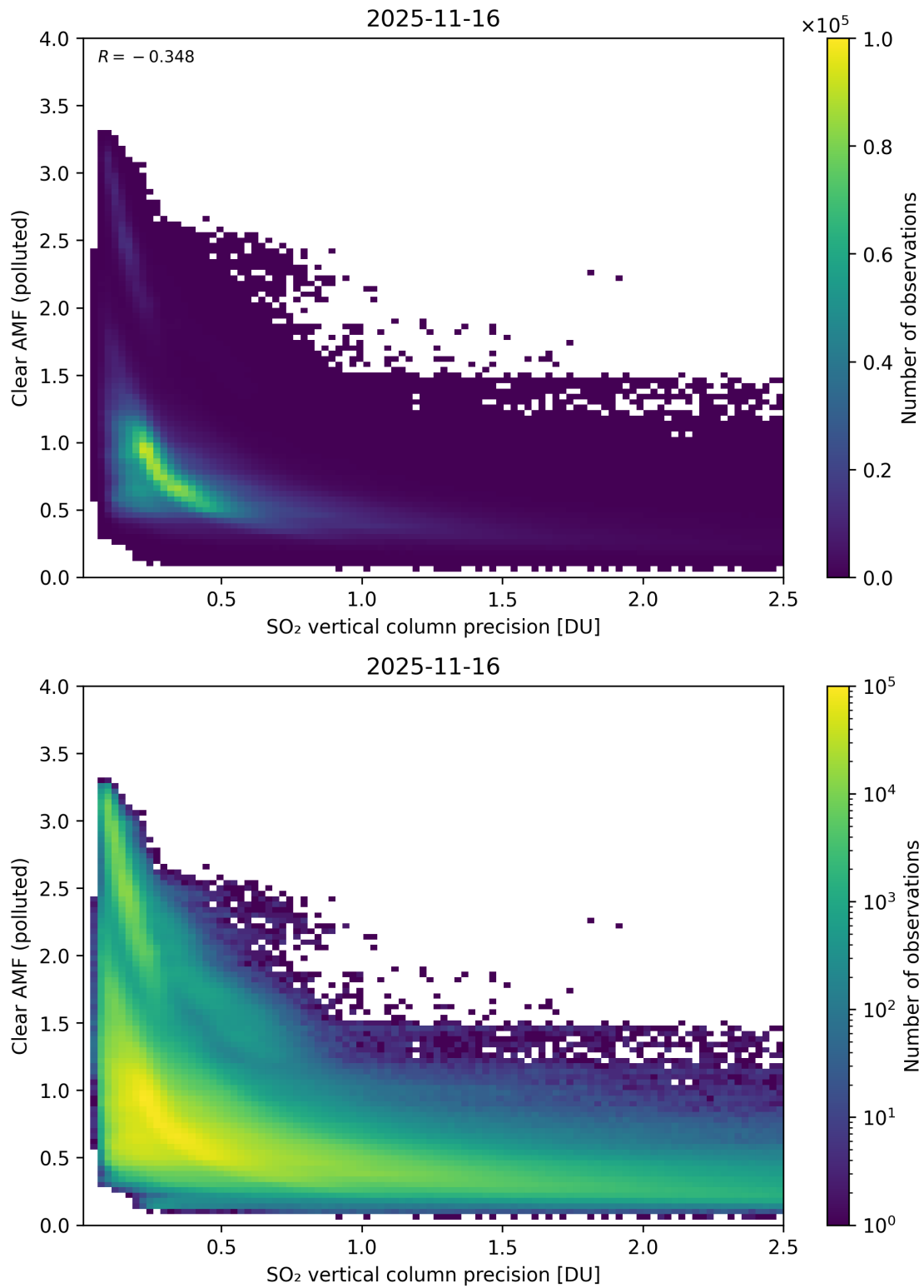
Figure 335: Scatter density plot of “SO 2 vertical column precision” against “Clear AMF (polluted)” for 2025-11-15 to 2025-11-17.
