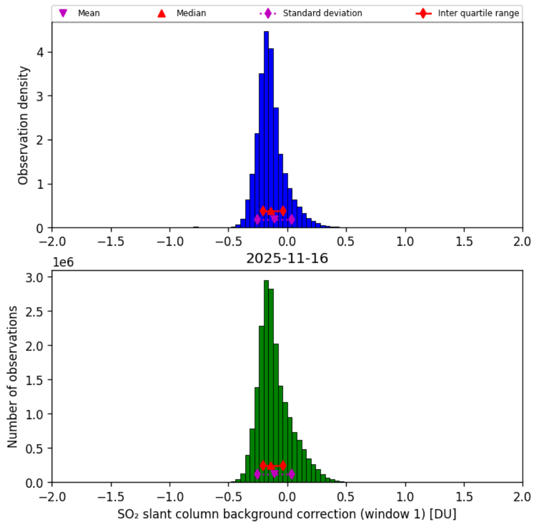
Figure 66: Histogram of “SO 2 slant column background correction (window 1)” for 2025-11-15 to 2025-11-17
