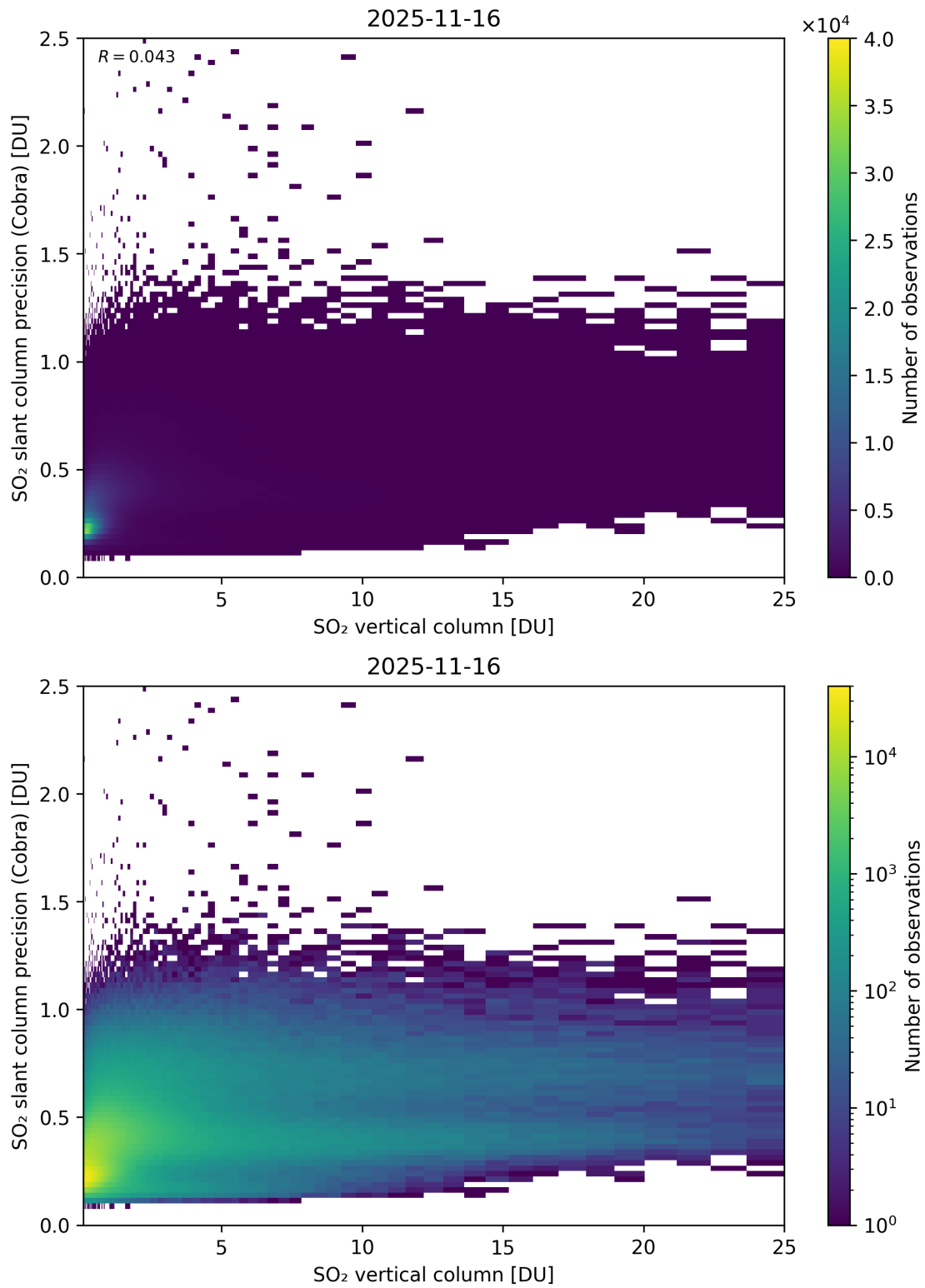
Figure 350: Scatter density plot of “SO 2 vertical column” against “SO 2 slant column precision (Cobra)” for 2025-11-15 to 2025-11-17.
