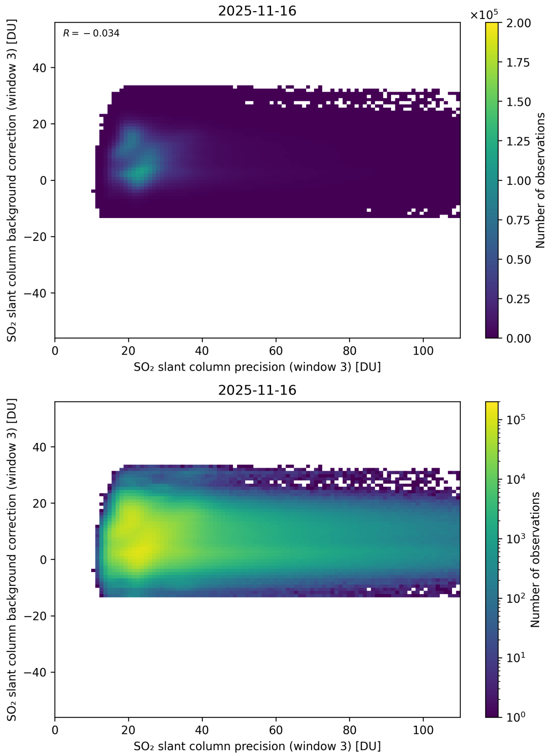
Figure 307: Scatter density plot of “SO 2 slant column precision (window 3)” against “SO 2 slant column background correction (window 3)” for 2025-11-15 to 2025-11-17.
