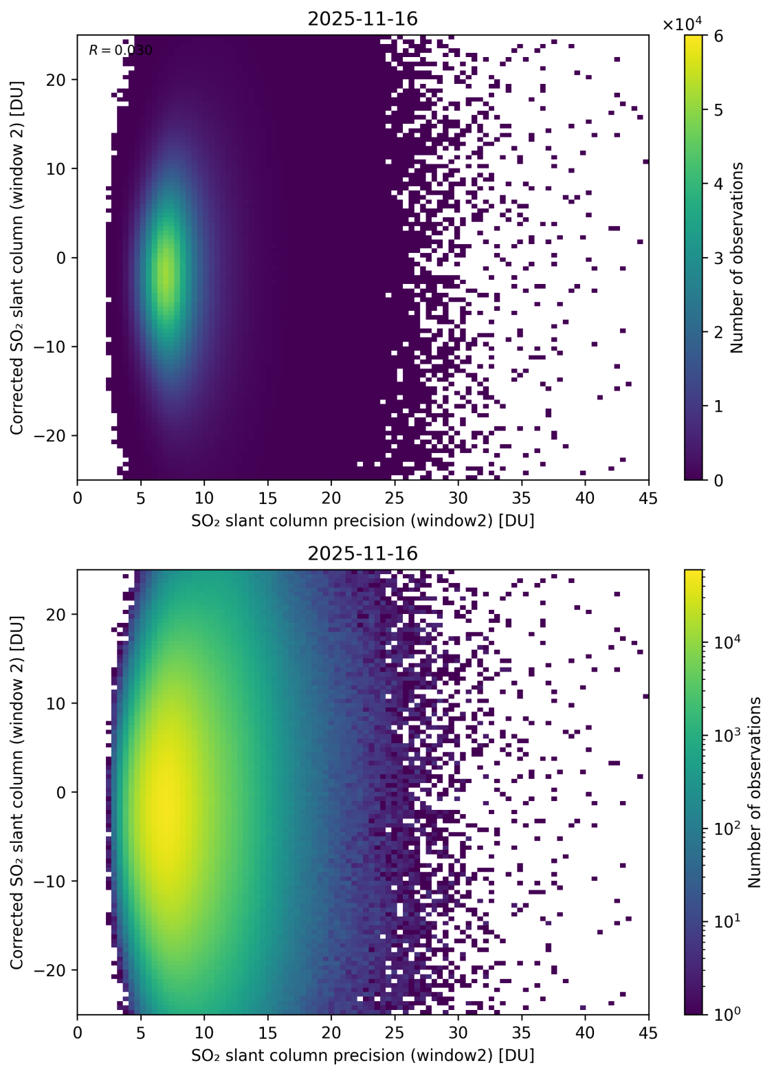
Figure 297: Scatter density plot of “SO 2 slant column precision (window2)” against “Corrected SO 2 slant column (window 2)” for 2025-11-15 to 2025-11-17.
