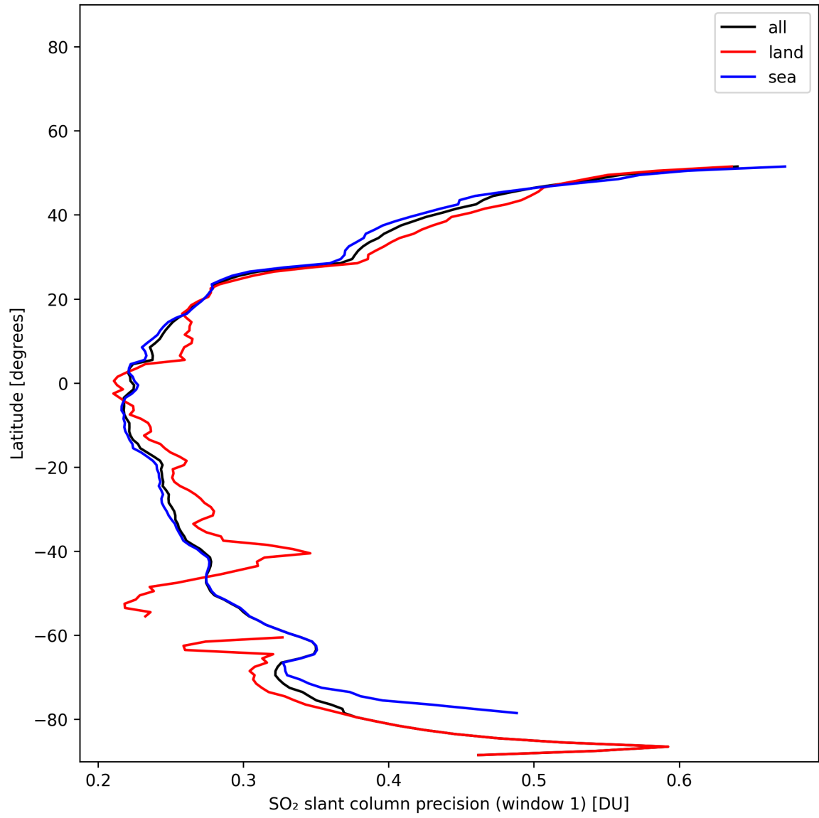
Figure 38: Zonal average of “SO 2 slant column precision (window 1)” for 2025-11-15 to 2025-11-17.
