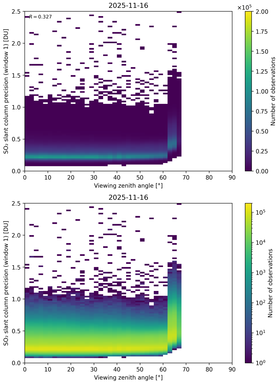
Figure 377: Scatter density plot of “Viewing zenith angle” against “SO 2 slant column precision (window 1)” for 2025-11-15 to 2025-11-17.
