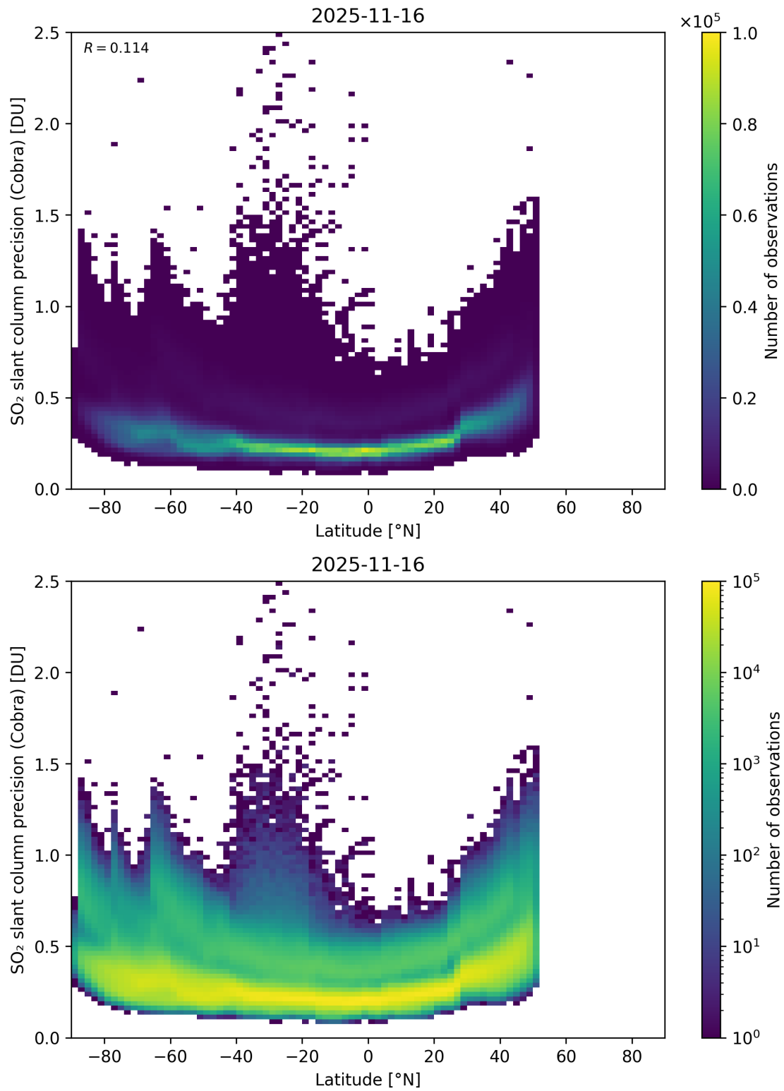
Figure 158: Scatter density plot of “Latitude” against “SO 2 slant column precision (Cobra)” for 2025-11-15 to 2025-11-17.
