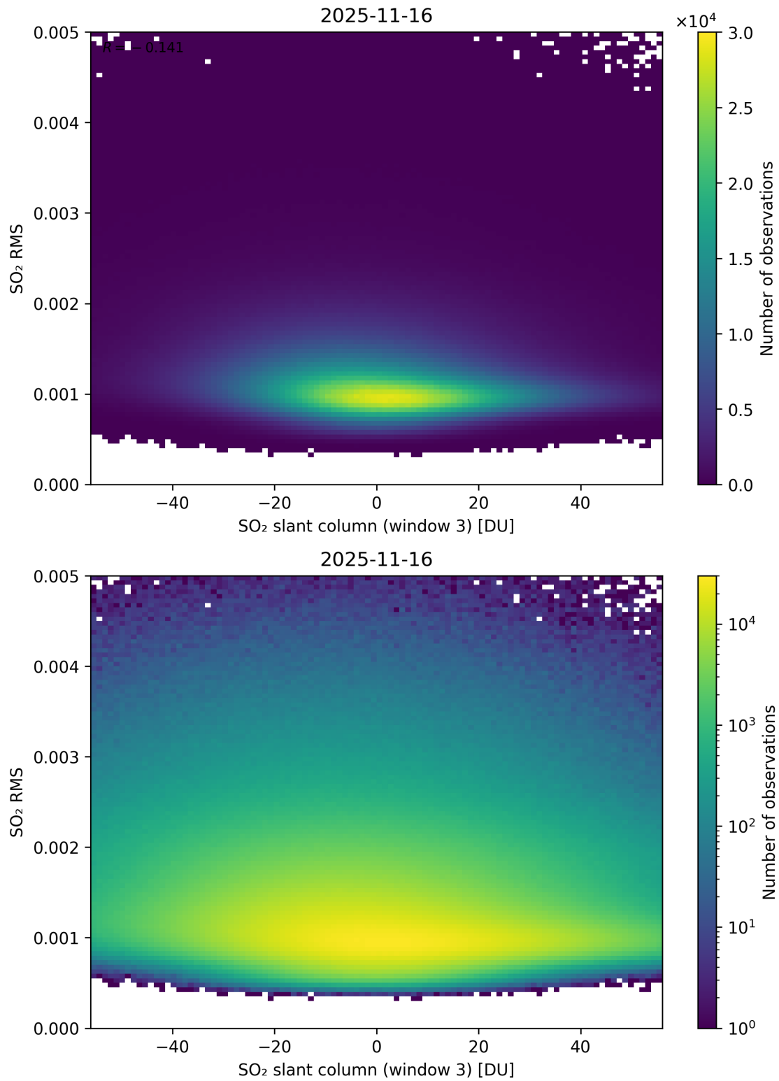
Figure 306: Scatter density plot of “SO 2 slant column (window 3)” against “SO 2 RMS” for 2025-11-15 to 2025-11-17.
