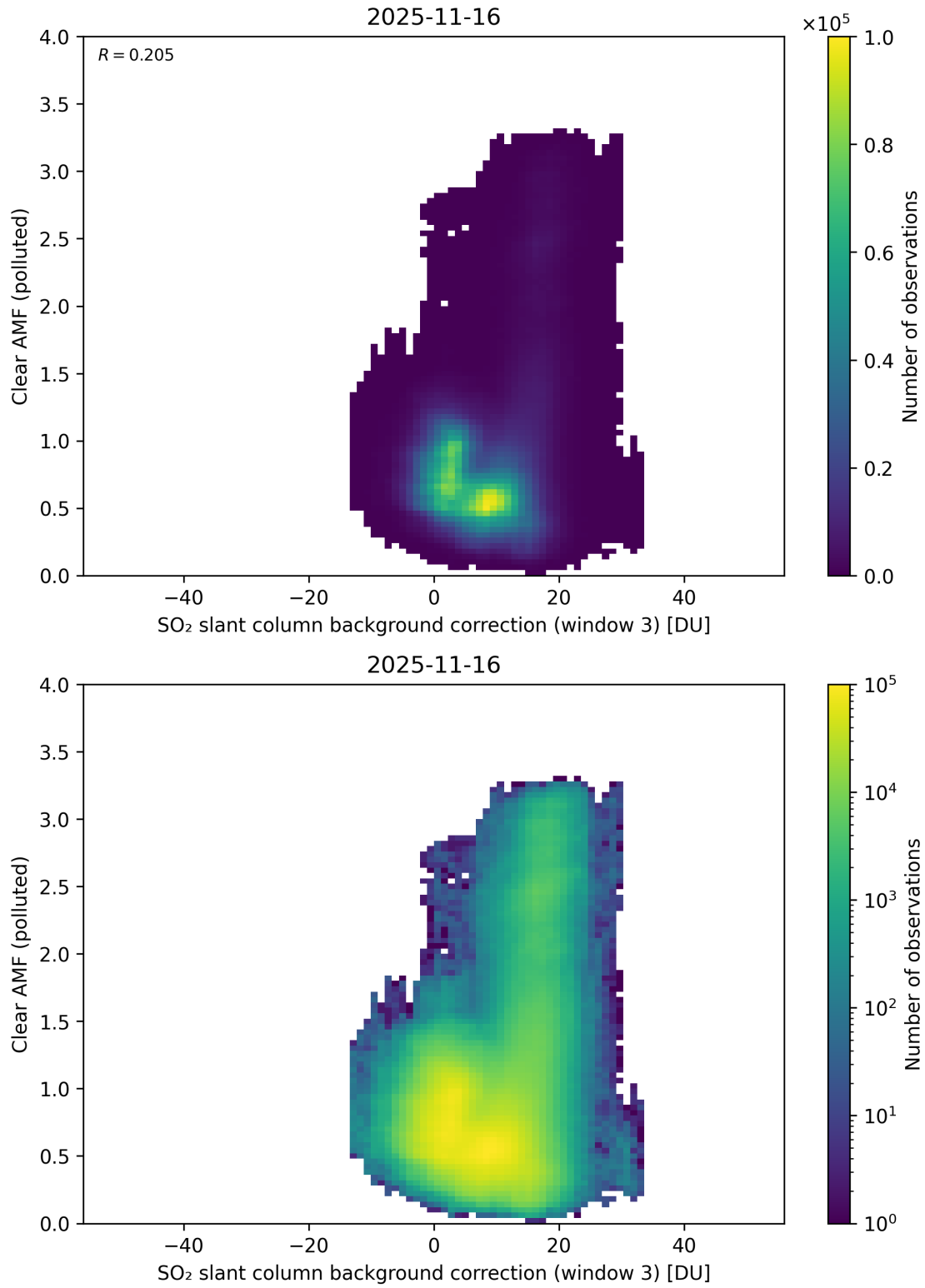
Figure 135: Scatter density plot of “SO 2 slant column background correction (window 3)” against “Clear AMF (polluted)” for 2025-11-15 to 2025-11-17.
