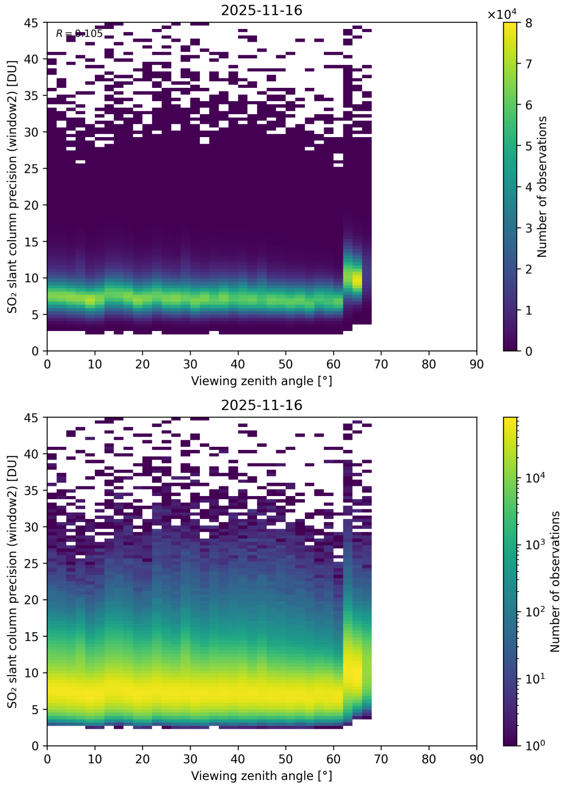
Figure 378: Scatter density plot of “Viewing zenith angle” against “SO 2 slant column precision (window2)” for 2025-11-15 to 2025-11-17.
