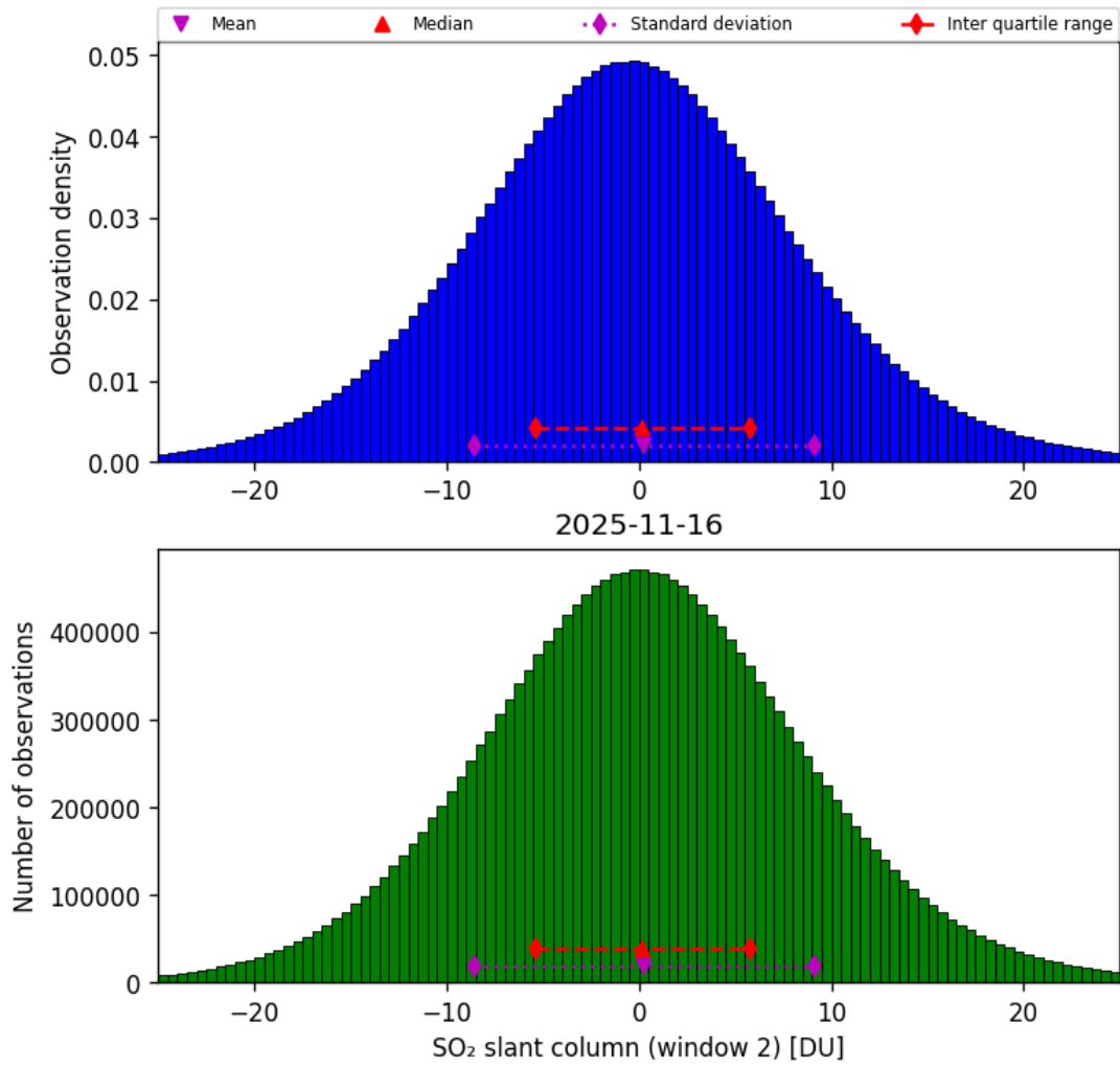
Figure 67: Histogram of “SO 2 slant column (window 2)” for 2025-11-15 to 2025-11-17
