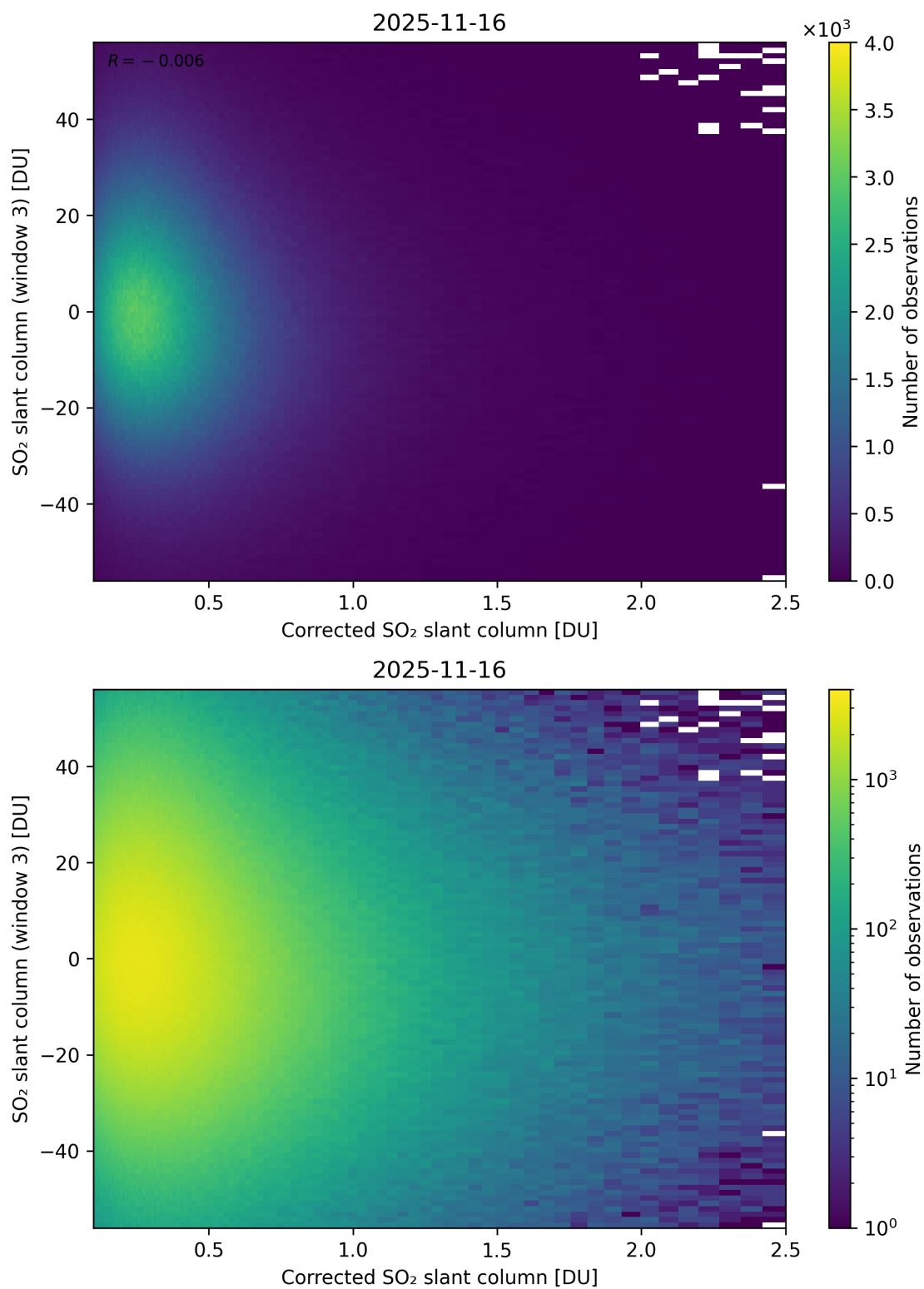
Figure 240: Scatter density plot of “Corrected SO 2 slant column” against “SO 2 slant column (window 3)” for 2025-11-15 to 2025-11-17.
