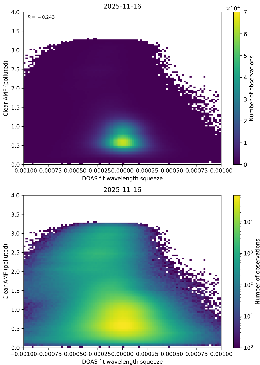
Figure 144: Scatter density plot of “DOAS fit wavelength squeeze” against “Clear AMF (polluted)” for 2025-11-15 to 2025-11-17.
