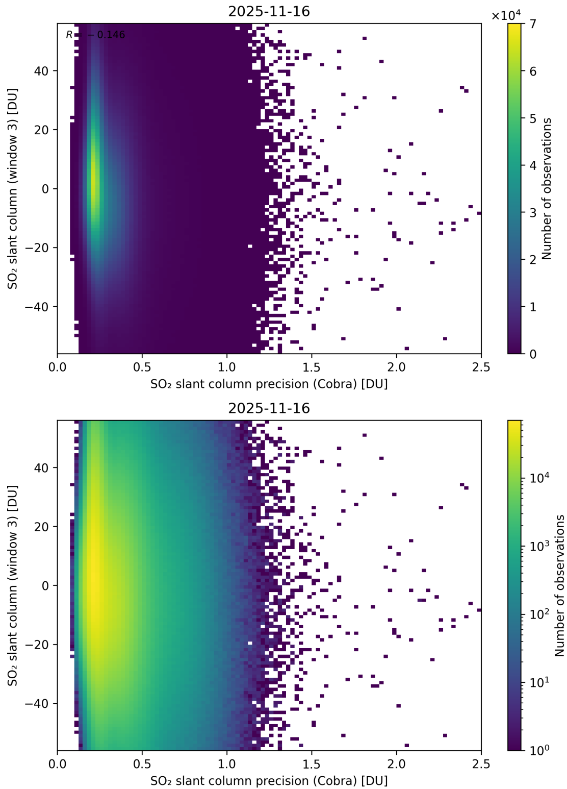
Figure 211: Scatter density plot of “SO 2 slant column precision (Cobra)” against “SO 2 slant column (window 3)” for 2025-11-15 to 2025-11-17.
