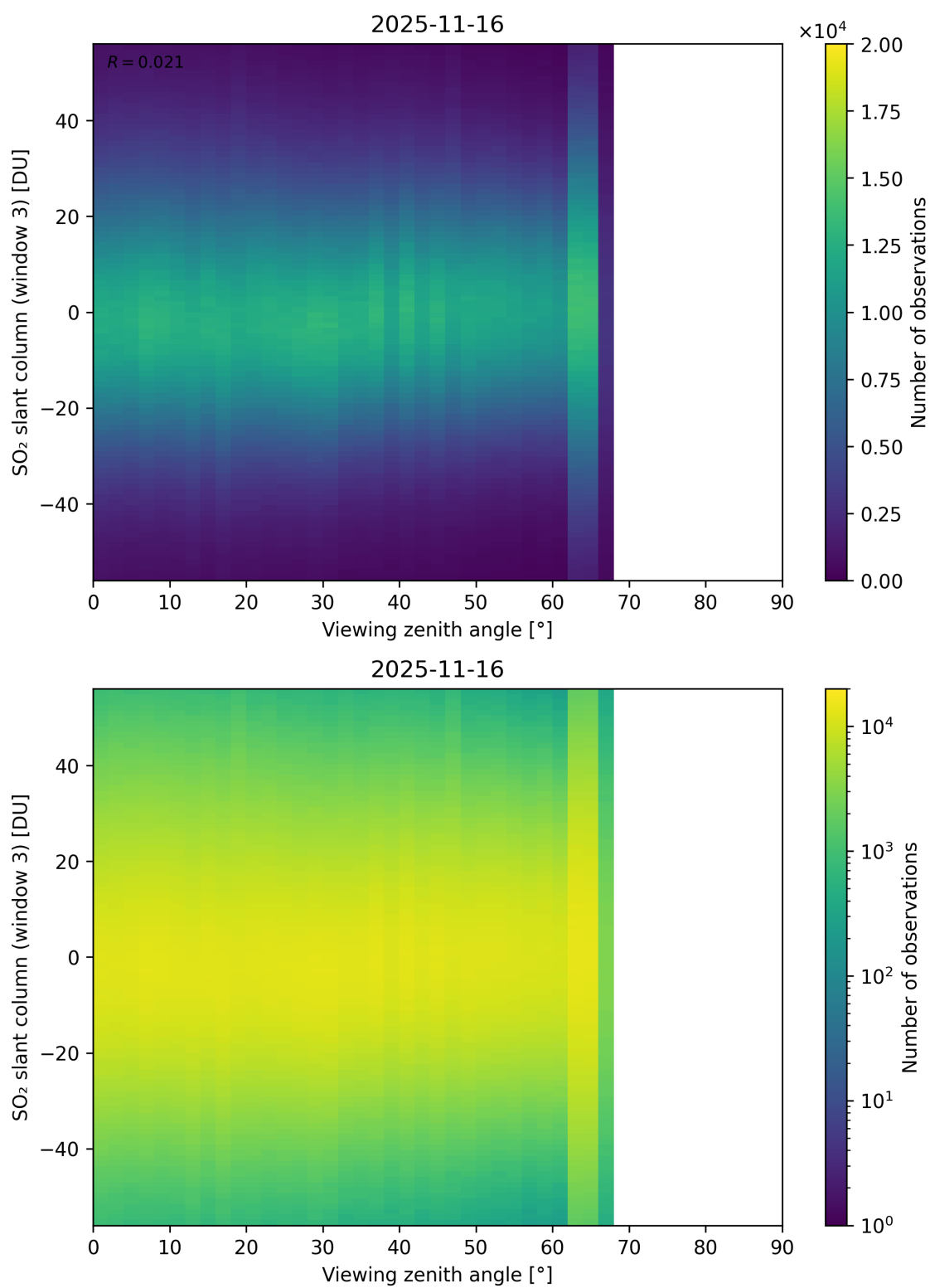
Figure 379: Scatter density plot of “Viewing zenith angle” against “SO 2 slant column (window 3)” for 2025-11-15 to 2025-11-17.
