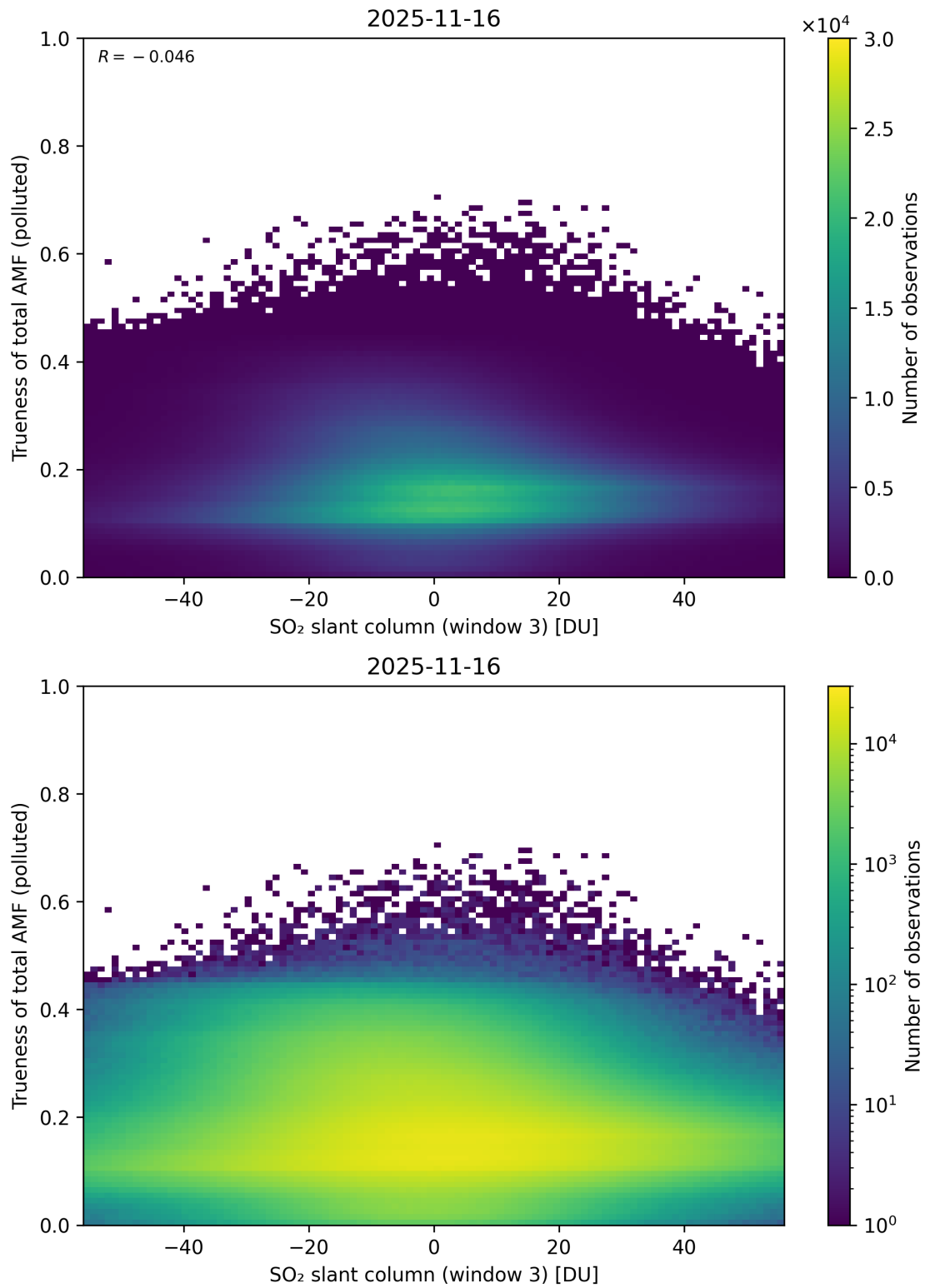
Figure 319: Scatter density plot of “SO 2 slant column (window 3)” against “Trueness of total AMF (polluted)” for 2025-11-15 to 2025-11-17.
