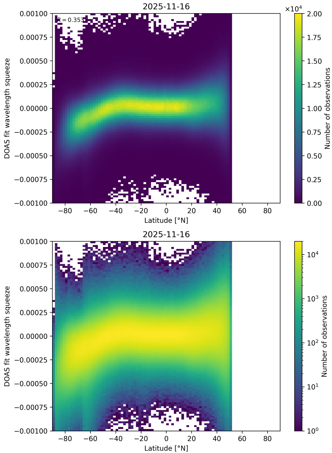
Figure 154: Scatter density plot of “Latitude” against “DOAS fit wavelength squeeze” for 2025-11-15 to 2025-11-17.
