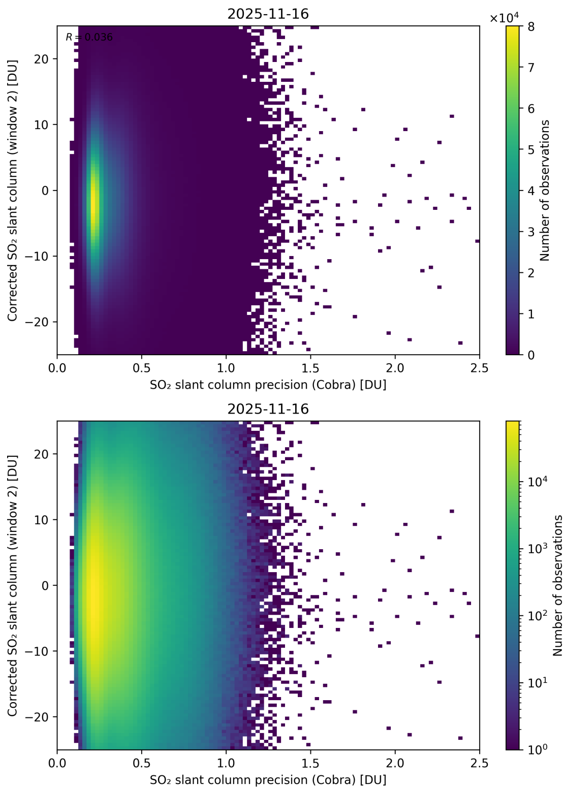
Figure 206: Scatter density plot of “SO 2 slant column precision (Cobra)” against “Corrected SO 2 slant column (window 2)” for 2025-11-15 to 2025-11-17.
