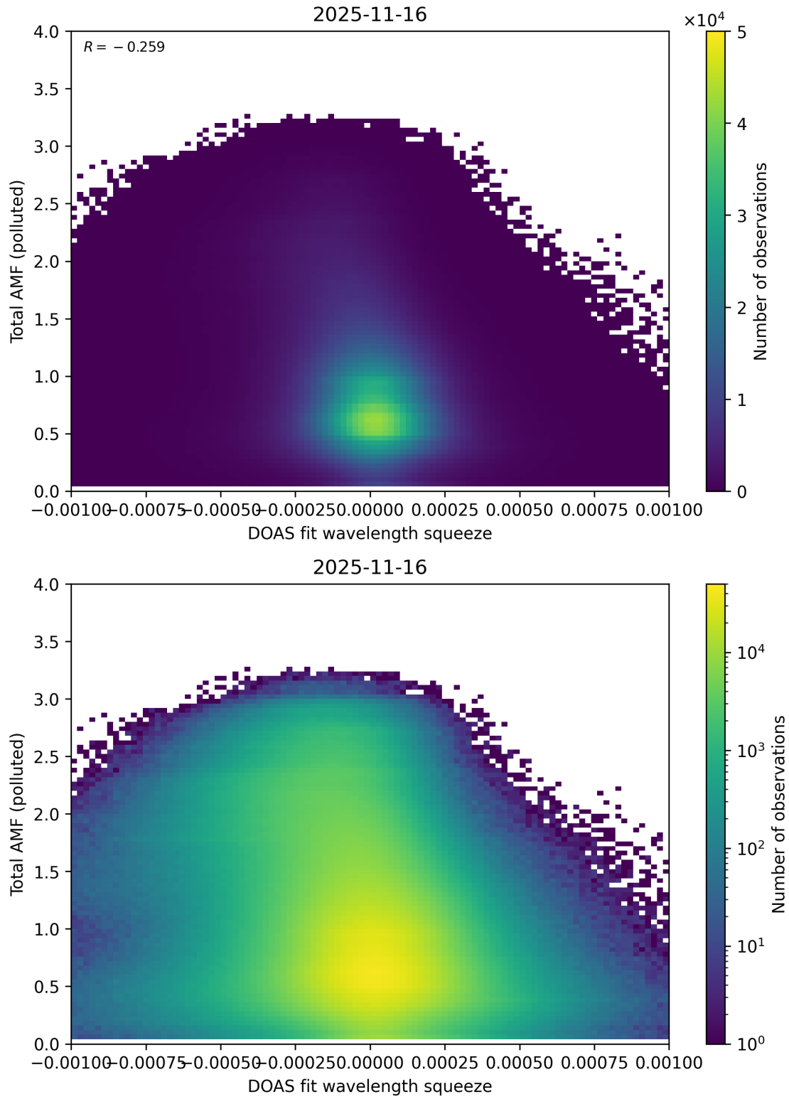
Figure 145: Scatter density plot of “DOAS fit wavelength squeeze” against “Total AMF (polluted)” for 2025-11-15 to 2025-11-17.
