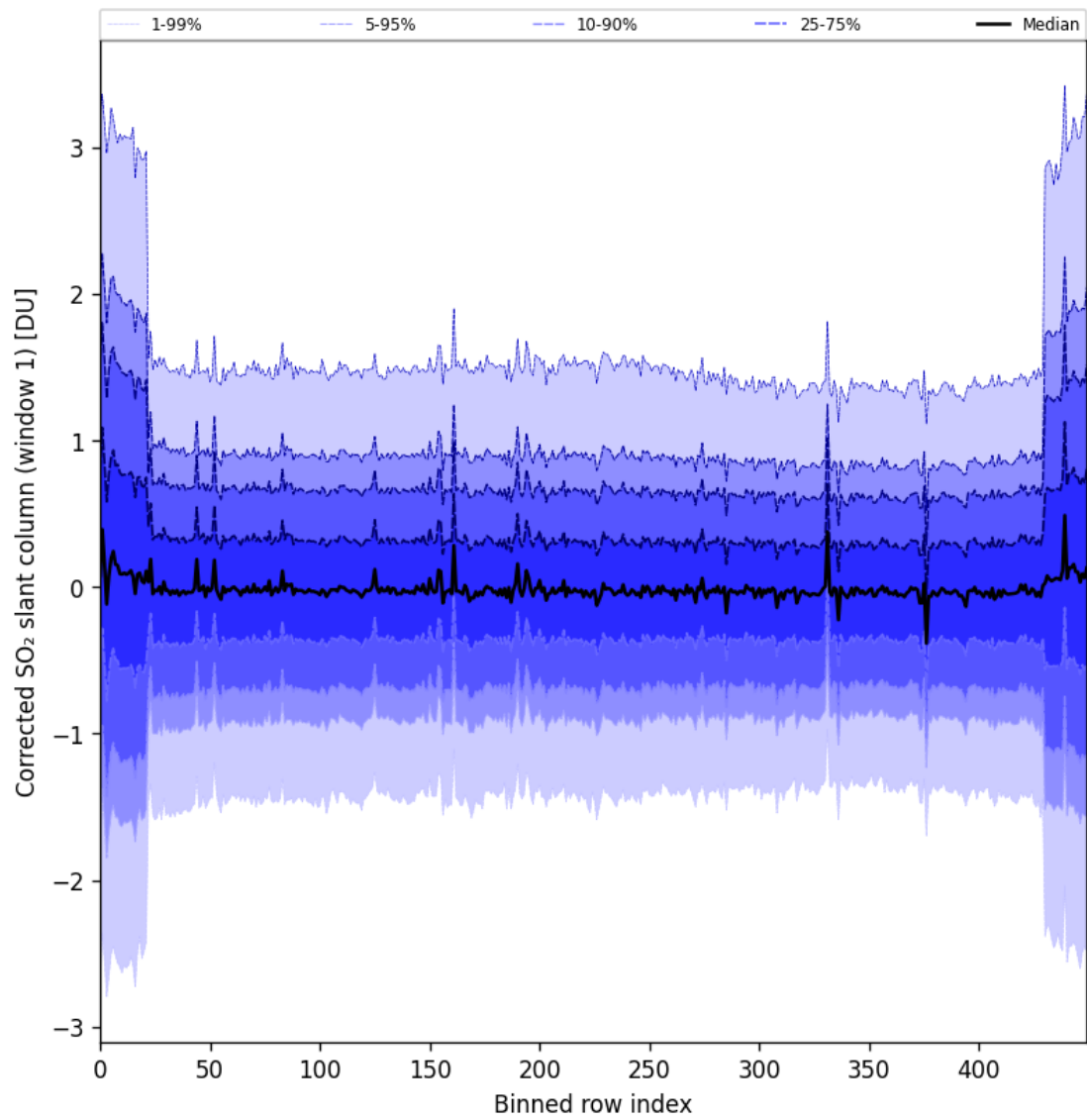
Figure 91: Along track statistics of “Corrected SO 2 slant column (window 1)” for 2025-11-15 to 2025-11-17
