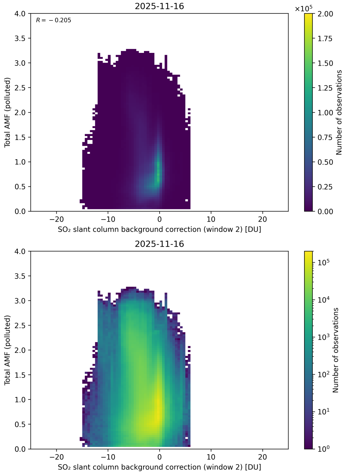
Figure 130: Scatter density plot of “SO 2 slant column background correction (window 2)” against “Total AMF (polluted)” for 2025-11-15 to 2025-11-17.
