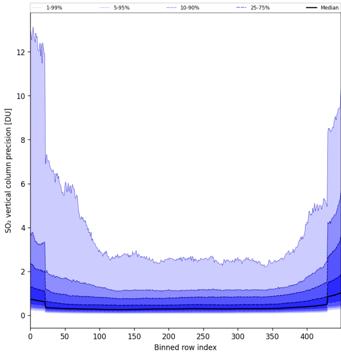
Figure 85: Along track statistics of “SO 2 vertical column precision” for 2025-11-15 to 2025-11-17
