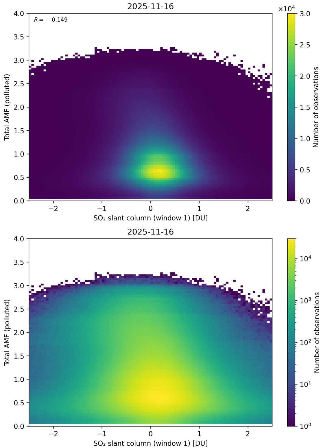
Figure 289: Scatter density plot of “SO 2 slant column (window 1)” against “Total AMF (polluted)” for 2025-11-15 to 2025-11-17.
