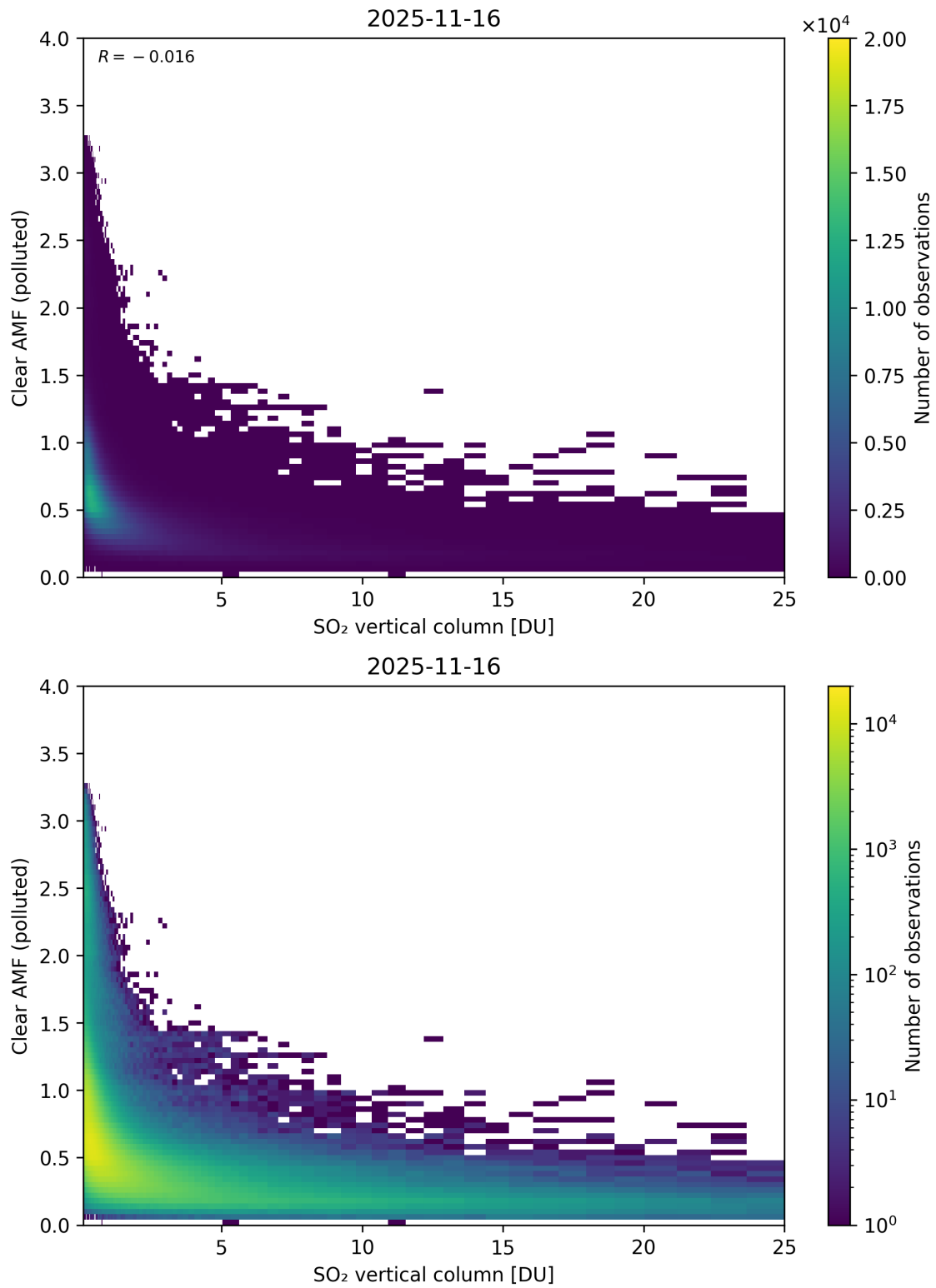
Figure 348: Scatter density plot of “SO 2 vertical column” against “Clear AMF (polluted)” for 2025-11-15 to 2025-11-17.
