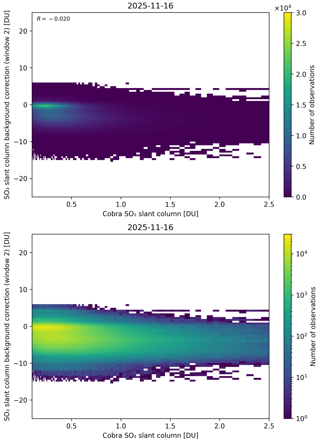
Figure 194: Scatter density plot of “Cobra SO 2 slant column” against “SO 2 slant column background correction (window 2)” for 2025-11-15 to 2025-11-17.
