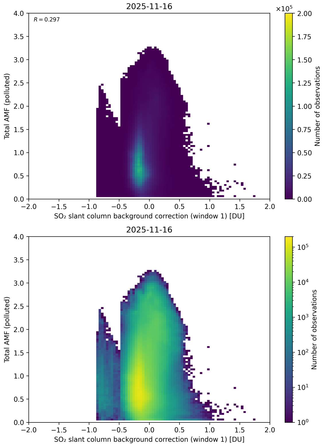
Figure 120: Scatter density plot of “SO 2 slant column background correction (window 1)” against “Total AMF (polluted)” for 2025-11-15 to 2025-11-17.
