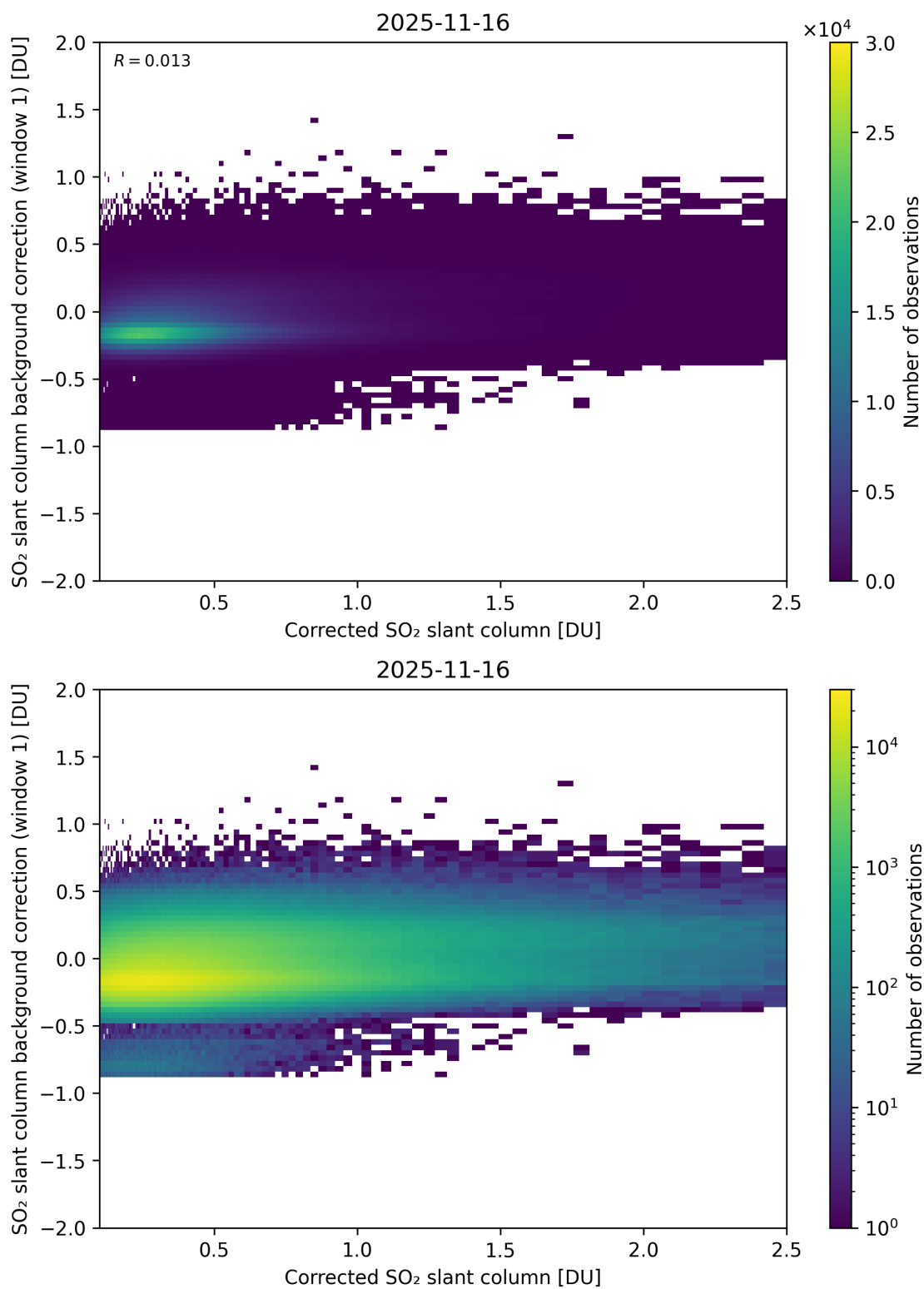
Figure 226: Scatter density plot of “Corrected SO 2 slant column” against “SO 2 slant column background correction (window 1)” for 2025-11-15 to 2025-11-17.
