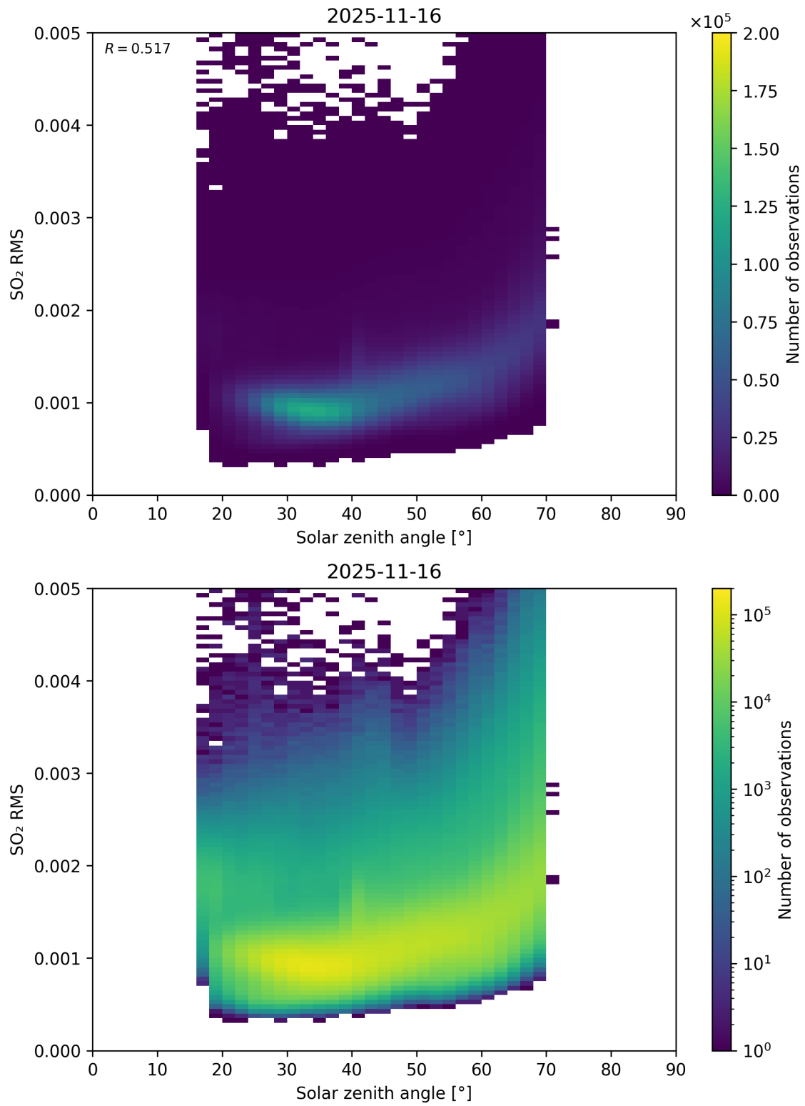
Figure 176: Scatter density plot of “Solar zenith angle” against “SO 2 RMS” for 2025-11-15 to 2025-11-17.
