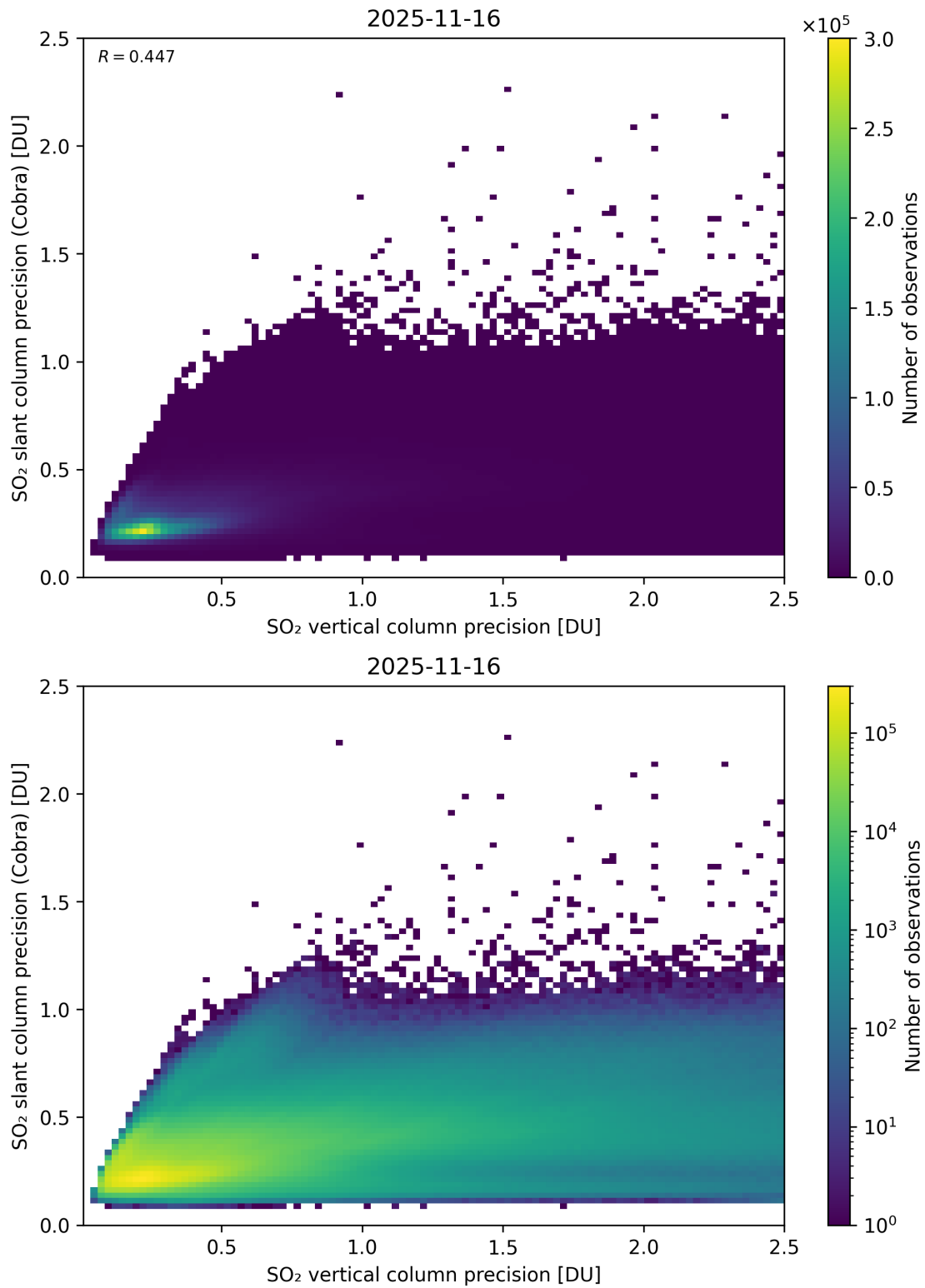
Figure 337: Scatter density plot of “SO 2 vertical column precision” against “SO 2 slant column precision (Cobra)” for 2025-11-15 to 2025-11-17.
