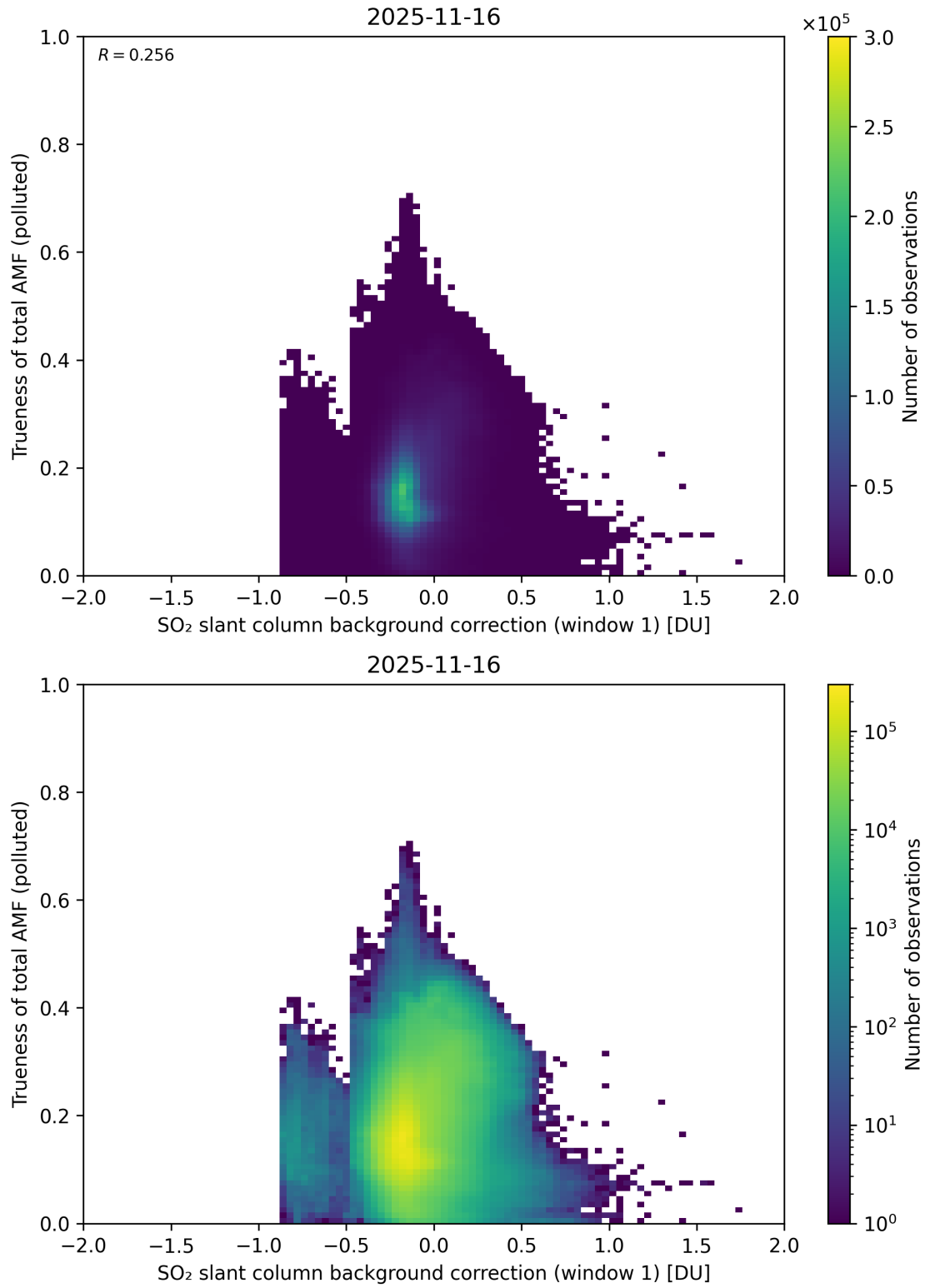
Figure 121: Scatter density plot of “SO 2 slant column background correction (window 1)” against “Trueness of total AMF (polluted)” for 2025-11-15 to 2025-11-17.
