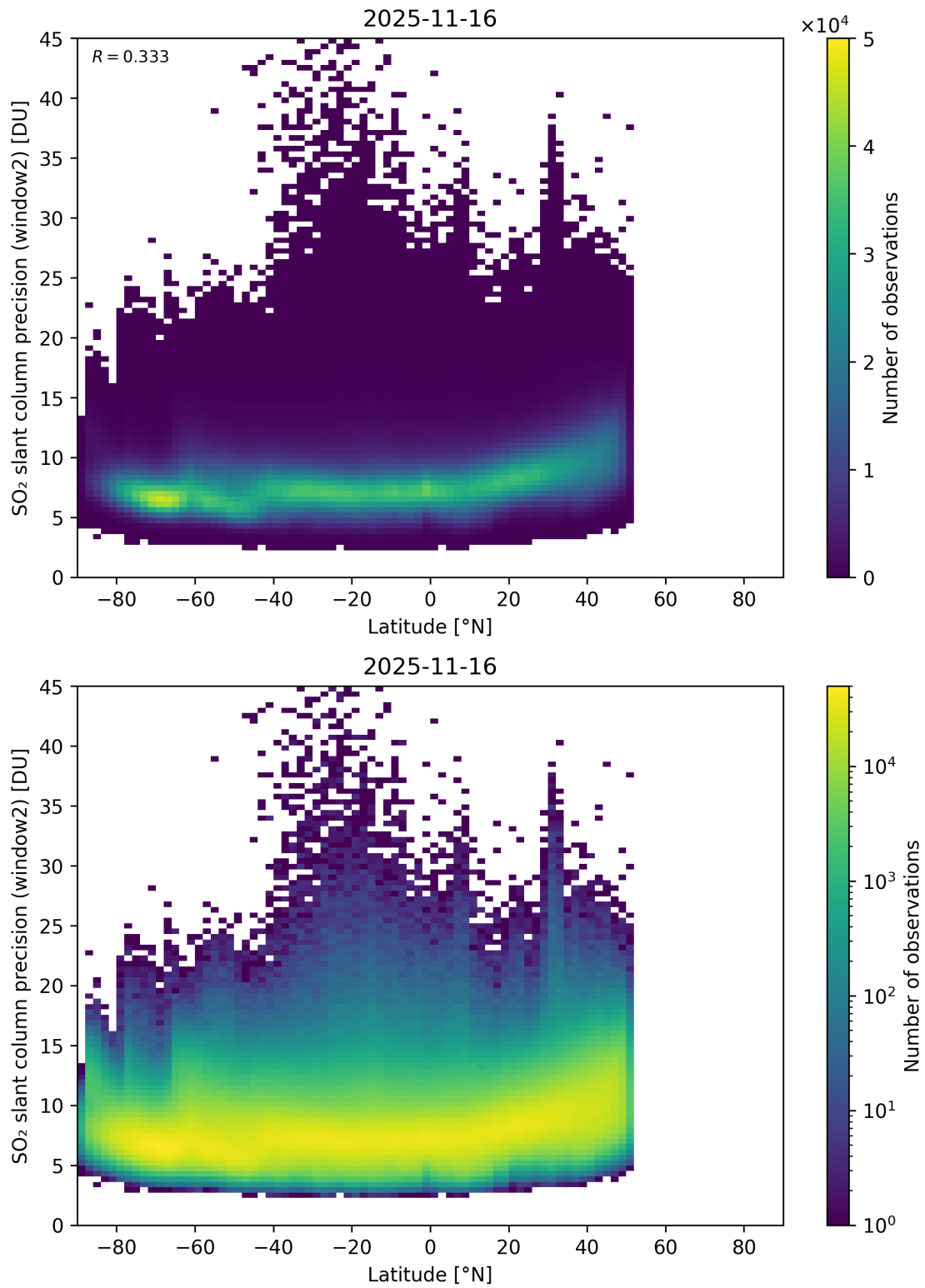
Figure 164: Scatter density plot of “Latitude” against “SO 2 slant column precision (window2)” for 2025-11-15 to 2025-11-17.
