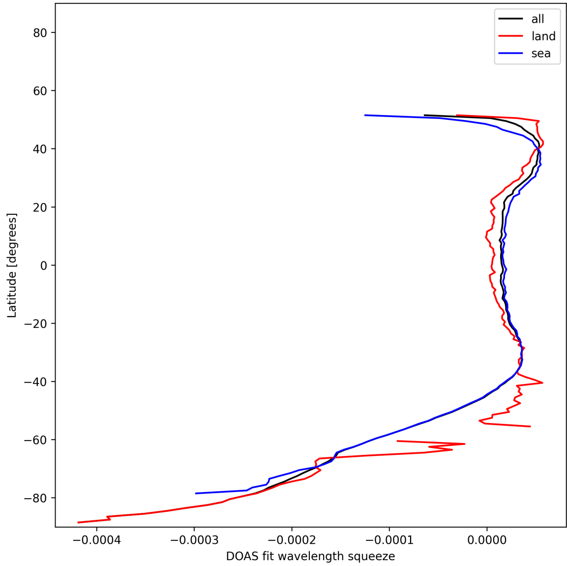
Figure 51: Zonal average of “DOAS fit wavelength squeeze” for 2025-11-15 to 2025-11-17.
