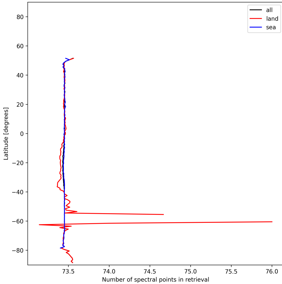
Figure 56: Zonal average of “Number of spectral points in retrieval” for 2025-11-15 to 2025-11-17.
