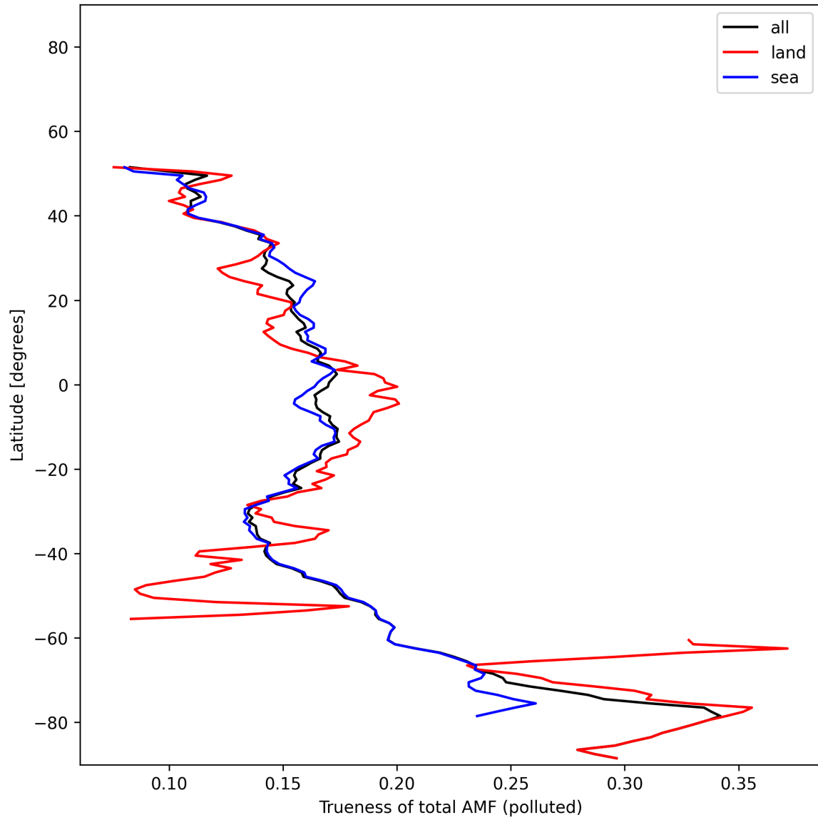
Figure 54: Zonal average of “Trueness of total AMF (polluted)” for 2025-11-15 to 2025-11-17.
