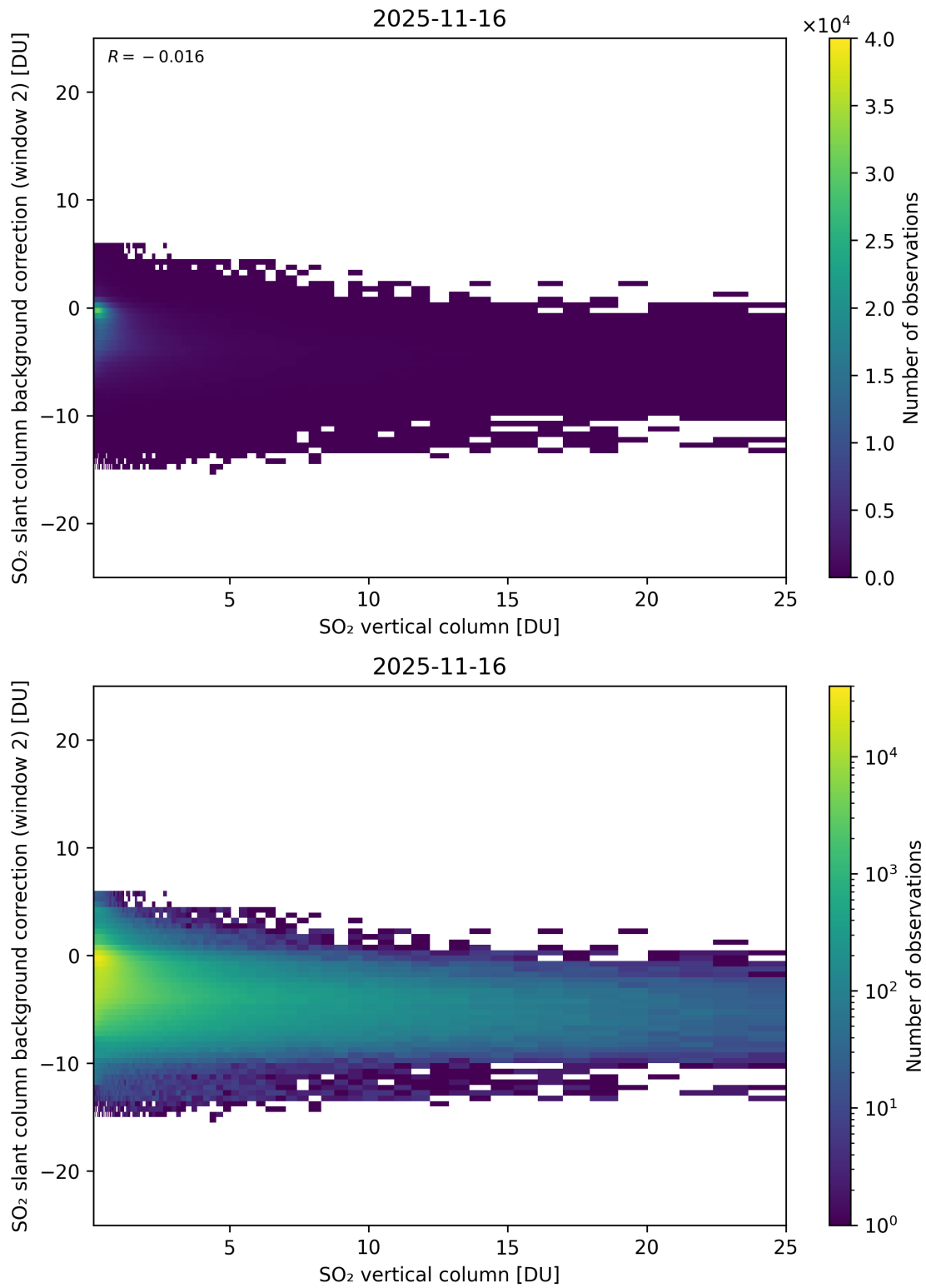
Figure 324: Scatter density plot of “SO 2 vertical column” against “SO 2 slant column background correction (window 2)” for 2025-11-15 to 2025-11-17.
