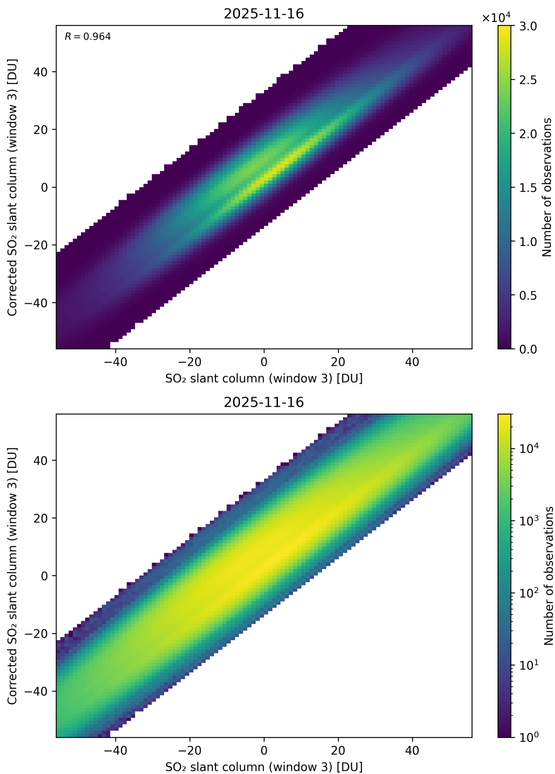
Figure 316: Scatter density plot of “SO 2 slant column (window 3)” against “Corrected SO 2 slant column (window 3)” for 2025-11-15 to 2025-11-17.
