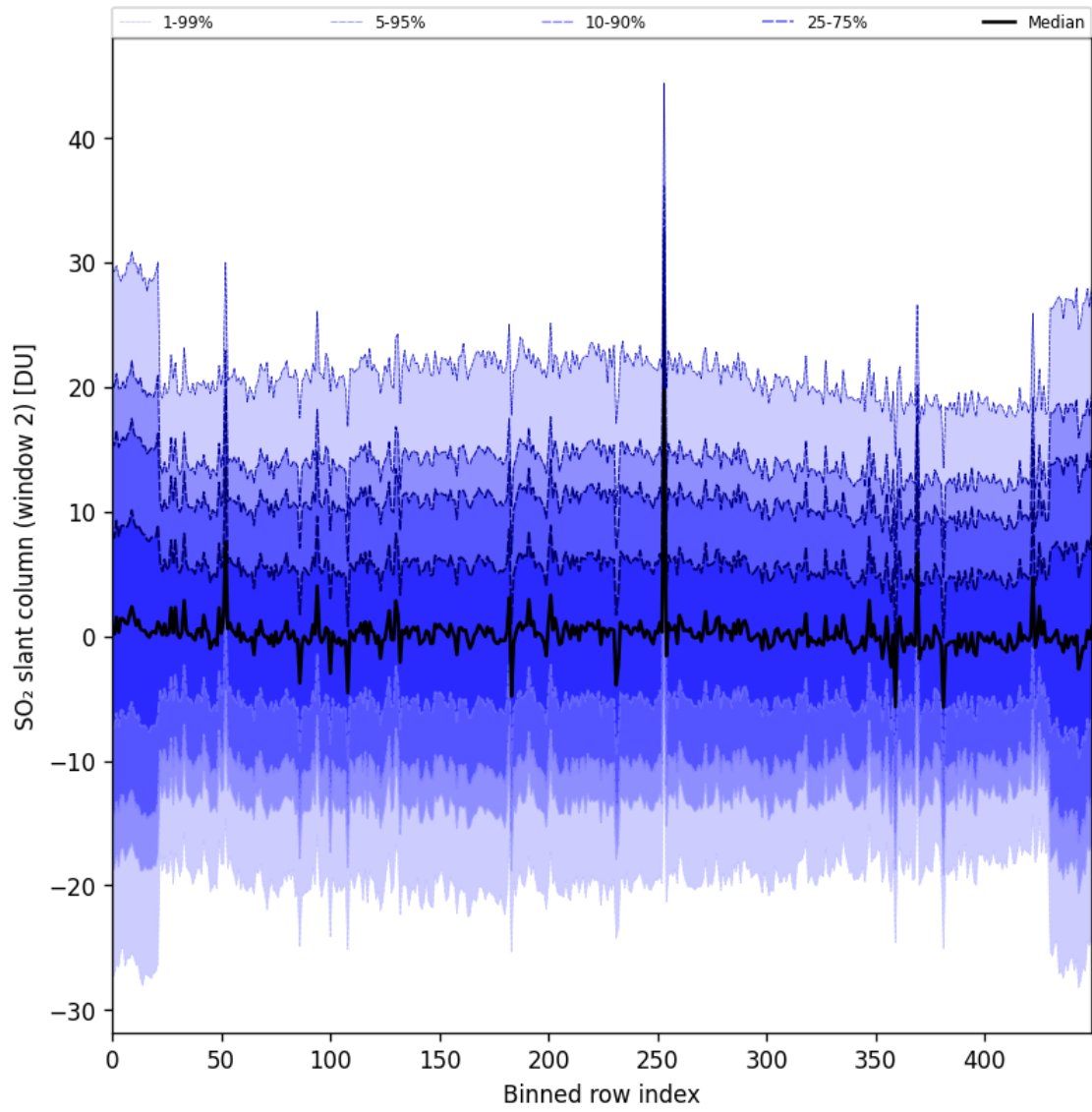
Figure 93: Along track statistics of “SO 2 slant column (window 2)” for 2025-11-15 to 2025-11-17
