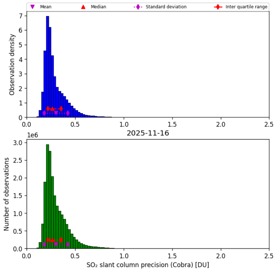
Figure 62: Histogram of “SO 2 slant column precision (Cobra)” for 2025-11-15 to 2025-11-17
