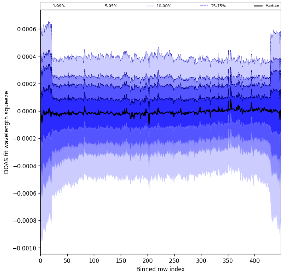
Figure 103: Along track statistics of “DOAS fit wavelength squeeze” for 2025-11-15 to 2025-11-17
