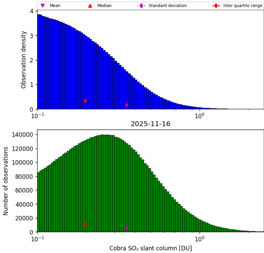
Figure 61: Histogram of “Cobra SO 2 slant column” for 2025-11-15 to 2025-11-17
