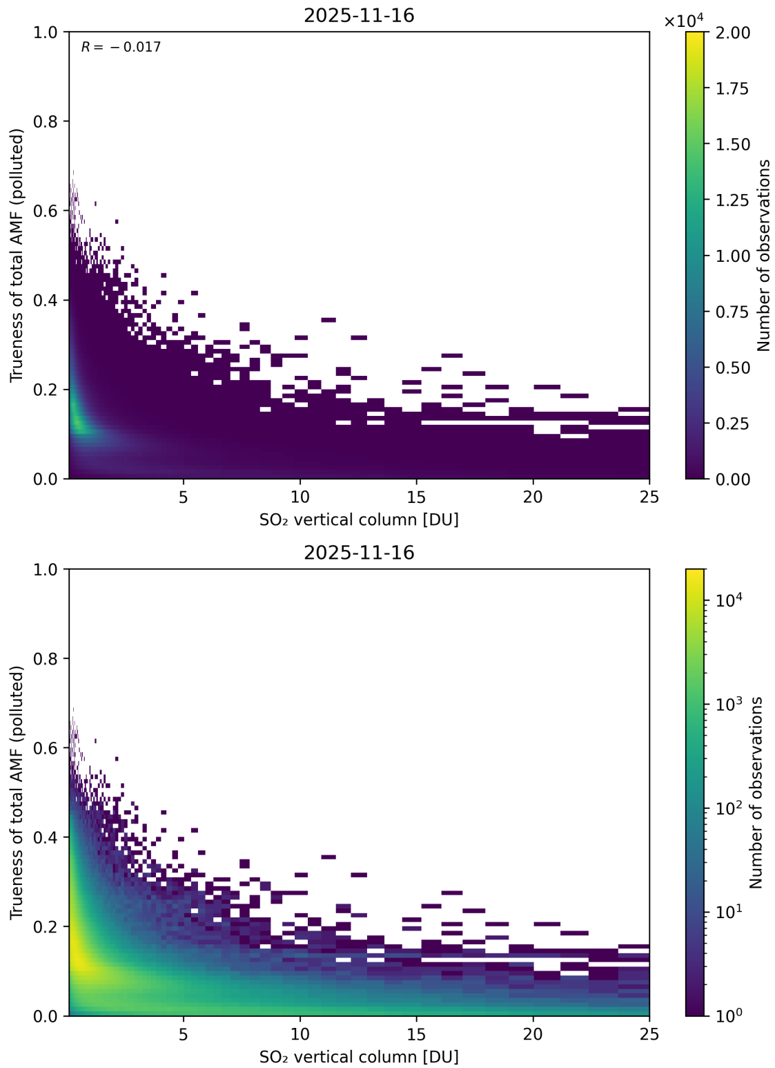
Figure 360: Scatter density plot of “SO 2 vertical column” against “Trueness of total AMF (polluted)” for 2025-11-15 to 2025-11-17.
