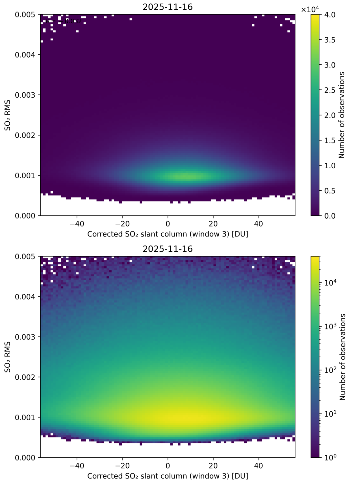
Figure 258: Scatter density plot of “Corrected SO 2 slant column (window 3)” against “SO 2 RMS” for 2025-11-15 to 2025-11-17.
