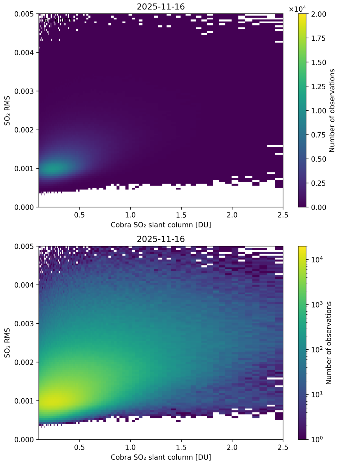
Figure 198: Scatter density plot of “Cobra SO 2 slant column” against “SO 2 RMS” for 2025-11-15 to 2025-11-17.
