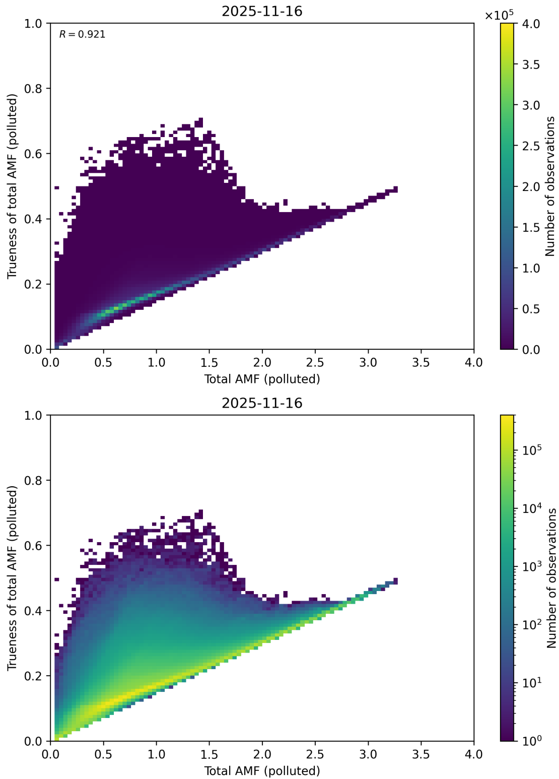
Figure 321: Scatter density plot of “Total AMF (polluted)” against “Trueness of total AMF (polluted)” for 2025-11-15 to 2025-11-17.
