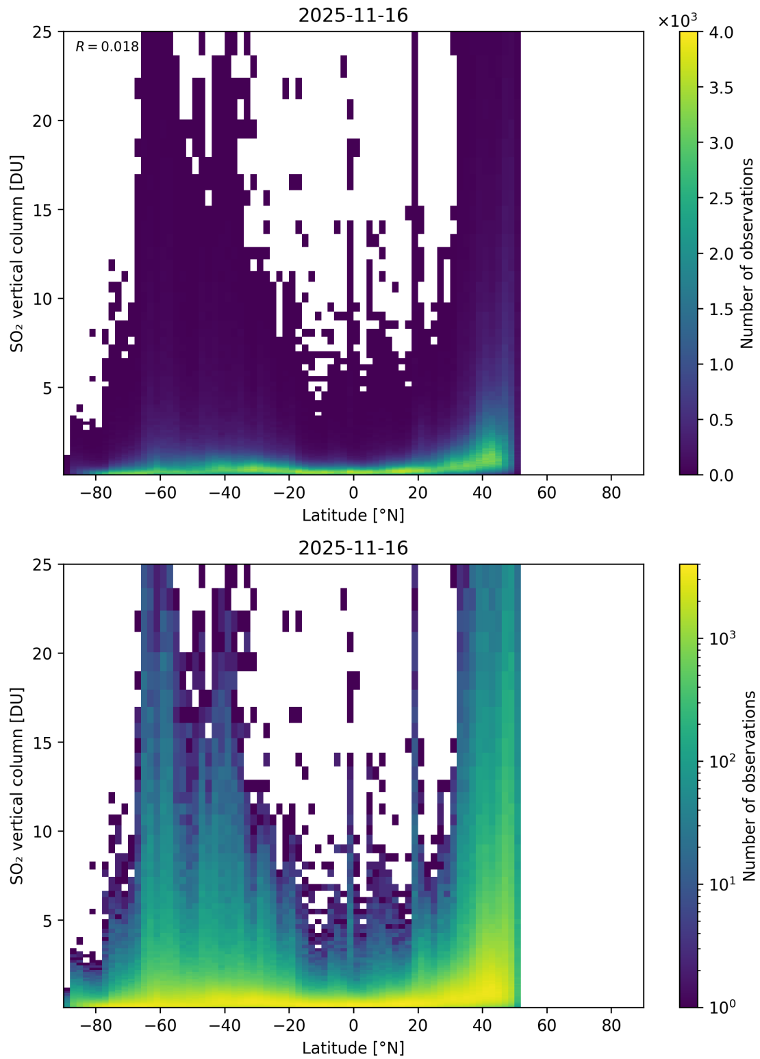
Figure 169: Scatter density plot of “Latitude” against “SO 2 vertical column” for 2025-11-15 to 2025-11-17.
