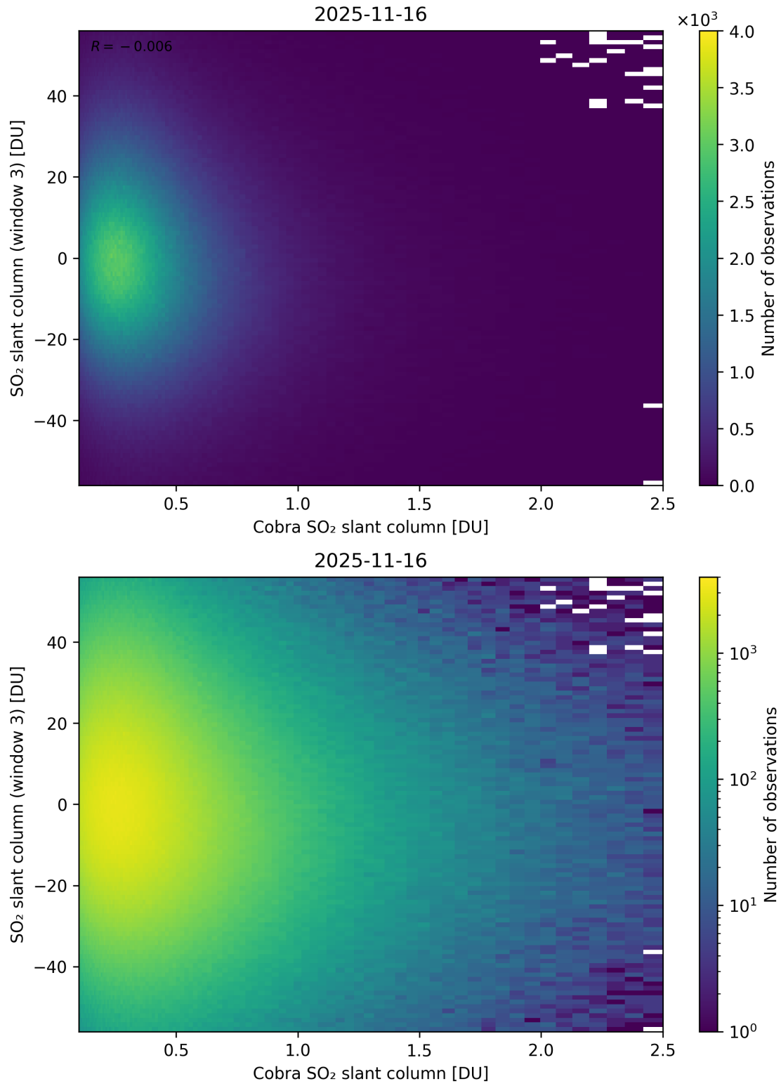
Figure 222: Scatter density plot of “Cobra SO 2 slant column” against “SO 2 slant column (window 3)” for 2025-11-15 to 2025-11-17.
