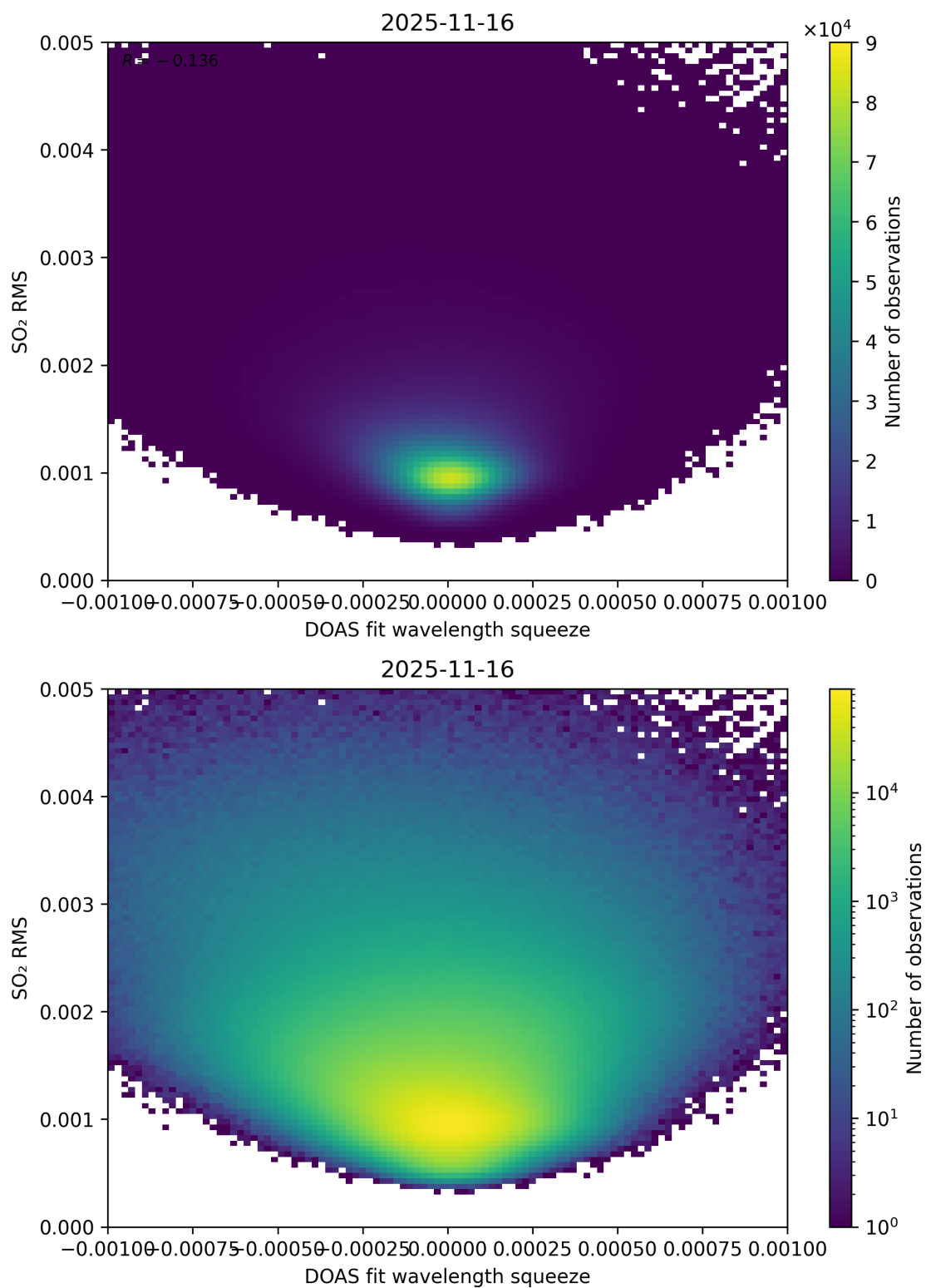
Figure 143: Scatter density plot of “DOAS fit wavelength squeeze” against “SO 2 RMS” for 2025-11-15 to 2025-11-17.
