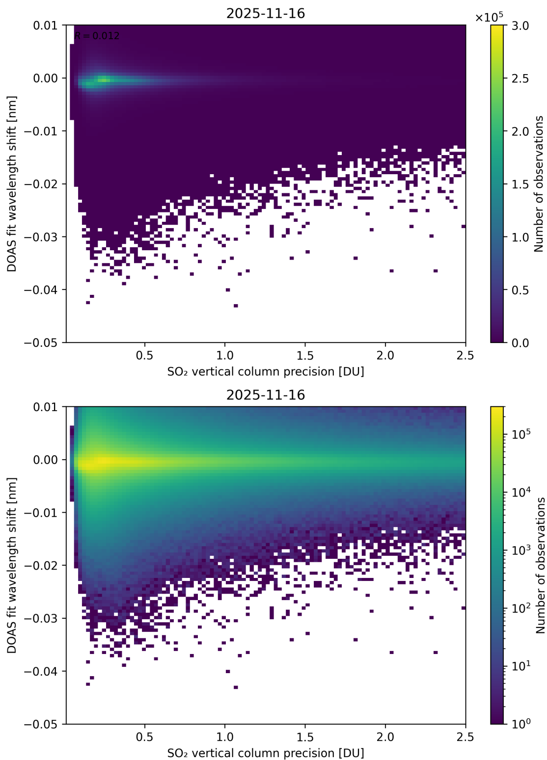
Figure 332: Scatter density plot of “SO 2 vertical column precision” against “DOAS fit wavelength shift” for 2025-11-15 to 2025-11-17.
