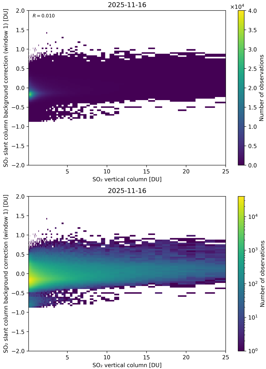
Figure 323: Scatter density plot of “SO 2 vertical column” against “SO 2 slant column background correction (window 1)” for 2025-11-15 to 2025-11-17.
