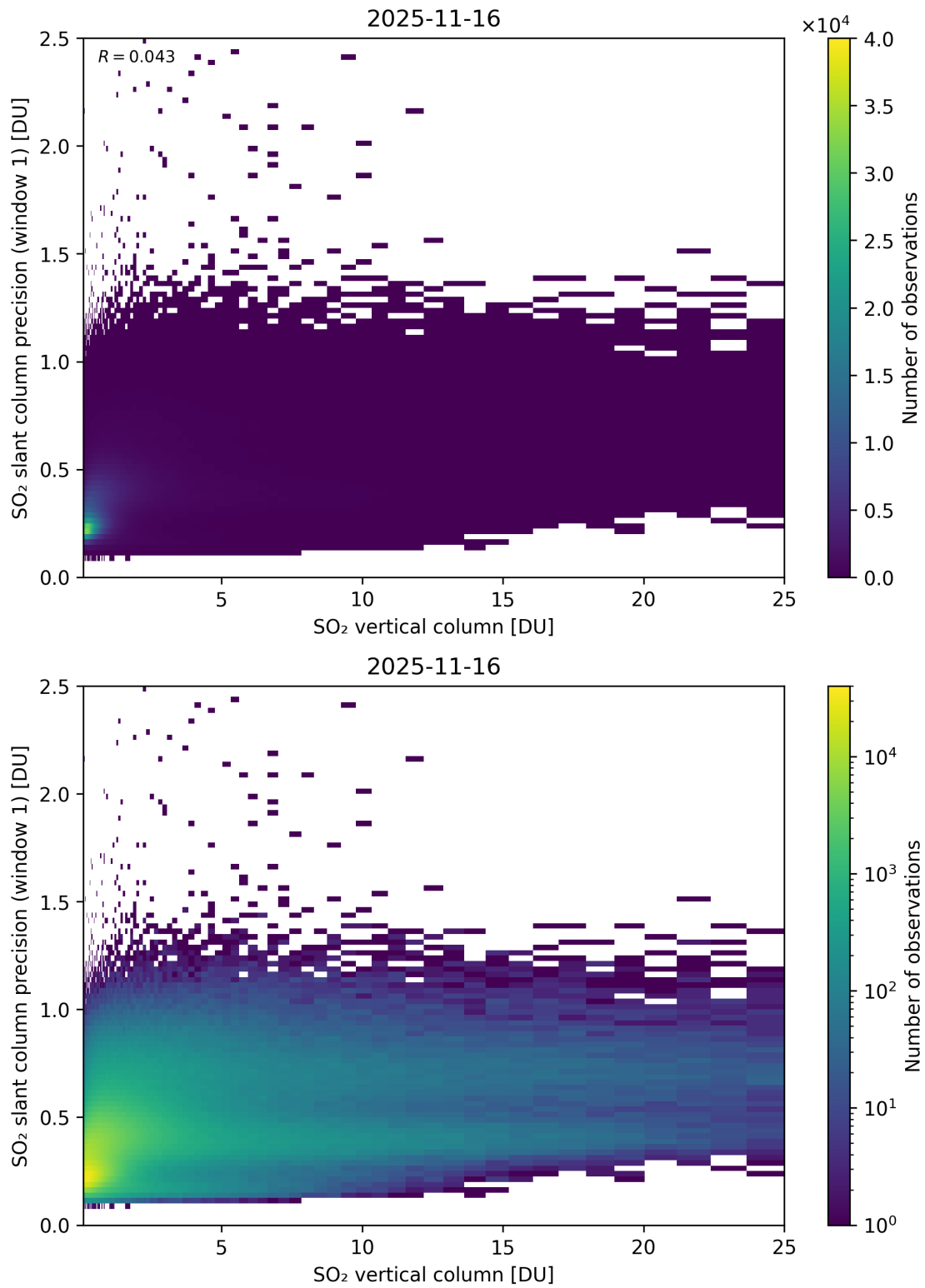
Figure 355: Scatter density plot of “SO 2 vertical column” against “SO 2 slant column precision (window 1)” for 2025-11-15 to 2025-11-17.
