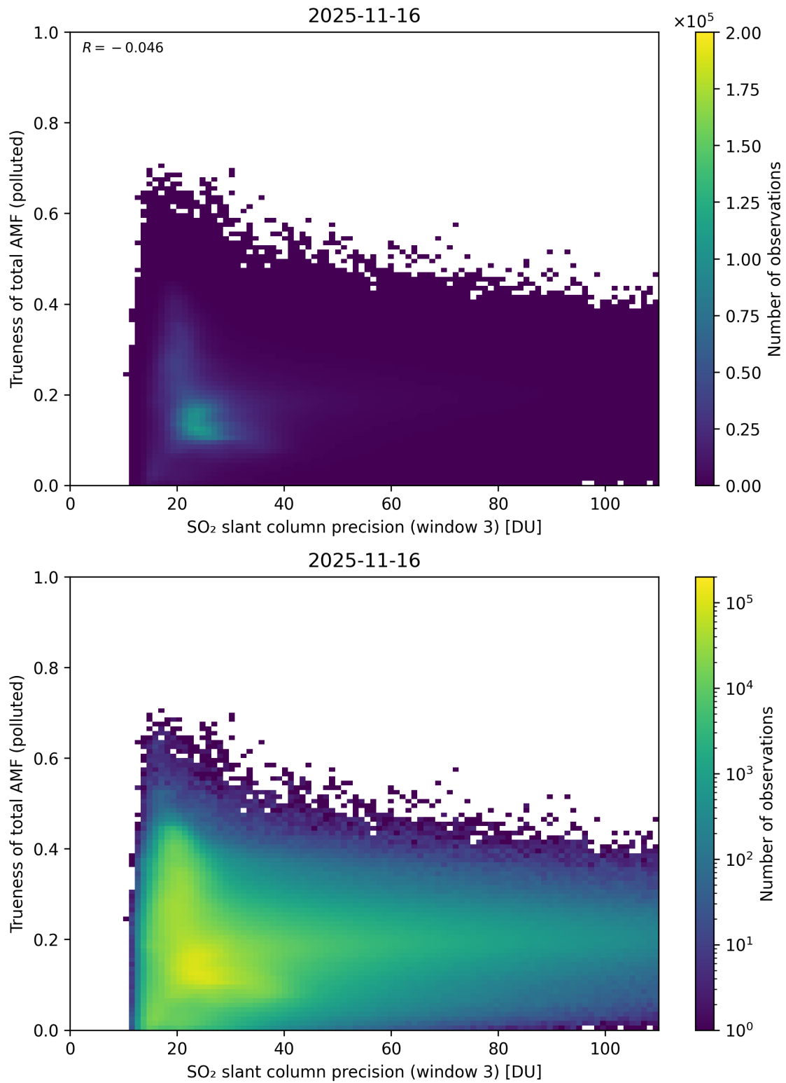
Figure 314: Scatter density plot of “SO 2 slant column precision (window 3)” against “Trueness of total AMF (polluted)” for 2025-11-15 to 2025-11-17.
