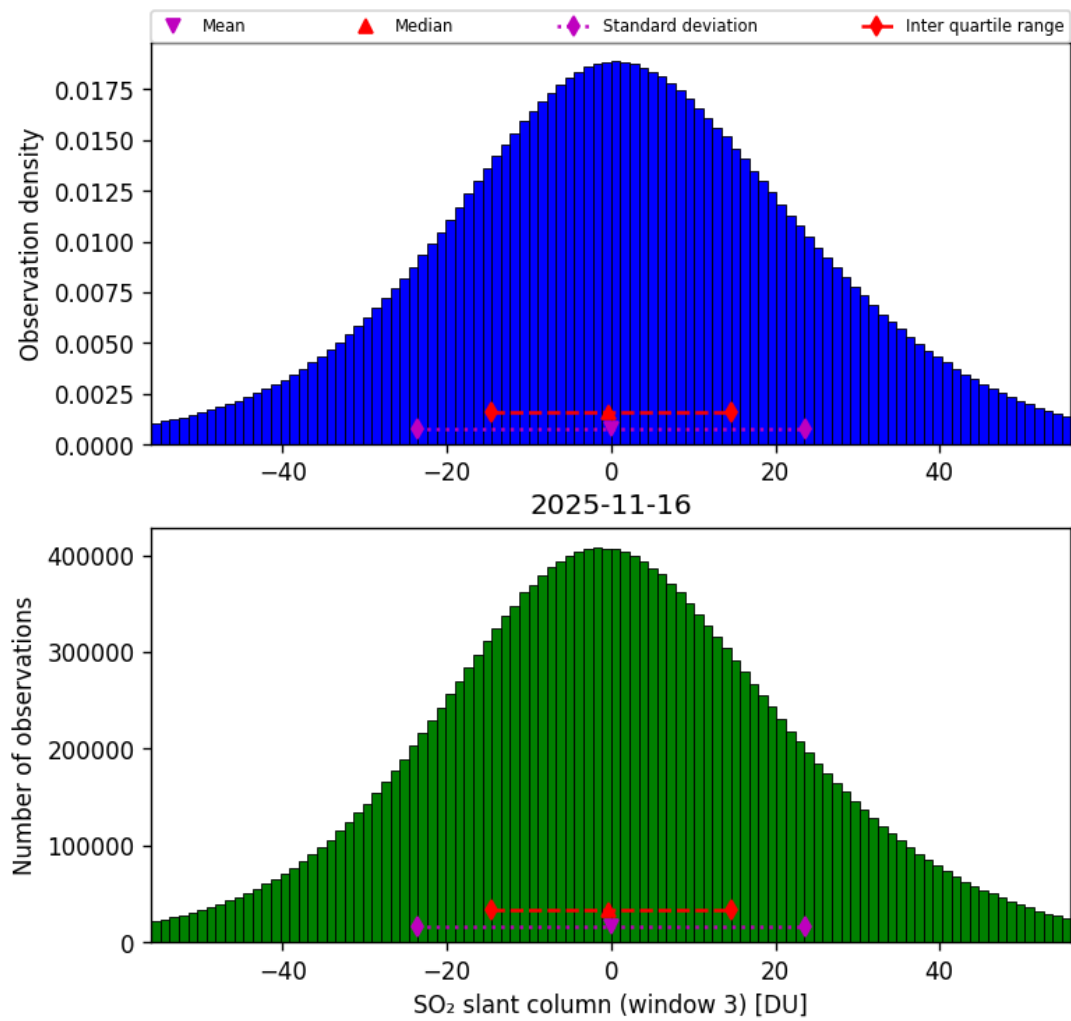
Figure 71: Histogram of “SO 2 slant column (window 3)” for 2025-11-15 to 2025-11-17
