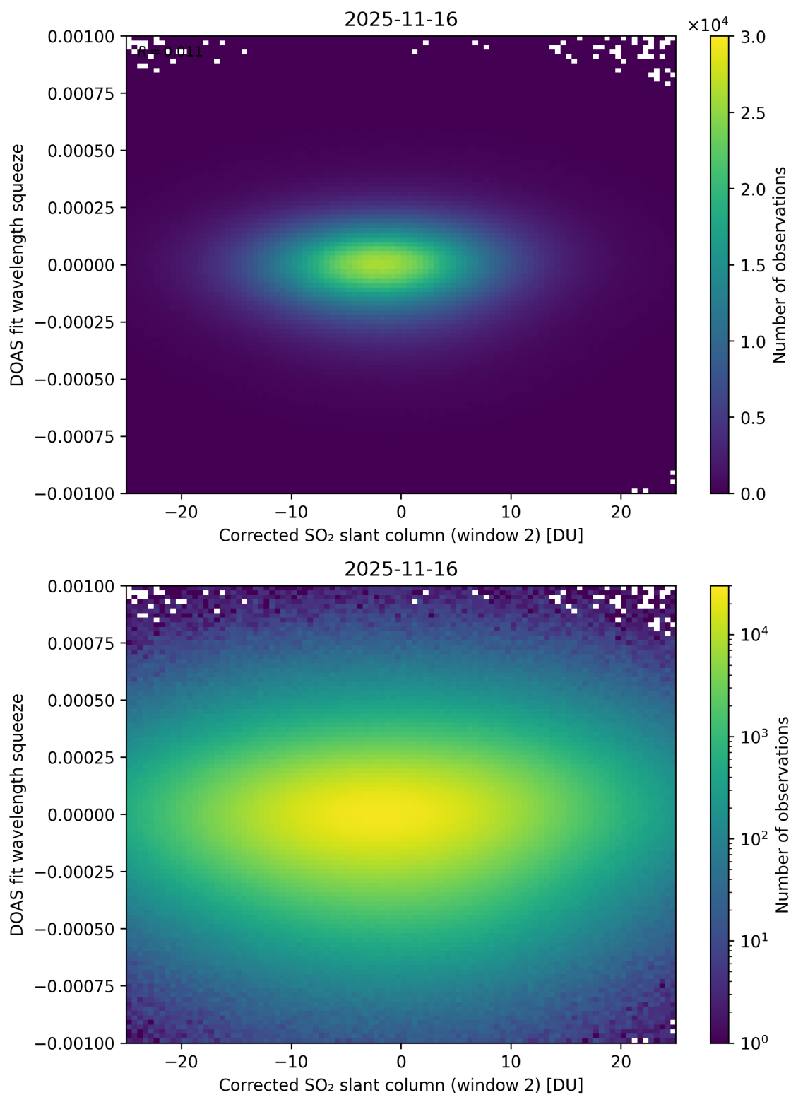
Figure 247: Scatter density plot of “Corrected SO 2 slant column (window 2)” against “DOAS fit wavelength squeeze” for 2025-11-15 to 2025-11-17.
