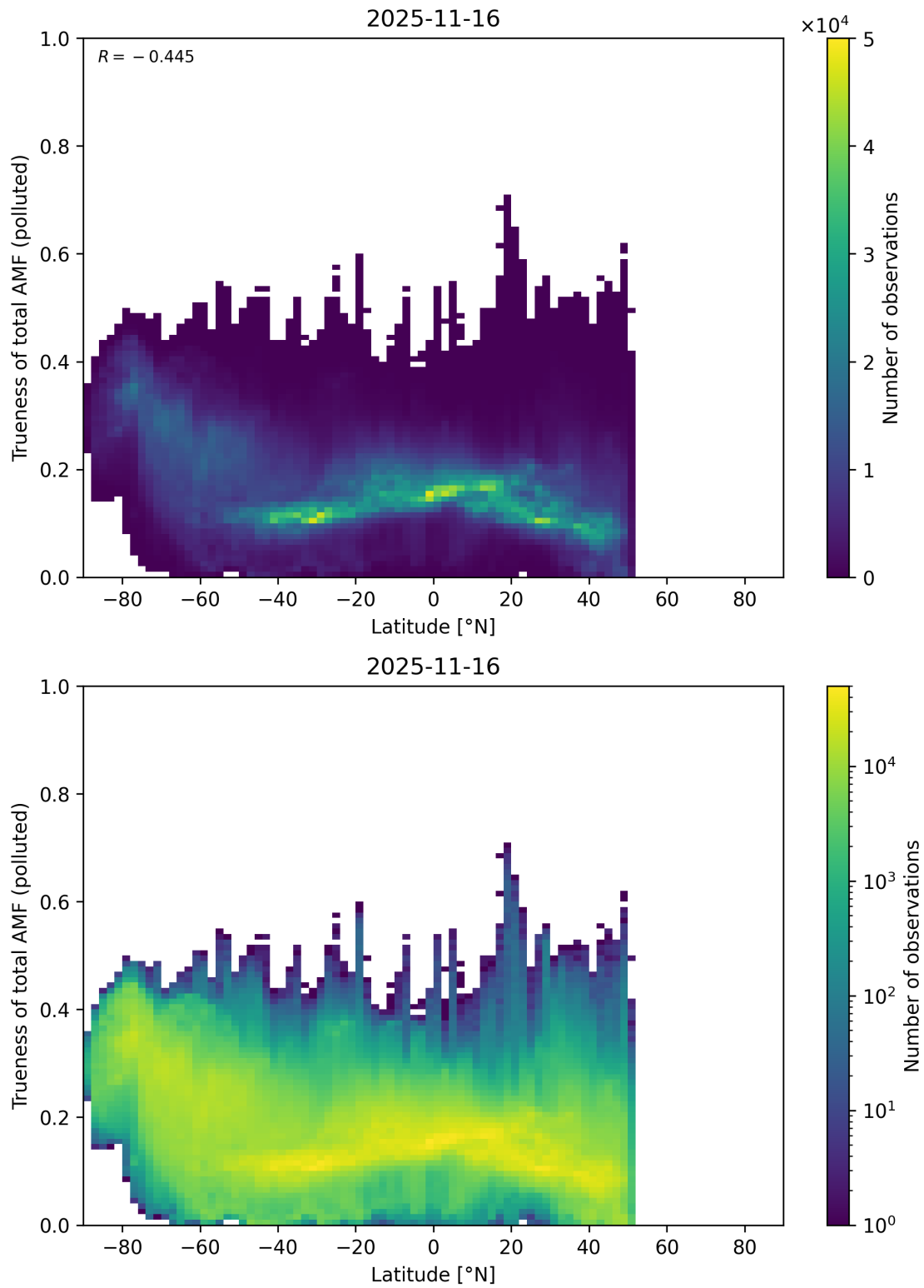
Figure 168: Scatter density plot of “Latitude” against “Trueness of total AMF (polluted)” for 2025-11-15 to 2025-11-17.
