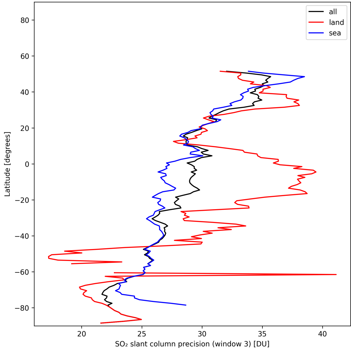
Figure 46: Zonal average of “SO 2 slant column precision (window 3)” for 2025-11-15 to 2025-11-17.
