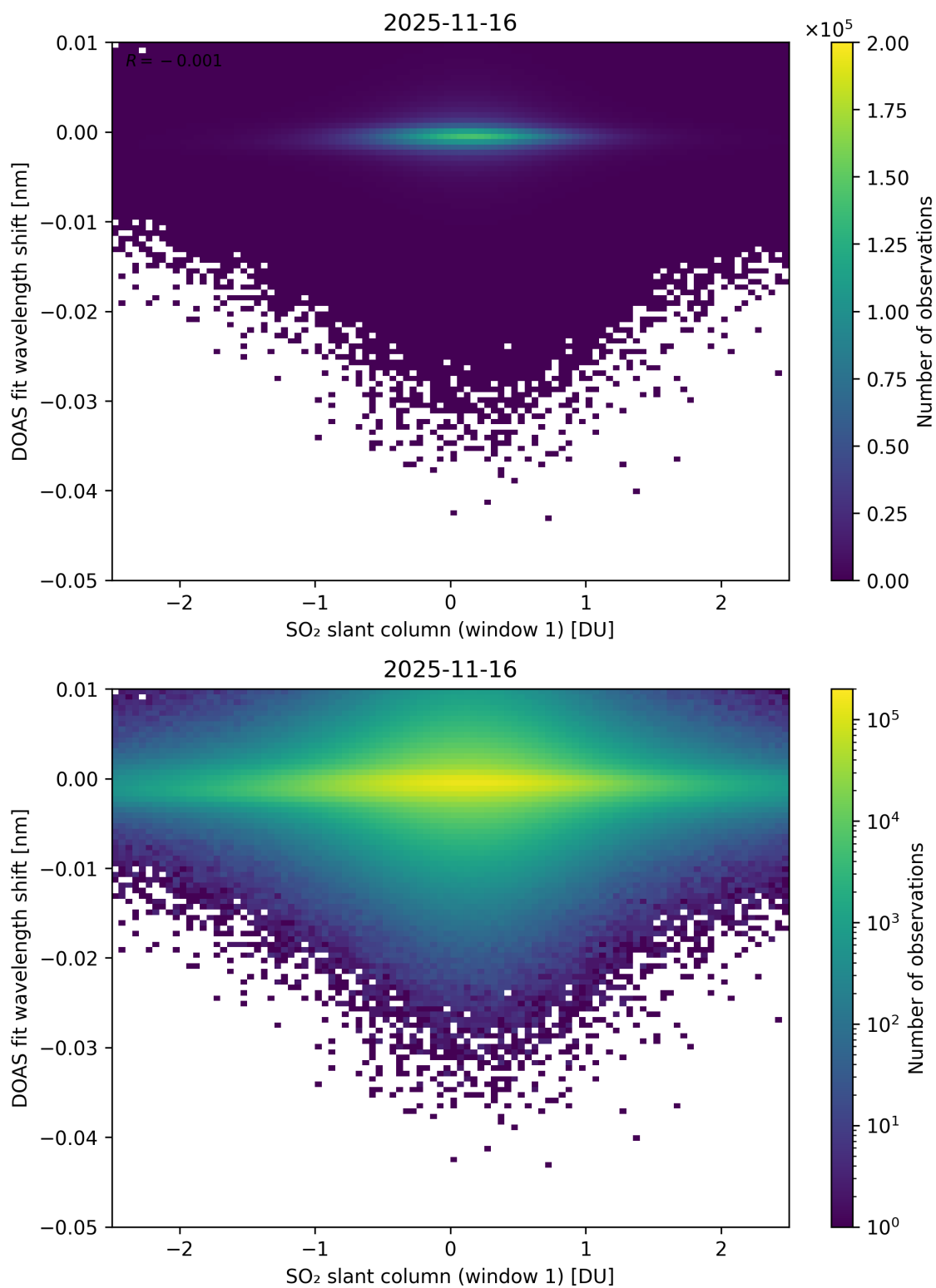
Figure 265: Scatter density plot of “SO 2 slant column (window 1)” against “DOAS fit wavelength shift” for 2025-11-15 to 2025-11-17.
