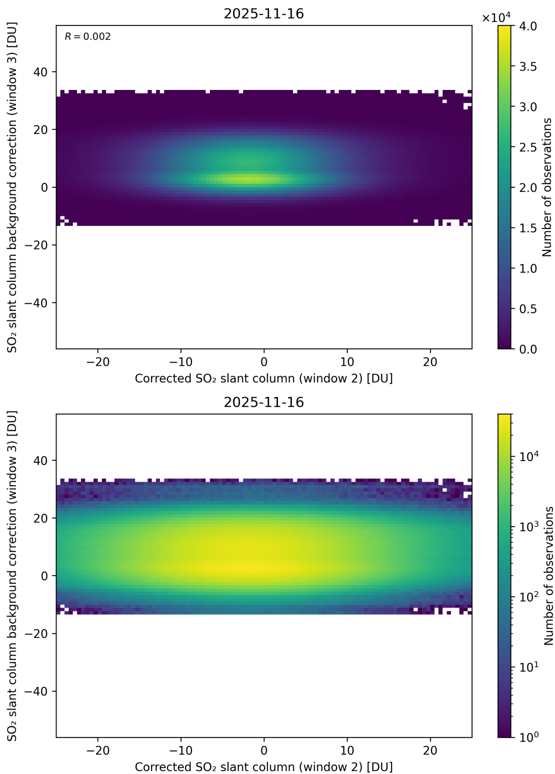
Figure 245: Scatter density plot of “Corrected SO 2 slant column (window 2)” against “SO 2 slant column background correction (window 3)” for 2025-11-15 to 2025-11-17.
