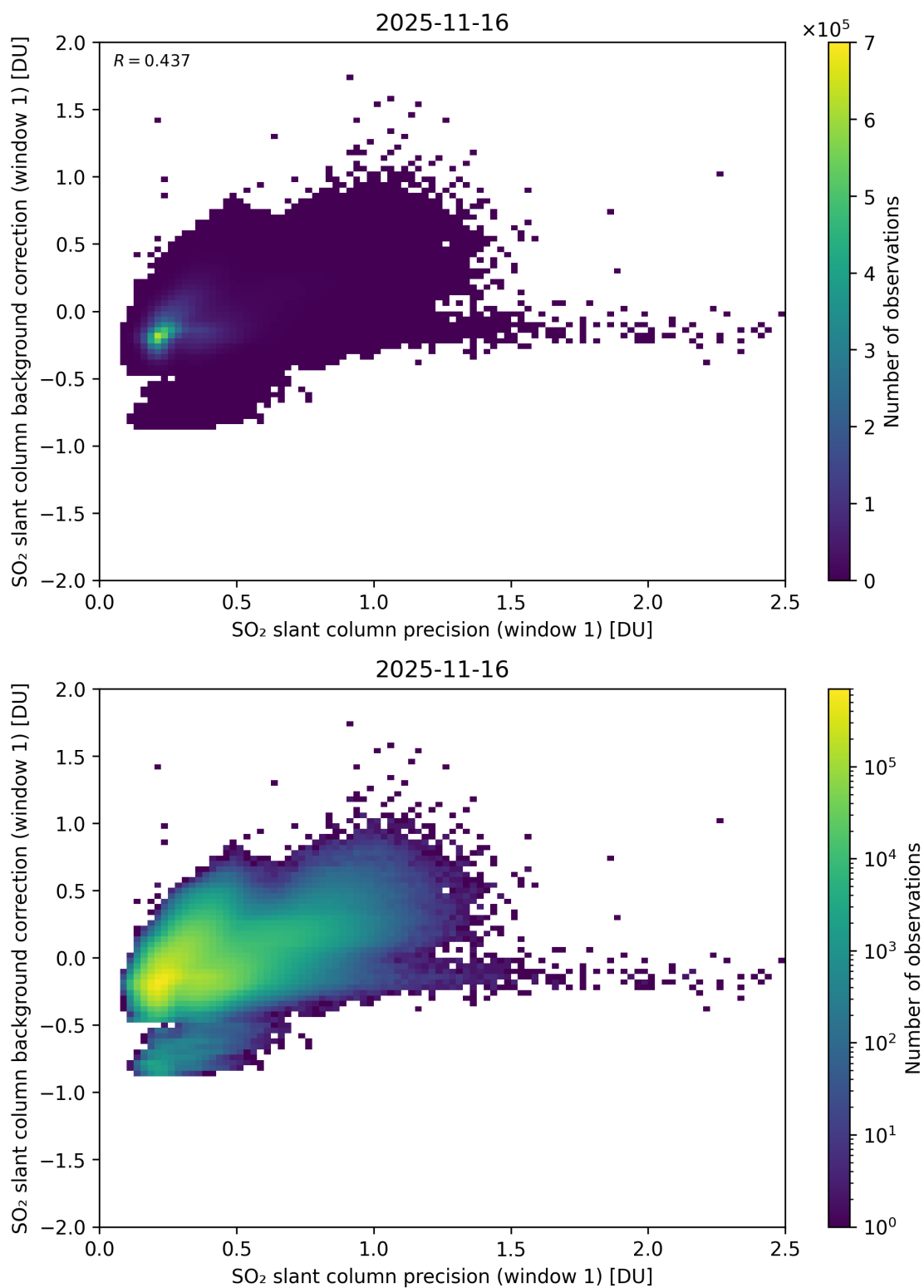
Figure 268: Scatter density plot of “SO 2 slant column precision (window 1)” against “SO 2 slant column background correction (window 1)” for 2025-11-15 to 2025-11-17.
