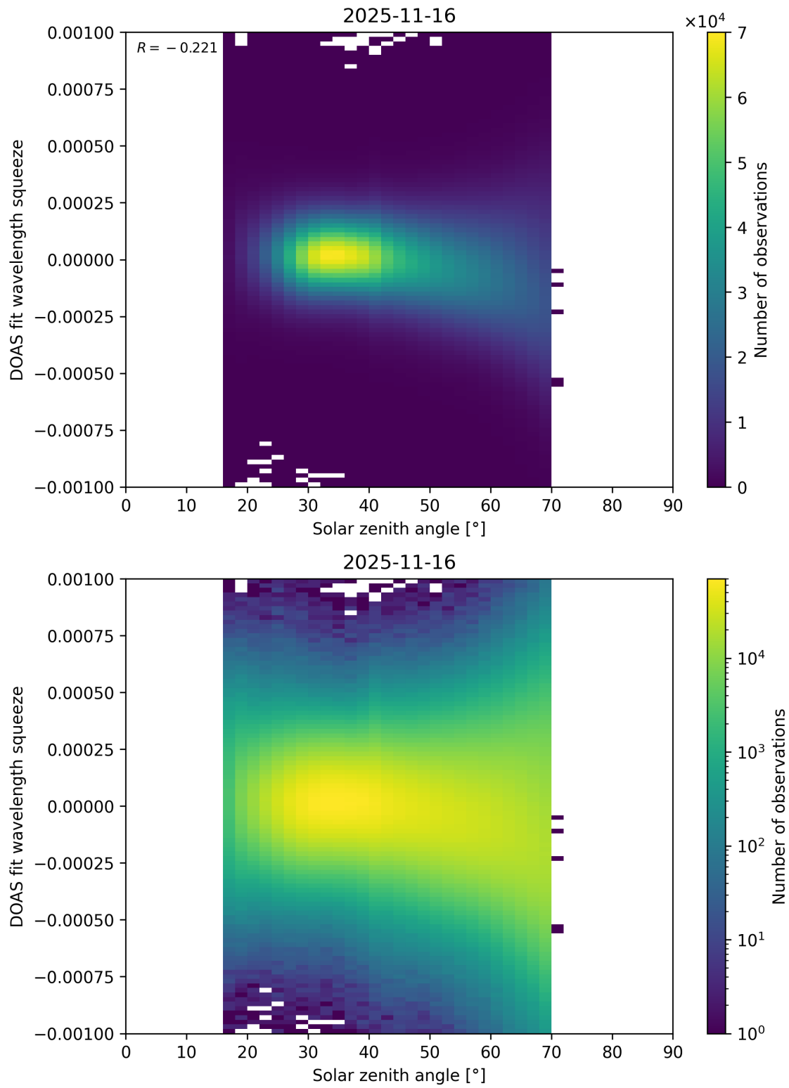
Figure 175: Scatter density plot of “Solar zenith angle” against “DOAS fit wavelength squeeze” for 2025-11-15 to 2025-11-17.
