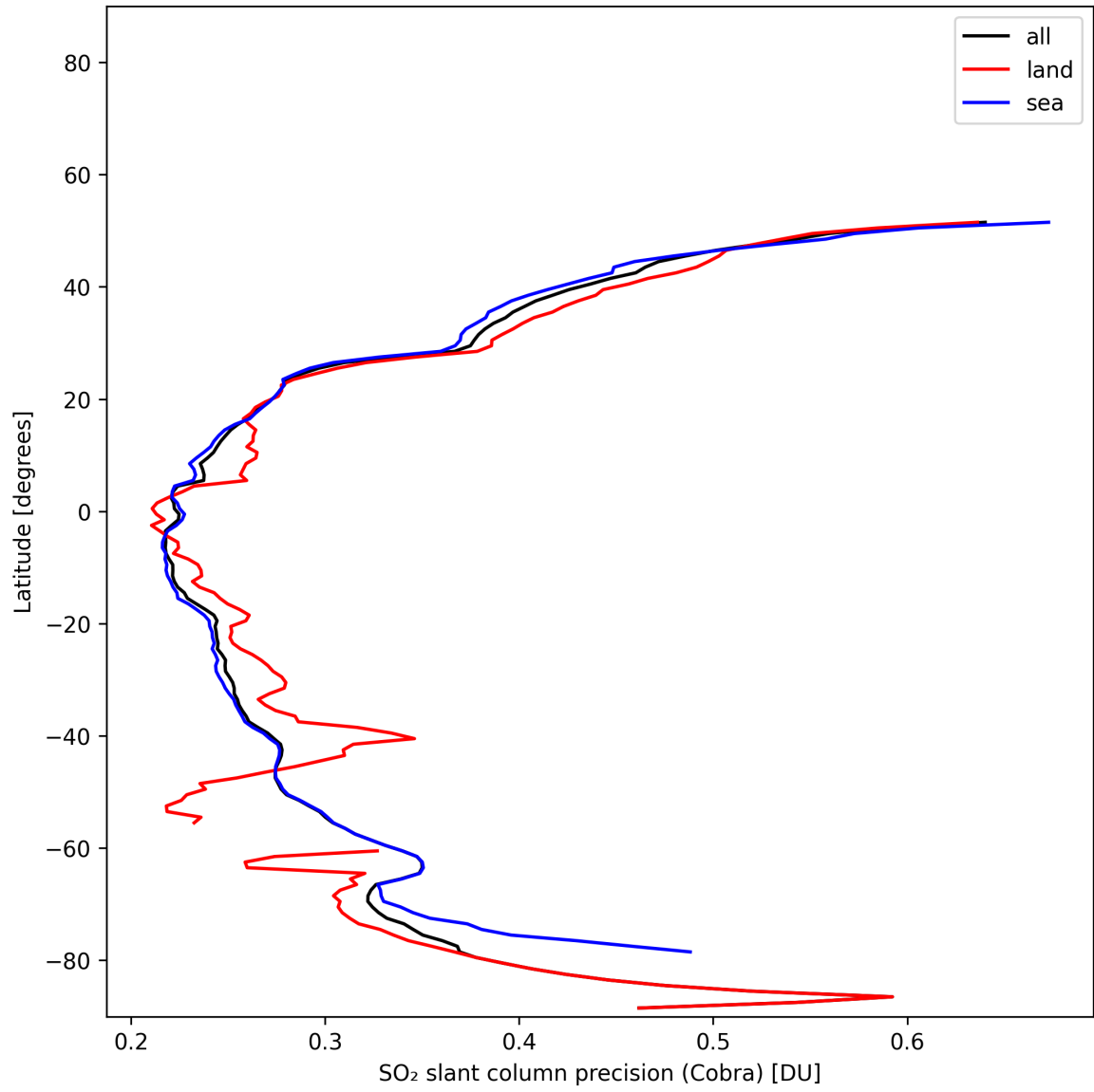
Figure 36: Zonal average of “SO 2 slant column precision (Cobra)” for 2025-11-15 to 2025-11-17.
