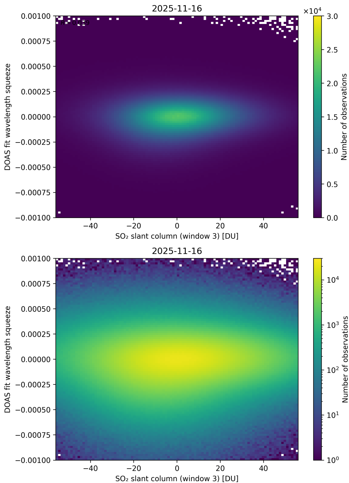
Figure 305: Scatter density plot of “SO 2 slant column (window 3)” against “DOAS fit wavelength squeeze” for 2025-11-15 to 2025-11-17.
