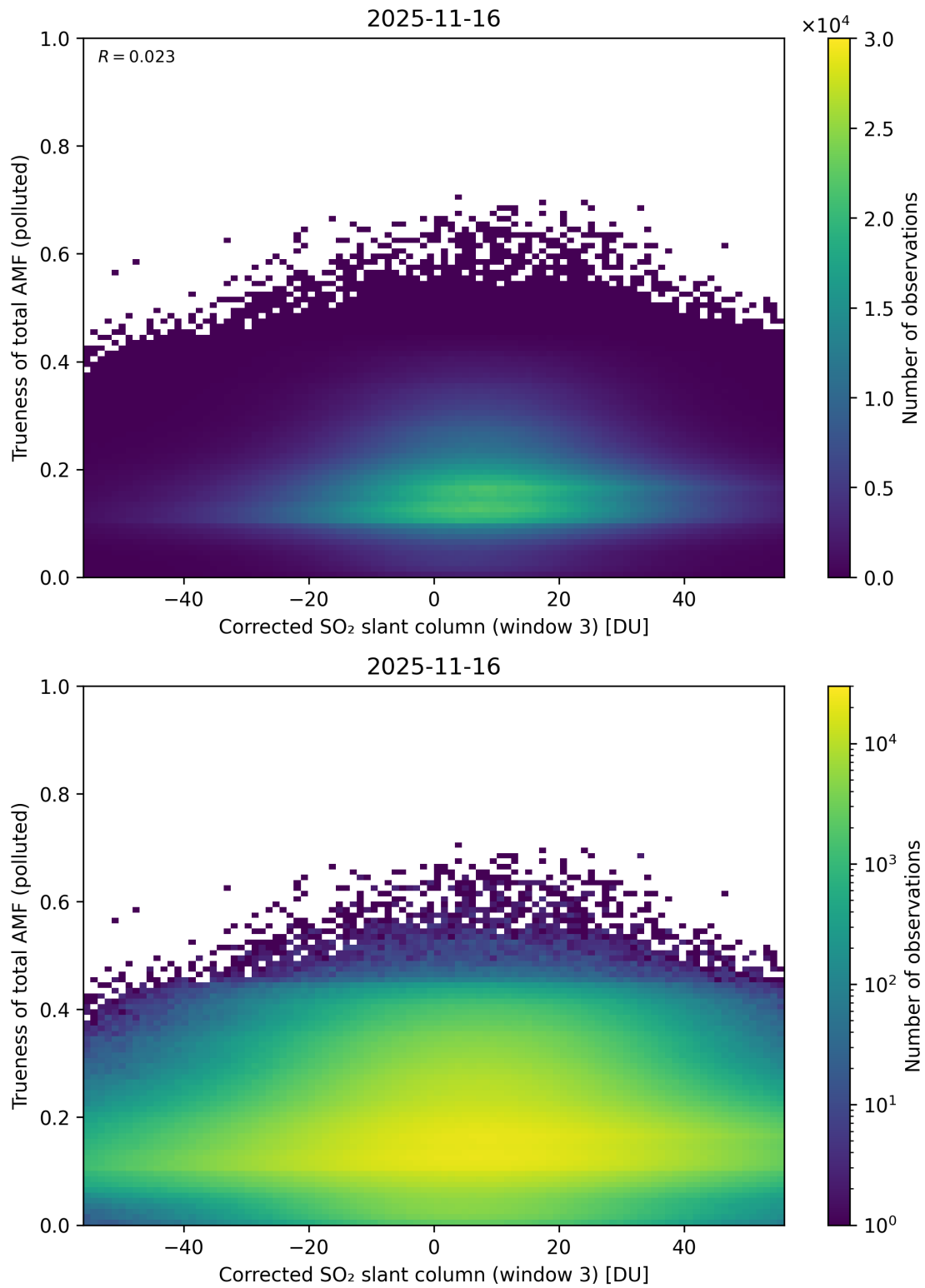
Figure 261: Scatter density plot of “Corrected SO 2 slant column (window 3)” against “Trueness of total AMF (polluted)” for 2025-11-15 to 2025-11-17.
