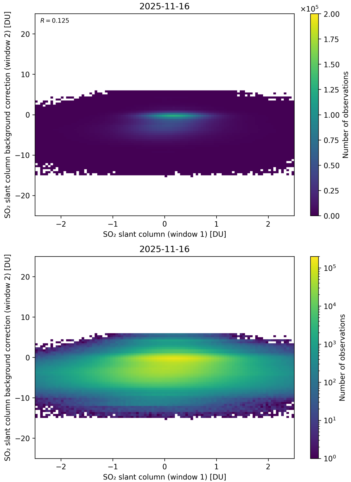
Figure 263: Scatter density plot of “SO 2 slant column (window 1)” against “SO 2 slant column background correction (window 2)” for 2025-11-15 to 2025-11-17.
