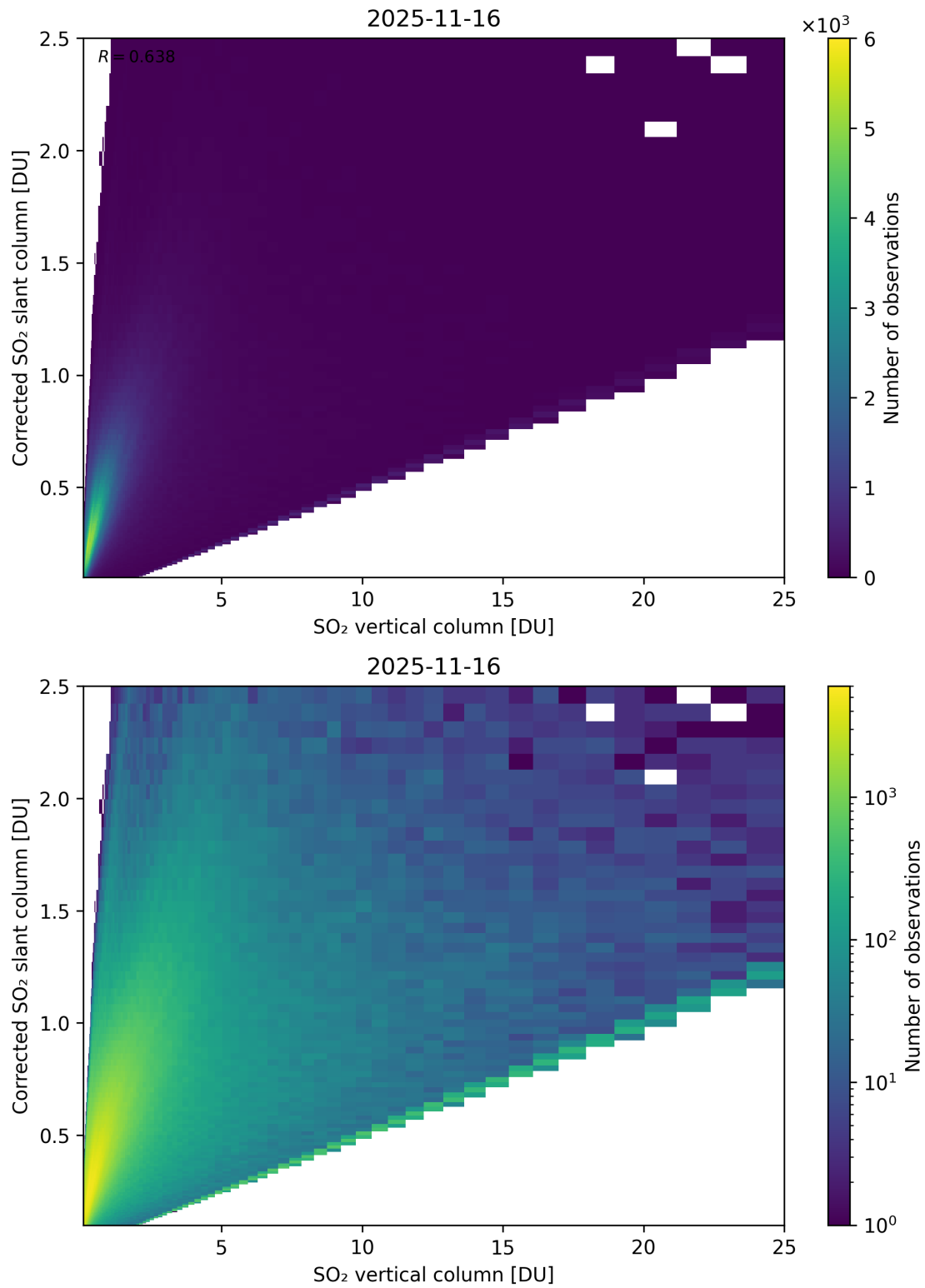
Figure 351: Scatter density plot of “SO 2 vertical column” against “Corrected SO 2 slant column” for 2025-11-15 to 2025-11-17.
