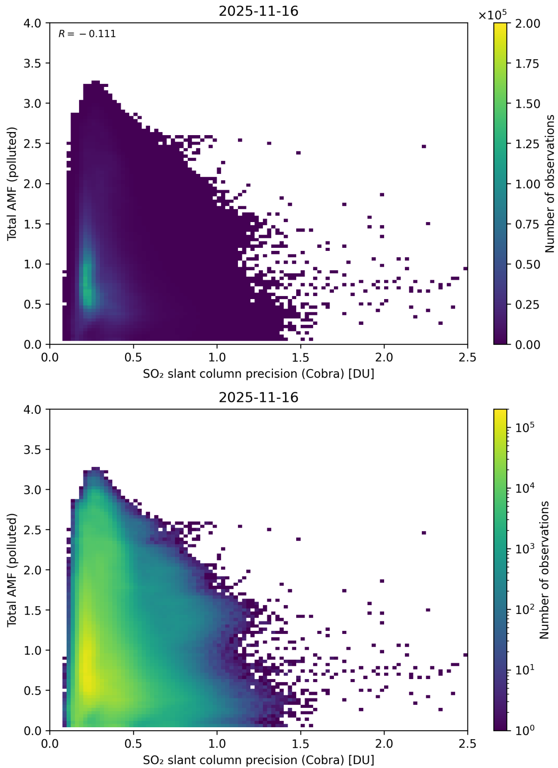
Figure 213: Scatter density plot of “SO 2 slant column precision (Cobra)” against “Total AMF (polluted)” for 2025-11-15 to 2025-11-17.
