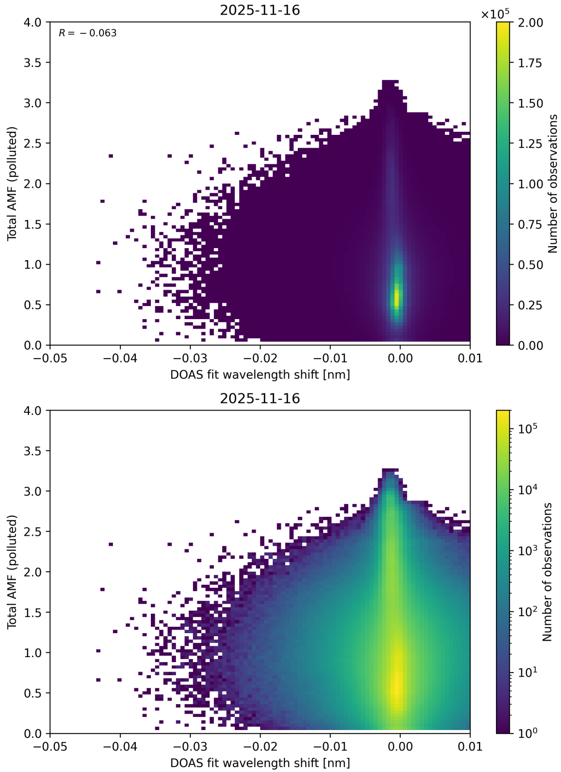
Figure 141: Scatter density plot of “DOAS fit wavelength shift” against “Total AMF (polluted)” for 2025-11-15 to 2025-11-17.
