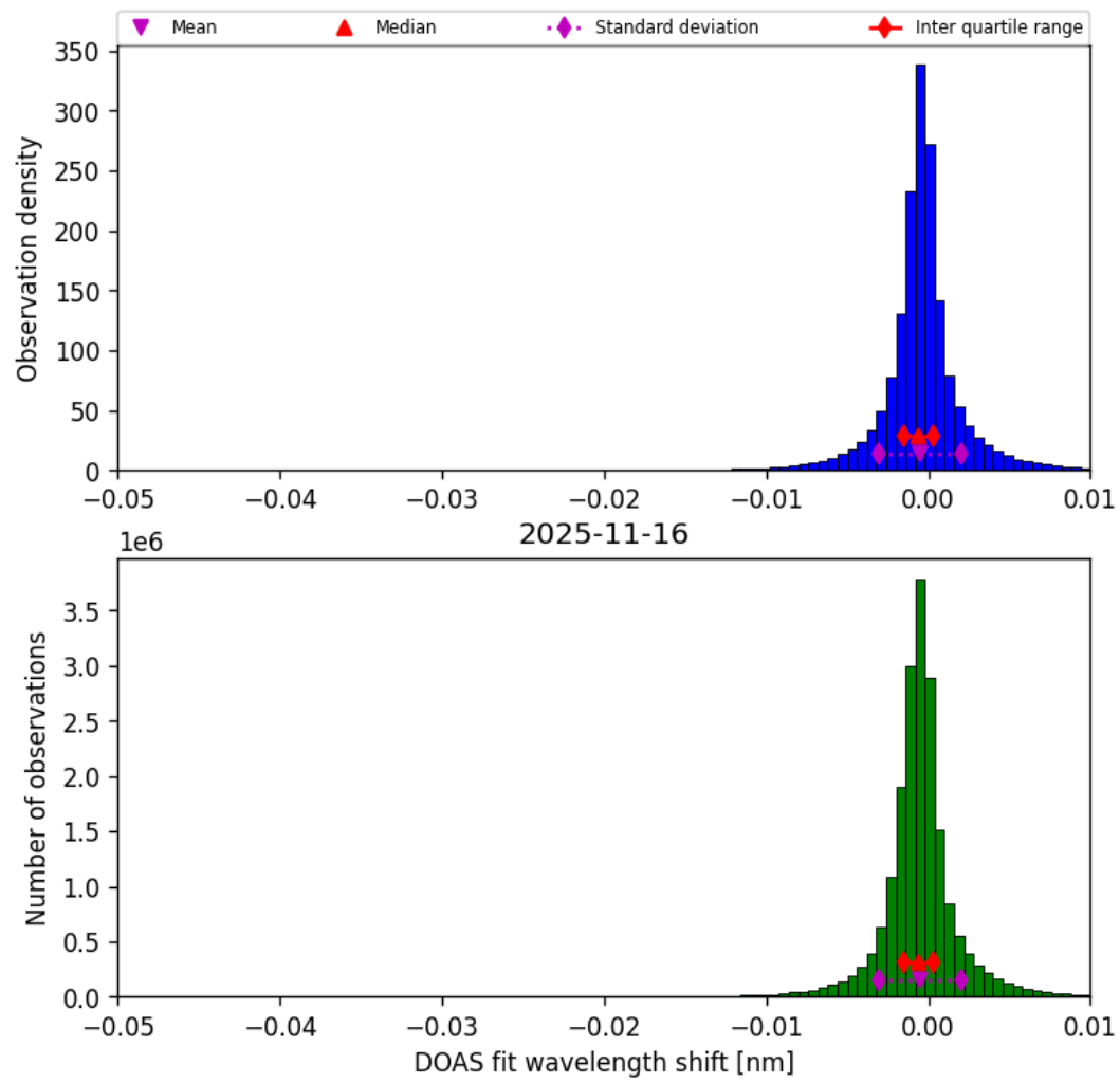
Figure 76: Histogram of “DOAS fit wavelength shift” for 2025-11-15 to 2025-11-17
