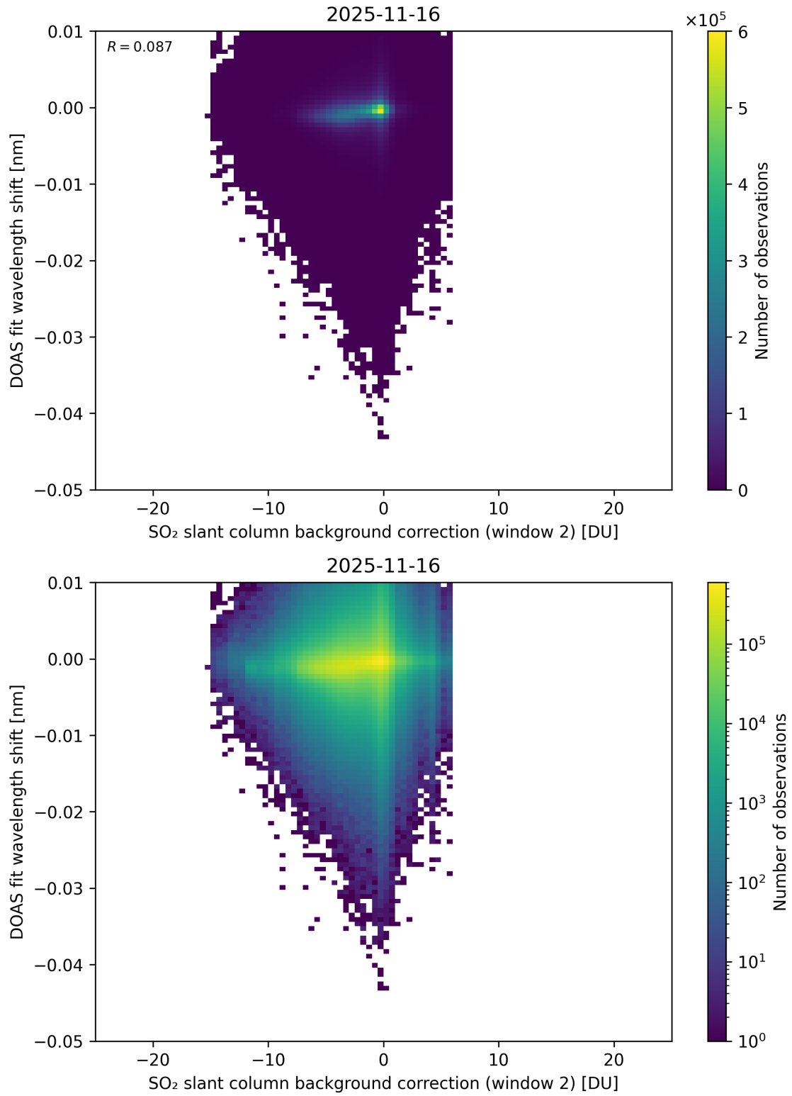
Figure 123: Scatter density plot of “SO 2 slant column background correction (window 2)” against “DOAS fit wavelength shift” for 2025-11-15 to 2025-11-17.
