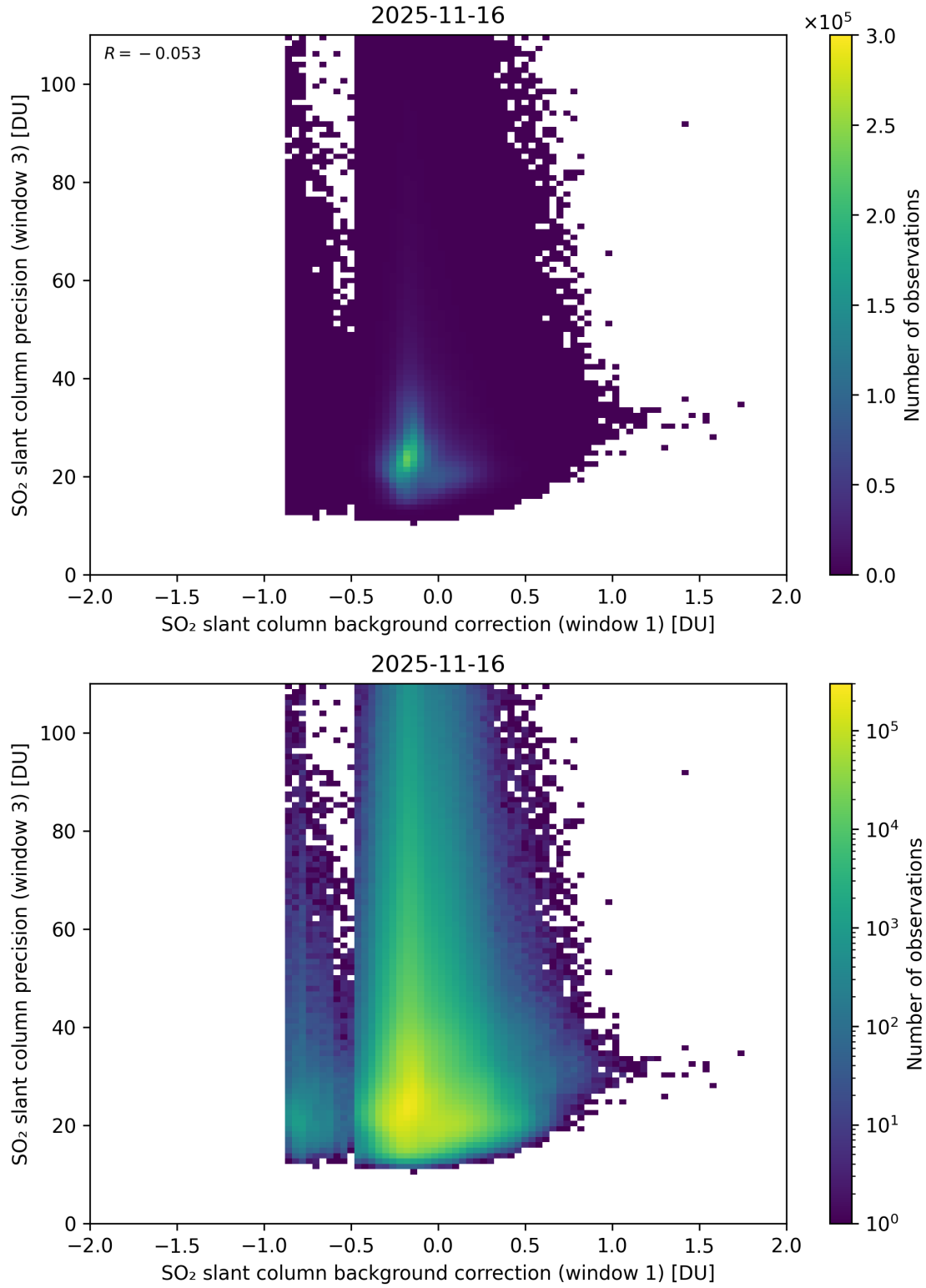
Figure 119: Scatter density plot of “SO 2 slant column background correction (window 1)” against “SO 2 slant column precision (window 3)” for 2025-11-15 to 2025-11-17.
