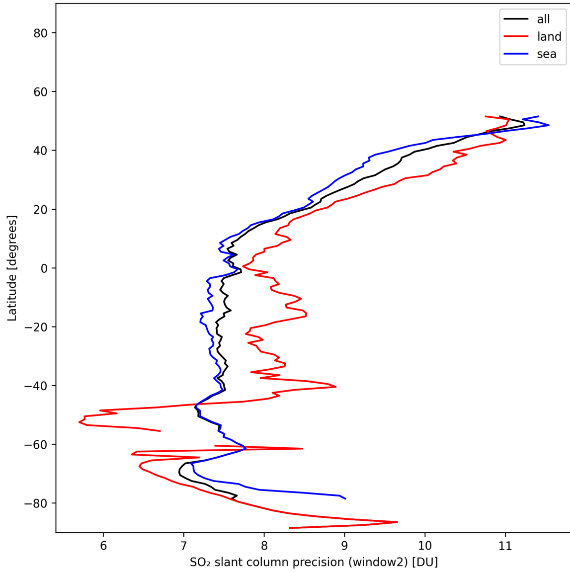
Figure 42: Zonal average of “SO 2 slant column precision (window2)” for 2025-11-15 to 2025-11-17.
