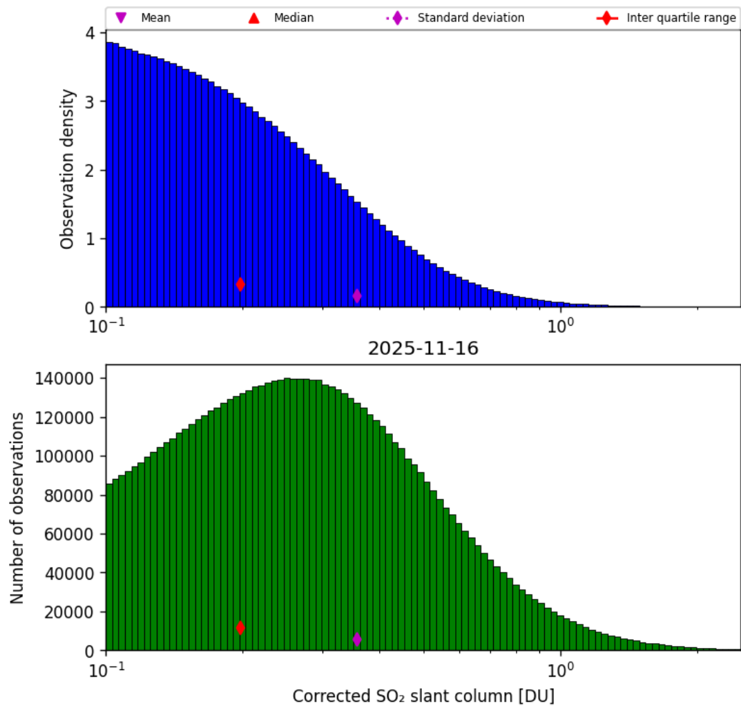
Figure 60: Histogram of “Corrected SO 2 slant column” for 2025-11-15 to 2025-11-17
