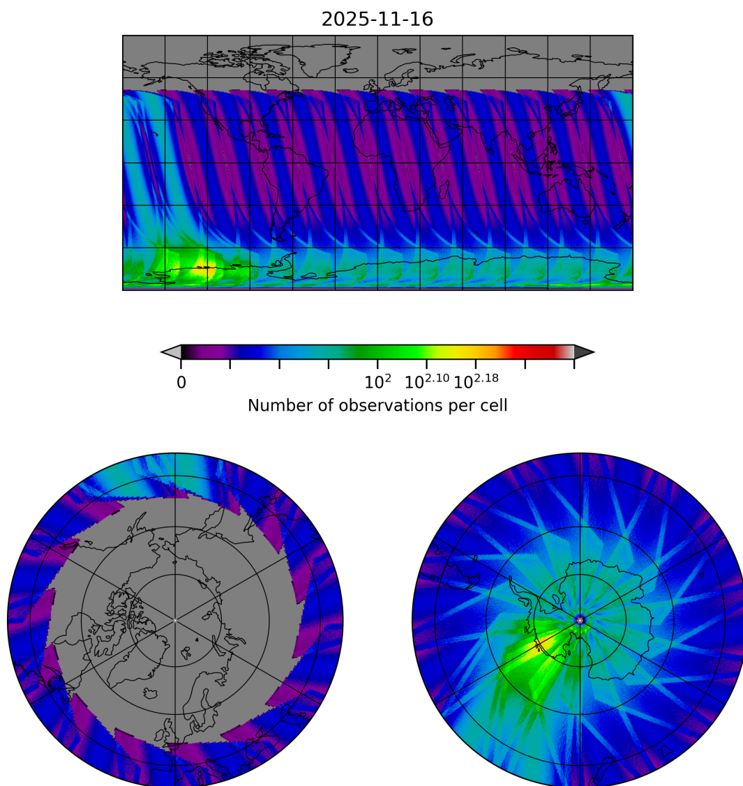
Figure 30: Map of the number of observations for 2025-11-15 to 2025-11-17
