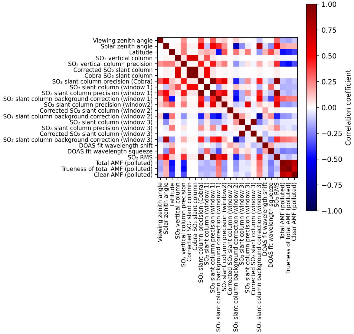
Figure 2: Map of correlation matrix for 2025-11-15 to 2025-11-17.
