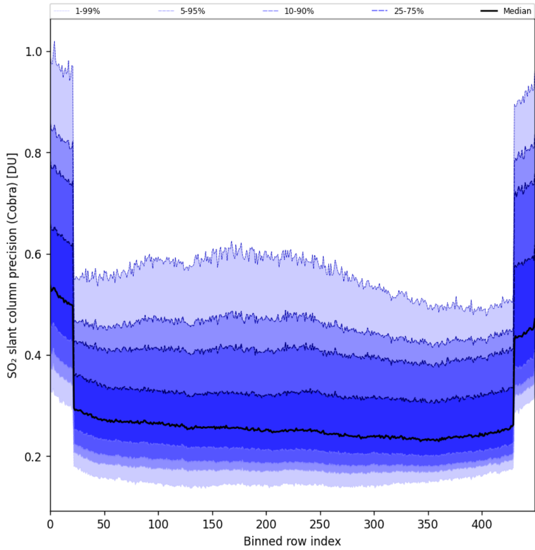
Figure 88: Along track statistics of “SO 2 slant column precision (Cobra)” for 2025-11-15 to 2025-11-17
