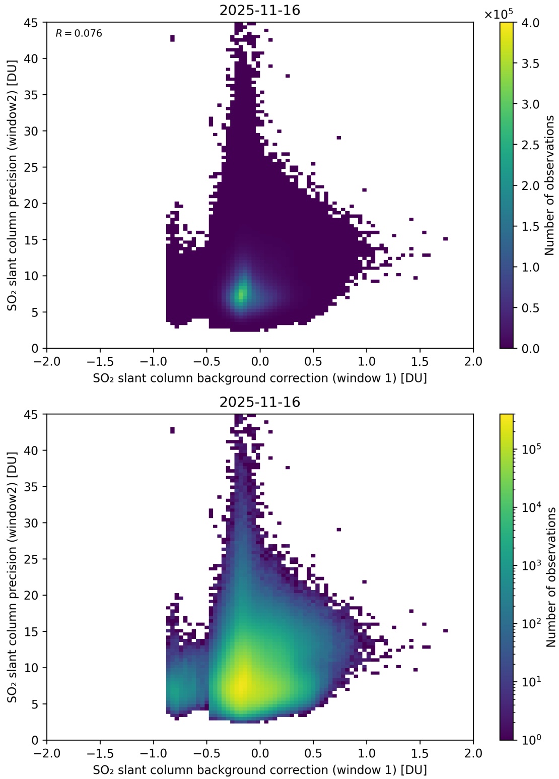
Figure 117: Scatter density plot of “SO 2 slant column background correction (window 1)” against “SO 2 slant column precision (window2)” for 2025-11-15 to 2025-11-17.
