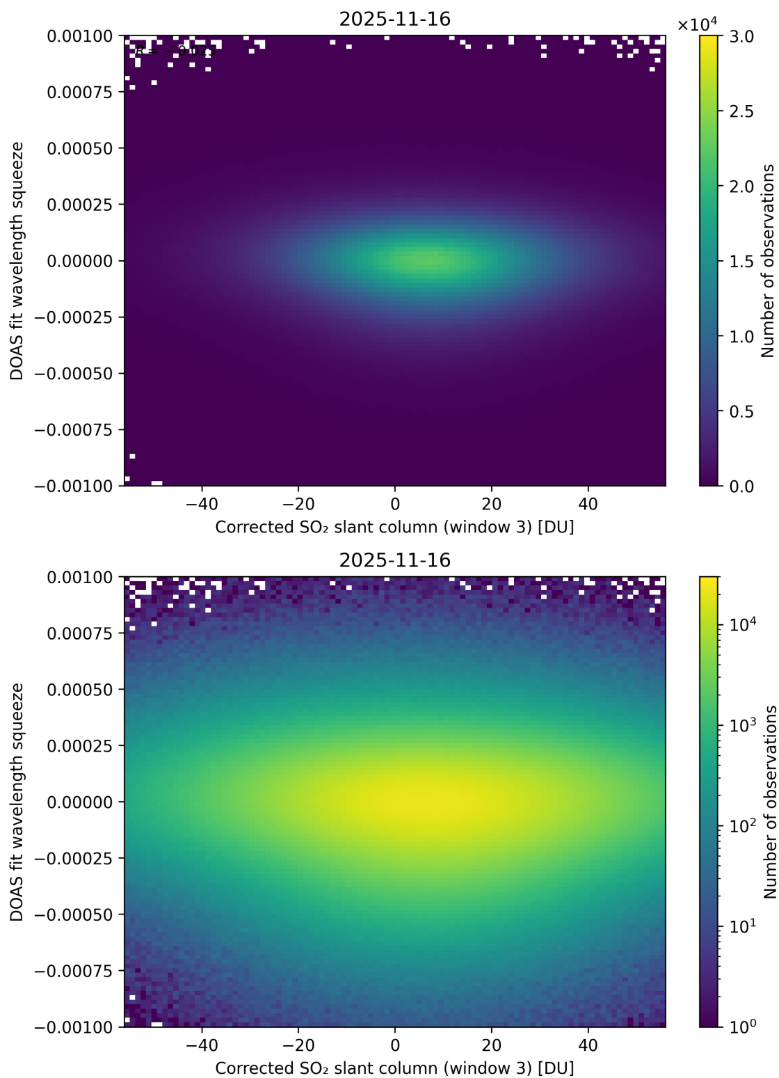
Figure 257: Scatter density plot of “Corrected SO 2 slant column (window 3)” against “DOAS fit wavelength squeeze” for 2025-11-15 to 2025-11-17.
