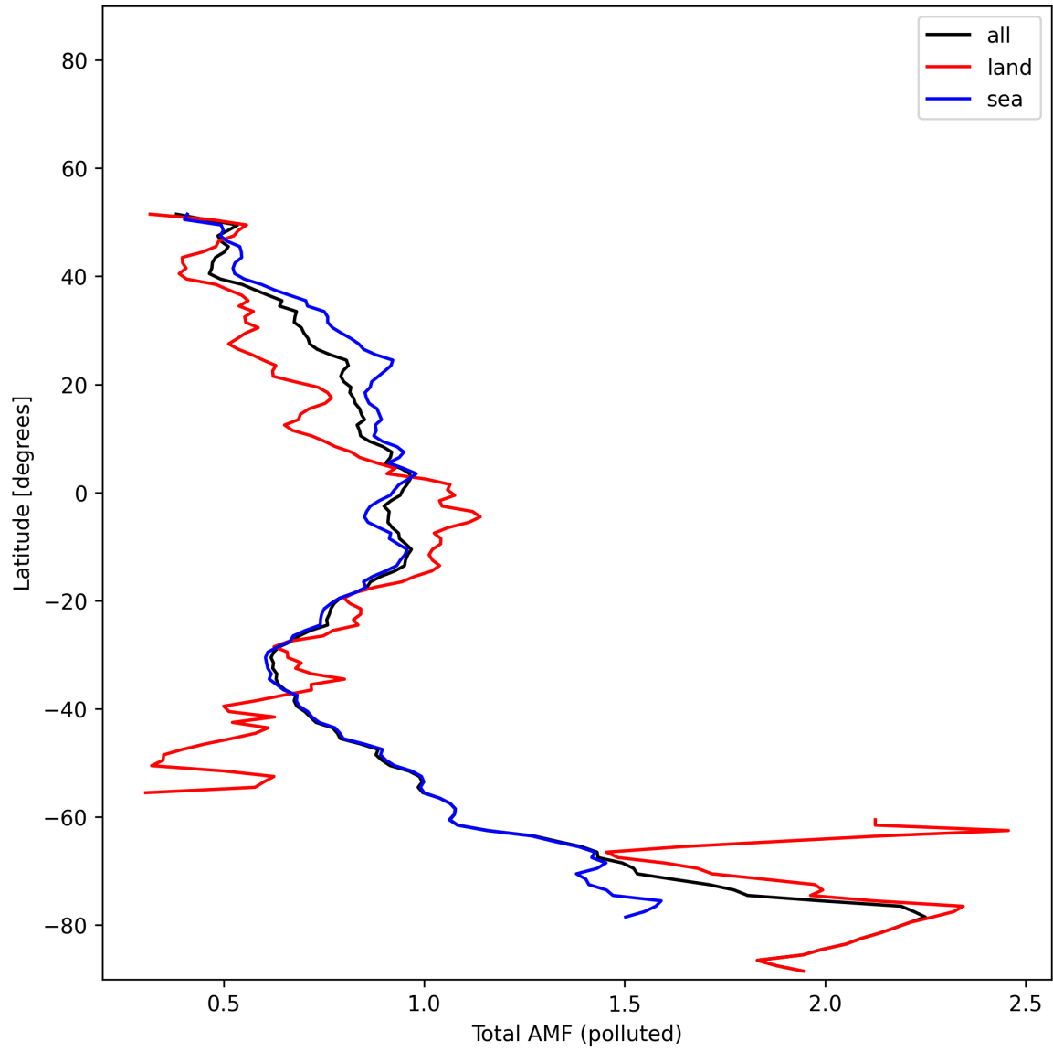
Figure 53: Zonal average of “Total AMF (polluted)” for 2025-11-15 to 2025-11-17.
