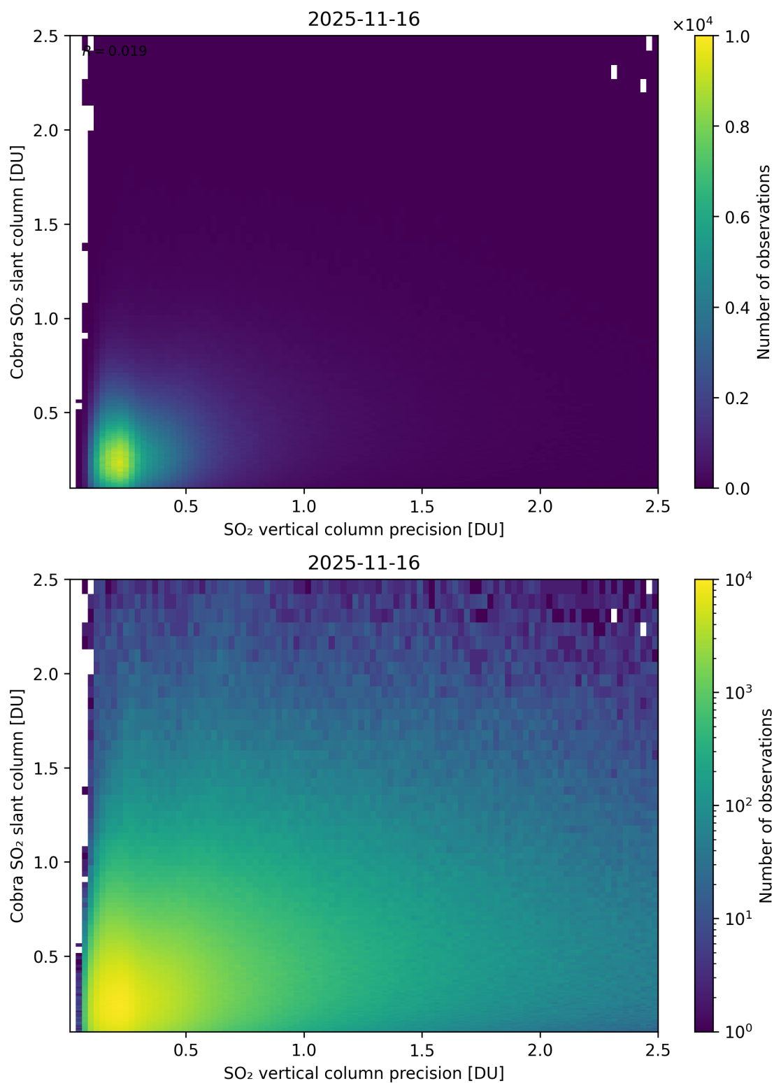
Figure 336: Scatter density plot of “SO 2 vertical column precision” against “Cobra SO 2 slant column” for 2025-11-15 to 2025-11-17.
