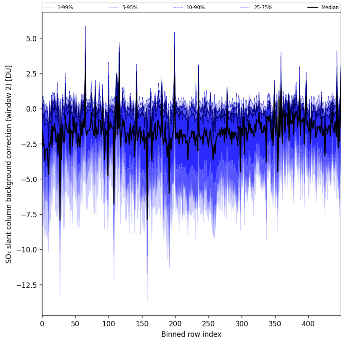
Figure 96: Along track statistics of “SO 2 slant column background correction (window 2)” for 2025-11-15 to 2025-11-17
