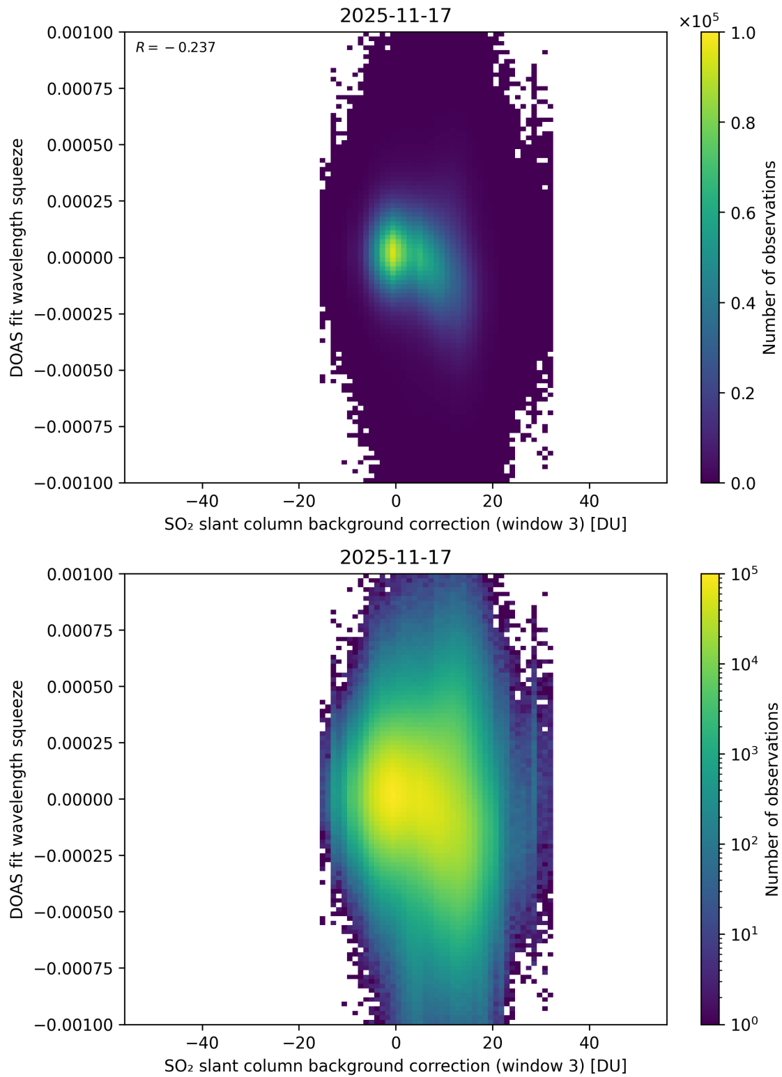
Figure 133: Scatter density plot of “SO 2 slant column background correction (window 3)” against “DOAS fit wavelength squeeze” for 2025-11-16 to 2025-11-18.
