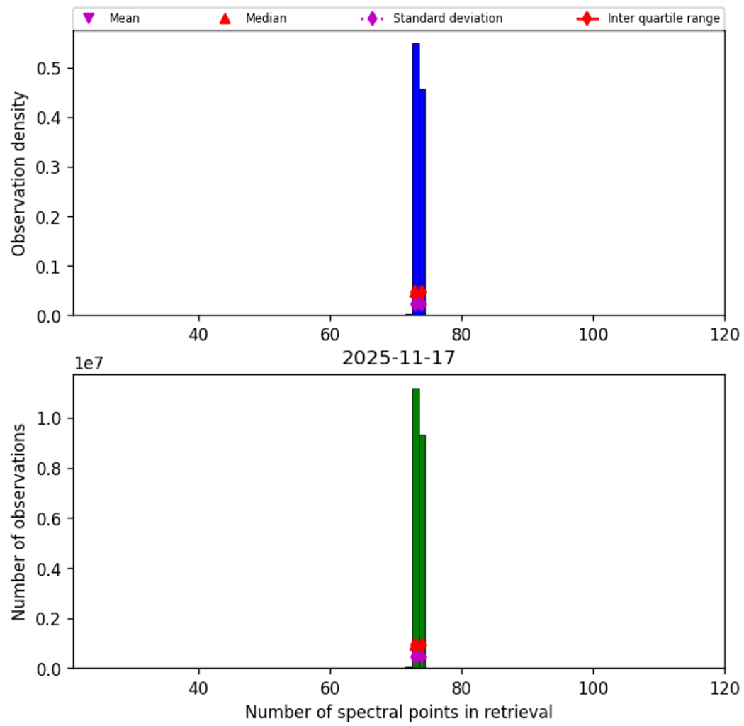
Figure 82: Histogram of “Number of spectral points in retrieval” for 2025-11-16 to 2025-11-18
