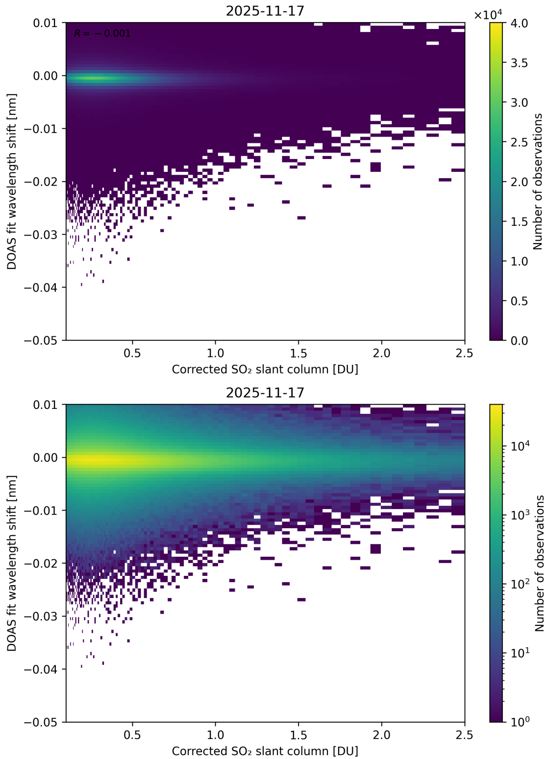
Figure 229: Scatter density plot of “Corrected SO 2 slant column” against “DOAS fit wavelength shift” for 2025-11-16 to 2025-11-18.
