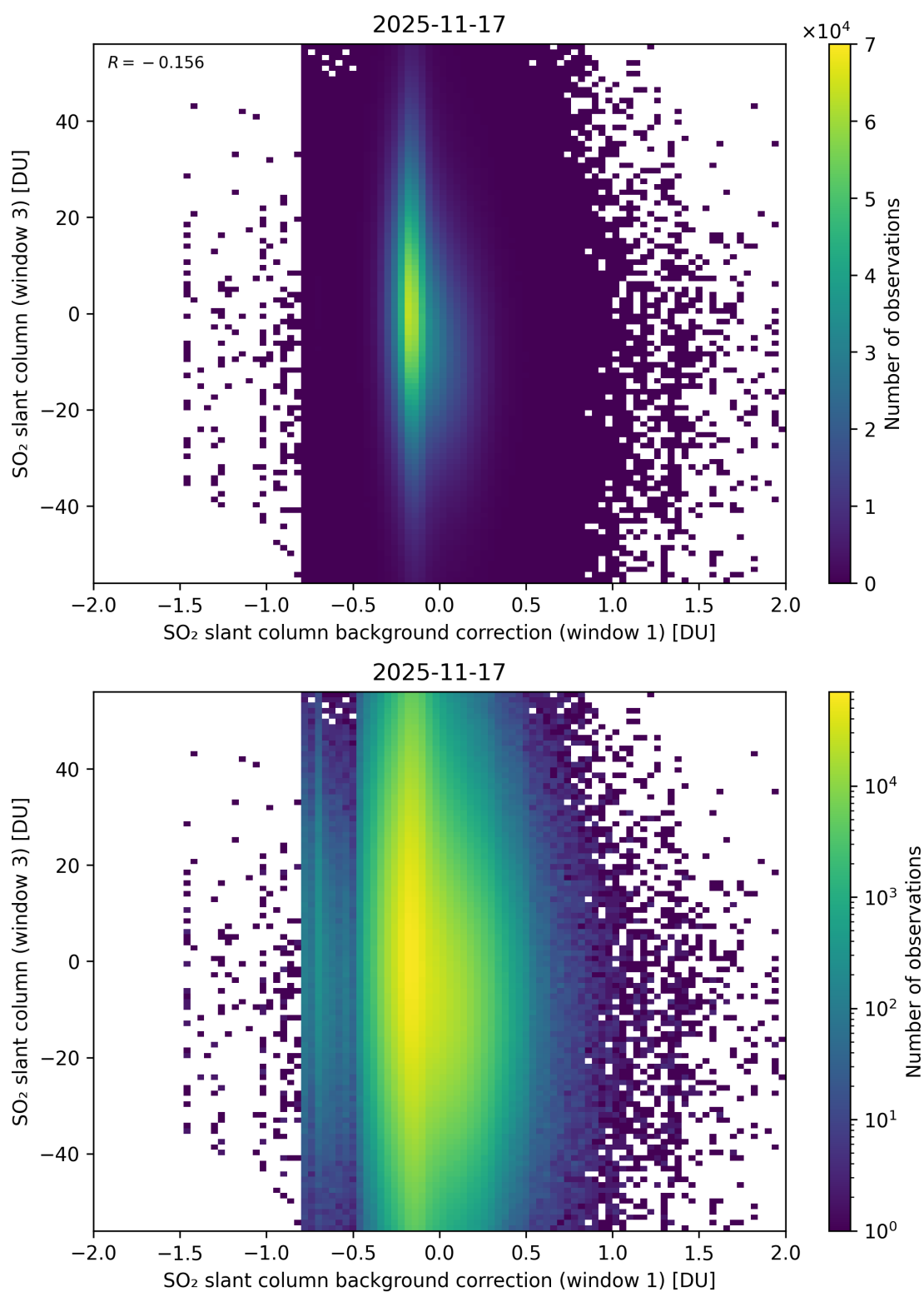
Figure 118: Scatter density plot of “SO 2 slant column background correction (window 1)” against “SO 2 slant column (window 3)” for 2025-11-16 to 2025-11-18.
