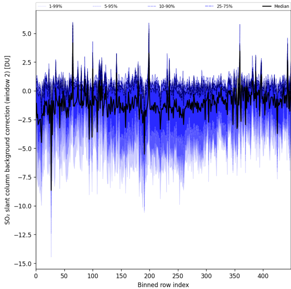
Figure 96: Along track statistics of “SO 2 slant column background correction (window 2)” for 2025-11-16 to 2025-11-18
