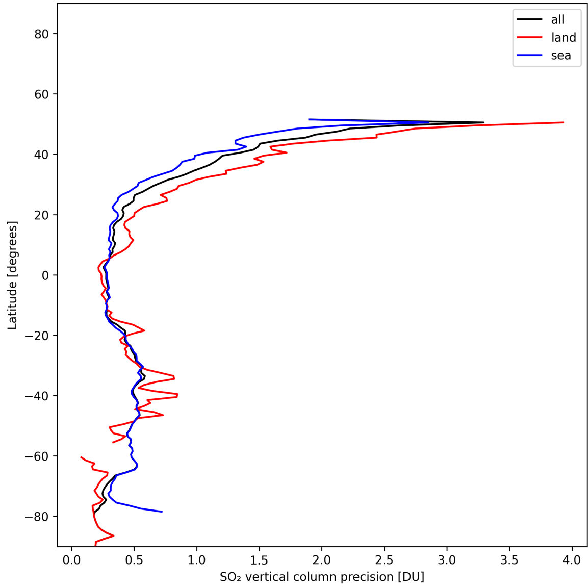
Figure 33: Zonal average of “SO 2 vertical column precision” for 2025-11-16 to 2025-11-18.
