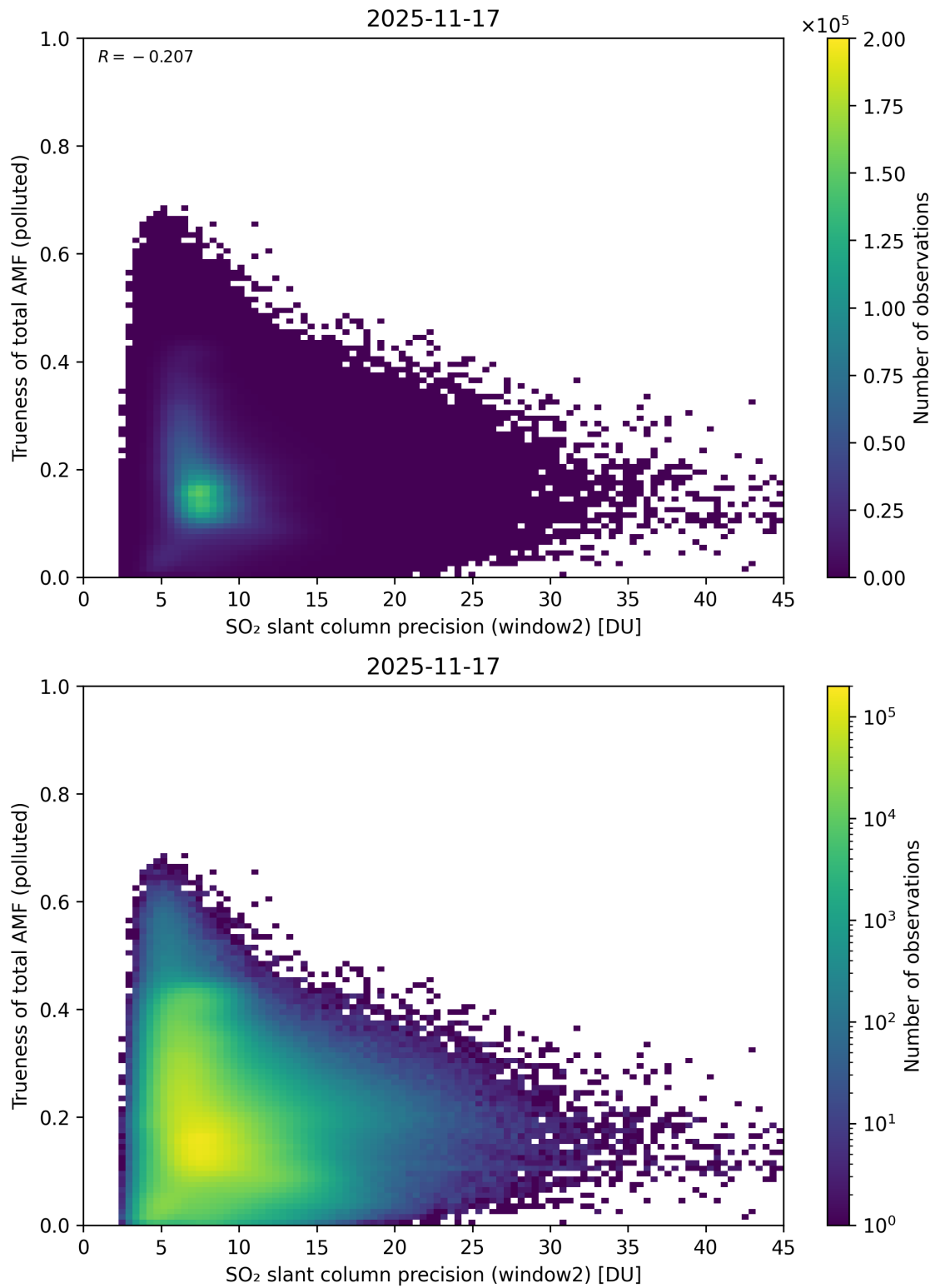
Figure 302: Scatter density plot of “SO 2 slant column precision (window2)” against “Trueness of total AMF (polluted)” for 2025-11-16 to 2025-11-18.
