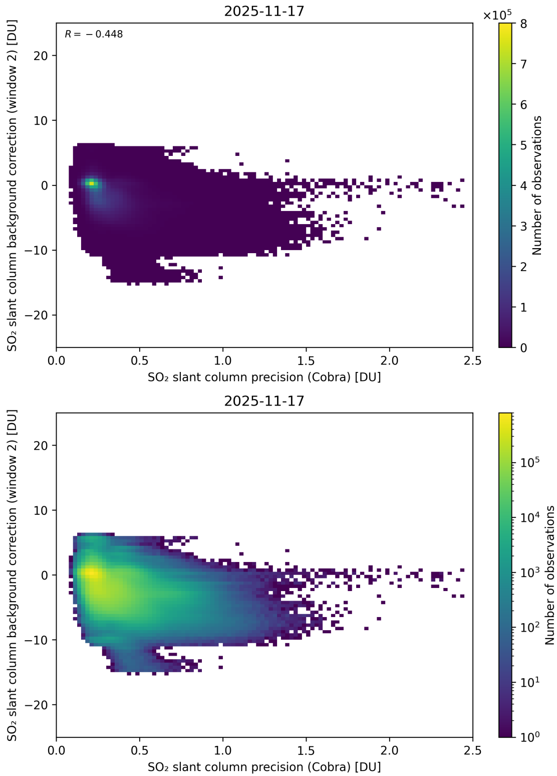
Figure 200: Scatter density plot of “SO 2 slant column precision (Cobra)” against “SO 2 slant column background correction (window 2)” for 2025-11-16 to 2025-11-18.
