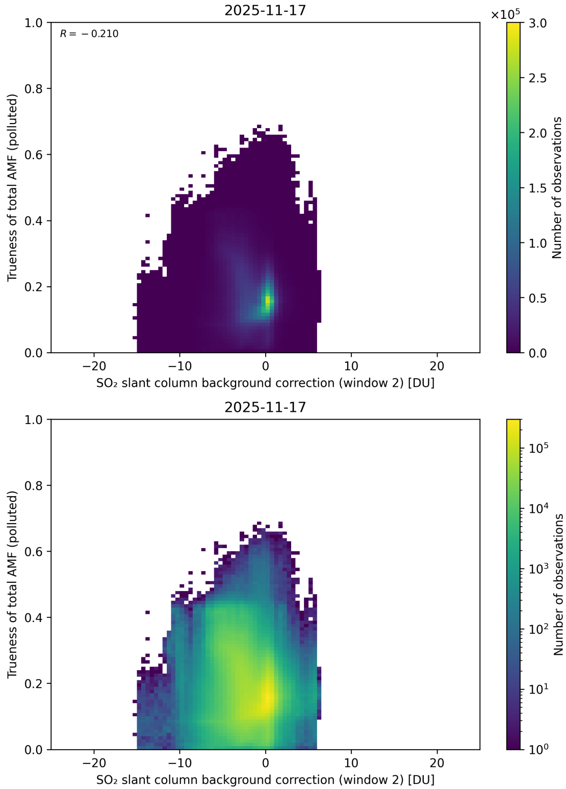
Figure 131: Scatter density plot of “SO 2 slant column background correction (window 2)” against “Trueness of total AMF (polluted)” for 2025-11-16 to 2025-11-18.
