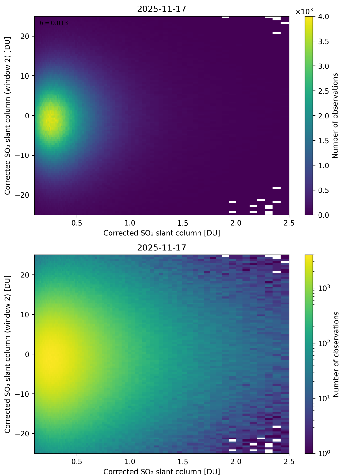
Figure 235: Scatter density plot of “Corrected SO 2 slant column” against “Corrected SO 2 slant column (window 2)” for 2025-11-16 to 2025-11-18.
