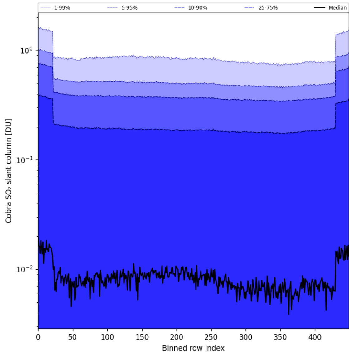
Figure 87: Along track statistics of “Cobra SO 2 slant column” for 2025-11-16 to 2025-11-18
