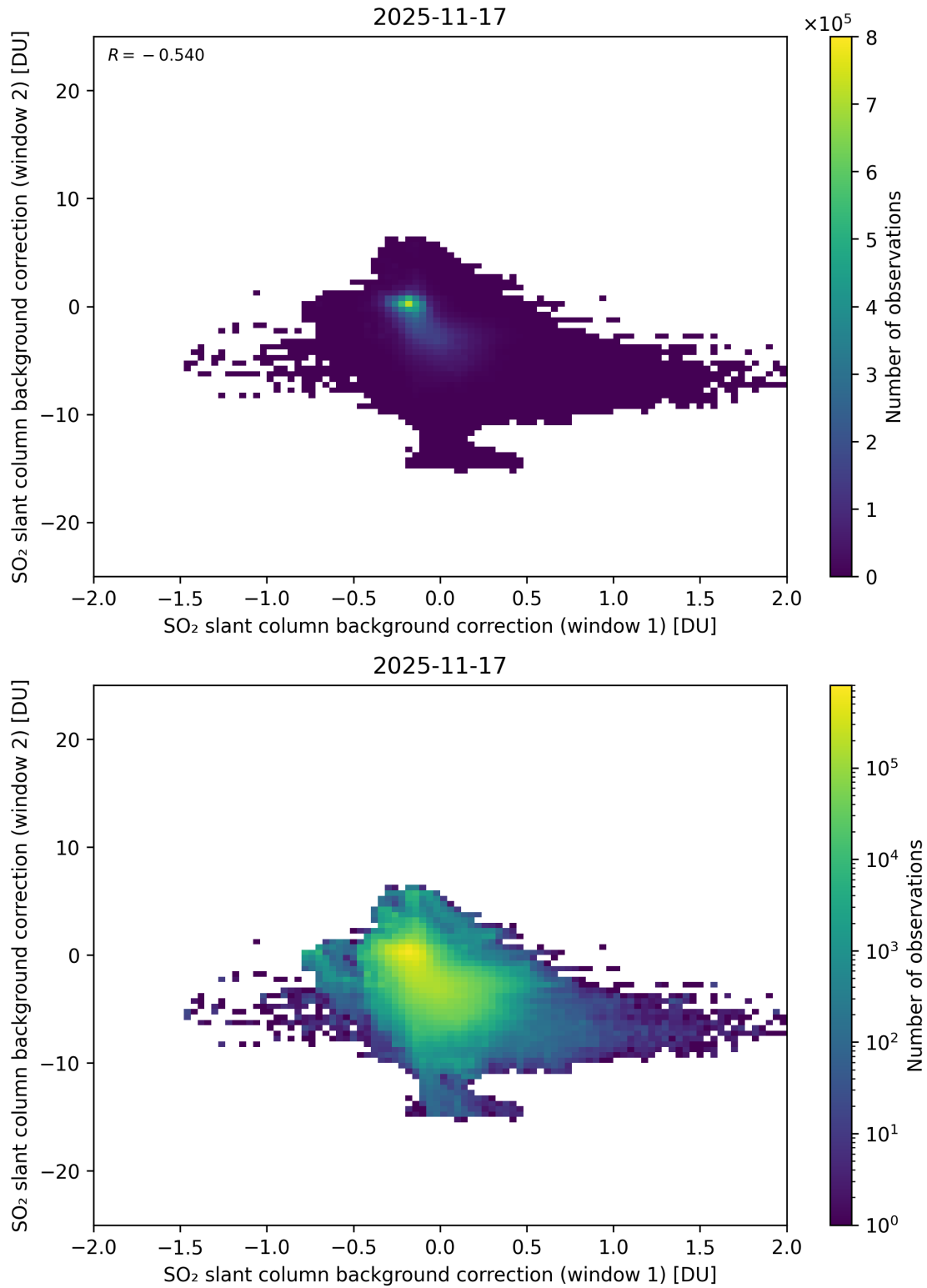
Figure 109: Scatter density plot of “SO 2 slant column background correction (window 1)” against “SO 2 slant column background correction (window 2)” for 2025-11-16 to 2025-11-18.
