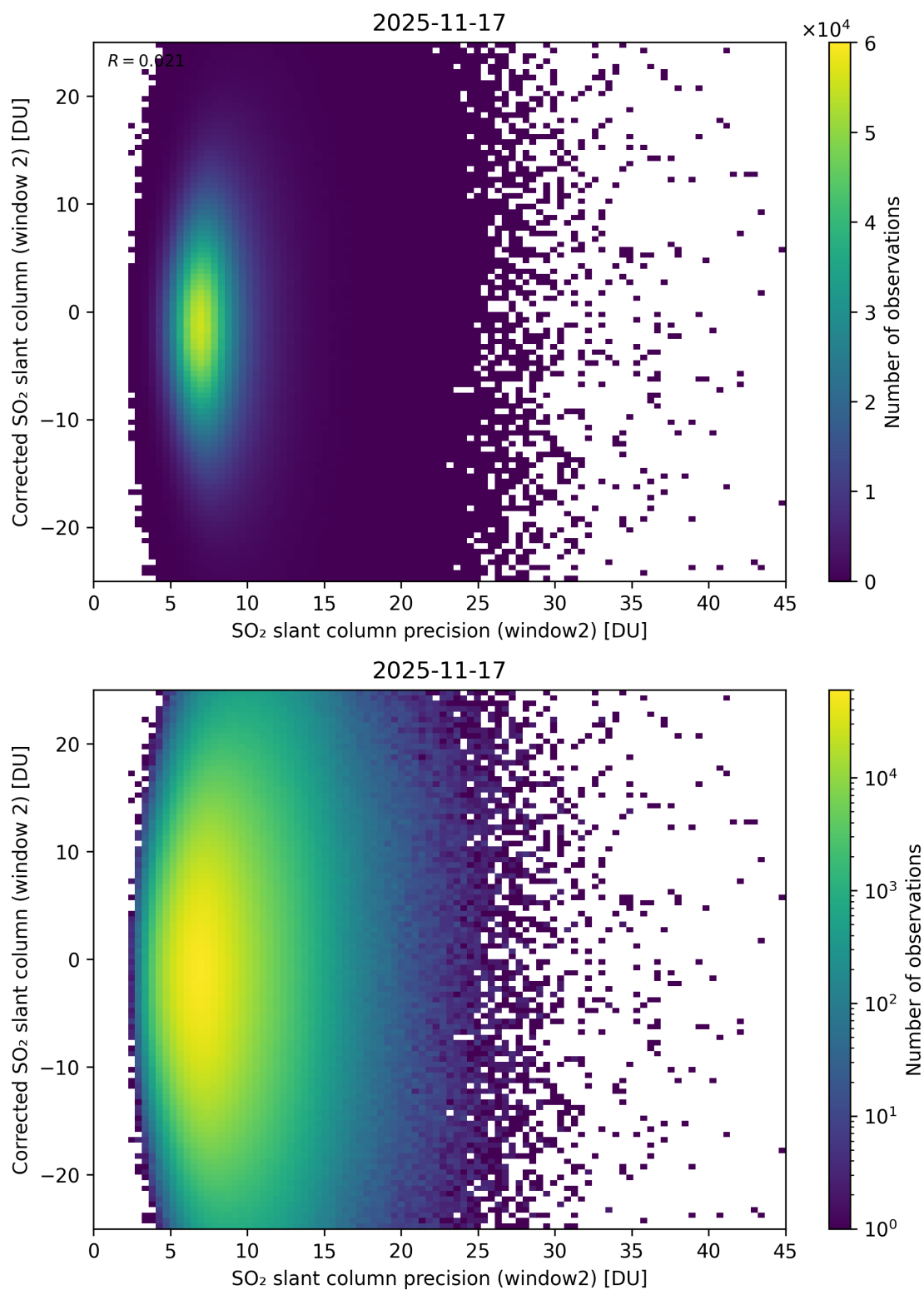
Figure 297: Scatter density plot of “SO 2 slant column precision (window2)” against “Corrected SO 2 slant column (window 2)” for 2025-11-16 to 2025-11-18.
