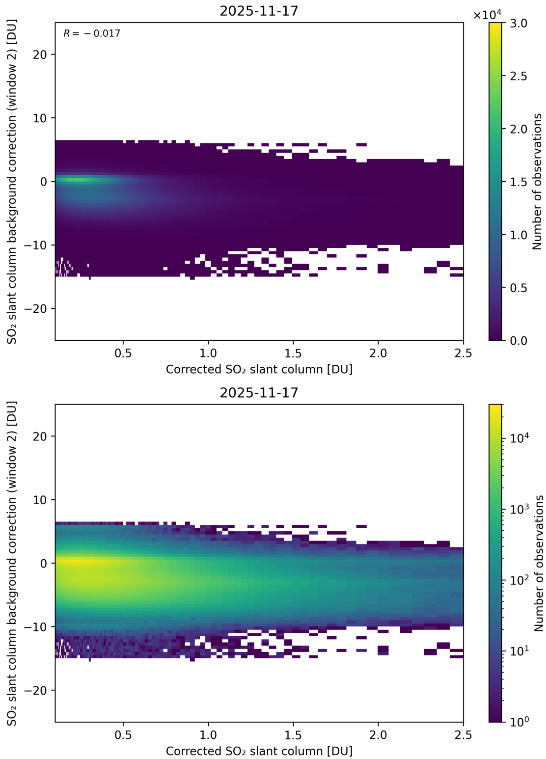
Figure 227: Scatter density plot of “Corrected SO 2 slant column” against “SO 2 slant column background correction (window 2)” for 2025-11-16 to 2025-11-18.
