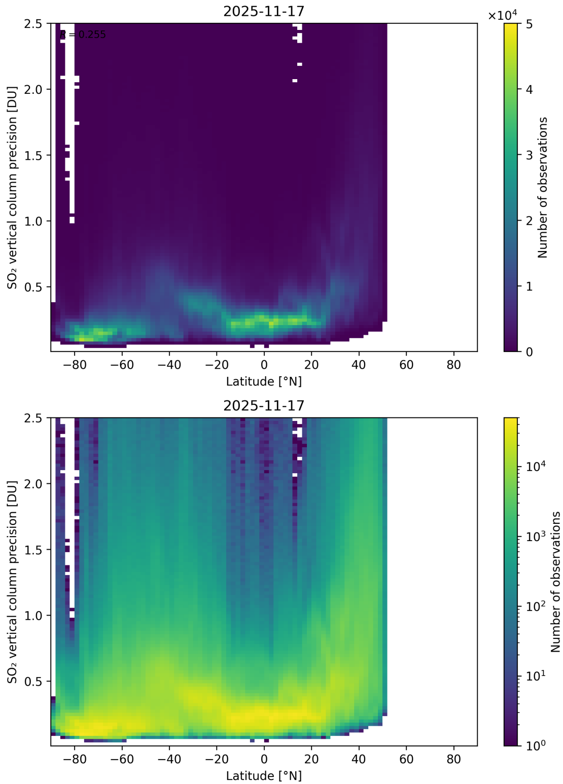
Figure 170: Scatter density plot of “Latitude” against “SO 2 vertical column precision” for 2025-11-16 to 2025-11-18.
