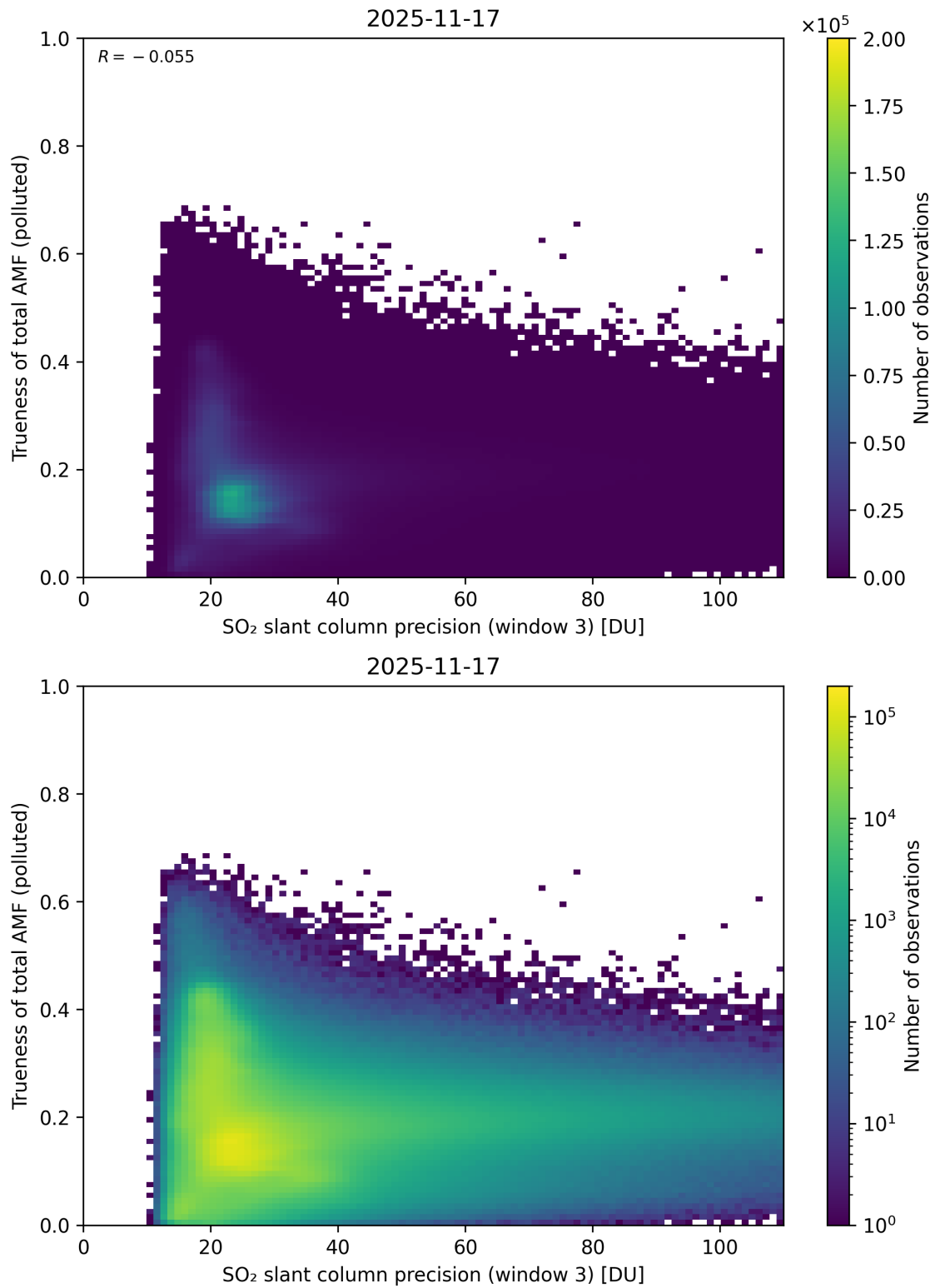
Figure 314: Scatter density plot of “SO 2 slant column precision (window 3)” against “Trueness of total AMF (polluted)” for 2025-11-16 to 2025-11-18.
