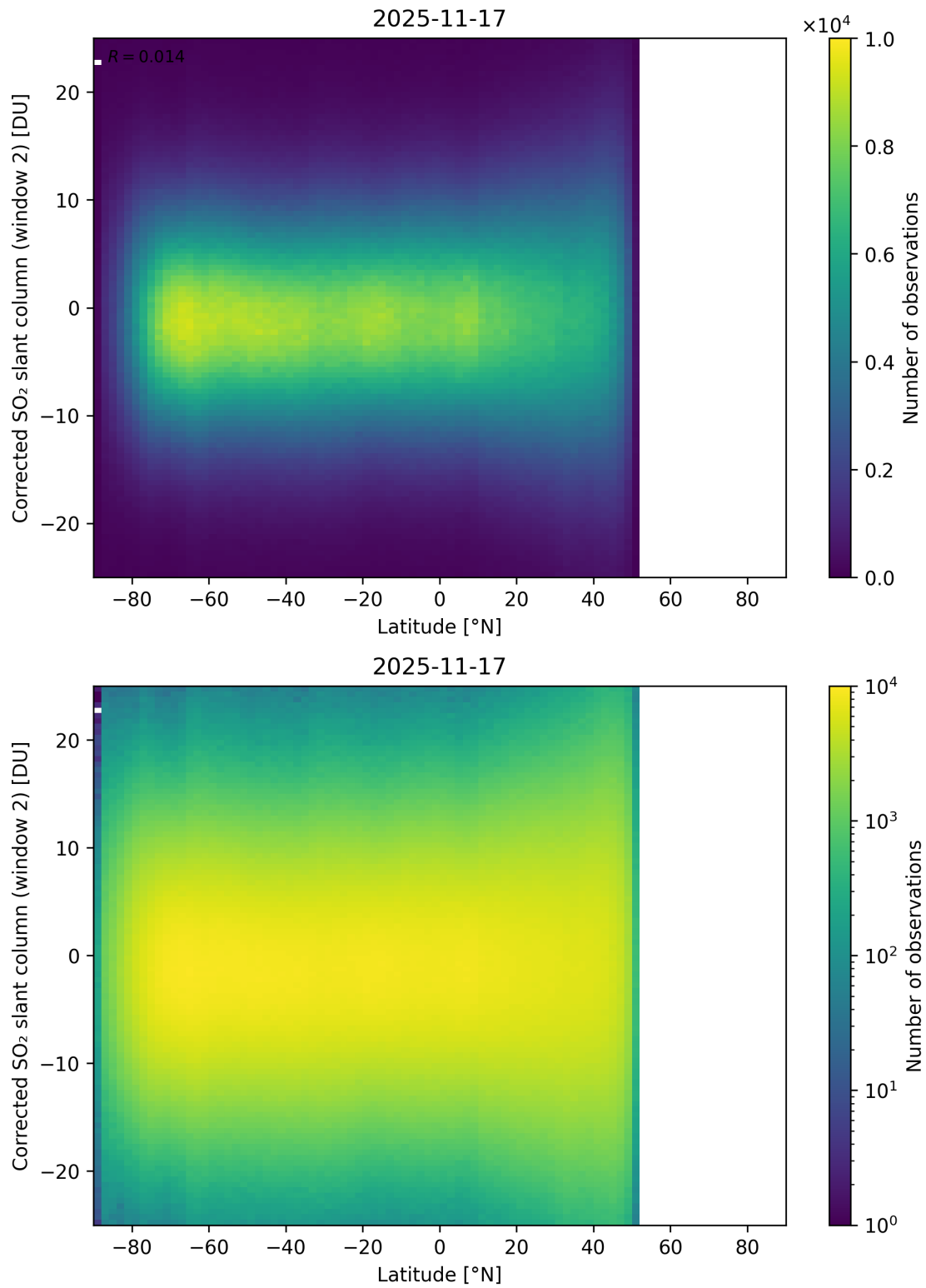
Figure 160: Scatter density plot of “Latitude” against “Corrected SO 2 slant column (window 2)” for 2025-11-16 to 2025-11-18.
