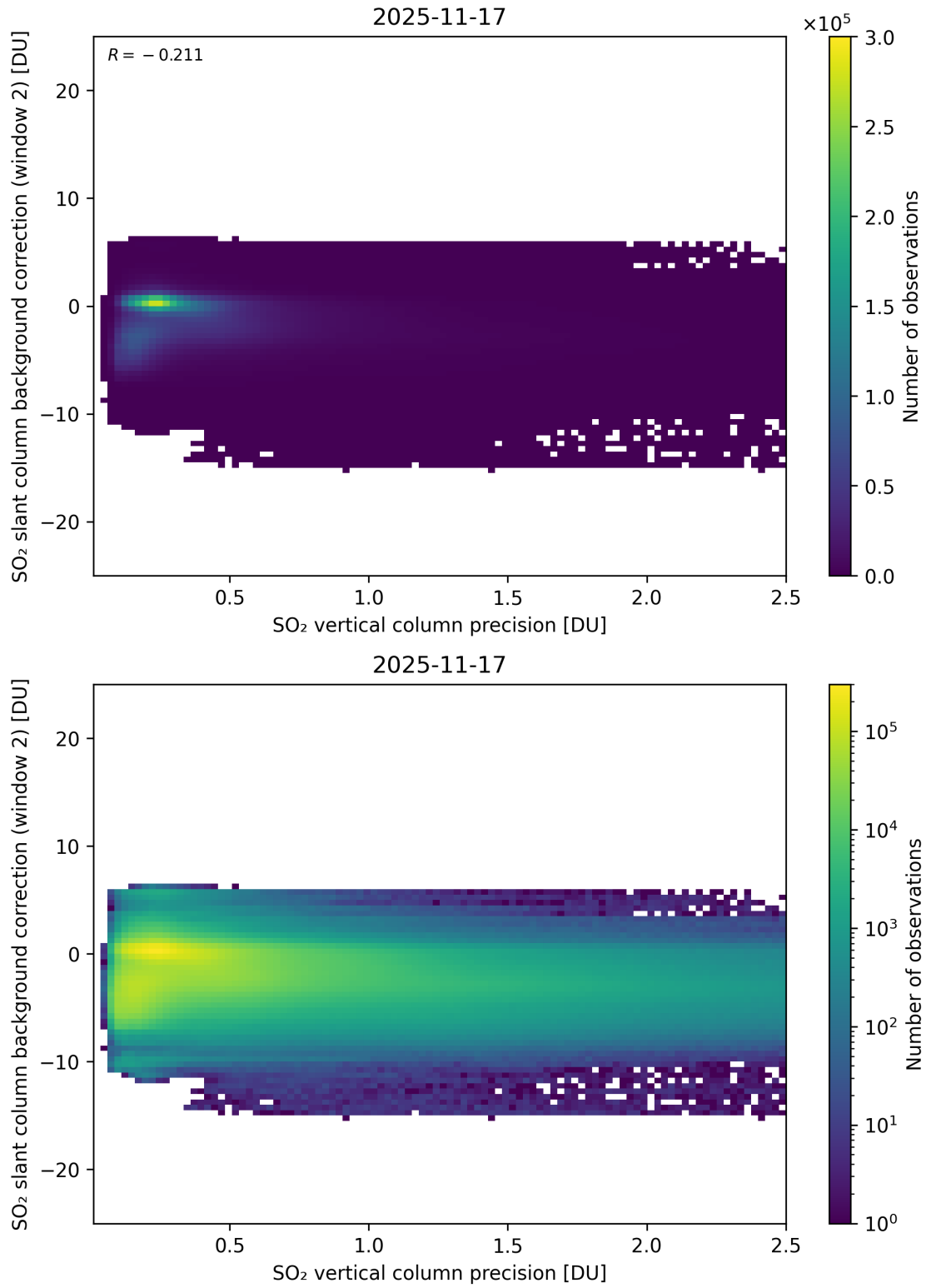
Figure 330: Scatter density plot of “SO 2 vertical column precision” against “SO 2 slant column background correction (window 2)” for 2025-11-16 to 2025-11-18.
