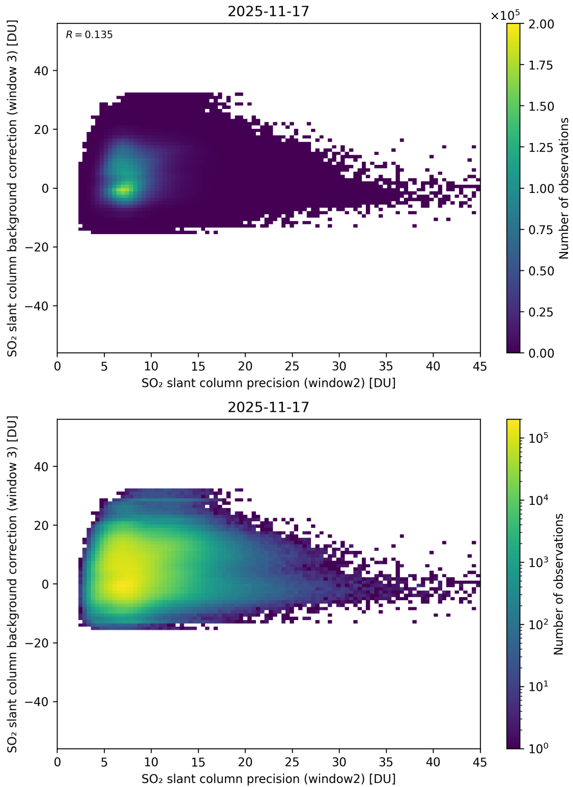
Figure 292: Scatter density plot of “SO 2 slant column precision (window2)” against “SO 2 slant column background correction (window 3)” for 2025-11-16 to 2025-11-18.
