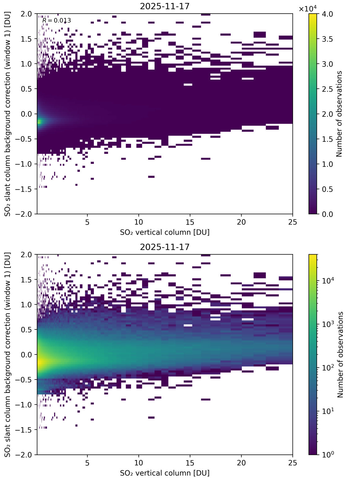
Figure 323: Scatter density plot of “SO 2 vertical column” against “SO 2 slant column background correction (window 1)” for 2025-11-16 to 2025-11-18.
