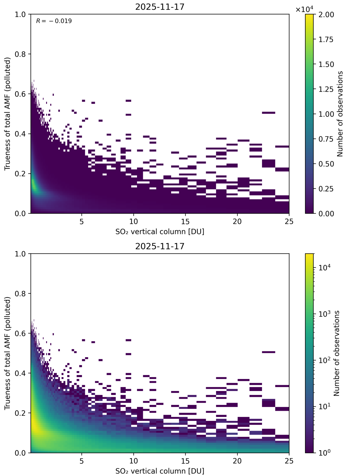
Figure 360: Scatter density plot of “SO 2 vertical column” against “Trueness of total AMF (polluted)” for 2025-11-16 to 2025-11-18.
