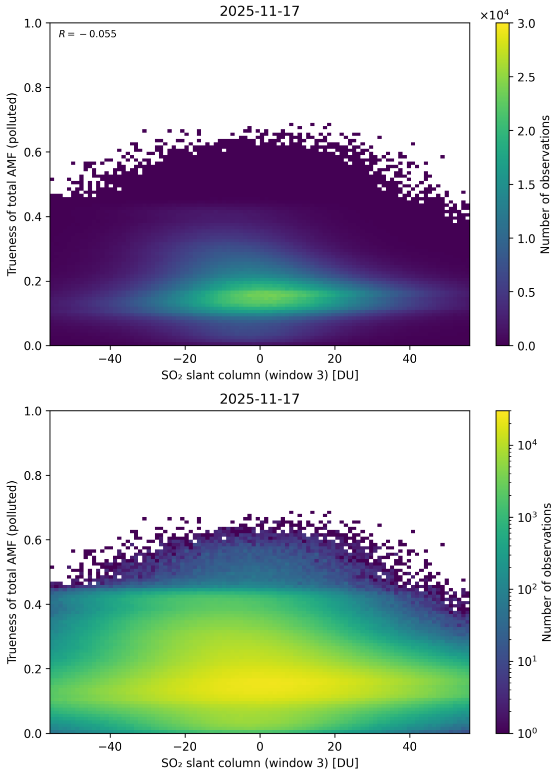
Figure 319: Scatter density plot of “SO 2 slant column (window 3)” against “Trueness of total AMF (polluted)” for 2025-11-16 to 2025-11-18.
