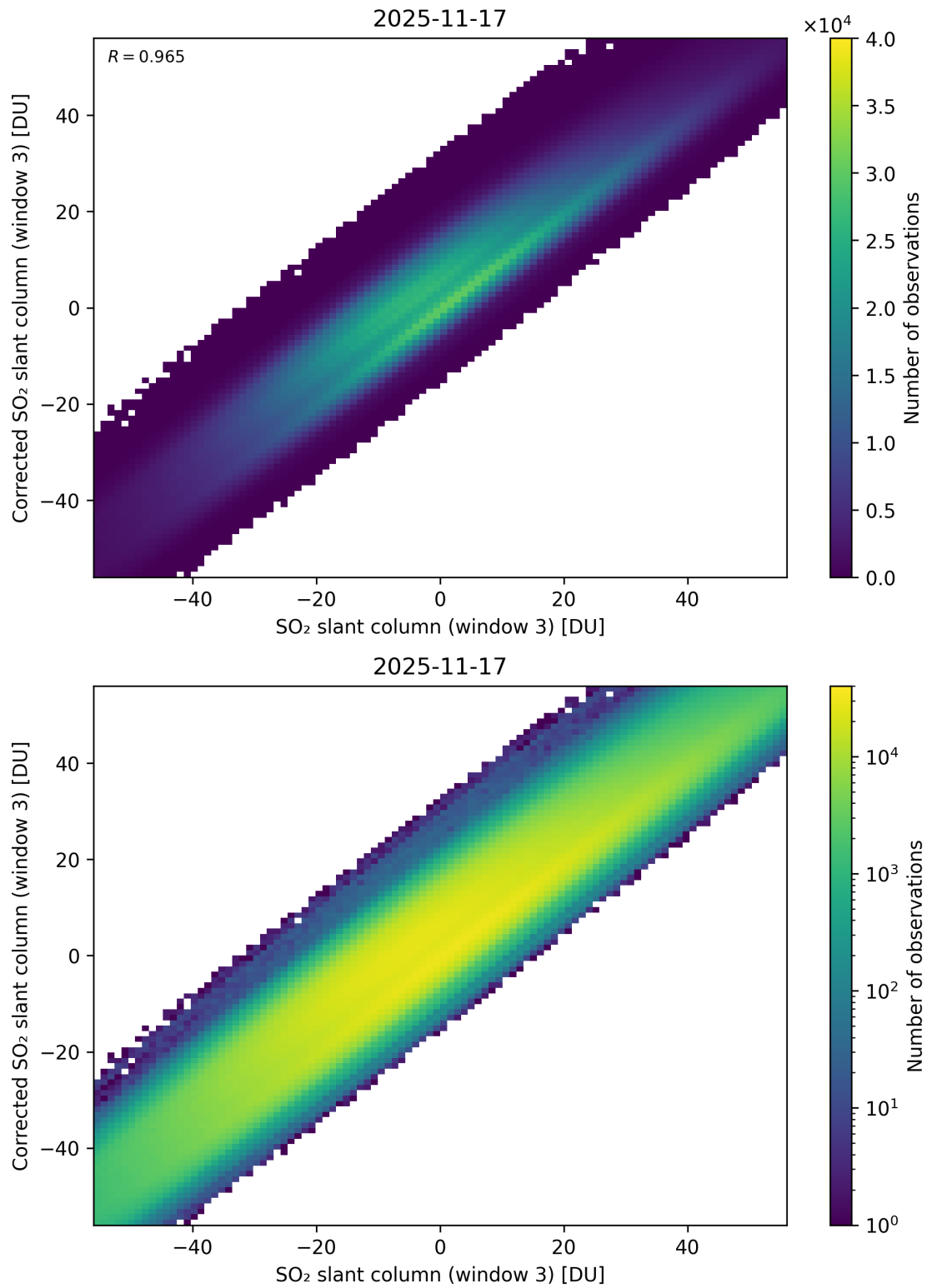
Figure 316: Scatter density plot of “SO 2 slant column (window 3)” against “Corrected SO 2 slant column (window 3)” for 2025-11-16 to 2025-11-18.
