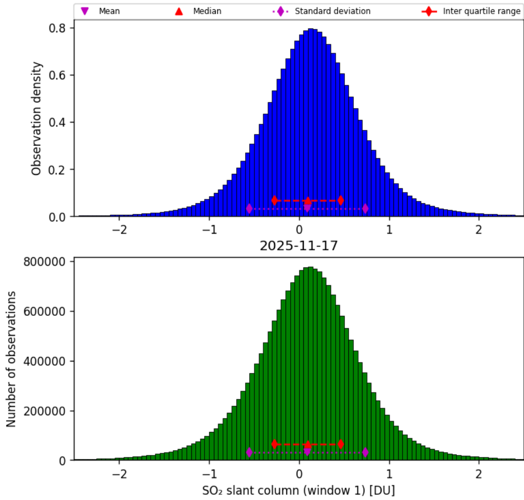
Figure 63: Histogram of “SO 2 slant column (window 1)” for 2025-11-16 to 2025-11-18
