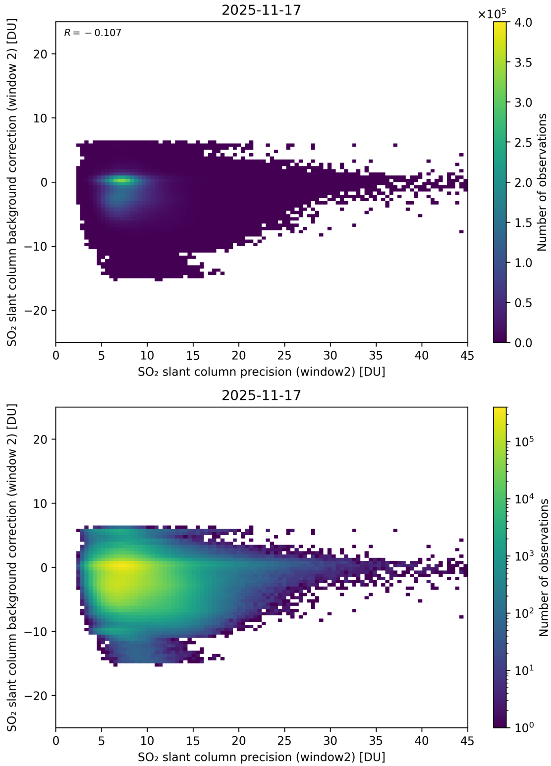
Figure 291: Scatter density plot of “SO 2 slant column precision (window2)” against “SO 2 slant column background correction (window 2)” for 2025-11-16 to 2025-11-18.
