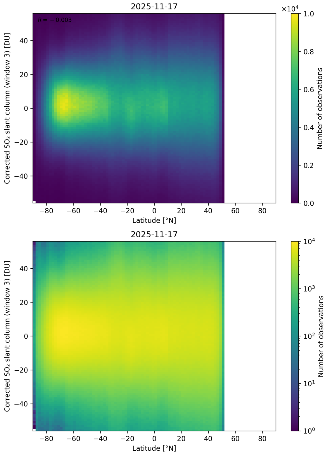
Figure 161: Scatter density plot of “Latitude” against “Corrected SO 2 slant column (window 3)” for 2025-11-16 to 2025-11-18.
