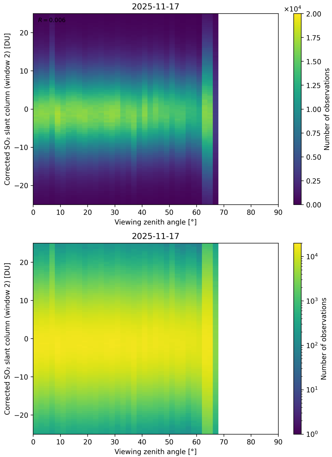
Figure 374: Scatter density plot of “Viewing zenith angle” against “Corrected SO 2 slant column (window 2)” for 2025-11-16 to 2025-11-18.
