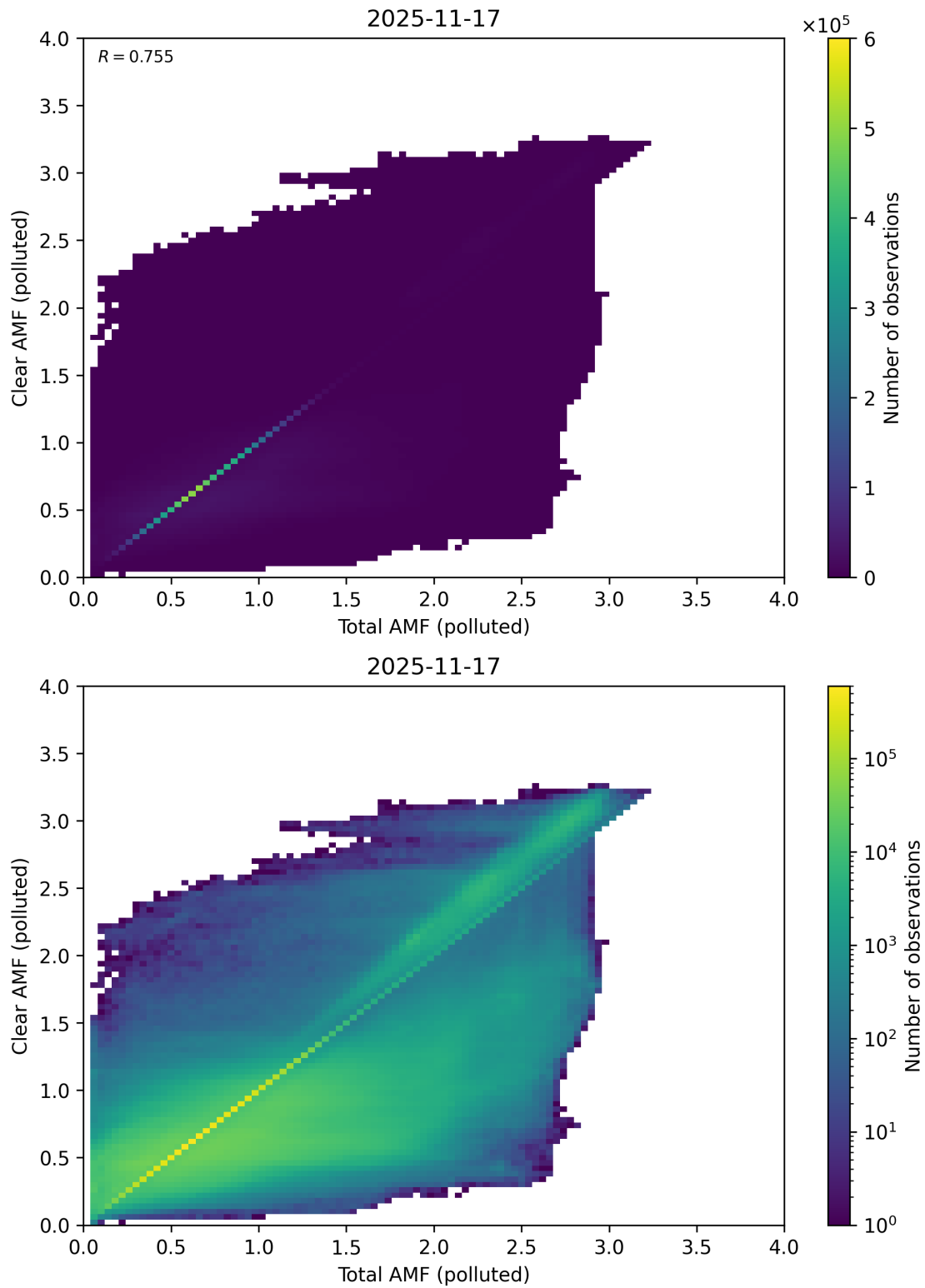
Figure 320: Scatter density plot of “Total AMF (polluted)” against “Clear AMF (polluted)” for 2025-11-16 to 2025-11-18.
