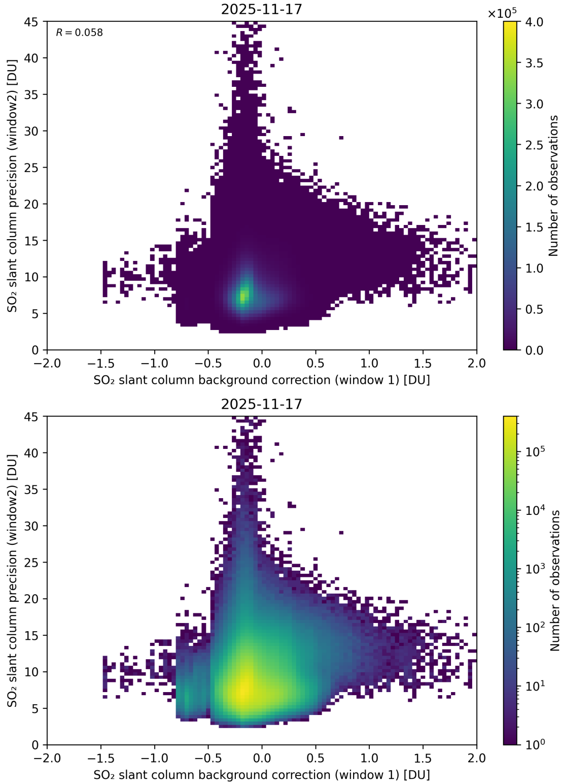
Figure 117: Scatter density plot of “SO 2 slant column background correction (window 1)” against “SO 2 slant column precision (window2)” for 2025-11-16 to 2025-11-18.
