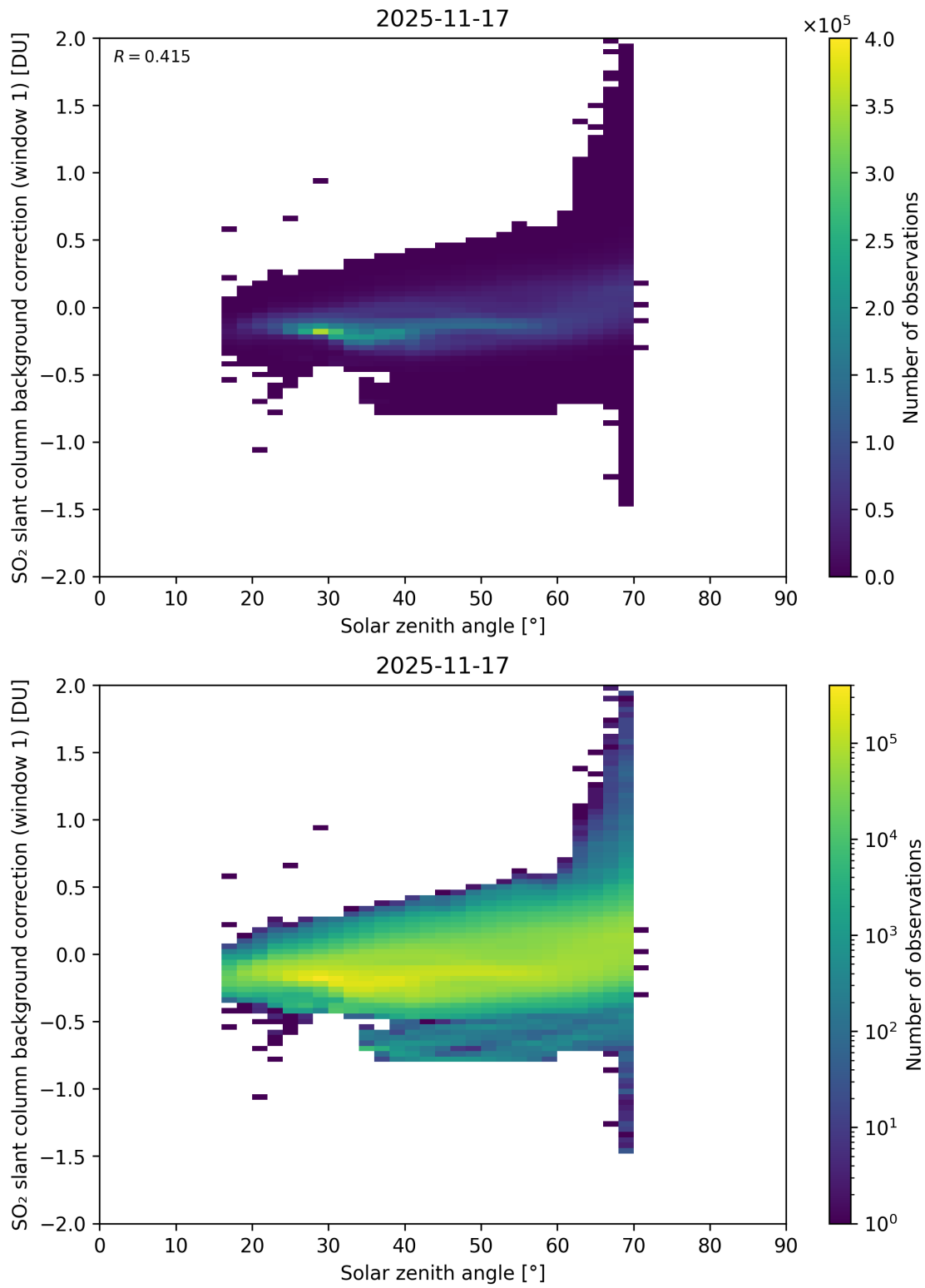
Figure 171: Scatter density plot of “Solar zenith angle” against “SO 2 slant column background correction (window 1)” for 2025-11-16 to 2025-11-18.
