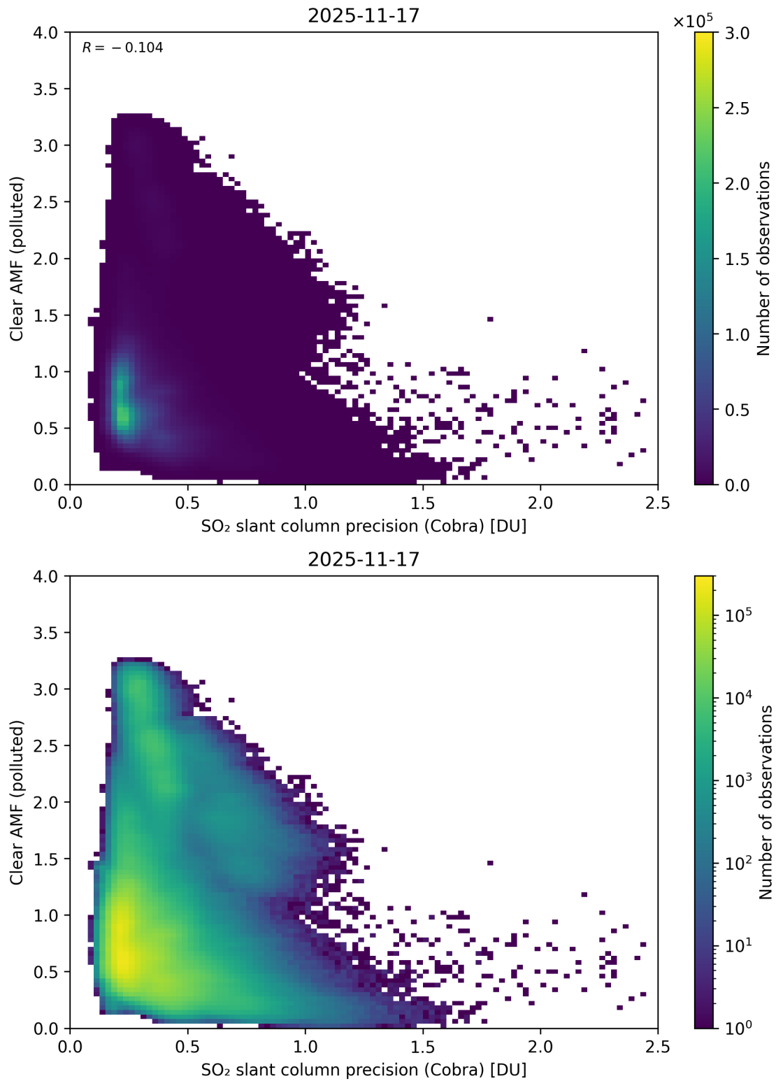
Figure 205: Scatter density plot of “SO 2 slant column precision (Cobra)” against “Clear AMF (polluted)” for 2025-11-16 to 2025-11-18.
