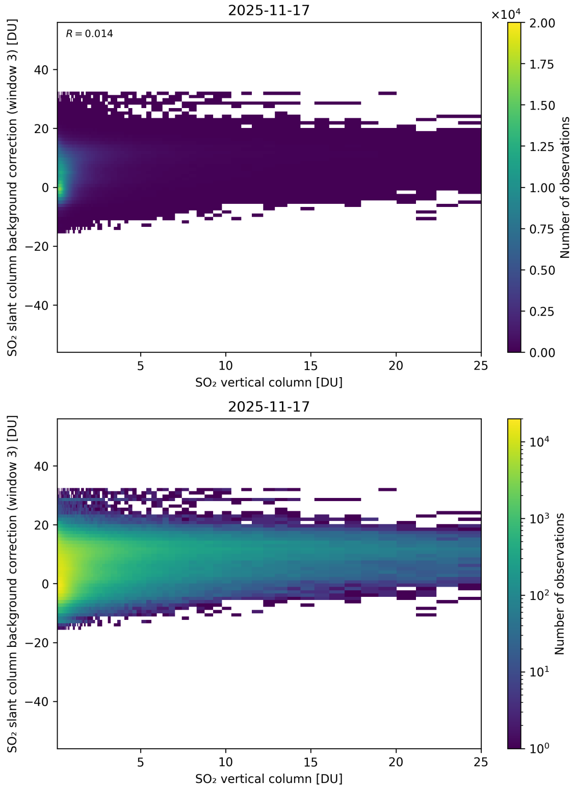
Figure 325: Scatter density plot of “SO 2 vertical column” against “SO 2 slant column background correction (window 3)” for 2025-11-16 to 2025-11-18.
