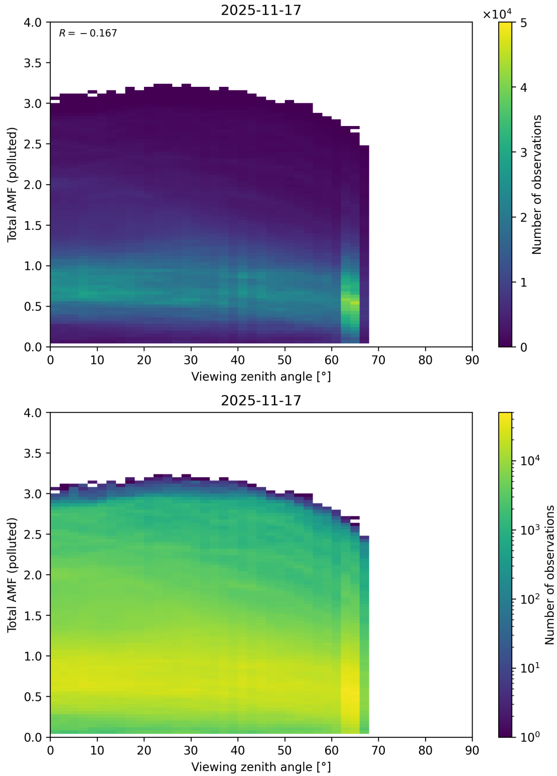
Figure 381: Scatter density plot of “Viewing zenith angle” against “Total AMF (polluted)” for 2025-11-16 to 2025-11-18.
