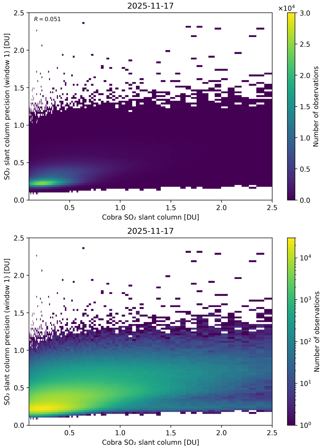
Figure 220: Scatter density plot of “Cobra SO 2 slant column” against “SO 2 slant column precision (window 1)” for 2025-11-16 to 2025-11-18.
