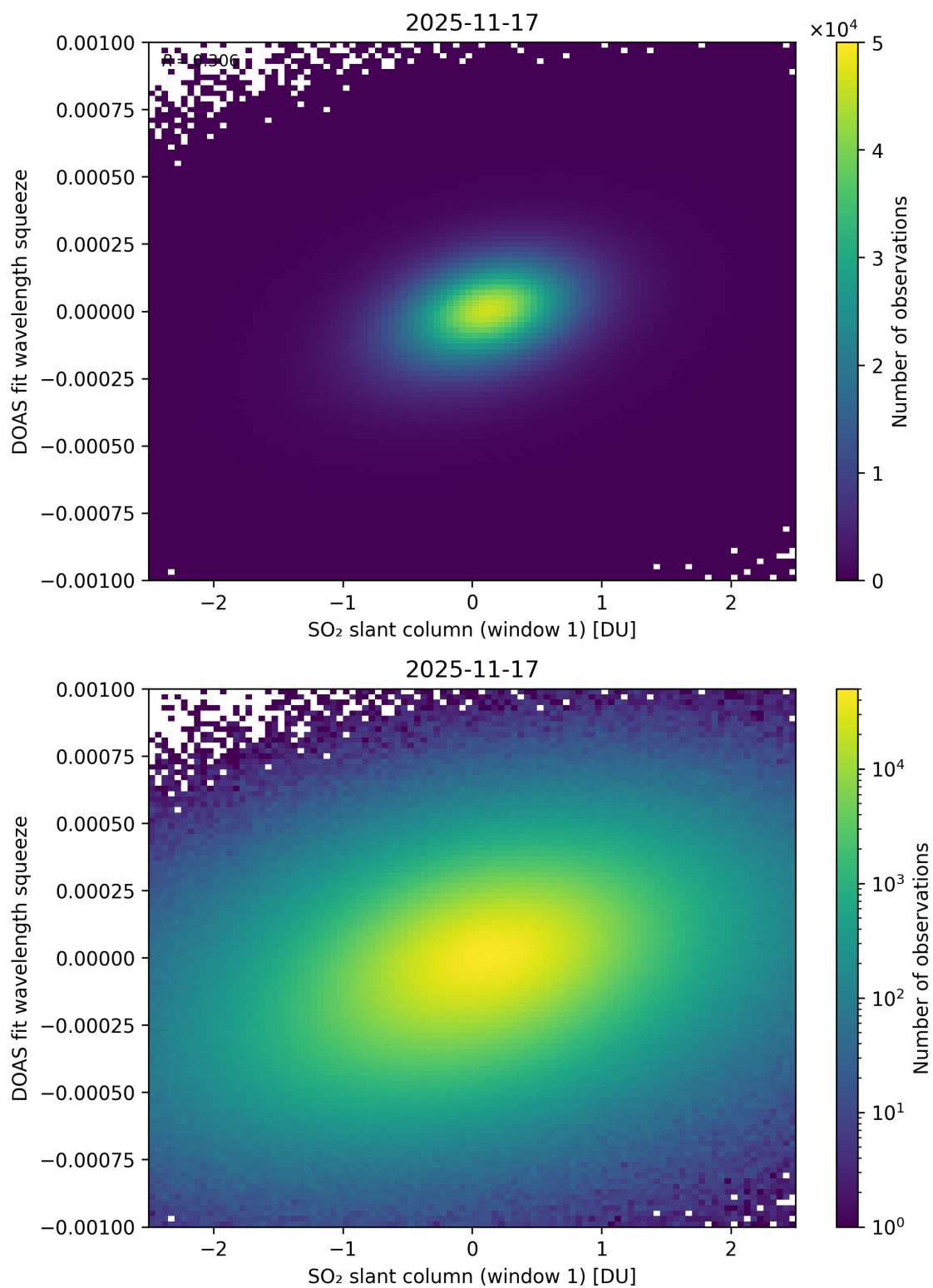
Figure 266: Scatter density plot of “SO 2 slant column (window 1)” against “DOAS fit wavelength squeeze” for 2025-11-16 to 2025-11-18.
