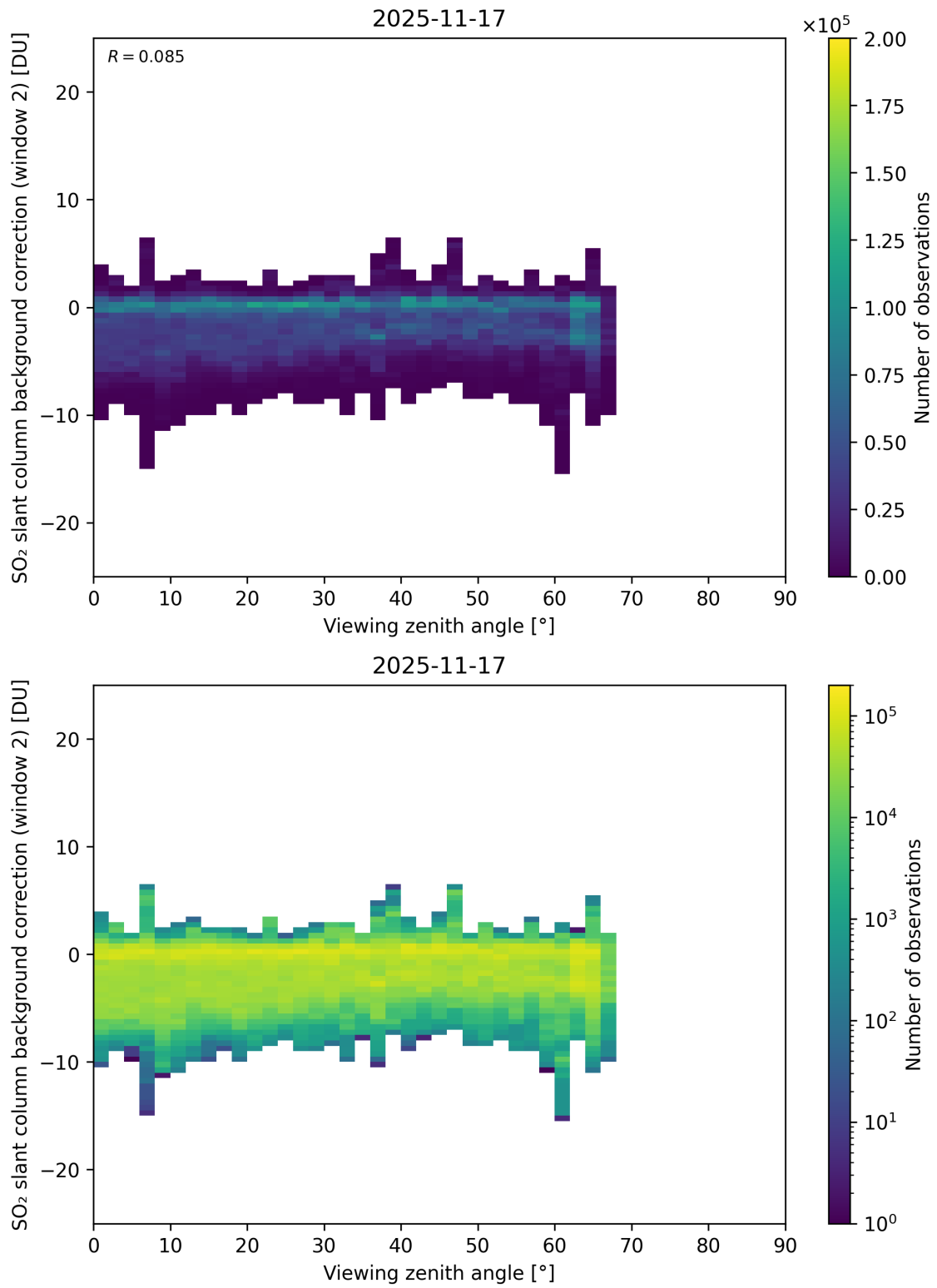
Figure 363: Scatter density plot of “Viewing zenith angle” against “SO 2 slant column background correction (window 2)” for 2025-11-16 to 2025-11-18.
