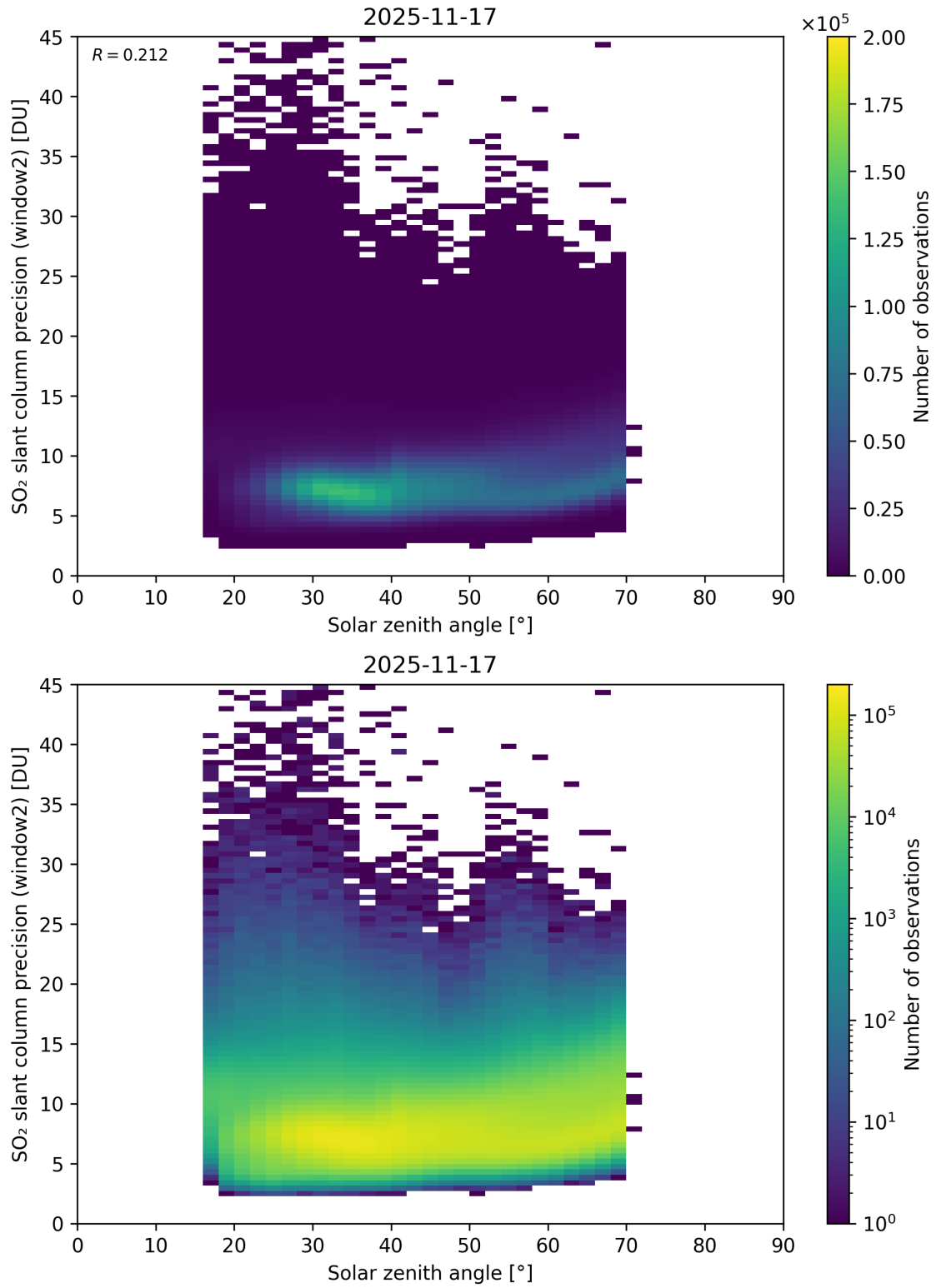
Figure 186: Scatter density plot of “Solar zenith angle” against “SO 2 slant column precision (window2)” for 2025-11-16 to 2025-11-18.
