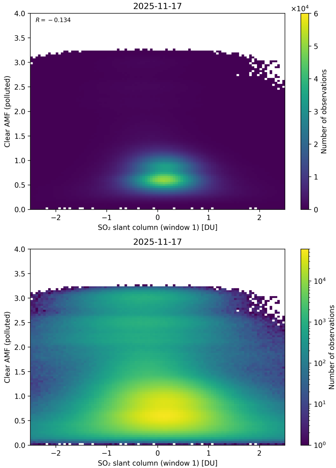
Figure 282: Scatter density plot of “SO 2 slant column (window 1)” against “Clear AMF (polluted)” for 2025-11-16 to 2025-11-18.
