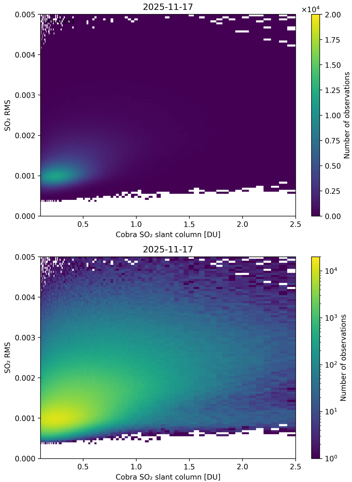
Figure 198: Scatter density plot of “Cobra SO 2 slant column” against “SO 2 RMS” for 2025-11-16 to 2025-11-18.
