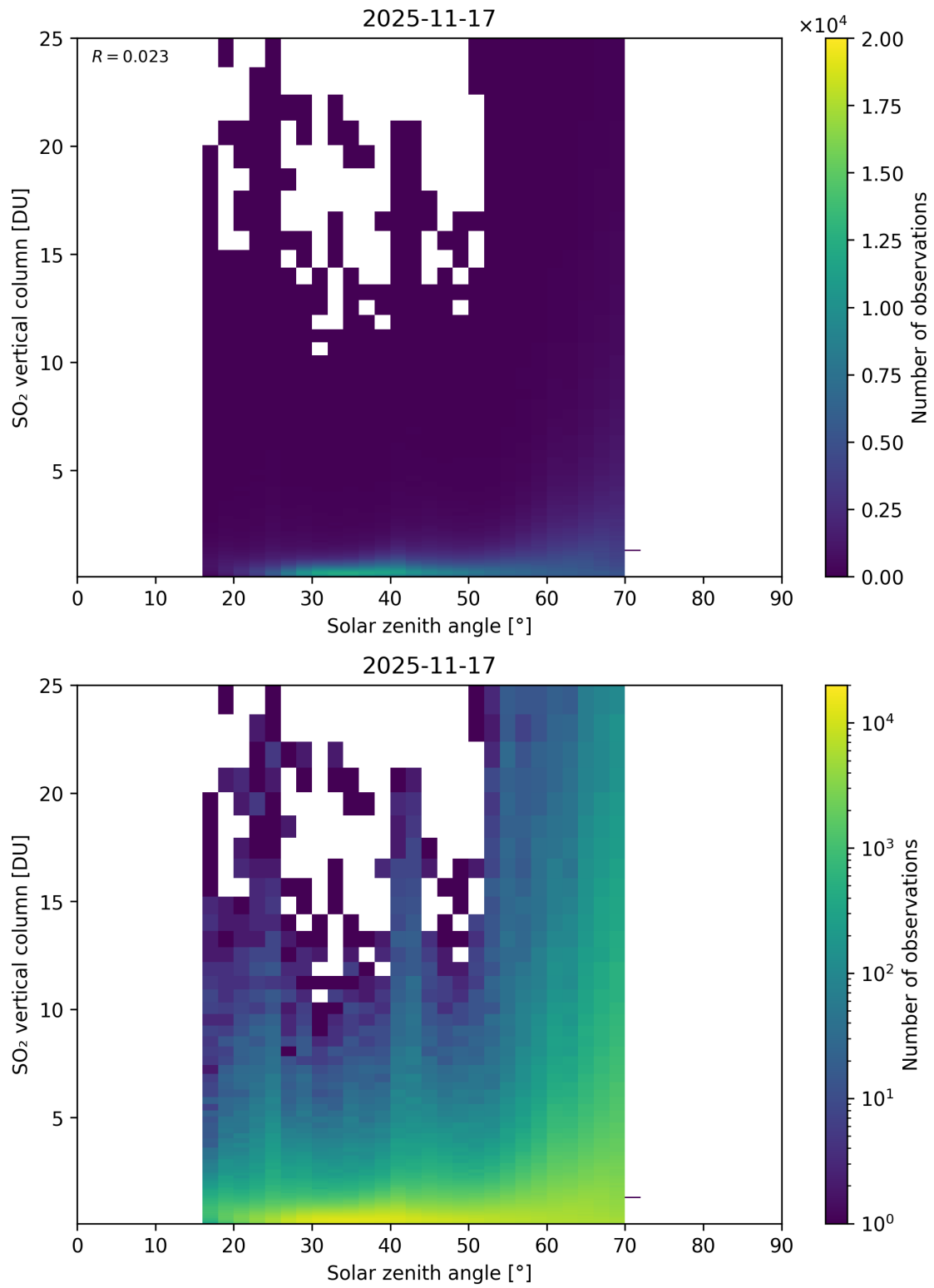
Figure 191: Scatter density plot of “Solar zenith angle” against “SO 2 vertical column” for 2025-11-16 to 2025-11-18.
