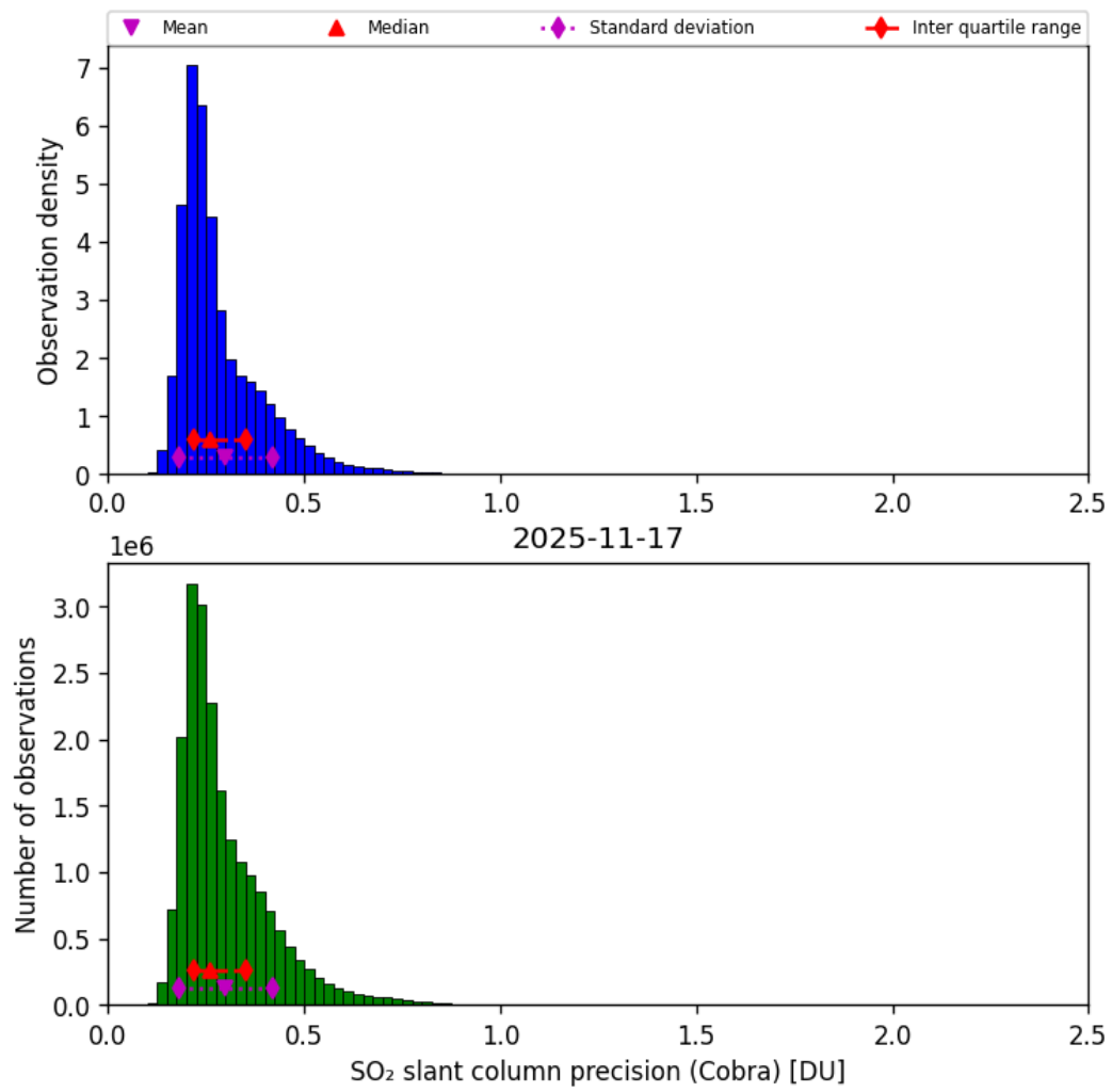
Figure 62: Histogram of “SO 2 slant column precision (Cobra)” for 2025-11-16 to 2025-11-18
