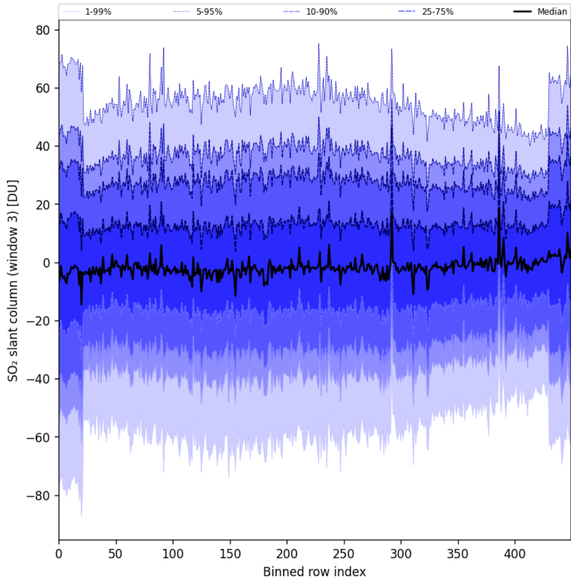
Figure 97: Along track statistics of “SO 2 slant column (window 3)” for 2025-11-16 to 2025-11-18
