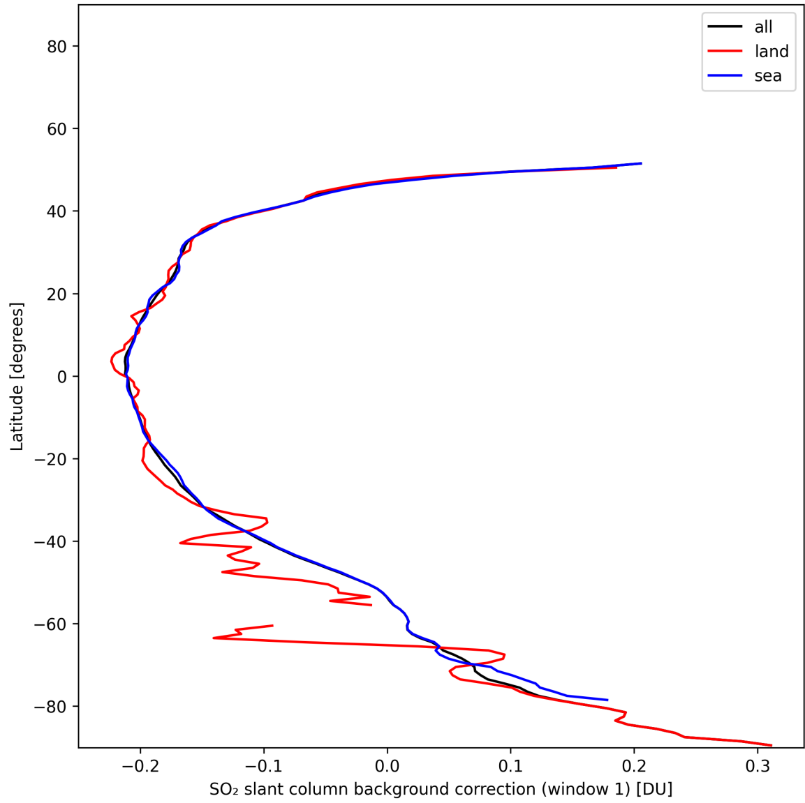
Figure 40: Zonal average of “SO 2 slant column background correction (window 1)” for 2025-11-16 to 2025-11-18.
