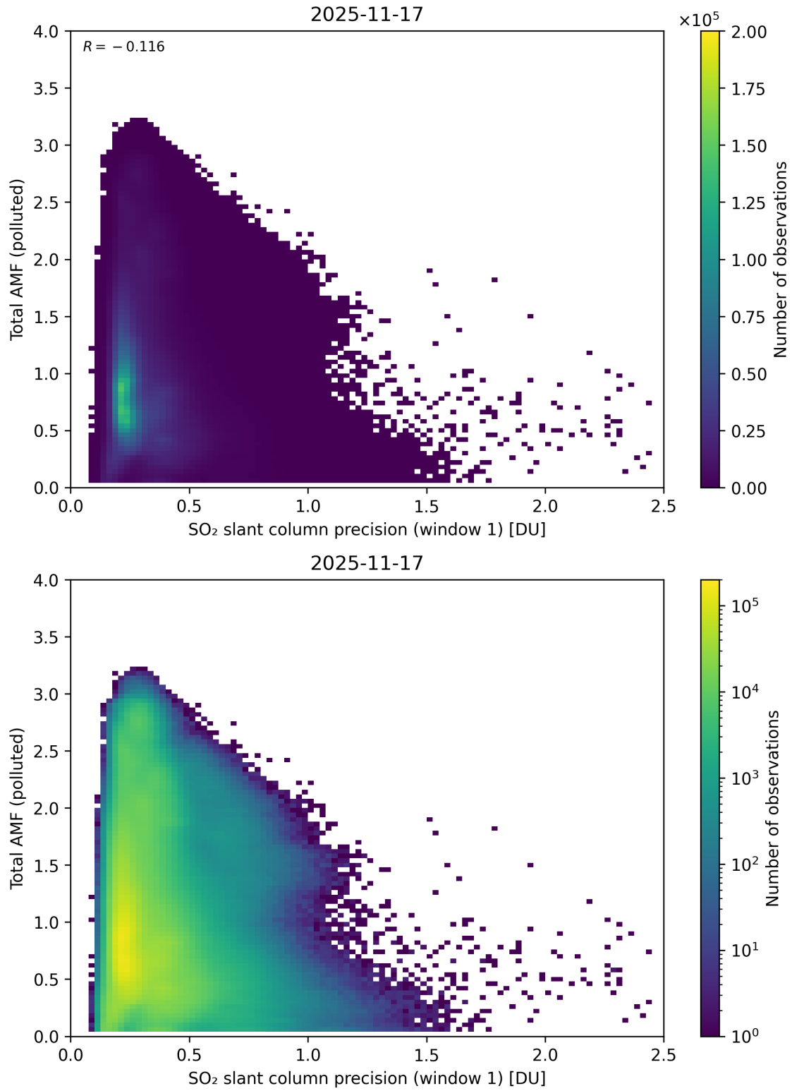
Figure 280: Scatter density plot of “SO 2 slant column precision (window 1)” against “Total AMF (polluted)” for 2025-11-16 to 2025-11-18.
