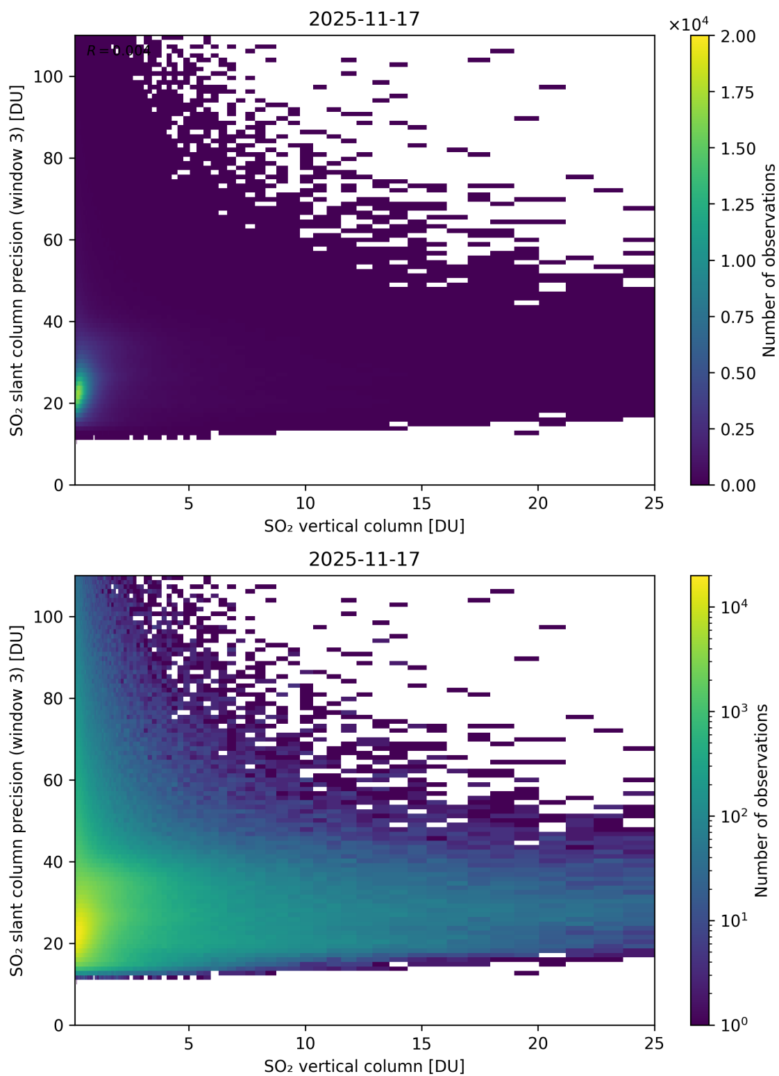
Figure 358: Scatter density plot of “SO 2 vertical column” against “SO 2 slant column precision (window 3)” for 2025-11-16 to 2025-11-18.
