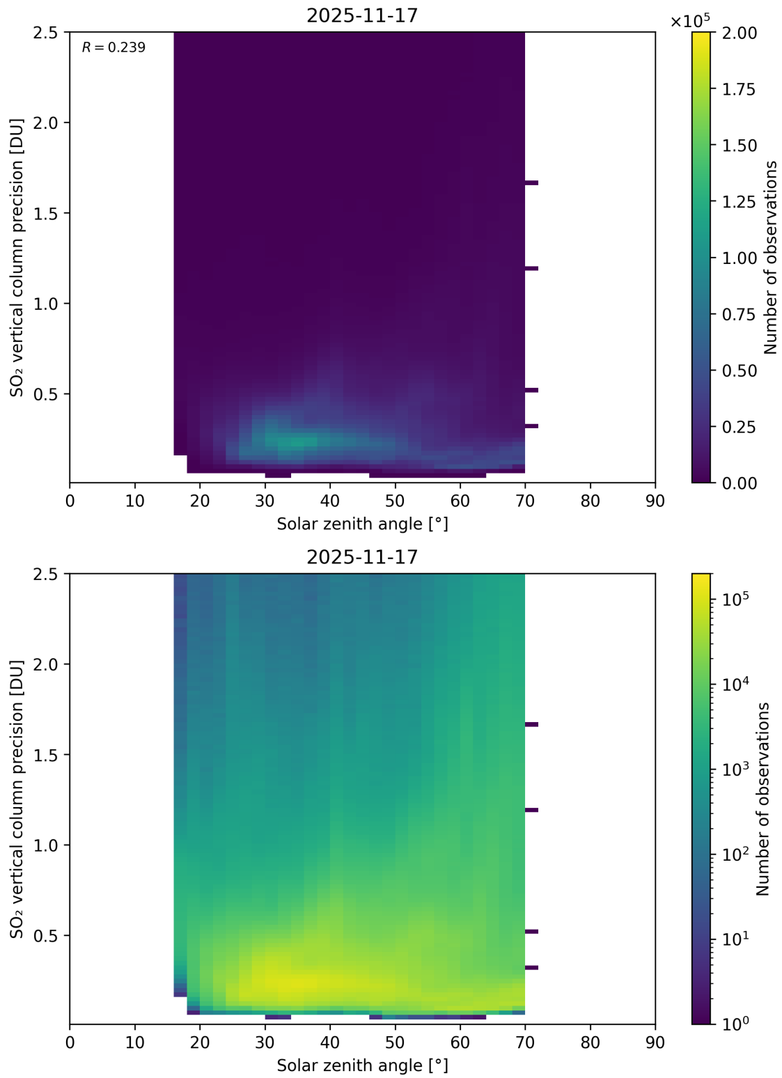
Figure 192: Scatter density plot of “Solar zenith angle” against “SO 2 vertical column precision” for 2025-11-16 to 2025-11-18.
