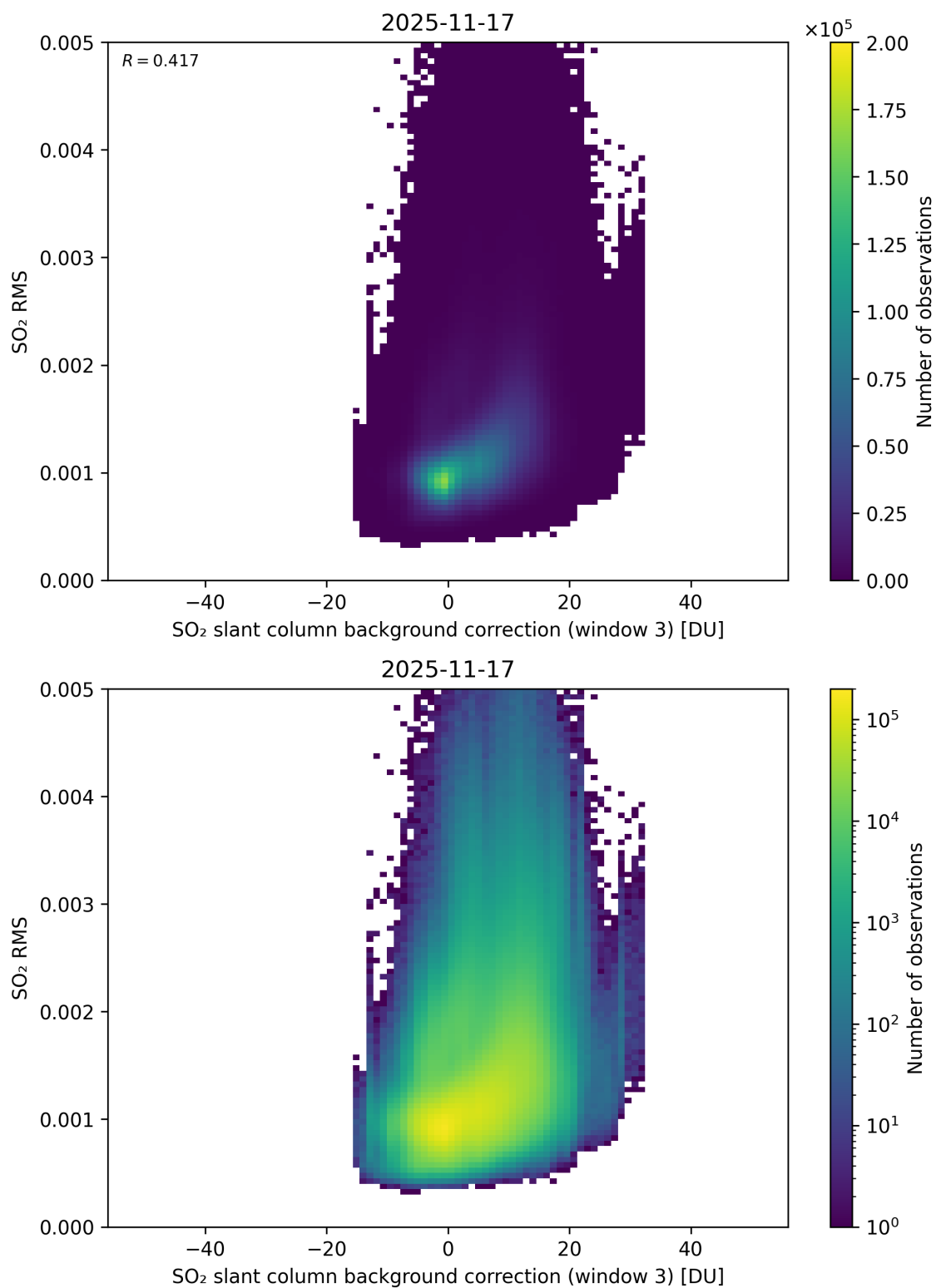
Figure 134: Scatter density plot of “SO 2 slant column background correction (window 3)” against “SO 2 RMS” for 2025-11-16 to 2025-11-18.
