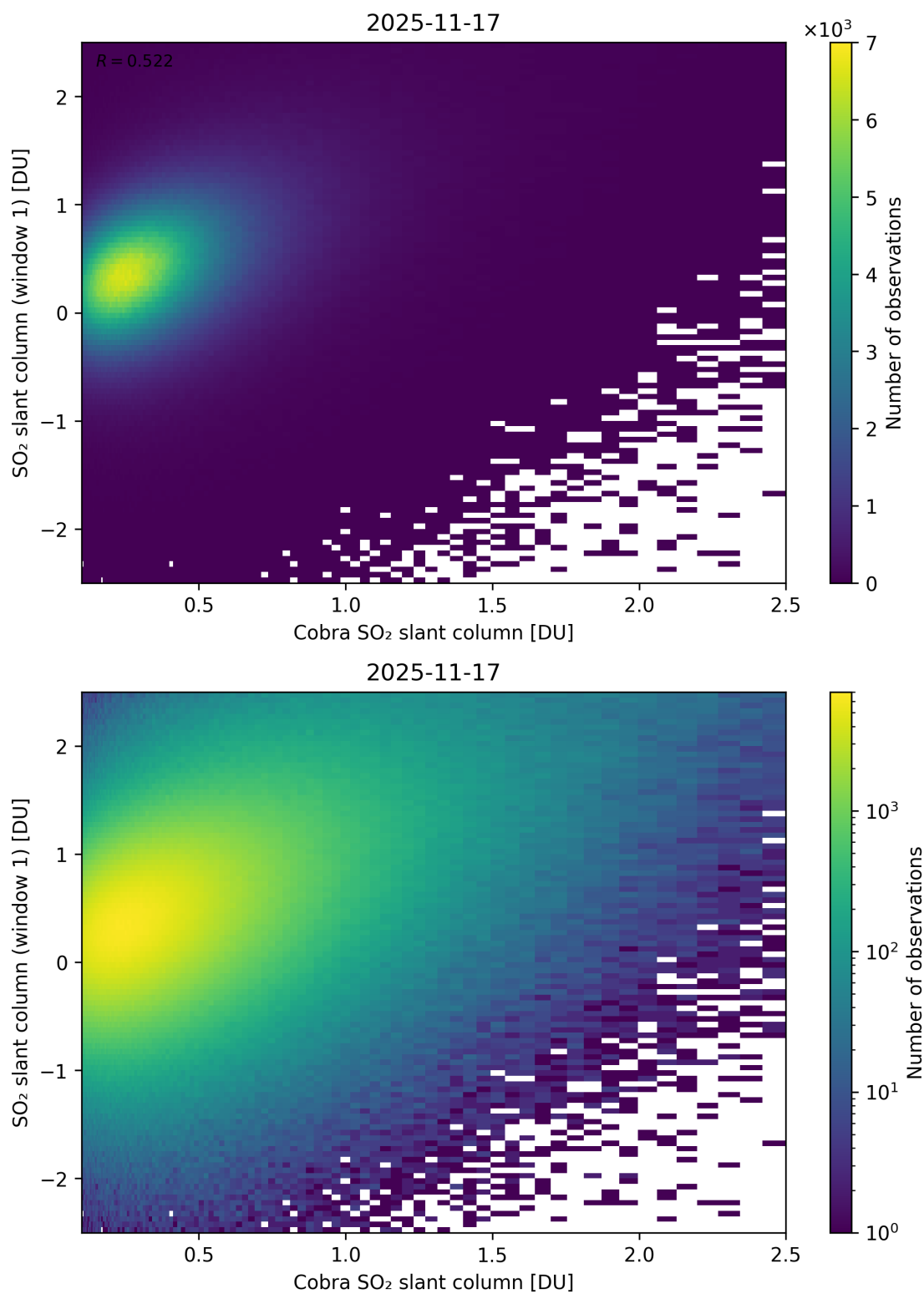
Figure 219: Scatter density plot of “Cobra SO 2 slant column” against “SO 2 slant column (window 1)” for 2025-11-16 to 2025-11-18.
