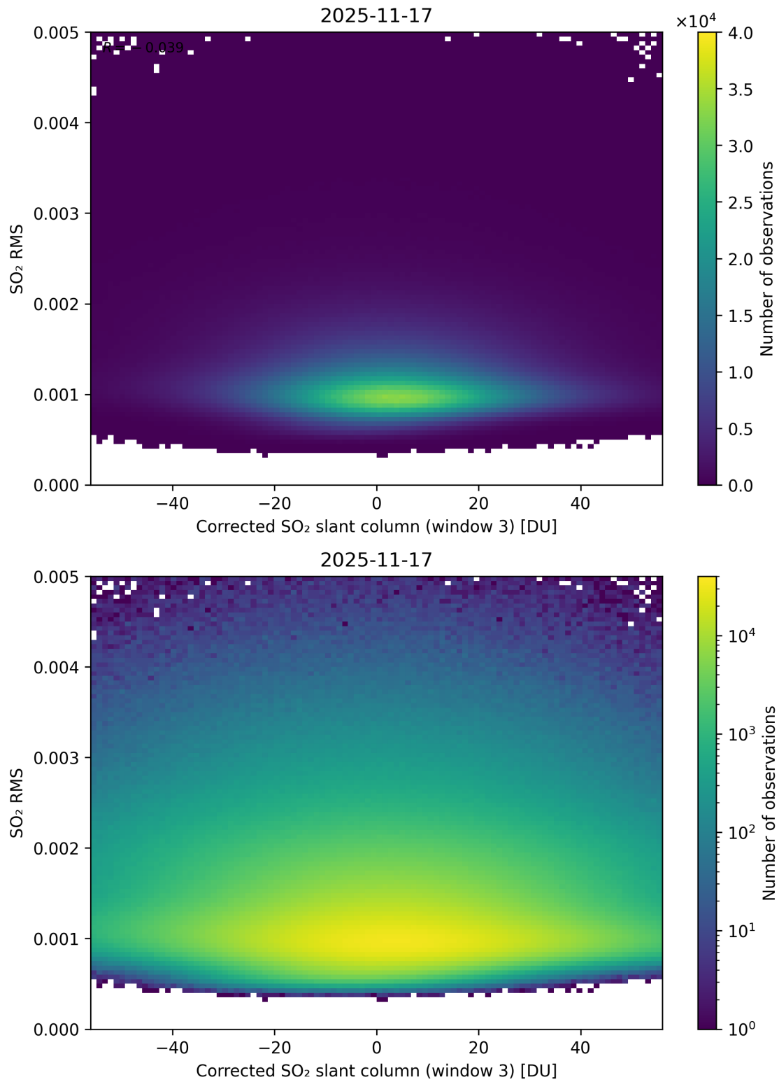
Figure 258: Scatter density plot of “Corrected SO 2 slant column (window 3)” against “SO 2 RMS” for 2025-11-16 to 2025-11-18.
