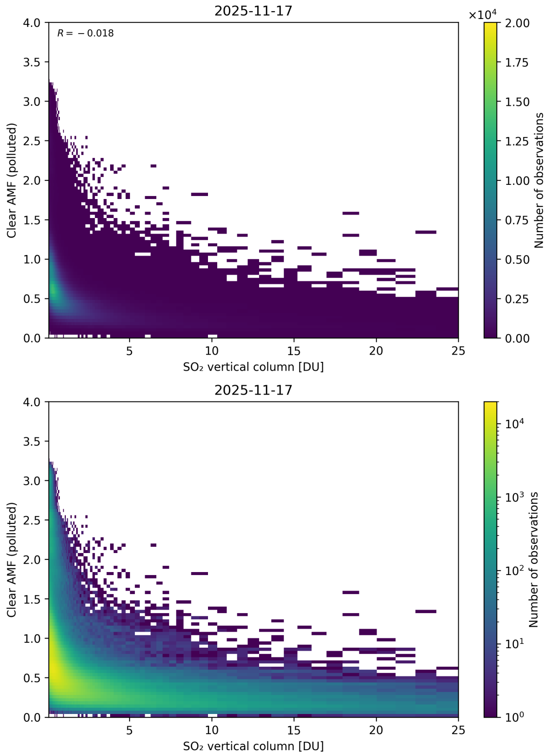
Figure 348: Scatter density plot of “SO 2 vertical column” against “Clear AMF (polluted)” for 2025-11-16 to 2025-11-18.
