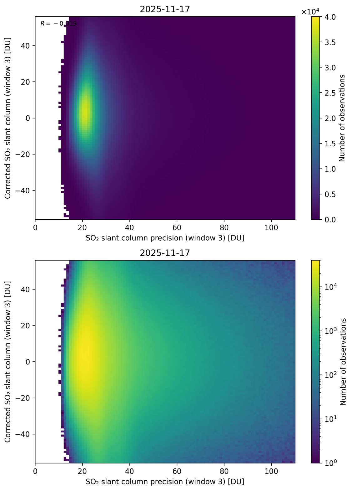
Figure 312: Scatter density plot of “SO 2 slant column precision (window 3)” against “Corrected SO 2 slant column (window 3)” for 2025-11-16 to 2025-11-18.
