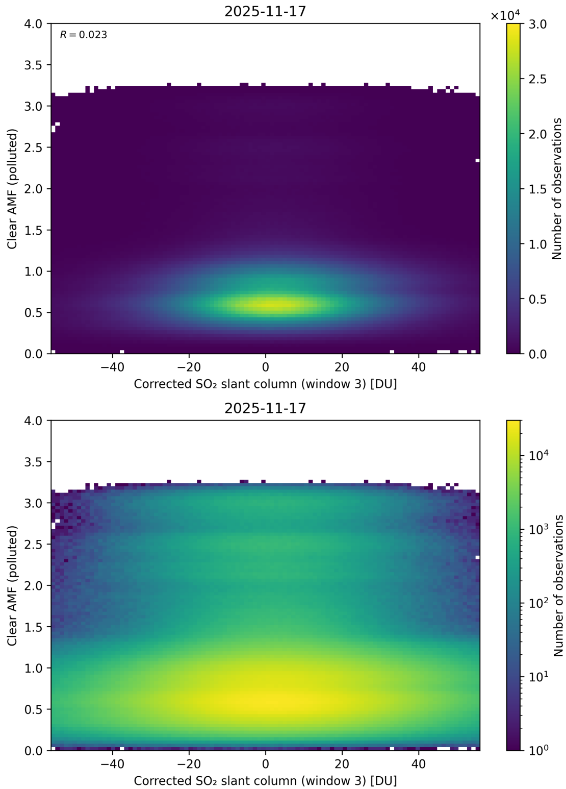
Figure 259: Scatter density plot of “Corrected SO 2 slant column (window 3)” against “Clear AMF (polluted)” for 2025-11-16 to 2025-11-18.
