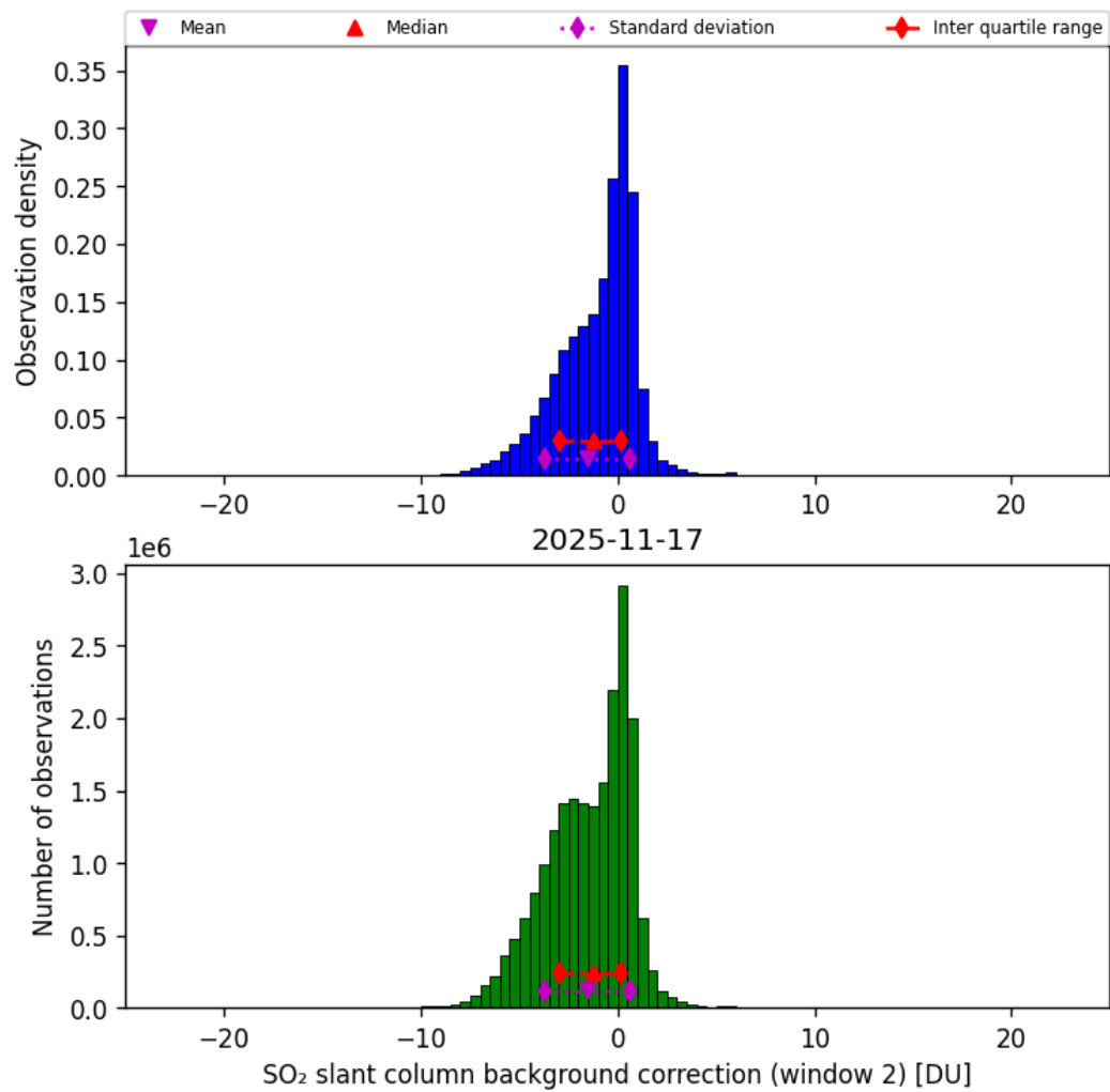
Figure 70: Histogram of “SO 2 slant column background correction (window 2)” for 2025-11-16 to 2025-11-18
