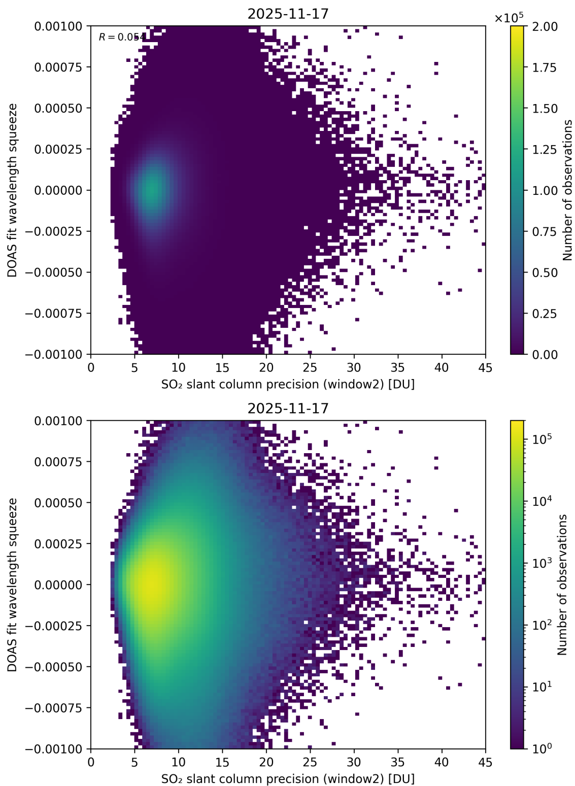
Figure 294: Scatter density plot of “SO 2 slant column precision (window2)” against “DOAS fit wavelength squeeze” for 2025-11-16 to 2025-11-18.
