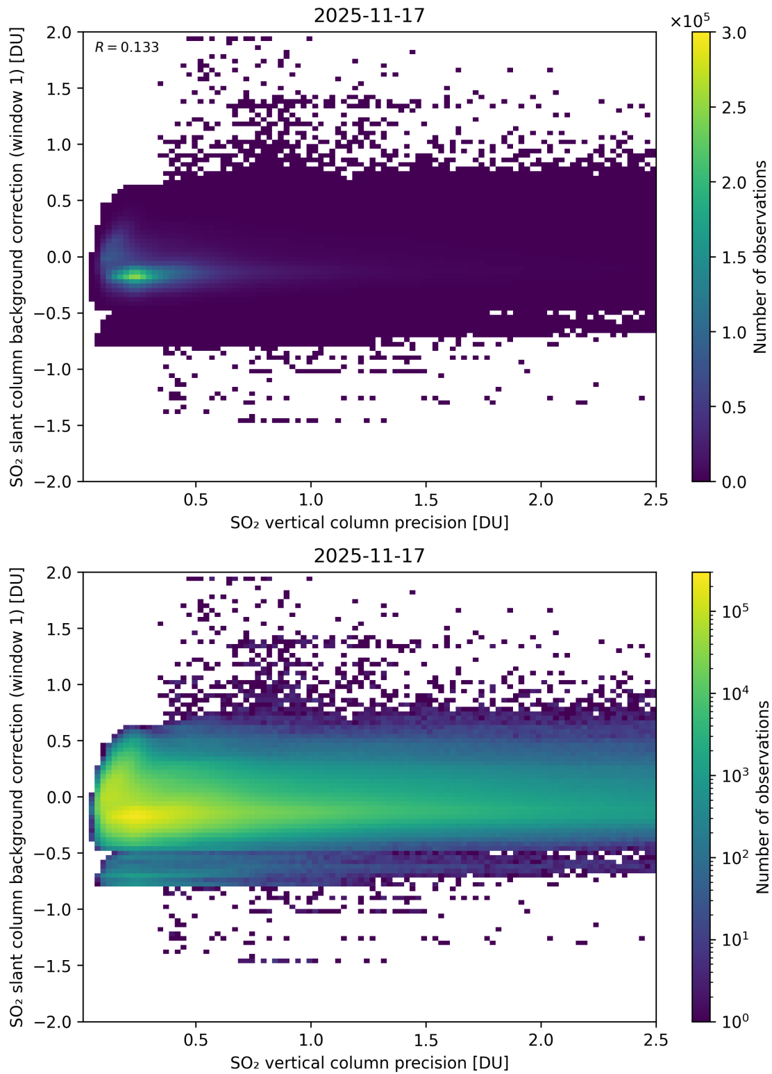
Figure 329: Scatter density plot of “SO 2 vertical column precision” against “SO 2 slant column background correction (window 1)” for 2025-11-16 to 2025-11-18.
