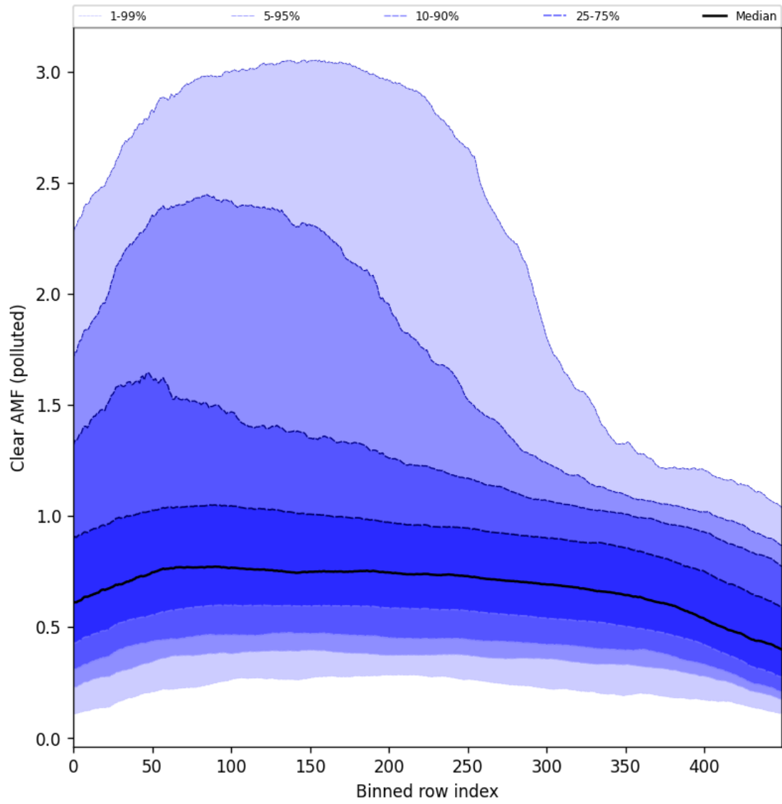
Figure 107: Along track statistics of “Clear AMF (polluted)” for 2025-11-16 to 2025-11-18
