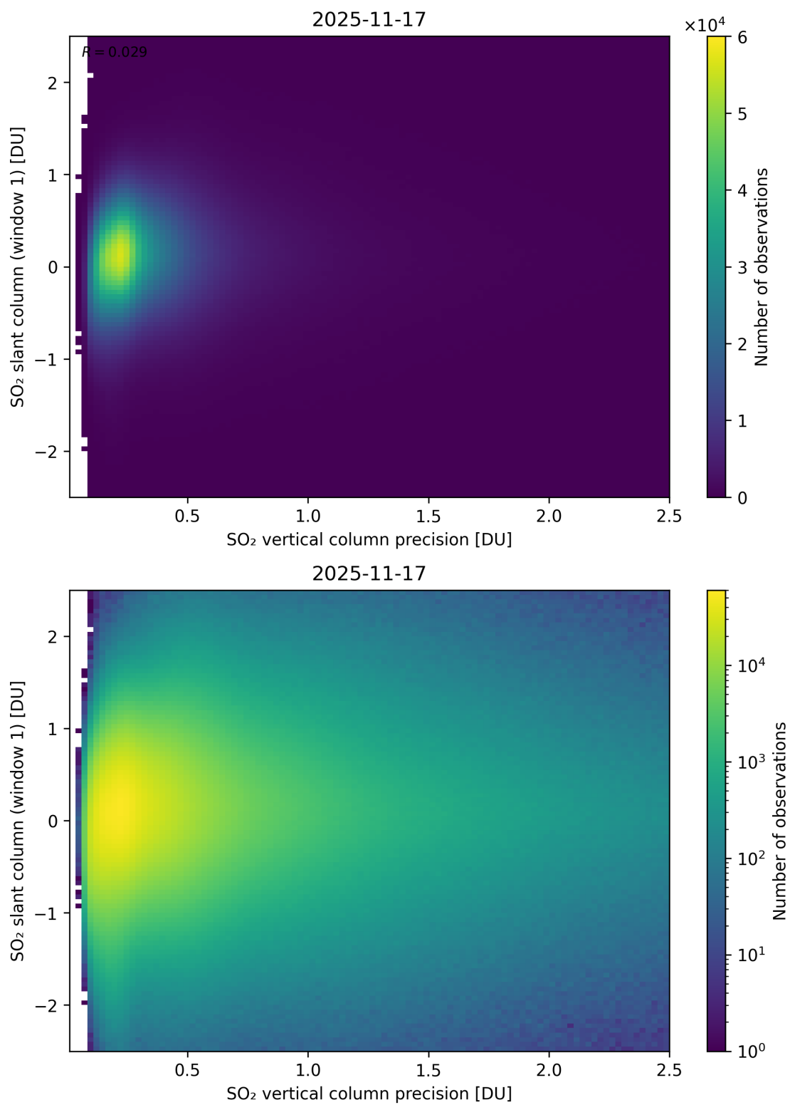
Figure 341: Scatter density plot of “SO 2 vertical column precision” against “SO 2 slant column (window 1)” for 2025-11-16 to 2025-11-18.
