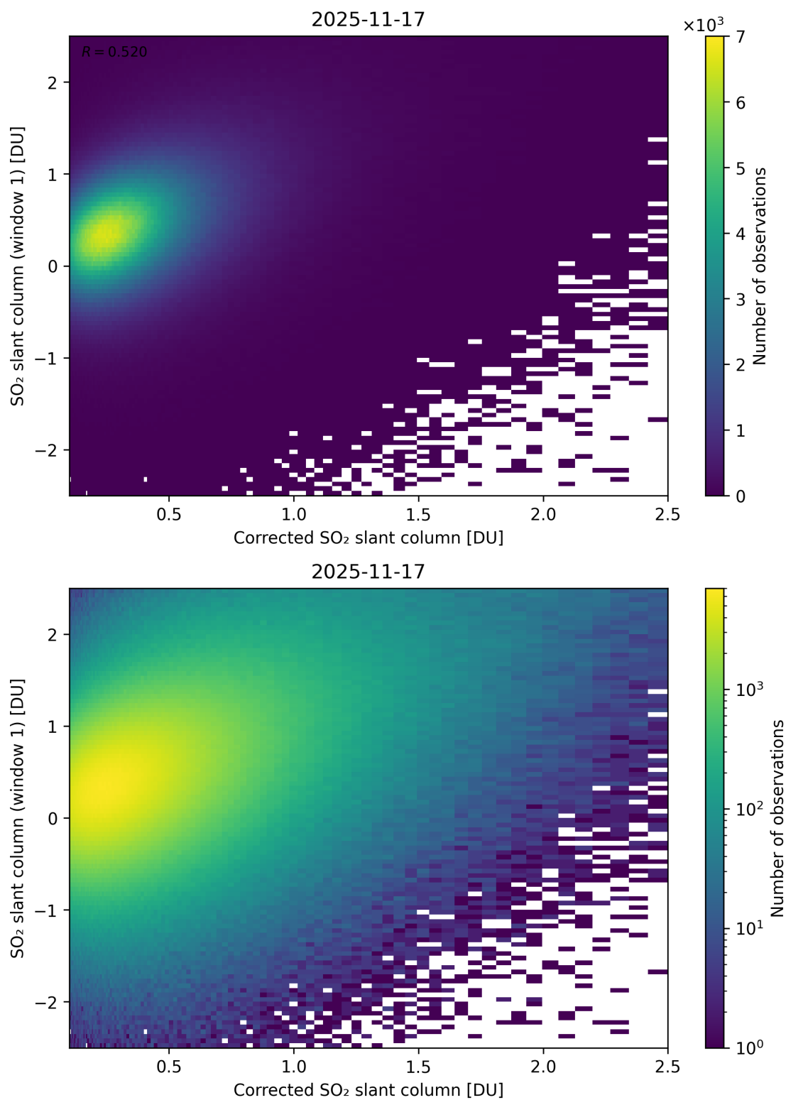
Figure 237: Scatter density plot of “Corrected SO 2 slant column” against “SO 2 slant column (window 1)” for 2025-11-16 to 2025-11-18.
