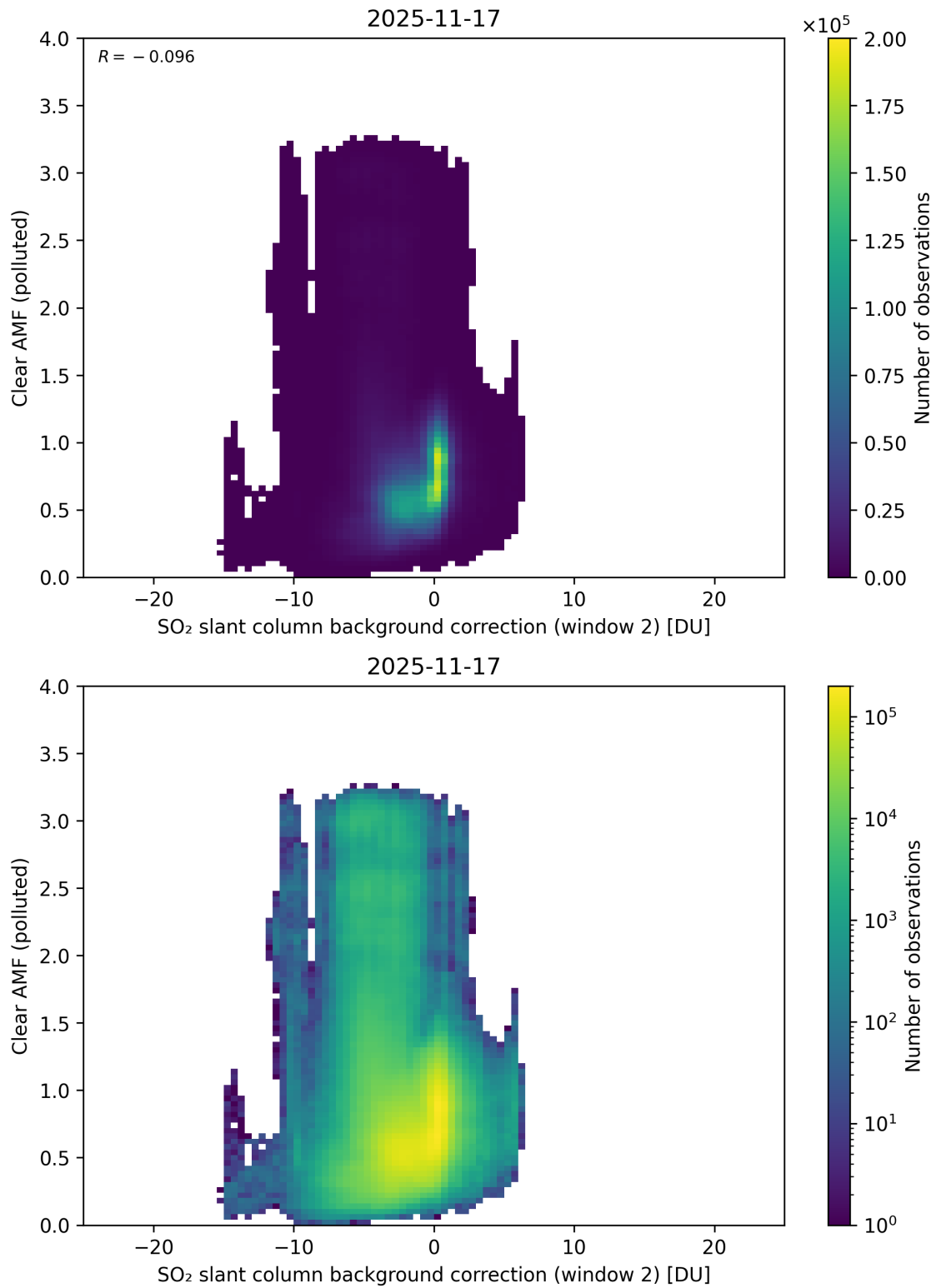
Figure 126: Scatter density plot of “SO 2 slant column background correction (window 2)” against “Clear AMF (polluted)” for 2025-11-16 to 2025-11-18.
