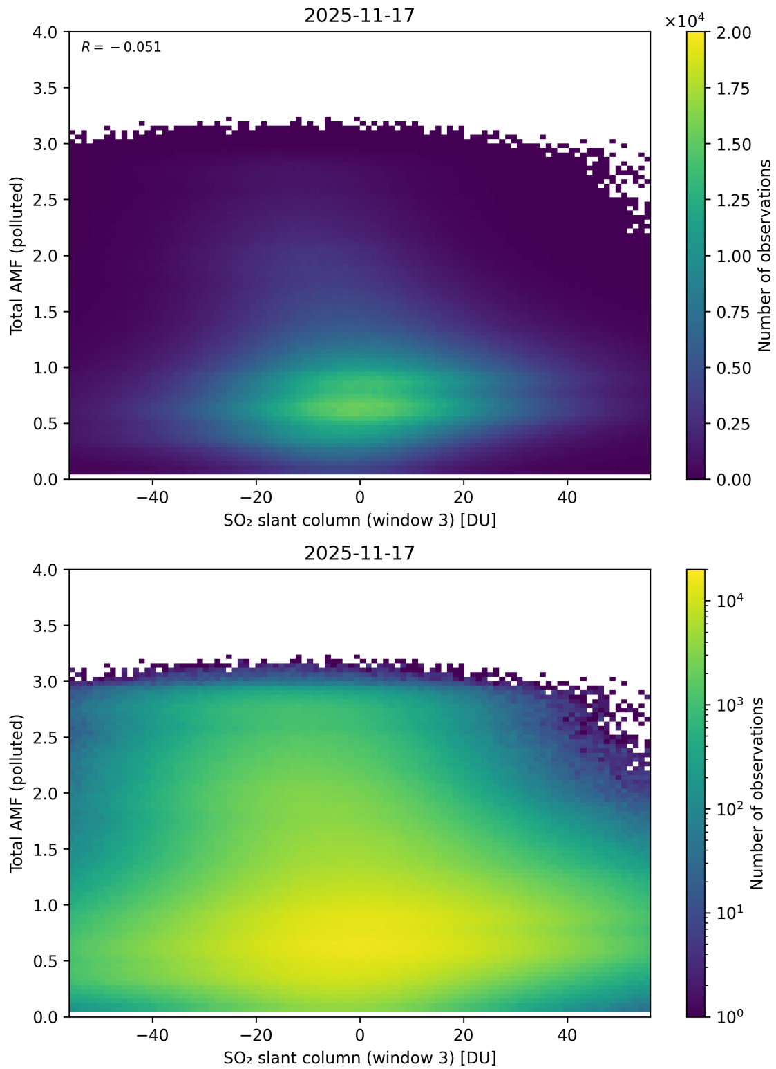
Figure 318: Scatter density plot of “SO 2 slant column (window 3)” against “Total AMF (polluted)” for 2025-11-16 to 2025-11-18.
