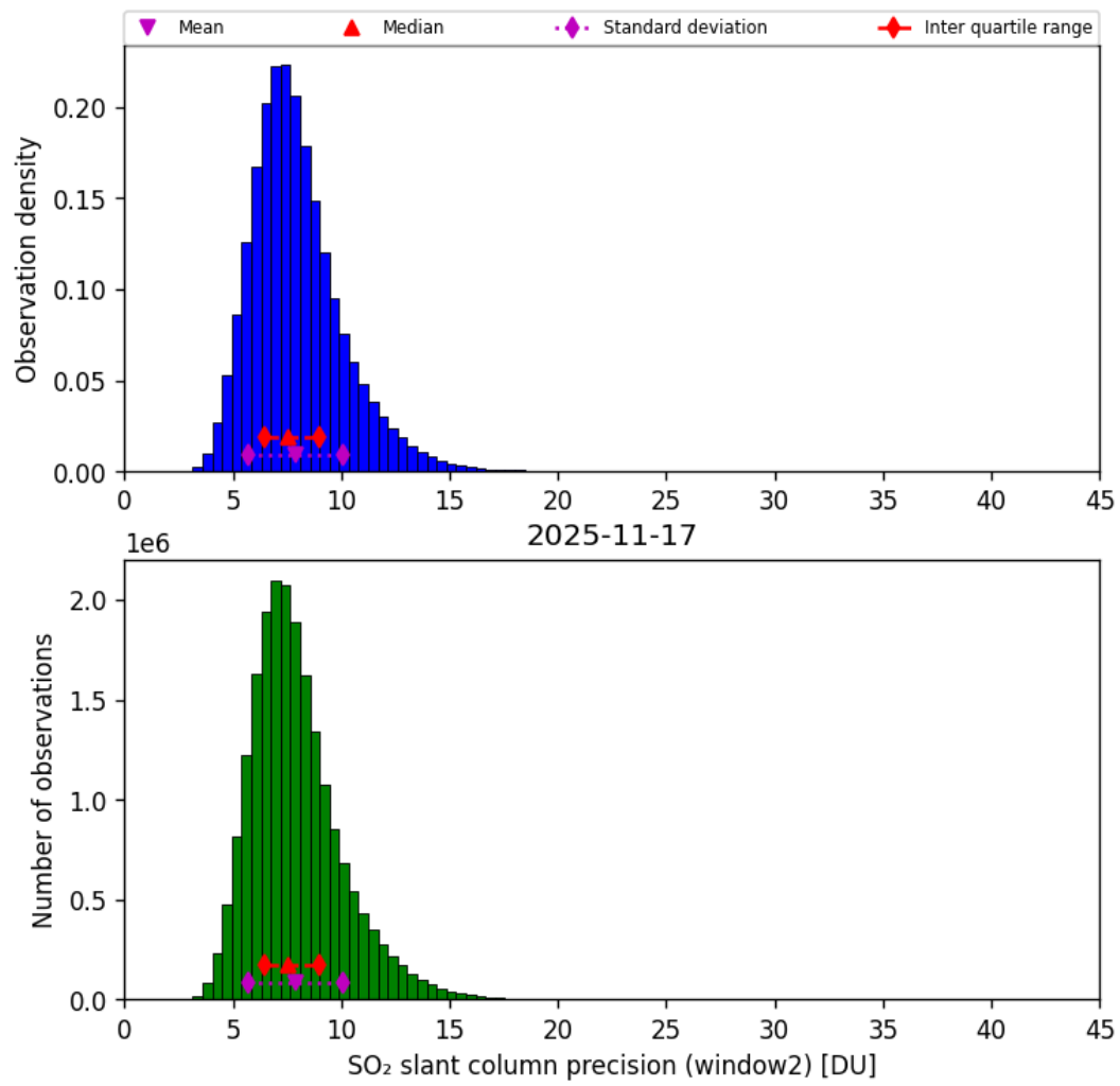
Figure 68: Histogram of “SO 2 slant column precision (window2)” for 2025-11-16 to 2025-11-18
