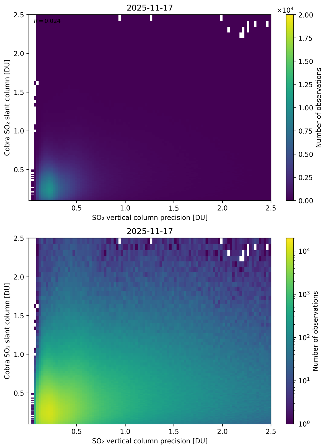
Figure 336: Scatter density plot of “SO 2 vertical column precision” against “Cobra SO 2 slant column” for 2025-11-16 to 2025-11-18.
