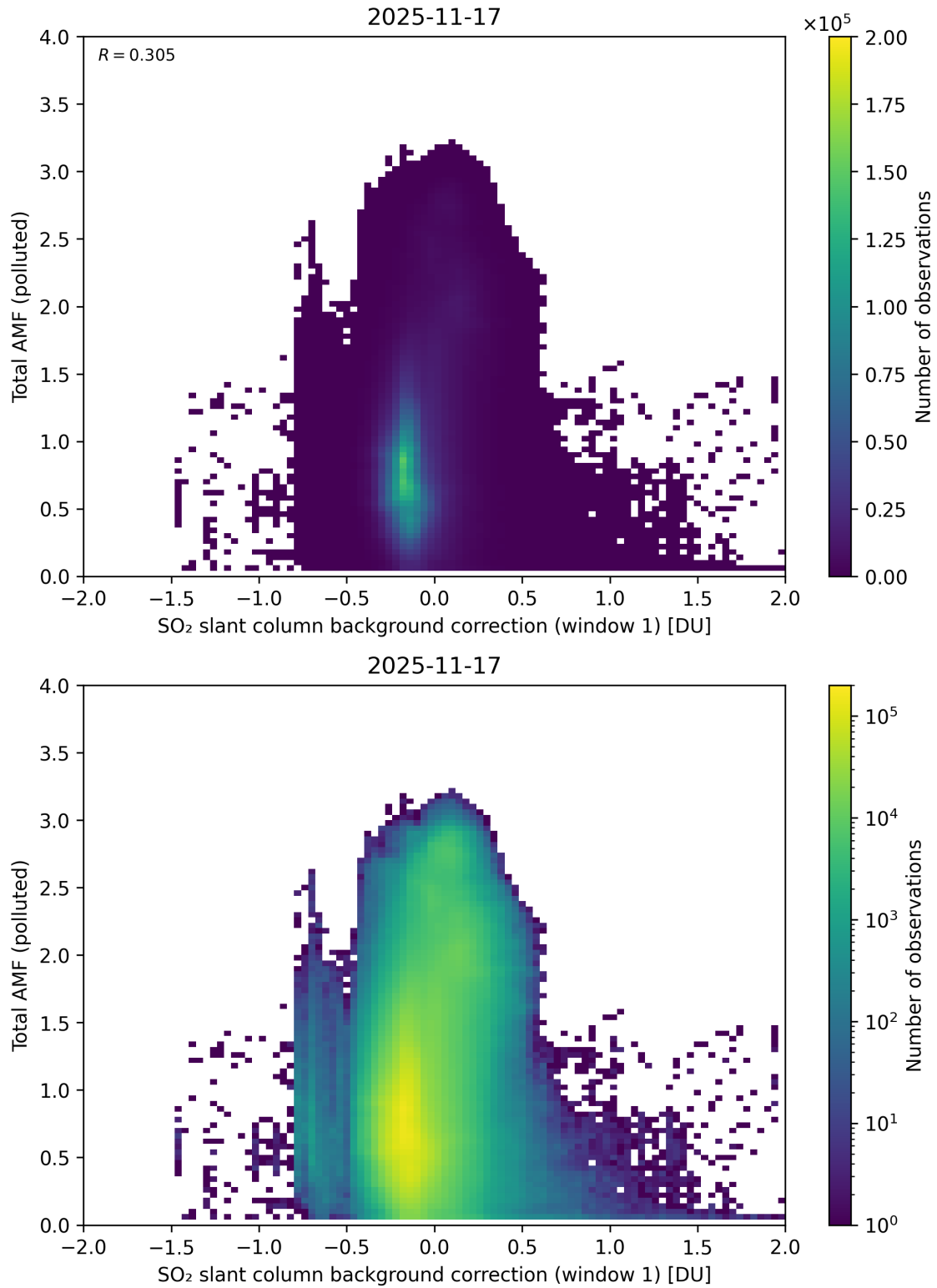
Figure 120: Scatter density plot of “SO 2 slant column background correction (window 1)” against “Total AMF (polluted)” for 2025-11-16 to 2025-11-18.
