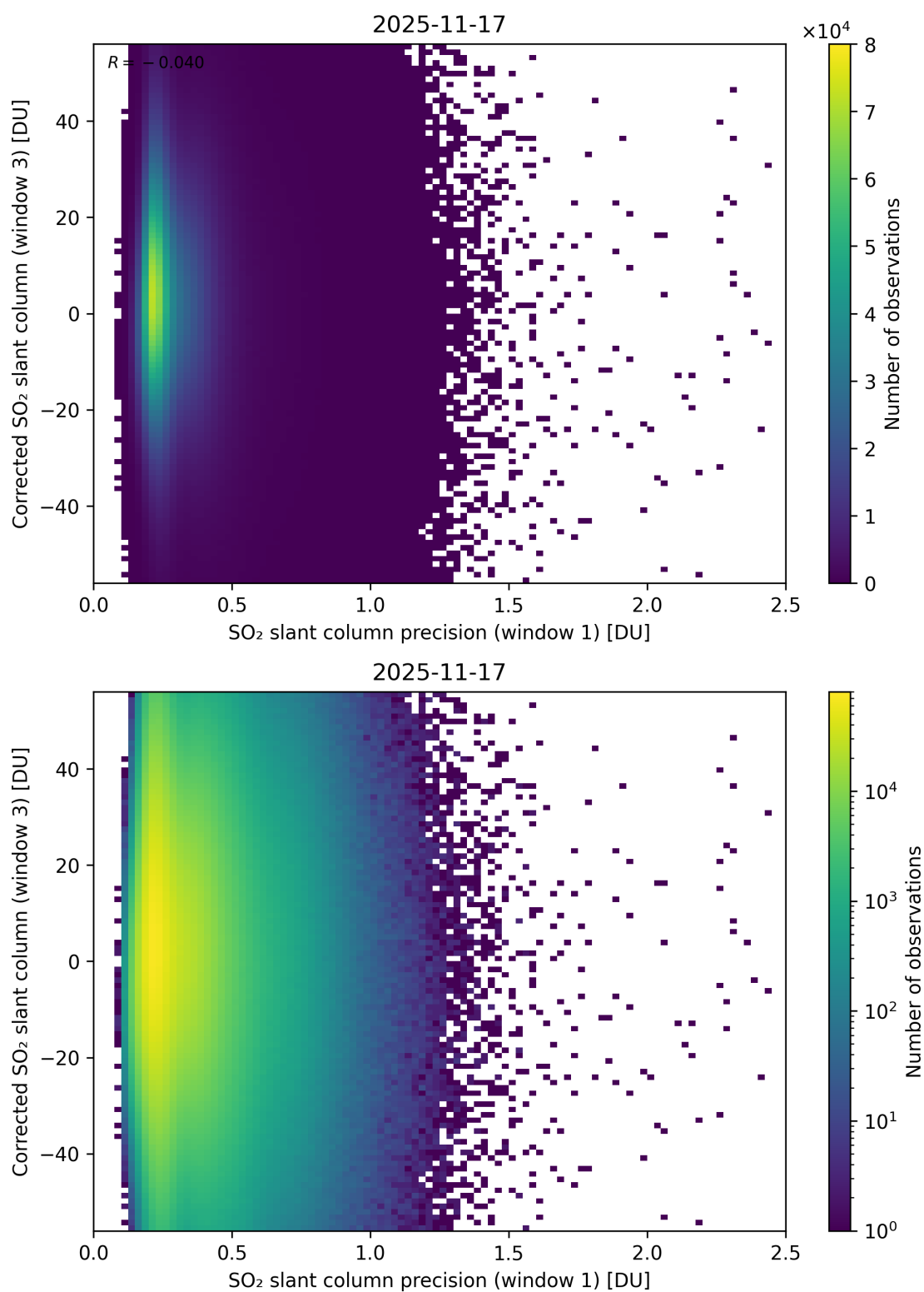
Figure 276: Scatter density plot of “SO 2 slant column precision (window 1)” against “Corrected SO 2 slant column (window 3)” for 2025-11-16 to 2025-11-18.
