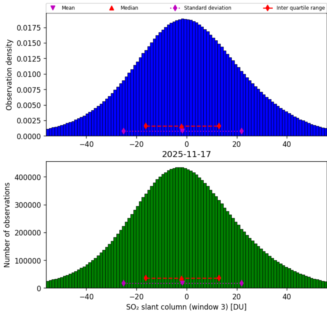
Figure 71: Histogram of “SO 2 slant column (window 3)” for 2025-11-16 to 2025-11-18
