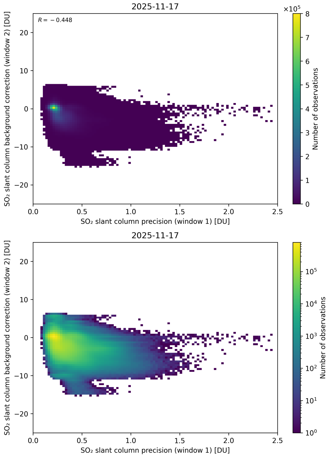
Figure 269: Scatter density plot of “SO 2 slant column precision (window 1)” against “SO 2 slant column background correction (window 2)” for 2025-11-16 to 2025-11-18.
