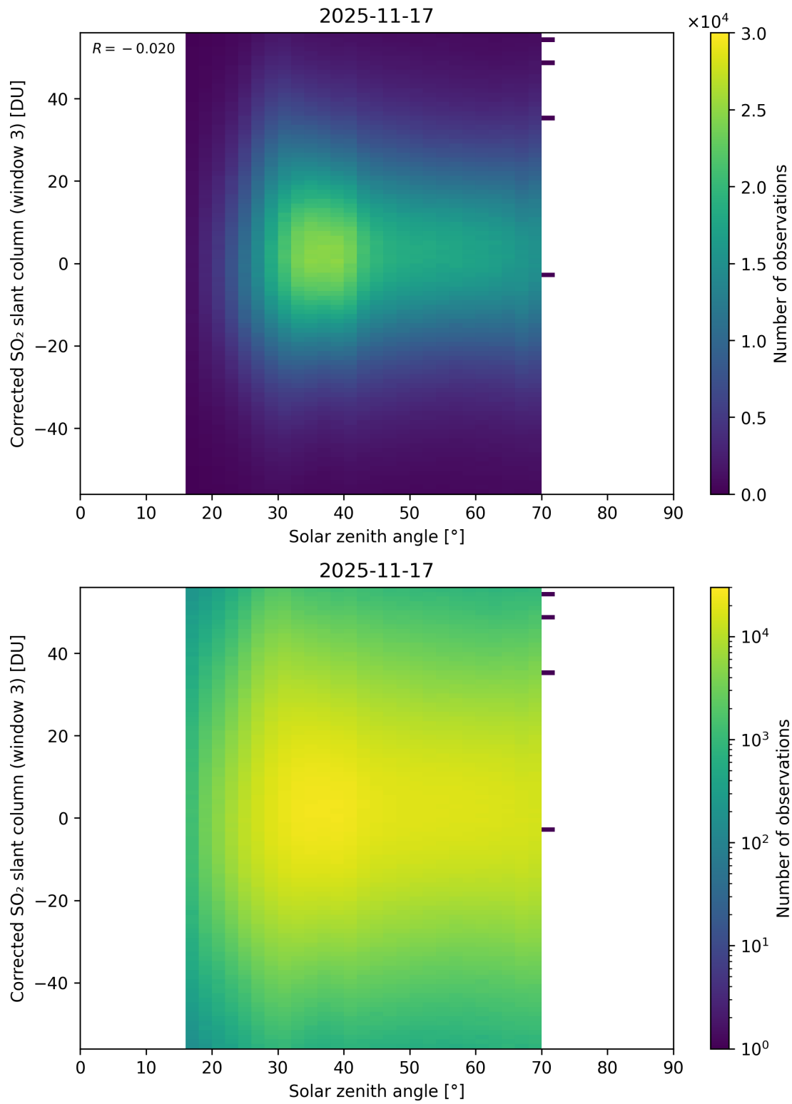
Figure 183: Scatter density plot of “Solar zenith angle” against “Corrected SO 2 slant column (window 3)” for 2025-11-16 to 2025-11-18.
