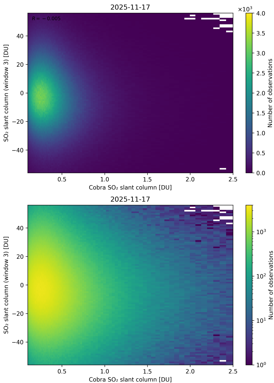
Figure 222: Scatter density plot of “Cobra SO 2 slant column” against “SO 2 slant column (window 3)” for 2025-11-16 to 2025-11-18.
