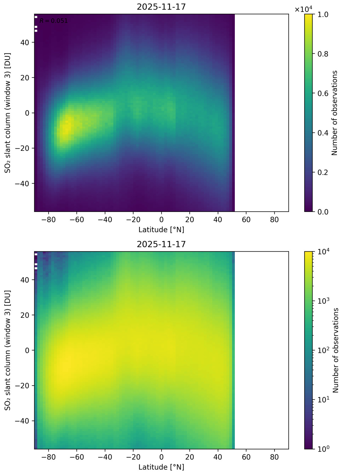
Figure 165: Scatter density plot of “Latitude” against “SO 2 slant column (window 3)” for 2025-11-16 to 2025-11-18.
