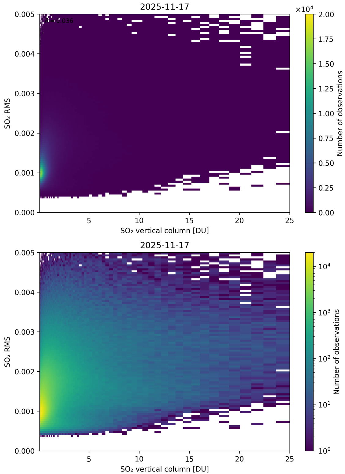
Figure 328: Scatter density plot of “SO 2 vertical column” against “SO 2 RMS” for 2025-11-16 to 2025-11-18.
