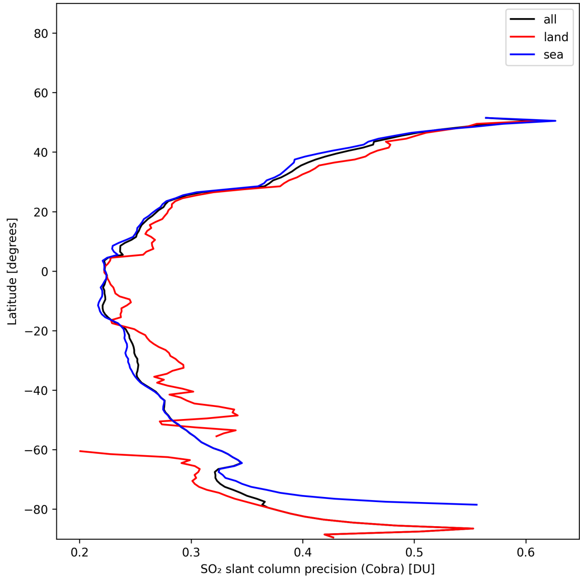
Figure 36: Zonal average of “SO 2 slant column precision (Cobra)” for 2025-11-16 to 2025-11-18.
