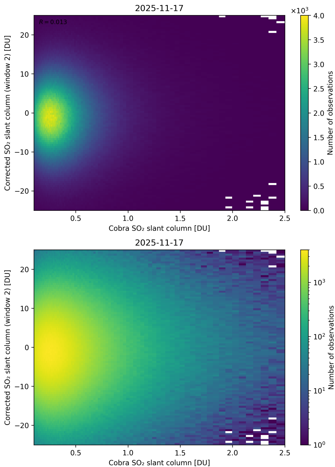
Figure 217: Scatter density plot of “Cobra SO 2 slant column” against “Corrected SO 2 slant column (window 2)” for 2025-11-16 to 2025-11-18.
