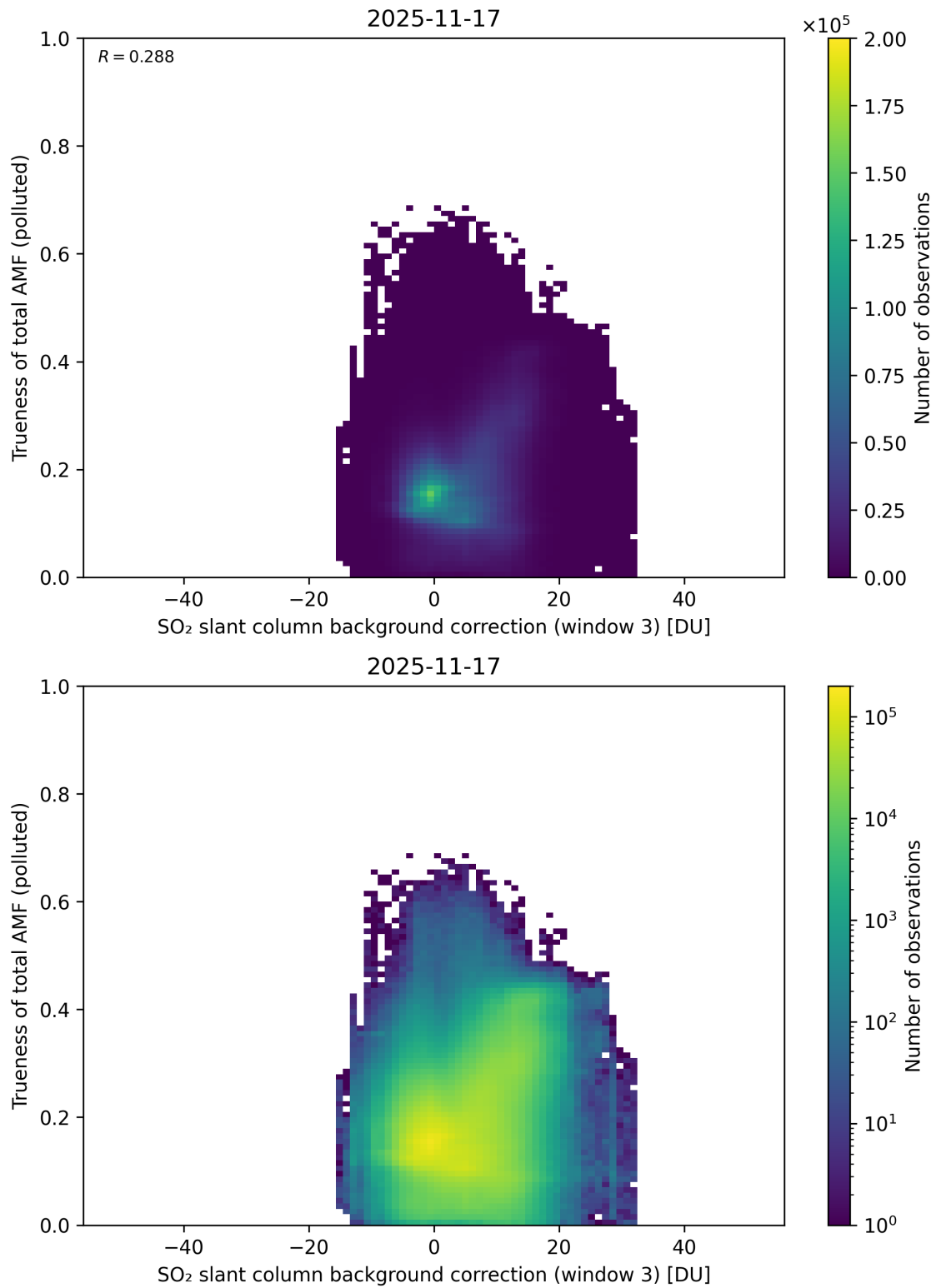
Figure 137: Scatter density plot of “SO 2 slant column background correction (window 3)” against “Trueness of total AMF (polluted)” for 2025-11-16 to 2025-11-18.
