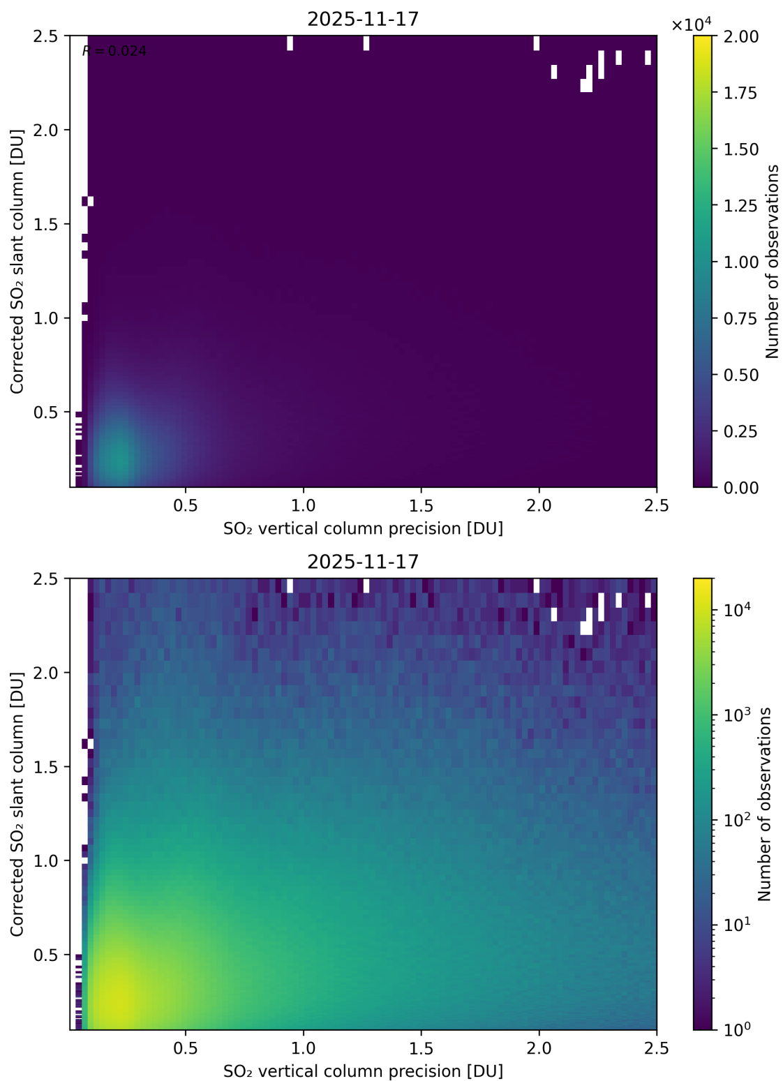
Figure 338: Scatter density plot of “SO 2 vertical column precision” against “Corrected SO 2 slant column” for 2025-11-16 to 2025-11-18.
