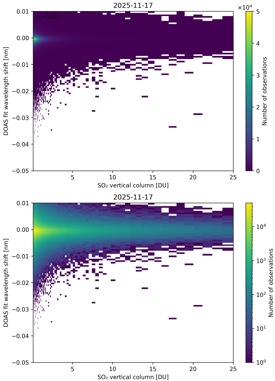
Figure 326: Scatter density plot of “SO 2 vertical column” against “DOAS fit wavelength shift” for 2025-11-16 to 2025-11-18.
