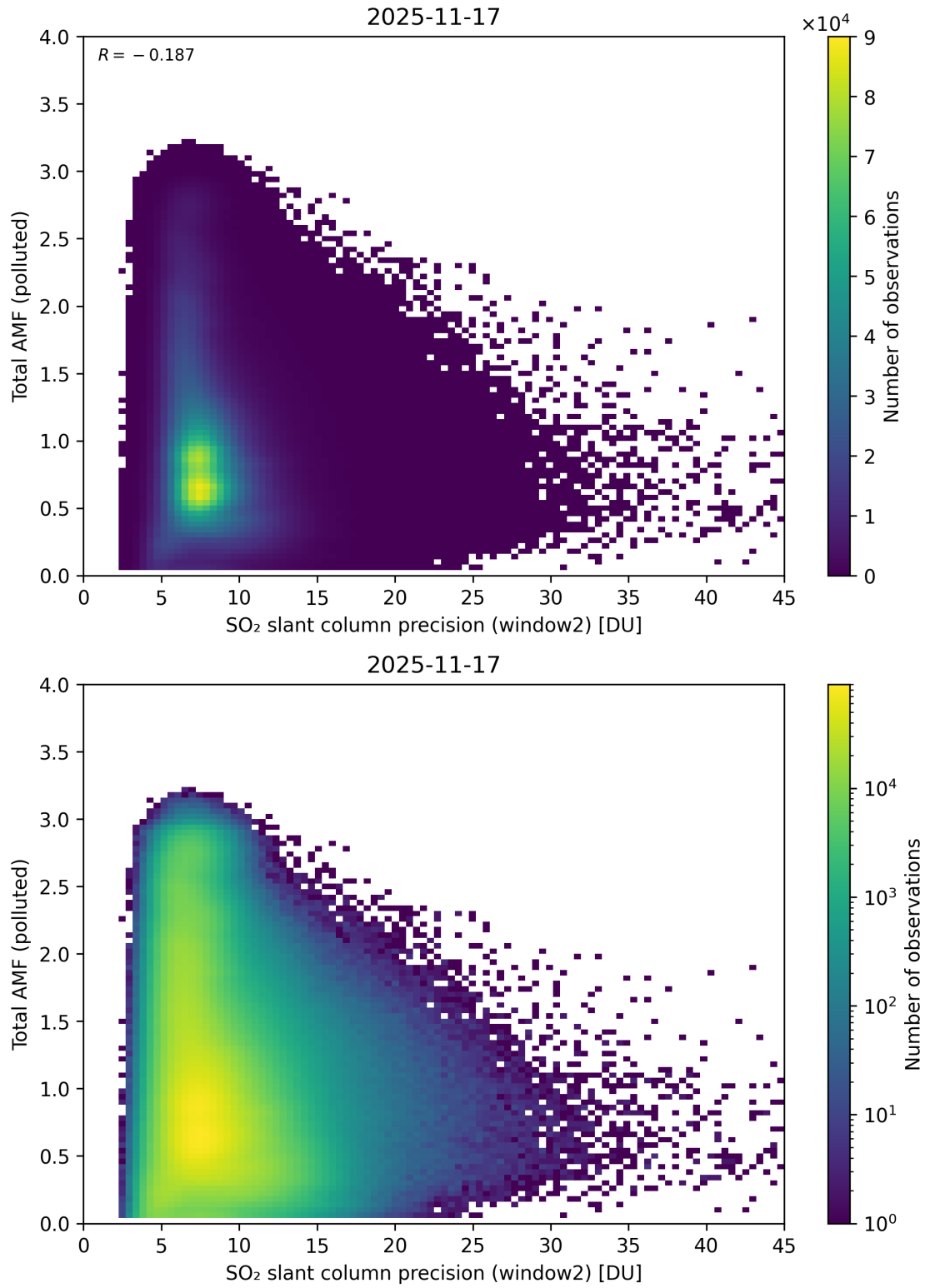
Figure 301: Scatter density plot of “SO 2 slant column precision (window2)” against “Total AMF (polluted)” for 2025-11-16 to 2025-11-18.
