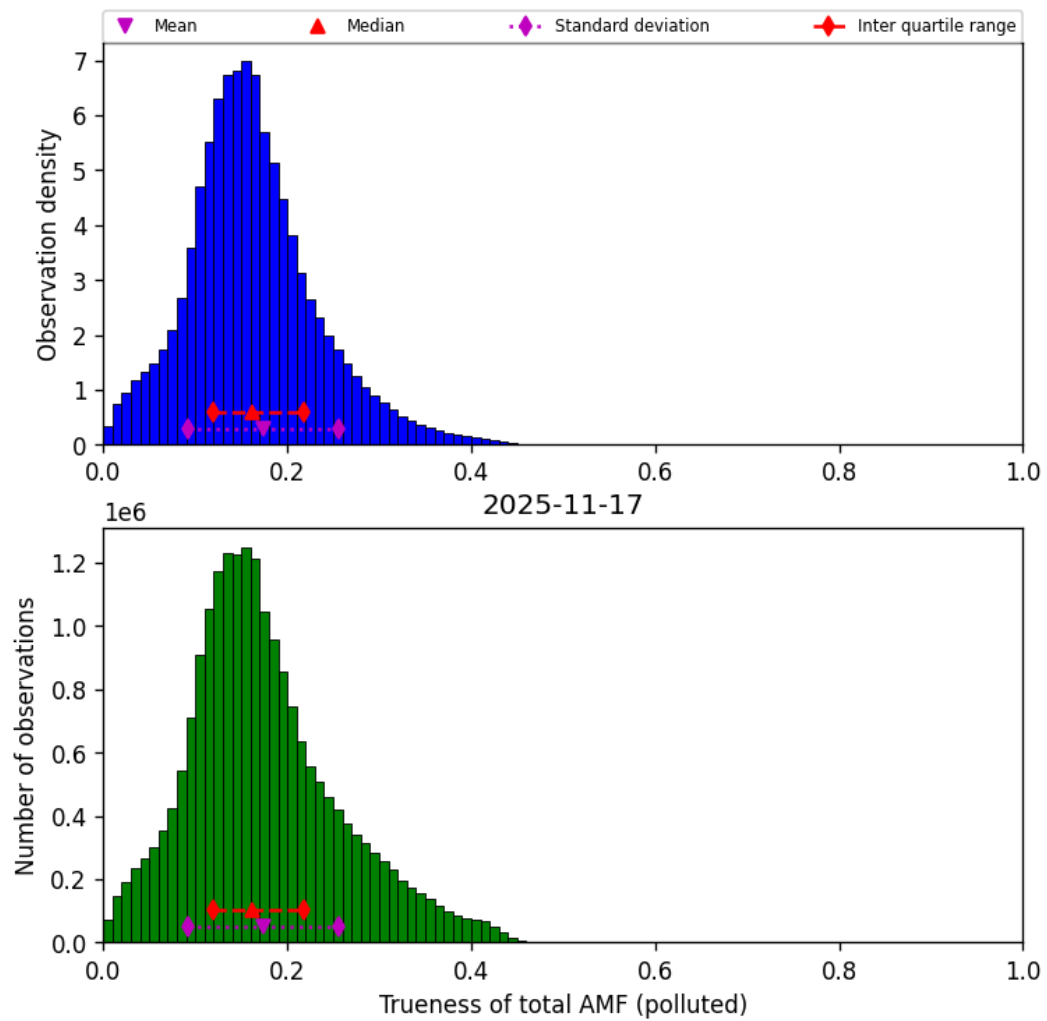
Figure 80: Histogram of “Trueness of total AMF (polluted)” for 2025-11-16 to 2025-11-18
