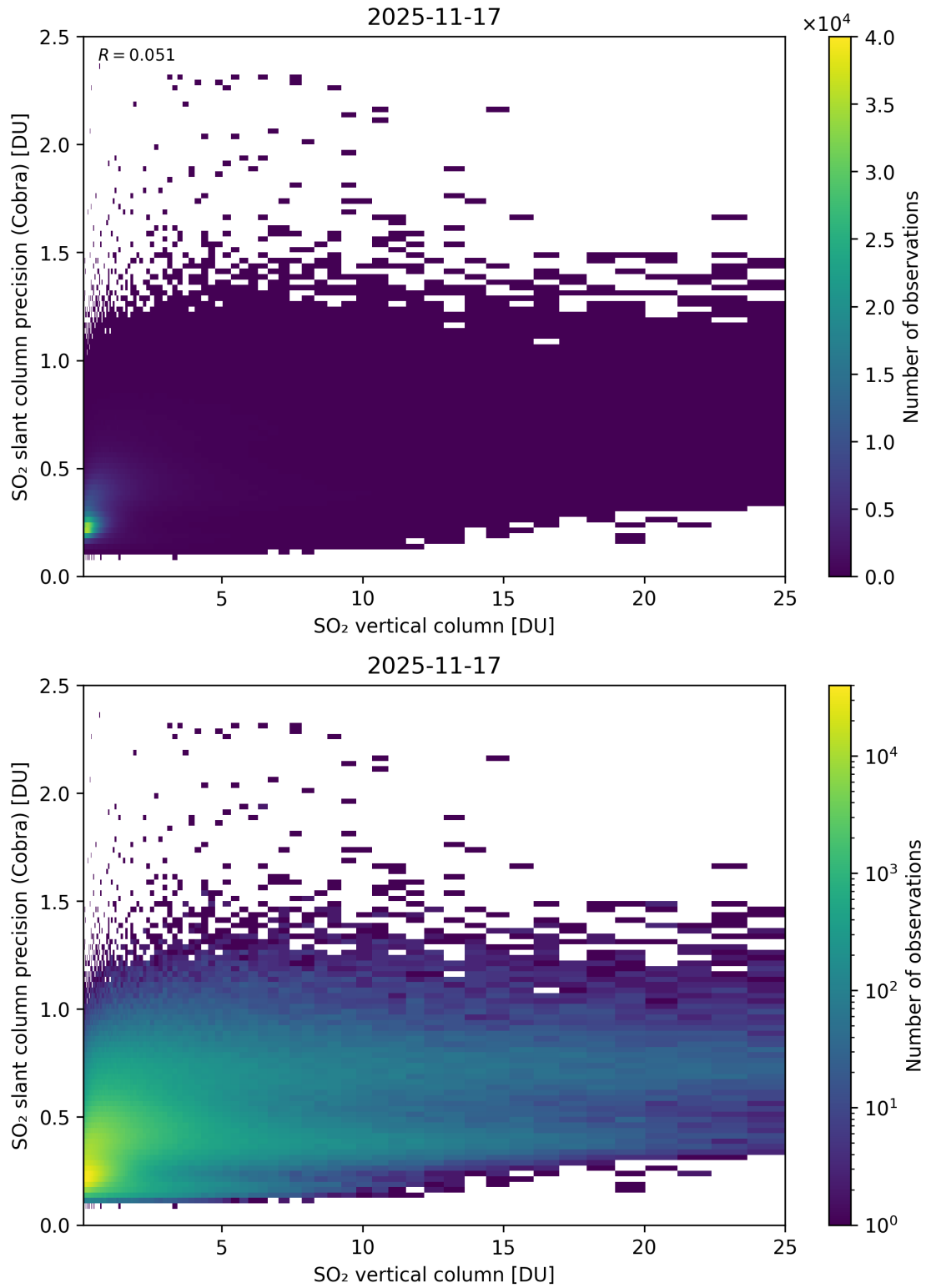
Figure 350: Scatter density plot of “SO 2 vertical column” against “SO 2 slant column precision (Cobra)” for 2025-11-16 to 2025-11-18.
