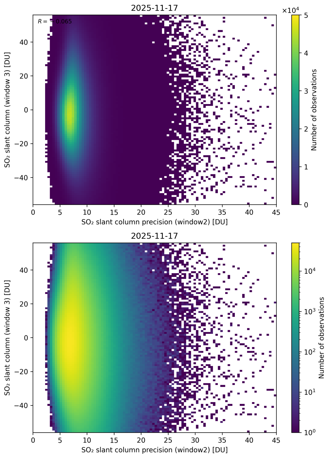
Figure 299: Scatter density plot of “SO 2 slant column precision (window2)” against “SO 2 slant column (window 3)” for 2025-11-16 to 2025-11-18.
