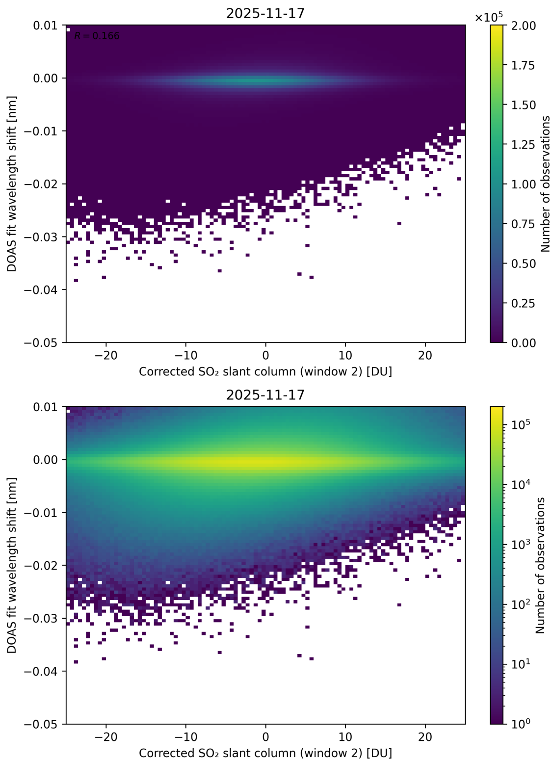
Figure 246: Scatter density plot of “Corrected SO 2 slant column (window 2)” against “DOAS fit wavelength shift” for 2025-11-16 to 2025-11-18.
