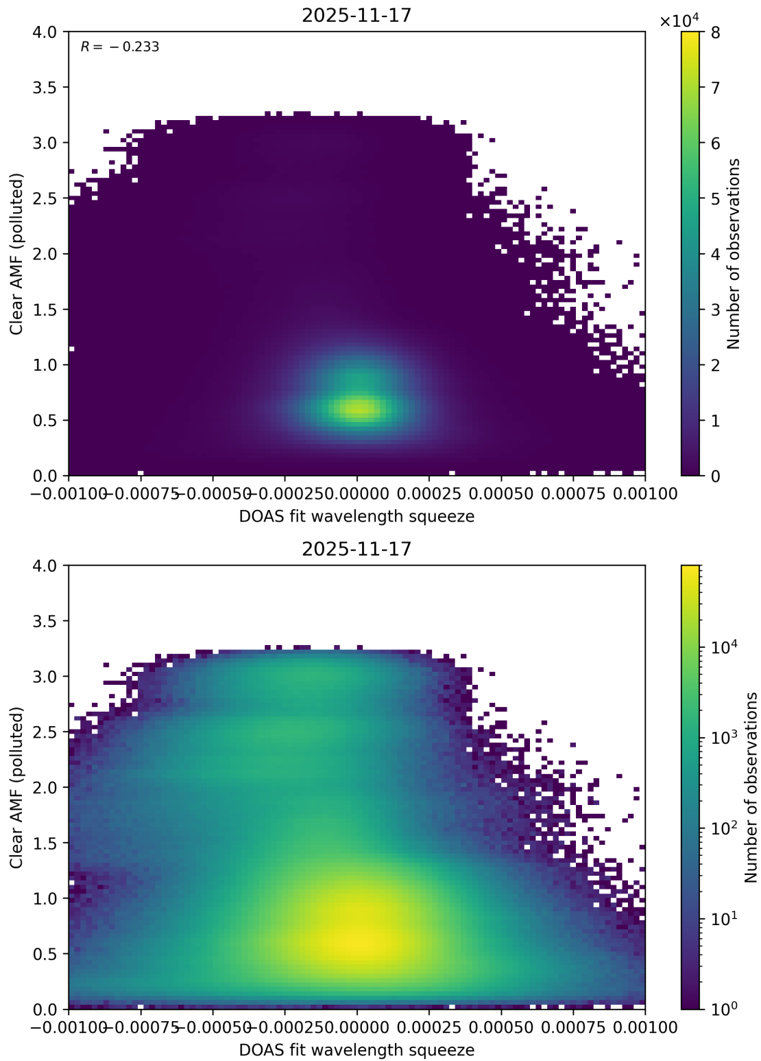
Figure 144: Scatter density plot of “DOAS fit wavelength squeeze” against “Clear AMF (polluted)” for 2025-11-16 to 2025-11-18.
