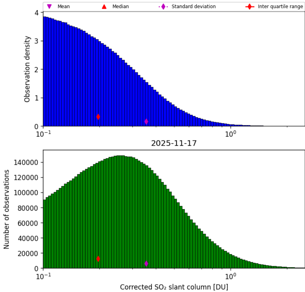
Figure 60: Histogram of “Corrected SO 2 slant column” for 2025-11-16 to 2025-11-18
