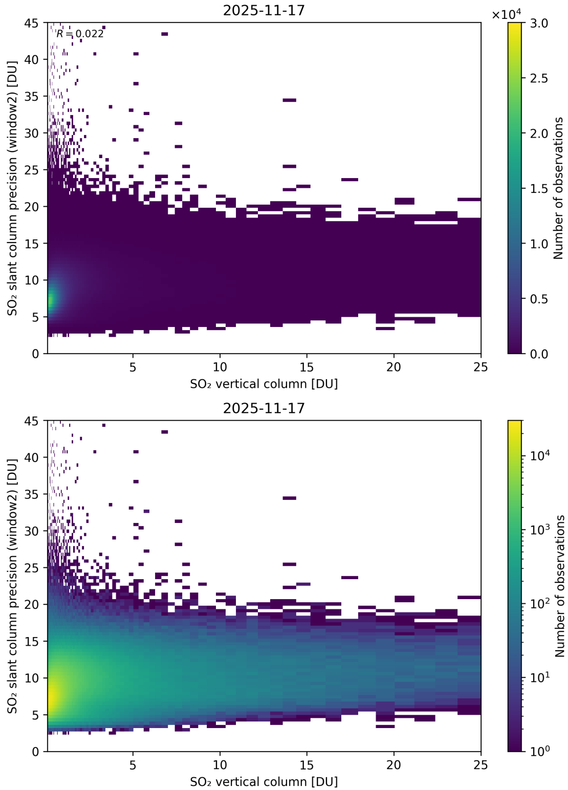
Figure 356: Scatter density plot of “SO 2 vertical column” against “SO 2 slant column precision (window2)” for 2025-11-16 to 2025-11-18.
