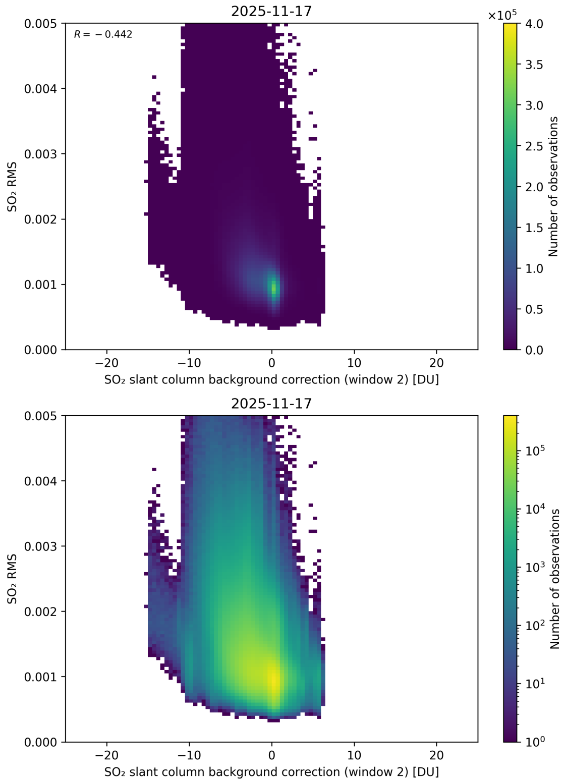
Figure 125: Scatter density plot of “SO 2 slant column background correction (window 2)” against “SO 2 RMS” for 2025-11-16 to 2025-11-18.
