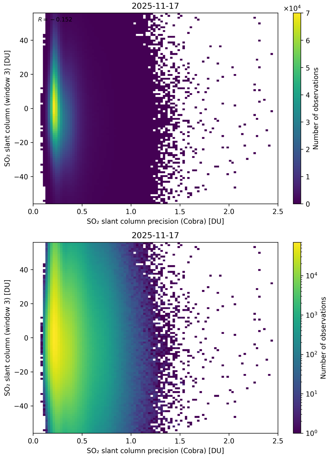
Figure 211: Scatter density plot of “SO 2 slant column precision (Cobra)” against “SO 2 slant column (window 3)” for 2025-11-16 to 2025-11-18.
