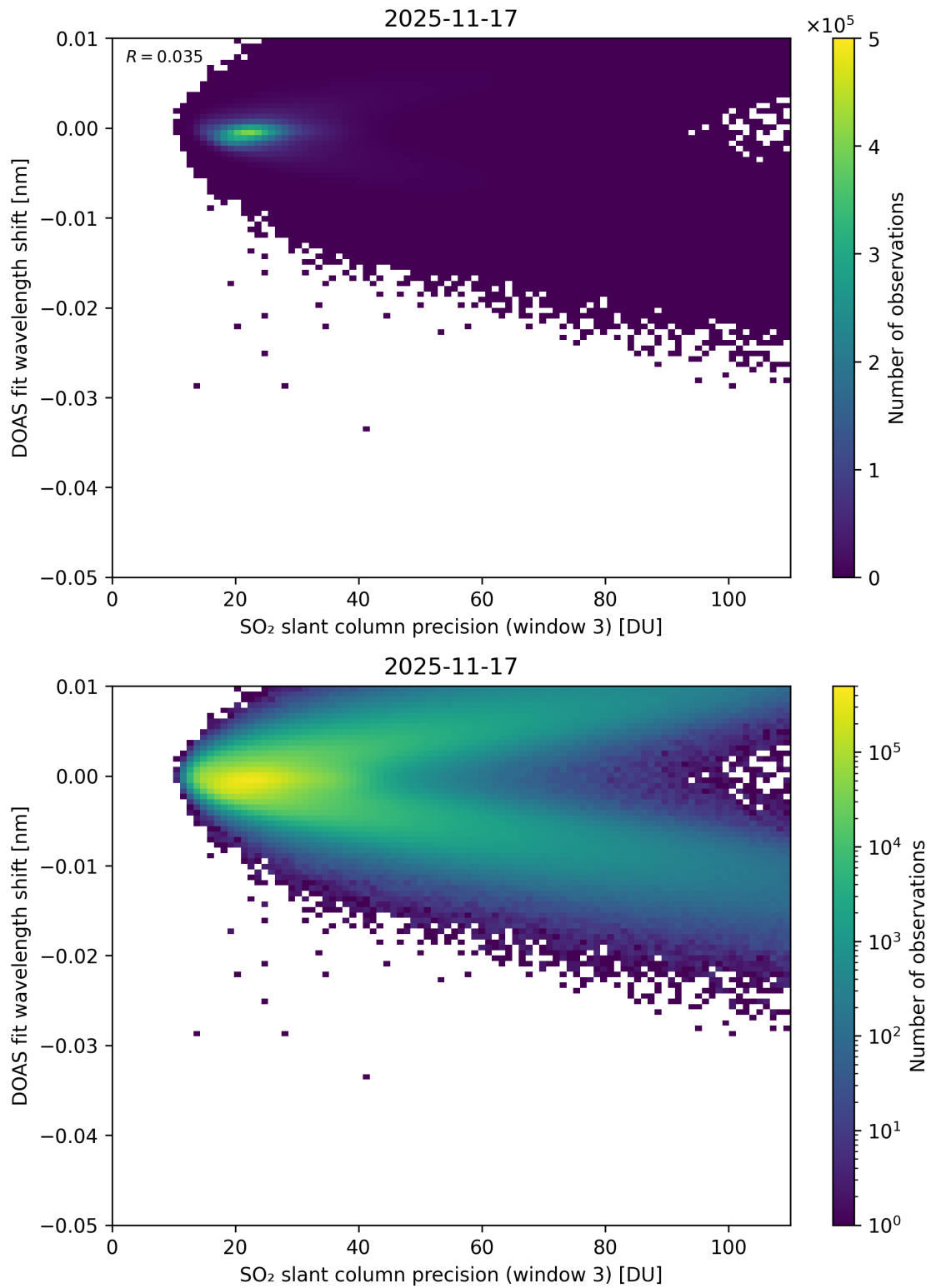
Figure 308: Scatter density plot of “SO 2 slant column precision (window 3)” against “DOAS fit wavelength shift” for 2025-11-16 to 2025-11-18.
