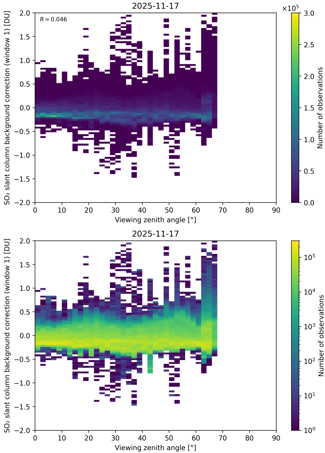
Figure 362: Scatter density plot of “Viewing zenith angle” against “SO 2 slant column background correction (window 1)” for 2025-11-16 to 2025-11-18.
