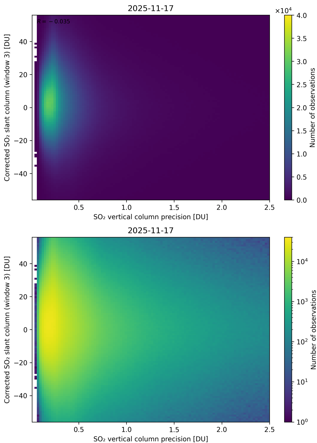
Figure 340: Scatter density plot of “SO 2 vertical column precision” against “Corrected SO 2 slant column (window 3)” for 2025-11-16 to 2025-11-18.
