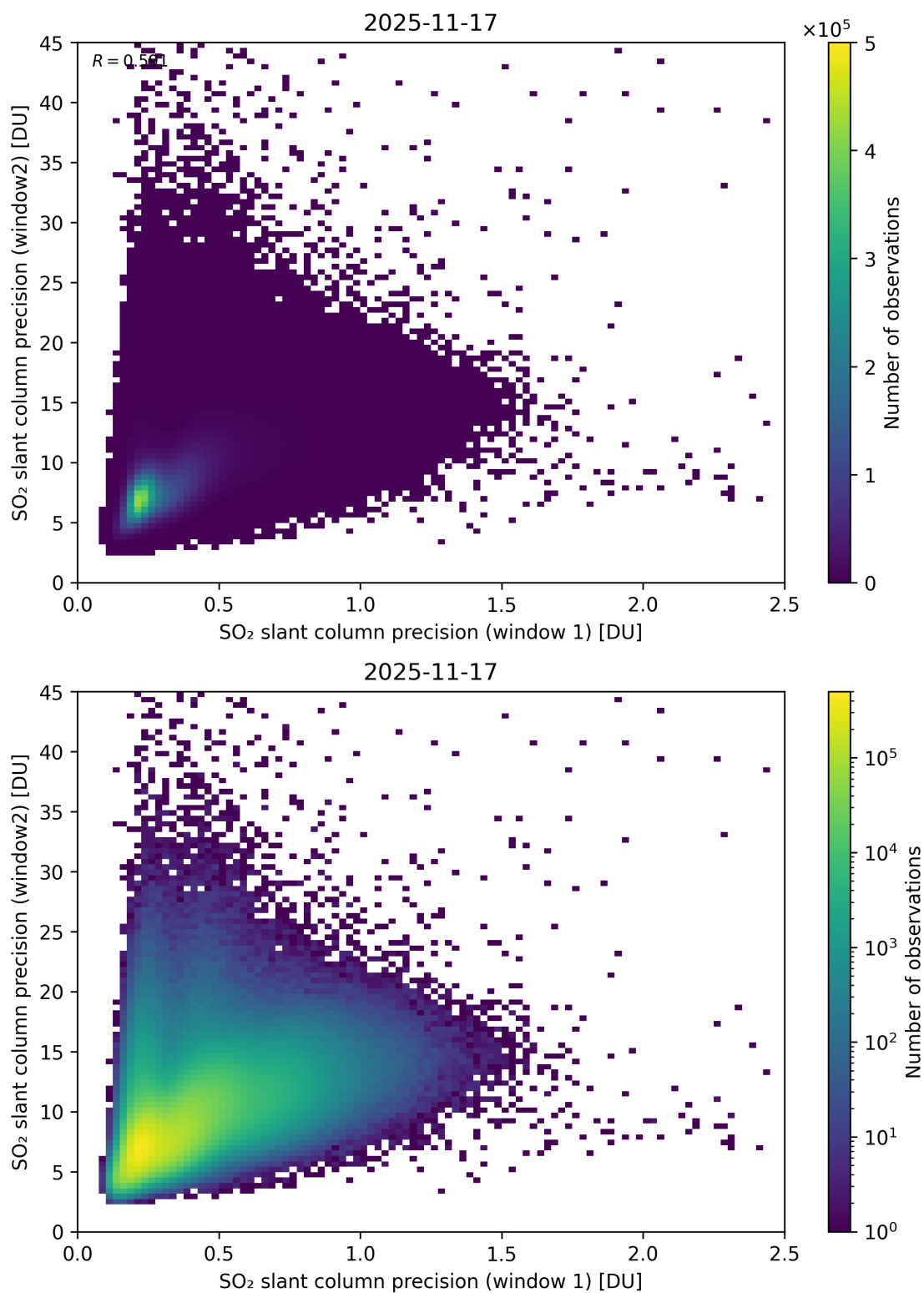
Figure 277: Scatter density plot of “SO 2 slant column precision (window 1)” against “SO 2 slant column precision (window2)” for 2025-11-16 to 2025-11-18.
