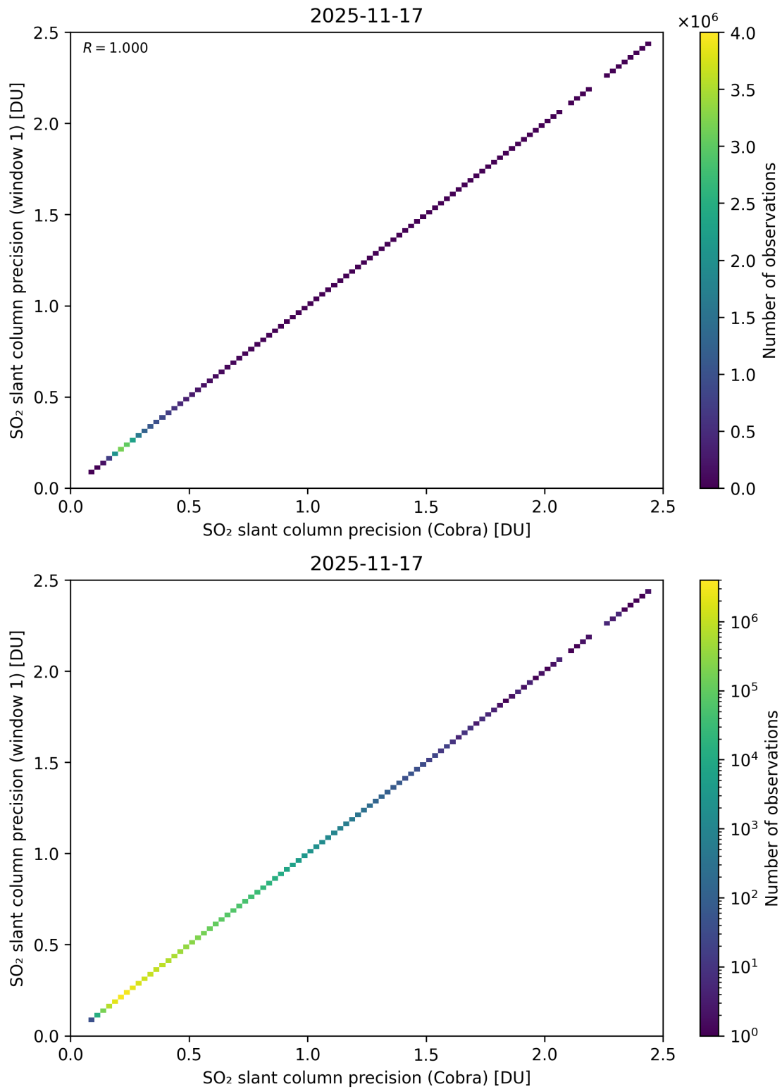
Figure 209: Scatter density plot of “SO 2 slant column precision (Cobra)” against “SO 2 slant column precision (window 1)” for 2025-11-16 to 2025-11-18.
