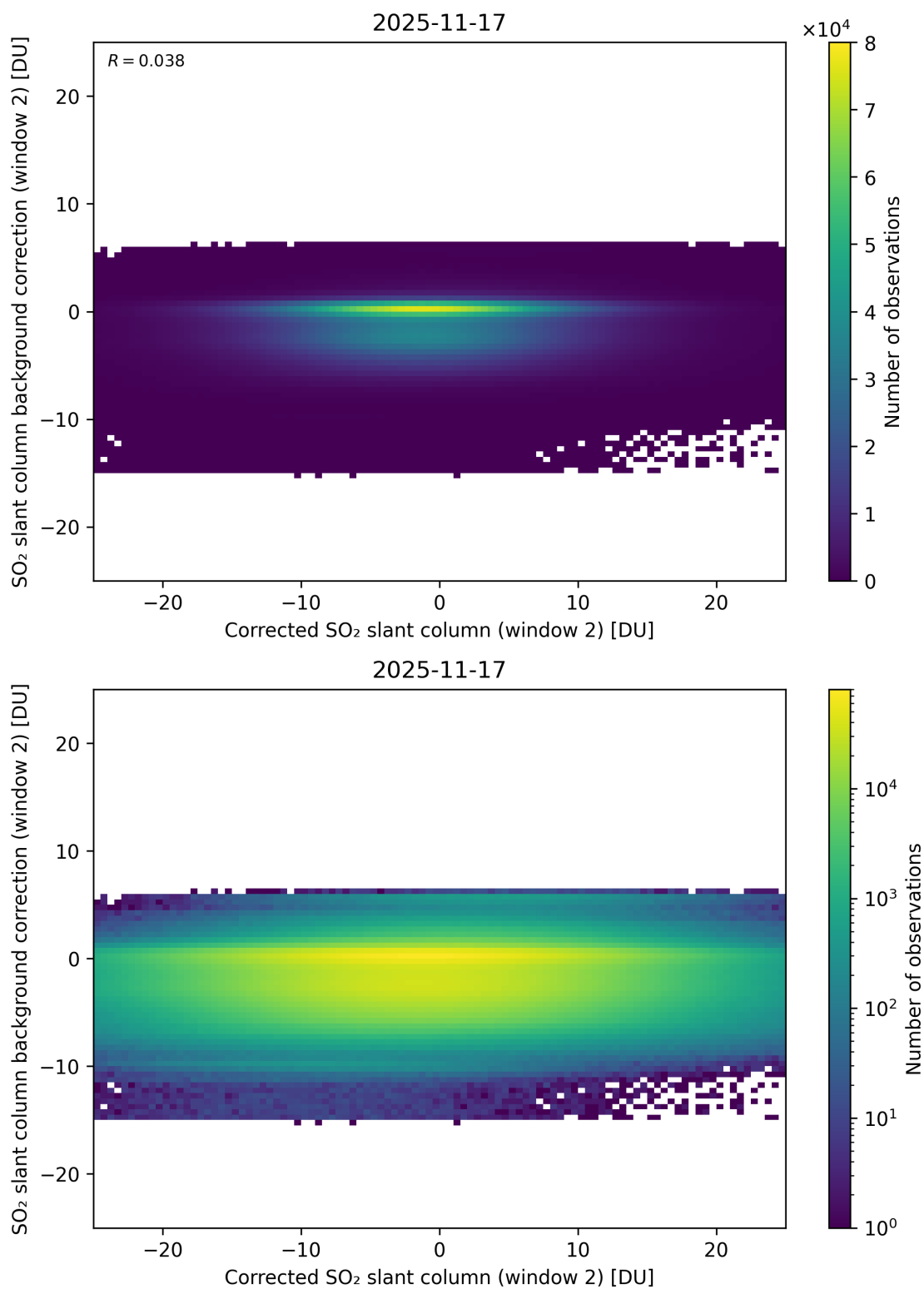
Figure 244: Scatter density plot of “Corrected SO 2 slant column (window 2)” against “SO 2 slant column background correction (window 2)” for 2025-11-16 to 2025-11-18.
