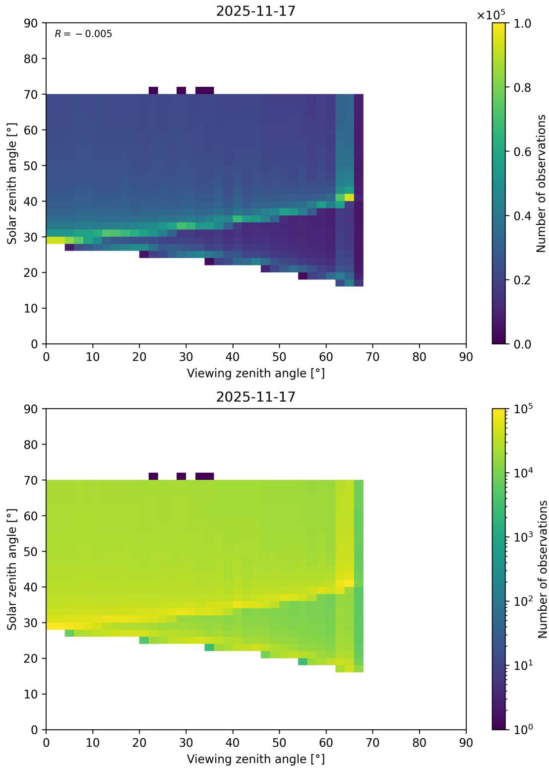
Figure 369: Scatter density plot of “Viewing zenith angle” against “Solar zenith angle” for 2025-11-16 to 2025-11-18.
