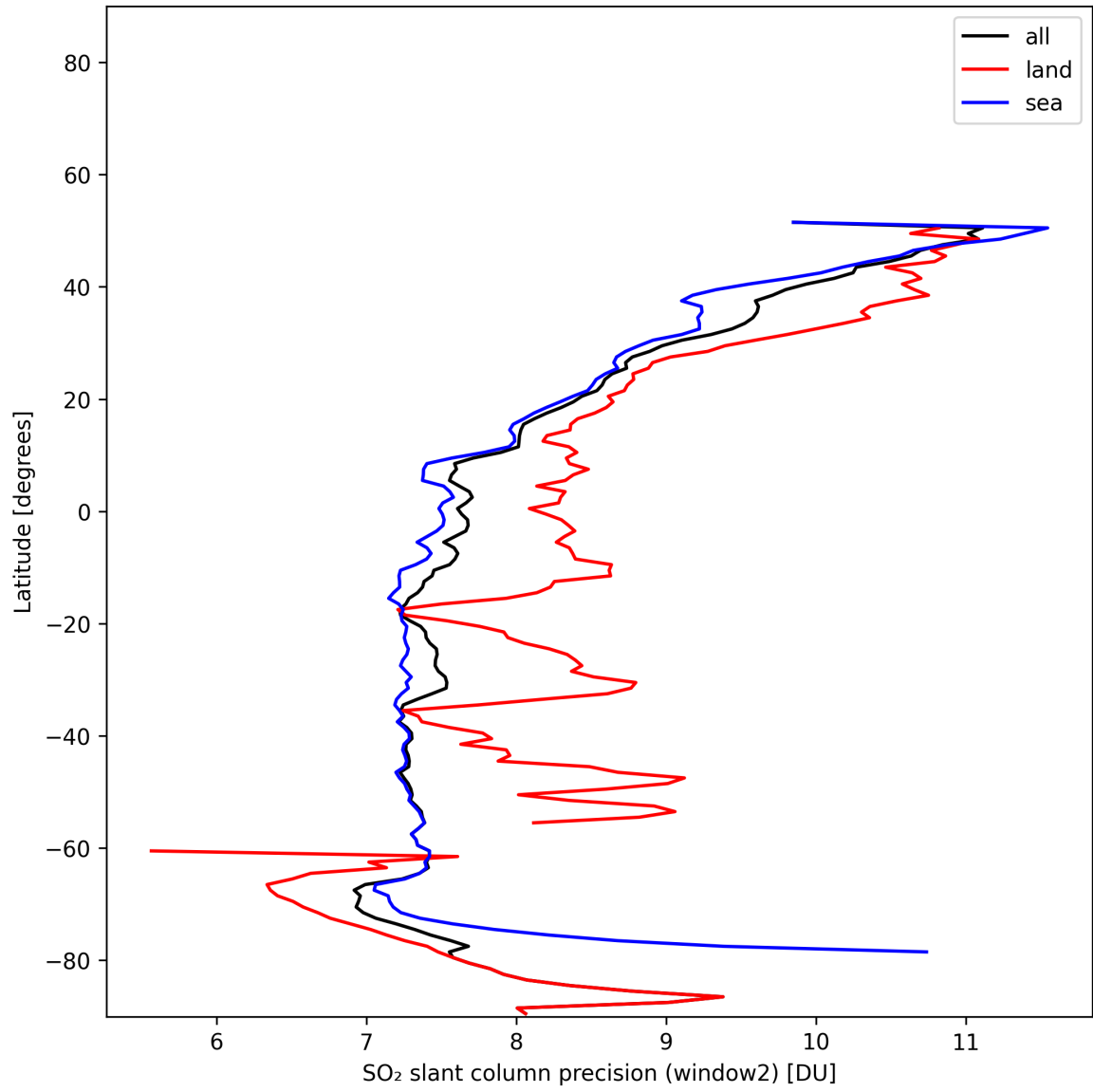
Figure 42: Zonal average of “SO 2 slant column precision (window2)” for 2025-11-16 to 2025-11-18.
