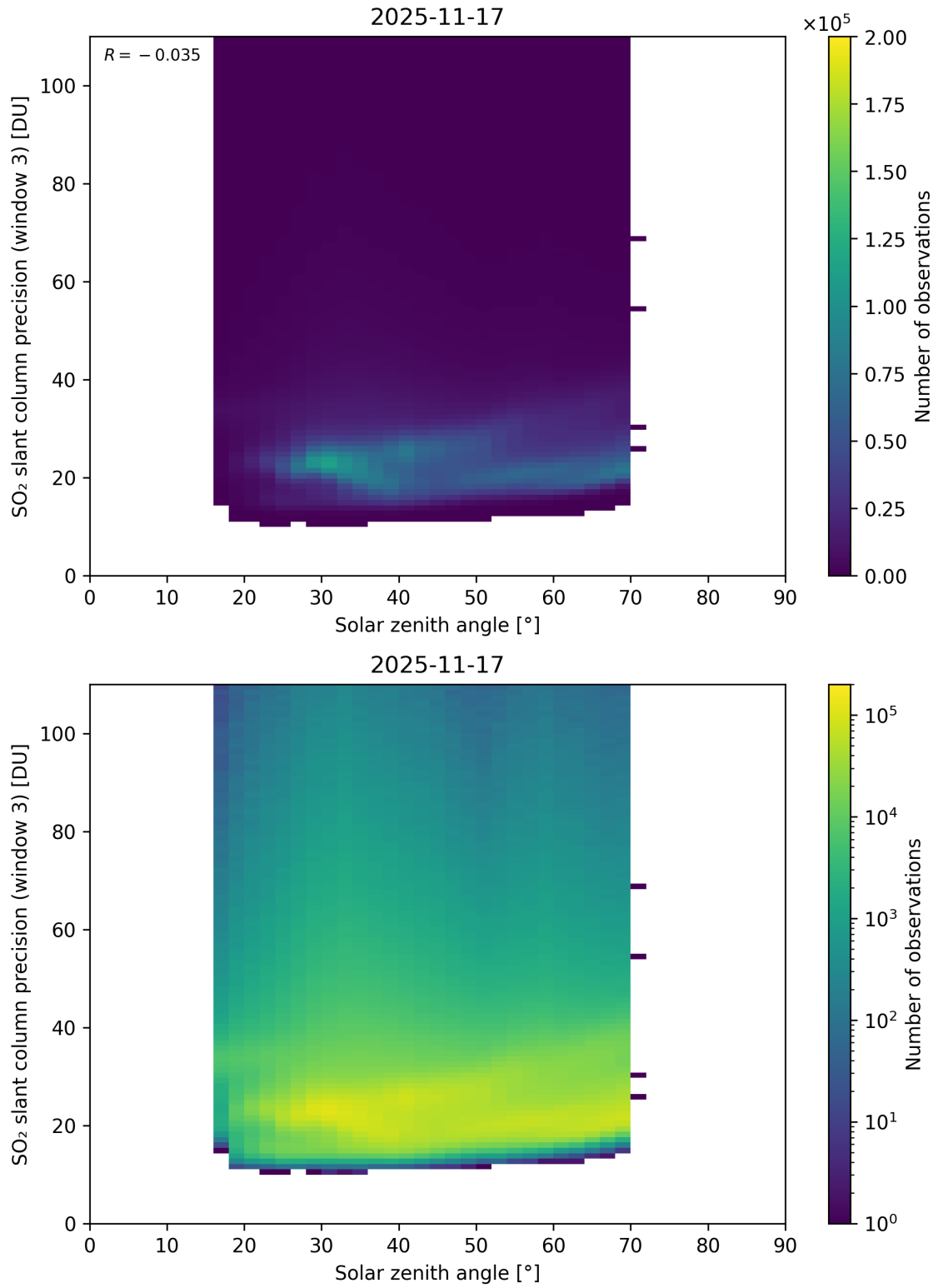
Figure 188: Scatter density plot of “Solar zenith angle” against “SO 2 slant column precision (window 3)” for 2025-11-16 to 2025-11-18.
