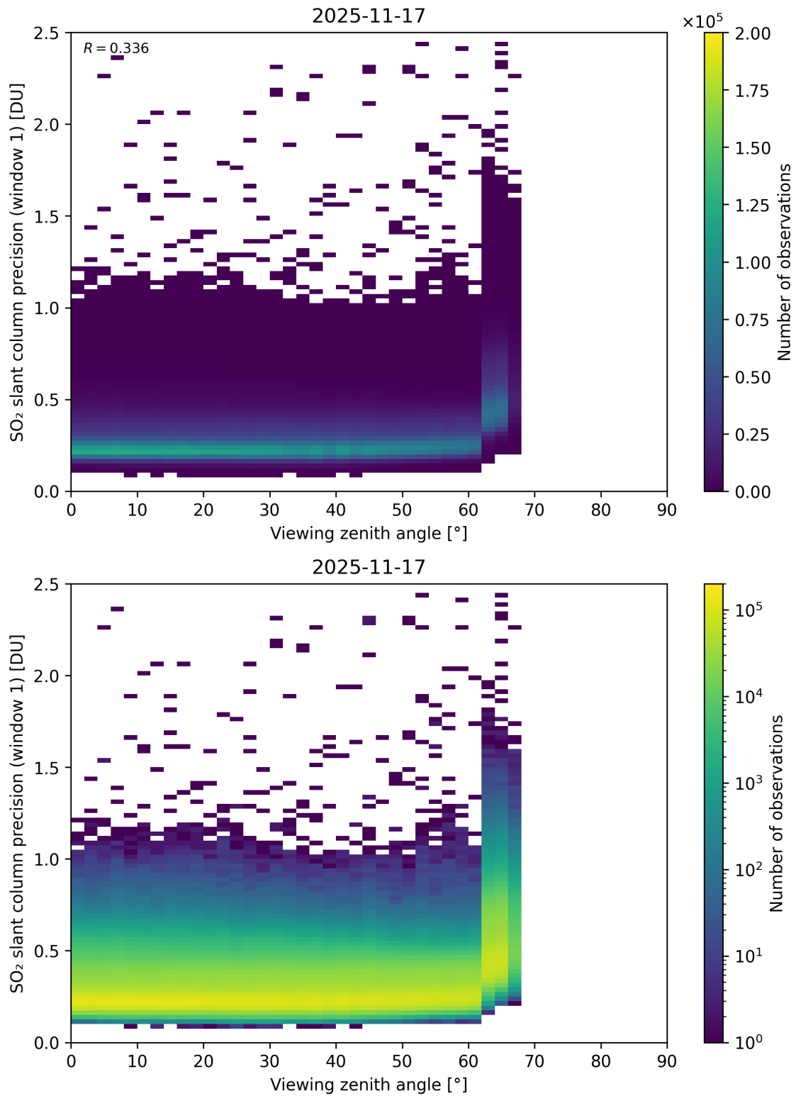
Figure 377: Scatter density plot of “Viewing zenith angle” against “SO 2 slant column precision (window 1)” for 2025-11-16 to 2025-11-18.
