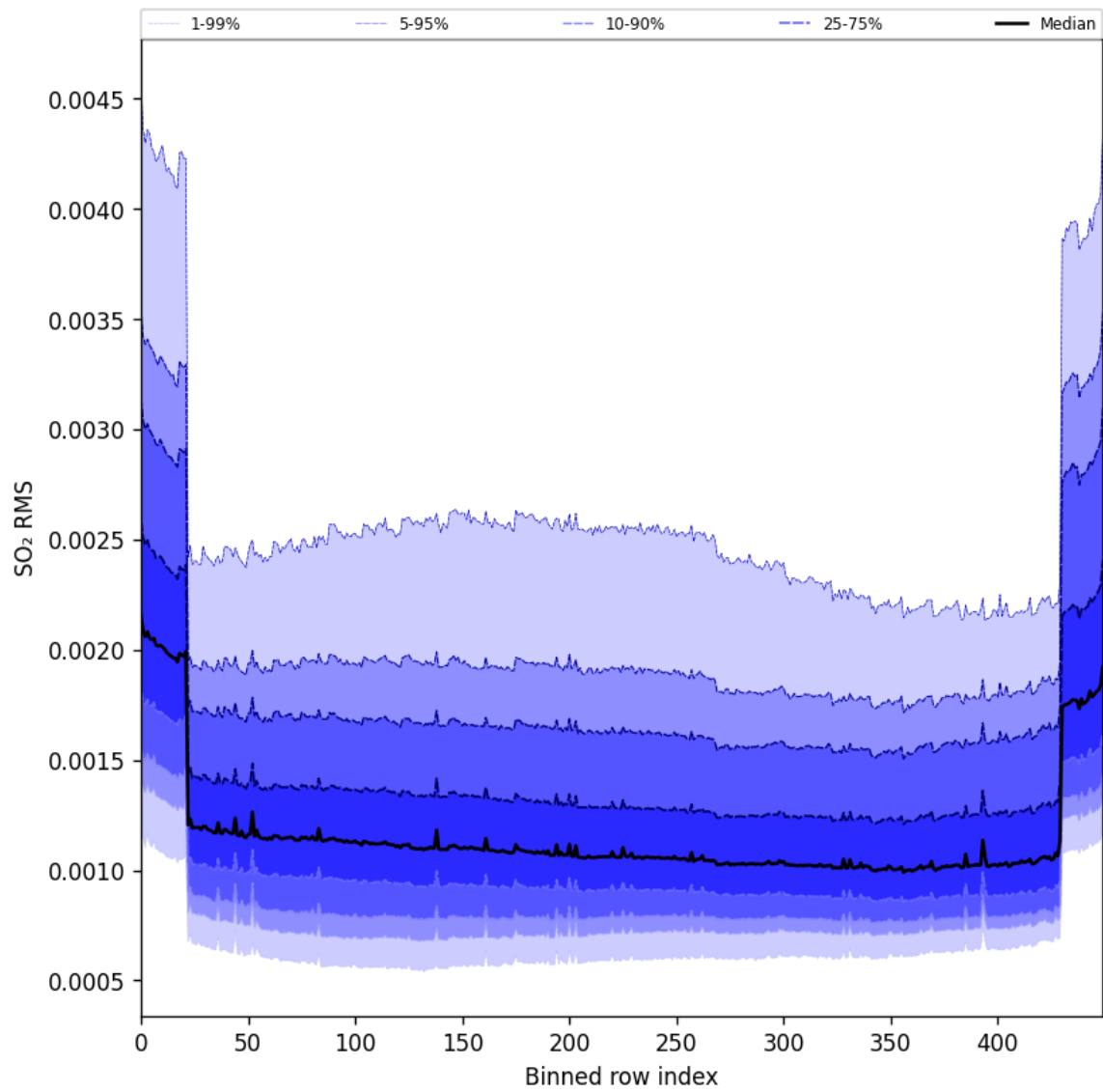
Figure 104: Along track statistics of “SO 2 RMS” for 2025-11-16 to 2025-11-18
