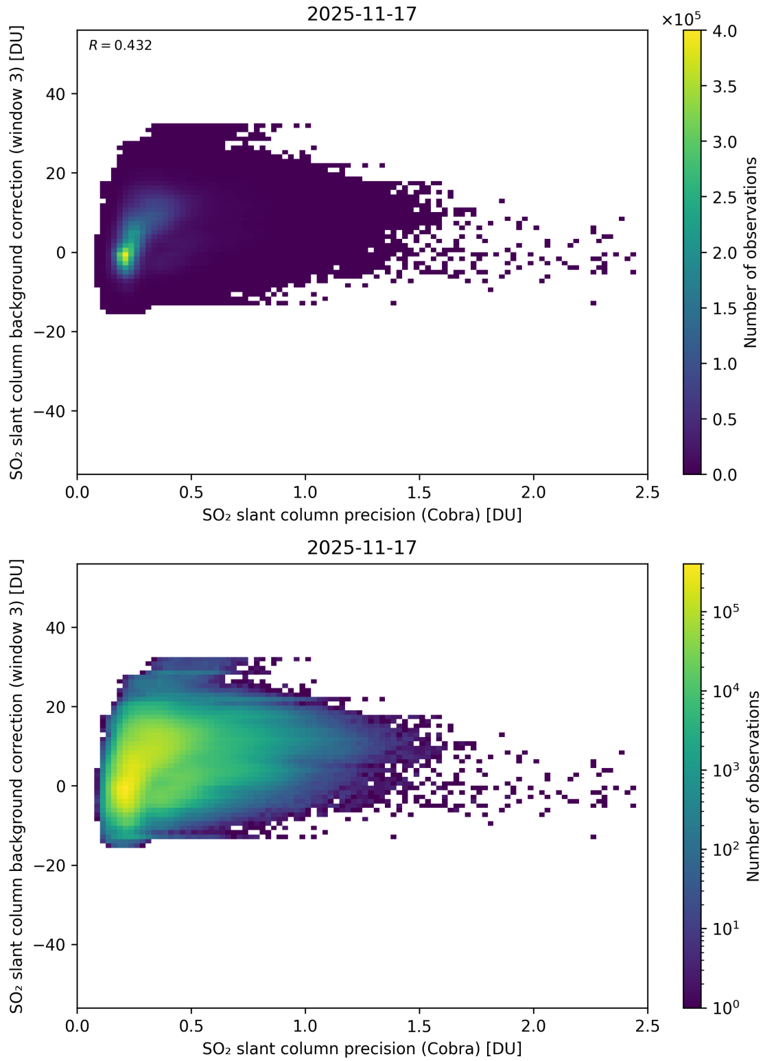
Figure 201: Scatter density plot of “SO 2 slant column precision (Cobra)” against “SO 2 slant column background correction (window 3)” for 2025-11-16 to 2025-11-18.
