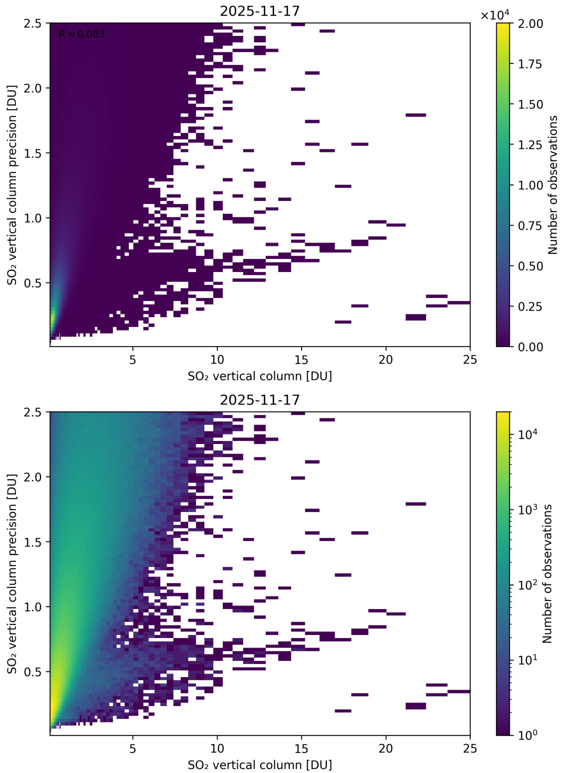
Figure 361: Scatter density plot of “SO 2 vertical column” against “SO 2 vertical column precision” for 2025-11-16 to 2025-11-18.
