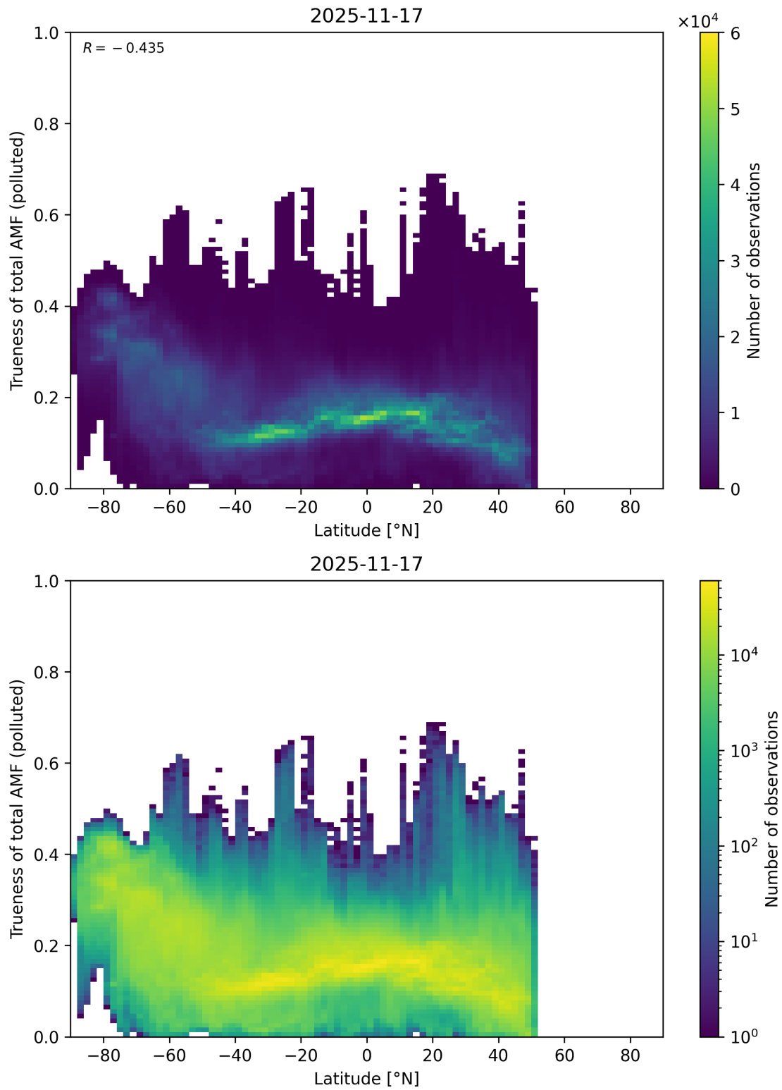
Figure 168: Scatter density plot of “Latitude” against “Trueness of total AMF (polluted)” for 2025-11-16 to 2025-11-18.
