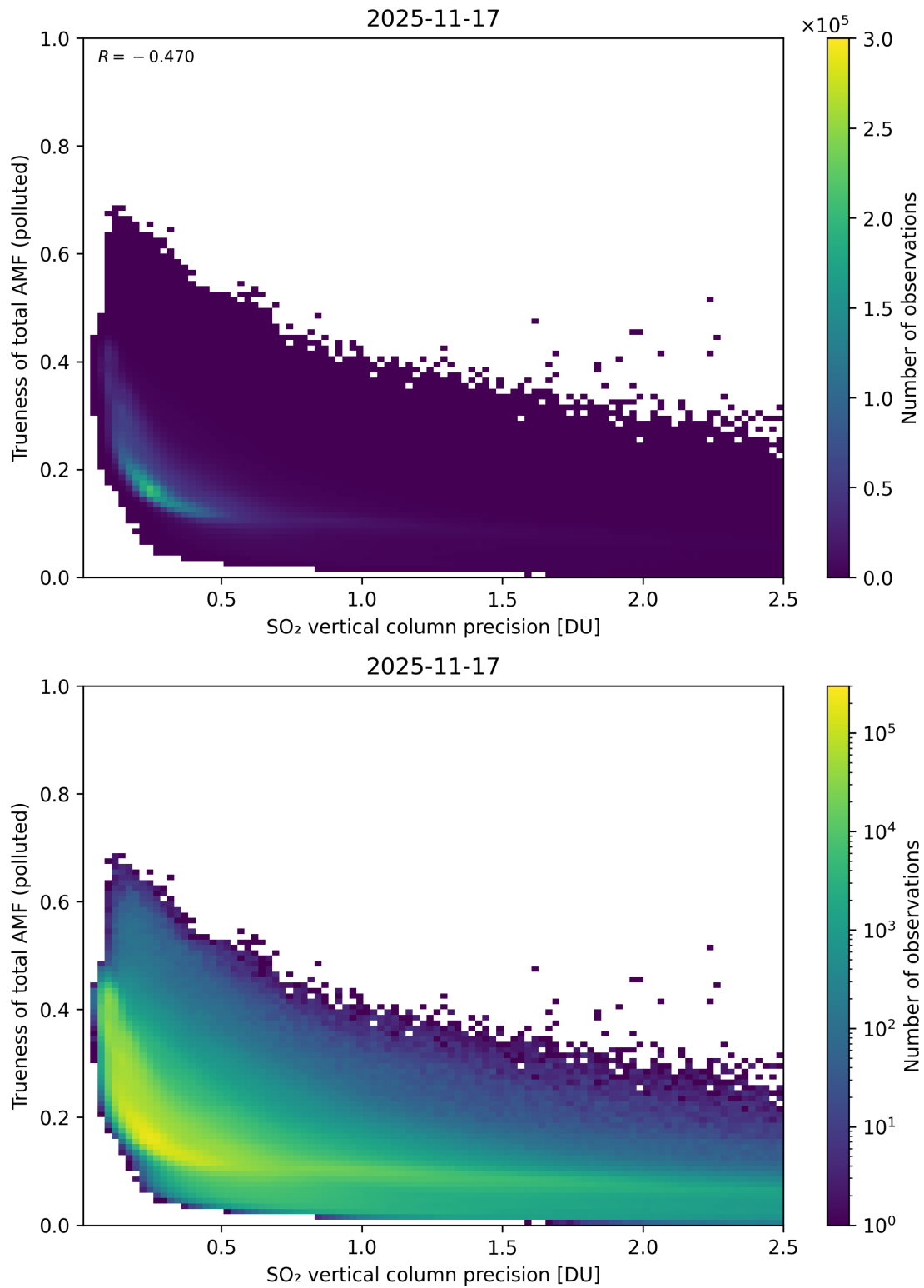
Figure 347: Scatter density plot of “SO 2 vertical column precision” against “Trueness of total AMF (polluted)” for 2025-11-16 to 2025-11-18.
