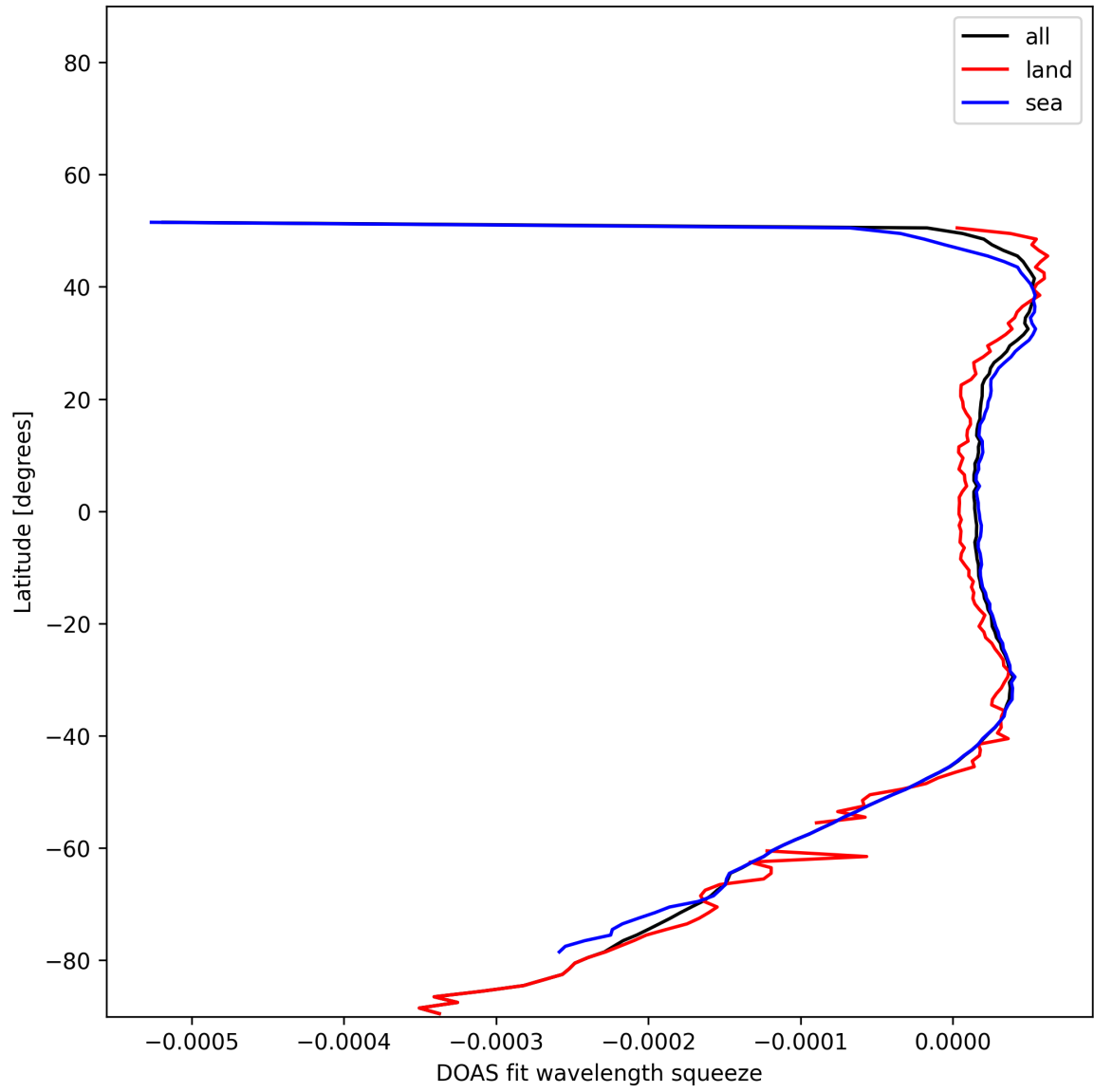
Figure 51: Zonal average of “DOAS fit wavelength squeeze” for 2025-11-16 to 2025-11-18.
