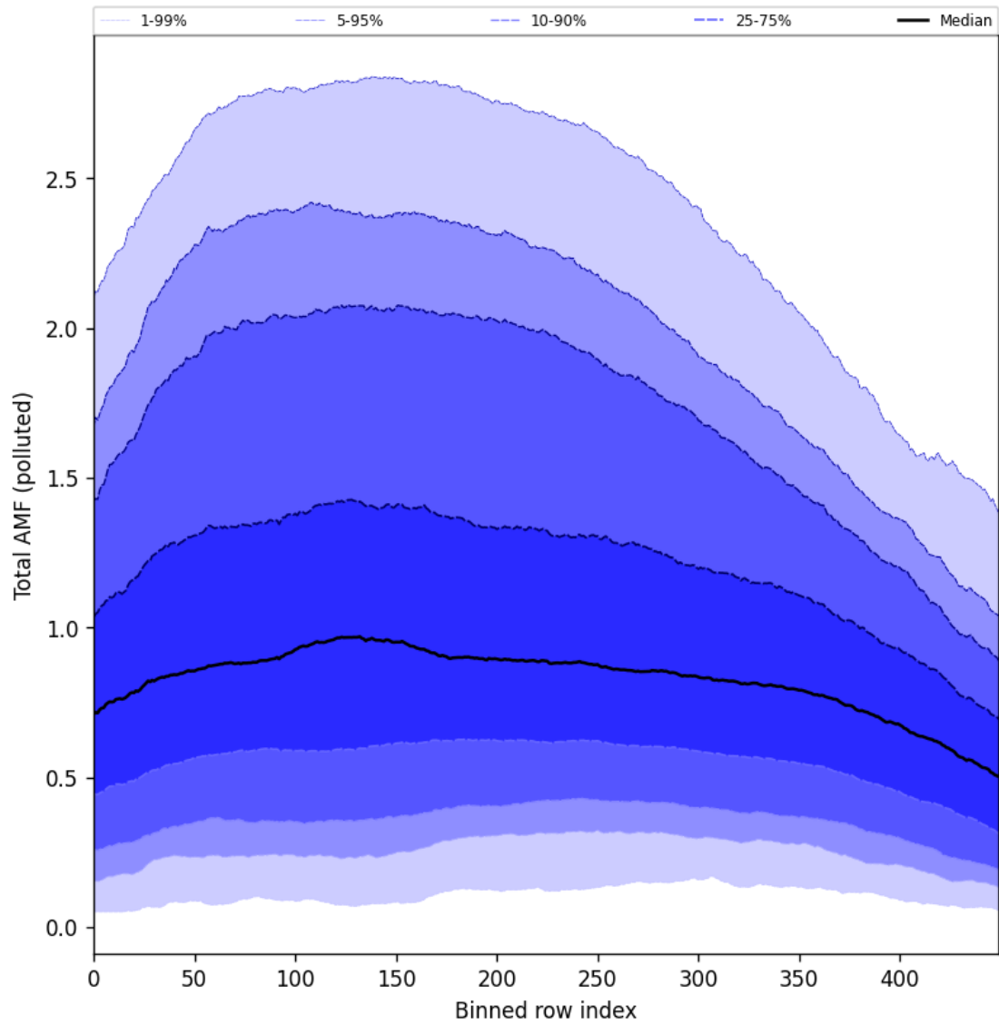
Figure 105: Along track statistics of “Total AMF (polluted)” for 2025-11-16 to 2025-11-18
