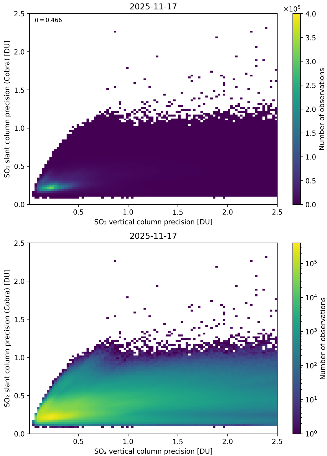
Figure 337: Scatter density plot of “SO 2 vertical column precision” against “SO 2 slant column precision (Cobra)” for 2025-11-16 to 2025-11-18.
