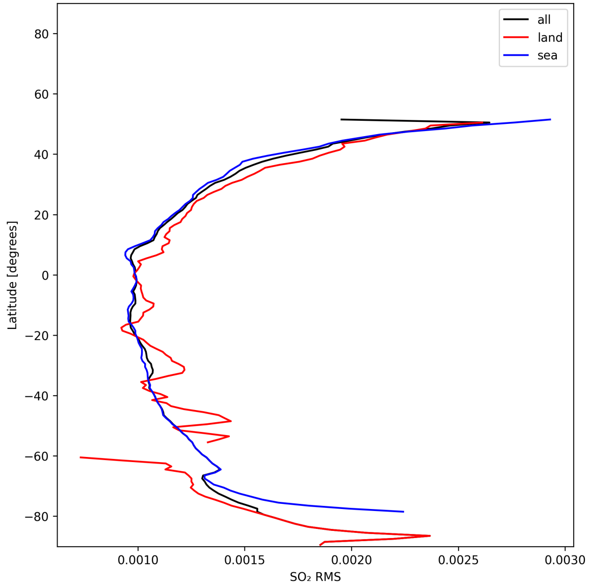
Figure 52: Zonal average of “SO 2 RMS” for 2025-11-16 to 2025-11-18.
