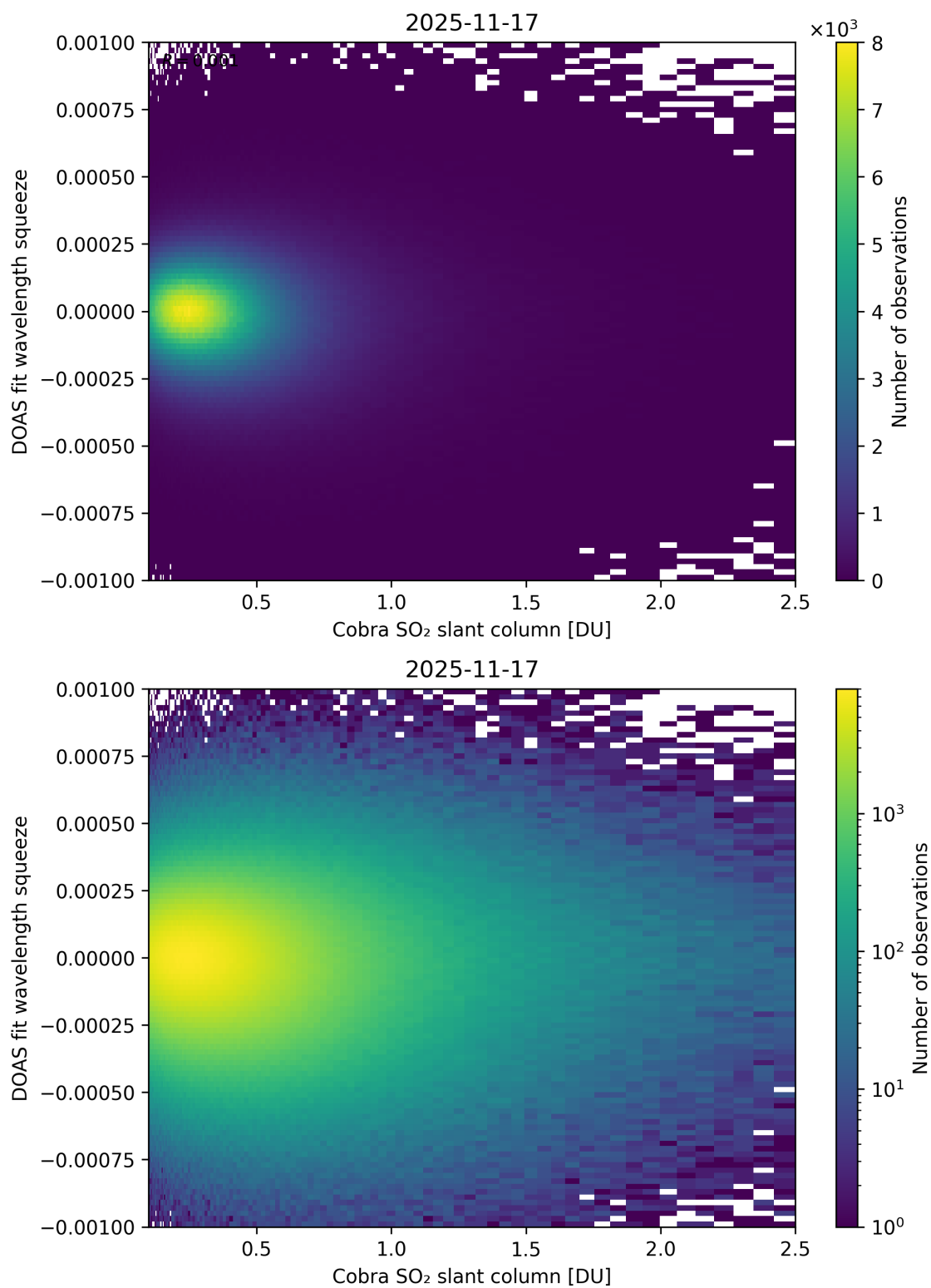
Figure 197: Scatter density plot of “Cobra SO 2 slant column” against “DOAS fit wavelength squeeze” for 2025-11-16 to 2025-11-18.
