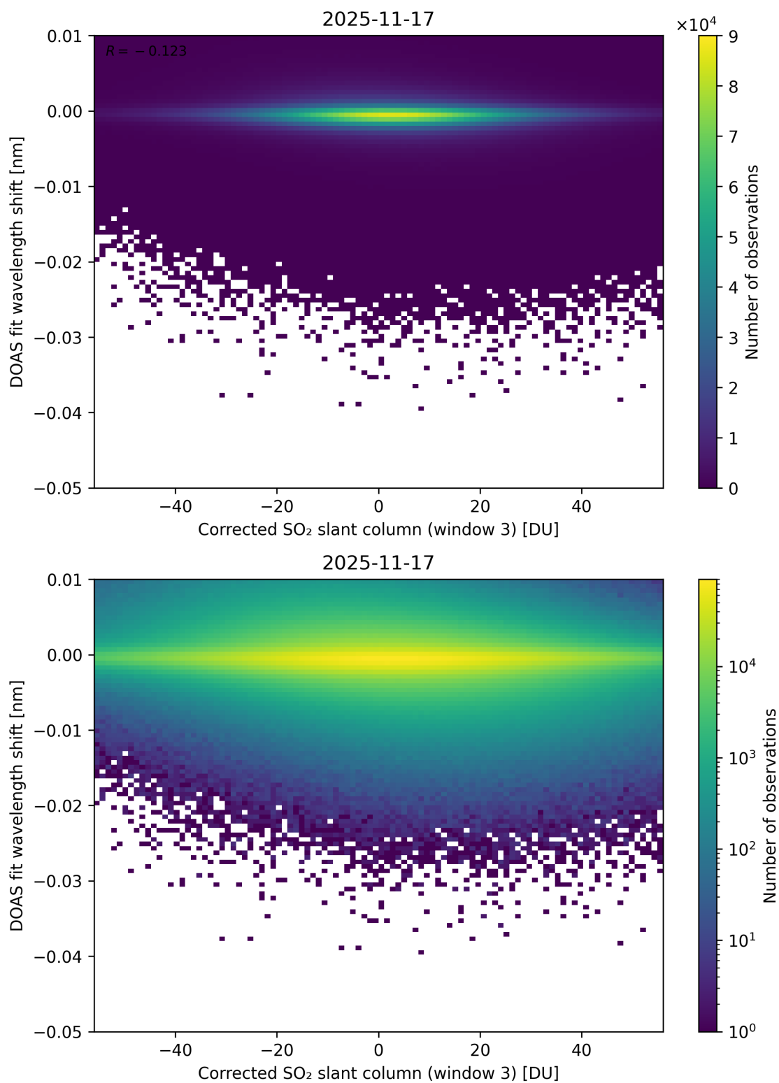
Figure 256: Scatter density plot of “Corrected SO 2 slant column (window 3)” against “DOAS fit wavelength shift” for 2025-11-16 to 2025-11-18.
