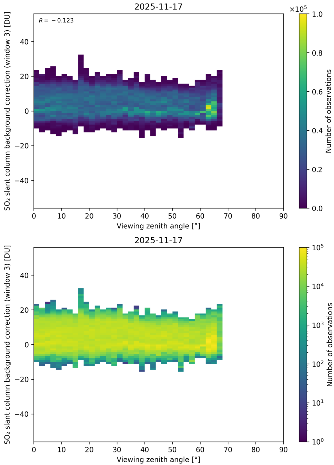
Figure 364: Scatter density plot of “Viewing zenith angle” against “SO 2 slant column background correction (window 3)” for 2025-11-16 to 2025-11-18.
