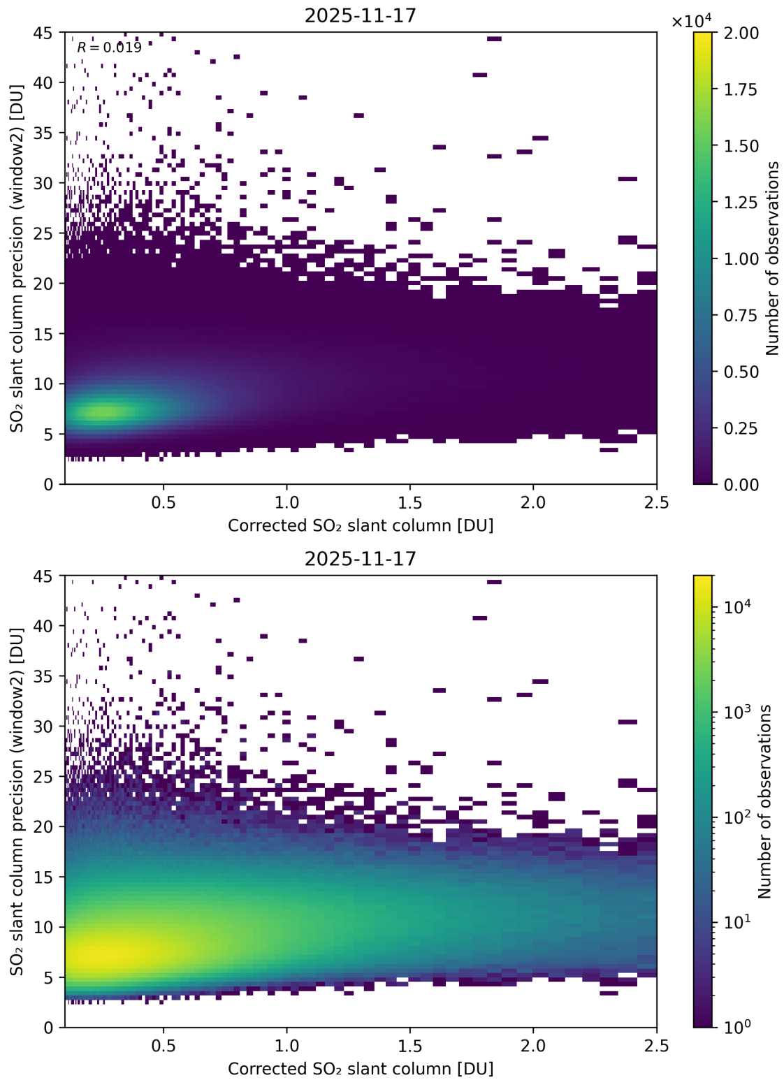
Figure 239: Scatter density plot of “Corrected SO 2 slant column” against “SO 2 slant column precision (window2)” for 2025-11-16 to 2025-11-18.
