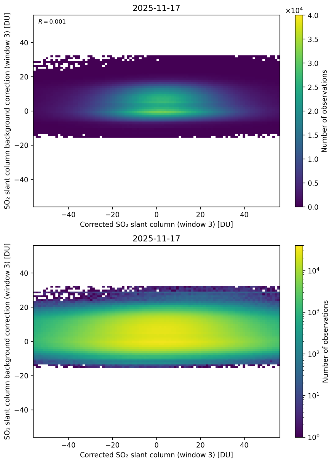
Figure 255: Scatter density plot of “Corrected SO 2 slant column (window 3)” against “SO 2 slant column background correction (window 3)” for 2025-11-16 to 2025-11-18.
