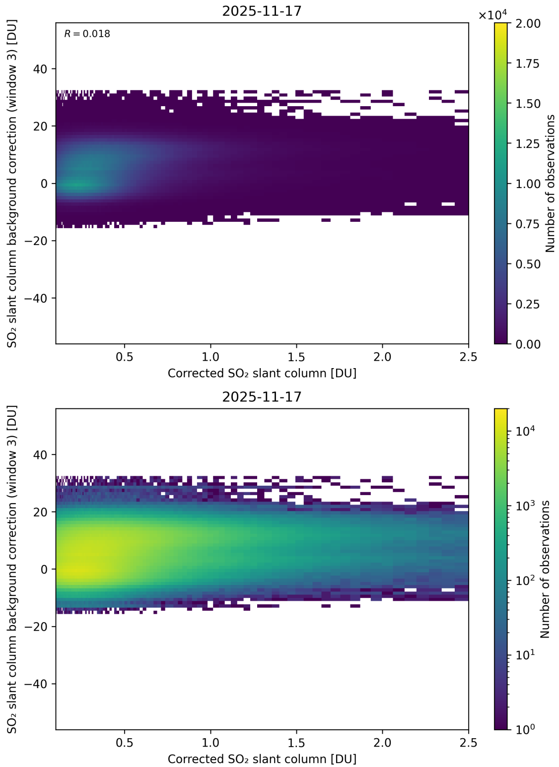
Figure 228: Scatter density plot of “Corrected SO 2 slant column” against “SO 2 slant column background correction (window 3)” for 2025-11-16 to 2025-11-18.
