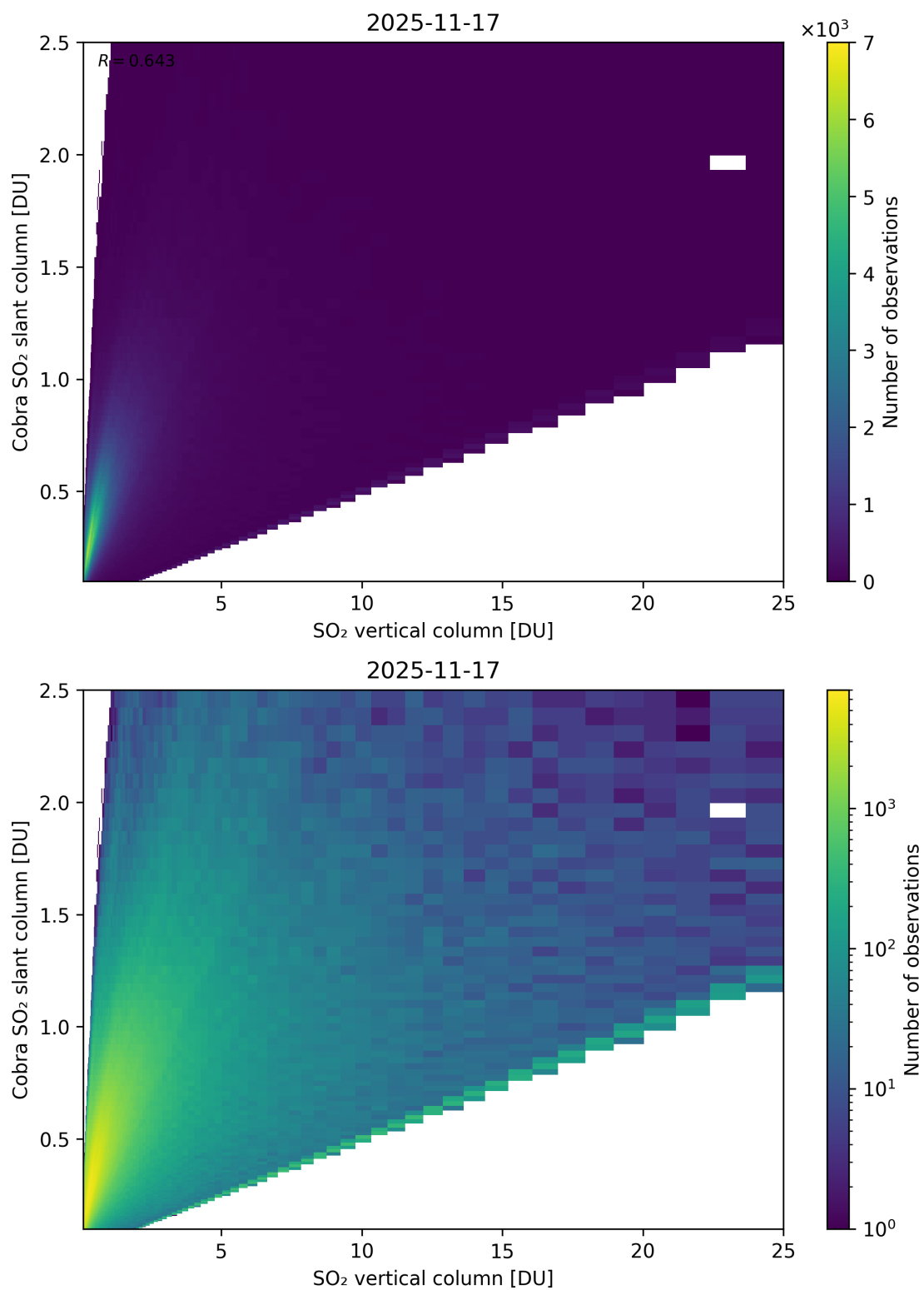
Figure 349: Scatter density plot of “SO 2 vertical column” against “Cobra SO 2 slant column” for 2025-11-16 to 2025-11-18.
