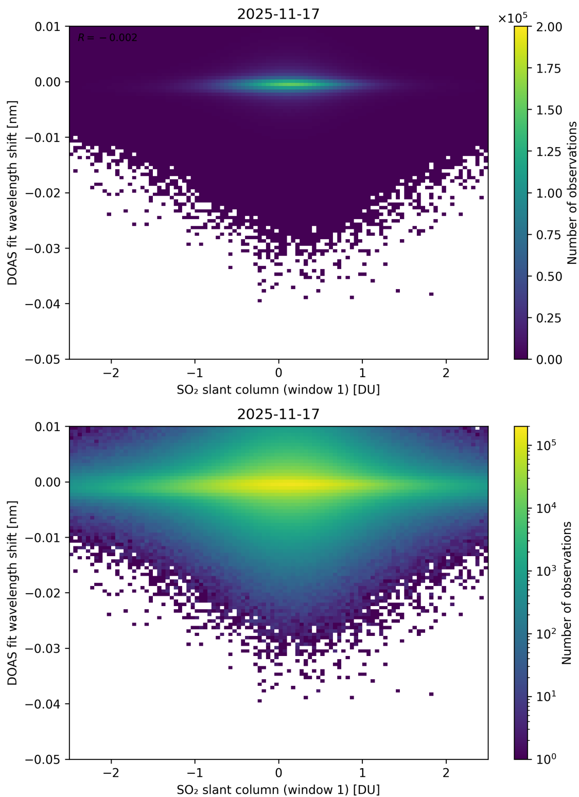
Figure 265: Scatter density plot of “SO 2 slant column (window 1)” against “DOAS fit wavelength shift” for 2025-11-16 to 2025-11-18.
