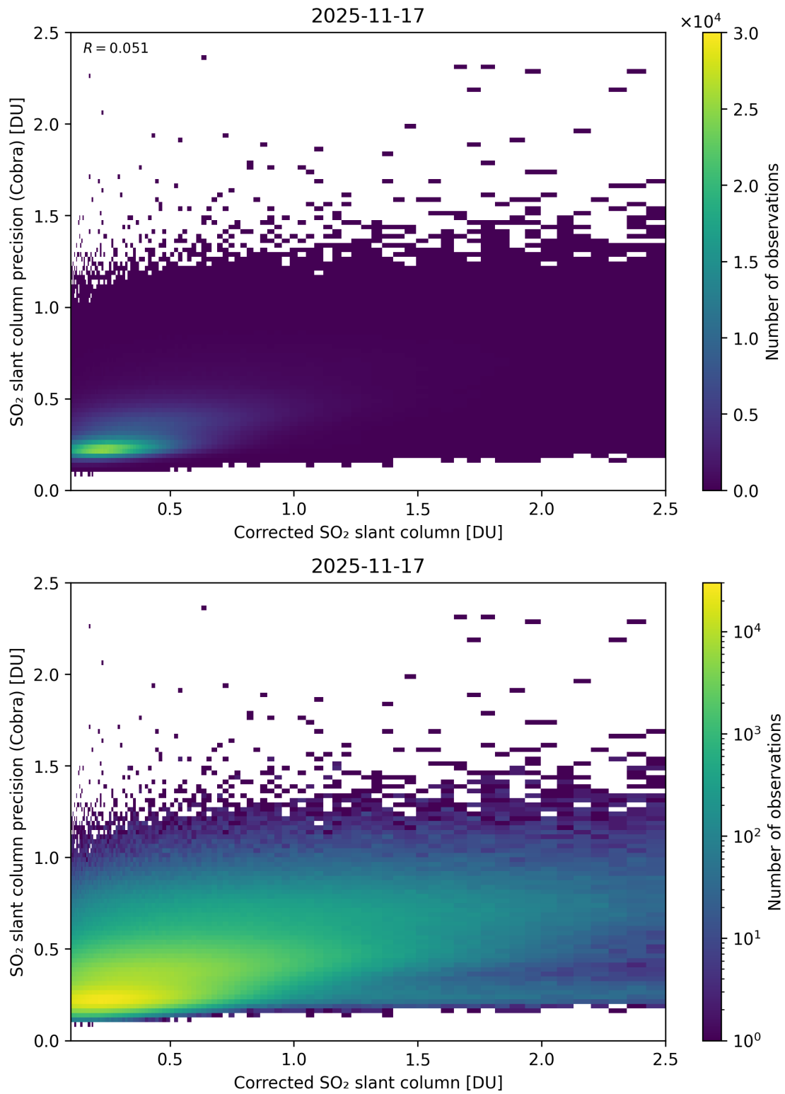
Figure 234: Scatter density plot of “Corrected SO 2 slant column” against “SO 2 slant column precision (Cobra)” for 2025-11-16 to 2025-11-18.
