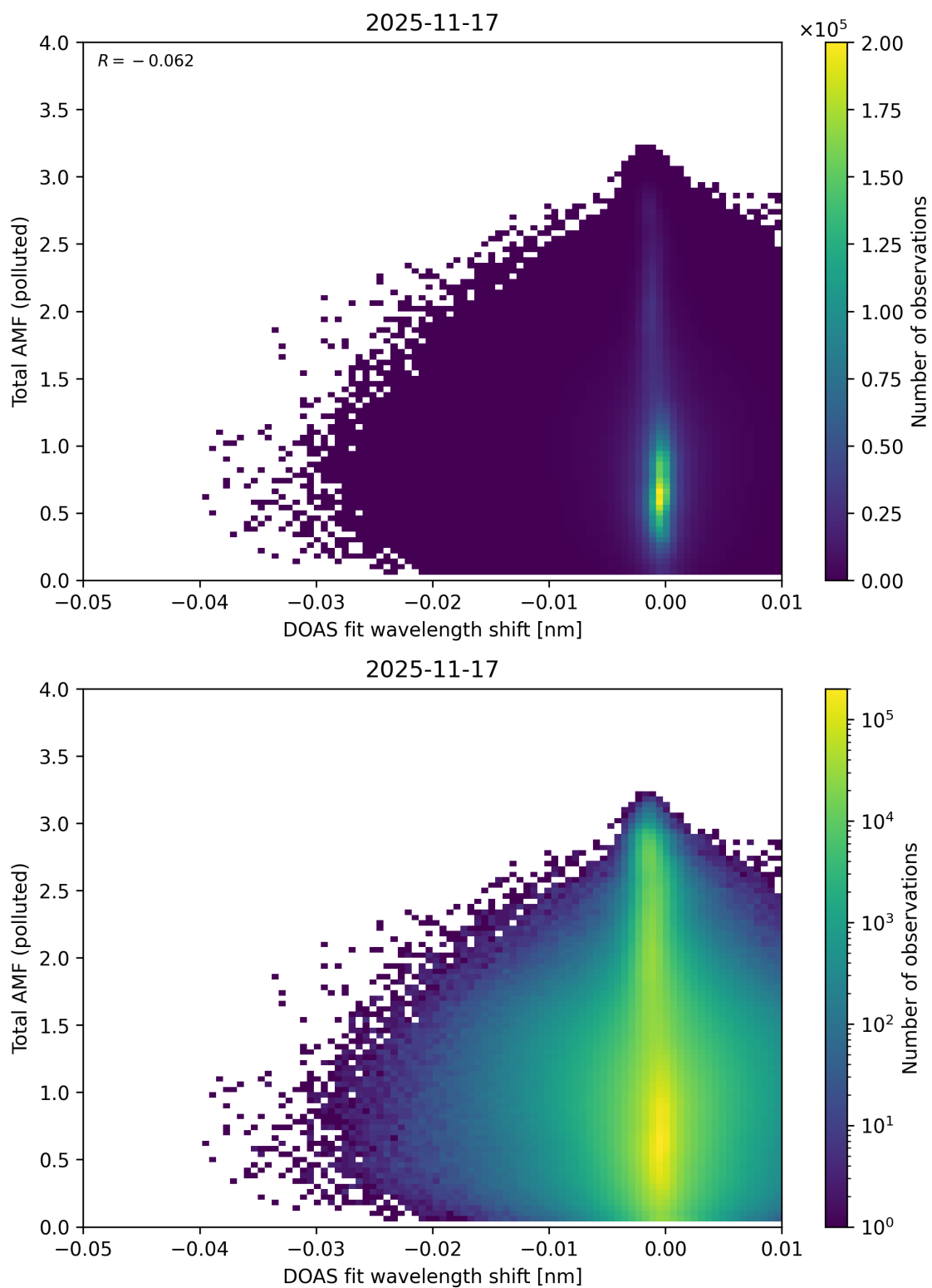
Figure 141: Scatter density plot of “DOAS fit wavelength shift” against “Total AMF (polluted)” for 2025-11-16 to 2025-11-18.
