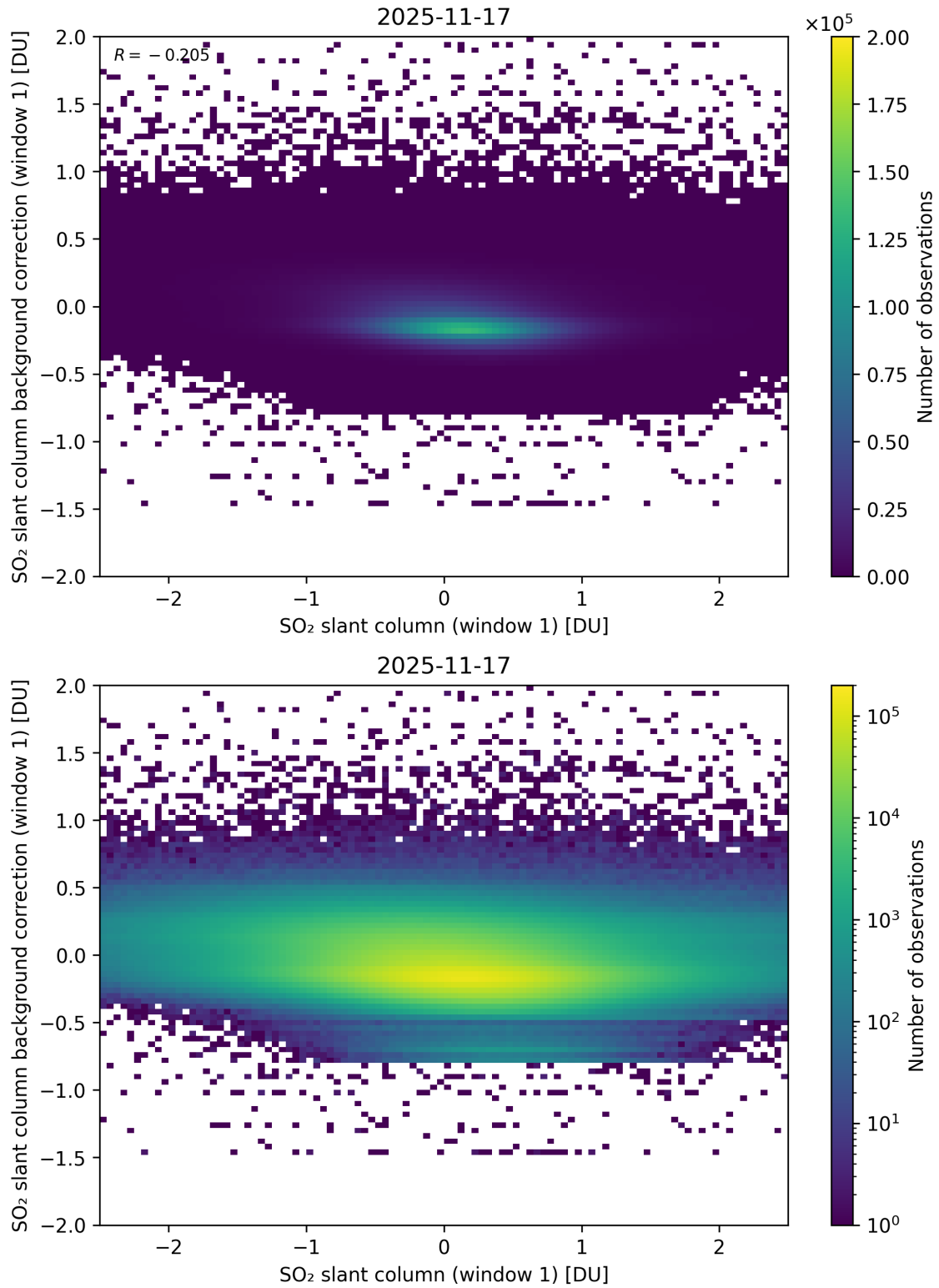
Figure 262: Scatter density plot of “SO 2 slant column (window 1)” against “SO 2 slant column background correction (window 1)” for 2025-11-16 to 2025-11-18.
