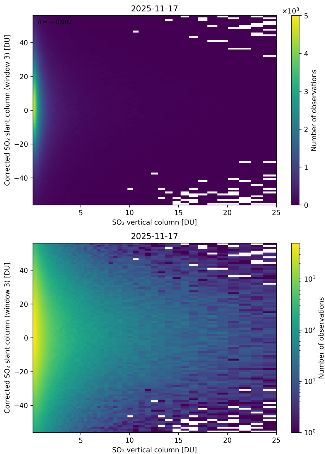
Figure 353: Scatter density plot of “SO 2 vertical column” against “Corrected SO 2 slant column (window 3)” for 2025-11-16 to 2025-11-18.
