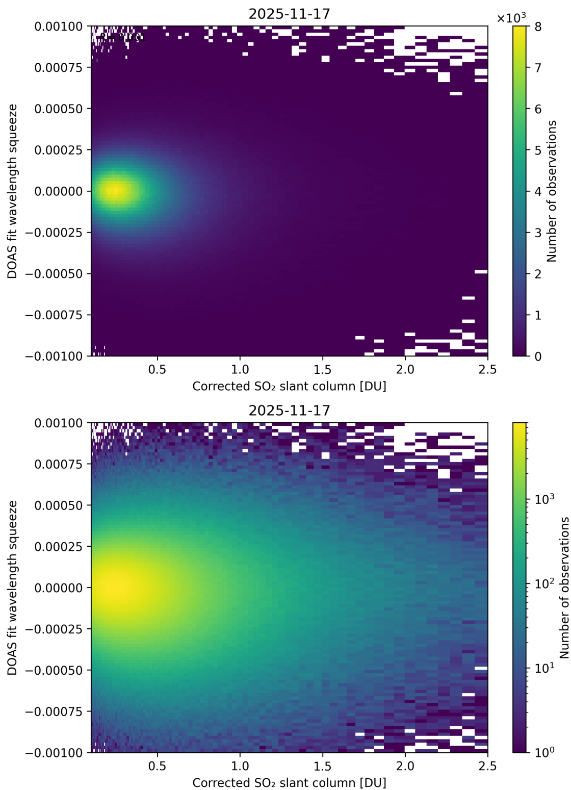
Figure 230: Scatter density plot of “Corrected SO 2 slant column” against “DOAS fit wavelength squeeze” for 2025-11-16 to 2025-11-18.
