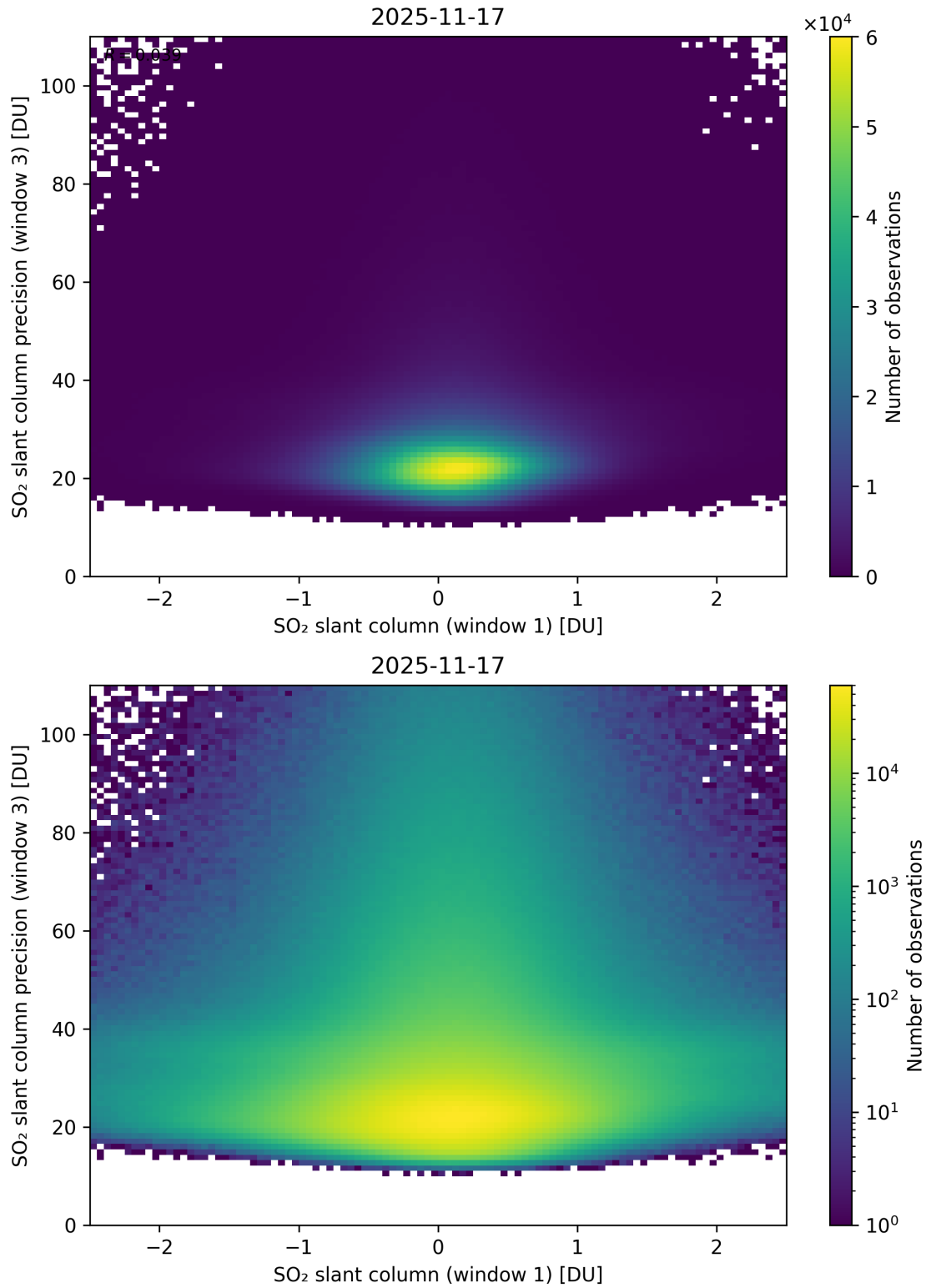
Figure 288: Scatter density plot of “SO 2 slant column (window 1)” against “SO 2 slant column precision (window 3)” for 2025-11-16 to 2025-11-18.
