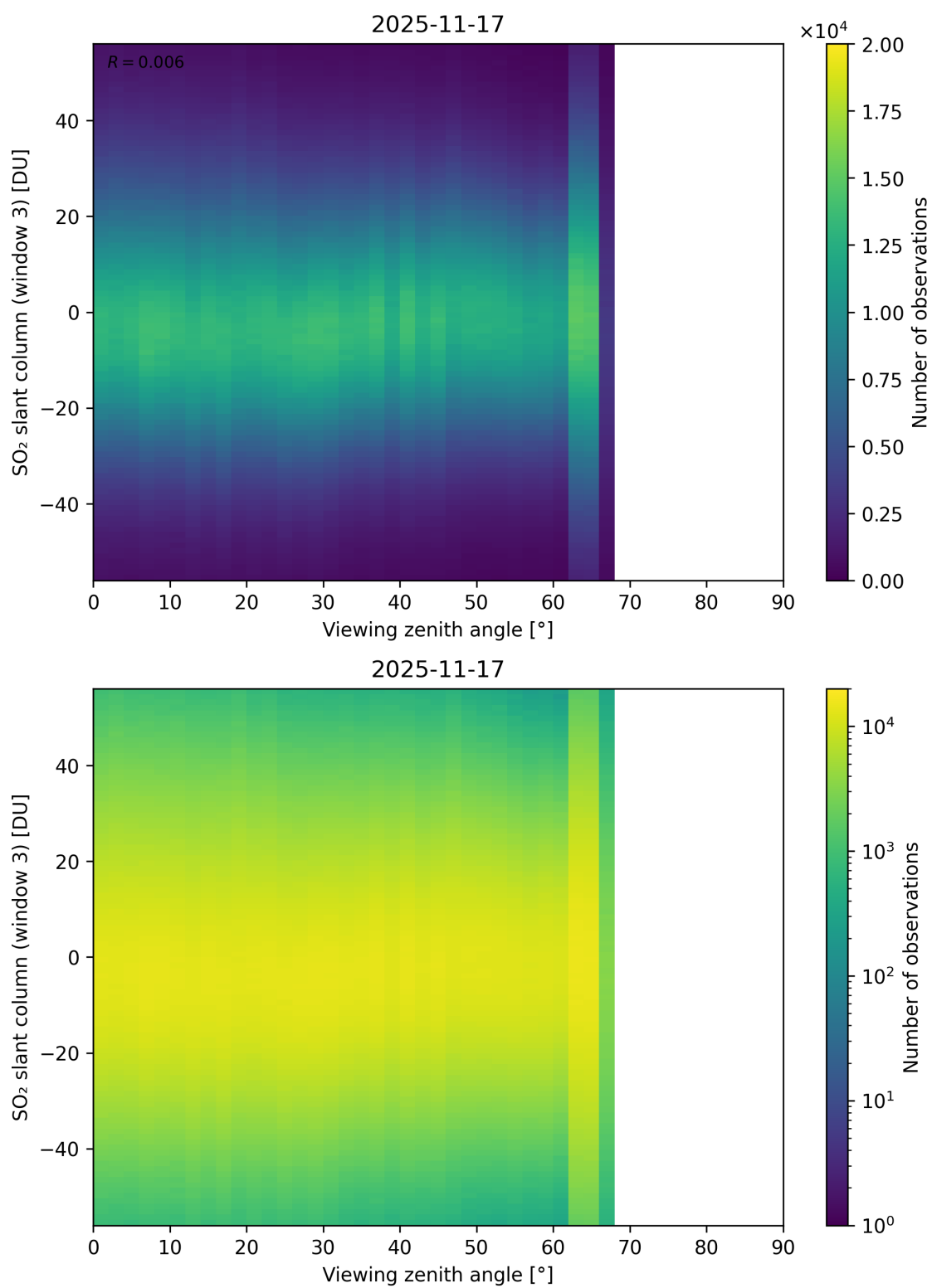
Figure 379: Scatter density plot of “Viewing zenith angle” against “SO 2 slant column (window 3)” for 2025-11-16 to 2025-11-18.
