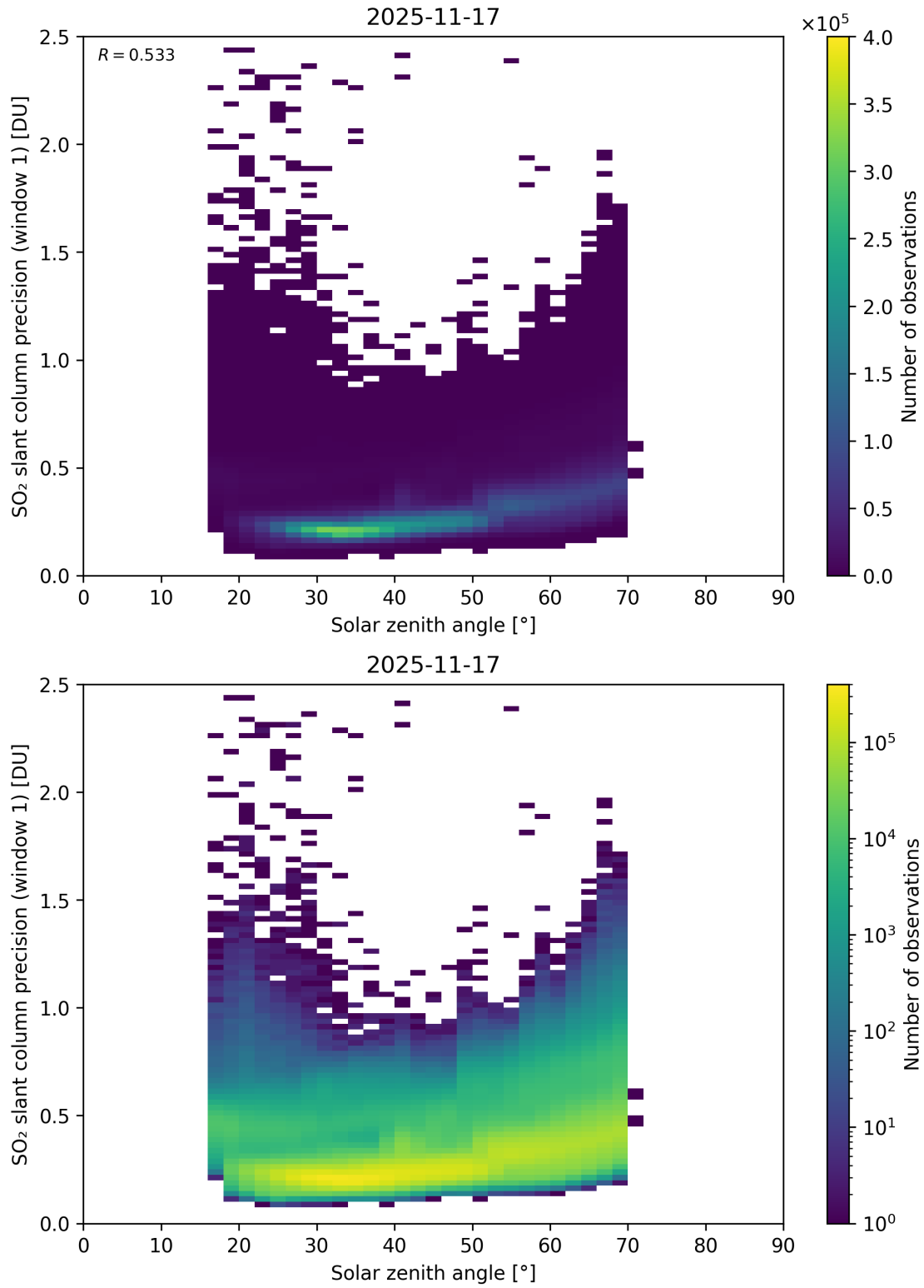
Figure 185: Scatter density plot of “Solar zenith angle” against “SO 2 slant column precision (window 1)” for 2025-11-16 to 2025-11-18.
