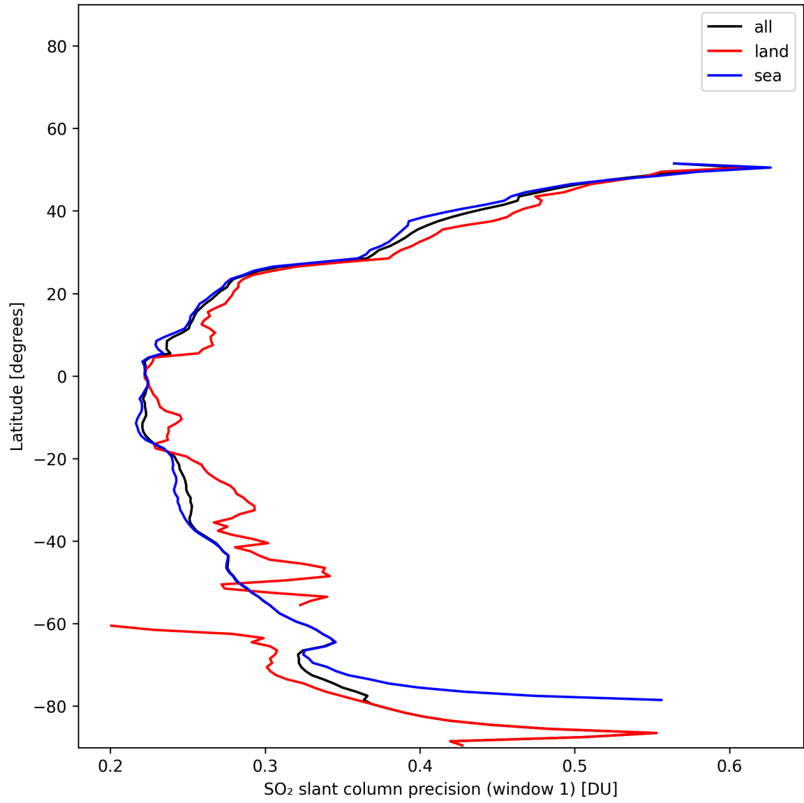
Figure 38: Zonal average of “SO 2 slant column precision (window 1)” for 2025-11-16 to 2025-11-18.
