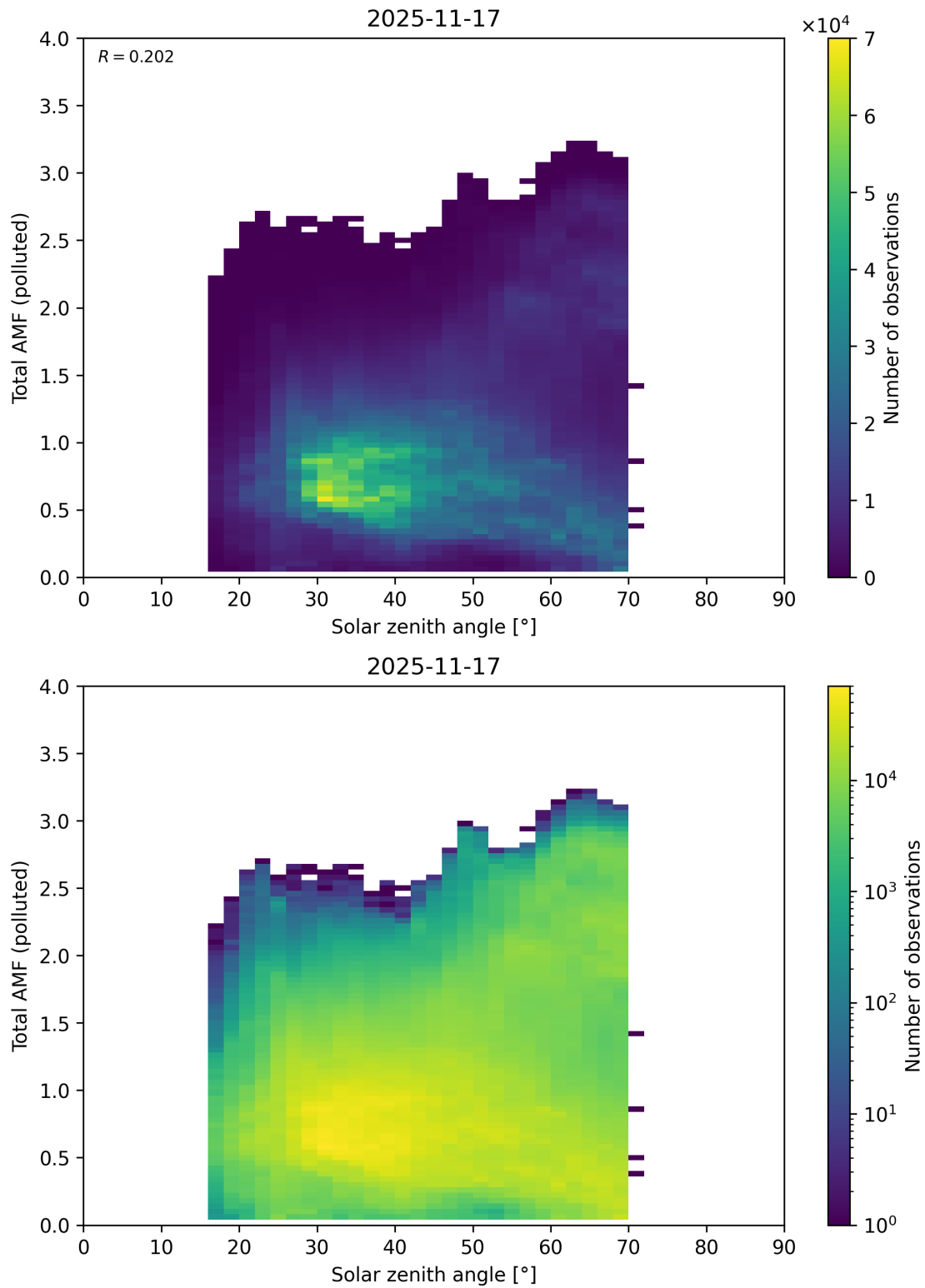
Figure 189: Scatter density plot of “Solar zenith angle” against “Total AMF (polluted)” for 2025-11-16 to 2025-11-18.
