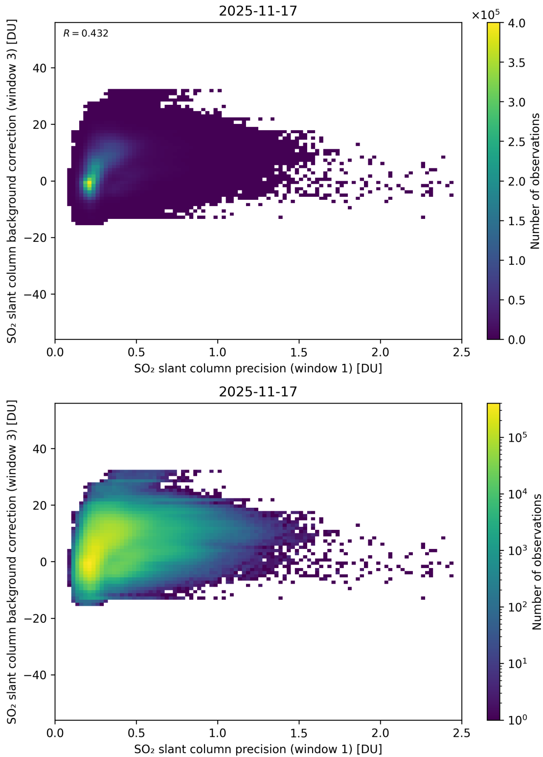
Figure 270: Scatter density plot of “SO 2 slant column precision (window 1)” against “SO 2 slant column background correction (window 3)” for 2025-11-16 to 2025-11-18.
