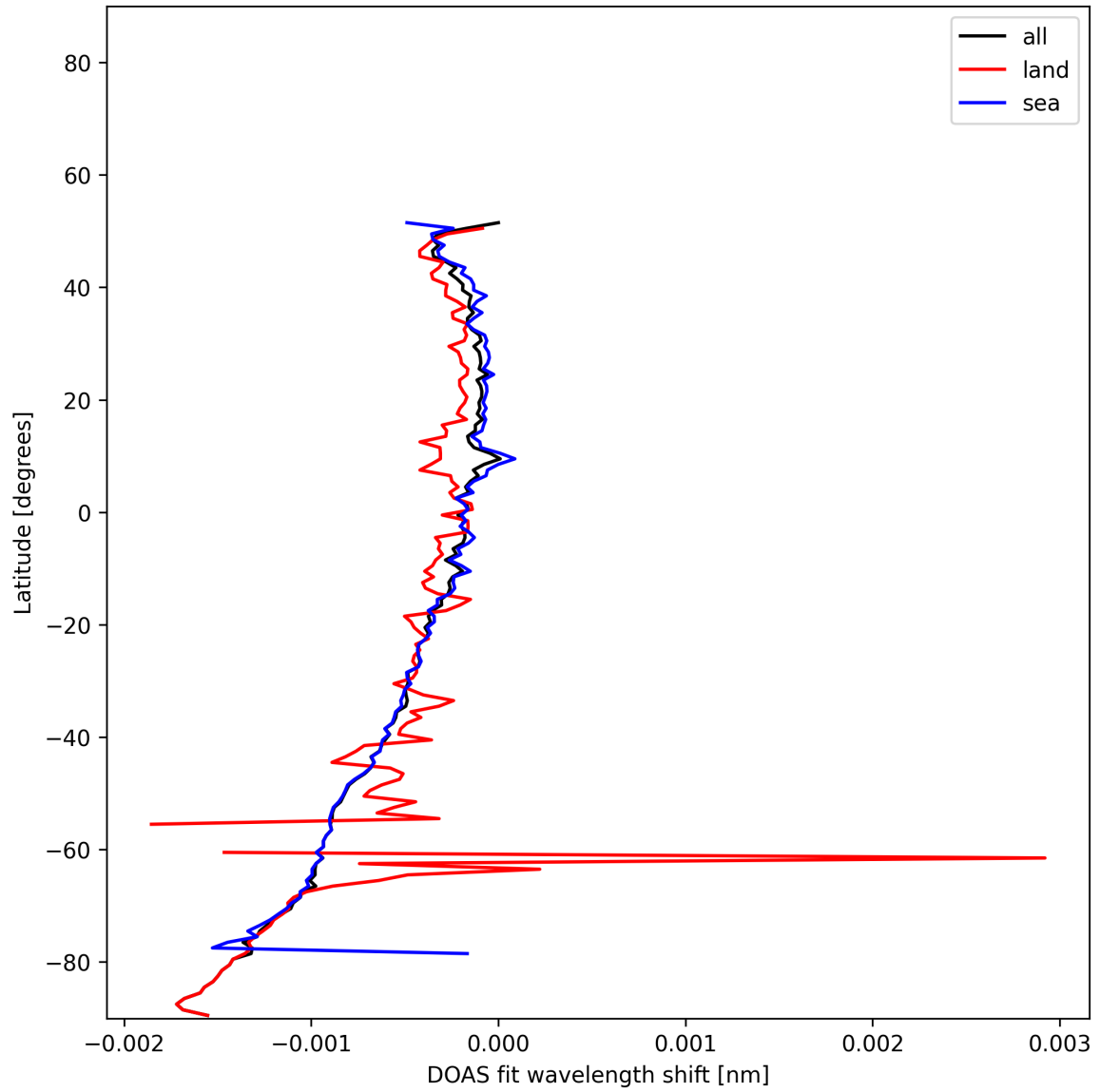
Figure 50: Zonal average of "DOAS fit wavelength shift" for 2025-11-16 to 2025-11-18.
