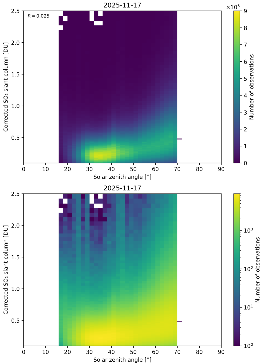
Figure 181: Scatter density plot of “Solar zenith angle” against “Corrected SO 2 slant column” for 2025-11-16 to 2025-11-18.
