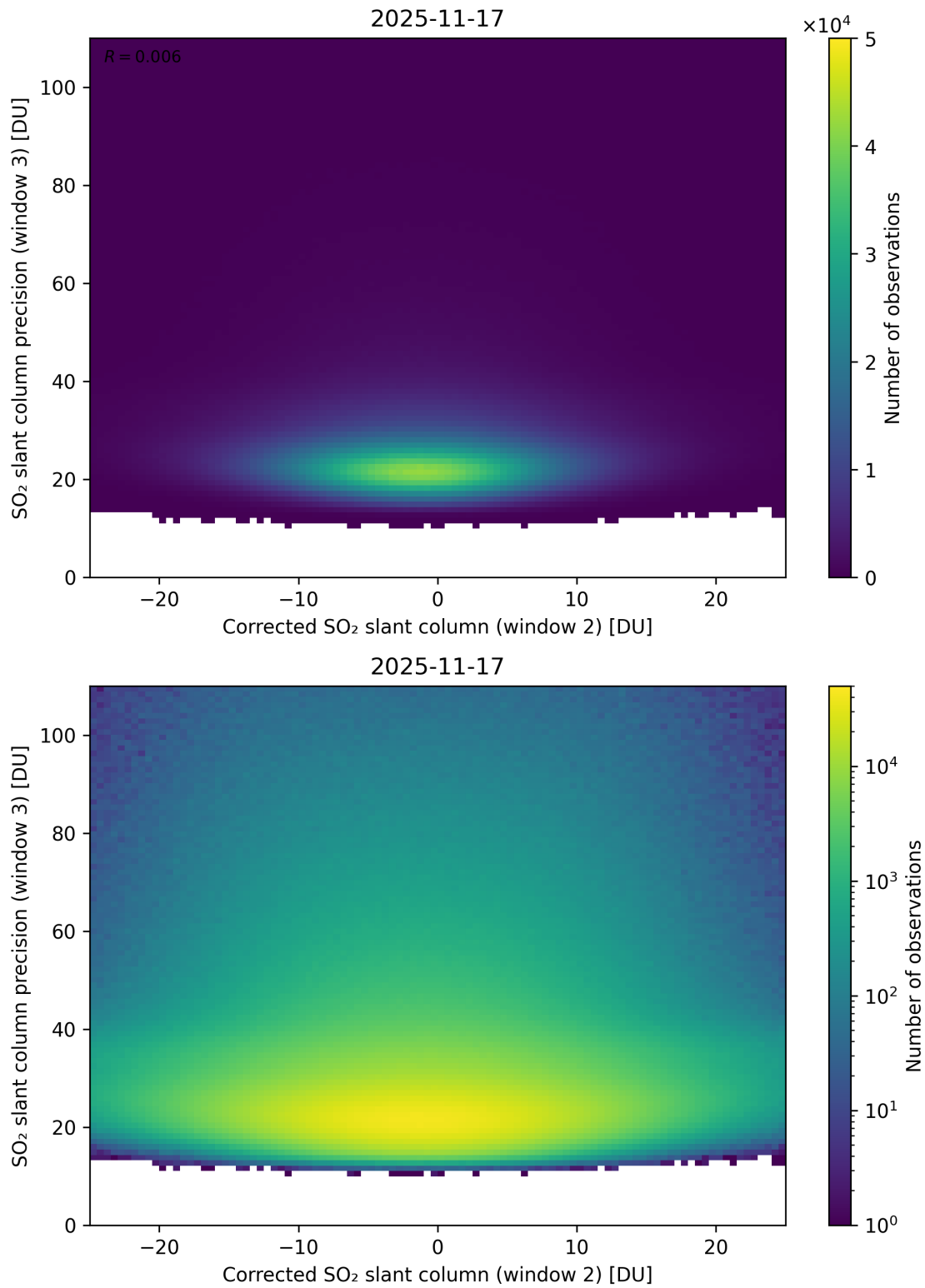
Figure 252: Scatter density plot of “Corrected SO 2 slant column (window 2)” against “SO 2 slant column precision (window 3)” for 2025-11-16 to 2025-11-18.
