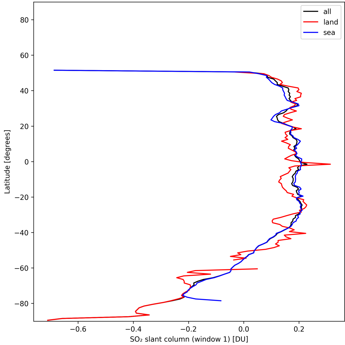
Figure 37: Zonal average of “SO 2 slant column (window 1)” for 2025-11-16 to 2025-11-18.
