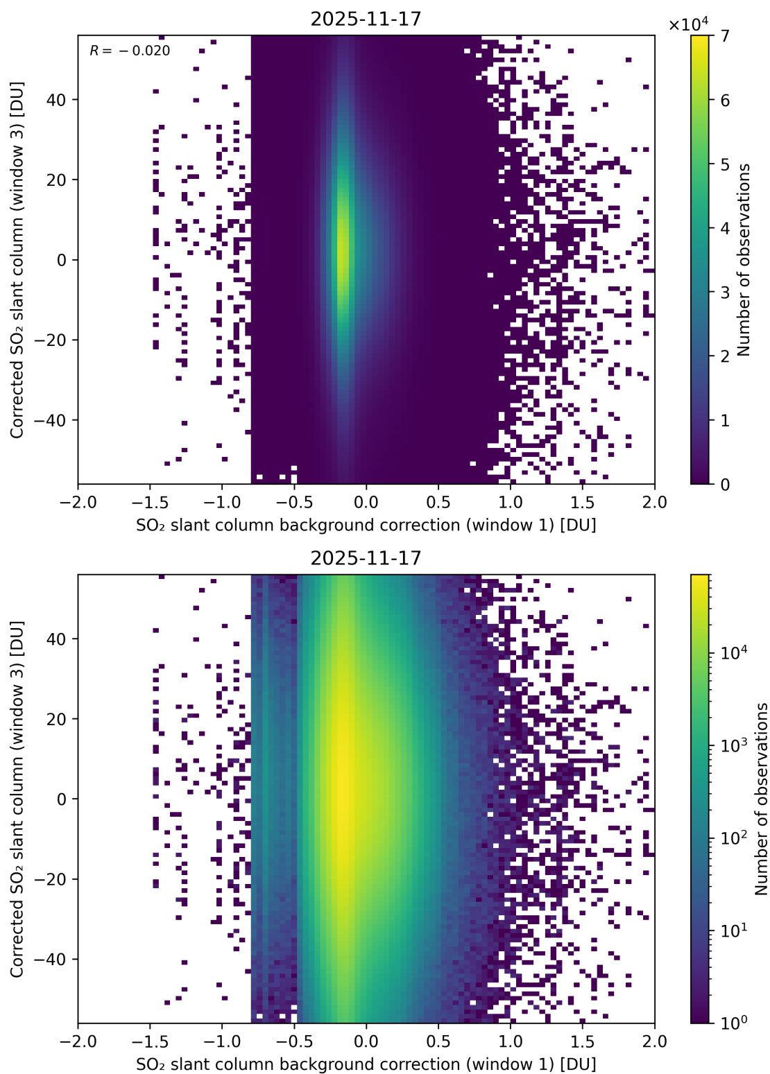
Figure 116: Scatter density plot of “SO 2 slant column background correction (window 1)” against “Corrected SO 2 slant column (window 3)” for 2025-11-16 to 2025-11-18.
