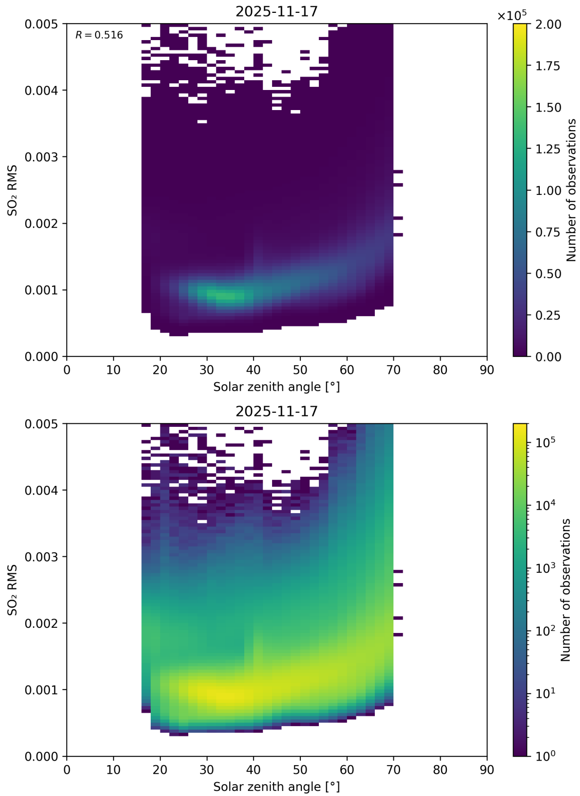
Figure 176: Scatter density plot of “Solar zenith angle” against “SO 2 RMS” for 2025-11-16 to 2025-11-18.
