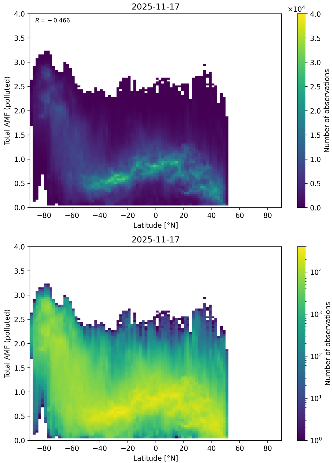
Figure 167: Scatter density plot of “Latitude” against “Total AMF (polluted)” for 2025-11-16 to 2025-11-18.
