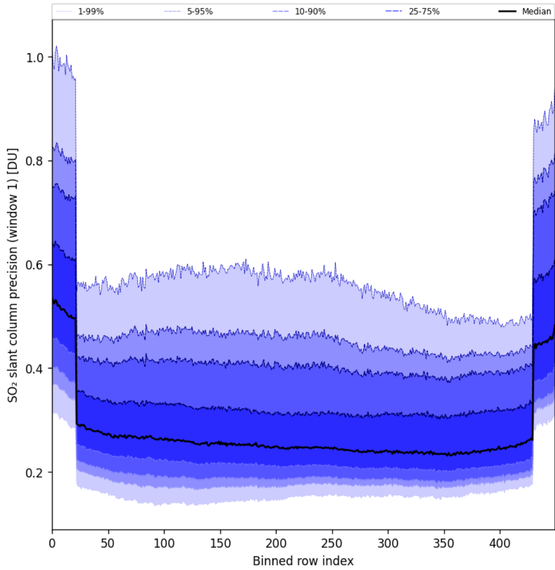
Figure 90: Along track statistics of “SO 2 slant column precision (window 1)” for 2025-11-16 to 2025-11-18
