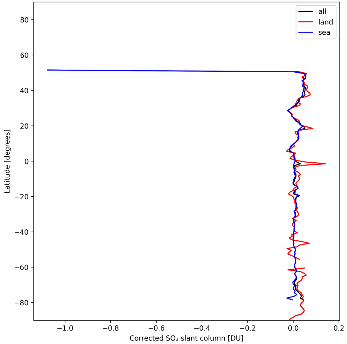
Figure 34: Zonal average of “Corrected SO 2 slant column” for 2025-11-16 to 2025-11-18.
