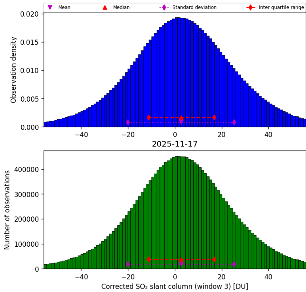
Figure 73: Histogram of "Corrected SO 2 slant column (window 3)" for 2025-11-16 to 2025-11-18
