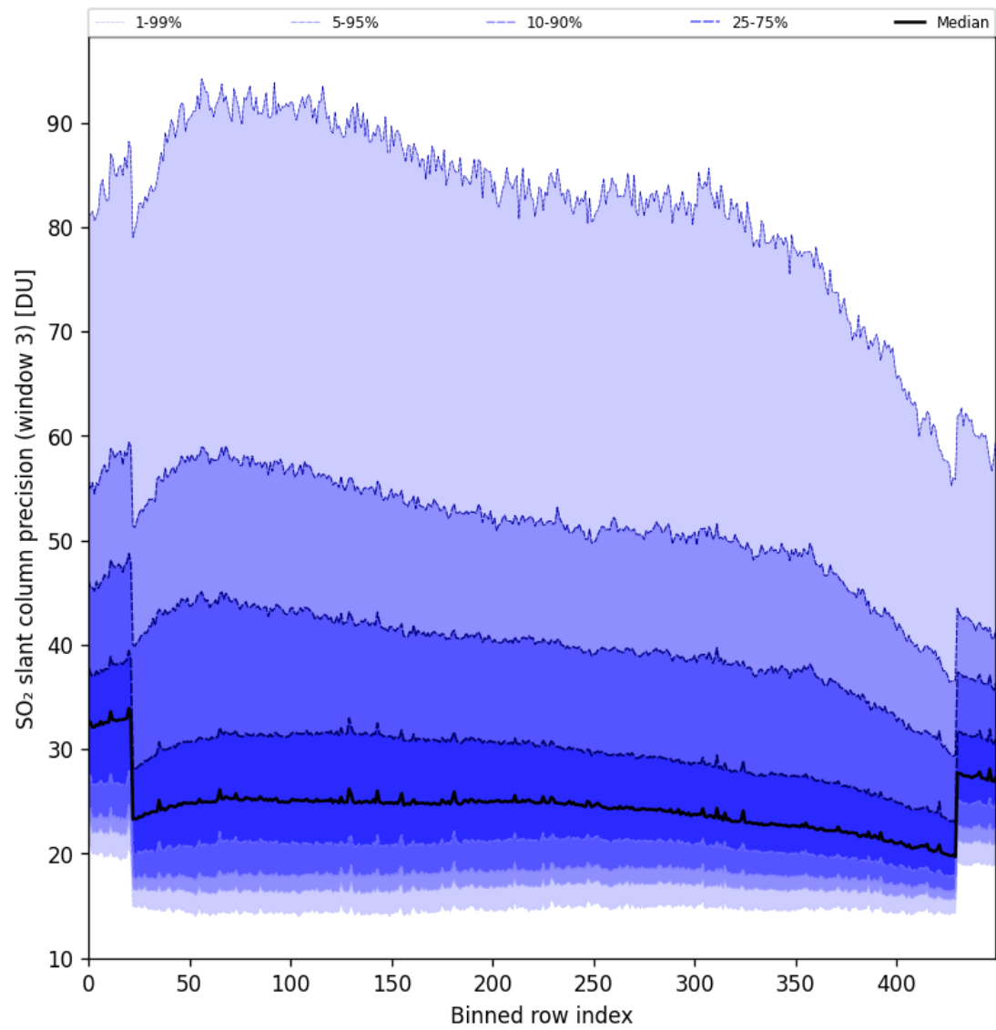
Figure 98: Along track statistics of “SO 2 slant column precision (window 3)” for 2025-11-16 to 2025-11-18
