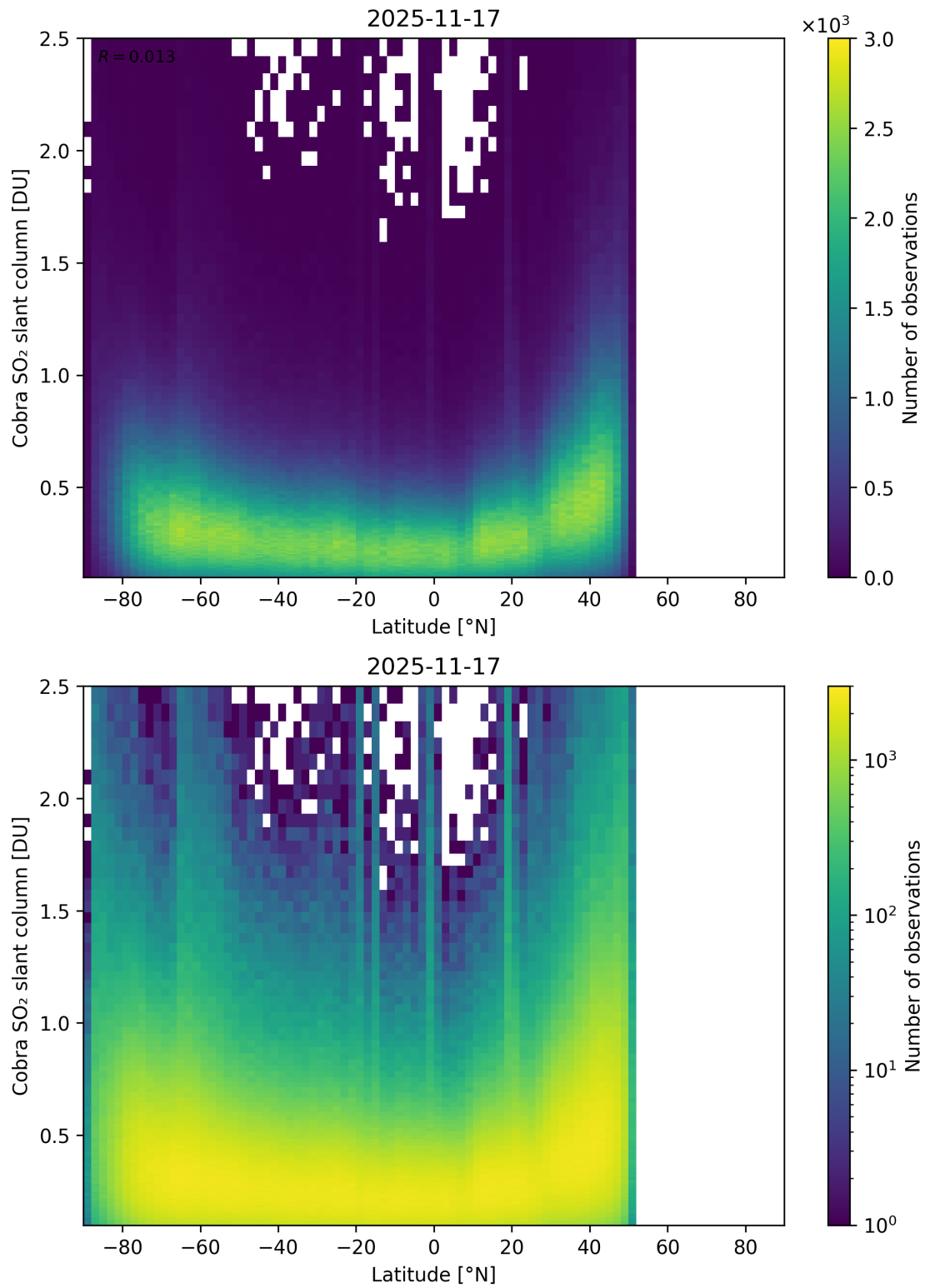
Figure 157: Scatter density plot of “Latitude” against “Cobra SO 2 slant column” for 2025-11-16 to 2025-11-18.
