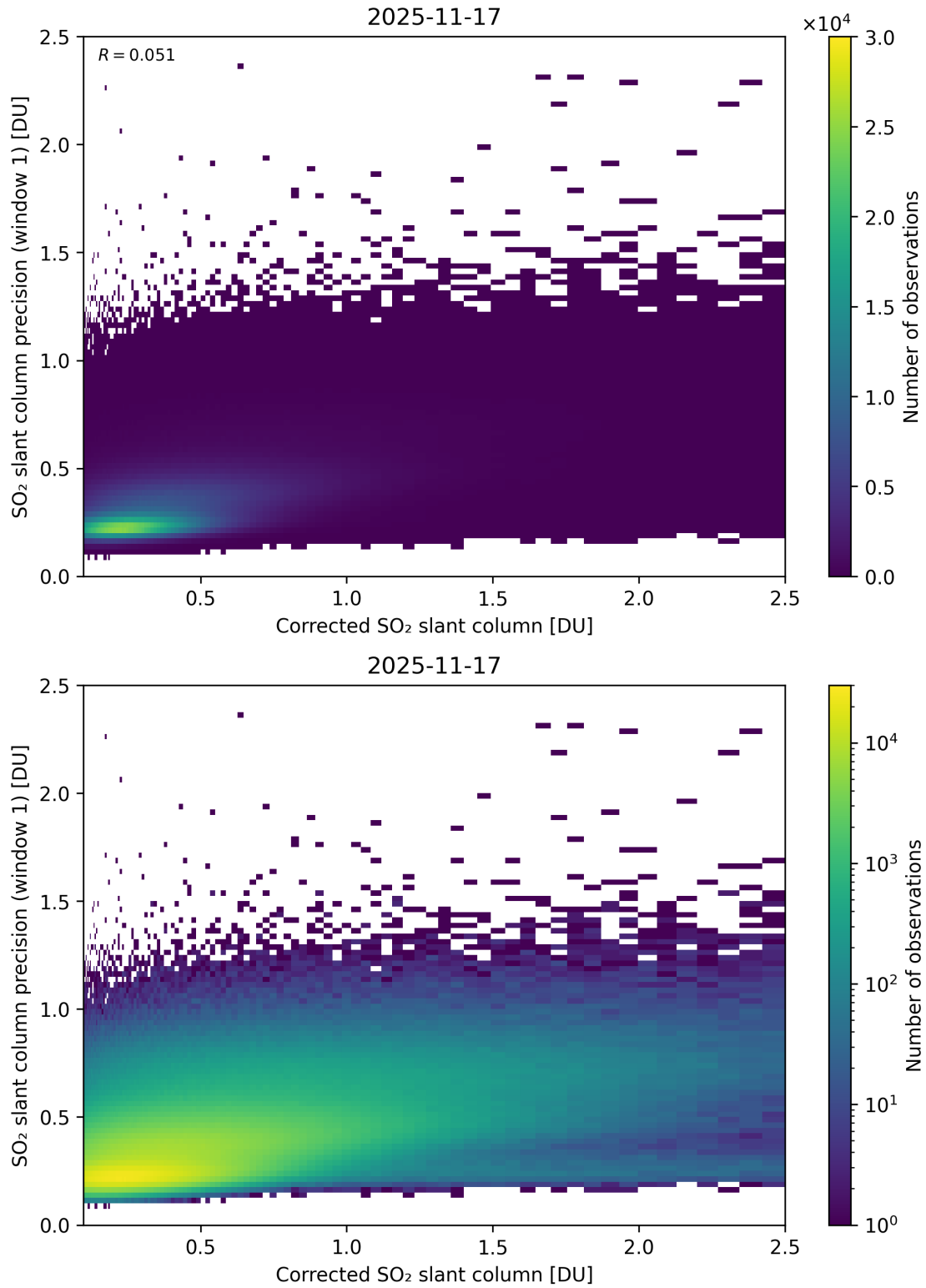
Figure 238: Scatter density plot of “Corrected SO 2 slant column” against “SO 2 slant column precision (window 1)” for 2025-11-16 to 2025-11-18.
