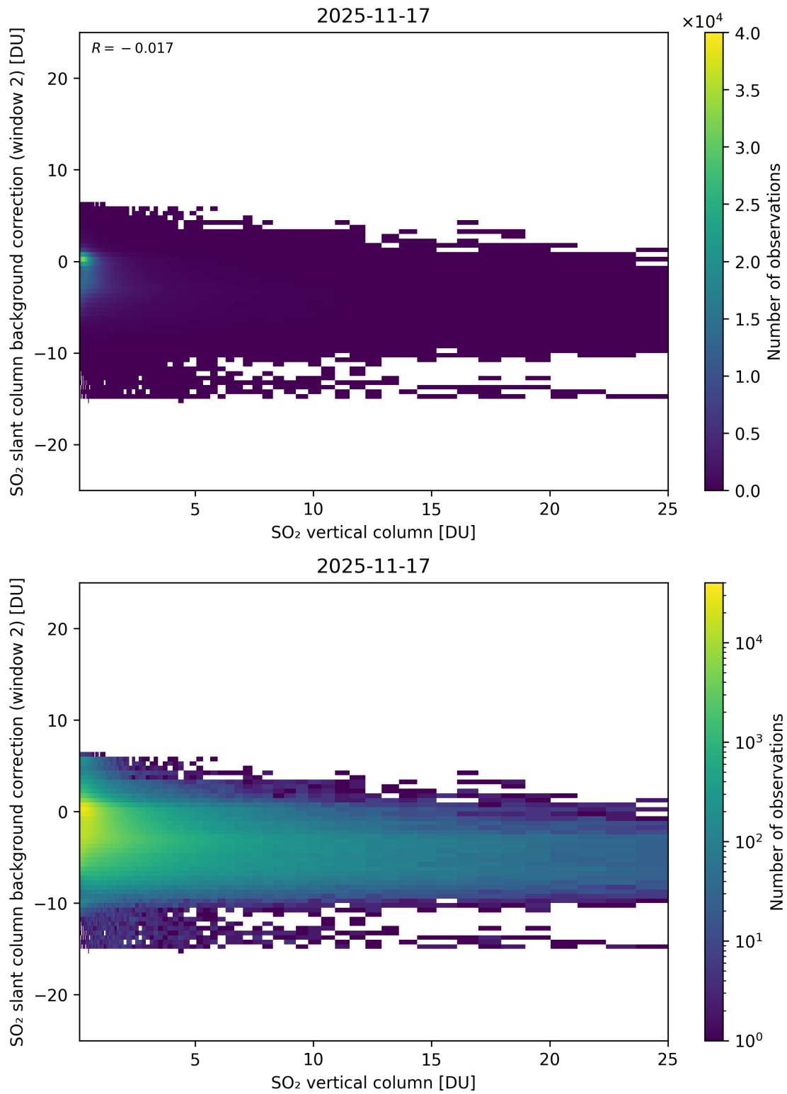
Figure 324: Scatter density plot of “SO 2 vertical column” against “SO 2 slant column background correction (window 2)” for 2025-11-16 to 2025-11-18.
