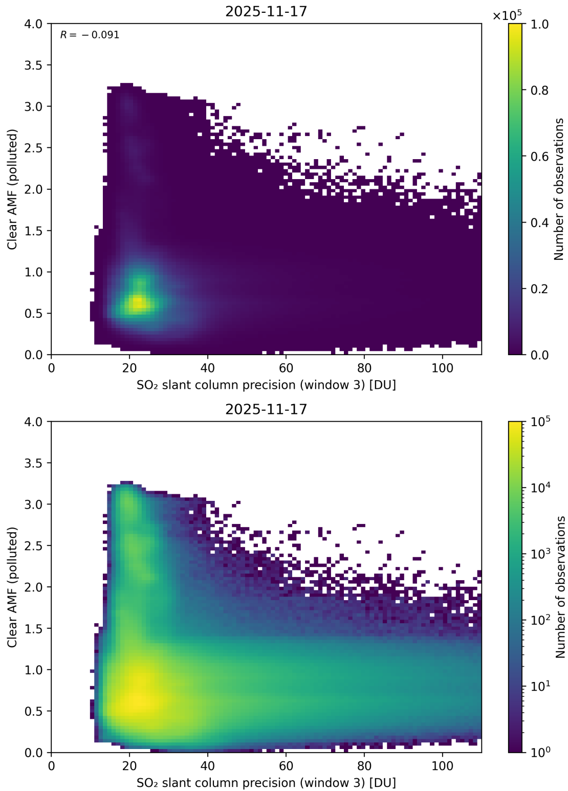
Figure 311: Scatter density plot of “SO 2 slant column precision (window 3)” against “Clear AMF (polluted)” for 2025-11-16 to 2025-11-18.
