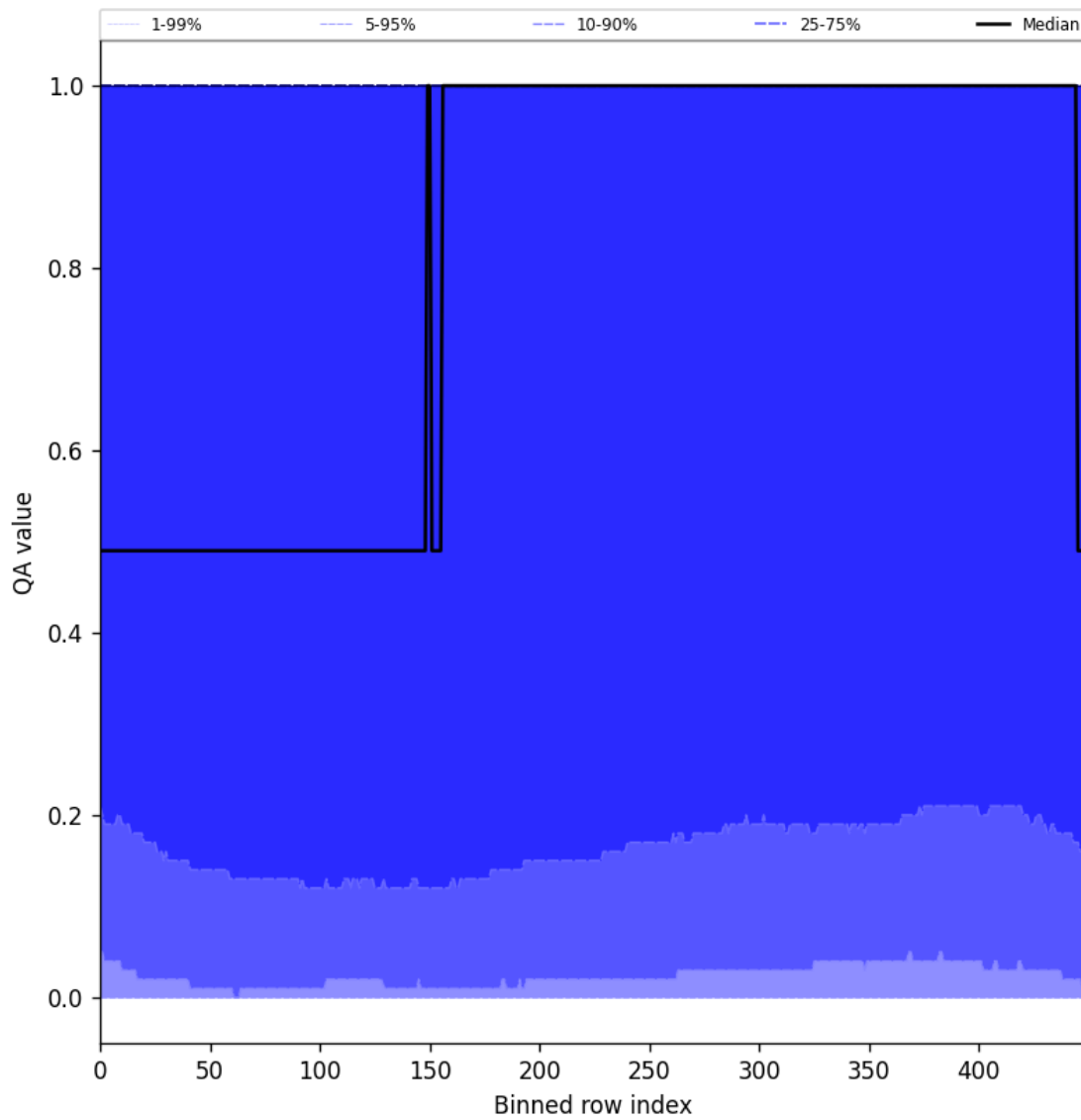
Figure 83: Along track statistics of “QA value” for 2025-11-16 to 2025-11-18
