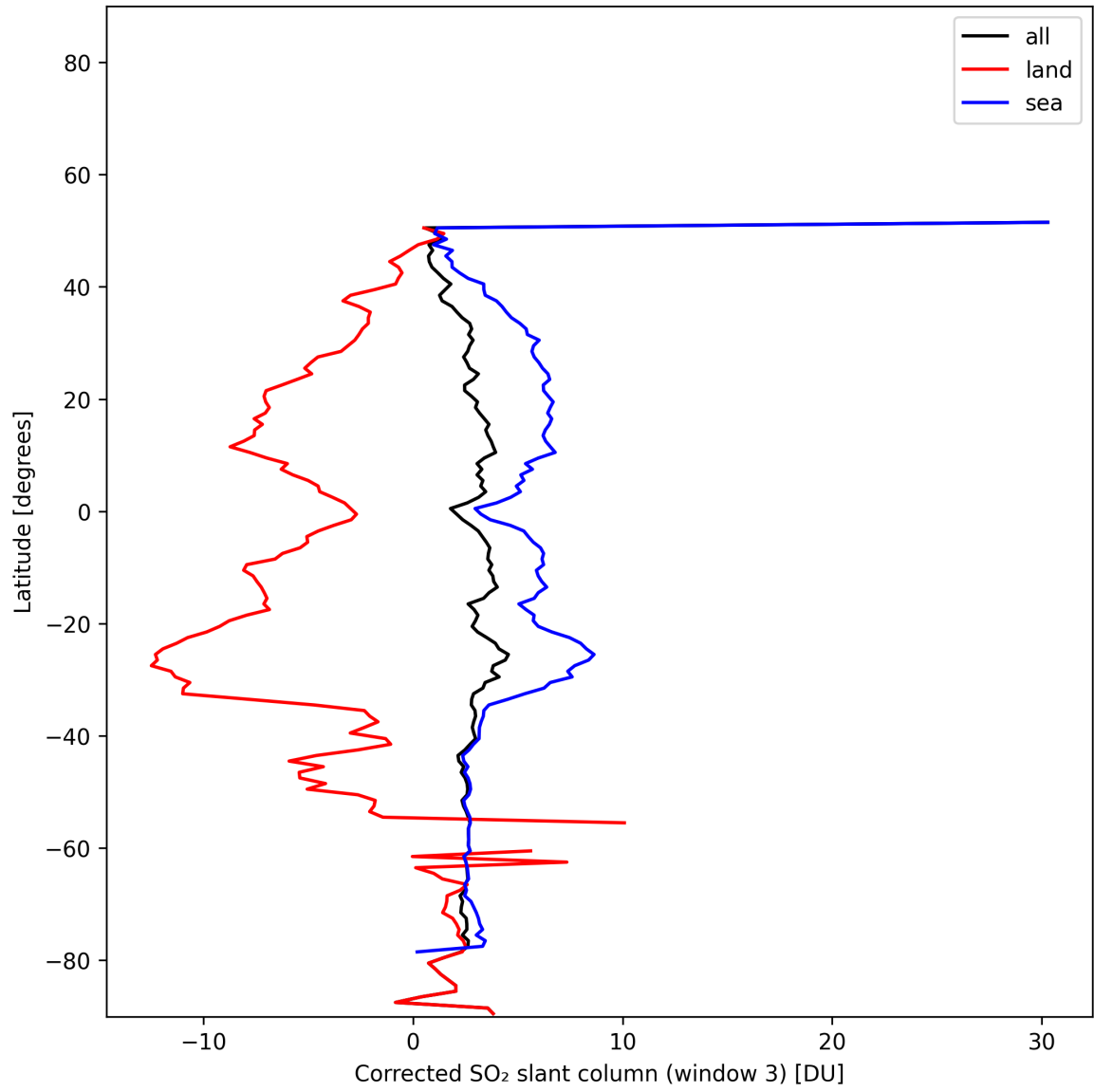
Figure 47: Zonal average of “Corrected SO 2 slant column (window 3)” for 2025-11-16 to 2025-11-18.
