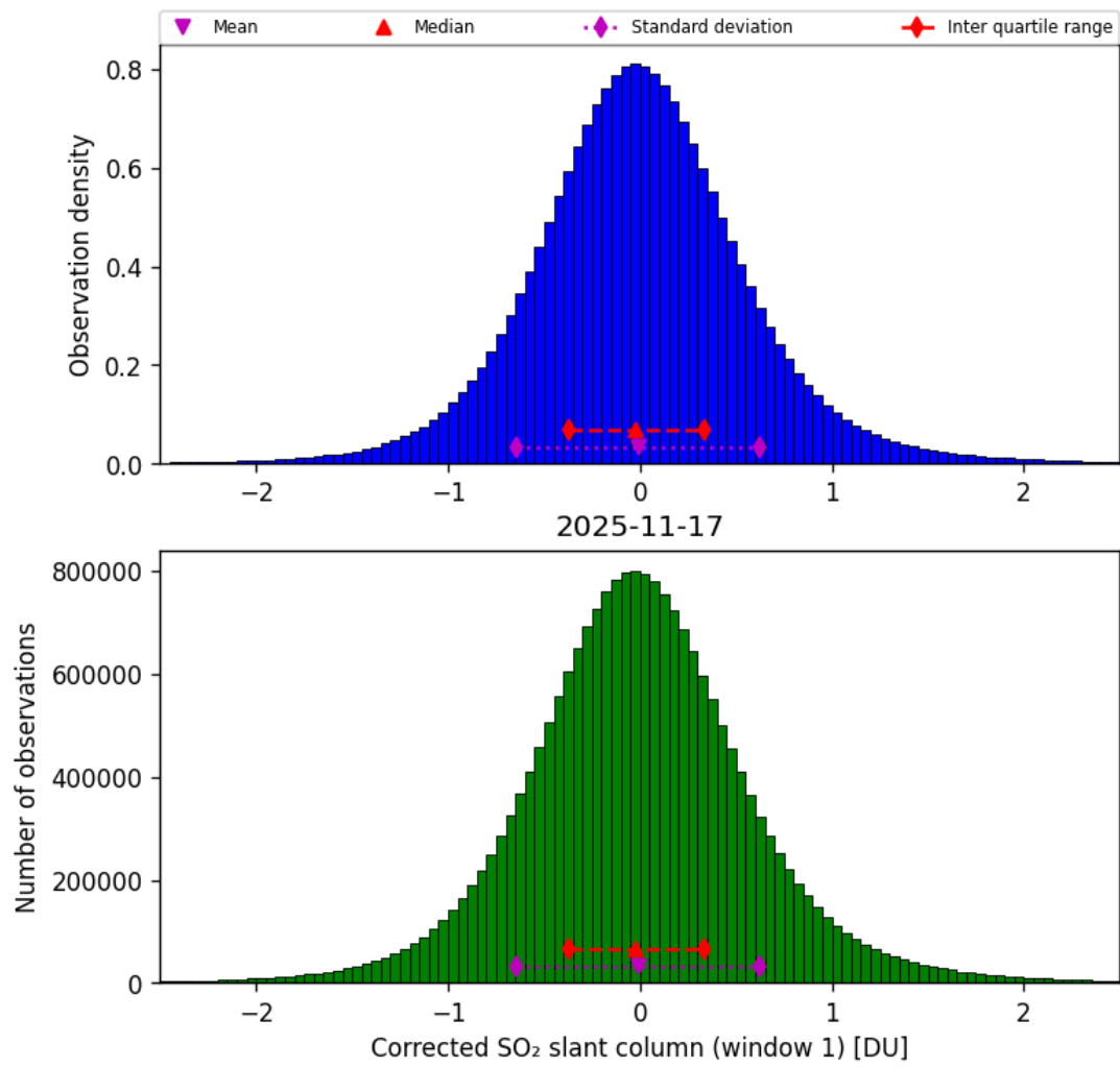
Figure 65: Histogram of “Corrected SO 2 slant column (window 1)” for 2025-11-16 to 2025-11-18
