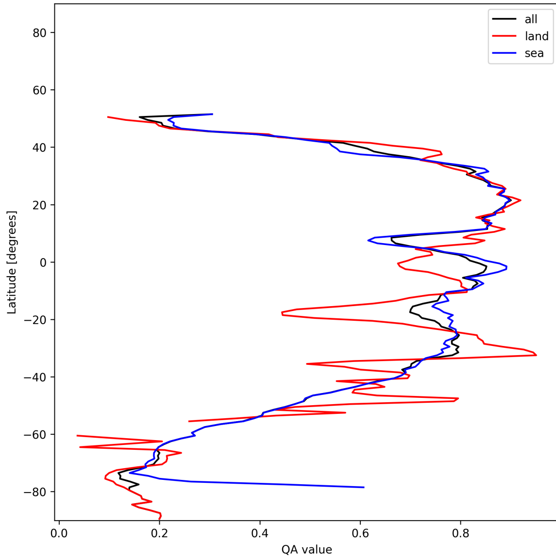
Figure 31: Zonal average of “QA value” for 2025-11-16 to 2025-11-18.
