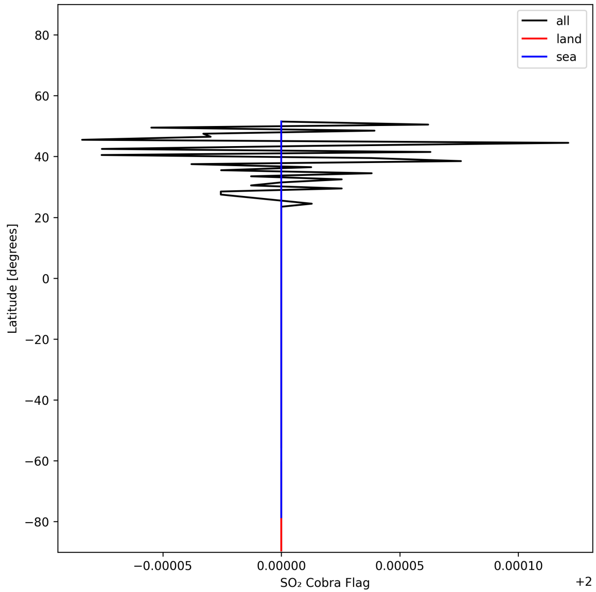
Figure 49: Zonal average of “SO 2 Cobra Flag” for 2025-11-16 to 2025-11-18.
