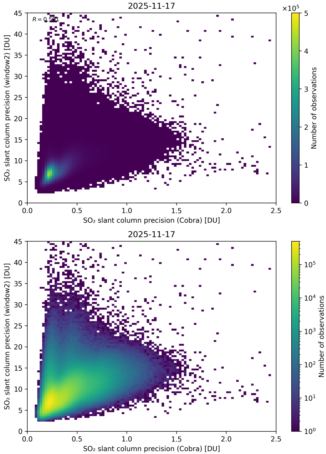
Figure 210: Scatter density plot of “SO 2 slant column precision (Cobra)” against “SO 2 slant column precision (window2)” for 2025-11-16 to 2025-11-18.
