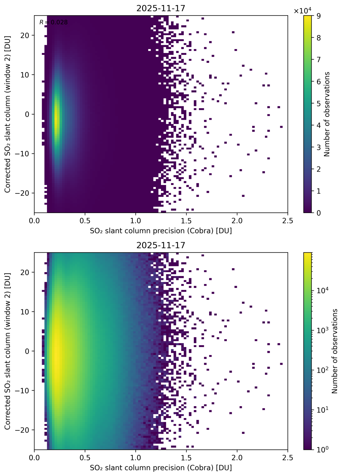
Figure 206: Scatter density plot of “SO 2 slant column precision (Cobra)” against “Corrected SO 2 slant column (window 2)” for 2025-11-16 to 2025-11-18.
