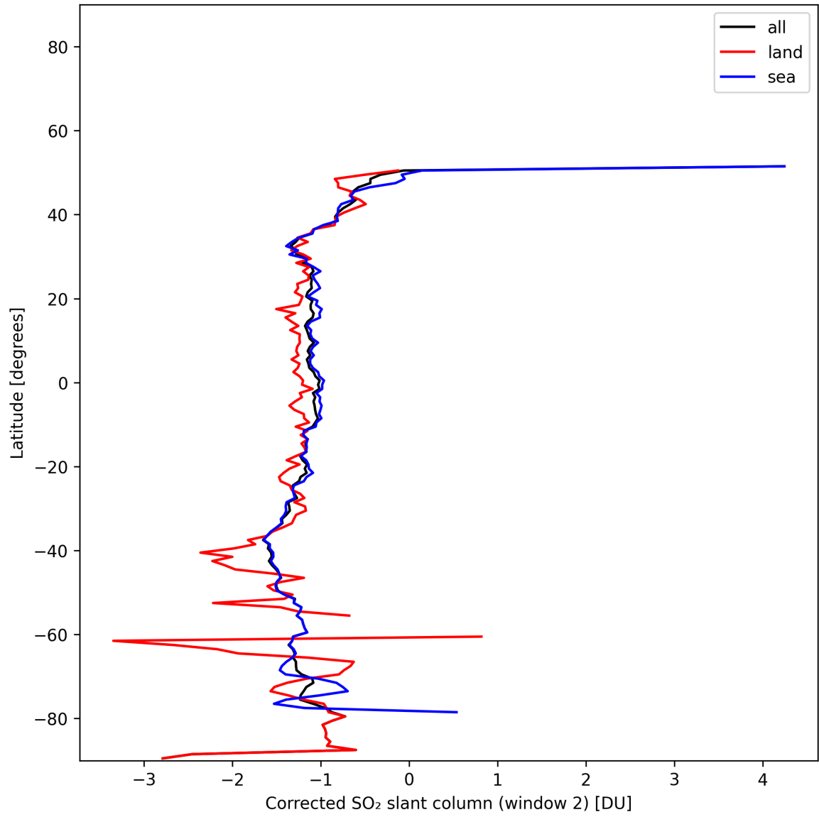
Figure 43: Zonal average of “Corrected SO 2 slant column (window 2)” for 2025-11-16 to 2025-11-18.
