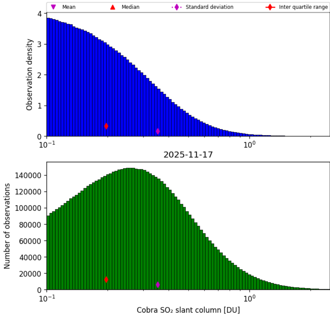
Figure 61: Histogram of “Cobra SO 2 slant column” for 2025-11-16 to 2025-11-18
