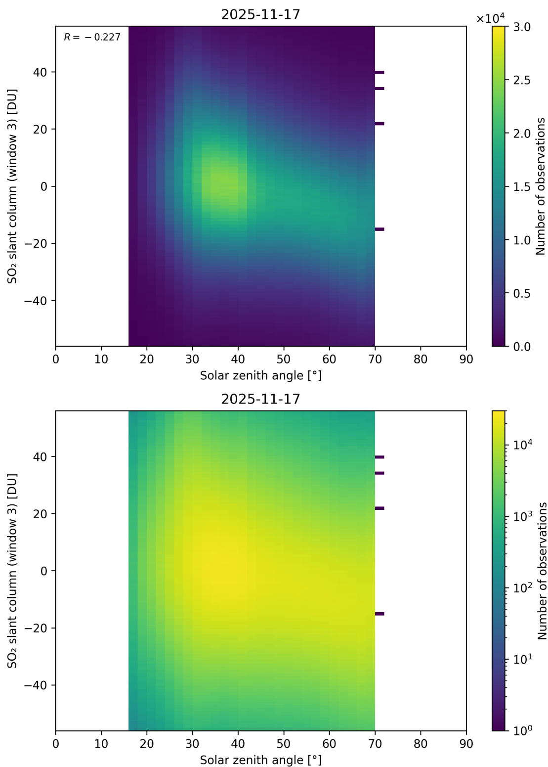
Figure 187: Scatter density plot of “Solar zenith angle” against “SO 2 slant column (window 3)” for 2025-11-16 to 2025-11-18.
