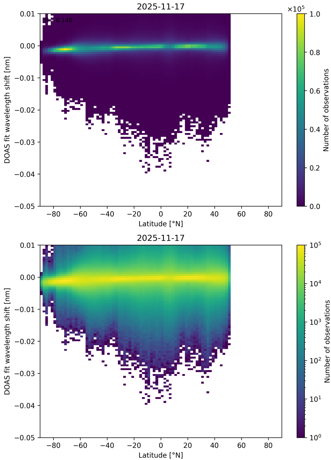
Figure 153: Scatter density plot of “Latitude” against “DOAS fit wavelength shift” for 2025-11-16 to 2025-11-18.
