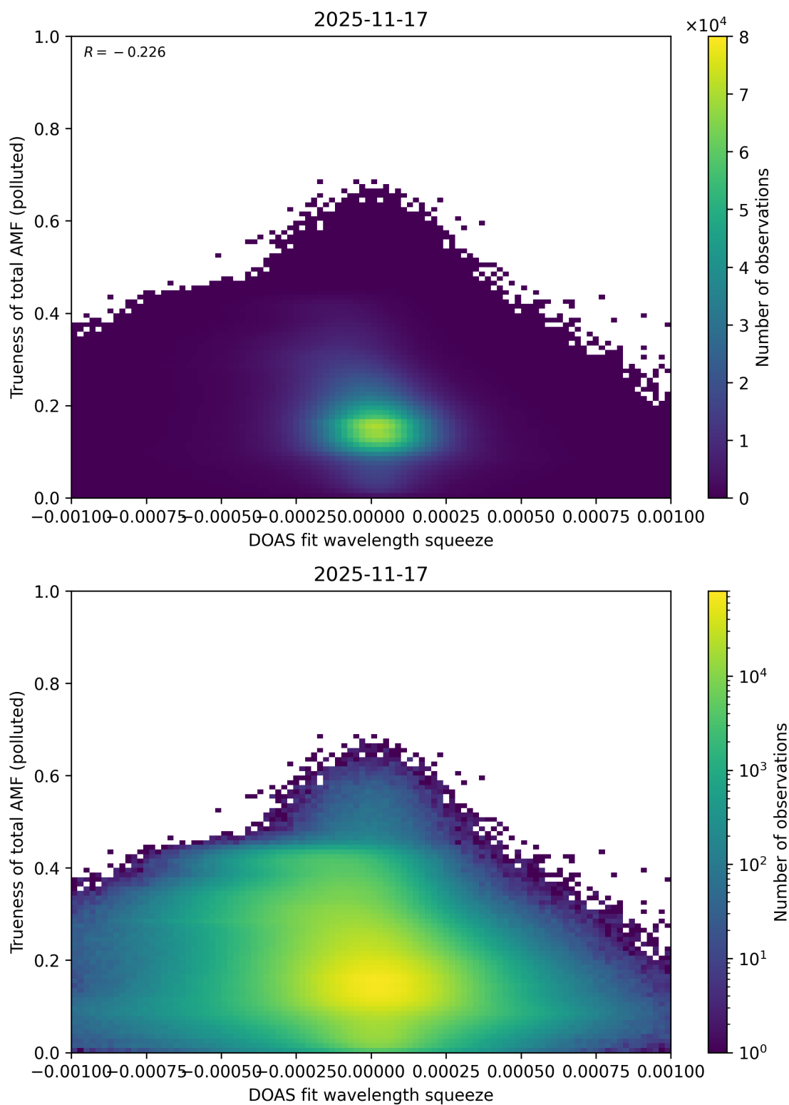
Figure 146: Scatter density plot of “DOAS fit wavelength squeeze” against “Trueness of total AMF (polluted)” for 2025-11-16 to 2025-11-18.
