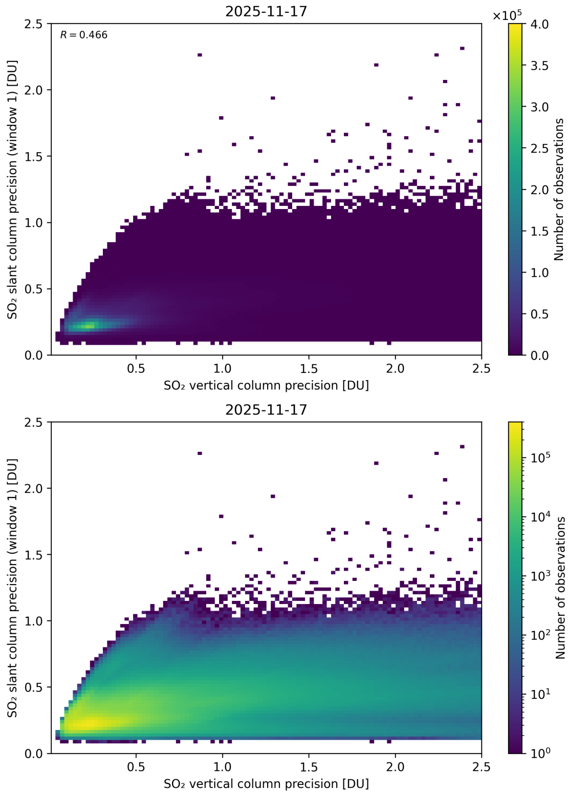
Figure 342: Scatter density plot of “SO 2 vertical column precision” against “SO 2 slant column precision (window 1)” for 2025-11-16 to 2025-11-18.
