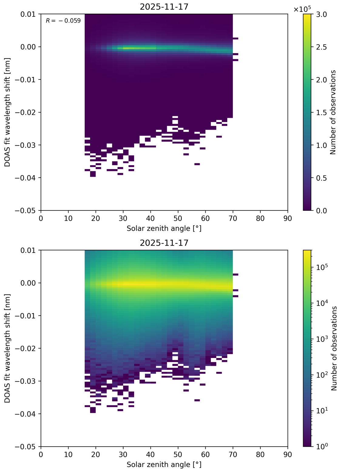
Figure 174: Scatter density plot of “Solar zenith angle” against “DOAS fit wavelength shift” for 2025-11-16 to 2025-11-18.
