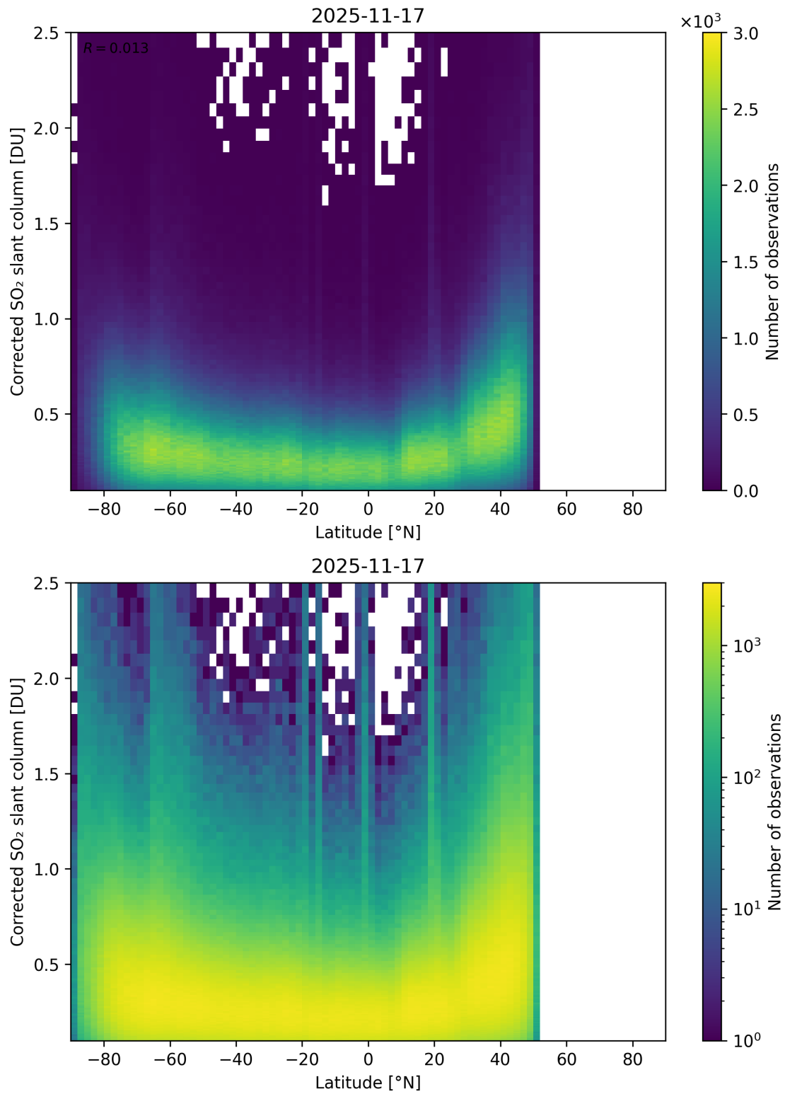
Figure 159: Scatter density plot of “Latitude” against “Corrected SO 2 slant column” for 2025-11-16 to 2025-11-18.
