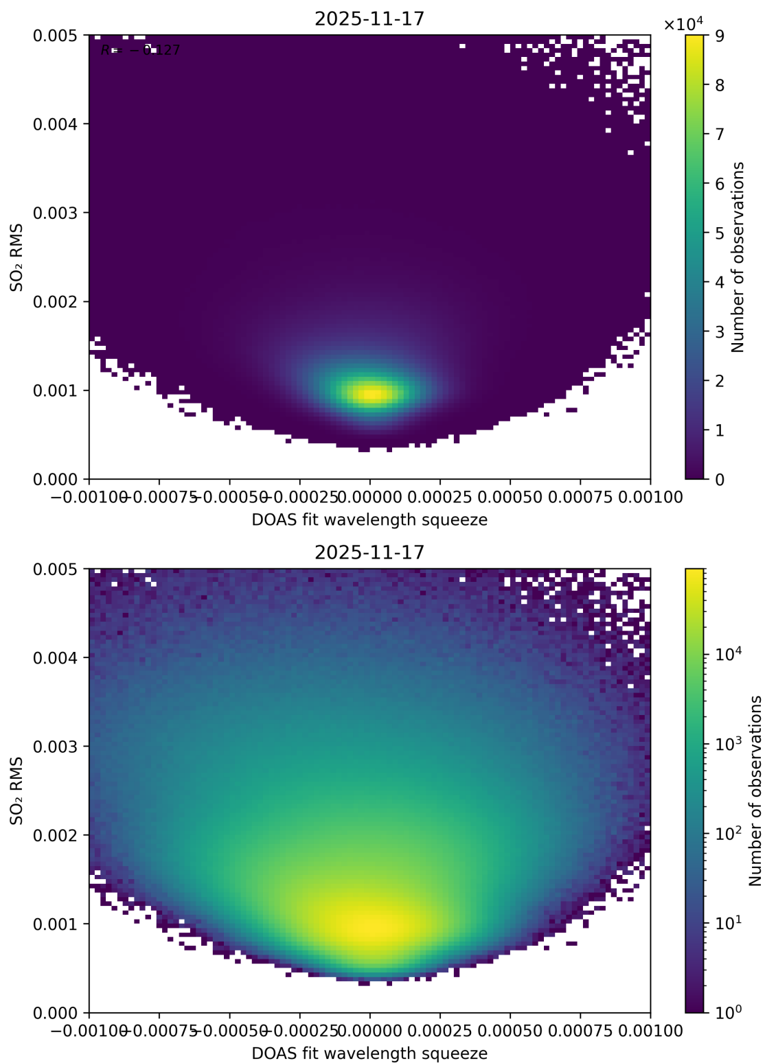
Figure 143: Scatter density plot of “DOAS fit wavelength squeeze” against “SO 2 RMS” for 2025-11-16 to 2025-11-18.
