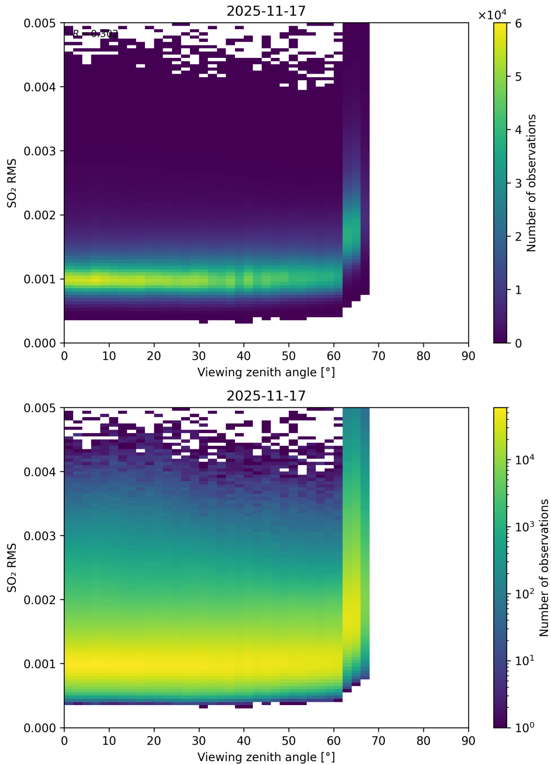
Figure 367: Scatter density plot of “Viewing zenith angle” against “SO 2 RMS” for 2025-11-16 to 2025-11-18.
