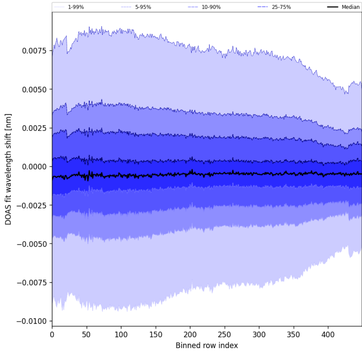
Figure 102: Along track statistics of “DOAS fit wavelength shift” for 2025-11-16 to 2025-11-18
