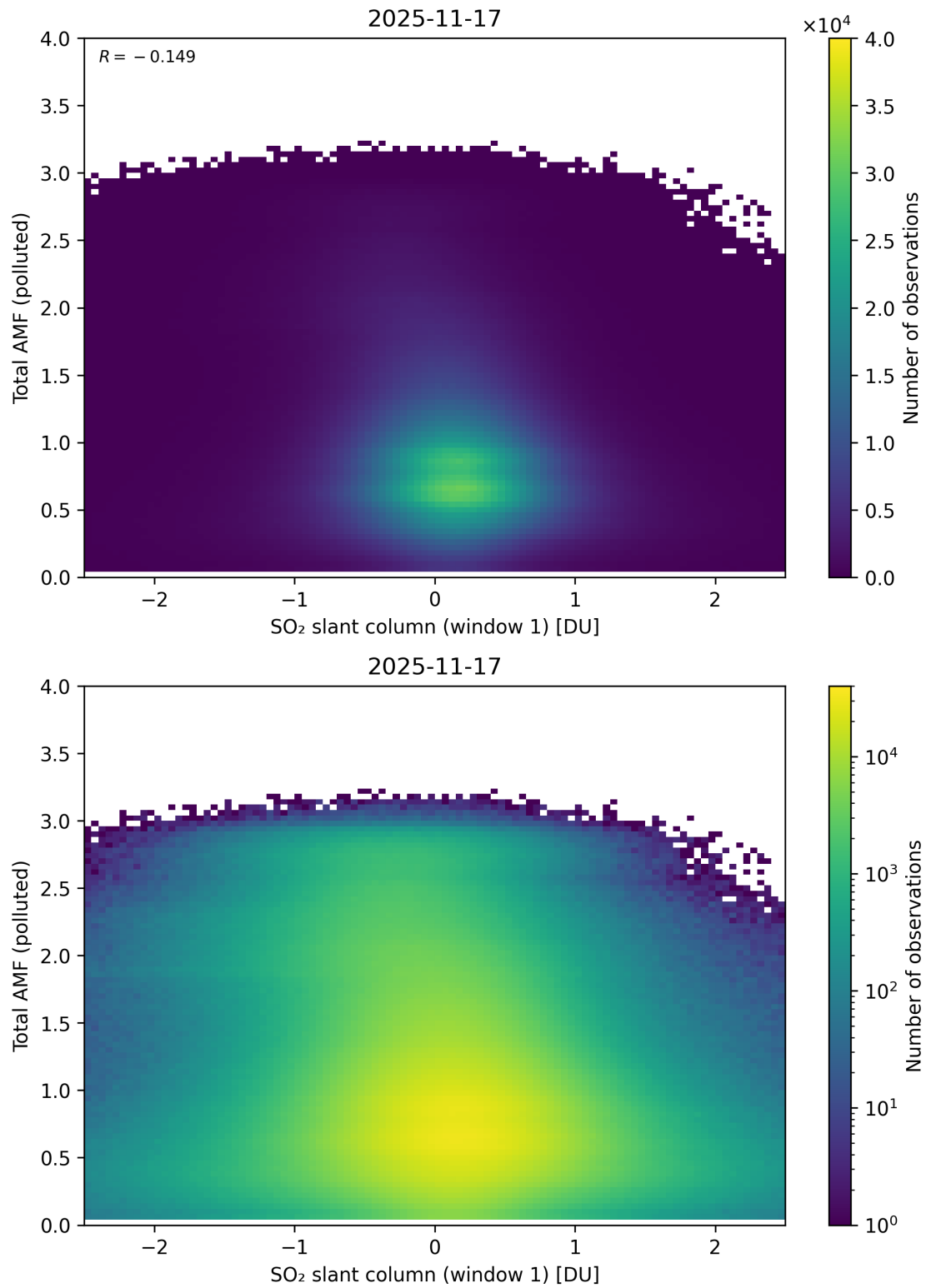
Figure 289: Scatter density plot of “SO 2 slant column (window 1)” against “Total AMF (polluted)” for 2025-11-16 to 2025-11-18.
