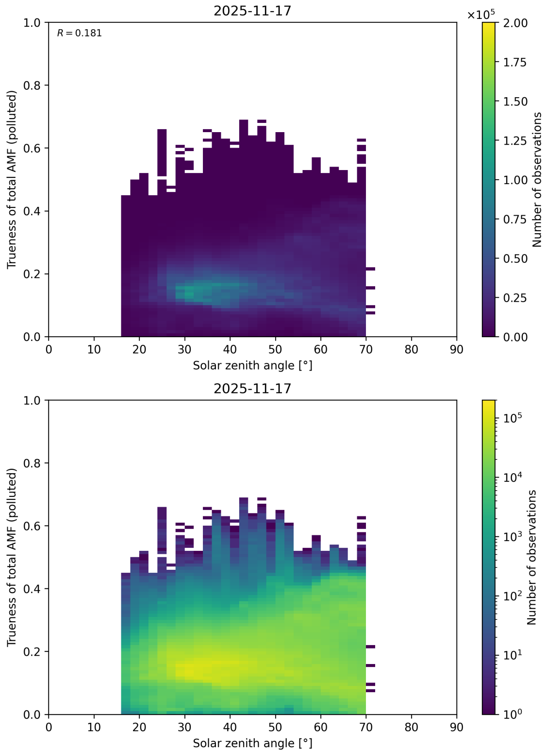
Figure 190: Scatter density plot of “Solar zenith angle” against “Trueness of total AMF (polluted)” for 2025-11-16 to 2025-11-18.
