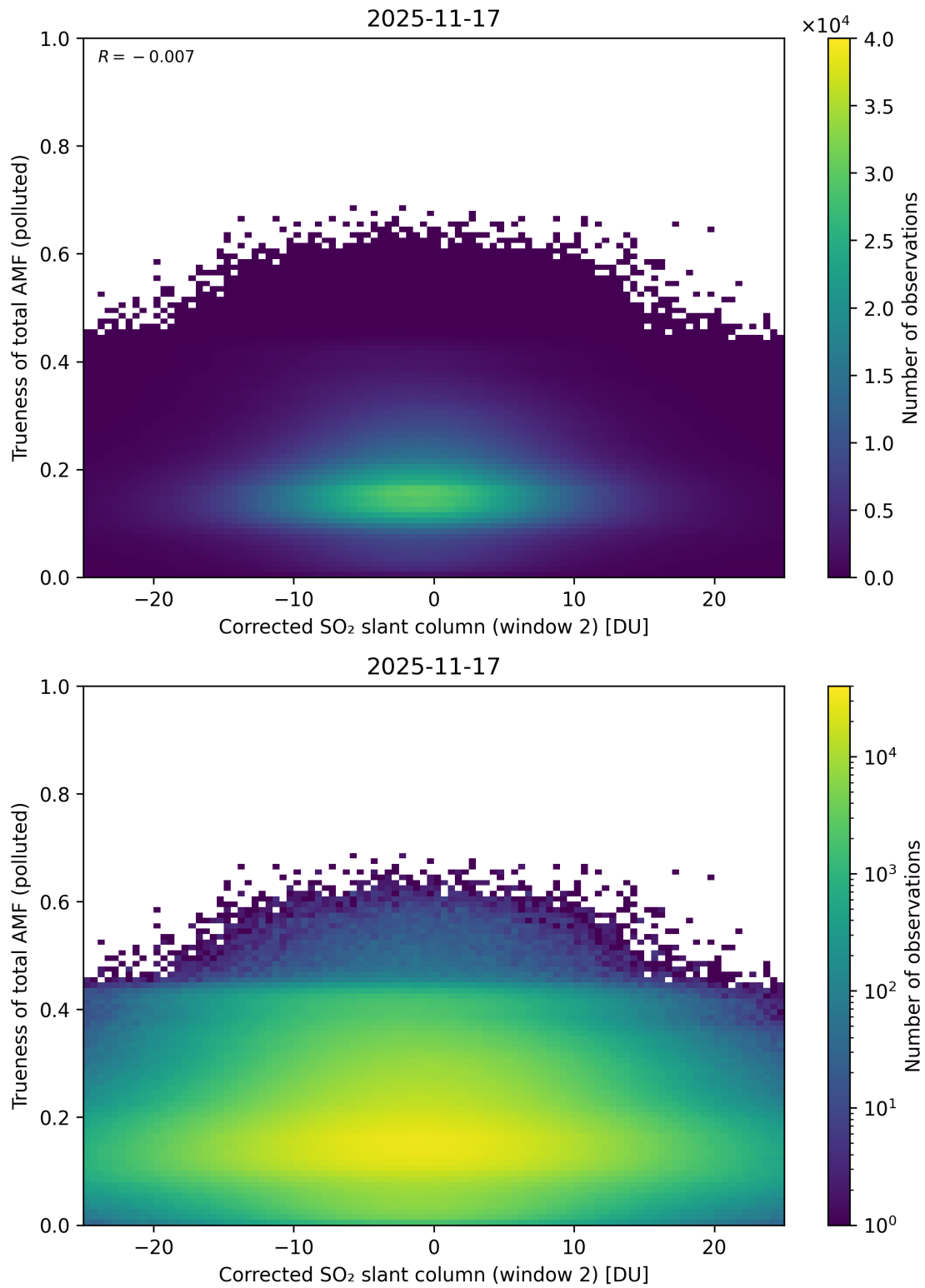
Figure 254: Scatter density plot of “Corrected SO 2 slant column (window 2)” against “Trueness of total AMF (polluted)” for 2025-11-16 to 2025-11-18.
