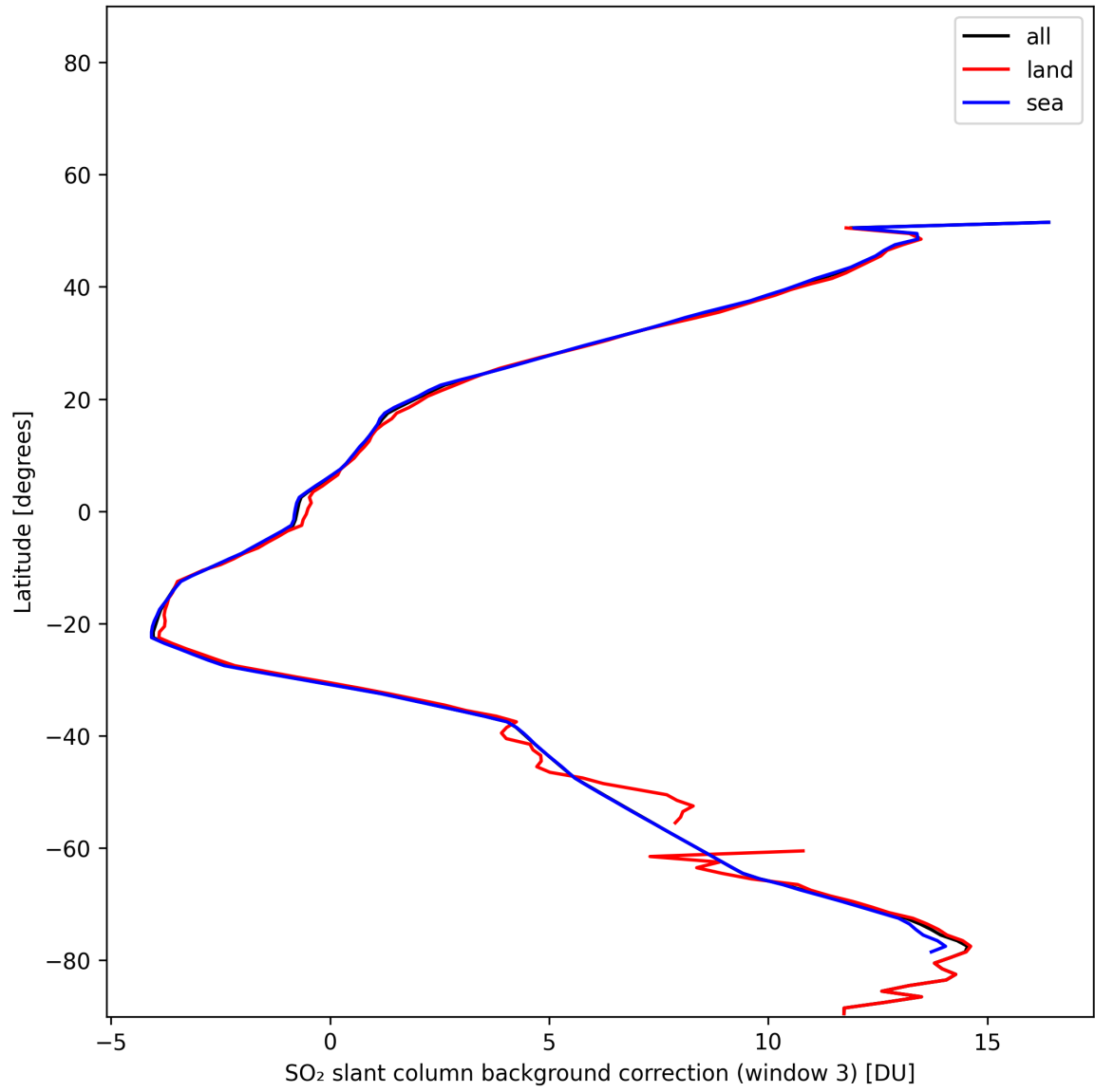
Figure 48: Zonal average of “SO 2 slant column background correction (window 3)” for 2025-11-16 to 2025-11-18.
