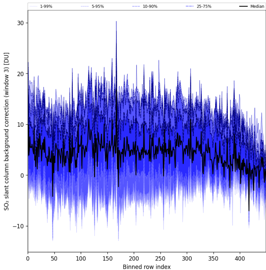
Figure 100: Along track statistics of “SO 2 slant column background correction (window 3)” for 2025-11-16 to 2025-11-18
