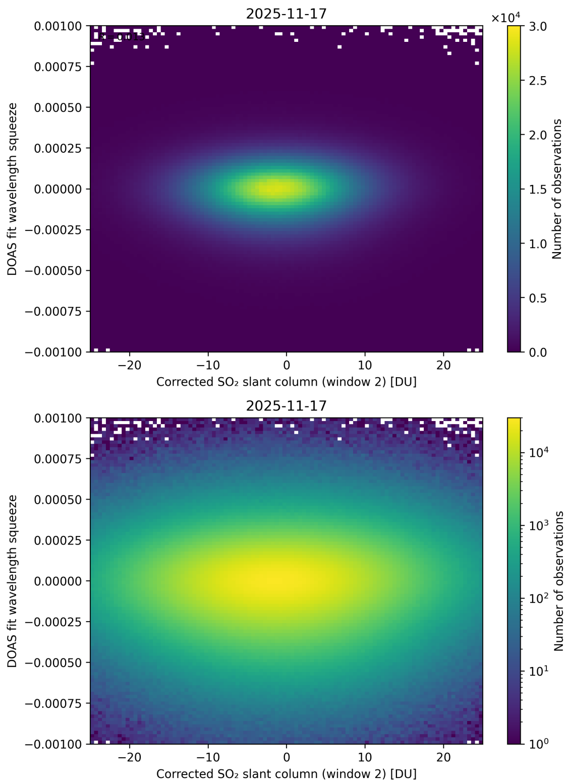
Figure 247: Scatter density plot of “Corrected SO 2 slant column (window 2)” against “DOAS fit wavelength squeeze” for 2025-11-16 to 2025-11-18.
