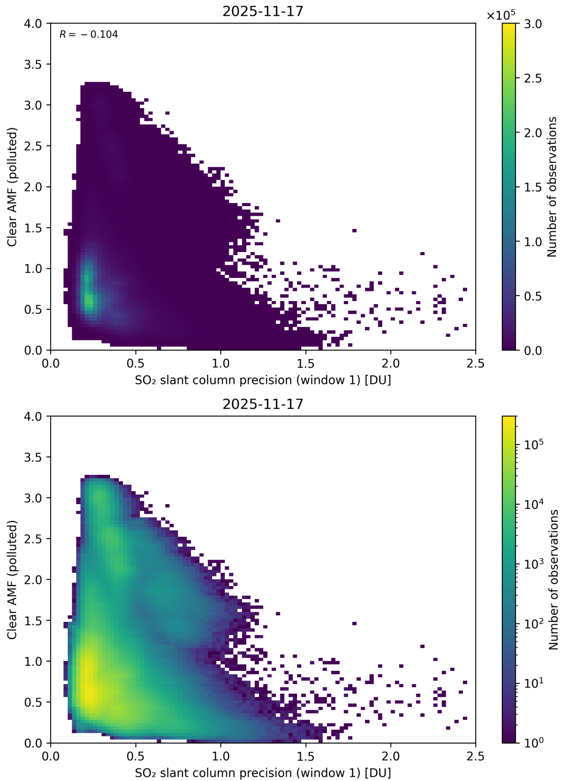
Figure 274: Scatter density plot of “SO 2 slant column precision (window 1)” against “Clear AMF (polluted)” for 2025-11-16 to 2025-11-18.
