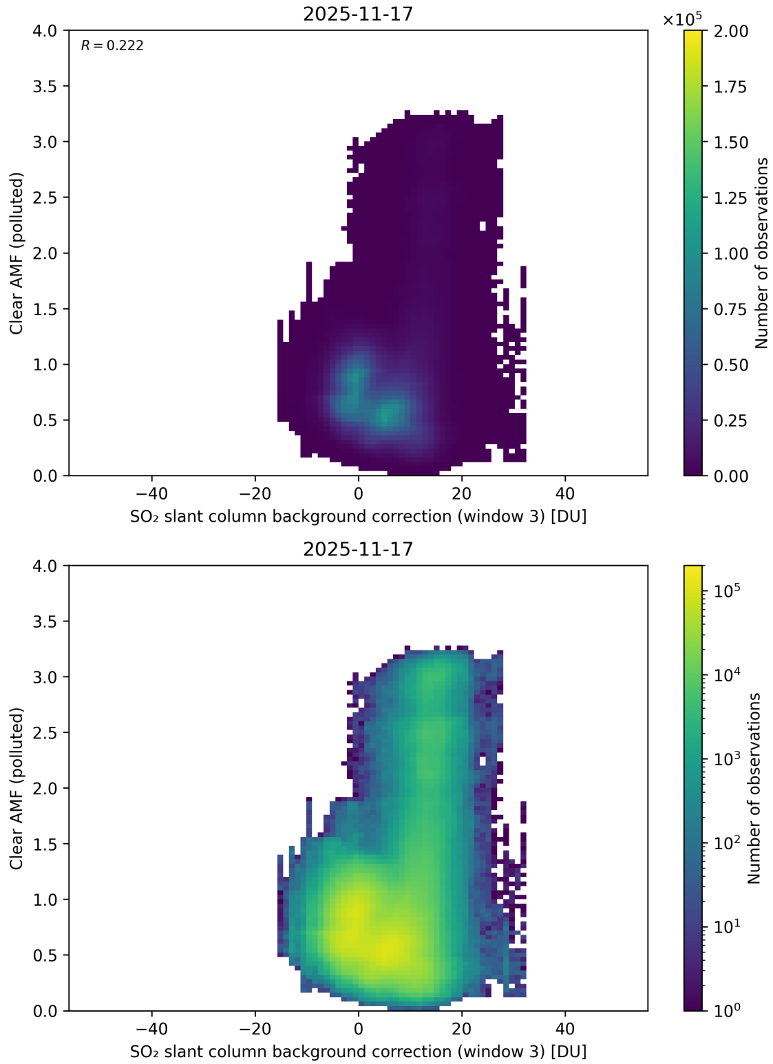
Figure 135: Scatter density plot of “SO 2 slant column background correction (window 3)” against “Clear AMF (polluted)” for 2025-11-16 to 2025-11-18.
