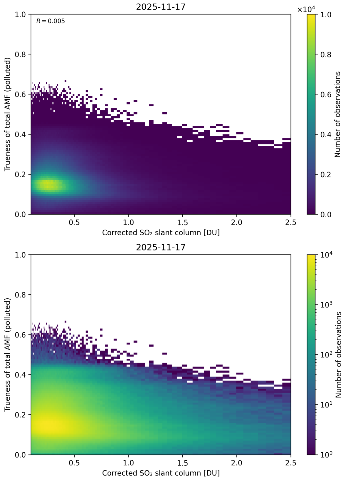
Figure 243: Scatter density plot of “Corrected SO 2 slant column” against “Trueness of total AMF (polluted)” for 2025-11-16 to 2025-11-18.
