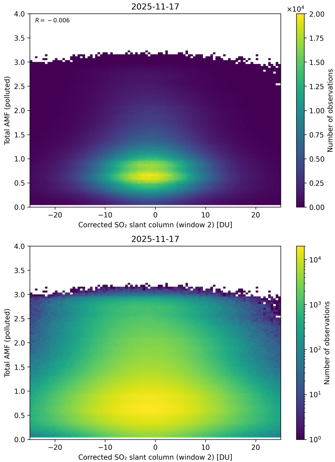
Figure 253: Scatter density plot of “Corrected SO 2 slant column (window 2)” against “Total AMF (polluted)” for 2025-11-16 to 2025-11-18.
