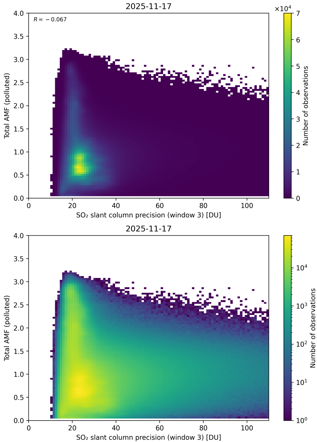
Figure 313: Scatter density plot of “SO 2 slant column precision (window 3)” against “Total AMF (polluted)” for 2025-11-16 to 2025-11-18.
