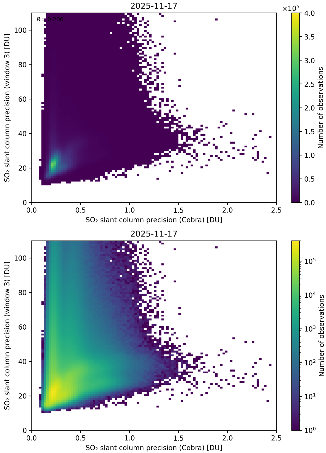
Figure 212: Scatter density plot of “SO 2 slant column precision (Cobra)” against “SO 2 slant column precision (window 3)” for 2025-11-16 to 2025-11-18.
