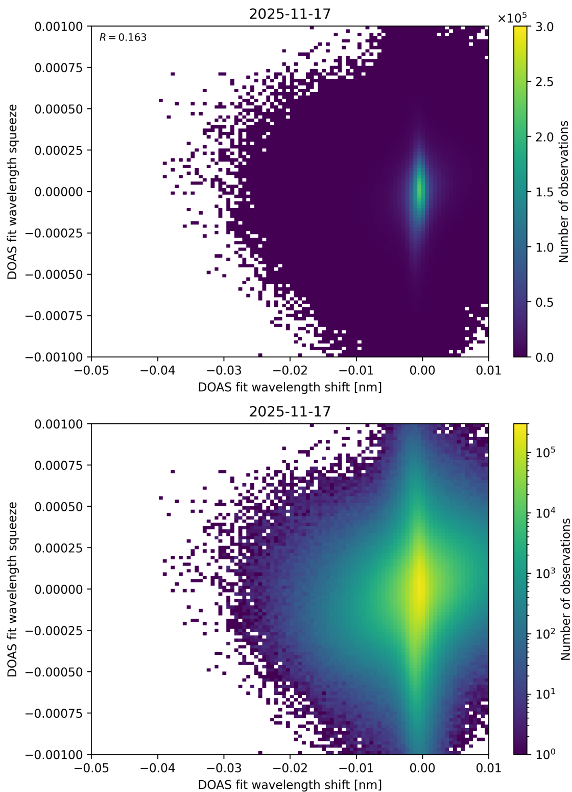
Figure 138: Scatter density plot of “DOAS fit wavelength shift” against “DOAS fit wavelength squeeze” for 2025-11-16 to 2025-11-18.
