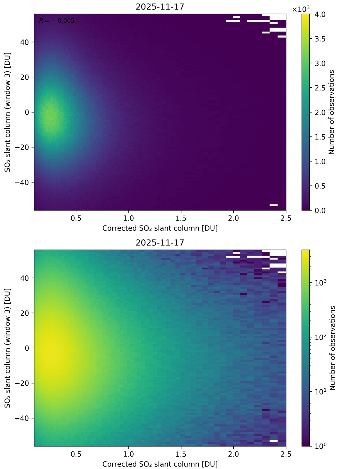
Figure 240: Scatter density plot of “Corrected SO 2 slant column” against “SO 2 slant column (window 3)” for 2025-11-16 to 2025-11-18.
