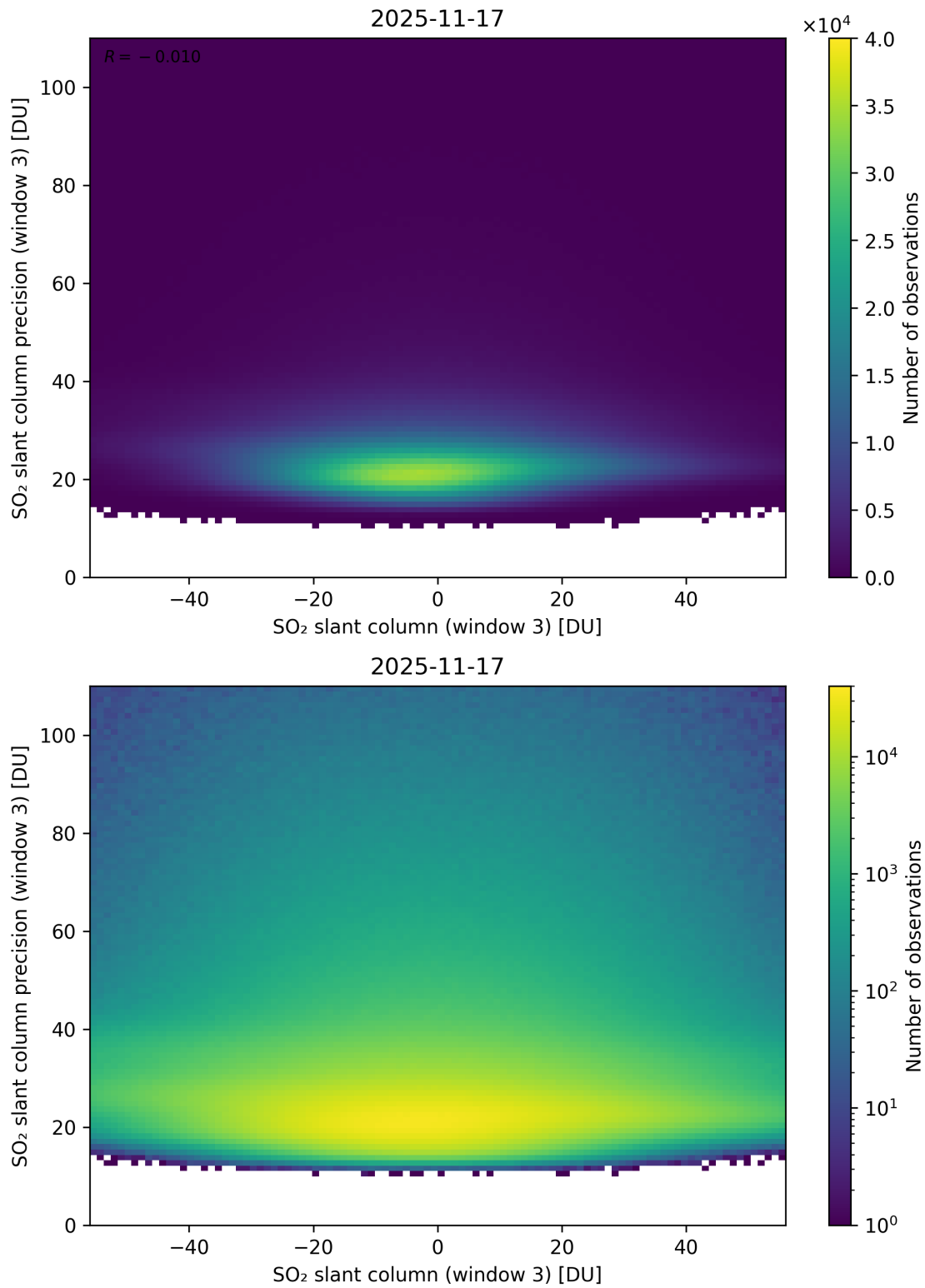
Figure 317: Scatter density plot of “SO 2 slant column (window 3)” against “SO 2 slant column precision (window 3)” for 2025-11-16 to 2025-11-18.
