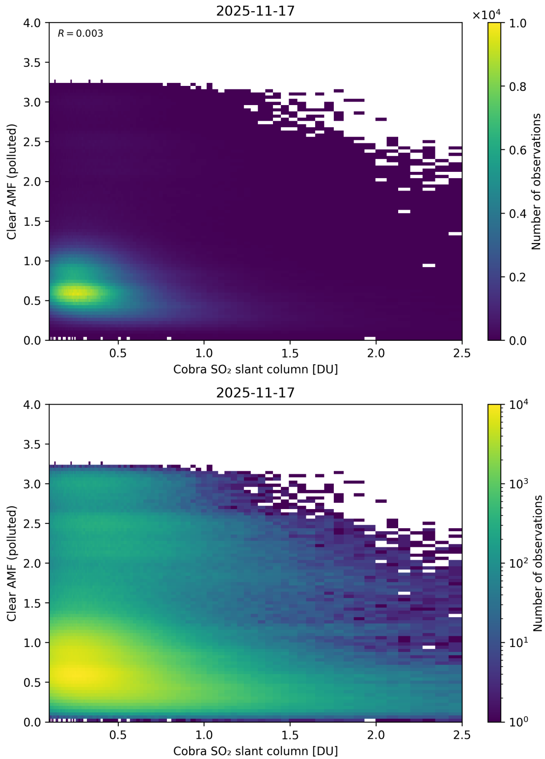
Figure 215: Scatter density plot of “Cobra SO 2 slant column” against “Clear AMF (polluted)” for 2025-11-16 to 2025-11-18.
