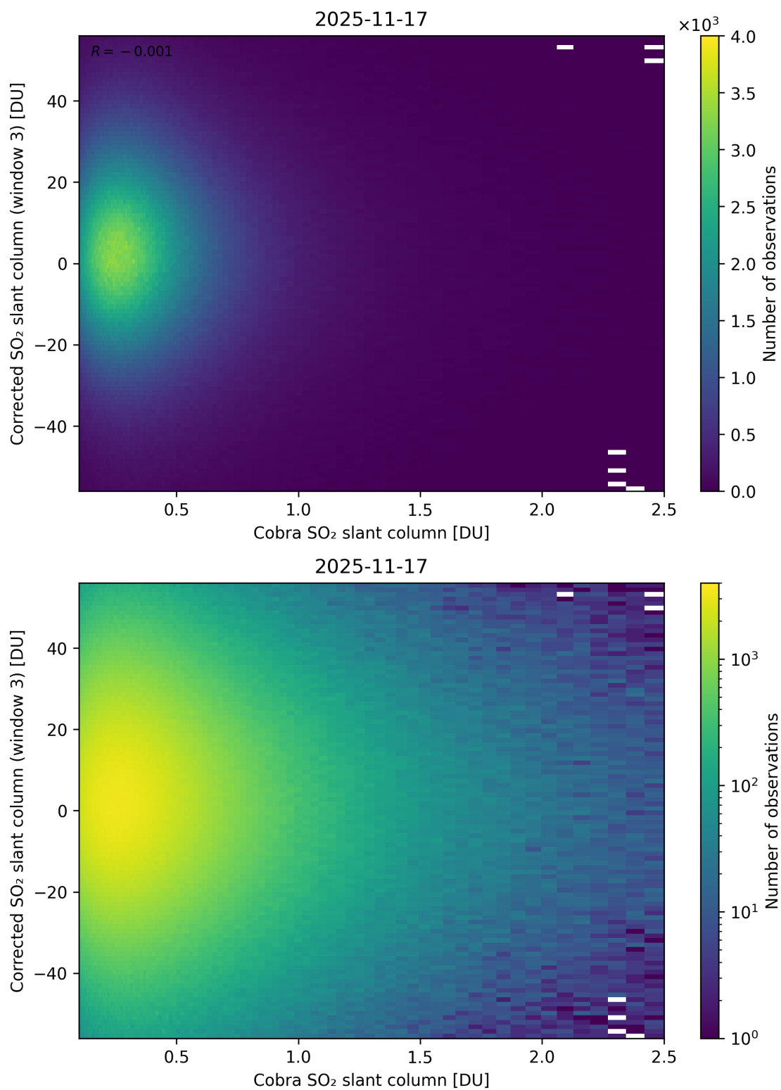
Figure 218: Scatter density plot of “Cobra SO 2 slant column” against “Corrected SO 2 slant column (window 3)” for 2025-11-16 to 2025-11-18.
