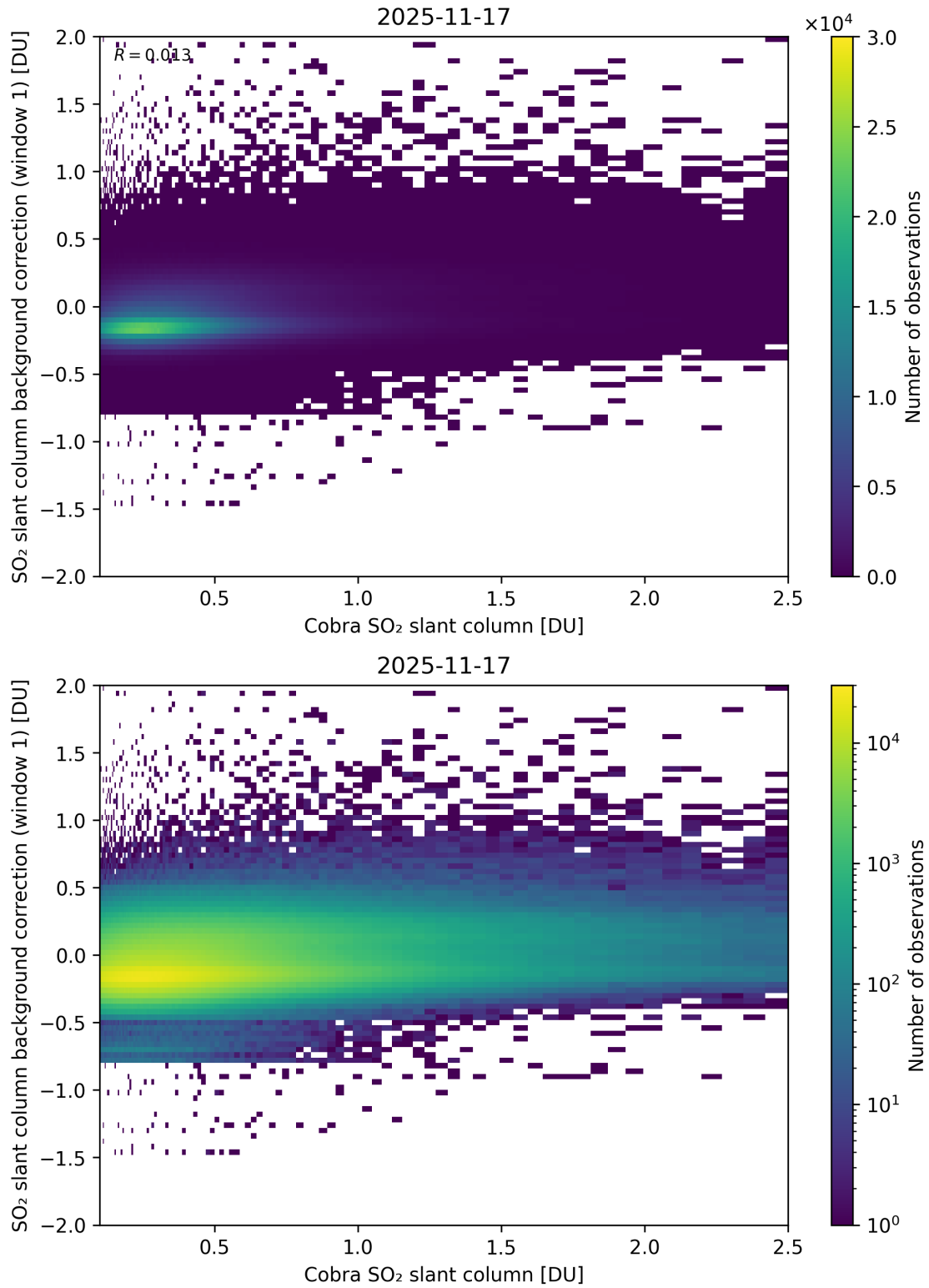
Figure 193: Scatter density plot of “Cobra SO 2 slant column” against “SO 2 slant column background correction (window 1)” for 2025-11-16 to 2025-11-18.
