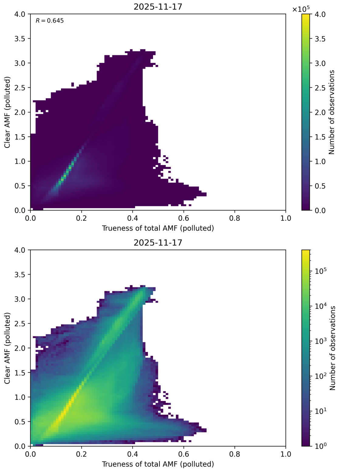
Figure 322: Scatter density plot of “Trueness of total AMF (polluted)” against “Clear AMF (polluted)” for 2025-11-16 to 2025-11-18.
