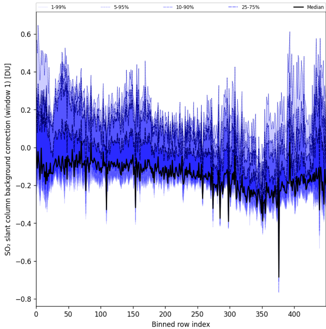
Figure 92: Along track statistics of “SO 2 slant column background correction (window 1)” for 2025-11-16 to 2025-11-18
