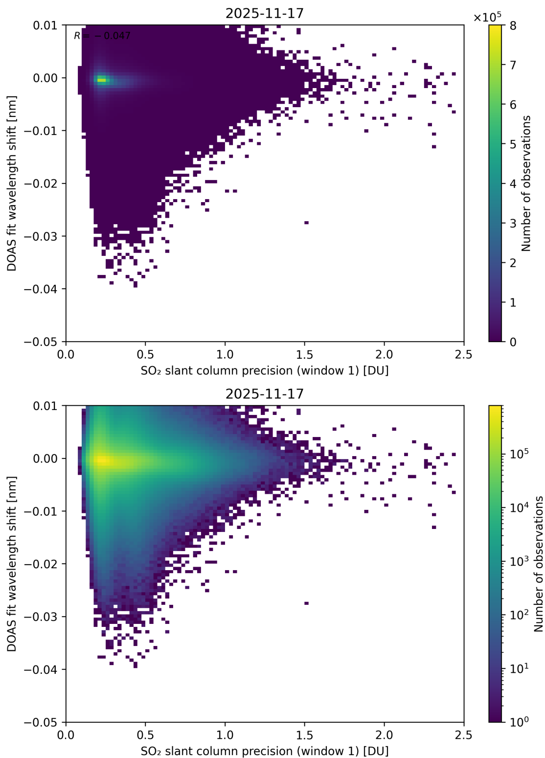
Figure 271: Scatter density plot of “SO 2 slant column precision (window 1)” against “DOAS fit wavelength shift” for 2025-11-16 to 2025-11-18.
