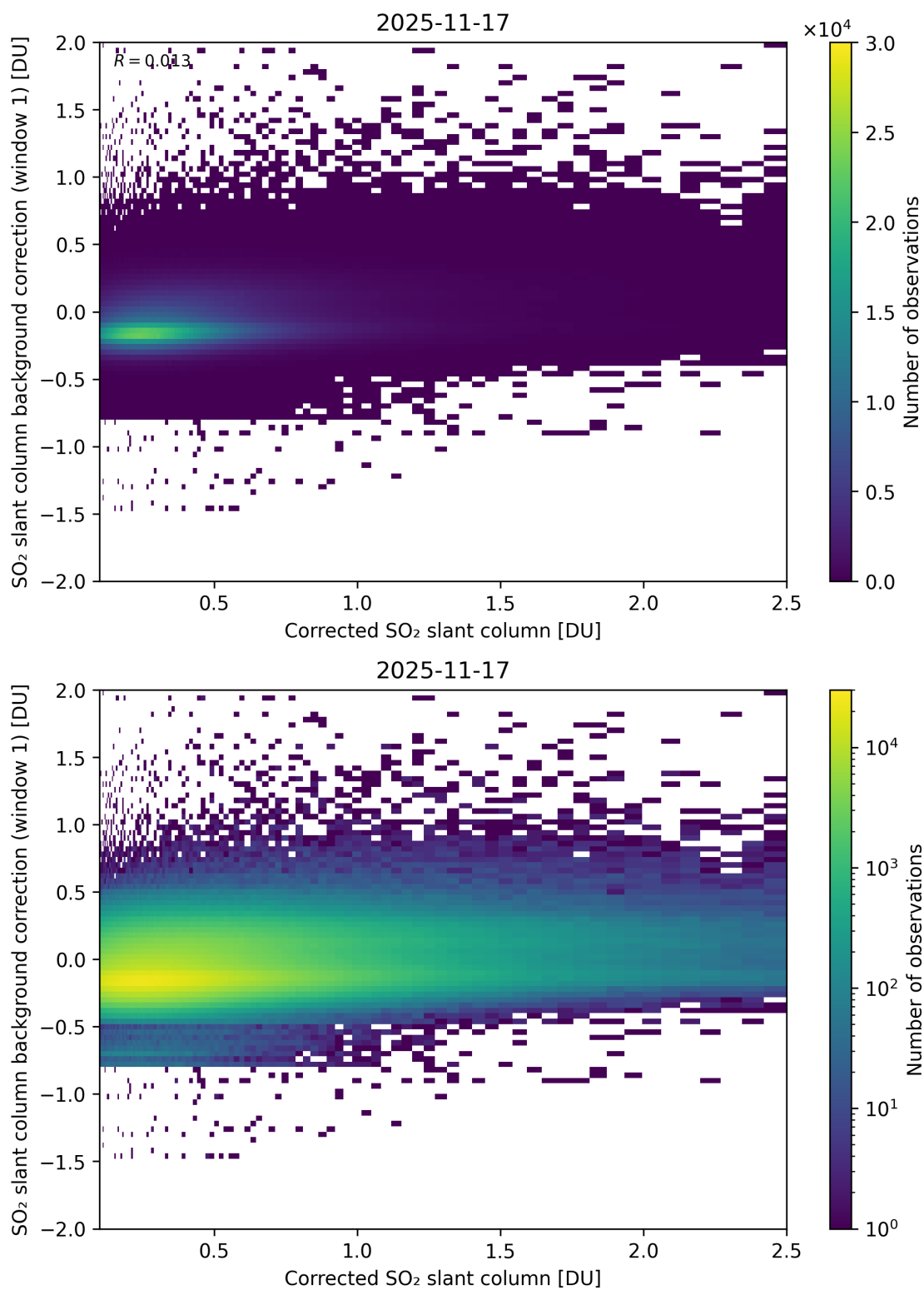
Figure 226: Scatter density plot of “Corrected SO 2 slant column” against “SO 2 slant column background correction (window 1)” for 2025-11-16 to 2025-11-18.
