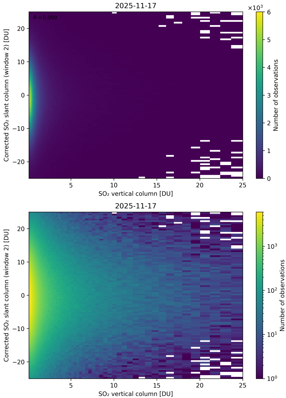
Figure 352: Scatter density plot of “SO 2 vertical column” against “Corrected SO 2 slant column (window 2)” for 2025-11-16 to 2025-11-18.
