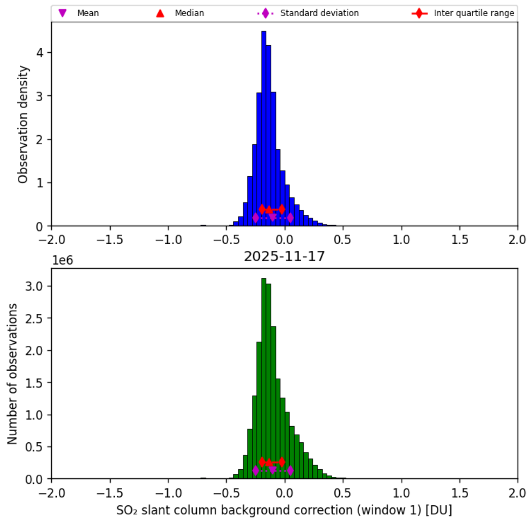
Figure 66: Histogram of “SO 2 slant column background correction (window 1)” for 2025-11-16 to 2025-11-18
