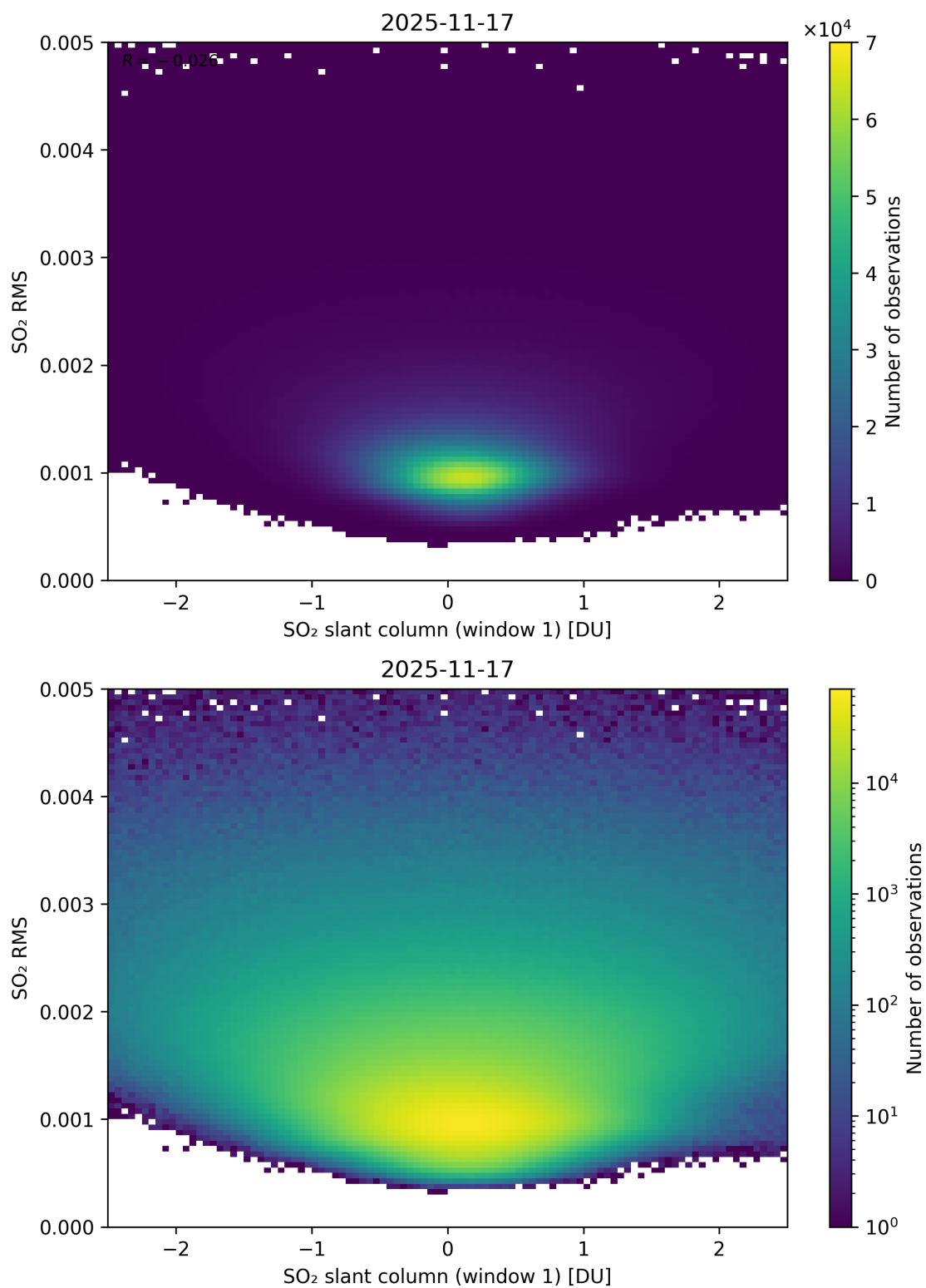
Figure 267: Scatter density plot of “SO 2 slant column (window 1)” against “SO 2 RMS” for 2025-11-16 to 2025-11-18.
