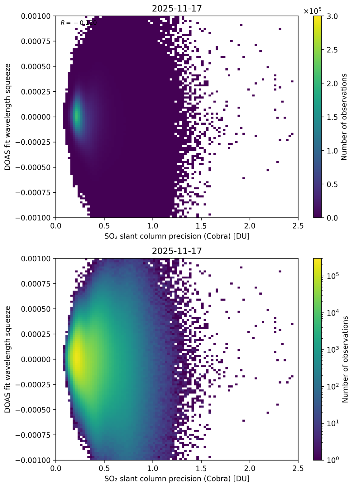
Figure 203: Scatter density plot of “SO 2 slant column precision (Cobra)” against “DOAS fit wavelength squeeze” for 2025-11-16 to 2025-11-18.
