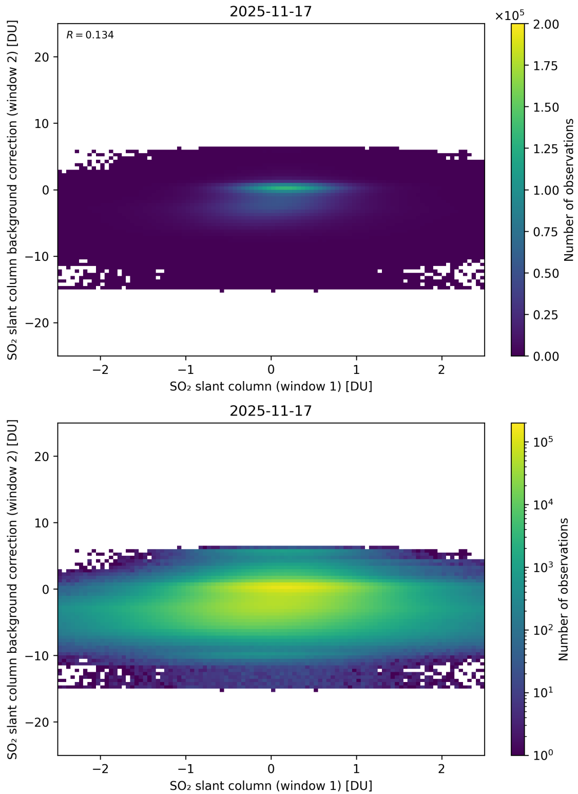
Figure 263: Scatter density plot of “SO 2 slant column (window 1)” against “SO 2 slant column background correction (window 2)” for 2025-11-16 to 2025-11-18.
