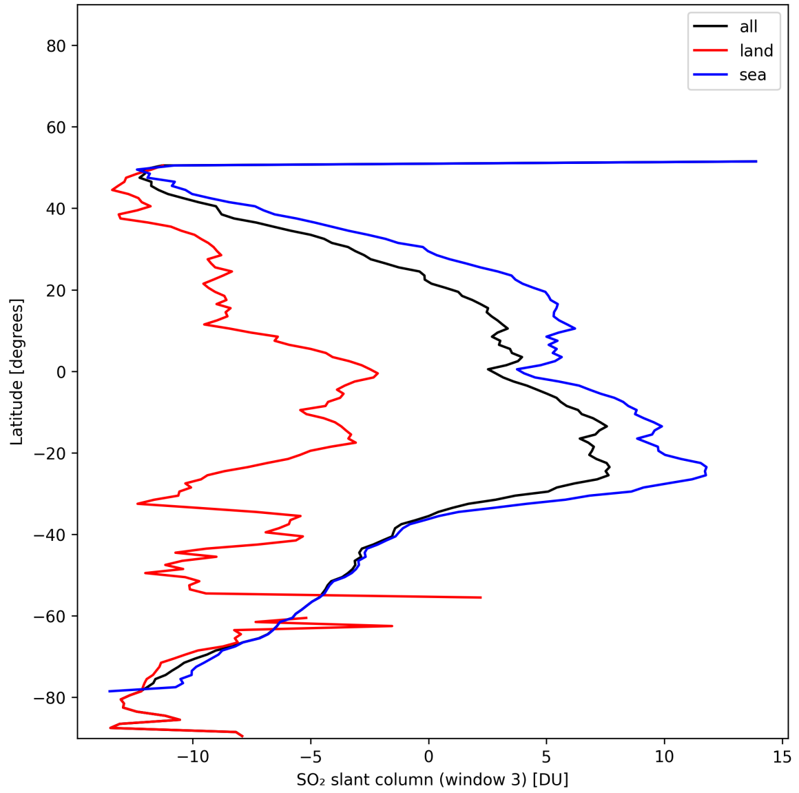
Figure 45: Zonal average of “SO 2 slant column (window 3)” for 2025-11-16 to 2025-11-18.
