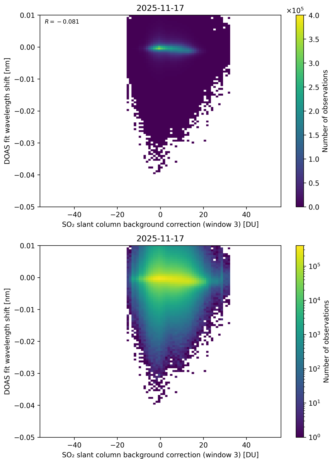
Figure 132: Scatter density plot of “SO 2 slant column background correction (window 3)” against “DOAS fit wavelength shift” for 2025-11-16 to 2025-11-18.
