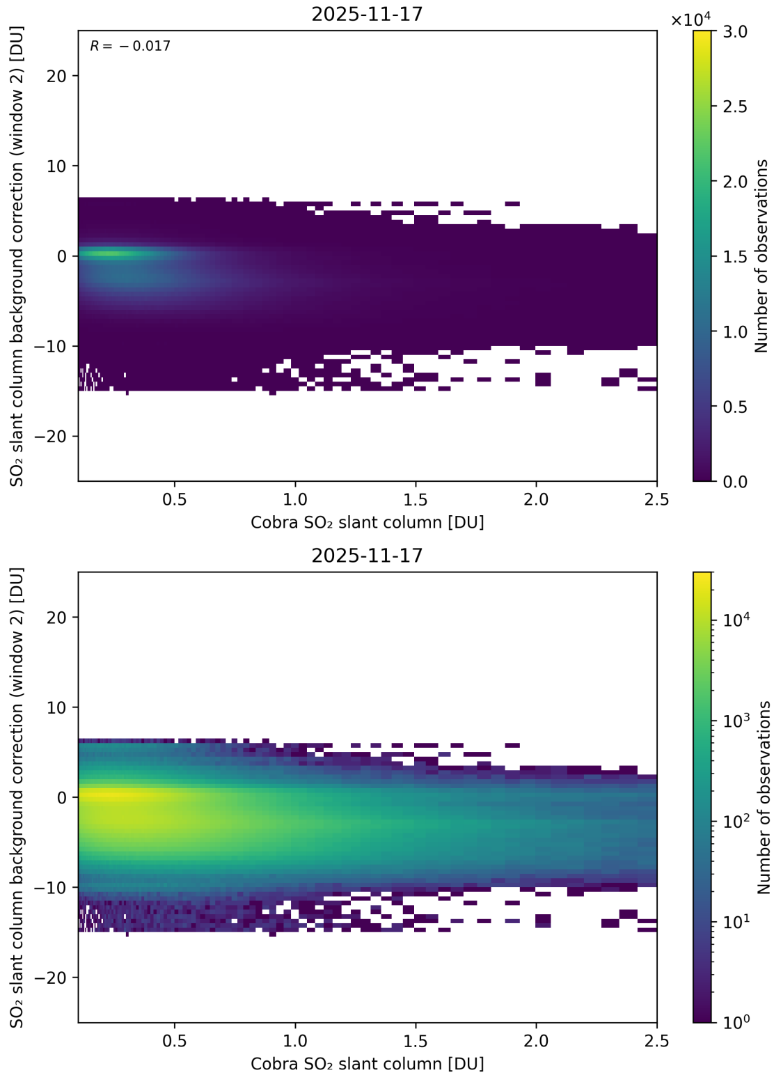
Figure 194: Scatter density plot of “Cobra SO 2 slant column” against “SO 2 slant column background correction (window 2)” for 2025-11-16 to 2025-11-18.
