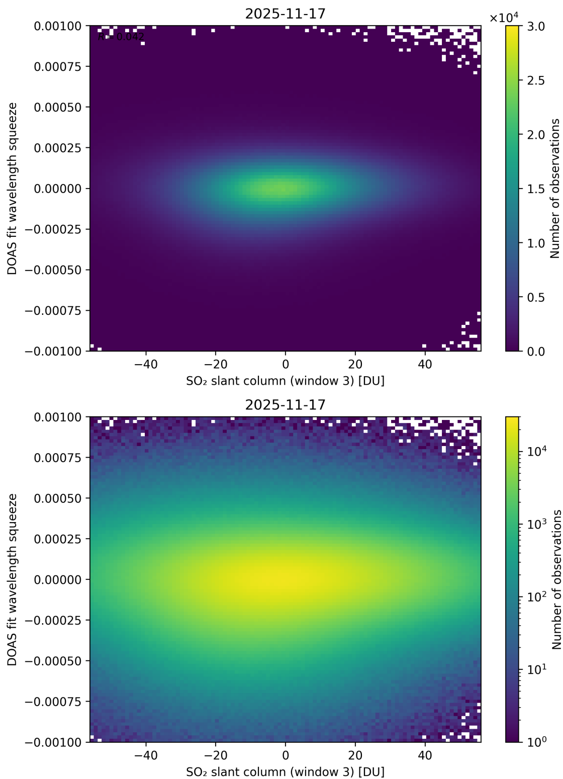
Figure 305: Scatter density plot of “SO 2 slant column (window 3)” against “DOAS fit wavelength squeeze” for 2025-11-16 to 2025-11-18.
