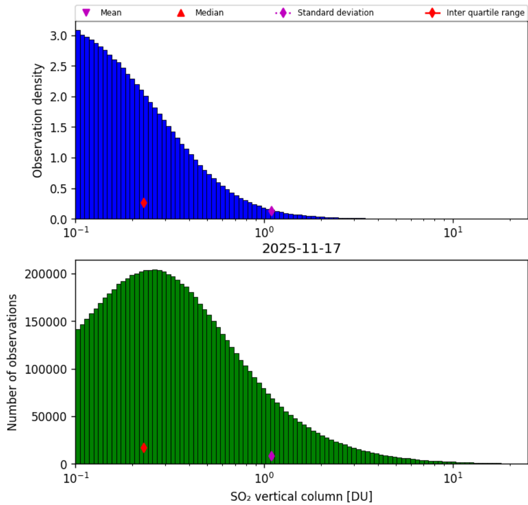
Figure 58: Histogram of “SO 2 vertical column” for 2025-11-16 to 2025-11-18
