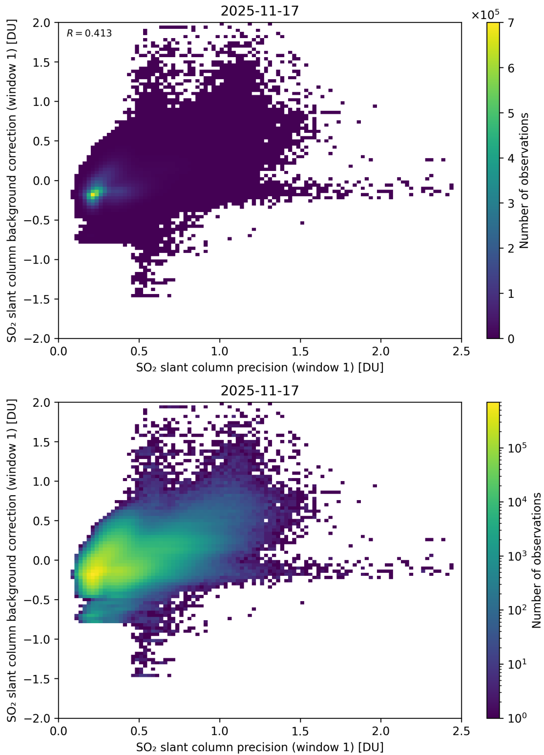
Figure 268: Scatter density plot of “SO 2 slant column precision (window 1)” against “SO 2 slant column background correction (window 1)” for 2025-11-16 to 2025-11-18.
