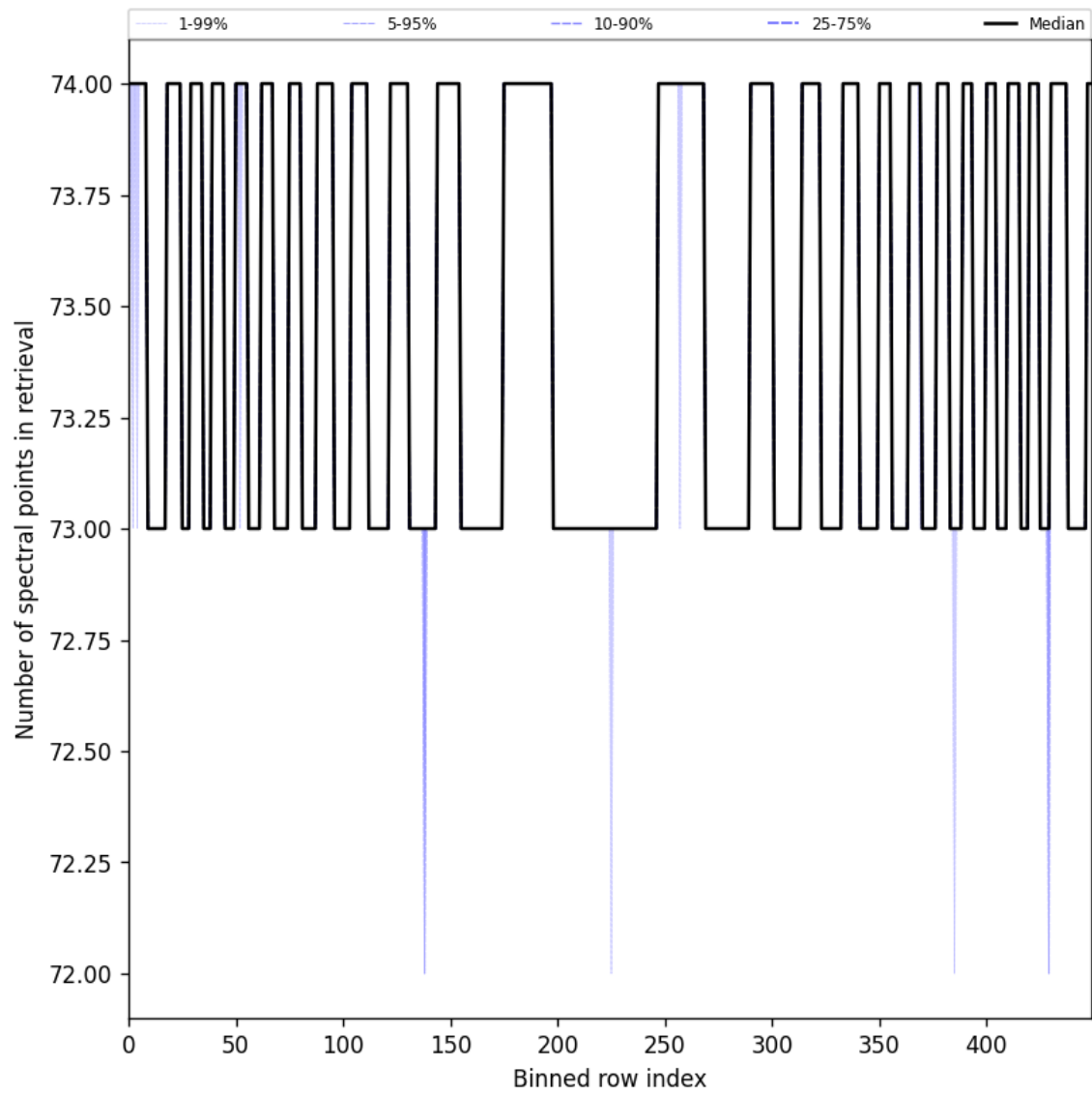
Figure 108: Along track statistics of “Number of spectral points in retrieval” for 2025-11-16 to 2025-11-18
