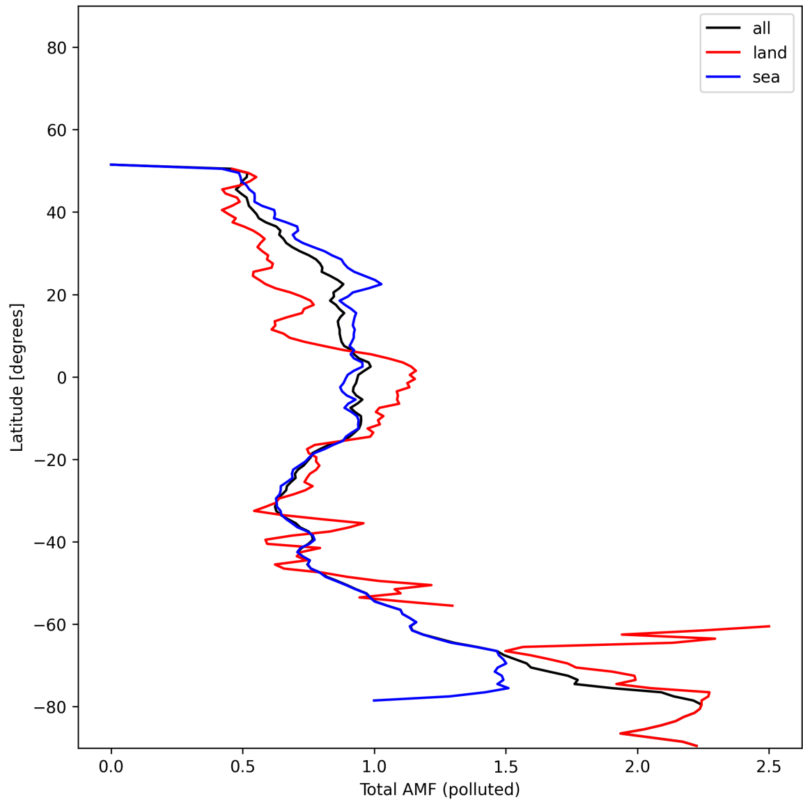
Figure 53: Zonal average of “Total AMF (polluted)” for 2025-11-16 to 2025-11-18.
