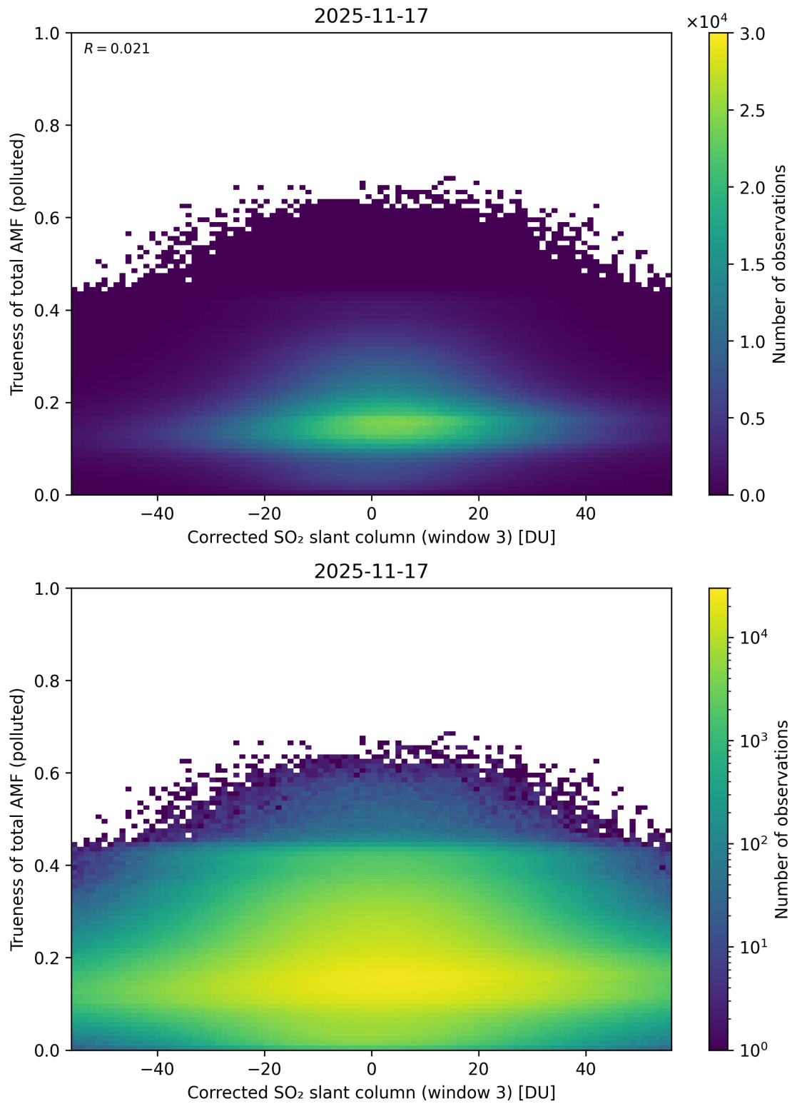
Figure 261: Scatter density plot of “Corrected SO 2 slant column (window 3)” against “Trueness of total AMF (polluted)” for 2025-11-16 to 2025-11-18.
