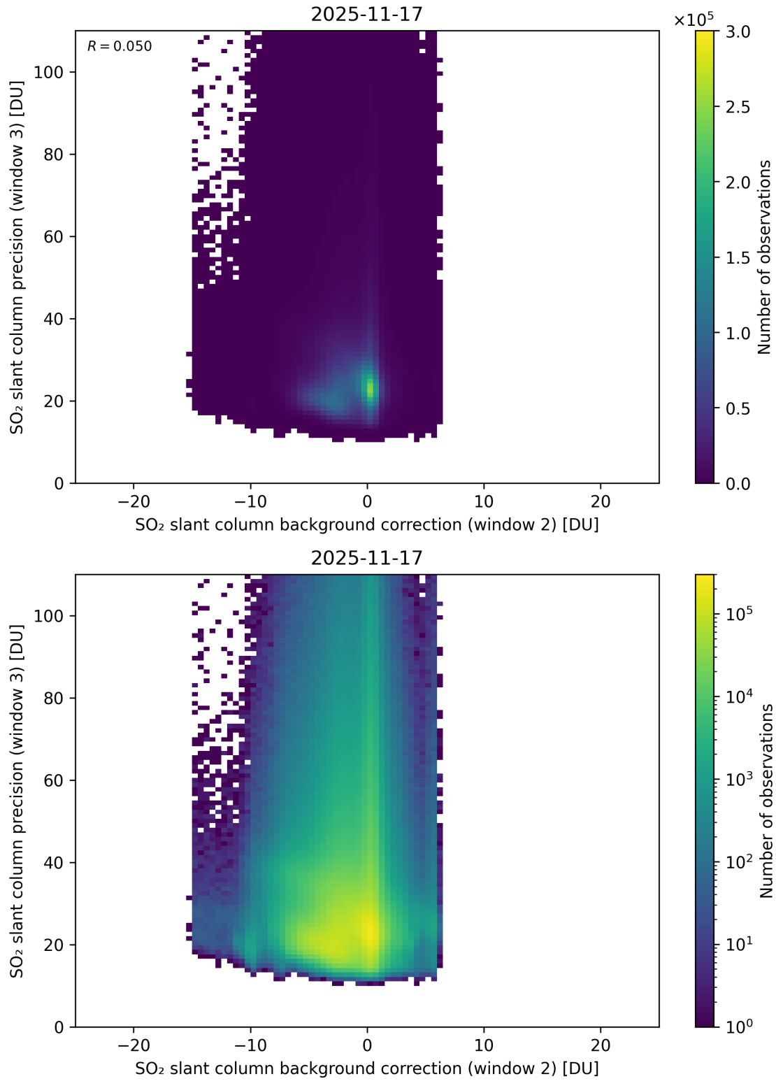
Figure 129: Scatter density plot of “SO 2 slant column background correction (window 2)” against “SO 2 slant column precision (window 3)” for 2025-11-16 to 2025-11-18.
