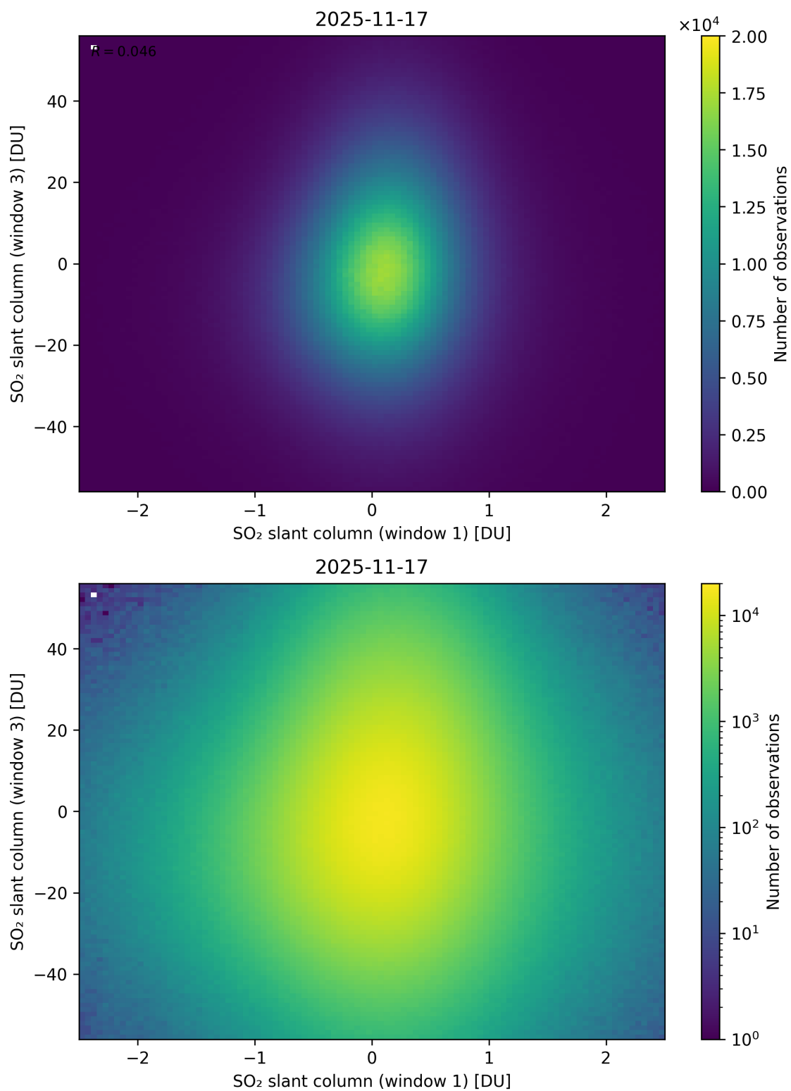
Figure 287: Scatter density plot of “SO 2 slant column (window 1)” against “SO 2 slant column (window 3)” for 2025-11-16 to 2025-11-18.
