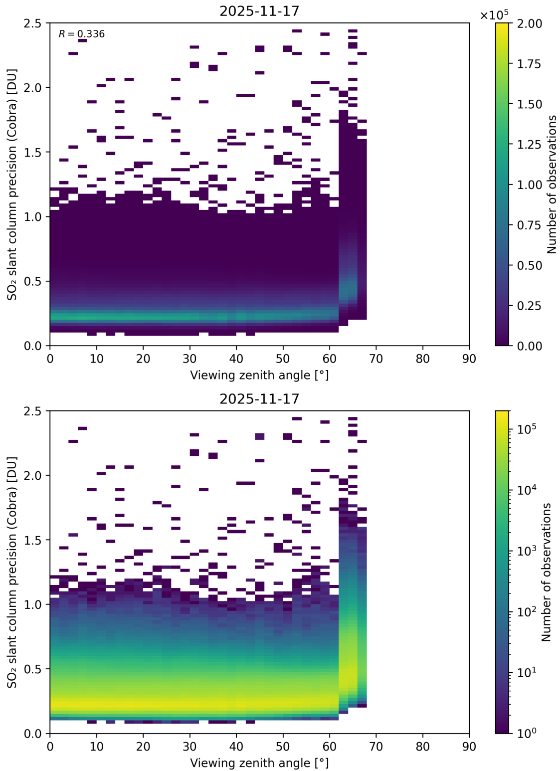
Figure 372: Scatter density plot of “Viewing zenith angle” against “SO 2 slant column precision (Cobra)” for 2025-11-16 to 2025-11-18.
