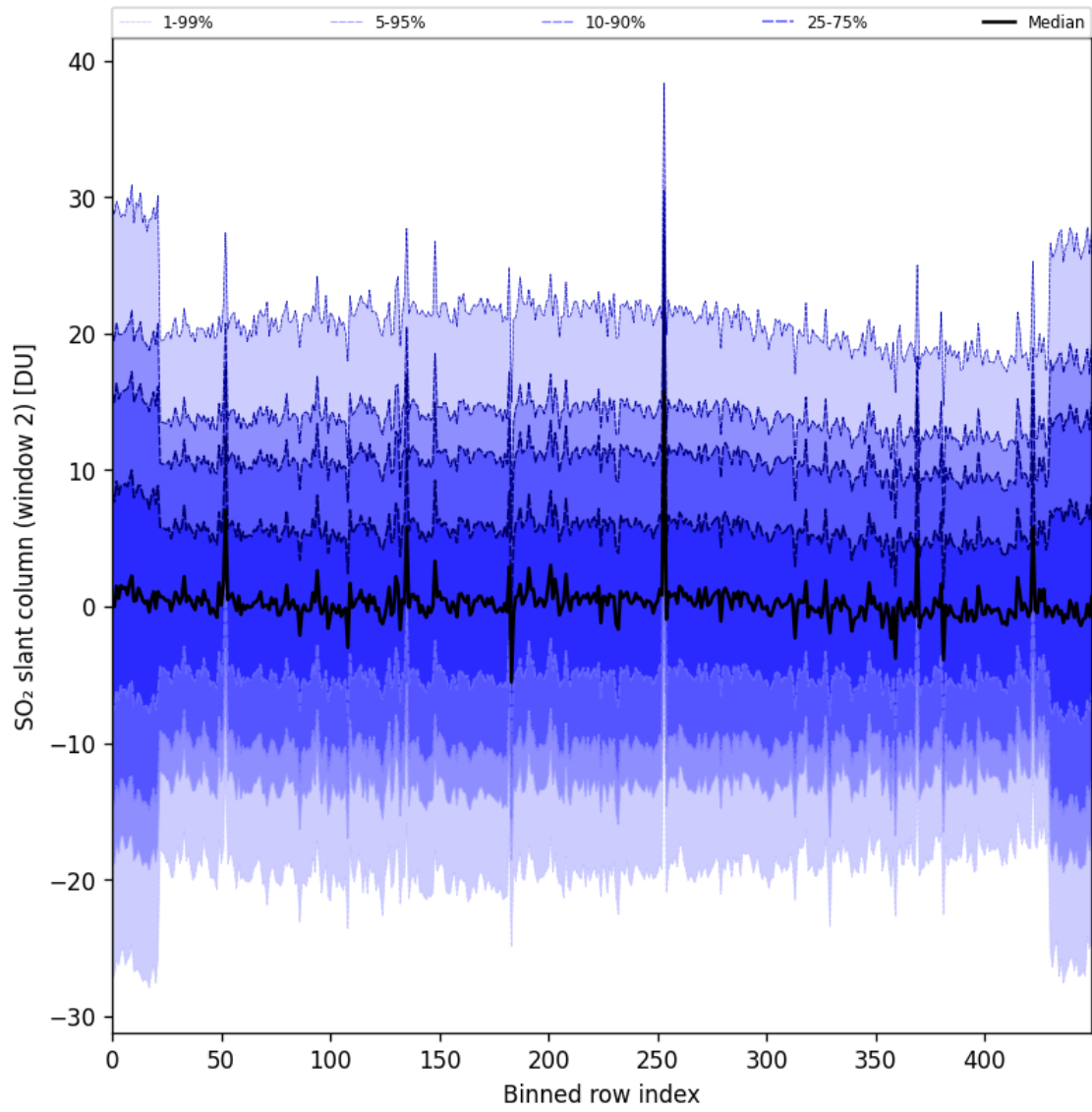
Figure 93: Along track statistics of “SO 2 slant column (window 2)” for 2025-11-16 to 2025-11-18
