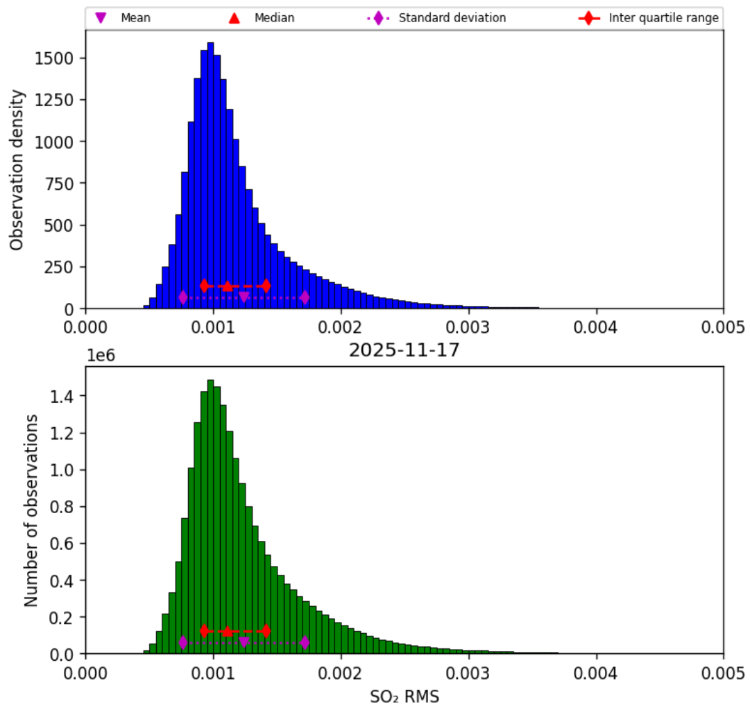
Figure 78: Histogram of “SO 2 RMS” for 2025-11-16 to 2025-11-18
