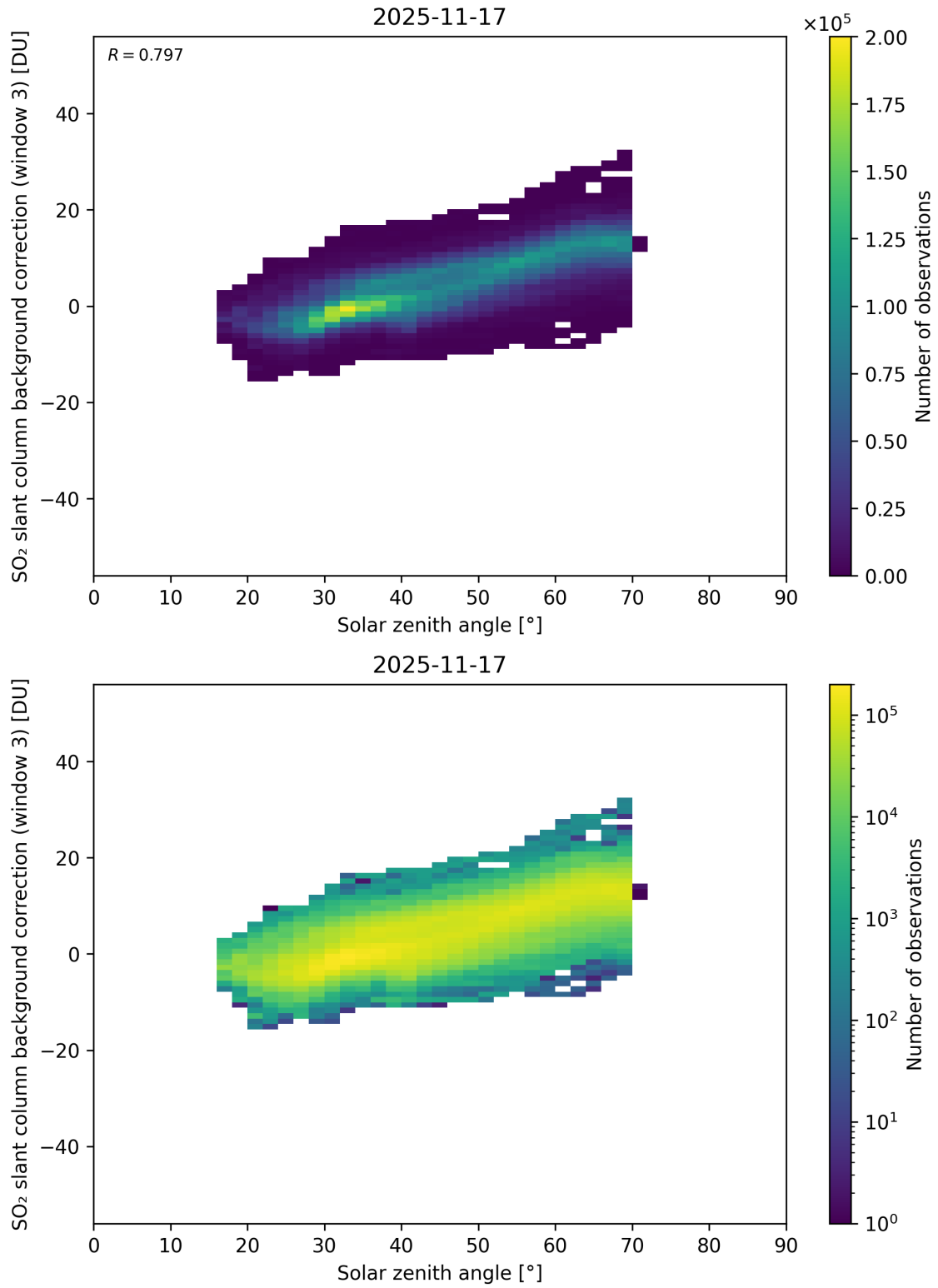
Figure 173: Scatter density plot of “Solar zenith angle” against “SO 2 slant column background correction (window 3)” for 2025-11-16 to 2025-11-18.
