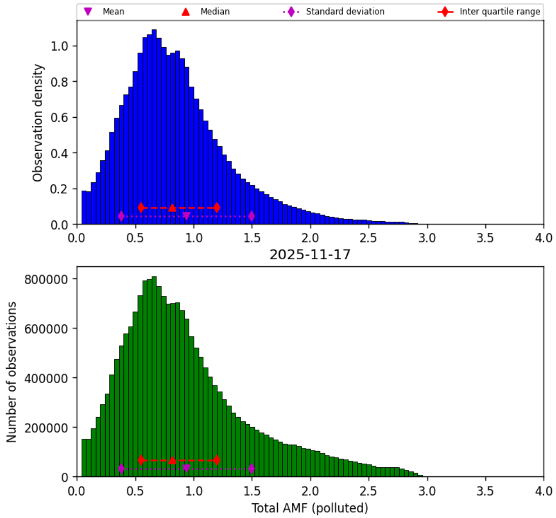
Figure 79: Histogram of “Total AMF (polluted)” for 2025-11-16 to 2025-11-18
