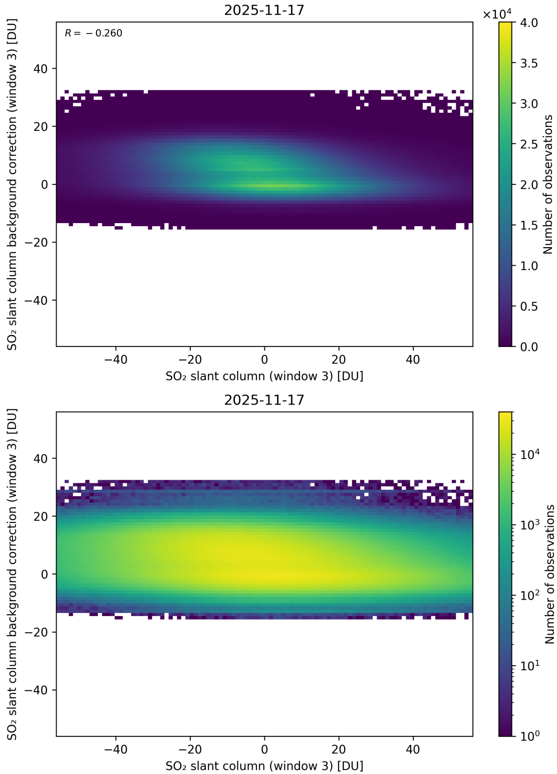
Figure 303: Scatter density plot of “SO 2 slant column (window 3)” against “SO 2 slant column background correction (window 3)” for 2025-11-16 to 2025-11-18.
