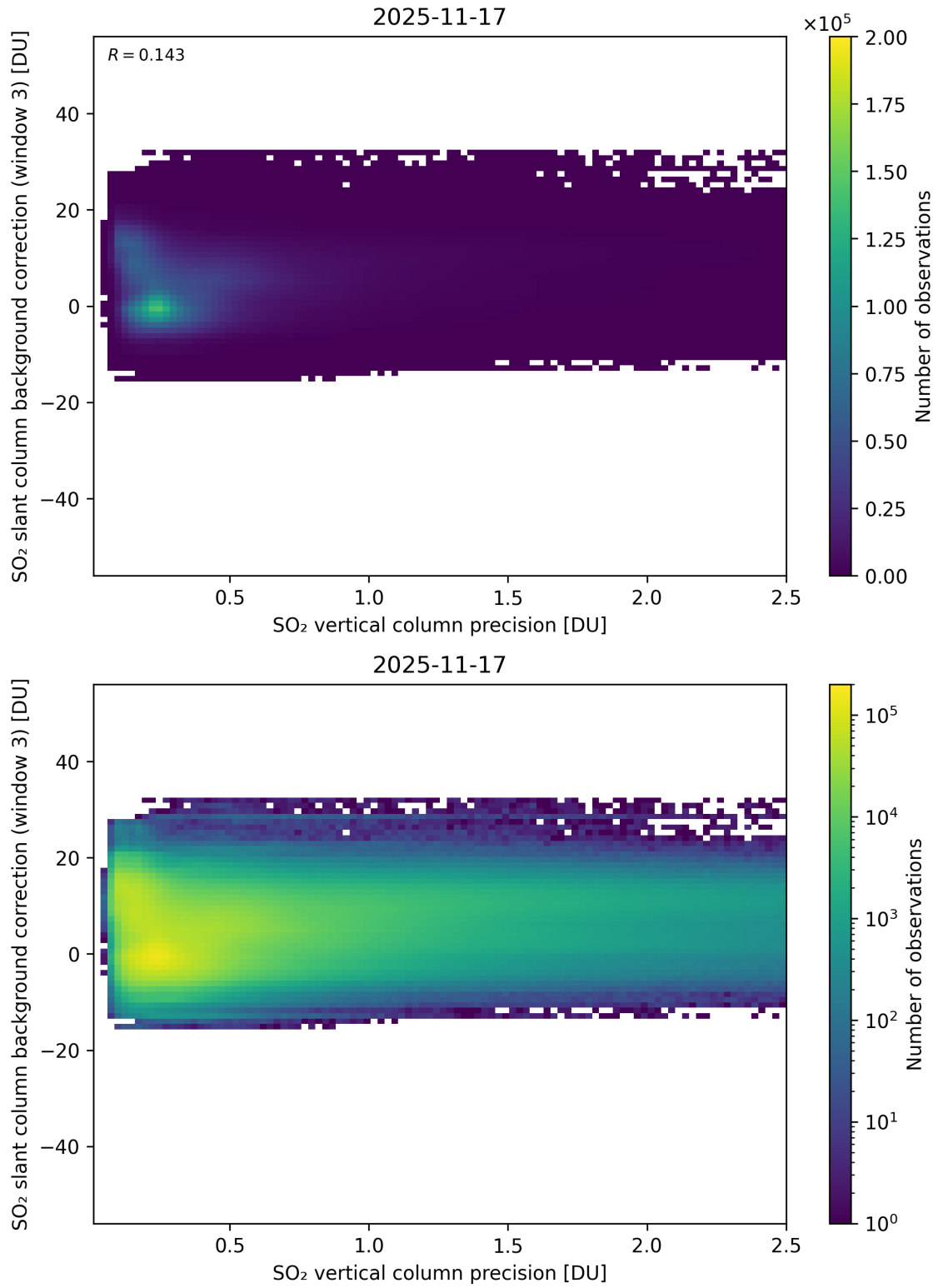
Figure 331: Scatter density plot of “SO 2 vertical column precision” against “SO 2 slant column background correction (window 3)” for 2025-11-16 to 2025-11-18.
