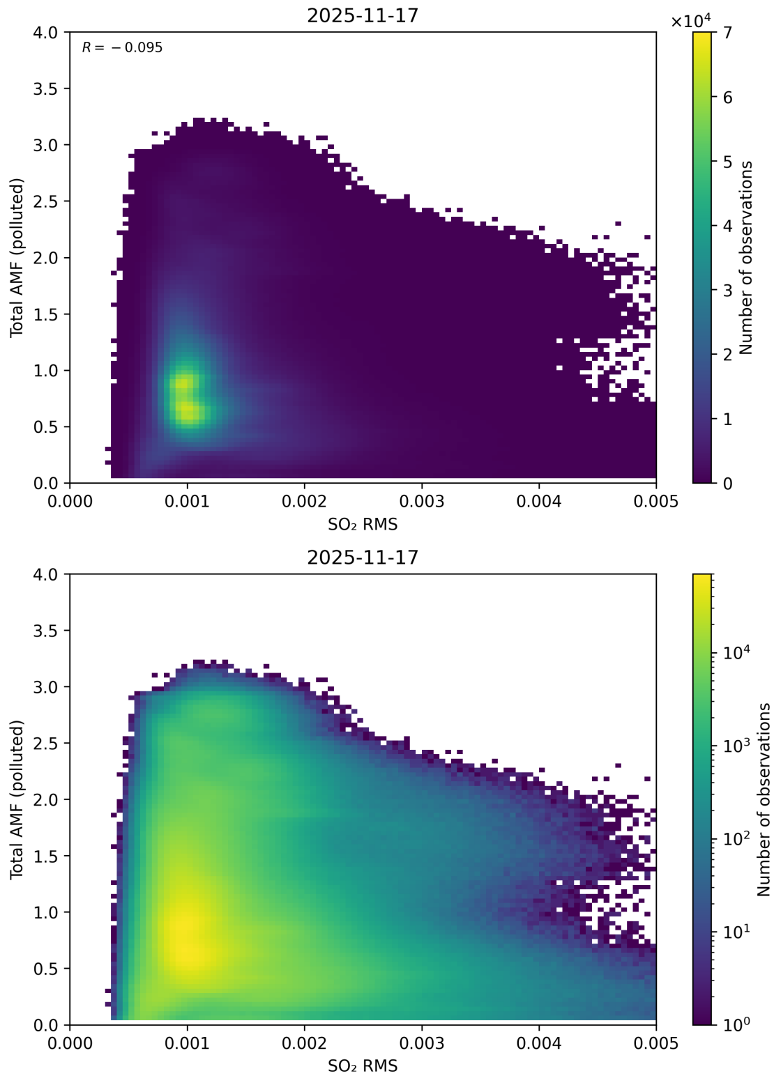
Figure 148: Scatter density plot of “SO 2 RMS” against “Total AMF (polluted)” for 2025-11-16 to 2025-11-18.
