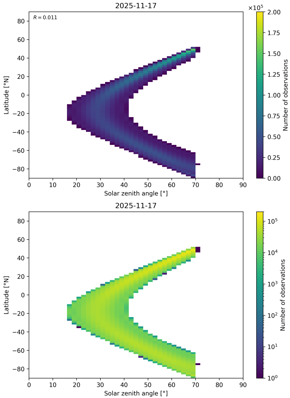
Figure 177: Scatter density plot of “Solar zenith angle” against “Latitude” for 2025-11-16 to 2025-11-18.
