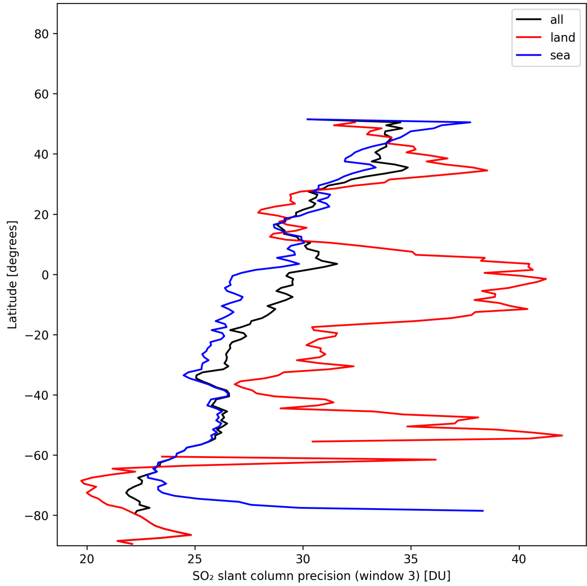
Figure 46: Zonal average of “SO 2 slant column precision (window 3)” for 2025-11-16 to 2025-11-18.
