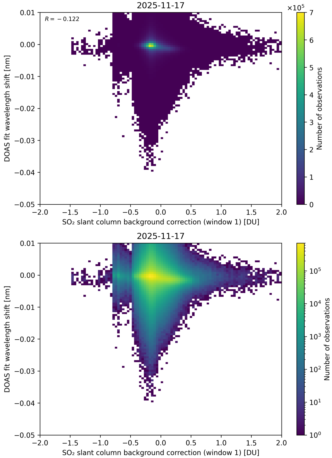
Figure 111: Scatter density plot of “SO 2 slant column background correction (window 1)” against “DOAS fit wavelength shift” for 2025-11-16 to 2025-11-18.
