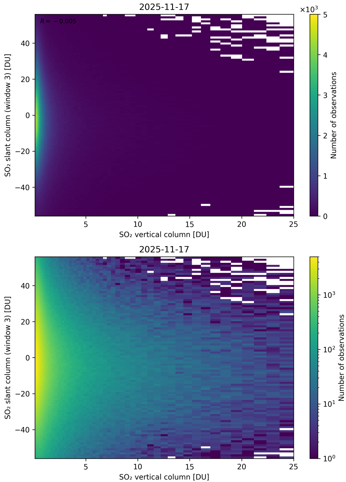
Figure 357: Scatter density plot of “SO 2 vertical column” against “SO 2 slant column (window 3)” for 2025-11-16 to 2025-11-18.
