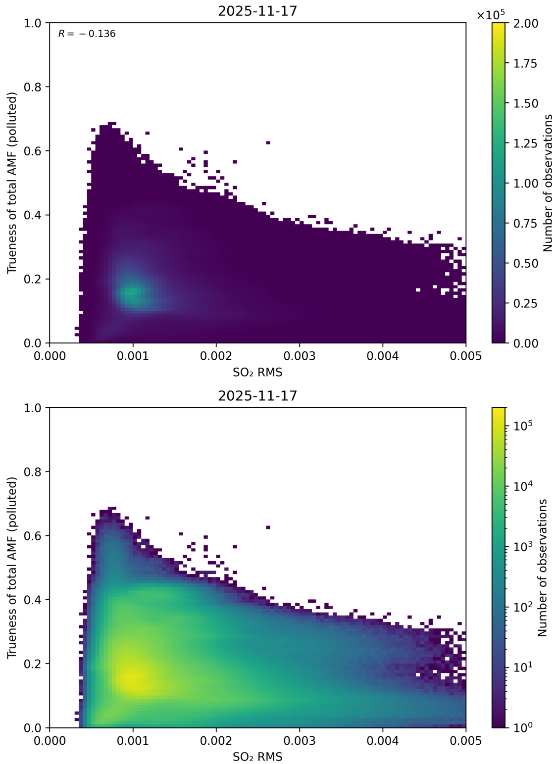
Figure 149: Scatter density plot of “SO 2 RMS” against “Trueness of total AMF (polluted)” for 2025-11-16 to 2025-11-18.
