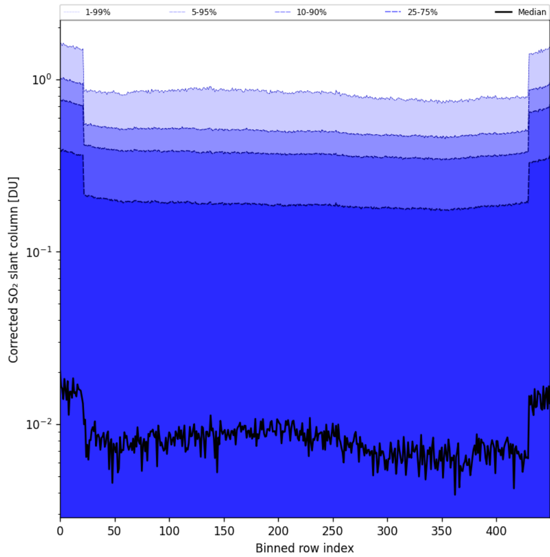
Figure 86: Along track statistics of "Corrected SO 2 slant column" for 2025-11-16 to 2025-11-18
