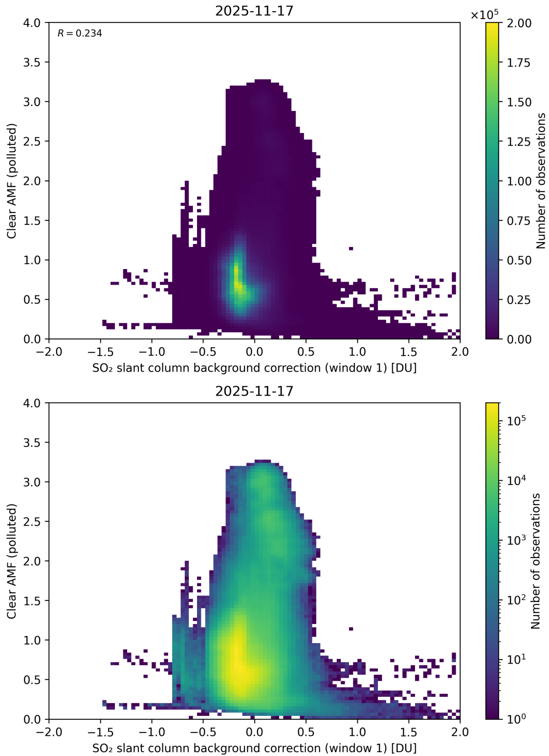
Figure 114: Scatter density plot of “SO 2 slant column background correction (window 1)” against “Clear AMF (polluted)” for 2025-11-16 to 2025-11-18.
