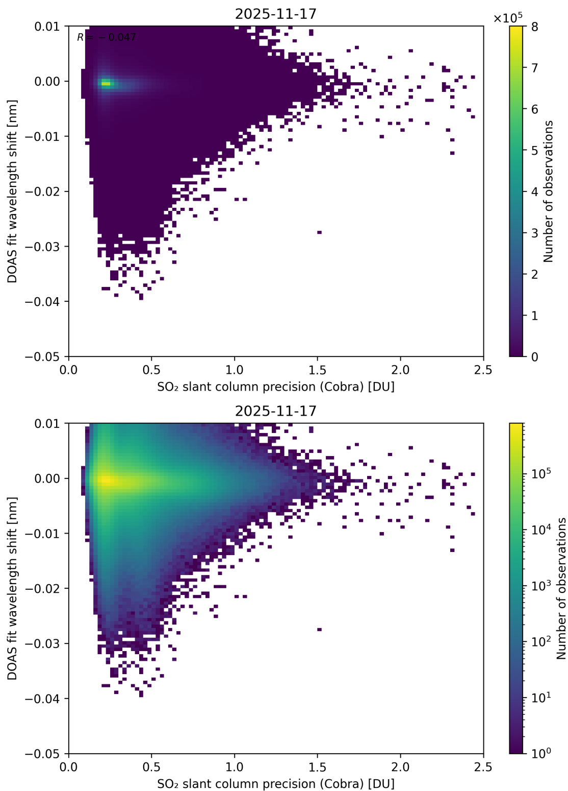
Figure 202: Scatter density plot of “SO 2 slant column precision (Cobra)” against “DOAS fit wavelength shift” for 2025-11-16 to 2025-11-18.
