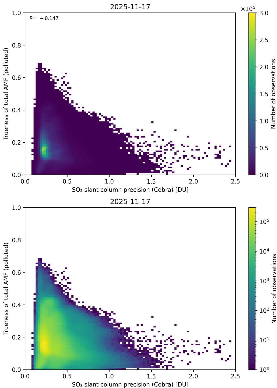
Figure 214: Scatter density plot of “SO 2 slant column precision (Cobra)” against “Trueness of total AMF (polluted)” for 2025-11-16 to 2025-11-18.
