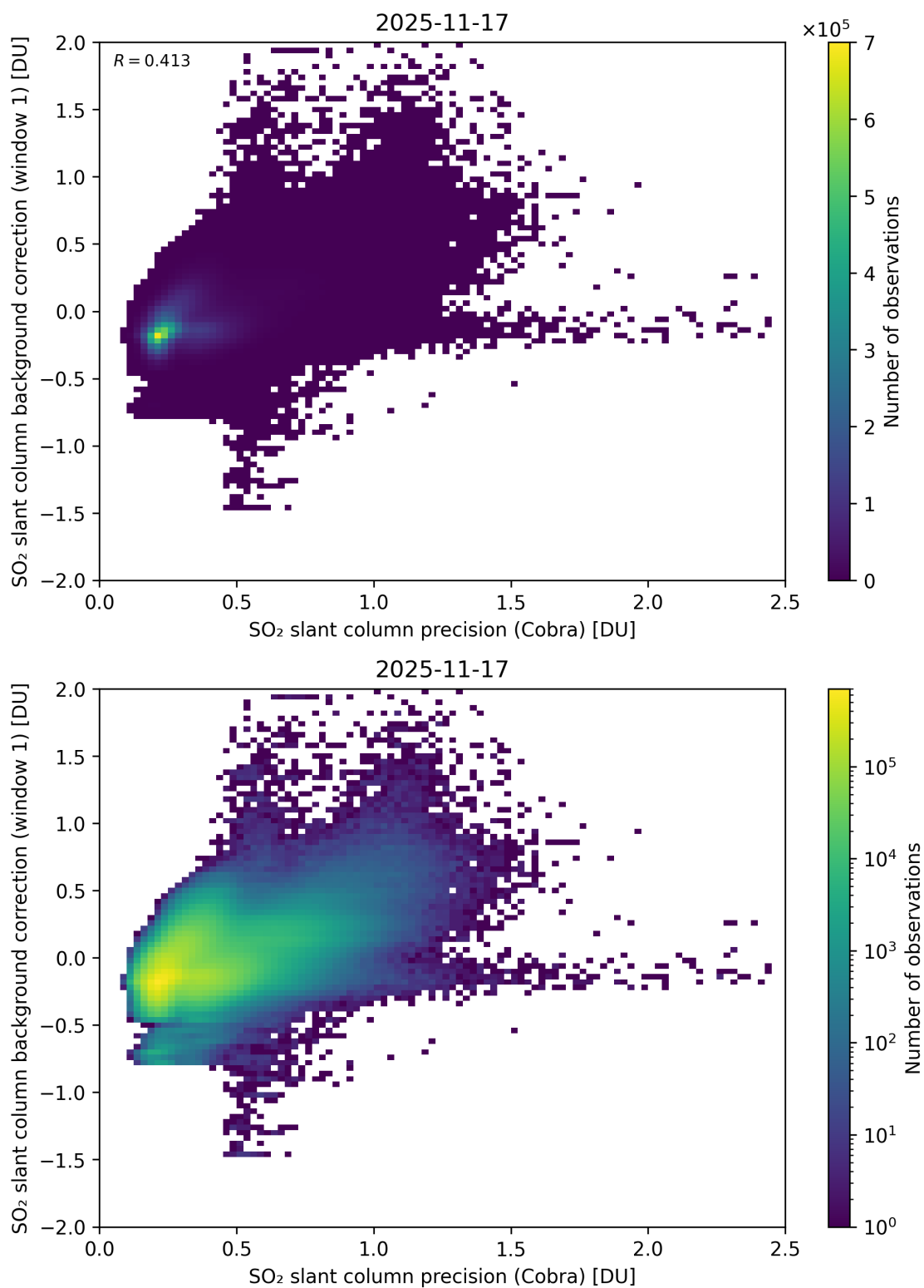
Figure 199: Scatter density plot of “SO 2 slant column precision (Cobra)” against “SO 2 slant column background correction (window 1)” for 2025-11-16 to 2025-11-18.
