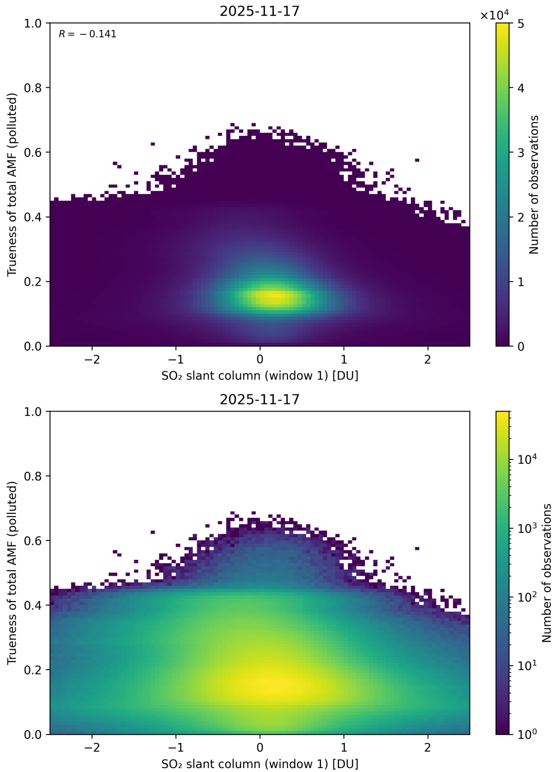
Figure 290: Scatter density plot of “SO 2 slant column (window 1)” against “Trueness of total AMF (polluted)” for 2025-11-16 to 2025-11-18.
