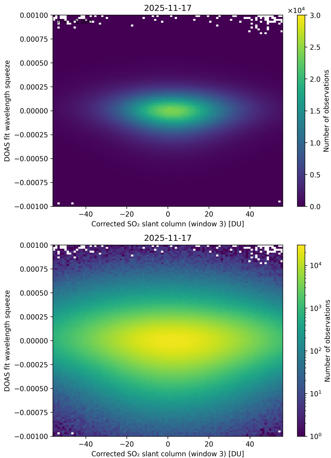
Figure 257: Scatter density plot of “Corrected SO 2 slant column (window 3)” against “DOAS fit wavelength squeeze” for 2025-11-16 to 2025-11-18.
