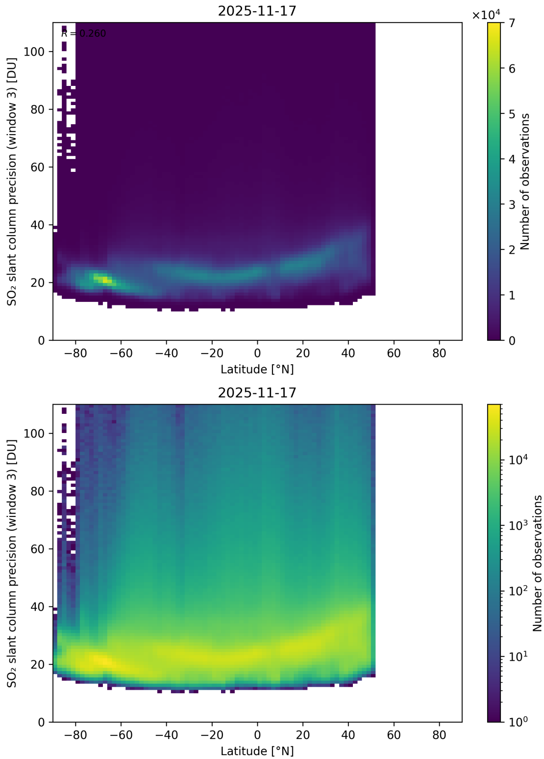
Figure 166: Scatter density plot of “Latitude” against “SO 2 slant column precision (window 3)” for 2025-11-16 to 2025-11-18.
