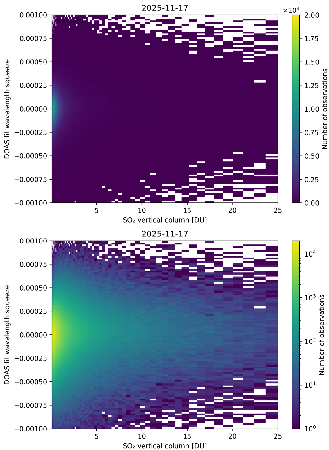
Figure 327: Scatter density plot of “SO 2 vertical column” against “DOAS fit wavelength squeeze” for 2025-11-16 to 2025-11-18.
