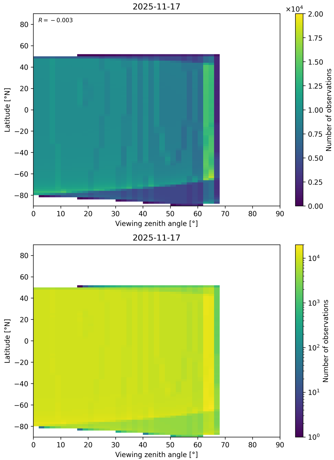
Figure 368: Scatter density plot of “Viewing zenith angle” against “Latitude” for 2025-11-16 to 2025-11-18.
