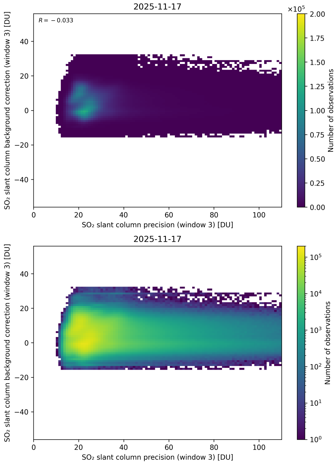
Figure 307: Scatter density plot of “SO 2 slant column precision (window 3)” against “SO 2 slant column background correction (window 3)” for 2025-11-16 to 2025-11-18.
