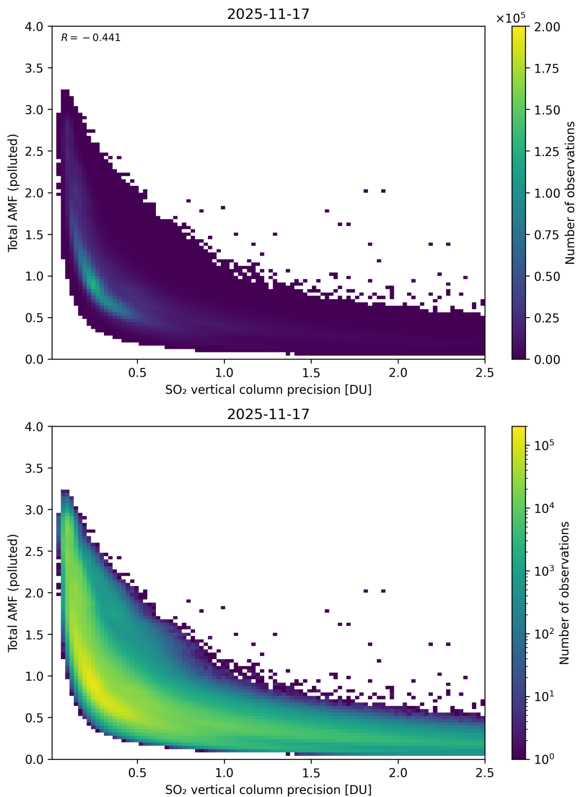
Figure 346: Scatter density plot of “SO 2 vertical column precision” against “Total AMF (polluted)” for 2025-11-16 to 2025-11-18.
