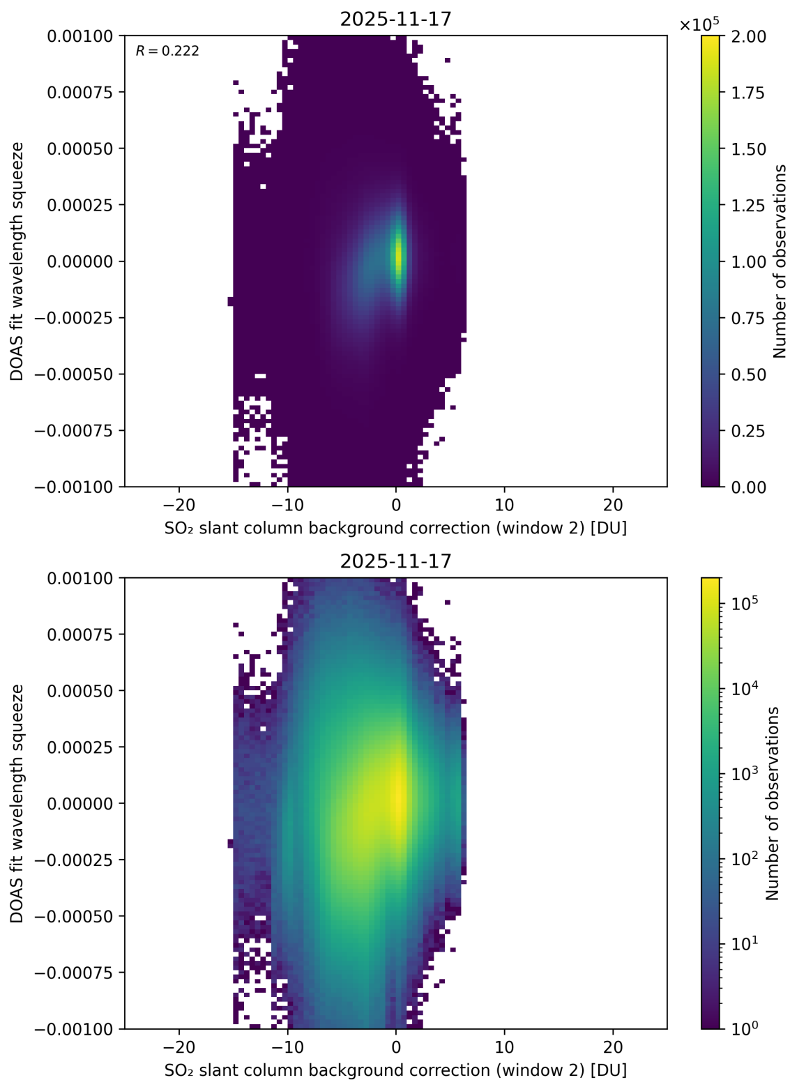
Figure 124: Scatter density plot of “SO 2 slant column background correction (window 2)” against “DOAS fit wavelength squeeze” for 2025-11-16 to 2025-11-18.
