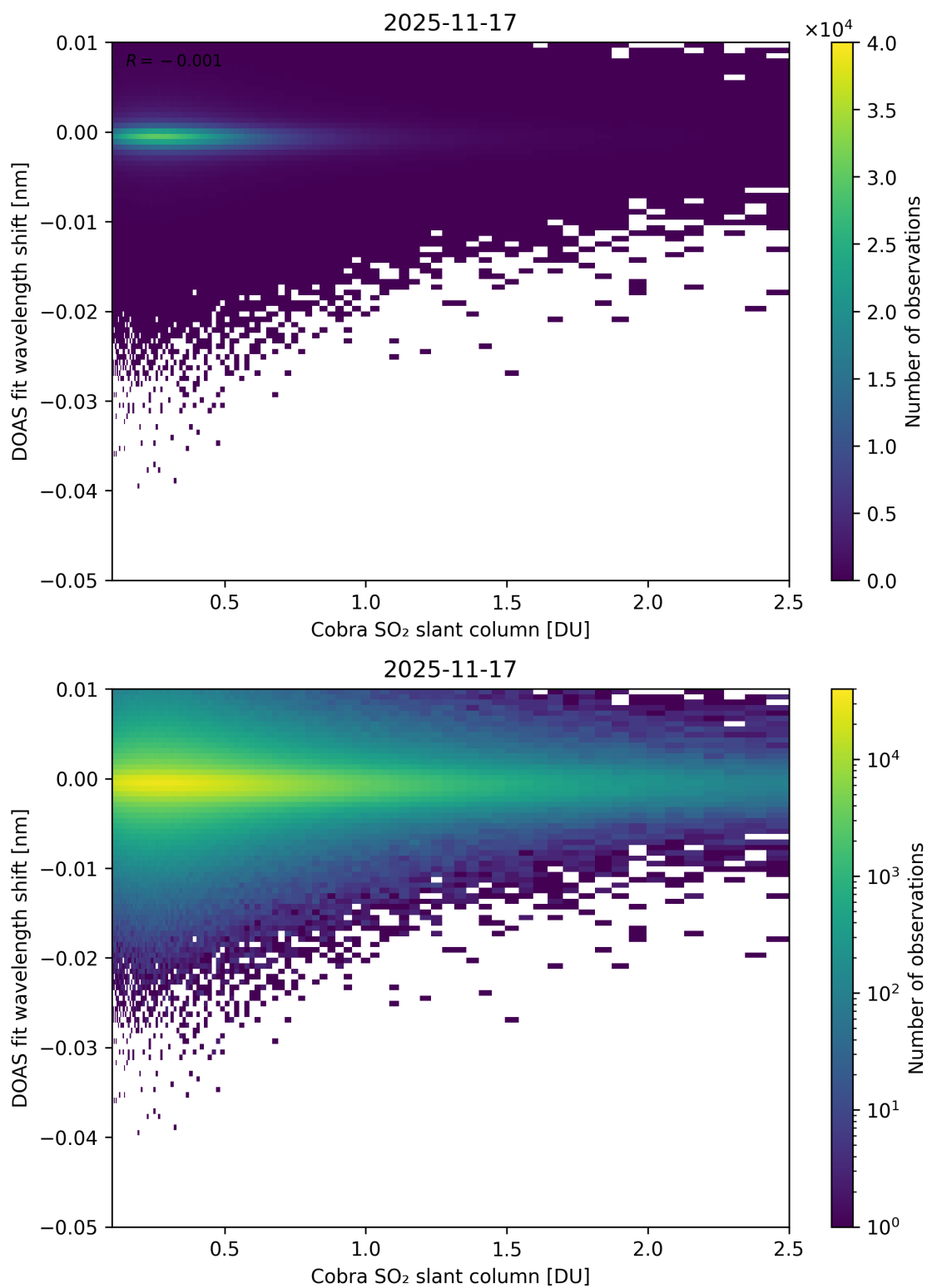
Figure 196: Scatter density plot of “Cobra SO 2 slant column” against “DOAS fit wavelength shift” for 2025-11-16 to 2025-11-18.
