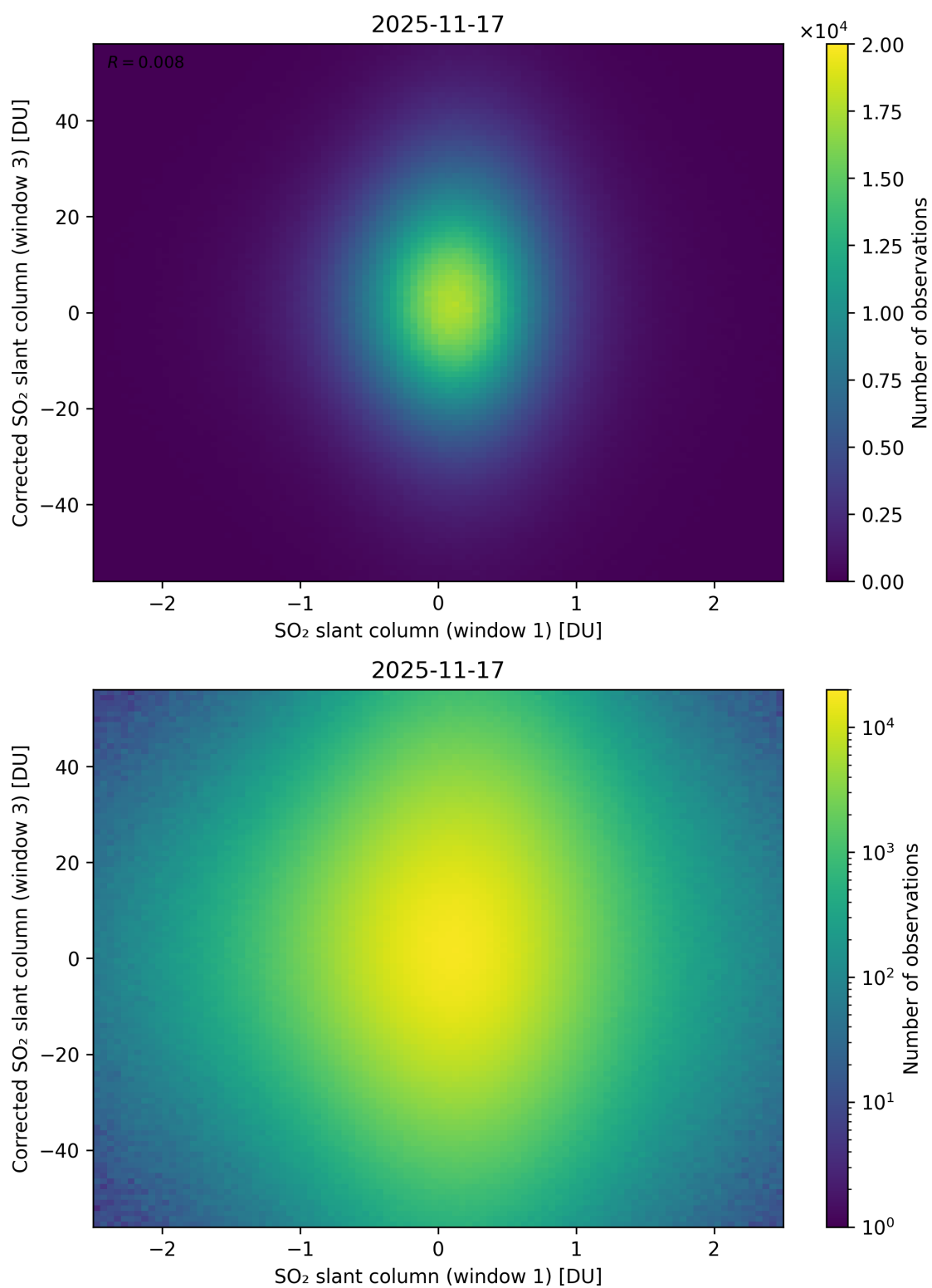
Figure 284: Scatter density plot of “SO 2 slant column (window 1)” against “Corrected SO 2 slant column (window 3)” for 2025-11-16 to 2025-11-18.
