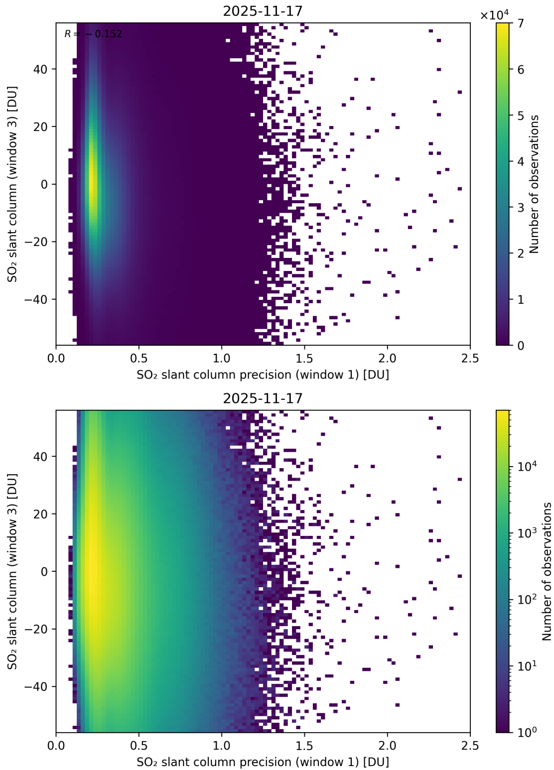
Figure 278: Scatter density plot of “SO 2 slant column precision (window 1)” against “SO 2 slant column (window 3)” for 2025-11-16 to 2025-11-18.
