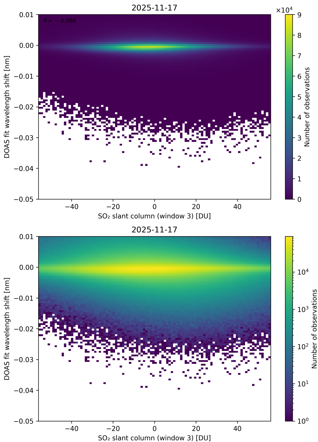
Figure 304: Scatter density plot of “SO 2 slant column (window 3)” against “DOAS fit wavelength shift” for 2025-11-16 to 2025-11-18.
