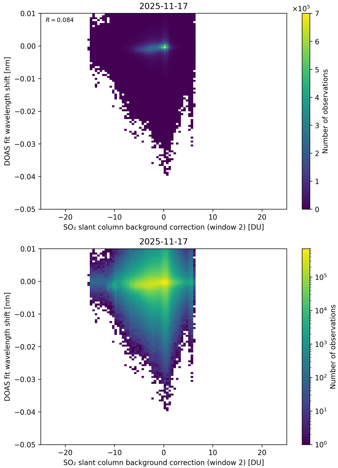
Figure 123: Scatter density plot of “SO 2 slant column background correction (window 2)” against “DOAS fit wavelength shift” for 2025-11-16 to 2025-11-18.
