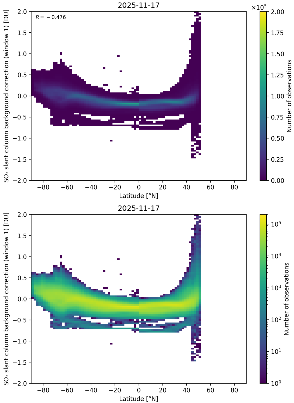
Figure 150: Scatter density plot of “Latitude” against “SO 2 slant column background correction (window 1)” for 2025-11-16 to 2025-11-18.
