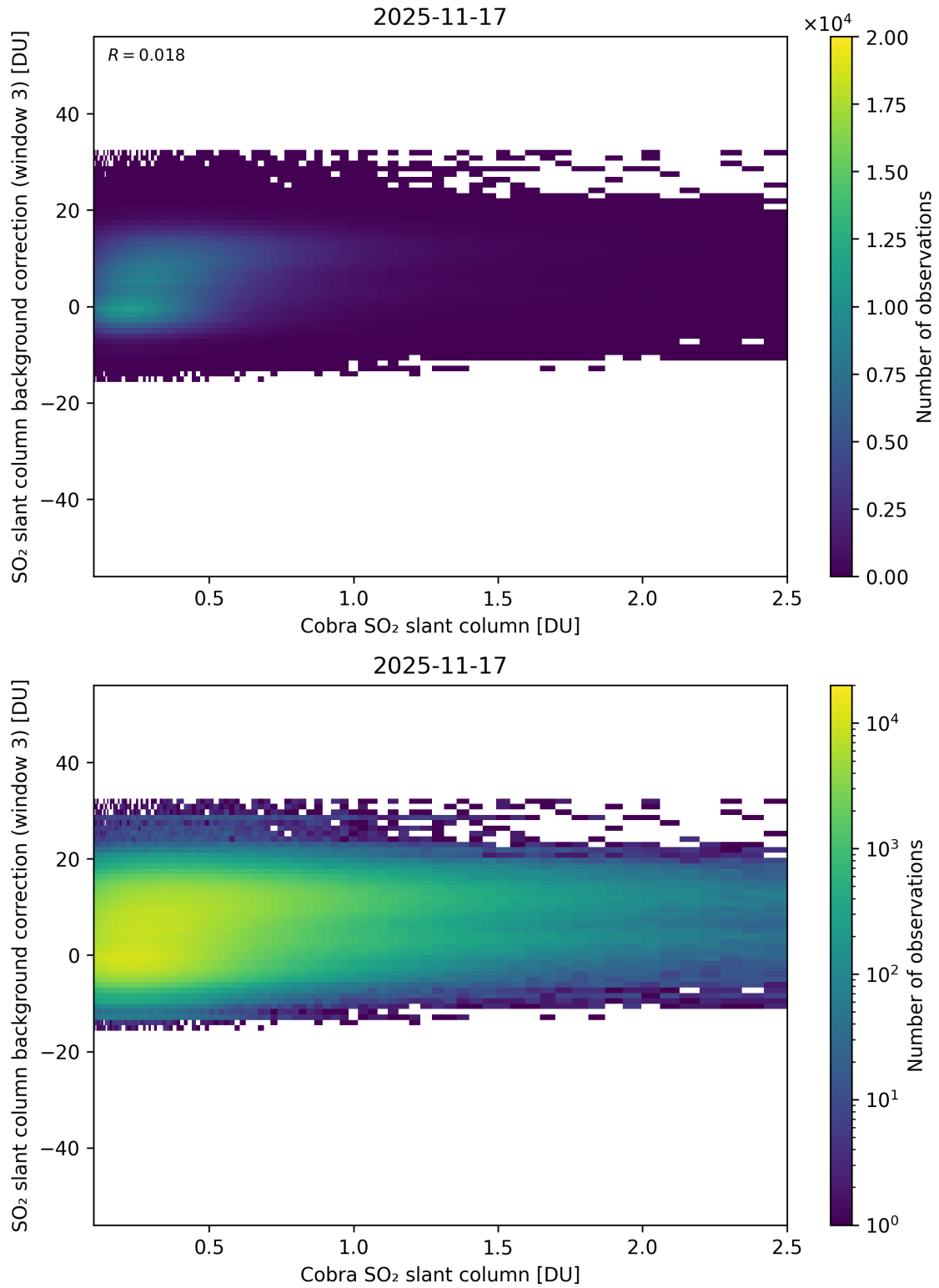
Figure 195: Scatter density plot of “Cobra SO 2 slant column” against “SO 2 slant column background correction (window 3)” for 2025-11-16 to 2025-11-18.
