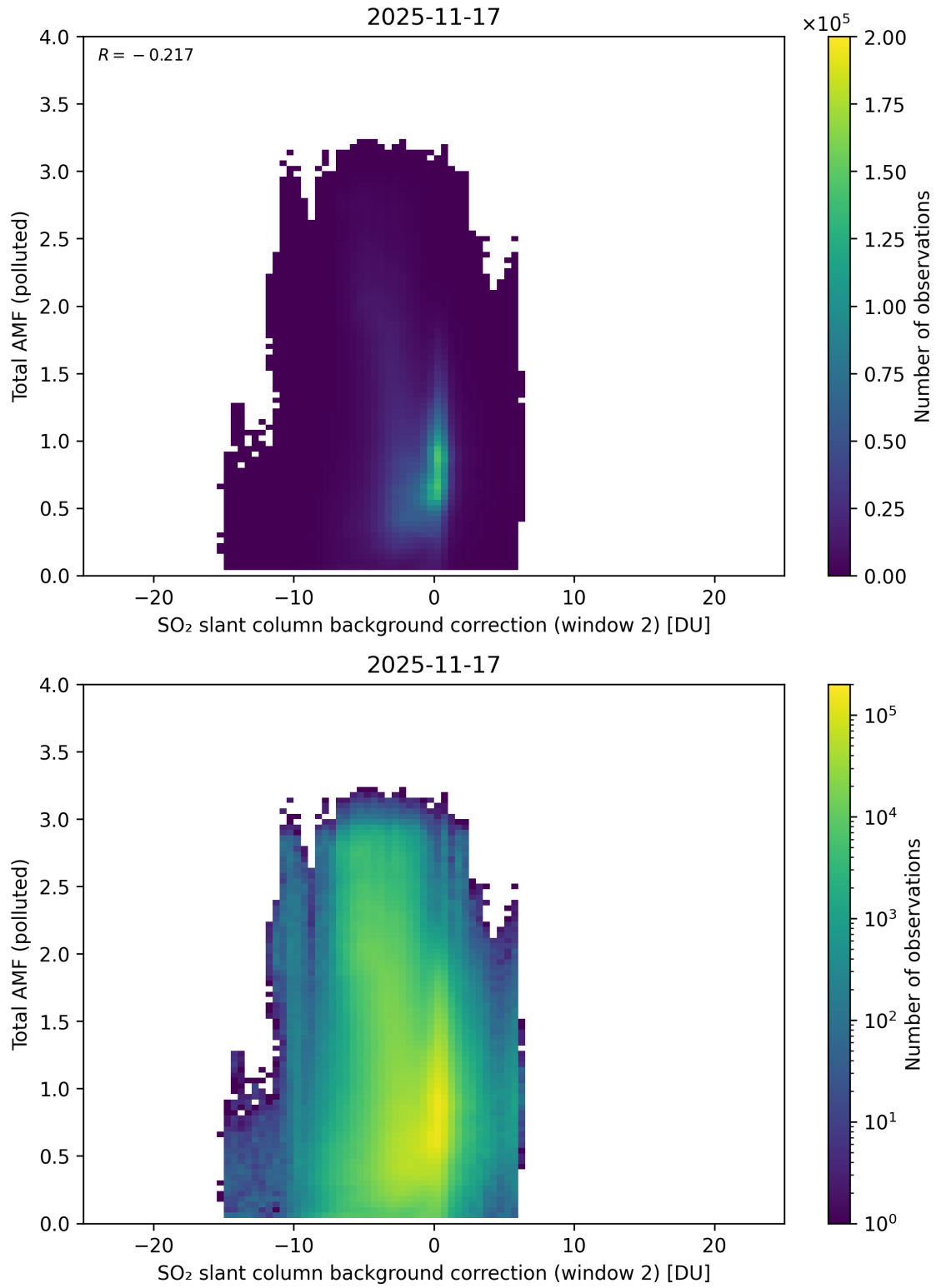
Figure 130: Scatter density plot of “SO 2 slant column background correction (window 2)” against “Total AMF (polluted)” for 2025-11-16 to 2025-11-18.
