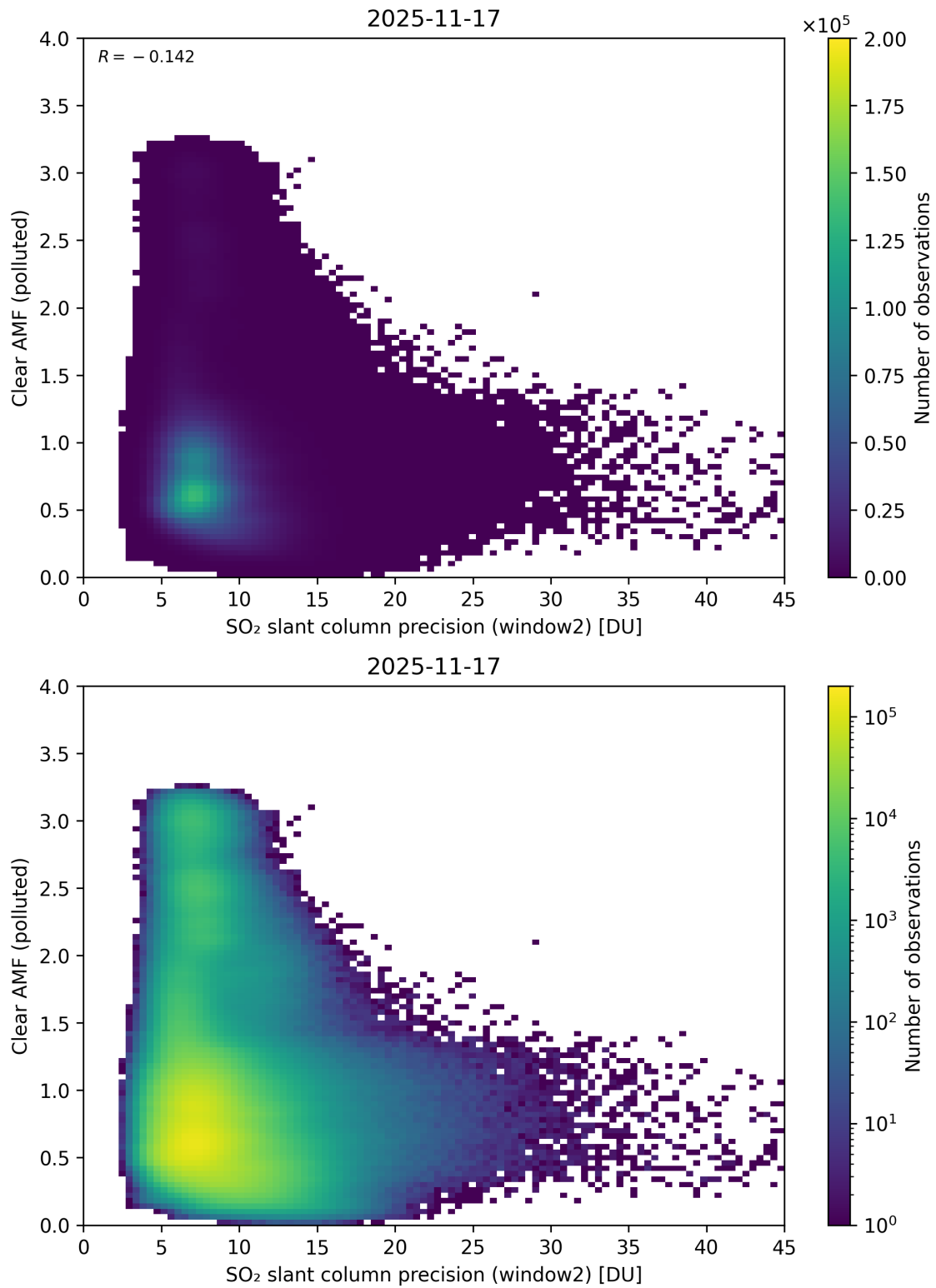
Figure 296: Scatter density plot of “SO 2 slant column precision (window2)” against “Clear AMF (polluted)” for 2025-11-16 to 2025-11-18.
