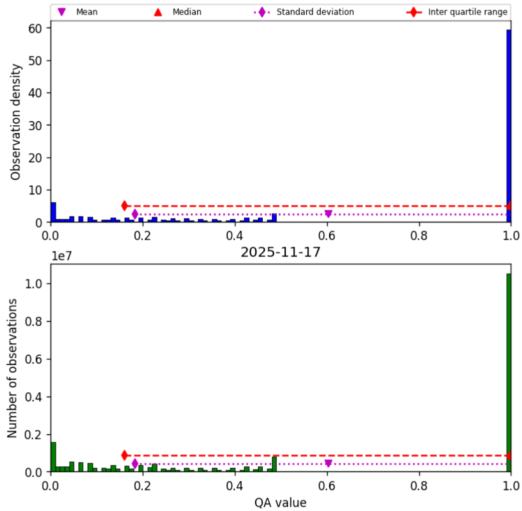
Figure 57: Histogram of “QA value” for 2025-11-16 to 2025-11-18
