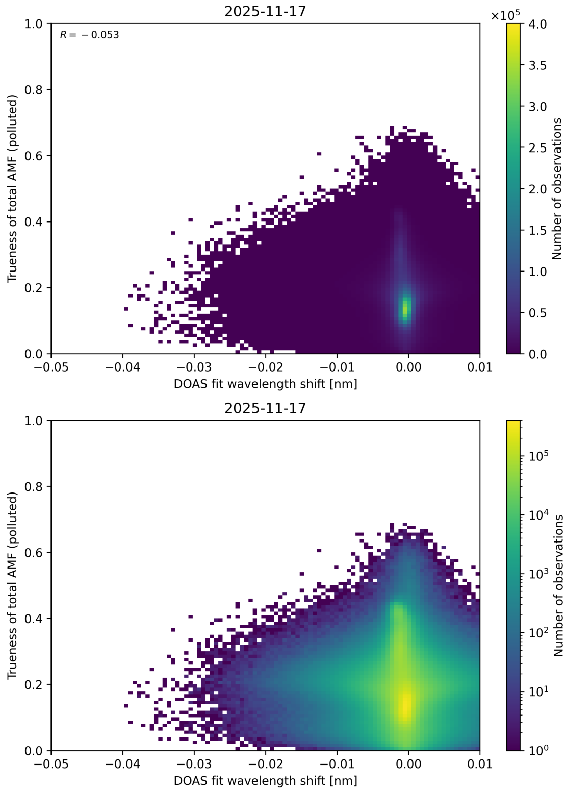
Figure 142: Scatter density plot of “DOAS fit wavelength shift” against “Trueness of total AMF (polluted)” for 2025-11-16 to 2025-11-18.
