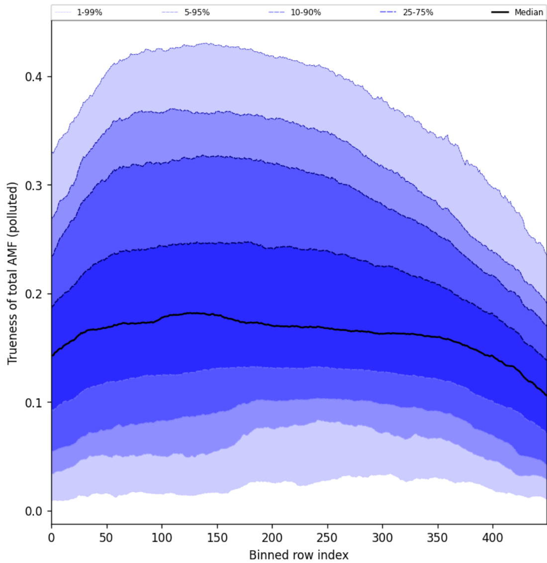
Figure 106: Along track statistics of “Trueness of total AMF (polluted)” for 2025-11-16 to 2025-11-18
