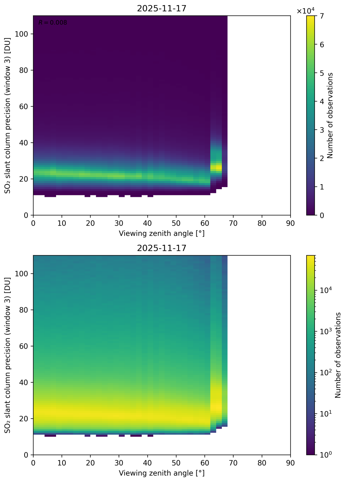
Figure 380: Scatter density plot of “Viewing zenith angle” against “SO 2 slant column precision (window 3)” for 2025-11-16 to 2025-11-18.
