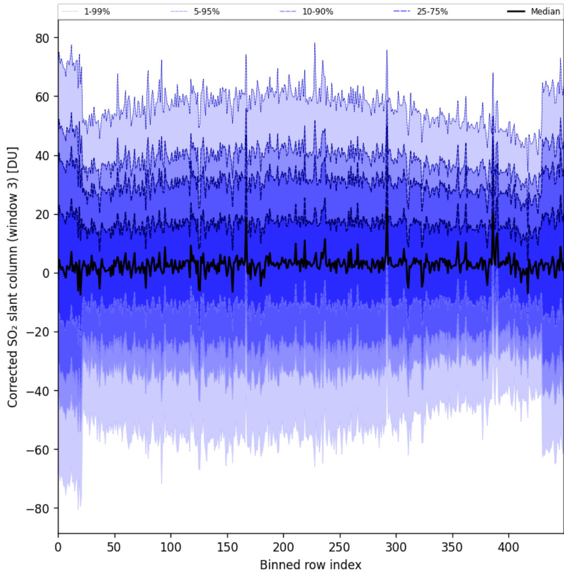
Figure 99: Along track statistics of “Corrected SO 2 slant column (window 3)” for 2025-11-16 to 2025-11-18
