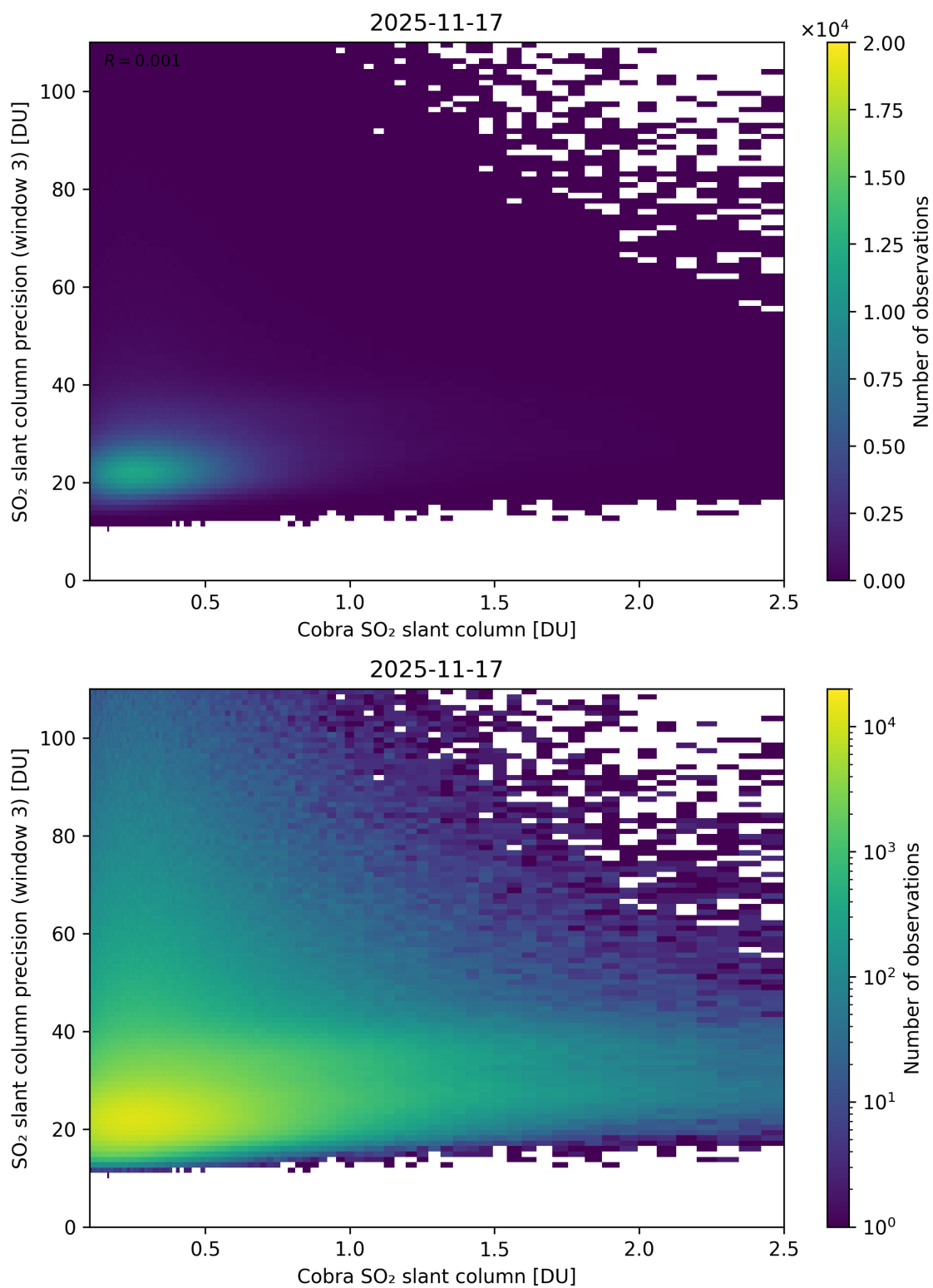
Figure 223: Scatter density plot of “Cobra SO 2 slant column” against “SO 2 slant column precision (window 3)” for 2025-11-16 to 2025-11-18.
