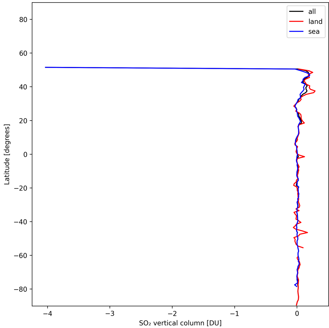
Figure 32: Zonal average of “SO 2 vertical column” for 2025-11-16 to 2025-11-18.
