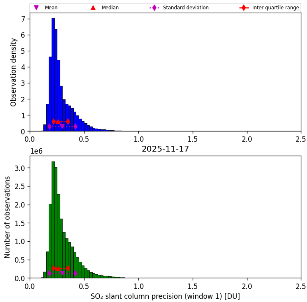
Figure 64: Histogram of “SO 2 slant column precision (window 1)” for 2025-11-16 to 2025-11-18
