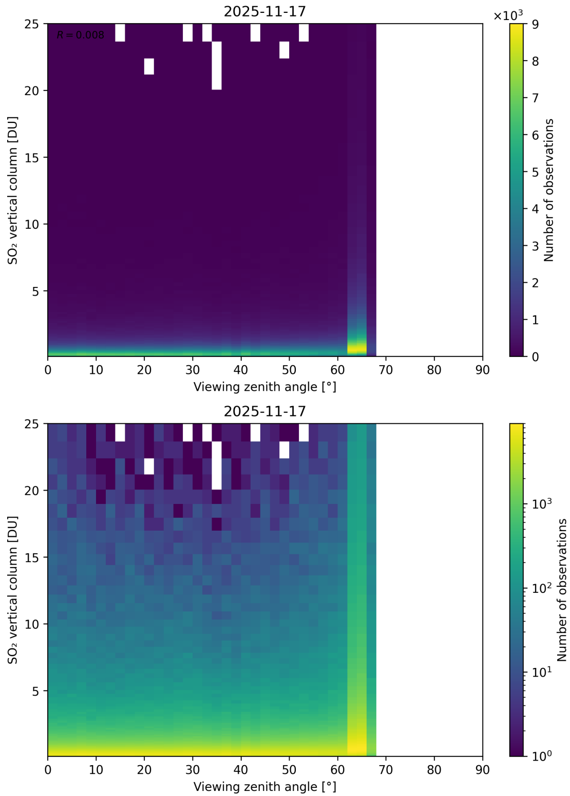
Figure 383: Scatter density plot of “Viewing zenith angle” against “SO 2 vertical column” for 2025-11-16 to 2025-11-18.
