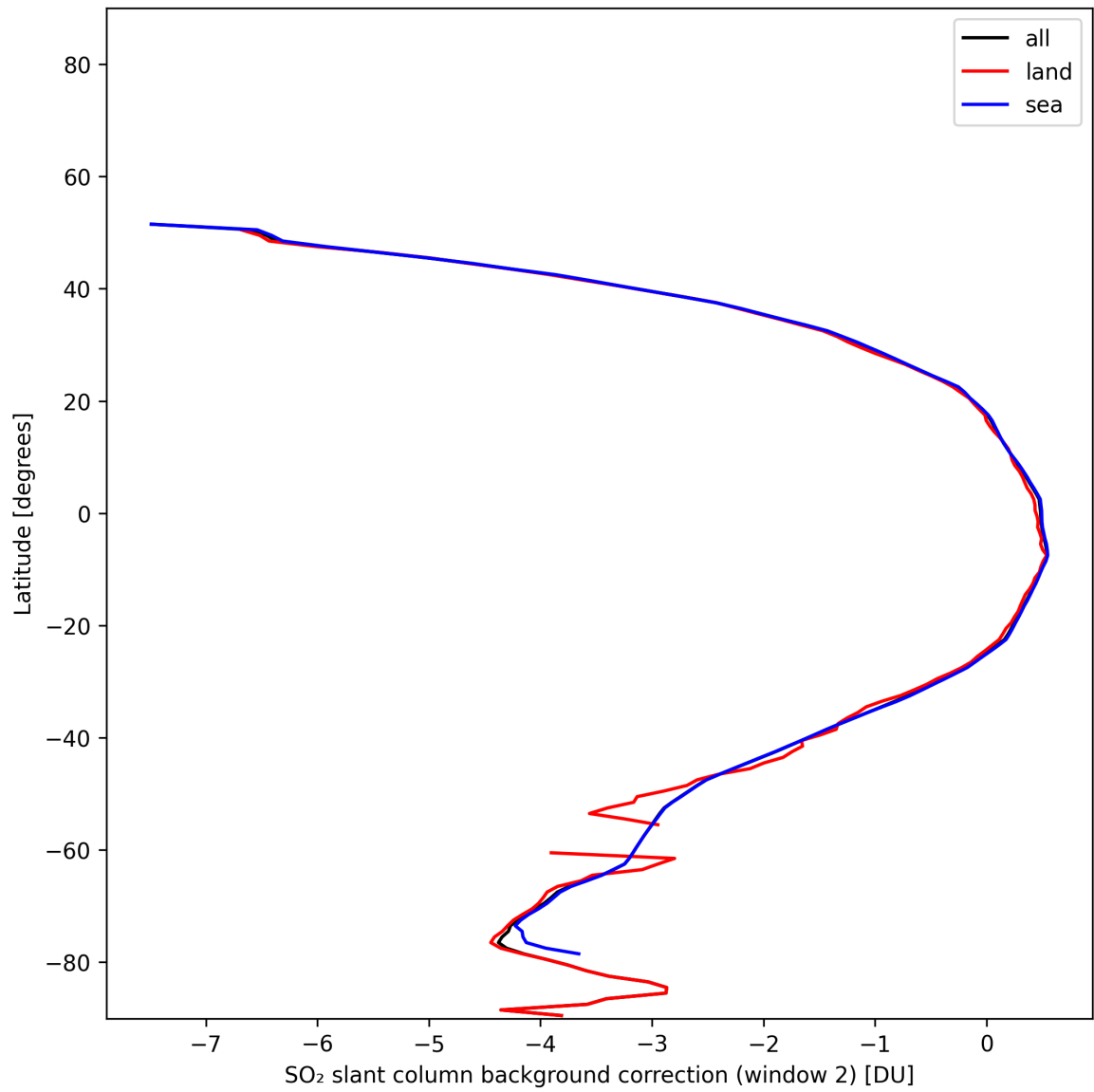
Figure 44: Zonal average of “SO 2 slant column background correction (window 2)” for 2025-11-16 to 2025-11-18.
