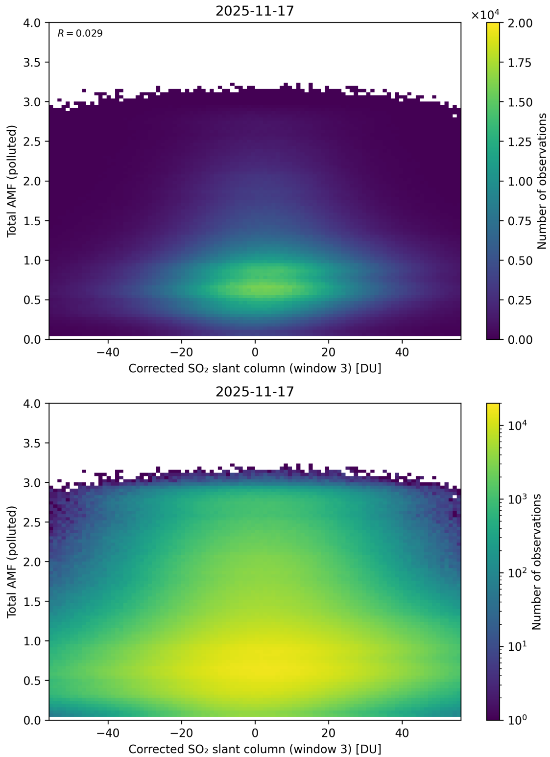
Figure 260: Scatter density plot of “Corrected SO 2 slant column (window 3)” against “Total AMF (polluted)” for 2025-11-16 to 2025-11-18.
