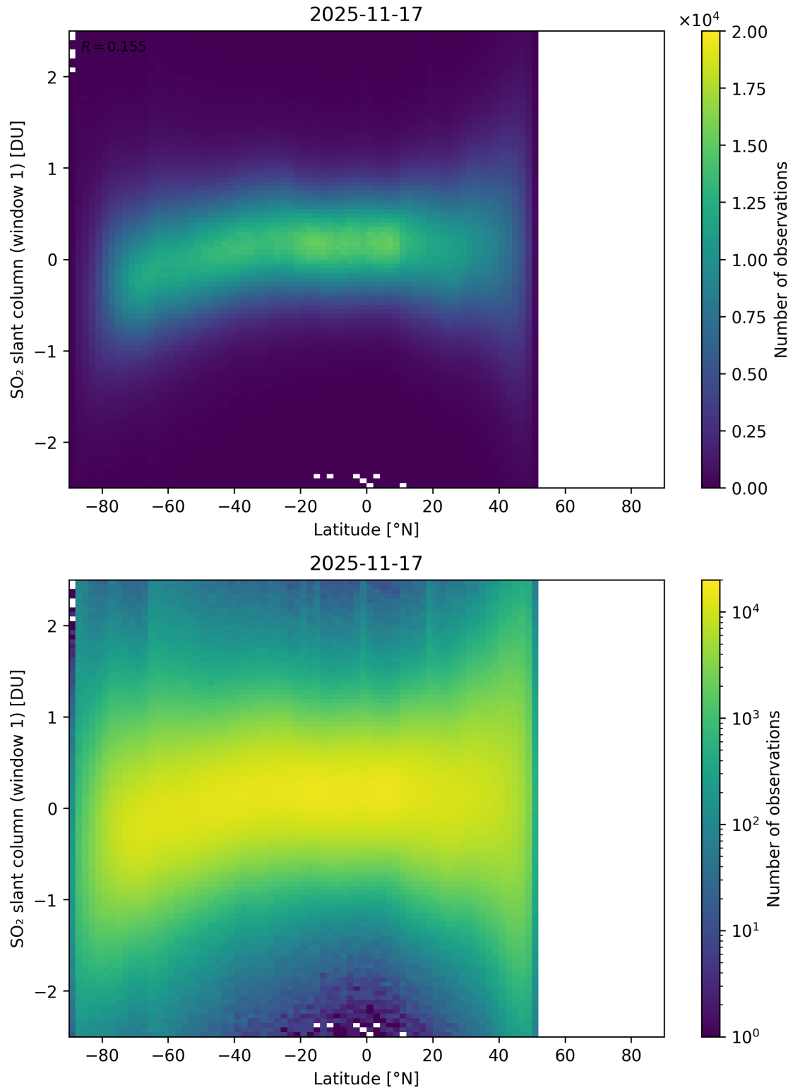
Figure 162: Scatter density plot of “Latitude” against “SO 2 slant column (window 1)” for 2025-11-16 to 2025-11-18.
