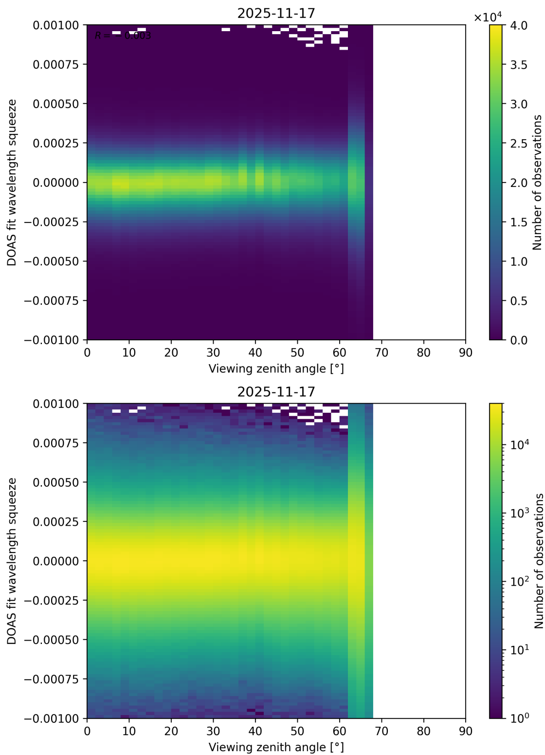
Figure 366: Scatter density plot of “Viewing zenith angle” against “DOAS fit wavelength squeeze” for 2025-11-16 to 2025-11-18.
