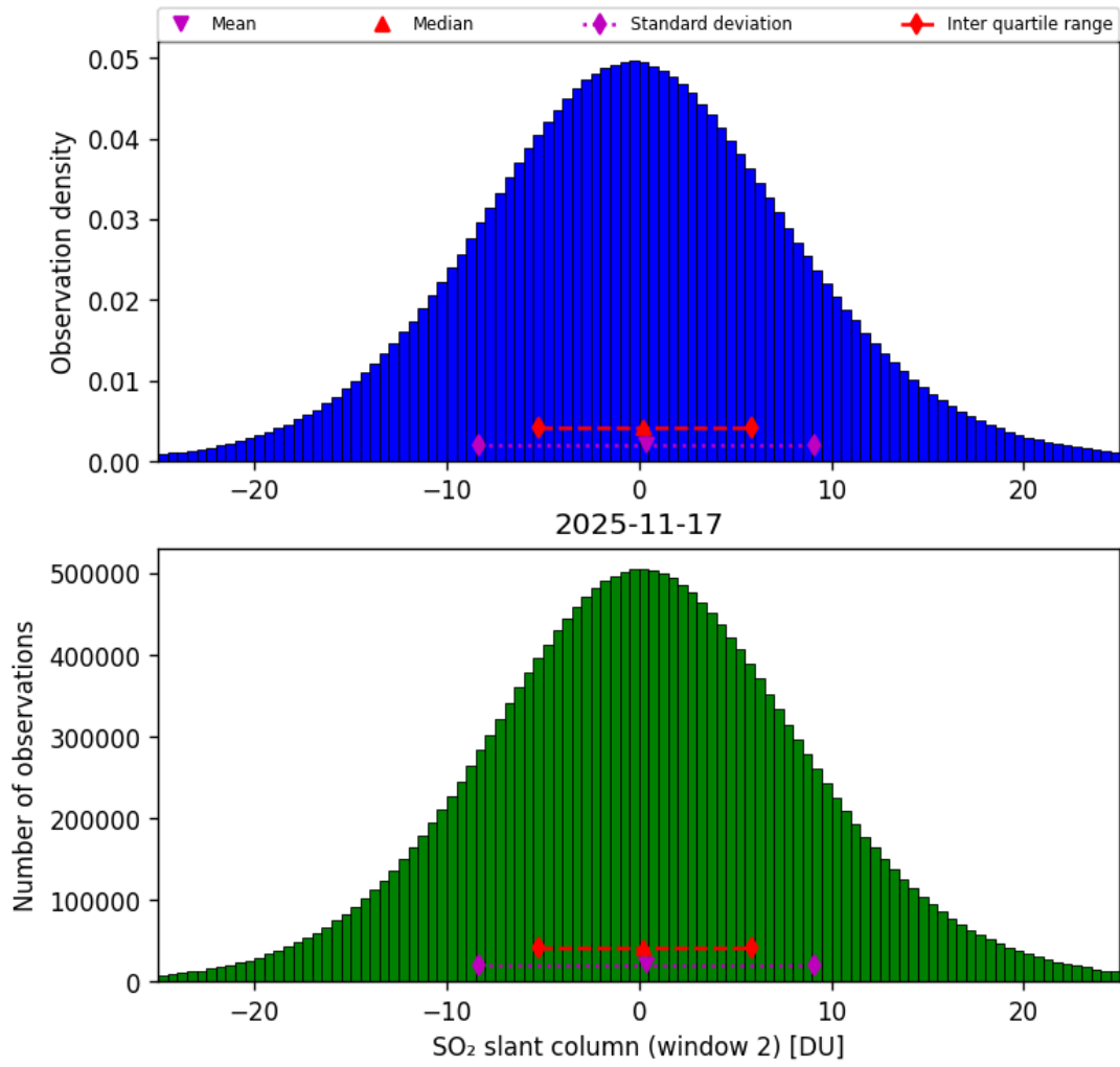
Figure 67: Histogram of “SO 2 slant column (window 2)” for 2025-11-16 to 2025-11-18
