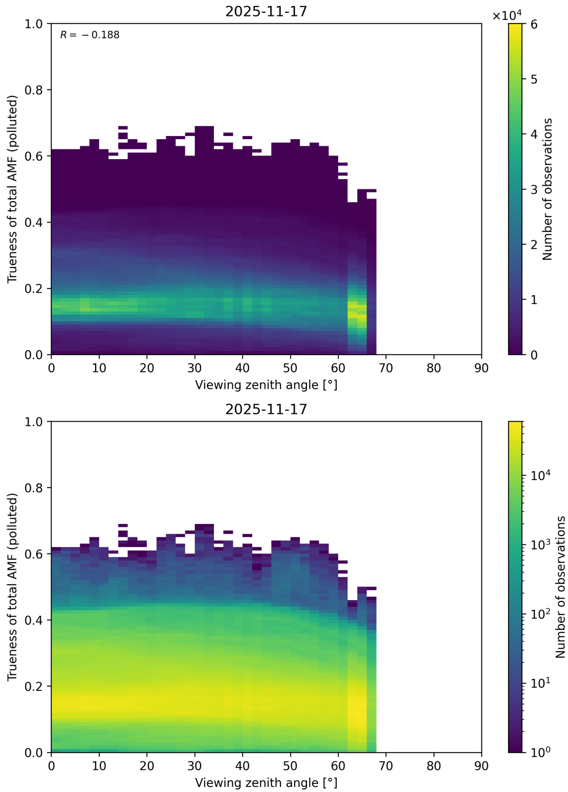
Figure 382: Scatter density plot of “Viewing zenith angle” against “Trueness of total AMF (polluted)” for 2025-11-16 to 2025-11-18.
