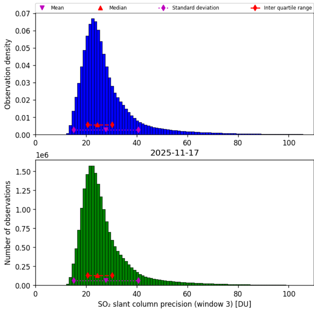
Figure 72: Histogram of “SO 2 slant column precision (window 3)” for 2025-11-16 to 2025-11-18
