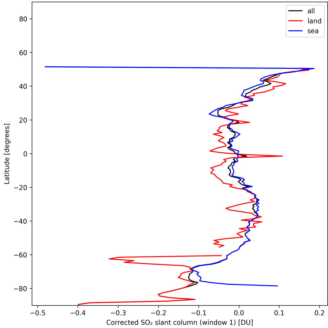
Figure 39: Zonal average of “Corrected SO 2 slant column (window 1)” for 2025-11-16 to 2025-11-18.
