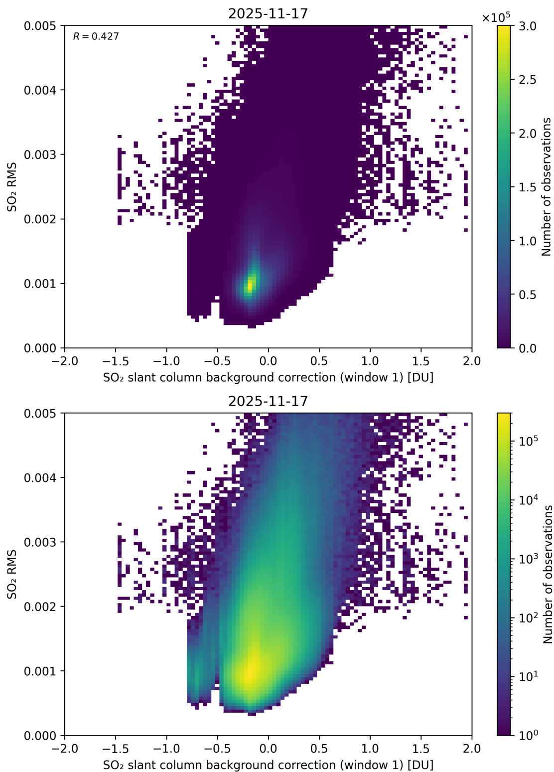
Figure 113: Scatter density plot of “SO 2 slant column background correction (window 1)” against “SO 2 RMS” for 2025-11-16 to 2025-11-18.
