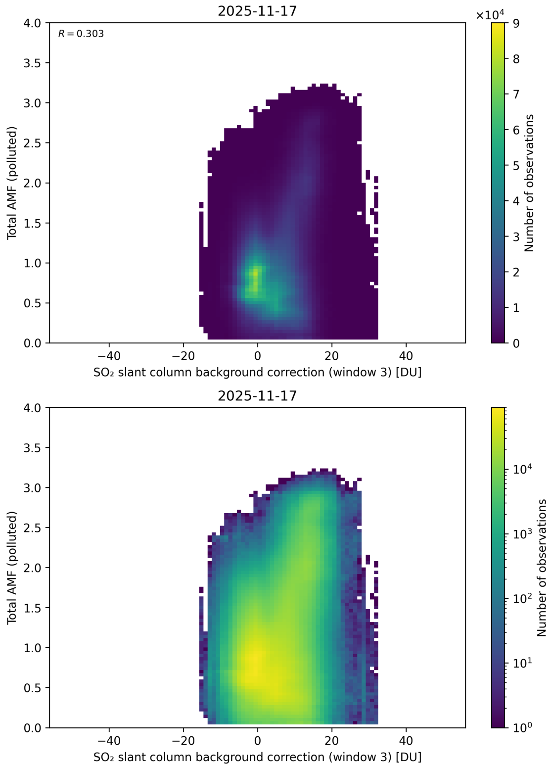
Figure 136: Scatter density plot of “SO 2 slant column background correction (window 3)” against “Total AMF (polluted)” for 2025-11-16 to 2025-11-18.
