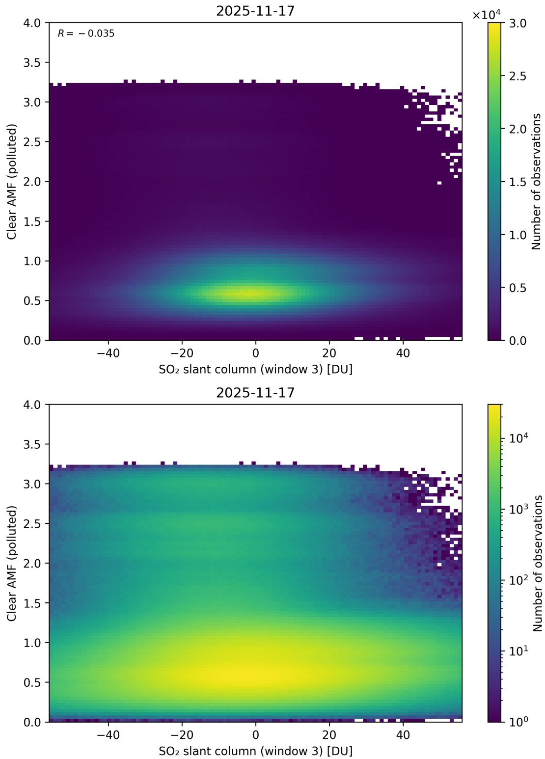
Figure 315: Scatter density plot of “SO 2 slant column (window 3)” against “Clear AMF (polluted)” for 2025-11-16 to 2025-11-18.
