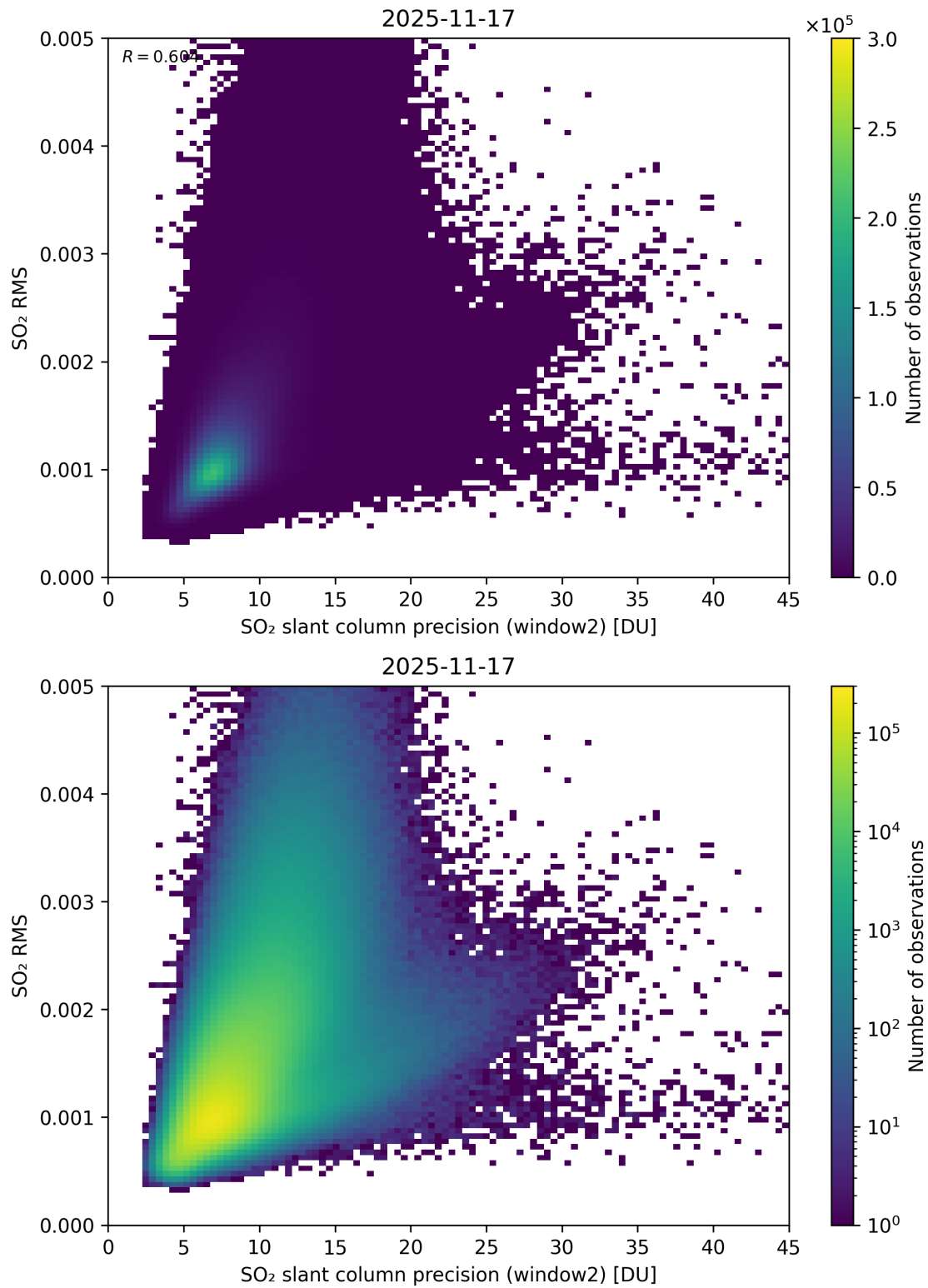
Figure 295: Scatter density plot of “SO 2 slant column precision (window2)” against “SO 2 RMS” for 2025-11-16 to 2025-11-18.
