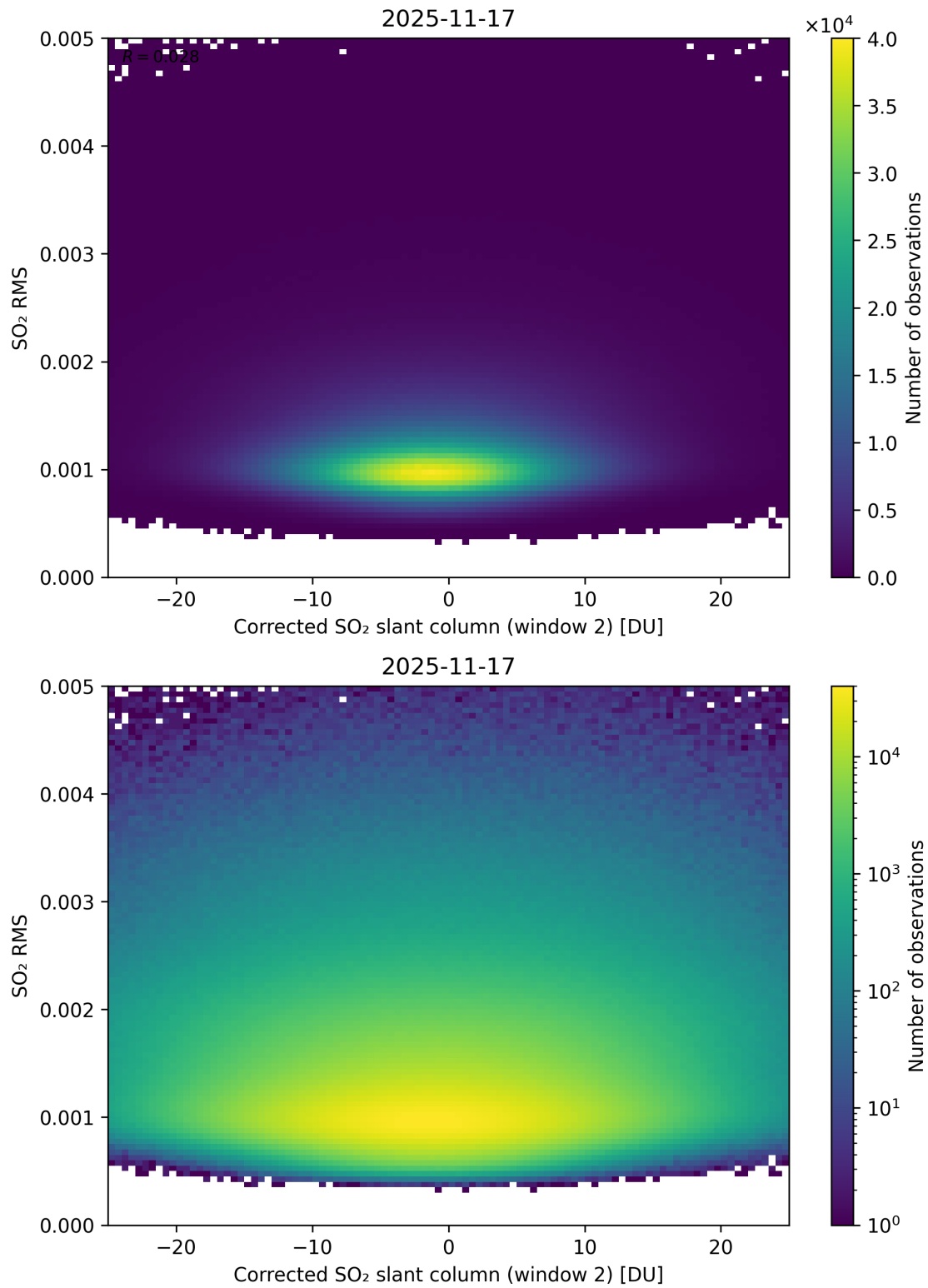
Figure 248: Scatter density plot of “Corrected SO 2 slant column (window 2)” against “SO 2 RMS” for 2025-11-16 to 2025-11-18.
