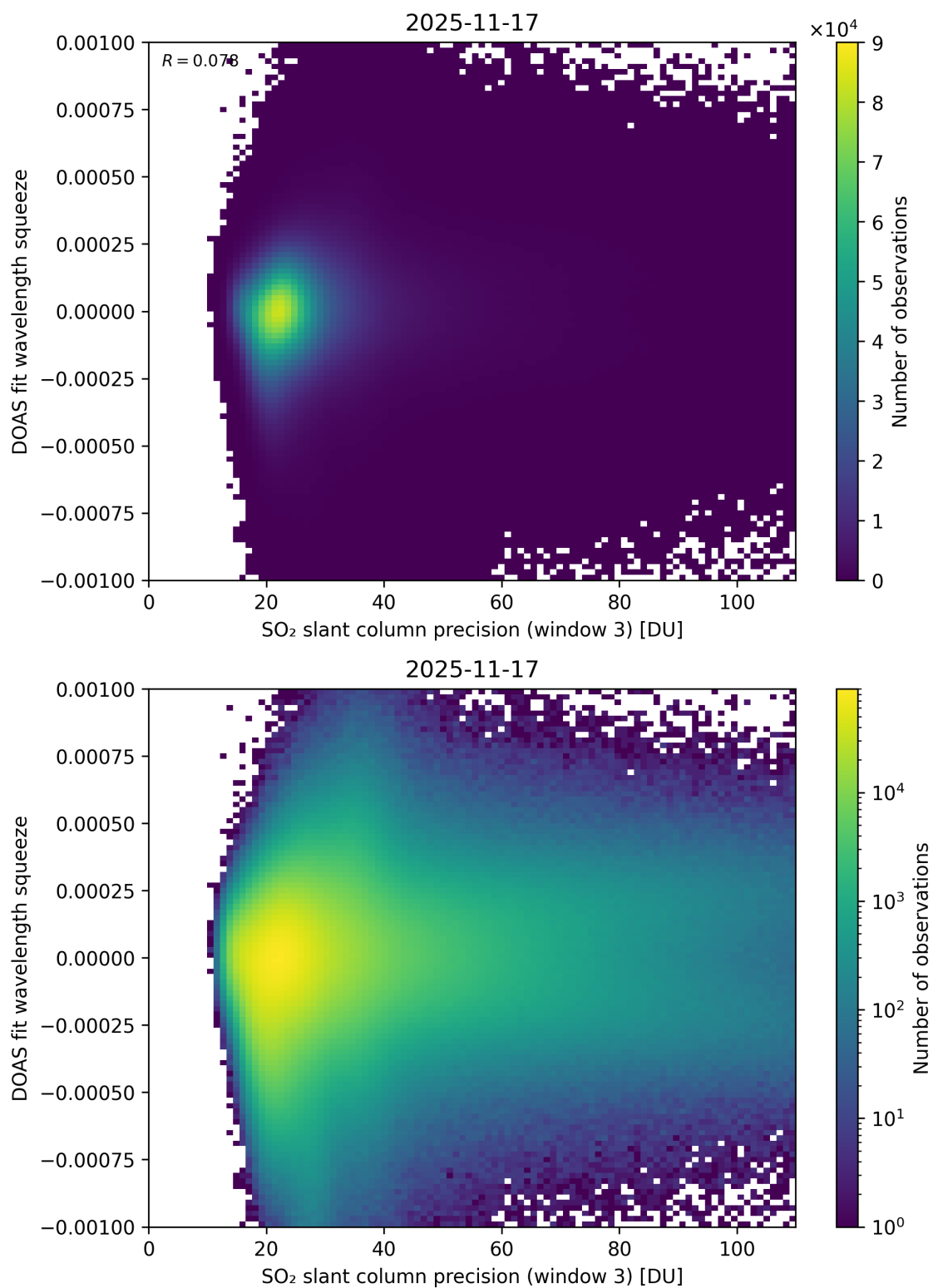
Figure 309: Scatter density plot of “SO 2 slant column precision (window 3)” against “DOAS fit wavelength squeeze” for 2025-11-16 to 2025-11-18.
