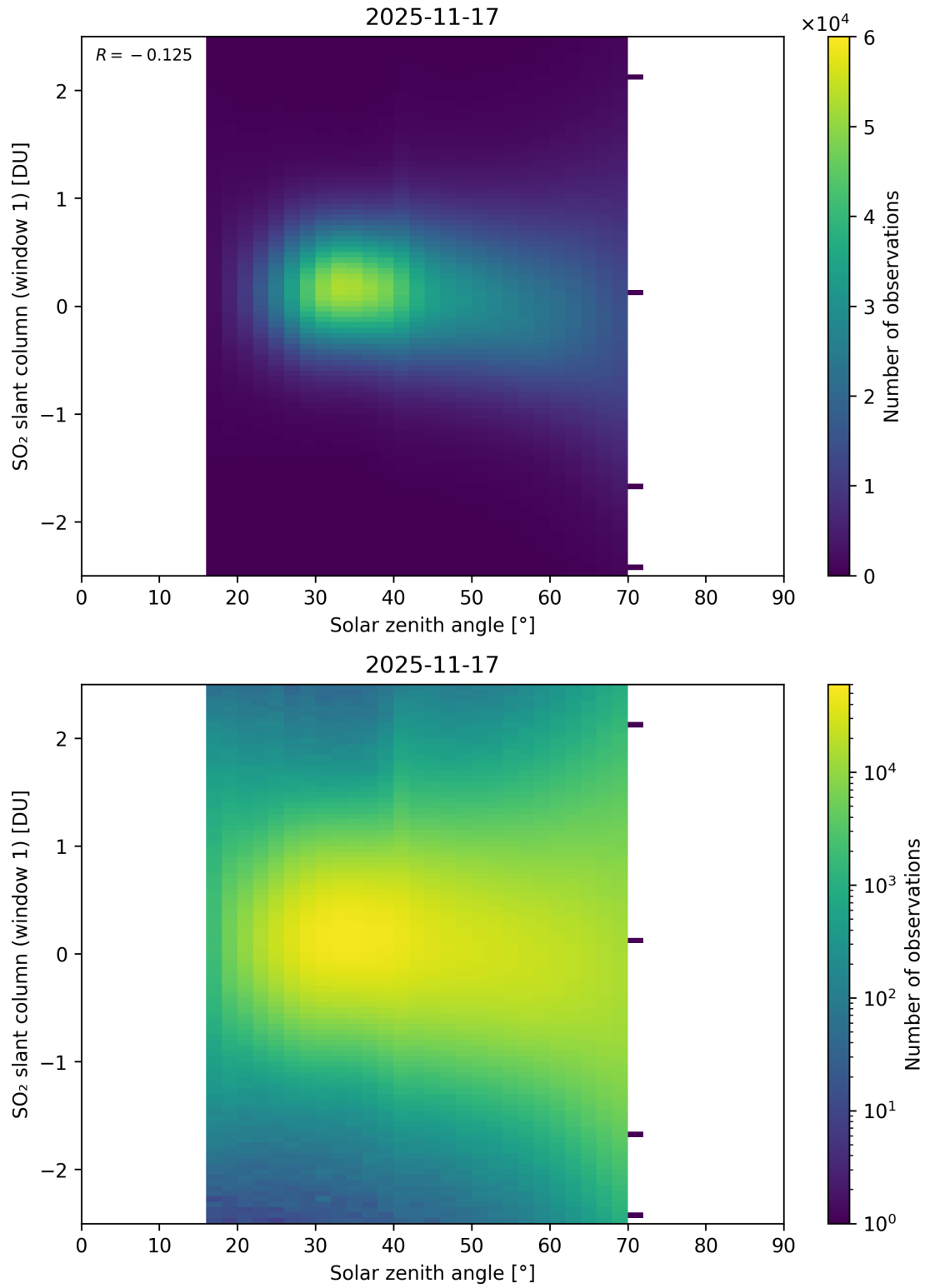
Figure 184: Scatter density plot of “Solar zenith angle” against “SO 2 slant column (window 1)” for 2025-11-16 to 2025-11-18.
