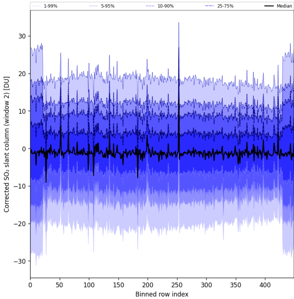
Figure 95: Along track statistics of “Corrected SO 2 slant column (window 2)” for 2025-11-16 to 2025-11-18
