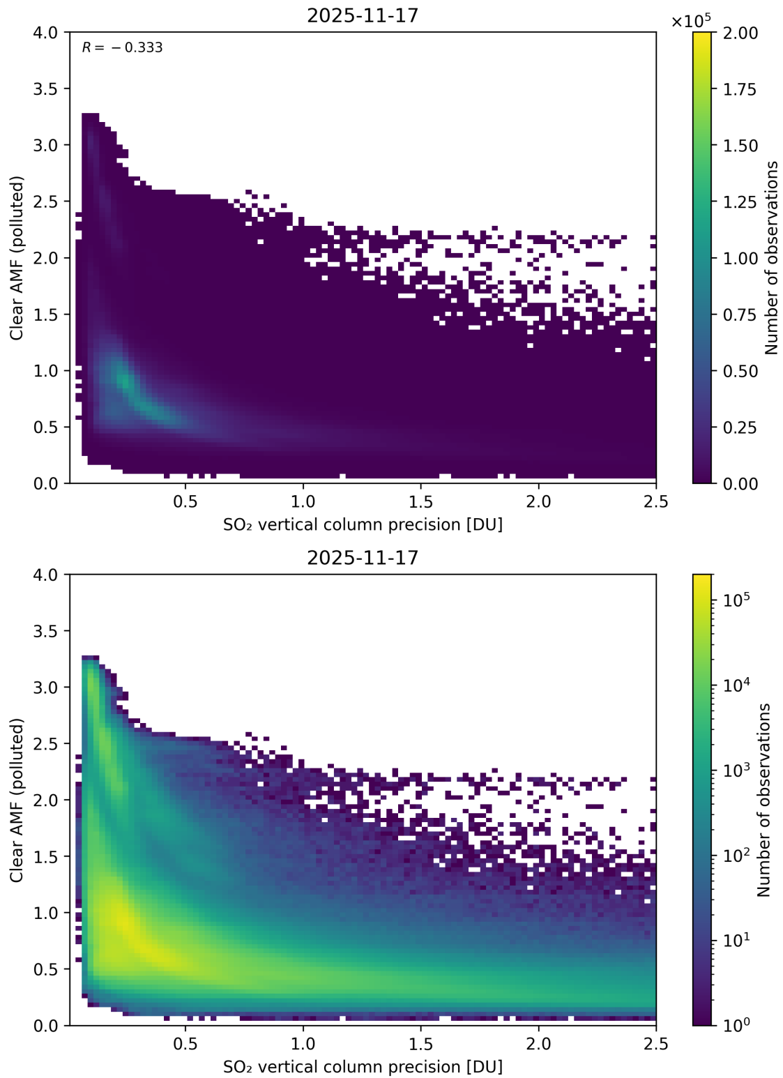
Figure 335: Scatter density plot of “SO 2 vertical column precision” against “Clear AMF (polluted)” for 2025-11-16 to 2025-11-18.
