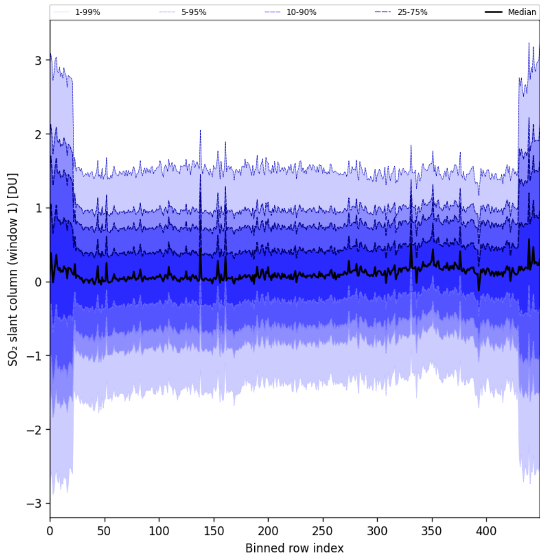
Figure 89: Along track statistics of “SO 2 slant column (window 1)” for 2025-11-16 to 2025-11-18
