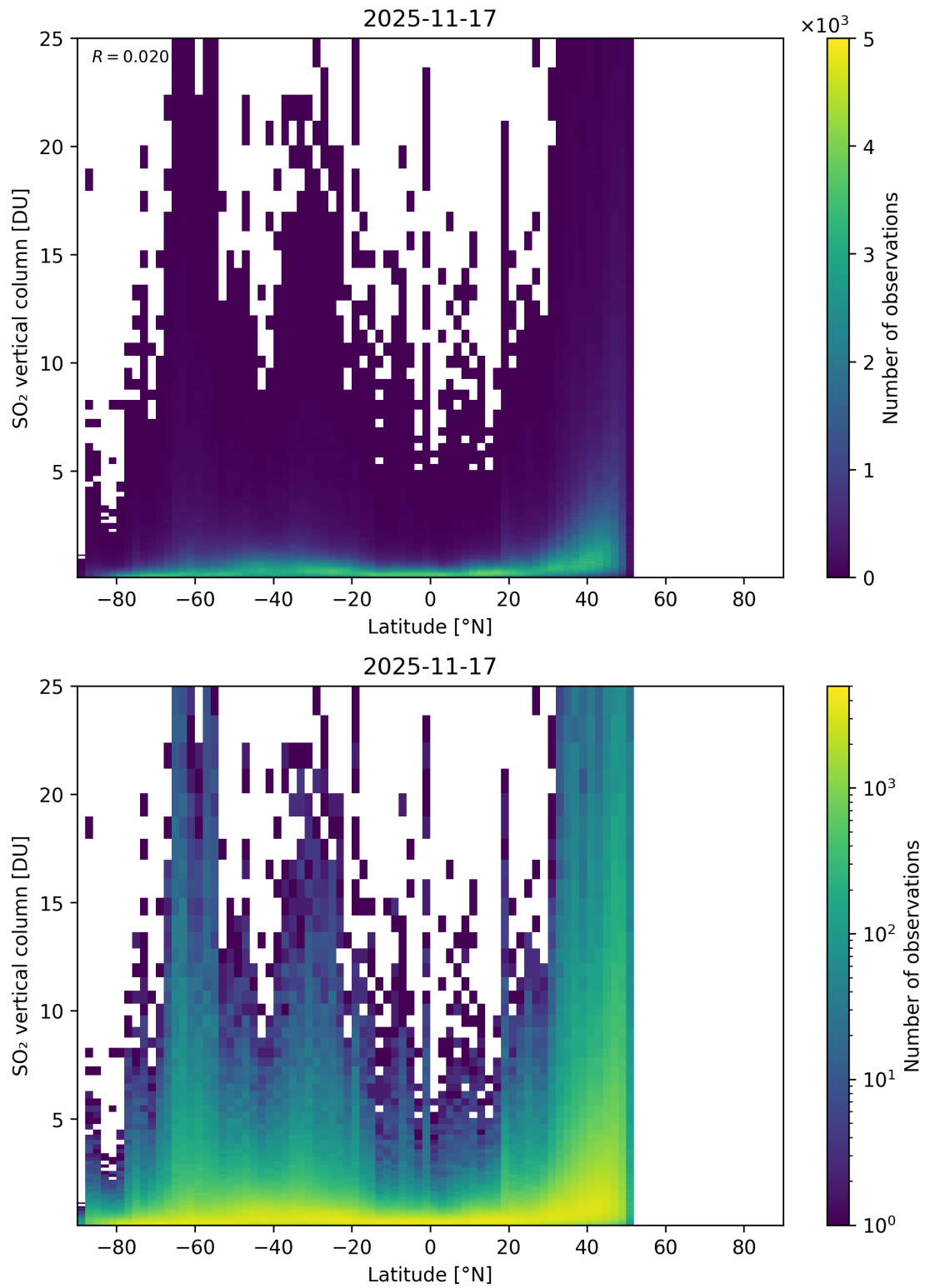
Figure 169: Scatter density plot of “Latitude” against “SO 2 vertical column” for 2025-11-16 to 2025-11-18.
