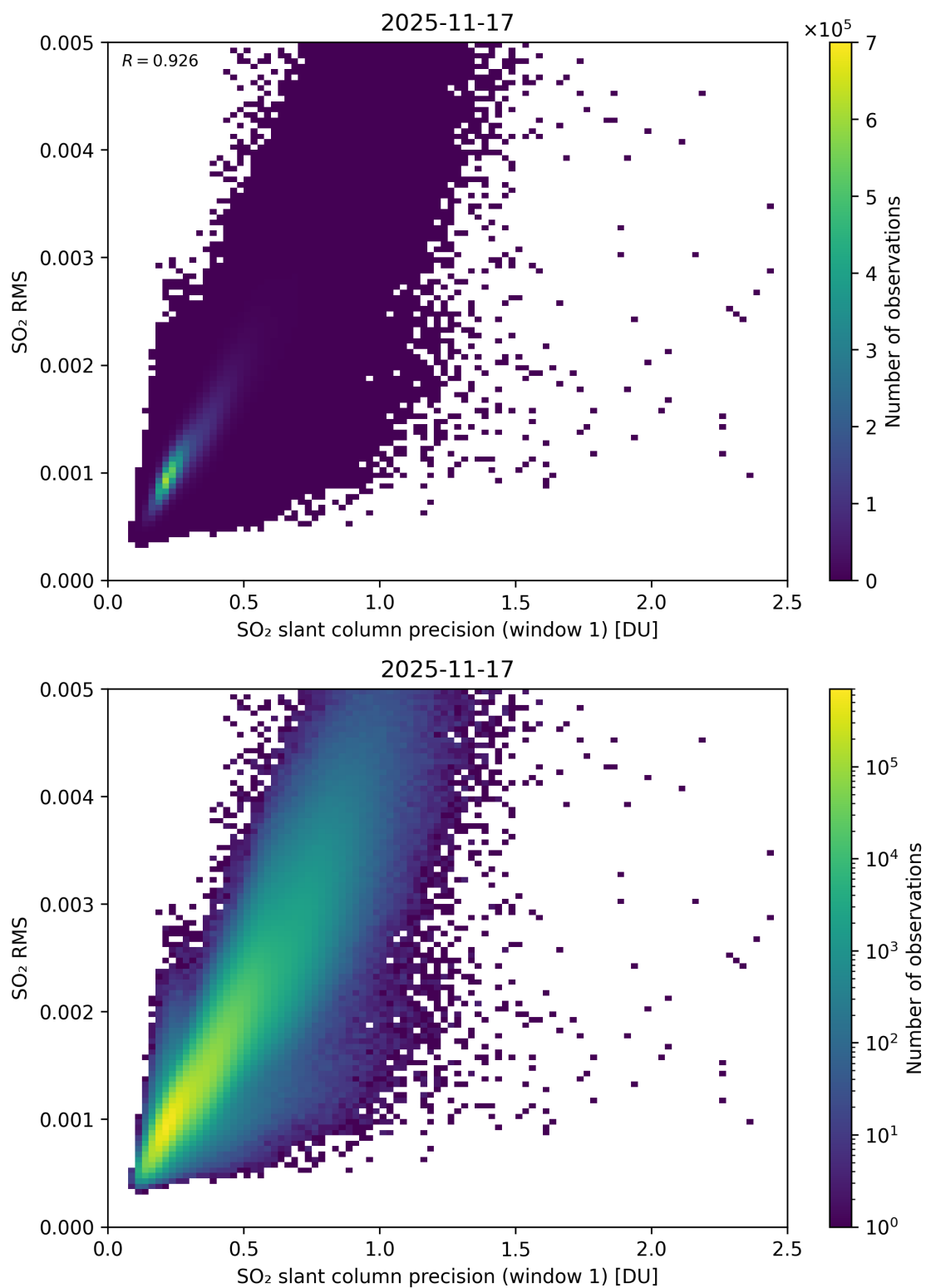
Figure 273: Scatter density plot of “SO 2 slant column precision (window 1)” against “SO 2 RMS” for 2025-11-16 to 2025-11-18.
