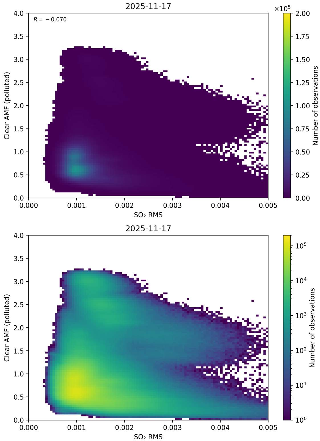
Figure 147: Scatter density plot of “SO 2 RMS” against “Clear AMF (polluted)” for 2025-11-16 to 2025-11-18.
