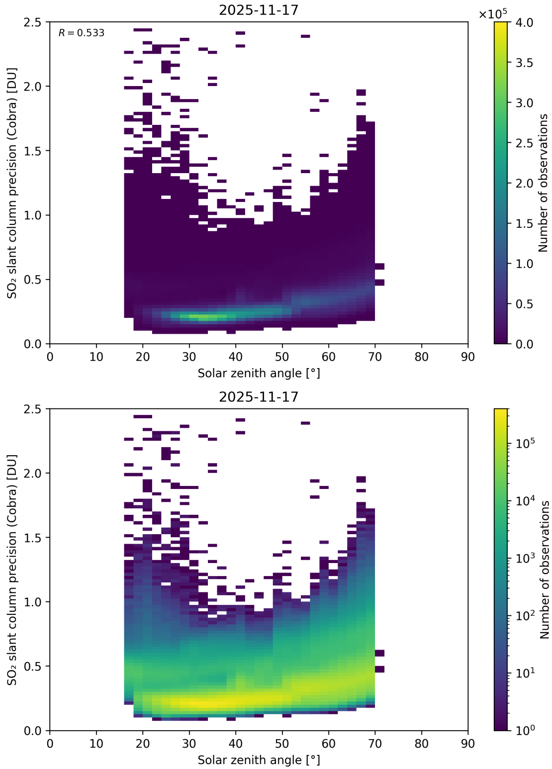
Figure 180: Scatter density plot of “Solar zenith angle” against “SO 2 slant column precision (Cobra)” for 2025-11-16 to 2025-11-18.
