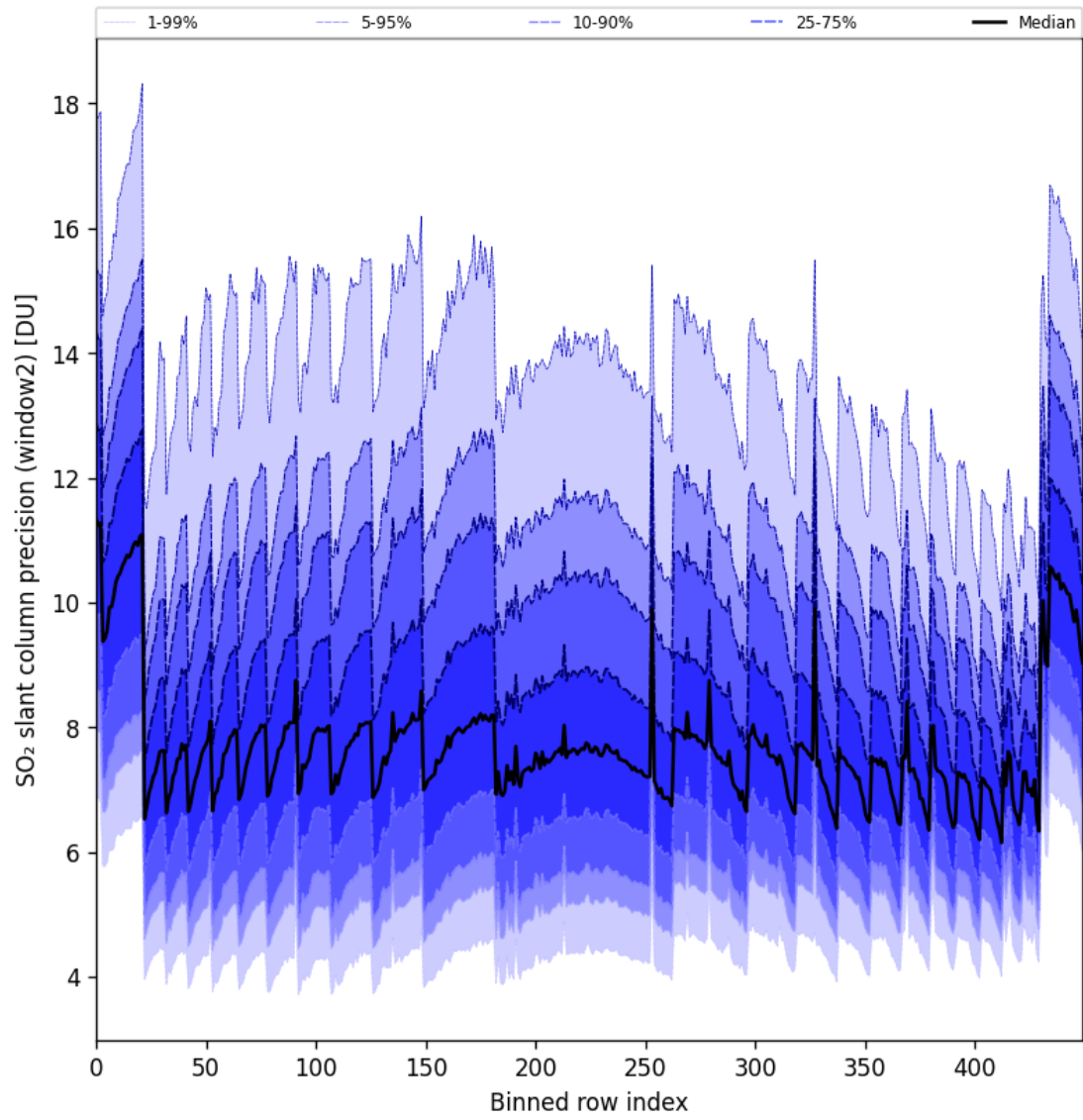
Figure 94: Along track statistics of “SO 2 slant column precision (window2)” for 2025-11-16 to 2025-11-18
