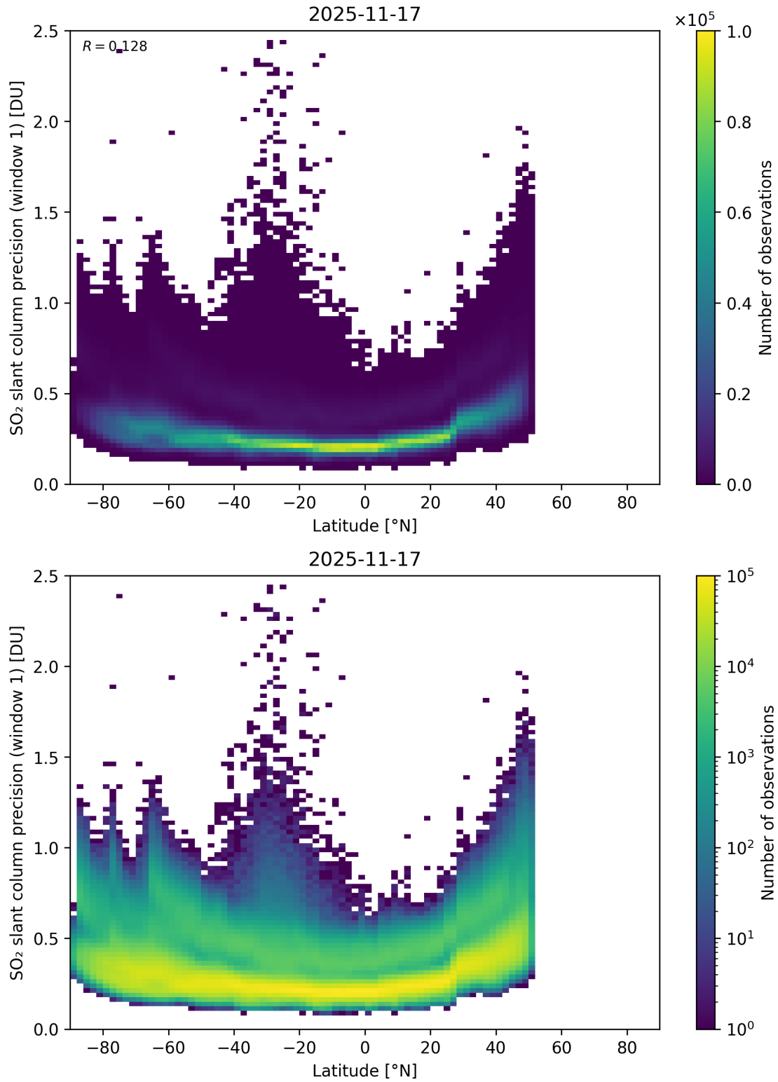
Figure 163: Scatter density plot of “Latitude” against “SO 2 slant column precision (window 1)” for 2025-11-16 to 2025-11-18.
