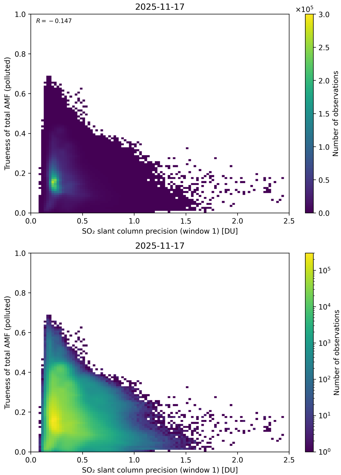
Figure 281: Scatter density plot of “SO 2 slant column precision (window 1)” against “Trueness of total AMF (polluted)” for 2025-11-16 to 2025-11-18.
