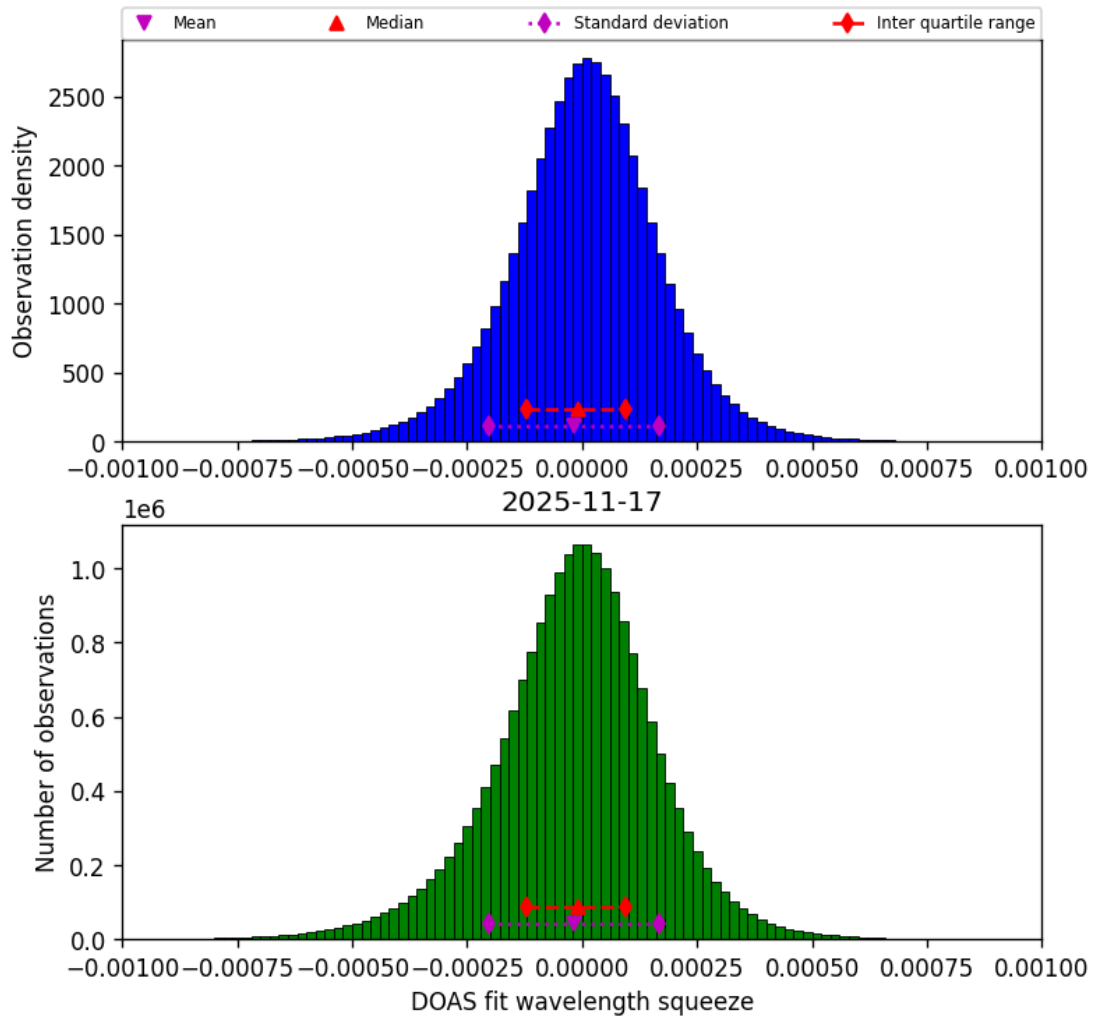
Figure 77: Histogram of “DOAS fit wavelength squeeze” for 2025-11-16 to 2025-11-18
