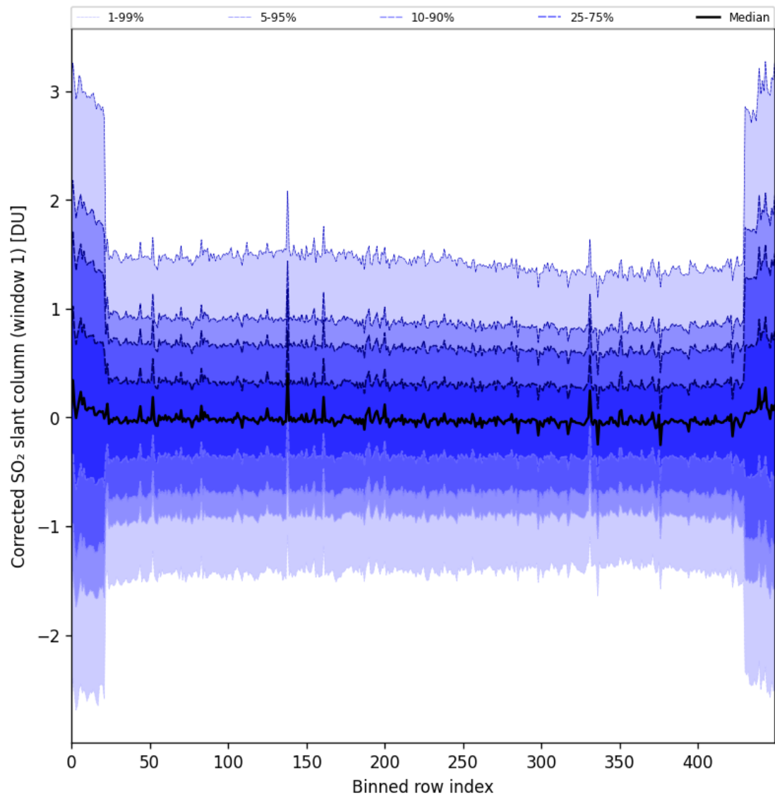
Figure 91: Along track statistics of “Corrected SO 2 slant column (window 1)” for 2025-11-16 to 2025-11-18
