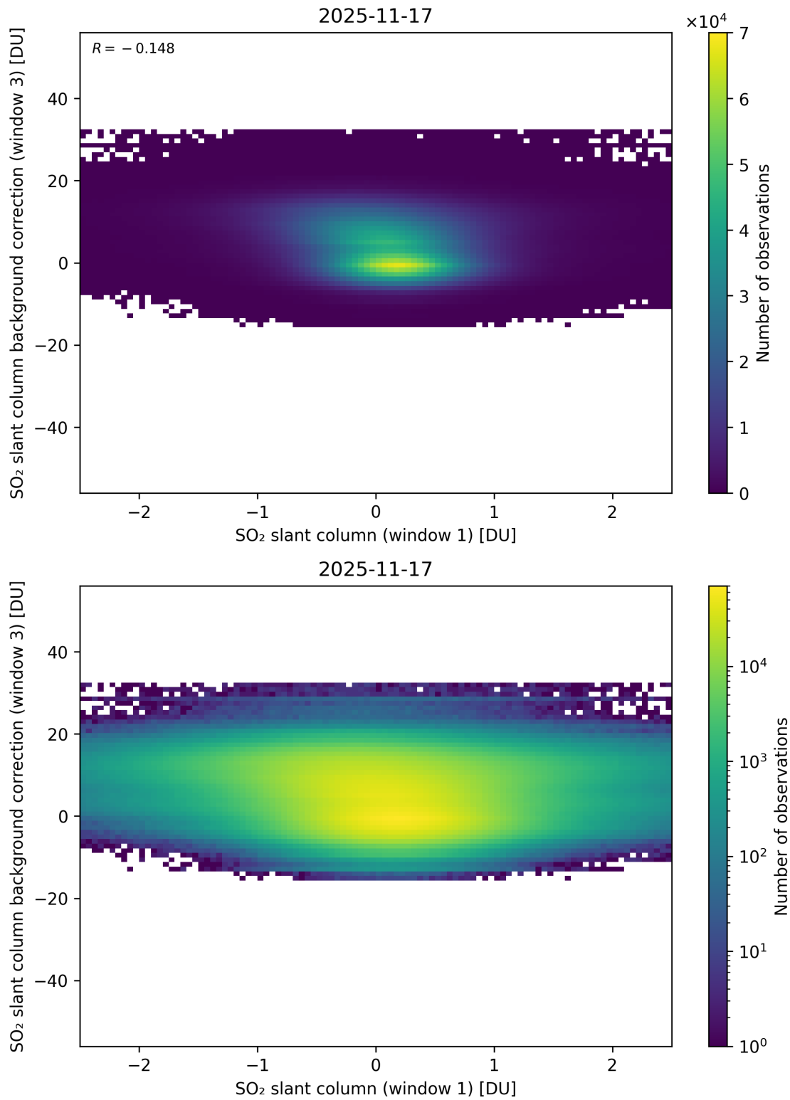
Figure 264: Scatter density plot of “SO 2 slant column (window 1)” against “SO 2 slant column background correction (window 3)” for 2025-11-16 to 2025-11-18.
