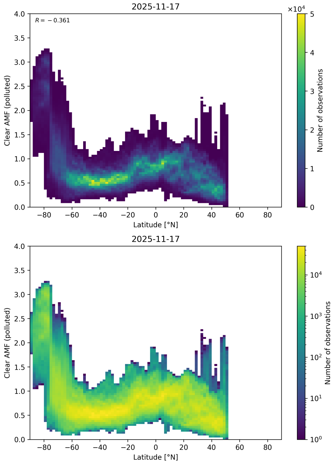
Figure 156: Scatter density plot of “Latitude” against “Clear AMF (polluted)” for 2025-11-16 to 2025-11-18.
