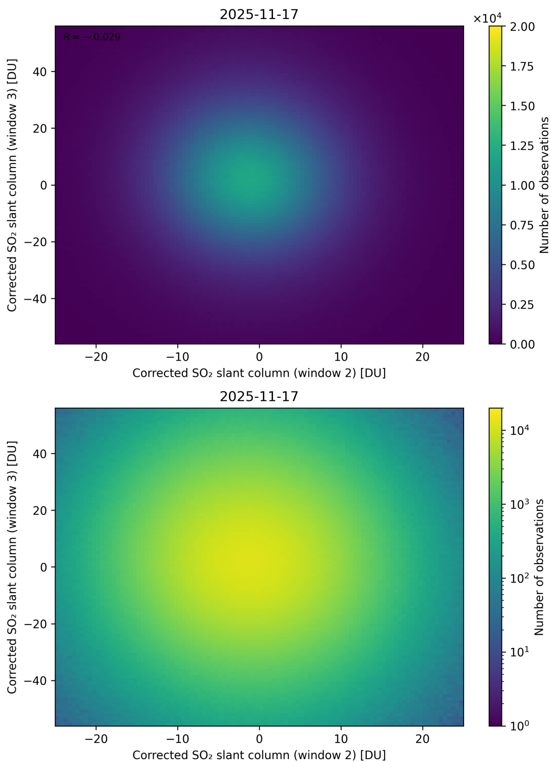
Figure 250: Scatter density plot of “Corrected SO 2 slant column (window 2)” against “Corrected SO 2 slant column (window 3)” for 2025-11-16 to 2025-11-18.
