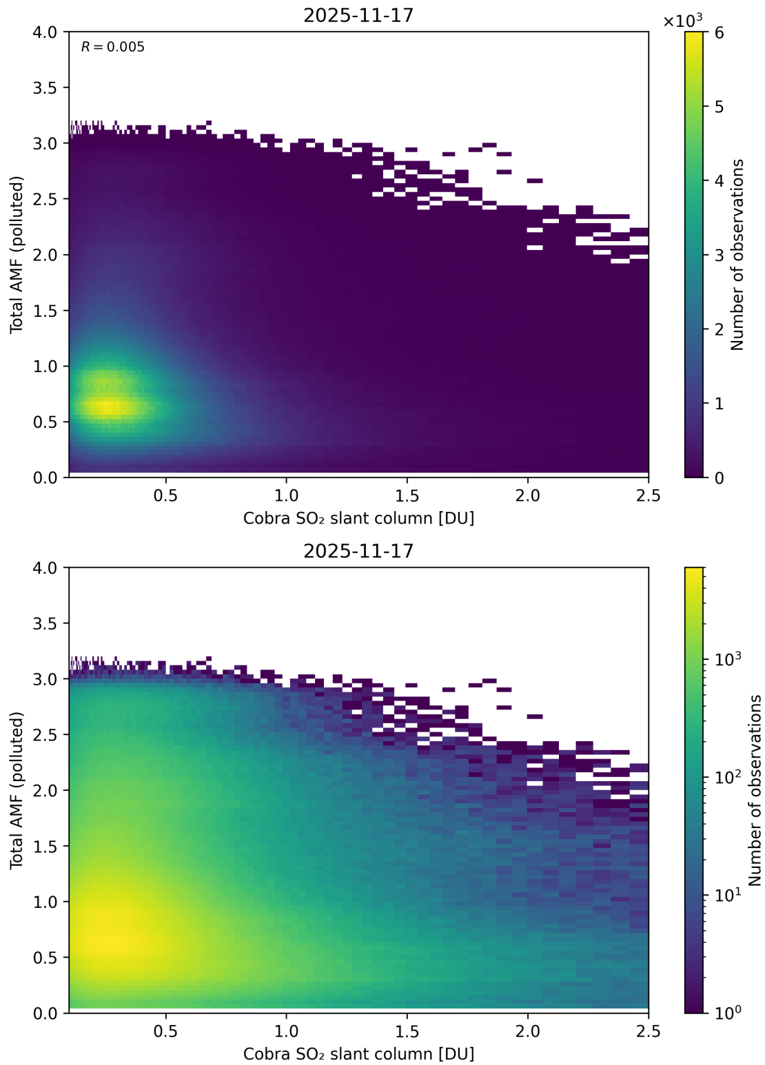
Figure 224: Scatter density plot of “Cobra SO 2 slant column” against “Total AMF (polluted)” for 2025-11-16 to 2025-11-18.
