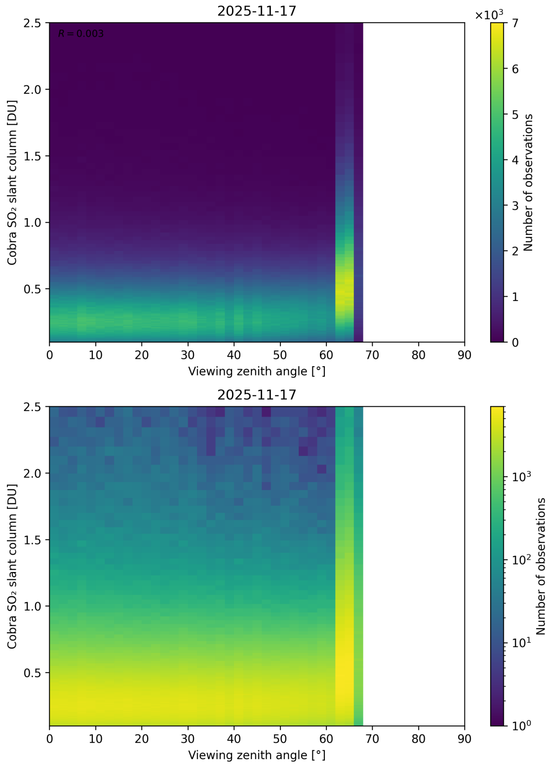
Figure 371: Scatter density plot of “Viewing zenith angle” against “Cobra SO 2 slant column” for 2025-11-16 to 2025-11-18.
