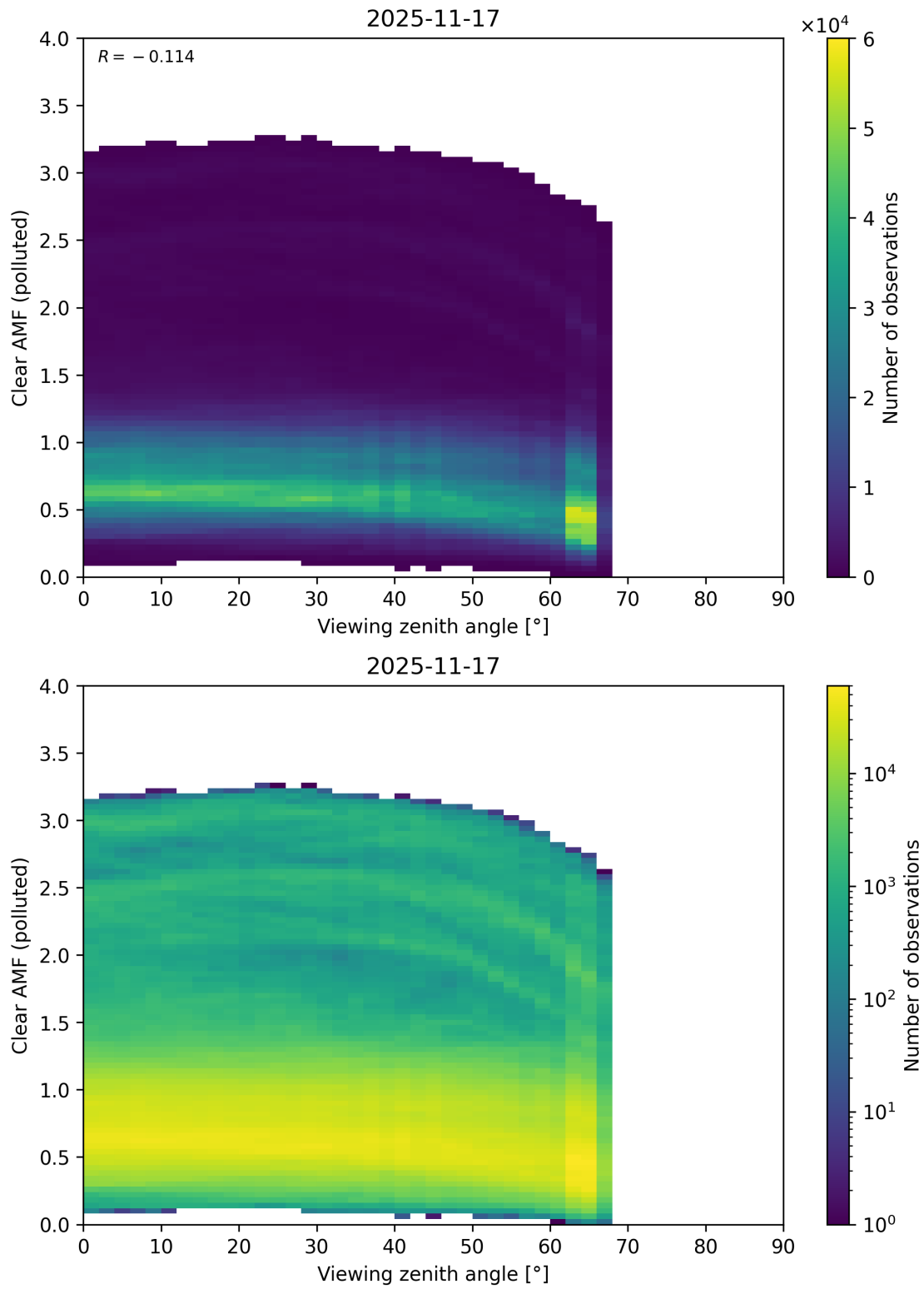
Figure 370: Scatter density plot of “Viewing zenith angle” against “Clear AMF (polluted)” for 2025-11-16 to 2025-11-18.
