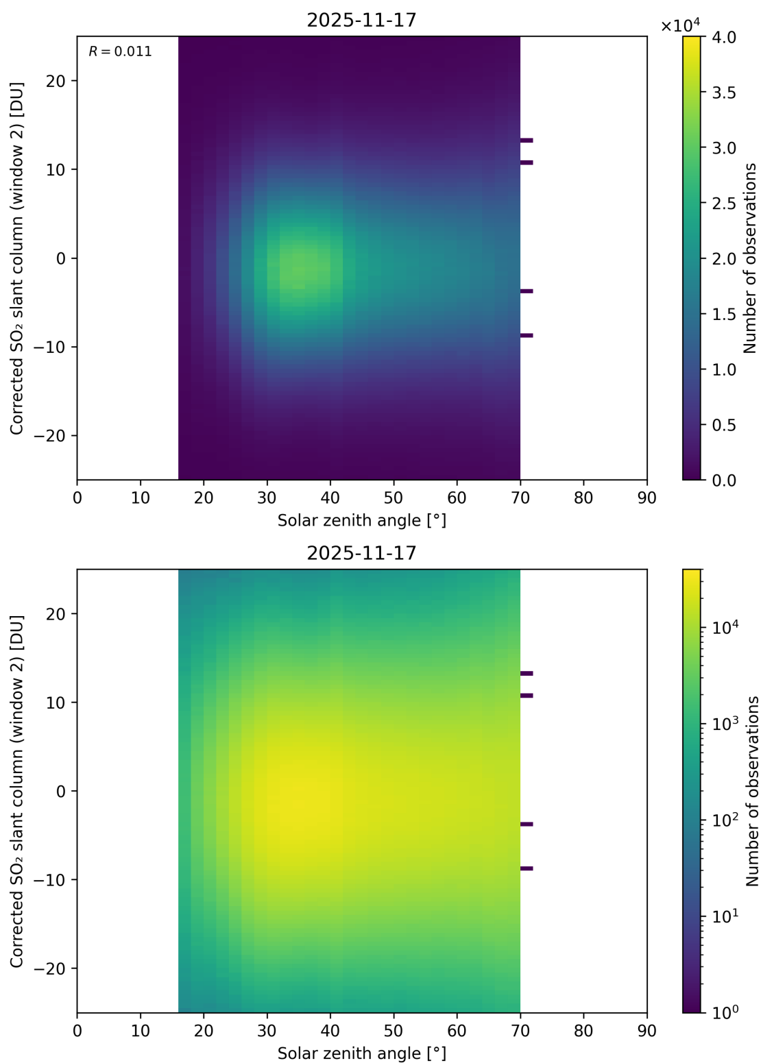
Figure 182: Scatter density plot of “Solar zenith angle” against “Corrected SO 2 slant column (window 2)” for 2025-11-16 to 2025-11-18.
