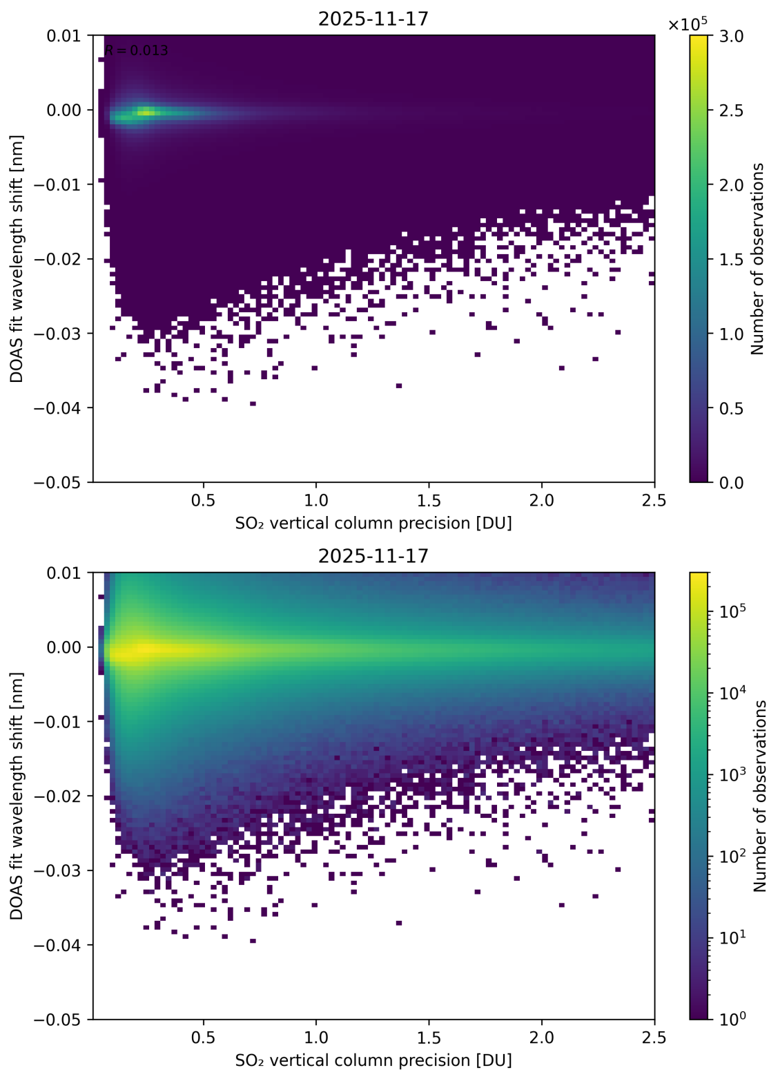
Figure 332: Scatter density plot of “SO 2 vertical column precision” against “DOAS fit wavelength shift” for 2025-11-16 to 2025-11-18.
