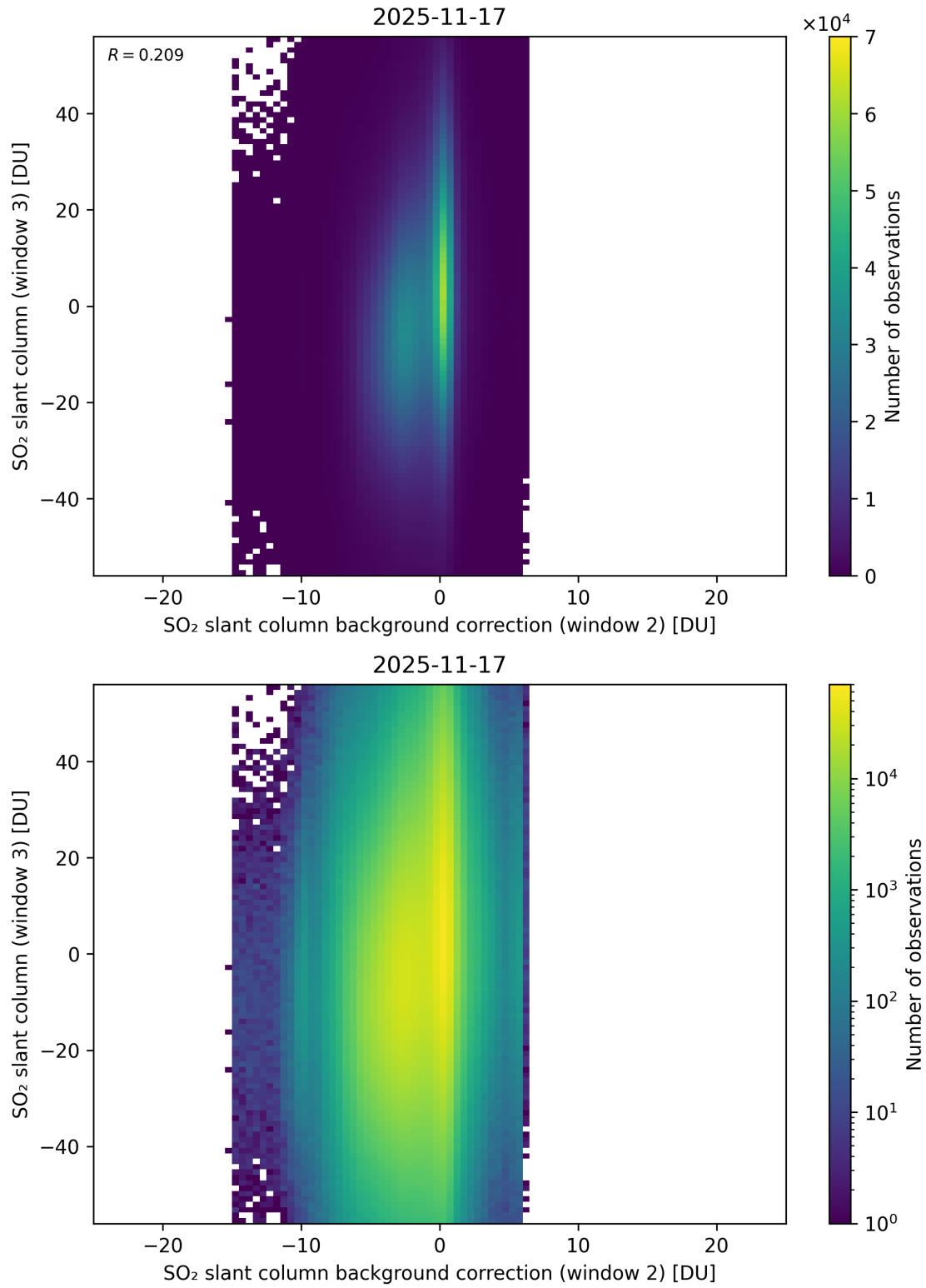
Figure 128: Scatter density plot of “SO 2 slant column background correction (window 2)” against “SO 2 slant column (window 3)” for 2025-11-16 to 2025-11-18.
