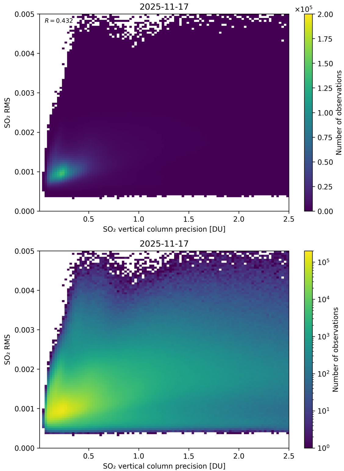
Figure 334: Scatter density plot of “SO 2 vertical column precision” against “SO 2 RMS” for 2025-11-16 to 2025-11-18.
