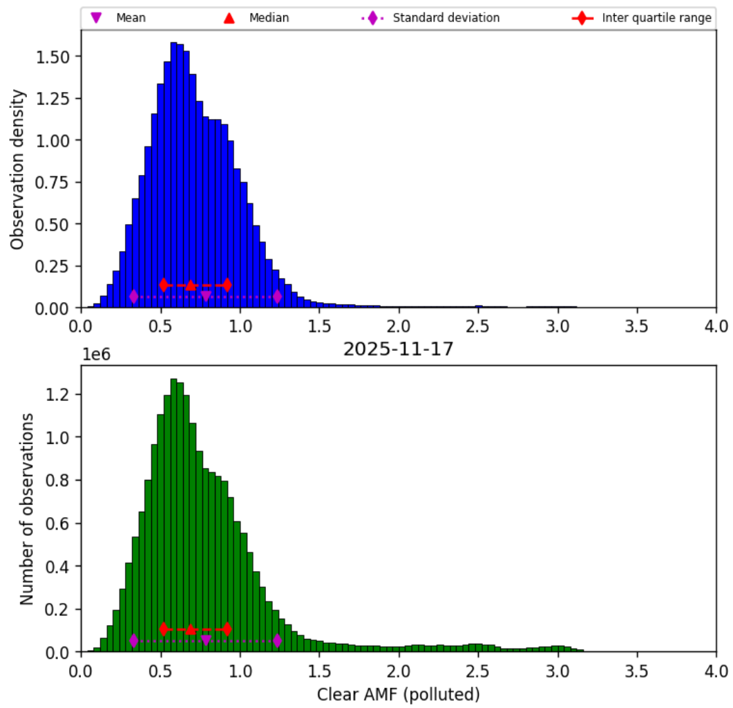
Figure 81: Histogram of “Clear AMF (polluted)” for 2025-11-16 to 2025-11-18
