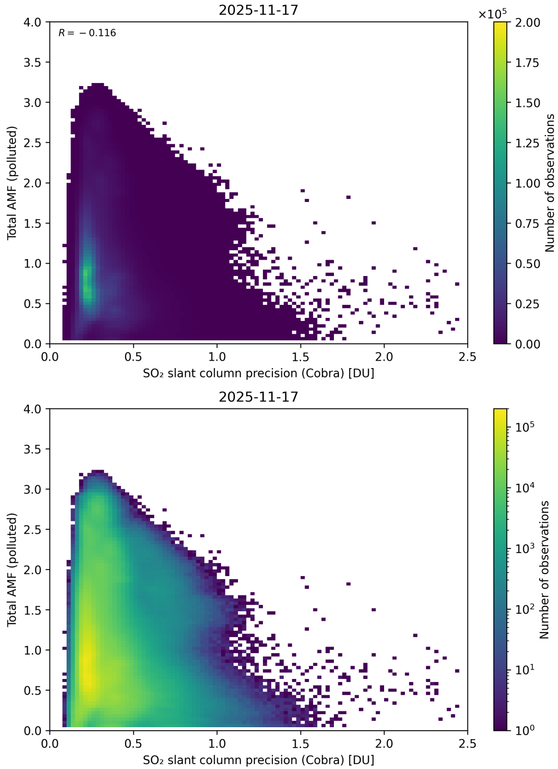
Figure 213: Scatter density plot of “SO 2 slant column precision (Cobra)” against “Total AMF (polluted)” for 2025-11-16 to 2025-11-18.
