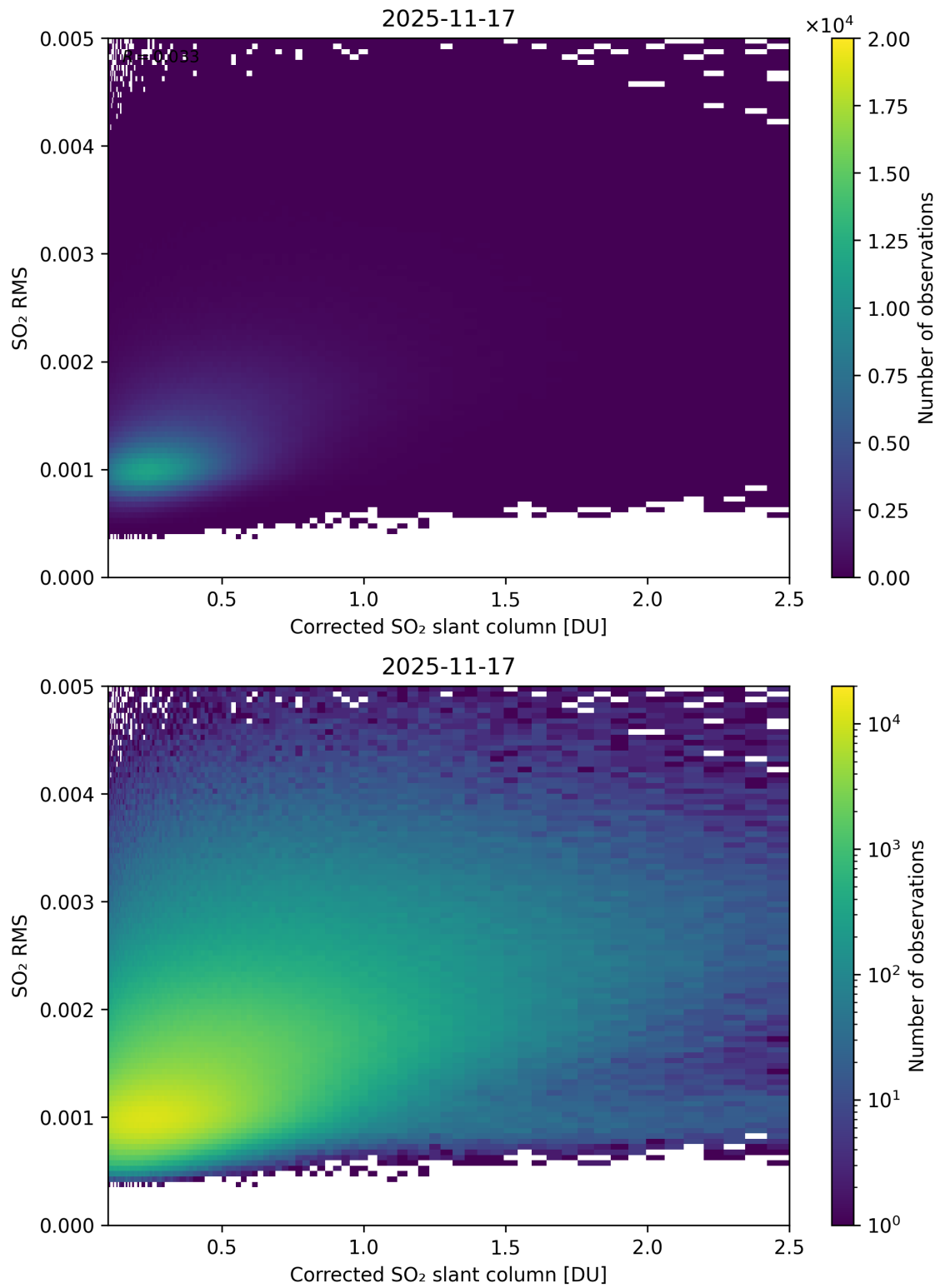
Figure 231: Scatter density plot of “Corrected SO 2 slant column” against “SO 2 RMS” for 2025-11-16 to 2025-11-18.
