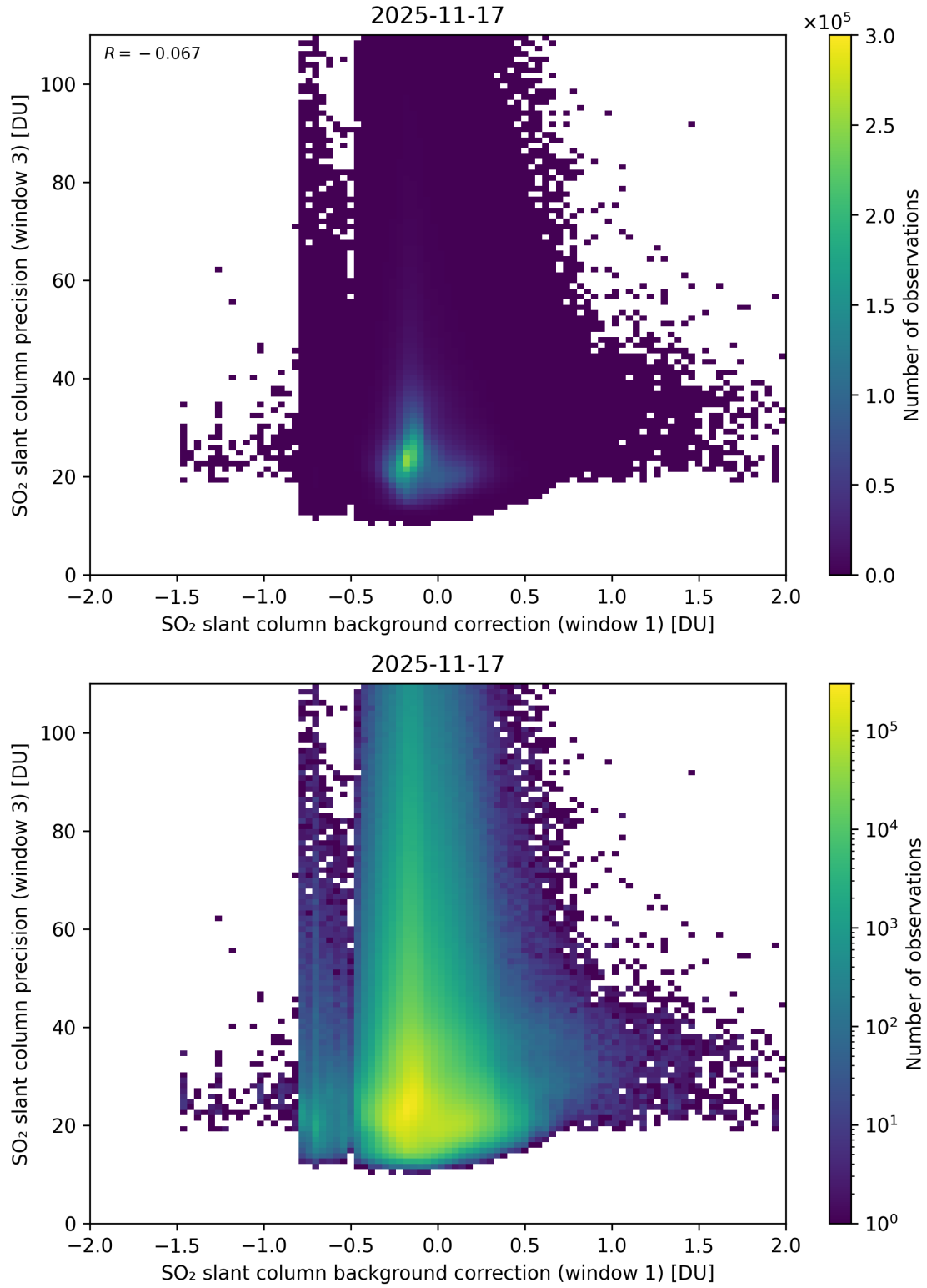
Figure 119: Scatter density plot of “SO 2 slant column background correction (window 1)” against “SO 2 slant column precision (window 3)” for 2025-11-16 to 2025-11-18.
