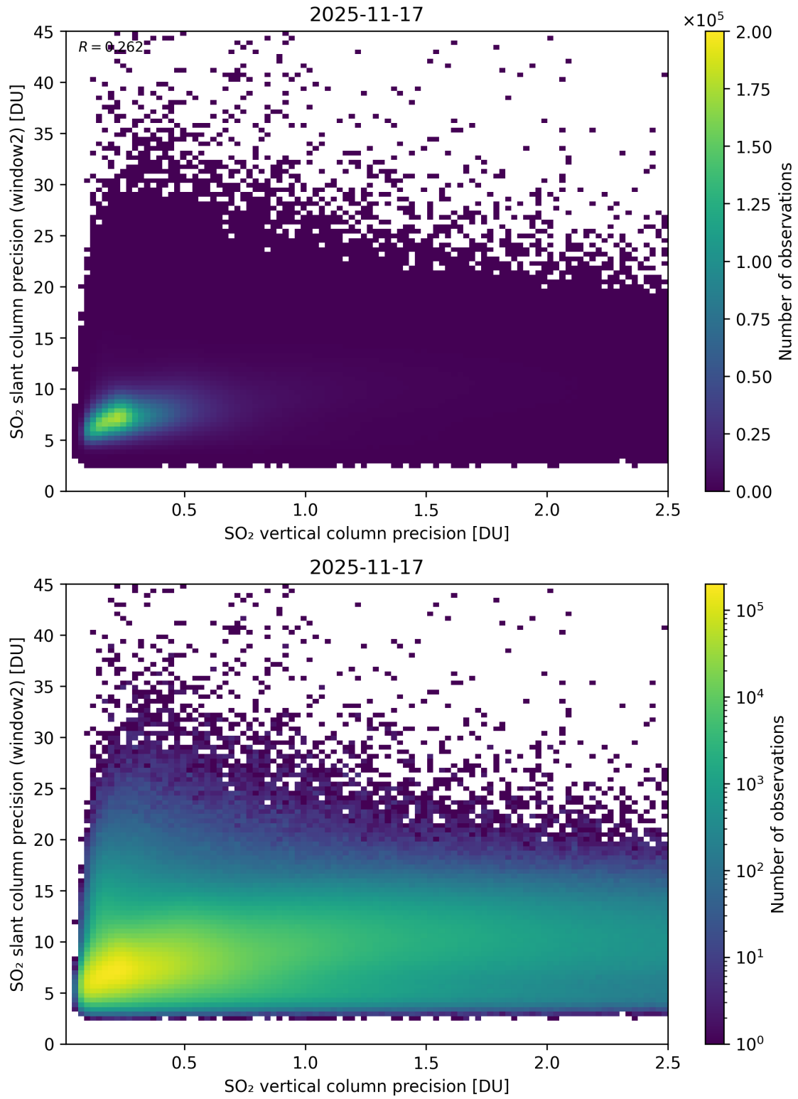
Figure 343: Scatter density plot of “SO 2 vertical column precision” against “SO 2 slant column precision (window2)” for 2025-11-16 to 2025-11-18.
