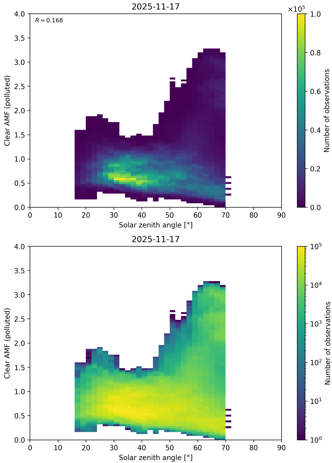
Figure 178: Scatter density plot of “Solar zenith angle” against “Clear AMF (polluted)” for 2025-11-16 to 2025-11-18.
