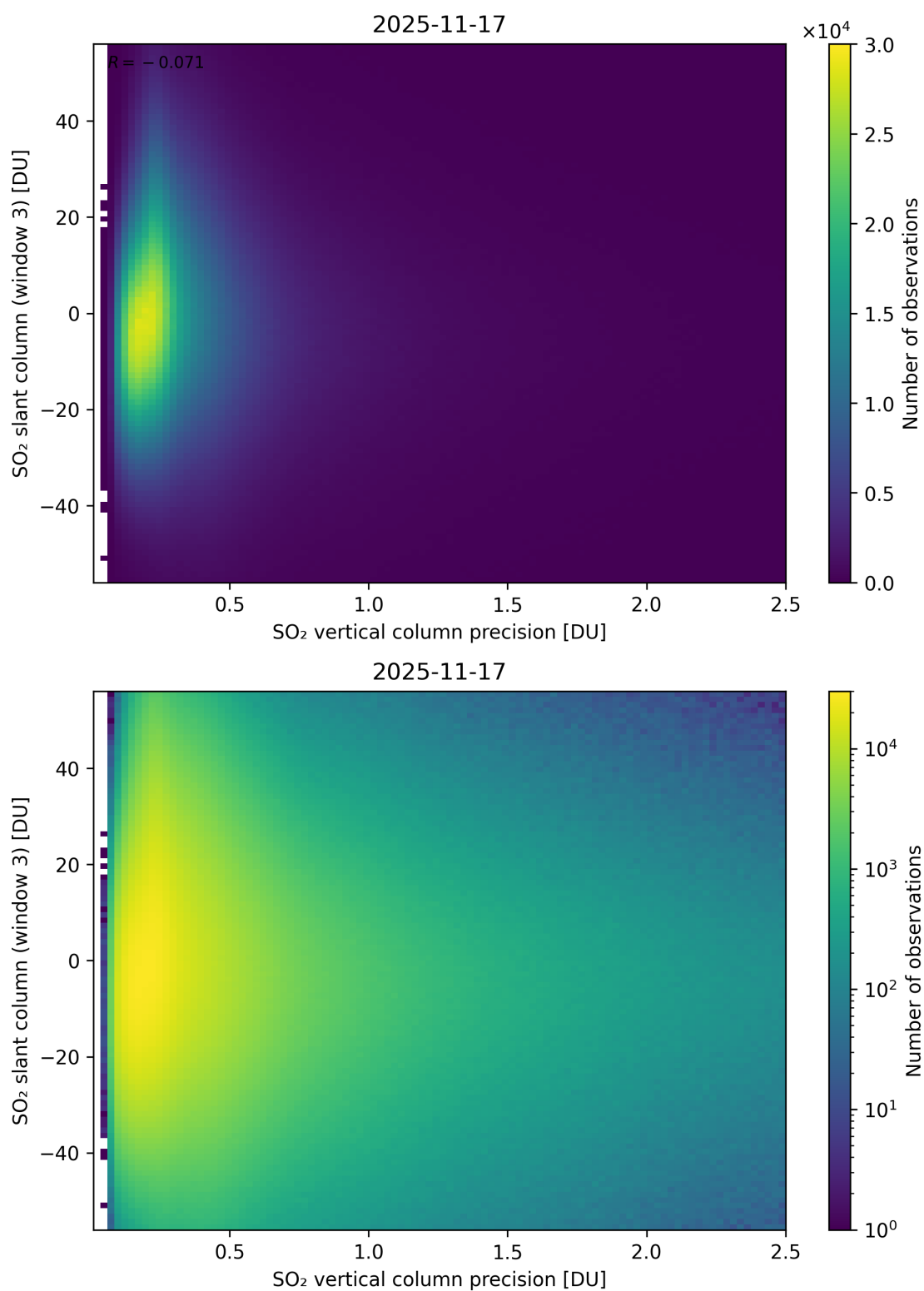
Figure 344: Scatter density plot of “SO 2 vertical column precision” against “SO 2 slant column (window 3)” for 2025-11-16 to 2025-11-18.
