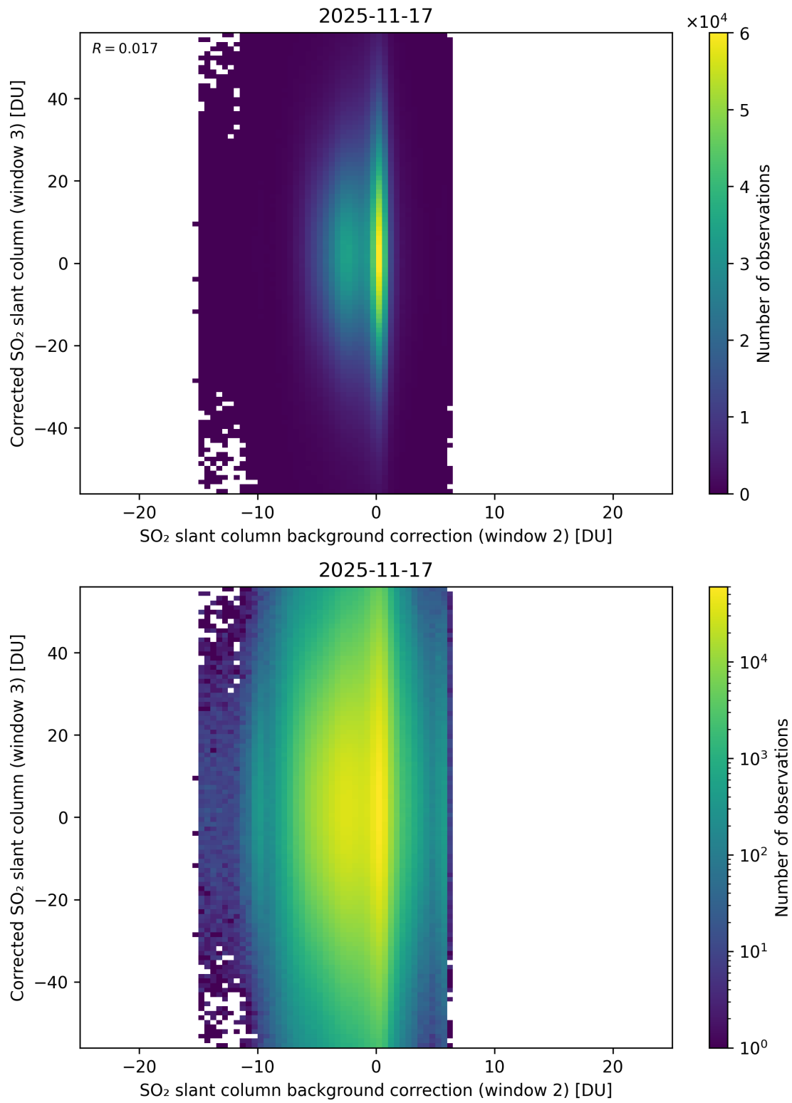
Figure 127: Scatter density plot of “SO 2 slant column background correction (window 2)” against “Corrected SO 2 slant column (window 3)” for 2025-11-16 to 2025-11-18.
