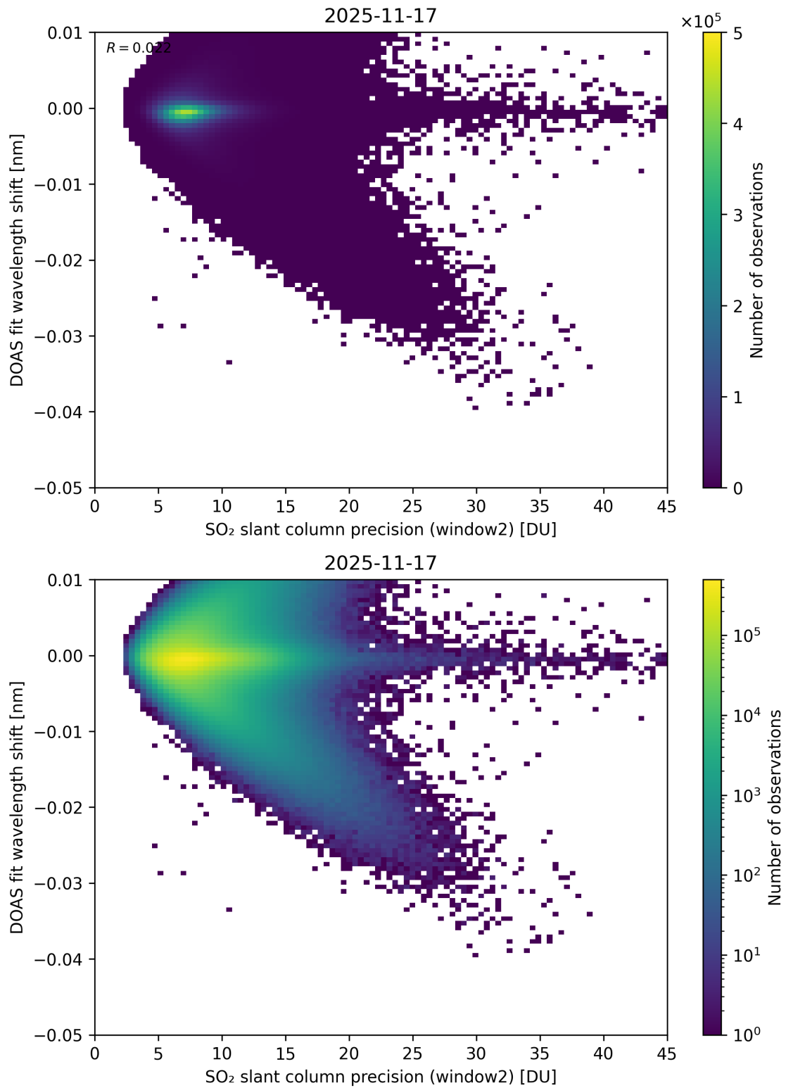
Figure 293: Scatter density plot of “SO 2 slant column precision (window2)” against “DOAS fit wavelength shift” for 2025-11-16 to 2025-11-18.
