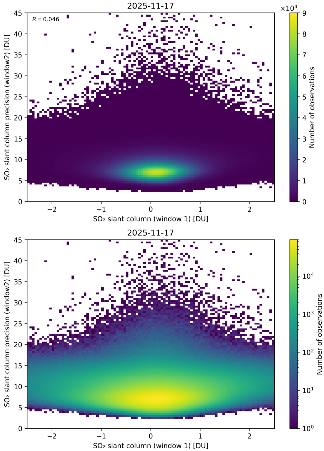
Figure 286: Scatter density plot of “SO 2 slant column (window 1)” against “SO 2 slant column precision (window2)” for 2025-11-16 to 2025-11-18.
