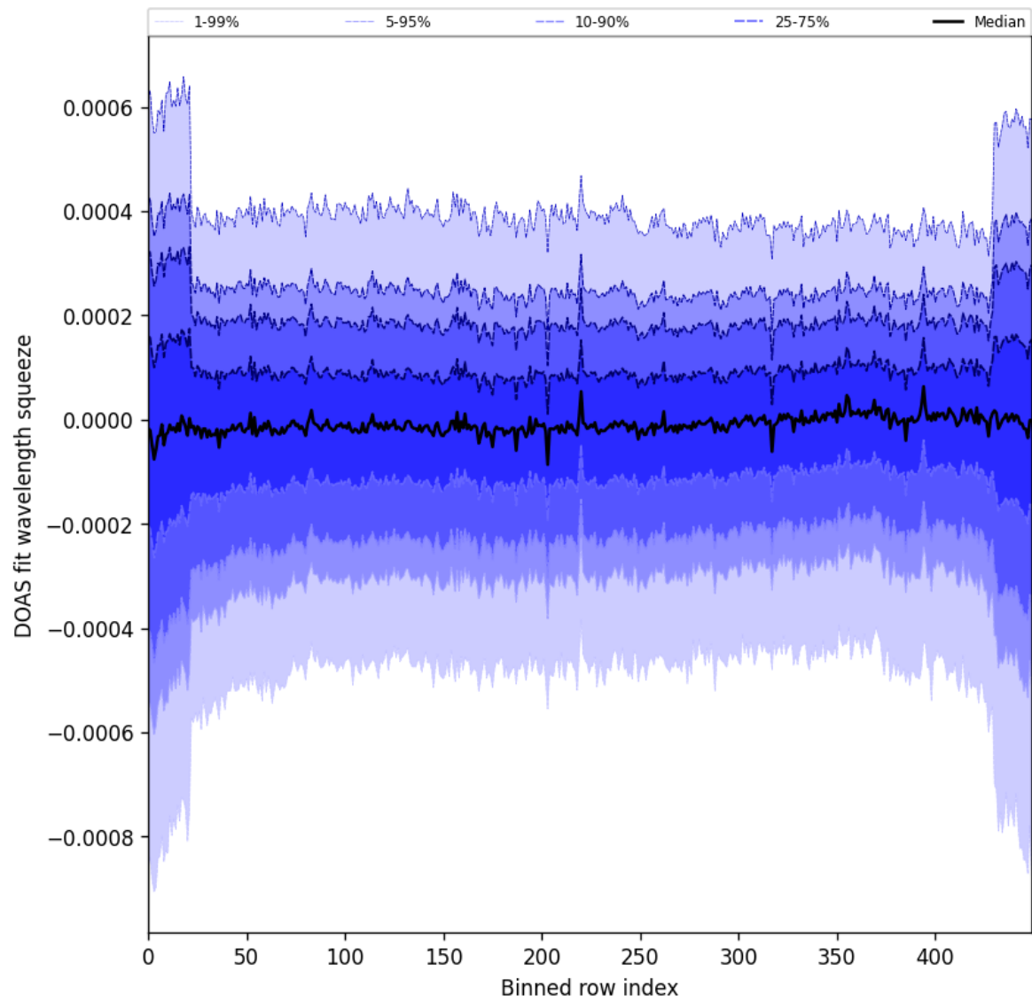
Figure 103: Along track statistics of “DOAS fit wavelength squeeze” for 2025-11-16 to 2025-11-18
