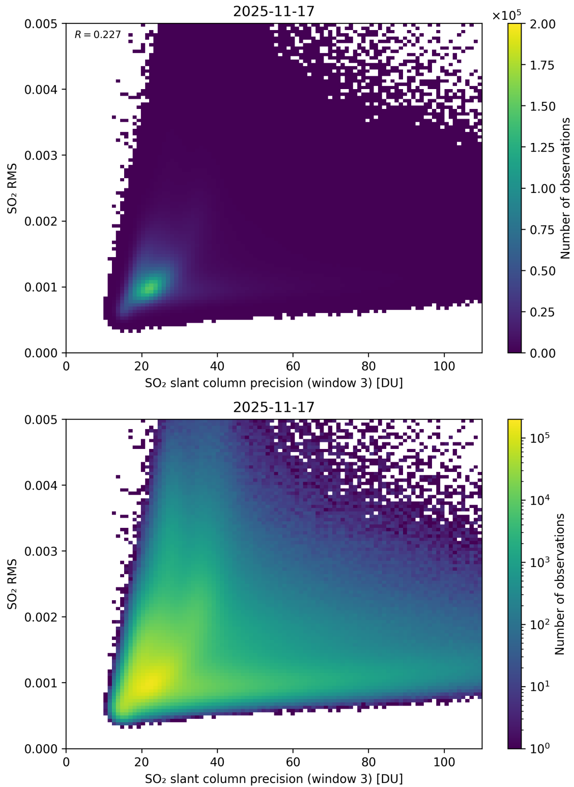
Figure 310: Scatter density plot of “SO 2 slant column precision (window 3)” against “SO 2 RMS” for 2025-11-16 to 2025-11-18.
