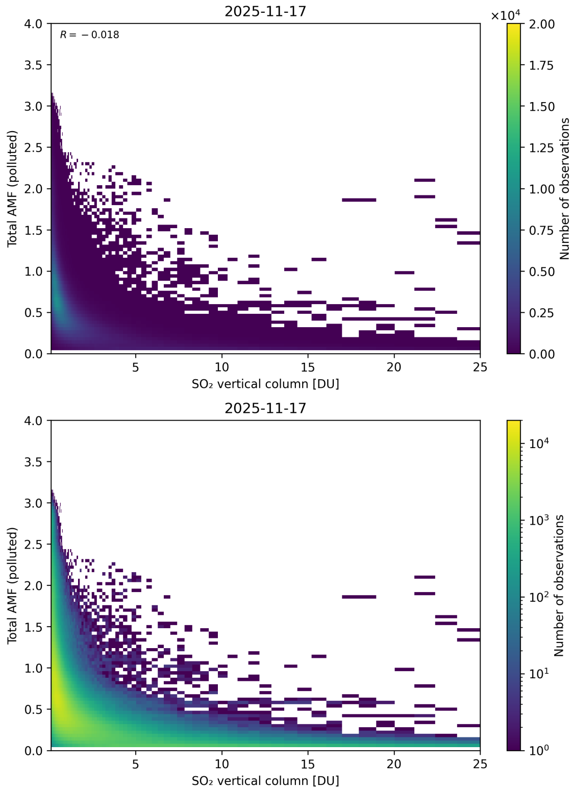
Figure 359: Scatter density plot of “SO 2 vertical column” against “Total AMF (polluted)” for 2025-11-16 to 2025-11-18.
