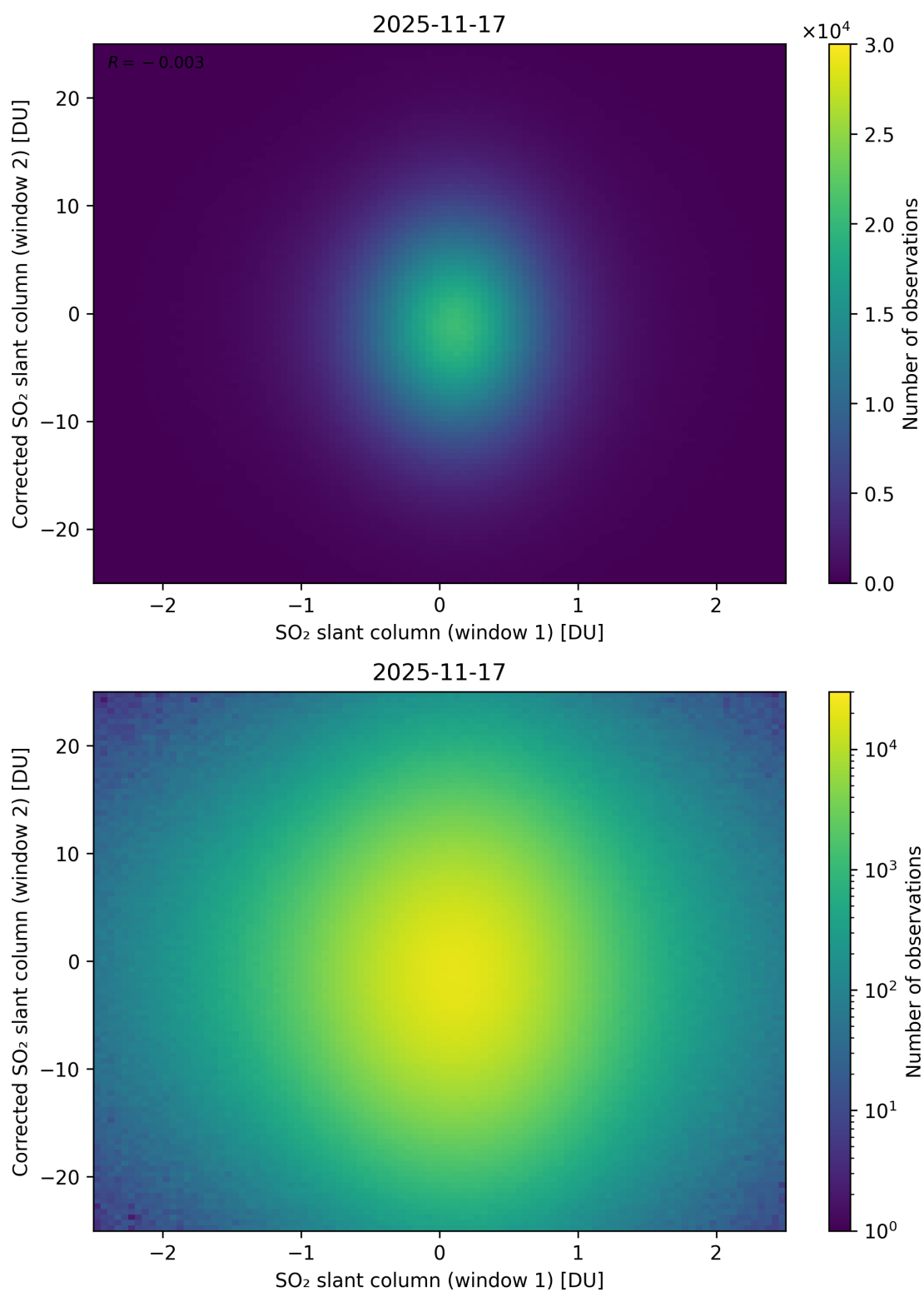
Figure 283: Scatter density plot of “SO 2 slant column (window 1)” against “Corrected SO 2 slant column (window 2)” for 2025-11-16 to 2025-11-18.
