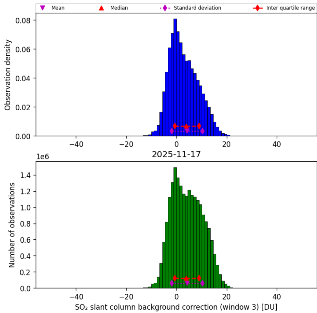
Figure 74: Histogram of “SO 2 slant column background correction (window 3)” for 2025-11-16 to 2025-11-18
