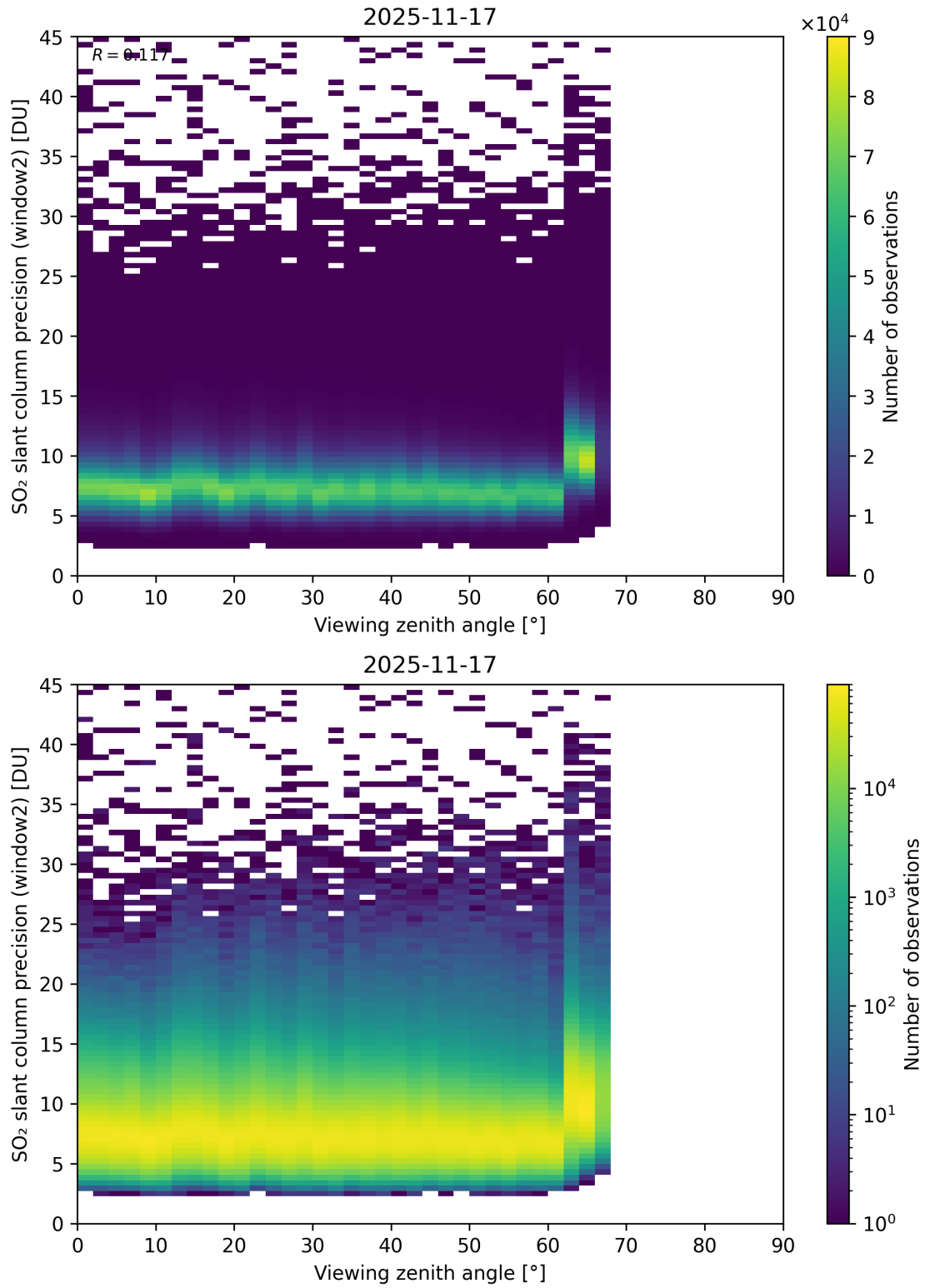
Figure 378: Scatter density plot of “Viewing zenith angle” against “SO 2 slant column precision (window2)” for 2025-11-16 to 2025-11-18.
