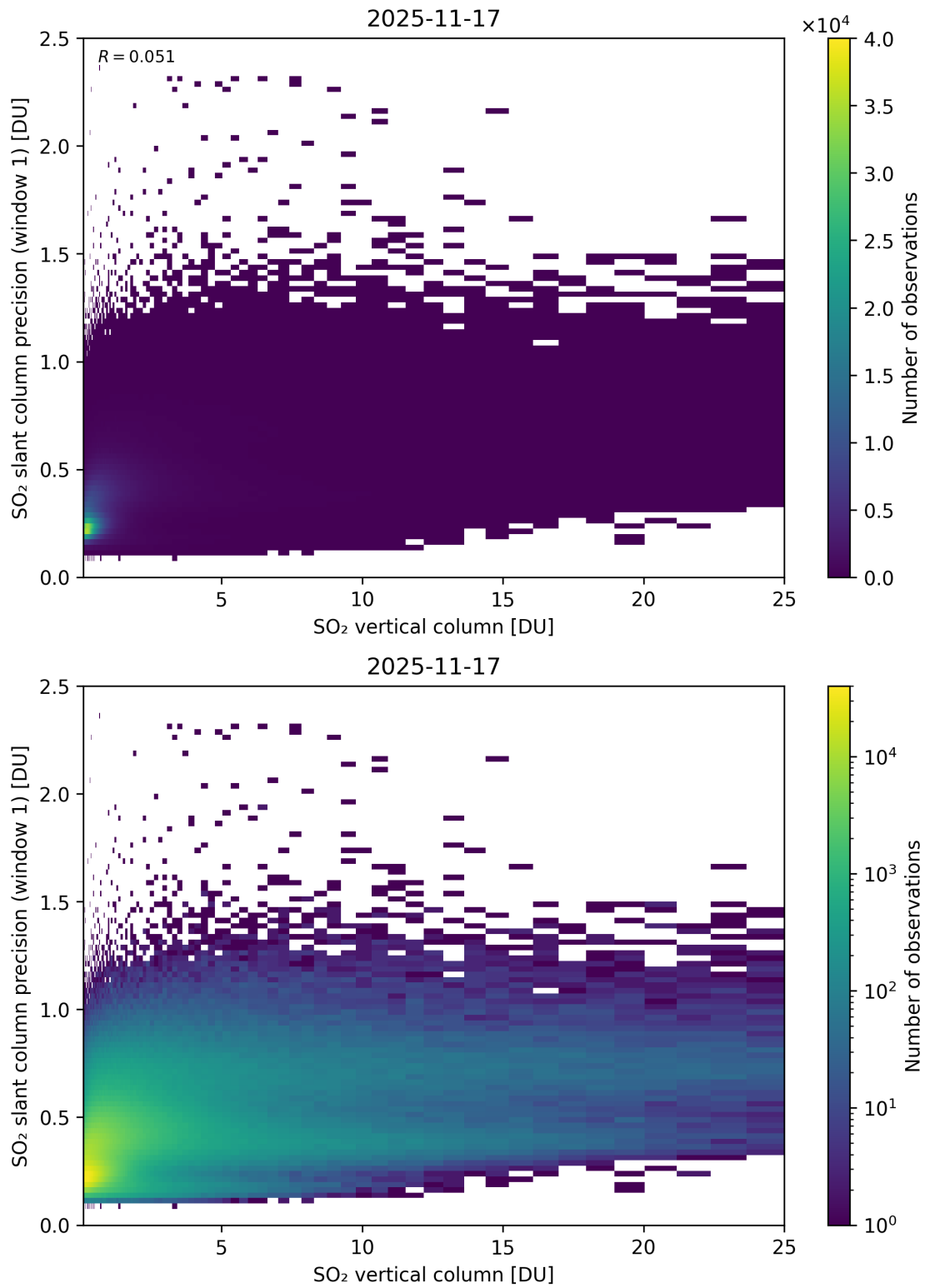
Figure 355: Scatter density plot of “SO 2 vertical column” against “SO 2 slant column precision (window 1)” for 2025-11-16 to 2025-11-18.
