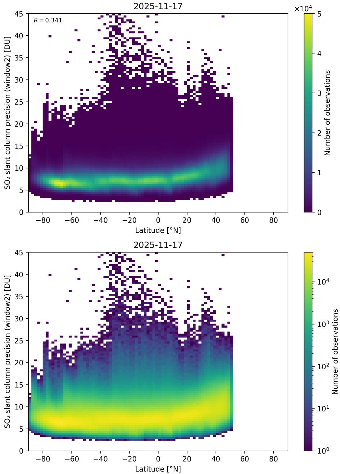
Figure 164: Scatter density plot of “Latitude” against “SO 2 slant column precision (window2)” for 2025-11-16 to 2025-11-18.
