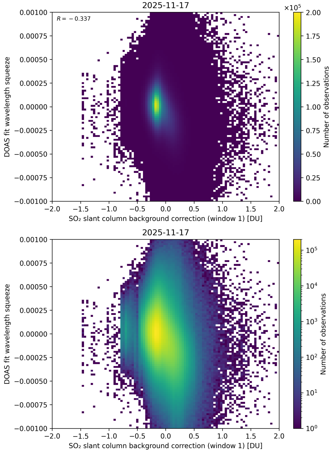
Figure 112: Scatter density plot of “SO 2 slant column background correction (window 1)” against “DOAS fit wavelength squeeze” for 2025-11-16 to 2025-11-18.
