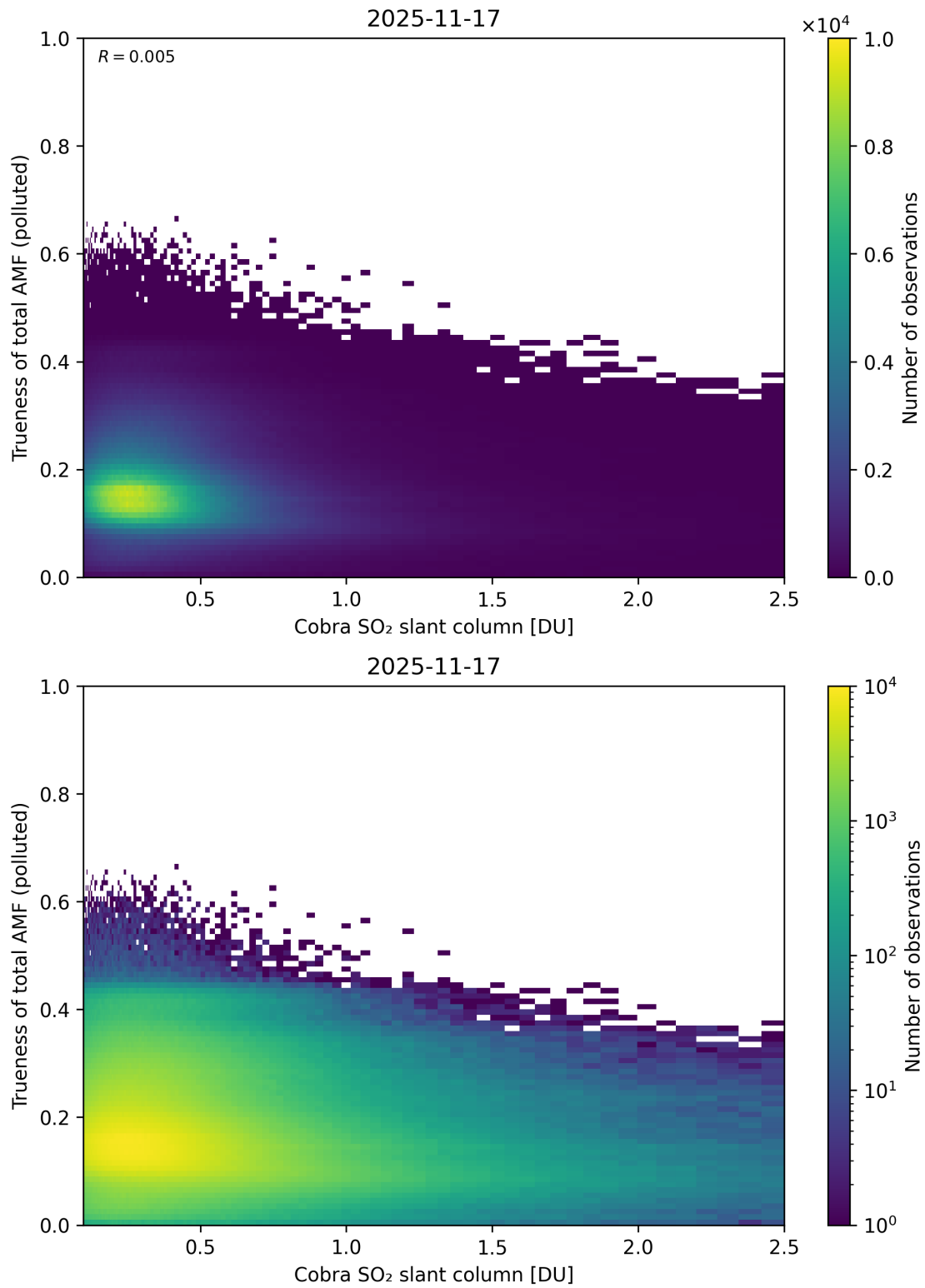
Figure 225: Scatter density plot of “Cobra SO 2 slant column” against “Trueness of total AMF (polluted)” for 2025-11-16 to 2025-11-18.
