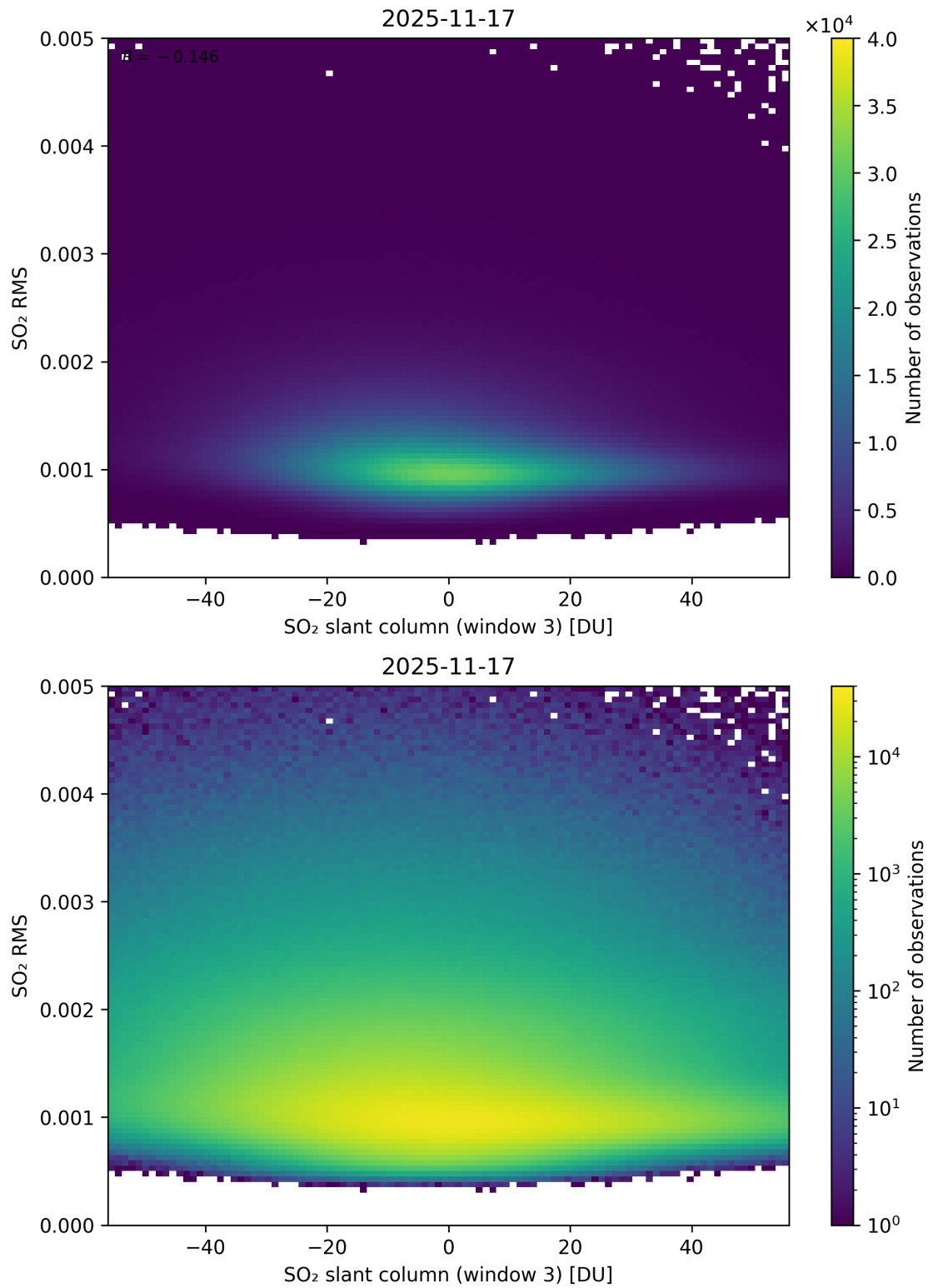
Figure 306: Scatter density plot of “SO 2 slant column (window 3)” against “SO 2 RMS” for 2025-11-16 to 2025-11-18.
