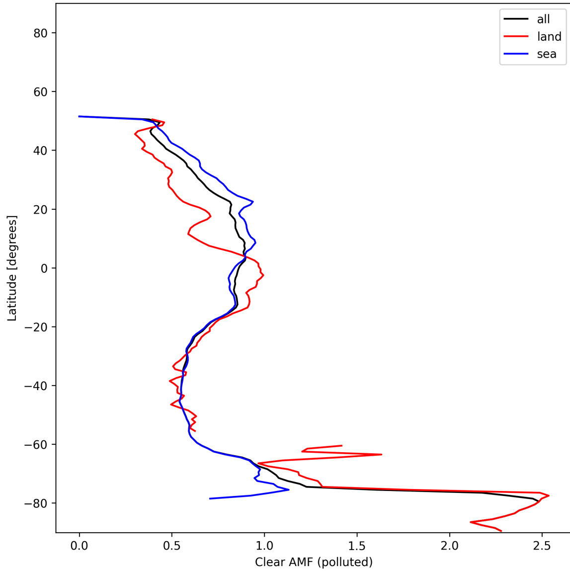
Figure 55: Zonal average of “Clear AMF (polluted)” for 2025-11-16 to 2025-11-18.
