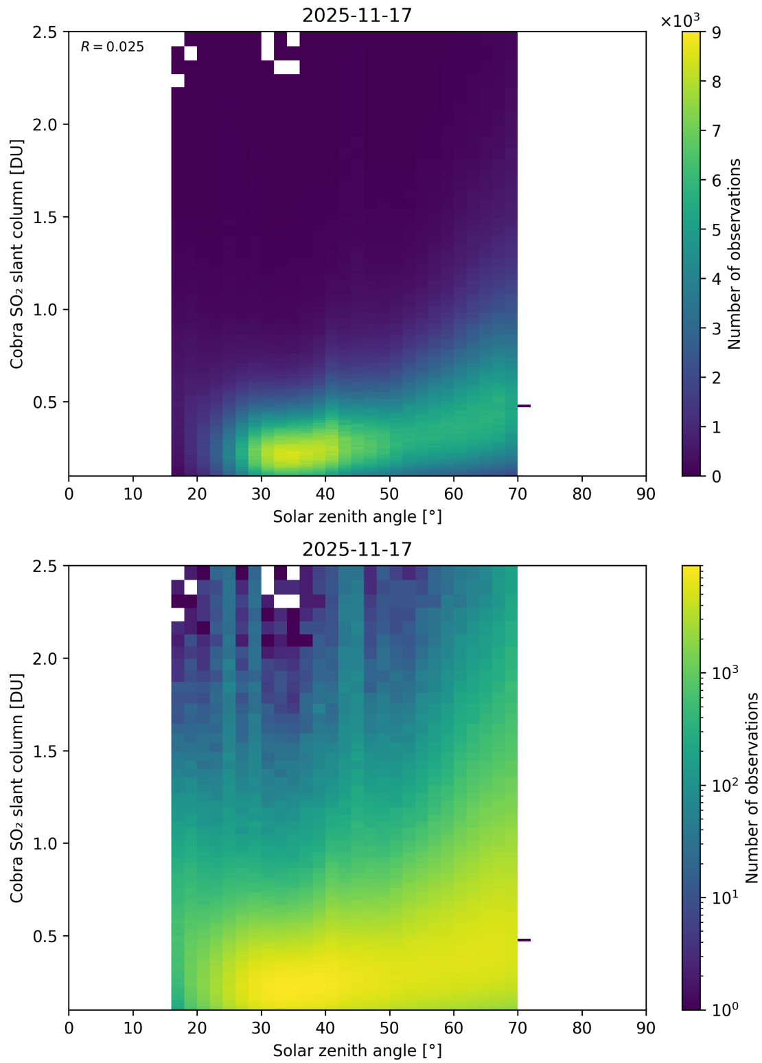
Figure 179: Scatter density plot of “Solar zenith angle” against “Cobra SO 2 slant column” for 2025-11-16 to 2025-11-18.
