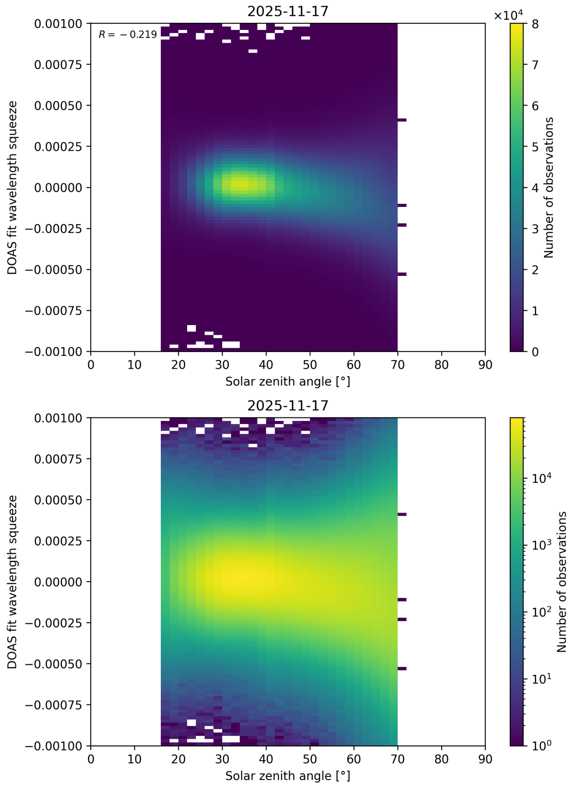
Figure 175: Scatter density plot of “Solar zenith angle” against “DOAS fit wavelength squeeze” for 2025-11-16 to 2025-11-18.
