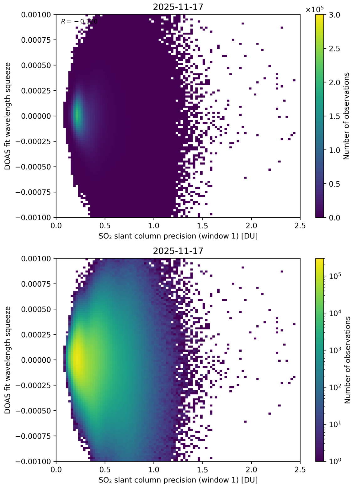
Figure 272: Scatter density plot of “SO 2 slant column precision (window 1)” against “DOAS fit wavelength squeeze” for 2025-11-16 to 2025-11-18.
