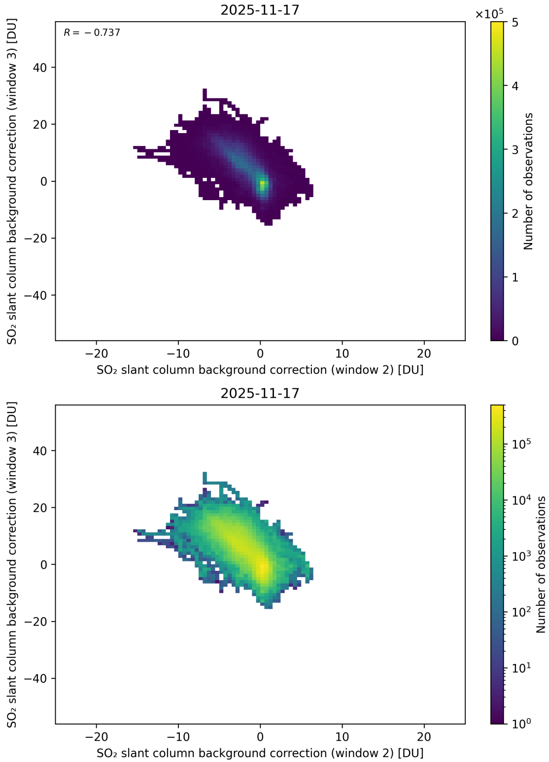
Figure 122: Scatter density plot of “SO 2 slant column background correction (window 2)” against “SO 2 slant column background correction (window 3)” for 2025-11-16 to 2025-11-18.
