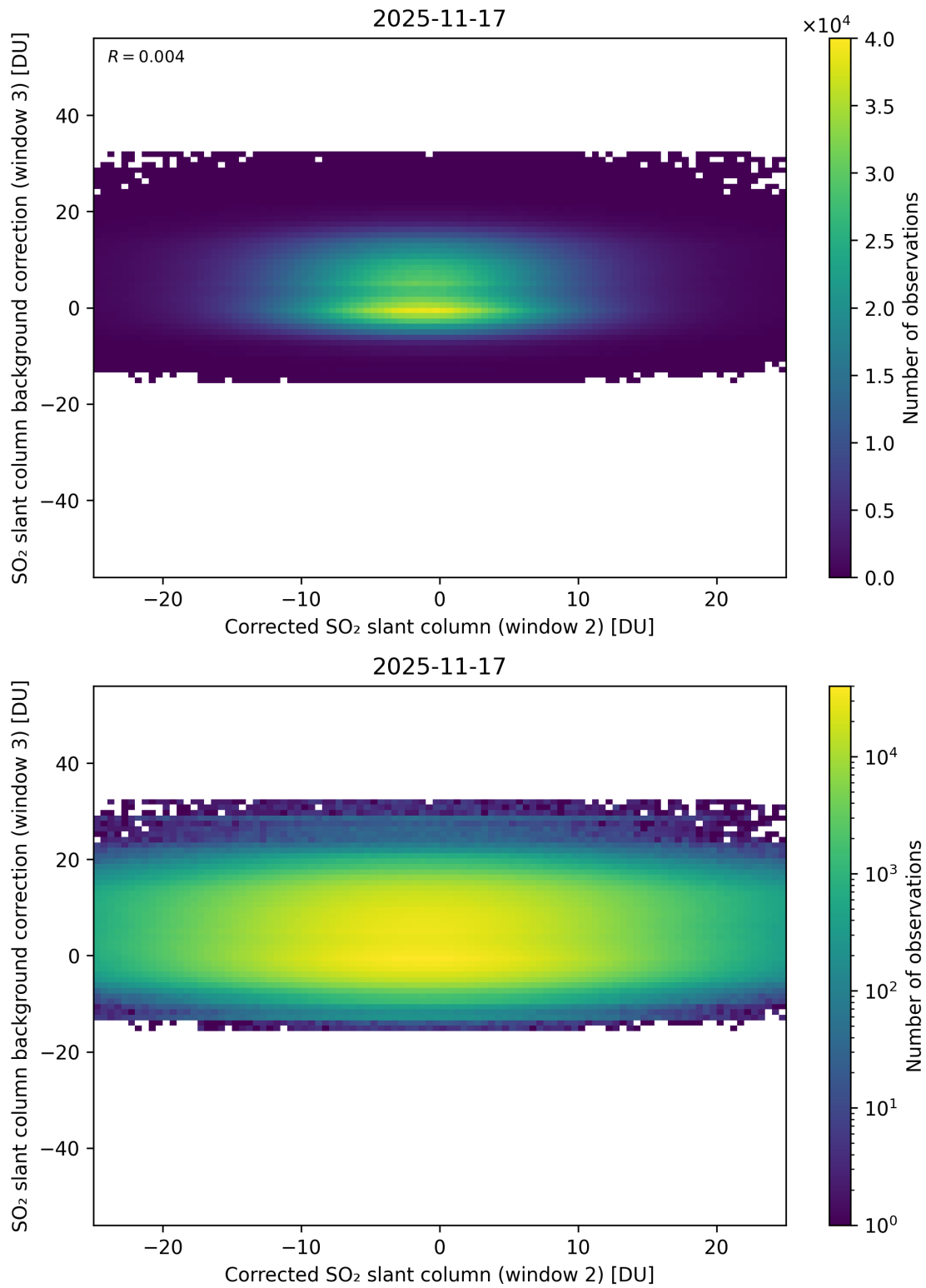
Figure 245: Scatter density plot of “Corrected SO 2 slant column (window 2)” against “SO 2 slant column background correction (window 3)” for 2025-11-16 to 2025-11-18.
