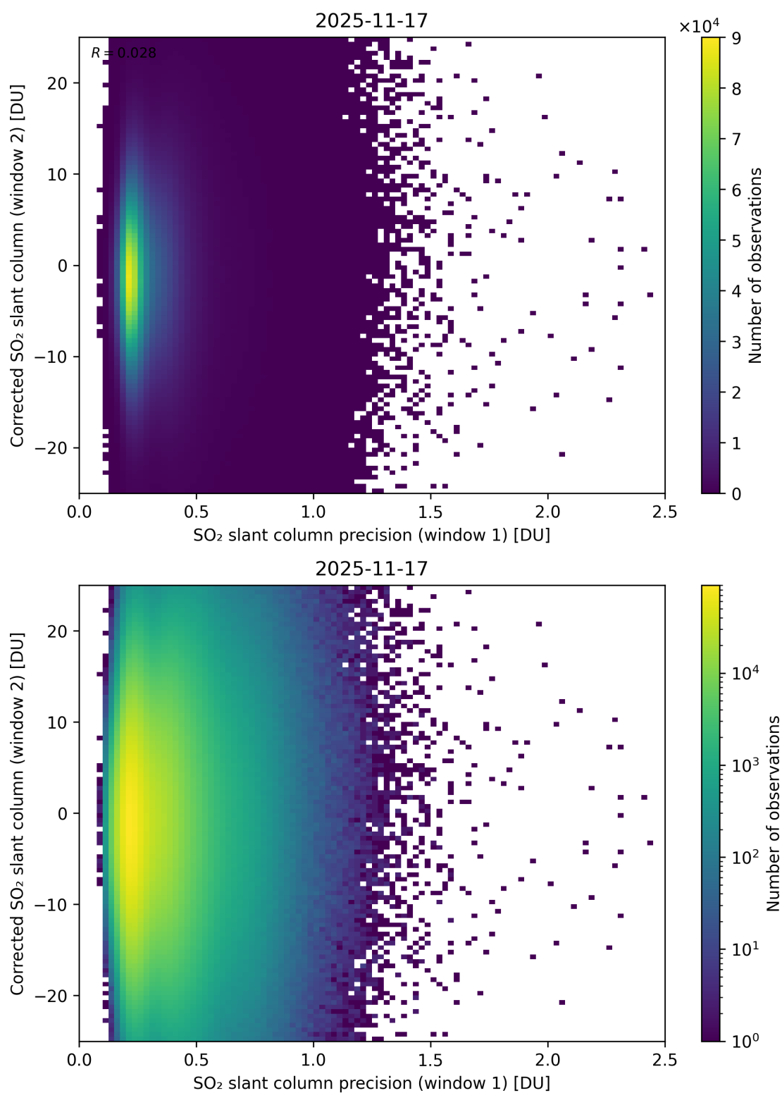
Figure 275: Scatter density plot of “SO 2 slant column precision (window 1)” against “Corrected SO 2 slant column (window 2)” for 2025-11-16 to 2025-11-18.
