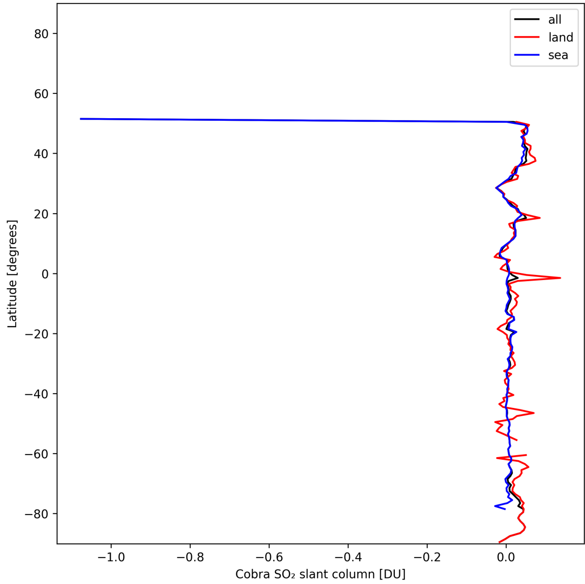
Figure 35: Zonal average of “Cobra SO 2 slant column” for 2025-11-16 to 2025-11-18.
