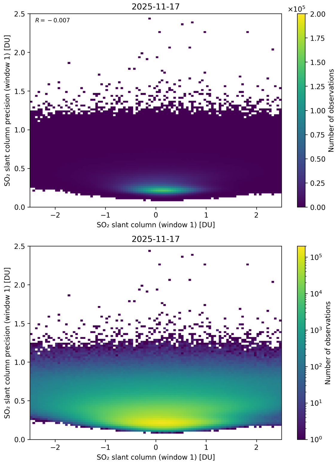
Figure 285: Scatter density plot of “SO 2 slant column (window 1)” against “SO 2 slant column precision (window 1)” for 2025-11-16 to 2025-11-18.
