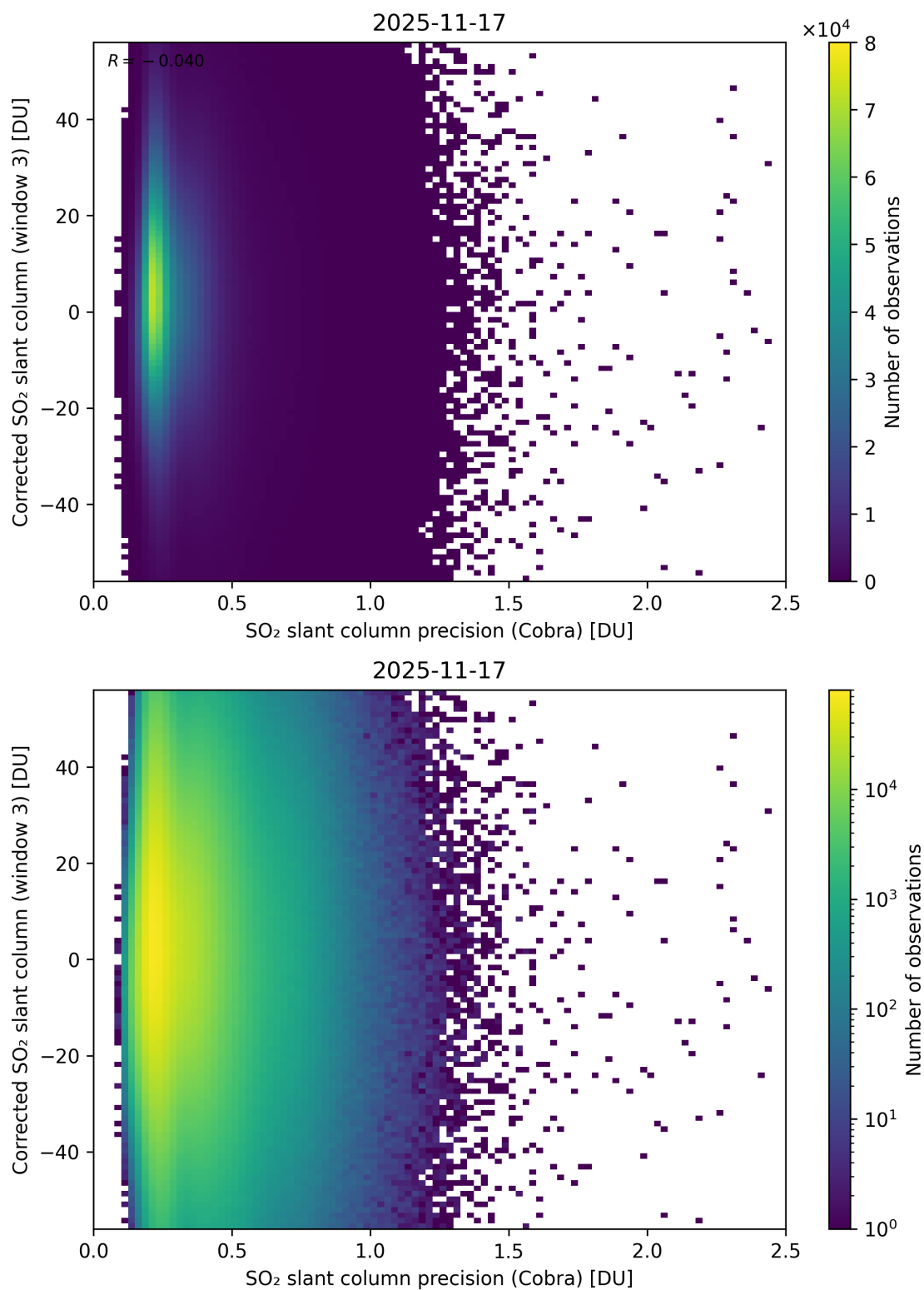
Figure 207: Scatter density plot of “SO 2 slant column precision (Cobra)” against “Corrected SO 2 slant column (window 3)” for 2025-11-16 to 2025-11-18.
