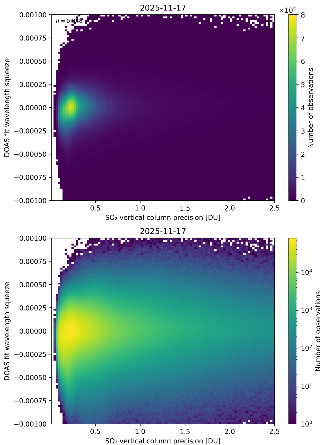
Figure 333: Scatter density plot of “SO 2 vertical column precision” against “DOAS fit wavelength squeeze” for 2025-11-16 to 2025-11-18.
