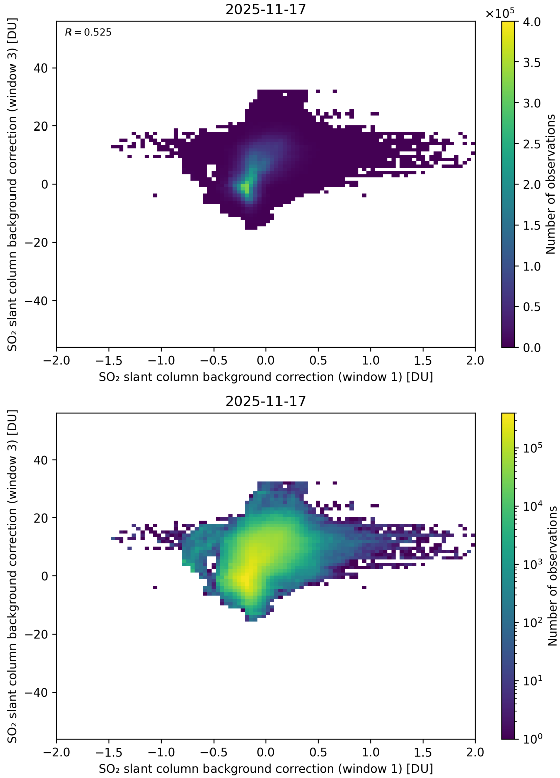
Figure 110: Scatter density plot of “SO 2 slant column background correction (window 1)” against “SO 2 slant column background correction (window 3)” for 2025-11-16 to 2025-11-18.
