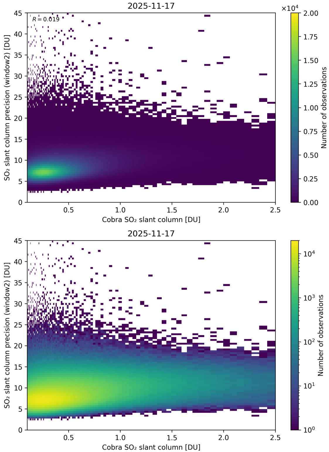
Figure 221: Scatter density plot of “Cobra SO 2 slant column” against “SO 2 slant column precision (window2)” for 2025-11-16 to 2025-11-18.
