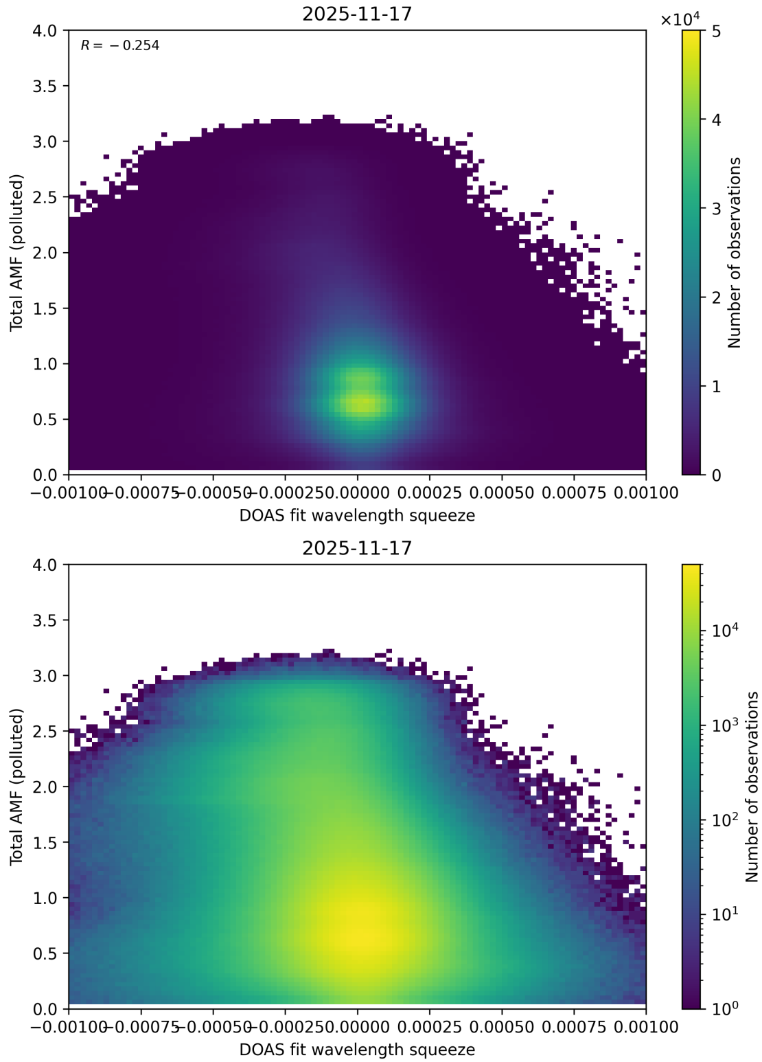
Figure 145: Scatter density plot of “DOAS fit wavelength squeeze” against “Total AMF (polluted)” for 2025-11-16 to 2025-11-18.
