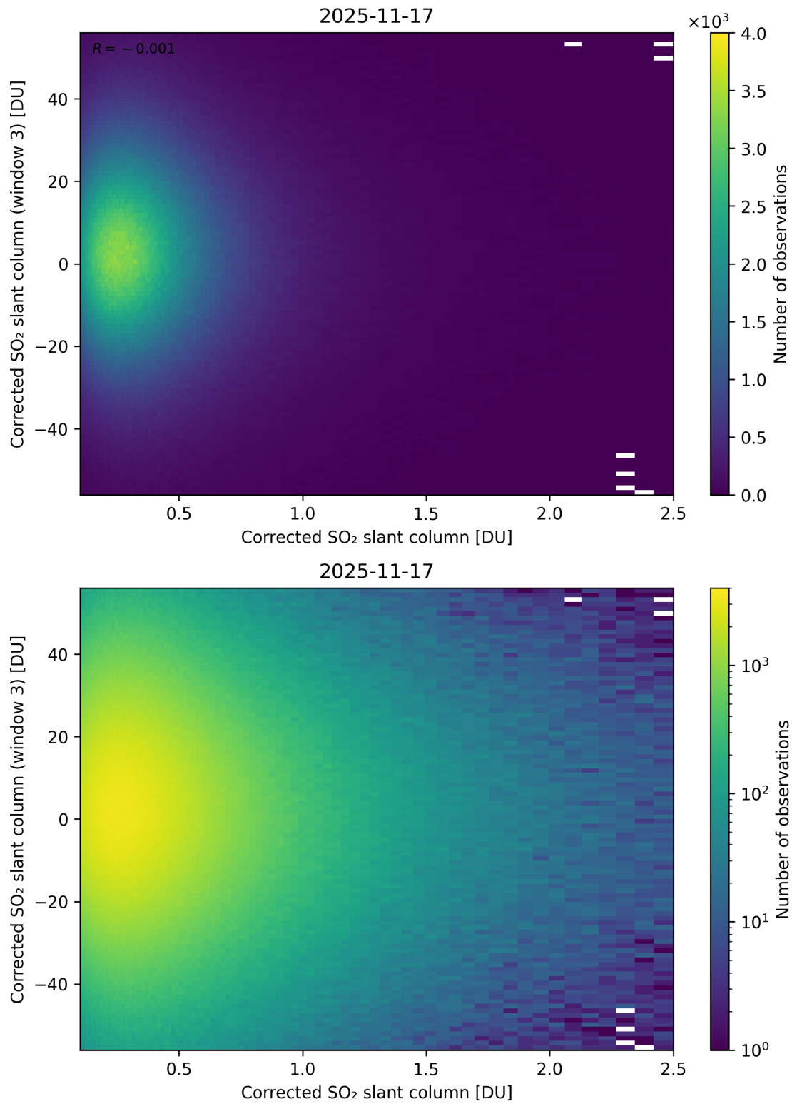
Figure 236: Scatter density plot of “Corrected SO 2 slant column” against “Corrected SO 2 slant column (window 3)” for 2025-11-16 to 2025-11-18.
