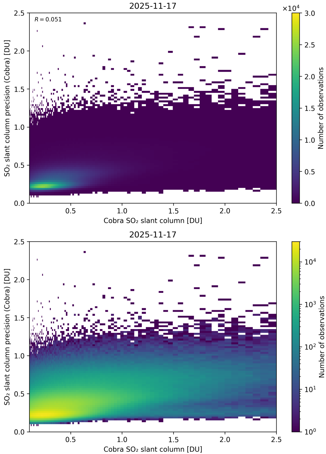
Figure 216: Scatter density plot of “Cobra SO 2 slant column” against “SO 2 slant column precision (Cobra)” for 2025-11-16 to 2025-11-18.
