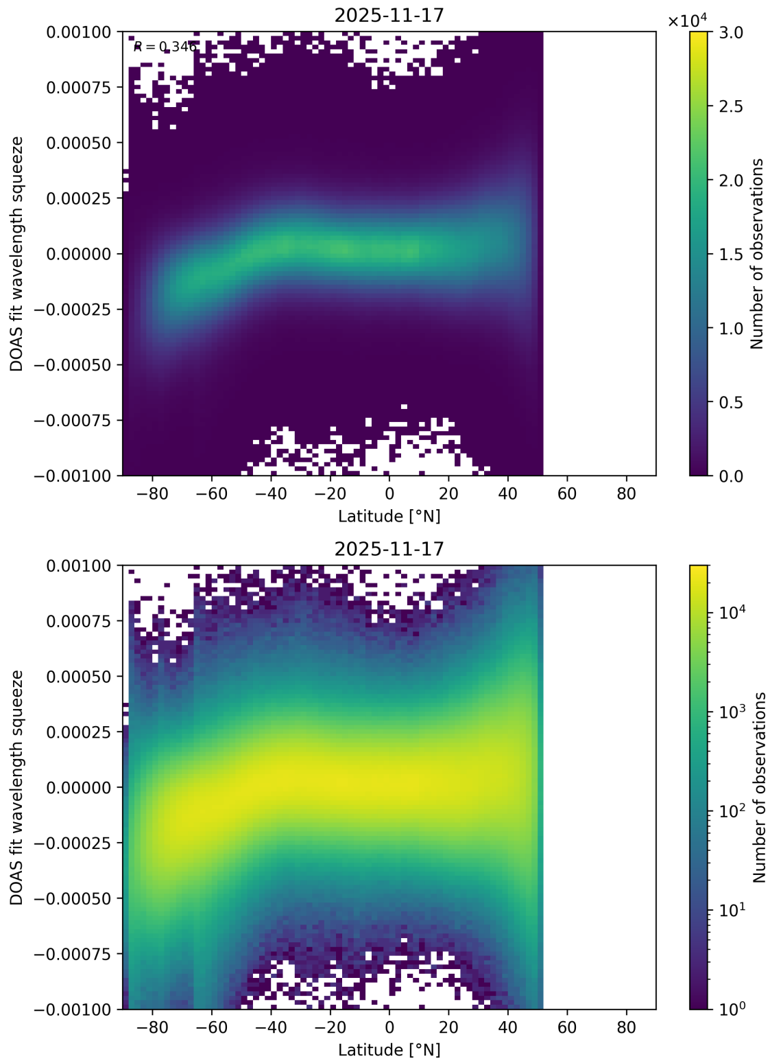
Figure 154: Scatter density plot of “Latitude” against “DOAS fit wavelength squeeze” for 2025-11-16 to 2025-11-18.
