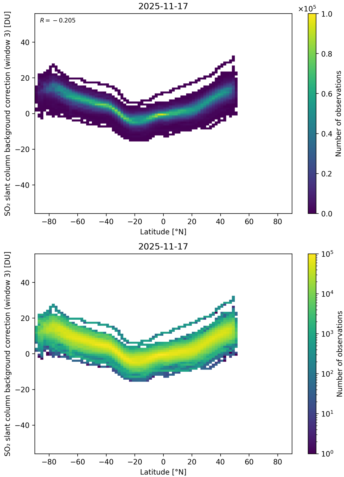
Figure 152: Scatter density plot of “Latitude” against “SO 2 slant column background correction (window 3)” for 2025-11-16 to 2025-11-18.
