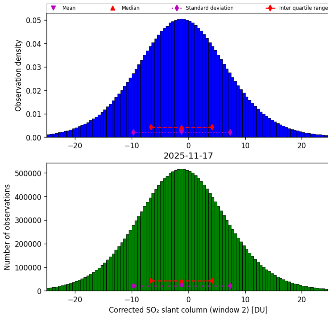
Figure 69: Histogram of “Corrected SO 2 slant column (window 2)” for 2025-11-16 to 2025-11-18
