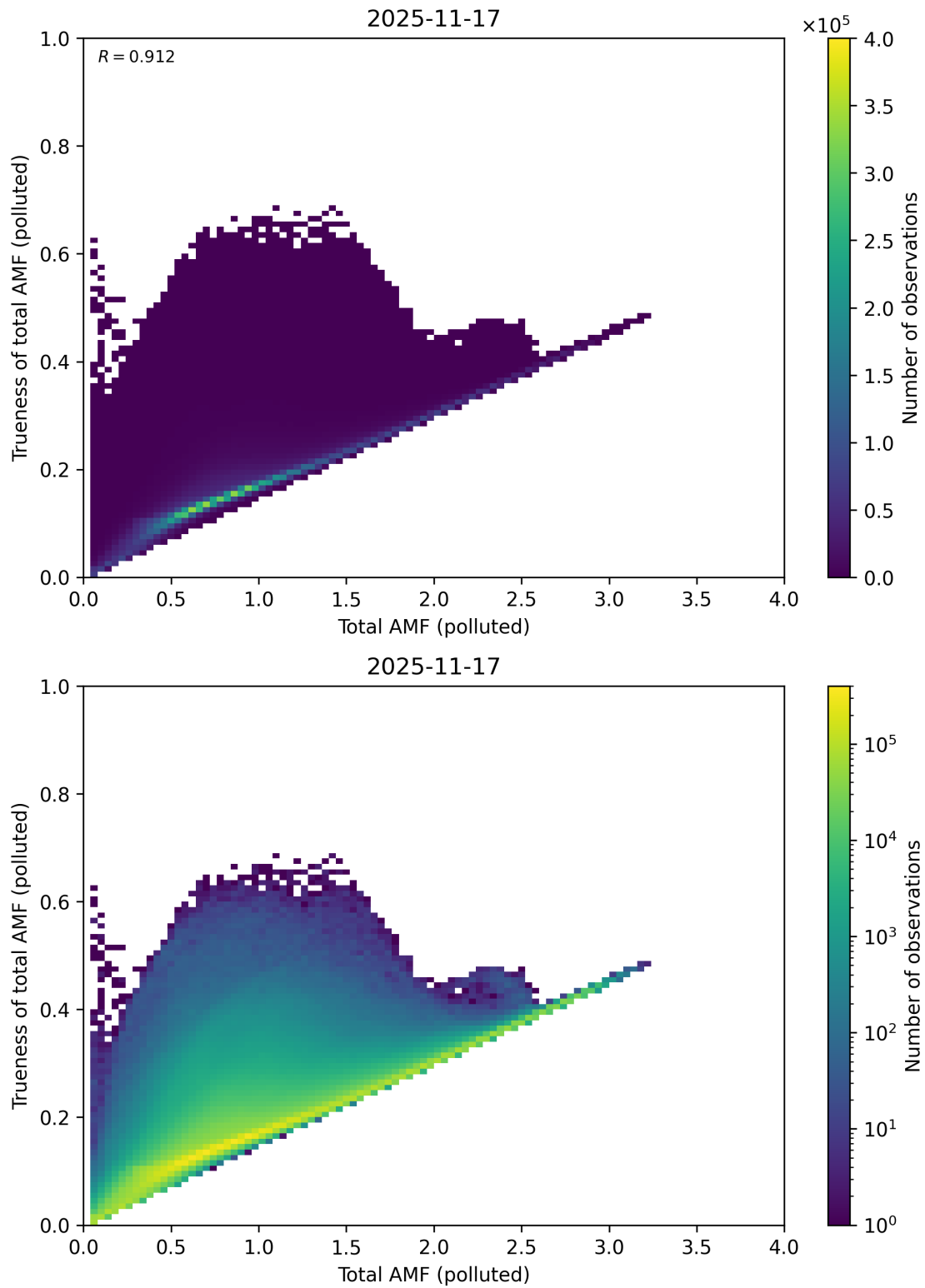
Figure 321: Scatter density plot of “Total AMF (polluted)” against “Trueness of total AMF (polluted)” for 2025-11-16 to 2025-11-18.
