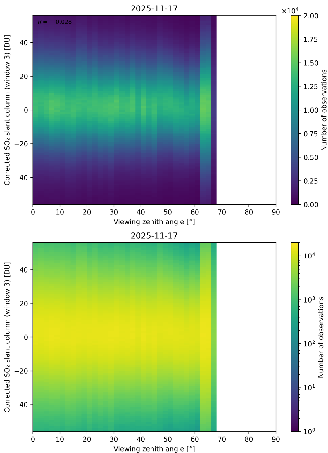
Figure 375: Scatter density plot of “Viewing zenith angle” against “Corrected SO 2 slant column (window 3)” for 2025-11-16 to 2025-11-18.
