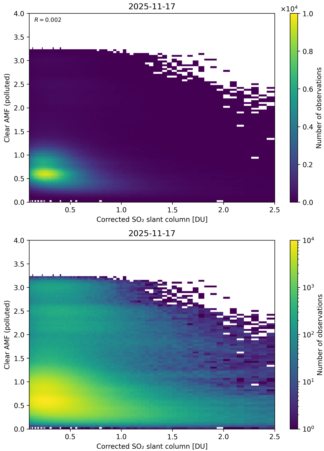
Figure 232: Scatter density plot of “Corrected SO 2 slant column” against “Clear AMF (polluted)” for 2025-11-16 to 2025-11-18.
