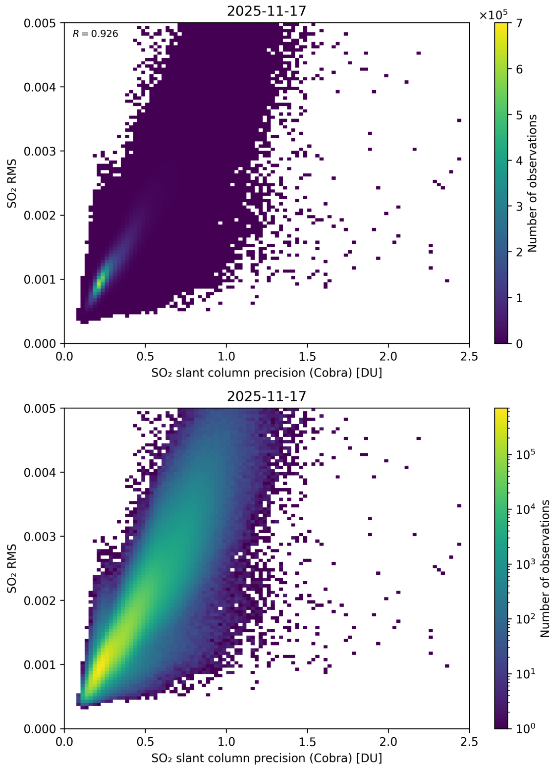
Figure 204: Scatter density plot of “SO 2 slant column precision (Cobra)” against “SO 2 RMS” for 2025-11-16 to 2025-11-18.
