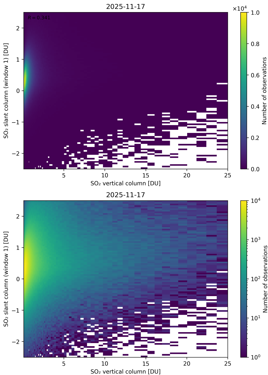
Figure 354: Scatter density plot of “SO 2 vertical column” against “SO 2 slant column (window 1)” for 2025-11-16 to 2025-11-18.
