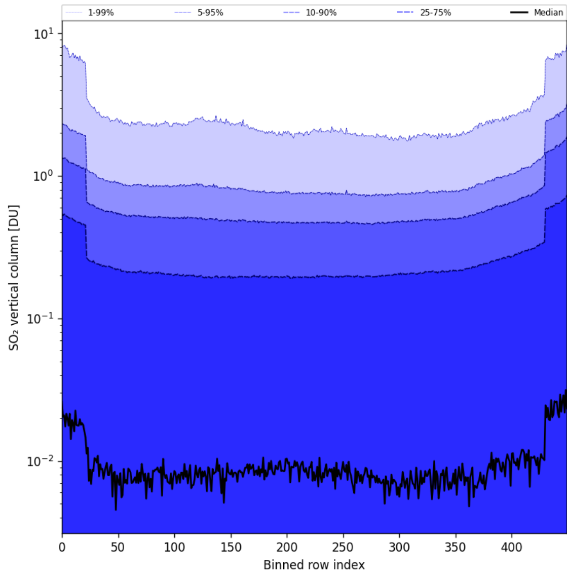
Figure 84: Along track statistics of “SO 2 vertical column” for 2025-11-16 to 2025-11-18
