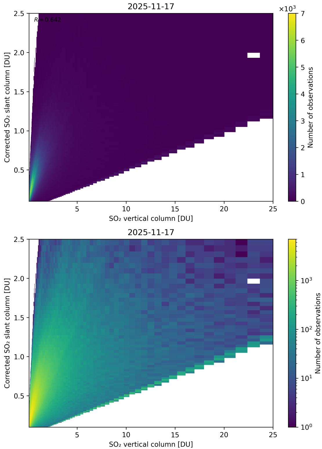
Figure 351: Scatter density plot of “SO 2 vertical column” against “Corrected SO 2 slant column” for 2025-11-16 to 2025-11-18.
