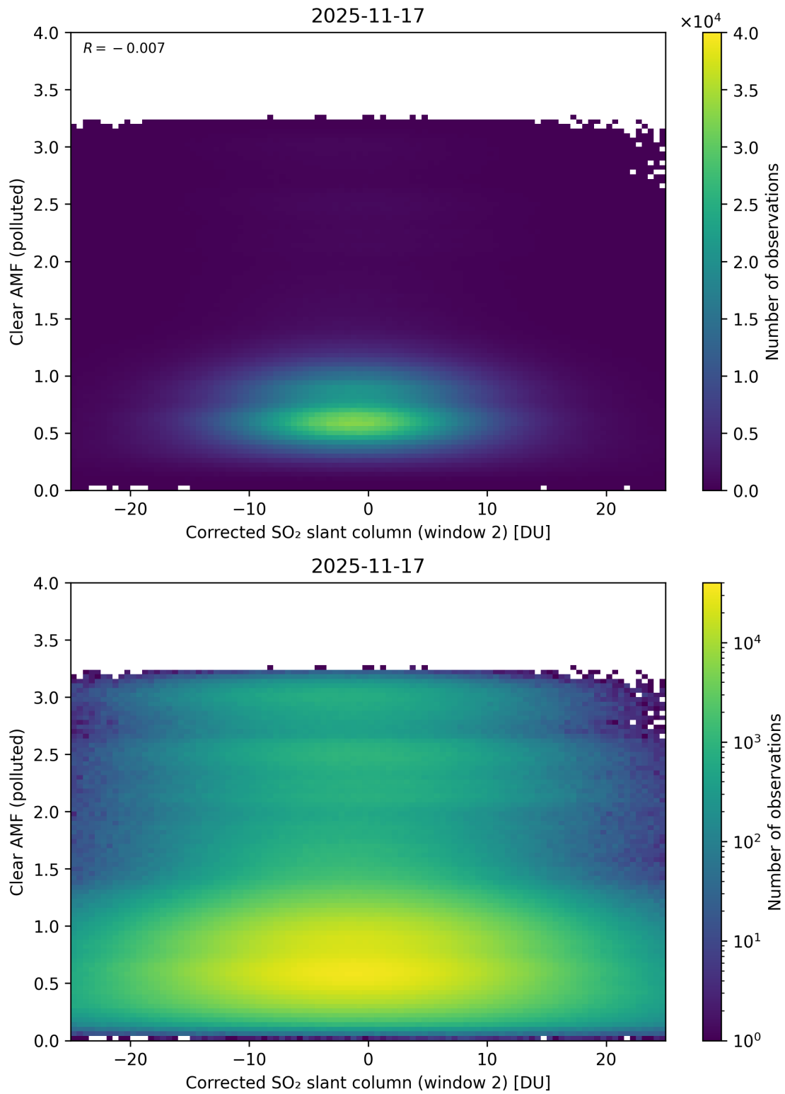
Figure 249: Scatter density plot of “Corrected SO 2 slant column (window 2)” against “Clear AMF (polluted)” for 2025-11-16 to 2025-11-18.
