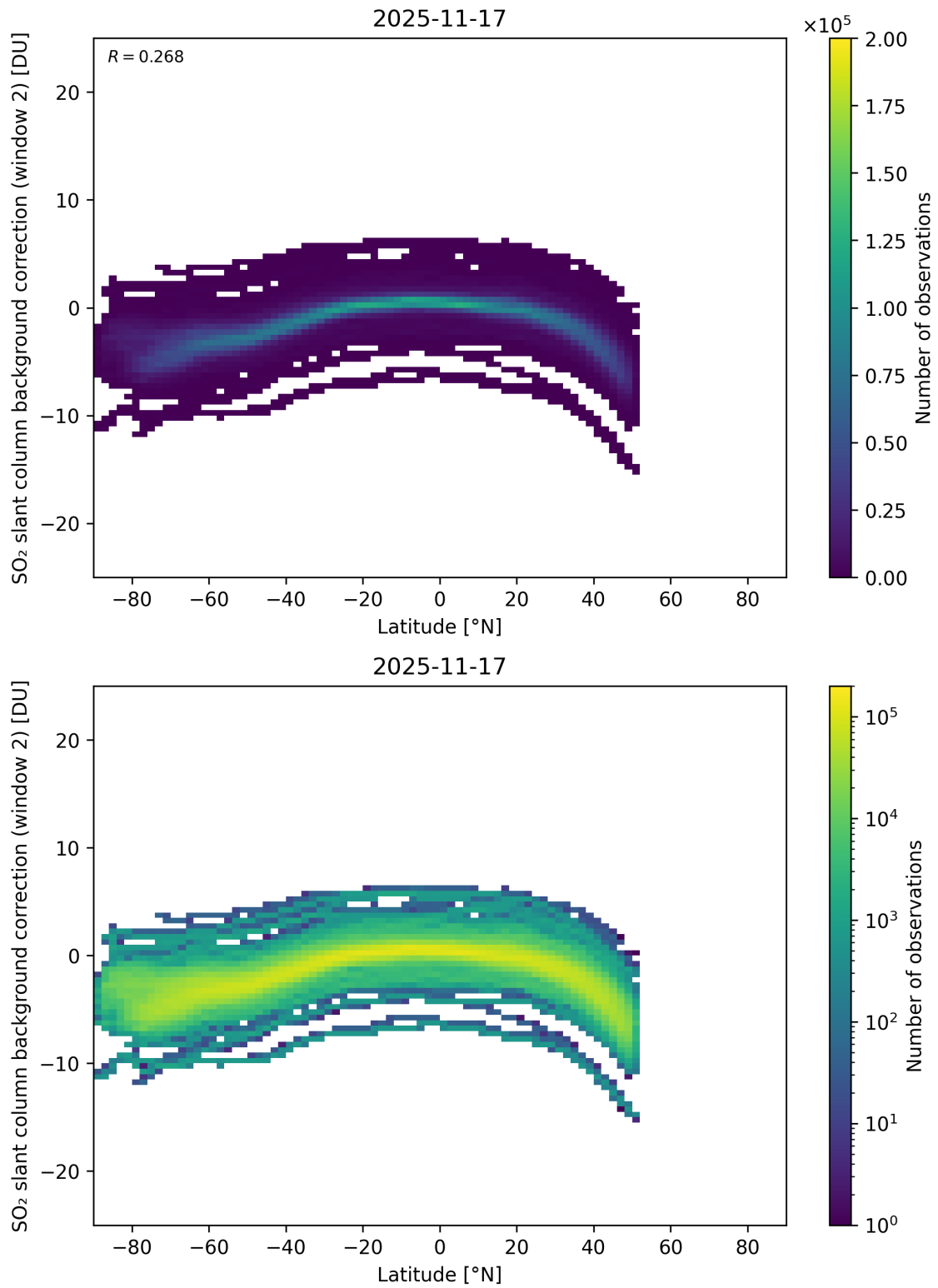
Figure 151: Scatter density plot of “Latitude” against “SO 2 slant column background correction (window 2)” for 2025-11-16 to 2025-11-18.
