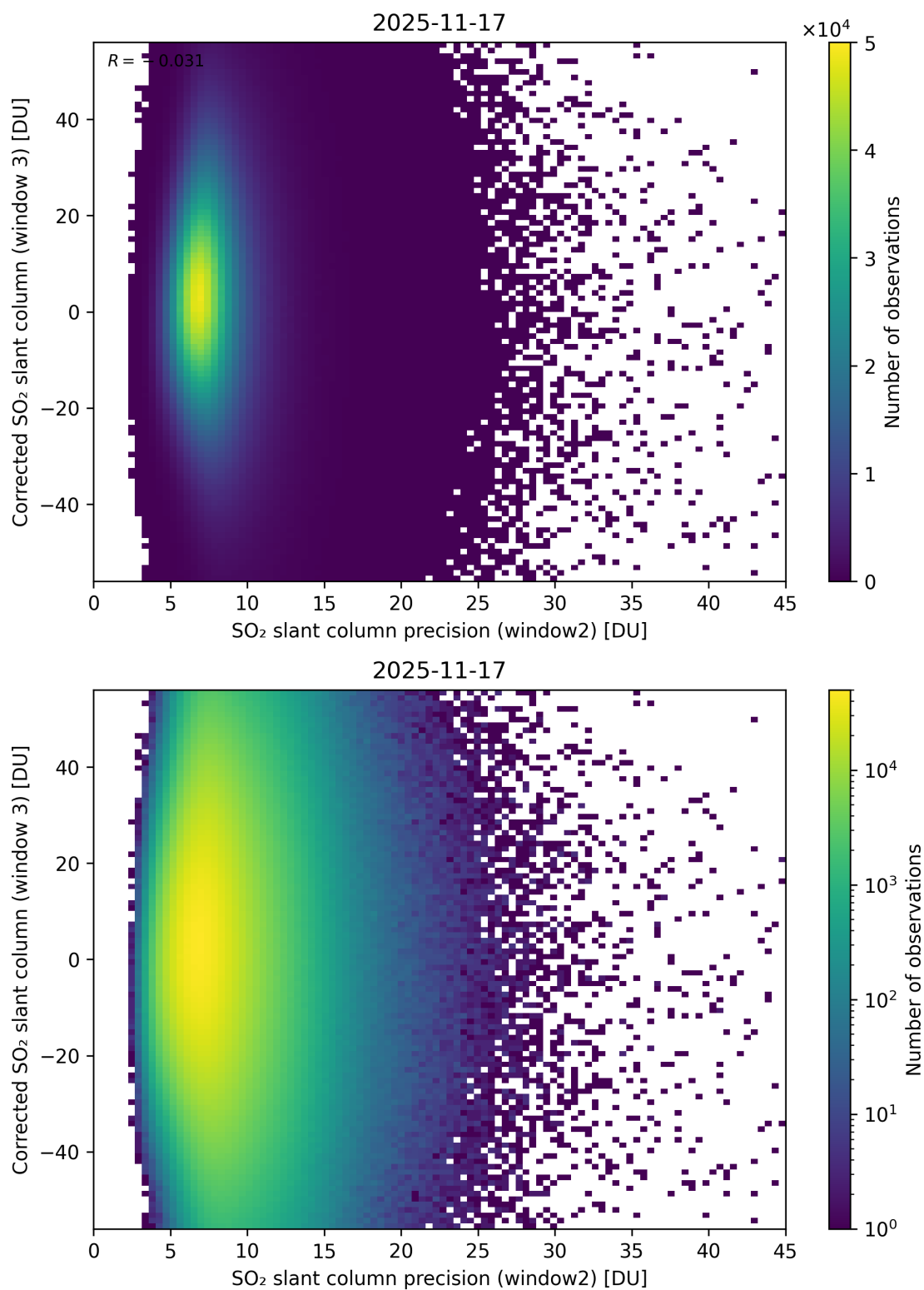
Figure 298: Scatter density plot of “SO 2 slant column precision (window2)” against “Corrected SO 2 slant column (window 3)” for 2025-11-16 to 2025-11-18.
