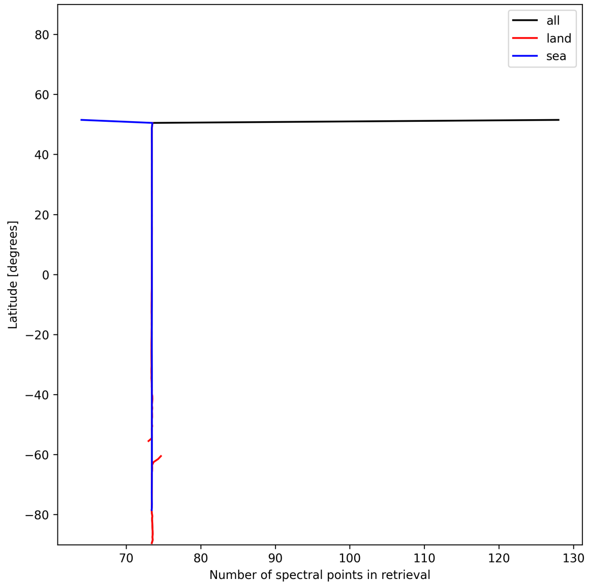
Figure 56: Zonal average of “Number of spectral points in retrieval” for 2025-11-16 to 2025-11-18.
