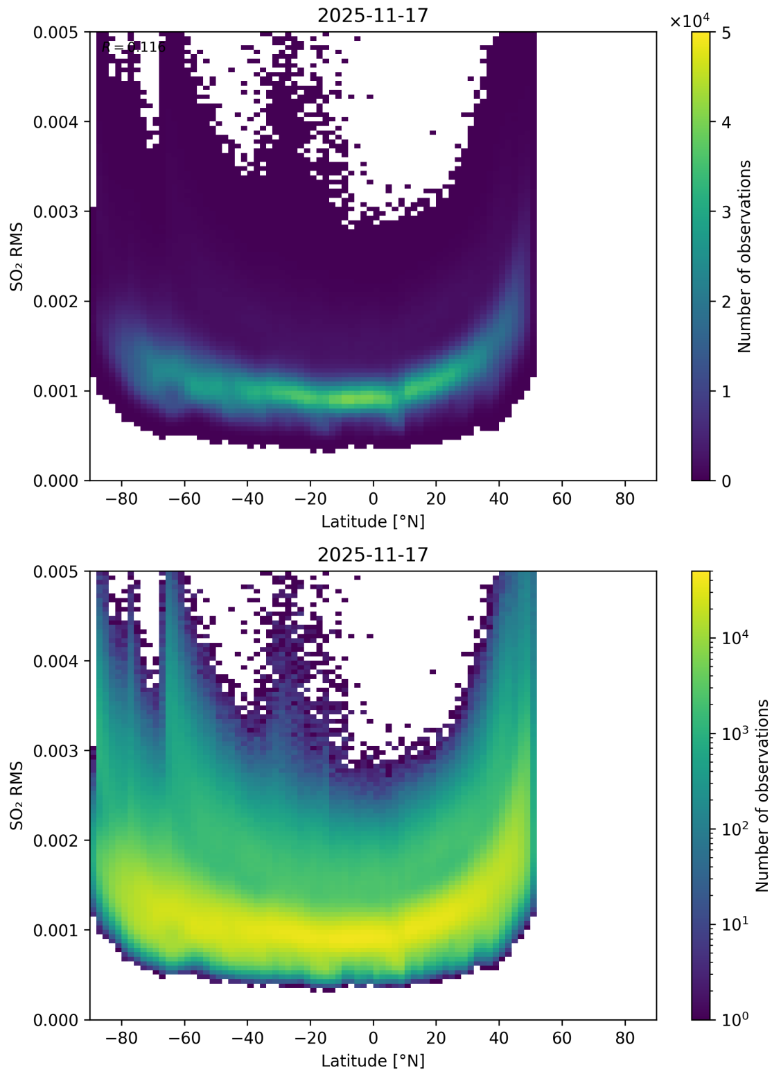
Figure 155: Scatter density plot of “Latitude” against “SO 2 RMS” for 2025-11-16 to 2025-11-18.
