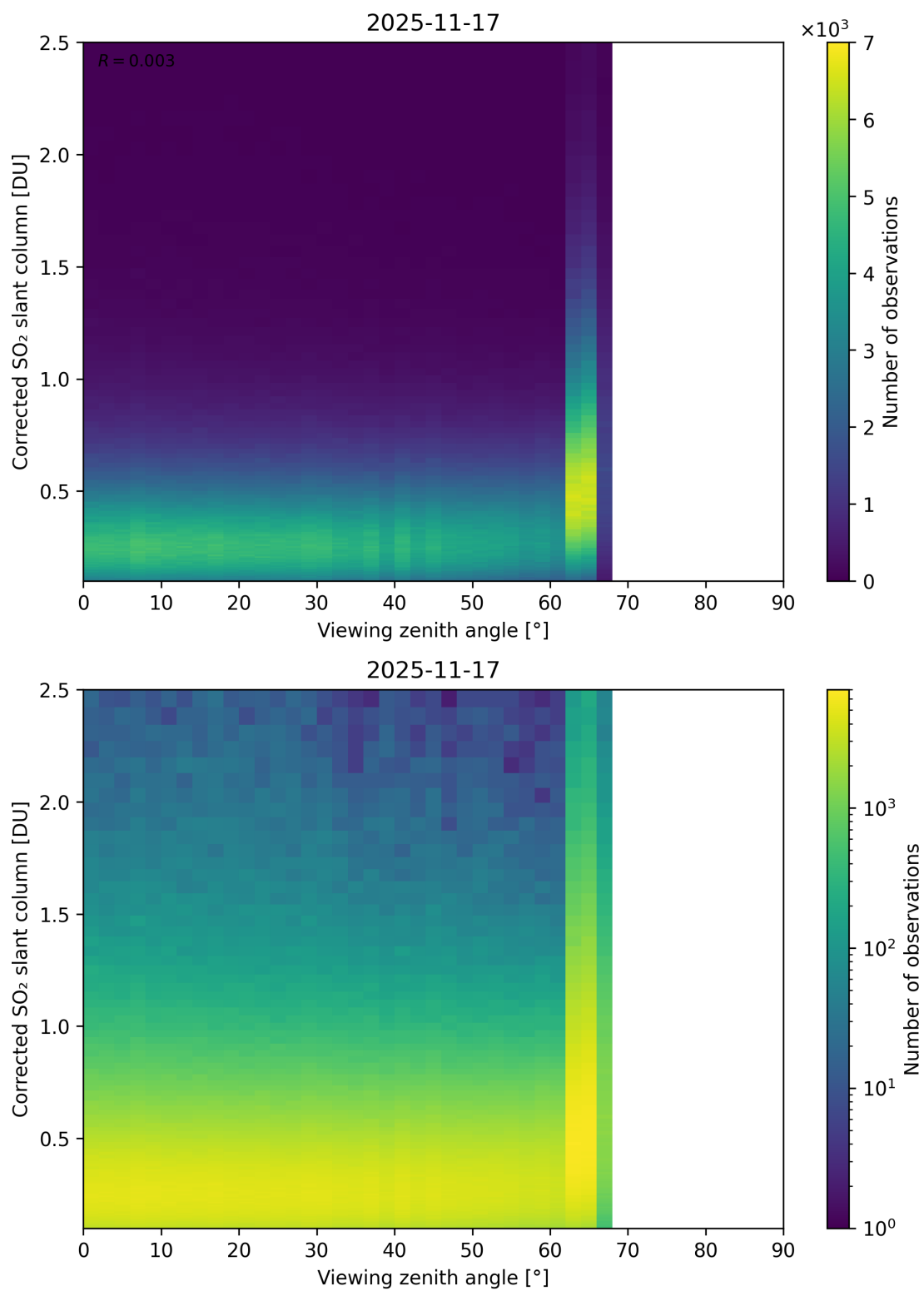
Figure 373: Scatter density plot of “Viewing zenith angle” against “Corrected SO 2 slant column” for 2025-11-16 to 2025-11-18.
