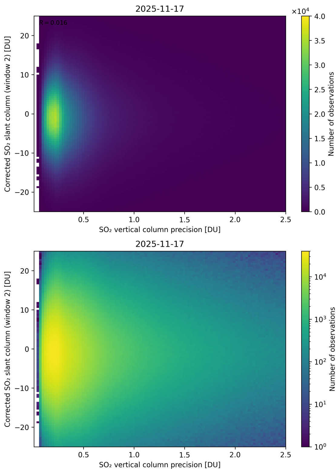
Figure 339: Scatter density plot of “SO 2 vertical column precision” against “Corrected SO 2 slant column (window 2)” for 2025-11-16 to 2025-11-18.
