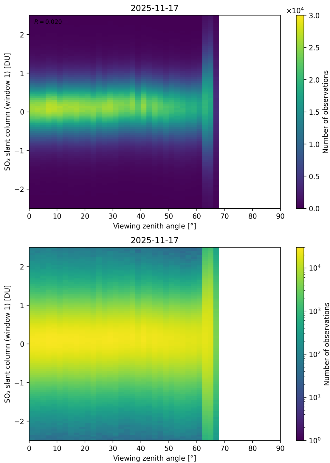
Figure 376: Scatter density plot of “Viewing zenith angle” against “SO 2 slant column (window 1)” for 2025-11-16 to 2025-11-18.
