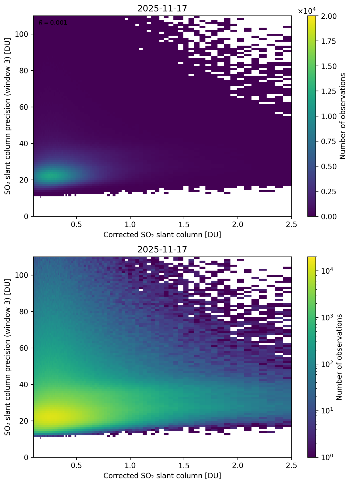
Figure 241: Scatter density plot of “Corrected SO 2 slant column” against “SO 2 slant column precision (window 3)” for 2025-11-16 to 2025-11-18.
