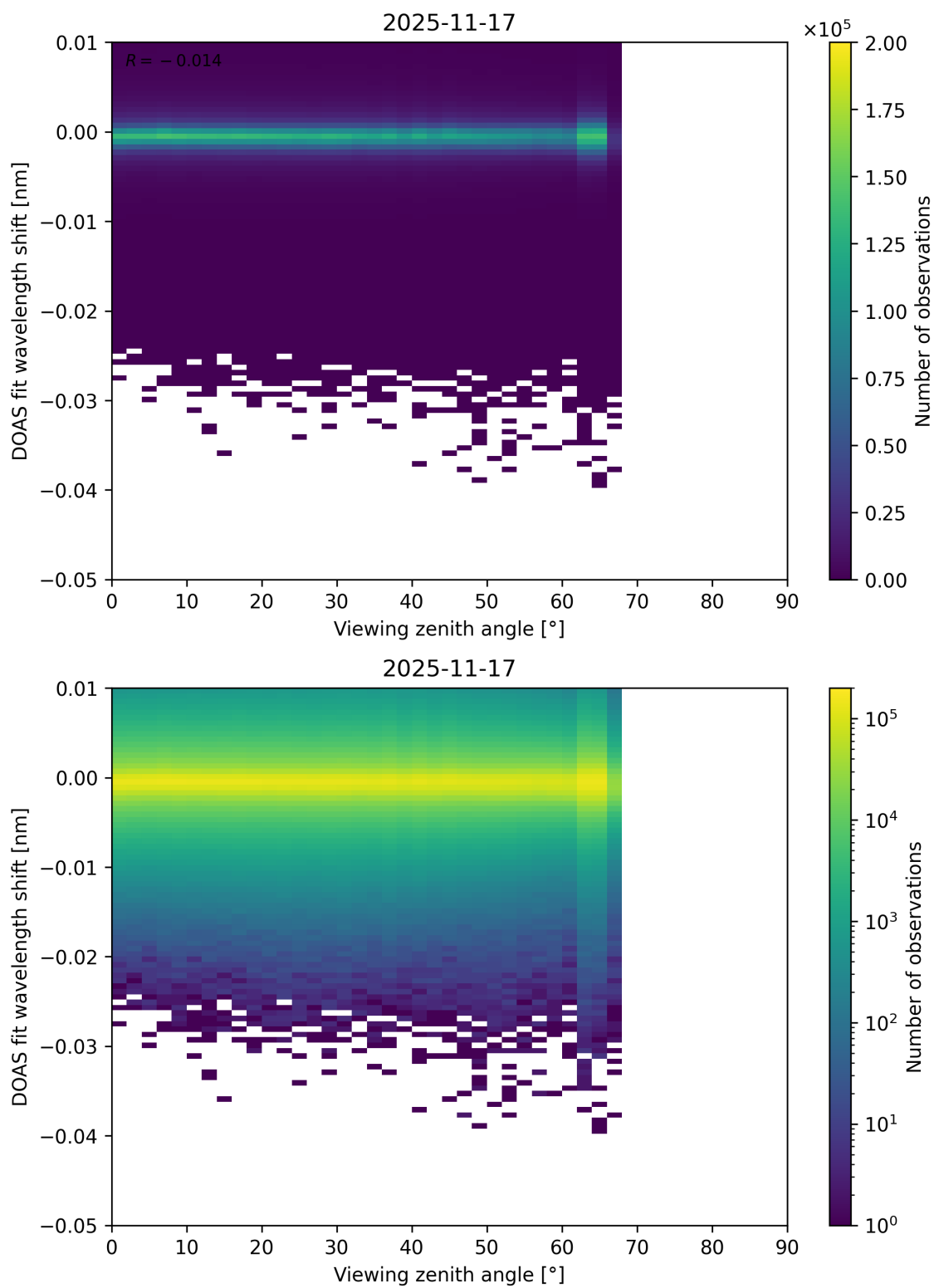
Figure 365: Scatter density plot of “Viewing zenith angle” against “DOAS fit wavelength shift” for 2025-11-16 to 2025-11-18.
