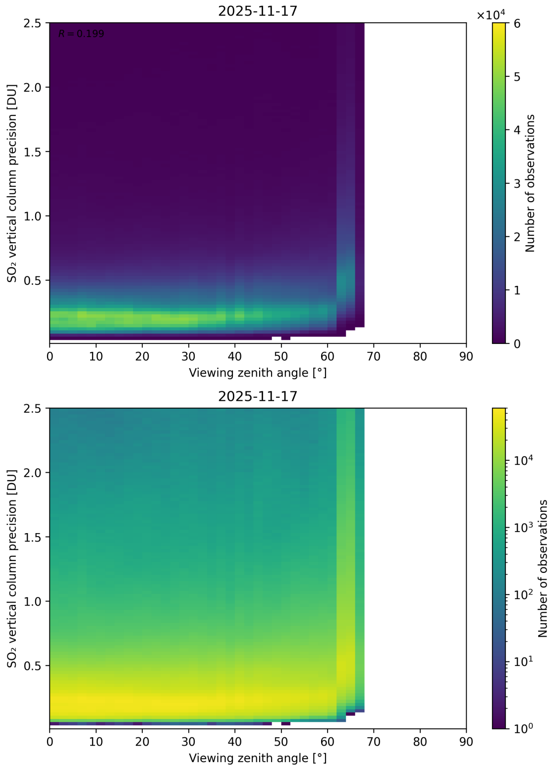
Figure 384: Scatter density plot of “Viewing zenith angle” against “SO 2 vertical column precision” for 2025-11-16 to 2025-11-18.
