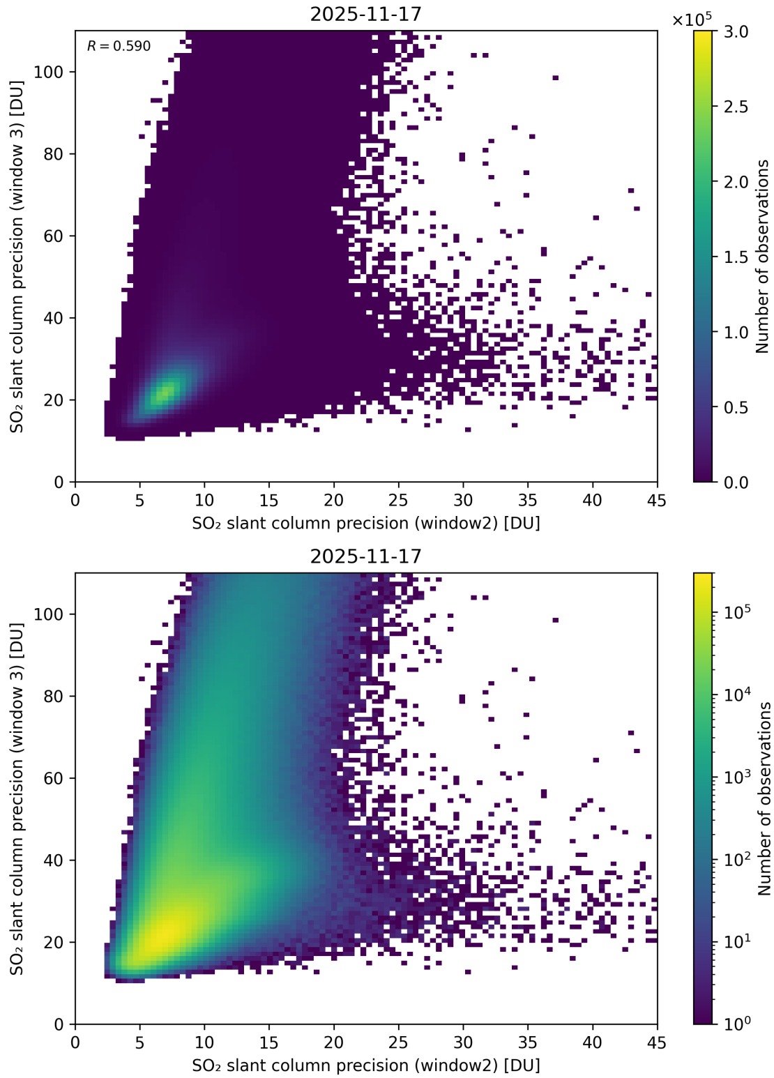
Figure 300: Scatter density plot of “SO 2 slant column precision (window2)” against “SO 2 slant column precision (window 3)” for 2025-11-16 to 2025-11-18.
