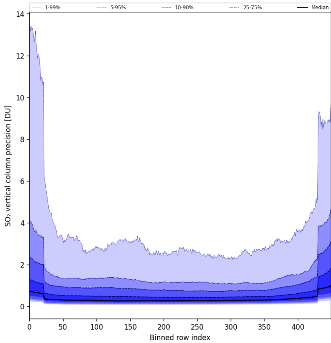
Figure 85: Along track statistics of “SO 2 vertical column precision” for 2025-11-16 to 2025-11-18
