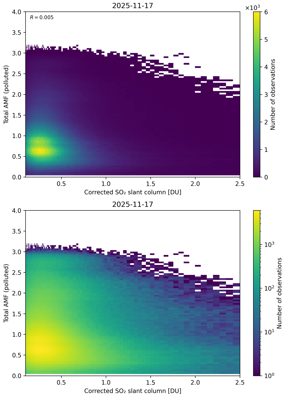
Figure 242: Scatter density plot of “Corrected SO 2 slant column” against “Total AMF (polluted)” for 2025-11-16 to 2025-11-18.
