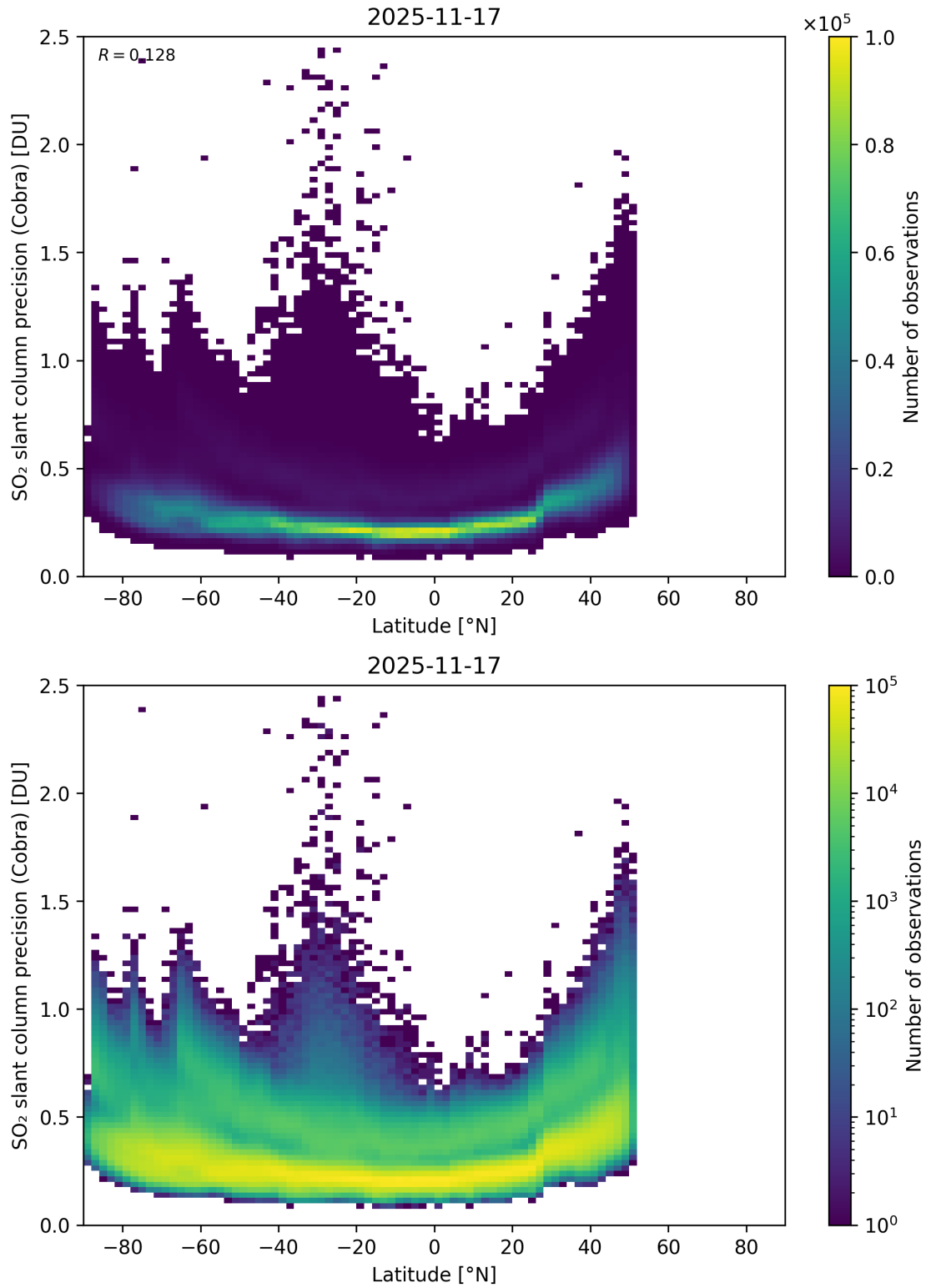
Figure 158: Scatter density plot of “Latitude” against “SO 2 slant column precision (Cobra)” for 2025-11-16 to 2025-11-18.
