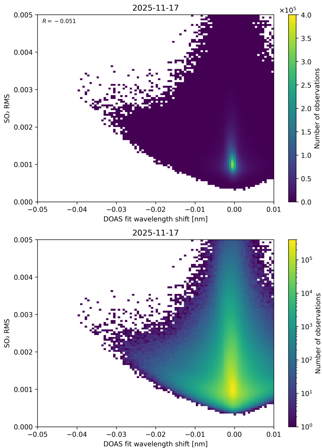
Figure 139: Scatter density plot of “DOAS fit wavelength shift” against “SO 2 RMS” for 2025-11-16 to 2025-11-18.
