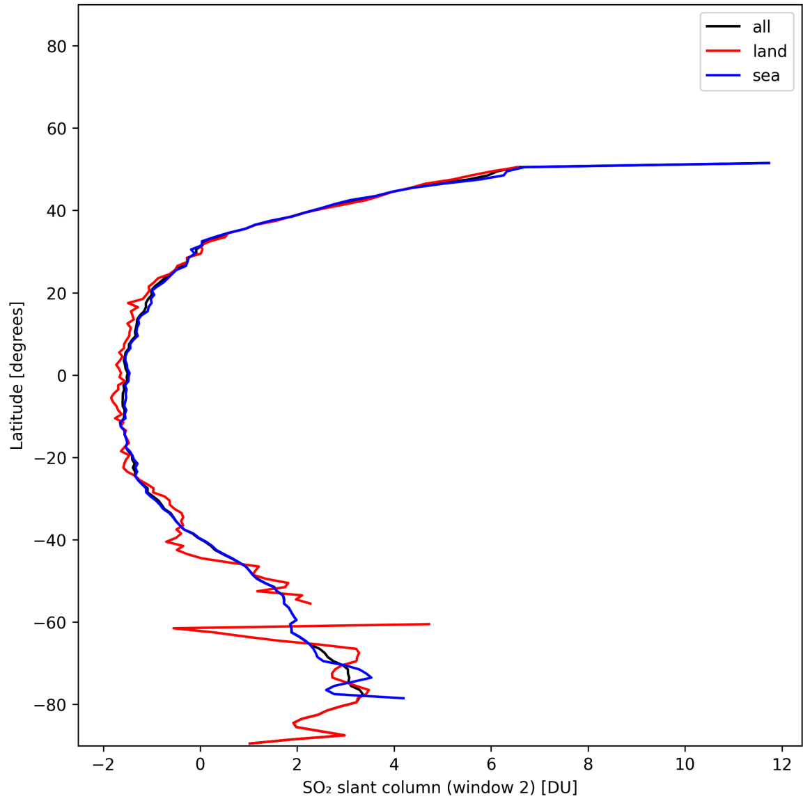
Figure 41: Zonal average of “SO 2 slant column (window 2)” for 2025-11-16 to 2025-11-18.
