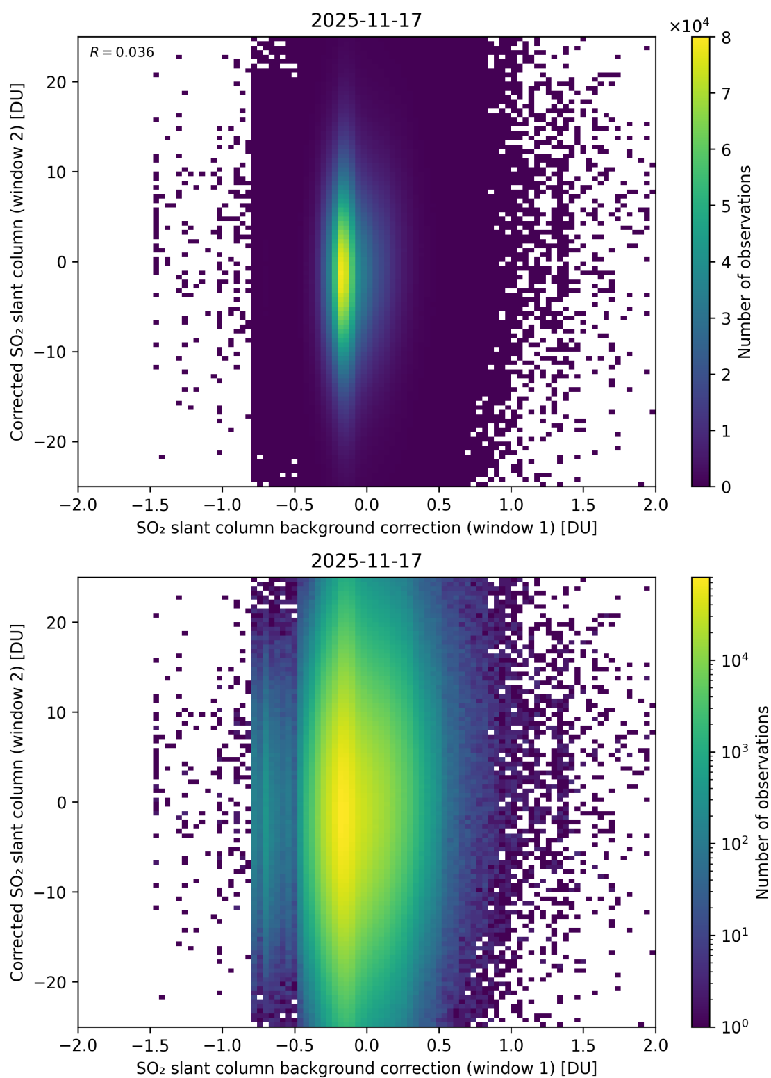
Figure 115: Scatter density plot of “SO 2 slant column background correction (window 1)” against “Corrected SO 2 slant column (window 2)” for 2025-11-16 to 2025-11-18.
