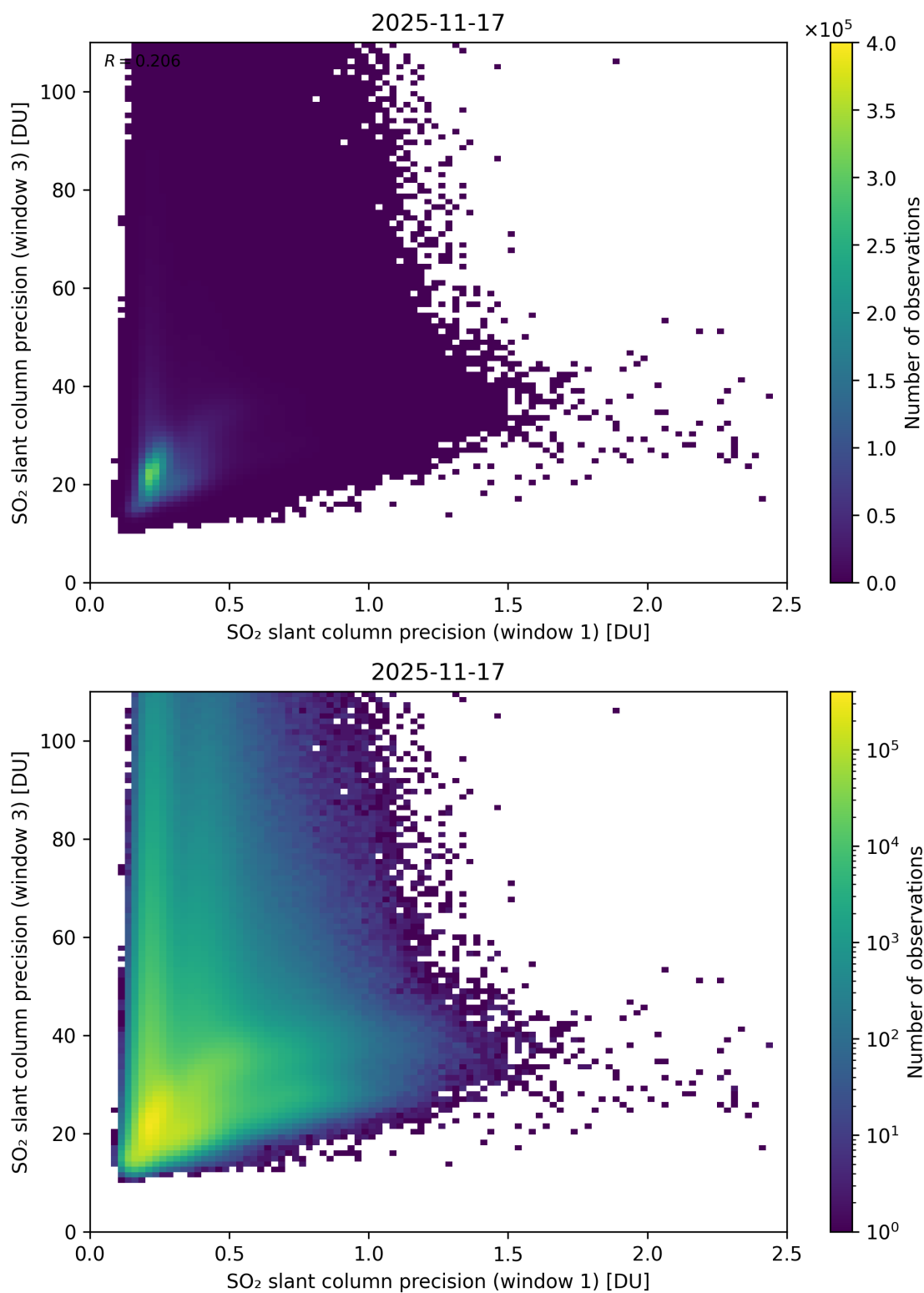
Figure 279: Scatter density plot of “SO 2 slant column precision (window 1)” against “SO 2 slant column precision (window 3)” for 2025-11-16 to 2025-11-18.
