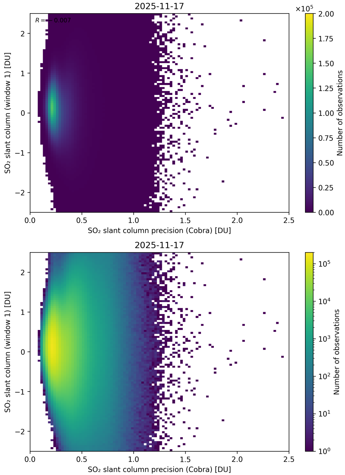
Figure 208: Scatter density plot of “SO 2 slant column precision (Cobra)” against “SO 2 slant column (window 1)” for 2025-11-16 to 2025-11-18.
