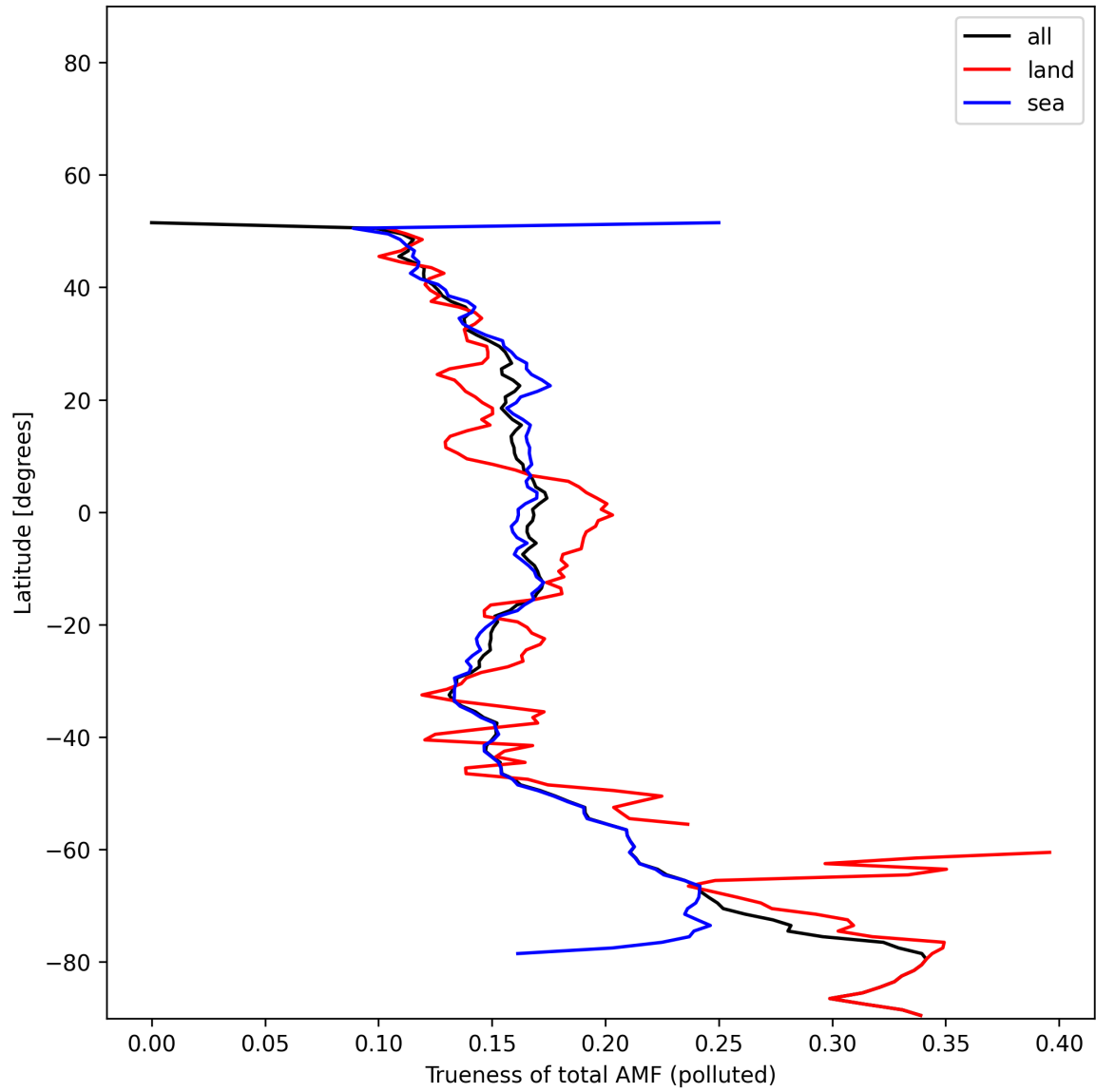
Figure 54: Zonal average of “Trueness of total AMF (polluted)” for 2025-11-16 to 2025-11-18.
