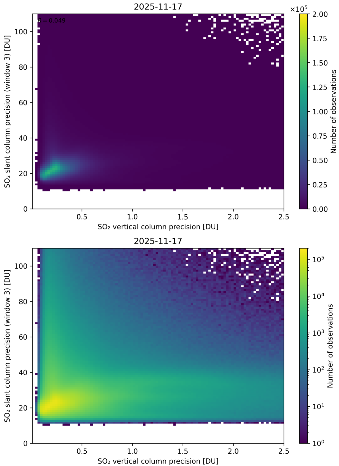
Figure 345: Scatter density plot of “SO 2 vertical column precision” against “SO 2 slant column precision (window 3)” for 2025-11-16 to 2025-11-18.
