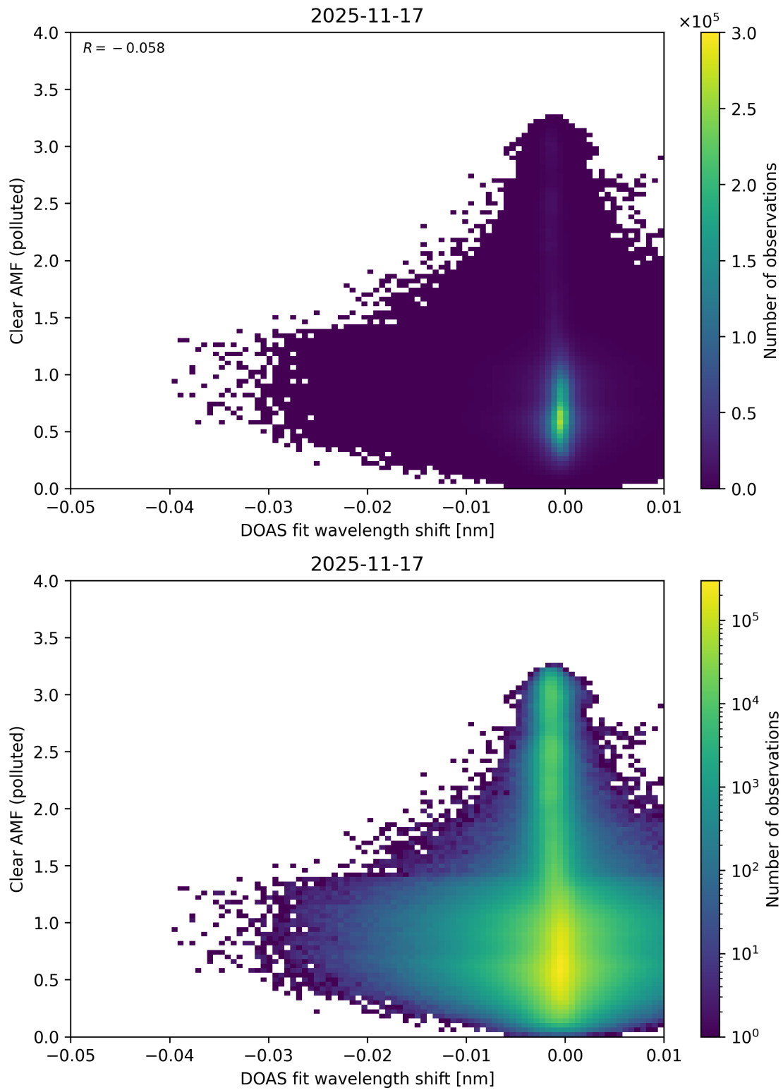
Figure 140: Scatter density plot of “DOAS fit wavelength shift” against “Clear AMF (polluted)” for 2025-11-16 to 2025-11-18.
