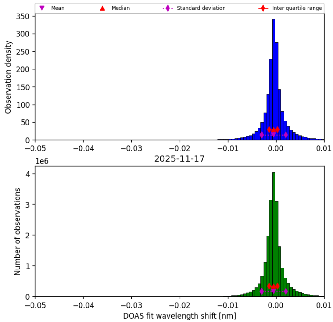
Figure 76: Histogram of “DOAS fit wavelength shift” for 2025-11-16 to 2025-11-18
