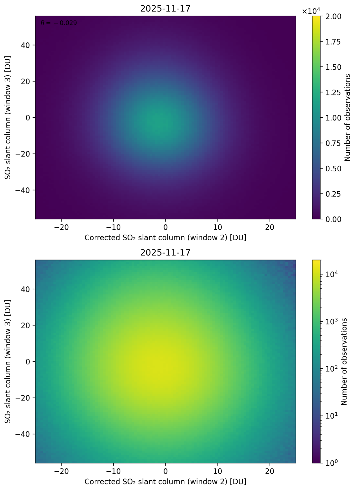
Figure 251: Scatter density plot of “Corrected SO 2 slant column (window 2)” against “SO 2 slant column (window 3)” for 2025-11-16 to 2025-11-18.
