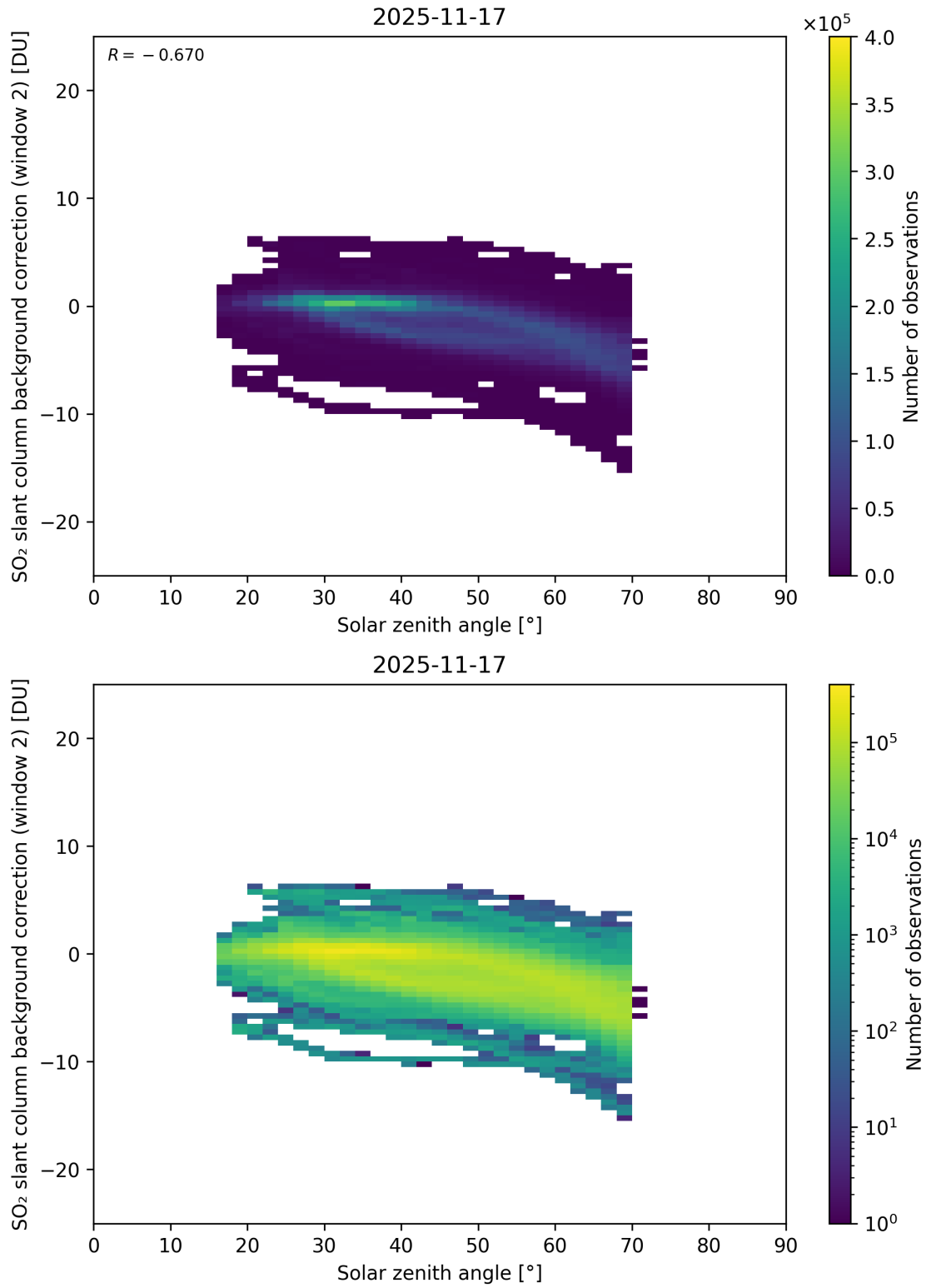
Figure 172: Scatter density plot of “Solar zenith angle” against “SO 2 slant column background correction (window 2)” for 2025-11-16 to 2025-11-18.
