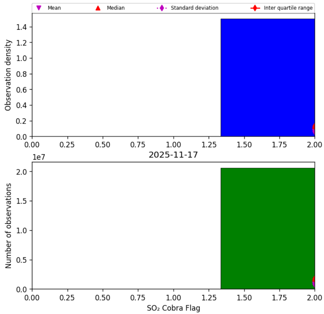
Figure 75: Histogram of “SO 2 Cobra Flag” for 2025-11-16 to 2025-11-18
