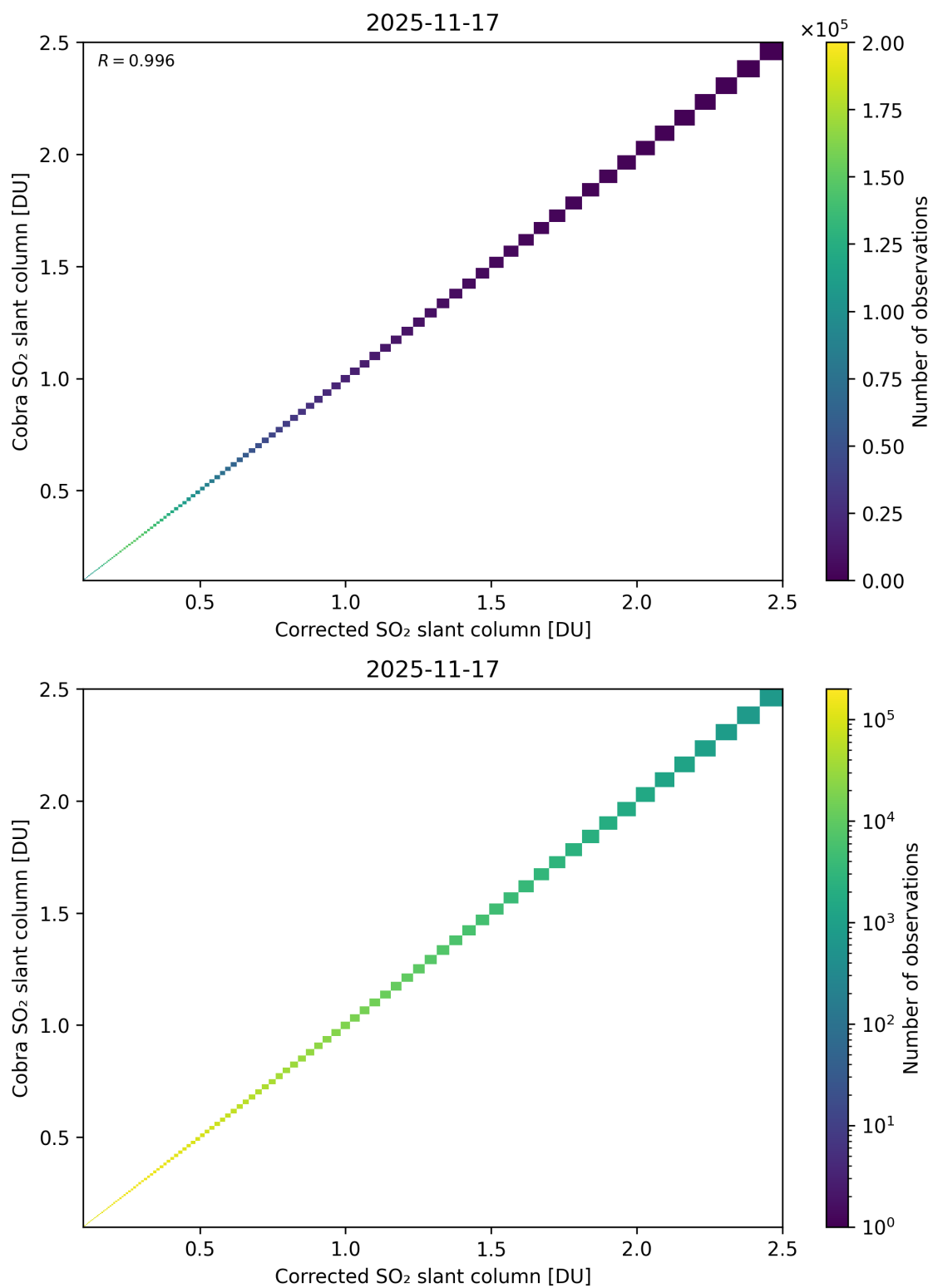
Figure 233: Scatter density plot of “Corrected SO 2 slant column” against “Cobra SO 2 slant column” for 2025-11-16 to 2025-11-18.
