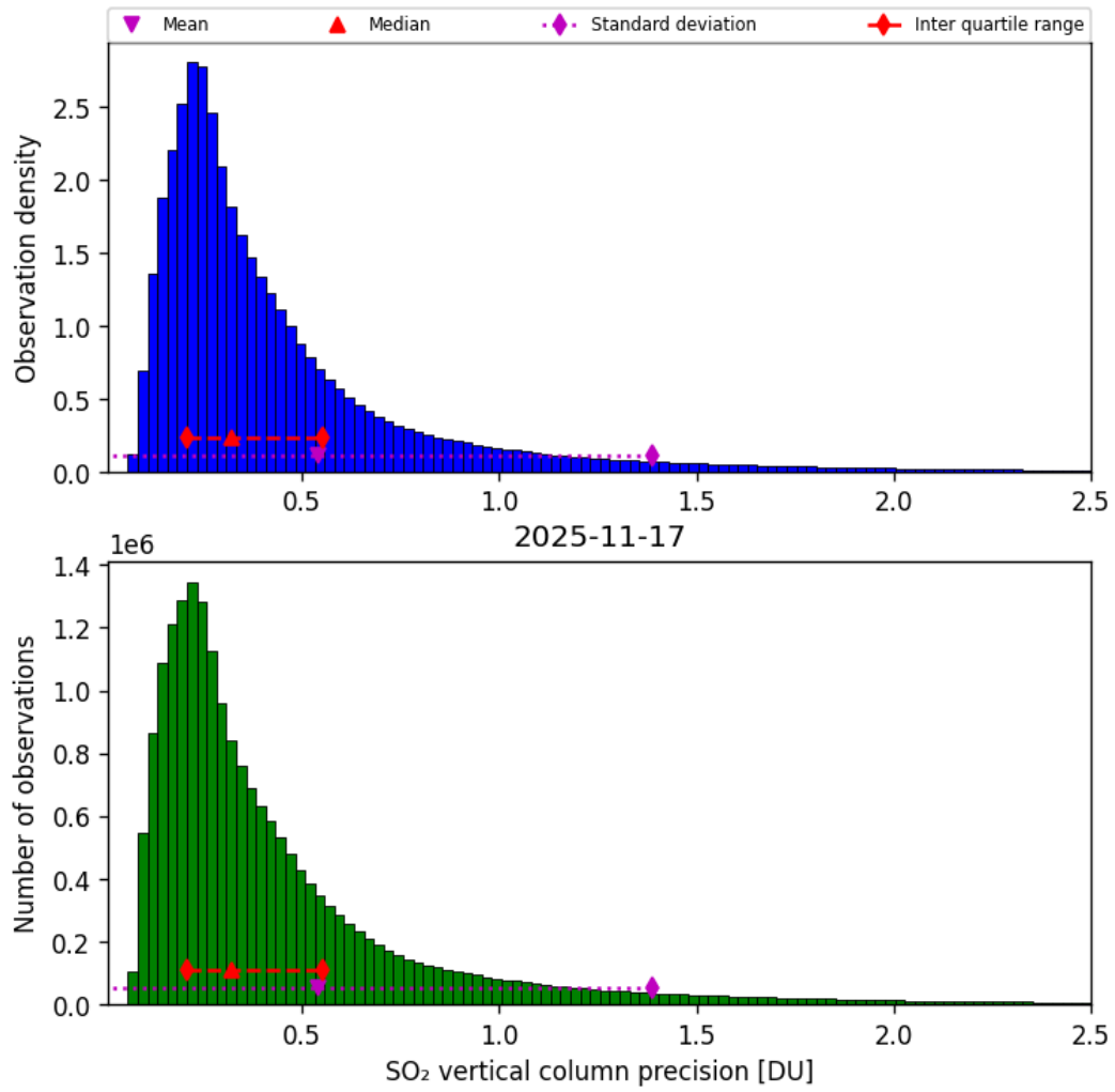
Figure 59: Histogram of “SO 2 vertical column precision” for 2025-11-16 to 2025-11-18
