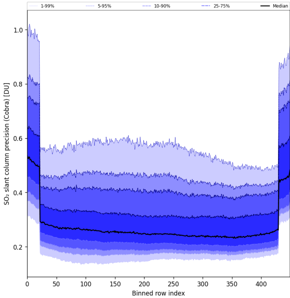
Figure 88: Along track statistics of “SO 2 slant column precision (Cobra)” for 2025-11-16 to 2025-11-18
