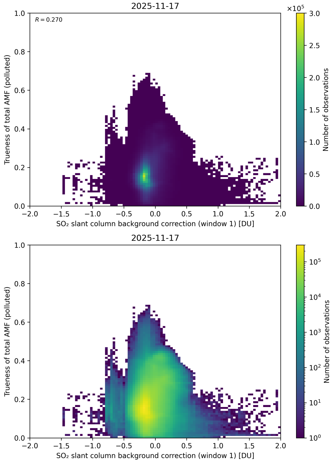
Figure 121: Scatter density plot of “SO 2 slant column background correction (window 1)” against “Trueness of total AMF (polluted)” for 2025-11-16 to 2025-11-18.
