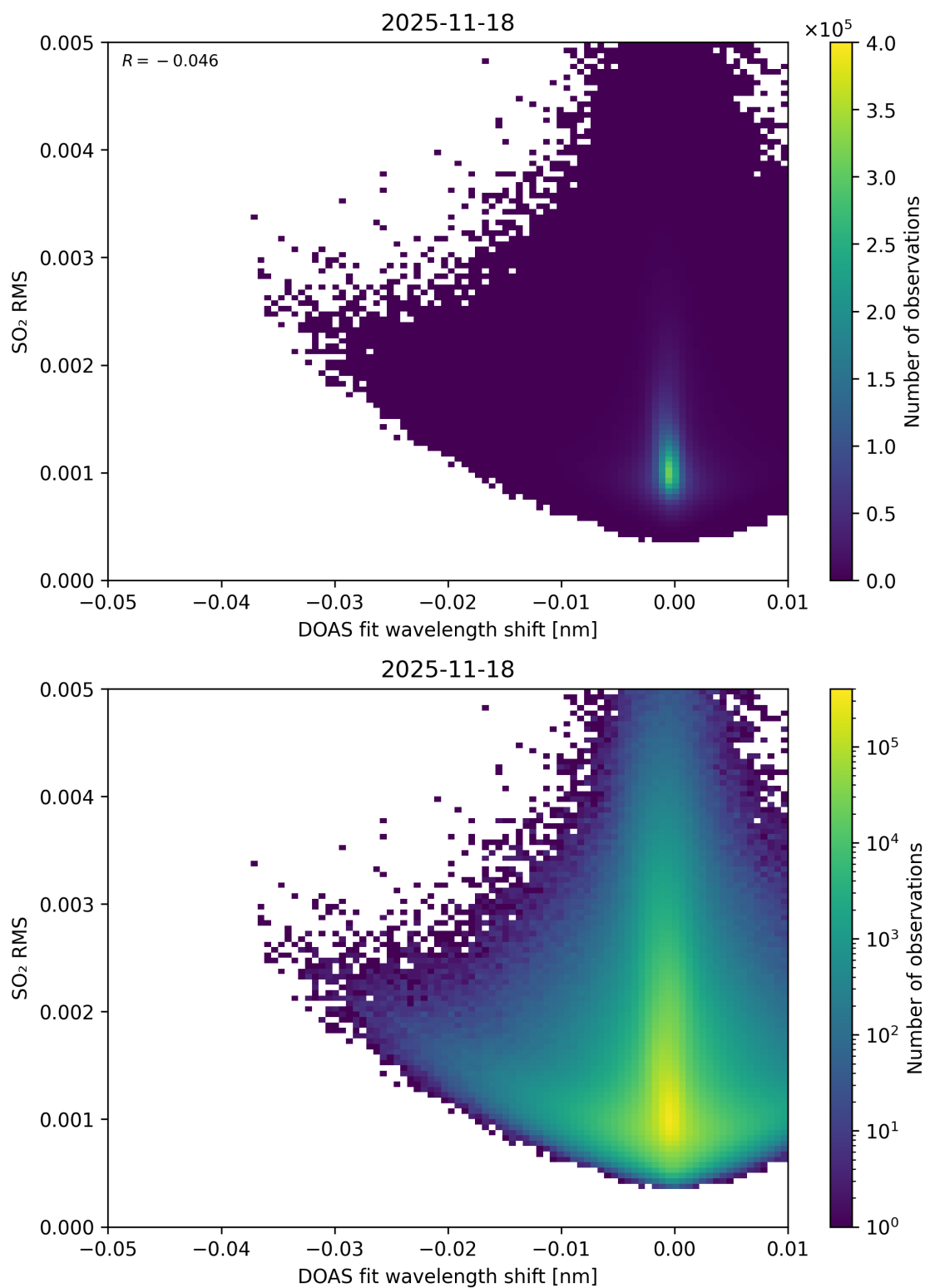
Figure 139: Scatter density plot of “DOAS fit wavelength shift” against “SO 2 RMS” for 2025-11-18 to 2025-11-19.
