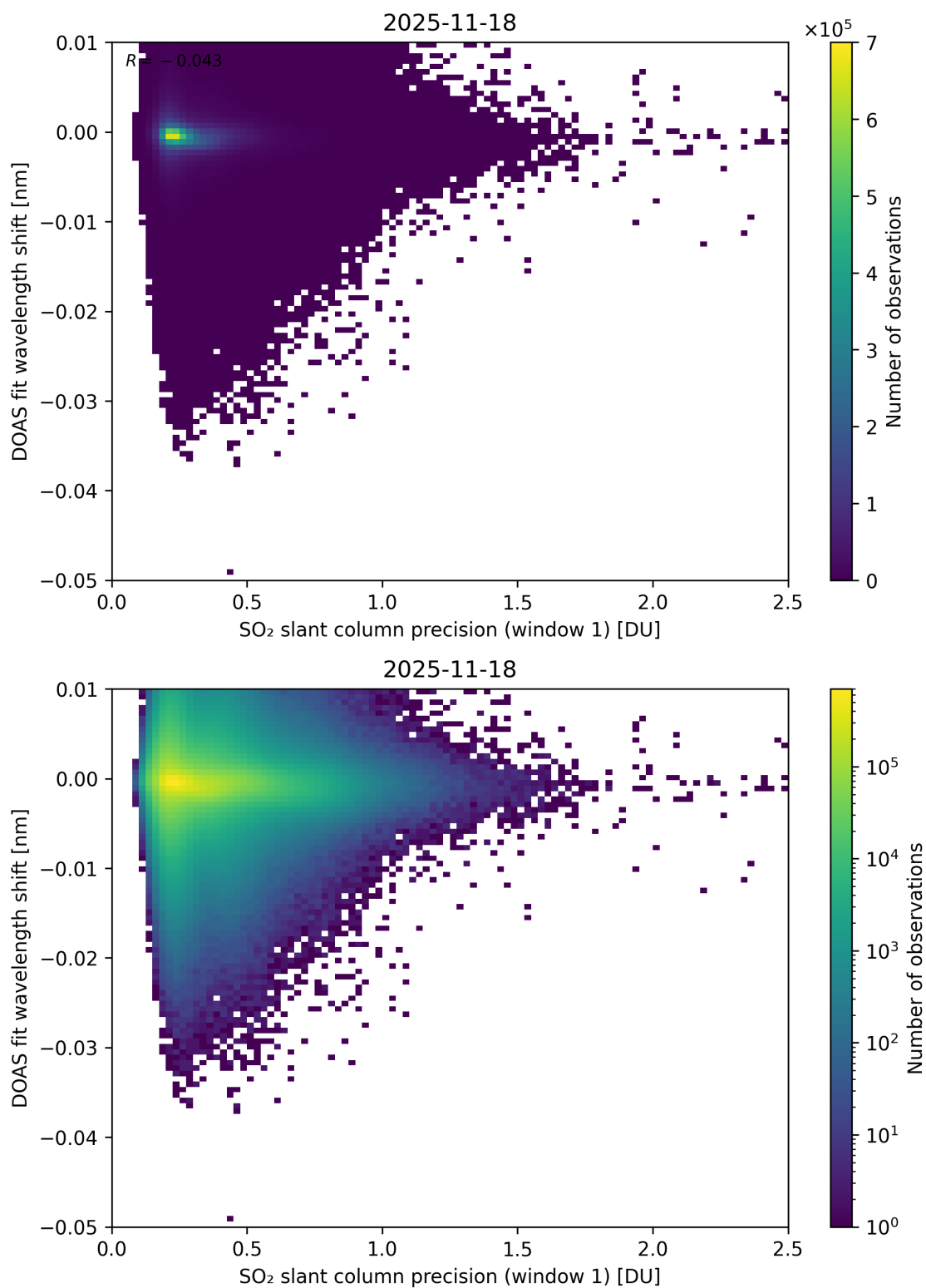
Figure 271: Scatter density plot of “SO 2 slant column precision (window 1)” against “DOAS fit wavelength shift” for 2025-11-18 to 2025-11-19.
