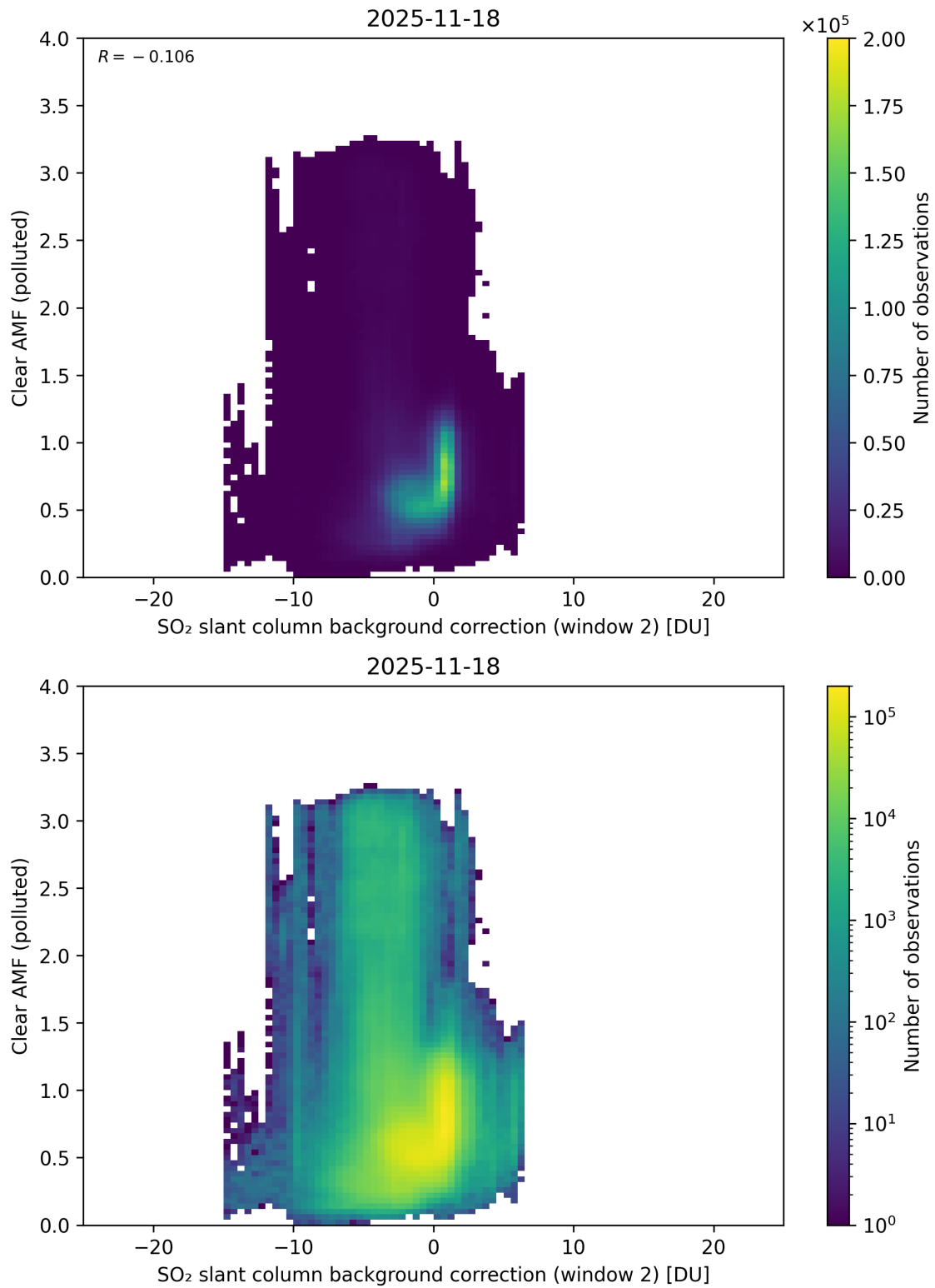
Figure 126: Scatter density plot of “SO 2 slant column background correction (window 2)” against “Clear AMF (polluted)” for 2025-11-18 to 2025-11-19.
