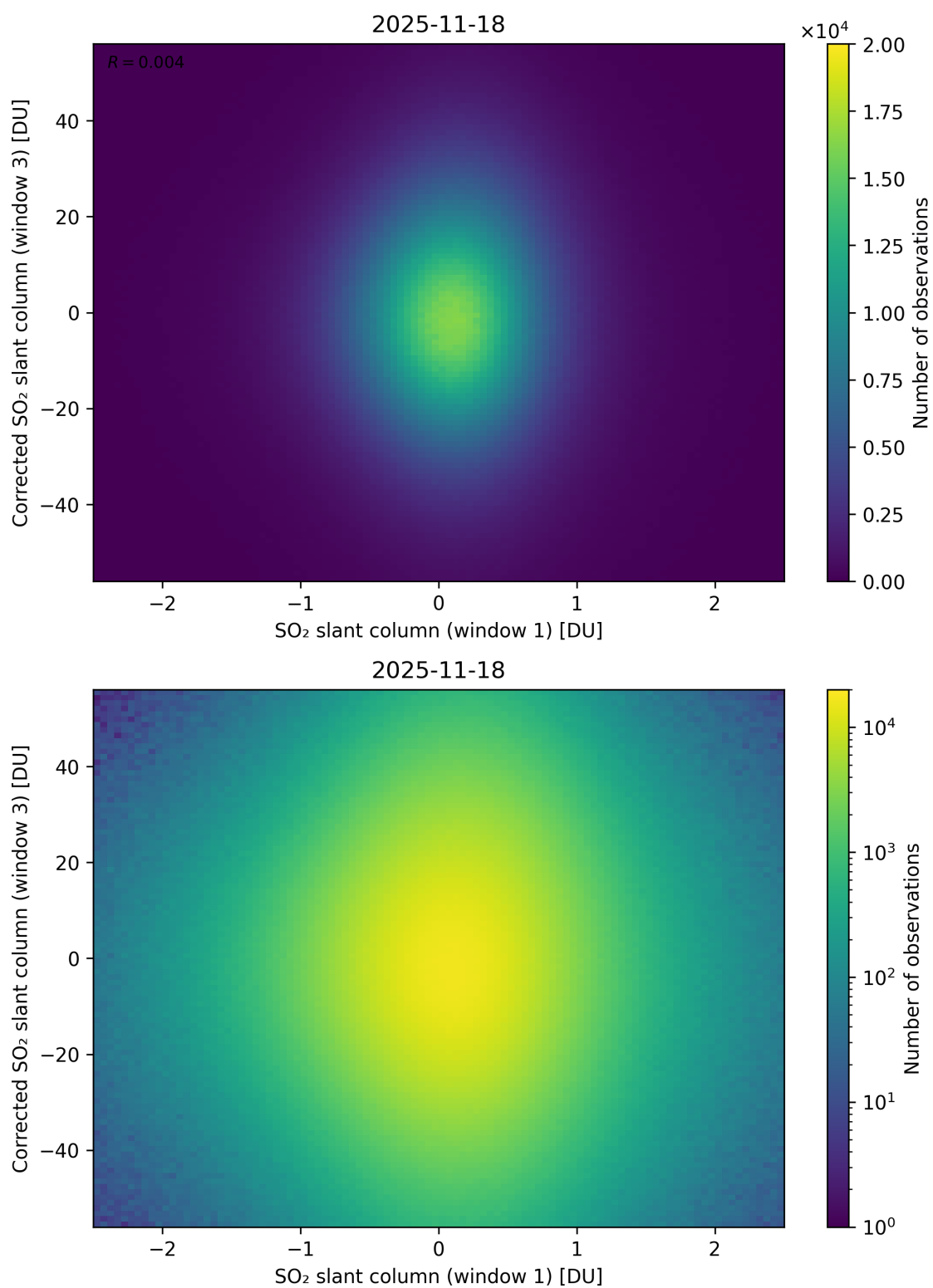
Figure 284: Scatter density plot of “SO 2 slant column (window 1)” against “Corrected SO 2 slant column (window 3)” for 2025-11-18 to 2025-11-19.
