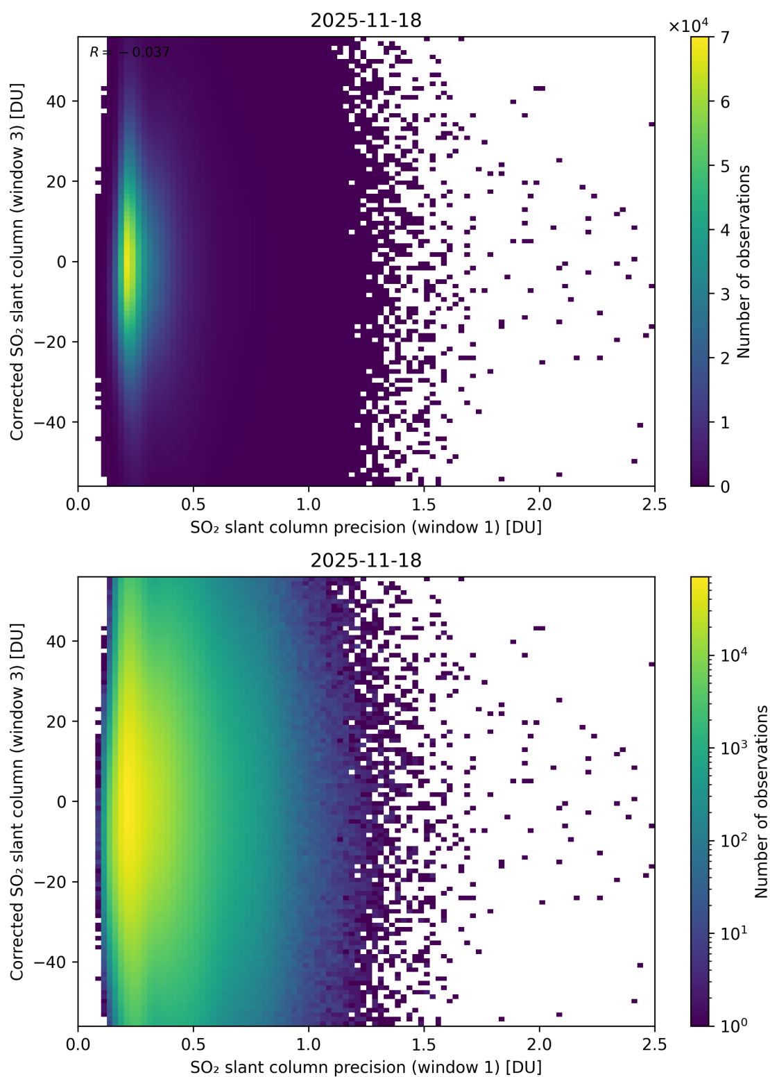
Figure 276: Scatter density plot of “SO 2 slant column precision (window 1)” against “Corrected SO 2 slant column (window 3)” for 2025-11-18 to 2025-11-19.
