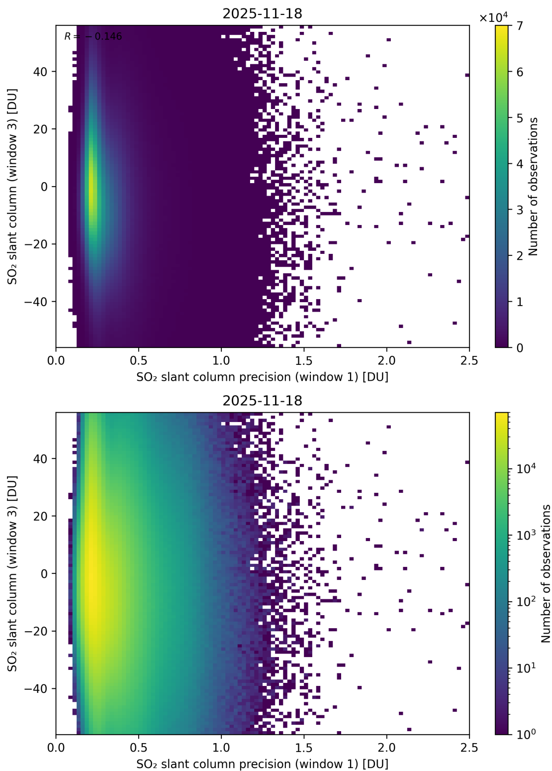
Figure 278: Scatter density plot of “SO 2 slant column precision (window 1)” against “SO 2 slant column (window 3)” for 2025-11-18 to 2025-11-19.
