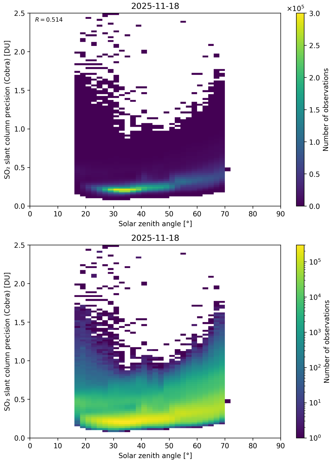
Figure 180: Scatter density plot of “Solar zenith angle” against “SO 2 slant column precision (Cobra)” for 2025-11-18 to 2025-11-19.
