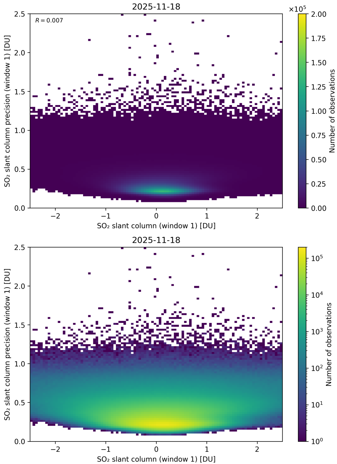
Figure 285: Scatter density plot of “SO 2 slant column (window 1)” against “SO 2 slant column precision (window 1)” for 2025-11-18 to 2025-11-19.
