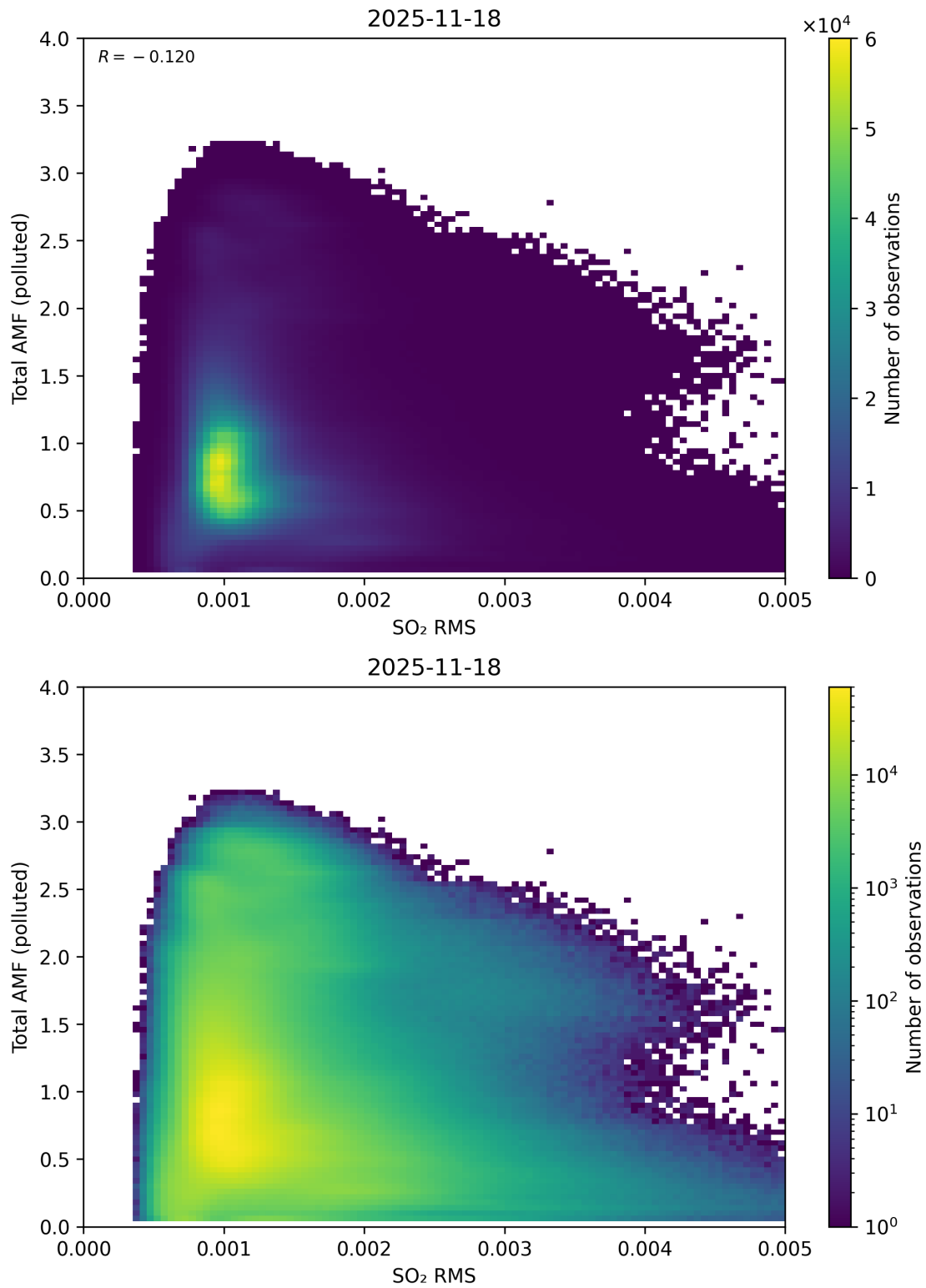
Figure 148: Scatter density plot of “SO 2 RMS” against “Total AMF (polluted)” for 2025-11-18 to 2025-11-19.
