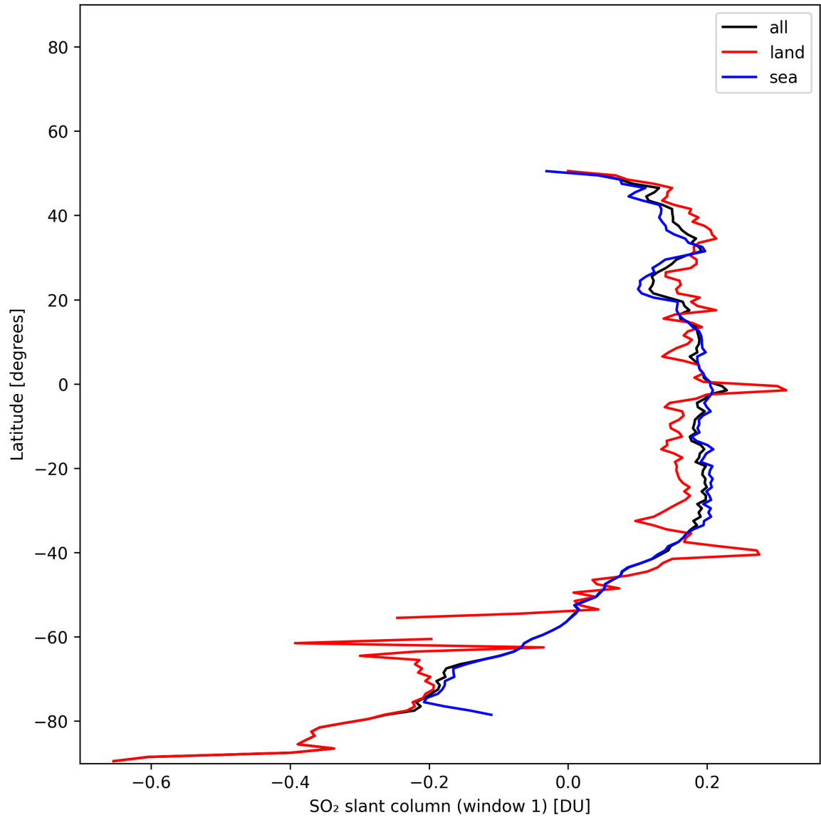
Figure 37: Zonal average of “SO 2 slant column (window 1)” for 2025-11-18 to 2025-11-19.
