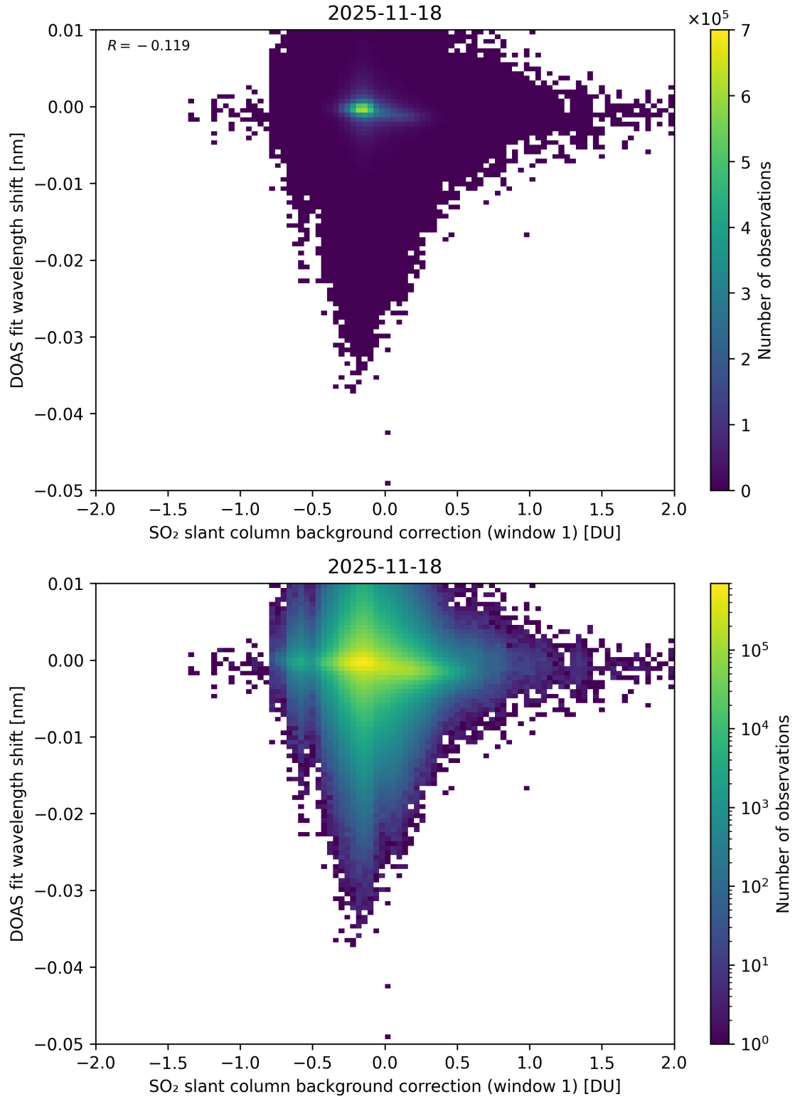
Figure 111: Scatter density plot of “SO 2 slant column background correction (window 1)” against “DOAS fit wavelength shift” for 2025-11-18 to 2025-11-19.
