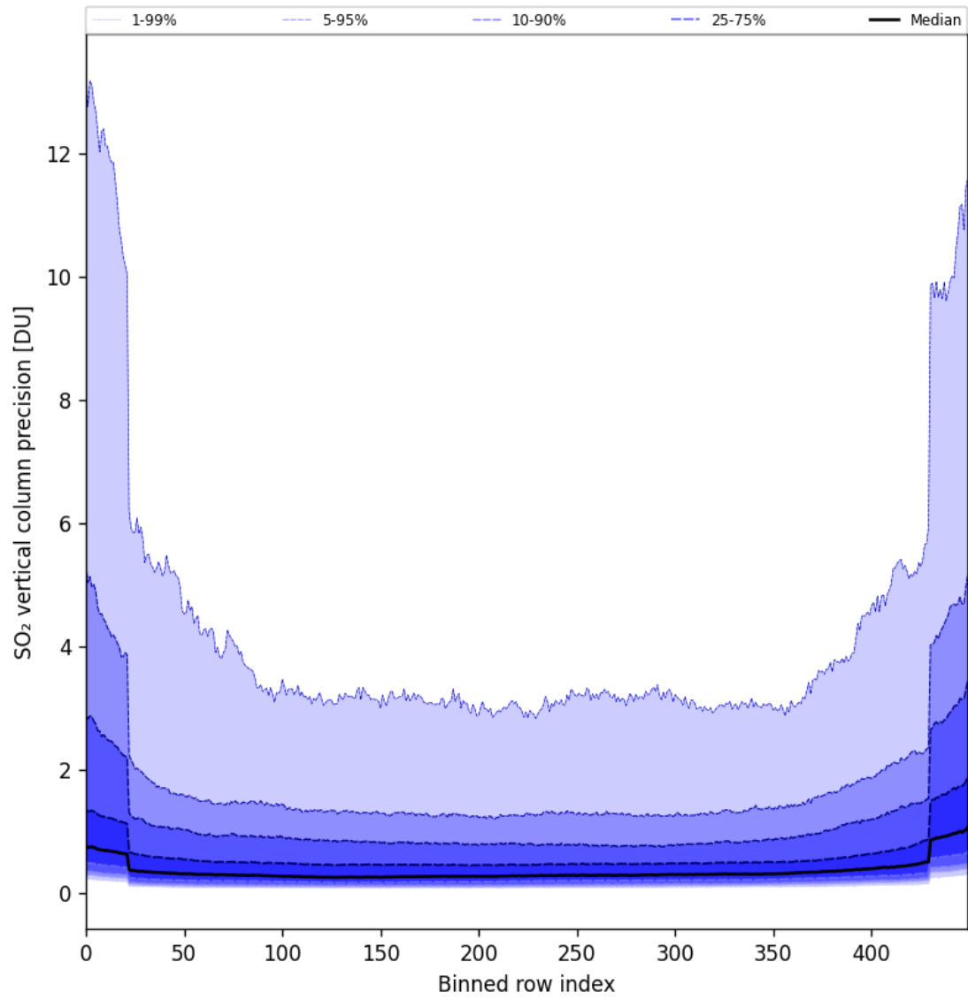
Figure 85: Along track statistics of “SO 2 vertical column precision” for 2025-11-18 to 2025-11-19
