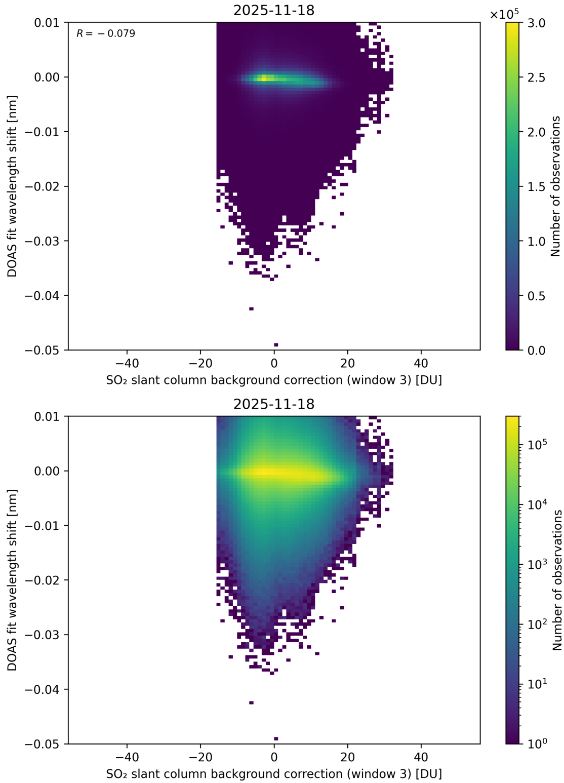
Figure 132: Scatter density plot of “SO 2 slant column background correction (window 3)” against “DOAS fit wavelength shift” for 2025-11-18 to 2025-11-19.
