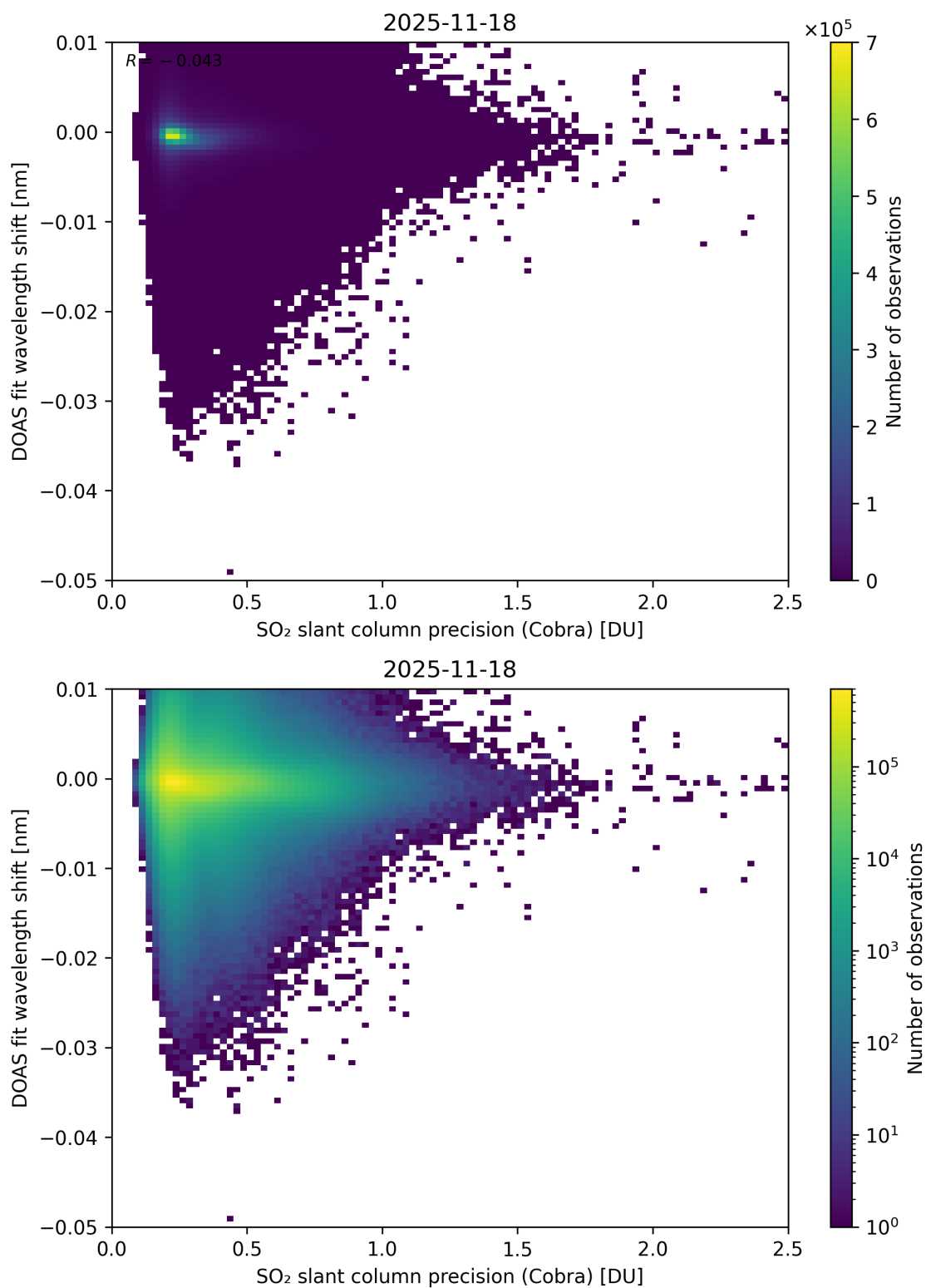
Figure 202: Scatter density plot of “SO 2 slant column precision (Cobra)” against “DOAS fit wavelength shift” for 2025-11-18 to 2025-11-19.
