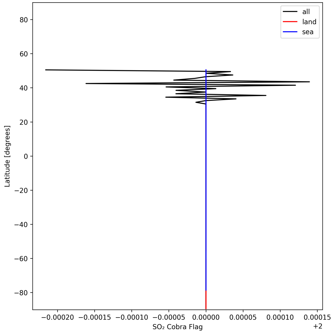
Figure 49: Zonal average of “SO 2 Cobra Flag” for 2025-11-18 to 2025-11-19.
