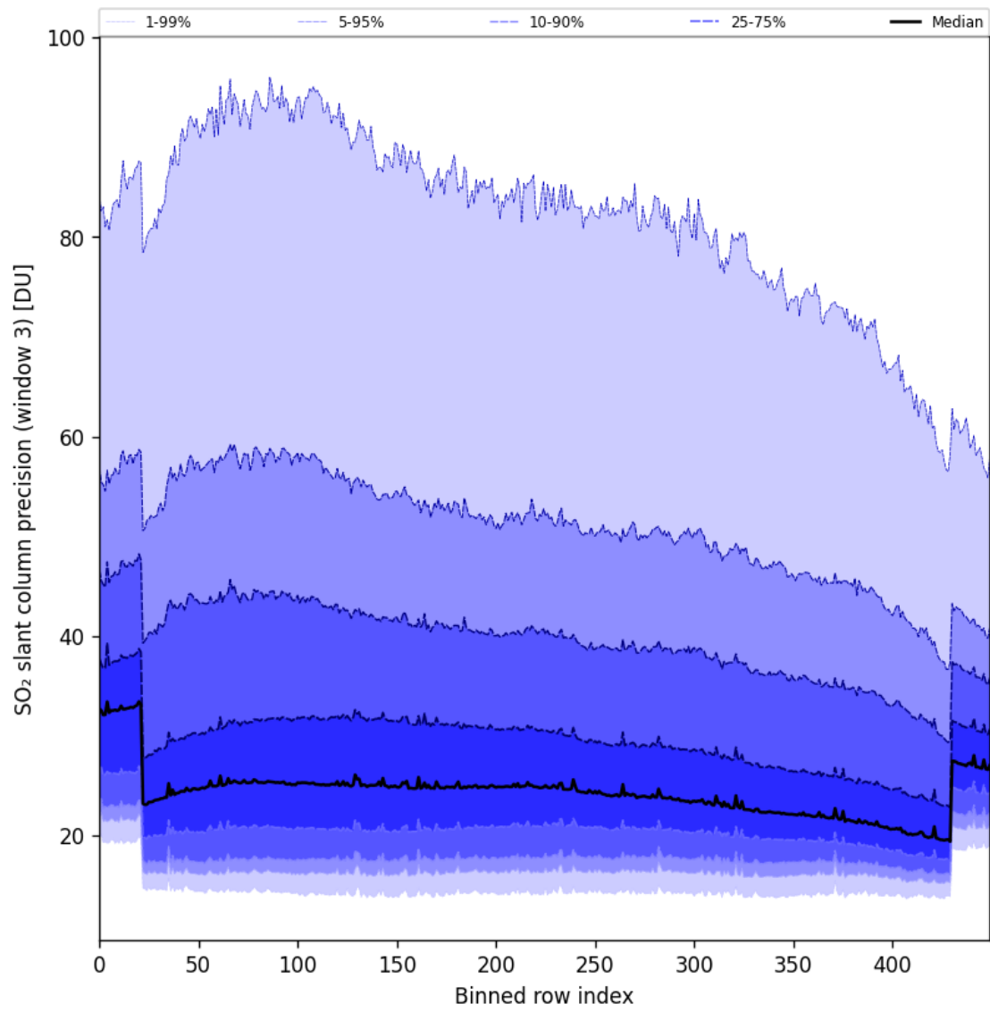
Figure 98: Along track statistics of “SO 2 slant column precision (window 3)” for 2025-11-18 to 2025-11-19
