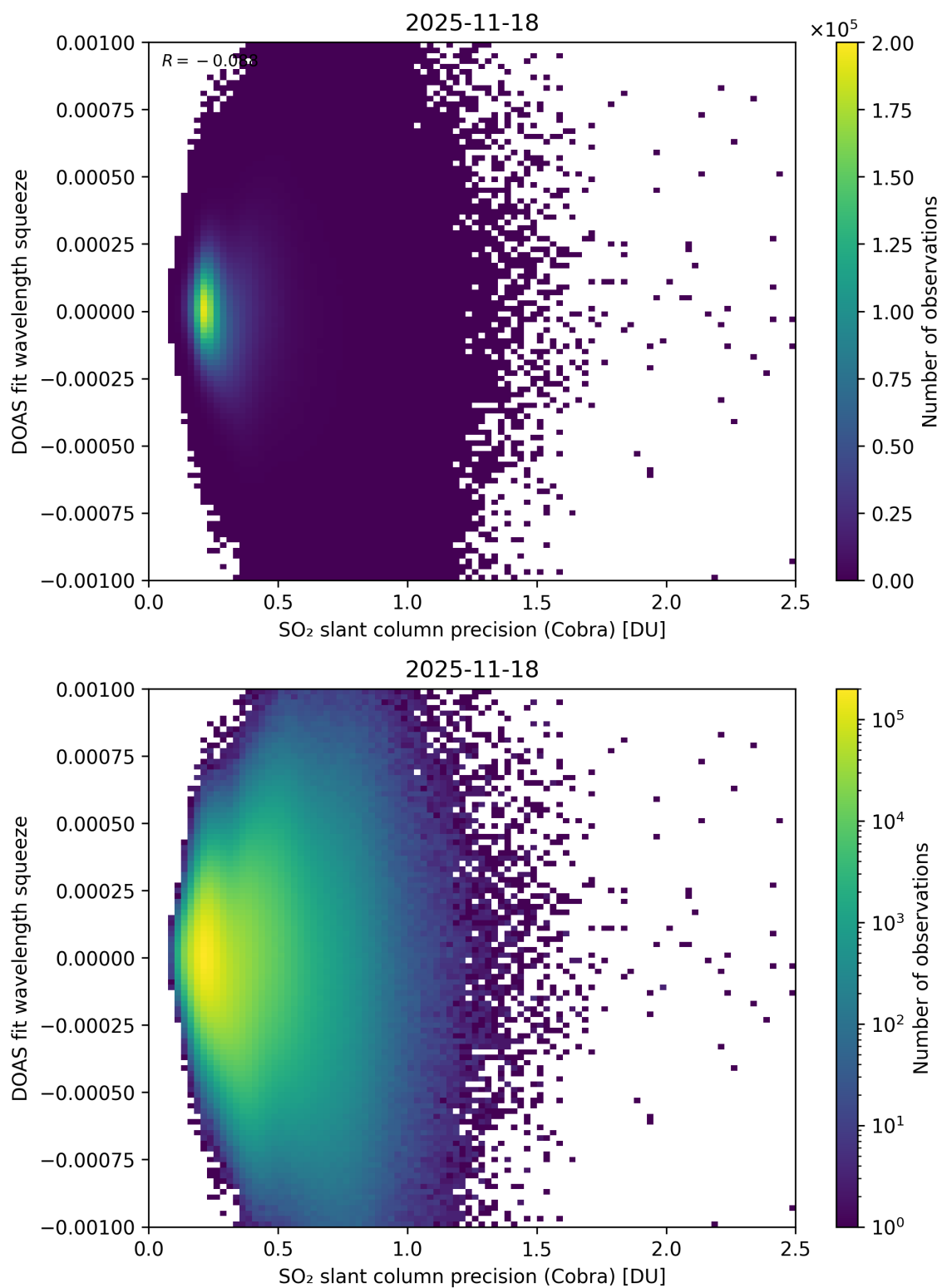
Figure 203: Scatter density plot of “SO 2 slant column precision (Cobra)” against “DOAS fit wavelength squeeze” for 2025-11-18 to 2025-11-19.
