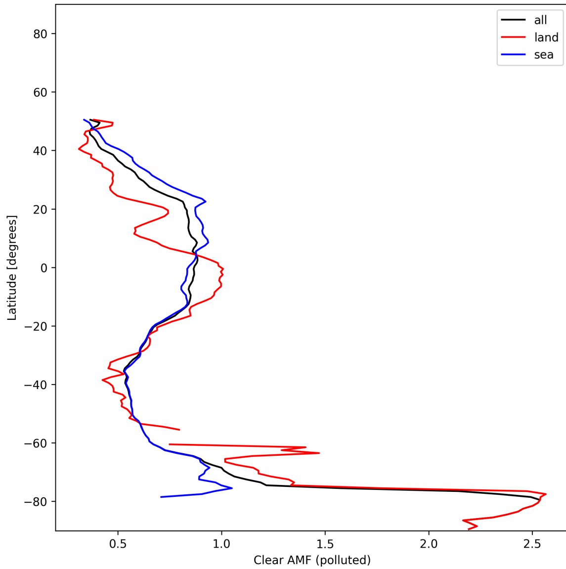
Figure 55: Zonal average of “Clear AMF (polluted)” for 2025-11-18 to 2025-11-19.
