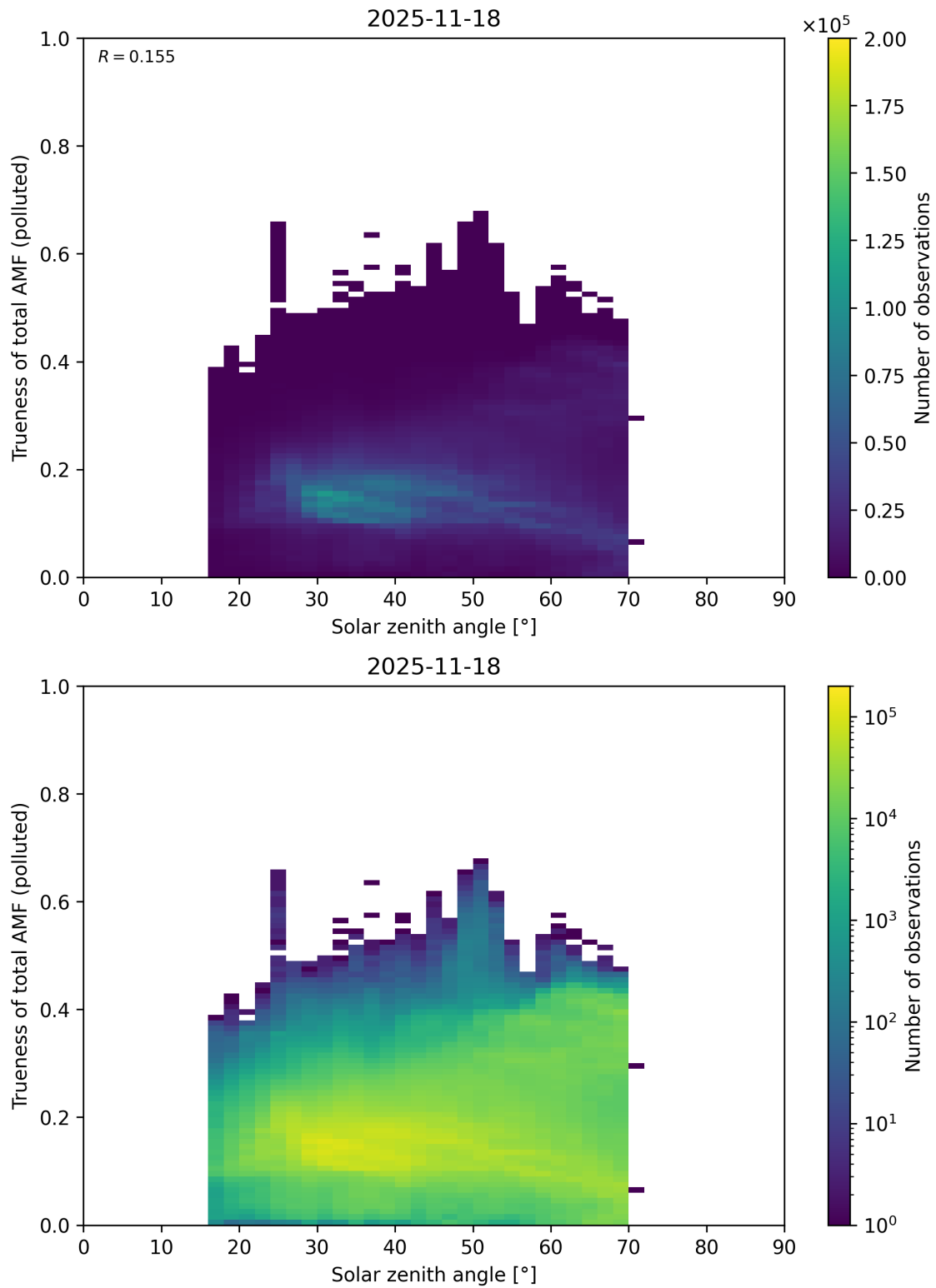
Figure 190: Scatter density plot of “Solar zenith angle” against “Trueness of total AMF (polluted)” for 2025-11-18 to 2025-11-19.
