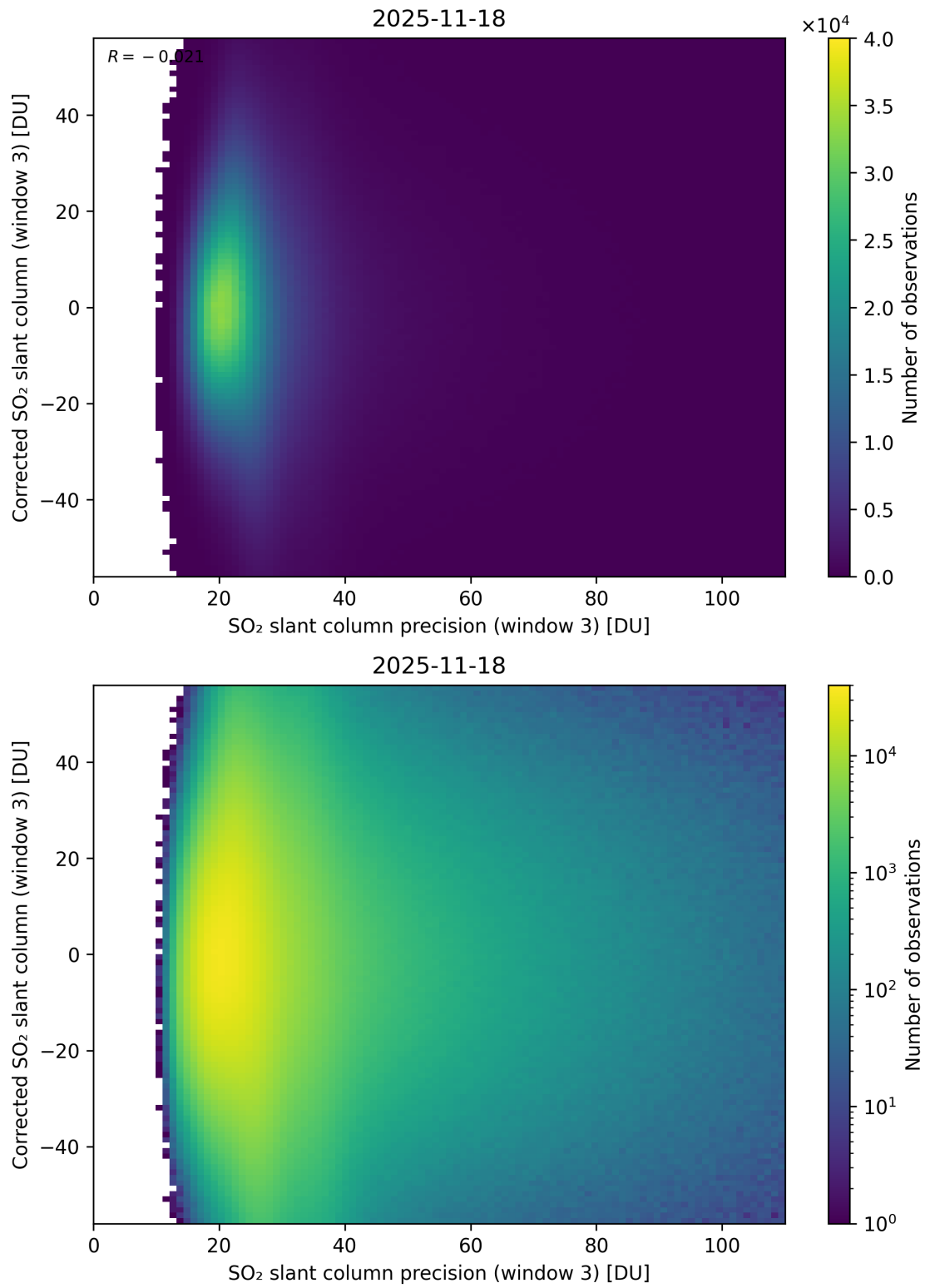
Figure 312: Scatter density plot of “SO 2 slant column precision (window 3)” against “Corrected SO 2 slant column (window 3)” for 2025-11-18 to 2025-11-19.
