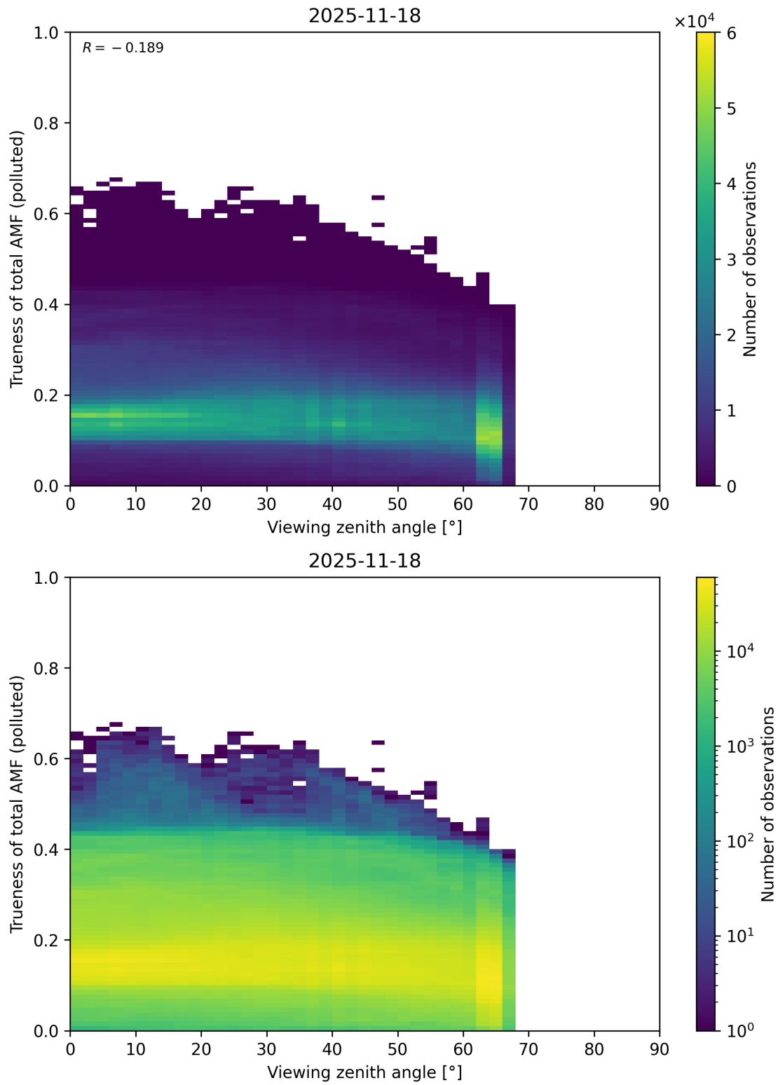
Figure 382: Scatter density plot of “Viewing zenith angle” against “Trueness of total AMF (polluted)” for 2025-11-18 to 2025-11-19.
