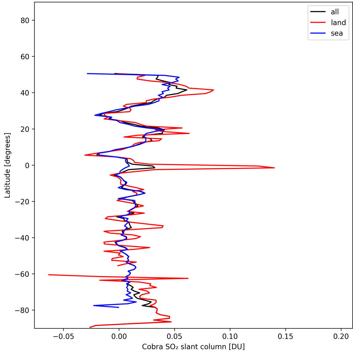
Figure 35: Zonal average of “Cobra SO 2 slant column” for 2025-11-18 to 2025-11-19.
