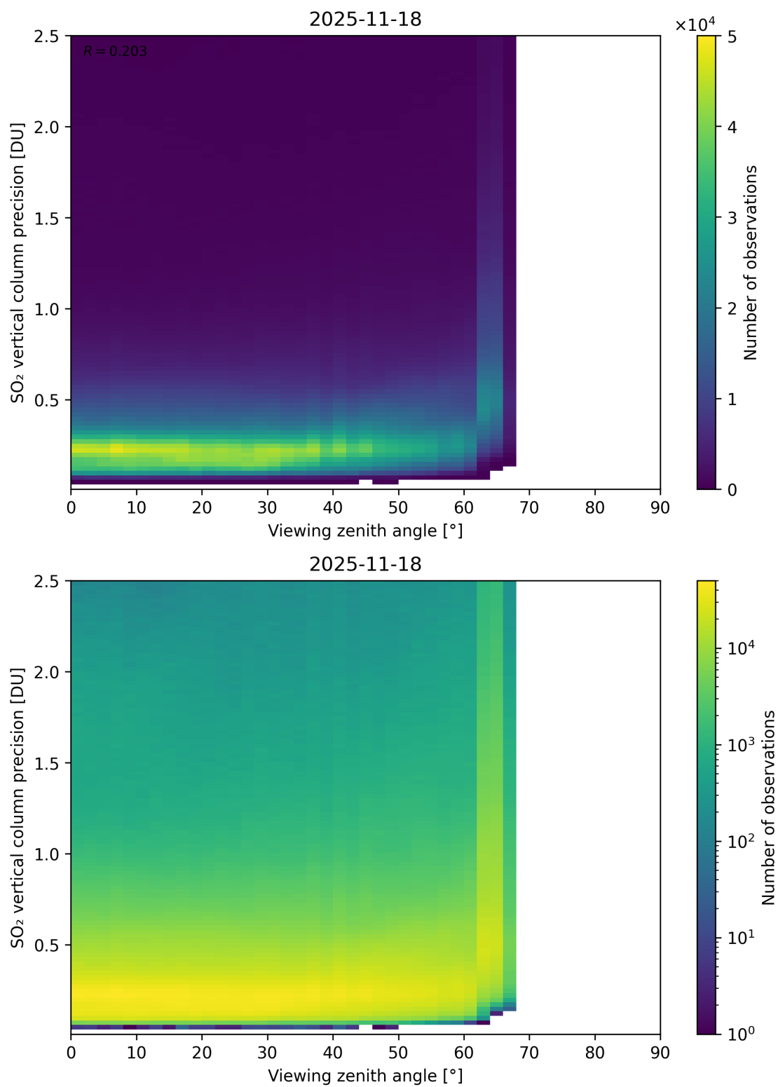
Figure 384: Scatter density plot of “Viewing zenith angle” against “SO 2 vertical column precision” for 2025-11-18 to 2025-11-19.
