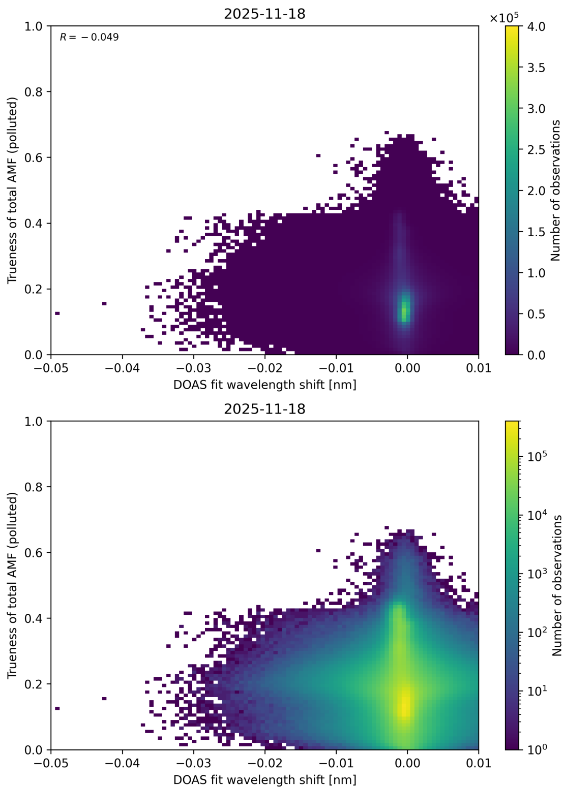
Figure 142: Scatter density plot of “DOAS fit wavelength shift” against “Trueness of total AMF (polluted)” for 2025-11-18 to 2025-11-19.
