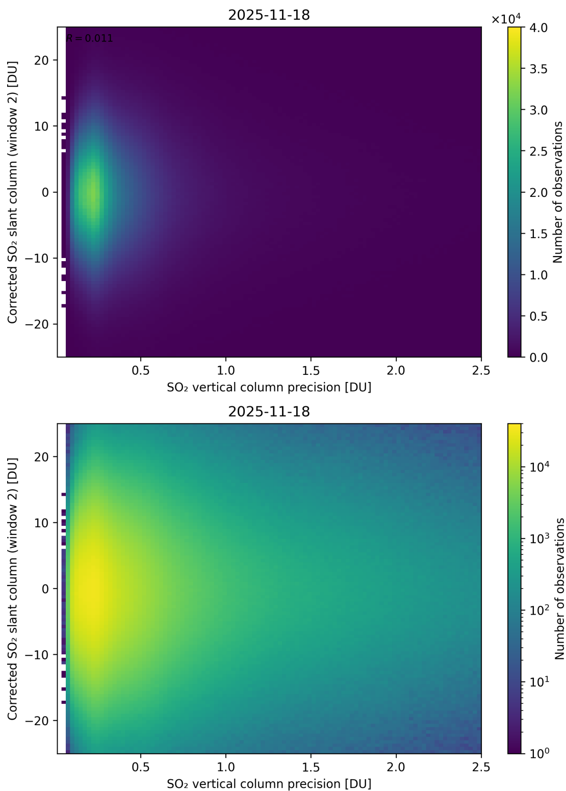
Figure 339: Scatter density plot of “SO 2 vertical column precision” against “Corrected SO 2 slant column (window 2)” for 2025-11-18 to 2025-11-19.
