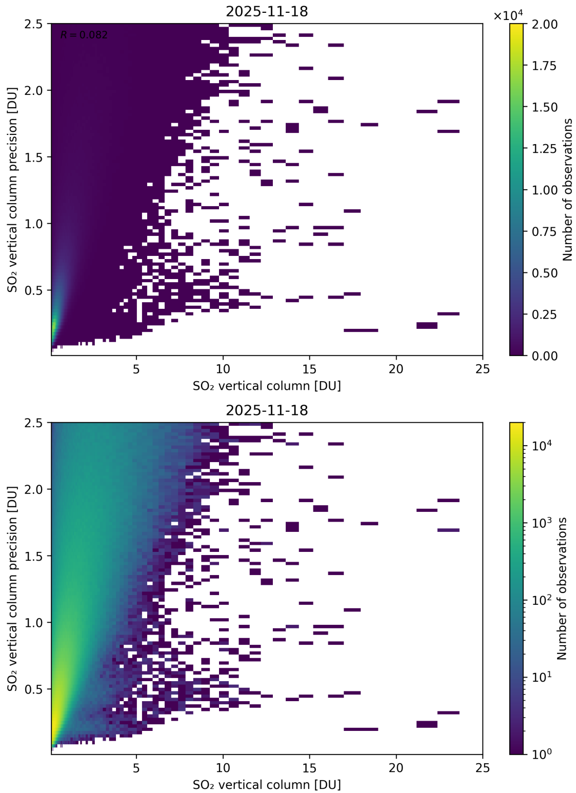
Figure 361: Scatter density plot of “SO 2 vertical column” against “SO 2 vertical column precision” for 2025-11-18 to 2025-11-19.
