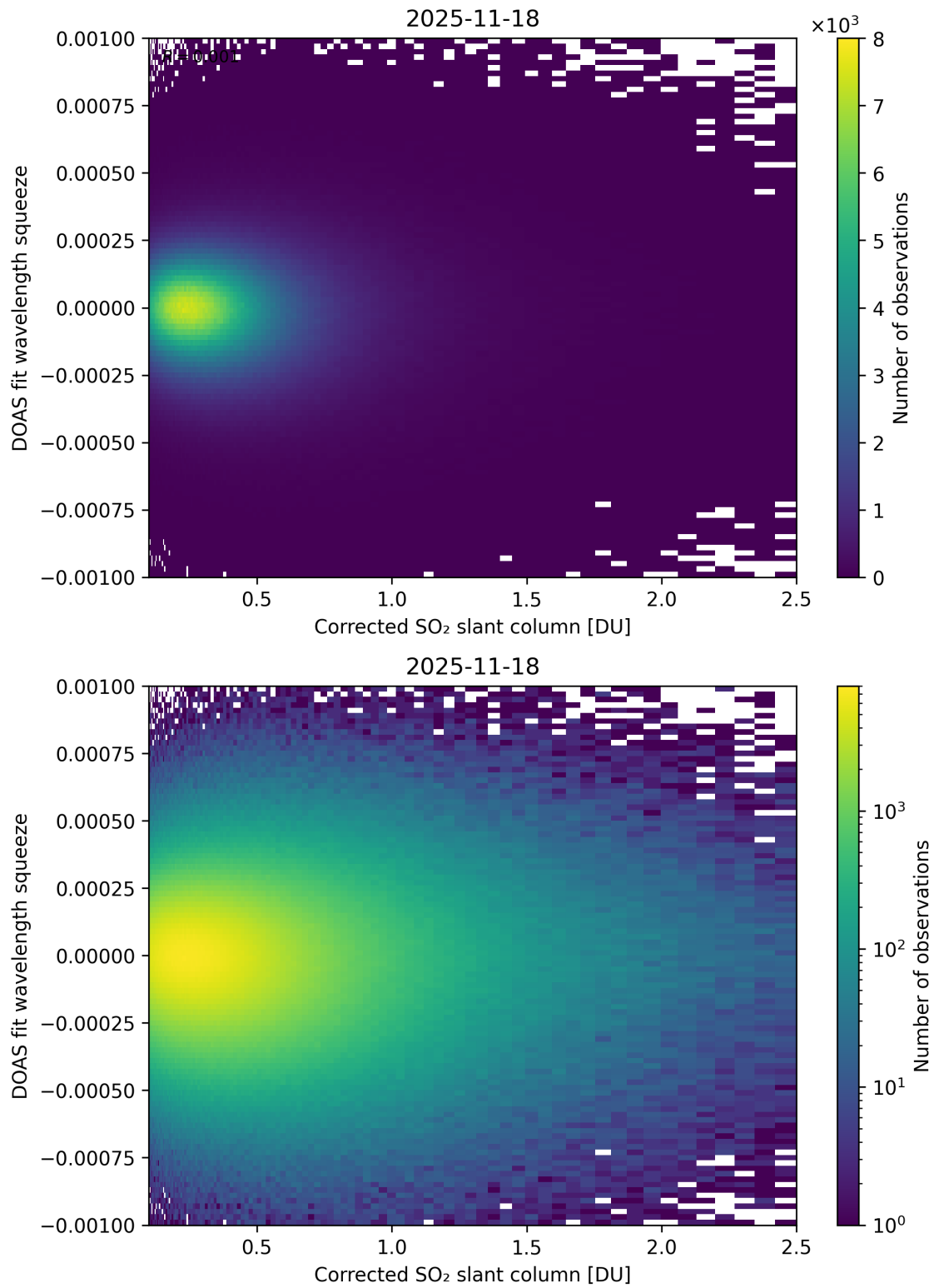
Figure 230: Scatter density plot of "Corrected SO 2 slant column" against "DOAS fit wavelength squeeze" for 2025-11-18 to 2025-11-19.
