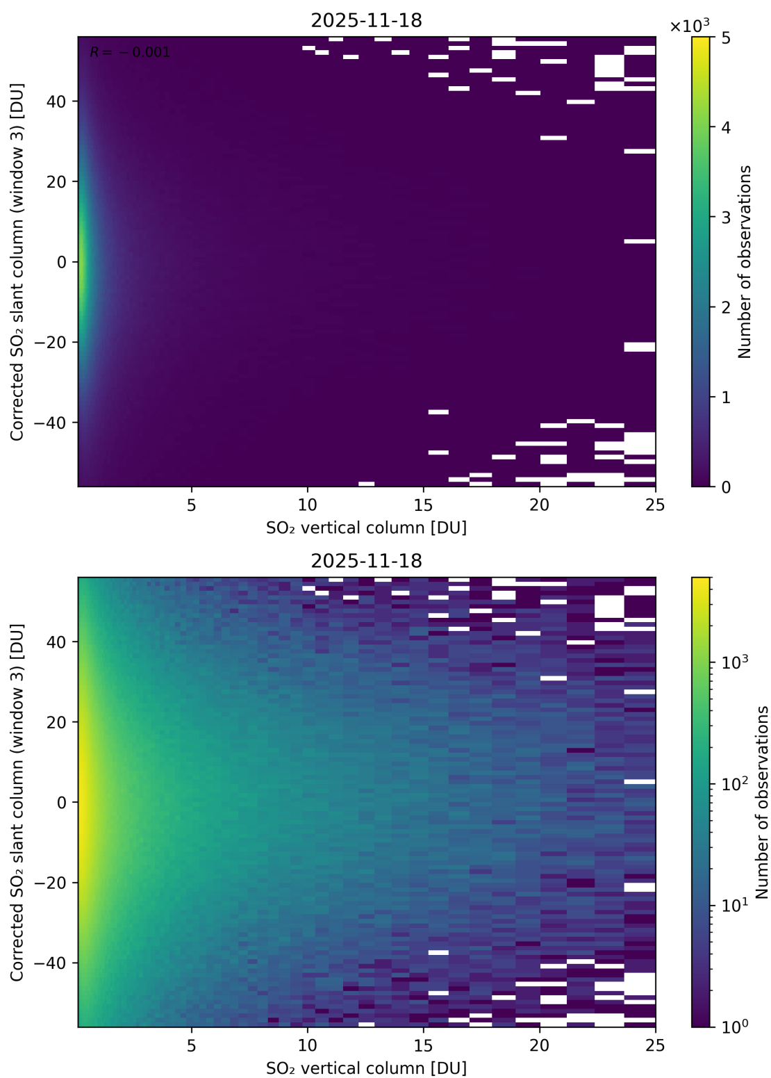
Figure 353: Scatter density plot of “SO 2 vertical column” against “Corrected SO 2 slant column (window 3)” for 2025-11-18 to 2025-11-19.
