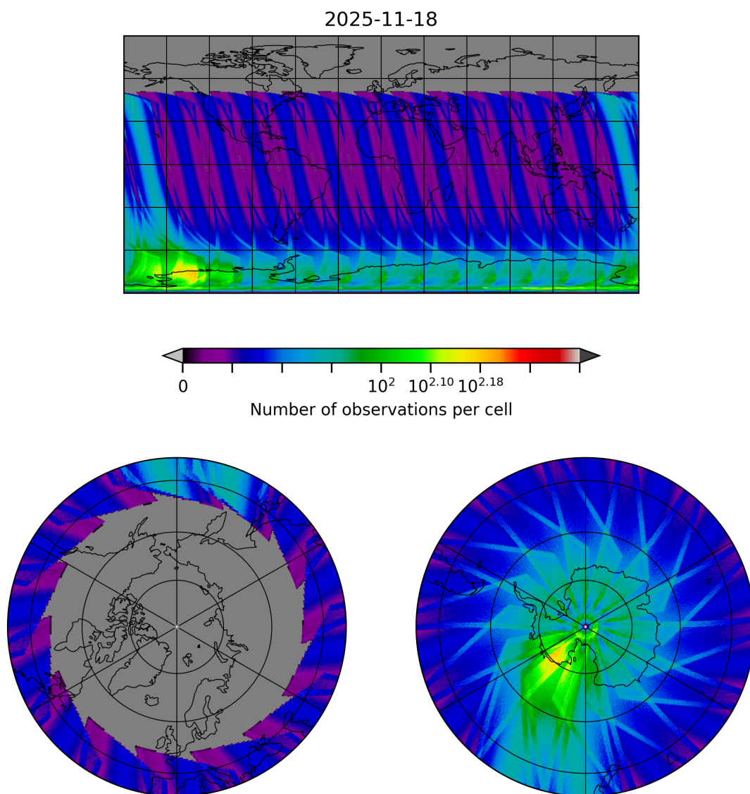
Figure 30: Map of the number of observations for 2025-11-18 to 2025-11-19
