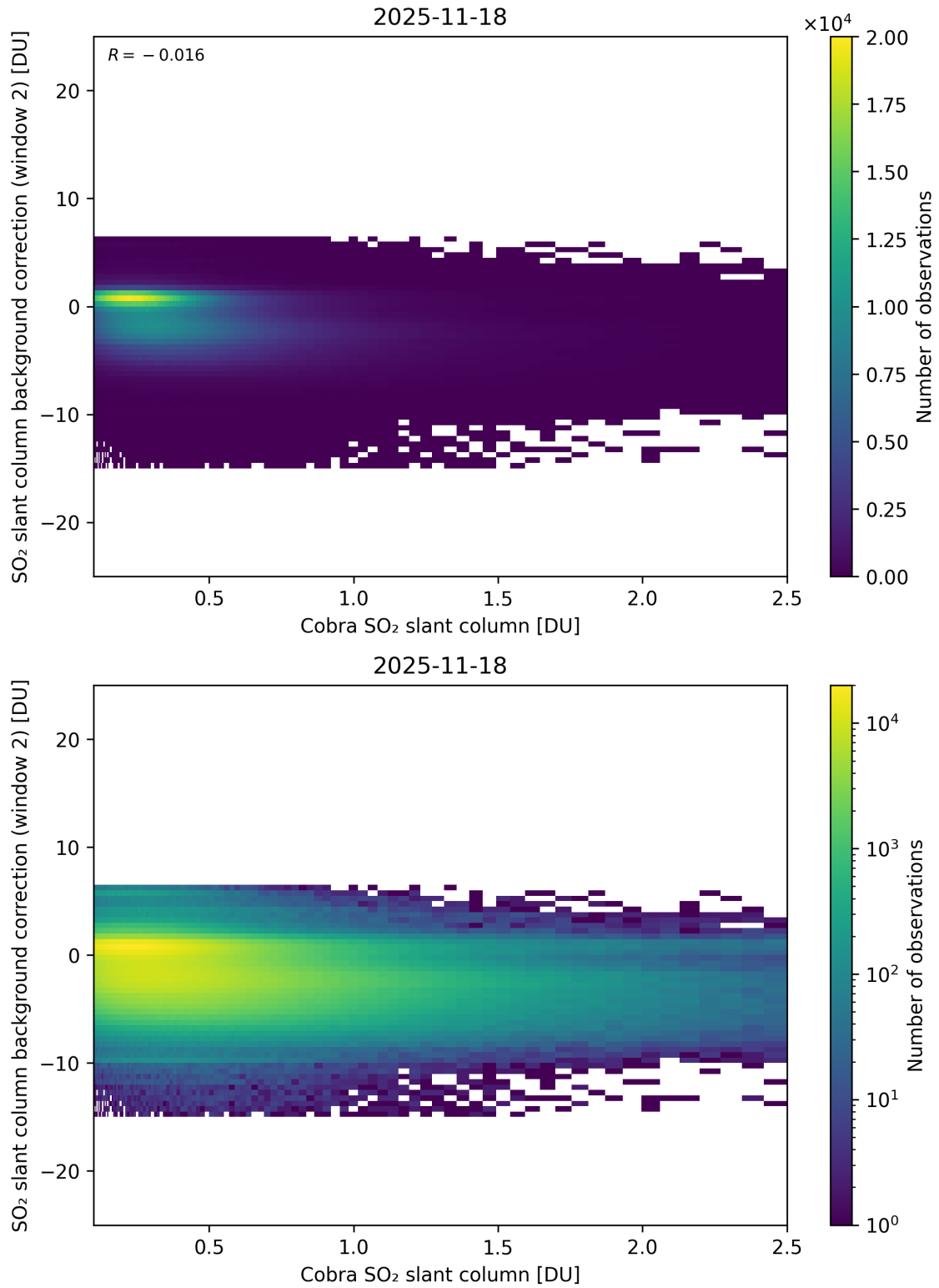
Figure 194: Scatter density plot of “Cobra SO 2 slant column” against “SO 2 slant column background correction (window 2)” for 2025-11-18 to 2025-11-19.
