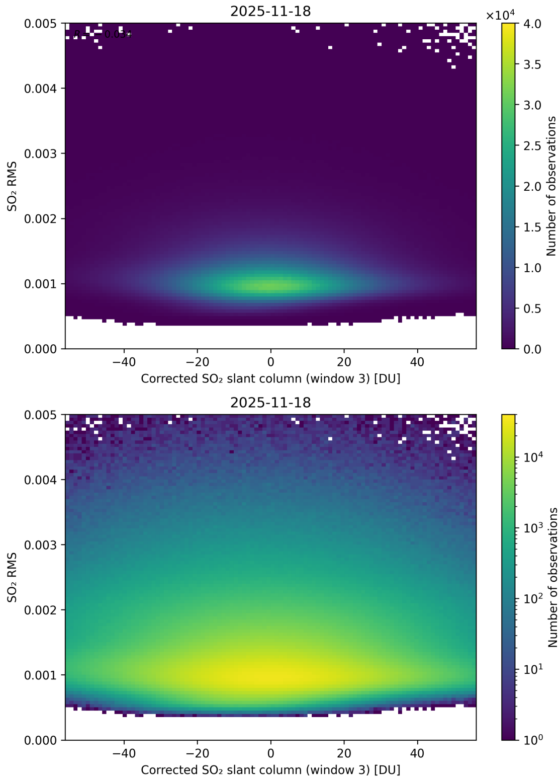
Figure 258: Scatter density plot of “Corrected SO 2 slant column (window 3)” against “SO 2 RMS” for 2025-11-18 to 2025-11-19.
