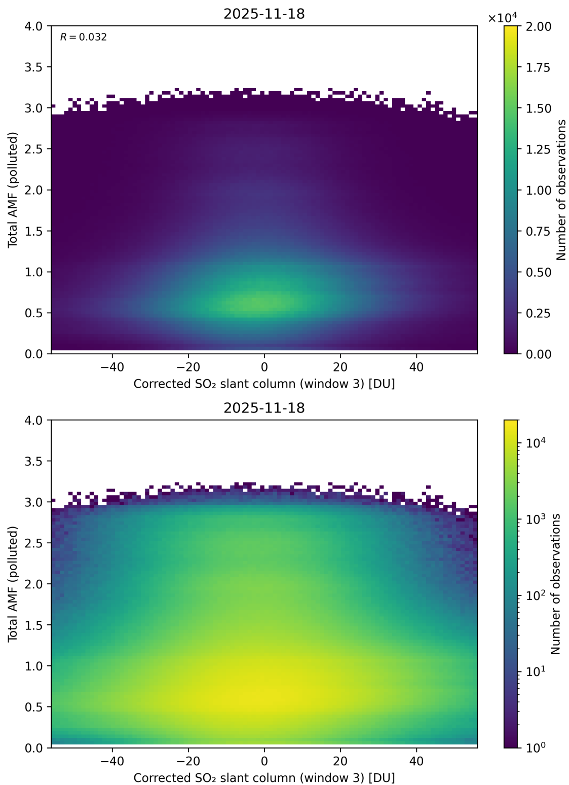
Figure 260: Scatter density plot of “Corrected SO 2 slant column (window 3)” against “Total AMF (polluted)” for 2025-11-18 to 2025-11-19.
