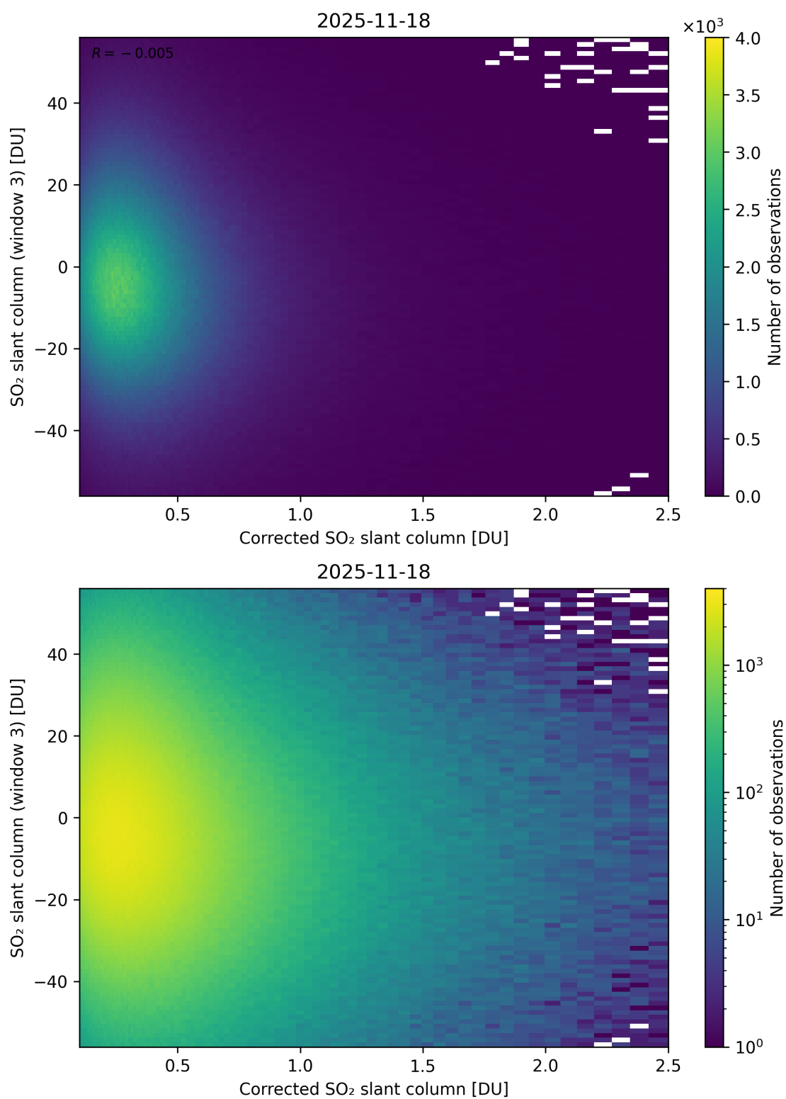
Figure 240: Scatter density plot of “Corrected SO 2 slant column” against “SO 2 slant column (window 3)” for 2025-11-18 to 2025-11-19.
