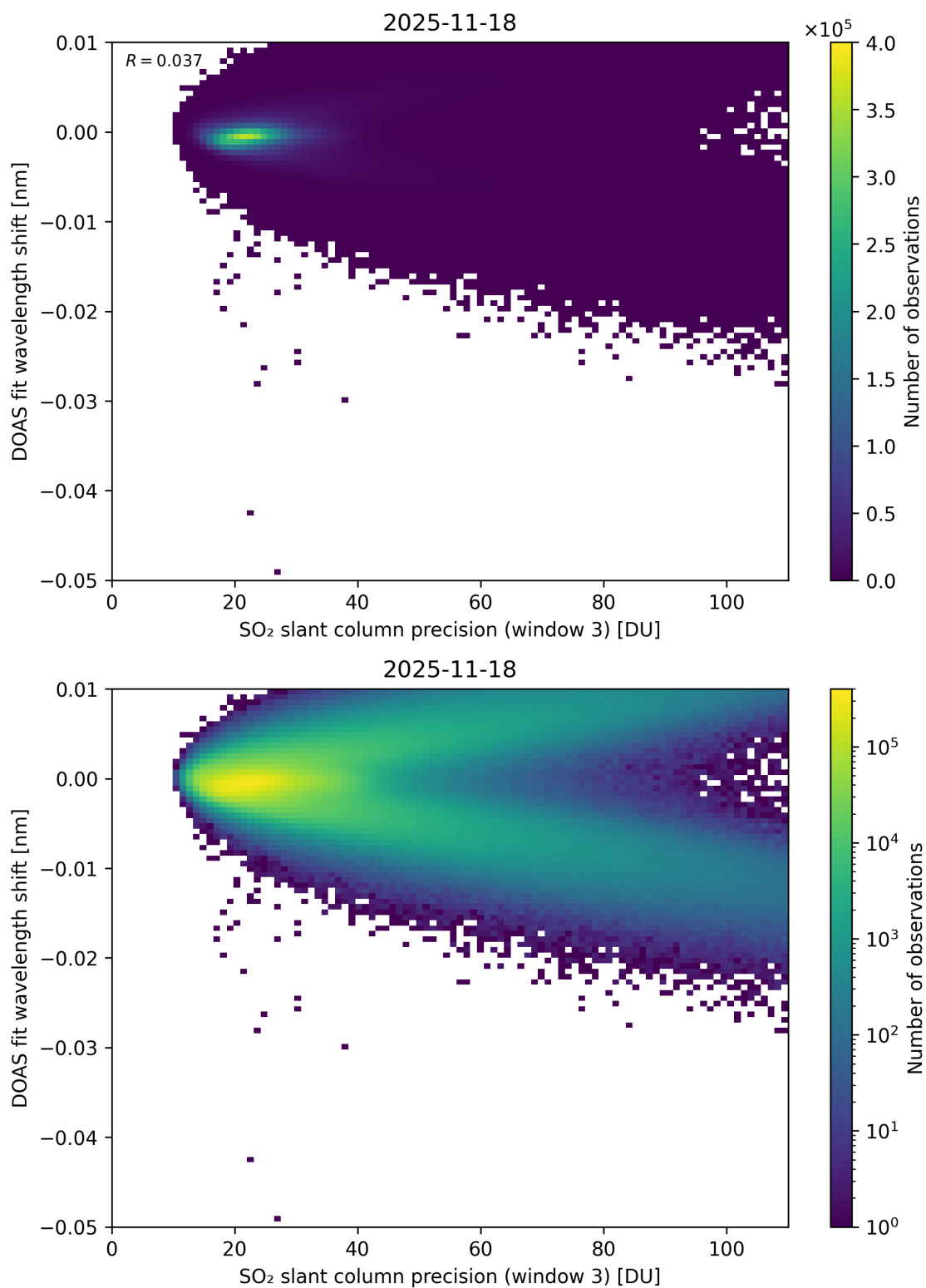
Figure 308: Scatter density plot of “SO 2 slant column precision (window 3)” against “DOAS fit wavelength shift” for 2025-11-18 to 2025-11-19.
