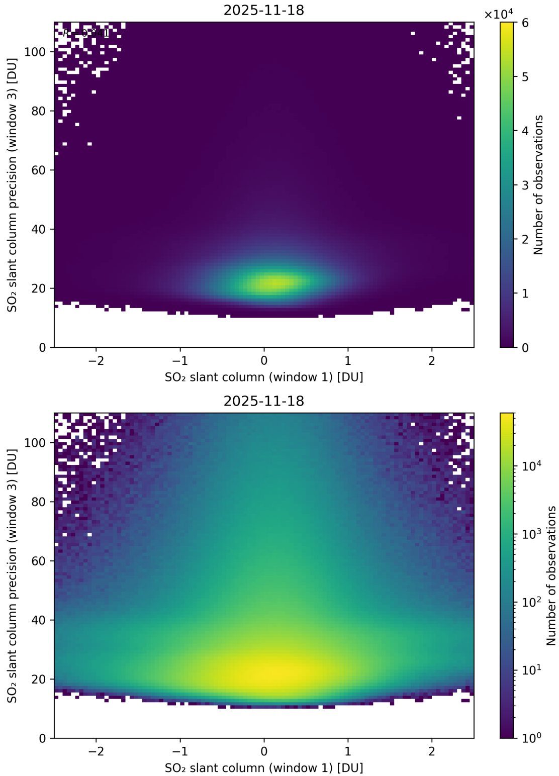
Figure 288: Scatter density plot of “SO 2 slant column (window 1)” against “SO 2 slant column precision (window 3)” for 2025-11-18 to 2025-11-19.
