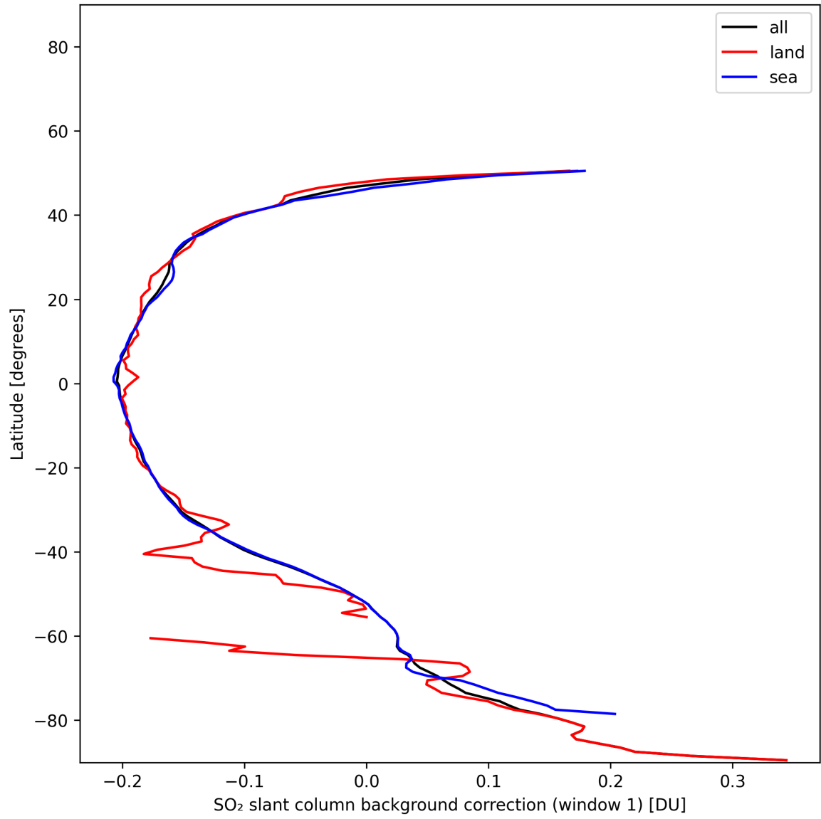
Figure 40: Zonal average of “SO 2 slant column background correction (window 1)” for 2025-11-18 to 2025-11-19.
