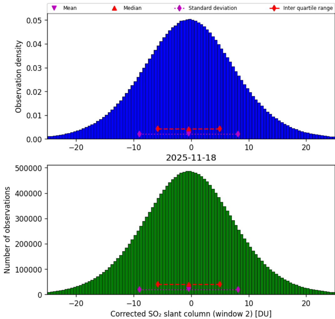
Figure 69: Histogram of “Corrected SO 2 slant column (window 2)” for 2025-11-18 to 2025-11-19
