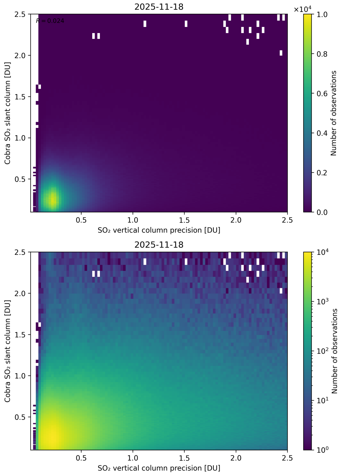
Figure 336: Scatter density plot of “SO 2 vertical column precision” against “Cobra SO 2 slant column” for 2025-11-18 to 2025-11-19.
