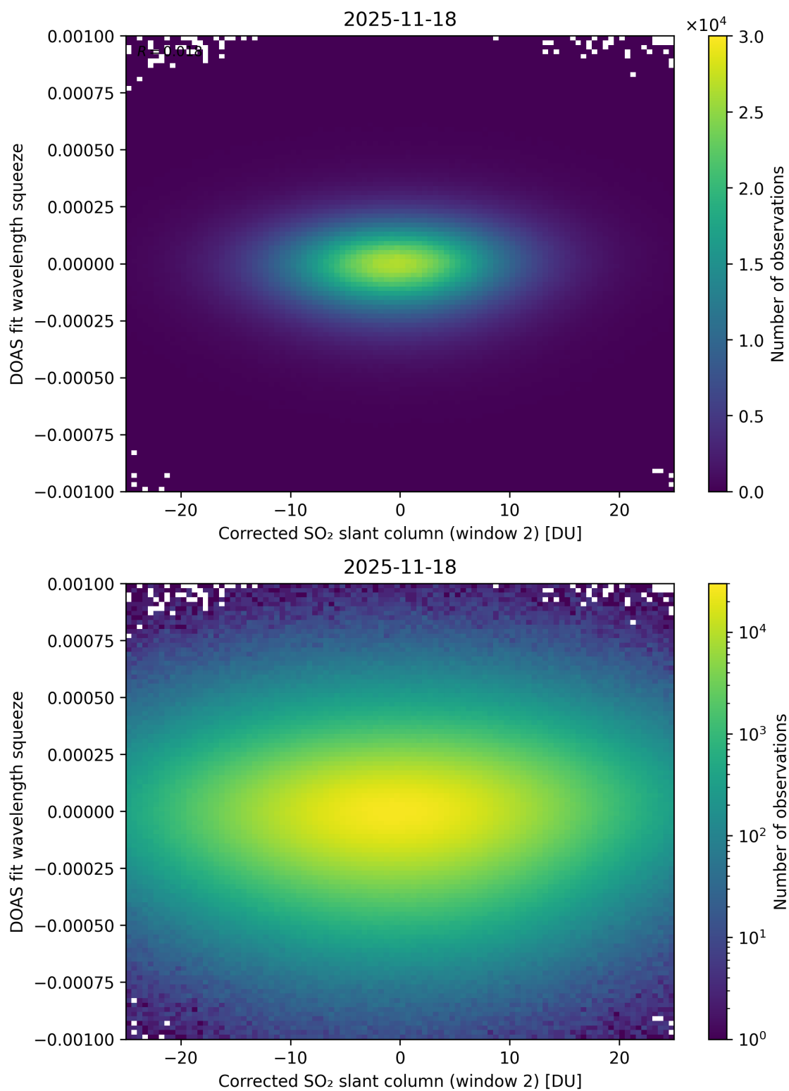
Figure 247: Scatter density plot of “Corrected SO 2 slant column (window 2)” against “DOAS fit wavelength squeeze” for 2025-11-18 to 2025-11-19.
