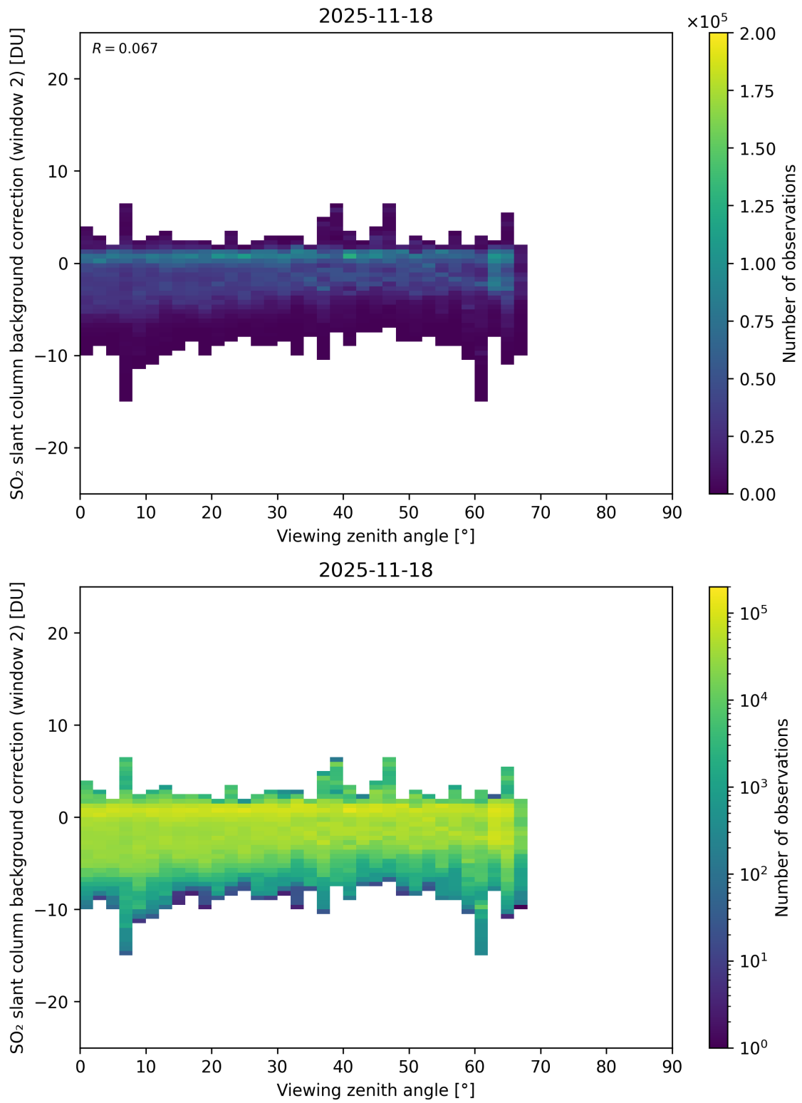
Figure 363: Scatter density plot of “Viewing zenith angle” against “SO 2 slant column background correction (window 2)” for 2025-11-18 to 2025-11-19.
