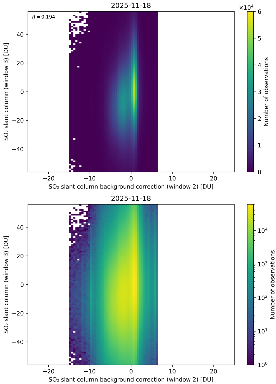
Figure 128: Scatter density plot of “SO 2 slant column background correction (window 2)” against “SO 2 slant column (window 3)” for 2025-11-18 to 2025-11-19.
