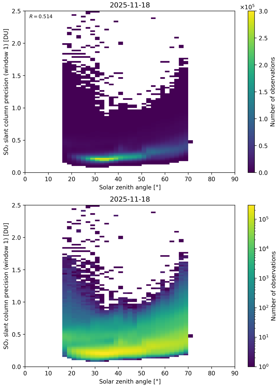
Figure 185: Scatter density plot of “Solar zenith angle” against “SO 2 slant column precision (window 1)” for 2025-11-18 to 2025-11-19.
