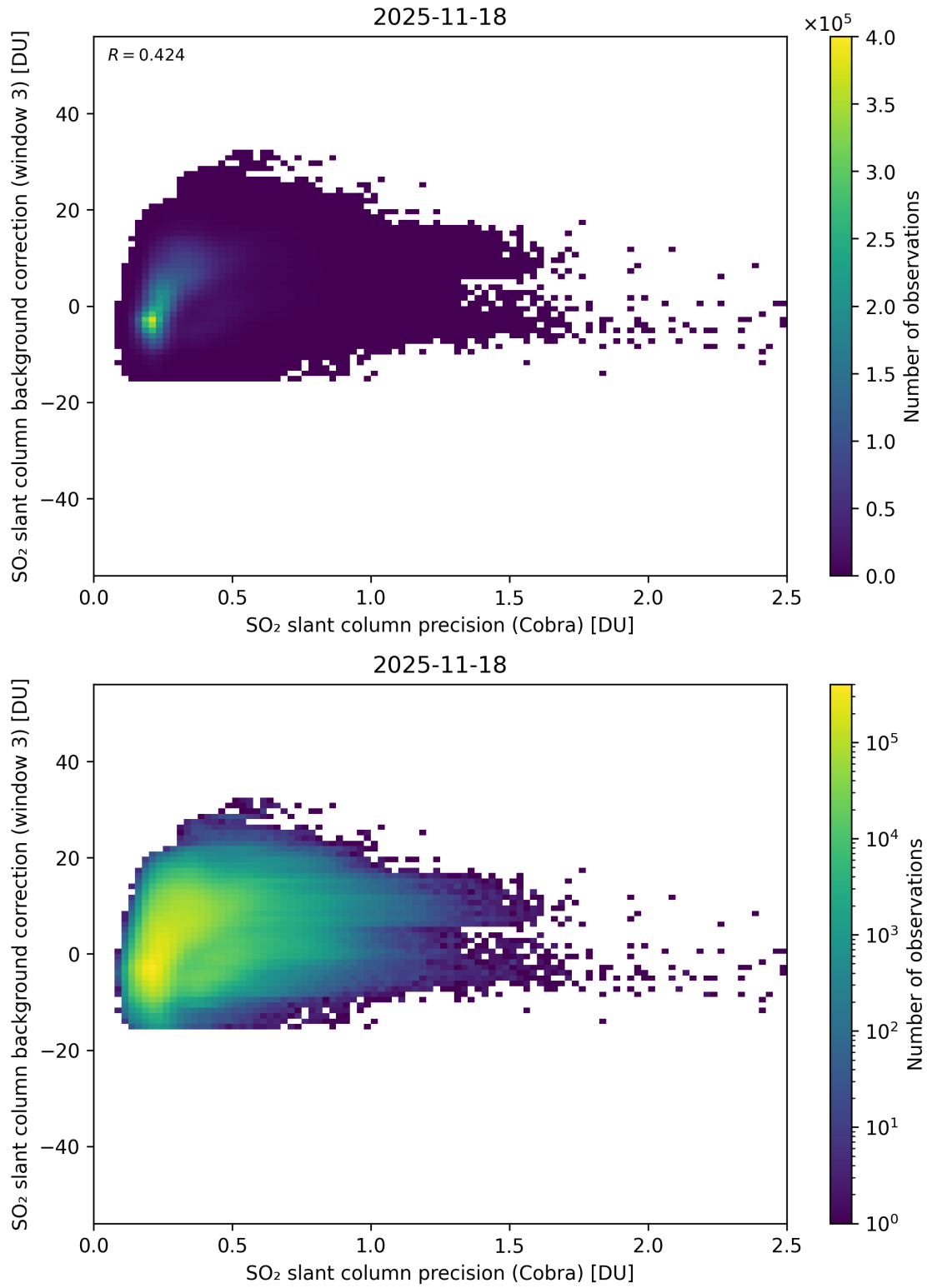
Figure 201: Scatter density plot of “SO 2 slant column precision (Cobra)” against “SO 2 slant column background correction (window 3)” for 2025-11-18 to 2025-11-19.
