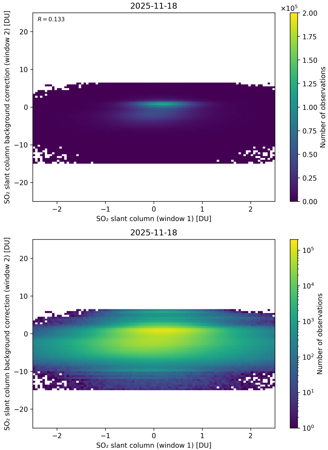
Figure 263: Scatter density plot of “SO 2 slant column (window 1)” against “SO 2 slant column background correction (window 2)” for 2025-11-18 to 2025-11-19.
