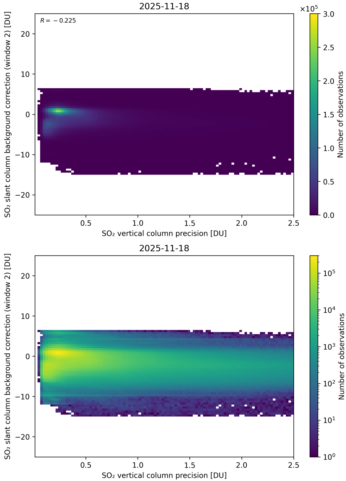
Figure 330: Scatter density plot of “SO 2 vertical column precision” against “SO 2 slant column background correction (window 2)” for 2025-11-18 to 2025-11-19.
