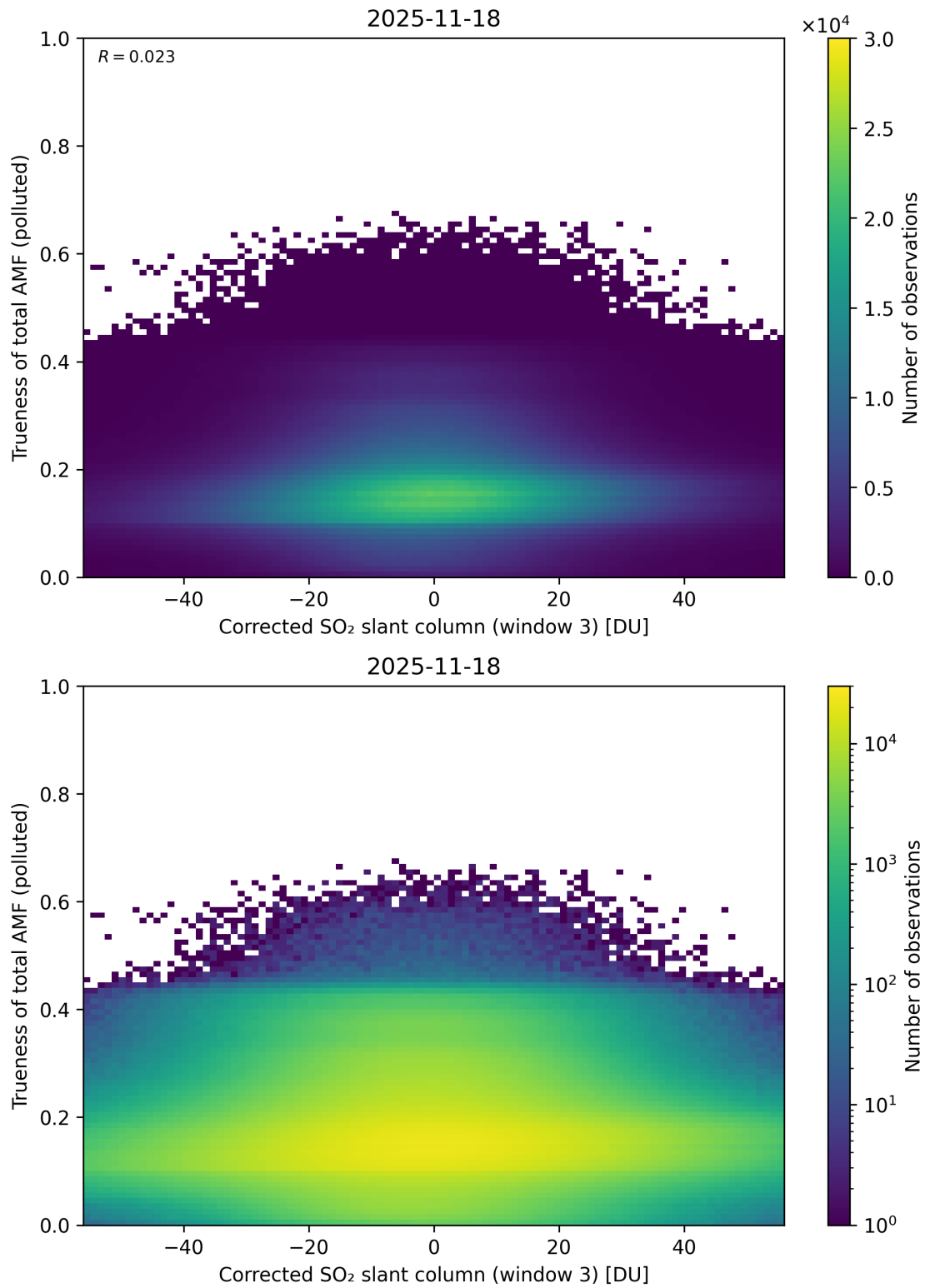
Figure 261: Scatter density plot of “Corrected SO 2 slant column (window 3)” against “Trueness of total AMF (polluted)” for 2025-11-18 to 2025-11-19.
