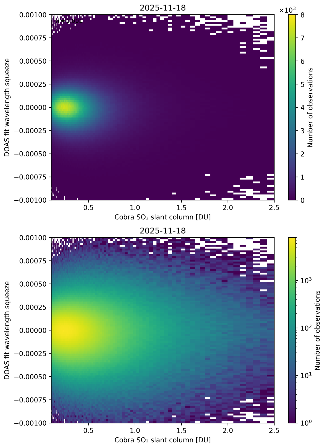
Figure 197: Scatter density plot of “Cobra SO 2 slant column” against “DOAS fit wavelength squeeze” for 2025-11-18 to 2025-11-19.
