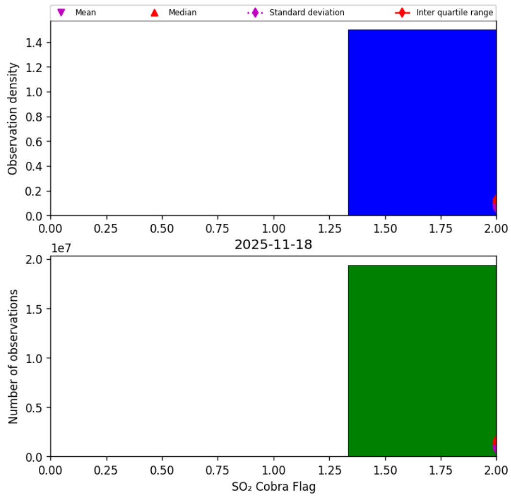
Figure 75: Histogram of “SO 2 Cobra Flag” for 2025-11-18 to 2025-11-19
