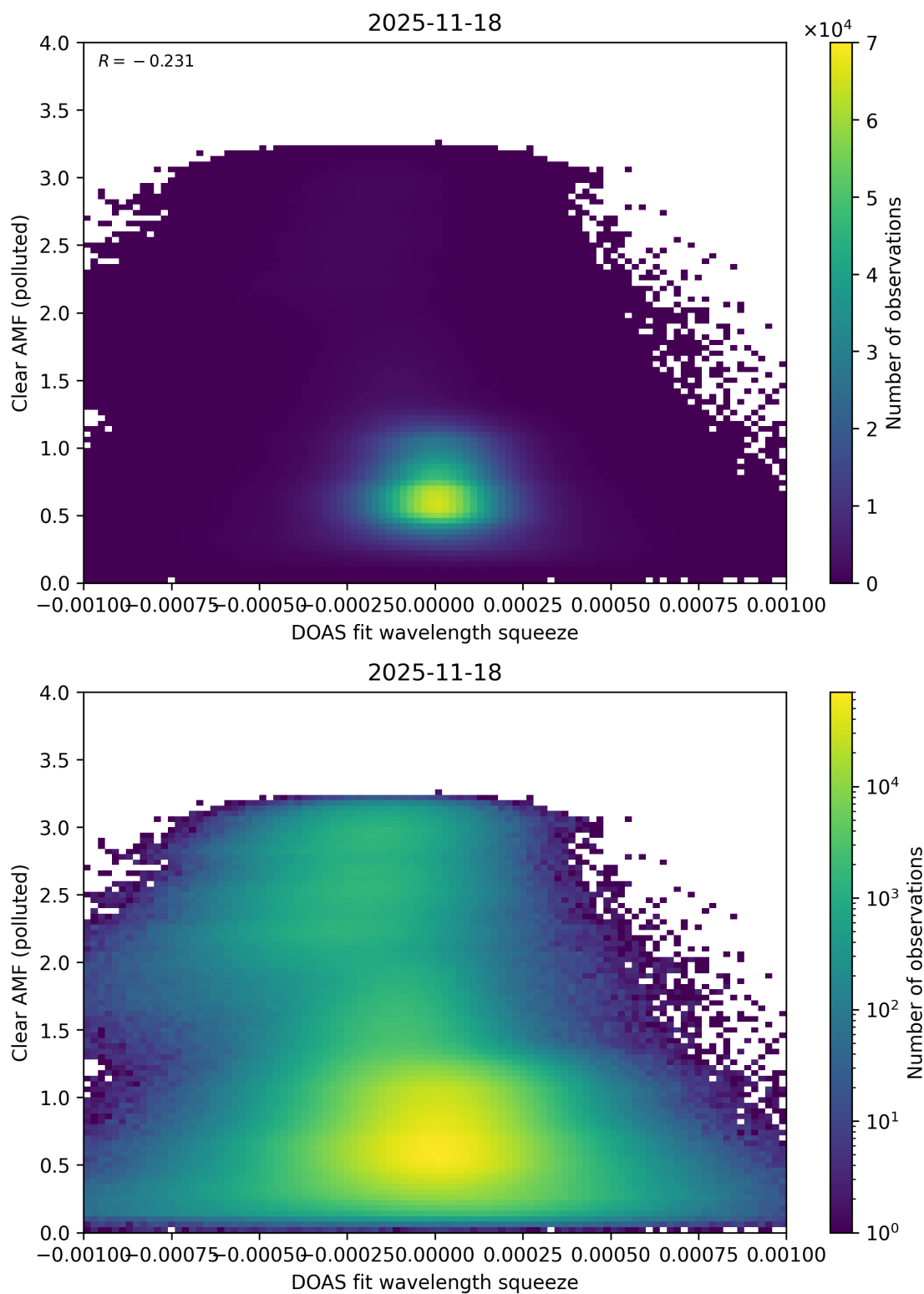
Figure 144: Scatter density plot of “DOAS fit wavelength squeeze” against “Clear AMF (polluted)” for 2025-11-18 to 2025-11-19.
