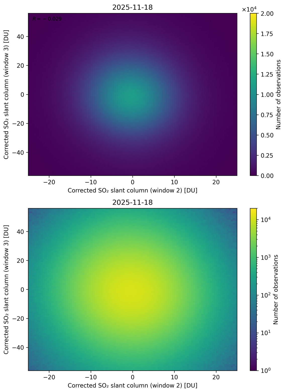
Figure 250: Scatter density plot of “Corrected SO 2 slant column (window 2)” against “Corrected SO 2 slant column (window 3)” for 2025-11-18 to 2025-11-19.
