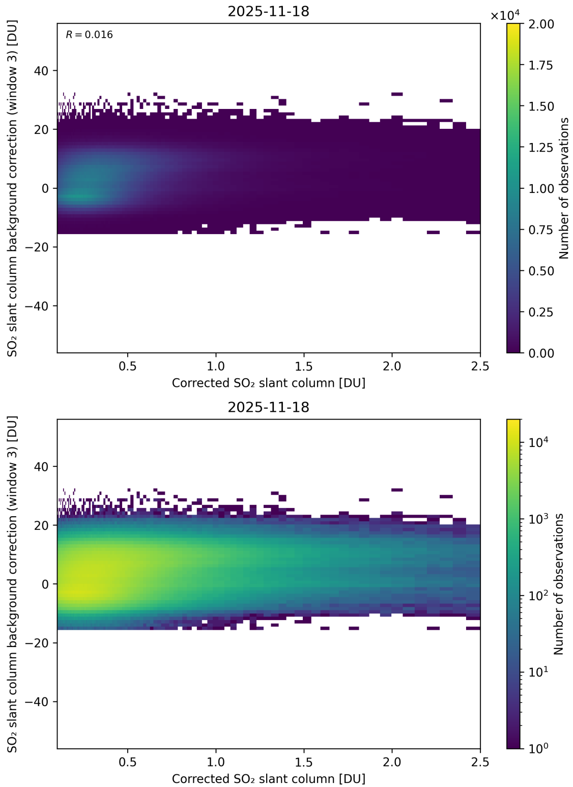
Figure 228: Scatter density plot of “Corrected SO 2 slant column” against “SO 2 slant column background correction (window 3)” for 2025-11-18 to 2025-11-19.
