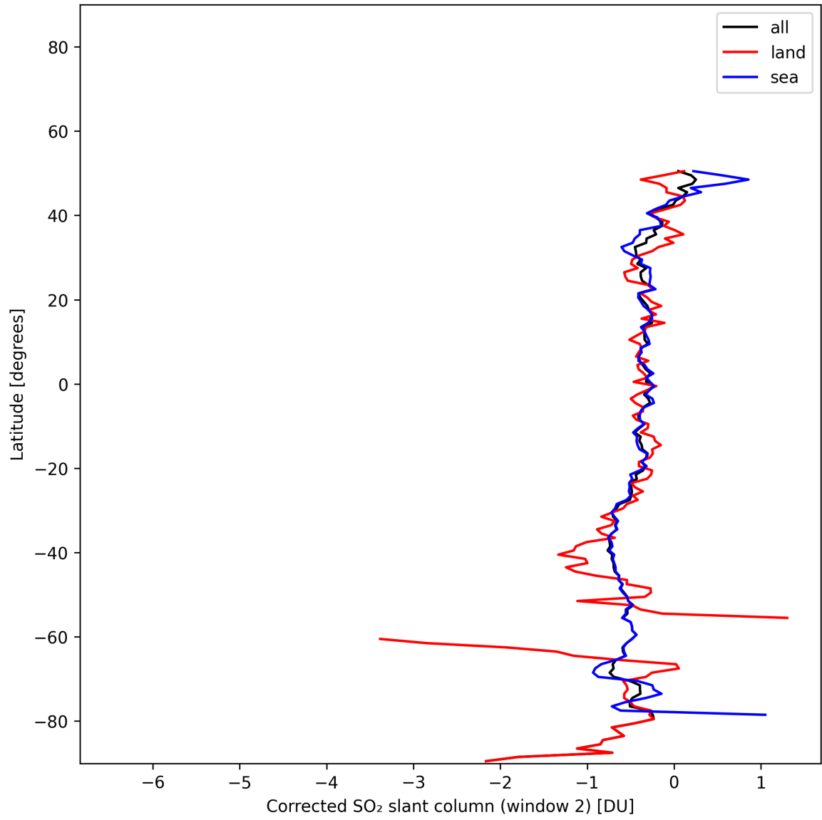
Figure 43: Zonal average of “Corrected SO 2 slant column (window 2)” for 2025-11-18 to 2025-11-19.
