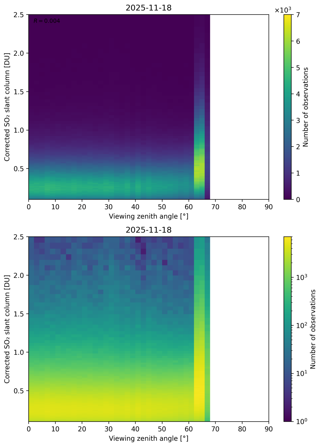
Figure 373: Scatter density plot of “Viewing zenith angle” against “Corrected SO 2 slant column” for 2025-11-18 to 2025-11-19.
