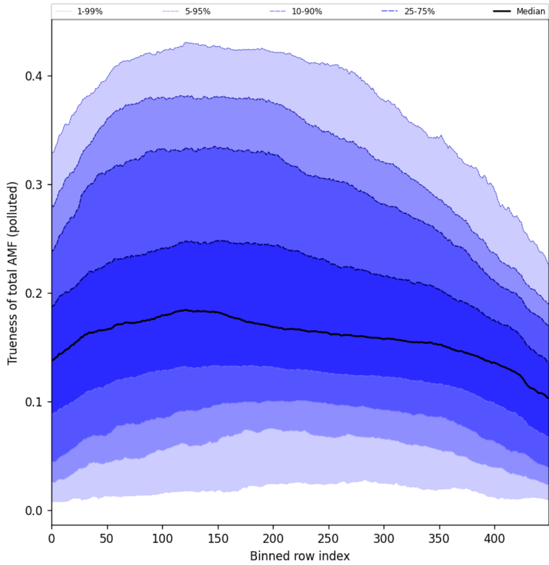
Figure 106: Along track statistics of “Trueness of total AMF (polluted)” for 2025-11-18 to 2025-11-19
