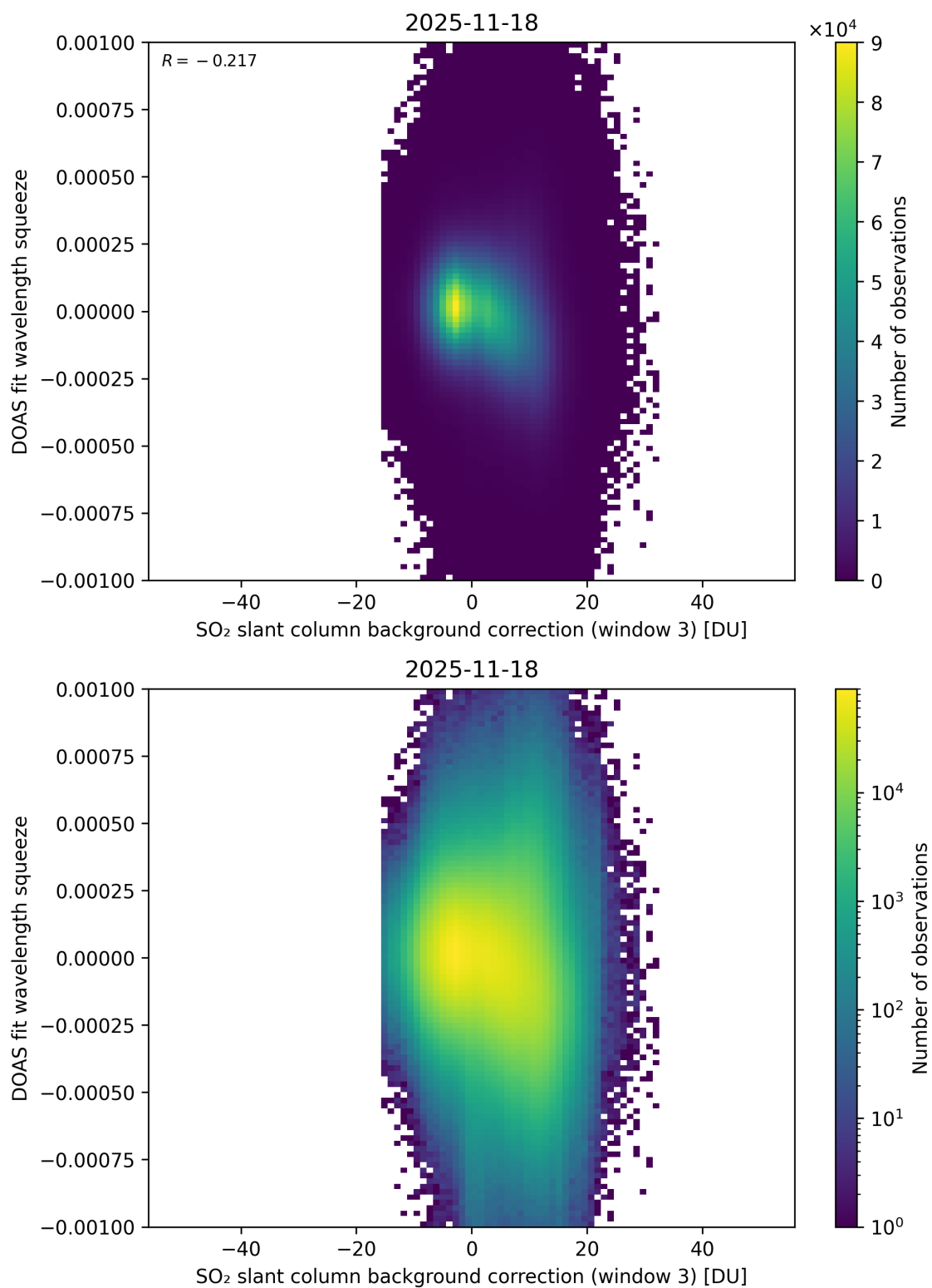
Figure 133: Scatter density plot of “SO 2 slant column background correction (window 3)” against “DOAS fit wavelength squeeze” for 2025-11-18 to 2025-11-19.
