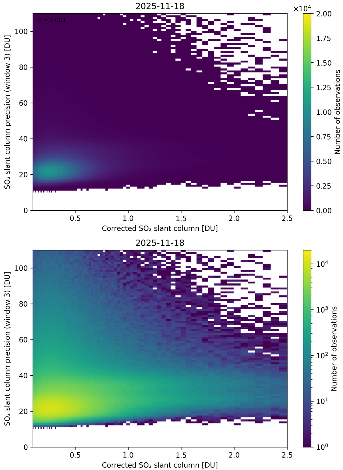
Figure 241: Scatter density plot of “Corrected SO 2 slant column” against “SO 2 slant column precision (window 3)” for 2025-11-18 to 2025-11-19.
