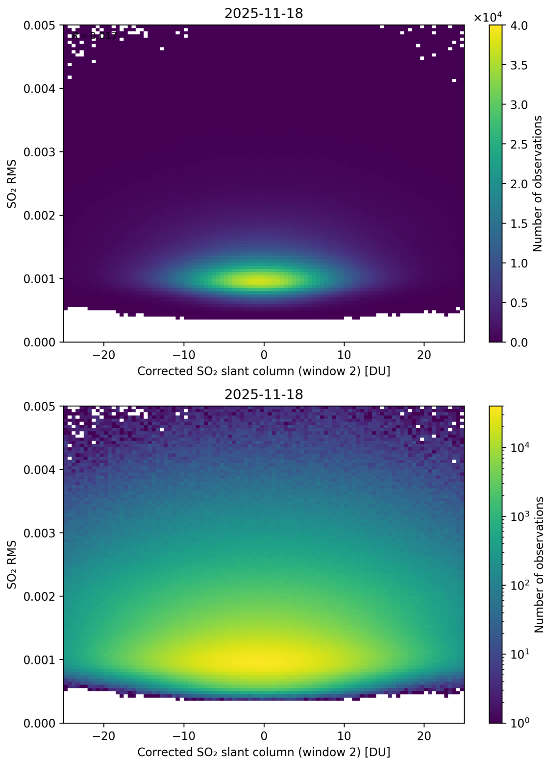
Figure 248: Scatter density plot of “Corrected SO 2 slant column (window 2)” against “SO 2 RMS” for 2025-11-18 to 2025-11-19.
