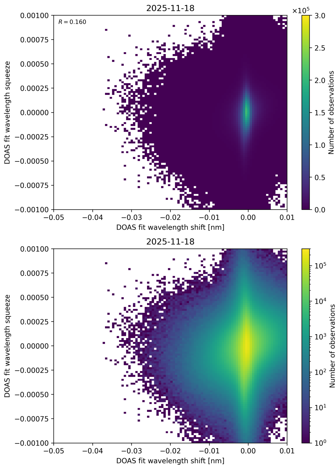
Figure 138: Scatter density plot of “DOAS fit wavelength shift” against “DOAS fit wavelength squeeze” for 2025-11-18 to 2025-11-19.
