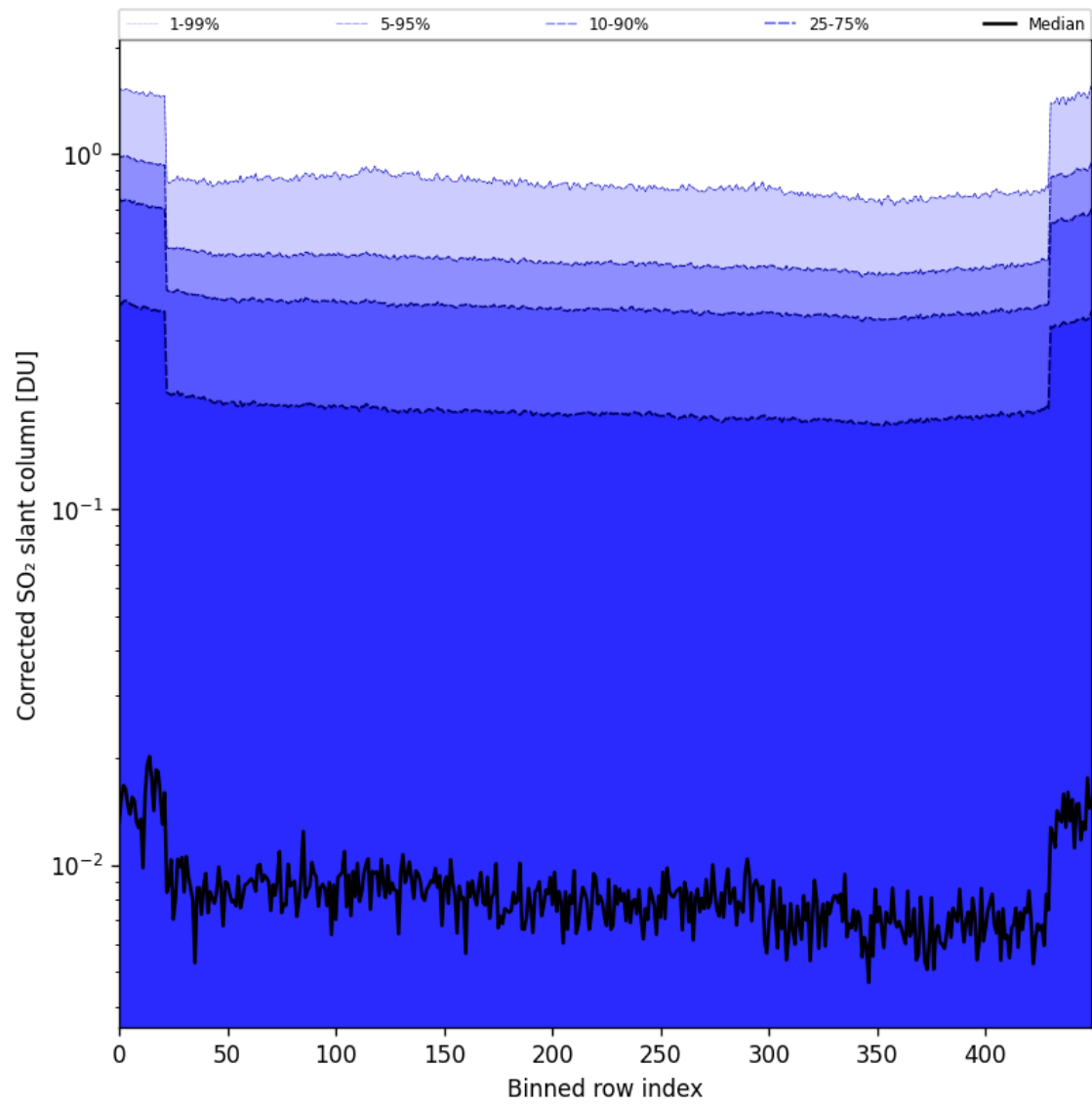
Figure 86: Along track statistics of “Corrected SO 2 slant column” for 2025-11-18 to 2025-11-19
