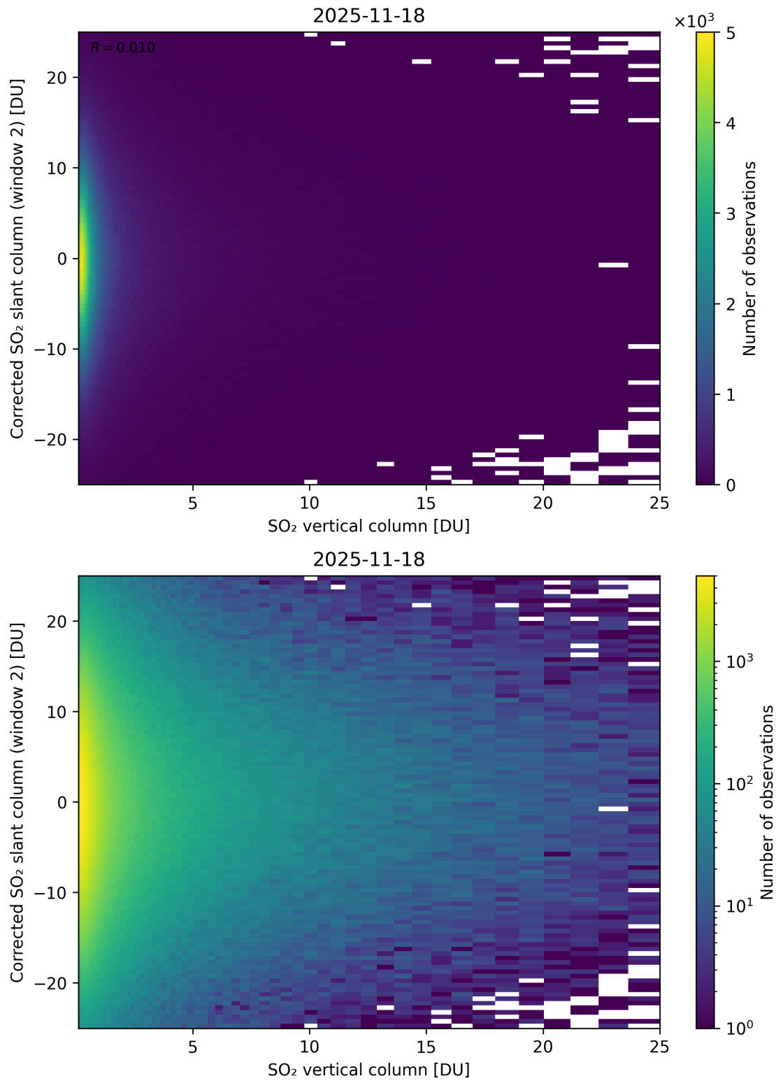
Figure 352: Scatter density plot of “SO 2 vertical column” against “Corrected SO 2 slant column (window 2)” for 2025-11-18 to 2025-11-19.
