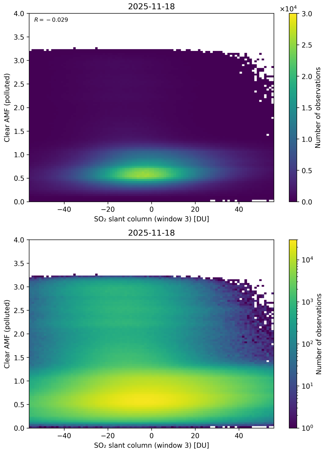
Figure 315: Scatter density plot of “SO 2 slant column (window 3)” against “Clear AMF (polluted)” for 2025-11-18 to 2025-11-19.
