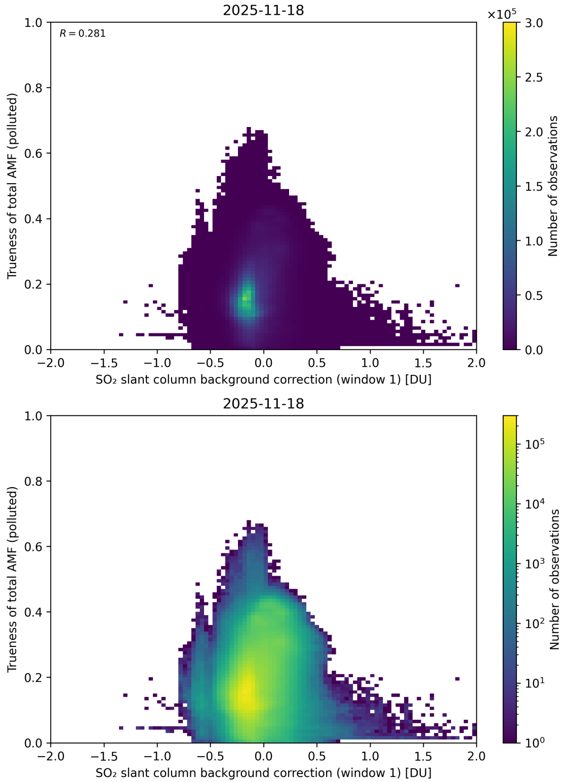
Figure 121: Scatter density plot of “SO 2 slant column background correction (window 1)” against “Trueness of total AMF (polluted)” for 2025-11-18 to 2025-11-19.
