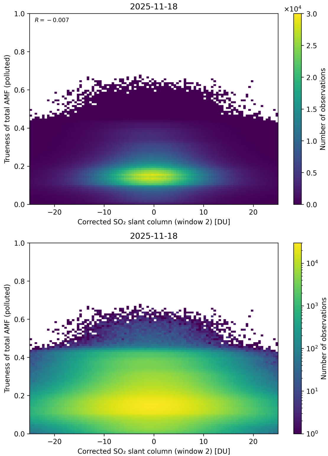
Figure 254: Scatter density plot of “Corrected SO 2 slant column (window 2)” against “Trueness of total AMF (polluted)” for 2025-11-18 to 2025-11-19.
