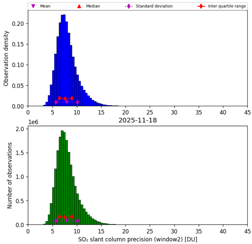
Figure 68: Histogram of “SO 2 slant column precision (window2)” for 2025-11-18 to 2025-11-19
