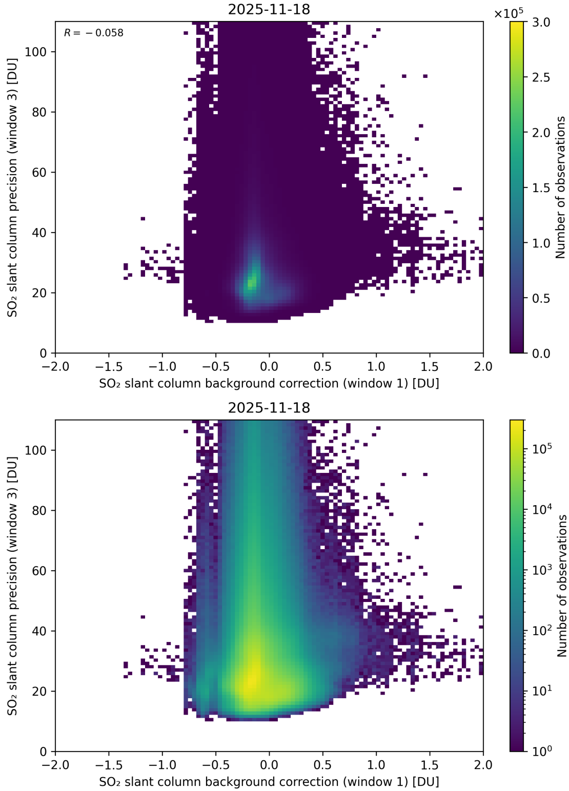
Figure 119: Scatter density plot of “SO 2 slant column background correction (window 1)” against “SO 2 slant column precision (window 3)” for 2025-11-18 to 2025-11-19.
