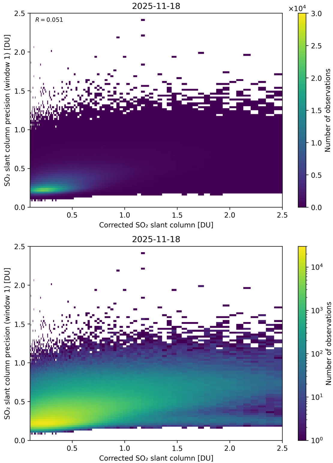
Figure 238: Scatter density plot of “Corrected SO 2 slant column” against “SO 2 slant column precision (window 1)” for 2025-11-18 to 2025-11-19.
