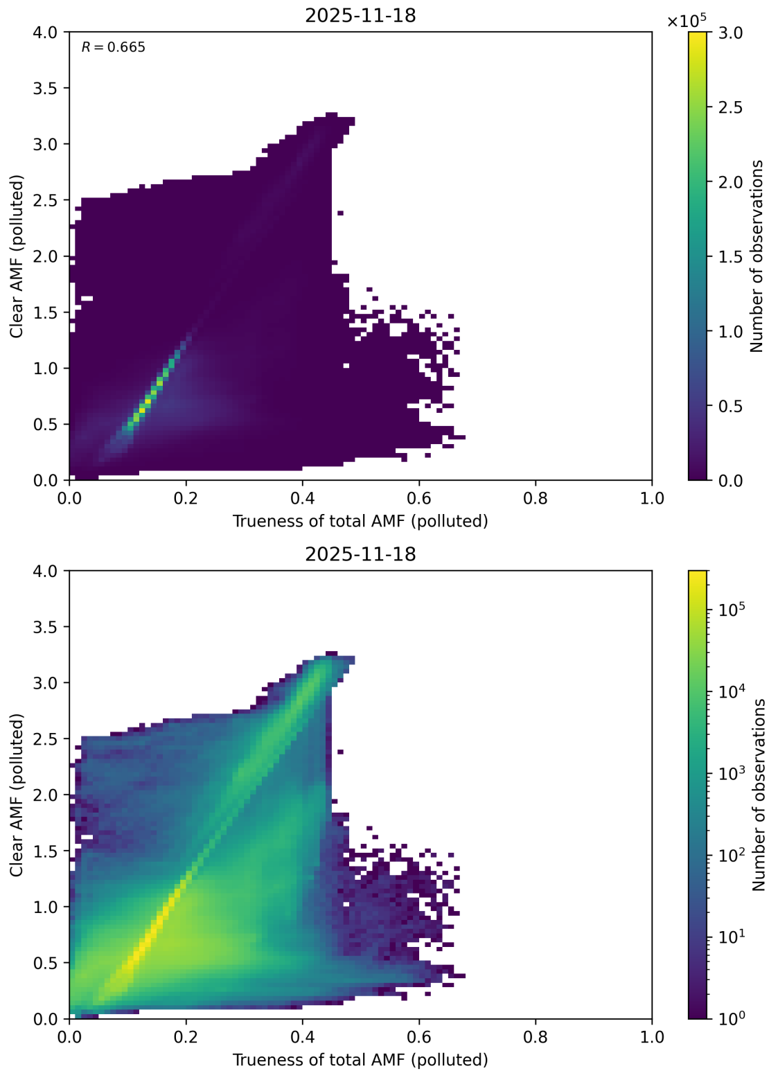
Figure 322: Scatter density plot of “Trueness of total AMF (polluted)” against “Clear AMF (polluted)” for 2025-11-18 to 2025-11-19.
