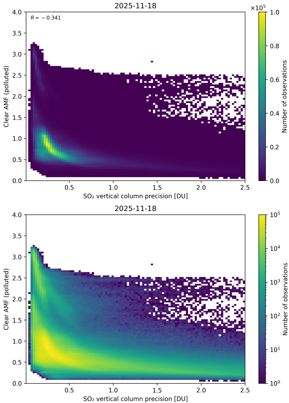
Figure 335: Scatter density plot of “SO 2 vertical column precision” against “Clear AMF (polluted)” for 2025-11-18 to 2025-11-19.
