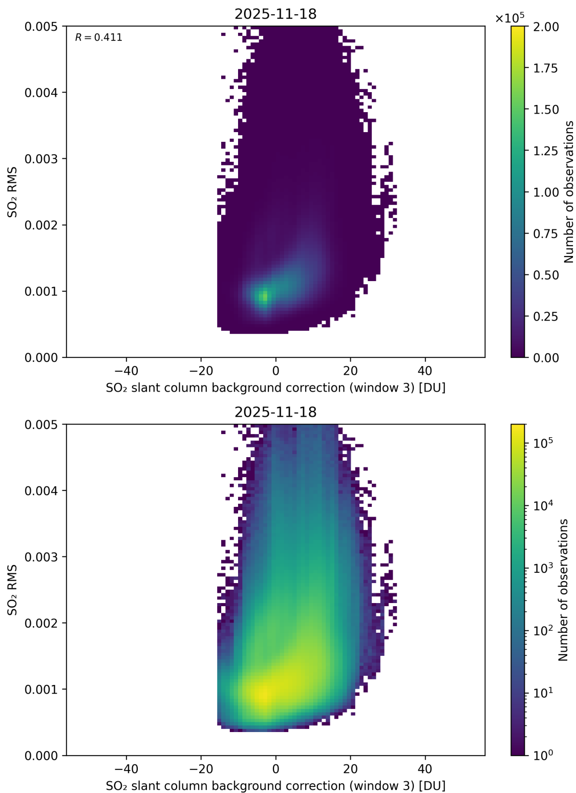
Figure 134: Scatter density plot of “SO 2 slant column background correction (window 3)” against “SO 2 RMS” for 2025-11-18 to 2025-11-19.
