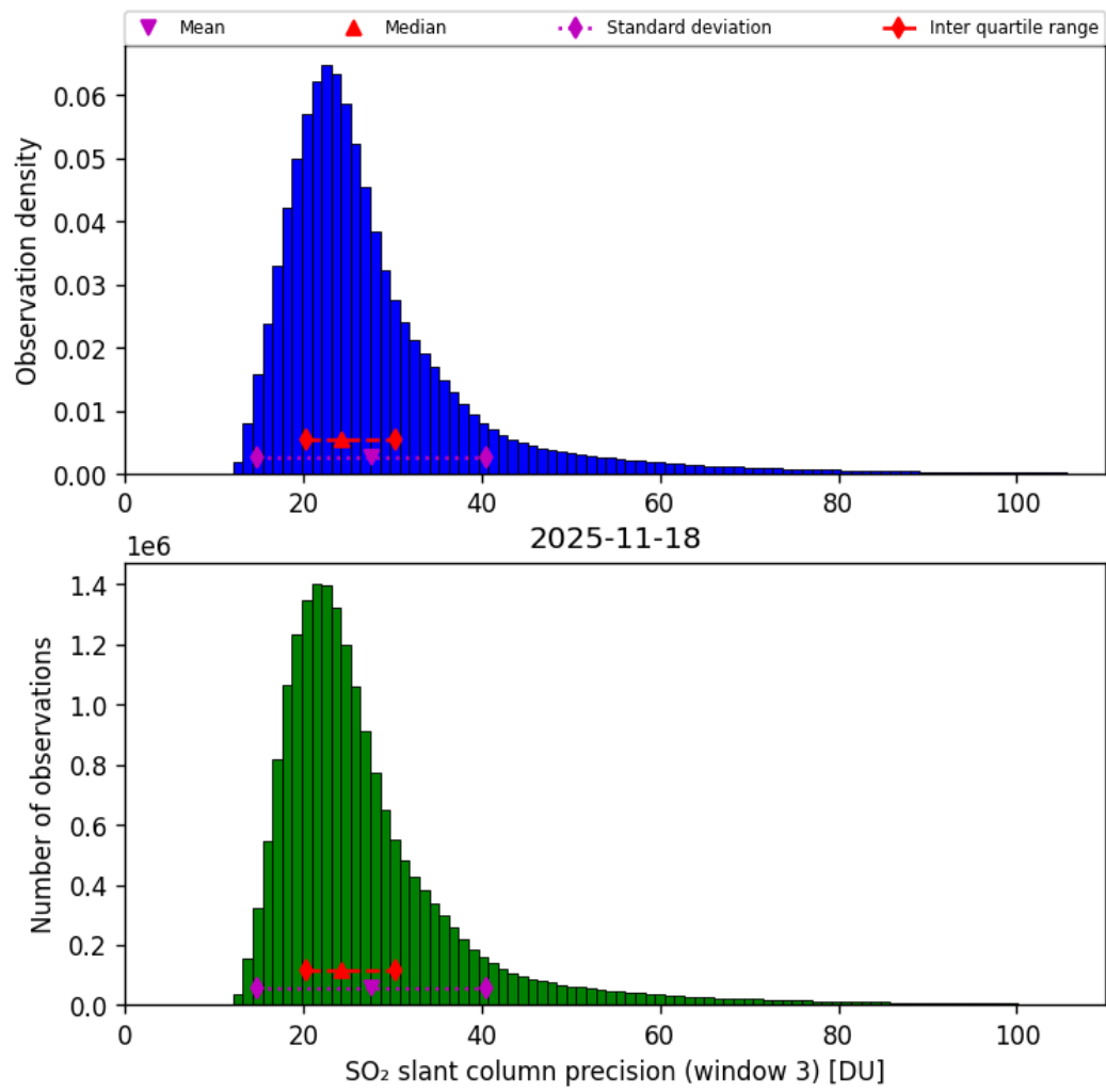
Figure 72: Histogram of “SO 2 slant column precision (window 3)” for 2025-11-18 to 2025-11-19
