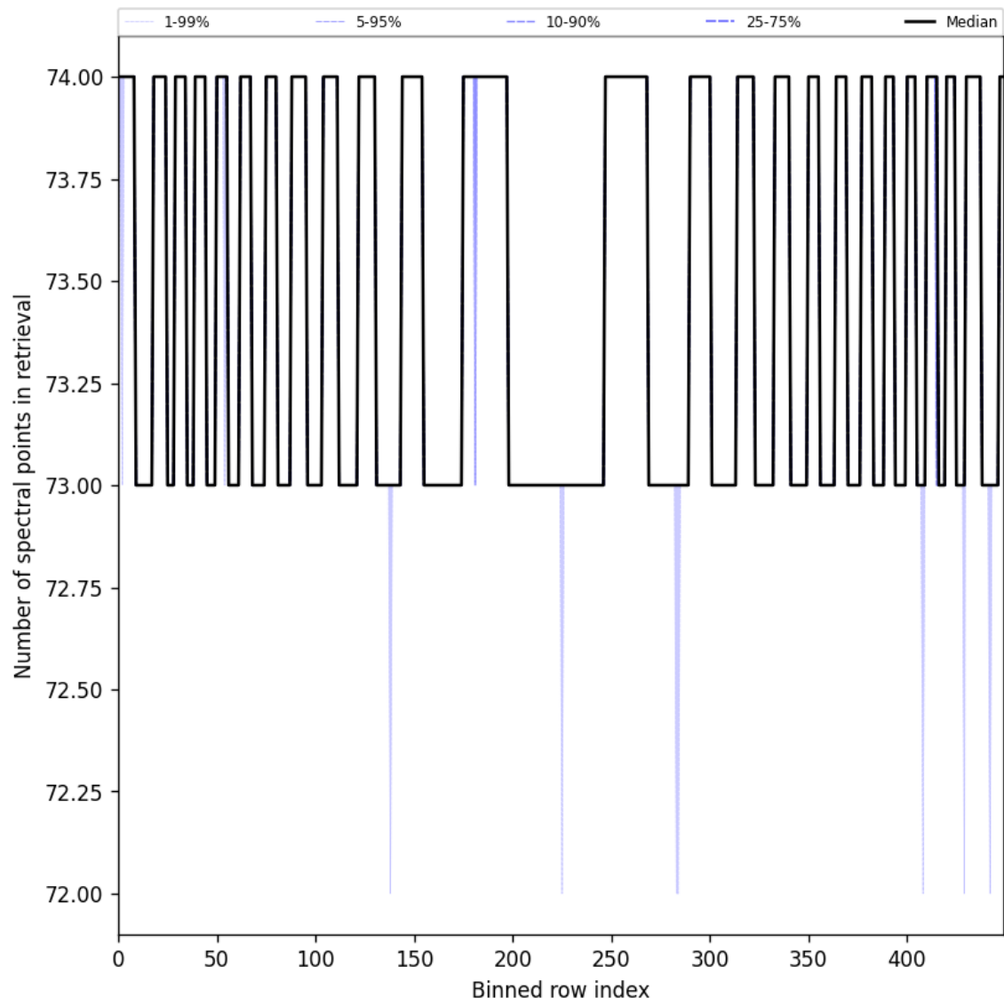
Figure 108: Along track statistics of “Number of spectral points in retrieval” for 2025-11-18 to 2025-11-19
