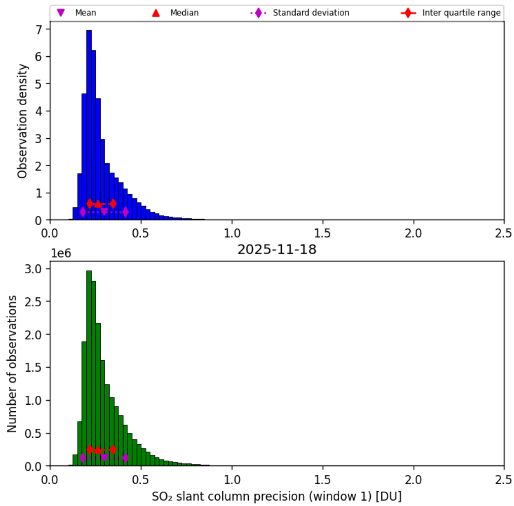
Figure 64: Histogram of “SO 2 slant column precision (window 1)” for 2025-11-18 to 2025-11-19
