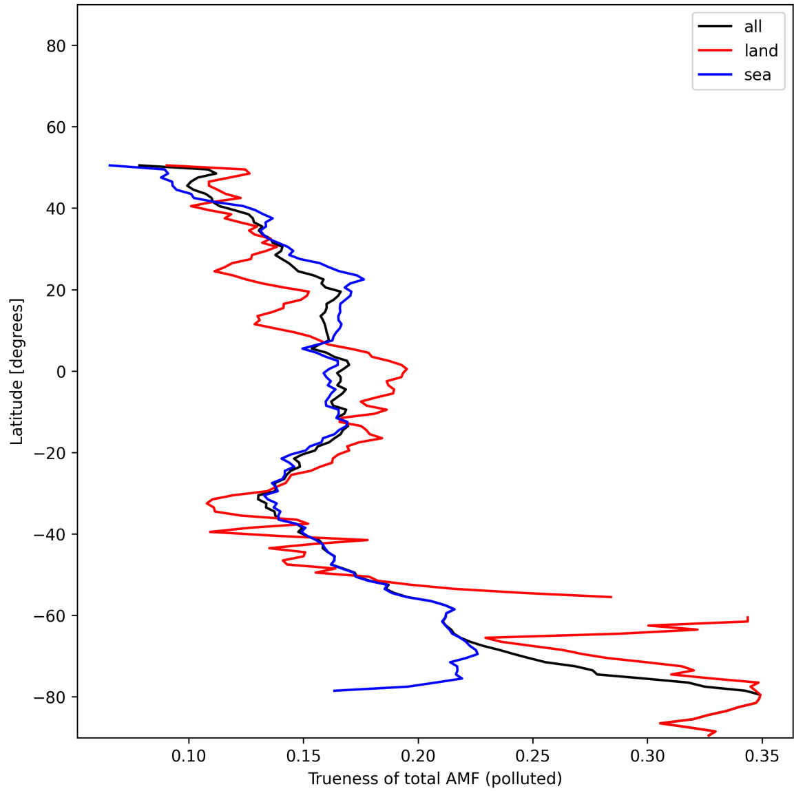
Figure 54: Zonal average of “Trueness of total AMF (polluted)” for 2025-11-18 to 2025-11-19.
