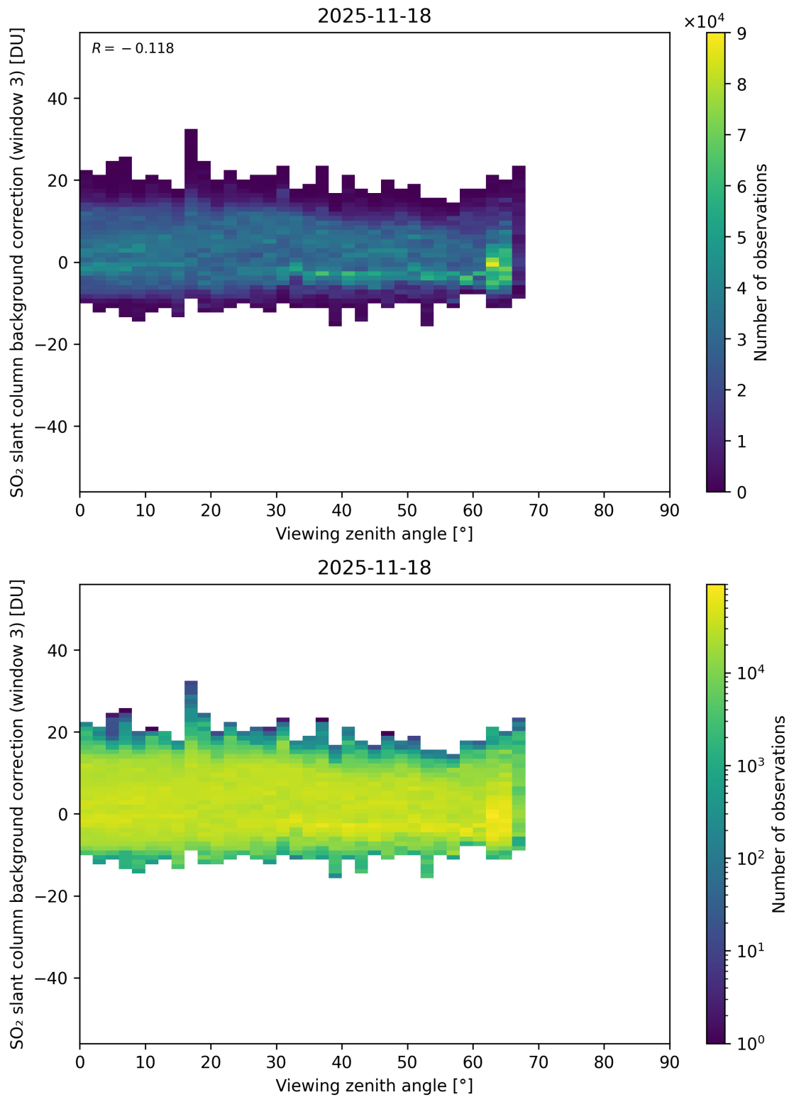
Figure 364: Scatter density plot of “Viewing zenith angle” against “SO 2 slant column background correction (window 3)” for 2025-11-18 to 2025-11-19.
