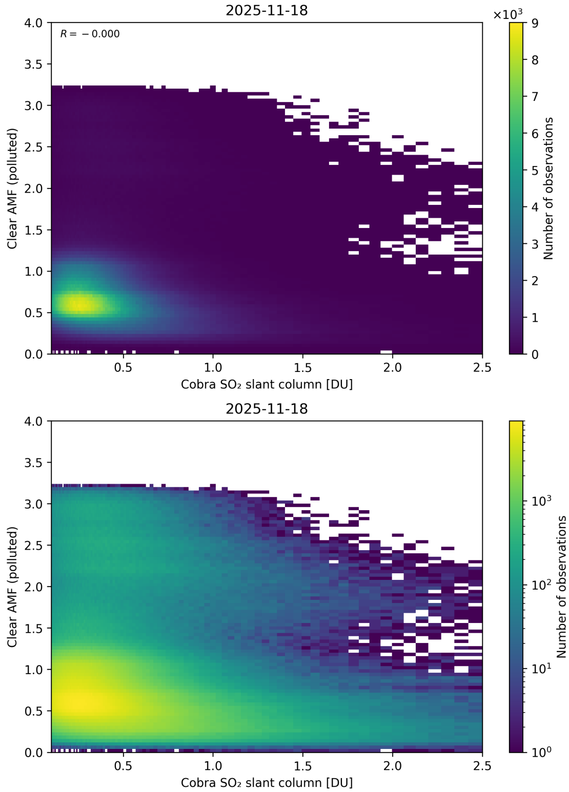
Figure 215: Scatter density plot of “Cobra SO 2 slant column” against “Clear AMF (polluted)” for 2025-11-18 to 2025-11-19.
