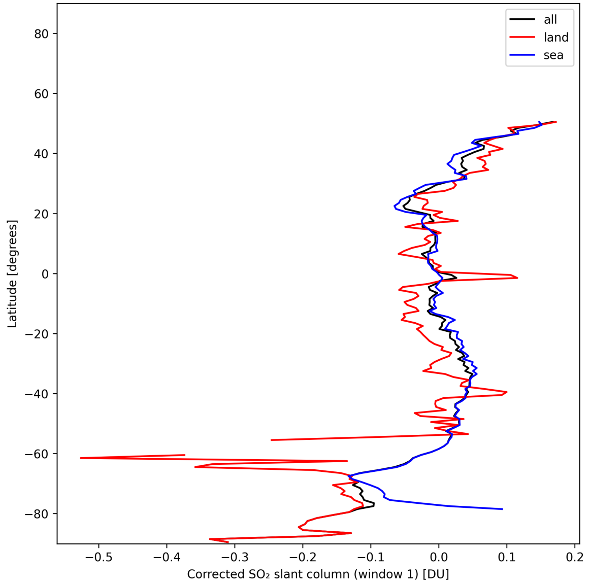
Figure 39: Zonal average of “Corrected SO 2 slant column (window 1)” for 2025-11-18 to 2025-11-19.
