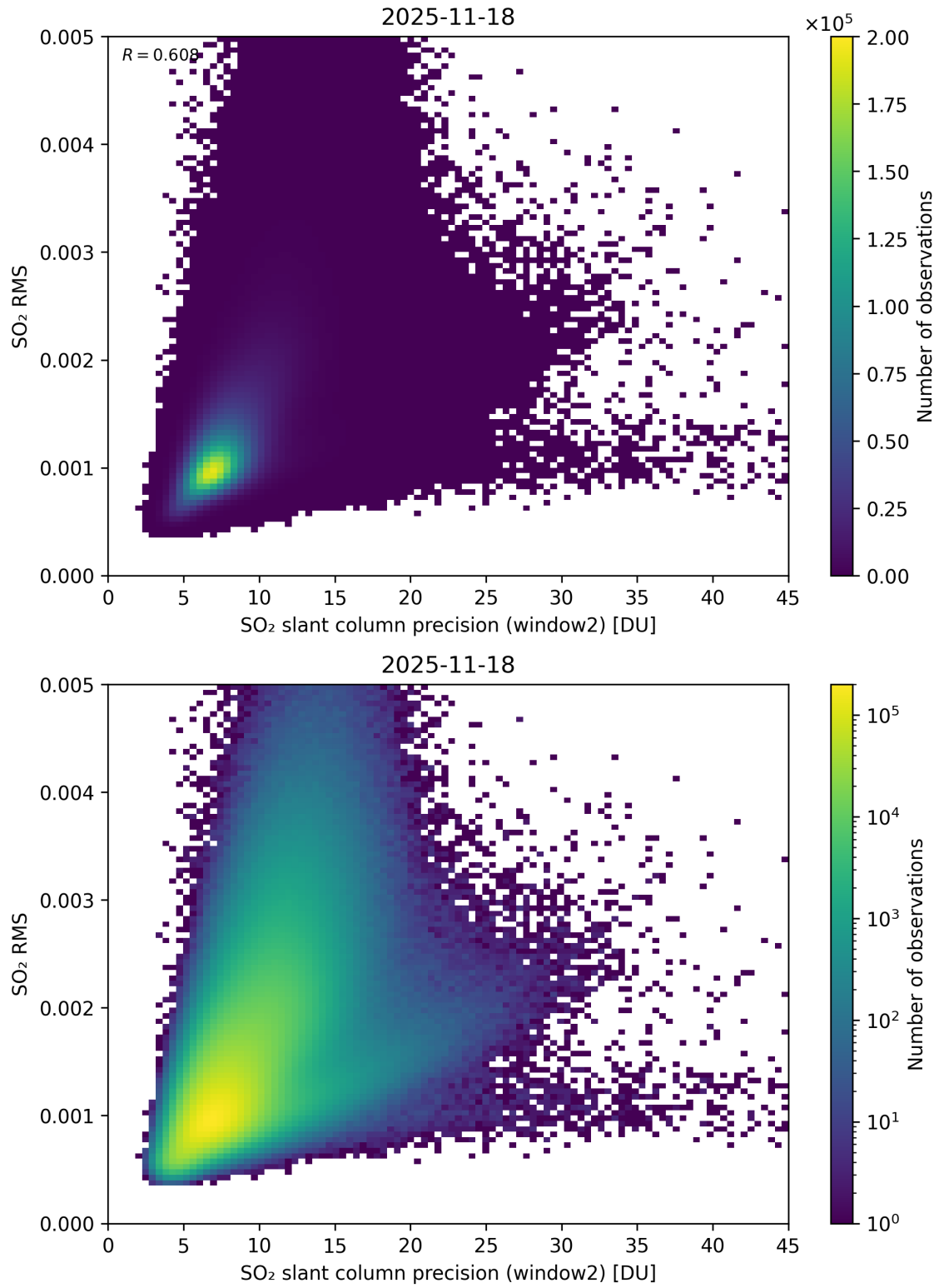
Figure 295: Scatter density plot of “SO 2 slant column precision (window2)” against “SO 2 RMS” for 2025-11-18 to 2025-11-19.
