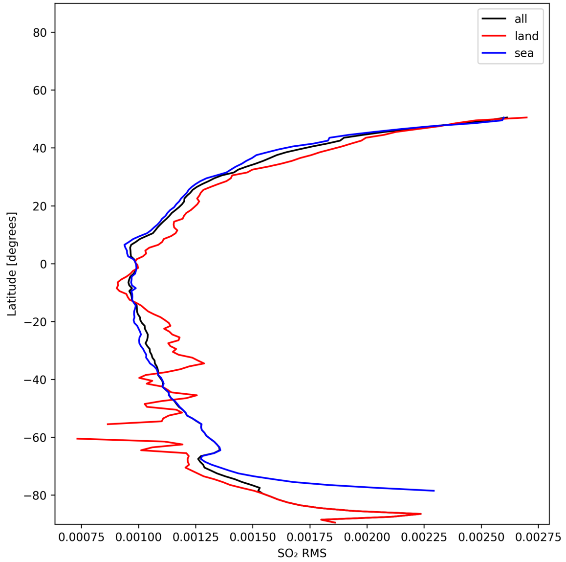
Figure 52: Zonal average of “SO 2 RMS” for 2025-11-18 to 2025-11-19.
