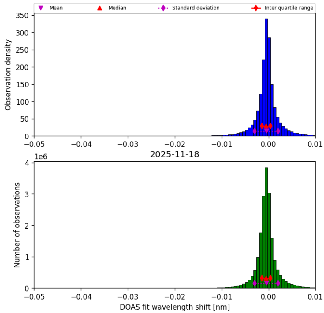
Figure 76: Histogram of “DOAS fit wavelength shift” for 2025-11-18 to 2025-11-19
