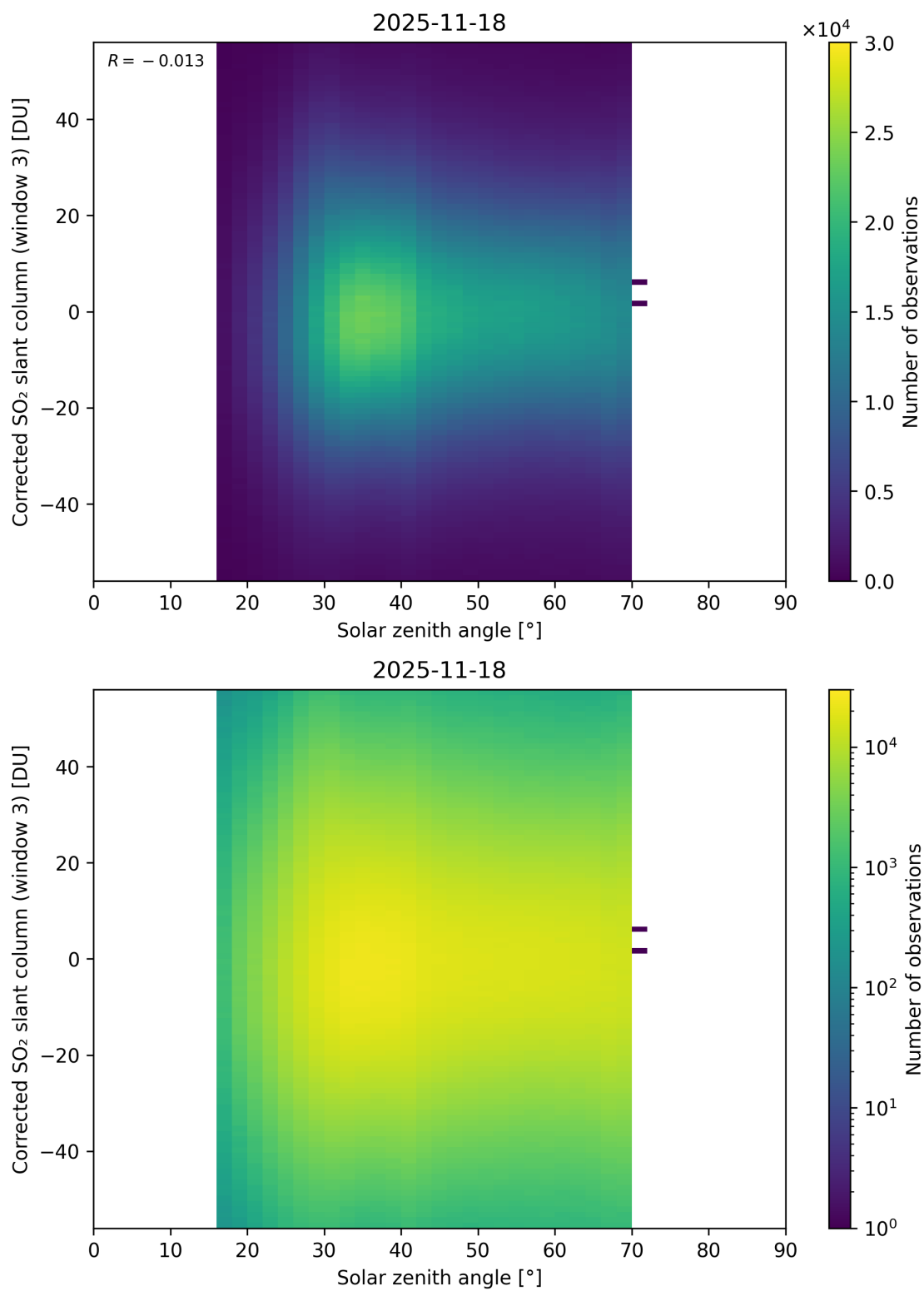
Figure 183: Scatter density plot of “Solar zenith angle” against “Corrected SO 2 slant column (window 3)” for 2025-11-18 to 2025-11-19.
