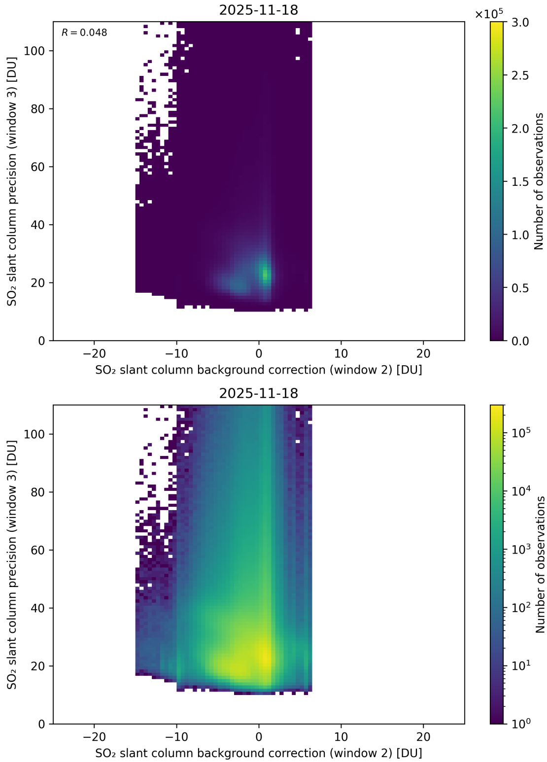
Figure 129: Scatter density plot of “SO 2 slant column background correction (window 2)” against “SO 2 slant column precision (window 3)” for 2025-11-18 to 2025-11-19.
