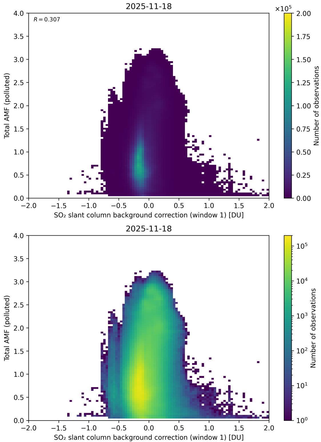
Figure 120: Scatter density plot of “SO 2 slant column background correction (window 1)” against “Total AMF (polluted)” for 2025-11-18 to 2025-11-19.
