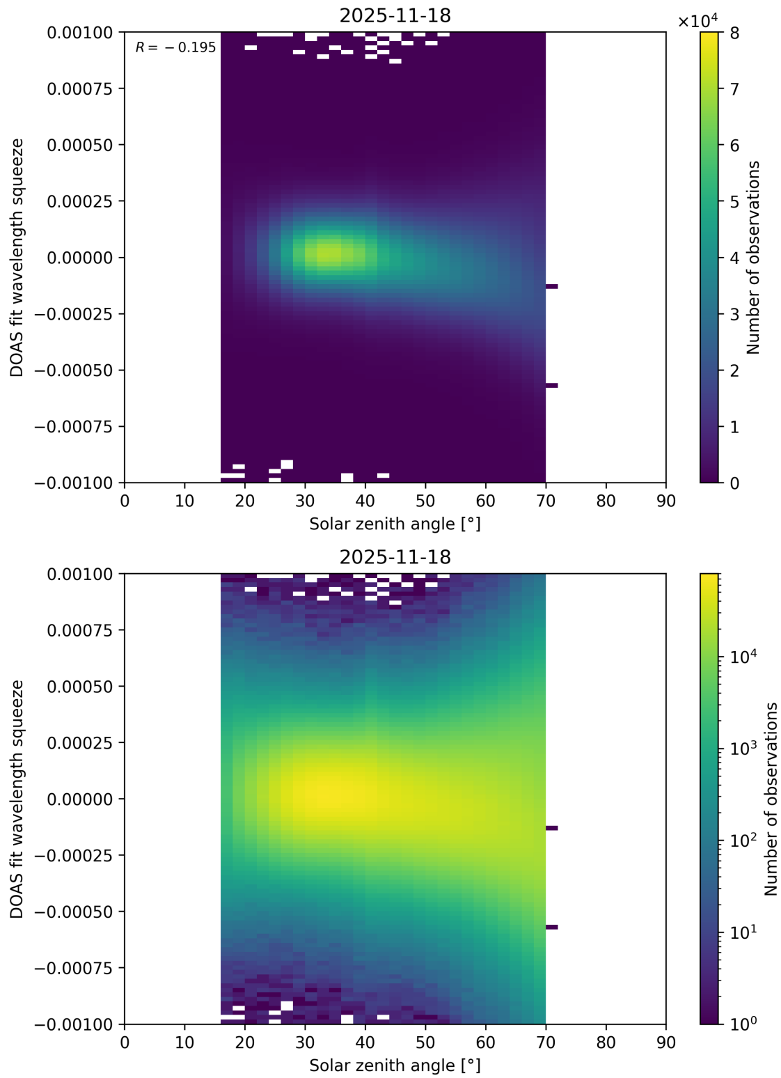
Figure 175: Scatter density plot of “Solar zenith angle” against “DOAS fit wavelength squeeze” for 2025-11-18 to 2025-11-19.
