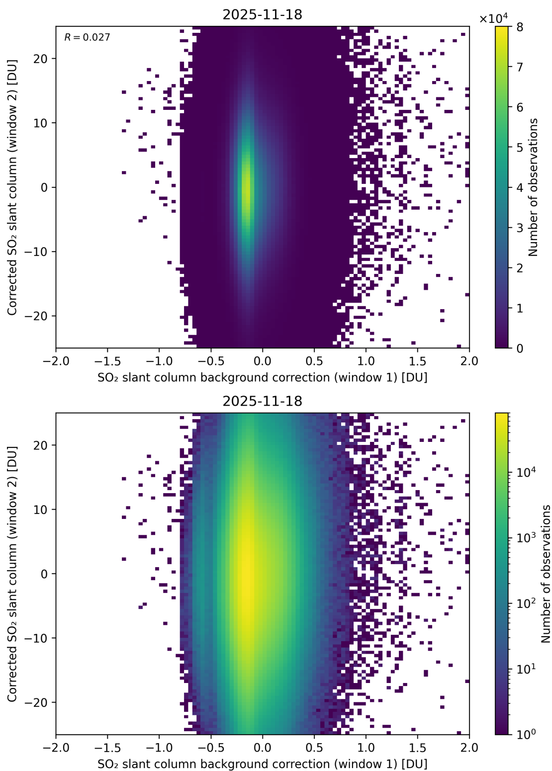
Figure 115: Scatter density plot of “SO 2 slant column background correction (window 1)” against “Corrected SO 2 slant column (window 2)” for 2025-11-18 to 2025-11-19.
