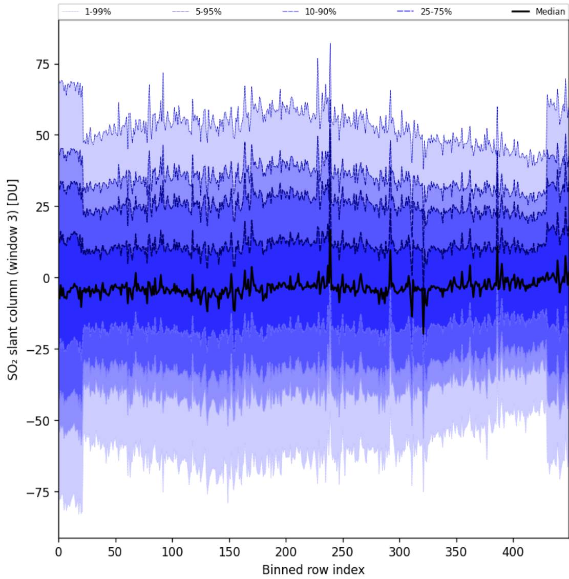
Figure 97: Along track statistics of “SO 2 slant column (window 3)” for 2025-11-18 to 2025-11-19
