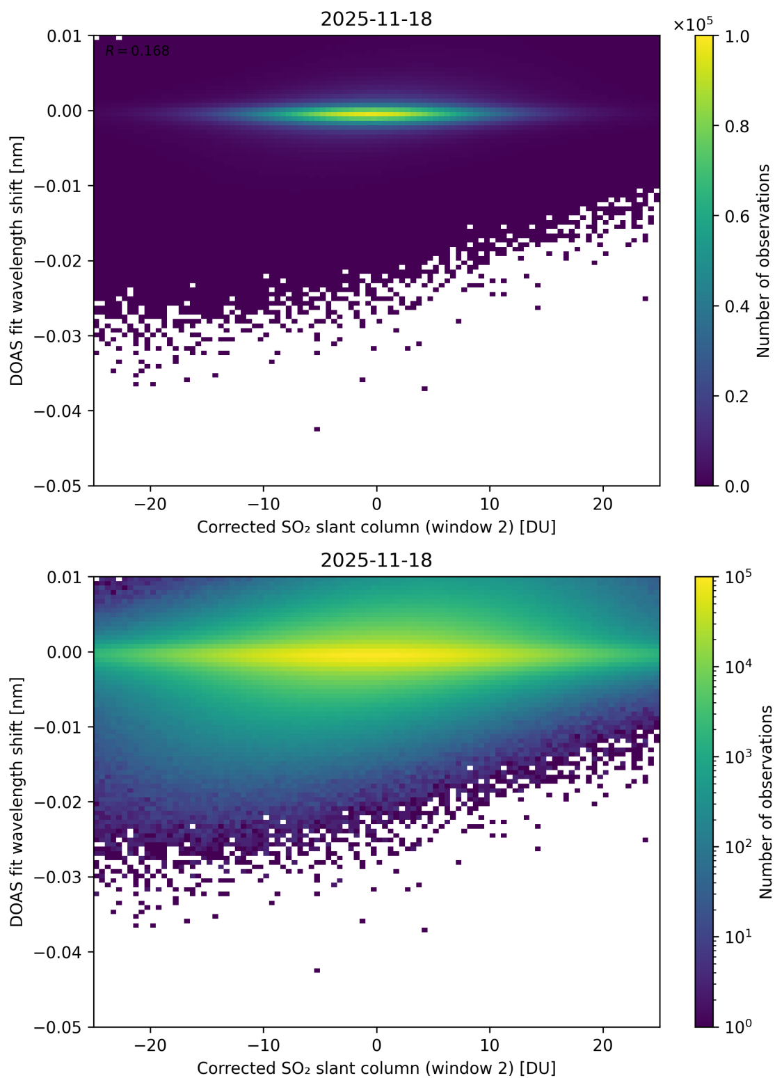
Figure 246: Scatter density plot of “Corrected SO 2 slant column (window 2)” against “DOAS fit wavelength shift” for 2025-11-18 to 2025-11-19.
