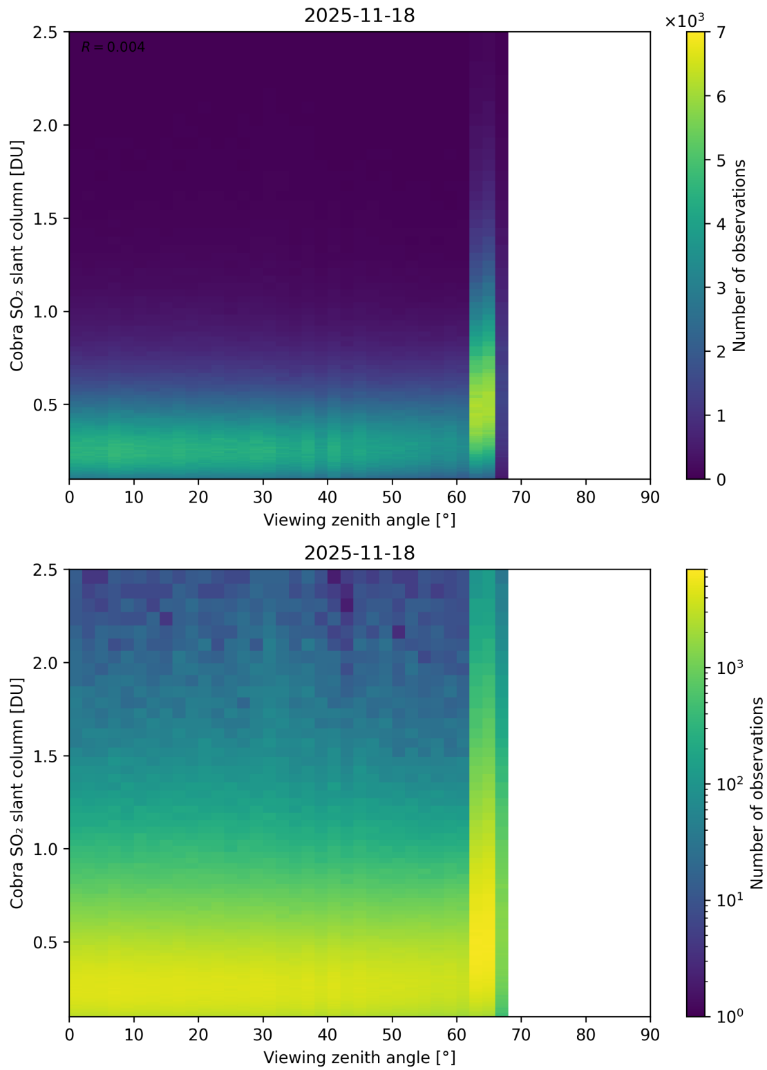
Figure 371: Scatter density plot of “Viewing zenith angle” against “Cobra SO 2 slant column” for 2025-11-18 to 2025-11-19.
