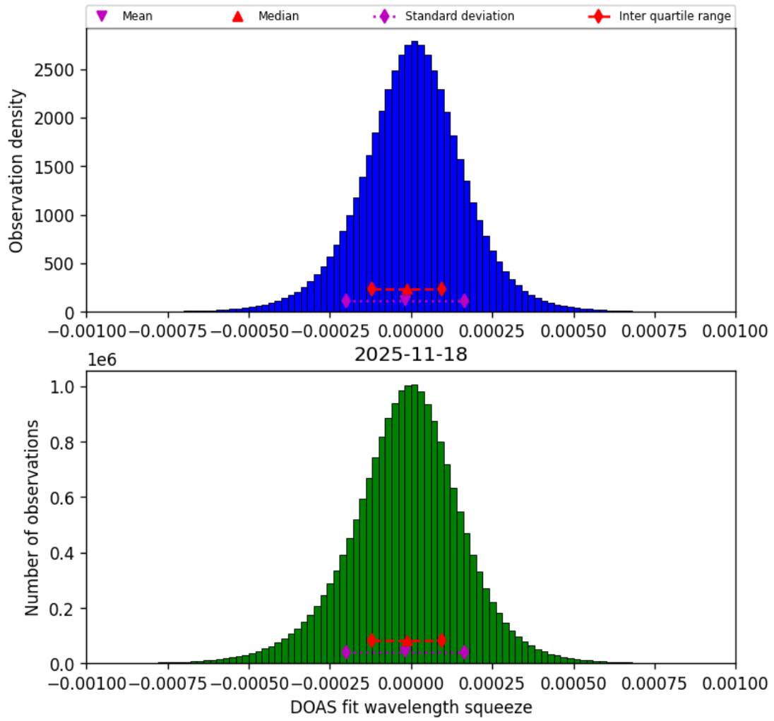
Figure 77: Histogram of “DOAS fit wavelength squeeze” for 2025-11-18 to 2025-11-19
