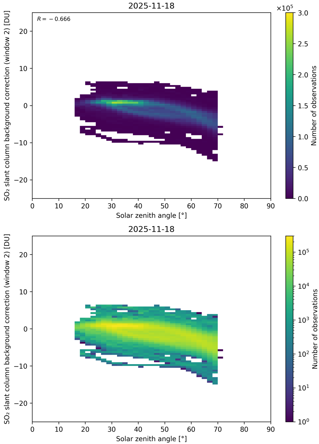
Figure 172: Scatter density plot of “Solar zenith angle” against “SO 2 slant column background correction (window 2)” for 2025-11-18 to 2025-11-19.
