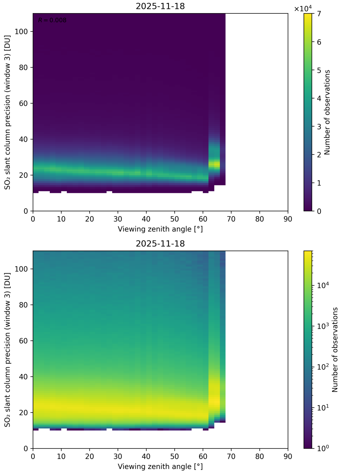
Figure 380: Scatter density plot of “Viewing zenith angle” against “SO 2 slant column precision (window 3)” for 2025-11-18 to 2025-11-19.
