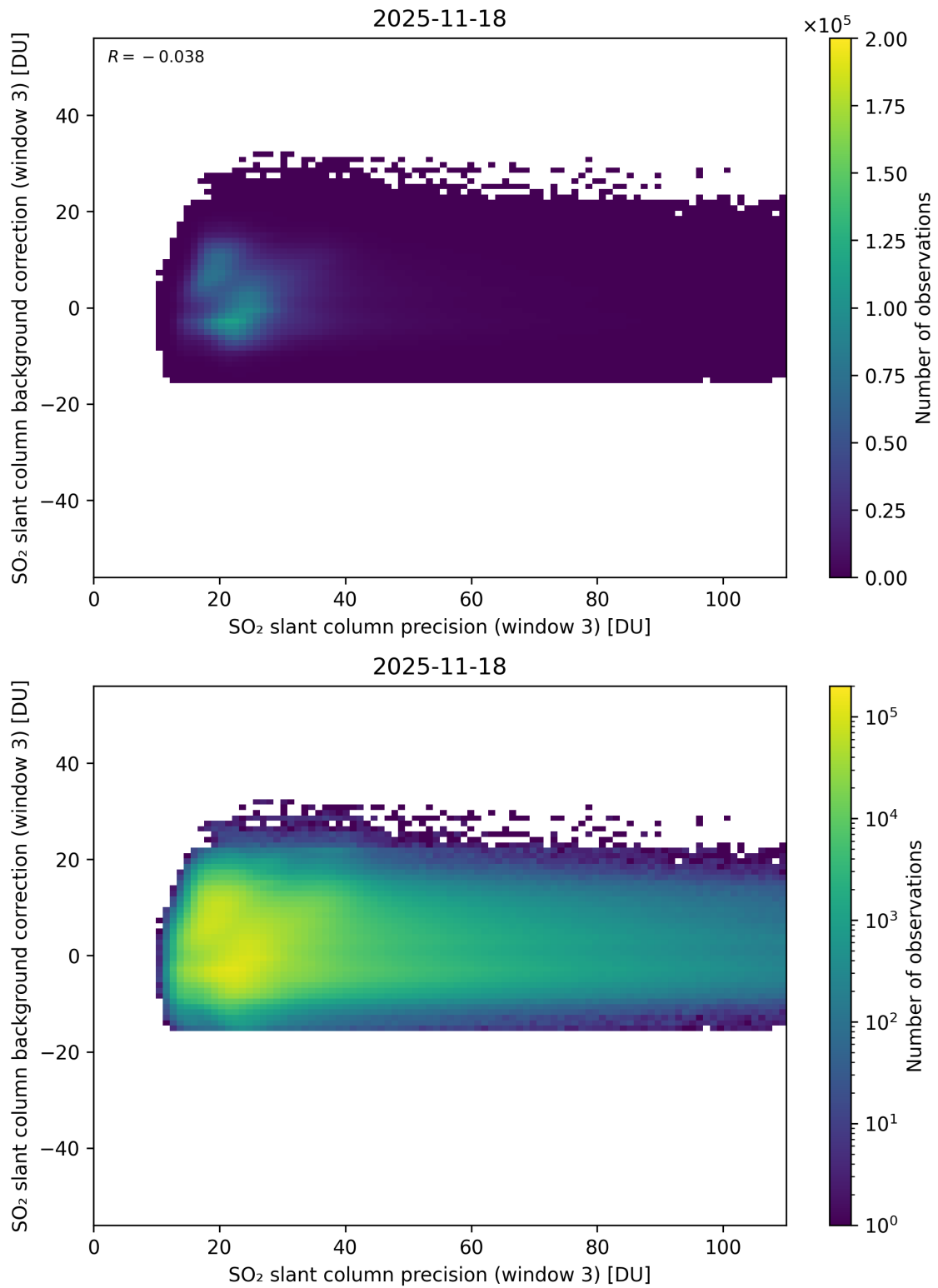
Figure 307: Scatter density plot of “SO 2 slant column precision (window 3)” against “SO 2 slant column background correction (window 3)” for 2025-11-18 to 2025-11-19.
