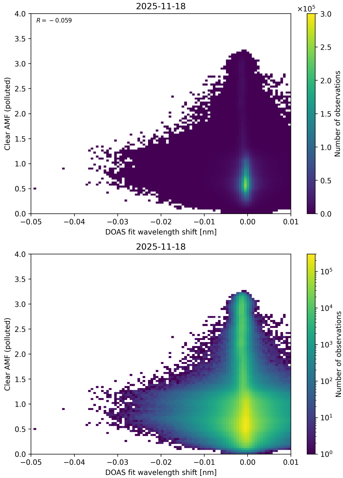
Figure 140: Scatter density plot of “DOAS fit wavelength shift” against “Clear AMF (polluted)” for 2025-11-18 to 2025-11-19.
