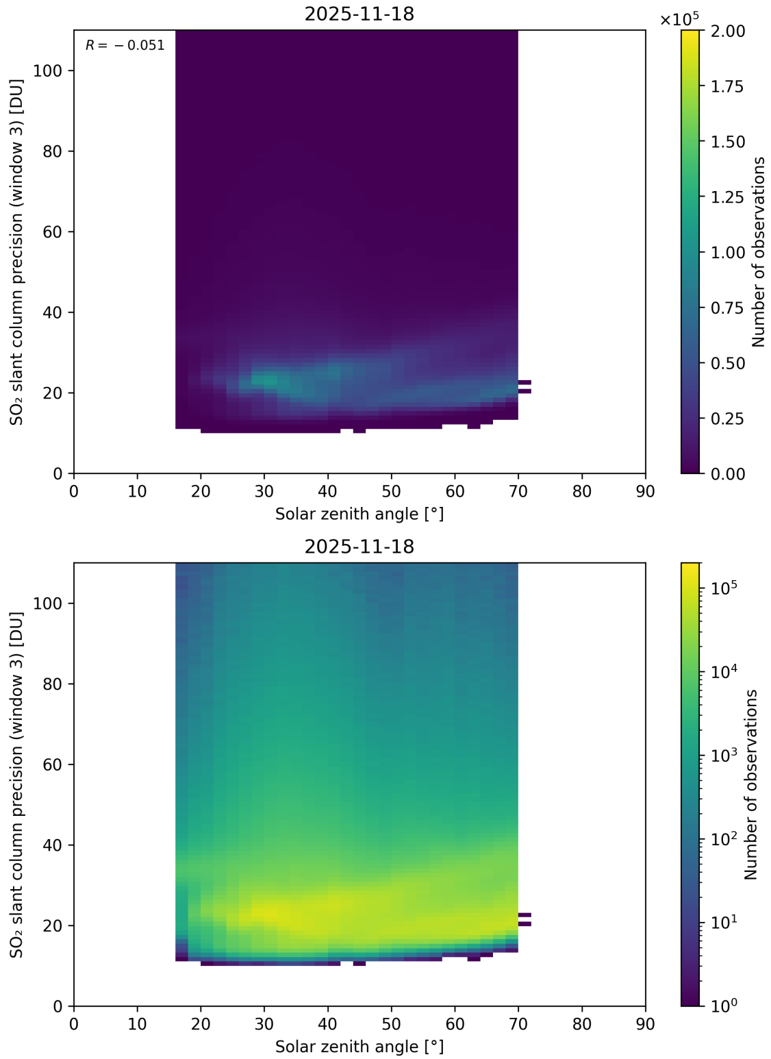
Figure 188: Scatter density plot of “Solar zenith angle” against “SO 2 slant column precision (window 3)” for 2025-11-18 to 2025-11-19.
