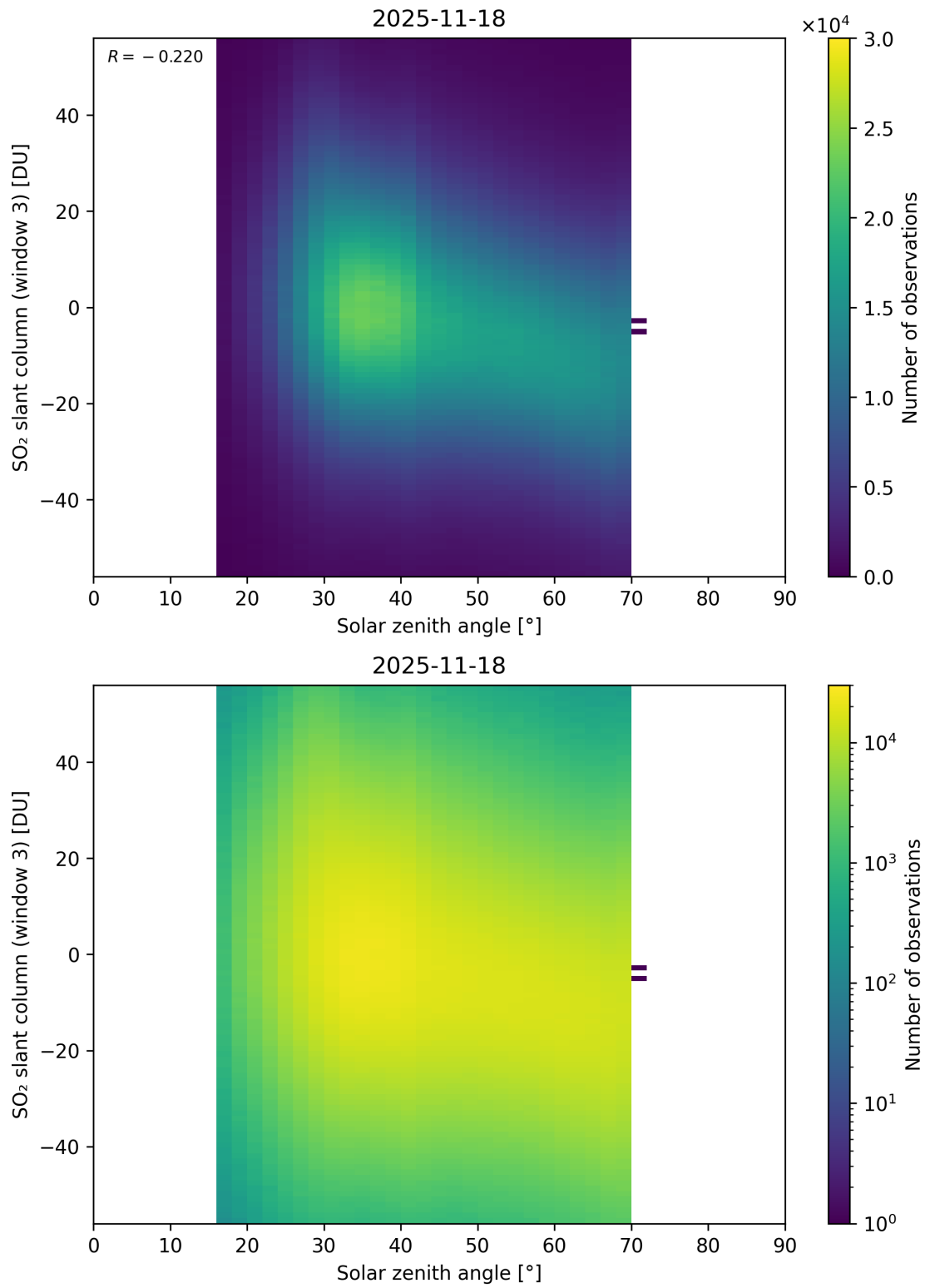
Figure 187: Scatter density plot of “Solar zenith angle” against “SO 2 slant column (window 3)” for 2025-11-18 to 2025-11-19.
