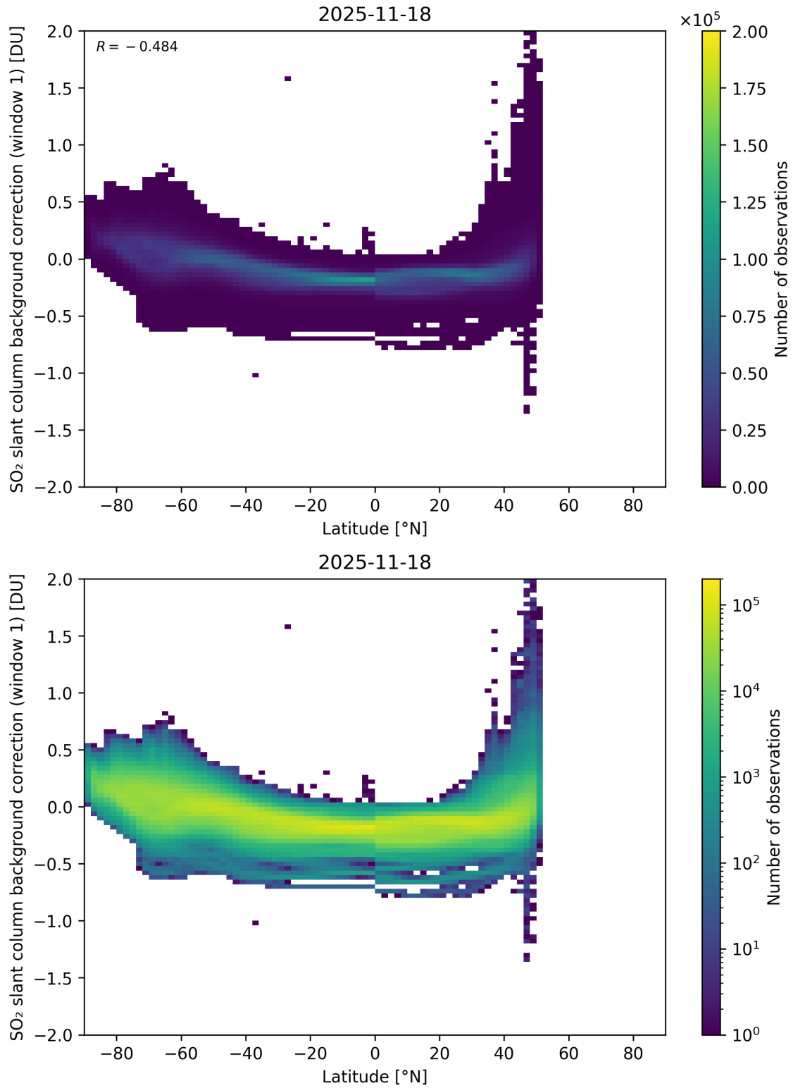
Figure 150: Scatter density plot of “Latitude” against “SO 2 slant column background correction (window 1)” for 2025-11-18 to 2025-11-19.
