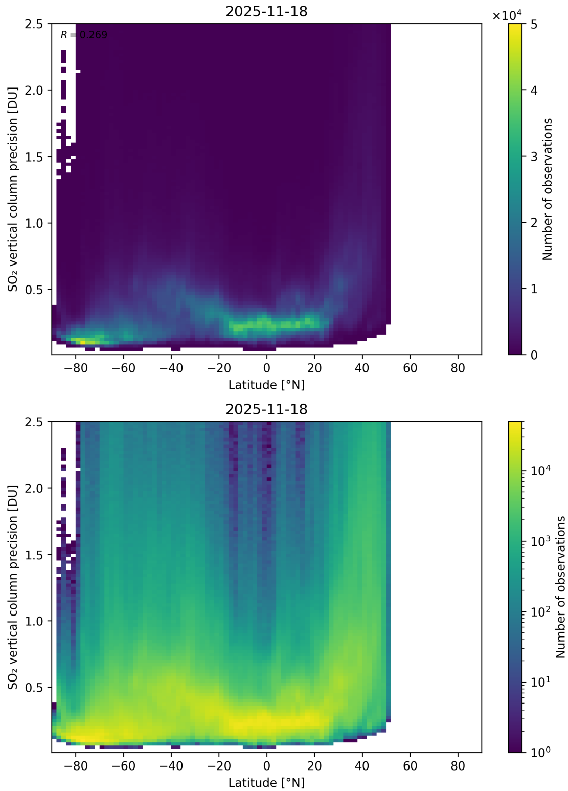
Figure 170: Scatter density plot of “Latitude” against “SO 2 vertical column precision” for 2025-11-18 to 2025-11-19.
