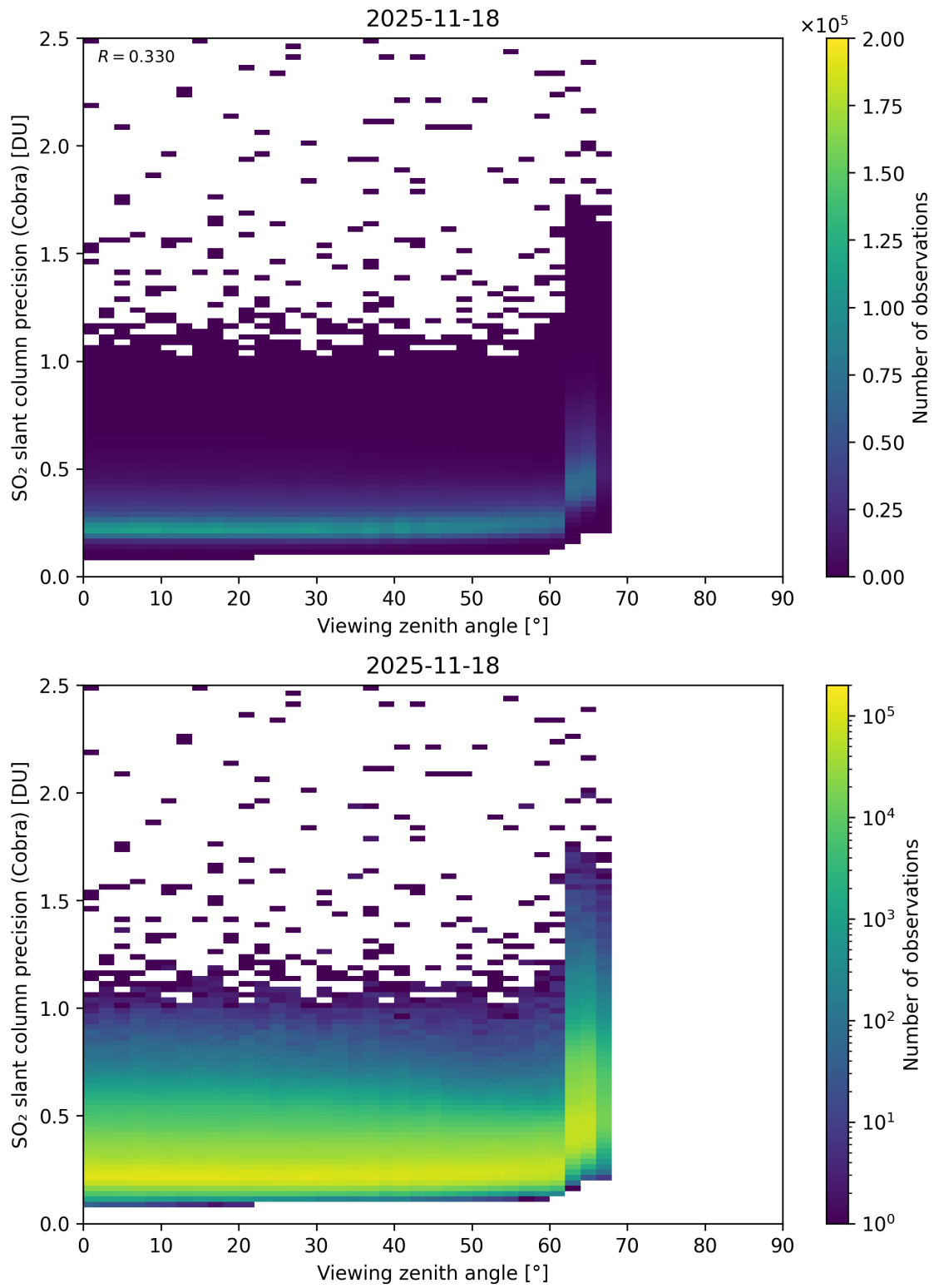
Figure 372: Scatter density plot of “Viewing zenith angle” against “SO 2 slant column precision (Cobra)” for 2025-11-18 to 2025-11-19.
