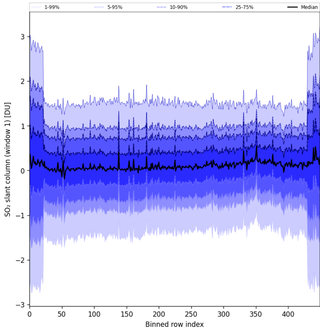
Figure 89: Along track statistics of "SO 2 slant column (window 1)" for 2025-11-18 to 2025-11-19
