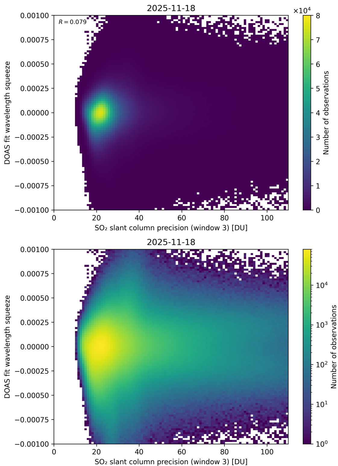
Figure 309: Scatter density plot of “SO 2 slant column precision (window 3)” against “DOAS fit wavelength squeeze” for 2025-11-18 to 2025-11-19.
