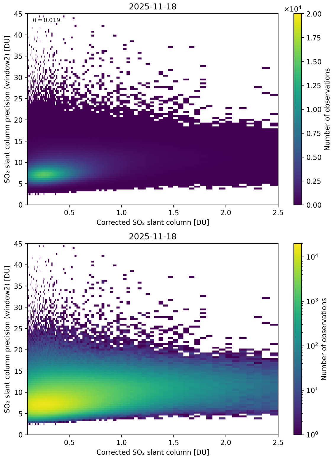
Figure 239: Scatter density plot of “Corrected SO 2 slant column” against “SO 2 slant column precision (window2)” for 2025-11-18 to 2025-11-19.
