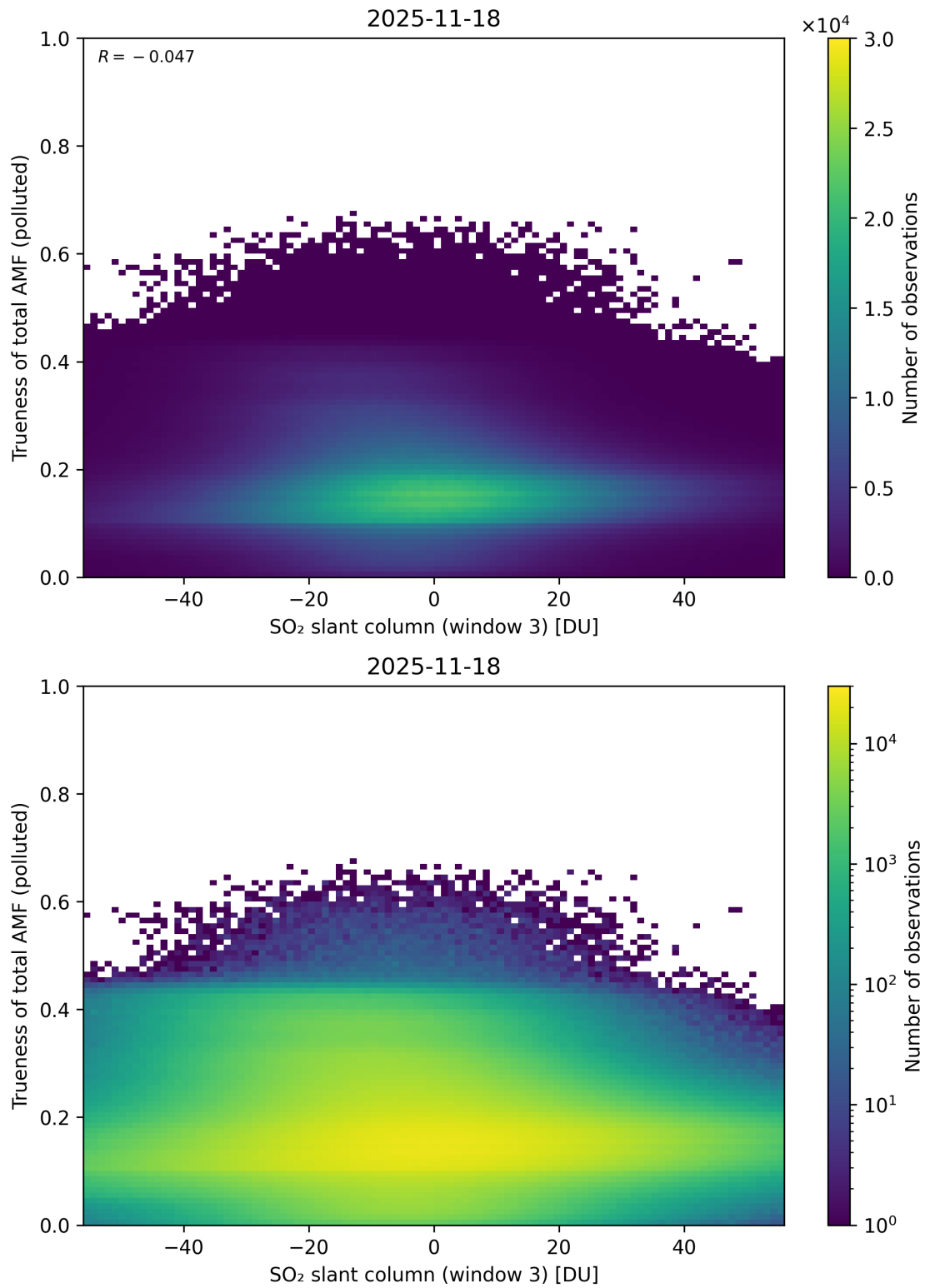
Figure 319: Scatter density plot of “SO 2 slant column (window 3)” against “Trueness of total AMF (polluted)” for 2025-11-18 to 2025-11-19.
