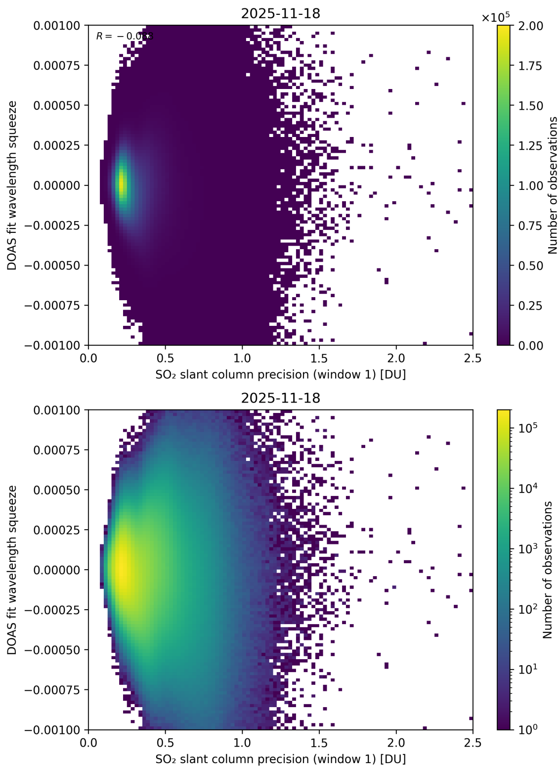
Figure 272: Scatter density plot of “SO 2 slant column precision (window 1)” against “DOAS fit wavelength squeeze” for 2025-11-18 to 2025-11-19.
