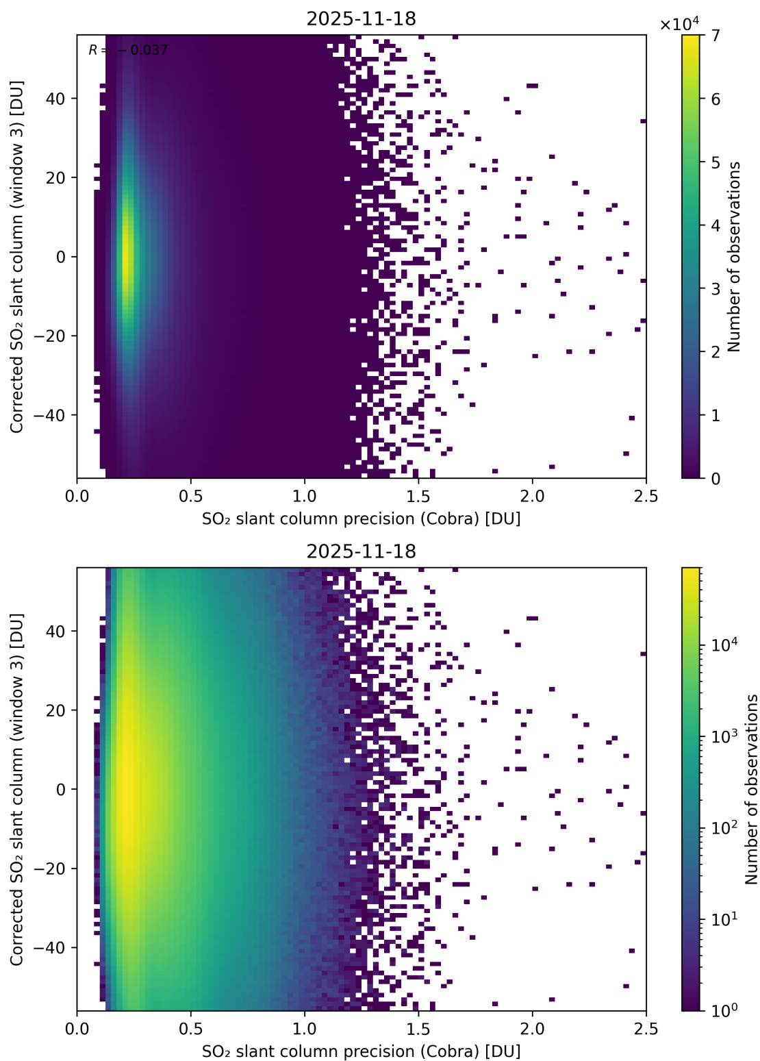
Figure 207: Scatter density plot of “SO 2 slant column precision (Cobra)” against “Corrected SO 2 slant column (window 3)” for 2025-11-18 to 2025-11-19.
