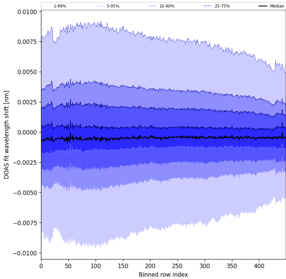
Figure 102: Along track statistics of “DOAS fit wavelength shift” for 2025-11-18 to 2025-11-19
