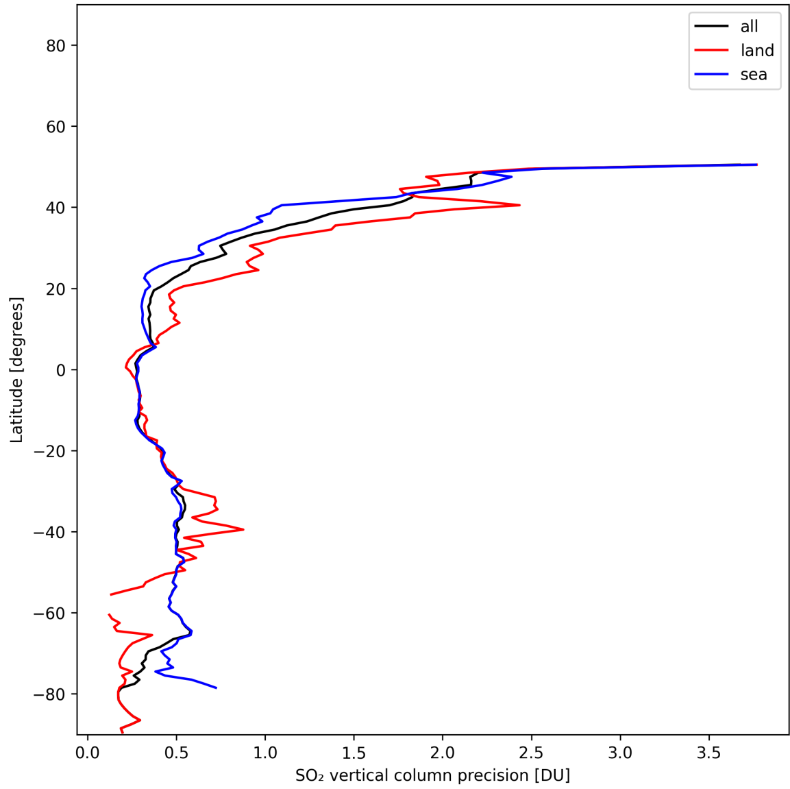
Figure 33: Zonal average of “SO 2 vertical column precision” for 2025-11-18 to 2025-11-19.
