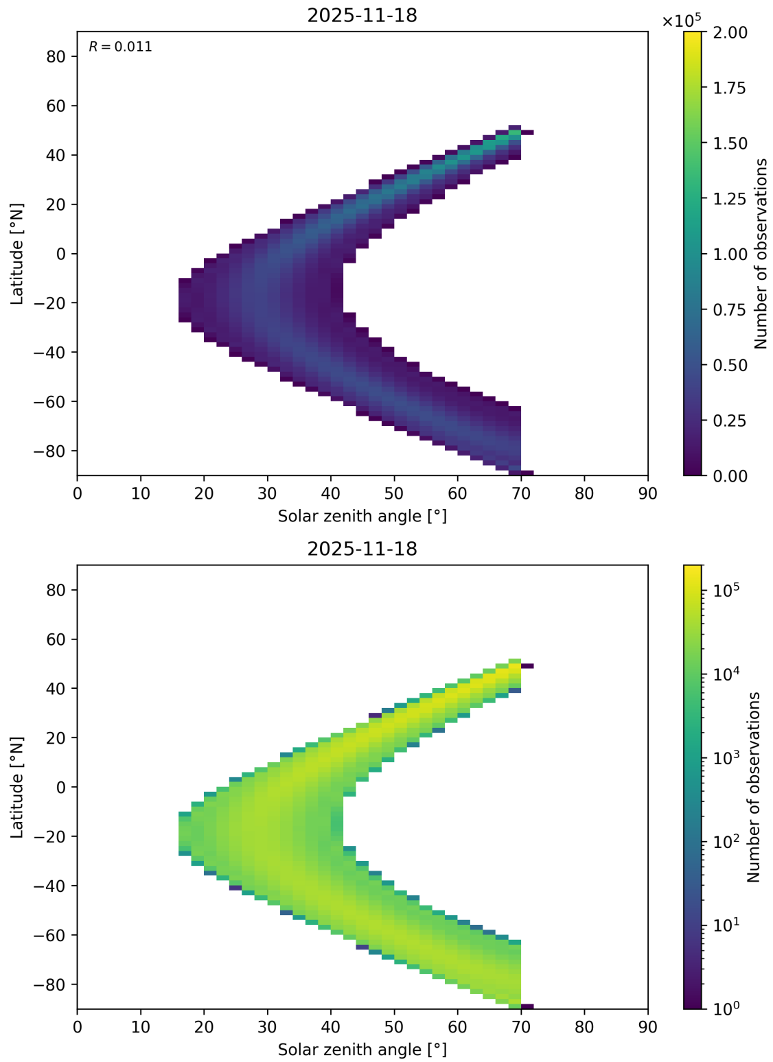
Figure 177: Scatter density plot of “Solar zenith angle” against “Latitude” for 2025-11-18 to 2025-11-19.
