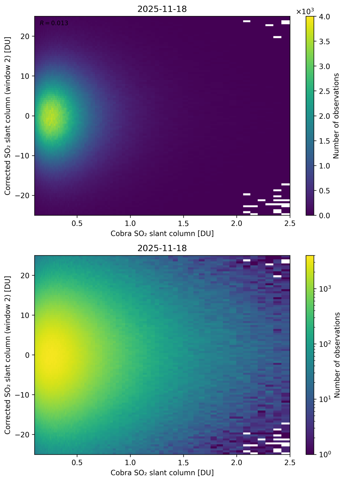
Figure 217: Scatter density plot of “Cobra SO 2 slant column” against “Corrected SO 2 slant column (window 2)” for 2025-11-18 to 2025-11-19.
