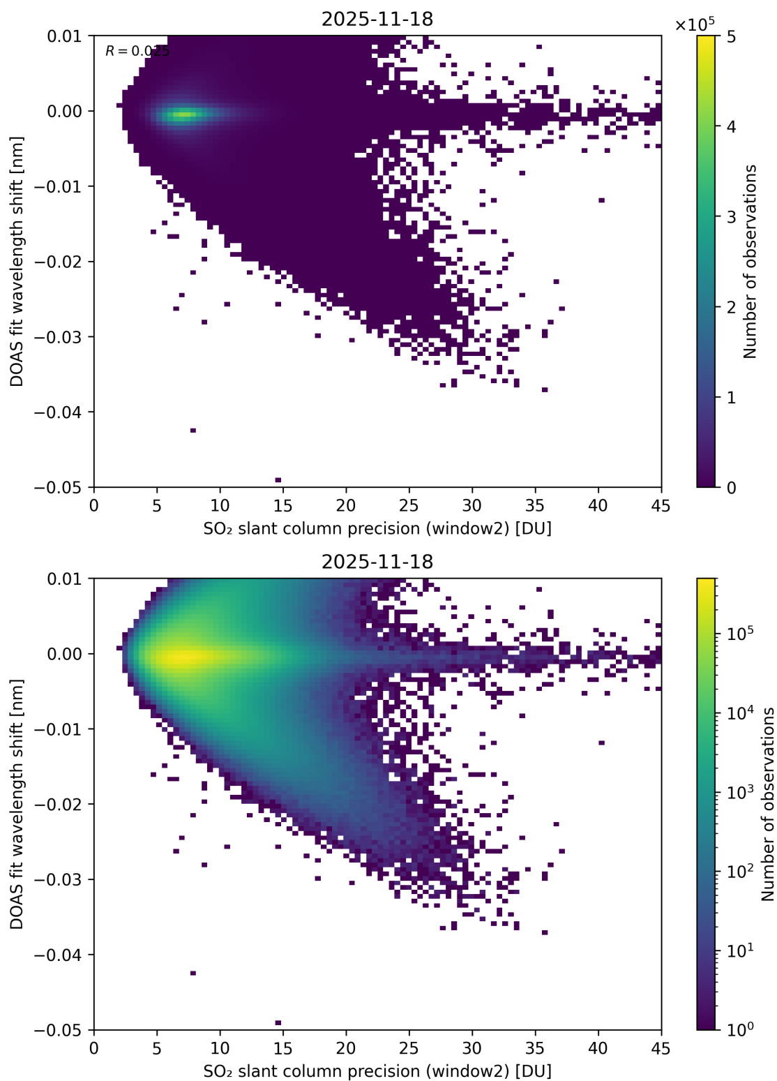
Figure 293: Scatter density plot of “SO 2 slant column precision (window2)” against “DOAS fit wavelength shift” for 2025-11-18 to 2025-11-19.
