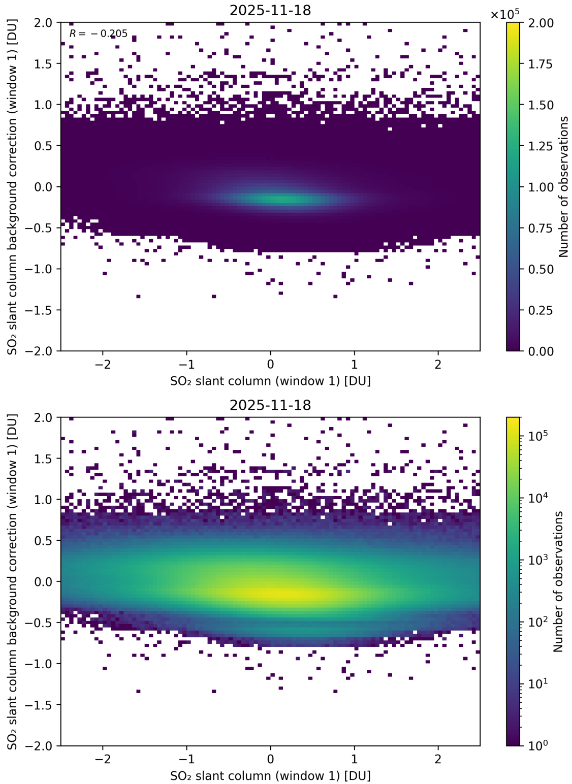
Figure 262: Scatter density plot of “SO 2 slant column (window 1)” against “SO 2 slant column background correction (window 1)” for 2025-11-18 to 2025-11-19.
