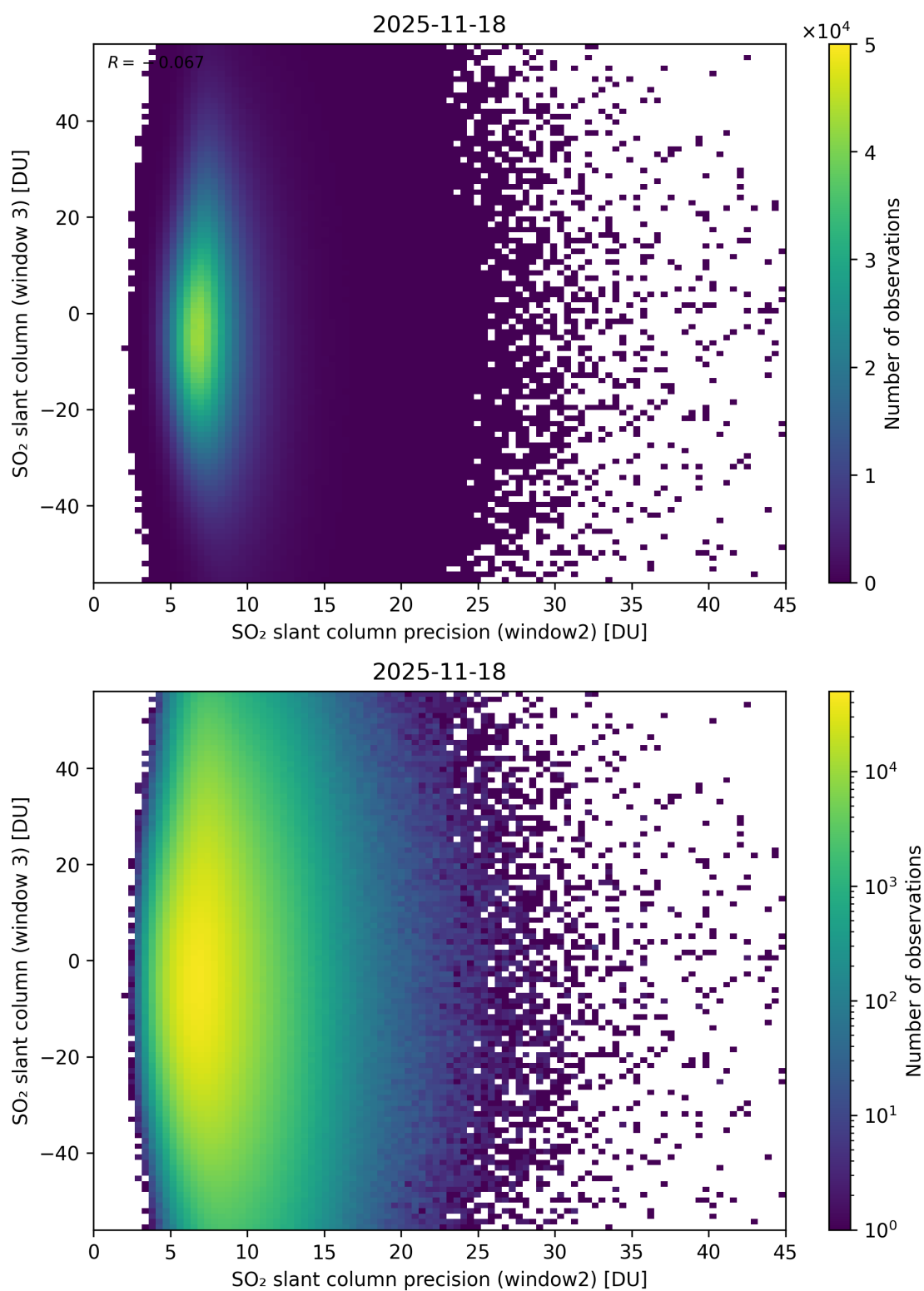
Figure 299: Scatter density plot of “SO 2 slant column precision (window2)” against “SO 2 slant column (window 3)” for 2025-11-18 to 2025-11-19.
