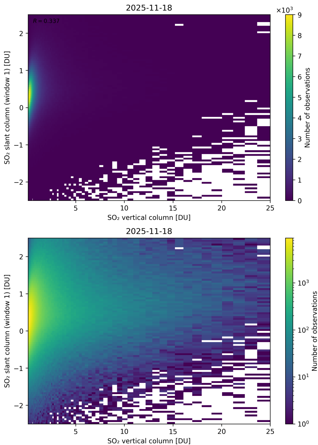
Figure 354: Scatter density plot of “SO 2 vertical column” against “SO 2 slant column (window 1)” for 2025-11-18 to 2025-11-19.
