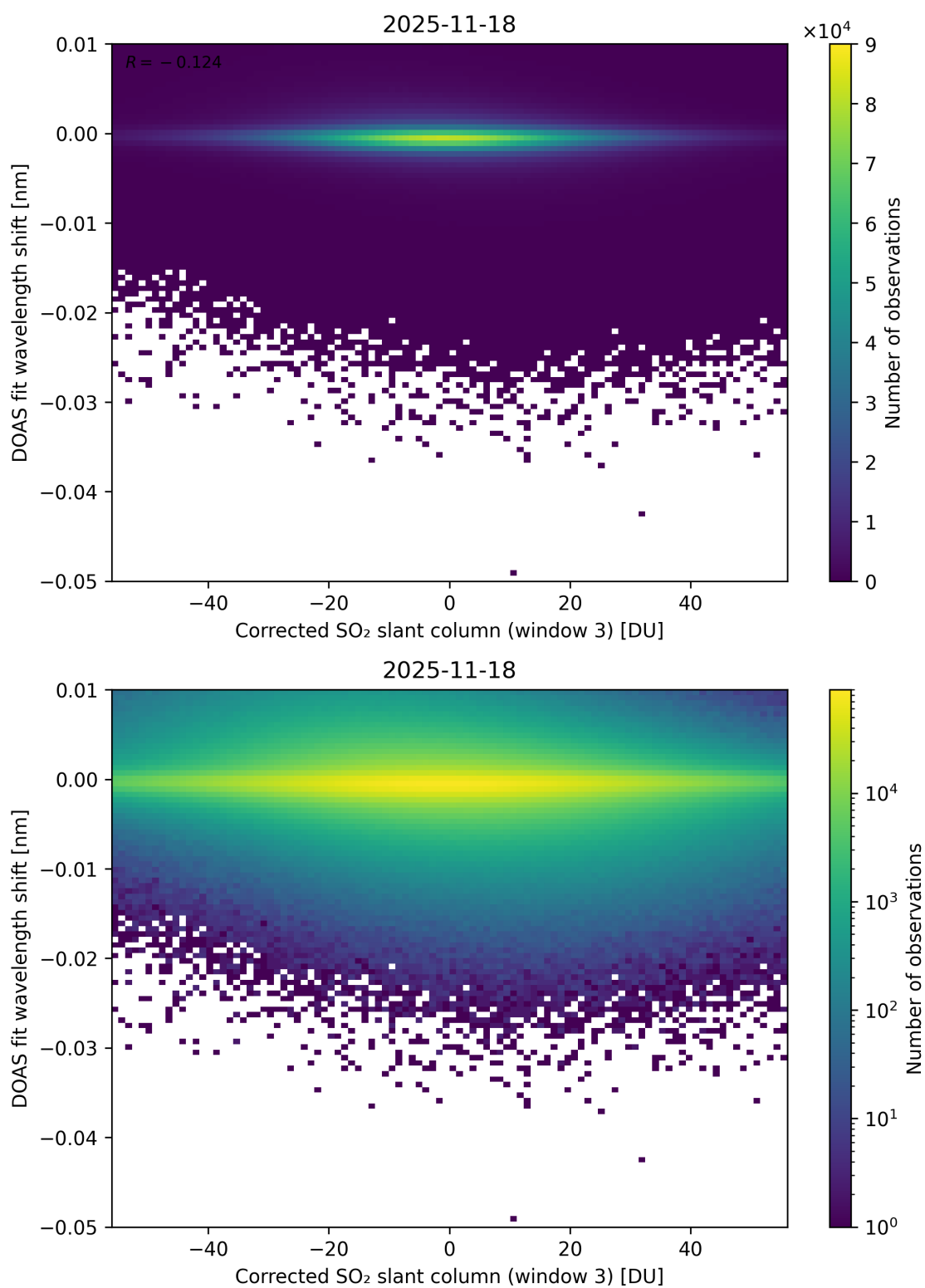
Figure 256: Scatter density plot of “Corrected SO 2 slant column (window 3)” against “DOAS fit wavelength shift” for 2025-11-18 to 2025-11-19.
