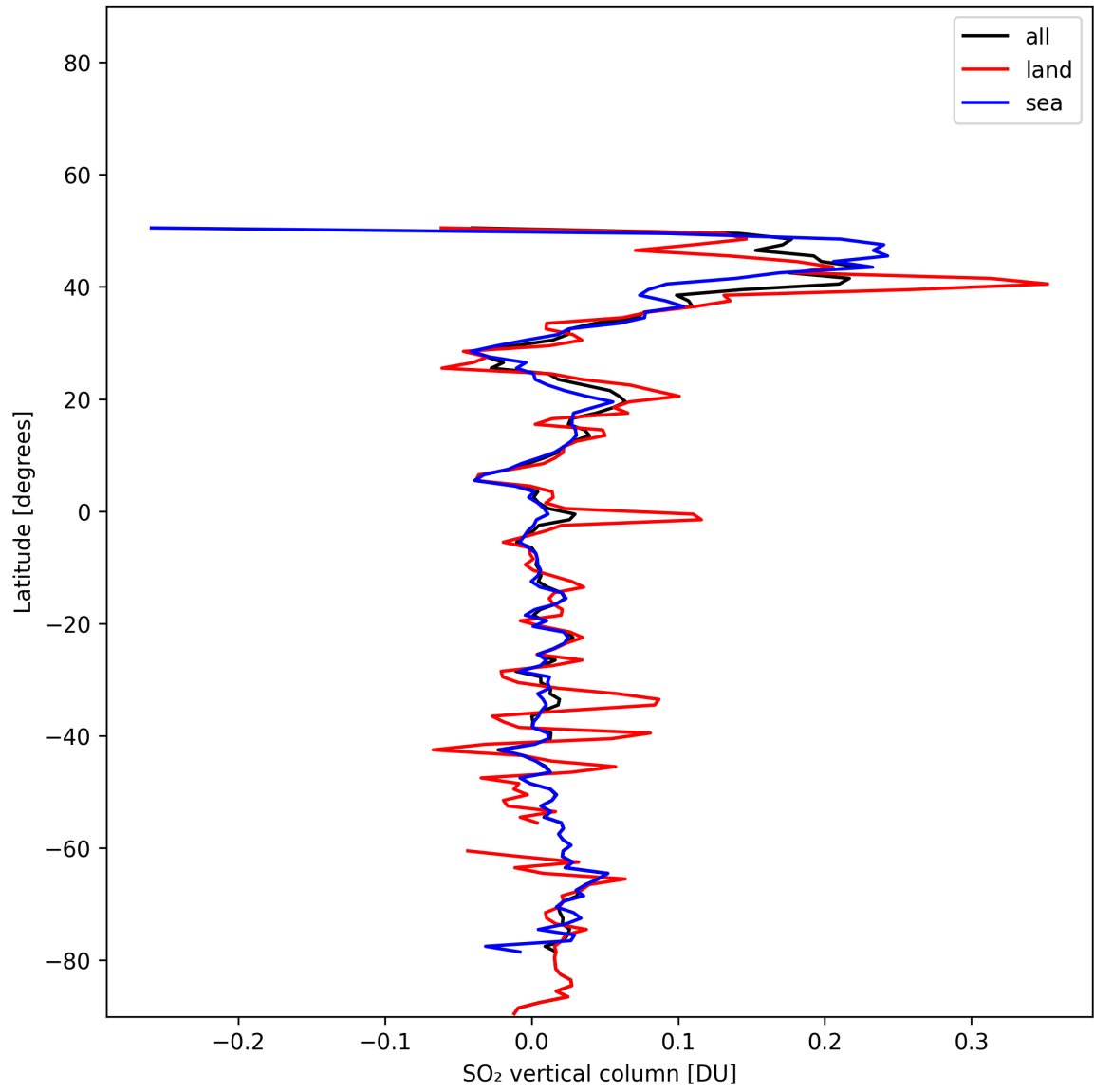
Figure 32: Zonal average of “SO 2 vertical column” for 2025-11-18 to 2025-11-19.
