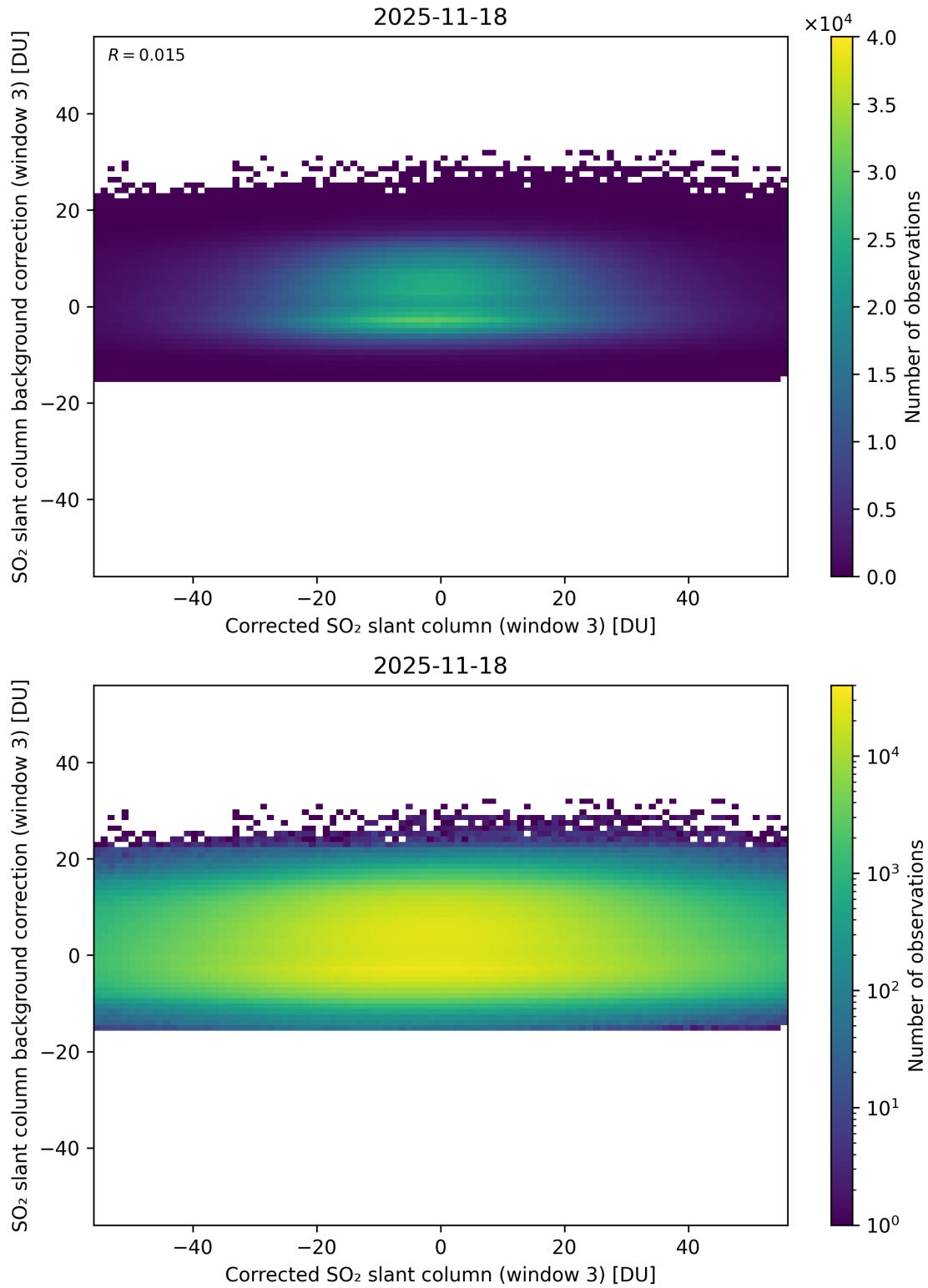
Figure 255: Scatter density plot of “Corrected SO 2 slant column (window 3)” against “SO 2 slant column background correction (window 3)” for 2025-11-18 to 2025-11-19.
