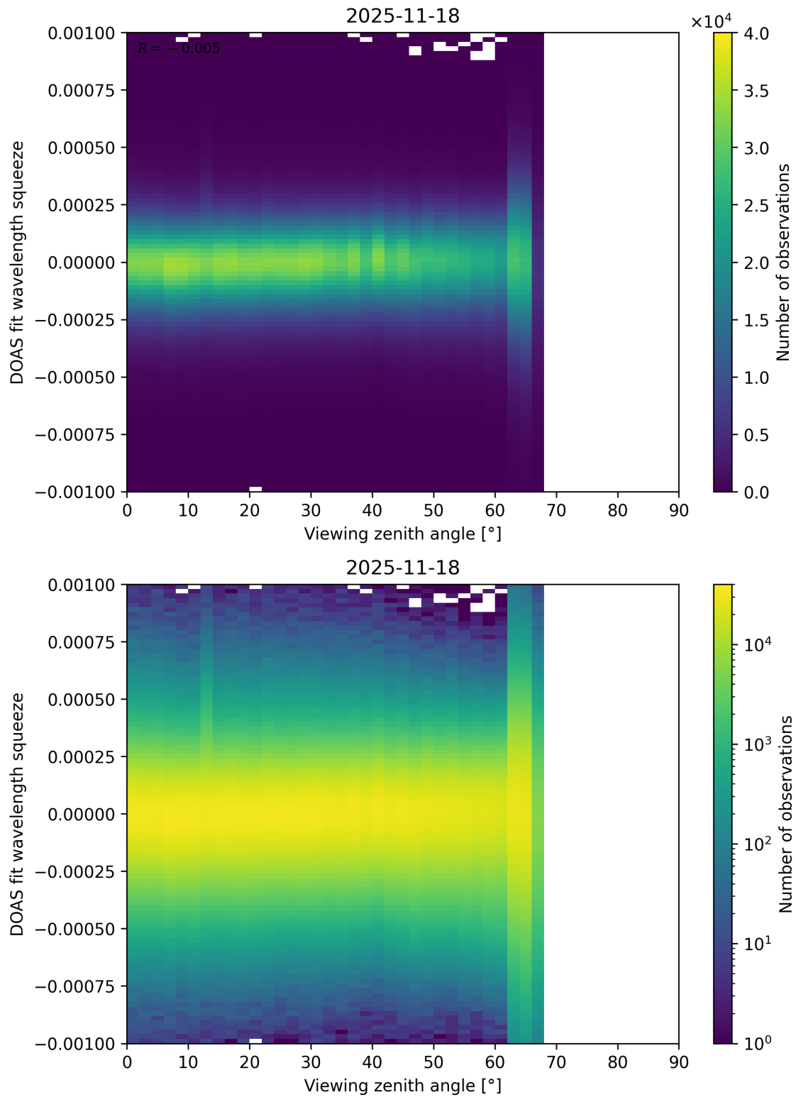
Figure 366: Scatter density plot of “Viewing zenith angle” against “DOAS fit wavelength squeeze” for 2025-11-18 to 2025-11-19.
