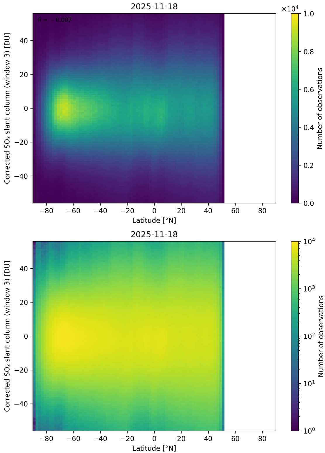
Figure 161: Scatter density plot of “Latitude” against “Corrected SO 2 slant column (window 3)” for 2025-11-18 to 2025-11-19.
