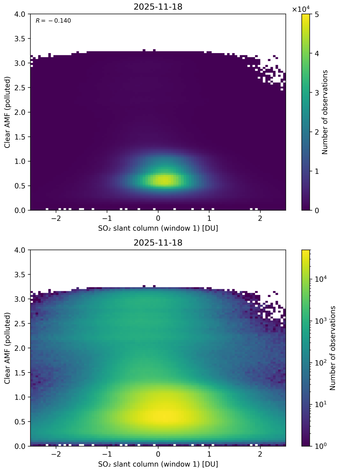
Figure 282: Scatter density plot of “SO 2 slant column (window 1)” against “Clear AMF (polluted)” for 2025-11-18 to 2025-11-19.
