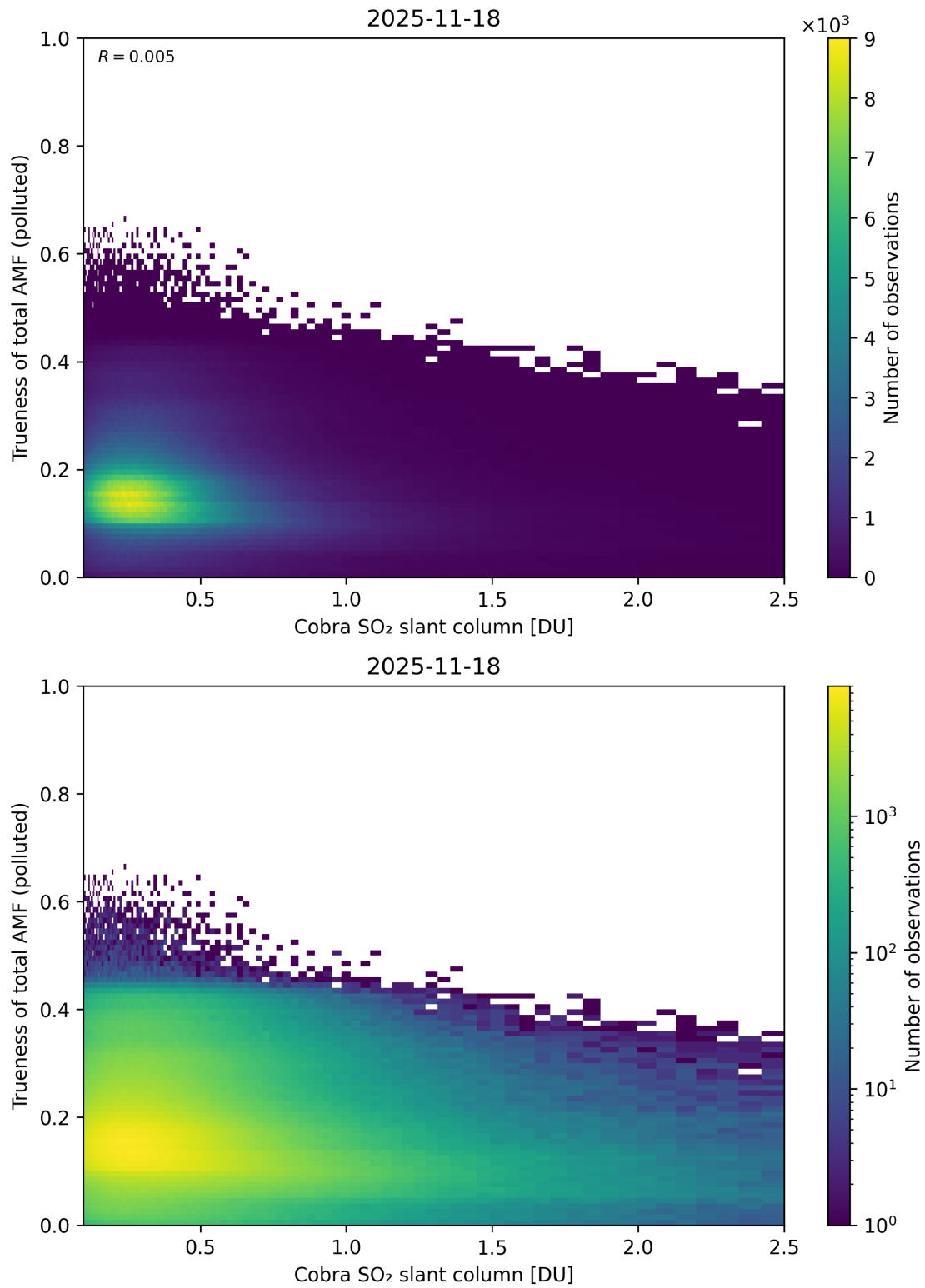
Figure 225: Scatter density plot of “Cobra SO 2 slant column” against “Trueness of total AMF (polluted)” for 2025-11-18 to 2025-11-19.
