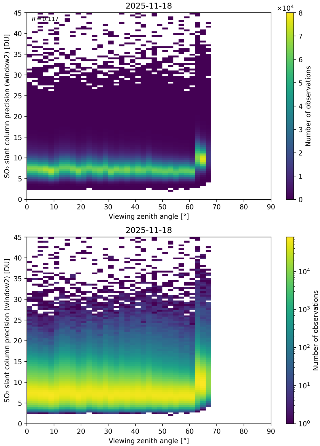
Figure 378: Scatter density plot of “Viewing zenith angle” against “SO 2 slant column precision (window2)” for 2025-11-18 to 2025-11-19.
