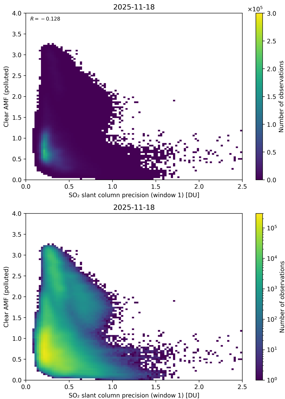
Figure 274: Scatter density plot of “SO 2 slant column precision (window 1)” against “Clear AMF (polluted)” for 2025-11-18 to 2025-11-19.
