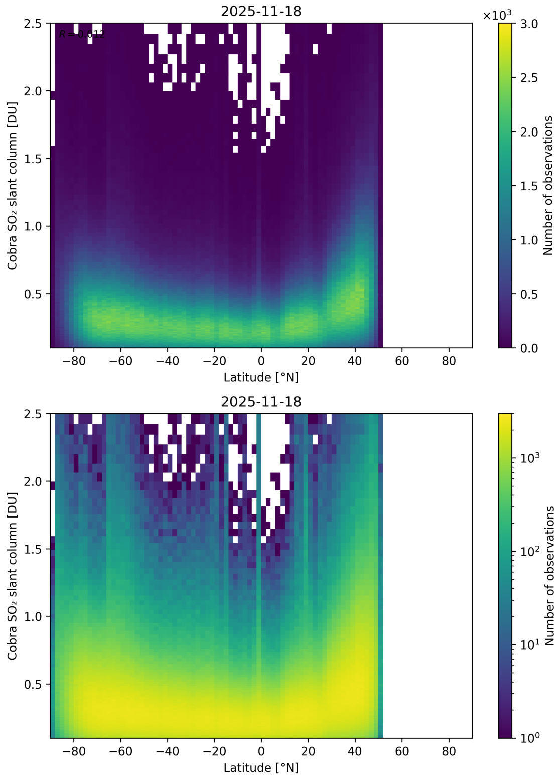
Figure 157: Scatter density plot of “Latitude” against “Cobra SO 2 slant column” for 2025-11-18 to 2025-11-19.
