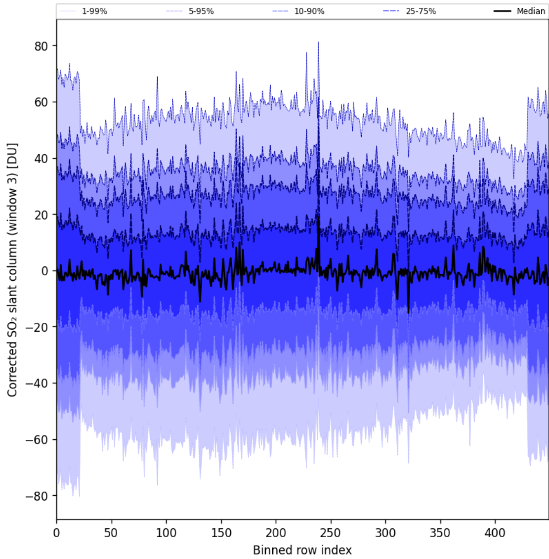
Figure 99: Along track statistics of “Corrected SO 2 slant column (window 3)” for 2025-11-18 to 2025-11-19
