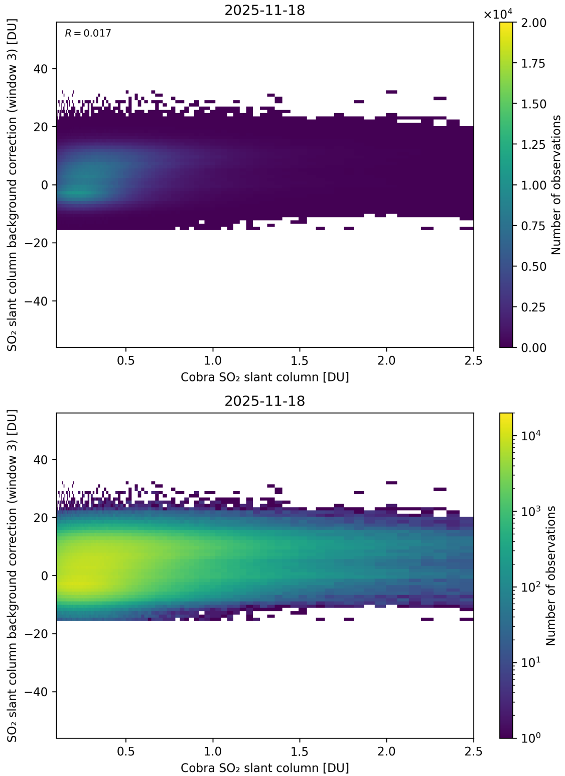
Figure 195: Scatter density plot of “Cobra SO 2 slant column” against “SO 2 slant column background correction (window 3)” for 2025-11-18 to 2025-11-19.
