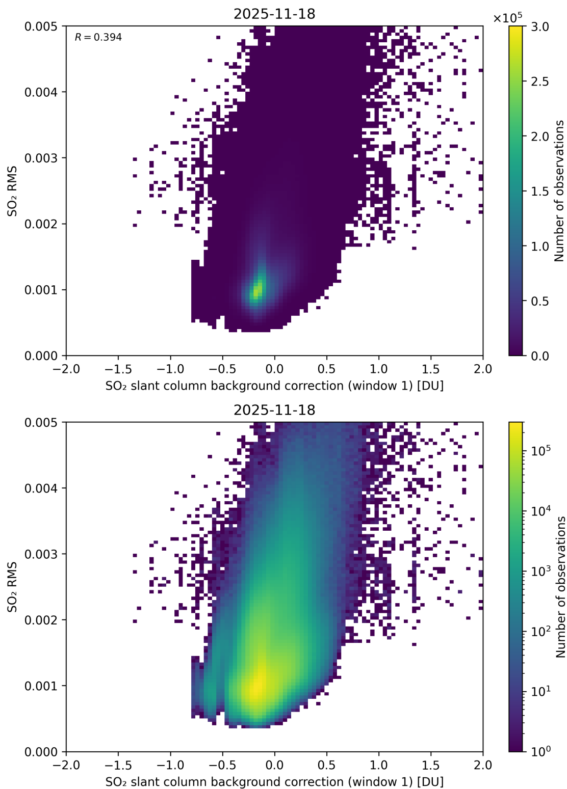
Figure 113: Scatter density plot of “SO 2 slant column background correction (window 1)” against “SO 2 RMS” for 2025-11-18 to 2025-11-19.
