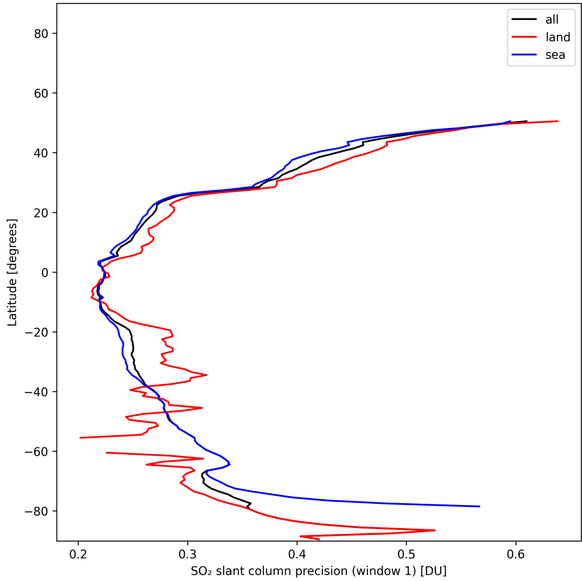
Figure 38: Zonal average of “SO 2 slant column precision (window 1)” for 2025-11-18 to 2025-11-19.
