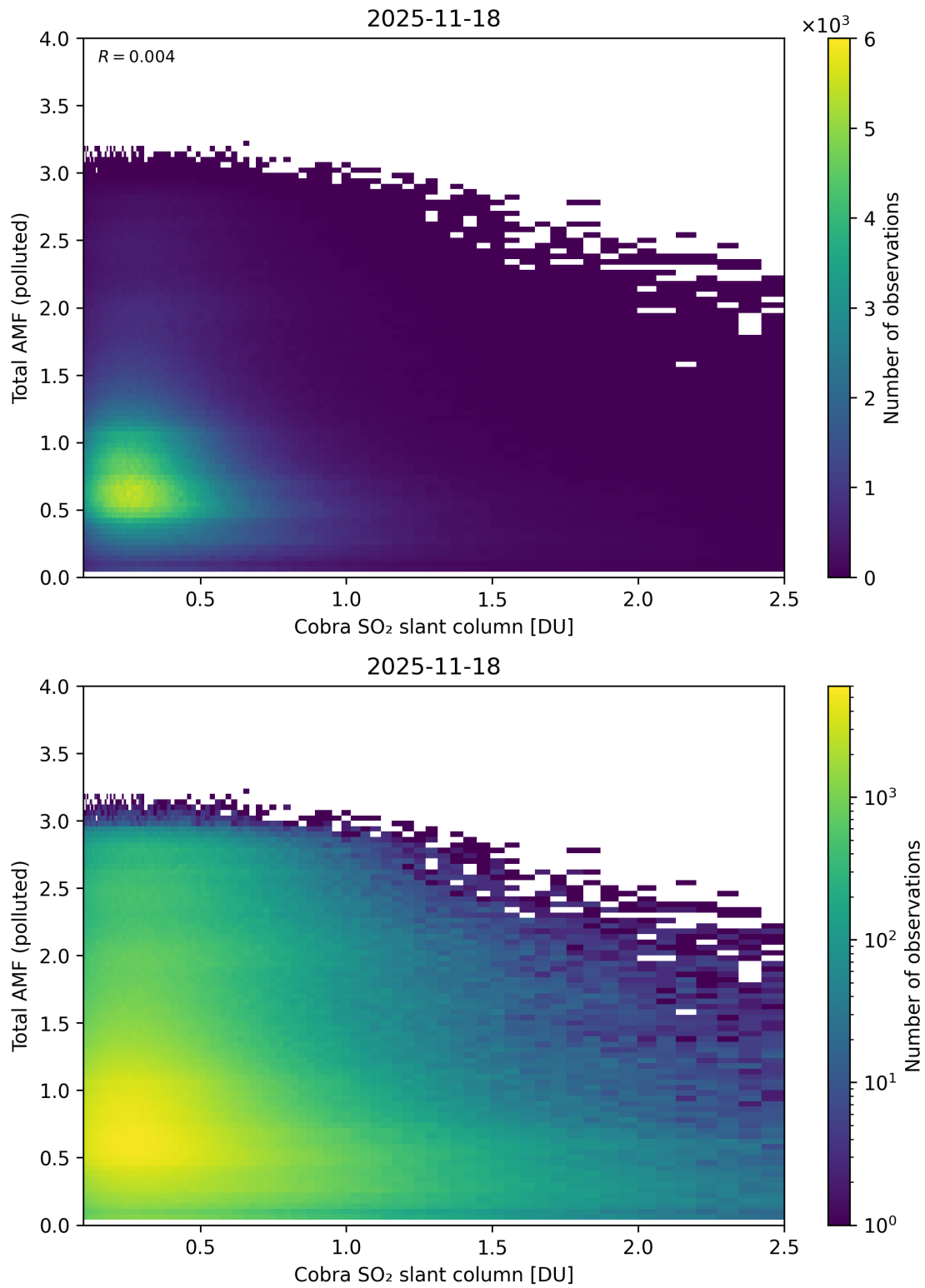
Figure 224: Scatter density plot of “Cobra SO 2 slant column” against “Total AMF (polluted)” for 2025-11-18 to 2025-11-19.
