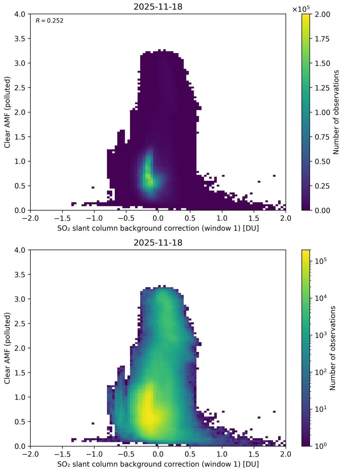
Figure 114: Scatter density plot of “SO 2 slant column background correction (window 1)” against “Clear AMF (polluted)” for 2025-11-18 to 2025-11-19.
