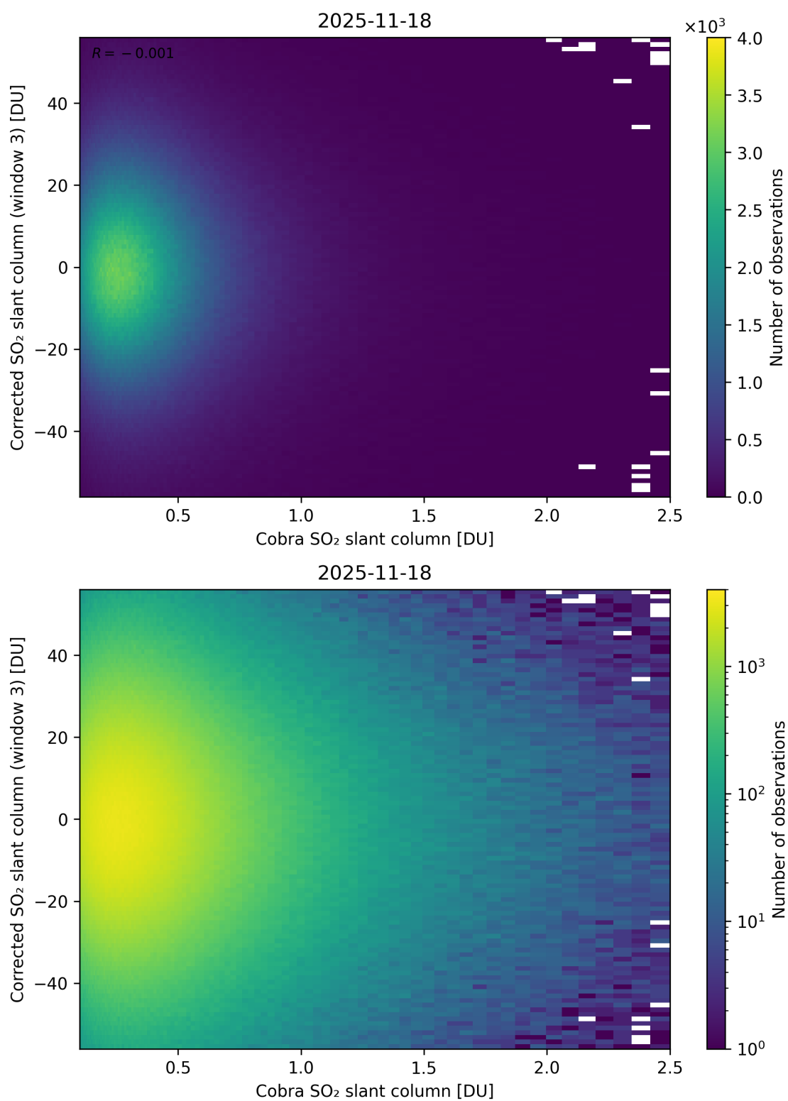
Figure 218: Scatter density plot of “Cobra SO 2 slant column” against “Corrected SO 2 slant column (window 3)” for 2025-11-18 to 2025-11-19.
