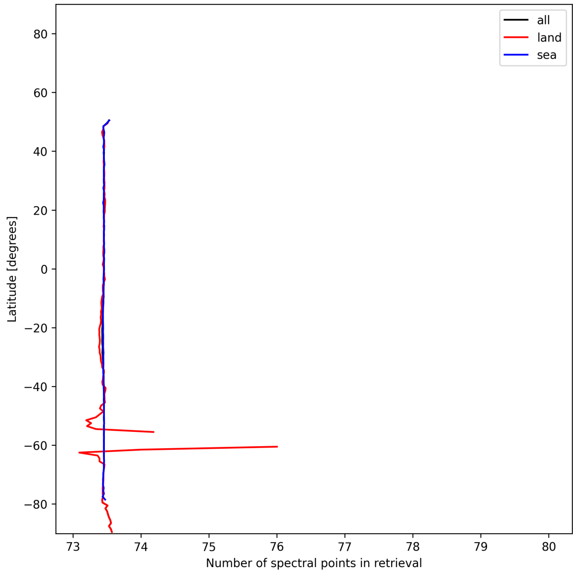
Figure 56: Zonal average of “Number of spectral points in retrieval” for 2025-11-18 to 2025-11-19.
