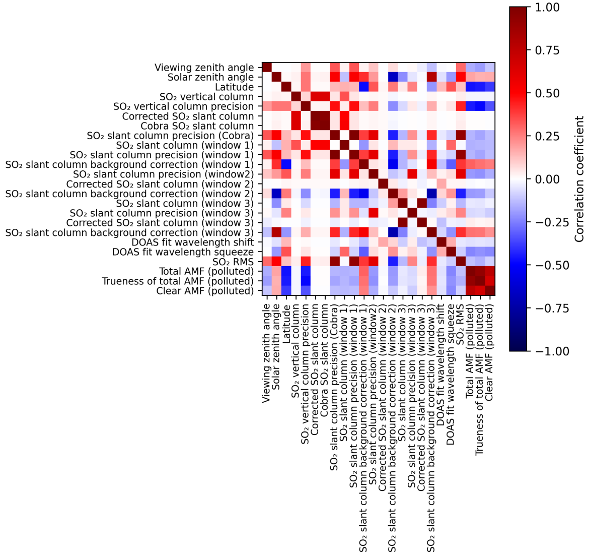
Figure 2: Map of correlation matrix for 2025-11-18 to 2025-11-19.
