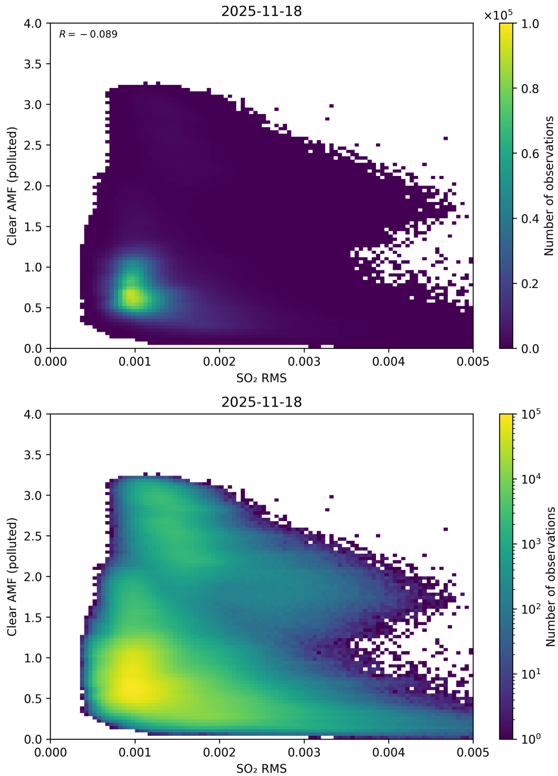
Figure 147: Scatter density plot of “SO 2 RMS” against “Clear AMF (polluted)” for 2025-11-18 to 2025-11-19.
