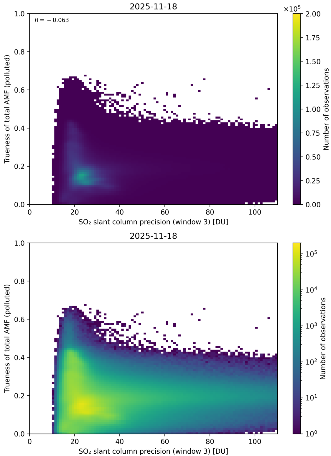
Figure 314: Scatter density plot of “SO 2 slant column precision (window 3)” against “Trueness of total AMF (polluted)” for 2025-11-18 to 2025-11-19.
