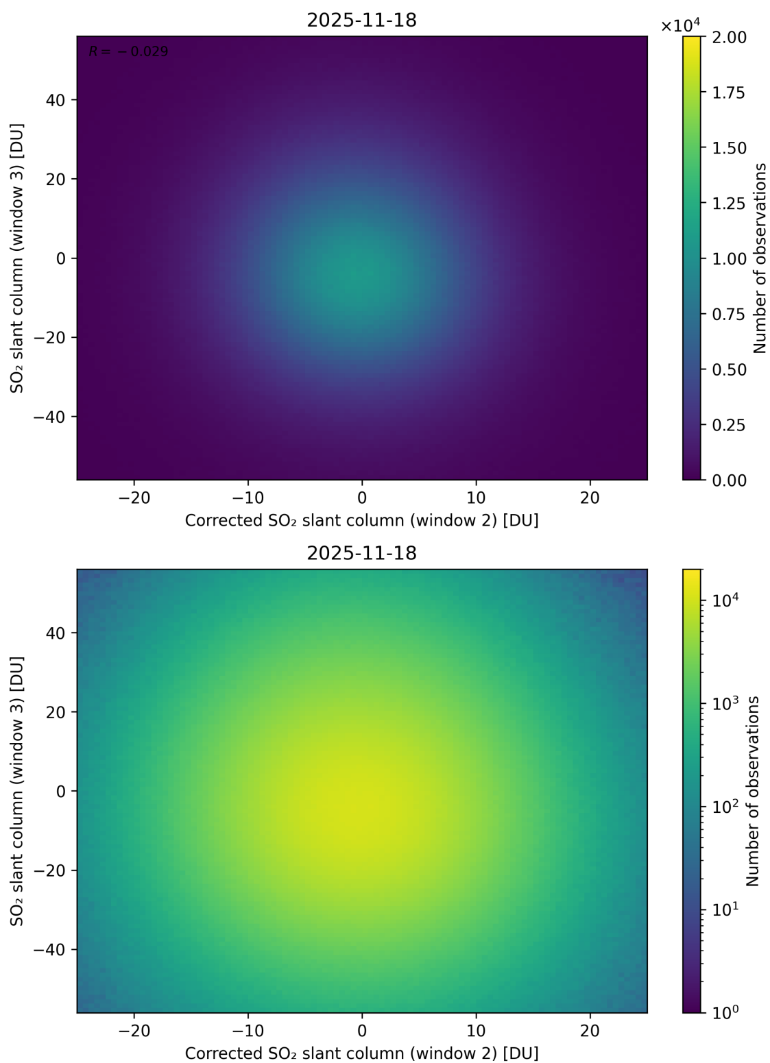
Figure 251: Scatter density plot of “Corrected SO 2 slant column (window 2)” against “SO 2 slant column (window 3)” for 2025-11-18 to 2025-11-19.
