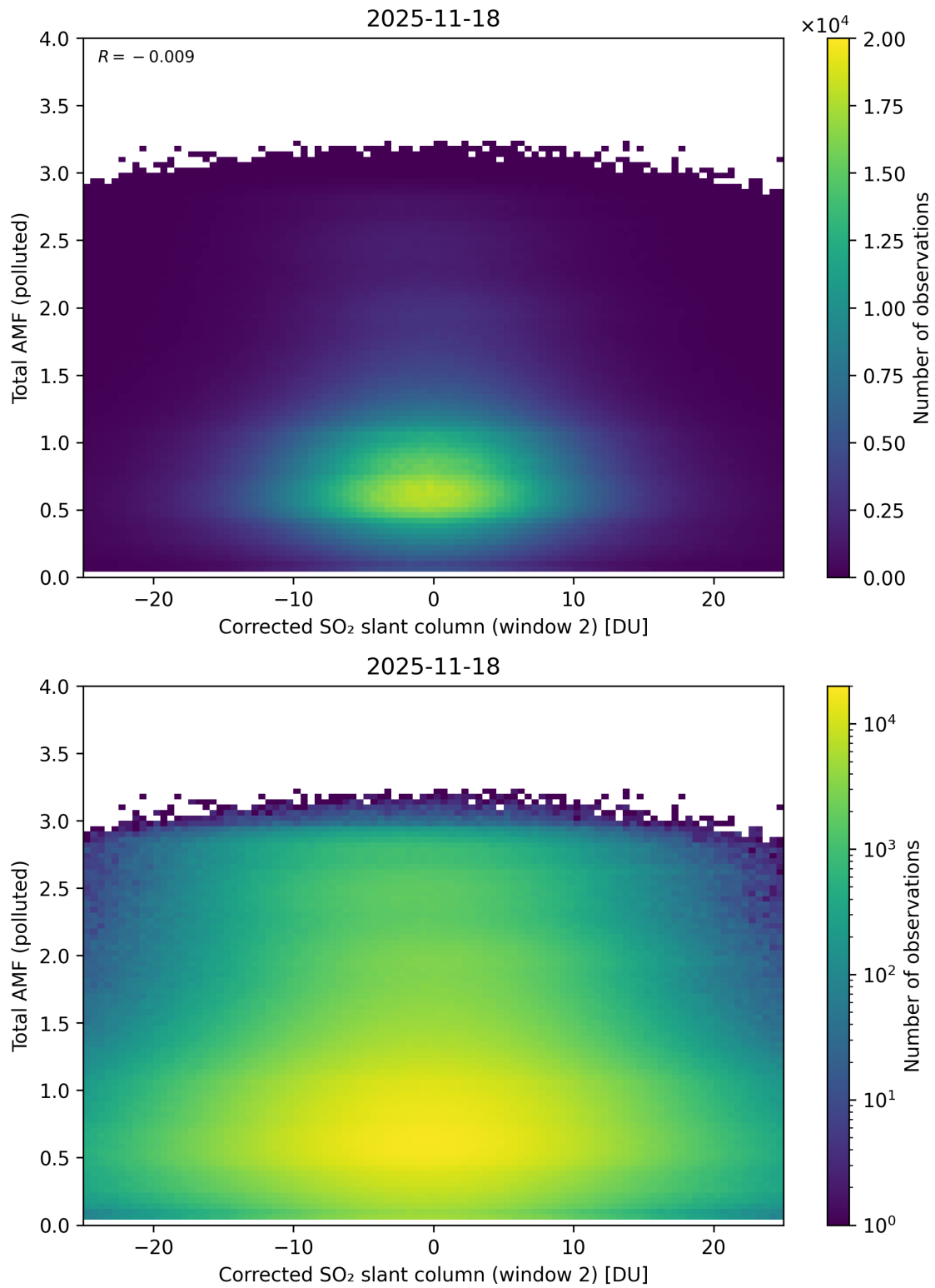
Figure 253: Scatter density plot of “Corrected SO 2 slant column (window 2)” against “Total AMF (polluted)” for 2025-11-18 to 2025-11-19.
