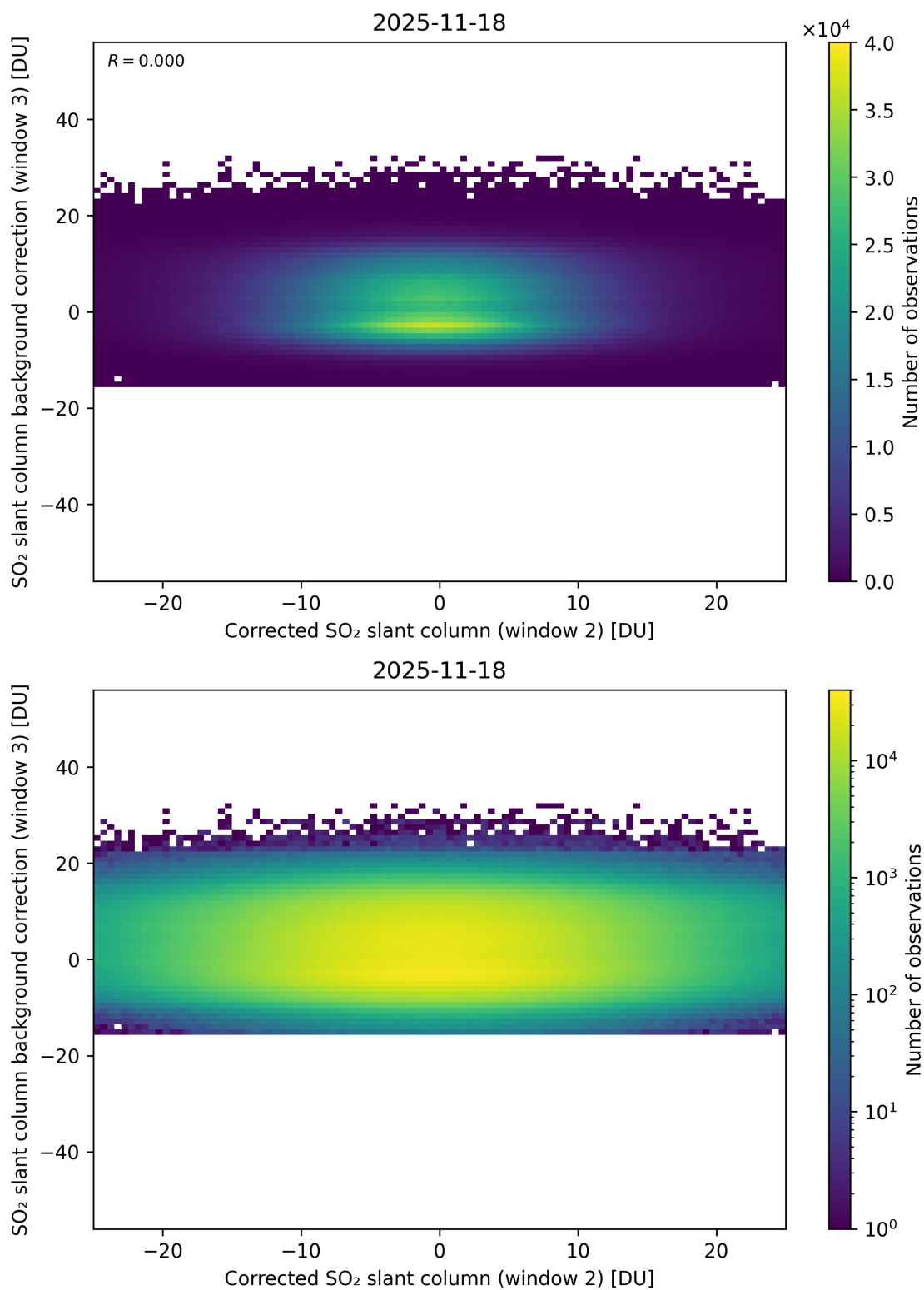
Figure 245: Scatter density plot of “Corrected SO 2 slant column (window 2)” against “SO 2 slant column background correction (window 3)” for 2025-11-18 to 2025-11-19.
