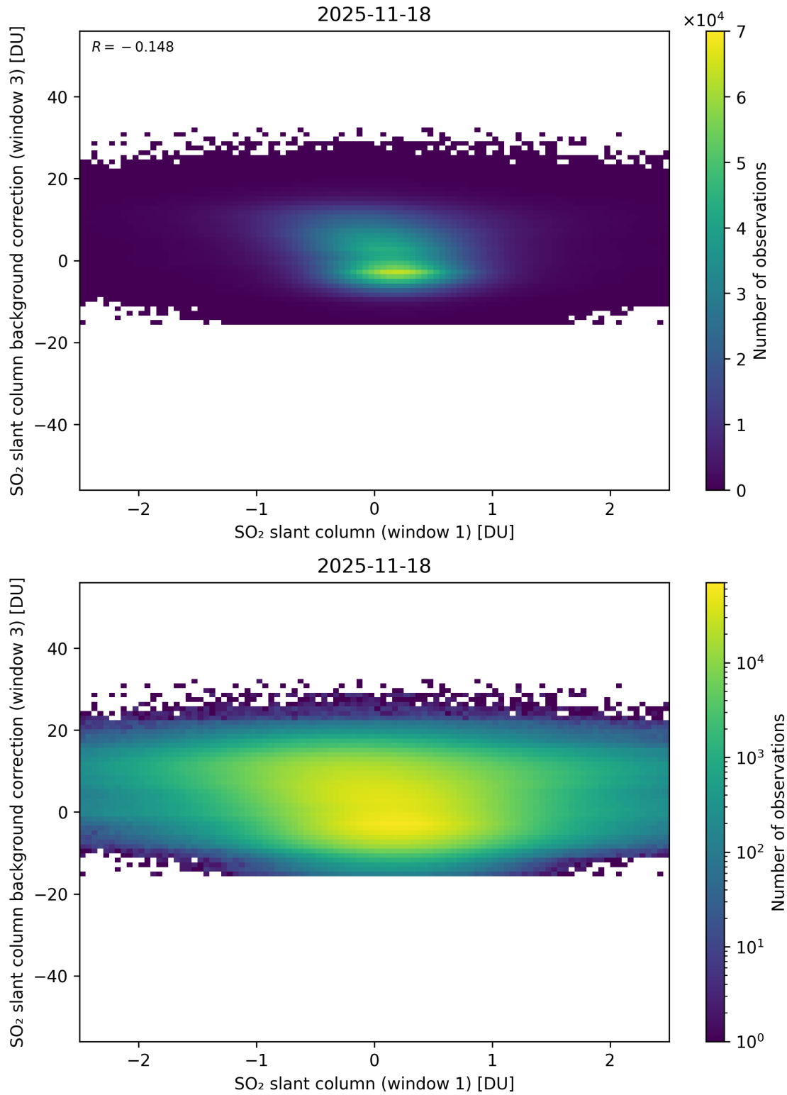
Figure 264: Scatter density plot of “SO 2 slant column (window 1)” against “SO 2 slant column background correction (window 3)” for 2025-11-18 to 2025-11-19.
