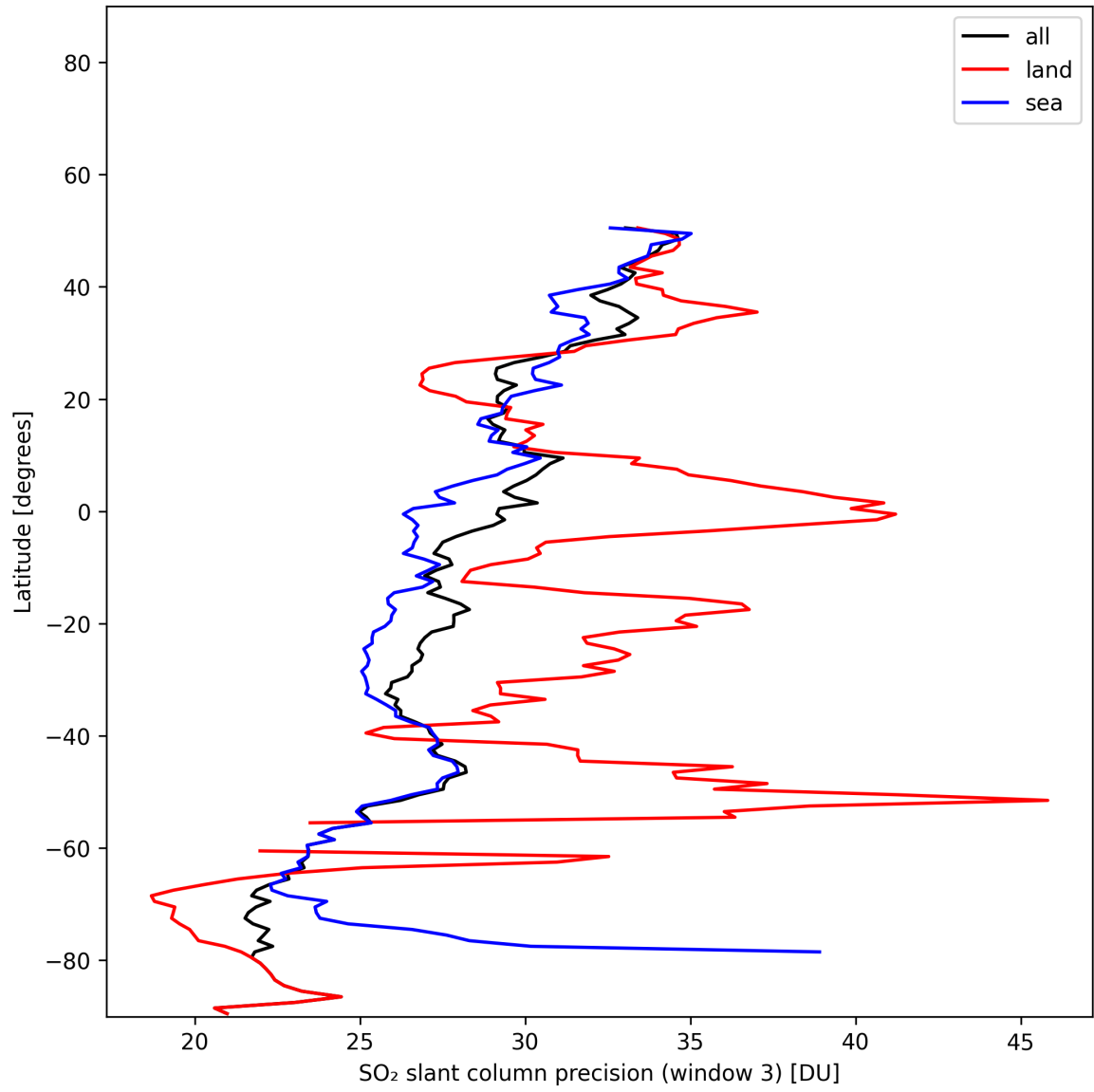
Figure 46: Zonal average of “SO 2 slant column precision (window 3)” for 2025-11-18 to 2025-11-19.
