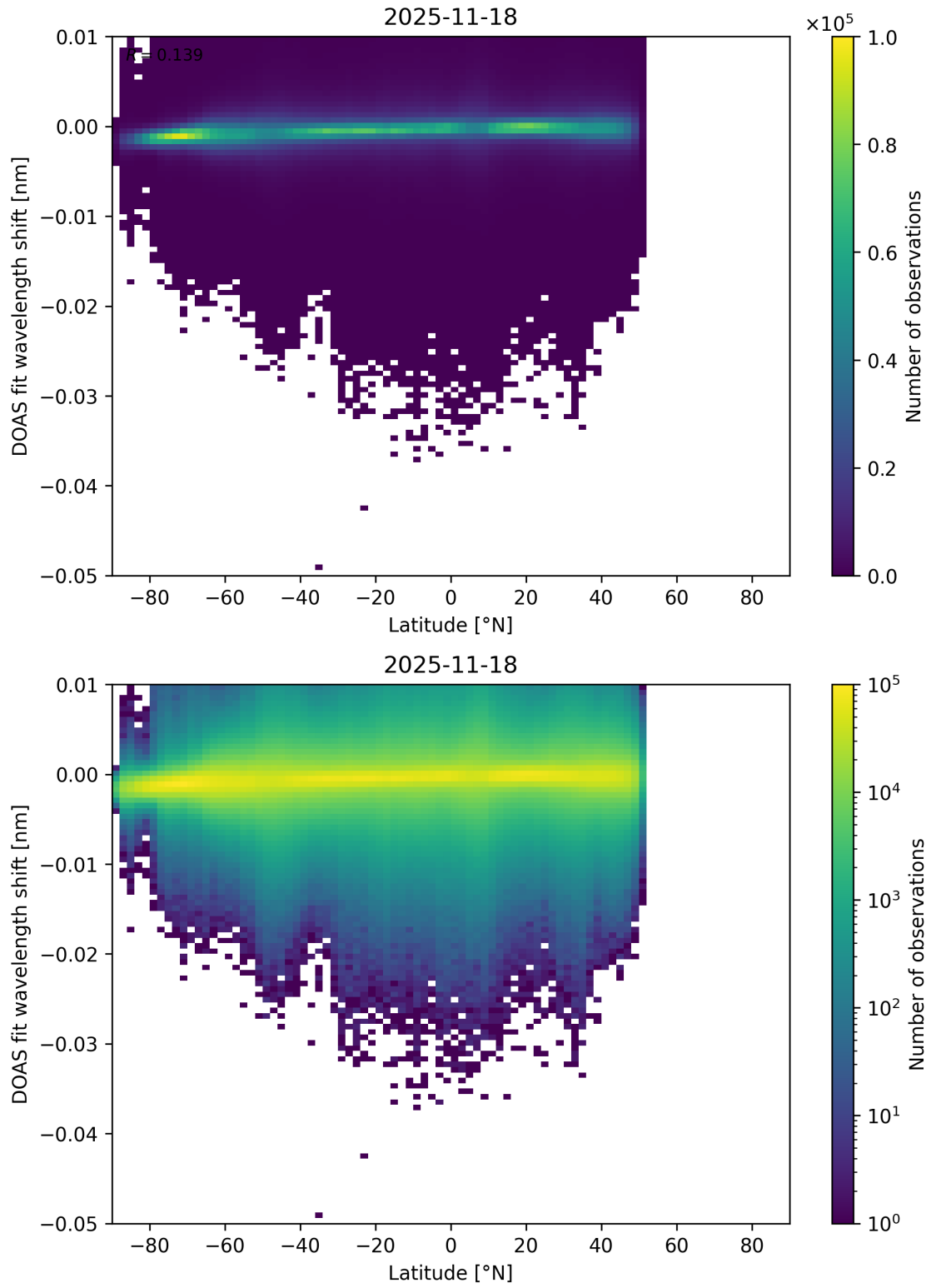
Figure 153: Scatter density plot of “Latitude” against “DOAS fit wavelength shift” for 2025-11-18 to 2025-11-19.
