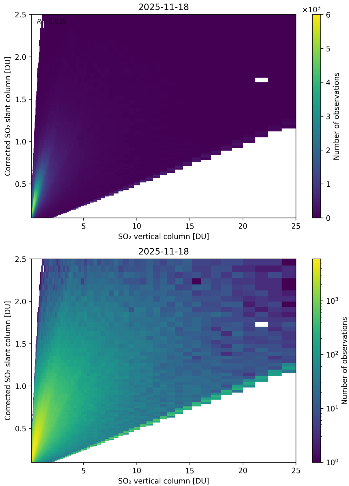
Figure 351: Scatter density plot of “SO 2 vertical column” against “Corrected SO 2 slant column” for 2025-11-18 to 2025-11-19.
