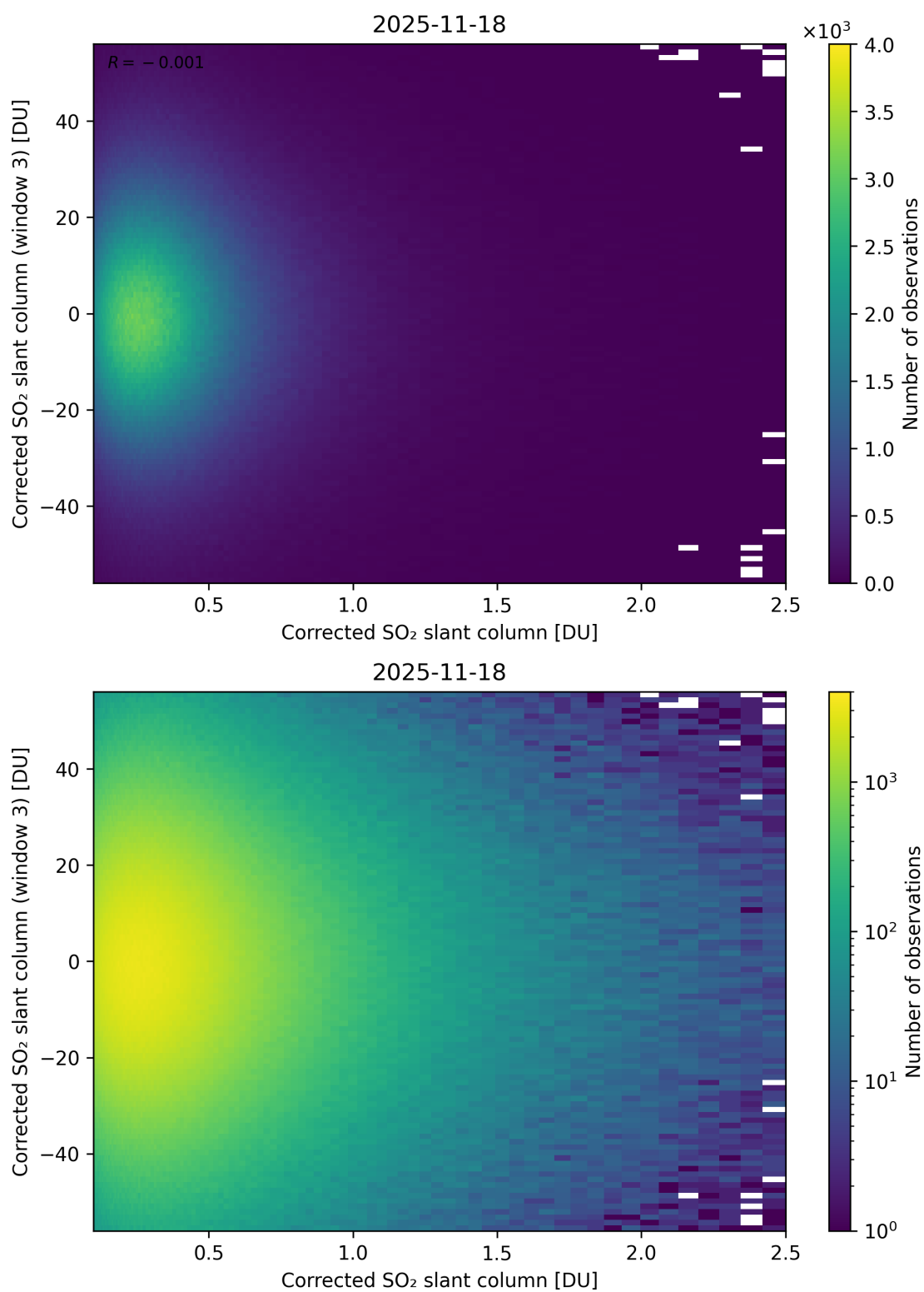
Figure 236: Scatter density plot of “Corrected SO 2 slant column” against “Corrected SO 2 slant column (window 3)” for 2025-11-18 to 2025-11-19.
