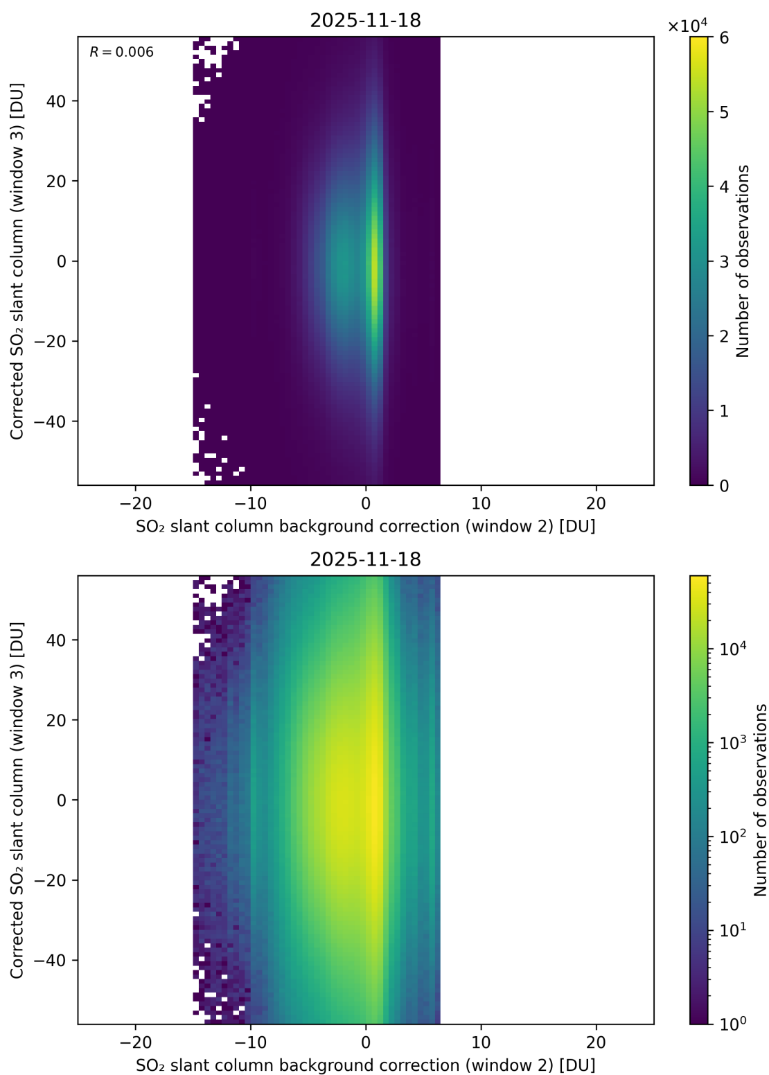
Figure 127: Scatter density plot of “SO 2 slant column background correction (window 2)” against “Corrected SO 2 slant column (window 3)” for 2025-11-18 to 2025-11-19.
