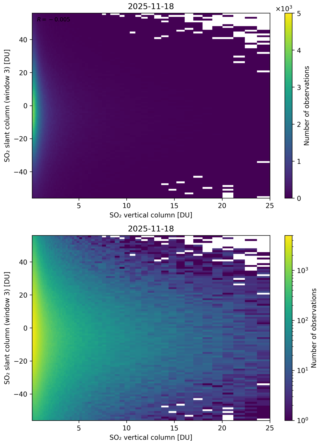
Figure 357: Scatter density plot of “SO 2 vertical column” against “SO 2 slant column (window 3)” for 2025-11-18 to 2025-11-19.
