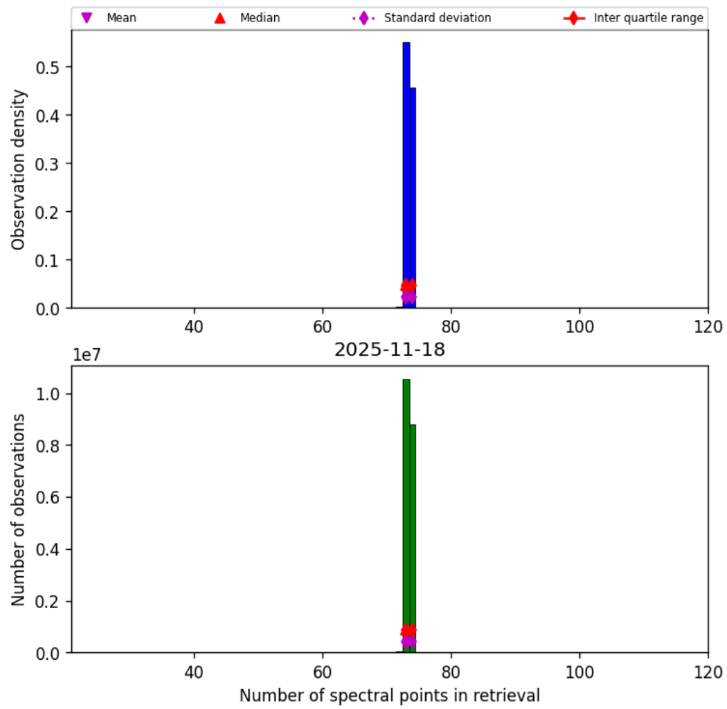
Figure 82: Histogram of "Number of spectral points in retrieval" for 2025-11-18 to 2025-11-19
