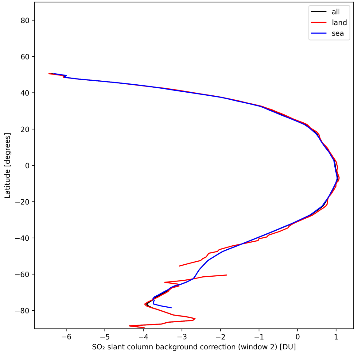
Figure 44: Zonal average of “SO 2 slant column background correction (window 2)” for 2025-11-18 to 2025-11-19.
