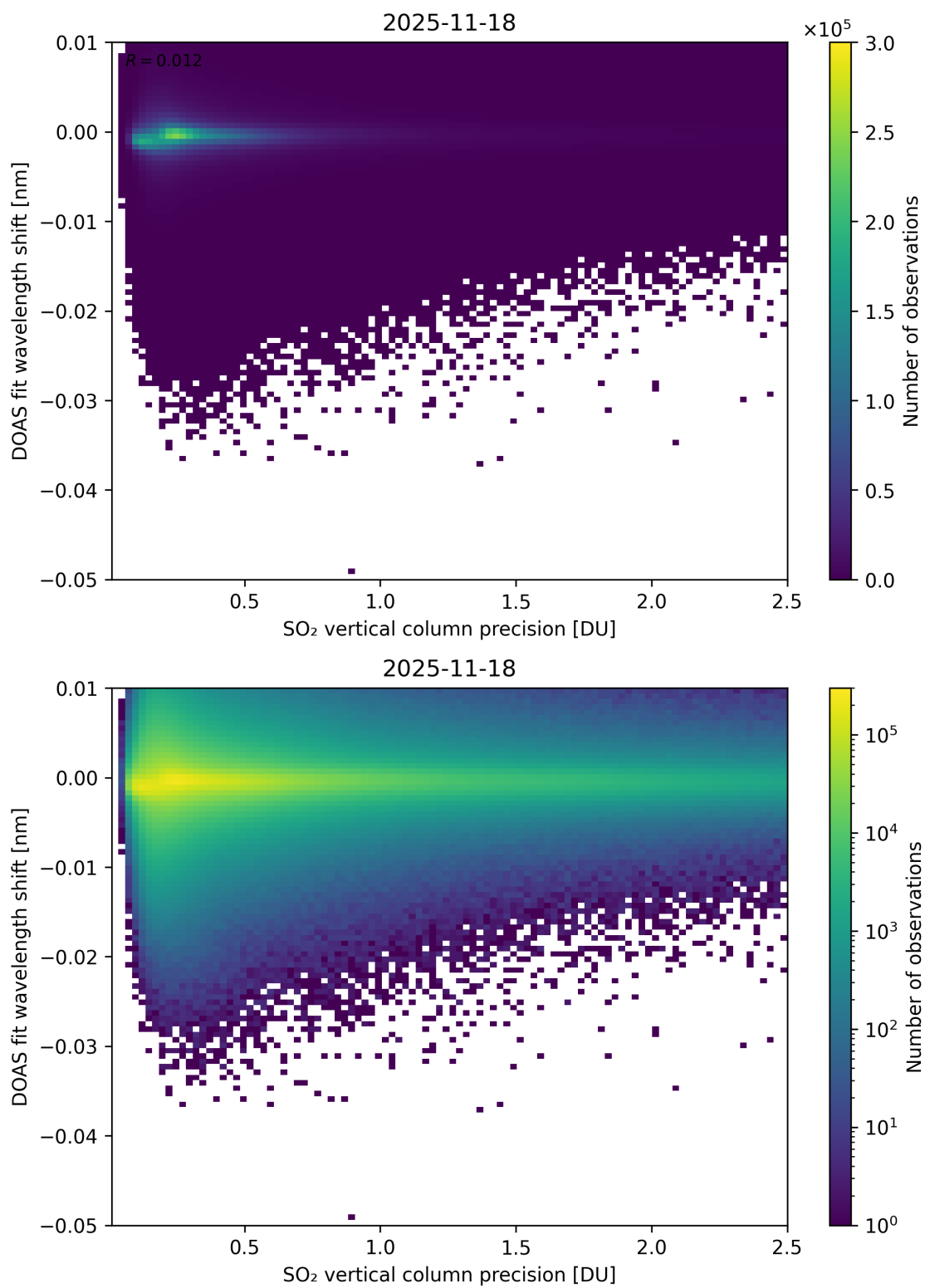
Figure 332: Scatter density plot of “SO 2 vertical column precision” against “DOAS fit wavelength shift” for 2025-11-18 to 2025-11-19.
