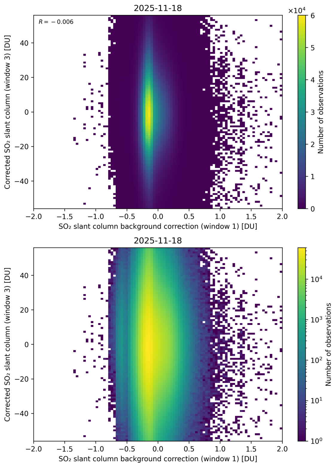
Figure 116: Scatter density plot of “SO 2 slant column background correction (window 1)” against “Corrected SO 2 slant column (window 3)” for 2025-11-18 to 2025-11-19.
