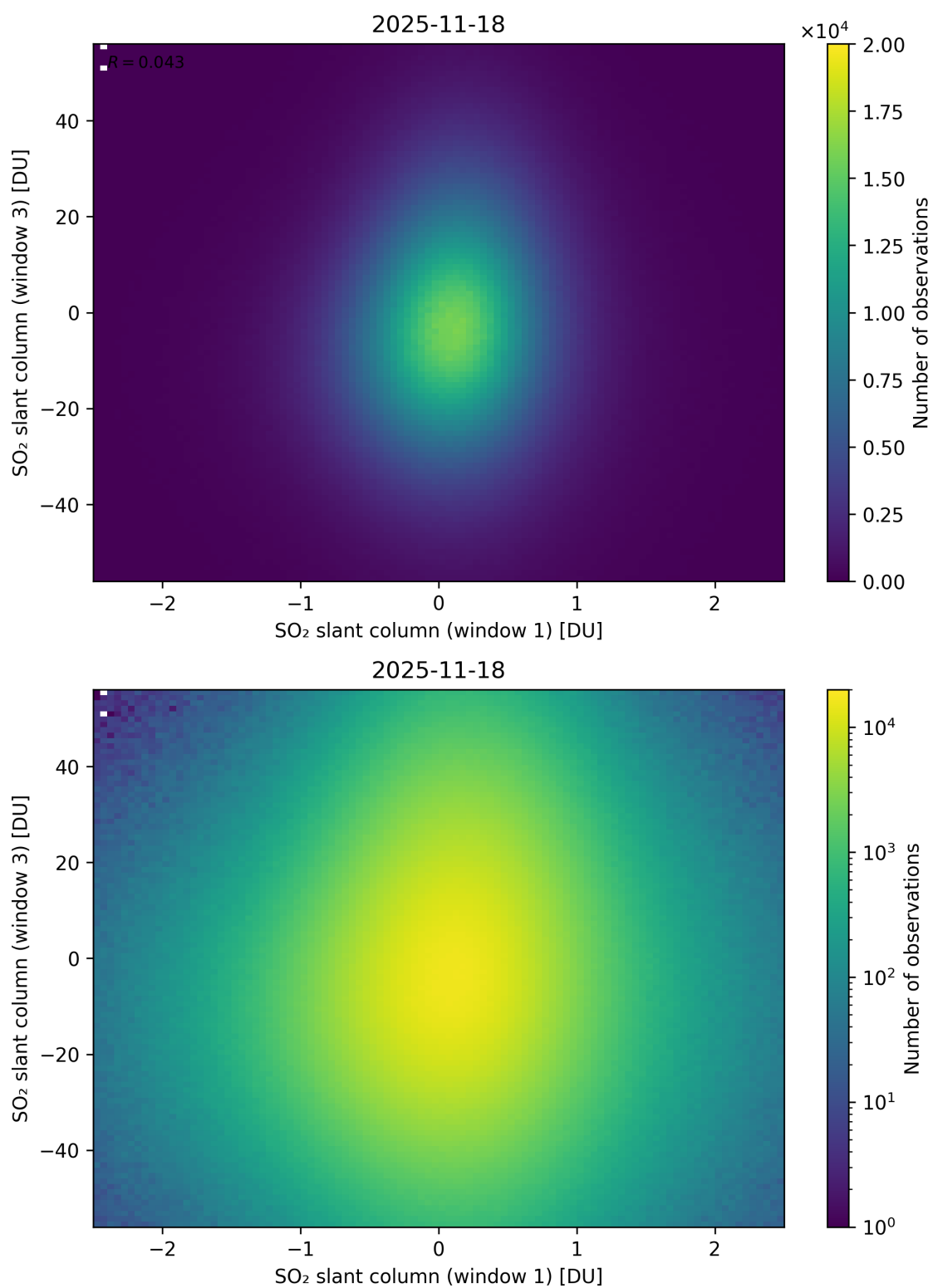
Figure 287: Scatter density plot of “SO 2 slant column (window 1)” against “SO 2 slant column (window 3)” for 2025-11-18 to 2025-11-19.
