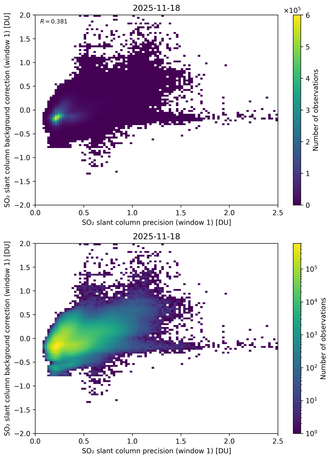
Figure 268: Scatter density plot of “SO 2 slant column precision (window 1)” against “SO 2 slant column background correction (window 1)” for 2025-11-18 to 2025-11-19.
