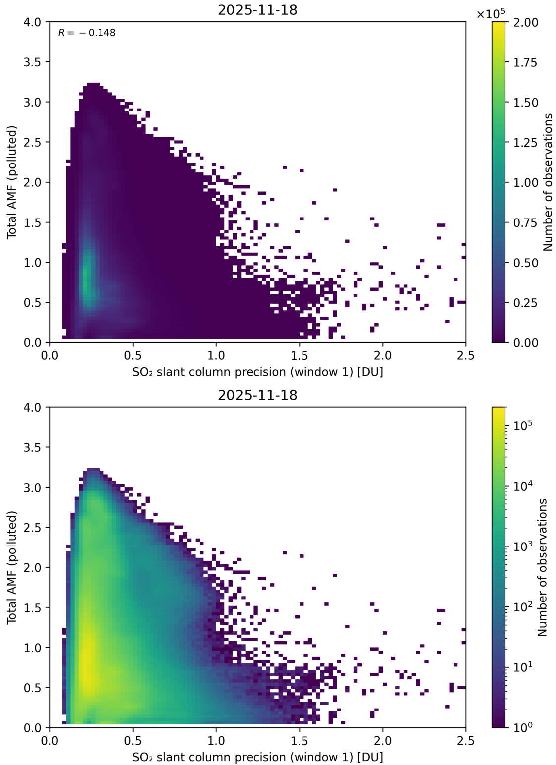
Figure 280: Scatter density plot of “SO 2 slant column precision (window 1)” against “Total AMF (polluted)” for 2025-11-18 to 2025-11-19.
