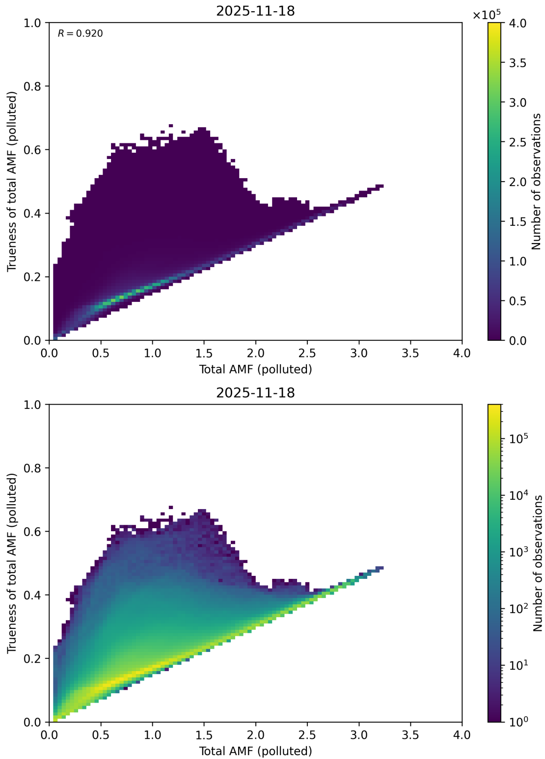
Figure 321: Scatter density plot of “Total AMF (polluted)” against “Trueness of total AMF (polluted)” for 2025-11-18 to 2025-11-19.
