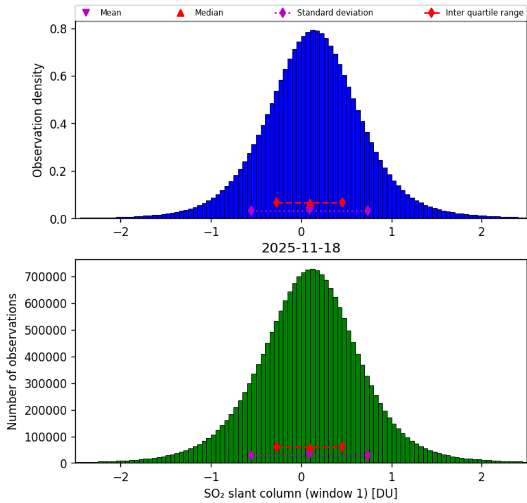
Figure 63: Histogram of “SO 2 slant column (window 1)” for 2025-11-18 to 2025-11-19
