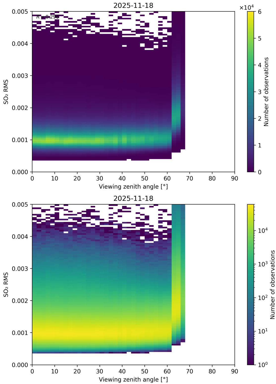
Figure 367: Scatter density plot of “Viewing zenith angle” against “SO 2 RMS” for 2025-11-18 to 2025-11-19.
