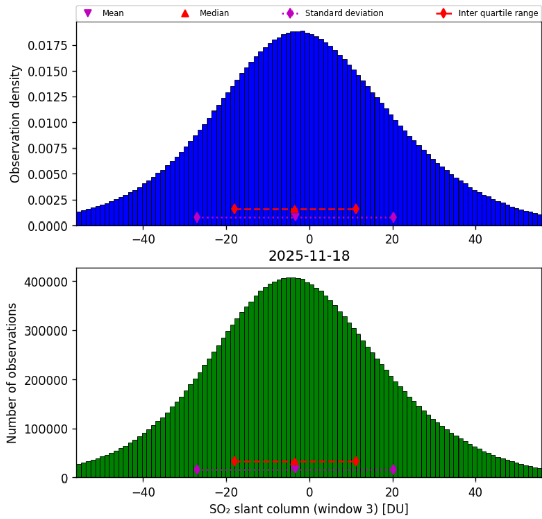
Figure 71: Histogram of “SO 2 slant column (window 3)” for 2025-11-18 to 2025-11-19
