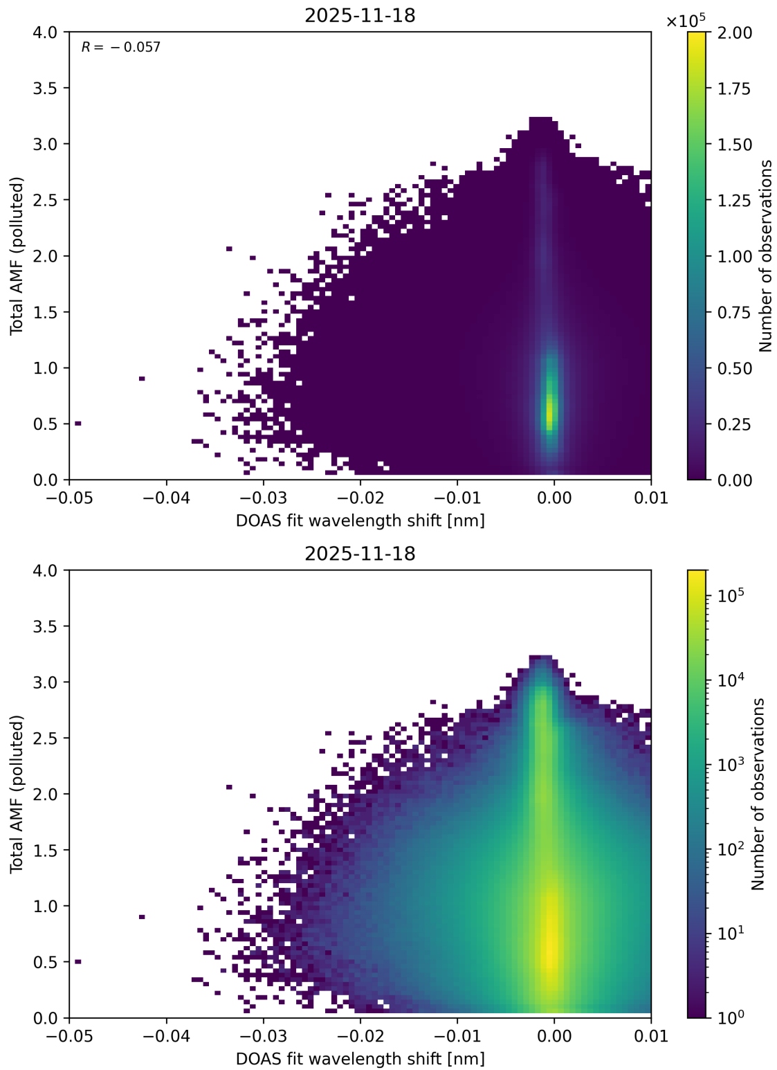
Figure 141: Scatter density plot of “DOAS fit wavelength shift” against “Total AMF (polluted)” for 2025-11-18 to 2025-11-19.
