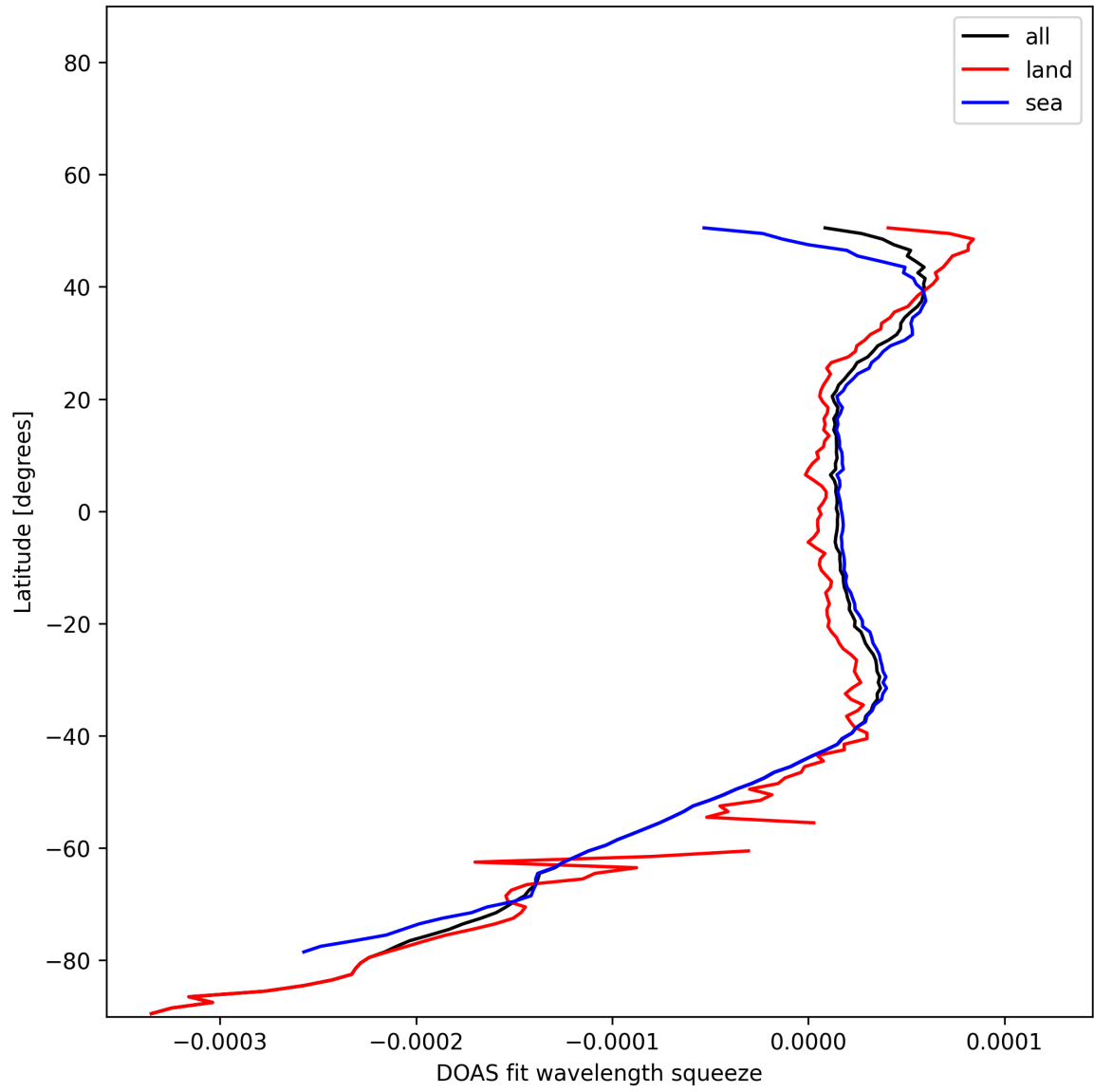
Figure 51: Zonal average of “DOAS fit wavelength squeeze” for 2025-11-18 to 2025-11-19.
