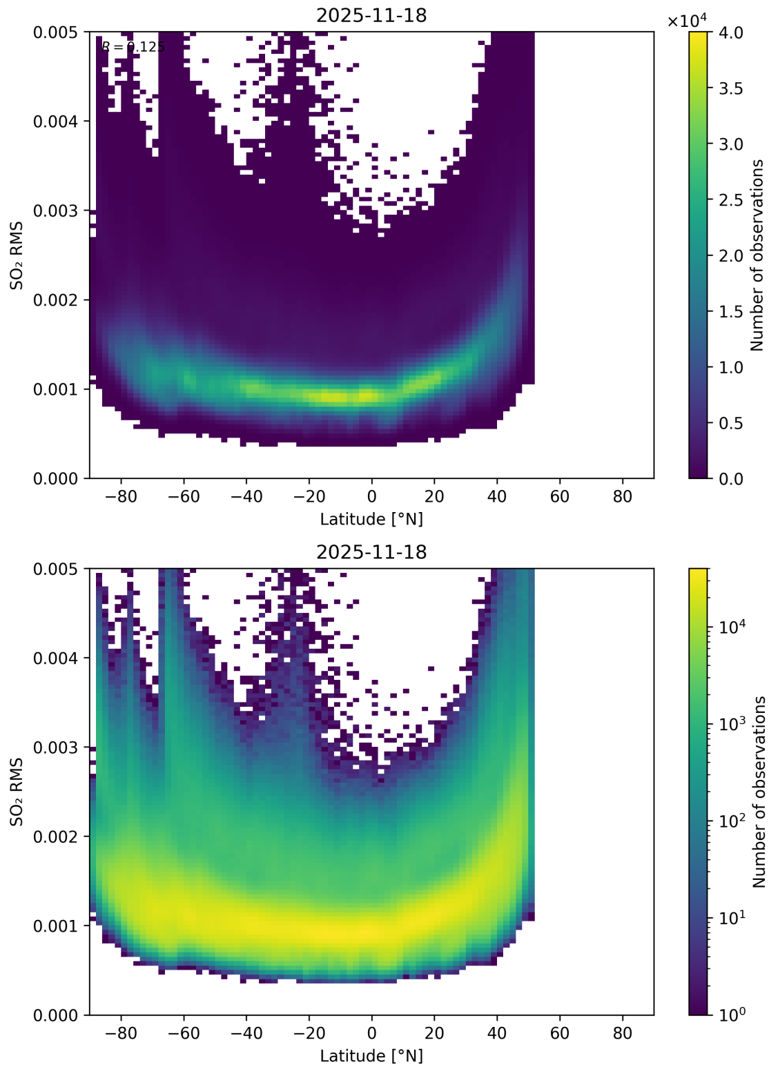
Figure 155: Scatter density plot of “Latitude” against “SO 2 RMS” for 2025-11-18 to 2025-11-19.
