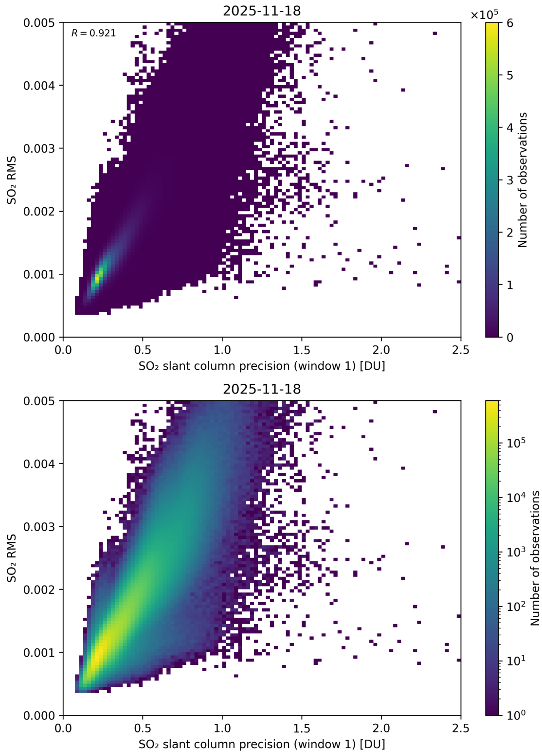
Figure 273: Scatter density plot of “SO 2 slant column precision (window 1)” against “SO 2 RMS” for 2025-11-18 to 2025-11-19.
