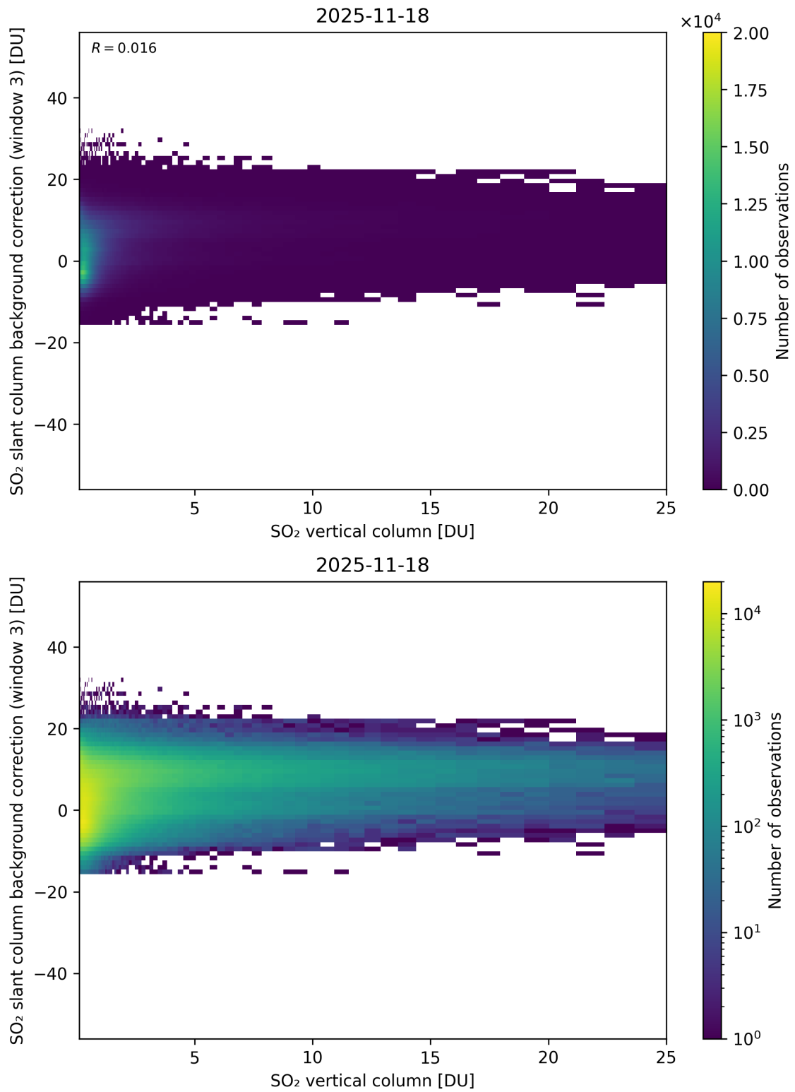
Figure 325: Scatter density plot of “SO 2 vertical column” against “SO 2 slant column background correction (window 3)” for 2025-11-18 to 2025-11-19.
