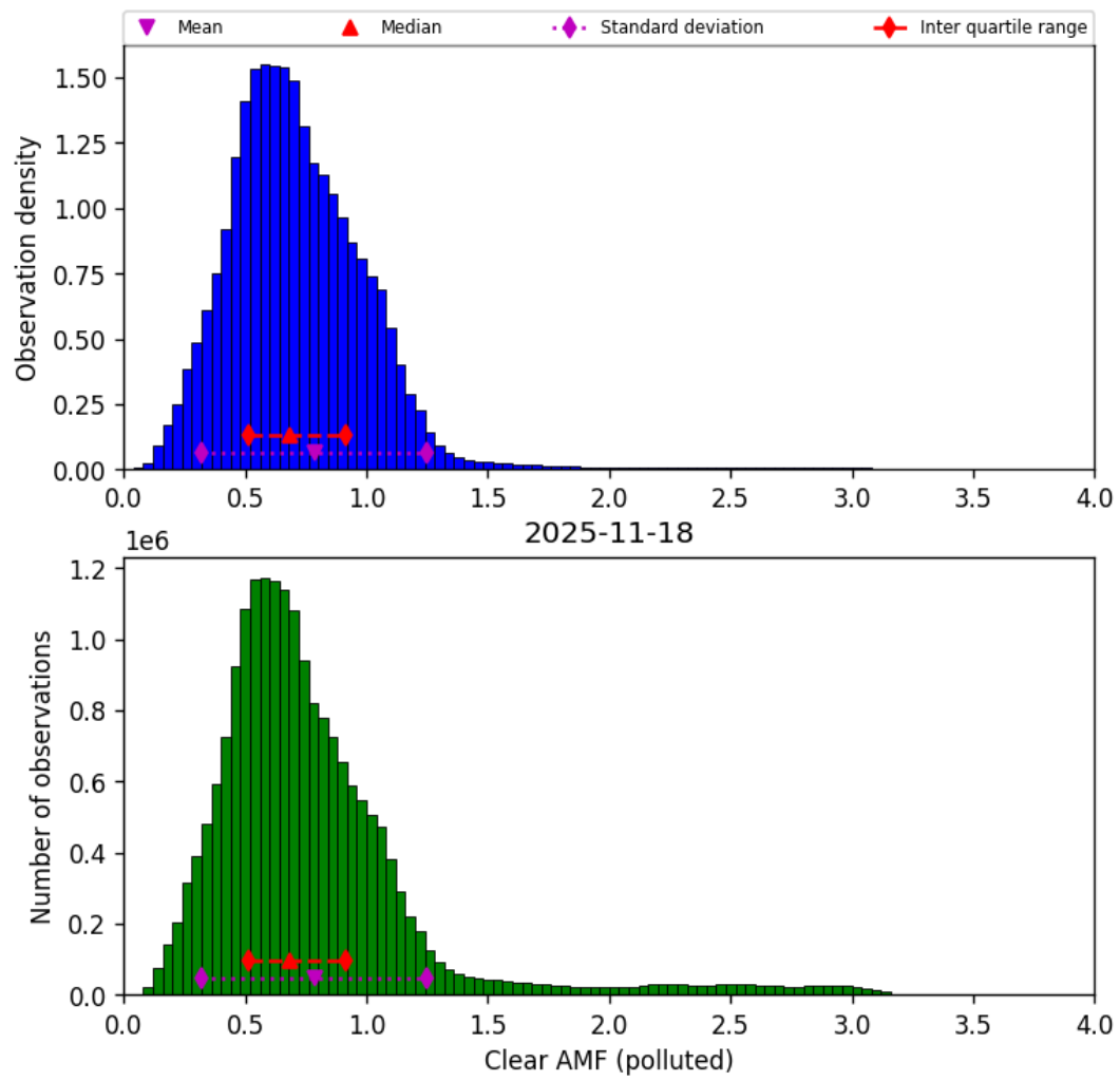
Figure 81: Histogram of “Clear AMF (polluted)” for 2025-11-18 to 2025-11-19
