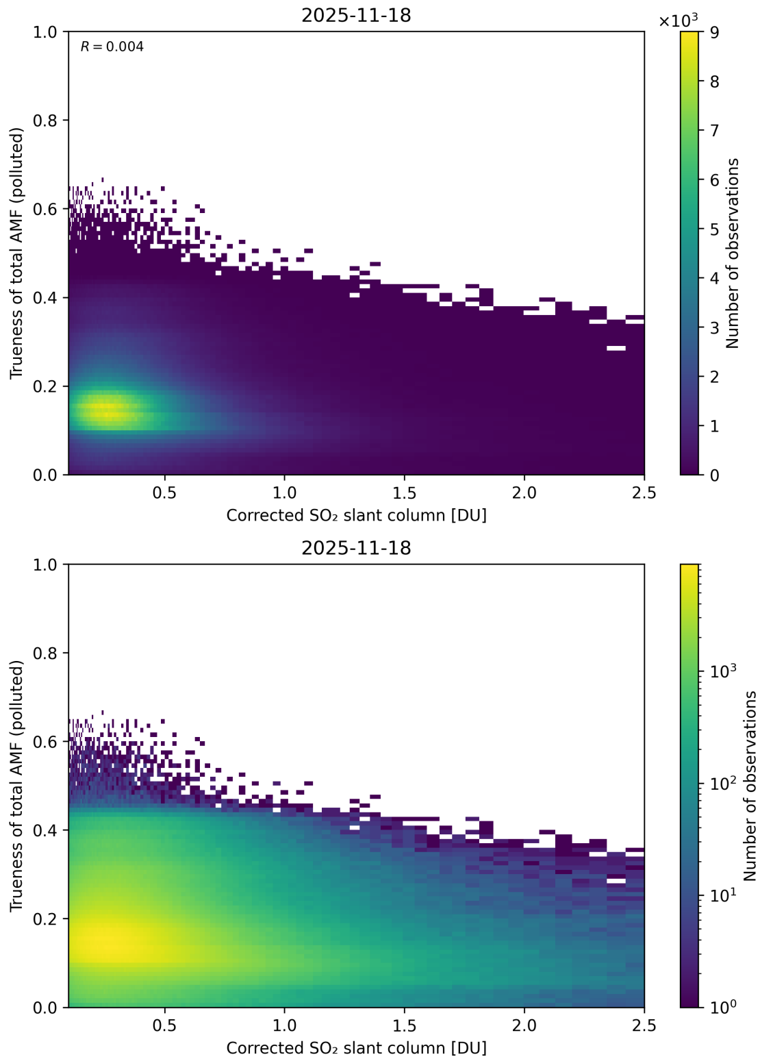
Figure 243: Scatter density plot of “Corrected SO 2 slant column” against “Trueness of total AMF (polluted)” for 2025-11-18 to 2025-11-19.
