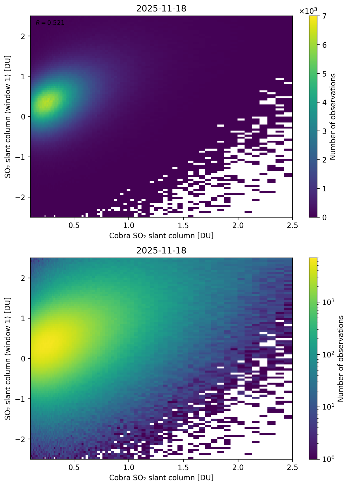
Figure 219: Scatter density plot of “Cobra SO 2 slant column” against “SO 2 slant column (window 1)” for 2025-11-18 to 2025-11-19.
