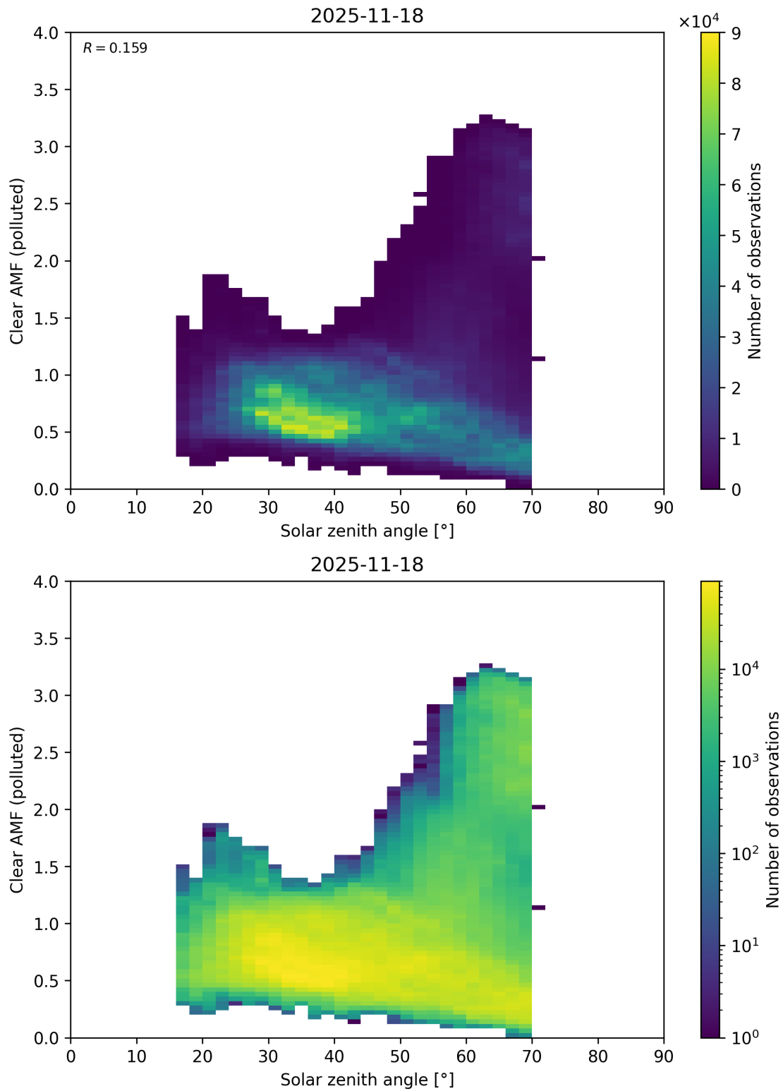
Figure 178: Scatter density plot of “Solar zenith angle” against “Clear AMF (polluted)” for 2025-11-18 to 2025-11-19.
