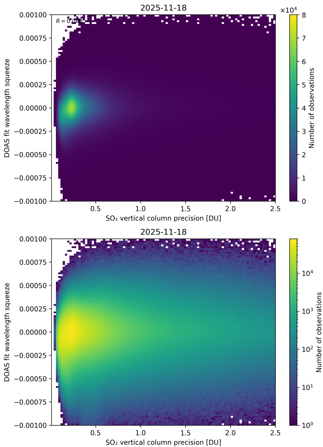
Figure 333: Scatter density plot of “SO 2 vertical column precision” against “DOAS fit wavelength squeeze” for 2025-11-18 to 2025-11-19.
