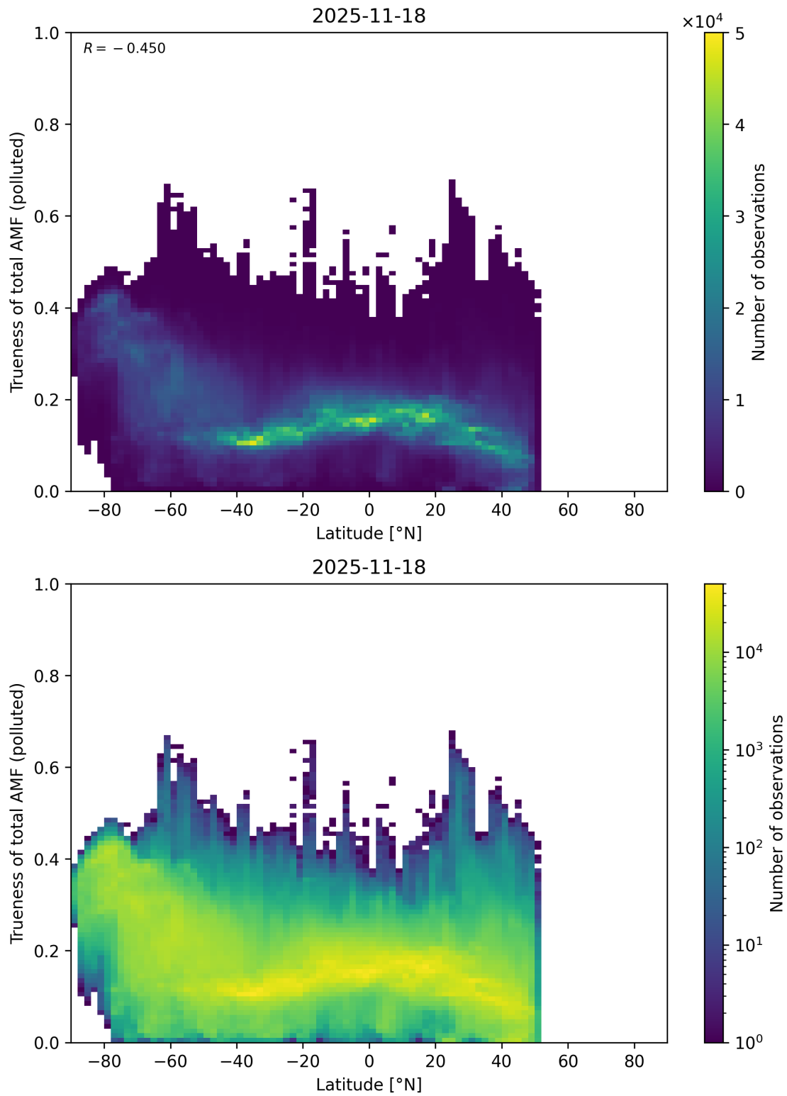
Figure 168: Scatter density plot of “Latitude” against “Trueness of total AMF (polluted)” for 2025-11-18 to 2025-11-19.
