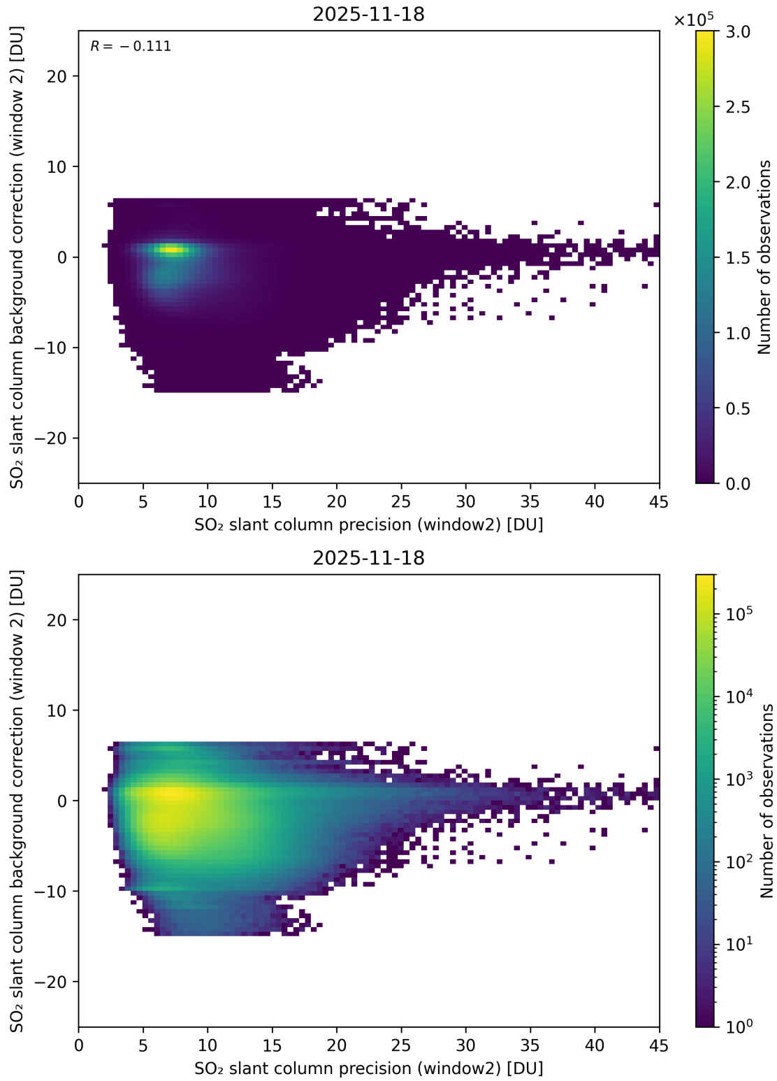
Figure 291: Scatter density plot of “SO 2 slant column precision (window2)” against “SO 2 slant column background correction (window 2)” for 2025-11-18 to 2025-11-19.
