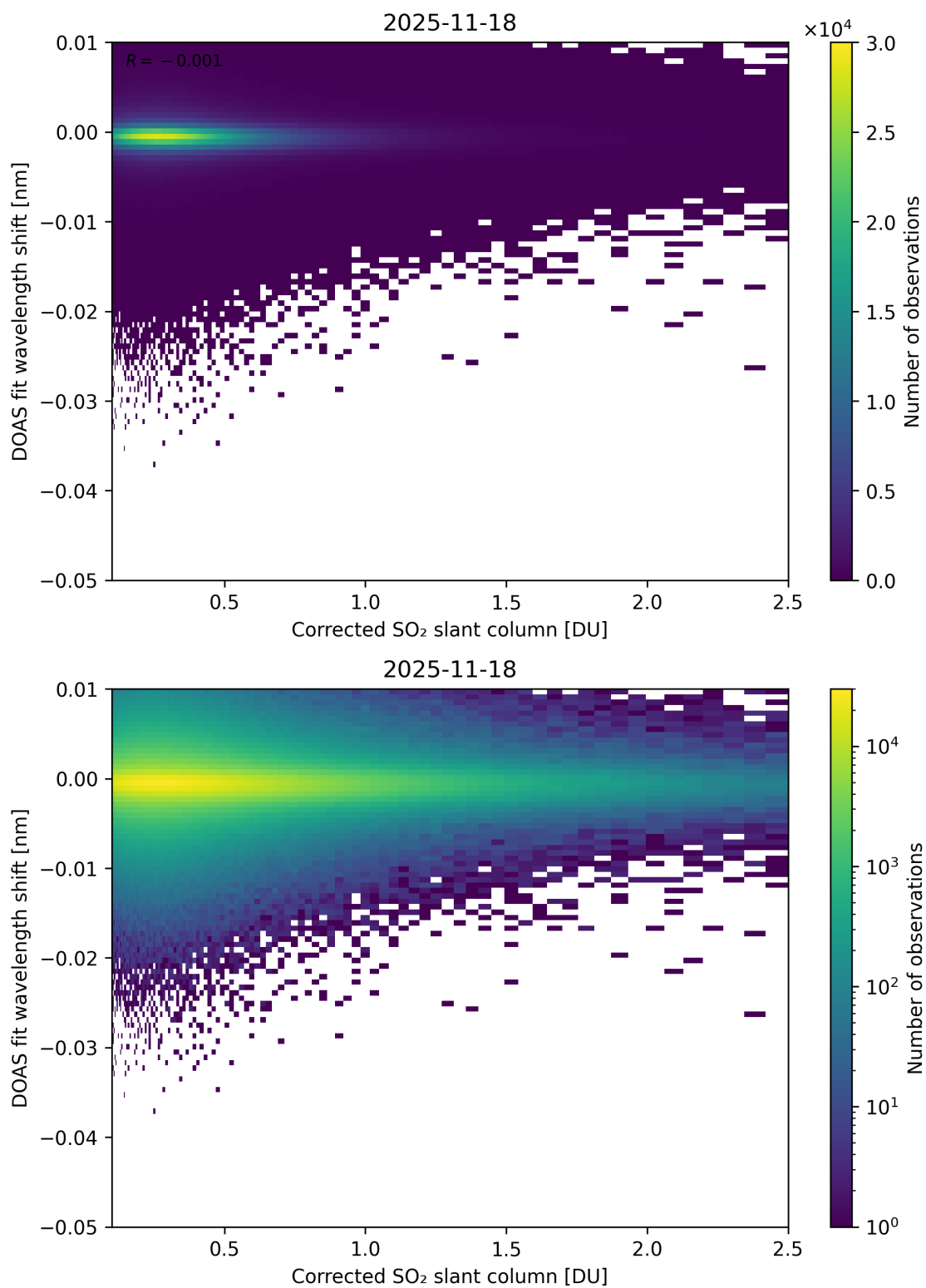
Figure 229: Scatter density plot of “Corrected SO 2 slant column” against “DOAS fit wavelength shift” for 2025-11-18 to 2025-11-19.
