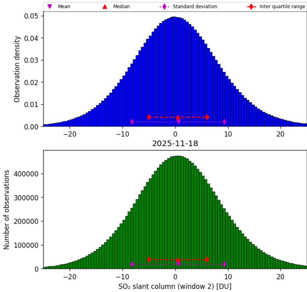
Figure 67: Histogram of “SO 2 slant column (window 2)” for 2025-11-18 to 2025-11-19
