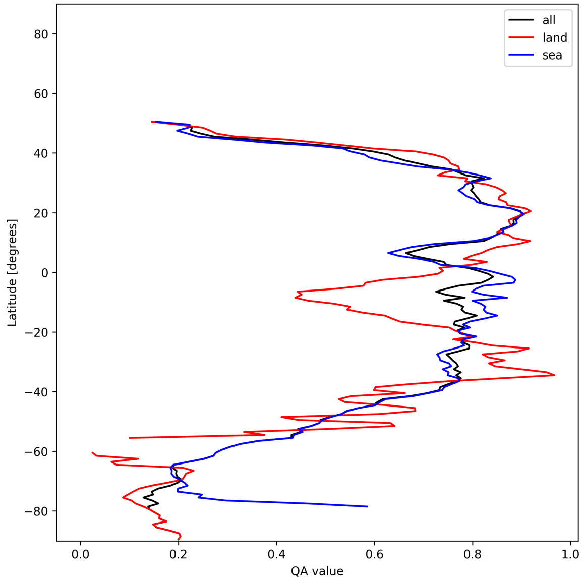
Figure 31: Zonal average of “QA value” for 2025-11-18 to 2025-11-19.
