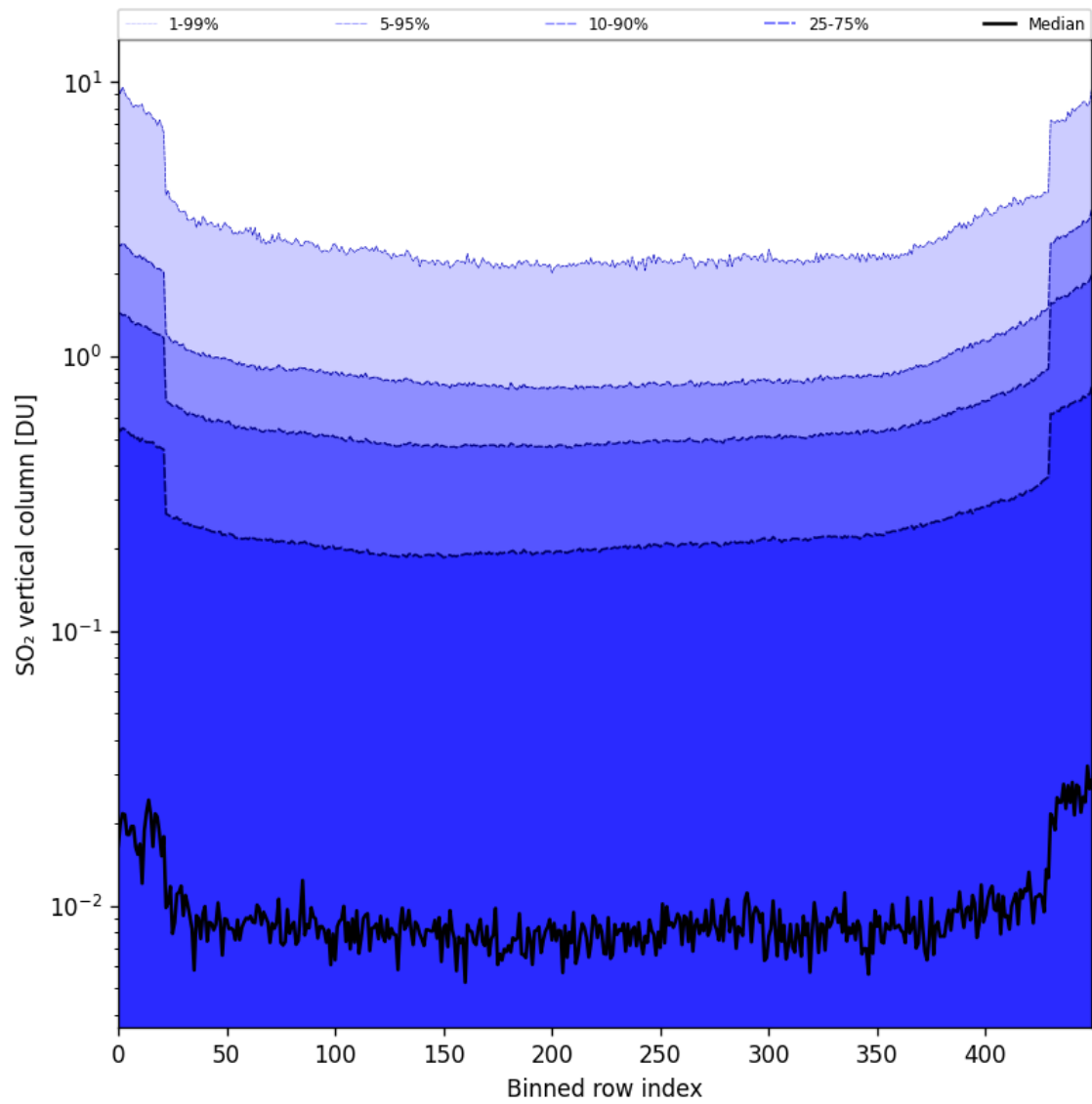
Figure 84: Along track statistics of “SO 2 vertical column” for 2025-11-18 to 2025-11-19
