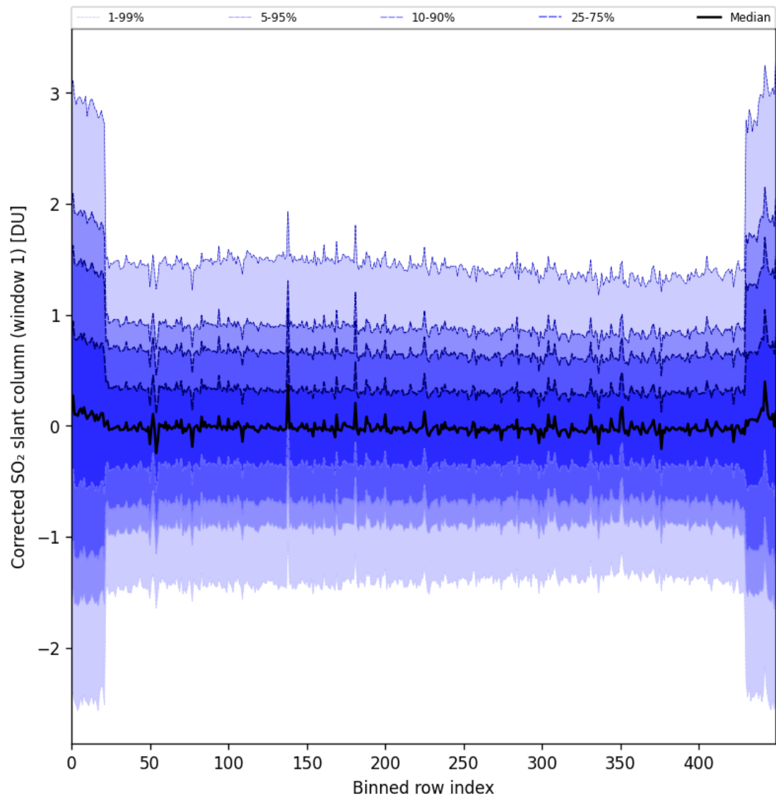
Figure 91: Along track statistics of “Corrected SO 2 slant column (window 1)” for 2025-11-18 to 2025-11-19
