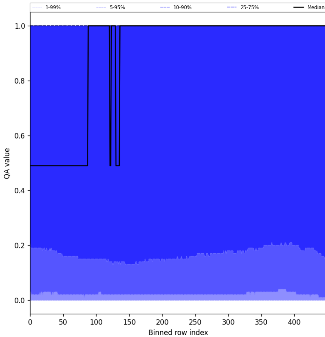
Figure 83: Along track statistics of “QA value” for 2025-11-18 to 2025-11-19
