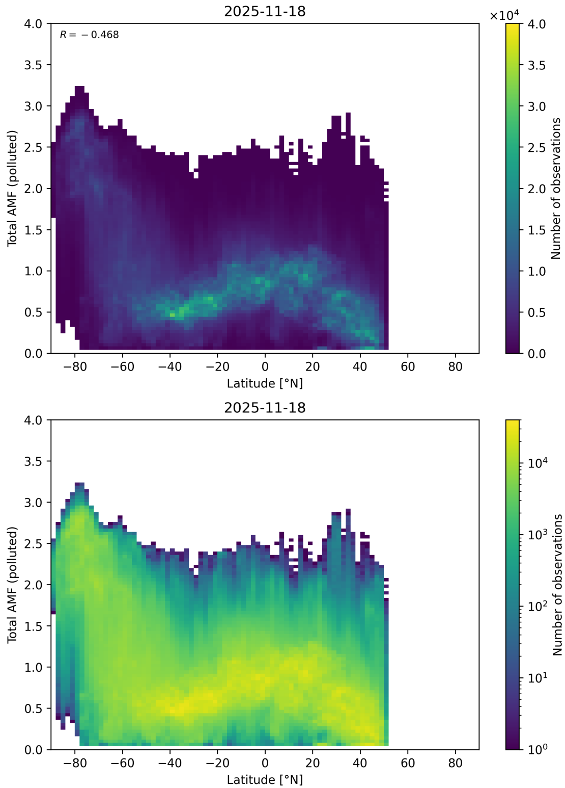
Figure 167: Scatter density plot of “Latitude” against “Total AMF (polluted)” for 2025-11-18 to 2025-11-19.
