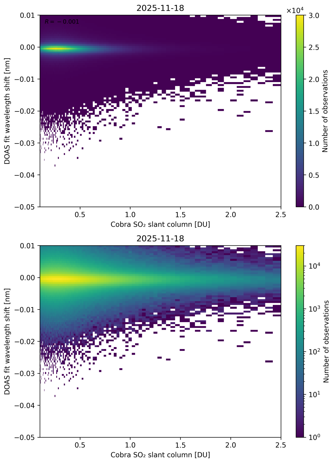
Figure 196: Scatter density plot of “Cobra SO 2 slant column” against “DOAS fit wavelength shift” for 2025-11-18 to 2025-11-19.
