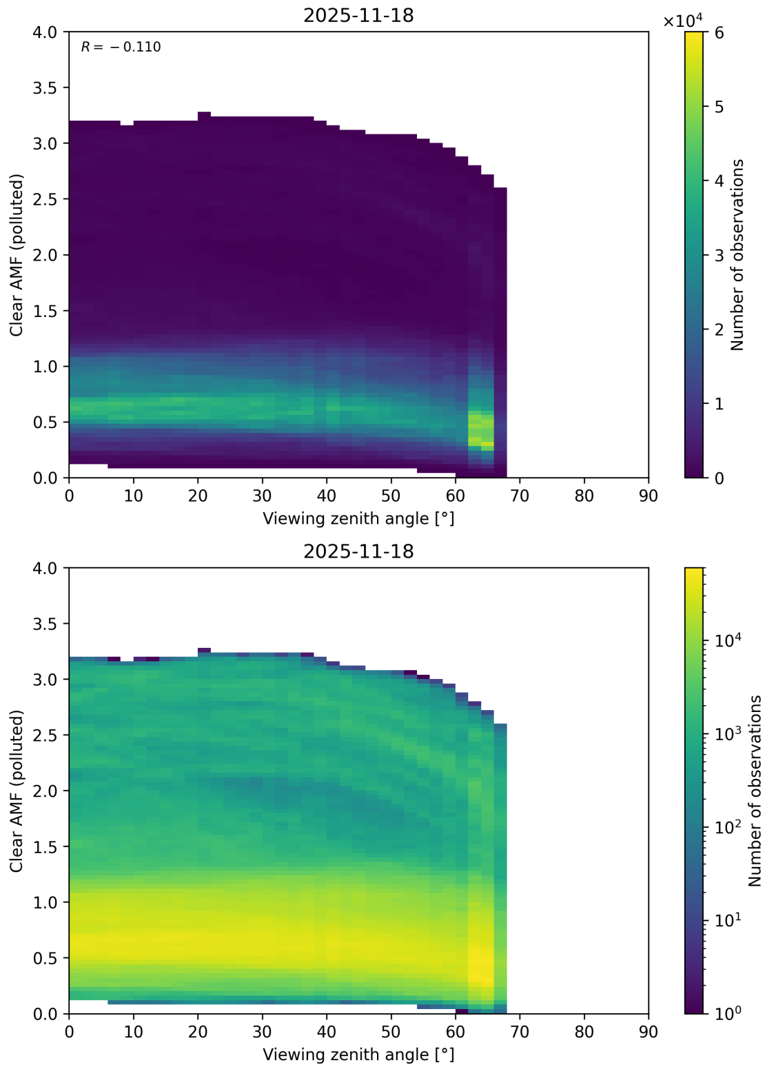
Figure 370: Scatter density plot of “Viewing zenith angle” against “Clear AMF (polluted)” for 2025-11-18 to 2025-11-19.
