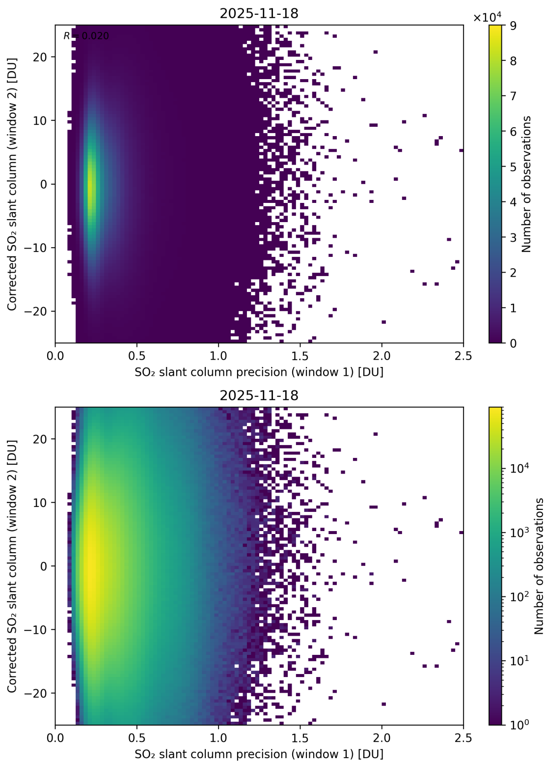
Figure 275: Scatter density plot of “SO 2 slant column precision (window 1)” against “Corrected SO 2 slant column (window 2)” for 2025-11-18 to 2025-11-19.
