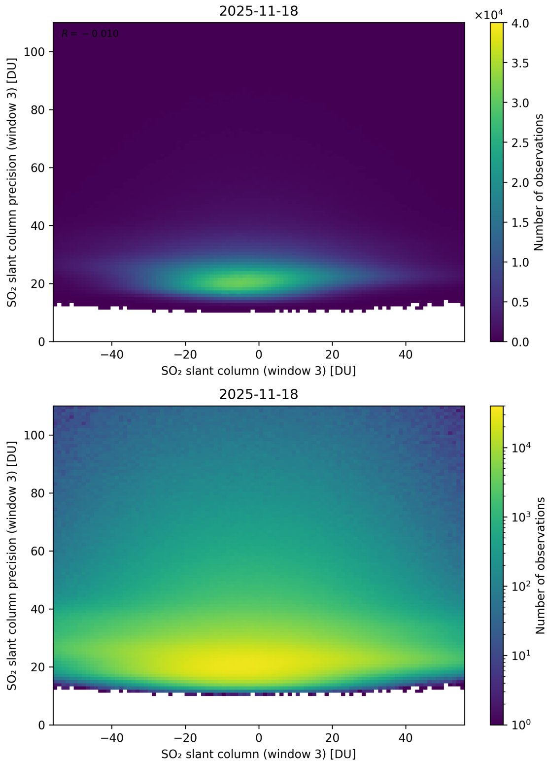
Figure 317: Scatter density plot of “SO 2 slant column (window 3)” against “SO 2 slant column precision (window 3)” for 2025-11-18 to 2025-11-19.
