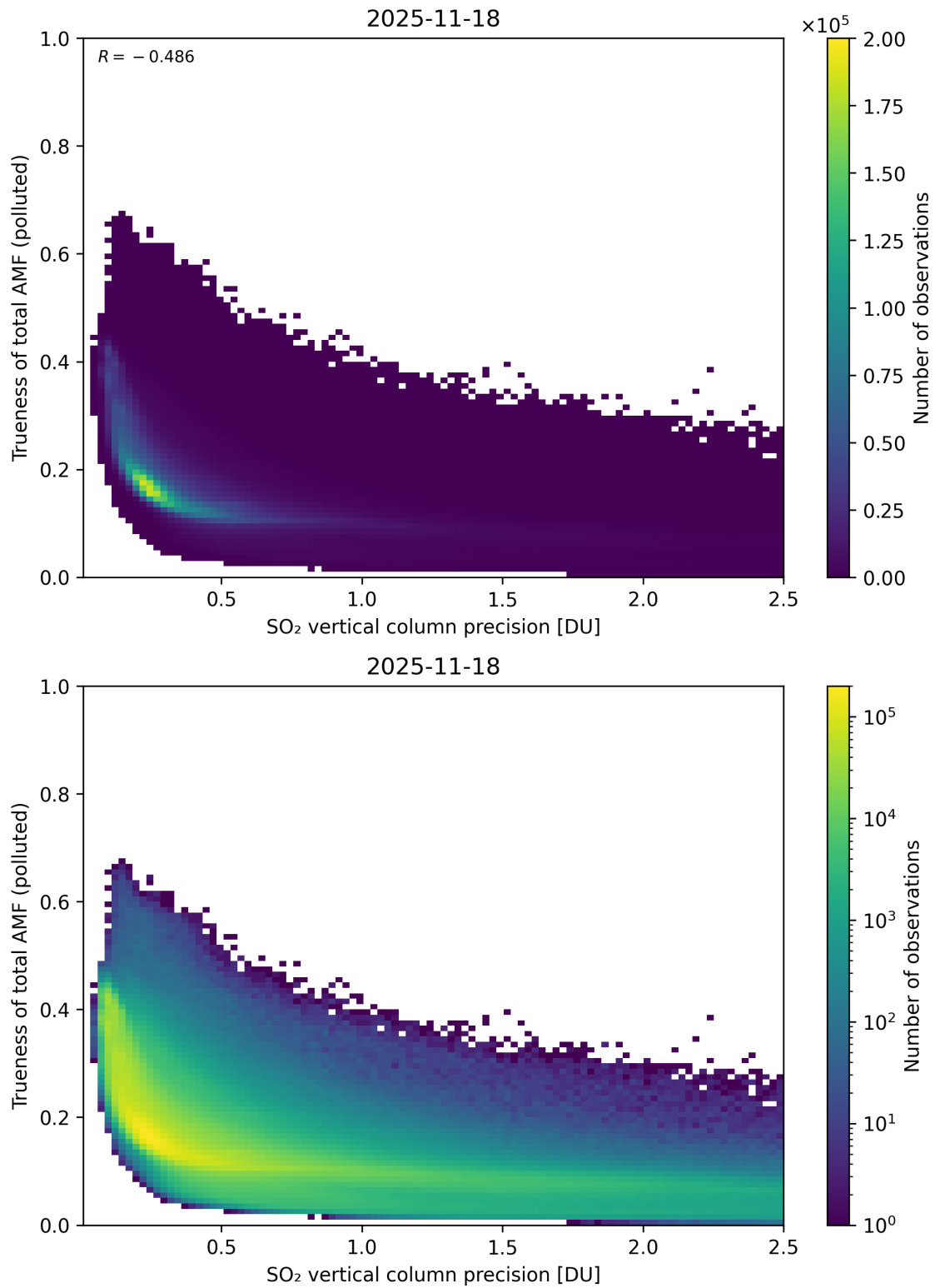
Figure 347: Scatter density plot of “SO 2 vertical column precision” against “Trueness of total AMF (polluted)” for 2025-11-18 to 2025-11-19.
