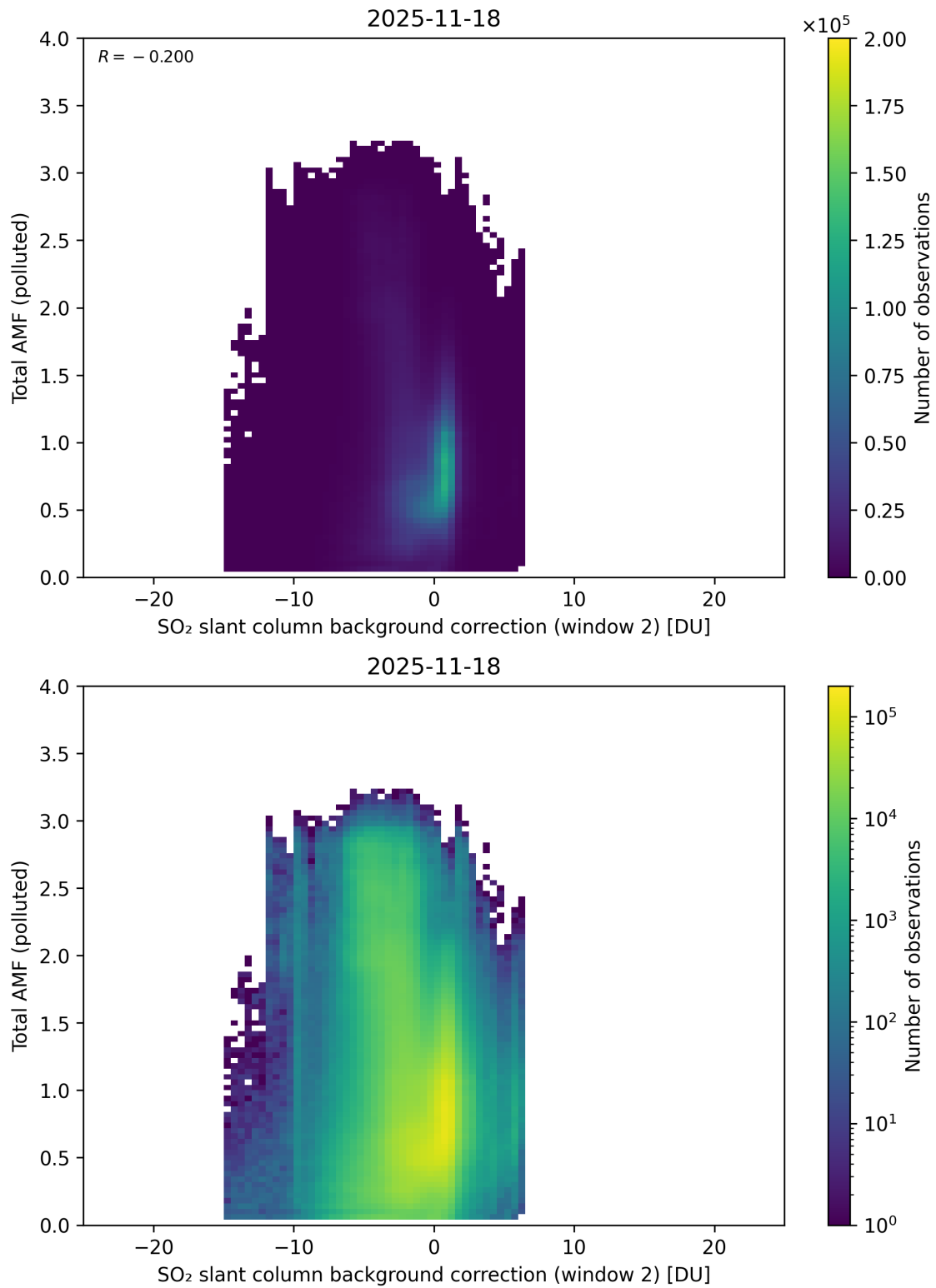
Figure 130: Scatter density plot of “SO 2 slant column background correction (window 2)” against “Total AMF (polluted)” for 2025-11-18 to 2025-11-19.
