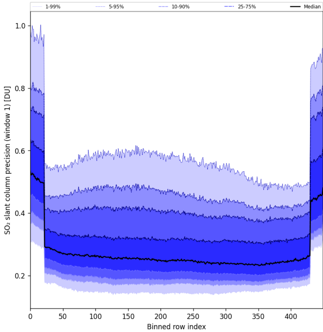
Figure 90: Along track statistics of “SO 2 slant column precision (window 1)” for 2025-11-18 to 2025-11-19
