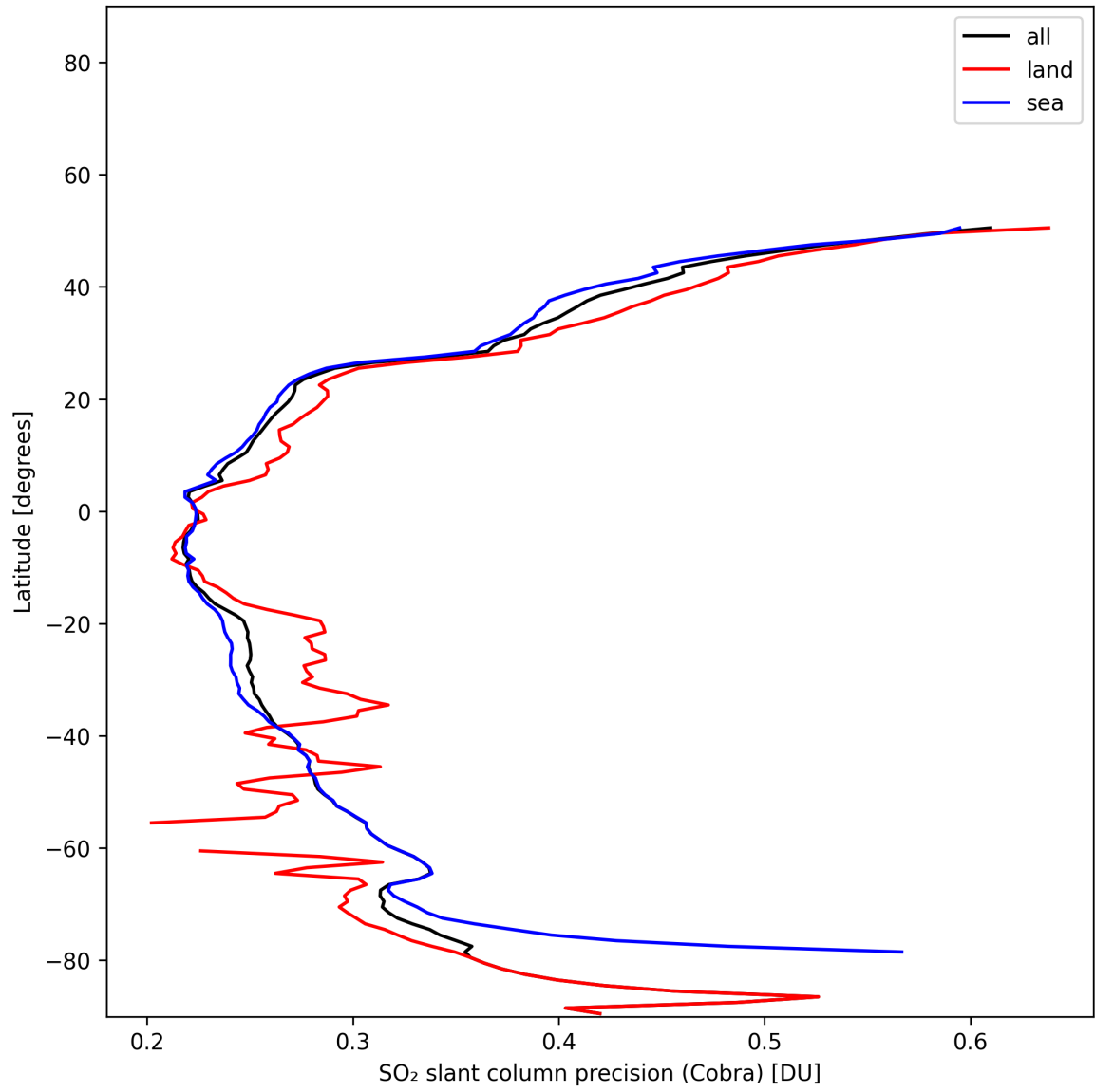
Figure 36: Zonal average of “SO 2 slant column precision (Cobra)” for 2025-11-18 to 2025-11-19.
