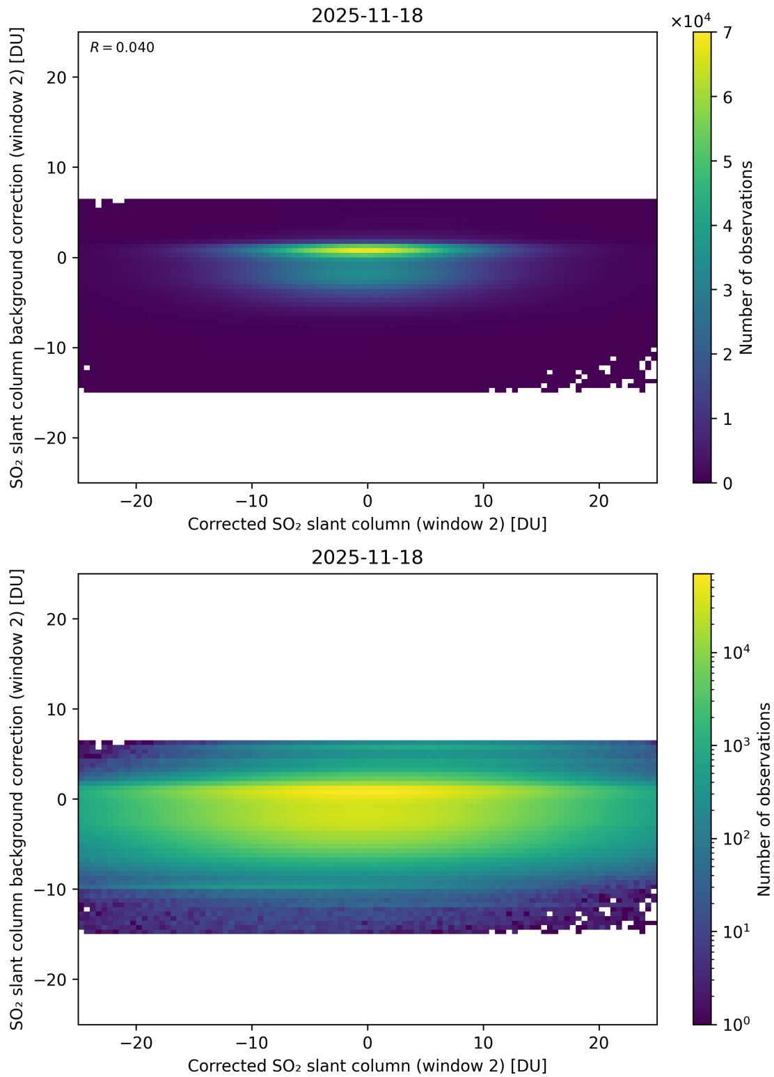
Figure 244: Scatter density plot of “Corrected SO 2 slant column (window 2)” against “SO 2 slant column background correction (window 2)” for 2025-11-18 to 2025-11-19.
