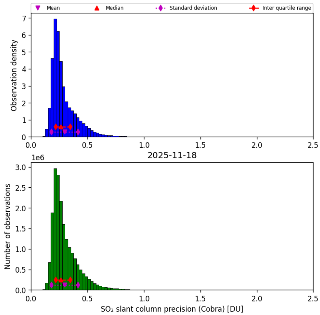
Figure 62: Histogram of “SO 2 slant column precision (Cobra)” for 2025-11-18 to 2025-11-19
