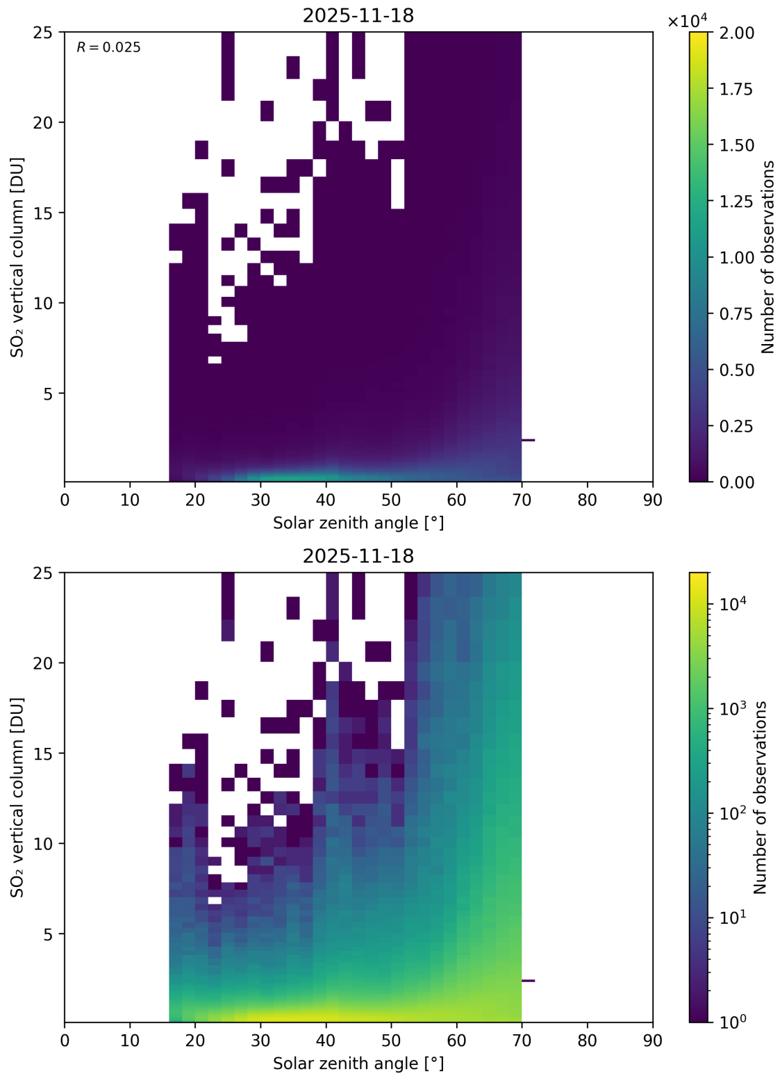
Figure 191: Scatter density plot of “Solar zenith angle” against “SO 2 vertical column” for 2025-11-18 to 2025-11-19.
