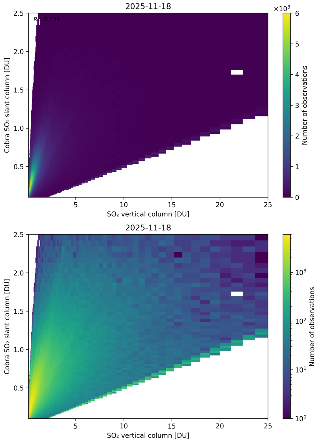
Figure 349: Scatter density plot of “SO 2 vertical column” against “Cobra SO 2 slant column” for 2025-11-18 to 2025-11-19.
