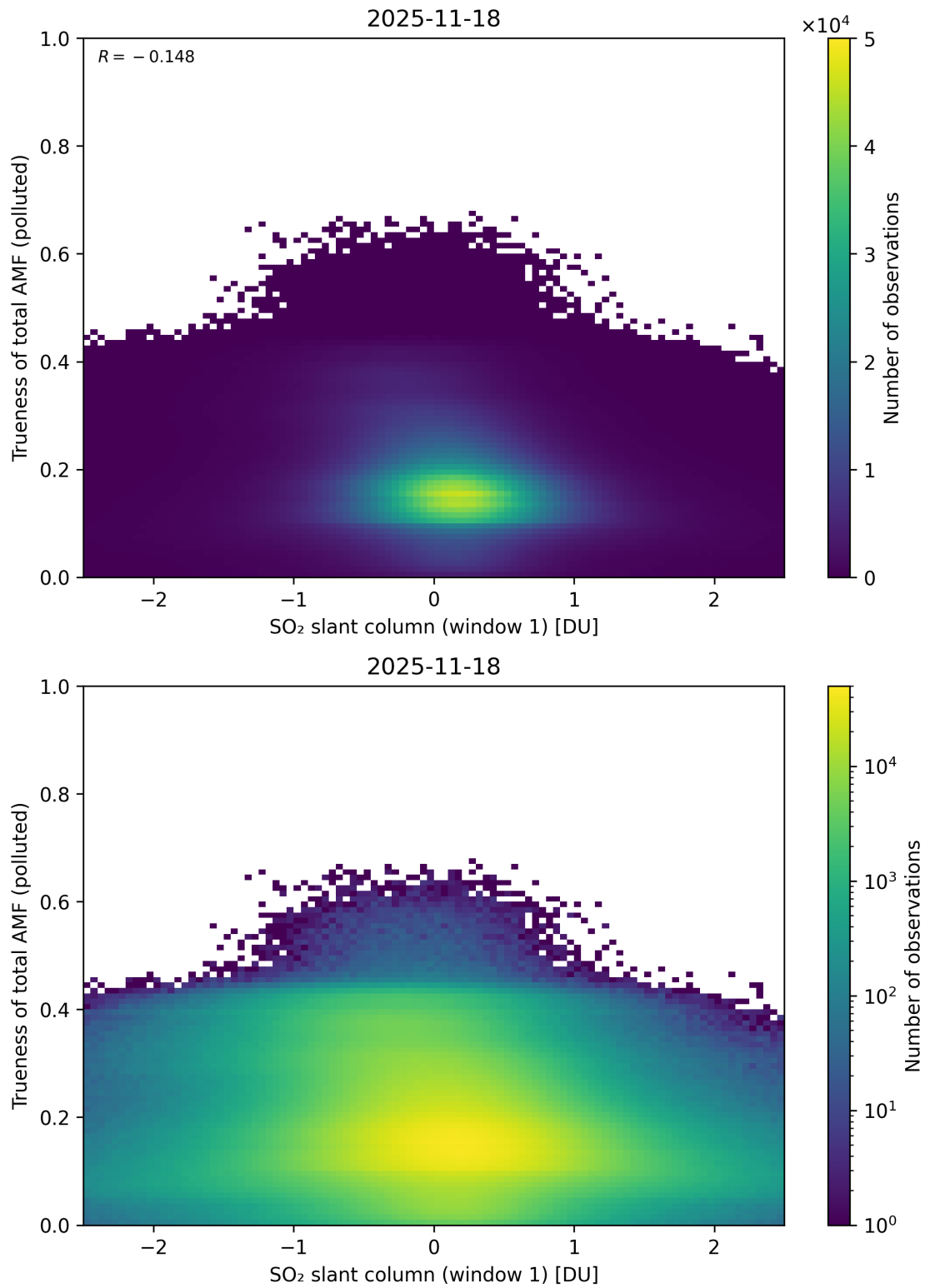
Figure 290: Scatter density plot of “SO 2 slant column (window 1)” against “Trueness of total AMF (polluted)” for 2025-11-18 to 2025-11-19.
