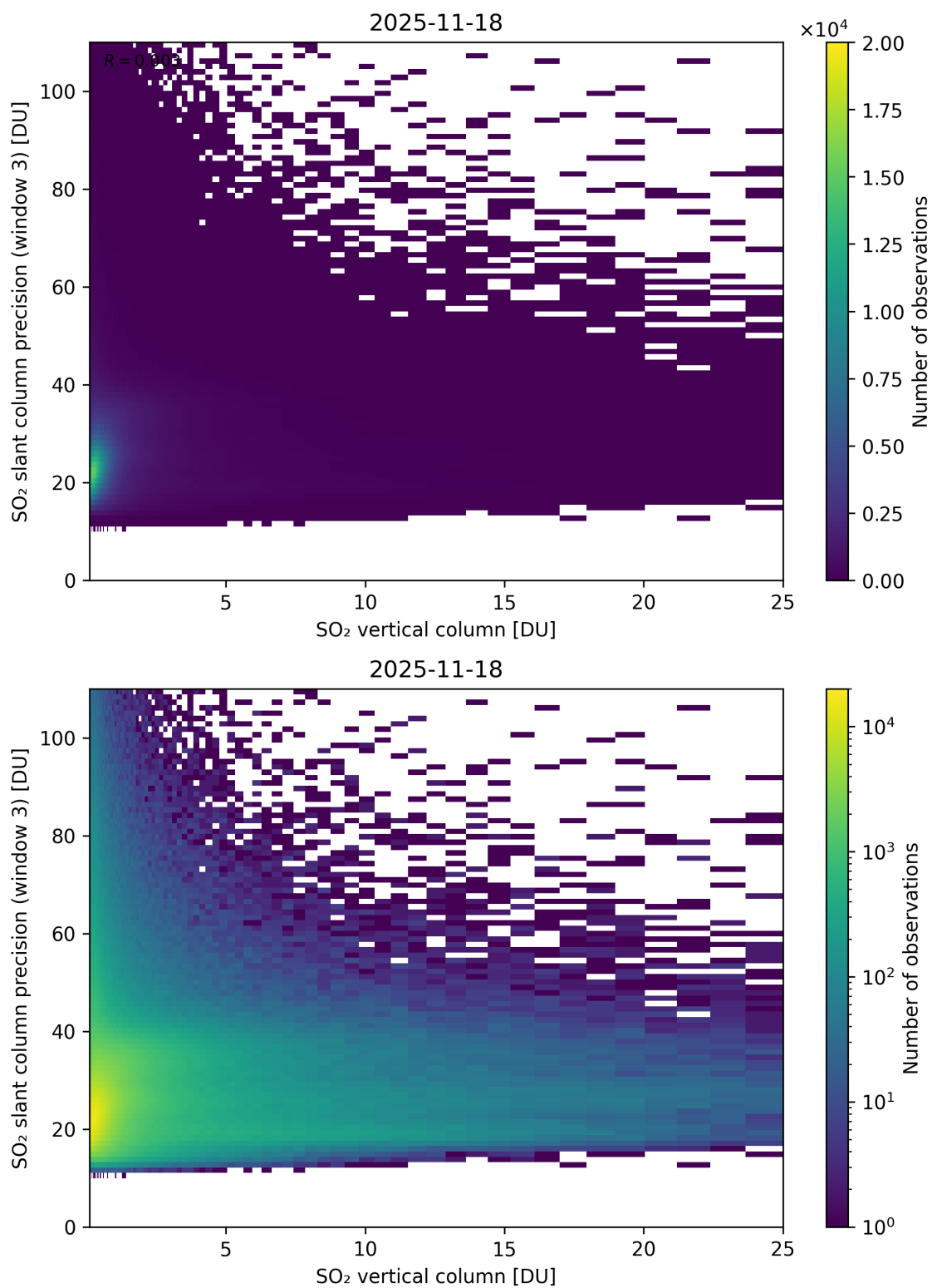
Figure 358: Scatter density plot of “SO 2 vertical column” against “SO 2 slant column precision (window 3)” for 2025-11-18 to 2025-11-19.
