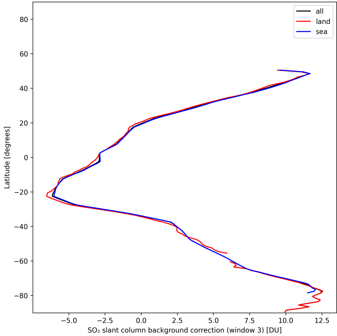
Figure 48: Zonal average of “SO 2 slant column background correction (window 3)” for 2025-11-18 to 2025-11-19.
