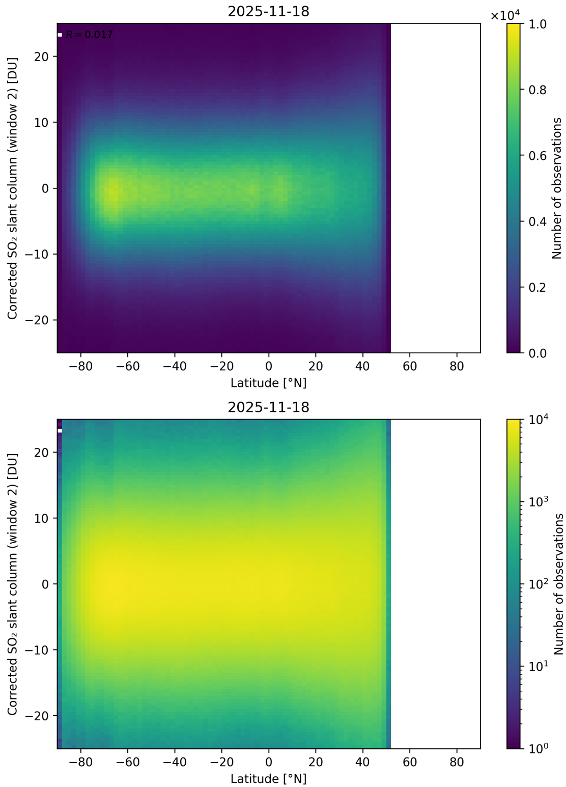
Figure 160: Scatter density plot of “Latitude” against “Corrected SO 2 slant column (window 2)” for 2025-11-18 to 2025-11-19.
