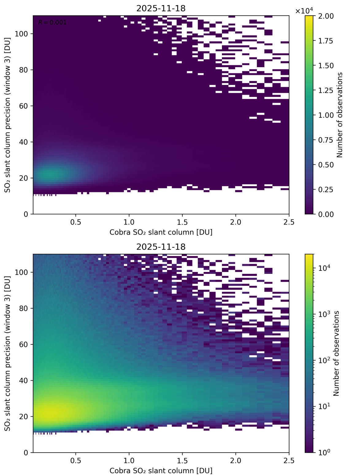
Figure 223: Scatter density plot of “Cobra SO 2 slant column” against “SO 2 slant column precision (window 3)” for 2025-11-18 to 2025-11-19.
