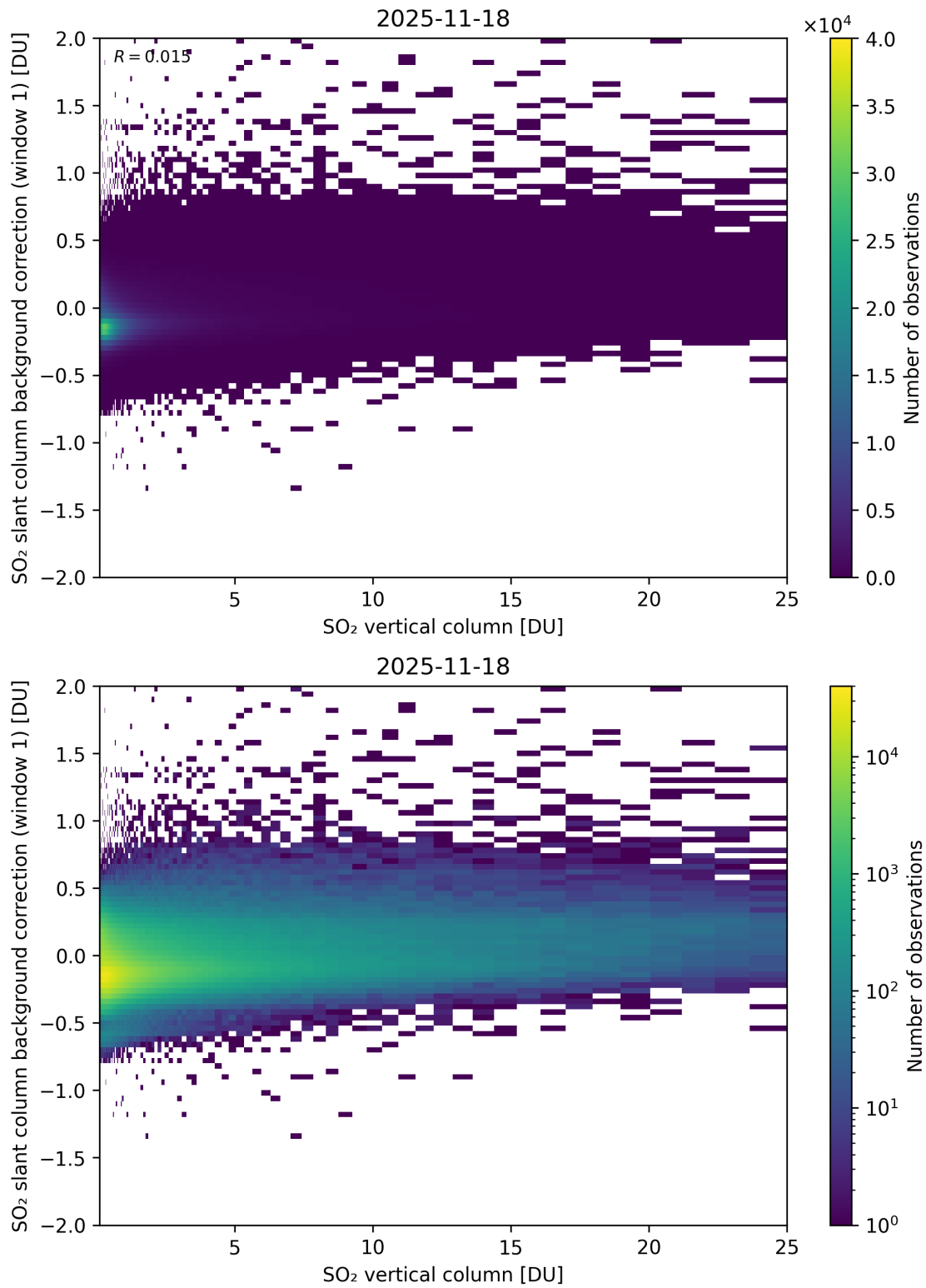
Figure 323: Scatter density plot of “SO 2 vertical column” against “SO 2 slant column background correction (window 1)” for 2025-11-18 to 2025-11-19.
