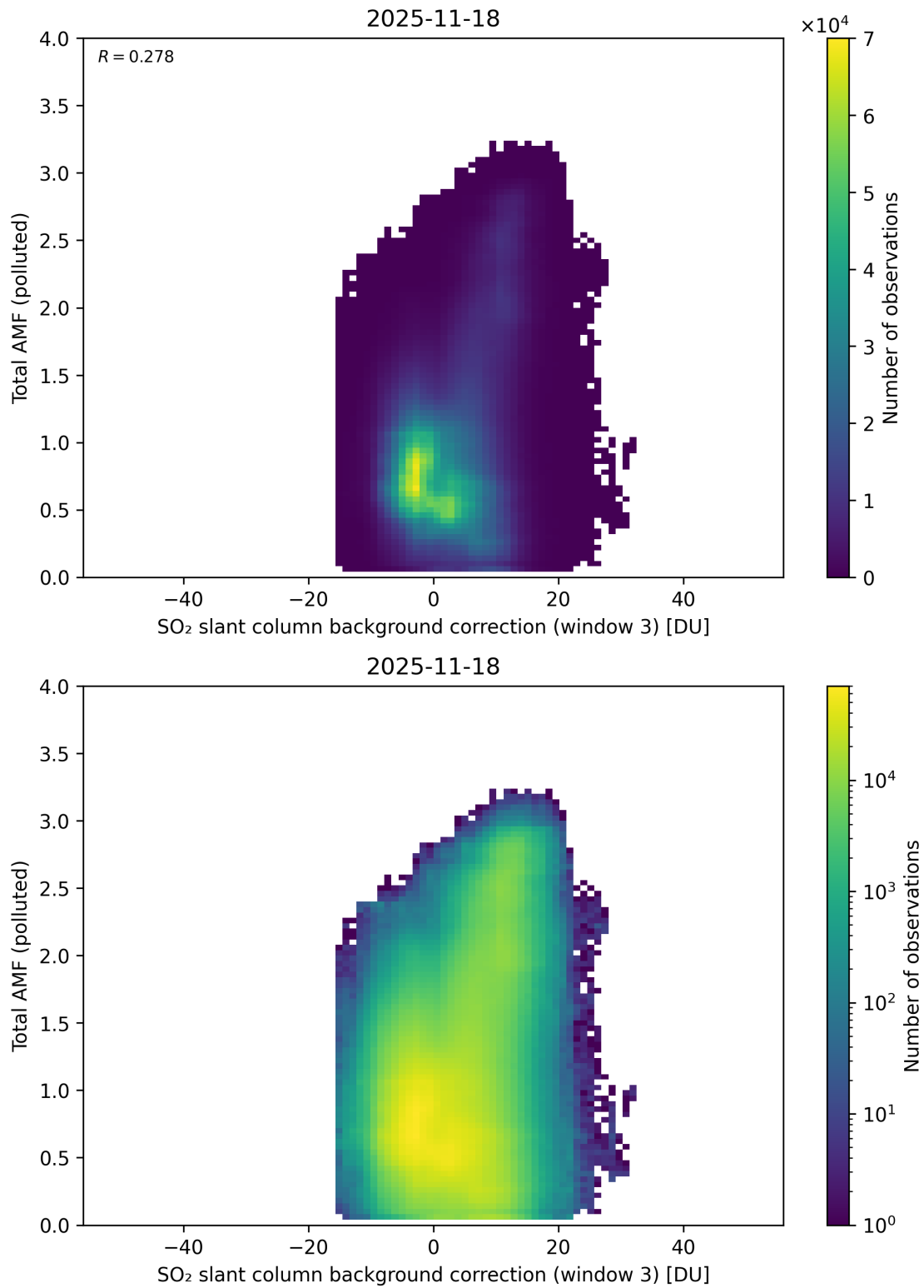
Figure 136: Scatter density plot of “SO 2 slant column background correction (window 3)” against “Total AMF (polluted)” for 2025-11-18 to 2025-11-19.
