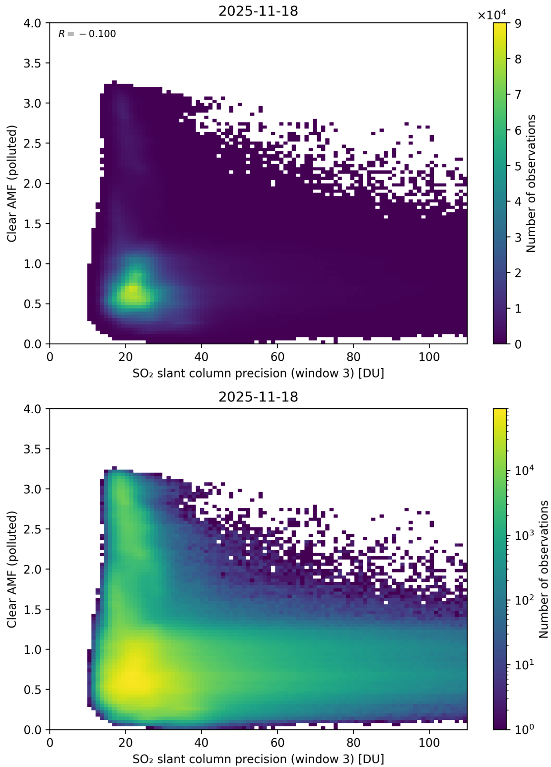
Figure 311: Scatter density plot of “SO 2 slant column precision (window 3)” against “Clear AMF (polluted)” for 2025-11-18 to 2025-11-19.
