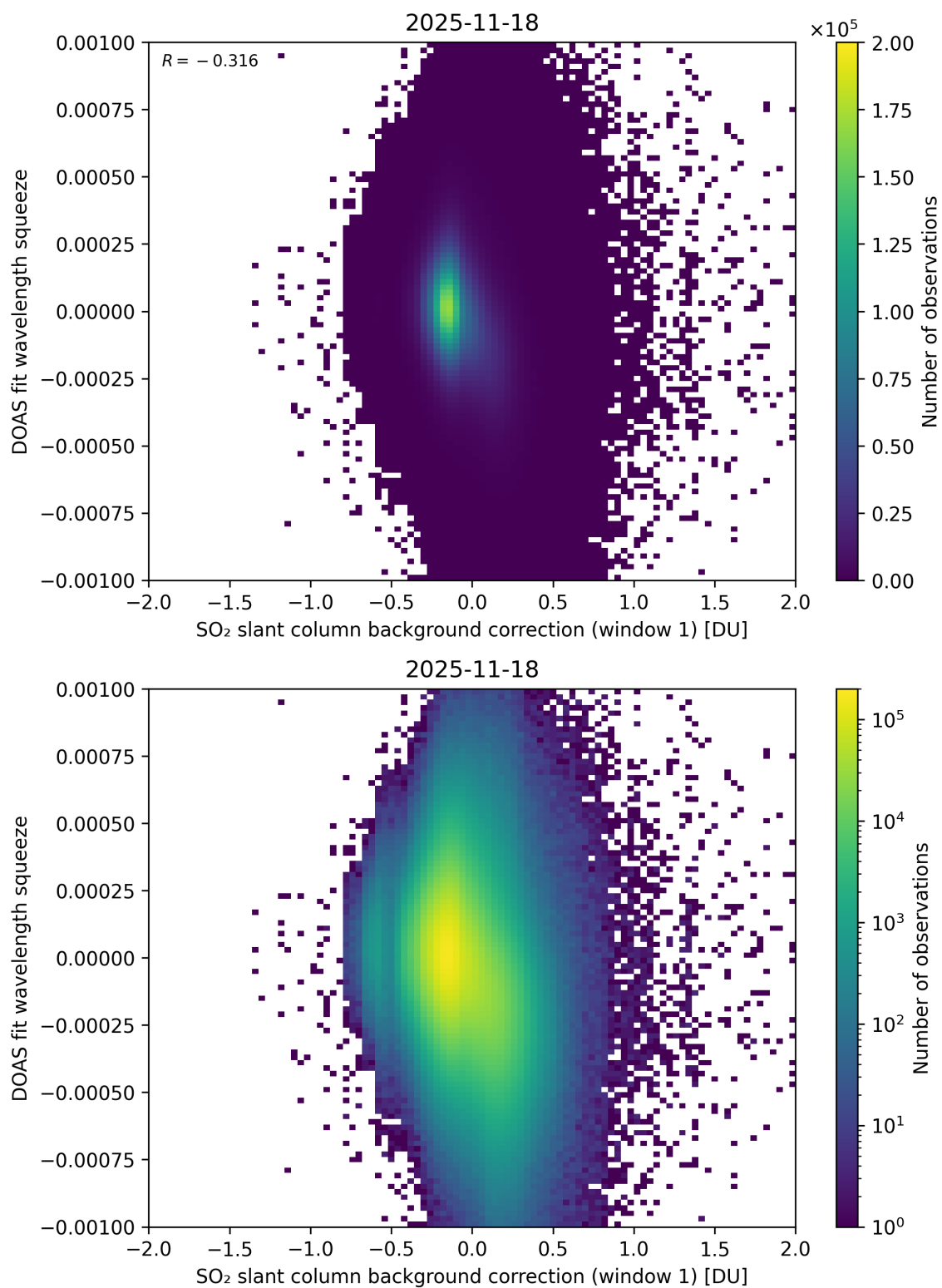
Figure 112: Scatter density plot of “SO 2 slant column background correction (window 1)” against “DOAS fit wavelength squeeze” for 2025-11-18 to 2025-11-19.
