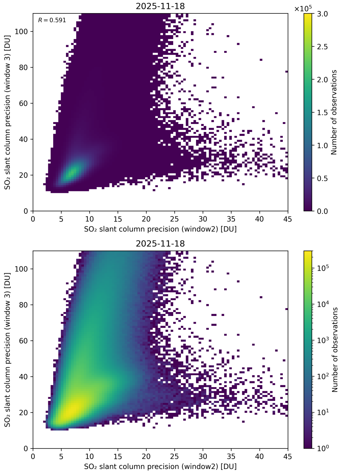
Figure 300: Scatter density plot of “SO 2 slant column precision (window2)” against “SO 2 slant column precision (window 3)” for 2025-11-18 to 2025-11-19.
