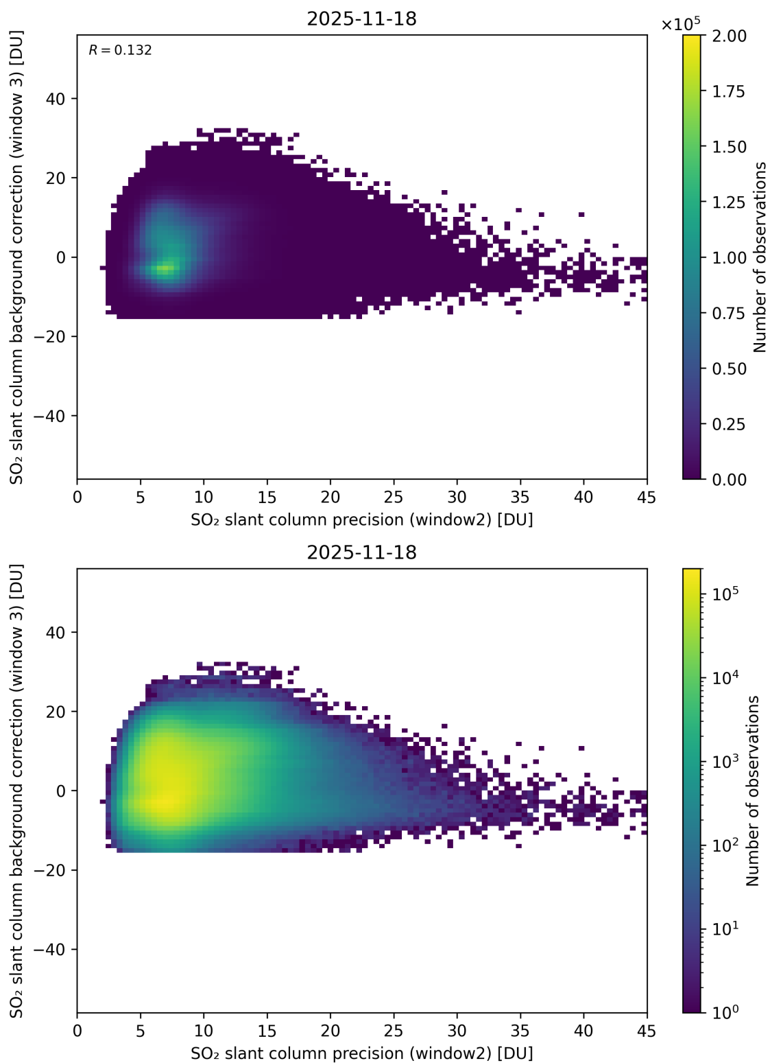
Figure 292: Scatter density plot of “SO 2 slant column precision (window2)” against “SO 2 slant column background correction (window 3)” for 2025-11-18 to 2025-11-19.
