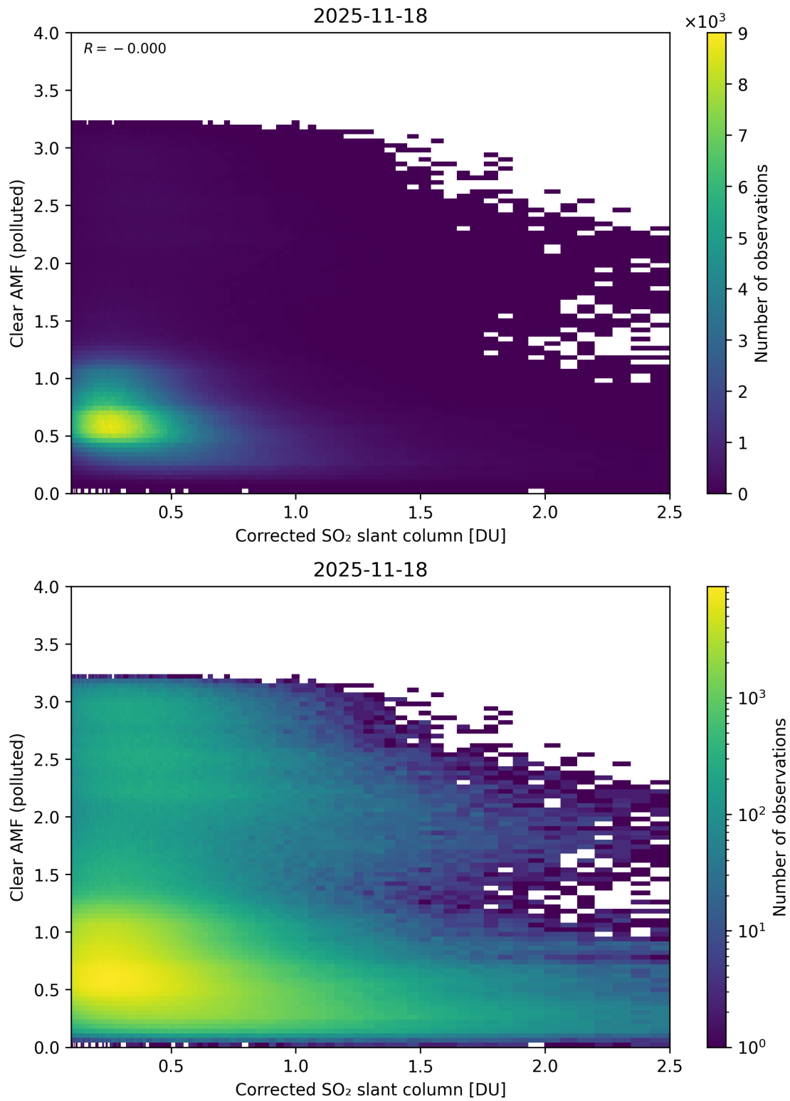
Figure 232: Scatter density plot of “Corrected SO 2 slant column” against “Clear AMF (polluted)” for 2025-11-18 to 2025-11-19.
