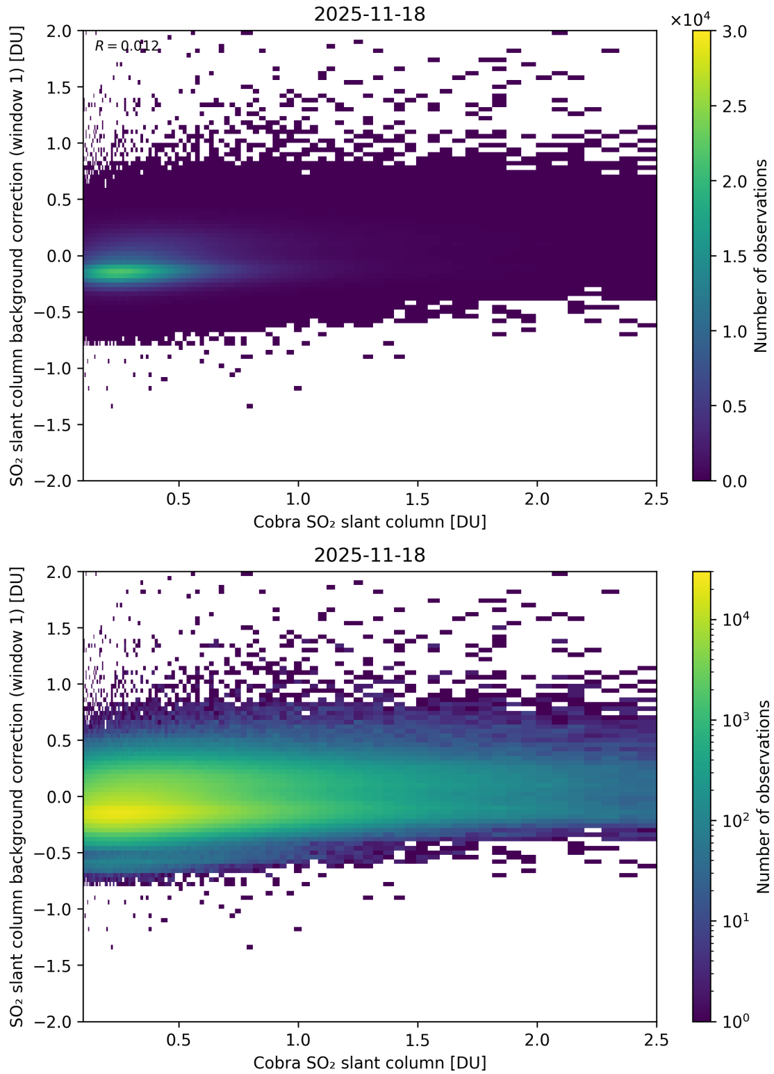
Figure 193: Scatter density plot of “Cobra SO 2 slant column” against “SO 2 slant column background correction (window 1)” for 2025-11-18 to 2025-11-19.
