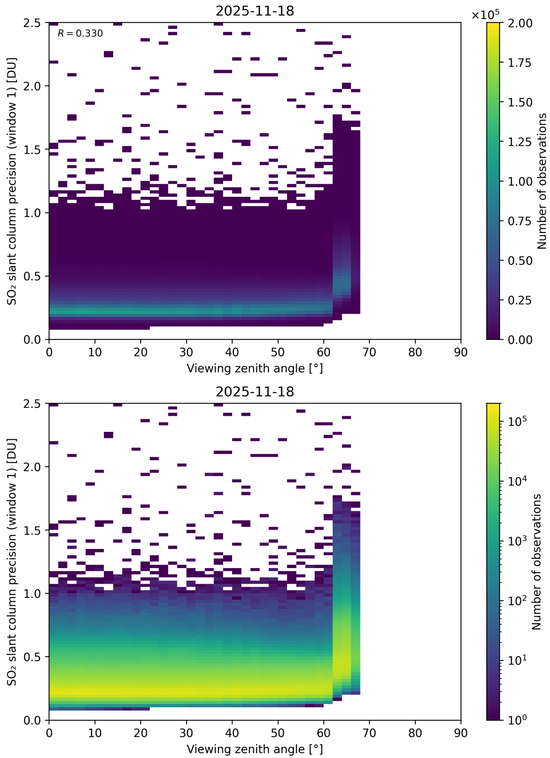
Figure 377: Scatter density plot of “Viewing zenith angle” against “SO 2 slant column precision (window 1)” for 2025-11-18 to 2025-11-19.
