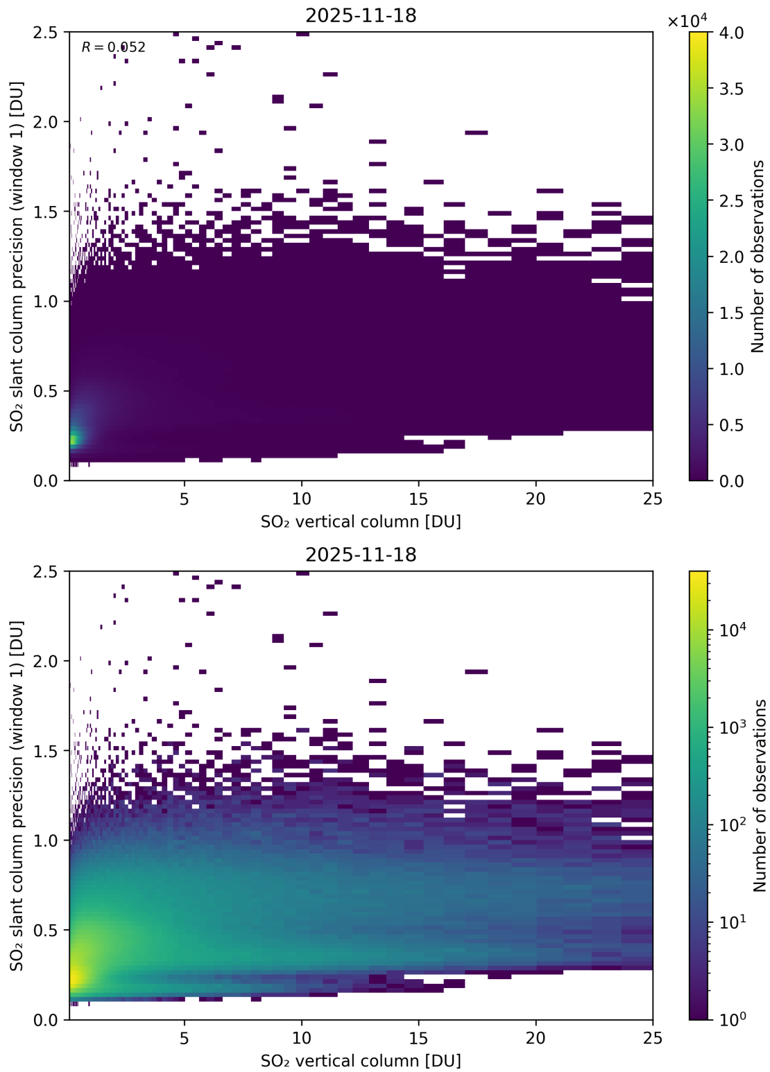
Figure 355: Scatter density plot of “SO 2 vertical column” against “SO 2 slant column precision (window 1)” for 2025-11-18 to 2025-11-19.
