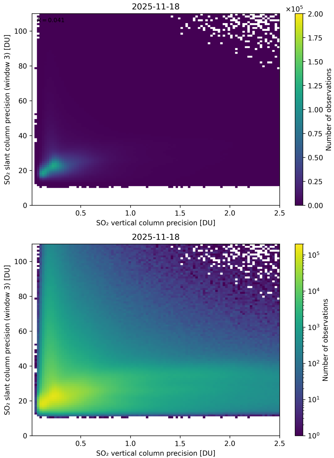
Figure 345: Scatter density plot of “SO 2 vertical column precision” against “SO 2 slant column precision (window 3)” for 2025-11-18 to 2025-11-19.
