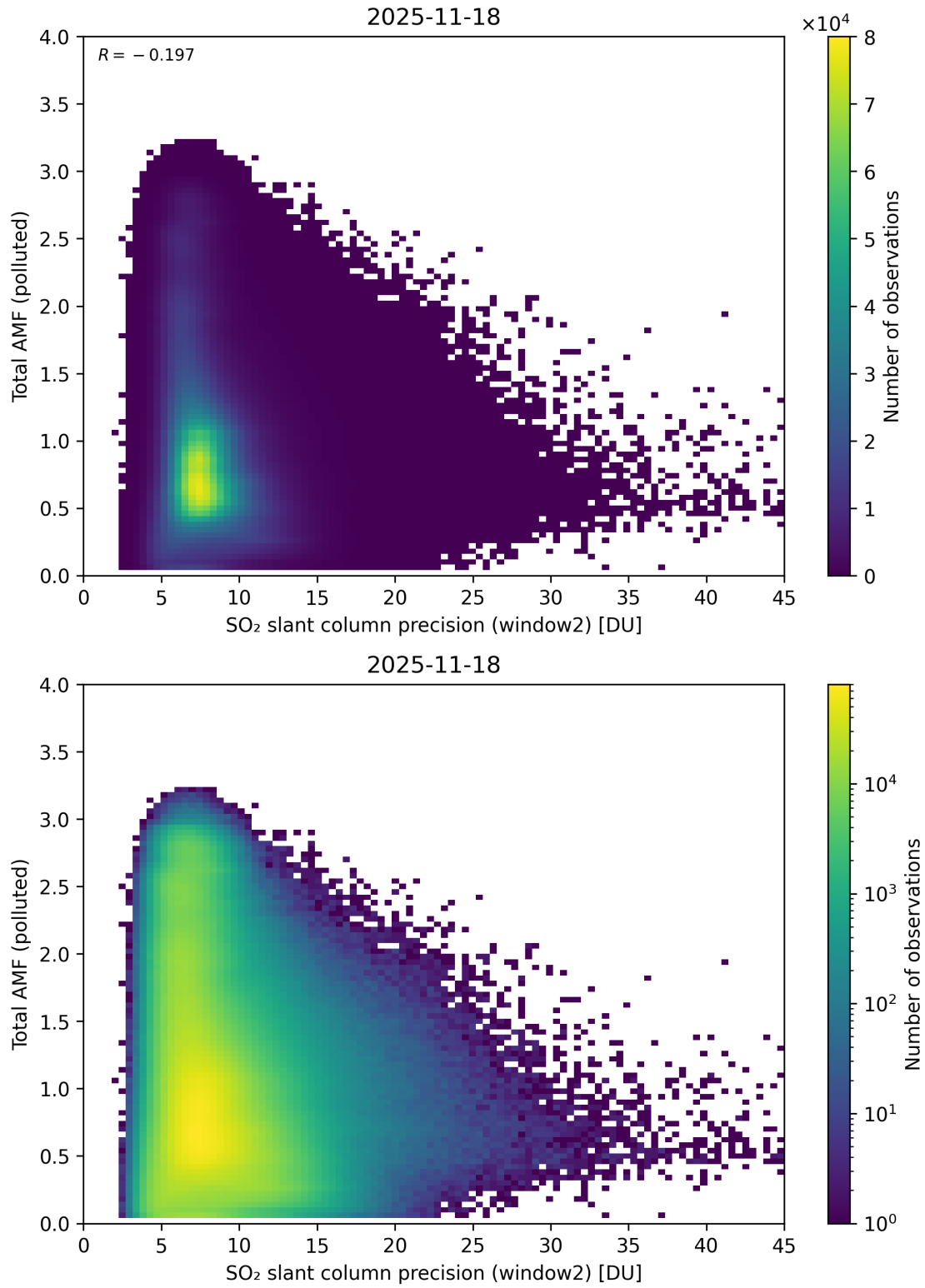
Figure 301: Scatter density plot of “SO 2 slant column precision (window2)” against “Total AMF (polluted)” for 2025-11-18 to 2025-11-19.
