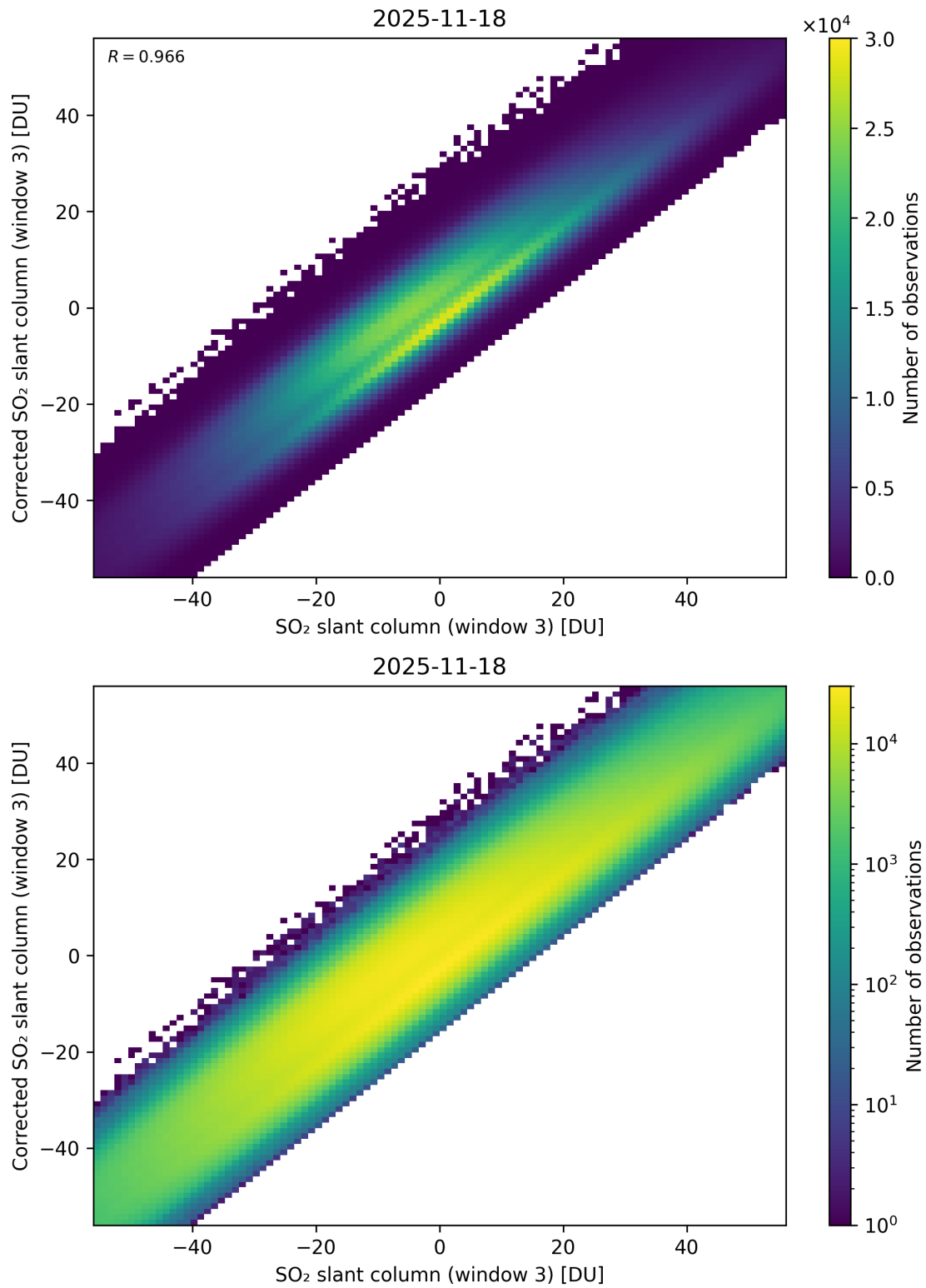
Figure 316: Scatter density plot of “SO 2 slant column (window 3)” against “Corrected SO 2 slant column (window 3)” for 2025-11-18 to 2025-11-19.
