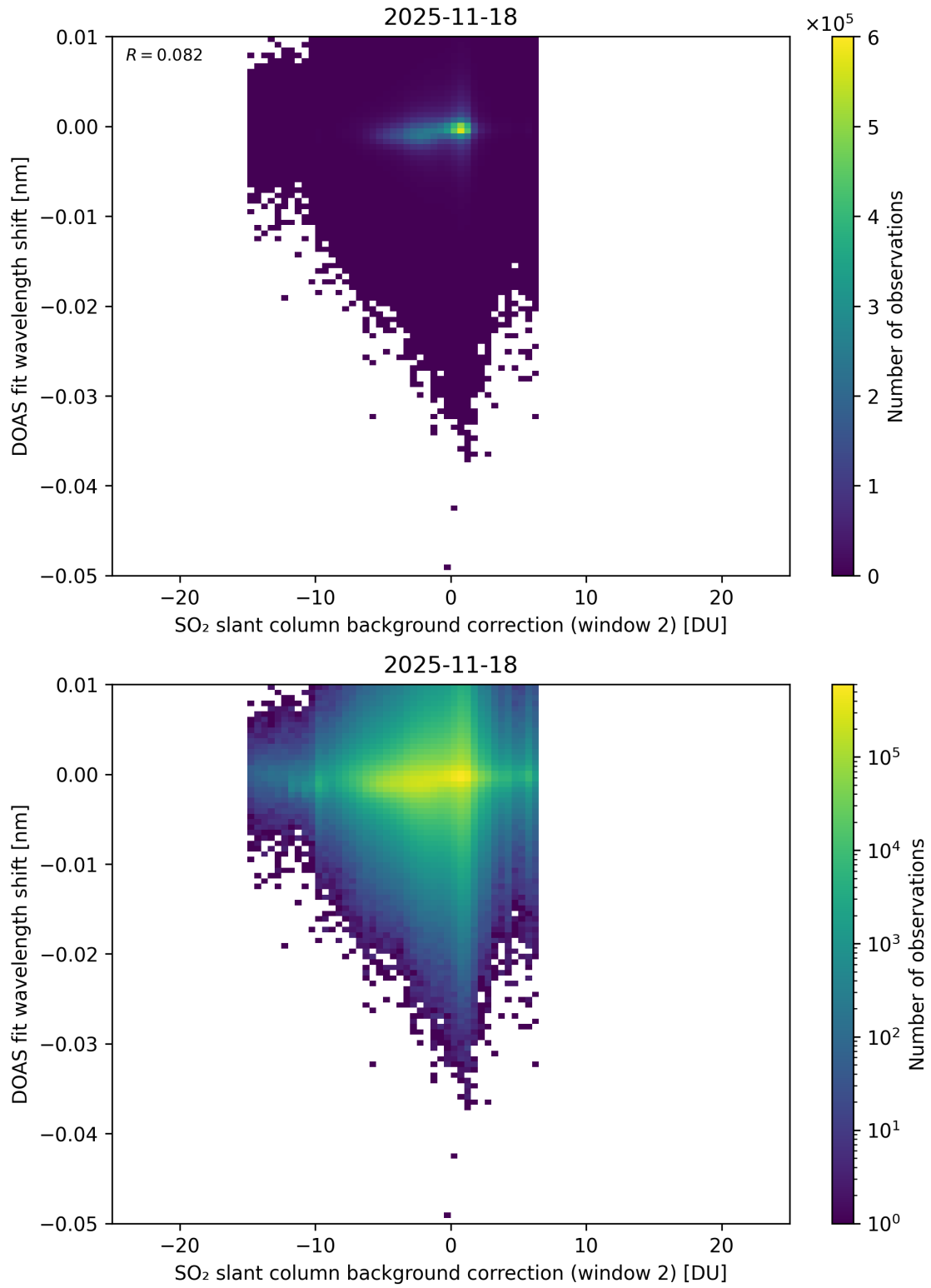
Figure 123: Scatter density plot of “SO 2 slant column background correction (window 2)” against “DOAS fit wavelength shift” for 2025-11-18 to 2025-11-19.
