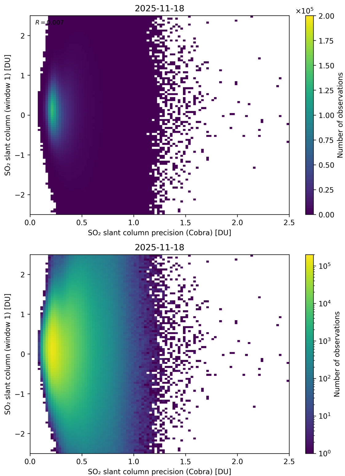
Figure 208: Scatter density plot of “SO 2 slant column precision (Cobra)” against “SO 2 slant column (window 1)” for 2025-11-18 to 2025-11-19.
