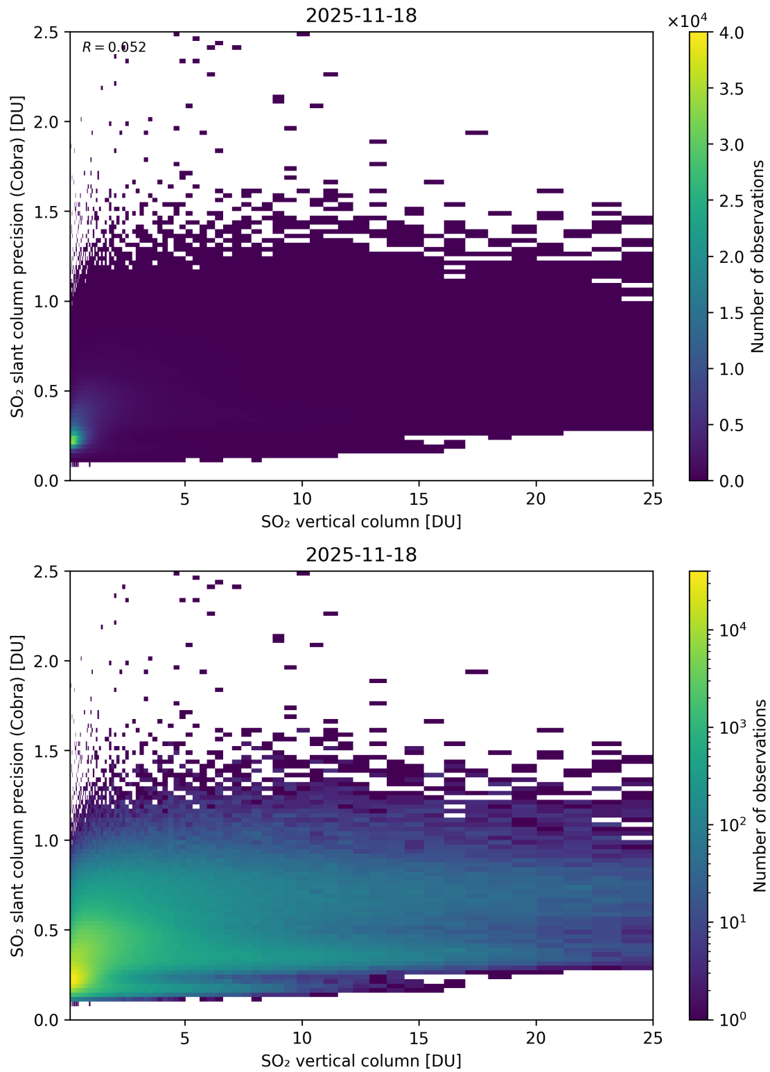
Figure 350: Scatter density plot of “SO 2 vertical column” against “SO 2 slant column precision (Cobra)” for 2025-11-18 to 2025-11-19.
