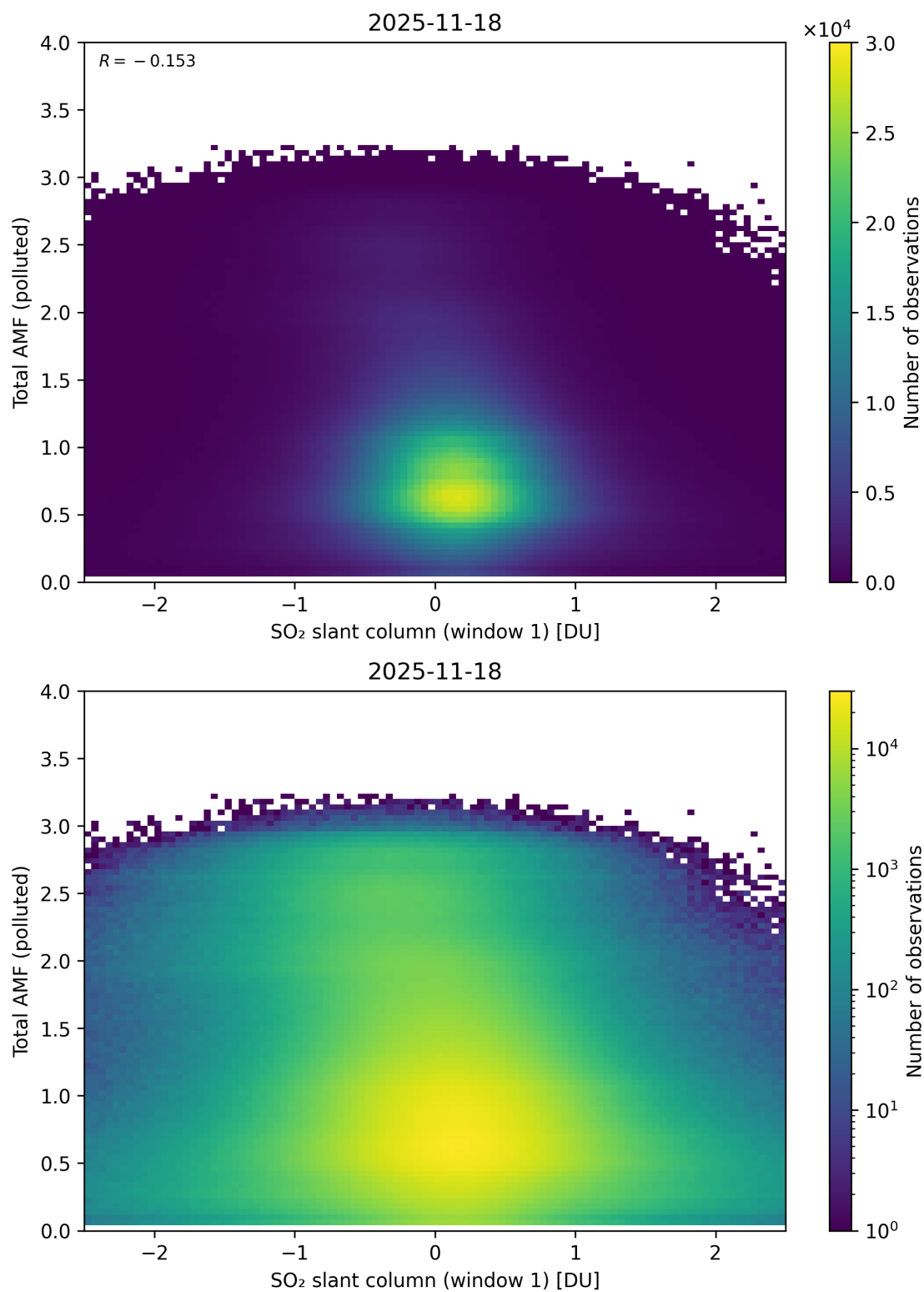
Figure 289: Scatter density plot of “SO 2 slant column (window 1)” against “Total AMF (polluted)” for 2025-11-18 to 2025-11-19.
