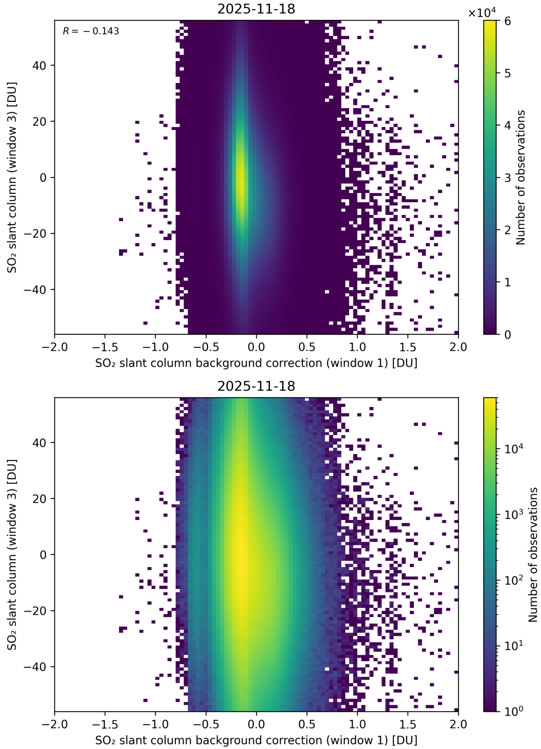
Figure 118: Scatter density plot of “SO 2 slant column background correction (window 1)” against “SO 2 slant column (window 3)” for 2025-11-18 to 2025-11-19.
