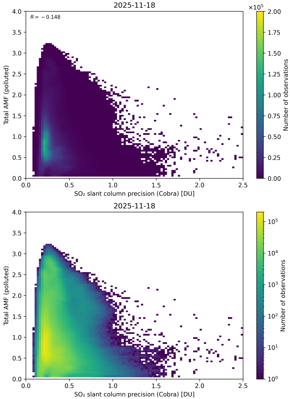
Figure 213: Scatter density plot of “SO 2 slant column precision (Cobra)” against “Total AMF (polluted)” for 2025-11-18 to 2025-11-19.
