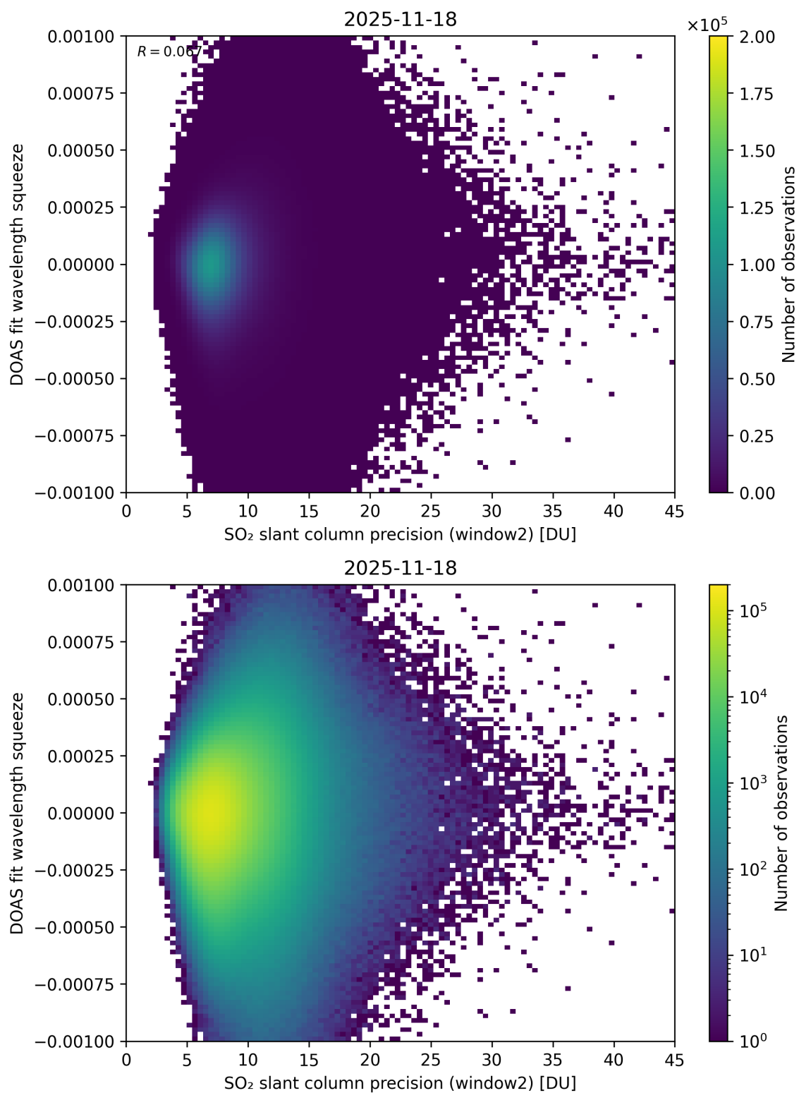
Figure 294: Scatter density plot of “SO 2 slant column precision (window2)” against “DOAS fit wavelength squeeze” for 2025-11-18 to 2025-11-19.
