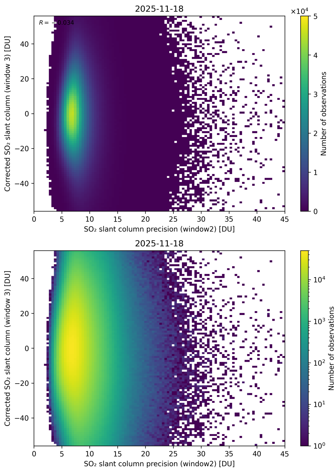
Figure 298: Scatter density plot of “SO 2 slant column precision (window2)” against “Corrected SO 2 slant column (window 3)” for 2025-11-18 to 2025-11-19.
