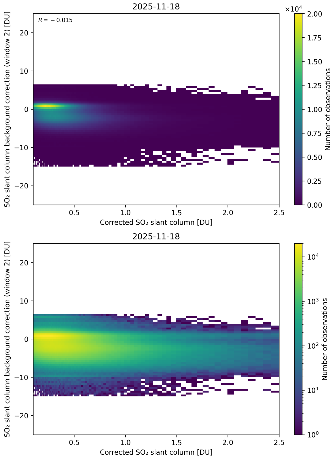
Figure 227: Scatter density plot of “Corrected SO 2 slant column” against “SO 2 slant column background correction (window 2)” for 2025-11-18 to 2025-11-19.
