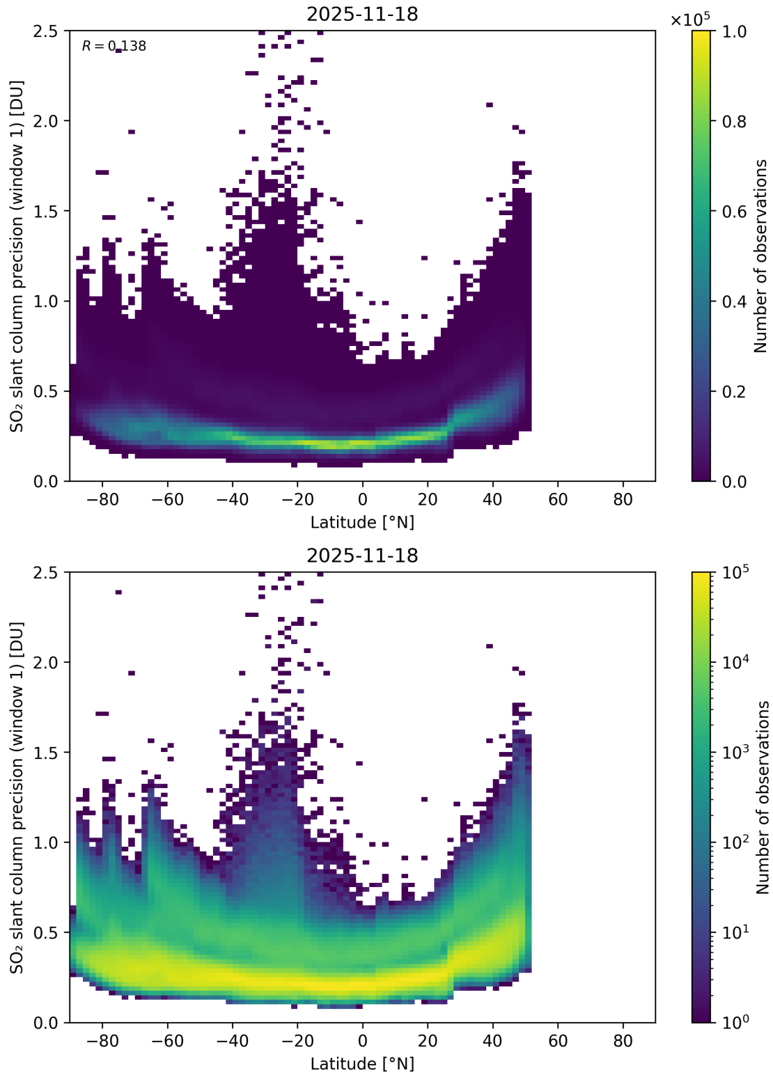
Figure 163: Scatter density plot of “Latitude” against “SO 2 slant column precision (window 1)” for 2025-11-18 to 2025-11-19.
