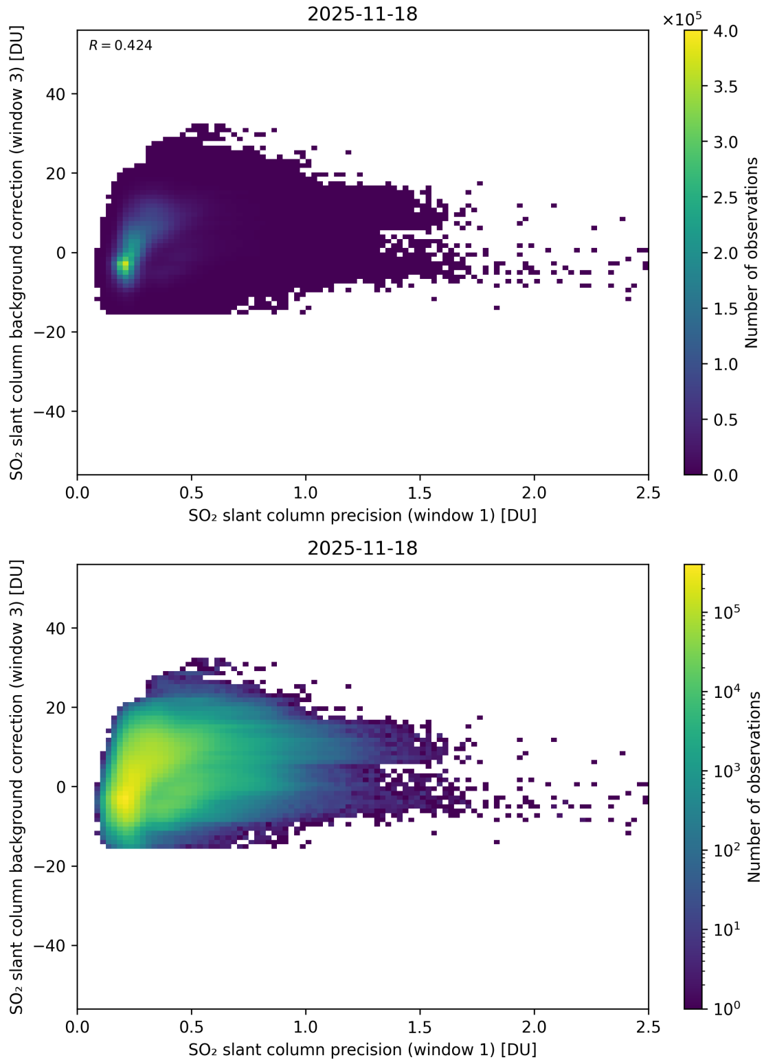
Figure 270: Scatter density plot of “SO 2 slant column precision (window 1)” against “SO 2 slant column background correction (window 3)” for 2025-11-18 to 2025-11-19.
