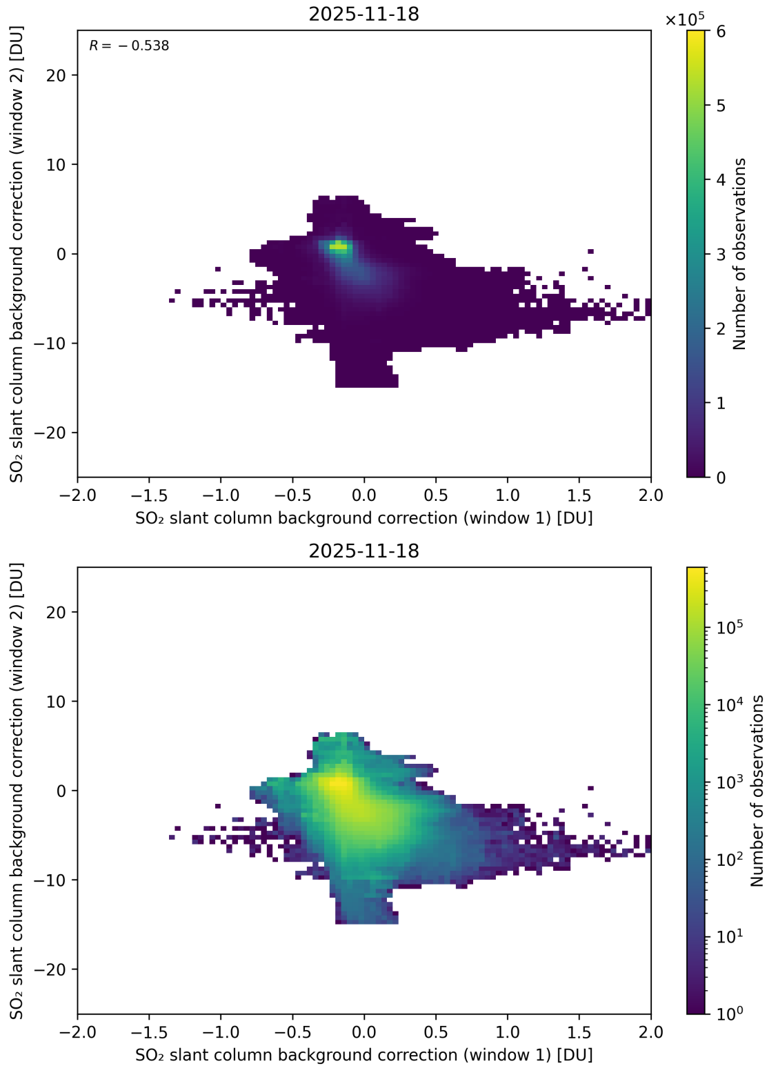
Figure 109: Scatter density plot of “SO 2 slant column background correction (window 1)” against “SO 2 slant column background correction (window 2)” for 2025-11-18 to 2025-11-19.
