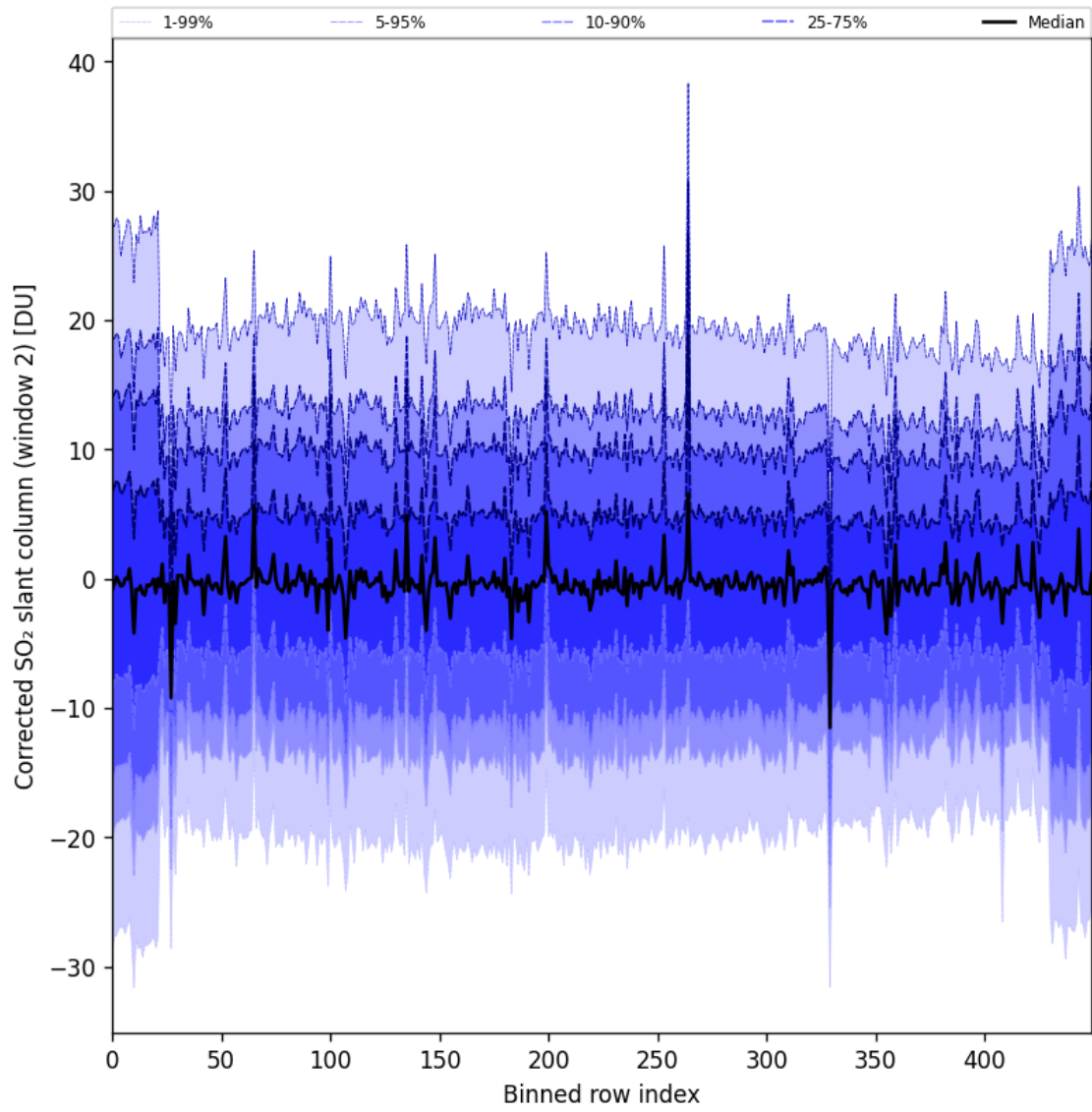
Figure 95: Along track statistics of “Corrected SO 2 slant column (window 2)” for 2025-11-18 to 2025-11-19
