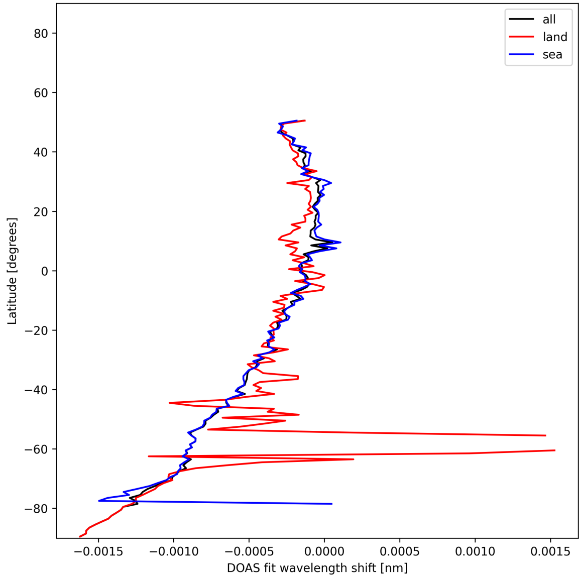
Figure 50: Zonal average of "DOAS fit wavelength shift" for 2025-11-18 to 2025-11-19.
