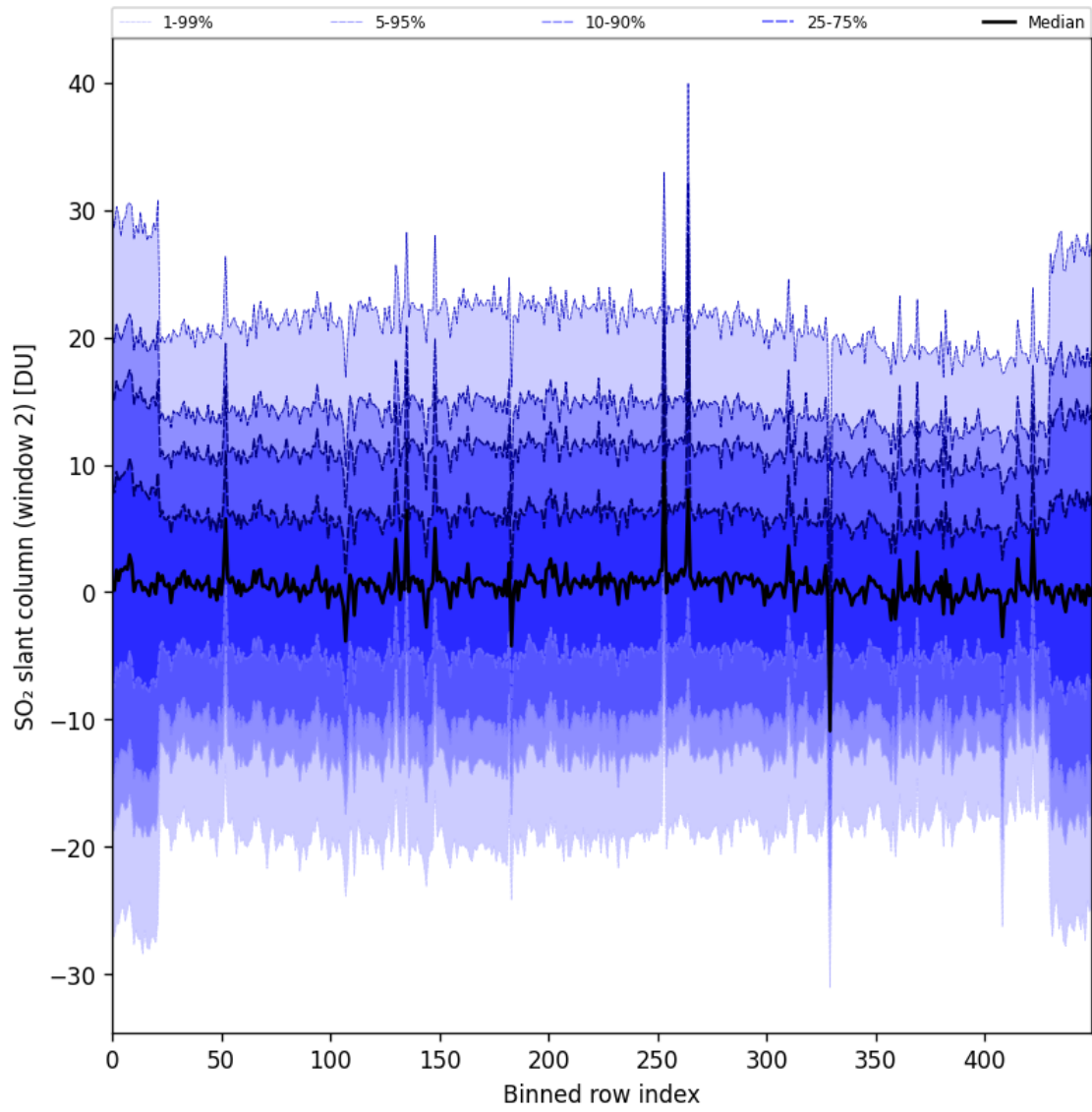
Figure 93: Along track statistics of “SO 2 slant column (window 2)” for 2025-11-18 to 2025-11-19
