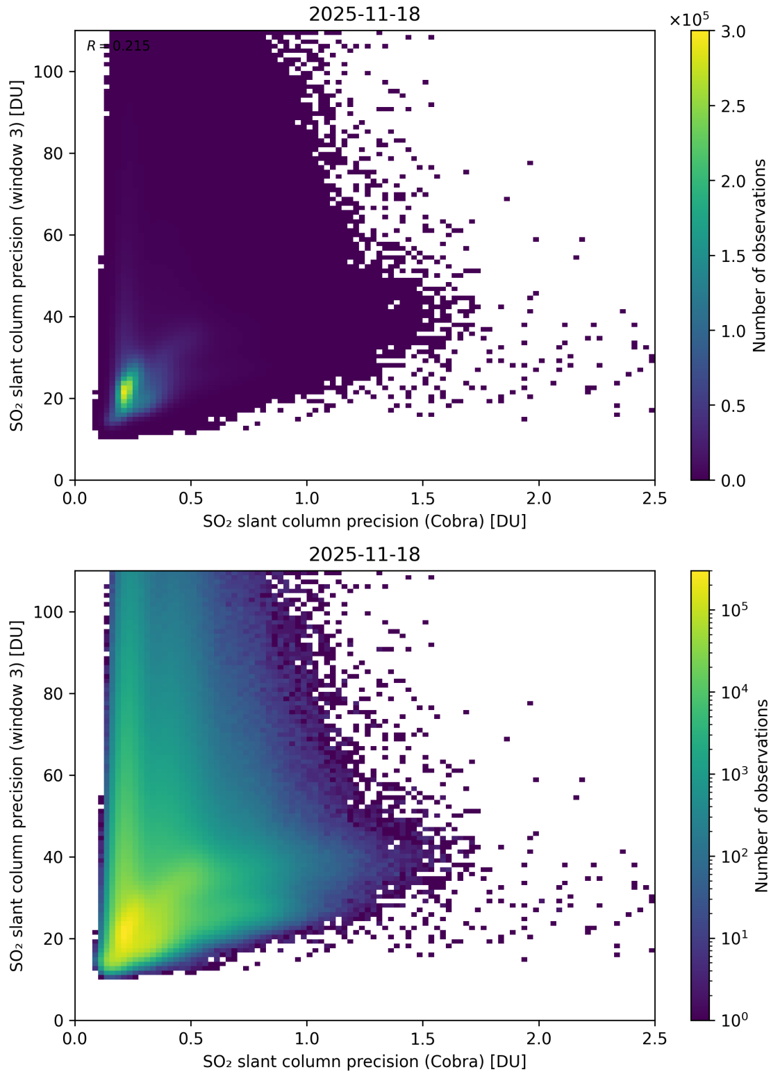
Figure 212: Scatter density plot of “SO 2 slant column precision (Cobra)” against “SO 2 slant column precision (window 3)” for 2025-11-18 to 2025-11-19.
