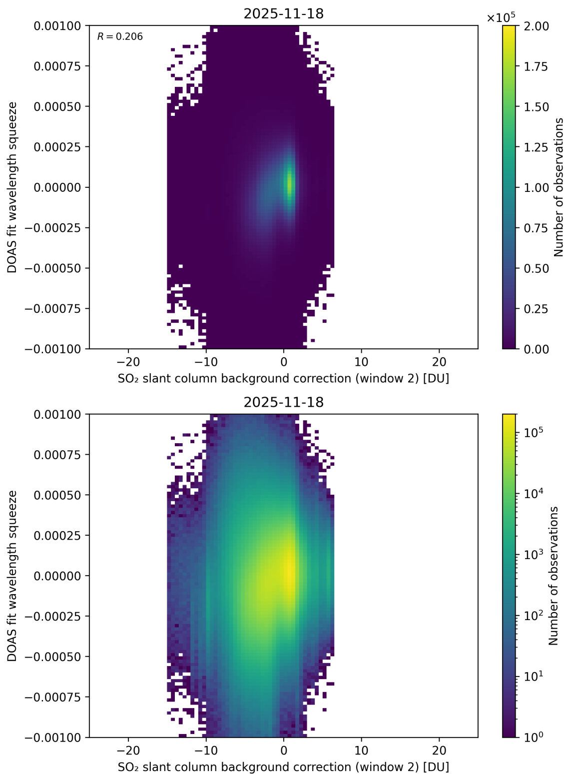
Figure 124: Scatter density plot of “SO 2 slant column background correction (window 2)” against “DOAS fit wavelength squeeze” for 2025-11-18 to 2025-11-19.
