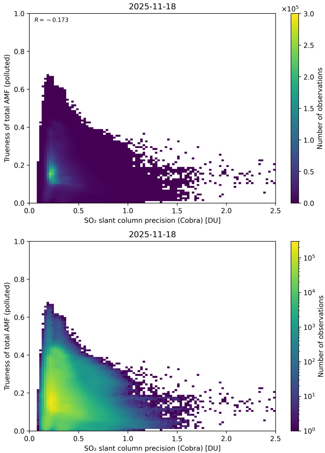
Figure 214: Scatter density plot of “SO 2 slant column precision (Cobra)” against “Trueness of total AMF (polluted)” for 2025-11-18 to 2025-11-19.
