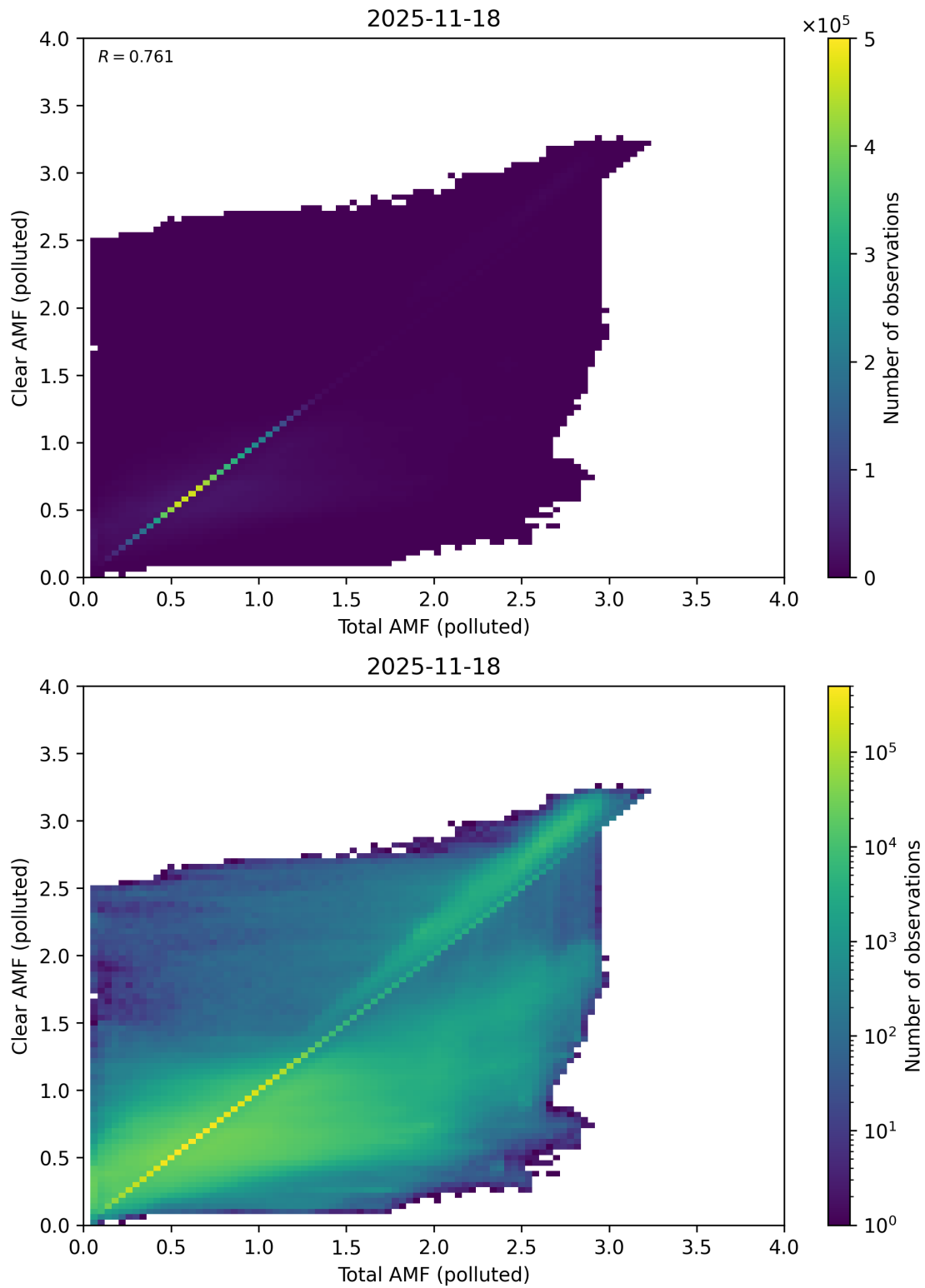
Figure 320: Scatter density plot of “Total AMF (polluted)” against “Clear AMF (polluted)” for 2025-11-18 to 2025-11-19.
