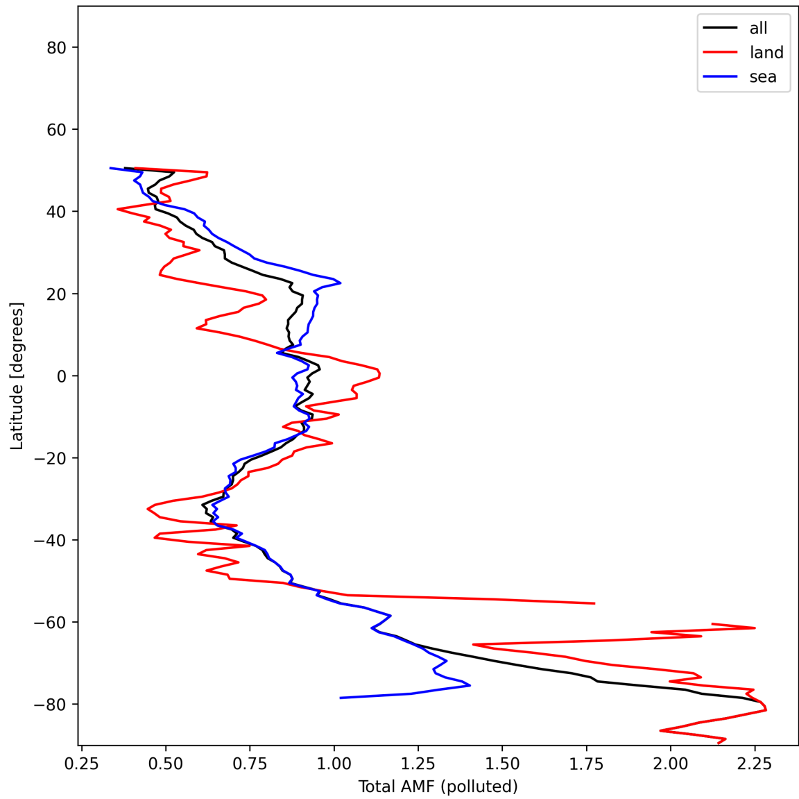
Figure 53: Zonal average of “Total AMF (polluted)” for 2025-11-18 to 2025-11-19.
