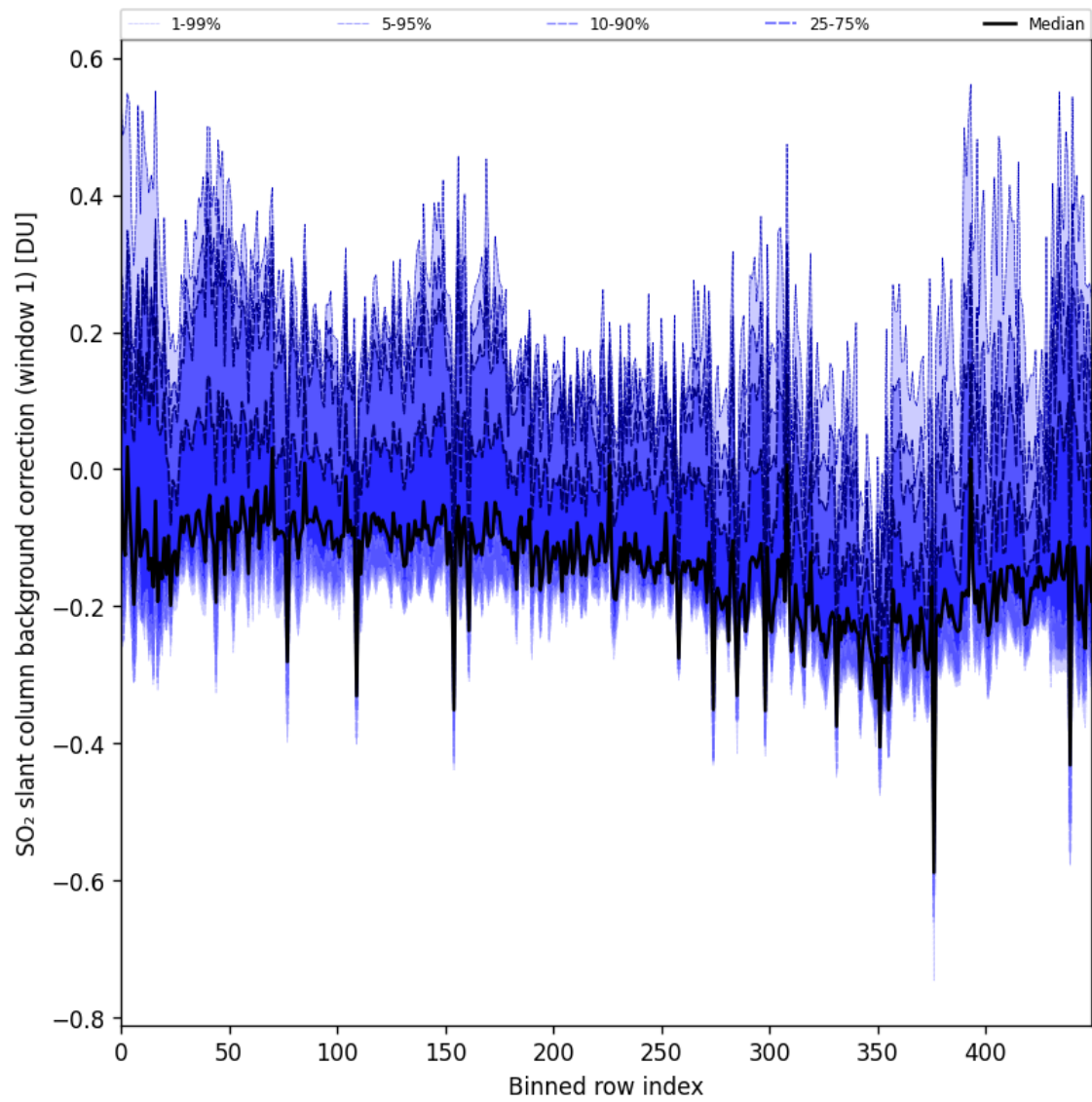
Figure 92: Along track statistics of “SO 2 slant column background correction (window 1)” for 2025-11-18 to 2025-11-19
