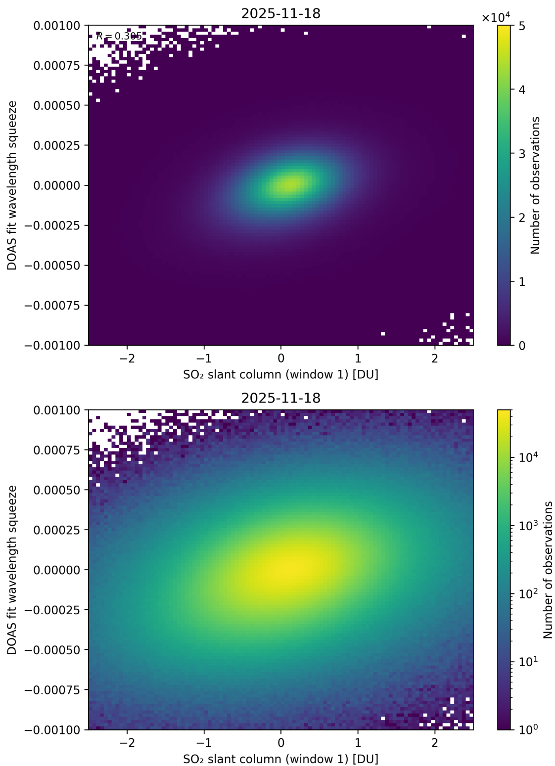
Figure 266: Scatter density plot of “SO 2 slant column (window 1)” against “DOAS fit wavelength squeeze” for 2025-11-18 to 2025-11-19.
