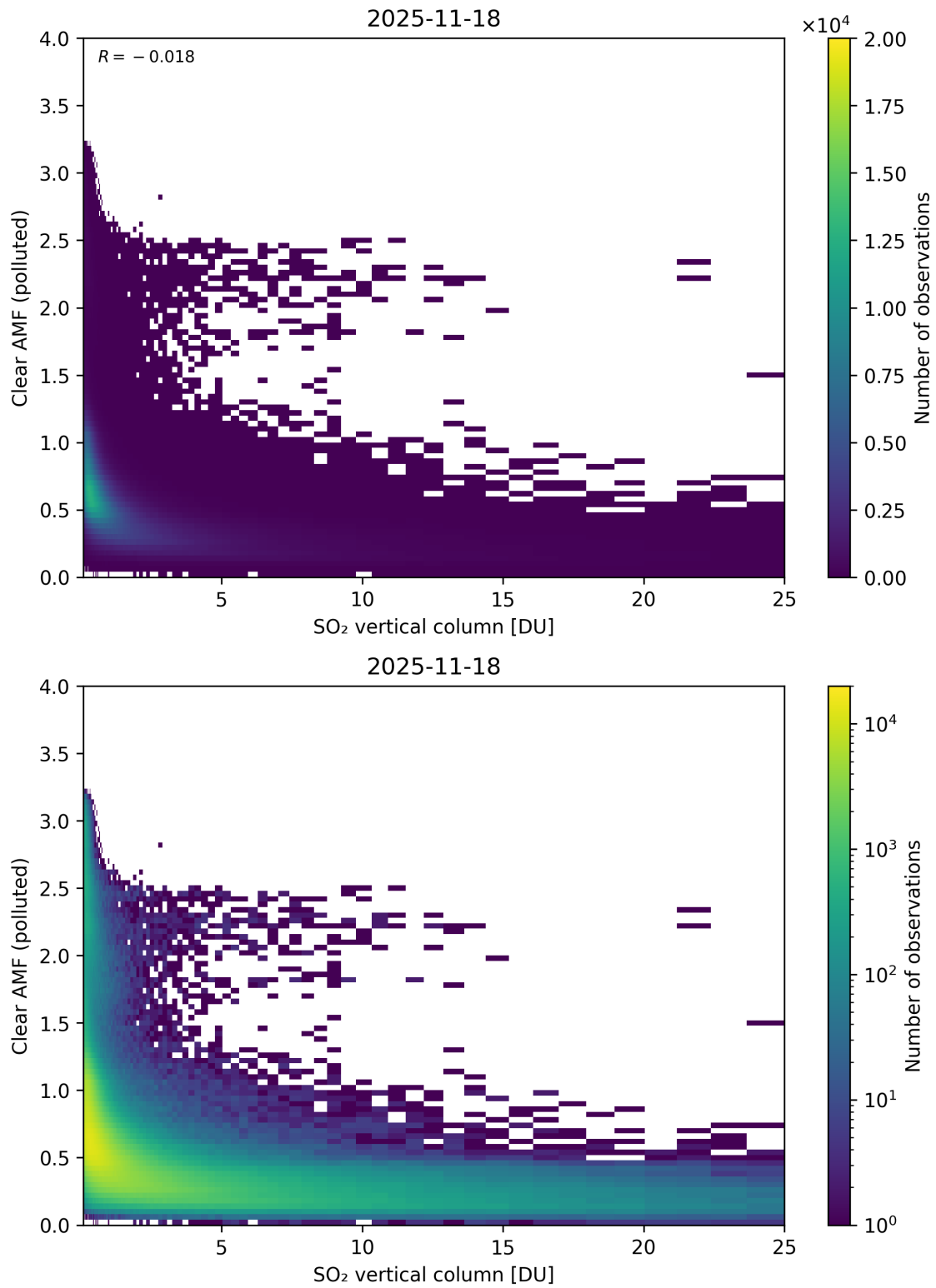
Figure 348: Scatter density plot of “SO 2 vertical column” against “Clear AMF (polluted)” for 2025-11-18 to 2025-11-19.
