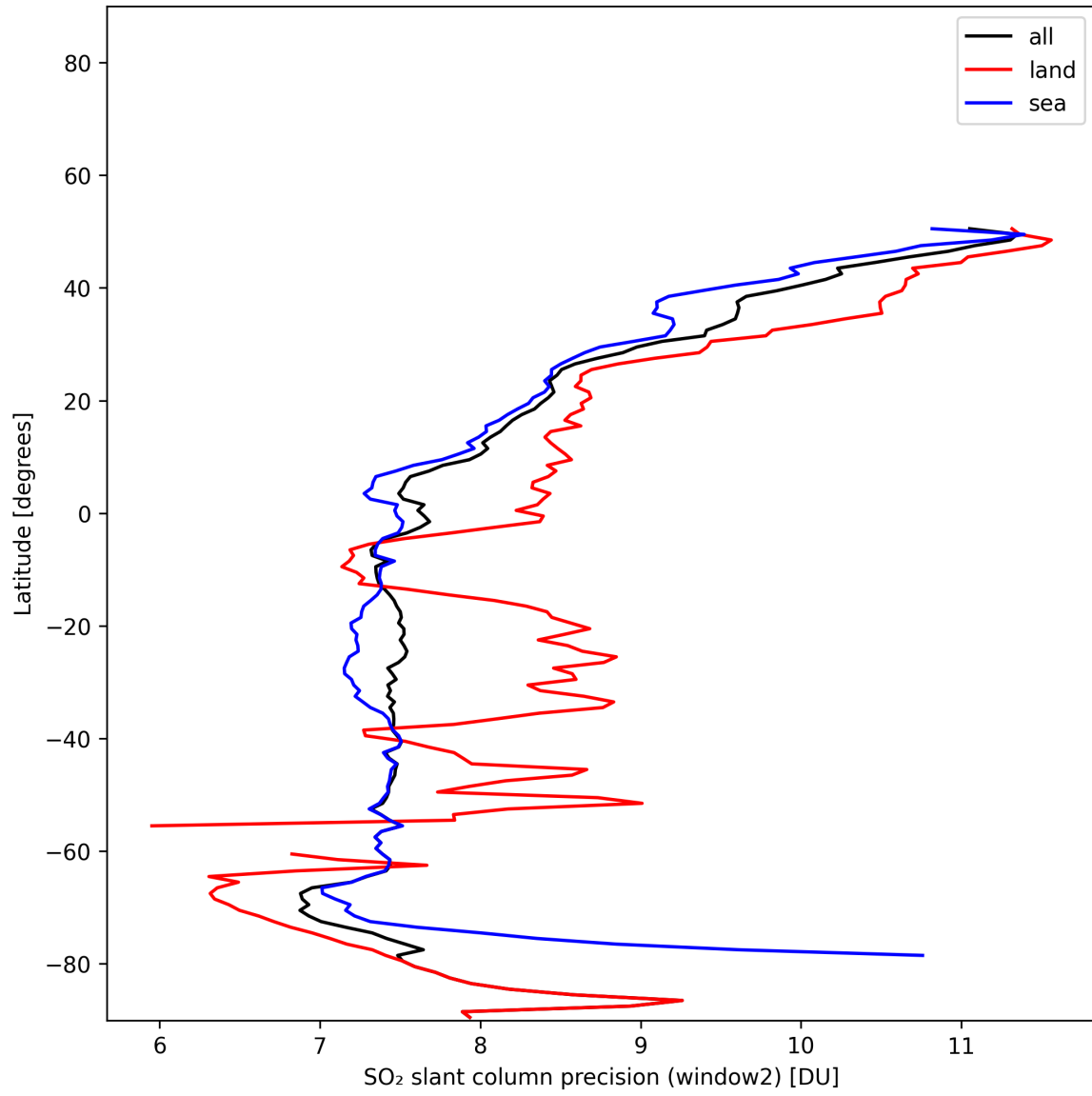
Figure 42: Zonal average of “SO 2 slant column precision (window2)” for 2025-11-18 to 2025-11-19.
