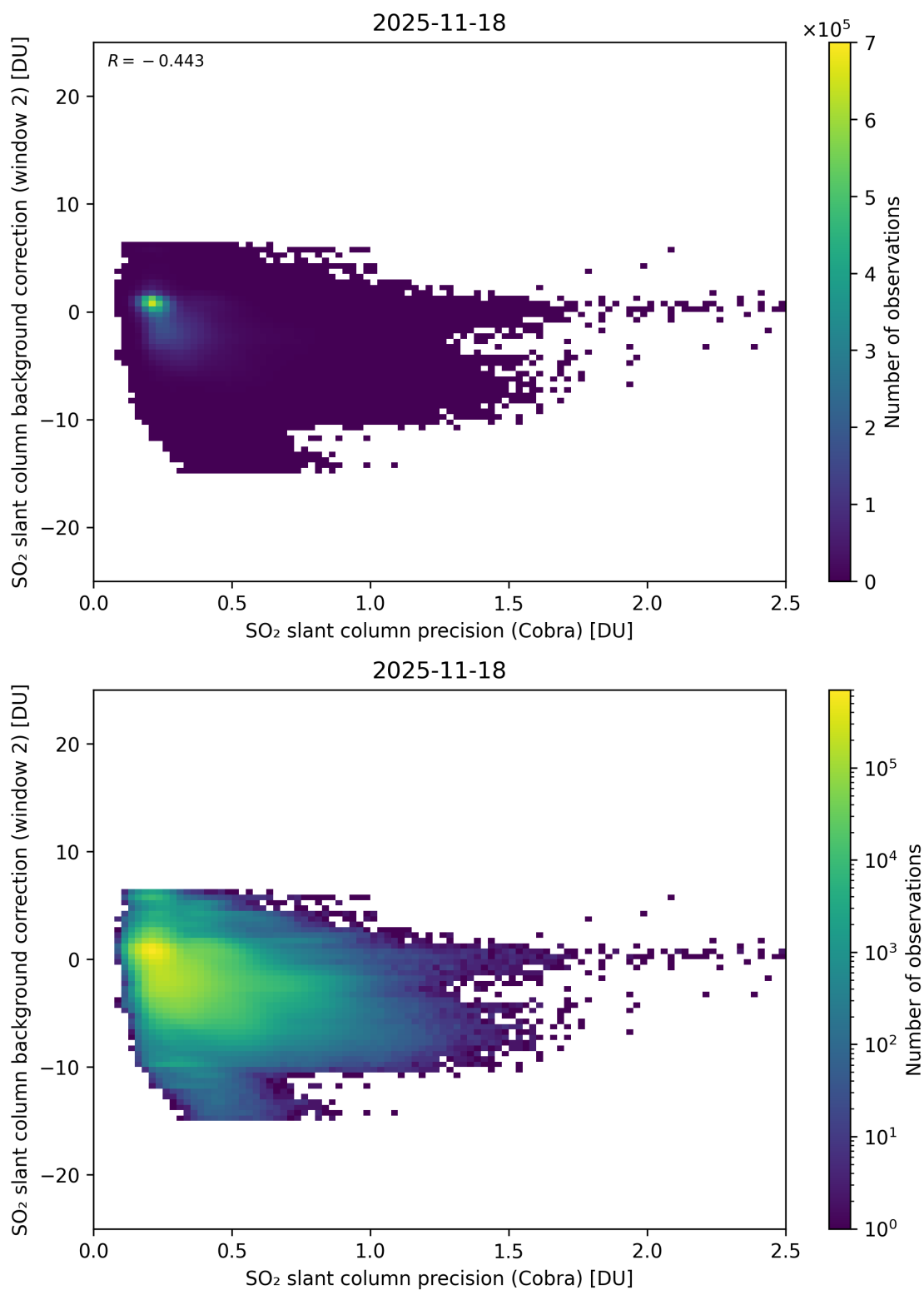
Figure 200: Scatter density plot of “SO 2 slant column precision (Cobra)” against “SO 2 slant column background correction (window 2)” for 2025-11-18 to 2025-11-19.
