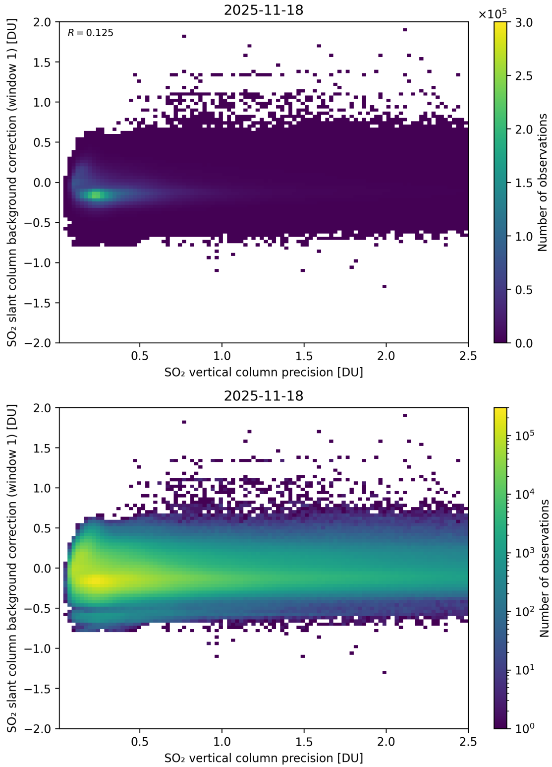
Figure 329: Scatter density plot of “SO 2 vertical column precision” against “SO 2 slant column background correction (window 1)” for 2025-11-18 to 2025-11-19.
