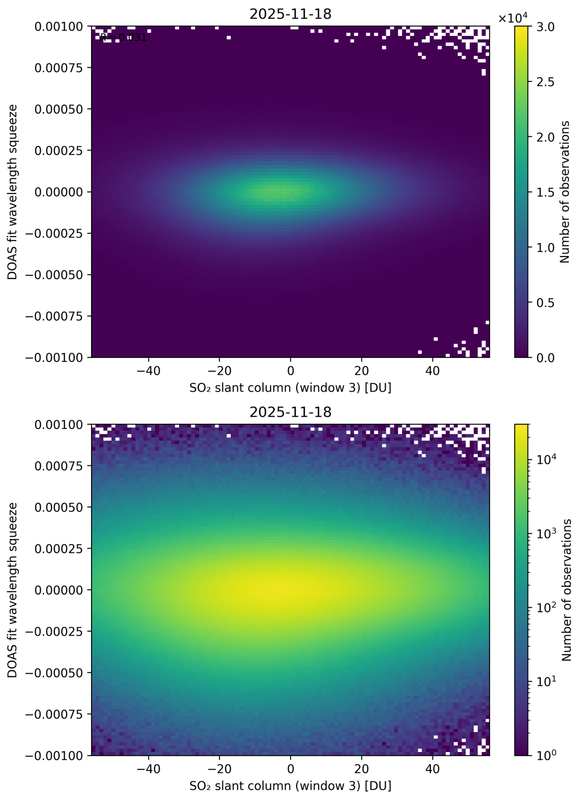
Figure 305: Scatter density plot of “SO 2 slant column (window 3)” against “DOAS fit wavelength squeeze” for 2025-11-18 to 2025-11-19.
