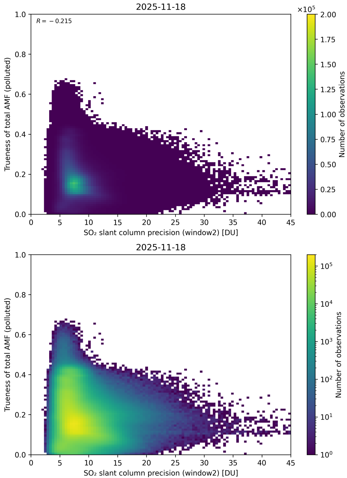
Figure 302: Scatter density plot of “SO 2 slant column precision (window2)” against “Trueness of total AMF (polluted)” for 2025-11-18 to 2025-11-19.
