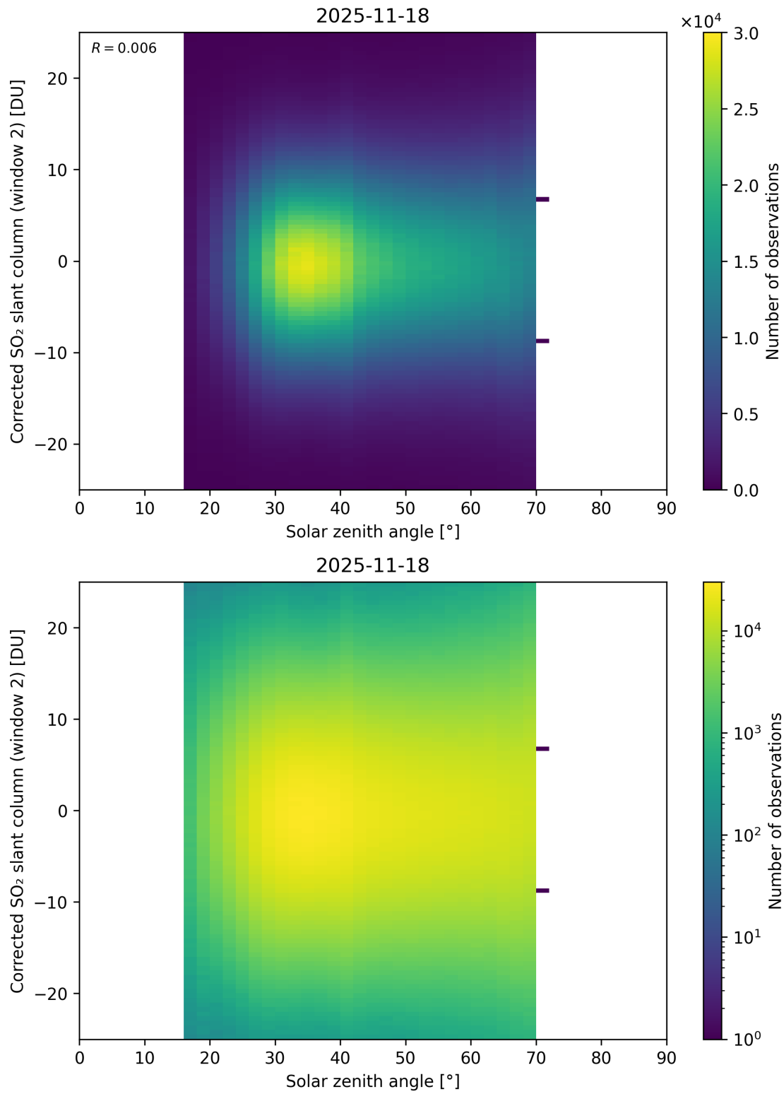
Figure 182: Scatter density plot of “Solar zenith angle” against “Corrected SO 2 slant column (window 2)” for 2025-11-18 to 2025-11-19.
