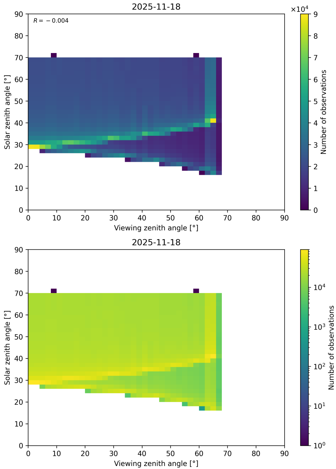
Figure 369: Scatter density plot of “Viewing zenith angle” against “Solar zenith angle” for 2025-11-18 to 2025-11-19.
