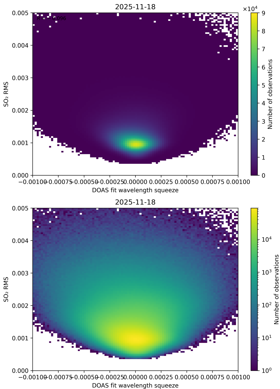
Figure 143: Scatter density plot of “DOAS fit wavelength squeeze” against “SO 2 RMS” for 2025-11-18 to 2025-11-19.
