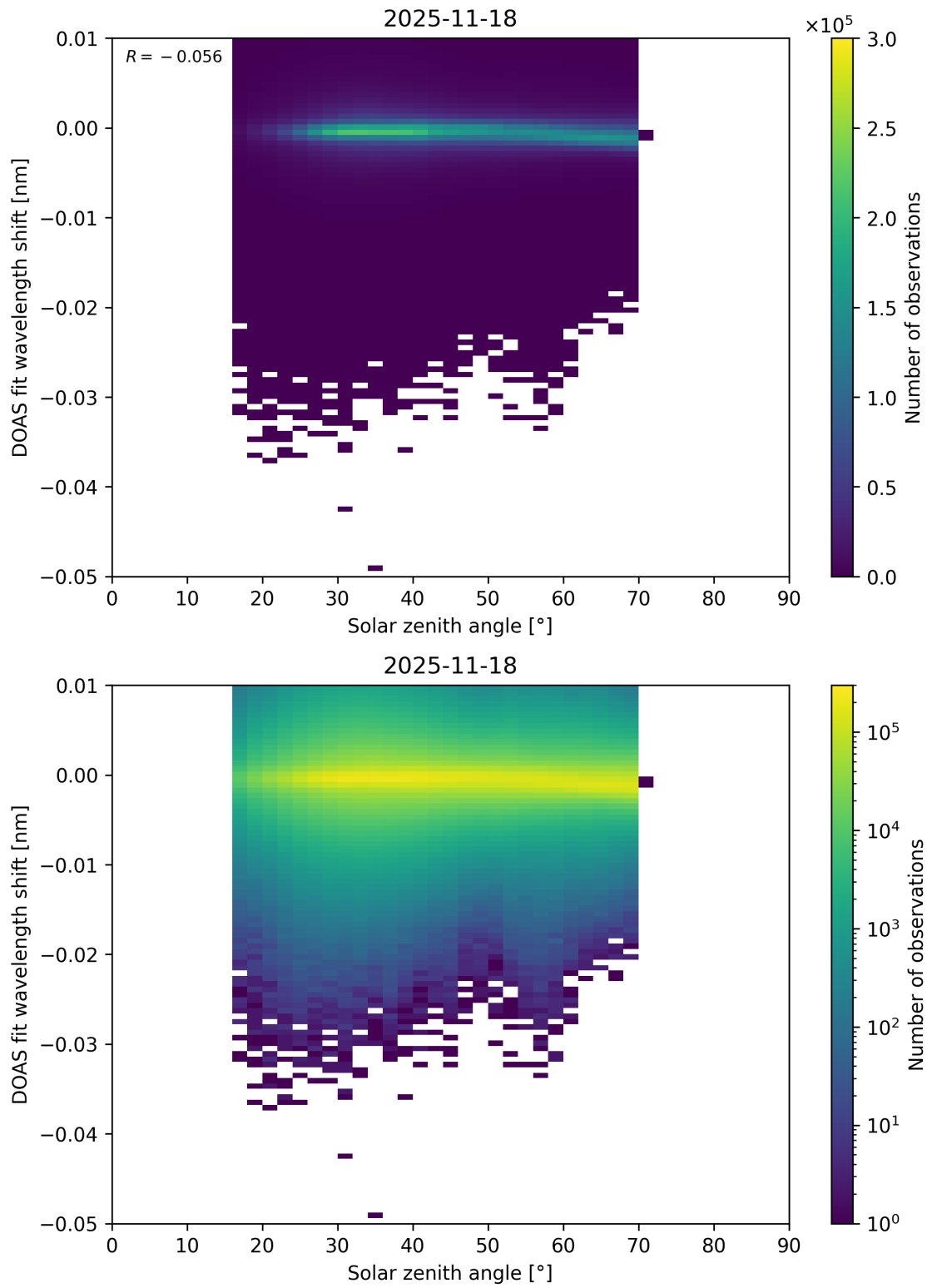
Figure 174: Scatter density plot of “Solar zenith angle” against “DOAS fit wavelength shift” for 2025-11-18 to 2025-11-19.
