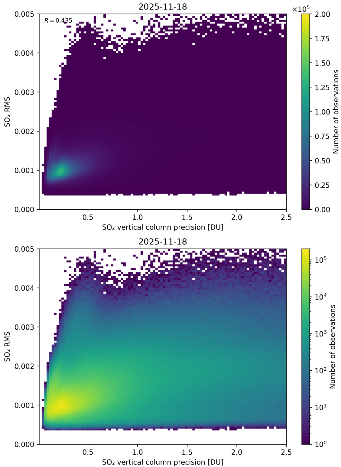
Figure 334: Scatter density plot of “SO 2 vertical column precision” against “SO 2 RMS” for 2025-11-18 to 2025-11-19.
