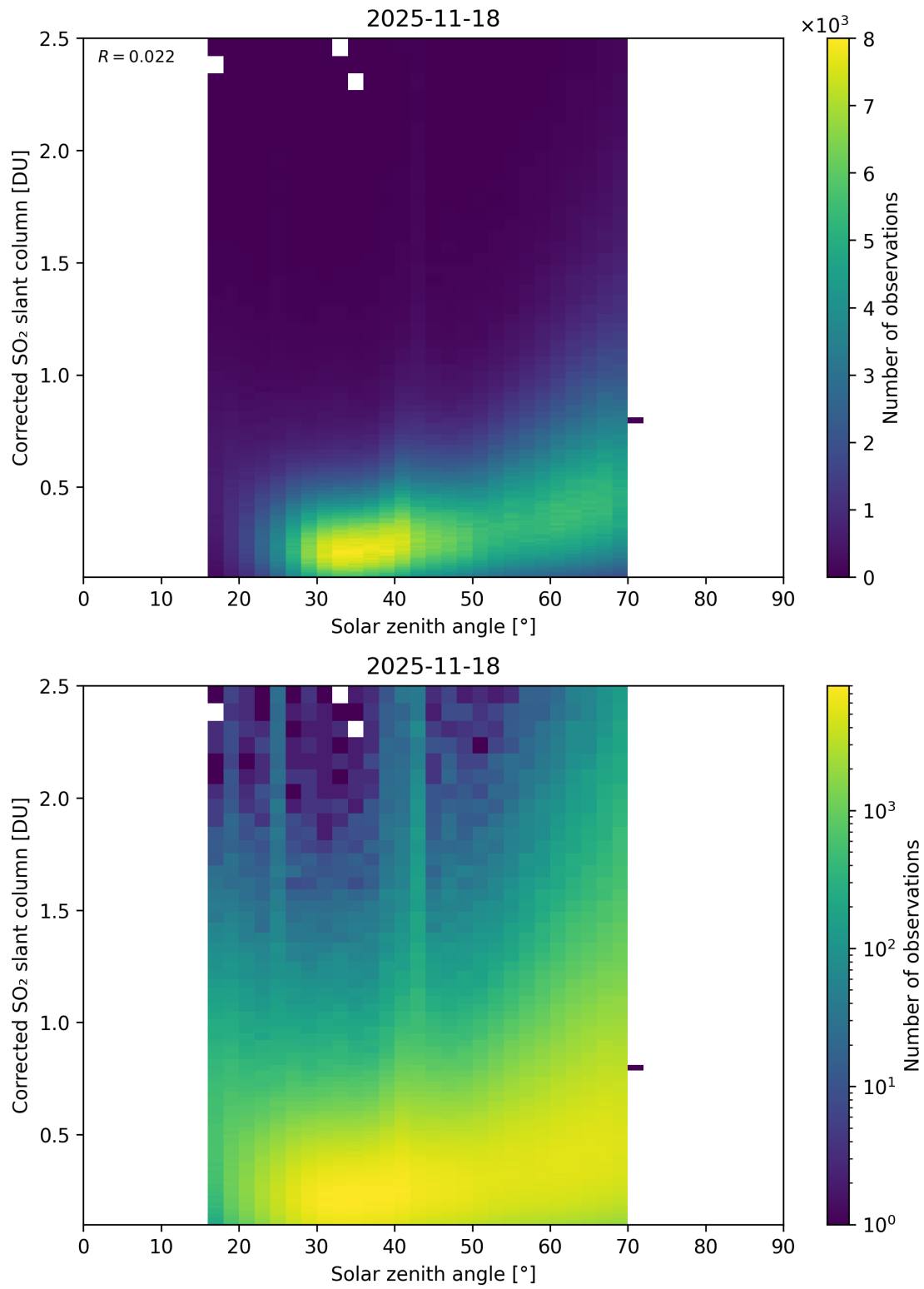
Figure 181: Scatter density plot of “Solar zenith angle” against “Corrected SO 2 slant column” for 2025-11-18 to 2025-11-19.
