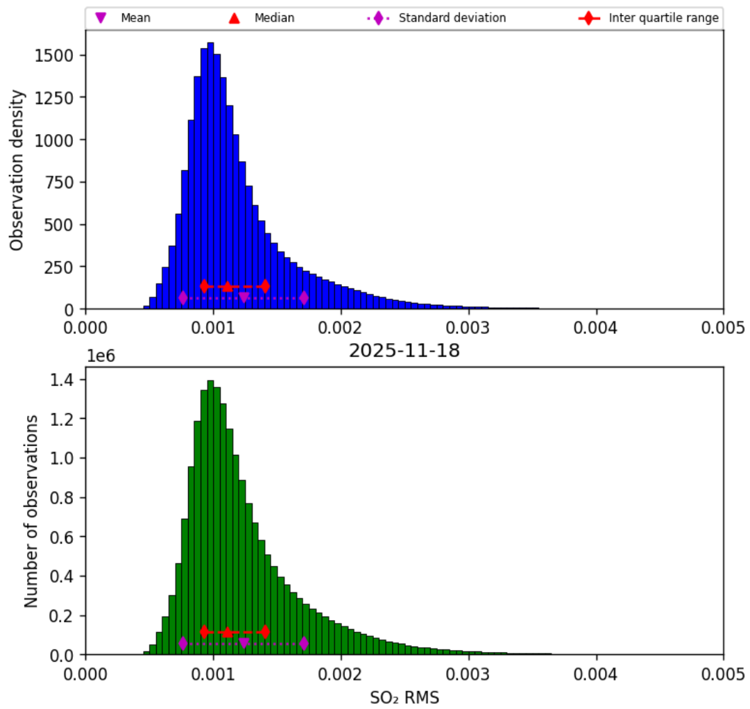
Figure 78: Histogram of “SO 2 RMS” for 2025-11-18 to 2025-11-19
