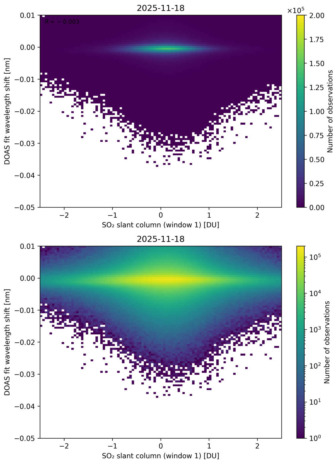
Figure 265: Scatter density plot of “SO 2 slant column (window 1)” against “DOAS fit wavelength shift” for 2025-11-18 to 2025-11-19.
