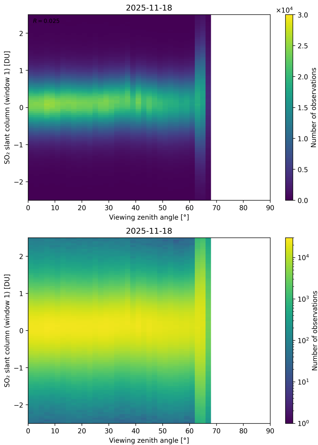
Figure 376: Scatter density plot of “Viewing zenith angle” against “SO 2 slant column (window 1)” for 2025-11-18 to 2025-11-19.
