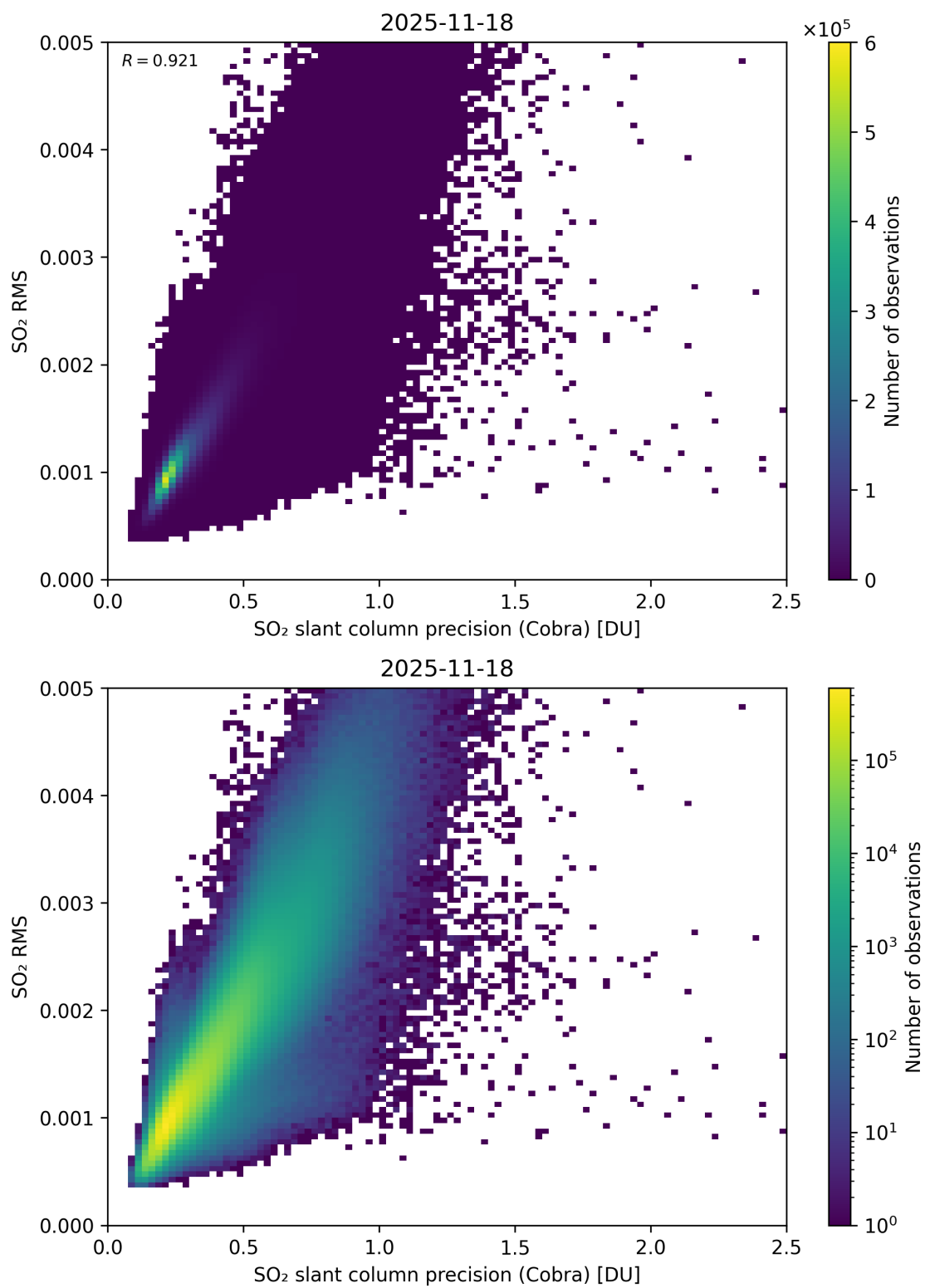
Figure 204: Scatter density plot of “SO 2 slant column precision (Cobra)” against “SO 2 RMS” for 2025-11-18 to 2025-11-19.
