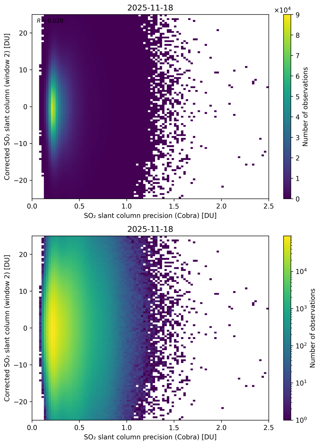
Figure 206: Scatter density plot of “SO 2 slant column precision (Cobra)” against “Corrected SO 2 slant column (window 2)” for 2025-11-18 to 2025-11-19.
