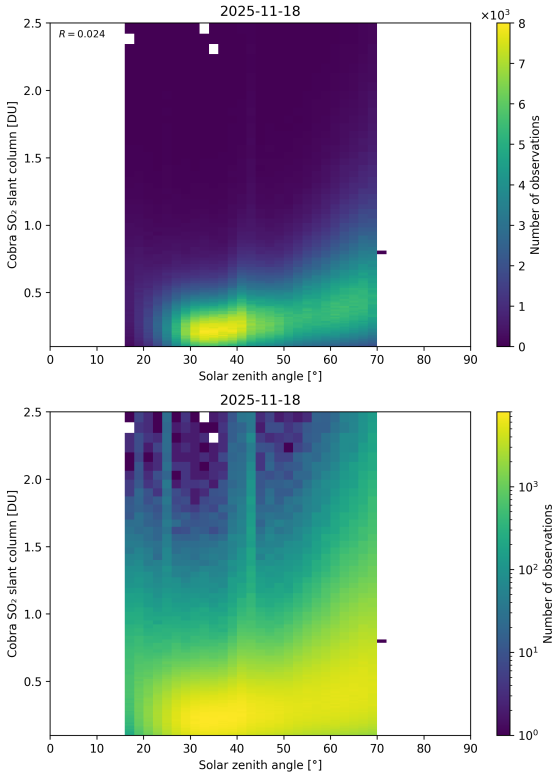
Figure 179: Scatter density plot of “Solar zenith angle” against “Cobra SO 2 slant column” for 2025-11-18 to 2025-11-19.
