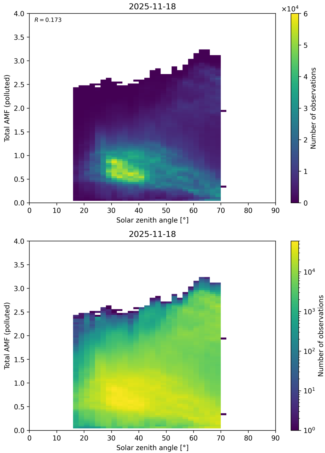
Figure 189: Scatter density plot of “Solar zenith angle” against “Total AMF (polluted)” for 2025-11-18 to 2025-11-19.
