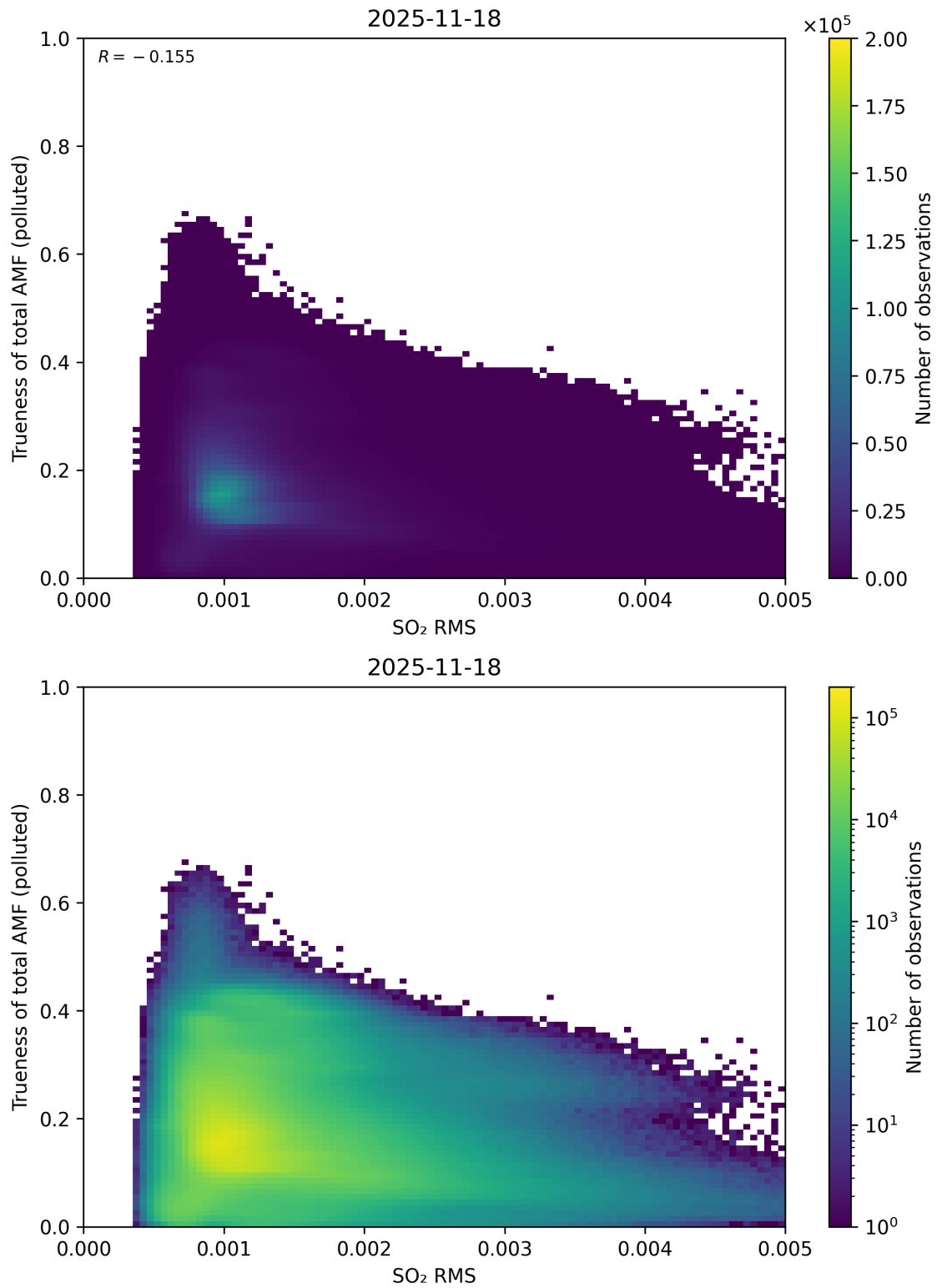
Figure 149: Scatter density plot of “SO 2 RMS” against “Trueness of total AMF (polluted)” for 2025-11-18 to 2025-11-19.
