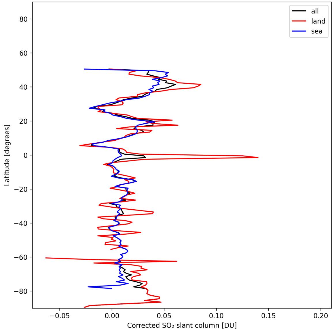
Figure 34: Zonal average of “Corrected SO 2 slant column” for 2025-11-18 to 2025-11-19.
