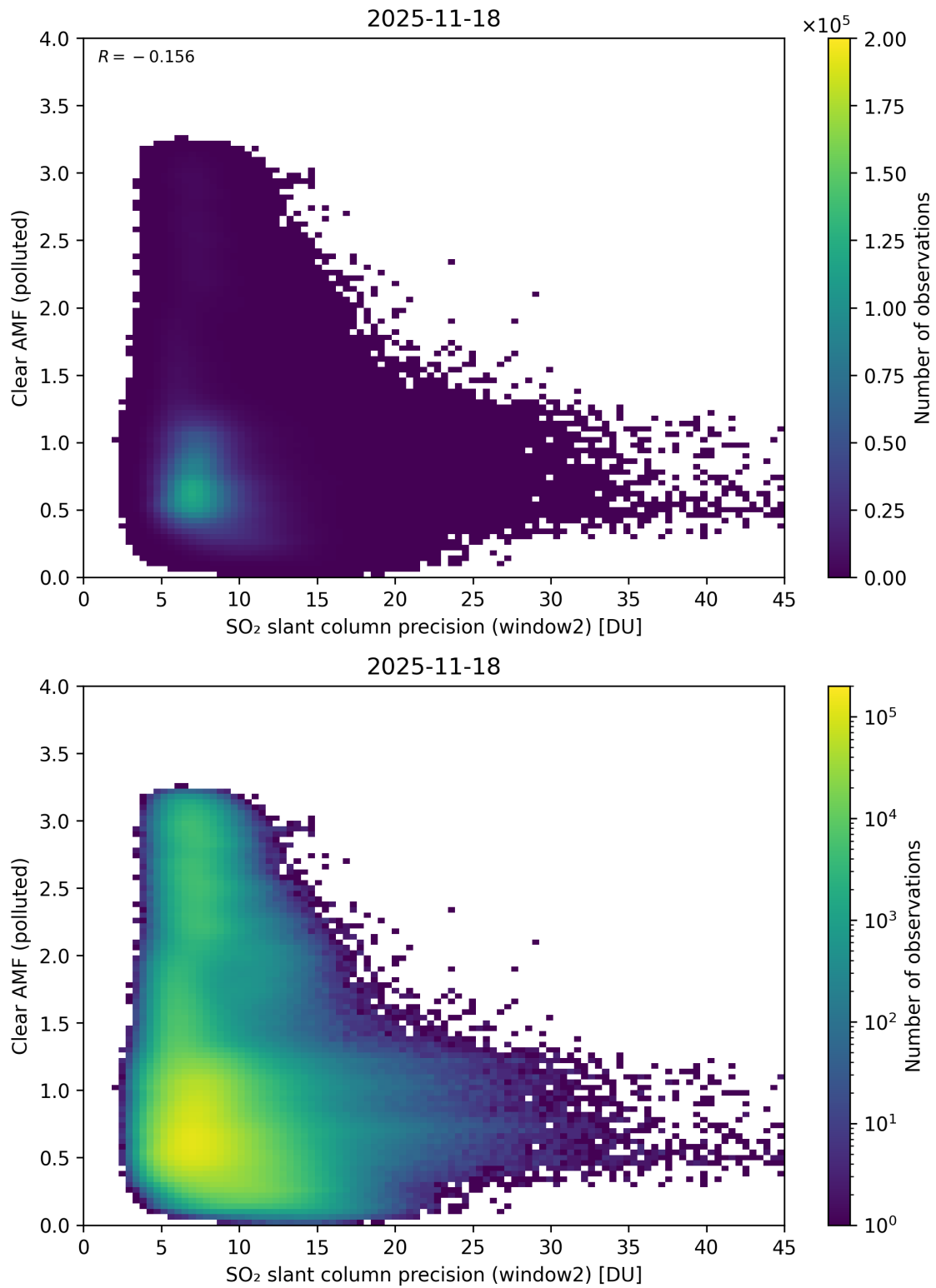
Figure 296: Scatter density plot of “SO 2 slant column precision (window2)” against “Clear AMF (polluted)” for 2025-11-18 to 2025-11-19.
