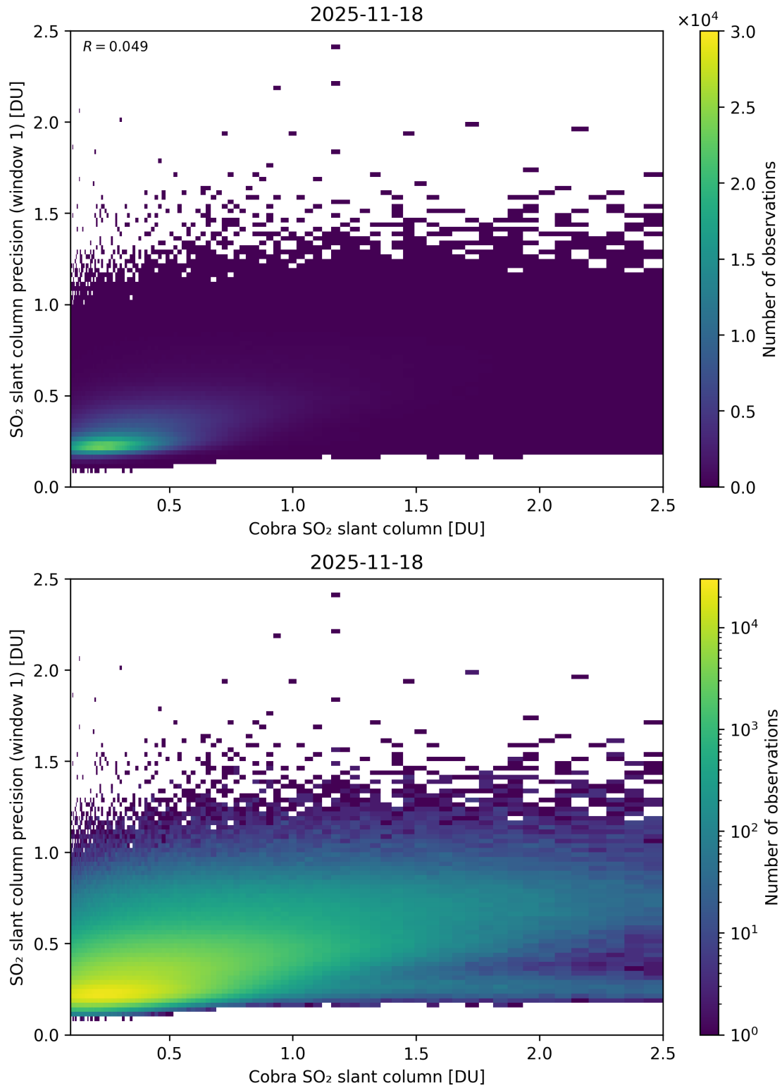
Figure 220: Scatter density plot of “Cobra SO 2 slant column” against “SO 2 slant column precision (window 1)” for 2025-11-18 to 2025-11-19.
