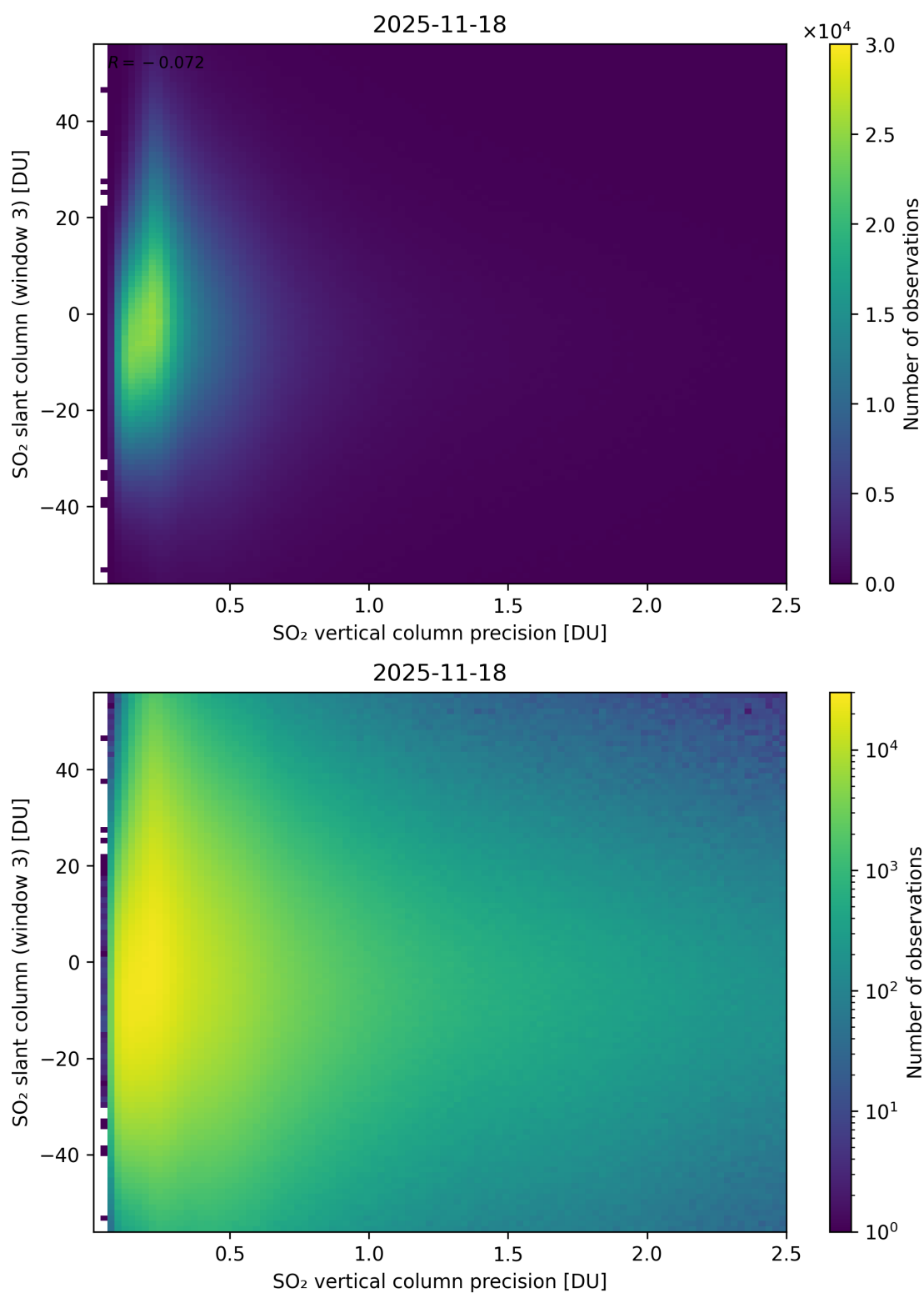
Figure 344: Scatter density plot of “SO 2 vertical column precision” against “SO 2 slant column (window 3)” for 2025-11-18 to 2025-11-19.
