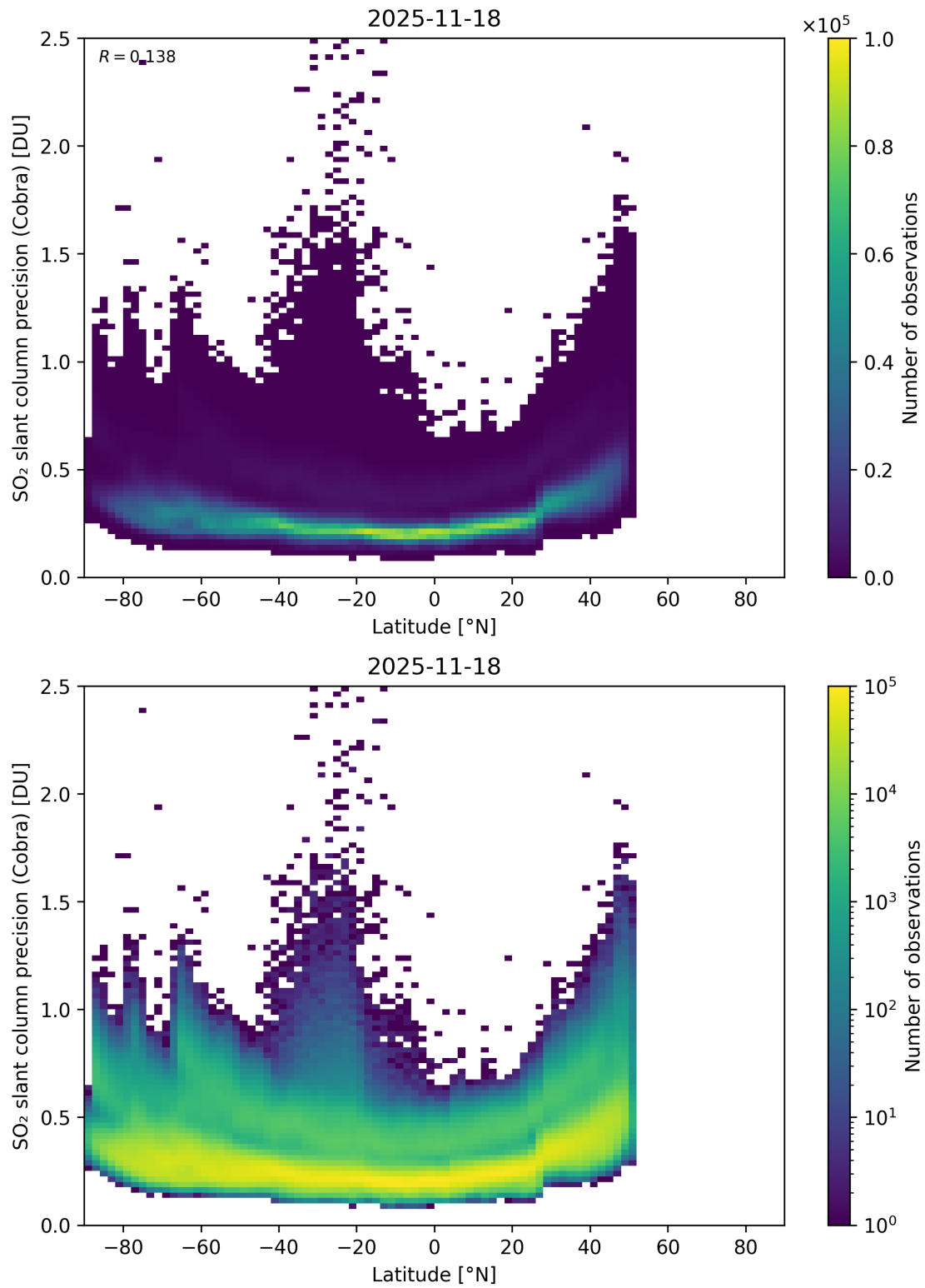
Figure 158: Scatter density plot of “Latitude” against “SO 2 slant column precision (Cobra)” for 2025-11-18 to 2025-11-19.
