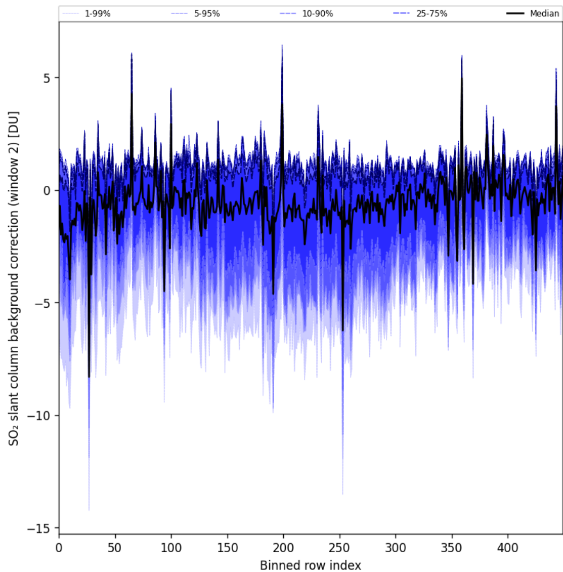
Figure 96: Along track statistics of “SO 2 slant column background correction (window 2)” for 2025-11-18 to 2025-11-19
