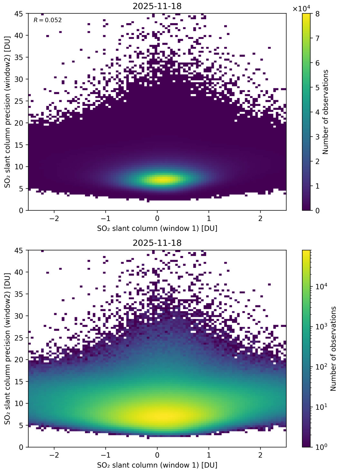
Figure 286: Scatter density plot of “SO 2 slant column (window 1)” against “SO 2 slant column precision (window2)” for 2025-11-18 to 2025-11-19.
