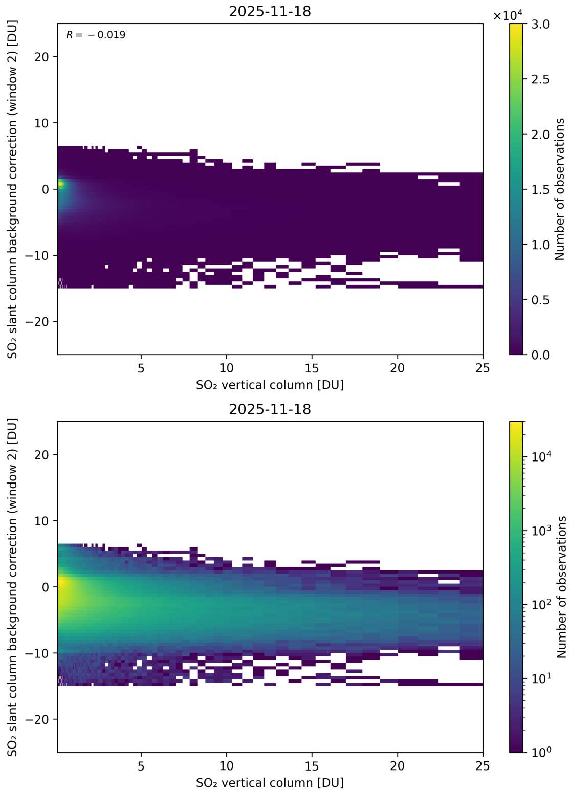
Figure 324: Scatter density plot of “SO 2 vertical column” against “SO 2 slant column background correction (window 2)” for 2025-11-18 to 2025-11-19.
