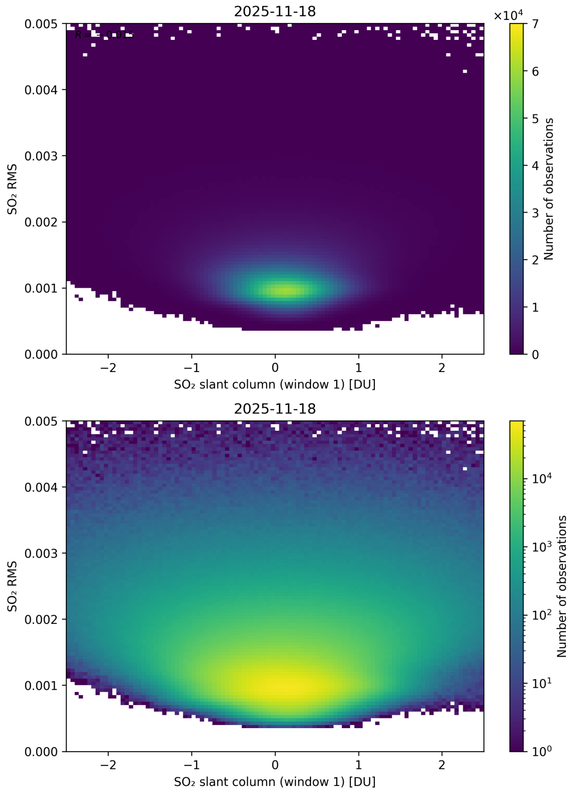
Figure 267: Scatter density plot of “SO 2 slant column (window 1)” against “SO 2 RMS” for 2025-11-18 to 2025-11-19.
