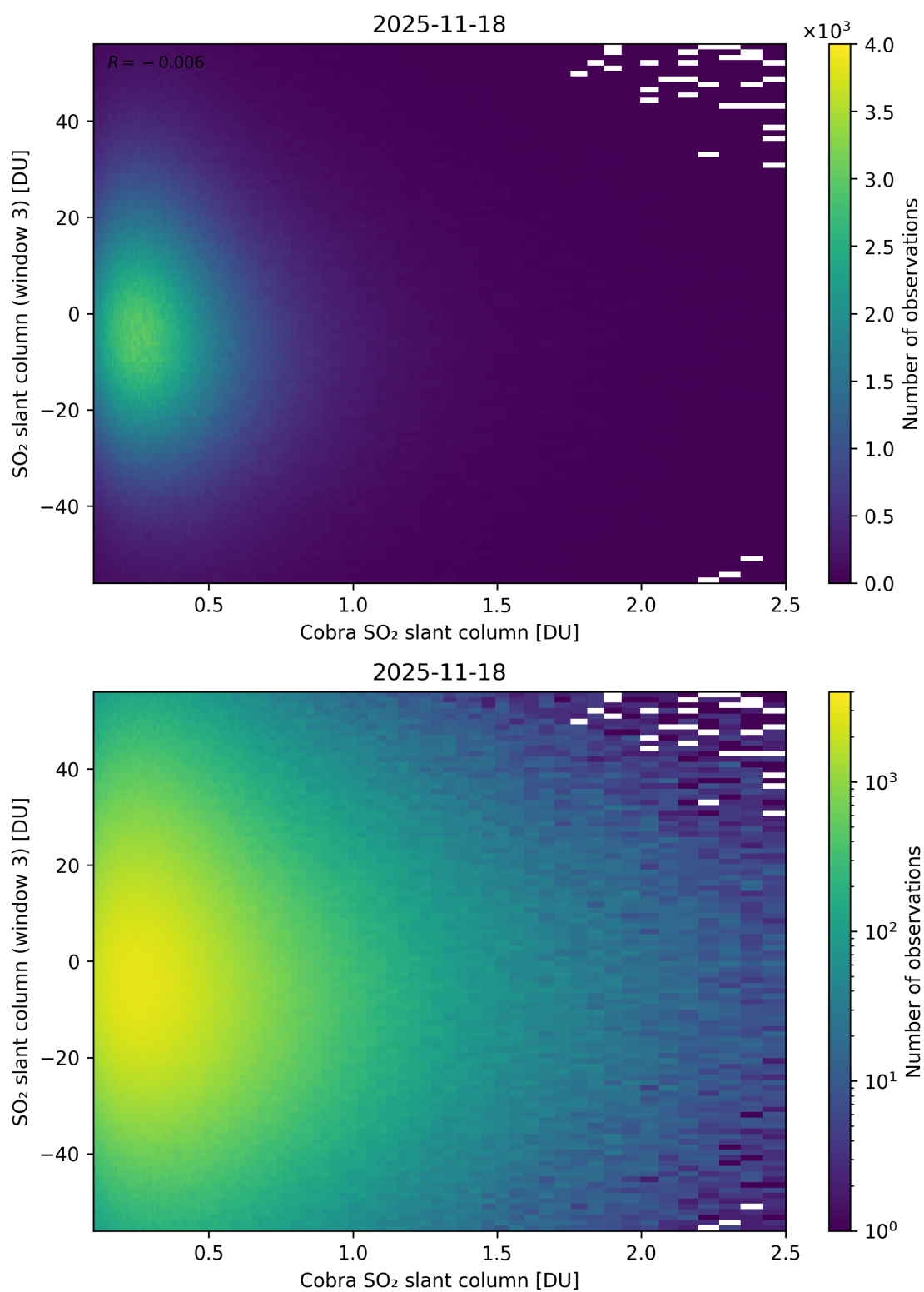
Figure 222: Scatter density plot of “Cobra SO 2 slant column” against “SO 2 slant column (window 3)” for 2025-11-18 to 2025-11-19.
