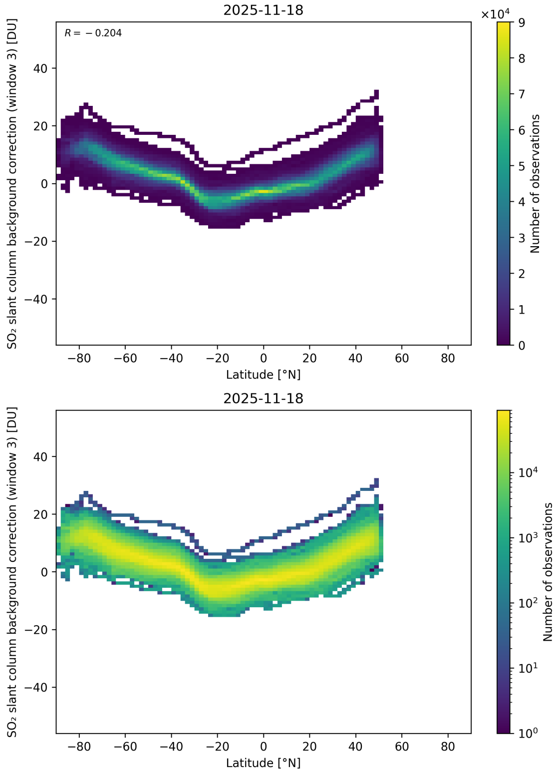
Figure 152: Scatter density plot of “Latitude” against “SO 2 slant column background correction (window 3)” for 2025-11-18 to 2025-11-19.
