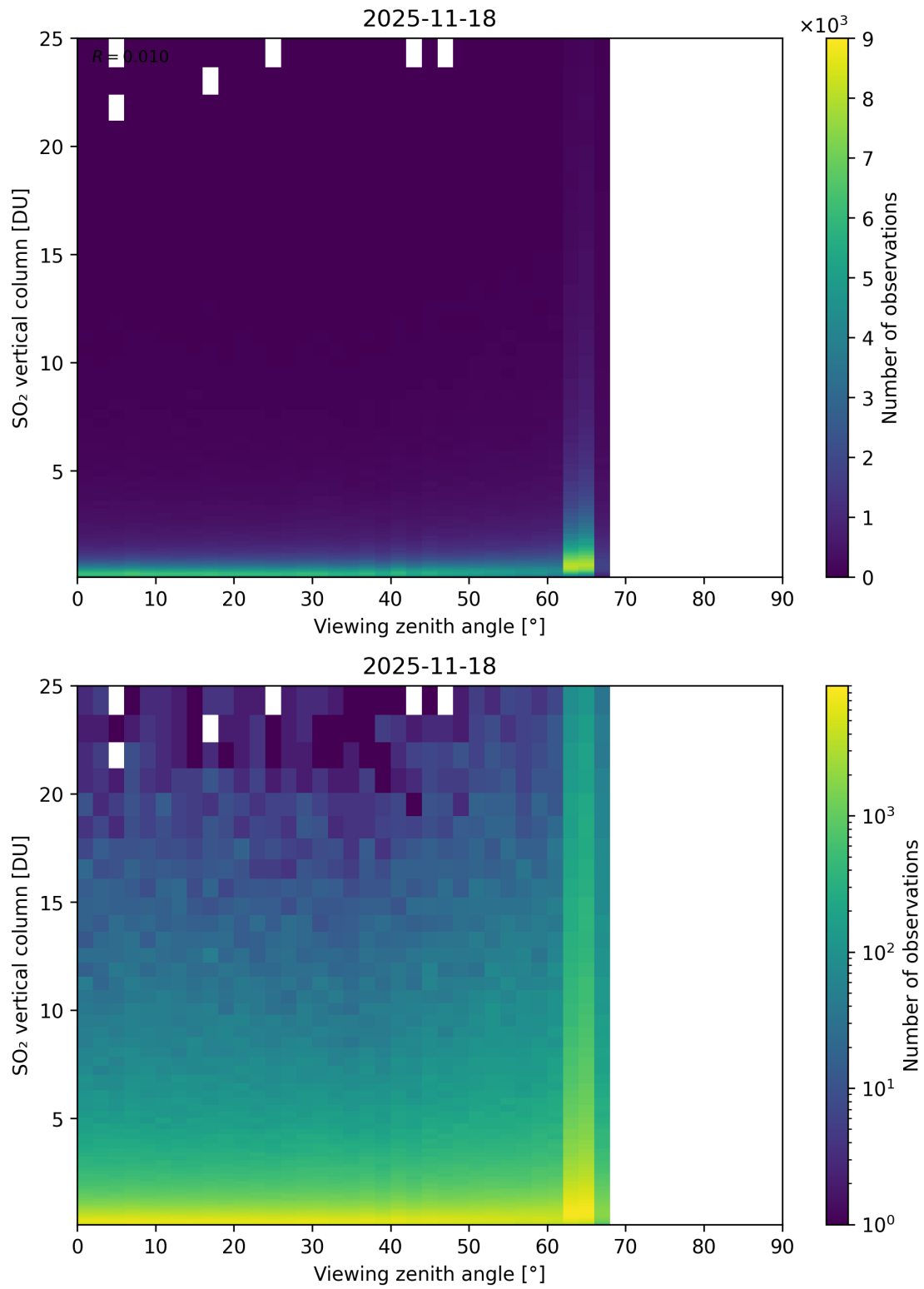
Figure 383: Scatter density plot of “Viewing zenith angle” against “SO 2 vertical column” for 2025-11-18 to 2025-11-19.
