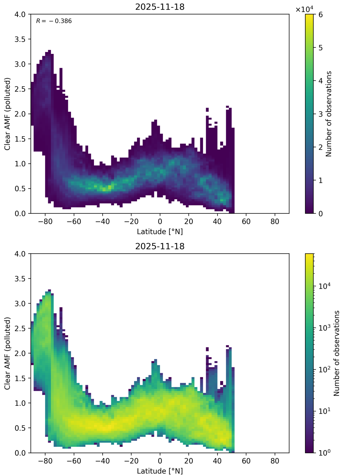
Figure 156: Scatter density plot of “Latitude” against “Clear AMF (polluted)” for 2025-11-18 to 2025-11-19.
