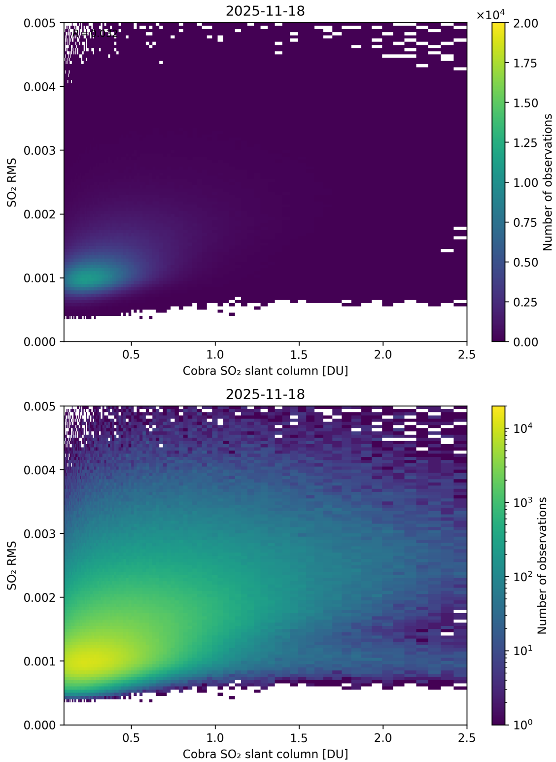
Figure 198: Scatter density plot of “Cobra SO 2 slant column” against “SO 2 RMS” for 2025-11-18 to 2025-11-19.
