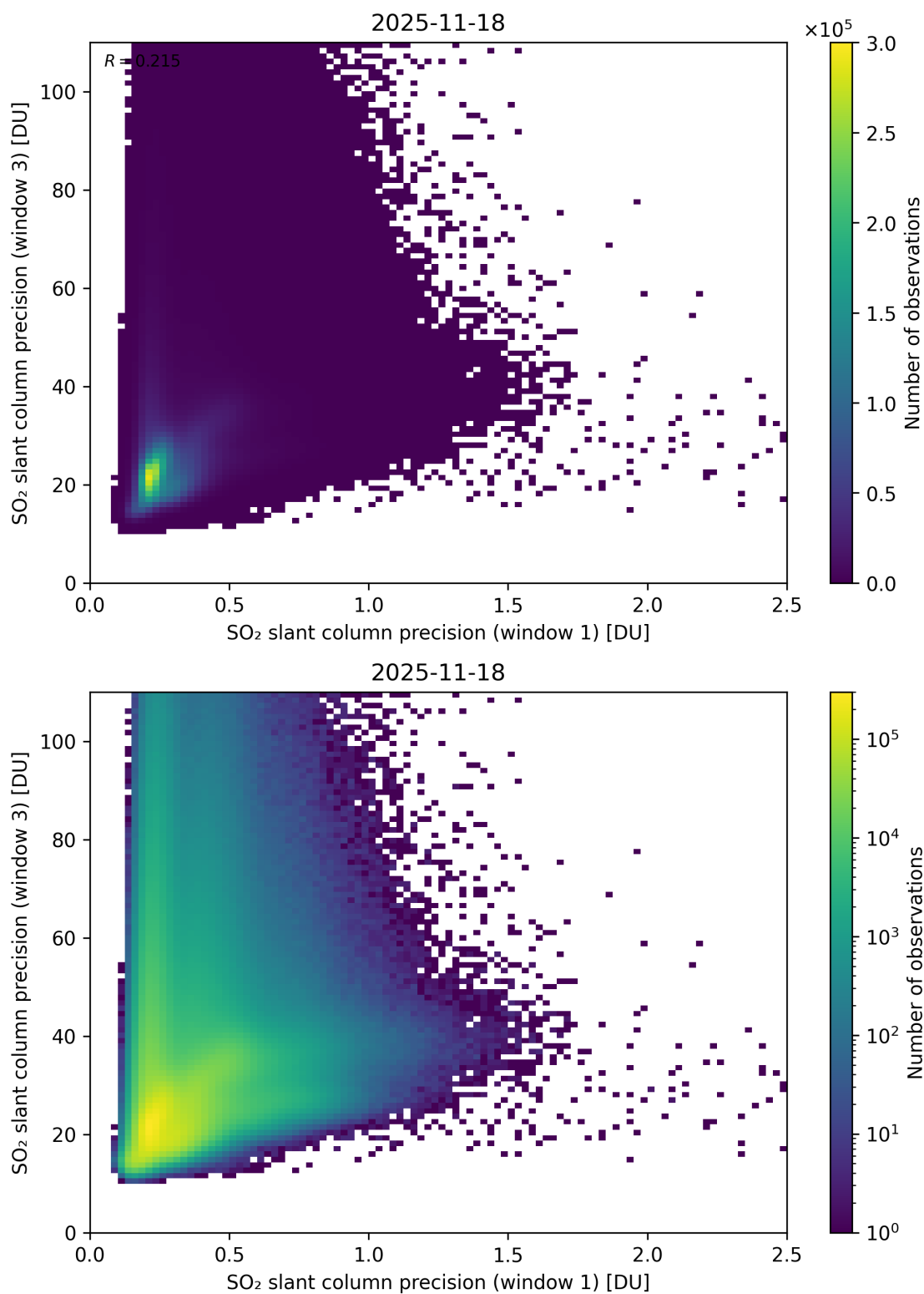
Figure 279: Scatter density plot of “SO 2 slant column precision (window 1)” against “SO 2 slant column precision (window 3)” for 2025-11-18 to 2025-11-19.
