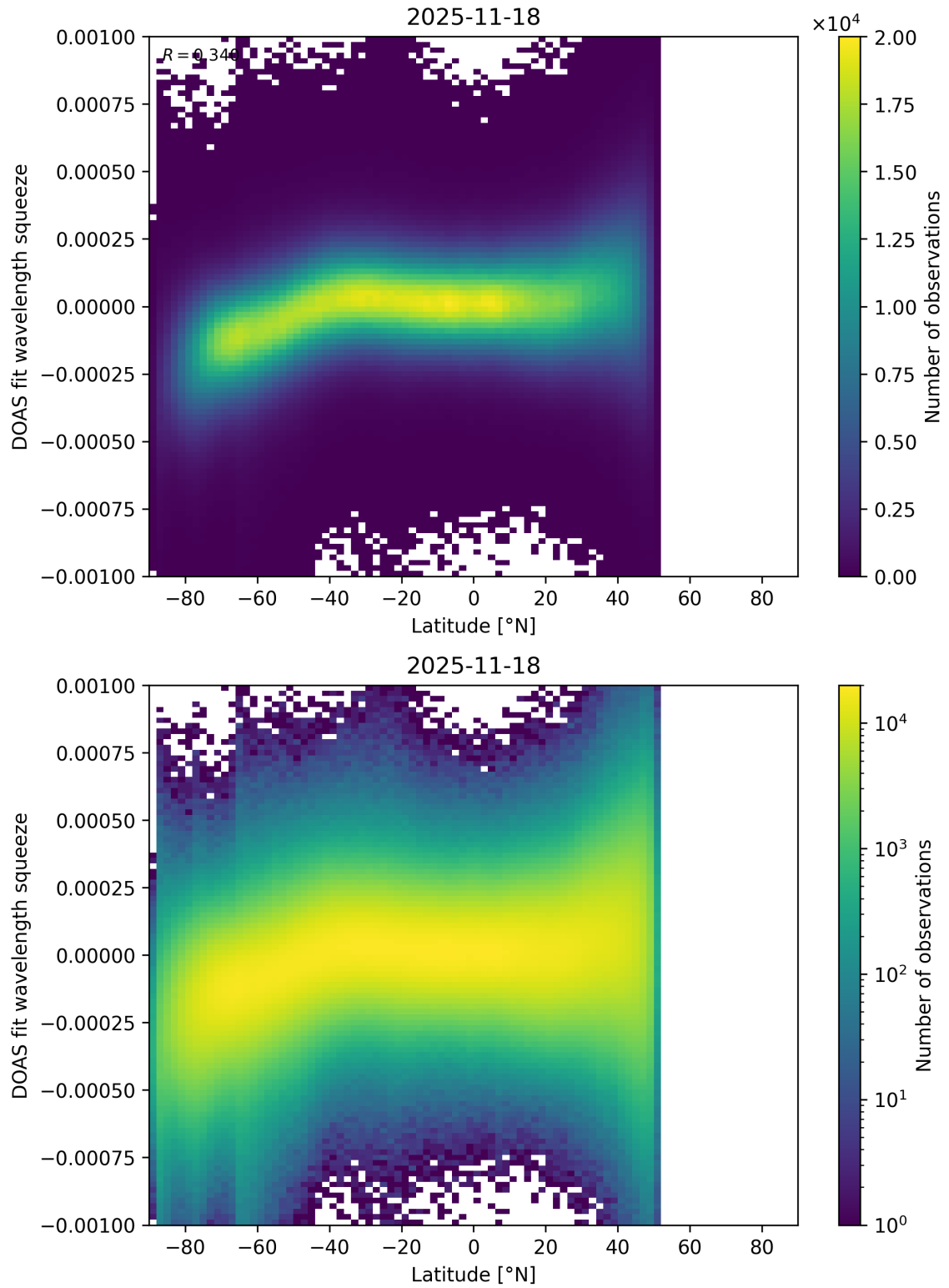
Figure 154: Scatter density plot of “Latitude” against “DOAS fit wavelength squeeze” for 2025-11-18 to 2025-11-19.
