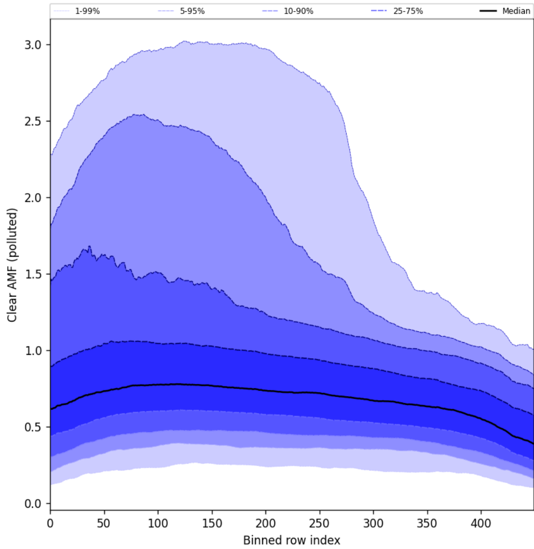
Figure 107: Along track statistics of “Clear AMF (polluted)” for 2025-11-18 to 2025-11-19
