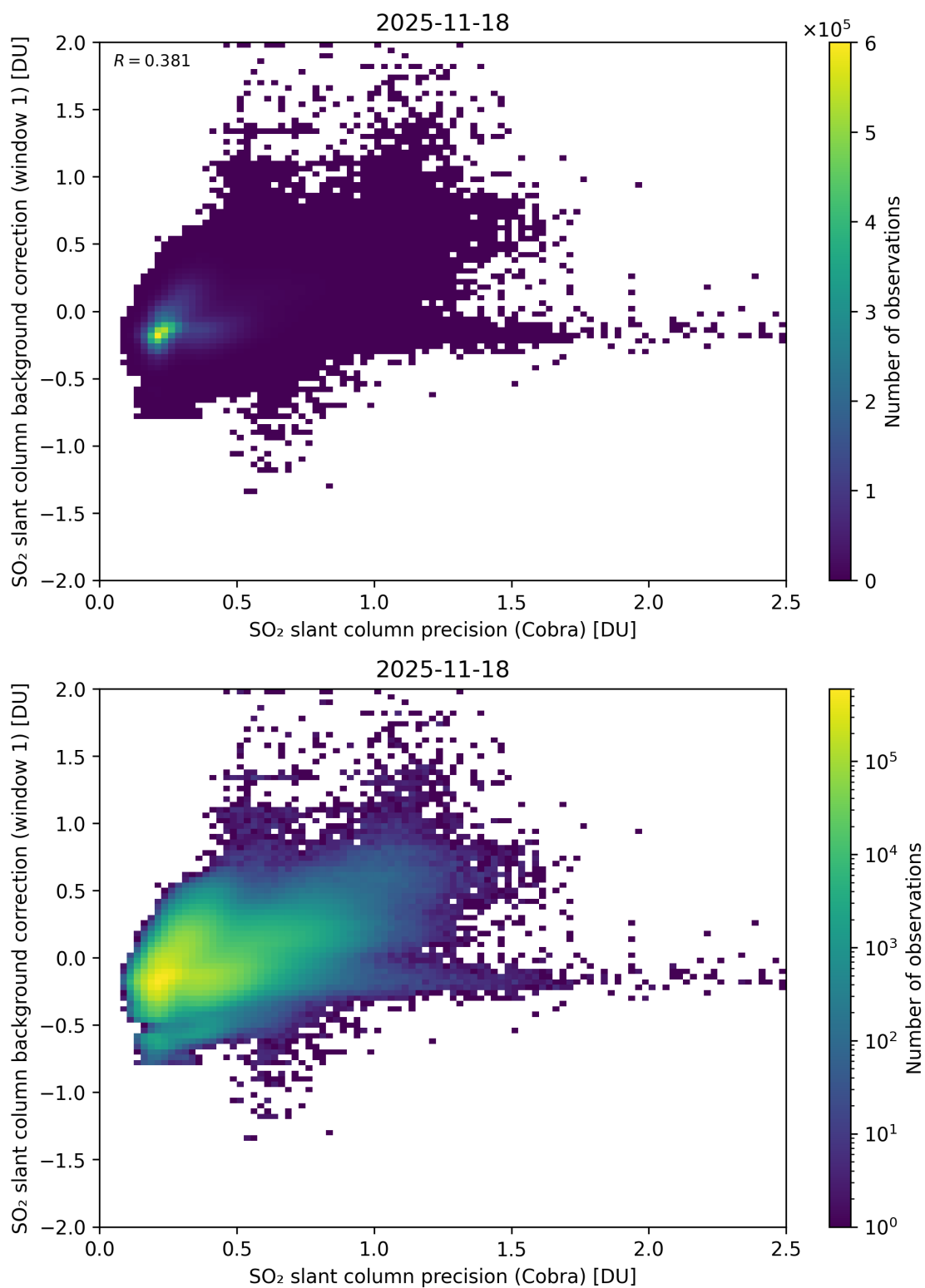
Figure 199: Scatter density plot of “SO 2 slant column precision (Cobra)” against “SO 2 slant column background correction (window 1)” for 2025-11-18 to 2025-11-19.
