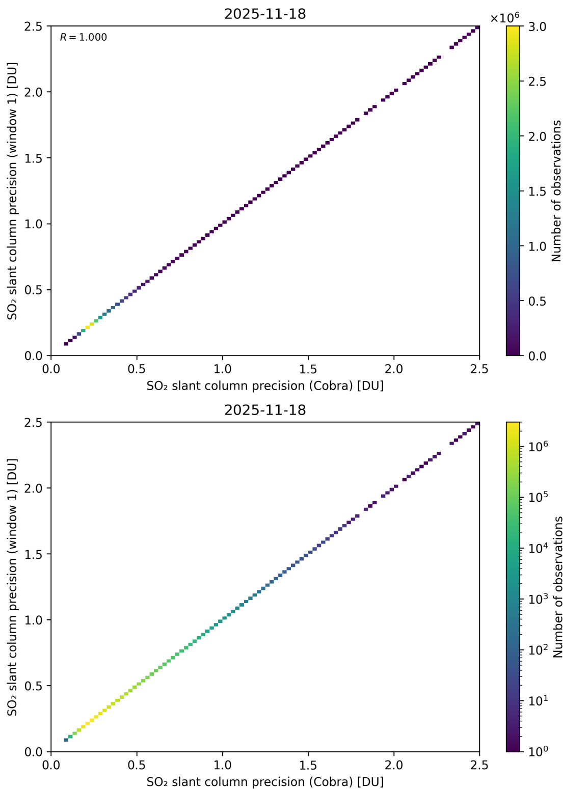
Figure 209: Scatter density plot of “SO 2 slant column precision (Cobra)” against “SO 2 slant column precision (window 1)” for 2025-11-18 to 2025-11-19.
