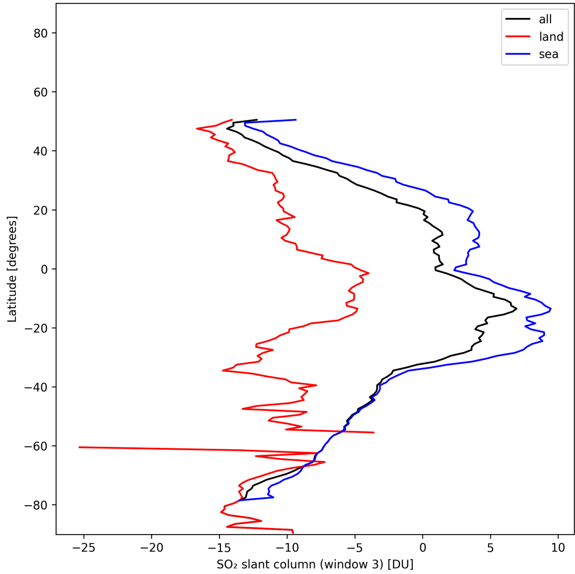
Figure 45: Zonal average of “SO 2 slant column (window 3)” for 2025-11-18 to 2025-11-19.
