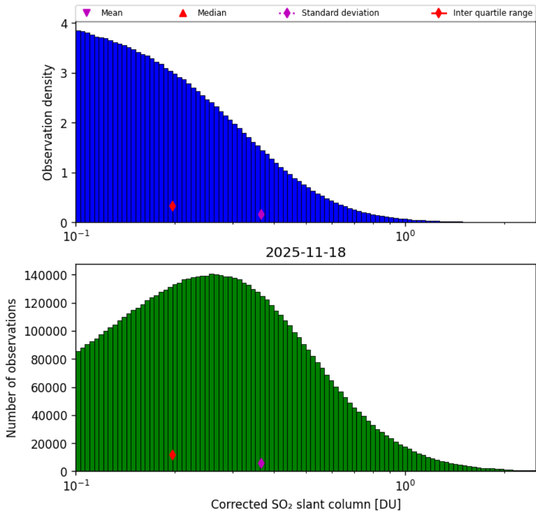
Figure 60: Histogram of “Corrected SO 2 slant column” for 2025-11-18 to 2025-11-19
