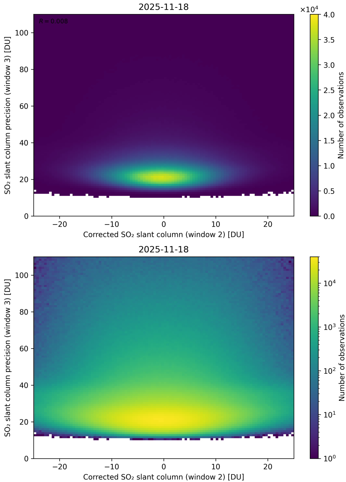
Figure 252: Scatter density plot of “Corrected SO 2 slant column (window 2)” against “SO 2 slant column precision (window 3)” for 2025-11-18 to 2025-11-19.
