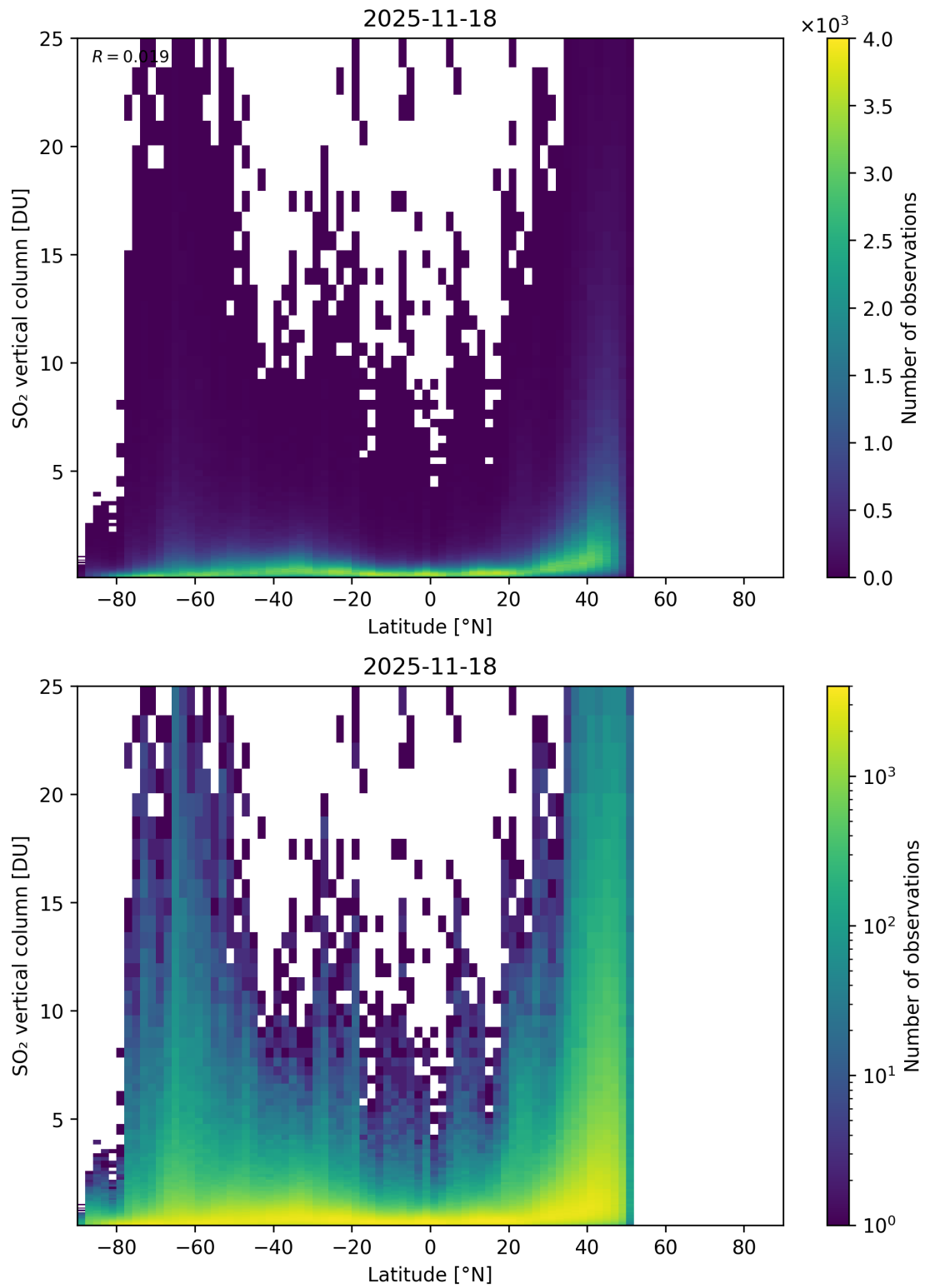
Figure 169: Scatter density plot of “Latitude” against “SO 2 vertical column” for 2025-11-18 to 2025-11-19.
