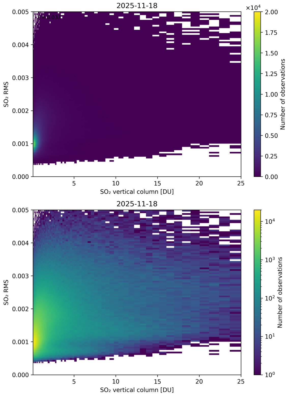
Figure 328: Scatter density plot of “SO 2 vertical column” against “SO 2 RMS” for 2025-11-18 to 2025-11-19.
