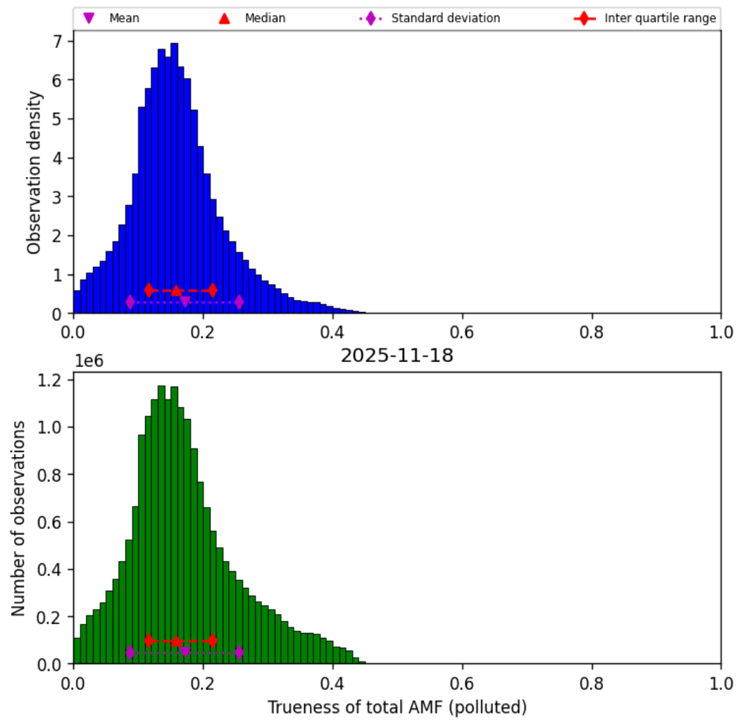
Figure 80: Histogram of “Trueness of total AMF (polluted)” for 2025-11-18 to 2025-11-19
