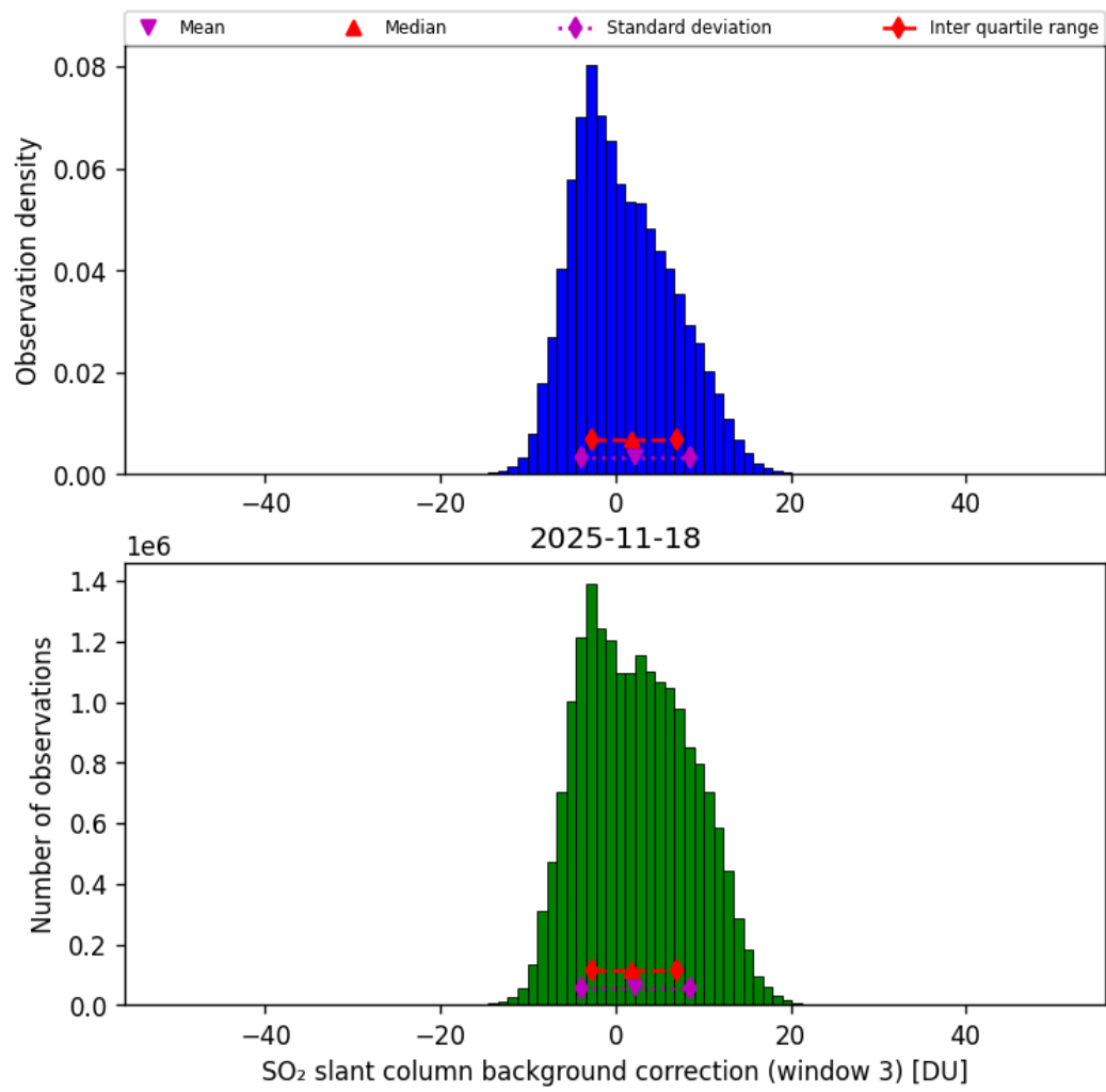
Figure 74: Histogram of “SO 2 slant column background correction (window 3)” for 2025-11-18 to 2025-11-19
