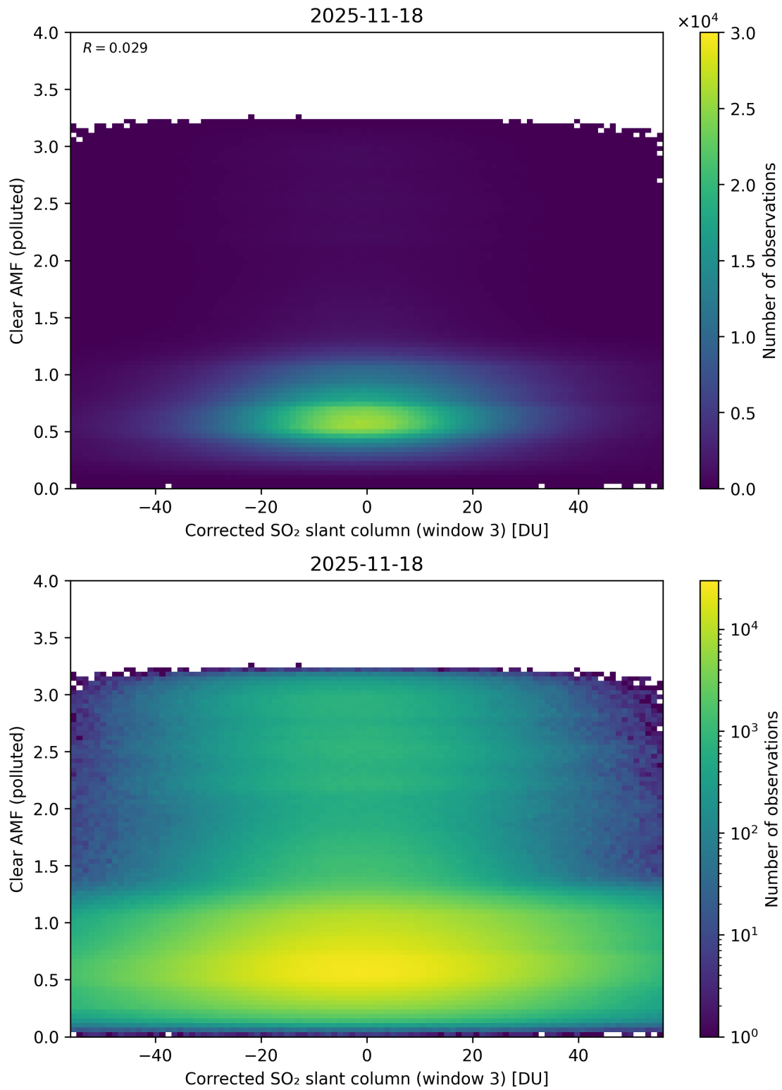
Figure 259: Scatter density plot of “Corrected SO 2 slant column (window 3)” against “Clear AMF (polluted)” for 2025-11-18 to 2025-11-19.
