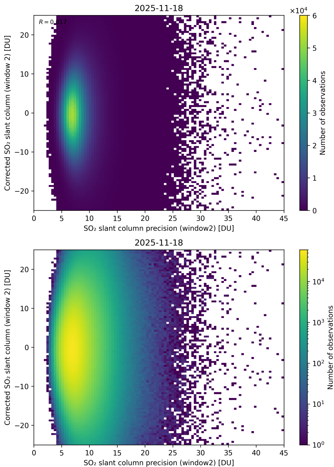
Figure 297: Scatter density plot of “SO 2 slant column precision (window2)” against “Corrected SO 2 slant column (window 2)” for 2025-11-18 to 2025-11-19.
