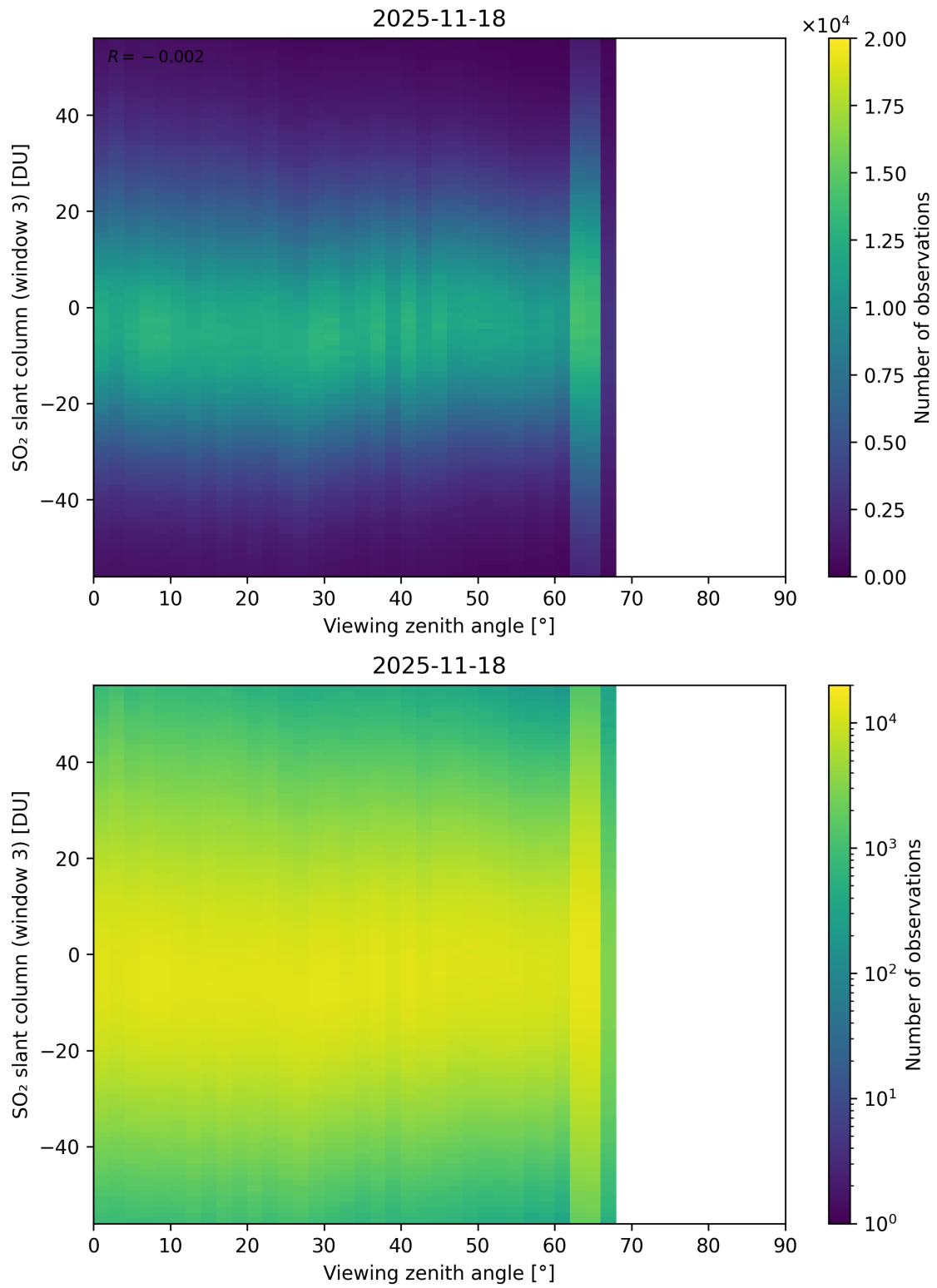
Figure 379: Scatter density plot of “Viewing zenith angle” against “SO 2 slant column (window 3)” for 2025-11-18 to 2025-11-19.
