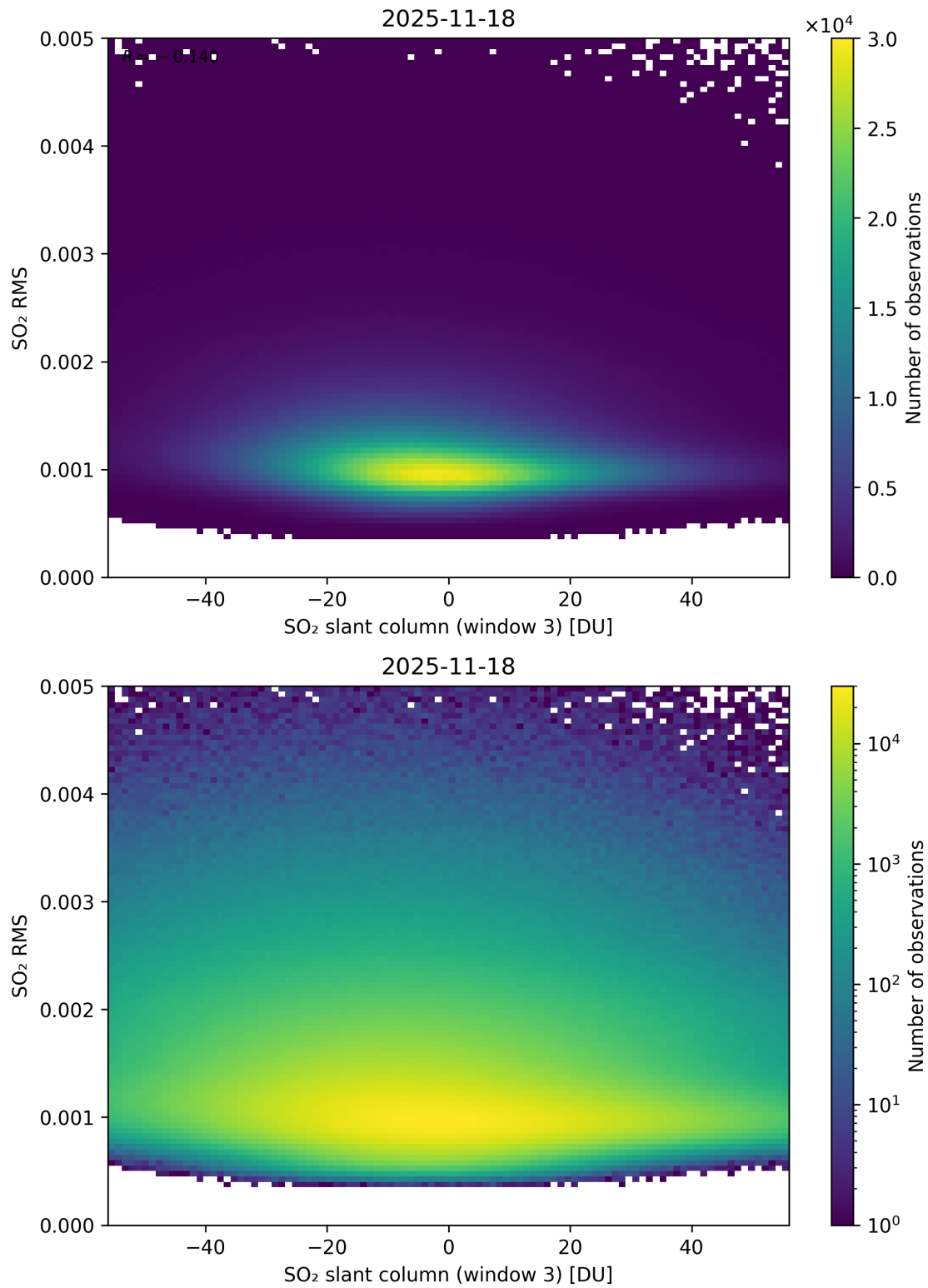
Figure 306: Scatter density plot of “SO 2 slant column (window 3)” against “SO 2 RMS” for 2025-11-18 to 2025-11-19.
