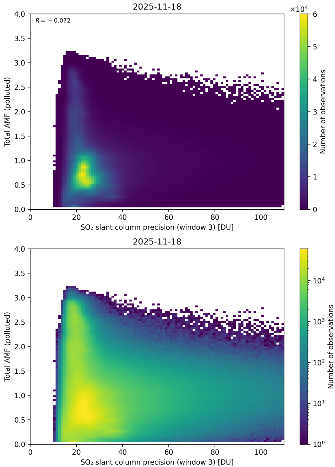
Figure 313: Scatter density plot of “SO 2 slant column precision (window 3)” against “Total AMF (polluted)” for 2025-11-18 to 2025-11-19.
