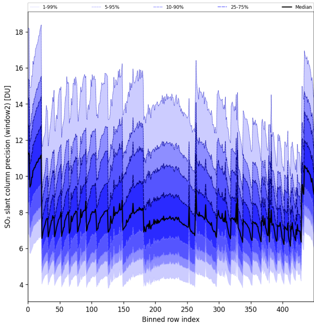
Figure 94: Along track statistics of “SO 2 slant column precision (window2)” for 2025-11-18 to 2025-11-19
