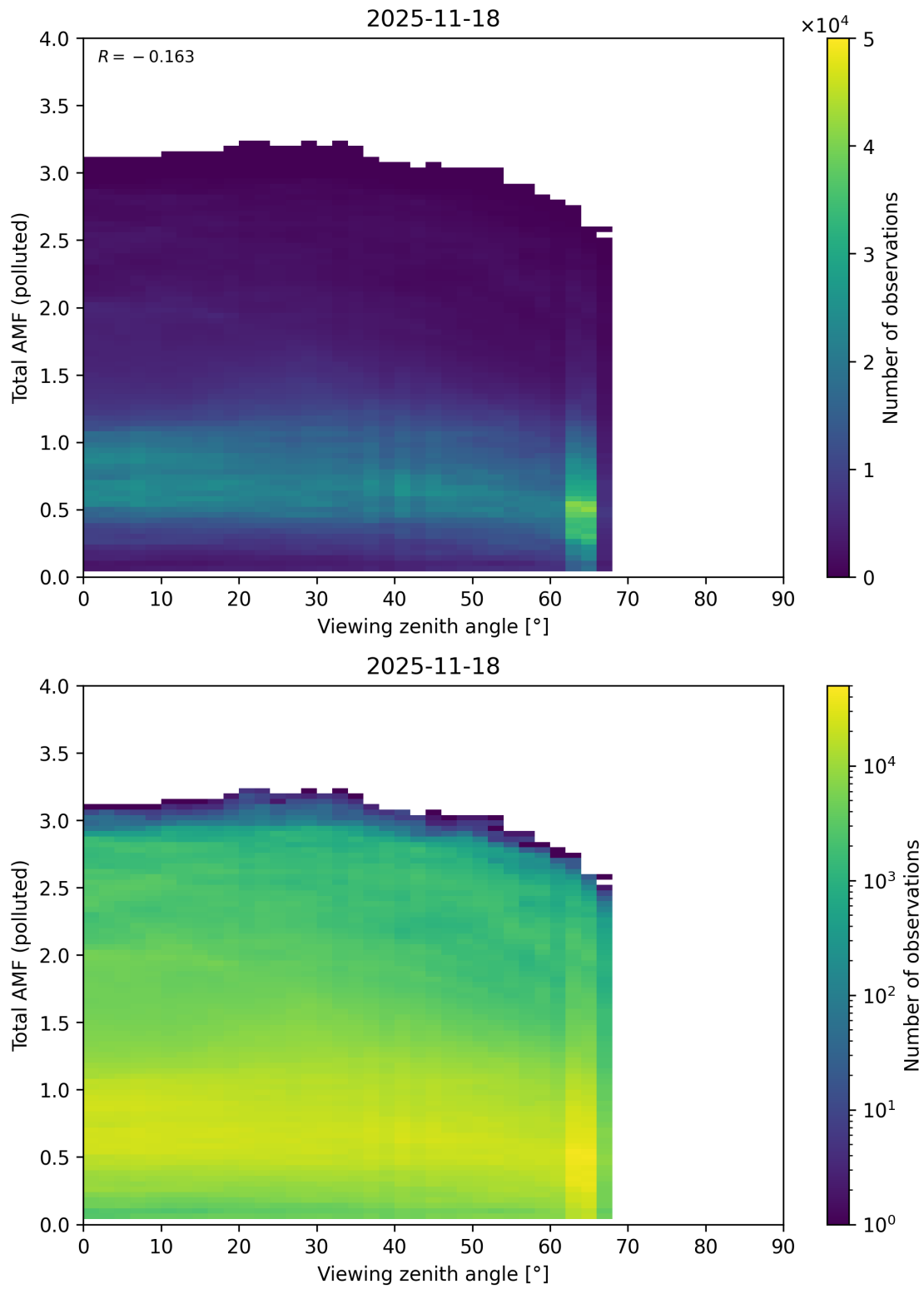
Figure 381: Scatter density plot of “Viewing zenith angle” against “Total AMF (polluted)” for 2025-11-18 to 2025-11-19.
