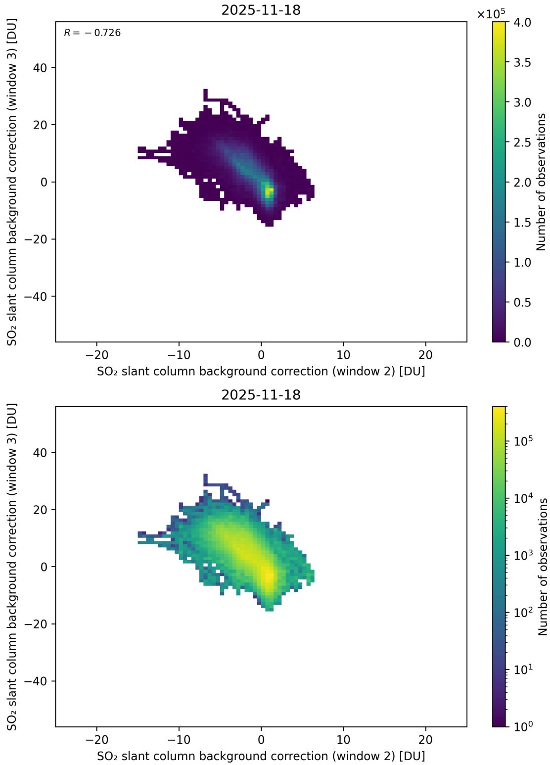
Figure 122: Scatter density plot of “SO 2 slant column background correction (window 2)” against “SO 2 slant column background correction (window 3)” for 2025-11-18 to 2025-11-19.
