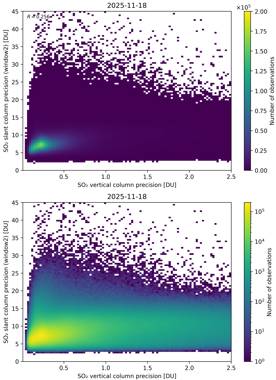
Figure 343: Scatter density plot of “SO 2 vertical column precision” against “SO 2 slant column precision (window2)” for 2025-11-18 to 2025-11-19.
