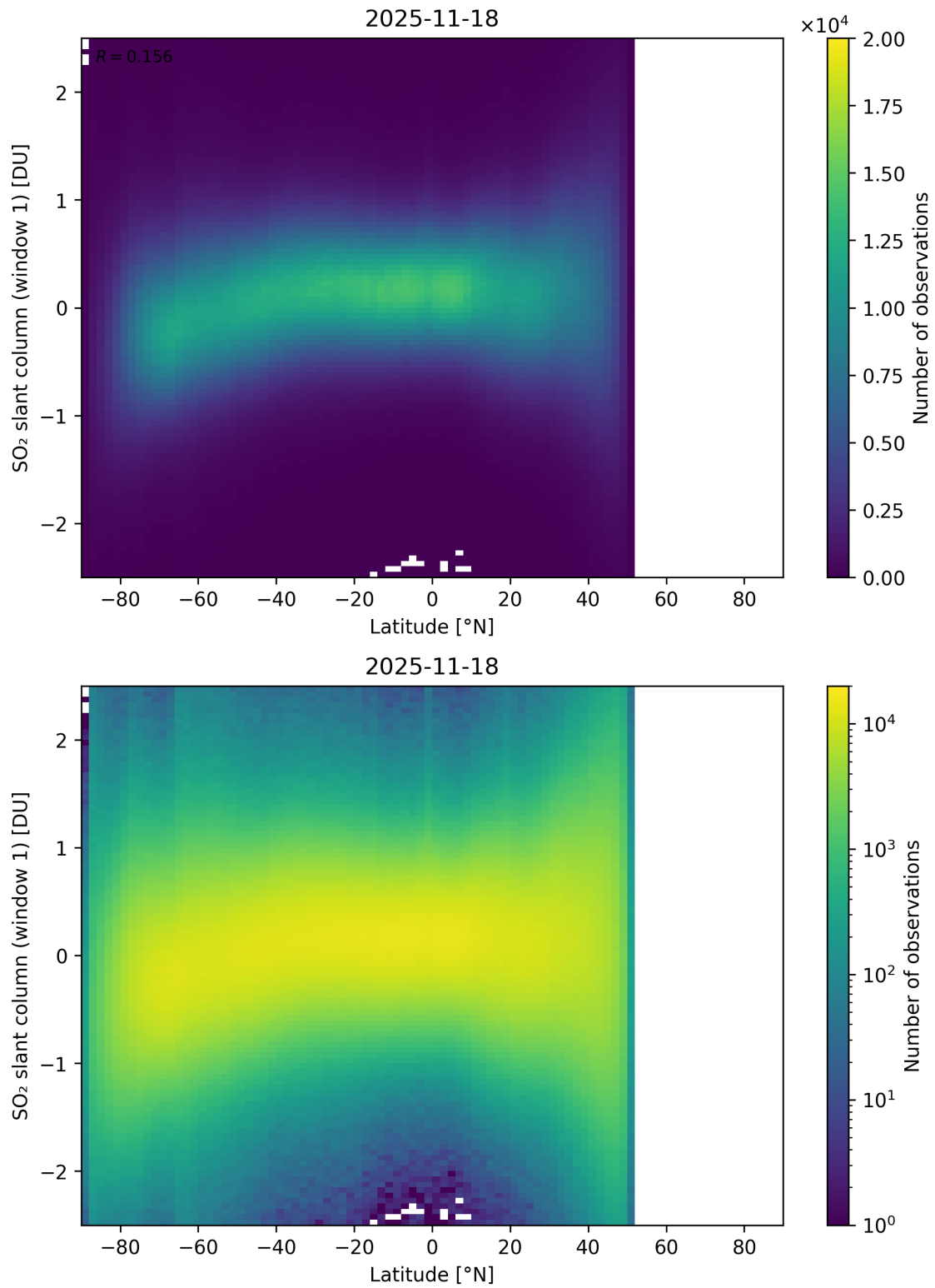
Figure 162: Scatter density plot of “Latitude” against “SO 2 slant column (window 1)” for 2025-11-18 to 2025-11-19.
