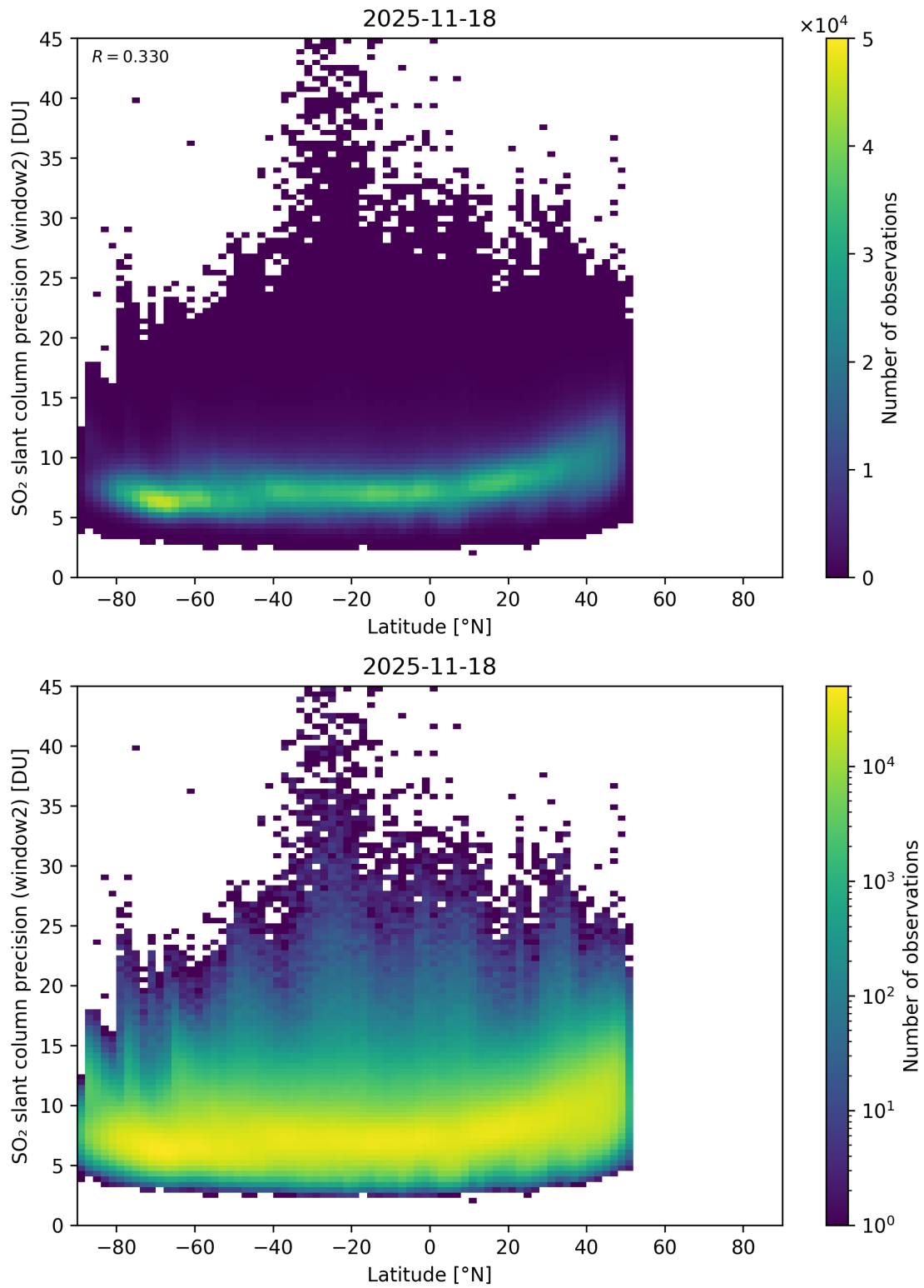
Figure 164: Scatter density plot of “Latitude” against “SO 2 slant column precision (window2)” for 2025-11-18 to 2025-11-19.
