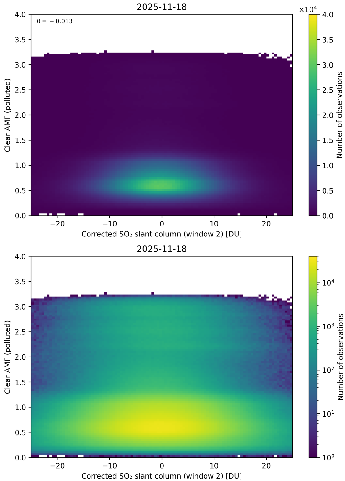
Figure 249: Scatter density plot of “Corrected SO 2 slant column (window 2)” against “Clear AMF (polluted)” for 2025-11-18 to 2025-11-19.
