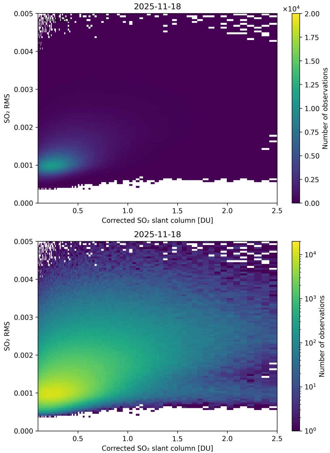
Figure 231: Scatter density plot of “Corrected SO 2 slant column” against “SO 2 RMS” for 2025-11-18 to 2025-11-19.
