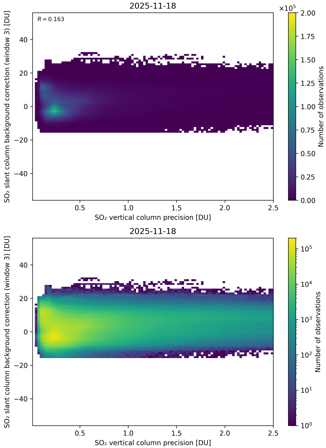
Figure 331: Scatter density plot of “SO 2 vertical column precision” against “SO 2 slant column background correction (window 3)” for 2025-11-18 to 2025-11-19.
