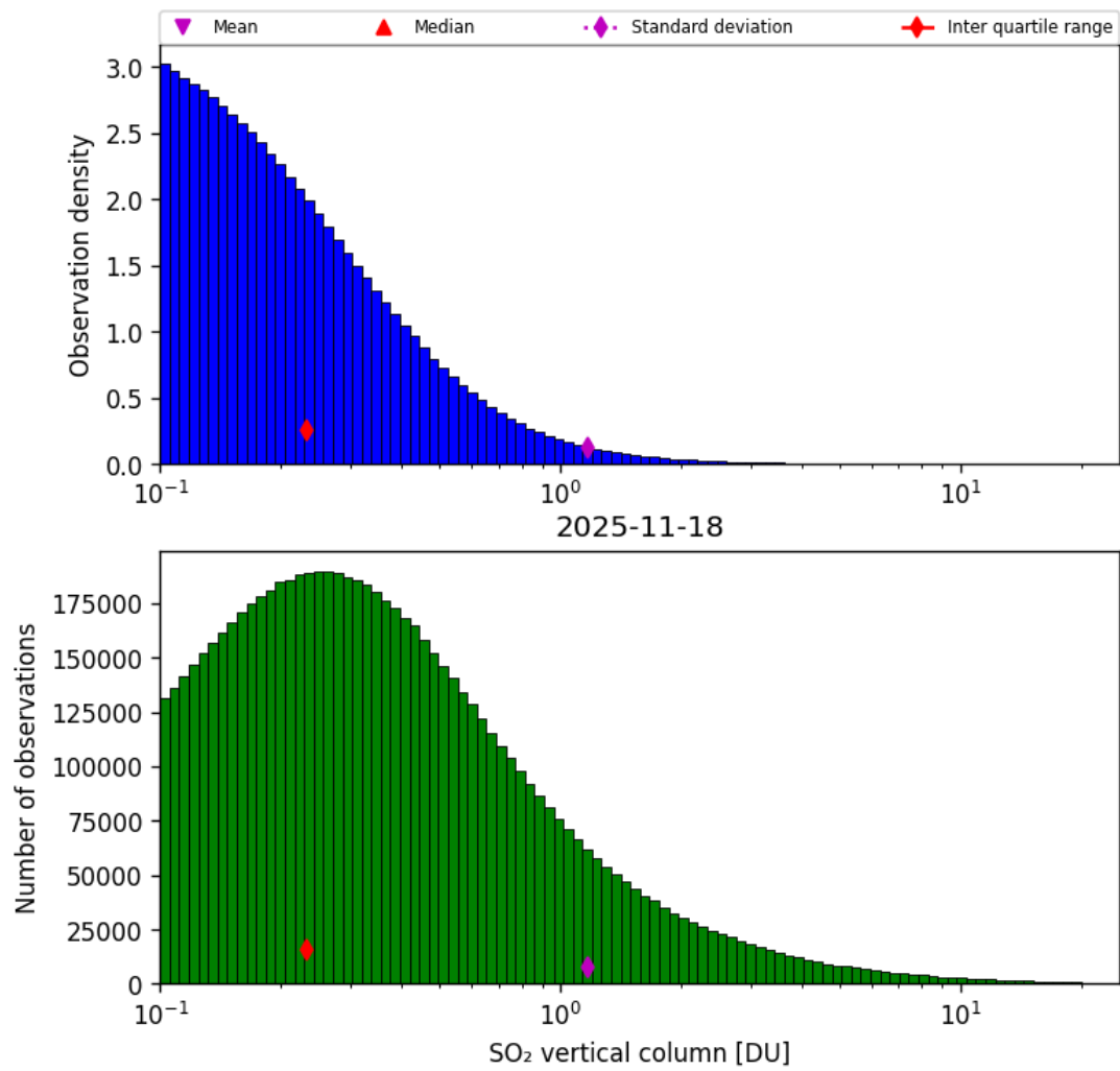
Figure 58: Histogram of “SO 2 vertical column” for 2025-11-18 to 2025-11-19
