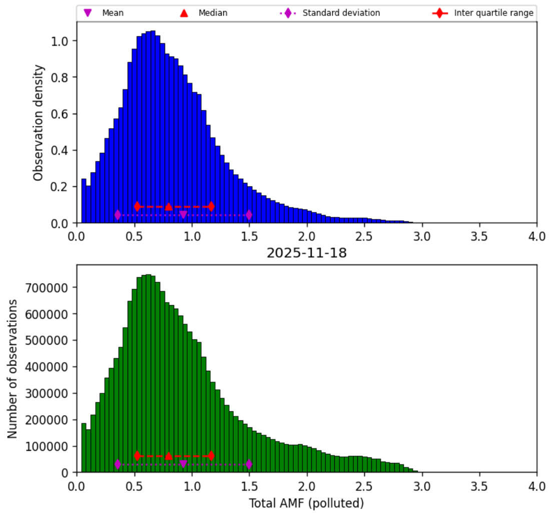
Figure 79: Histogram of “Total AMF (polluted)” for 2025-11-18 to 2025-11-19
