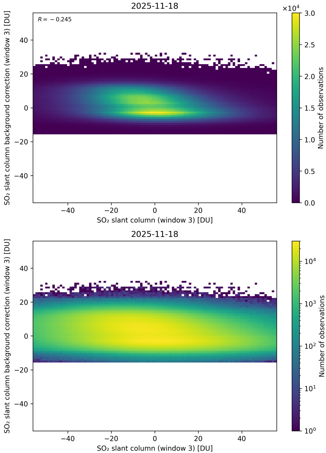
Figure 303: Scatter density plot of “SO 2 slant column (window 3)” against “SO 2 slant column background correction (window 3)” for 2025-11-18 to 2025-11-19.
