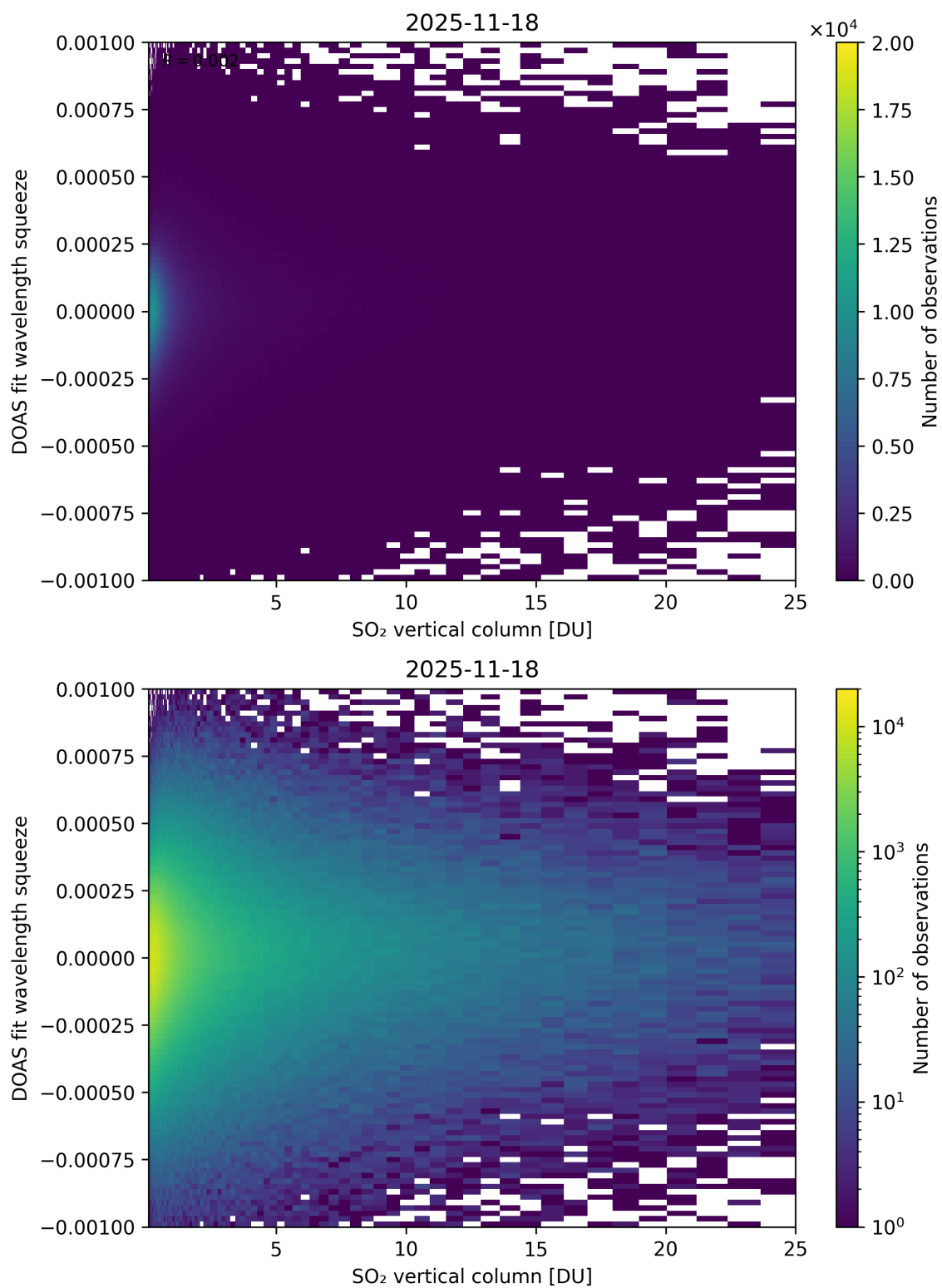
Figure 327: Scatter density plot of “SO 2 vertical column” against “DOAS fit wavelength squeeze” for 2025-11-18 to 2025-11-19.
