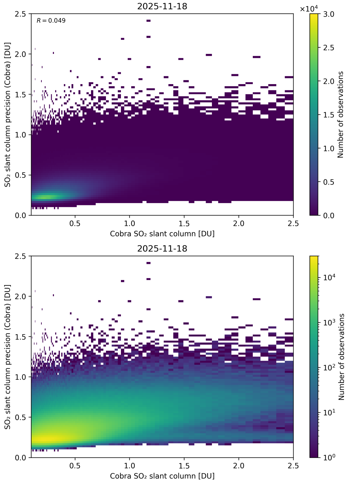
Figure 216: Scatter density plot of “Cobra SO 2 slant column” against “SO 2 slant column precision (Cobra)” for 2025-11-18 to 2025-11-19.
