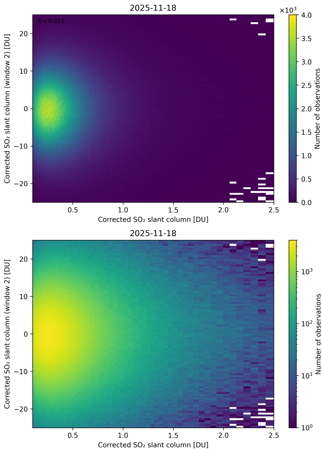
Figure 235: Scatter density plot of “Corrected SO 2 slant column” against “Corrected SO 2 slant column (window 2)” for 2025-11-18 to 2025-11-19.
