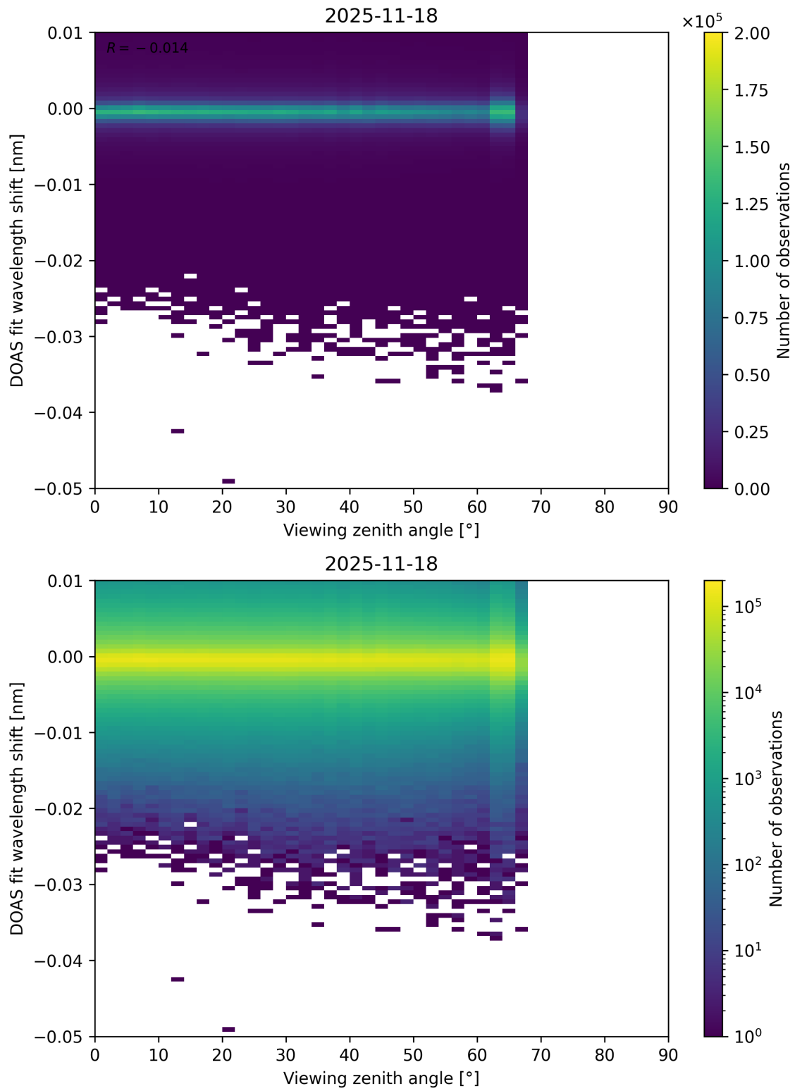
Figure 365: Scatter density plot of “Viewing zenith angle” against “DOAS fit wavelength shift” for 2025-11-18 to 2025-11-19.
