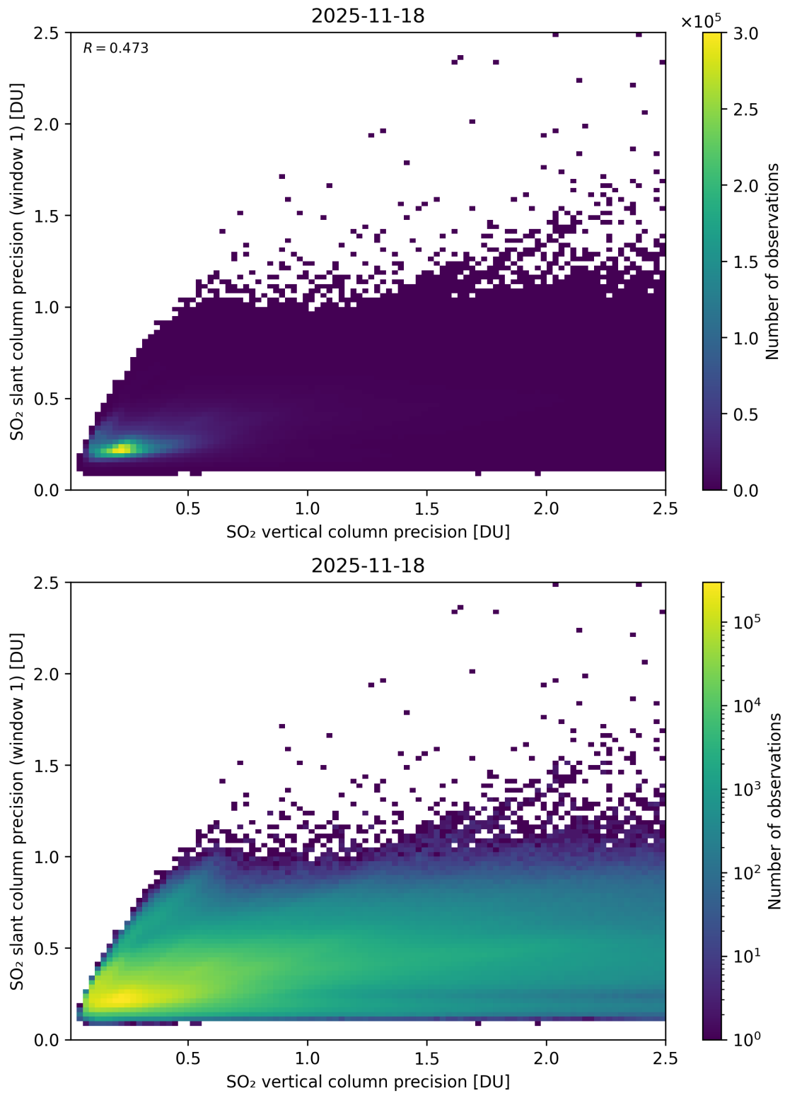
Figure 342: Scatter density plot of “SO 2 vertical column precision” against “SO 2 slant column precision (window 1)” for 2025-11-18 to 2025-11-19.
