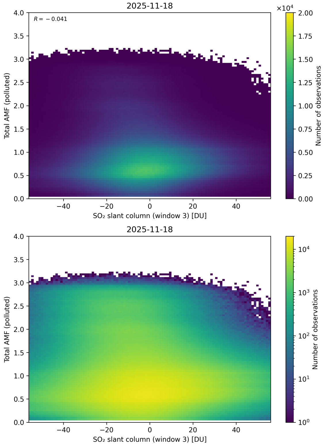
Figure 318: Scatter density plot of “SO 2 slant column (window 3)” against “Total AMF (polluted)” for 2025-11-18 to 2025-11-19.
