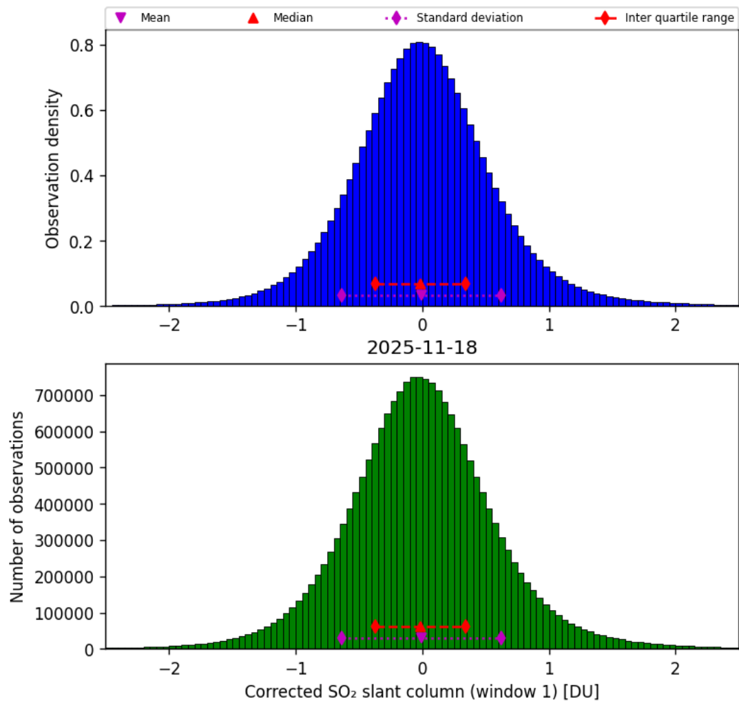
Figure 65: Histogram of “Corrected SO 2 slant column (window 1)” for 2025-11-18 to 2025-11-19
