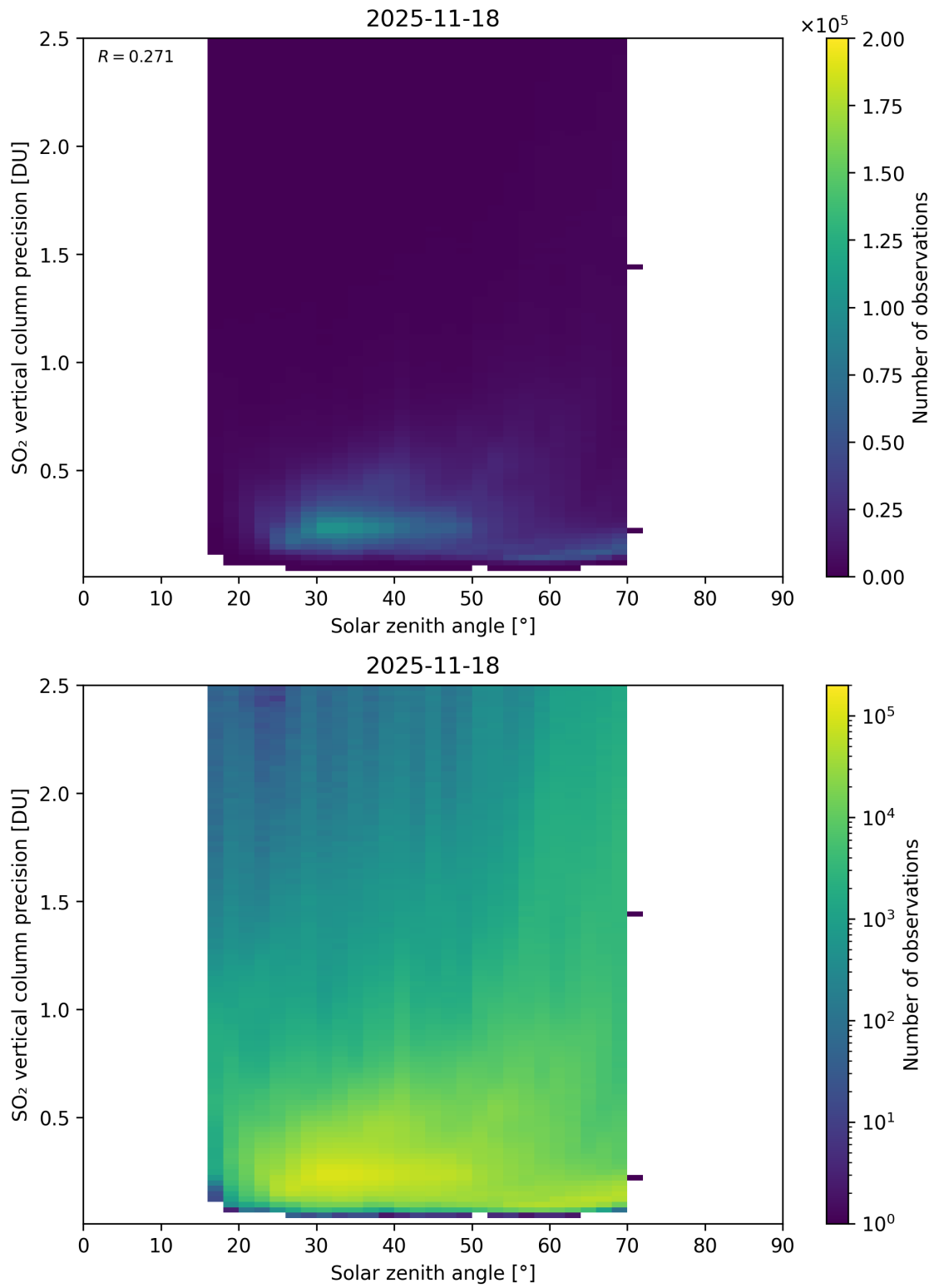
Figure 192: Scatter density plot of “Solar zenith angle” against “SO 2 vertical column precision” for 2025-11-18 to 2025-11-19.
