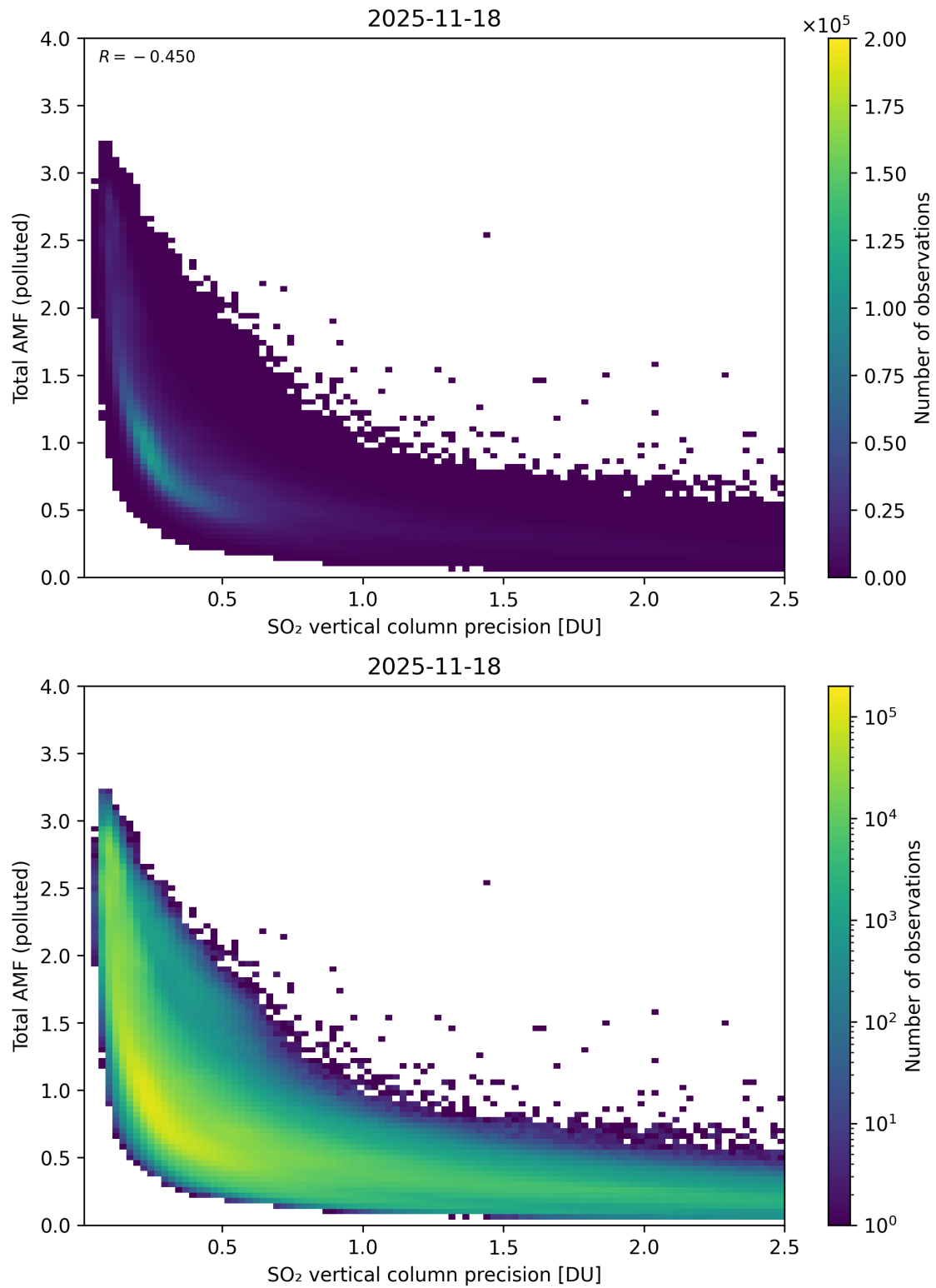
Figure 346: Scatter density plot of “SO 2 vertical column precision” against “Total AMF (polluted)” for 2025-11-18 to 2025-11-19.
