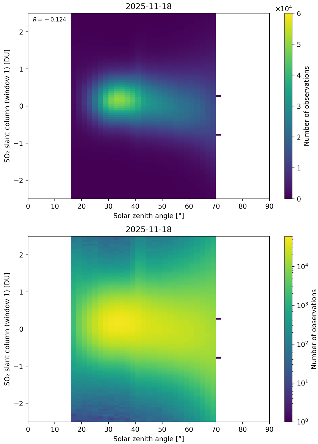
Figure 184: Scatter density plot of “Solar zenith angle” against “SO 2 slant column (window 1)” for 2025-11-18 to 2025-11-19.
