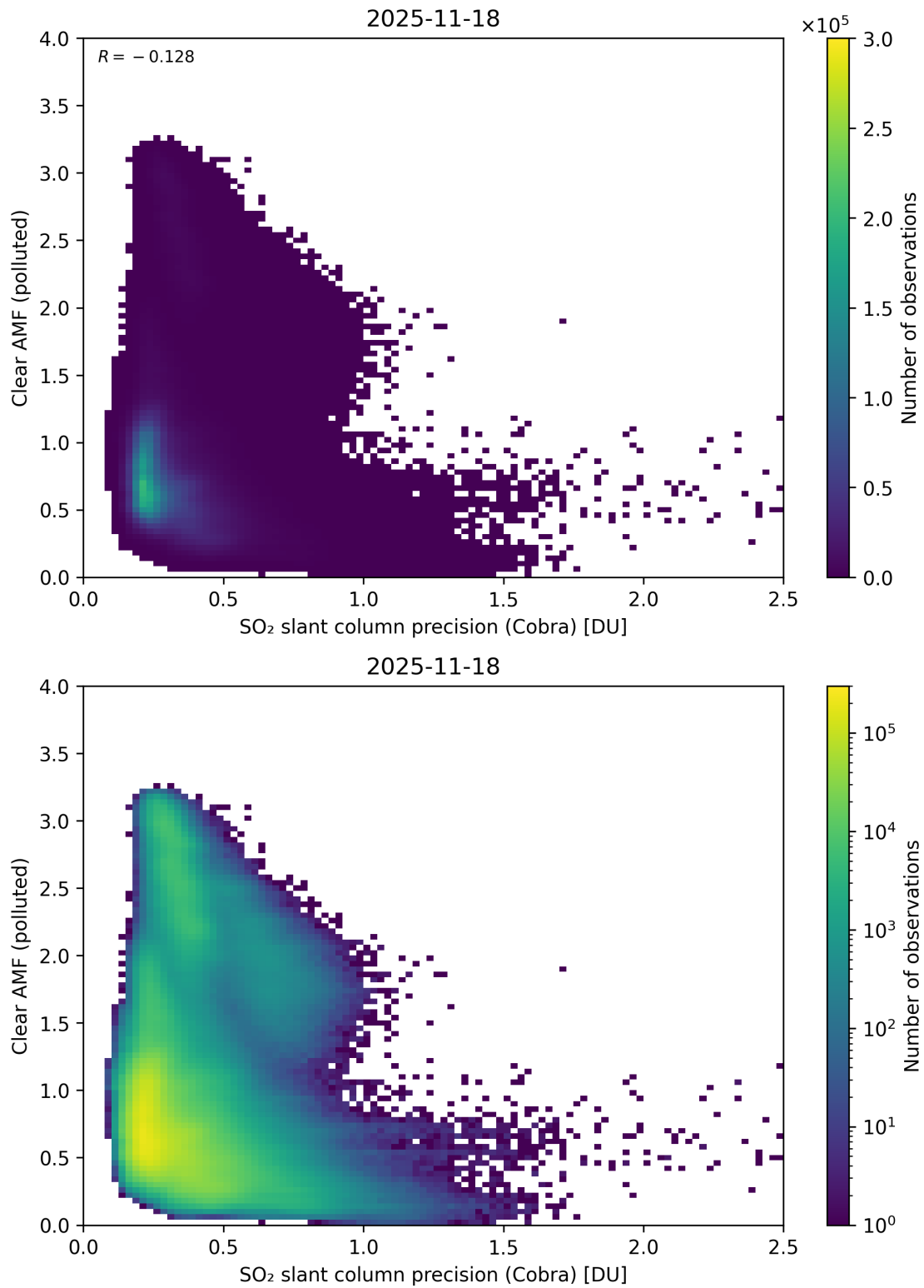
Figure 205: Scatter density plot of “SO 2 slant column precision (Cobra)” against “Clear AMF (polluted)” for 2025-11-18 to 2025-11-19.
