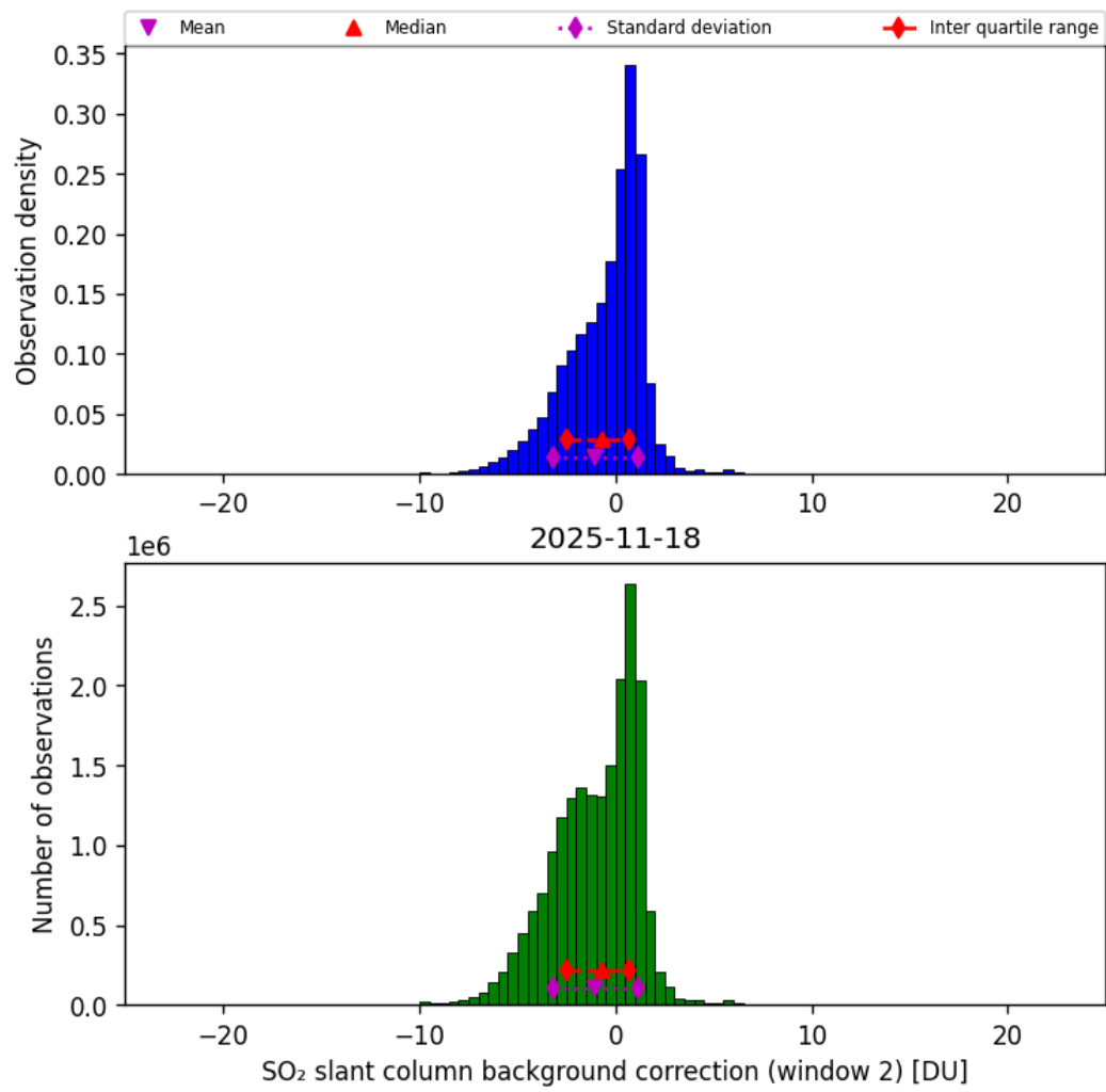
Figure 70: Histogram of “SO 2 slant column background correction (window 2)” for 2025-11-18 to 2025-11-19
