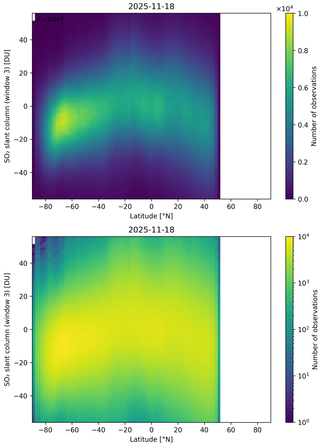
Figure 165: Scatter density plot of “Latitude” against “SO 2 slant column (window 3)” for 2025-11-18 to 2025-11-19.
