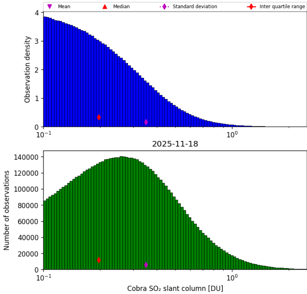
Figure 61: Histogram of “Cobra SO 2 slant column” for 2025-11-18 to 2025-11-19
