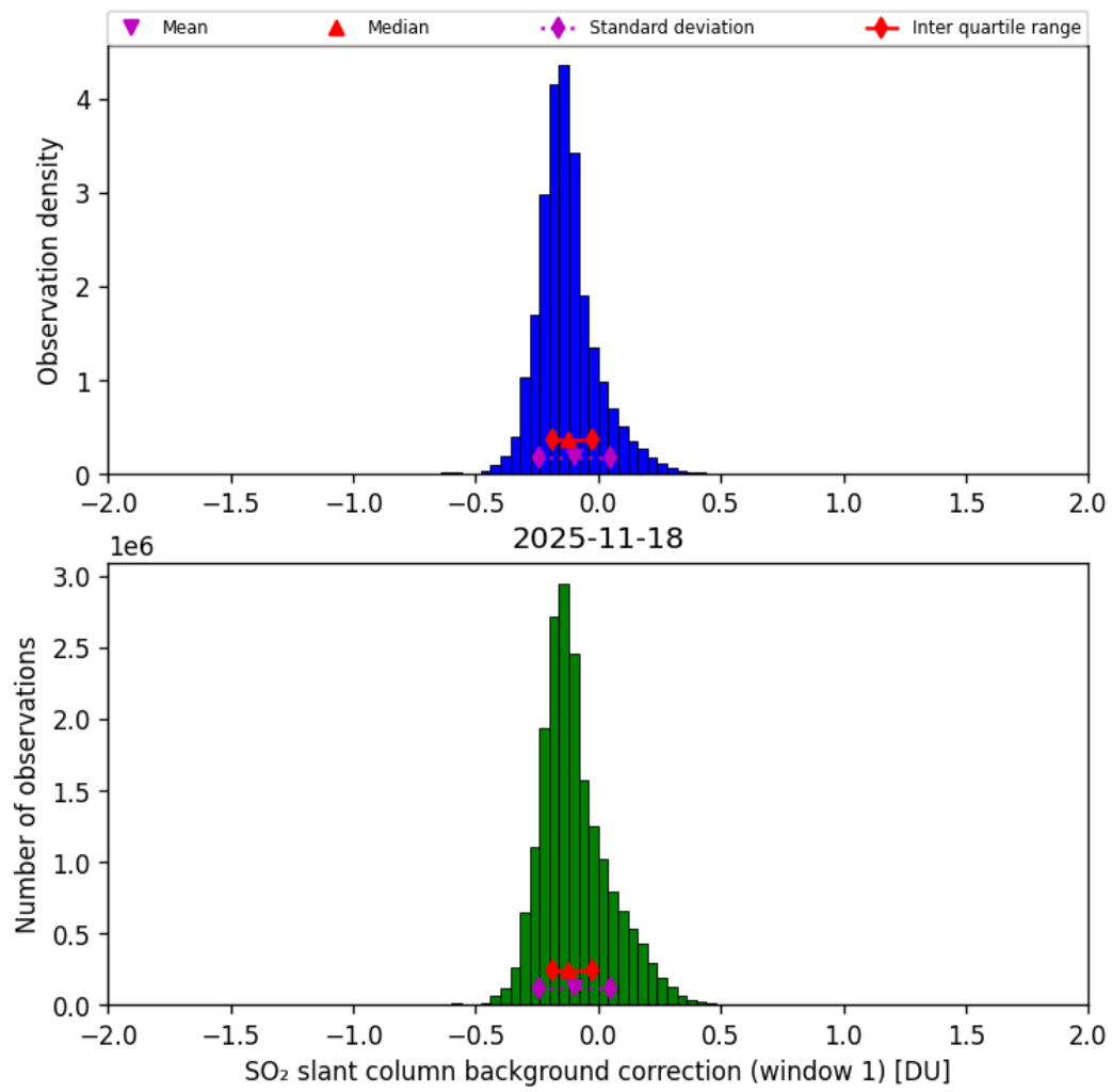
Figure 66: Histogram of “SO 2 slant column background correction (window 1)” for 2025-11-18 to 2025-11-19
