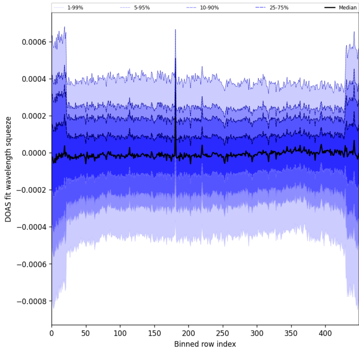
Figure 103: Along track statistics of “DOAS fit wavelength squeeze” for 2025-11-18 to 2025-11-19
