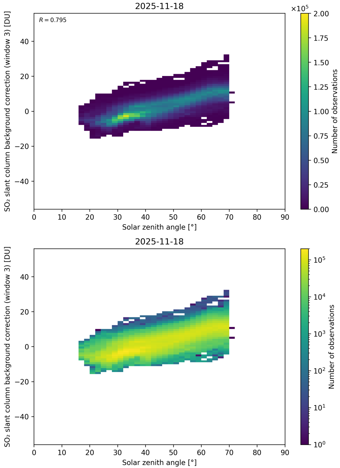
Figure 173: Scatter density plot of “Solar zenith angle” against “SO 2 slant column background correction (window 3)” for 2025-11-18 to 2025-11-19.
