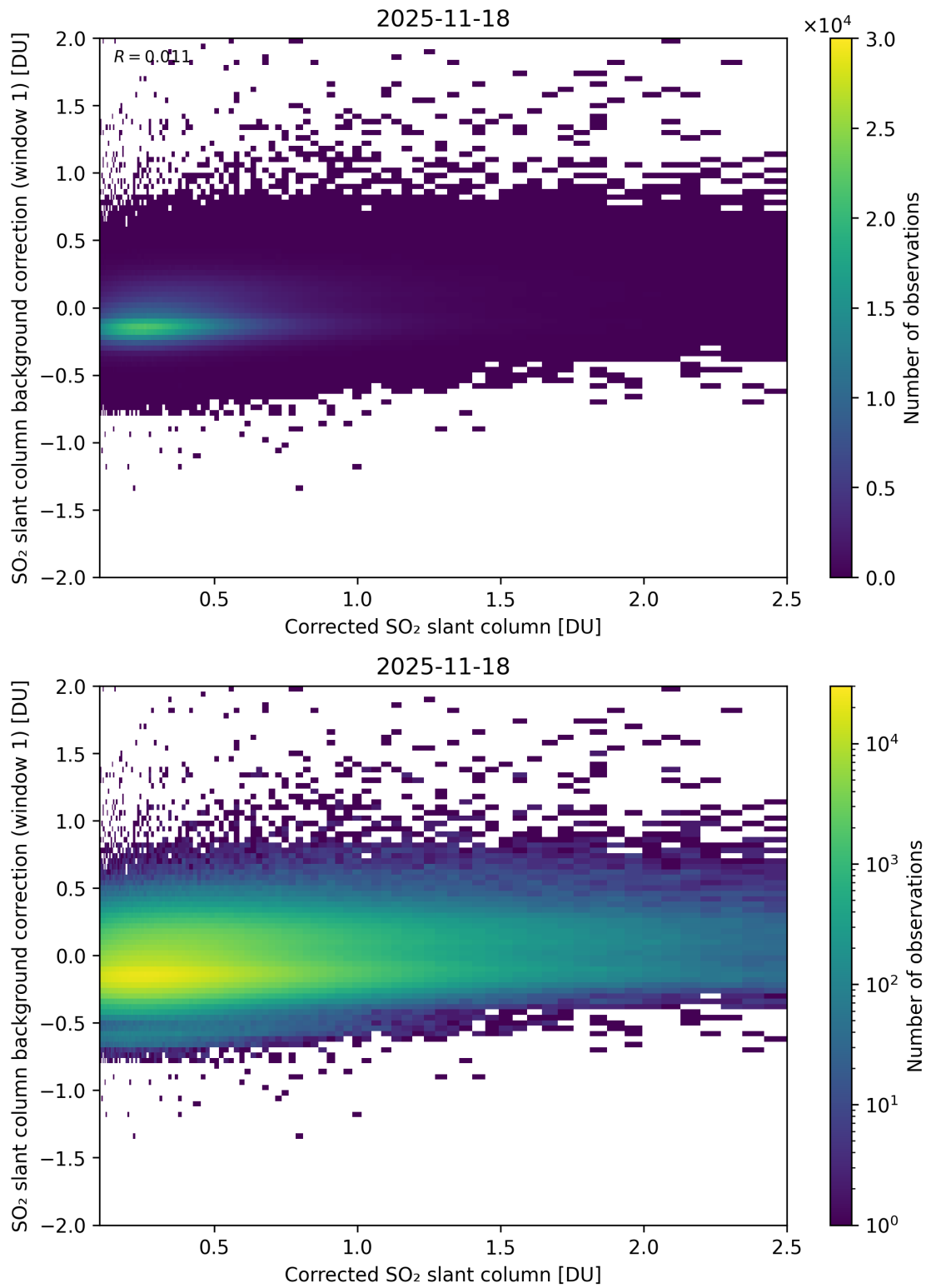
Figure 226: Scatter density plot of “Corrected SO 2 slant column” against “SO 2 slant column background correction (window 1)” for 2025-11-18 to 2025-11-19.
