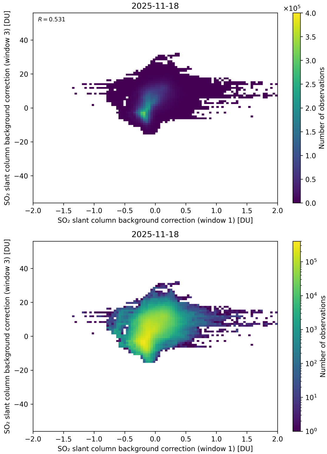
Figure 110: Scatter density plot of “SO 2 slant column background correction (window 1)” against “SO 2 slant column background correction (window 3)” for 2025-11-18 to 2025-11-19.
