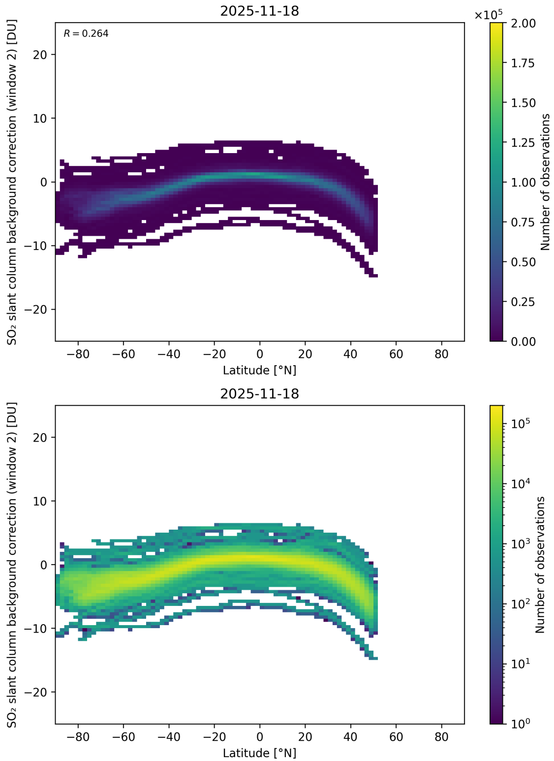
Figure 151: Scatter density plot of “Latitude” against “SO 2 slant column background correction (window 2)” for 2025-11-18 to 2025-11-19.
