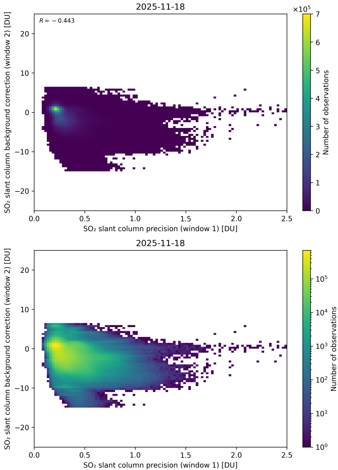
Figure 269: Scatter density plot of “SO 2 slant column precision (window 1)” against “SO 2 slant column background correction (window 2)” for 2025-11-18 to 2025-11-19.
