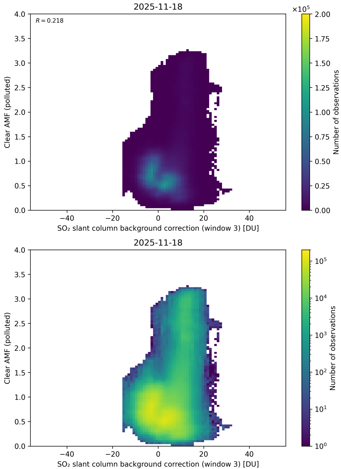
Figure 135: Scatter density plot of “SO 2 slant column background correction (window 3)” against “Clear AMF (polluted)” for 2025-11-18 to 2025-11-19.
