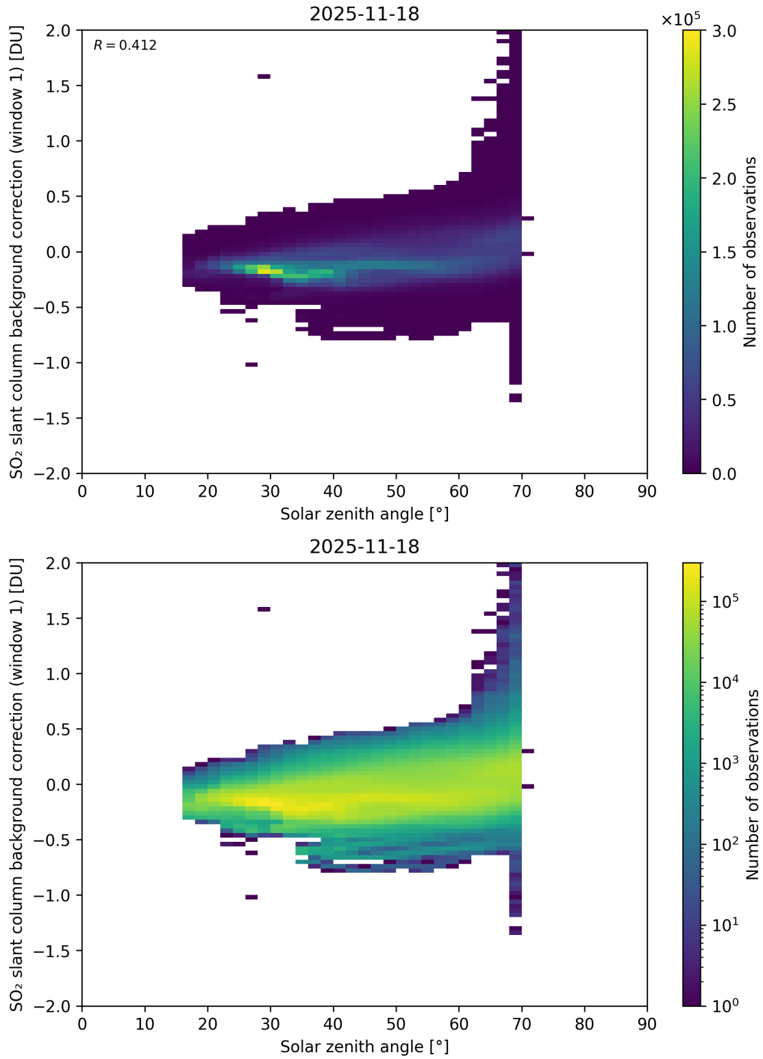
Figure 171: Scatter density plot of “Solar zenith angle” against “SO 2 slant column background correction (window 1)” for 2025-11-18 to 2025-11-19.
