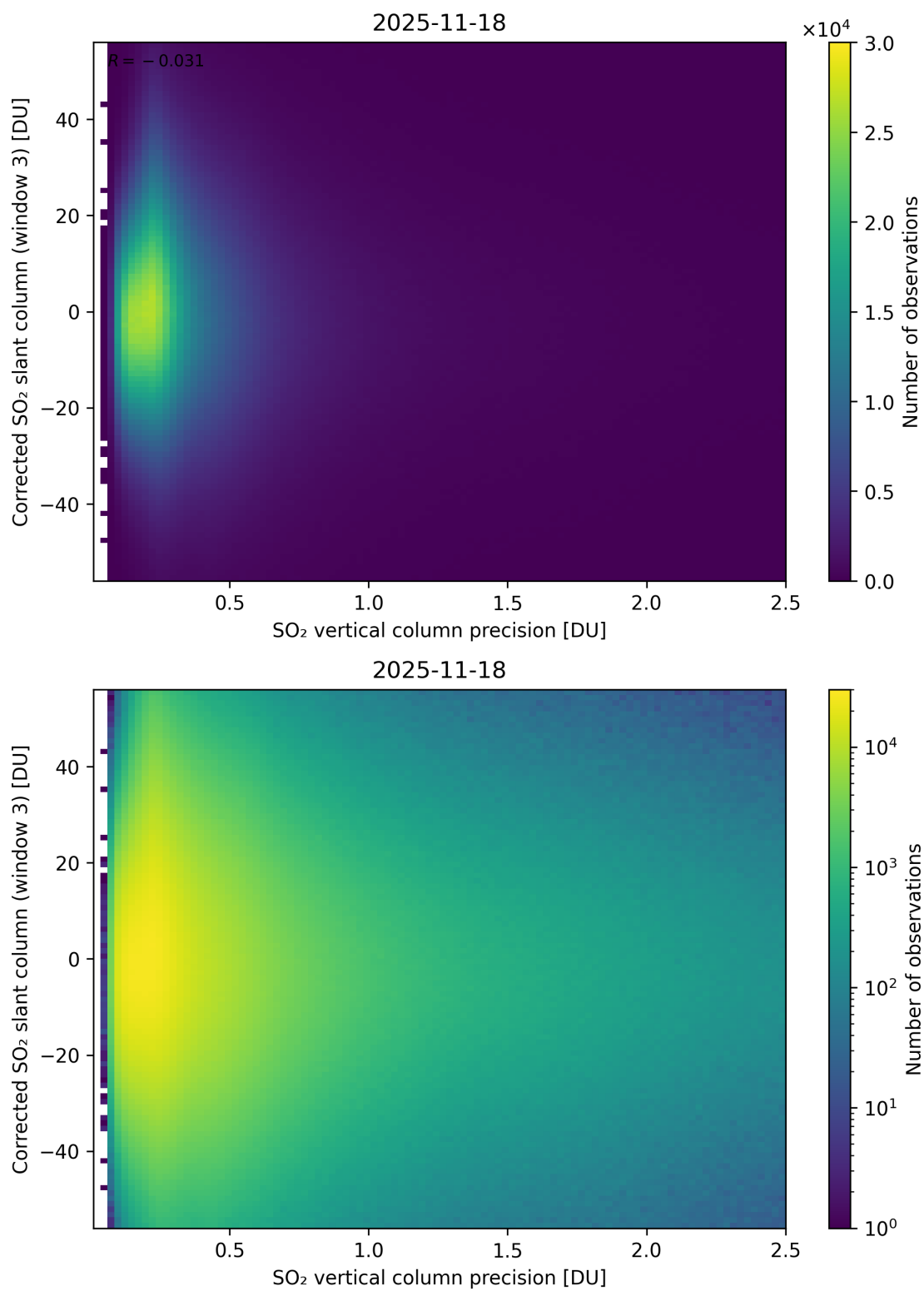
Figure 340: Scatter density plot of “SO 2 vertical column precision” against “Corrected SO 2 slant column (window 3)” for 2025-11-18 to 2025-11-19.
