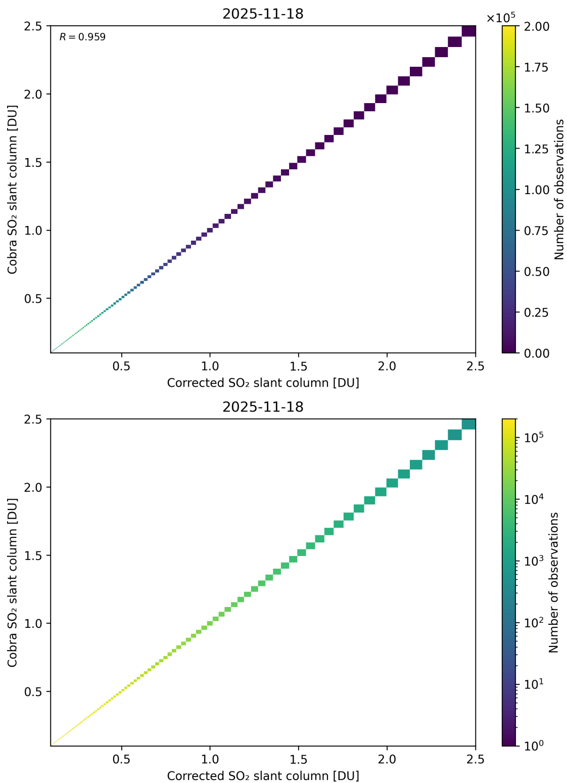
Figure 233: Scatter density plot of “Corrected SO 2 slant column” against “Cobra SO 2 slant column” for 2025-11-18 to 2025-11-19.
