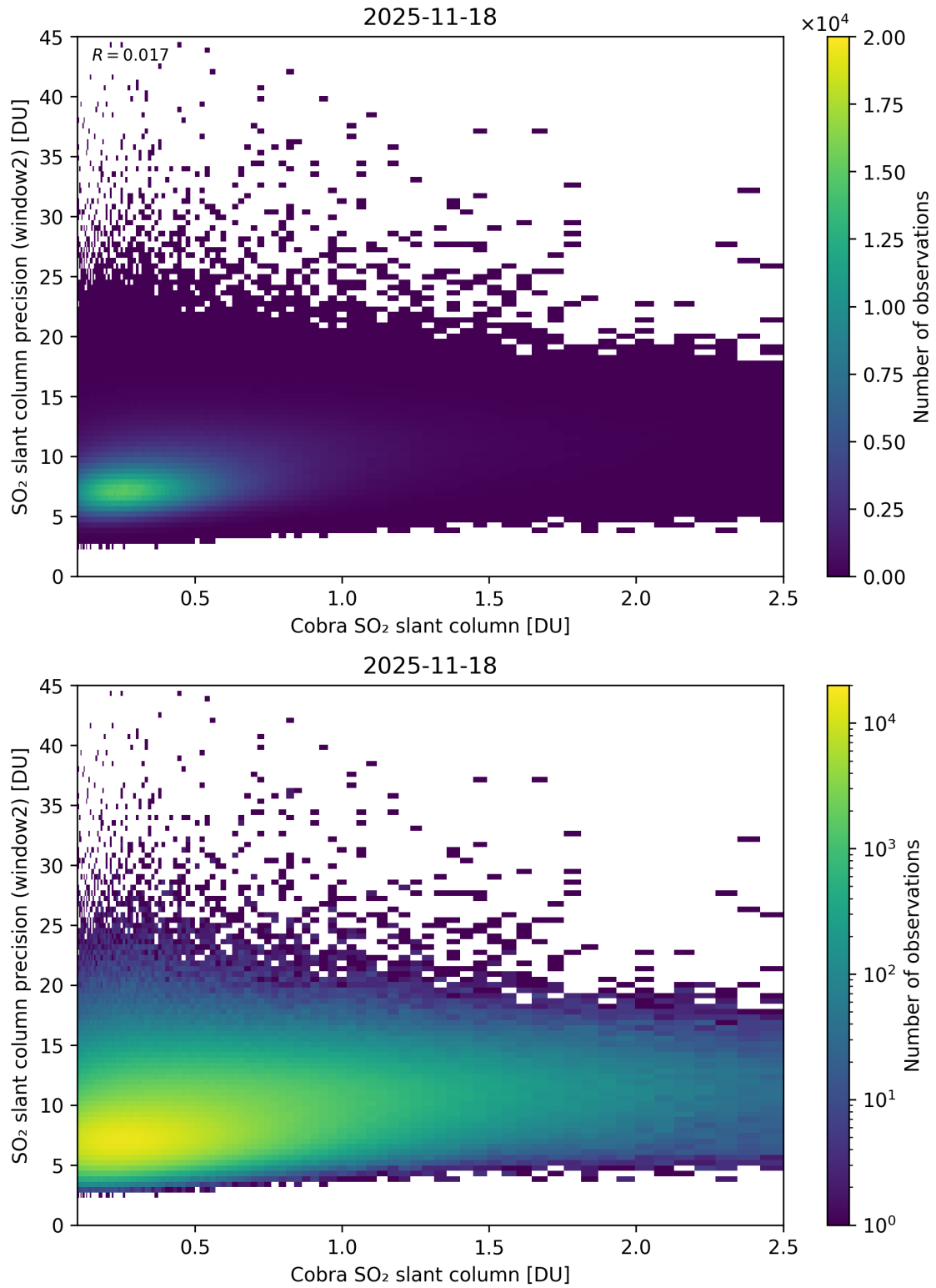
Figure 221: Scatter density plot of “Cobra SO 2 slant column” against “SO 2 slant column precision (window2)” for 2025-11-18 to 2025-11-19.
