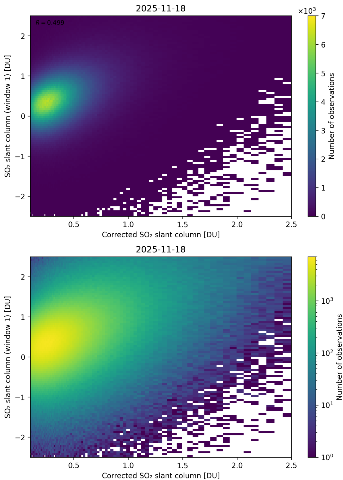
Figure 237: Scatter density plot of “Corrected SO 2 slant column” against “SO 2 slant column (window 1)” for 2025-11-18 to 2025-11-19.
