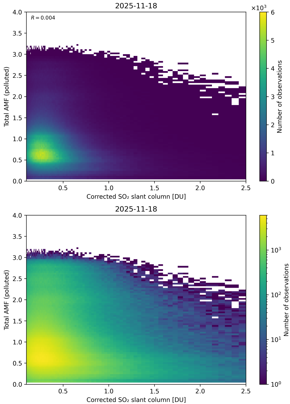
Figure 242: Scatter density plot of “Corrected SO 2 slant column” against “Total AMF (polluted)” for 2025-11-18 to 2025-11-19.
