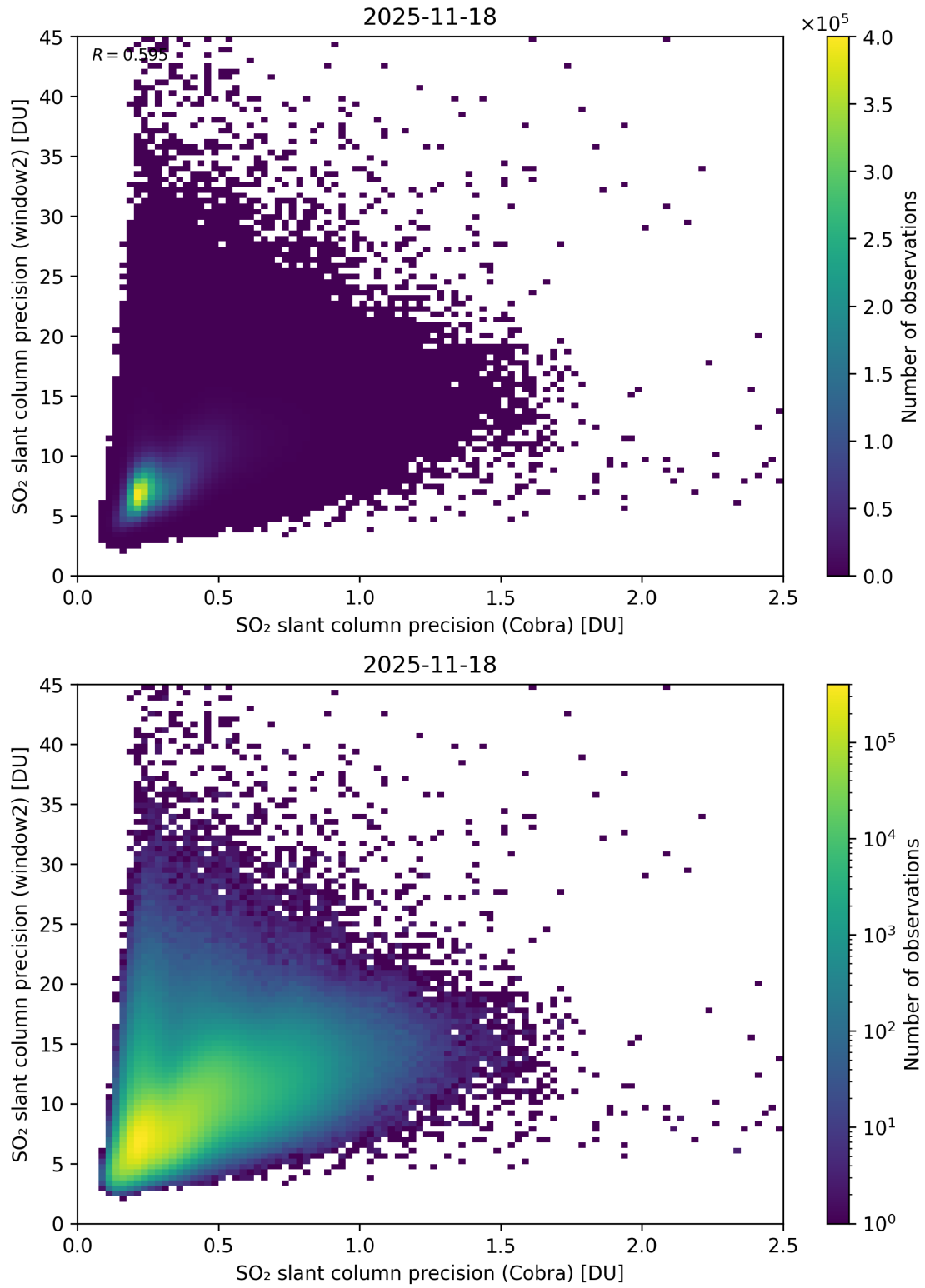
Figure 210: Scatter density plot of “SO 2 slant column precision (Cobra)” against “SO 2 slant column precision (window2)” for 2025-11-18 to 2025-11-19.
