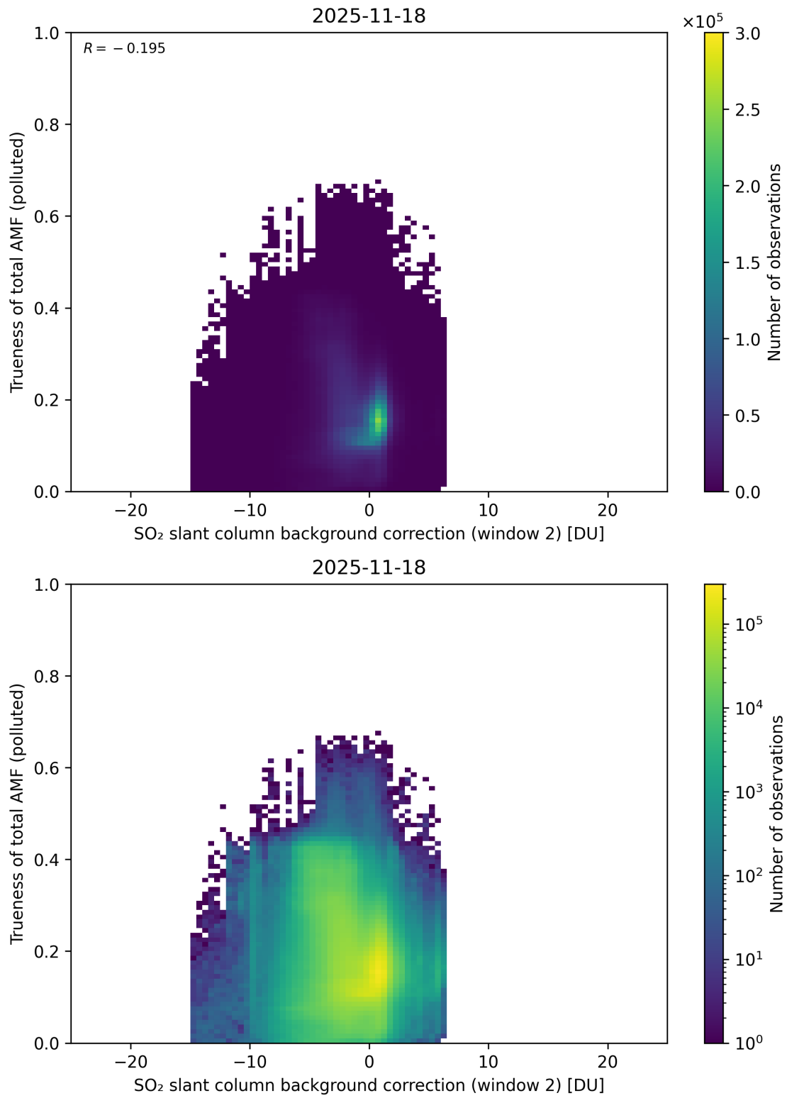
Figure 131: Scatter density plot of “SO 2 slant column background correction (window 2)” against “Trueness of total AMF (polluted)” for 2025-11-18 to 2025-11-19.
