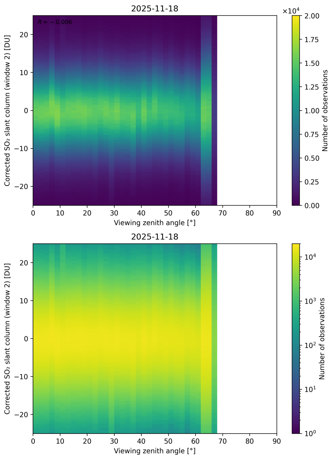
Figure 374: Scatter density plot of “Viewing zenith angle” against “Corrected SO 2 slant column (window 2)” for 2025-11-18 to 2025-11-19.
