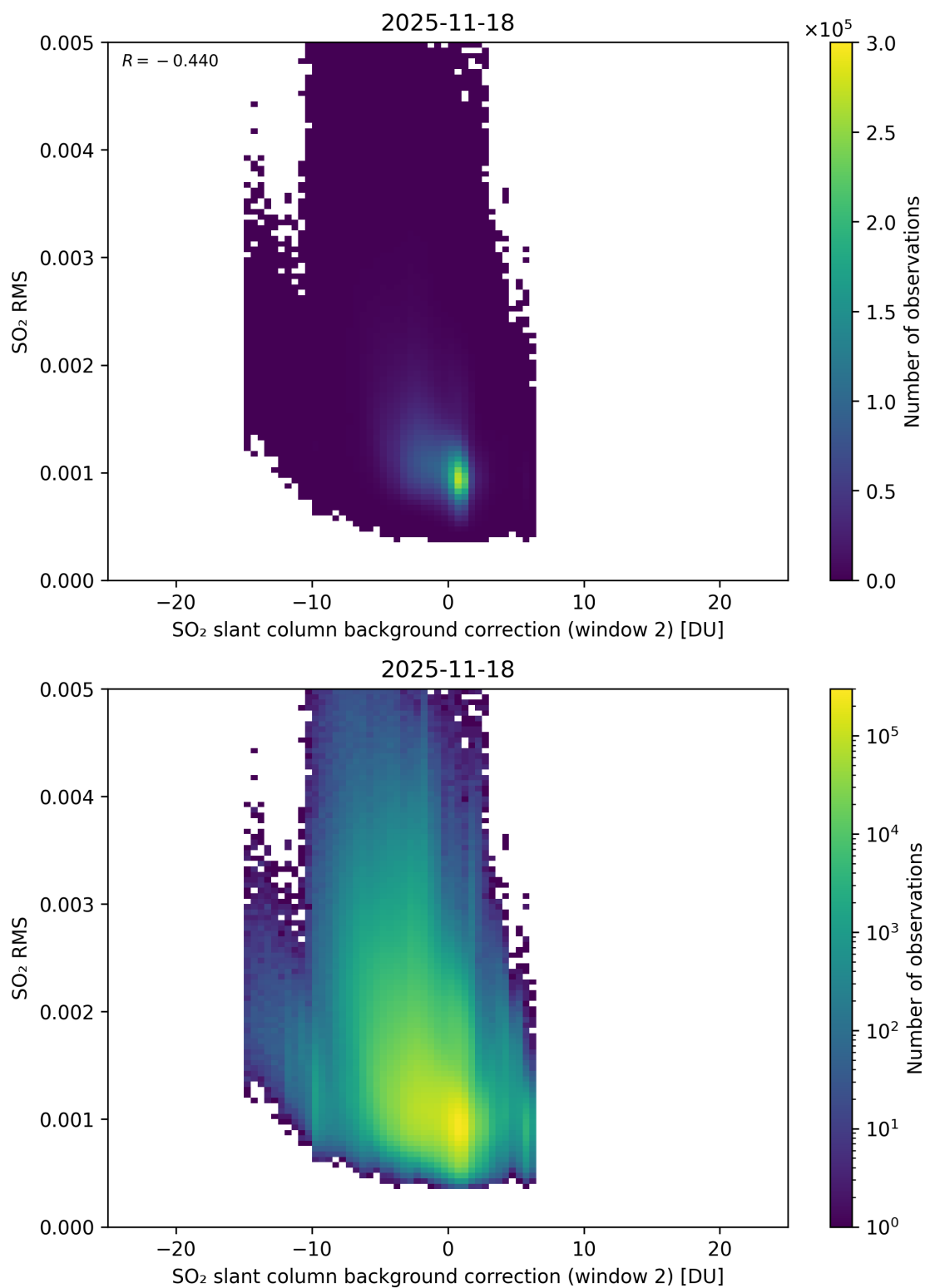
Figure 125: Scatter density plot of “SO 2 slant column background correction (window 2)” against “SO 2 RMS” for 2025-11-18 to 2025-11-19.
