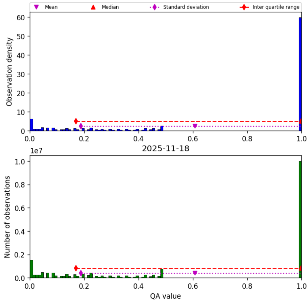
Figure 57: Histogram of “QA value” for 2025-11-18 to 2025-11-19
