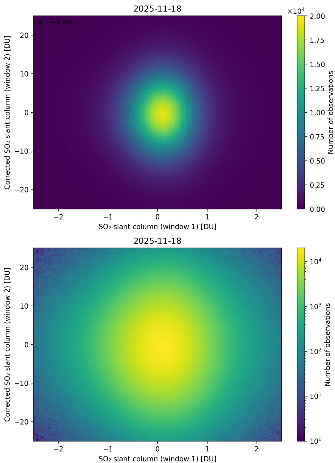
Figure 283: Scatter density plot of “SO 2 slant column (window 1)” against “Corrected SO 2 slant column (window 2)” for 2025-11-18 to 2025-11-19.
