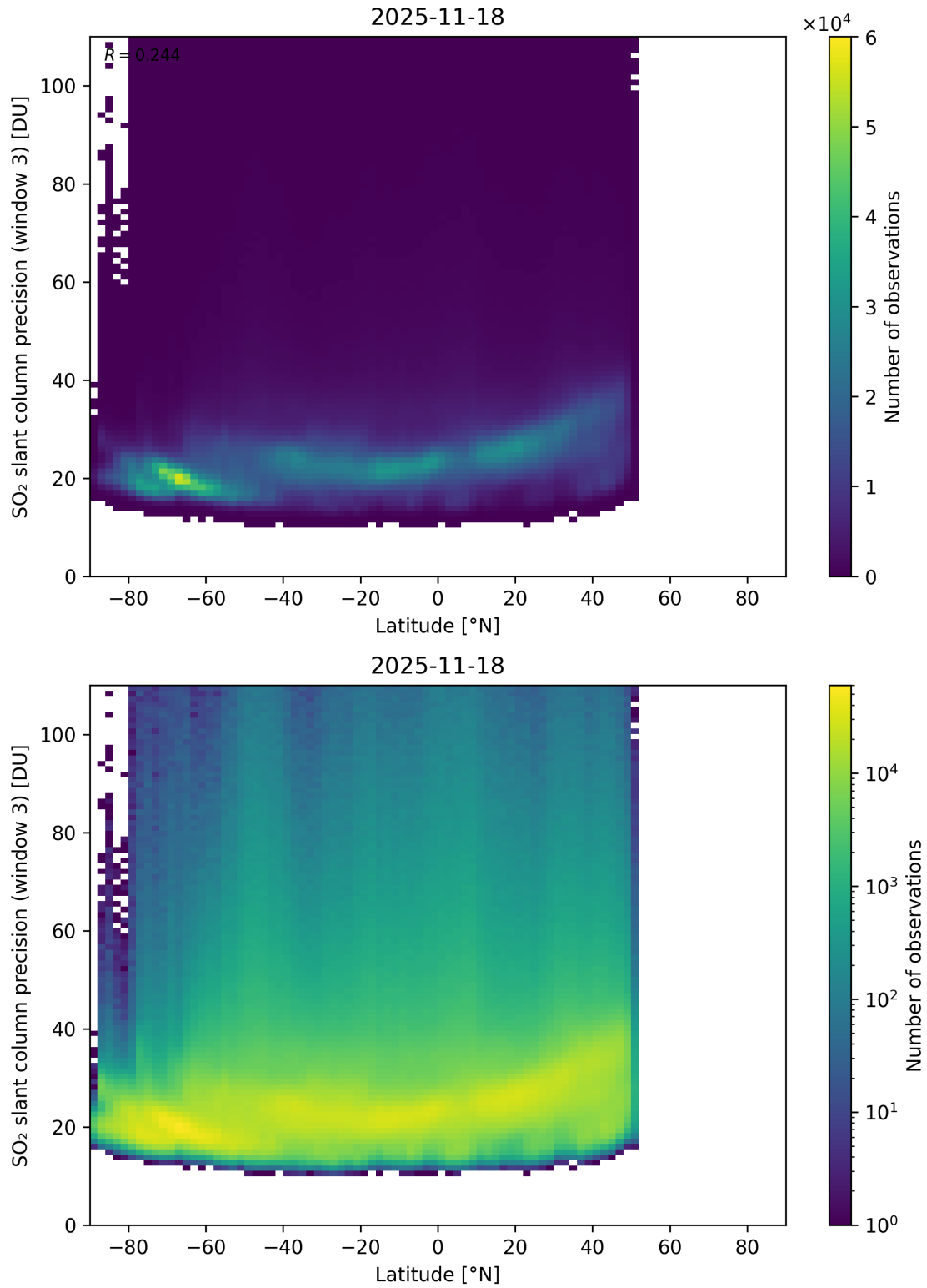
Figure 166: Scatter density plot of “Latitude” against “SO 2 slant column precision (window 3)” for 2025-11-18 to 2025-11-19.
