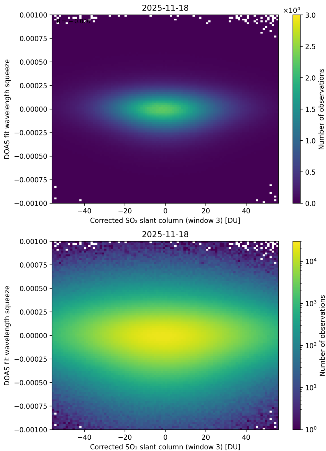
Figure 257: Scatter density plot of “Corrected SO 2 slant column (window 3)” against “DOAS fit wavelength squeeze” for 2025-11-18 to 2025-11-19.
