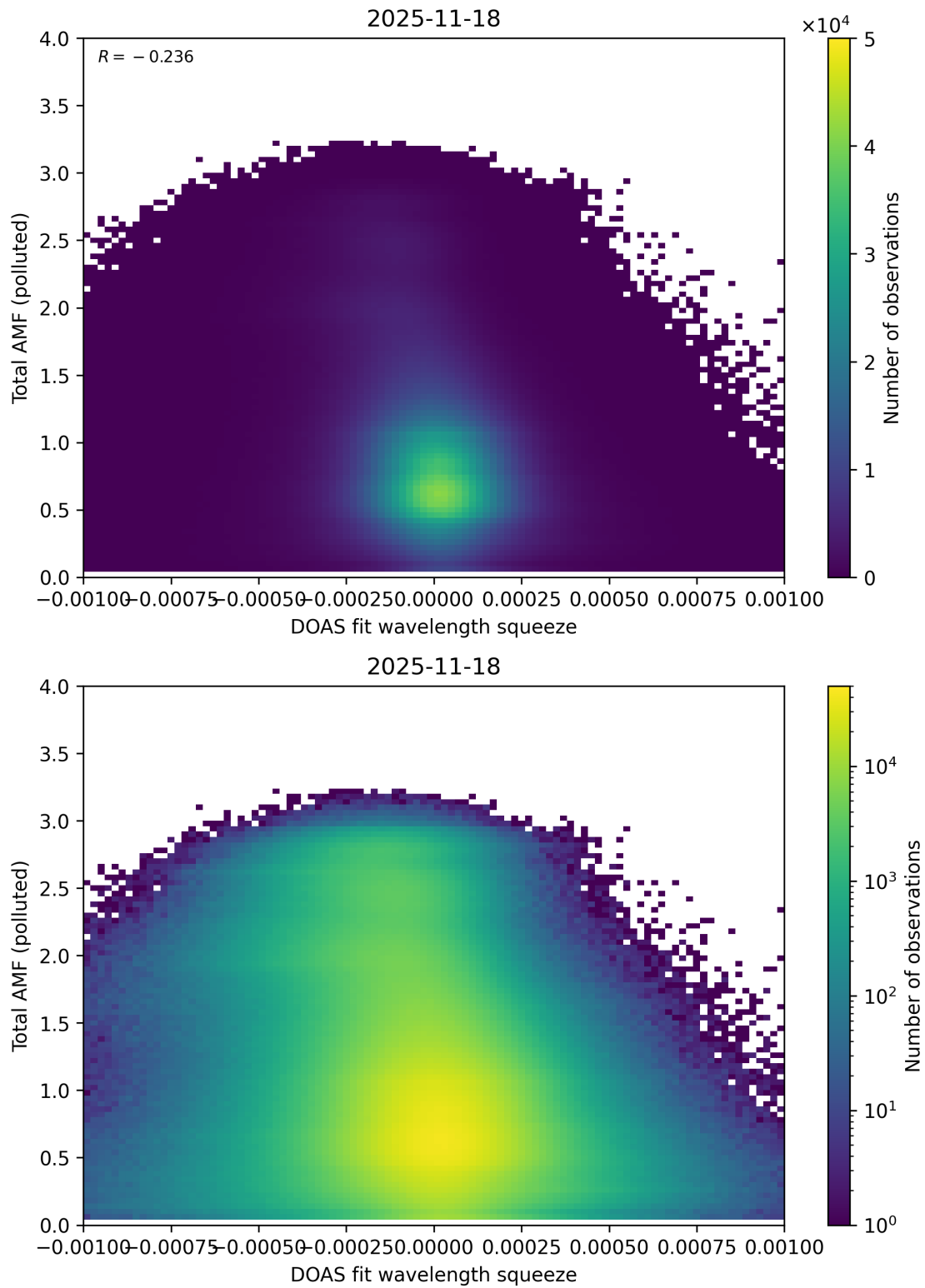
Figure 145: Scatter density plot of “DOAS fit wavelength squeeze” against “Total AMF (polluted)” for 2025-11-18 to 2025-11-19.
