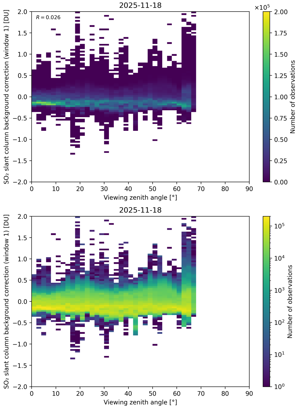
Figure 362: Scatter density plot of “Viewing zenith angle” against “SO 2 slant column background correction (window 1)” for 2025-11-18 to 2025-11-19.
