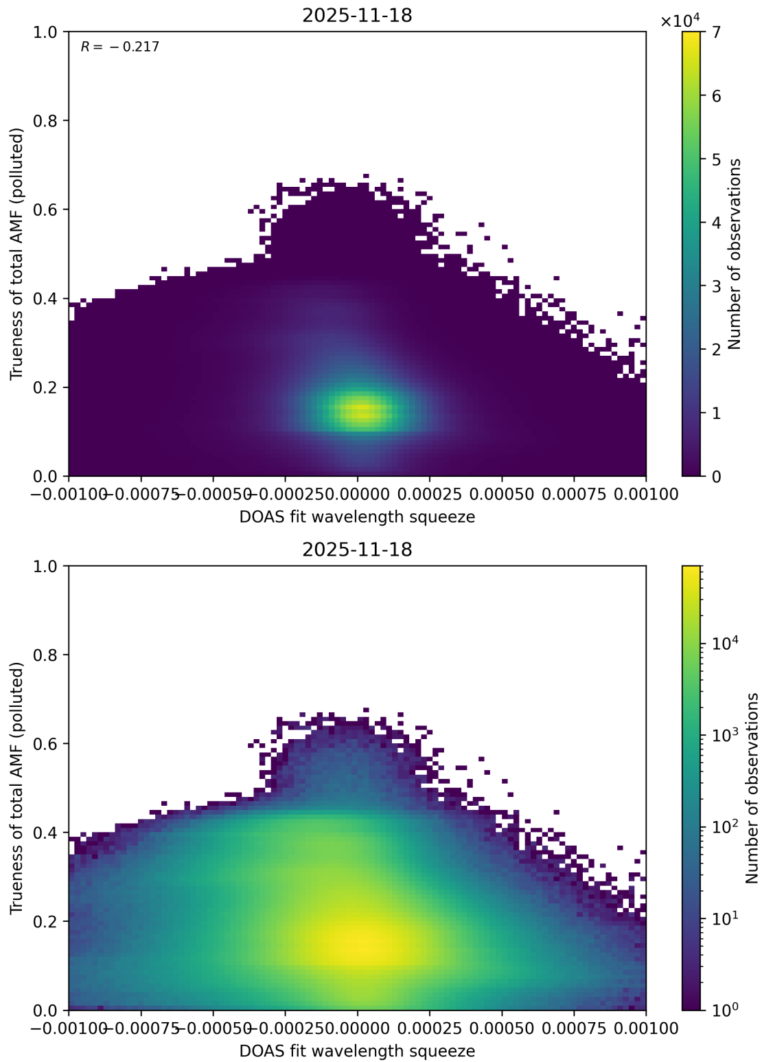
Figure 146: Scatter density plot of “DOAS fit wavelength squeeze” against “Trueness of total AMF (polluted)” for 2025-11-18 to 2025-11-19.
