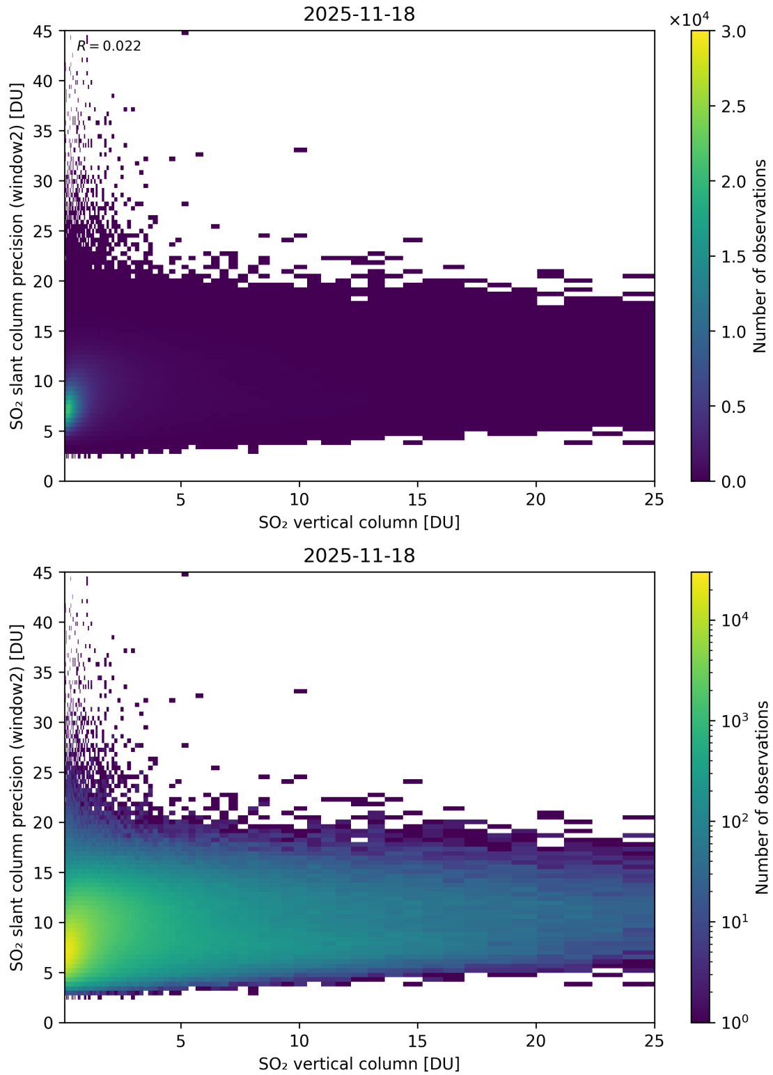
Figure 356: Scatter density plot of “SO 2 vertical column” against “SO 2 slant column precision (window2)” for 2025-11-18 to 2025-11-19.
