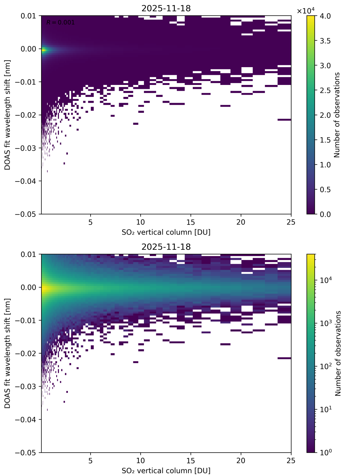
Figure 326: Scatter density plot of “SO 2 vertical column” against “DOAS fit wavelength shift” for 2025-11-18 to 2025-11-19.
