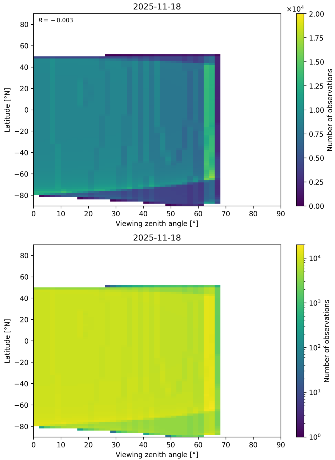
Figure 368: Scatter density plot of “Viewing zenith angle” against “Latitude” for 2025-11-18 to 2025-11-19.
