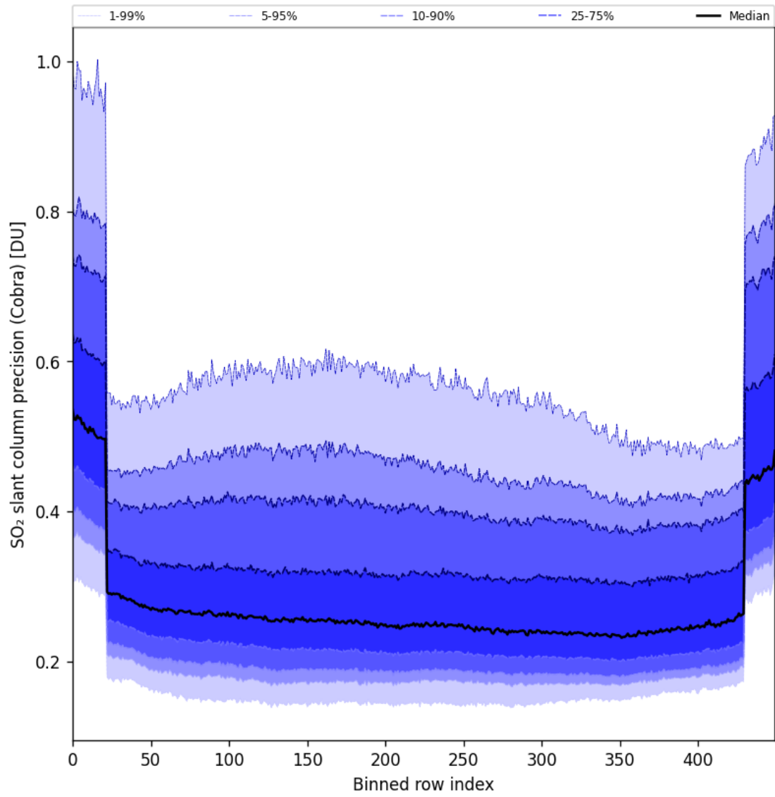
Figure 88: Along track statistics of “SO 2 slant column precision (Cobra)” for 2025-11-18 to 2025-11-19
