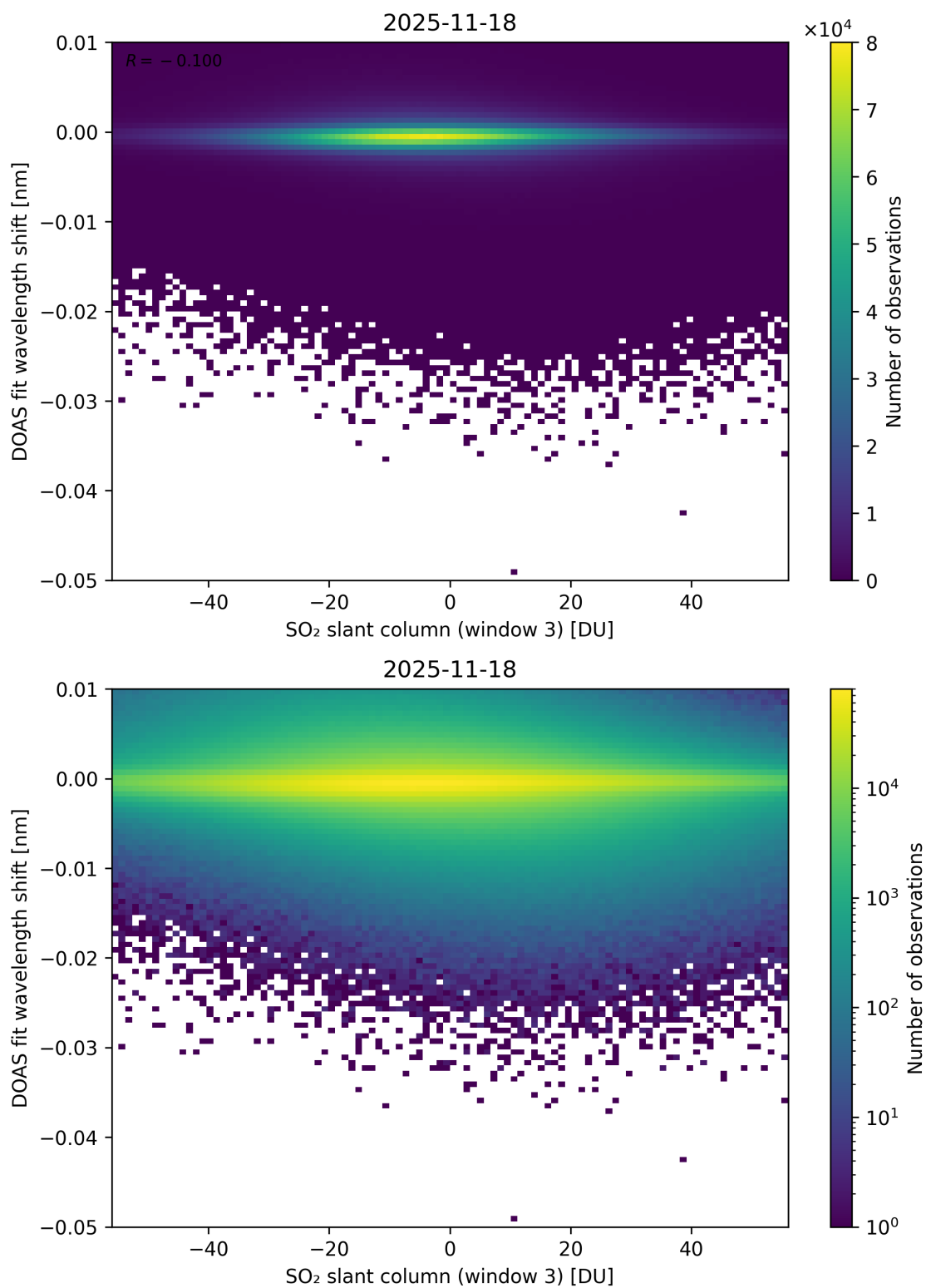
Figure 304: Scatter density plot of “SO 2 slant column (window 3)” against “DOAS fit wavelength shift” for 2025-11-18 to 2025-11-19.
