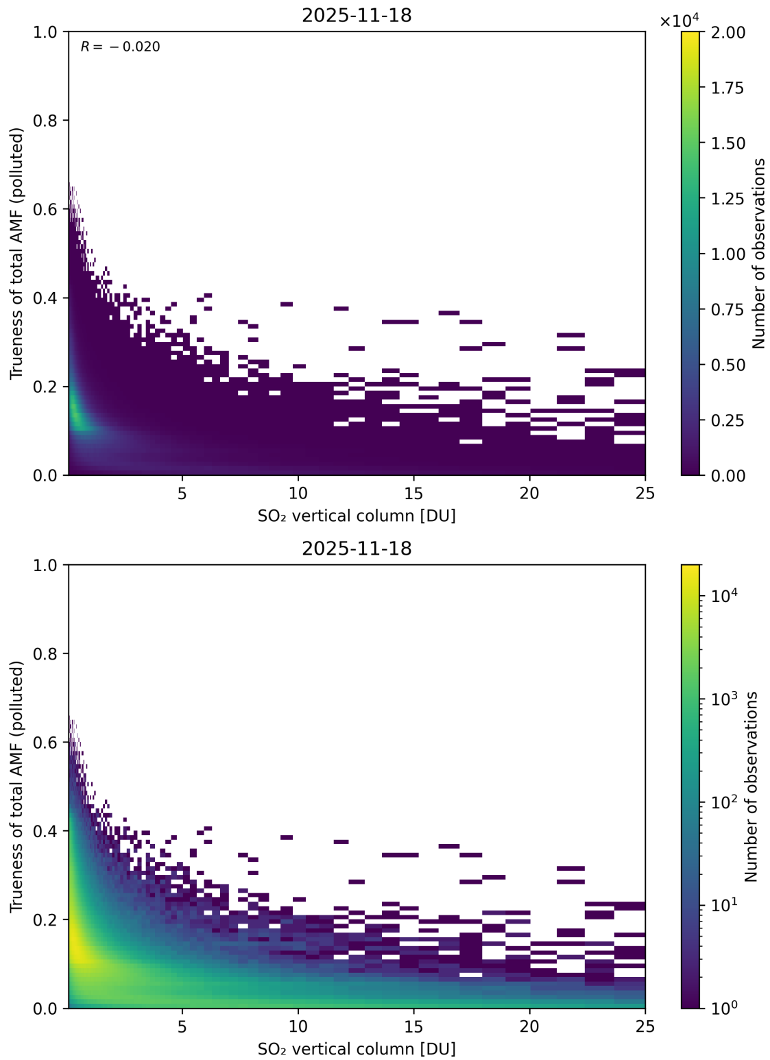
Figure 360: Scatter density plot of “SO 2 vertical column” against “Trueness of total AMF (polluted)” for 2025-11-18 to 2025-11-19.
