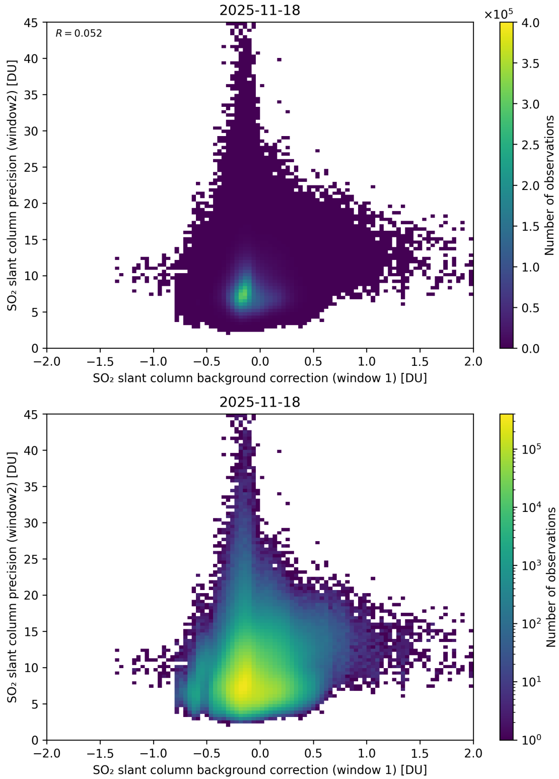
Figure 117: Scatter density plot of “SO 2 slant column background correction (window 1)” against “SO 2 slant column precision (window2)” for 2025-11-18 to 2025-11-19.
