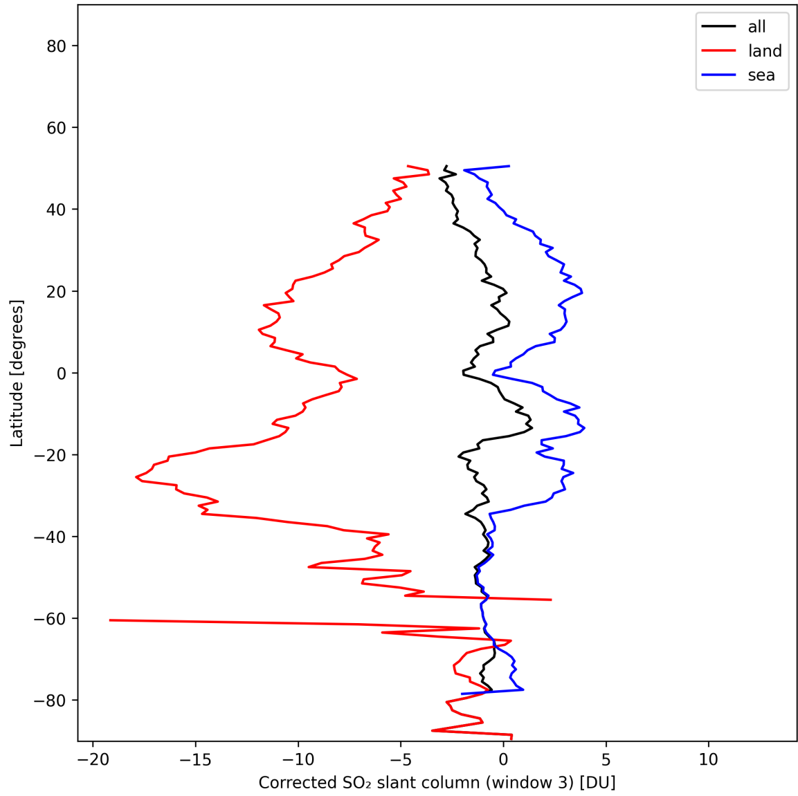
Figure 47: Zonal average of “Corrected SO 2 slant column (window 3)” for 2025-11-18 to 2025-11-19.
