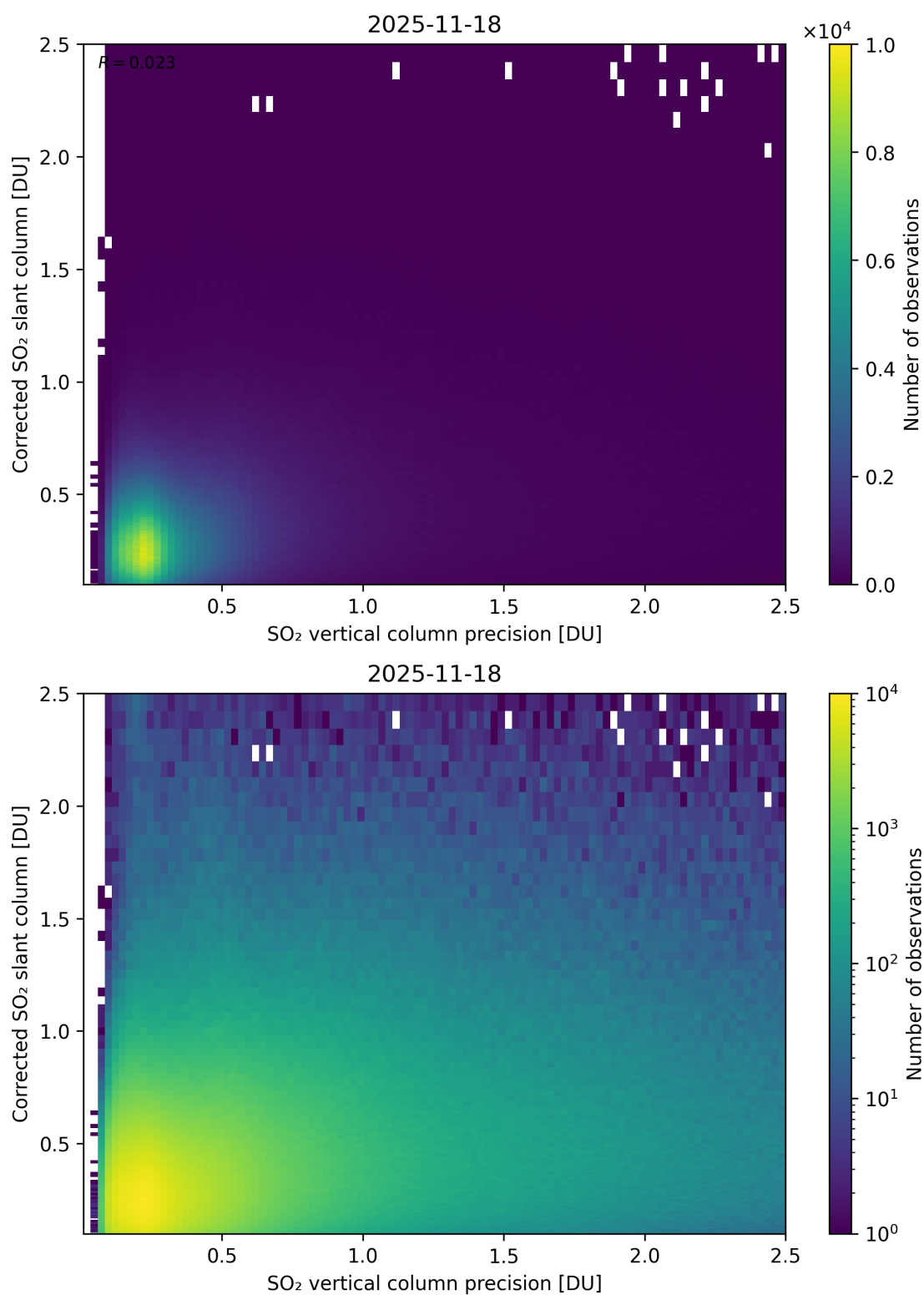
Figure 338: Scatter density plot of “SO 2 vertical column precision” against “Corrected SO 2 slant column” for 2025-11-18 to 2025-11-19.
