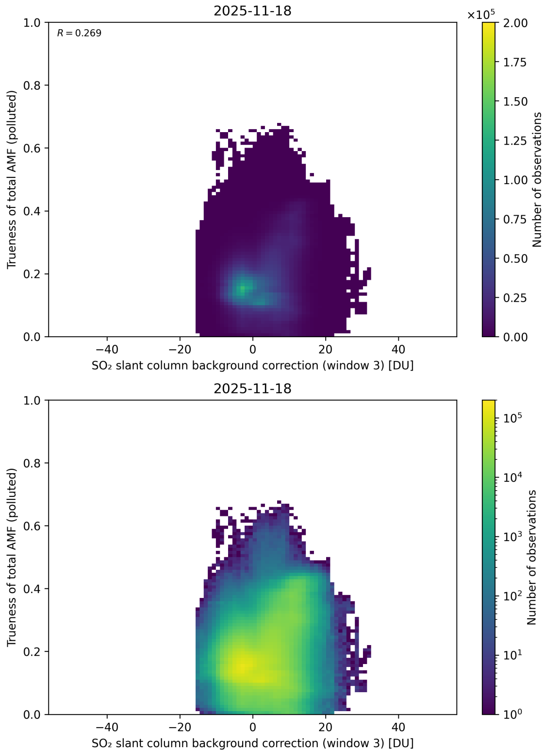
Figure 137: Scatter density plot of “SO 2 slant column background correction (window 3)” against “Trueness of total AMF (polluted)” for 2025-11-18 to 2025-11-19.
