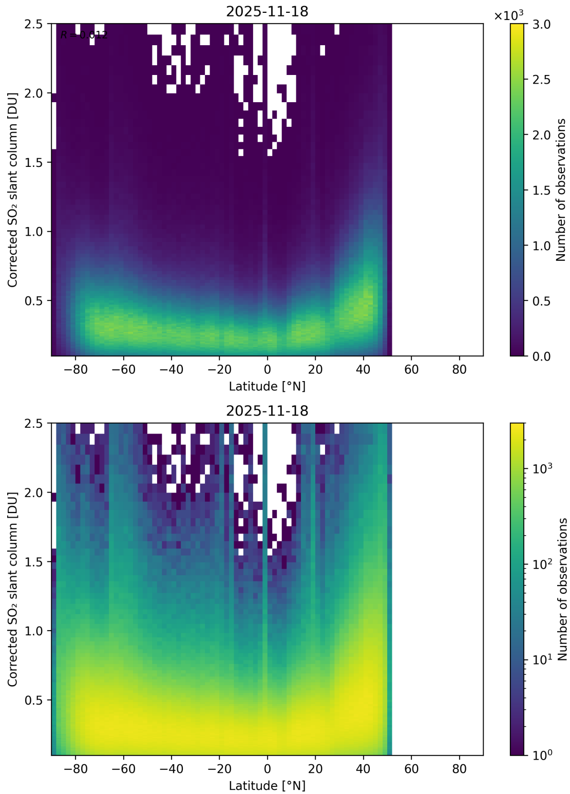
Figure 159: Scatter density plot of “Latitude” against “Corrected SO 2 slant column” for 2025-11-18 to 2025-11-19.
