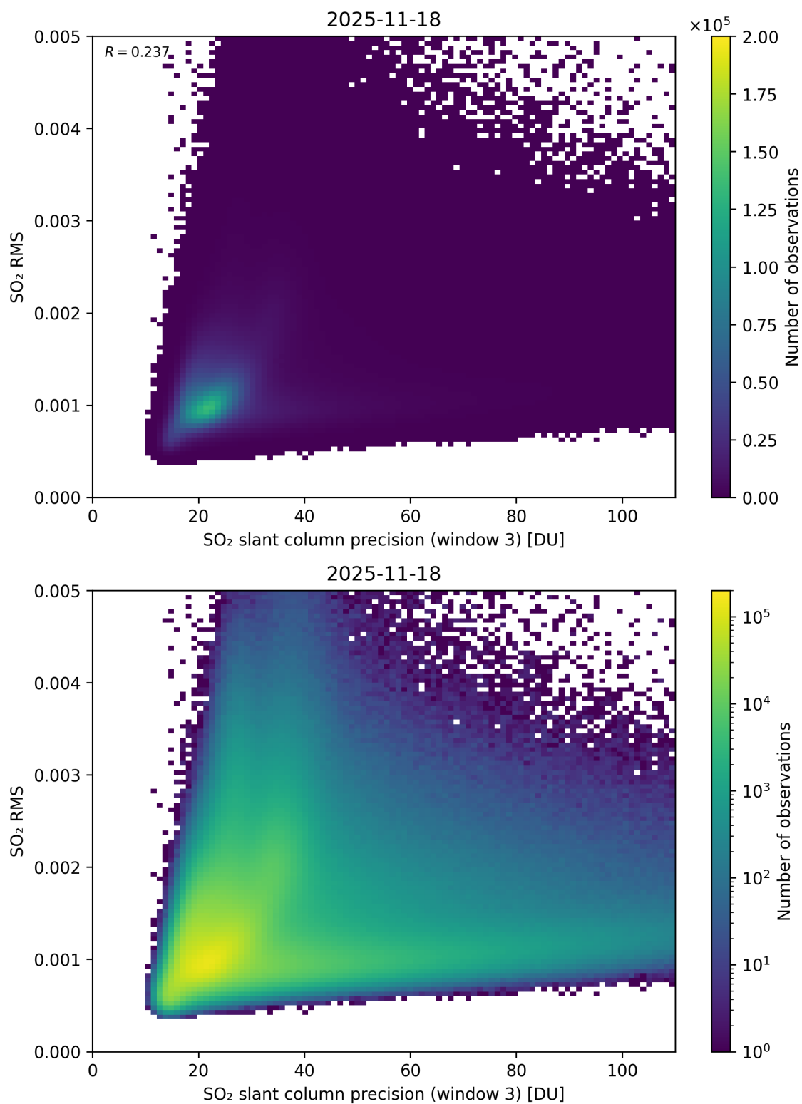
Figure 310: Scatter density plot of “SO 2 slant column precision (window 3)” against “SO 2 RMS” for 2025-11-18 to 2025-11-19.
