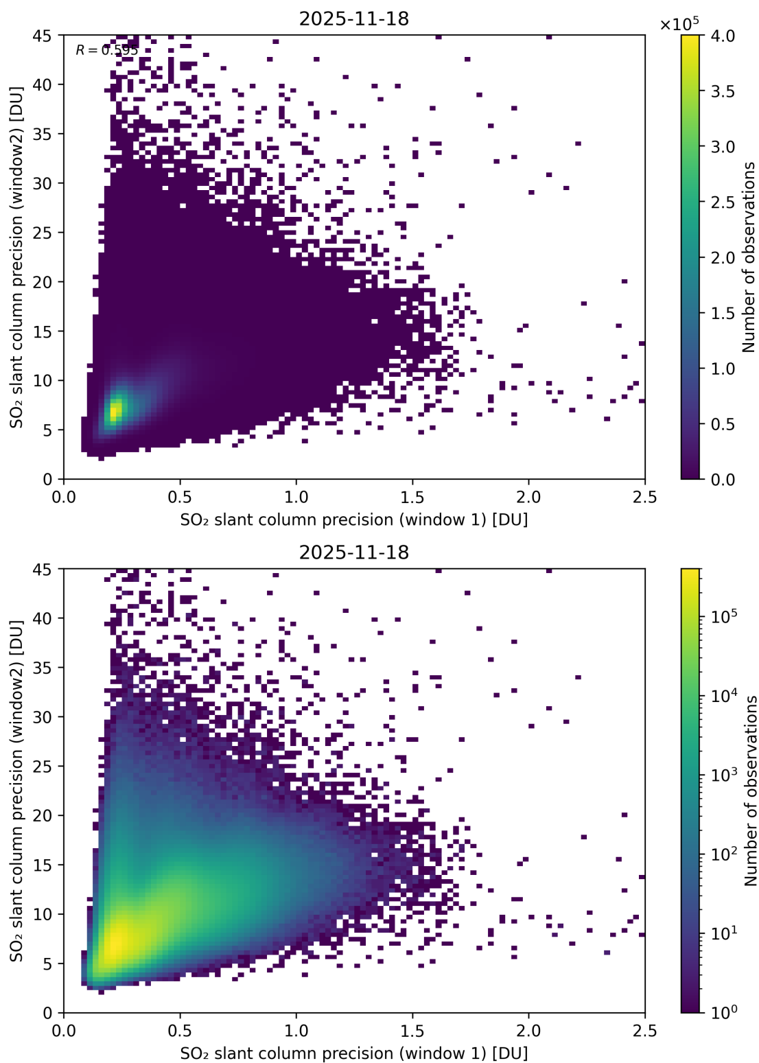
Figure 277: Scatter density plot of “SO 2 slant column precision (window 1)” against “SO 2 slant column precision (window2)” for 2025-11-18 to 2025-11-19.
