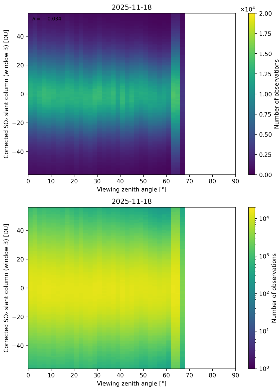
Figure 375: Scatter density plot of “Viewing zenith angle” against “Corrected SO 2 slant column (window 3)” for 2025-11-18 to 2025-11-19.
