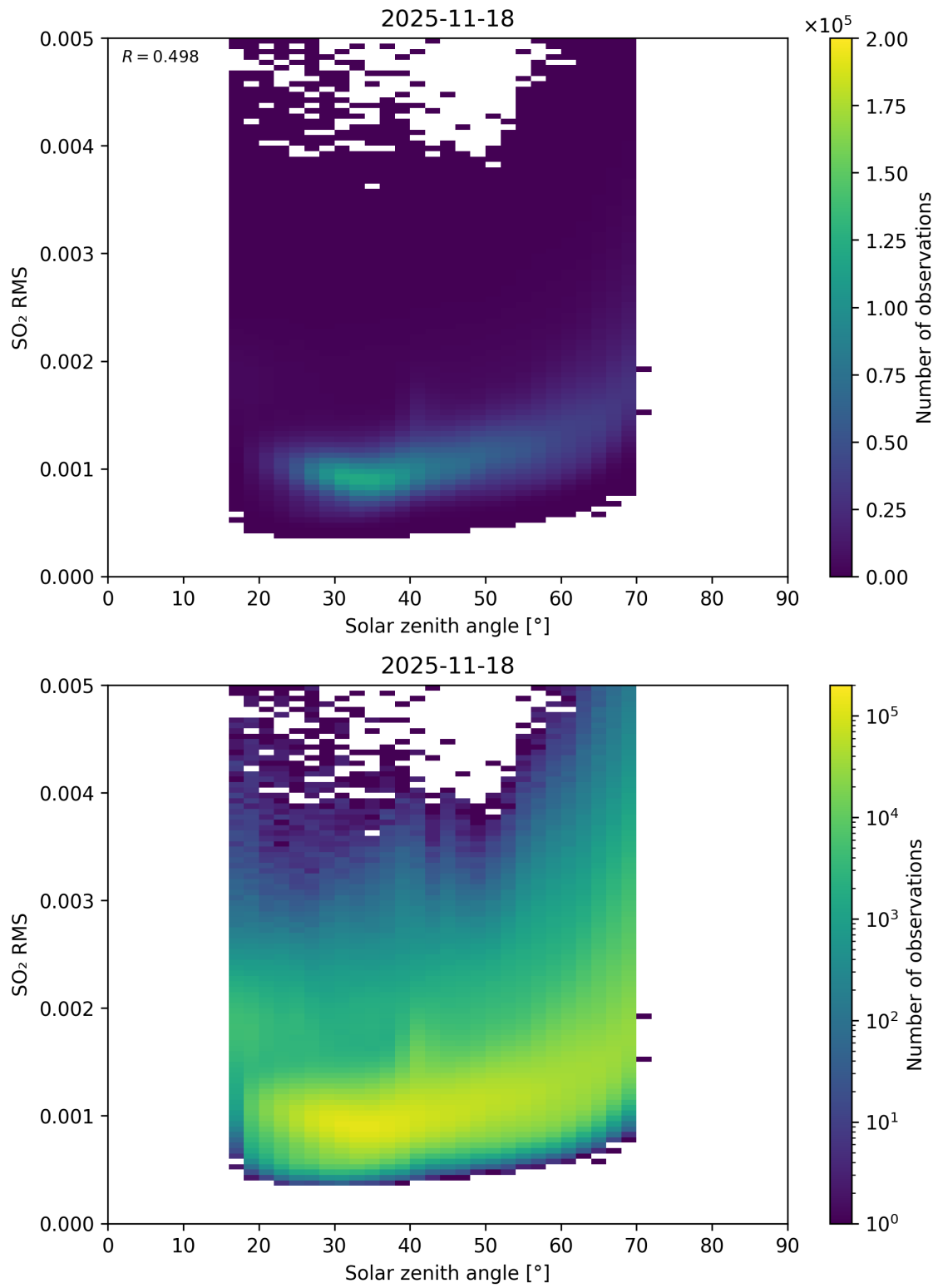
Figure 176: Scatter density plot of “Solar zenith angle” against “SO 2 RMS” for 2025-11-18 to 2025-11-19.
