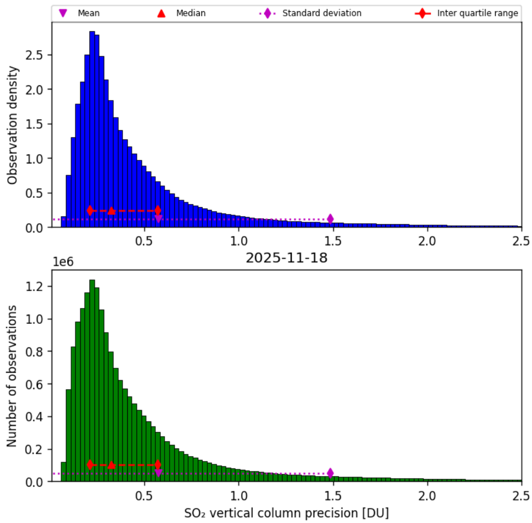
Figure 59: Histogram of “SO 2 vertical column precision” for 2025-11-18 to 2025-11-19
