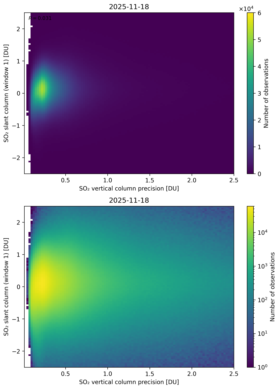
Figure 341: Scatter density plot of “SO 2 vertical column precision” against “SO 2 slant column (window 1)” for 2025-11-18 to 2025-11-19.
