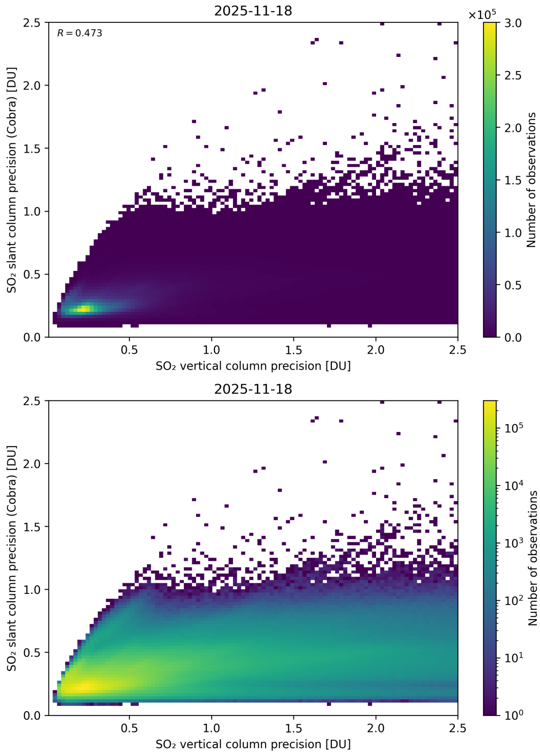
Figure 337: Scatter density plot of “SO 2 vertical column precision” against “SO 2 slant column precision (Cobra)” for 2025-11-18 to 2025-11-19.
