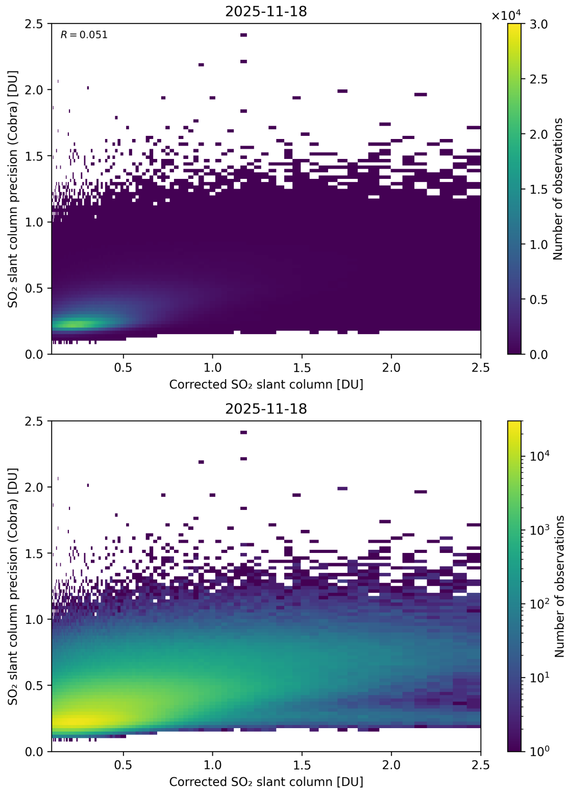
Figure 234: Scatter density plot of “Corrected SO 2 slant column” against “SO 2 slant column precision (Cobra)” for 2025-11-18 to 2025-11-19.
