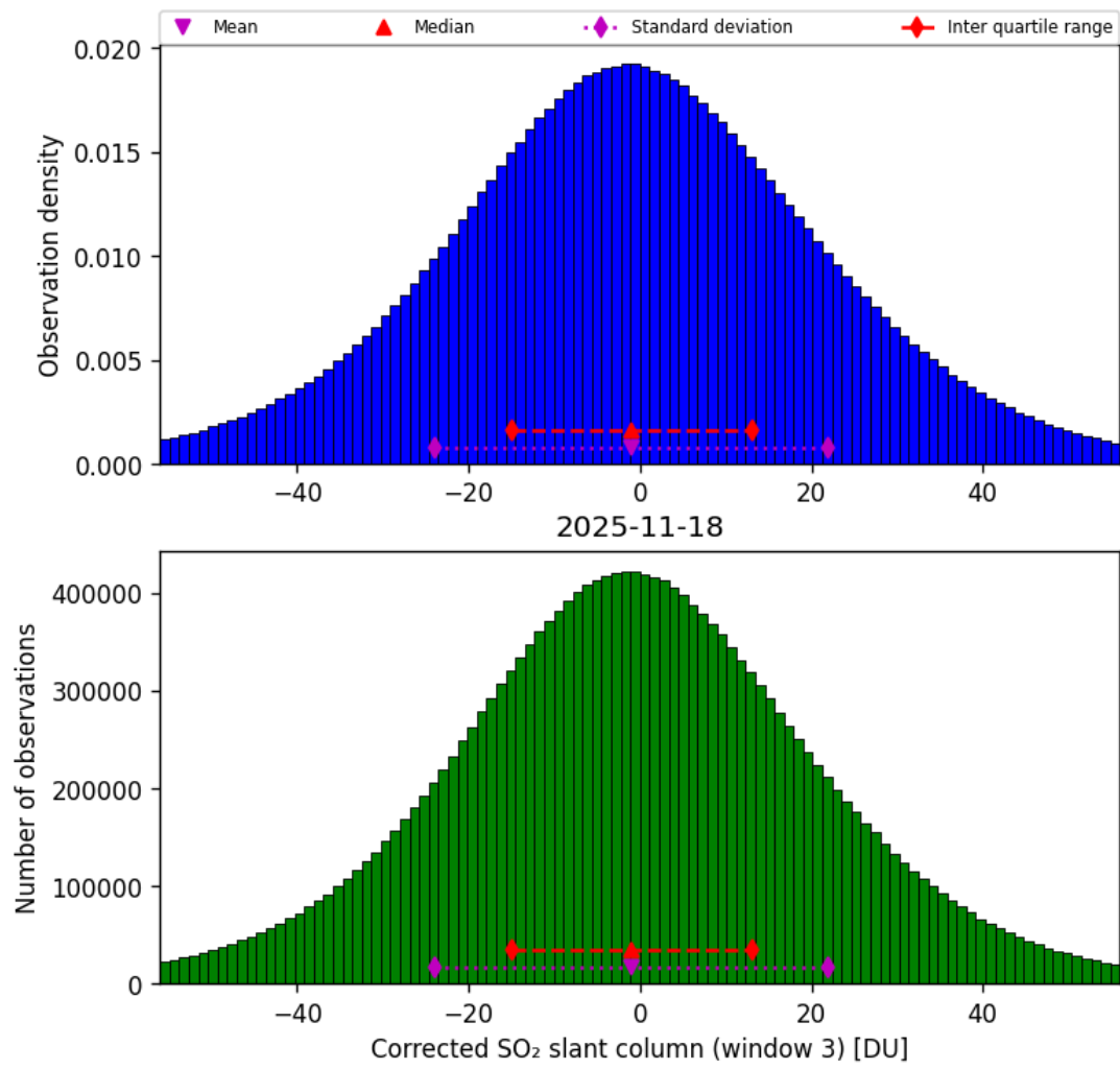
Figure 73: Histogram of “Corrected SO 2 slant column (window 3)” for 2025-11-18 to 2025-11-19
