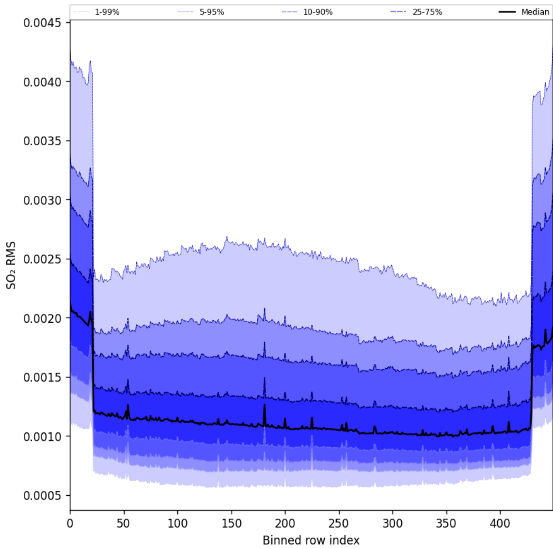
Figure 104: Along track statistics of “SO 2 RMS” for 2025-11-18 to 2025-11-19
