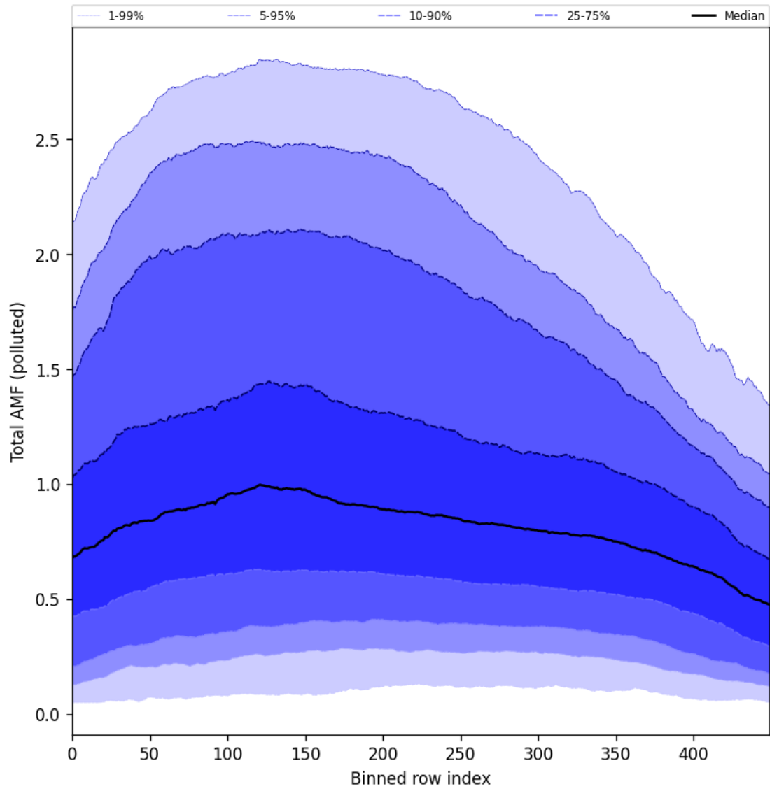
Figure 105: Along track statistics of “Total AMF (polluted)” for 2025-11-18 to 2025-11-19
