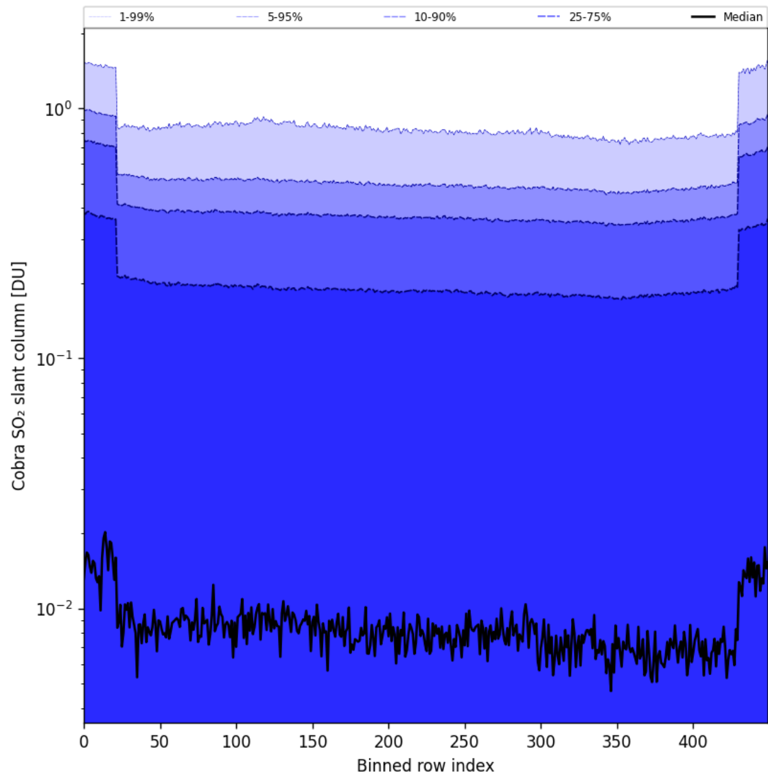
Figure 87: Along track statistics of “Cobra SO 2 slant column” for 2025-11-18 to 2025-11-19
