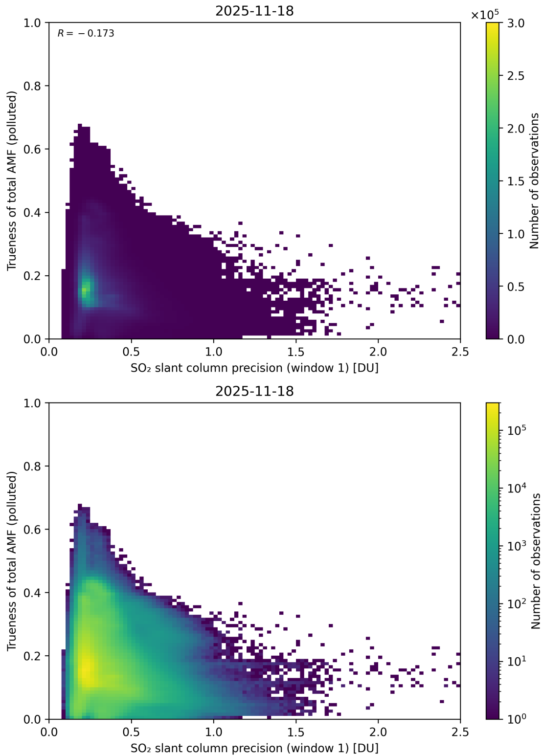
Figure 281: Scatter density plot of “SO 2 slant column precision (window 1)” against “Trueness of total AMF (polluted)” for 2025-11-18 to 2025-11-19.
