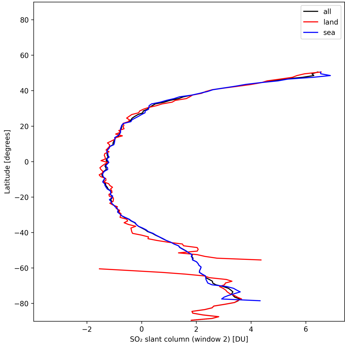
Figure 41: Zonal average of “SO 2 slant column (window 2)” for 2025-11-18 to 2025-11-19.
