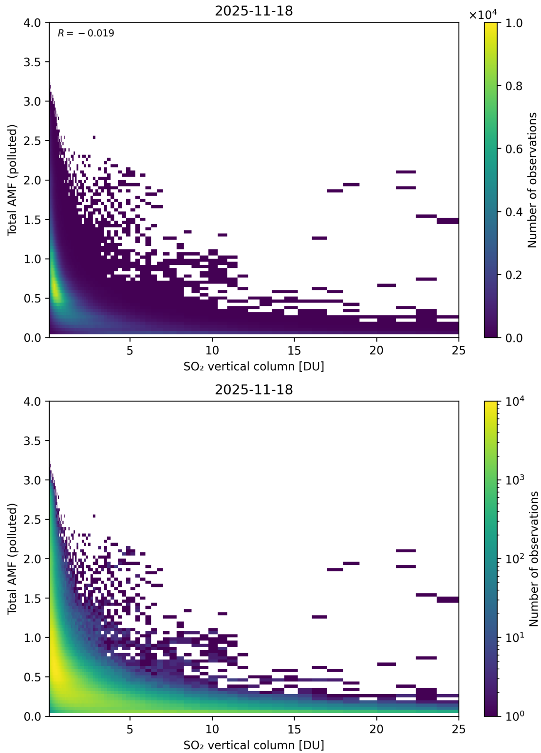
Figure 359: Scatter density plot of “SO 2 vertical column” against “Total AMF (polluted)” for 2025-11-18 to 2025-11-19.
