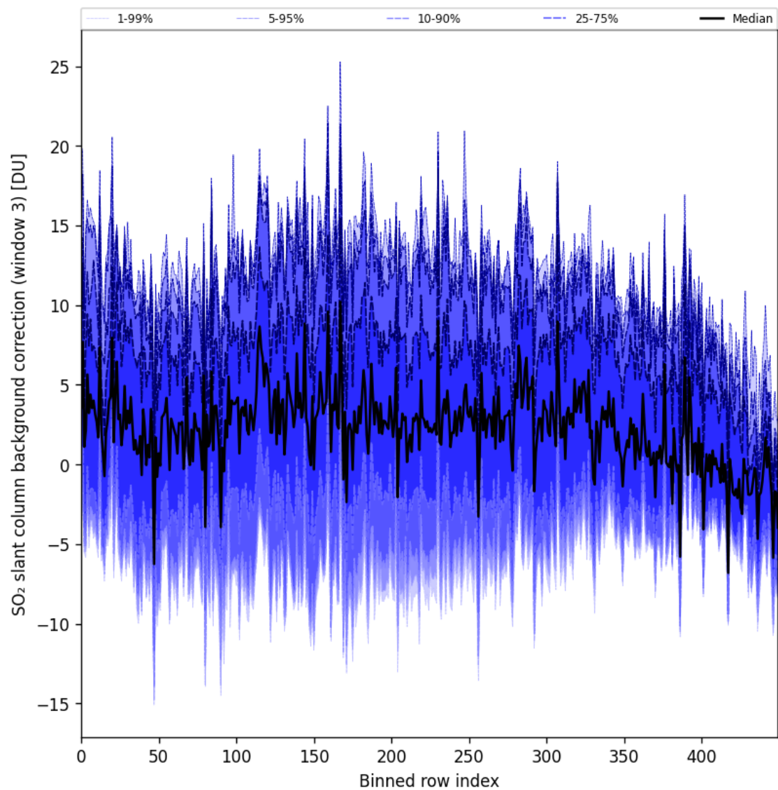
Figure 100: Along track statistics of “SO 2 slant column background correction (window 3)” for 2025-11-18 to 2025-11-19
