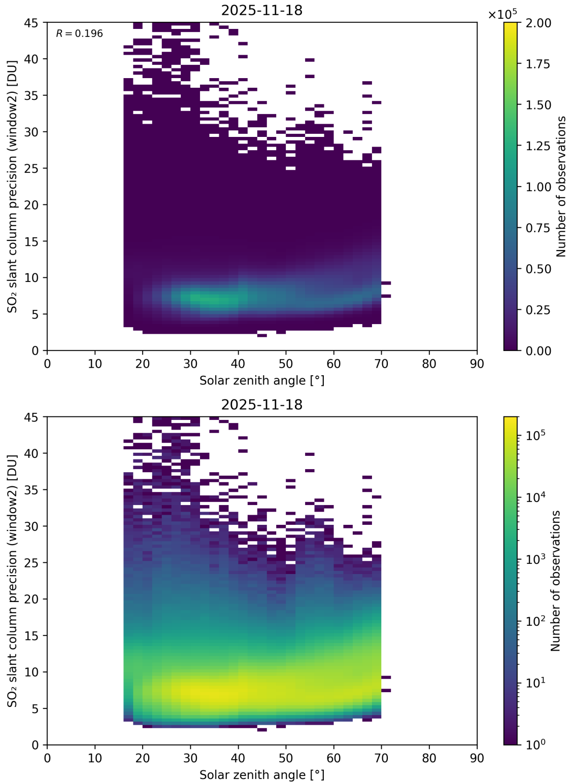
Figure 186: Scatter density plot of “Solar zenith angle” against “SO 2 slant column precision (window2)” for 2025-11-18 to 2025-11-19.
