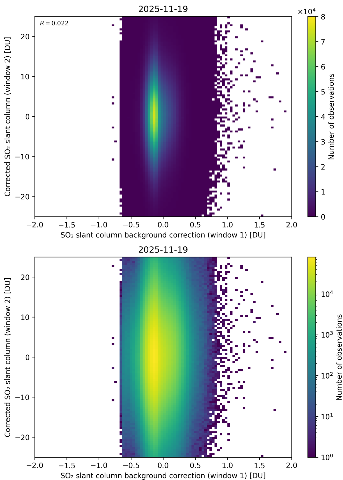
Figure 115: Scatter density plot of “SO 2 slant column background correction (window 1)” against “Corrected SO 2 slant column (window 2)” for 2025-11-18 to 2025-11-20.
