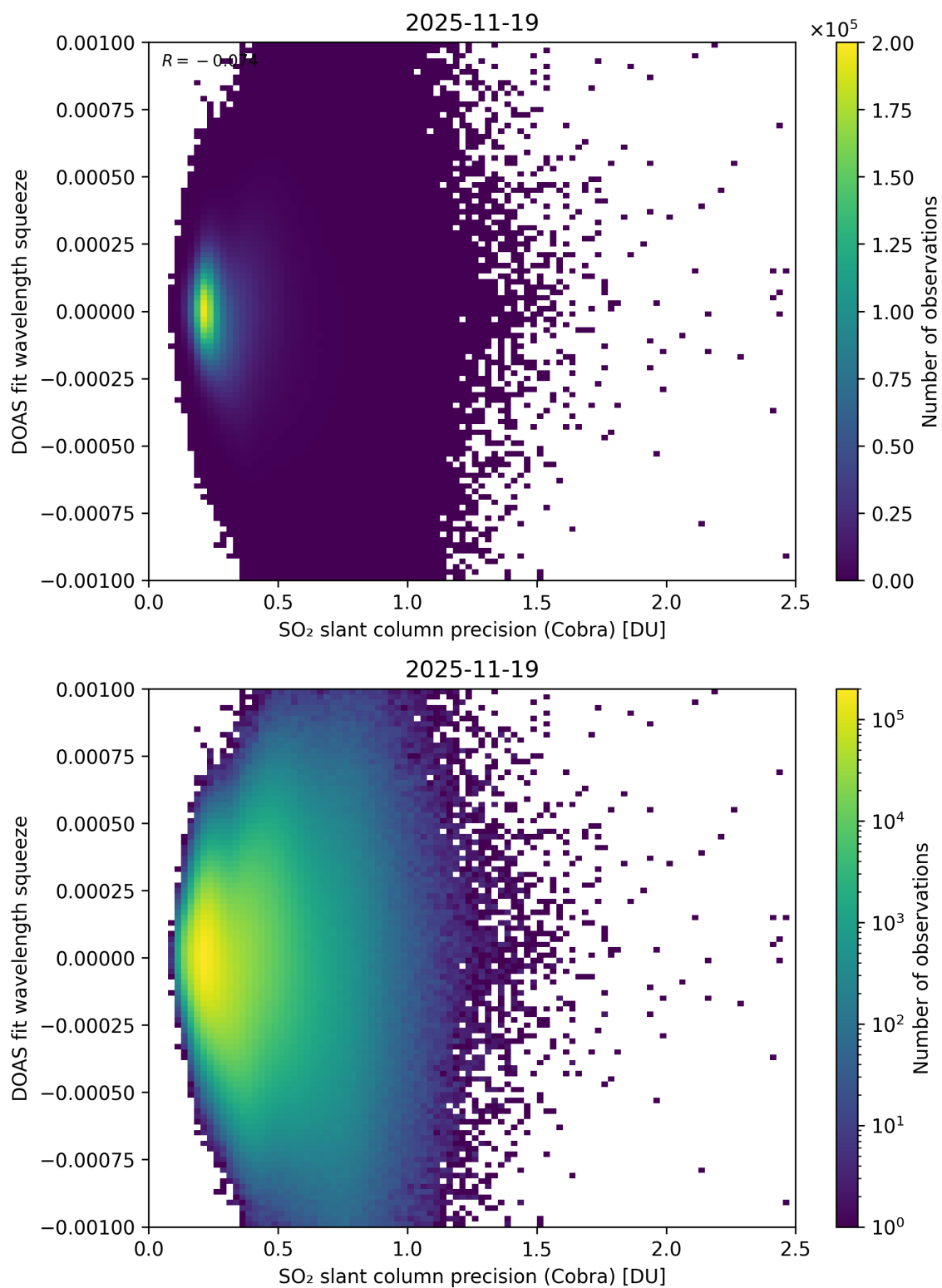
Figure 203: Scatter density plot of “SO 2 slant column precision (Cobra)” against “DOAS fit wavelength squeeze” for 2025-11-18 to 2025-11-20.
