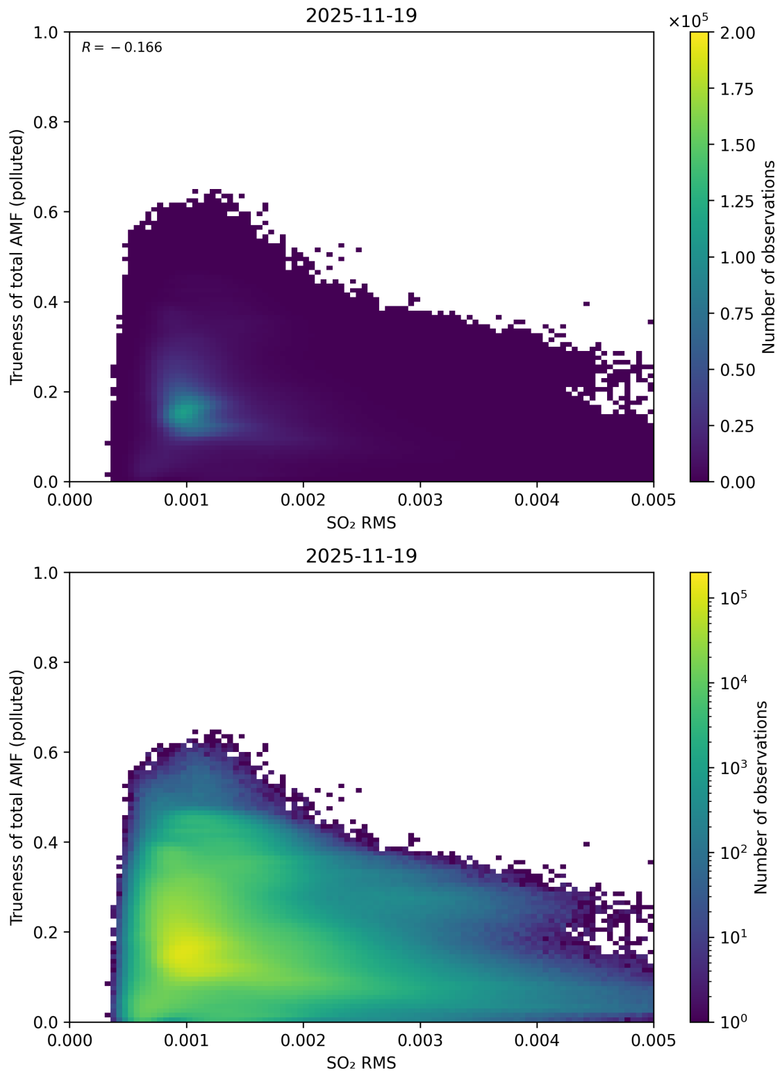
Figure 149: Scatter density plot of “SO 2 RMS” against “Trueness of total AMF (polluted)” for 2025-11-18 to 2025-11-20.
