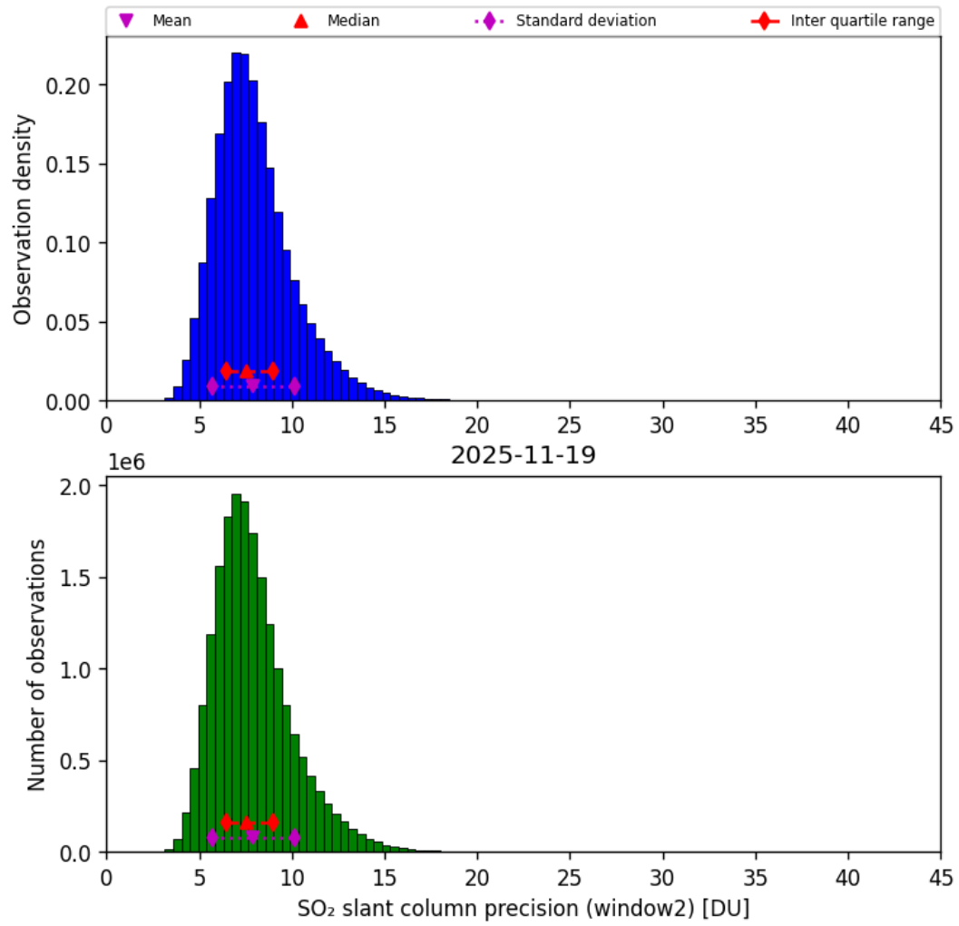
Figure 68: Histogram of “SO 2 slant column precision (window2)” for 2025-11-18 to 2025-11-20
