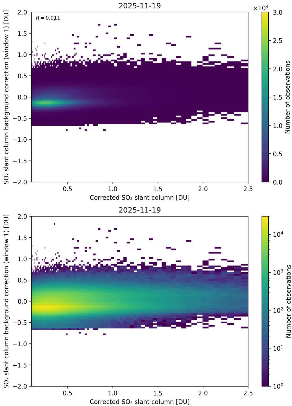
Figure 226: Scatter density plot of “Corrected SO 2 slant column” against “SO 2 slant column background correction (window 1)” for 2025-11-18 to 2025-11-20.
