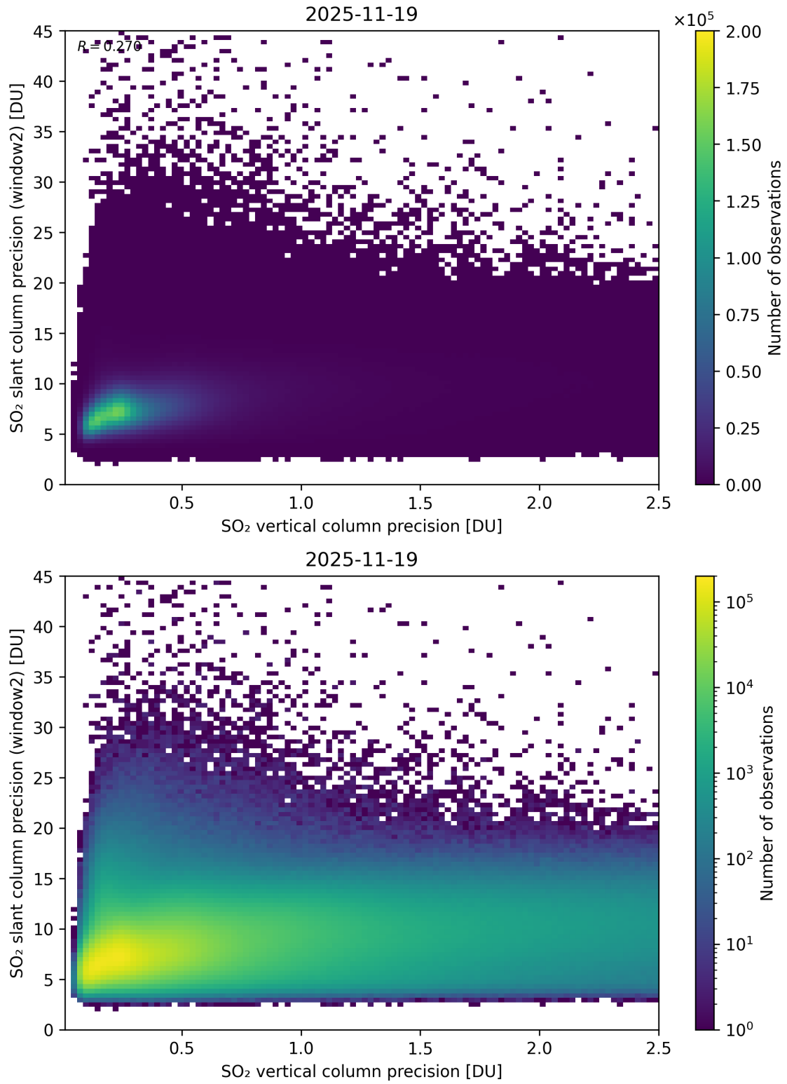
Figure 343: Scatter density plot of “SO 2 vertical column precision” against “SO 2 slant column precision (window2)” for 2025-11-18 to 2025-11-20.
