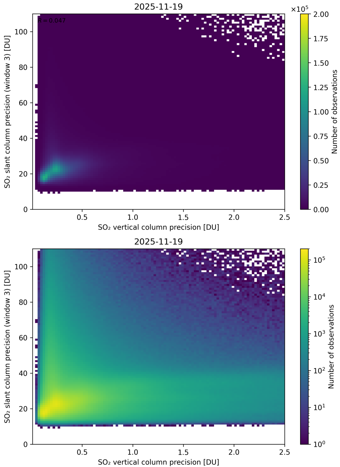
Figure 345: Scatter density plot of “SO 2 vertical column precision” against “SO 2 slant column precision (window 3)” for 2025-11-18 to 2025-11-20.
