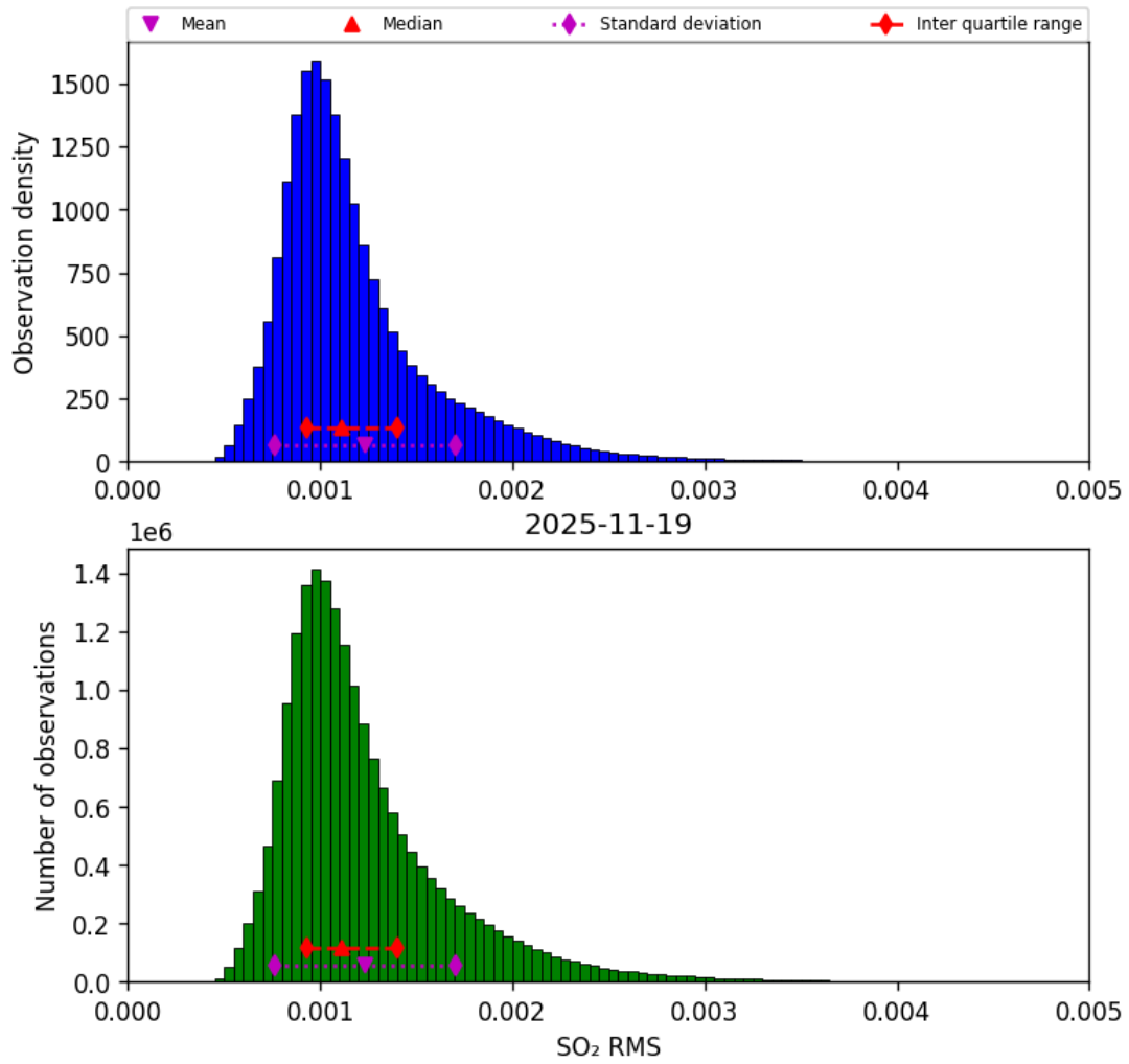
Figure 78: Histogram of “SO 2 RMS” for 2025-11-18 to 2025-11-20
