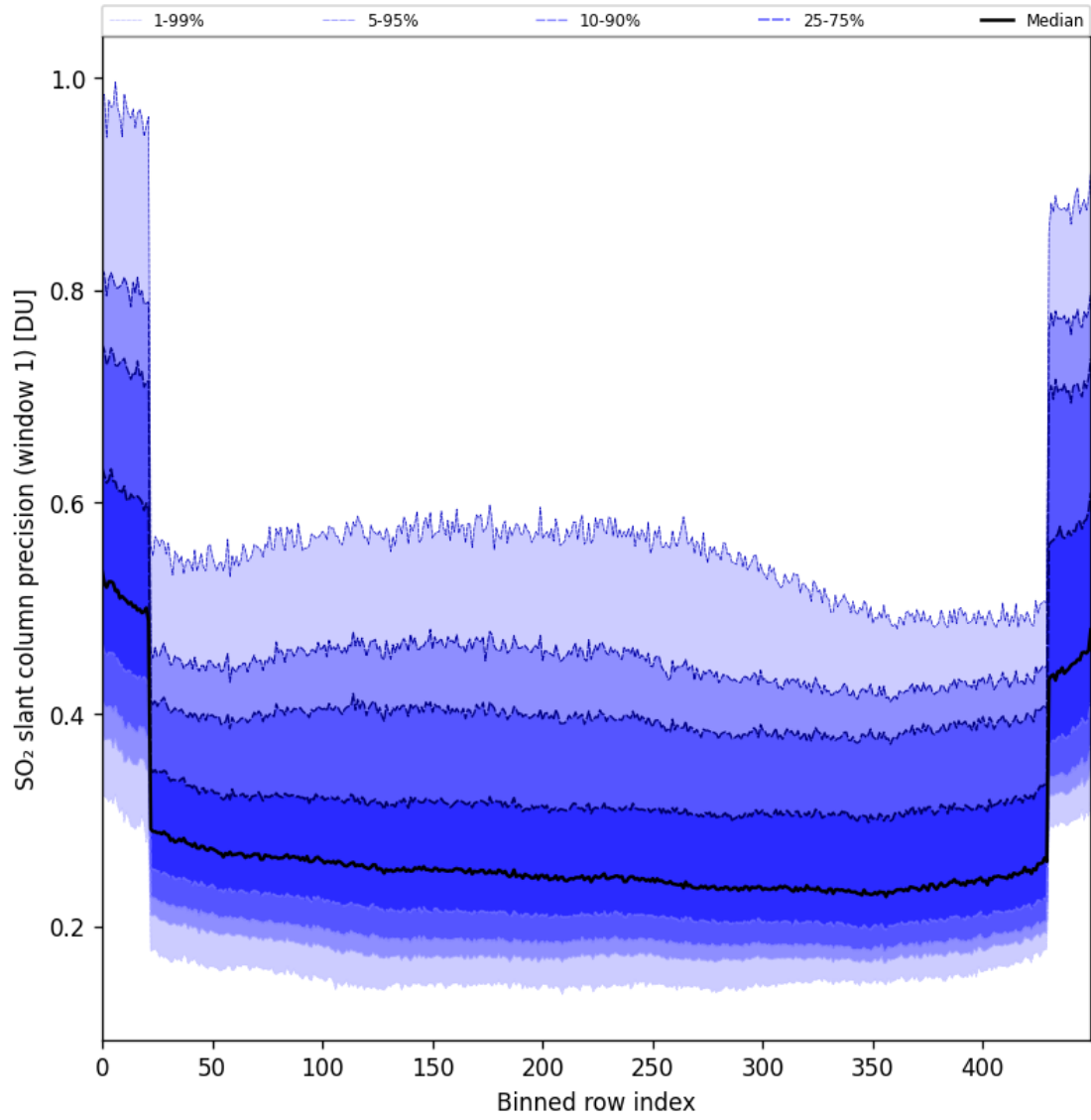
Figure 90: Along track statistics of “SO 2 slant column precision (window 1)” for 2025-11-18 to 2025-11-20
