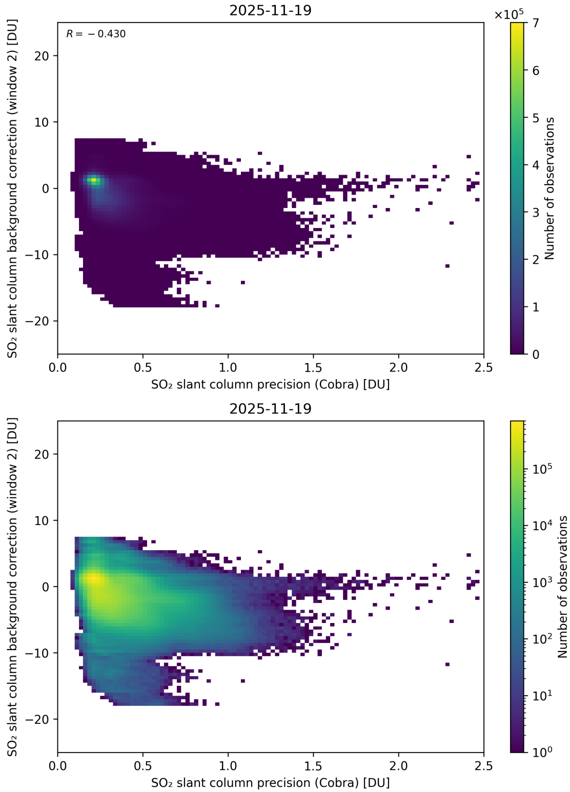
Figure 200: Scatter density plot of “SO 2 slant column precision (Cobra)” against “SO 2 slant column background correction (window 2)” for 2025-11-18 to 2025-11-20.
