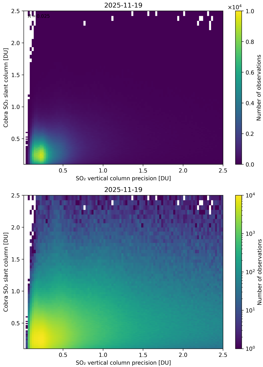
Figure 336: Scatter density plot of “SO 2 vertical column precision” against “Cobra SO 2 slant column” for 2025-11-18 to 2025-11-20.
