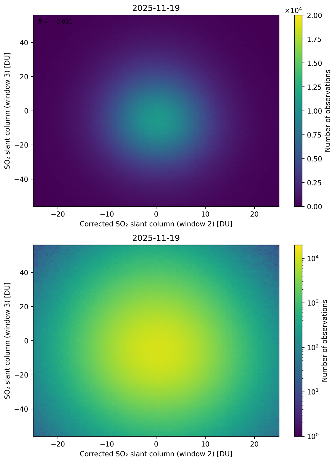
Figure 251: Scatter density plot of “Corrected SO 2 slant column (window 2)” against “SO 2 slant column (window 3)” for 2025-11-18 to 2025-11-20.
