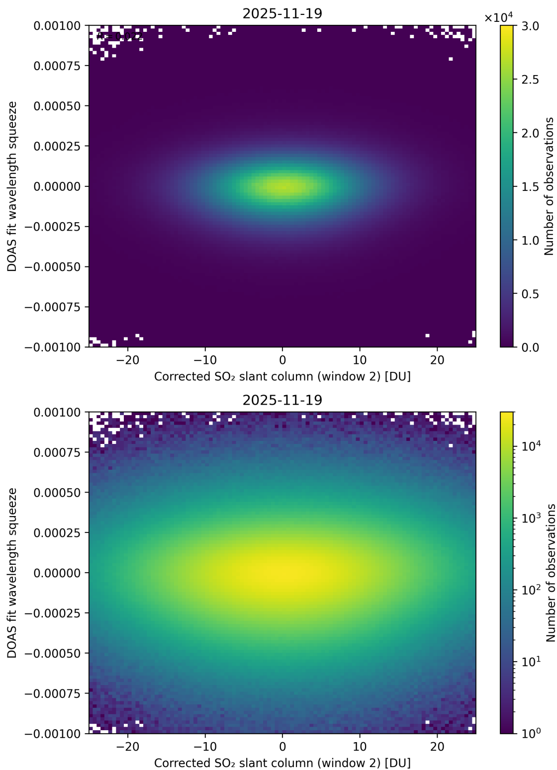
Figure 247: Scatter density plot of “Corrected SO 2 slant column (window 2)” against “DOAS fit wavelength squeeze” for 2025-11-18 to 2025-11-20.
