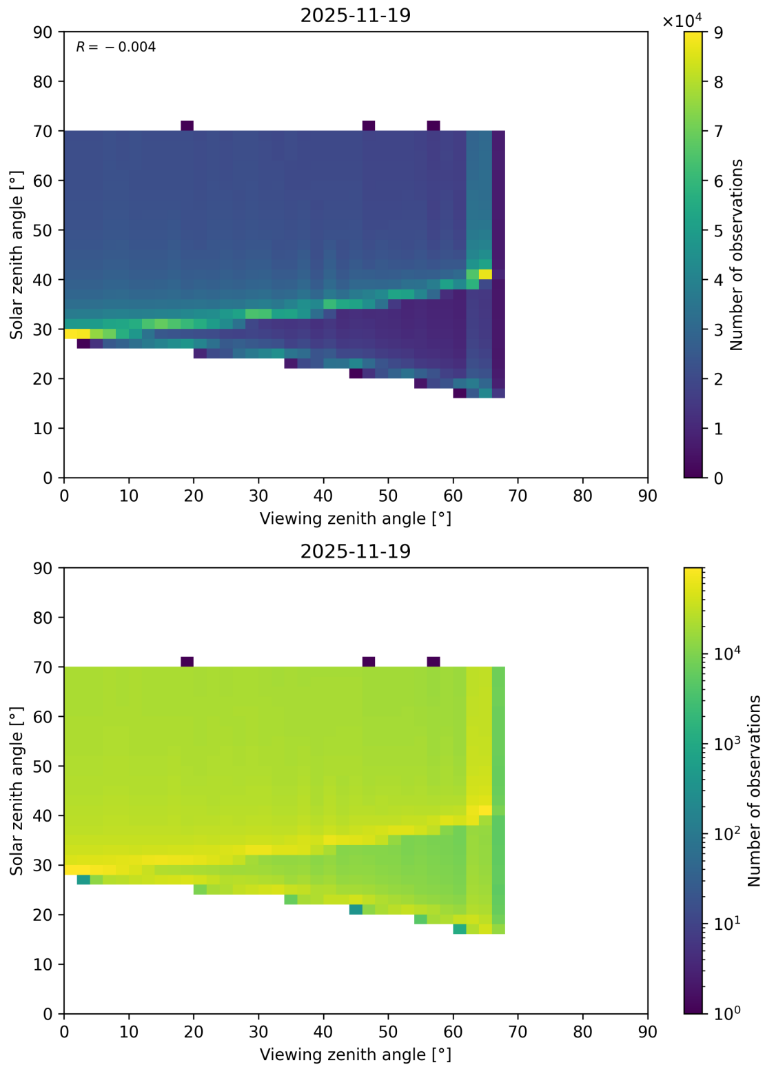
Figure 369: Scatter density plot of “Viewing zenith angle” against “Solar zenith angle” for 2025-11-18 to 2025-11-20.
