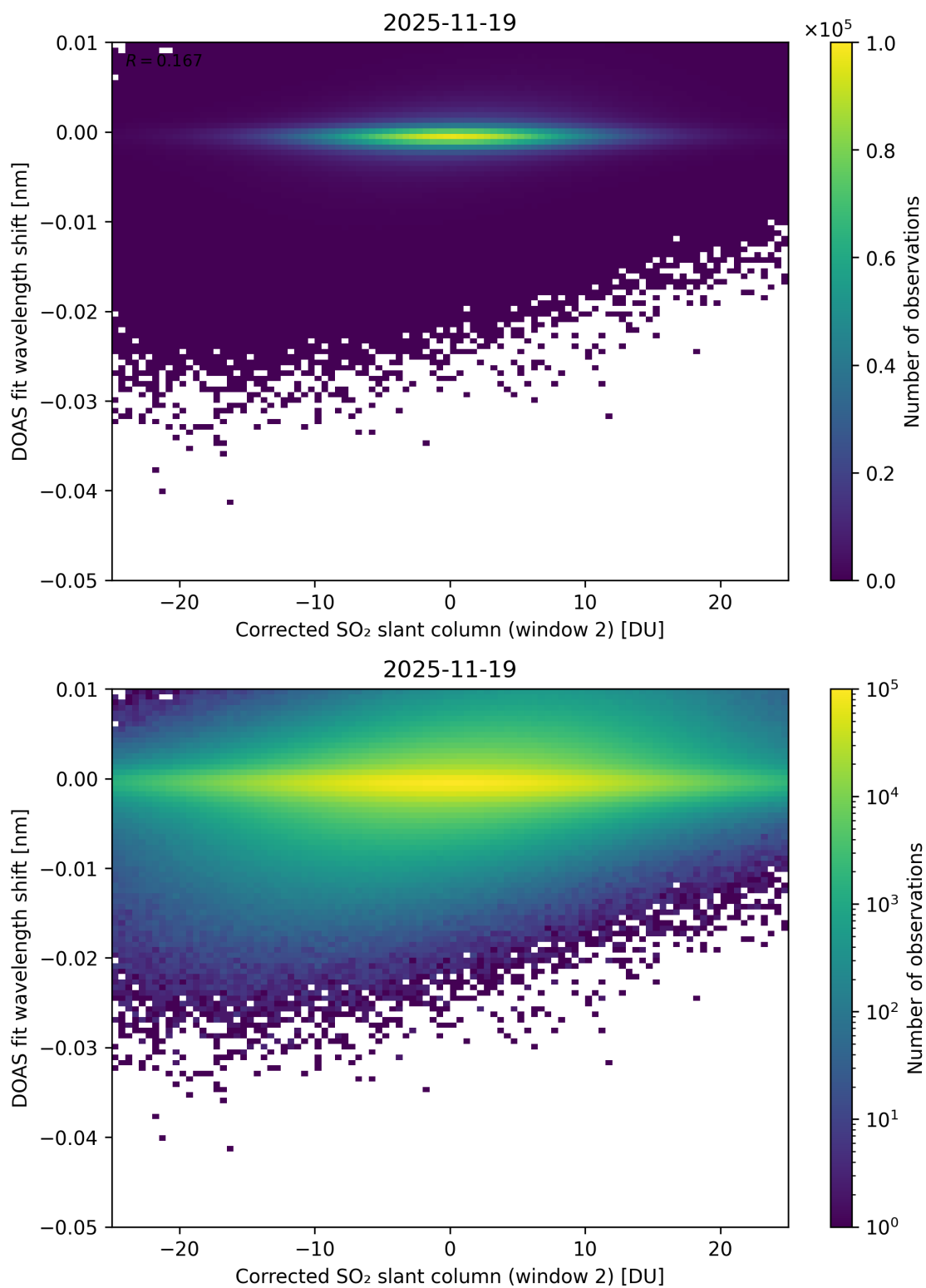
Figure 246: Scatter density plot of “Corrected SO 2 slant column (window 2)” against “DOAS fit wavelength shift” for 2025-11-18 to 2025-11-20.
