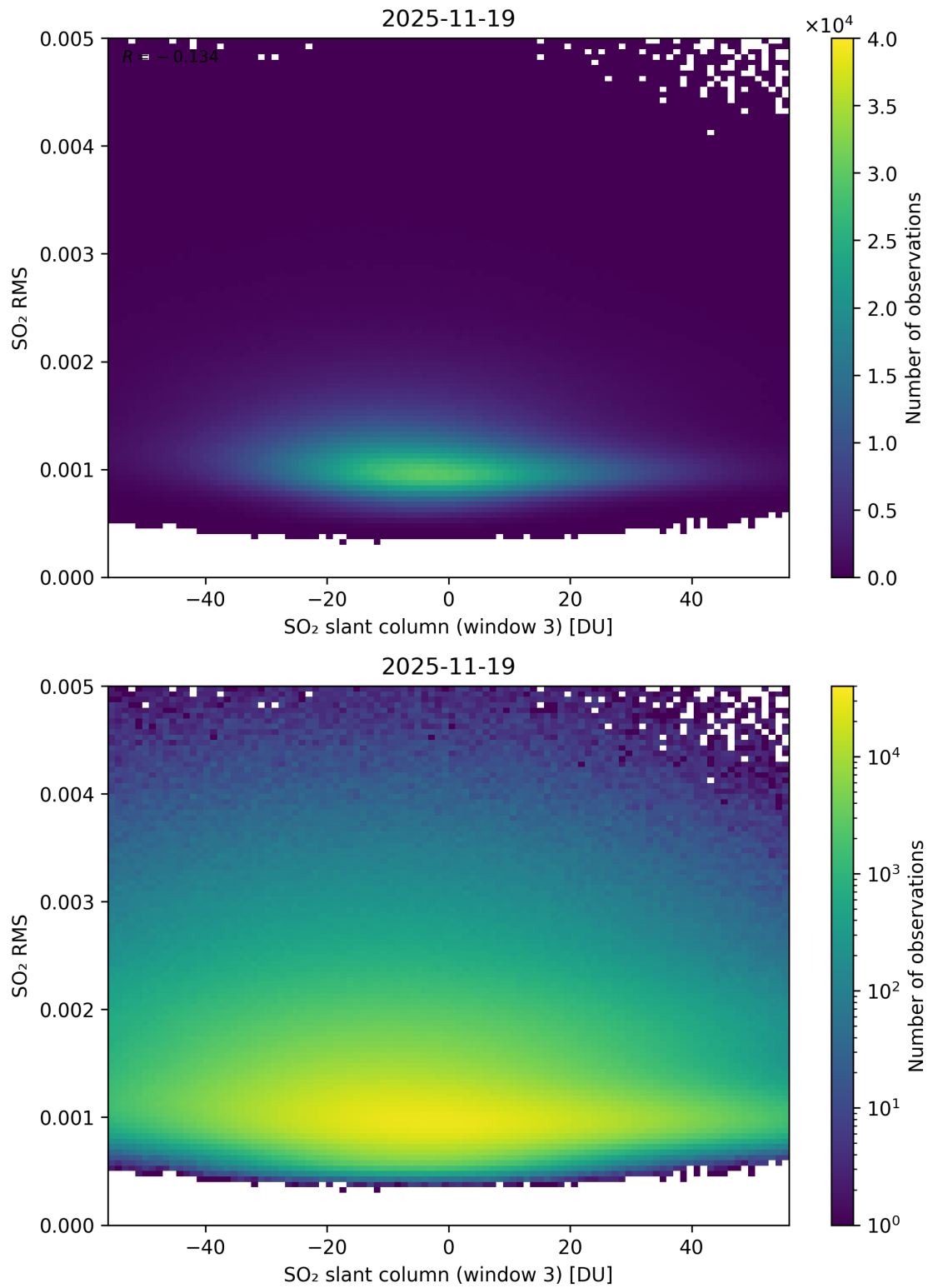
Figure 306: Scatter density plot of “SO 2 slant column (window 3)” against “SO 2 RMS” for 2025-11-18 to 2025-11-20.
