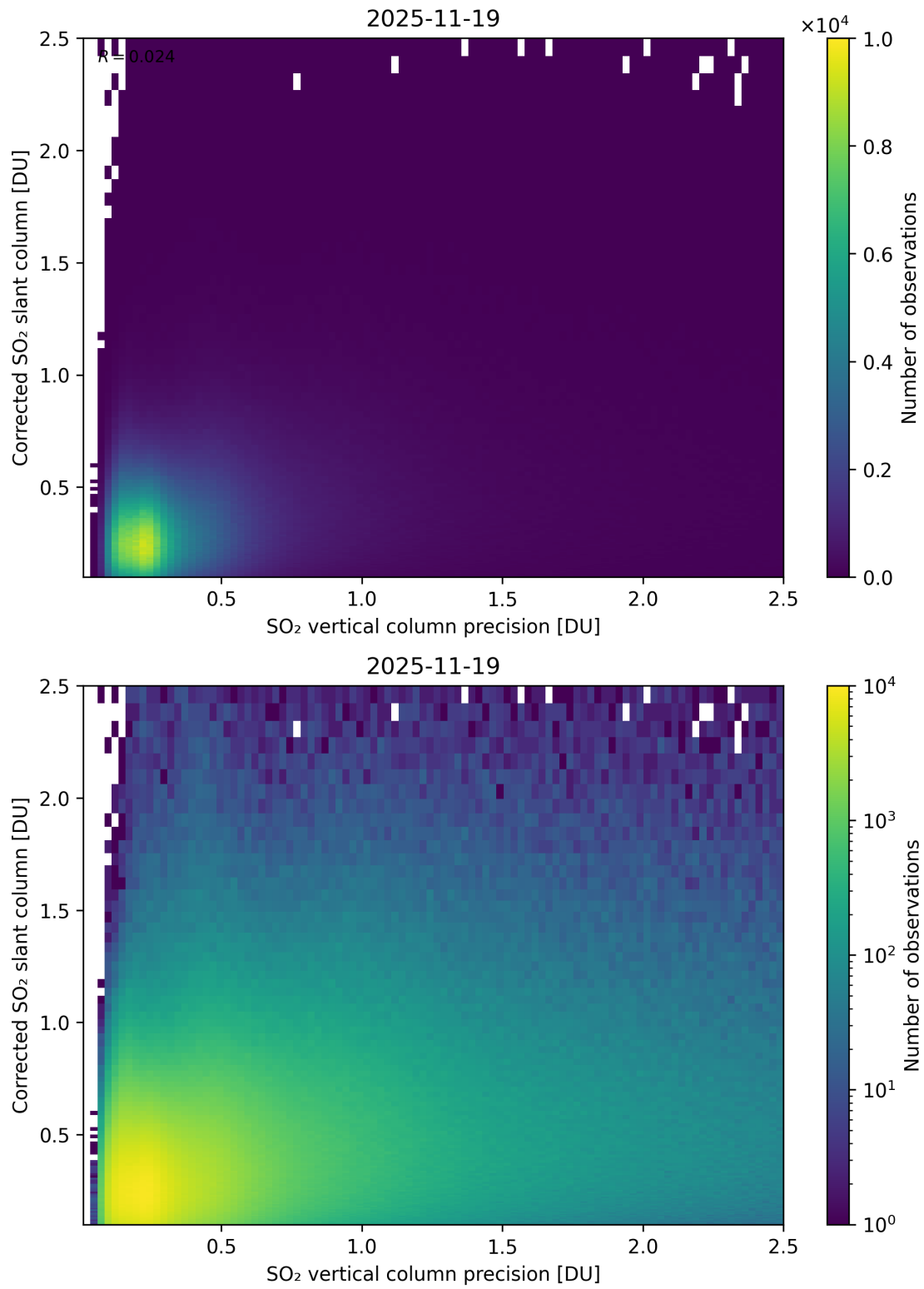
Figure 338: Scatter density plot of “SO 2 vertical column precision” against “Corrected SO 2 slant column” for 2025-11-18 to 2025-11-20.
