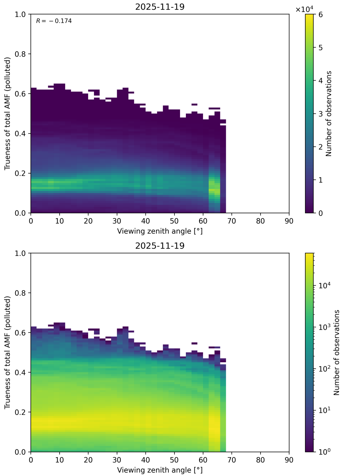
Figure 382: Scatter density plot of “Viewing zenith angle” against “Trueness of total AMF (polluted)” for 2025-11-18 to 2025-11-20.
