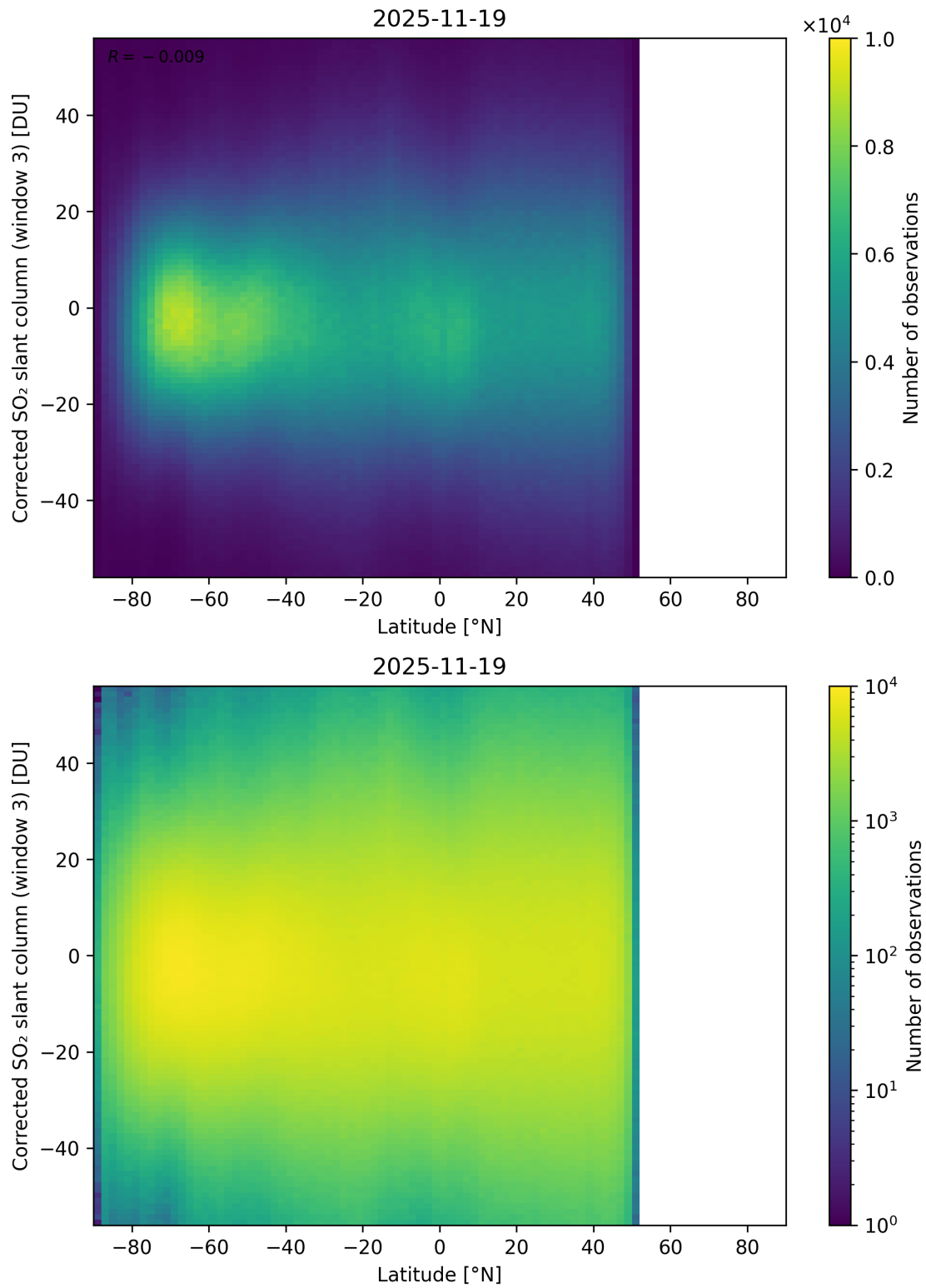
Figure 161: Scatter density plot of “Latitude” against “Corrected SO 2 slant column (window 3)” for 2025-11-18 to 2025-11-20.
