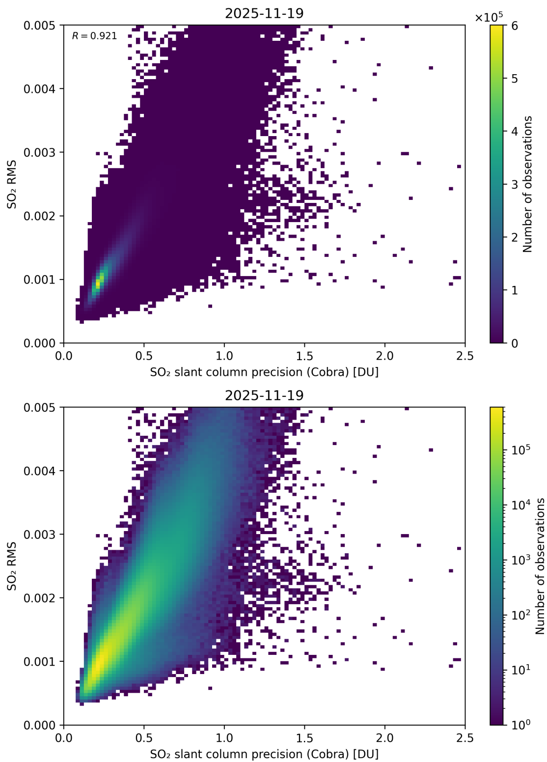
Figure 204: Scatter density plot of “SO 2 slant column precision (Cobra)” against “SO 2 RMS” for 2025-11-18 to 2025-11-20.
