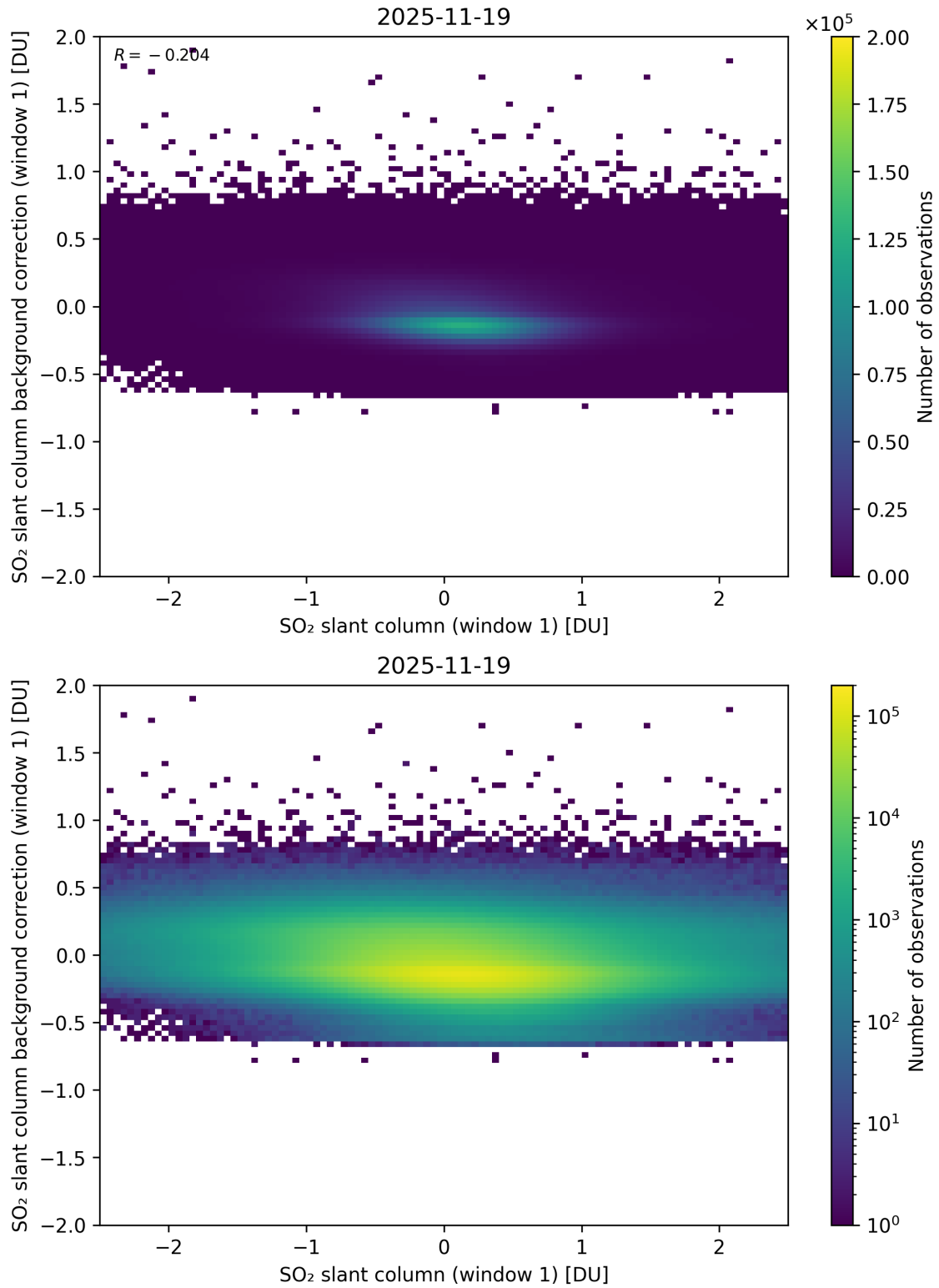
Figure 262: Scatter density plot of “SO 2 slant column (window 1)” against “SO 2 slant column background correction (window 1)” for 2025-11-18 to 2025-11-20.
