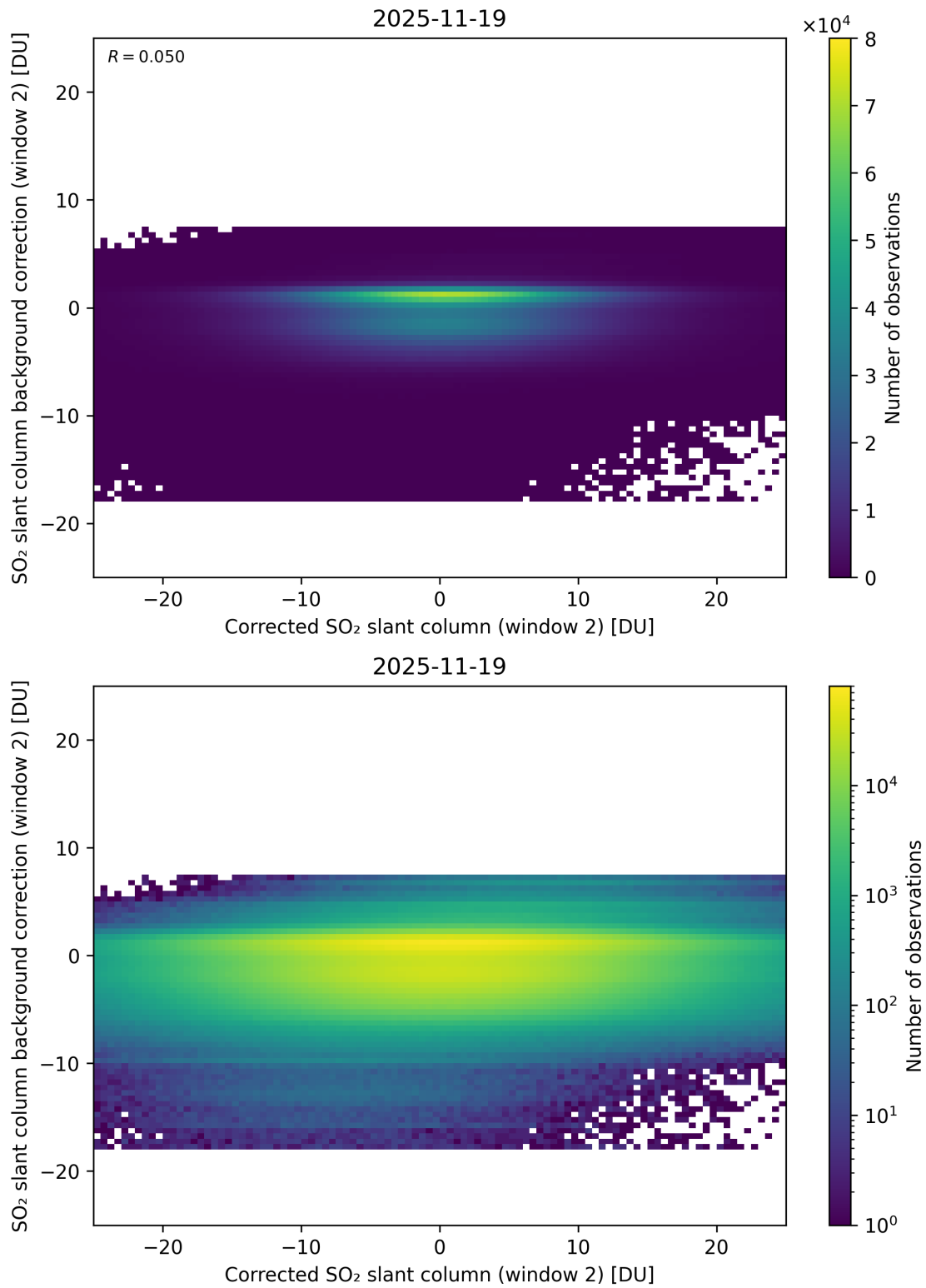
Figure 244: Scatter density plot of “Corrected SO 2 slant column (window 2)” against “SO 2 slant column background correction (window 2)” for 2025-11-18 to 2025-11-20.
