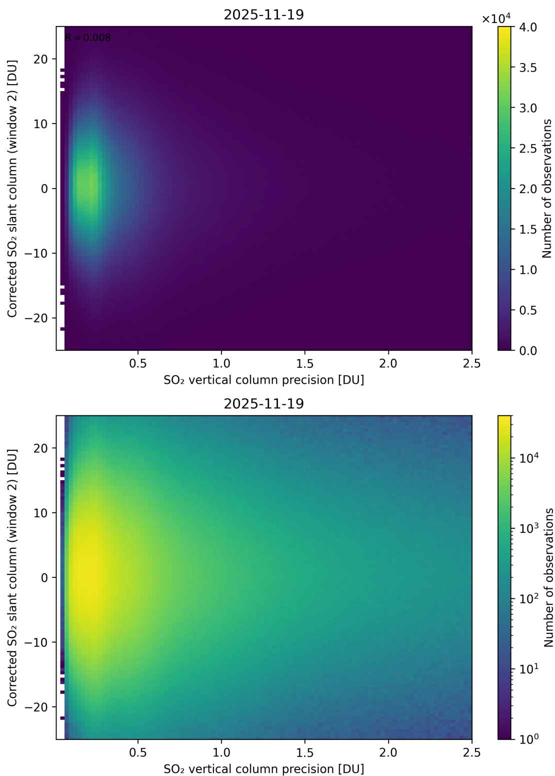
Figure 339: Scatter density plot of “SO 2 vertical column precision” against “Corrected SO 2 slant column (window 2)” for 2025-11-18 to 2025-11-20.
