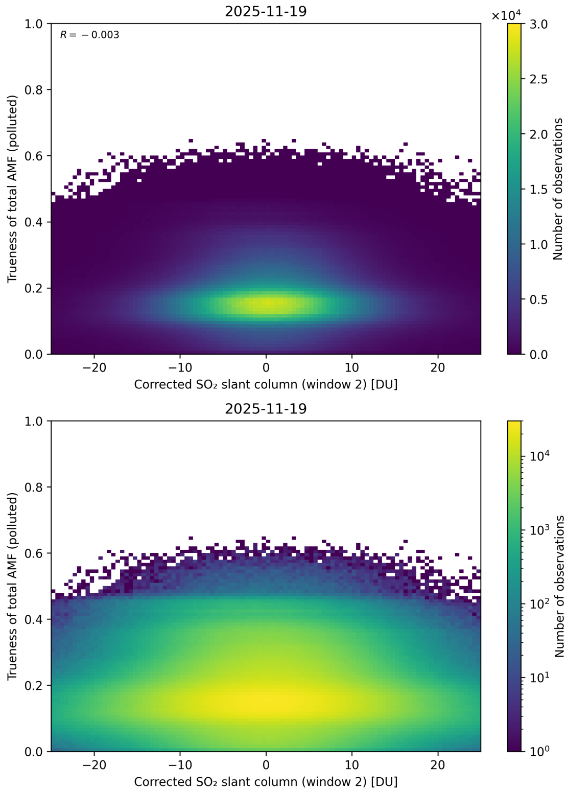
Figure 254: Scatter density plot of “Corrected SO 2 slant column (window 2)” against “Trueness of total AMF (polluted)” for 2025-11-18 to 2025-11-20.
