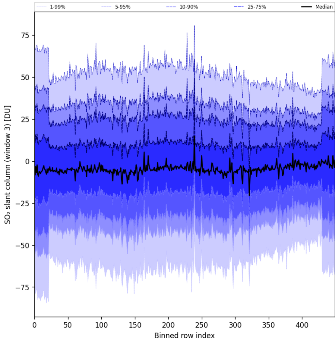
Figure 97: Along track statistics of “SO 2 slant column (window 3)” for 2025-11-18 to 2025-11-20
