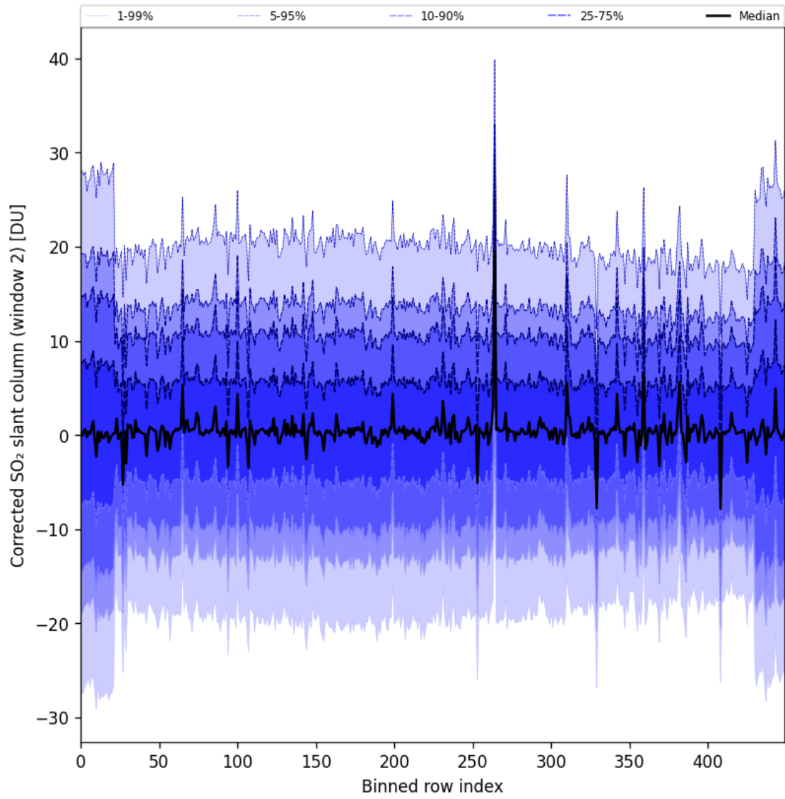
Figure 95: Along track statistics of “Corrected SO 2 slant column (window 2)” for 2025-11-18 to 2025-11-20
