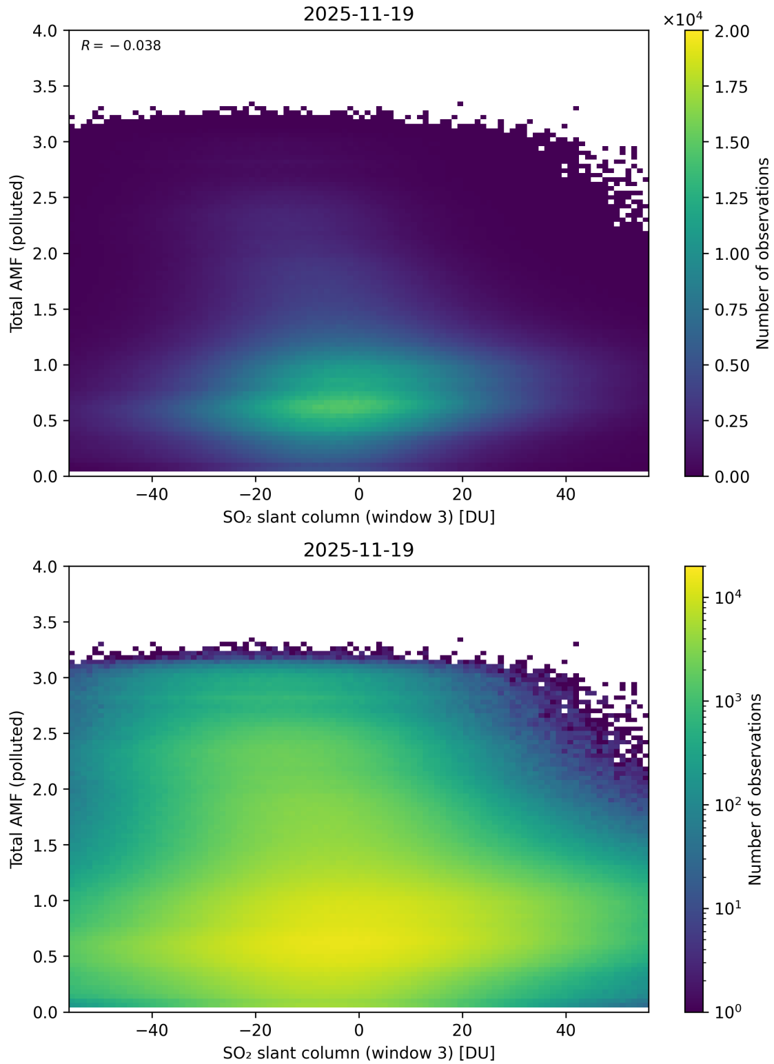
Figure 318: Scatter density plot of “SO 2 slant column (window 3)” against “Total AMF (polluted)” for 2025-11-18 to 2025-11-20.
