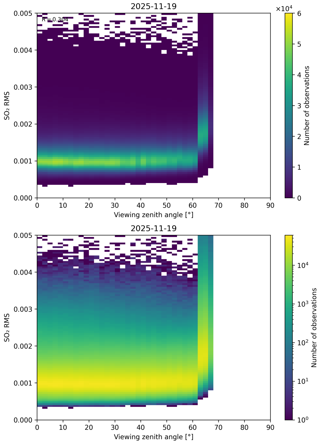
Figure 367: Scatter density plot of “Viewing zenith angle” against “SO 2 RMS” for 2025-11-18 to 2025-11-20.
