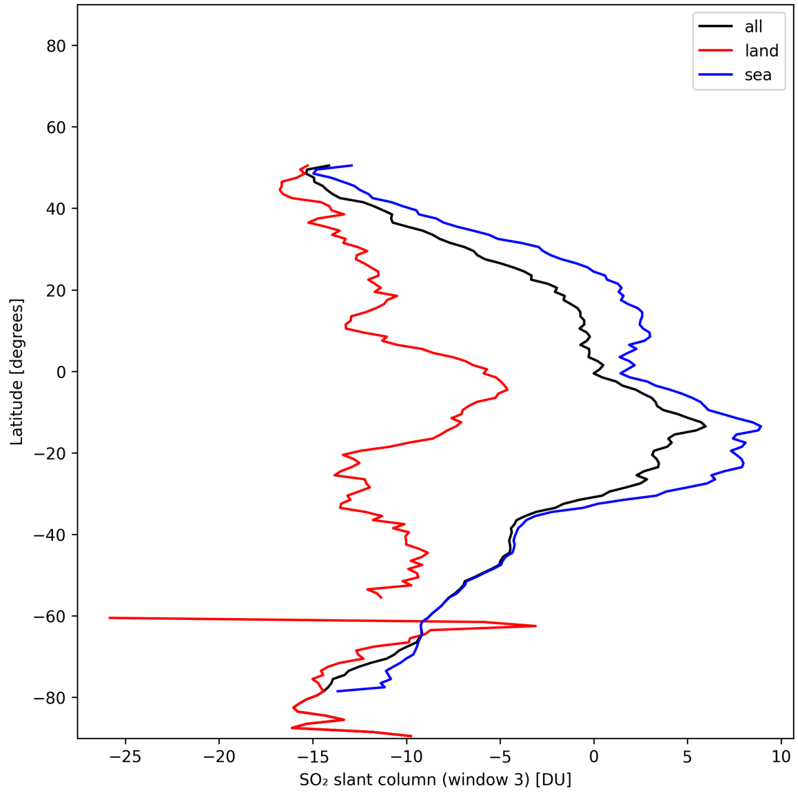
Figure 45: Zonal average of “SO 2 slant column (window 3)” for 2025-11-18 to 2025-11-20.
