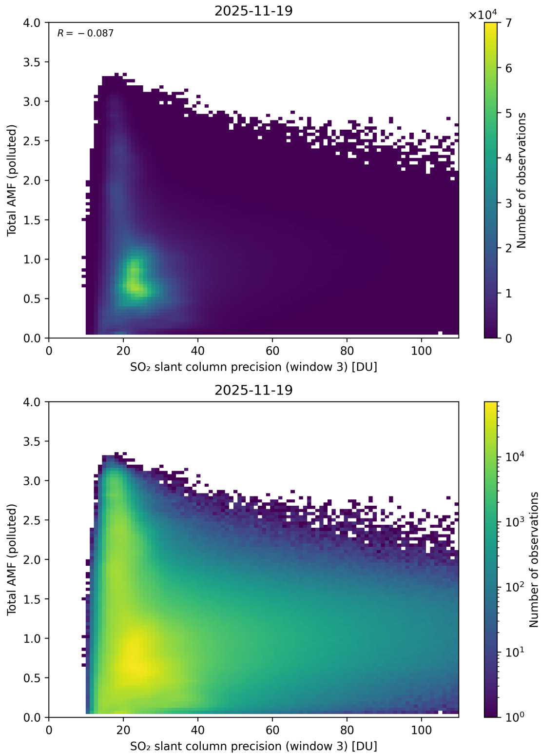
Figure 313: Scatter density plot of “SO 2 slant column precision (window 3)” against “Total AMF (polluted)” for 2025-11-18 to 2025-11-20.
