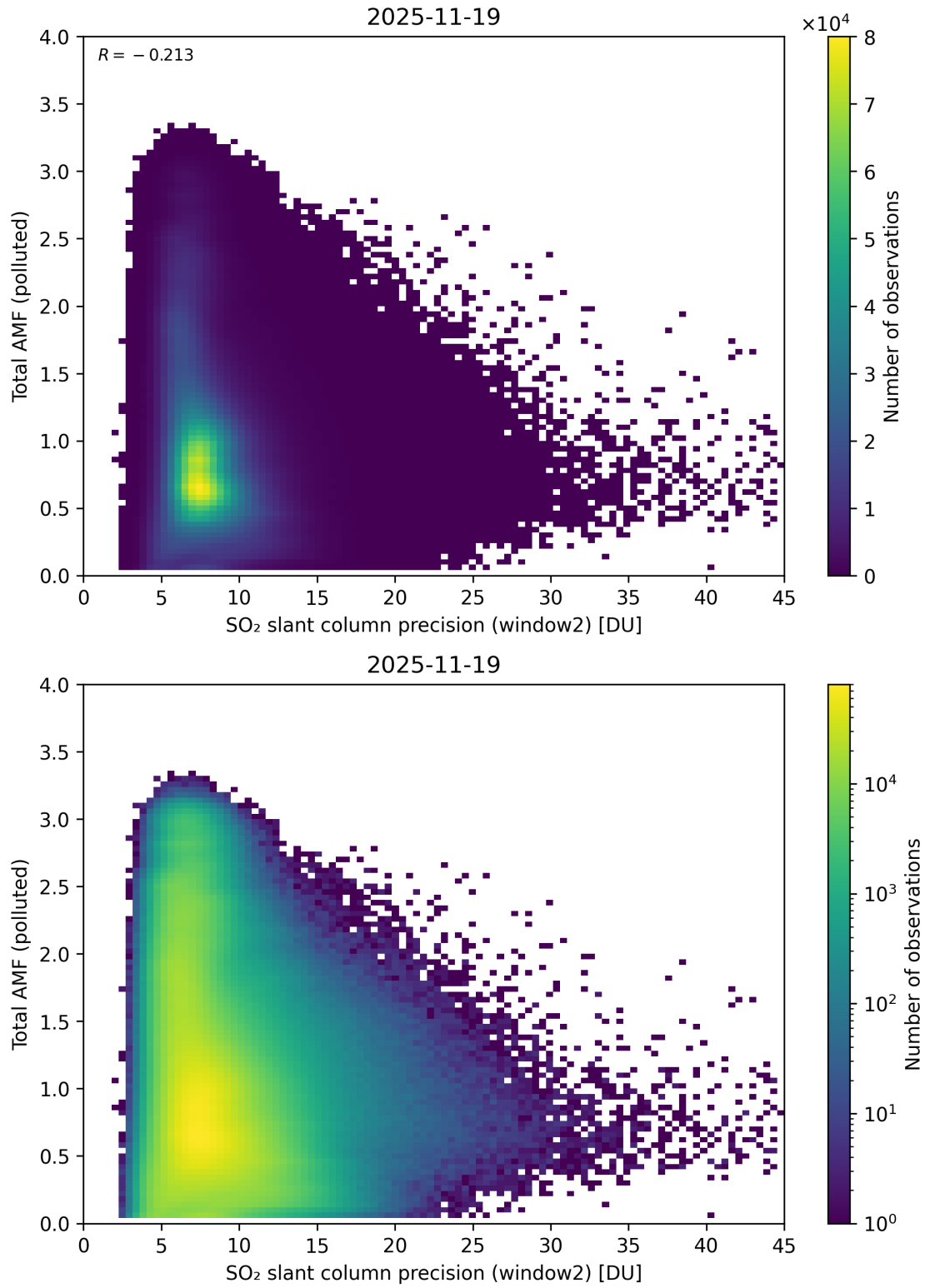
Figure 301: Scatter density plot of “SO 2 slant column precision (window2)” against “Total AMF (polluted)” for 2025-11-18 to 2025-11-20.
