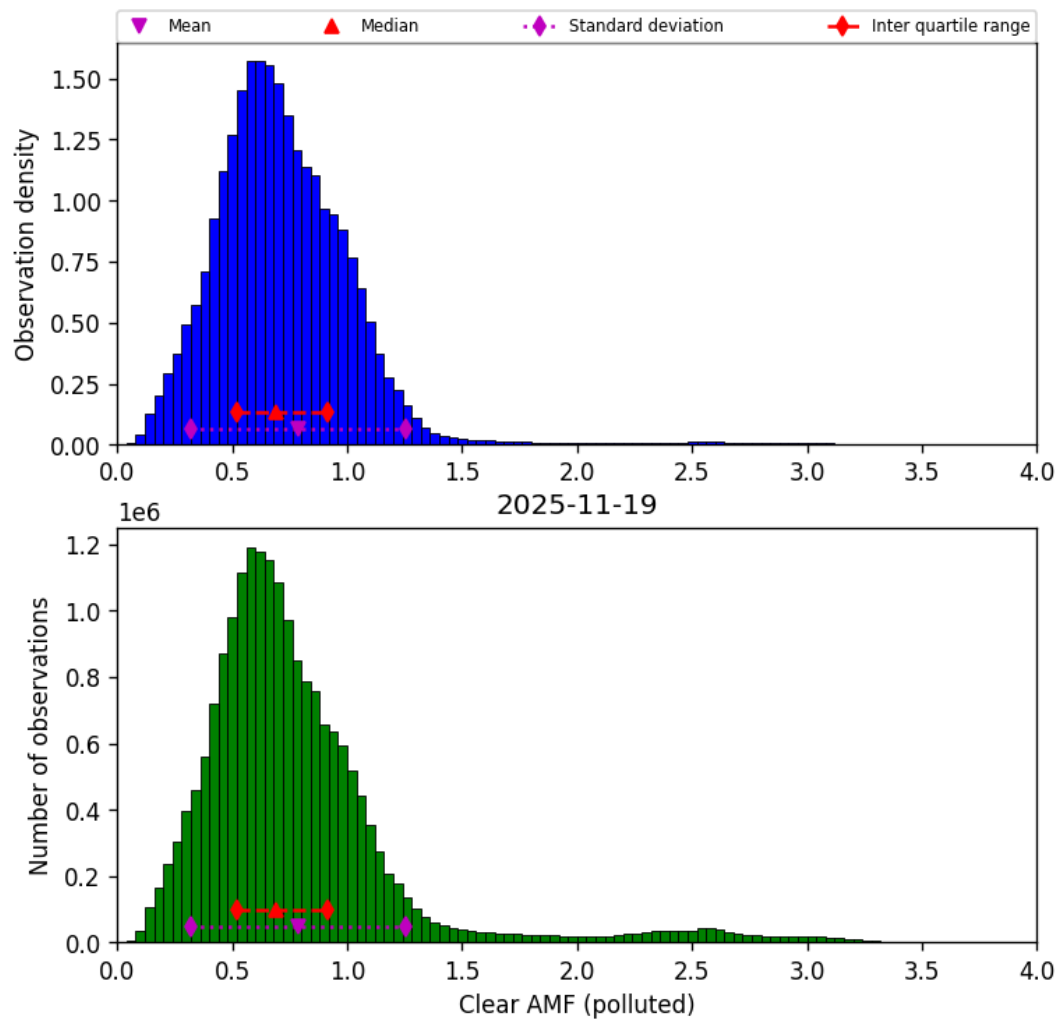
Figure 81: Histogram of “Clear AMF (polluted)” for 2025-11-18 to 2025-11-20
