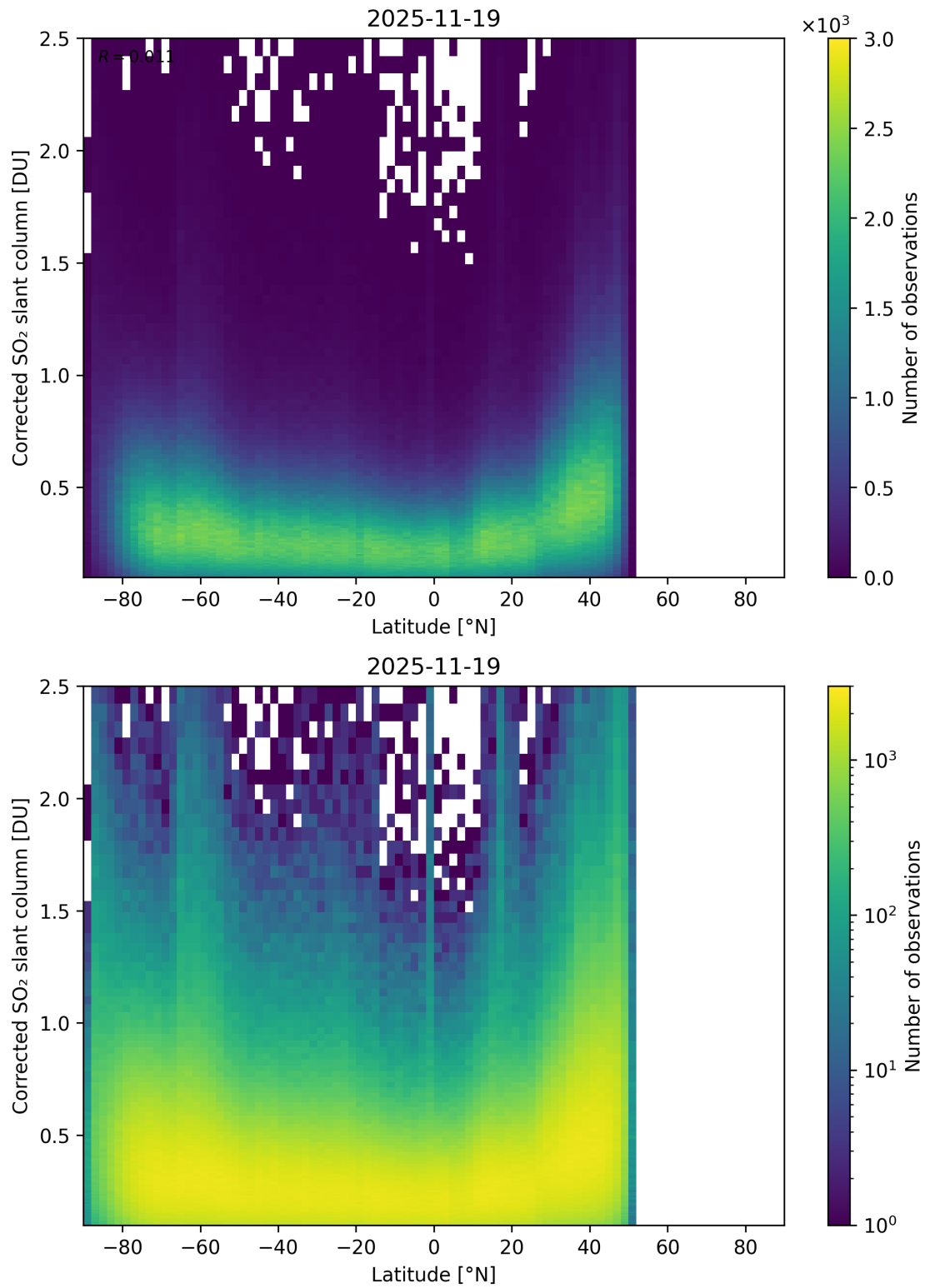
Figure 159: Scatter density plot of “Latitude” against “Corrected SO 2 slant column” for 2025-11-18 to 2025-11-20.
