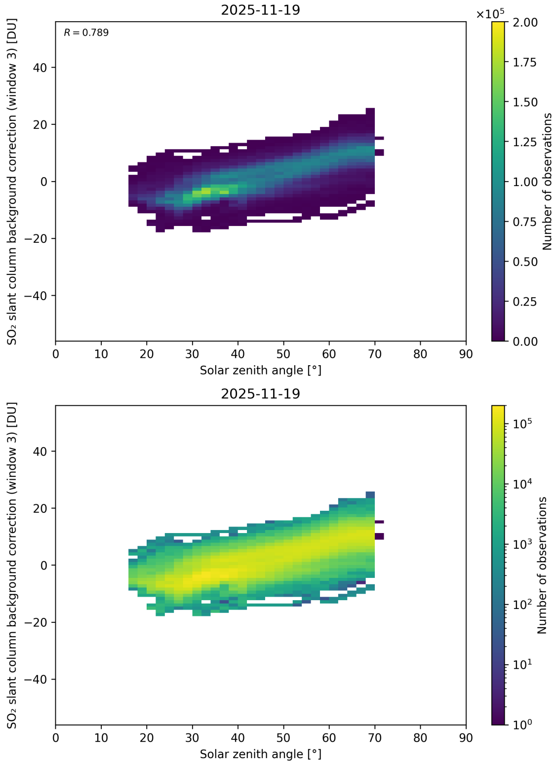
Figure 173: Scatter density plot of “Solar zenith angle” against “SO 2 slant column background correction (window 3)” for 2025-11-18 to 2025-11-20.
