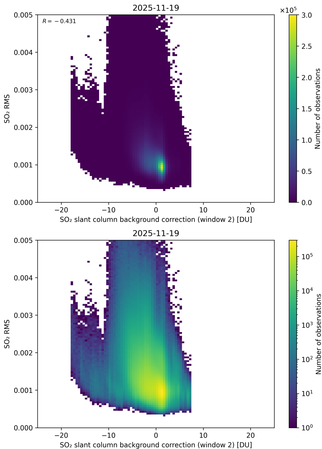
Figure 125: Scatter density plot of “SO 2 slant column background correction (window 2)” against “SO 2 RMS” for 2025-11-18 to 2025-11-20.
