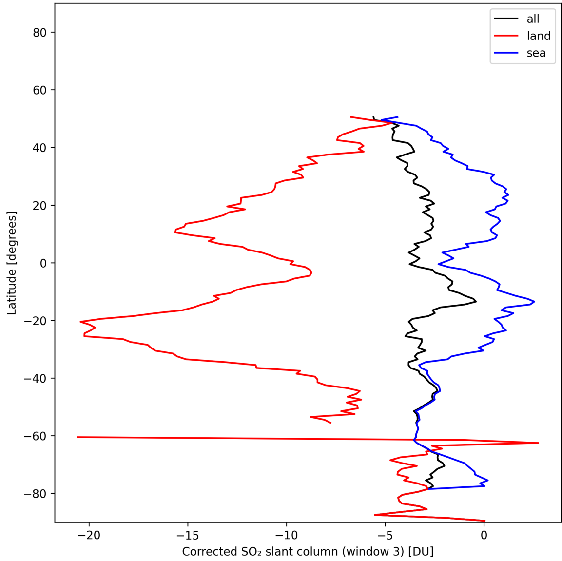
Figure 47: Zonal average of “Corrected SO 2 slant column (window 3)” for 2025-11-18 to 2025-11-20.
