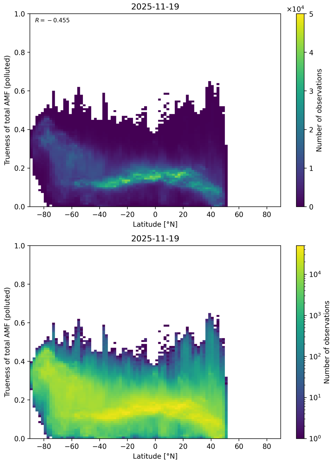
Figure 168: Scatter density plot of “Latitude” against “Trueness of total AMF (polluted)” for 2025-11-18 to 2025-11-20.
