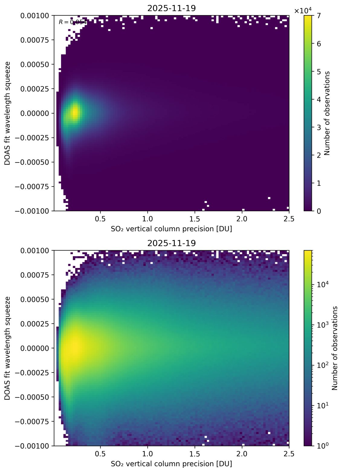
Figure 333: Scatter density plot of “SO 2 vertical column precision” against “DOAS fit wavelength squeeze” for 2025-11-18 to 2025-11-20.
