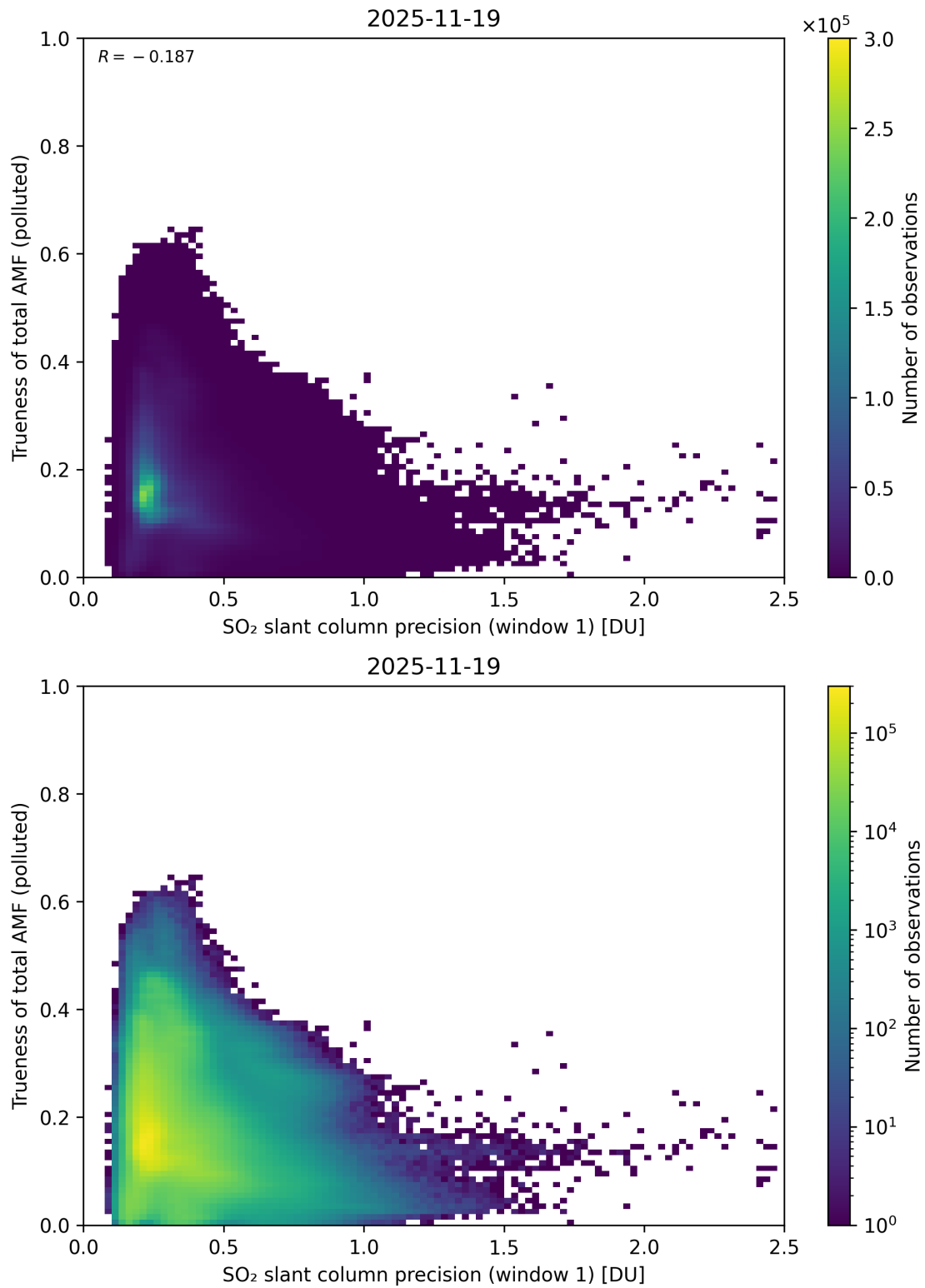
Figure 281: Scatter density plot of “SO 2 slant column precision (window 1)” against “Trueness of total AMF (polluted)” for 2025-11-18 to 2025-11-20.
