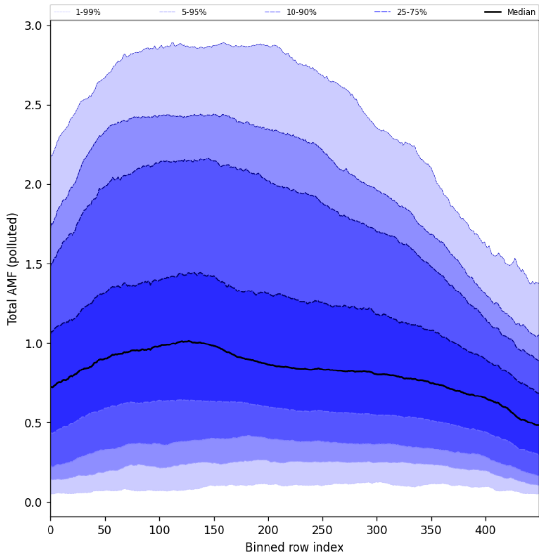
Figure 105: Along track statistics of “Total AMF (polluted)” for 2025-11-18 to 2025-11-20
