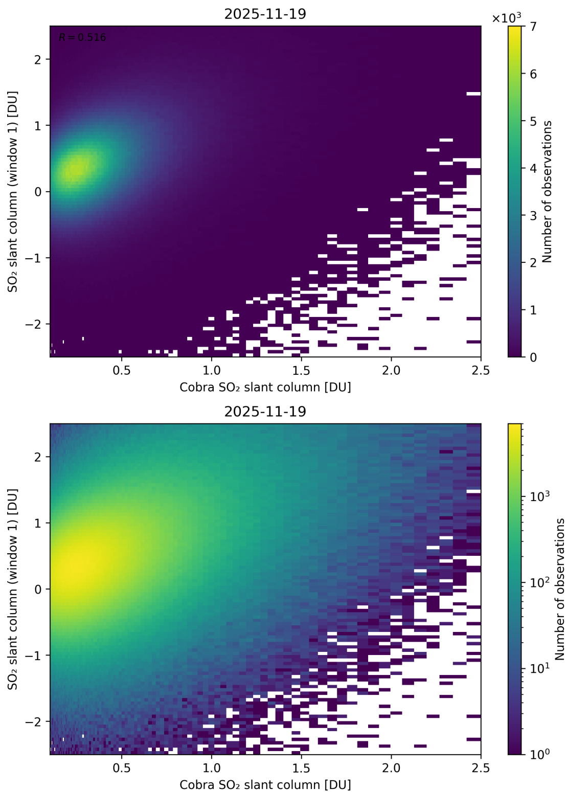
Figure 219: Scatter density plot of “Cobra SO 2 slant column” against “SO 2 slant column (window 1)” for 2025-11-18 to 2025-11-20.
