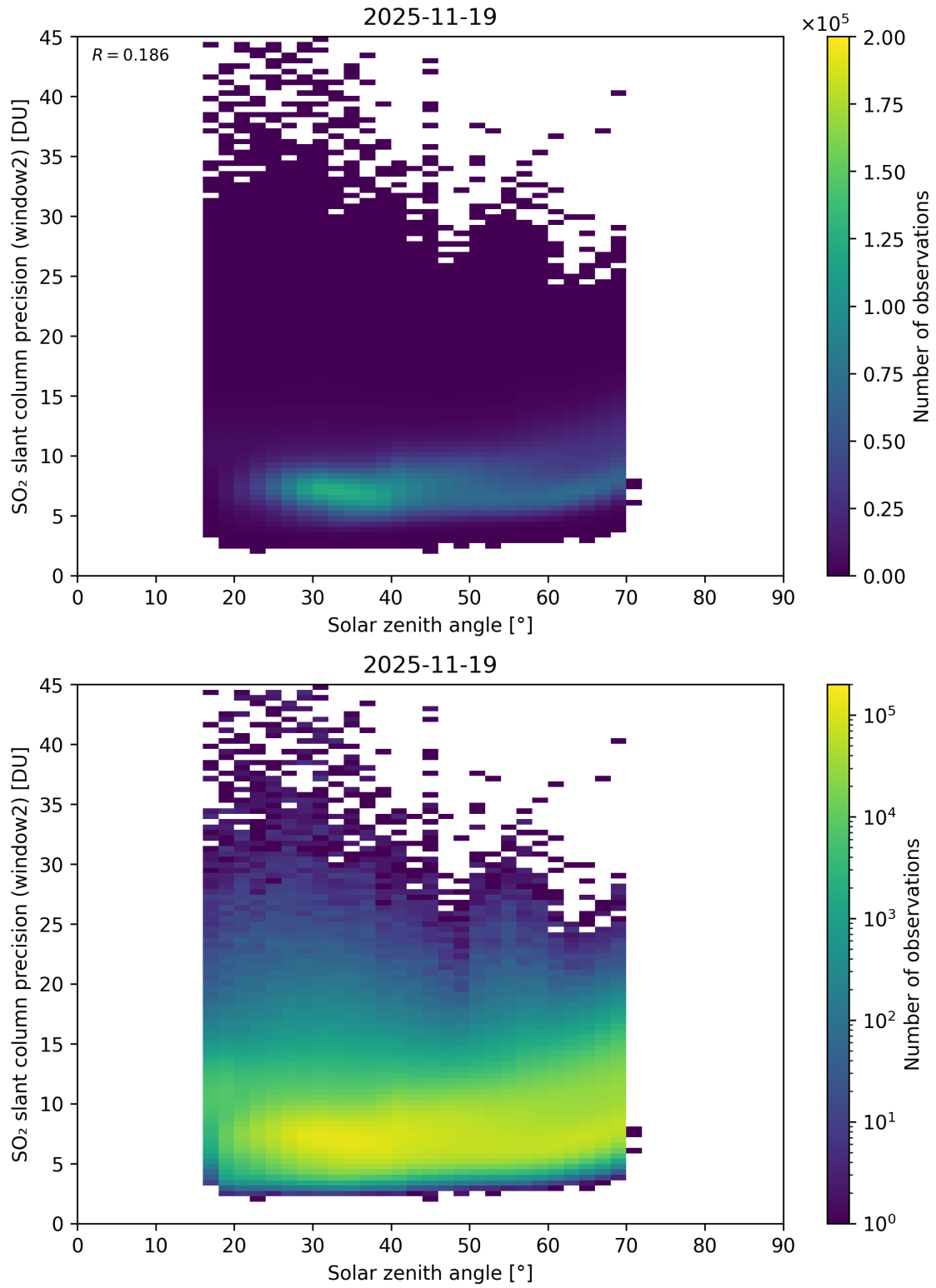
Figure 186: Scatter density plot of “Solar zenith angle” against “SO 2 slant column precision (window2)” for 2025-11-18 to 2025-11-20.
