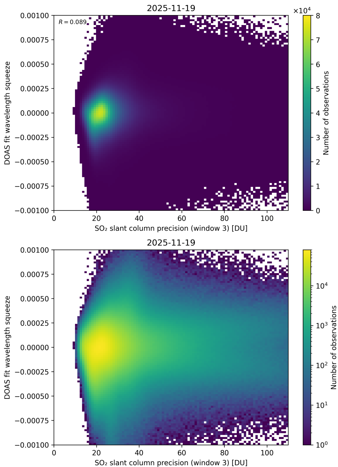
Figure 309: Scatter density plot of “SO 2 slant column precision (window 3)” against “DOAS fit wavelength squeeze” for 2025-11-18 to 2025-11-20.
