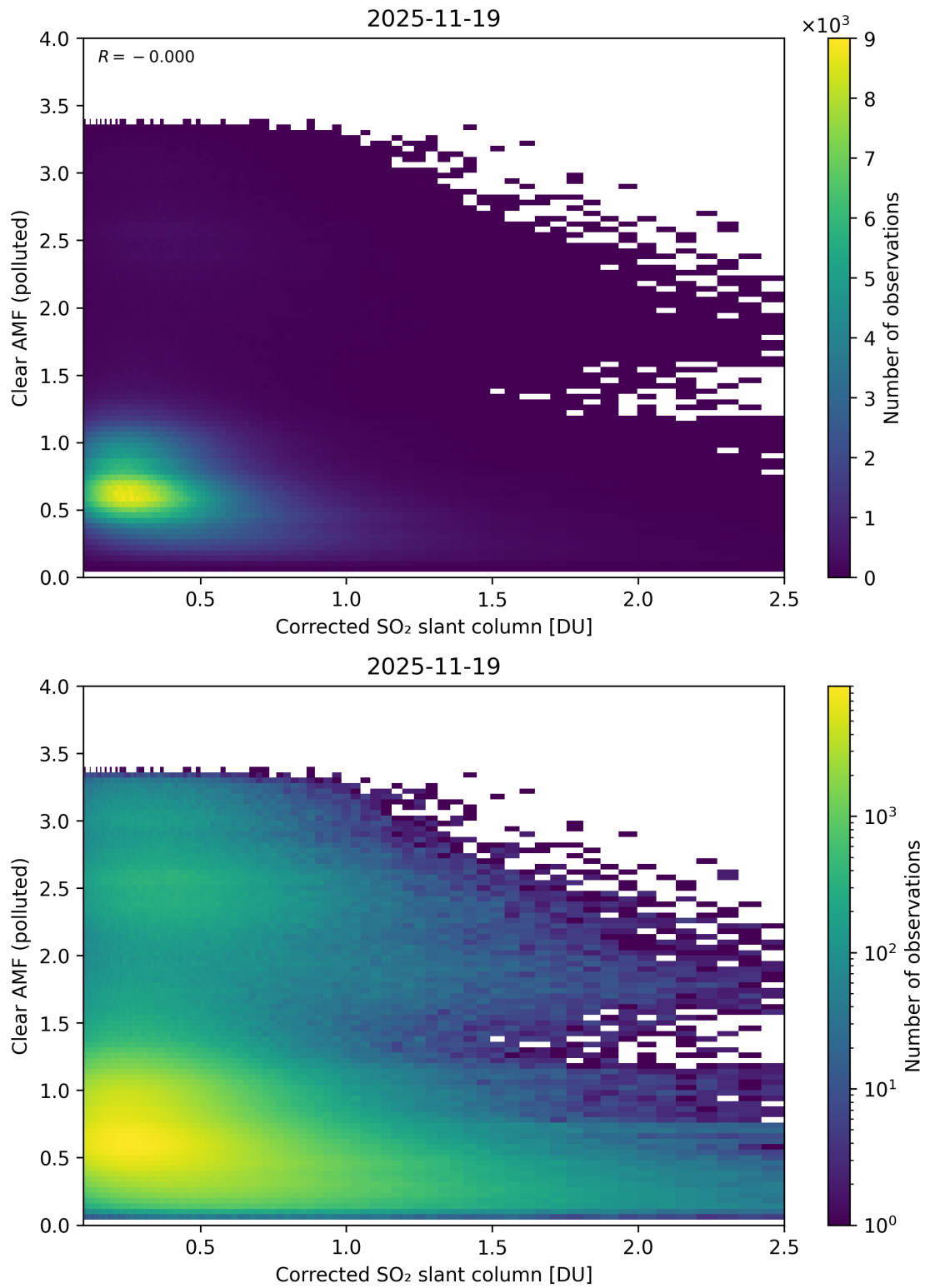
Figure 232: Scatter density plot of “Corrected SO 2 slant column” against “Clear AMF (polluted)” for 2025-11-18 to 2025-11-20.
