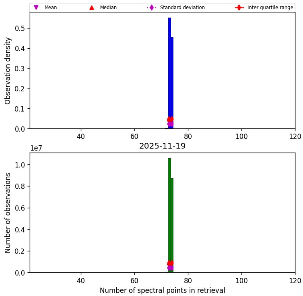
Figure 82: Histogram of “Number of spectral points in retrieval” for 2025-11-18 to 2025-11-20
