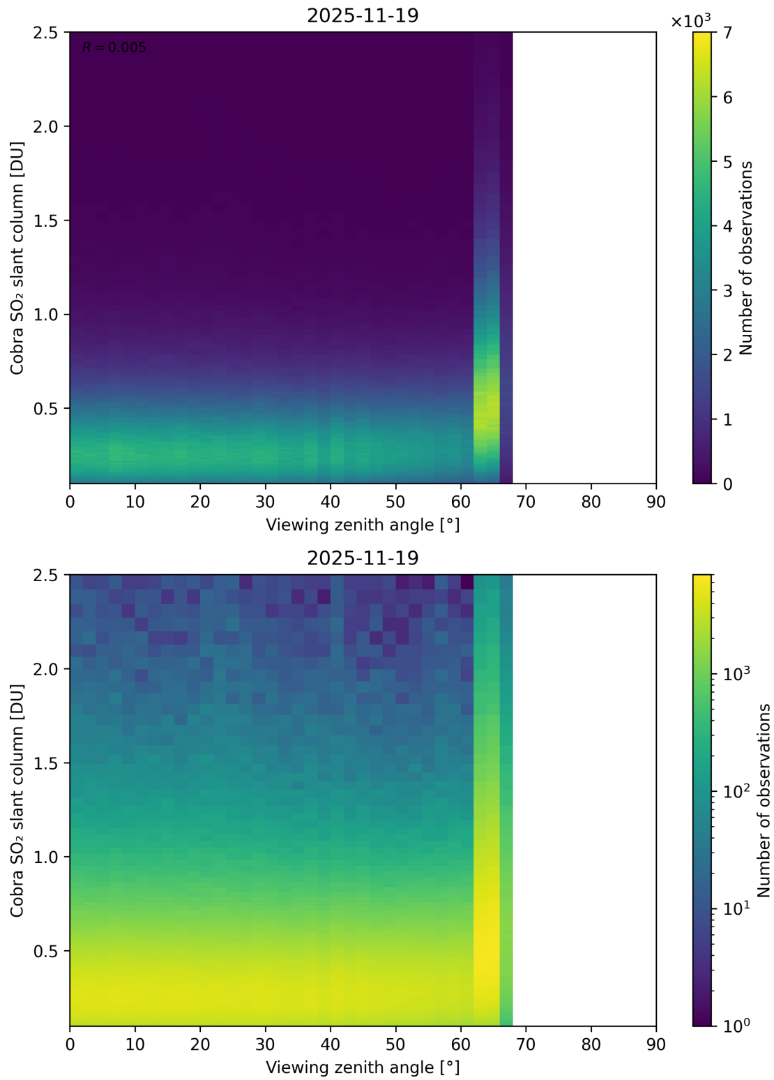
Figure 371: Scatter density plot of “Viewing zenith angle” against “Cobra SO 2 slant column” for 2025-11-18 to 2025-11-20.
