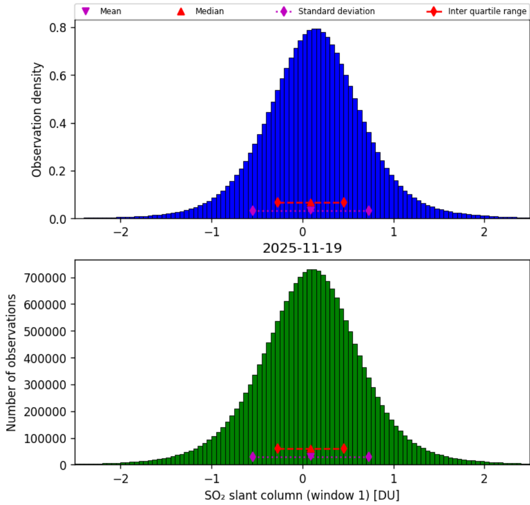
Figure 63: Histogram of “SO 2 slant column (window 1)” for 2025-11-18 to 2025-11-20
