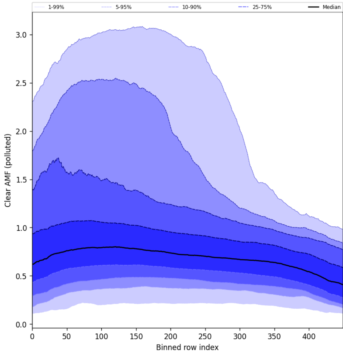
Figure 107: Along track statistics of “Clear AMF (polluted)” for 2025-11-18 to 2025-11-20
