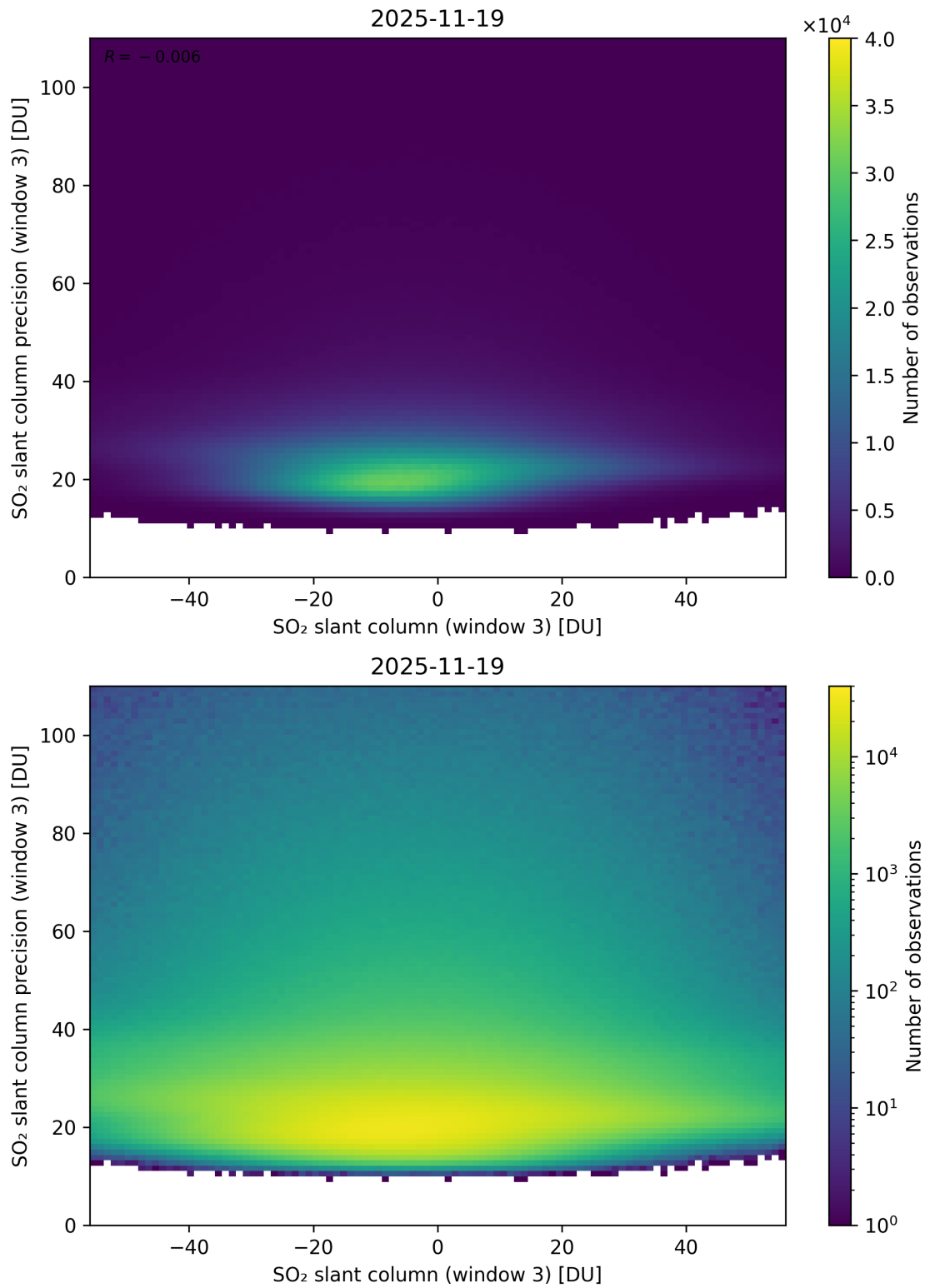
Figure 317: Scatter density plot of “SO 2 slant column (window 3)” against “SO 2 slant column precision (window 3)” for 2025-11-18 to 2025-11-20.
