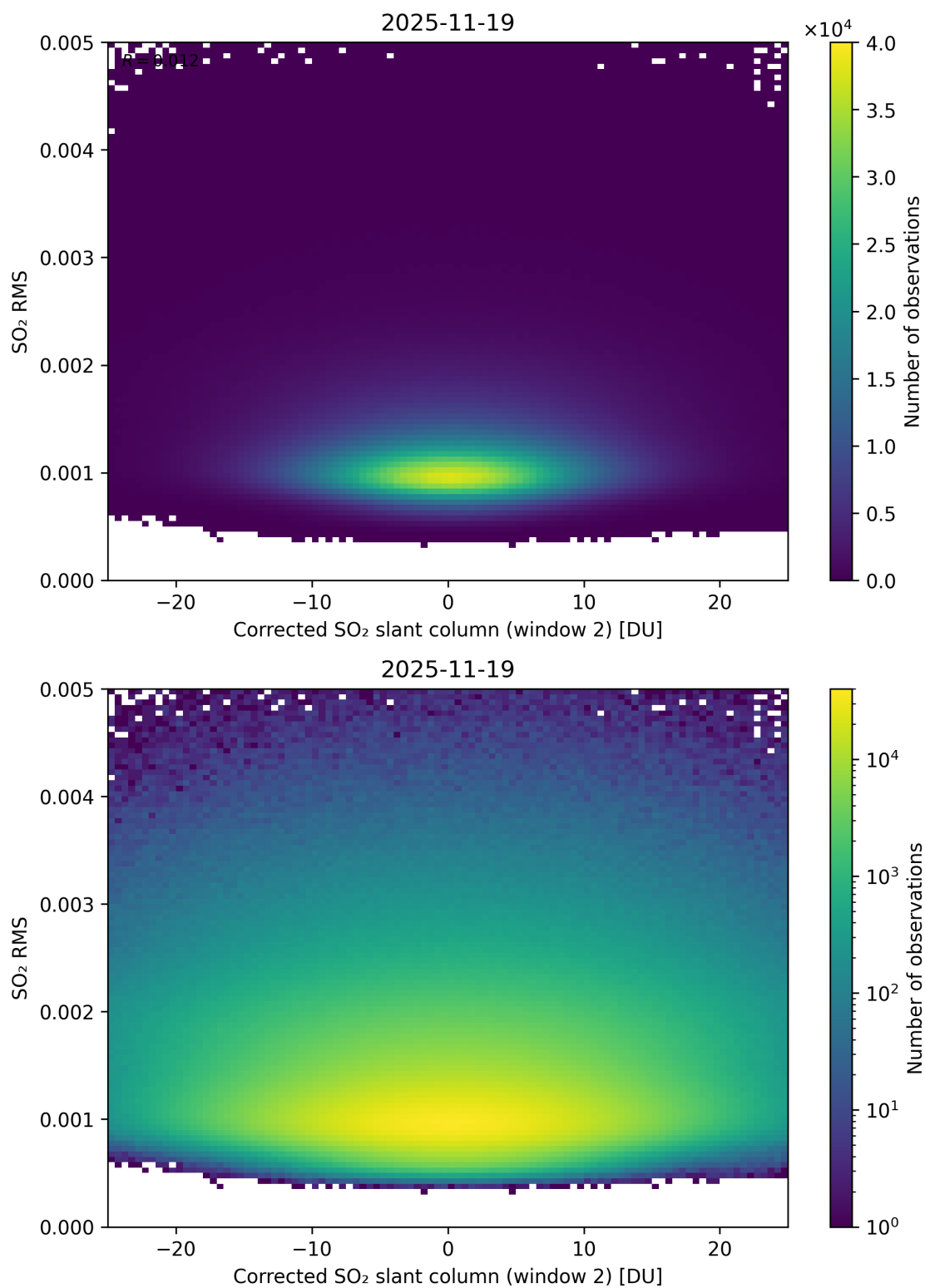
Figure 248: Scatter density plot of “Corrected SO 2 slant column (window 2)” against “SO 2 RMS” for 2025-11-18 to 2025-11-20.
