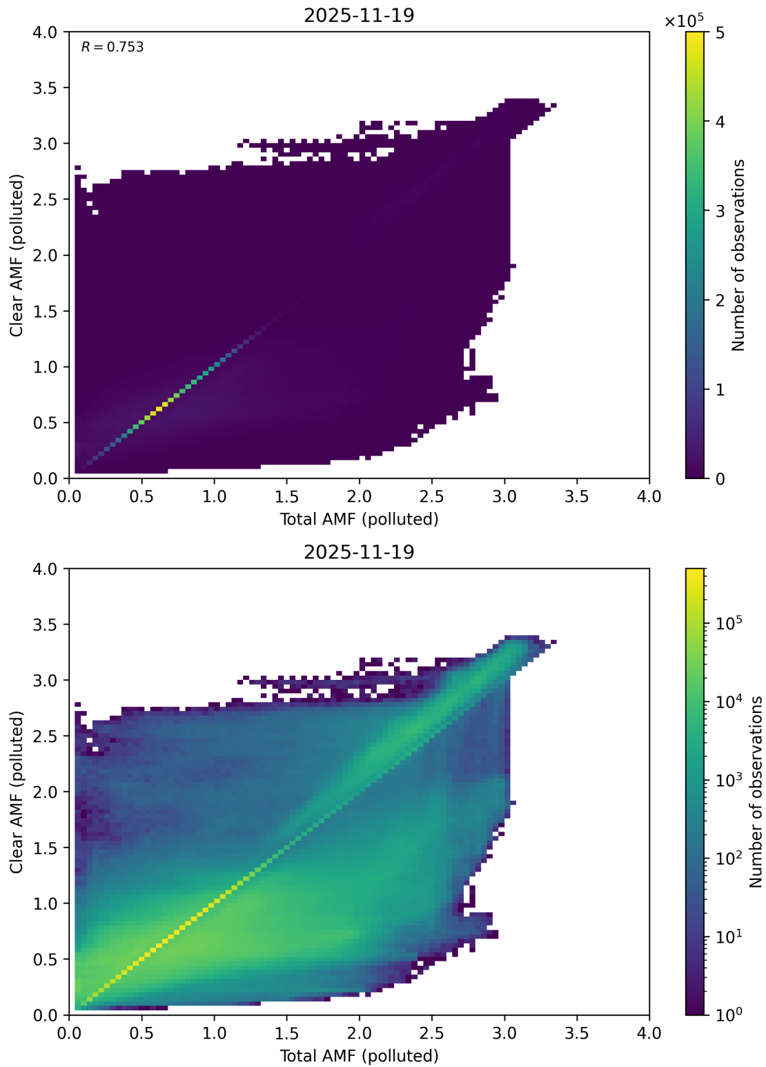
Figure 320: Scatter density plot of “Total AMF (polluted)” against “Clear AMF (polluted)” for 2025-11-18 to 2025-11-20.
