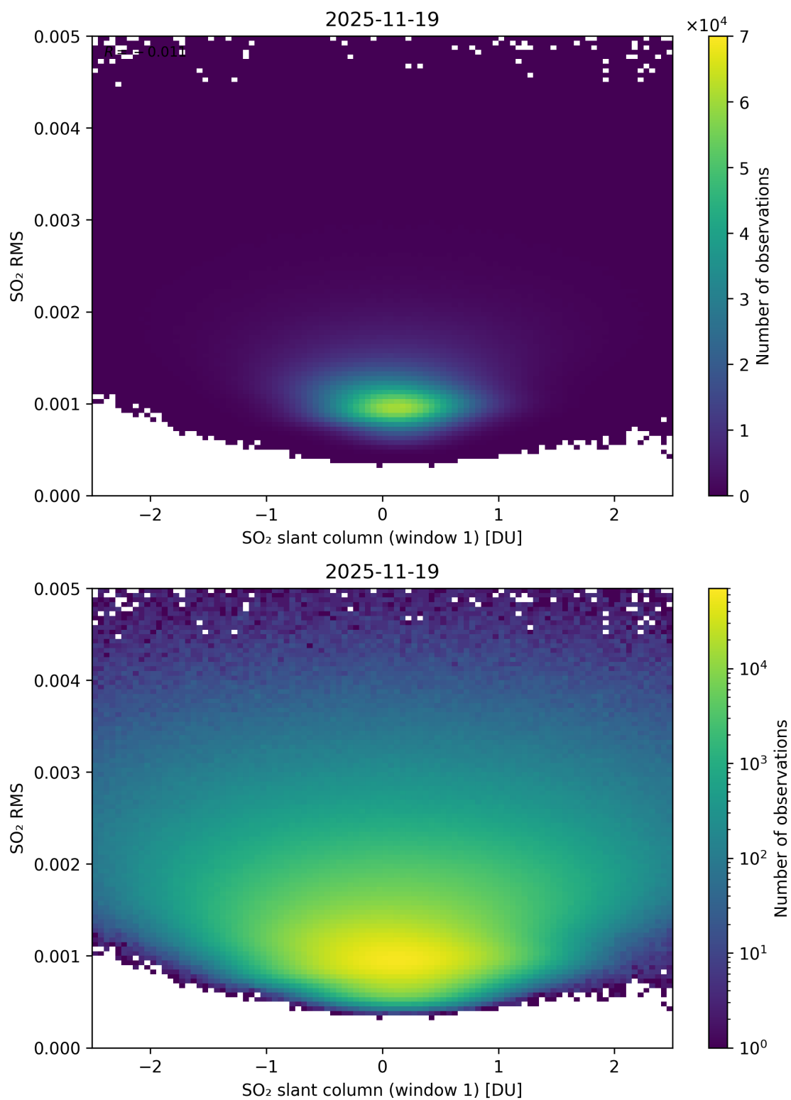
Figure 267: Scatter density plot of “SO 2 slant column (window 1)” against “SO 2 RMS” for 2025-11-18 to 2025-11-20.
