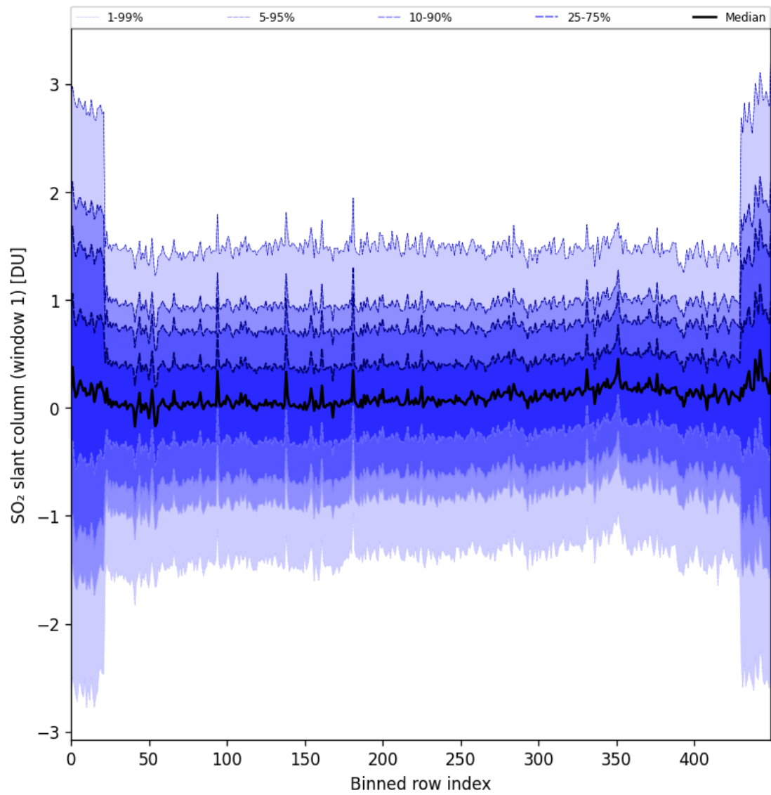
Figure 89: Along track statistics of “SO 2 slant column (window 1)” for 2025-11-18 to 2025-11-20
