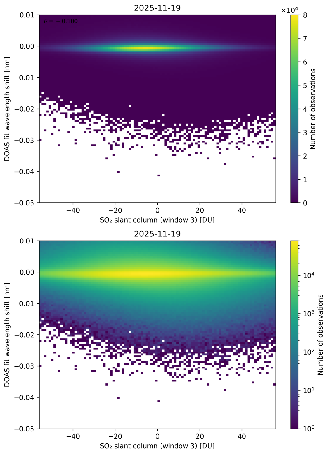
Figure 304: Scatter density plot of “SO 2 slant column (window 3)” against “DOAS fit wavelength shift” for 2025-11-18 to 2025-11-20.
