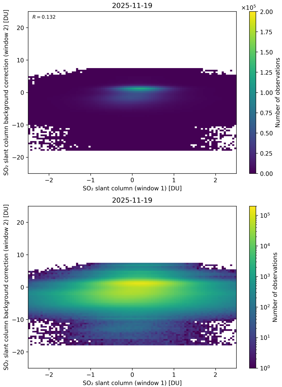
Figure 263: Scatter density plot of “SO 2 slant column (window 1)” against “SO 2 slant column background correction (window 2)” for 2025-11-18 to 2025-11-20.
