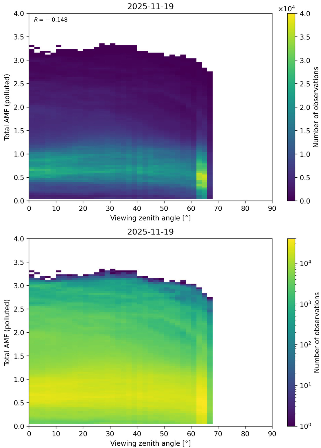
Figure 381: Scatter density plot of “Viewing zenith angle” against “Total AMF (polluted)” for 2025-11-18 to 2025-11-20.
