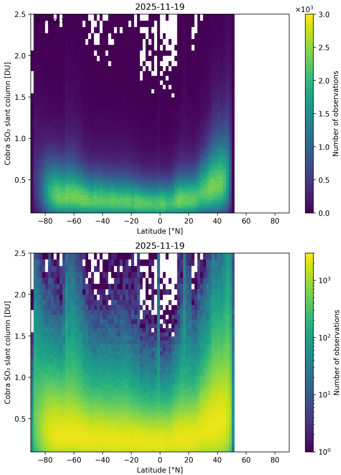
Figure 157: Scatter density plot of “Latitude” against “Cobra SO 2 slant column” for 2025-11-18 to 2025-11-20.
