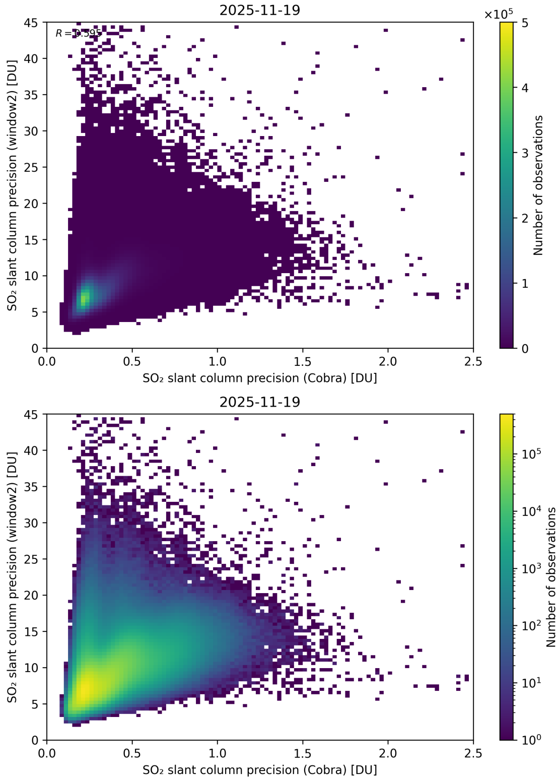
Figure 210: Scatter density plot of “SO 2 slant column precision (Cobra)” against “SO 2 slant column precision (window2)” for 2025-11-18 to 2025-11-20.
