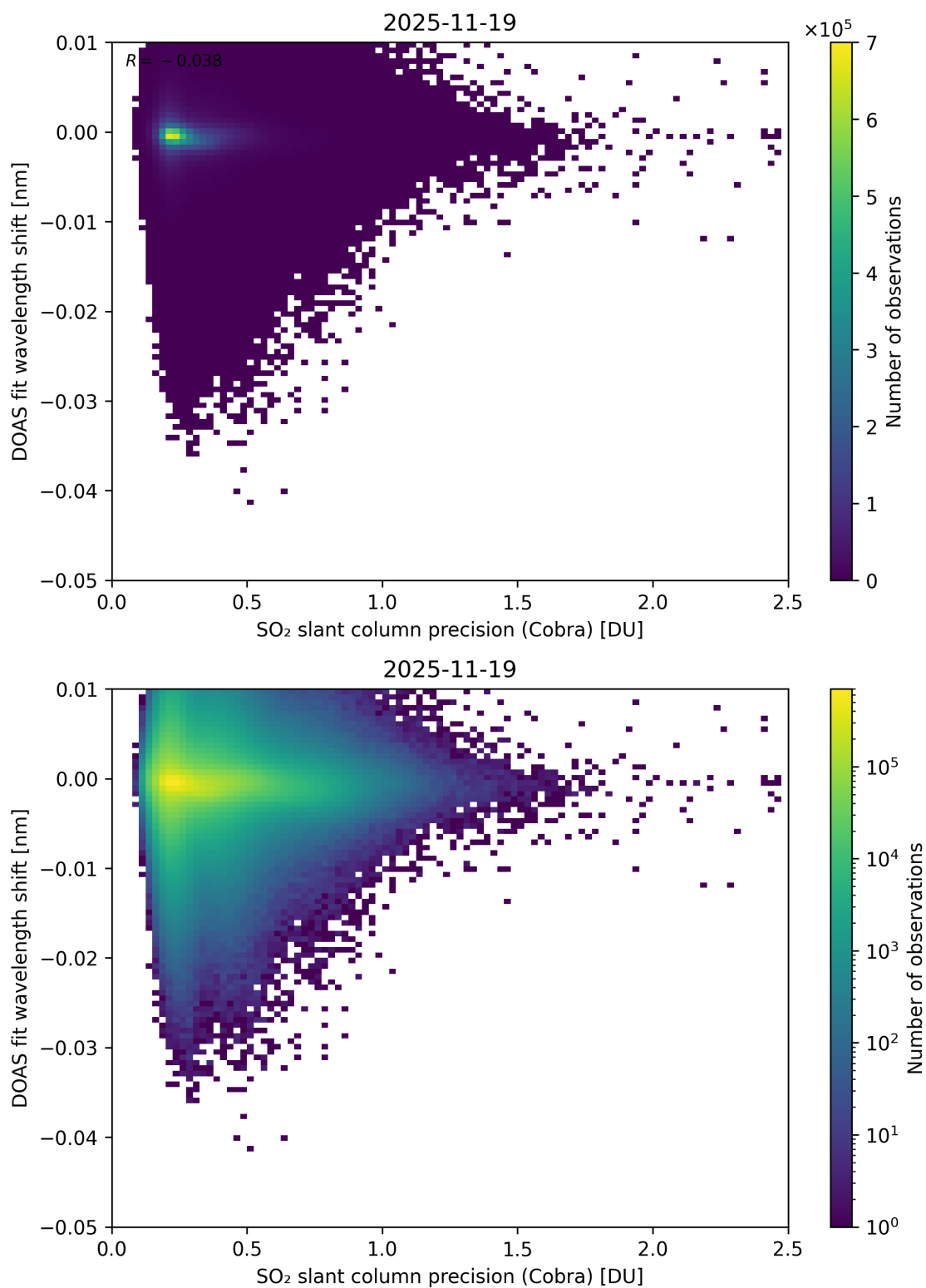
Figure 202: Scatter density plot of “SO 2 slant column precision (Cobra)” against “DOAS fit wavelength shift” for 2025-11-18 to 2025-11-20.
