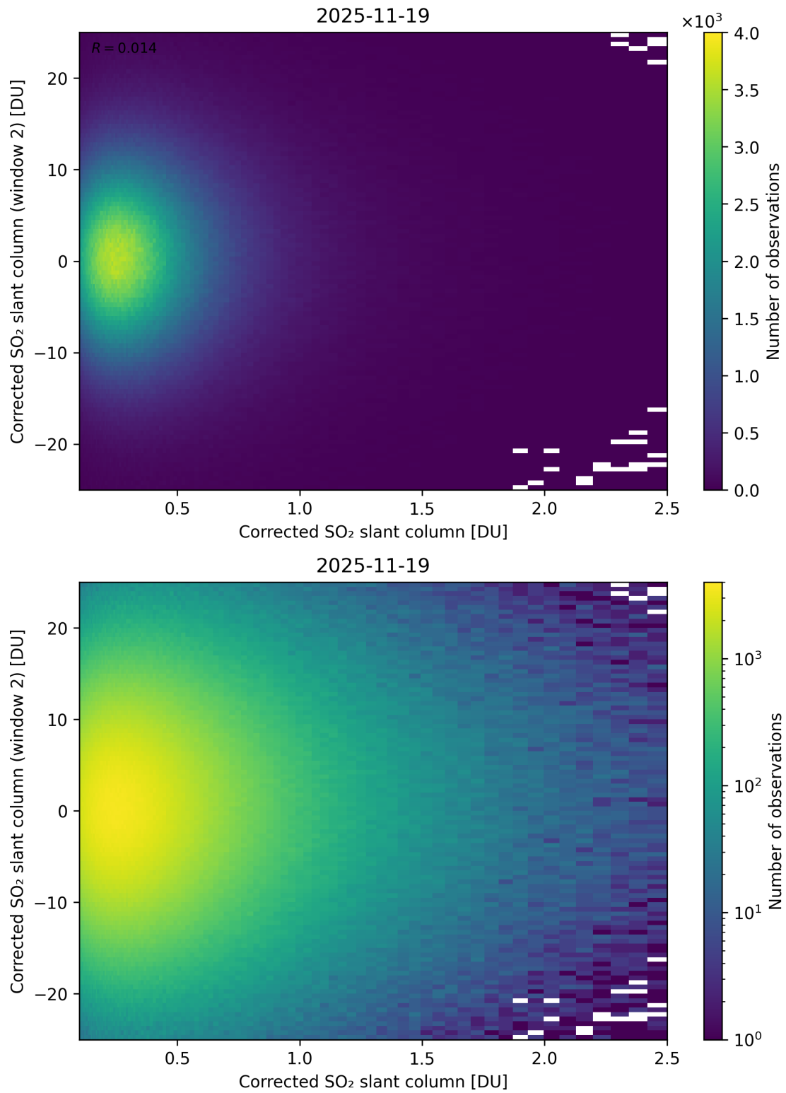
Figure 235: Scatter density plot of “Corrected SO 2 slant column” against “Corrected SO 2 slant column (window 2)” for 2025-11-18 to 2025-11-20.
