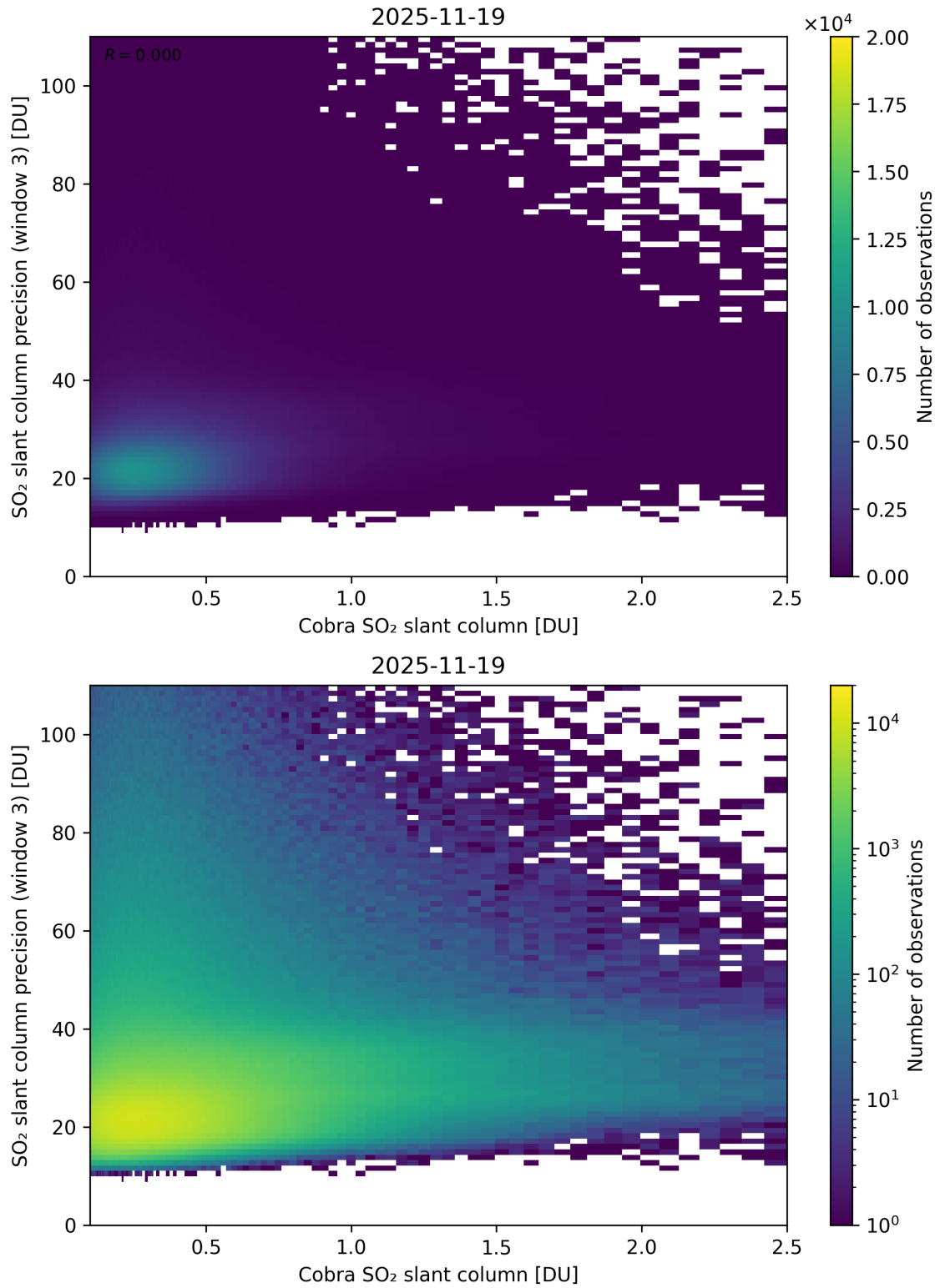
Figure 223: Scatter density plot of “Cobra SO 2 slant column” against “SO 2 slant column precision (window 3)” for 2025-11-18 to 2025-11-20.
