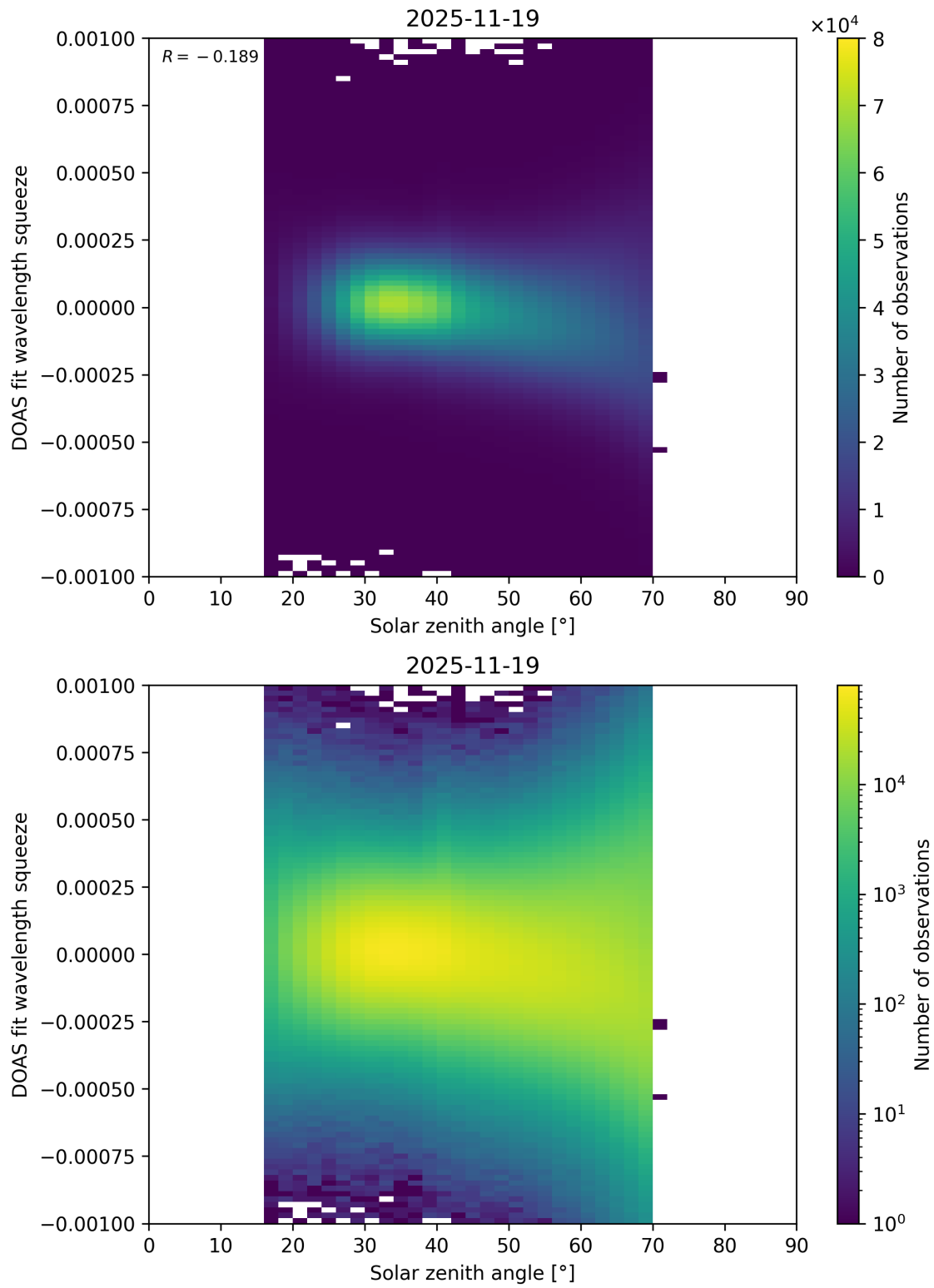
Figure 175: Scatter density plot of “Solar zenith angle” against “DOAS fit wavelength squeeze” for 2025-11-18 to 2025-11-20.
