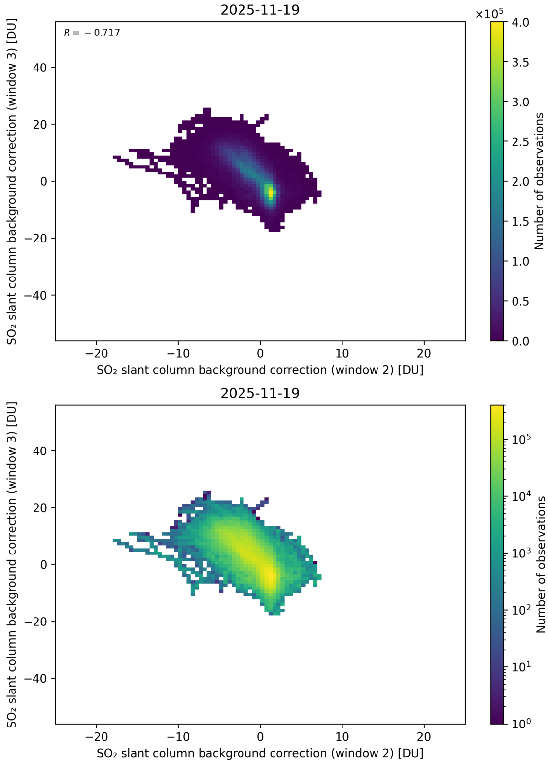
Figure 122: Scatter density plot of “SO 2 slant column background correction (window 2)” against “SO 2 slant column background correction (window 3)” for 2025-11-18 to 2025-11-20.
