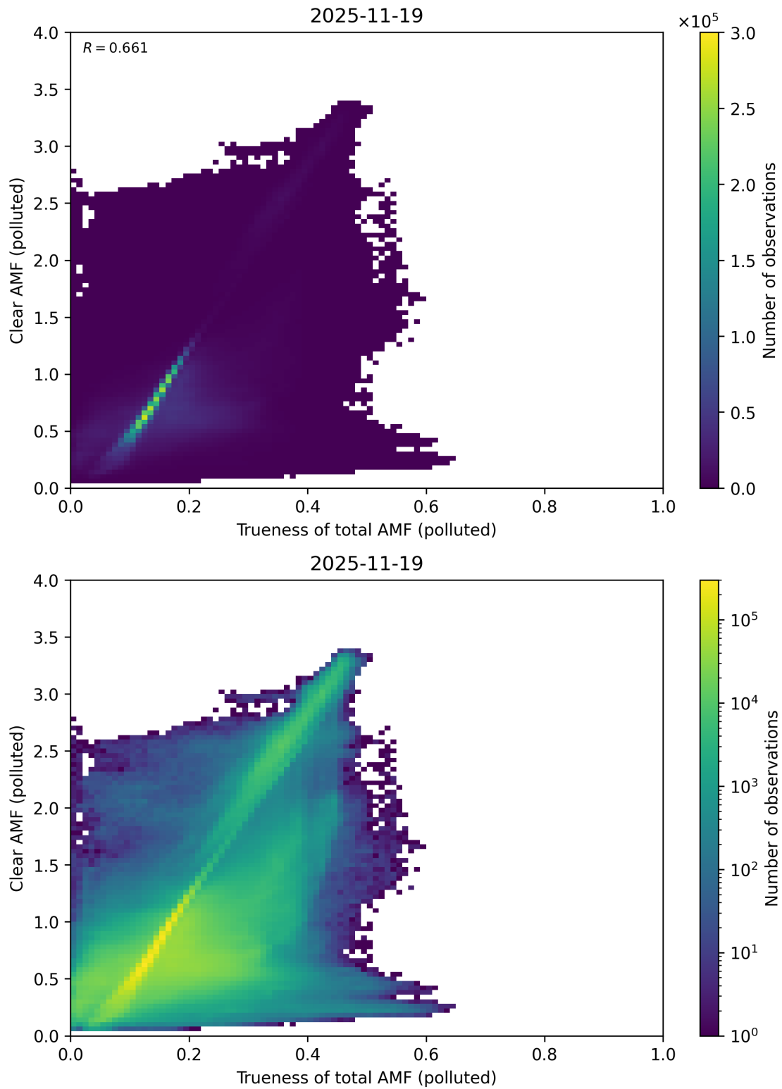
Figure 322: Scatter density plot of “Trueness of total AMF (polluted)” against “Clear AMF (polluted)” for 2025-11-18 to 2025-11-20.
