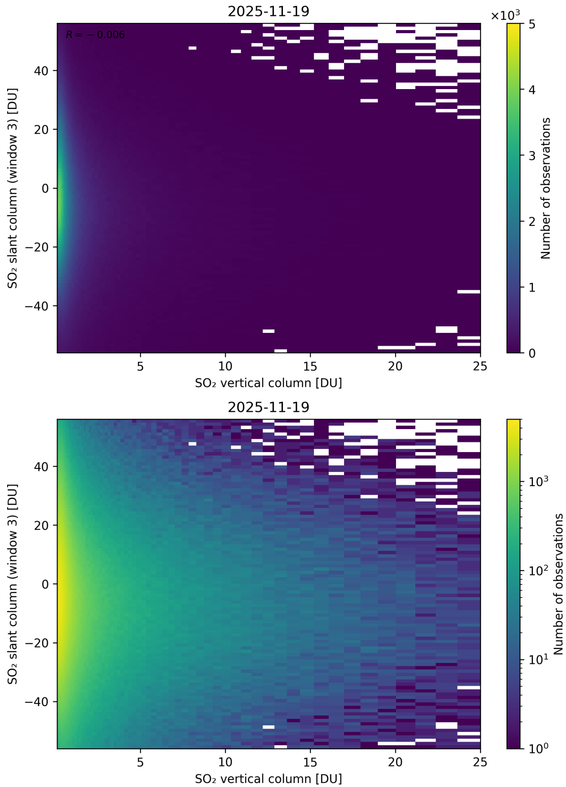
Figure 357: Scatter density plot of “SO 2 vertical column” against “SO 2 slant column (window 3)” for 2025-11-18 to 2025-11-20.
