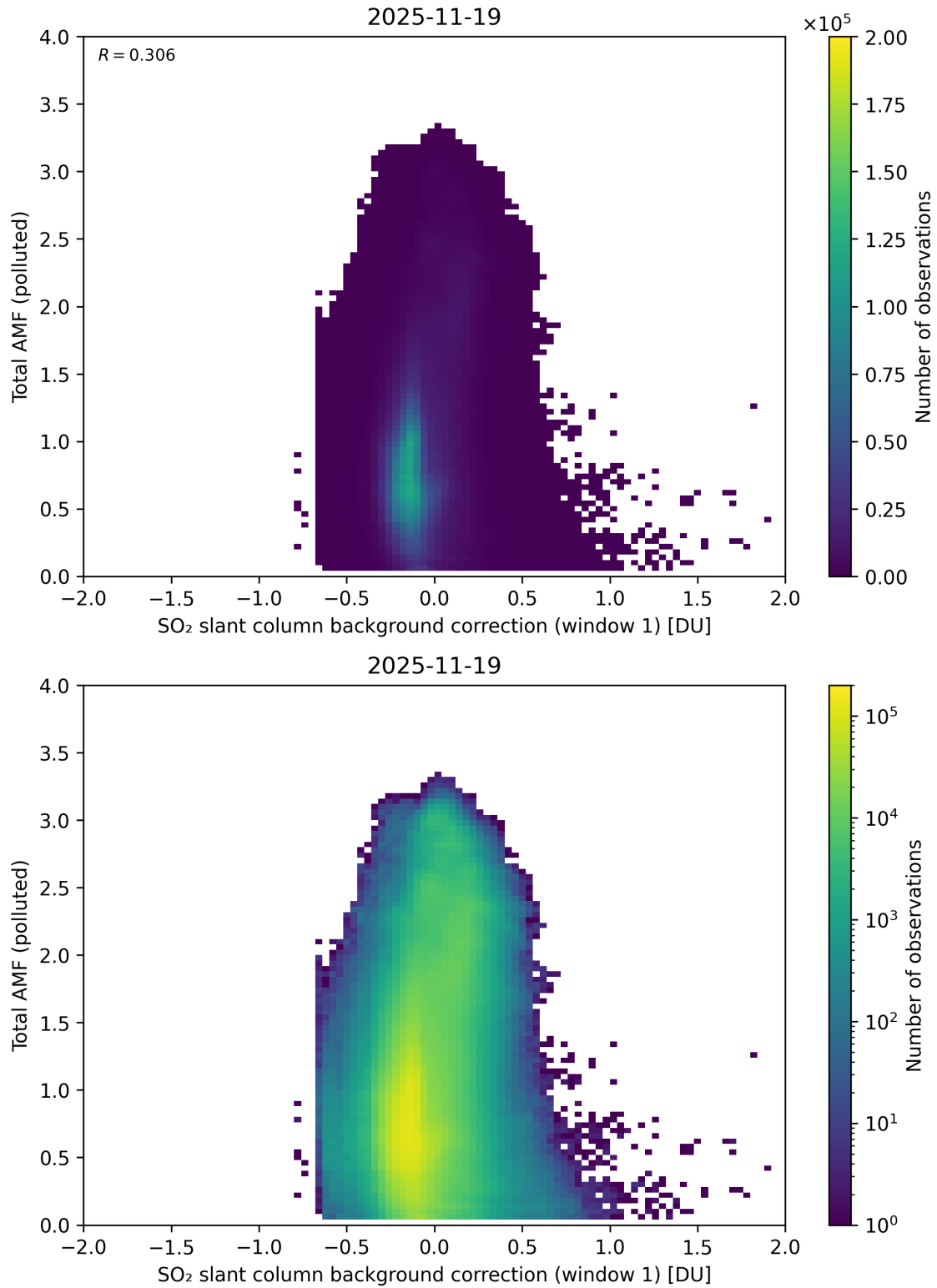
Figure 120: Scatter density plot of “SO 2 slant column background correction (window 1)” against “Total AMF (polluted)” for 2025-11-18 to 2025-11-20.
