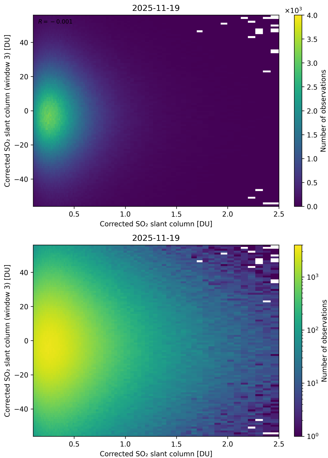
Figure 236: Scatter density plot of “Corrected SO 2 slant column” against “Corrected SO 2 slant column (window 3)” for 2025-11-18 to 2025-11-20.
