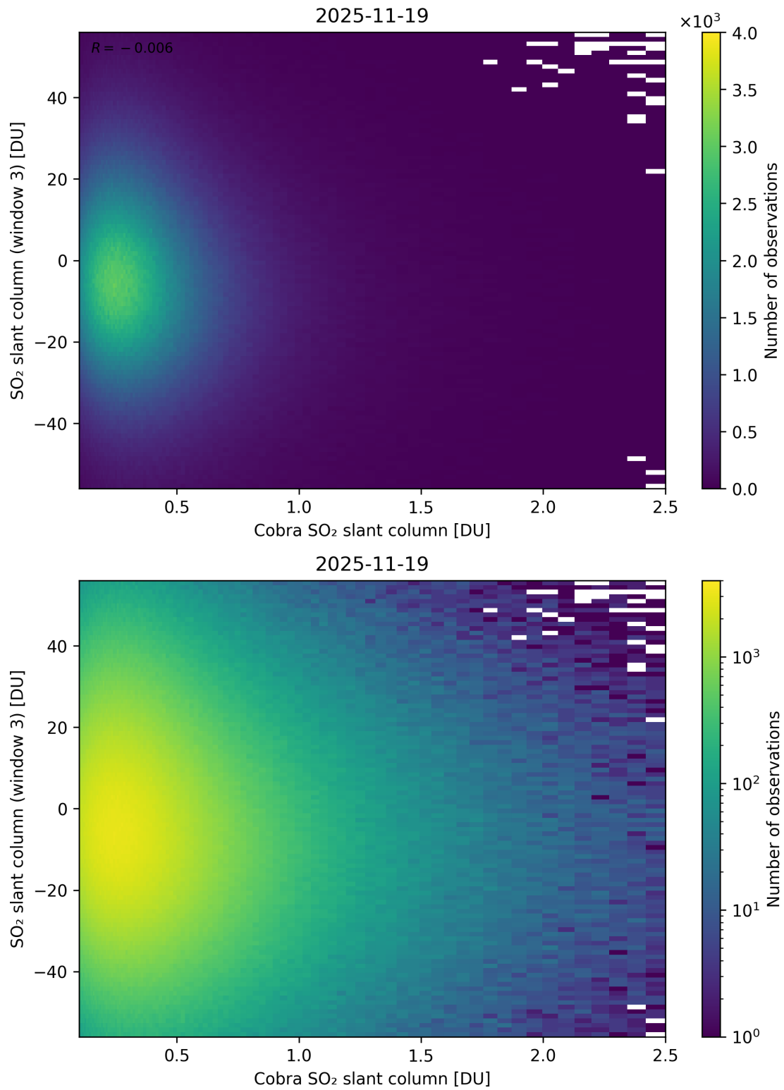
Figure 222: Scatter density plot of “Cobra SO 2 slant column” against “SO 2 slant column (window 3)” for 2025-11-18 to 2025-11-20.
