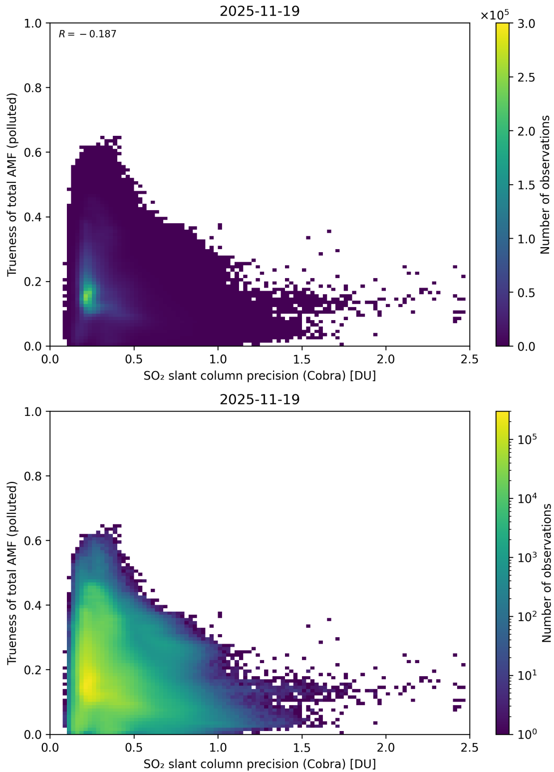
Figure 214: Scatter density plot of “SO 2 slant column precision (Cobra)” against “Trueness of total AMF (polluted)” for 2025-11-18 to 2025-11-20.
