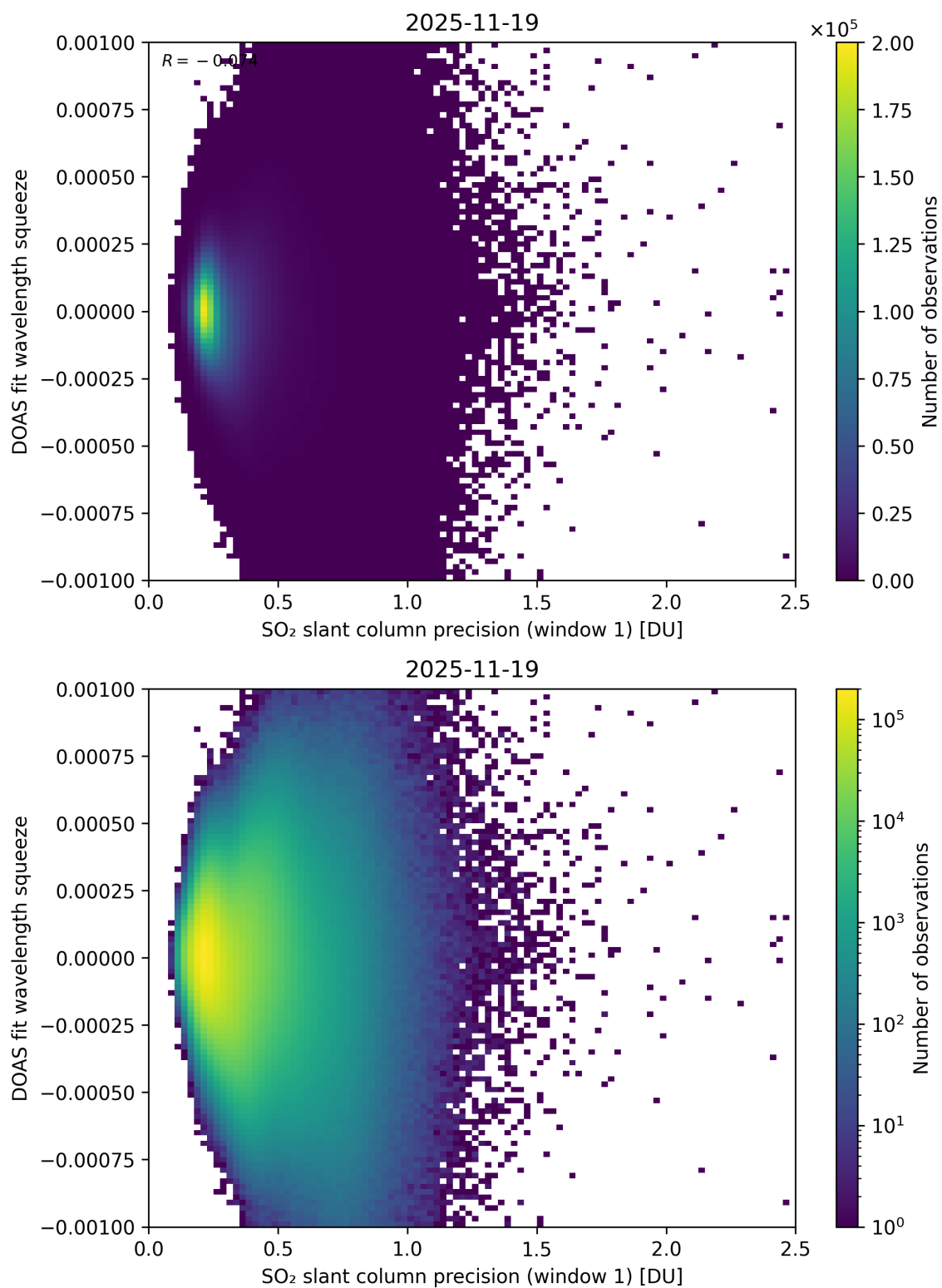
Figure 272: Scatter density plot of “SO 2 slant column precision (window 1)” against “DOAS fit wavelength squeeze” for 2025-11-18 to 2025-11-20.
