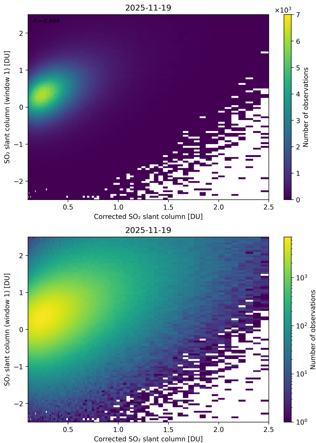
Figure 237: Scatter density plot of “Corrected SO 2 slant column” against “SO 2 slant column (window 1)” for 2025-11-18 to 2025-11-20.
