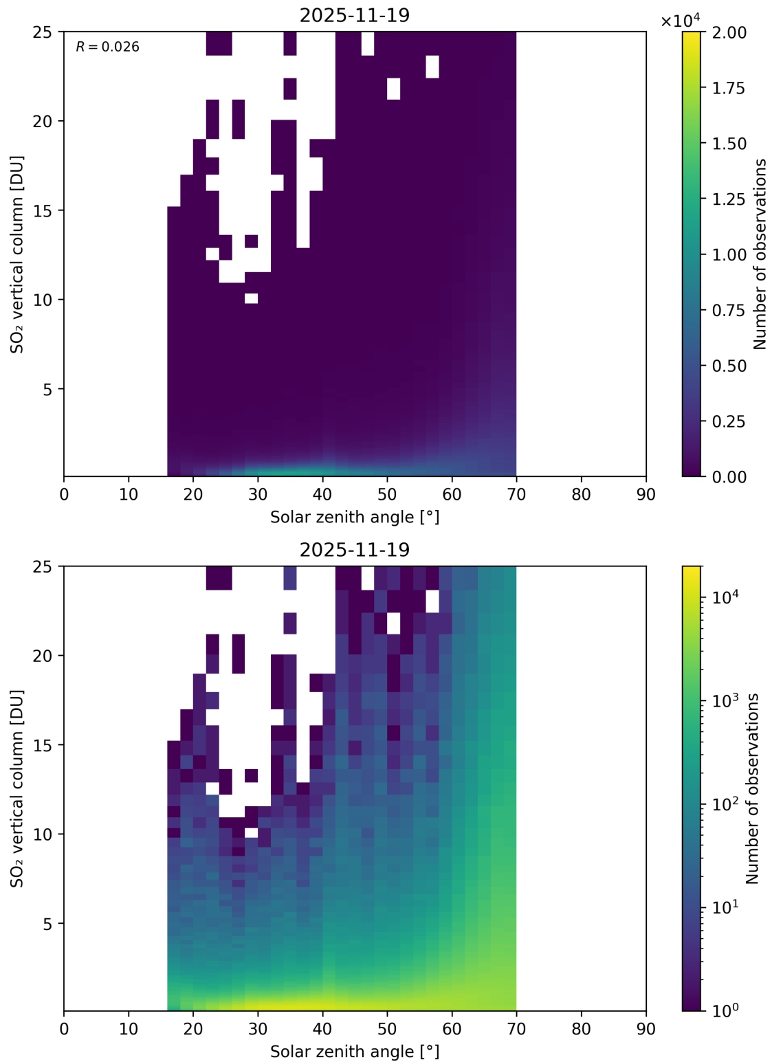
Figure 191: Scatter density plot of “Solar zenith angle” against “SO 2 vertical column” for 2025-11-18 to 2025-11-20.
