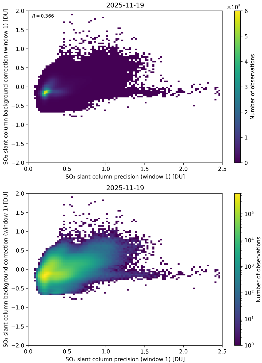
Figure 268: Scatter density plot of “SO 2 slant column precision (window 1)” against “SO 2 slant column background correction (window 1)” for 2025-11-18 to 2025-11-20.
