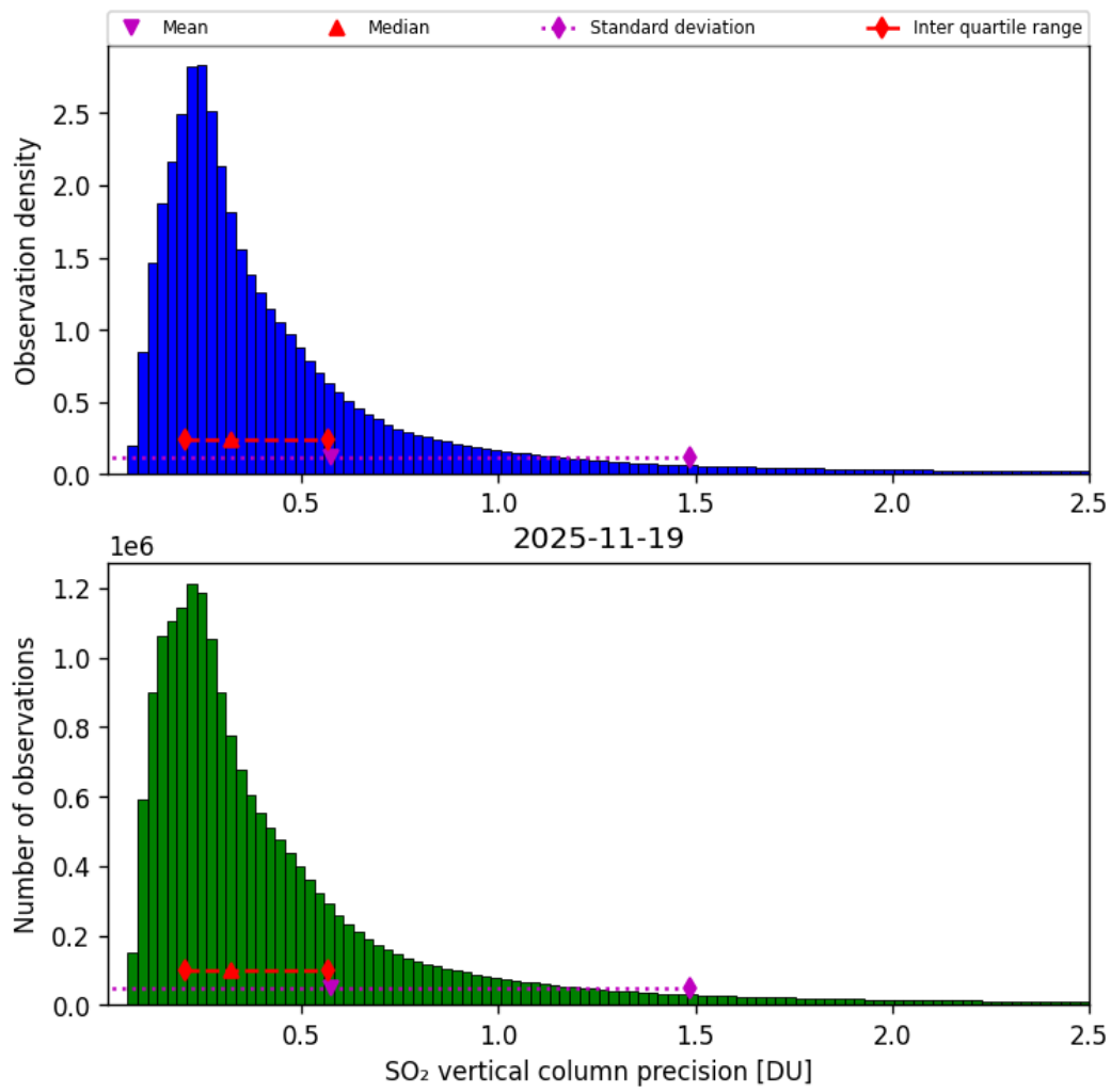
Figure 59: Histogram of “SO 2 vertical column precision” for 2025-11-18 to 2025-11-20
