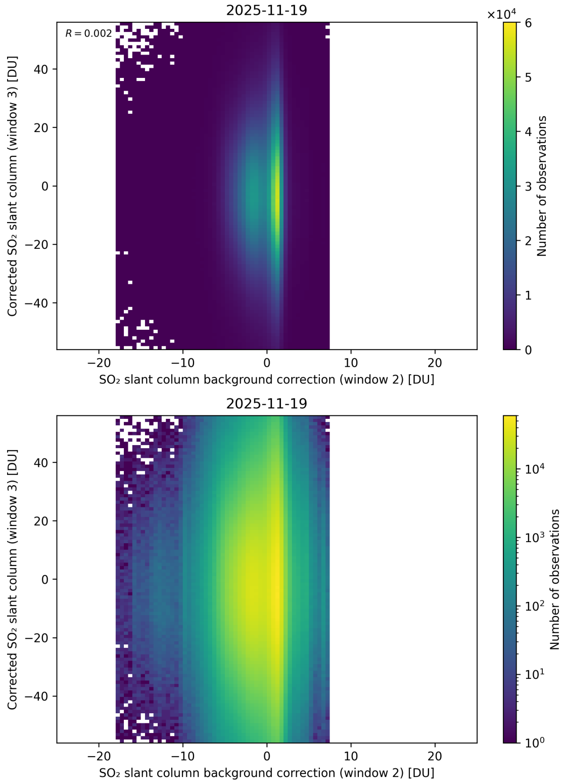
Figure 127: Scatter density plot of “SO 2 slant column background correction (window 2)” against “Corrected SO 2 slant column (window 3)” for 2025-11-18 to 2025-11-20.
