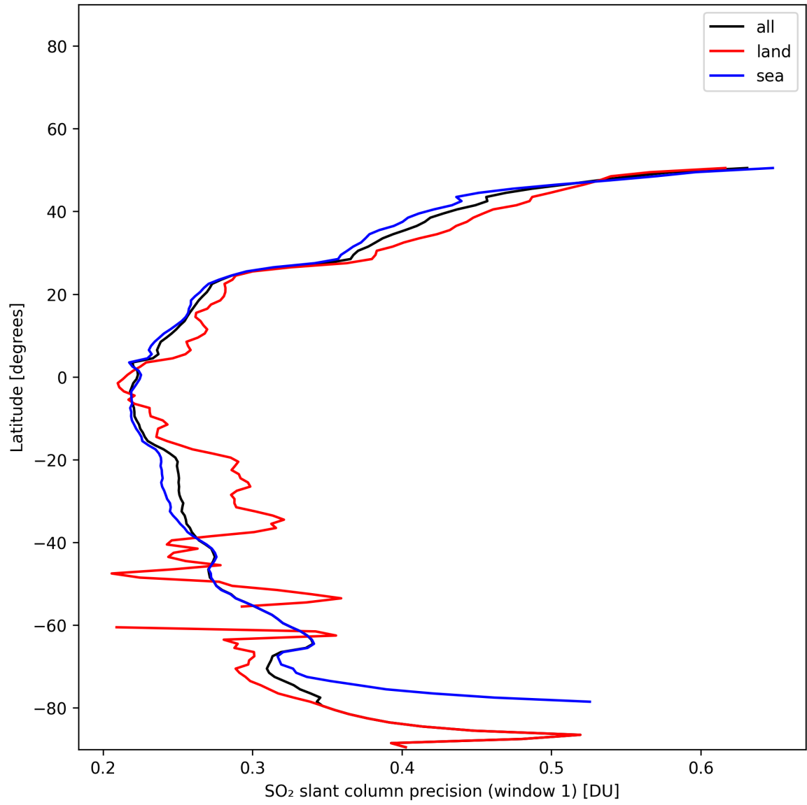
Figure 38: Zonal average of “SO 2 slant column precision (window 1)” for 2025-11-18 to 2025-11-20.
