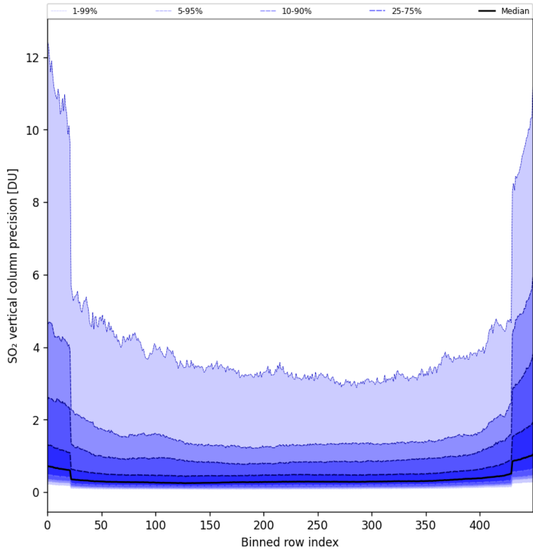
Figure 85: Along track statistics of “SO 2 vertical column precision” for 2025-11-18 to 2025-11-20
