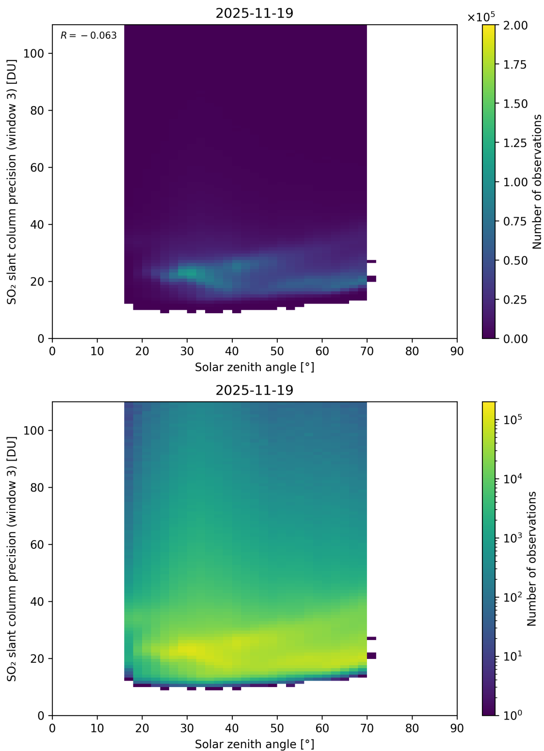
Figure 188: Scatter density plot of “Solar zenith angle” against “SO 2 slant column precision (window 3)” for 2025-11-18 to 2025-11-20.
