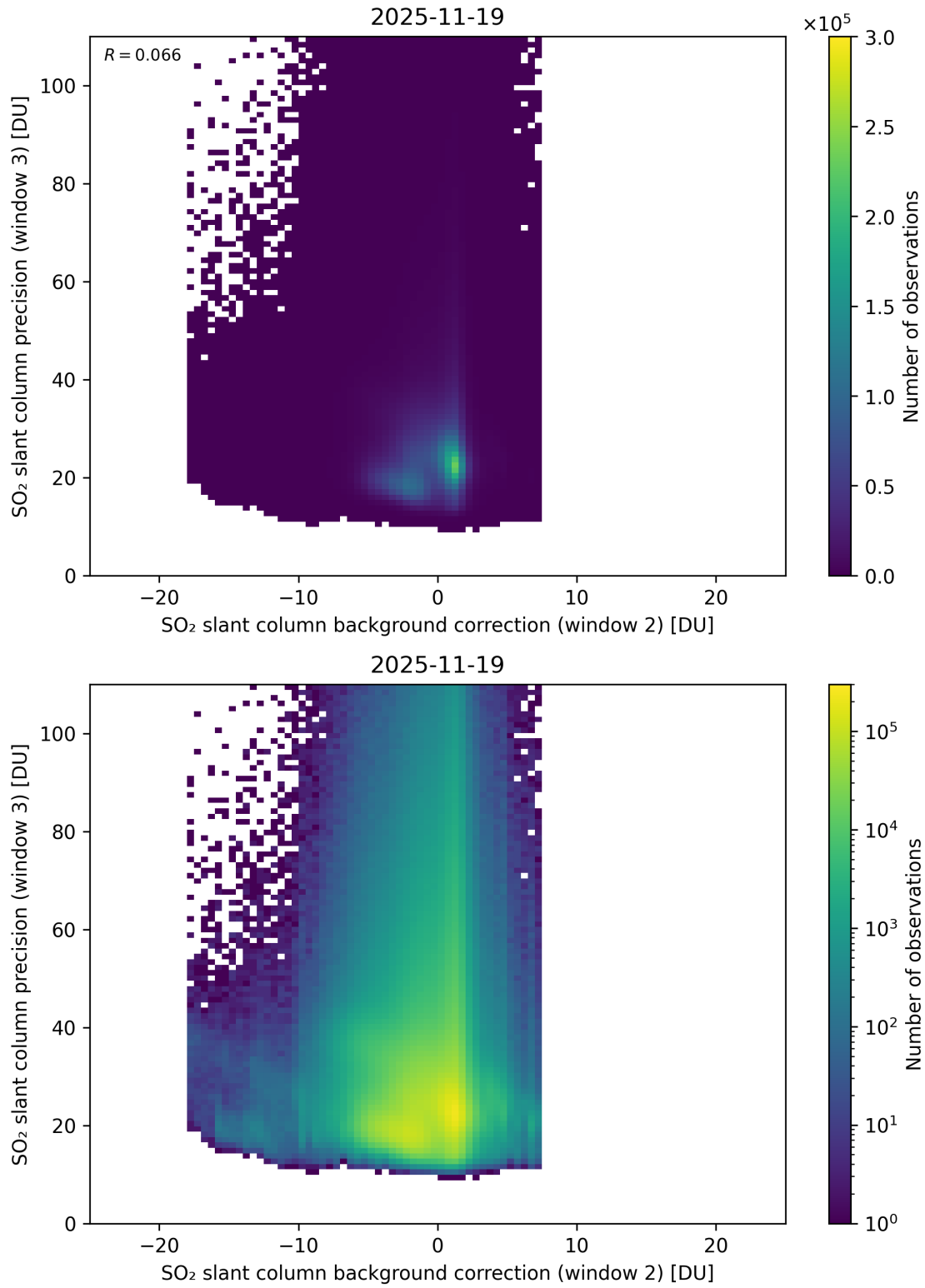
Figure 129: Scatter density plot of “SO 2 slant column background correction (window 2)” against “SO 2 slant column precision (window 3)” for 2025-11-18 to 2025-11-20.
