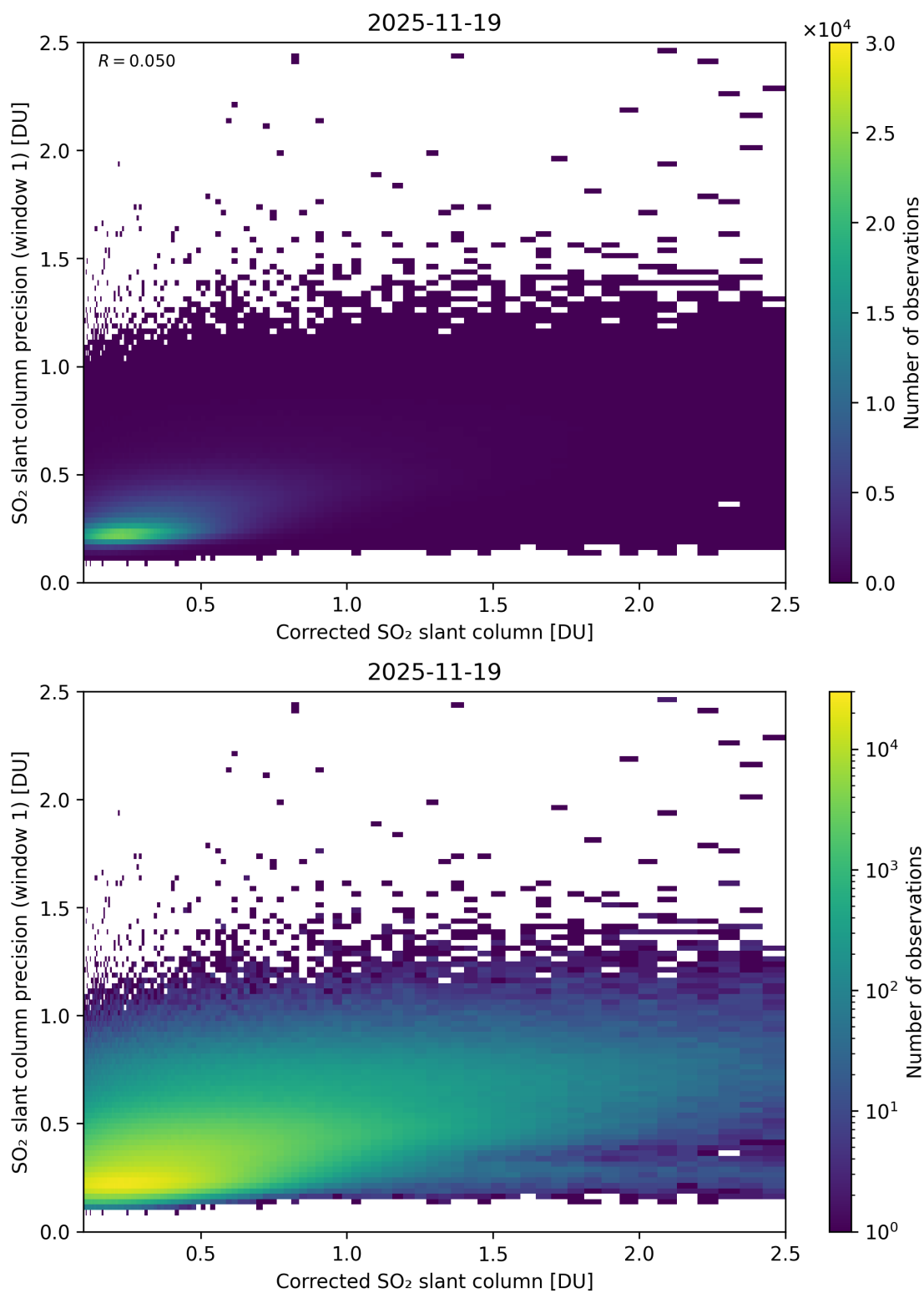
Figure 238: Scatter density plot of “Corrected SO 2 slant column” against “SO 2 slant column precision (window 1)” for 2025-11-18 to 2025-11-20.
