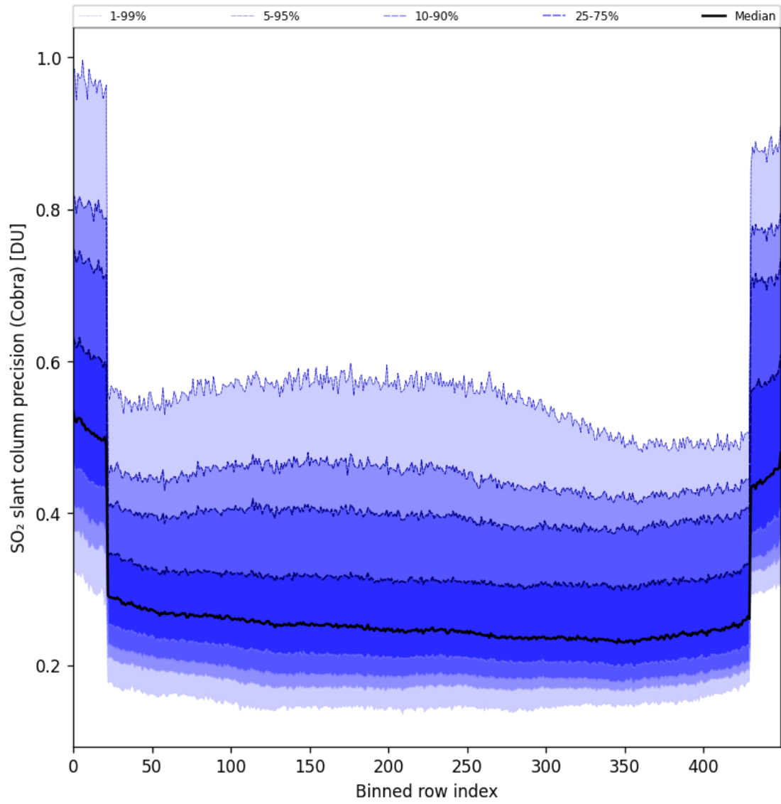
Figure 88: Along track statistics of “SO 2 slant column precision (Cobra)” for 2025-11-18 to 2025-11-20
