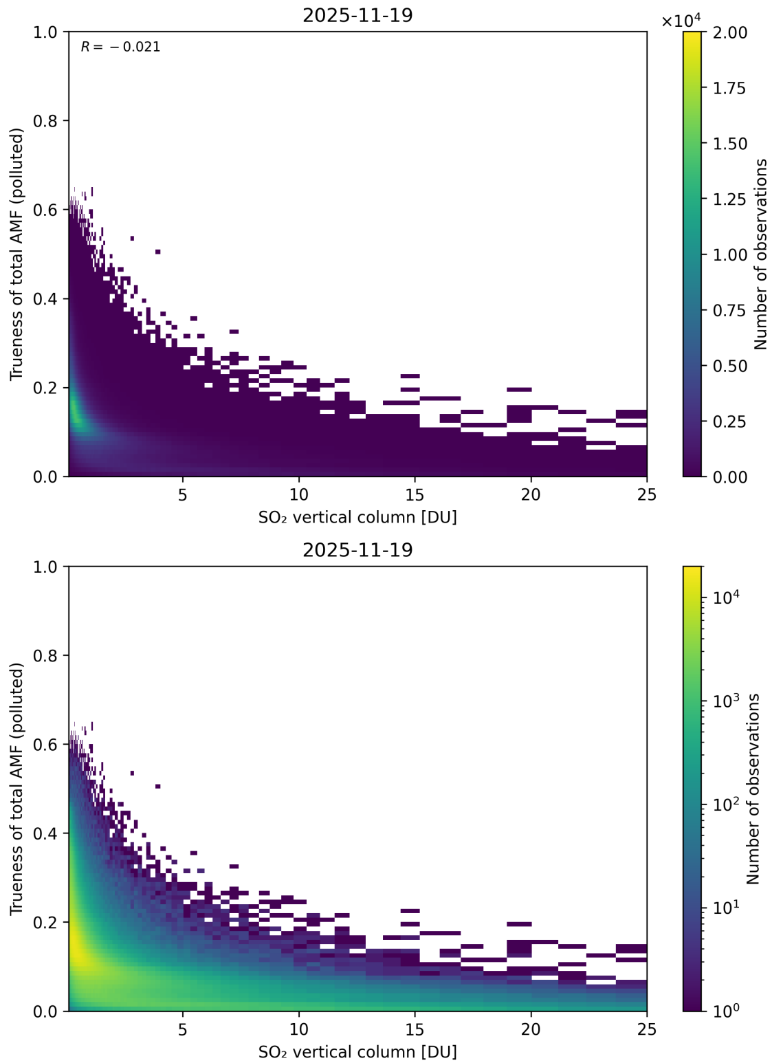
Figure 360: Scatter density plot of “SO 2 vertical column” against “Trueness of total AMF (polluted)” for 2025-11-18 to 2025-11-20.
