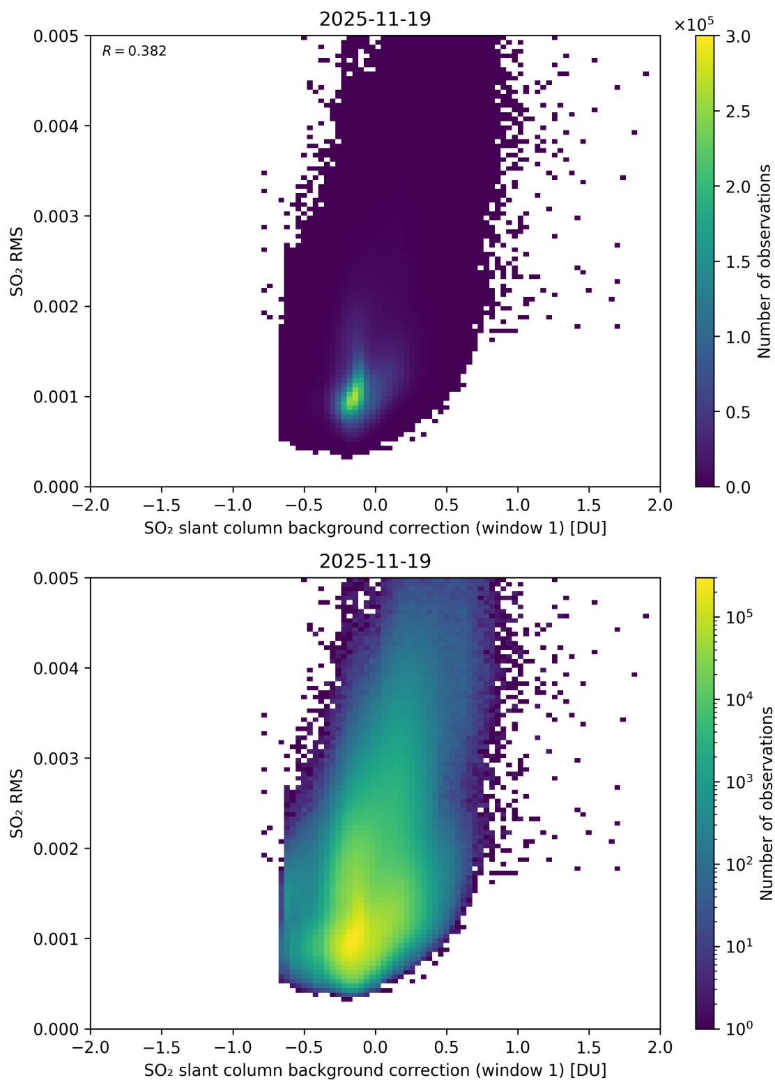
Figure 113: Scatter density plot of “SO 2 slant column background correction (window 1)” against “SO 2 RMS” for 2025-11-18 to 2025-11-20.
