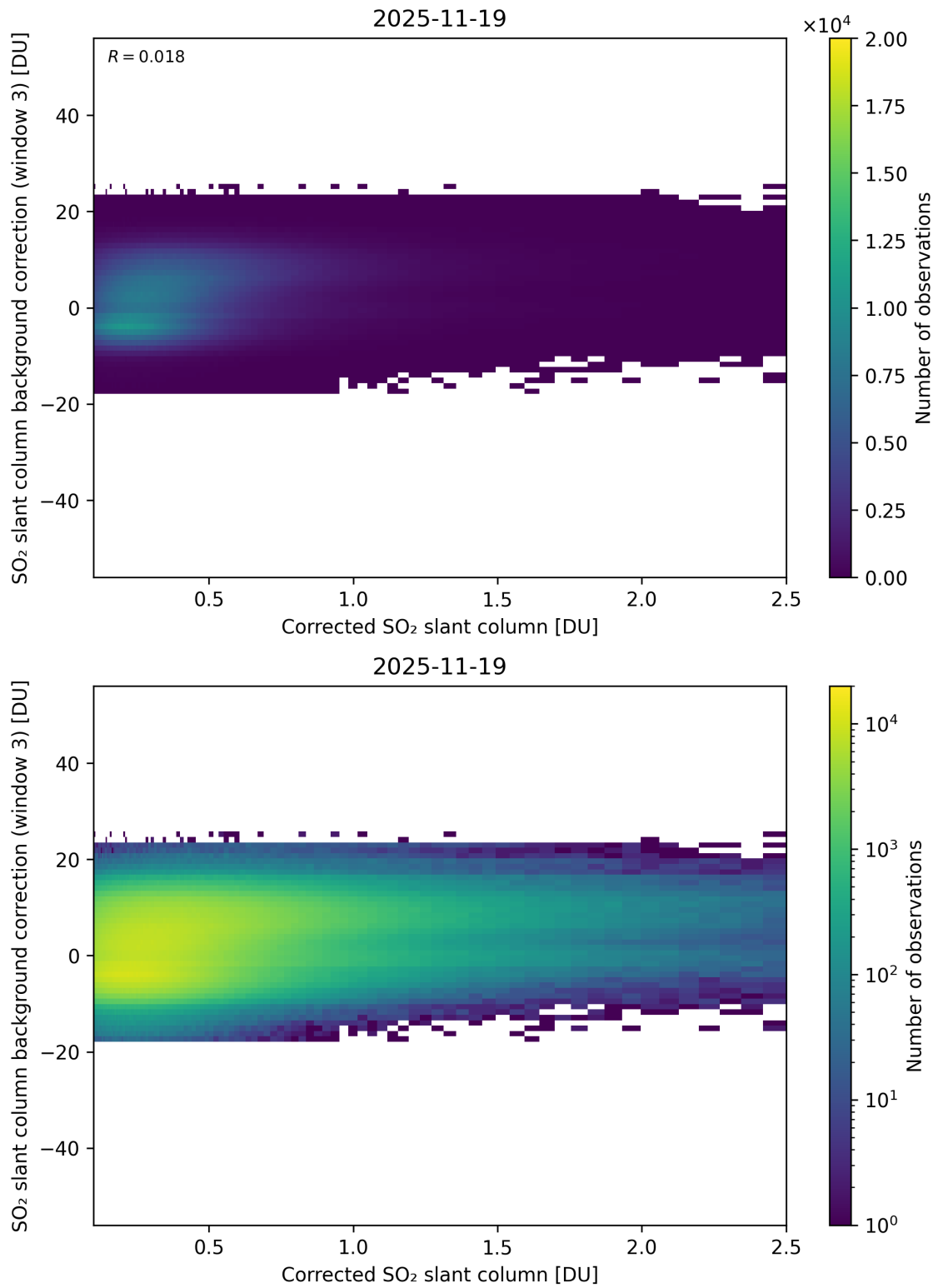
Figure 228: Scatter density plot of “Corrected SO 2 slant column” against “SO 2 slant column background correction (window 3)” for 2025-11-18 to 2025-11-20.
