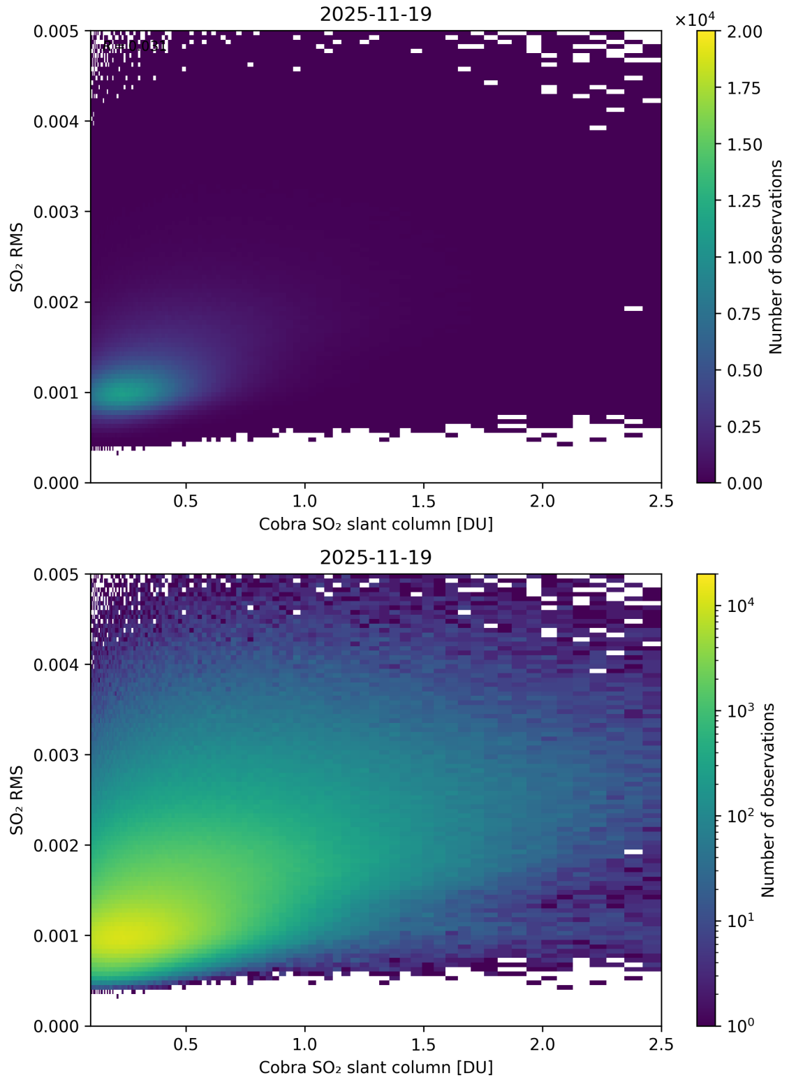
Figure 198: Scatter density plot of “Cobra SO 2 slant column” against “SO 2 RMS” for 2025-11-18 to 2025-11-20.
