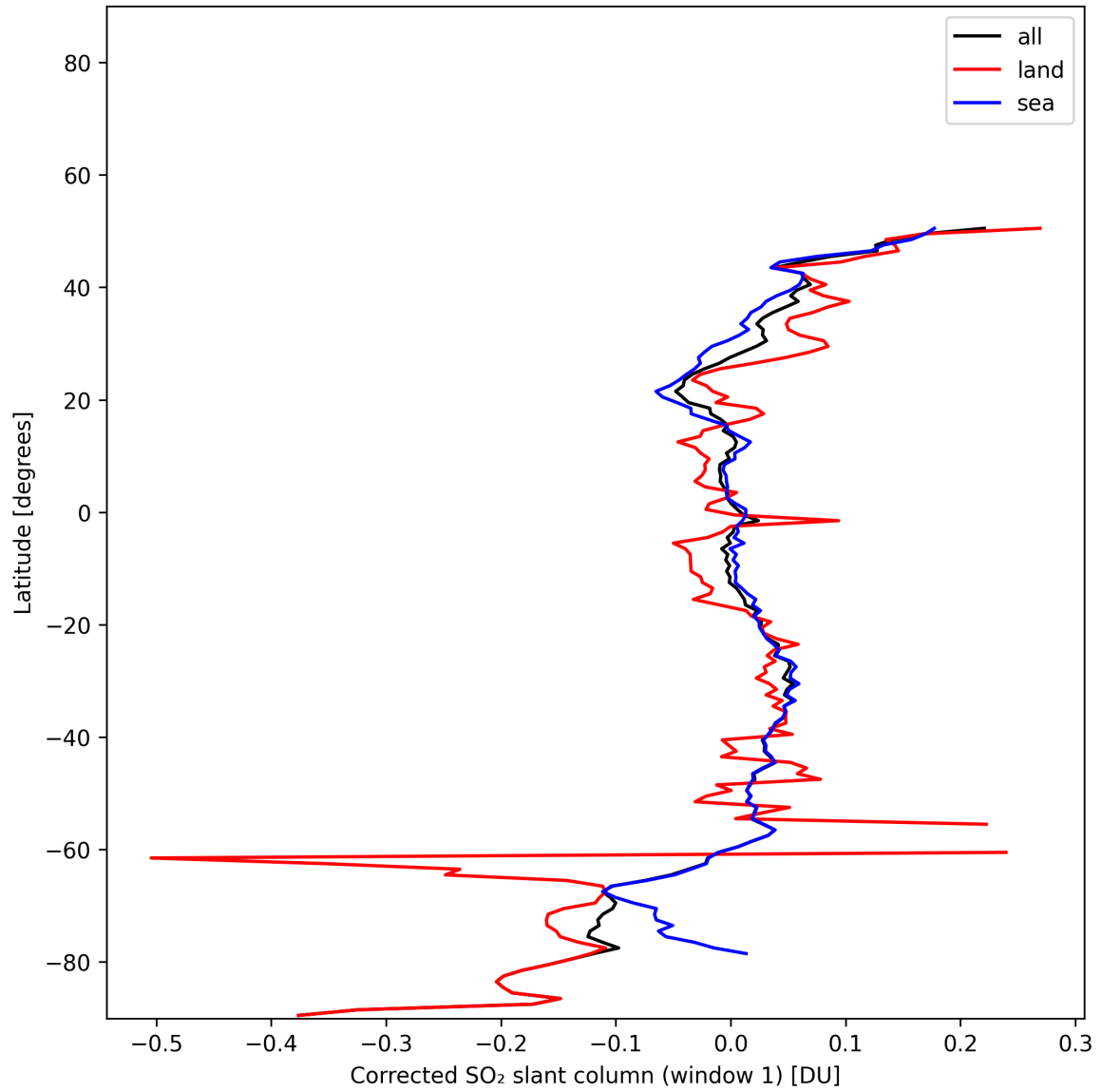
Figure 39: Zonal average of “Corrected SO 2 slant column (window 1)” for 2025-11-18 to 2025-11-20.
