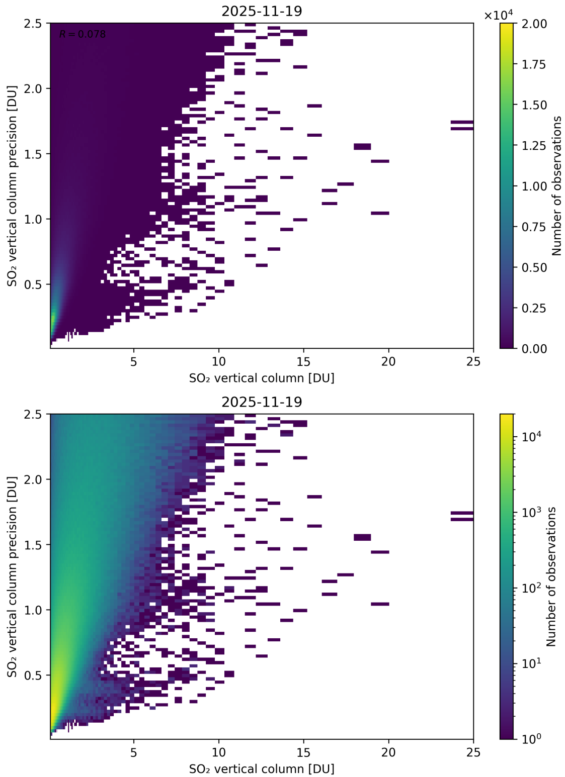
Figure 361: Scatter density plot of “SO 2 vertical column” against “SO 2 vertical column precision” for 2025-11-18 to 2025-11-20.
