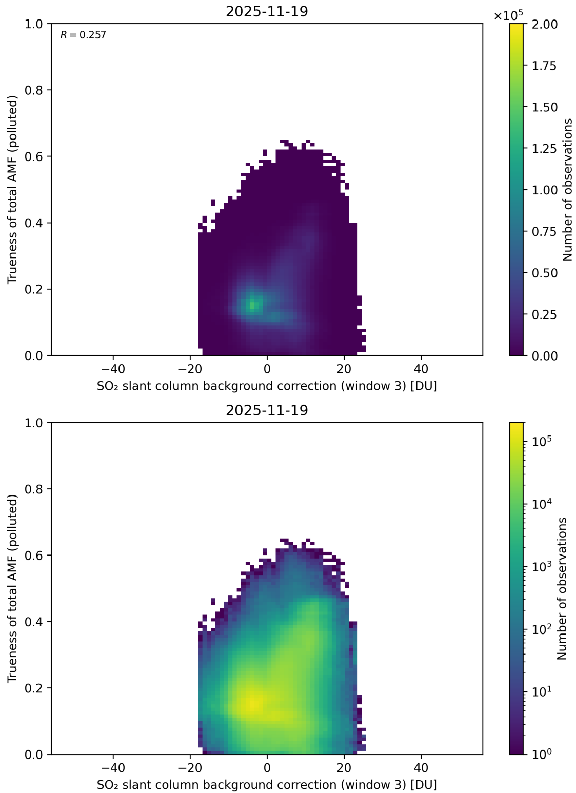
Figure 137: Scatter density plot of “SO 2 slant column background correction (window 3)” against “Trueness of total AMF (polluted)” for 2025-11-18 to 2025-11-20.
