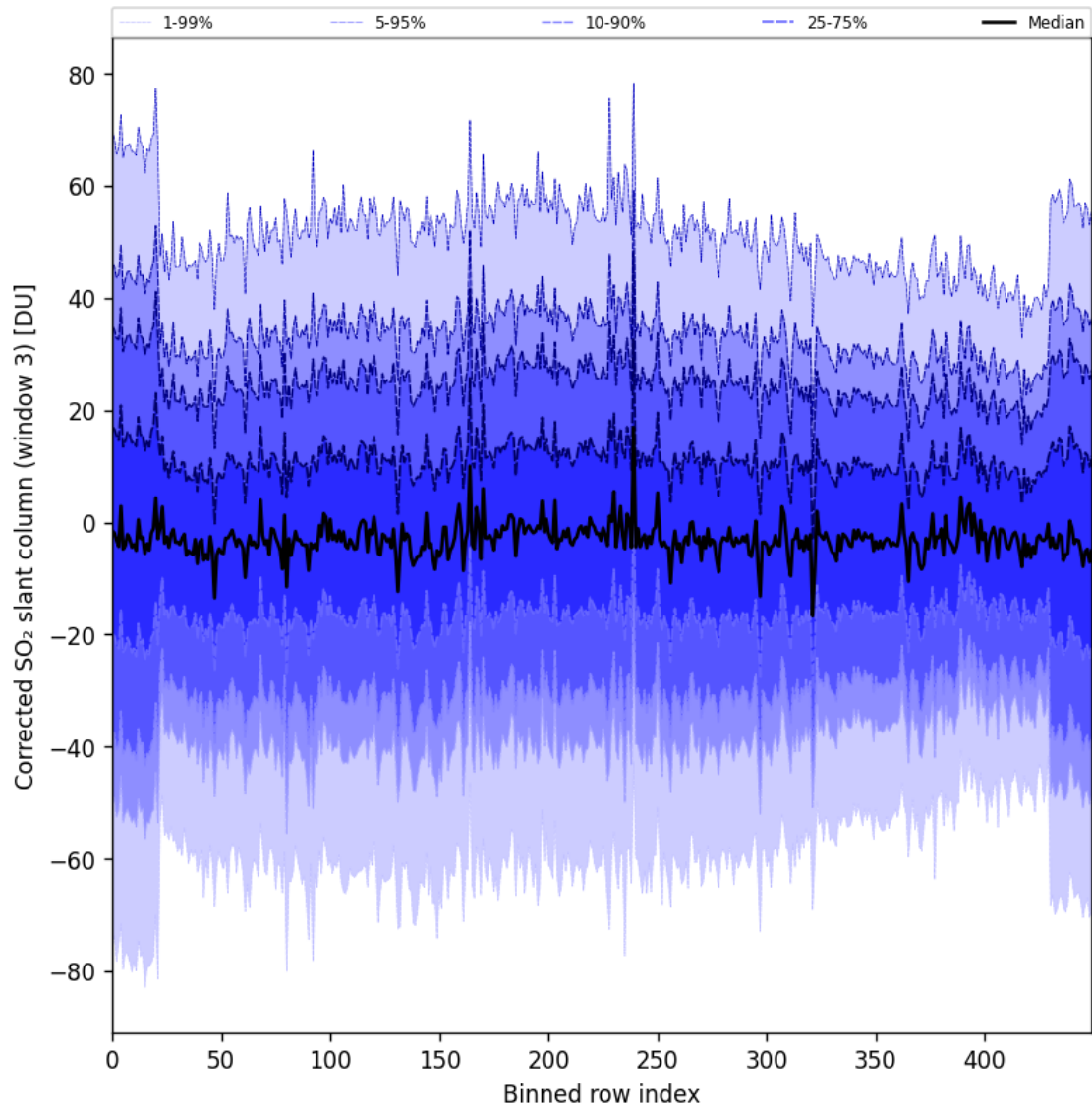
Figure 99: Along track statistics of “Corrected SO 2 slant column (window 3)” for 2025-11-18 to 2025-11-20
