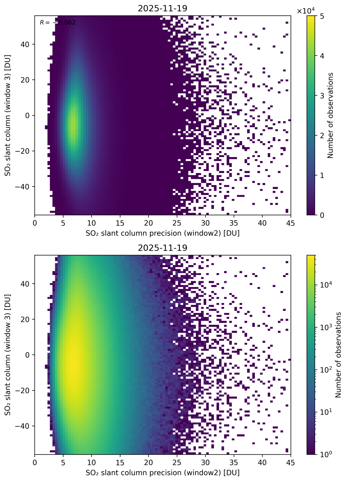
Figure 299: Scatter density plot of “SO 2 slant column precision (window2)” against “SO 2 slant column (window 3)” for 2025-11-18 to 2025-11-20.
