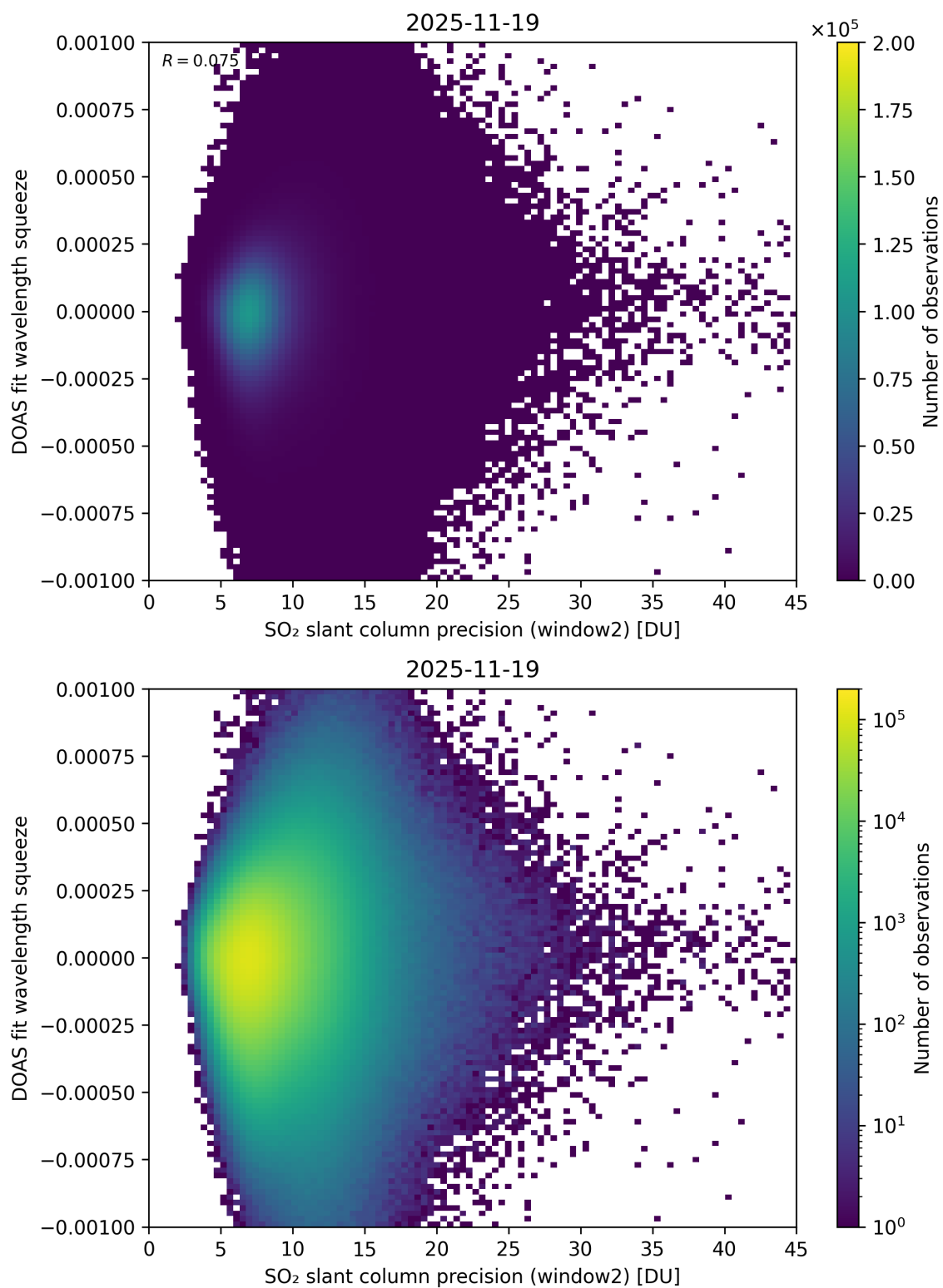
Figure 294: Scatter density plot of “SO 2 slant column precision (window2)” against “DOAS fit wavelength squeeze” for 2025-11-18 to 2025-11-20.
