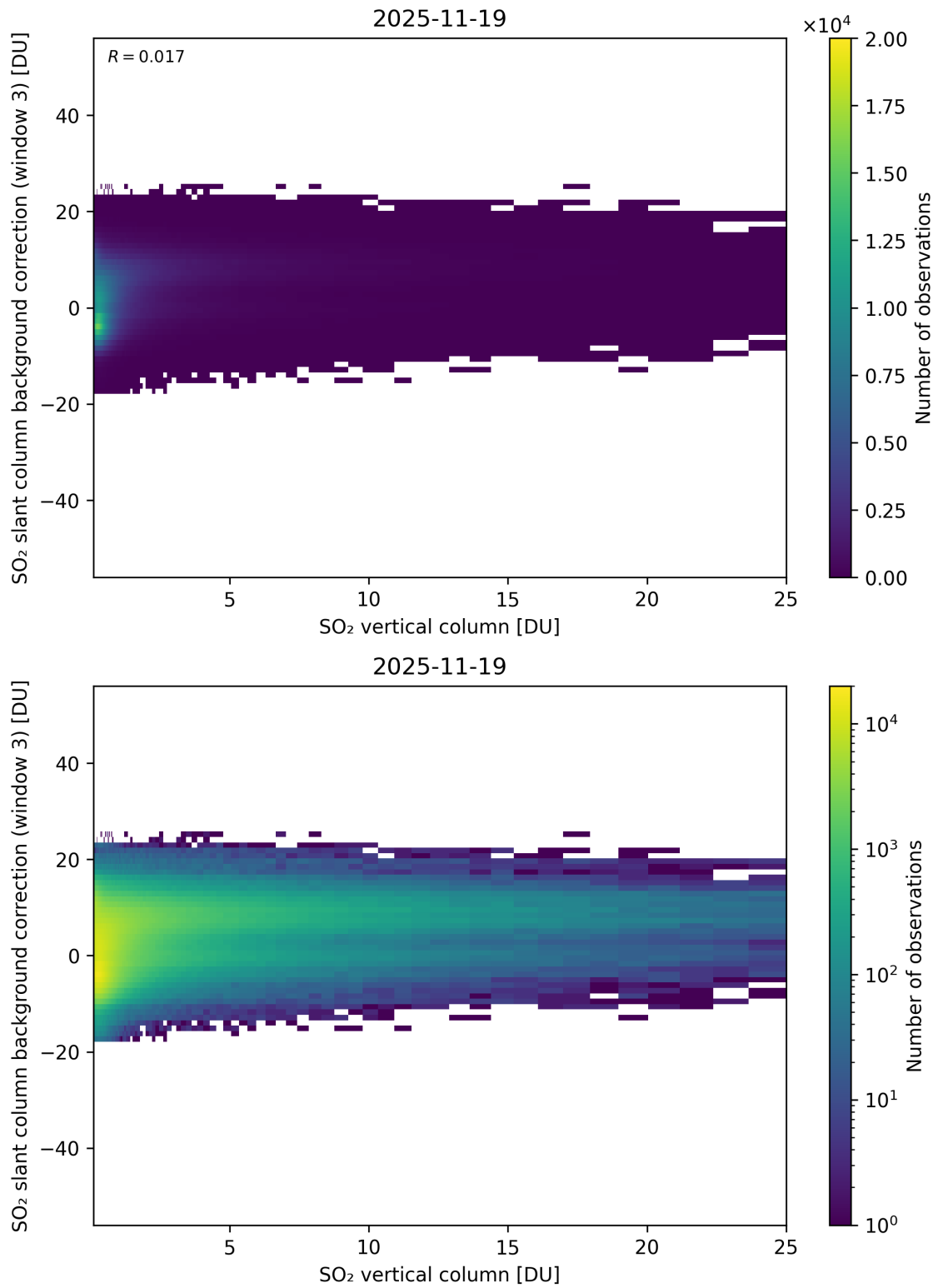
Figure 325: Scatter density plot of “SO 2 vertical column” against “SO 2 slant column background correction (window 3)” for 2025-11-18 to 2025-11-20.
