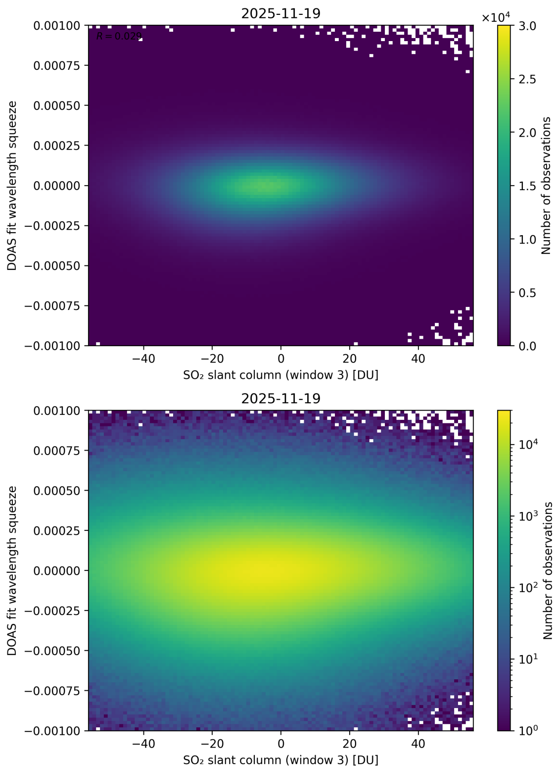
Figure 305: Scatter density plot of “SO 2 slant column (window 3)” against “DOAS fit wavelength squeeze” for 2025-11-18 to 2025-11-20.
