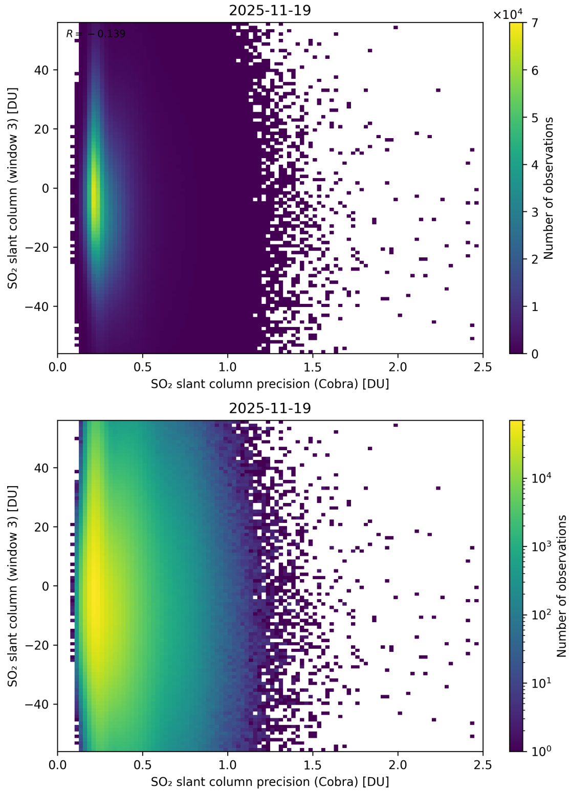
Figure 211: Scatter density plot of “SO 2 slant column precision (Cobra)” against “SO 2 slant column (window 3)” for 2025-11-18 to 2025-11-20.
