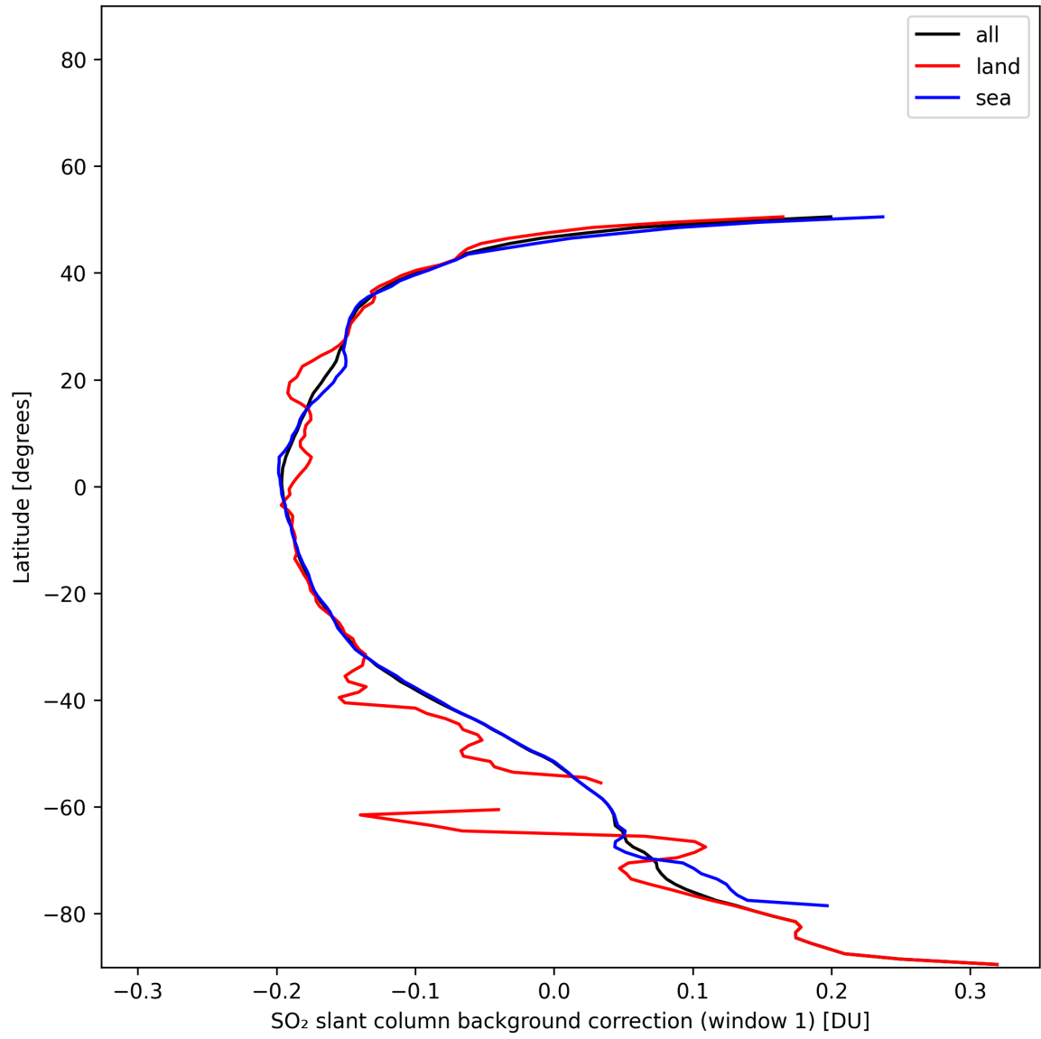
Figure 40: Zonal average of “SO 2 slant column background correction (window 1)” for 2025-11-18 to 2025-11-20.
