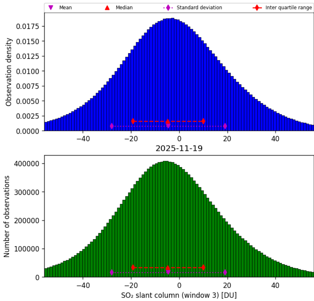
Figure 71: Histogram of “SO 2 slant column (window 3)” for 2025-11-18 to 2025-11-20
