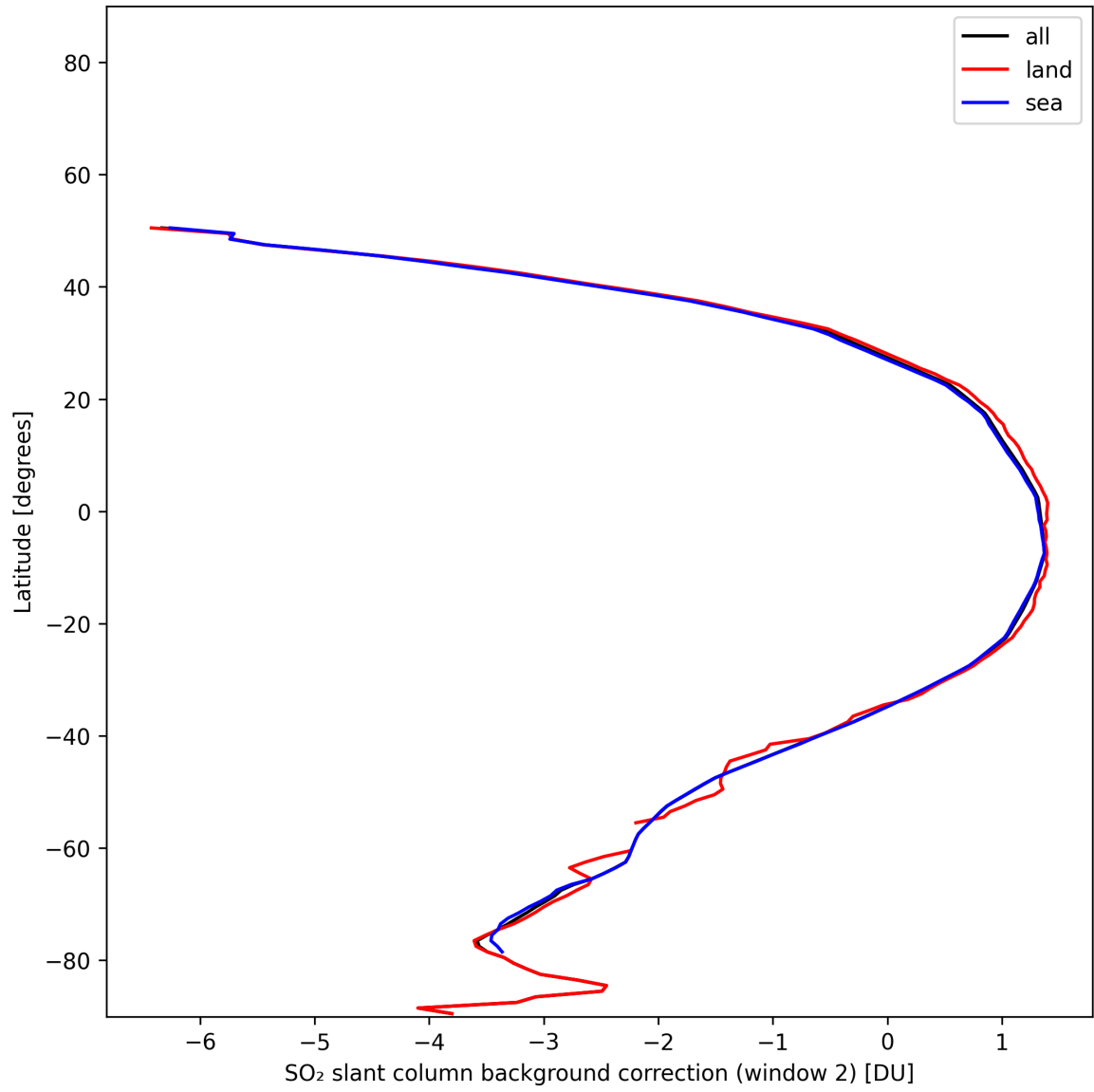
Figure 44: Zonal average of “SO 2 slant column background correction (window 2)” for 2025-11-18 to 2025-11-20.
