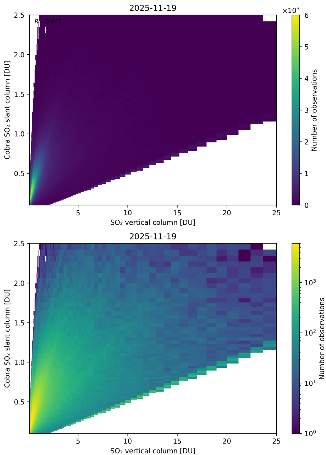
Figure 349: Scatter density plot of “SO 2 vertical column” against “Cobra SO 2 slant column” for 2025-11-18 to 2025-11-20.
