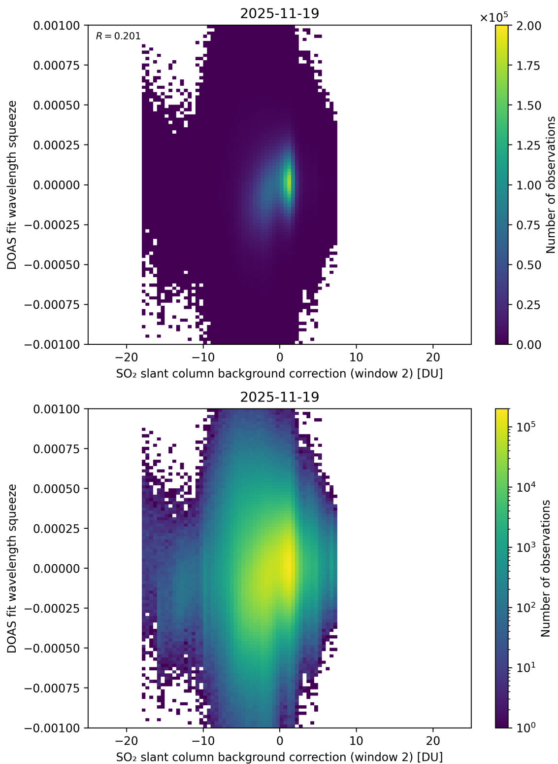
Figure 124: Scatter density plot of “SO 2 slant column background correction (window 2)” against “DOAS fit wavelength squeeze” for 2025-11-18 to 2025-11-20.
