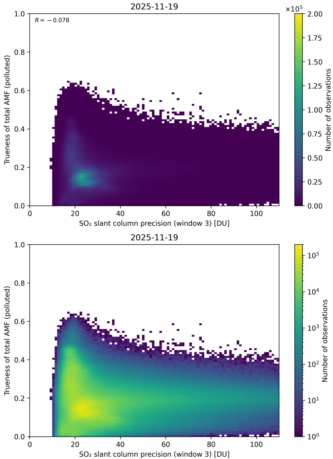
Figure 314: Scatter density plot of “SO 2 slant column precision (window 3)” against “Trueness of total AMF (polluted)” for 2025-11-18 to 2025-11-20.
