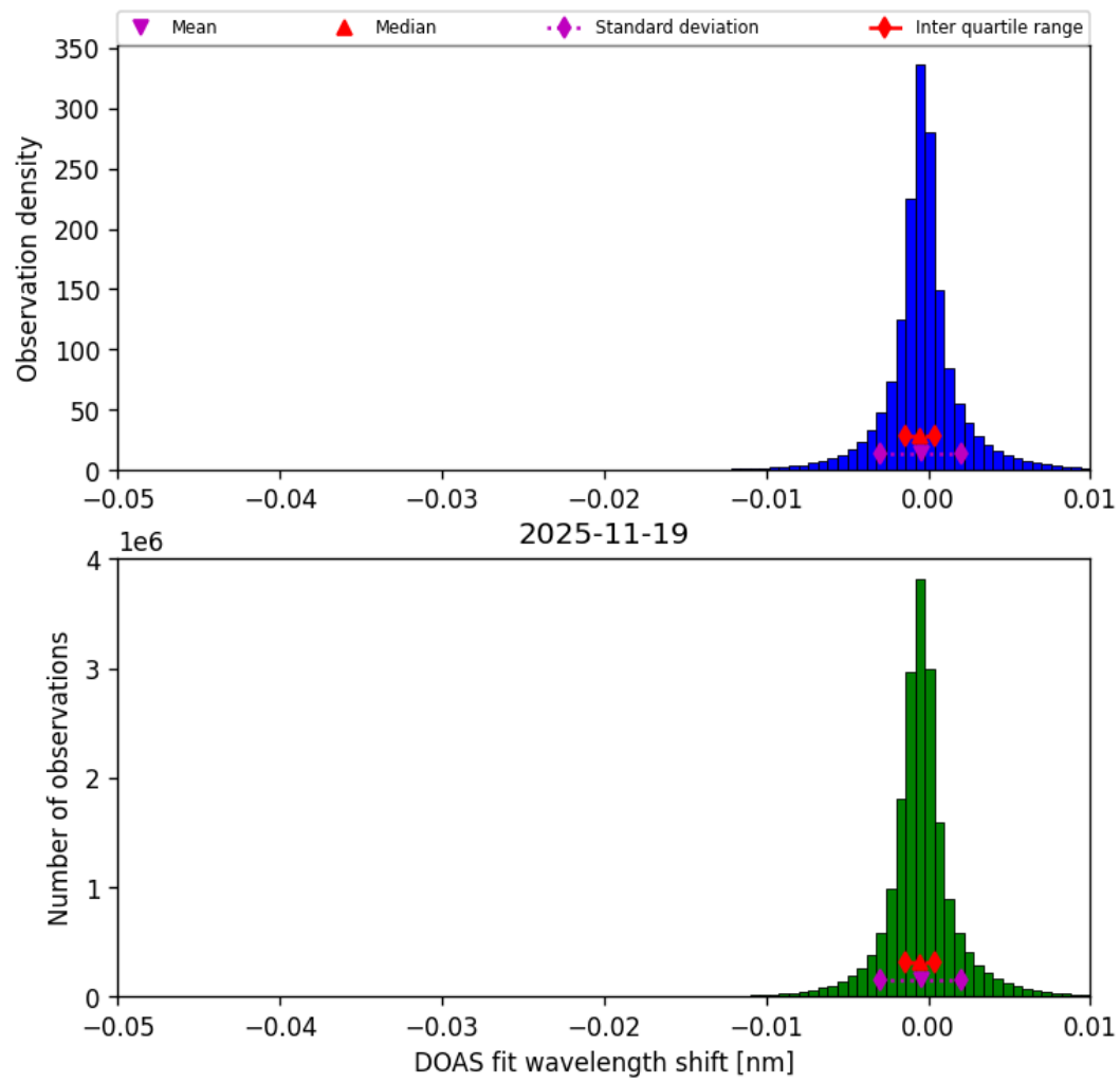
Figure 76: Histogram of “DOAS fit wavelength shift” for 2025-11-18 to 2025-11-20
