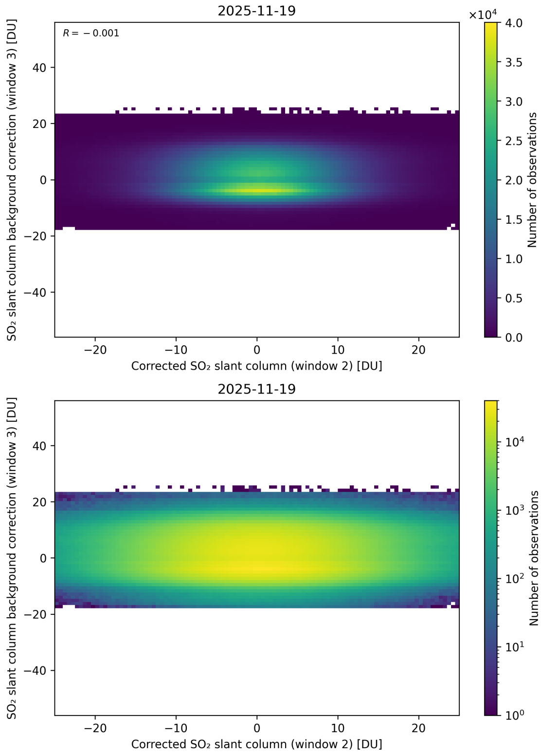
Figure 245: Scatter density plot of “Corrected SO 2 slant column (window 2)” against “SO 2 slant column background correction (window 3)” for 2025-11-18 to 2025-11-20.
