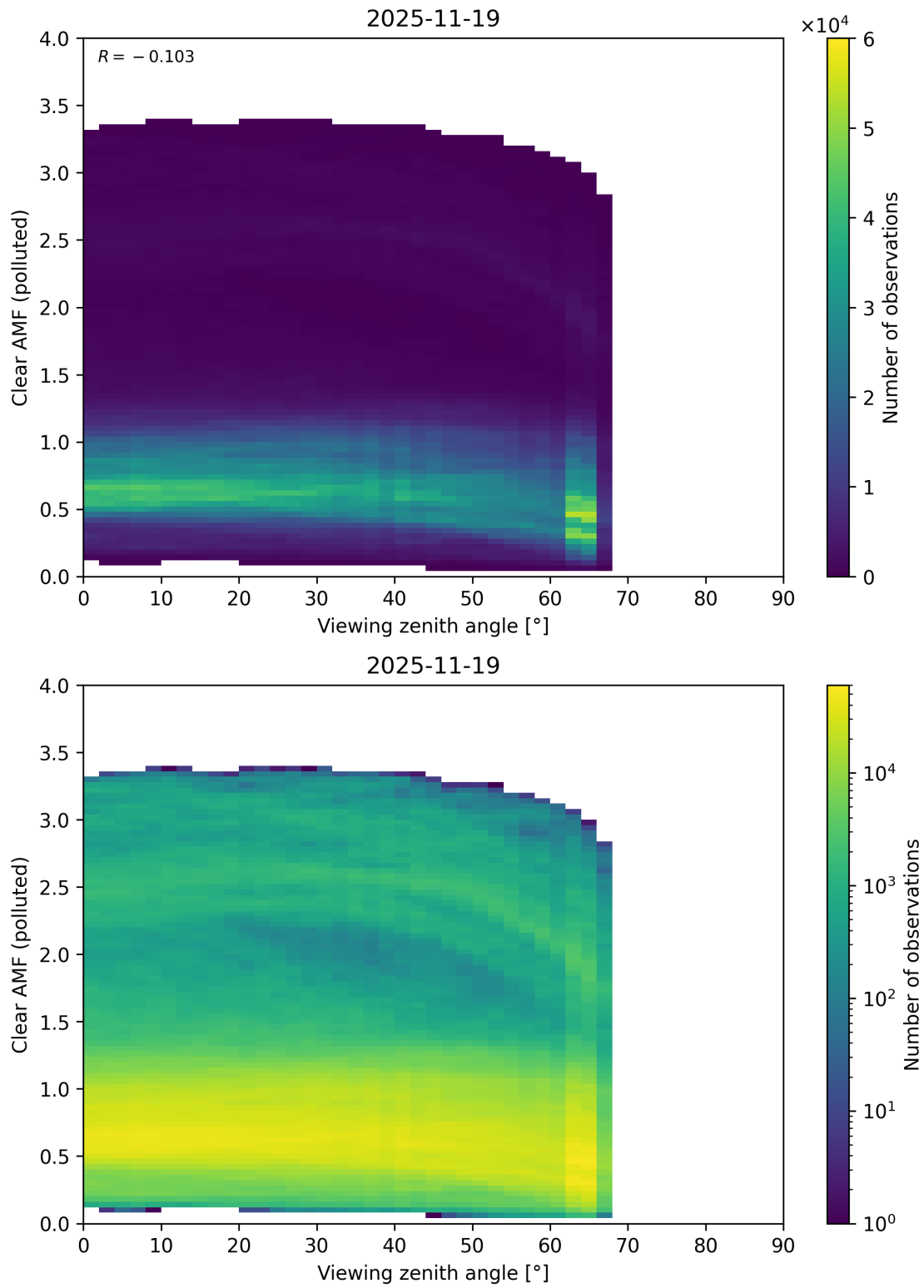
Figure 370: Scatter density plot of “Viewing zenith angle” against “Clear AMF (polluted)” for 2025-11-18 to 2025-11-20.
