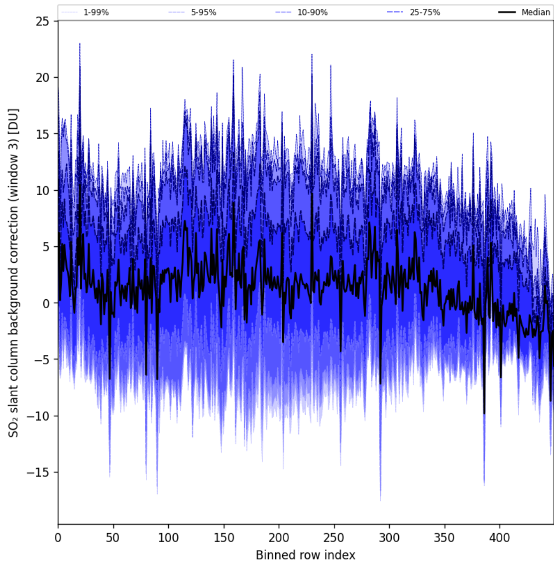
Figure 100: Along track statistics of “SO 2 slant column background correction (window 3)” for 2025-11-18 to 2025-11-20
