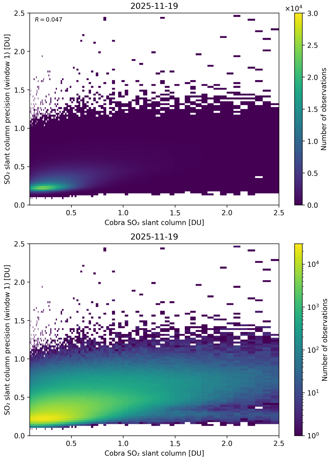
Figure 220: Scatter density plot of “Cobra SO 2 slant column” against “SO 2 slant column precision (window 1)” for 2025-11-18 to 2025-11-20.
