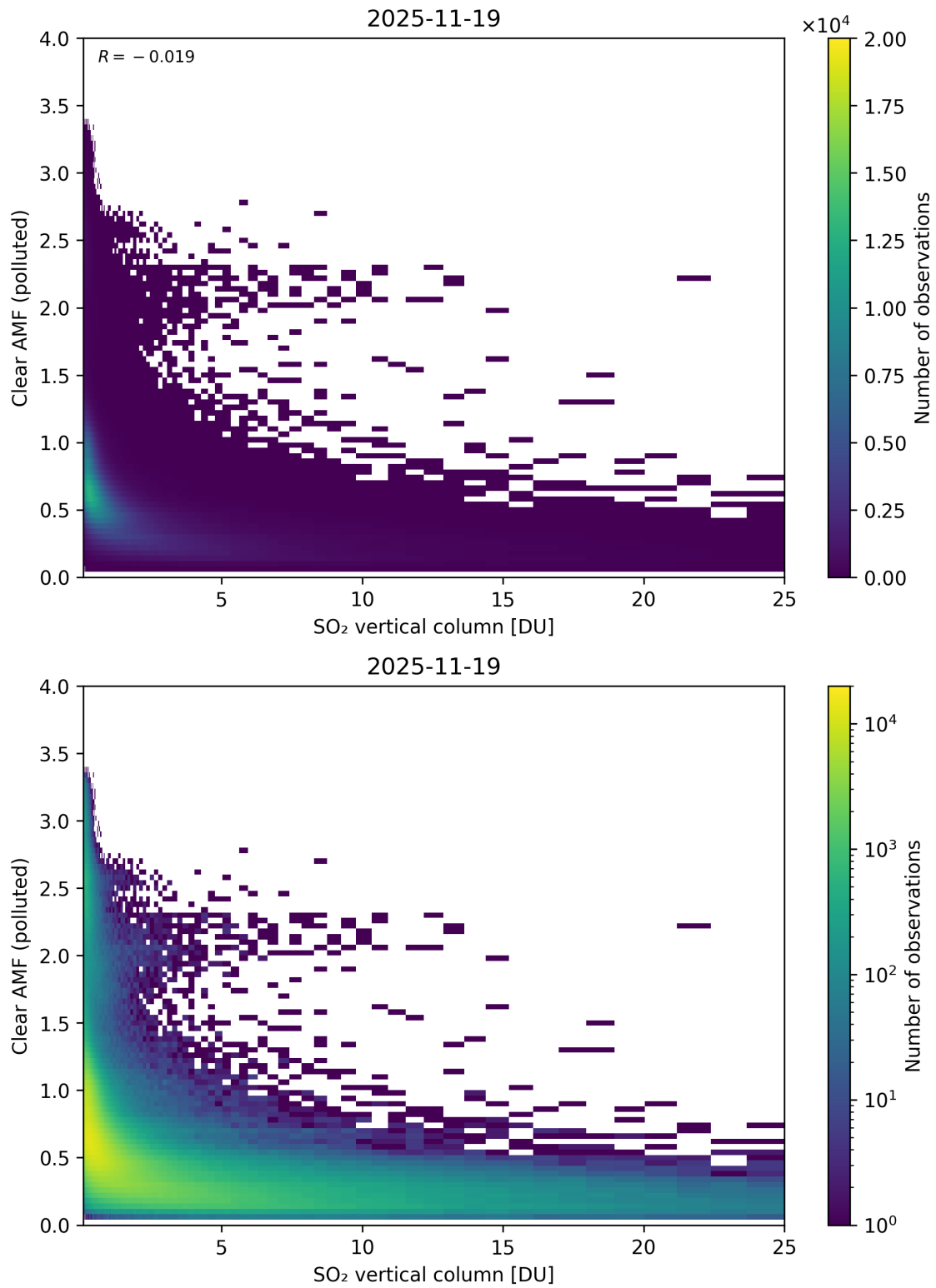
Figure 348: Scatter density plot of “SO 2 vertical column” against “Clear AMF (polluted)” for 2025-11-18 to 2025-11-20.
