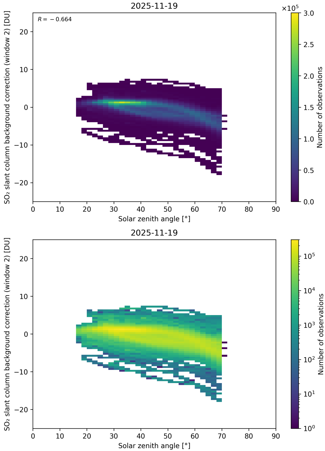
Figure 172: Scatter density plot of “Solar zenith angle” against “SO 2 slant column background correction (window 2)” for 2025-11-18 to 2025-11-20.
