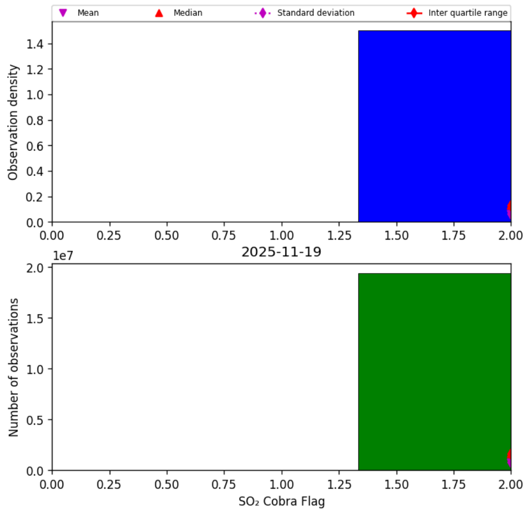
Figure 75: Histogram of "SO 2 Cobra Flag" for 2025-11-18 to 2025-11-20
