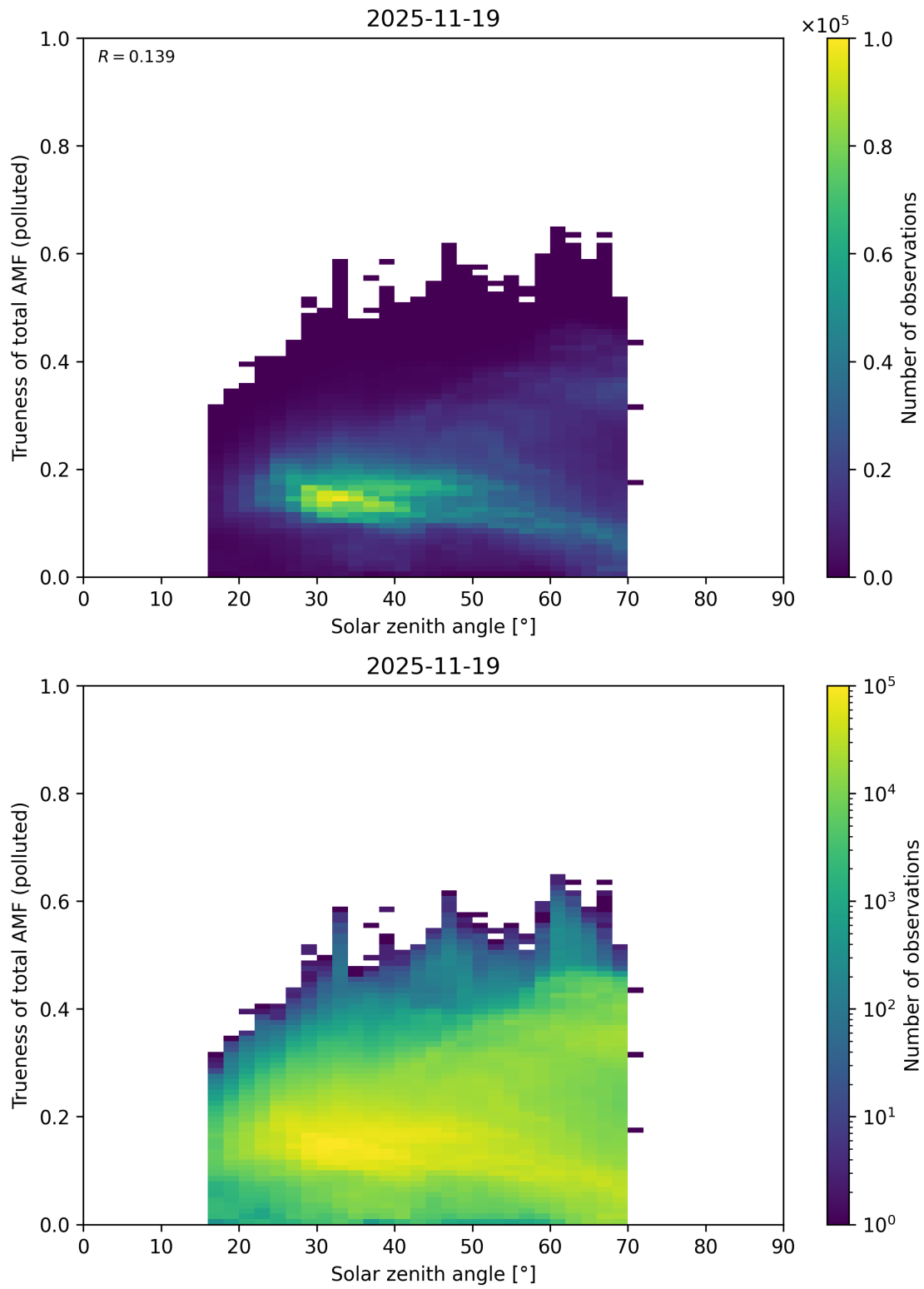
Figure 190: Scatter density plot of “Solar zenith angle” against “Trueness of total AMF (polluted)” for 2025-11-18 to 2025-11-20.
