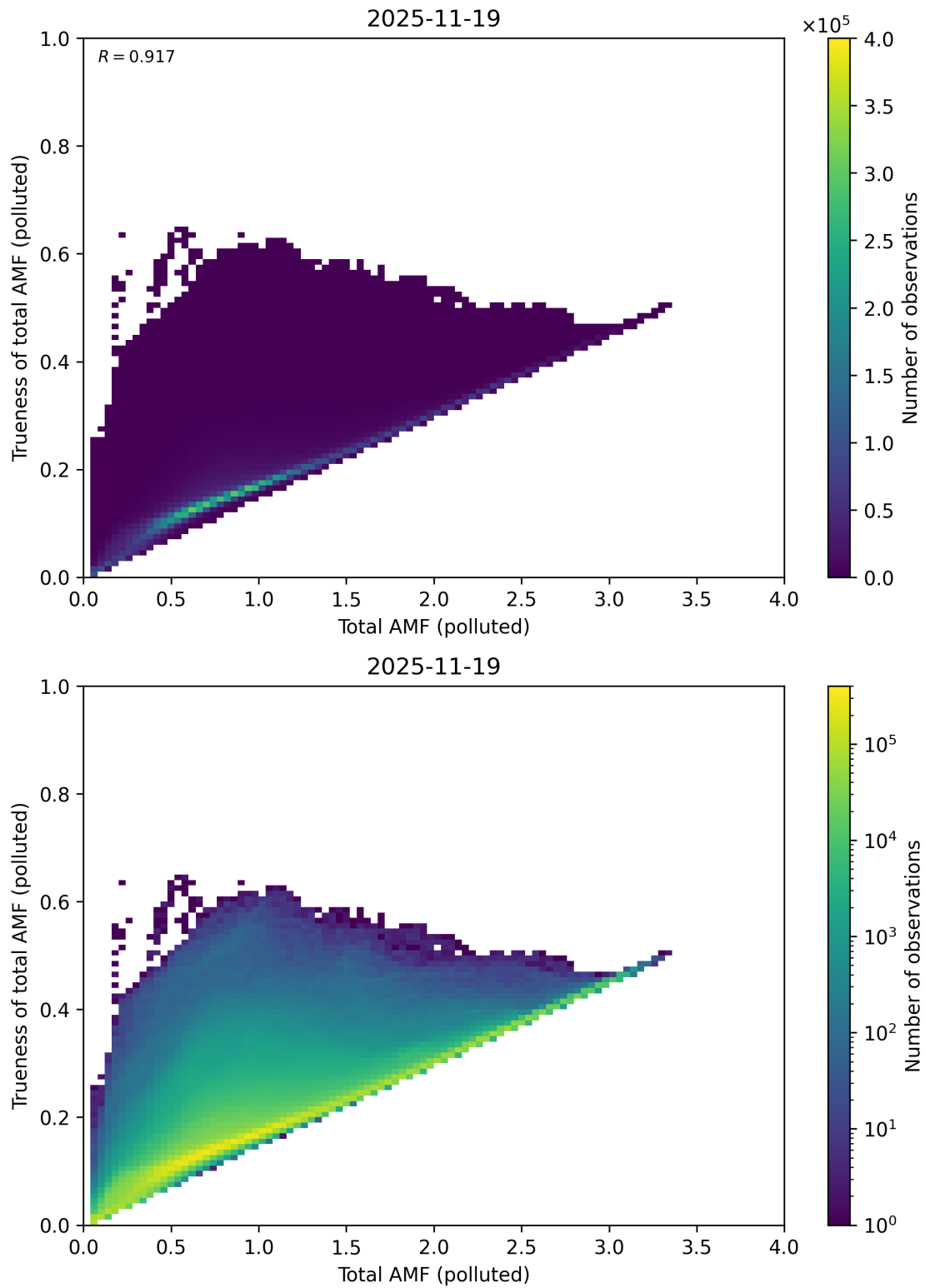
Figure 321: Scatter density plot of “Total AMF (polluted)” against “Trueness of total AMF (polluted)” for 2025-11-18 to 2025-11-20.
