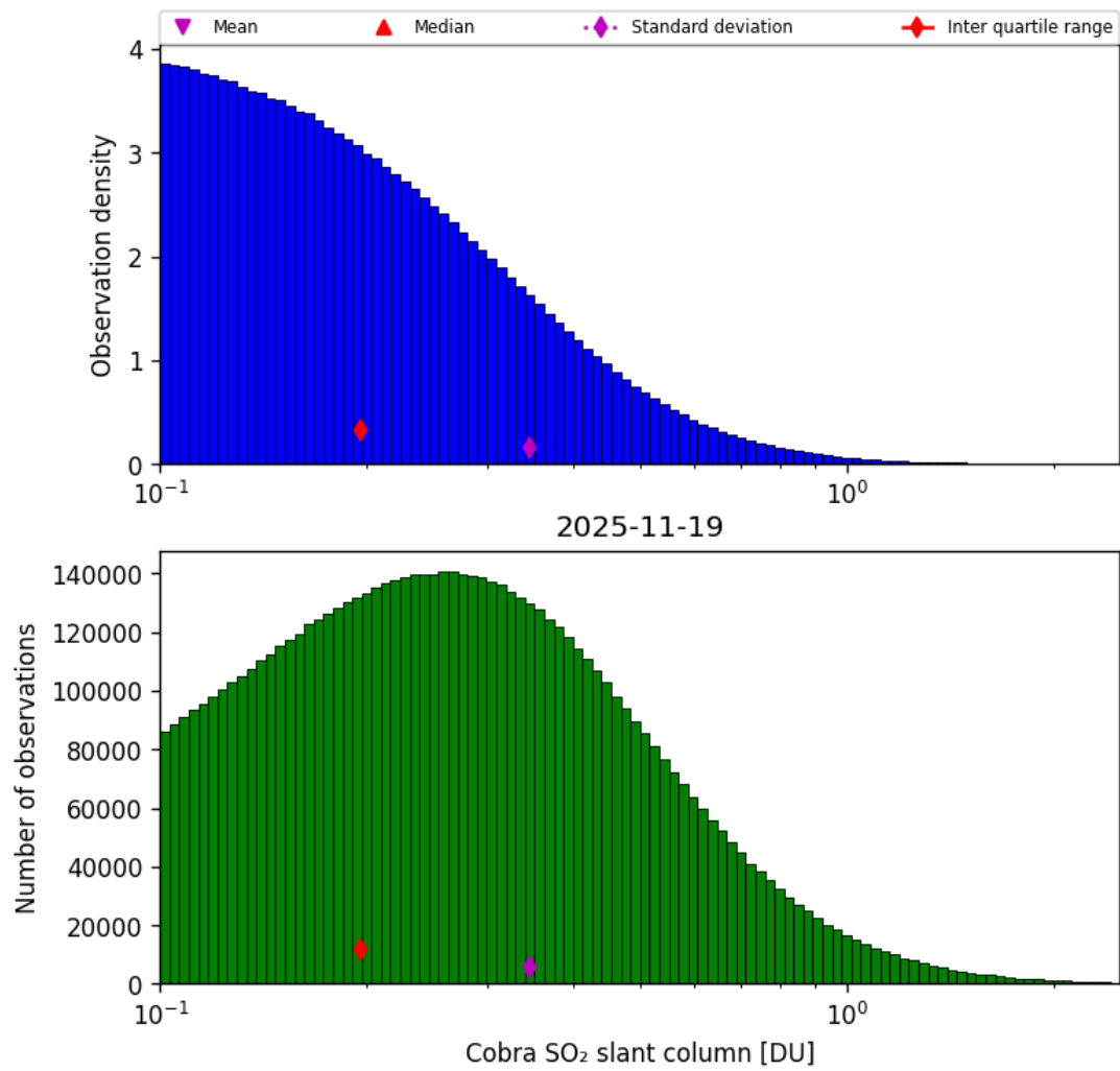
Figure 61: Histogram of “Cobra SO 2 slant column” for 2025-11-18 to 2025-11-20
