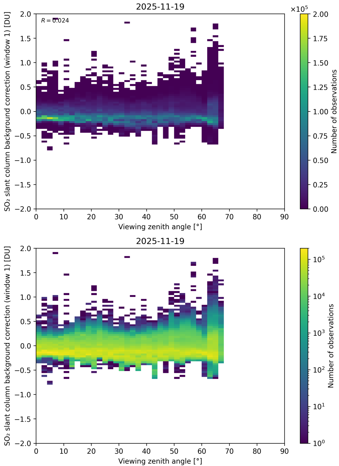
Figure 362: Scatter density plot of “Viewing zenith angle” against “SO 2 slant column background correction (window 1)” for 2025-11-18 to 2025-11-20.
