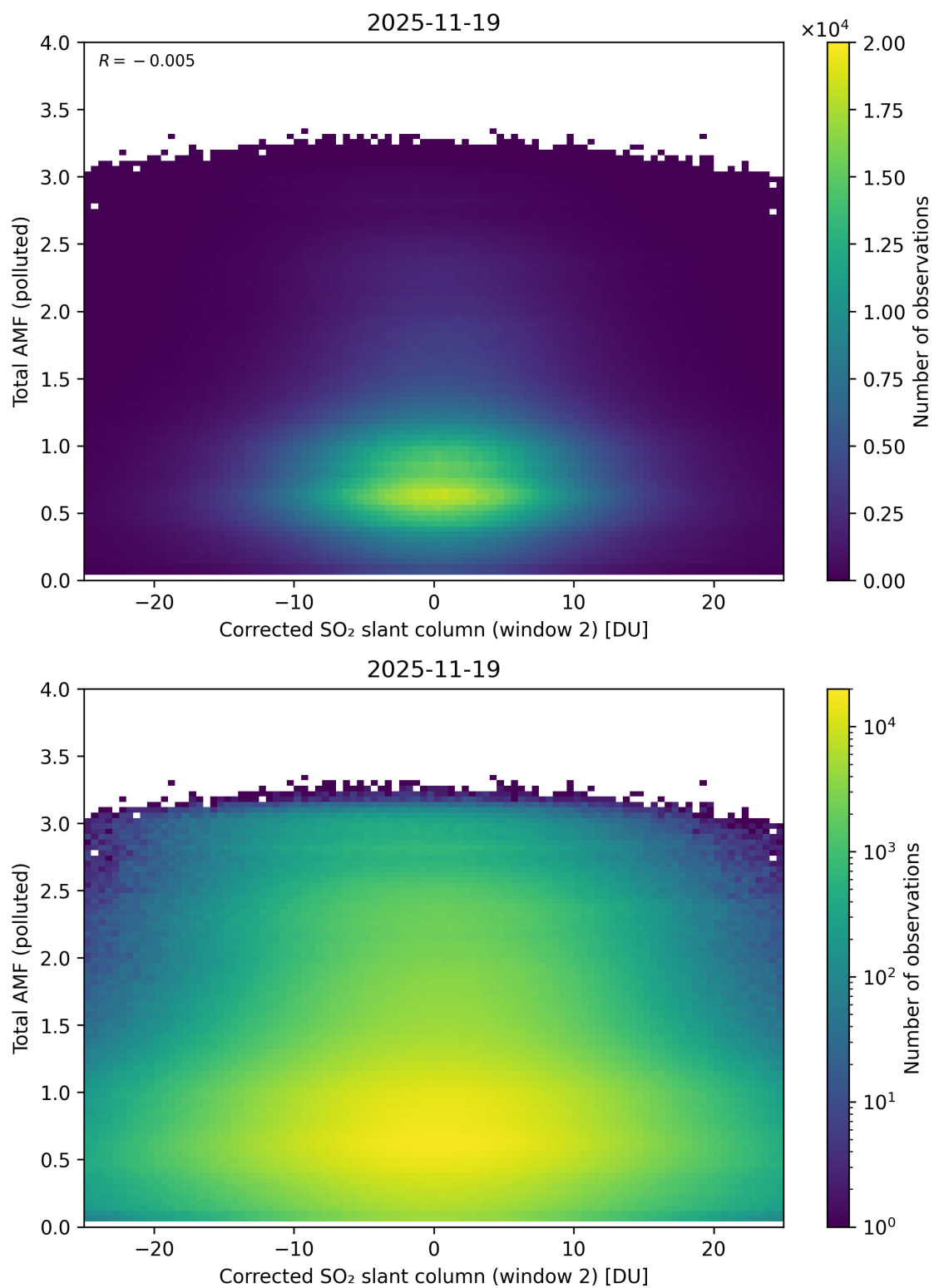
Figure 253: Scatter density plot of “Corrected SO 2 slant column (window 2)” against “Total AMF (polluted)” for 2025-11-18 to 2025-11-20.
