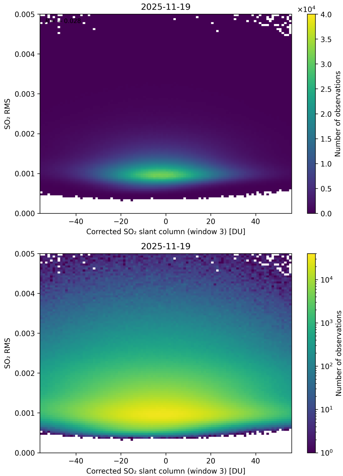
Figure 258: Scatter density plot of “Corrected SO 2 slant column (window 3)” against “SO 2 RMS” for 2025-11-18 to 2025-11-20.
