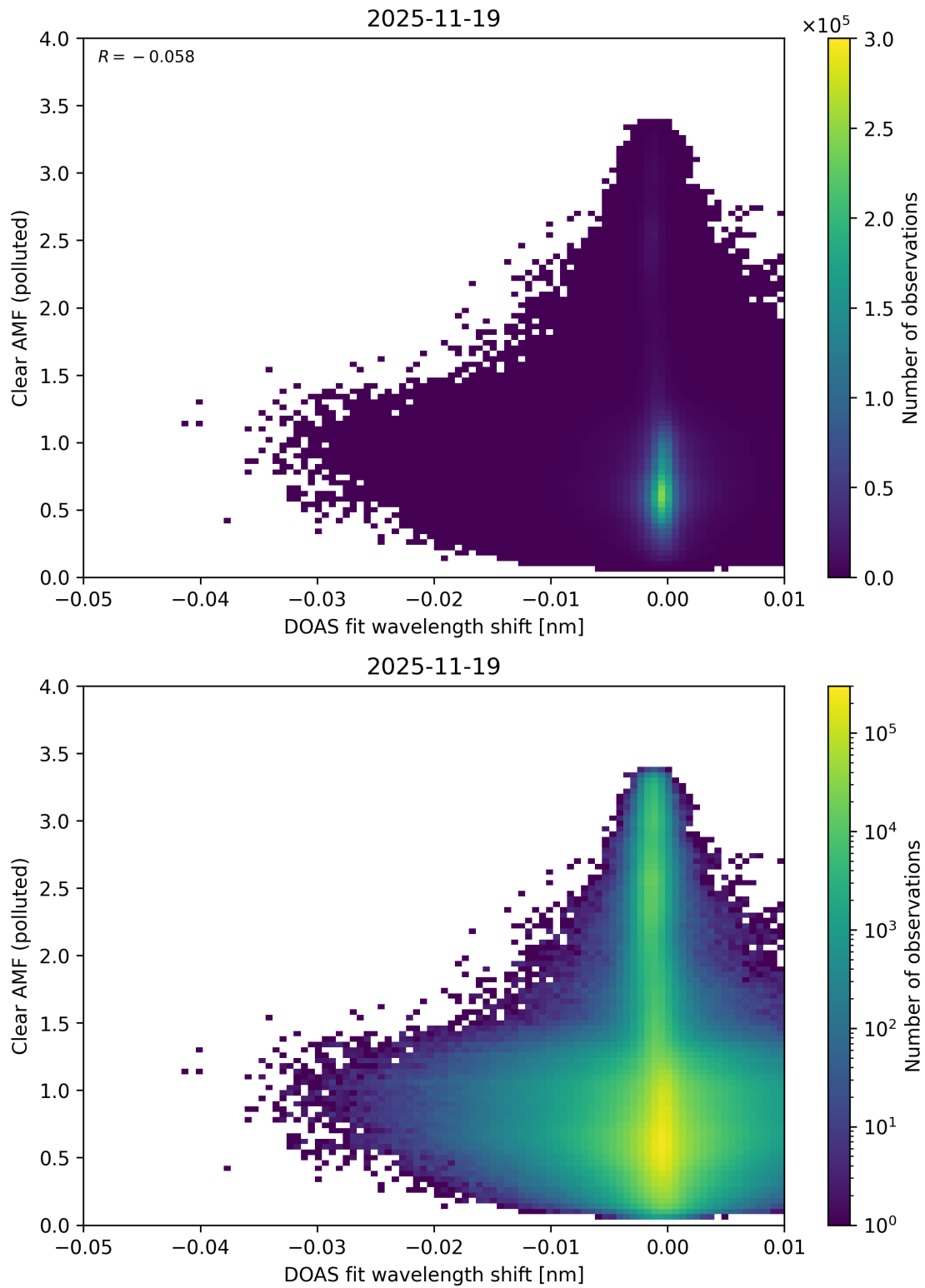
Figure 140: Scatter density plot of “DOAS fit wavelength shift” against “Clear AMF (polluted)” for 2025-11-18 to 2025-11-20.
