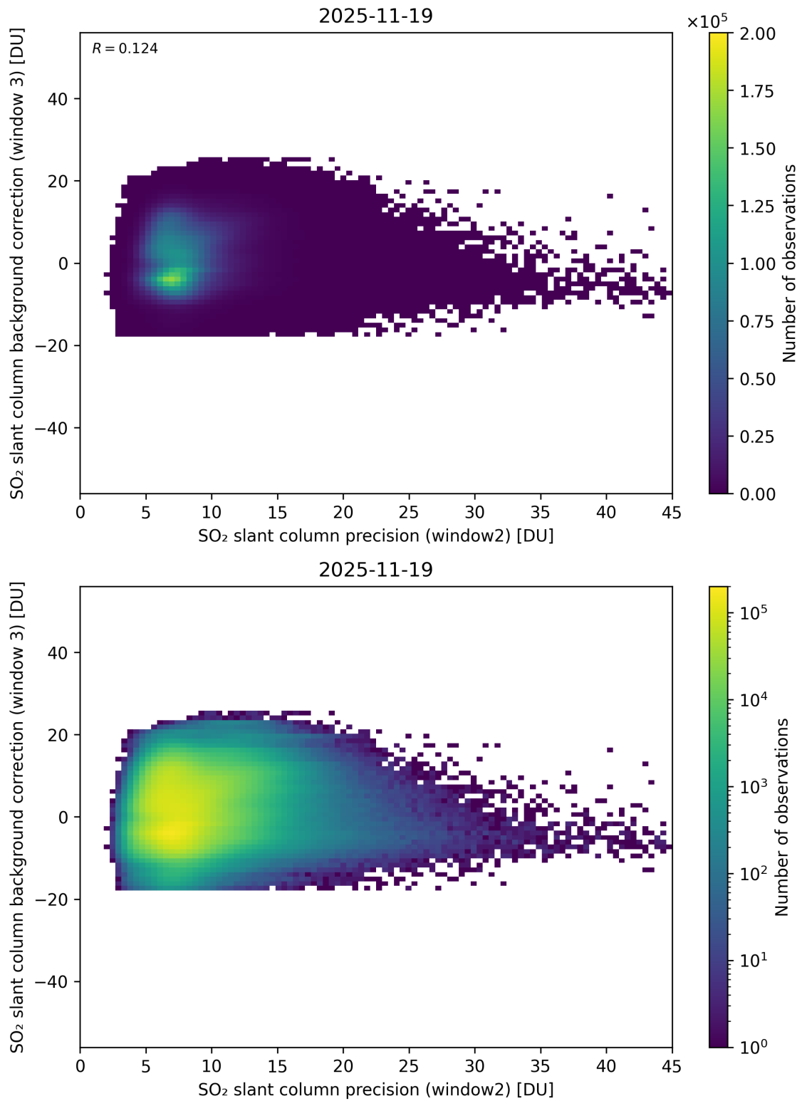
Figure 292: Scatter density plot of “SO 2 slant column precision (window2)” against “SO 2 slant column background correction (window 3)” for 2025-11-18 to 2025-11-20.
