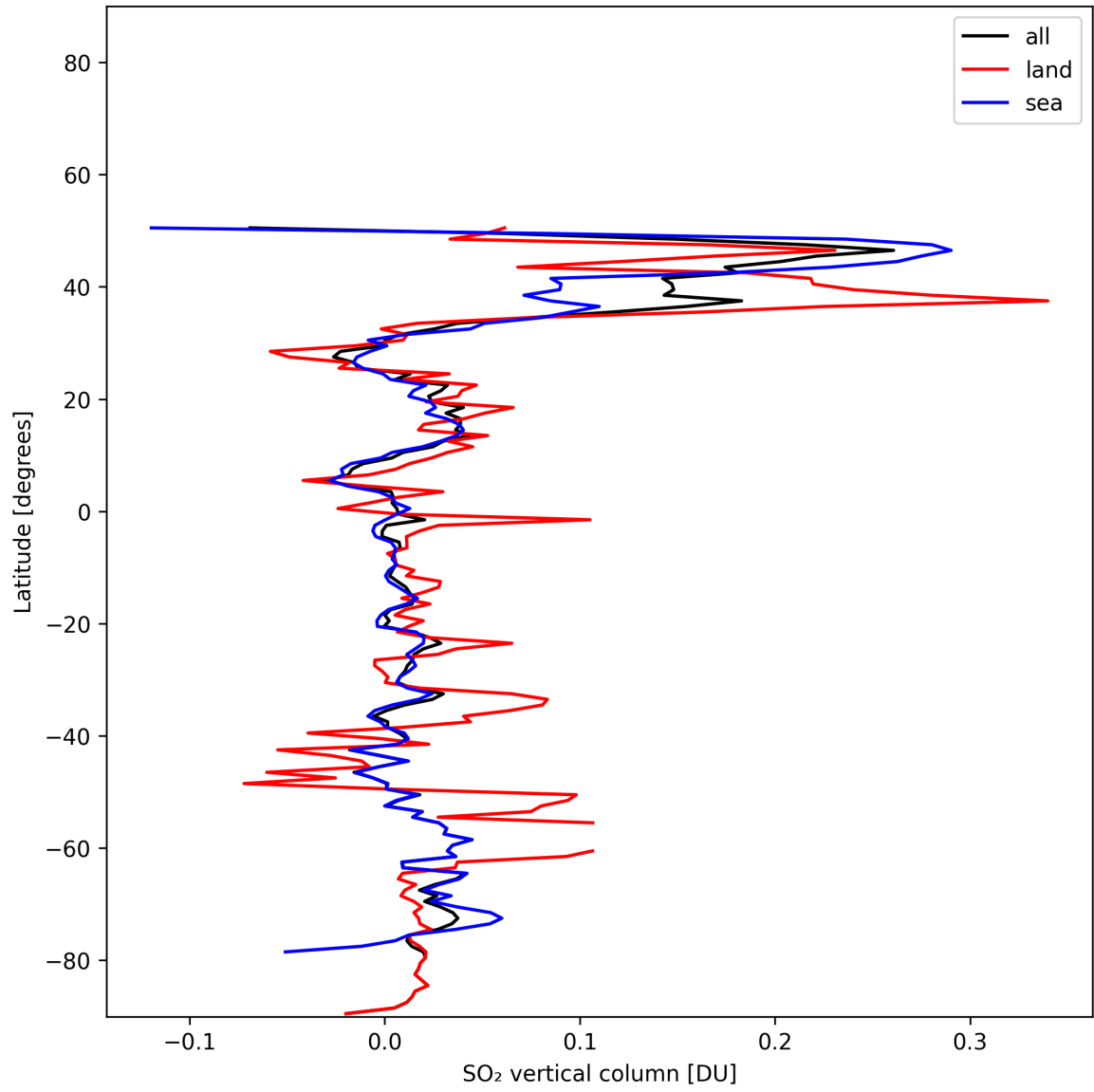
Figure 32: Zonal average of “SO 2 vertical column” for 2025-11-18 to 2025-11-20.
