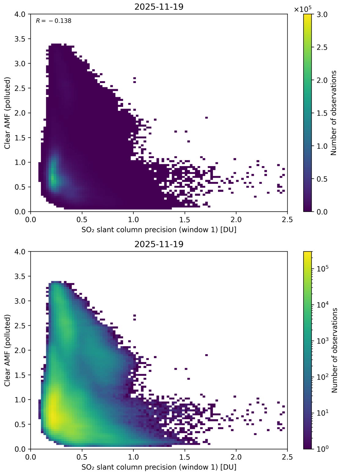
Figure 274: Scatter density plot of “SO 2 slant column precision (window 1)” against “Clear AMF (polluted)” for 2025-11-18 to 2025-11-20.
