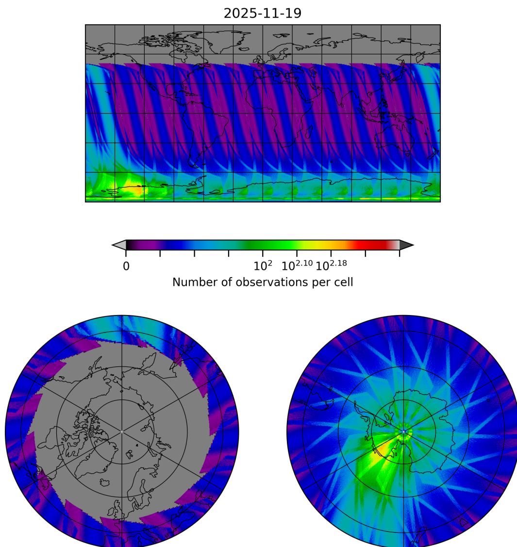
Figure 30: Map of the number of observations for 2025-11-18 to 2025-11-20
