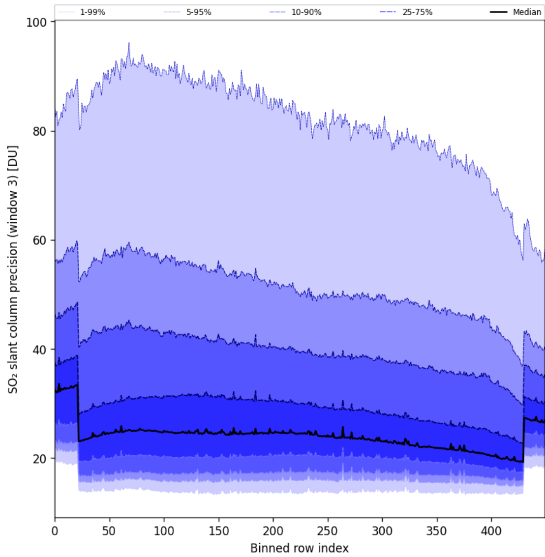
Figure 98: Along track statistics of “SO 2 slant column precision (window 3)” for 2025-11-18 to 2025-11-20
