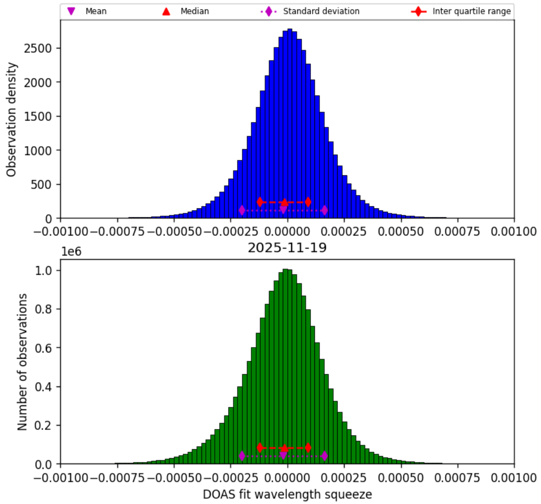
Figure 77: Histogram of “DOAS fit wavelength squeeze” for 2025-11-18 to 2025-11-20
