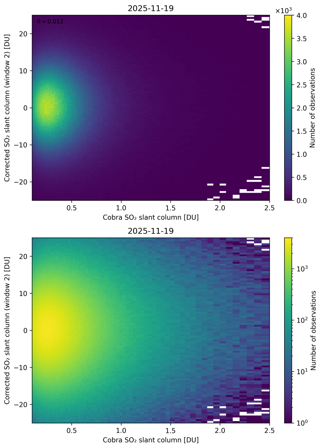
Figure 217: Scatter density plot of “Cobra SO 2 slant column” against “Corrected SO 2 slant column (window 2)” for 2025-11-18 to 2025-11-20.
