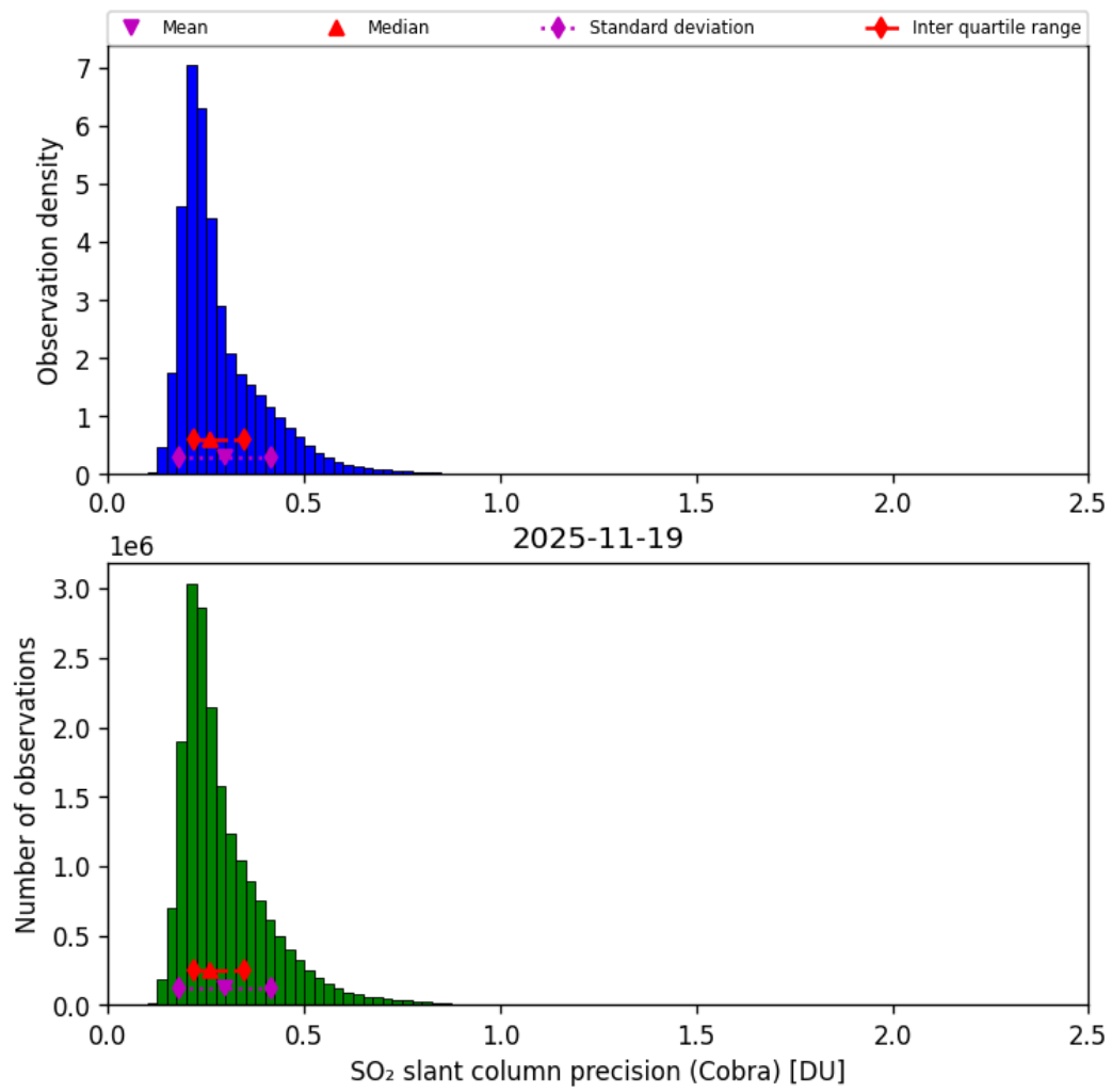
Figure 62: Histogram of “SO 2 slant column precision (Cobra)” for 2025-11-18 to 2025-11-20
