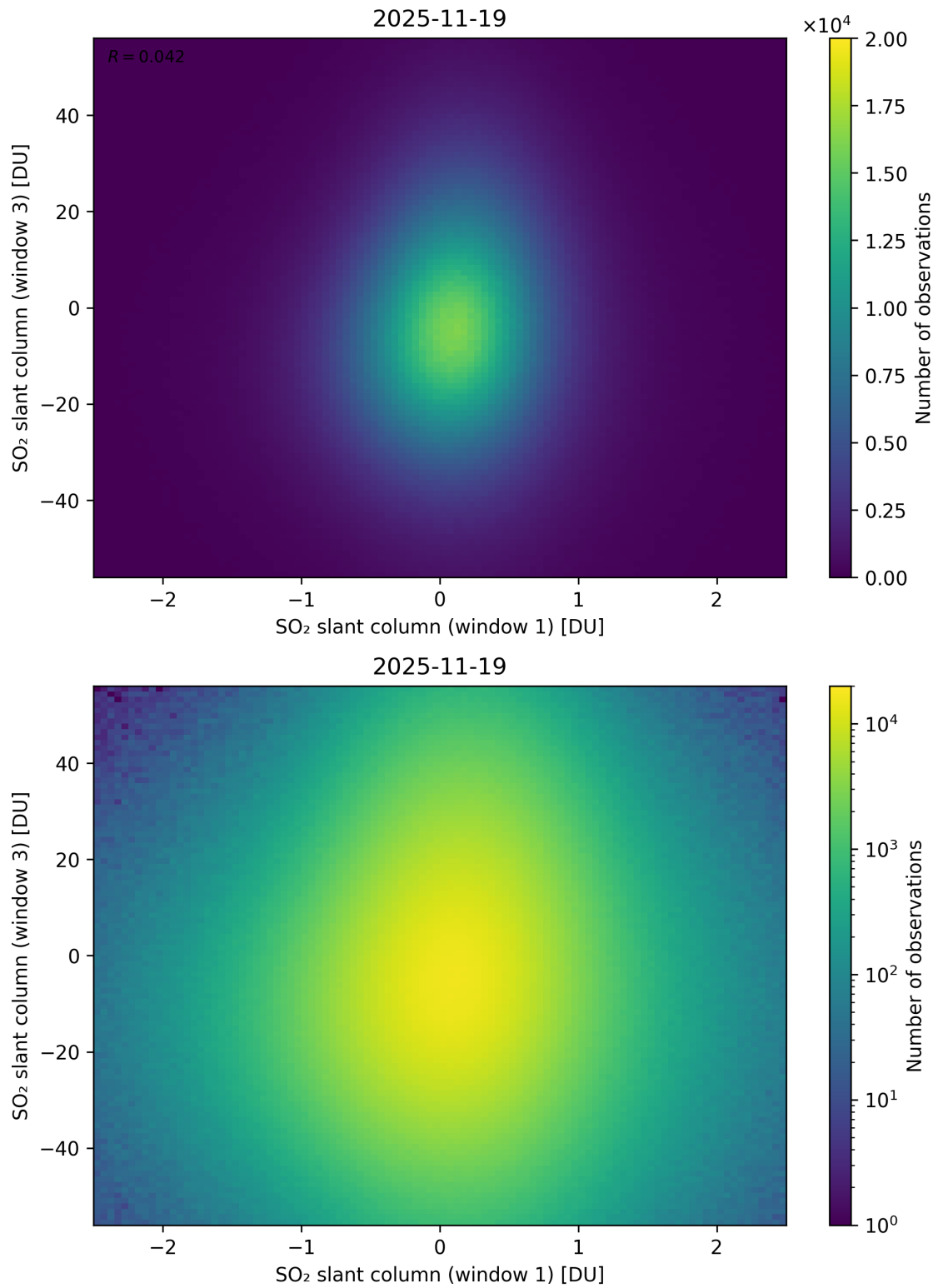
Figure 287: Scatter density plot of “SO 2 slant column (window 1)” against “SO 2 slant column (window 3)” for 2025-11-18 to 2025-11-20.
