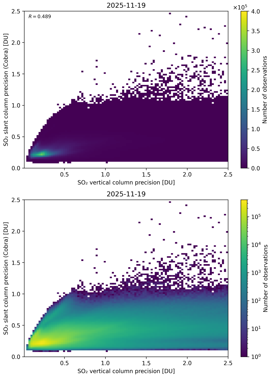
Figure 337: Scatter density plot of “SO 2 vertical column precision” against “SO 2 slant column precision (Cobra)” for 2025-11-18 to 2025-11-20.
