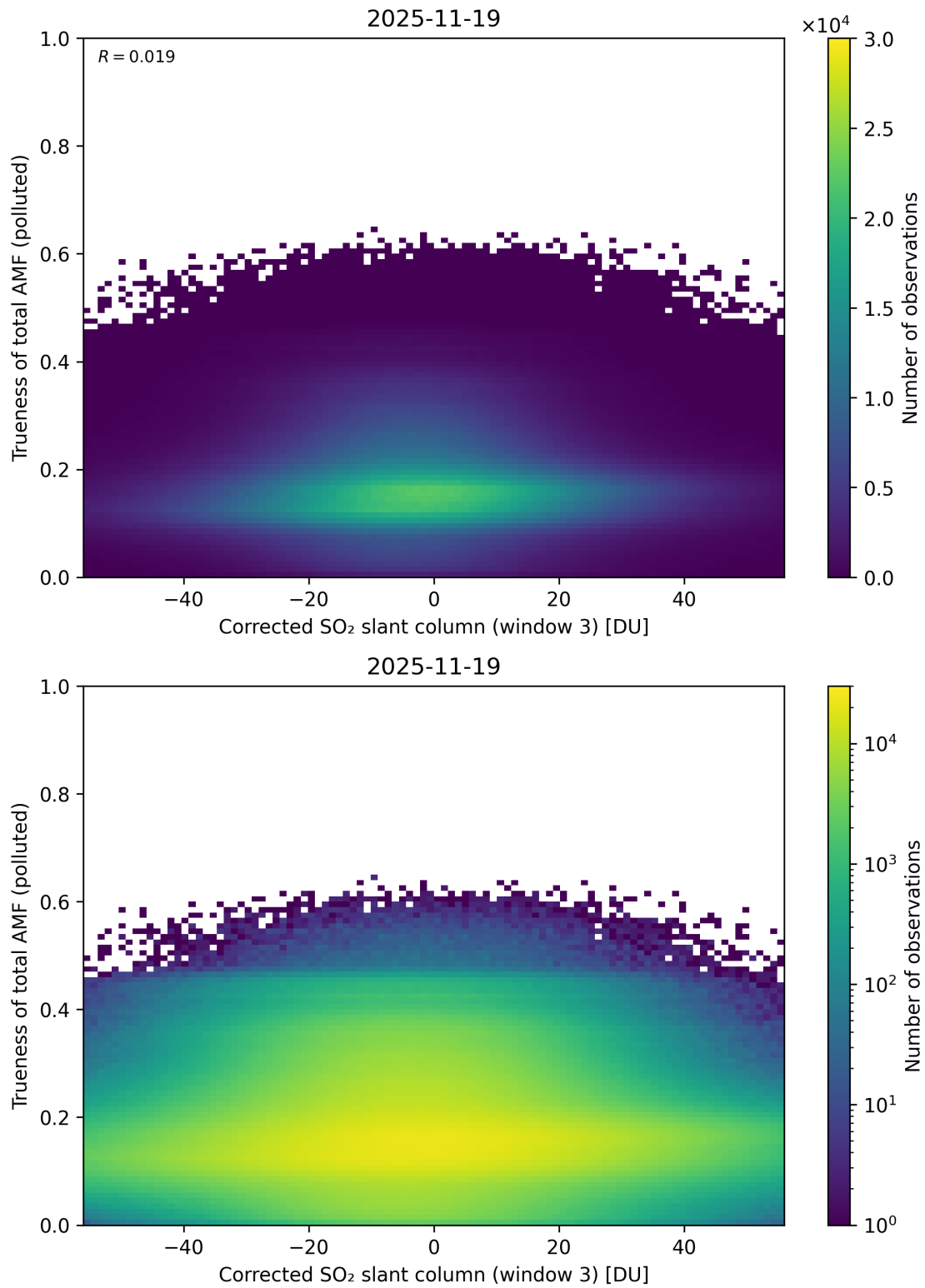
Figure 261: Scatter density plot of “Corrected SO 2 slant column (window 3)” against “Trueness of total AMF (polluted)” for 2025-11-18 to 2025-11-20.
