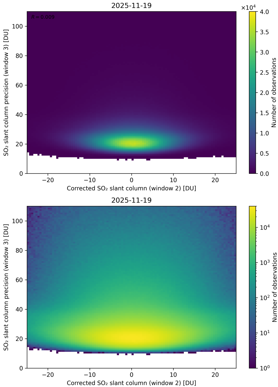
Figure 252: Scatter density plot of “Corrected SO 2 slant column (window 2)” against “SO 2 slant column precision (window 3)” for 2025-11-18 to 2025-11-20.
