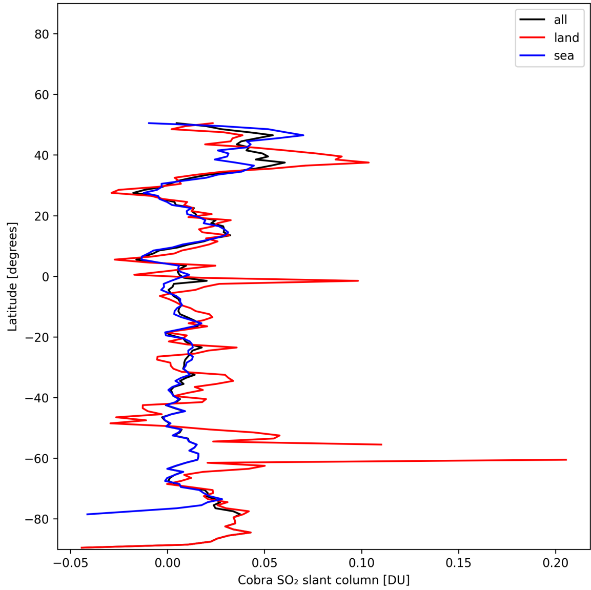
Figure 35: Zonal average of “Cobra SO 2 slant column” for 2025-11-18 to 2025-11-20.
