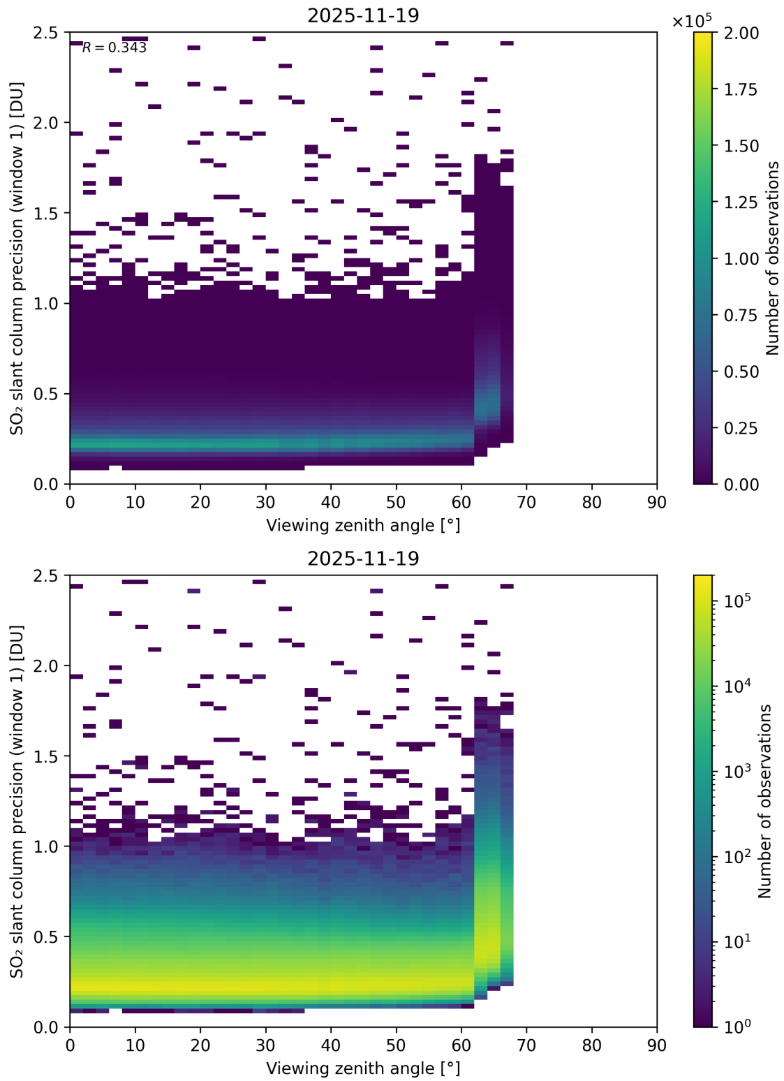
Figure 377: Scatter density plot of “Viewing zenith angle” against “SO 2 slant column precision (window 1)” for 2025-11-18 to 2025-11-20.
