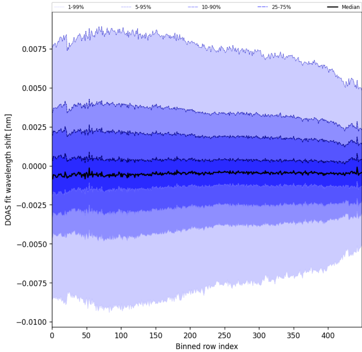
Figure 102: Along track statistics of “DOAS fit wavelength shift” for 2025-11-18 to 2025-11-20
