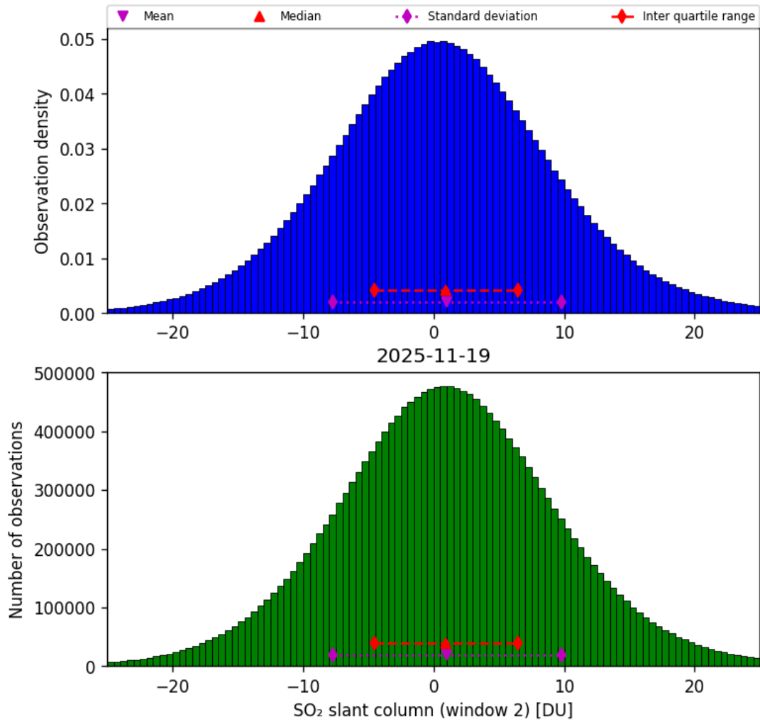
Figure 67: Histogram of “SO 2 slant column (window 2)” for 2025-11-18 to 2025-11-20
