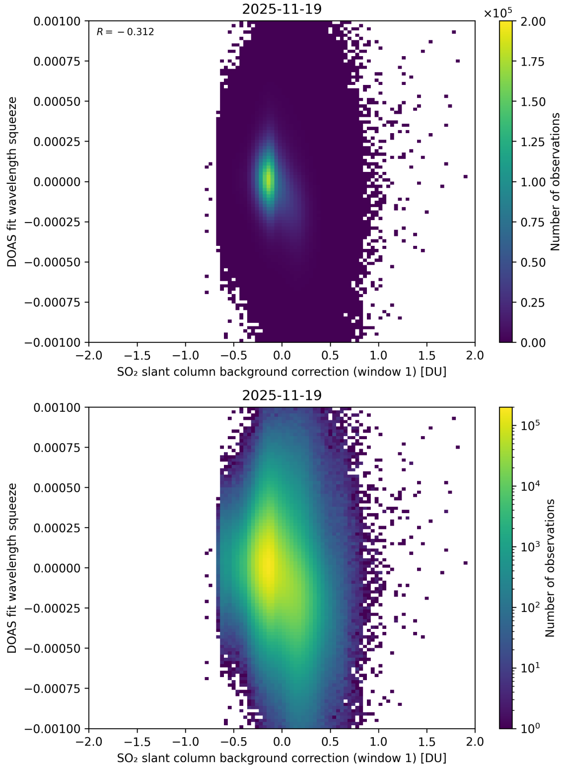
Figure 112: Scatter density plot of “SO 2 slant column background correction (window 1)” against “DOAS fit wavelength squeeze” for 2025-11-18 to 2025-11-20.
