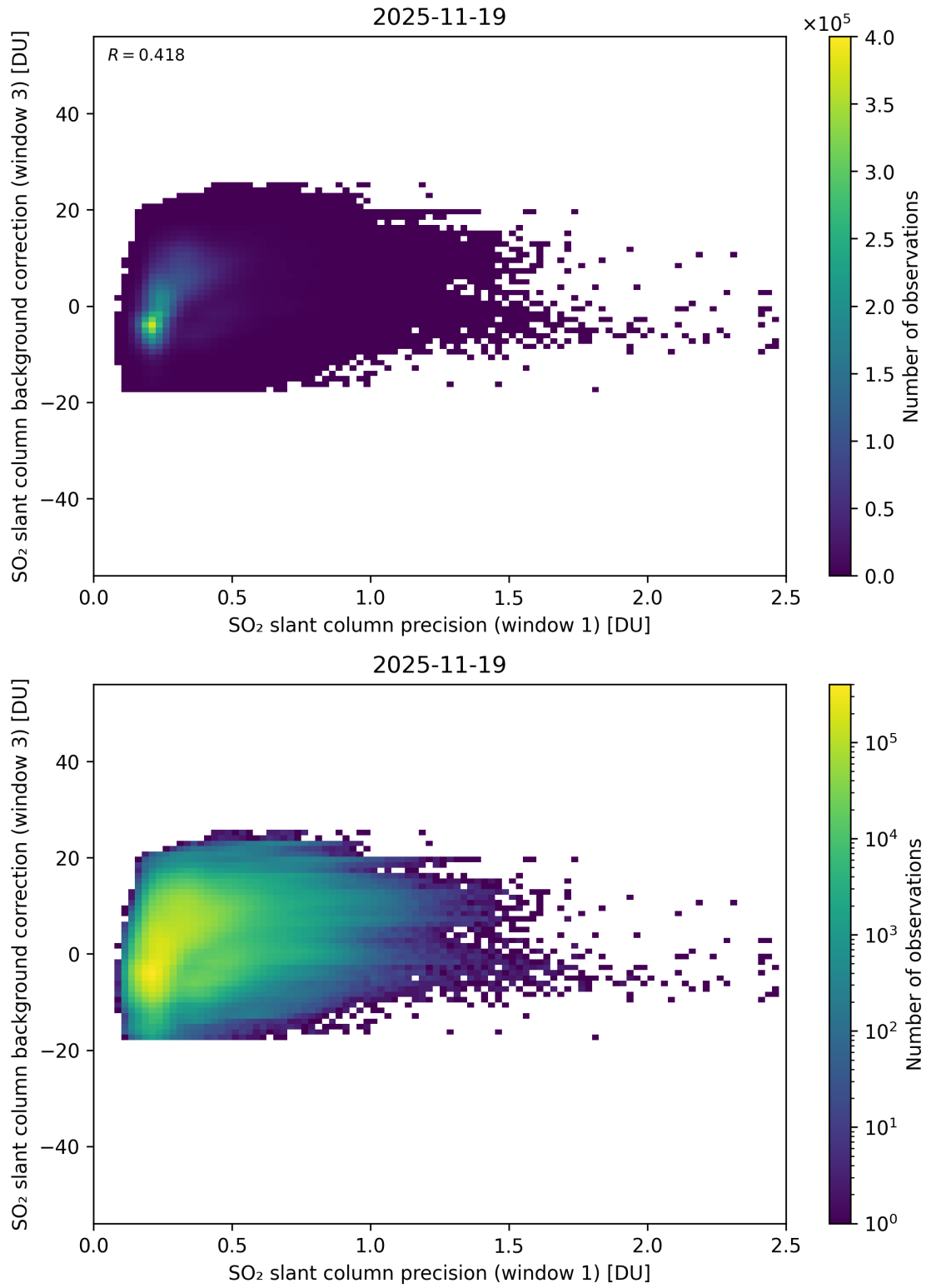
Figure 270: Scatter density plot of “SO 2 slant column precision (window 1)” against “SO 2 slant column background correction (window 3)” for 2025-11-18 to 2025-11-20.
