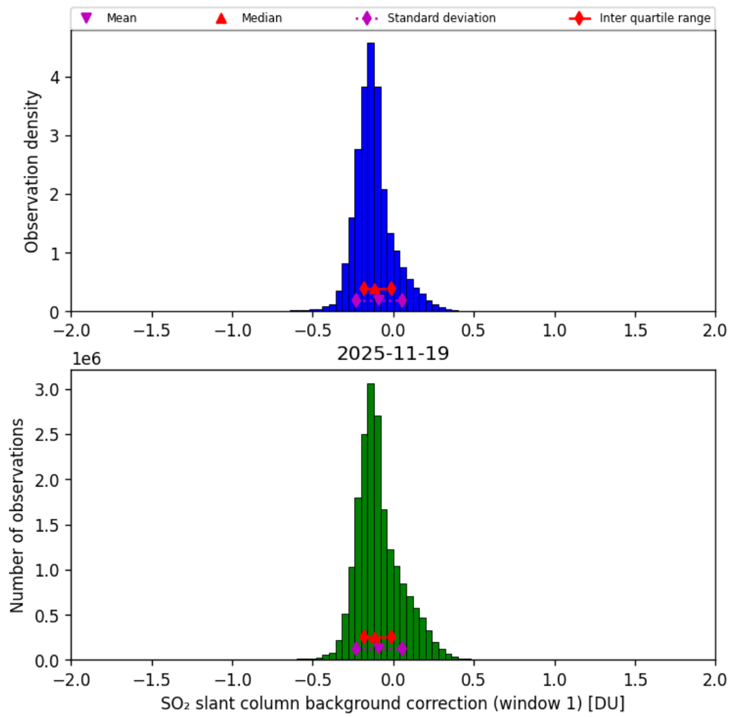
Figure 66: Histogram of “SO 2 slant column background correction (window 1)” for 2025-11-18 to 2025-11-20
