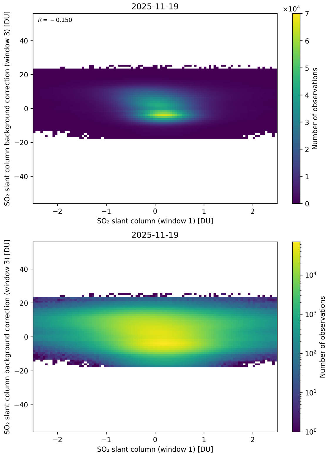
Figure 264: Scatter density plot of “SO 2 slant column (window 1)” against “SO 2 slant column background correction (window 3)” for 2025-11-18 to 2025-11-20.
