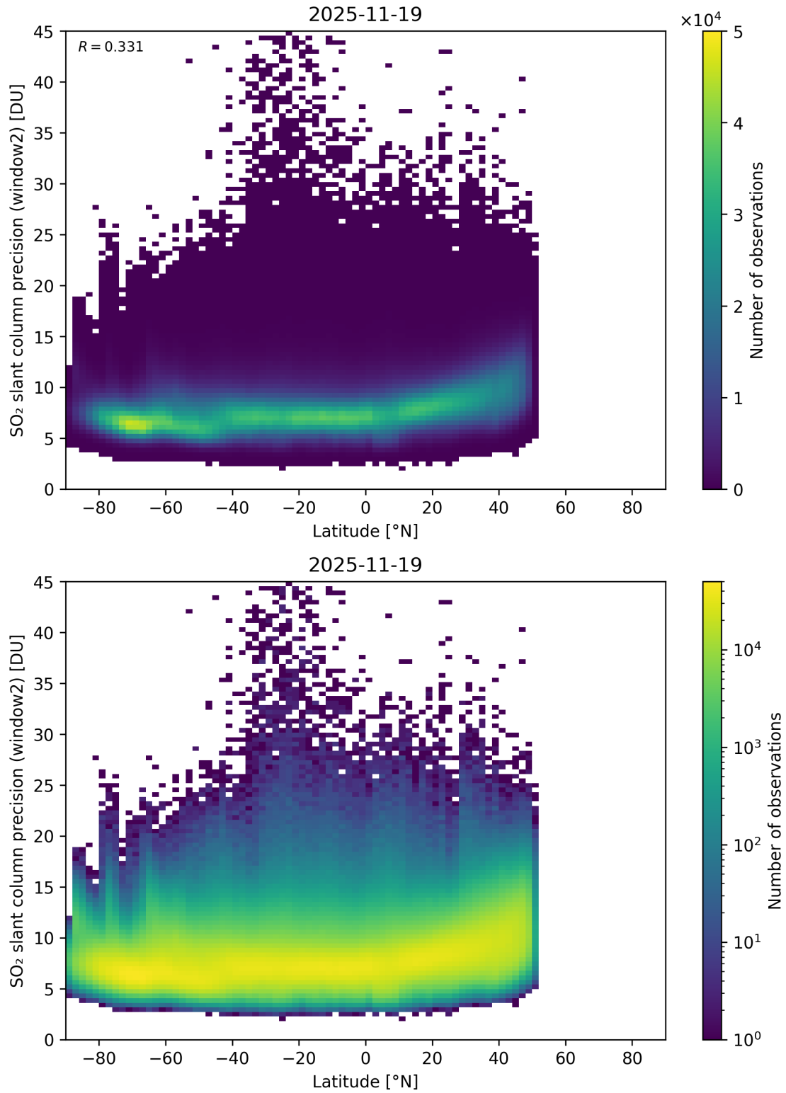
Figure 164: Scatter density plot of “Latitude” against “SO 2 slant column precision (window2)” for 2025-11-18 to 2025-11-20.
