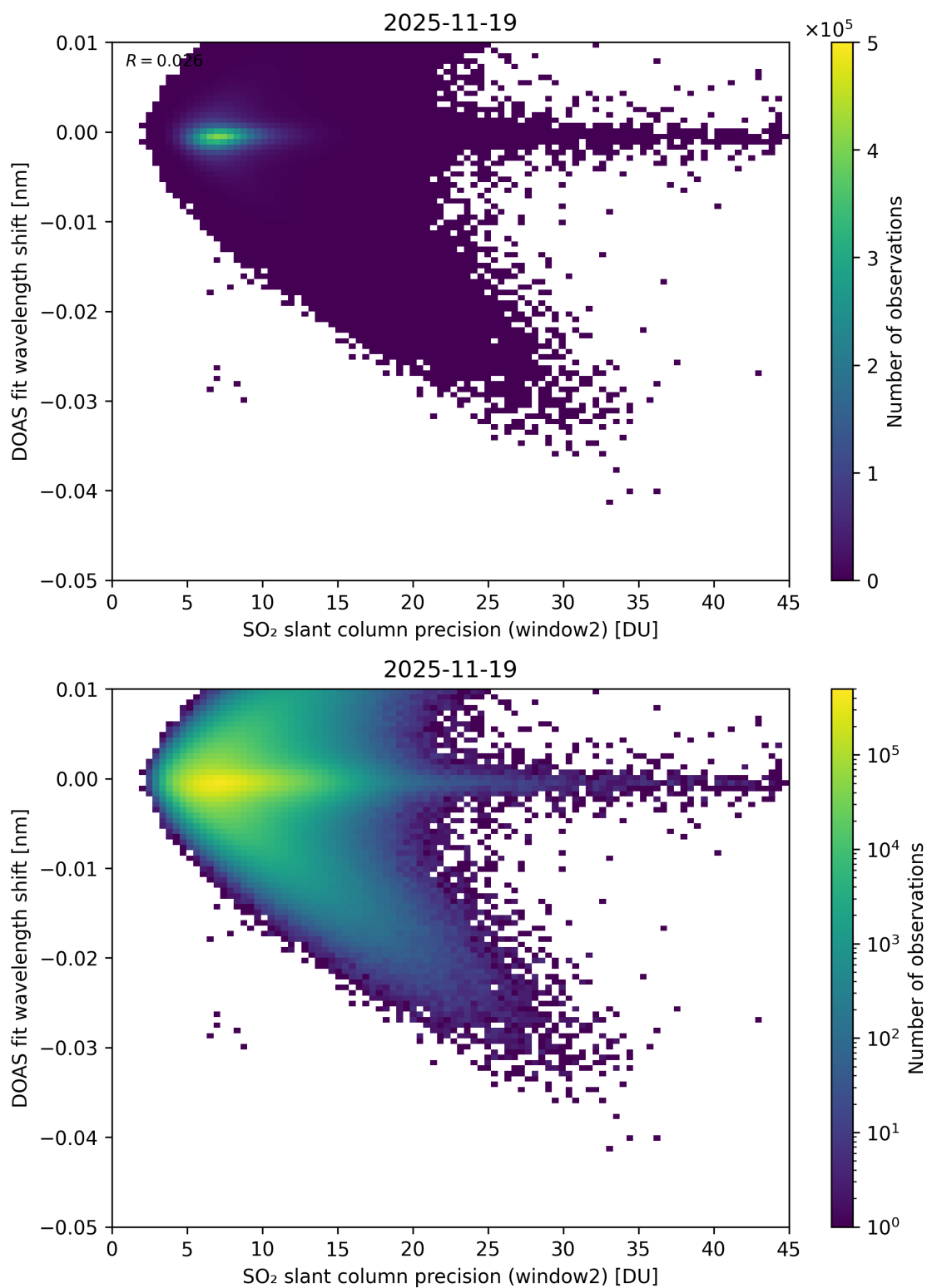
Figure 293: Scatter density plot of “SO 2 slant column precision (window2)” against “DOAS fit wavelength shift” for 2025-11-18 to 2025-11-20.
