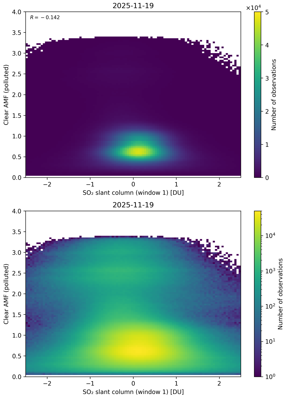
Figure 282: Scatter density plot of “SO 2 slant column (window 1)” against “Clear AMF (polluted)” for 2025-11-18 to 2025-11-20.
