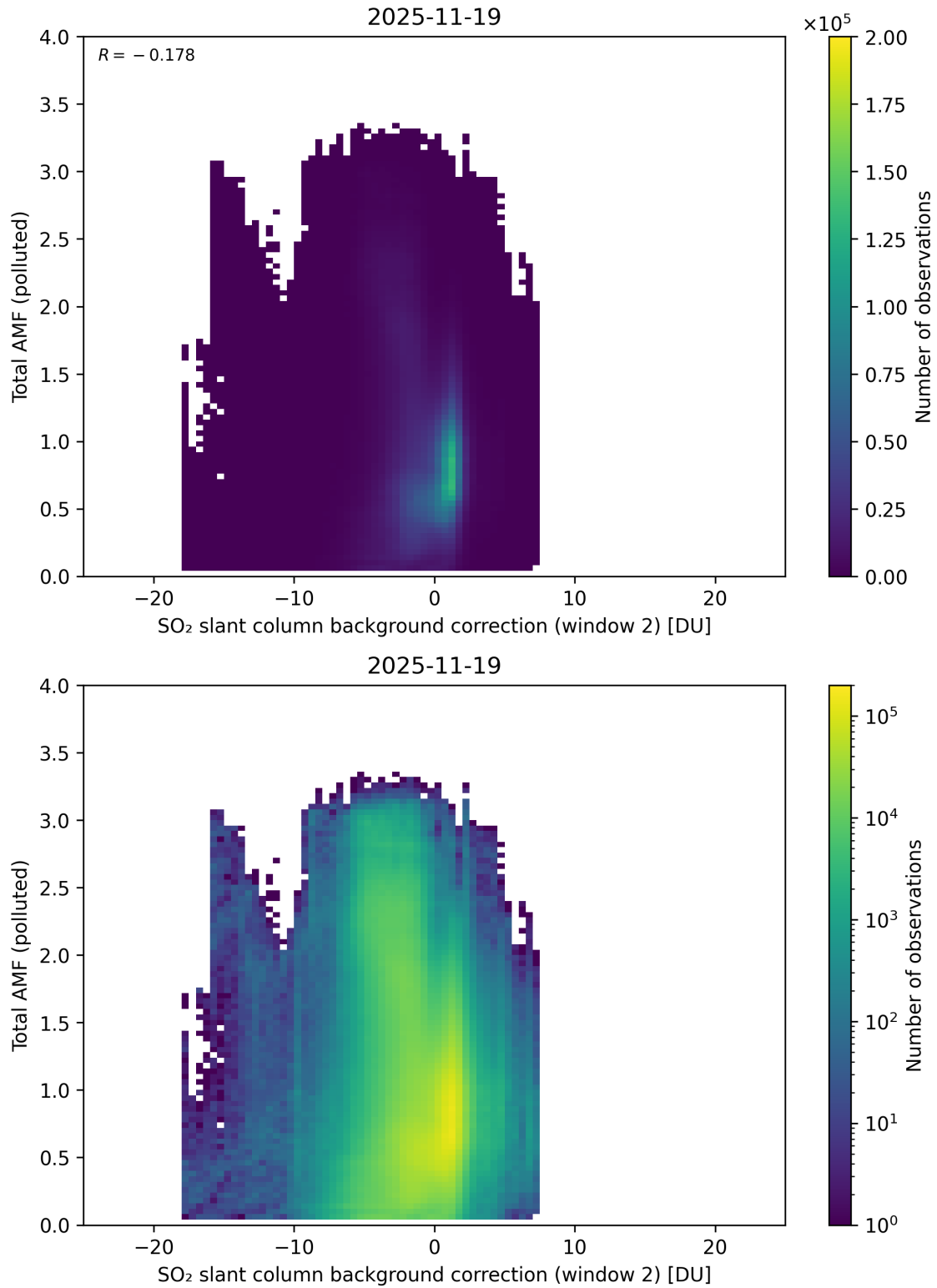
Figure 130: Scatter density plot of “SO 2 slant column background correction (window 2)” against “Total AMF (polluted)” for 2025-11-18 to 2025-11-20.
