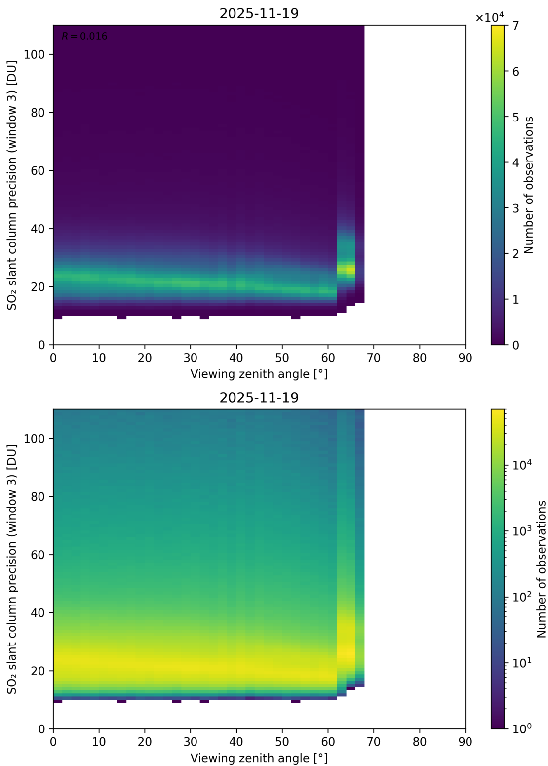
Figure 380: Scatter density plot of “Viewing zenith angle” against “SO 2 slant column precision (window 3)” for 2025-11-18 to 2025-11-20.
