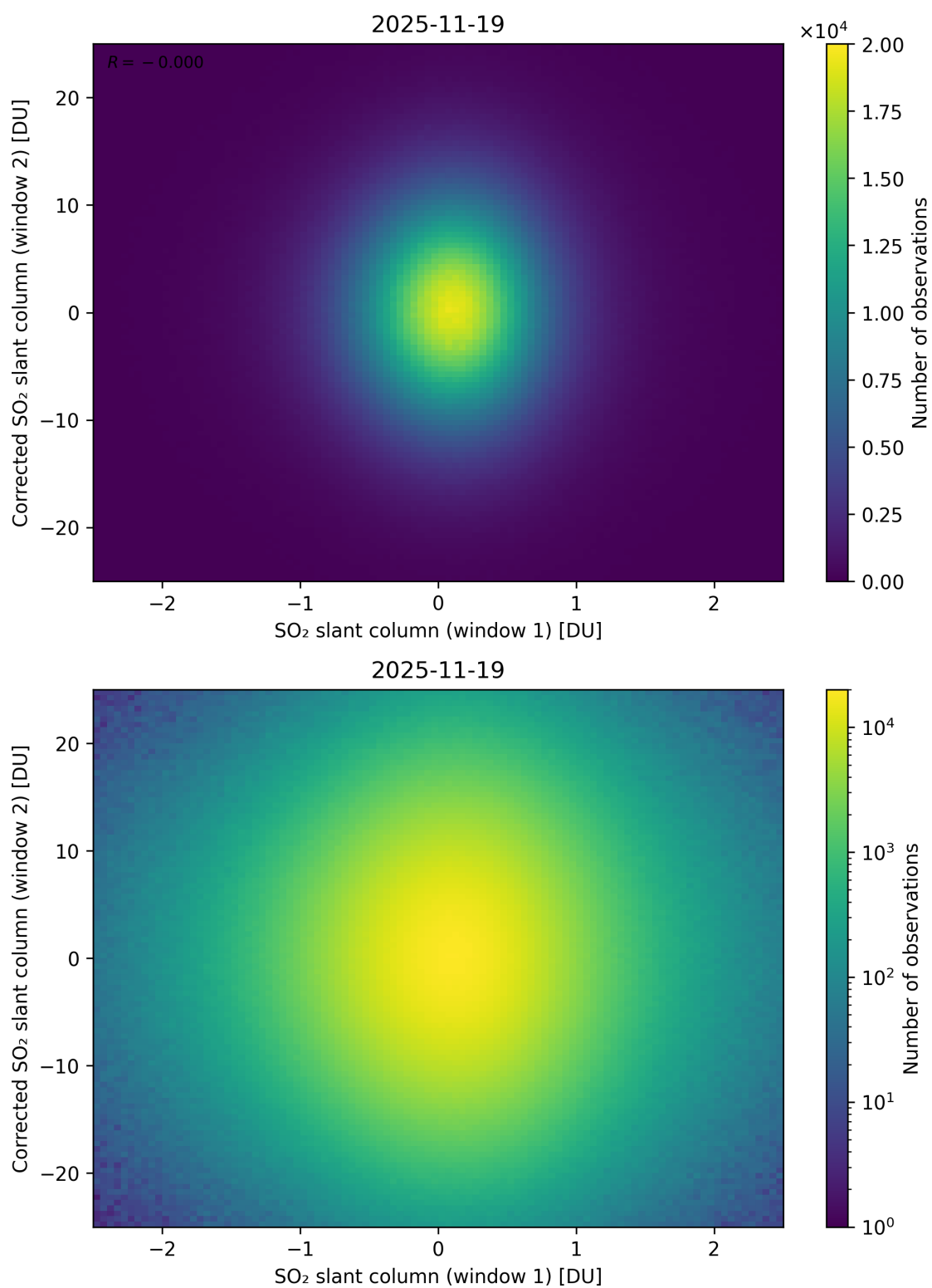
Figure 283: Scatter density plot of “SO 2 slant column (window 1)” against “Corrected SO 2 slant column (window 2)” for 2025-11-18 to 2025-11-20.
