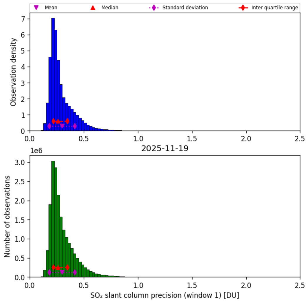
Figure 64: Histogram of “SO 2 slant column precision (window 1)” for 2025-11-18 to 2025-11-20
