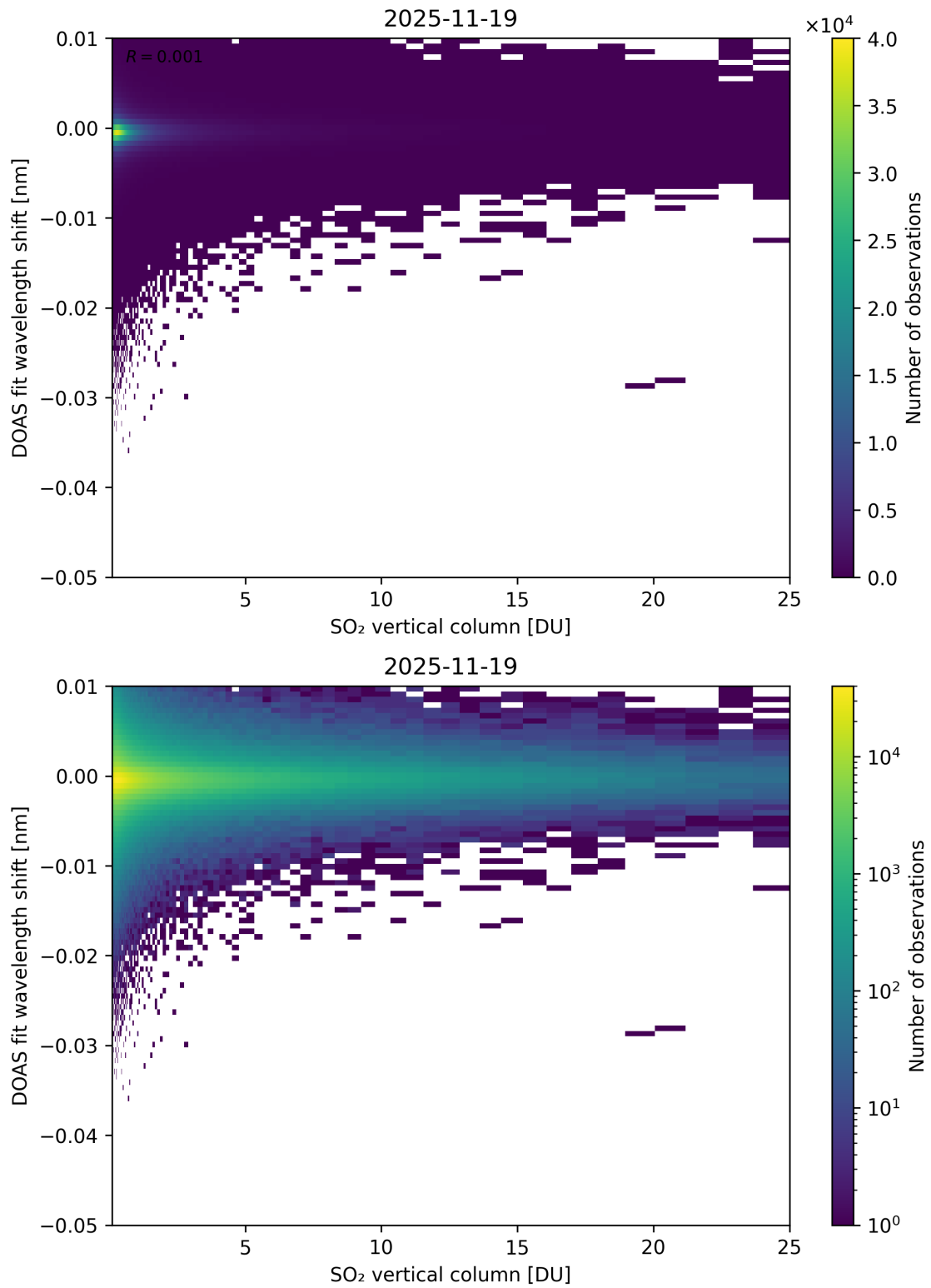
Figure 326: Scatter density plot of “SO 2 vertical column” against “DOAS fit wavelength shift” for 2025-11-18 to 2025-11-20.
