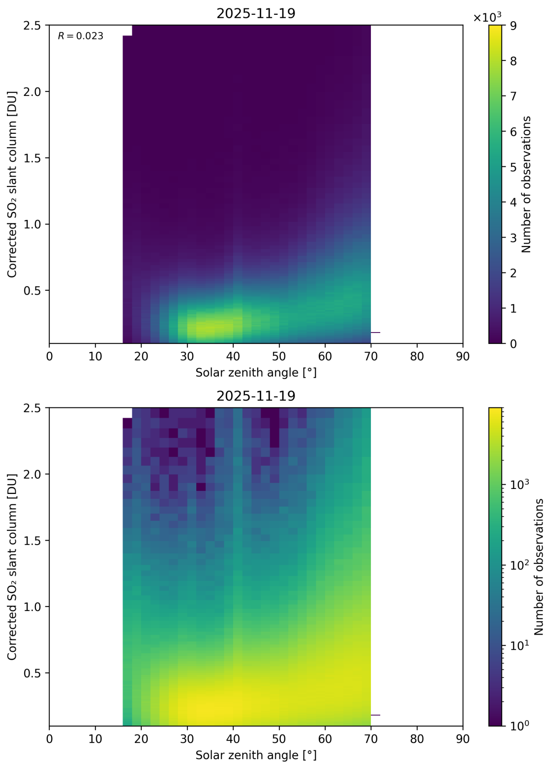
Figure 181: Scatter density plot of “Solar zenith angle” against “Corrected SO 2 slant column” for 2025-11-18 to 2025-11-20.
