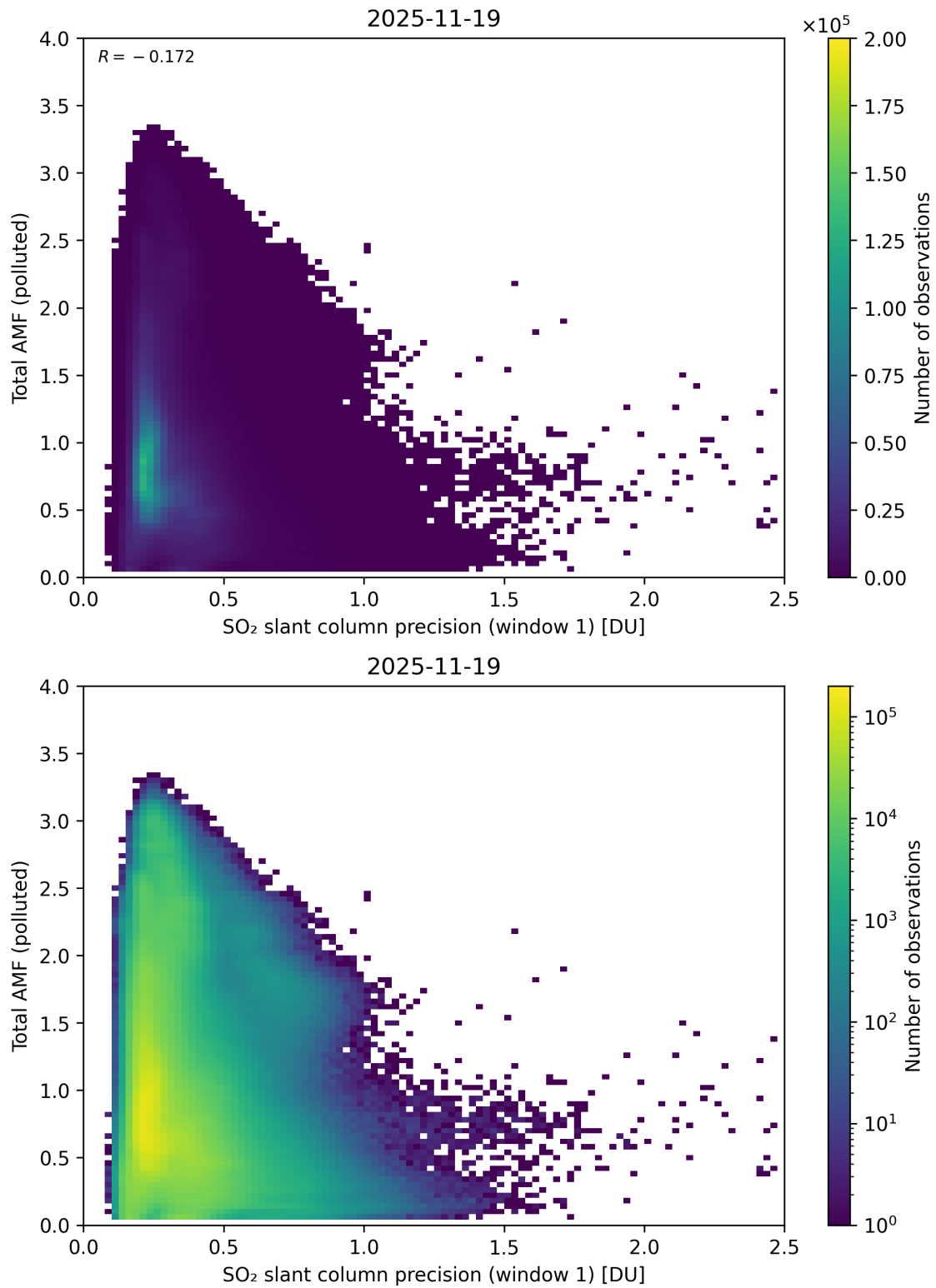
Figure 280: Scatter density plot of “SO 2 slant column precision (window 1)” against “Total AMF (polluted)” for 2025-11-18 to 2025-11-20.
