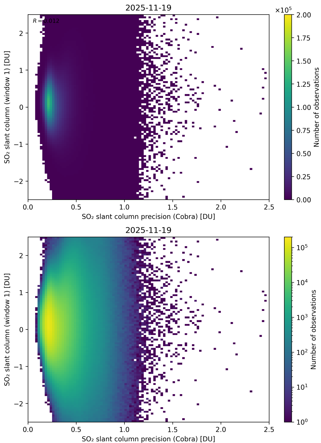
Figure 208: Scatter density plot of “SO 2 slant column precision (Cobra)” against “SO 2 slant column (window 1)” for 2025-11-18 to 2025-11-20.
