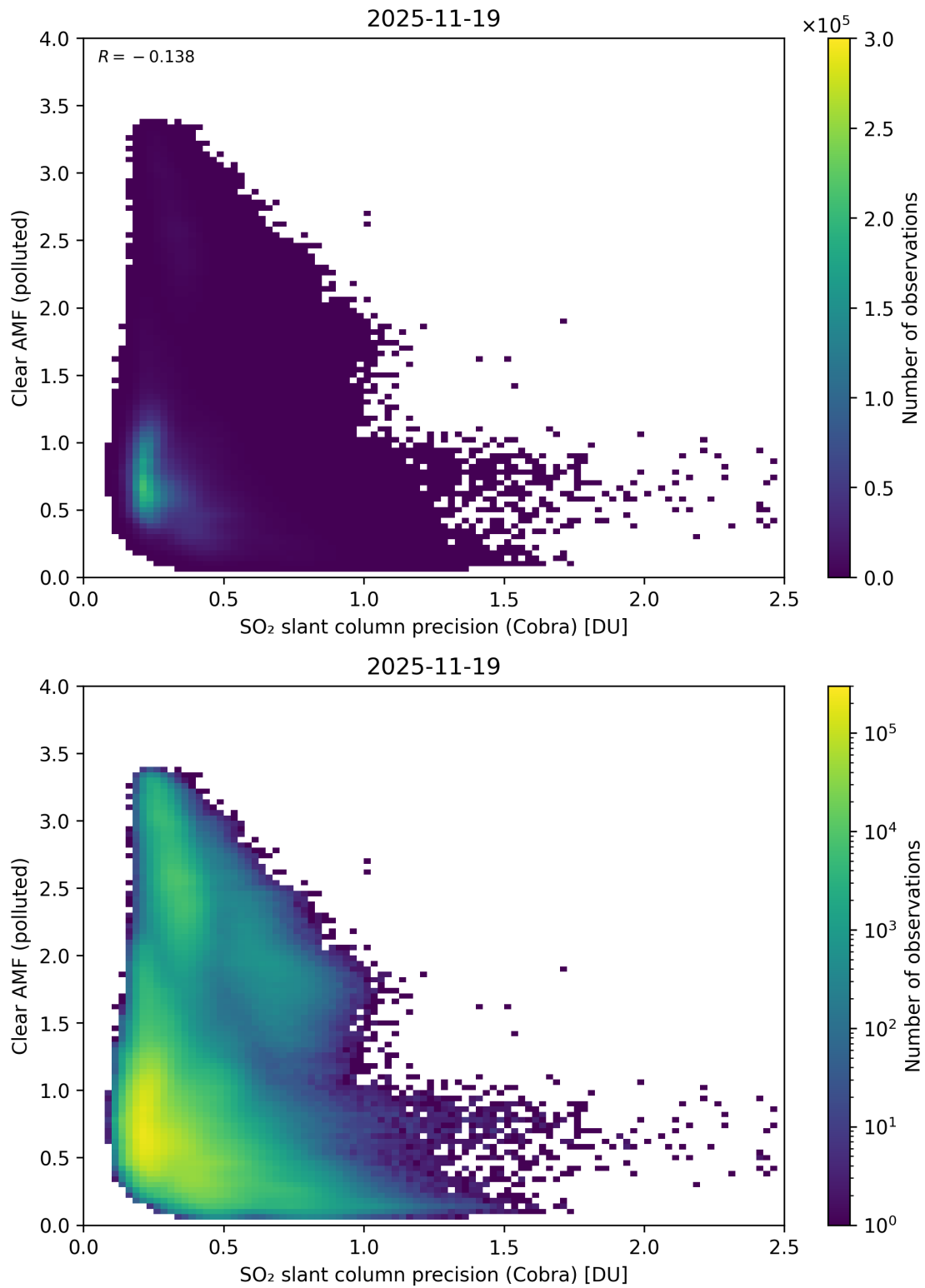
Figure 205: Scatter density plot of “SO 2 slant column precision (Cobra)” against “Clear AMF (polluted)” for 2025-11-18 to 2025-11-20.
