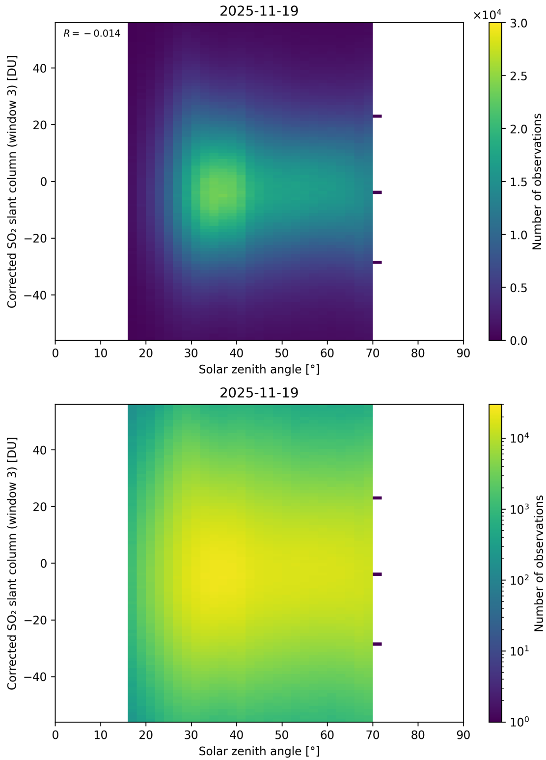
Figure 183: Scatter density plot of “Solar zenith angle” against “Corrected SO 2 slant column (window 3)” for 2025-11-18 to 2025-11-20.
