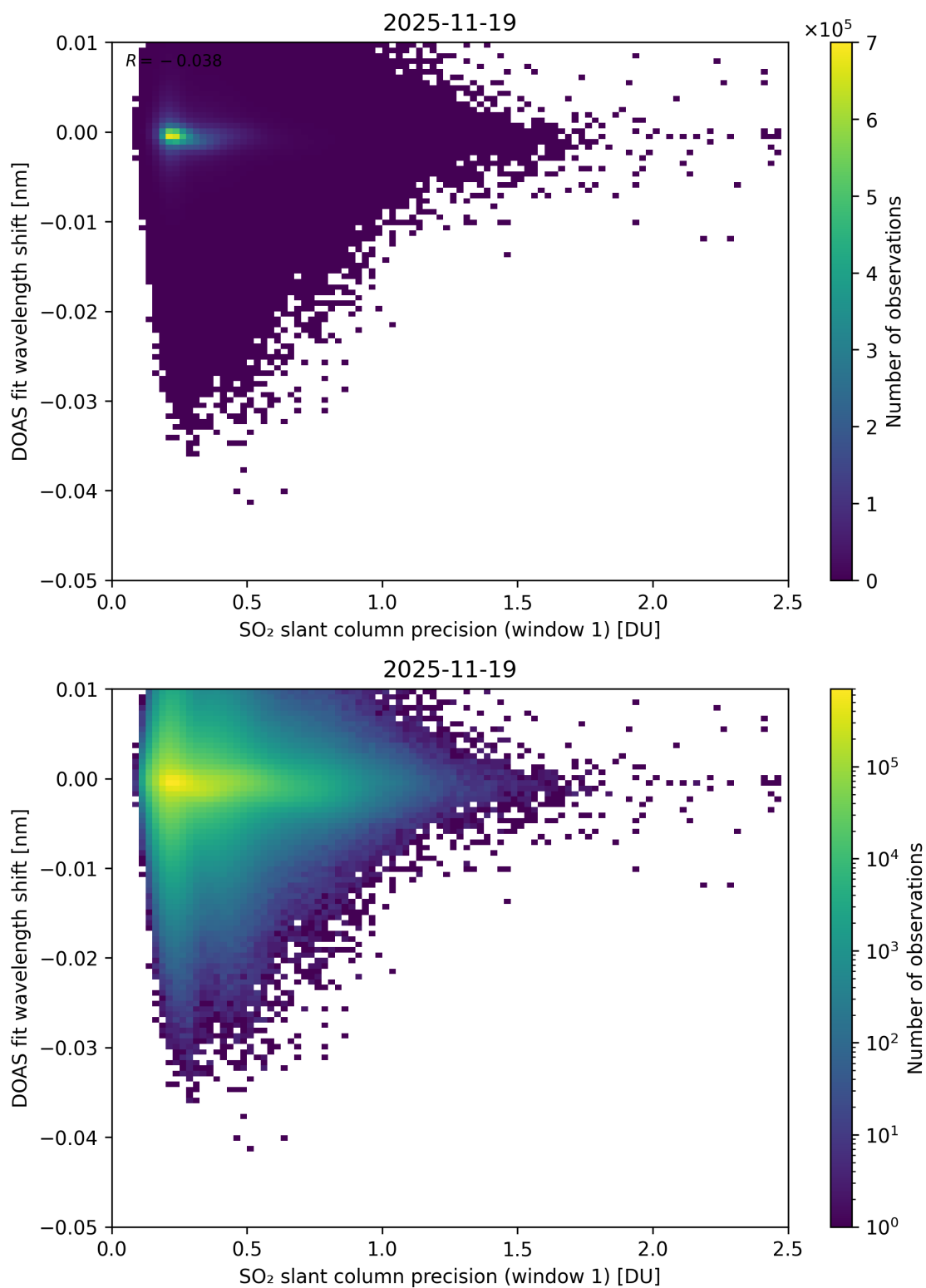
Figure 271: Scatter density plot of “SO 2 slant column precision (window 1)” against “DOAS fit wavelength shift” for 2025-11-18 to 2025-11-20.
