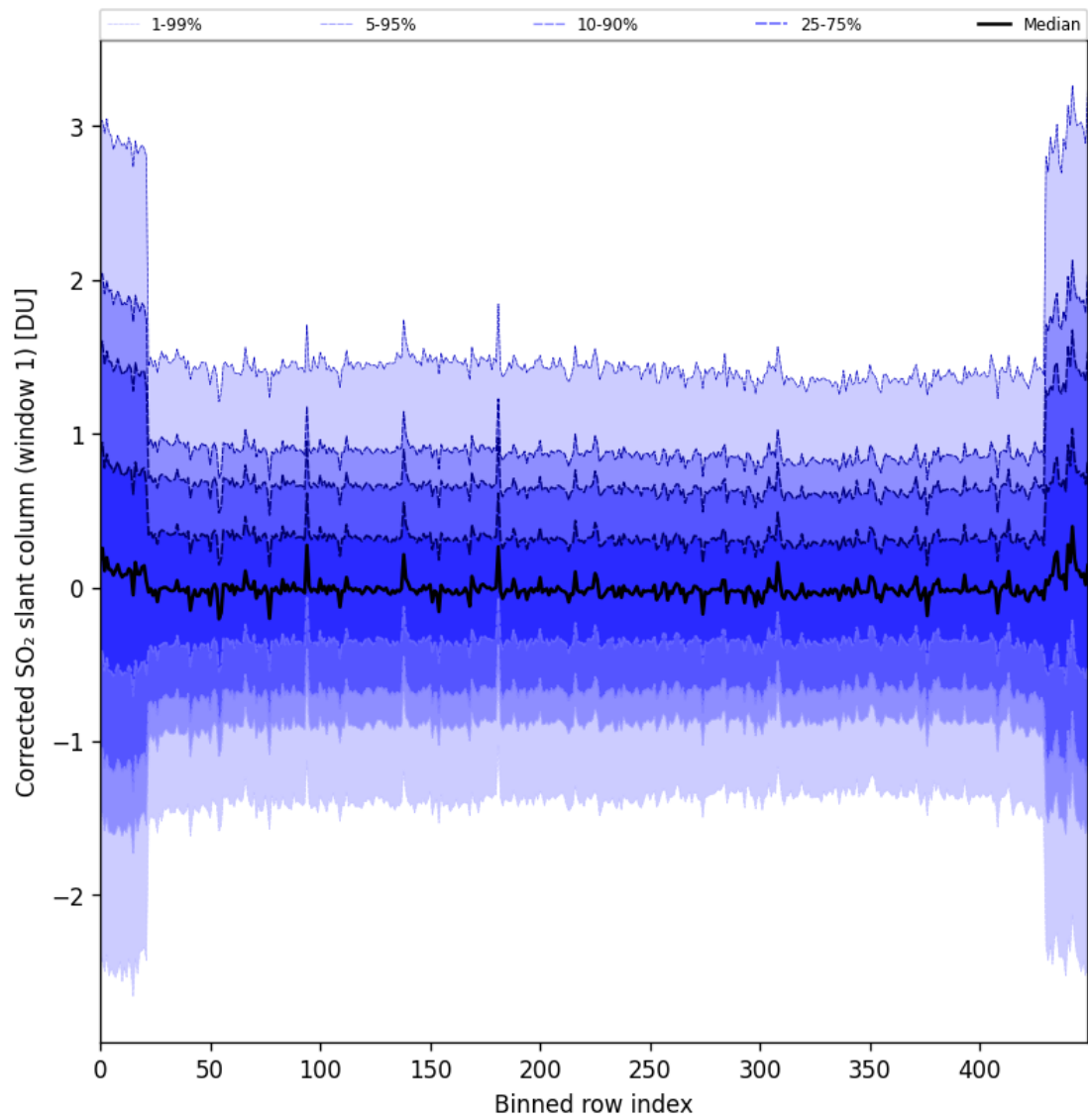
Figure 91: Along track statistics of “Corrected SO 2 slant column (window 1)” for 2025-11-18 to 2025-11-20
