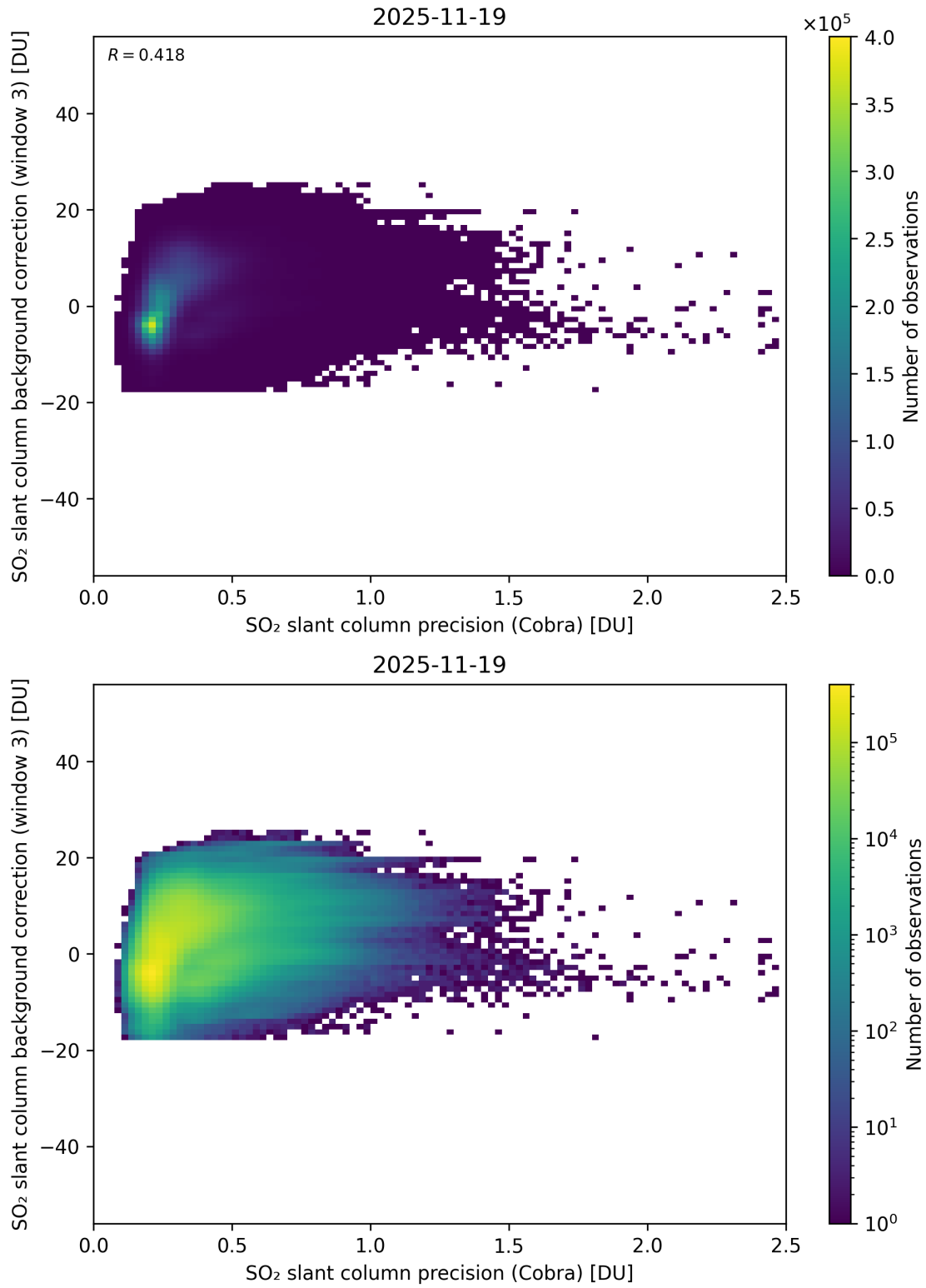
Figure 201: Scatter density plot of “SO 2 slant column precision (Cobra)” against “SO 2 slant column background correction (window 3)” for 2025-11-18 to 2025-11-20.
