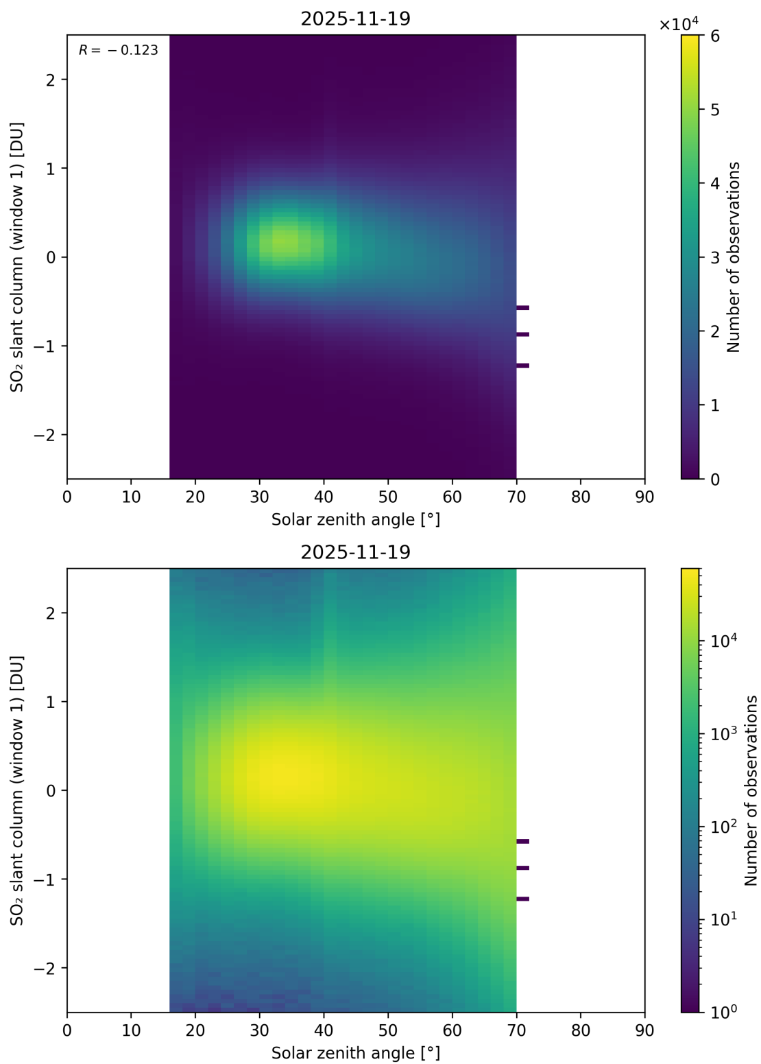
Figure 184: Scatter density plot of “Solar zenith angle” against “SO 2 slant column (window 1)” for 2025-11-18 to 2025-11-20.
