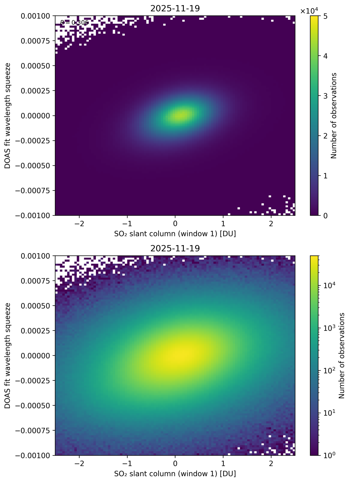
Figure 266: Scatter density plot of “SO 2 slant column (window 1)” against “DOAS fit wavelength squeeze” for 2025-11-18 to 2025-11-20.
