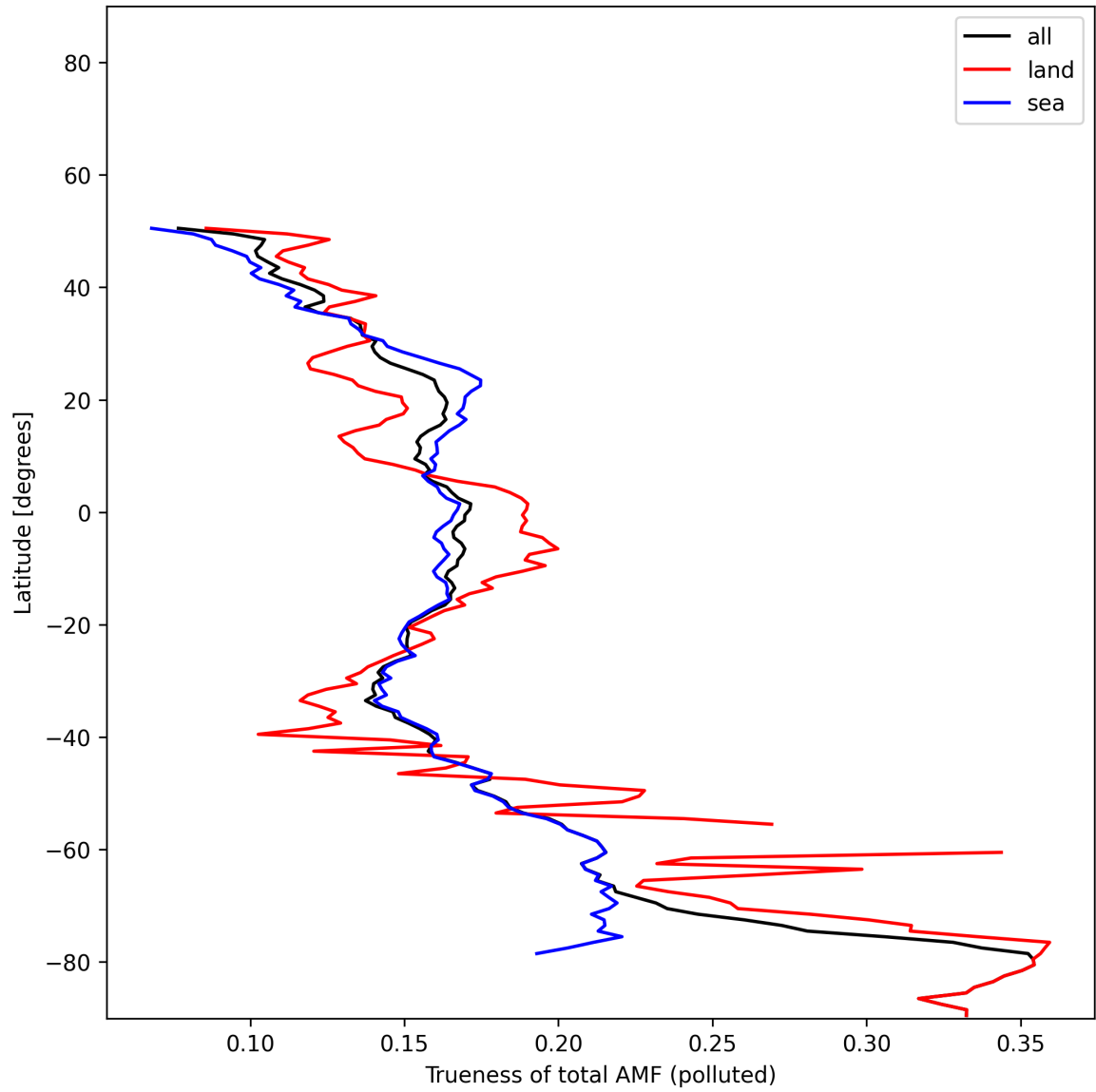
Figure 54: Zonal average of “Trueness of total AMF (polluted)” for 2025-11-18 to 2025-11-20.
