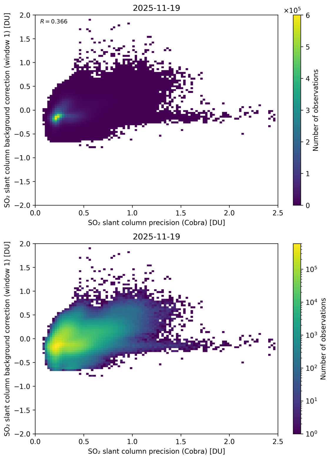
Figure 199: Scatter density plot of “SO 2 slant column precision (Cobra)” against “SO 2 slant column background correction (window 1)” for 2025-11-18 to 2025-11-20.
