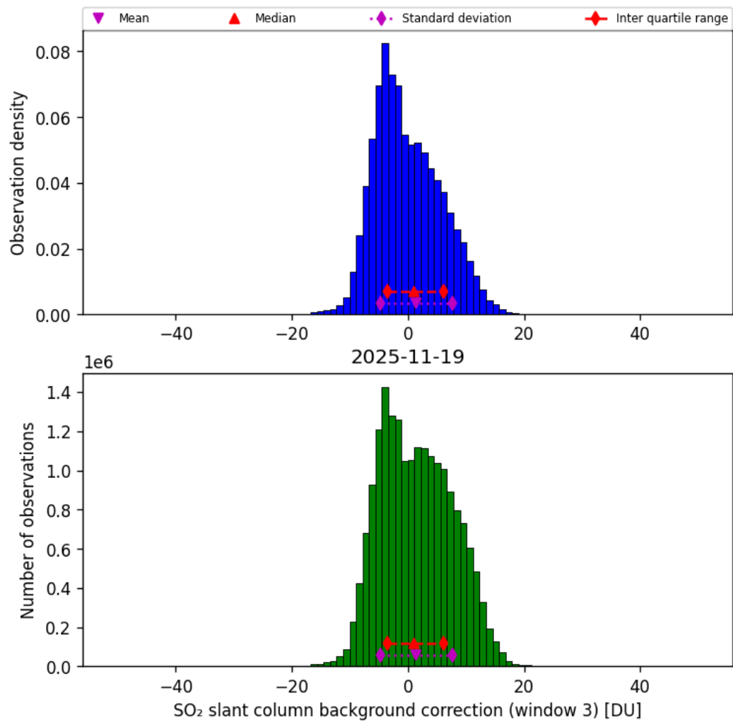
Figure 74: Histogram of “SO 2 slant column background correction (window 3)” for 2025-11-18 to 2025-11-20
