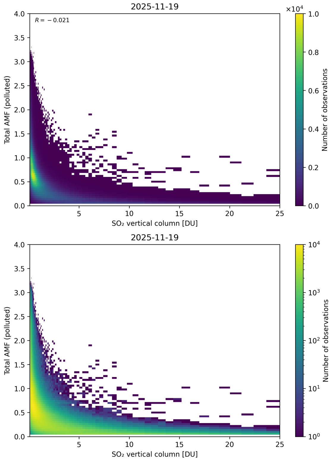
Figure 359: Scatter density plot of “SO 2 vertical column” against “Total AMF (polluted)” for 2025-11-18 to 2025-11-20.
