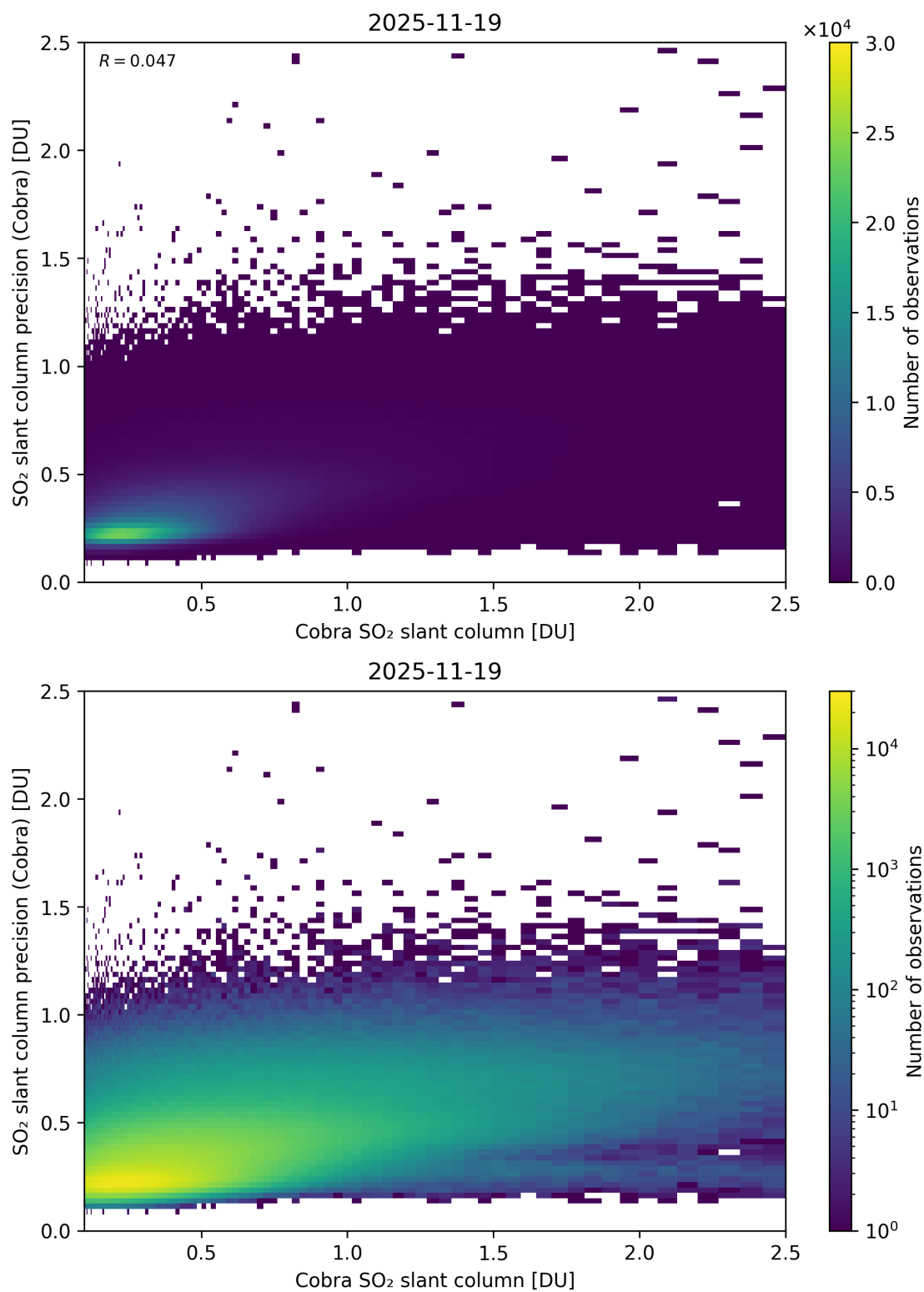
Figure 216: Scatter density plot of “Cobra SO 2 slant column” against “SO 2 slant column precision (Cobra)” for 2025-11-18 to 2025-11-20.
