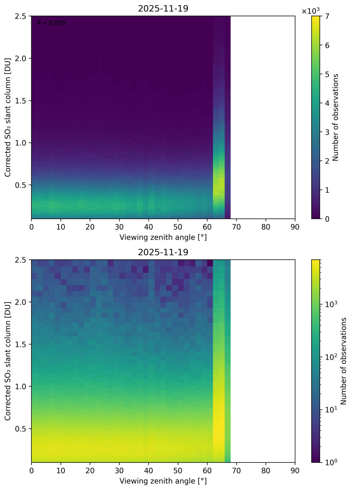
Figure 373: Scatter density plot of “Viewing zenith angle” against “Corrected SO 2 slant column” for 2025-11-18 to 2025-11-20.
