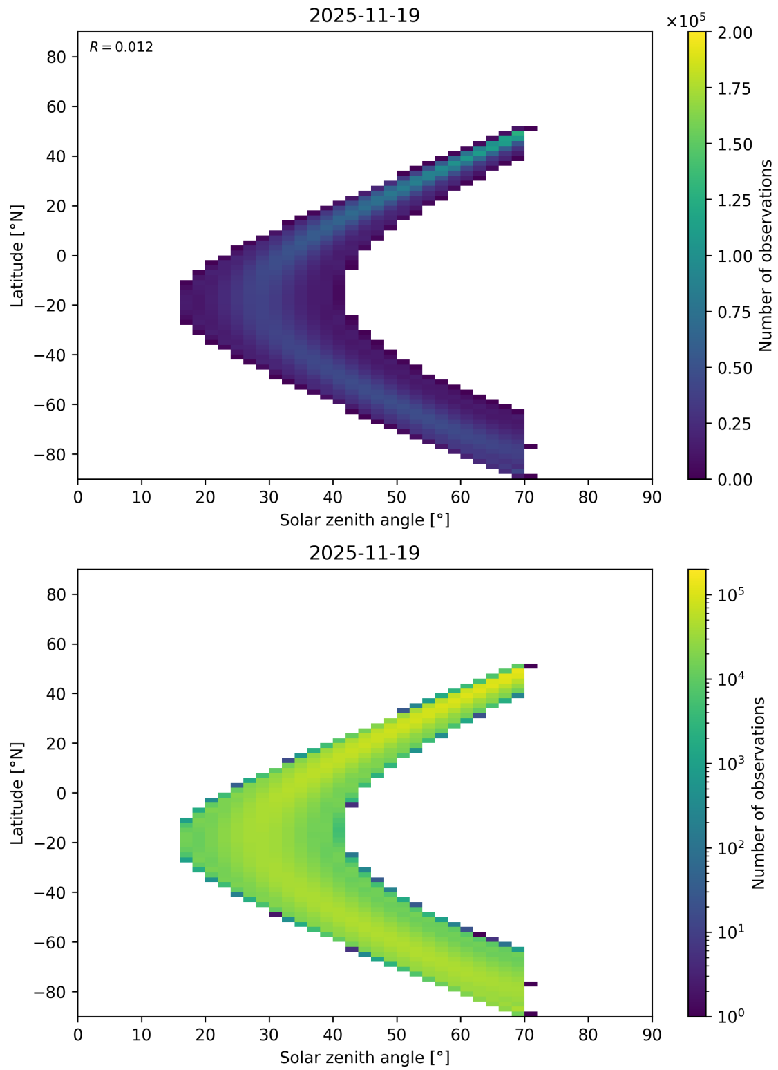
Figure 177: Scatter density plot of “Solar zenith angle” against “Latitude” for 2025-11-18 to 2025-11-20.
