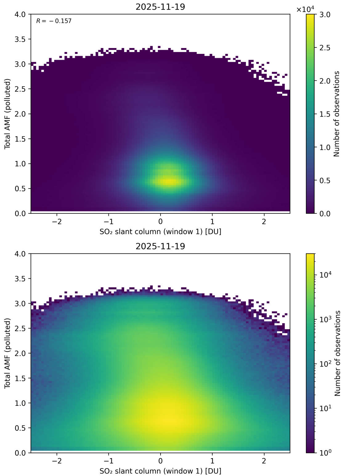
Figure 289: Scatter density plot of “SO 2 slant column (window 1)” against “Total AMF (polluted)” for 2025-11-18 to 2025-11-20.
