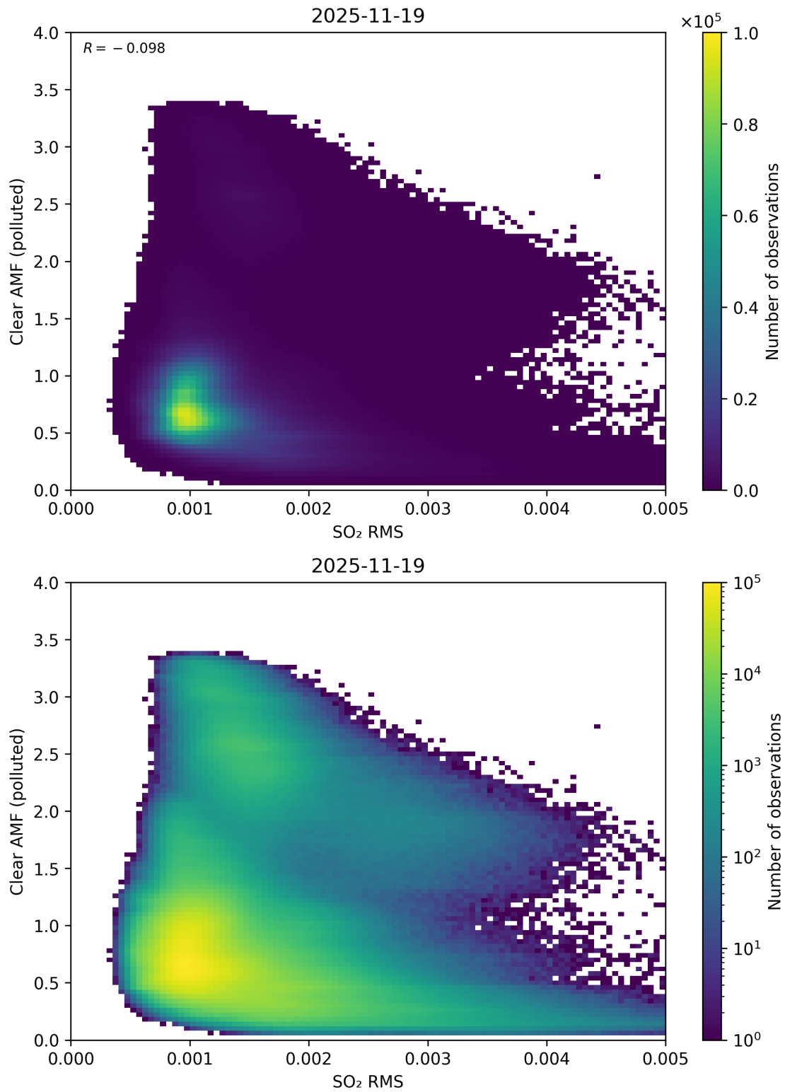
Figure 147: Scatter density plot of “SO 2 RMS” against “Clear AMF (polluted)” for 2025-11-18 to 2025-11-20.
