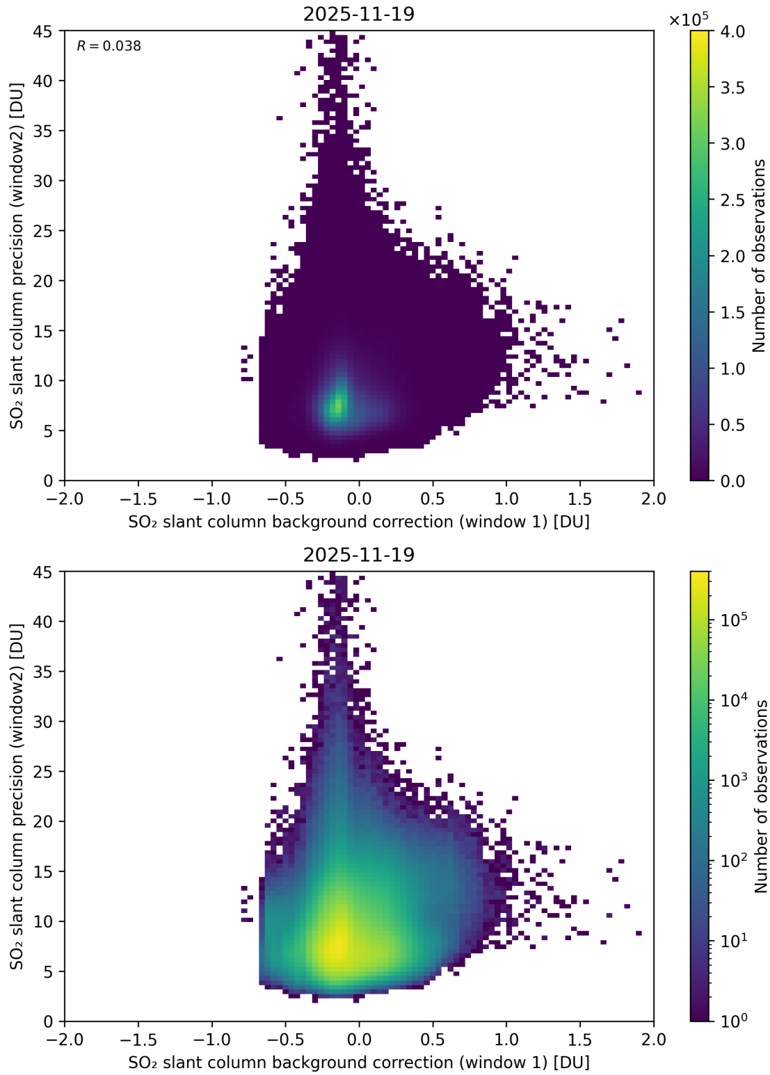
Figure 117: Scatter density plot of “SO 2 slant column background correction (window 1)” against “SO 2 slant column precision (window2)” for 2025-11-18 to 2025-11-20.
