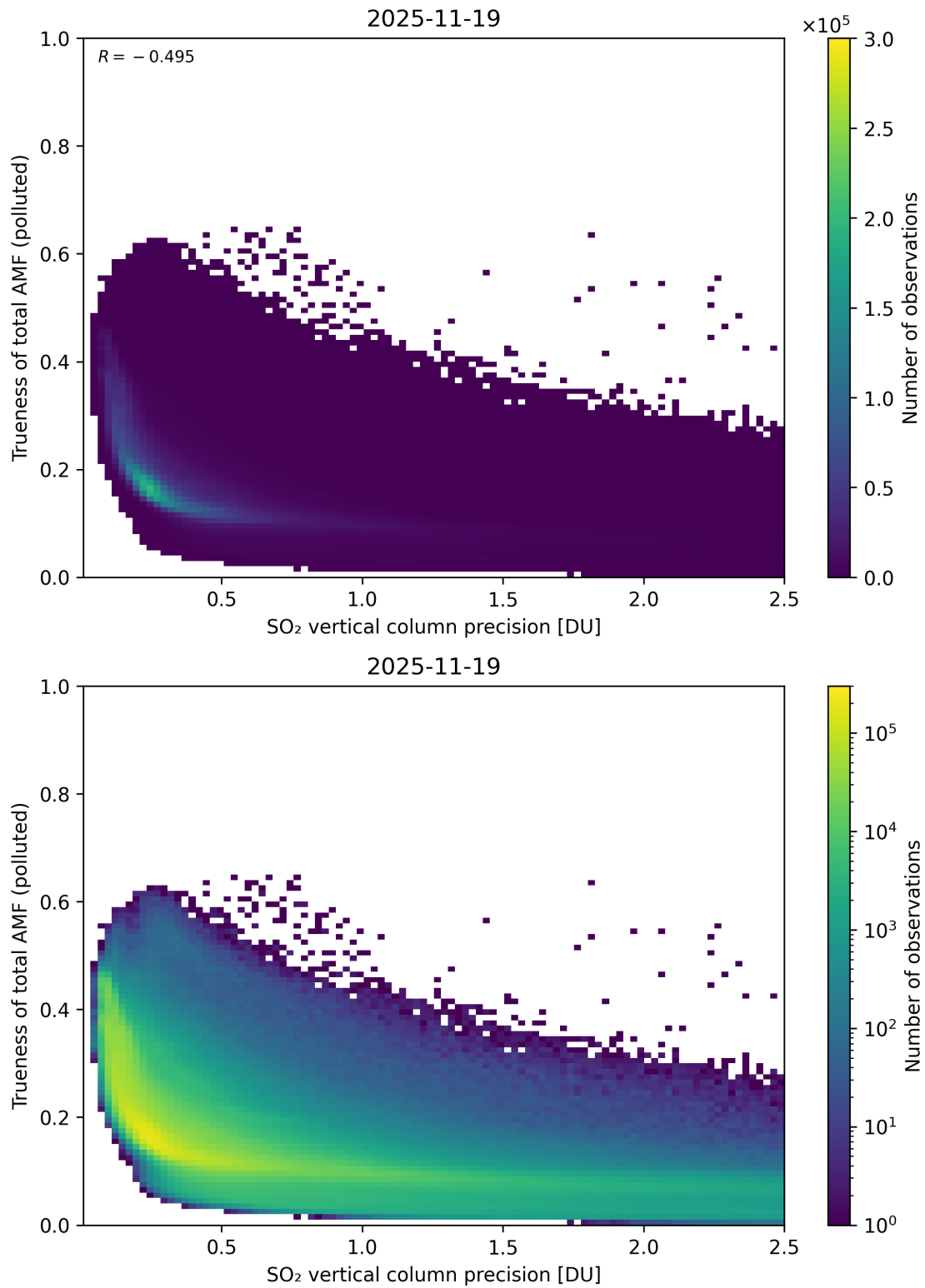
Figure 347: Scatter density plot of “SO 2 vertical column precision” against “Trueness of total AMF (polluted)” for 2025-11-18 to 2025-11-20.
