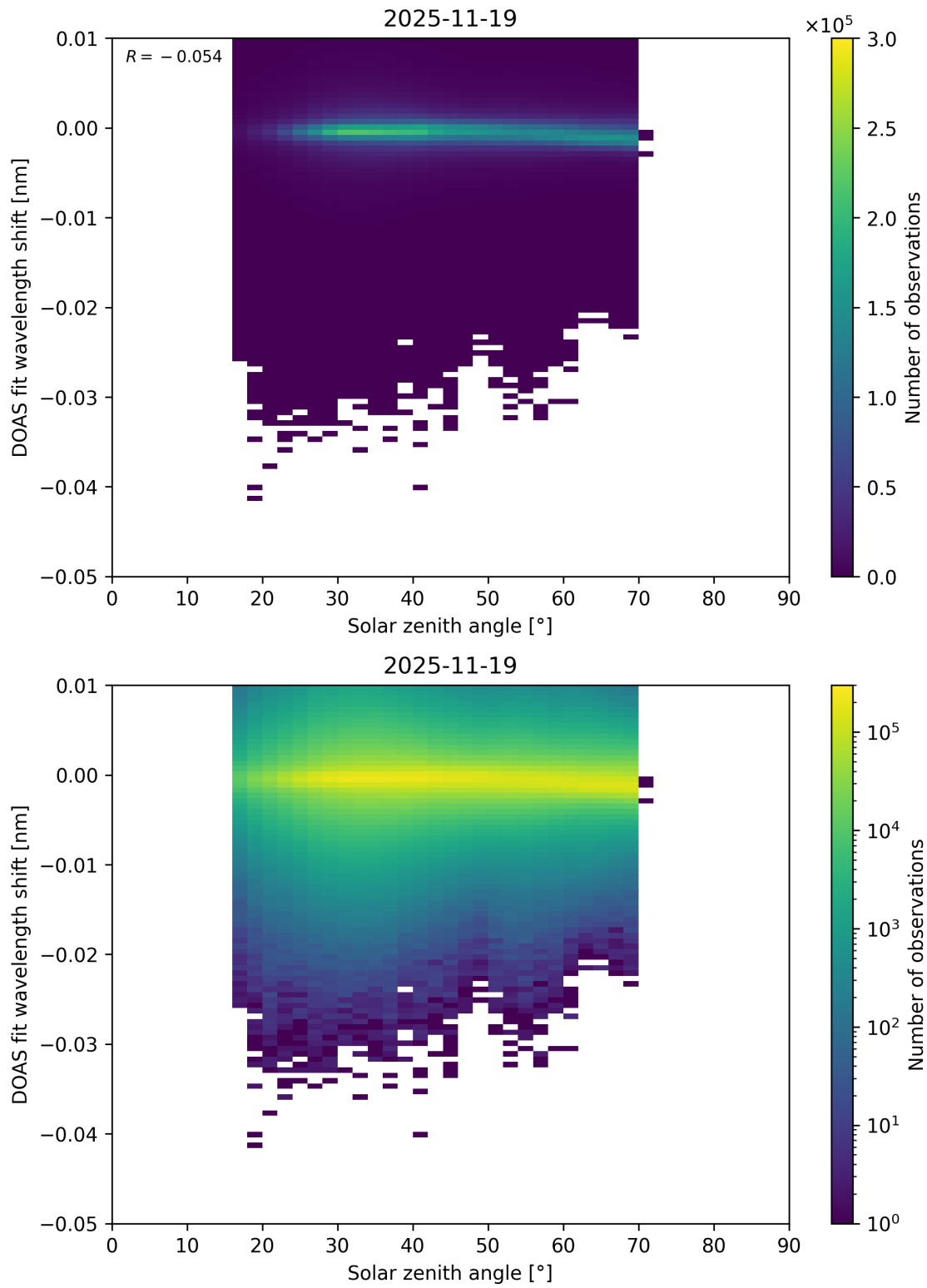
Figure 174: Scatter density plot of “Solar zenith angle” against “DOAS fit wavelength shift” for 2025-11-18 to 2025-11-20.
