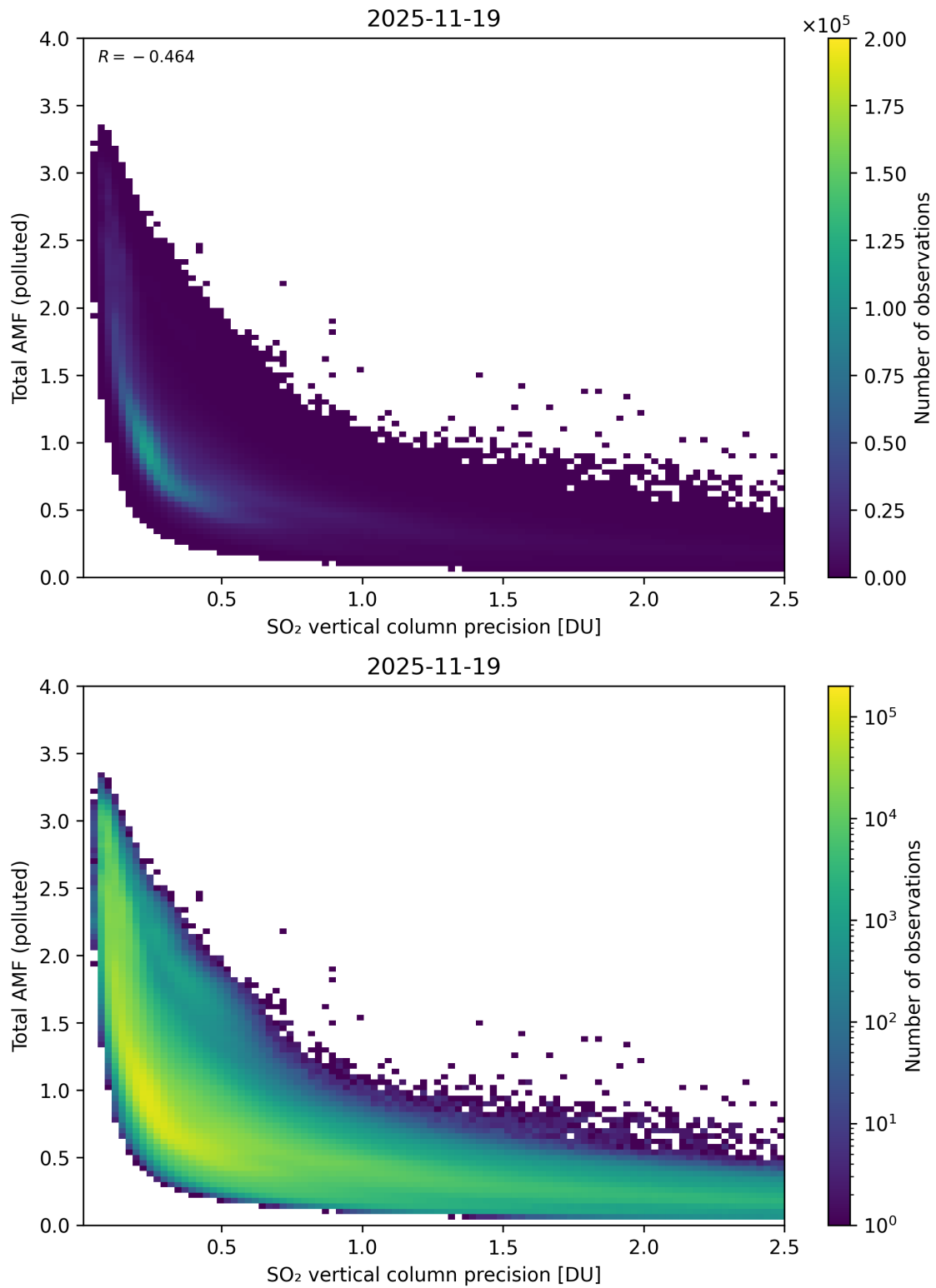
Figure 346: Scatter density plot of “SO 2 vertical column precision” against “Total AMF (polluted)” for 2025-11-18 to 2025-11-20.
