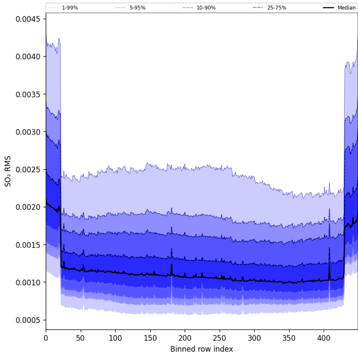
Figure 104: Along track statistics of “SO 2 RMS” for 2025-11-18 to 2025-11-20
