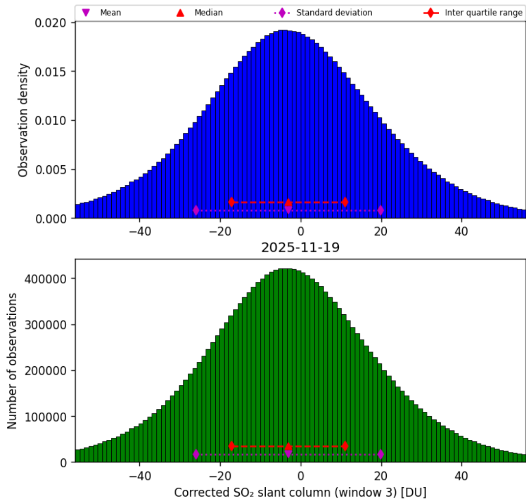
Figure 73: Histogram of “Corrected SO 2 slant column (window 3)” for 2025-11-18 to 2025-11-20
