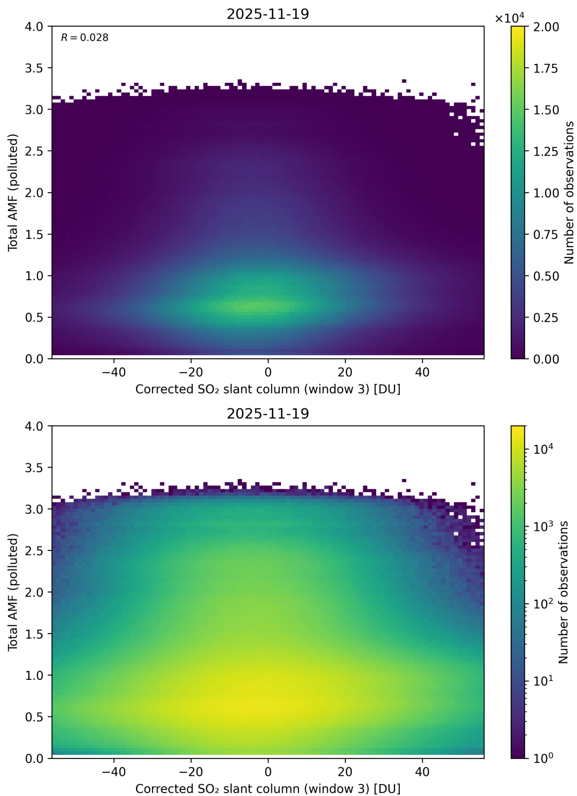
Figure 260: Scatter density plot of “Corrected SO 2 slant column (window 3)” against “Total AMF (polluted)” for 2025-11-18 to 2025-11-20.
