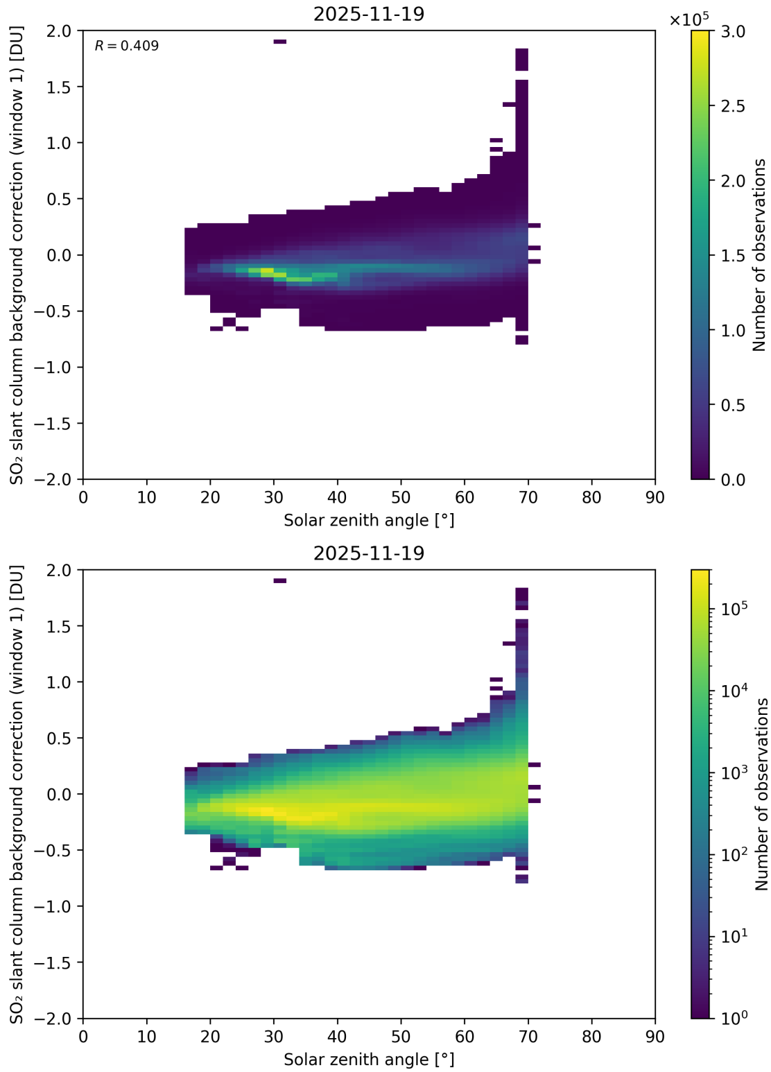
Figure 171: Scatter density plot of “Solar zenith angle” against “SO 2 slant column background correction (window 1)” for 2025-11-18 to 2025-11-20.
