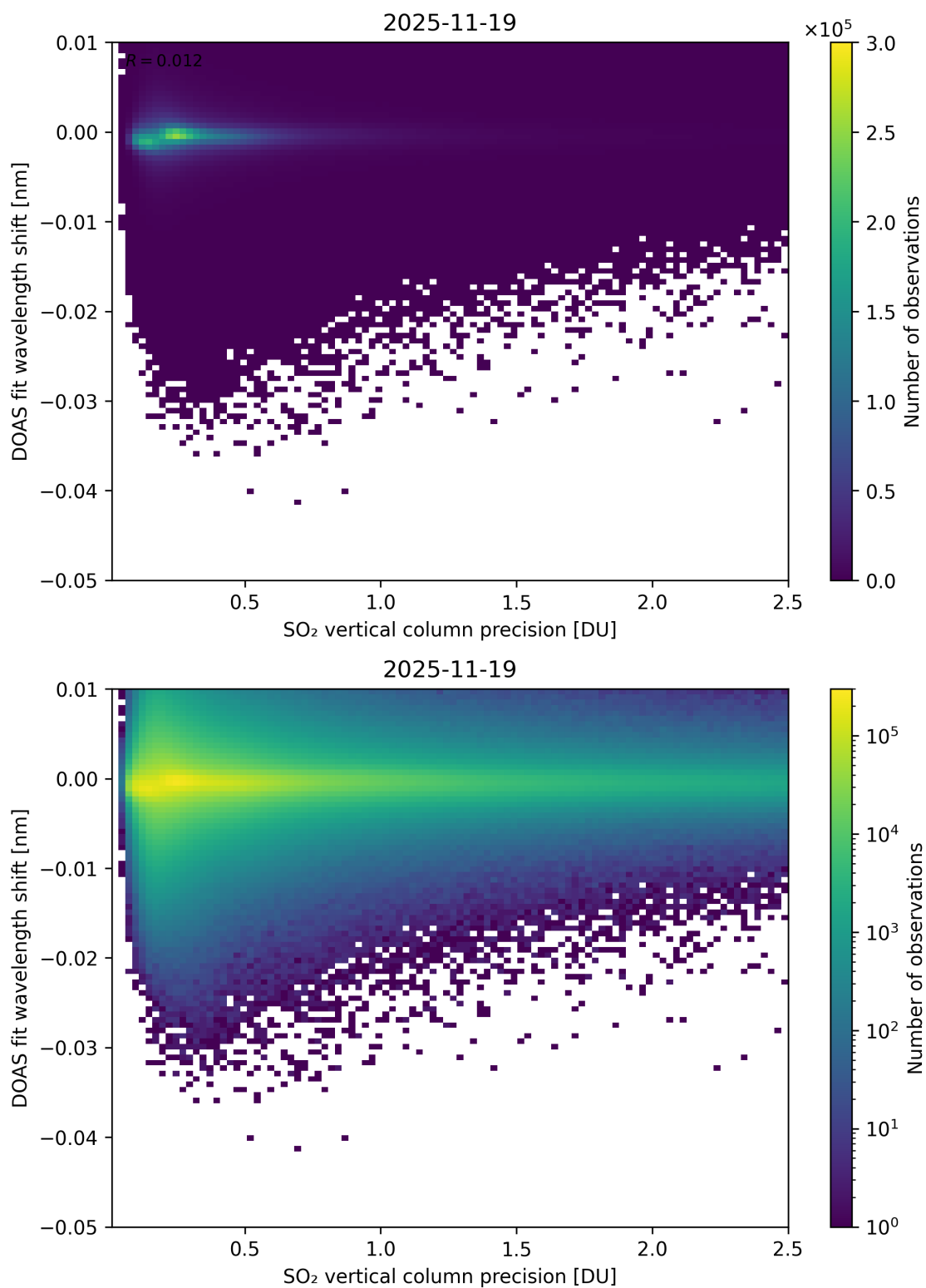
Figure 332: Scatter density plot of “SO 2 vertical column precision” against “DOAS fit wavelength shift” for 2025-11-18 to 2025-11-20.
