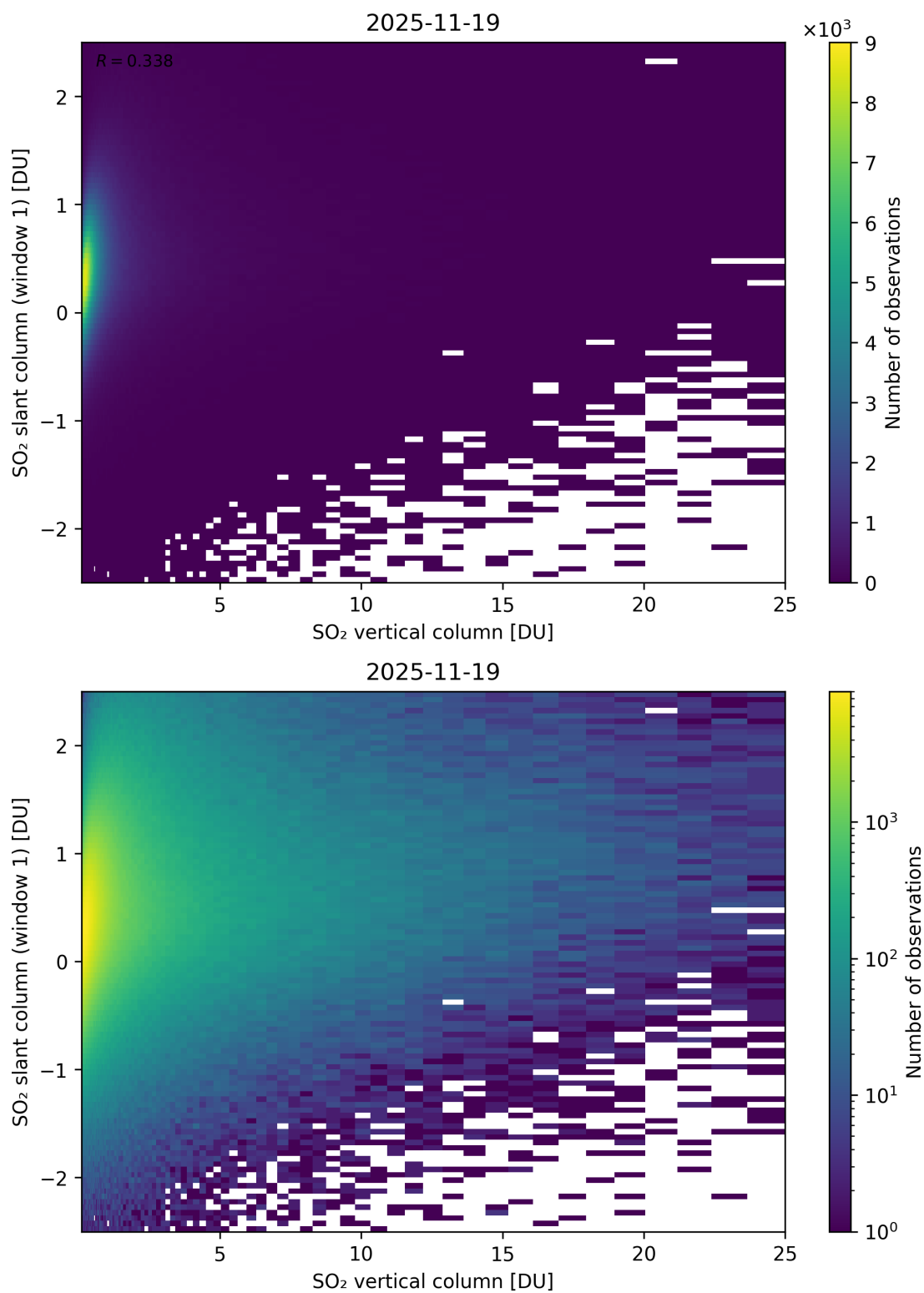
Figure 354: Scatter density plot of “SO 2 vertical column” against “SO 2 slant column (window 1)” for 2025-11-18 to 2025-11-20.
