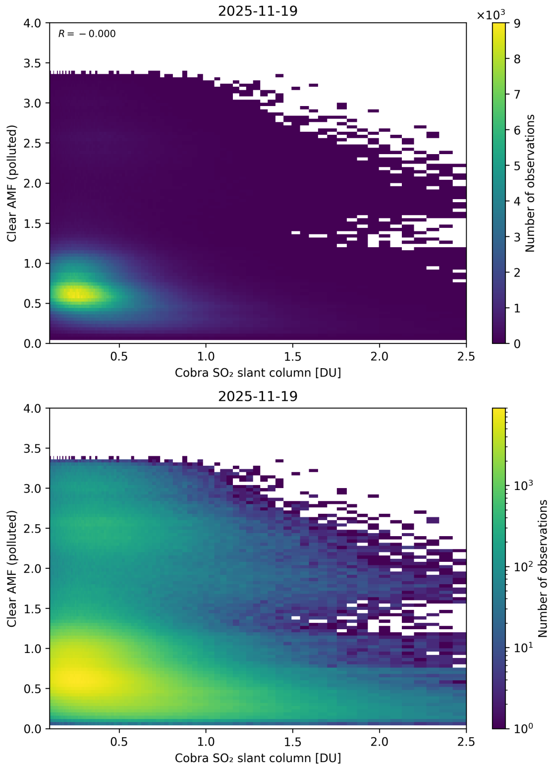
Figure 215: Scatter density plot of “Cobra SO 2 slant column” against “Clear AMF (polluted)” for 2025-11-18 to 2025-11-20.
