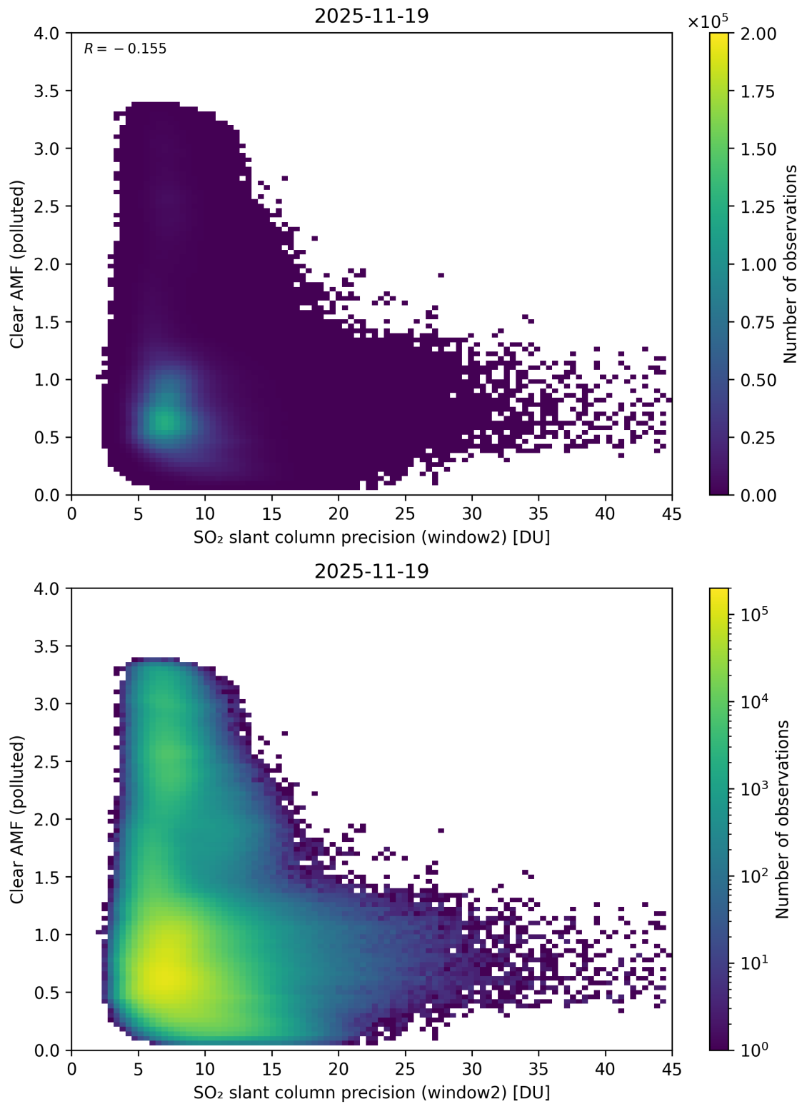
Figure 296: Scatter density plot of “SO 2 slant column precision (window2)” against “Clear AMF (polluted)” for 2025-11-18 to 2025-11-20.
