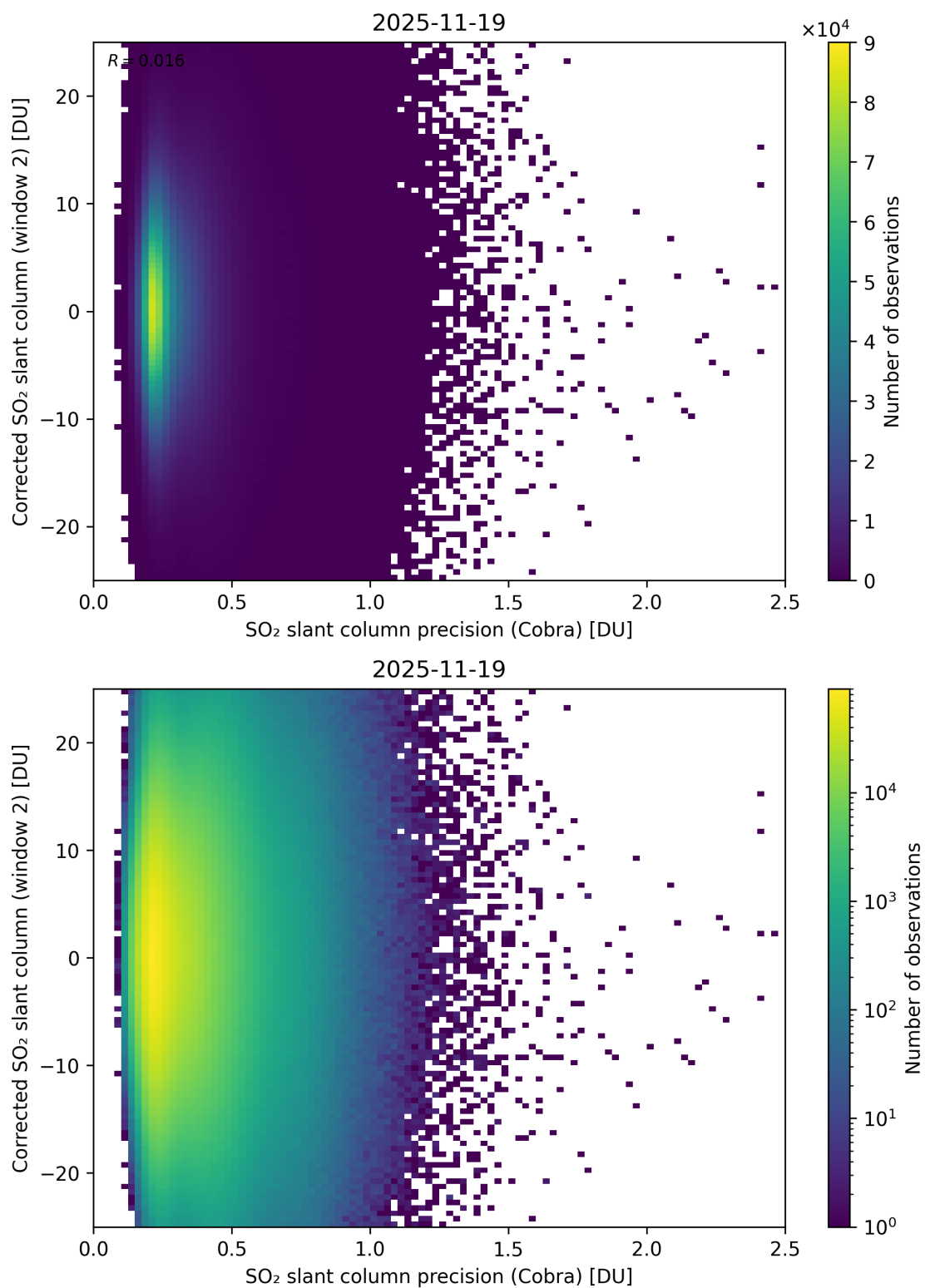
Figure 206: Scatter density plot of “SO 2 slant column precision (Cobra)” against “Corrected SO 2 slant column (window 2)” for 2025-11-18 to 2025-11-20.
