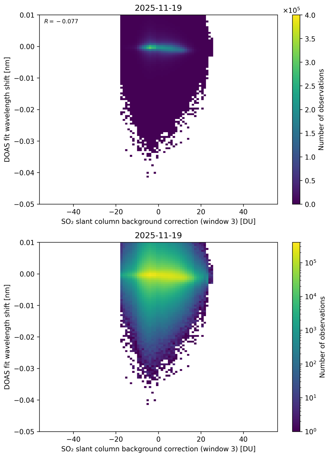
Figure 132: Scatter density plot of “SO 2 slant column background correction (window 3)” against “DOAS fit wavelength shift” for 2025-11-18 to 2025-11-20.
