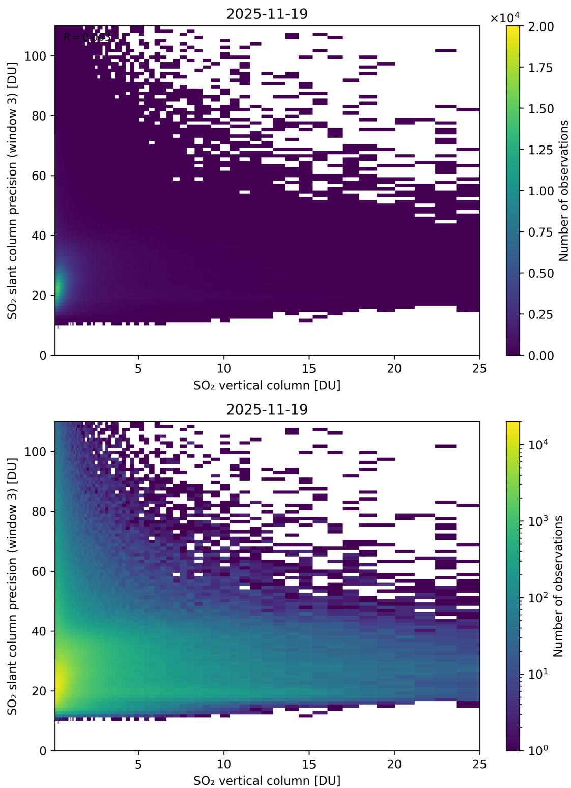
Figure 358: Scatter density plot of “SO 2 vertical column” against “SO 2 slant column precision (window 3)” for 2025-11-18 to 2025-11-20.
