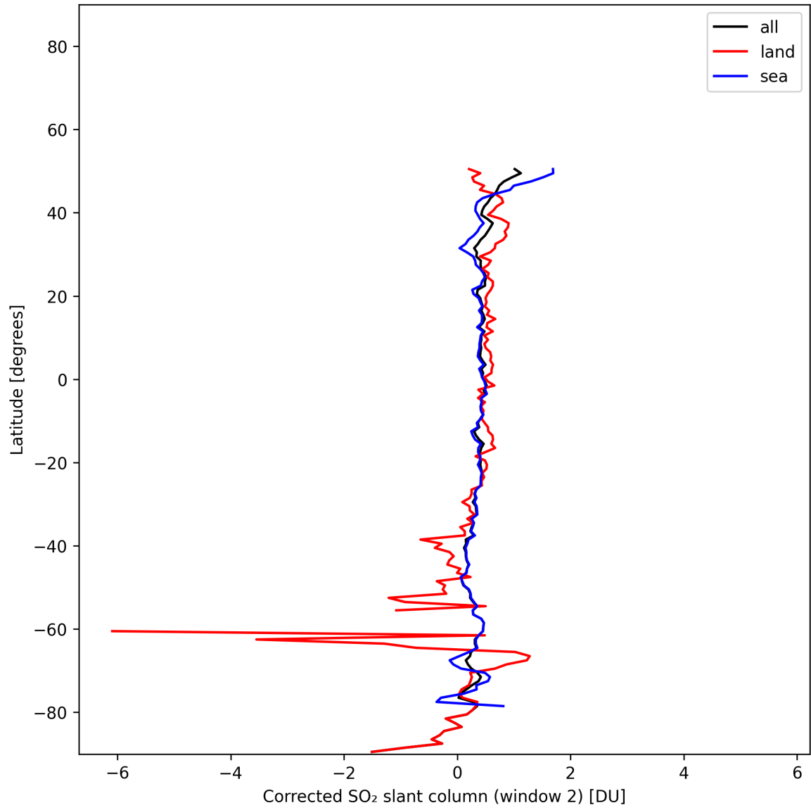
Figure 43: Zonal average of “Corrected SO 2 slant column (window 2)” for 2025-11-18 to 2025-11-20.
