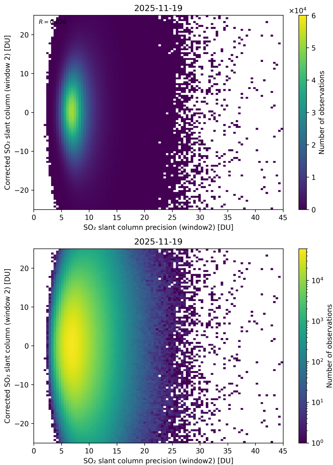
Figure 297: Scatter density plot of “SO 2 slant column precision (window2)” against “Corrected SO 2 slant column (window 2)” for 2025-11-18 to 2025-11-20.
