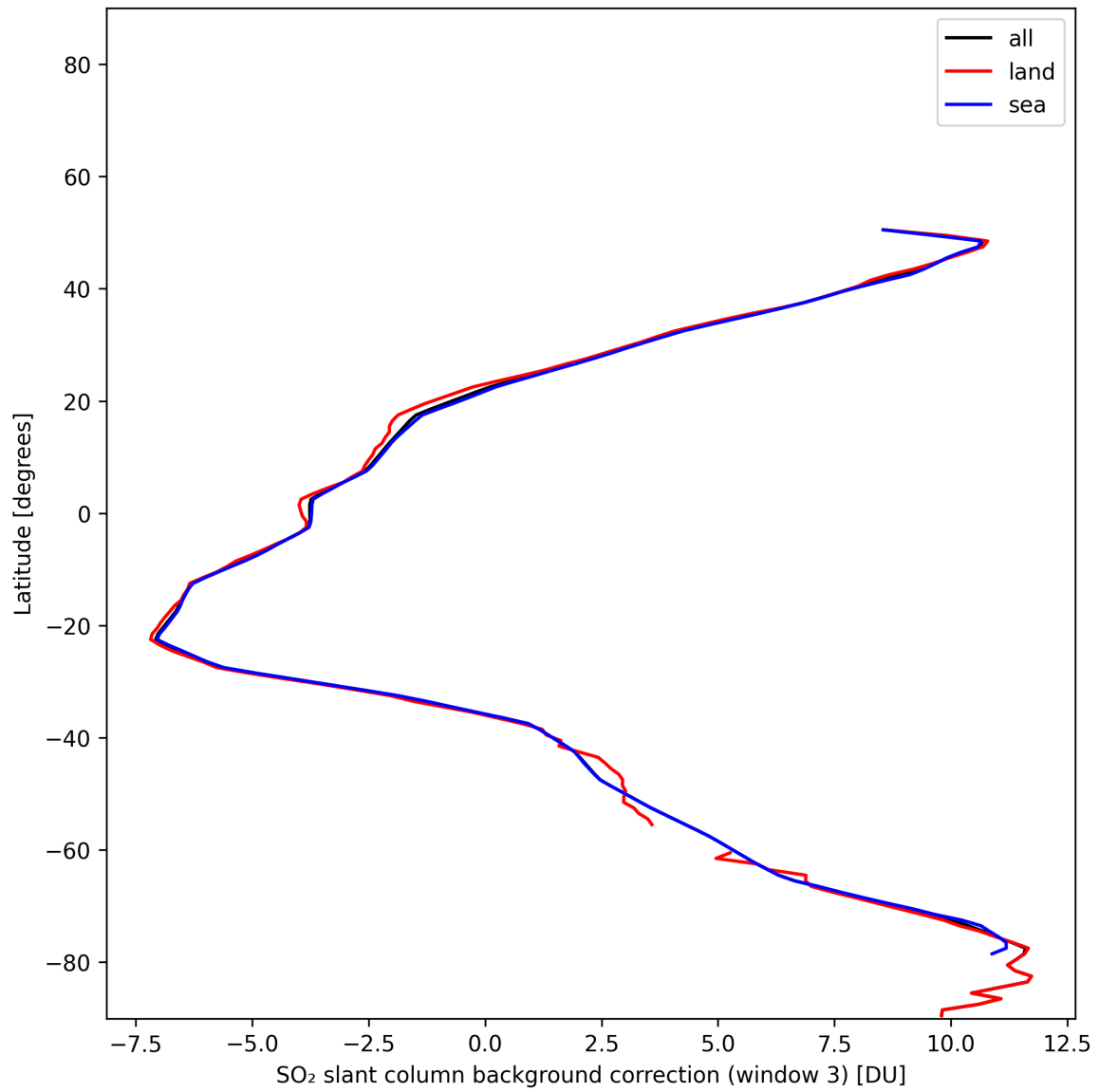
Figure 48: Zonal average of “SO 2 slant column background correction (window 3)” for 2025-11-18 to 2025-11-20.
