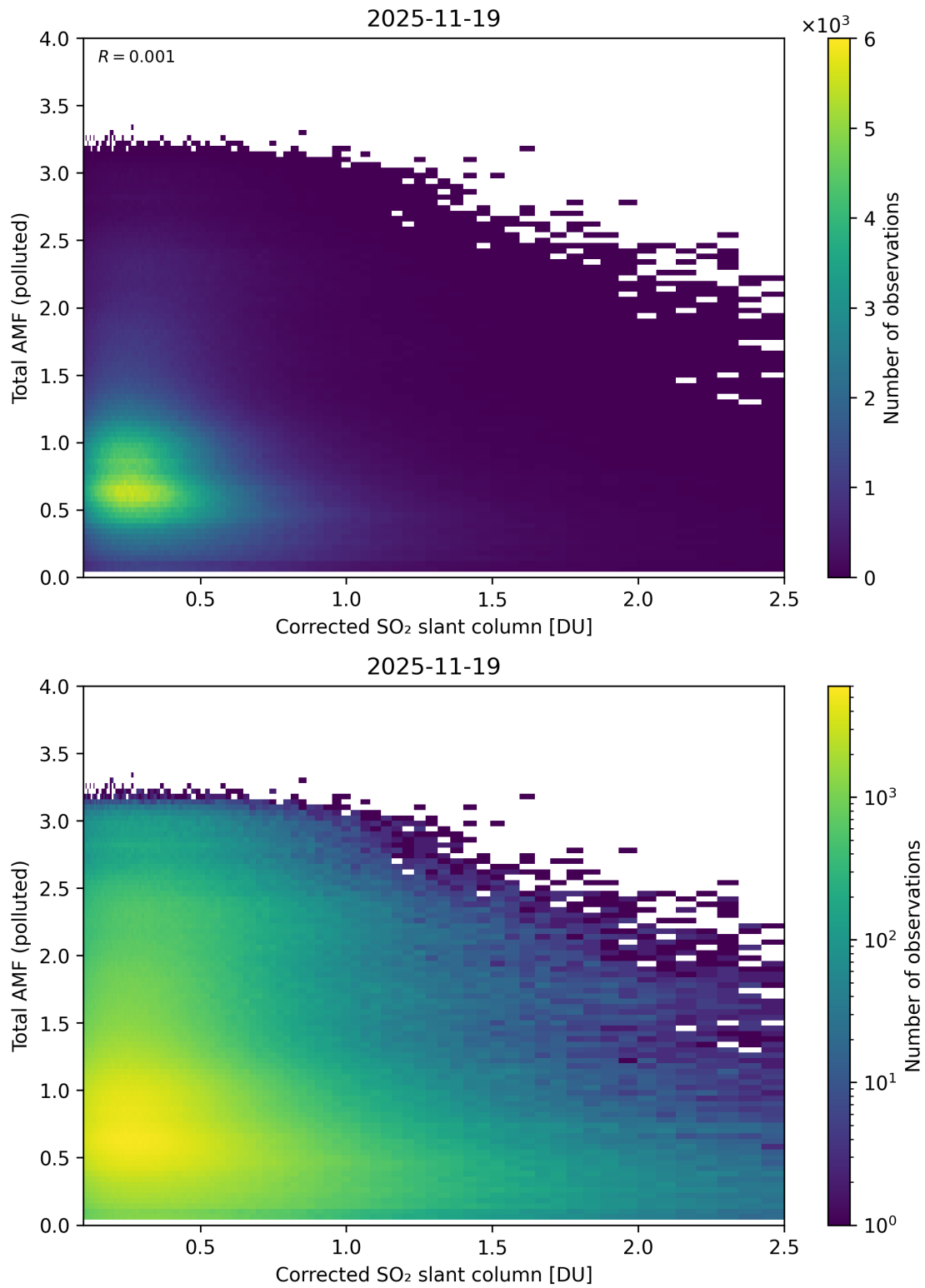
Figure 242: Scatter density plot of “Corrected SO 2 slant column” against “Total AMF (polluted)” for 2025-11-18 to 2025-11-20.
