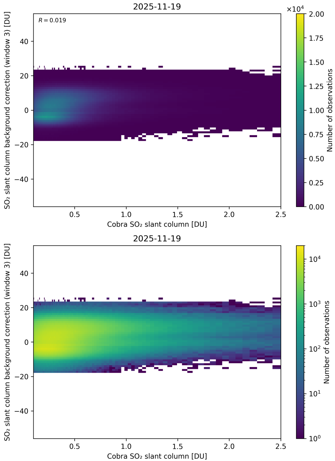
Figure 195: Scatter density plot of “Cobra SO 2 slant column” against “SO 2 slant column background correction (window 3)” for 2025-11-18 to 2025-11-20.
