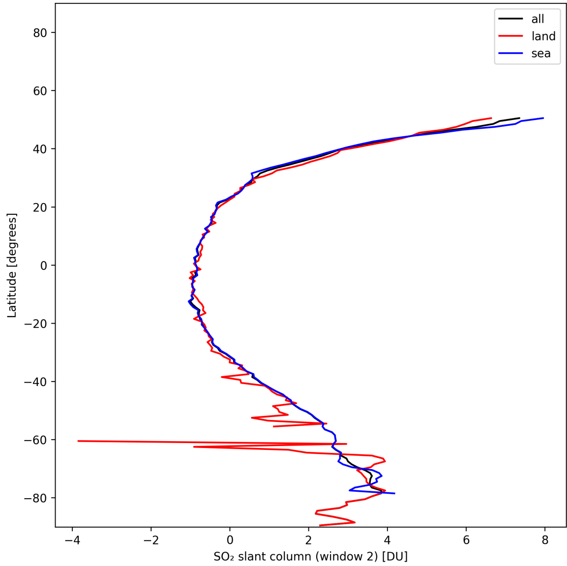
Figure 41: Zonal average of “SO 2 slant column (window 2)” for 2025-11-18 to 2025-11-20.
