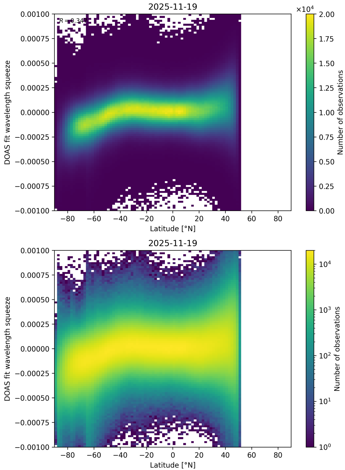
Figure 154: Scatter density plot of “Latitude” against “DOAS fit wavelength squeeze” for 2025-11-18 to 2025-11-20.
