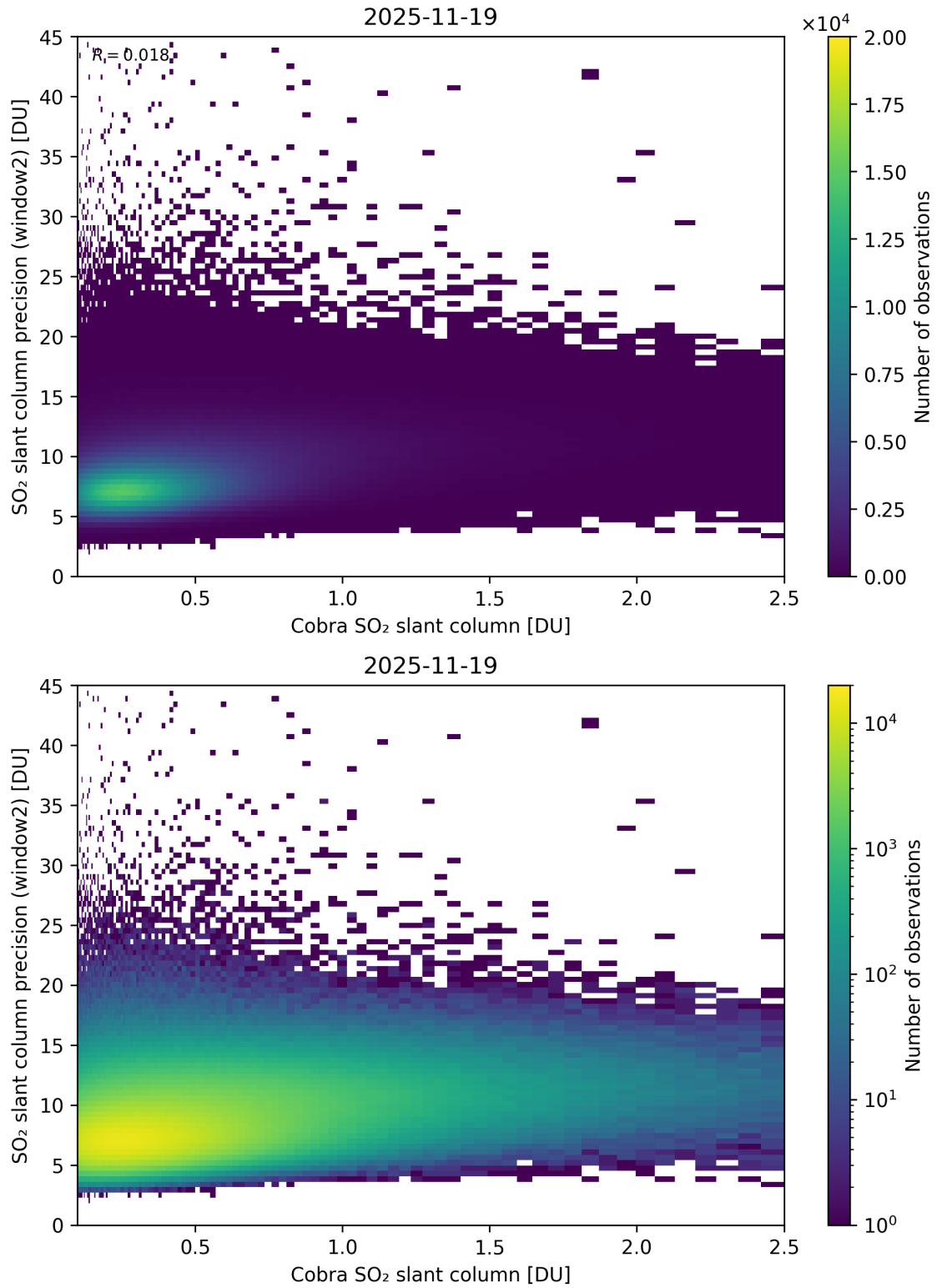
Figure 221: Scatter density plot of “Cobra SO 2 slant column” against “SO 2 slant column precision (window2)” for 2025-11-18 to 2025-11-20.
