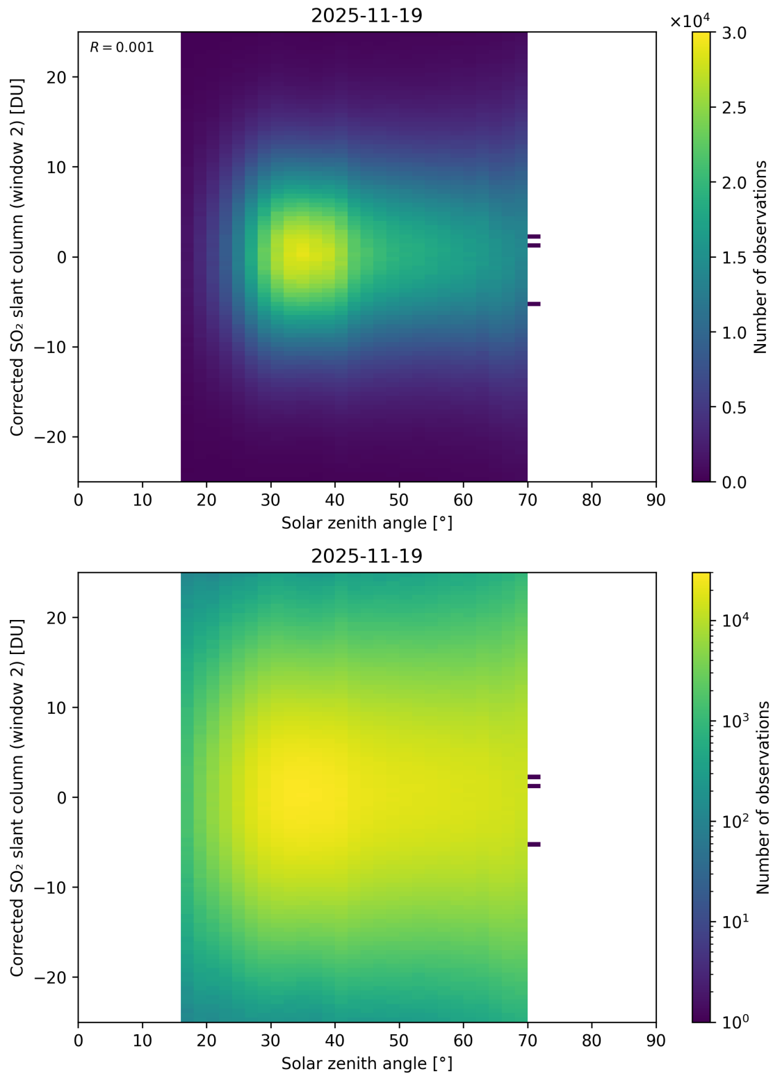
Figure 182: Scatter density plot of “Solar zenith angle” against “Corrected SO 2 slant column (window 2)” for 2025-11-18 to 2025-11-20.
