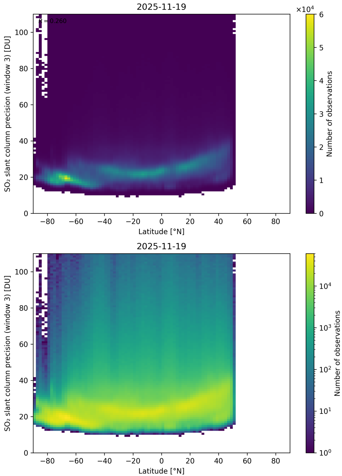
Figure 166: Scatter density plot of “Latitude” against “SO 2 slant column precision (window 3)” for 2025-11-18 to 2025-11-20.
