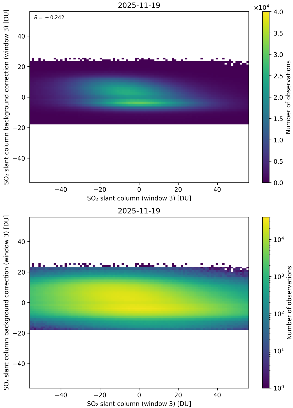
Figure 303: Scatter density plot of “SO 2 slant column (window 3)” against “SO 2 slant column background correction (window 3)” for 2025-11-18 to 2025-11-20.
