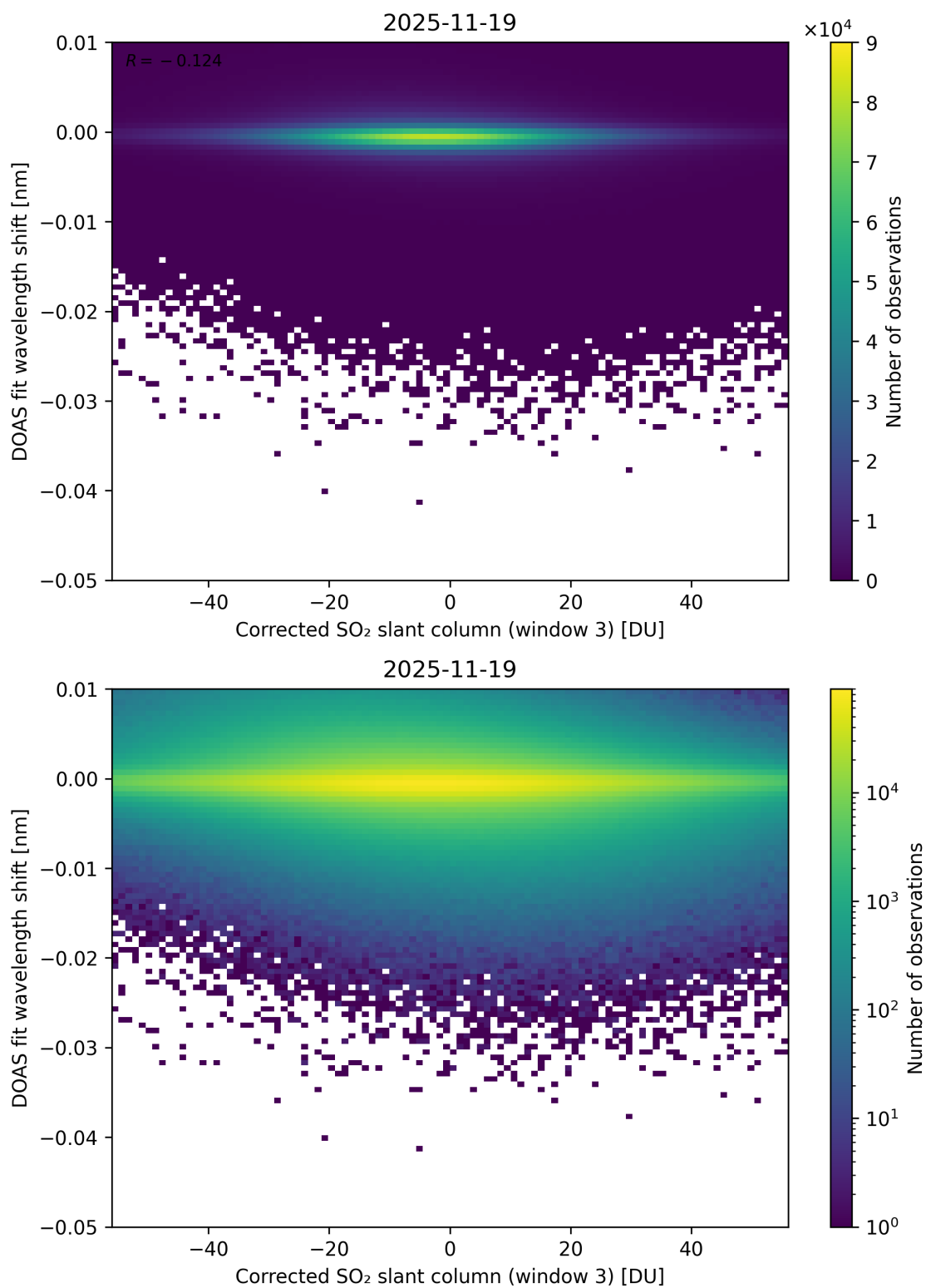
Figure 256: Scatter density plot of “Corrected SO 2 slant column (window 3)” against “DOAS fit wavelength shift” for 2025-11-18 to 2025-11-20.
