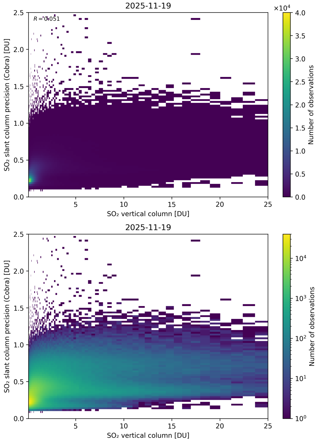
Figure 350: Scatter density plot of “SO 2 vertical column” against “SO 2 slant column precision (Cobra)” for 2025-11-18 to 2025-11-20.
