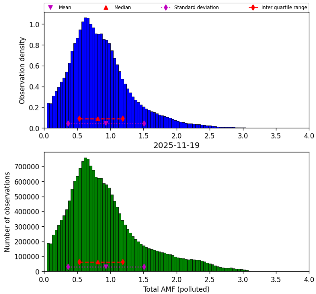
Figure 79: Histogram of “Total AMF (polluted)” for 2025-11-18 to 2025-11-20
