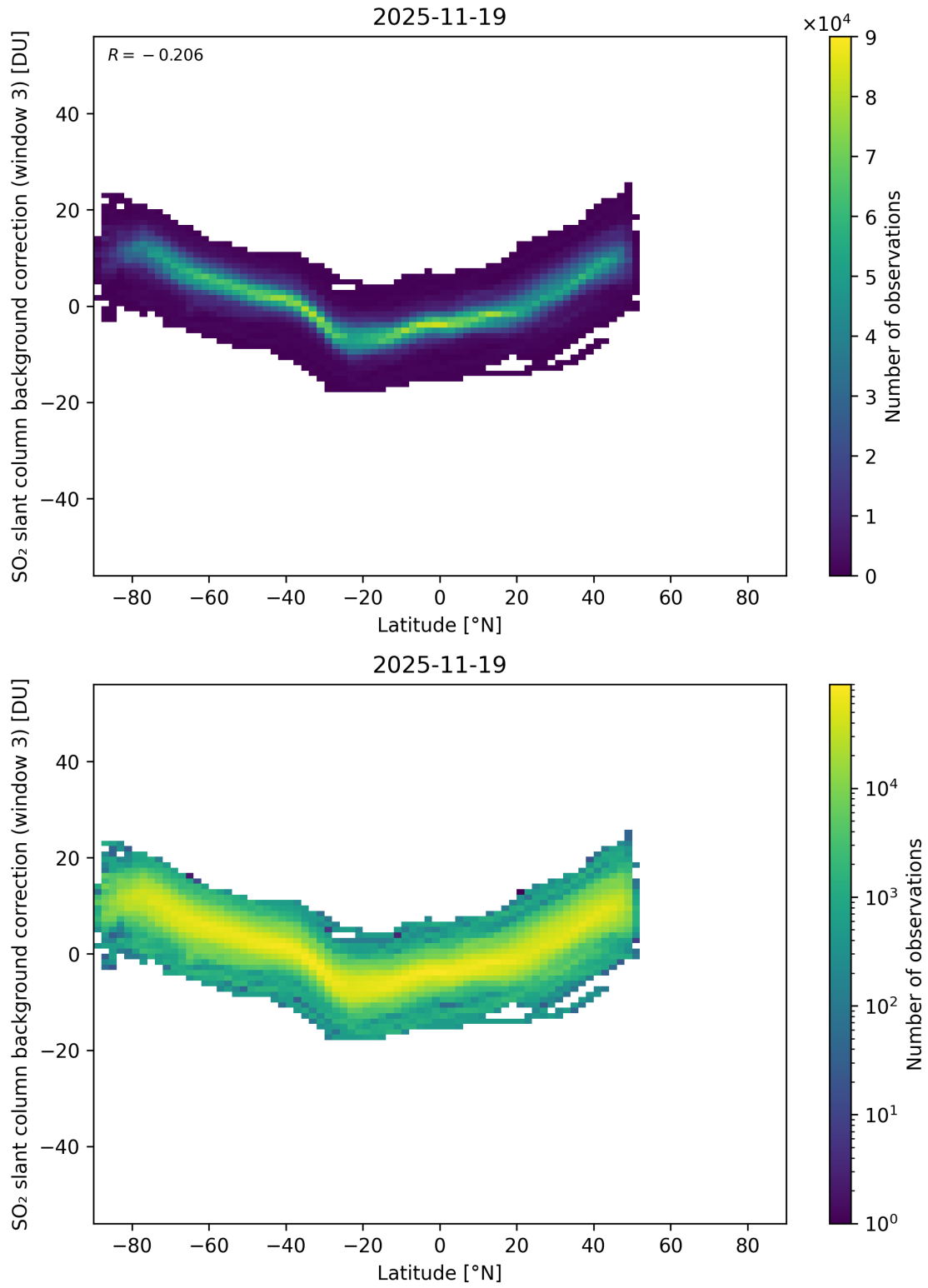
Figure 152: Scatter density plot of “Latitude” against “SO 2 slant column background correction (window 3)” for 2025-11-18 to 2025-11-20.
