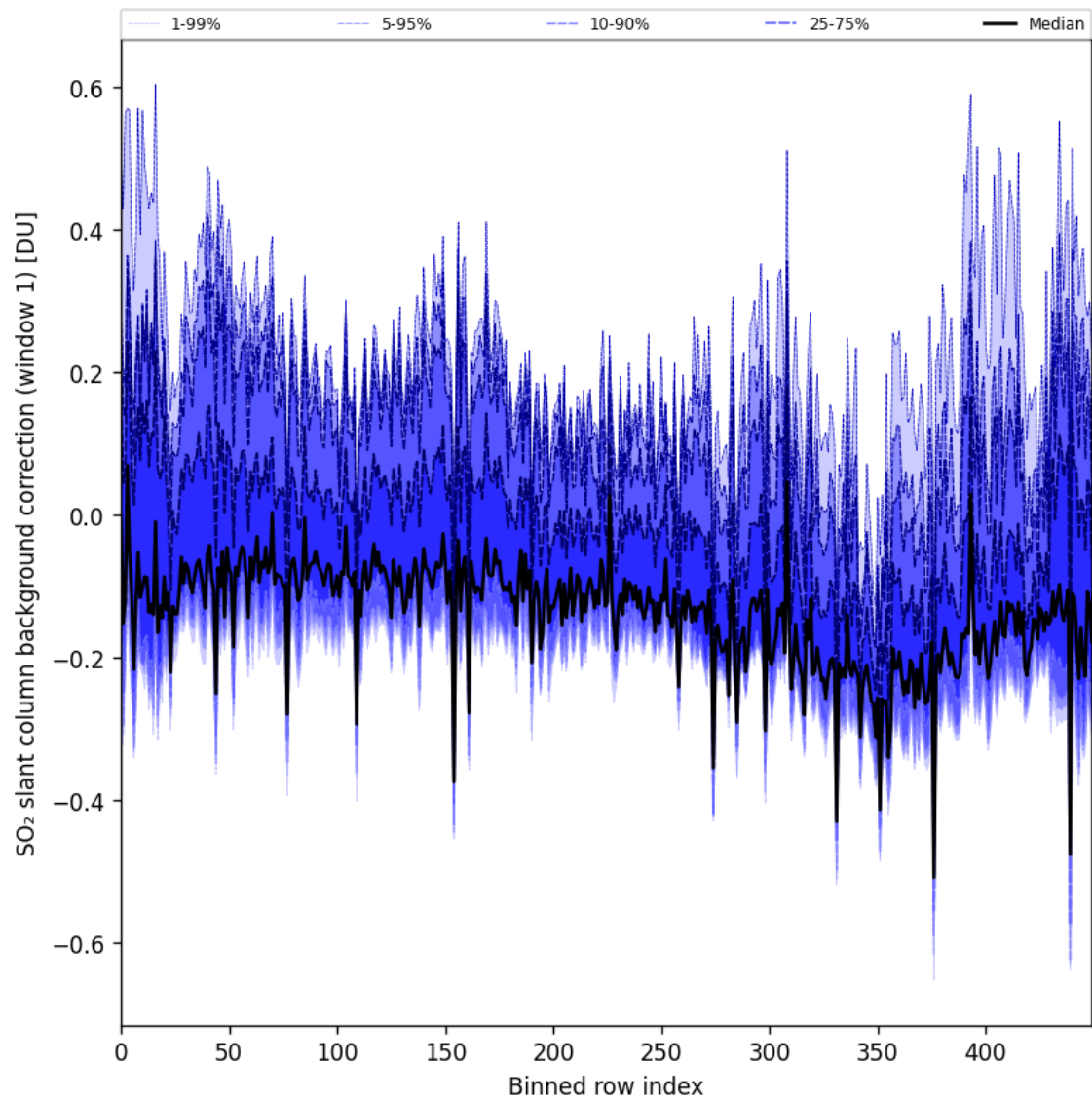
Figure 92: Along track statistics of “SO 2 slant column background correction (window 1)” for 2025-11-18 to 2025-11-20
