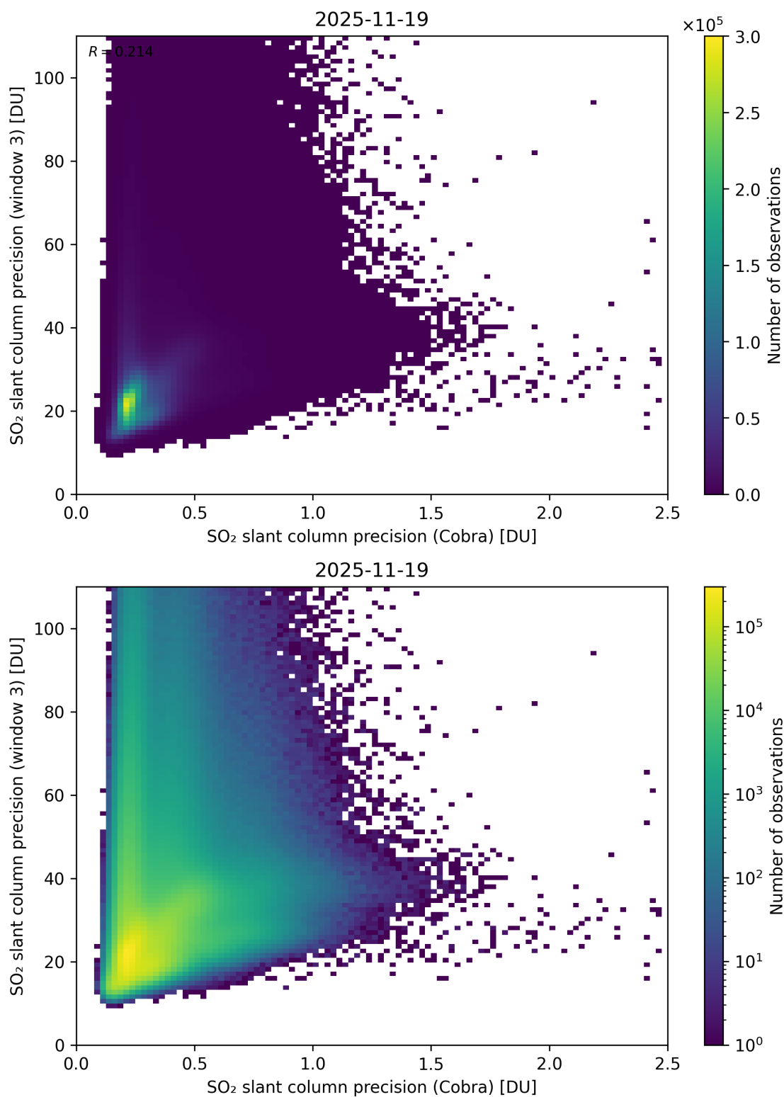
Figure 212: Scatter density plot of “SO 2 slant column precision (Cobra)” against “SO 2 slant column precision (window 3)” for 2025-11-18 to 2025-11-20.
