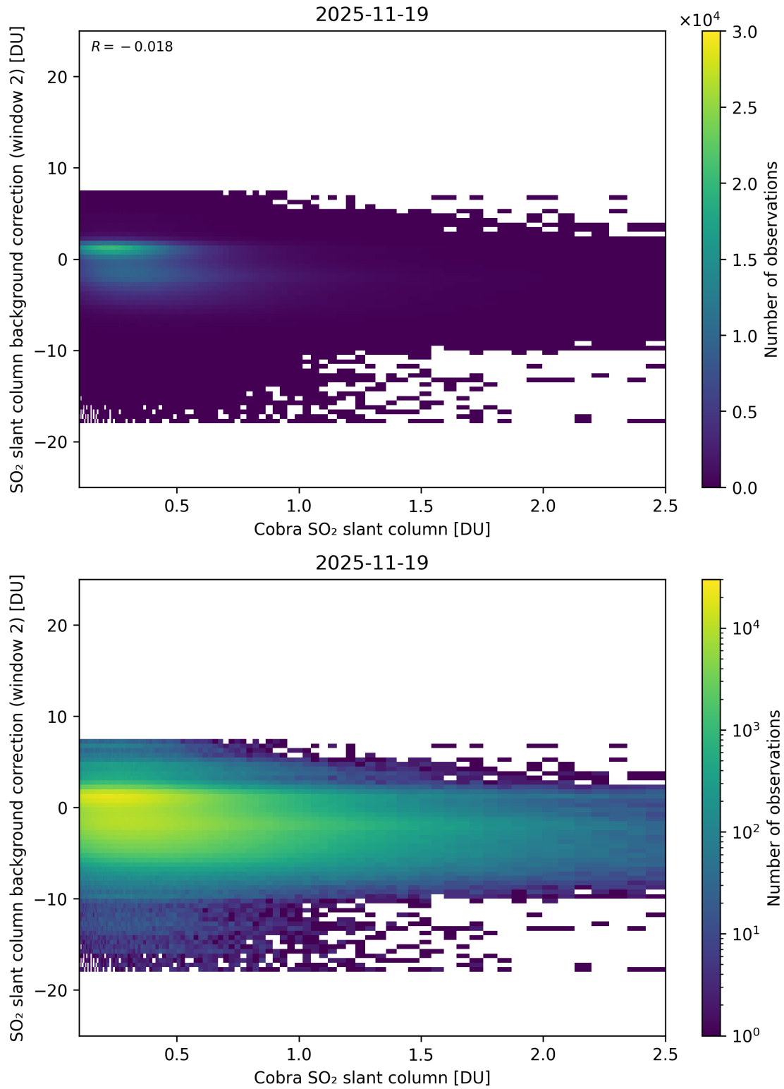
Figure 194: Scatter density plot of “Cobra SO 2 slant column” against “SO 2 slant column background correction (window 2)” for 2025-11-18 to 2025-11-20.
