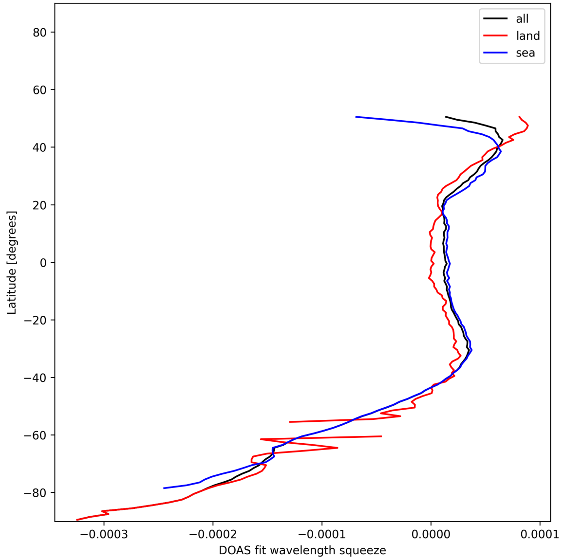
Figure 51: Zonal average of “DOAS fit wavelength squeeze” for 2025-11-18 to 2025-11-20.
