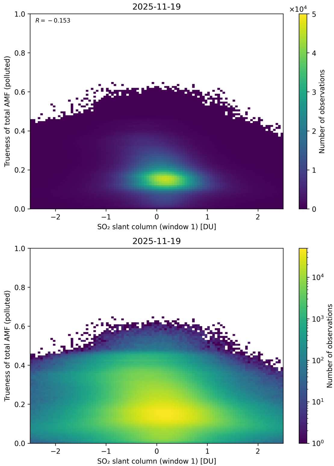
Figure 290: Scatter density plot of “SO 2 slant column (window 1)” against “Trueness of total AMF (polluted)” for 2025-11-18 to 2025-11-20.
