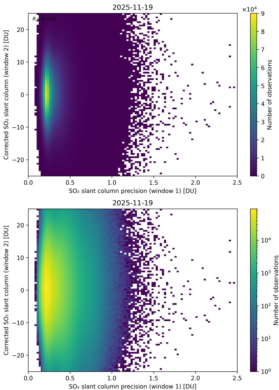
Figure 275: Scatter density plot of “SO 2 slant column precision (window 1)” against “Corrected SO 2 slant column (window 2)” for 2025-11-18 to 2025-11-20.
