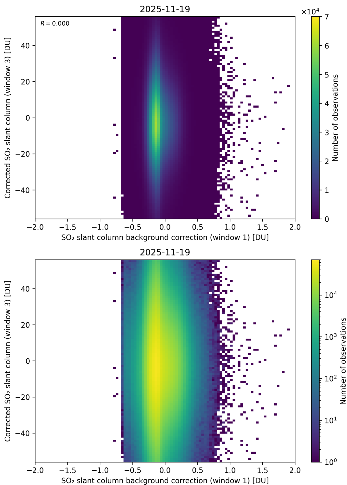
Figure 116: Scatter density plot of “SO 2 slant column background correction (window 1)” against “Corrected SO 2 slant column (window 3)” for 2025-11-18 to 2025-11-20.
