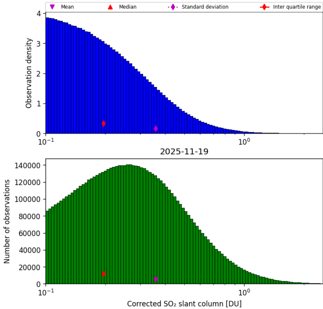
Figure 60: Histogram of “Corrected SO 2 slant column” for 2025-11-18 to 2025-11-20
