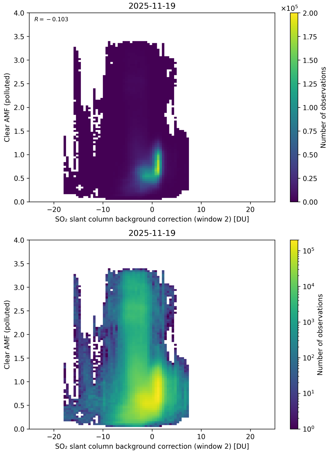
Figure 126: Scatter density plot of “SO 2 slant column background correction (window 2)” against “Clear AMF (polluted)” for 2025-11-18 to 2025-11-20.
