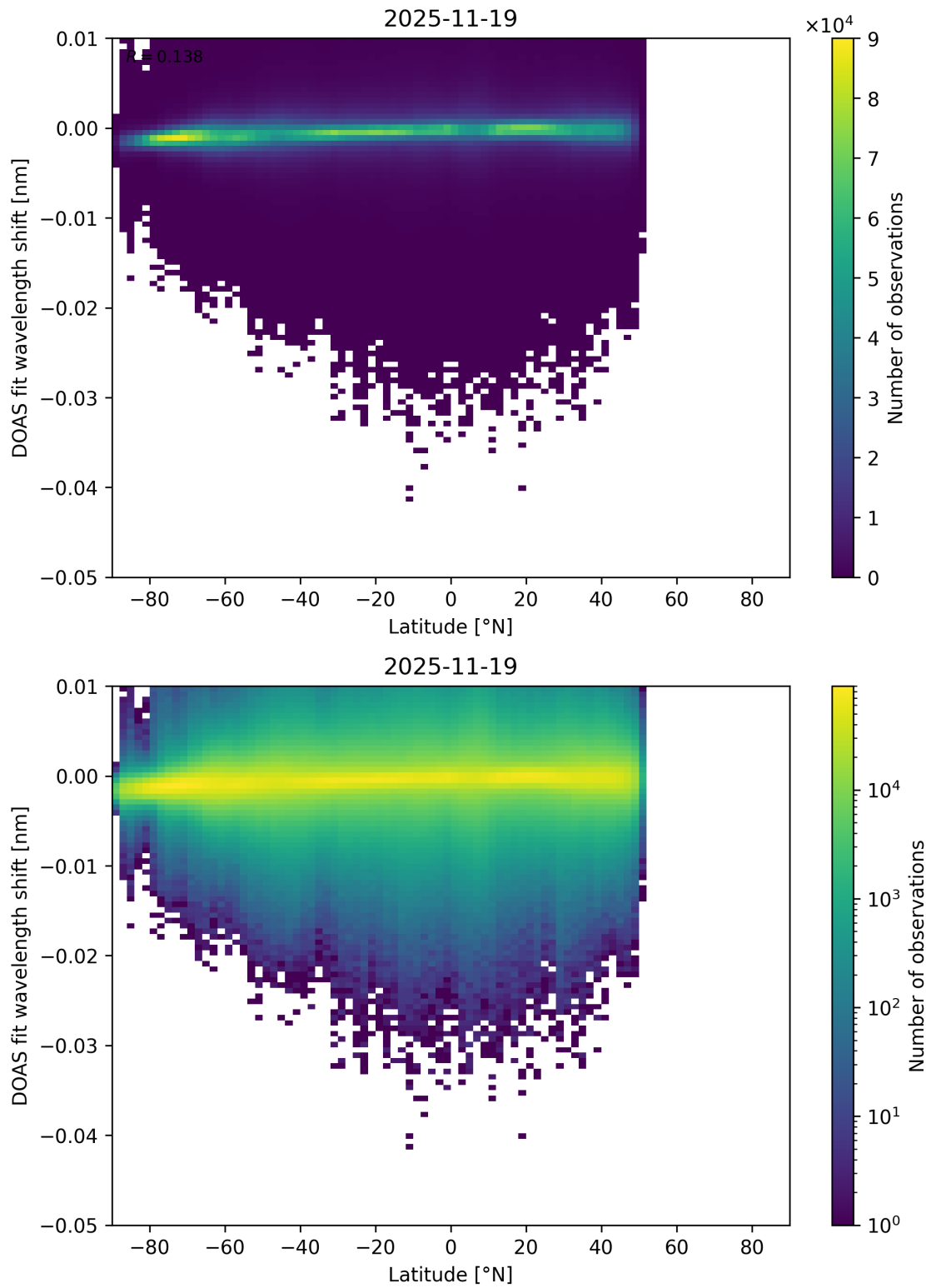
Figure 153: Scatter density plot of “Latitude” against “DOAS fit wavelength shift” for 2025-11-18 to 2025-11-20.
