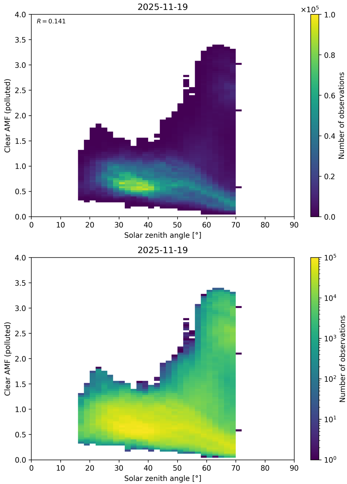
Figure 178: Scatter density plot of “Solar zenith angle” against “Clear AMF (polluted)” for 2025-11-18 to 2025-11-20.
