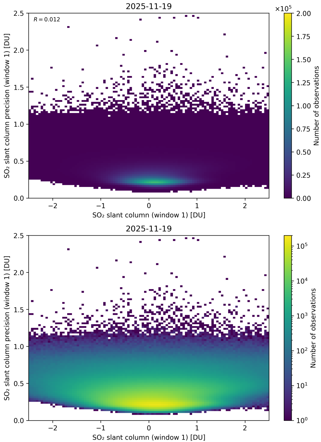
Figure 285: Scatter density plot of “SO 2 slant column (window 1)” against “SO 2 slant column precision (window 1)” for 2025-11-18 to 2025-11-20.
