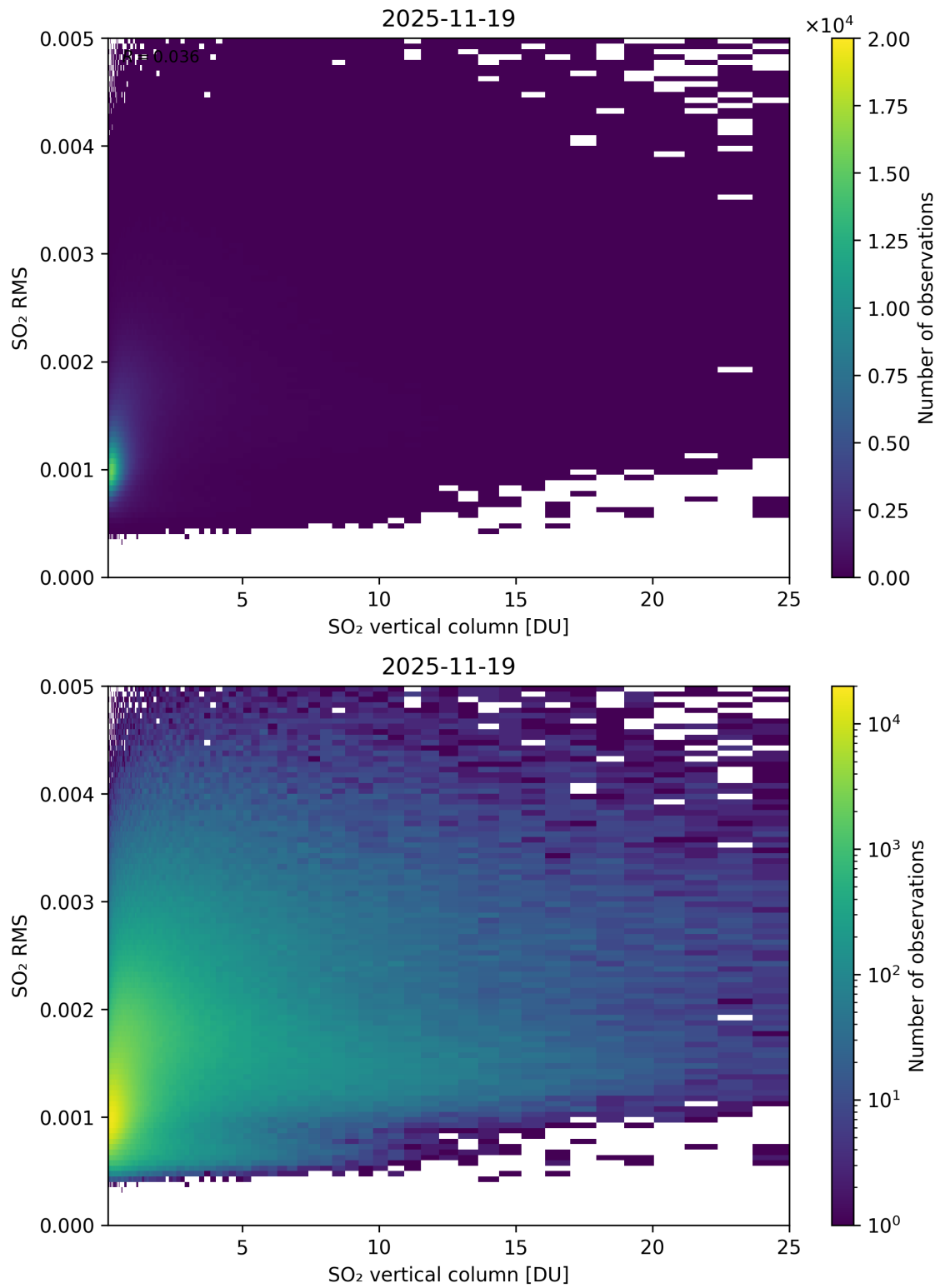
Figure 328: Scatter density plot of “SO 2 vertical column” against “SO 2 RMS” for 2025-11-18 to 2025-11-20.
