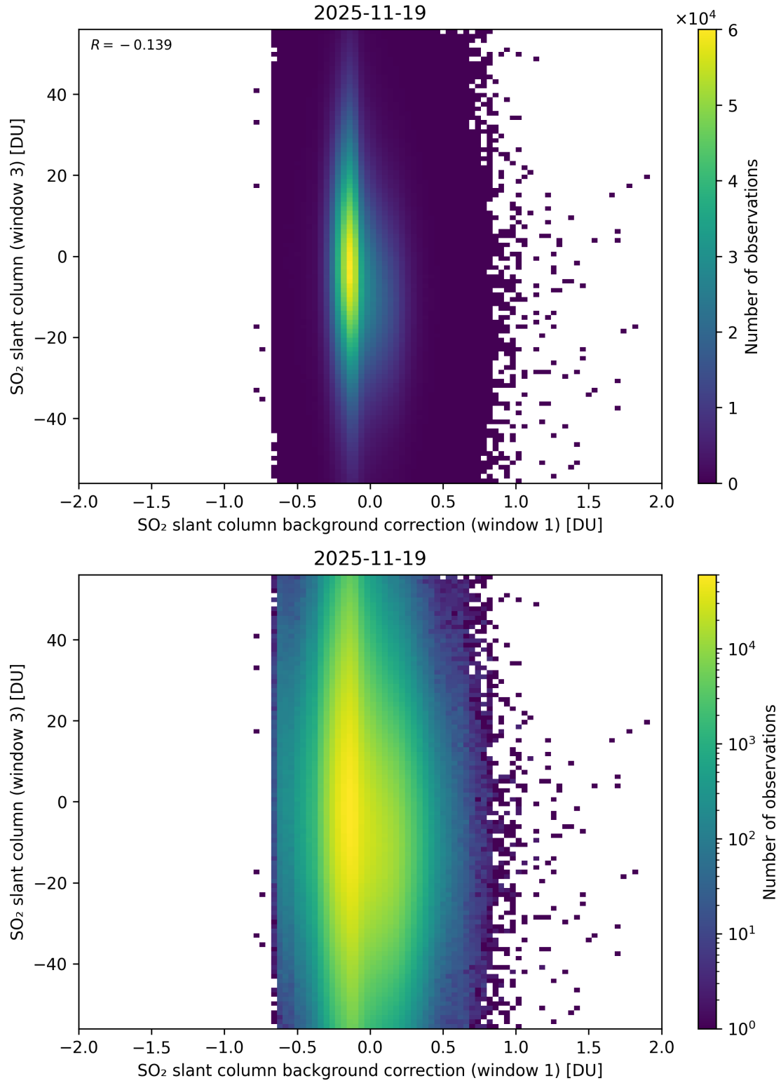
Figure 118: Scatter density plot of “SO 2 slant column background correction (window 1)” against “SO 2 slant column (window 3)” for 2025-11-18 to 2025-11-20.
