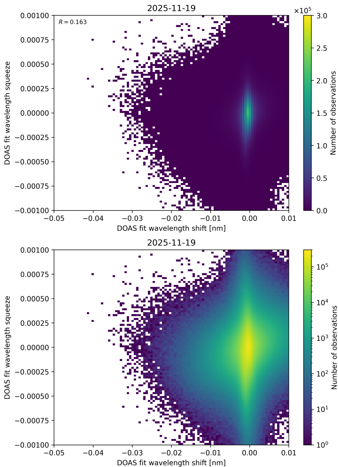
Figure 138: Scatter density plot of “DOAS fit wavelength shift” against “DOAS fit wavelength squeeze” for 2025-11-18 to 2025-11-20.
