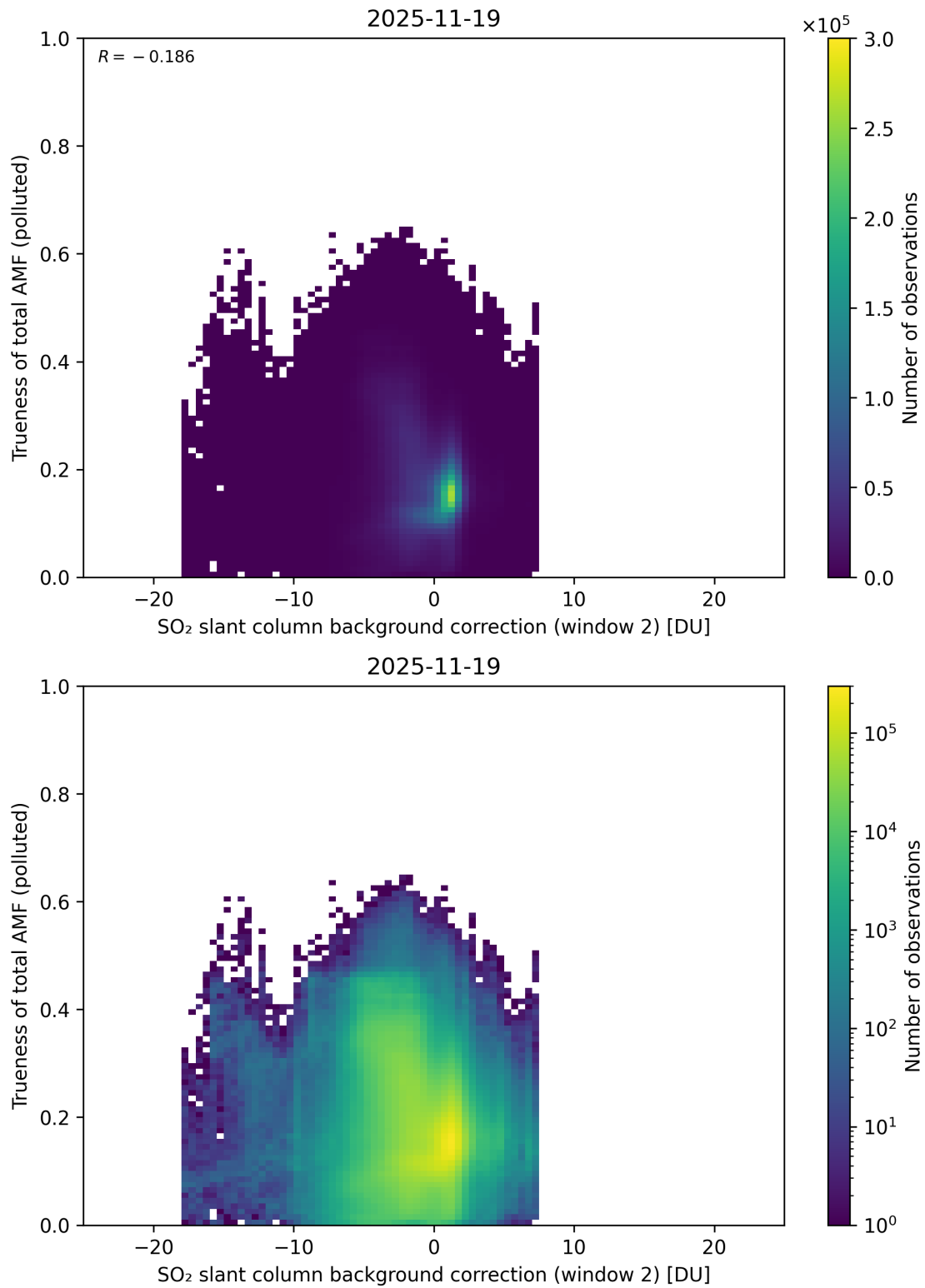
Figure 131: Scatter density plot of “SO 2 slant column background correction (window 2)” against “Trueness of total AMF (polluted)” for 2025-11-18 to 2025-11-20.
