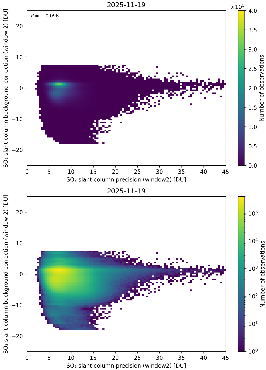
Figure 291: Scatter density plot of “SO 2 slant column precision (window2)” against “SO 2 slant column background correction (window 2)” for 2025-11-18 to 2025-11-20.
