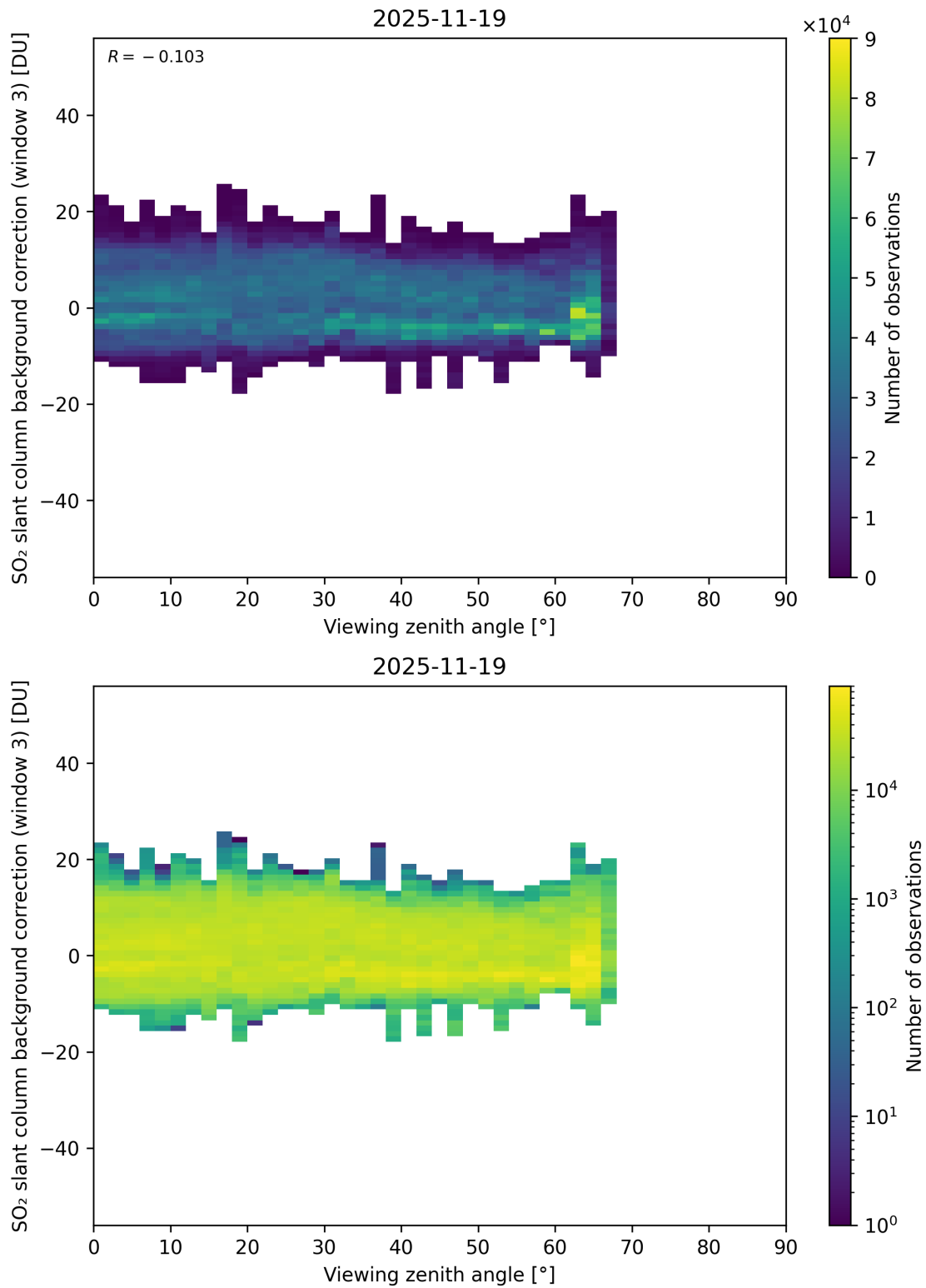
Figure 364: Scatter density plot of “Viewing zenith angle” against “SO 2 slant column background correction (window 3)” for 2025-11-18 to 2025-11-20.
