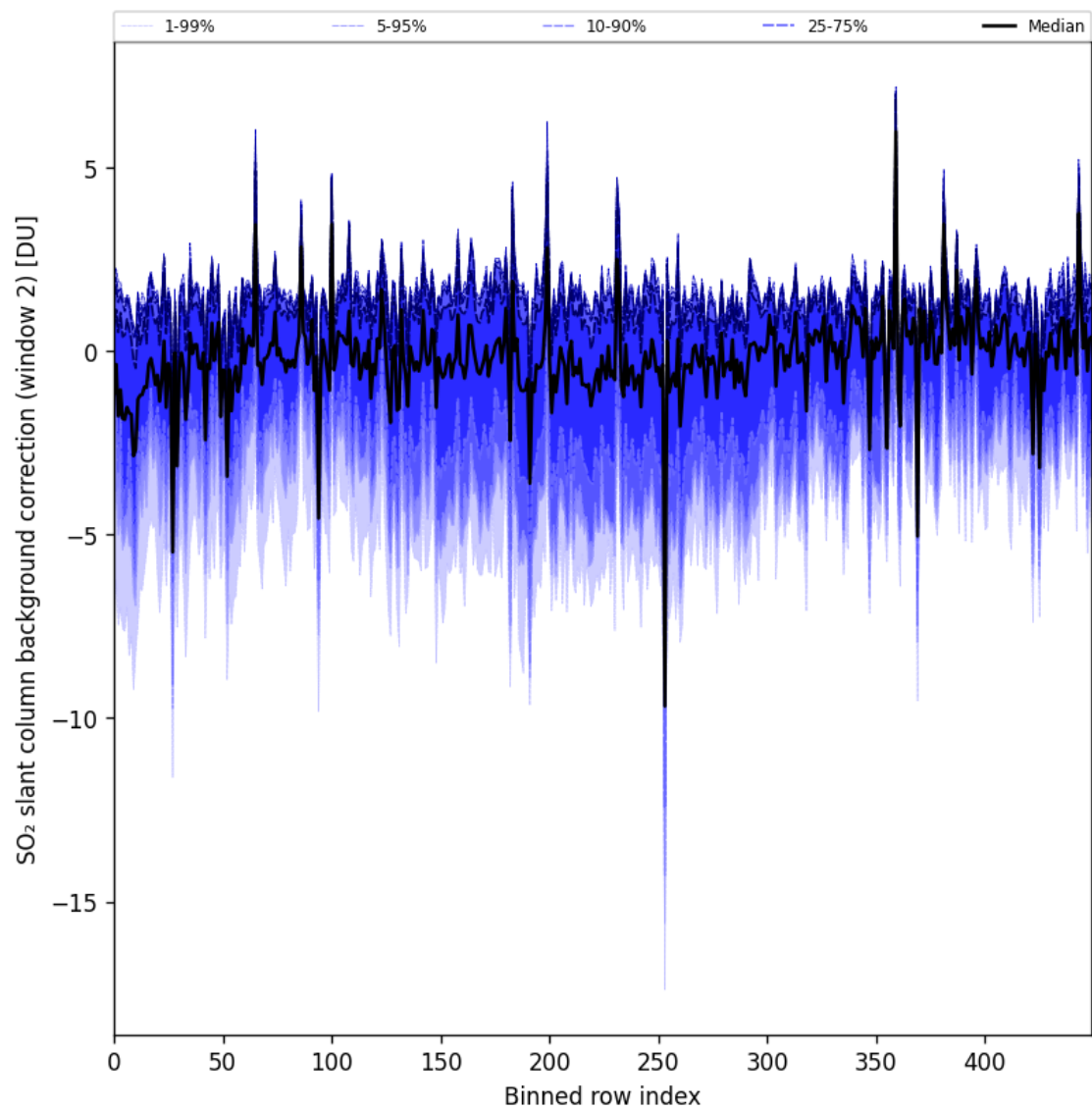
Figure 96: Along track statistics of “SO 2 slant column background correction (window 2)” for 2025-11-18 to 2025-11-20
