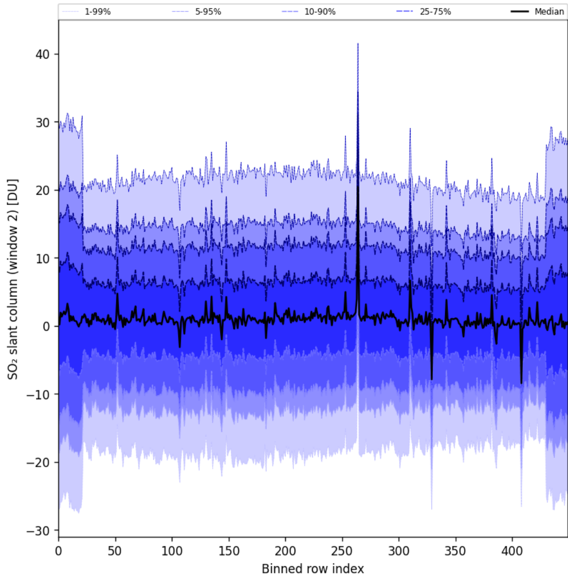
Figure 93: Along track statistics of “SO 2 slant column (window 2)” for 2025-11-18 to 2025-11-20
