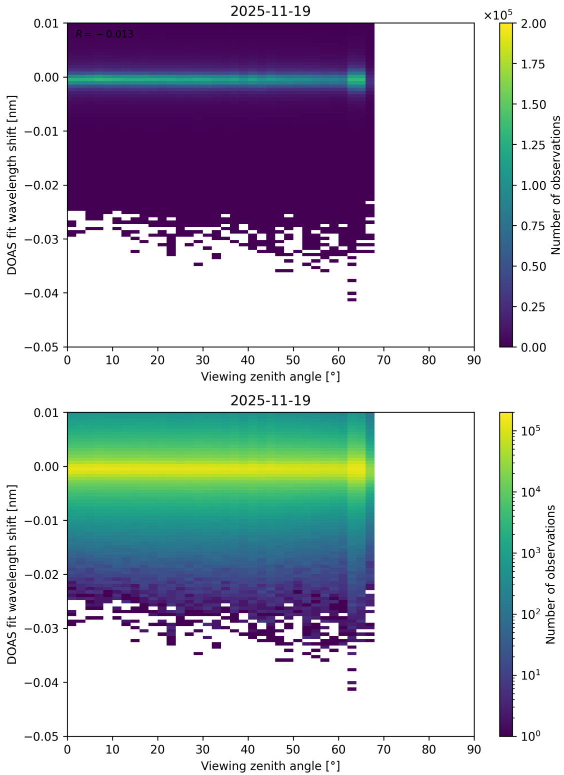
Figure 365: Scatter density plot of “Viewing zenith angle” against “DOAS fit wavelength shift” for 2025-11-18 to 2025-11-20.
