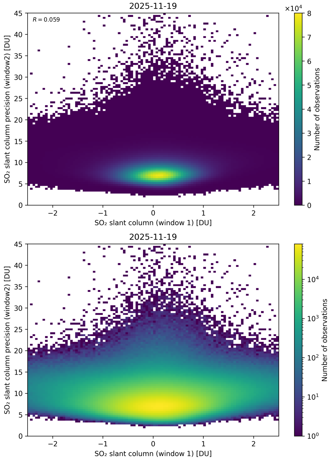
Figure 286: Scatter density plot of “SO 2 slant column (window 1)” against “SO 2 slant column precision (window2)” for 2025-11-18 to 2025-11-20.
