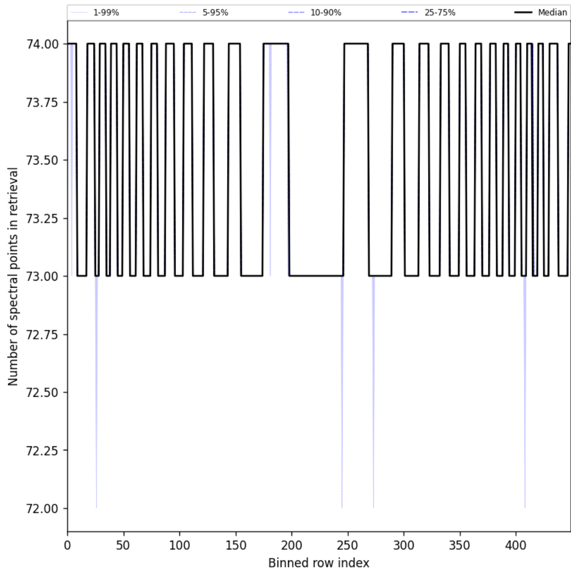
Figure 108: Along track statistics of “Number of spectral points in retrieval” for 2025-11-18 to 2025-11-20
