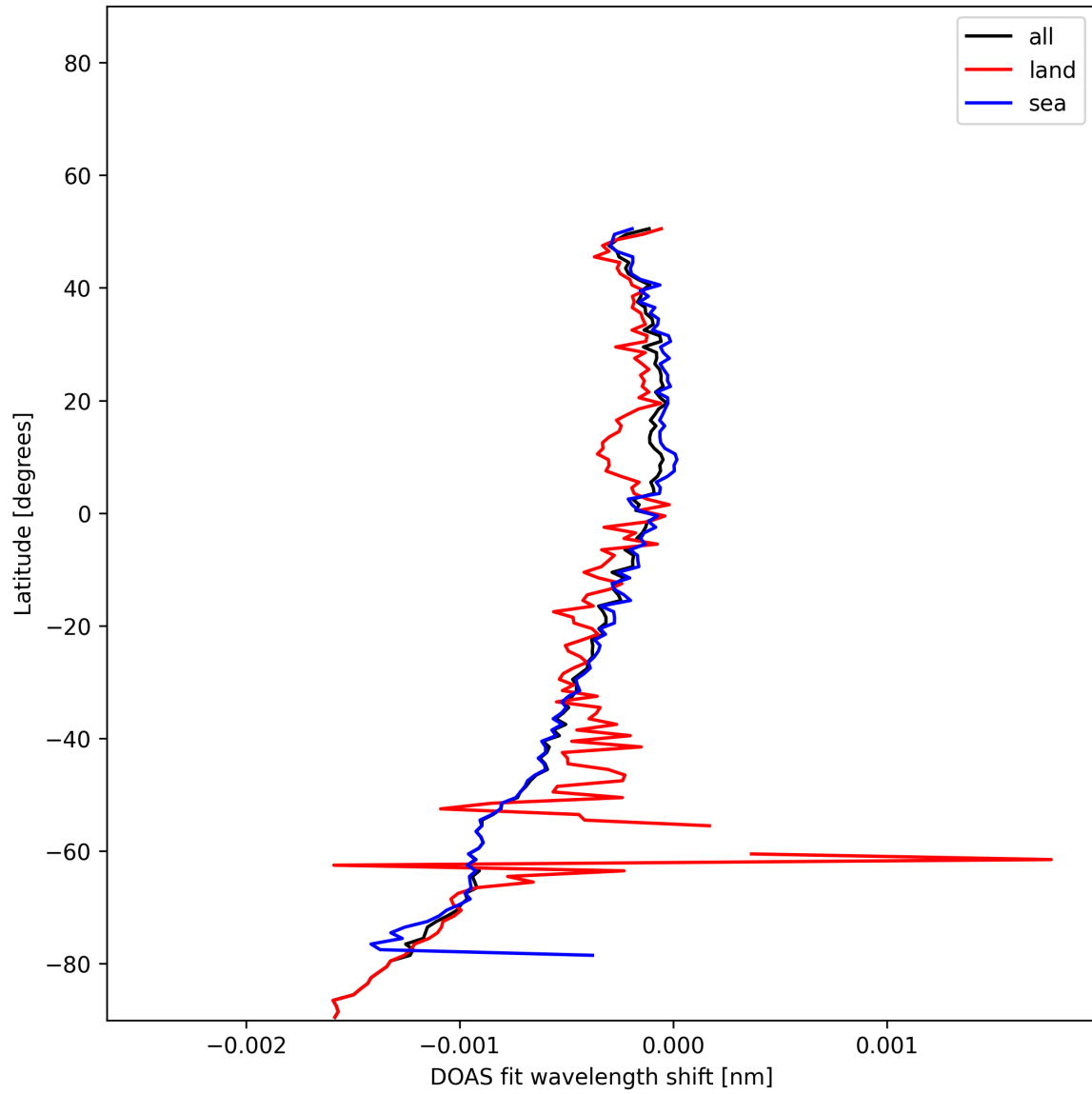
Figure 50: Zonal average of "DOAS fit wavelength shift" for 2025-11-18 to 2025-11-20.
