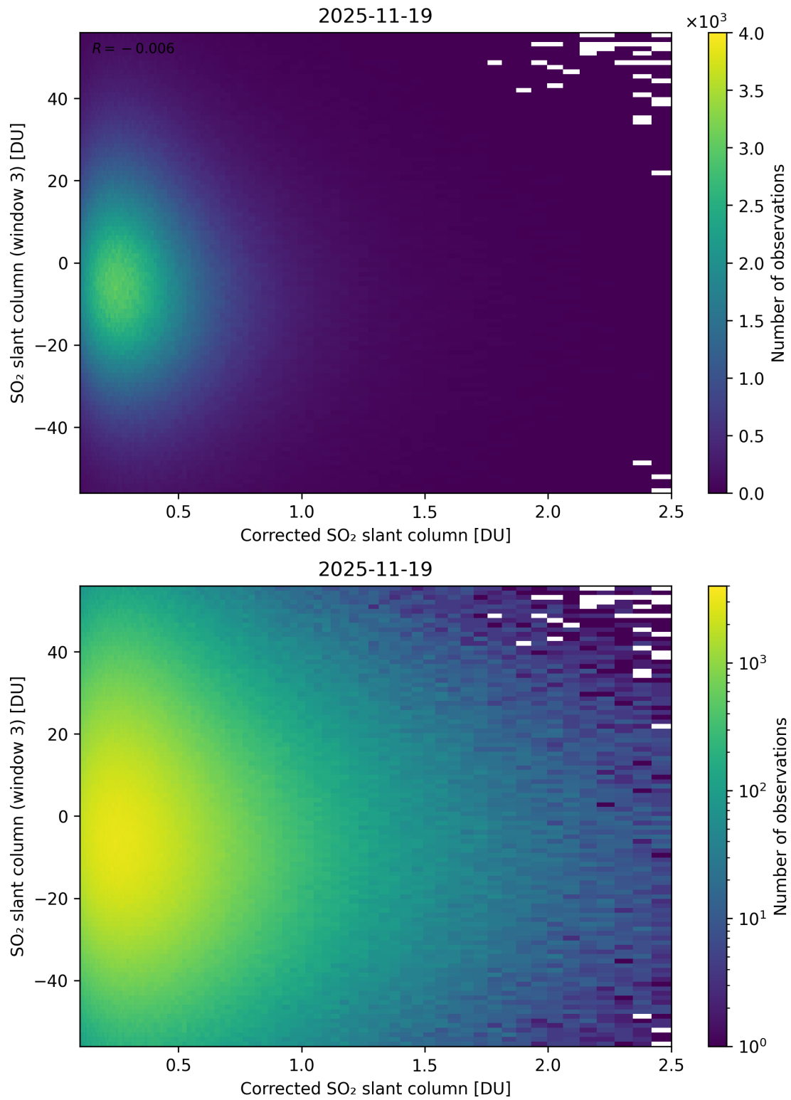
Figure 240: Scatter density plot of “Corrected SO 2 slant column” against “SO 2 slant column (window 3)” for 2025-11-18 to 2025-11-20.
