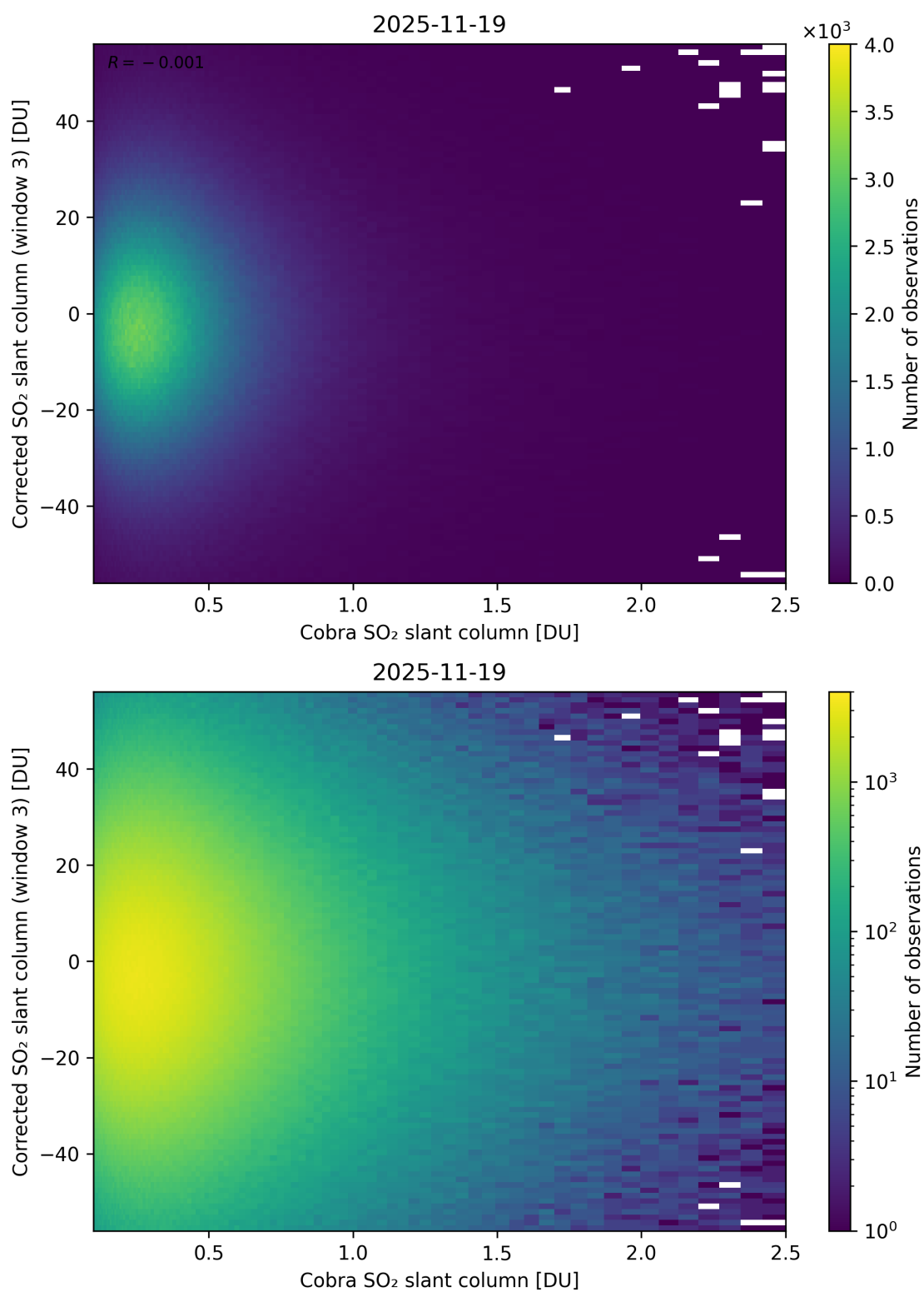
Figure 218: Scatter density plot of “Cobra SO 2 slant column” against “Corrected SO 2 slant column (window 3)” for 2025-11-18 to 2025-11-20.
