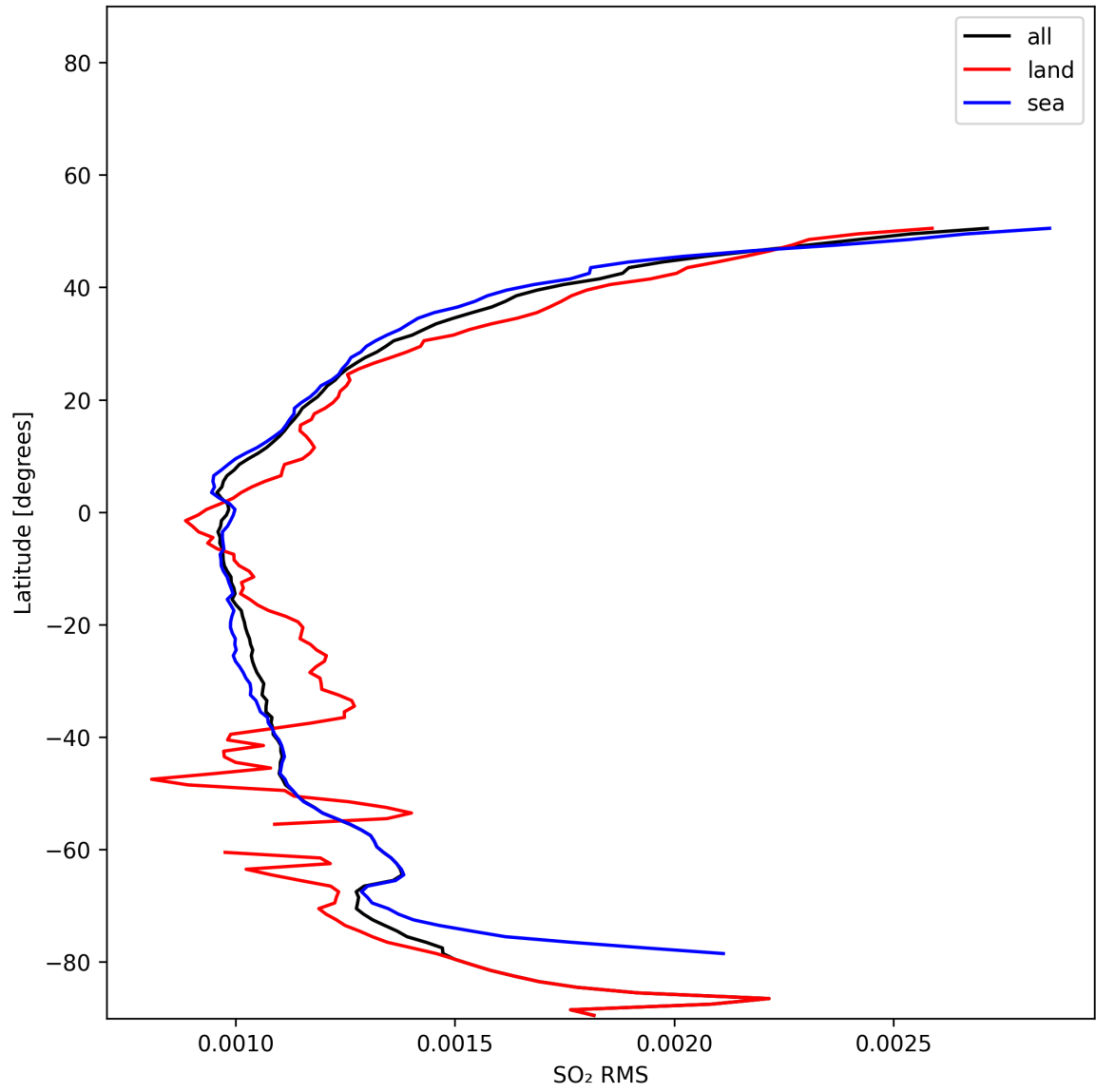
Figure 52: Zonal average of “SO 2 RMS” for 2025-11-18 to 2025-11-20.
