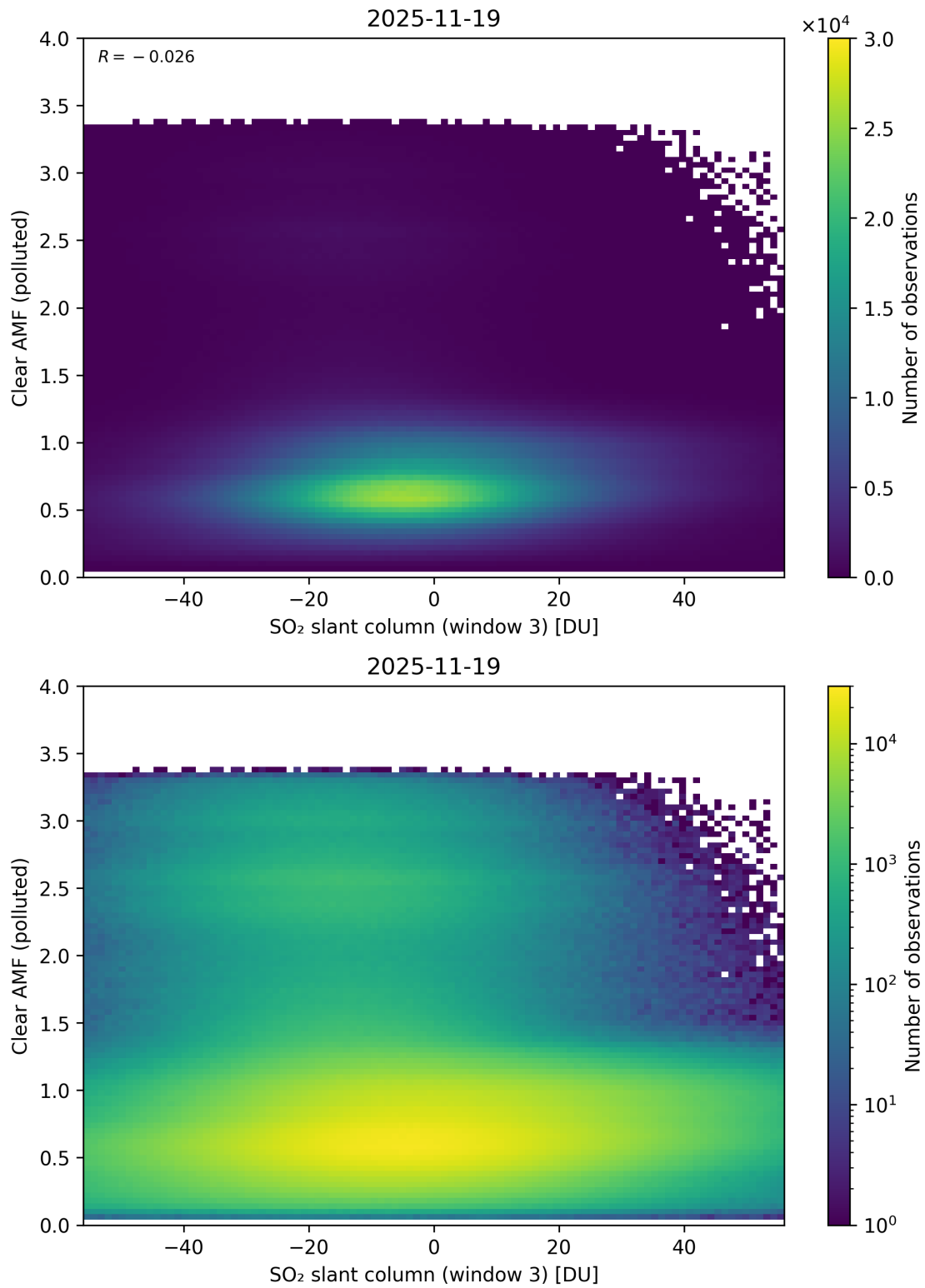
Figure 315: Scatter density plot of “SO 2 slant column (window 3)” against “Clear AMF (polluted)” for 2025-11-18 to 2025-11-20.
