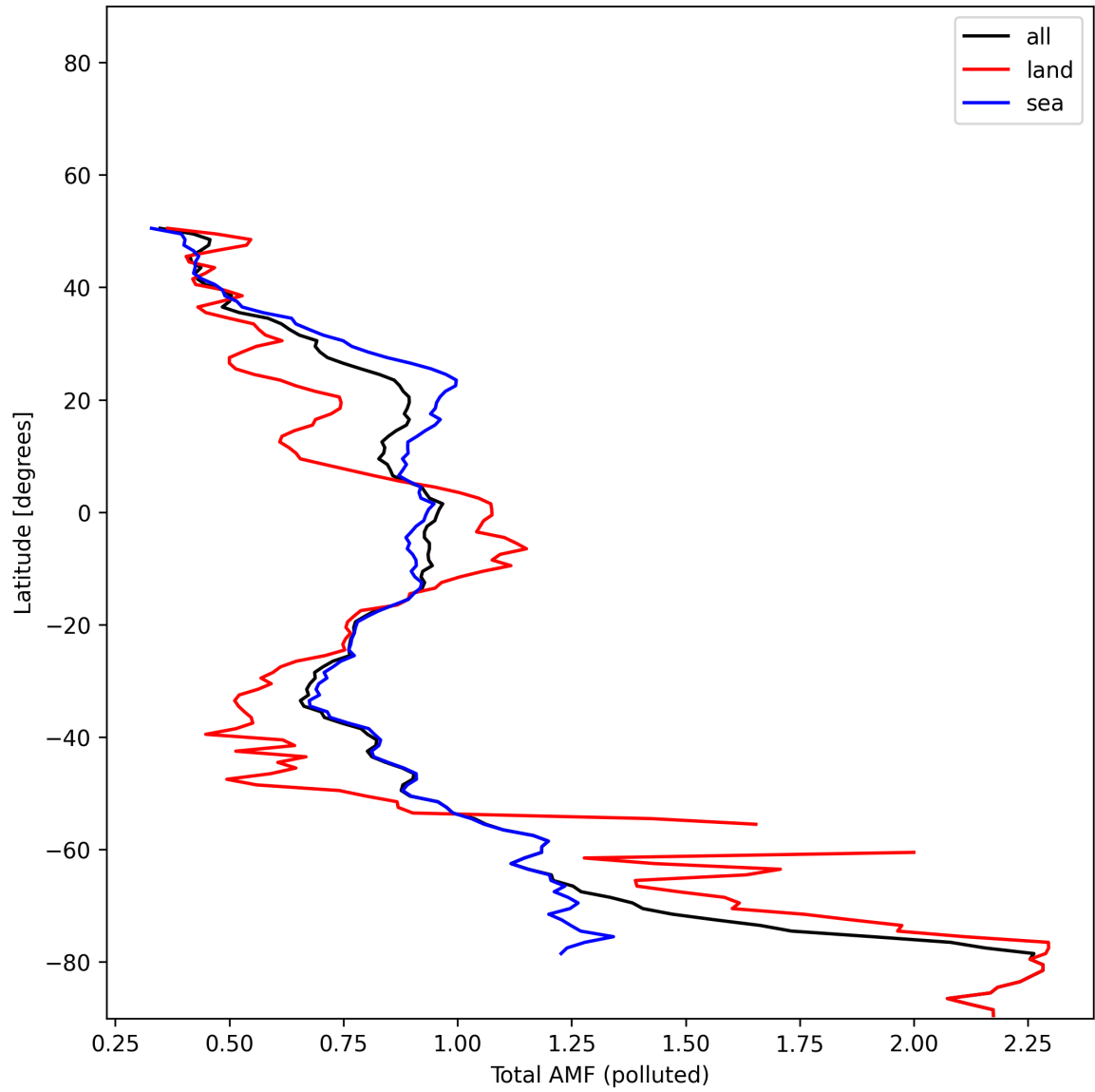
Figure 53: Zonal average of “Total AMF (polluted)” for 2025-11-18 to 2025-11-20.
