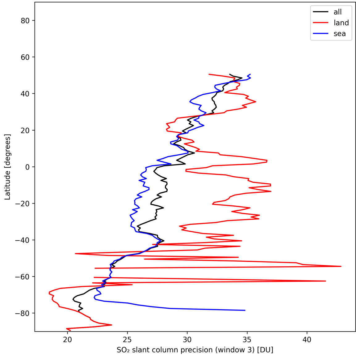
Figure 46: Zonal average of “SO 2 slant column precision (window 3)” for 2025-11-18 to 2025-11-20.
