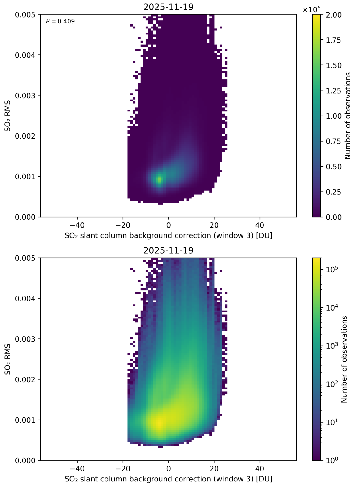
Figure 134: Scatter density plot of “SO 2 slant column background correction (window 3)” against “SO 2 RMS” for 2025-11-18 to 2025-11-20.
