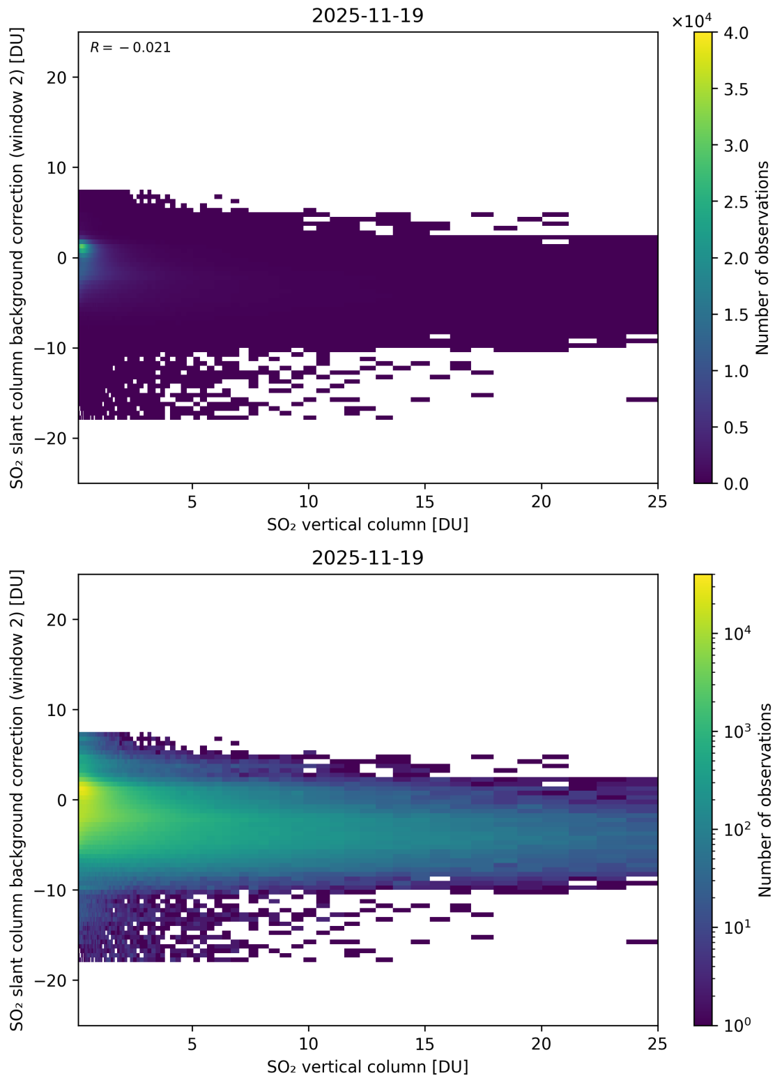
Figure 324: Scatter density plot of “SO 2 vertical column” against “SO 2 slant column background correction (window 2)” for 2025-11-18 to 2025-11-20.
