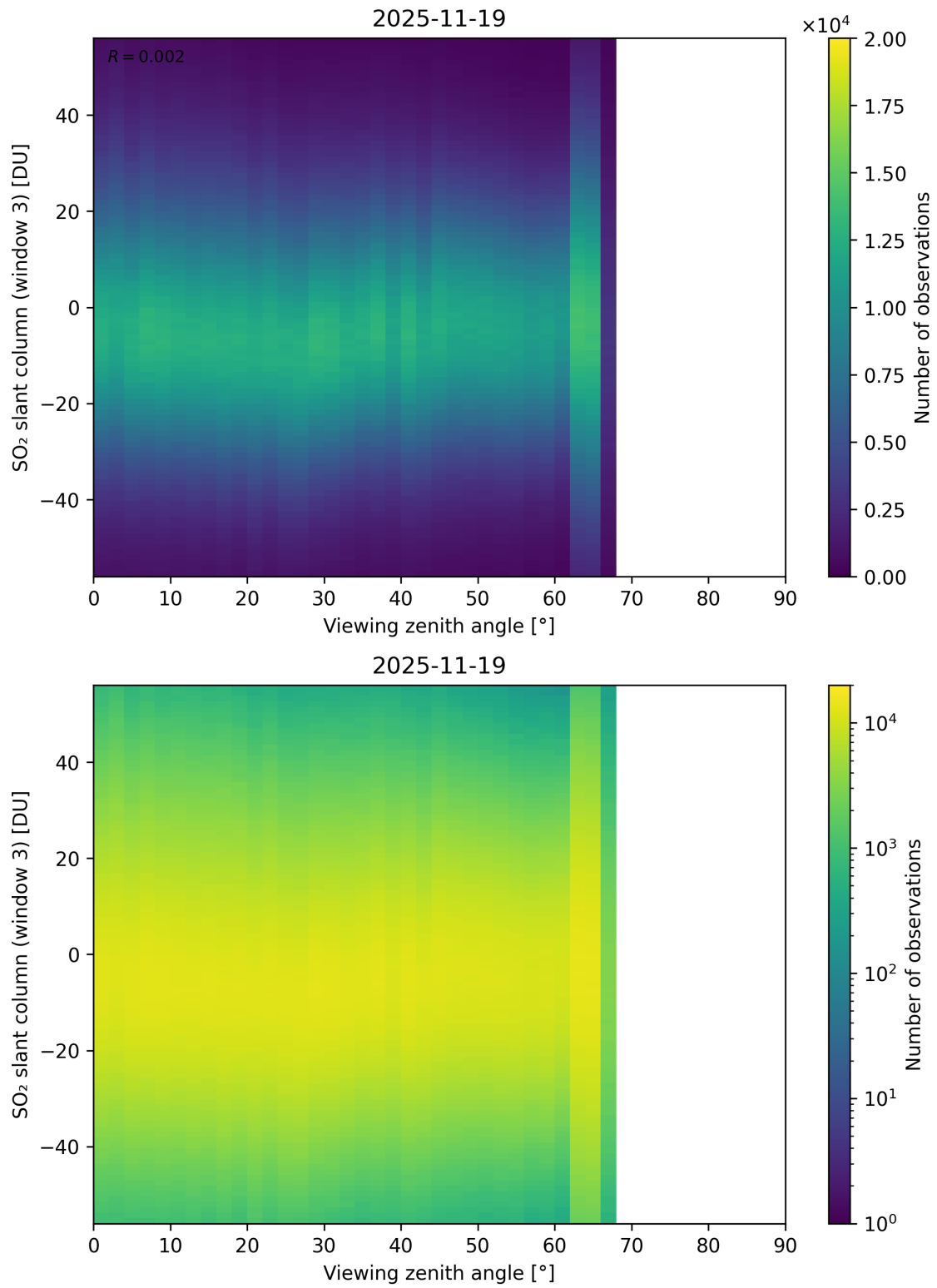
Figure 379: Scatter density plot of “Viewing zenith angle” against “SO 2 slant column (window 3)” for 2025-11-18 to 2025-11-20.
