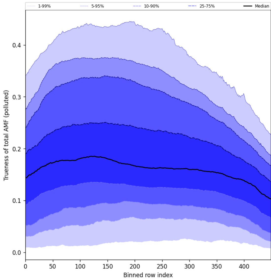
Figure 106: Along track statistics of “Trueness of total AMF (polluted)” for 2025-11-18 to 2025-11-20
