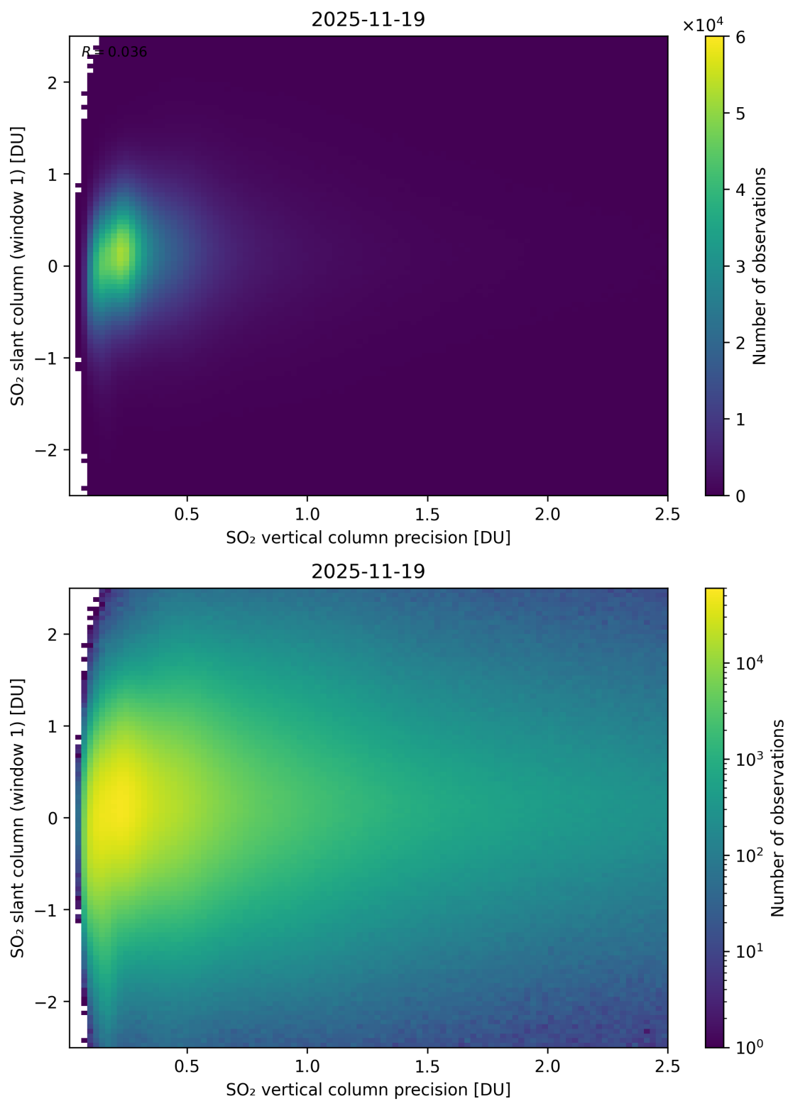
Figure 341: Scatter density plot of “SO 2 vertical column precision” against “SO 2 slant column (window 1)” for 2025-11-18 to 2025-11-20.
