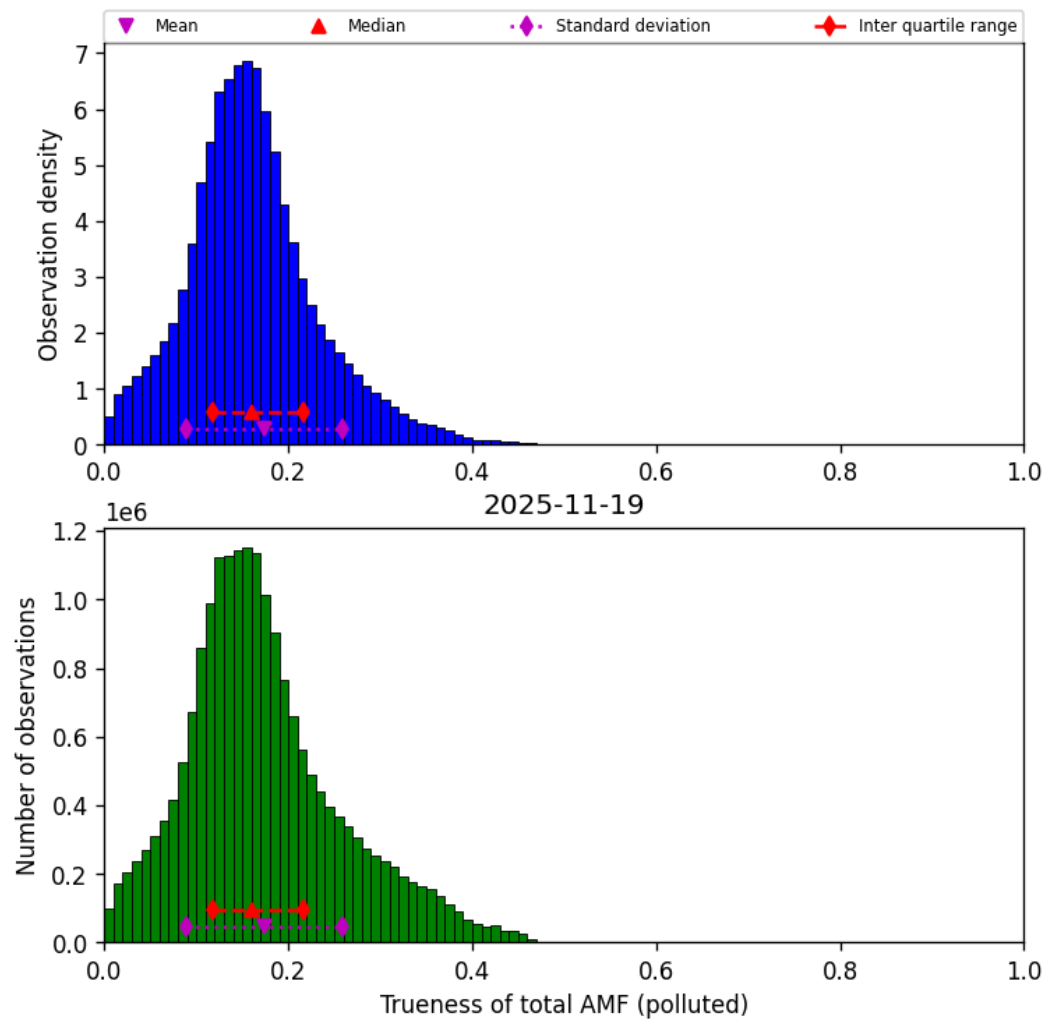
Figure 80: Histogram of “Trueness of total AMF (polluted)” for 2025-11-18 to 2025-11-20
