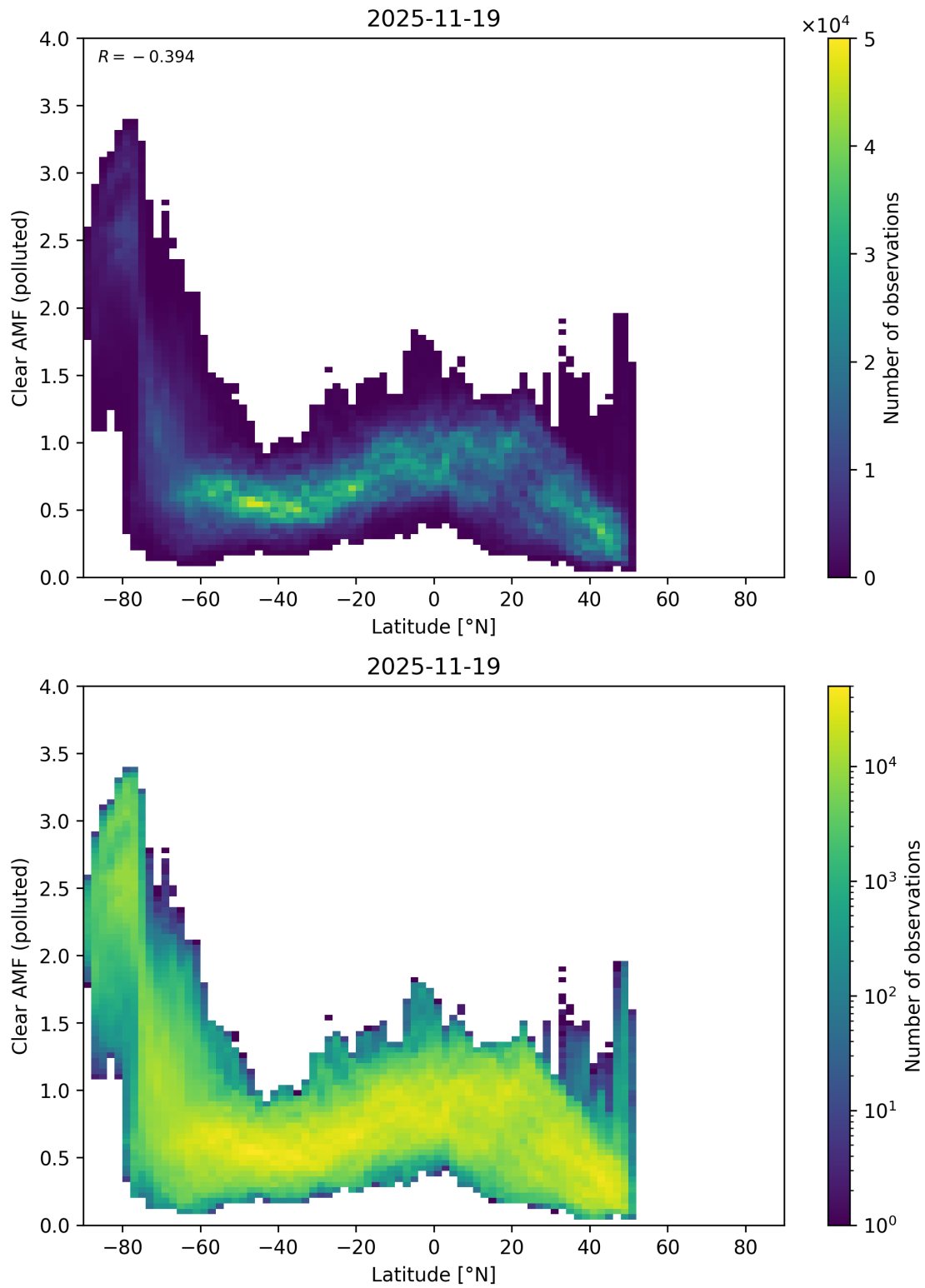
Figure 156: Scatter density plot of “Latitude” against “Clear AMF (polluted)” for 2025-11-18 to 2025-11-20.
