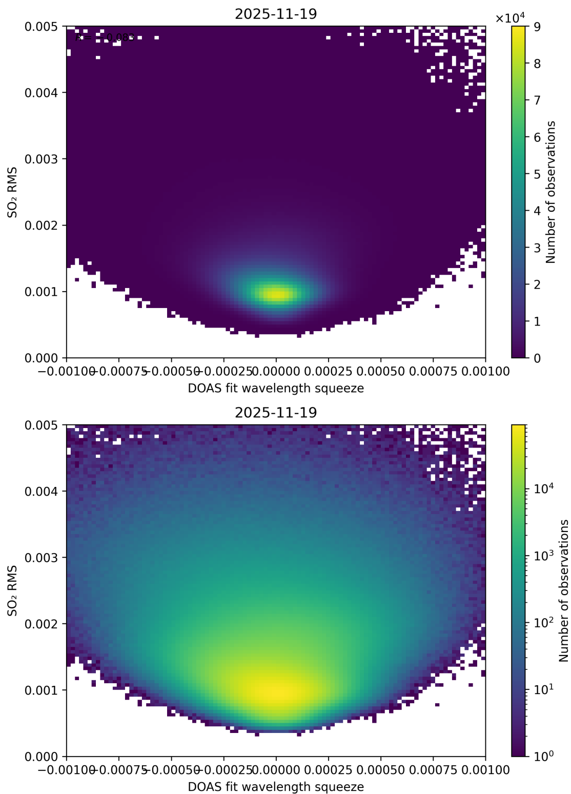
Figure 143: Scatter density plot of “DOAS fit wavelength squeeze” against “SO 2 RMS” for 2025-11-18 to 2025-11-20.
