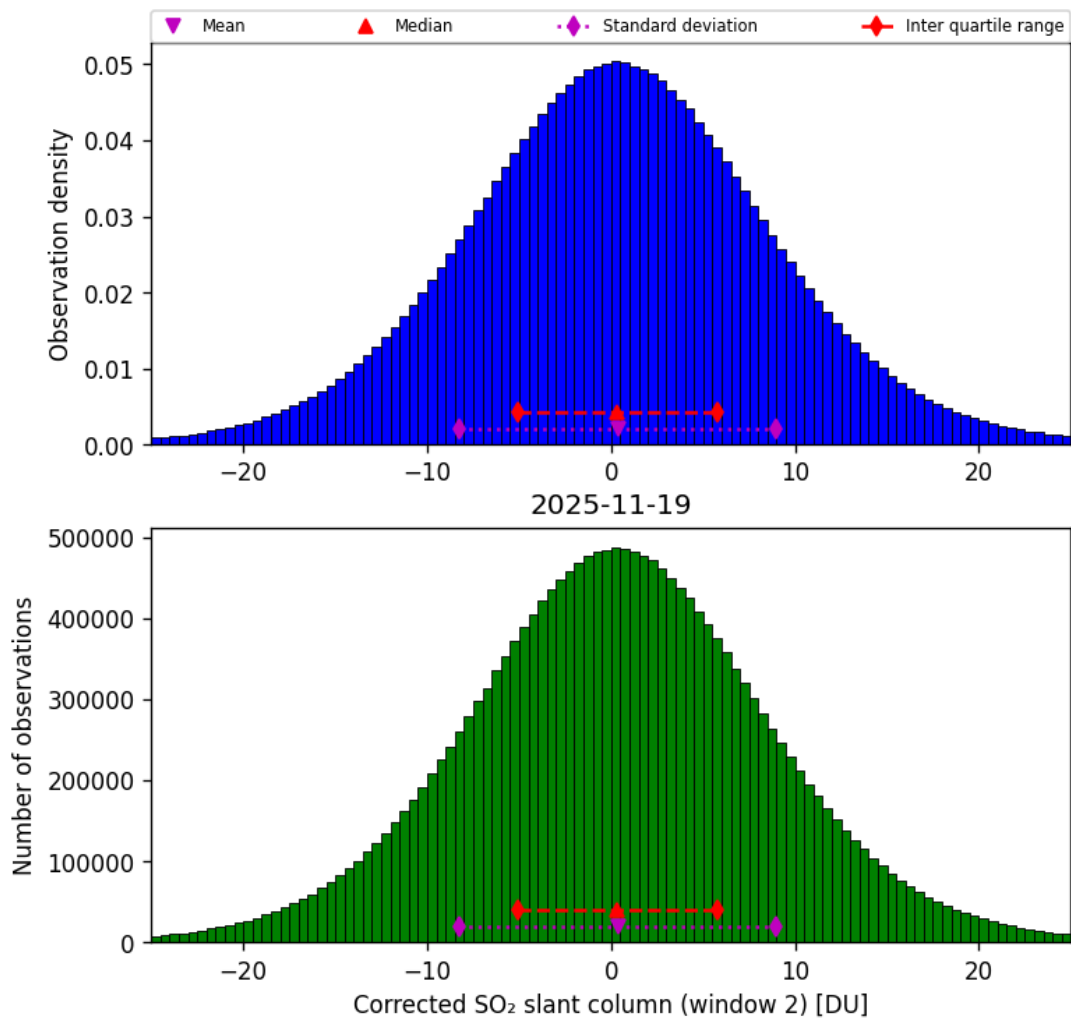
Figure 69: Histogram of “Corrected SO 2 slant column (window 2)” for 2025-11-18 to 2025-11-20
