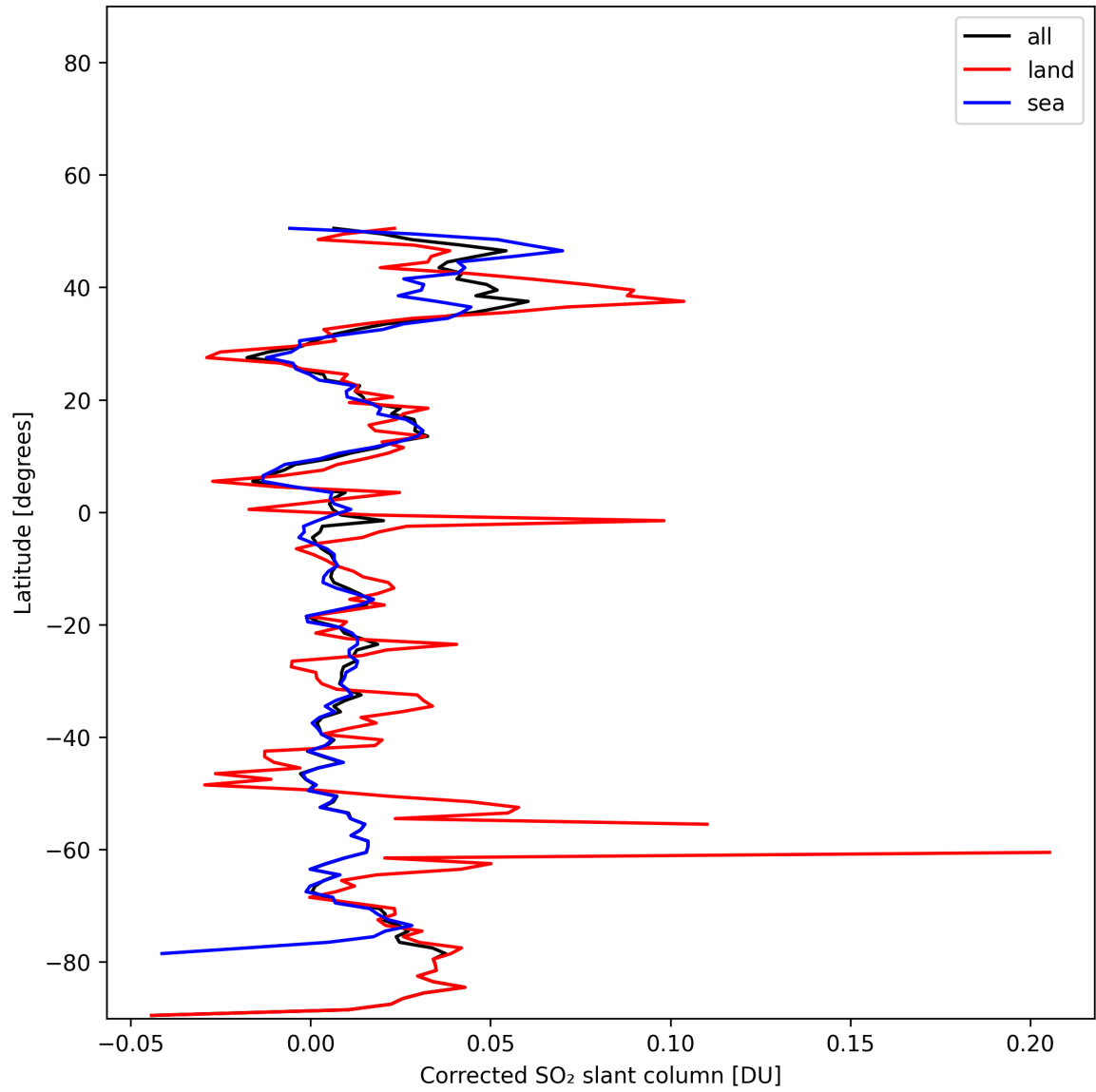
Figure 34: Zonal average of “Corrected SO 2 slant column” for 2025-11-18 to 2025-11-20.
