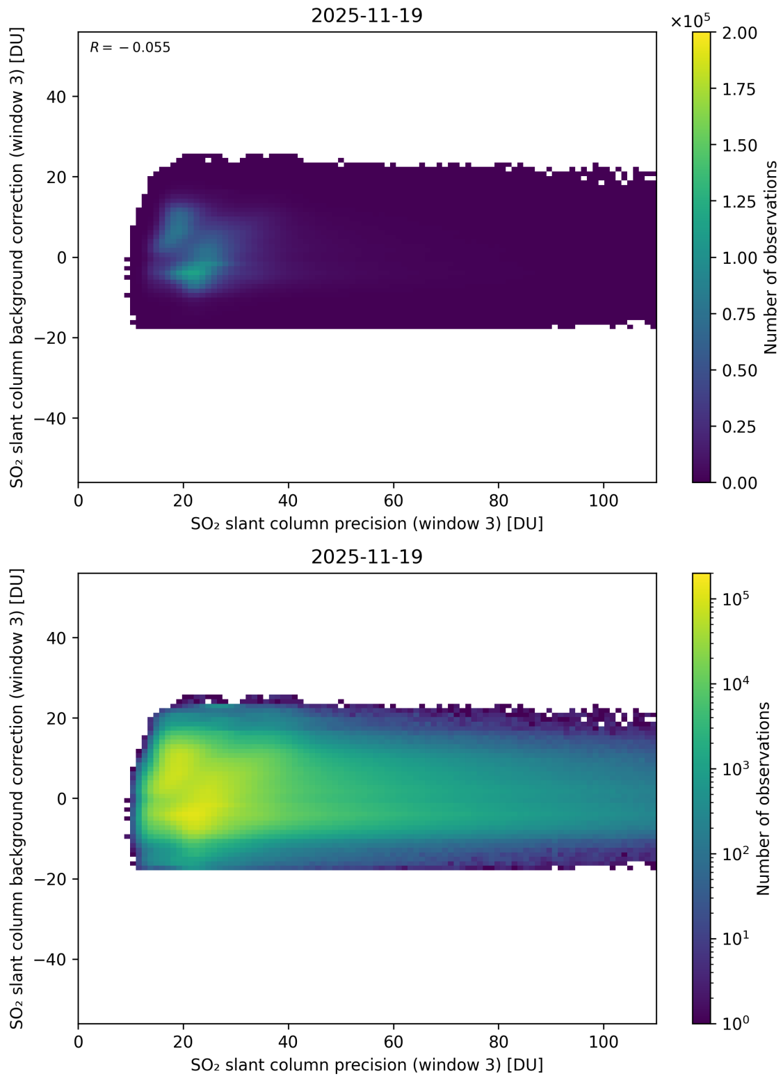
Figure 307: Scatter density plot of “SO 2 slant column precision (window 3)” against “SO 2 slant column background correction (window 3)” for 2025-11-18 to 2025-11-20.
