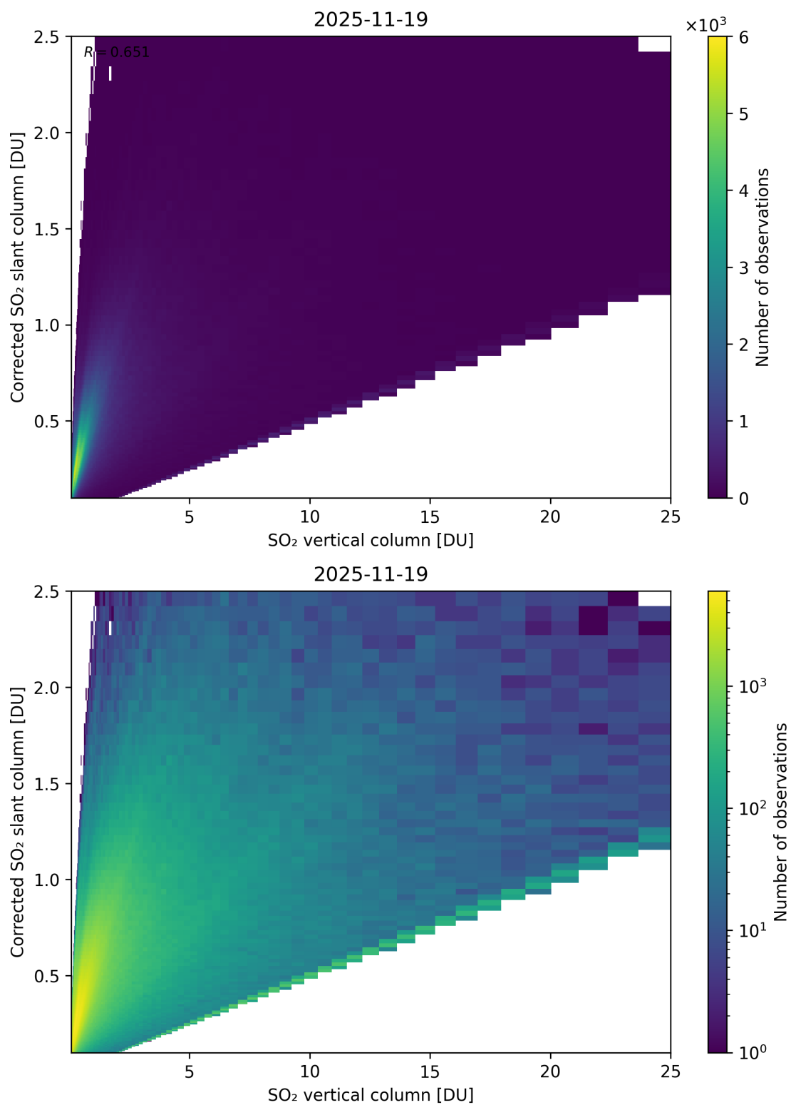
Figure 351: Scatter density plot of “SO 2 vertical column” against “Corrected SO 2 slant column” for 2025-11-18 to 2025-11-20.
