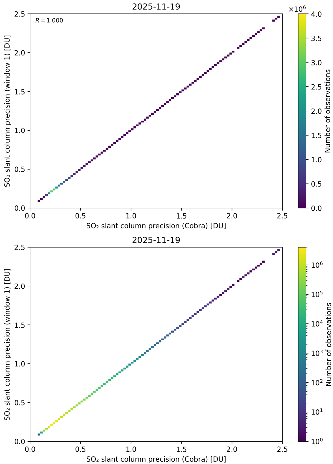
Figure 209: Scatter density plot of “SO 2 slant column precision (Cobra)” against “SO 2 slant column precision (window 1)” for 2025-11-18 to 2025-11-20.
