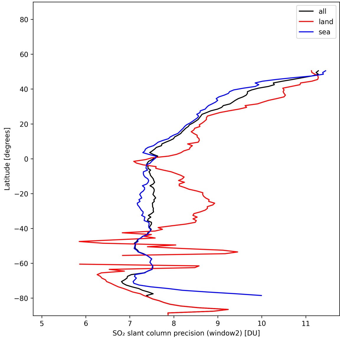
Figure 42: Zonal average of “SO 2 slant column precision (window2)” for 2025-11-18 to 2025-11-20.
