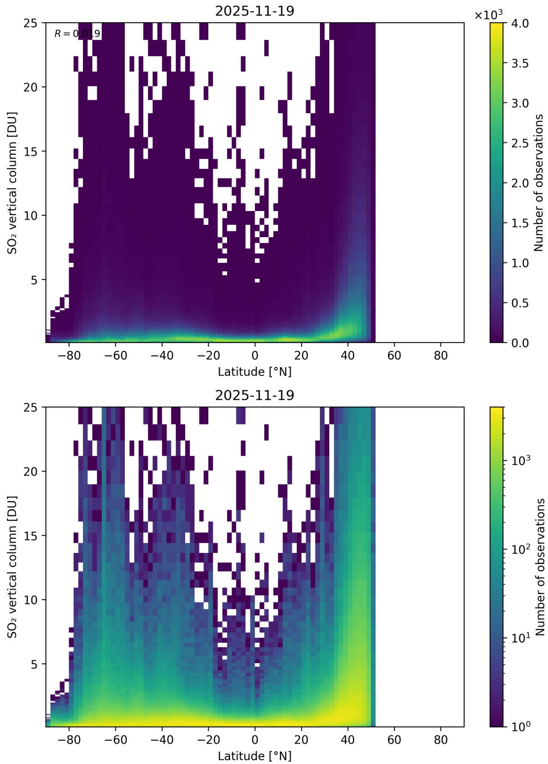
Figure 169: Scatter density plot of “Latitude” against “SO 2 vertical column” for 2025-11-18 to 2025-11-20.
