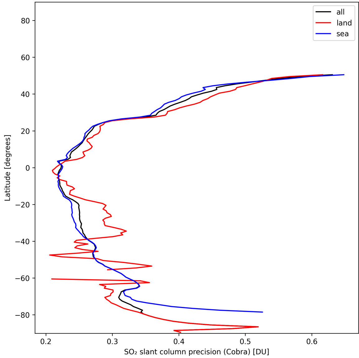
Figure 36: Zonal average of “SO 2 slant column precision (Cobra)” for 2025-11-18 to 2025-11-20.
