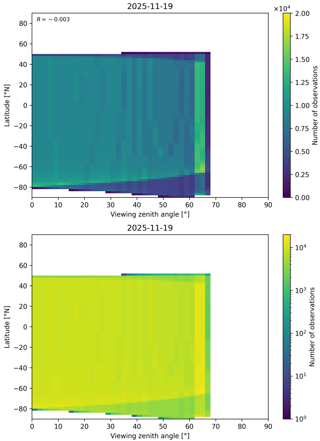
Figure 368: Scatter density plot of “Viewing zenith angle” against “Latitude” for 2025-11-18 to 2025-11-20.
