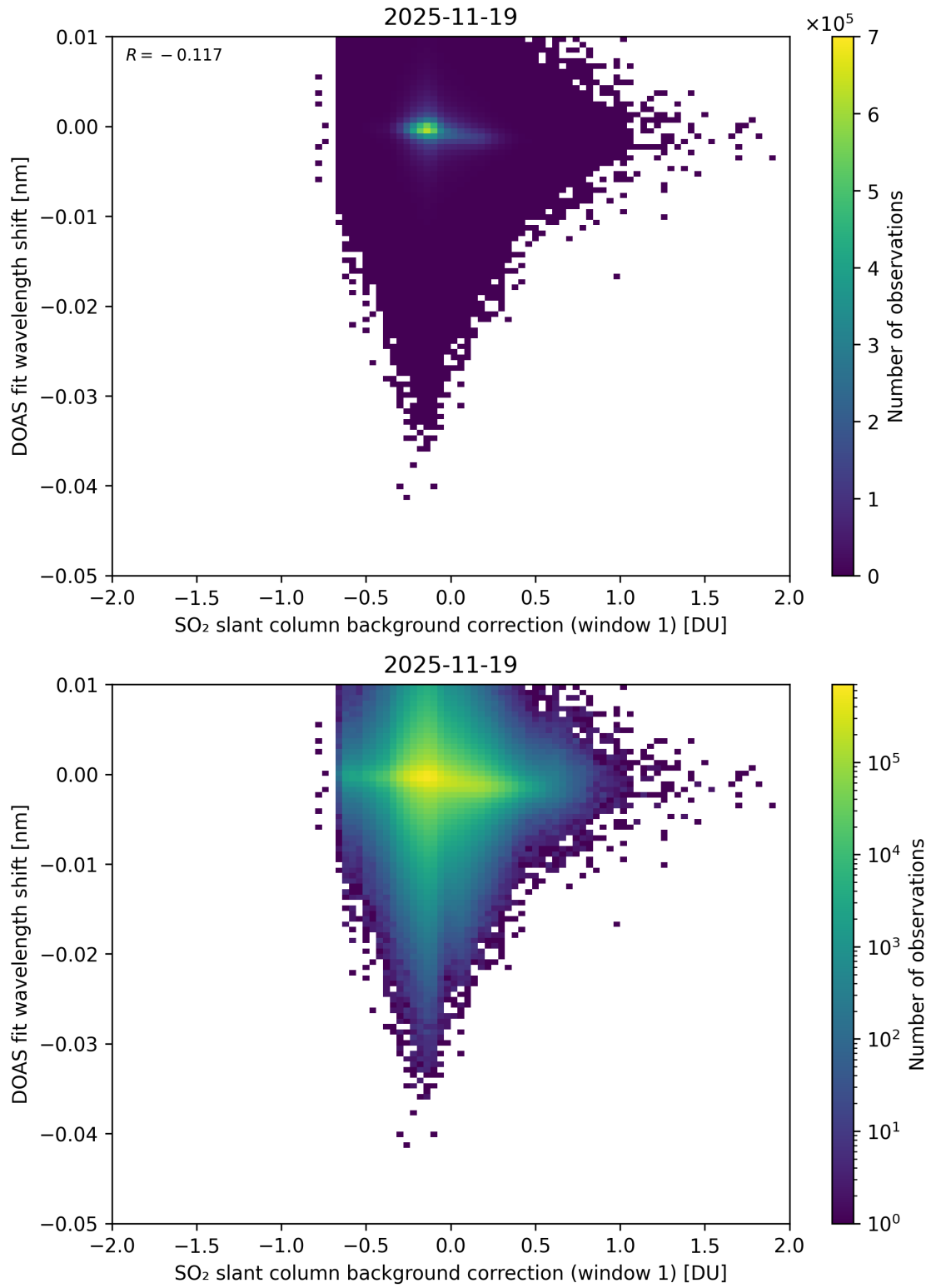
Figure 111: Scatter density plot of “SO 2 slant column background correction (window 1)” against “DOAS fit wavelength shift” for 2025-11-18 to 2025-11-20.
