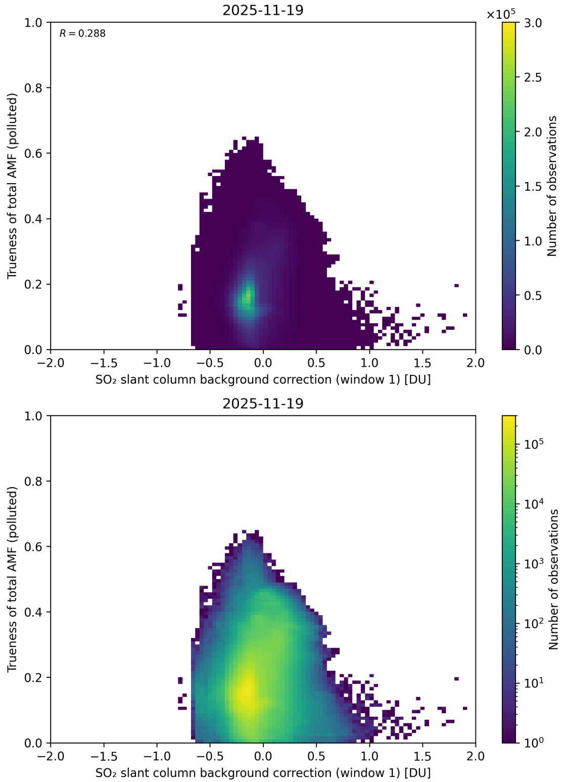
Figure 121: Scatter density plot of “SO 2 slant column background correction (window 1)” against “Trueness of total AMF (polluted)” for 2025-11-18 to 2025-11-20.
