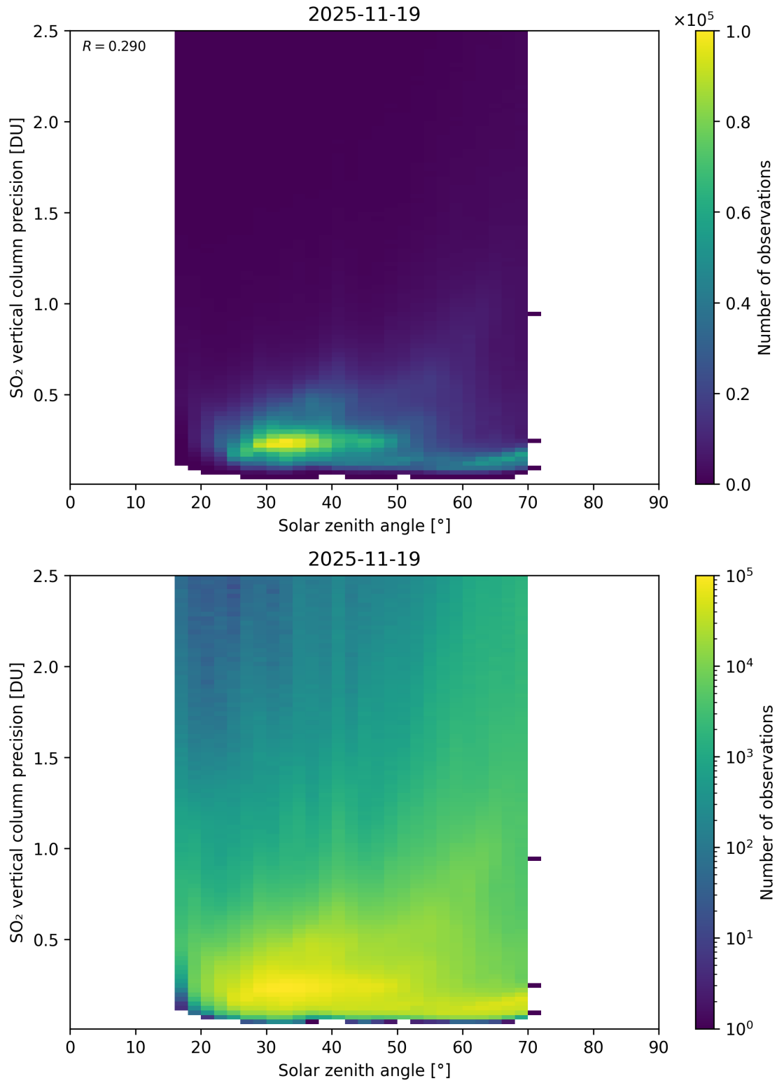
Figure 192: Scatter density plot of “Solar zenith angle” against “SO 2 vertical column precision” for 2025-11-18 to 2025-11-20.
