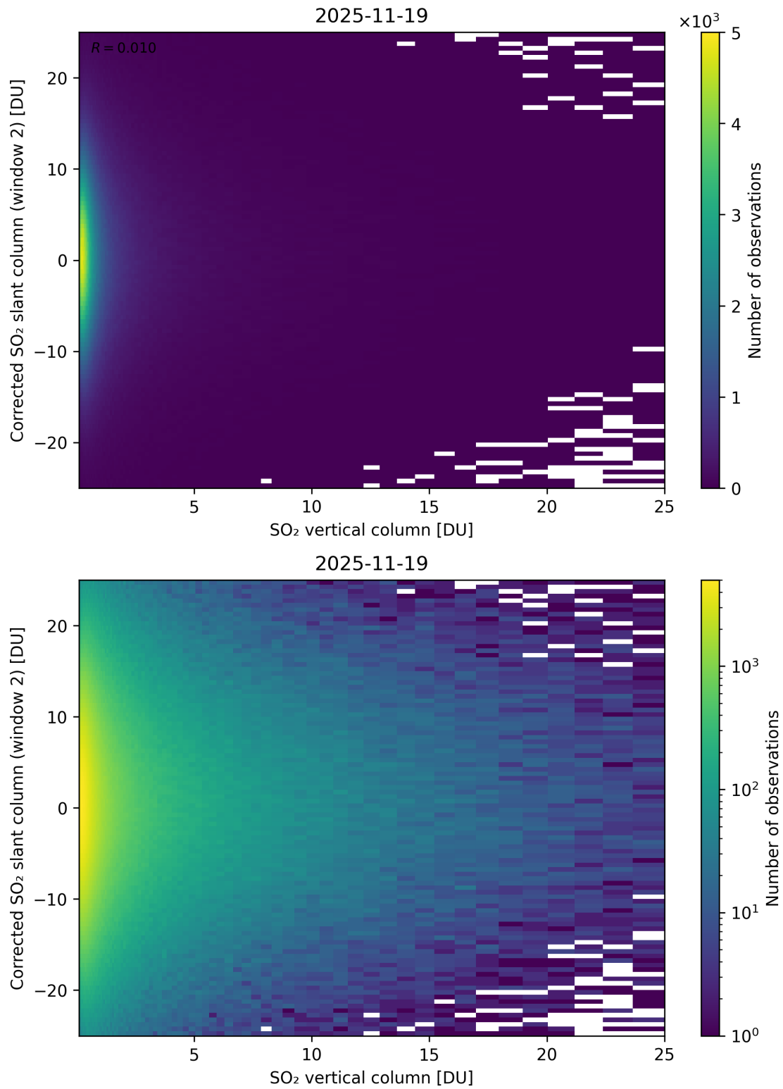
Figure 352: Scatter density plot of “SO 2 vertical column” against “Corrected SO 2 slant column (window 2)” for 2025-11-18 to 2025-11-20.
