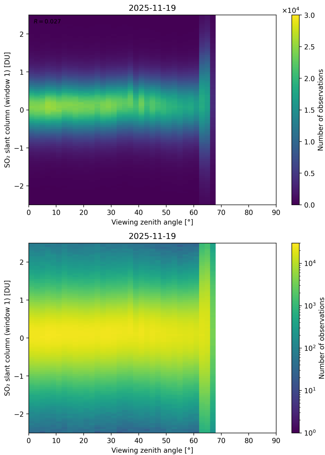
Figure 376: Scatter density plot of “Viewing zenith angle” against “SO 2 slant column (window 1)” for 2025-11-18 to 2025-11-20.
