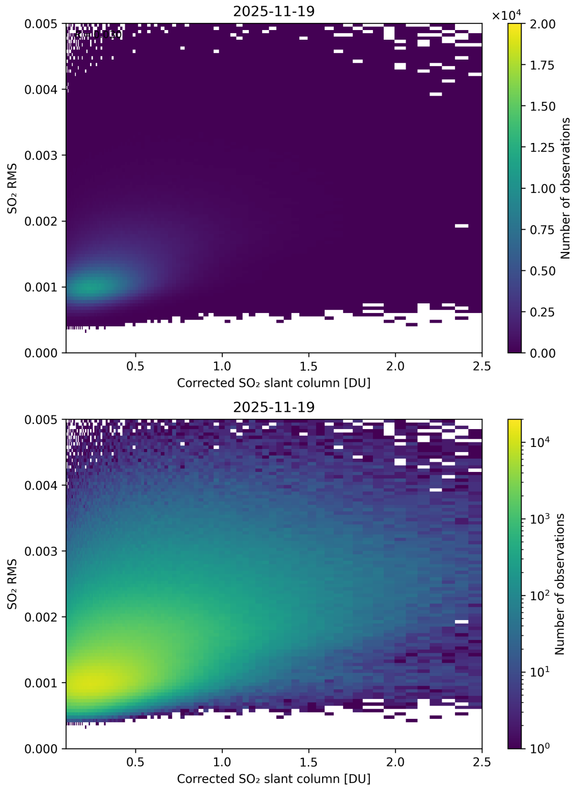
Figure 231: Scatter density plot of “Corrected SO 2 slant column” against “SO 2 RMS” for 2025-11-18 to 2025-11-20.
