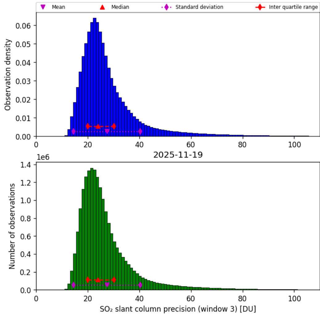
Figure 72: Histogram of “SO 2 slant column precision (window 3)” for 2025-11-18 to 2025-11-20
