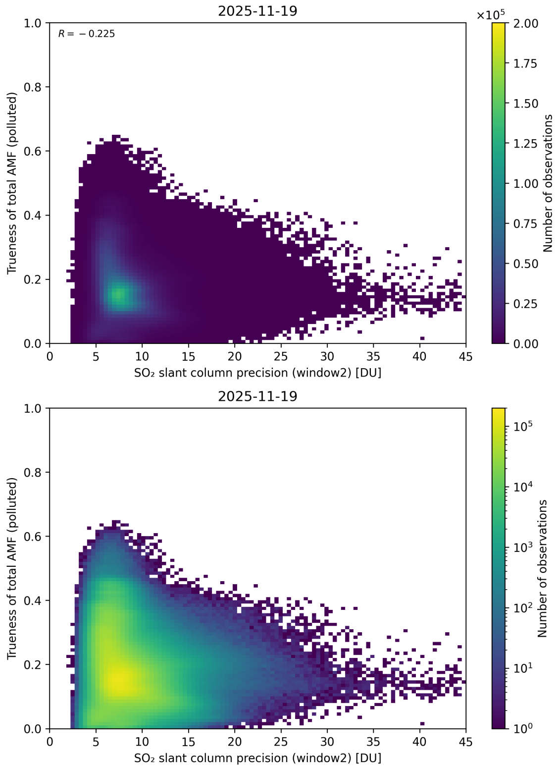
Figure 302: Scatter density plot of “SO 2 slant column precision (window2)” against “Trueness of total AMF (polluted)” for 2025-11-18 to 2025-11-20.
