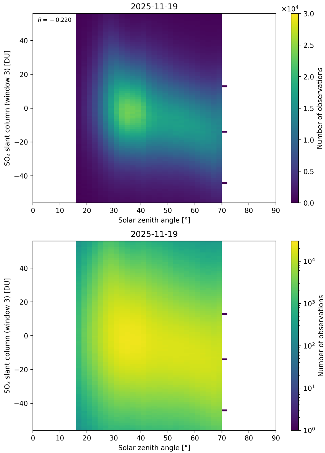
Figure 187: Scatter density plot of “Solar zenith angle” against “SO 2 slant column (window 3)” for 2025-11-18 to 2025-11-20.
