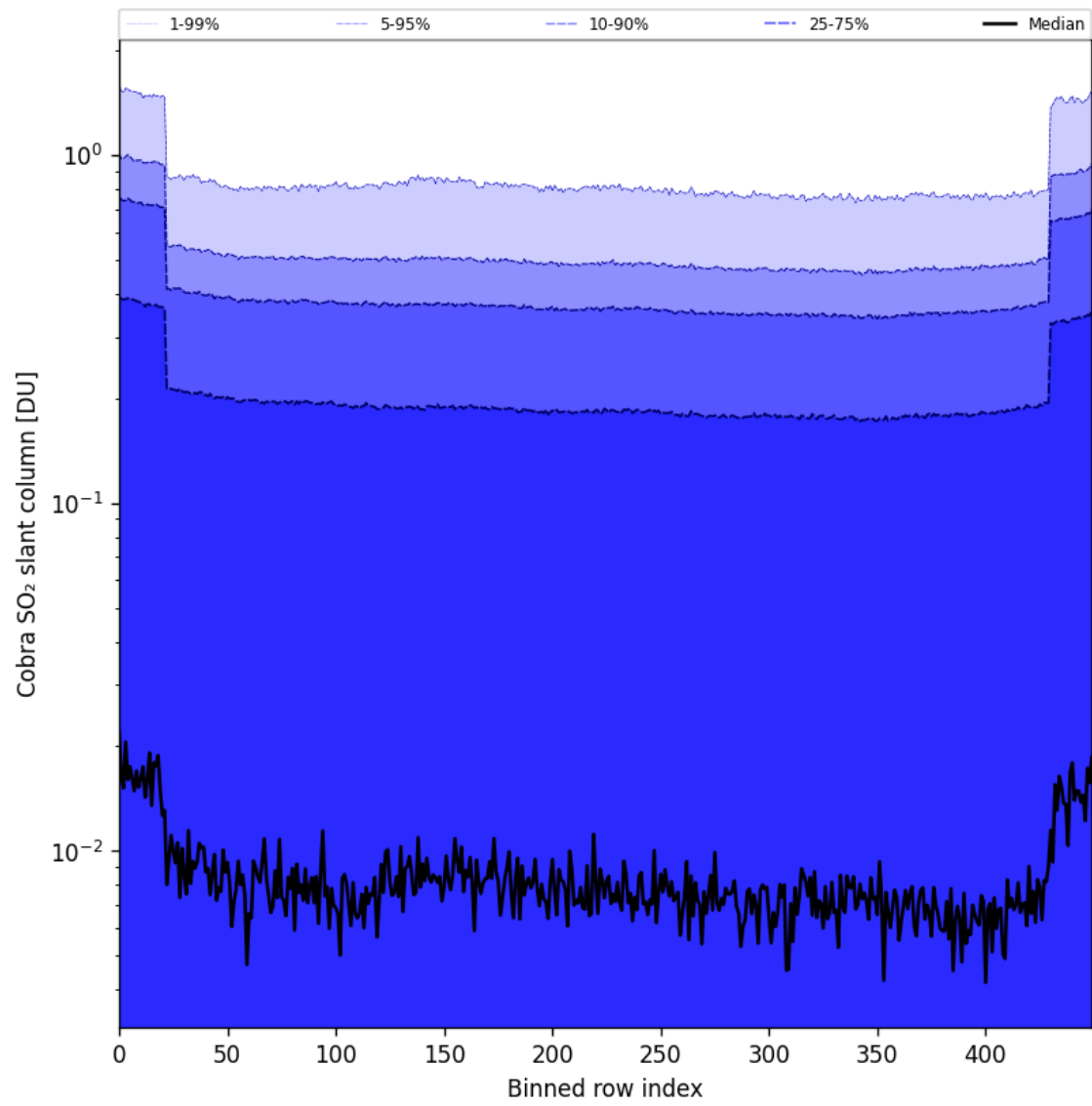
Figure 87: Along track statistics of "Cobra SO 2 slant column" for 2025-11-18 to 2025-11-20
