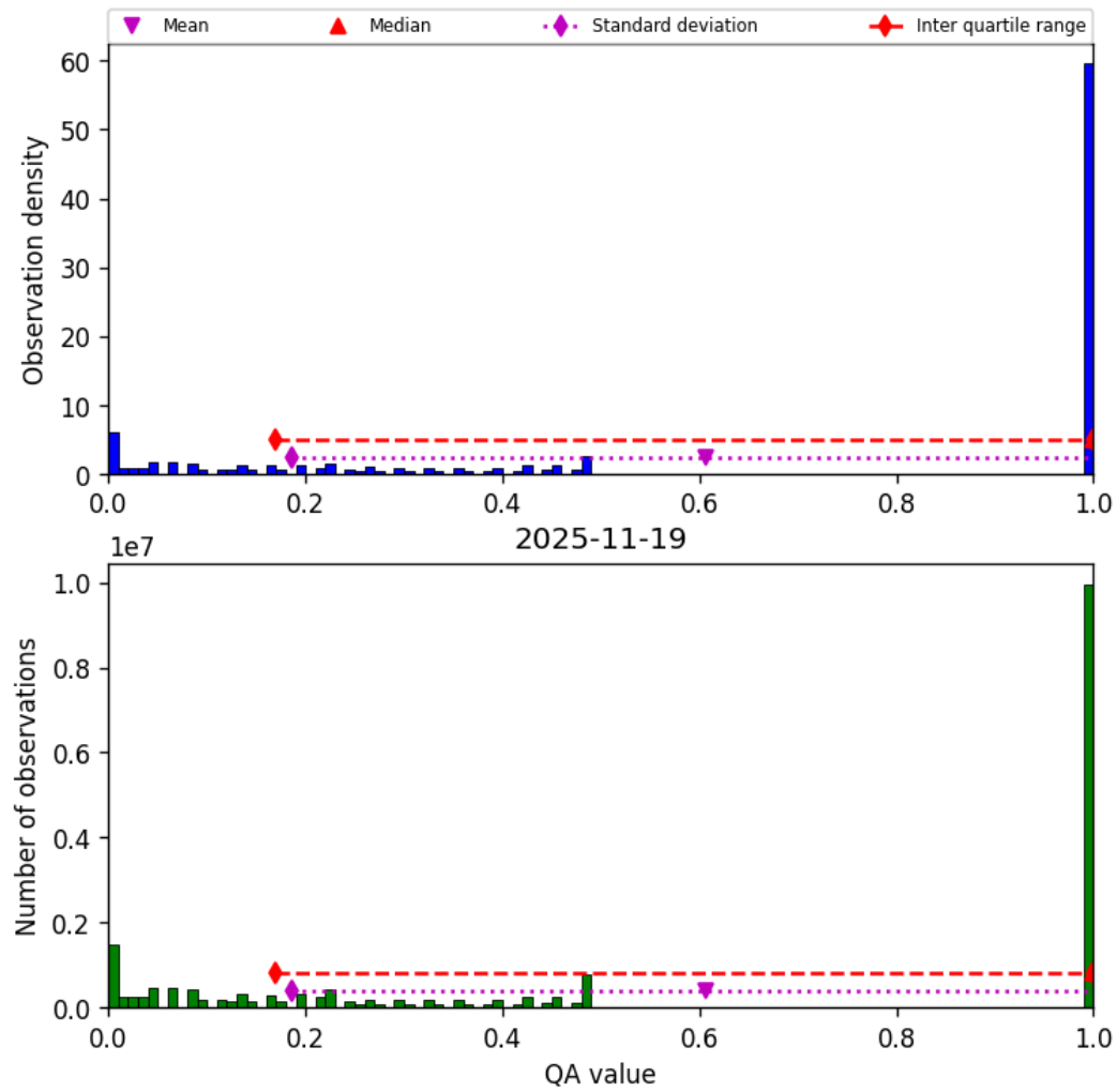
Figure 57: Histogram of “QA value” for 2025-11-18 to 2025-11-20
