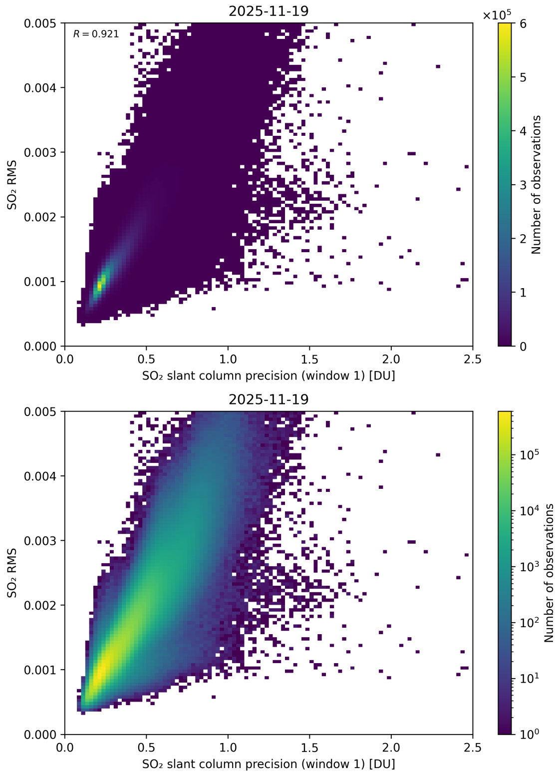
Figure 273: Scatter density plot of “SO 2 slant column precision (window 1)” against “SO 2 RMS” for 2025-11-18 to 2025-11-20.
