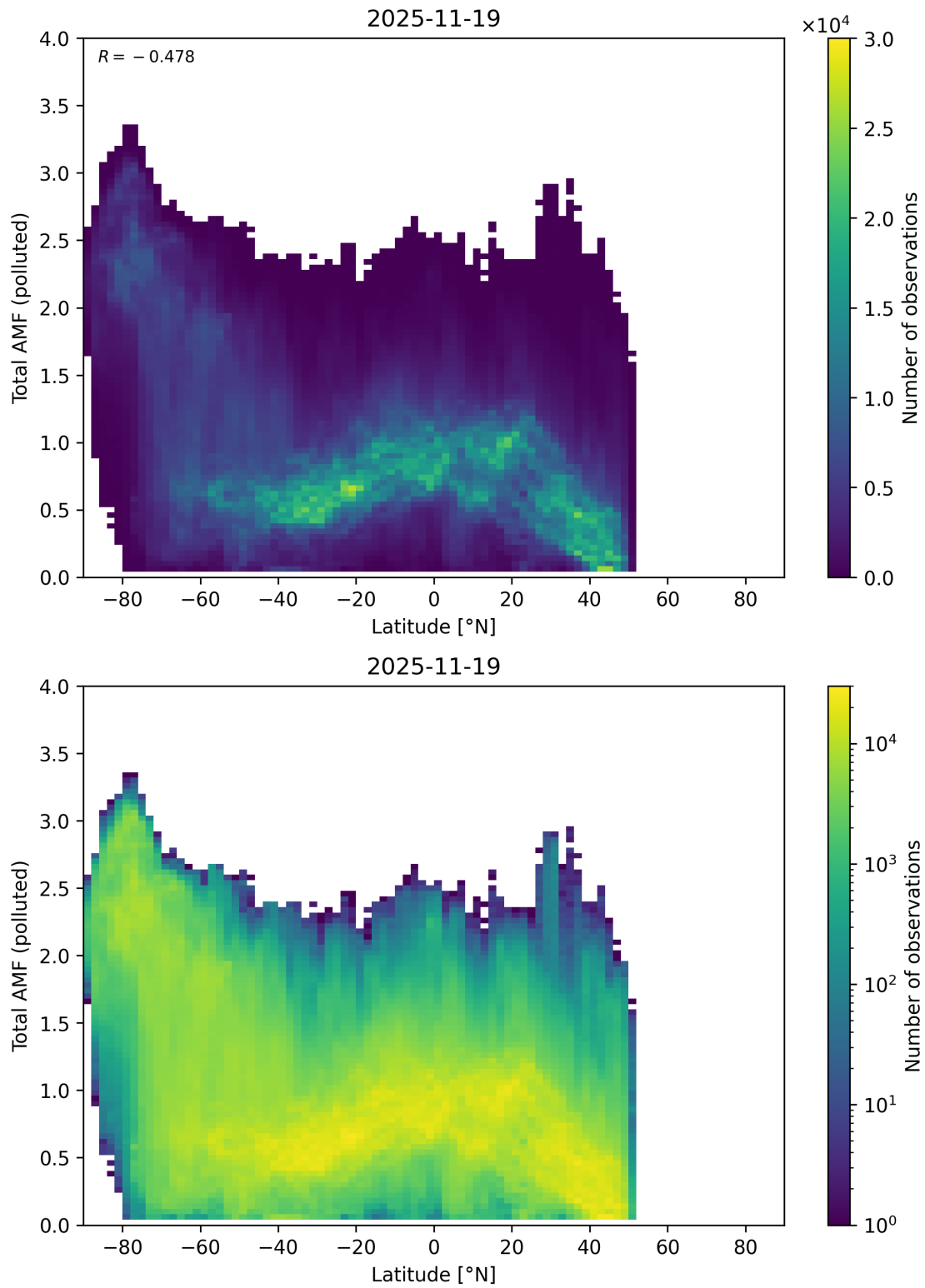
Figure 167: Scatter density plot of “Latitude” against “Total AMF (polluted)” for 2025-11-18 to 2025-11-20.
