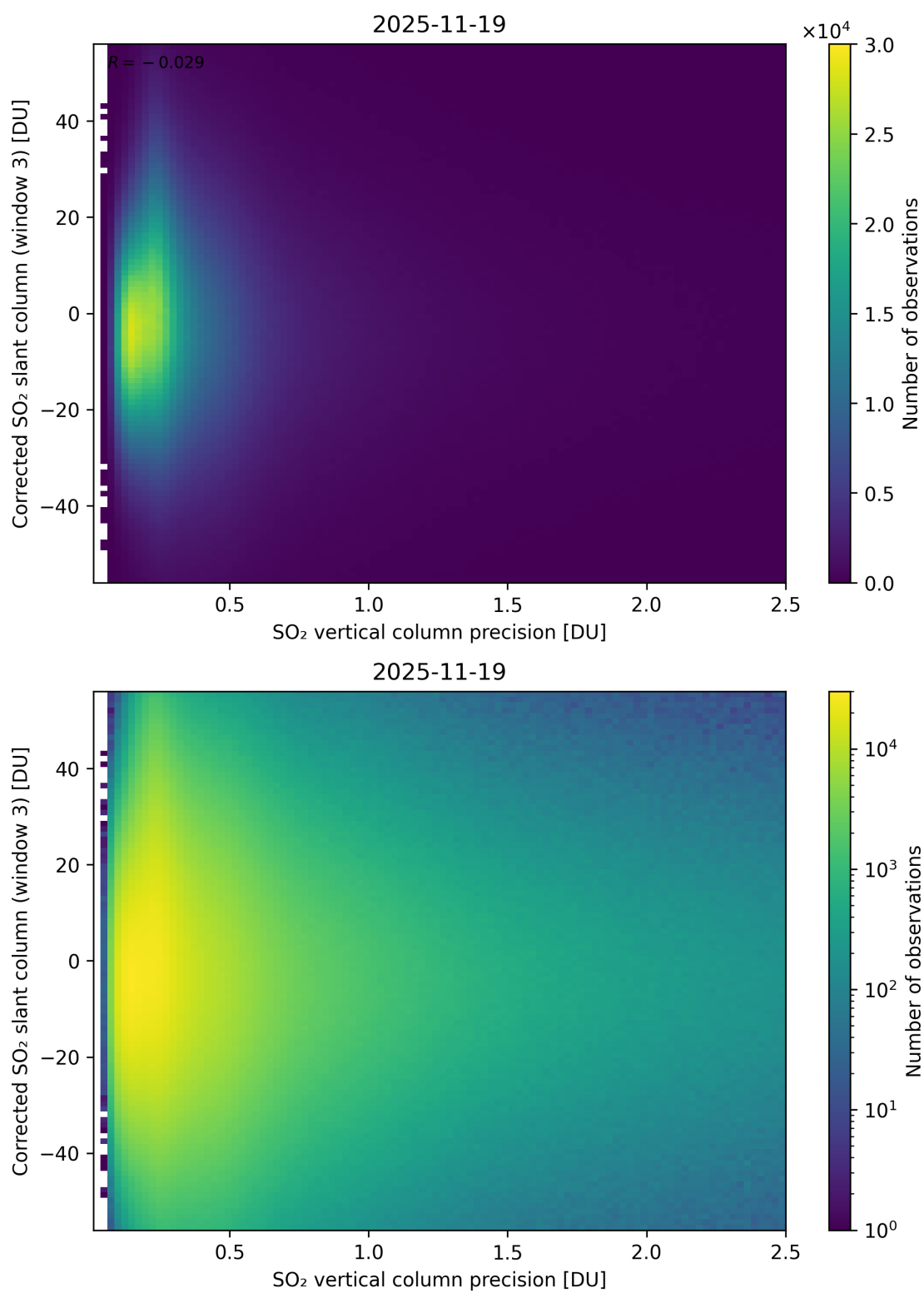
Figure 340: Scatter density plot of “SO 2 vertical column precision” against “Corrected SO 2 slant column (window 3)” for 2025-11-18 to 2025-11-20.
