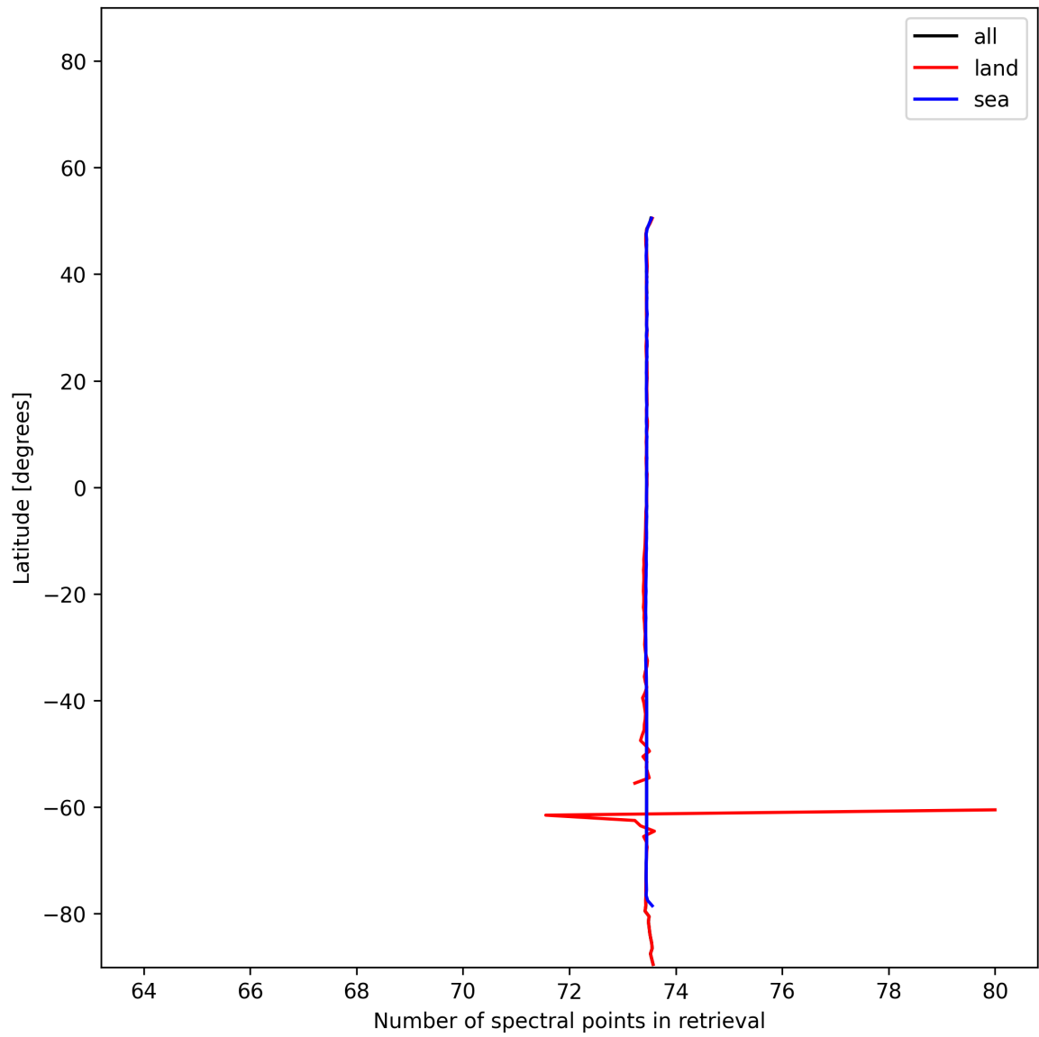
Figure 56: Zonal average of “Number of spectral points in retrieval” for 2025-11-18 to 2025-11-20.
