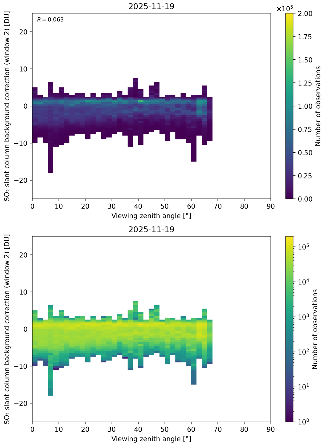
Figure 363: Scatter density plot of “Viewing zenith angle” against “SO 2 slant column background correction (window 2)” for 2025-11-18 to 2025-11-20.
