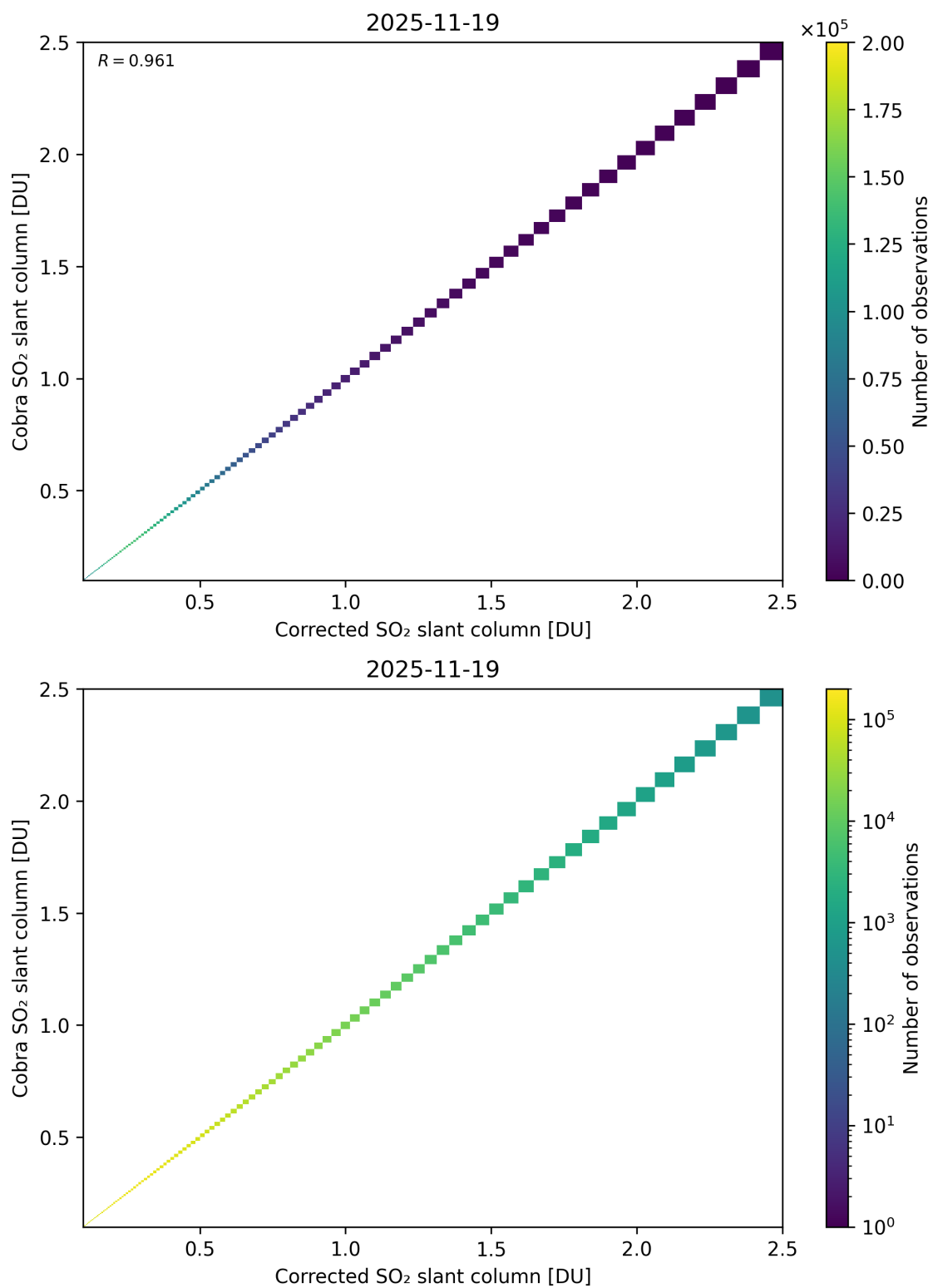
Figure 233: Scatter density plot of “Corrected SO 2 slant column” against “Cobra SO 2 slant column” for 2025-11-18 to 2025-11-20.
