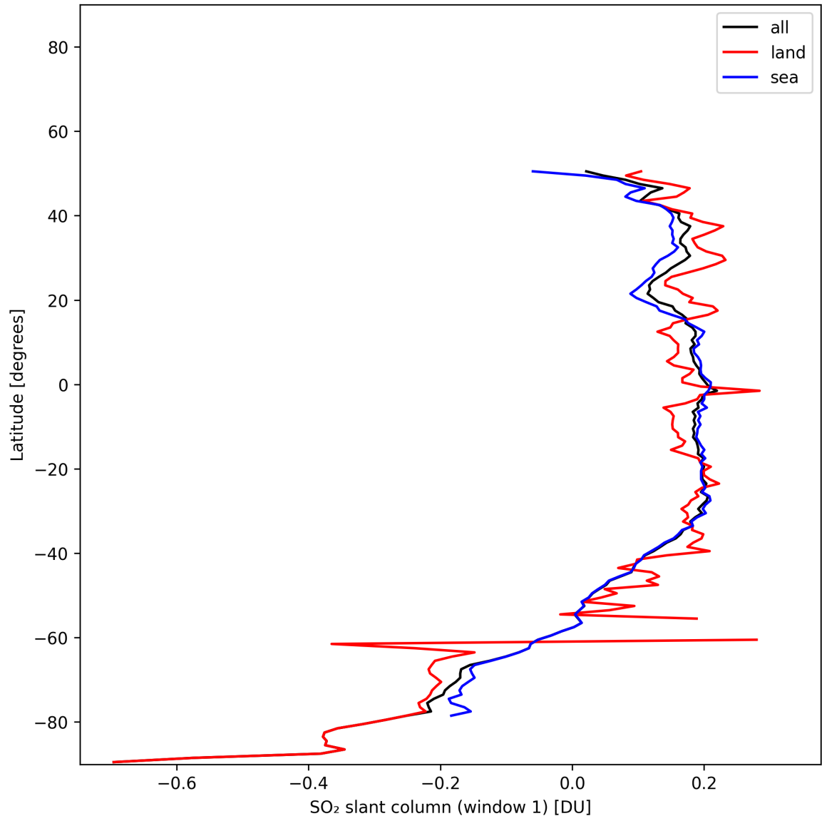
Figure 37: Zonal average of “SO 2 slant column (window 1)” for 2025-11-18 to 2025-11-20.
