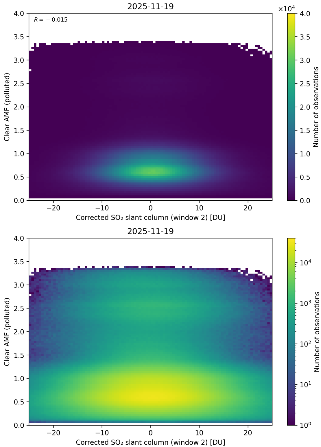
Figure 249: Scatter density plot of “Corrected SO 2 slant column (window 2)” against “Clear AMF (polluted)” for 2025-11-18 to 2025-11-20.
