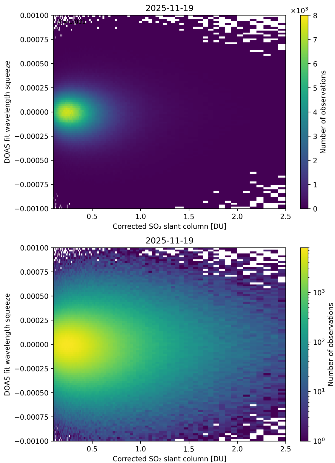
Figure 230: Scatter density plot of “Corrected SO 2 slant column” against “DOAS fit wavelength squeeze” for 2025-11-18 to 2025-11-20.
