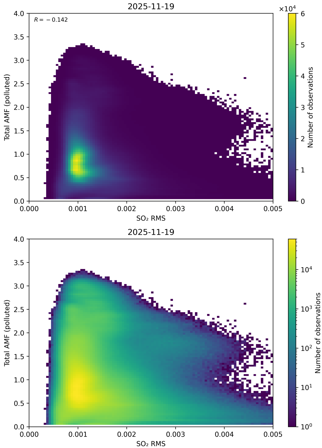
Figure 148: Scatter density plot of “SO 2 RMS” against “Total AMF (polluted)” for 2025-11-18 to 2025-11-20.
