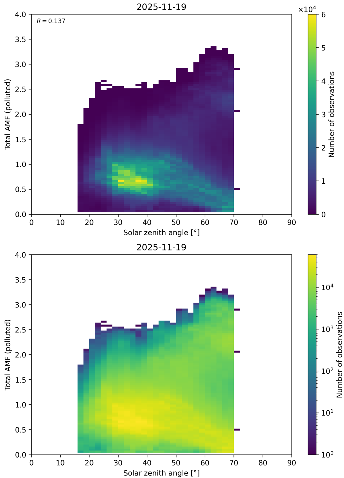
Figure 189: Scatter density plot of “Solar zenith angle” against “Total AMF (polluted)” for 2025-11-18 to 2025-11-20.
