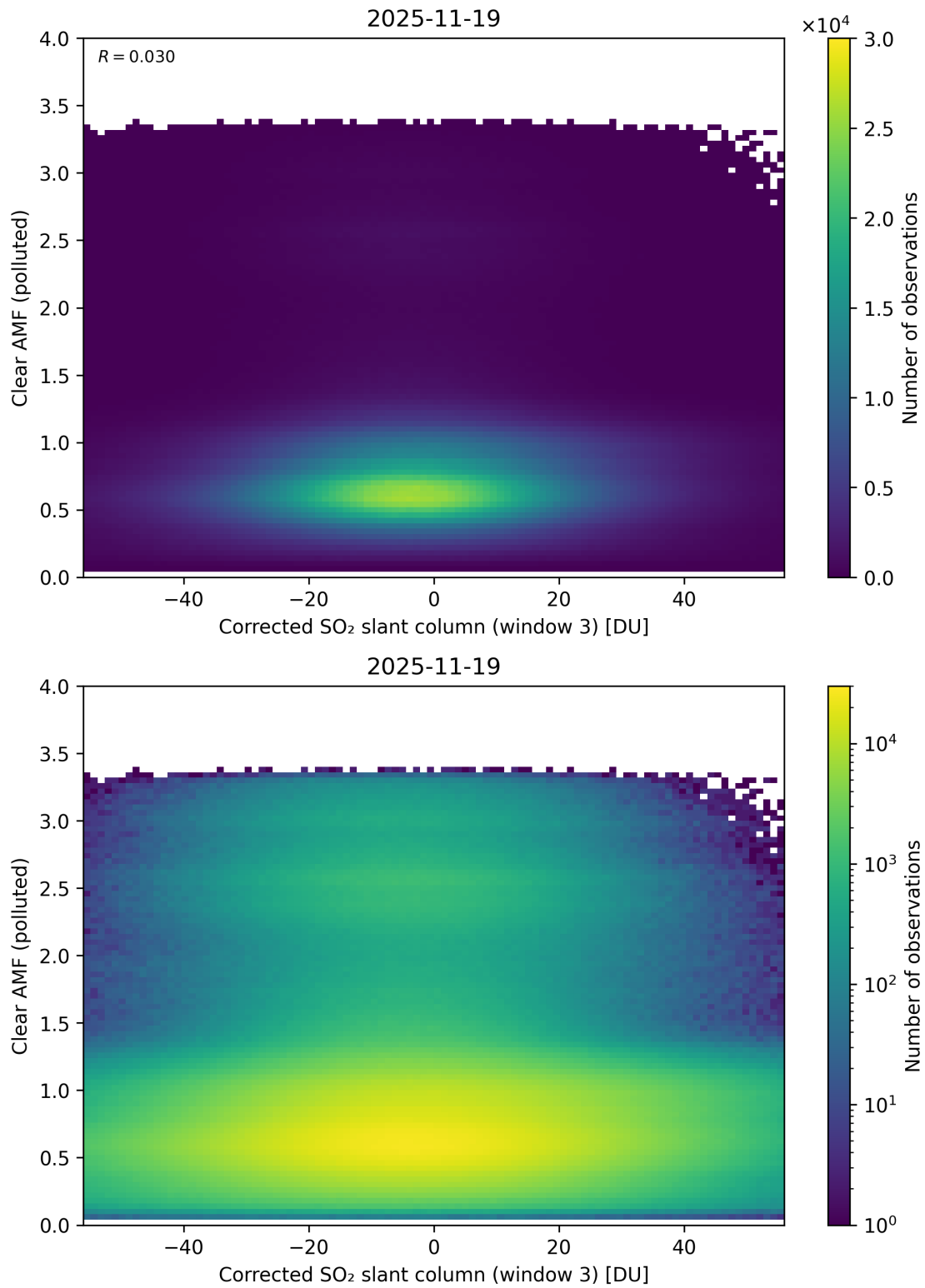
Figure 259: Scatter density plot of “Corrected SO 2 slant column (window 3)” against “Clear AMF (polluted)” for 2025-11-18 to 2025-11-20.
