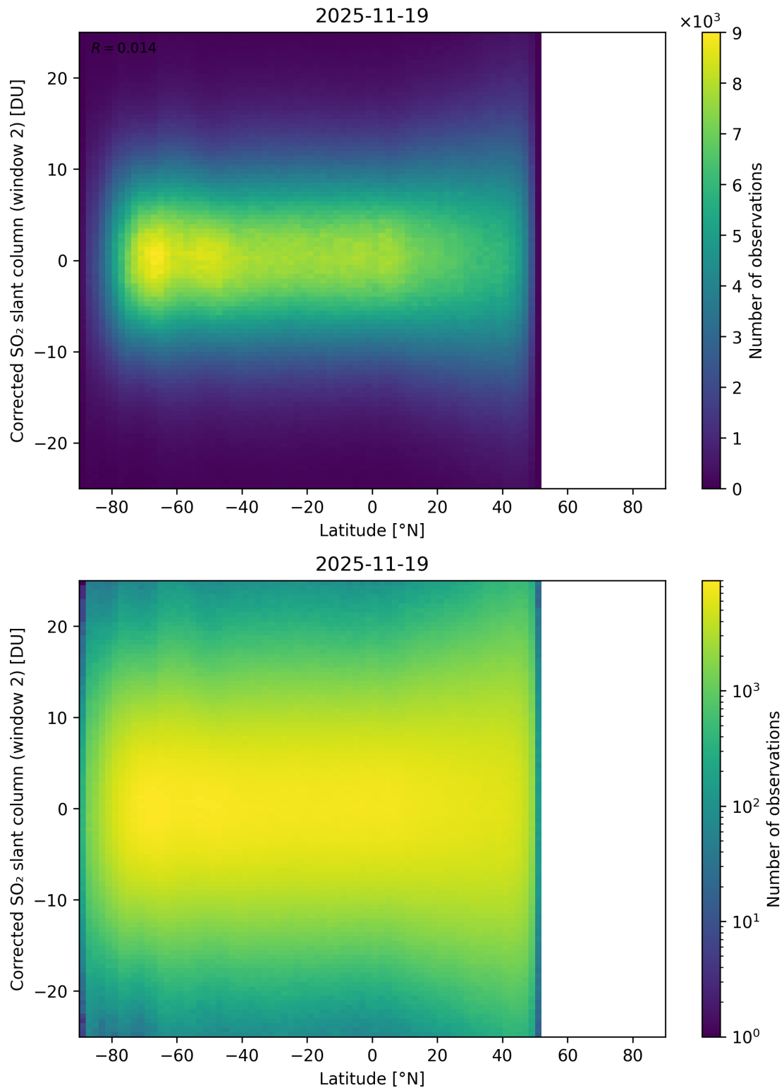
Figure 160: Scatter density plot of “Latitude” against “Corrected SO 2 slant column (window 2)” for 2025-11-18 to 2025-11-20.
