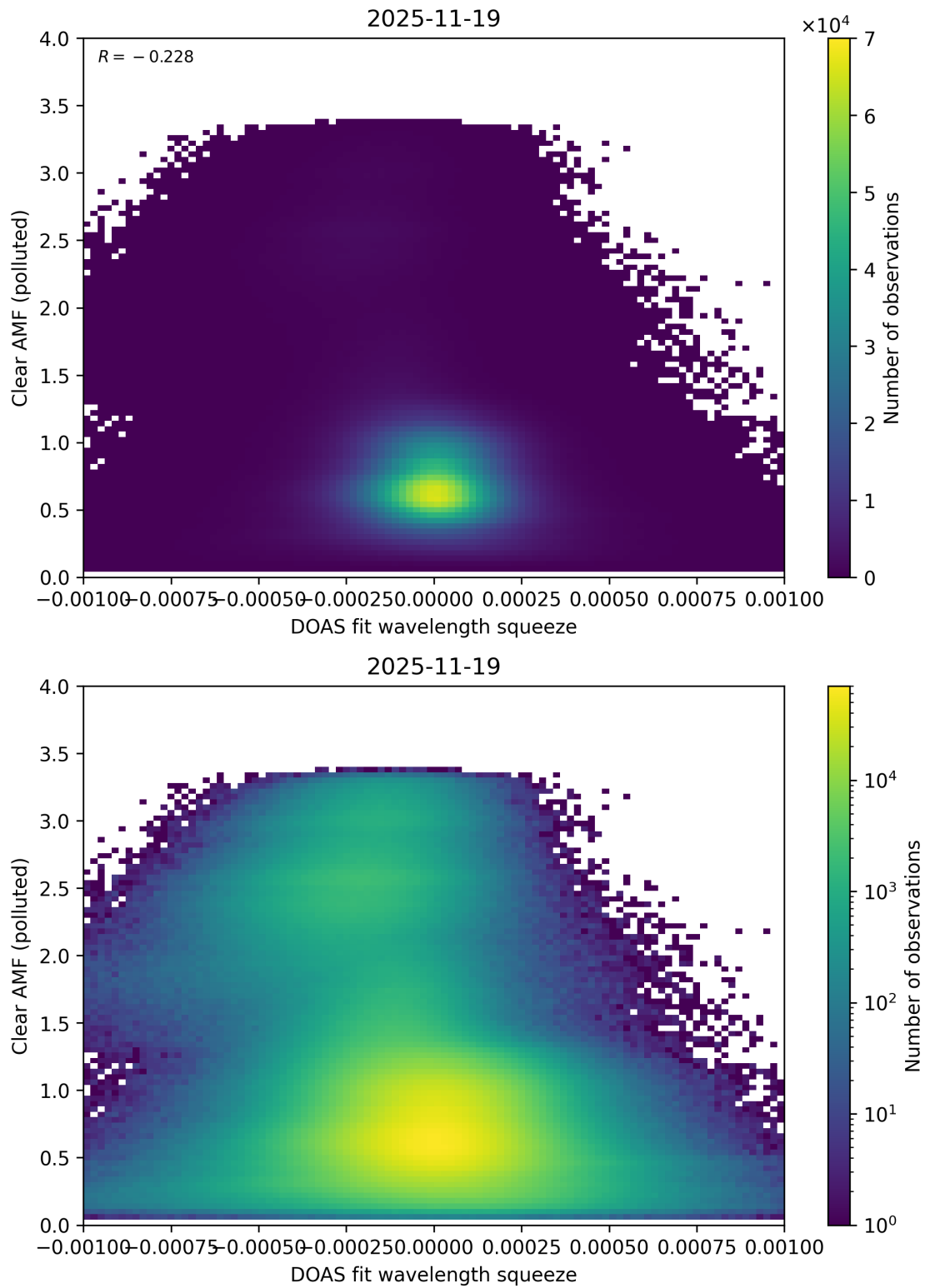
Figure 144: Scatter density plot of “DOAS fit wavelength squeeze” against “Clear AMF (polluted)” for 2025-11-18 to 2025-11-20.
