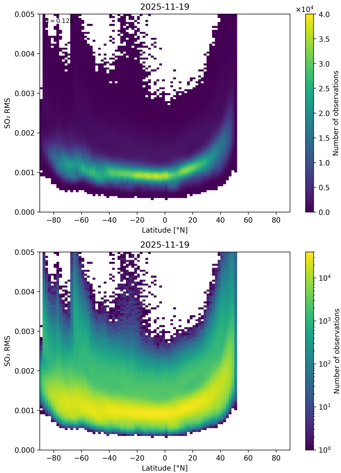
Figure 155: Scatter density plot of “Latitude” against “SO 2 RMS” for 2025-11-18 to 2025-11-20.
