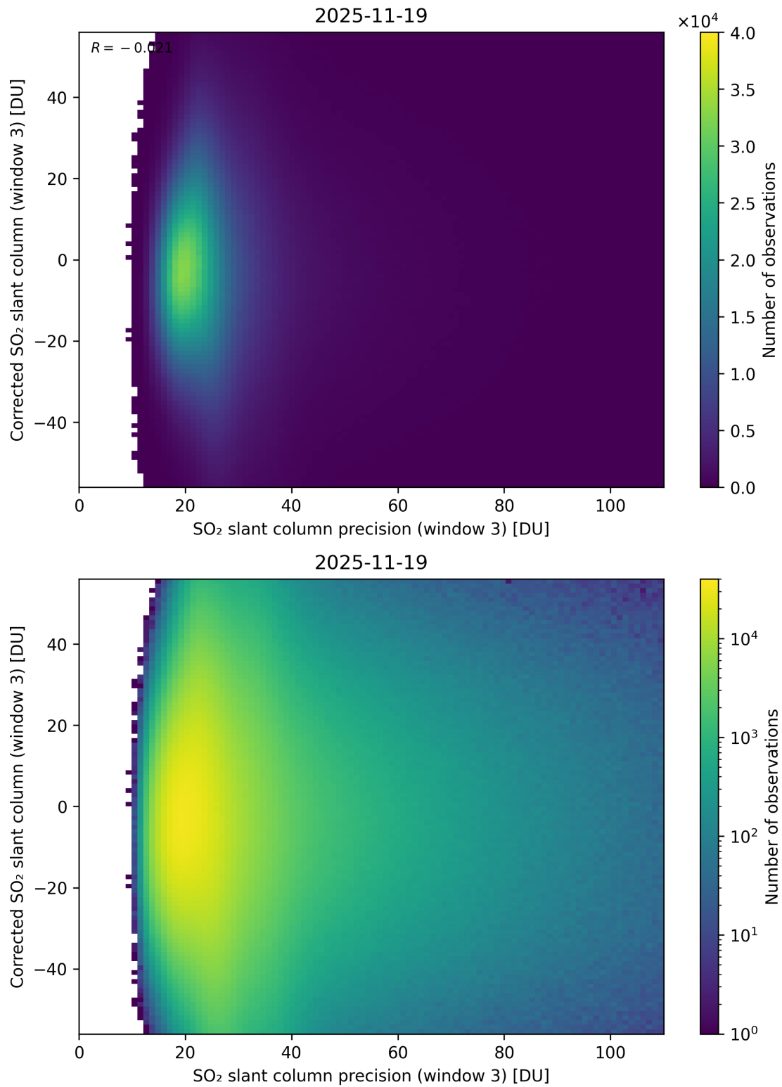
Figure 312: Scatter density plot of “SO 2 slant column precision (window 3)” against “Corrected SO 2 slant column (window 3)” for 2025-11-18 to 2025-11-20.
