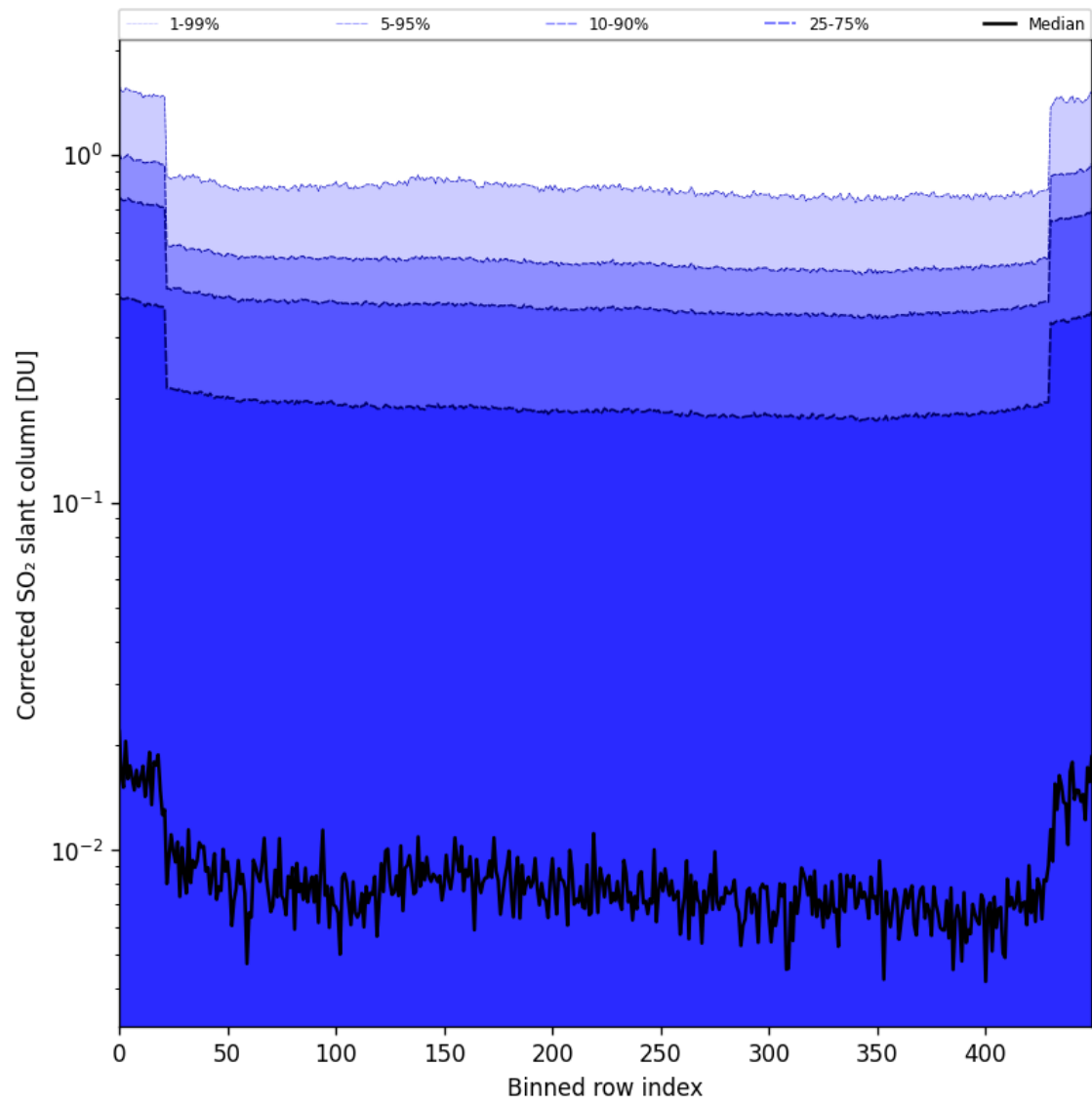
Figure 86: Along track statistics of “Corrected SO 2 slant column” for 2025-11-18 to 2025-11-20
