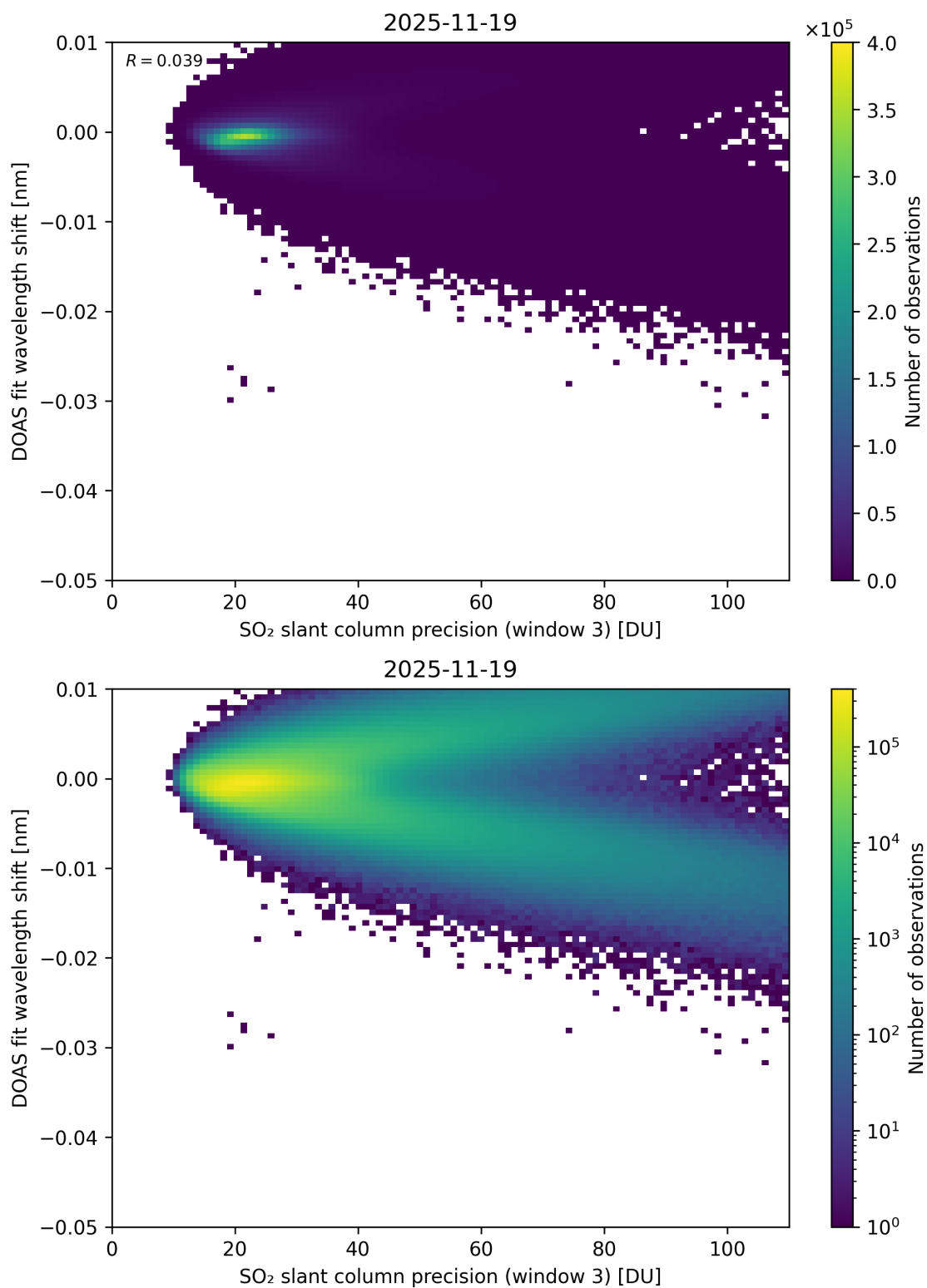
Figure 308: Scatter density plot of “SO 2 slant column precision (window 3)” against “DOAS fit wavelength shift” for 2025-11-18 to 2025-11-20.
