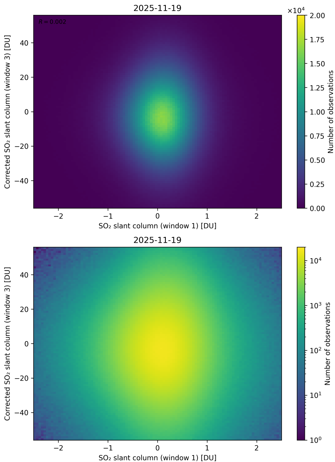
Figure 284: Scatter density plot of “SO 2 slant column (window 1)” against “Corrected SO 2 slant column (window 3)” for 2025-11-18 to 2025-11-20.
