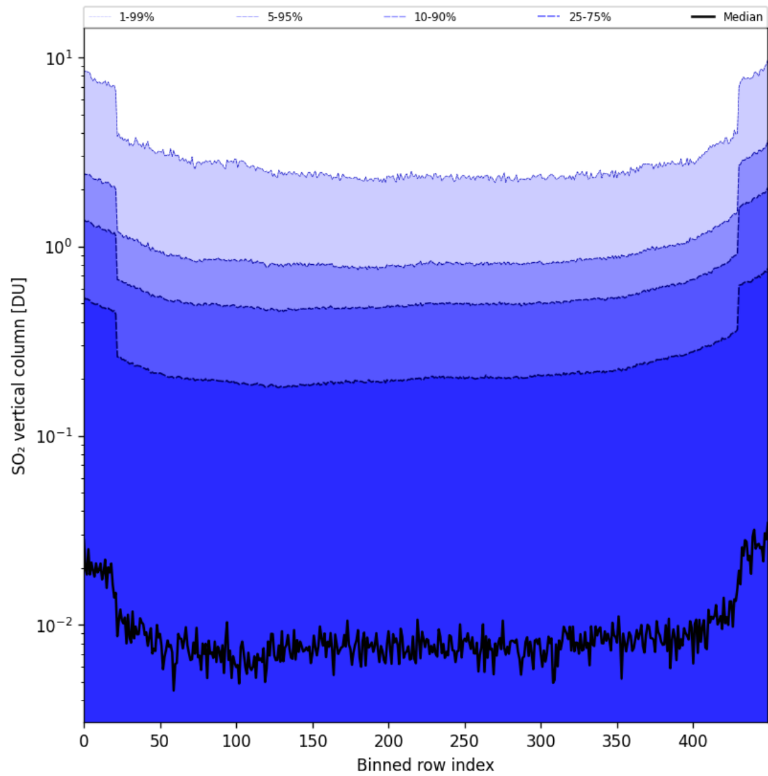
Figure 84: Along track statistics of “SO 2 vertical column” for 2025-11-18 to 2025-11-20
