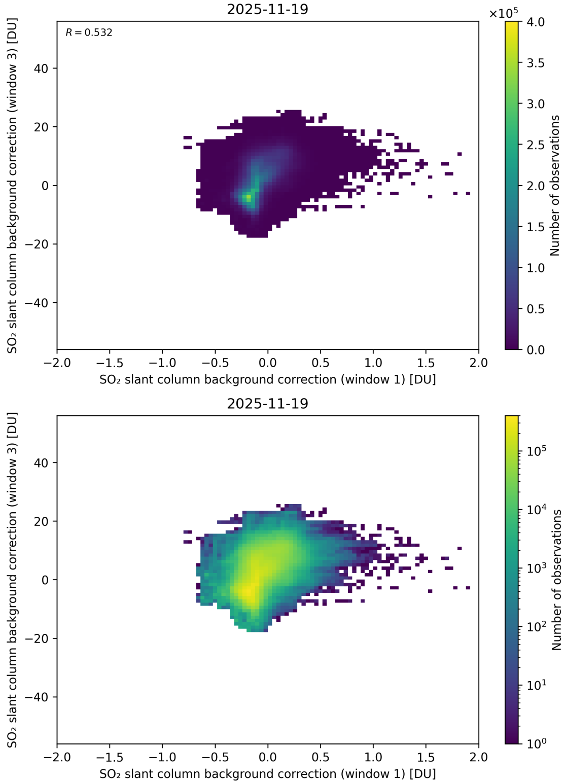
Figure 110: Scatter density plot of “SO 2 slant column background correction (window 1)” against “SO 2 slant column background correction (window 3)” for 2025-11-18 to 2025-11-20.
