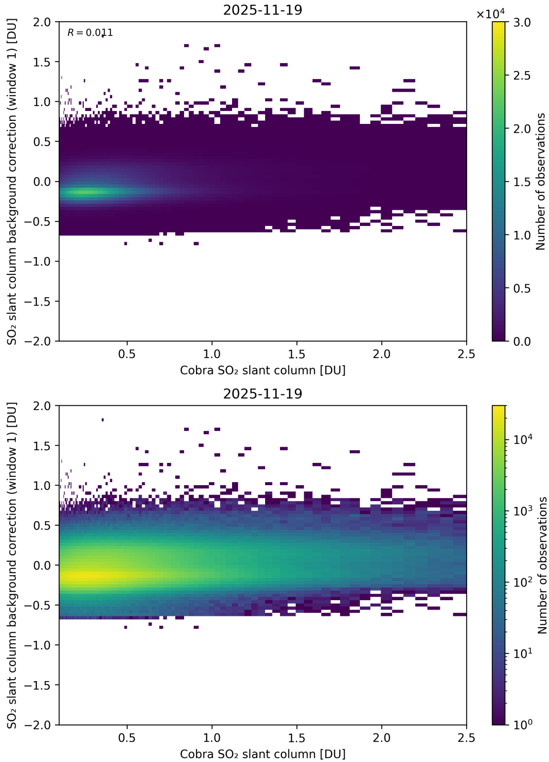
Figure 193: Scatter density plot of “Cobra SO 2 slant column” against “SO 2 slant column background correction (window 1)” for 2025-11-18 to 2025-11-20.
