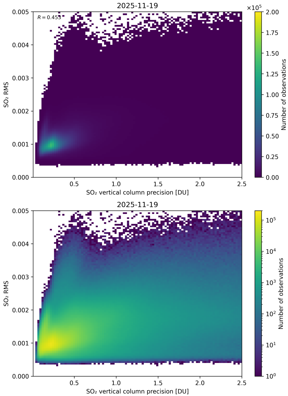
Figure 334: Scatter density plot of “SO 2 vertical column precision” against “SO 2 RMS” for 2025-11-18 to 2025-11-20.
