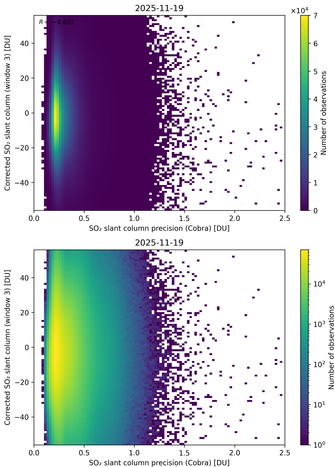
Figure 207: Scatter density plot of “SO 2 slant column precision (Cobra)” against “Corrected SO 2 slant column (window 3)” for 2025-11-18 to 2025-11-20.
