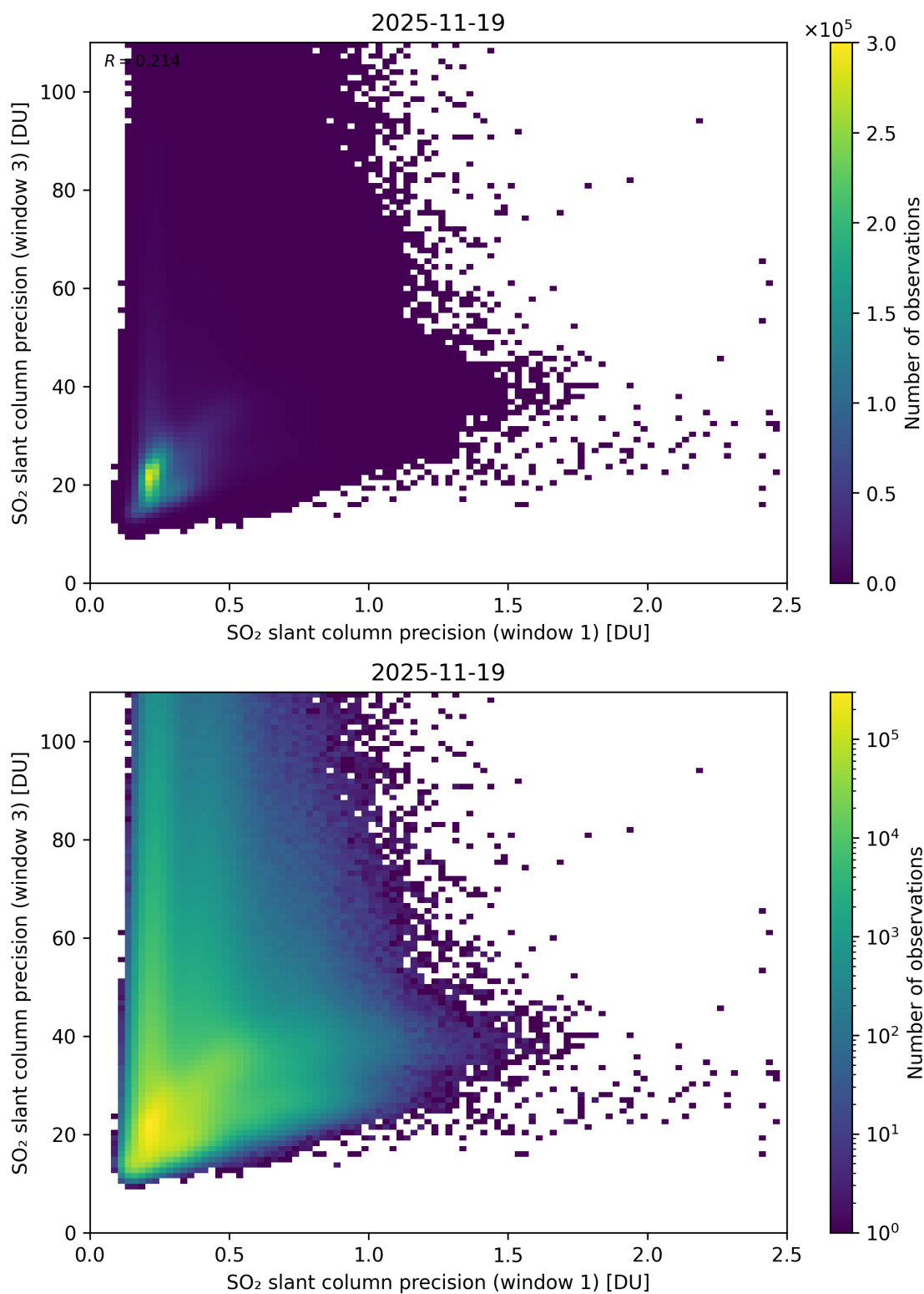
Figure 279: Scatter density plot of “SO 2 slant column precision (window 1)” against “SO 2 slant column precision (window 3)” for 2025-11-18 to 2025-11-20.
