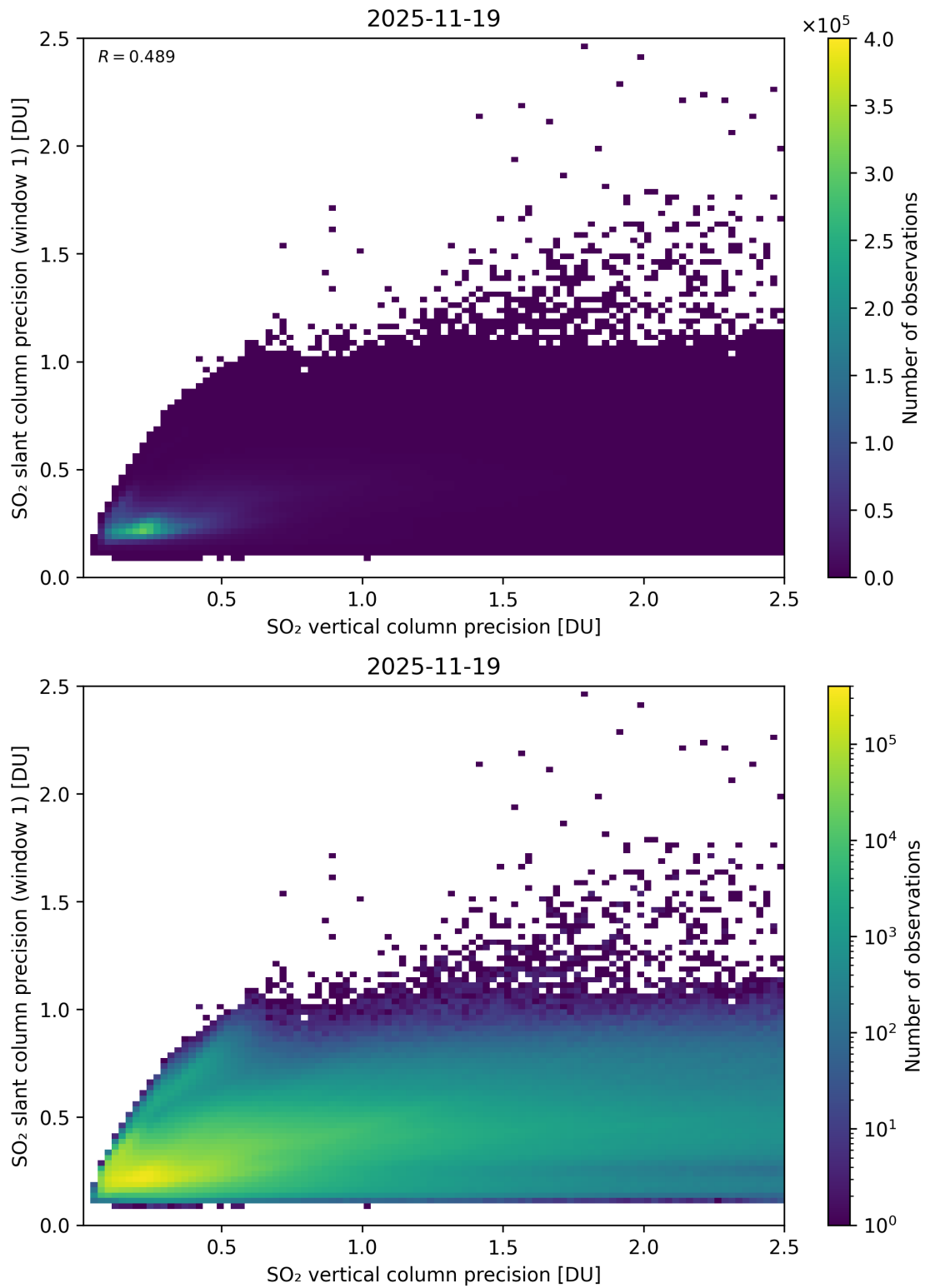
Figure 342: Scatter density plot of “SO 2 vertical column precision” against “SO 2 slant column precision (window 1)” for 2025-11-18 to 2025-11-20.
