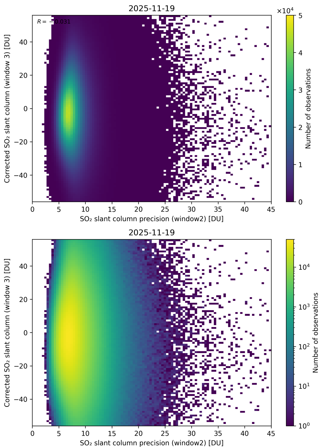
Figure 298: Scatter density plot of “SO 2 slant column precision (window2)” against “Corrected SO 2 slant column (window 3)” for 2025-11-18 to 2025-11-20.
