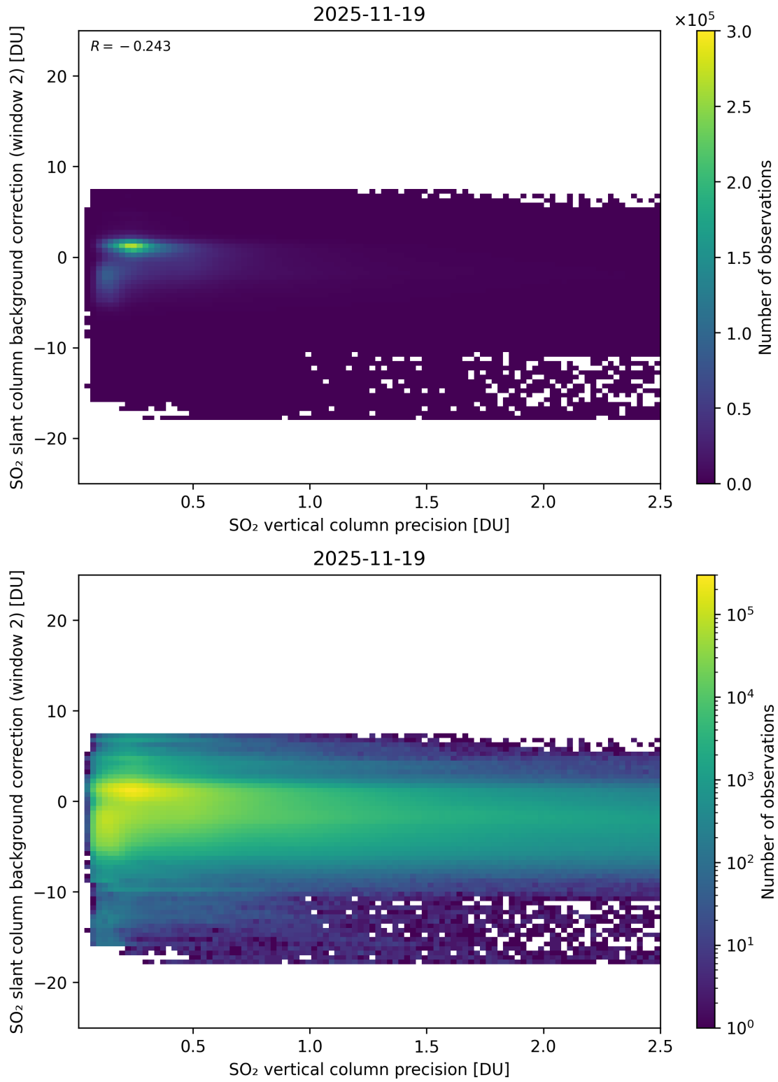
Figure 330: Scatter density plot of “SO 2 vertical column precision” against “SO 2 slant column background correction (window 2)” for 2025-11-18 to 2025-11-20.
