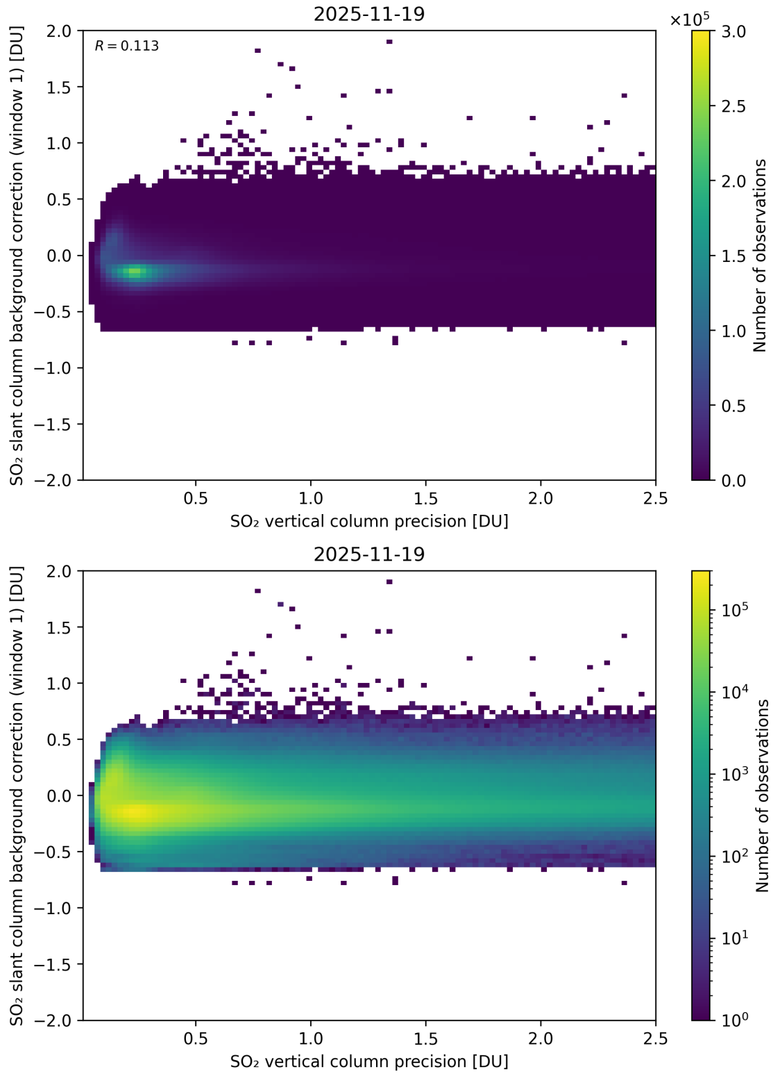
Figure 329: Scatter density plot of “SO 2 vertical column precision” against “SO 2 slant column background correction (window 1)” for 2025-11-18 to 2025-11-20.
