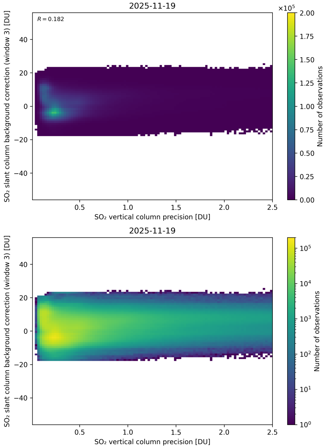
Figure 331: Scatter density plot of “SO 2 vertical column precision” against “SO 2 slant column background correction (window 3)” for 2025-11-18 to 2025-11-20.
