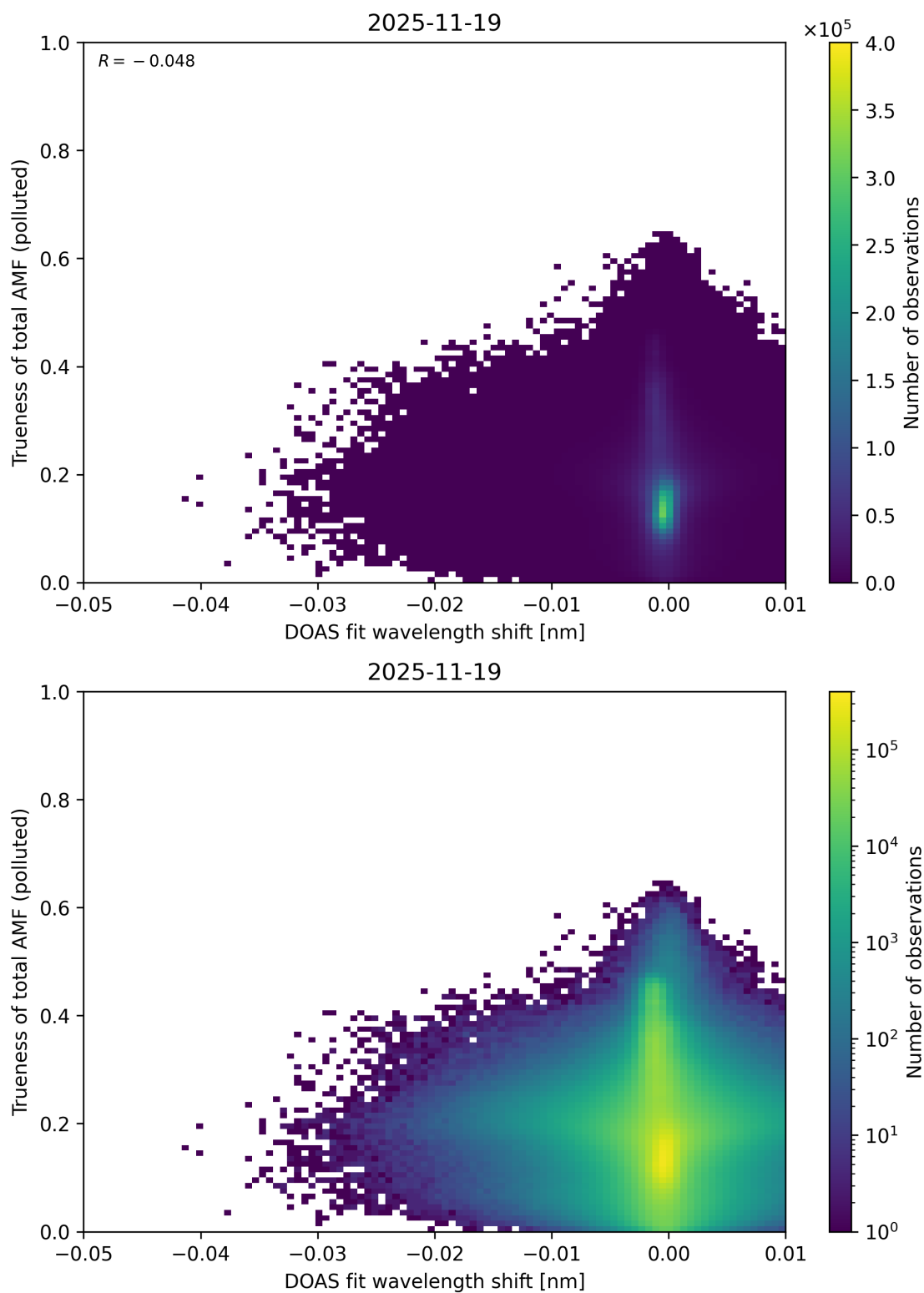
Figure 142: Scatter density plot of “DOAS fit wavelength shift” against “Trueness of total AMF (polluted)” for 2025-11-18 to 2025-11-20.
