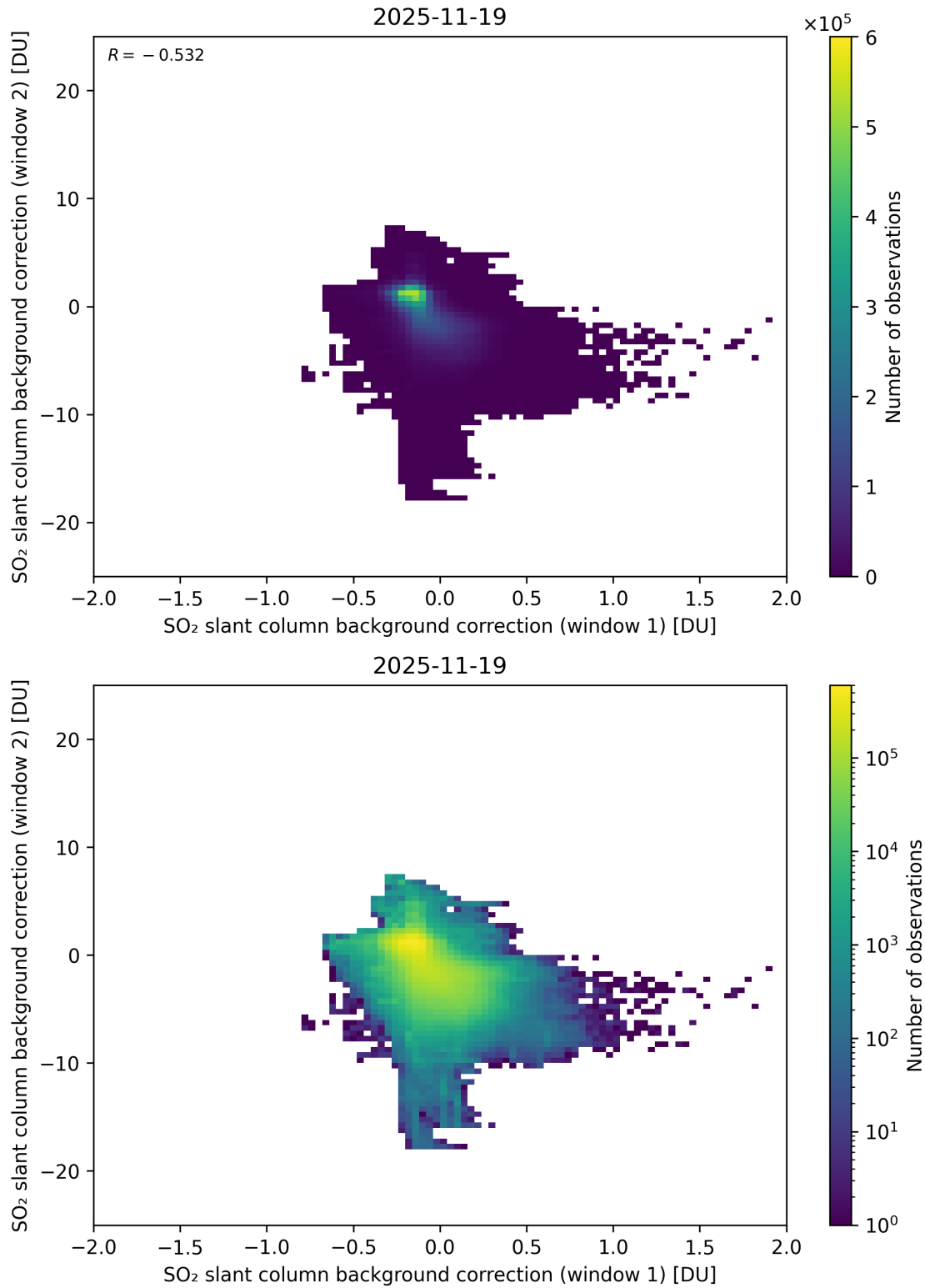
Figure 109: Scatter density plot of “SO 2 slant column background correction (window 1)” against “SO 2 slant column background correction (window 2)” for 2025-11-18 to 2025-11-20.
