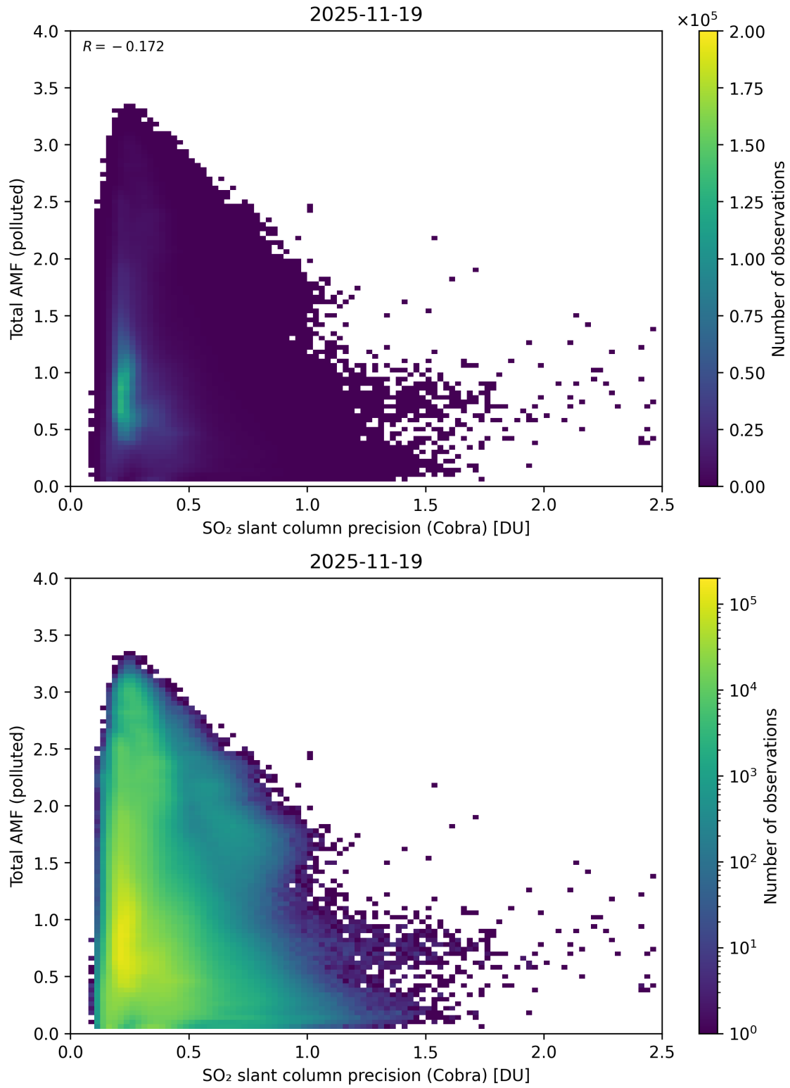
Figure 213: Scatter density plot of “SO 2 slant column precision (Cobra)” against “Total AMF (polluted)” for 2025-11-18 to 2025-11-20.
