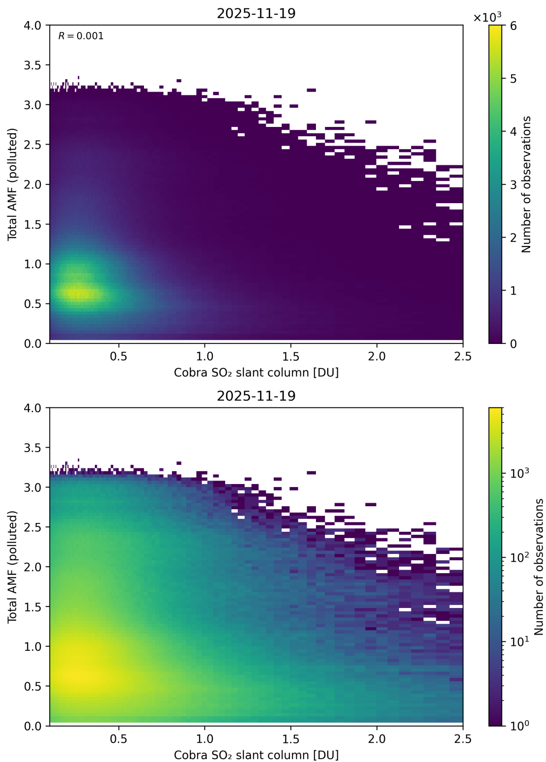
Figure 224: Scatter density plot of “Cobra SO 2 slant column” against “Total AMF (polluted)” for 2025-11-18 to 2025-11-20.
