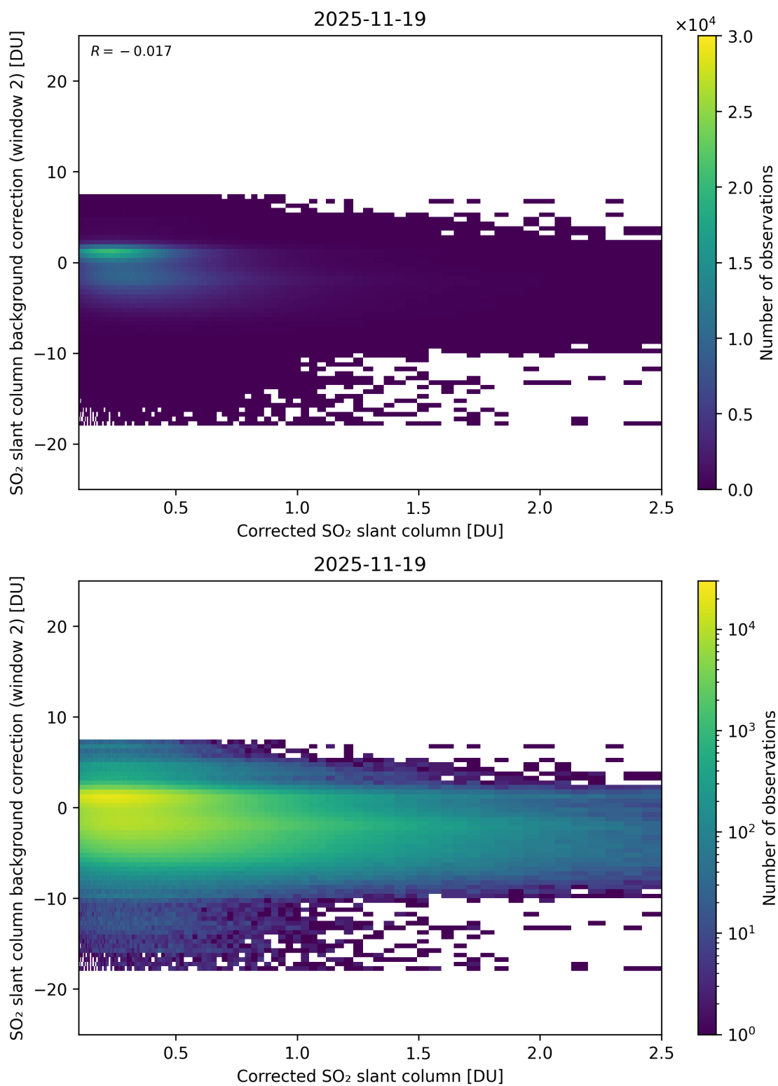
Figure 227: Scatter density plot of “Corrected SO 2 slant column” against “SO 2 slant column background correction (window 2)” for 2025-11-18 to 2025-11-20.
