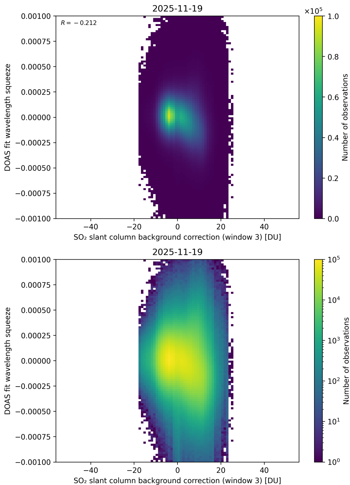
Figure 133: Scatter density plot of “SO 2 slant column background correction (window 3)” against “DOAS fit wavelength squeeze” for 2025-11-18 to 2025-11-20.
