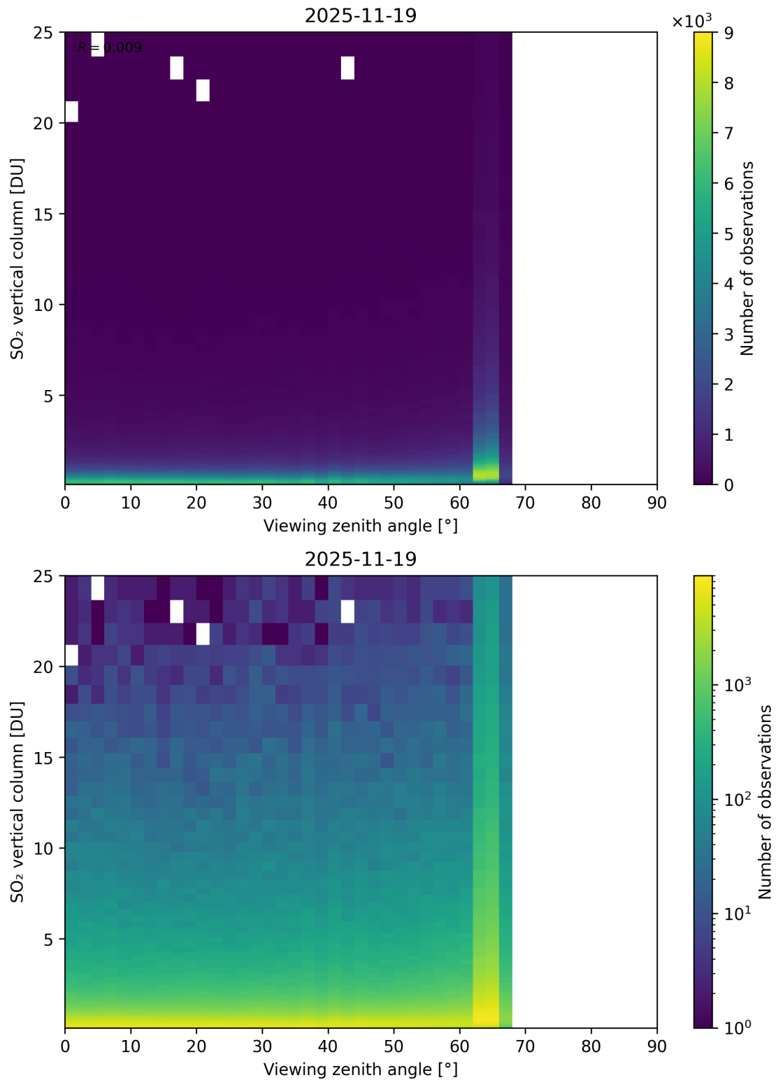
Figure 383: Scatter density plot of “Viewing zenith angle” against “SO 2 vertical column” for 2025-11-18 to 2025-11-20.
