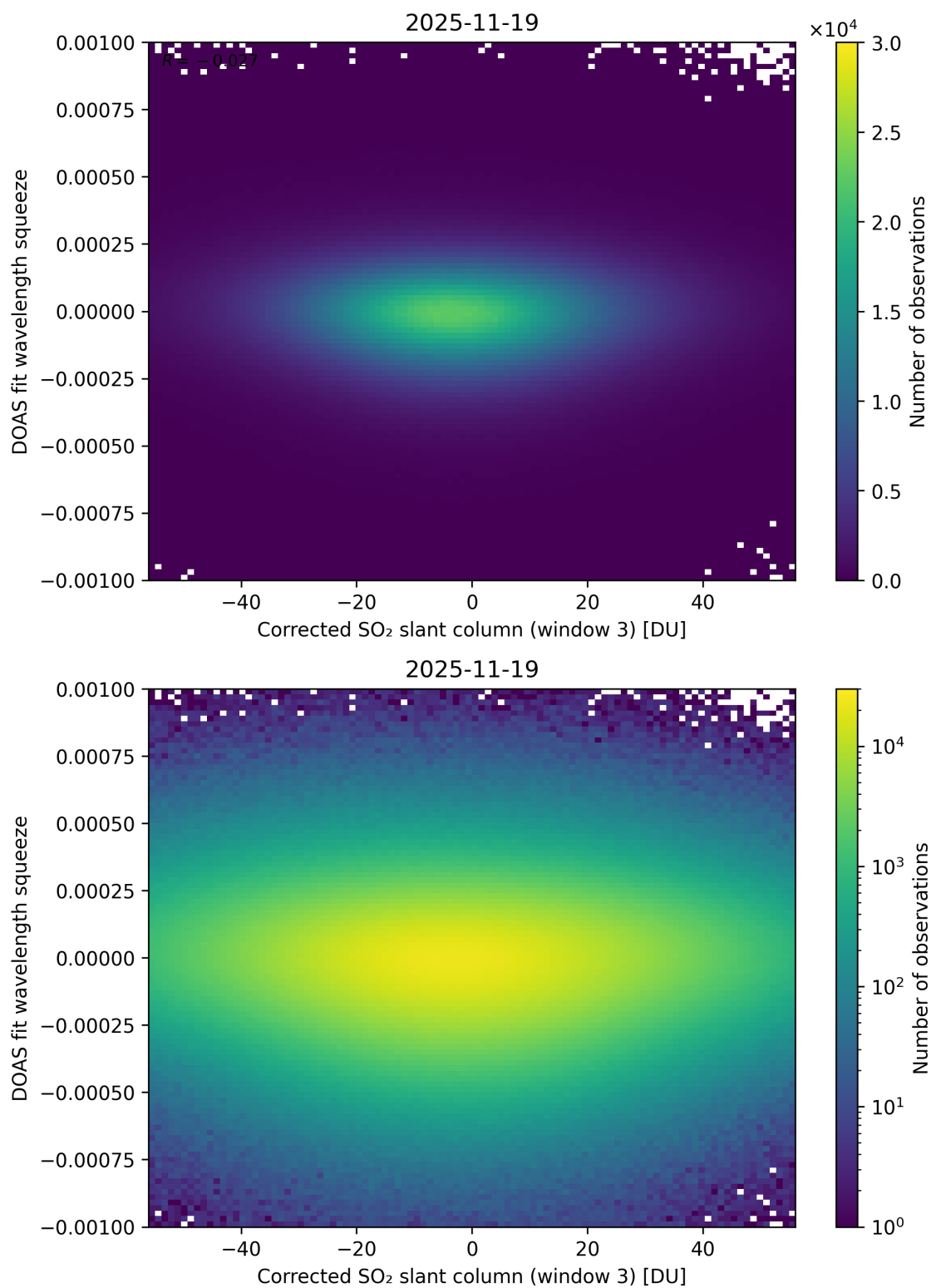
Figure 257: Scatter density plot of “Corrected SO 2 slant column (window 3)” against “DOAS fit wavelength squeeze” for 2025-11-18 to 2025-11-20.
