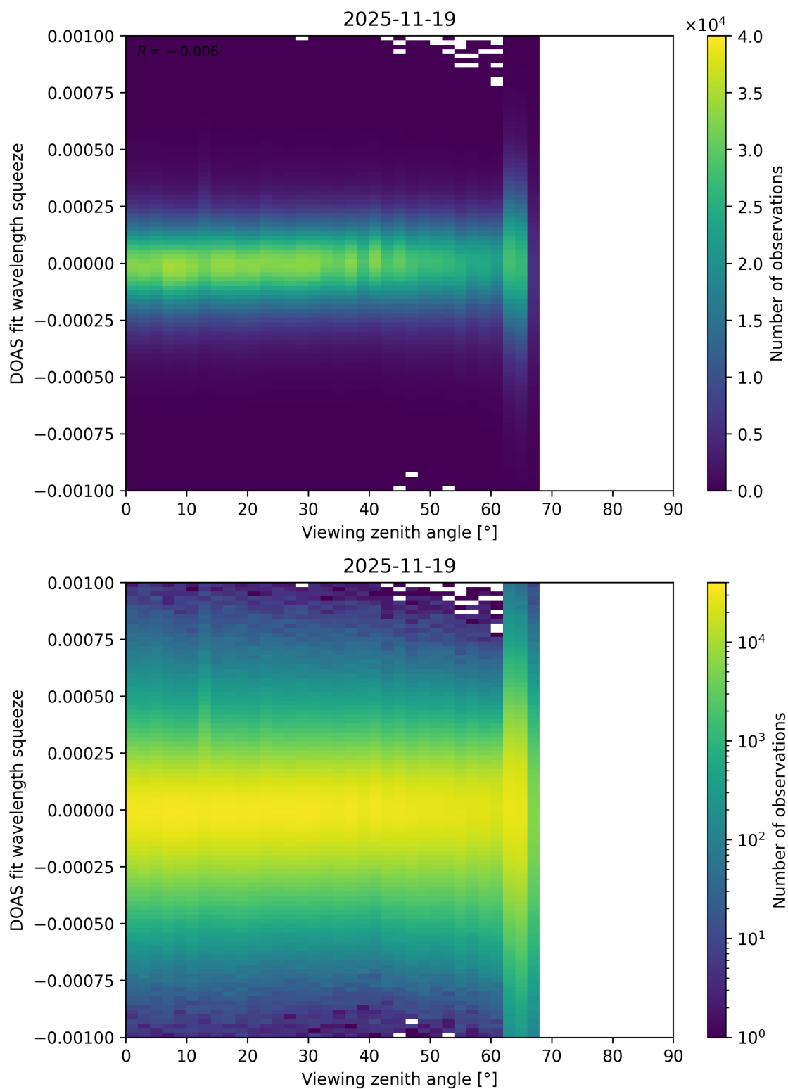
Figure 366: Scatter density plot of “Viewing zenith angle” against “DOAS fit wavelength squeeze” for 2025-11-18 to 2025-11-20.
