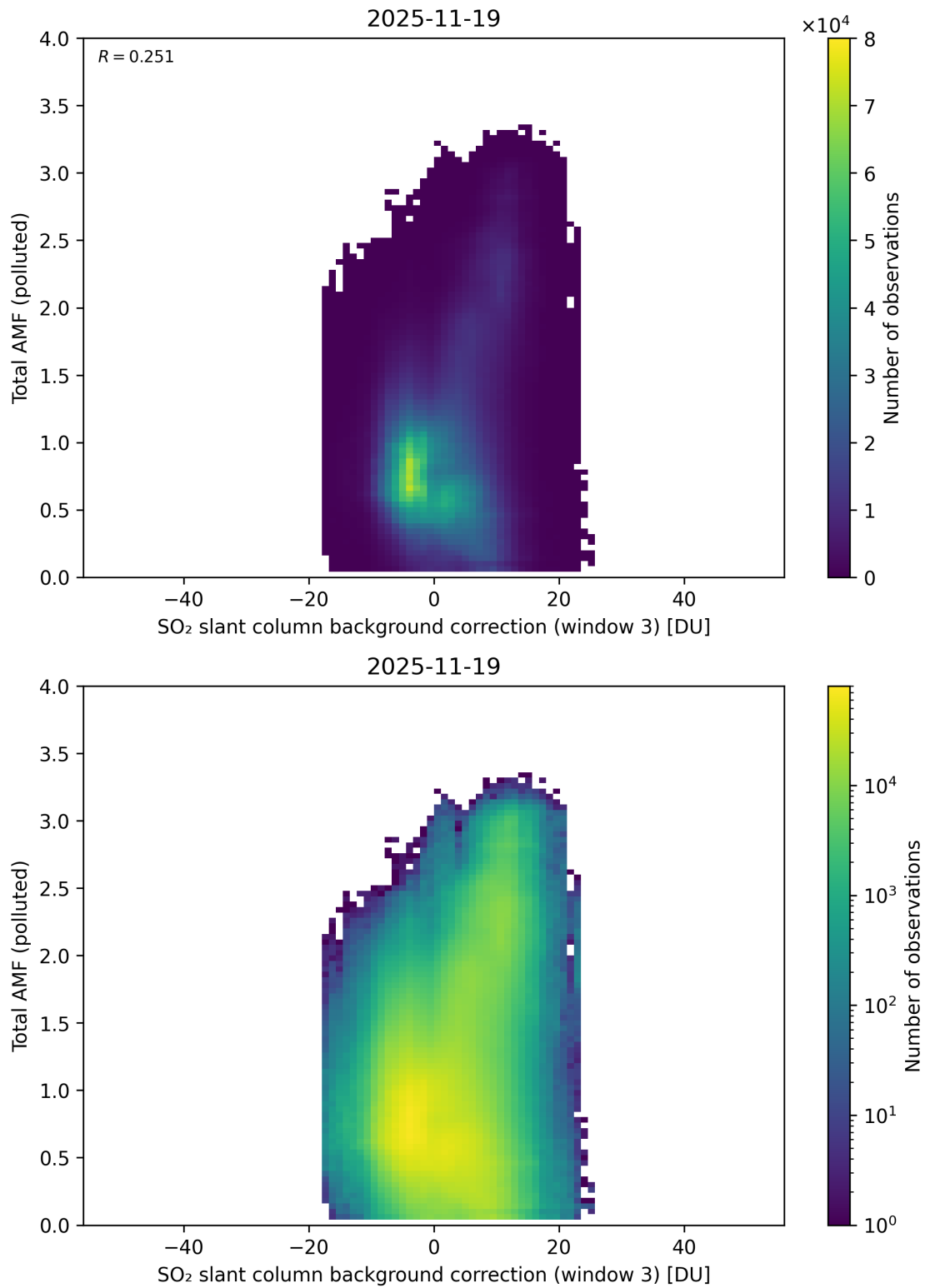
Figure 136: Scatter density plot of “SO 2 slant column background correction (window 3)” against “Total AMF (polluted)” for 2025-11-18 to 2025-11-20.
