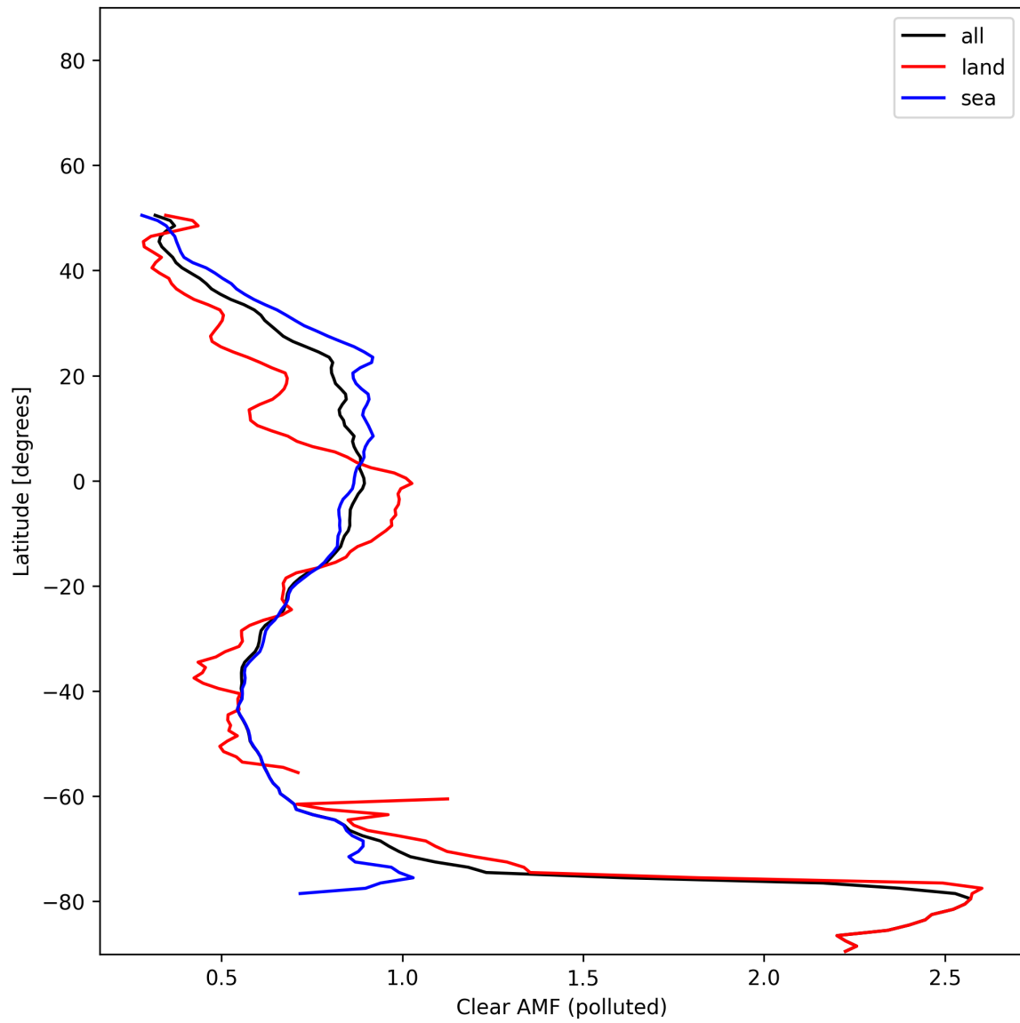
Figure 55: Zonal average of “Clear AMF (polluted)” for 2025-11-18 to 2025-11-20.
