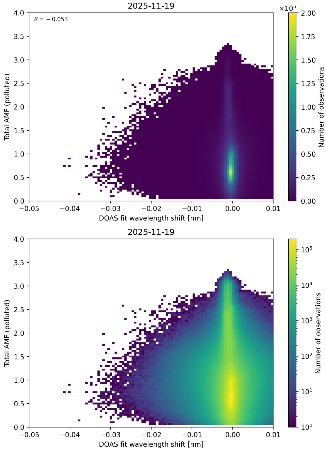
Figure 141: Scatter density plot of “DOAS fit wavelength shift” against “Total AMF (polluted)” for 2025-11-18 to 2025-11-20.
