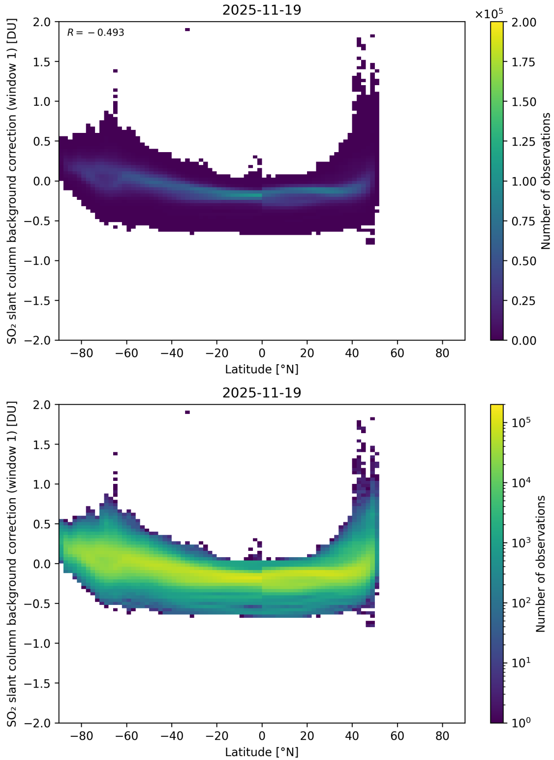
Figure 150: Scatter density plot of “Latitude” against “SO 2 slant column background correction (window 1)” for 2025-11-18 to 2025-11-20.
