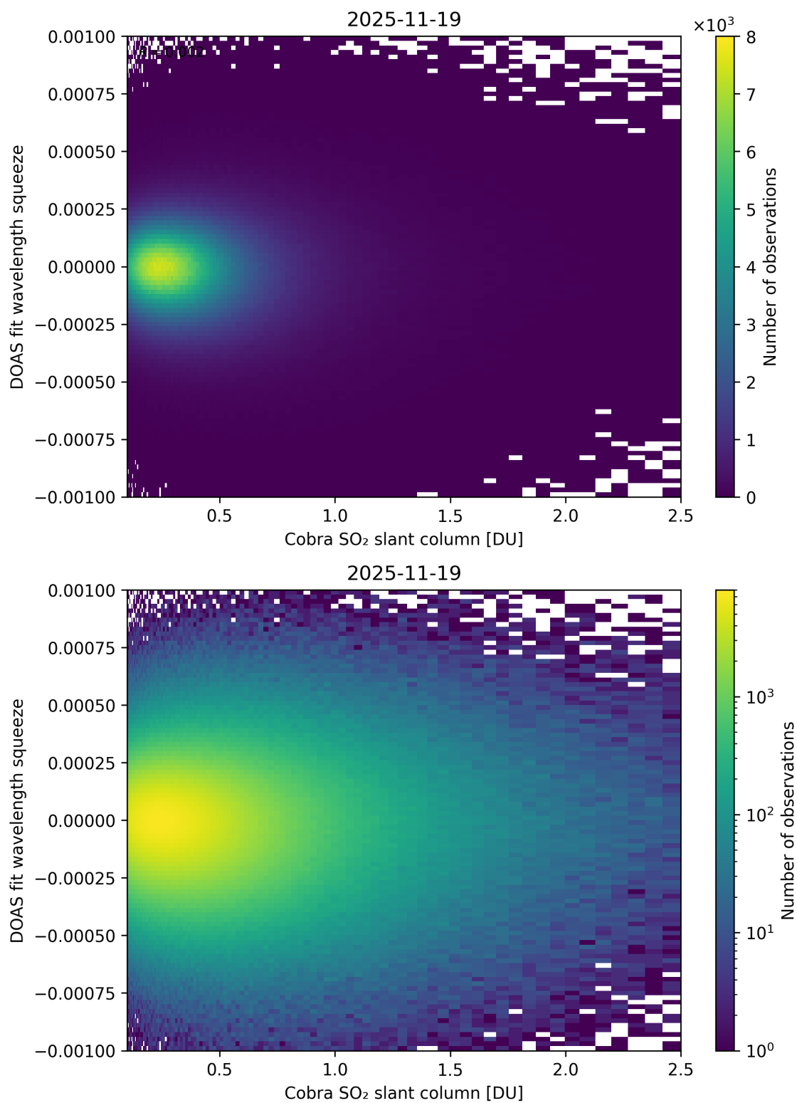
Figure 197: Scatter density plot of “Cobra SO 2 slant column” against “DOAS fit wavelength squeeze” for 2025-11-18 to 2025-11-20.
