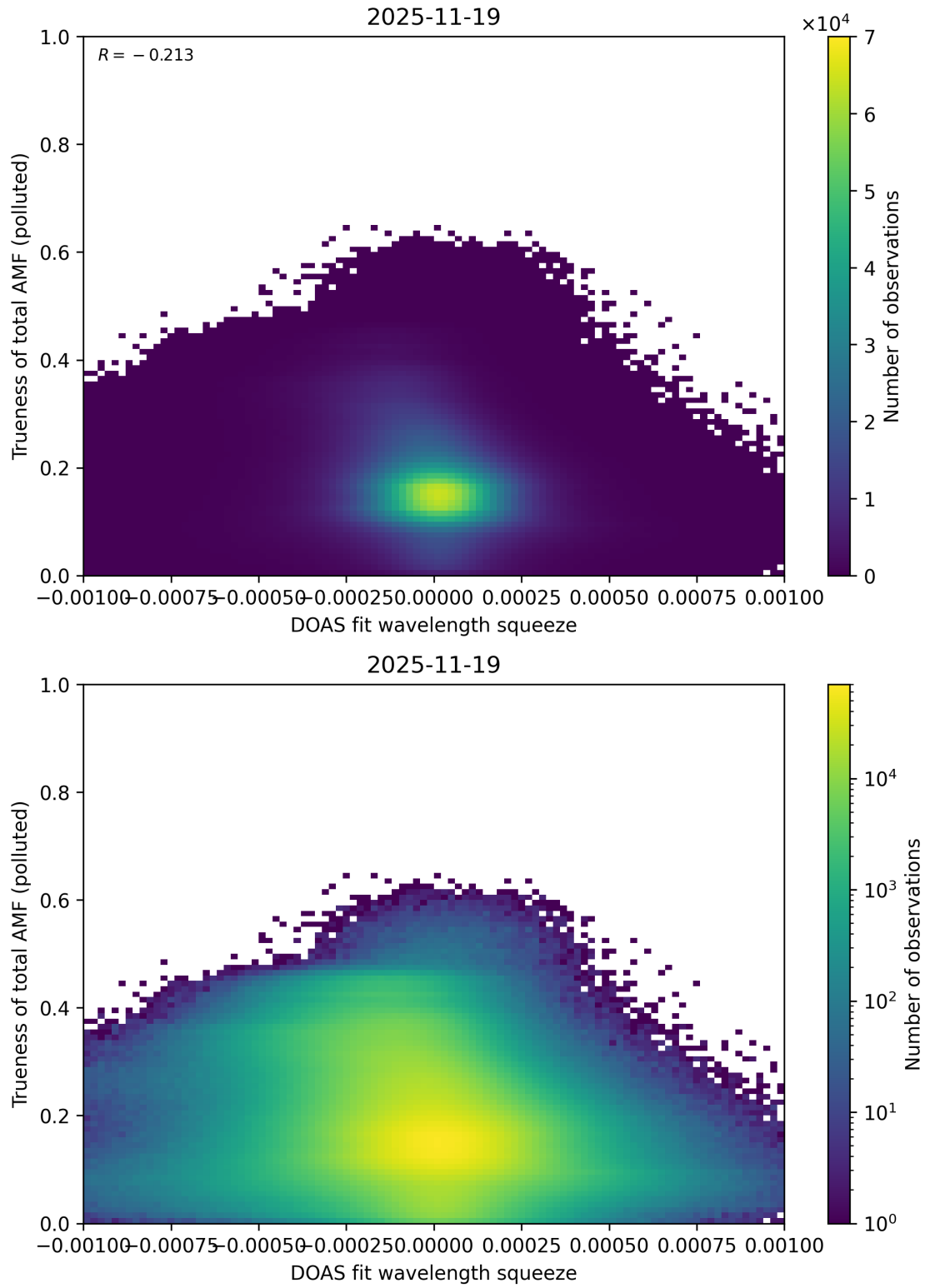
Figure 146: Scatter density plot of “DOAS fit wavelength squeeze” against “Trueness of total AMF (polluted)” for 2025-11-18 to 2025-11-20.
