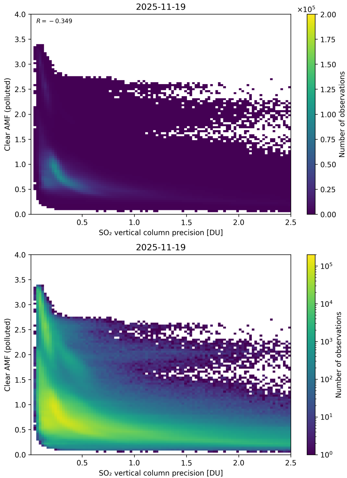
Figure 335: Scatter density plot of “SO 2 vertical column precision” against “Clear AMF (polluted)” for 2025-11-18 to 2025-11-20.
