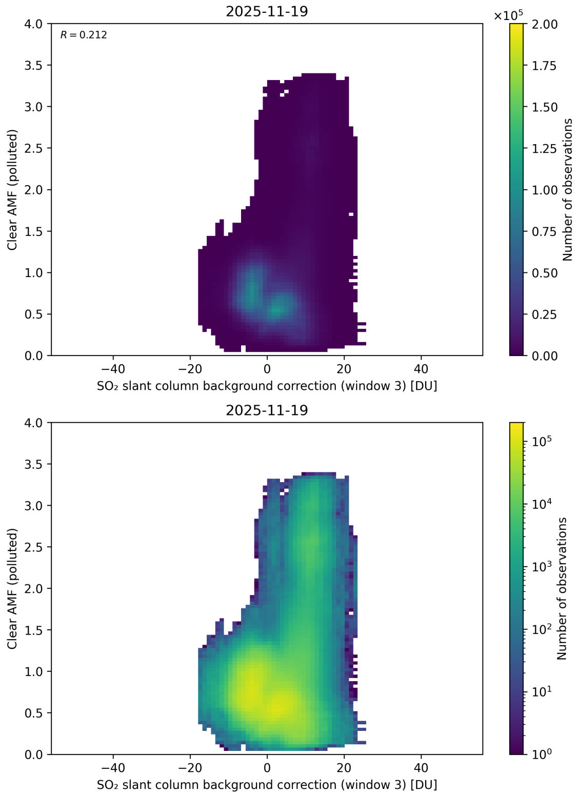
Figure 135: Scatter density plot of “SO 2 slant column background correction (window 3)” against “Clear AMF (polluted)” for 2025-11-18 to 2025-11-20.
