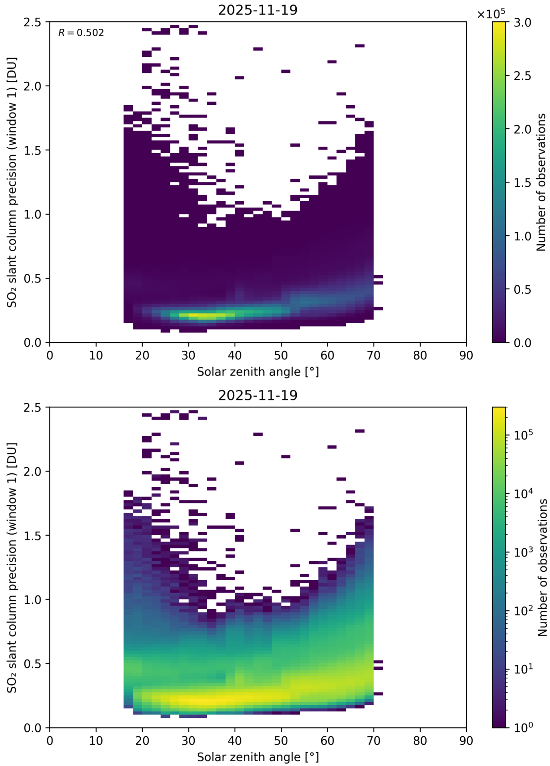
Figure 185: Scatter density plot of “Solar zenith angle” against “SO 2 slant column precision (window 1)” for 2025-11-18 to 2025-11-20.
