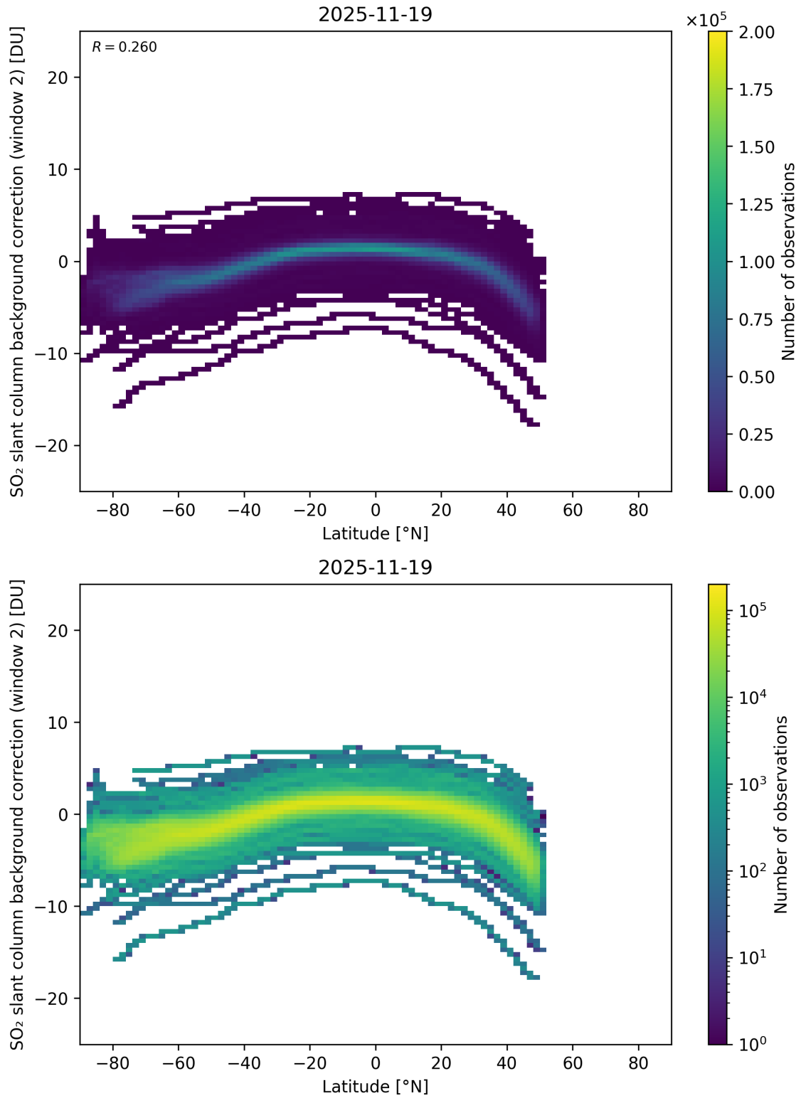
Figure 151: Scatter density plot of “Latitude” against “SO 2 slant column background correction (window 2)” for 2025-11-18 to 2025-11-20.
