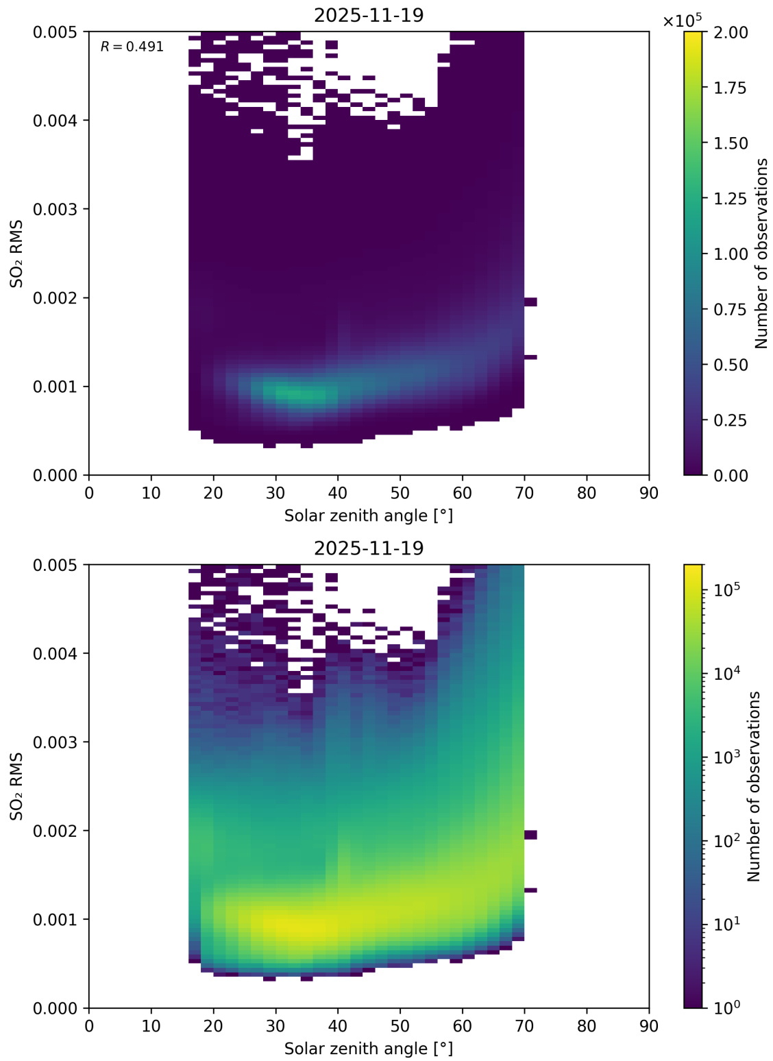
Figure 176: Scatter density plot of “Solar zenith angle” against “SO 2 RMS” for 2025-11-18 to 2025-11-20.
