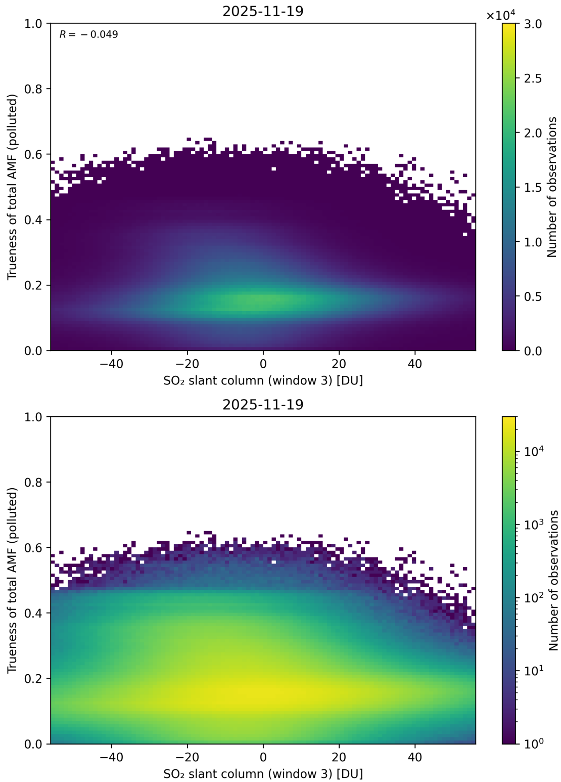
Figure 319: Scatter density plot of “SO 2 slant column (window 3)” against “Trueness of total AMF (polluted)” for 2025-11-18 to 2025-11-20.
