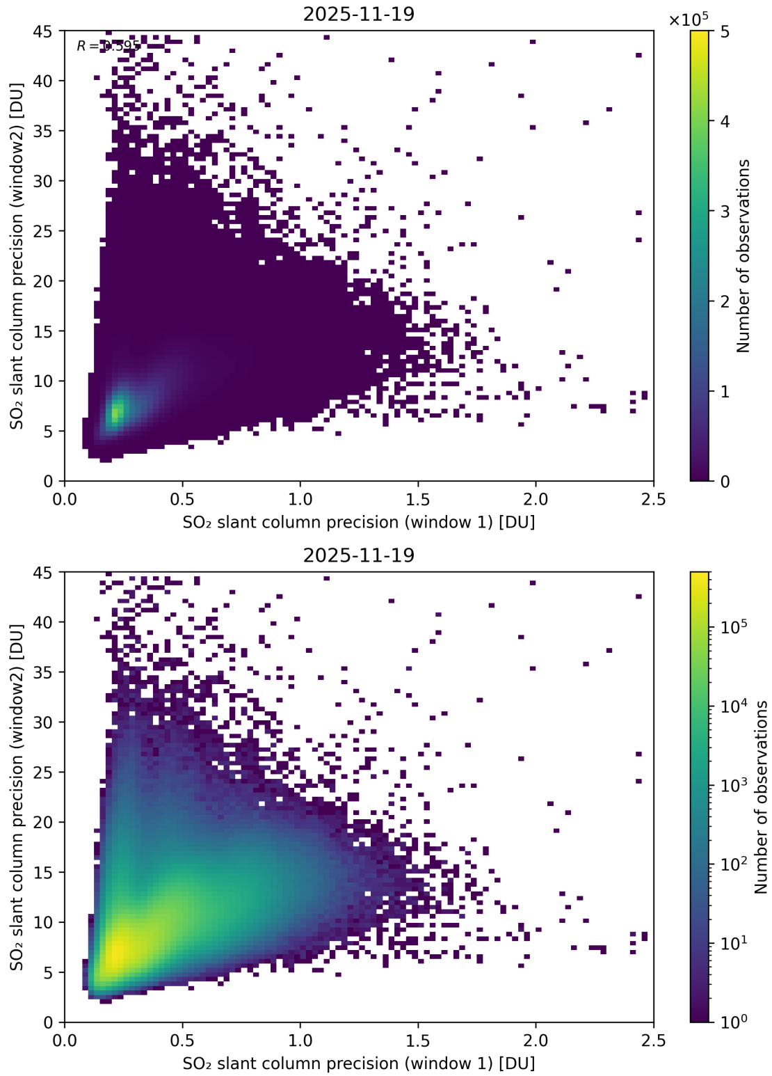
Figure 277: Scatter density plot of “SO 2 slant column precision (window 1)” against “SO 2 slant column precision (window2)” for 2025-11-18 to 2025-11-20.
