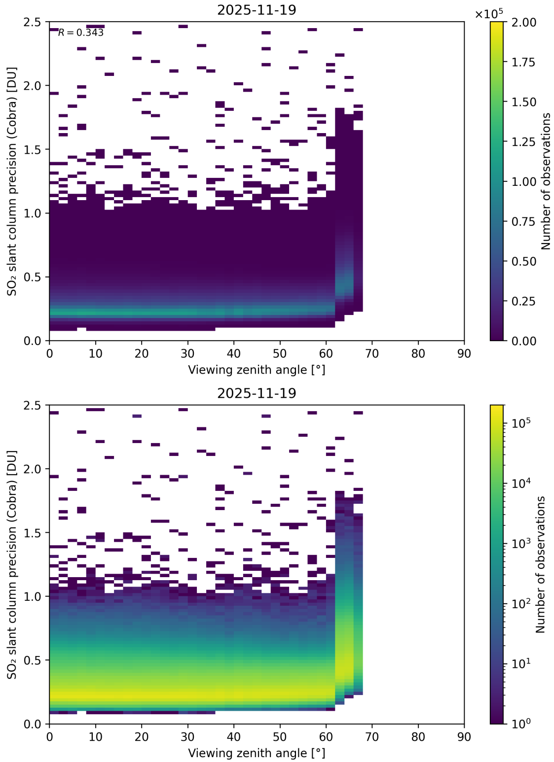
Figure 372: Scatter density plot of “Viewing zenith angle” against “SO 2 slant column precision (Cobra)” for 2025-11-18 to 2025-11-20.
