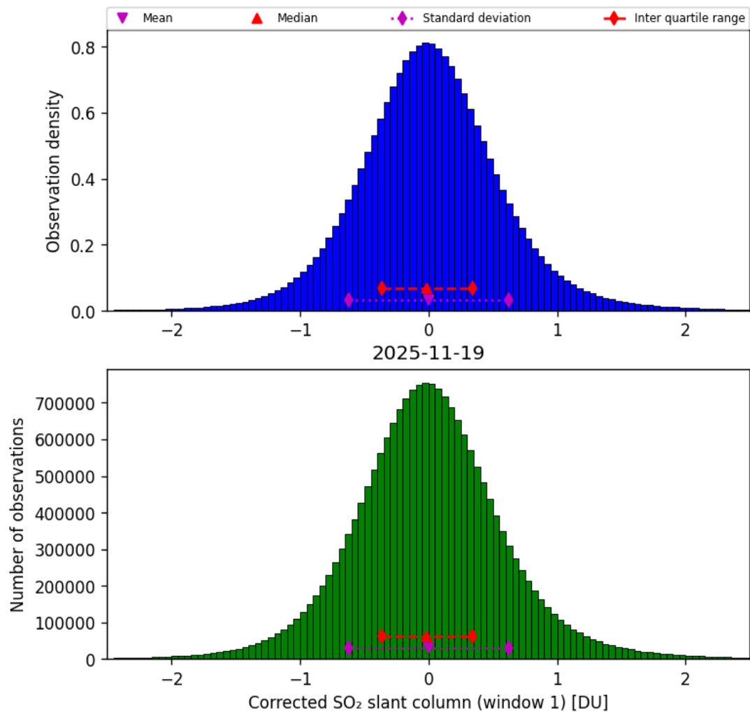
Figure 65: Histogram of “Corrected SO 2 slant column (window 1)” for 2025-11-18 to 2025-11-20
