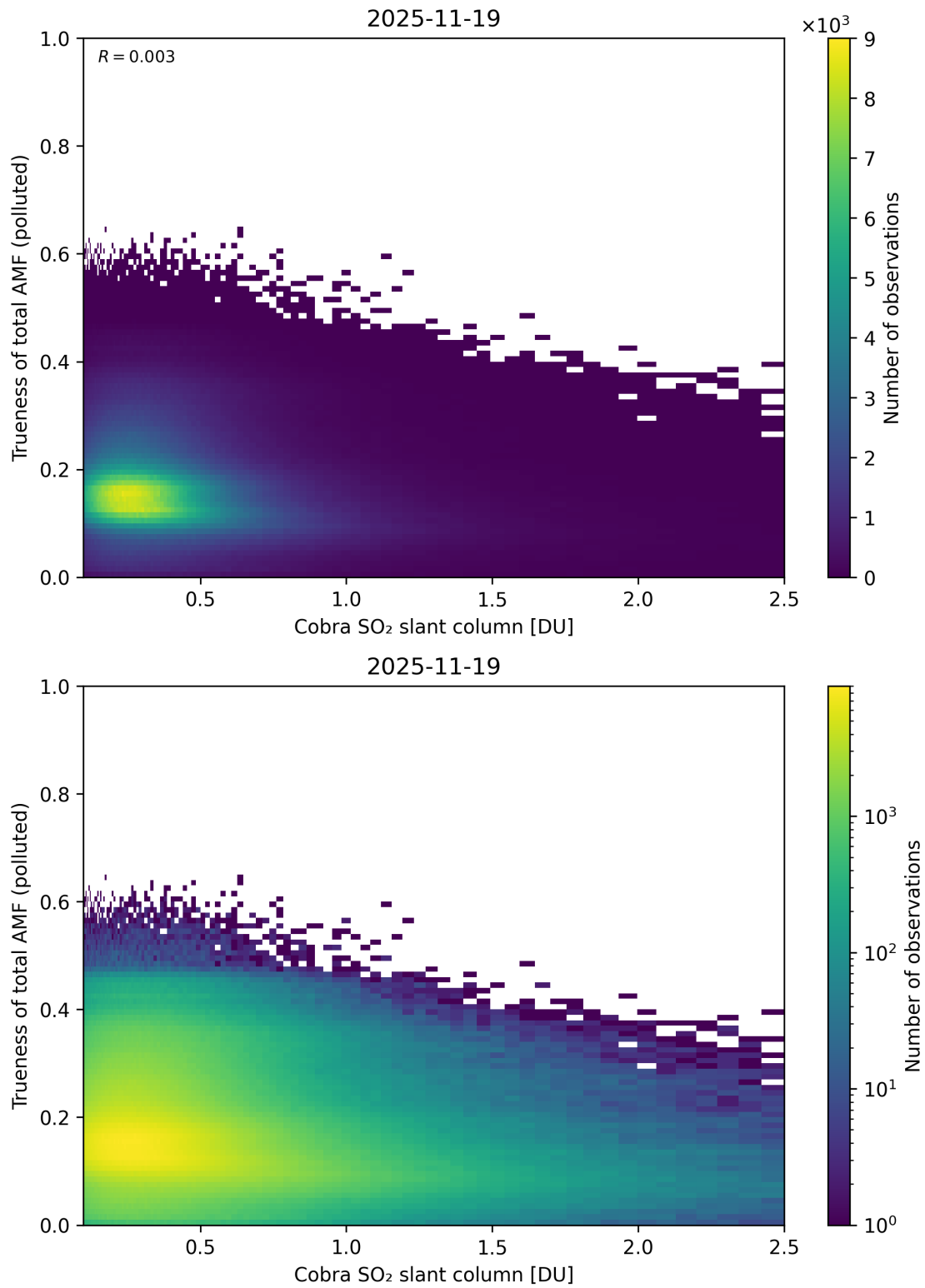
Figure 225: Scatter density plot of “Cobra SO 2 slant column” against “Trueness of total AMF (polluted)” for 2025-11-18 to 2025-11-20.
