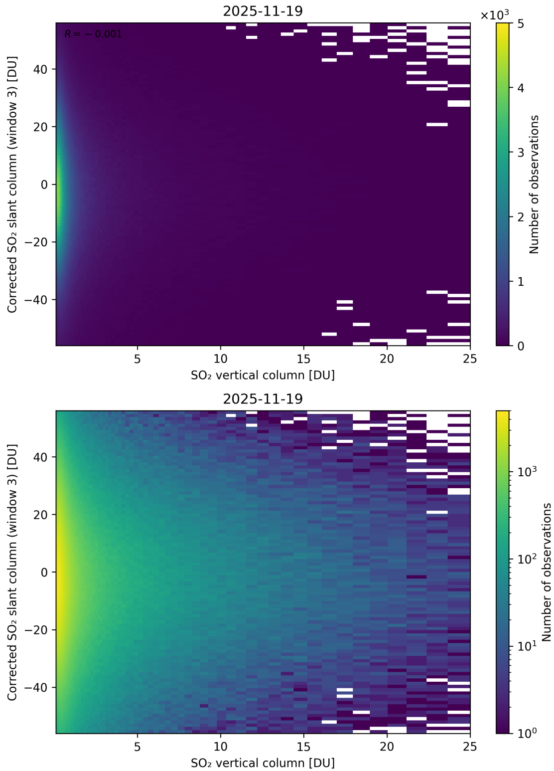
Figure 353: Scatter density plot of “SO 2 vertical column” against “Corrected SO 2 slant column (window 3)” for 2025-11-18 to 2025-11-20.
