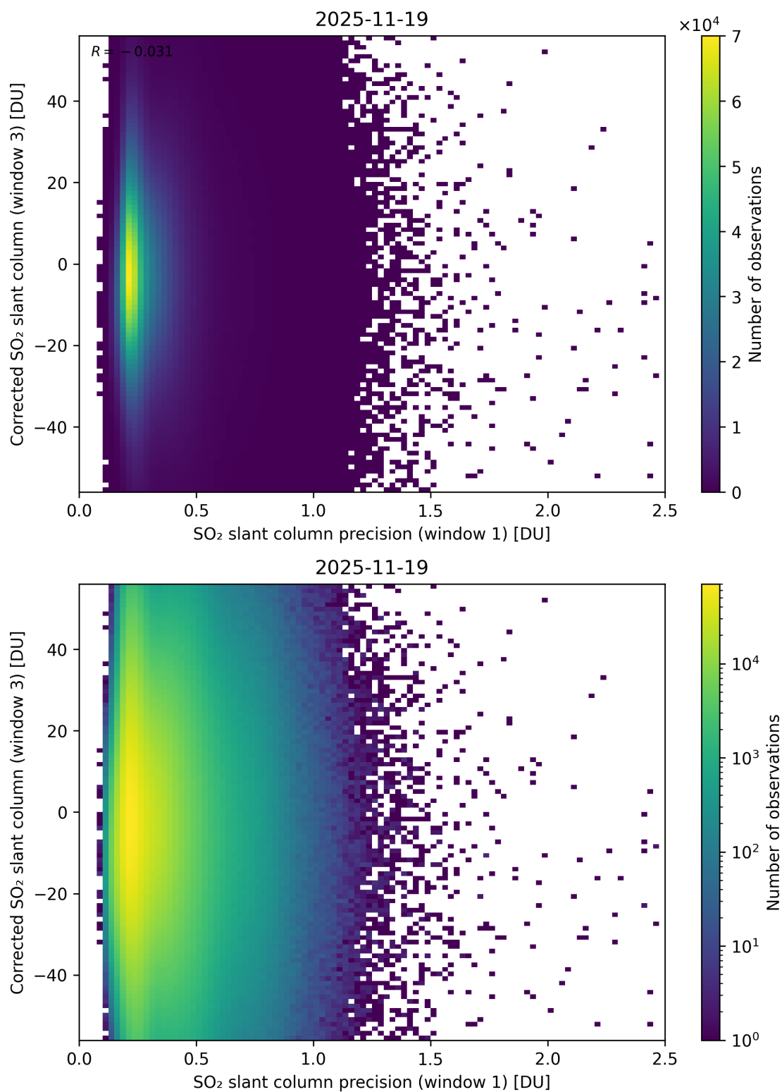
Figure 276: Scatter density plot of “SO 2 slant column precision (window 1)” against “Corrected SO 2 slant column (window 3)” for 2025-11-18 to 2025-11-20.
