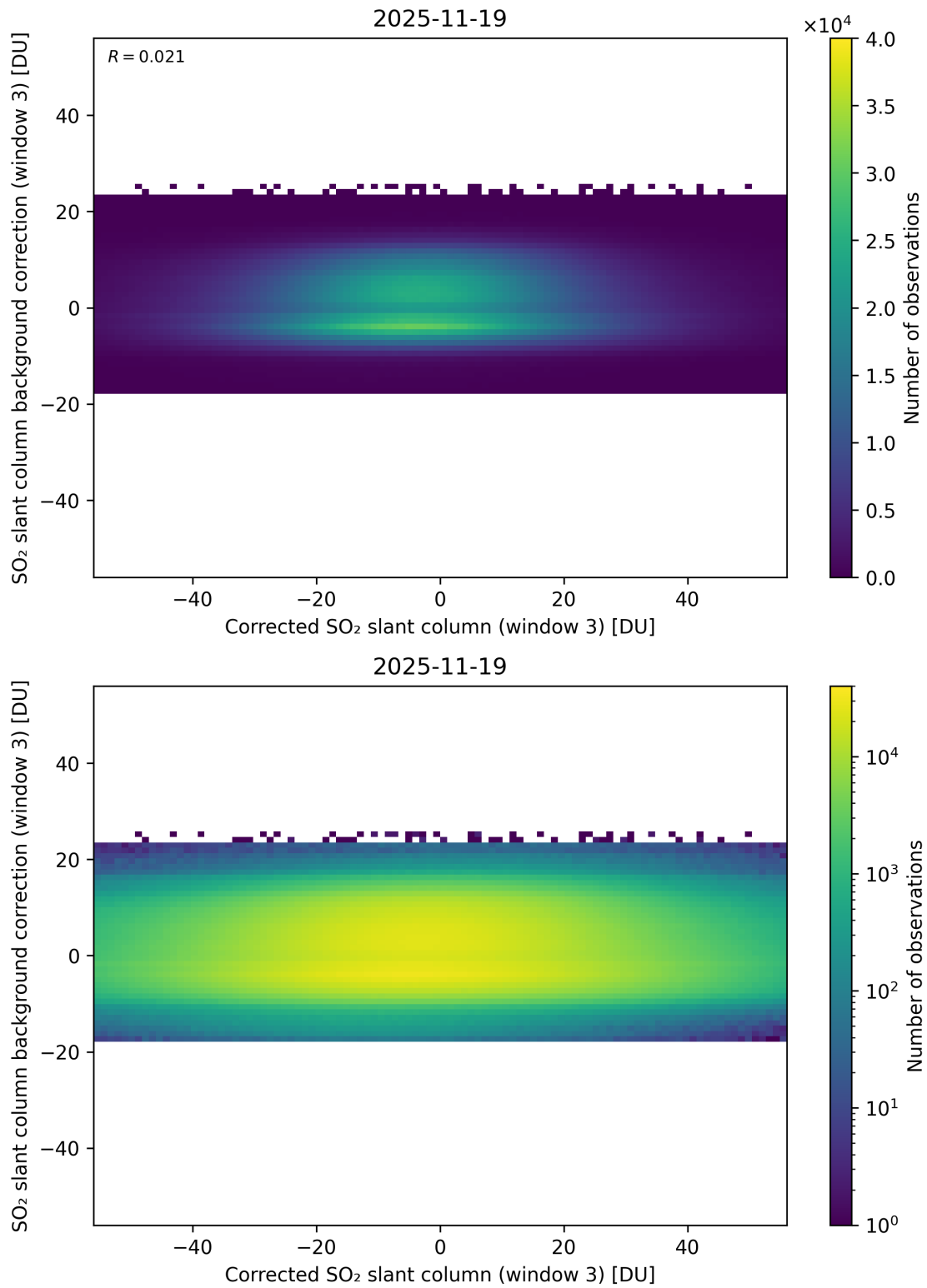
Figure 255: Scatter density plot of “Corrected SO 2 slant column (window 3)” against “SO 2 slant column background correction (window 3)” for 2025-11-18 to 2025-11-20.
