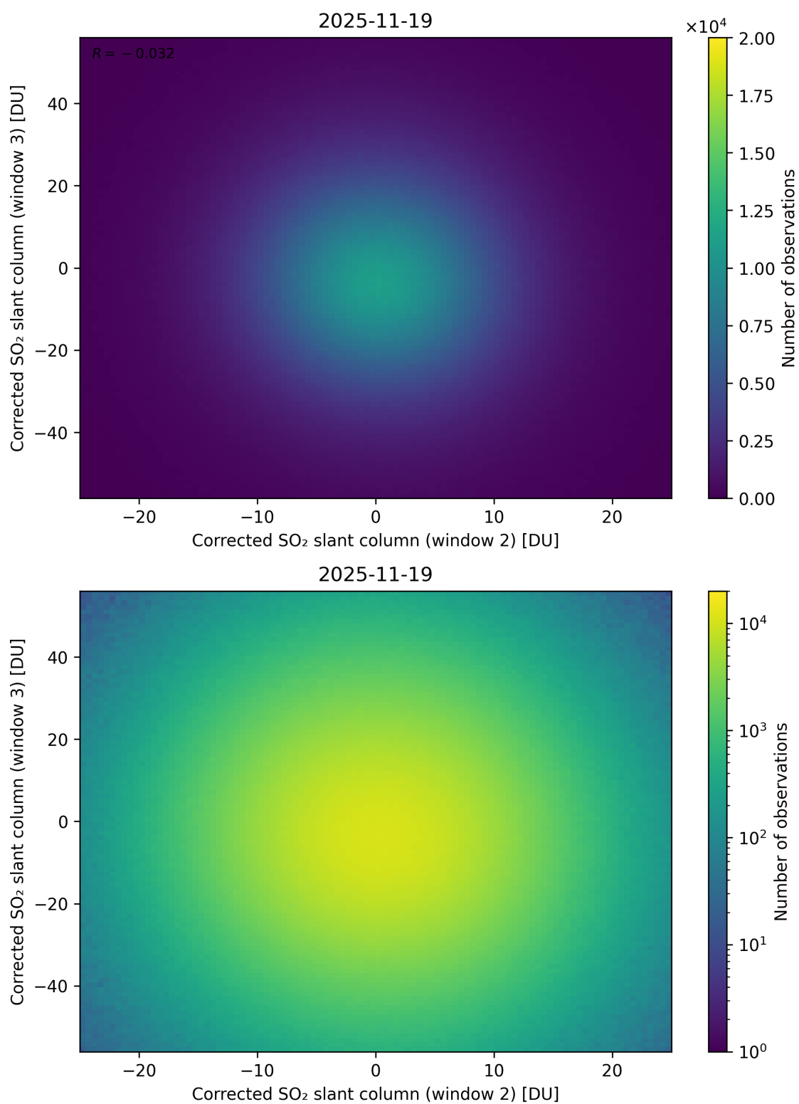
Figure 250: Scatter density plot of “Corrected SO 2 slant column (window 2)” against “Corrected SO 2 slant column (window 3)” for 2025-11-18 to 2025-11-20.
