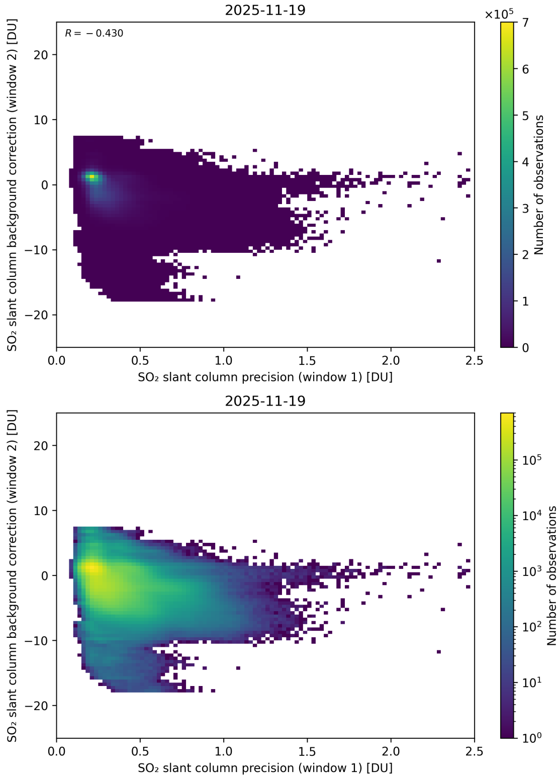
Figure 269: Scatter density plot of “SO 2 slant column precision (window 1)” against “SO 2 slant column background correction (window 2)” for 2025-11-18 to 2025-11-20.
