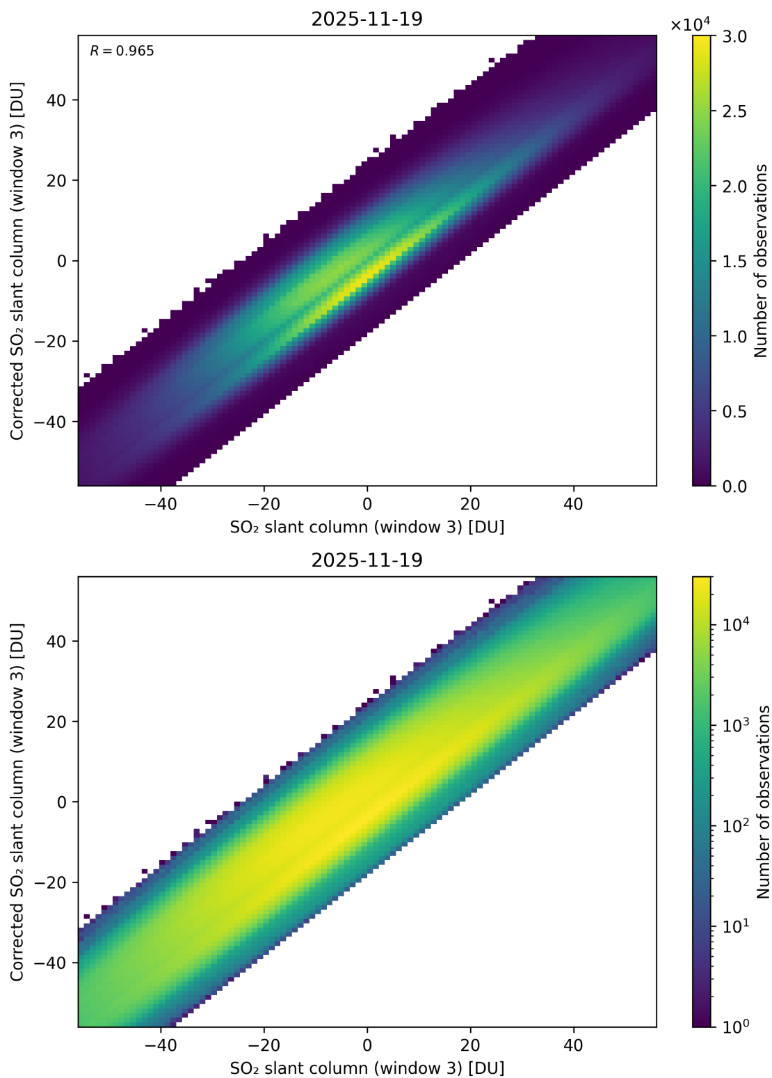
Figure 316: Scatter density plot of “SO 2 slant column (window 3)” against “Corrected SO 2 slant column (window 3)” for 2025-11-18 to 2025-11-20.
