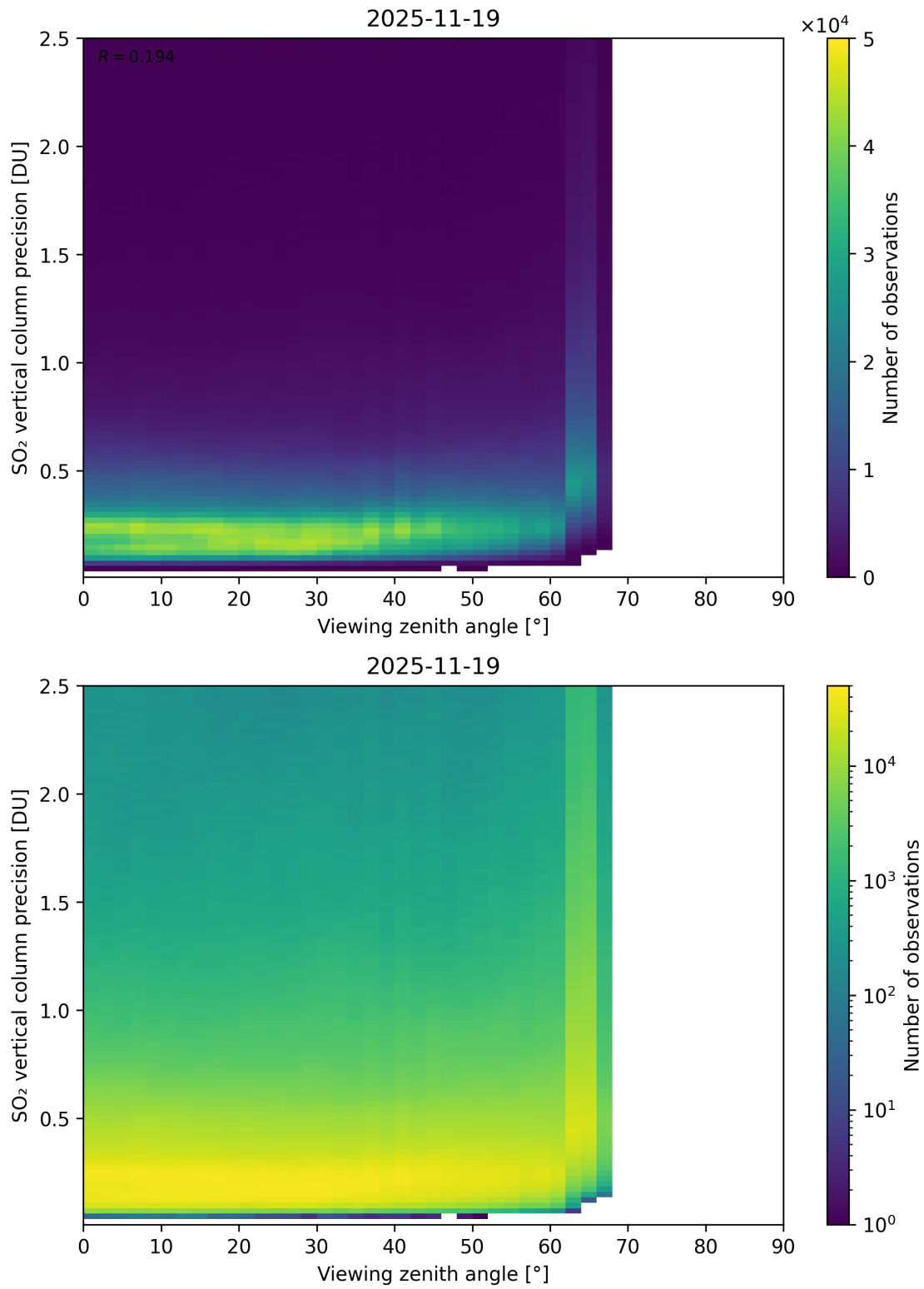
Figure 384: Scatter density plot of “Viewing zenith angle” against “SO 2 vertical column precision” for 2025-11-18 to 2025-11-20.
