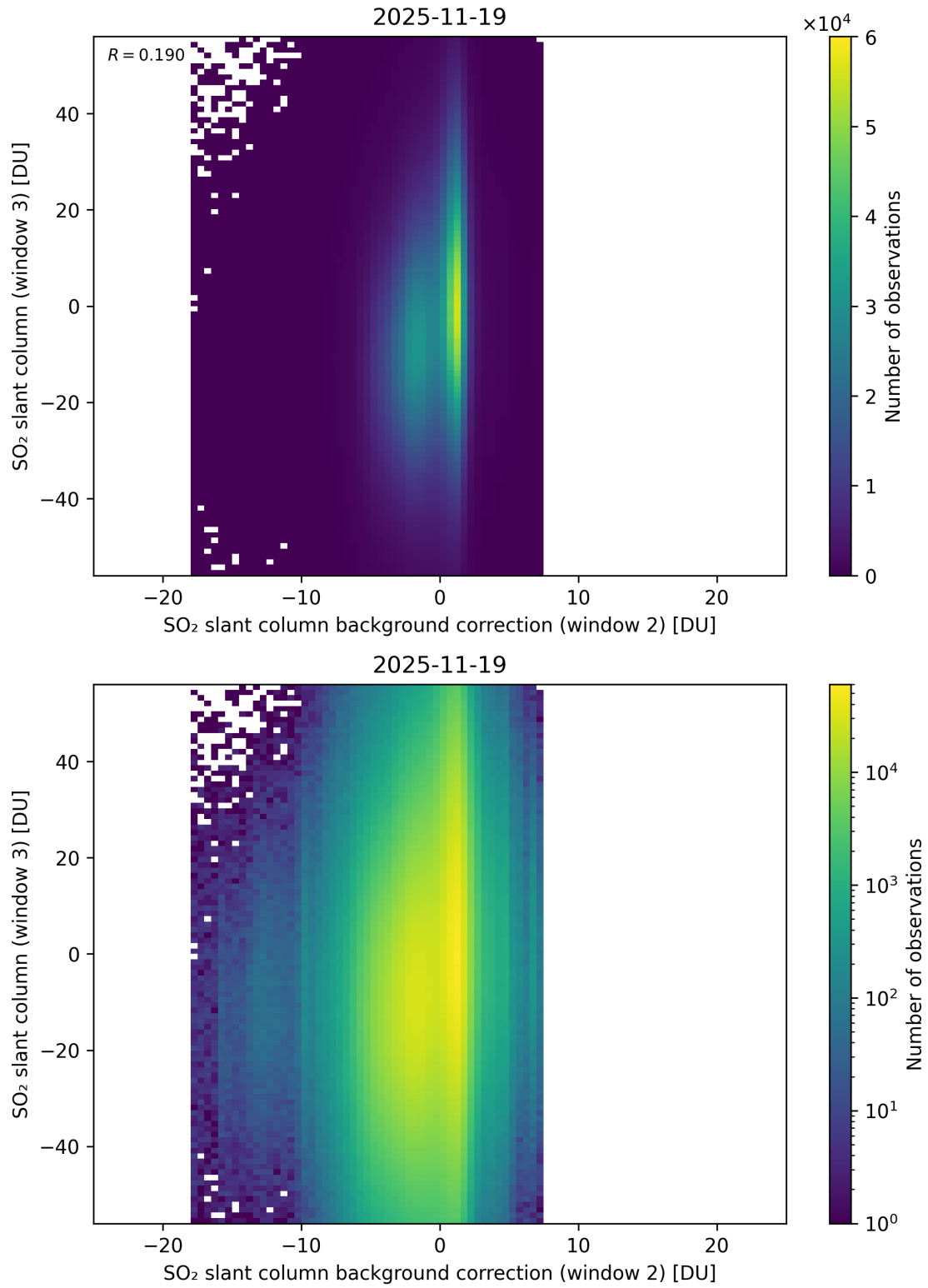
Figure 128: Scatter density plot of “SO 2 slant column background correction (window 2)” against “SO 2 slant column (window 3)” for 2025-11-18 to 2025-11-20.
