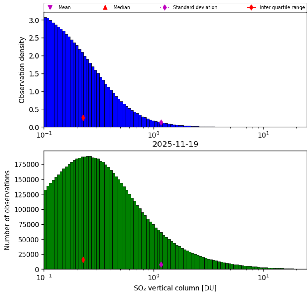
Figure 58: Histogram of “SO 2 vertical column” for 2025-11-18 to 2025-11-20
