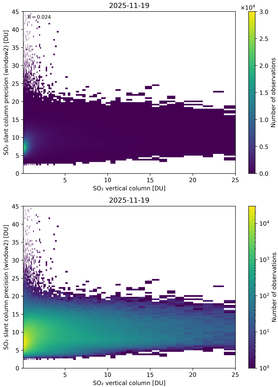
Figure 356: Scatter density plot of “SO 2 vertical column” against “SO 2 slant column precision (window2)” for 2025-11-18 to 2025-11-20.
