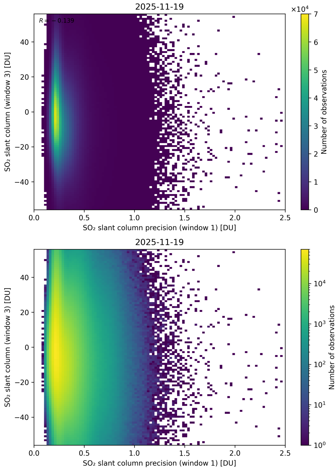
Figure 278: Scatter density plot of “SO 2 slant column precision (window 1)” against “SO 2 slant column (window 3)” for 2025-11-18 to 2025-11-20.
