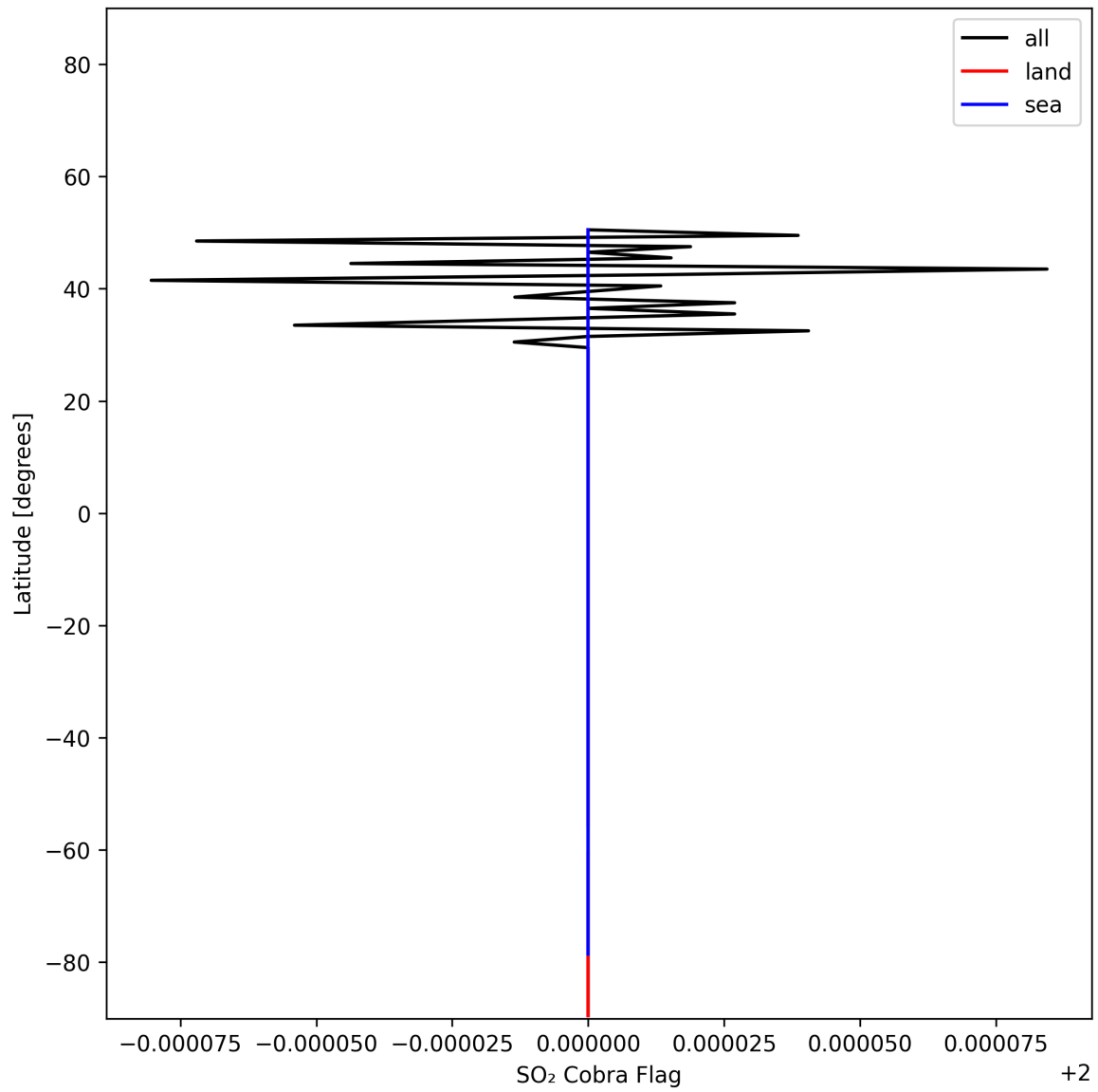
Figure 49: Zonal average of "SO 2 Cobra Flag" for 2025-11-18 to 2025-11-20.
