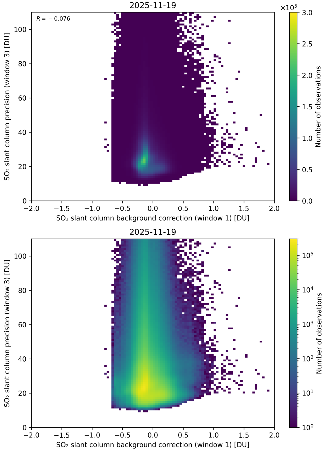
Figure 119: Scatter density plot of “SO 2 slant column background correction (window 1)” against “SO 2 slant column precision (window 3)” for 2025-11-18 to 2025-11-20.
