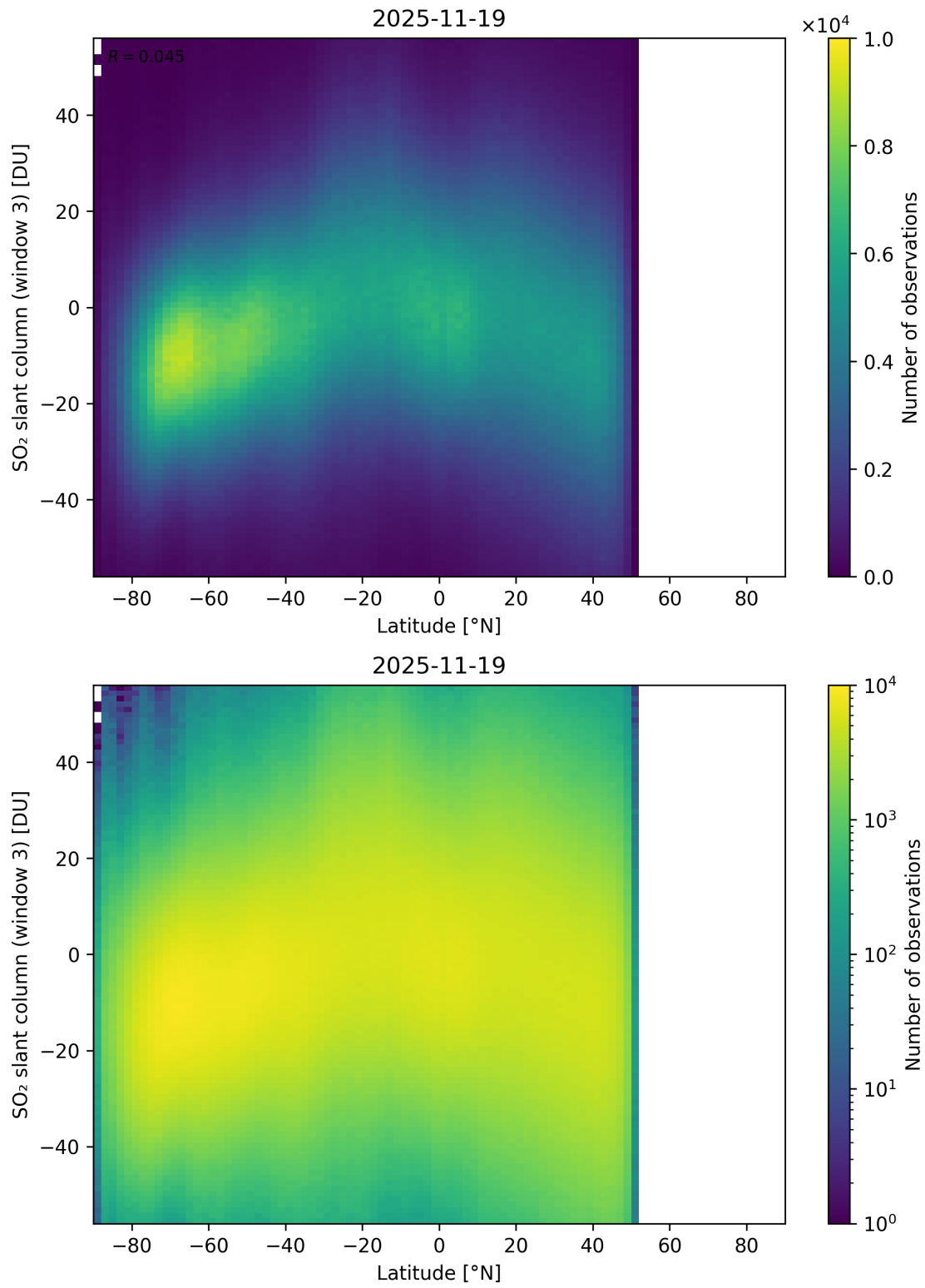
Figure 165: Scatter density plot of “Latitude” against “SO 2 slant column (window 3)” for 2025-11-18 to 2025-11-20.
