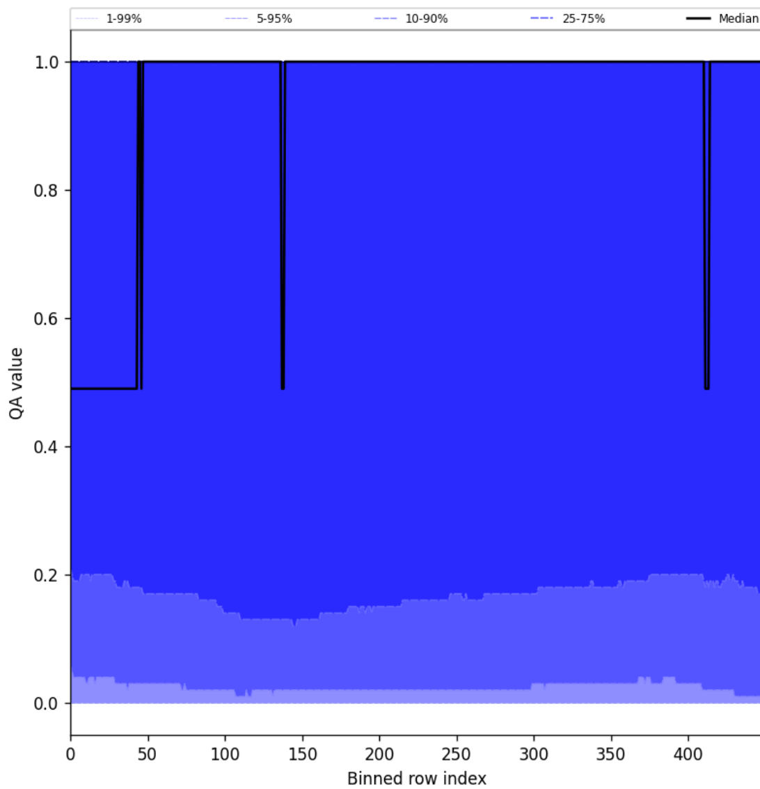
Figure 83: Along track statistics of “QA value” for 2025-11-18 to 2025-11-20
