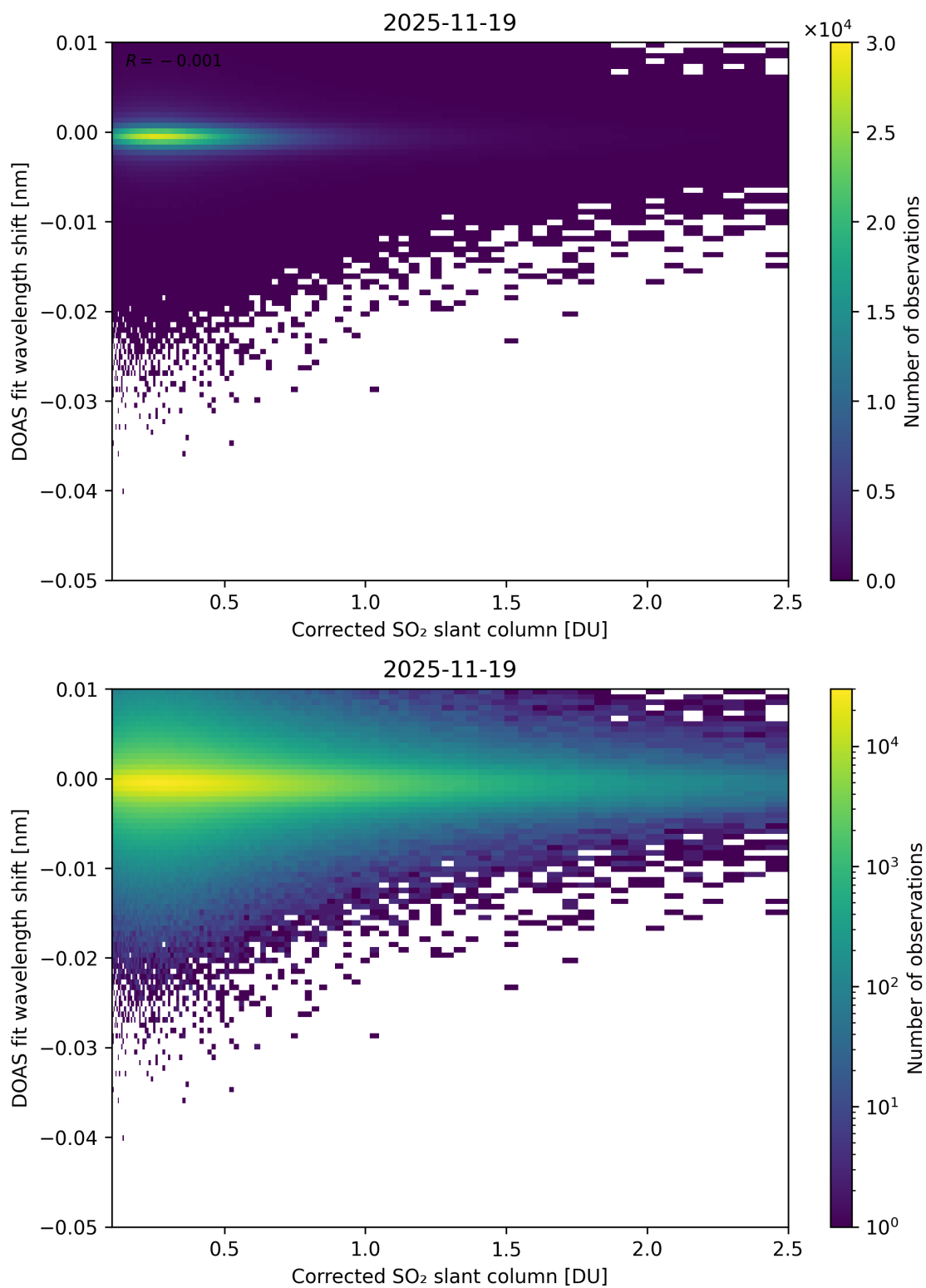
Figure 229: Scatter density plot of “Corrected SO 2 slant column” against “DOAS fit wavelength shift” for 2025-11-18 to 2025-11-20.
