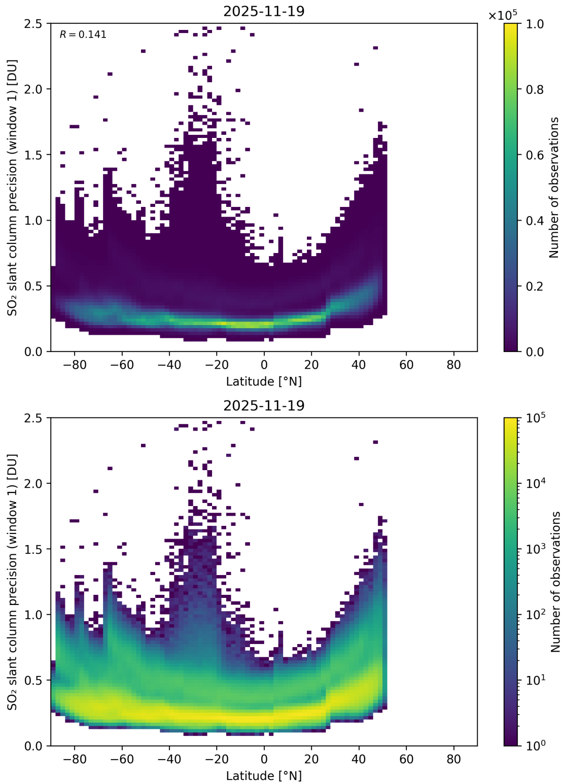
Figure 163: Scatter density plot of “Latitude” against “SO 2 slant column precision (window 1)” for 2025-11-18 to 2025-11-20.
