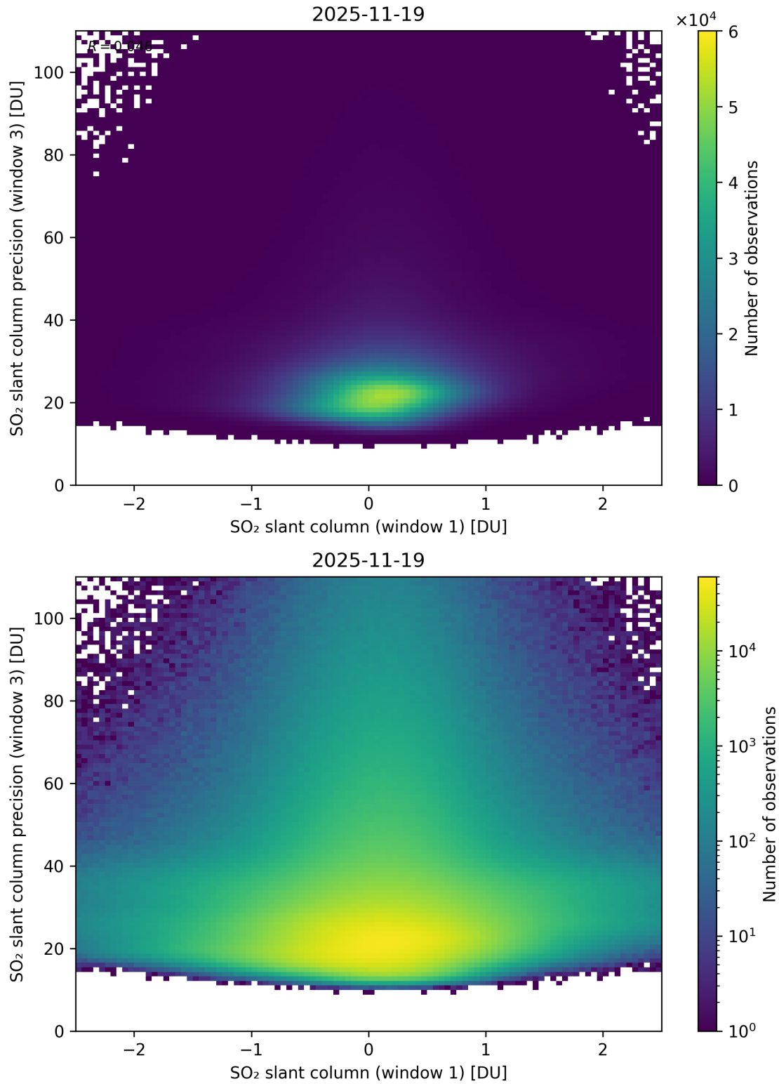
Figure 288: Scatter density plot of “SO 2 slant column (window 1)” against “SO 2 slant column precision (window 3)” for 2025-11-18 to 2025-11-20.
