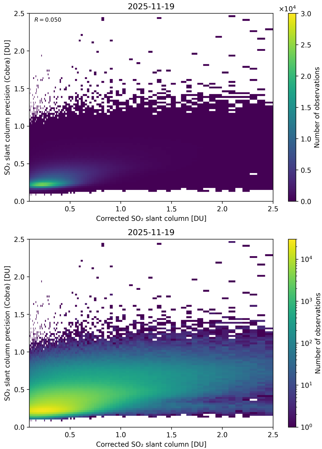
Figure 234: Scatter density plot of “Corrected SO 2 slant column” against “SO 2 slant column precision (Cobra)” for 2025-11-18 to 2025-11-20.
