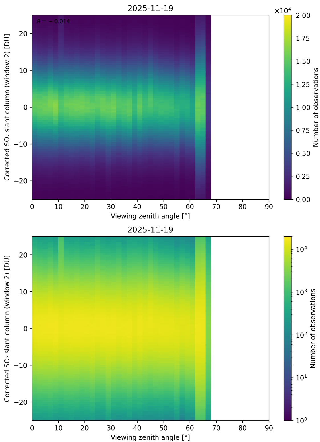
Figure 374: Scatter density plot of “Viewing zenith angle” against “Corrected SO 2 slant column (window 2)” for 2025-11-18 to 2025-11-20.
