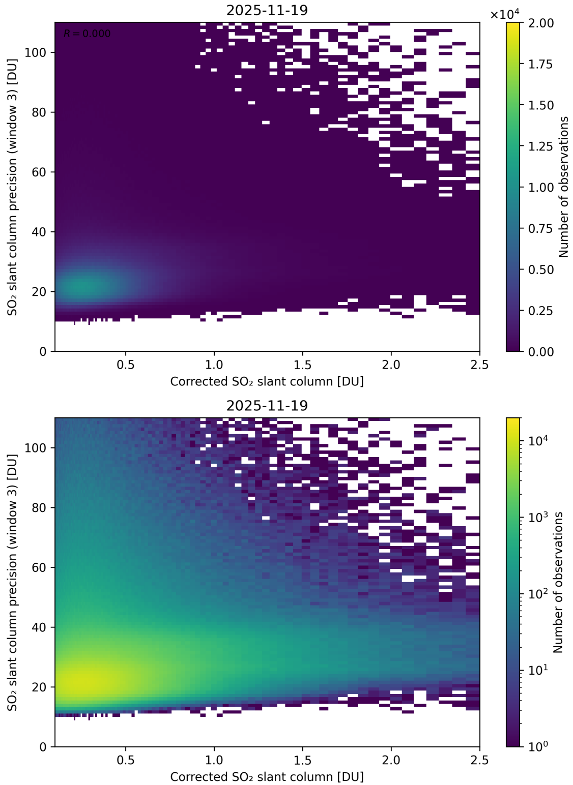
Figure 241: Scatter density plot of “Corrected SO 2 slant column” against “SO 2 slant column precision (window 3)” for 2025-11-18 to 2025-11-20.
