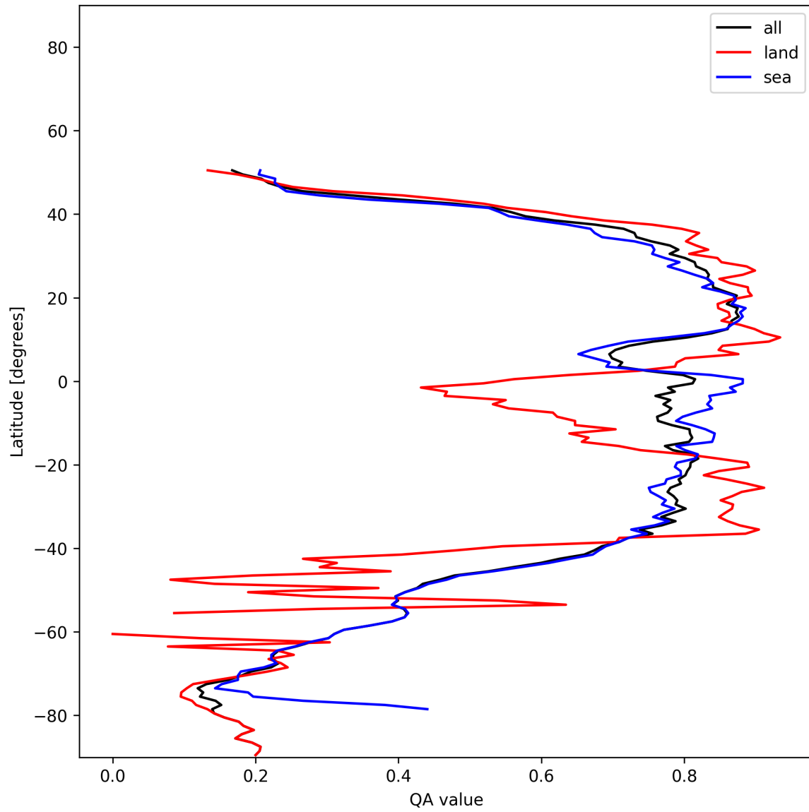
Figure 31: Zonal average of “QA value” for 2025-11-18 to 2025-11-20.
