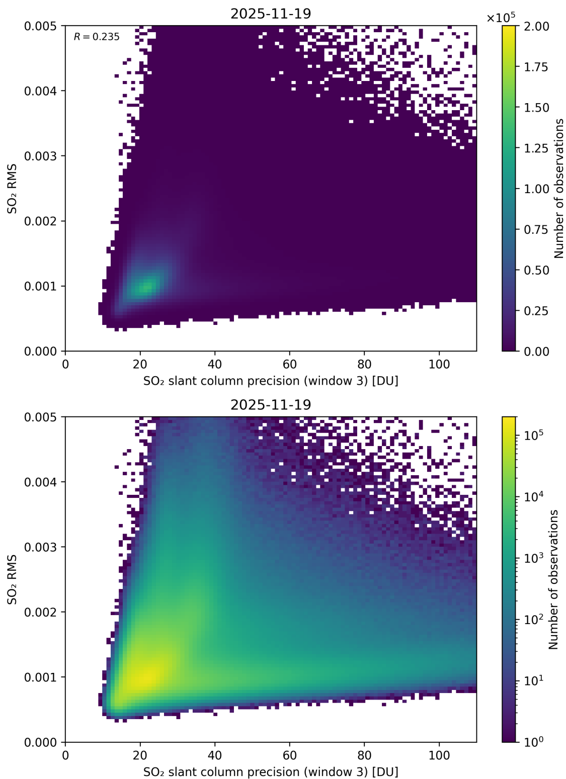
Figure 310: Scatter density plot of “SO 2 slant column precision (window 3)” against “SO 2 RMS” for 2025-11-18 to 2025-11-20.
