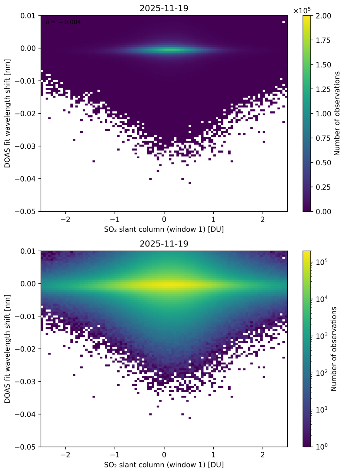
Figure 265: Scatter density plot of “SO 2 slant column (window 1)” against “DOAS fit wavelength shift” for 2025-11-18 to 2025-11-20.
