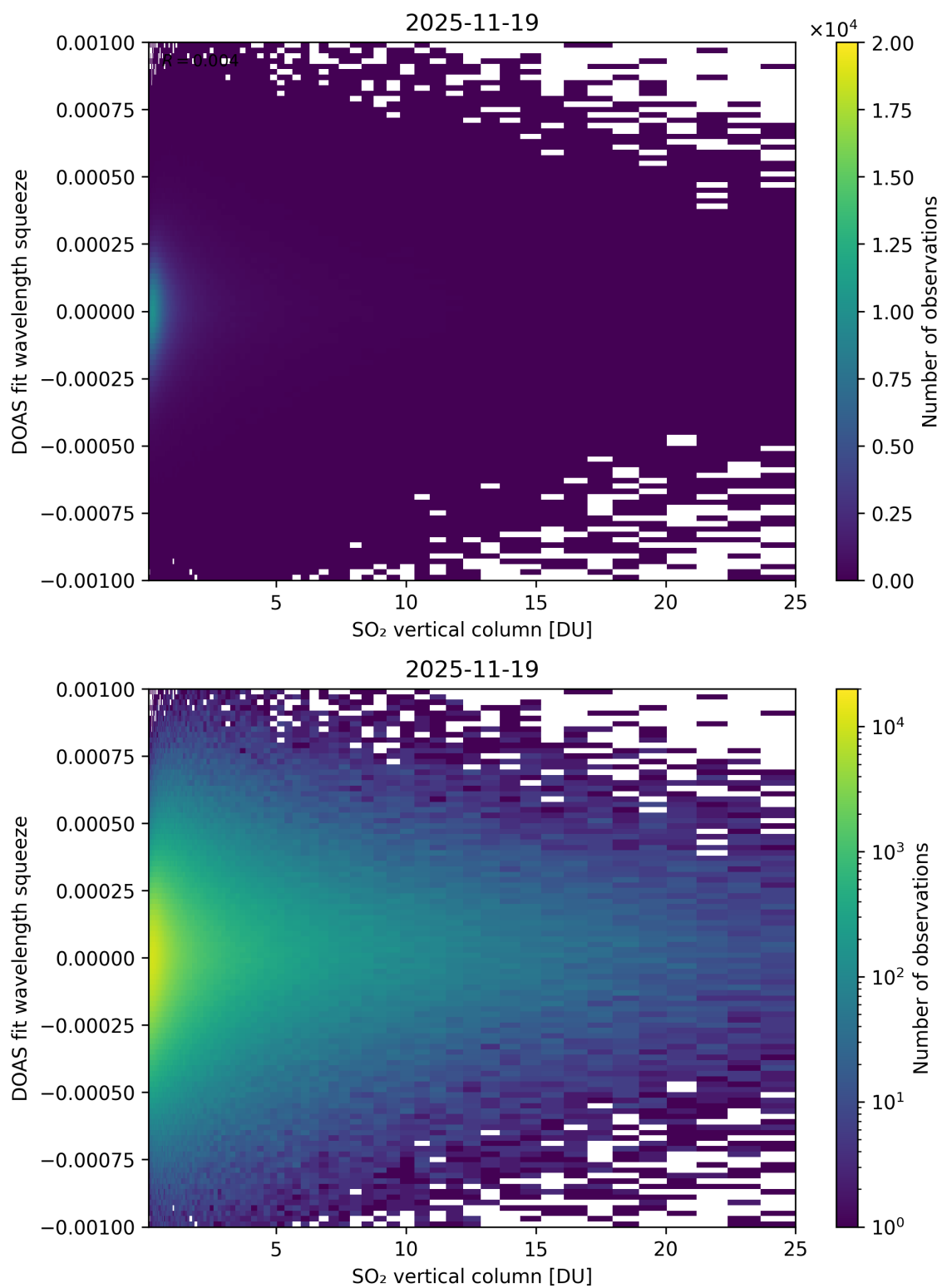
Figure 327: Scatter density plot of “SO 2 vertical column” against “DOAS fit wavelength squeeze” for 2025-11-18 to 2025-11-20.
