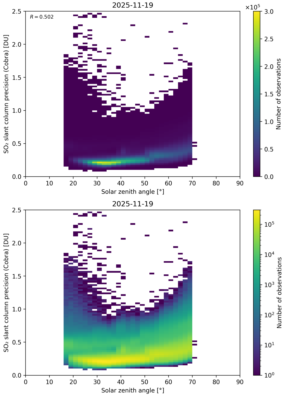
Figure 180: Scatter density plot of “Solar zenith angle” against “SO 2 slant column precision (Cobra)” for 2025-11-18 to 2025-11-20.
