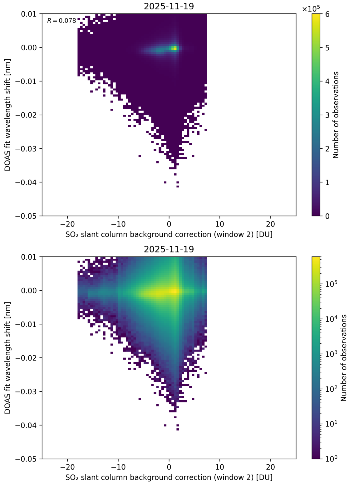
Figure 123: Scatter density plot of “SO 2 slant column background correction (window 2)” against “DOAS fit wavelength shift” for 2025-11-18 to 2025-11-20.
