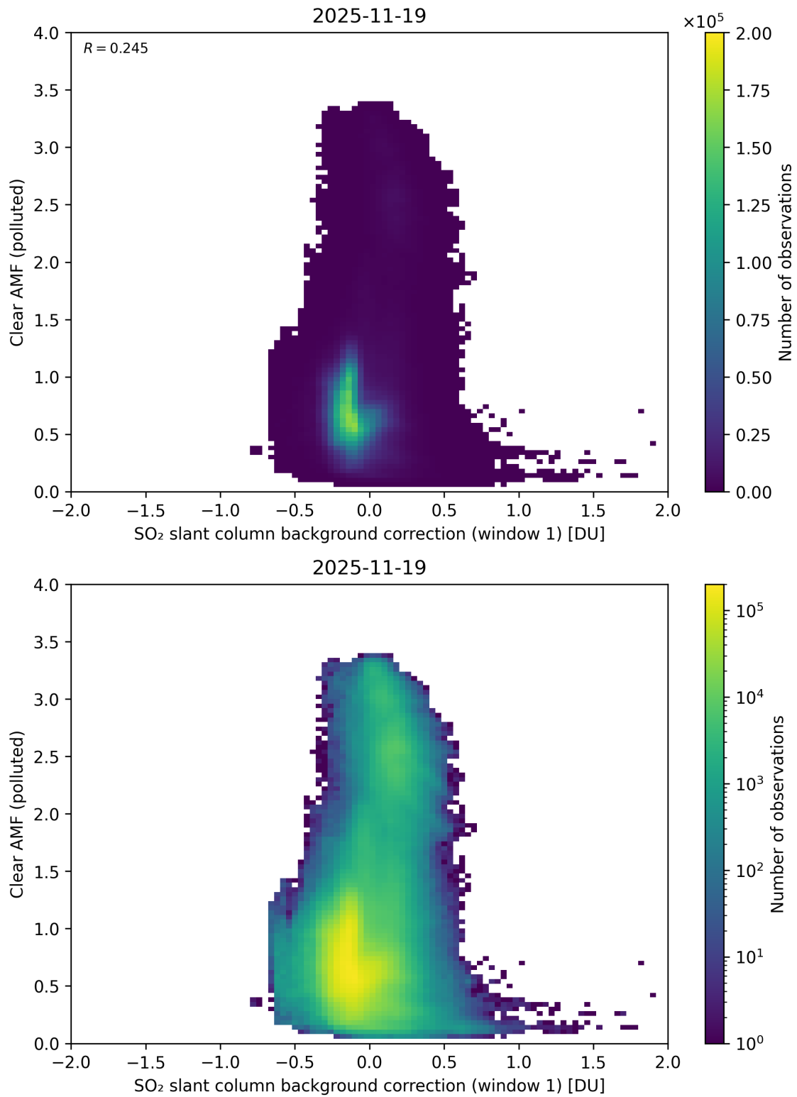
Figure 114: Scatter density plot of “SO 2 slant column background correction (window 1)” against “Clear AMF (polluted)” for 2025-11-18 to 2025-11-20.
