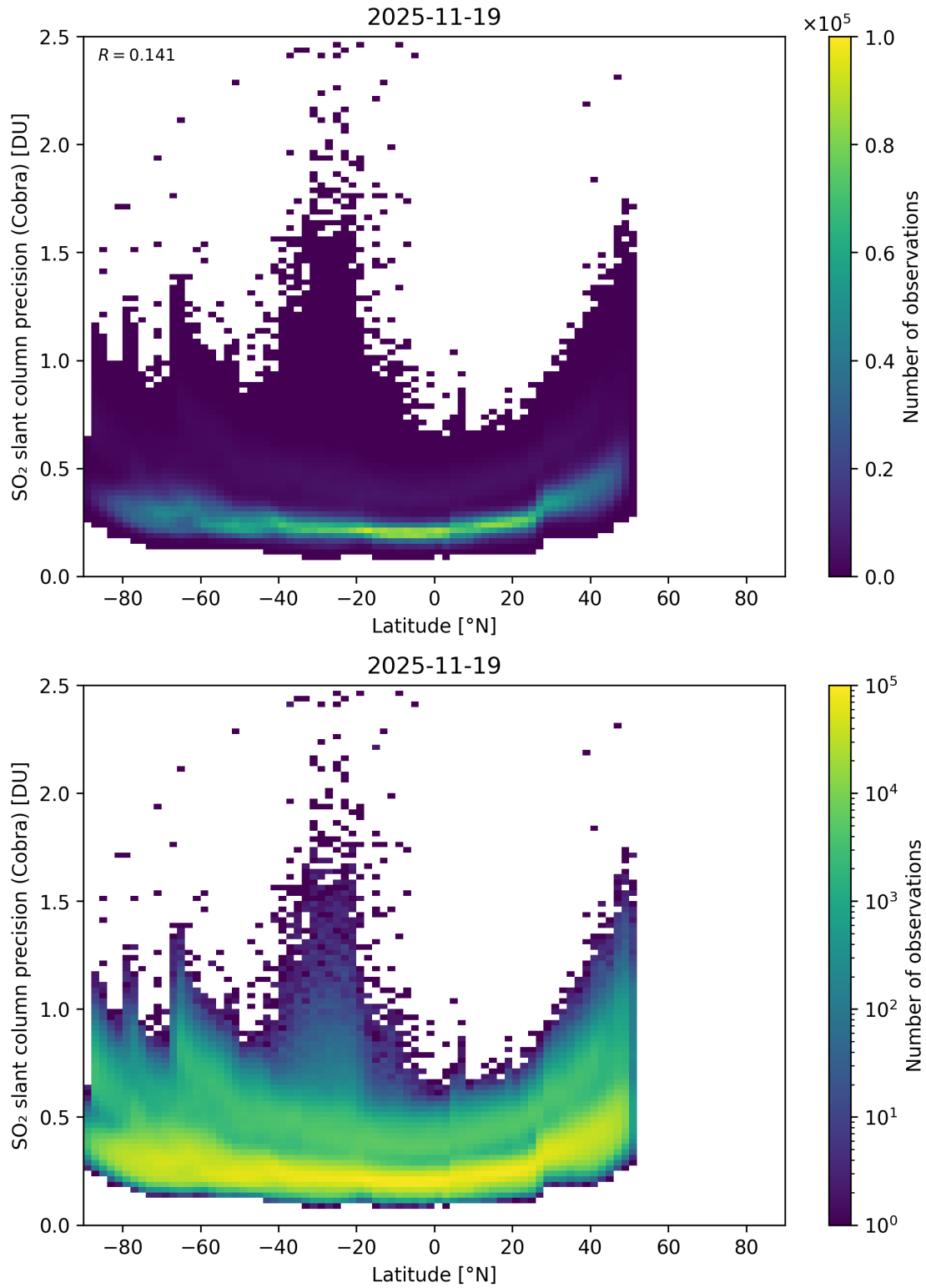
Figure 158: Scatter density plot of “Latitude” against “SO 2 slant column precision (Cobra)” for 2025-11-18 to 2025-11-20.
