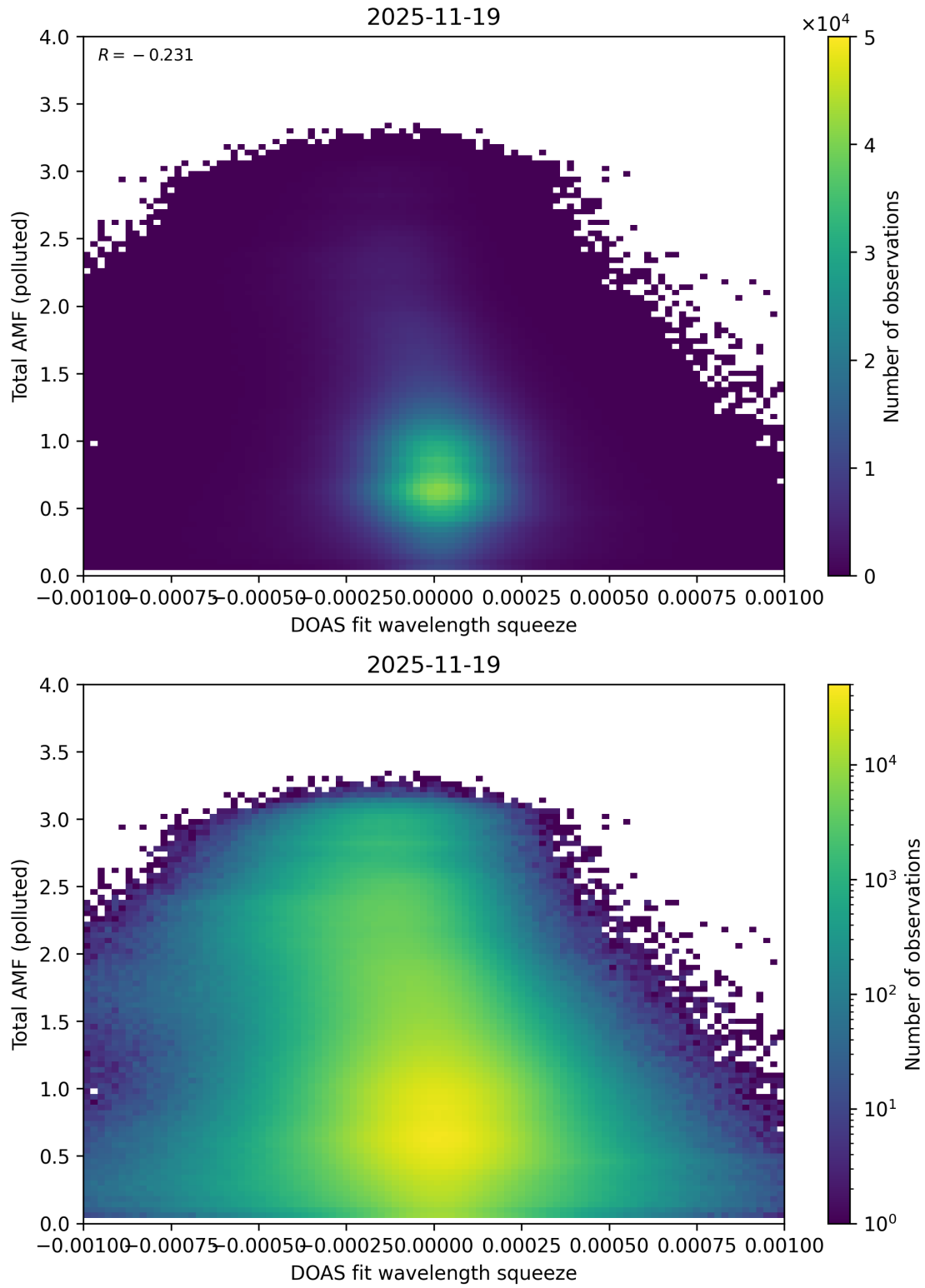
Figure 145: Scatter density plot of “DOAS fit wavelength squeeze” against “Total AMF (polluted)” for 2025-11-18 to 2025-11-20.
