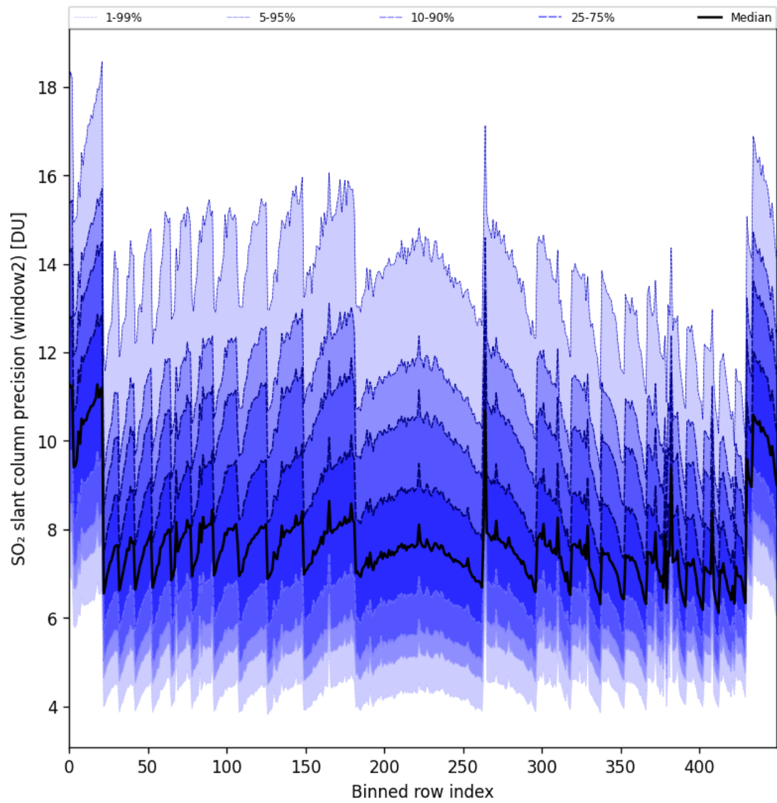
Figure 94: Along track statistics of “SO 2 slant column precision (window2)” for 2025-11-18 to 2025-11-20
