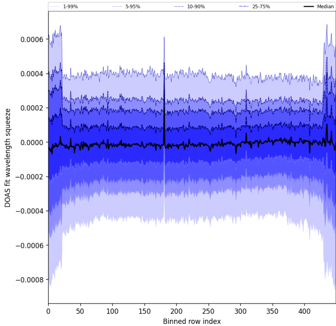
Figure 103: Along track statistics of “DOAS fit wavelength squeeze” for 2025-11-18 to 2025-11-20
