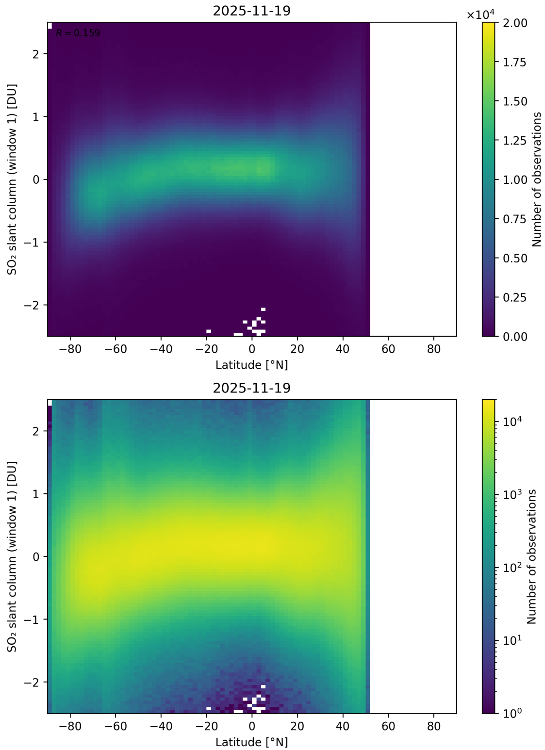
Figure 162: Scatter density plot of “Latitude” against “SO 2 slant column (window 1)” for 2025-11-18 to 2025-11-20.
