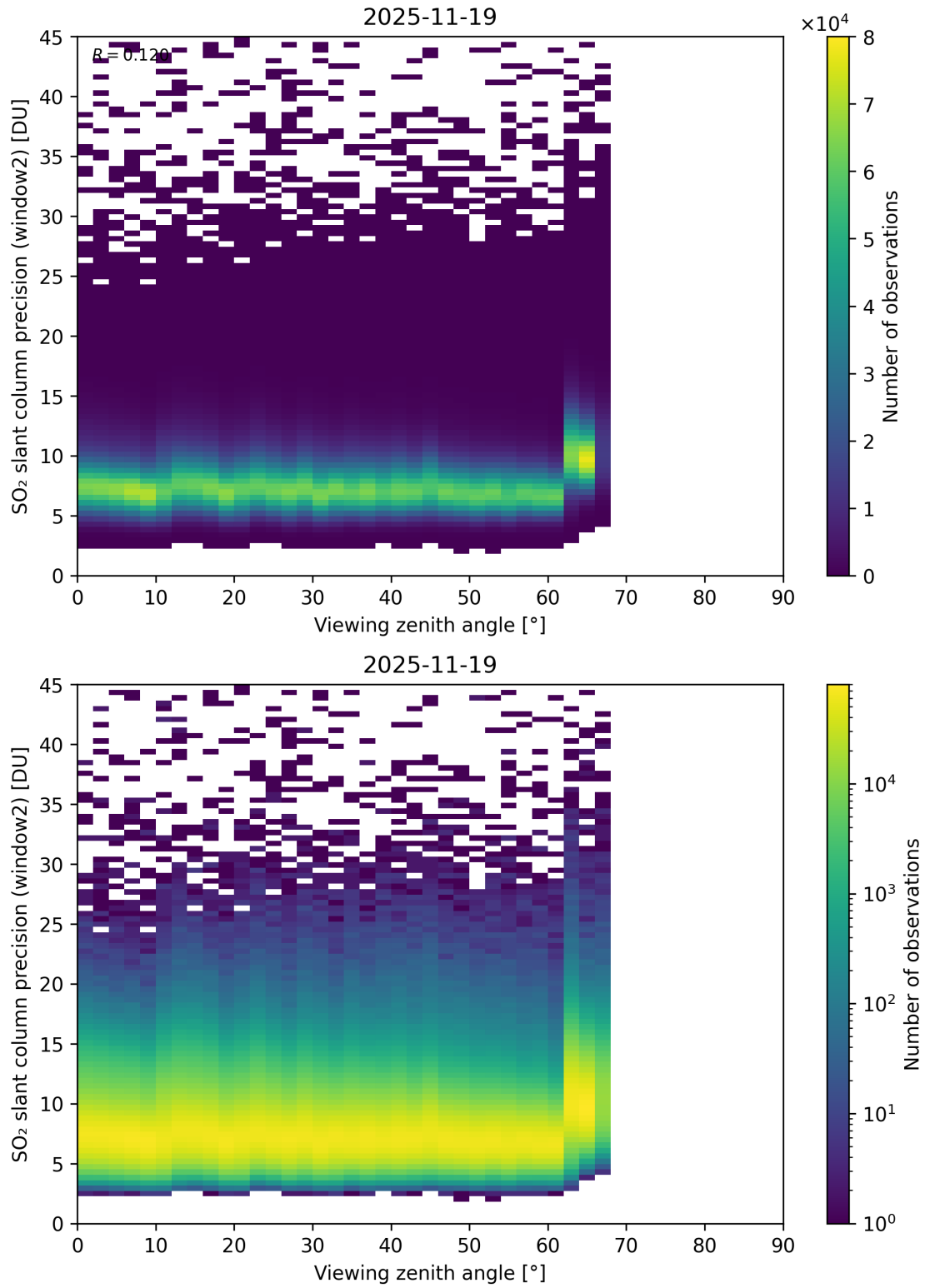
Figure 378: Scatter density plot of “Viewing zenith angle” against “SO 2 slant column precision (window2)” for 2025-11-18 to 2025-11-20.
