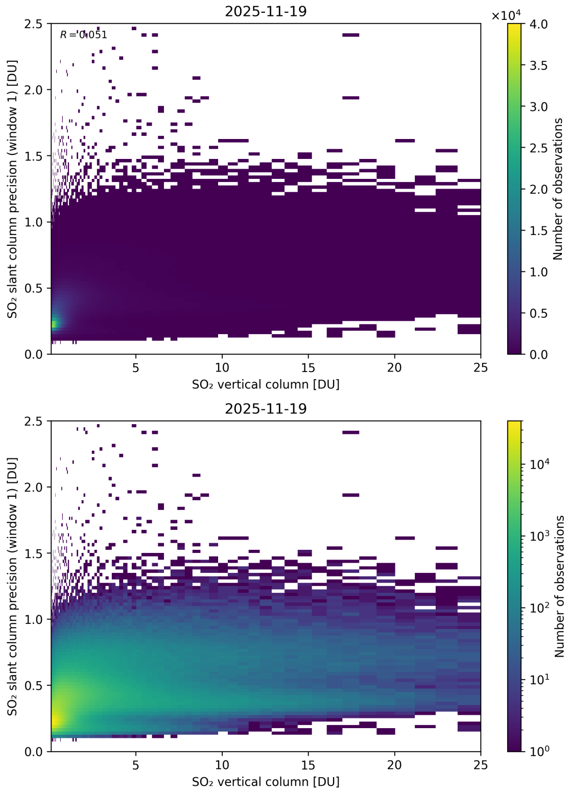
Figure 355: Scatter density plot of “SO 2 vertical column” against “SO 2 slant column precision (window 1)” for 2025-11-18 to 2025-11-20.
