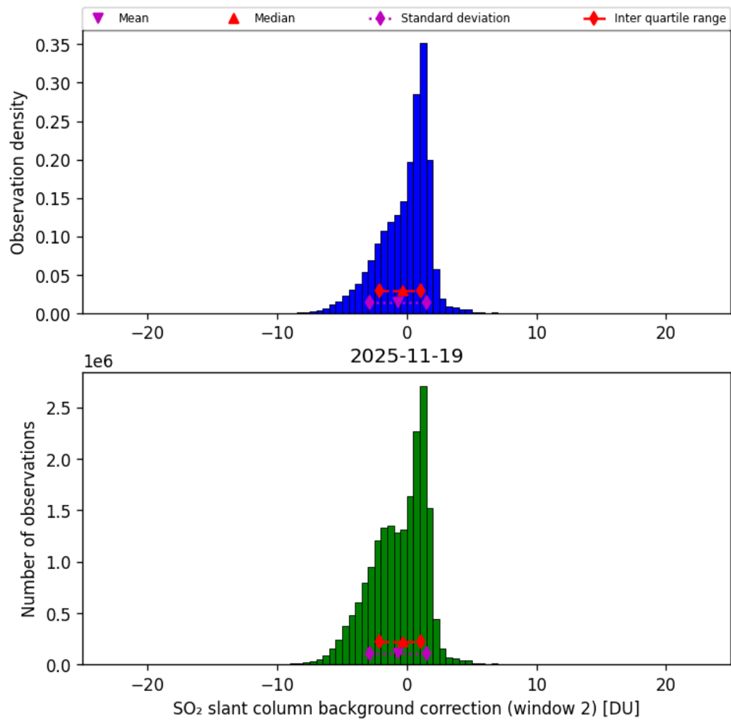
Figure 70: Histogram of “SO 2 slant column background correction (window 2)” for 2025-11-18 to 2025-11-20
