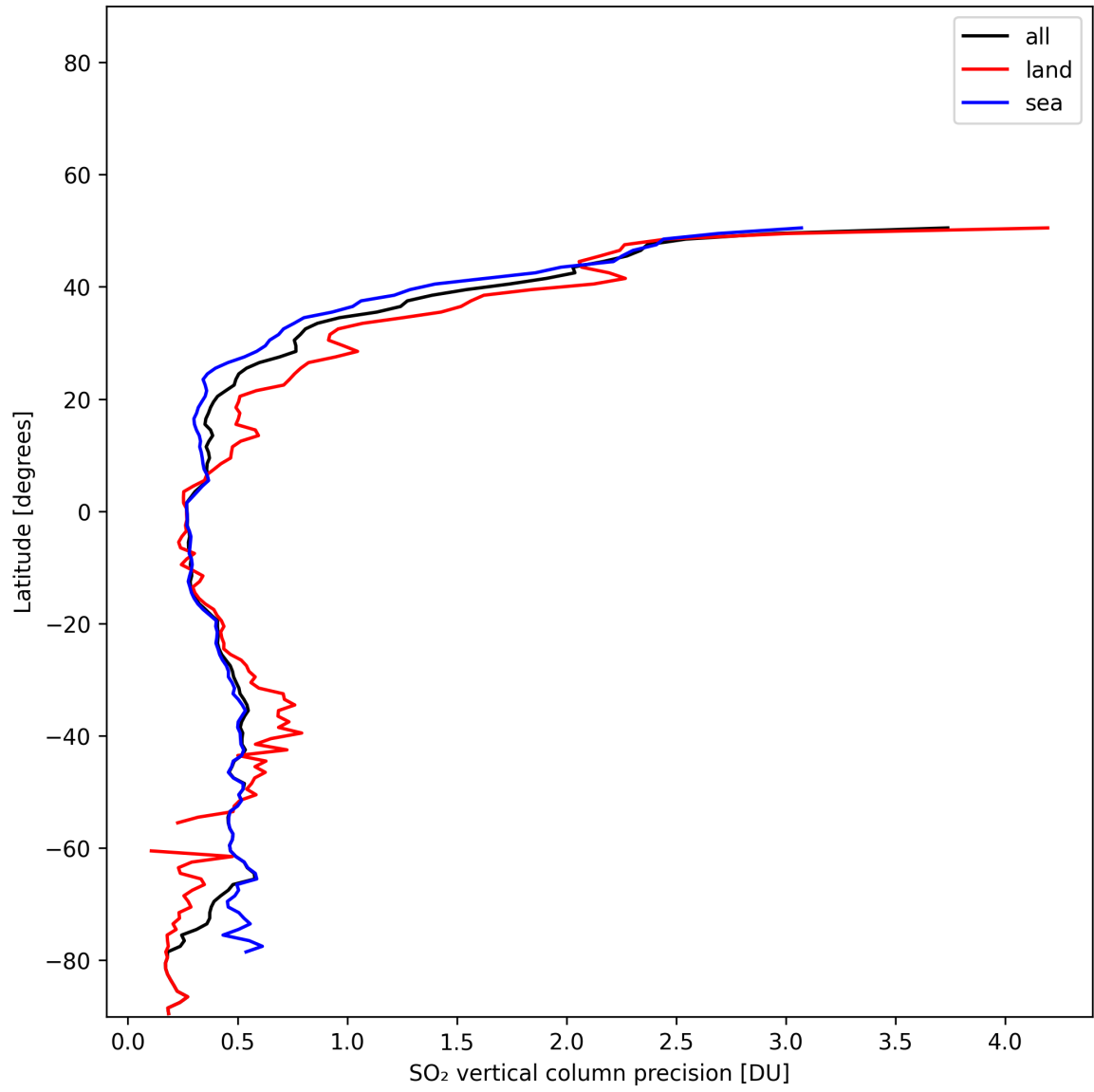
Figure 33: Zonal average of “SO 2 vertical column precision” for 2025-11-18 to 2025-11-20.
