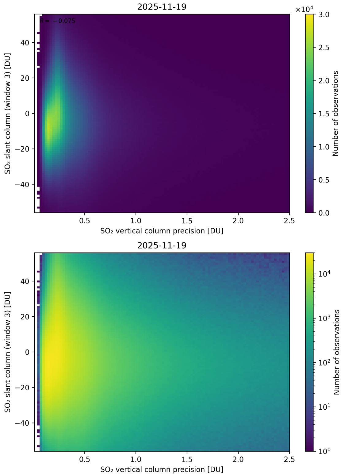
Figure 344: Scatter density plot of “SO 2 vertical column precision” against “SO 2 slant column (window 3)” for 2025-11-18 to 2025-11-20.
