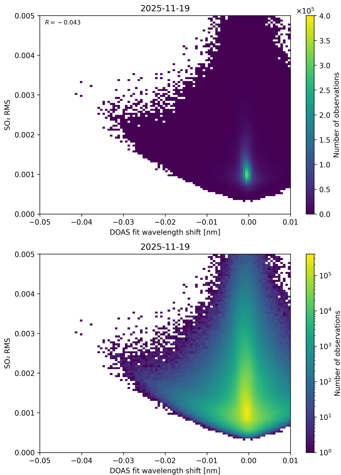
Figure 139: Scatter density plot of “DOAS fit wavelength shift” against “SO 2 RMS” for 2025-11-18 to 2025-11-20.
