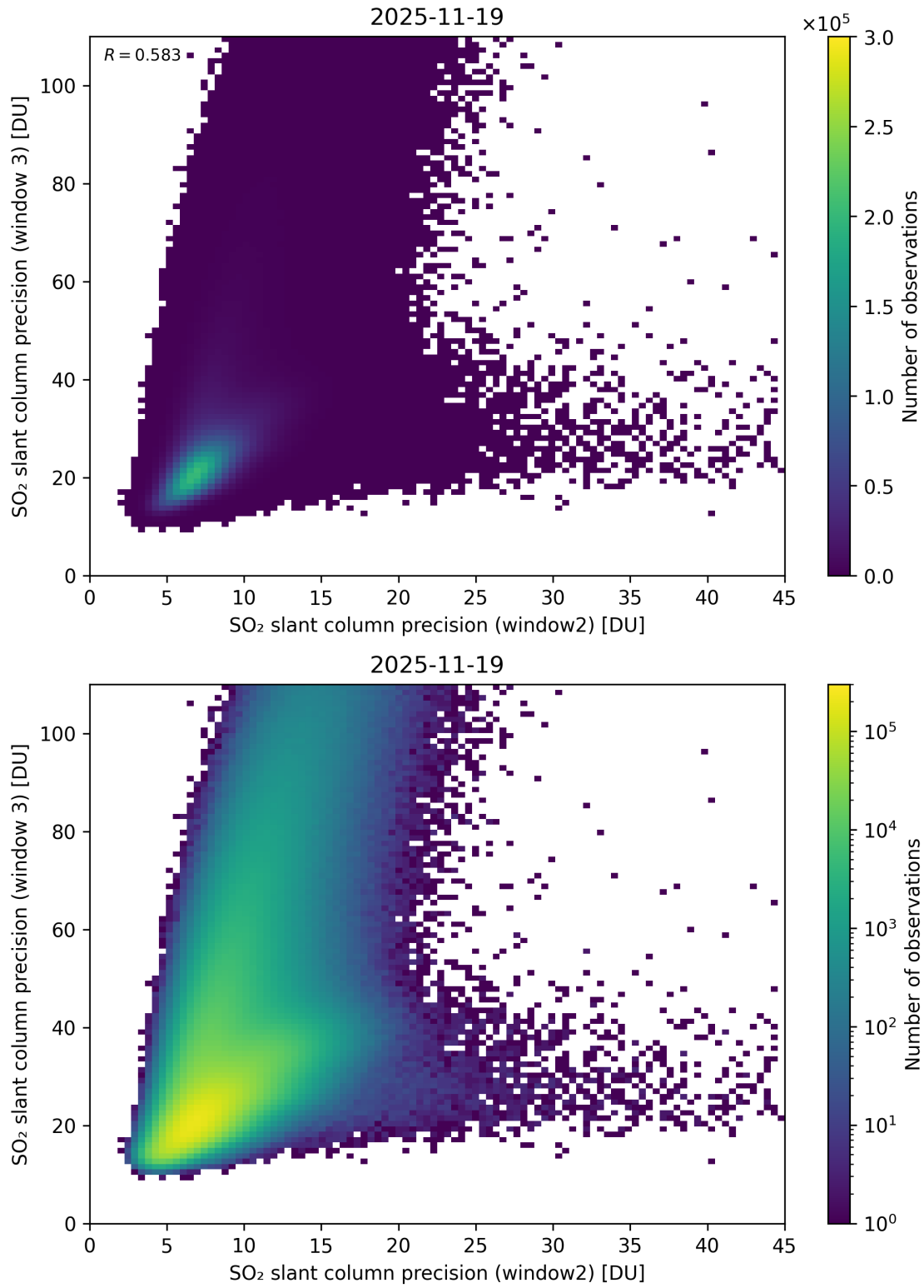
Figure 300: Scatter density plot of “SO 2 slant column precision (window2)” against “SO 2 slant column precision (window 3)” for 2025-11-18 to 2025-11-20.
