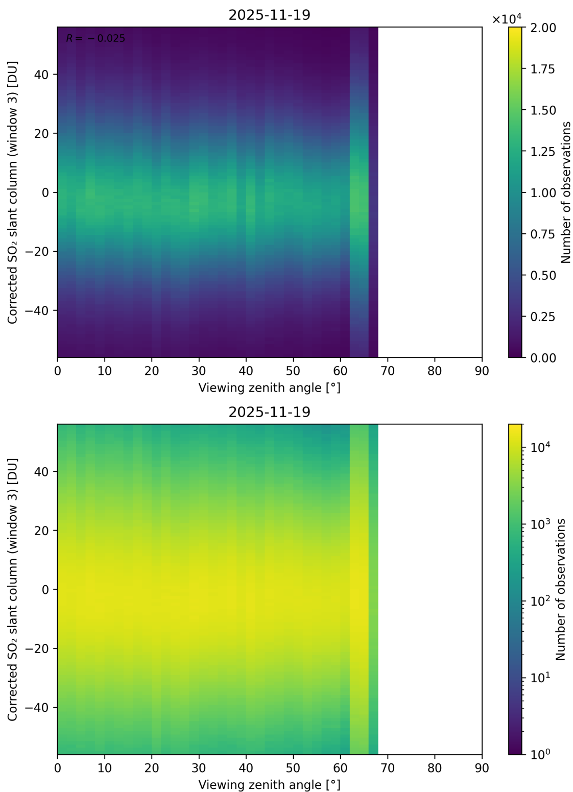
Figure 375: Scatter density plot of “Viewing zenith angle” against “Corrected SO 2 slant column (window 3)” for 2025-11-18 to 2025-11-20.
