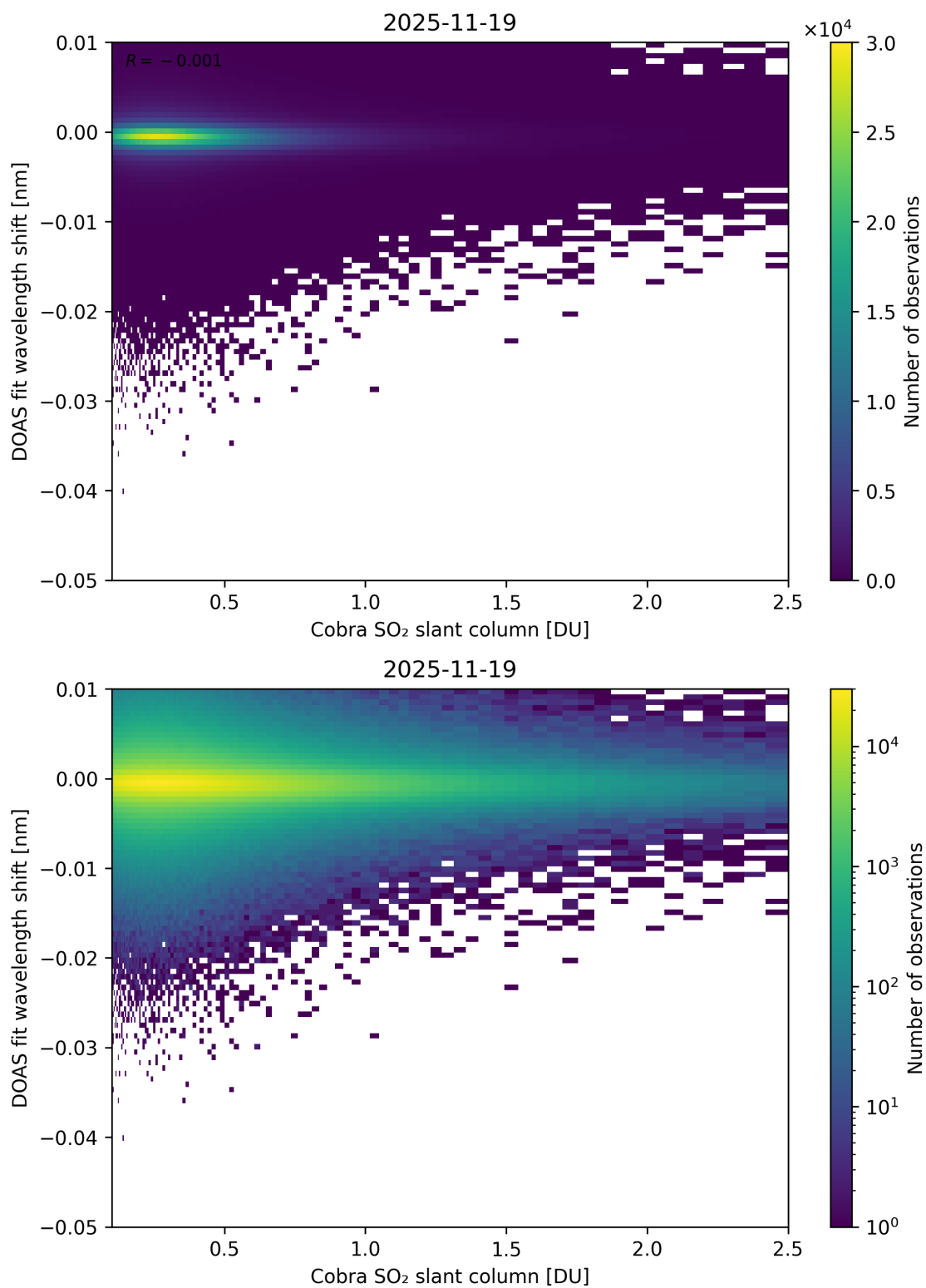
Figure 196: Scatter density plot of “Cobra SO 2 slant column” against “DOAS fit wavelength shift” for 2025-11-18 to 2025-11-20.
