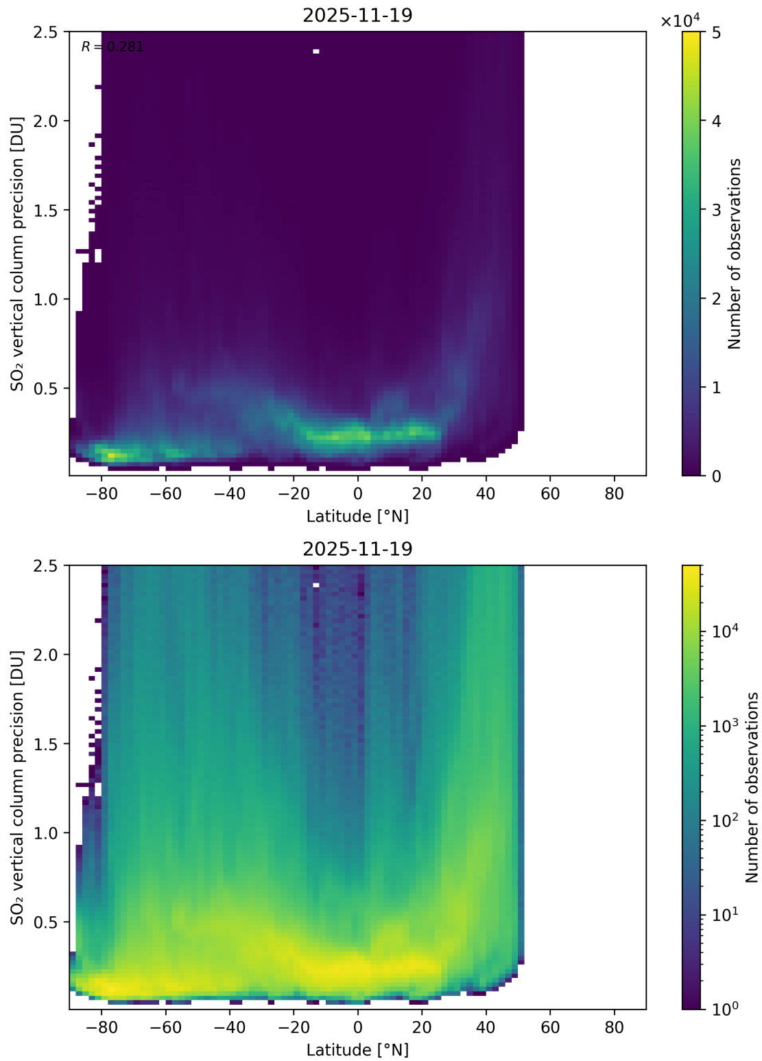
Figure 170: Scatter density plot of “Latitude” against “SO 2 vertical column precision” for 2025-11-18 to 2025-11-20.
