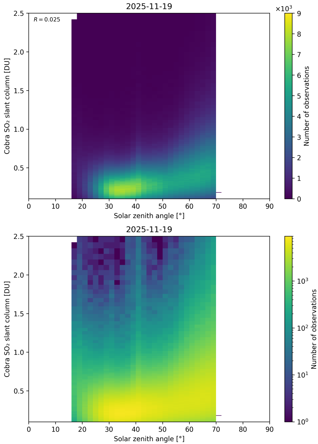
Figure 179: Scatter density plot of “Solar zenith angle” against “Cobra SO 2 slant column” for 2025-11-18 to 2025-11-20.
