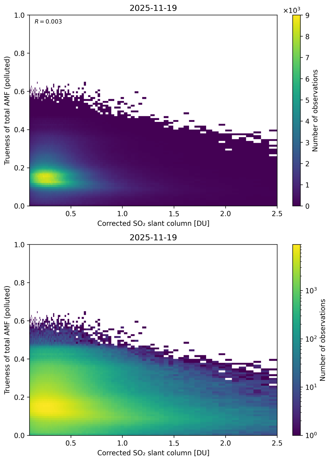
Figure 243: Scatter density plot of “Corrected SO 2 slant column” against “Trueness of total AMF (polluted)” for 2025-11-18 to 2025-11-20.
