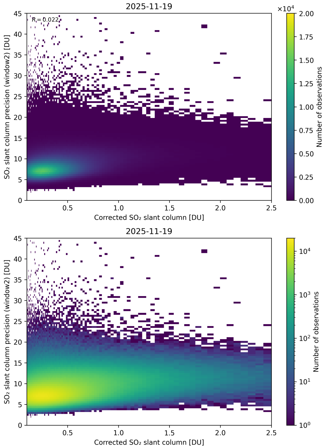
Figure 239: Scatter density plot of “Corrected SO 2 slant column” against “SO 2 slant column precision (window2)” for 2025-11-18 to 2025-11-20.
