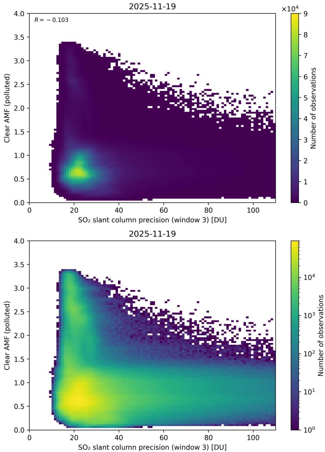
Figure 311: Scatter density plot of “SO 2 slant column precision (window 3)” against “Clear AMF (polluted)” for 2025-11-18 to 2025-11-20.
