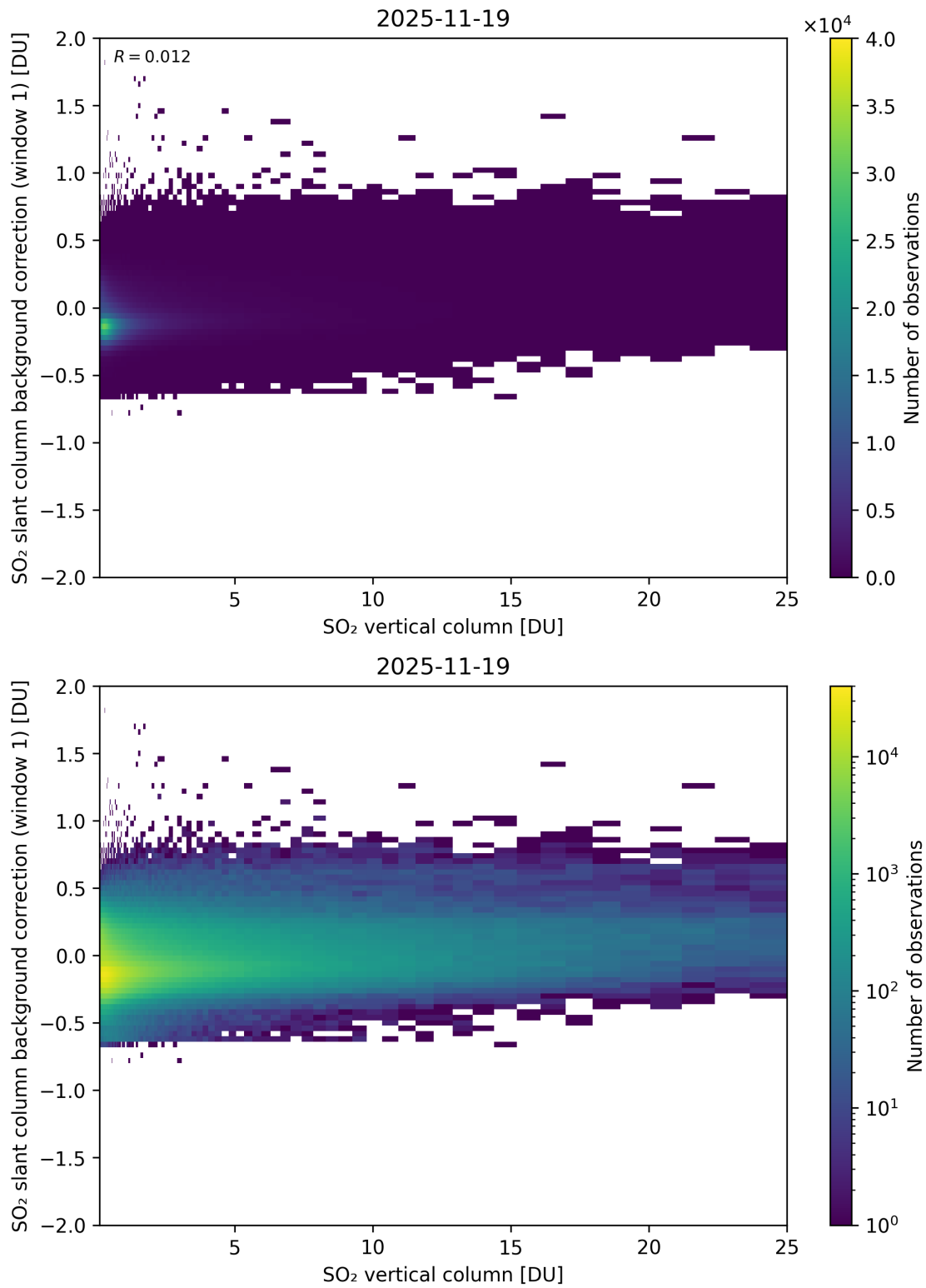
Figure 323: Scatter density plot of “SO 2 vertical column” against “SO 2 slant column background correction (window 1)” for 2025-11-18 to 2025-11-20.
