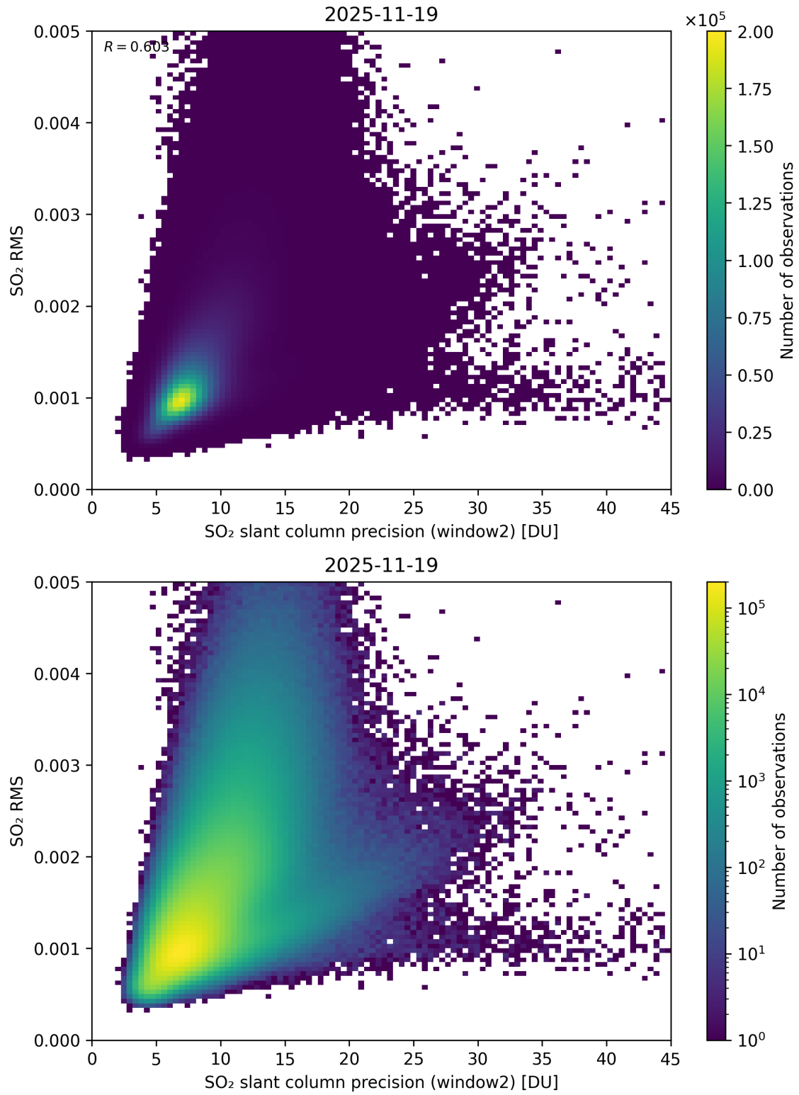
Figure 295: Scatter density plot of “SO 2 slant column precision (window2)” against “SO 2 RMS” for 2025-11-18 to 2025-11-20.
