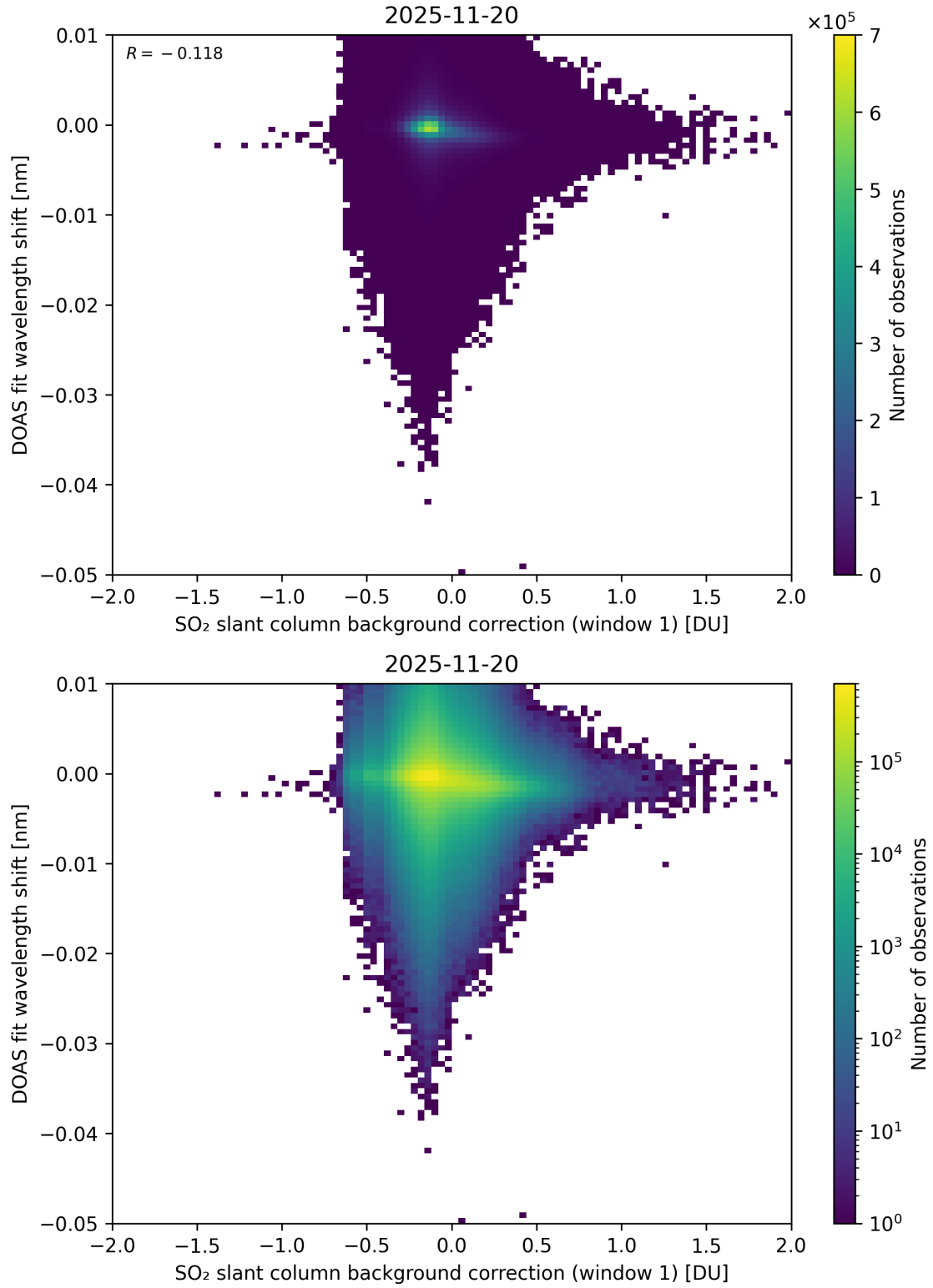
Figure 111: Scatter density plot of “SO 2 slant column background correction (window 1)” against “DOAS fit wavelength shift” for 2025-11-19 to 2025-11-21.
