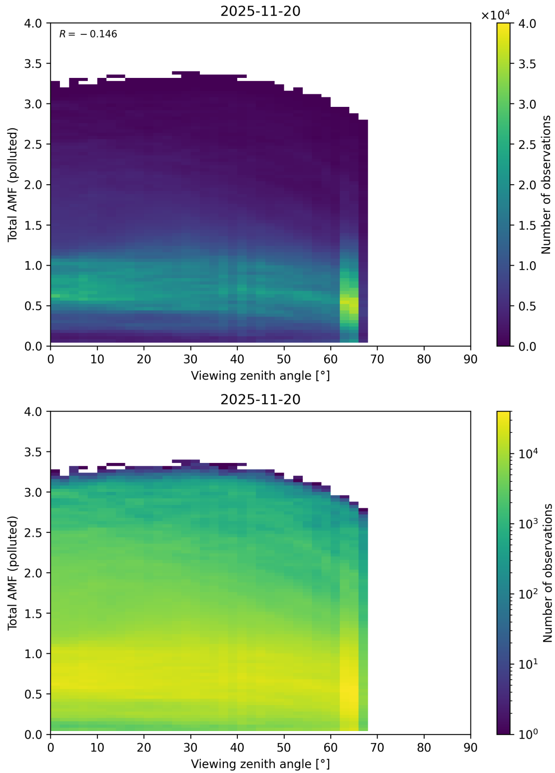
Figure 381: Scatter density plot of “Viewing zenith angle” against “Total AMF (polluted)” for 2025-11-19 to 2025-11-21.
