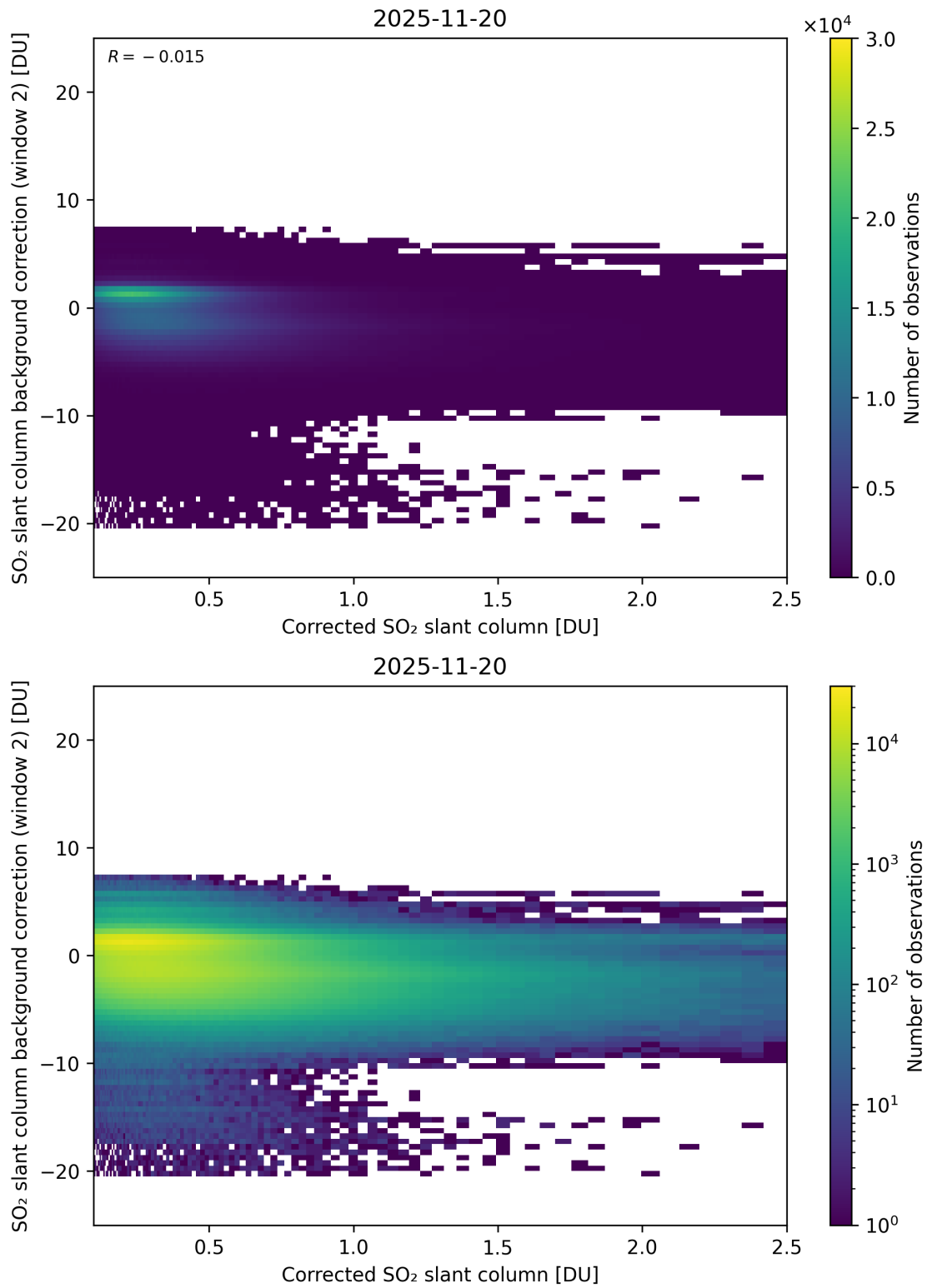
Figure 227: Scatter density plot of “Corrected SO 2 slant column” against “SO 2 slant column background correction (window 2)” for 2025-11-19 to 2025-11-21.
