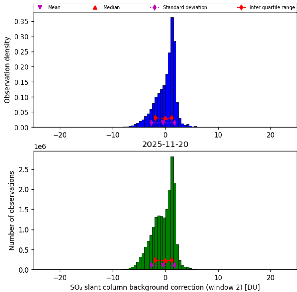
Figure 70: Histogram of “SO 2 slant column background correction (window 2)” for 2025-11-19 to 2025-11-21
