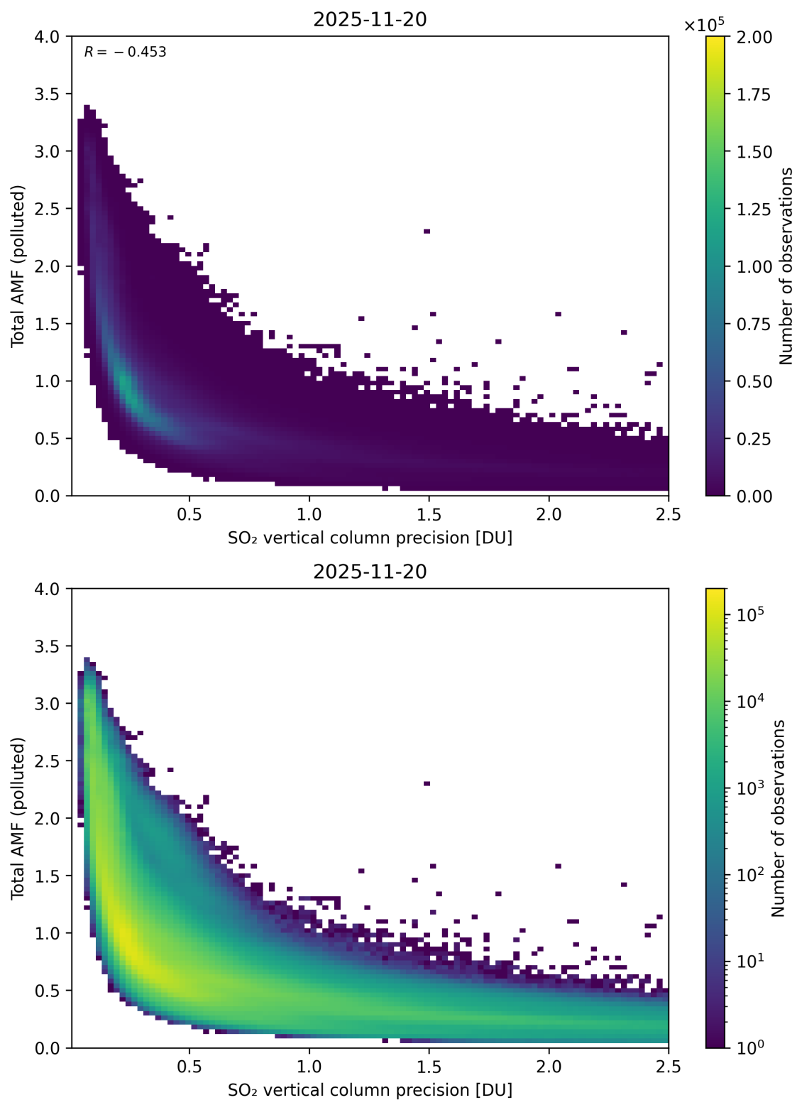
Figure 346: Scatter density plot of “SO 2 vertical column precision” against “Total AMF (polluted)” for 2025-11-19 to 2025-11-21.
