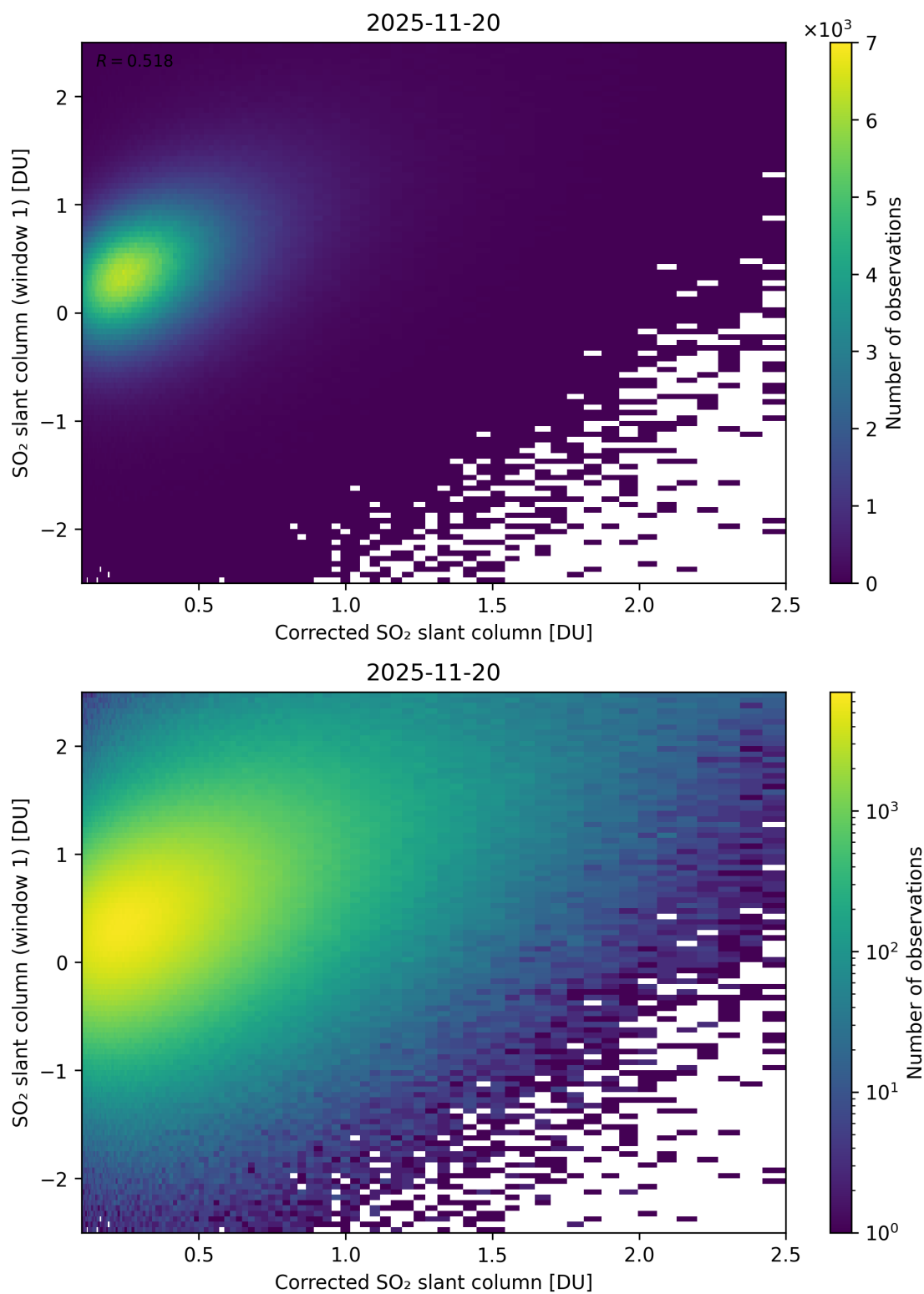
Figure 237: Scatter density plot of “Corrected SO 2 slant column” against “SO 2 slant column (window 1)” for 2025-11-19 to 2025-11-21.
