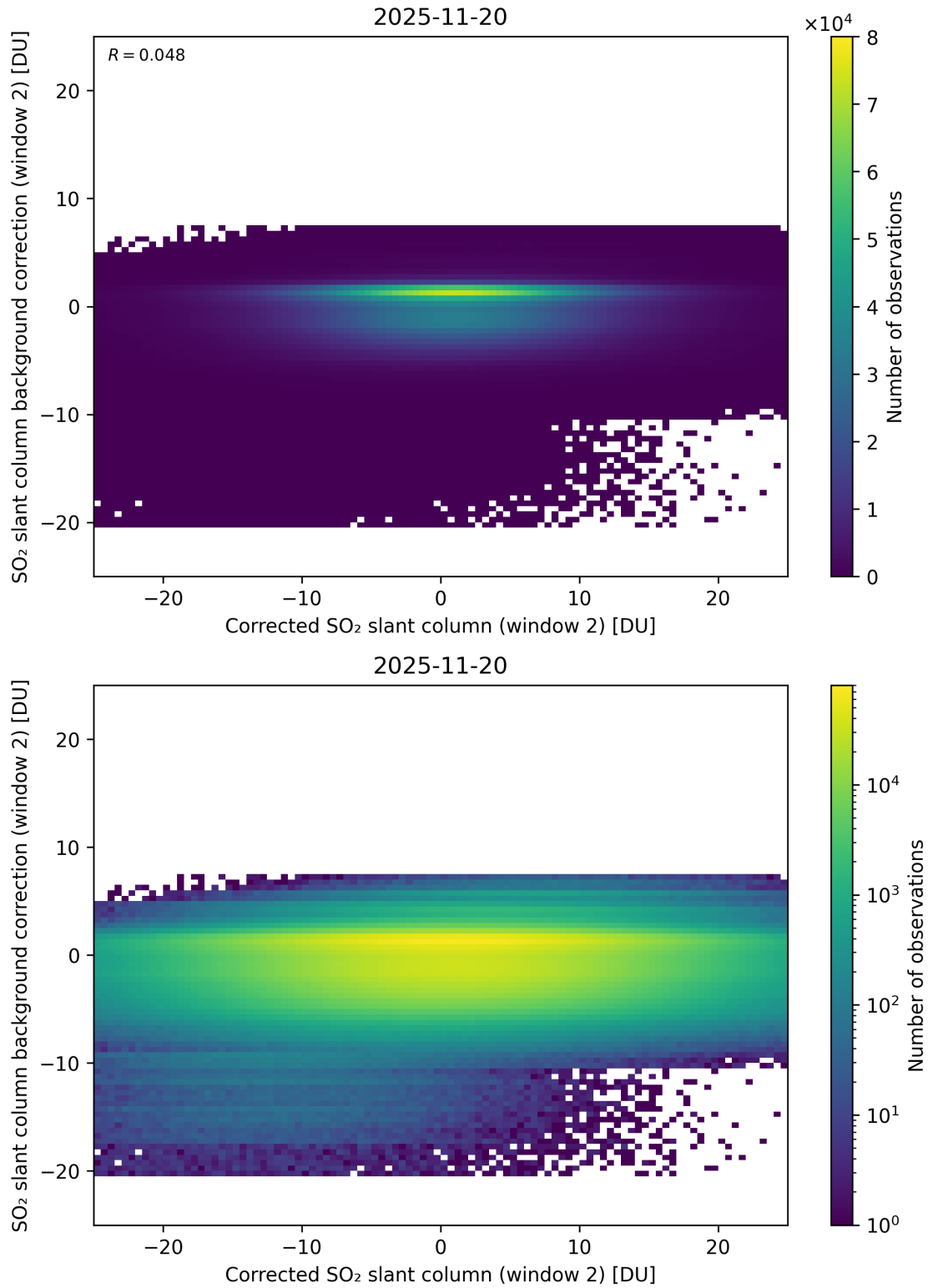
Figure 244: Scatter density plot of “Corrected SO 2 slant column (window 2)” against “SO 2 slant column background correction (window 2)” for 2025-11-19 to 2025-11-21.
