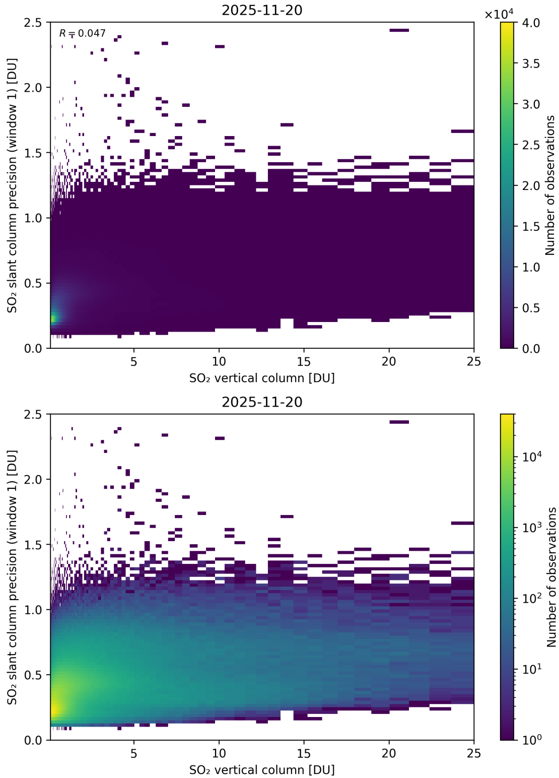
Figure 355: Scatter density plot of “SO 2 vertical column” against “SO 2 slant column precision (window 1)” for 2025-11-19 to 2025-11-21.
