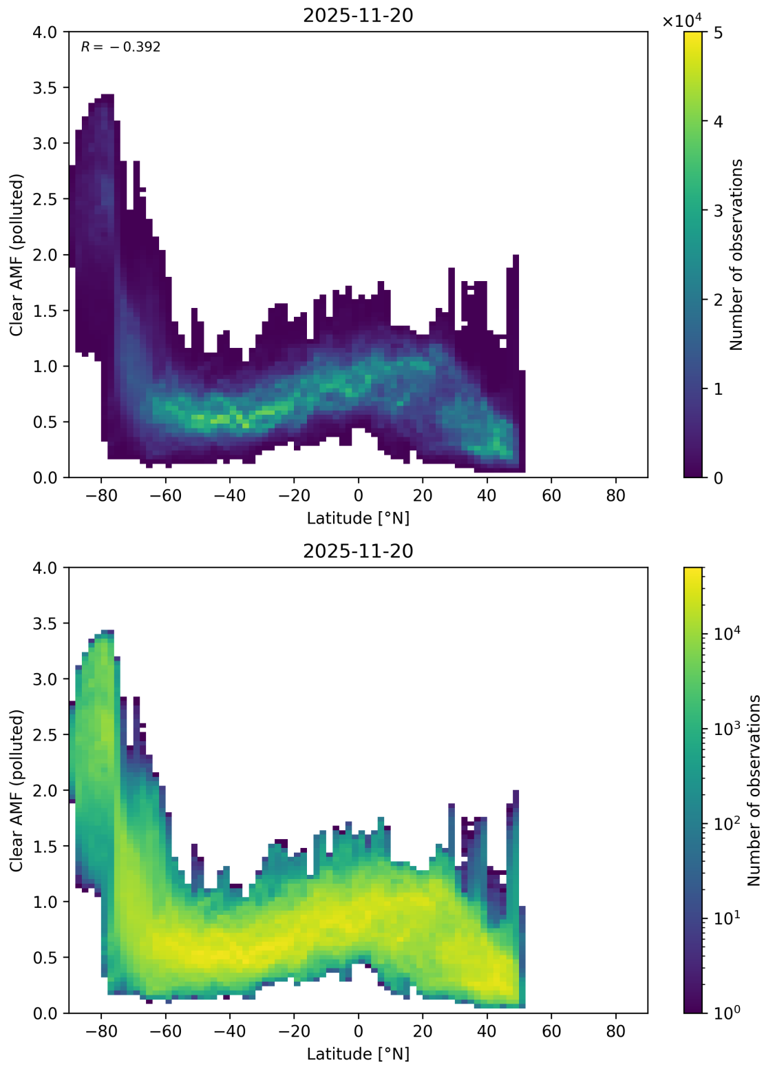
Figure 156: Scatter density plot of “Latitude” against “Clear AMF (polluted)” for 2025-11-19 to 2025-11-21.
