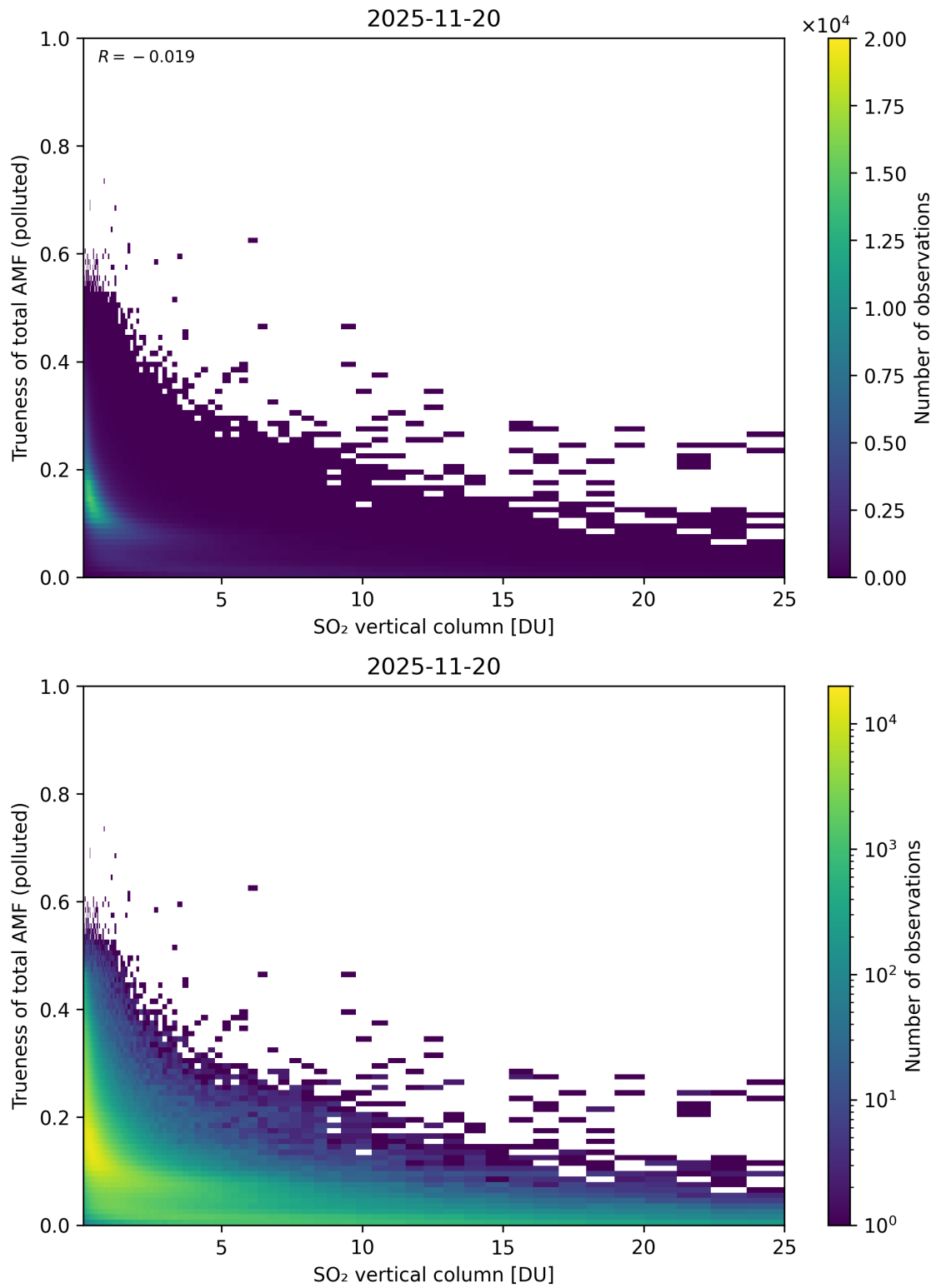
Figure 360: Scatter density plot of “SO 2 vertical column” against “Trueness of total AMF (polluted)” for 2025-11-19 to 2025-11-21.
