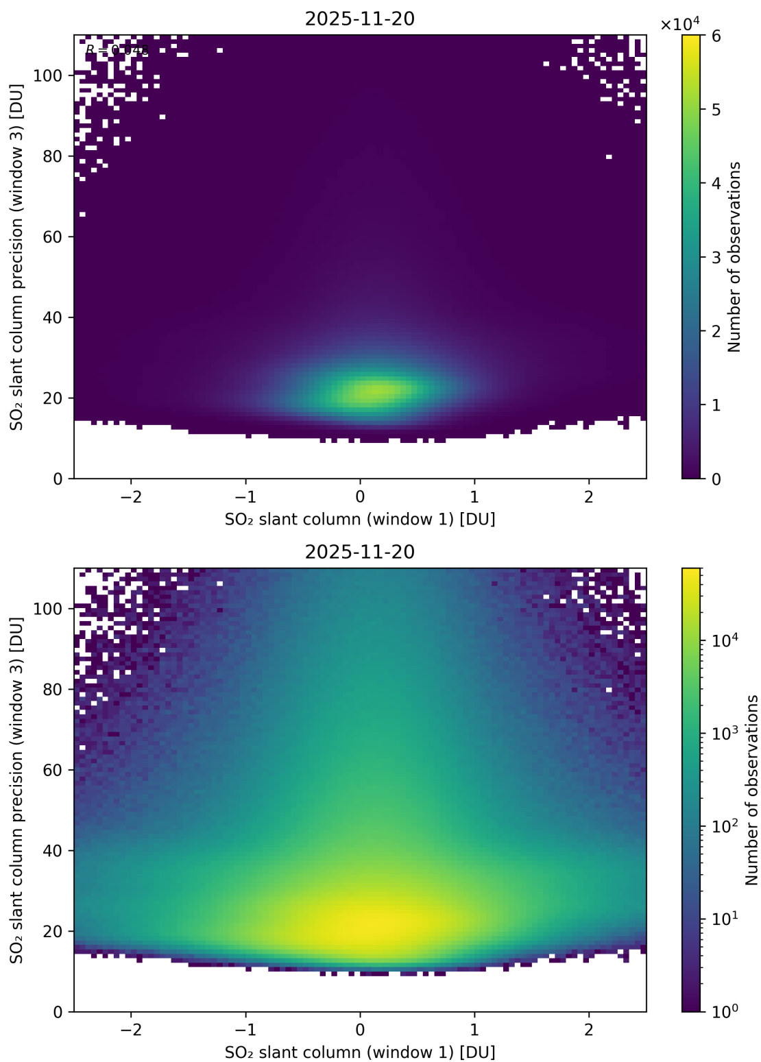
Figure 288: Scatter density plot of “SO 2 slant column (window 1)” against “SO 2 slant column precision (window 3)” for 2025-11-19 to 2025-11-21.
