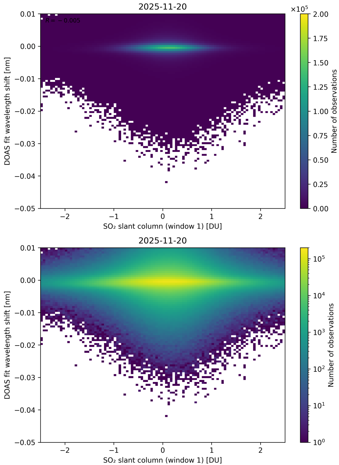
Figure 265: Scatter density plot of “SO 2 slant column (window 1)” against “DOAS fit wavelength shift” for 2025-11-19 to 2025-11-21.
