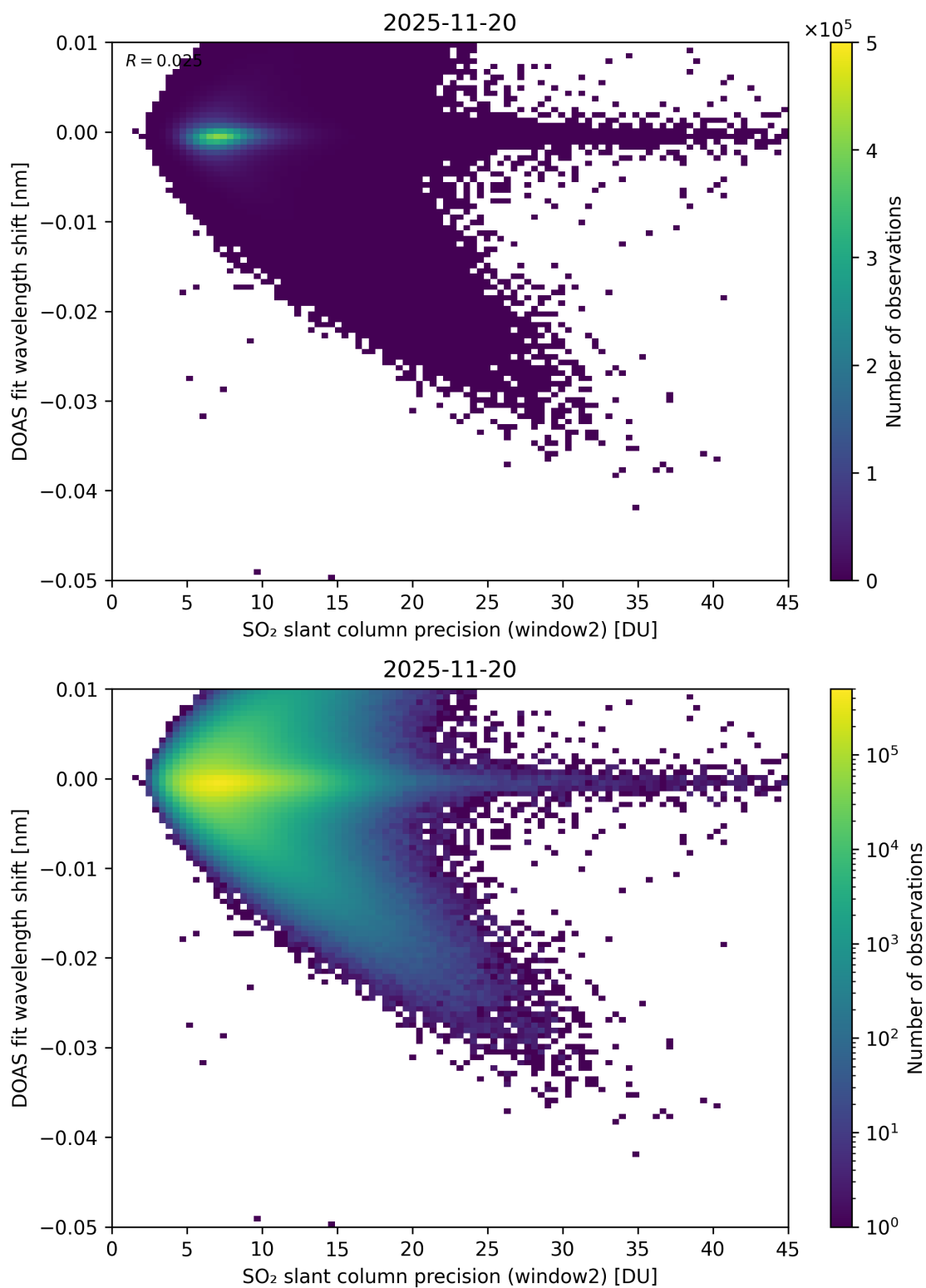
Figure 293: Scatter density plot of “SO 2 slant column precision (window2)” against “DOAS fit wavelength shift” for 2025-11-19 to 2025-11-21.
