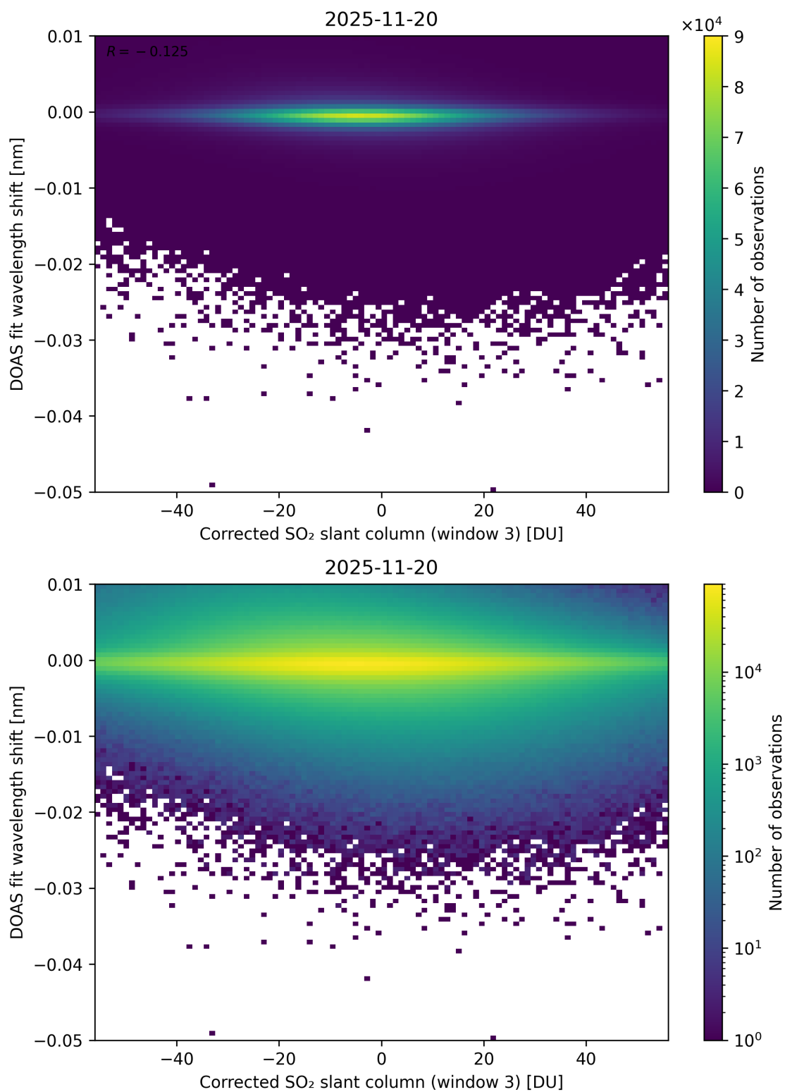
Figure 256: Scatter density plot of “Corrected SO 2 slant column (window 3)” against “DOAS fit wavelength shift” for 2025-11-19 to 2025-11-21.
