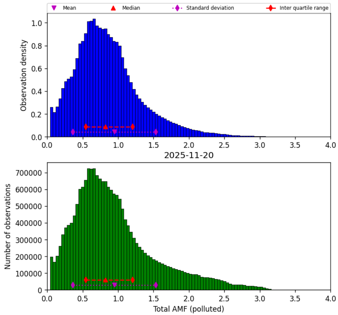
Figure 79: Histogram of “Total AMF (polluted)” for 2025-11-19 to 2025-11-21
