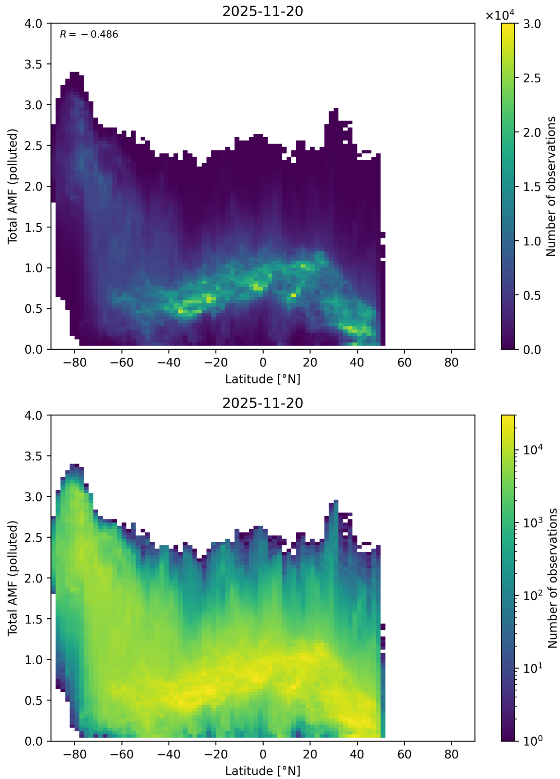
Figure 167: Scatter density plot of “Latitude” against “Total AMF (polluted)” for 2025-11-19 to 2025-11-21.
