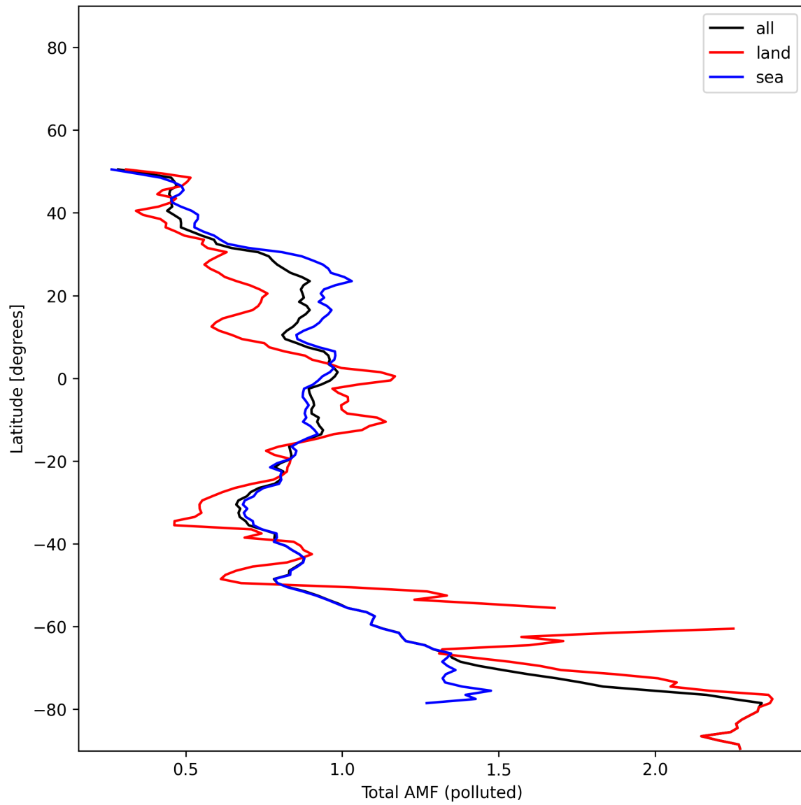
Figure 53: Zonal average of “Total AMF (polluted)” for 2025-11-19 to 2025-11-21.
