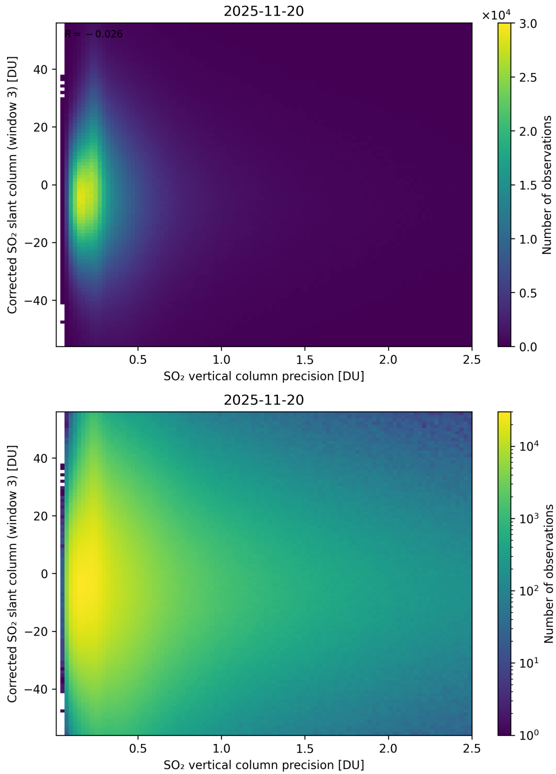
Figure 340: Scatter density plot of “SO 2 vertical column precision” against “Corrected SO 2 slant column (window 3)” for 2025-11-19 to 2025-11-21.
