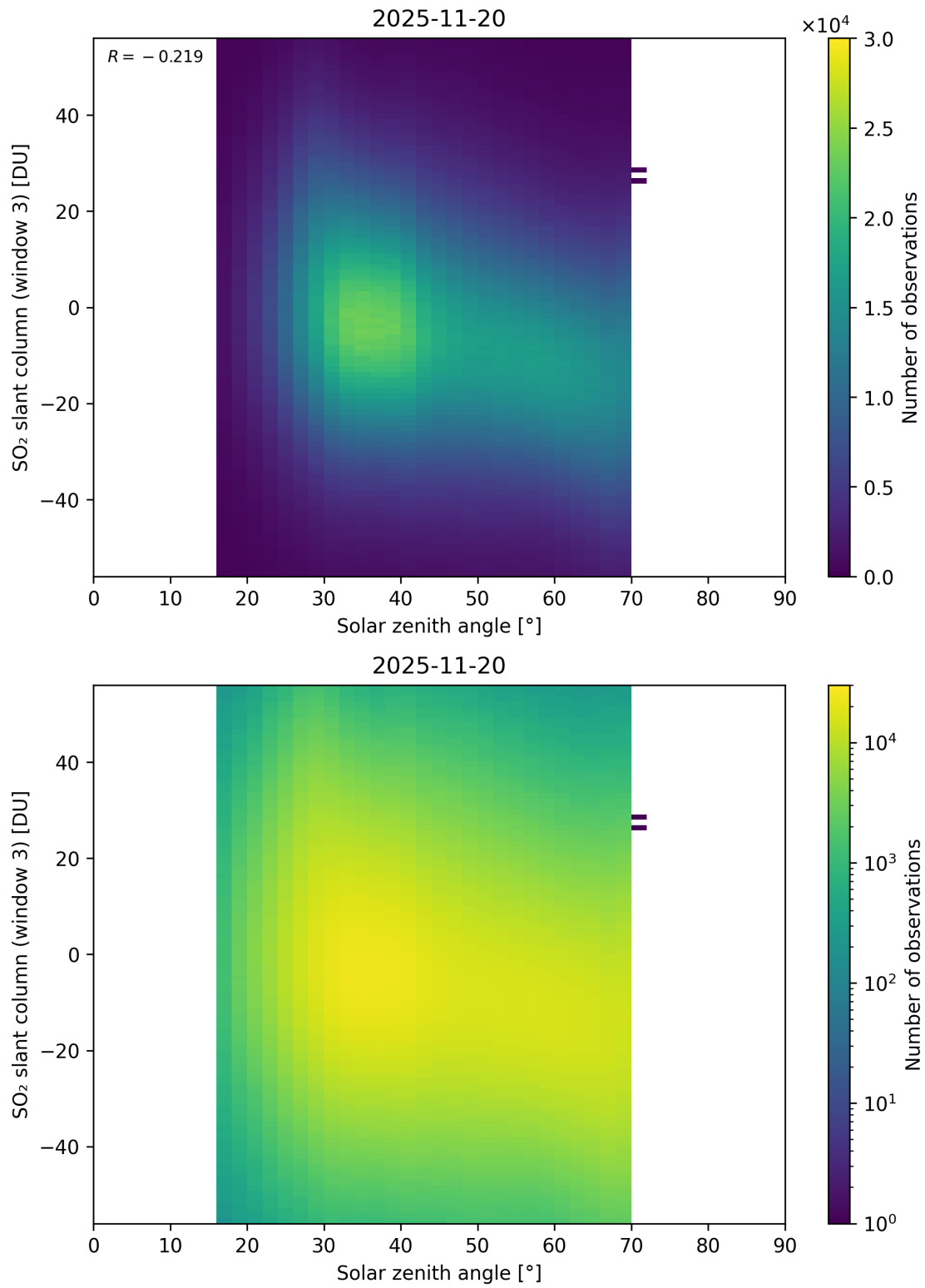
Figure 187: Scatter density plot of “Solar zenith angle” against “SO 2 slant column (window 3)” for 2025-11-19 to 2025-11-21.
