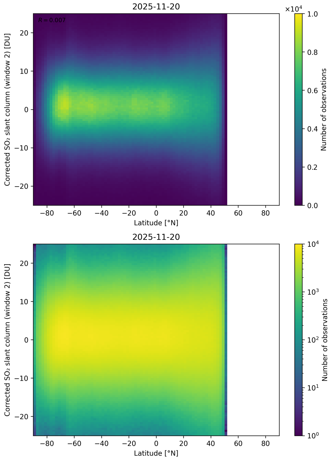
Figure 160: Scatter density plot of “Latitude” against “Corrected SO 2 slant column (window 2)” for 2025-11-19 to 2025-11-21.
