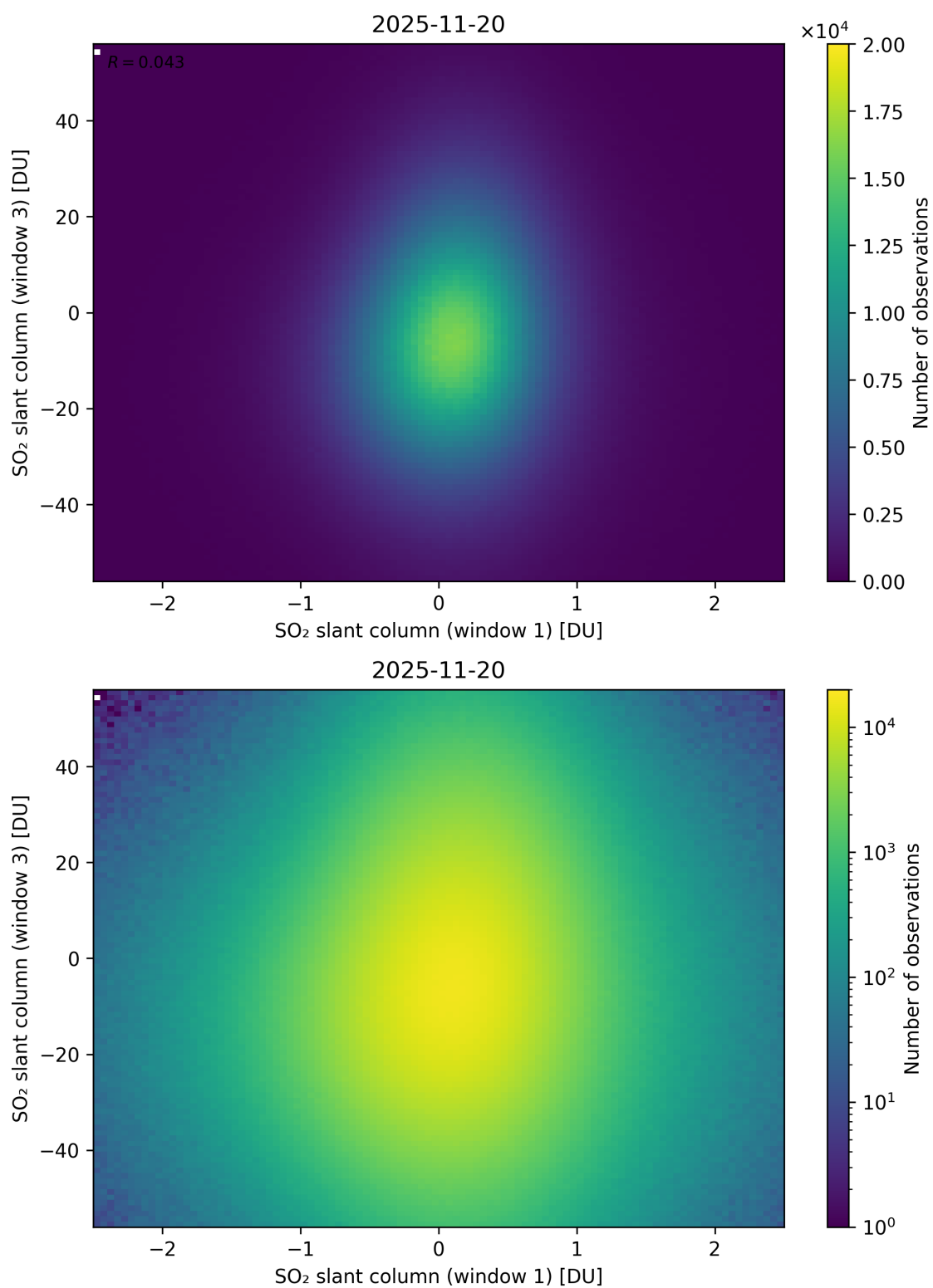
Figure 287: Scatter density plot of “SO 2 slant column (window 1)” against “SO 2 slant column (window 3)” for 2025-11-19 to 2025-11-21.
