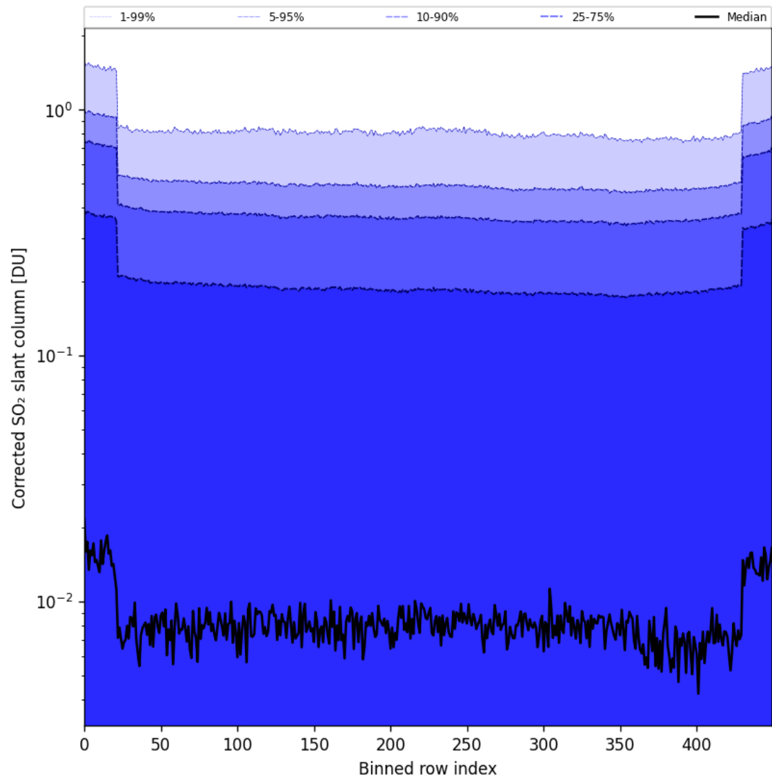
Figure 86: Along track statistics of “Corrected SO 2 slant column” for 2025-11-19 to 2025-11-21
