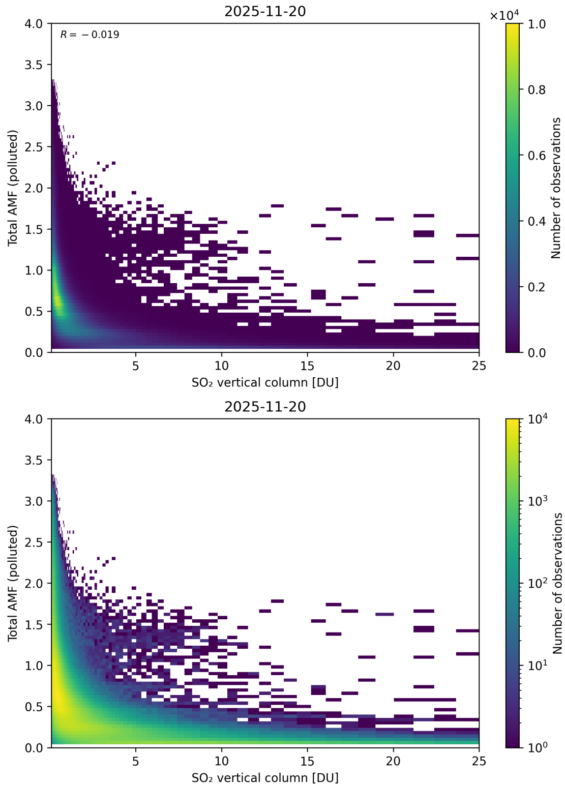
Figure 359: Scatter density plot of “SO 2 vertical column” against “Total AMF (polluted)” for 2025-11-19 to 2025-11-21.
