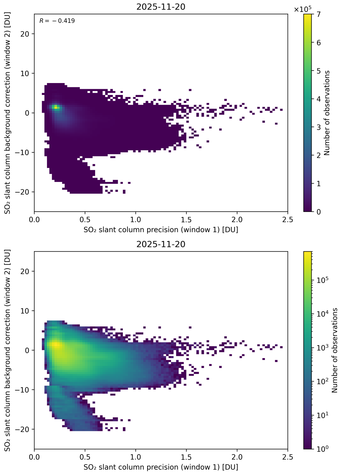
Figure 269: Scatter density plot of “SO 2 slant column precision (window 1)” against “SO 2 slant column background correction (window 2)” for 2025-11-19 to 2025-11-21.
