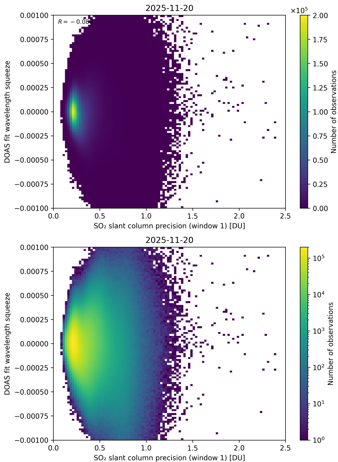
Figure 272: Scatter density plot of “SO 2 slant column precision (window 1)” against “DOAS fit wavelength squeeze” for 2025-11-19 to 2025-11-21.
