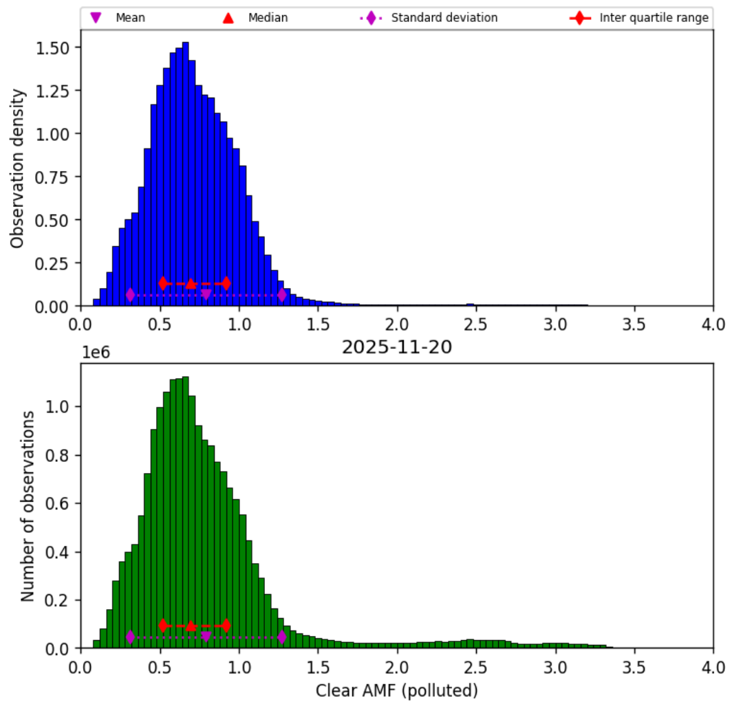
Figure 81: Histogram of “Clear AMF (polluted)” for 2025-11-19 to 2025-11-21
