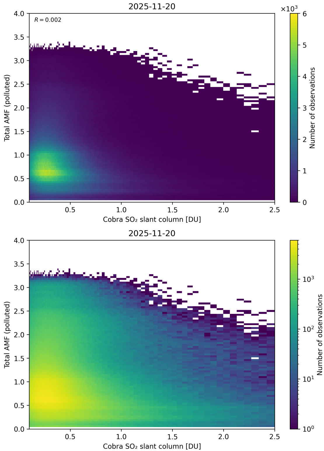
Figure 224: Scatter density plot of “Cobra SO 2 slant column” against “Total AMF (polluted)” for 2025-11-19 to 2025-11-21.
