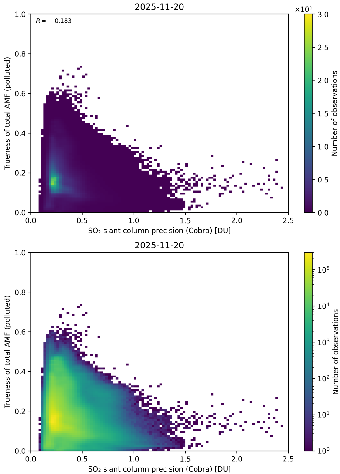
Figure 214: Scatter density plot of “SO 2 slant column precision (Cobra)” against “Trueness of total AMF (polluted)” for 2025-11-19 to 2025-11-21.
