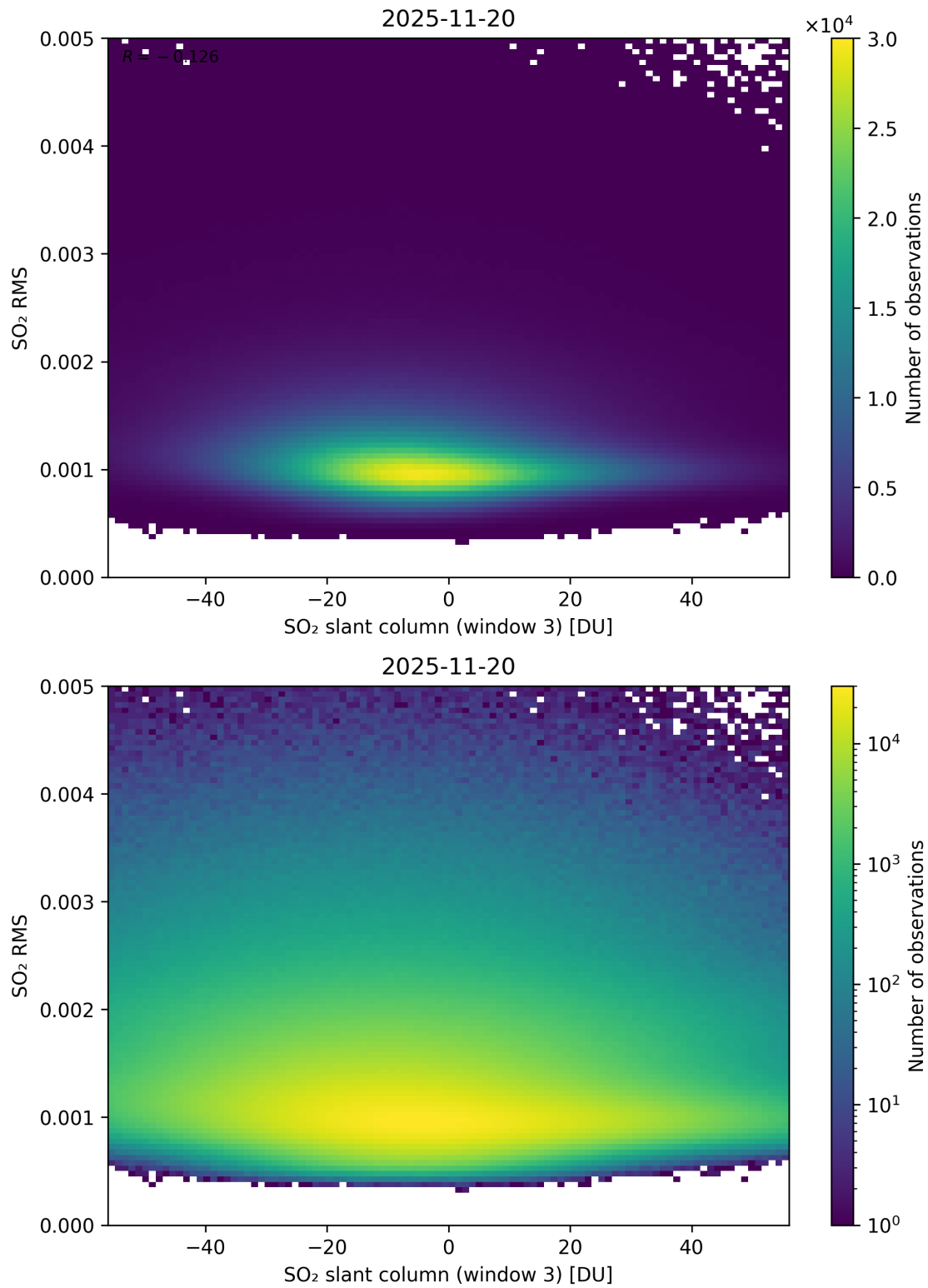
Figure 306: Scatter density plot of “SO 2 slant column (window 3)” against “SO 2 RMS” for 2025-11-19 to 2025-11-21.
