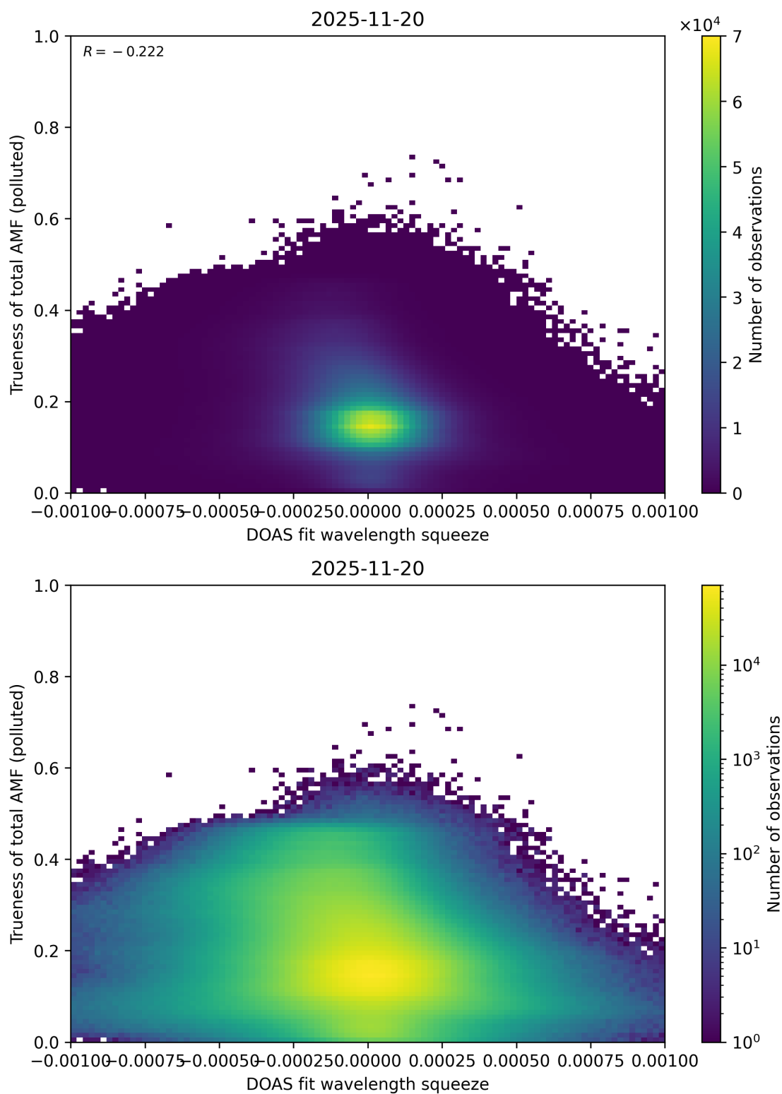
Figure 146: Scatter density plot of “DOAS fit wavelength squeeze” against “Trueness of total AMF (polluted)” for 2025-11-19 to 2025-11-21.
