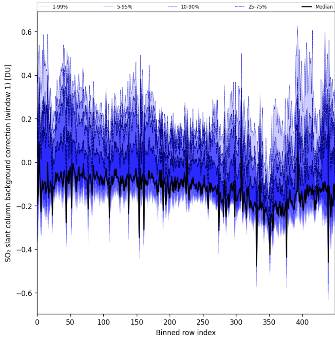
Figure 92: Along track statistics of “SO 2 slant column background correction (window 1)” for 2025-11-19 to 2025-11-21
