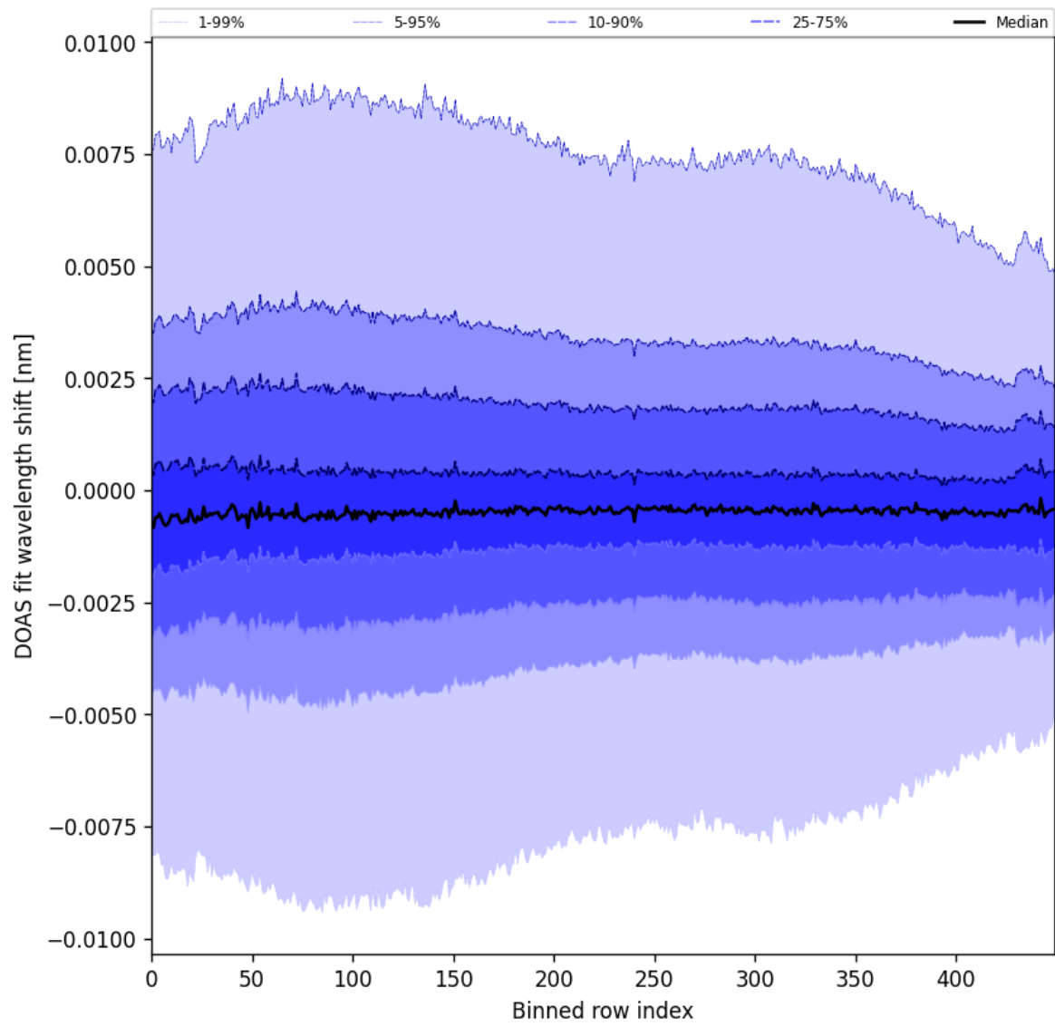
Figure 102: Along track statistics of “DOAS fit wavelength shift” for 2025-11-19 to 2025-11-21
