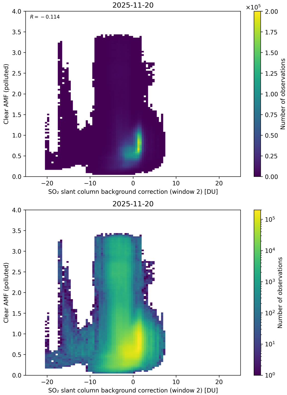
Figure 126: Scatter density plot of “SO 2 slant column background correction (window 2)” against “Clear AMF (polluted)” for 2025-11-19 to 2025-11-21.
