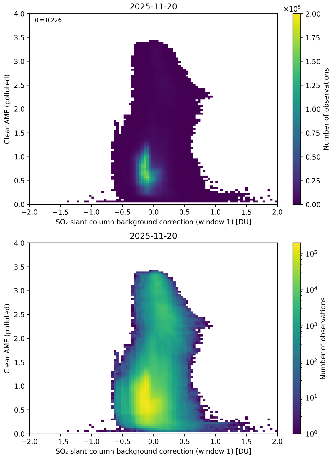
Figure 114: Scatter density plot of “SO 2 slant column background correction (window 1)” against “Clear AMF (polluted)” for 2025-11-19 to 2025-11-21.
