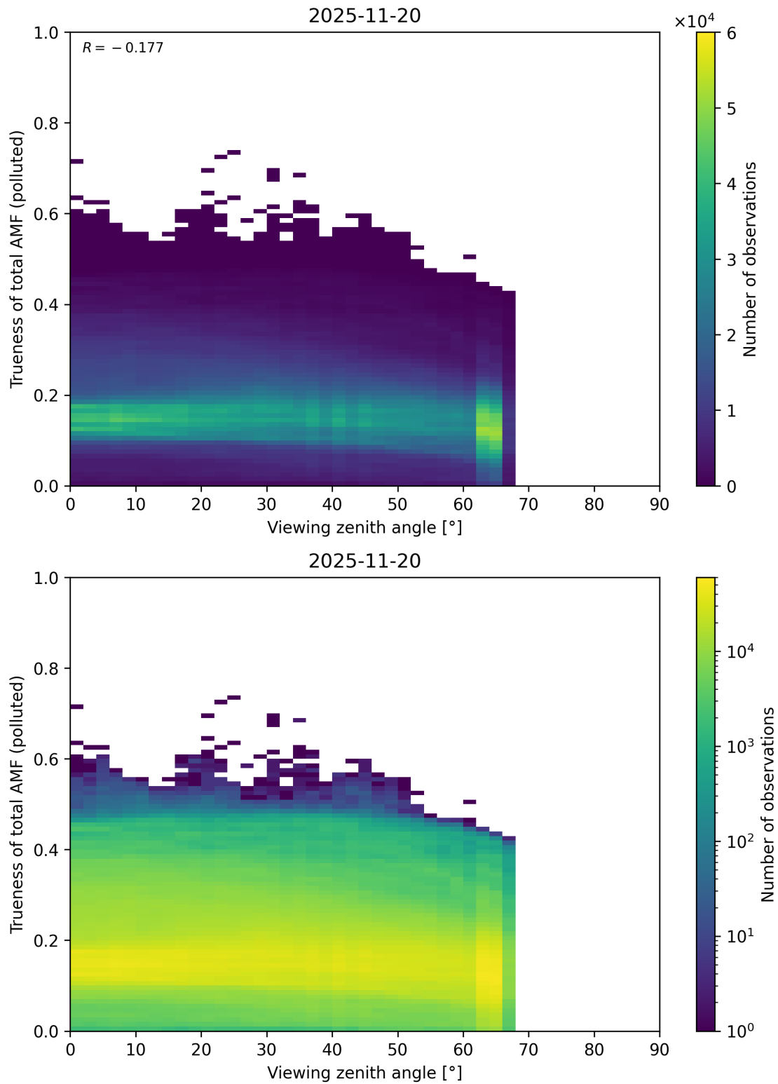
Figure 382: Scatter density plot of “Viewing zenith angle” against “Trueness of total AMF (polluted)” for 2025-11-19 to 2025-11-21.
