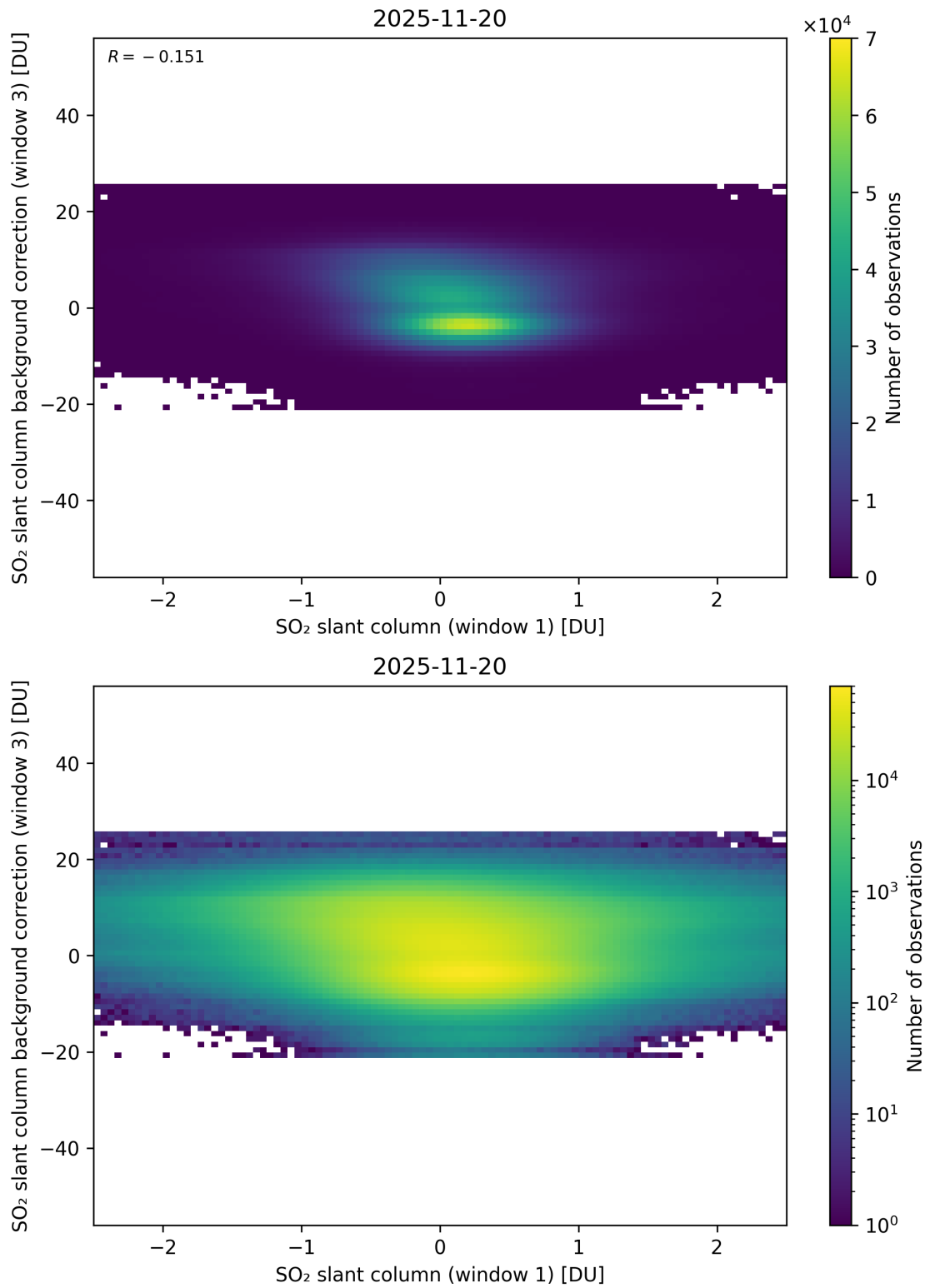
Figure 264: Scatter density plot of “SO 2 slant column (window 1)” against “SO 2 slant column background correction (window 3)” for 2025-11-19 to 2025-11-21.
