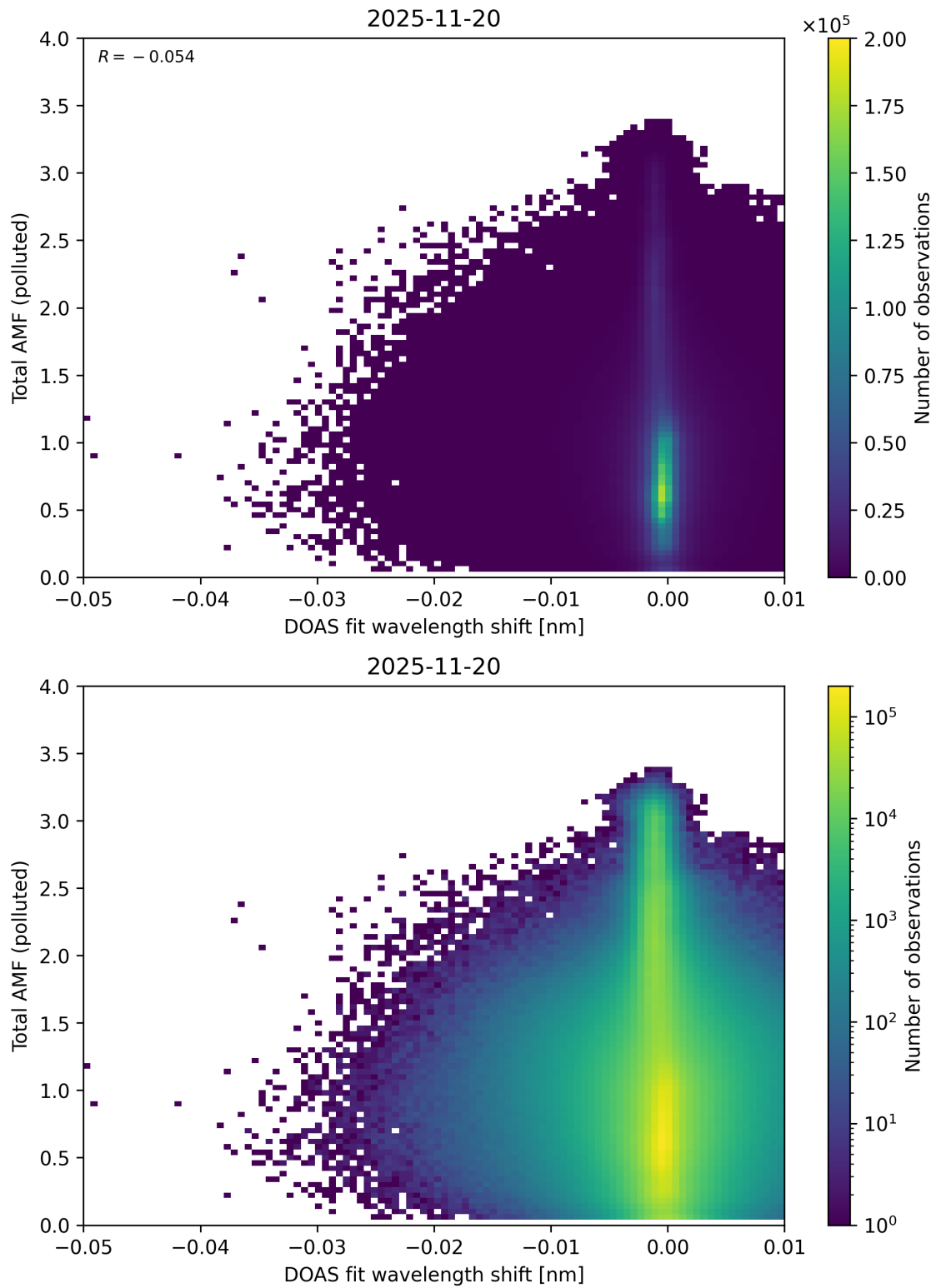
Figure 141: Scatter density plot of “DOAS fit wavelength shift” against “Total AMF (polluted)” for 2025-11-19 to 2025-11-21.
