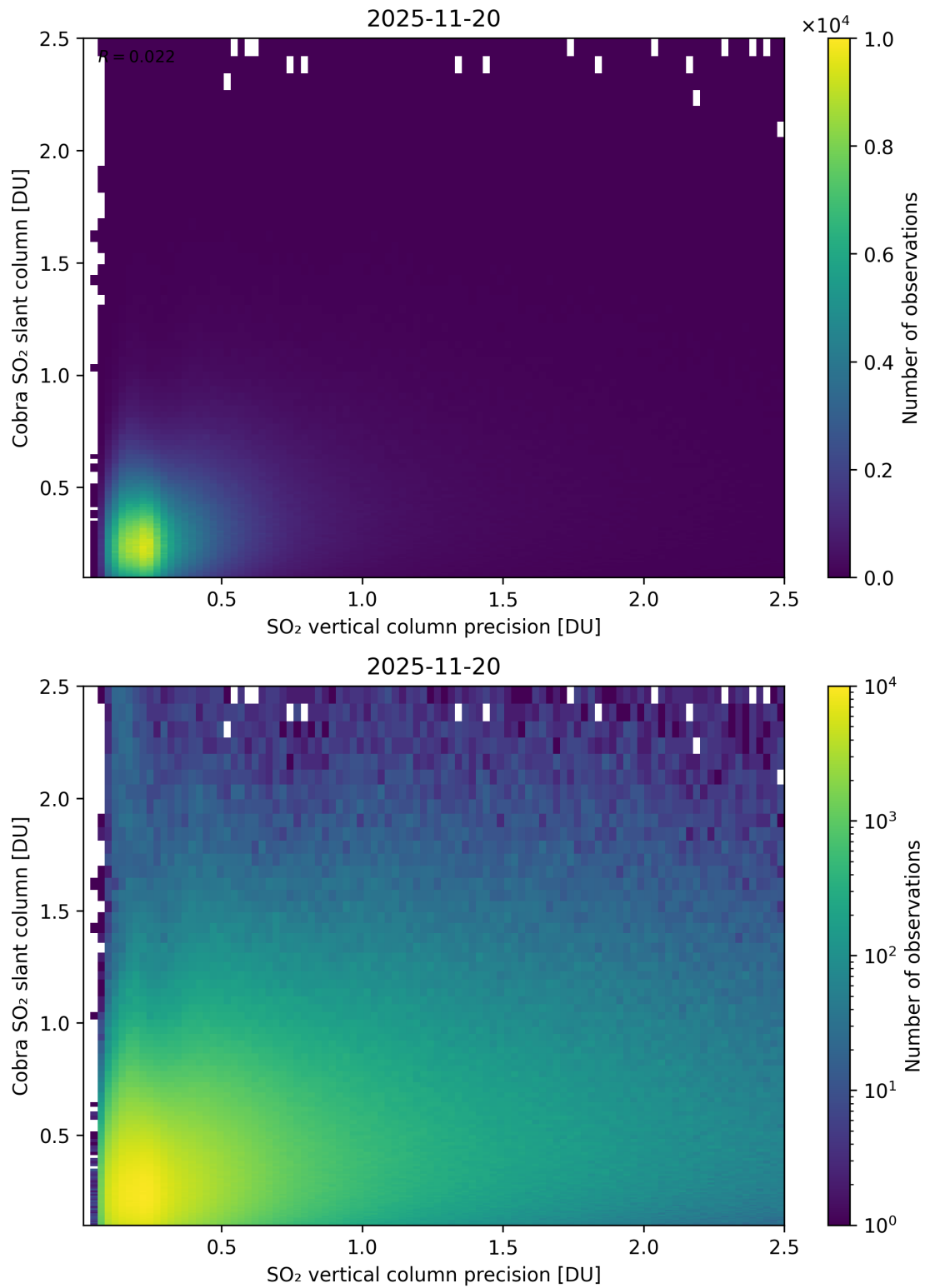
Figure 336: Scatter density plot of “SO 2 vertical column precision” against “Cobra SO 2 slant column” for 2025-11-19 to 2025-11-21.
