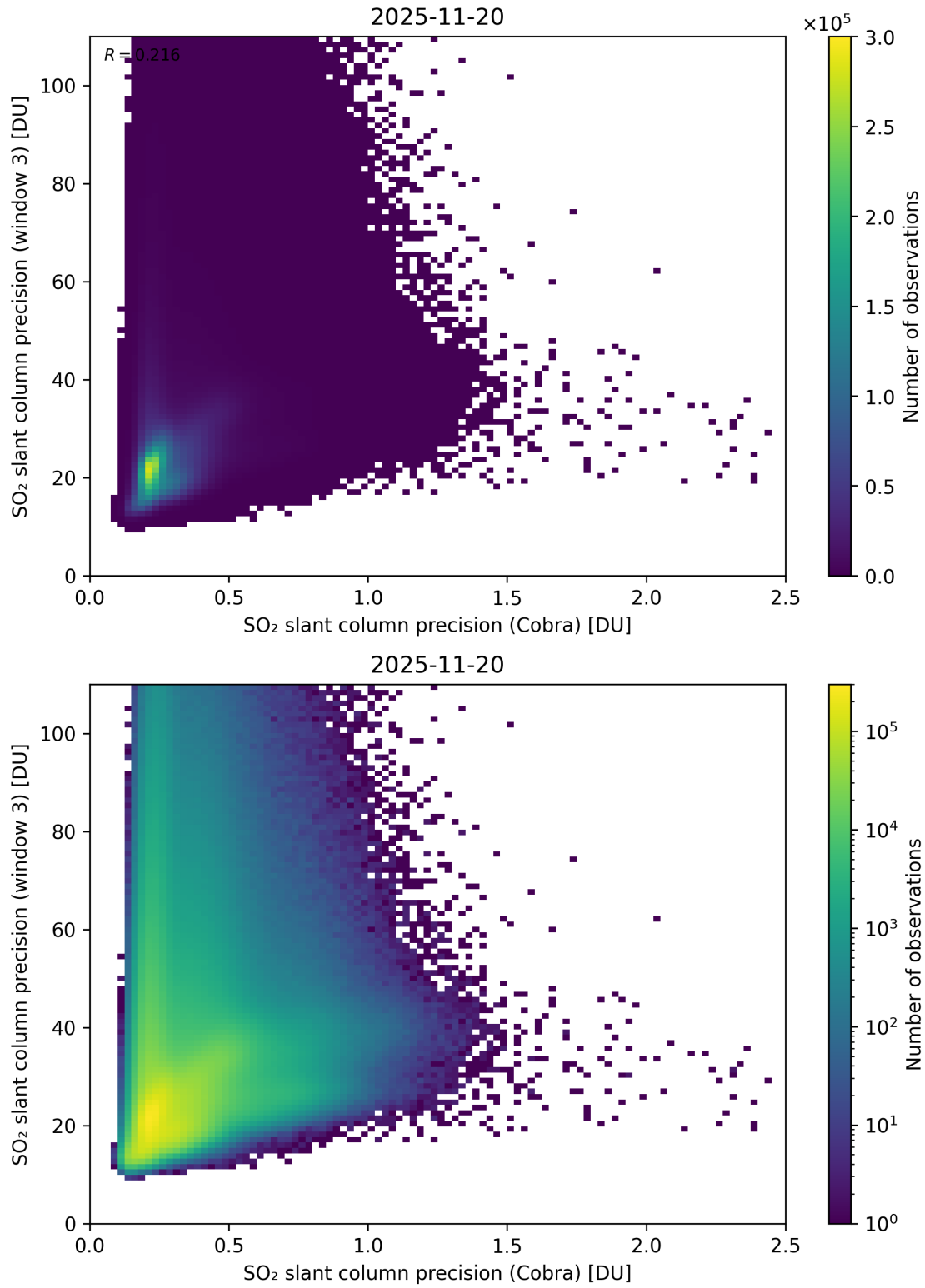
Figure 212: Scatter density plot of “SO 2 slant column precision (Cobra)” against “SO 2 slant column precision (window 3)” for 2025-11-19 to 2025-11-21.
