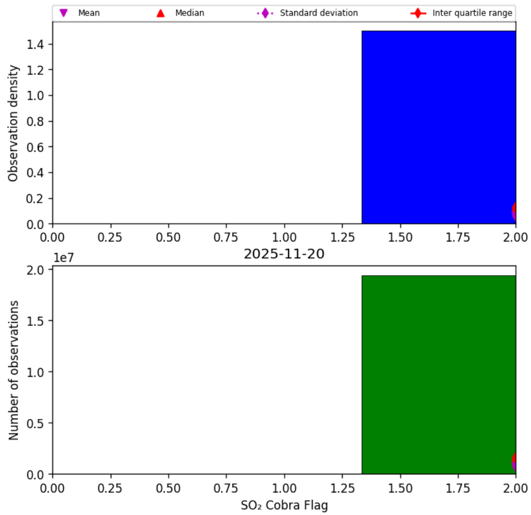
Figure 75: Histogram of “SO 2 Cobra Flag” for 2025-11-19 to 2025-11-21
