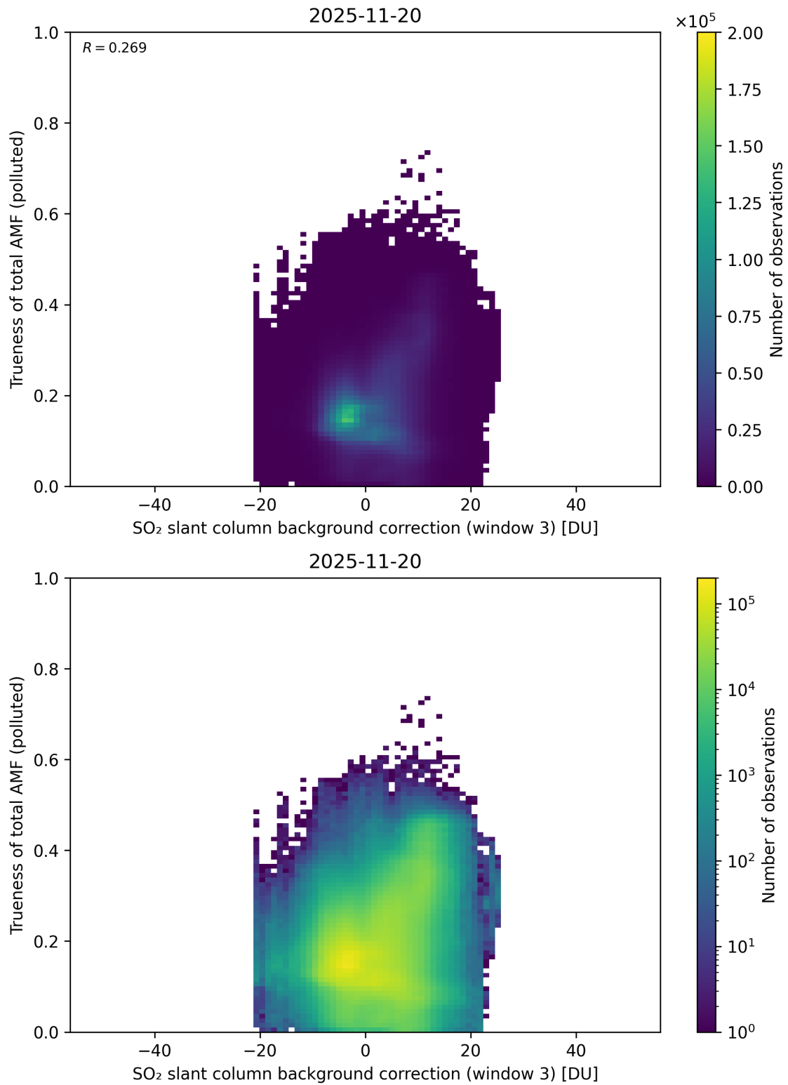
Figure 137: Scatter density plot of “SO 2 slant column background correction (window 3)” against “Trueness of total AMF (polluted)” for 2025-11-19 to 2025-11-21.
