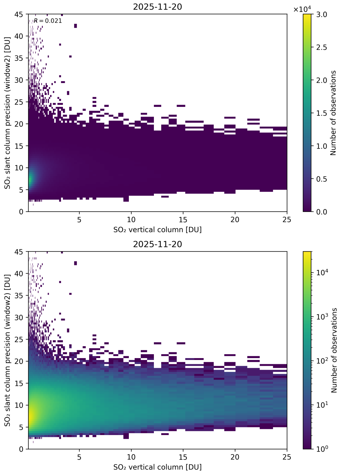
Figure 356: Scatter density plot of “SO 2 vertical column” against “SO 2 slant column precision (window2)” for 2025-11-19 to 2025-11-21.
