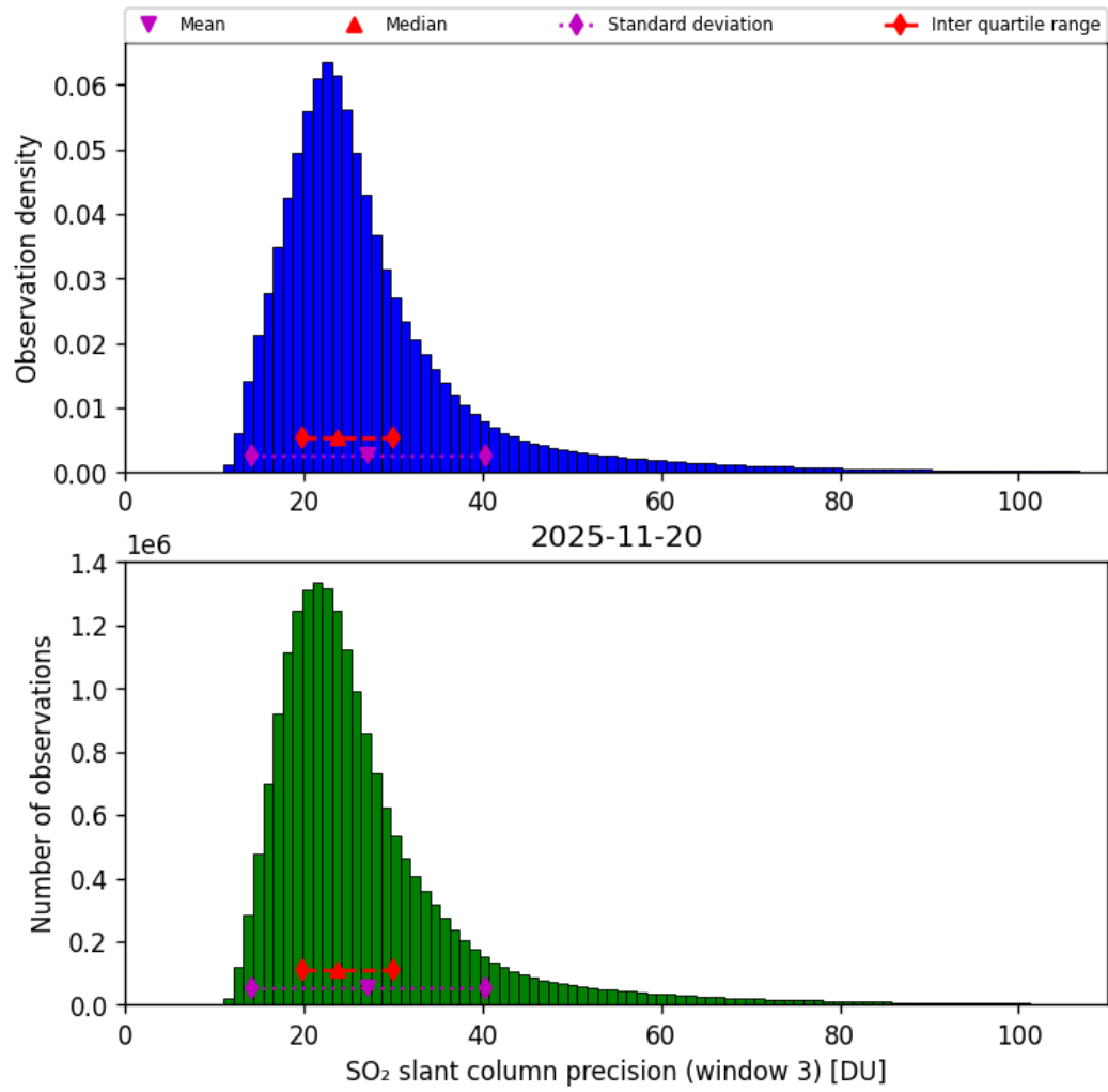
Figure 72: Histogram of “SO 2 slant column precision (window 3)” for 2025-11-19 to 2025-11-21
