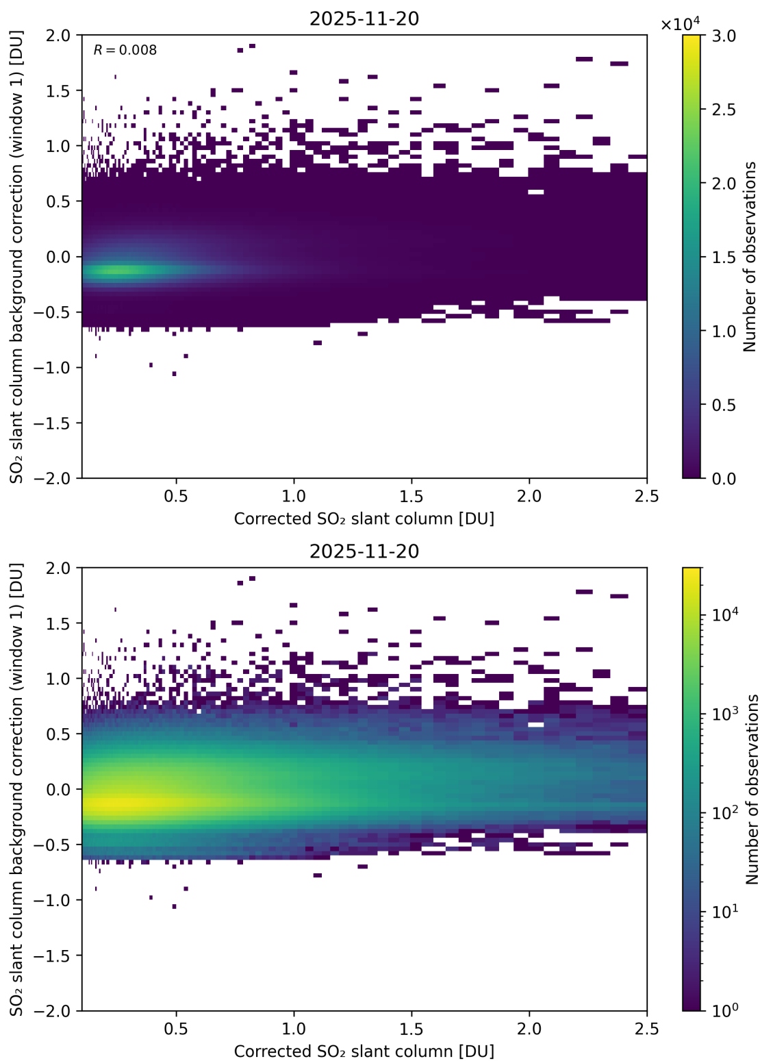
Figure 226: Scatter density plot of “Corrected SO 2 slant column” against “SO 2 slant column background correction (window 1)” for 2025-11-19 to 2025-11-21.
