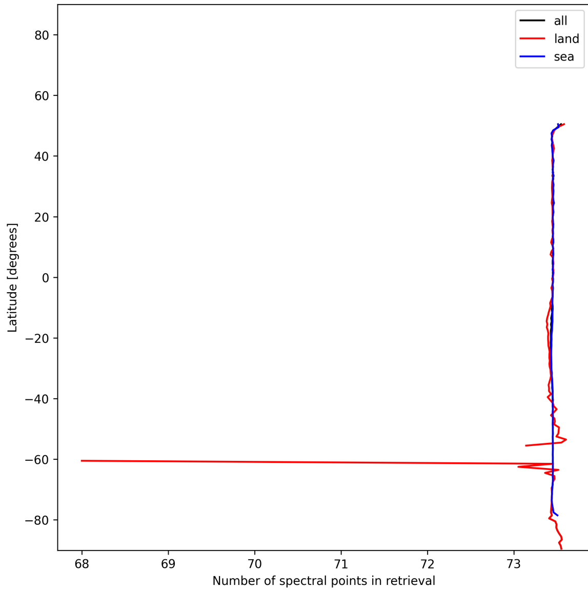
Figure 56: Zonal average of “Number of spectral points in retrieval” for 2025-11-19 to 2025-11-21.
