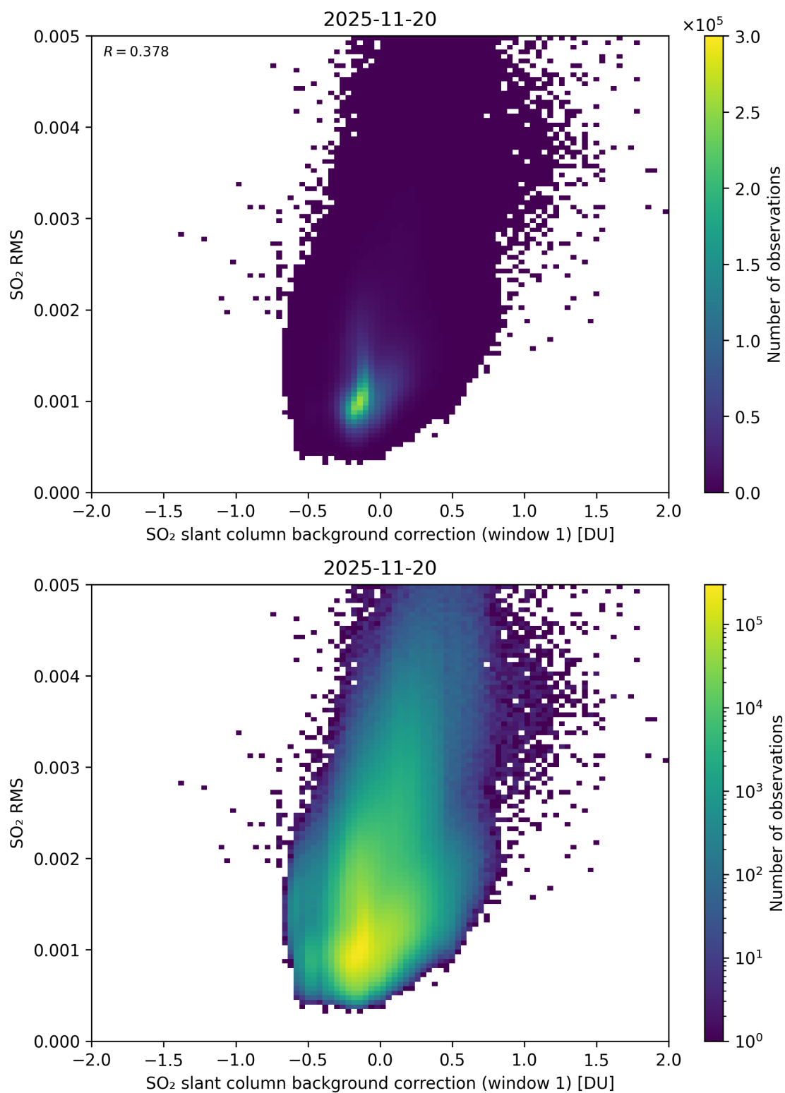
Figure 113: Scatter density plot of “SO 2 slant column background correction (window 1)” against “SO 2 RMS” for 2025-11-19 to 2025-11-21.
