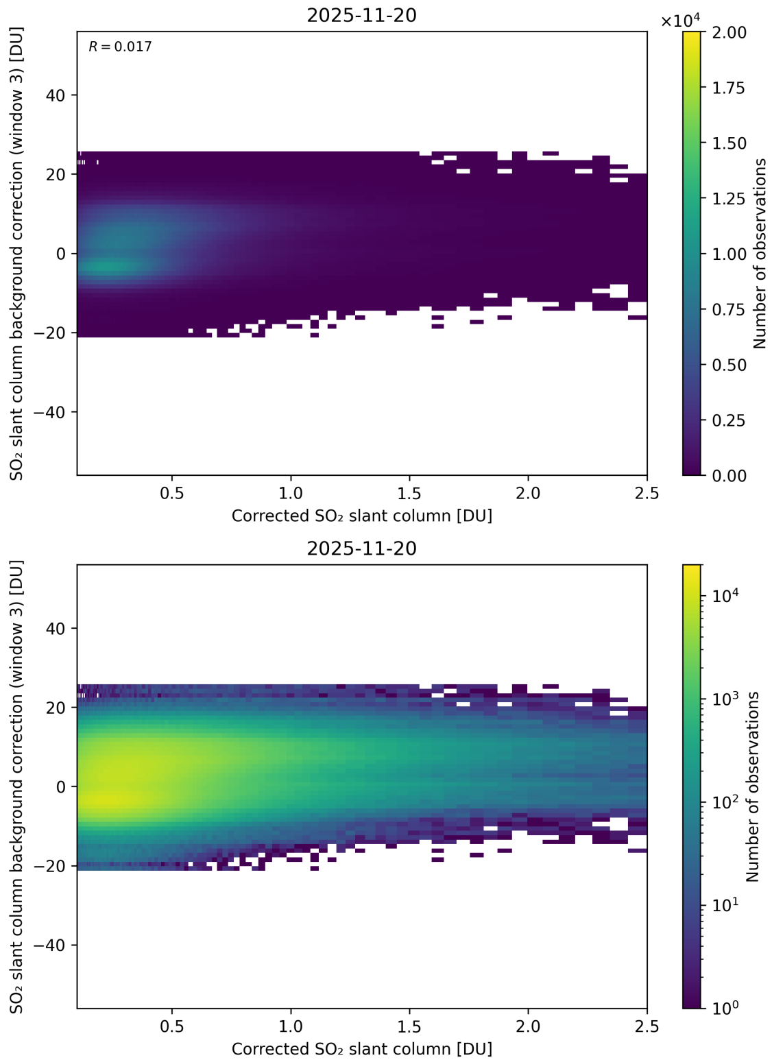
Figure 228: Scatter density plot of “Corrected SO 2 slant column” against “SO 2 slant column background correction (window 3)” for 2025-11-19 to 2025-11-21.
