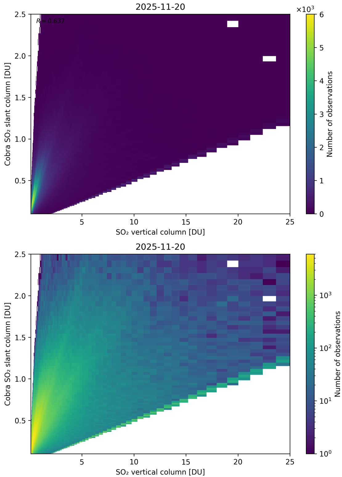
Figure 349: Scatter density plot of “SO 2 vertical column” against “Cobra SO 2 slant column” for 2025-11-19 to 2025-11-21.
