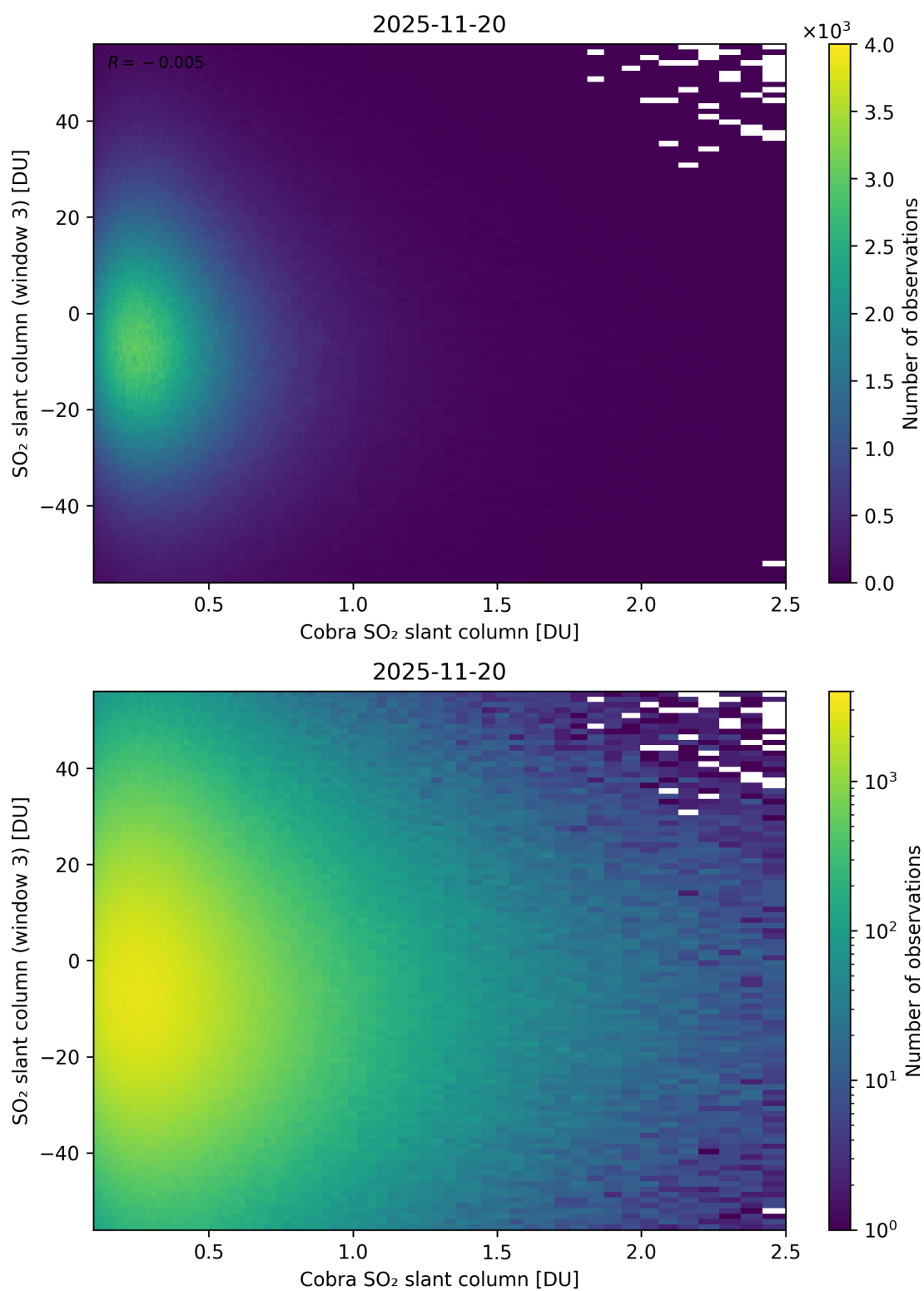
Figure 222: Scatter density plot of “Cobra SO 2 slant column” against “SO 2 slant column (window 3)” for 2025-11-19 to 2025-11-21.
