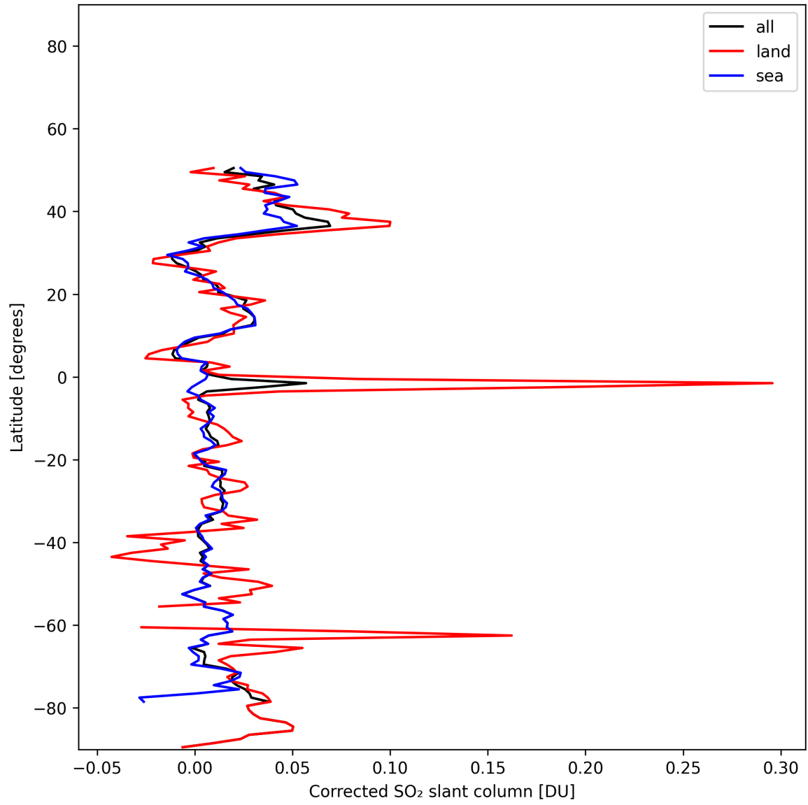
Figure 34: Zonal average of “Corrected SO 2 slant column” for 2025-11-19 to 2025-11-21.
