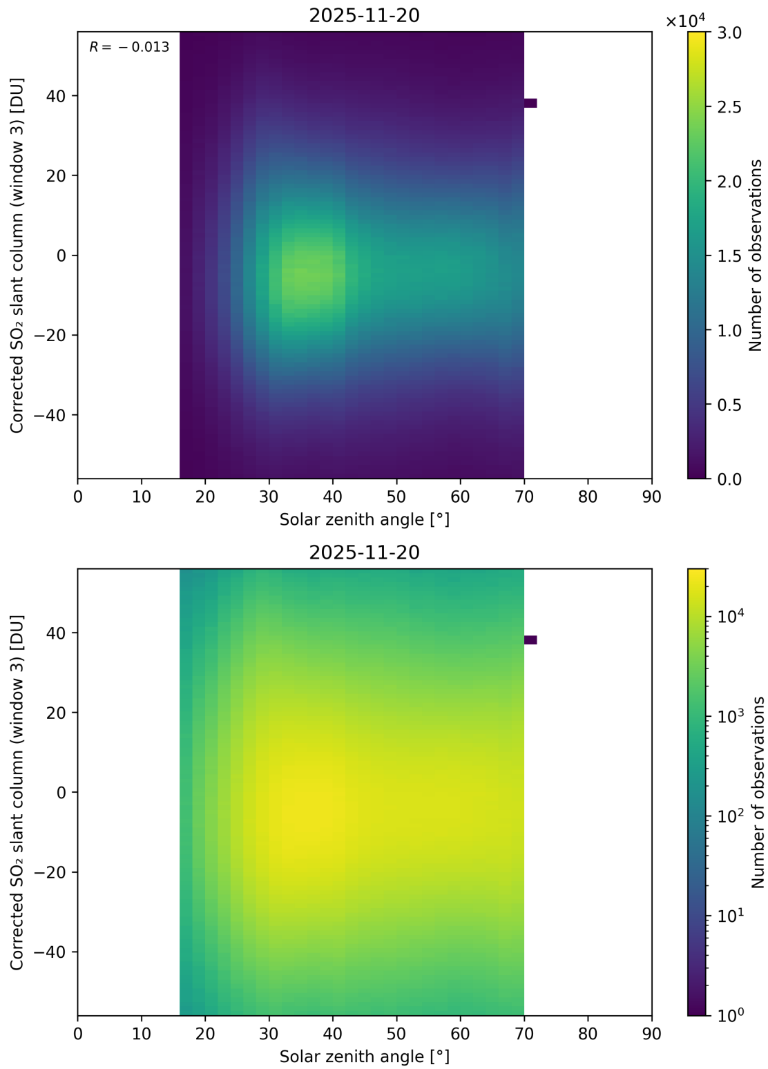
Figure 183: Scatter density plot of “Solar zenith angle” against “Corrected SO 2 slant column (window 3)” for 2025-11-19 to 2025-11-21.
