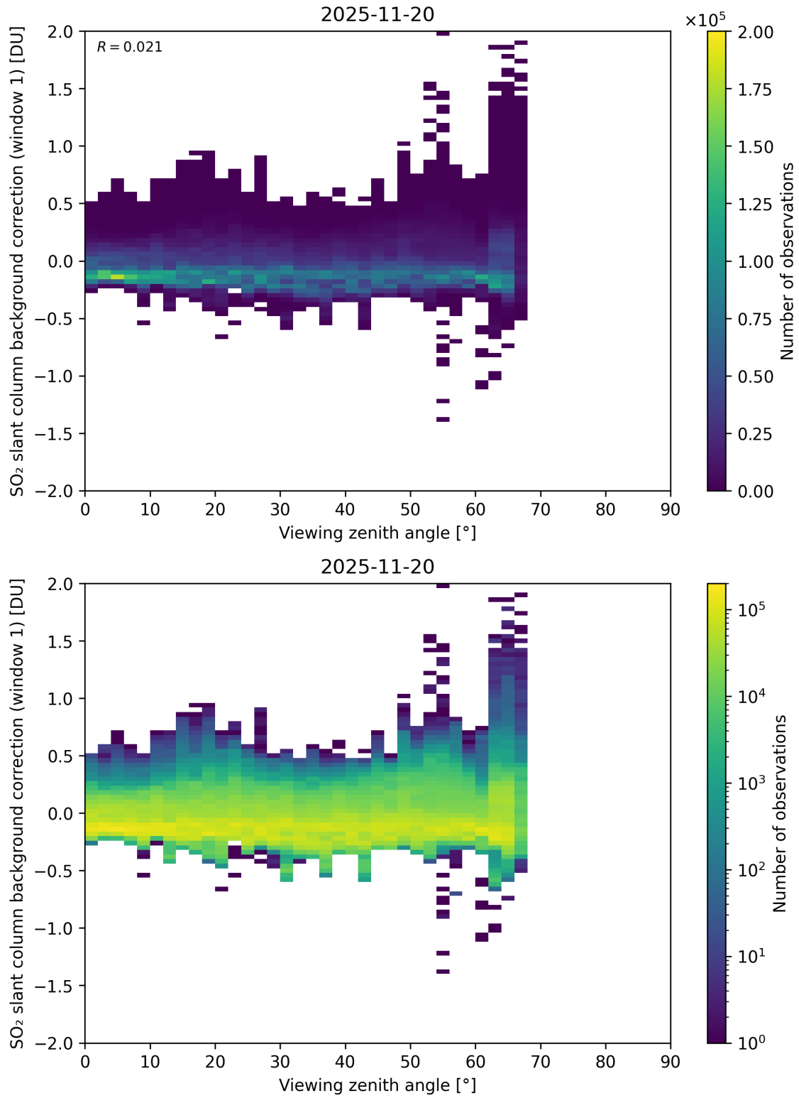
Figure 362: Scatter density plot of “Viewing zenith angle” against “SO 2 slant column background correction (window 1)” for 2025-11-19 to 2025-11-21.
