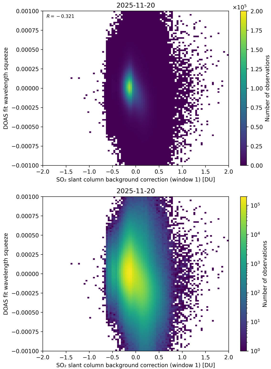
Figure 112: Scatter density plot of “SO 2 slant column background correction (window 1)” against “DOAS fit wavelength squeeze” for 2025-11-19 to 2025-11-21.
