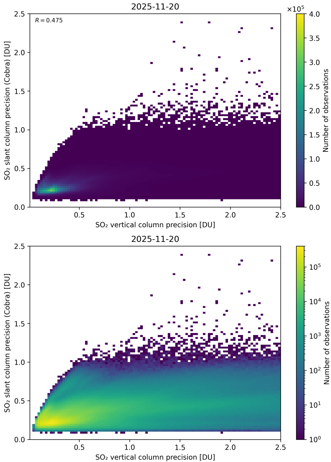
Figure 337: Scatter density plot of “SO 2 vertical column precision” against “SO 2 slant column precision (Cobra)” for 2025-11-19 to 2025-11-21.
