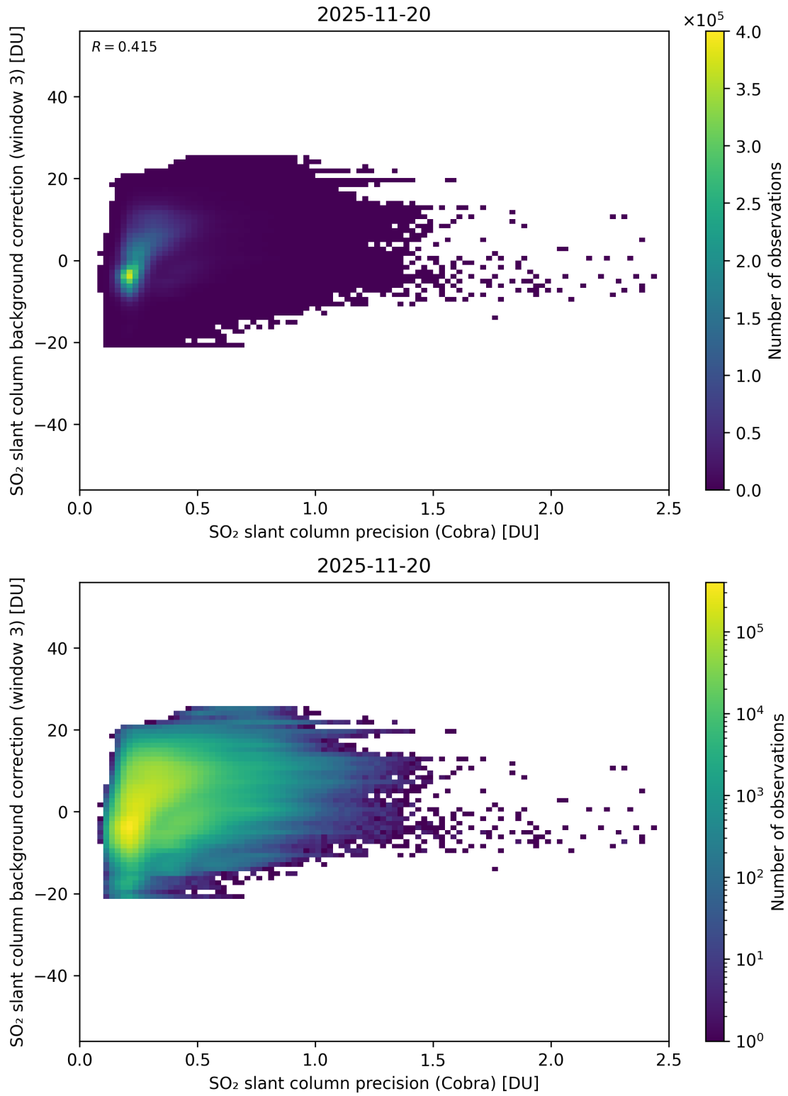
Figure 201: Scatter density plot of “SO 2 slant column precision (Cobra)” against “SO 2 slant column background correction (window 3)” for 2025-11-19 to 2025-11-21.
