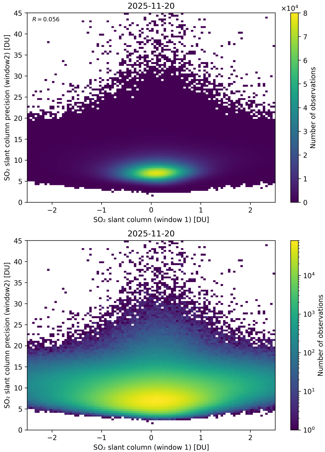
Figure 286: Scatter density plot of “SO 2 slant column (window 1)” against “SO 2 slant column precision (window2)” for 2025-11-19 to 2025-11-21.
