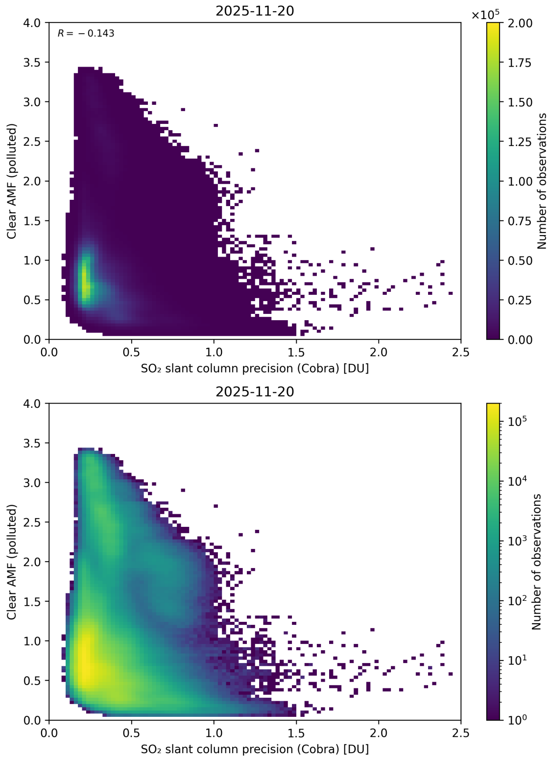
Figure 205: Scatter density plot of “SO 2 slant column precision (Cobra)” against “Clear AMF (polluted)” for 2025-11-19 to 2025-11-21.
