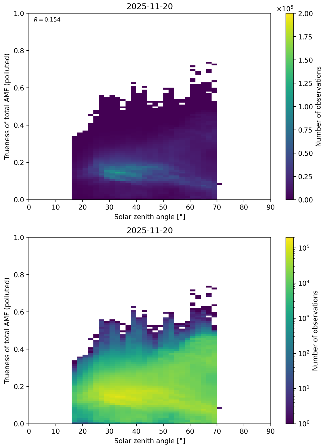
Figure 190: Scatter density plot of “Solar zenith angle” against “Trueness of total AMF (polluted)” for 2025-11-19 to 2025-11-21.
