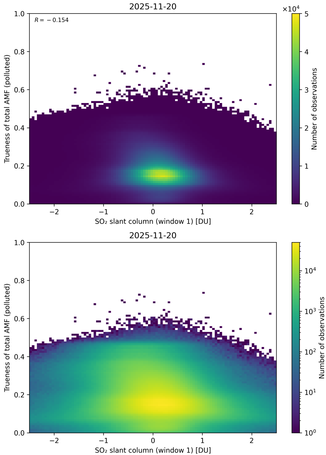
Figure 290: Scatter density plot of “SO 2 slant column (window 1)” against “Trueness of total AMF (polluted)” for 2025-11-19 to 2025-11-21.
