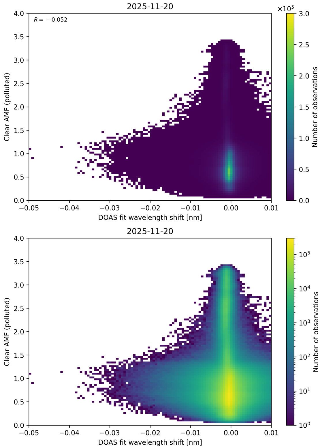
Figure 140: Scatter density plot of “DOAS fit wavelength shift” against “Clear AMF (polluted)” for 2025-11-19 to 2025-11-21.
