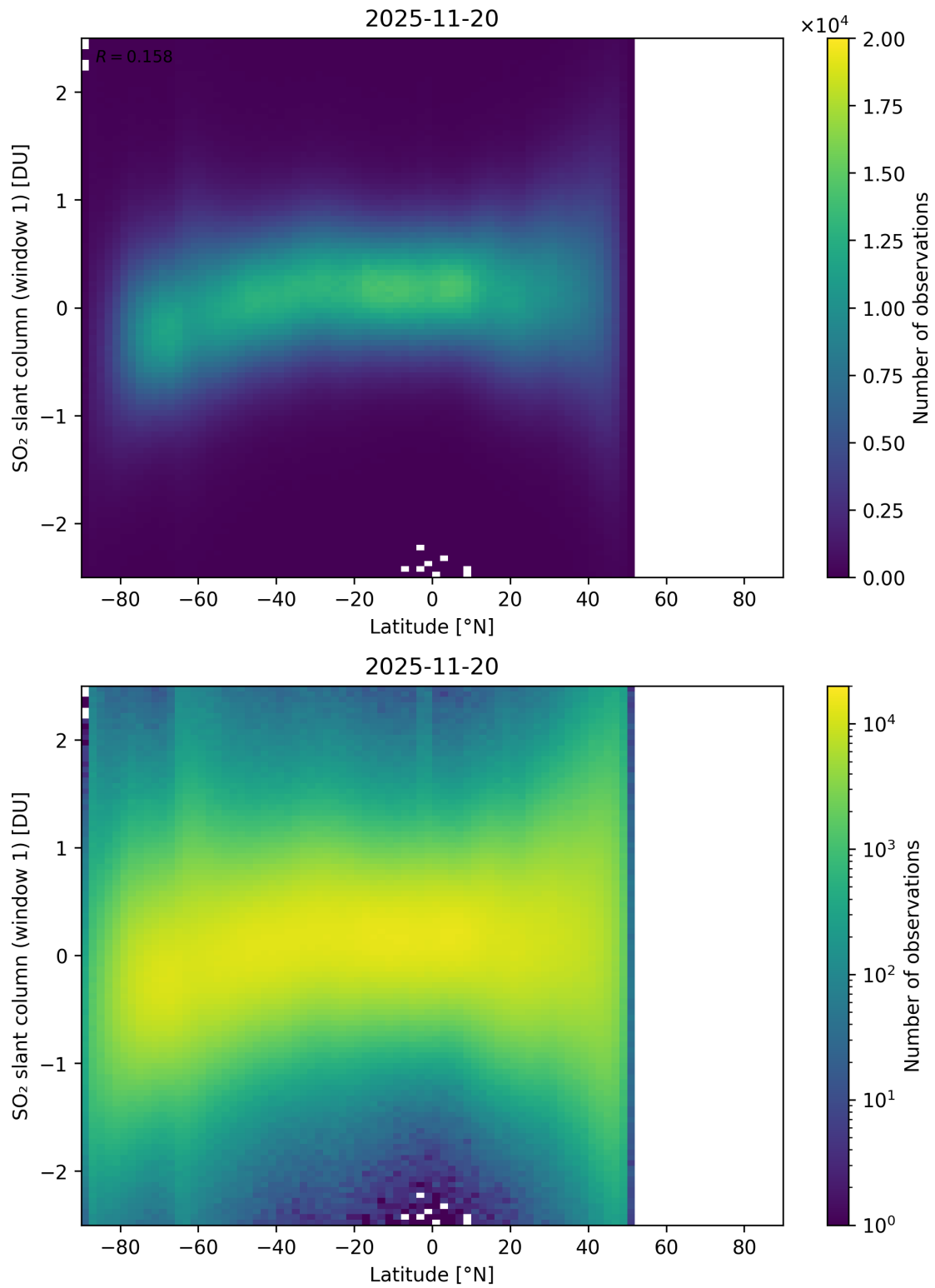
Figure 162: Scatter density plot of “Latitude” against “SO 2 slant column (window 1)” for 2025-11-19 to 2025-11-21.
