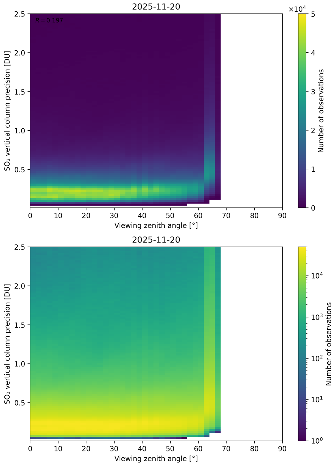
Figure 384: Scatter density plot of “Viewing zenith angle” against “SO 2 vertical column precision” for 2025-11-19 to 2025-11-21.
