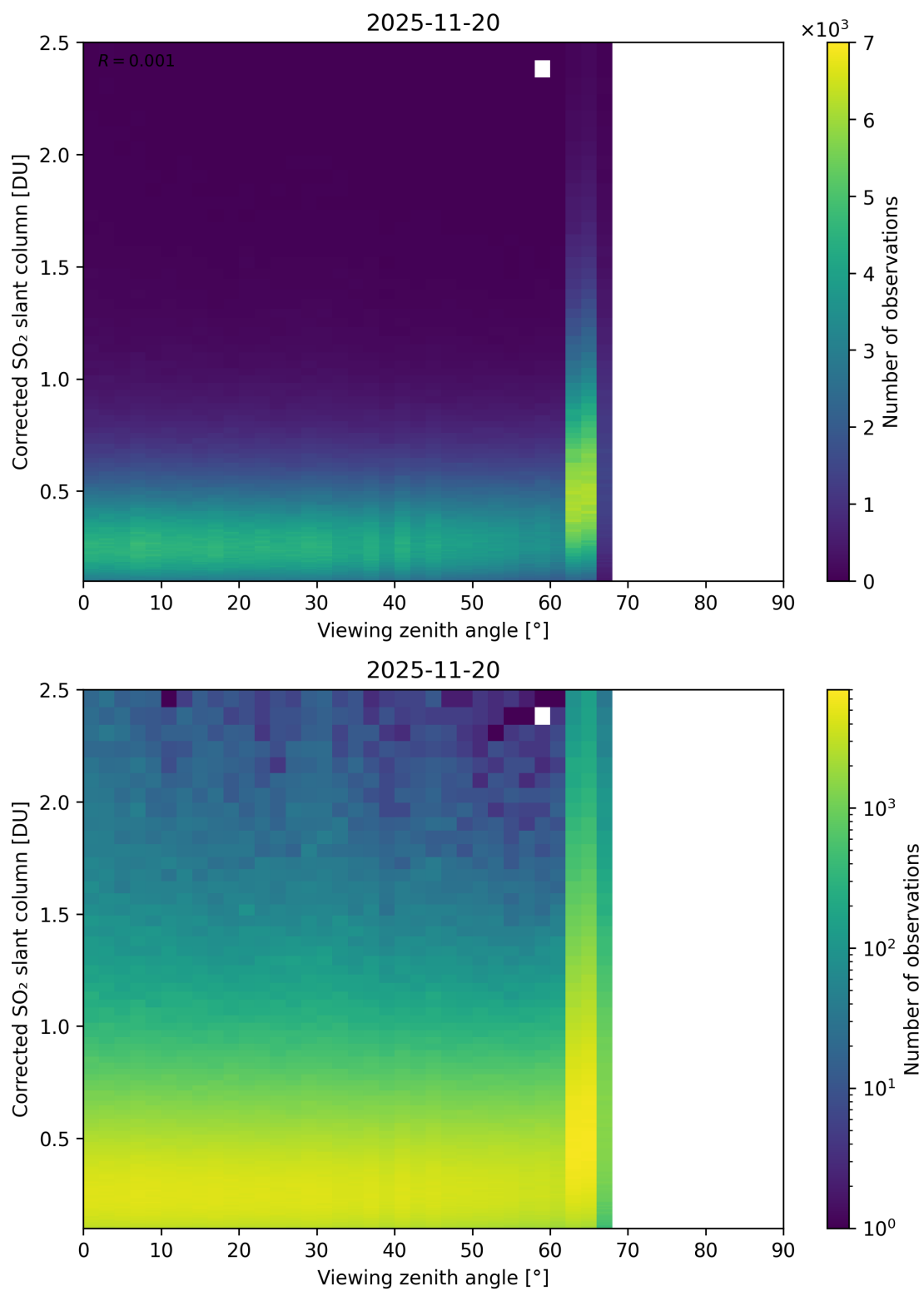
Figure 373: Scatter density plot of “Viewing zenith angle” against “Corrected SO 2 slant column” for 2025-11-19 to 2025-11-21.
