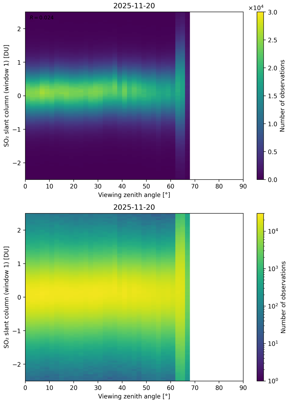
Figure 376: Scatter density plot of “Viewing zenith angle” against “SO 2 slant column (window 1)” for 2025-11-19 to 2025-11-21.
