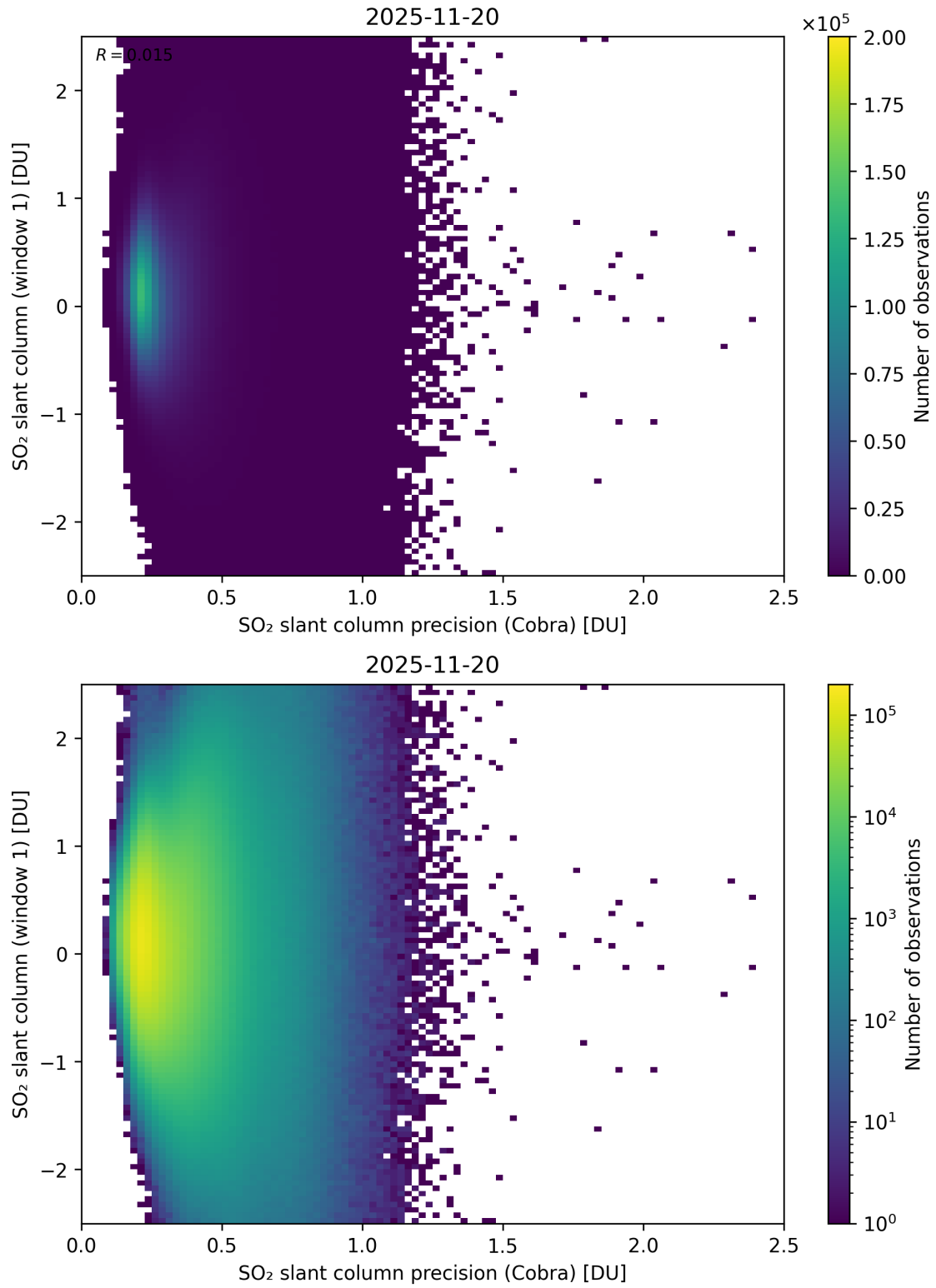
Figure 208: Scatter density plot of “SO 2 slant column precision (Cobra)” against “SO 2 slant column (window 1)” for 2025-11-19 to 2025-11-21.
