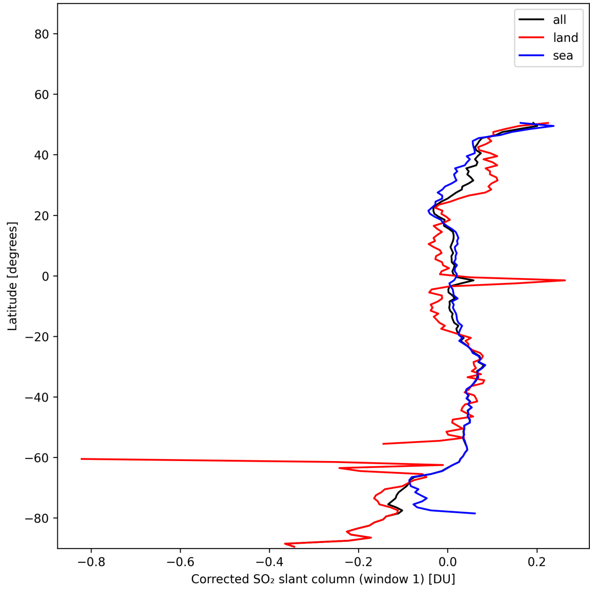
Figure 39: Zonal average of “Corrected SO 2 slant column (window 1)” for 2025-11-19 to 2025-11-21.
