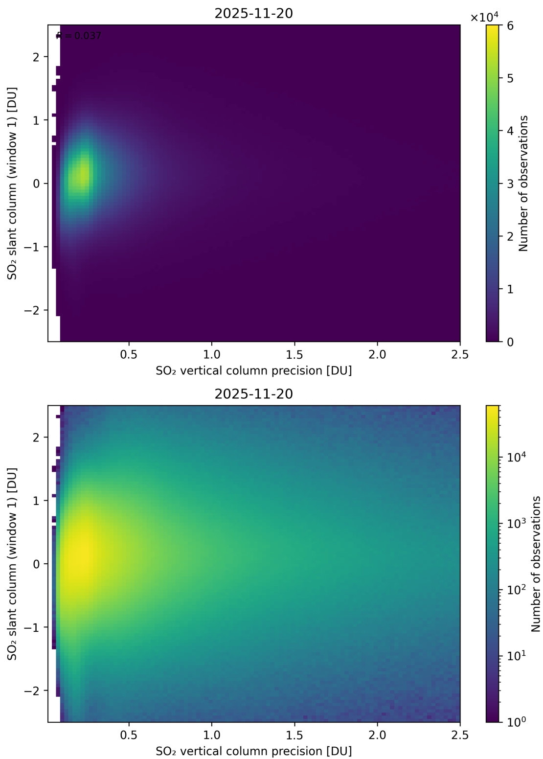
Figure 341: Scatter density plot of “SO 2 vertical column precision” against “SO 2 slant column (window 1)” for 2025-11-19 to 2025-11-21.
