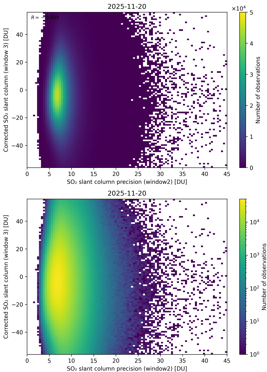
Figure 298: Scatter density plot of “SO 2 slant column precision (window2)” against “Corrected SO 2 slant column (window 3)” for 2025-11-19 to 2025-11-21.
