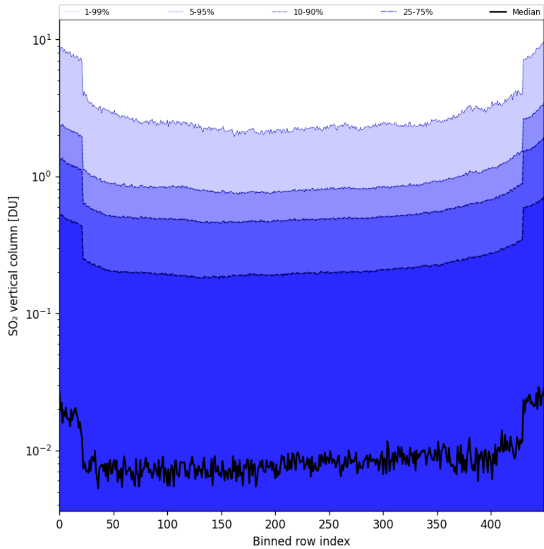
Figure 84: Along track statistics of “SO 2 vertical column” for 2025-11-19 to 2025-11-21
