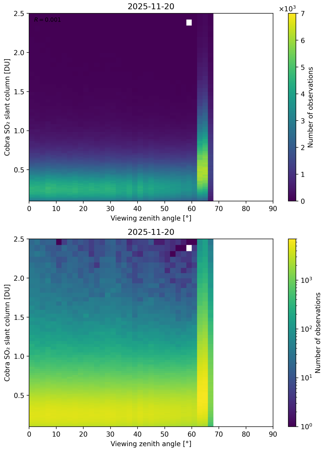
Figure 371: Scatter density plot of “Viewing zenith angle” against “Cobra SO 2 slant column” for 2025-11-19 to 2025-11-21.
