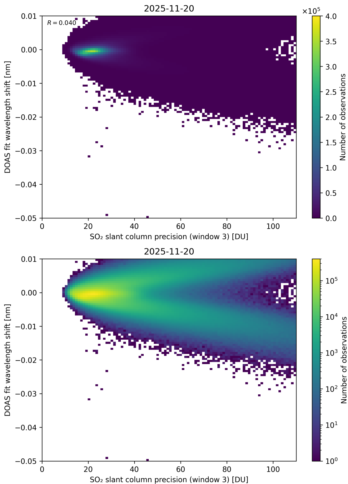
Figure 308: Scatter density plot of “SO 2 slant column precision (window 3)” against “DOAS fit wavelength shift” for 2025-11-19 to 2025-11-21.
