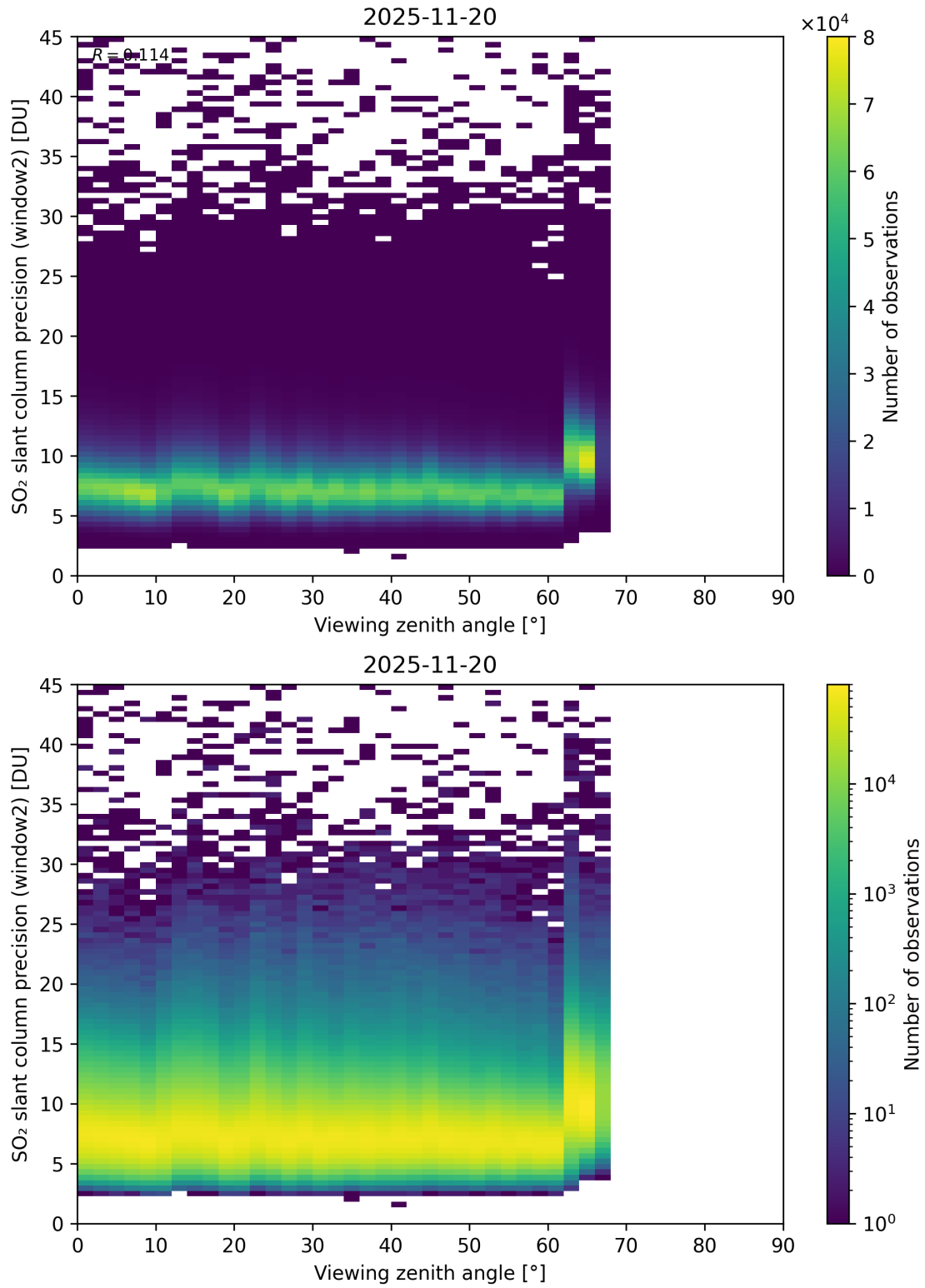
Figure 378: Scatter density plot of “Viewing zenith angle” against “SO 2 slant column precision (window2)” for 2025-11-19 to 2025-11-21.
