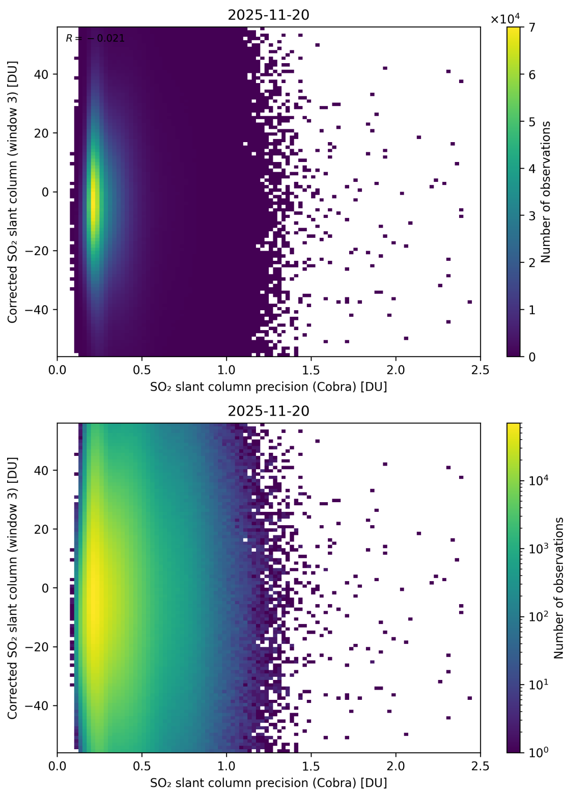
Figure 207: Scatter density plot of “SO 2 slant column precision (Cobra)” against “Corrected SO 2 slant column (window 3)” for 2025-11-19 to 2025-11-21.
