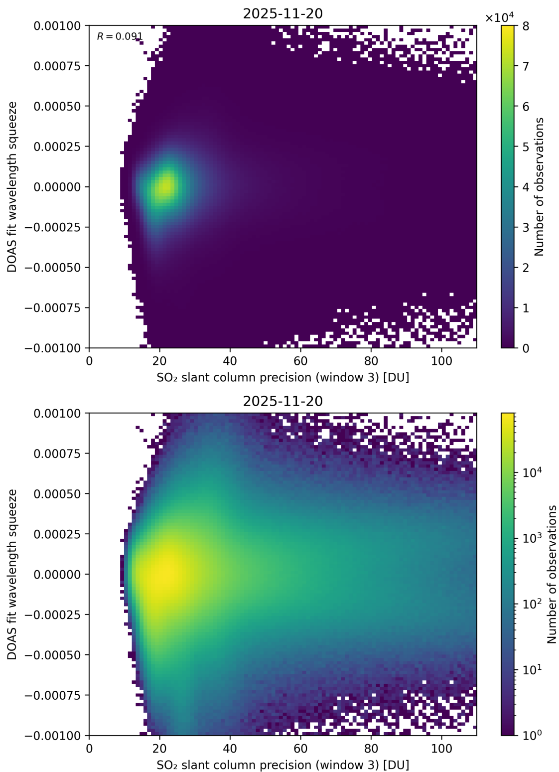
Figure 309: Scatter density plot of “SO 2 slant column precision (window 3)” against “DOAS fit wavelength squeeze” for 2025-11-19 to 2025-11-21.
