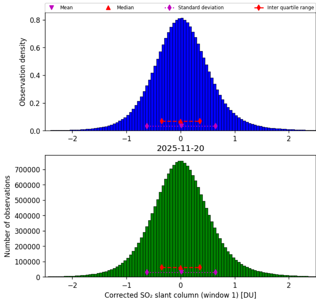
Figure 65: Histogram of “Corrected SO 2 slant column (window 1)” for 2025-11-19 to 2025-11-21
