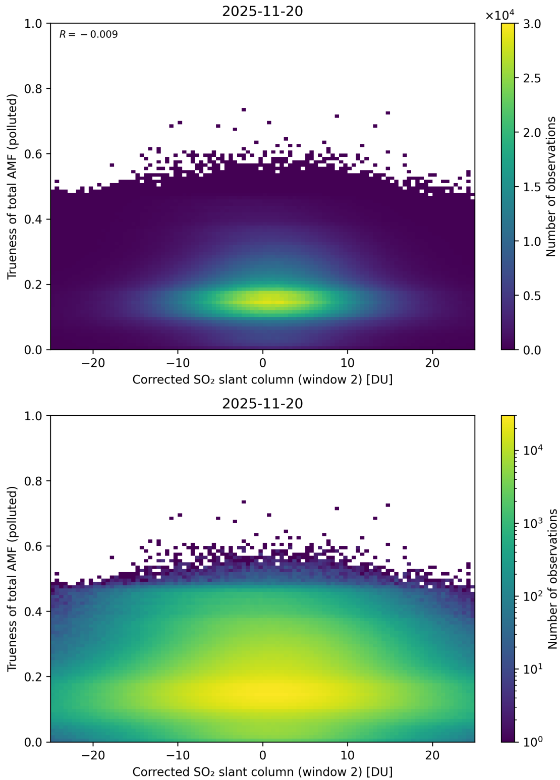
Figure 254: Scatter density plot of “Corrected SO 2 slant column (window 2)” against “Trueness of total AMF (polluted)” for 2025-11-19 to 2025-11-21.
