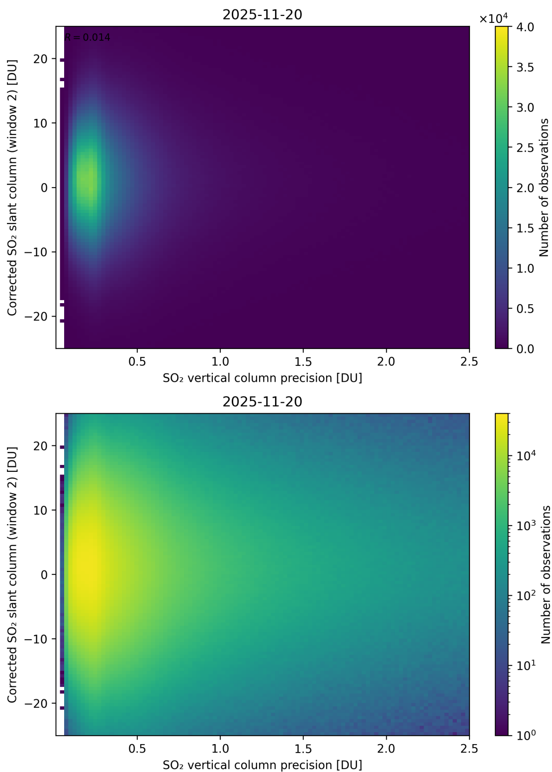
Figure 339: Scatter density plot of “SO 2 vertical column precision” against “Corrected SO 2 slant column (window 2)” for 2025-11-19 to 2025-11-21.
