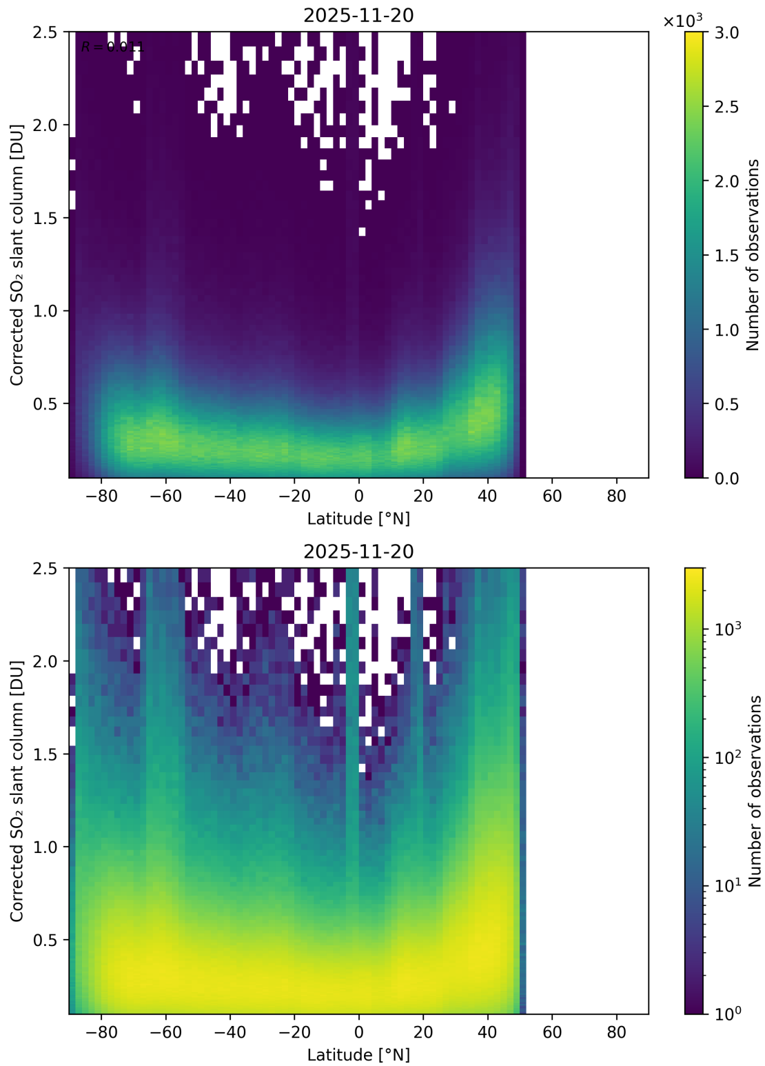
Figure 159: Scatter density plot of “Latitude” against “Corrected SO 2 slant column” for 2025-11-19 to 2025-11-21.
