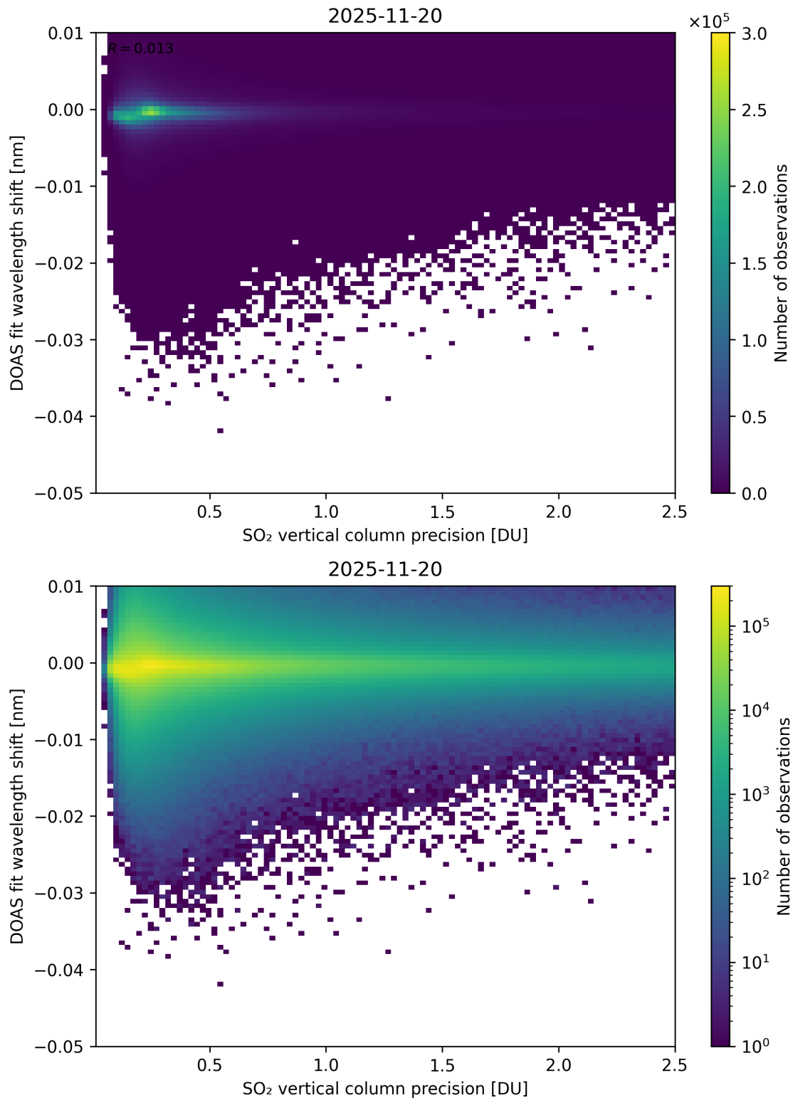
Figure 332: Scatter density plot of “SO 2 vertical column precision” against “DOAS fit wavelength shift” for 2025-11-19 to 2025-11-21.
