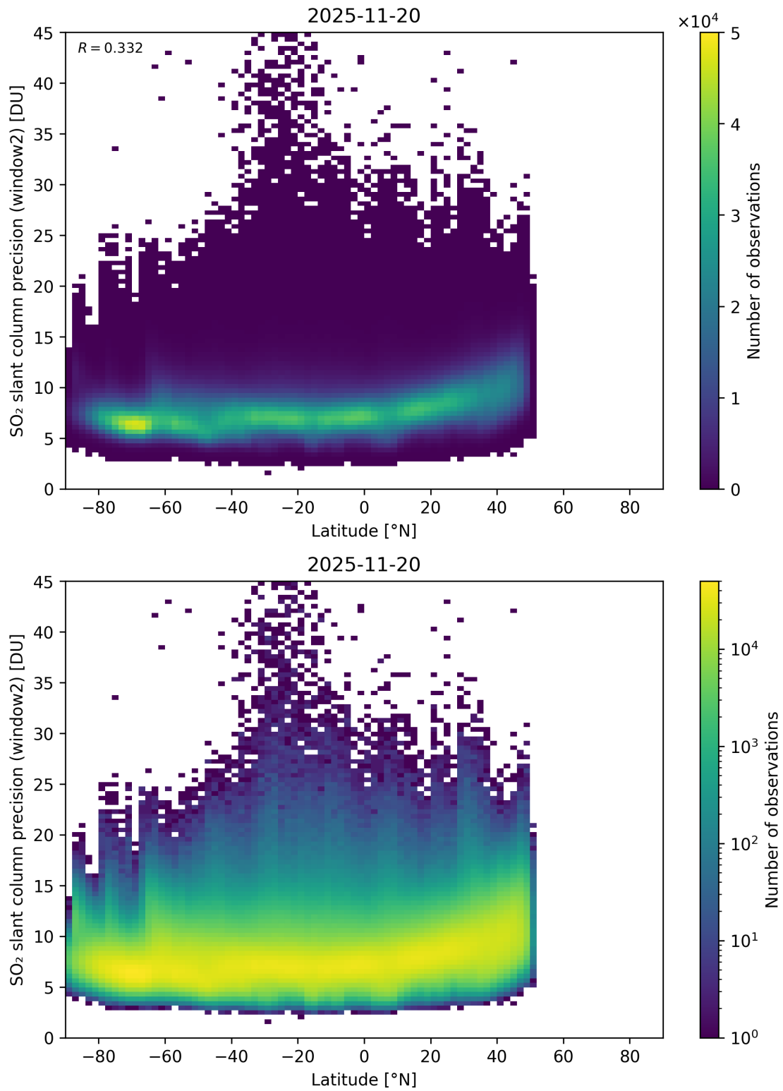
Figure 164: Scatter density plot of “Latitude” against “SO 2 slant column precision (window2)” for 2025-11-19 to 2025-11-21.
