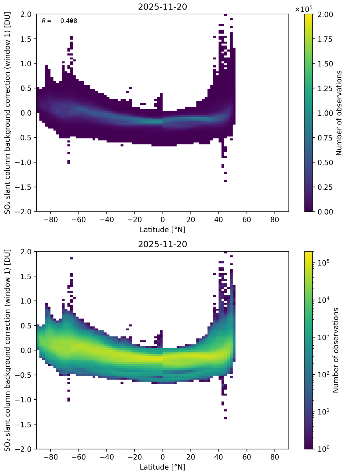
Figure 150: Scatter density plot of “Latitude” against “SO 2 slant column background correction (window 1)” for 2025-11-19 to 2025-11-21.
