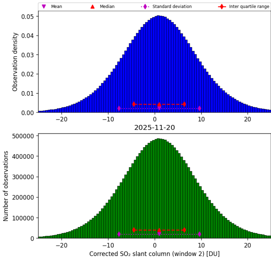
Figure 69: Histogram of “Corrected SO 2 slant column (window 2)” for 2025-11-19 to 2025-11-21
