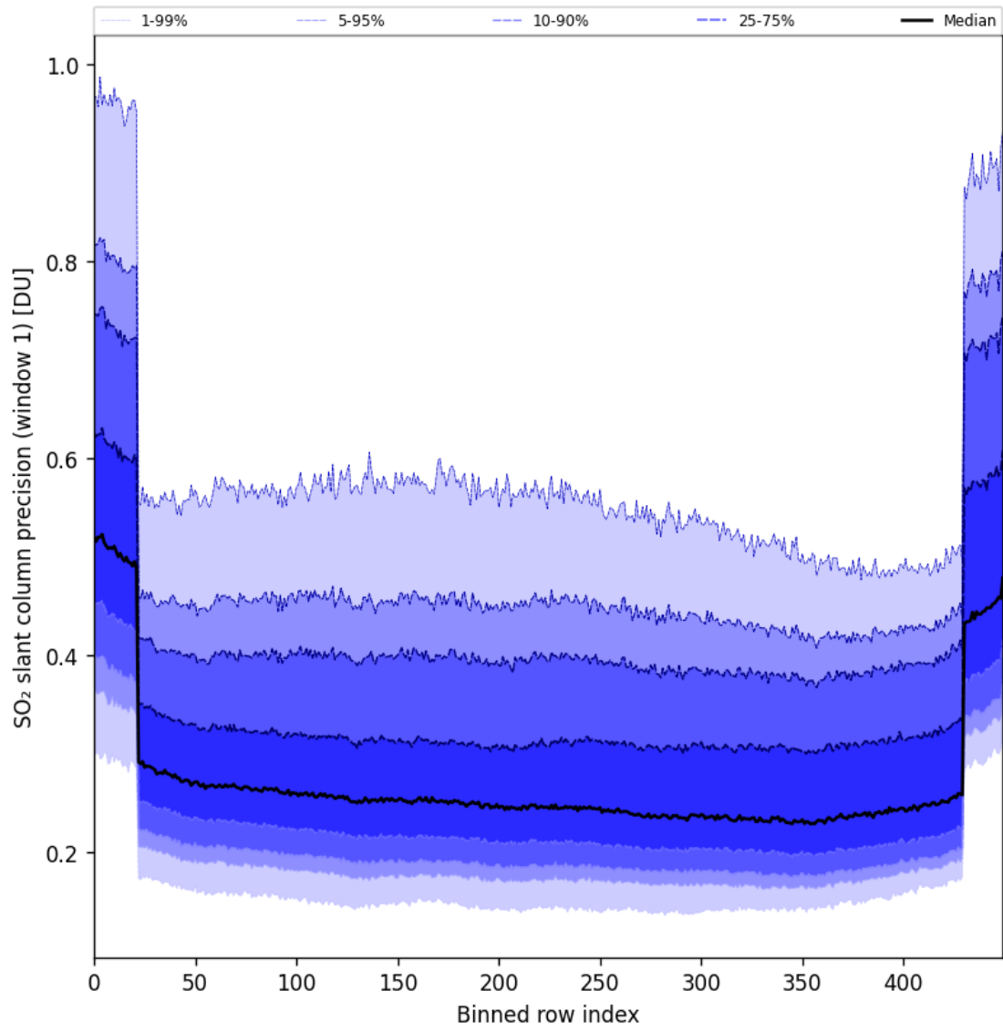
Figure 90: Along track statistics of “SO 2 slant column precision (window 1)” for 2025-11-19 to 2025-11-21
