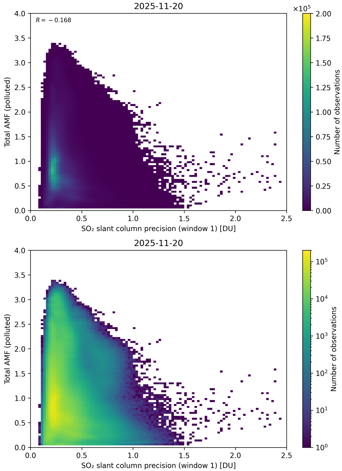
Figure 280: Scatter density plot of “SO 2 slant column precision (window 1)” against “Total AMF (polluted)” for 2025-11-19 to 2025-11-21.
