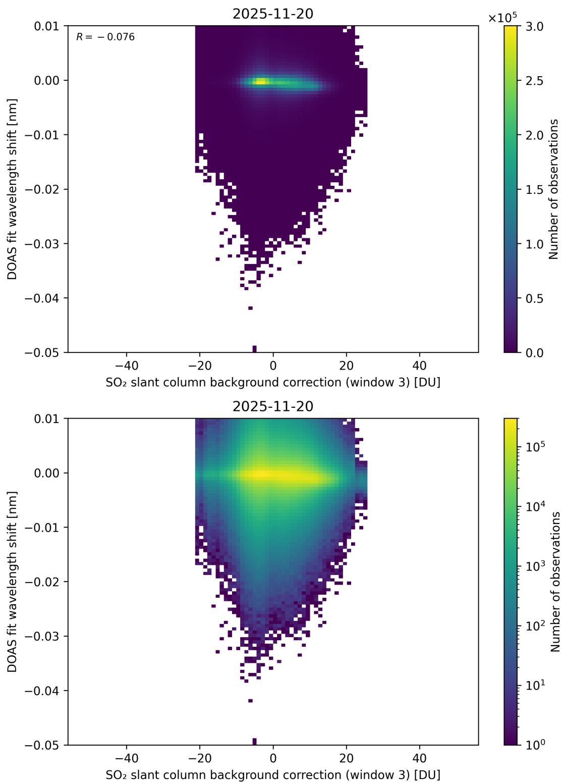
Figure 132: Scatter density plot of “SO 2 slant column background correction (window 3)” against “DOAS fit wavelength shift” for 2025-11-19 to 2025-11-21.
