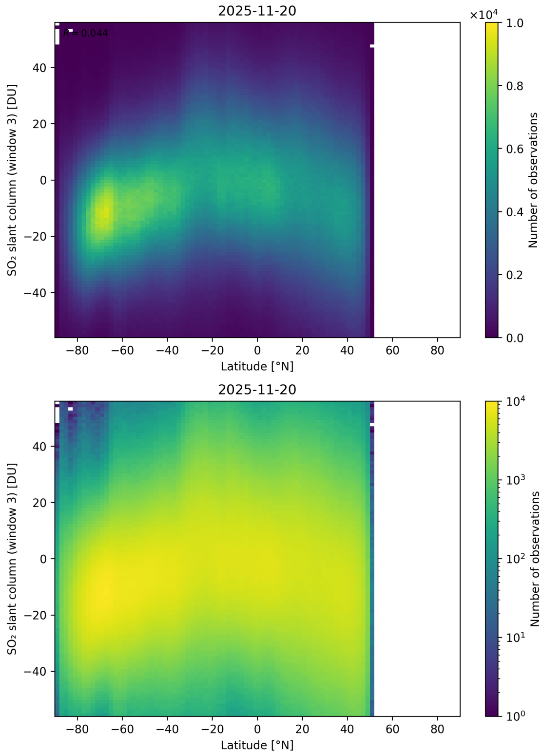
Figure 165: Scatter density plot of “Latitude” against “SO 2 slant column (window 3)” for 2025-11-19 to 2025-11-21.
