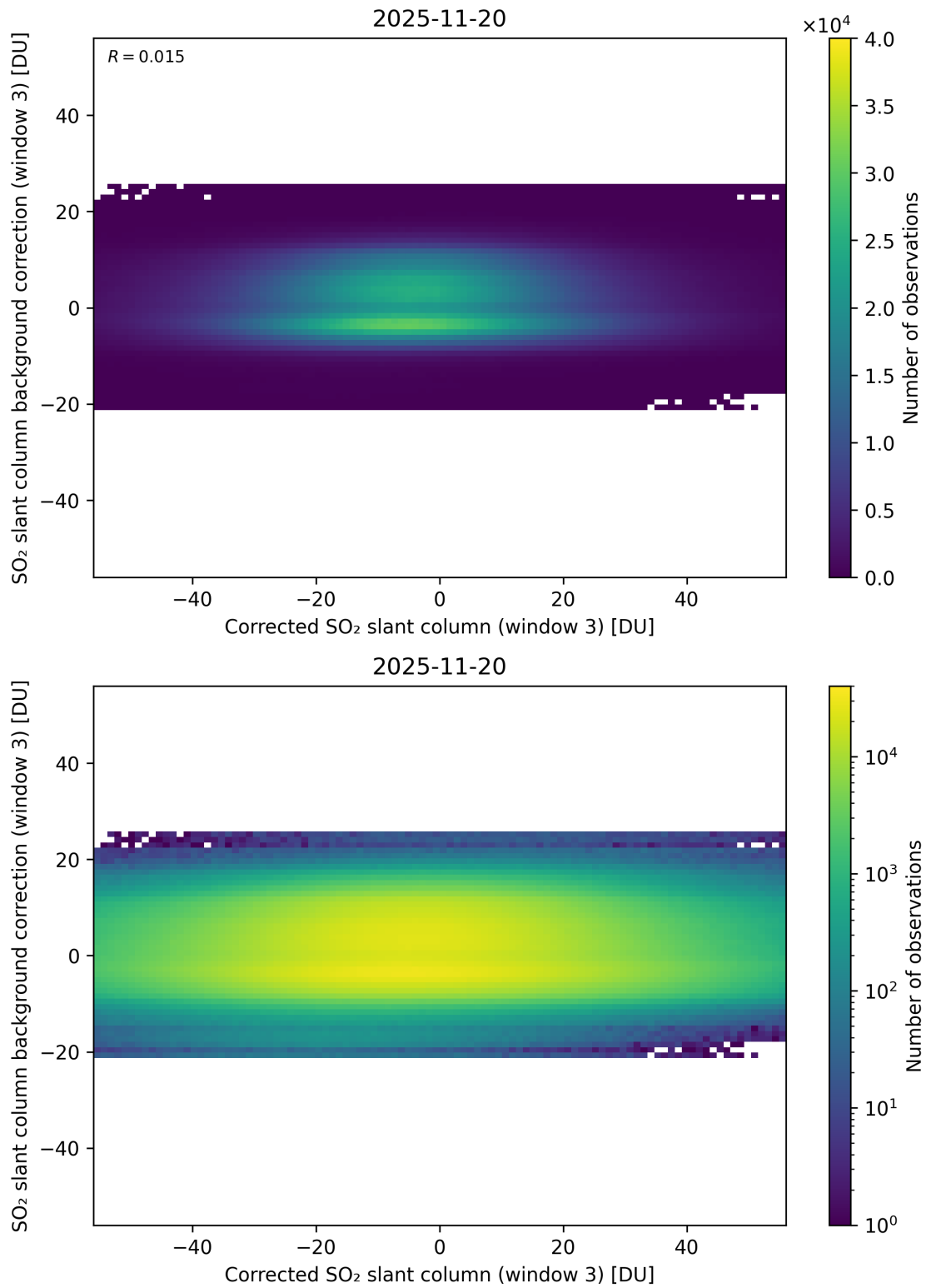
Figure 255: Scatter density plot of “Corrected SO 2 slant column (window 3)” against “SO 2 slant column background correction (window 3)” for 2025-11-19 to 2025-11-21.
