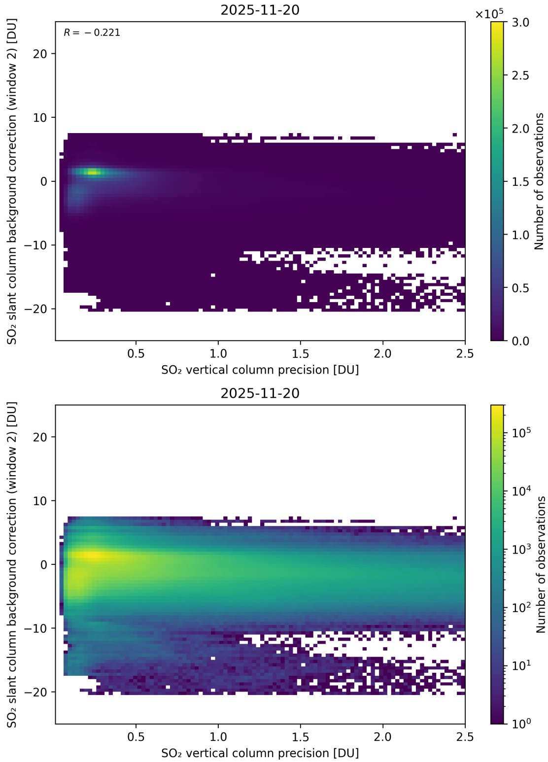
Figure 330: Scatter density plot of “SO 2 vertical column precision” against “SO 2 slant column background correction (window 2)” for 2025-11-19 to 2025-11-21.
