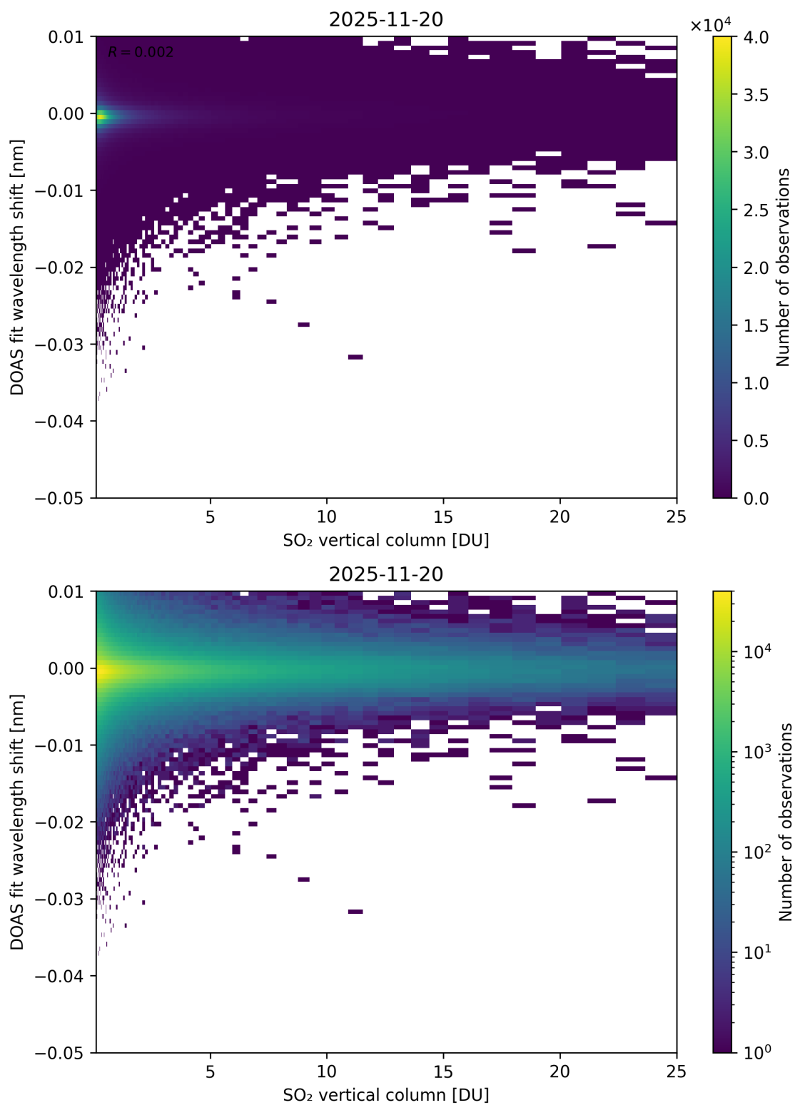
Figure 326: Scatter density plot of “SO 2 vertical column” against “DOAS fit wavelength shift” for 2025-11-19 to 2025-11-21.
