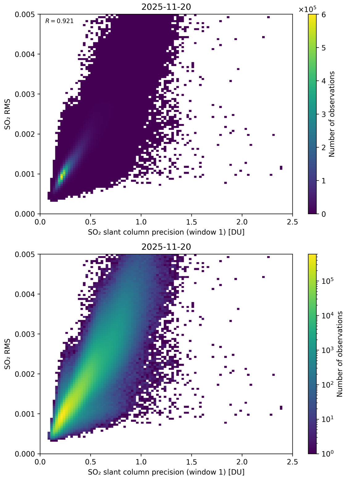
Figure 273: Scatter density plot of “SO 2 slant column precision (window 1)” against “SO 2 RMS” for 2025-11-19 to 2025-11-21.
