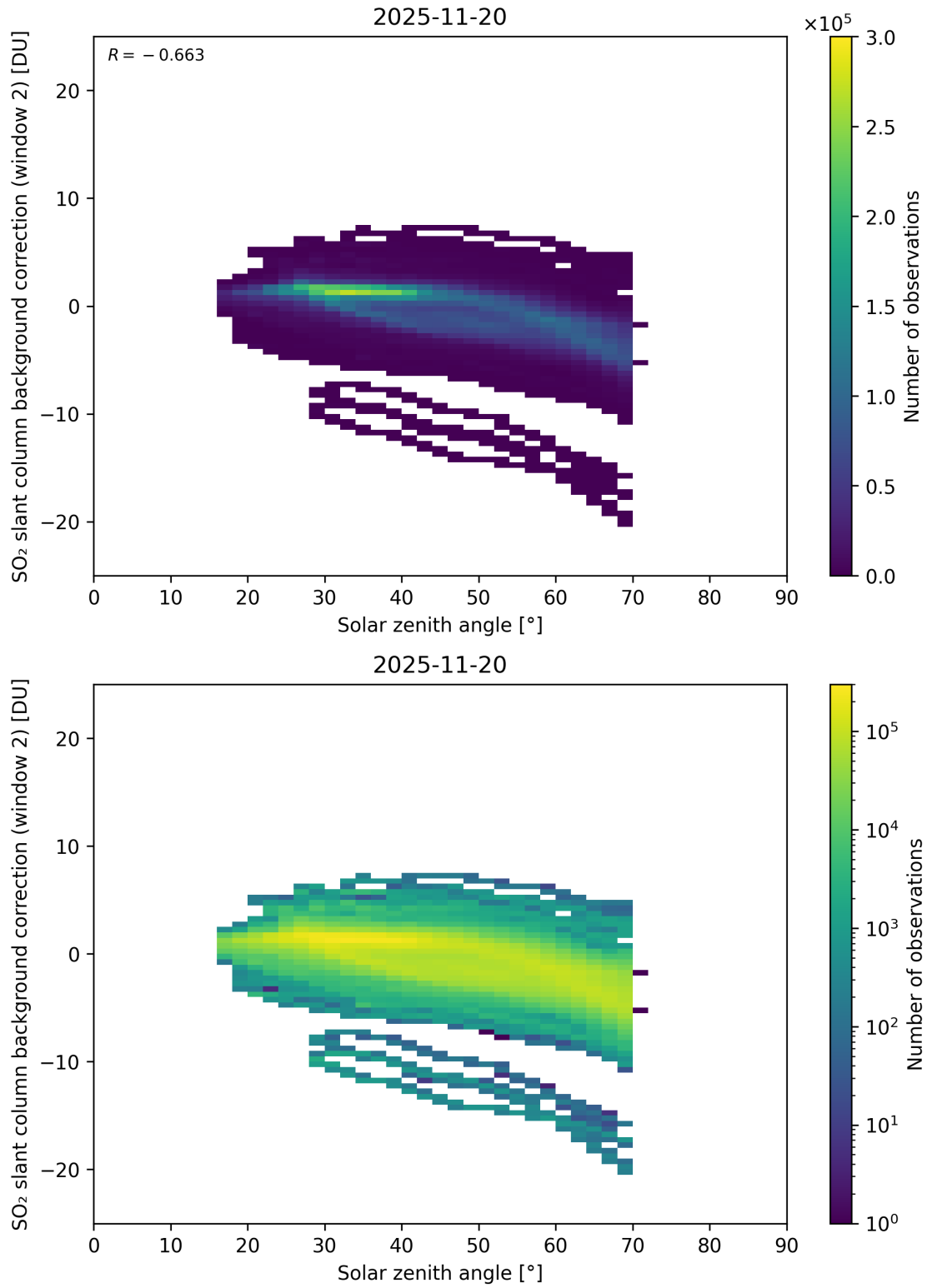
Figure 172: Scatter density plot of “Solar zenith angle” against “SO 2 slant column background correction (window 2)” for 2025-11-19 to 2025-11-21.
