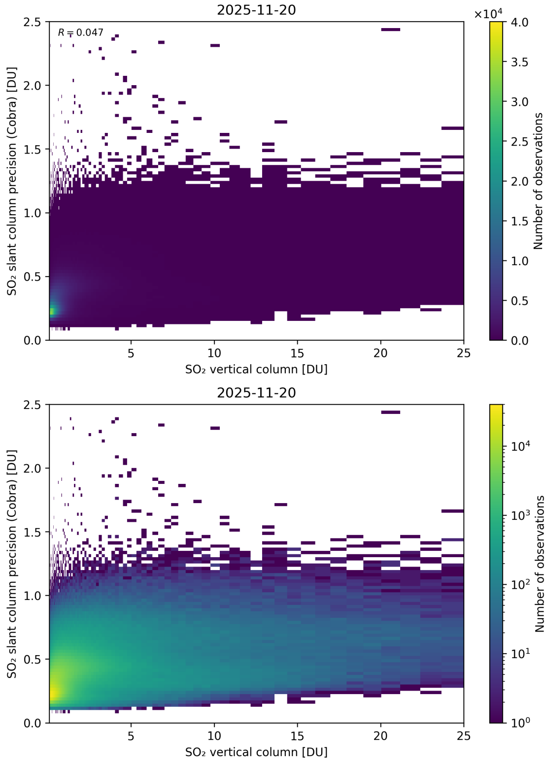
Figure 350: Scatter density plot of “SO 2 vertical column” against “SO 2 slant column precision (Cobra)” for 2025-11-19 to 2025-11-21.
