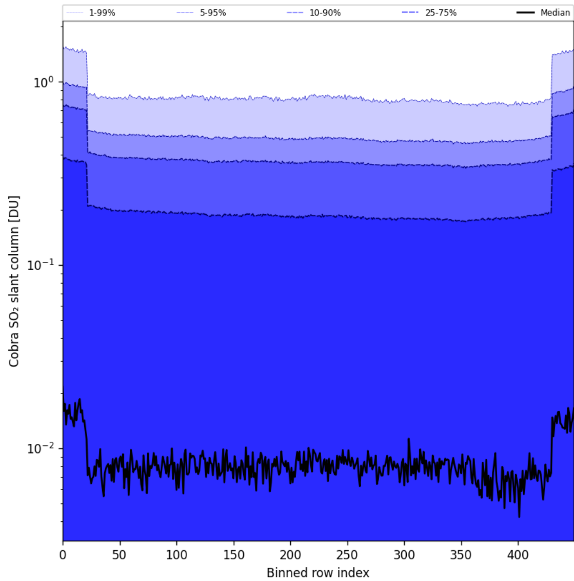
Figure 87: Along track statistics of “Cobra SO 2 slant column” for 2025-11-19 to 2025-11-21
