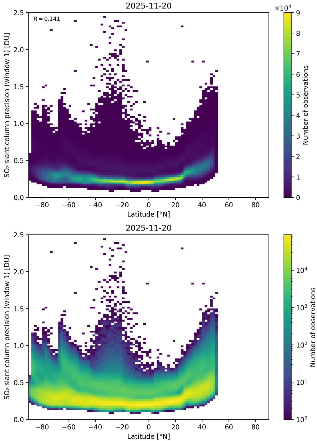
Figure 163: Scatter density plot of “Latitude” against “SO 2 slant column precision (window 1)” for 2025-11-19 to 2025-11-21.
