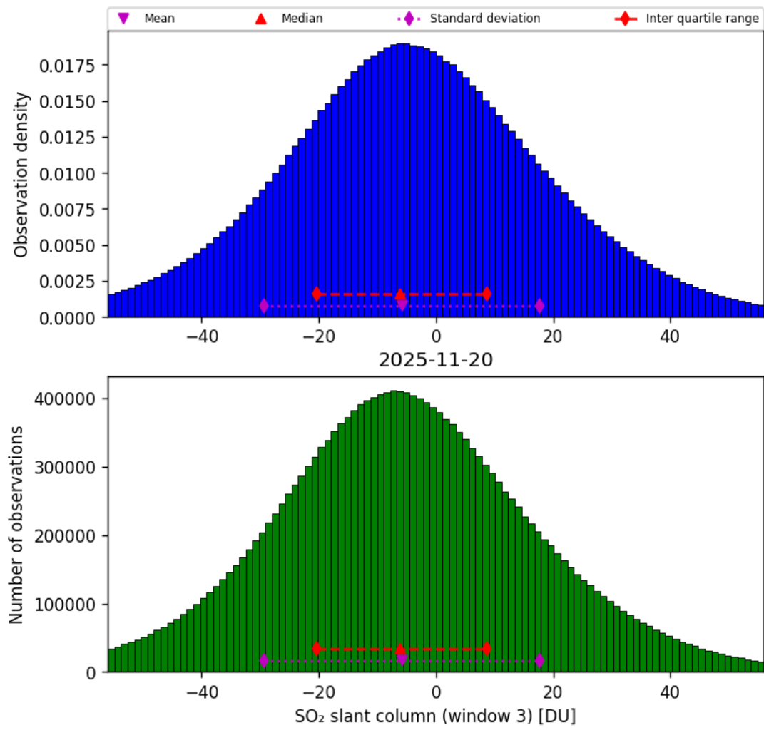
Figure 71: Histogram of “SO 2 slant column (window 3)” for 2025-11-19 to 2025-11-21
