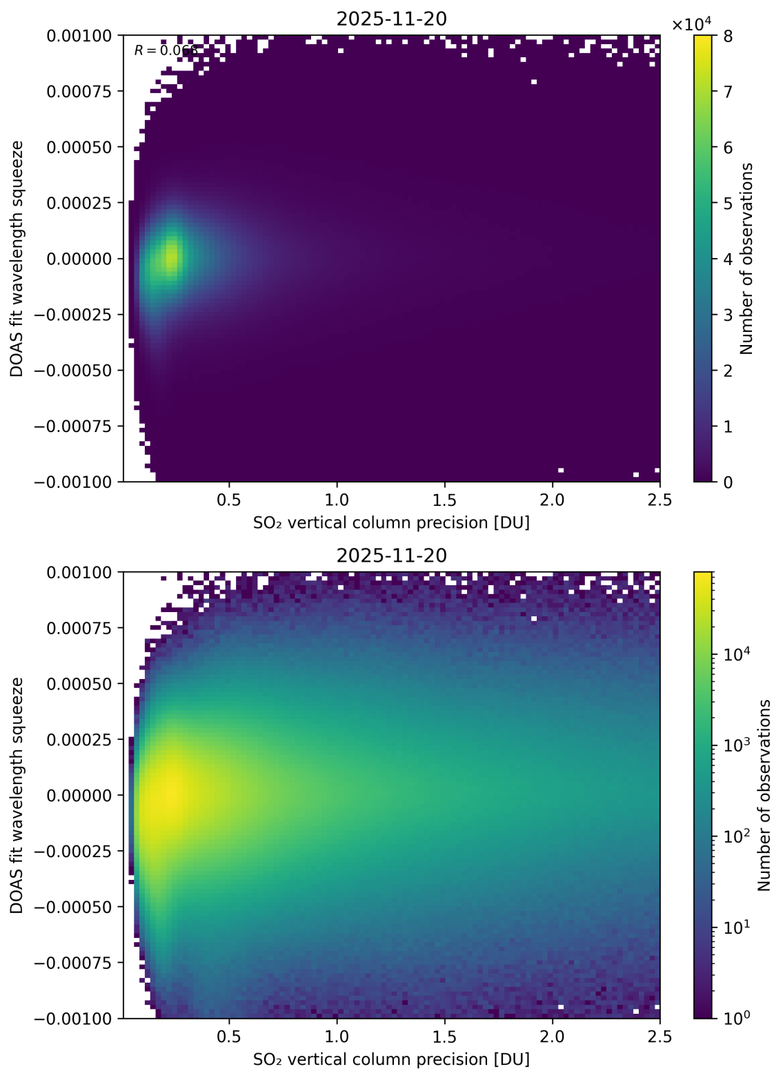
Figure 333: Scatter density plot of “SO 2 vertical column precision” against “DOAS fit wavelength squeeze” for 2025-11-19 to 2025-11-21.
