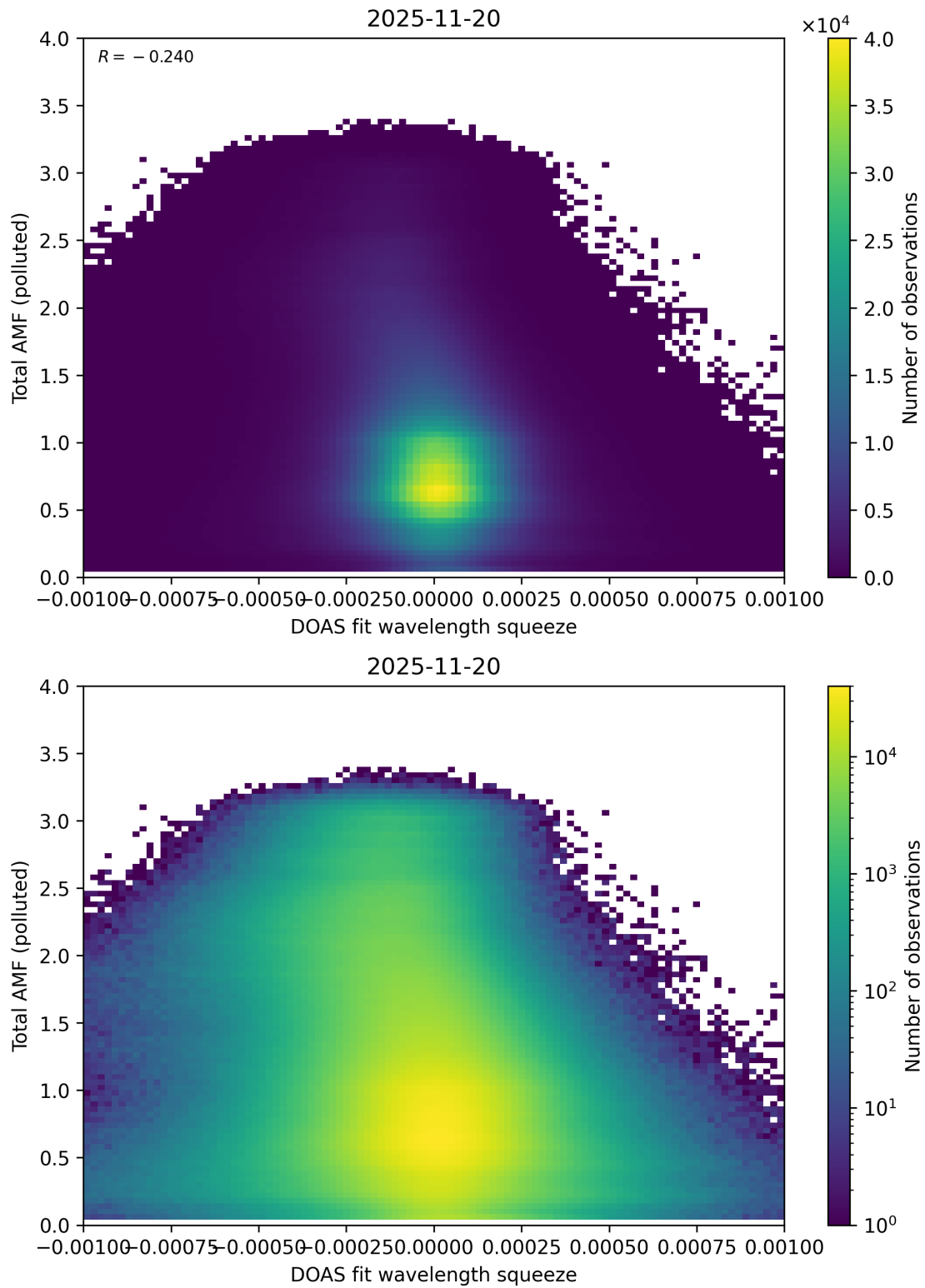
Figure 145: Scatter density plot of “DOAS fit wavelength squeeze” against “Total AMF (polluted)” for 2025-11-19 to 2025-11-21.
