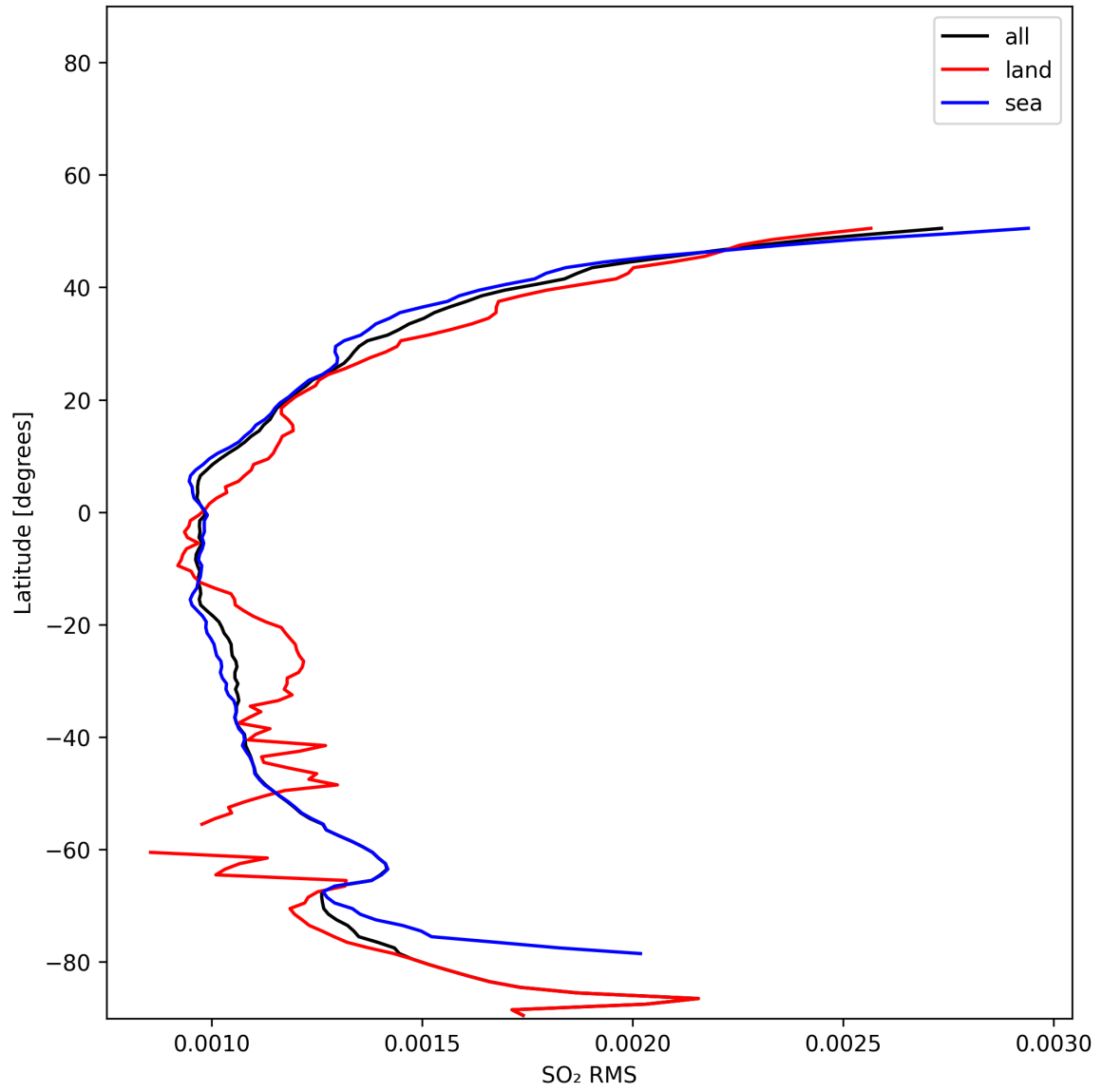
Figure 52: Zonal average of “SO 2 RMS” for 2025-11-19 to 2025-11-21.
