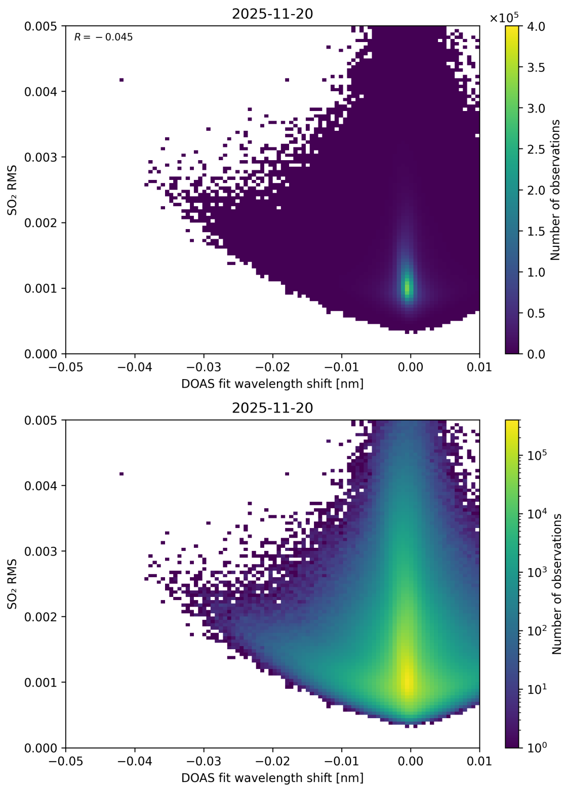
Figure 139: Scatter density plot of “DOAS fit wavelength shift” against “SO 2 RMS” for 2025-11-19 to 2025-11-21.
