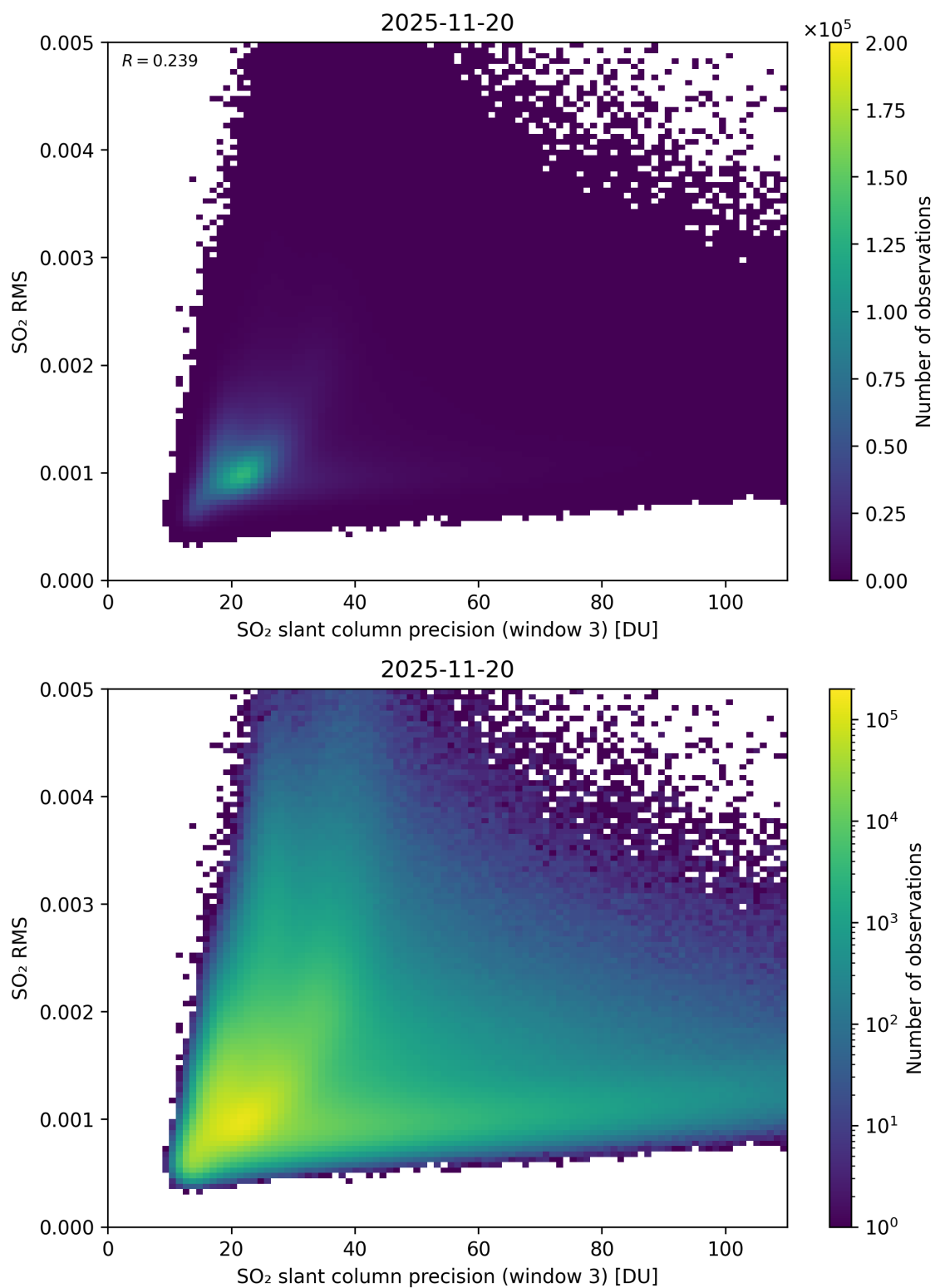
Figure 310: Scatter density plot of “SO 2 slant column precision (window 3)” against “SO 2 RMS” for 2025-11-19 to 2025-11-21.
