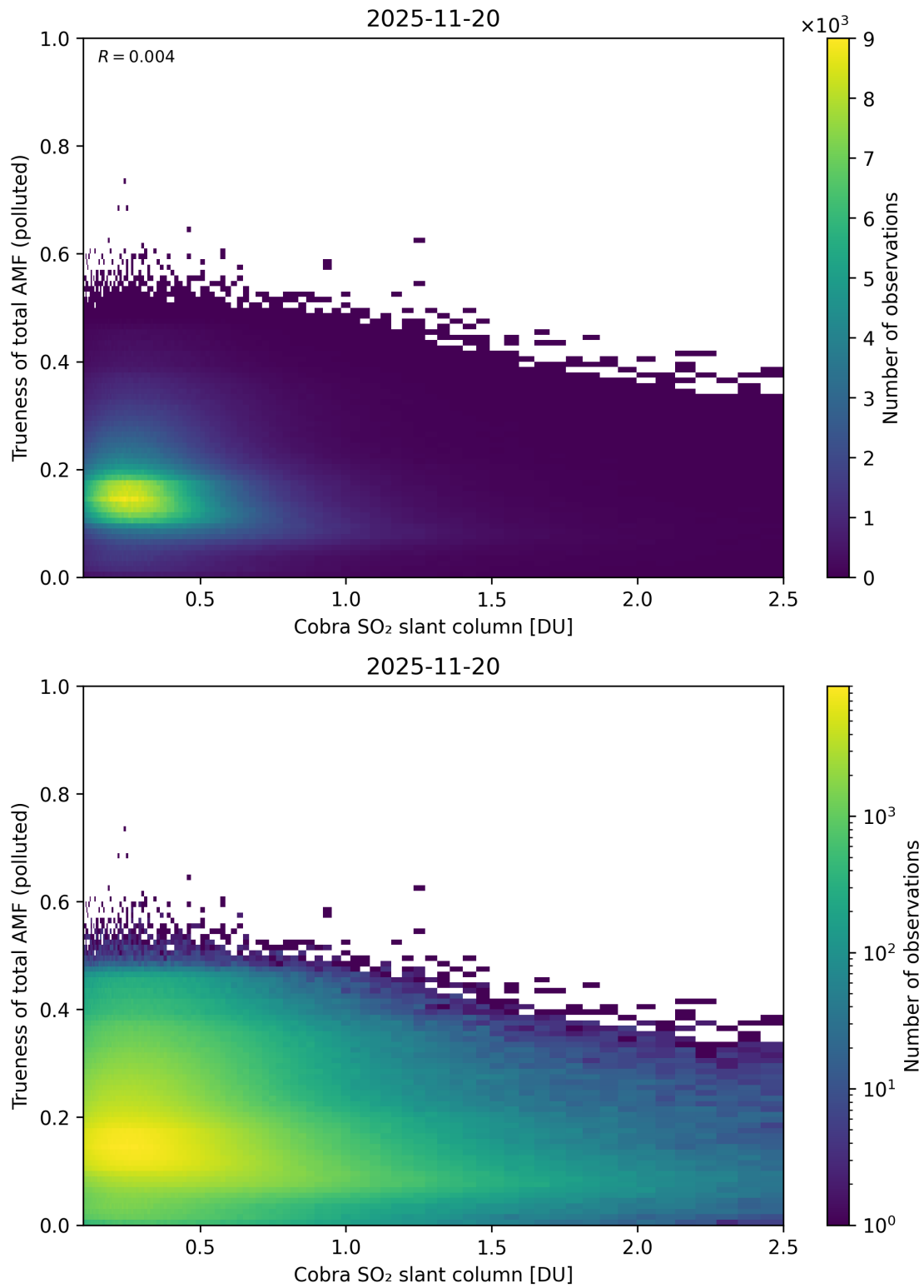
Figure 225: Scatter density plot of “Cobra SO 2 slant column” against “Trueness of total AMF (polluted)” for 2025-11-19 to 2025-11-21.
