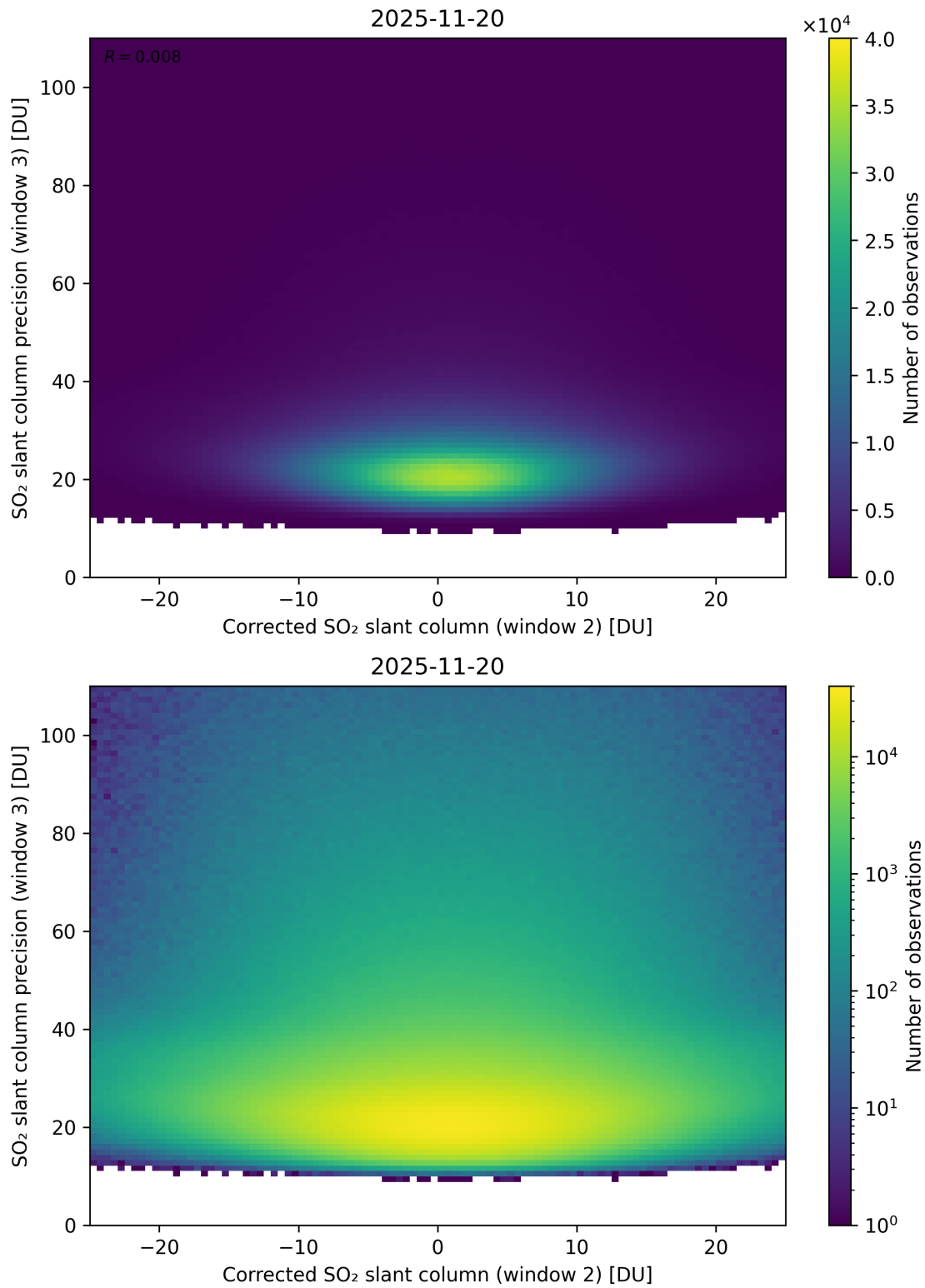
Figure 252: Scatter density plot of “Corrected SO 2 slant column (window 2)” against “SO 2 slant column precision (window 3)” for 2025-11-19 to 2025-11-21.
