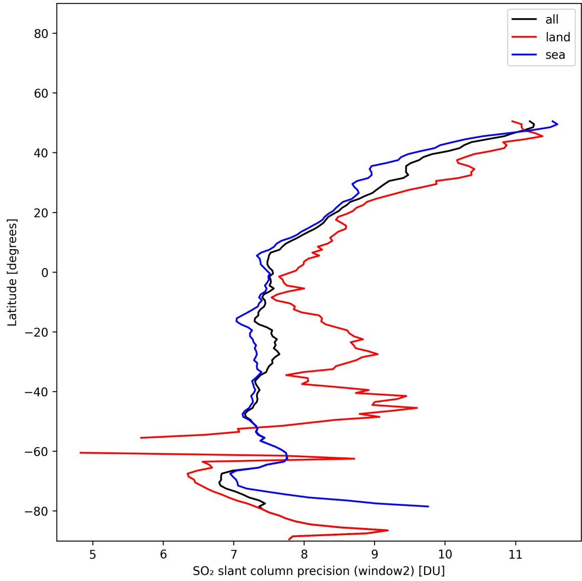
Figure 42: Zonal average of “SO 2 slant column precision (window2)” for 2025-11-19 to 2025-11-21.
