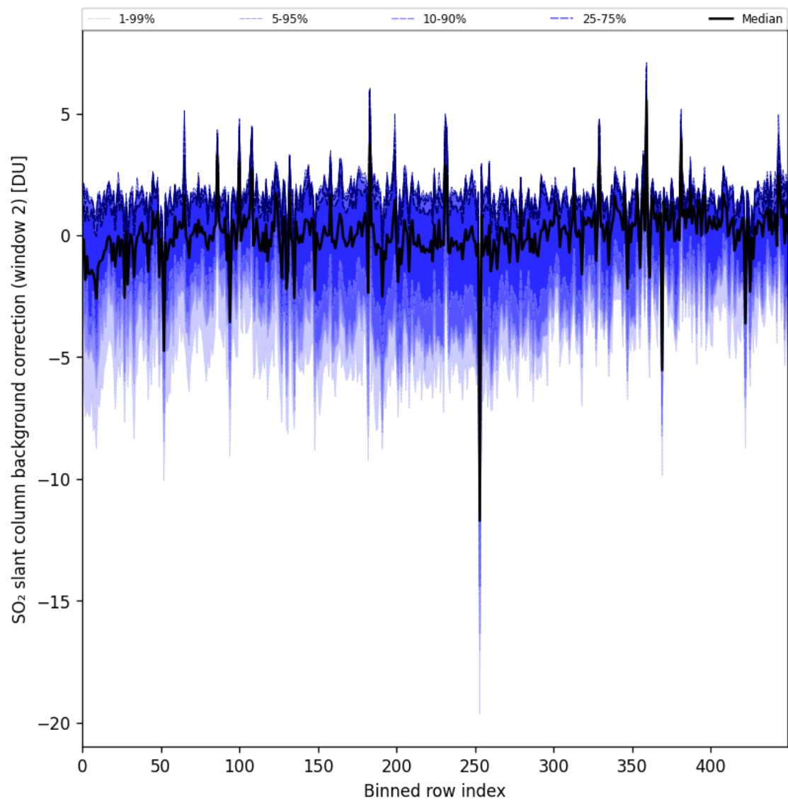
Figure 96: Along track statistics of “SO 2 slant column background correction (window 2)” for 2025-11-19 to 2025-11-21
