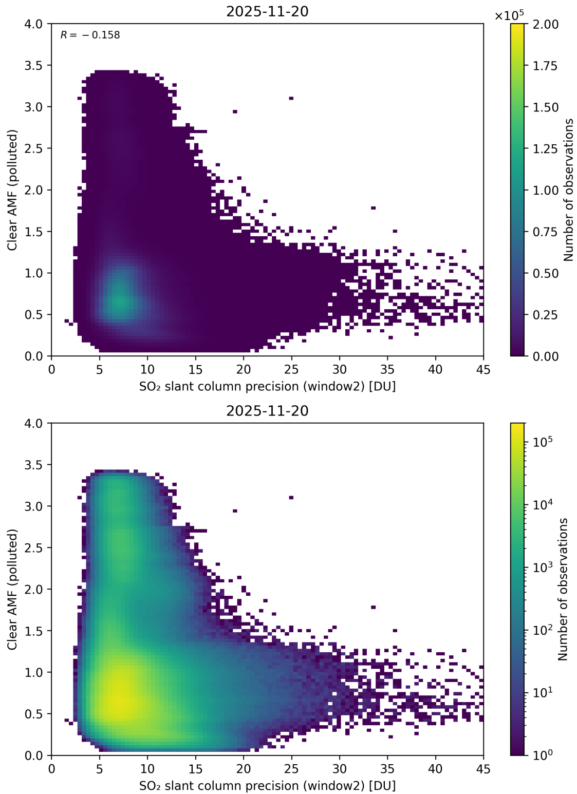
Figure 296: Scatter density plot of “SO 2 slant column precision (window2)” against “Clear AMF (polluted)” for 2025-11-19 to 2025-11-21.
