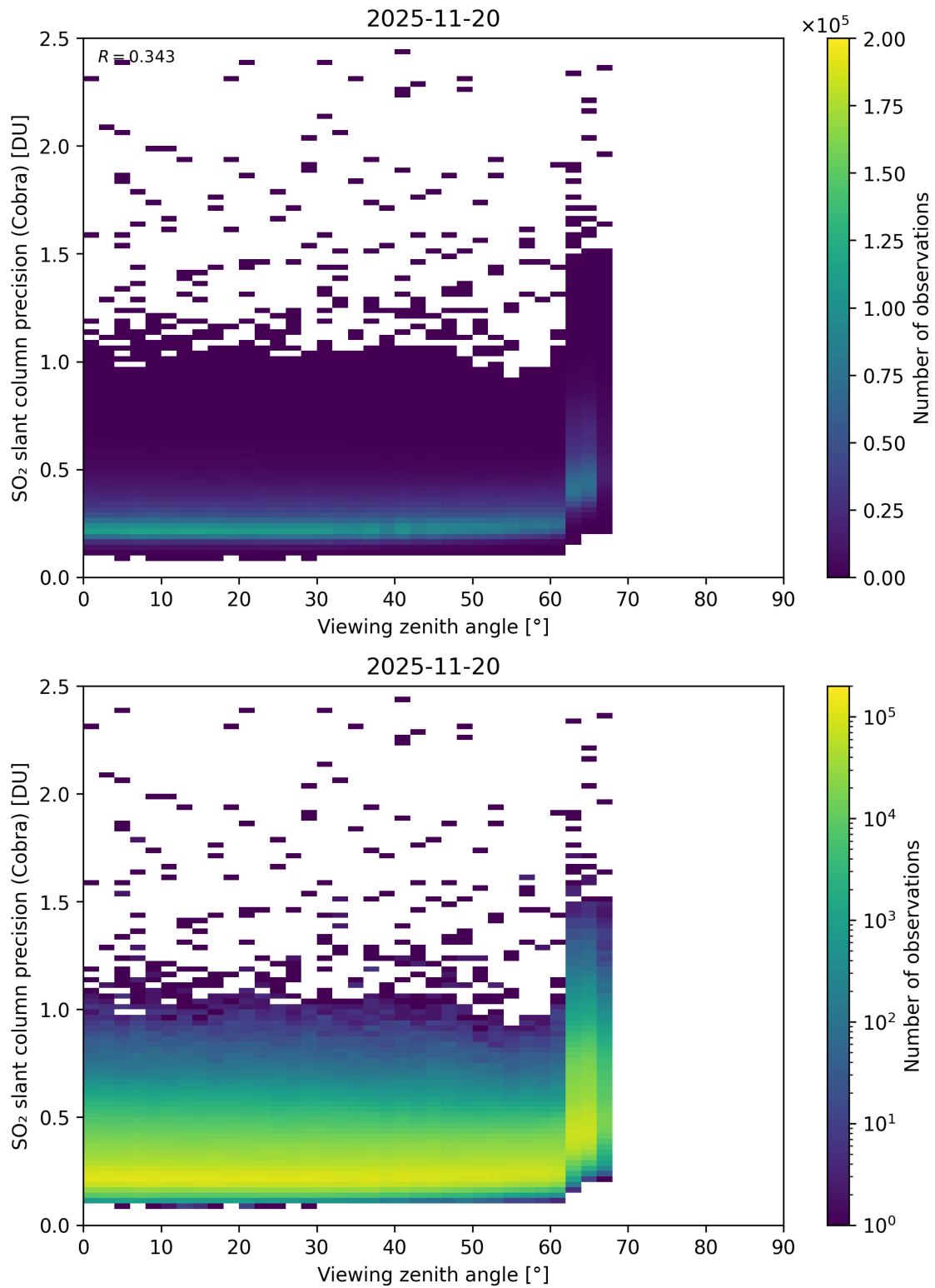
Figure 372: Scatter density plot of “Viewing zenith angle” against “SO 2 slant column precision (Cobra)” for 2025-11-19 to 2025-11-21.
