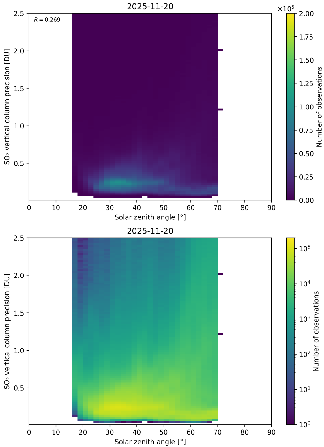
Figure 192: Scatter density plot of “Solar zenith angle” against “SO 2 vertical column precision” for 2025-11-19 to 2025-11-21.
