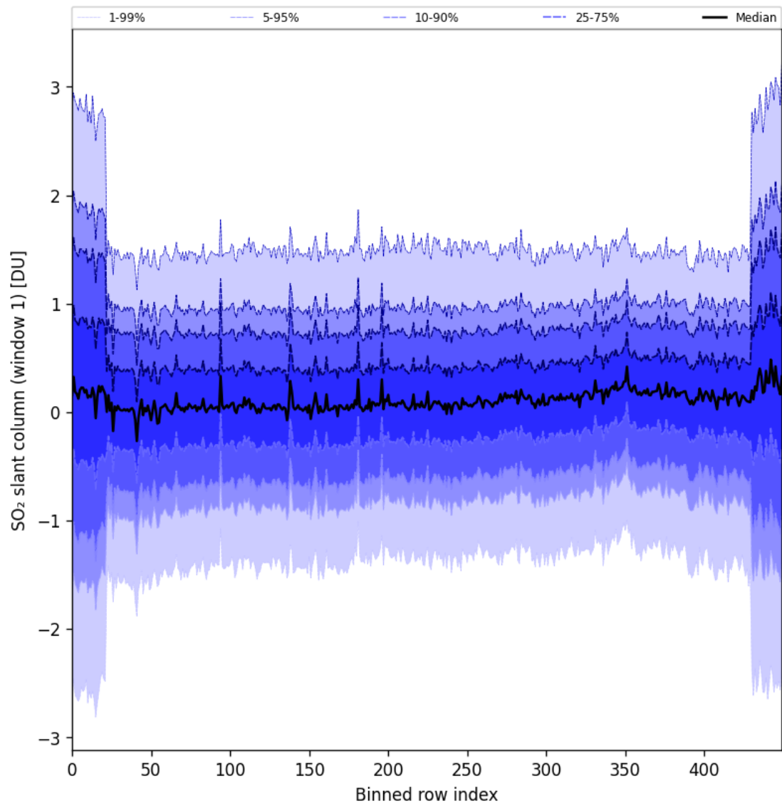
Figure 89: Along track statistics of “SO 2 slant column (window 1)” for 2025-11-19 to 2025-11-21
