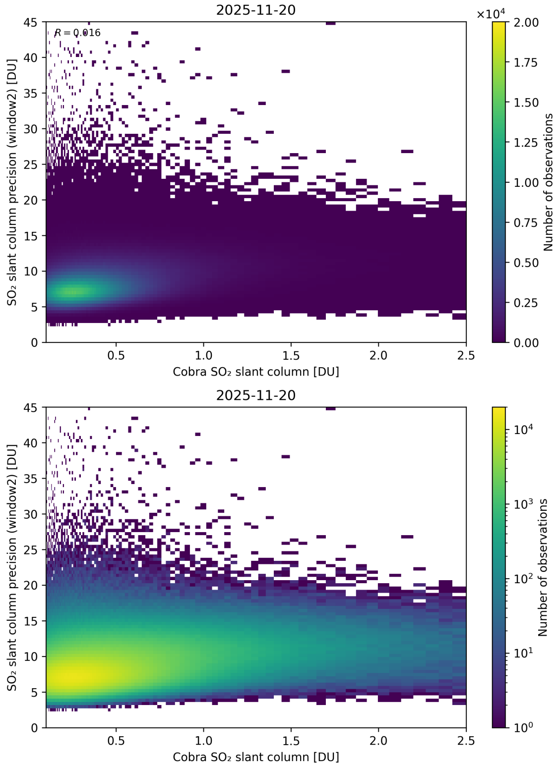
Figure 221: Scatter density plot of “Cobra SO 2 slant column” against “SO 2 slant column precision (window2)” for 2025-11-19 to 2025-11-21.
