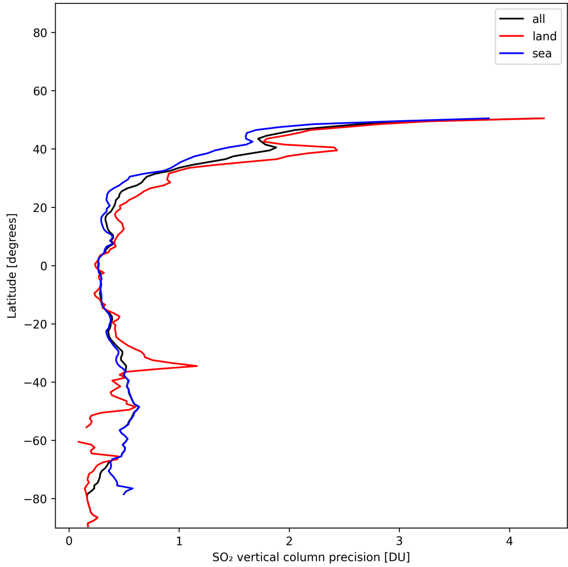
Figure 33: Zonal average of “SO 2 vertical column precision” for 2025-11-19 to 2025-11-21.
