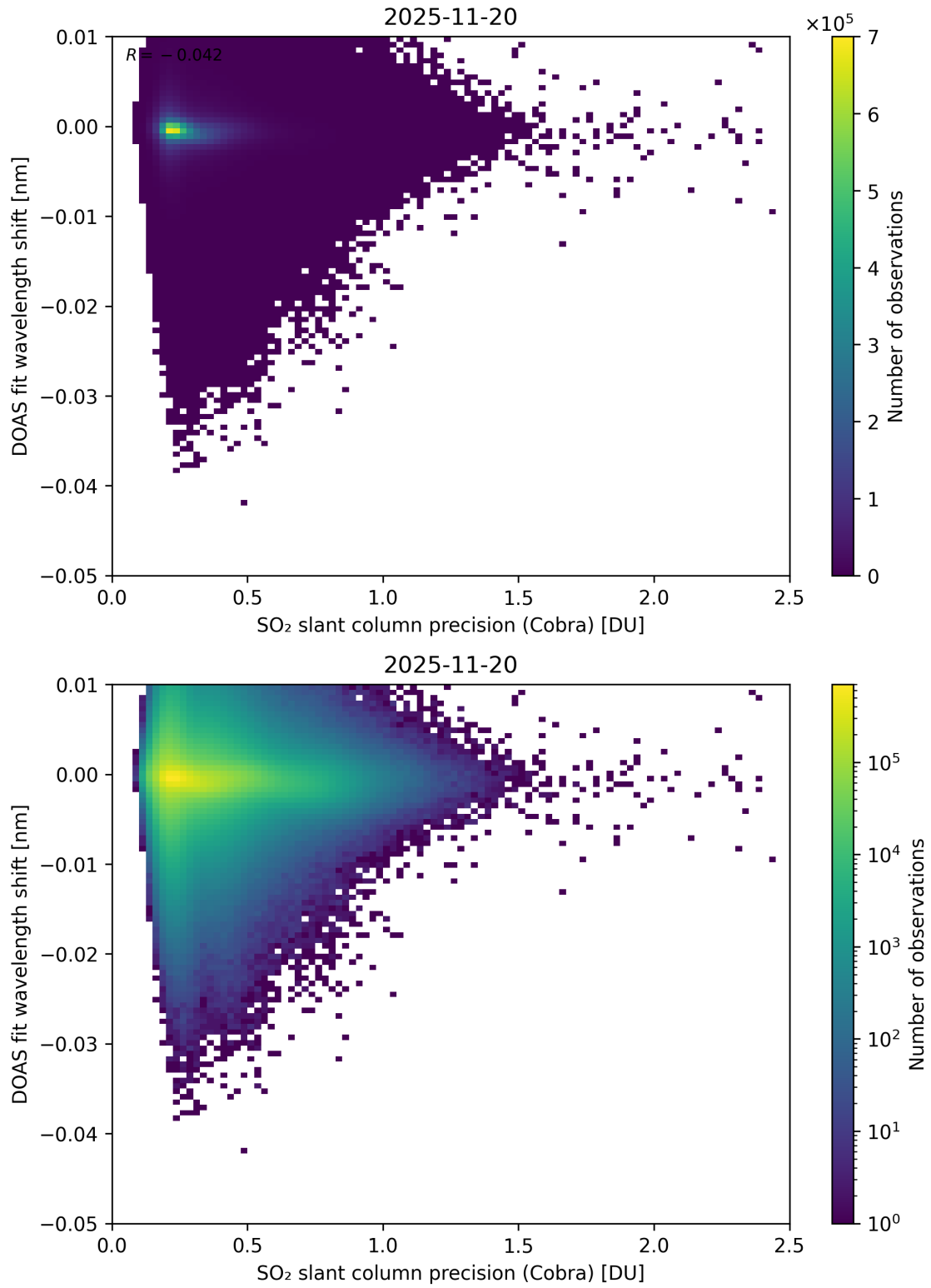
Figure 202: Scatter density plot of “SO 2 slant column precision (Cobra)” against “DOAS fit wavelength shift” for 2025-11-19 to 2025-11-21.
