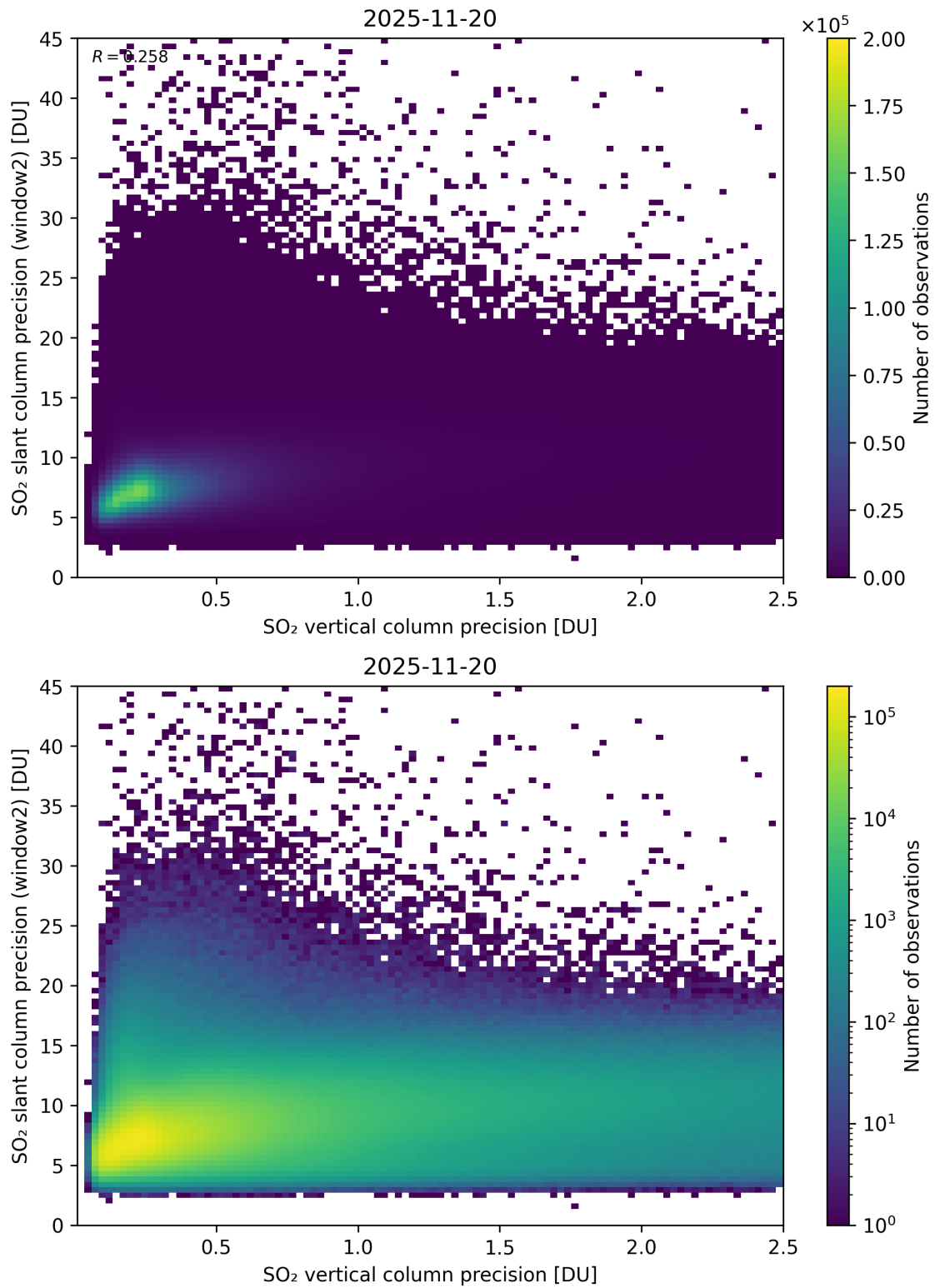
Figure 343: Scatter density plot of “SO 2 vertical column precision” against “SO 2 slant column precision (window2)” for 2025-11-19 to 2025-11-21.
