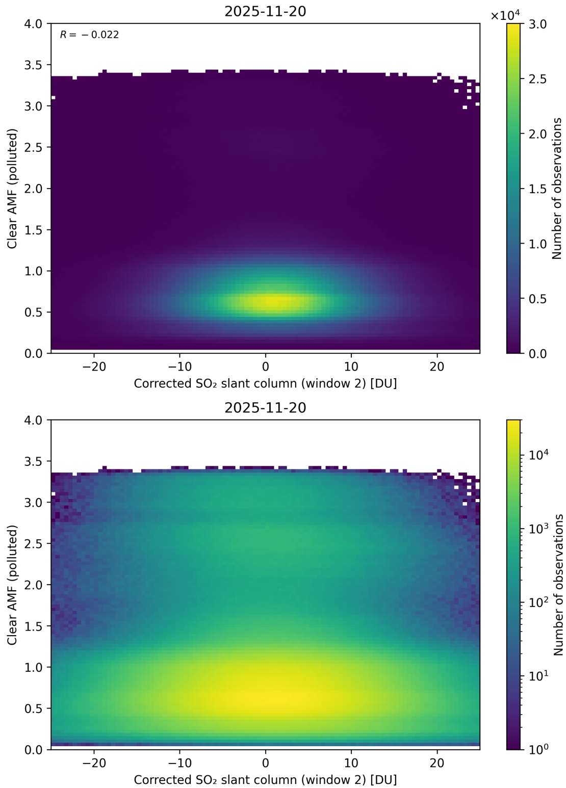
Figure 249: Scatter density plot of “Corrected SO 2 slant column (window 2)” against “Clear AMF (polluted)” for 2025-11-19 to 2025-11-21.
