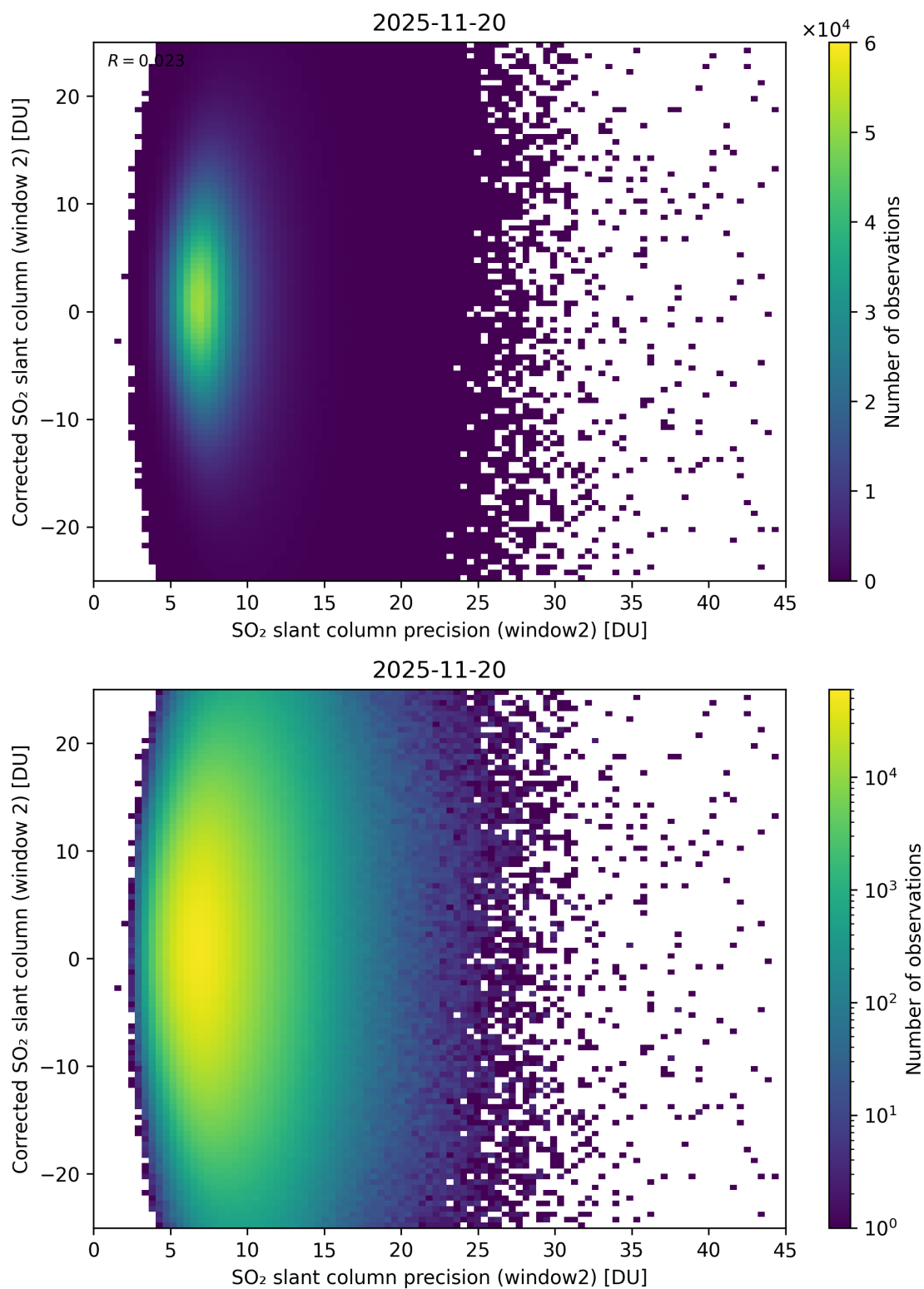
Figure 297: Scatter density plot of “SO 2 slant column precision (window2)” against “Corrected SO 2 slant column (window 2)” for 2025-11-19 to 2025-11-21.
