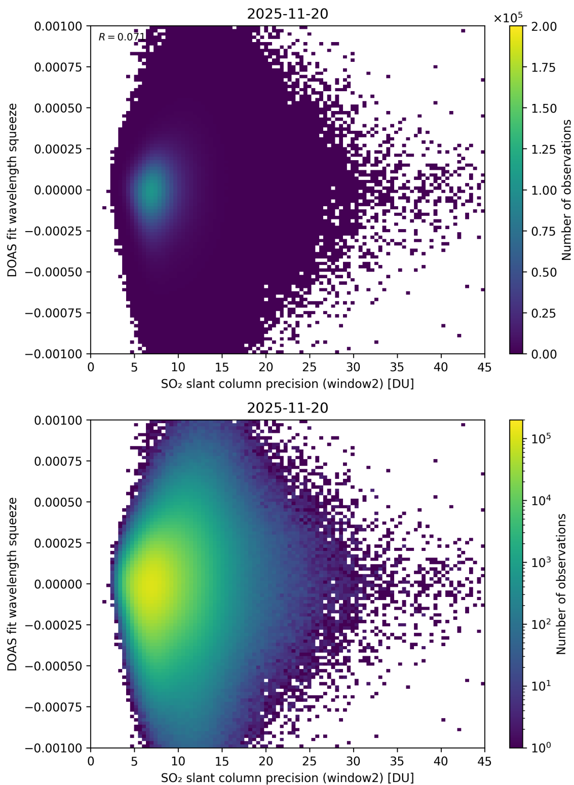
Figure 294: Scatter density plot of “SO 2 slant column precision (window2)” against “DOAS fit wavelength squeeze” for 2025-11-19 to 2025-11-21.
