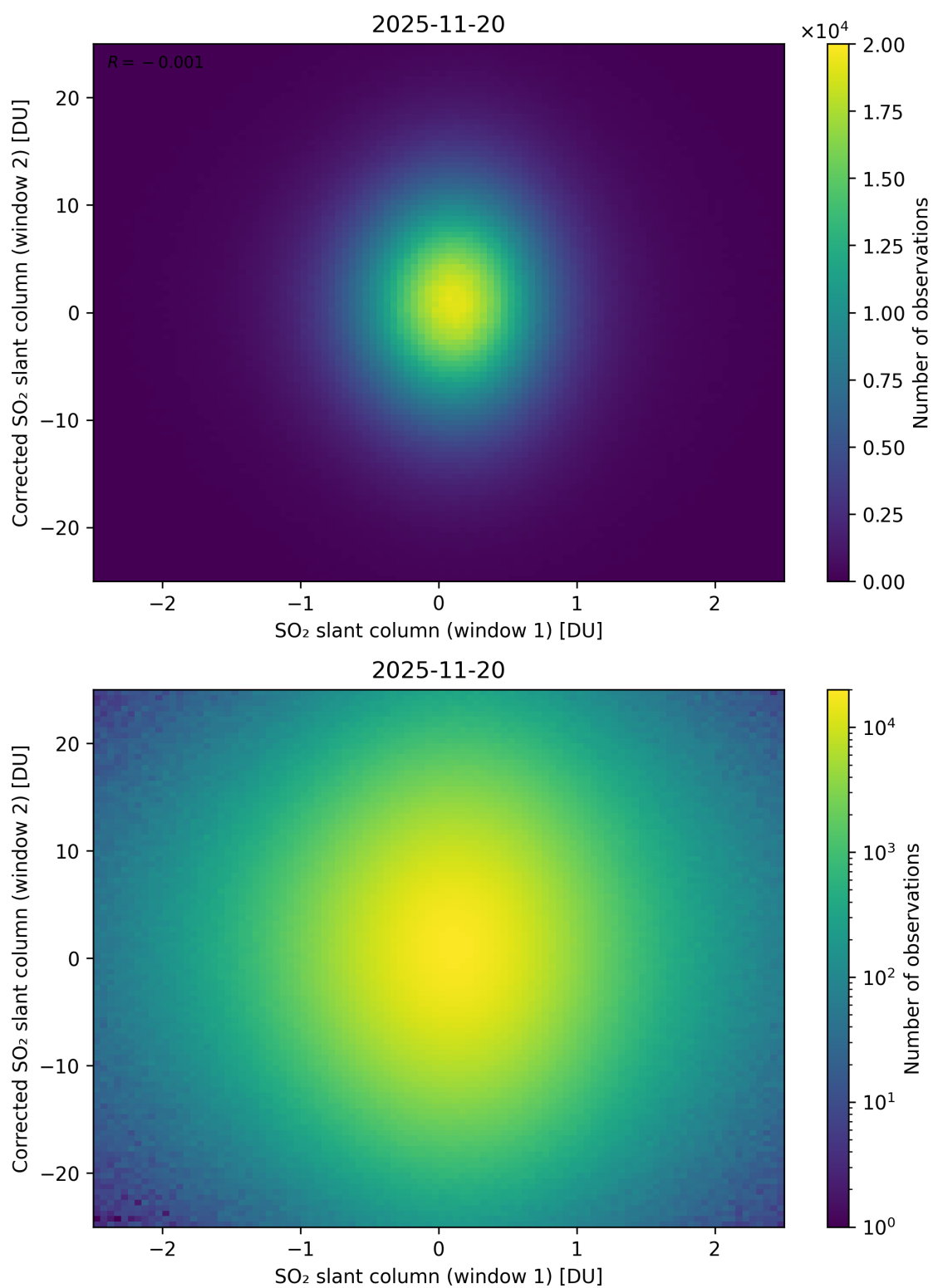
Figure 283: Scatter density plot of “SO 2 slant column (window 1)” against “Corrected SO 2 slant column (window 2)” for 2025-11-19 to 2025-11-21.
