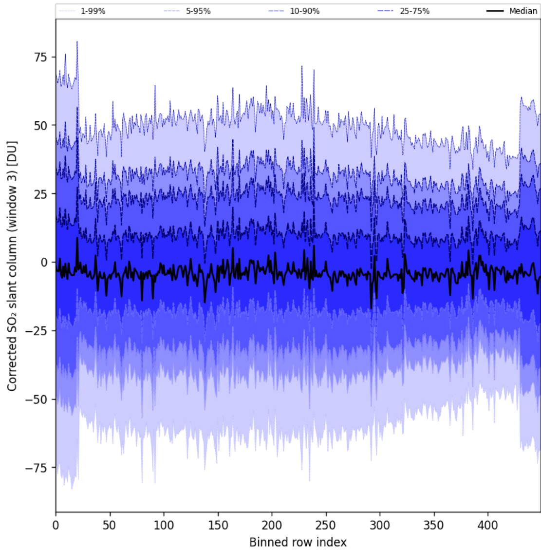
Figure 99: Along track statistics of “Corrected SO 2 slant column (window 3)” for 2025-11-19 to 2025-11-21
