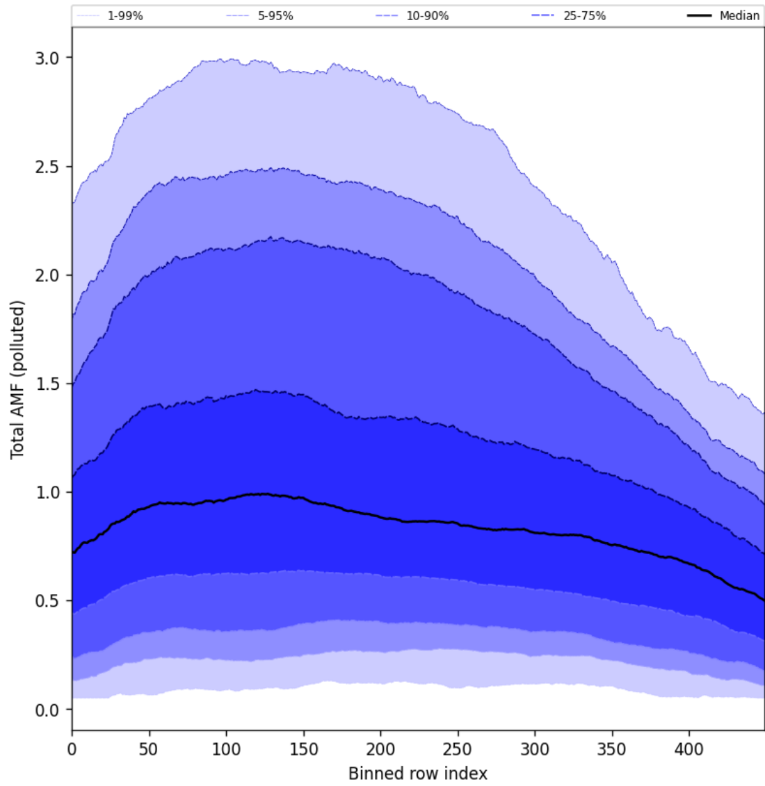
Figure 105: Along track statistics of “Total AMF (polluted)” for 2025-11-19 to 2025-11-21
