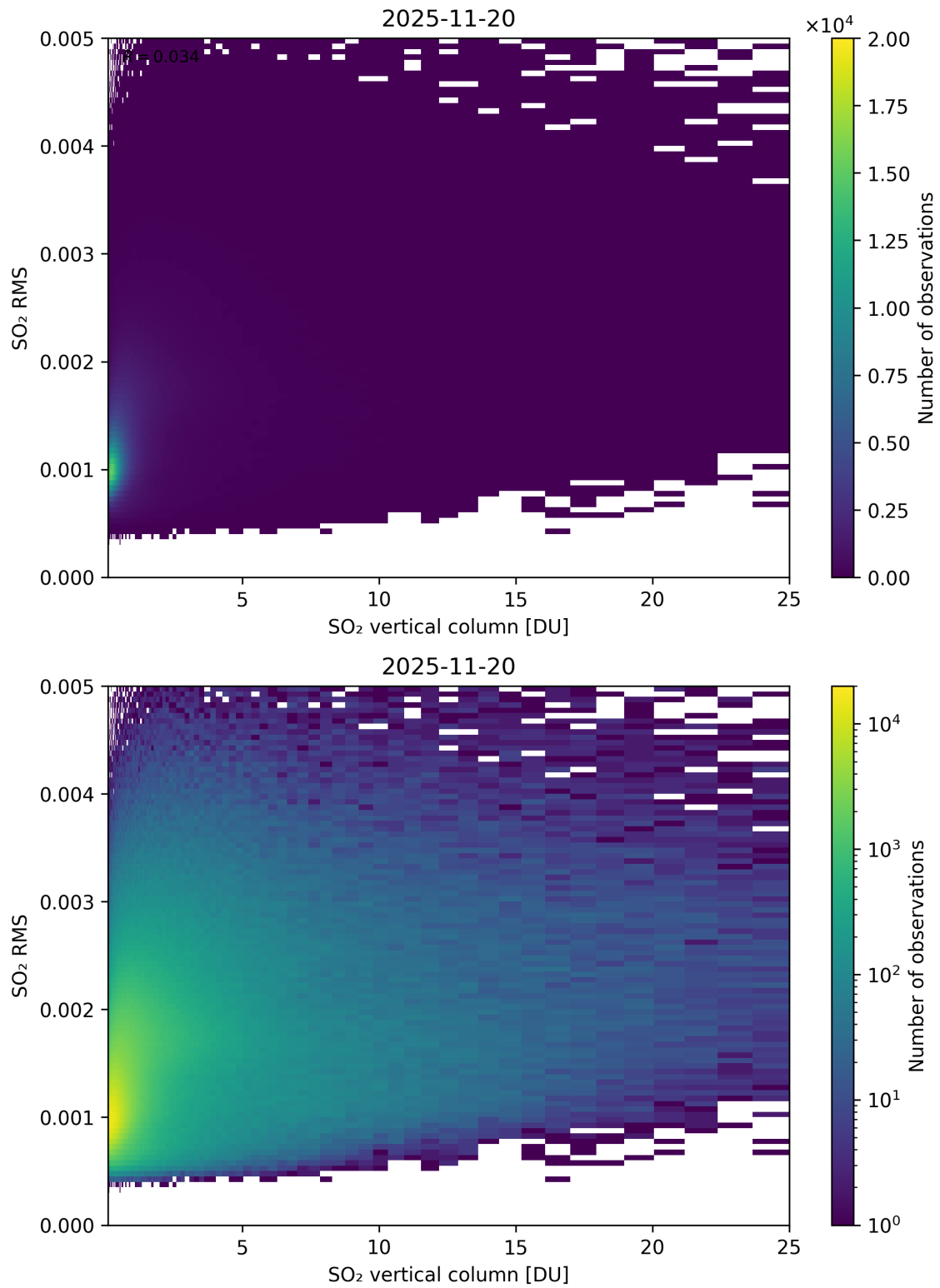
Figure 328: Scatter density plot of “SO 2 vertical column” against “SO 2 RMS” for 2025-11-19 to 2025-11-21.
