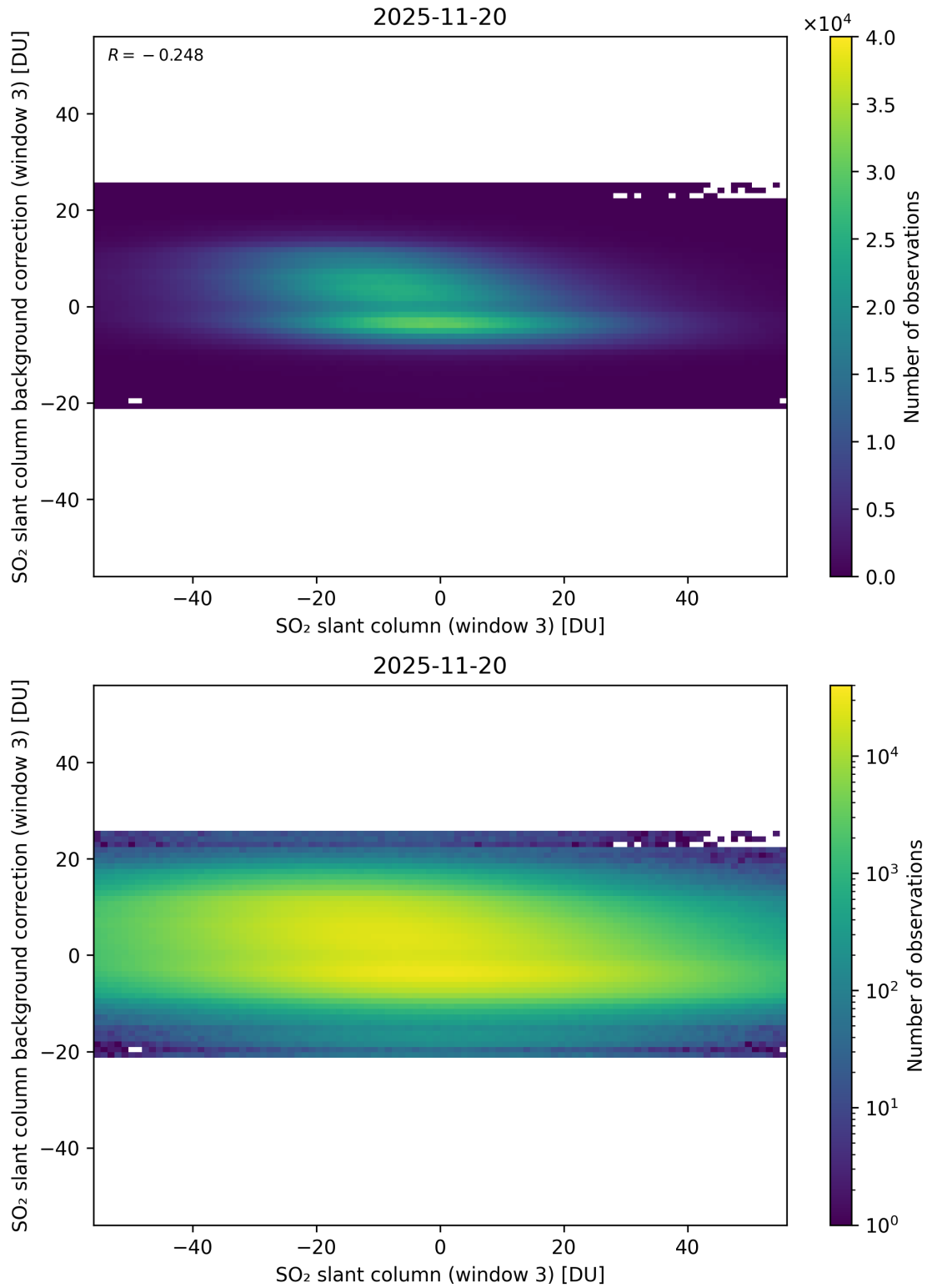
Figure 303: Scatter density plot of “SO 2 slant column (window 3)” against “SO 2 slant column background correction (window 3)” for 2025-11-19 to 2025-11-21.
