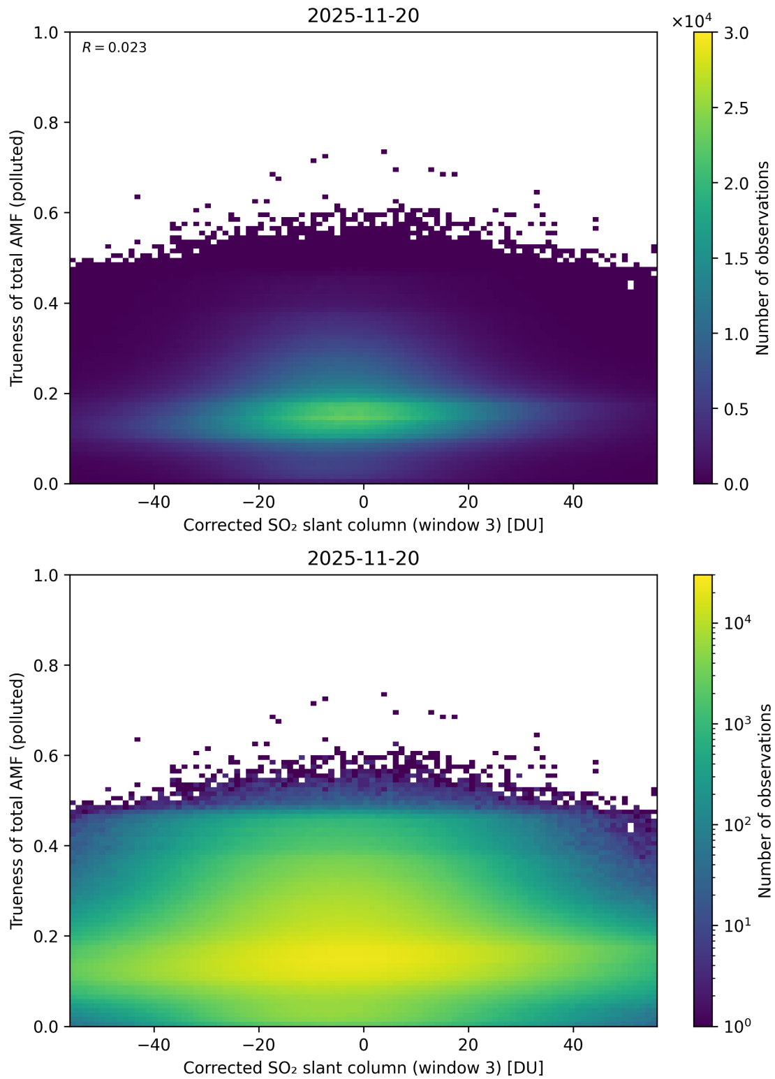
Figure 261: Scatter density plot of “Corrected SO 2 slant column (window 3)” against “Trueness of total AMF (polluted)” for 2025-11-19 to 2025-11-21.
