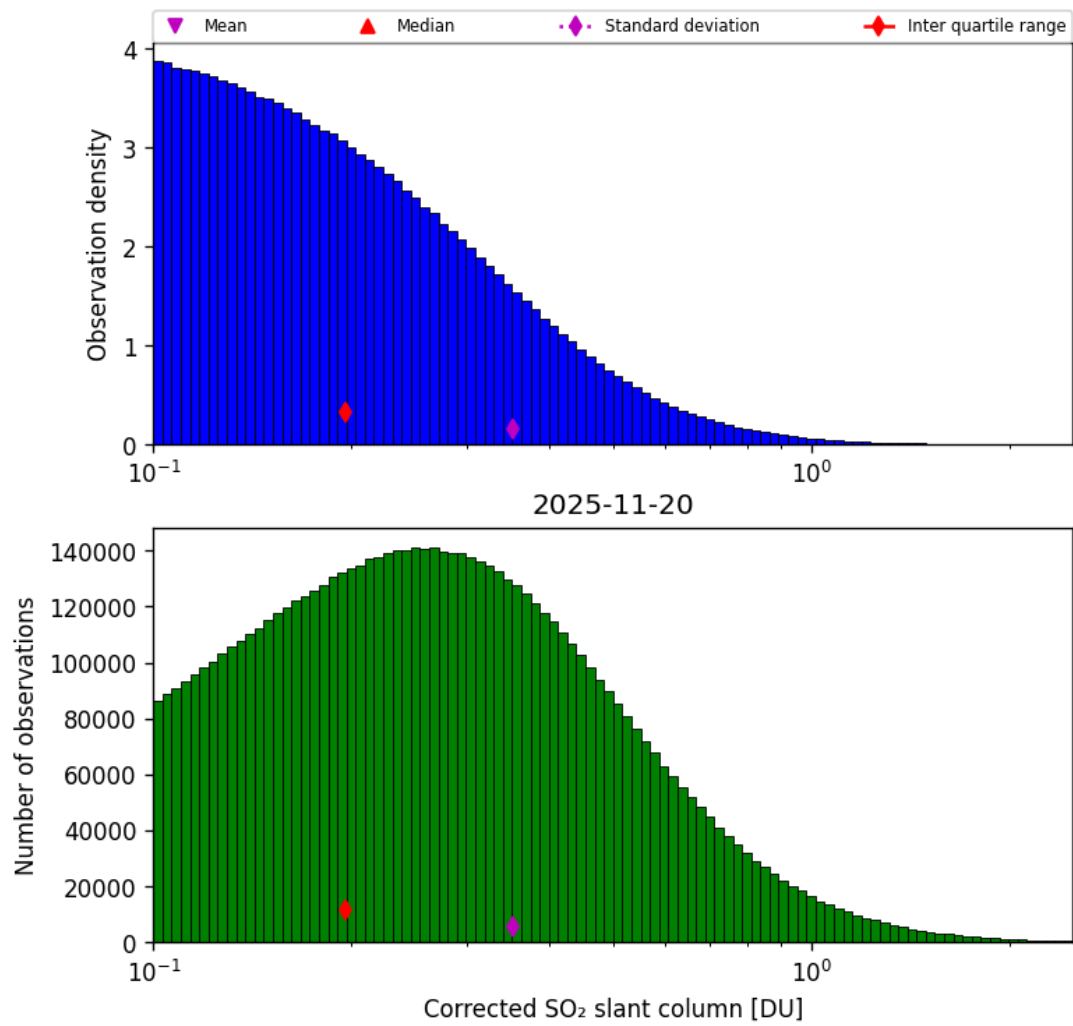
Figure 60: Histogram of “Corrected SO 2 slant column” for 2025-11-19 to 2025-11-21
