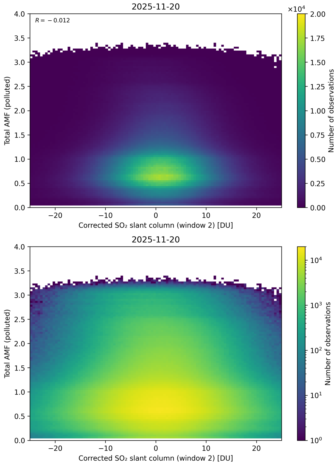
Figure 253: Scatter density plot of “Corrected SO 2 slant column (window 2)” against “Total AMF (polluted)” for 2025-11-19 to 2025-11-21.
