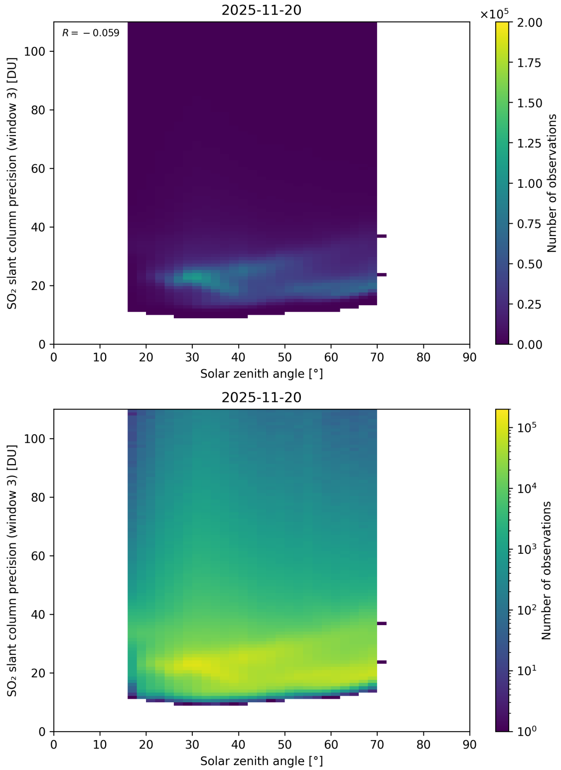
Figure 188: Scatter density plot of “Solar zenith angle” against “SO 2 slant column precision (window 3)” for 2025-11-19 to 2025-11-21.
