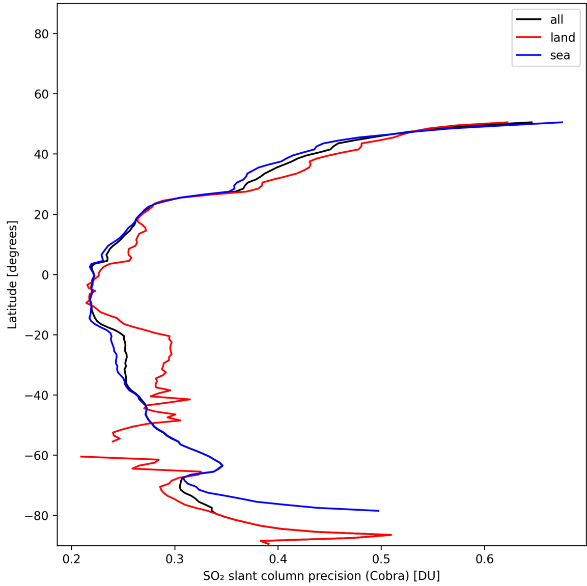
Figure 36: Zonal average of “SO 2 slant column precision (Cobra)” for 2025-11-19 to 2025-11-21.
