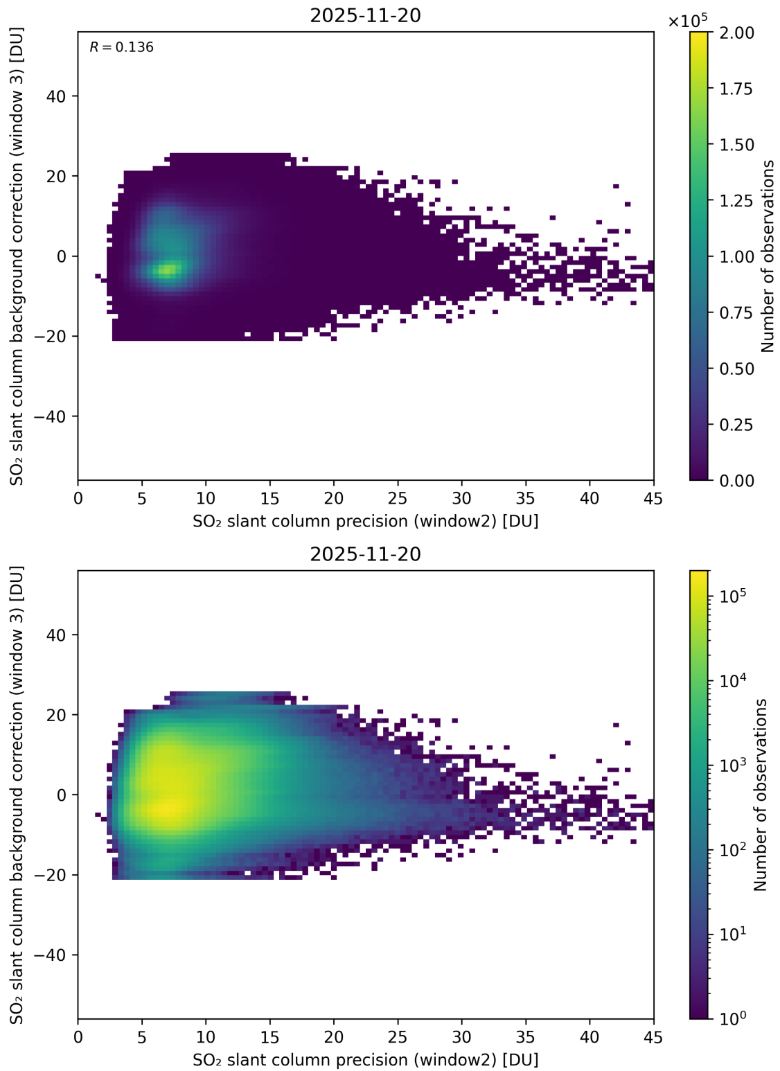
Figure 292: Scatter density plot of “SO 2 slant column precision (window2)” against “SO 2 slant column background correction (window 3)” for 2025-11-19 to 2025-11-21.
