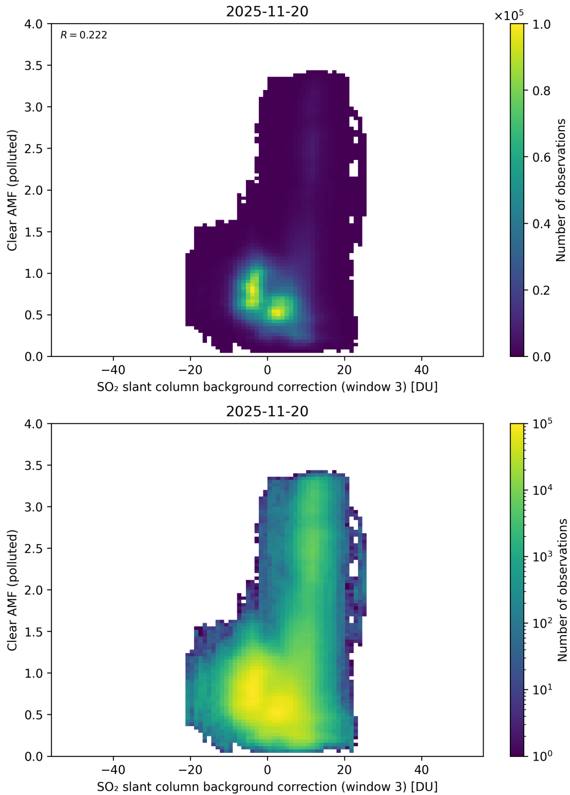
Figure 135: Scatter density plot of “SO 2 slant column background correction (window 3)” against “Clear AMF (polluted)” for 2025-11-19 to 2025-11-21.
