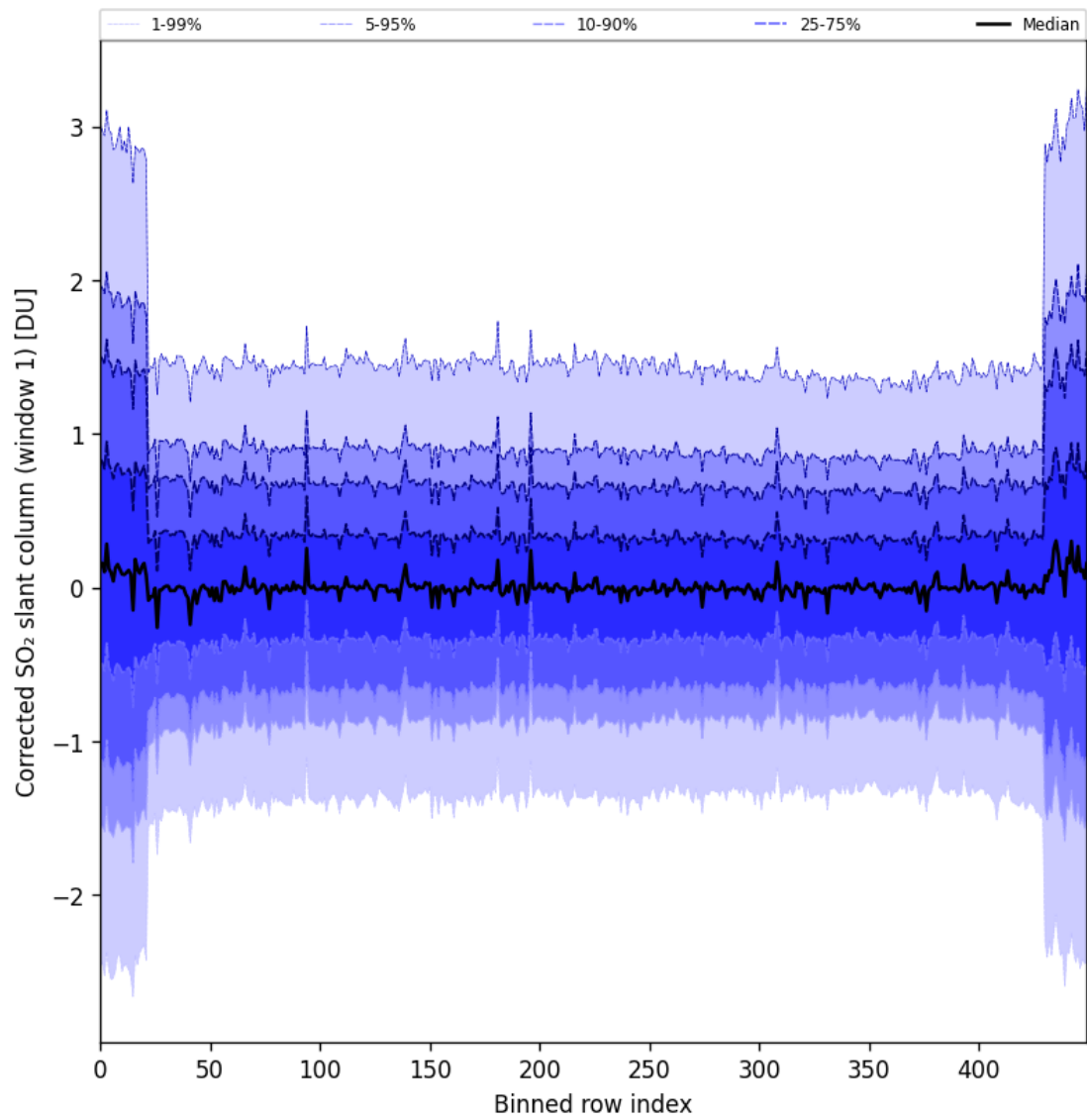
Figure 91: Along track statistics of “Corrected SO 2 slant column (window 1)” for 2025-11-19 to 2025-11-21
