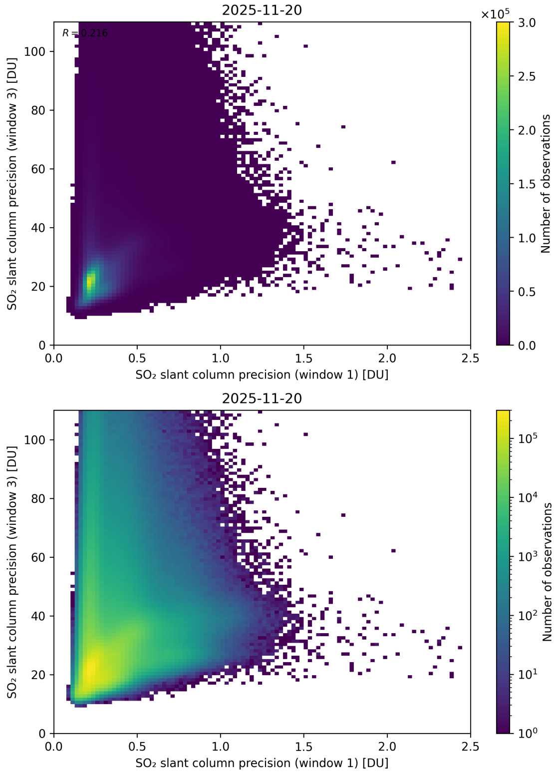
Figure 279: Scatter density plot of “SO 2 slant column precision (window 1)” against “SO 2 slant column precision (window 3)” for 2025-11-19 to 2025-11-21.
