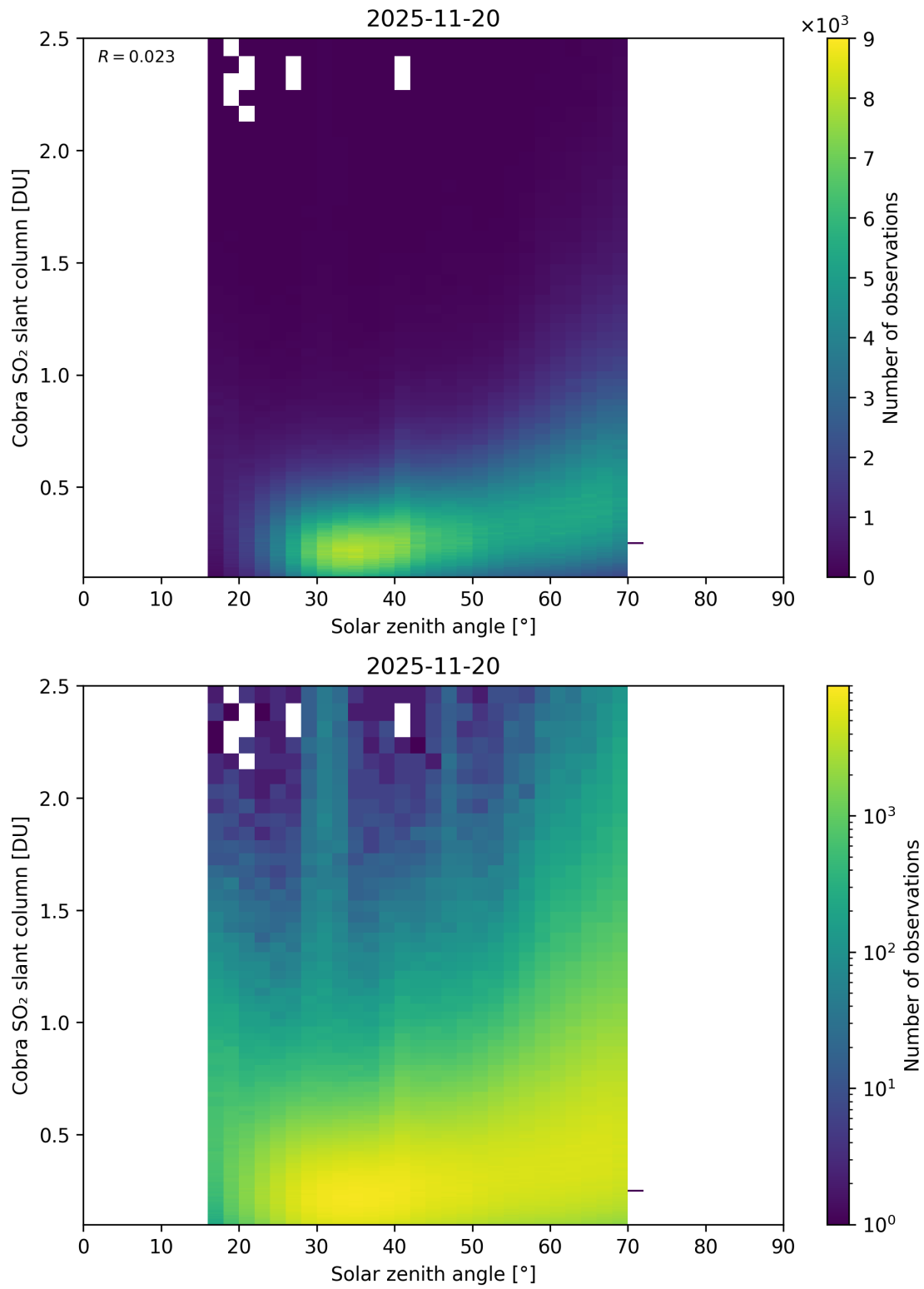
Figure 179: Scatter density plot of “Solar zenith angle” against “Cobra SO 2 slant column” for 2025-11-19 to 2025-11-21.
