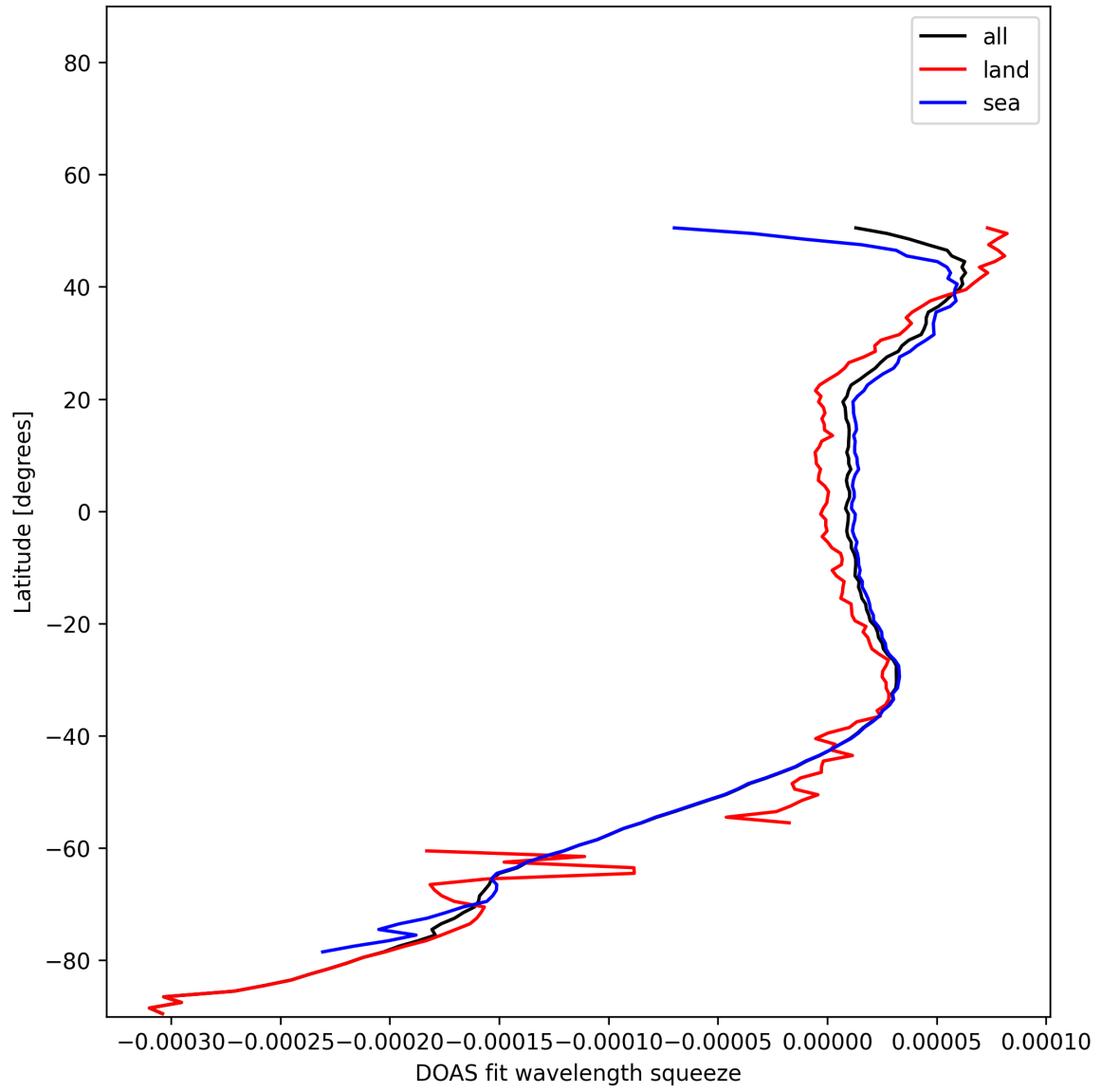
Figure 51: Zonal average of “DOAS fit wavelength squeeze” for 2025-11-19 to 2025-11-21.
