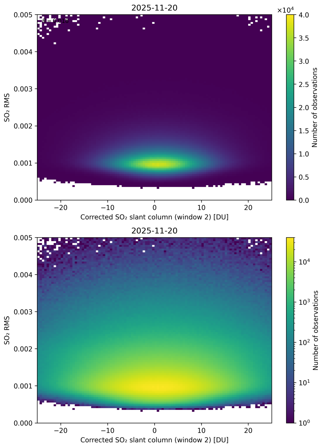
Figure 248: Scatter density plot of “Corrected SO 2 slant column (window 2)” against “SO 2 RMS” for 2025-11-19 to 2025-11-21.
