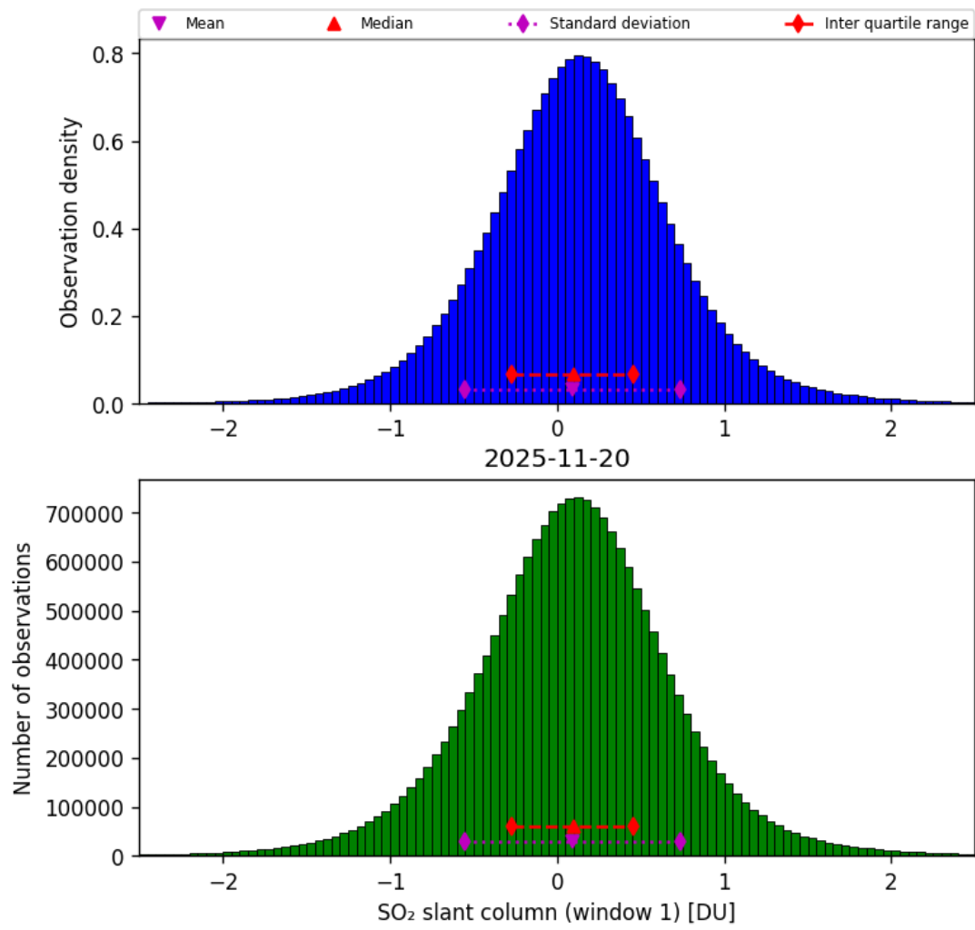
Figure 63: Histogram of “SO 2 slant column (window 1)” for 2025-11-19 to 2025-11-21
