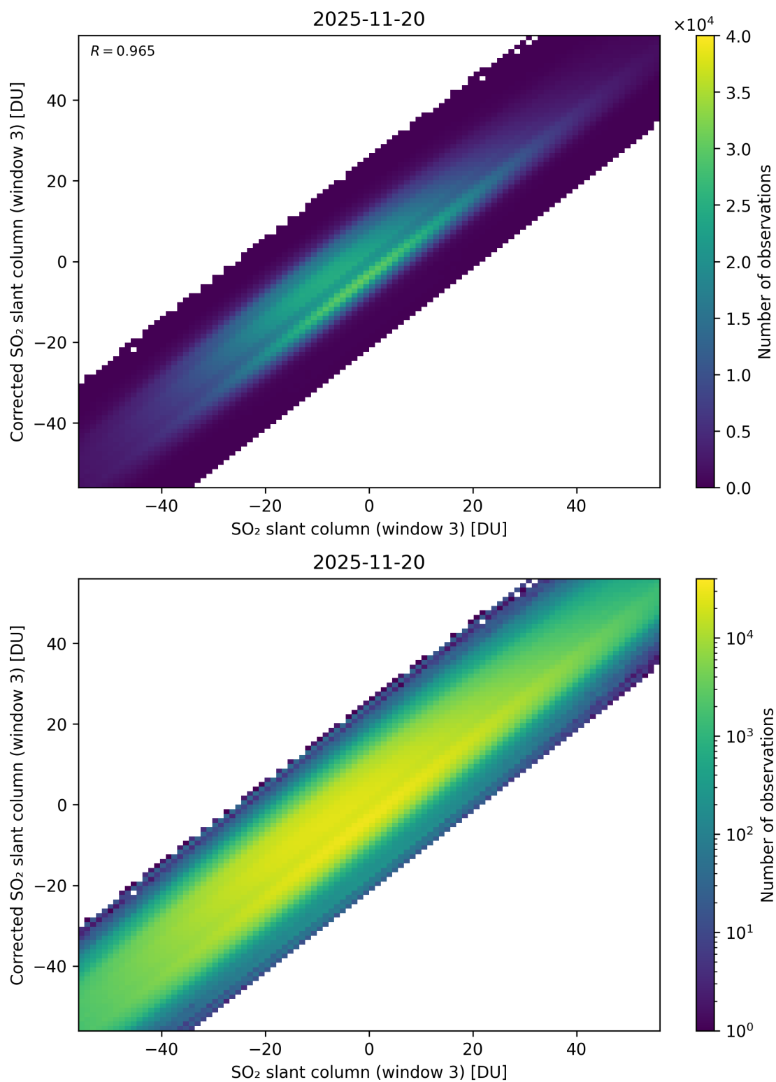
Figure 316: Scatter density plot of “SO 2 slant column (window 3)” against “Corrected SO 2 slant column (window 3)” for 2025-11-19 to 2025-11-21.
