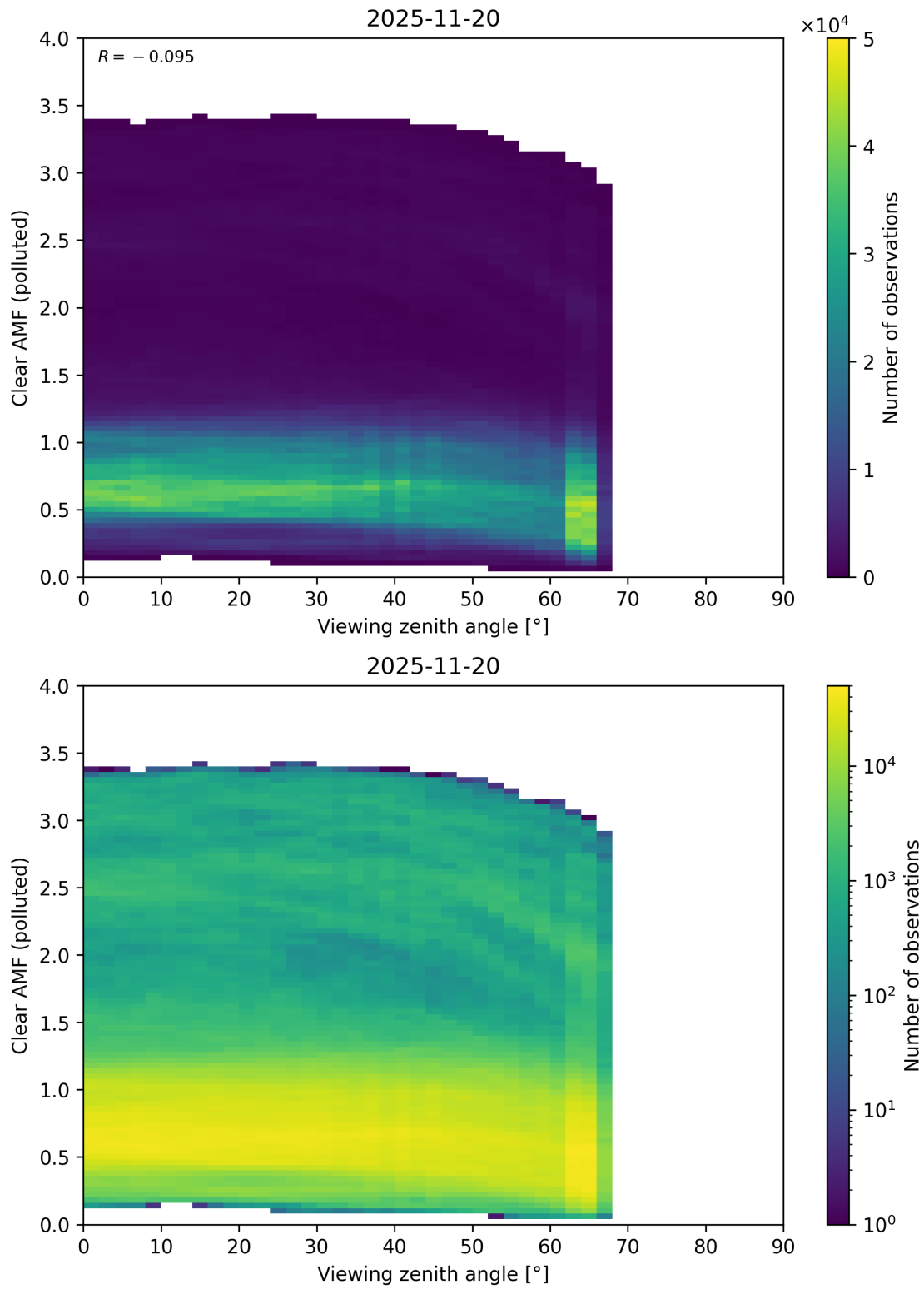
Figure 370: Scatter density plot of “Viewing zenith angle” against “Clear AMF (polluted)” for 2025-11-19 to 2025-11-21.
