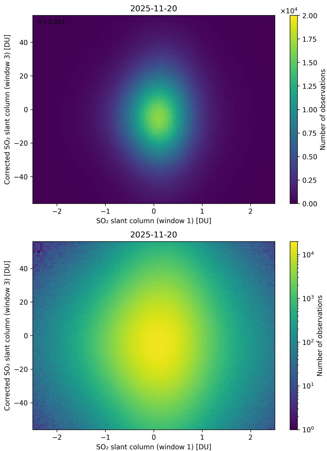
Figure 284: Scatter density plot of “SO 2 slant column (window 1)” against “Corrected SO 2 slant column (window 3)” for 2025-11-19 to 2025-11-21.
