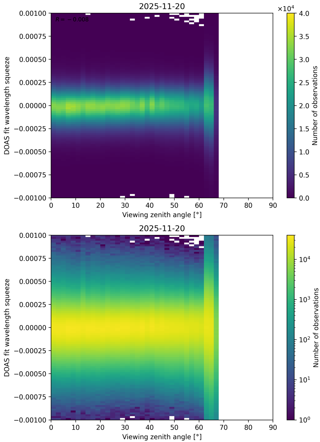
Figure 366: Scatter density plot of “Viewing zenith angle” against “DOAS fit wavelength squeeze” for 2025-11-19 to 2025-11-21.
