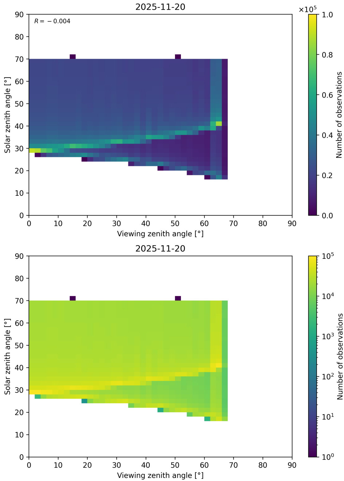
Figure 369: Scatter density plot of “Viewing zenith angle” against “Solar zenith angle” for 2025-11-19 to 2025-11-21.
