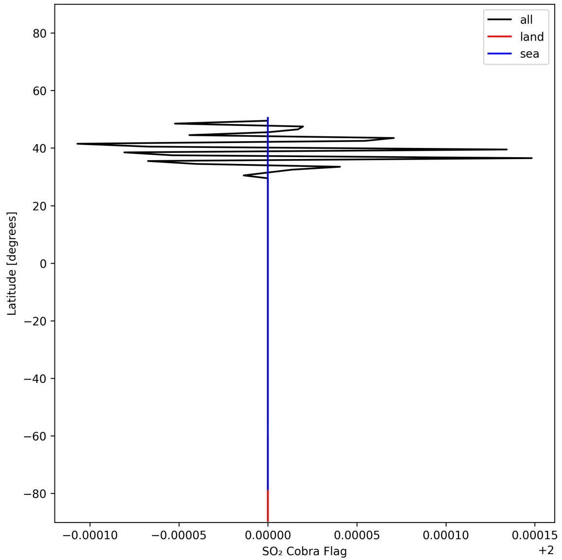
Figure 49: Zonal average of “SO 2 Cobra Flag” for 2025-11-19 to 2025-11-21.
