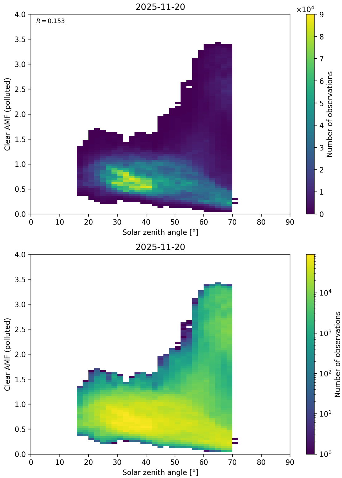
Figure 178: Scatter density plot of “Solar zenith angle” against “Clear AMF (polluted)” for 2025-11-19 to 2025-11-21.
