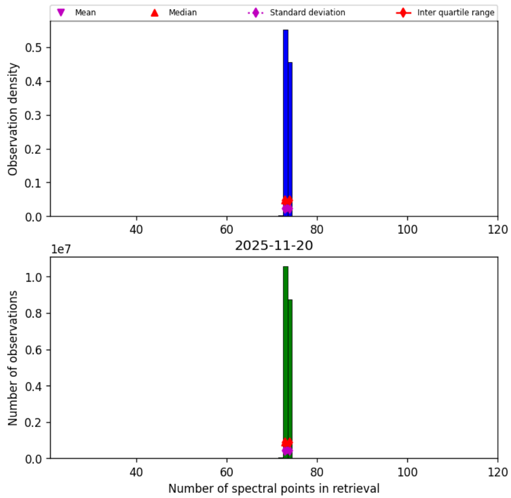
Figure 82: Histogram of “Number of spectral points in retrieval” for 2025-11-19 to 2025-11-21
