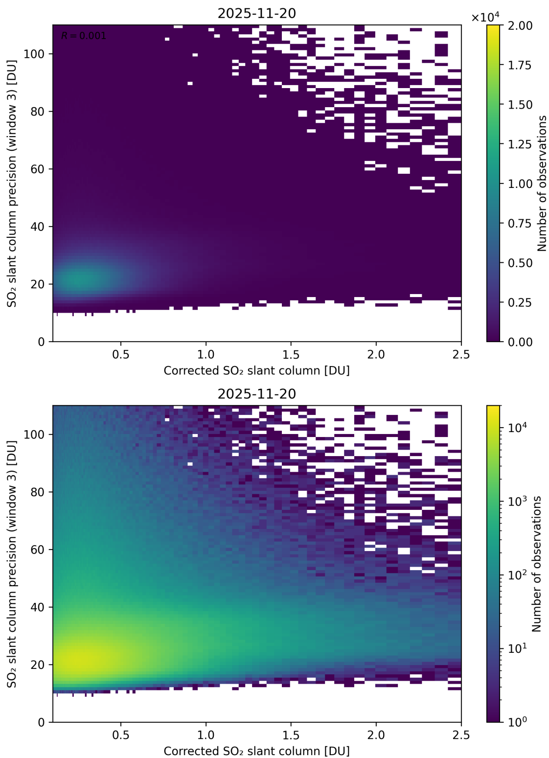
Figure 241: Scatter density plot of “Corrected SO 2 slant column” against “SO 2 slant column precision (window 3)” for 2025-11-19 to 2025-11-21.
