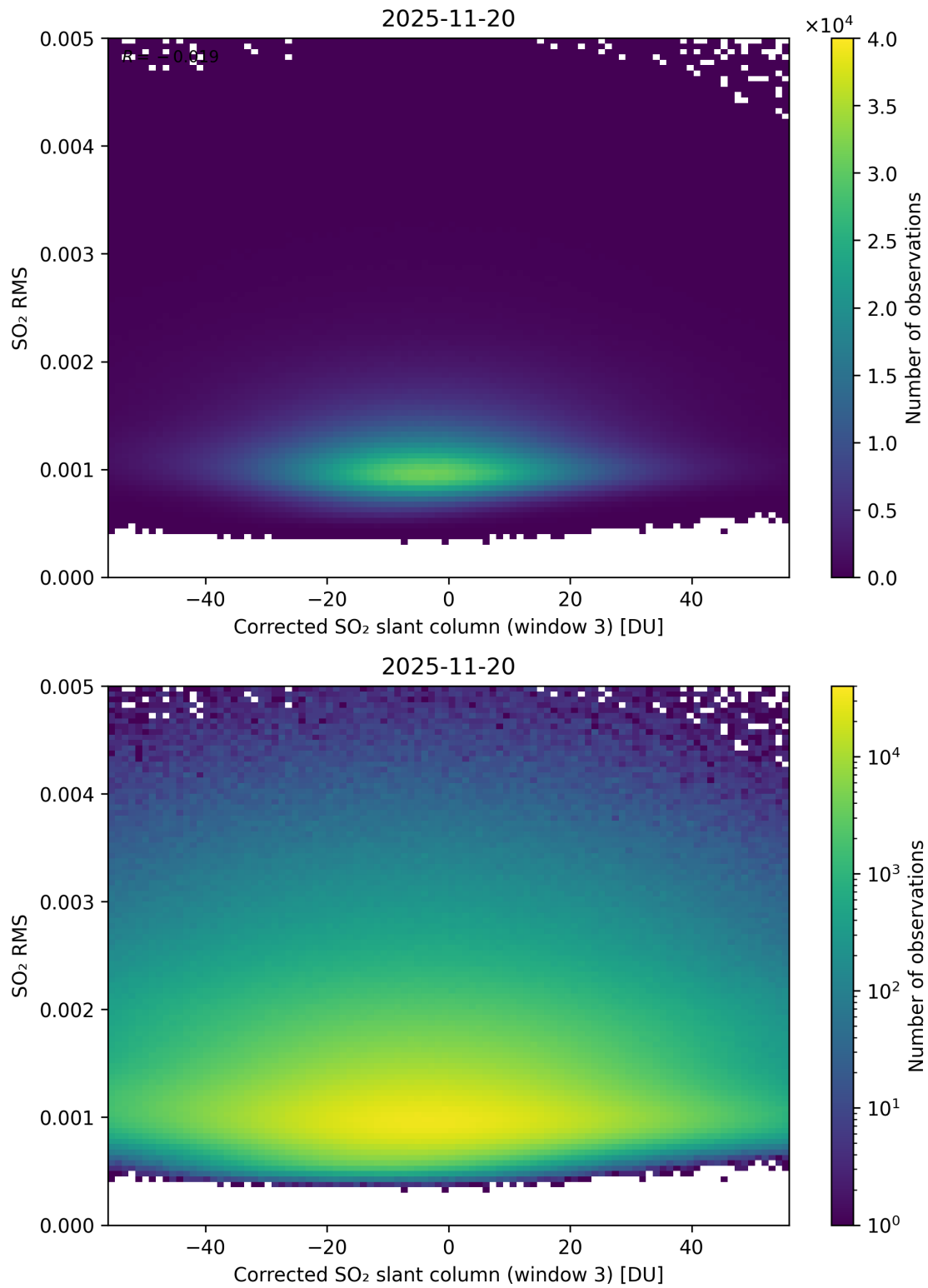
Figure 258: Scatter density plot of “Corrected SO 2 slant column (window 3)” against “SO 2 RMS” for 2025-11-19 to 2025-11-21.
