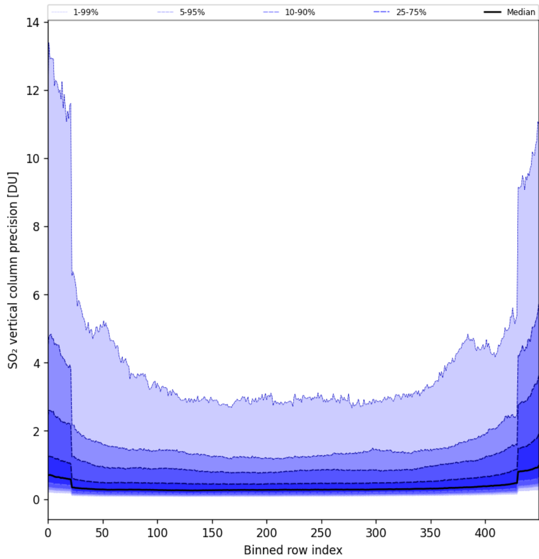
Figure 85: Along track statistics of “SO 2 vertical column precision” for 2025-11-19 to 2025-11-21
