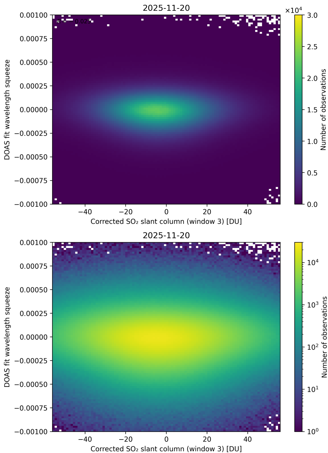
Figure 257: Scatter density plot of “Corrected SO 2 slant column (window 3)” against “DOAS fit wavelength squeeze” for 2025-11-19 to 2025-11-21.
