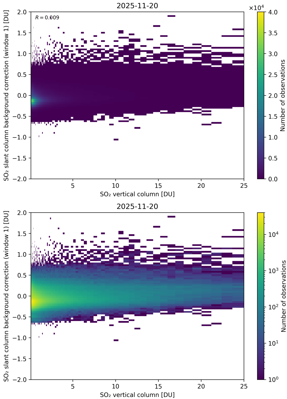
Figure 323: Scatter density plot of “SO 2 vertical column” against “SO 2 slant column background correction (window 1)” for 2025-11-19 to 2025-11-21.
