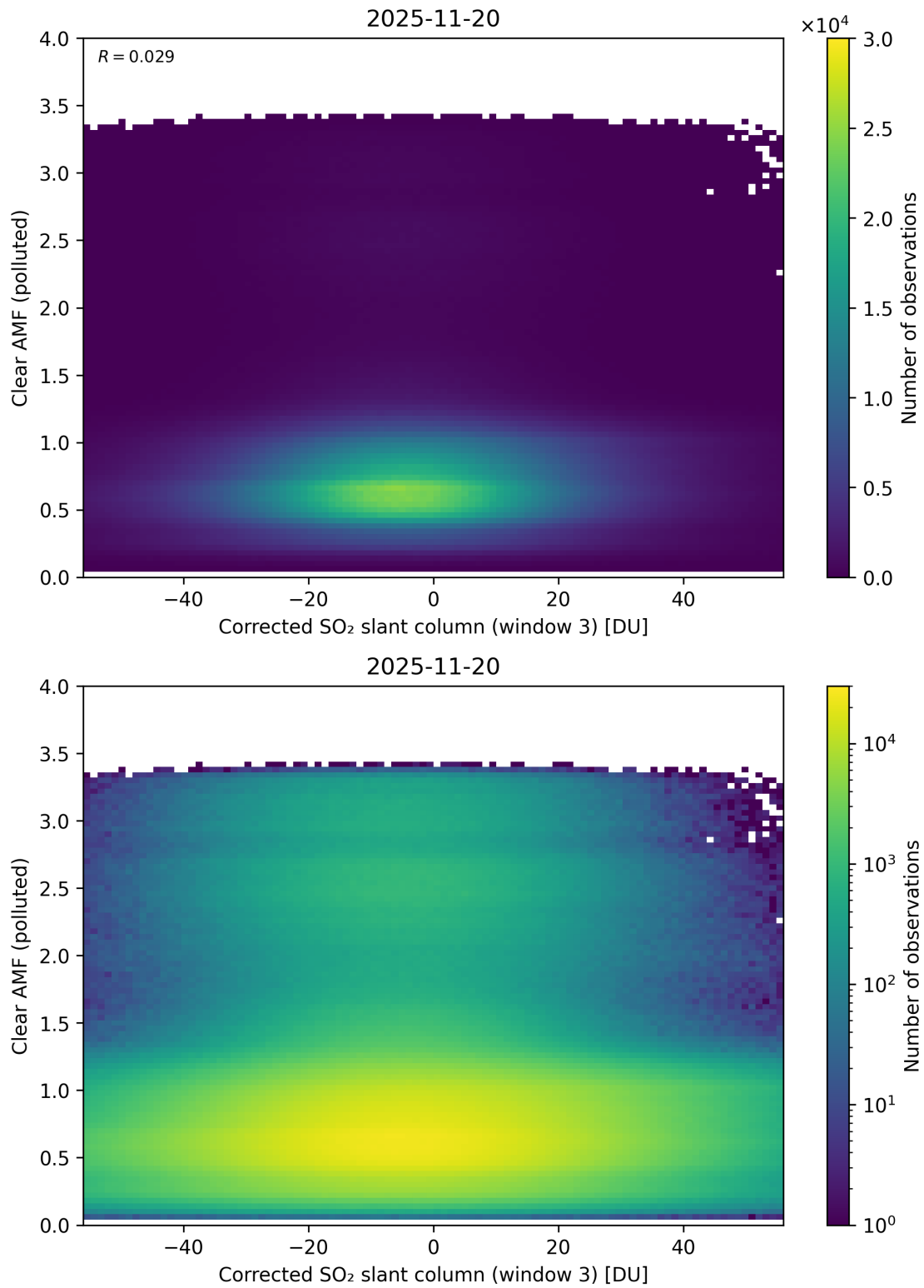
Figure 259: Scatter density plot of “Corrected SO 2 slant column (window 3)” against “Clear AMF (polluted)” for 2025-11-19 to 2025-11-21.
