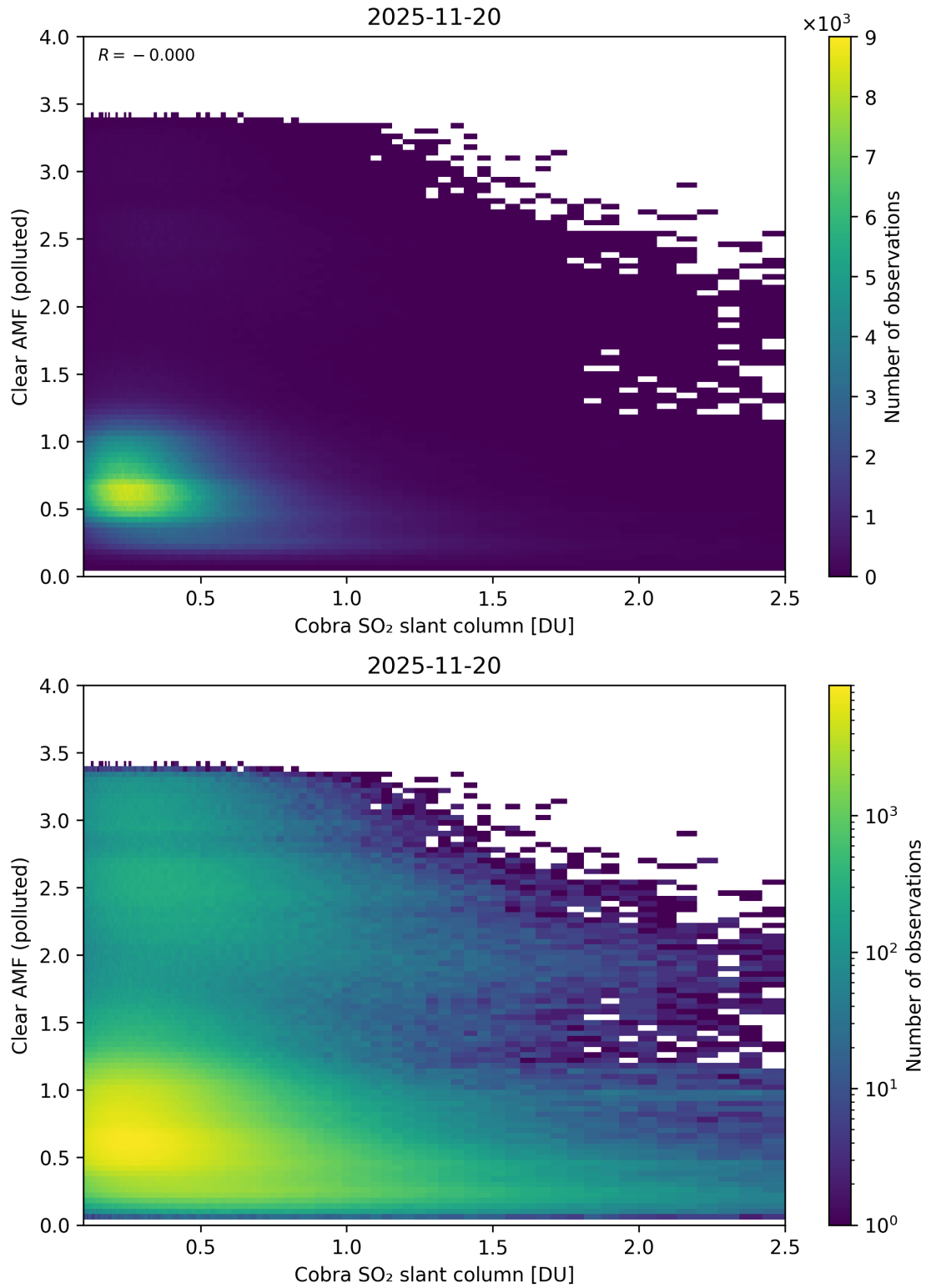
Figure 215: Scatter density plot of “Cobra SO 2 slant column” against “Clear AMF (polluted)” for 2025-11-19 to 2025-11-21.
