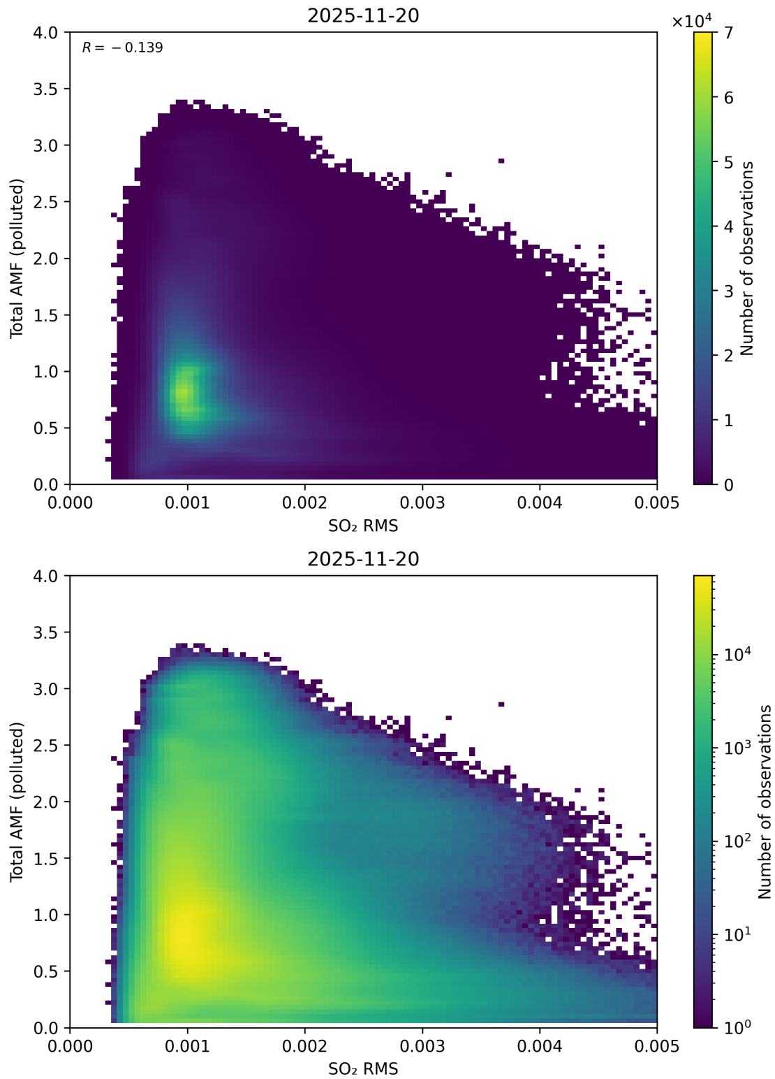
Figure 148: Scatter density plot of “SO 2 RMS” against “Total AMF (polluted)” for 2025-11-19 to 2025-11-21.
