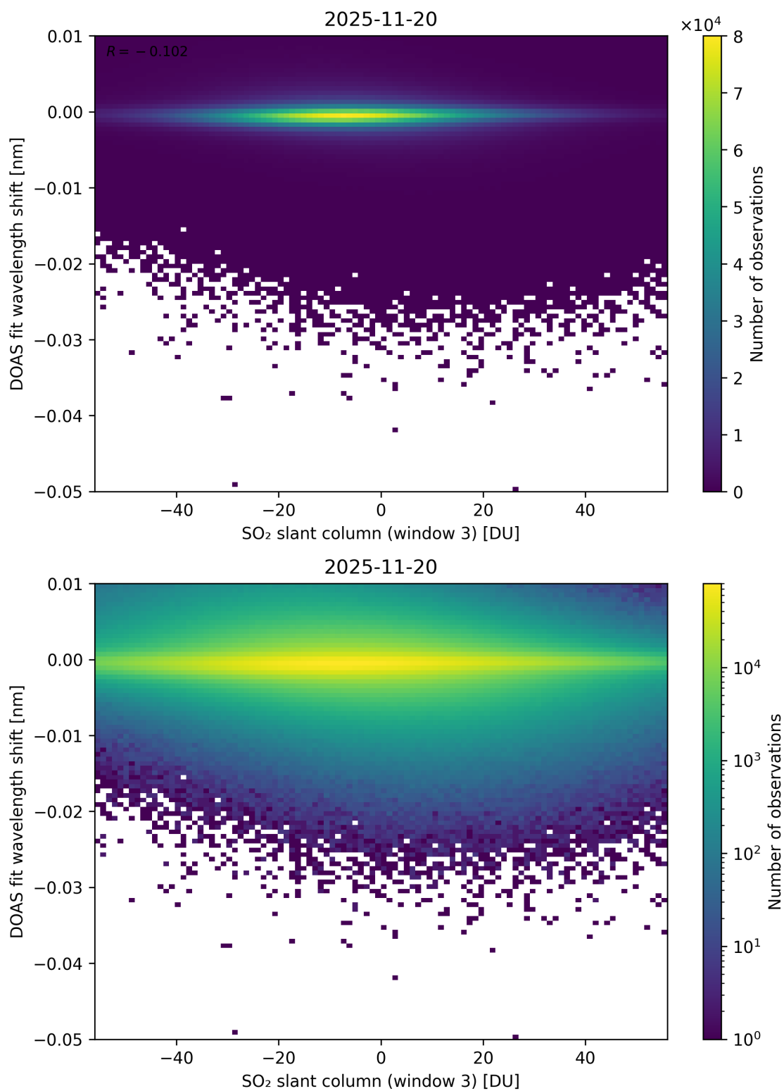
Figure 304: Scatter density plot of “SO 2 slant column (window 3)” against “DOAS fit wavelength shift” for 2025-11-19 to 2025-11-21.
