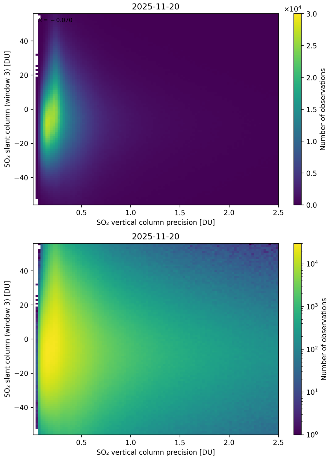
Figure 344: Scatter density plot of “SO 2 vertical column precision” against “SO 2 slant column (window 3)” for 2025-11-19 to 2025-11-21.
