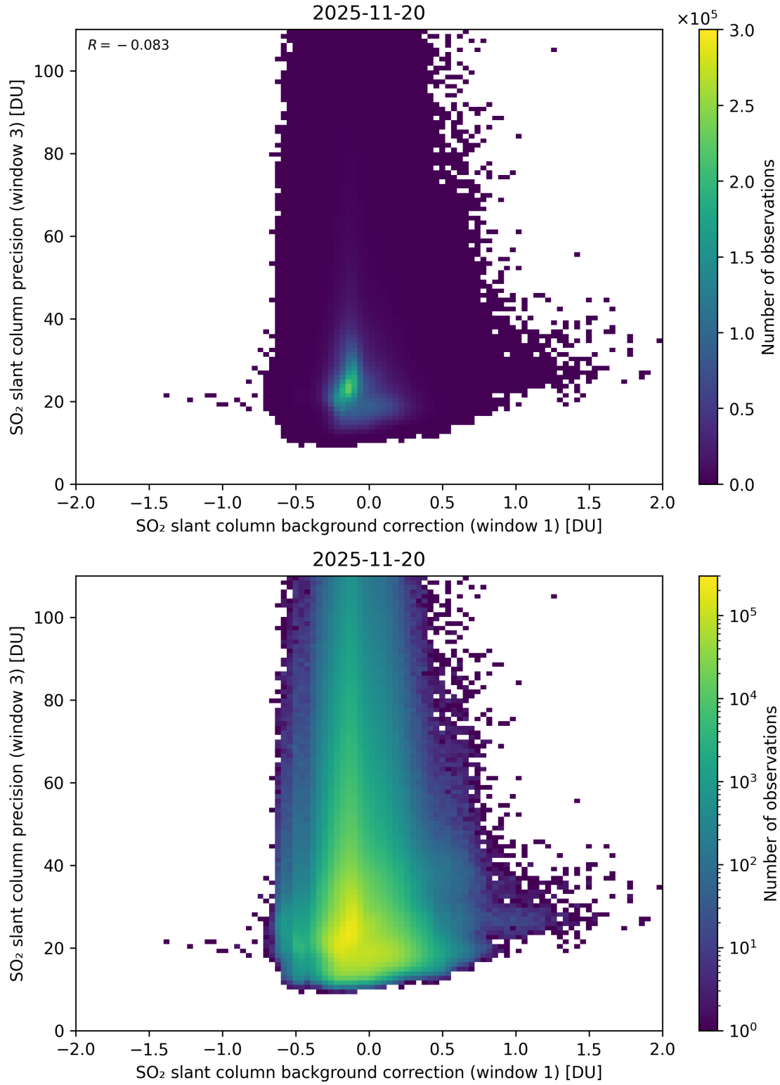
Figure 119: Scatter density plot of “SO 2 slant column background correction (window 1)” against “SO 2 slant column precision (window 3)” for 2025-11-19 to 2025-11-21.
