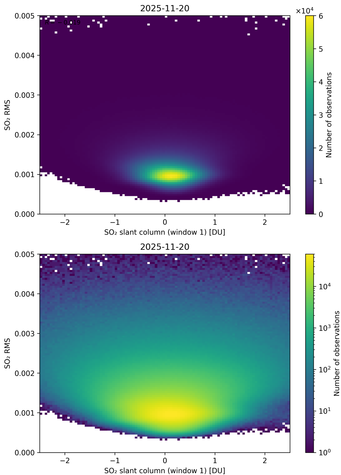
Figure 267: Scatter density plot of “SO 2 slant column (window 1)” against “SO 2 RMS” for 2025-11-19 to 2025-11-21.
