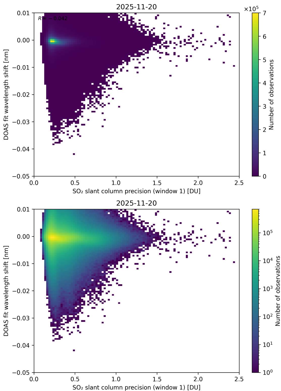
Figure 271: Scatter density plot of “SO 2 slant column precision (window 1)” against “DOAS fit wavelength shift” for 2025-11-19 to 2025-11-21.
