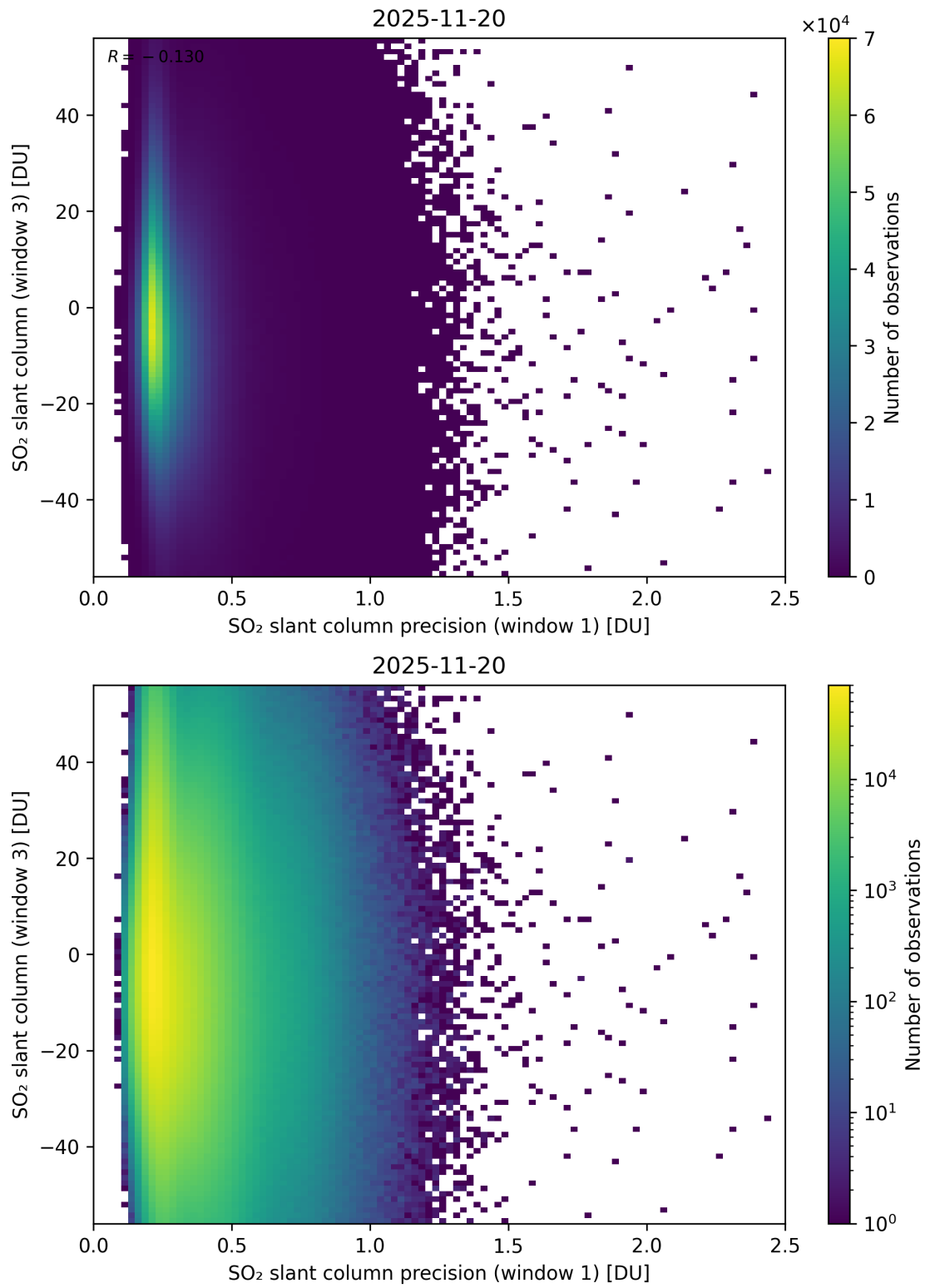
Figure 278: Scatter density plot of “SO 2 slant column precision (window 1)” against “SO 2 slant column (window 3)” for 2025-11-19 to 2025-11-21.
