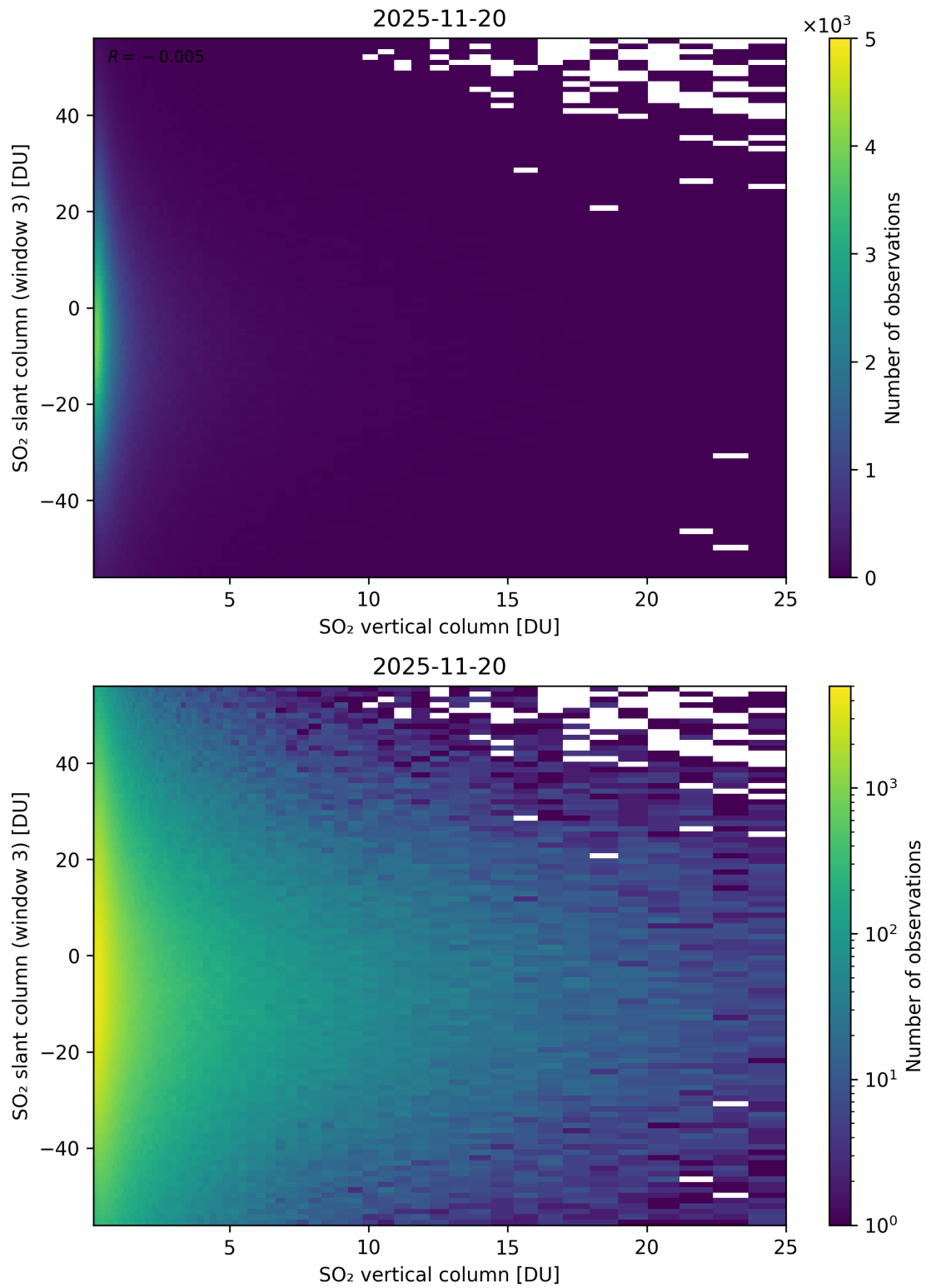
Figure 357: Scatter density plot of “SO 2 vertical column” against “SO 2 slant column (window 3)” for 2025-11-19 to 2025-11-21.
