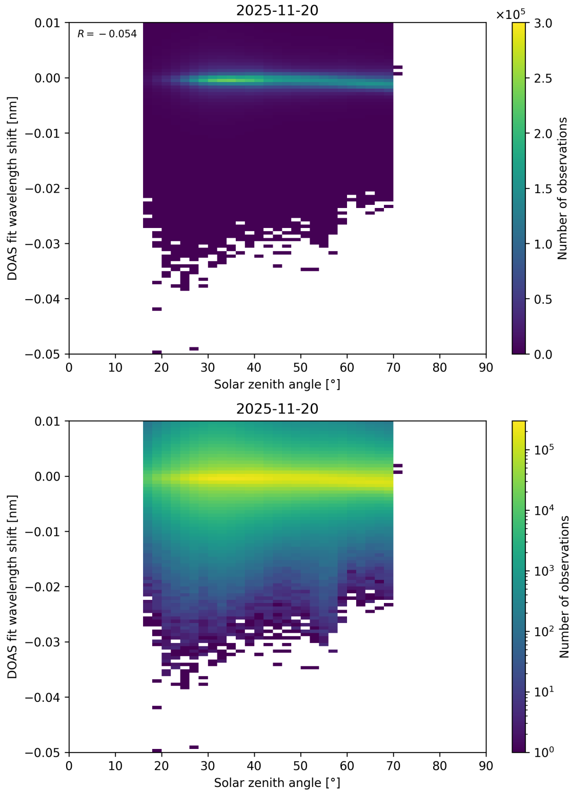
Figure 174: Scatter density plot of “Solar zenith angle” against “DOAS fit wavelength shift” for 2025-11-19 to 2025-11-21.
