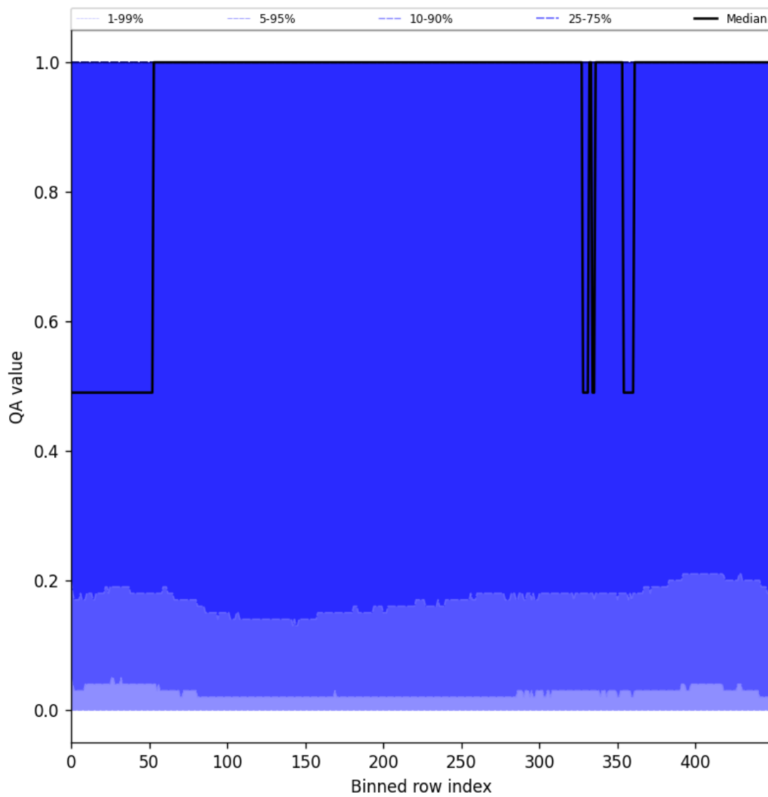
Figure 83: Along track statistics of “QA value” for 2025-11-19 to 2025-11-21
