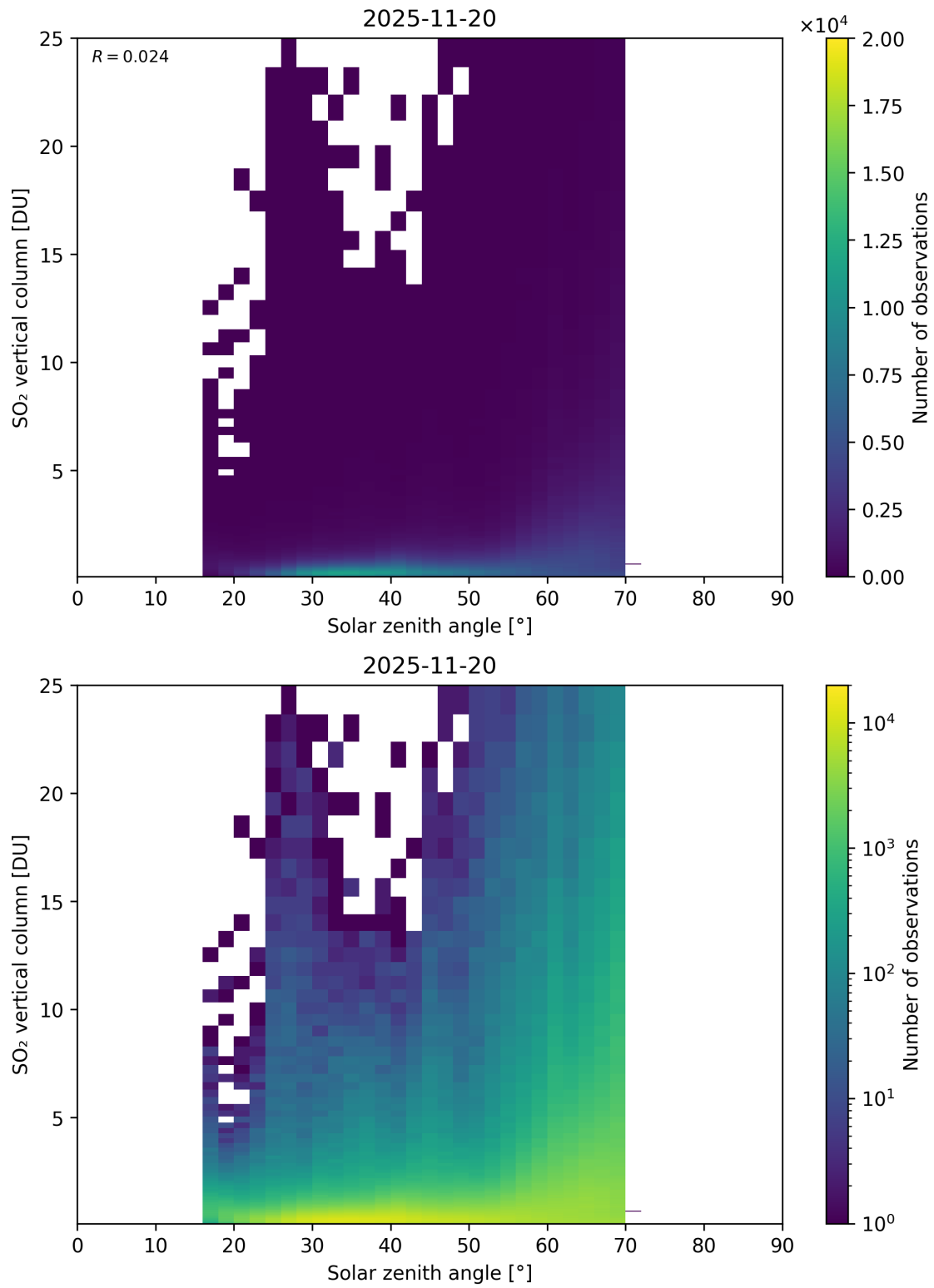
Figure 191: Scatter density plot of “Solar zenith angle” against “SO 2 vertical column” for 2025-11-19 to 2025-11-21.
