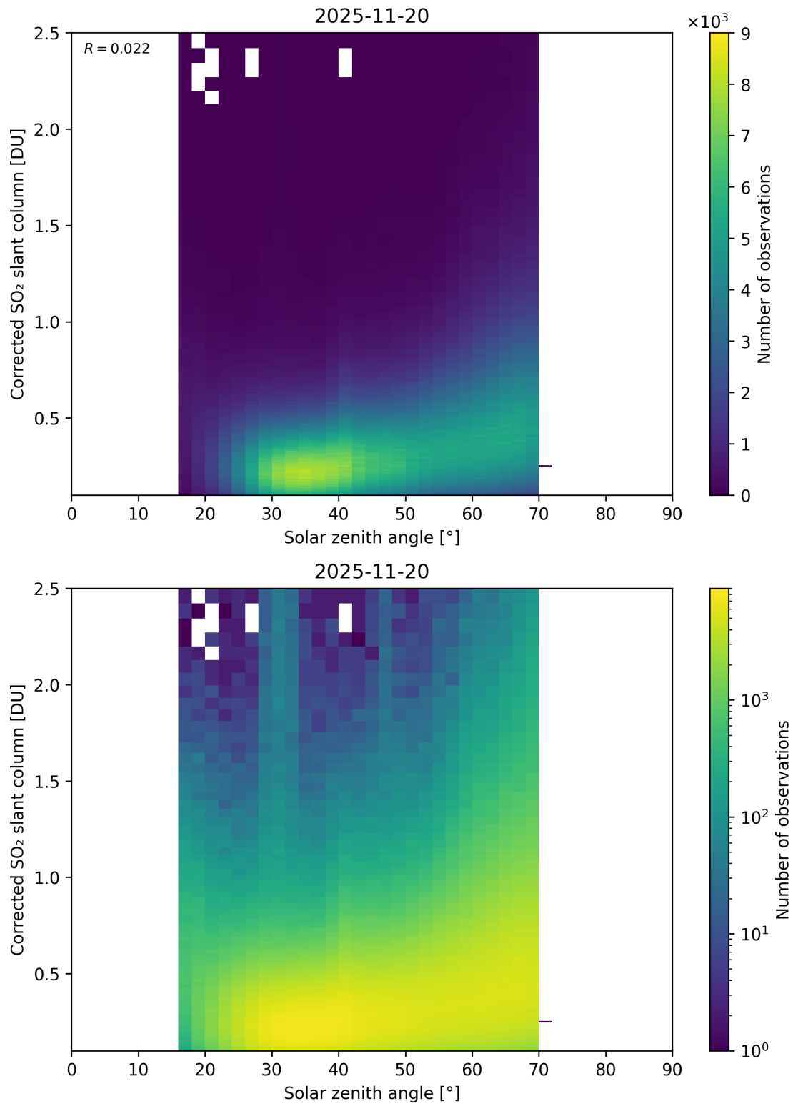
Figure 181: Scatter density plot of “Solar zenith angle” against “Corrected SO 2 slant column” for 2025-11-19 to 2025-11-21.
