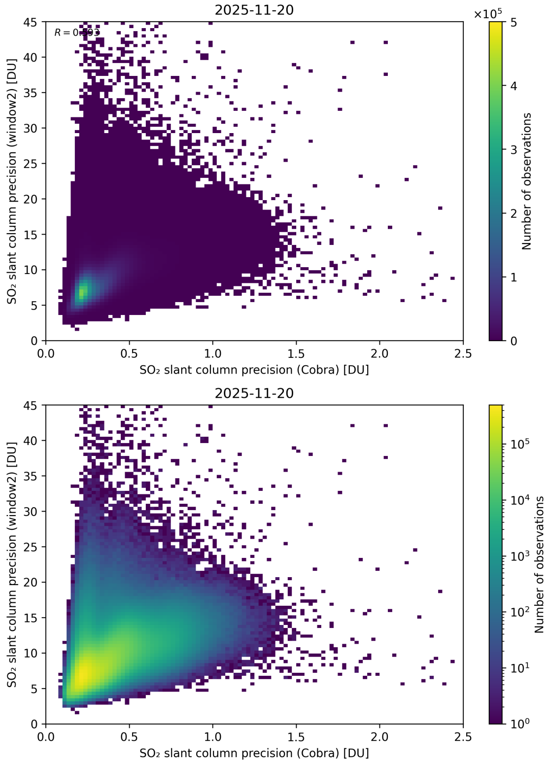
Figure 210: Scatter density plot of “SO 2 slant column precision (Cobra)” against “SO 2 slant column precision (window2)” for 2025-11-19 to 2025-11-21.
