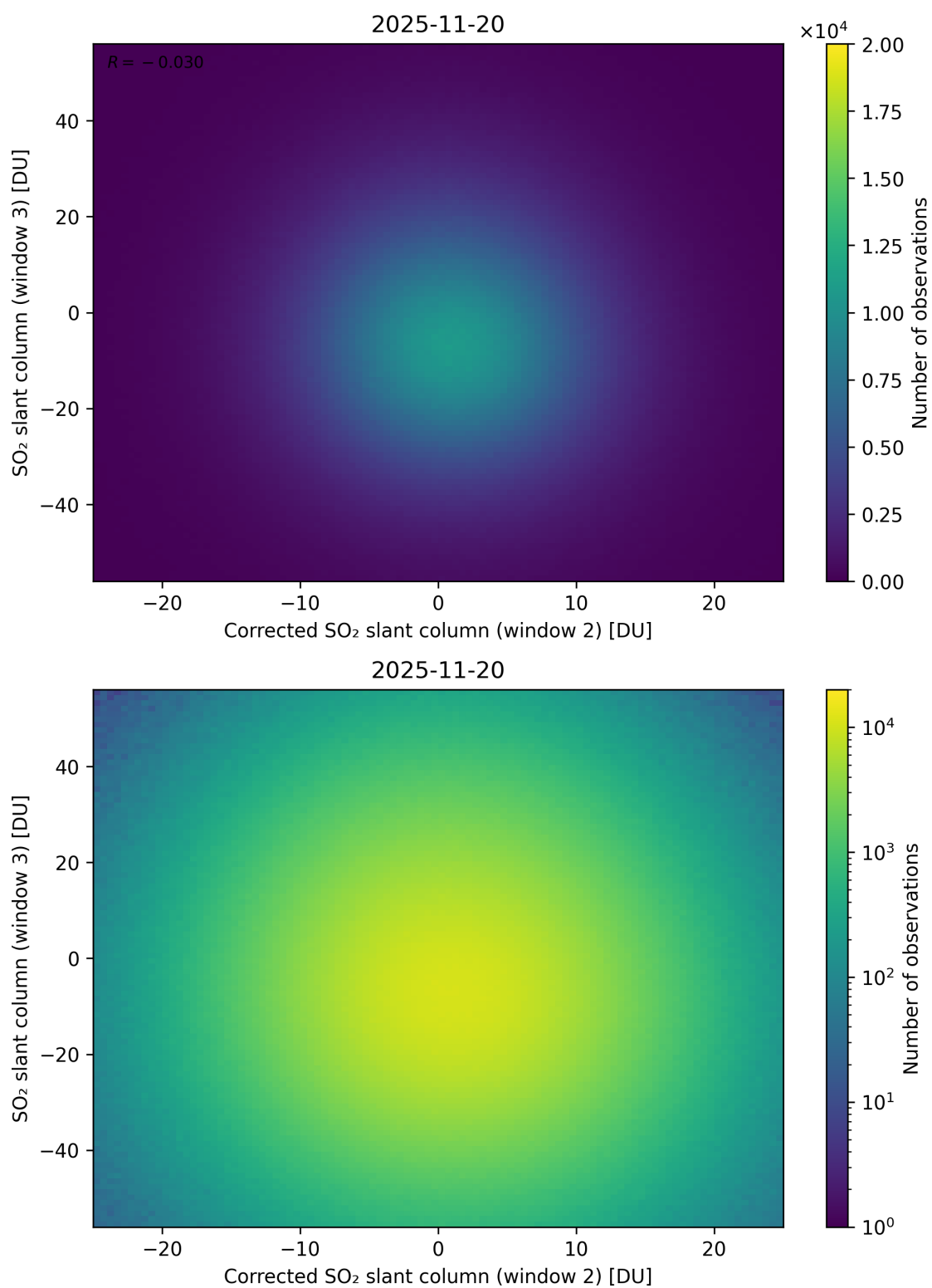
Figure 251: Scatter density plot of “Corrected SO 2 slant column (window 2)” against “SO 2 slant column (window 3)” for 2025-11-19 to 2025-11-21.
