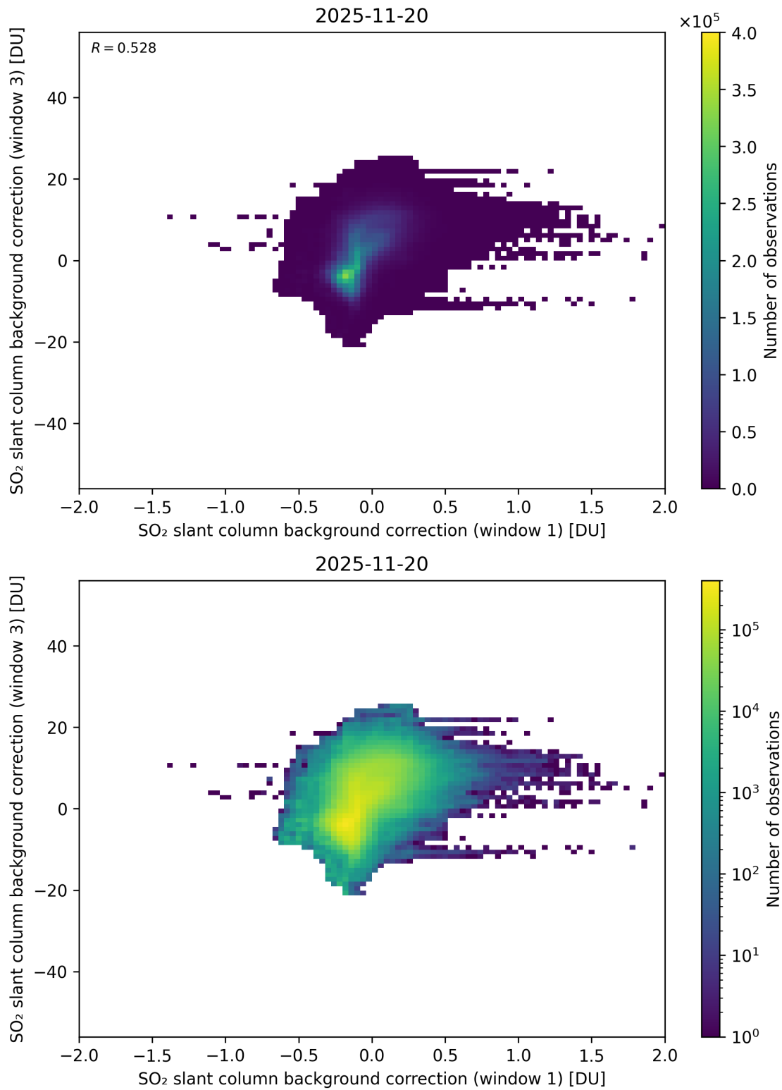
Figure 110: Scatter density plot of “SO 2 slant column background correction (window 1)” against “SO 2 slant column background correction (window 3)” for 2025-11-19 to 2025-11-21.
