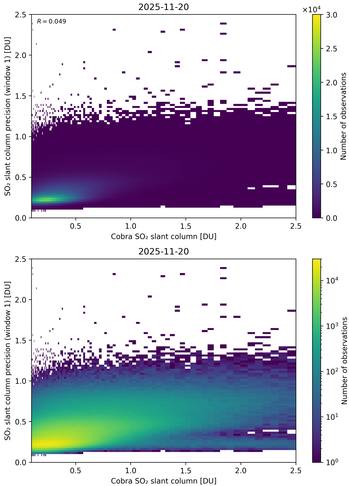
Figure 220: Scatter density plot of “Cobra SO 2 slant column” against “SO 2 slant column precision (window 1)” for 2025-11-19 to 2025-11-21.
