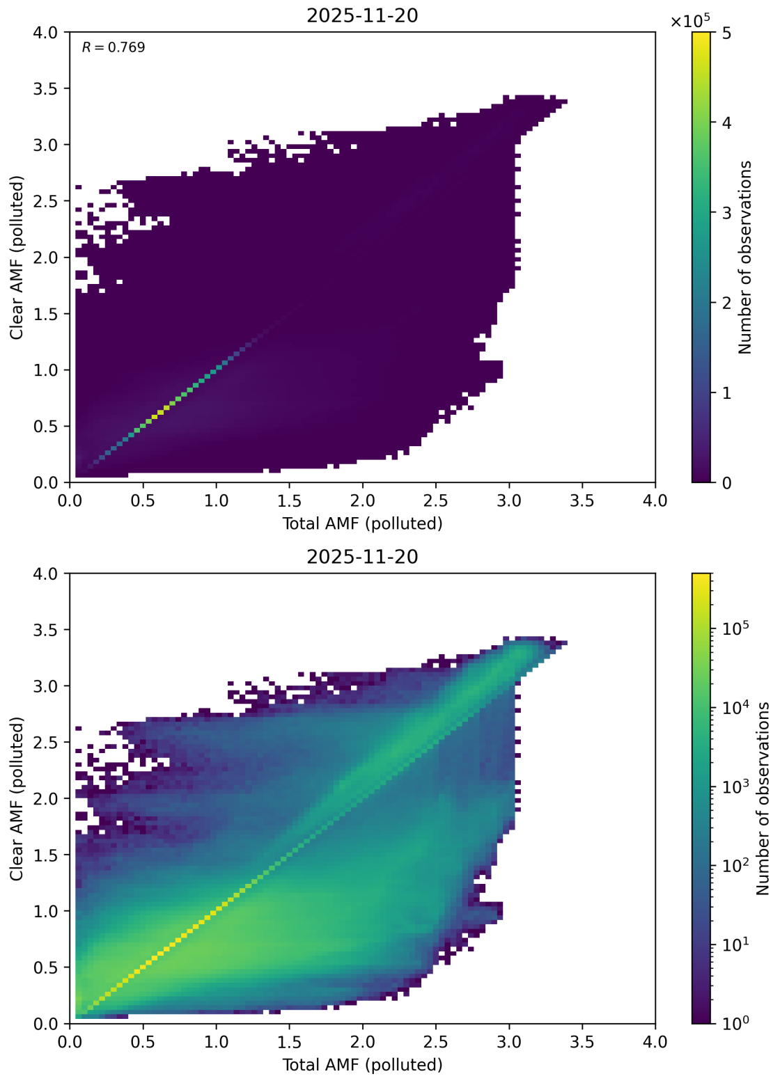
Figure 320: Scatter density plot of “Total AMF (polluted)” against “Clear AMF (polluted)” for 2025-11-19 to 2025-11-21.
