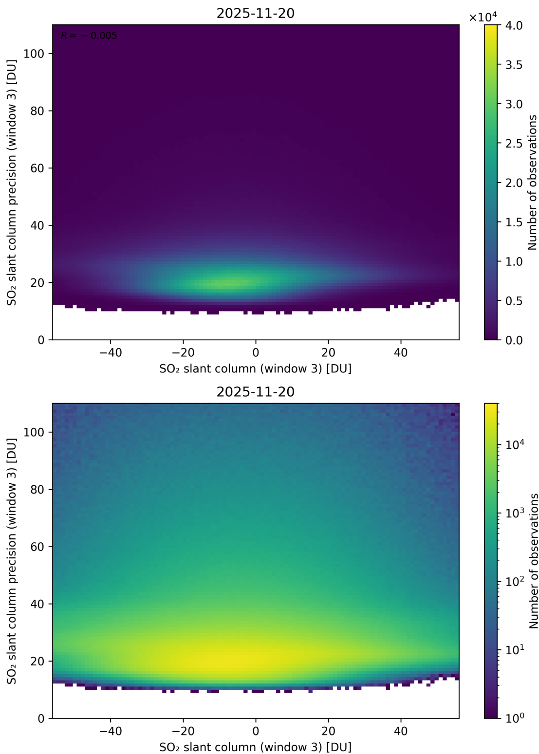
Figure 317: Scatter density plot of “SO 2 slant column (window 3)” against “SO 2 slant column precision (window 3)” for 2025-11-19 to 2025-11-21.
