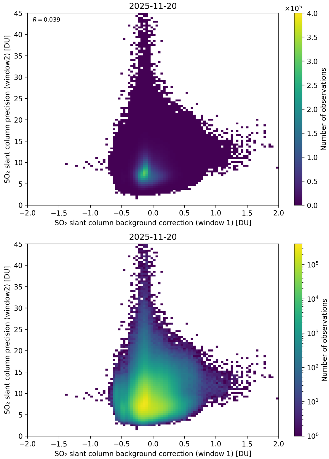
Figure 117: Scatter density plot of “SO 2 slant column background correction (window 1)” against “SO 2 slant column precision (window2)” for 2025-11-19 to 2025-11-21.
