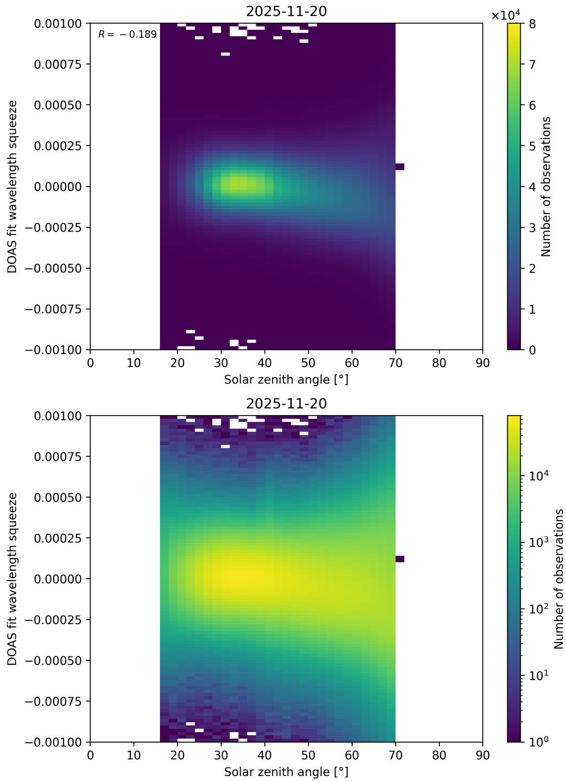
Figure 175: Scatter density plot of “Solar zenith angle” against “DOAS fit wavelength squeeze” for 2025-11-19 to 2025-11-21.
