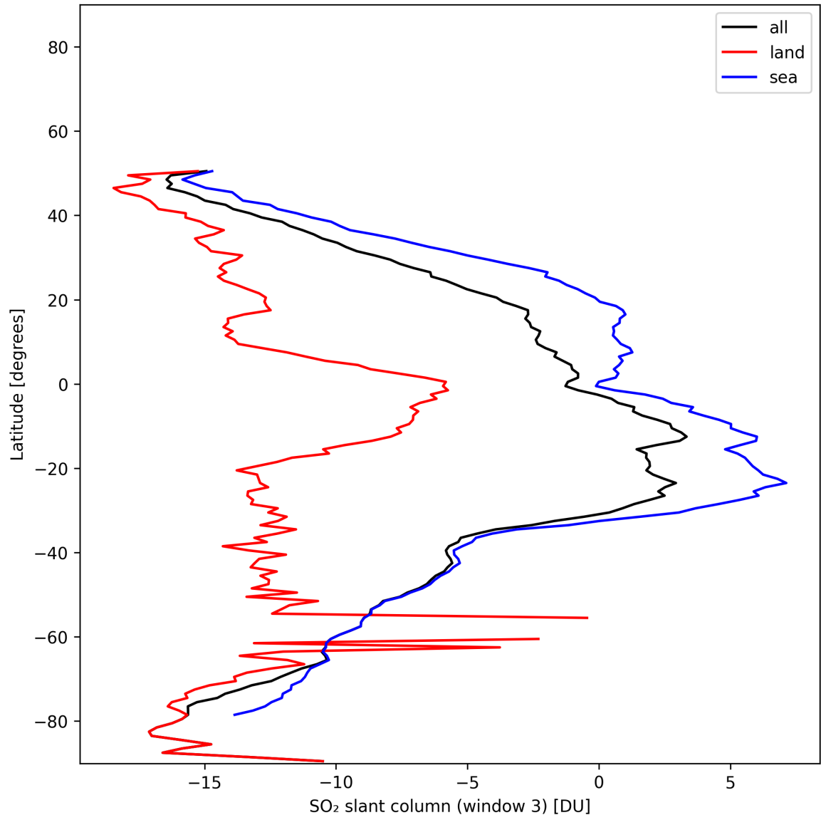
Figure 45: Zonal average of “SO 2 slant column (window 3)” for 2025-11-19 to 2025-11-21.
