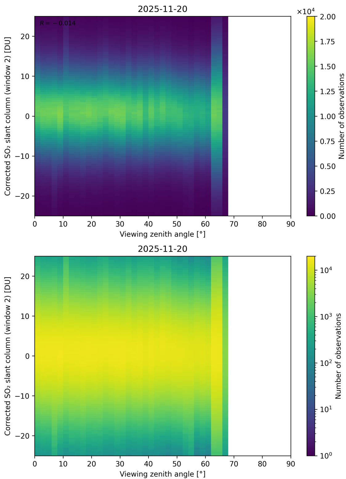
Figure 374: Scatter density plot of “Viewing zenith angle” against “Corrected SO 2 slant column (window 2)” for 2025-11-19 to 2025-11-21.
