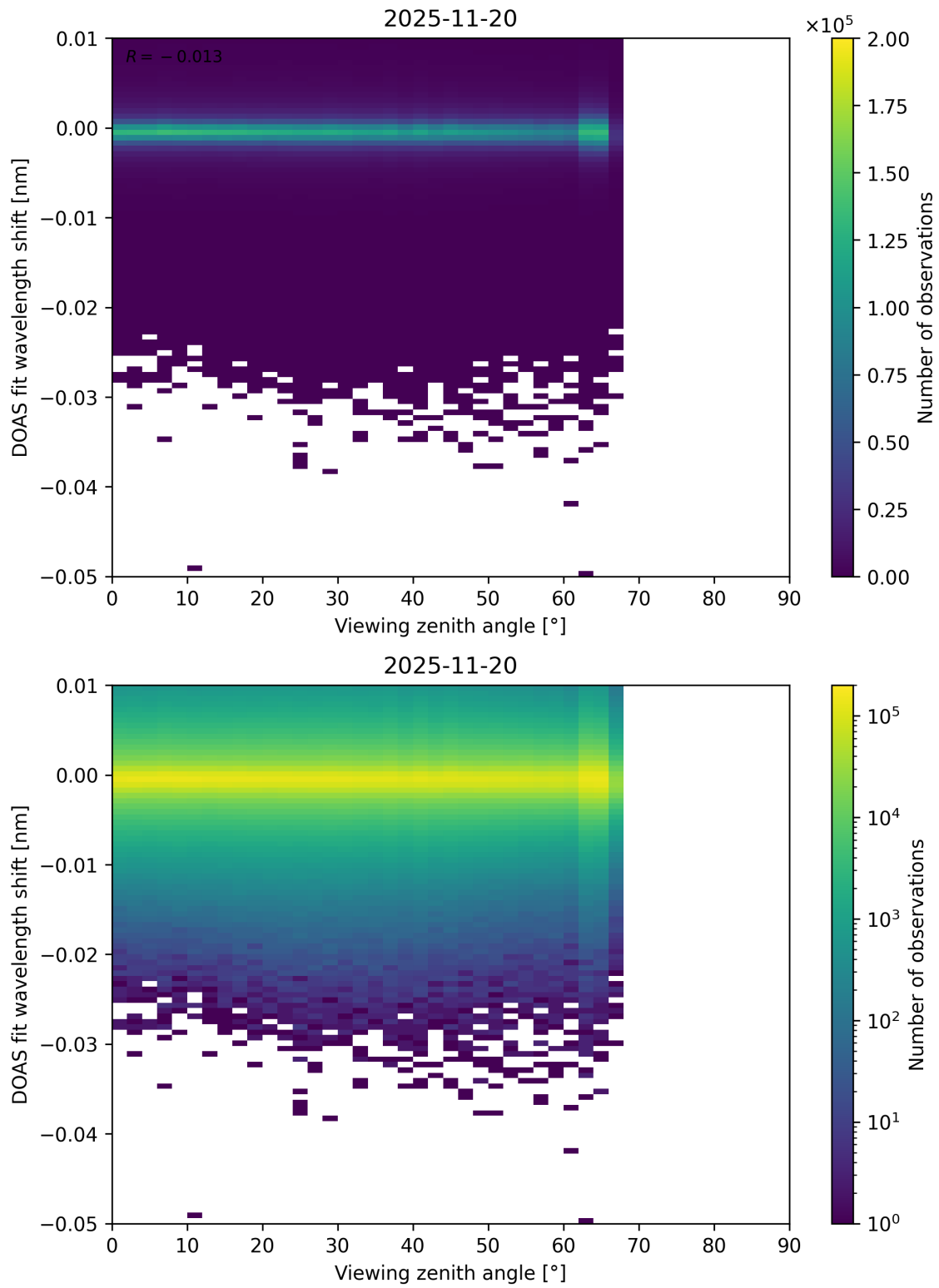
Figure 365: Scatter density plot of “Viewing zenith angle” against “DOAS fit wavelength shift” for 2025-11-19 to 2025-11-21.
