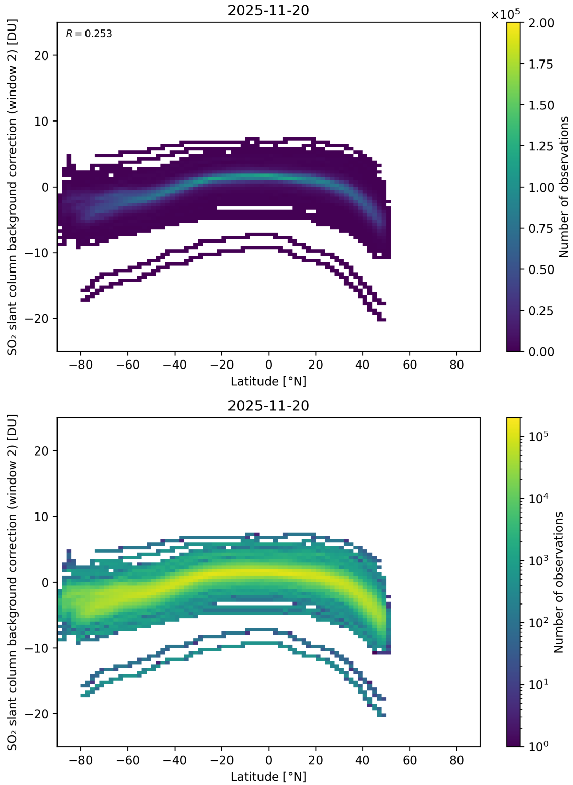
Figure 151: Scatter density plot of “Latitude” against “SO 2 slant column background correction (window 2)” for 2025-11-19 to 2025-11-21.
