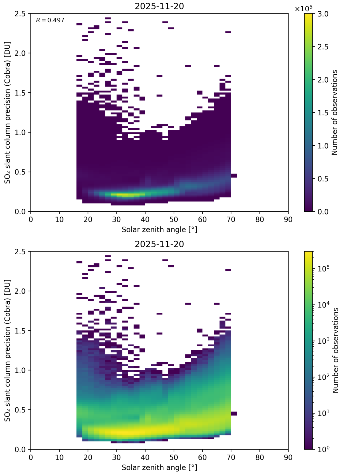
Figure 180: Scatter density plot of “Solar zenith angle” against “SO 2 slant column precision (Cobra)” for 2025-11-19 to 2025-11-21.
