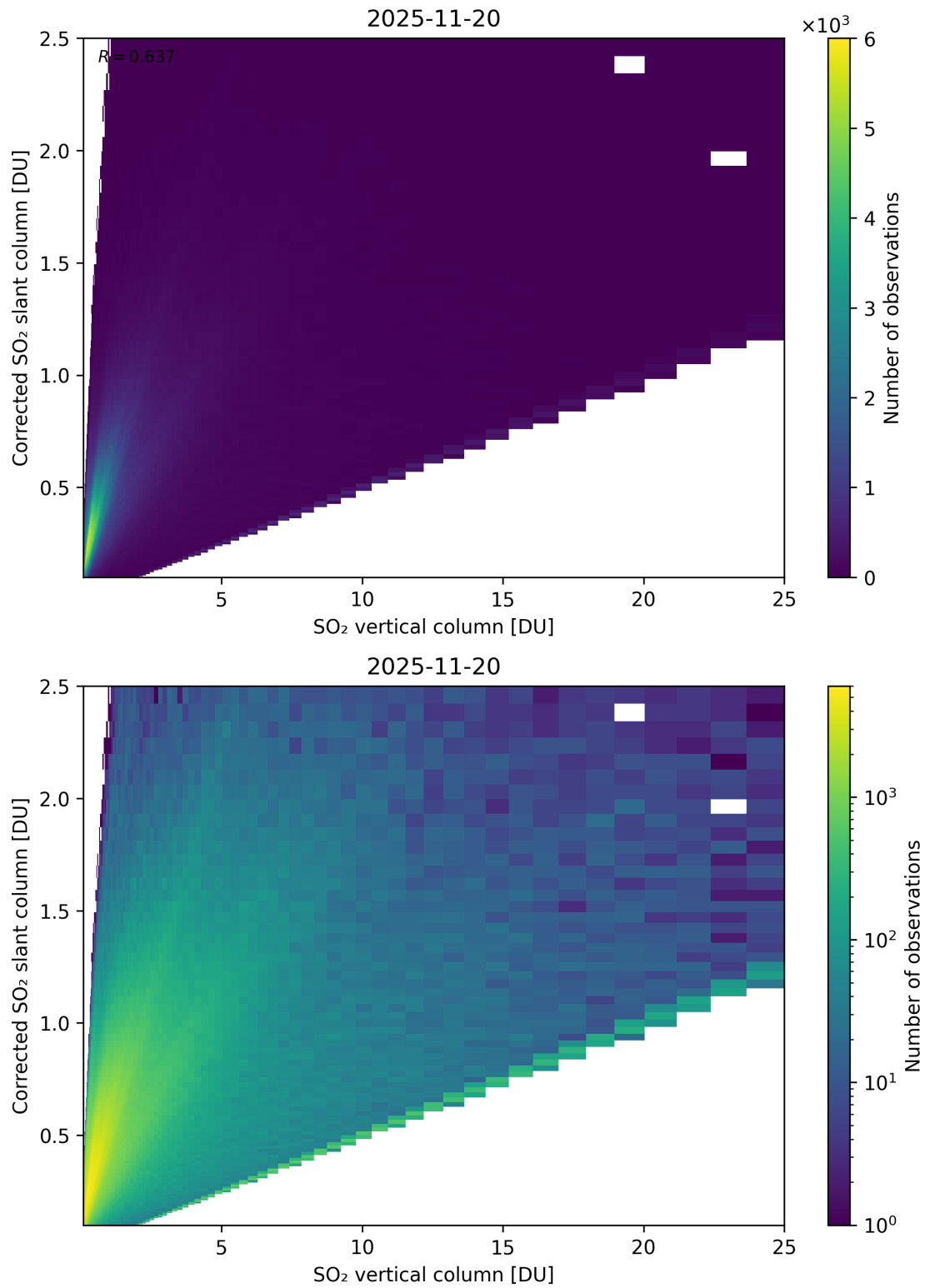
Figure 351: Scatter density plot of “SO 2 vertical column” against “Corrected SO 2 slant column” for 2025-11-19 to 2025-11-21.
