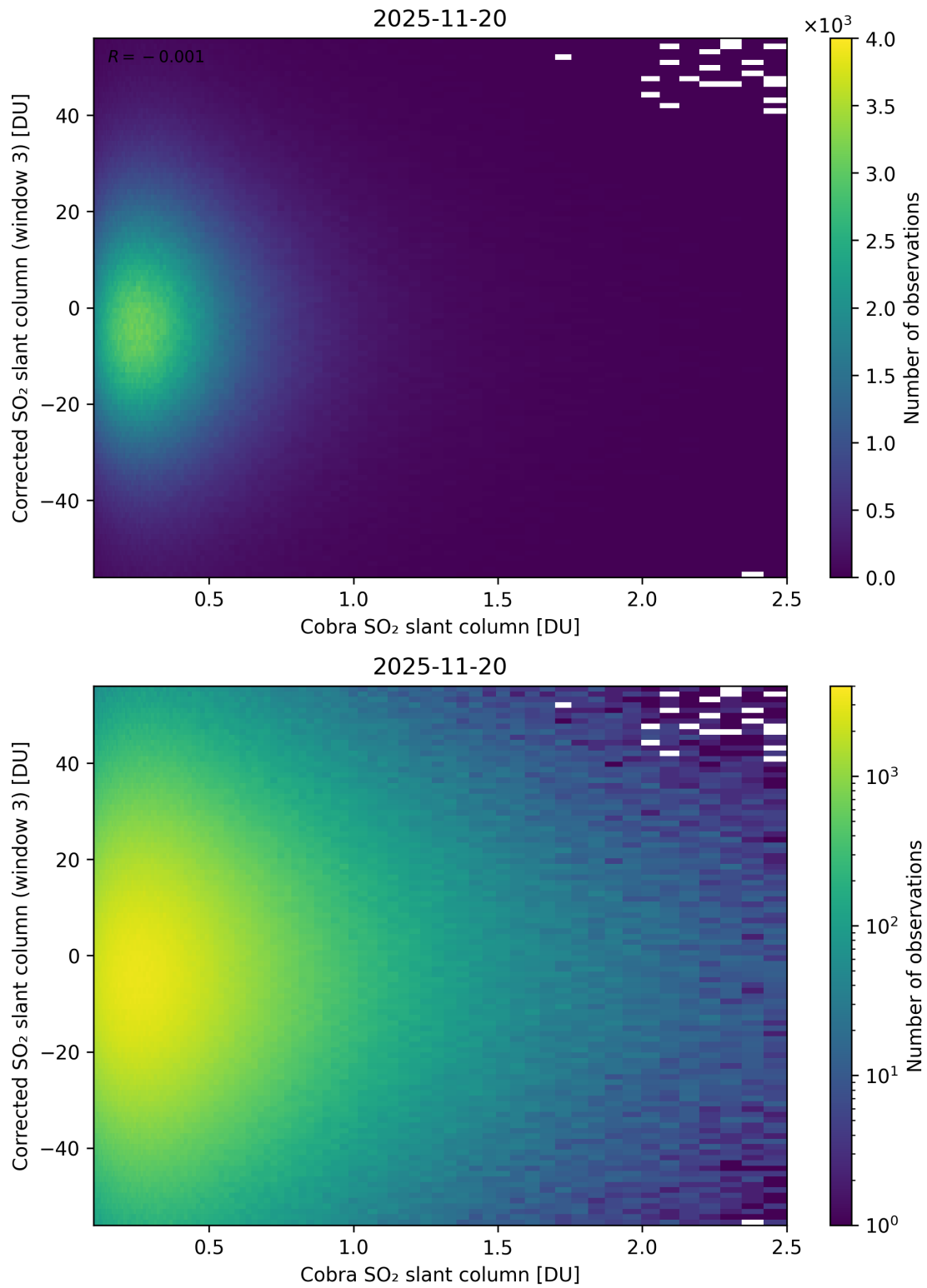
Figure 218: Scatter density plot of “Cobra SO 2 slant column” against “Corrected SO 2 slant column (window 3)” for 2025-11-19 to 2025-11-21.
