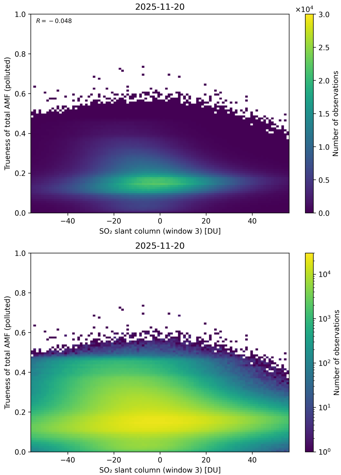
Figure 319: Scatter density plot of “SO 2 slant column (window 3)” against “Trueness of total AMF (polluted)” for 2025-11-19 to 2025-11-21.
