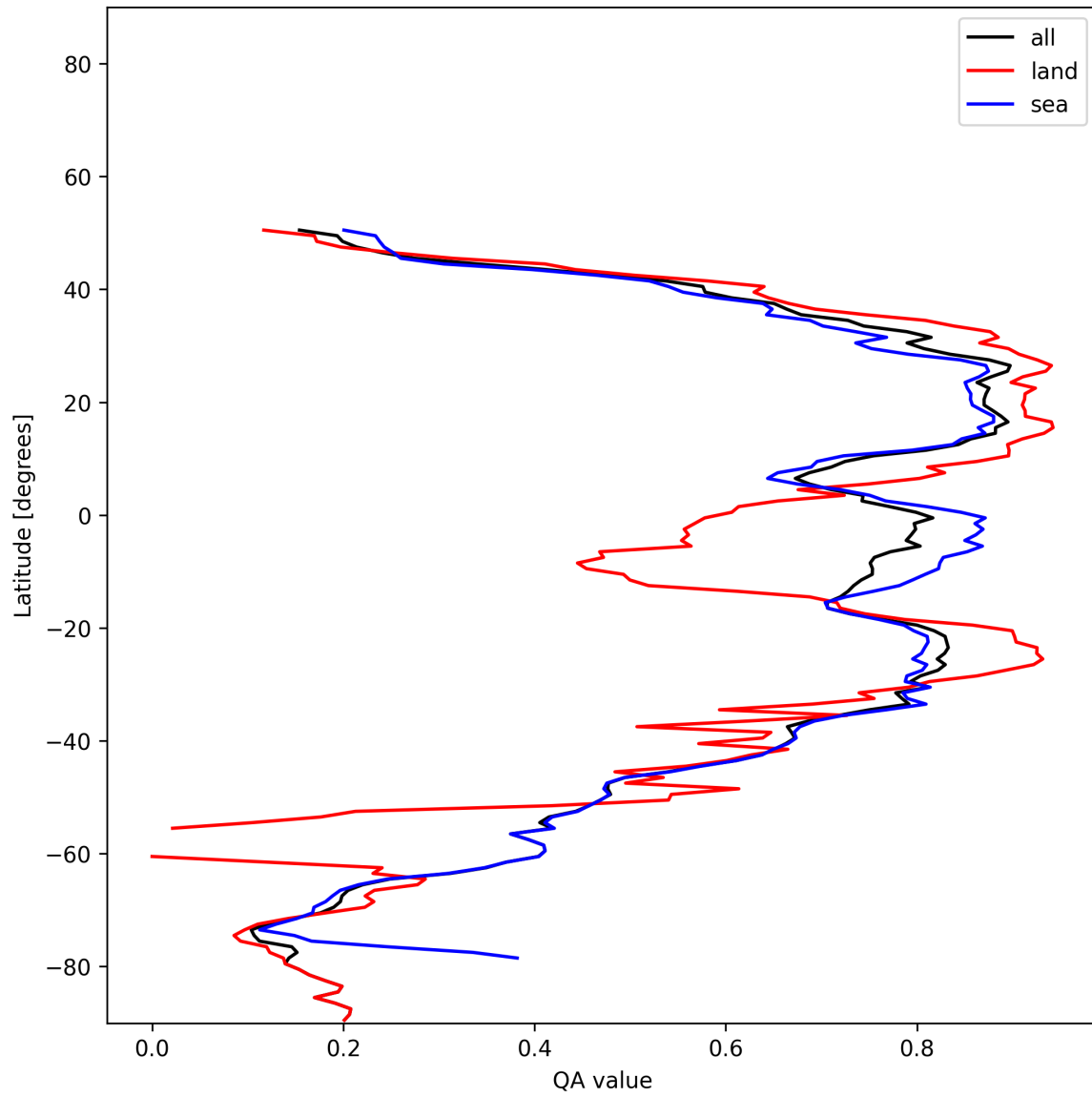
Figure 31: Zonal average of “QA value” for 2025-11-19 to 2025-11-21.
