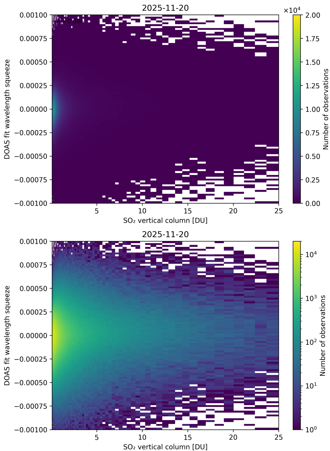
Figure 327: Scatter density plot of “SO 2 vertical column” against “DOAS fit wavelength squeeze” for 2025-11-19 to 2025-11-21.
