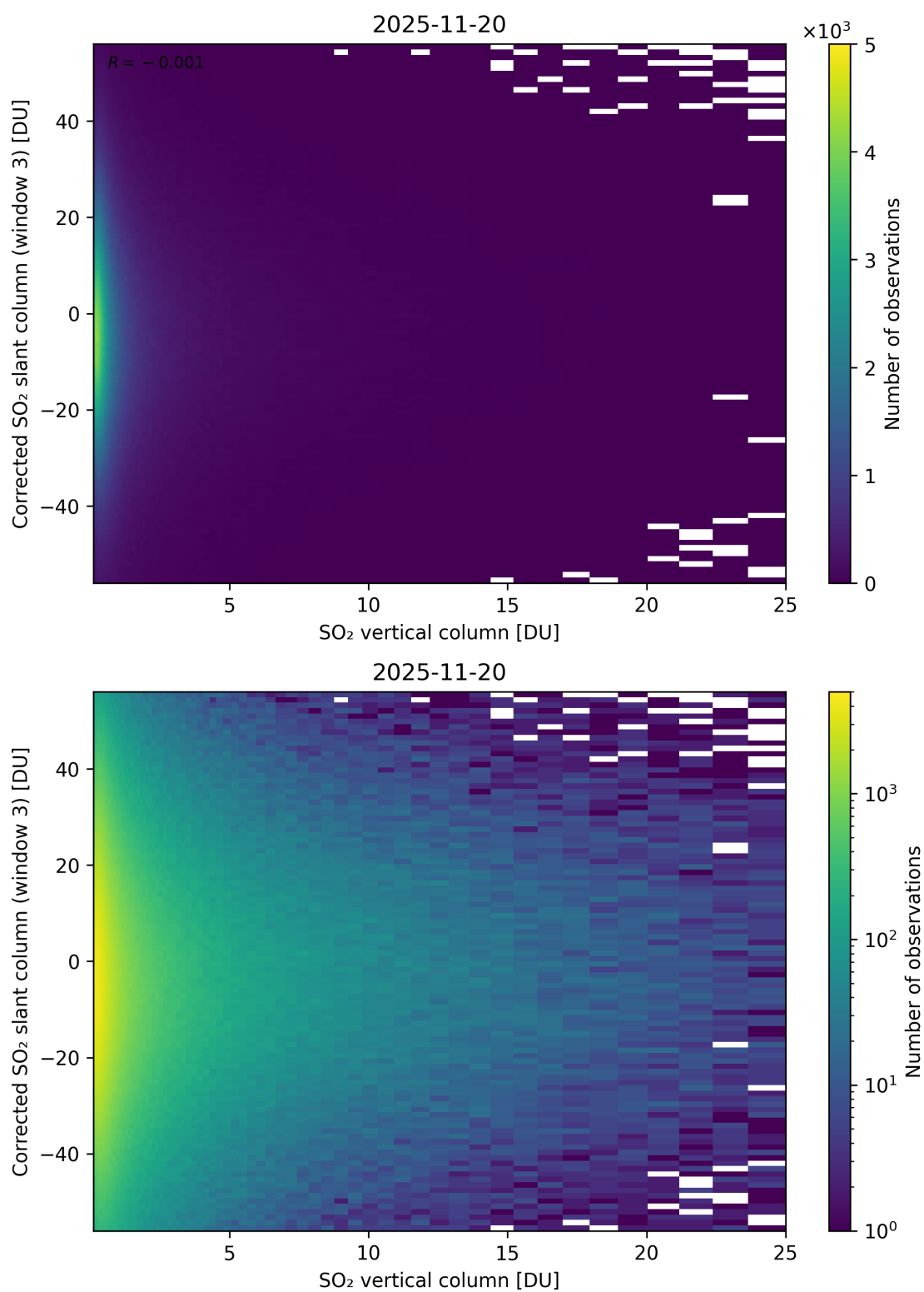
Figure 353: Scatter density plot of “SO 2 vertical column” against “Corrected SO 2 slant column (window 3)” for 2025-11-19 to 2025-11-21.
