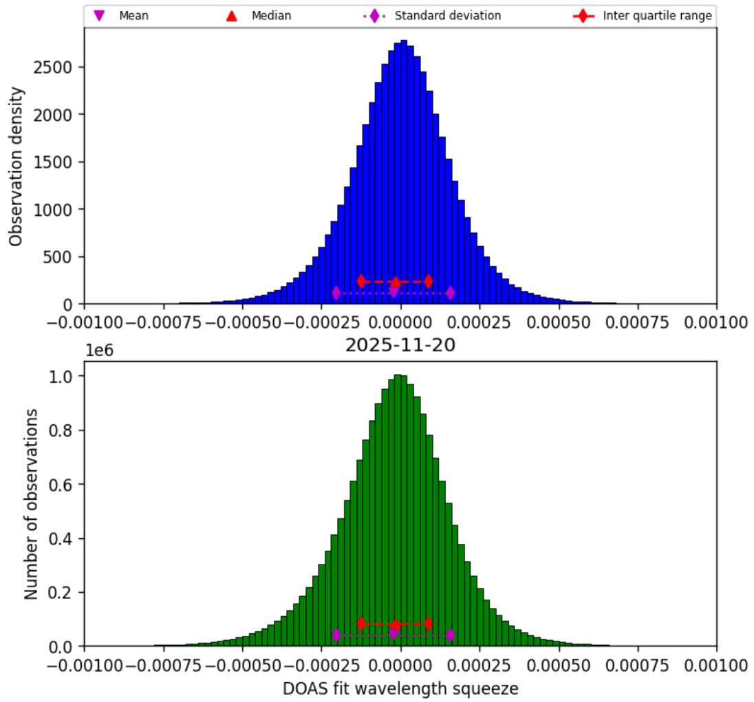
Figure 77: Histogram of “DOAS fit wavelength squeeze” for 2025-11-19 to 2025-11-21
