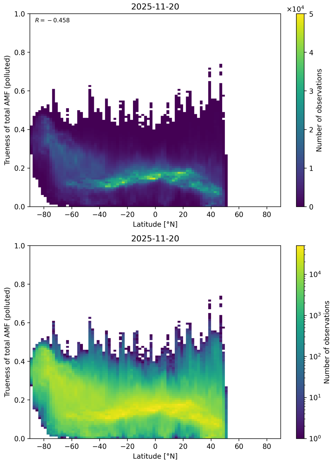
Figure 168: Scatter density plot of “Latitude” against “Trueness of total AMF (polluted)” for 2025-11-19 to 2025-11-21.
