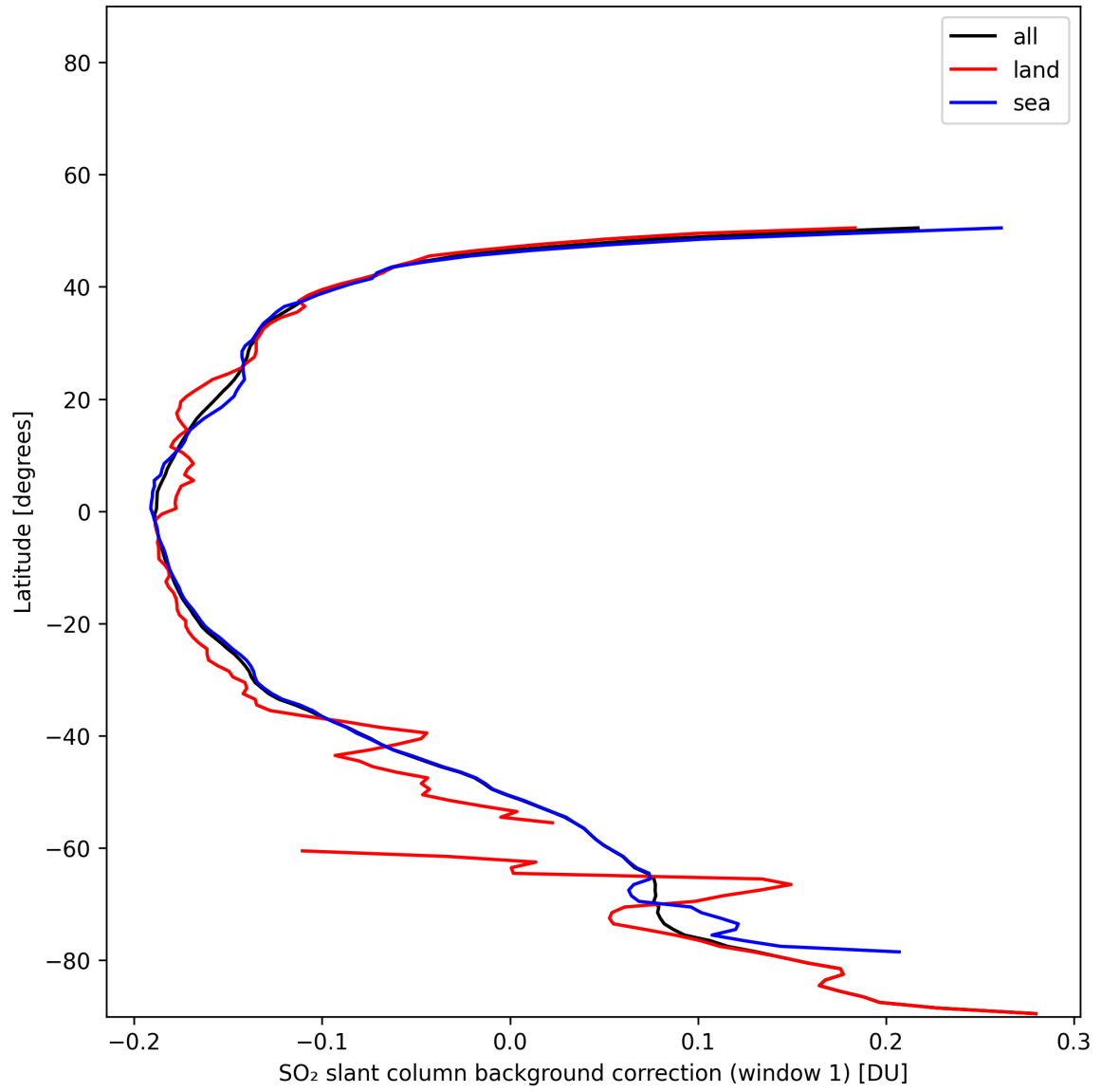
Figure 40: Zonal average of “SO 2 slant column background correction (window 1)” for 2025-11-19 to 2025-11-21.
