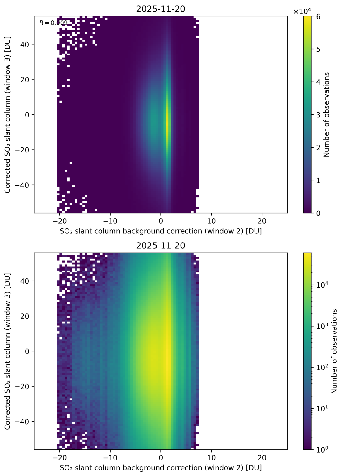
Figure 127: Scatter density plot of “SO 2 slant column background correction (window 2)” against “Corrected SO 2 slant column (window 3)” for 2025-11-19 to 2025-11-21.
