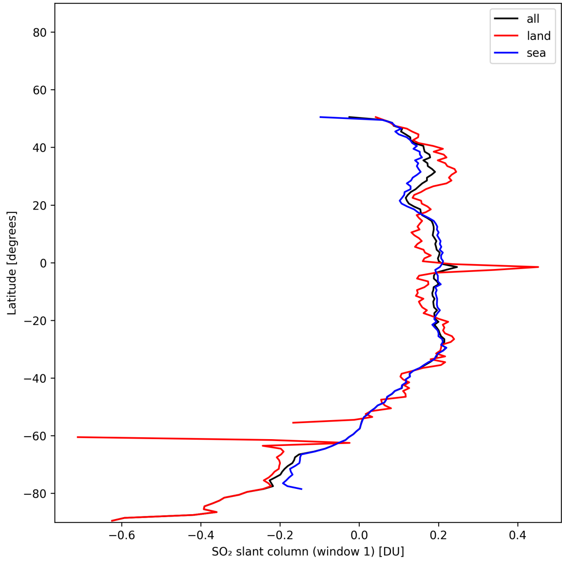
Figure 37: Zonal average of “SO 2 slant column (window 1)” for 2025-11-19 to 2025-11-21.
