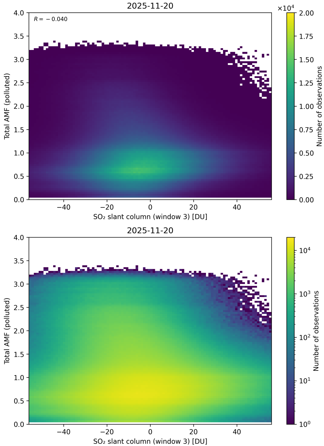
Figure 318: Scatter density plot of “SO 2 slant column (window 3)” against “Total AMF (polluted)” for 2025-11-19 to 2025-11-21.
