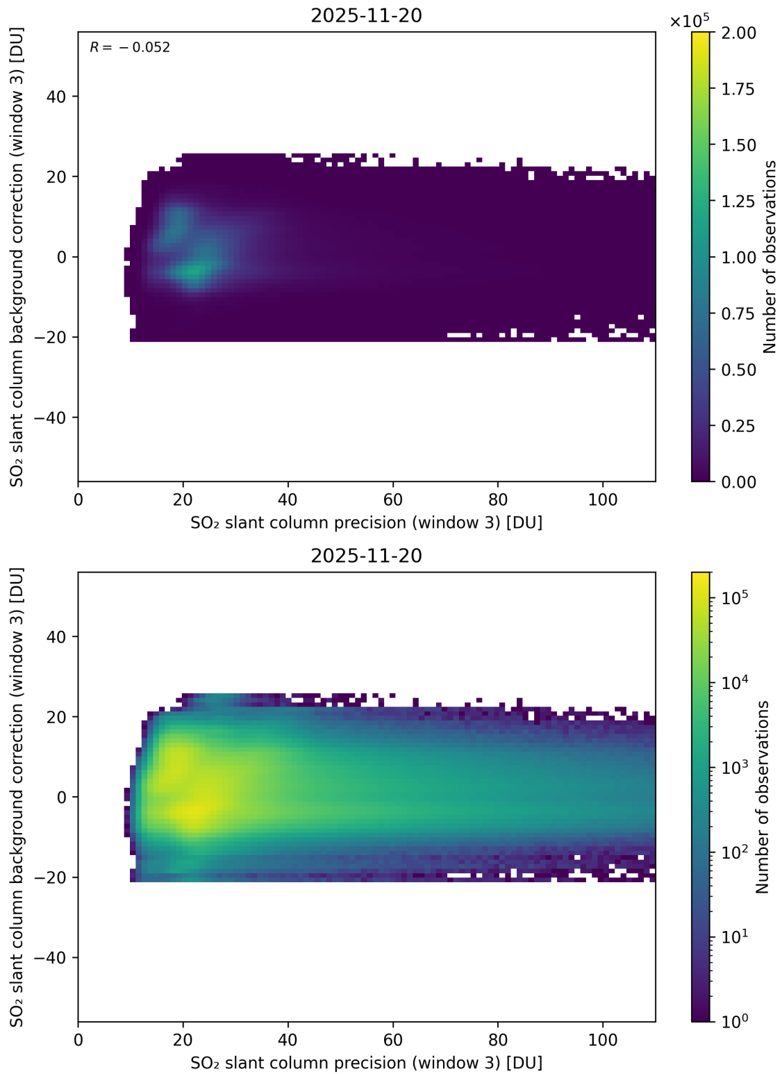
Figure 307: Scatter density plot of “SO 2 slant column precision (window 3)” against “SO 2 slant column background correction (window 3)” for 2025-11-19 to 2025-11-21.
