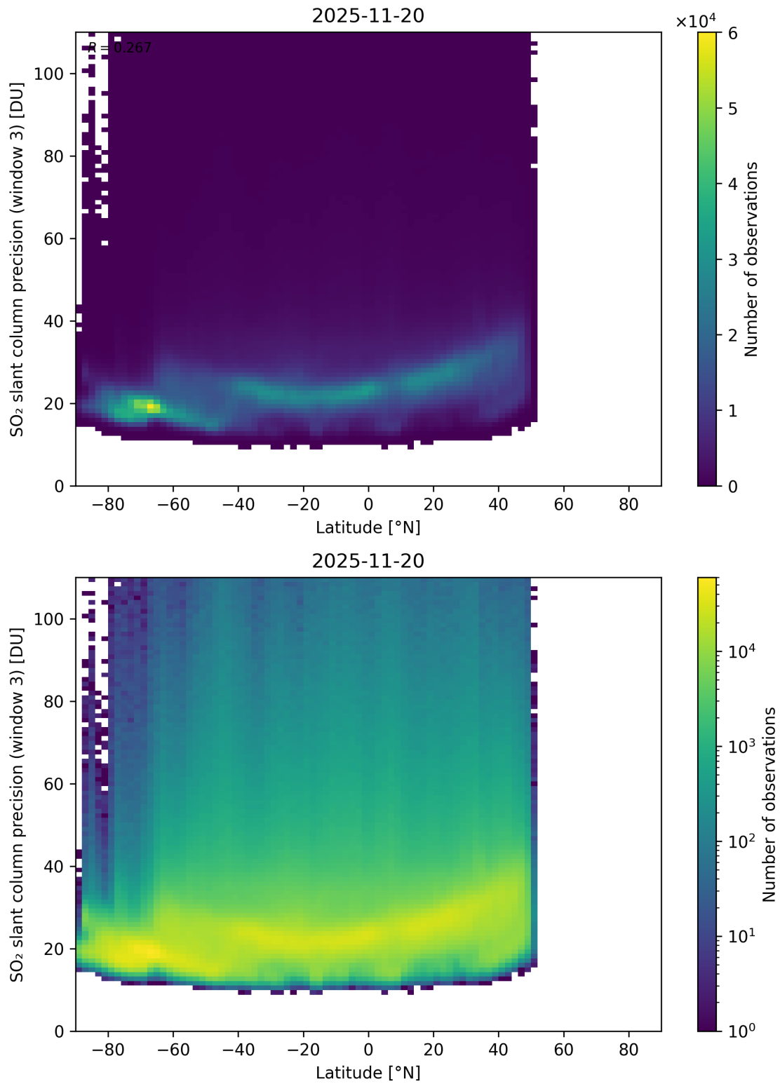
Figure 166: Scatter density plot of “Latitude” against “SO 2 slant column precision (window 3)” for 2025-11-19 to 2025-11-21.
