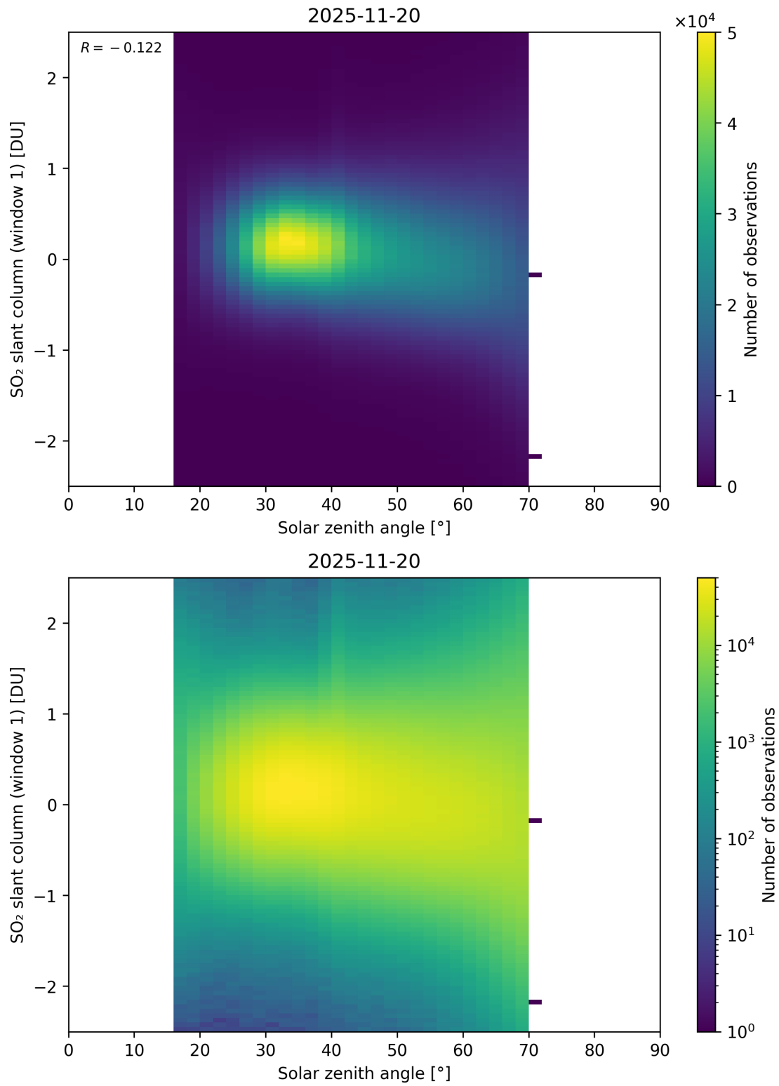
Figure 184: Scatter density plot of “Solar zenith angle” against “SO 2 slant column (window 1)” for 2025-11-19 to 2025-11-21.
