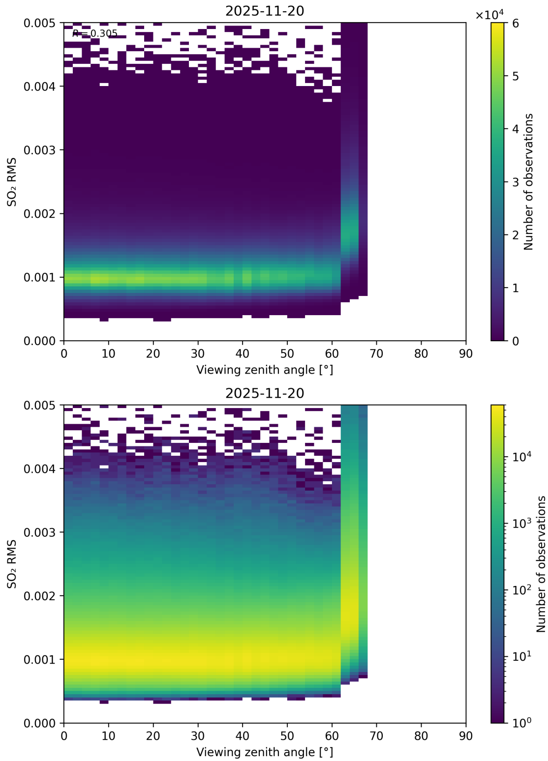
Figure 367: Scatter density plot of “Viewing zenith angle” against “SO 2 RMS” for 2025-11-19 to 2025-11-21.
