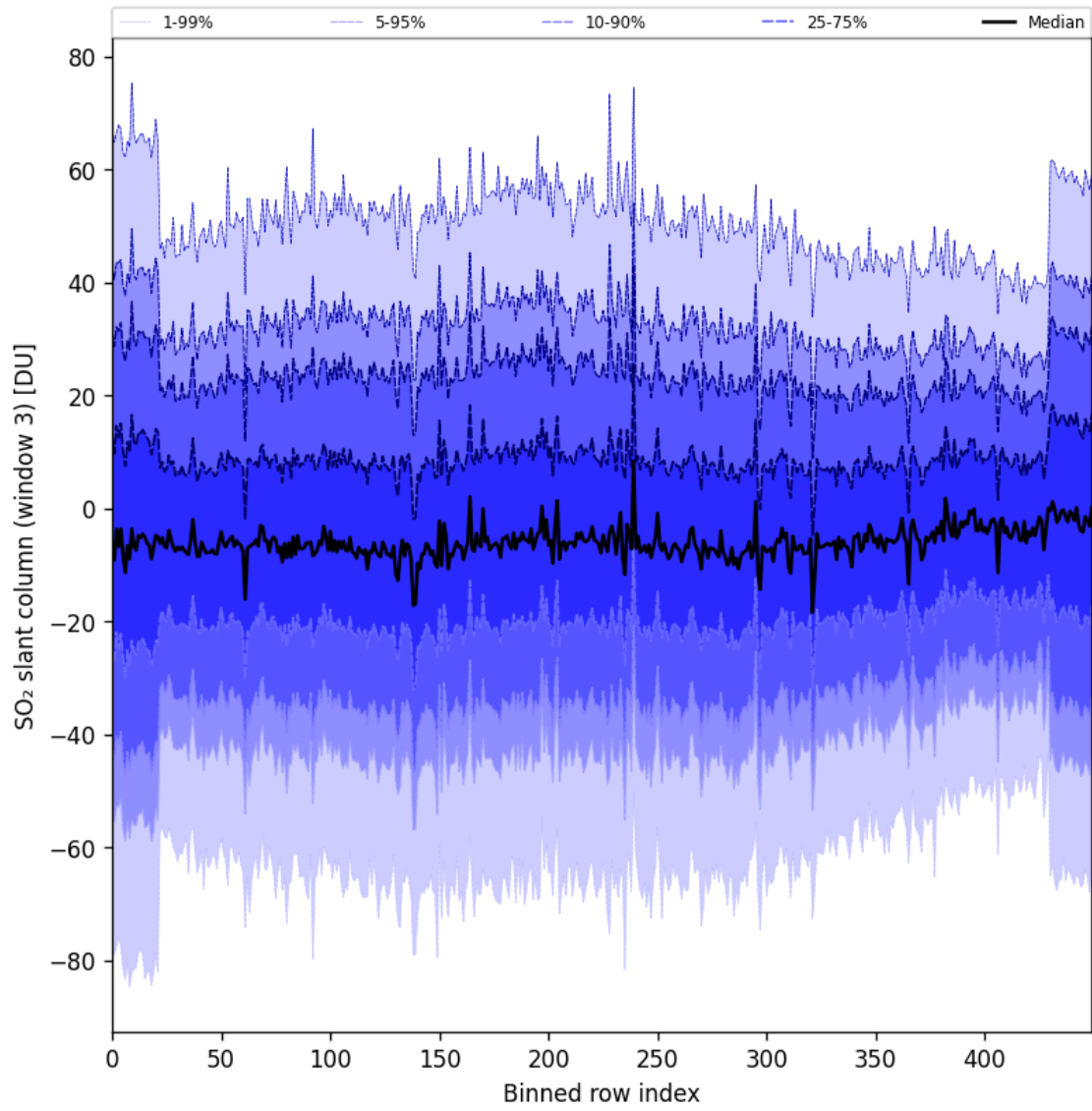
Figure 97: Along track statistics of “SO 2 slant column (window 3)” for 2025-11-19 to 2025-11-21
