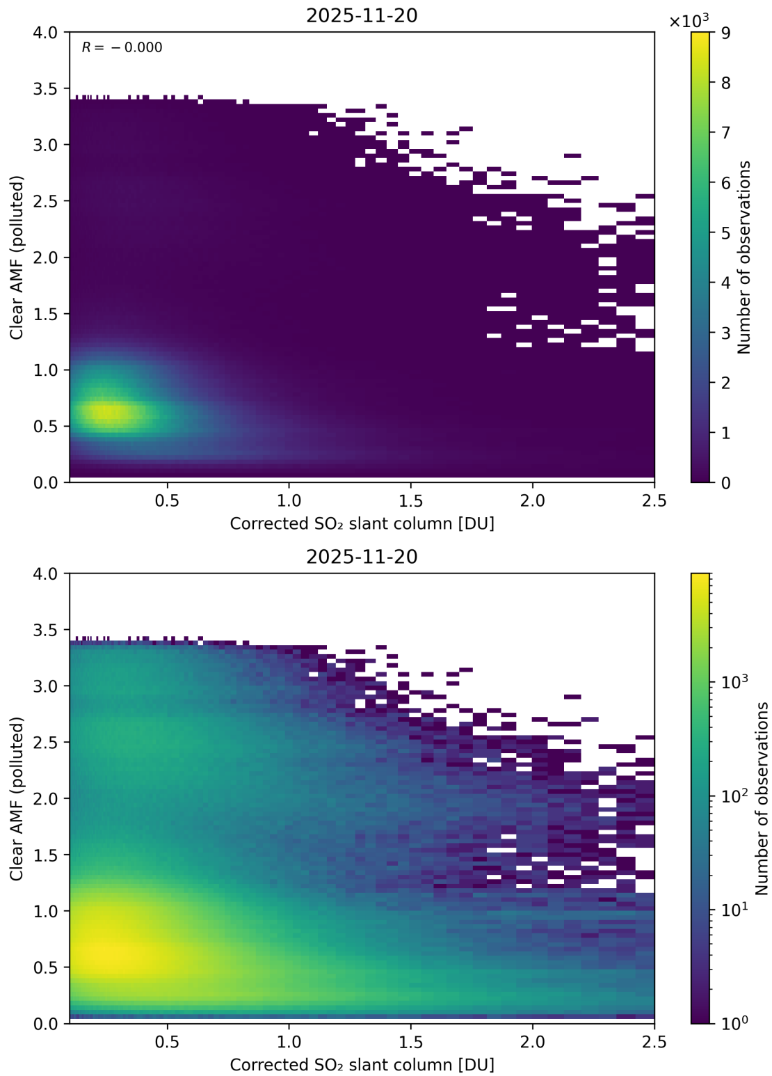
Figure 232: Scatter density plot of “Corrected SO 2 slant column” against “Clear AMF (polluted)” for 2025-11-19 to 2025-11-21.
