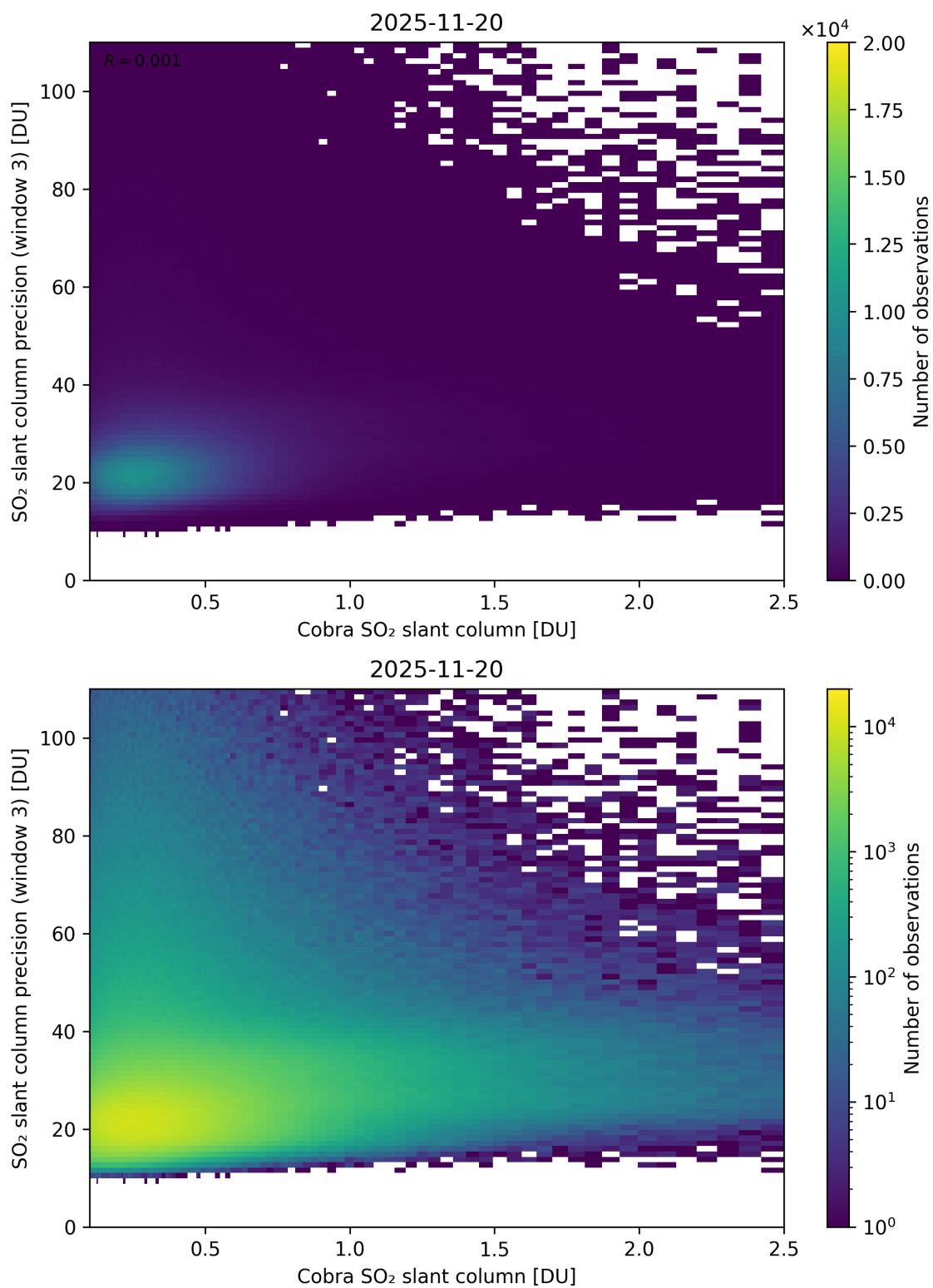
Figure 223: Scatter density plot of “Cobra SO 2 slant column” against “SO 2 slant column precision (window 3)” for 2025-11-19 to 2025-11-21.
