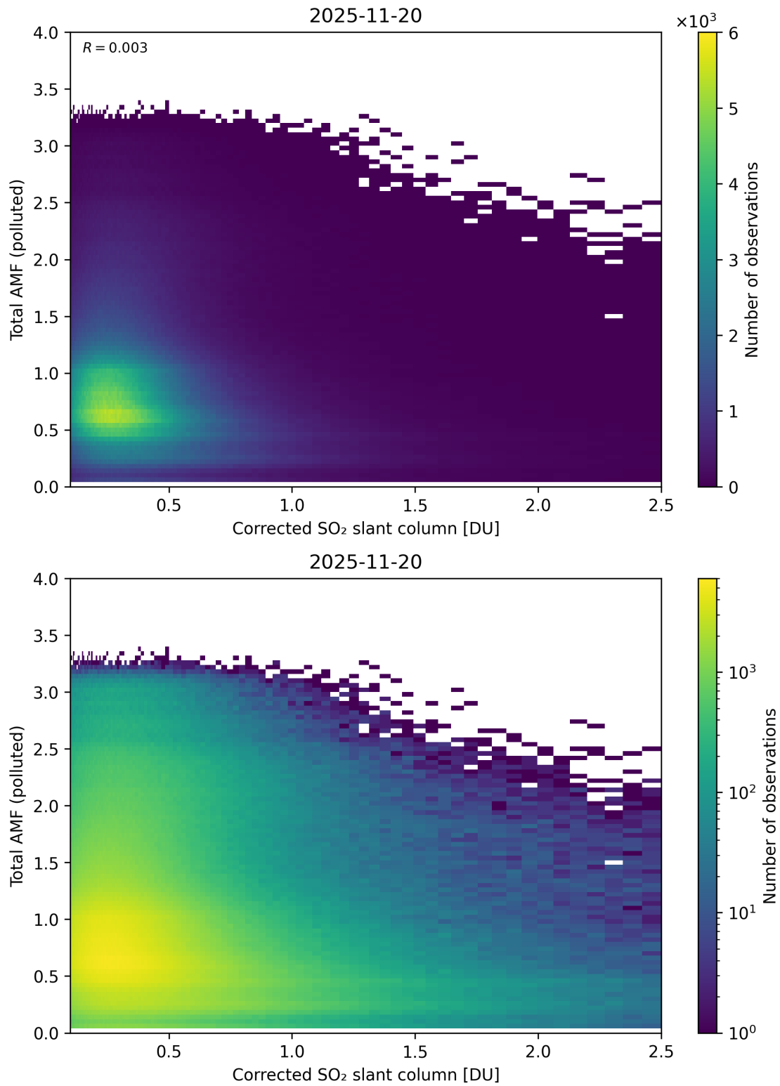
Figure 242: Scatter density plot of “Corrected SO 2 slant column” against “Total AMF (polluted)” for 2025-11-19 to 2025-11-21.
