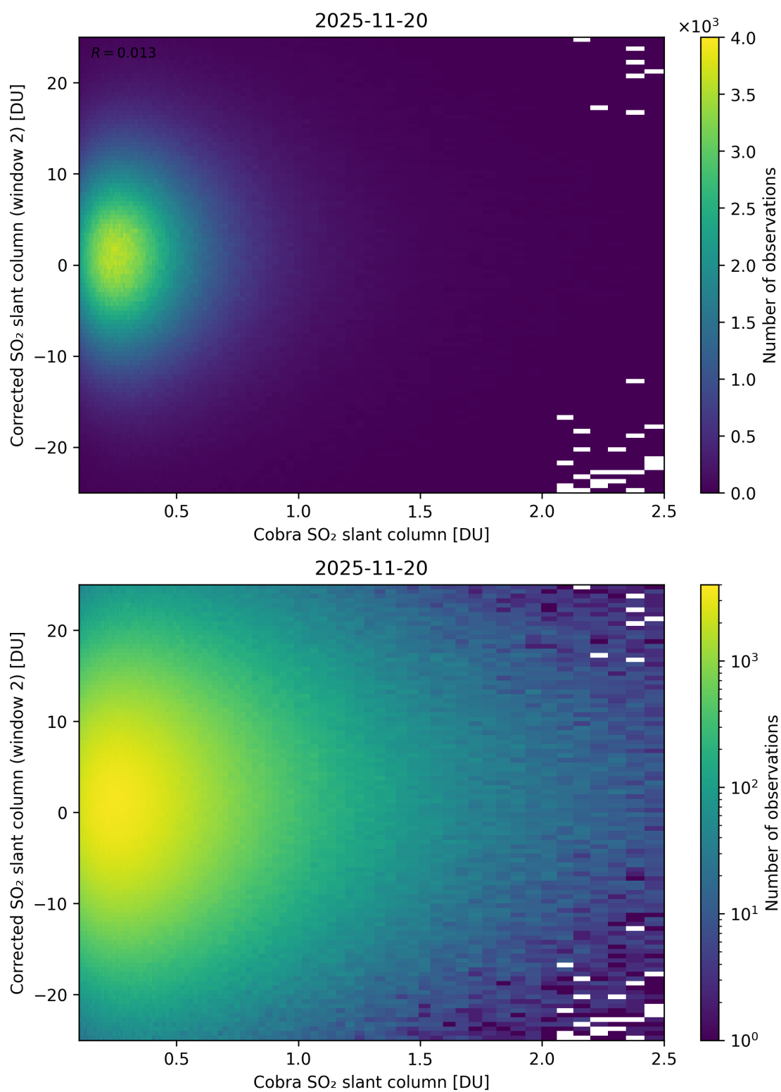
Figure 217: Scatter density plot of “Cobra SO 2 slant column” against “Corrected SO 2 slant column (window 2)” for 2025-11-19 to 2025-11-21.
