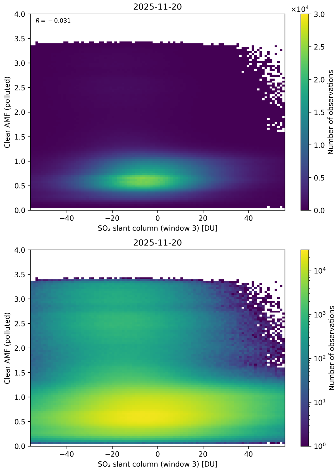
Figure 315: Scatter density plot of “SO 2 slant column (window 3)” against “Clear AMF (polluted)” for 2025-11-19 to 2025-11-21.
