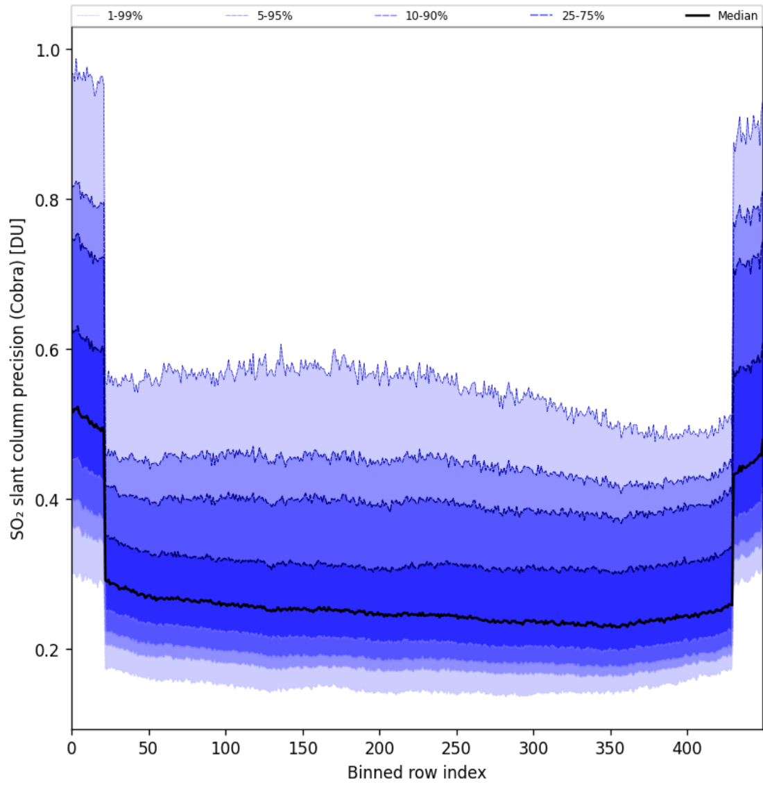
Figure 88: Along track statistics of “SO 2 slant column precision (Cobra)” for 2025-11-19 to 2025-11-21
