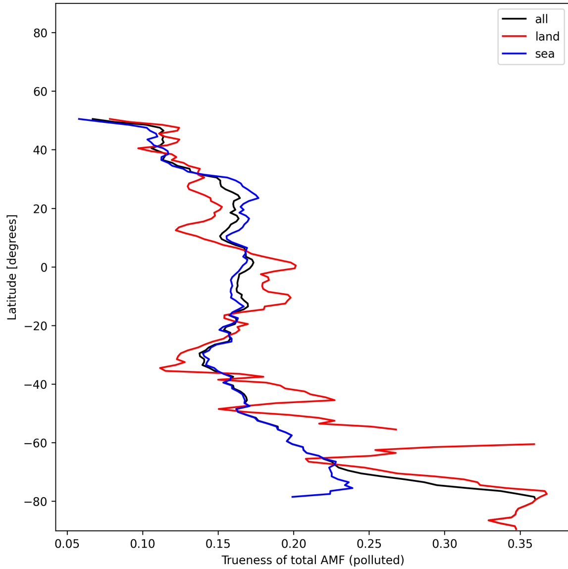
Figure 54: Zonal average of “Trueness of total AMF (polluted)” for 2025-11-19 to 2025-11-21.
