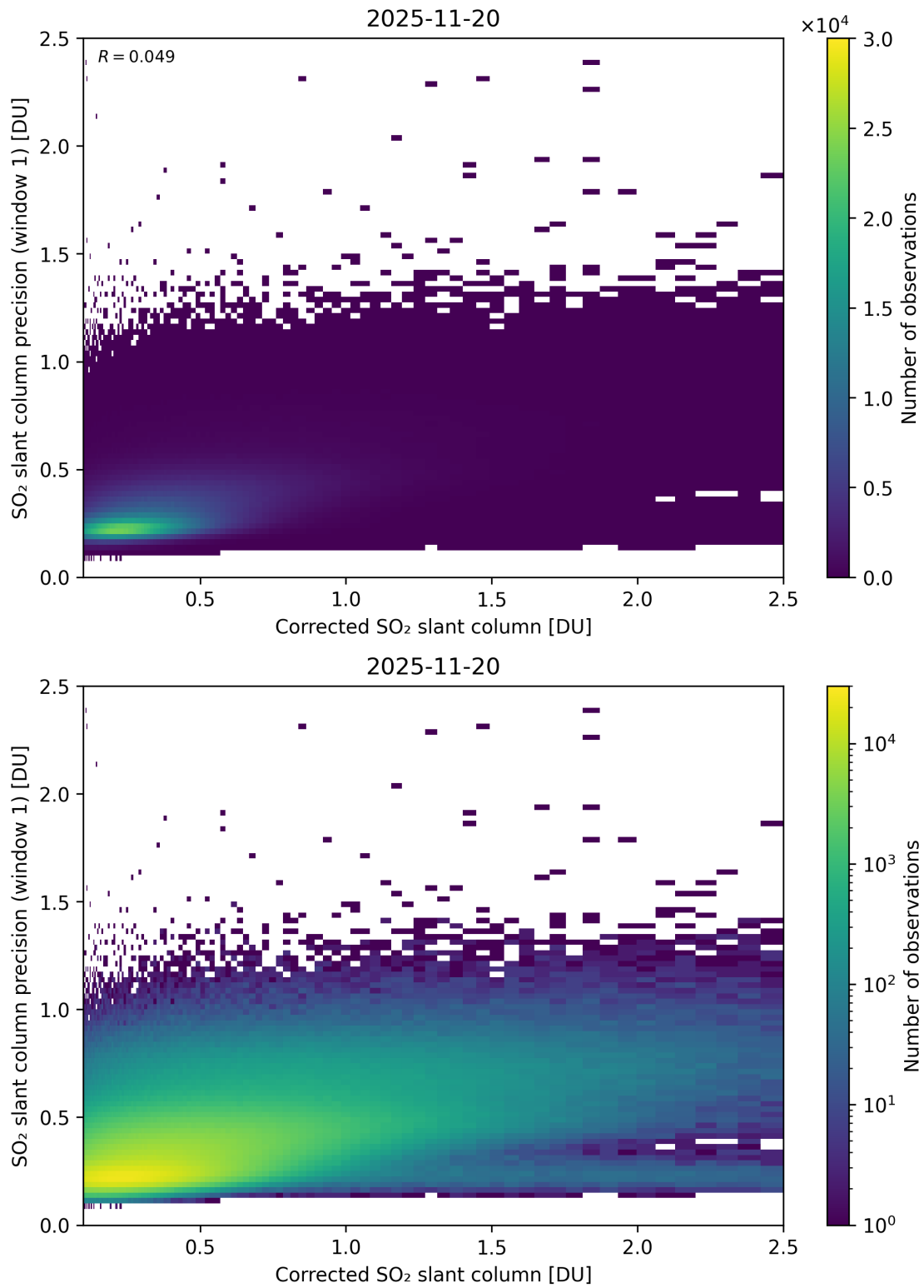
Figure 238: Scatter density plot of “Corrected SO 2 slant column” against “SO 2 slant column precision (window 1)” for 2025-11-19 to 2025-11-21.
