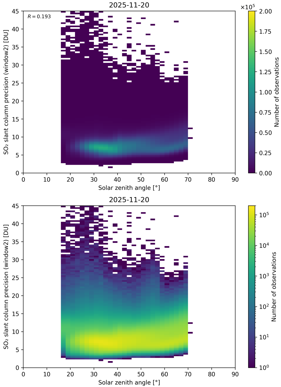
Figure 186: Scatter density plot of “Solar zenith angle” against “SO 2 slant column precision (window2)” for 2025-11-19 to 2025-11-21.
