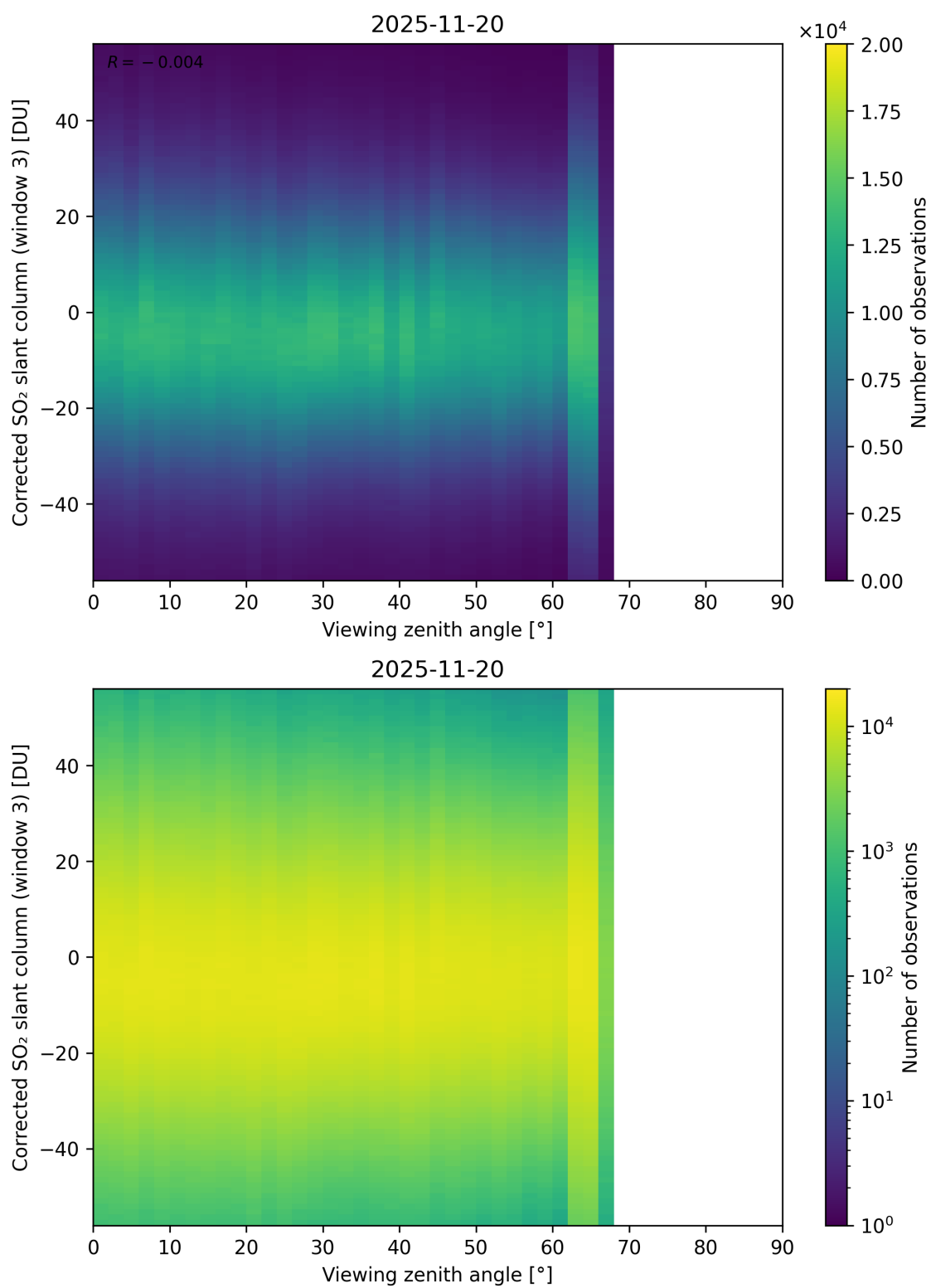
Figure 375: Scatter density plot of “Viewing zenith angle” against “Corrected SO 2 slant column (window 3)” for 2025-11-19 to 2025-11-21.
