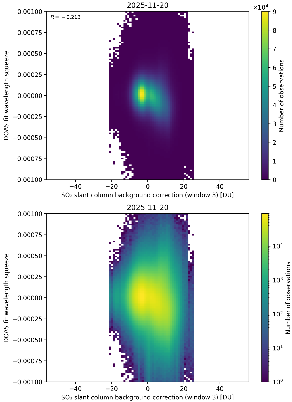
Figure 133: Scatter density plot of “SO 2 slant column background correction (window 3)” against “DOAS fit wavelength squeeze” for 2025-11-19 to 2025-11-21.
