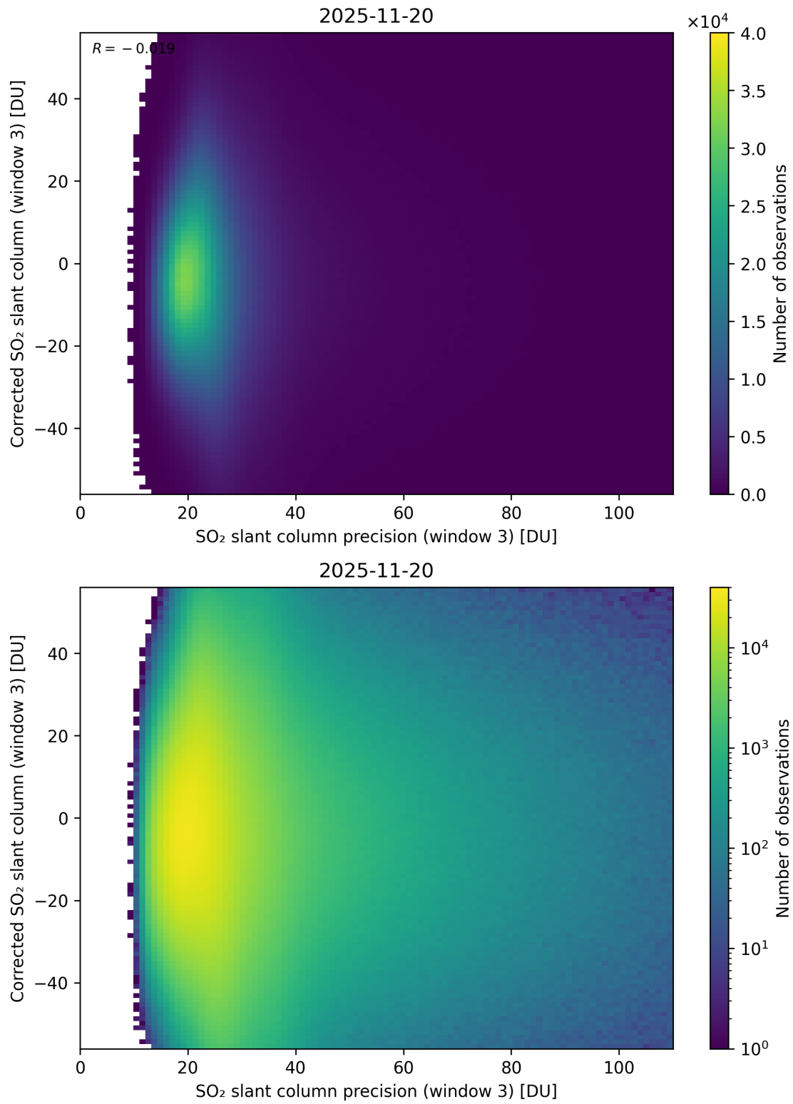
Figure 312: Scatter density plot of “SO 2 slant column precision (window 3)” against “Corrected SO 2 slant column (window 3)” for 2025-11-19 to 2025-11-21.
