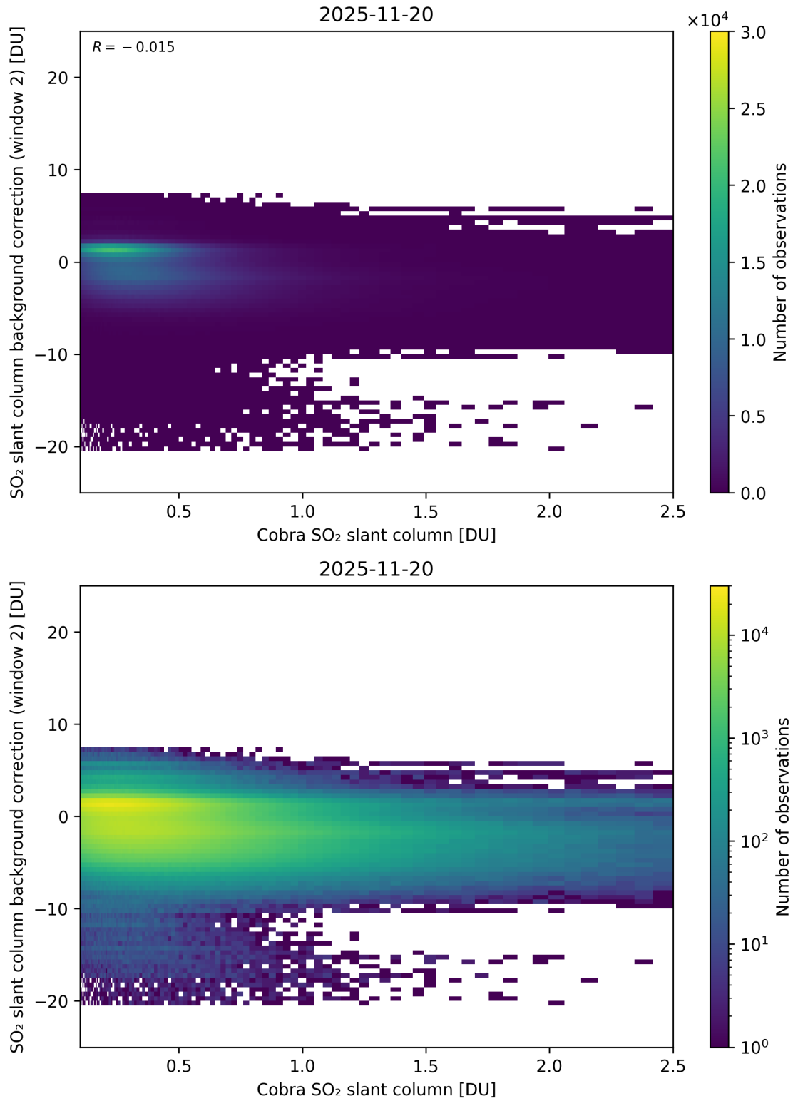
Figure 194: Scatter density plot of “Cobra SO 2 slant column” against “SO 2 slant column background correction (window 2)” for 2025-11-19 to 2025-11-21.
