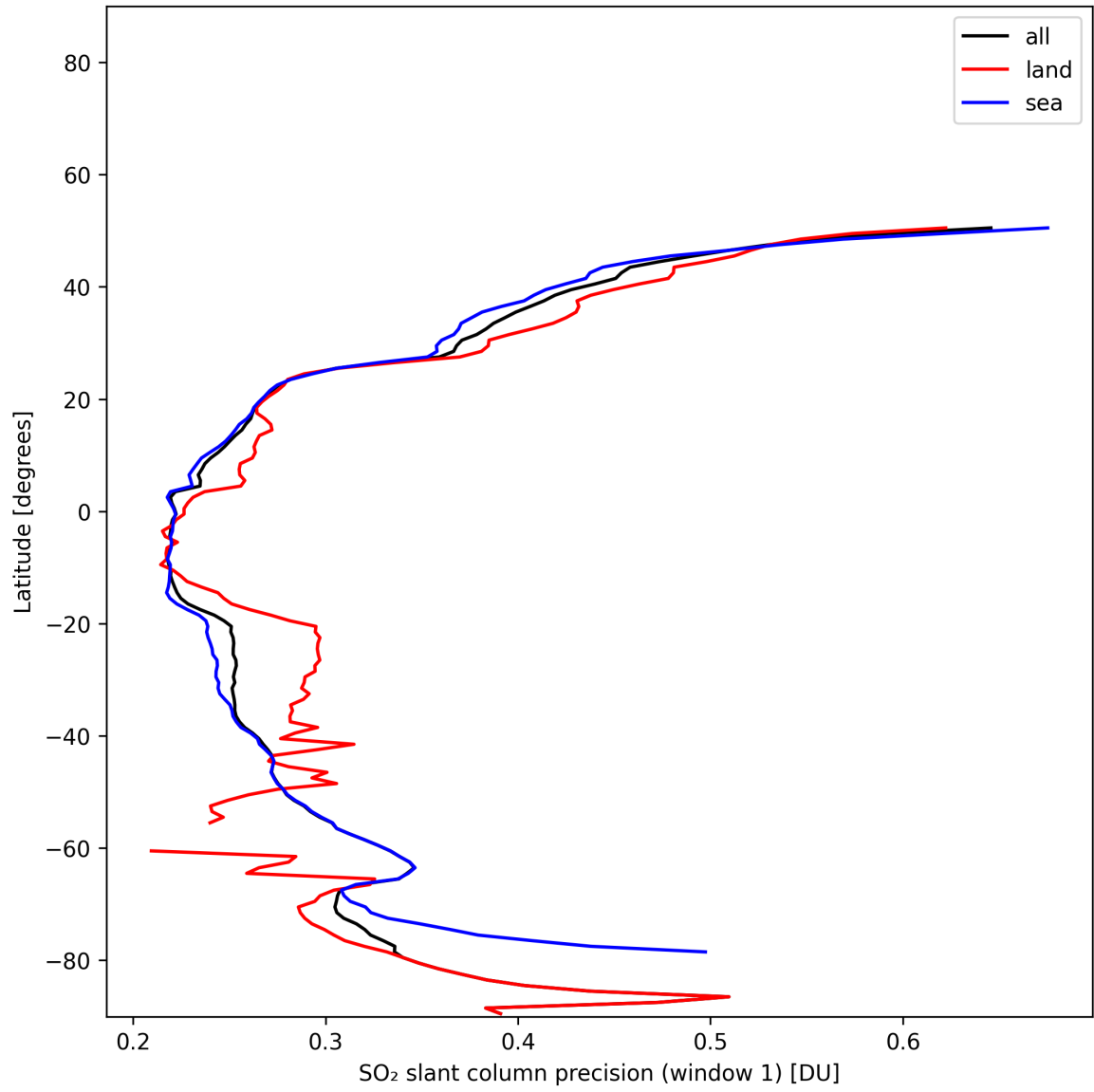
Figure 38: Zonal average of “SO 2 slant column precision (window 1)” for 2025-11-19 to 2025-11-21.
