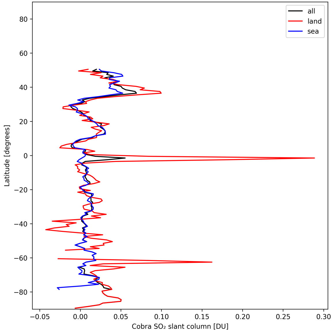
Figure 35: Zonal average of “Cobra SO 2 slant column” for 2025-11-19 to 2025-11-21.
