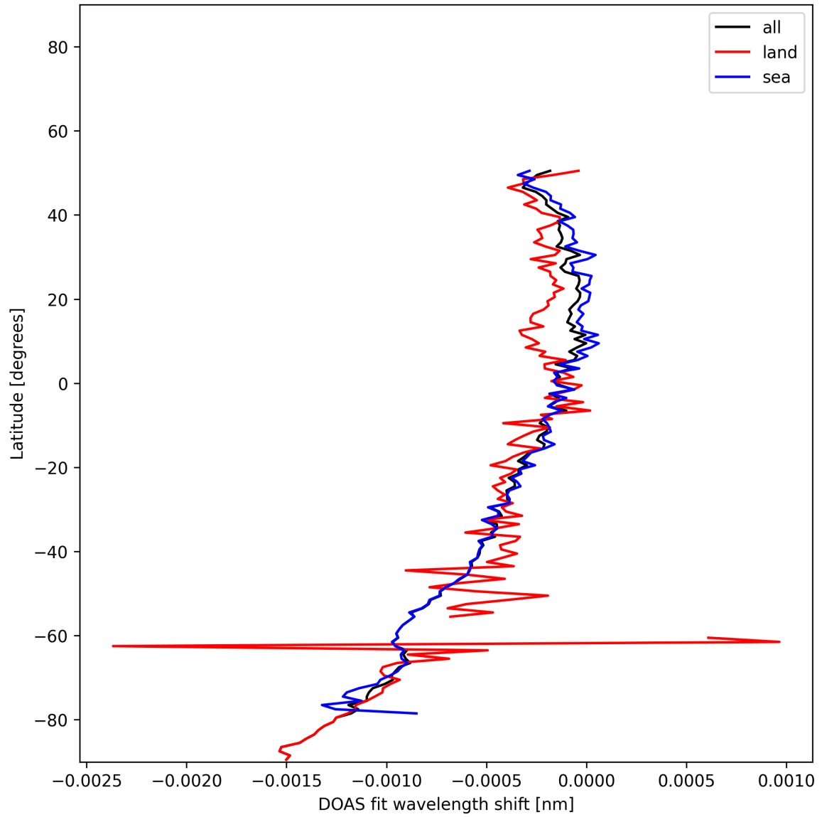
Figure 50: Zonal average of “DOAS fit wavelength shift” for 2025-11-19 to 2025-11-21.
