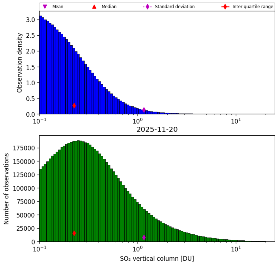
Figure 58: Histogram of “SO 2 vertical column” for 2025-11-19 to 2025-11-21
