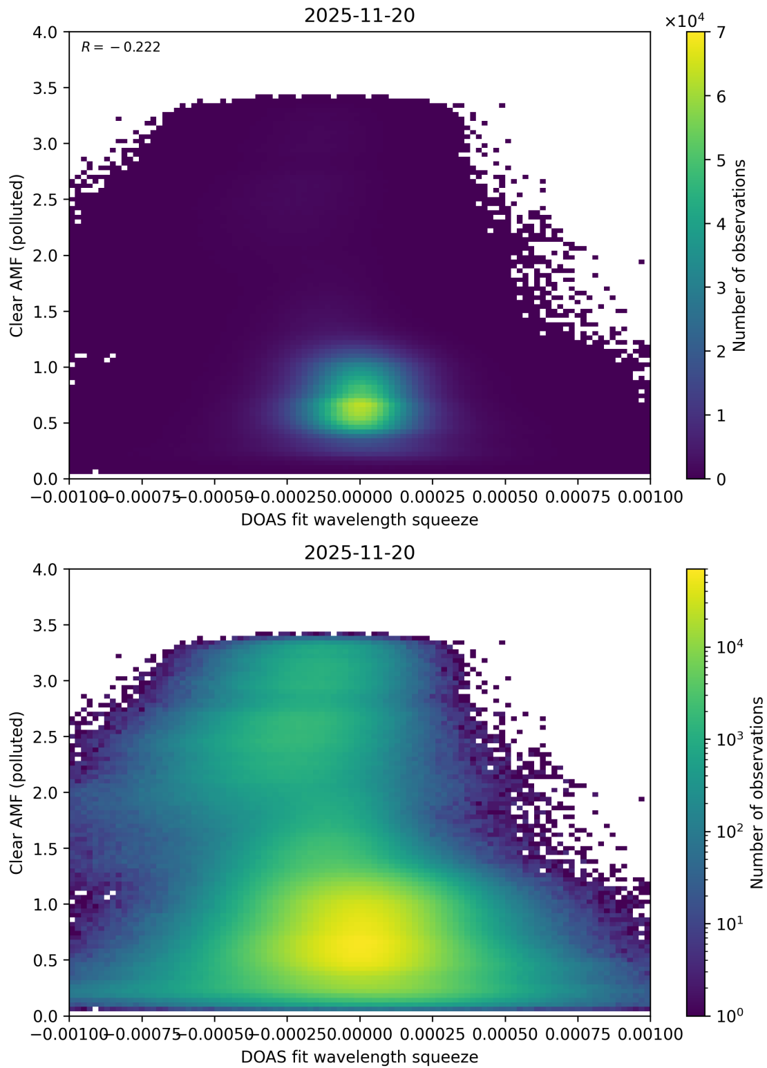
Figure 144: Scatter density plot of “DOAS fit wavelength squeeze” against “Clear AMF (polluted)” for 2025-11-19 to 2025-11-21.
