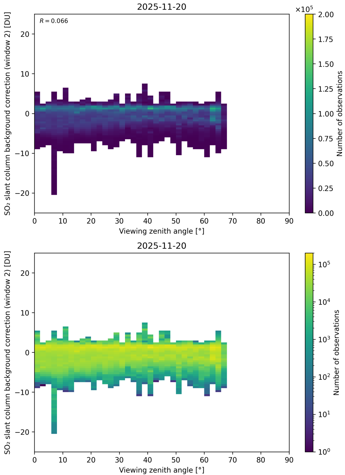
Figure 363: Scatter density plot of “Viewing zenith angle” against “SO 2 slant column background correction (window 2)” for 2025-11-19 to 2025-11-21.
