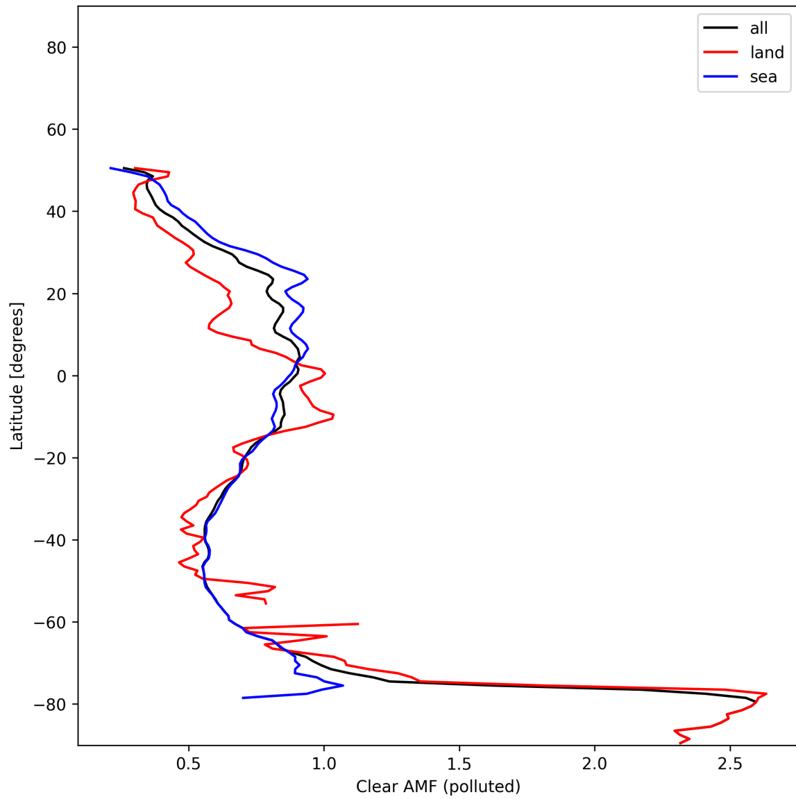
Figure 55: Zonal average of “Clear AMF (polluted)” for 2025-11-19 to 2025-11-21.
