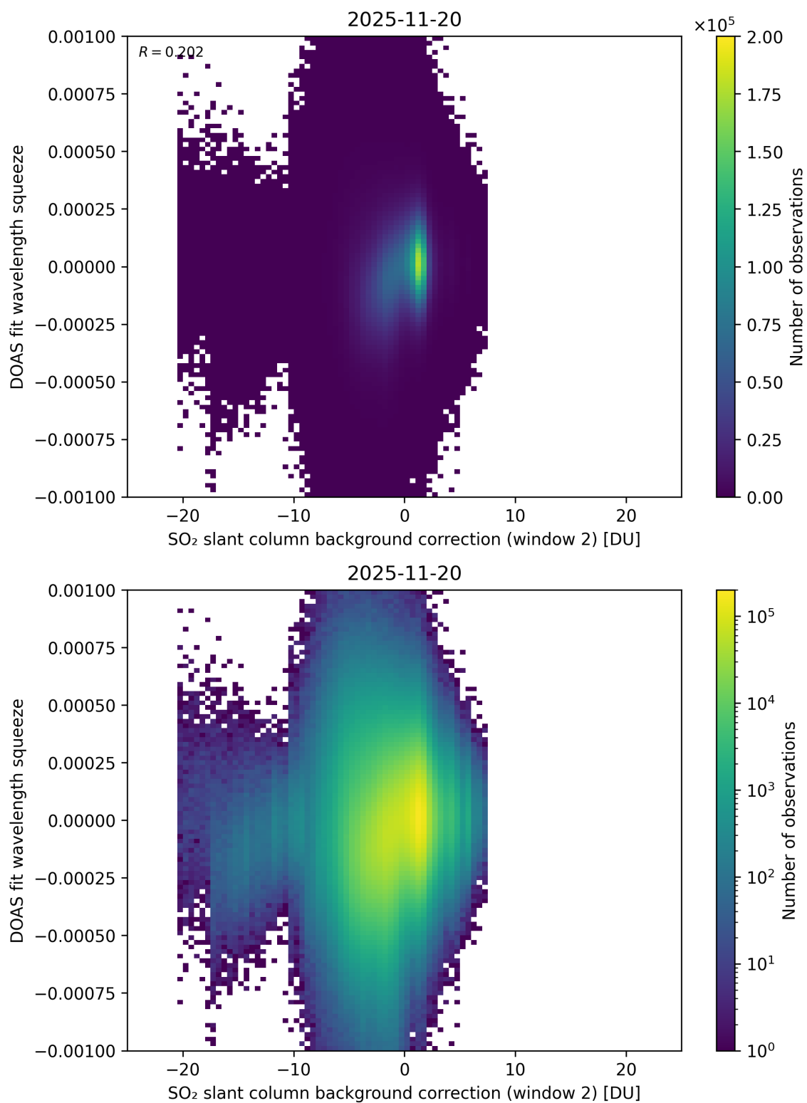
Figure 124: Scatter density plot of “SO 2 slant column background correction (window 2)” against “DOAS fit wavelength squeeze” for 2025-11-19 to 2025-11-21.
