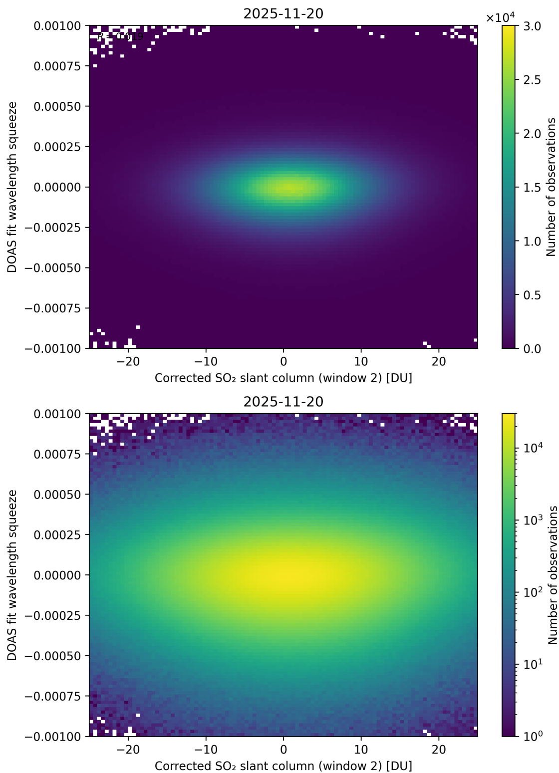
Figure 247: Scatter density plot of “Corrected SO 2 slant column (window 2)” against “DOAS fit wavelength squeeze” for 2025-11-19 to 2025-11-21.
