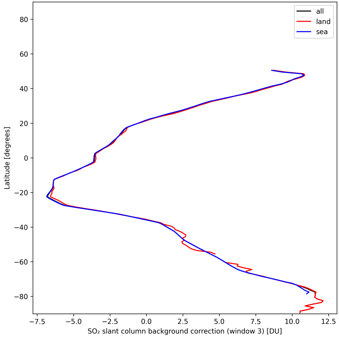
Figure 48: Zonal average of “SO 2 slant column background correction (window 3)” for 2025-11-19 to 2025-11-21.
