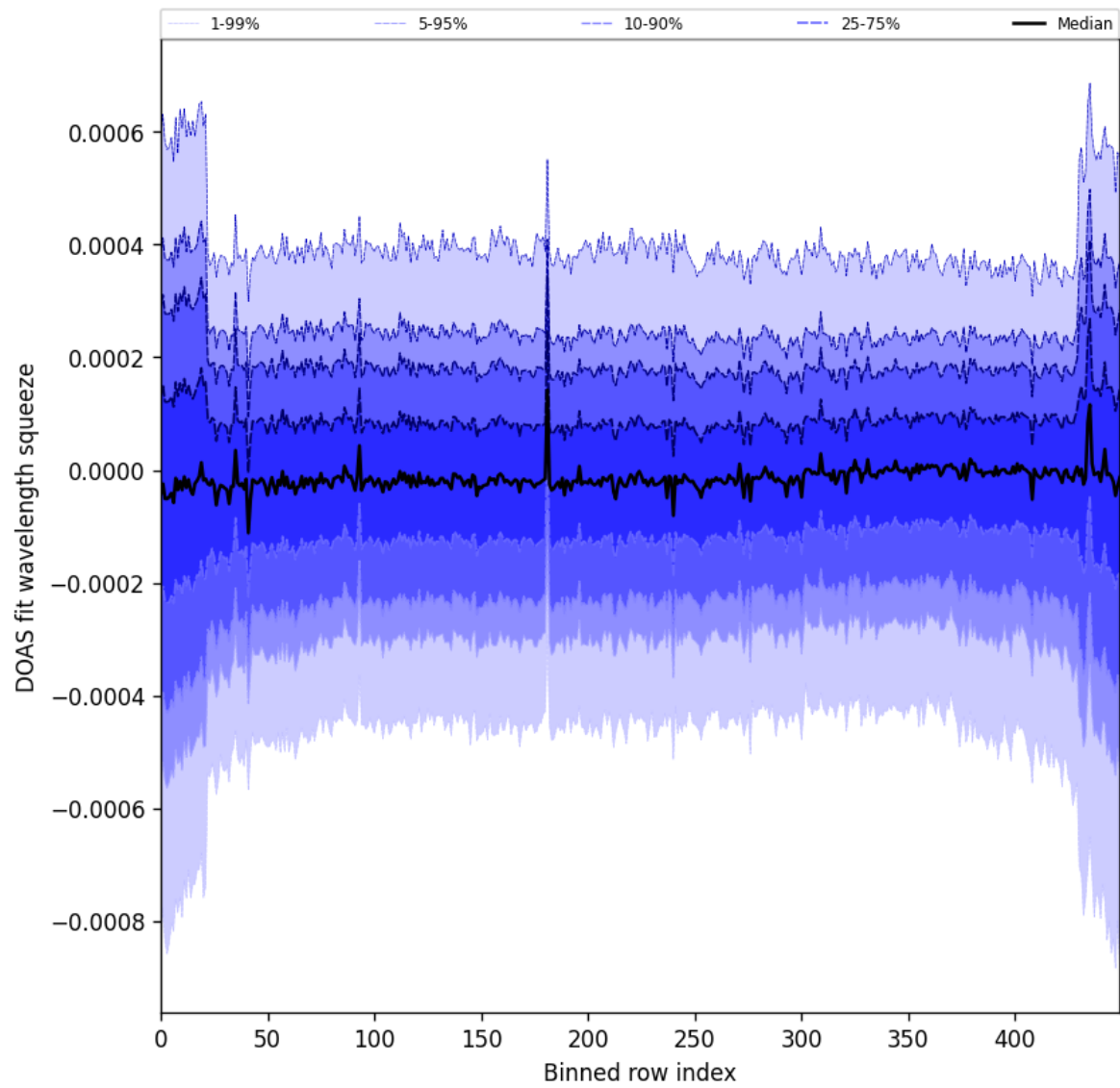
Figure 103: Along track statistics of “DOAS fit wavelength squeeze” for 2025-11-19 to 2025-11-21
