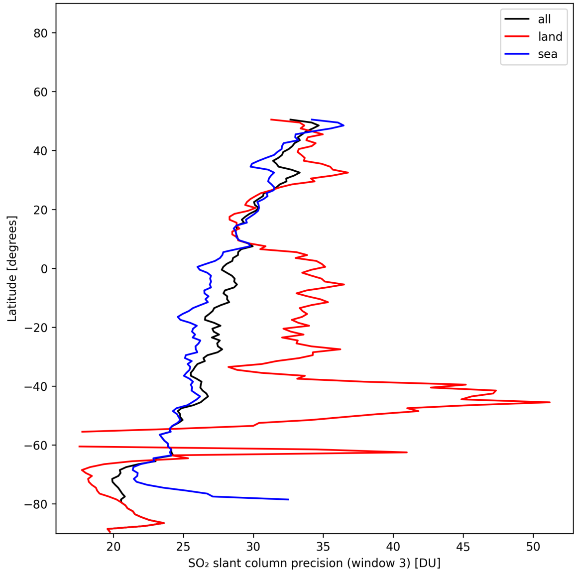
Figure 46: Zonal average of “SO 2 slant column precision (window 3)” for 2025-11-19 to 2025-11-21.
