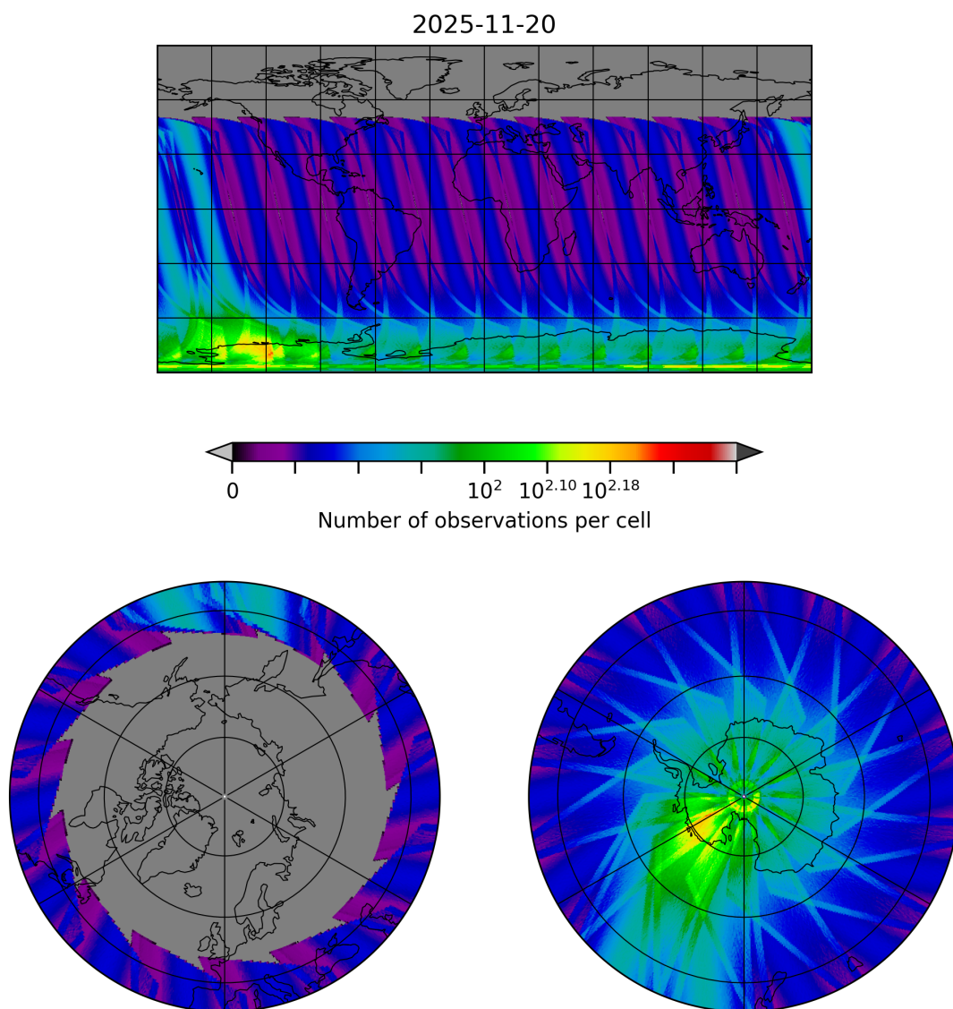
Figure 30: Map of the number of observations for 2025-11-19 to 2025-11-21
