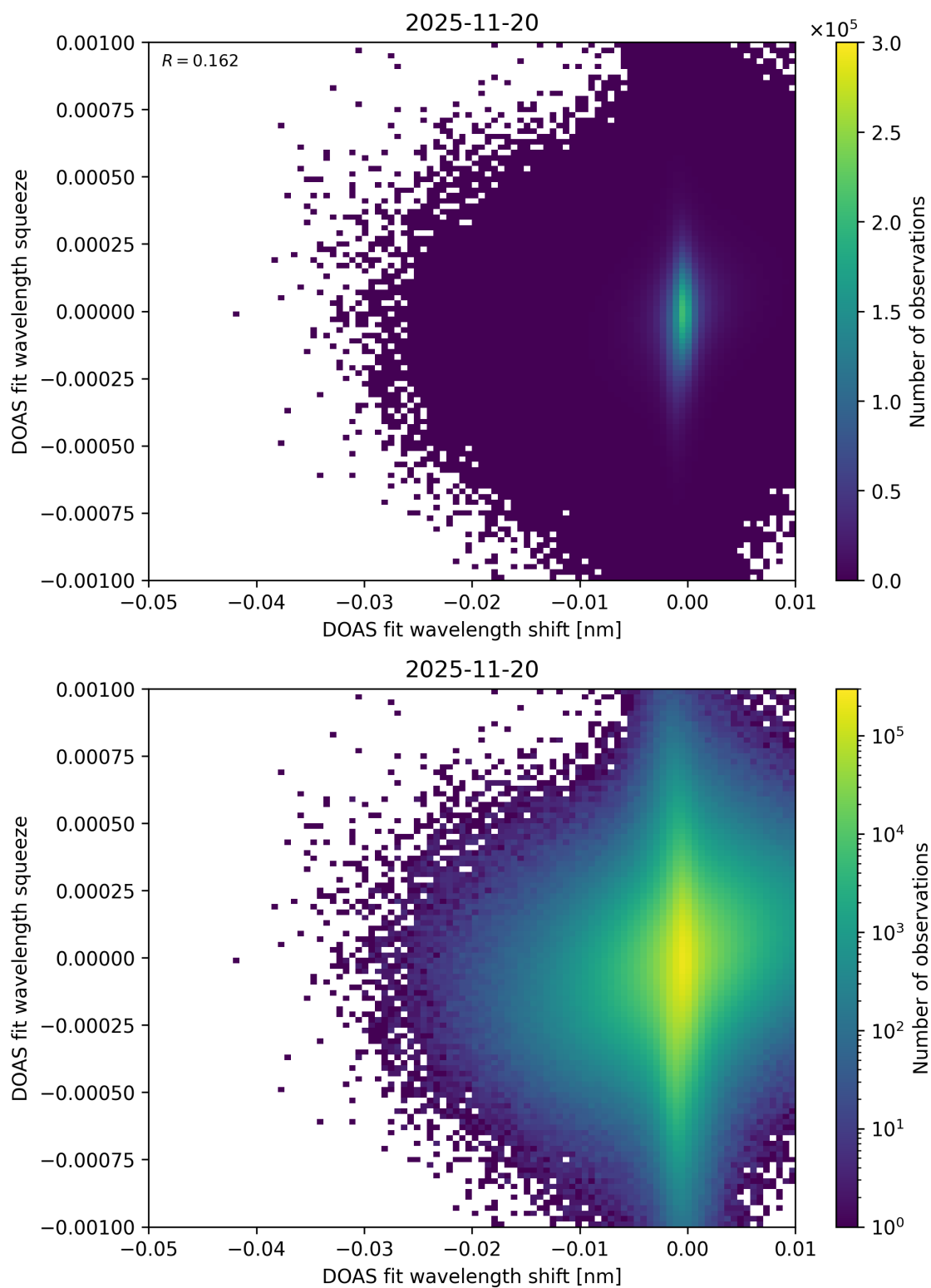
Figure 138: Scatter density plot of “DOAS fit wavelength shift” against “DOAS fit wavelength squeeze” for 2025-11-19 to 2025-11-21.
