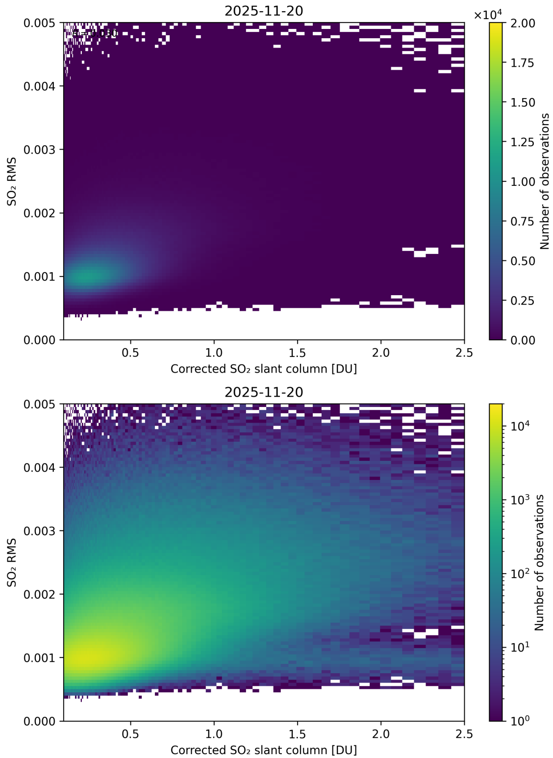
Figure 231: Scatter density plot of “Corrected SO 2 slant column” against “SO 2 RMS” for 2025-11-19 to 2025-11-21.
