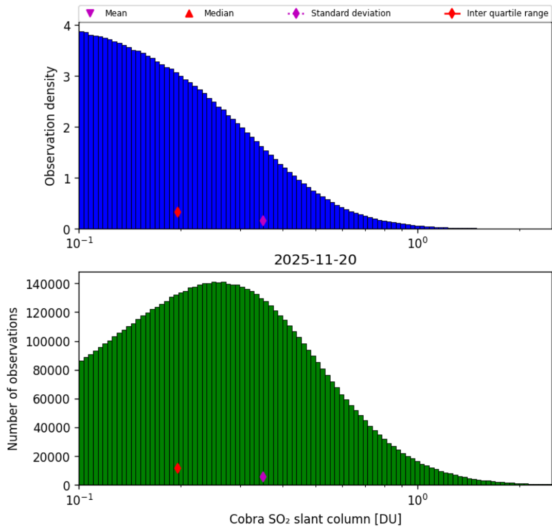
Figure 61: Histogram of “Cobra SO 2 slant column” for 2025-11-19 to 2025-11-21
