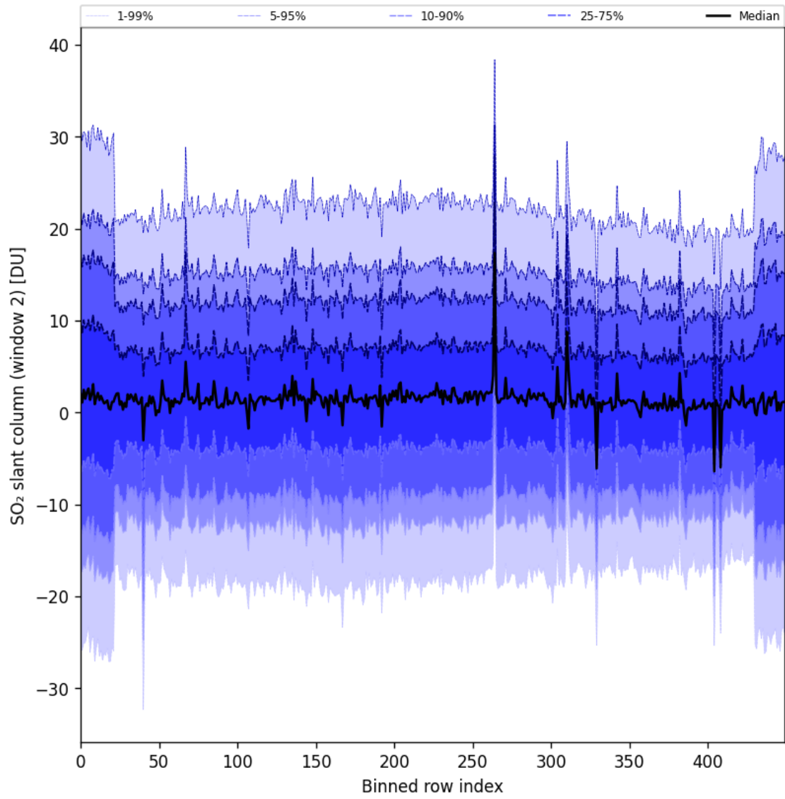
Figure 93: Along track statistics of “SO 2 slant column (window 2)” for 2025-11-19 to 2025-11-21
