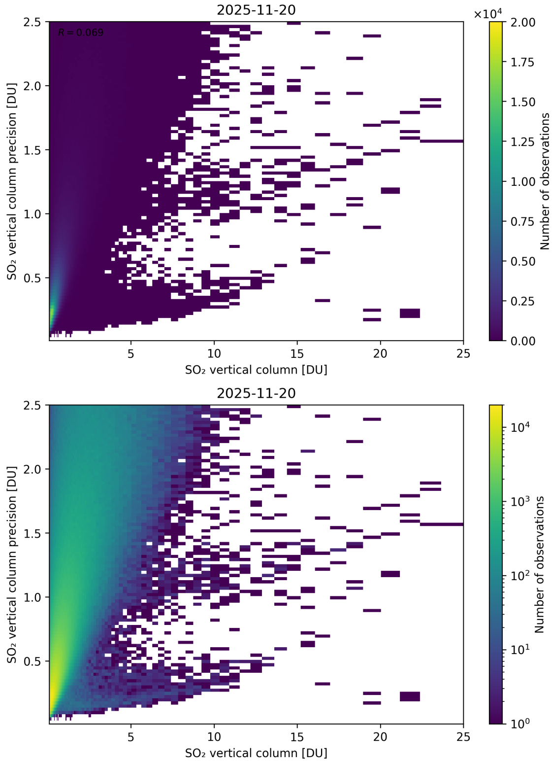
Figure 361: Scatter density plot of “SO 2 vertical column” against “SO 2 vertical column precision” for 2025-11-19 to 2025-11-21.
