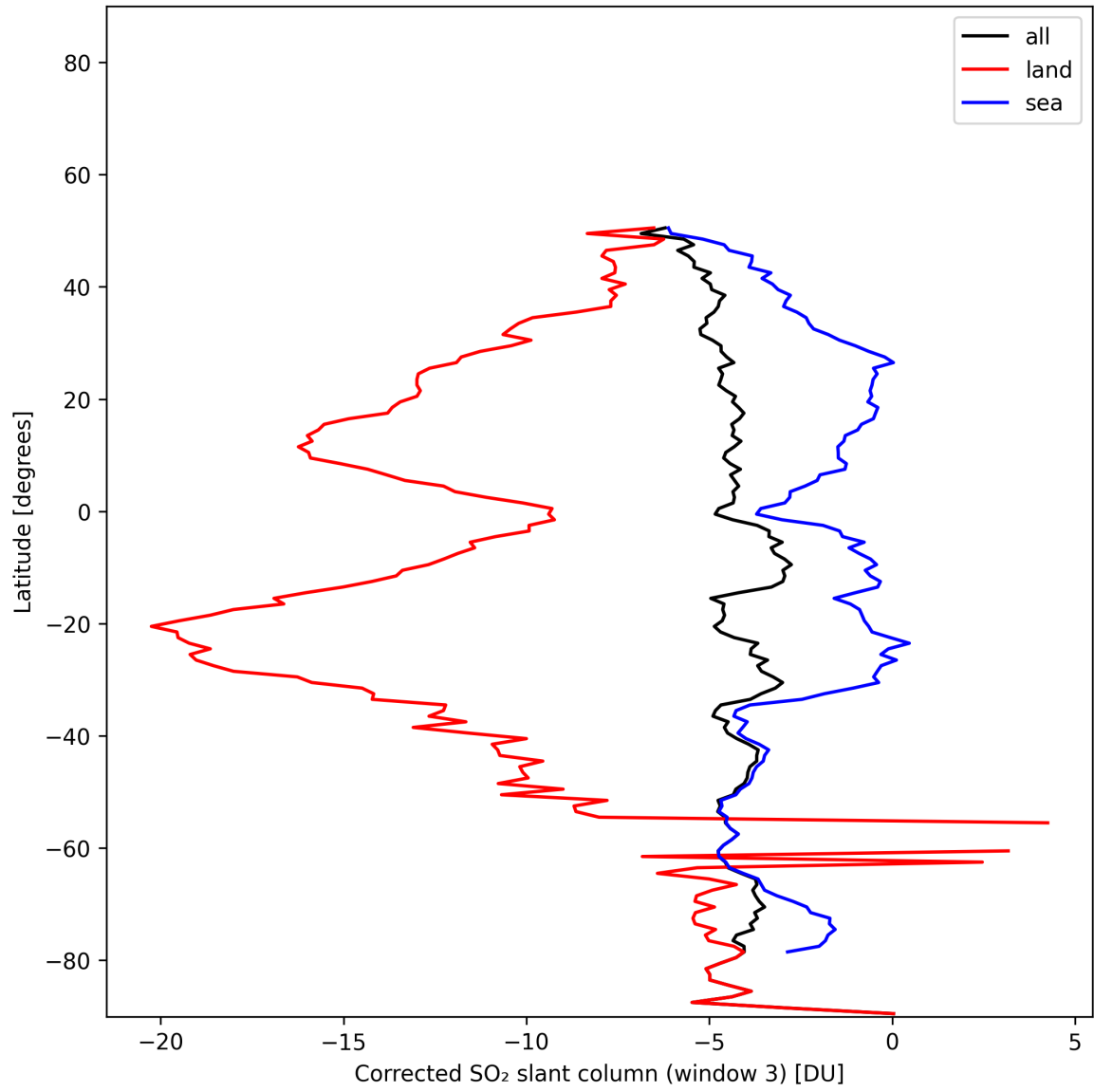
Figure 47: Zonal average of “Corrected SO 2 slant column (window 3)” for 2025-11-19 to 2025-11-21.
