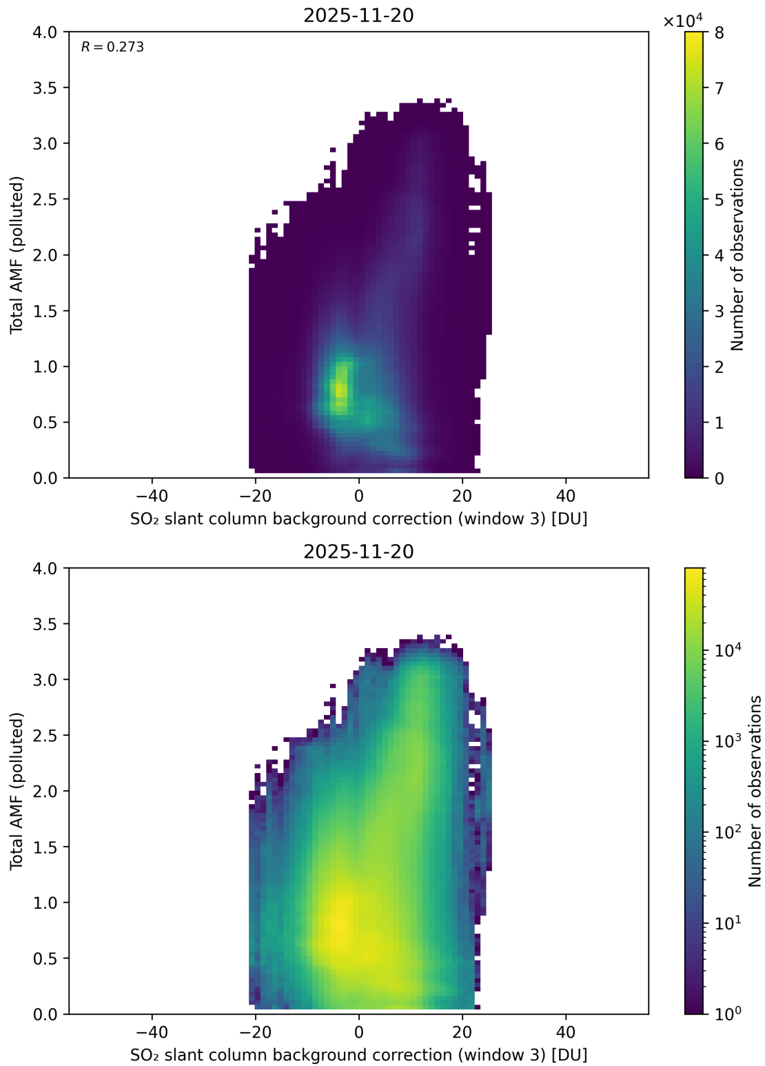
Figure 136: Scatter density plot of “SO 2 slant column background correction (window 3)” against “Total AMF (polluted)” for 2025-11-19 to 2025-11-21.
