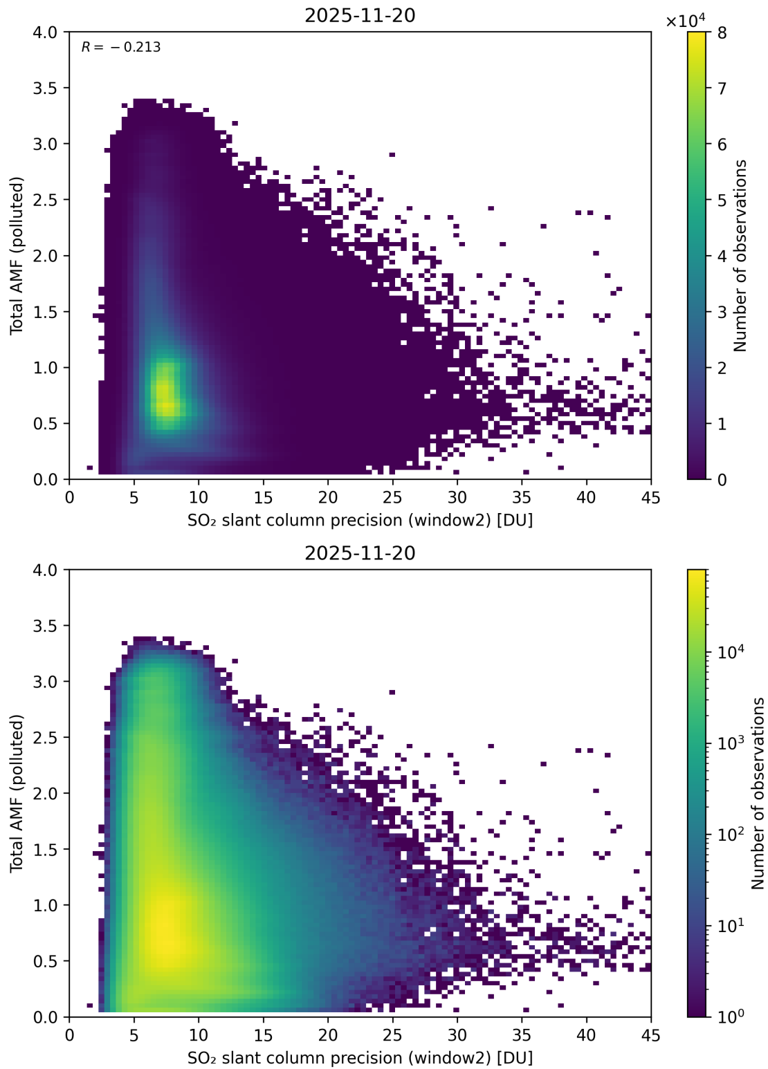
Figure 301: Scatter density plot of “SO 2 slant column precision (window2)” against “Total AMF (polluted)” for 2025-11-19 to 2025-11-21.
