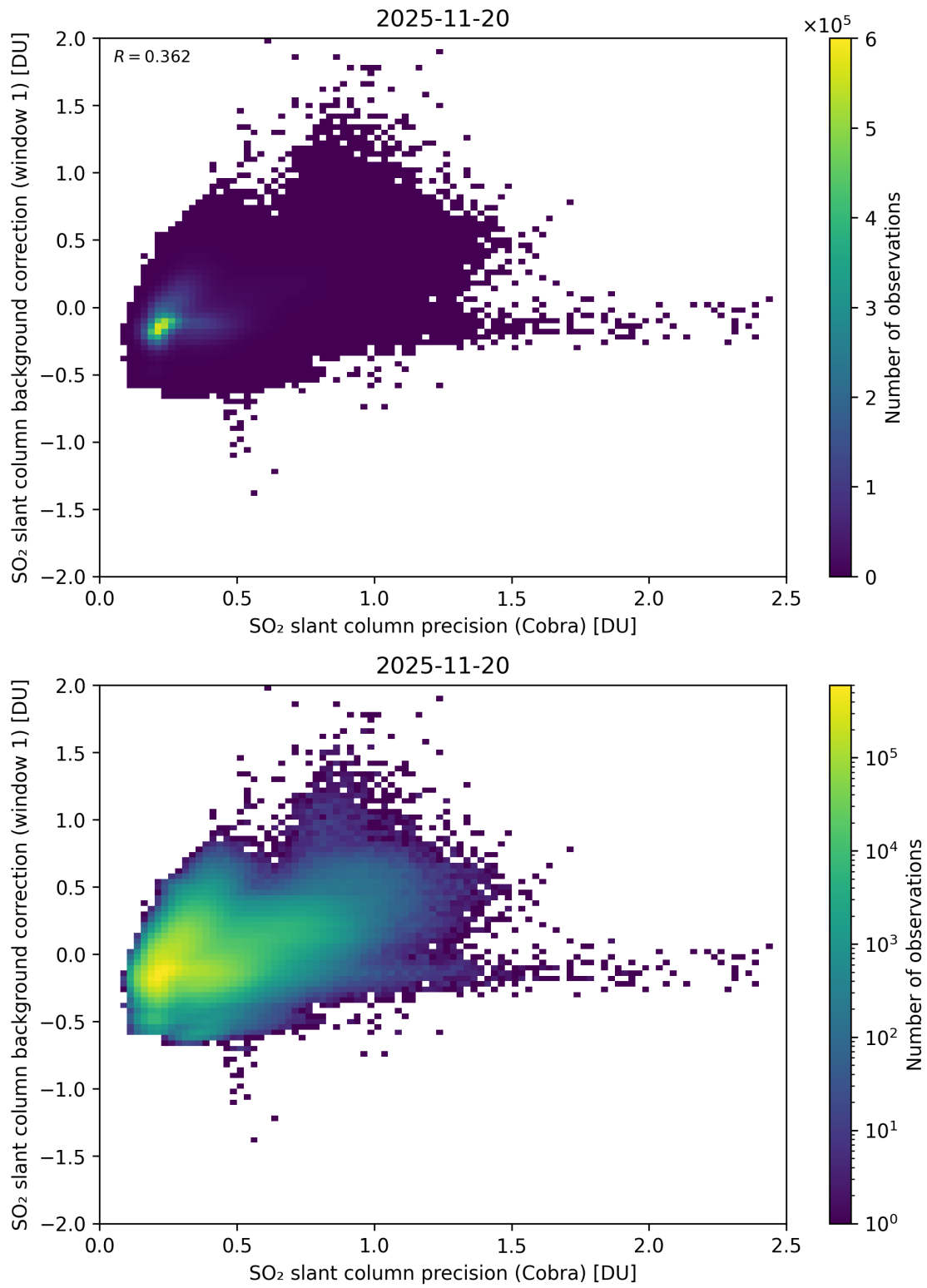
Figure 199: Scatter density plot of “SO 2 slant column precision (Cobra)” against “SO 2 slant column background correction (window 1)” for 2025-11-19 to 2025-11-21.
