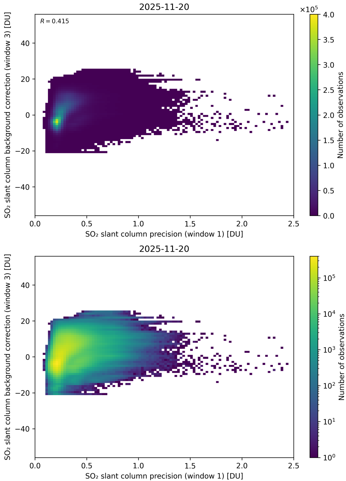
Figure 270: Scatter density plot of “SO 2 slant column precision (window 1)” against “SO 2 slant column background correction (window 3)” for 2025-11-19 to 2025-11-21.
