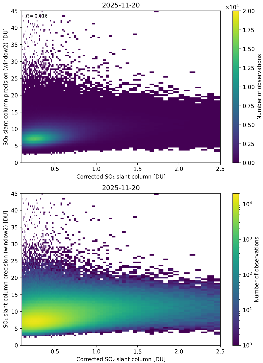
Figure 239: Scatter density plot of “Corrected SO 2 slant column” against “SO 2 slant column precision (window2)” for 2025-11-19 to 2025-11-21.
