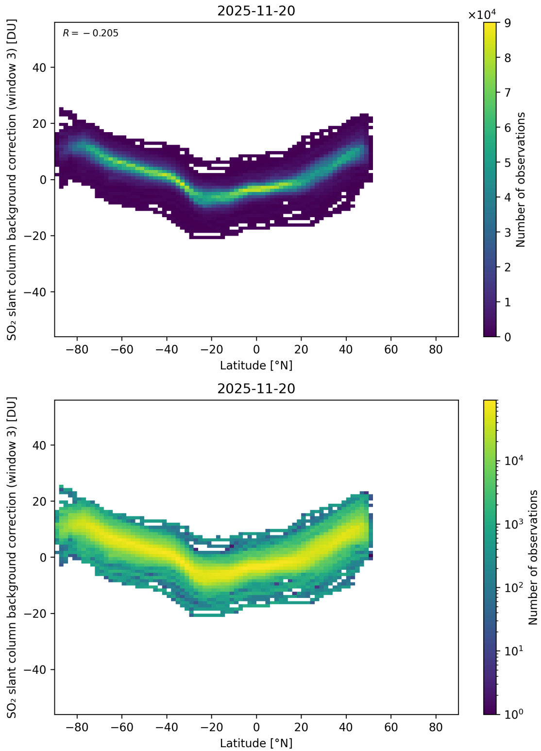
Figure 152: Scatter density plot of “Latitude” against “SO 2 slant column background correction (window 3)” for 2025-11-19 to 2025-11-21.
