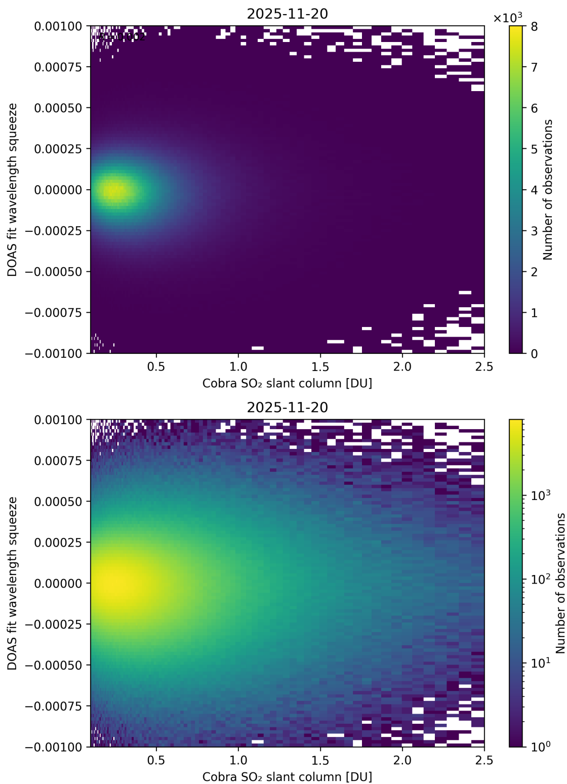
Figure 197: Scatter density plot of “Cobra SO 2 slant column” against “DOAS fit wavelength squeeze” for 2025-11-19 to 2025-11-21.
