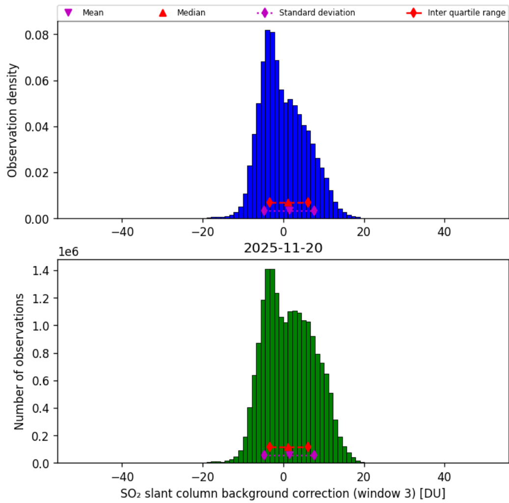
Figure 74: Histogram of “SO 2 slant column background correction (window 3)” for 2025-11-19 to 2025-11-21
