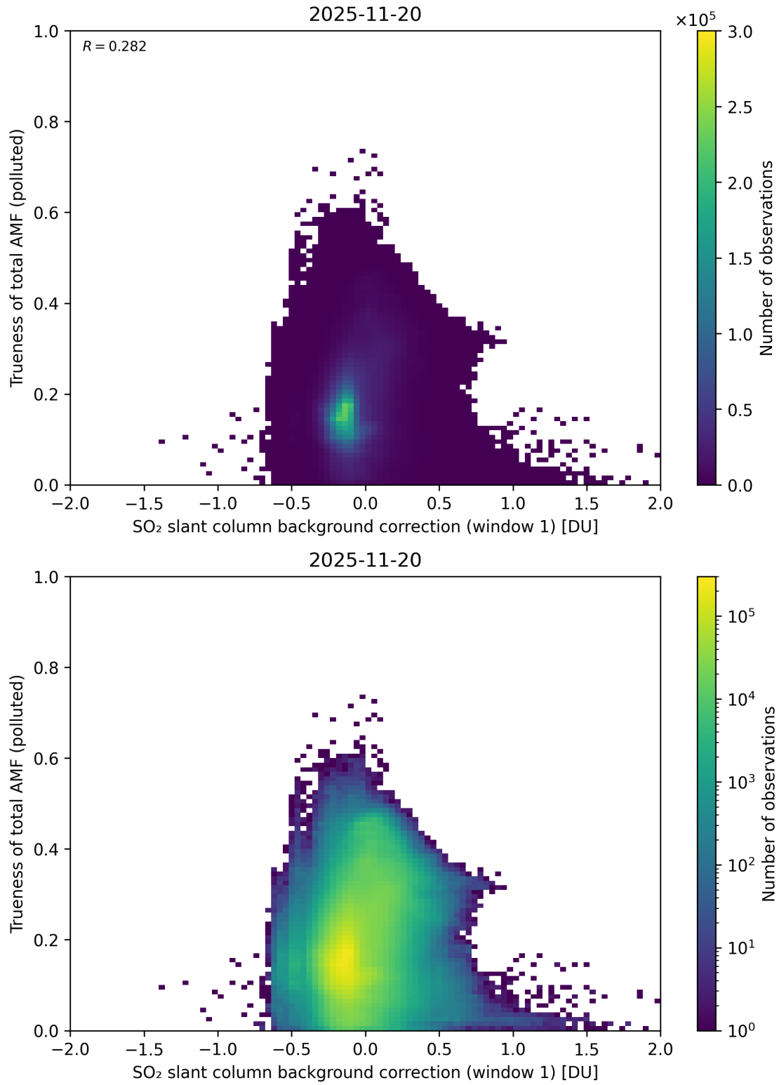
Figure 121: Scatter density plot of “SO 2 slant column background correction (window 1)” against “Trueness of total AMF (polluted)” for 2025-11-19 to 2025-11-21.
