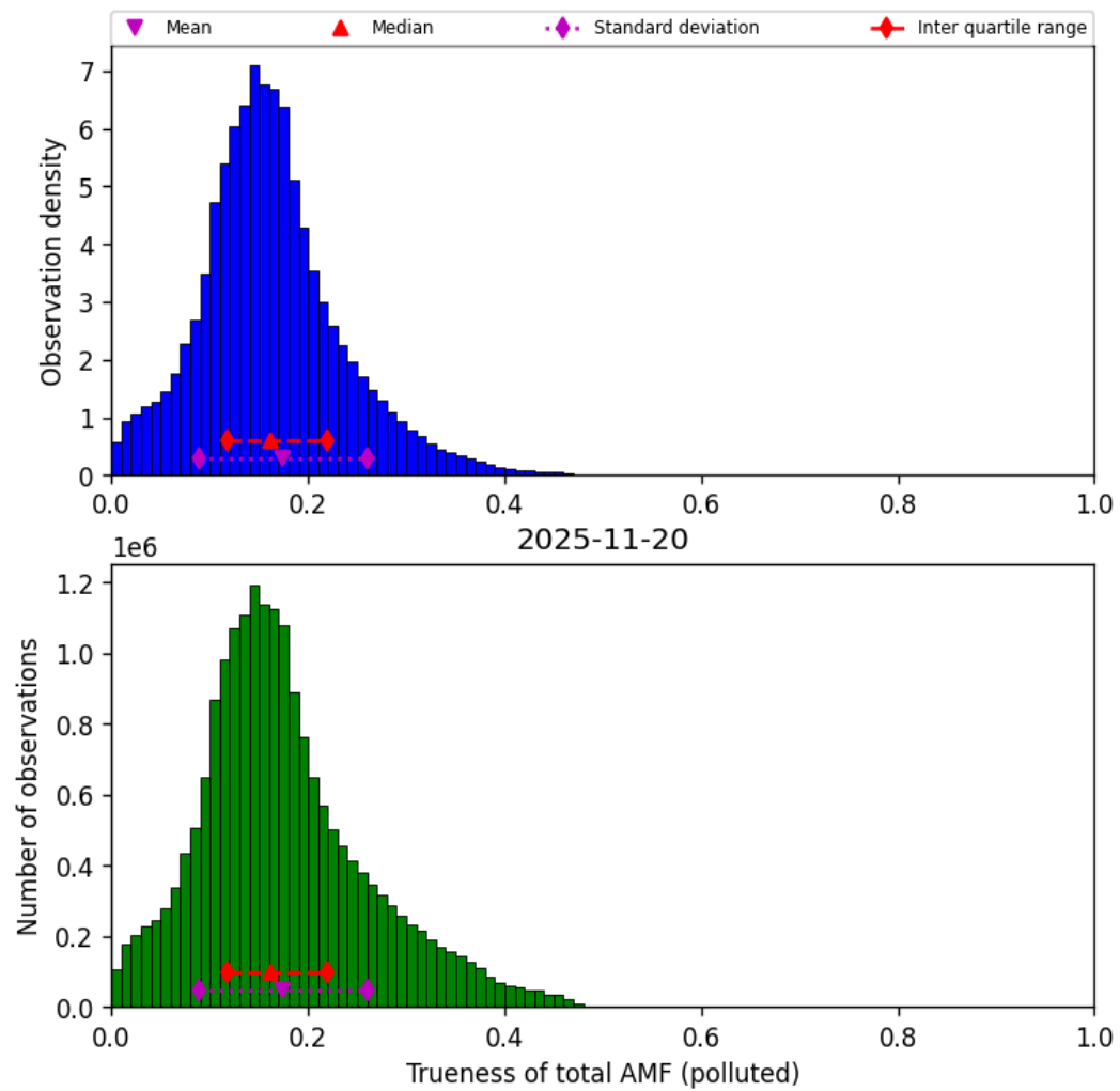
Figure 80: Histogram of “Trueness of total AMF (polluted)” for 2025-11-19 to 2025-11-21
