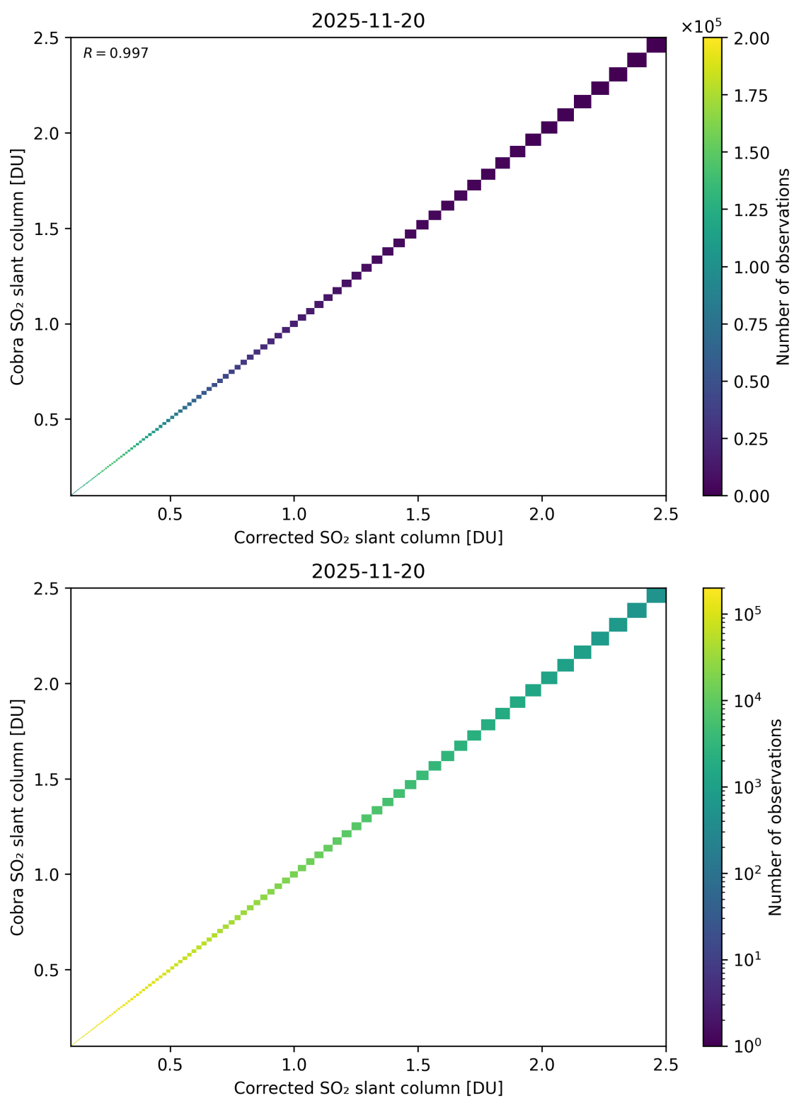
Figure 233: Scatter density plot of “Corrected SO 2 slant column” against “Cobra SO 2 slant column” for 2025-11-19 to 2025-11-21.
