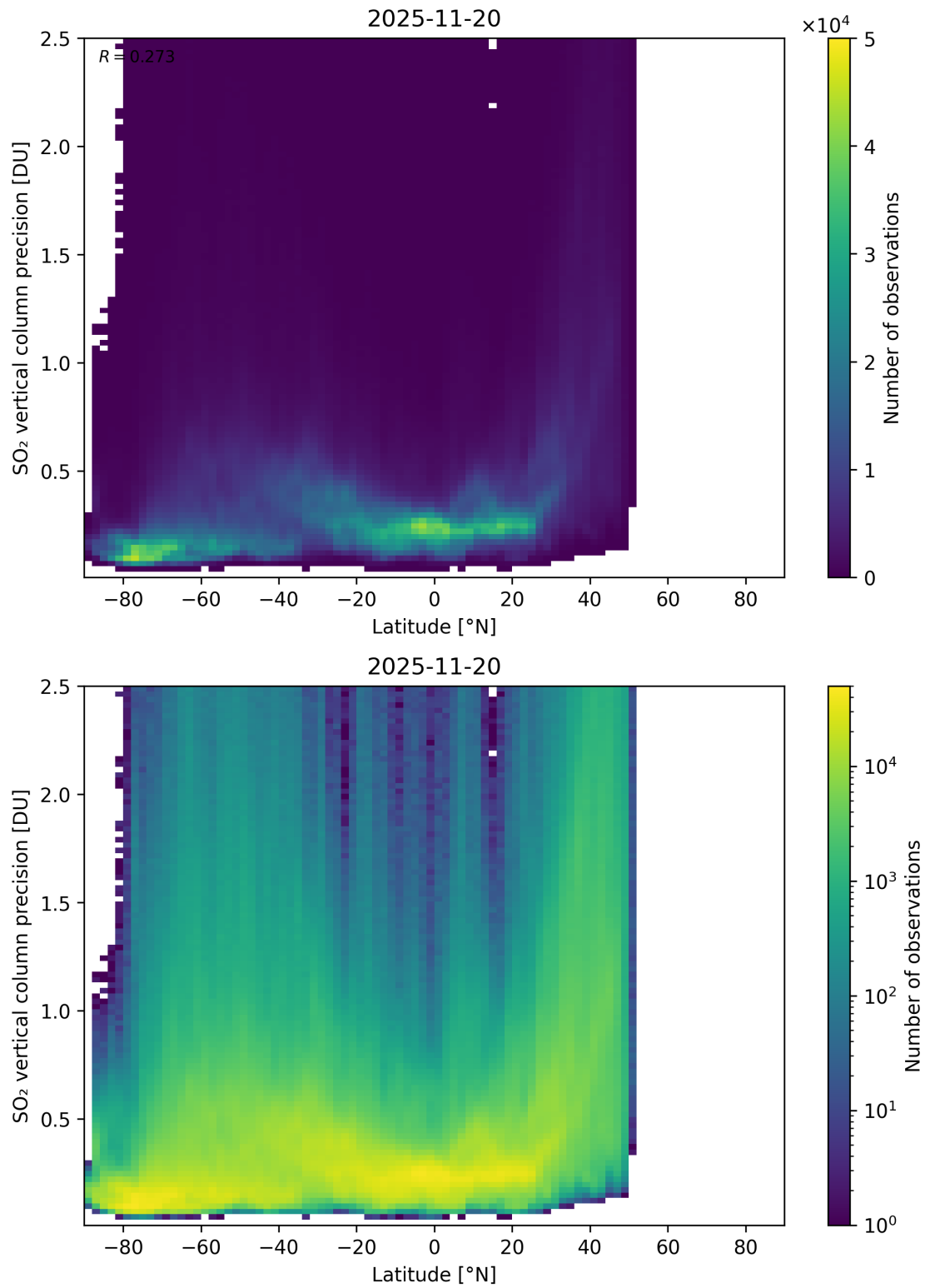
Figure 170: Scatter density plot of “Latitude” against “SO 2 vertical column precision” for 2025-11-19 to 2025-11-21.
