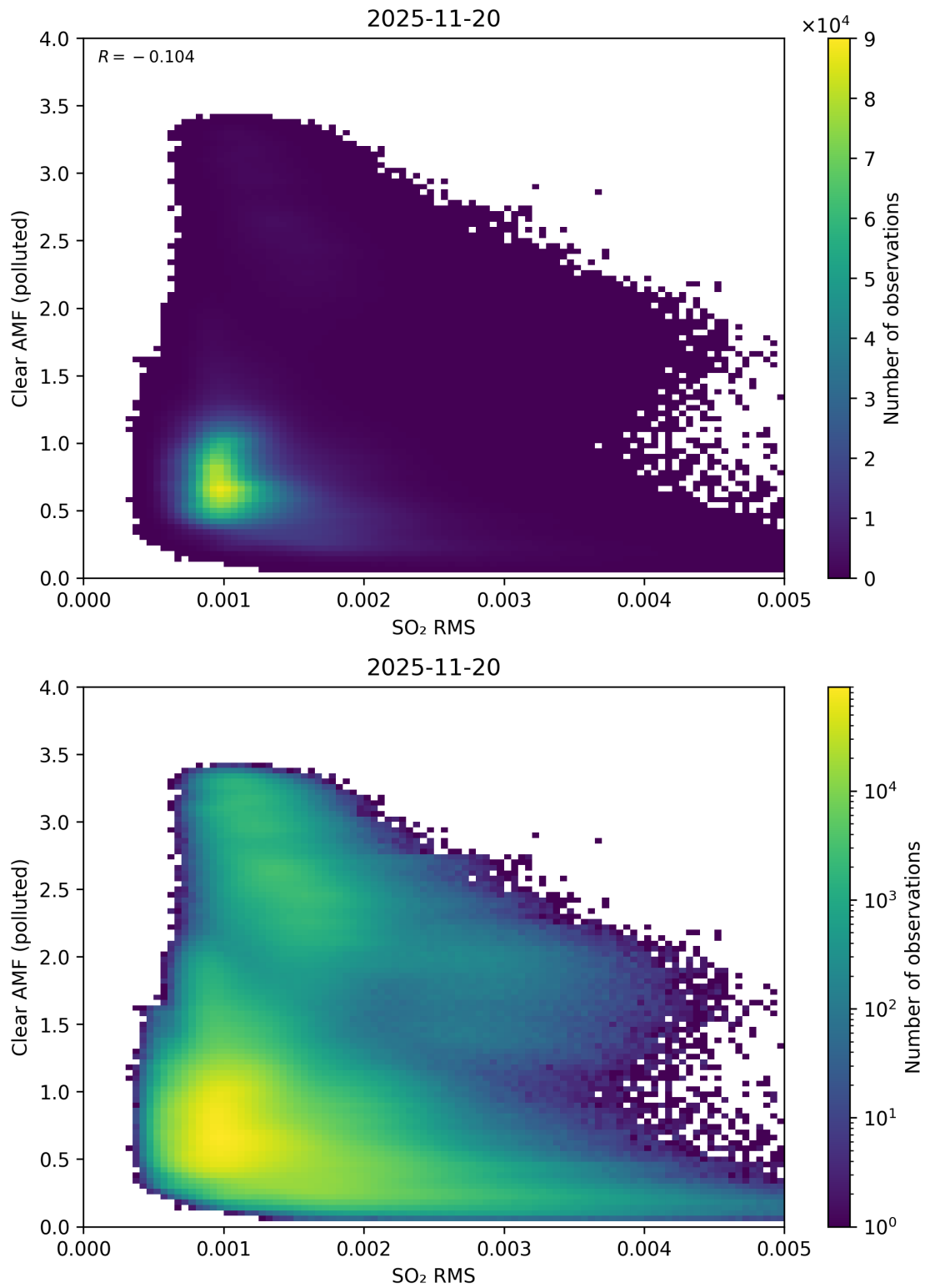
Figure 147: Scatter density plot of “SO 2 RMS” against “Clear AMF (polluted)” for 2025-11-19 to 2025-11-21.
