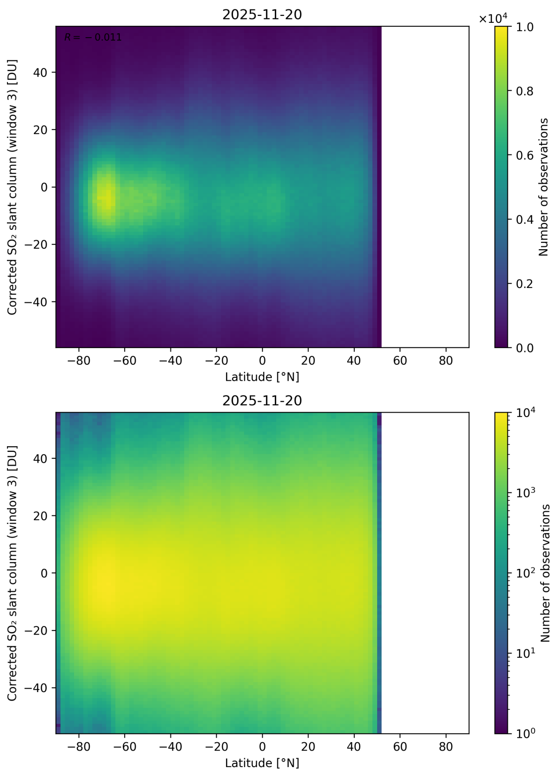
Figure 161: Scatter density plot of “Latitude” against “Corrected SO 2 slant column (window 3)” for 2025-11-19 to 2025-11-21.
