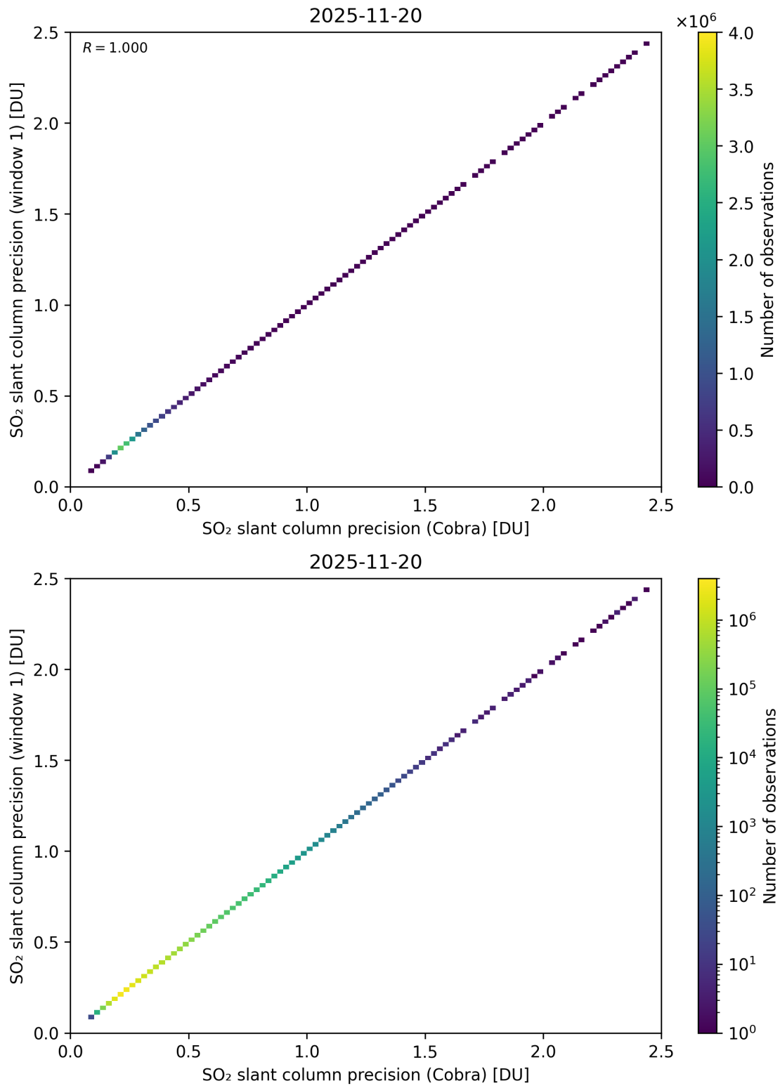
Figure 209: Scatter density plot of “SO 2 slant column precision (Cobra)” against “SO 2 slant column precision (window 1)” for 2025-11-19 to 2025-11-21.
