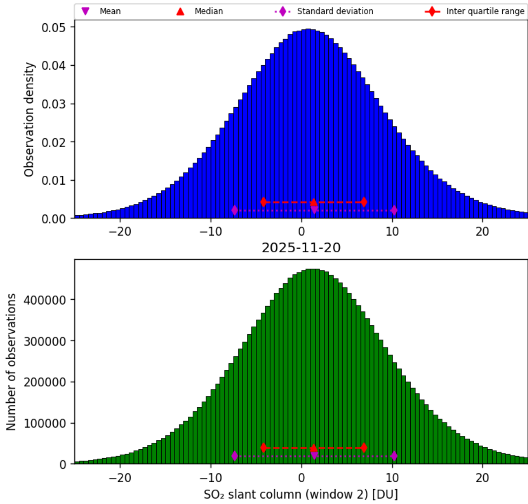
Figure 67: Histogram of “SO 2 slant column (window 2)” for 2025-11-19 to 2025-11-21
