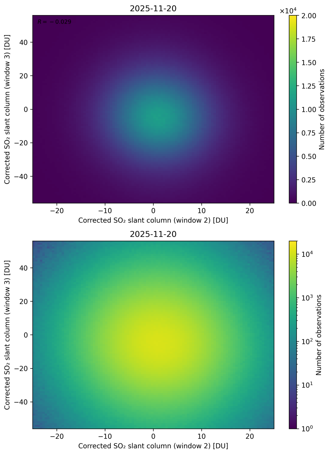
Figure 250: Scatter density plot of “Corrected SO 2 slant column (window 2)” against “Corrected SO 2 slant column (window 3)” for 2025-11-19 to 2025-11-21.
