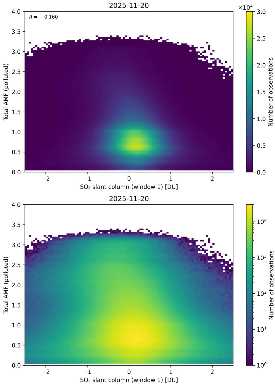
Figure 289: Scatter density plot of “SO 2 slant column (window 1)” against “Total AMF (polluted)” for 2025-11-19 to 2025-11-21.
