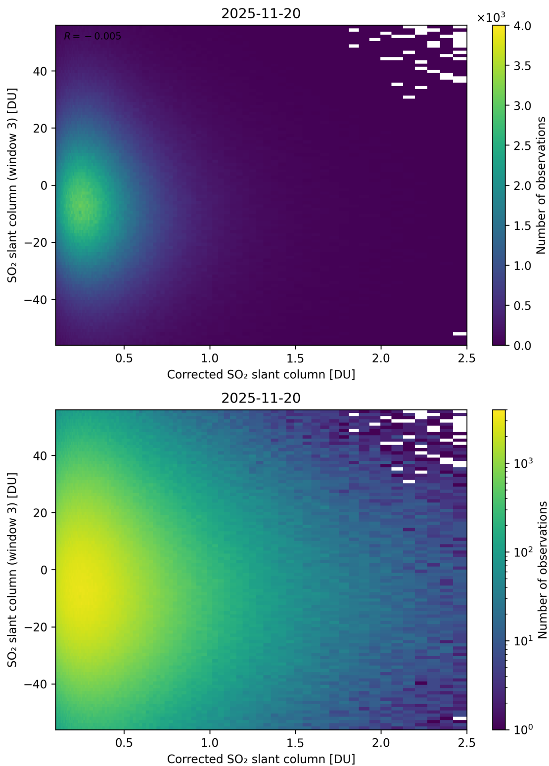
Figure 240: Scatter density plot of “Corrected SO 2 slant column” against “SO 2 slant column (window 3)” for 2025-11-19 to 2025-11-21.
