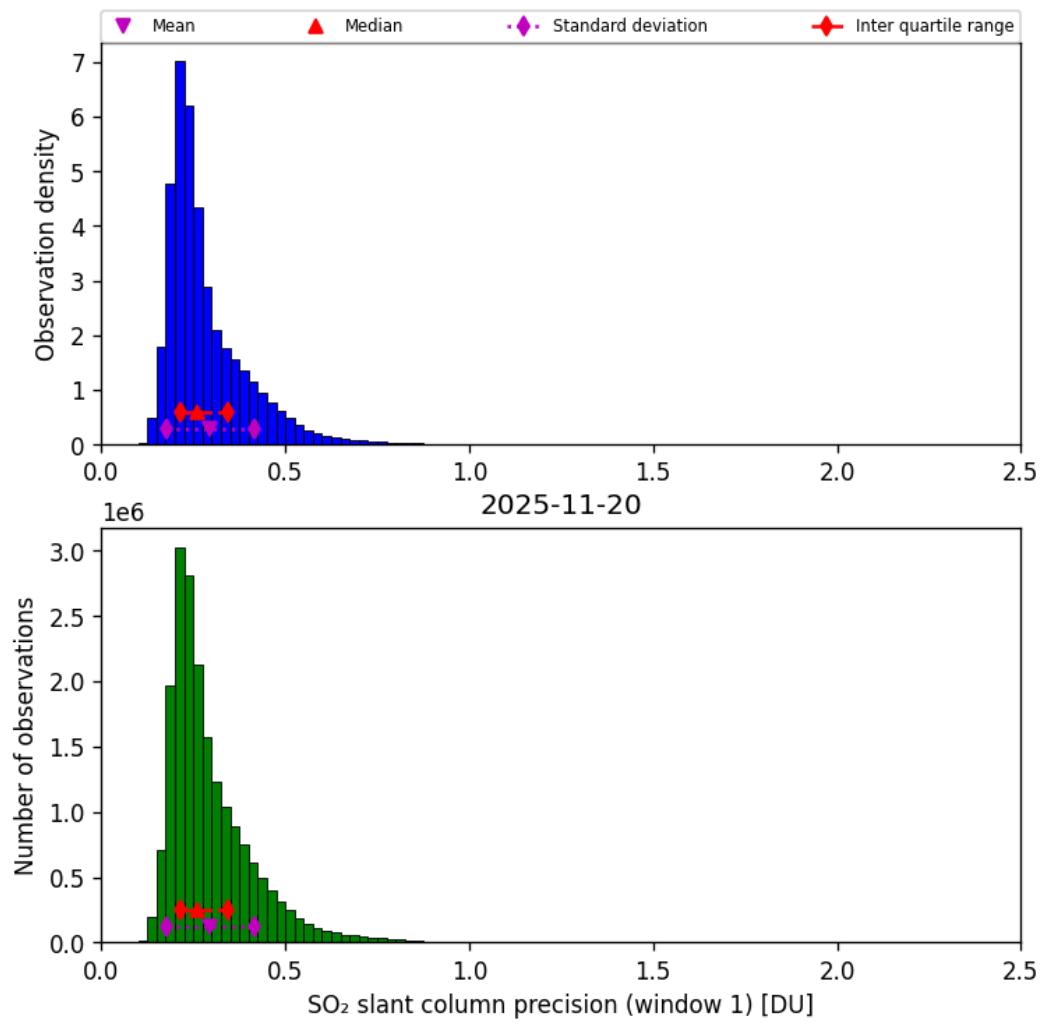
Figure 64: Histogram of “SO 2 slant column precision (window 1)” for 2025-11-19 to 2025-11-21
