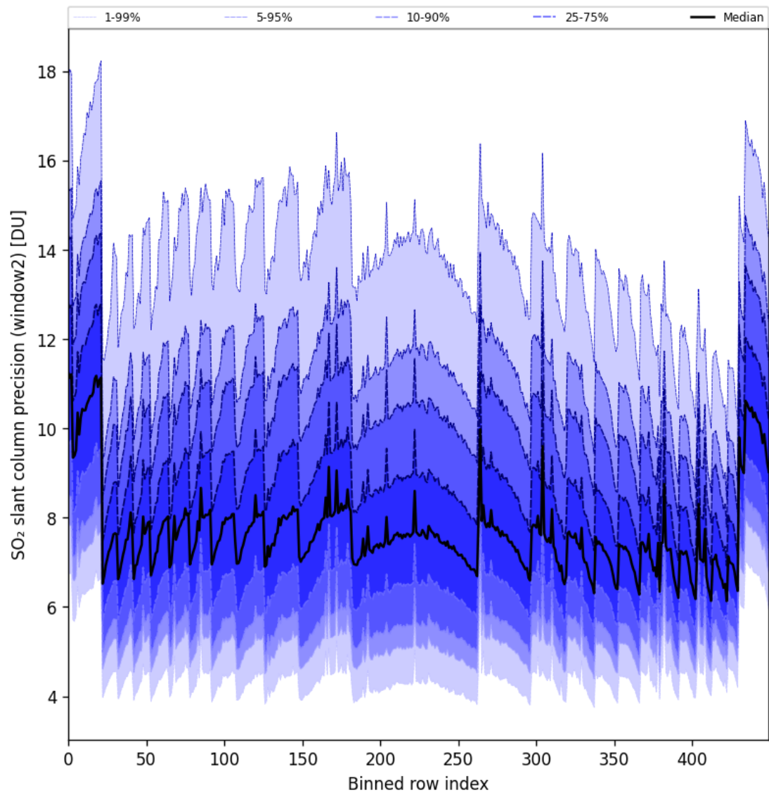
Figure 94: Along track statistics of “SO 2 slant column precision (window2)” for 2025-11-19 to 2025-11-21
