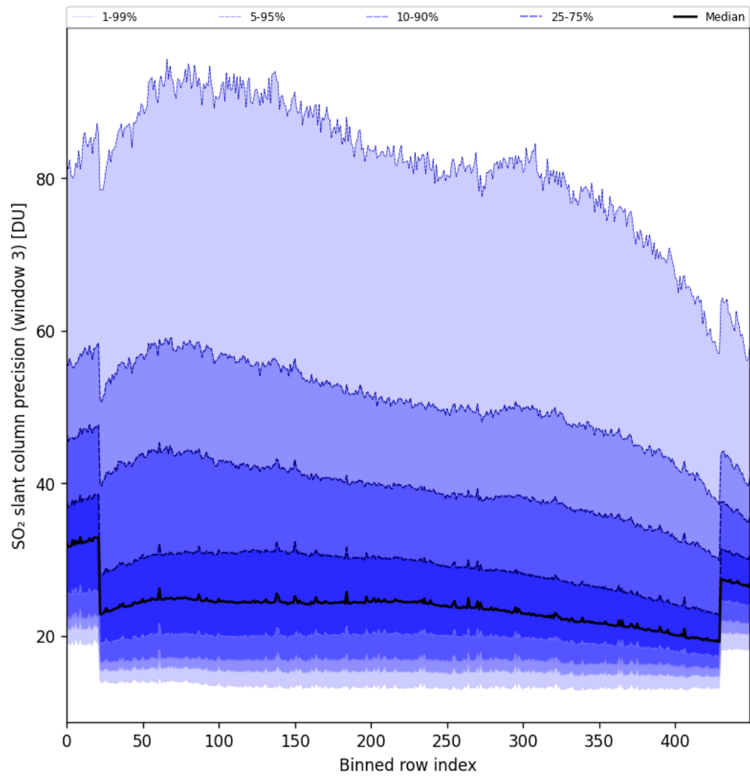
Figure 98: Along track statistics of “SO 2 slant column precision (window 3)” for 2025-11-19 to 2025-11-21
