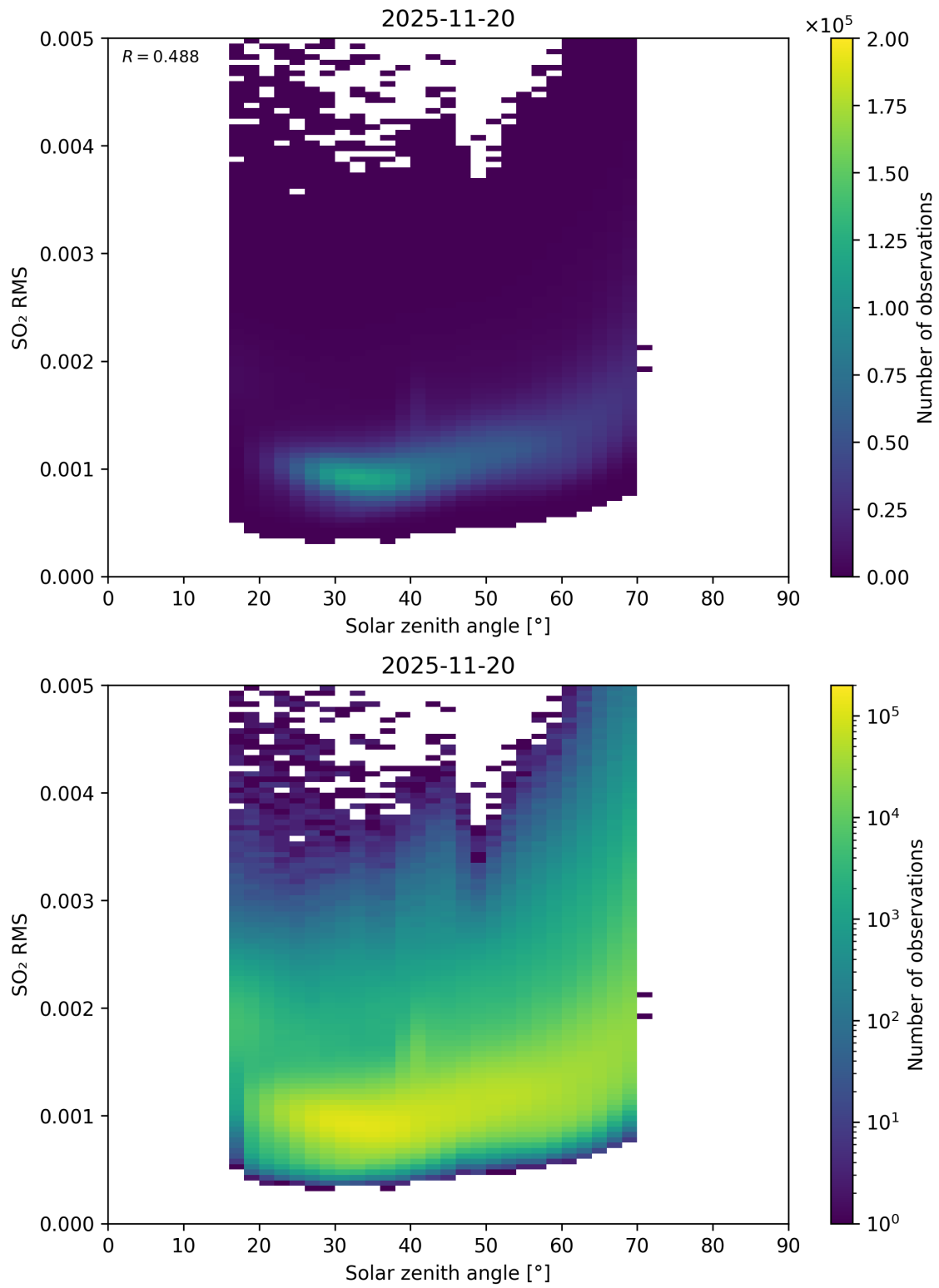
Figure 176: Scatter density plot of “Solar zenith angle” against “SO 2 RMS” for 2025-11-19 to 2025-11-21.
