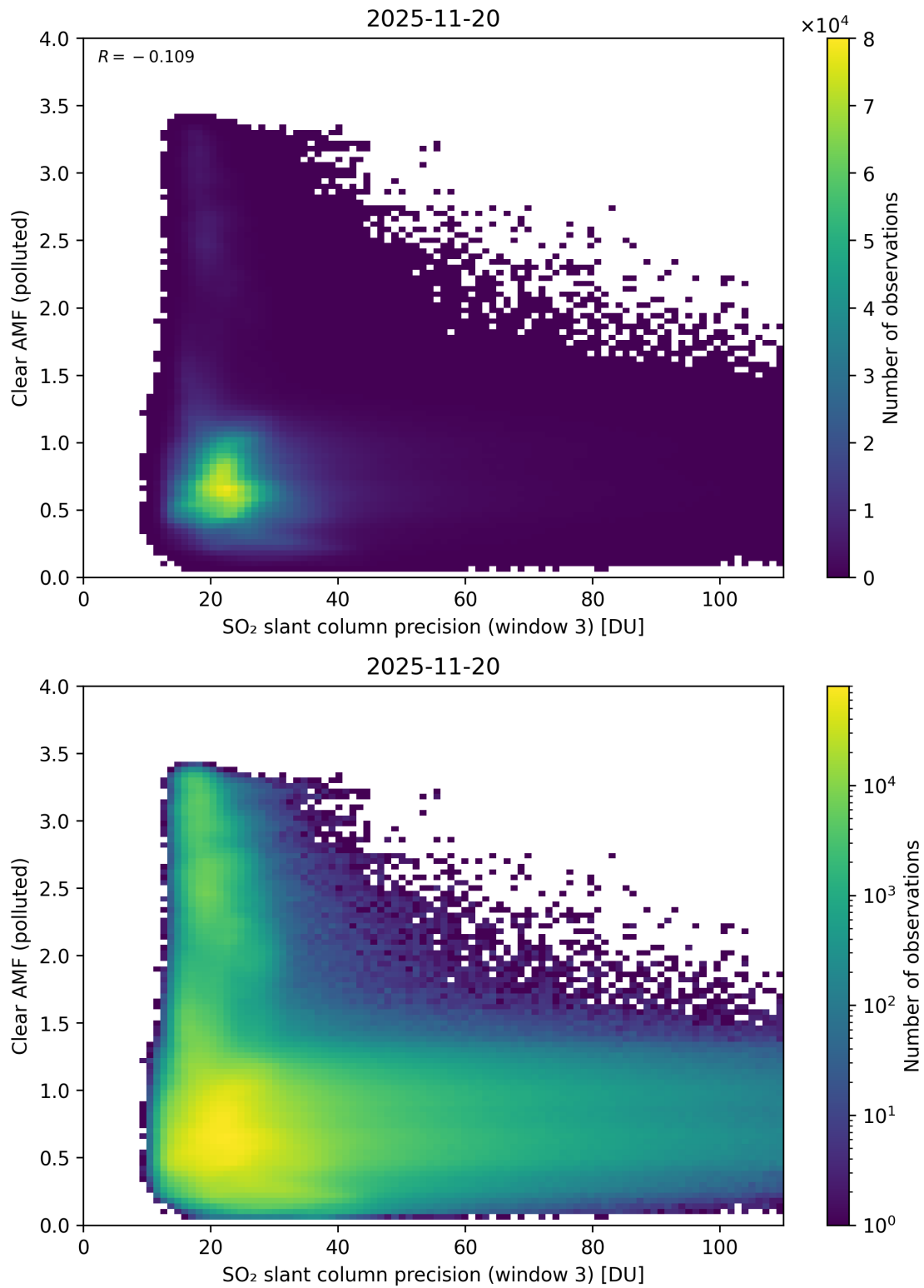
Figure 311: Scatter density plot of “SO 2 slant column precision (window 3)” against “Clear AMF (polluted)” for 2025-11-19 to 2025-11-21.
