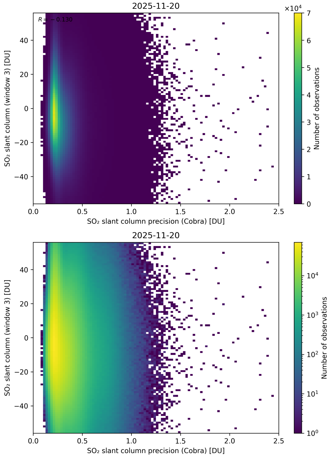
Figure 211: Scatter density plot of “SO 2 slant column precision (Cobra)” against “SO 2 slant column (window 3)” for 2025-11-19 to 2025-11-21.
