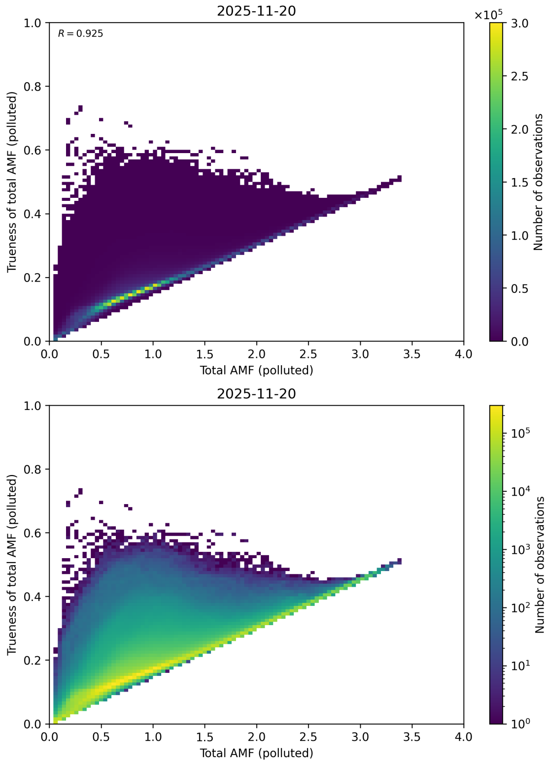
Figure 321: Scatter density plot of “Total AMF (polluted)” against “Trueness of total AMF (polluted)” for 2025-11-19 to 2025-11-21.
