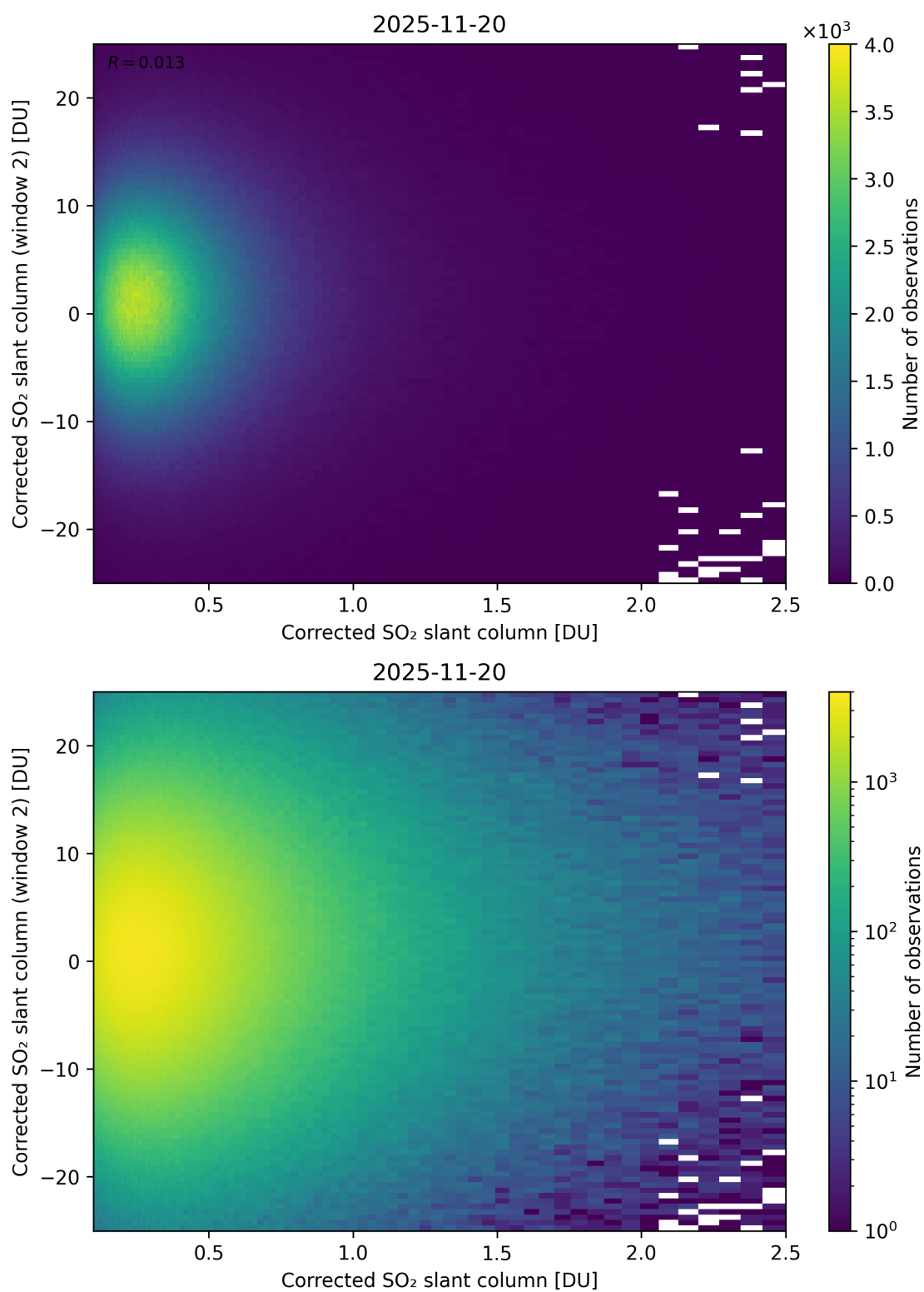
Figure 235: Scatter density plot of “Corrected SO 2 slant column” against “Corrected SO 2 slant column (window 2)” for 2025-11-19 to 2025-11-21.
