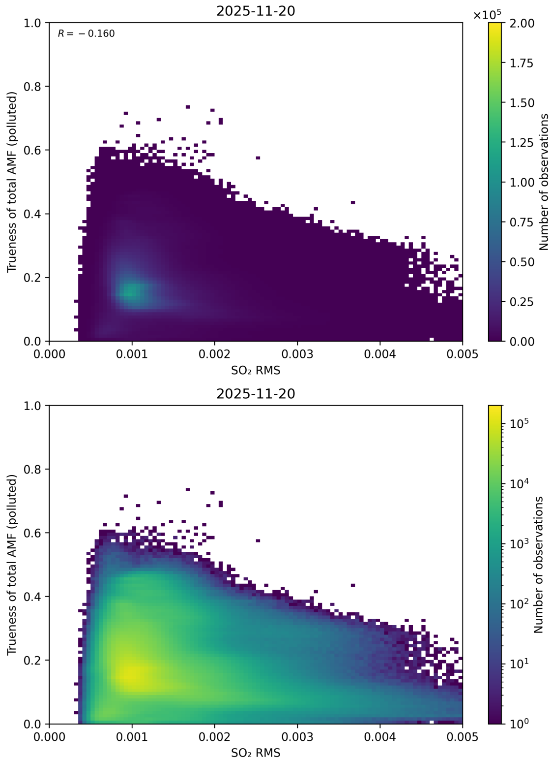
Figure 149: Scatter density plot of “SO 2 RMS” against “Trueness of total AMF (polluted)” for 2025-11-19 to 2025-11-21.
