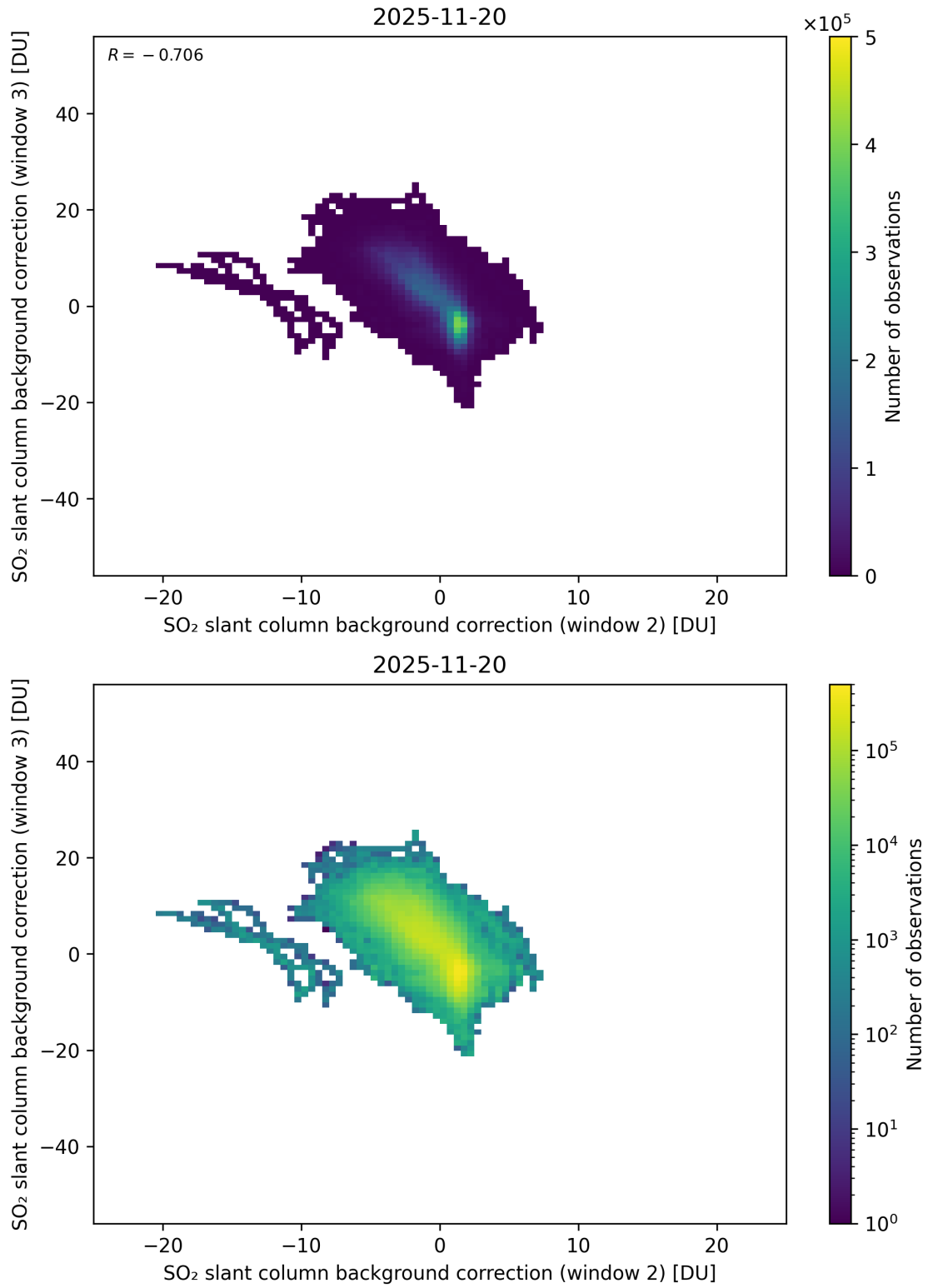
Figure 122: Scatter density plot of “SO 2 slant column background correction (window 2)” against “SO 2 slant column background correction (window 3)” for 2025-11-19 to 2025-11-21.
