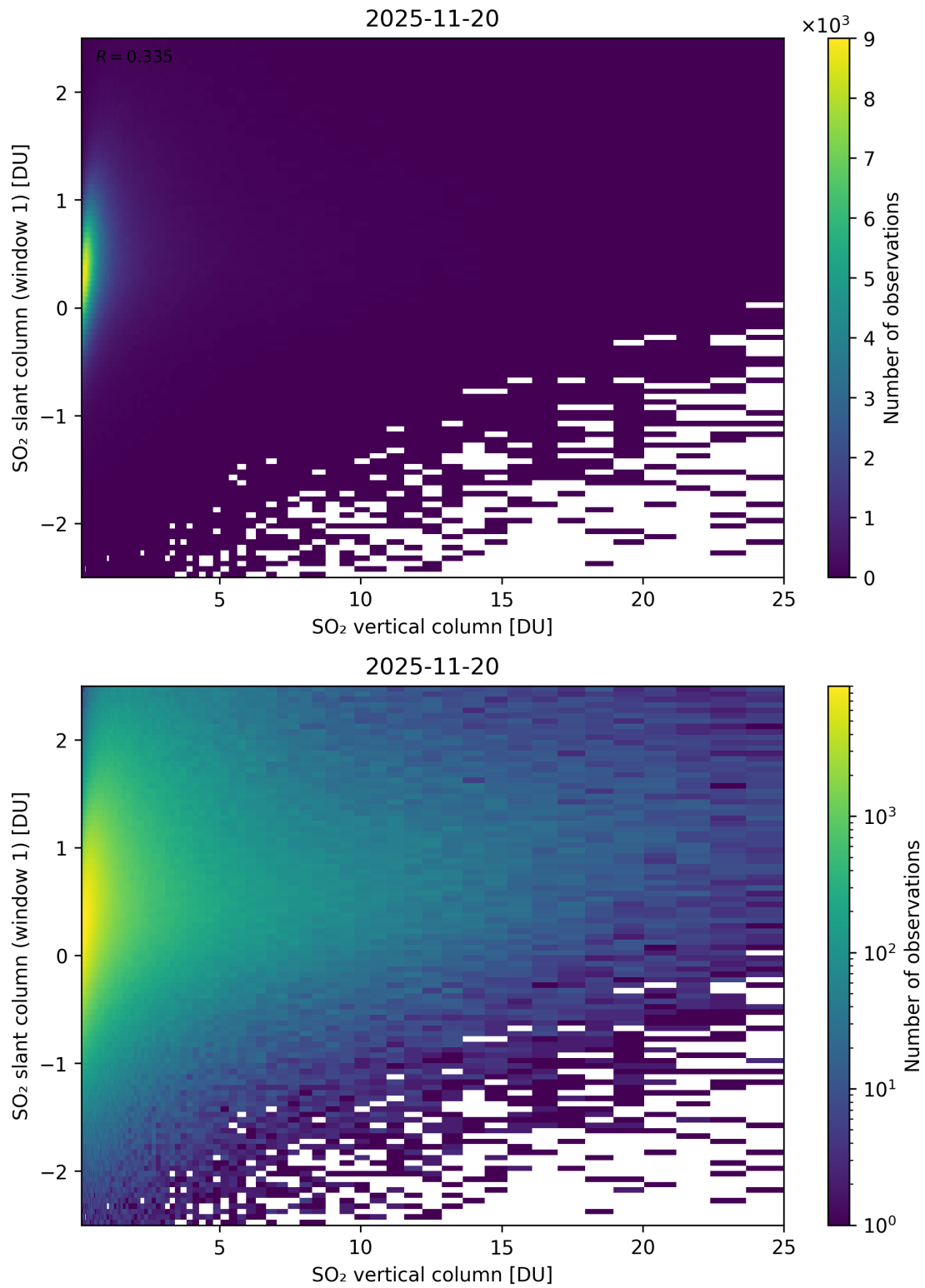
Figure 354: Scatter density plot of “SO 2 vertical column” against “SO 2 slant column (window 1)” for 2025-11-19 to 2025-11-21.
