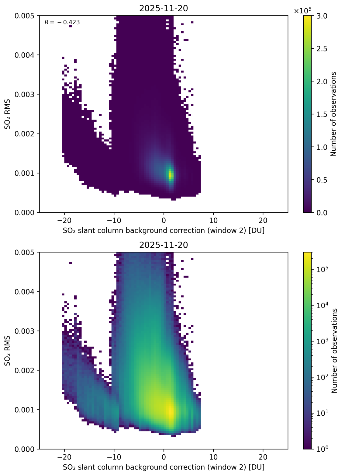
Figure 125: Scatter density plot of “SO 2 slant column background correction (window 2)” against “SO 2 RMS” for 2025-11-19 to 2025-11-21.
