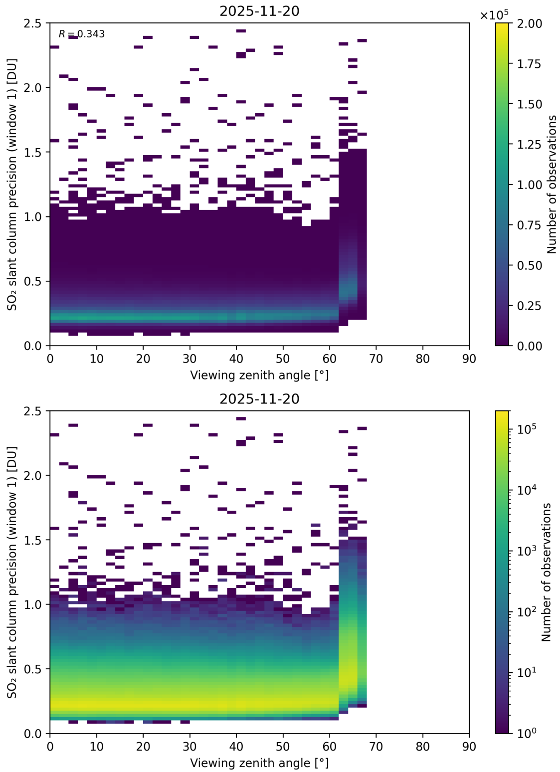
Figure 377: Scatter density plot of “Viewing zenith angle” against “SO 2 slant column precision (window 1)” for 2025-11-19 to 2025-11-21.
