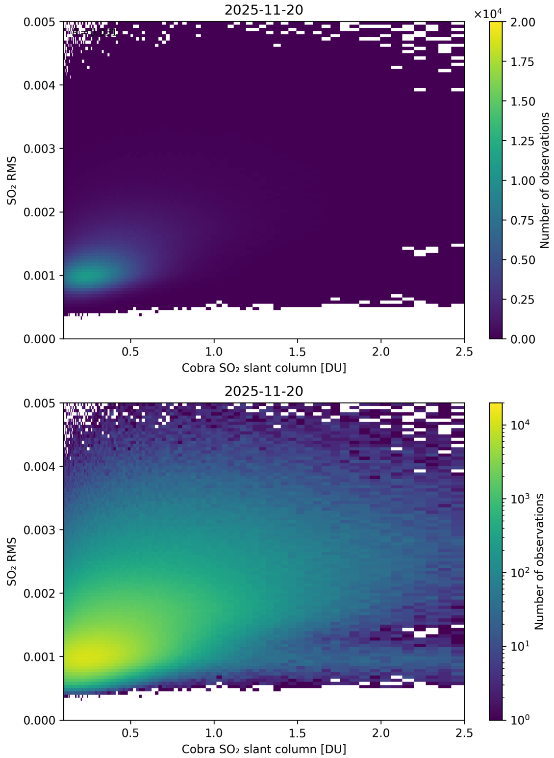
Figure 198: Scatter density plot of “Cobra SO 2 slant column” against “SO 2 RMS” for 2025-11-19 to 2025-11-21.
