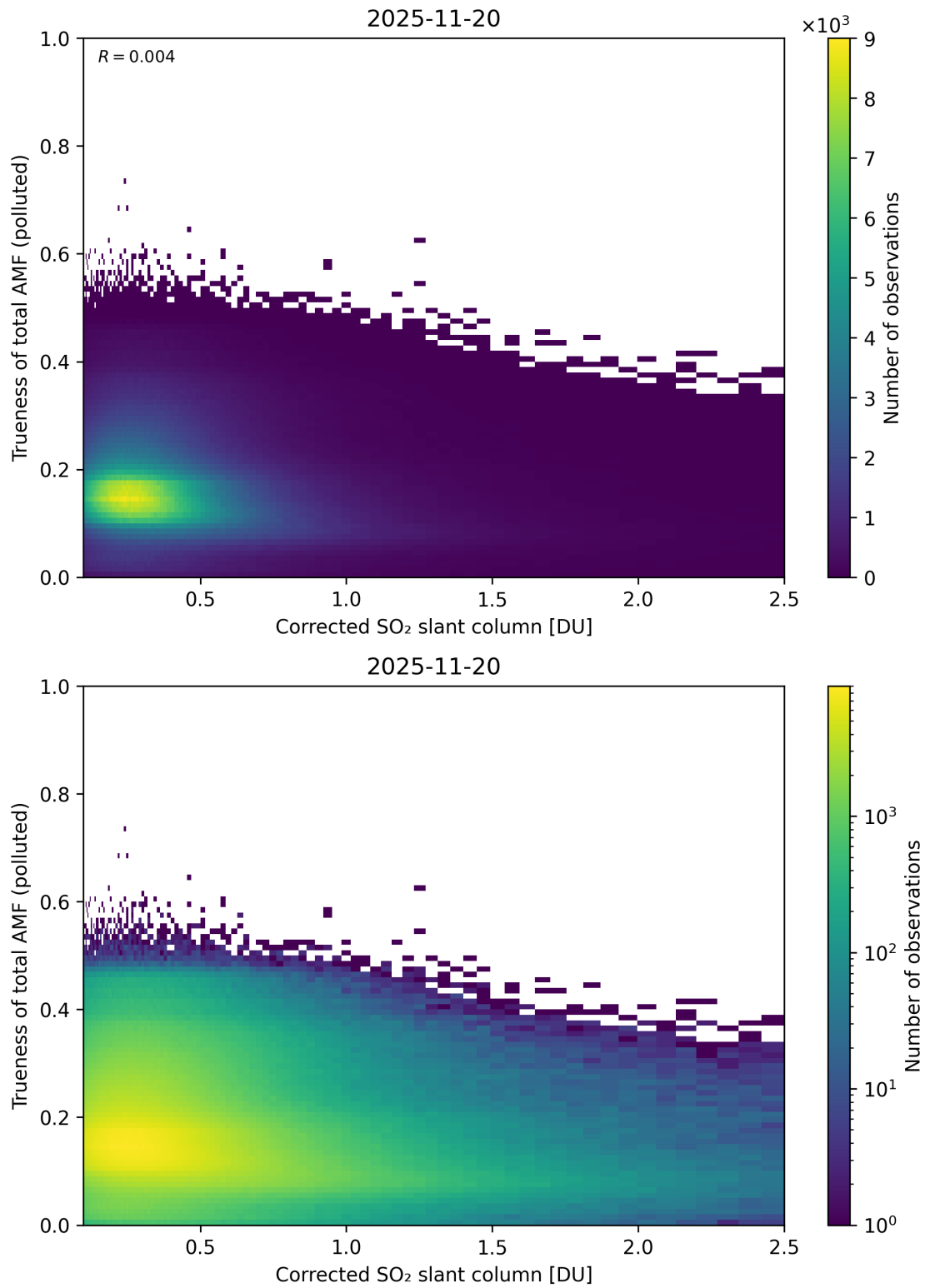
Figure 243: Scatter density plot of “Corrected SO 2 slant column” against “Trueness of total AMF (polluted)” for 2025-11-19 to 2025-11-21.
