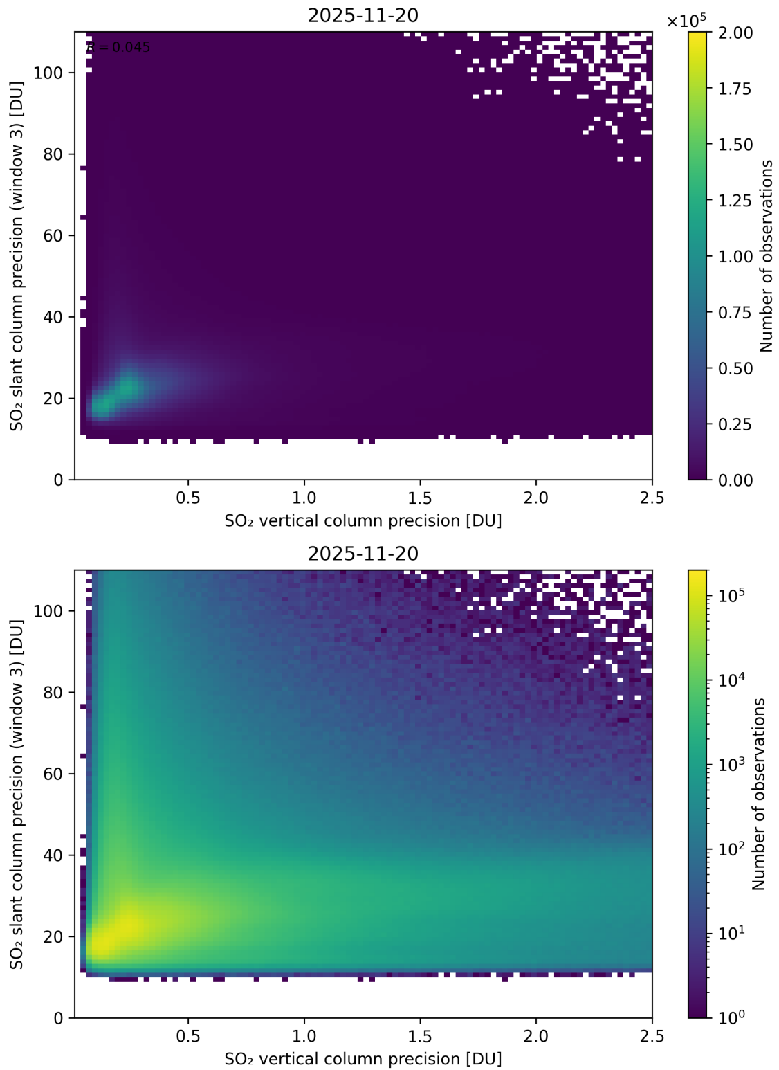
Figure 345: Scatter density plot of “SO 2 vertical column precision” against “SO 2 slant column precision (window 3)” for 2025-11-19 to 2025-11-21.
