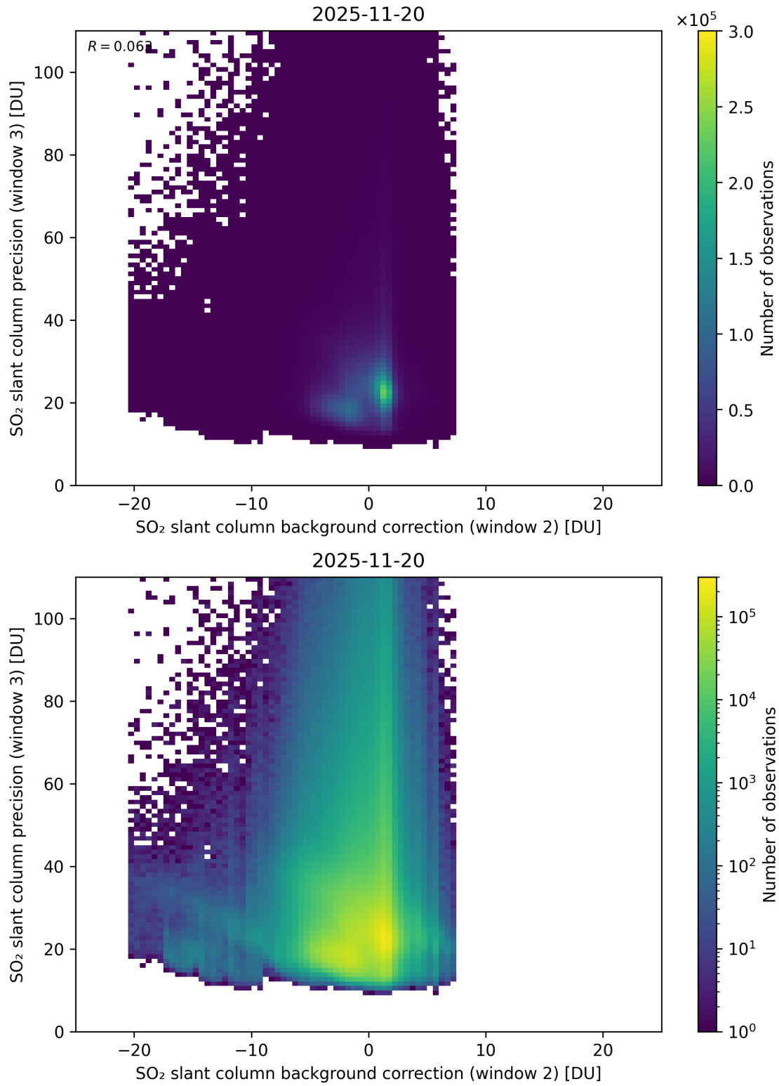
Figure 129: Scatter density plot of “SO 2 slant column background correction (window 2)” against “SO 2 slant column precision (window 3)” for 2025-11-19 to 2025-11-21.
