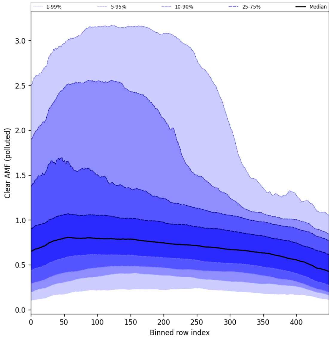
Figure 107: Along track statistics of “Clear AMF (polluted)” for 2025-11-19 to 2025-11-21
