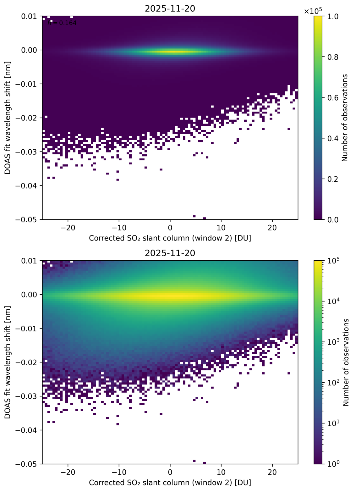
Figure 246: Scatter density plot of “Corrected SO 2 slant column (window 2)” against “DOAS fit wavelength shift” for 2025-11-19 to 2025-11-21.
