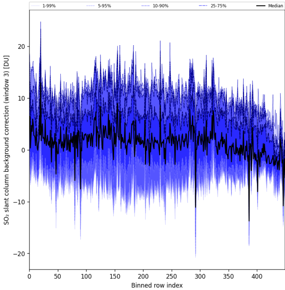
Figure 100: Along track statistics of "SO 2 slant column background correction (window 3)" for 2025-11-19 to 2025-11-21
