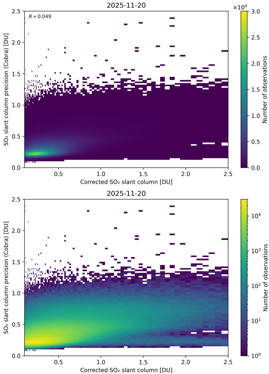
Figure 234: Scatter density plot of “Corrected SO 2 slant column” against “SO 2 slant column precision (Cobra)” for 2025-11-19 to 2025-11-21.
