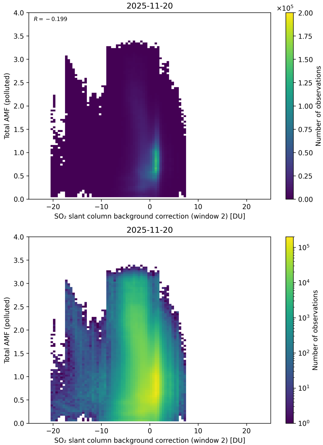
Figure 130: Scatter density plot of “SO 2 slant column background correction (window 2)” against “Total AMF (polluted)” for 2025-11-19 to 2025-11-21.
