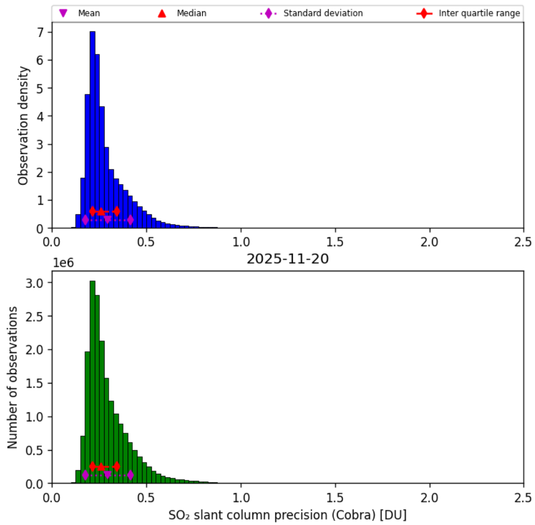
Figure 62: Histogram of “SO 2 slant column precision (Cobra)” for 2025-11-19 to 2025-11-21
