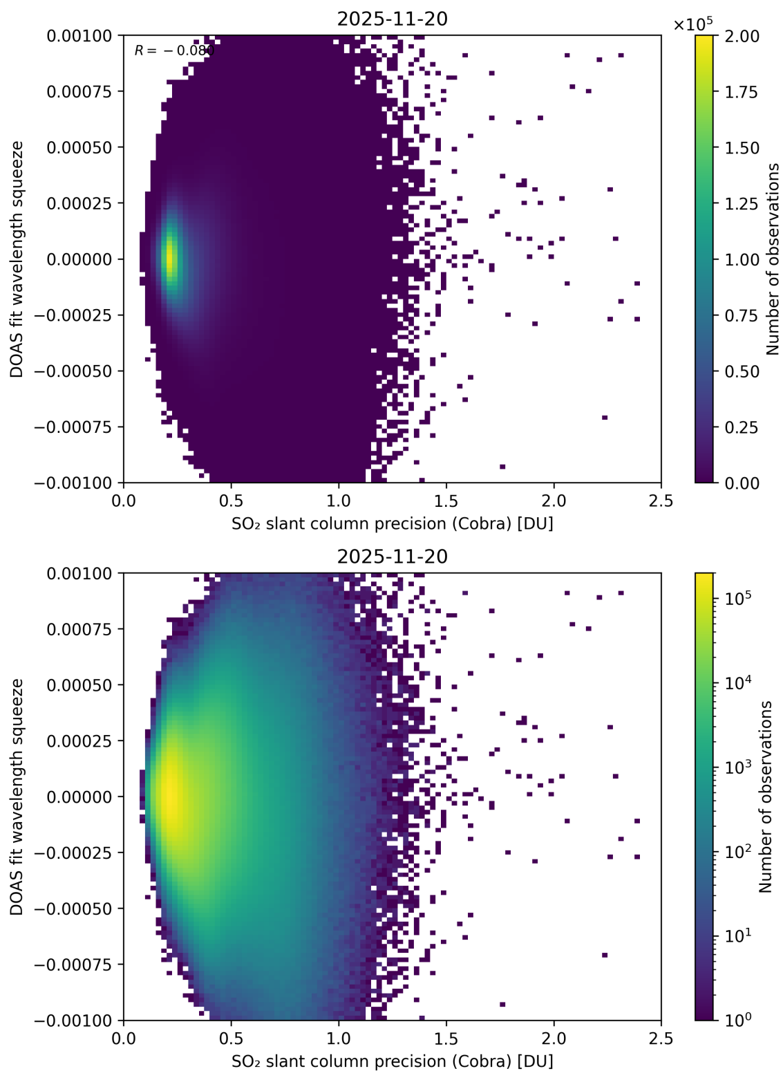
Figure 203: Scatter density plot of “SO 2 slant column precision (Cobra)” against “DOAS fit wavelength squeeze” for 2025-11-19 to 2025-11-21.
