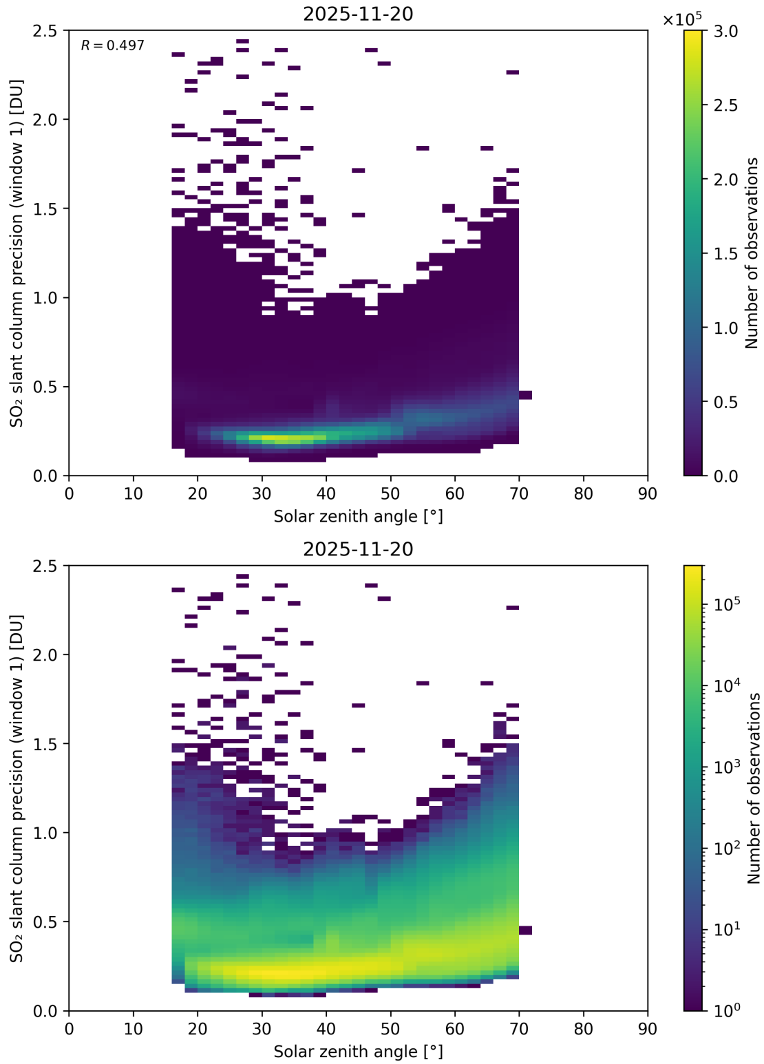
Figure 185: Scatter density plot of “Solar zenith angle” against “SO 2 slant column precision (window 1)” for 2025-11-19 to 2025-11-21.
