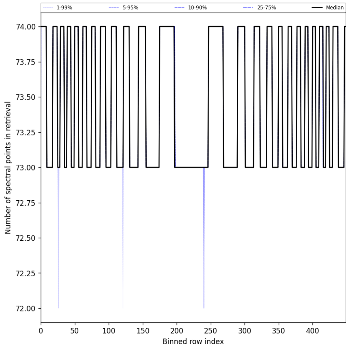
Figure 108: Along track statistics of “Number of spectral points in retrieval” for 2025-11-19 to 2025-11-21
