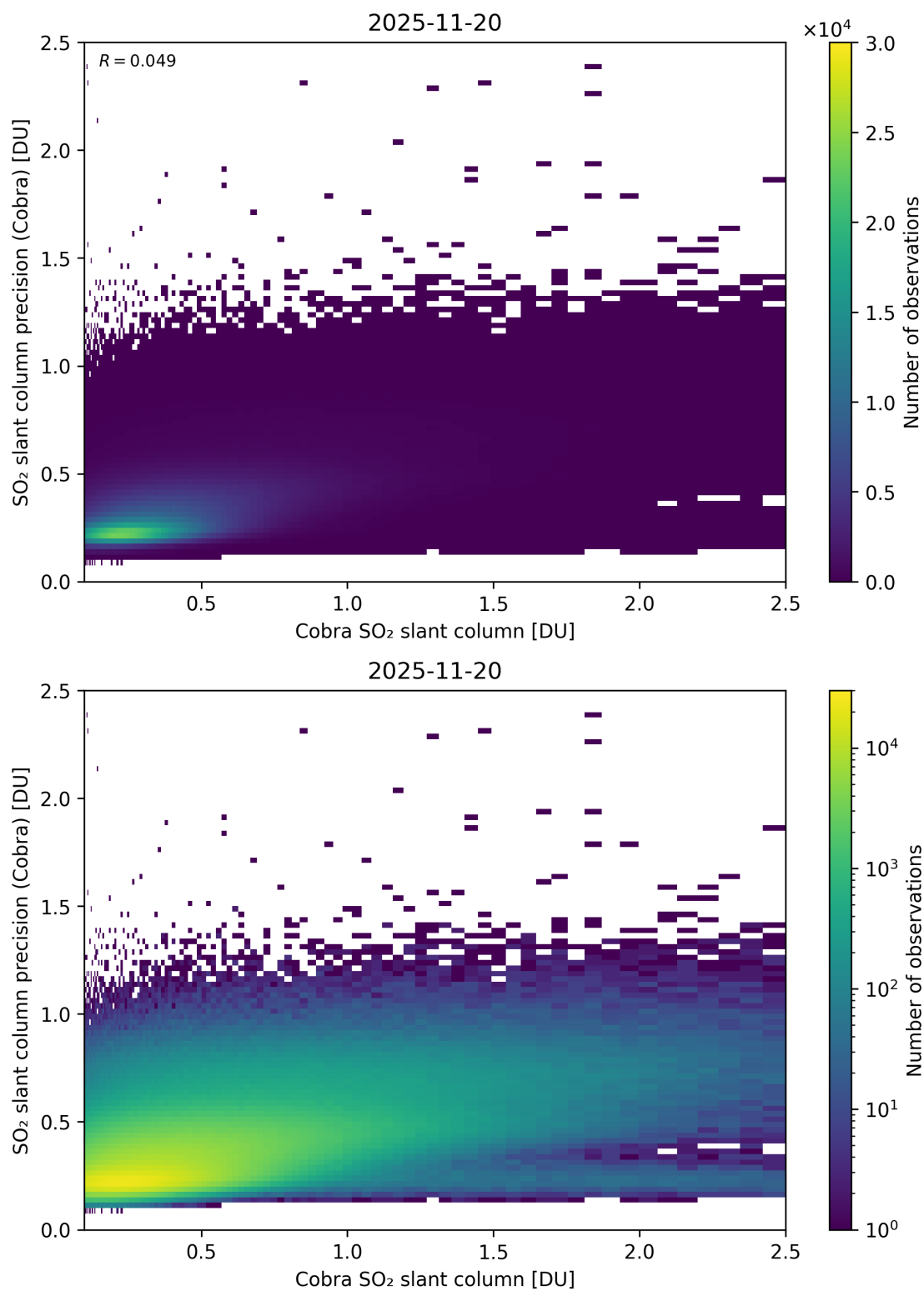
Figure 216: Scatter density plot of “Cobra SO 2 slant column” against “SO 2 slant column precision (Cobra)” for 2025-11-19 to 2025-11-21.
