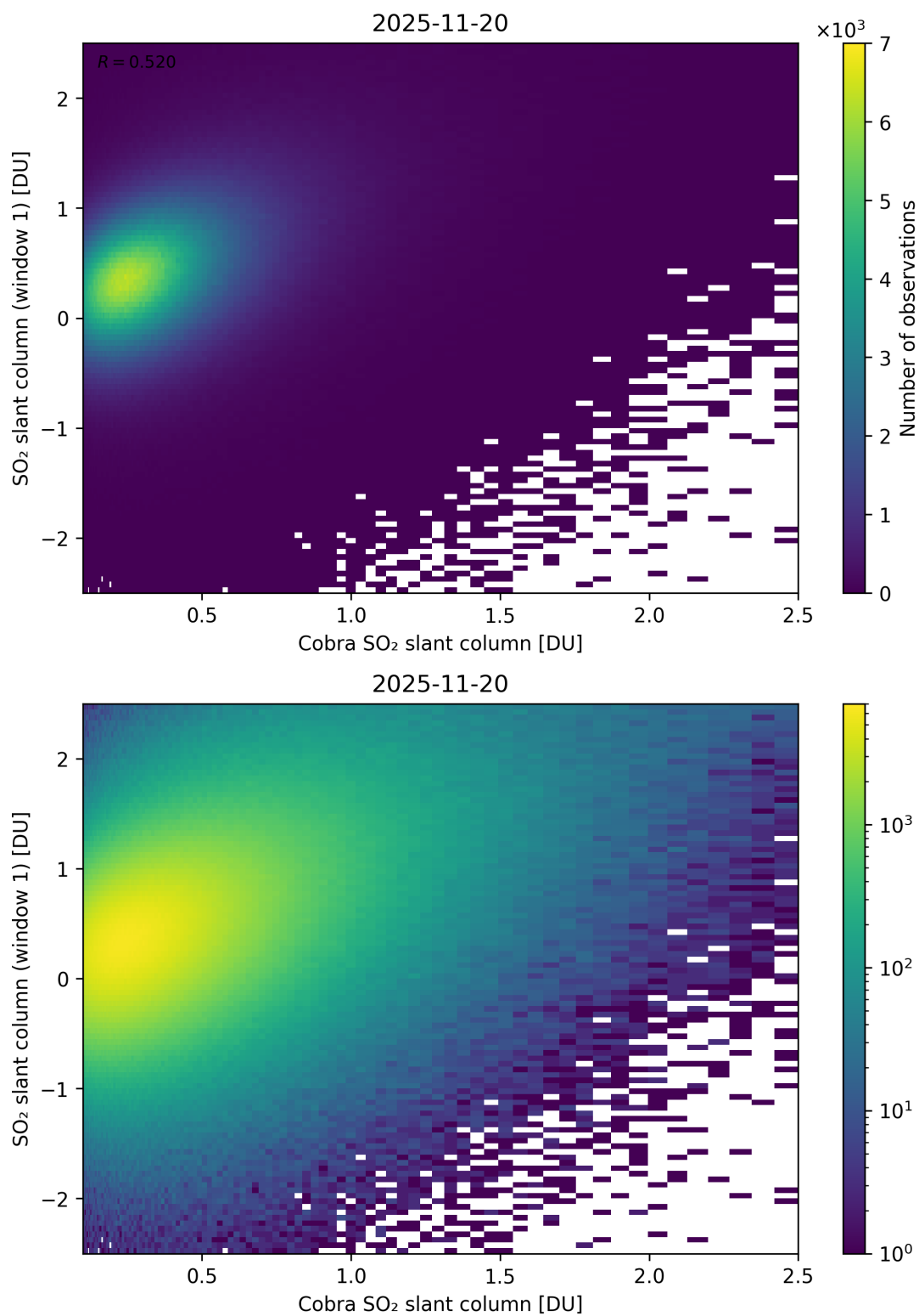
Figure 219: Scatter density plot of “Cobra SO 2 slant column” against “SO 2 slant column (window 1)” for 2025-11-19 to 2025-11-21.
