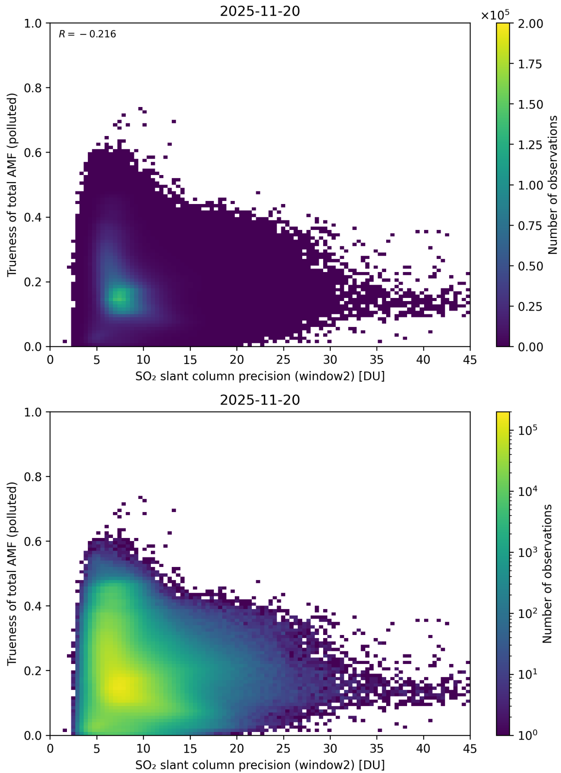
Figure 302: Scatter density plot of “SO 2 slant column precision (window2)” against “Trueness of total AMF (polluted)” for 2025-11-19 to 2025-11-21.
