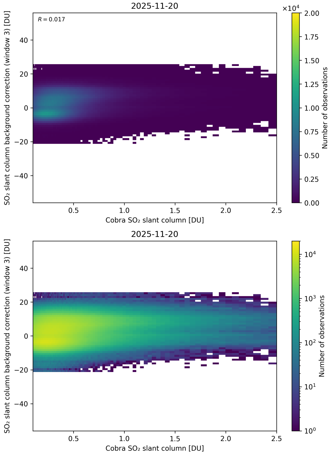
Figure 195: Scatter density plot of “Cobra SO 2 slant column” against “SO 2 slant column background correction (window 3)” for 2025-11-19 to 2025-11-21.
