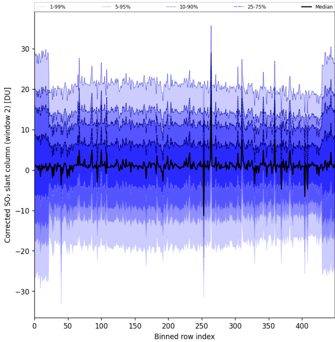
Figure 95: Along track statistics of “Corrected SO 2 slant column (window 2)” for 2025-11-19 to 2025-11-21
