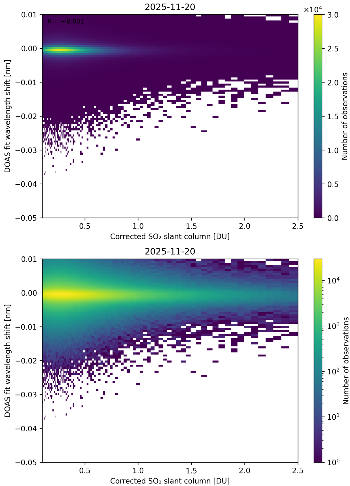
Figure 229: Scatter density plot of “Corrected SO 2 slant column” against “DOAS fit wavelength shift” for 2025-11-19 to 2025-11-21.
