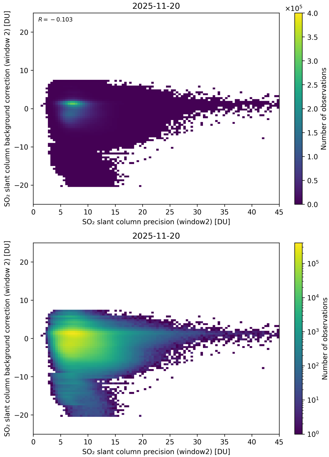
Figure 291: Scatter density plot of “SO 2 slant column precision (window2)” against “SO 2 slant column background correction (window 2)” for 2025-11-19 to 2025-11-21.
