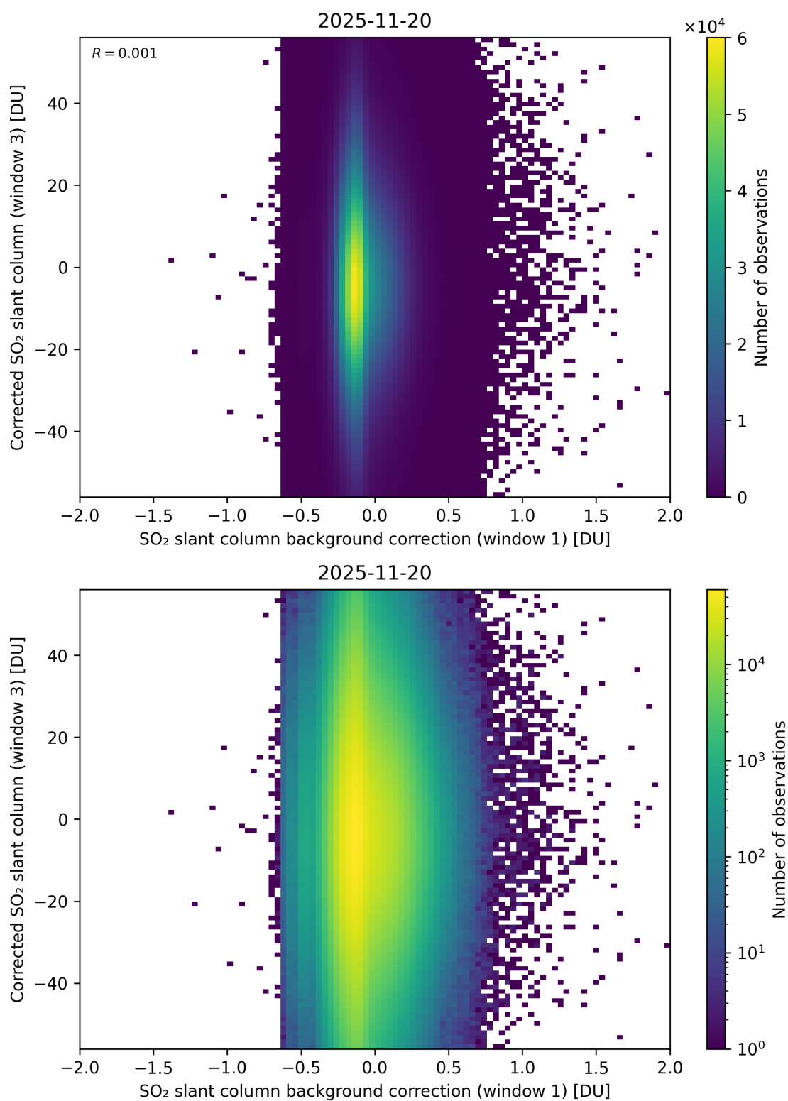
Figure 116: Scatter density plot of “SO 2 slant column background correction (window 1)” against “Corrected SO 2 slant column (window 3)” for 2025-11-19 to 2025-11-21.
