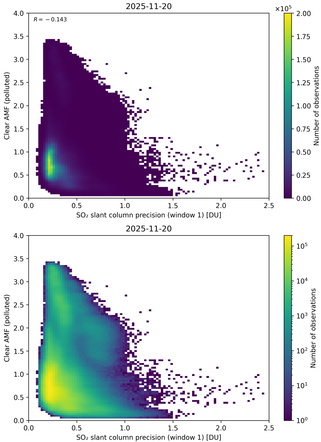
Figure 274: Scatter density plot of “SO 2 slant column precision (window 1)” against “Clear AMF (polluted)” for 2025-11-19 to 2025-11-21.
