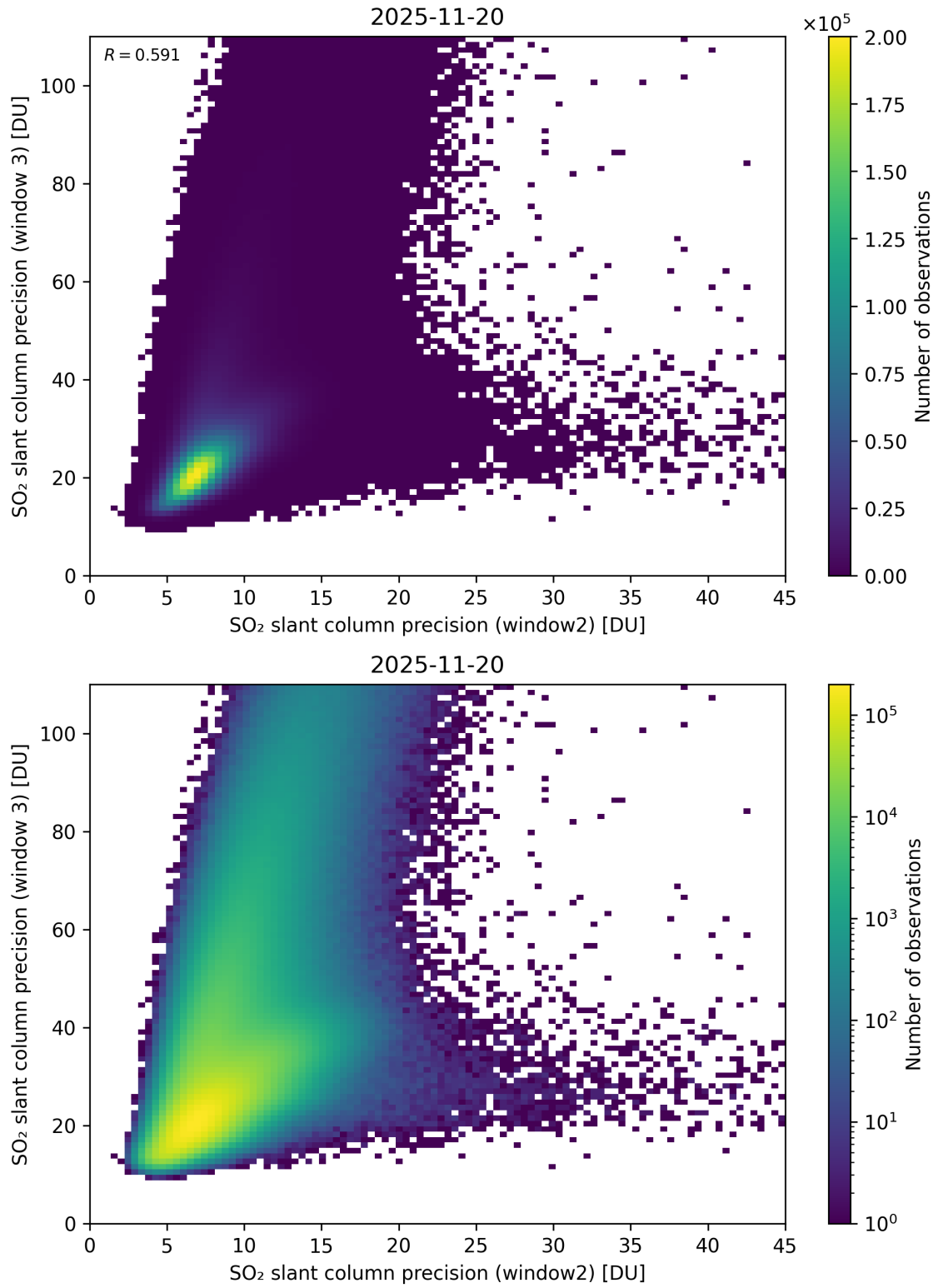
Figure 300: Scatter density plot of “SO 2 slant column precision (window2)” against “SO 2 slant column precision (window 3)” for 2025-11-19 to 2025-11-21.
