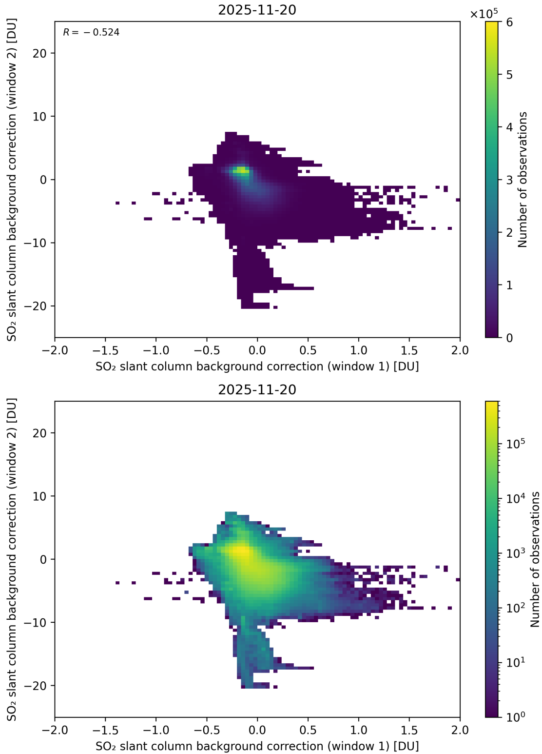
Figure 109: Scatter density plot of “SO 2 slant column background correction (window 1)” against “SO 2 slant column background correction (window 2)” for 2025-11-19 to 2025-11-21.
