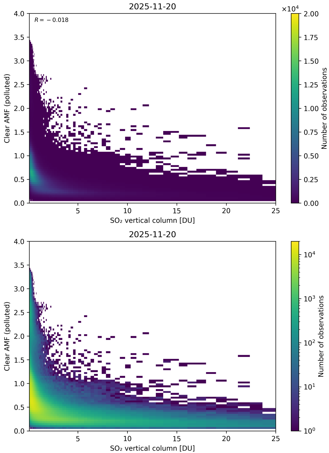
Figure 348: Scatter density plot of “SO 2 vertical column” against “Clear AMF (polluted)” for 2025-11-19 to 2025-11-21.
