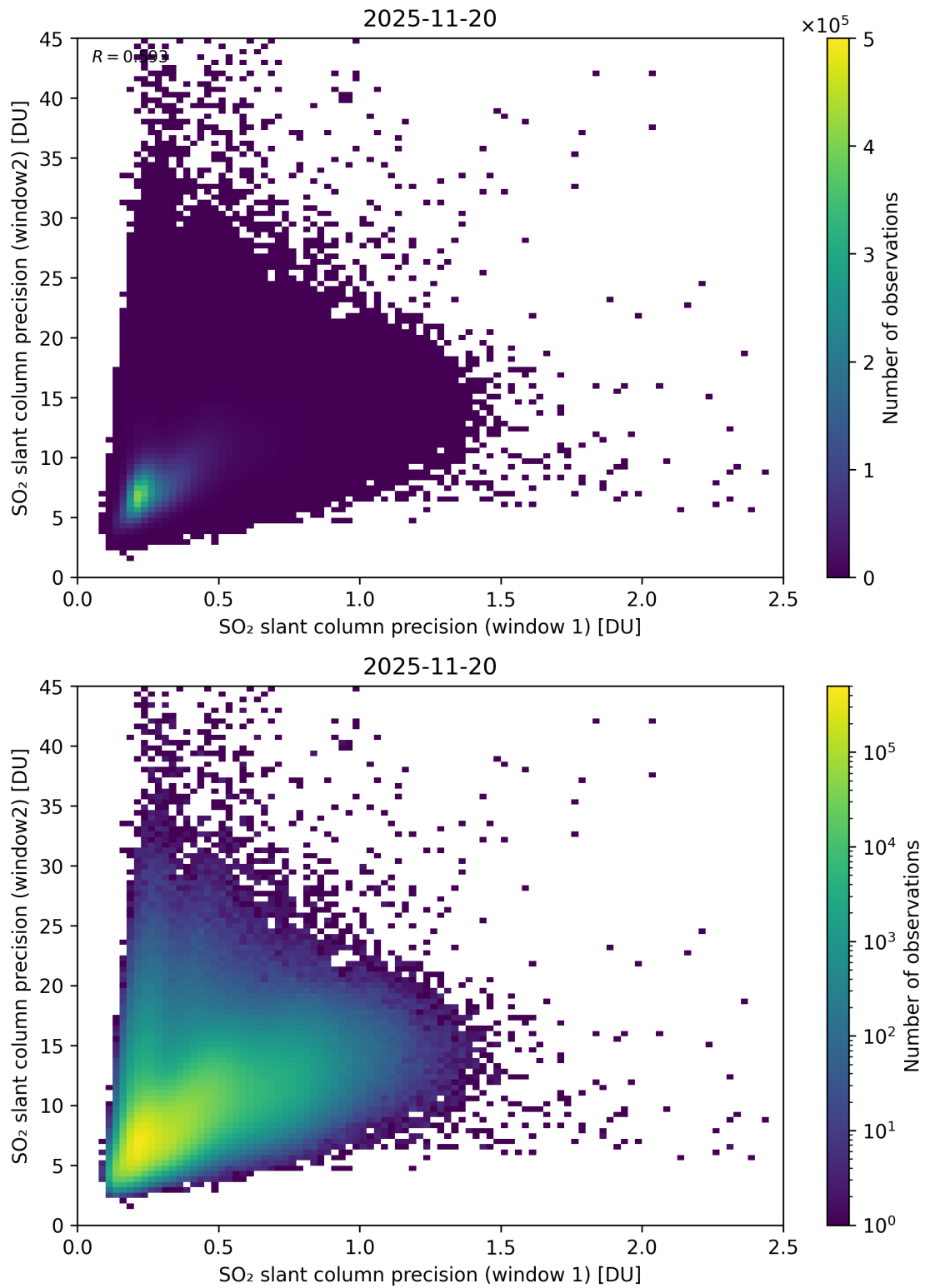
Figure 277: Scatter density plot of “SO 2 slant column precision (window 1)” against “SO 2 slant column precision (window2)” for 2025-11-19 to 2025-11-21.
