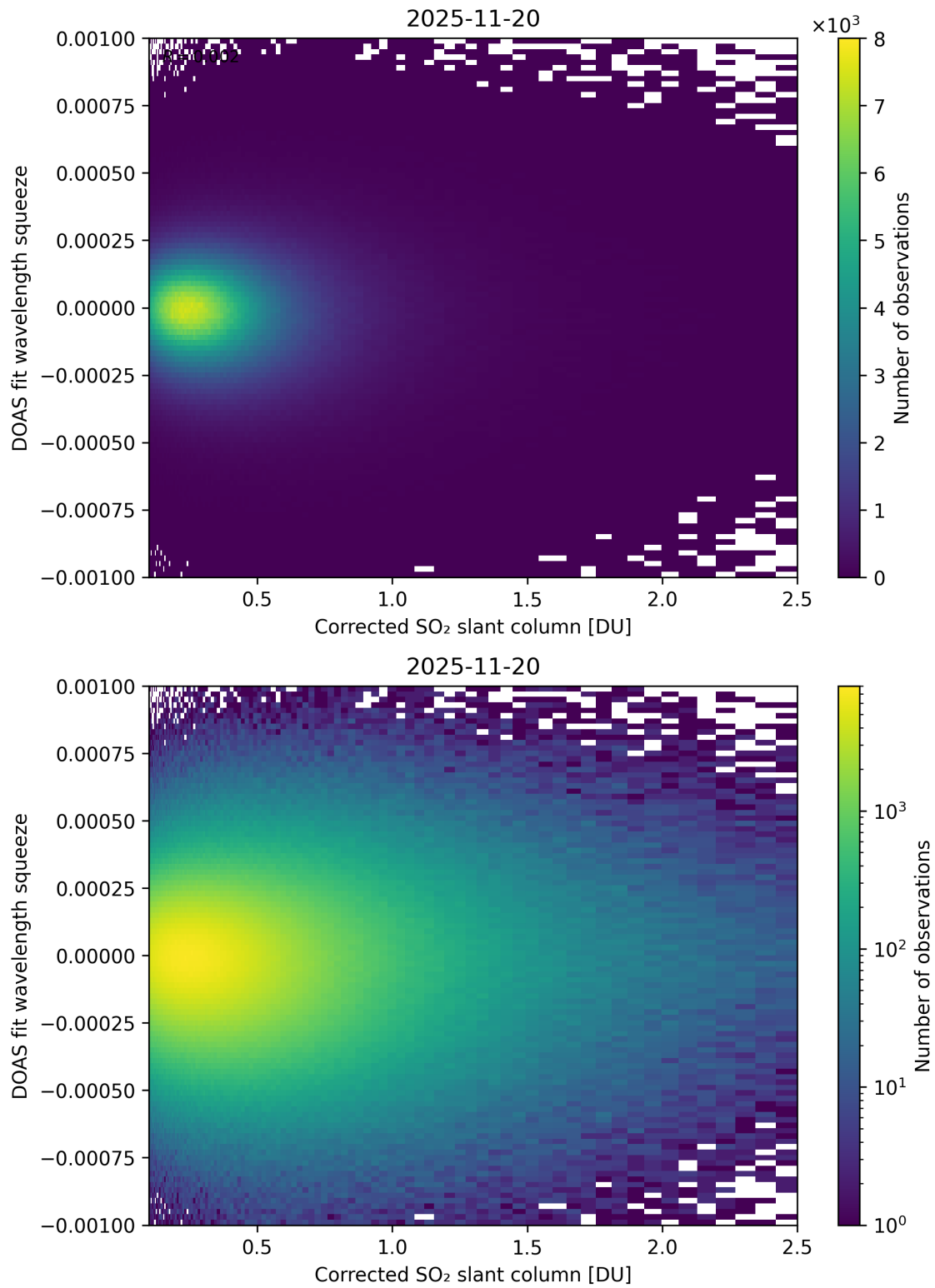
Figure 230: Scatter density plot of “Corrected SO 2 slant column” against “DOAS fit wavelength squeeze” for 2025-11-19 to 2025-11-21.
