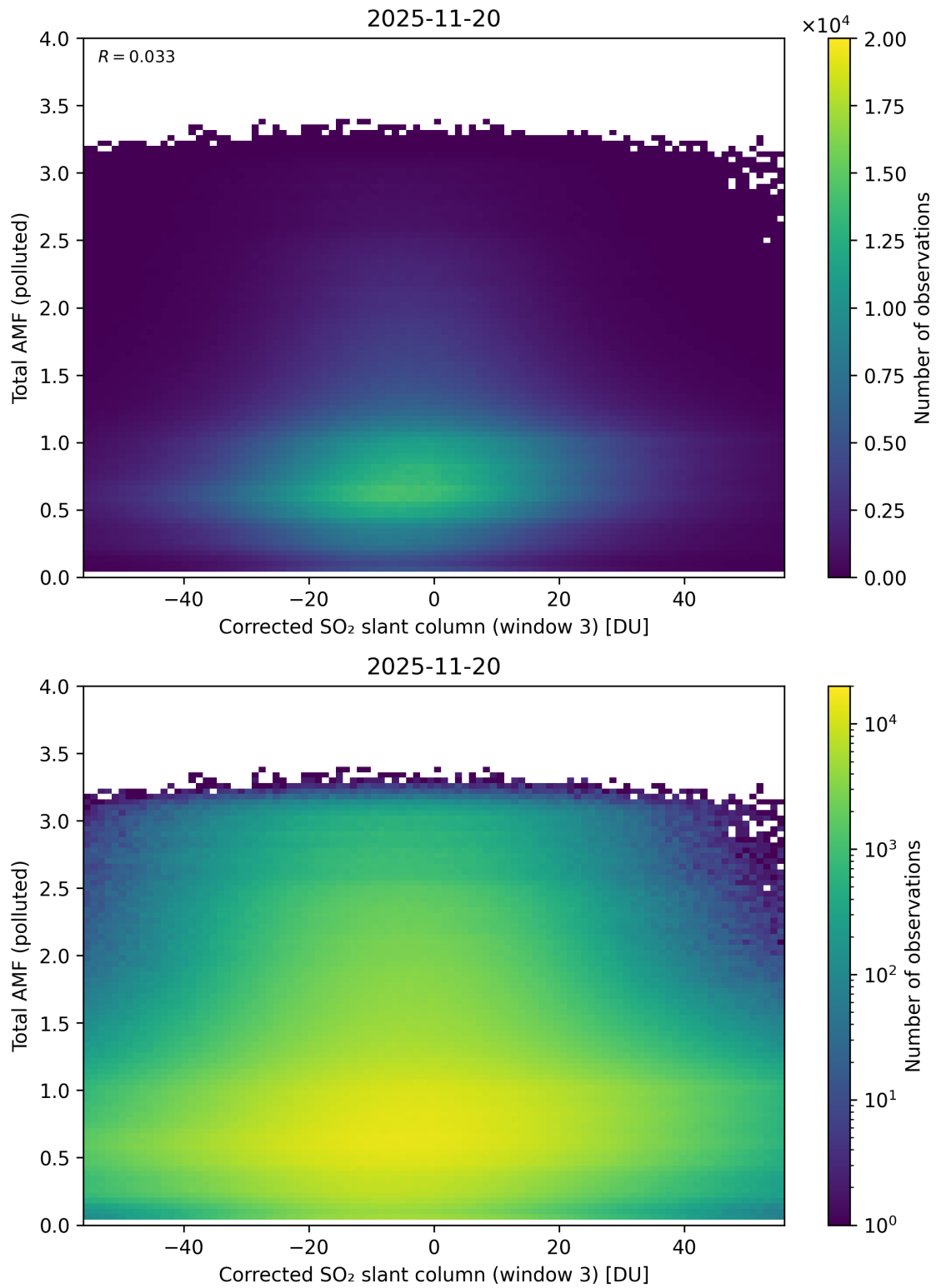
Figure 260: Scatter density plot of “Corrected SO 2 slant column (window 3)” against “Total AMF (polluted)” for 2025-11-19 to 2025-11-21.
