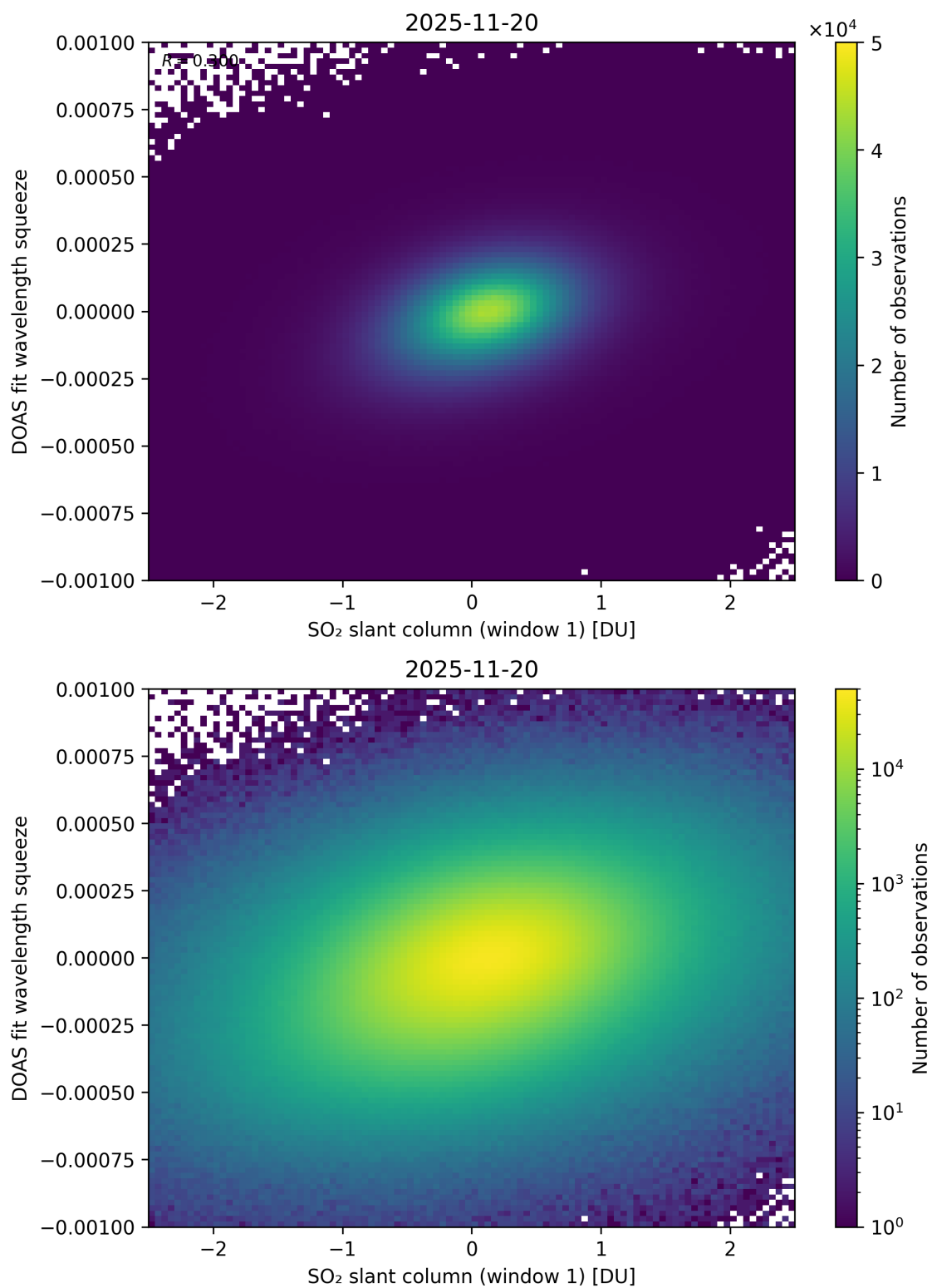
Figure 266: Scatter density plot of “SO 2 slant column (window 1)” against “DOAS fit wavelength squeeze” for 2025-11-19 to 2025-11-21.
