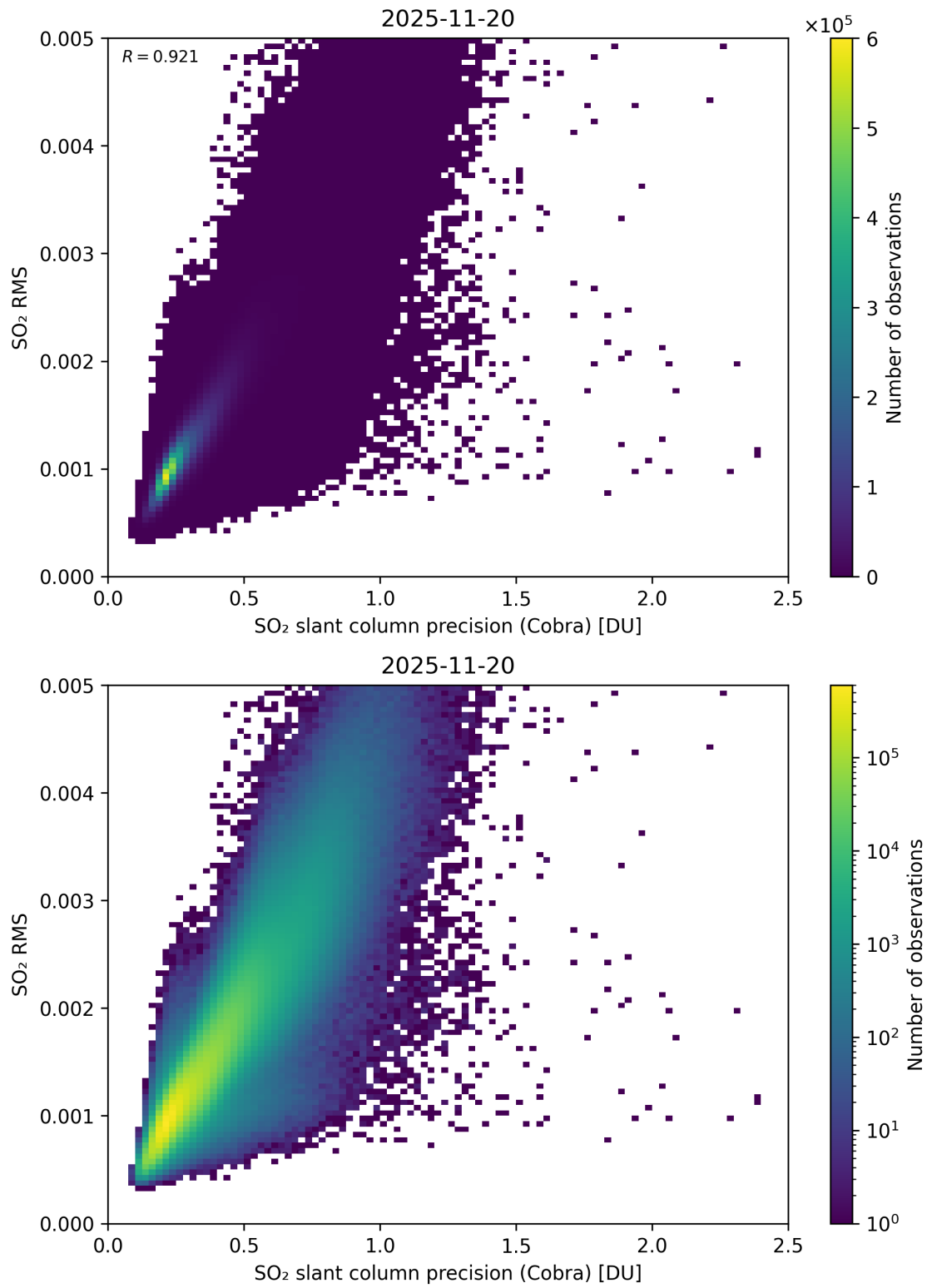
Figure 204: Scatter density plot of “SO 2 slant column precision (Cobra)” against “SO 2 RMS” for 2025-11-19 to 2025-11-21.
