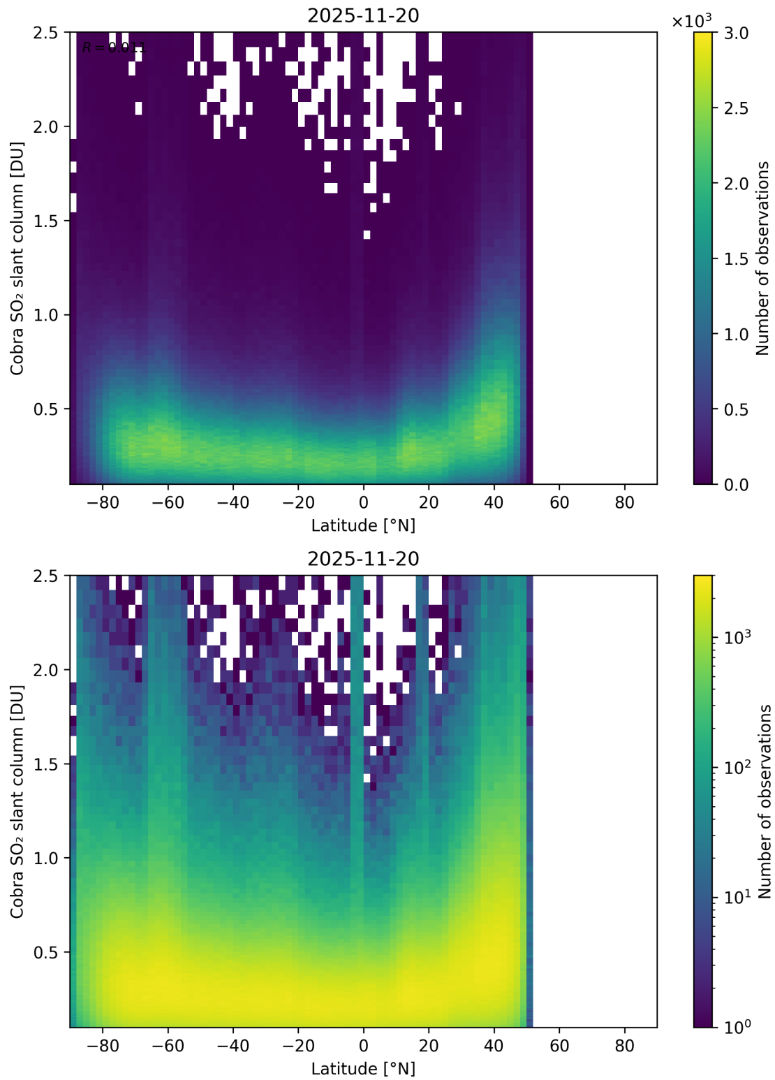
Figure 157: Scatter density plot of “Latitude” against “Cobra SO 2 slant column” for 2025-11-19 to 2025-11-21.
