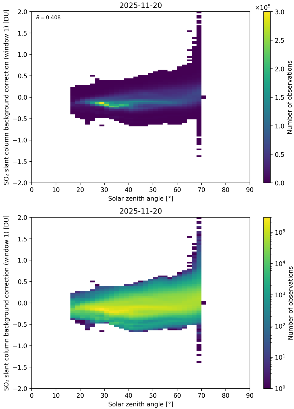
Figure 171: Scatter density plot of “Solar zenith angle” against “SO 2 slant column background correction (window 1)” for 2025-11-19 to 2025-11-21.
