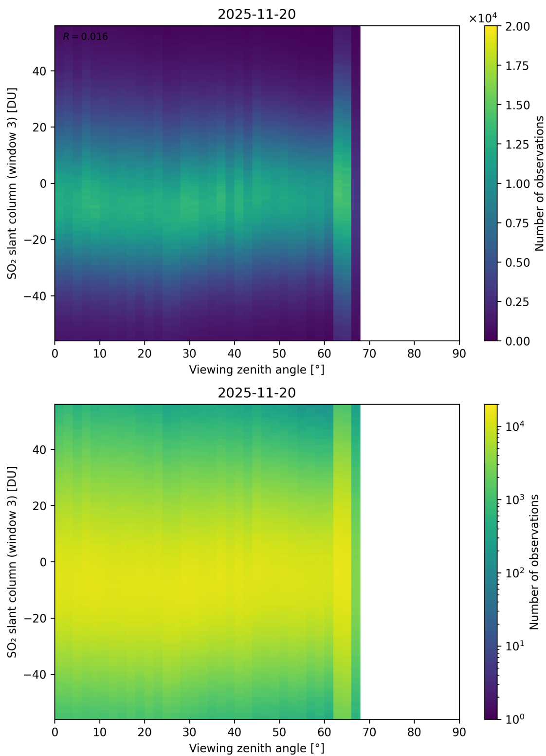
Figure 379: Scatter density plot of “Viewing zenith angle” against “SO 2 slant column (window 3)” for 2025-11-19 to 2025-11-21.
