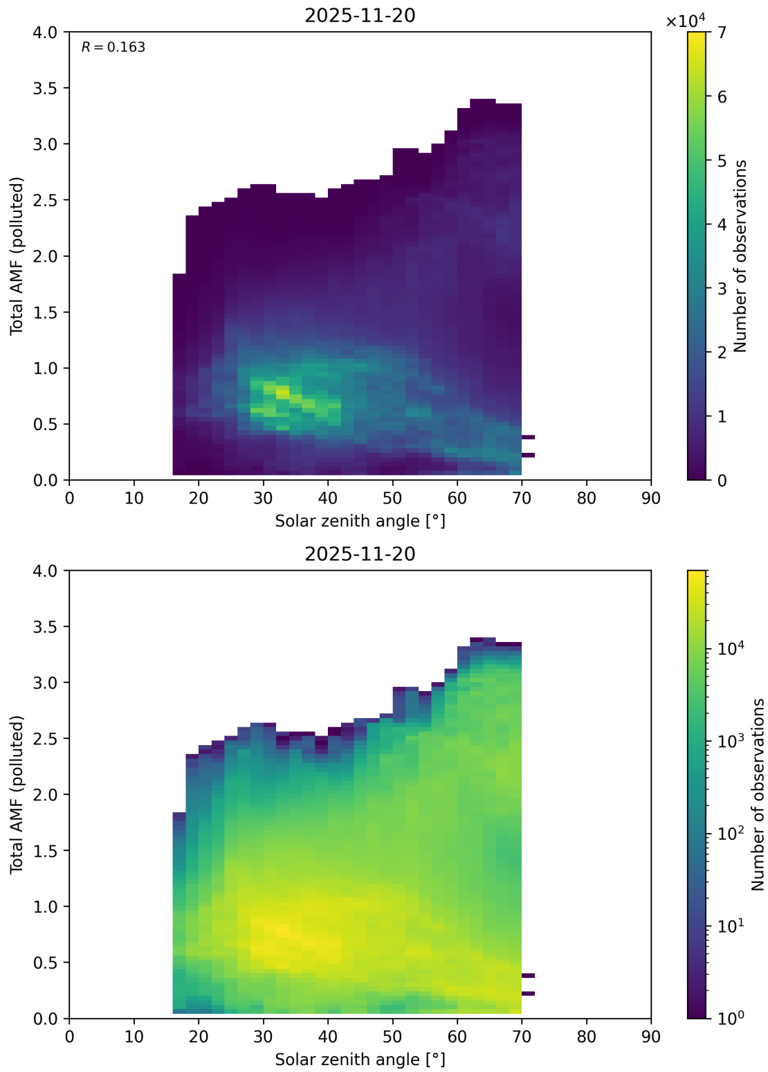
Figure 189: Scatter density plot of “Solar zenith angle” against “Total AMF (polluted)” for 2025-11-19 to 2025-11-21.
