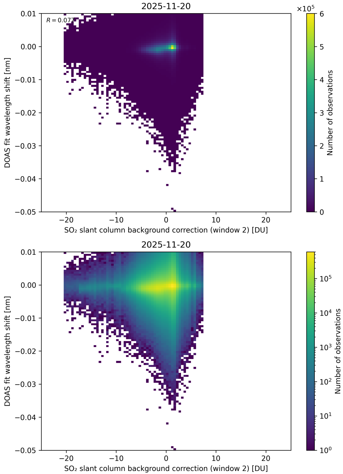
Figure 123: Scatter density plot of “SO 2 slant column background correction (window 2)” against “DOAS fit wavelength shift” for 2025-11-19 to 2025-11-21.
