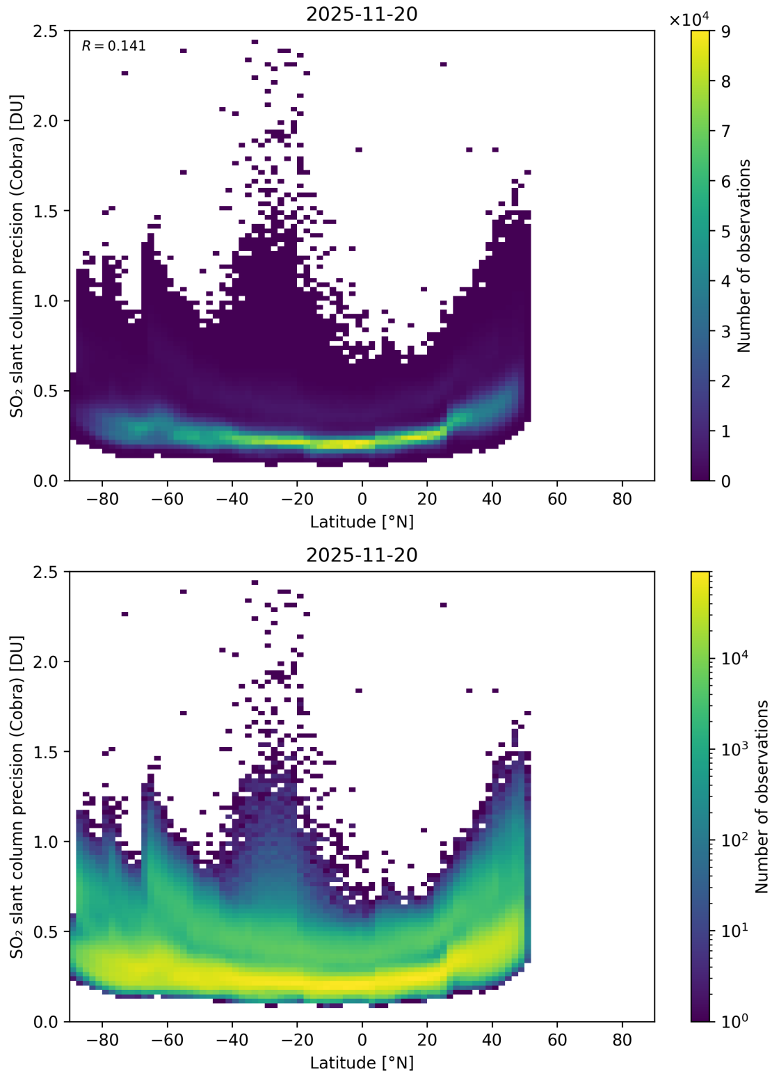
Figure 158: Scatter density plot of “Latitude” against “SO 2 slant column precision (Cobra)” for 2025-11-19 to 2025-11-21.
