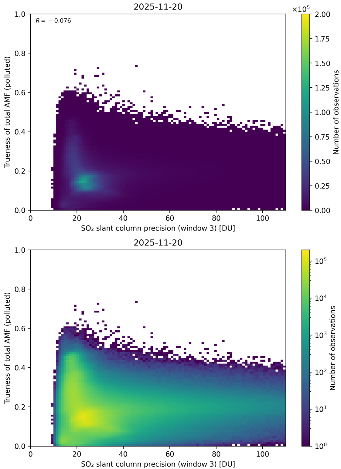
Figure 314: Scatter density plot of “SO 2 slant column precision (window 3)” against “Trueness of total AMF (polluted)” for 2025-11-19 to 2025-11-21.
