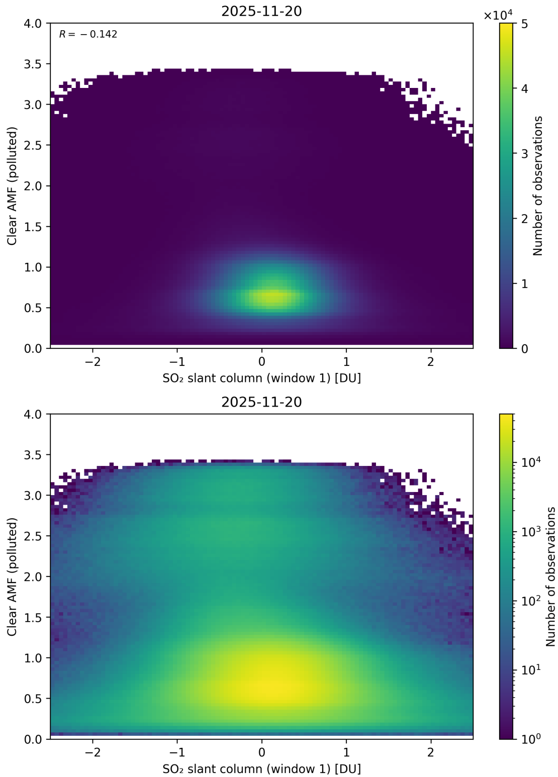
Figure 282: Scatter density plot of “SO 2 slant column (window 1)” against “Clear AMF (polluted)” for 2025-11-19 to 2025-11-21.
