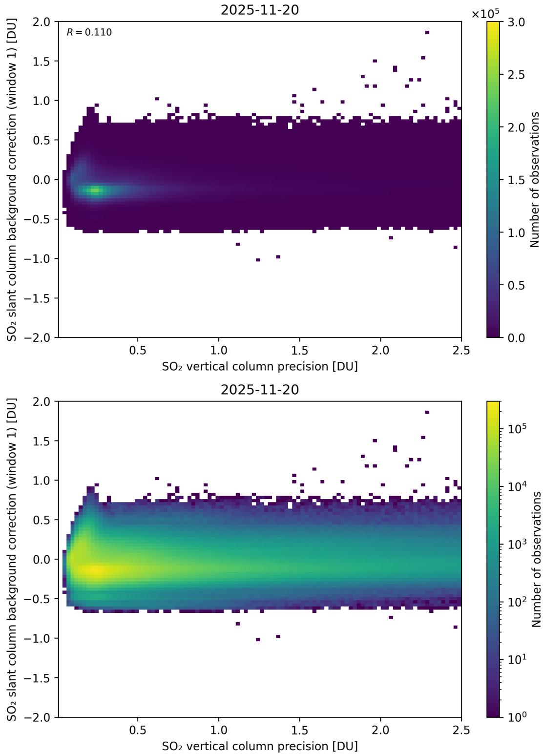
Figure 329: Scatter density plot of “SO 2 vertical column precision” against “SO 2 slant column background correction (window 1)” for 2025-11-19 to 2025-11-21.
