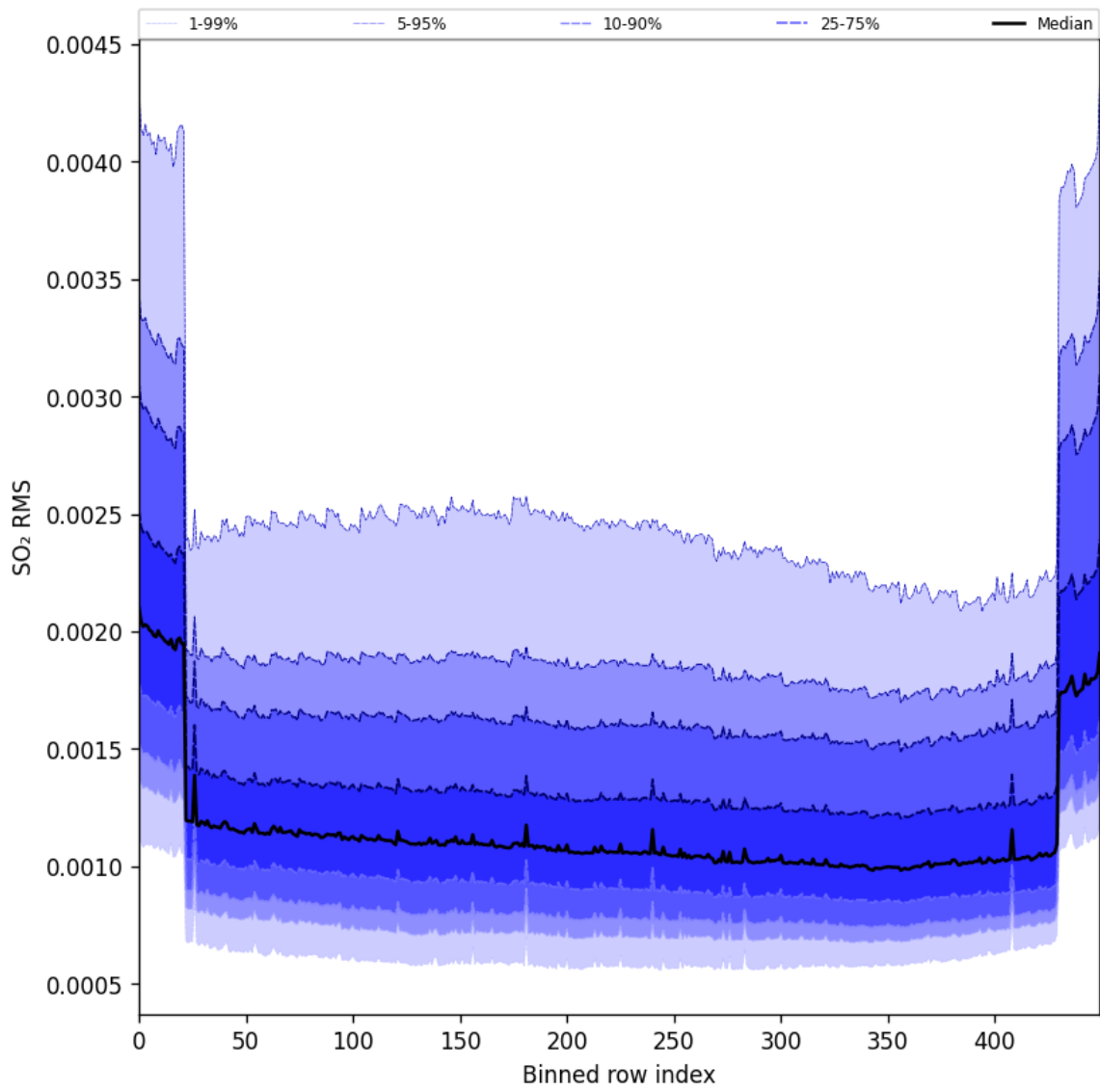
Figure 104: Along track statistics of “SO 2 RMS” for 2025-11-19 to 2025-11-21
