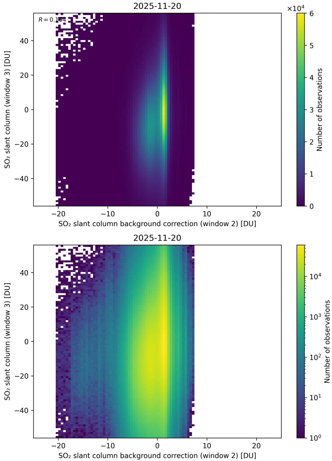
Figure 128: Scatter density plot of “SO 2 slant column background correction (window 2)” against “SO 2 slant column (window 3)” for 2025-11-19 to 2025-11-21.
