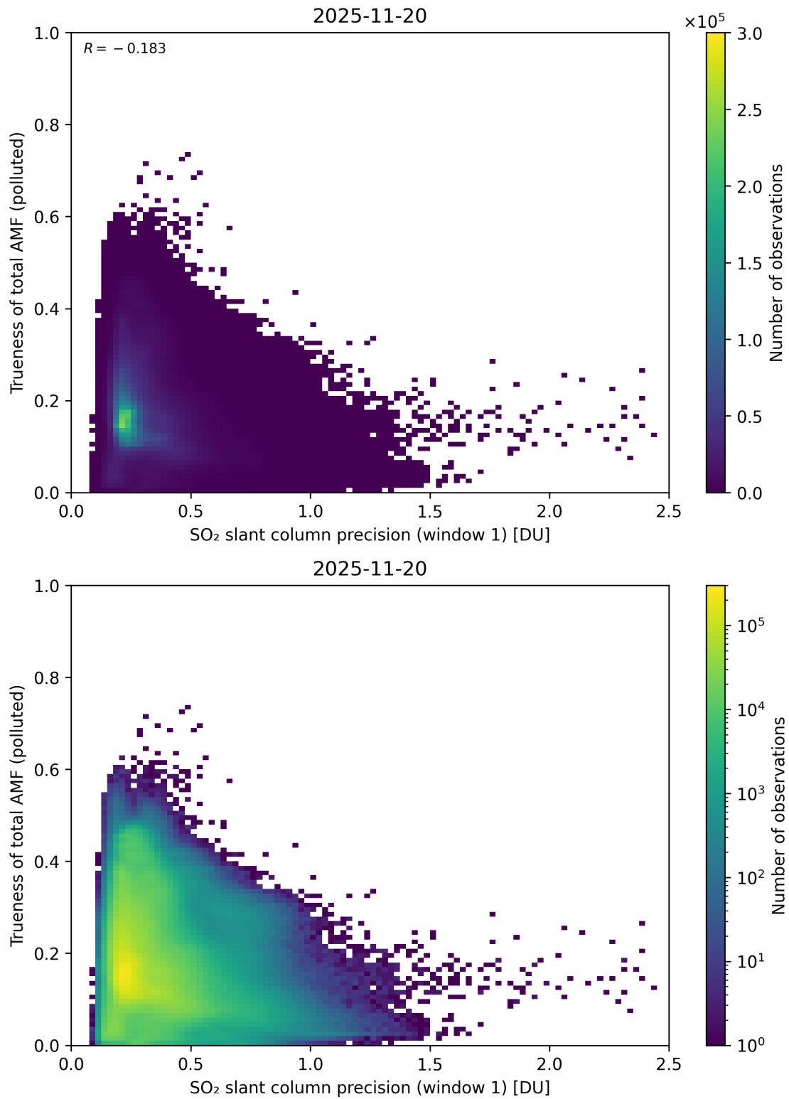
Figure 281: Scatter density plot of “SO 2 slant column precision (window 1)” against “Trueness of total AMF (polluted)” for 2025-11-19 to 2025-11-21.
