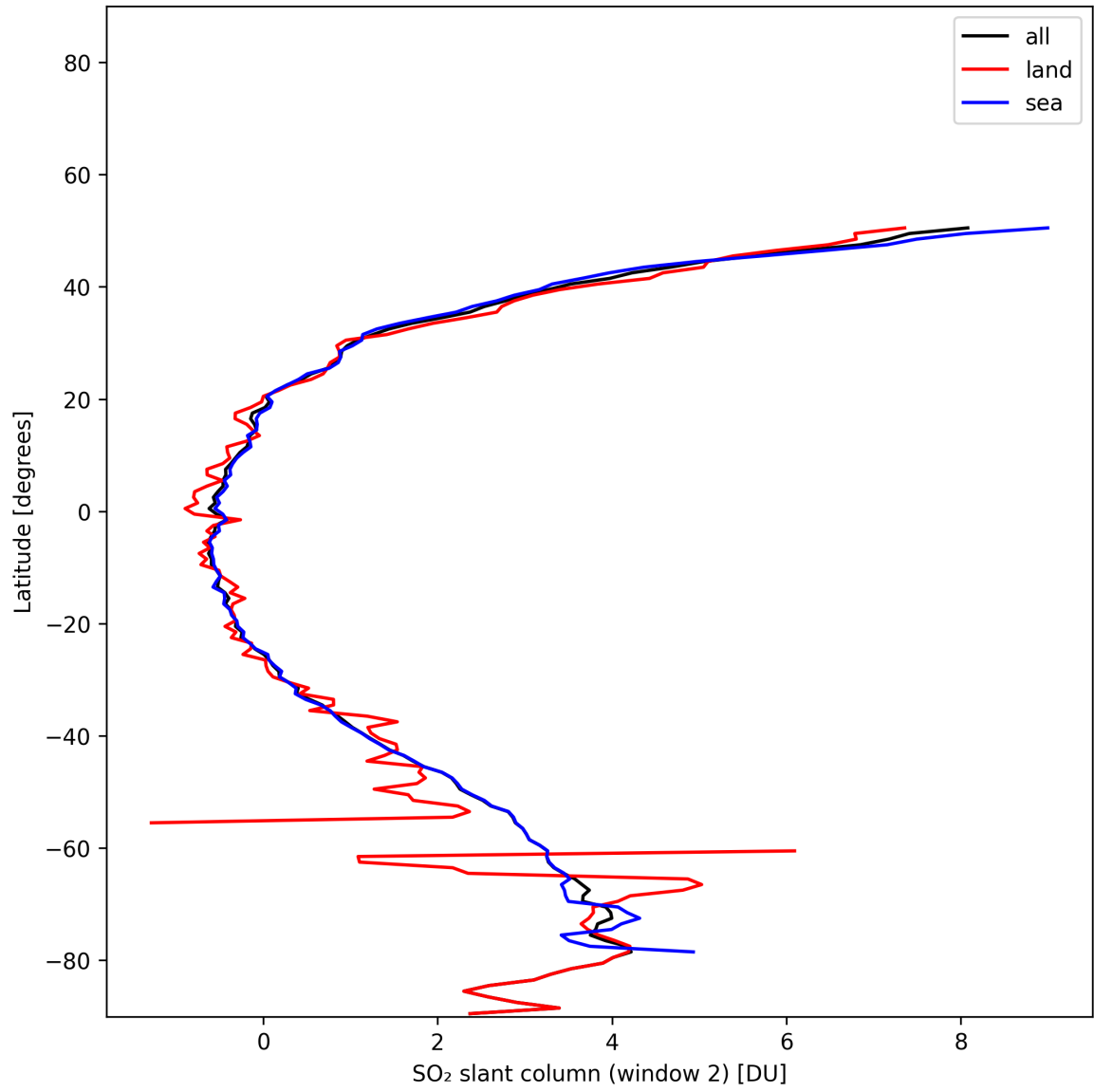
Figure 41: Zonal average of “SO 2 slant column (window 2)” for 2025-11-19 to 2025-11-21.
