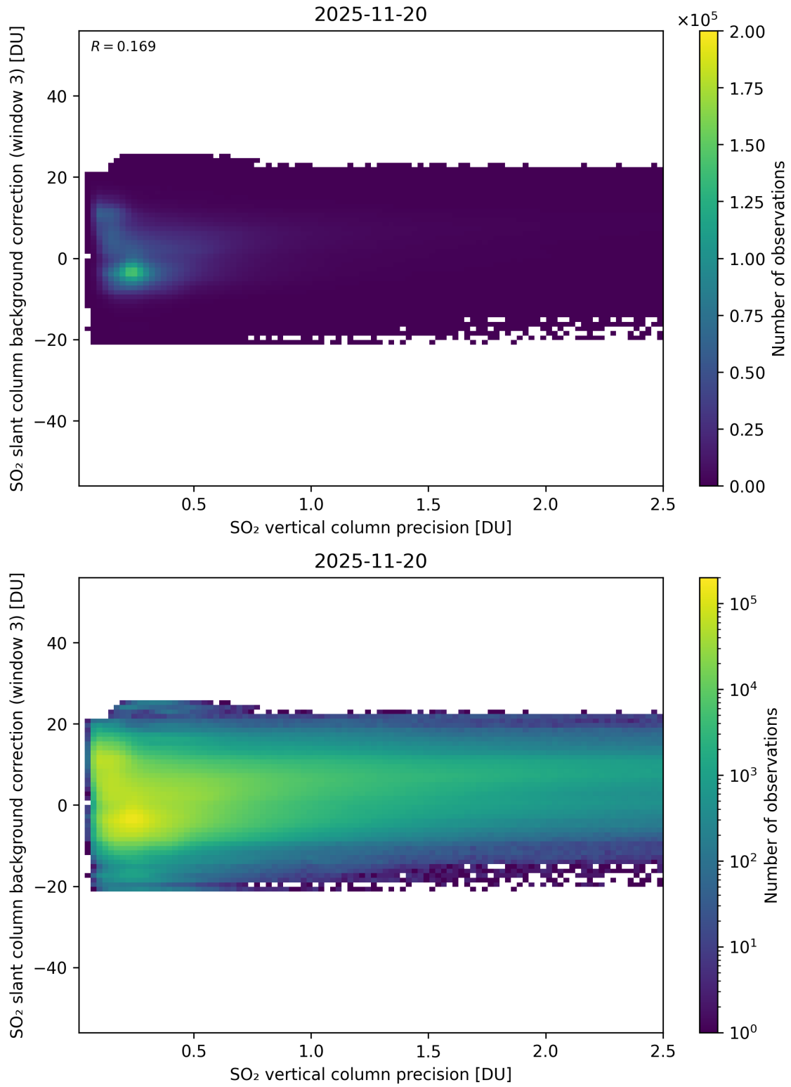
Figure 331: Scatter density plot of “SO 2 vertical column precision” against “SO 2 slant column background correction (window 3)” for 2025-11-19 to 2025-11-21.
