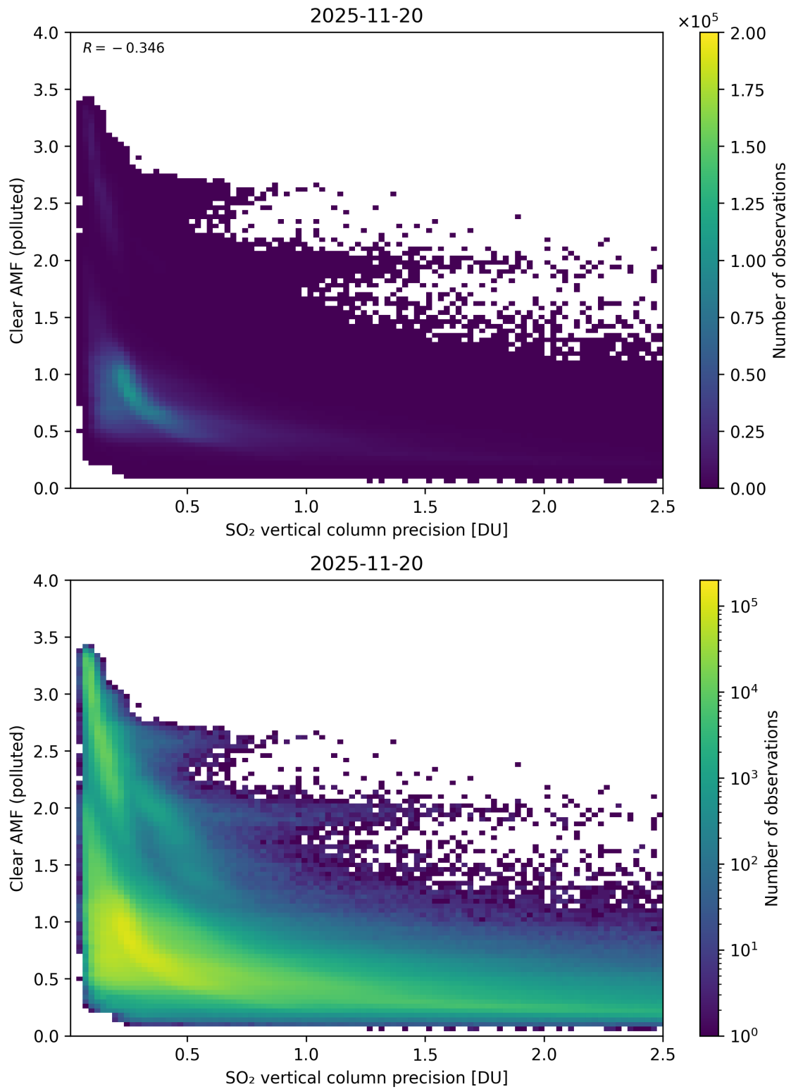
Figure 335: Scatter density plot of “SO 2 vertical column precision” against “Clear AMF (polluted)” for 2025-11-19 to 2025-11-21.
