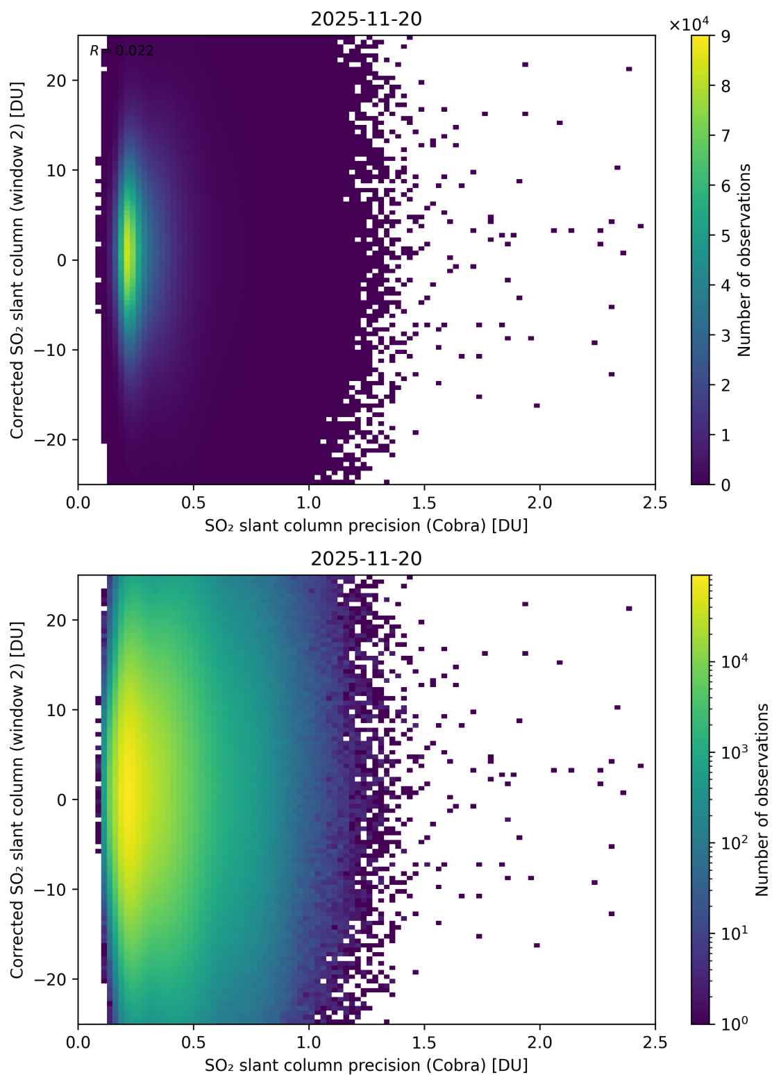
Figure 206: Scatter density plot of “SO 2 slant column precision (Cobra)” against “Corrected SO 2 slant column (window 2)” for 2025-11-19 to 2025-11-21.
