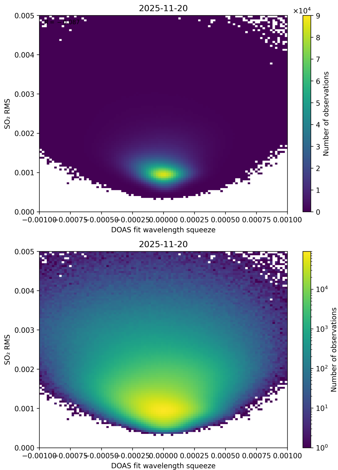
Figure 143: Scatter density plot of “DOAS fit wavelength squeeze” against “SO 2 RMS” for 2025-11-19 to 2025-11-21.
