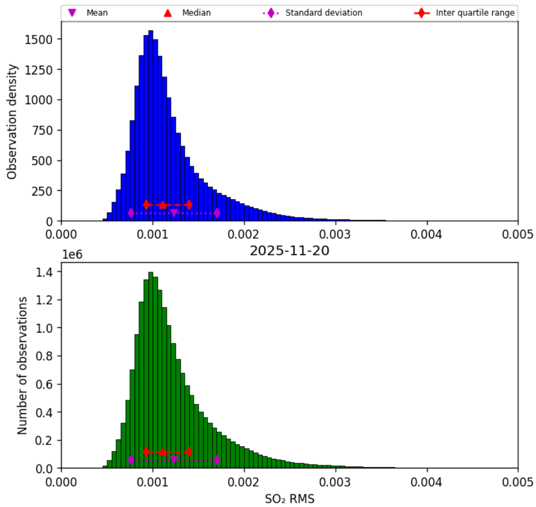
Figure 78: Histogram of “SO 2 RMS” for 2025-11-19 to 2025-11-21
