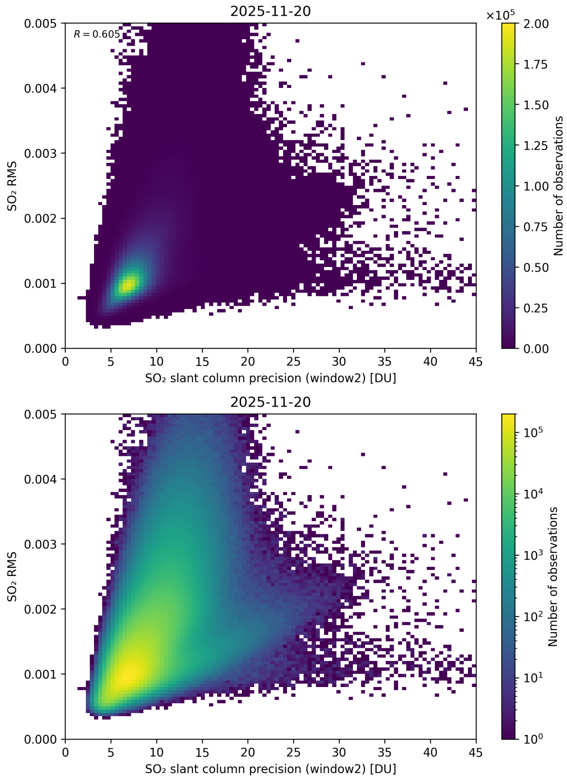
Figure 295: Scatter density plot of “SO 2 slant column precision (window2)” against “SO 2 RMS” for 2025-11-19 to 2025-11-21.
