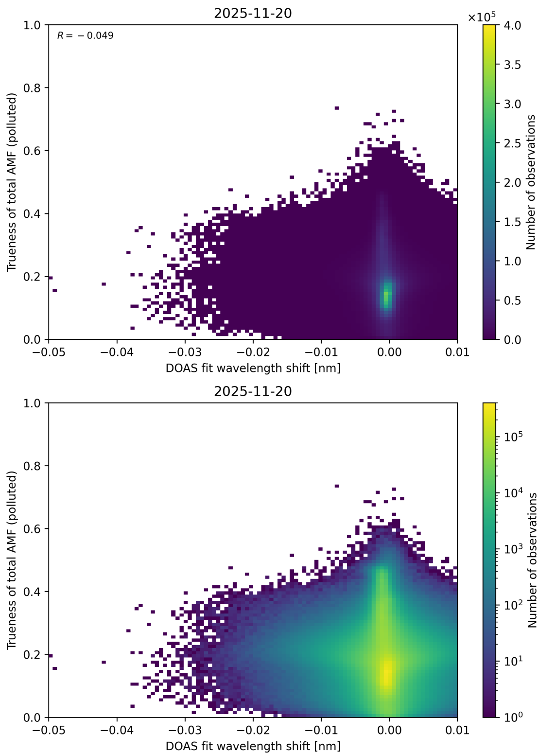
Figure 142: Scatter density plot of “DOAS fit wavelength shift” against “Trueness of total AMF (polluted)” for 2025-11-19 to 2025-11-21.
