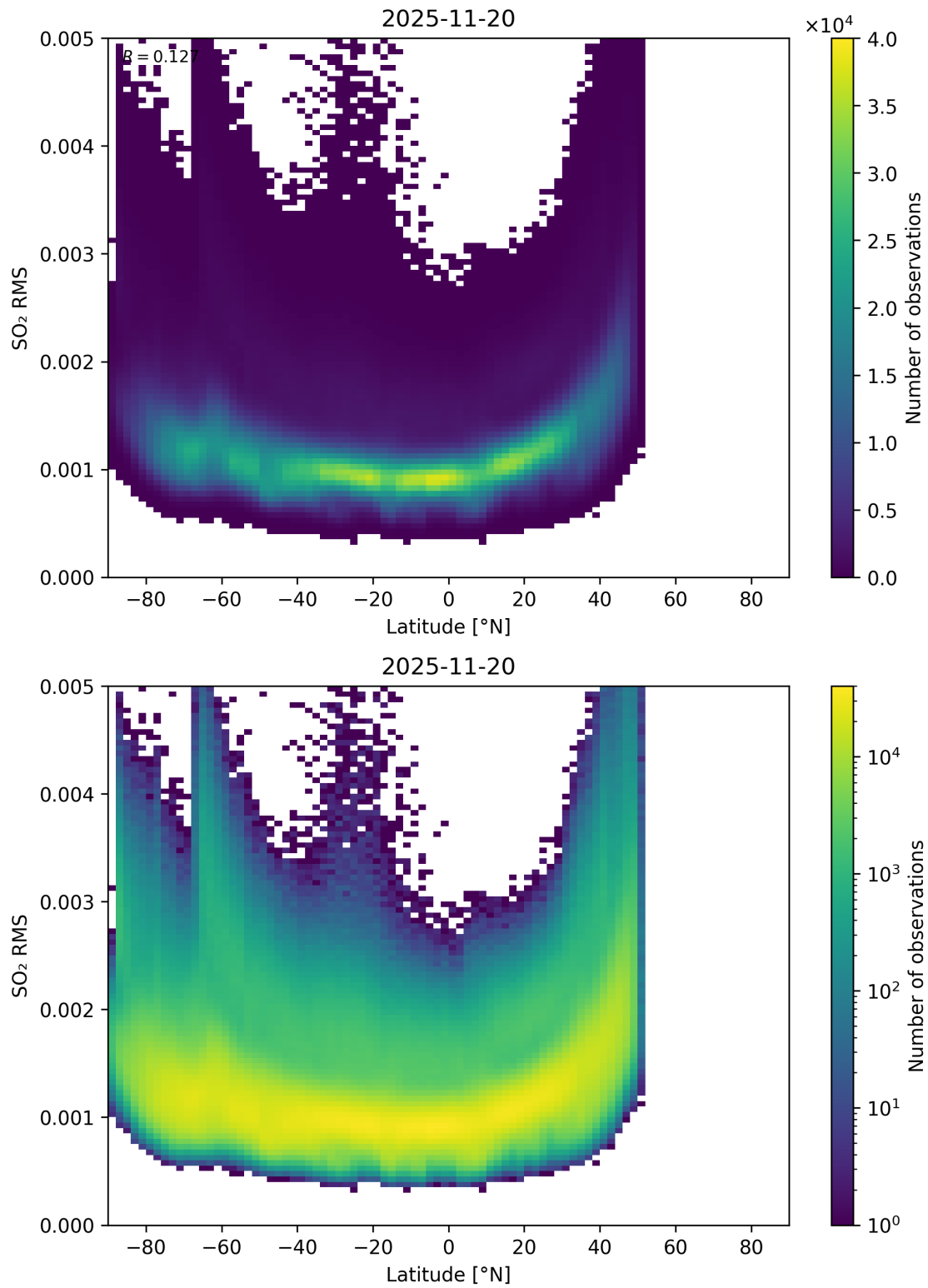
Figure 155: Scatter density plot of “Latitude” against “SO 2 RMS” for 2025-11-19 to 2025-11-21.
