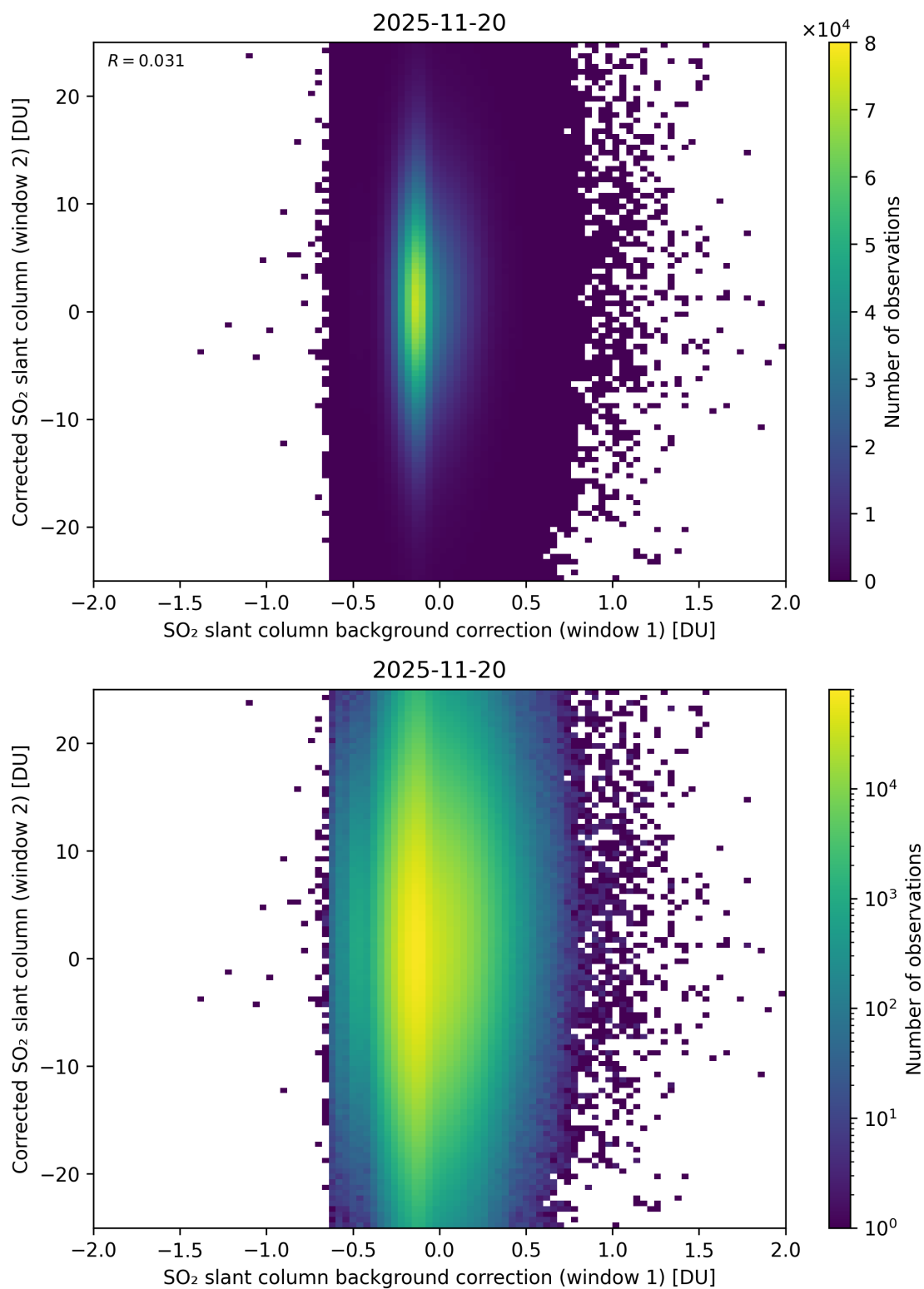
Figure 115: Scatter density plot of “SO 2 slant column background correction (window 1)” against “Corrected SO 2 slant column (window 2)” for 2025-11-19 to 2025-11-21.
