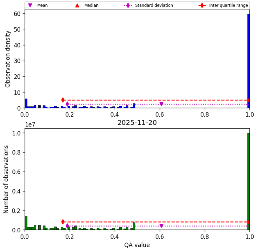
Figure 57: Histogram of “QA value” for 2025-11-19 to 2025-11-21
