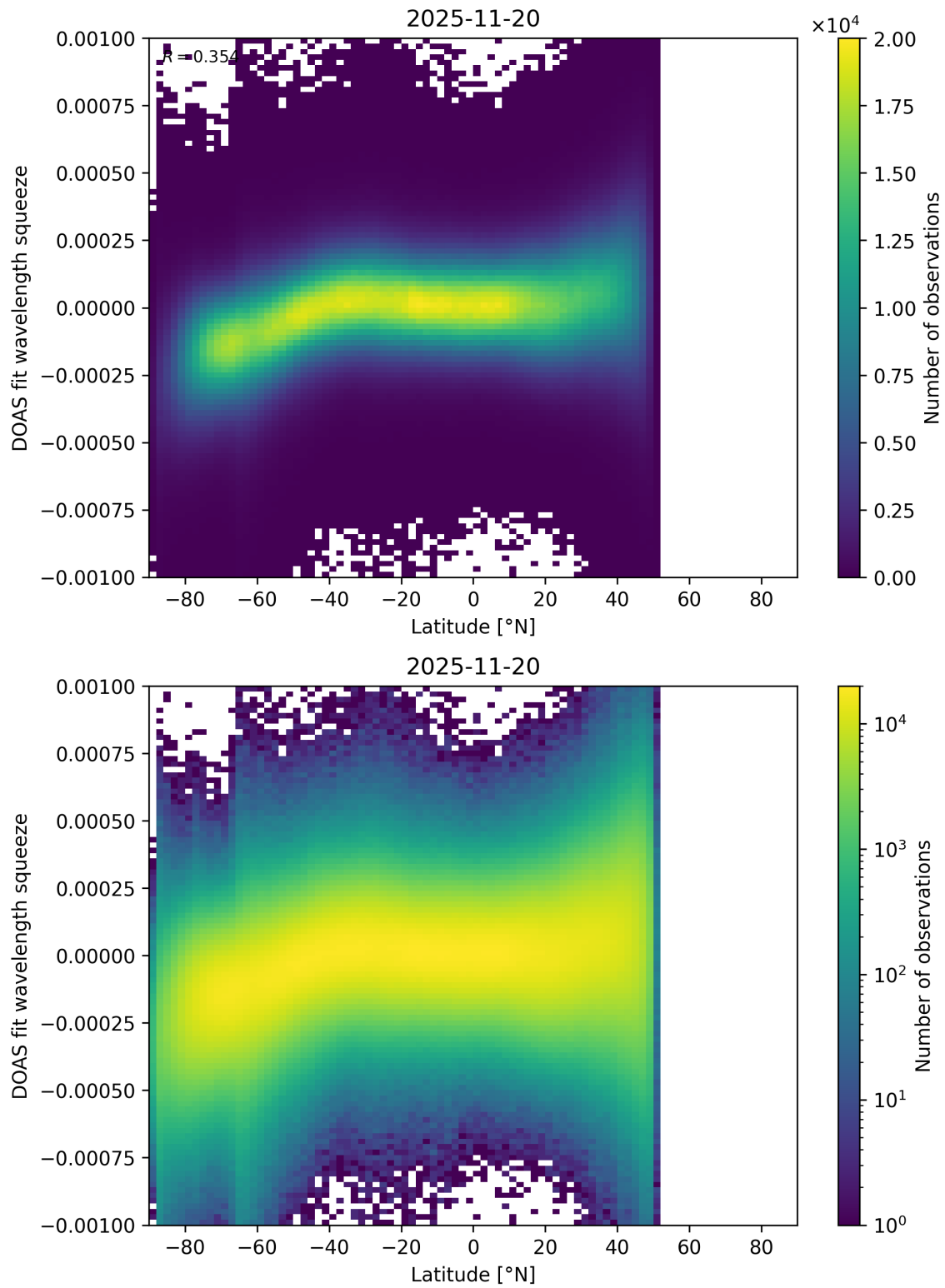
Figure 154: Scatter density plot of “Latitude” against “DOAS fit wavelength squeeze” for 2025-11-19 to 2025-11-21.
