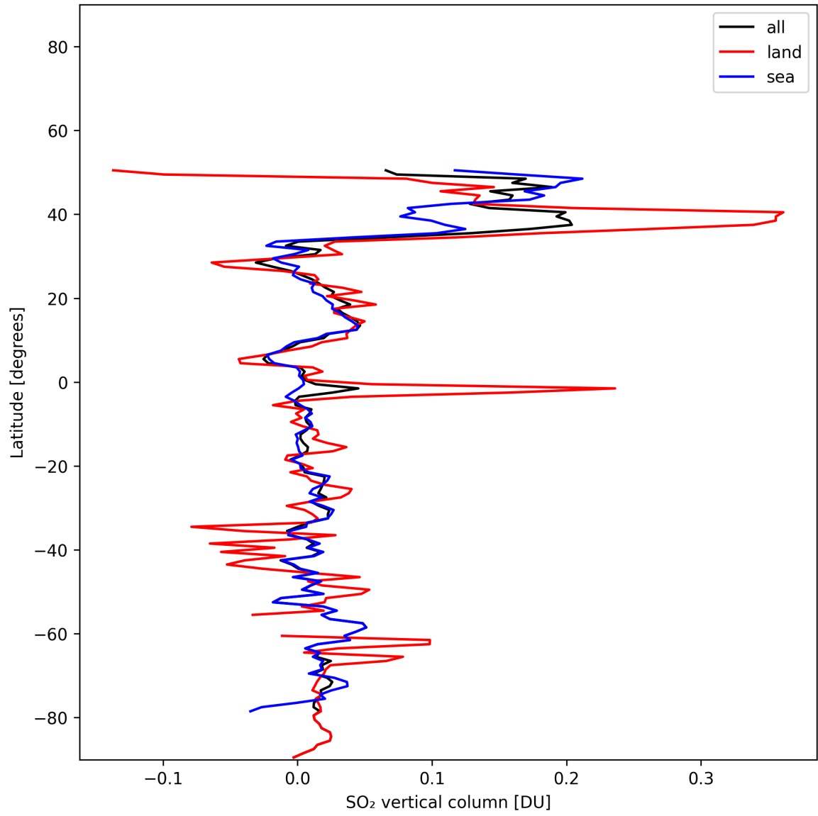
Figure 32: Zonal average of “SO 2 vertical column” for 2025-11-19 to 2025-11-21.
