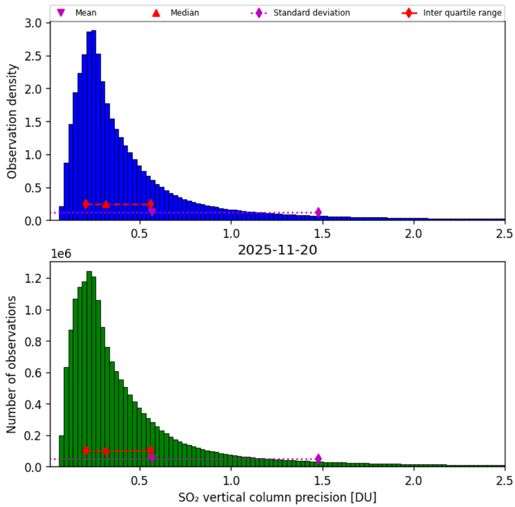
Figure 59: Histogram of “SO 2 vertical column precision” for 2025-11-19 to 2025-11-21
