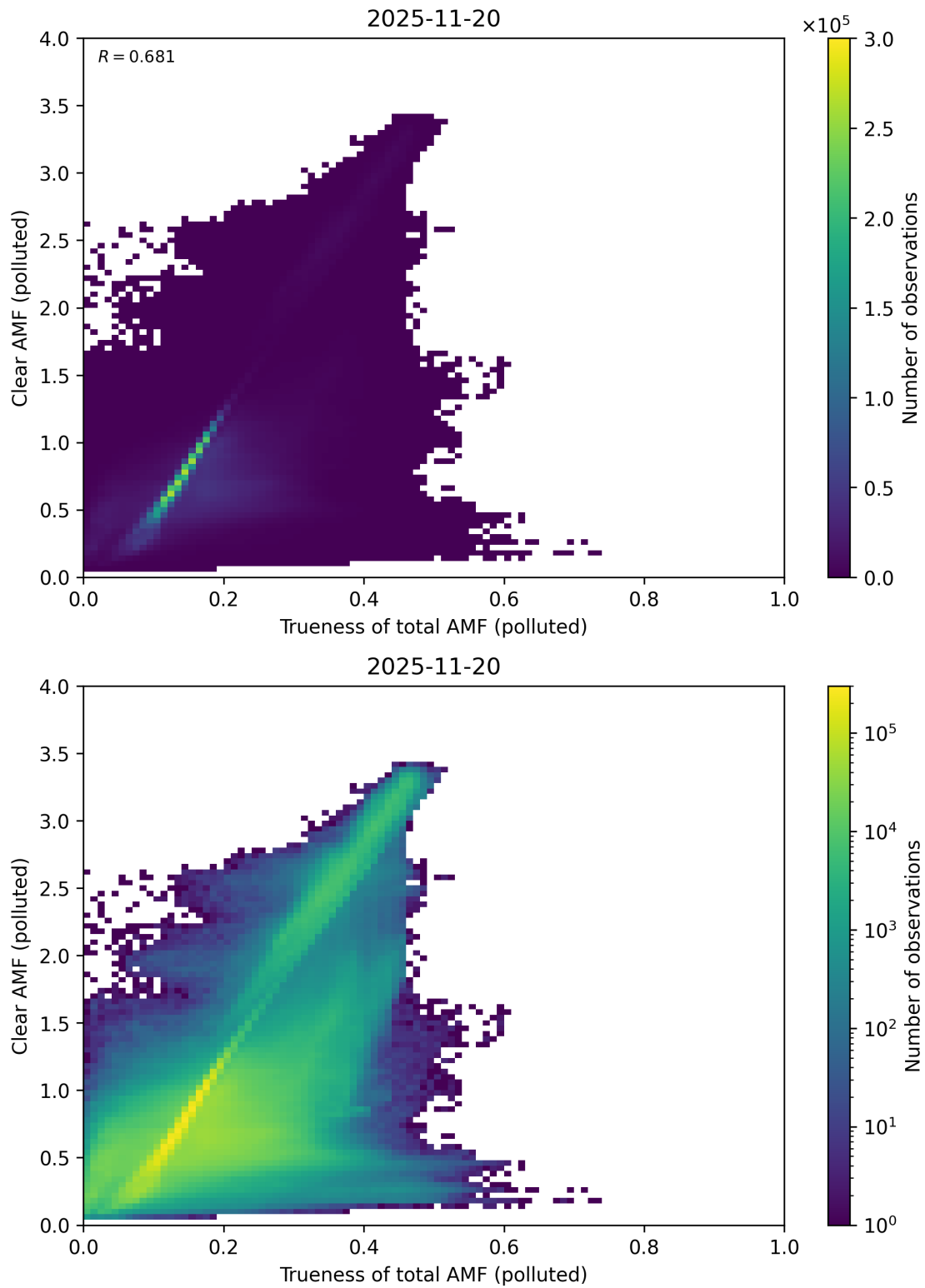
Figure 322: Scatter density plot of “Trueness of total AMF (polluted)” against “Clear AMF (polluted)” for 2025-11-19 to 2025-11-21.
