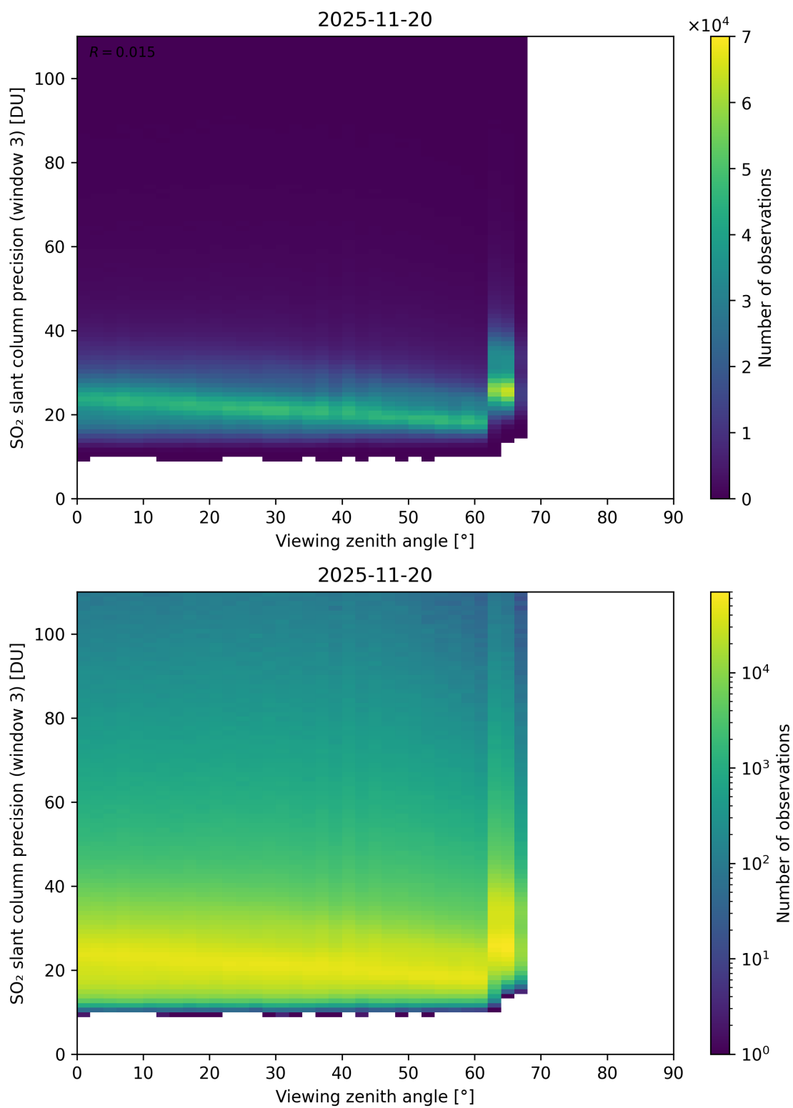
Figure 380: Scatter density plot of “Viewing zenith angle” against “SO 2 slant column precision (window 3)” for 2025-11-19 to 2025-11-21.
