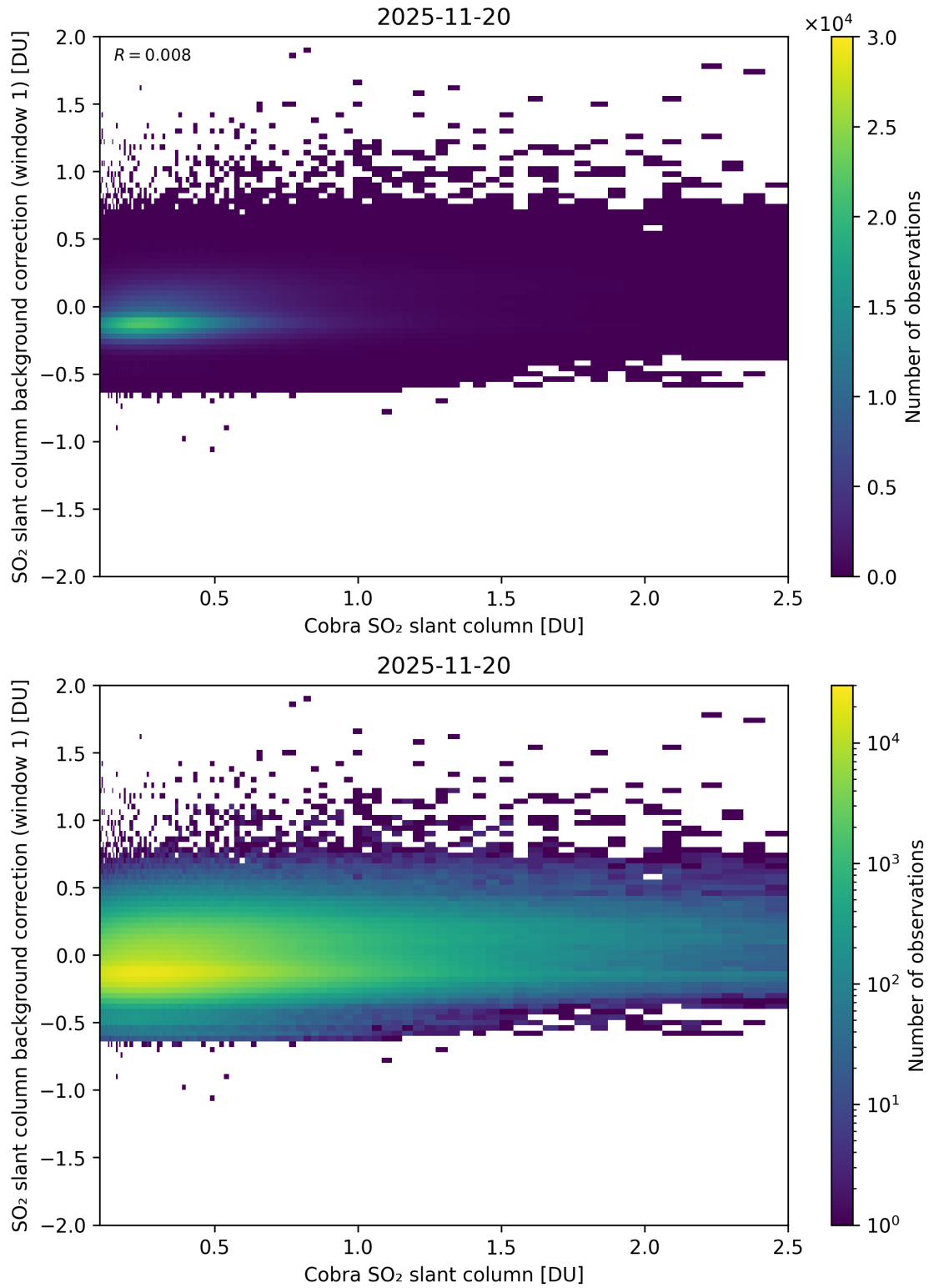
Figure 193: Scatter density plot of “Cobra SO 2 slant column” against “SO 2 slant column background correction (window 1)” for 2025-11-19 to 2025-11-21.
