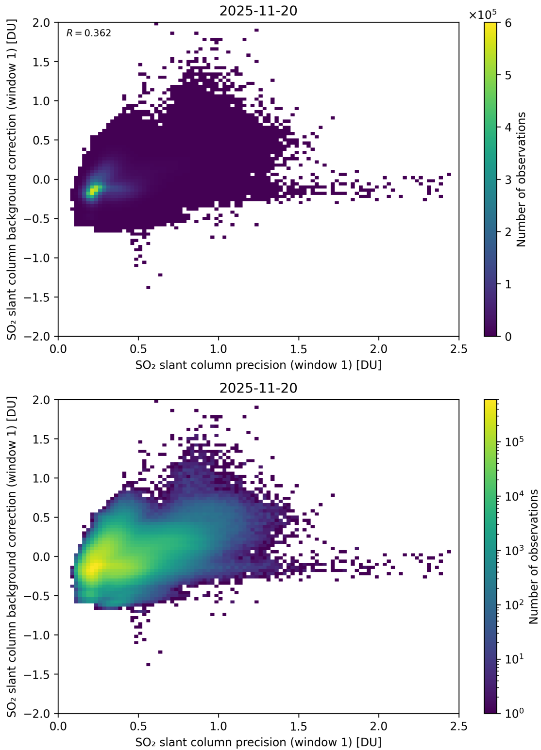
Figure 268: Scatter density plot of “SO 2 slant column precision (window 1)” against “SO 2 slant column background correction (window 1)” for 2025-11-19 to 2025-11-21.
