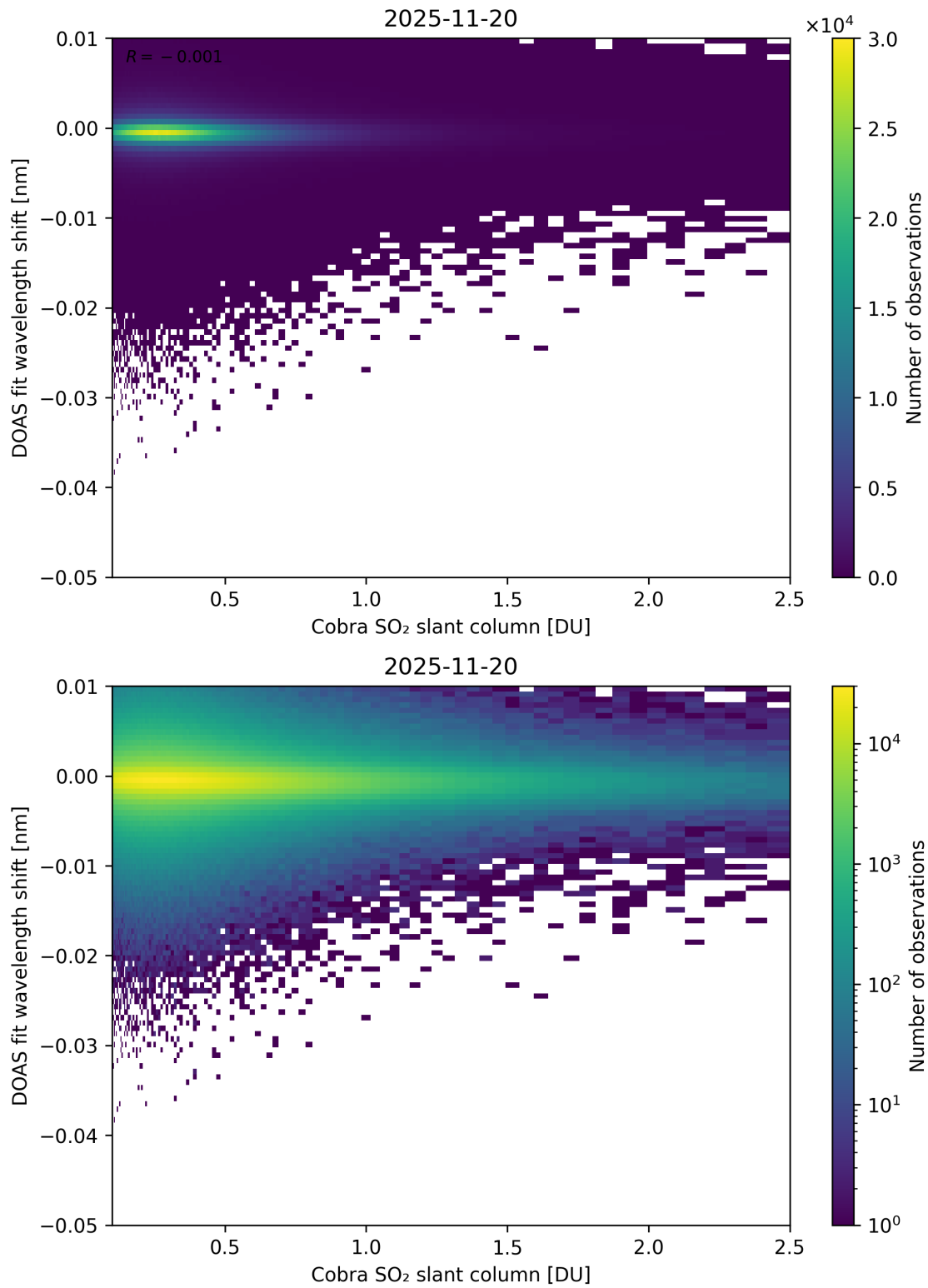
Figure 196: Scatter density plot of “Cobra SO 2 slant column” against “DOAS fit wavelength shift” for 2025-11-19 to 2025-11-21.
