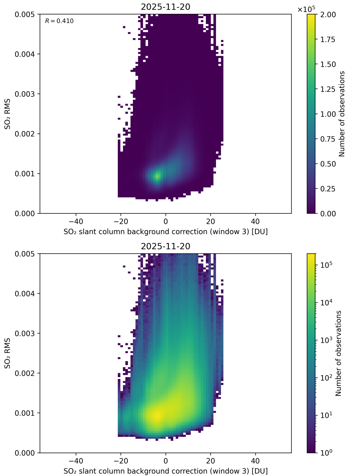
Figure 134: Scatter density plot of “SO 2 slant column background correction (window 3)” against “SO 2 RMS” for 2025-11-19 to 2025-11-21.
