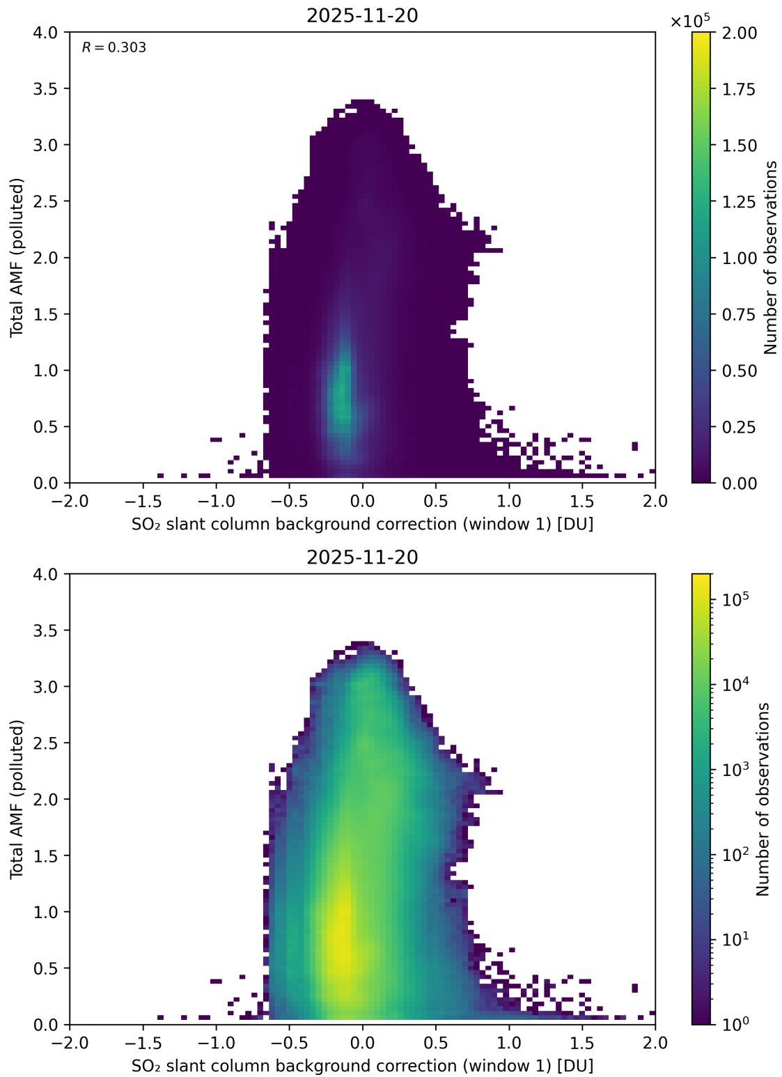
Figure 120: Scatter density plot of “SO 2 slant column background correction (window 1)” against “Total AMF (polluted)” for 2025-11-19 to 2025-11-21.
