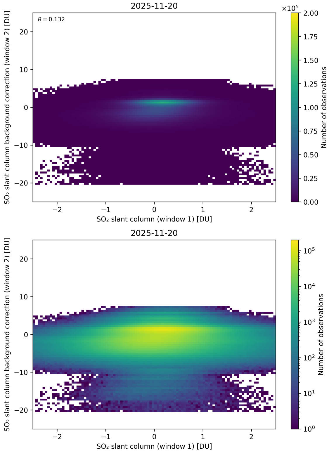
Figure 263: Scatter density plot of “SO 2 slant column (window 1)” against “SO 2 slant column background correction (window 2)” for 2025-11-19 to 2025-11-21.
