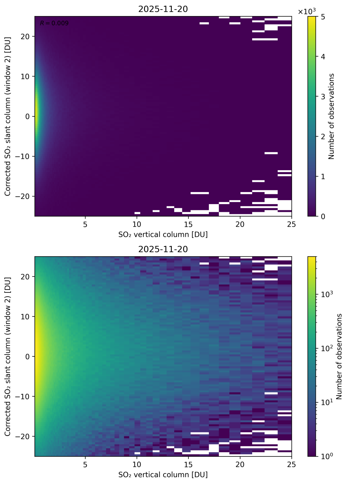
Figure 352: Scatter density plot of “SO 2 vertical column” against “Corrected SO 2 slant column (window 2)” for 2025-11-19 to 2025-11-21.
