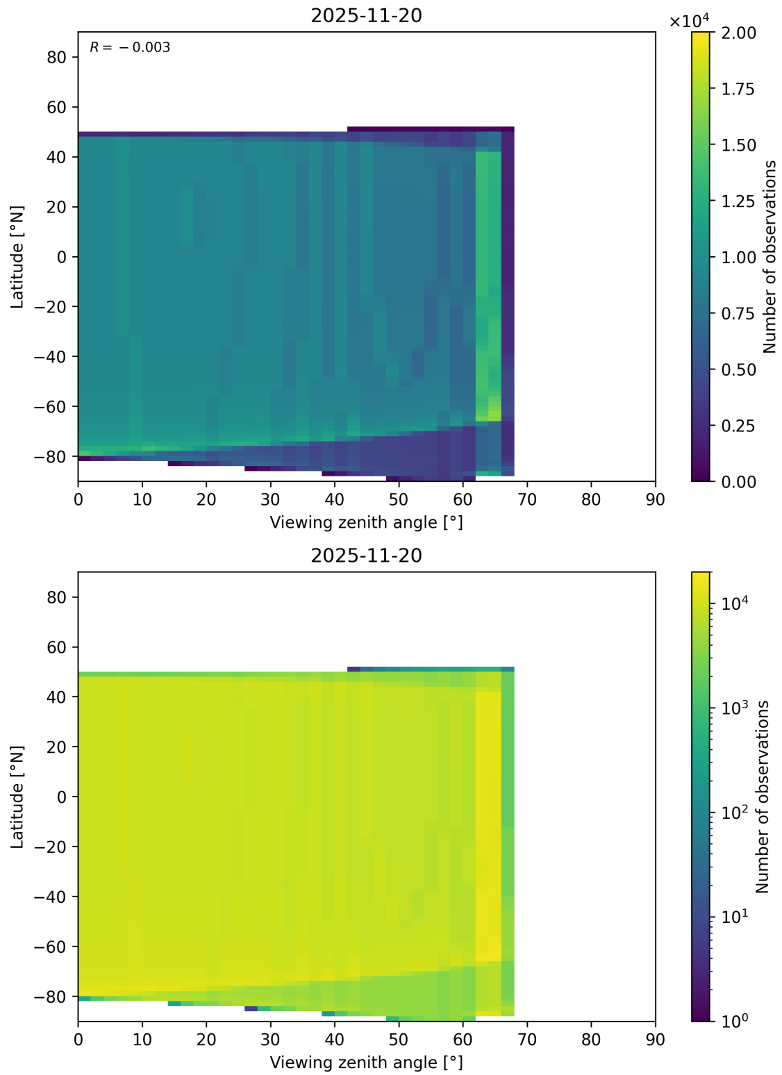
Figure 368: Scatter density plot of “Viewing zenith angle” against “Latitude” for 2025-11-19 to 2025-11-21.
