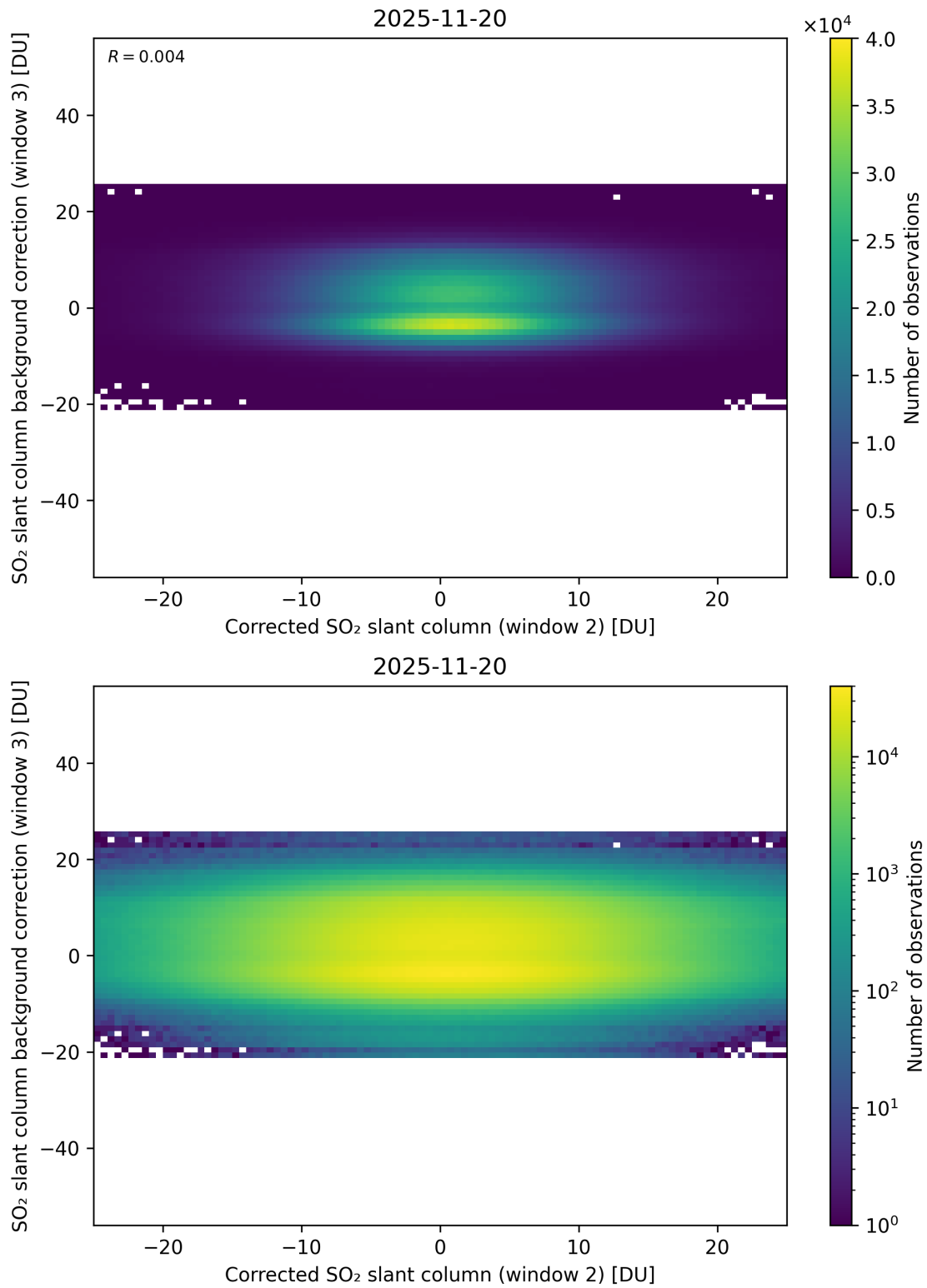
Figure 245: Scatter density plot of “Corrected SO 2 slant column (window 2)” against “SO 2 slant column background correction (window 3)” for 2025-11-19 to 2025-11-21.
