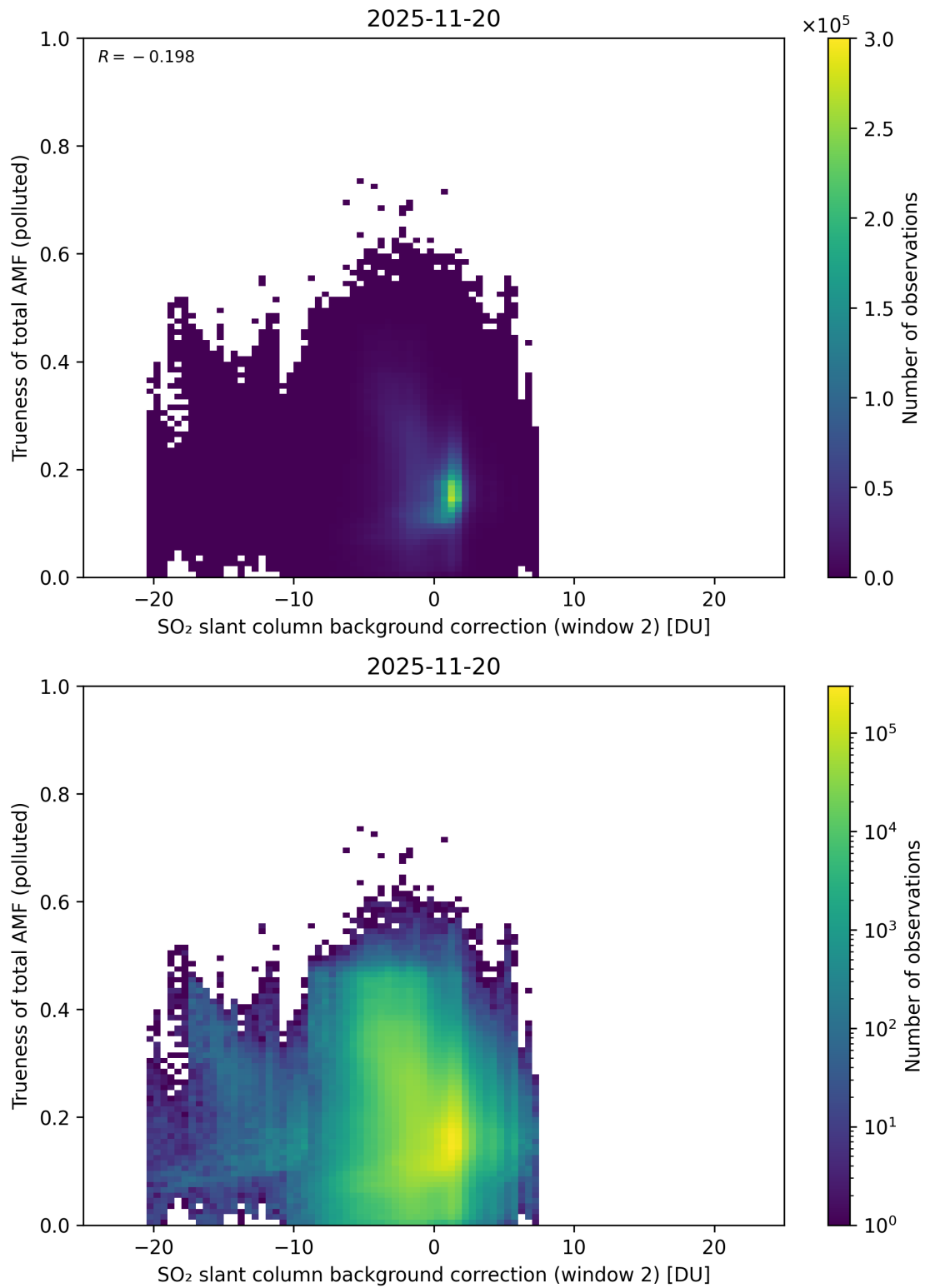
Figure 131: Scatter density plot of “SO 2 slant column background correction (window 2)” against “Trueness of total AMF (polluted)” for 2025-11-19 to 2025-11-21.
