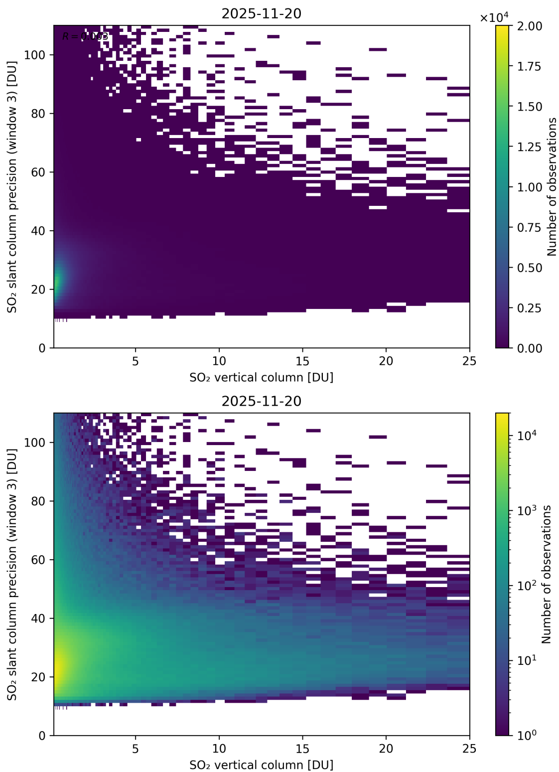
Figure 358: Scatter density plot of “SO 2 vertical column” against “SO 2 slant column precision (window 3)” for 2025-11-19 to 2025-11-21.
