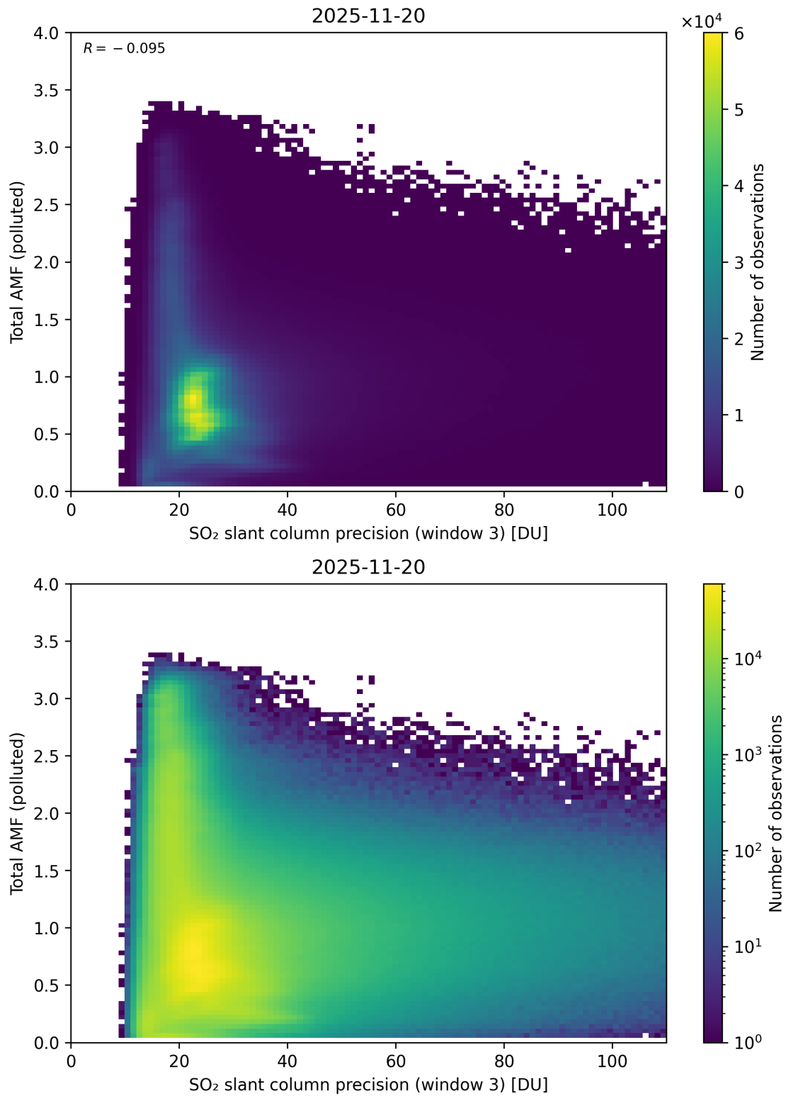
Figure 313: Scatter density plot of “SO 2 slant column precision (window 3)” against “Total AMF (polluted)” for 2025-11-19 to 2025-11-21.
