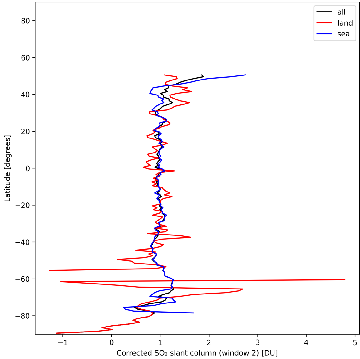
Figure 43: Zonal average of "Corrected SO 2 slant column (window 2)" for 2025-11-19 to 2025-11-21.
