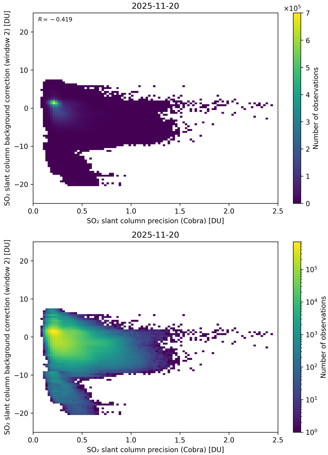
Figure 200: Scatter density plot of “SO 2 slant column precision (Cobra)” against “SO 2 slant column background correction (window 2)” for 2025-11-19 to 2025-11-21.
