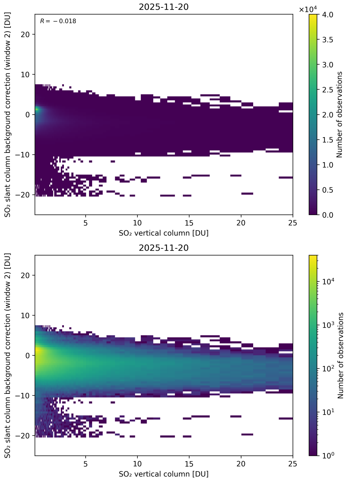
Figure 324: Scatter density plot of “SO 2 vertical column” against “SO 2 slant column background correction (window 2)” for 2025-11-19 to 2025-11-21.
