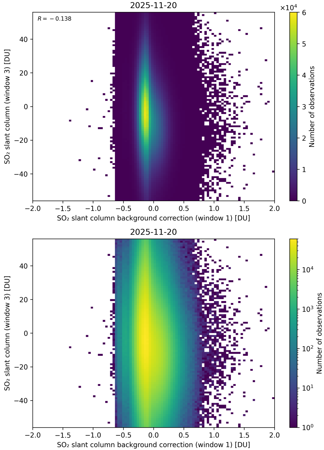
Figure 118: Scatter density plot of “SO 2 slant column background correction (window 1)” against “SO 2 slant column (window 3)” for 2025-11-19 to 2025-11-21.
