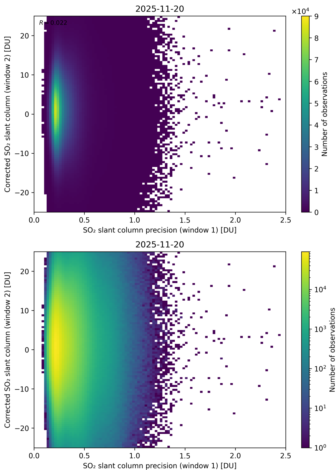
Figure 275: Scatter density plot of “SO 2 slant column precision (window 1)” against “Corrected SO 2 slant column (window 2)” for 2025-11-19 to 2025-11-21.
