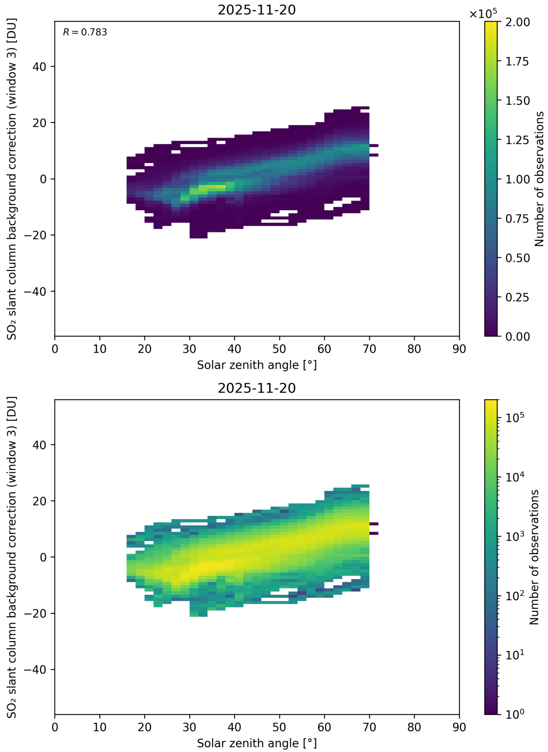
Figure 173: Scatter density plot of “Solar zenith angle” against “SO 2 slant column background correction (window 3)” for 2025-11-19 to 2025-11-21.
