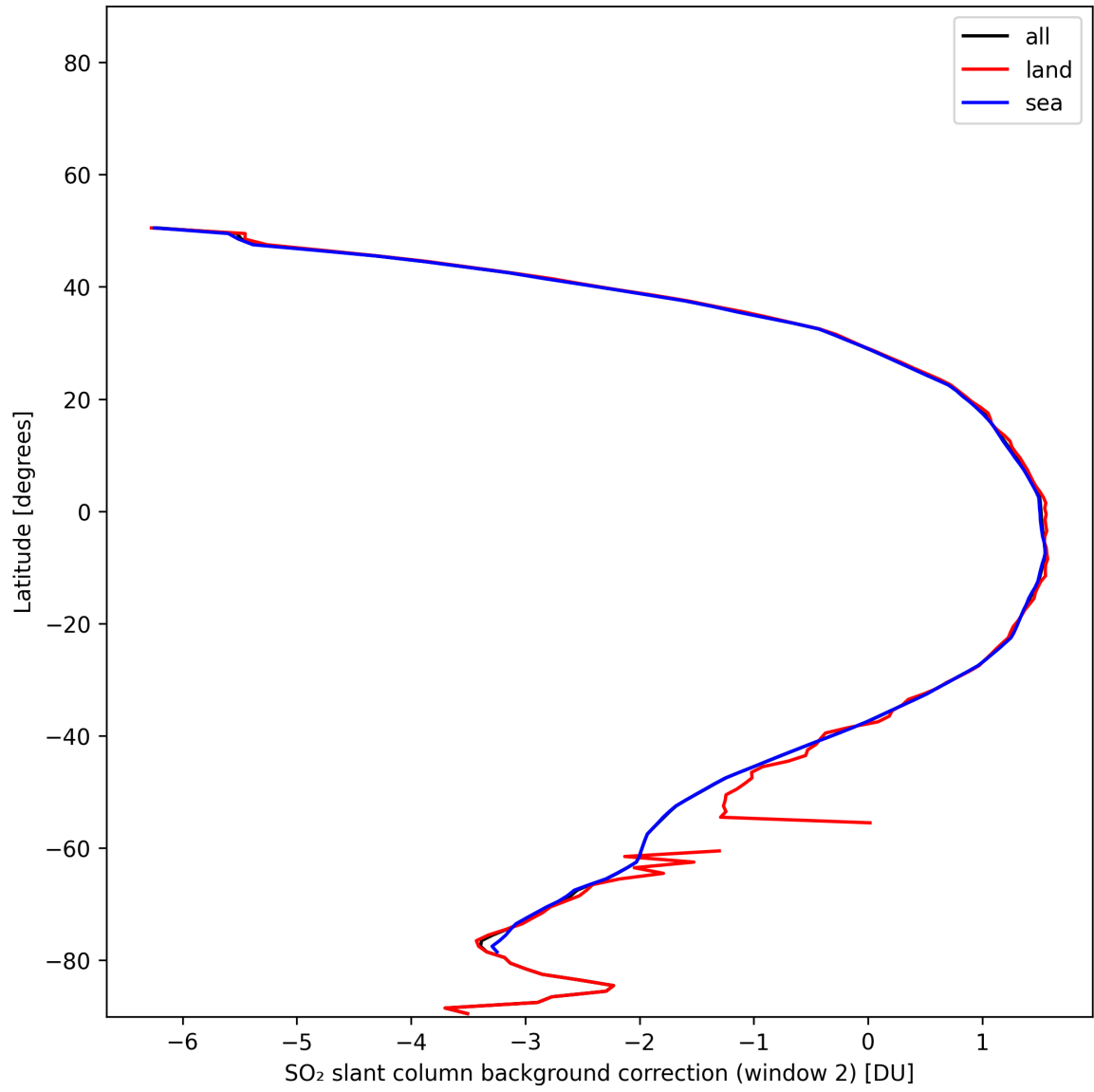
Figure 44: Zonal average of “SO 2 slant column background correction (window 2)” for 2025-11-19 to 2025-11-21.
