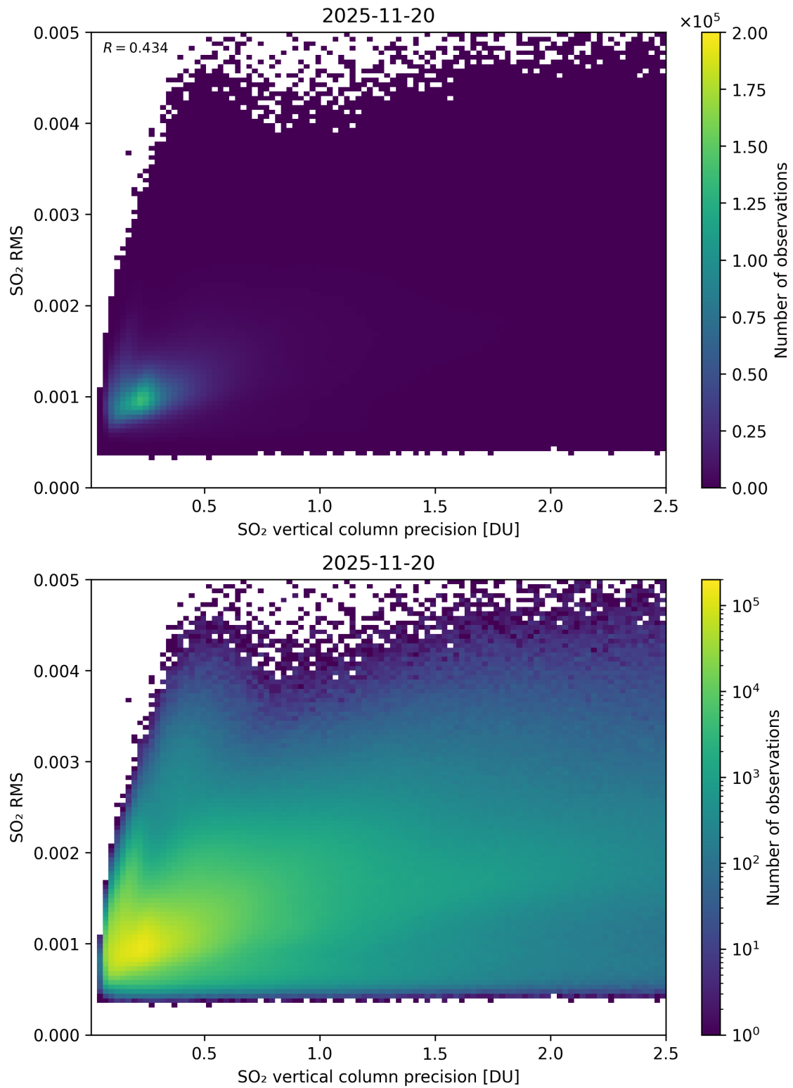
Figure 334: Scatter density plot of “SO 2 vertical column precision” against “SO 2 RMS” for 2025-11-19 to 2025-11-21.
