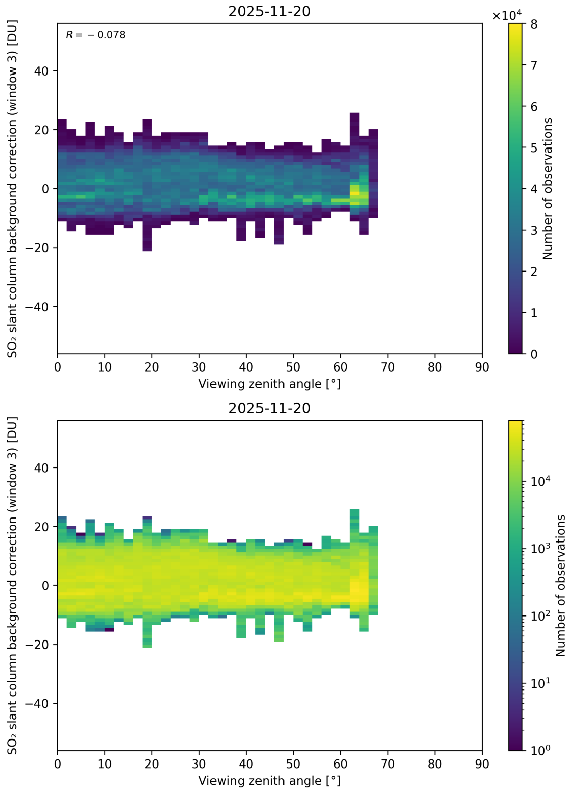
Figure 364: Scatter density plot of “Viewing zenith angle” against “SO 2 slant column background correction (window 3)” for 2025-11-19 to 2025-11-21.
