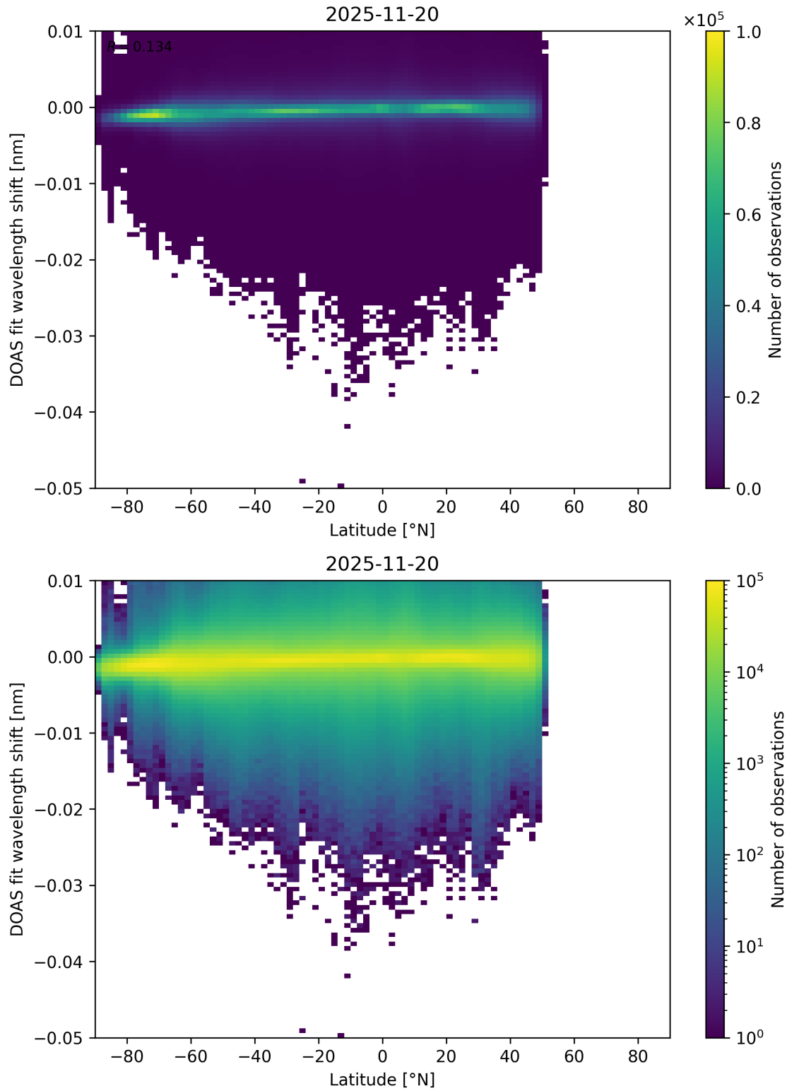
Figure 153: Scatter density plot of “Latitude” against “DOAS fit wavelength shift” for 2025-11-19 to 2025-11-21.
