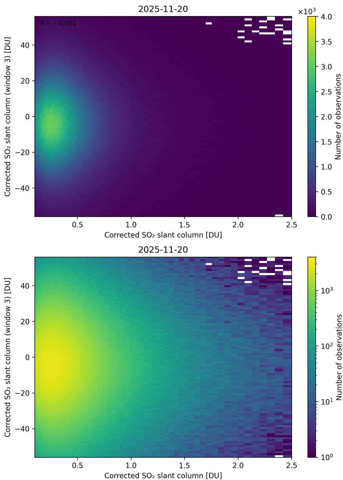
Figure 236: Scatter density plot of “Corrected SO 2 slant column” against “Corrected SO 2 slant column (window 3)” for 2025-11-19 to 2025-11-21.
