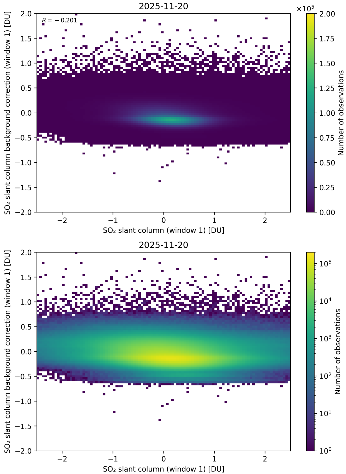
Figure 262: Scatter density plot of “SO 2 slant column (window 1)” against “SO 2 slant column background correction (window 1)” for 2025-11-19 to 2025-11-21.
