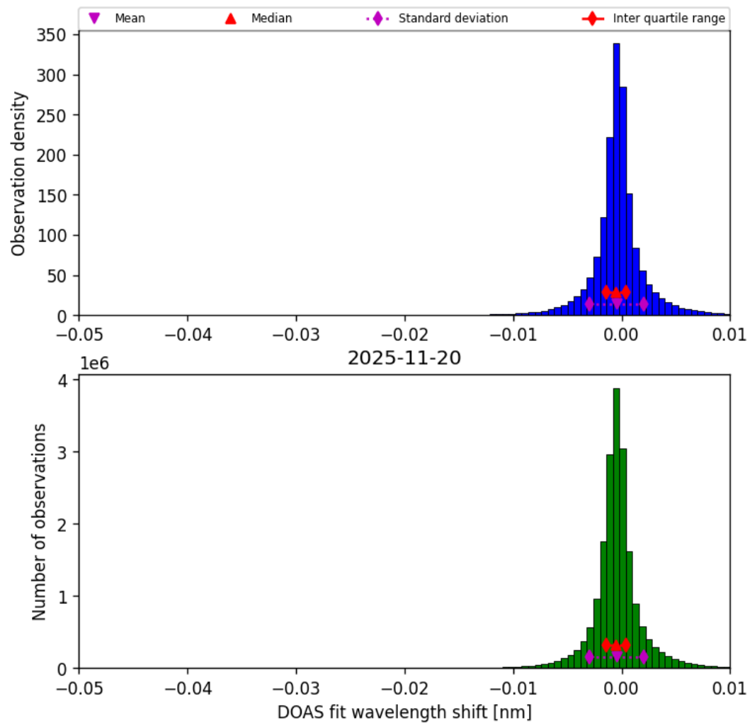
Figure 76: Histogram of “DOAS fit wavelength shift” for 2025-11-19 to 2025-11-21
