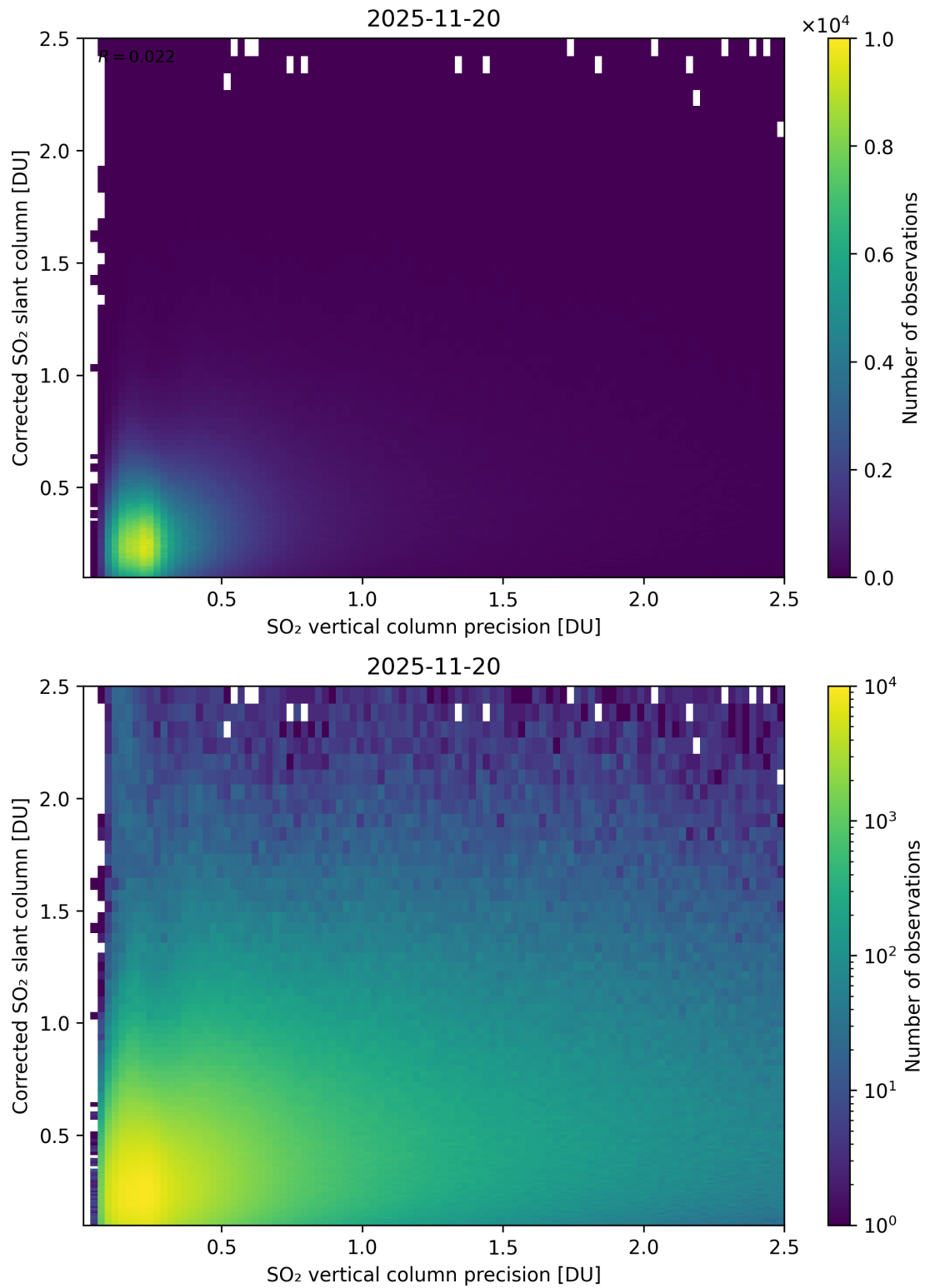
Figure 338: Scatter density plot of “SO 2 vertical column precision” against “Corrected SO 2 slant column” for 2025-11-19 to 2025-11-21.
