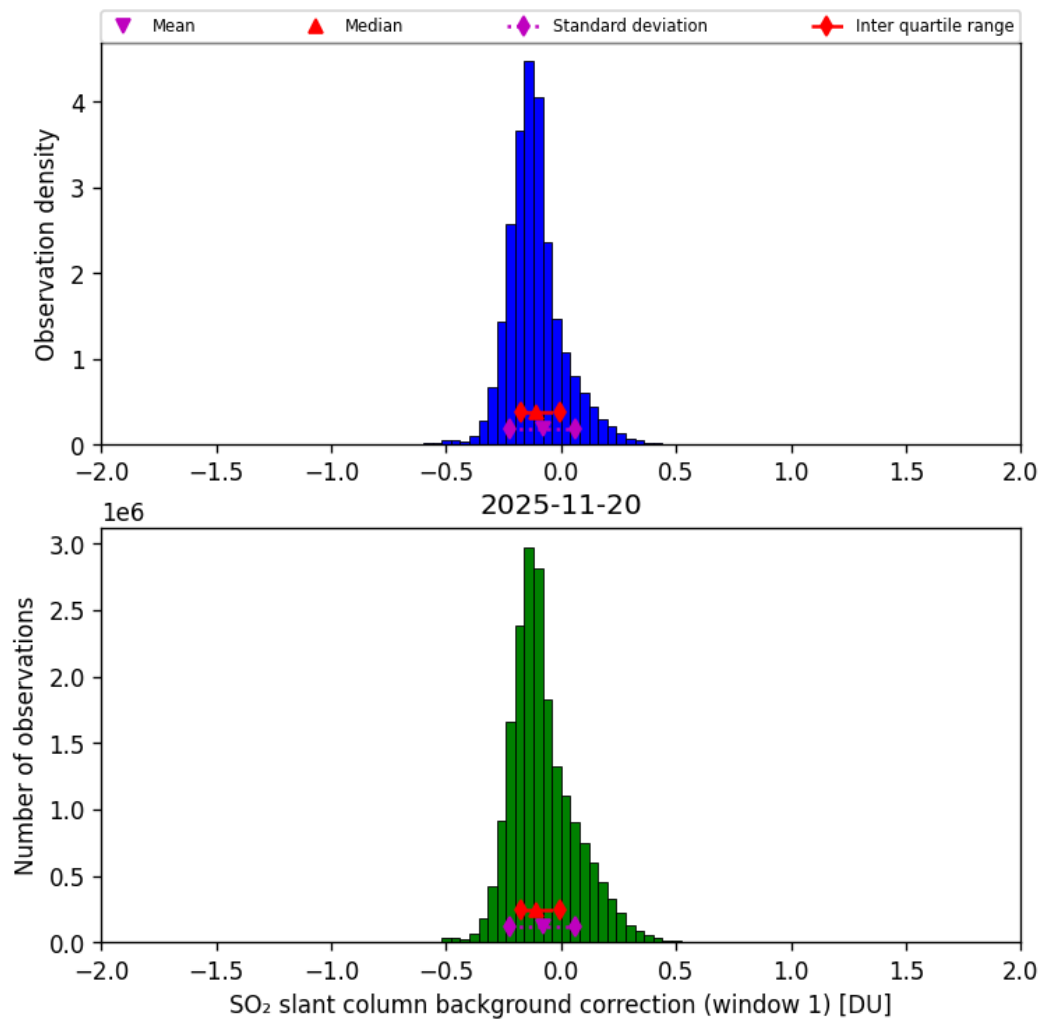
Figure 66: Histogram of “SO 2 slant column background correction (window 1)” for 2025-11-19 to 2025-11-21
