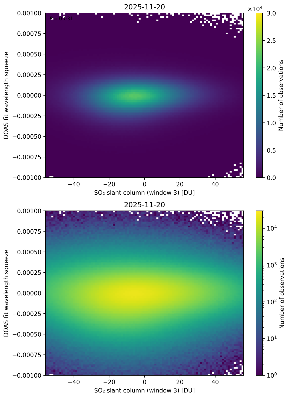
Figure 305: Scatter density plot of “SO 2 slant column (window 3)” against “DOAS fit wavelength squeeze” for 2025-11-19 to 2025-11-21.
