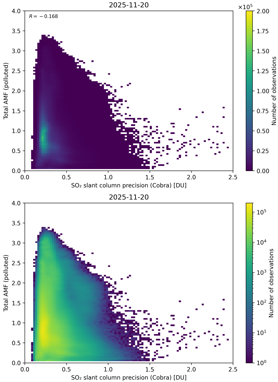
Figure 213: Scatter density plot of “SO 2 slant column precision (Cobra)” against “Total AMF (polluted)” for 2025-11-19 to 2025-11-21.
