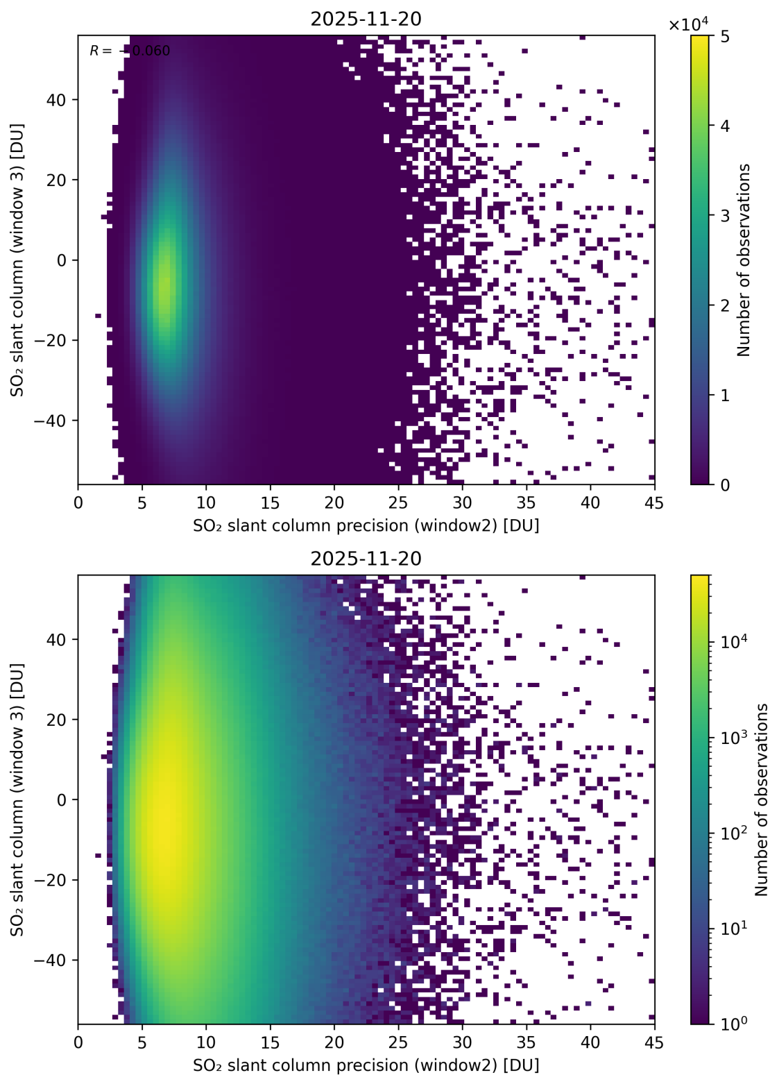
Figure 299: Scatter density plot of “SO 2 slant column precision (window2)” against “SO 2 slant column (window 3)” for 2025-11-19 to 2025-11-21.
