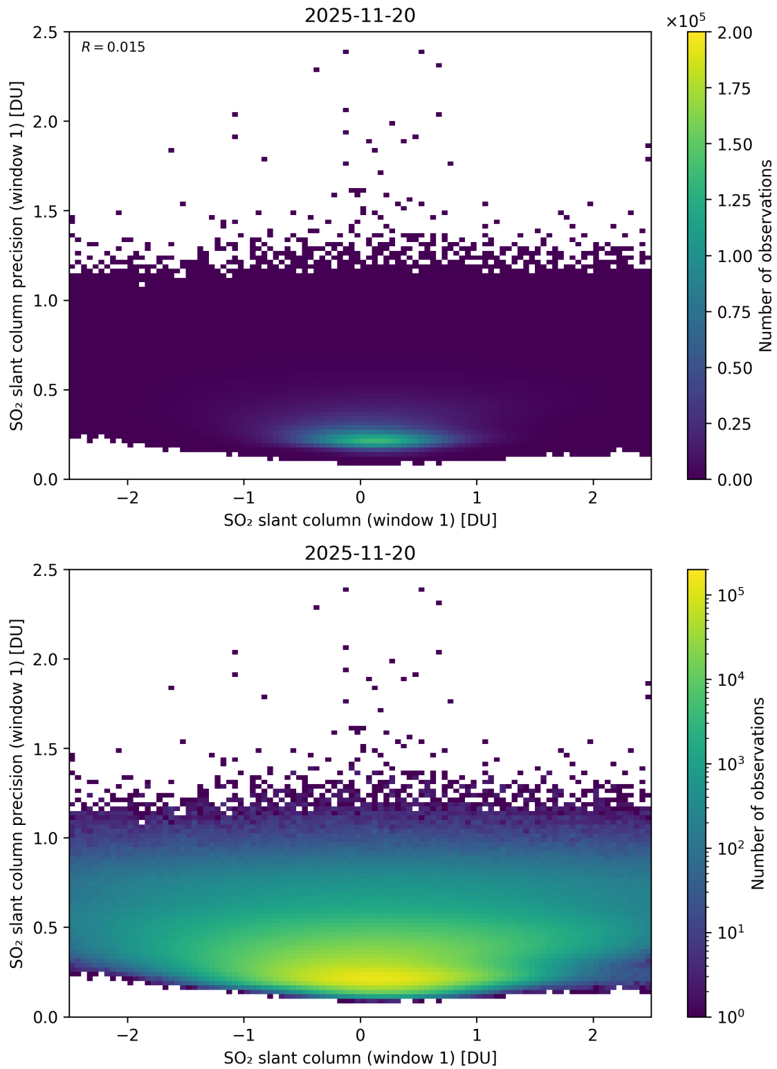
Figure 285: Scatter density plot of “SO 2 slant column (window 1)” against “SO 2 slant column precision (window 1)” for 2025-11-19 to 2025-11-21.
