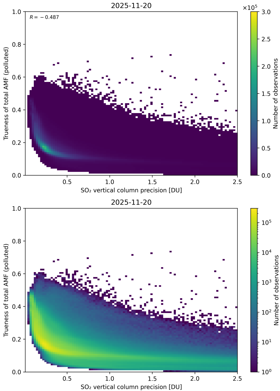
Figure 347: Scatter density plot of “SO 2 vertical column precision” against “Trueness of total AMF (polluted)” for 2025-11-19 to 2025-11-21.
