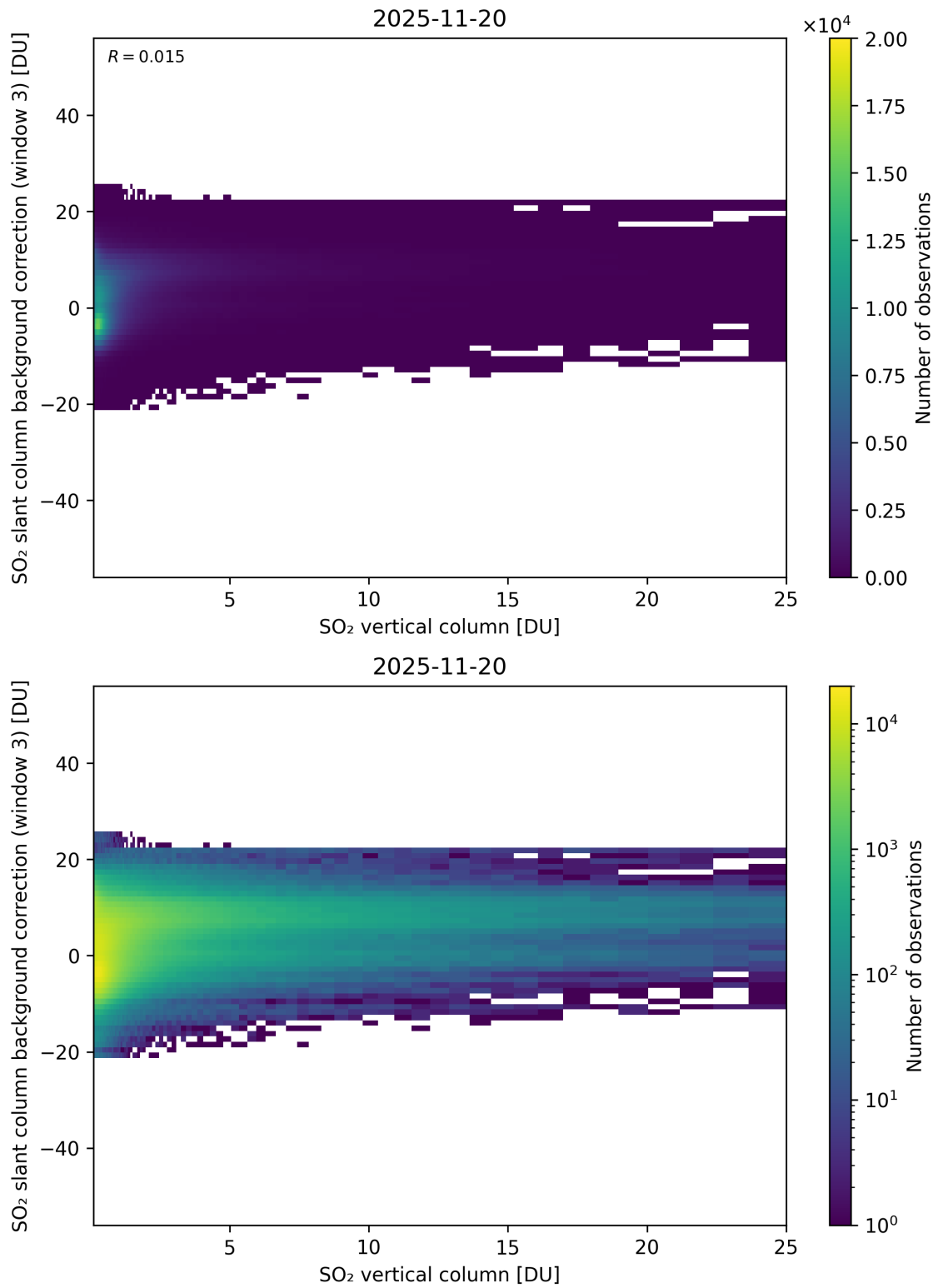
Figure 325: Scatter density plot of “SO 2 vertical column” against “SO 2 slant column background correction (window 3)” for 2025-11-19 to 2025-11-21.
