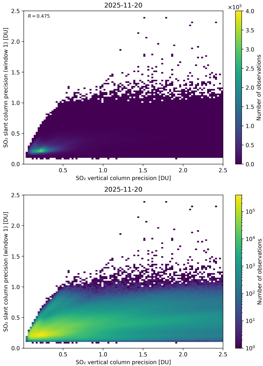
Figure 342: Scatter density plot of “SO 2 vertical column precision” against “SO 2 slant column precision (window 1)” for 2025-11-19 to 2025-11-21.
