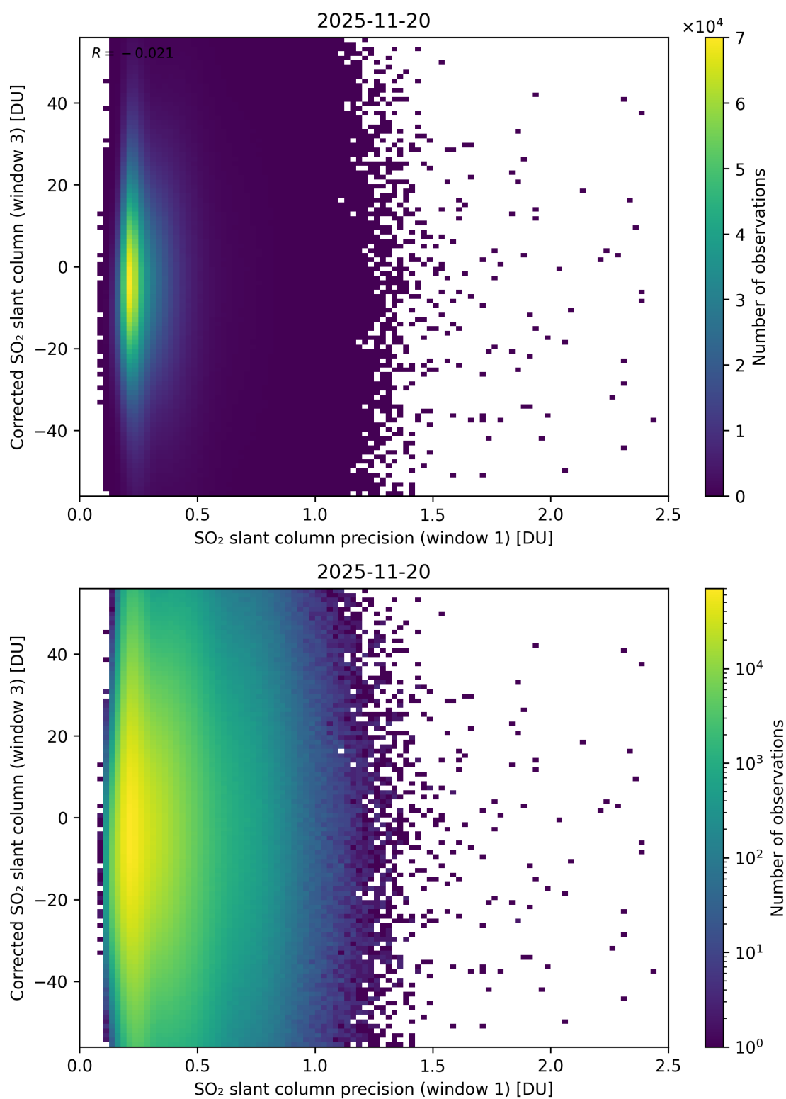
Figure 276: Scatter density plot of “SO 2 slant column precision (window 1)” against “Corrected SO 2 slant column (window 3)” for 2025-11-19 to 2025-11-21.
