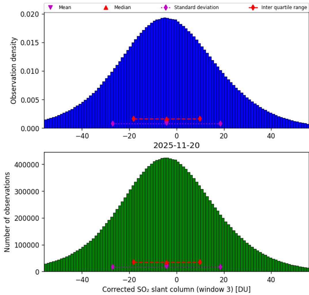
Figure 73: Histogram of “Corrected SO 2 slant column (window 3)” for 2025-11-19 to 2025-11-21
