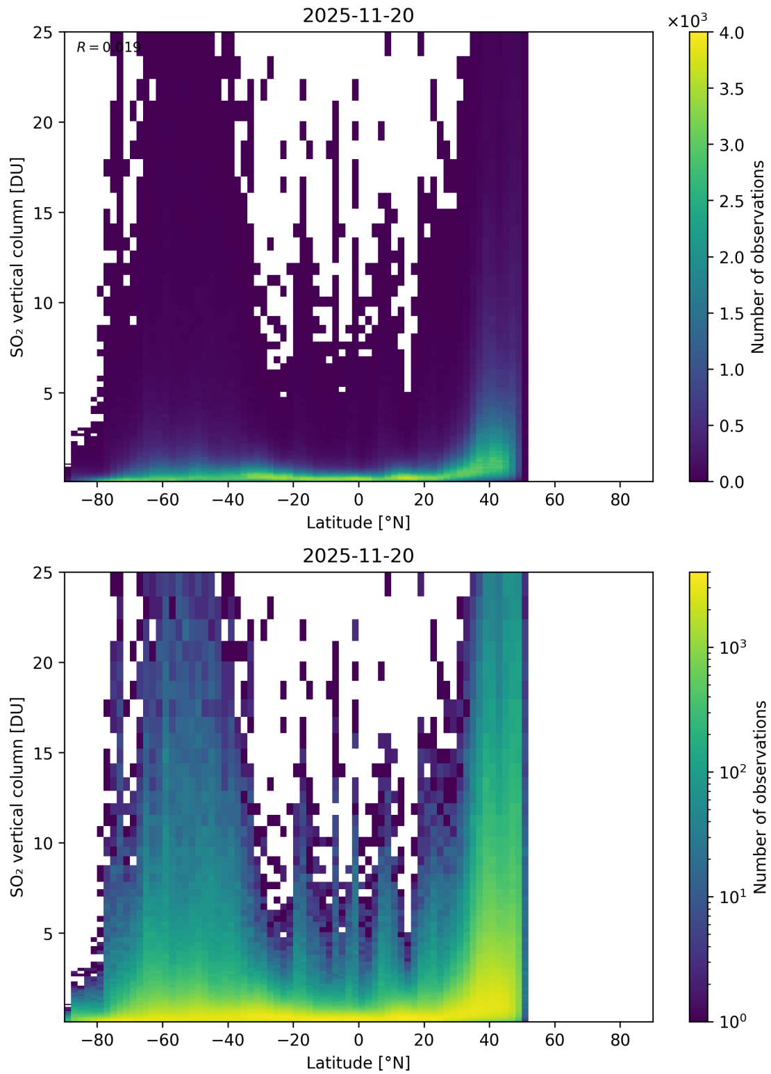
Figure 169: Scatter density plot of “Latitude” against “SO 2 vertical column” for 2025-11-19 to 2025-11-21.
