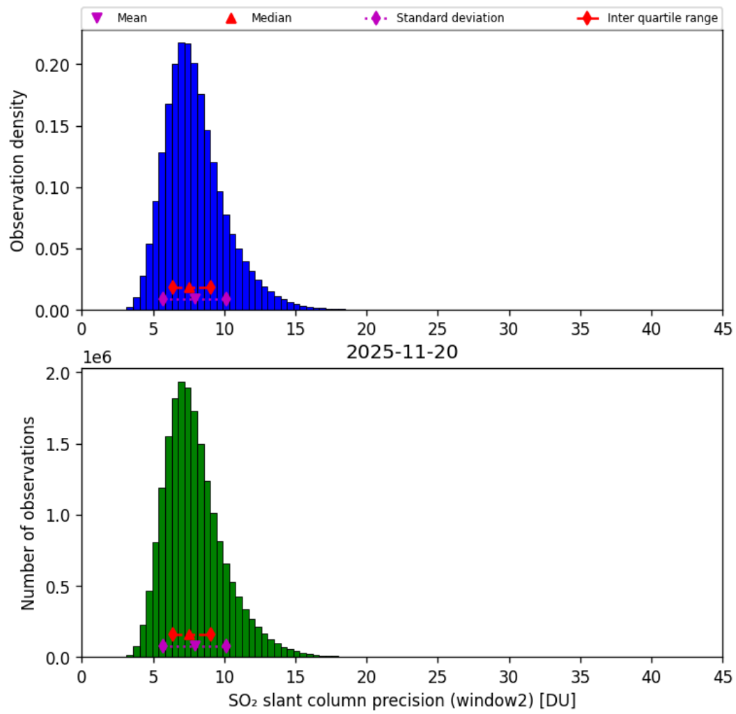
Figure 68: Histogram of “SO 2 slant column precision (window2)” for 2025-11-19 to 2025-11-21
