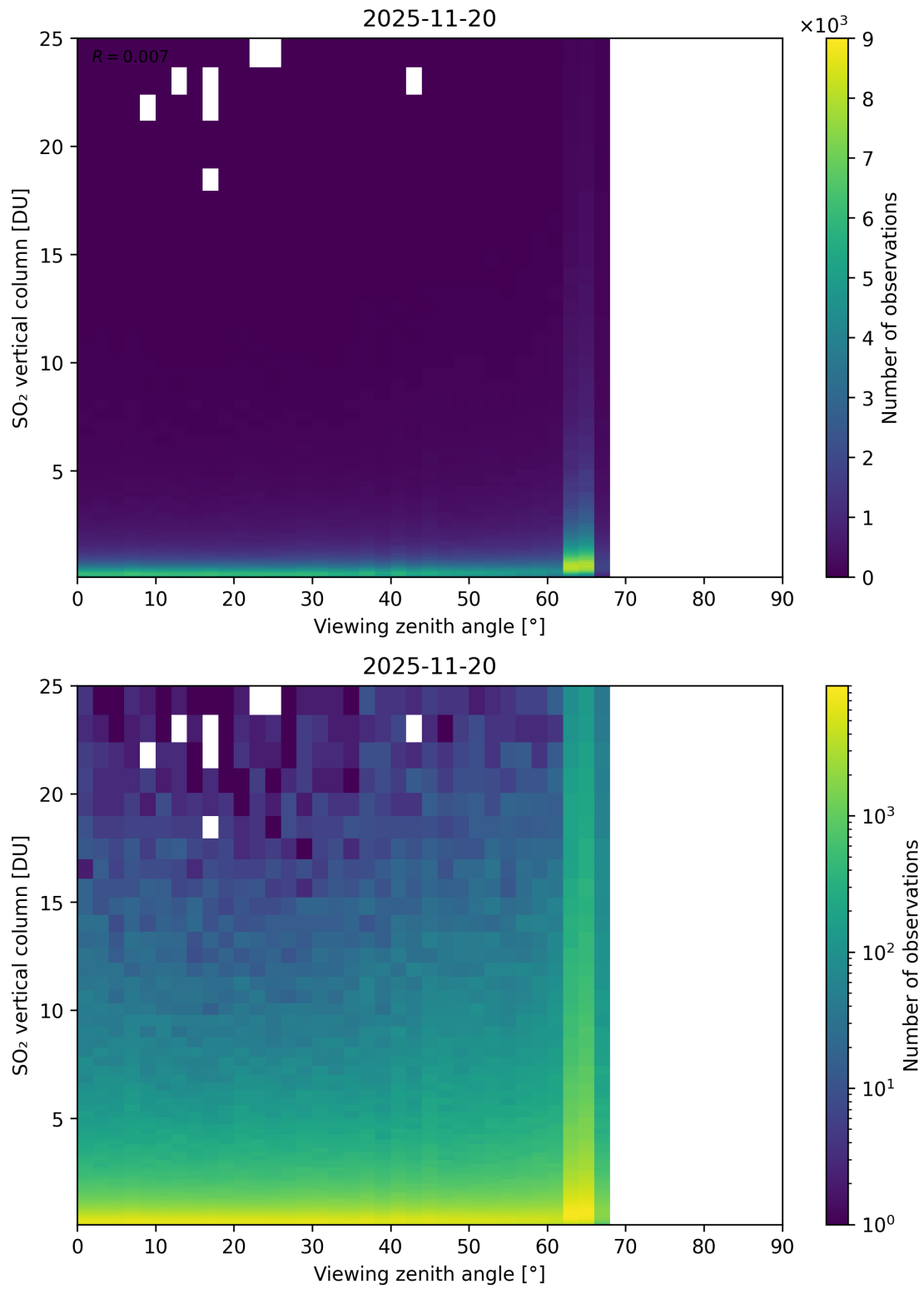
Figure 383: Scatter density plot of “Viewing zenith angle” against “SO 2 vertical column” for 2025-11-19 to 2025-11-21.
