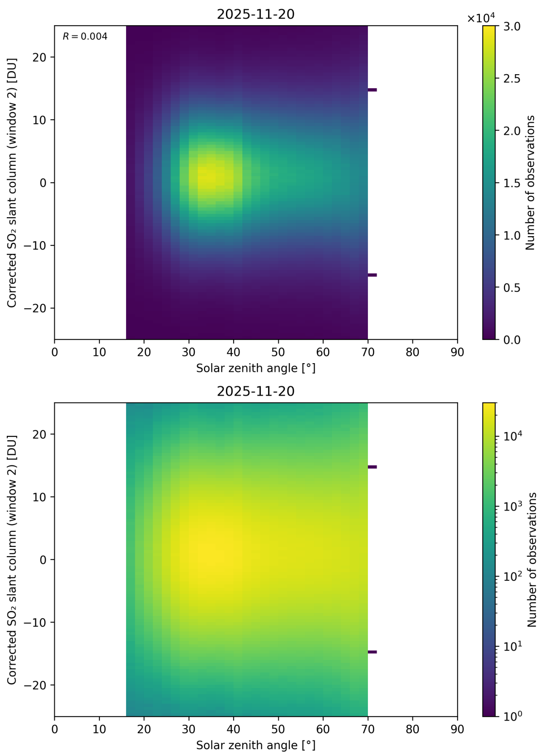
Figure 182: Scatter density plot of “Solar zenith angle” against “Corrected SO 2 slant column (window 2)” for 2025-11-19 to 2025-11-21.
