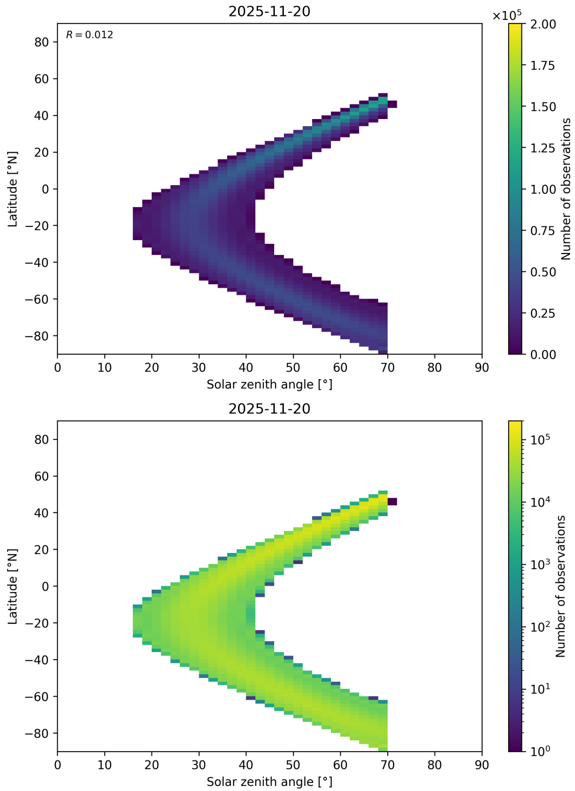
Figure 177: Scatter density plot of “Solar zenith angle” against “Latitude” for 2025-11-19 to 2025-11-21.
