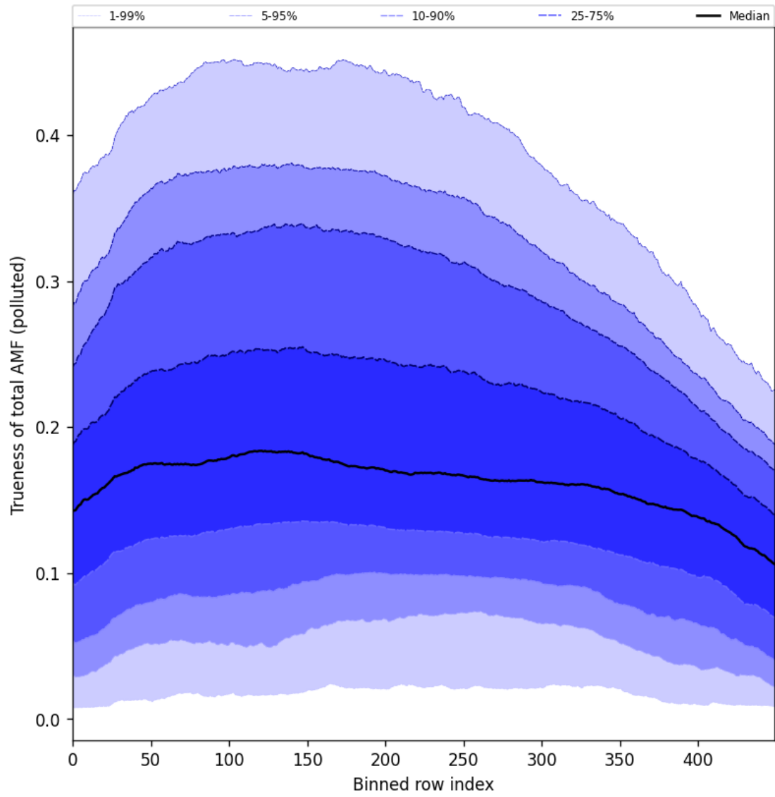
Figure 106: Along track statistics of “Trueness of total AMF (polluted)” for 2025-11-19 to 2025-11-21
