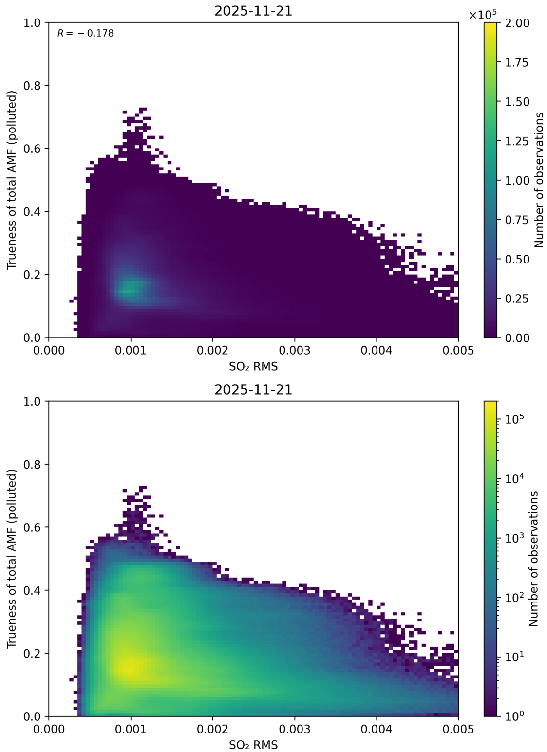
Figure 149: Scatter density plot of “SO 2 RMS” against “Trueness of total AMF (polluted)” for 2025-11-20 to 2025-11-22.
