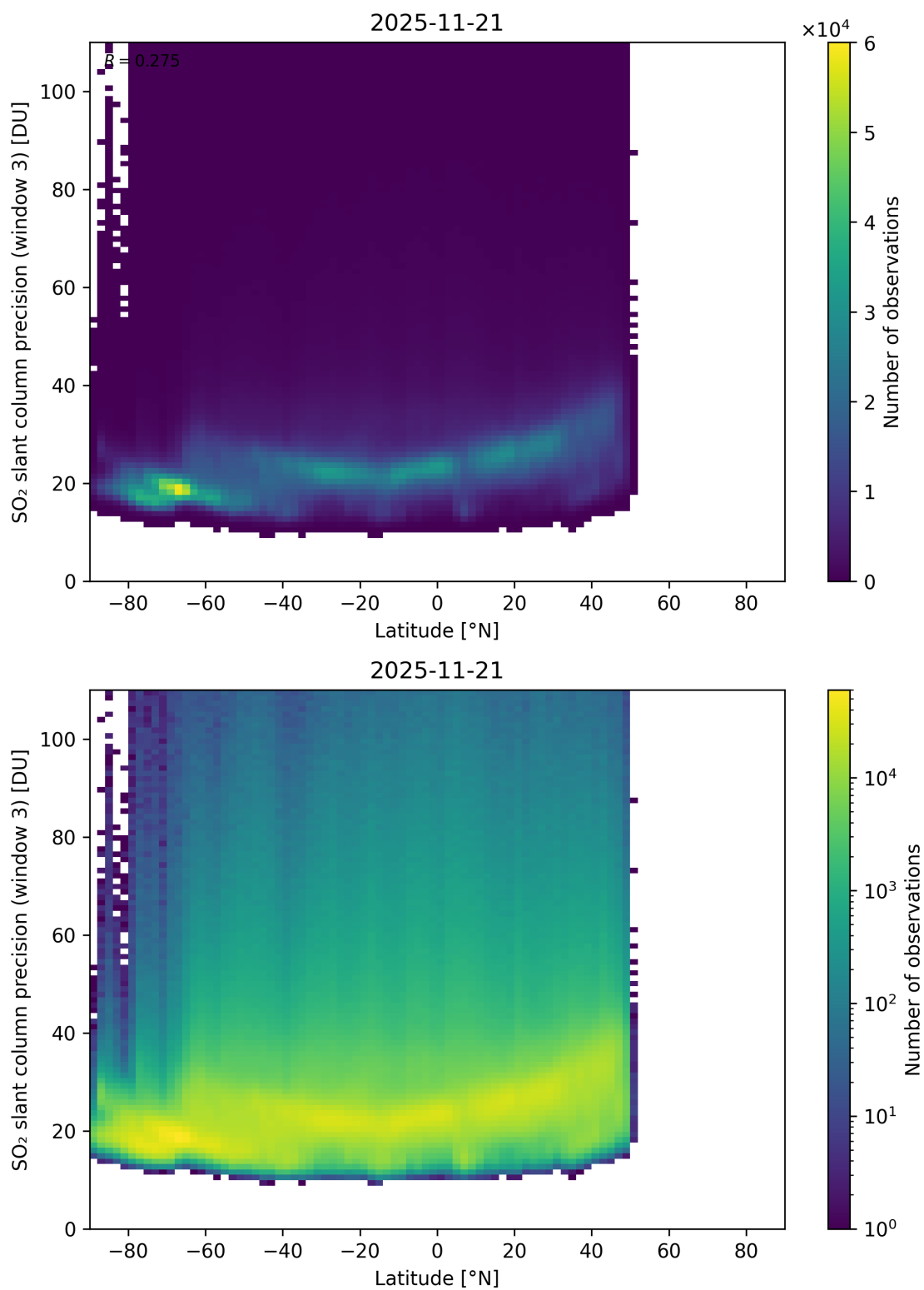
Figure 166: Scatter density plot of “Latitude” against “SO 2 slant column precision (window 3)” for 2025-11-20 to 2025-11-22.
