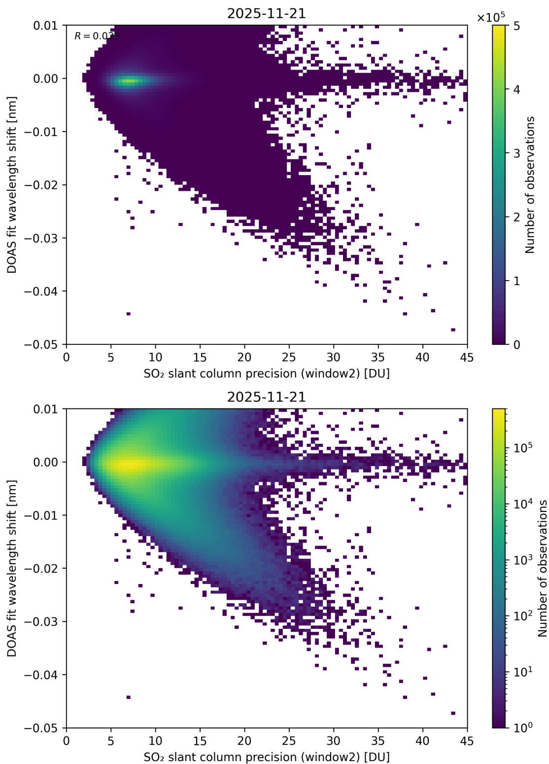
Figure 293: Scatter density plot of “SO 2 slant column precision (window2)” against “DOAS fit wavelength shift” for 2025-11-20 to 2025-11-22.
