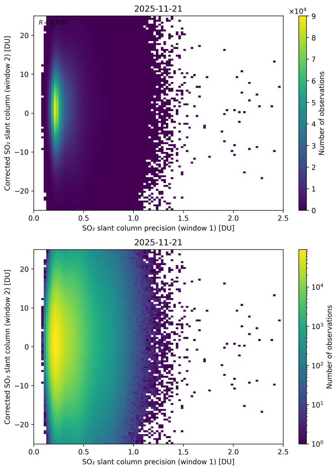
Figure 275: Scatter density plot of “SO 2 slant column precision (window 1)” against “Corrected SO 2 slant column (window 2)” for 2025-11-20 to 2025-11-22.
