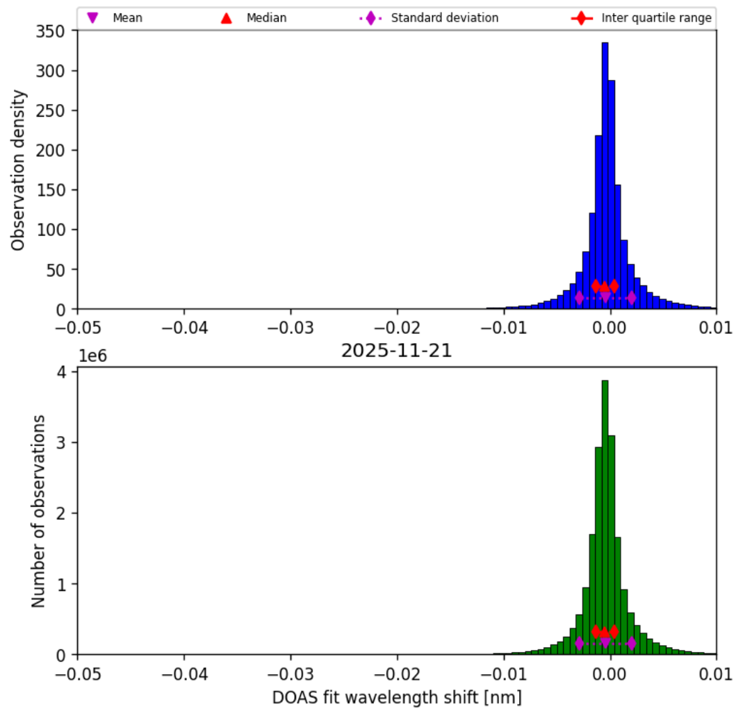
Figure 76: Histogram of “DOAS fit wavelength shift” for 2025-11-20 to 2025-11-22
