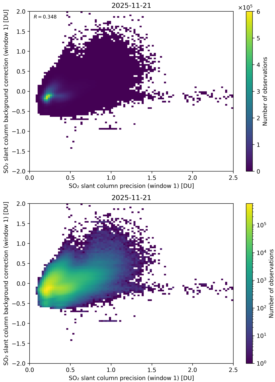
Figure 268: Scatter density plot of “SO 2 slant column precision (window 1)” against “SO 2 slant column background correction (window 1)” for 2025-11-20 to 2025-11-22.
