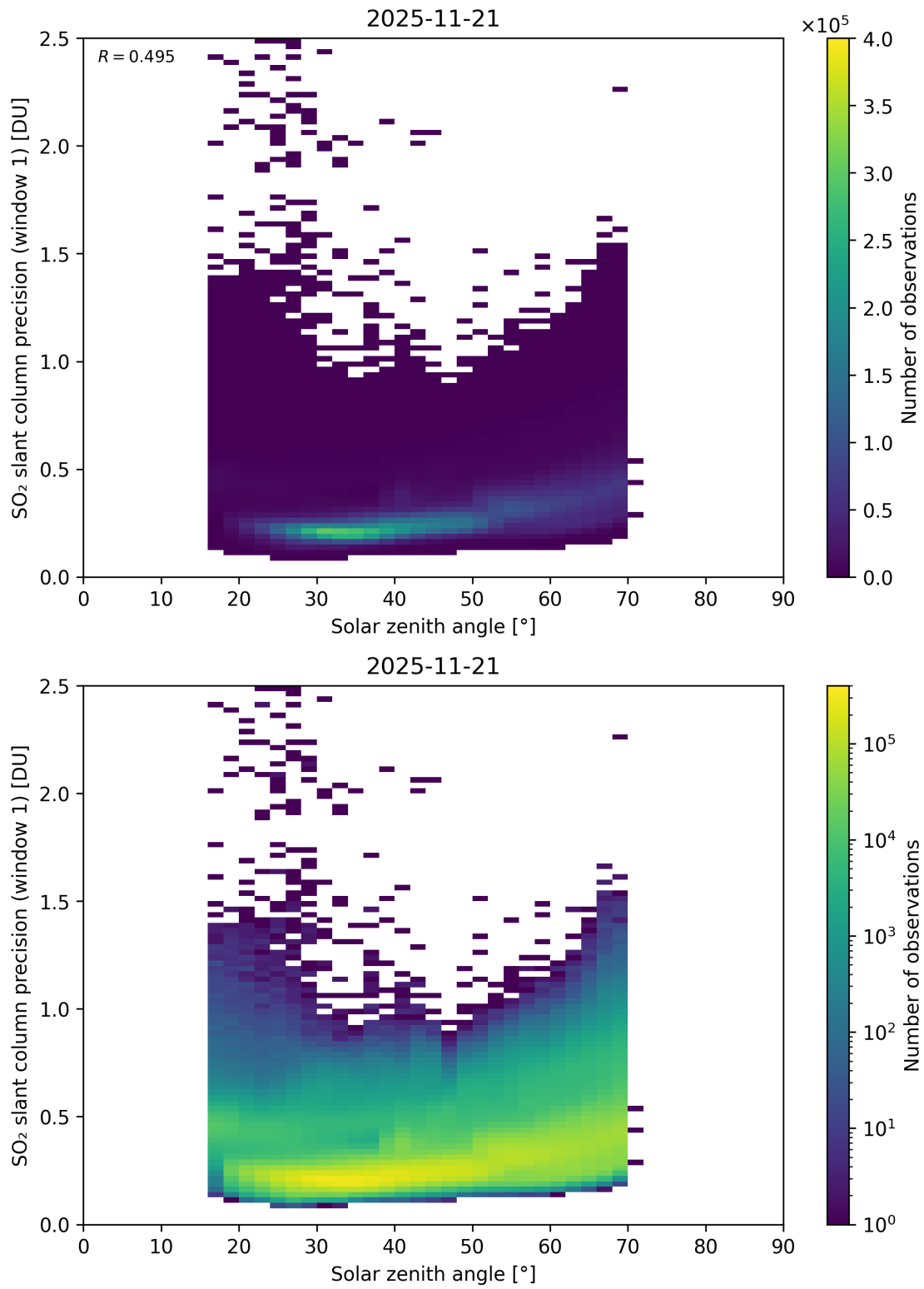
Figure 185: Scatter density plot of “Solar zenith angle” against “SO 2 slant column precision (window 1)” for 2025-11-20 to 2025-11-22.
