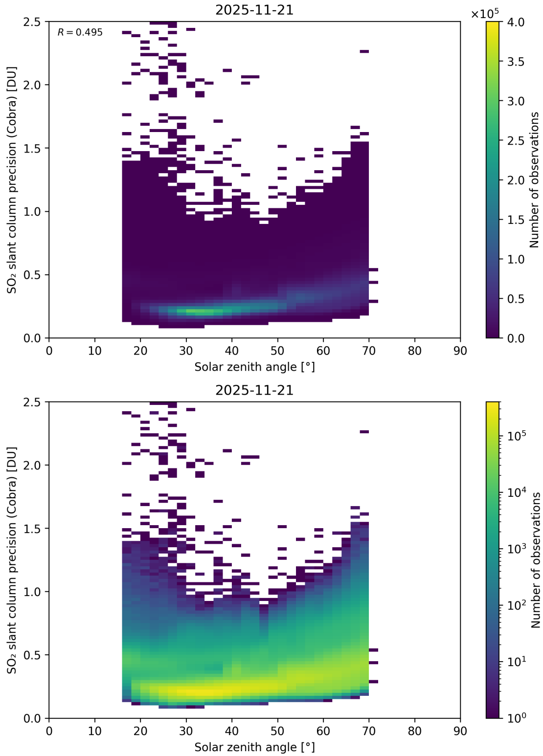
Figure 180: Scatter density plot of “Solar zenith angle” against “SO 2 slant column precision (Cobra)” for 2025-11-20 to 2025-11-22.
