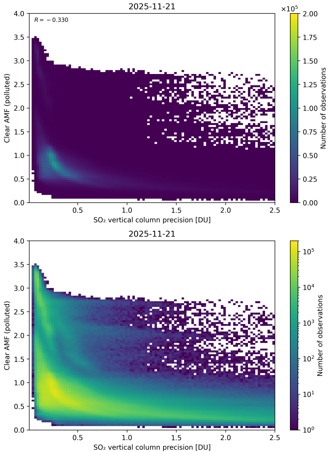
Figure 335: Scatter density plot of “SO 2 vertical column precision” against “Clear AMF (polluted)” for 2025-11-20 to 2025-11-22.
