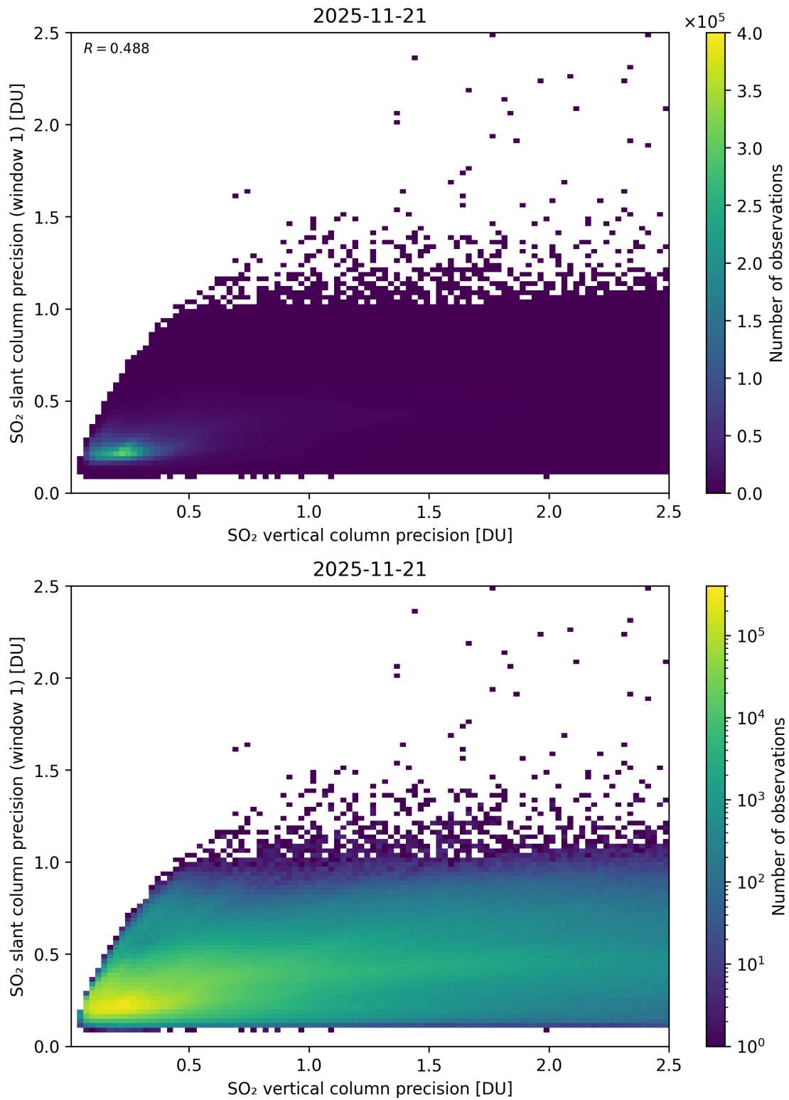
Figure 342: Scatter density plot of “SO 2 vertical column precision” against “SO 2 slant column precision (window 1)” for 2025-11-20 to 2025-11-22.
