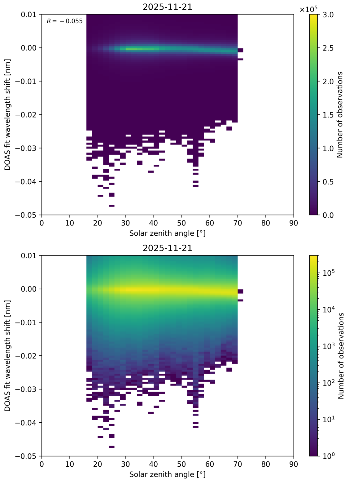
Figure 174: Scatter density plot of “Solar zenith angle” against “DOAS fit wavelength shift” for 2025-11-20 to 2025-11-22.
