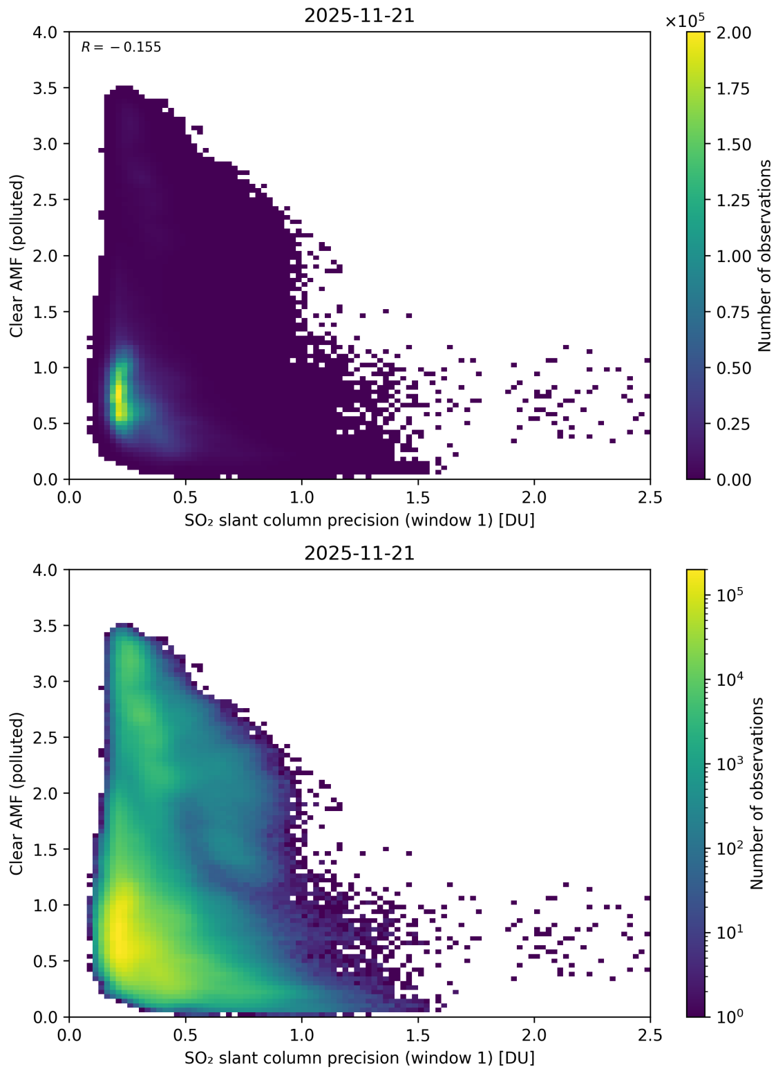
Figure 274: Scatter density plot of “SO 2 slant column precision (window 1)” against “Clear AMF (polluted)” for 2025-11-20 to 2025-11-22.
