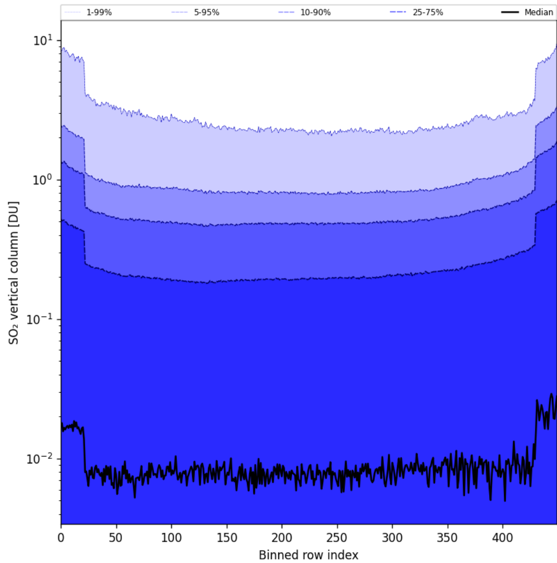
Figure 84: Along track statistics of “SO 2 vertical column” for 2025-11-20 to 2025-11-22
