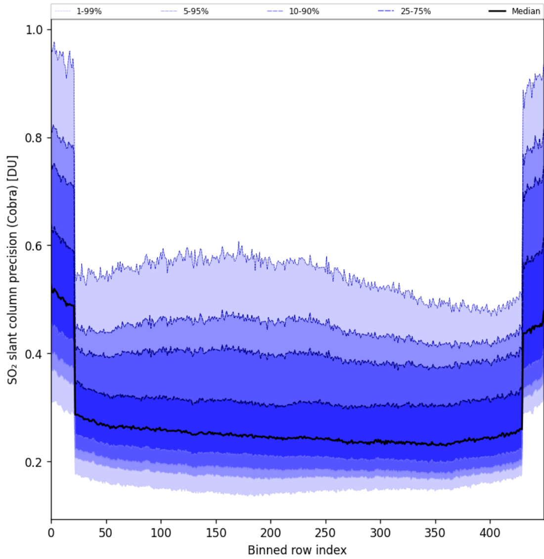
Figure 88: Along track statistics of “SO 2 slant column precision (Cobra)” for 2025-11-20 to 2025-11-22
