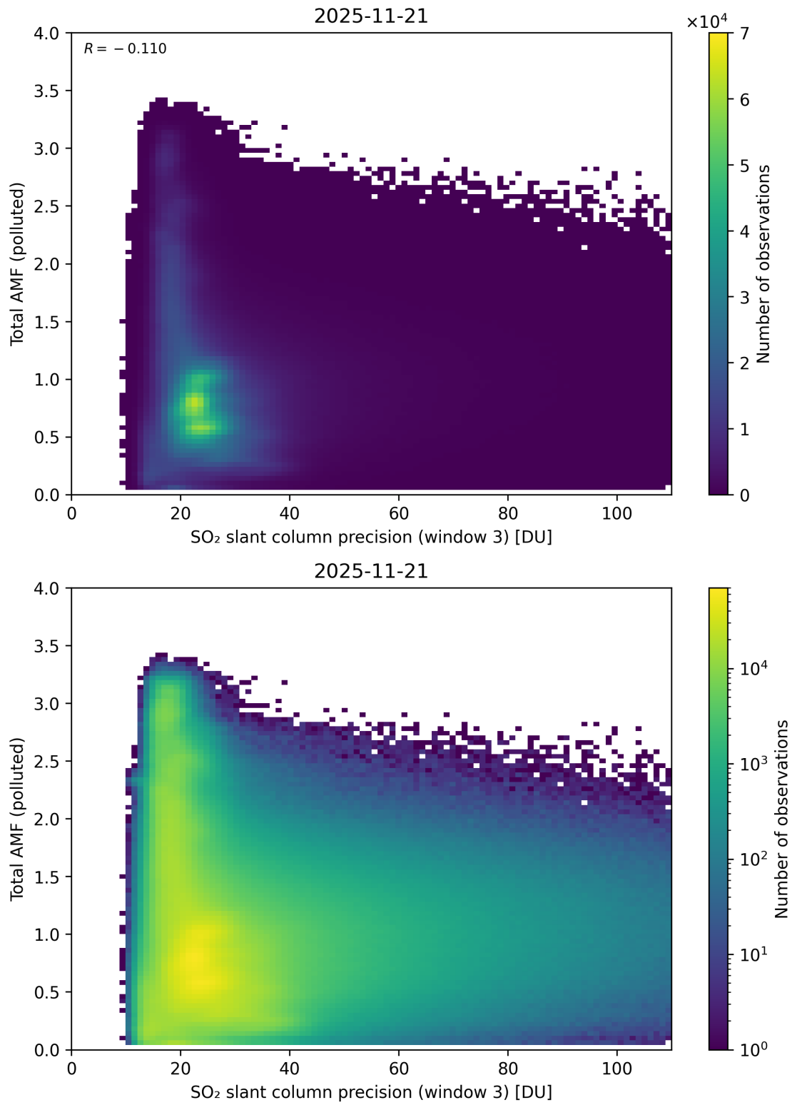
Figure 313: Scatter density plot of “SO 2 slant column precision (window 3)” against “Total AMF (polluted)” for 2025-11-20 to 2025-11-22.
