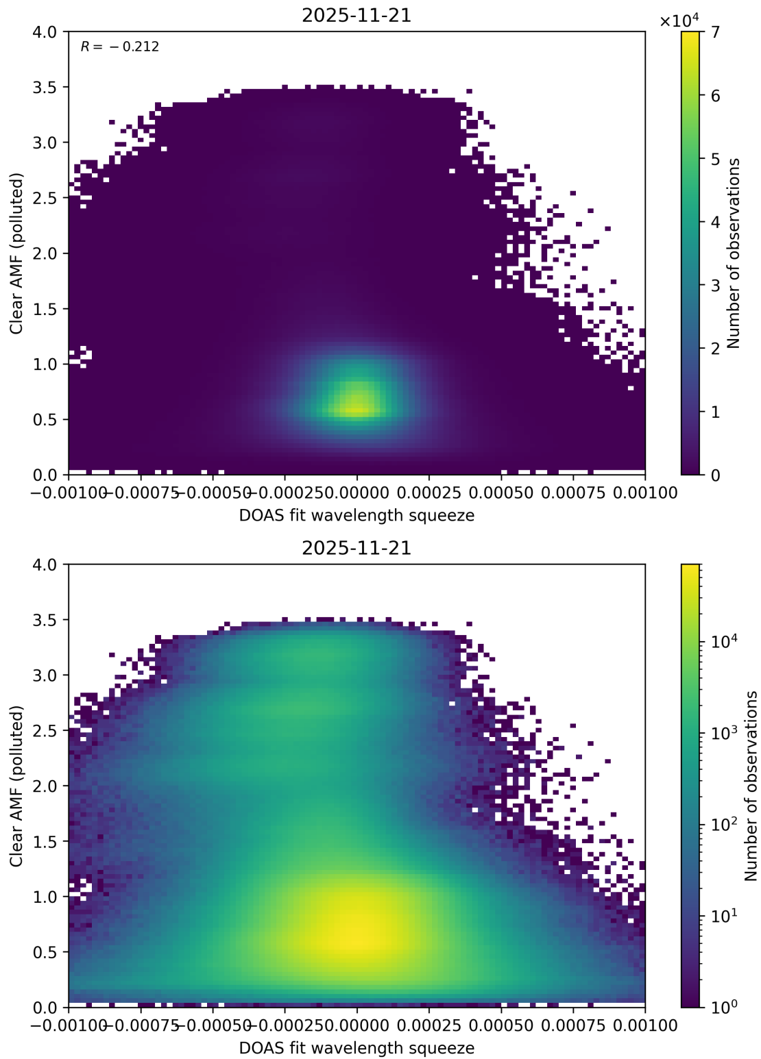
Figure 144: Scatter density plot of “DOAS fit wavelength squeeze” against “Clear AMF (polluted)” for 2025-11-20 to 2025-11-22.
