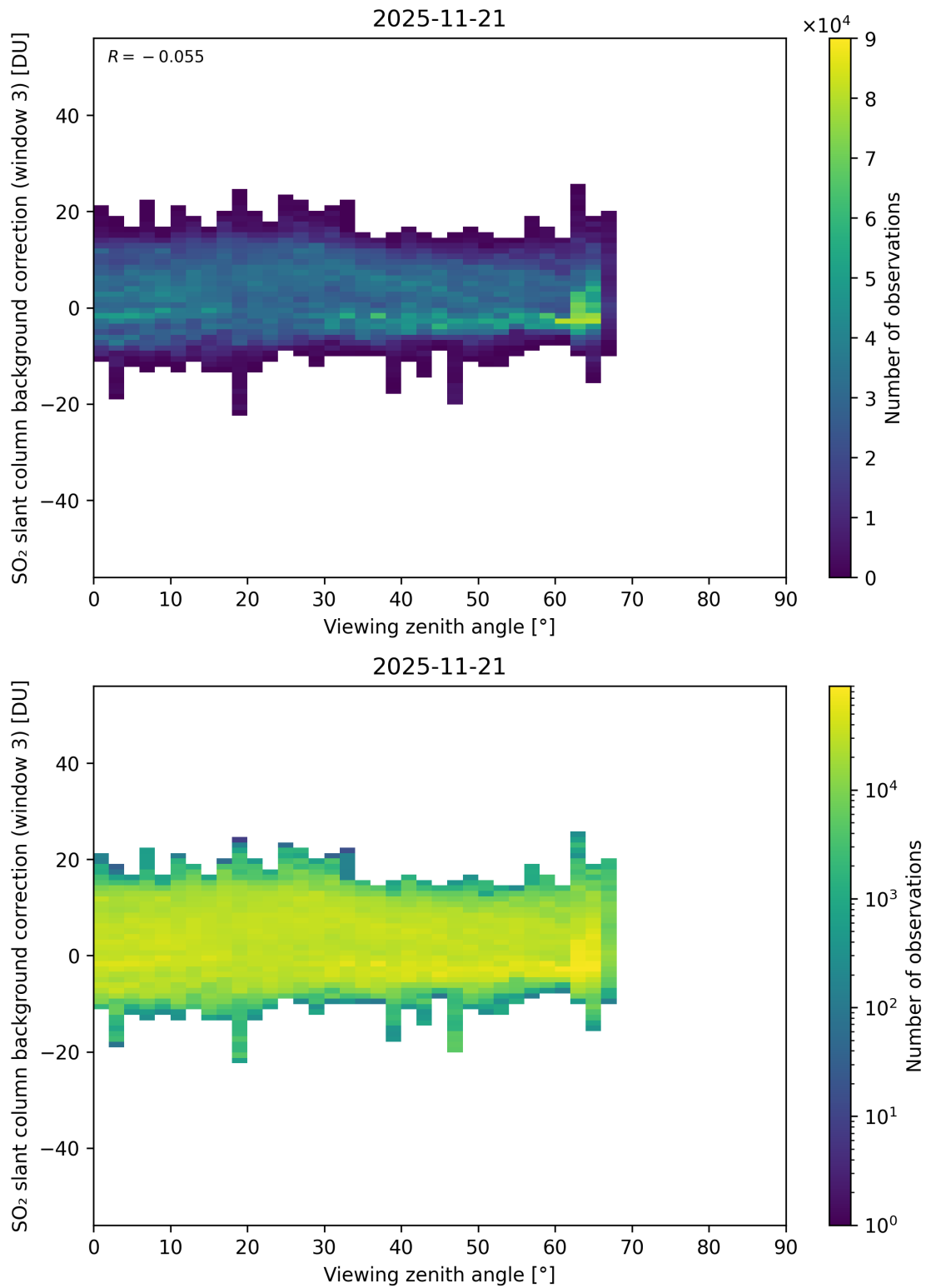
Figure 364: Scatter density plot of “Viewing zenith angle” against “SO 2 slant column background correction (window 3)” for 2025-11-20 to 2025-11-22.
