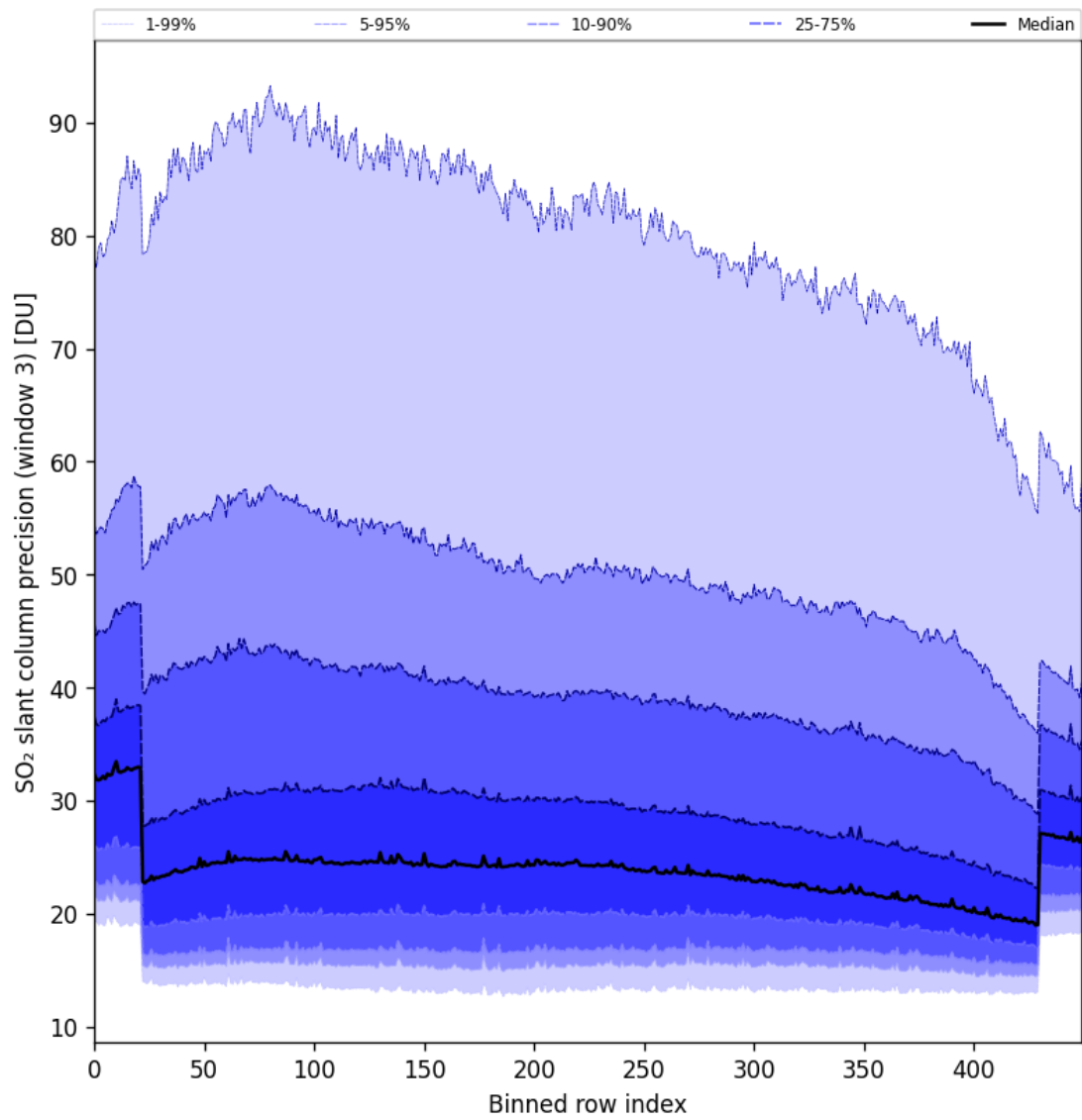
Figure 98: Along track statistics of “SO 2 slant column precision (window 3)” for 2025-11-20 to 2025-11-22
