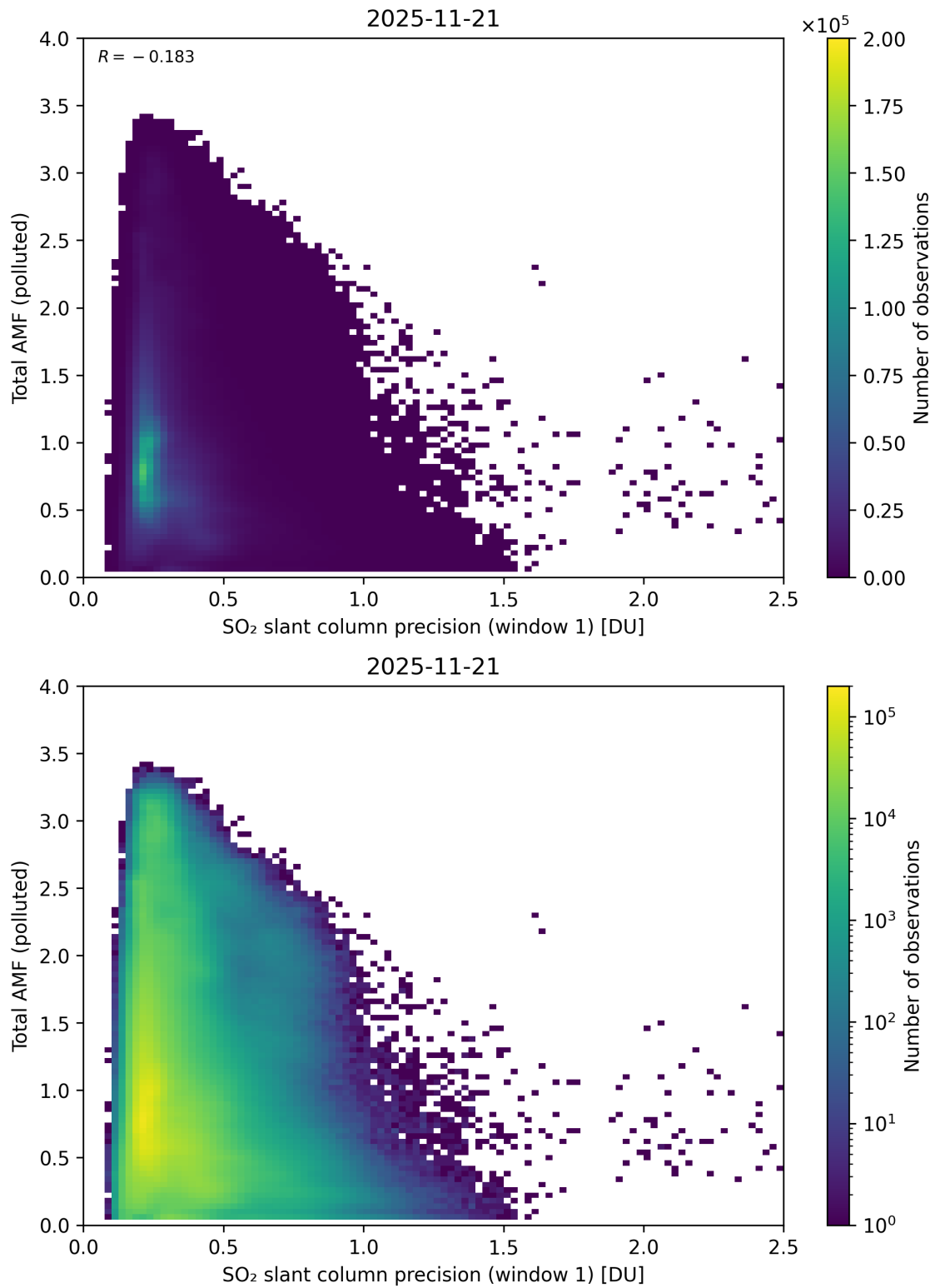
Figure 280: Scatter density plot of “SO 2 slant column precision (window 1)” against “Total AMF (polluted)” for 2025-11-20 to 2025-11-22.
