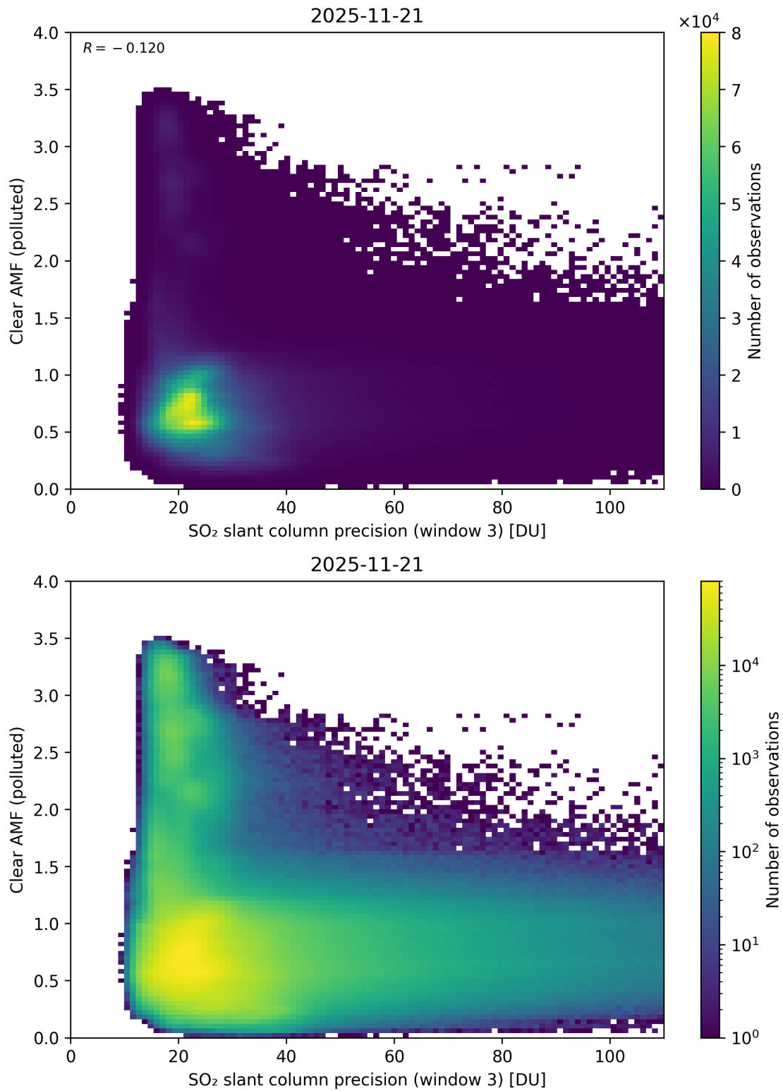
Figure 311: Scatter density plot of “SO 2 slant column precision (window 3)” against “Clear AMF (polluted)” for 2025-11-20 to 2025-11-22.
