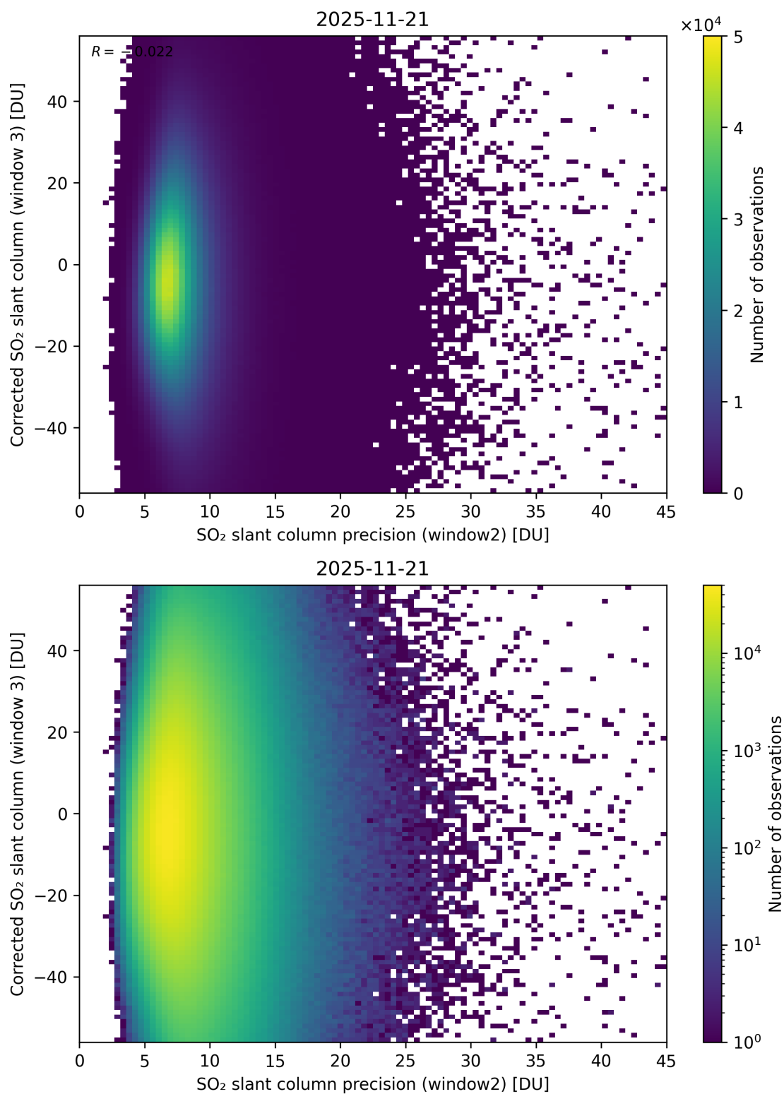
Figure 298: Scatter density plot of “SO 2 slant column precision (window2)” against “Corrected SO 2 slant column (window 3)” for 2025-11-20 to 2025-11-22.
