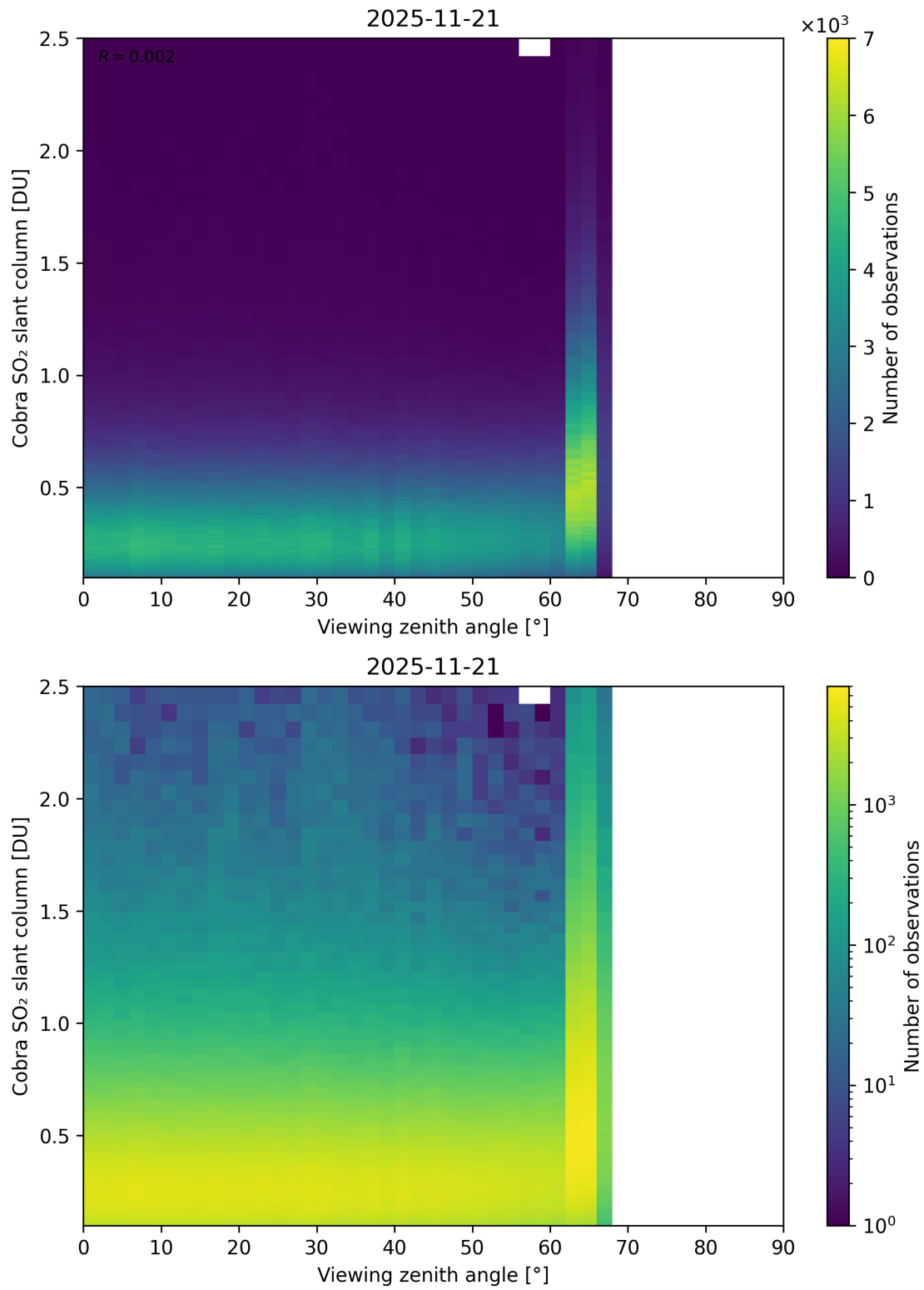
Figure 371: Scatter density plot of “Viewing zenith angle” against “Cobra SO 2 slant column” for 2025-11-20 to 2025-11-22.
