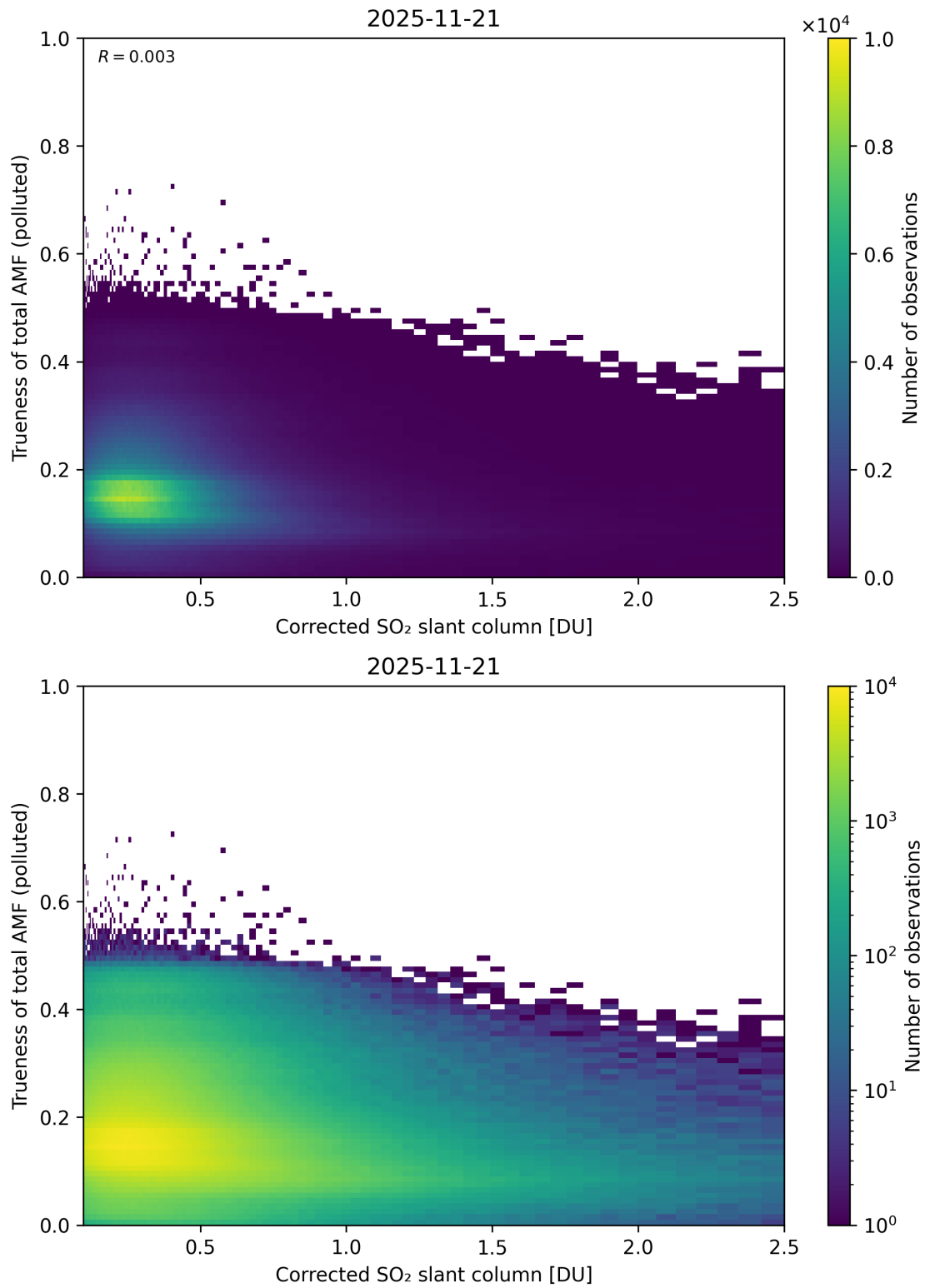
Figure 243: Scatter density plot of “Corrected SO 2 slant column” against “Trueness of total AMF (polluted)” for 2025-11-20 to 2025-11-22.
