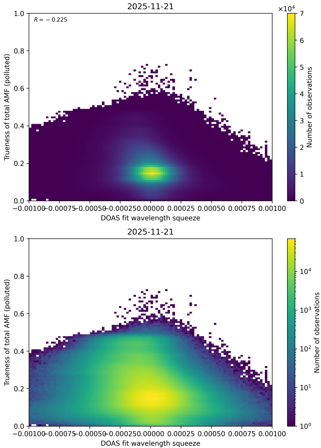
Figure 146: Scatter density plot of “DOAS fit wavelength squeeze” against “Trueness of total AMF (polluted)” for 2025-11-20 to 2025-11-22.
