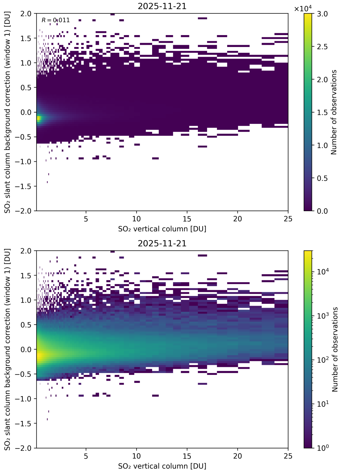
Figure 323: Scatter density plot of “SO 2 vertical column” against “SO 2 slant column background correction (window 1)” for 2025-11-20 to 2025-11-22.
