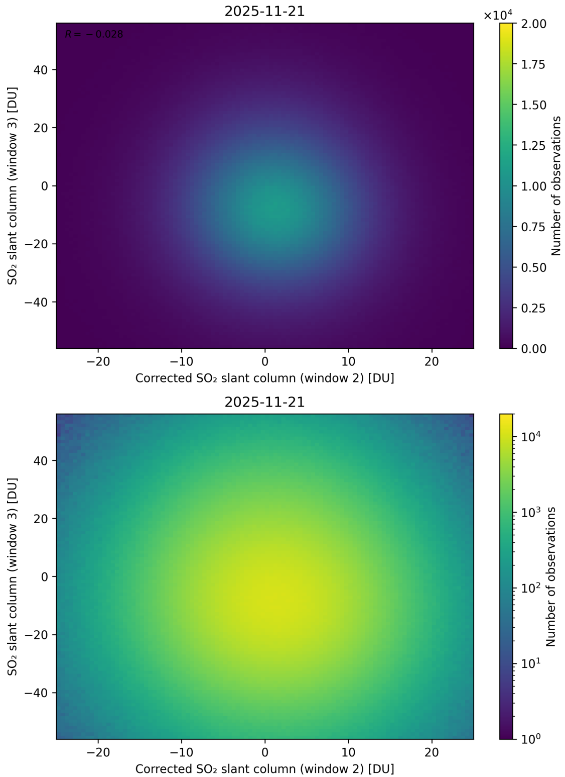
Figure 251: Scatter density plot of “Corrected SO 2 slant column (window 2)” against “SO 2 slant column (window 3)” for 2025-11-20 to 2025-11-22.
