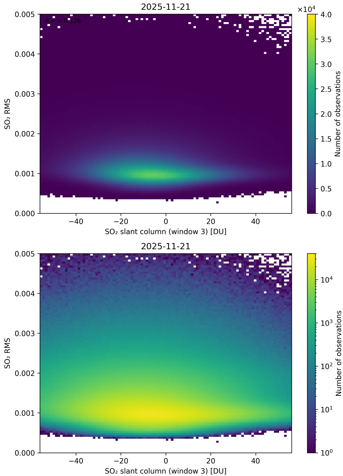
Figure 306: Scatter density plot of “SO 2 slant column (window 3)” against “SO 2 RMS” for 2025-11-20 to 2025-11-22.
