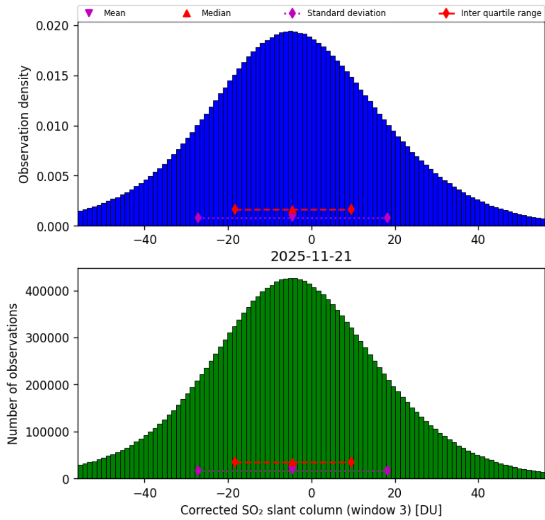
Figure 73: Histogram of “Corrected SO 2 slant column (window 3)” for 2025-11-20 to 2025-11-22
