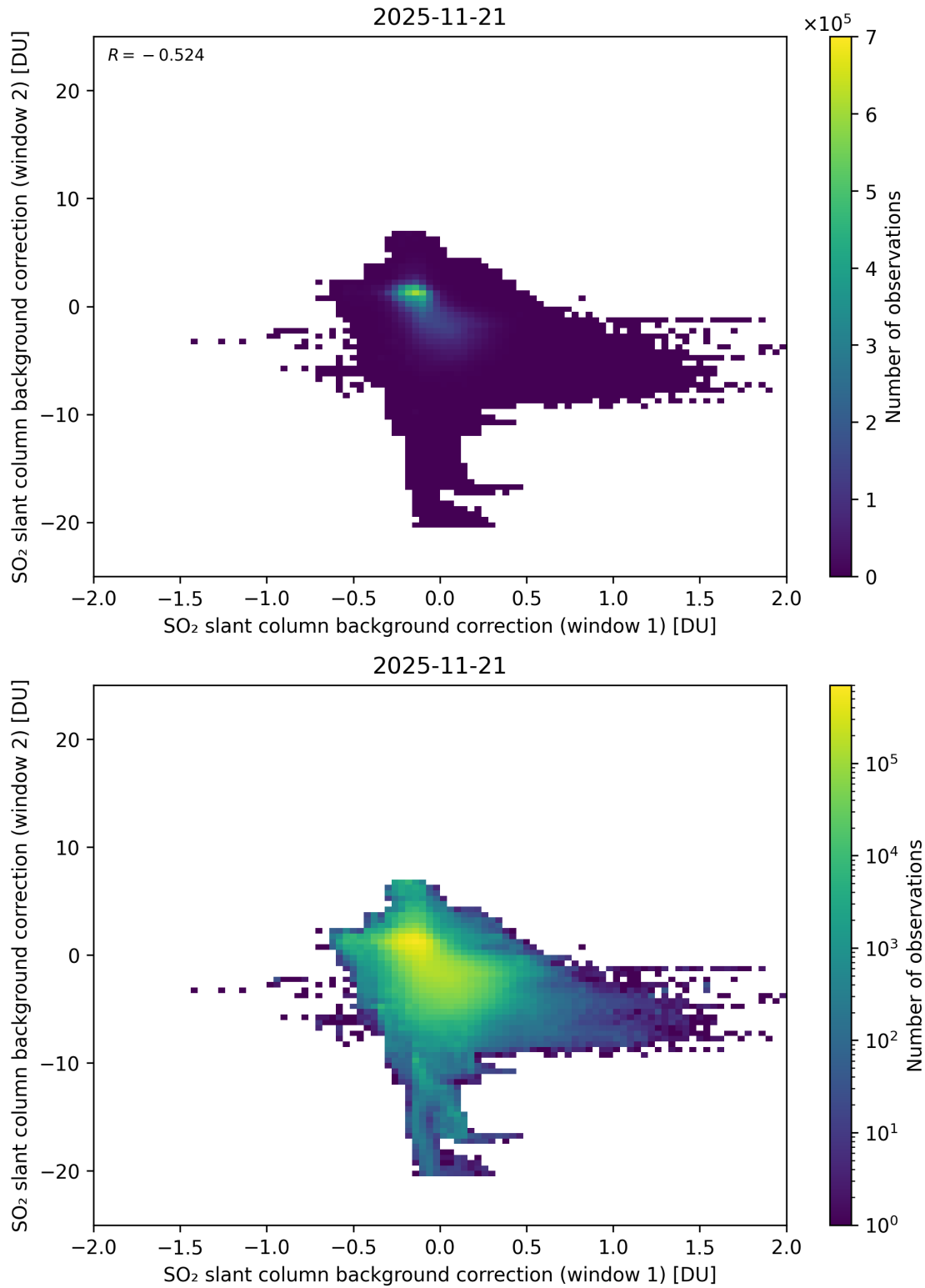
Figure 109: Scatter density plot of “SO 2 slant column background correction (window 1)” against “SO 2 slant column background correction (window 2)” for 2025-11-20 to 2025-11-22.
