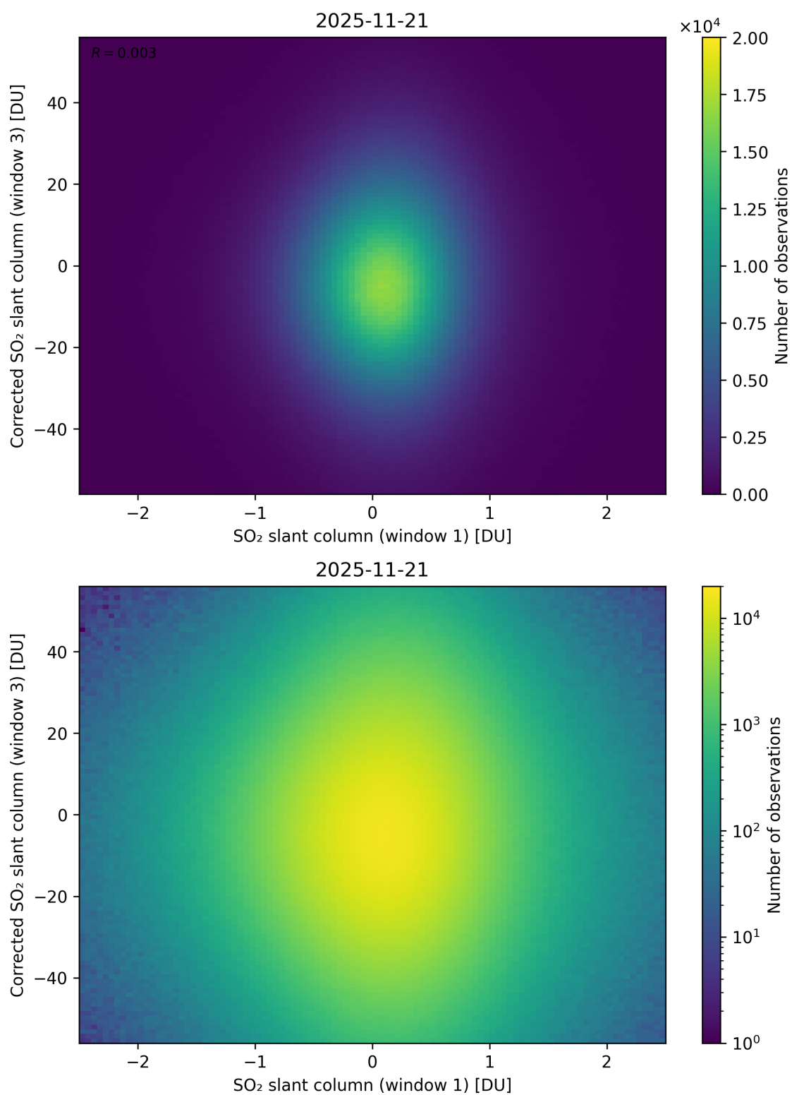
Figure 284: Scatter density plot of “SO 2 slant column (window 1)” against “Corrected SO 2 slant column (window 3)” for 2025-11-20 to 2025-11-22.
