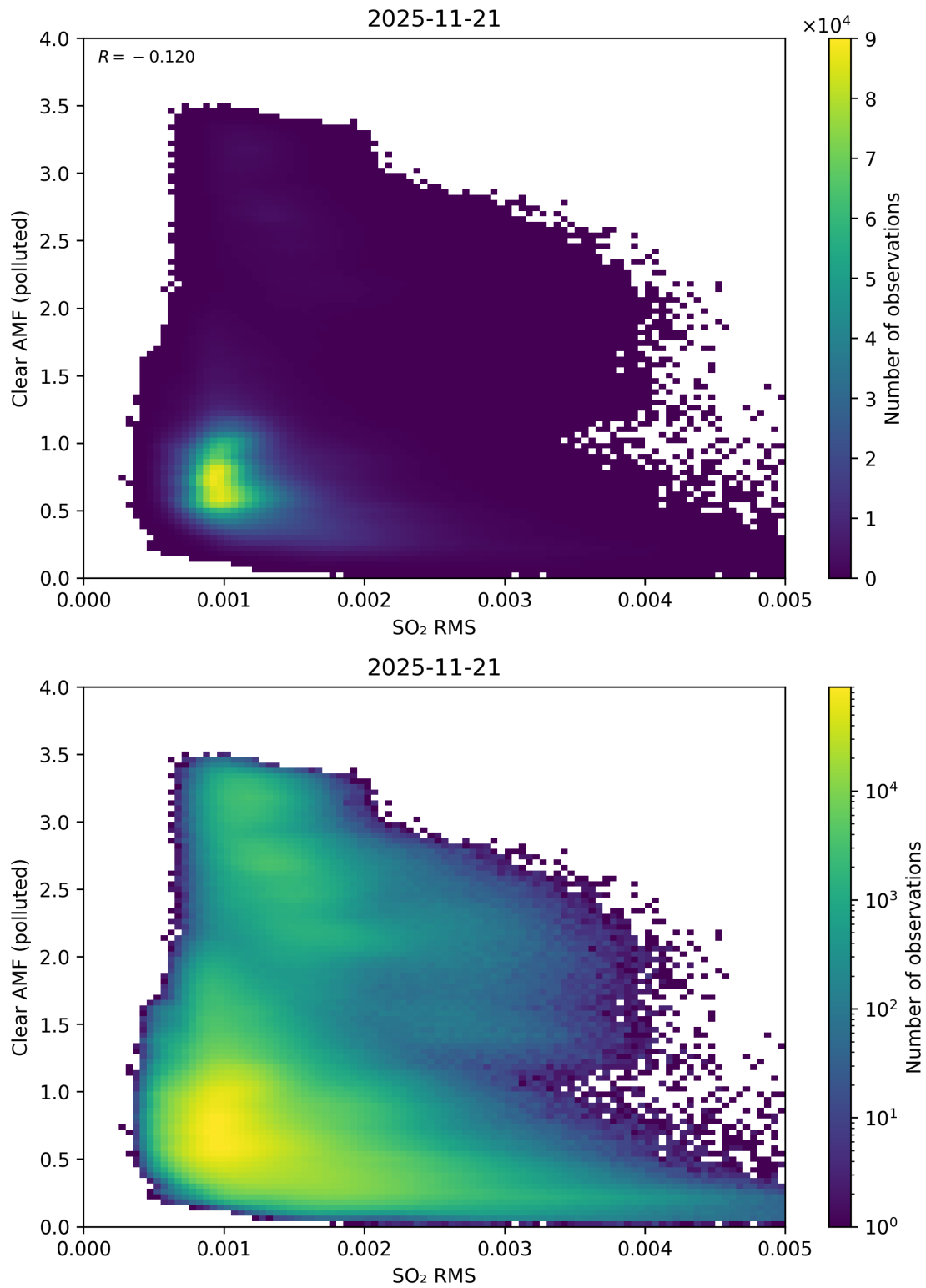
Figure 147: Scatter density plot of “SO 2 RMS” against “Clear AMF (polluted)” for 2025-11-20 to 2025-11-22.
