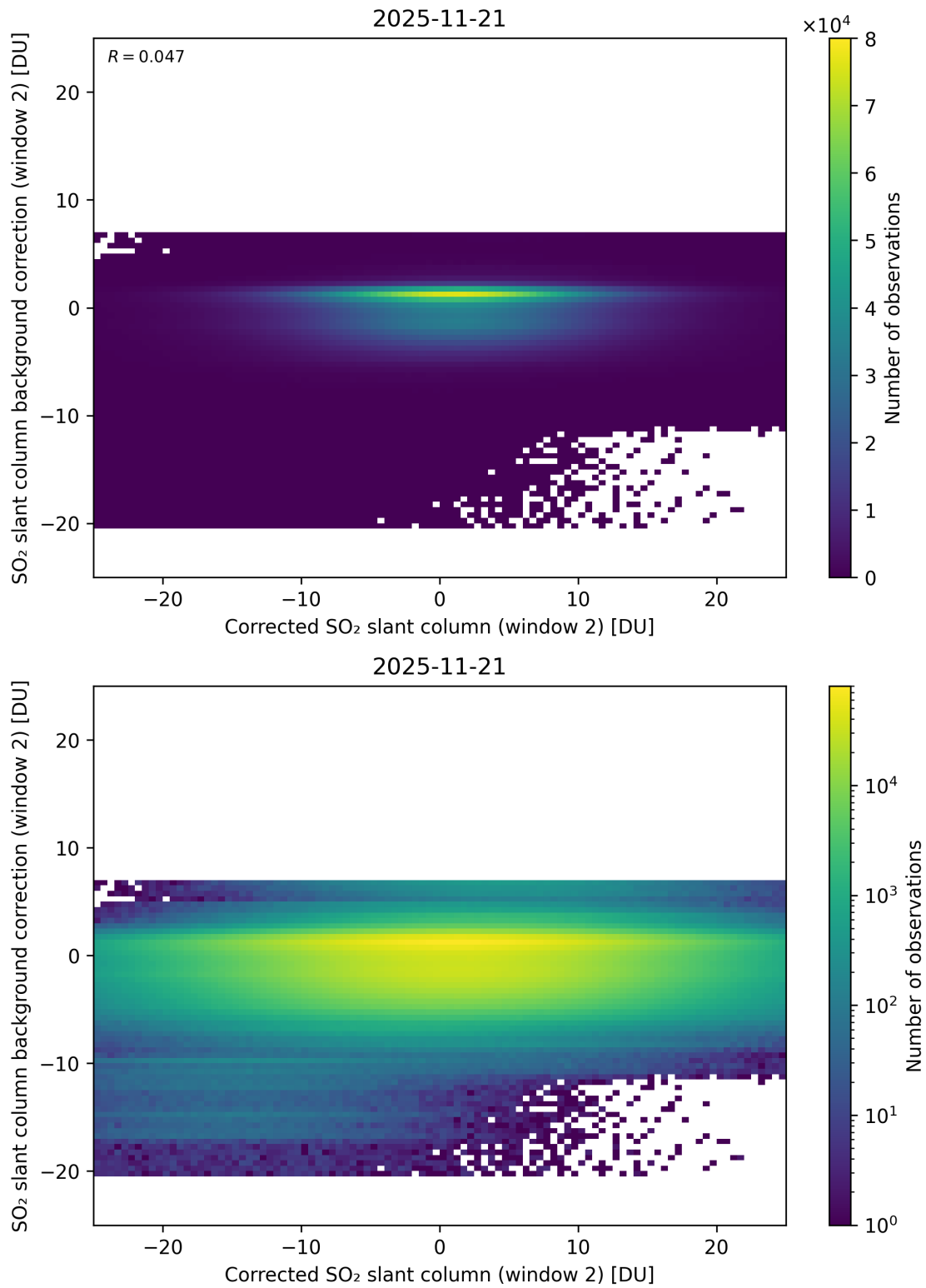
Figure 244: Scatter density plot of “Corrected SO 2 slant column (window 2)” against “SO 2 slant column background correction (window 2)” for 2025-11-20 to 2025-11-22.
