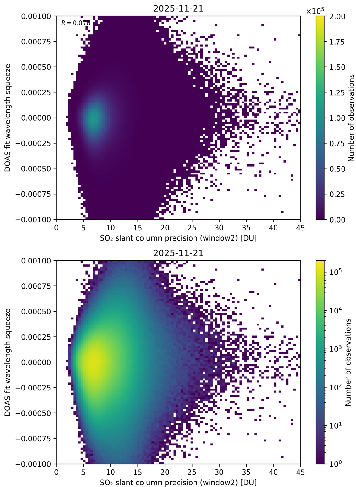
Figure 294: Scatter density plot of “SO 2 slant column precision (window2)” against “DOAS fit wavelength squeeze” for 2025-11-20 to 2025-11-22.
