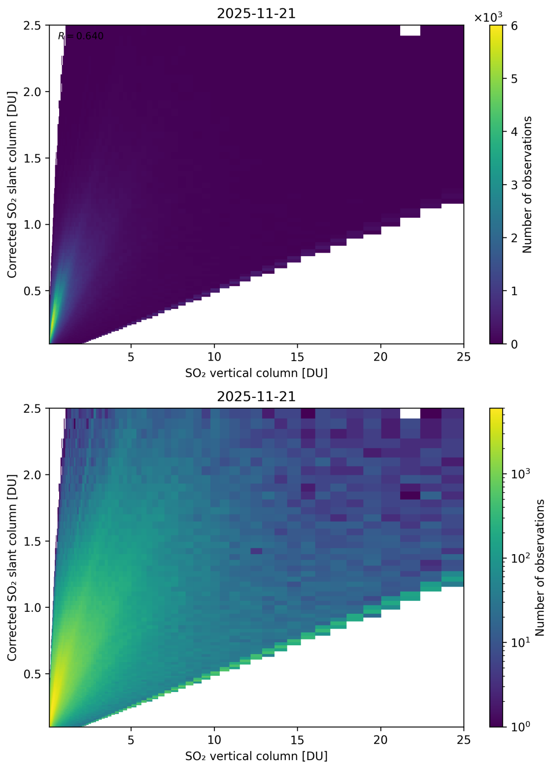
Figure 351: Scatter density plot of “SO 2 vertical column” against “Corrected SO 2 slant column” for 2025-11-20 to 2025-11-22.
