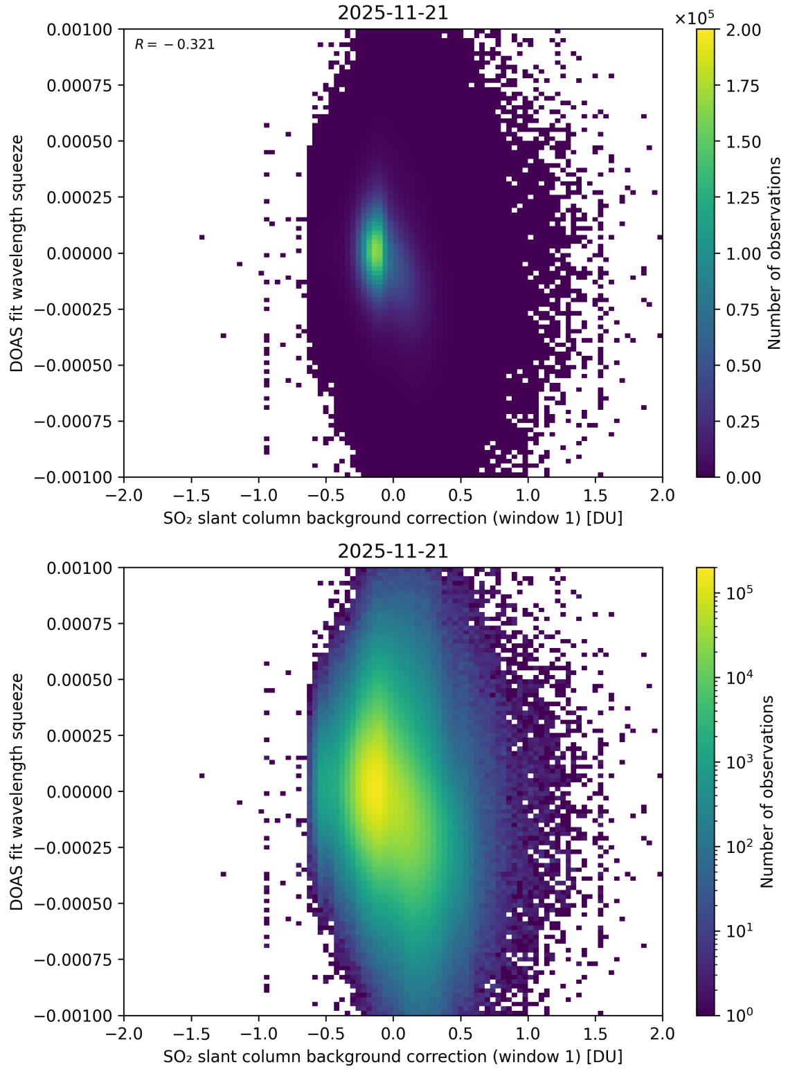
Figure 112: Scatter density plot of “SO 2 slant column background correction (window 1)” against “DOAS fit wavelength squeeze” for 2025-11-20 to 2025-11-22.
