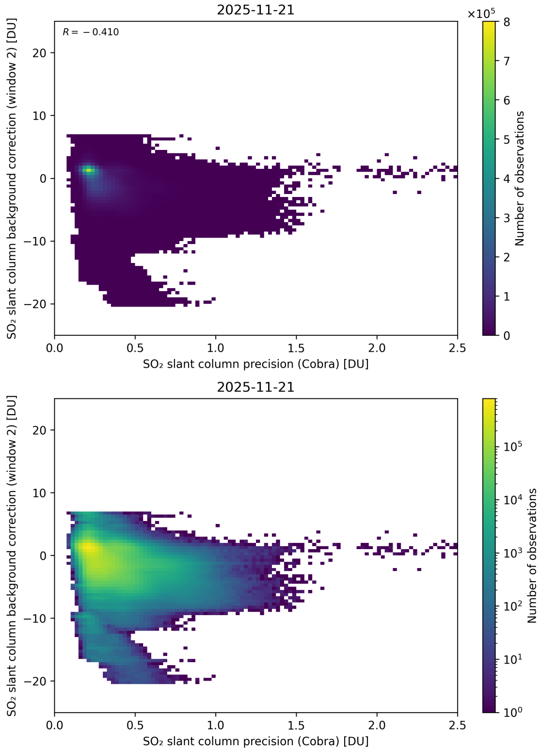
Figure 200: Scatter density plot of “SO 2 slant column precision (Cobra)” against “SO 2 slant column background correction (window 2)” for 2025-11-20 to 2025-11-22.
