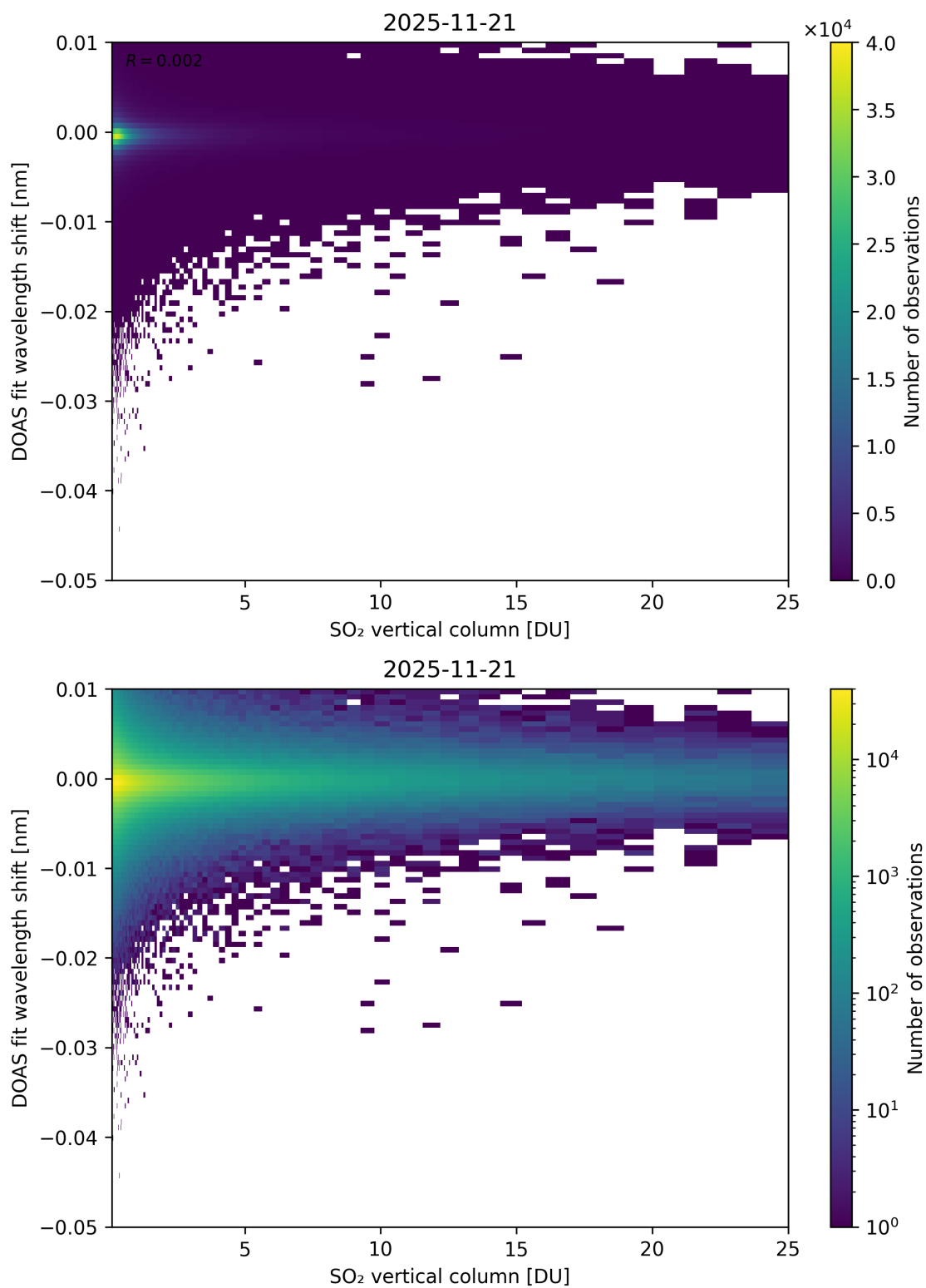
Figure 326: Scatter density plot of “SO 2 vertical column” against “DOAS fit wavelength shift” for 2025-11-20 to 2025-11-22.
