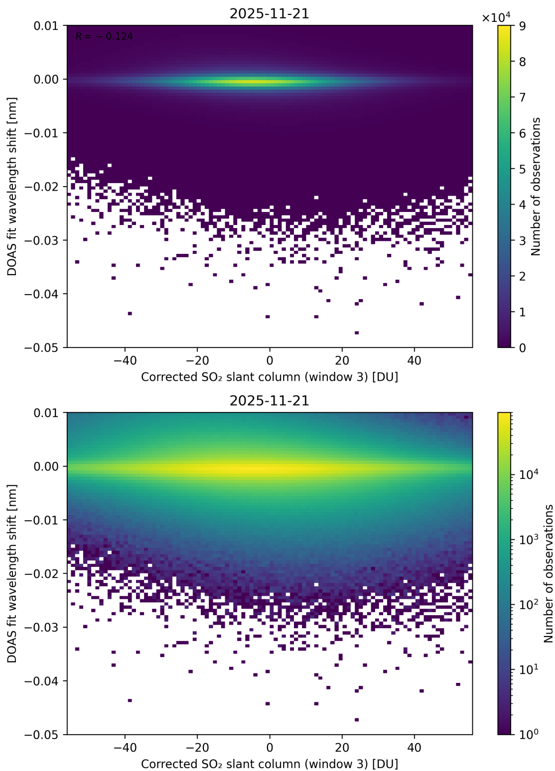
Figure 256: Scatter density plot of “Corrected SO 2 slant column (window 3)” against “DOAS fit wavelength shift” for 2025-11-20 to 2025-11-22.
