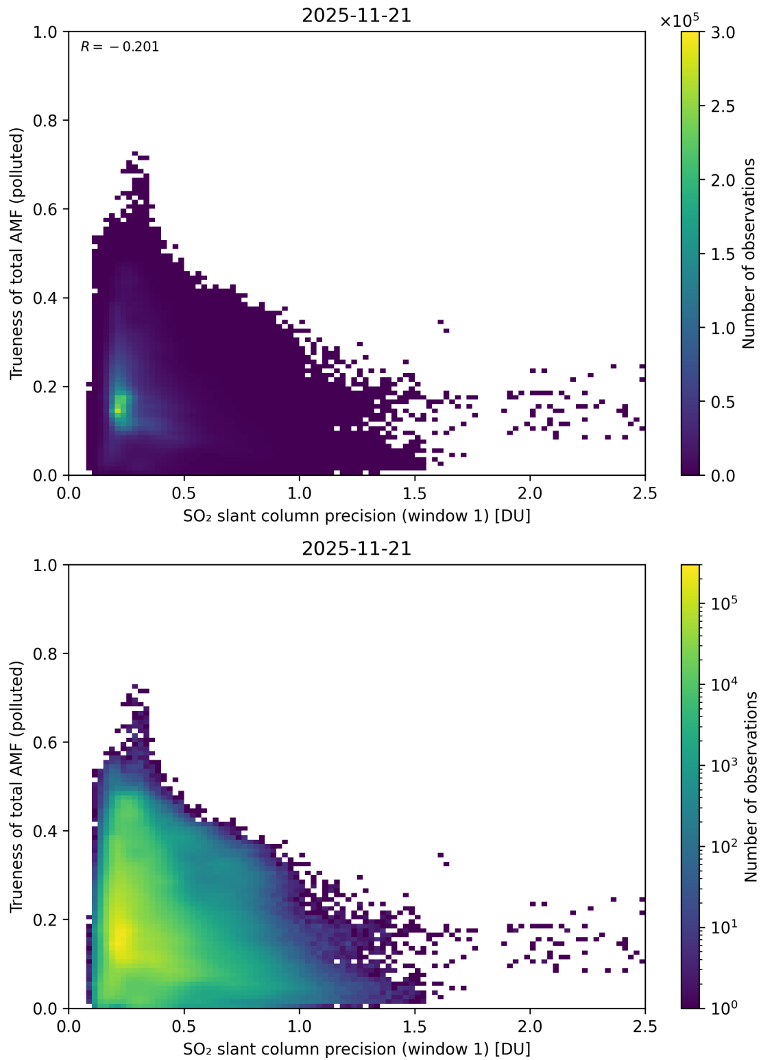
Figure 281: Scatter density plot of “SO 2 slant column precision (window 1)” against “Trueness of total AMF (polluted)” for 2025-11-20 to 2025-11-22.
