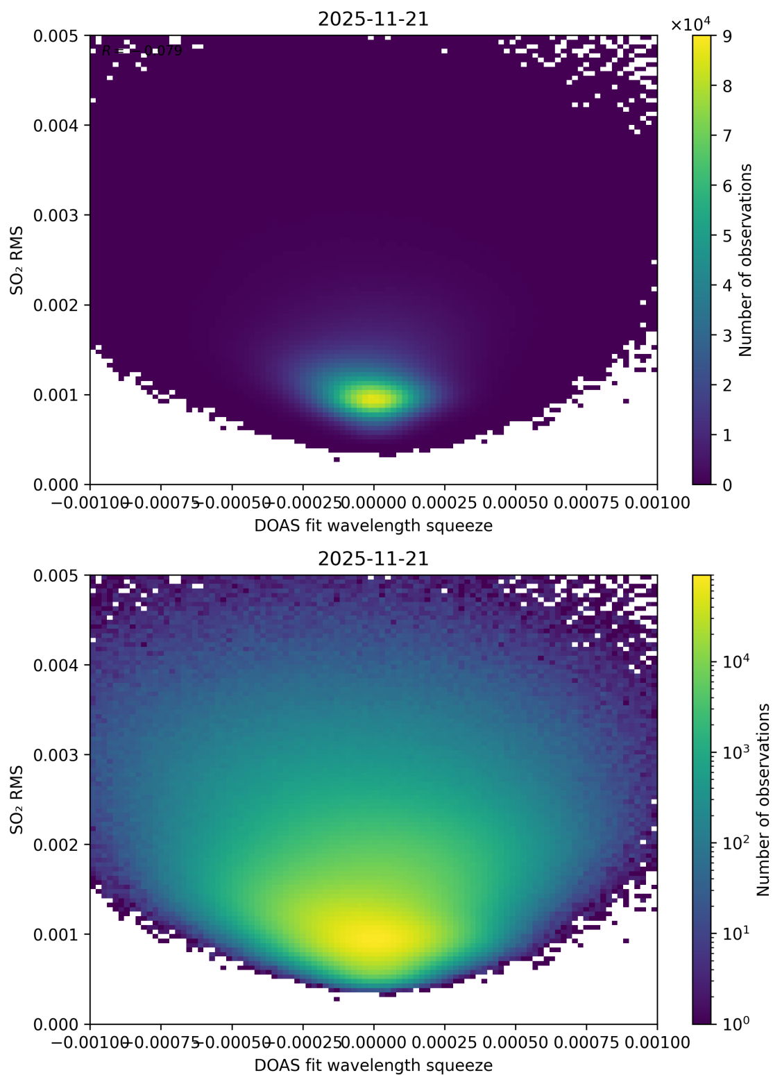
Figure 143: Scatter density plot of “DOAS fit wavelength squeeze” against “SO 2 RMS” for 2025-11-20 to 2025-11-22.
