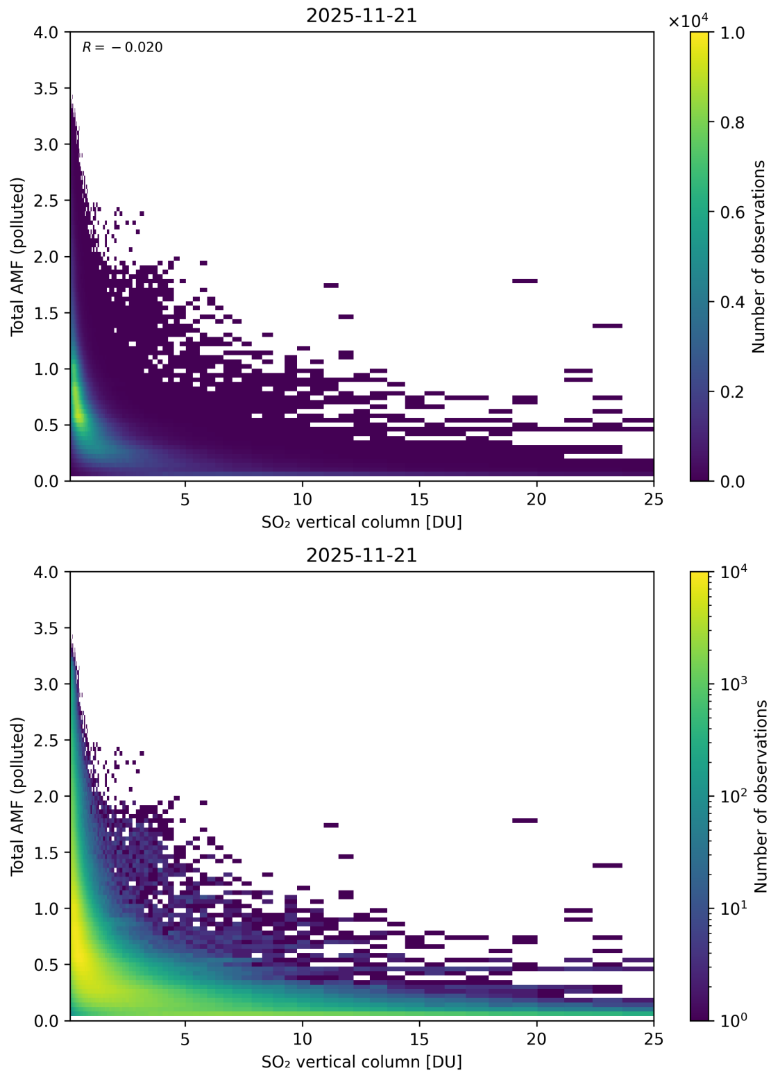
Figure 359: Scatter density plot of “SO 2 vertical column” against “Total AMF (polluted)” for 2025-11-20 to 2025-11-22.
