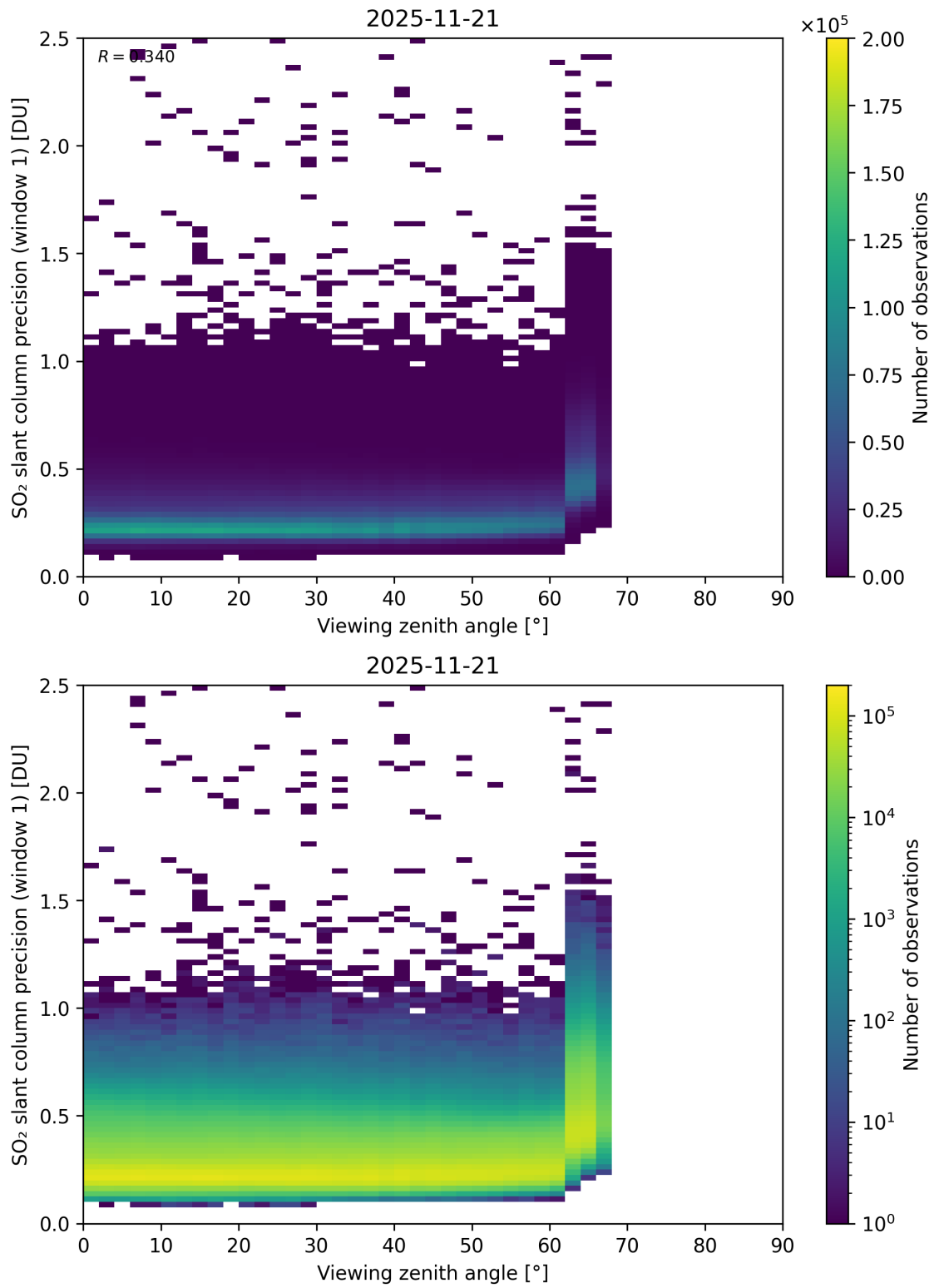
Figure 377: Scatter density plot of “Viewing zenith angle” against “SO 2 slant column precision (window 1)” for 2025-11-20 to 2025-11-22.
