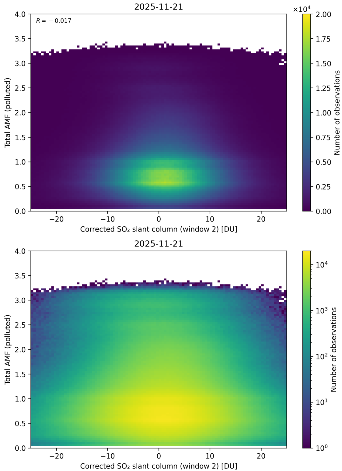
Figure 253: Scatter density plot of “Corrected SO 2 slant column (window 2)” against “Total AMF (polluted)” for 2025-11-20 to 2025-11-22.
