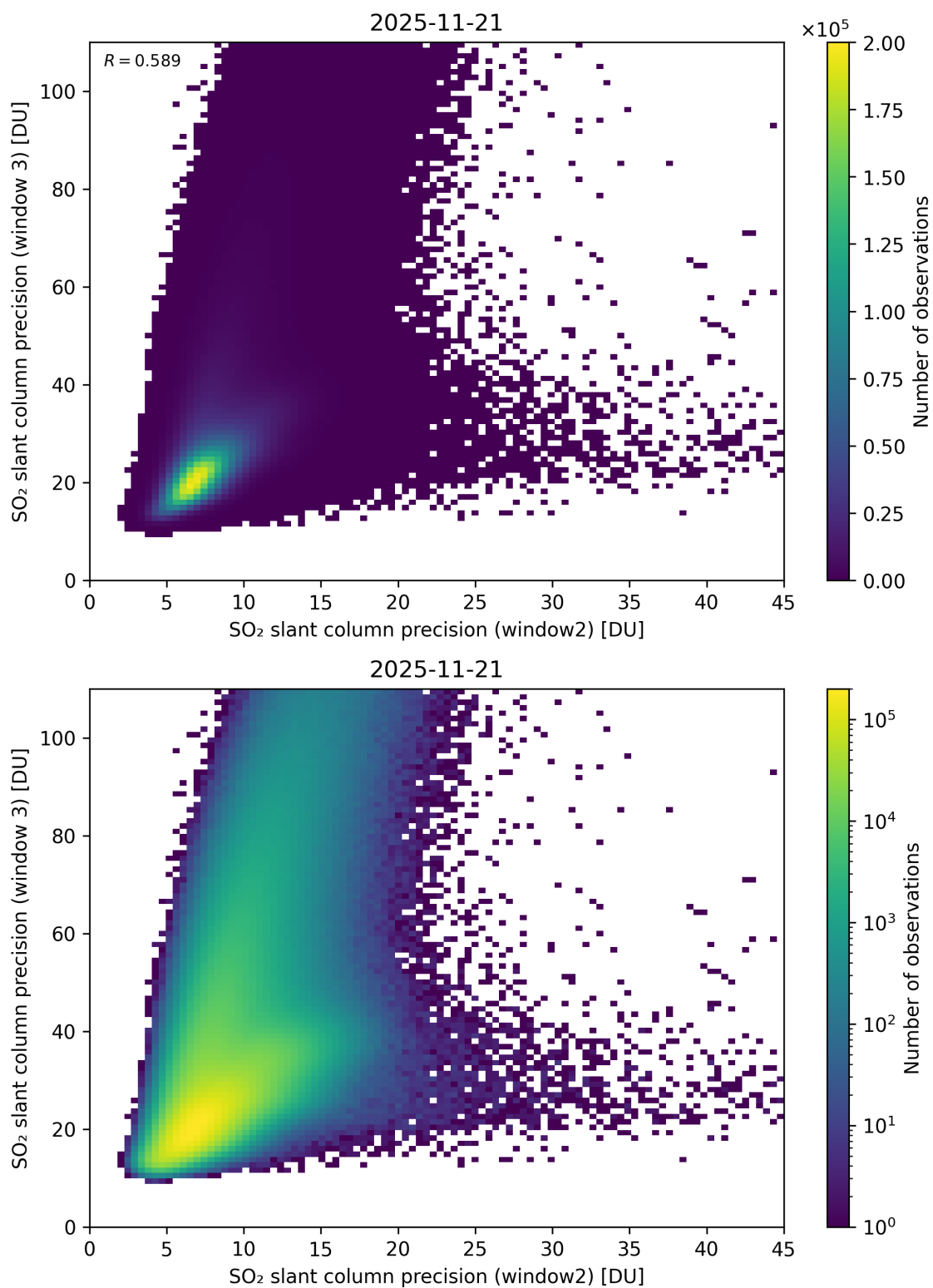
Figure 300: Scatter density plot of “SO 2 slant column precision (window2)” against “SO 2 slant column precision (window 3)” for 2025-11-20 to 2025-11-22.
