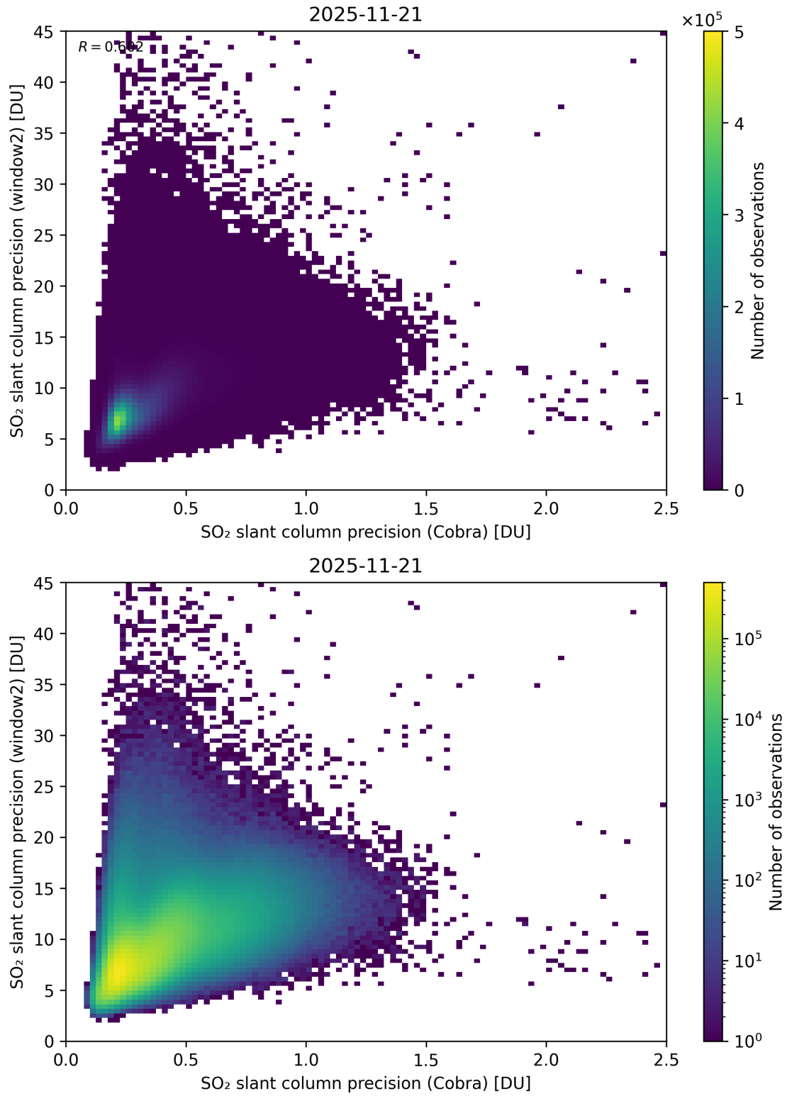
Figure 210: Scatter density plot of “SO 2 slant column precision (Cobra)” against “SO 2 slant column precision (window2)” for 2025-11-20 to 2025-11-22.
