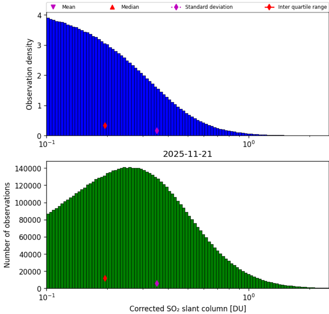
Figure 60: Histogram of “Corrected SO 2 slant column” for 2025-11-20 to 2025-11-22
