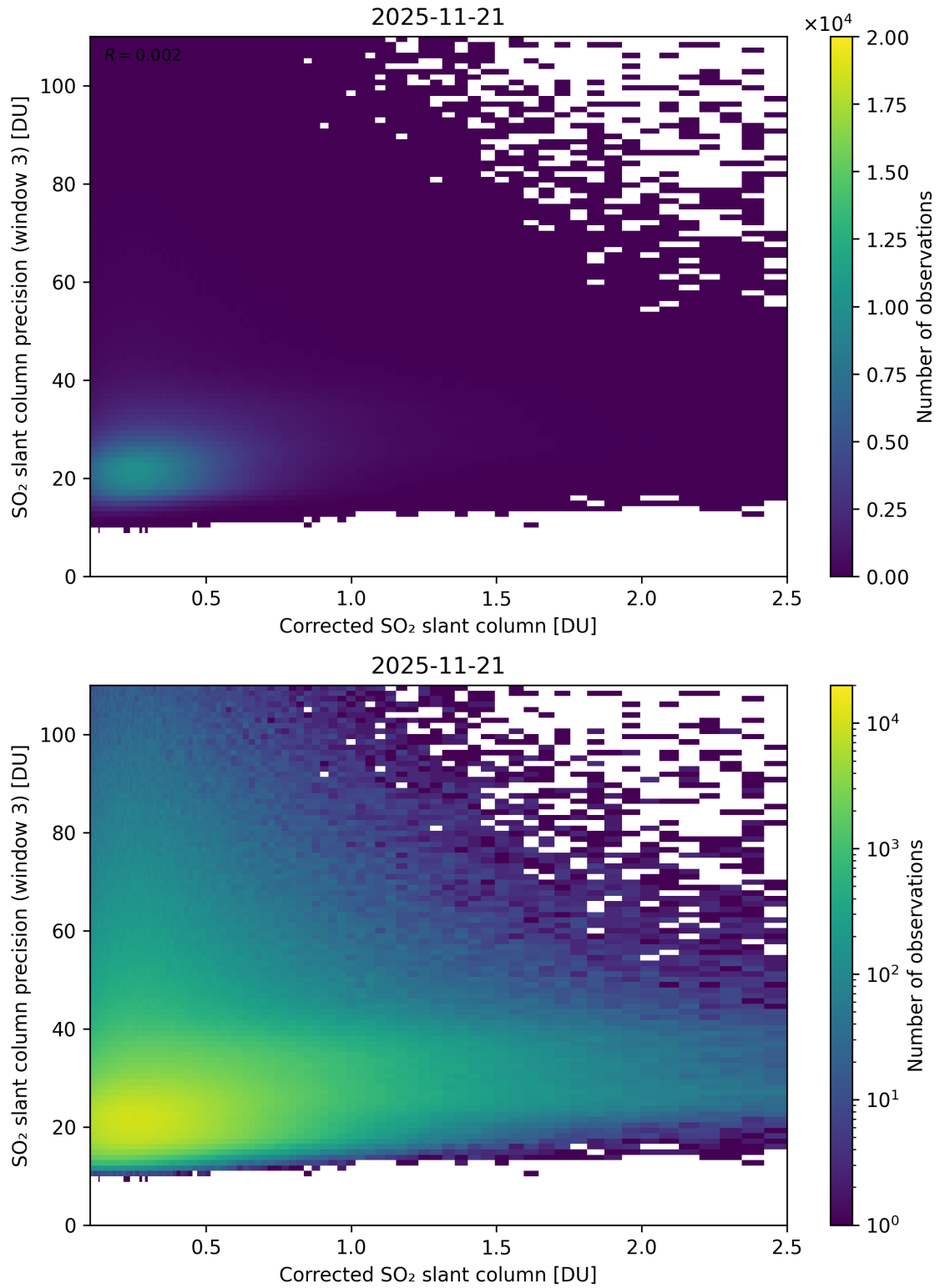
Figure 241: Scatter density plot of “Corrected SO 2 slant column” against “SO 2 slant column precision (window 3)” for 2025-11-20 to 2025-11-22.
