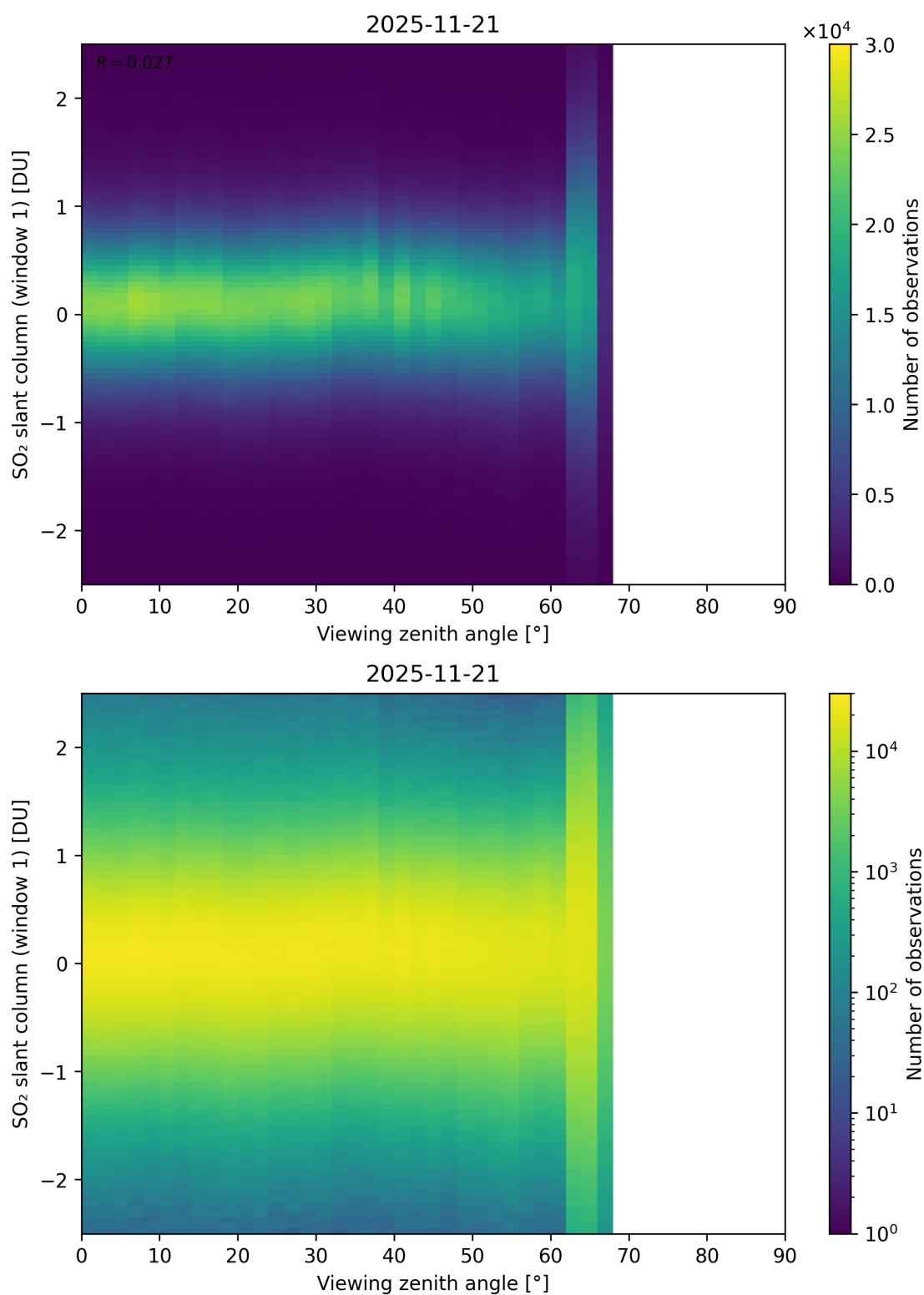
Figure 376: Scatter density plot of “Viewing zenith angle” against “SO 2 slant column (window 1)” for 2025-11-20 to 2025-11-22.
