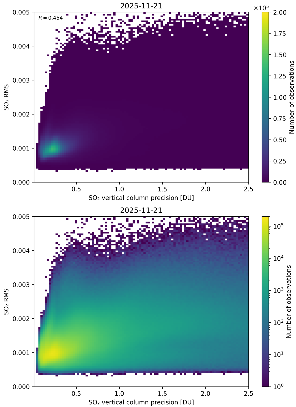
Figure 334: Scatter density plot of “SO 2 vertical column precision” against “SO 2 RMS” for 2025-11-20 to 2025-11-22.
