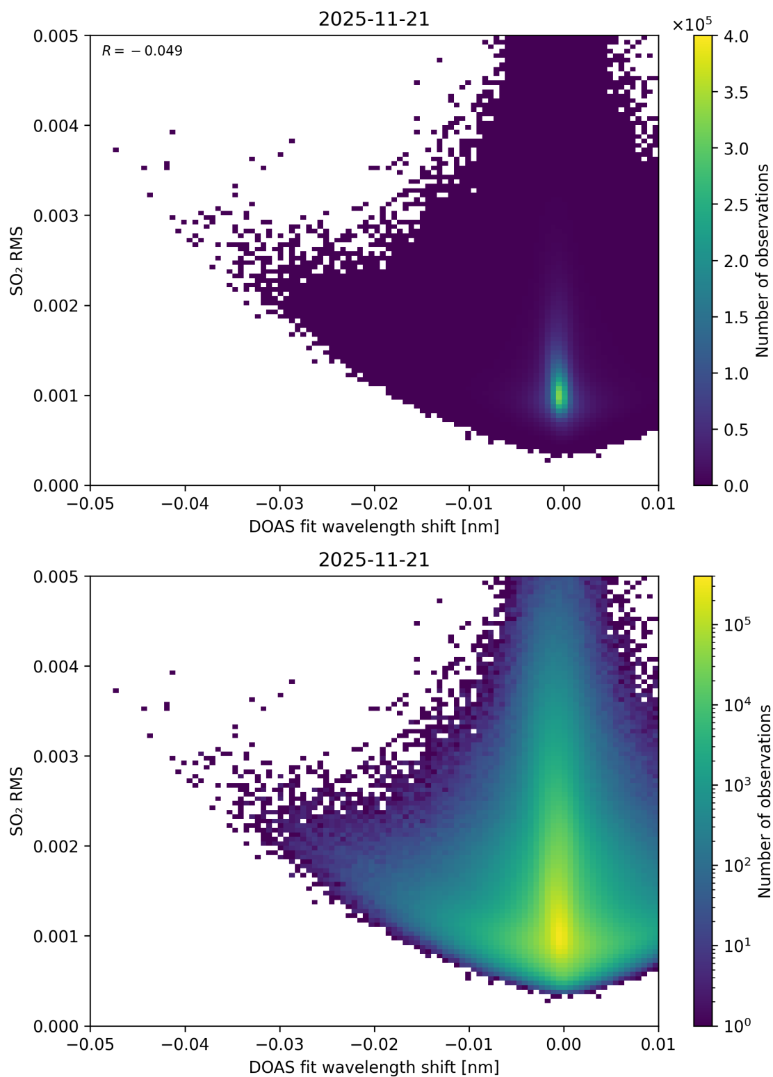
Figure 139: Scatter density plot of “DOAS fit wavelength shift” against “SO 2 RMS” for 2025-11-20 to 2025-11-22.
