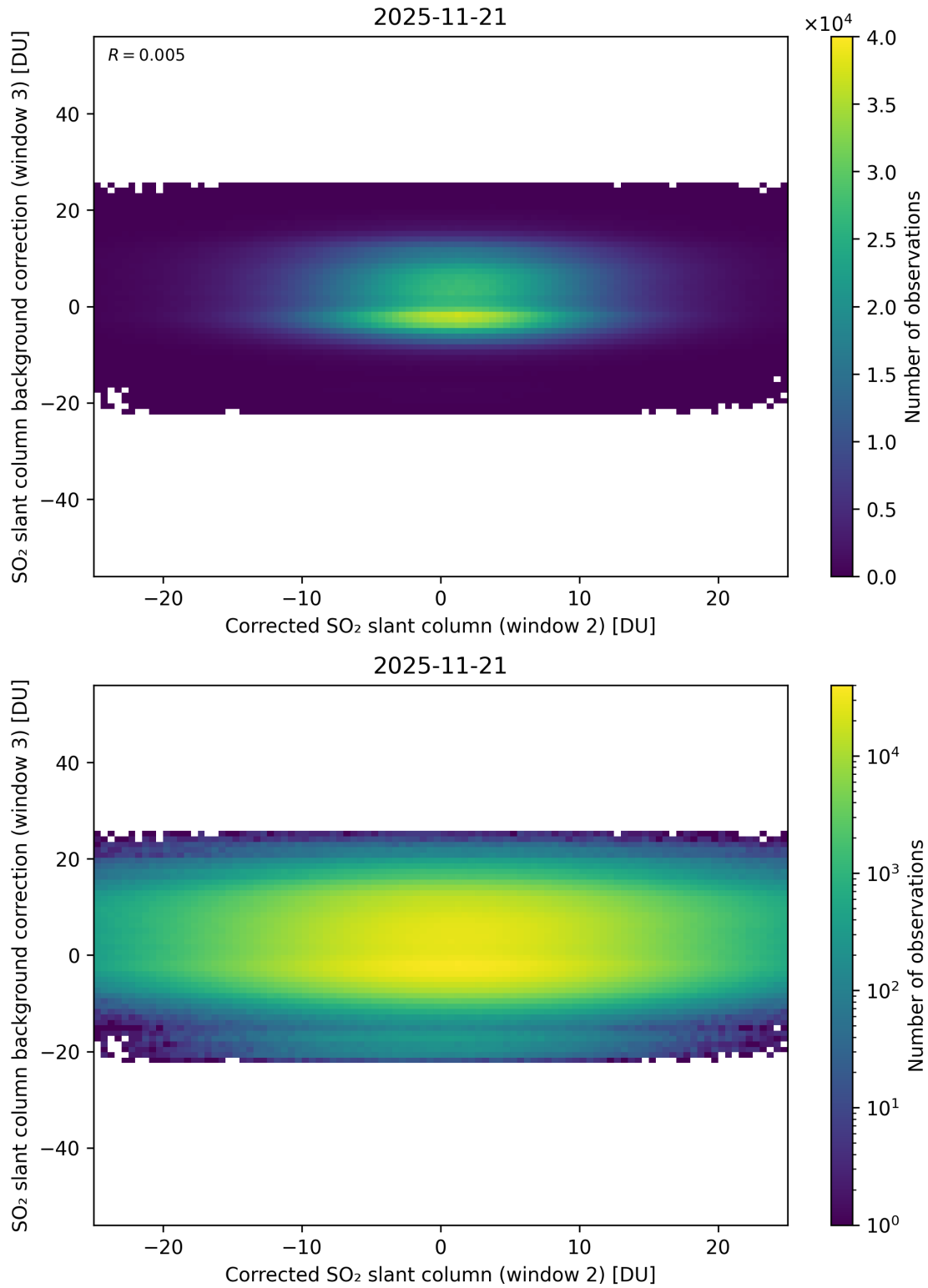
Figure 245: Scatter density plot of “Corrected SO 2 slant column (window 2)” against “SO 2 slant column background correction (window 3)” for 2025-11-20 to 2025-11-22.
