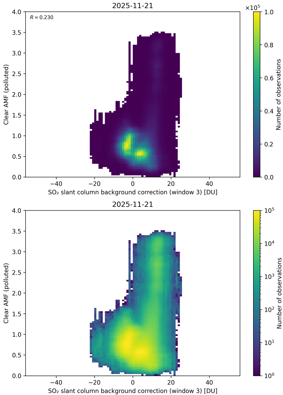
Figure 135: Scatter density plot of “SO 2 slant column background correction (window 3)” against “Clear AMF (polluted)” for 2025-11-20 to 2025-11-22.
