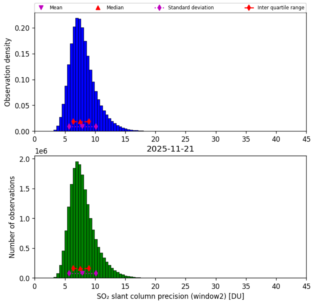
Figure 68: Histogram of “SO 2 slant column precision (window2)” for 2025-11-20 to 2025-11-22
