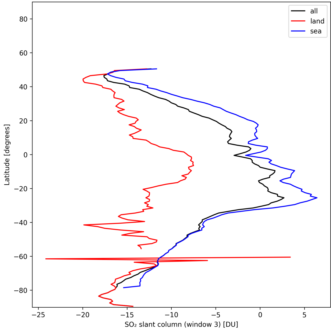
Figure 45: Zonal average of “SO 2 slant column (window 3)” for 2025-11-20 to 2025-11-22.
