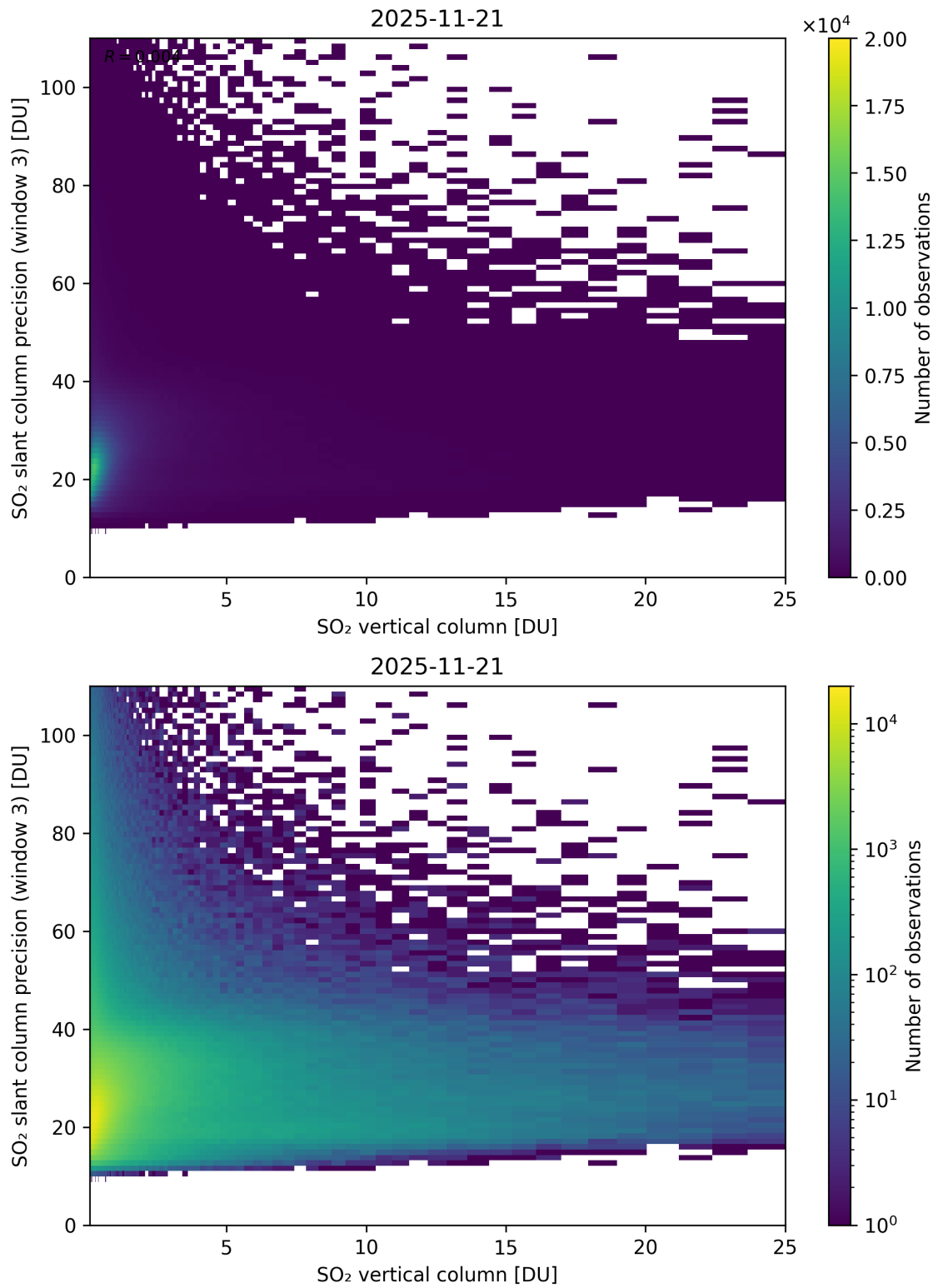
Figure 358: Scatter density plot of “SO 2 vertical column” against “SO 2 slant column precision (window 3)” for 2025-11-20 to 2025-11-22.
