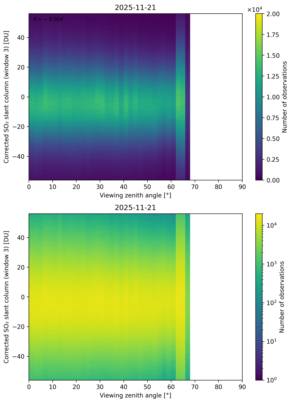
Figure 375: Scatter density plot of “Viewing zenith angle” against “Corrected SO 2 slant column (window 3)” for 2025-11-20 to 2025-11-22.
