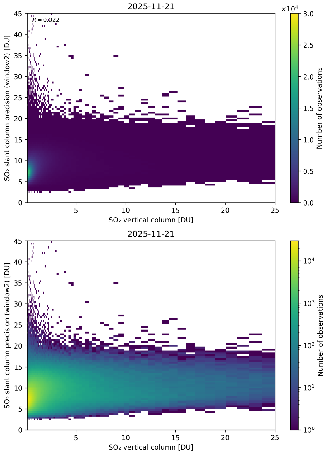
Figure 356: Scatter density plot of “SO 2 vertical column” against “SO 2 slant column precision (window2)” for 2025-11-20 to 2025-11-22.
