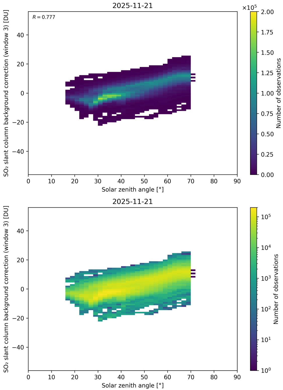
Figure 173: Scatter density plot of “Solar zenith angle” against “SO 2 slant column background correction (window 3)” for 2025-11-20 to 2025-11-22.
