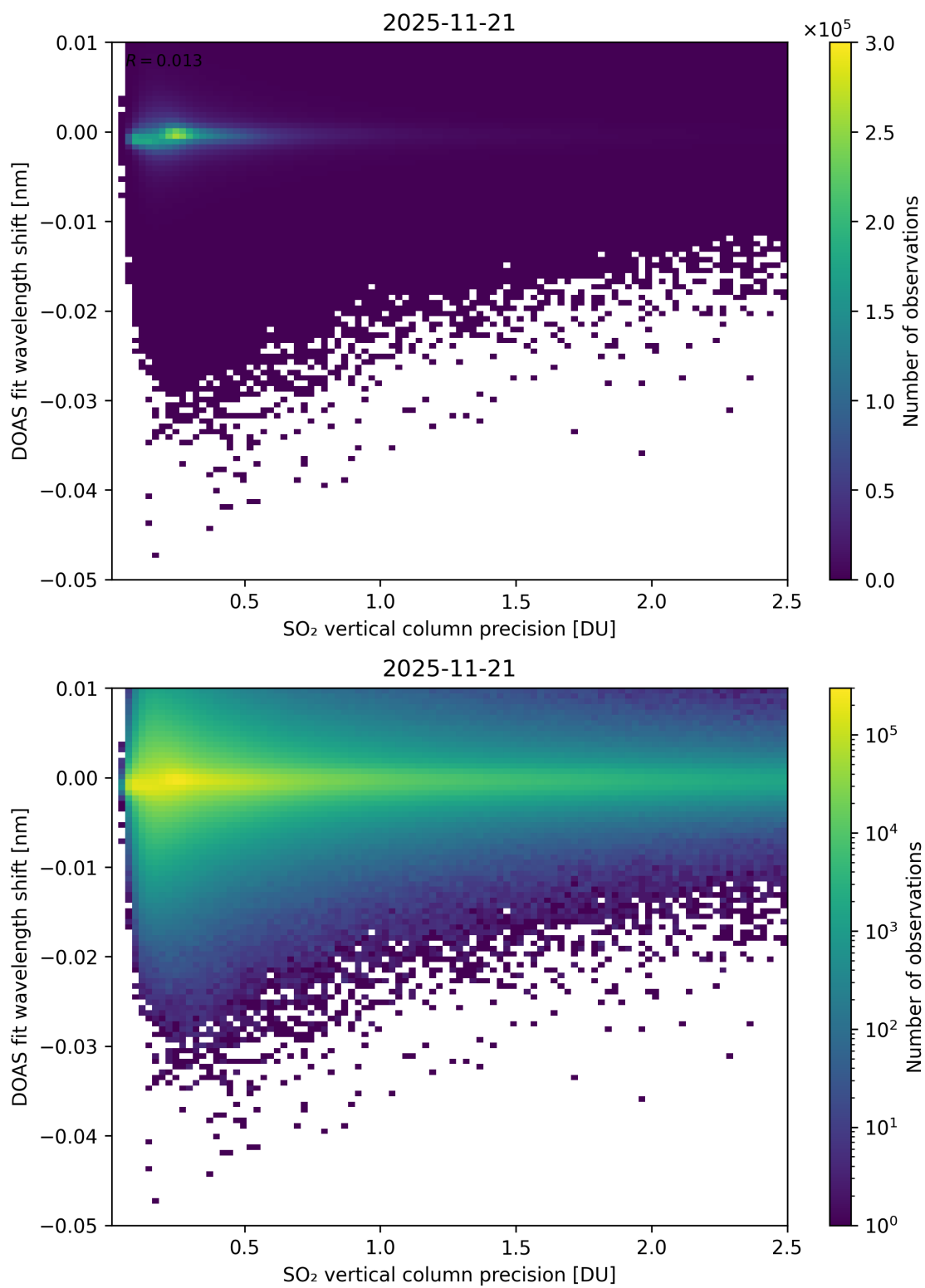
Figure 332: Scatter density plot of “SO 2 vertical column precision” against “DOAS fit wavelength shift” for 2025-11-20 to 2025-11-22.
