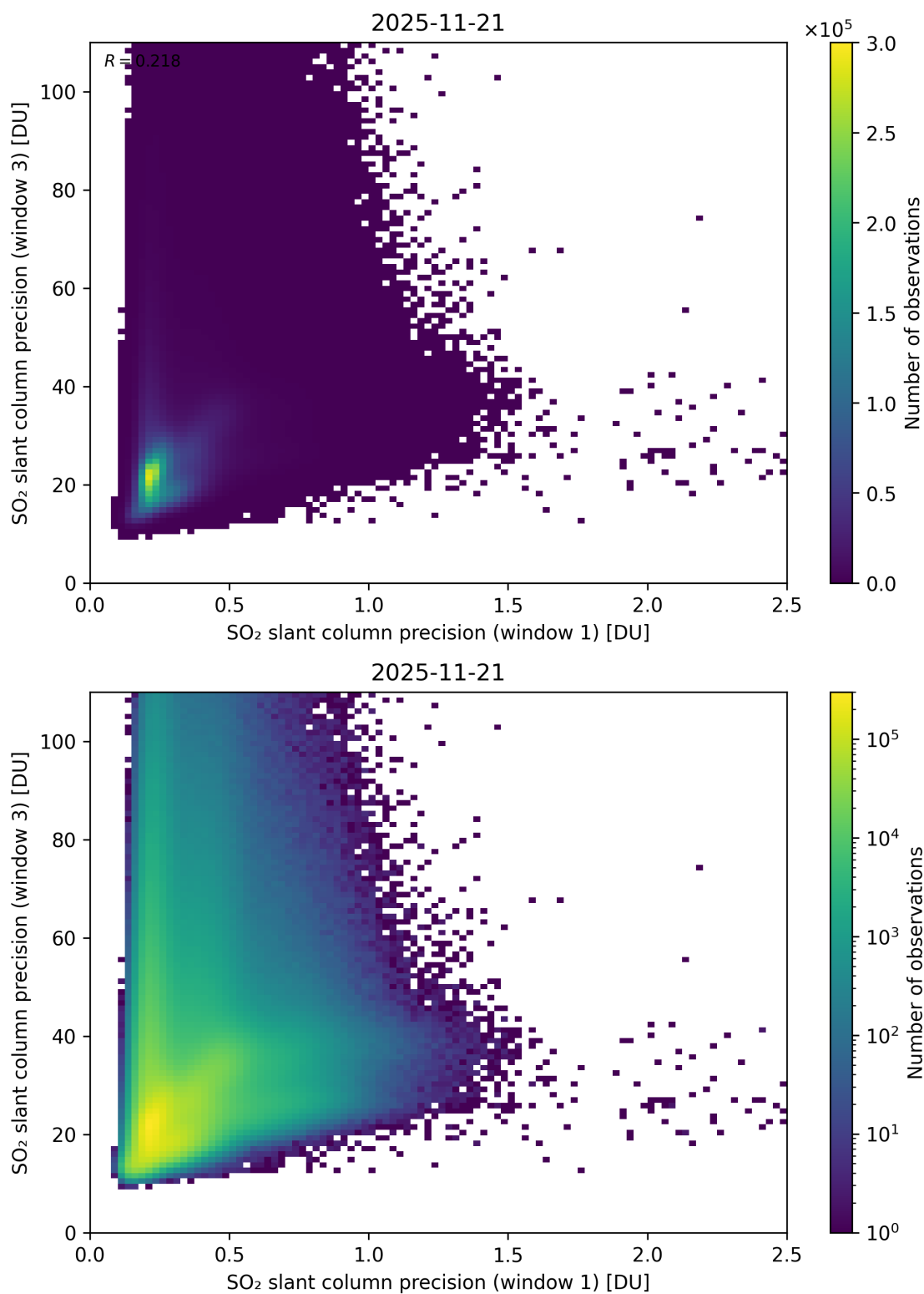
Figure 279: Scatter density plot of “SO 2 slant column precision (window 1)” against “SO 2 slant column precision (window 3)” for 2025-11-20 to 2025-11-22.
