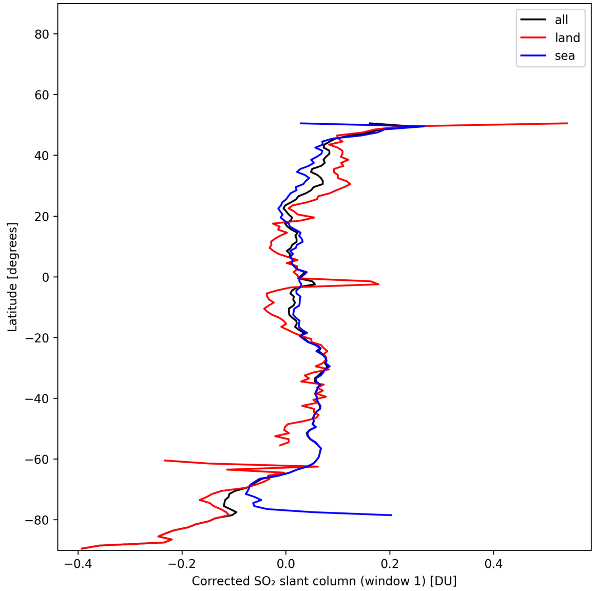
Figure 39: Zonal average of “Corrected SO 2 slant column (window 1)” for 2025-11-20 to 2025-11-22.
