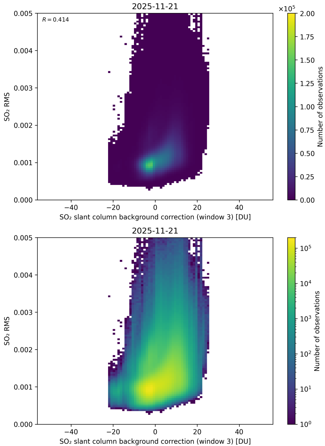
Figure 134: Scatter density plot of “SO 2 slant column background correction (window 3)” against “SO 2 RMS” for 2025-11-20 to 2025-11-22.
