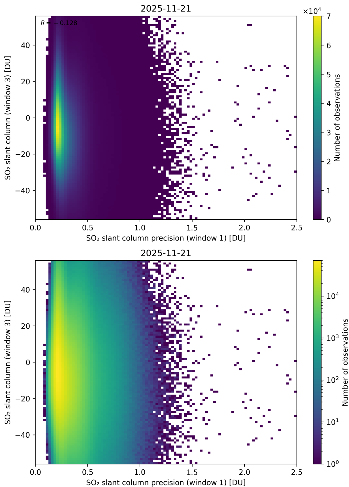
Figure 278: Scatter density plot of “SO 2 slant column precision (window 1)” against “SO 2 slant column (window 3)” for 2025-11-20 to 2025-11-22.
