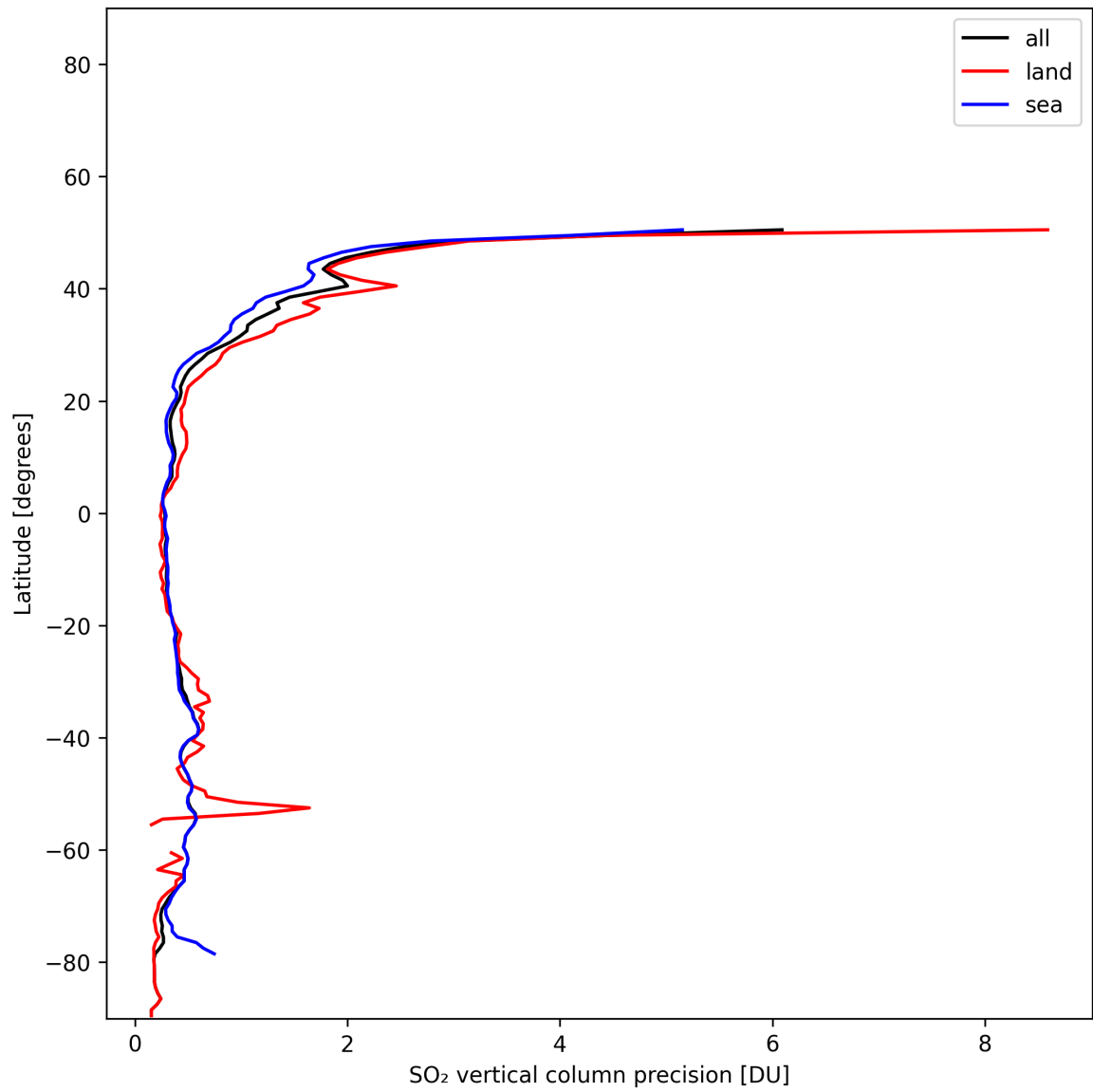
Figure 33: Zonal average of “SO 2 vertical column precision” for 2025-11-20 to 2025-11-22.
