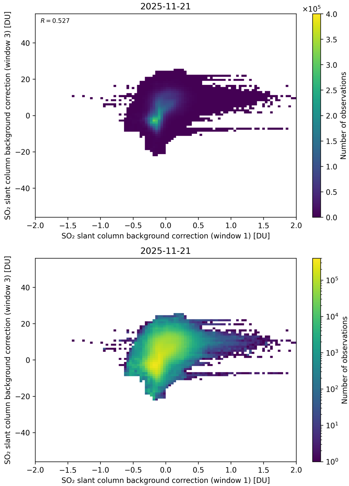
Figure 110: Scatter density plot of “SO 2 slant column background correction (window 1)” against “SO 2 slant column background correction (window 3)” for 2025-11-20 to 2025-11-22.
