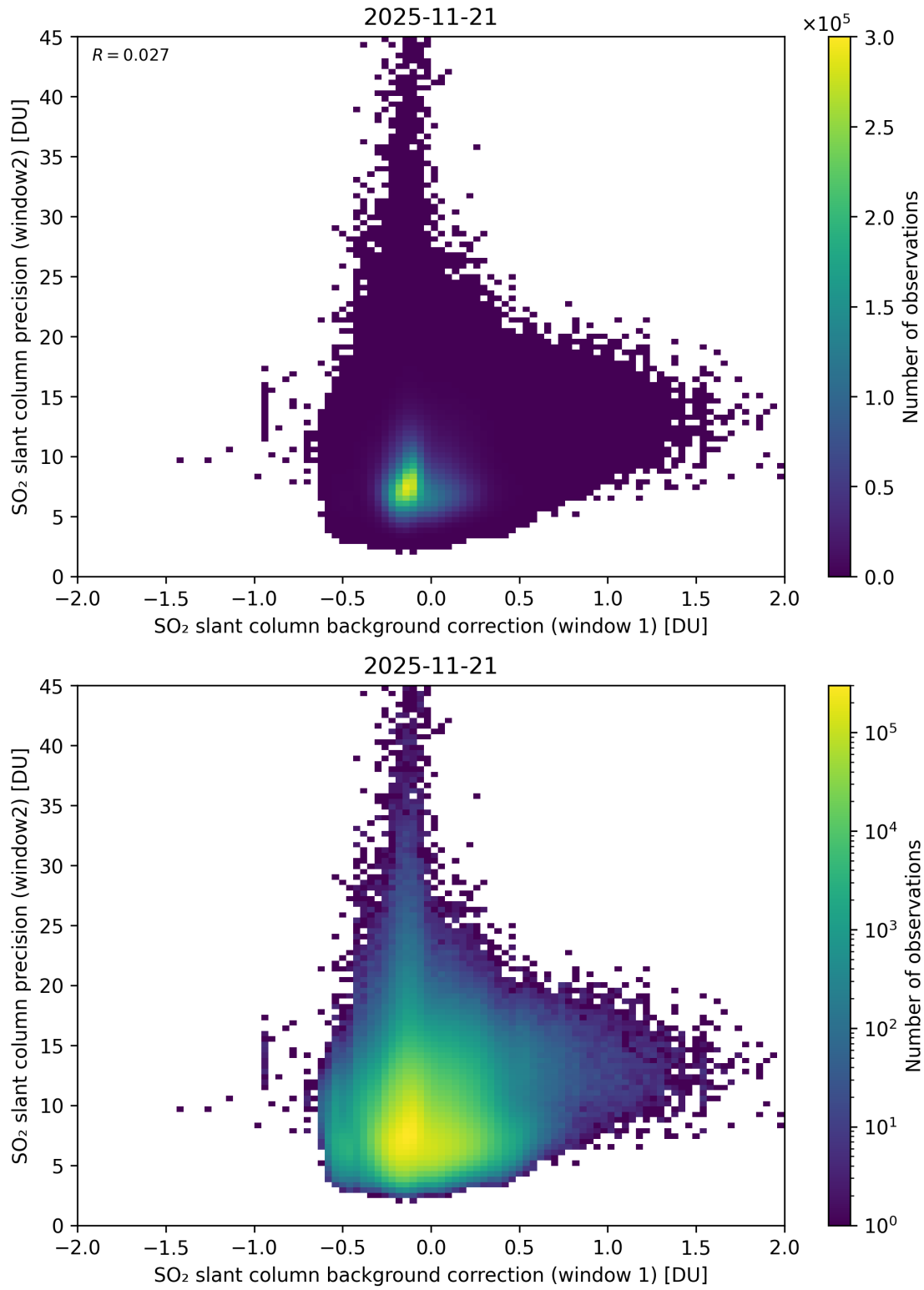
Figure 117: Scatter density plot of “SO 2 slant column background correction (window 1)” against “SO 2 slant column precision (window2)” for 2025-11-20 to 2025-11-22.
