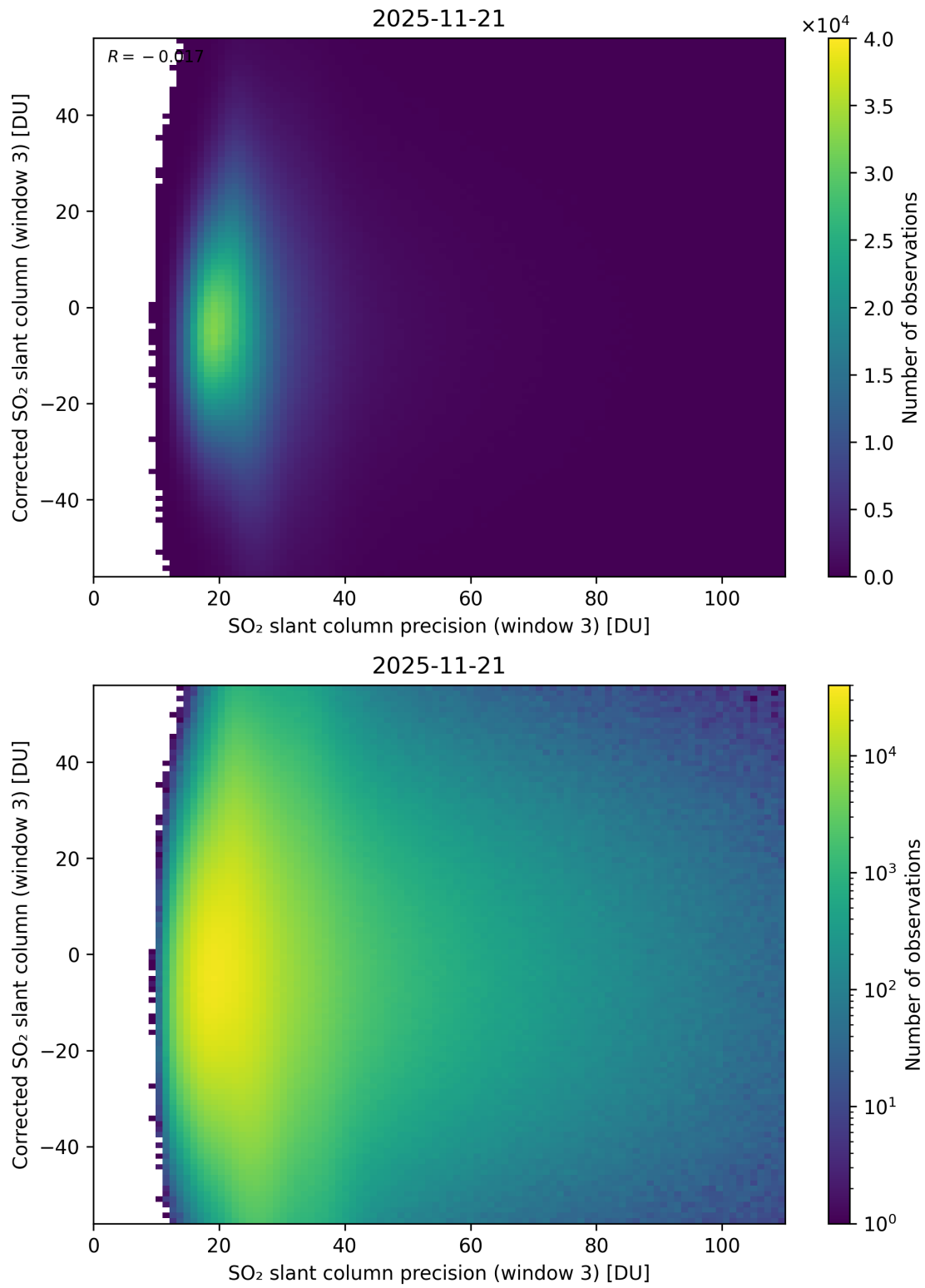
Figure 312: Scatter density plot of “SO 2 slant column precision (window 3)” against “Corrected SO 2 slant column (window 3)” for 2025-11-20 to 2025-11-22.
