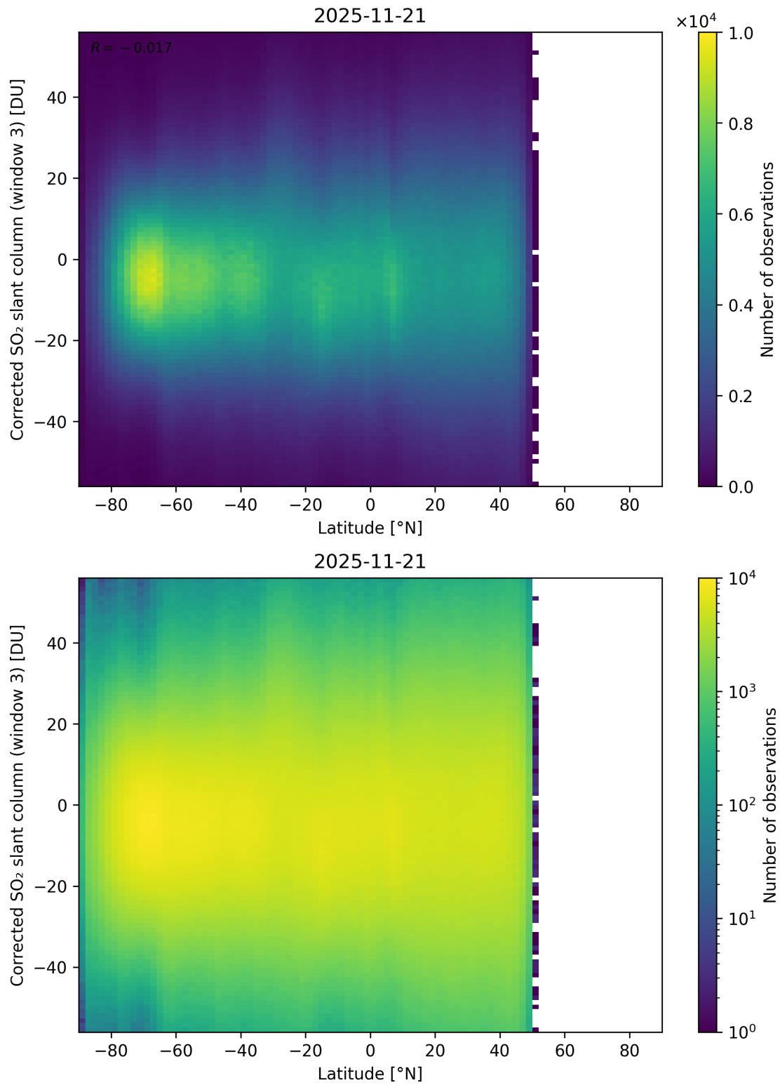
Figure 161: Scatter density plot of “Latitude” against “Corrected SO 2 slant column (window 3)” for 2025-11-20 to 2025-11-22.
