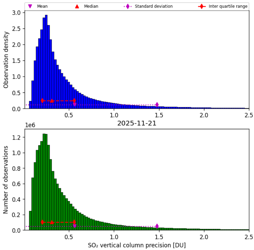
Figure 59: Histogram of "SO 2 vertical column precision" for 2025-11-20 to 2025-11-22
