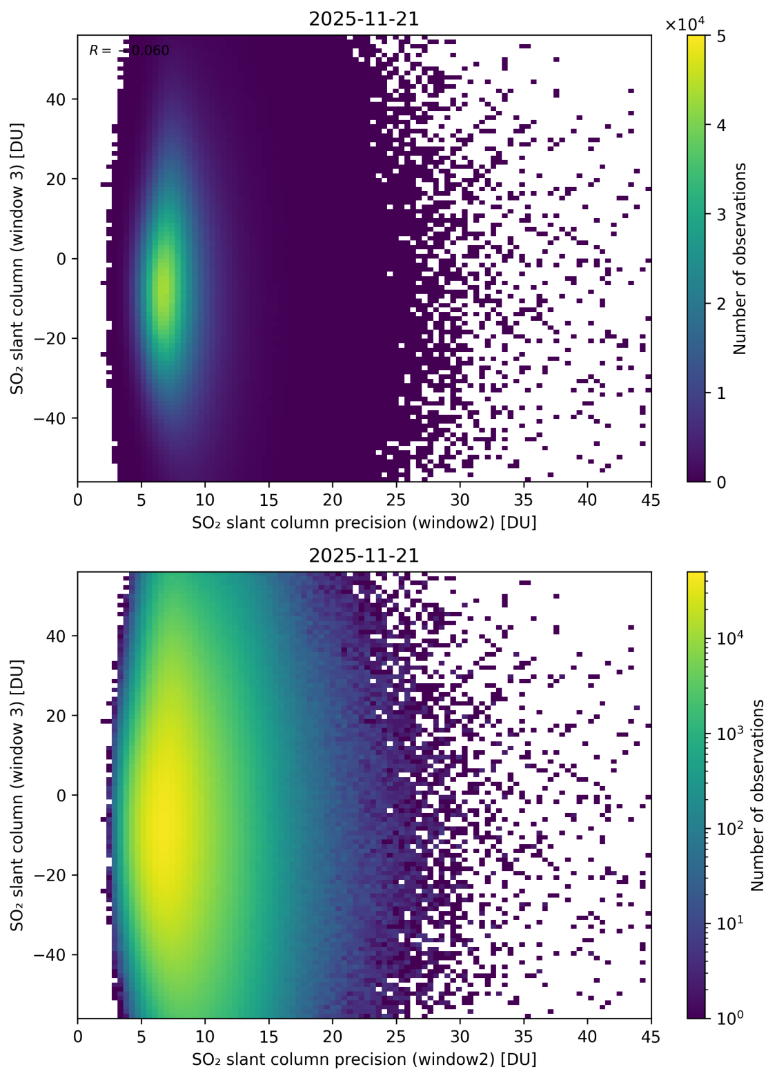
Figure 299: Scatter density plot of “SO 2 slant column precision (window2)” against “SO 2 slant column (window 3)” for 2025-11-20 to 2025-11-22.
