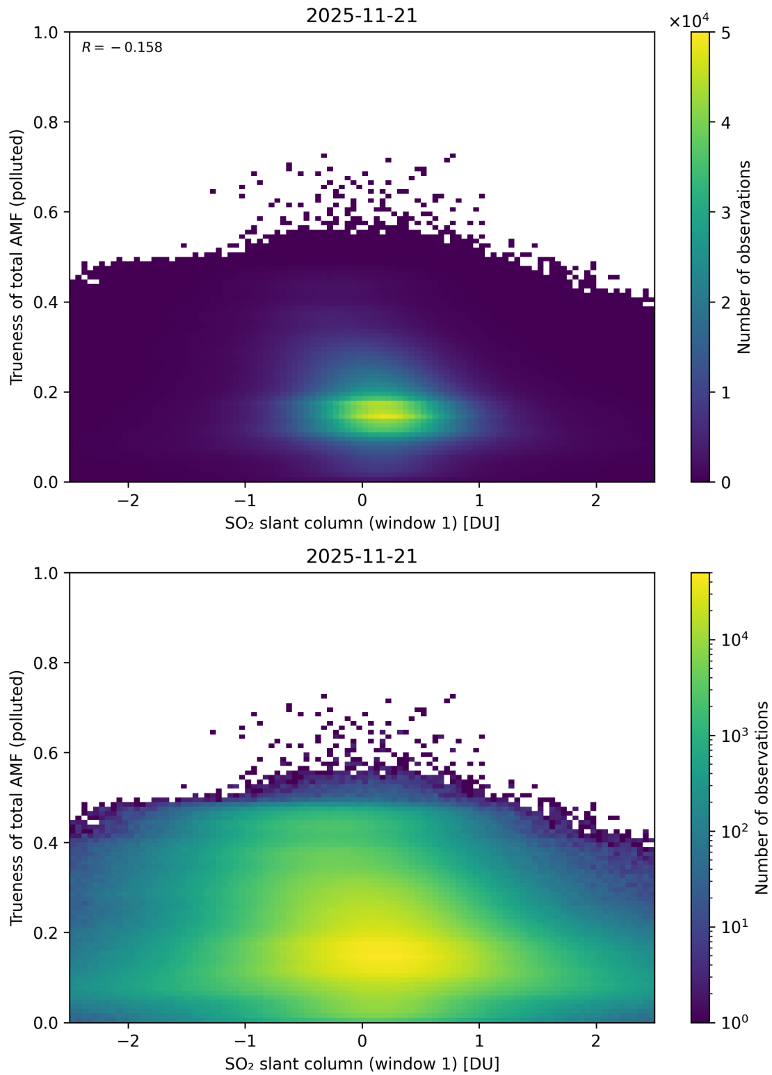
Figure 290: Scatter density plot of “SO 2 slant column (window 1)” against “Trueness of total AMF (polluted)” for 2025-11-20 to 2025-11-22.
