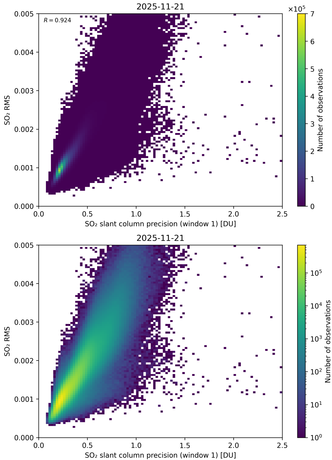
Figure 273: Scatter density plot of “SO 2 slant column precision (window 1)” against “SO 2 RMS” for 2025-11-20 to 2025-11-22.
