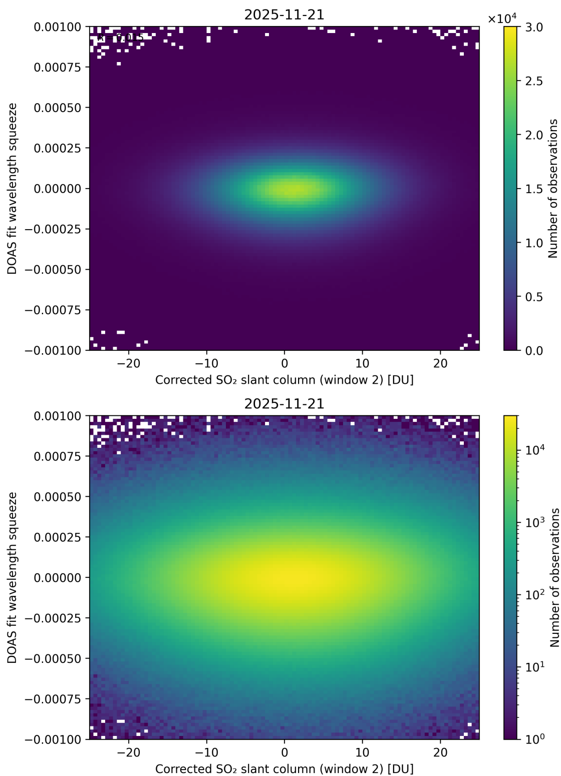
Figure 247: Scatter density plot of “Corrected SO 2 slant column (window 2)” against “DOAS fit wavelength squeeze” for 2025-11-20 to 2025-11-22.
