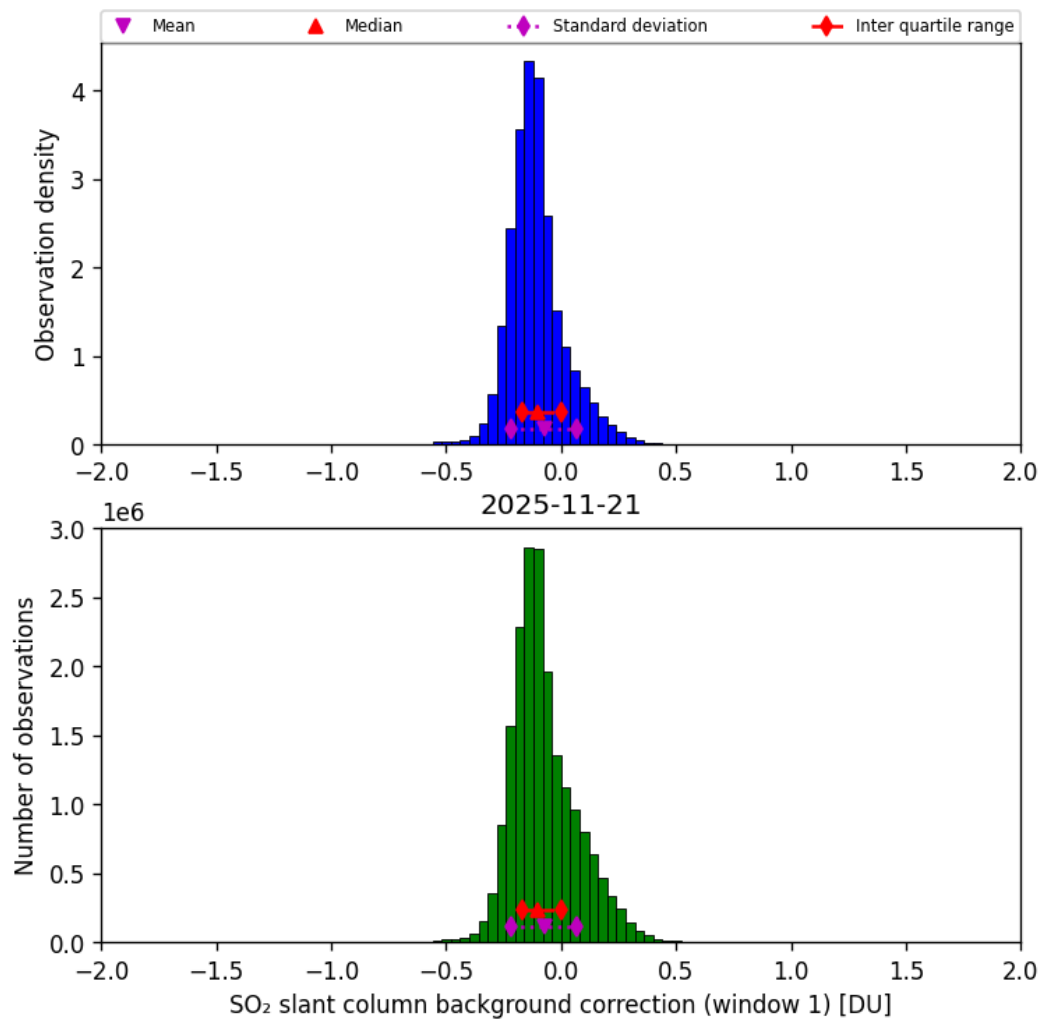
Figure 66: Histogram of “SO 2 slant column background correction (window 1)” for 2025-11-20 to 2025-11-22
