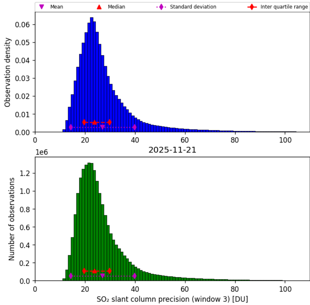
Figure 72: Histogram of “SO 2 slant column precision (window 3)” for 2025-11-20 to 2025-11-22
