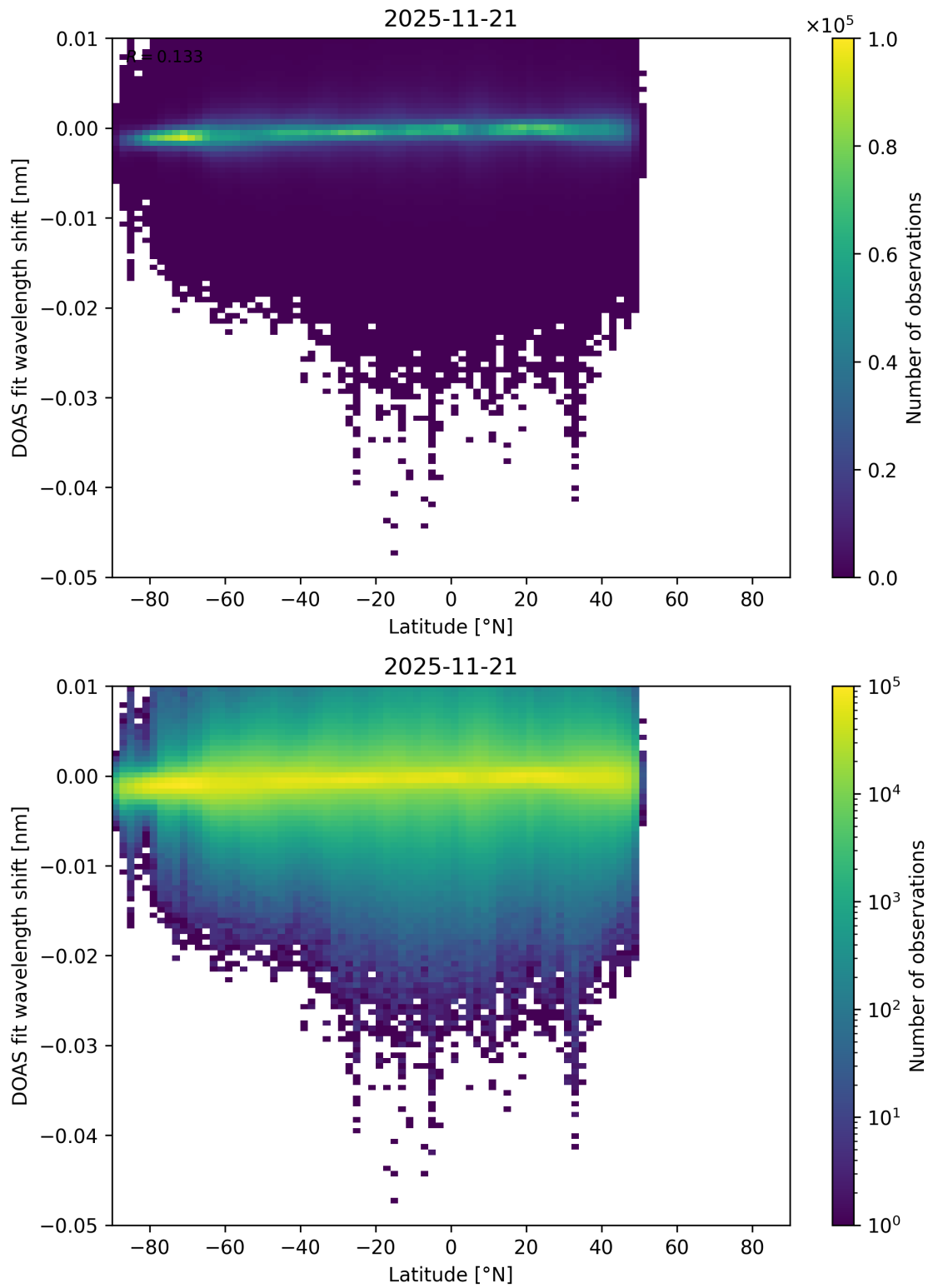
Figure 153: Scatter density plot of “Latitude” against “DOAS fit wavelength shift” for 2025-11-20 to 2025-11-22.
