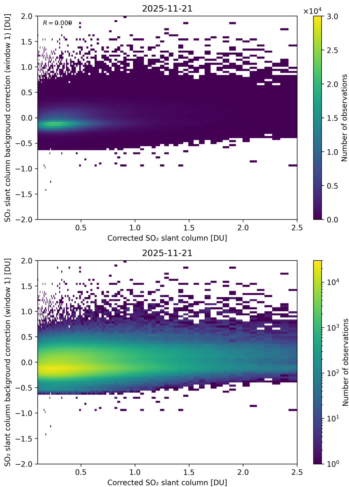
Figure 226: Scatter density plot of “Corrected SO 2 slant column” against “SO 2 slant column background correction (window 1)” for 2025-11-20 to 2025-11-22.
