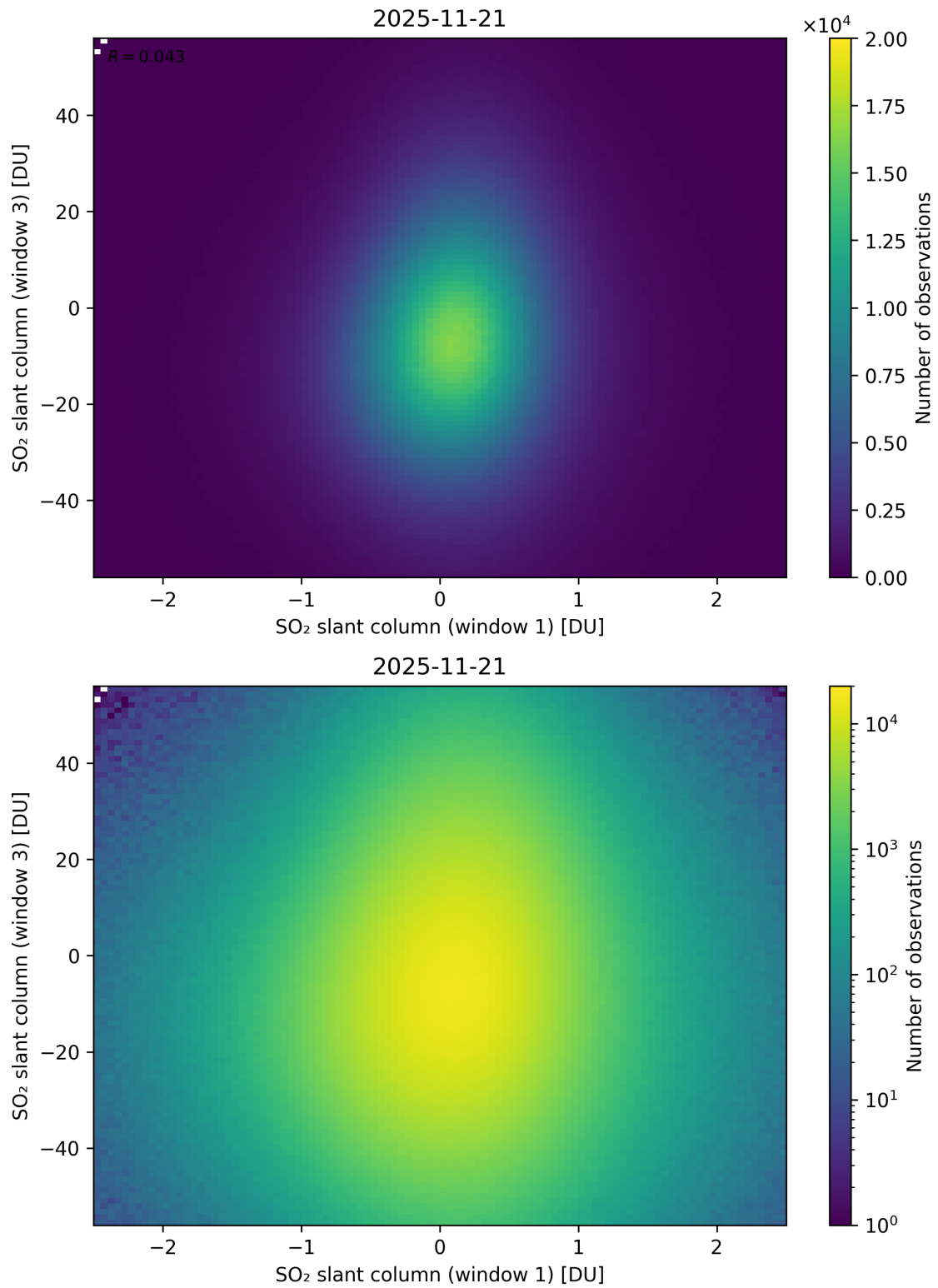
Figure 287: Scatter density plot of “SO 2 slant column (window 1)” against “SO 2 slant column (window 3)” for 2025-11-20 to 2025-11-22.
