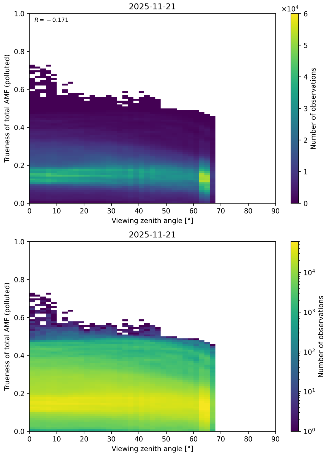
Figure 382: Scatter density plot of “Viewing zenith angle” against “Trueness of total AMF (polluted)” for 2025-11-20 to 2025-11-22.
