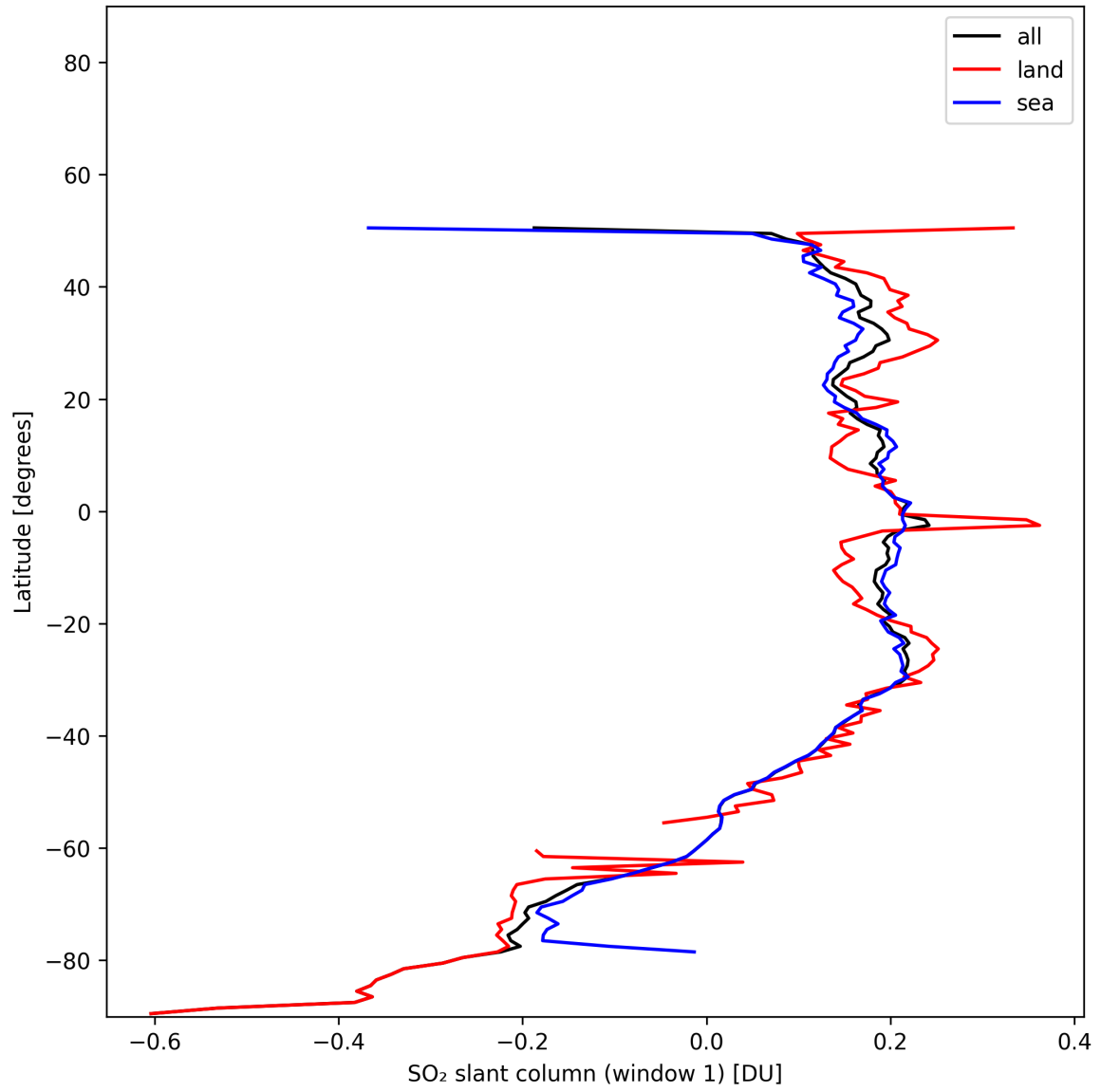
Figure 37: Zonal average of “SO 2 slant column (window 1)” for 2025-11-20 to 2025-11-22.
