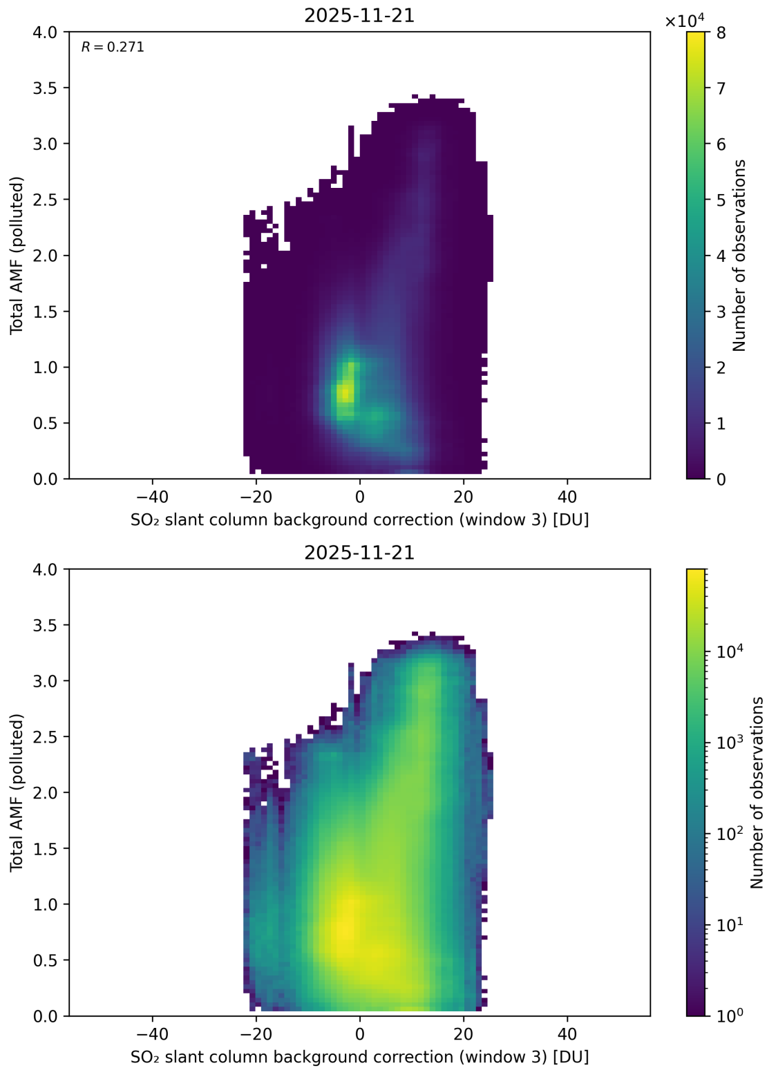
Figure 136: Scatter density plot of “SO 2 slant column background correction (window 3)” against “Total AMF (polluted)” for 2025-11-20 to 2025-11-22.
