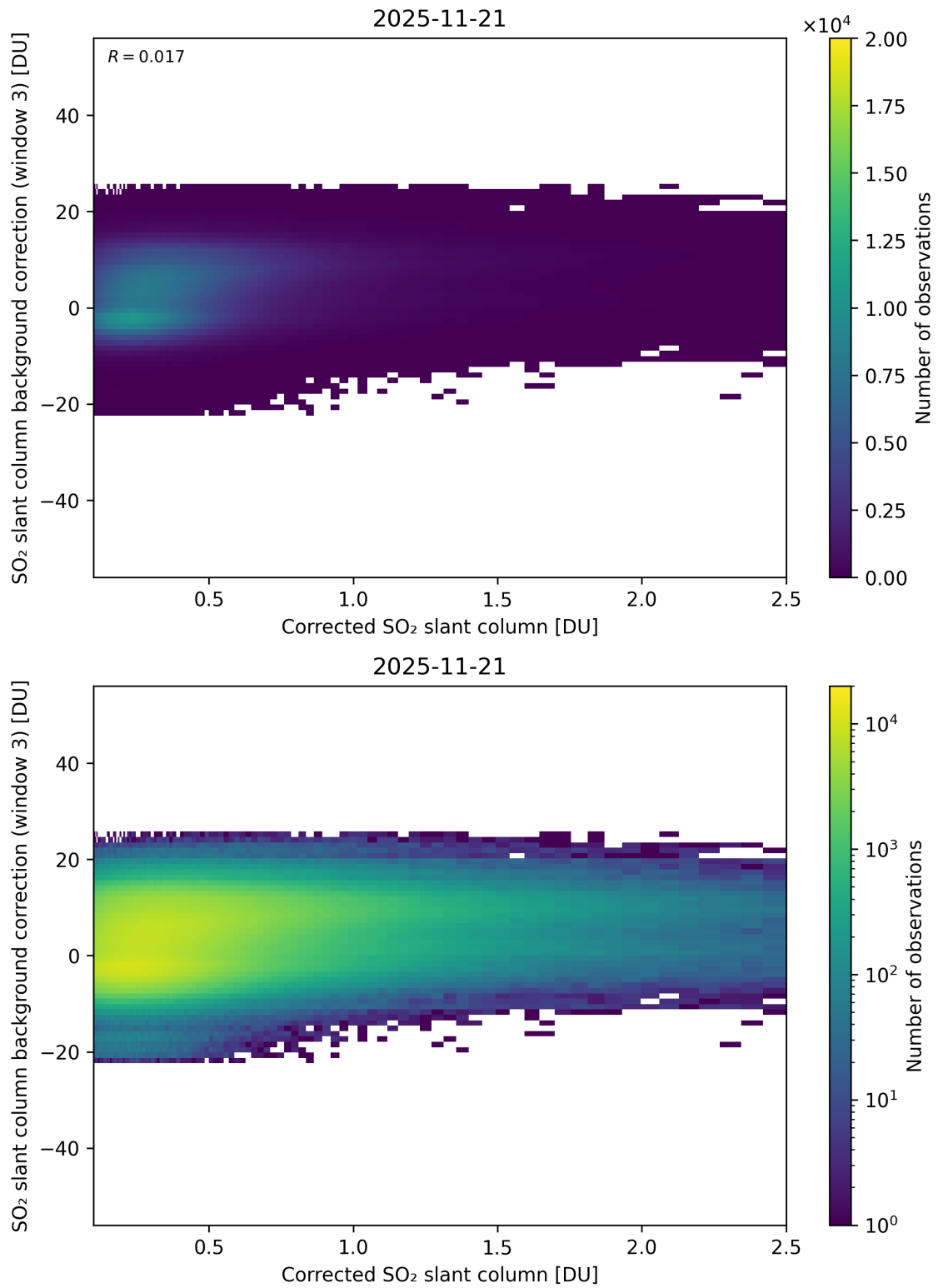
Figure 228: Scatter density plot of “Corrected SO 2 slant column” against “SO 2 slant column background correction (window 3)” for 2025-11-20 to 2025-11-22.
