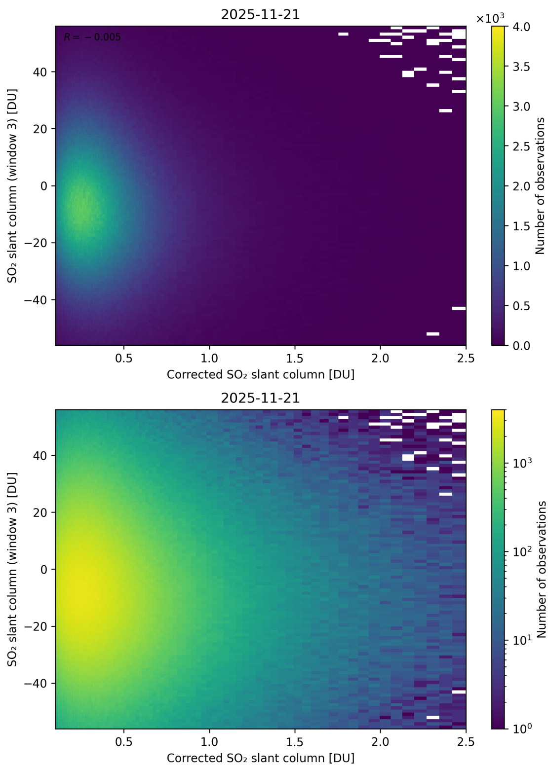
Figure 240: Scatter density plot of “Corrected SO 2 slant column” against “SO 2 slant column (window 3)” for 2025-11-20 to 2025-11-22.
