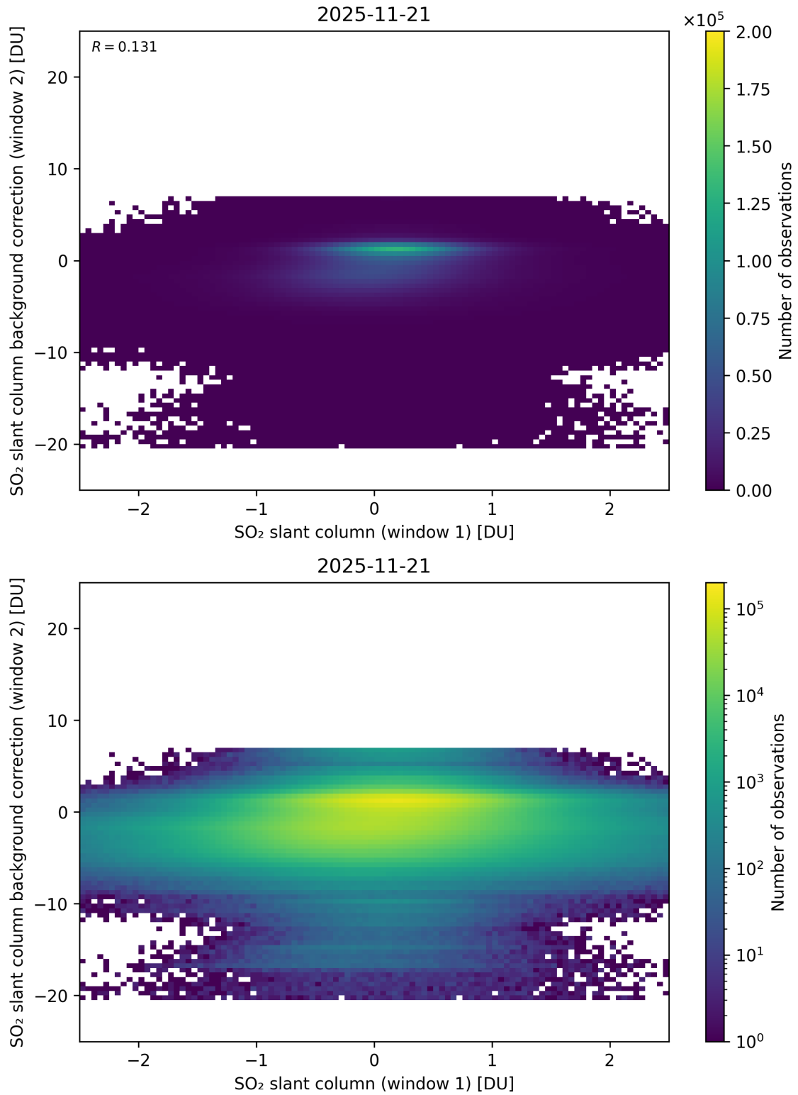
Figure 263: Scatter density plot of “SO 2 slant column (window 1)” against “SO 2 slant column background correction (window 2)” for 2025-11-20 to 2025-11-22.
