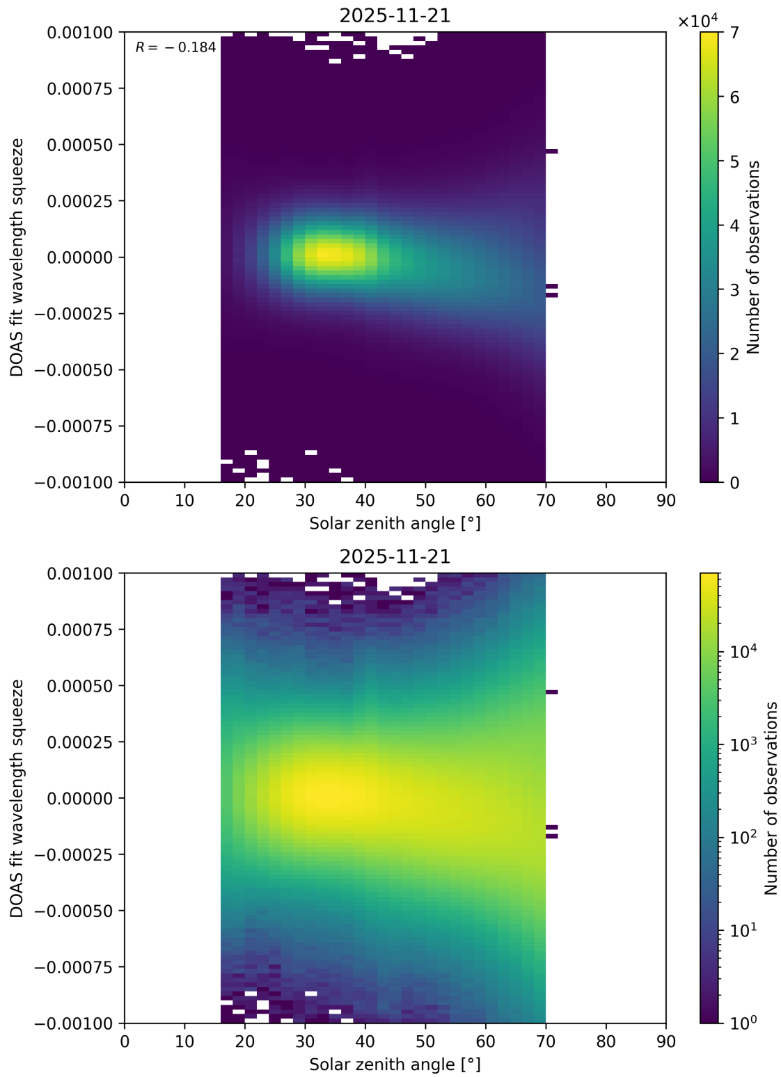
Figure 175: Scatter density plot of “Solar zenith angle” against “DOAS fit wavelength squeeze” for 2025-11-20 to 2025-11-22.
