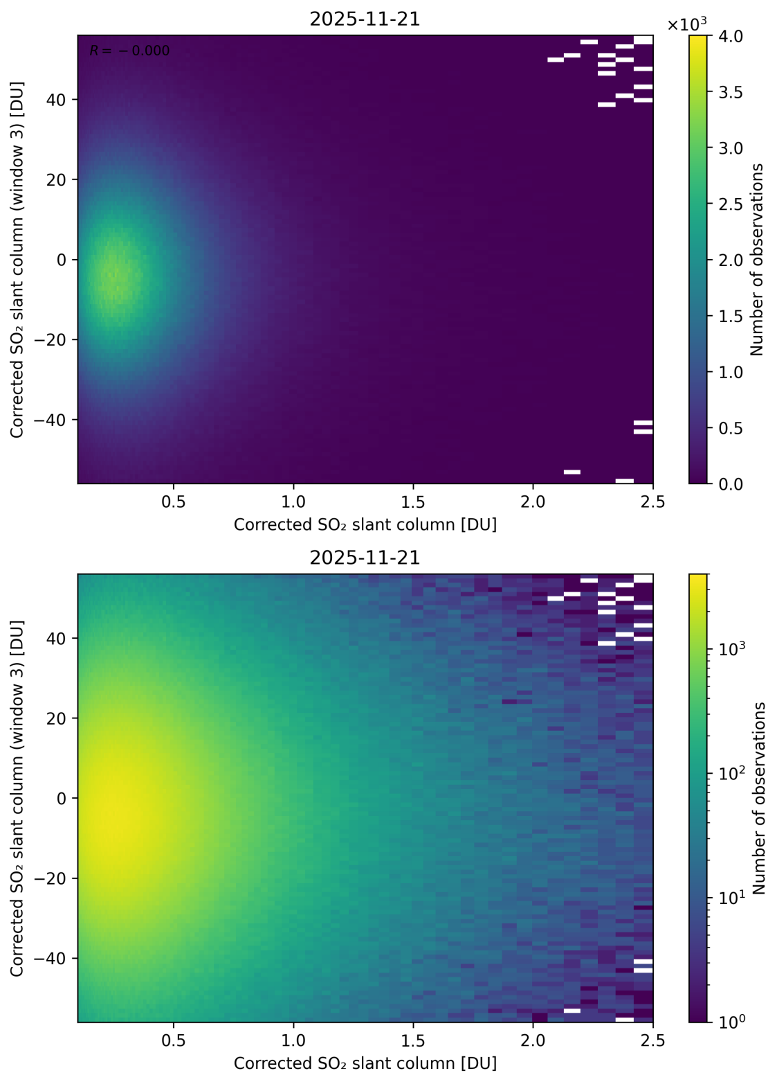
Figure 236: Scatter density plot of “Corrected SO 2 slant column” against “Corrected SO 2 slant column (window 3)” for 2025-11-20 to 2025-11-22.
