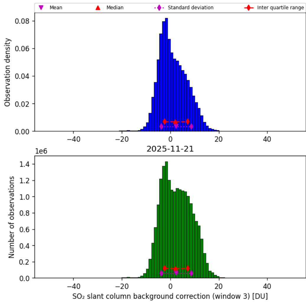
Figure 74: Histogram of “SO 2 slant column background correction (window 3)” for 2025-11-20 to 2025-11-22
