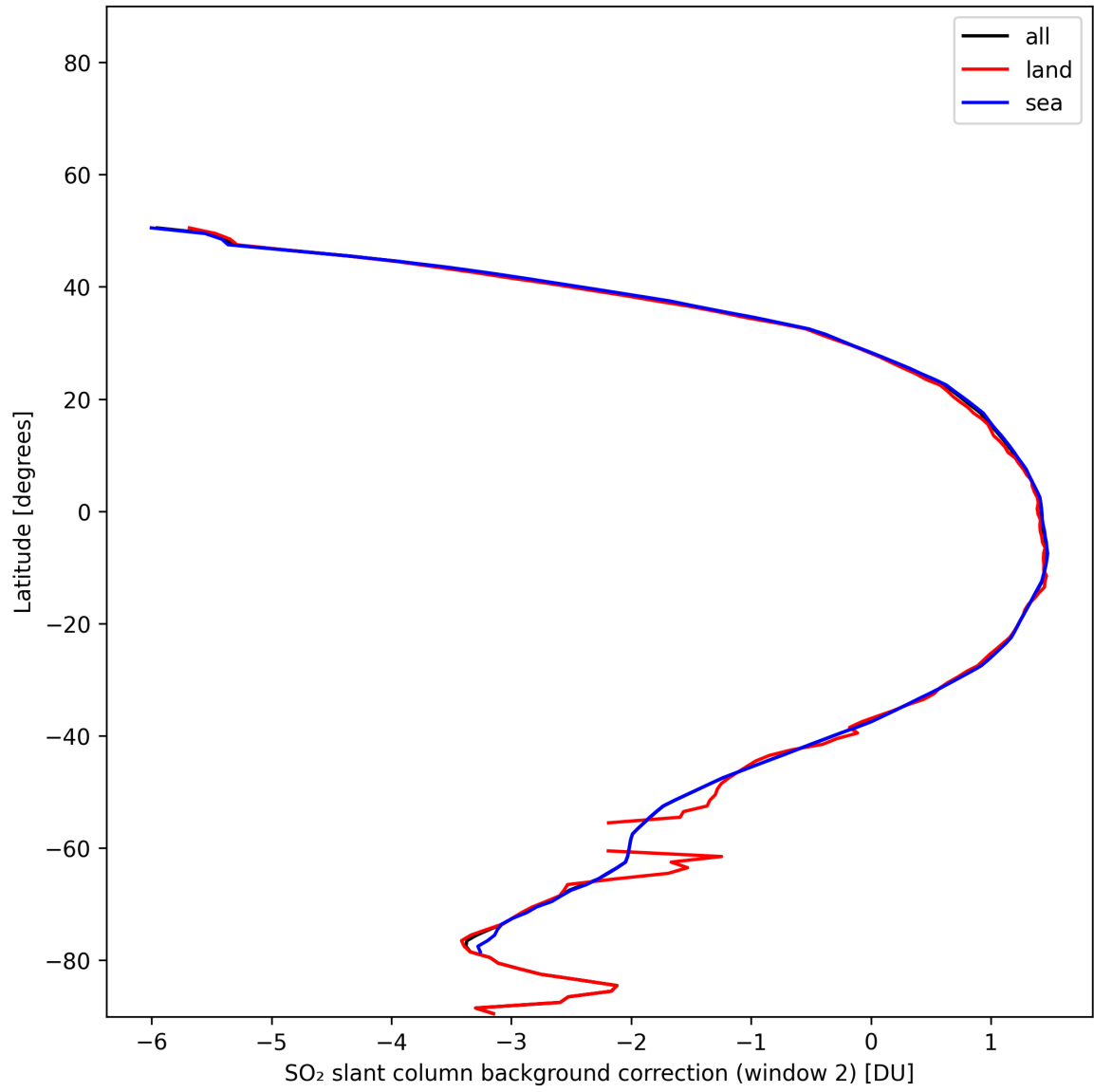
Figure 44: Zonal average of “SO 2 slant column background correction (window 2)” for 2025-11-20 to 2025-11-22.
