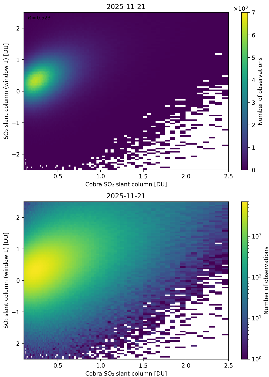
Figure 219: Scatter density plot of “Cobra SO 2 slant column” against “SO 2 slant column (window 1)” for 2025-11-20 to 2025-11-22.
