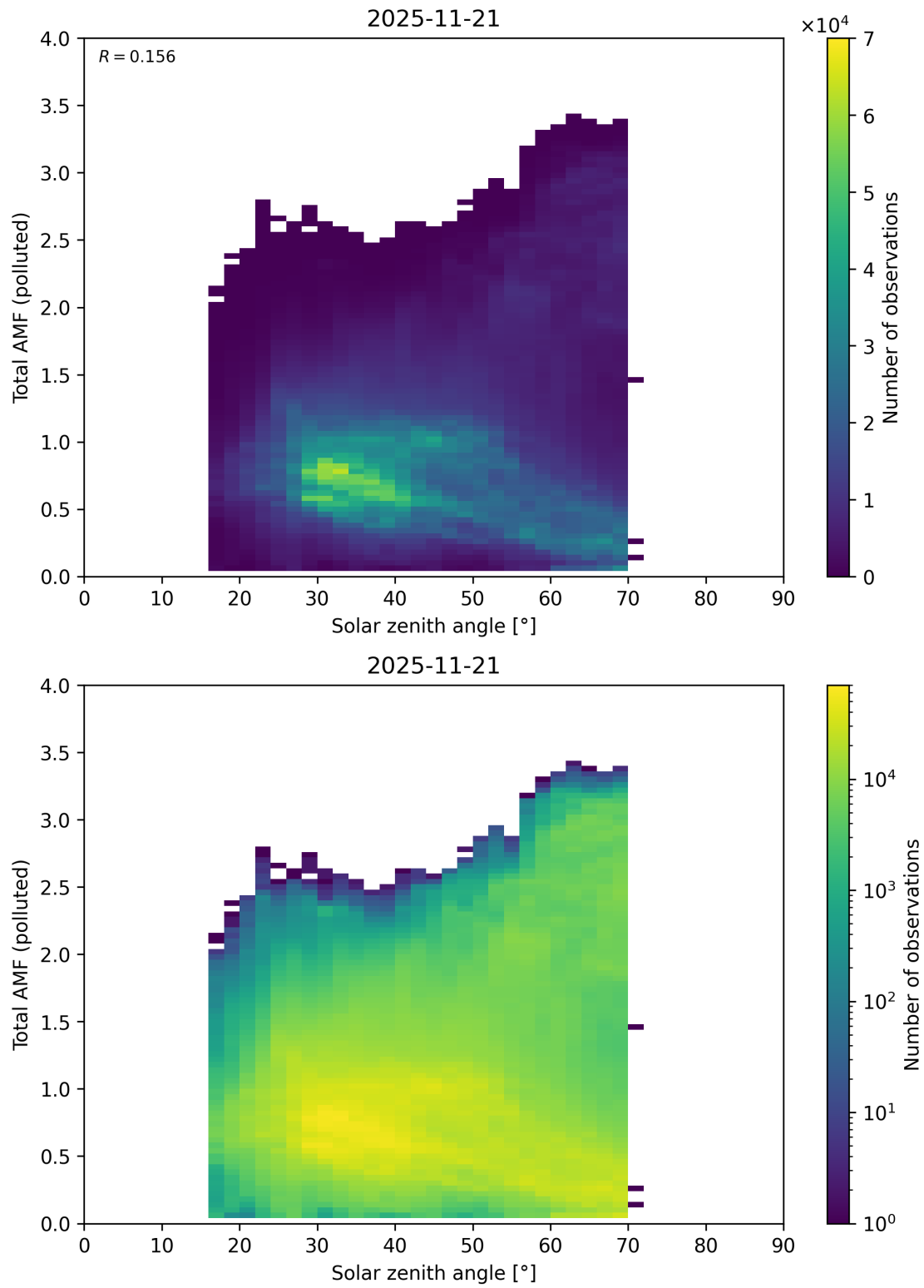
Figure 189: Scatter density plot of “Solar zenith angle” against “Total AMF (polluted)” for 2025-11-20 to 2025-11-22.
