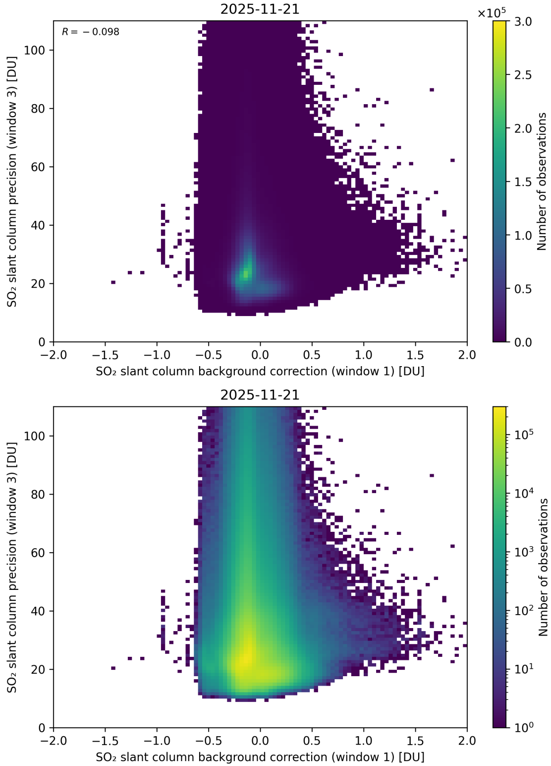
Figure 119: Scatter density plot of “SO 2 slant column background correction (window 1)” against “SO 2 slant column precision (window 3)” for 2025-11-20 to 2025-11-22.
