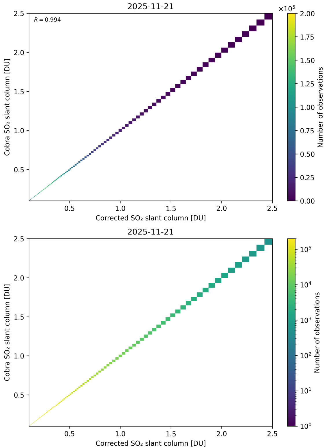
Figure 233: Scatter density plot of “Corrected SO 2 slant column” against “Cobra SO 2 slant column” for 2025-11-20 to 2025-11-22.
