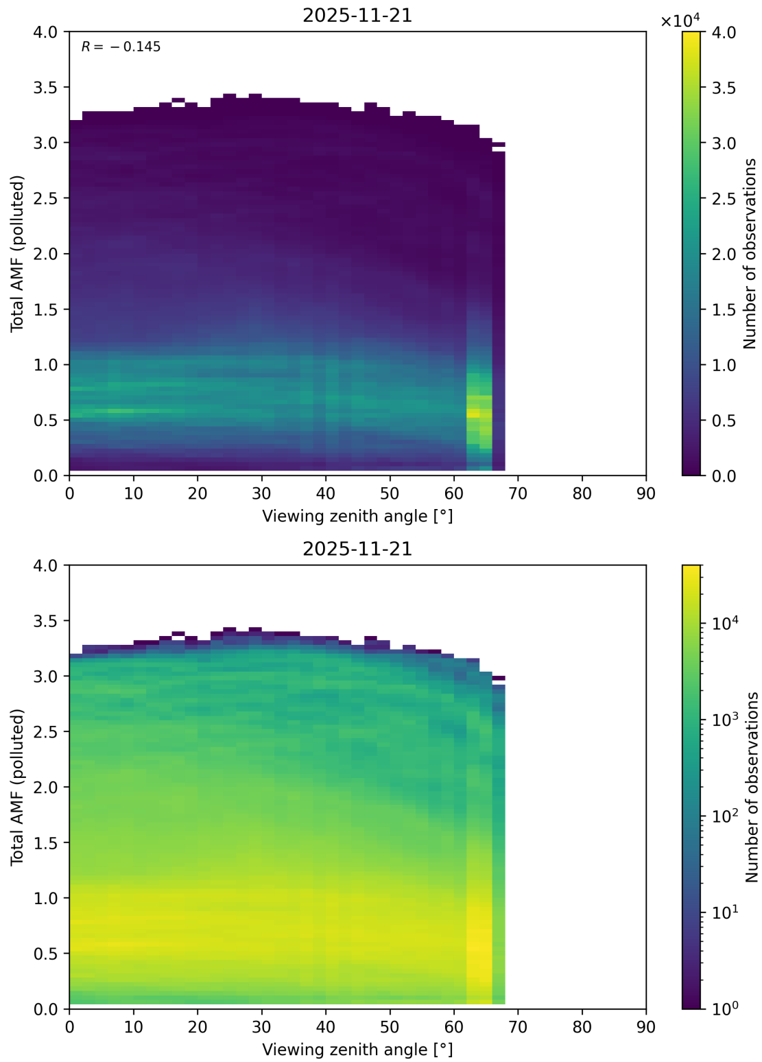
Figure 381: Scatter density plot of “Viewing zenith angle” against “Total AMF (polluted)” for 2025-11-20 to 2025-11-22.
