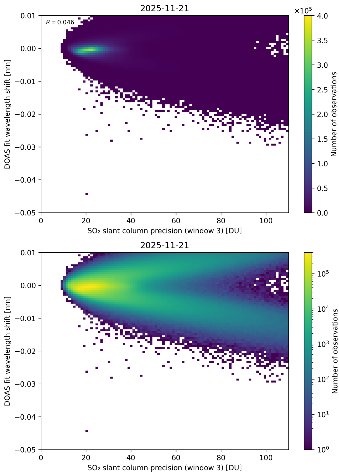
Figure 308: Scatter density plot of “SO 2 slant column precision (window 3)” against “DOAS fit wavelength shift” for 2025-11-20 to 2025-11-22.
