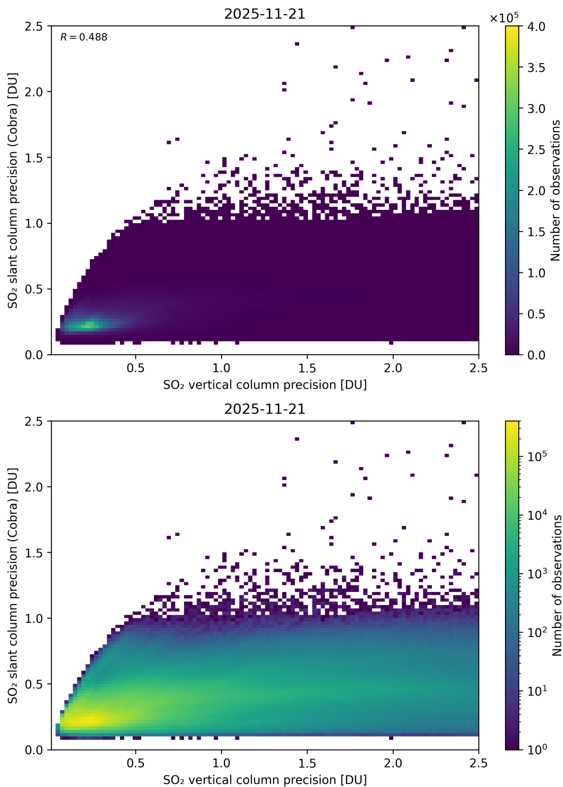
Figure 337: Scatter density plot of “SO 2 vertical column precision” against “SO 2 slant column precision (Cobra)” for 2025-11-20 to 2025-11-22.
