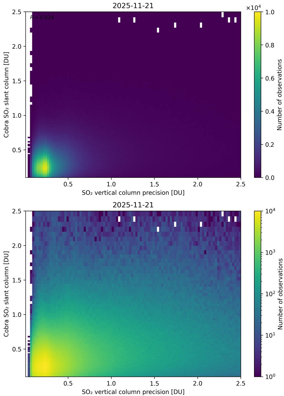
Figure 336: Scatter density plot of “SO 2 vertical column precision” against “Cobra SO 2 slant column” for 2025-11-20 to 2025-11-22.
