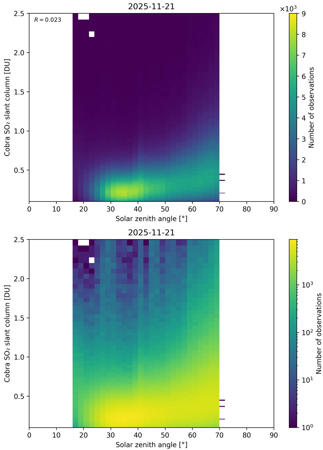
Figure 179: Scatter density plot of “Solar zenith angle” against “Cobra SO 2 slant column” for 2025-11-20 to 2025-11-22.
