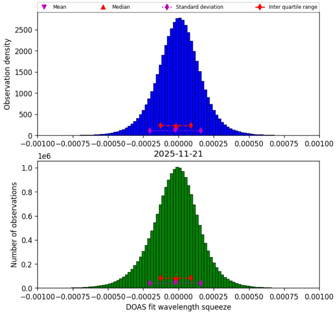
Figure 77: Histogram of “DOAS fit wavelength squeeze” for 2025-11-20 to 2025-11-22
