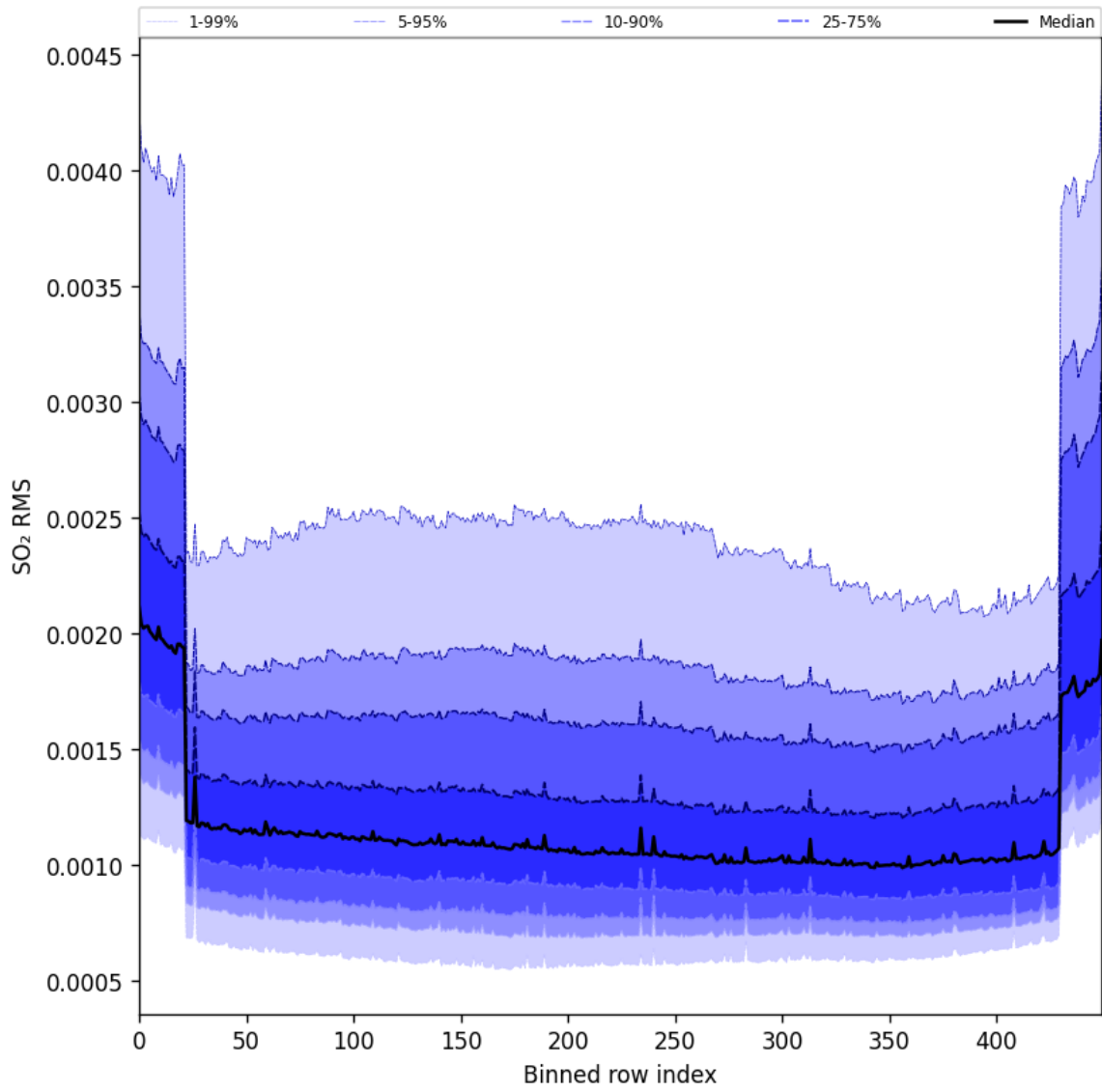
Figure 104: Along track statistics of “SO 2 RMS” for 2025-11-20 to 2025-11-22
