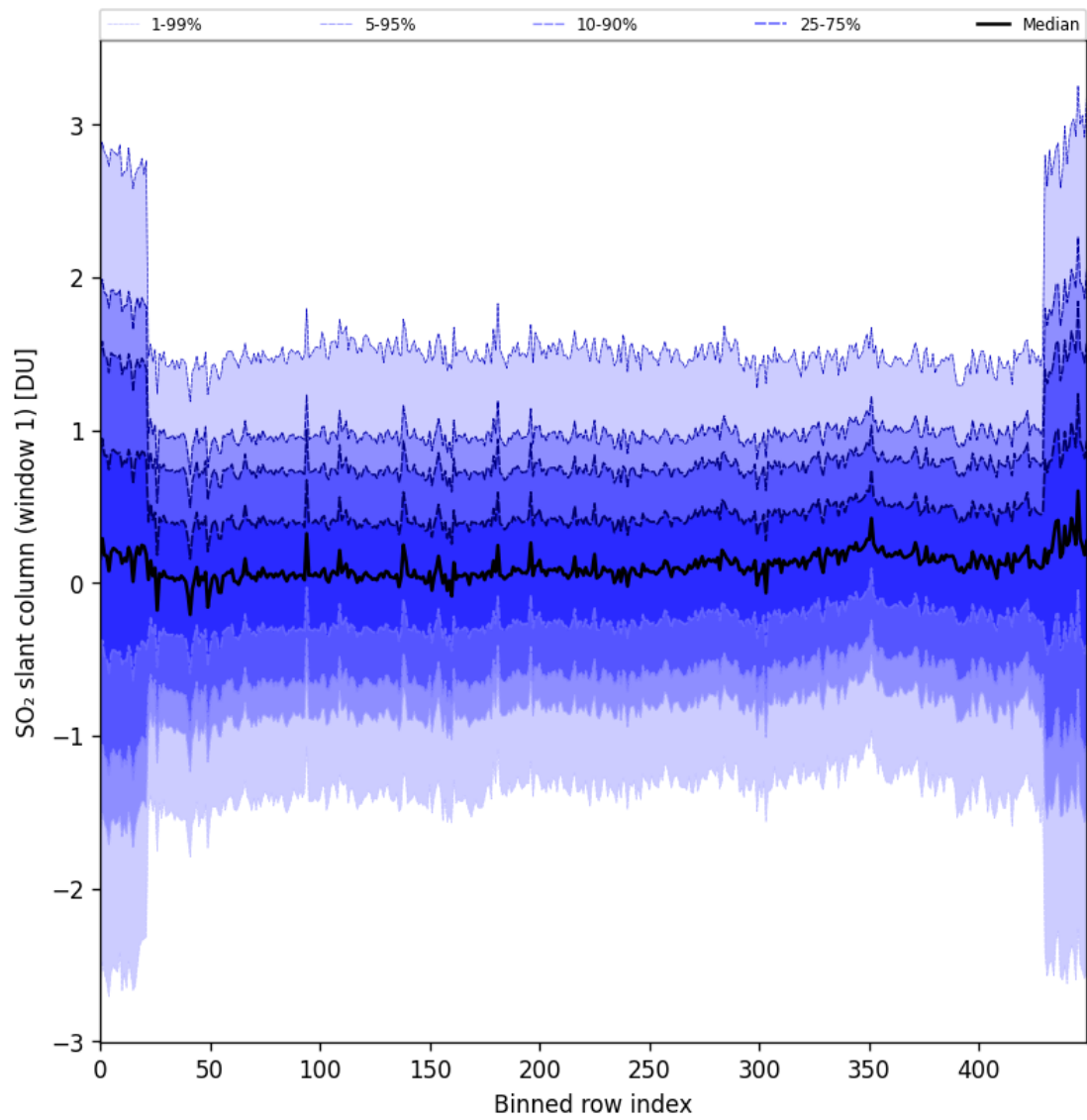
Figure 89: Along track statistics of “SO 2 slant column (window 1)” for 2025-11-20 to 2025-11-22
