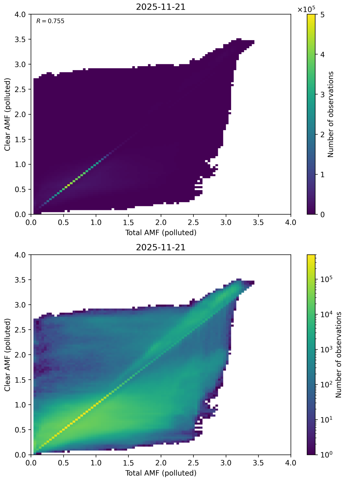
Figure 320: Scatter density plot of “Total AMF (polluted)” against “Clear AMF (polluted)” for 2025-11-20 to 2025-11-22.
