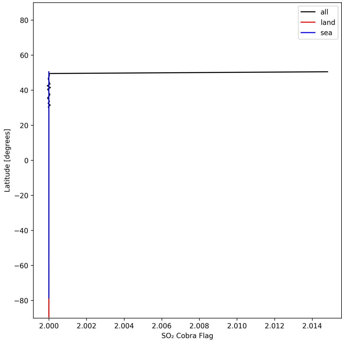
Figure 49: Zonal average of “SO 2 Cobra Flag” for 2025-11-20 to 2025-11-22.
