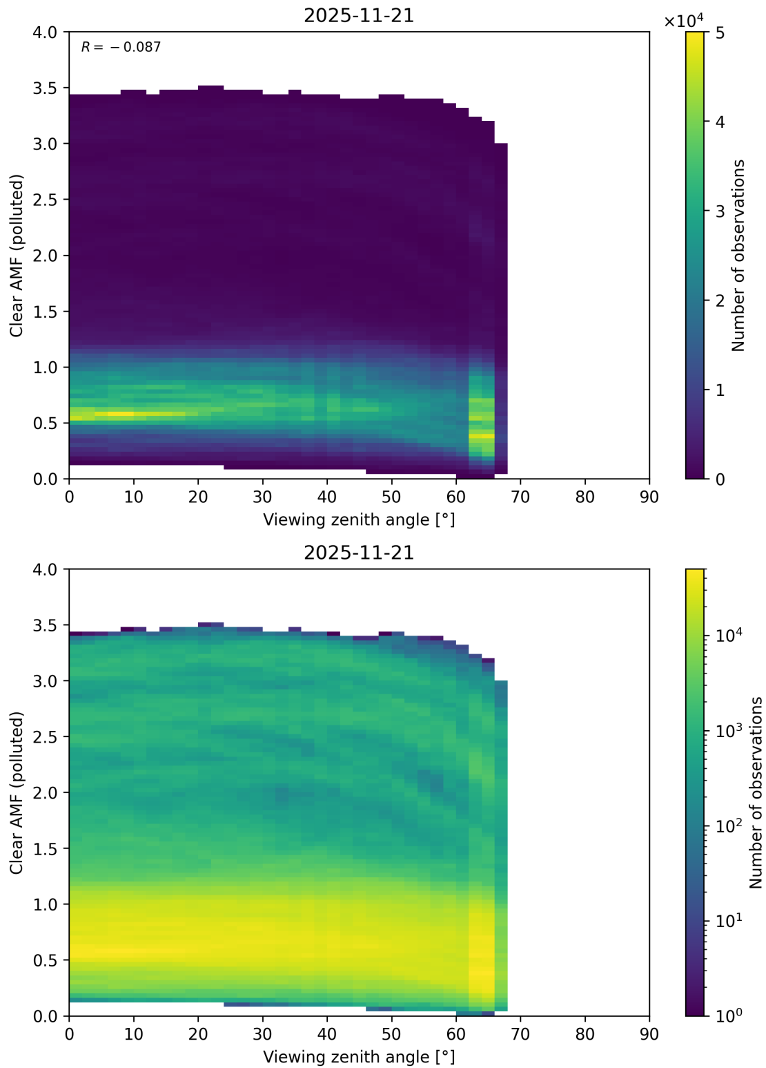
Figure 370: Scatter density plot of “Viewing zenith angle” against “Clear AMF (polluted)” for 2025-11-20 to 2025-11-22.
