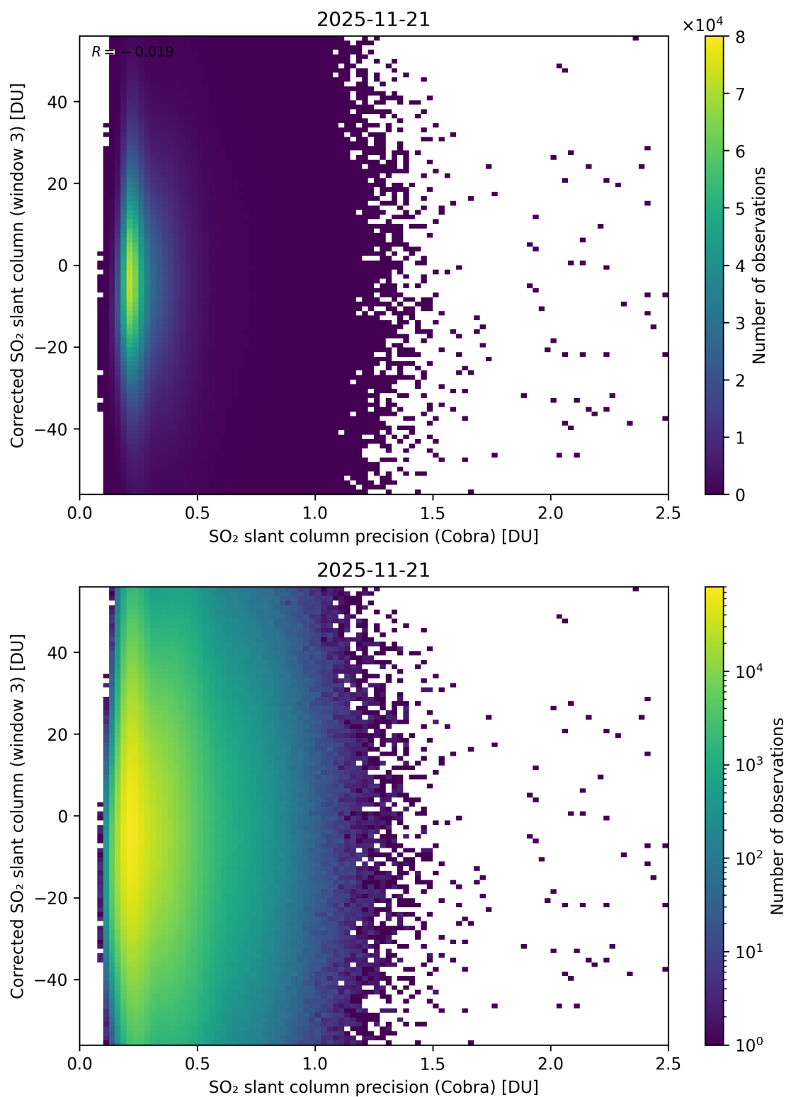
Figure 207: Scatter density plot of “SO 2 slant column precision (Cobra)” against “Corrected SO 2 slant column (window 3)” for 2025-11-20 to 2025-11-22.
