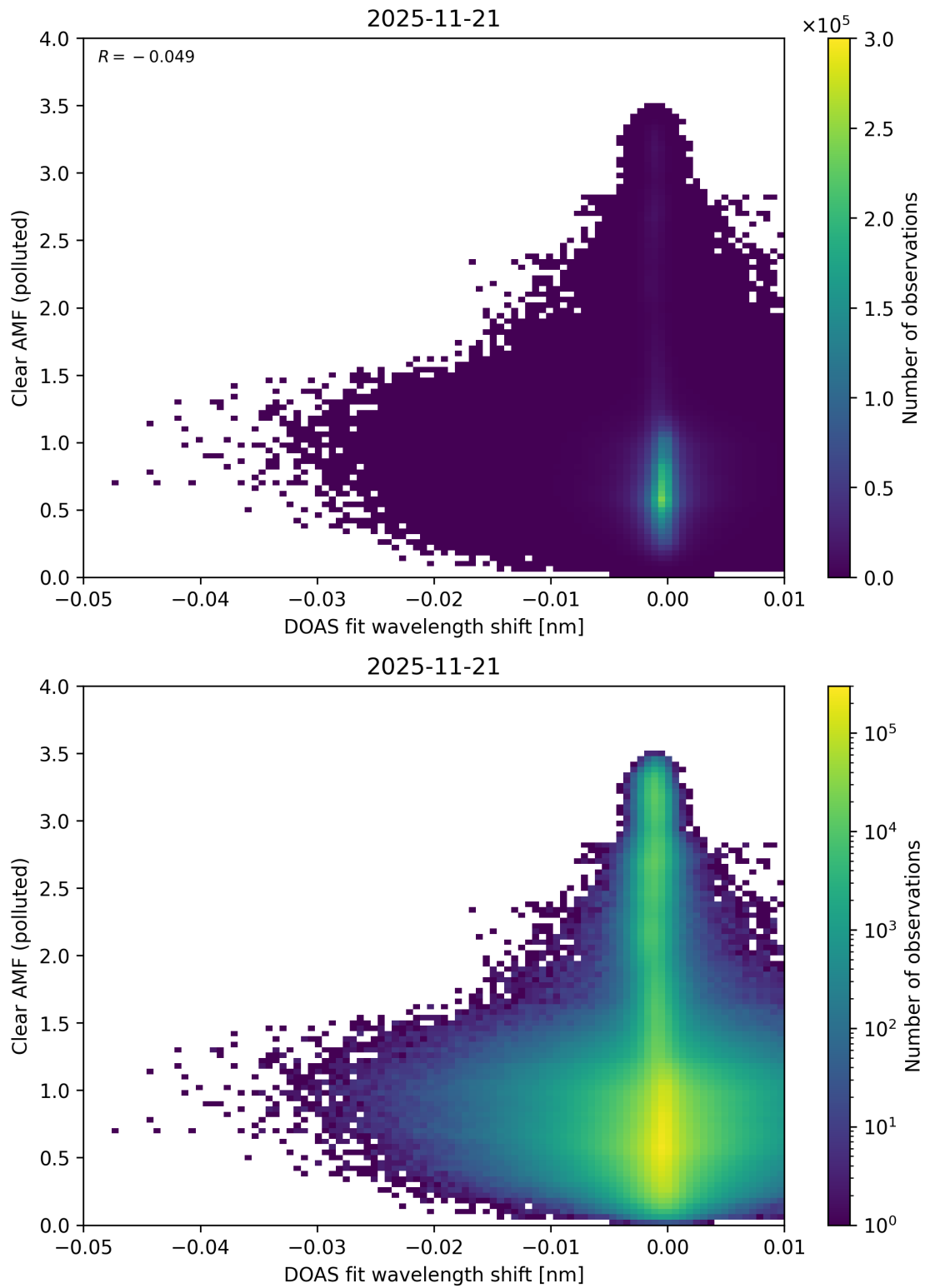
Figure 140: Scatter density plot of “DOAS fit wavelength shift” against “Clear AMF (polluted)” for 2025-11-20 to 2025-11-22.
