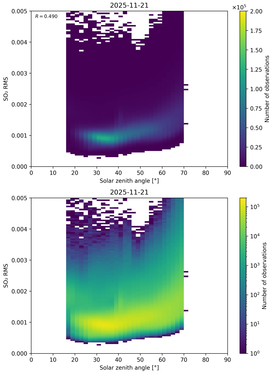
Figure 176: Scatter density plot of “Solar zenith angle” against “SO 2 RMS” for 2025-11-20 to 2025-11-22.
