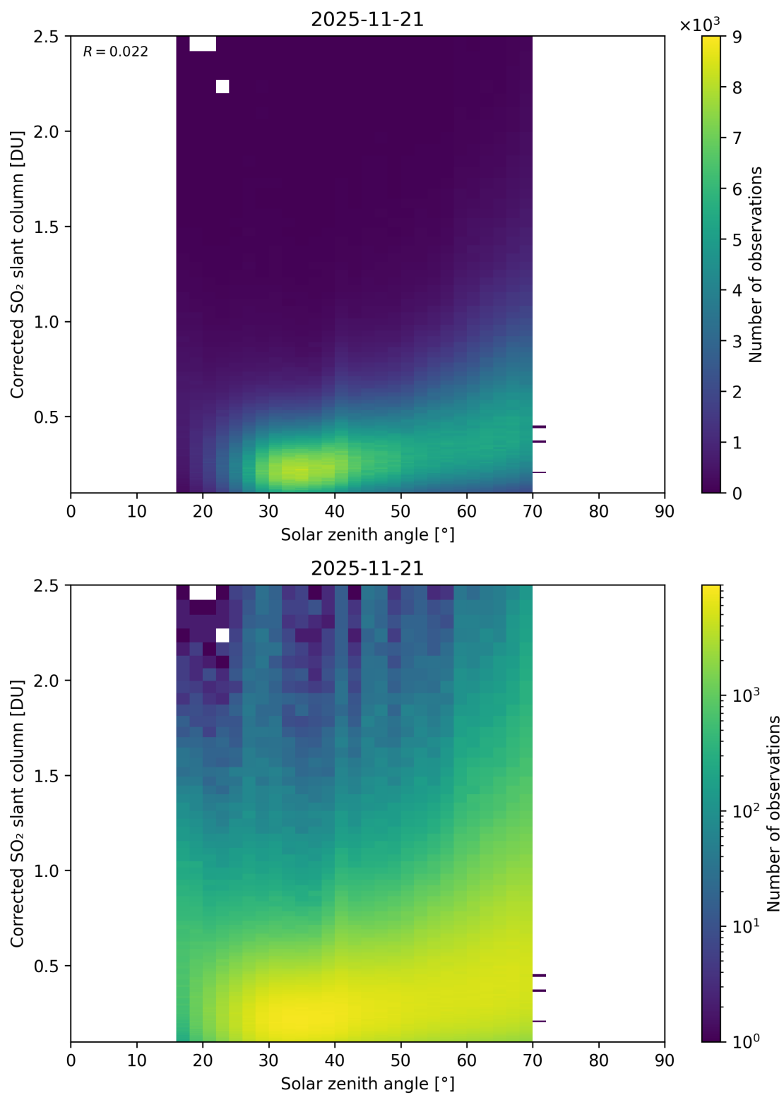
Figure 181: Scatter density plot of “Solar zenith angle” against “Corrected SO 2 slant column” for 2025-11-20 to 2025-11-22.
