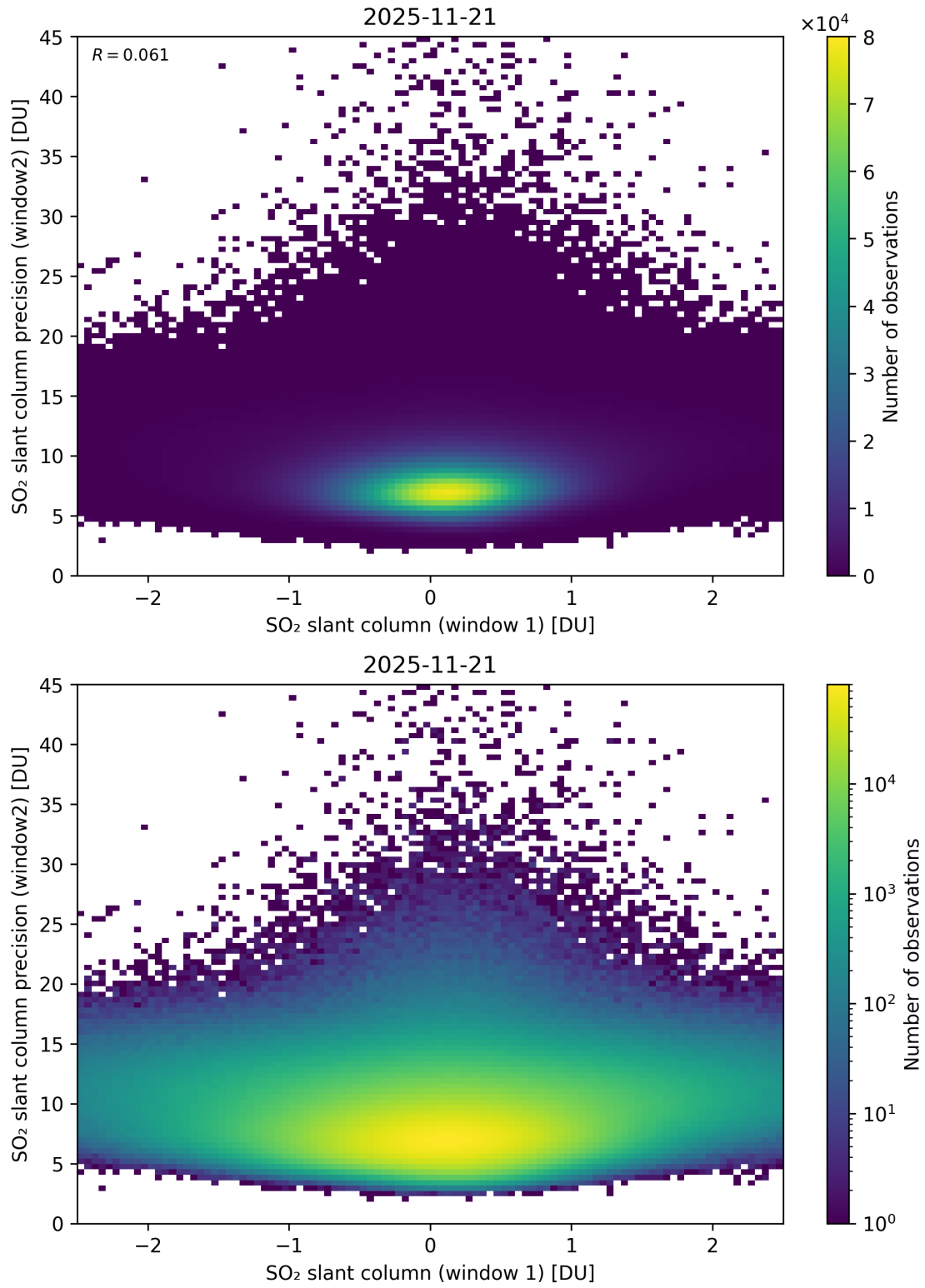
Figure 286: Scatter density plot of “SO 2 slant column (window 1)” against “SO 2 slant column precision (window2)” for 2025-11-20 to 2025-11-22.
