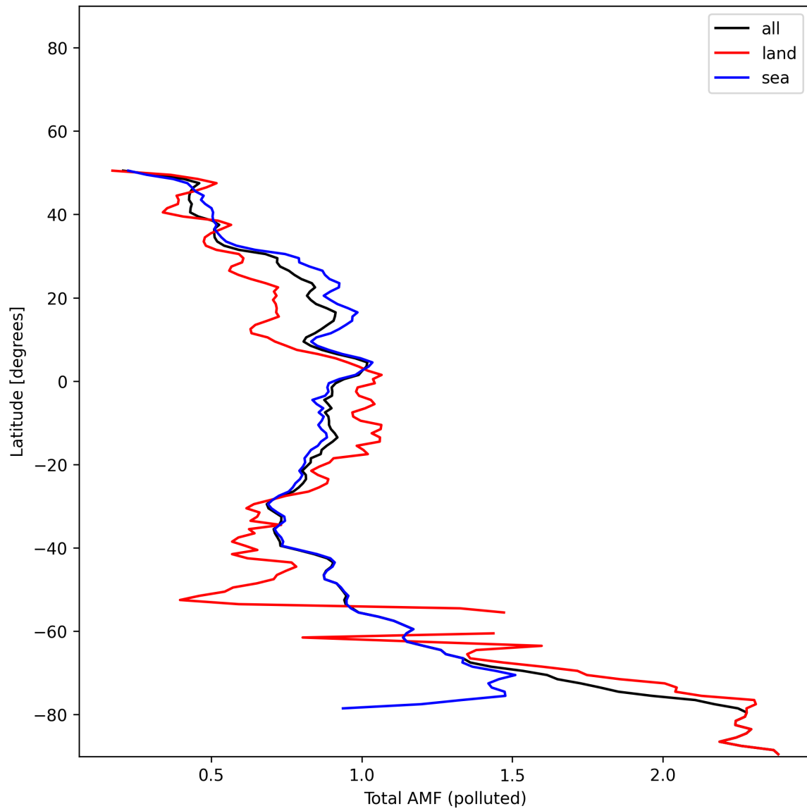
Figure 53: Zonal average of “Total AMF (polluted)” for 2025-11-20 to 2025-11-22.
