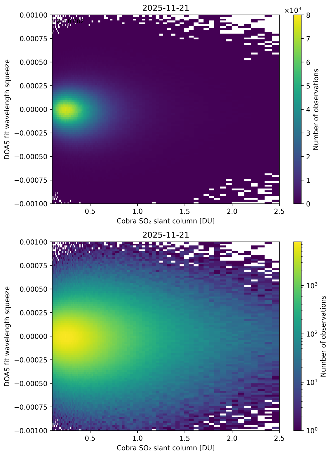
Figure 197: Scatter density plot of “Cobra SO 2 slant column” against “DOAS fit wavelength squeeze” for 2025-11-20 to 2025-11-22.
