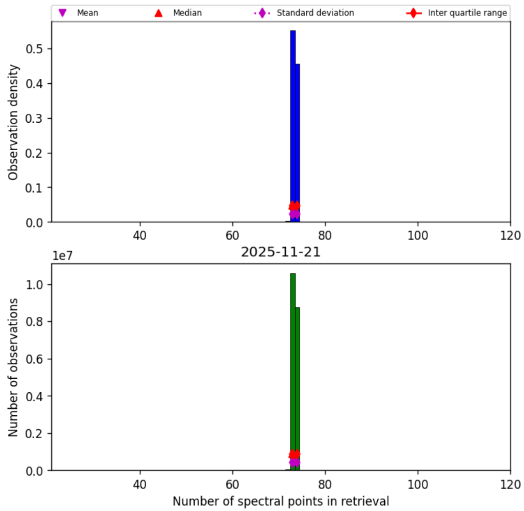
Figure 82: Histogram of “Number of spectral points in retrieval” for 2025-11-20 to 2025-11-22
