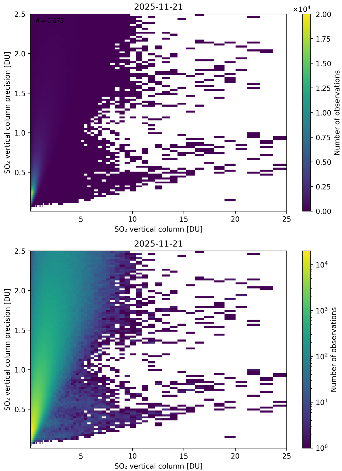
Figure 361: Scatter density plot of “SO 2 vertical column” against “SO 2 vertical column precision” for 2025-11-20 to 2025-11-22.
