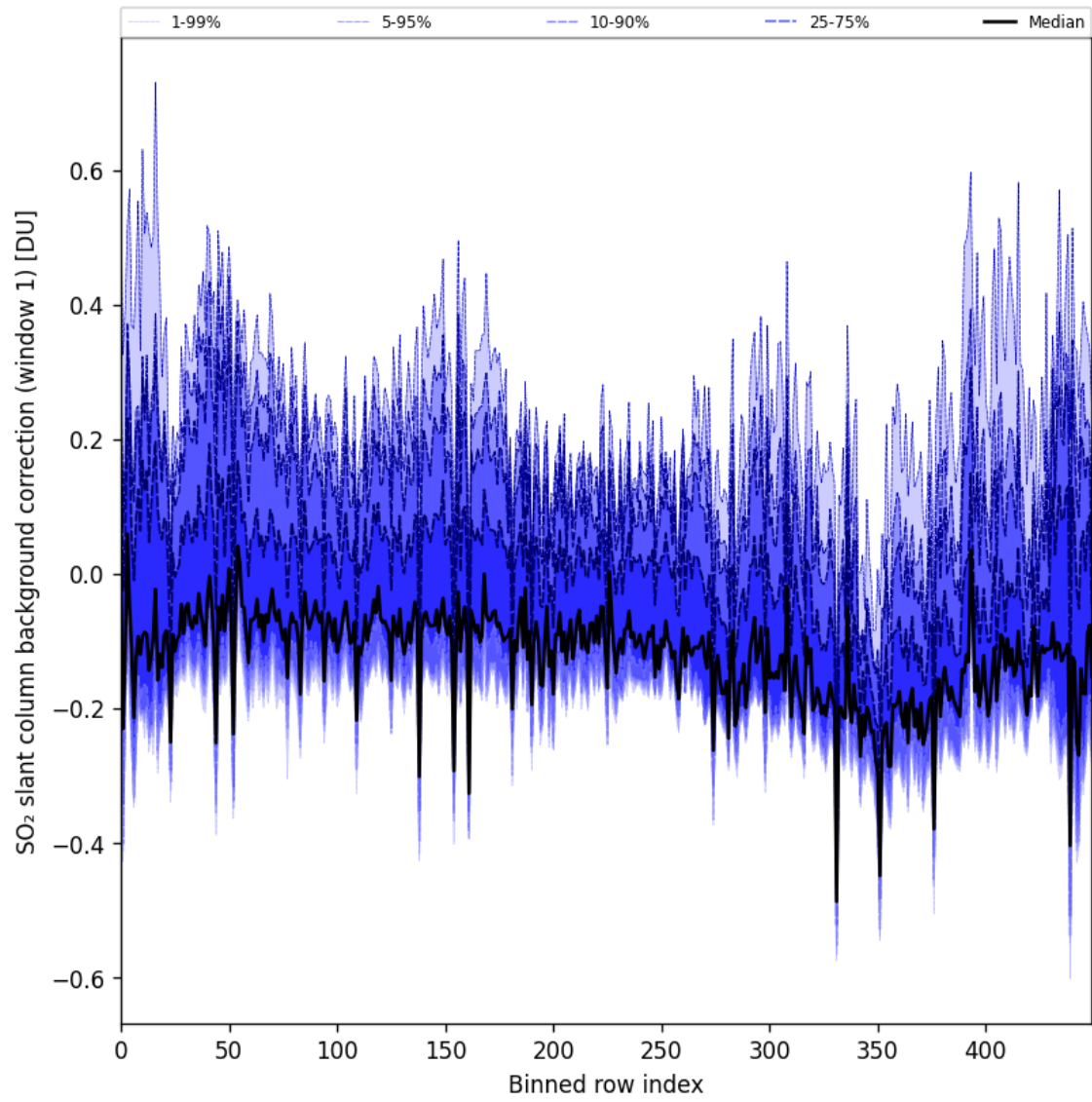
Figure 92: Along track statistics of “SO 2 slant column background correction (window 1)” for 2025-11-20 to 2025-11-22
