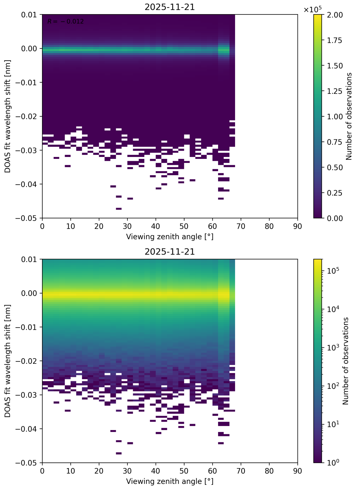
Figure 365: Scatter density plot of “Viewing zenith angle” against “DOAS fit wavelength shift” for 2025-11-20 to 2025-11-22.
