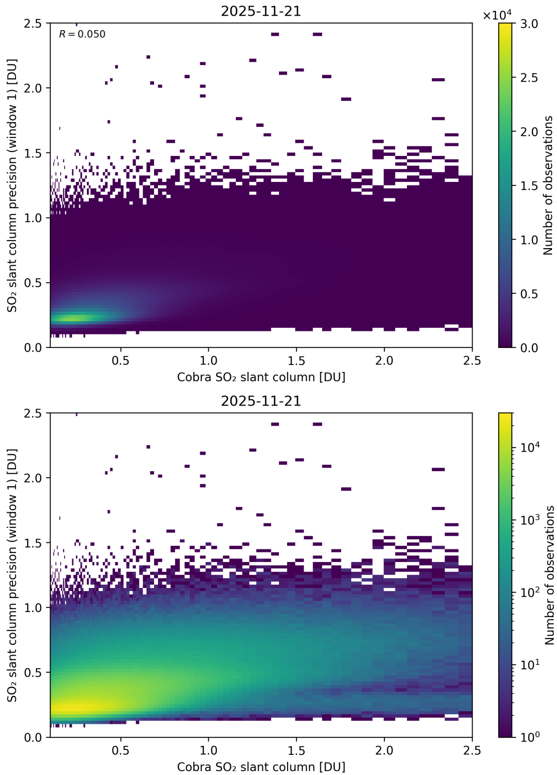
Figure 220: Scatter density plot of “Cobra SO 2 slant column” against “SO 2 slant column precision (window 1)” for 2025-11-20 to 2025-11-22.
