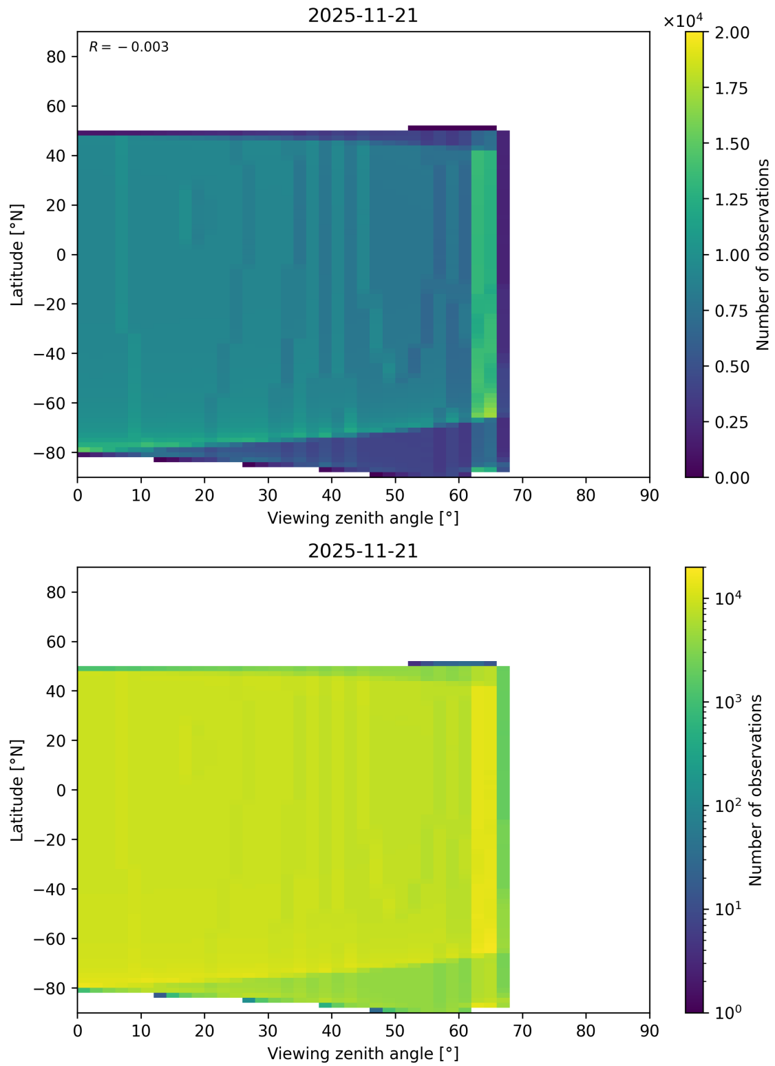
Figure 368: Scatter density plot of “Viewing zenith angle” against “Latitude” for 2025-11-20 to 2025-11-22.
