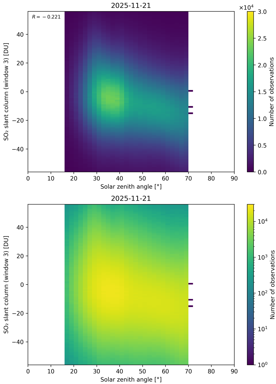
Figure 187: Scatter density plot of “Solar zenith angle” against “SO 2 slant column (window 3)” for 2025-11-20 to 2025-11-22.
