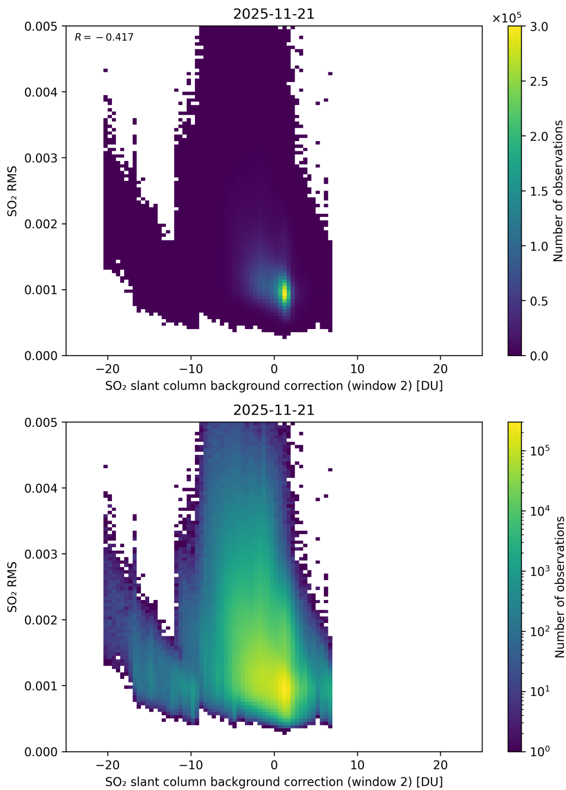
Figure 125: Scatter density plot of “SO 2 slant column background correction (window 2)” against “SO 2 RMS” for 2025-11-20 to 2025-11-22.
