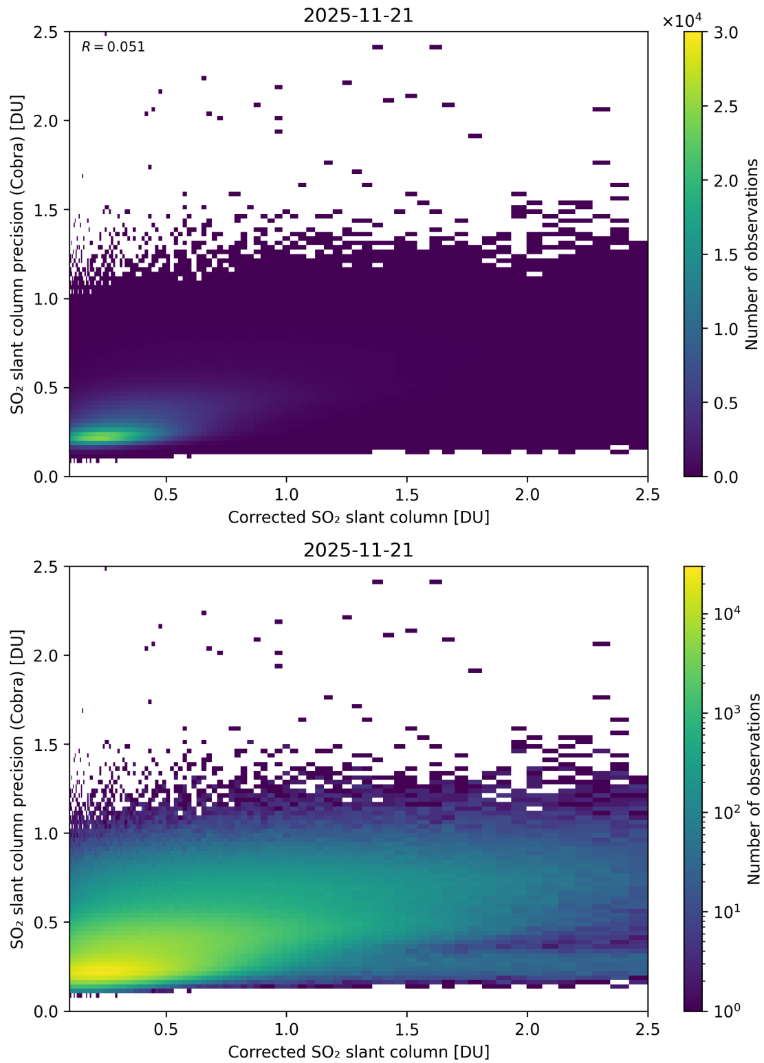
Figure 234: Scatter density plot of “Corrected SO 2 slant column” against “SO 2 slant column precision (Cobra)” for 2025-11-20 to 2025-11-22.
