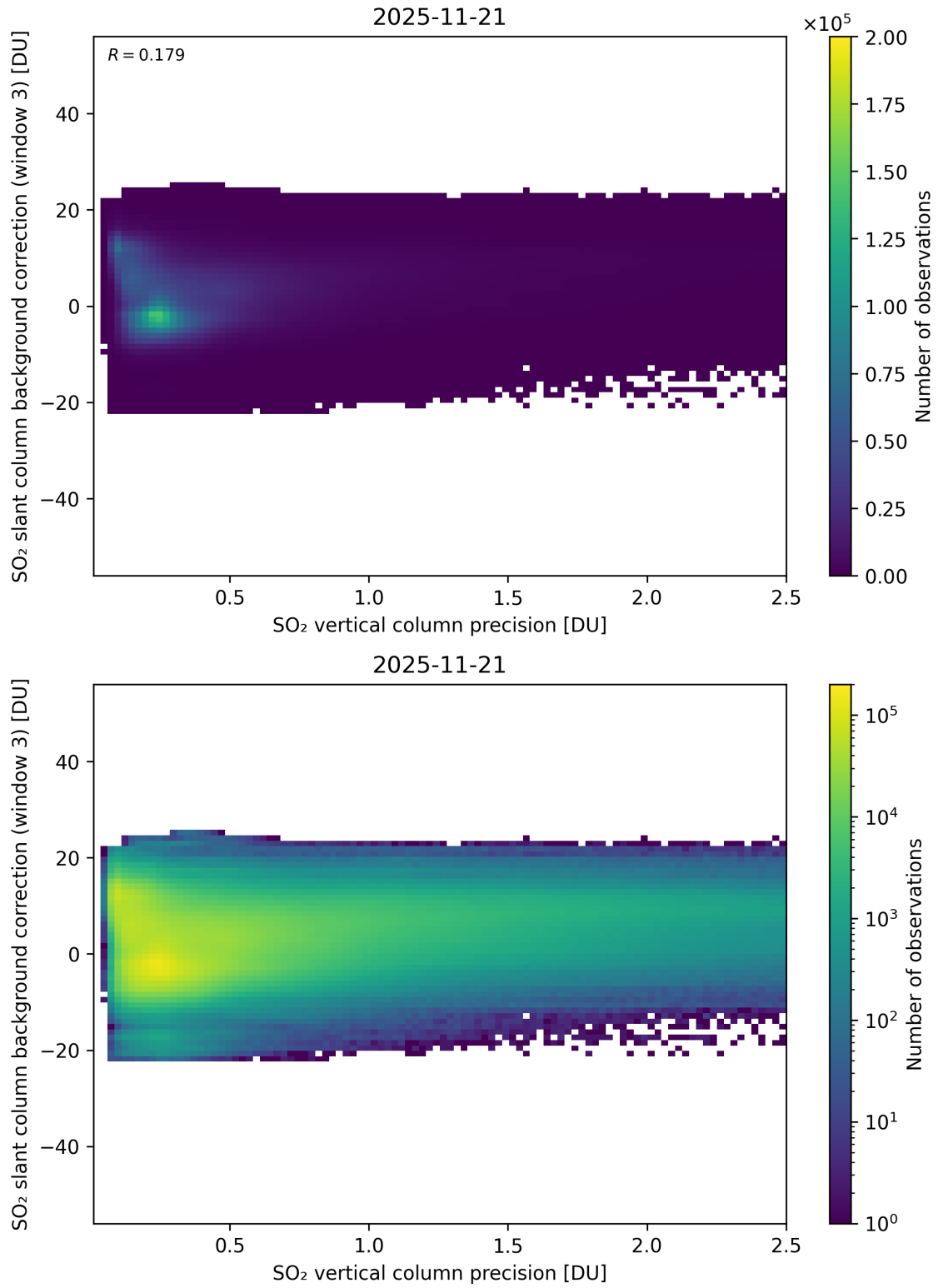
Figure 331: Scatter density plot of “SO 2 vertical column precision” against “SO 2 slant column background correction (window 3)” for 2025-11-20 to 2025-11-22.
