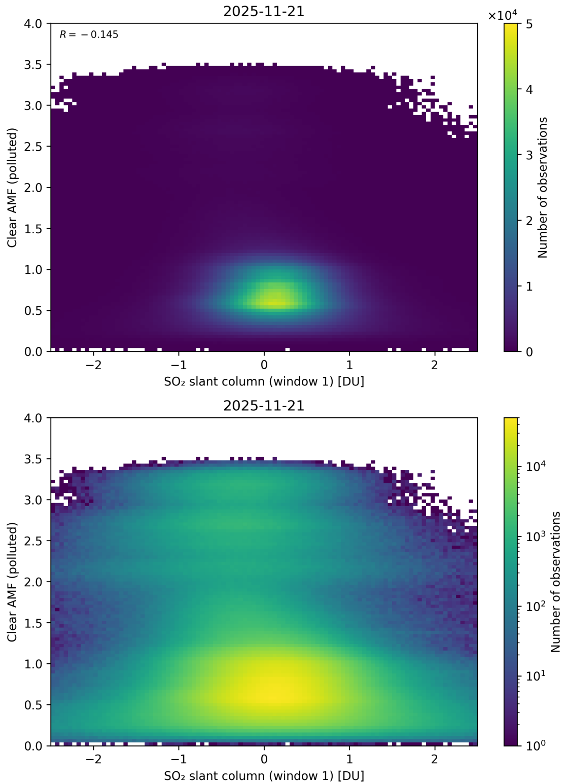
Figure 282: Scatter density plot of “SO 2 slant column (window 1)” against “Clear AMF (polluted)” for 2025-11-20 to 2025-11-22.
