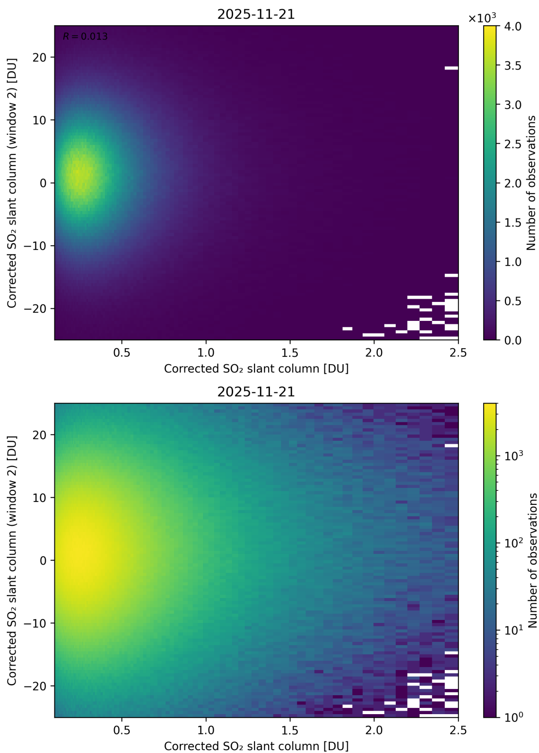
Figure 235: Scatter density plot of “Corrected SO 2 slant column” against “Corrected SO 2 slant column (window 2)” for 2025-11-20 to 2025-11-22.
