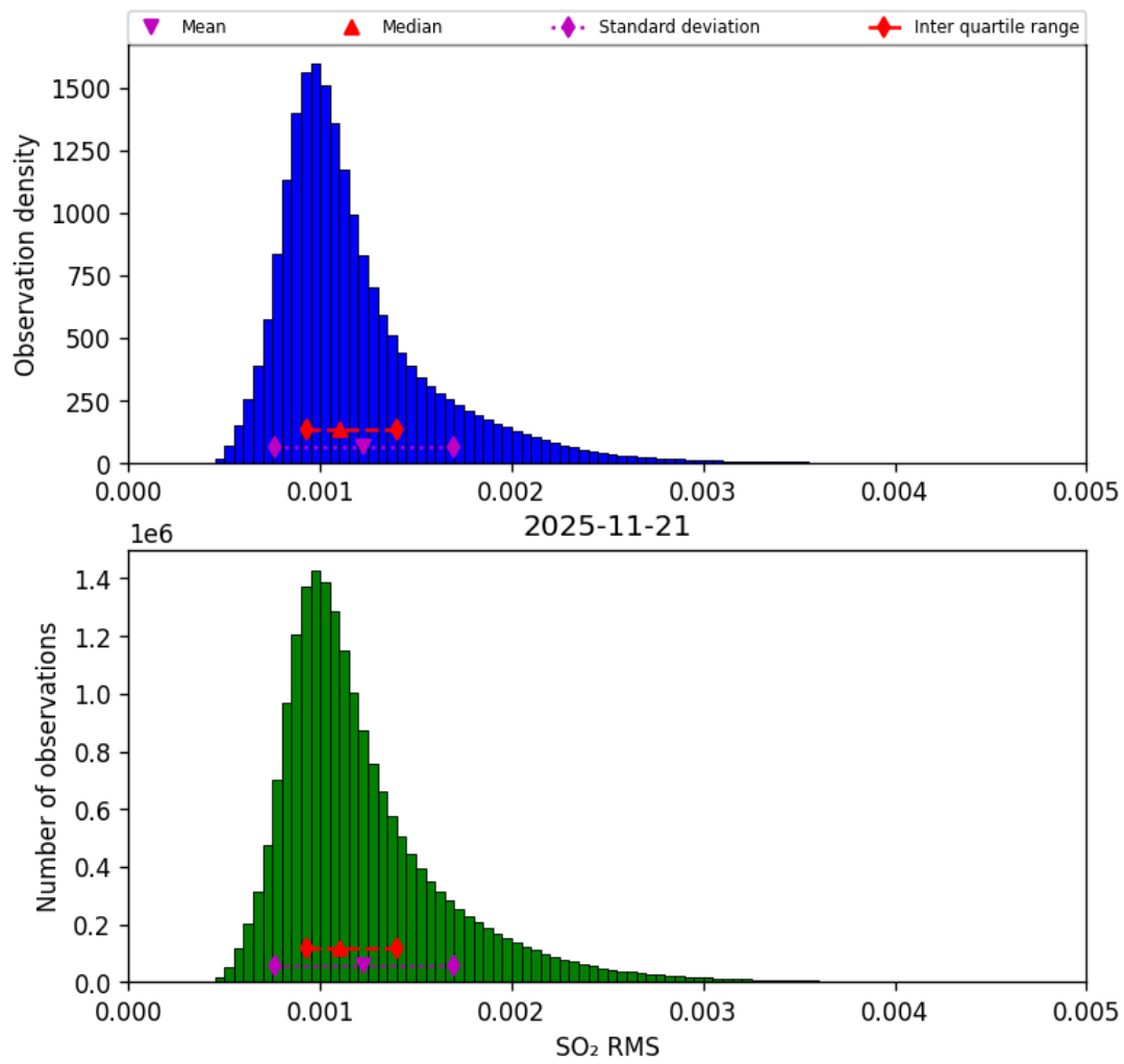
Figure 78: Histogram of “SO 2 RMS” for 2025-11-20 to 2025-11-22
