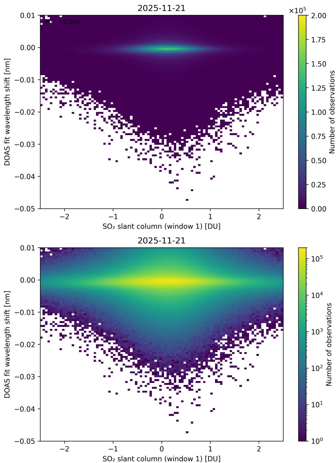
Figure 265: Scatter density plot of “SO 2 slant column (window 1)” against “DOAS fit wavelength shift” for 2025-11-20 to 2025-11-22.
