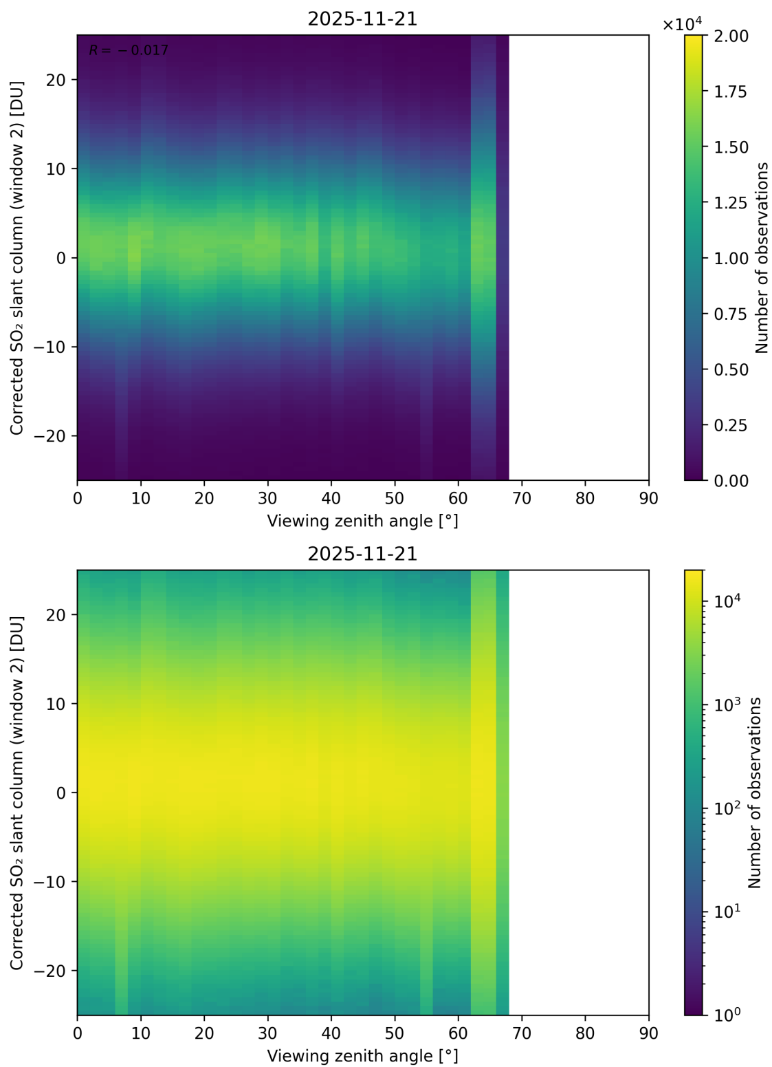
Figure 374: Scatter density plot of “Viewing zenith angle” against “Corrected SO 2 slant column (window 2)” for 2025-11-20 to 2025-11-22.
