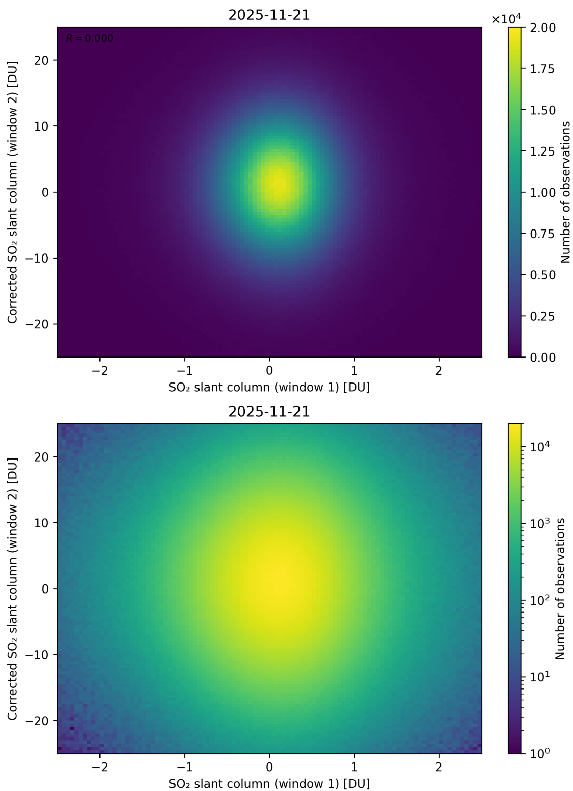
Figure 283: Scatter density plot of “SO 2 slant column (window 1)” against “Corrected SO 2 slant column (window 2)” for 2025-11-20 to 2025-11-22.
