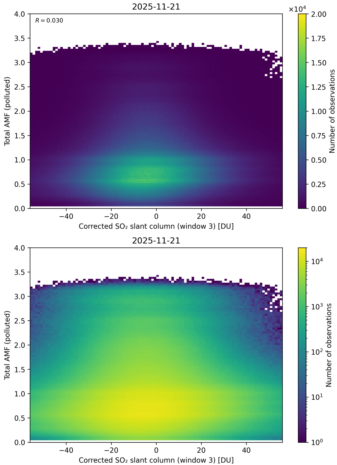
Figure 260: Scatter density plot of “Corrected SO 2 slant column (window 3)” against “Total AMF (polluted)” for 2025-11-20 to 2025-11-22.
