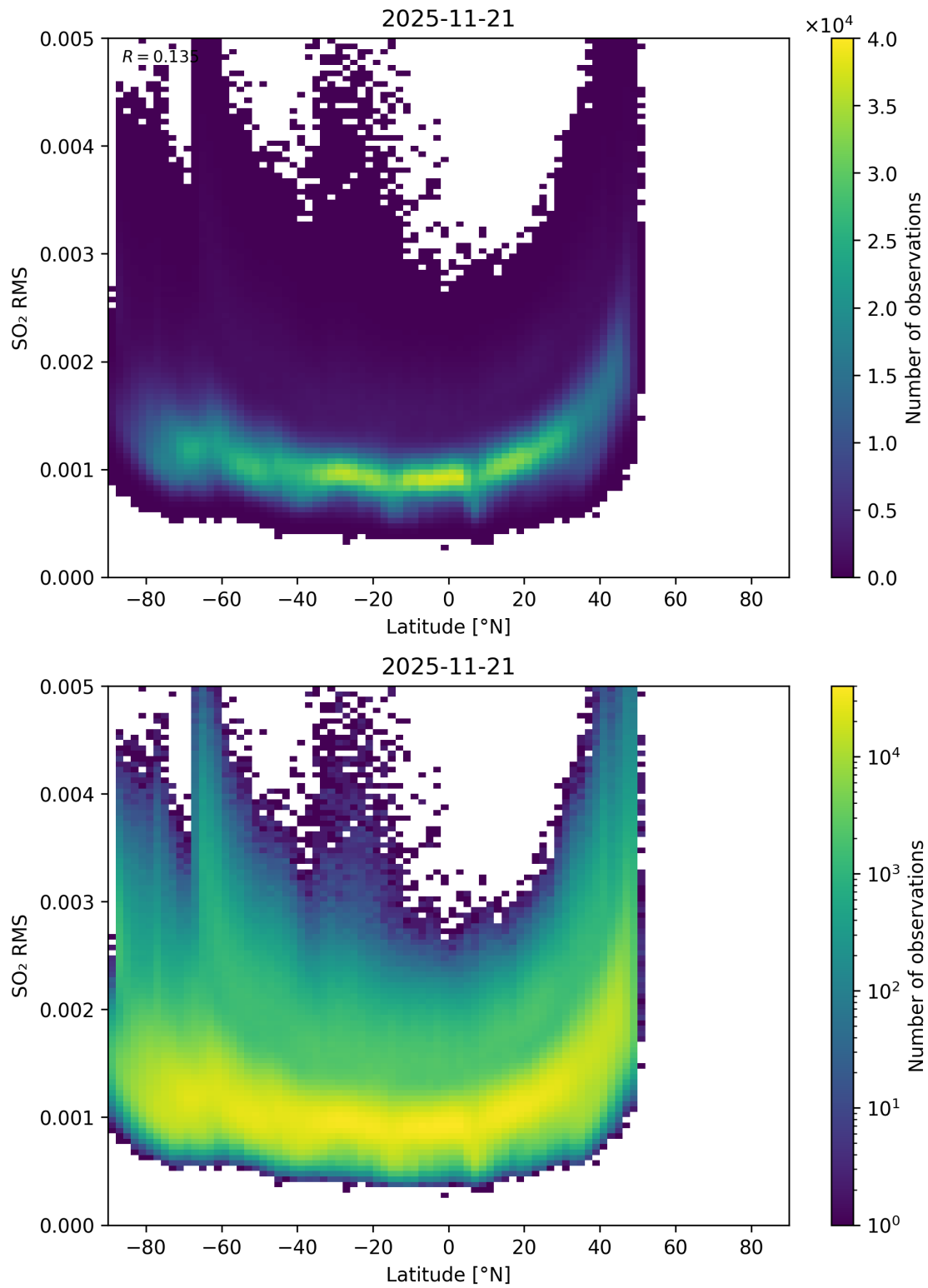
Figure 155: Scatter density plot of “Latitude” against “SO 2 RMS” for 2025-11-20 to 2025-11-22.
