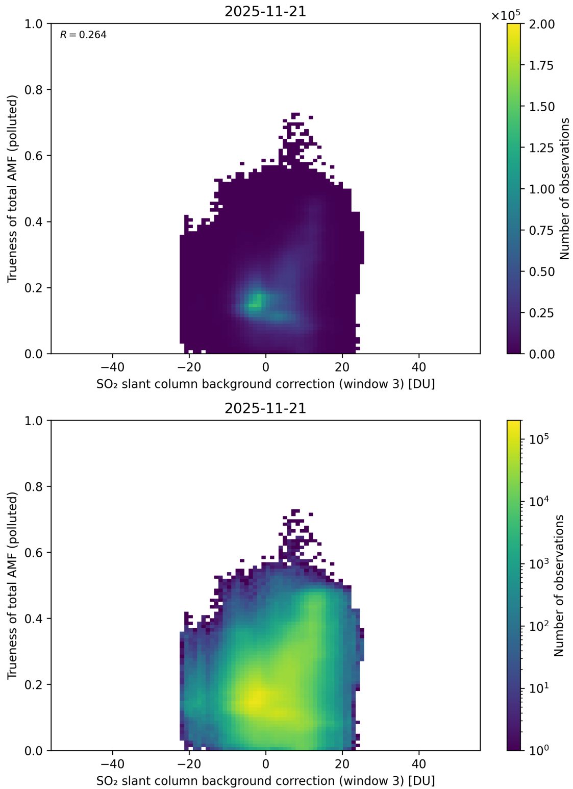
Figure 137: Scatter density plot of “SO 2 slant column background correction (window 3)” against “Trueness of total AMF (polluted)” for 2025-11-20 to 2025-11-22.
