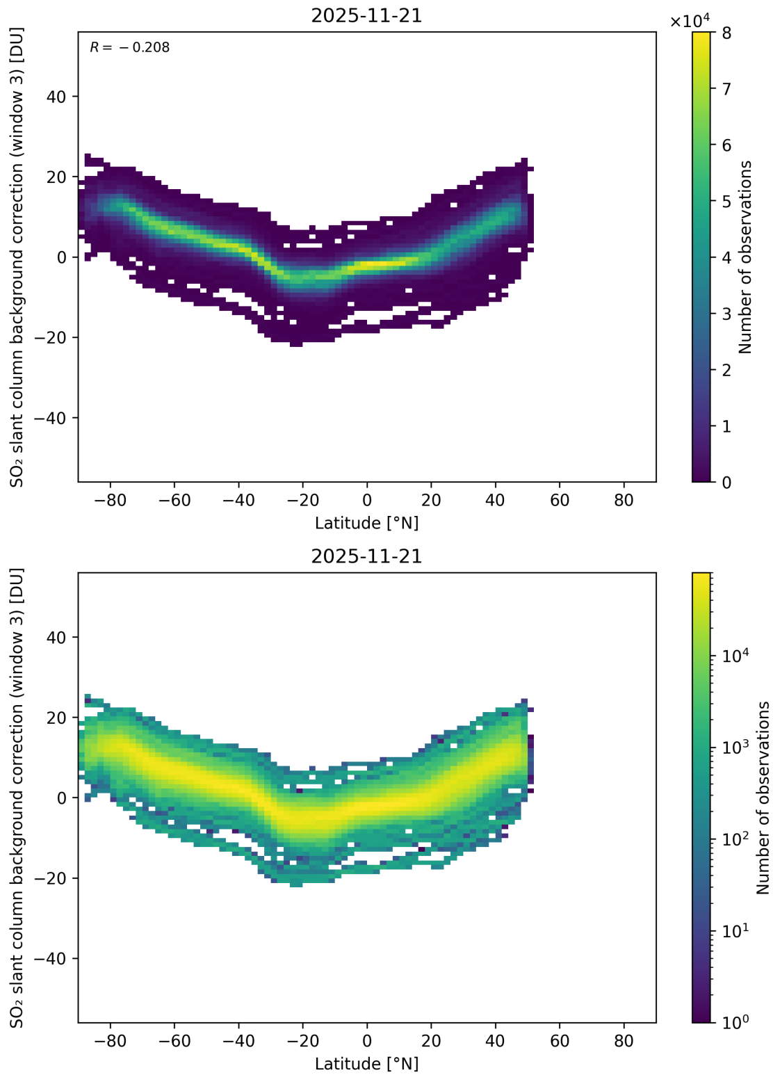
Figure 152: Scatter density plot of “Latitude” against “SO 2 slant column background correction (window 3)” for 2025-11-20 to 2025-11-22.
