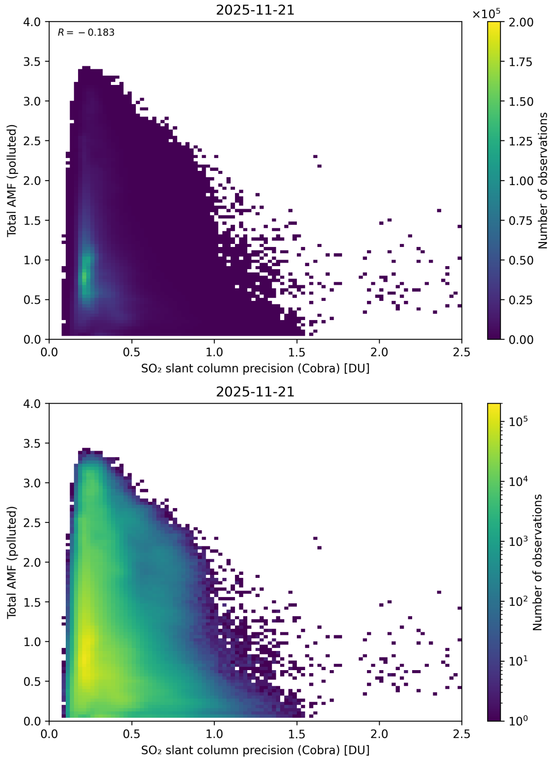
Figure 213: Scatter density plot of “SO 2 slant column precision (Cobra)” against “Total AMF (polluted)” for 2025-11-20 to 2025-11-22.
