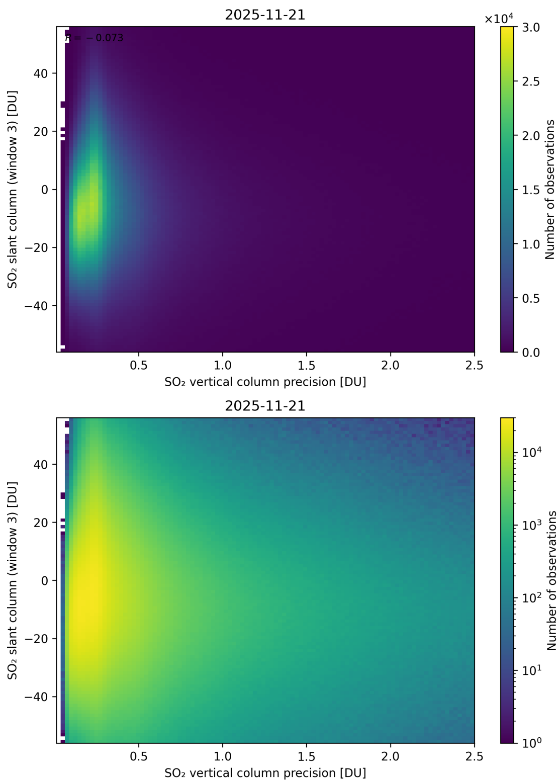
Figure 344: Scatter density plot of “SO 2 vertical column precision” against “SO 2 slant column (window 3)” for 2025-11-20 to 2025-11-22.
