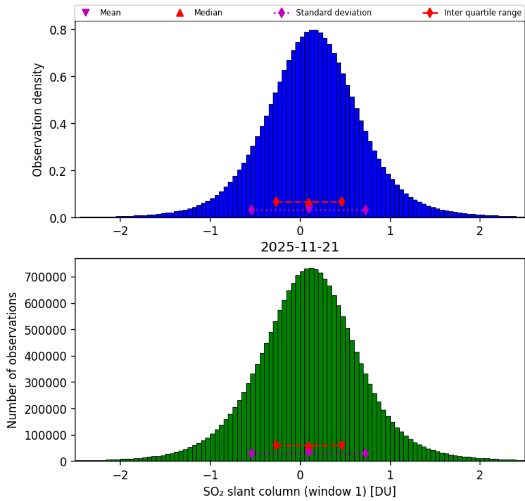
Figure 63: Histogram of “SO 2 slant column (window 1)” for 2025-11-20 to 2025-11-22
