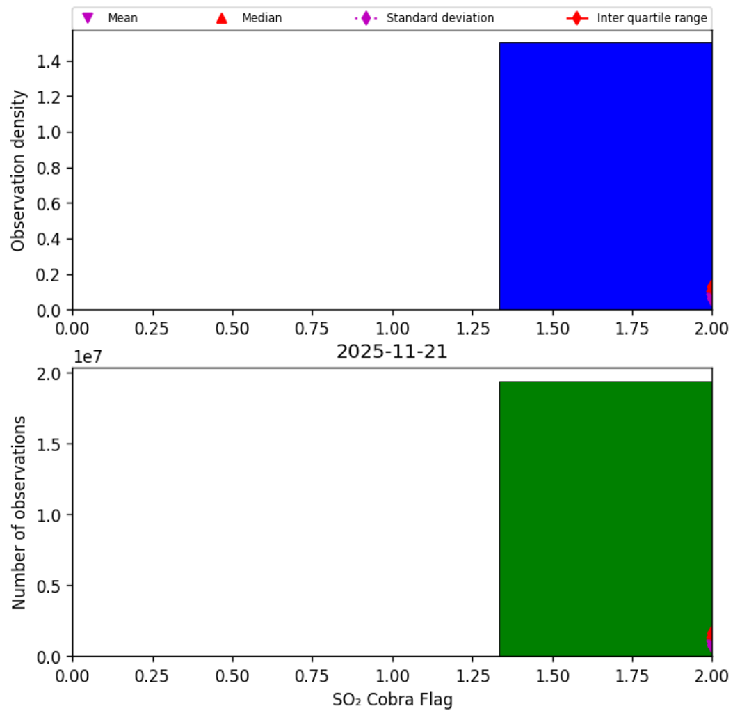
Figure 75: Histogram of “SO 2 Cobra Flag” for 2025-11-20 to 2025-11-22
