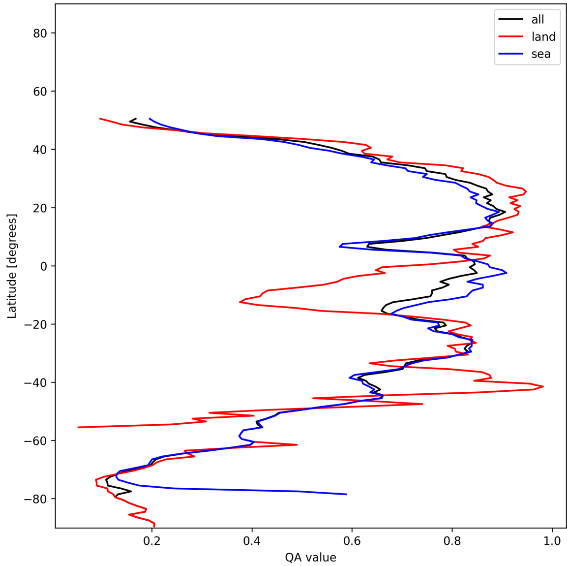
Figure 31: Zonal average of “QA value” for 2025-11-20 to 2025-11-22.
