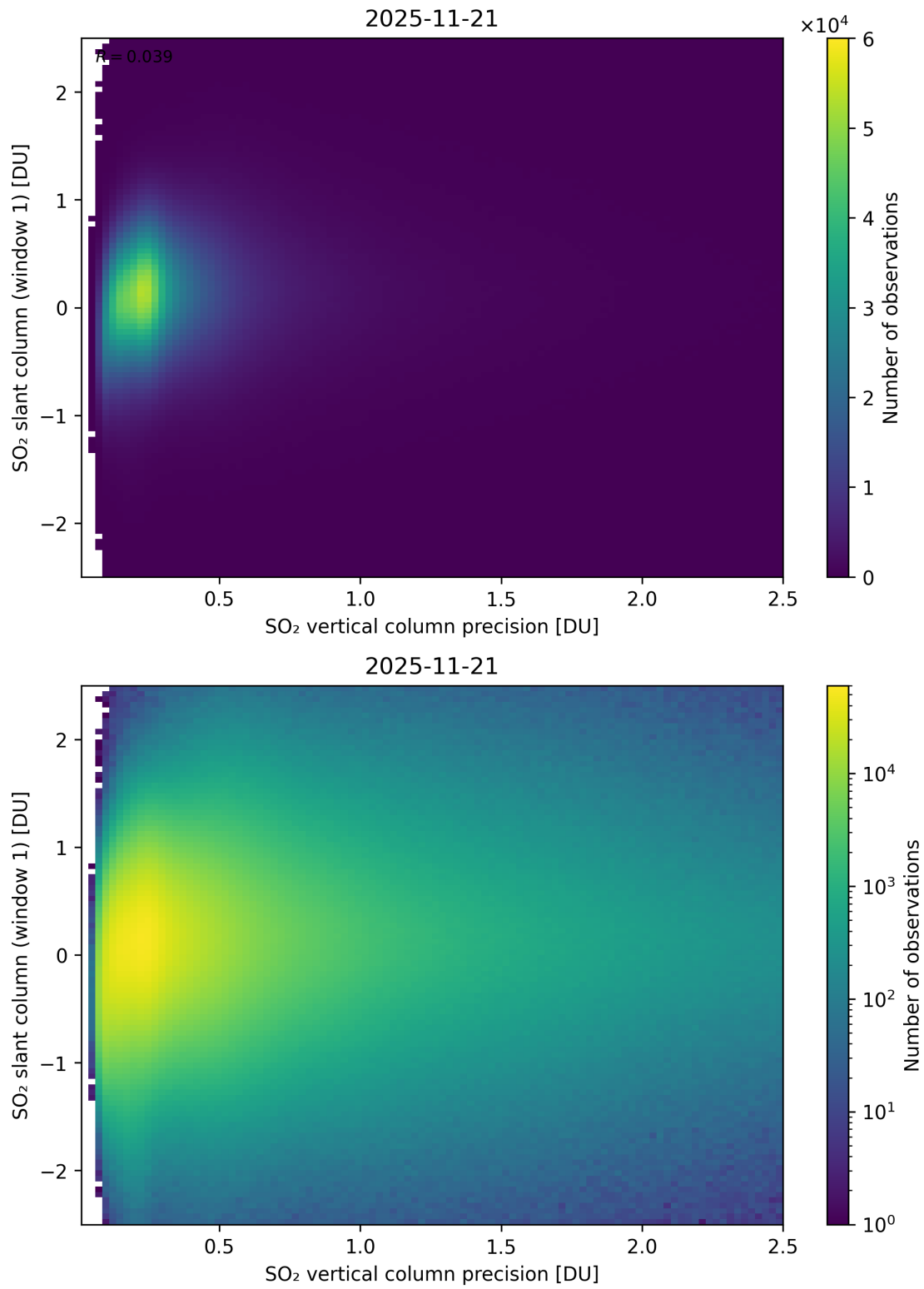
Figure 341: Scatter density plot of “SO 2 vertical column precision” against “SO 2 slant column (window 1)” for 2025-11-20 to 2025-11-22.
