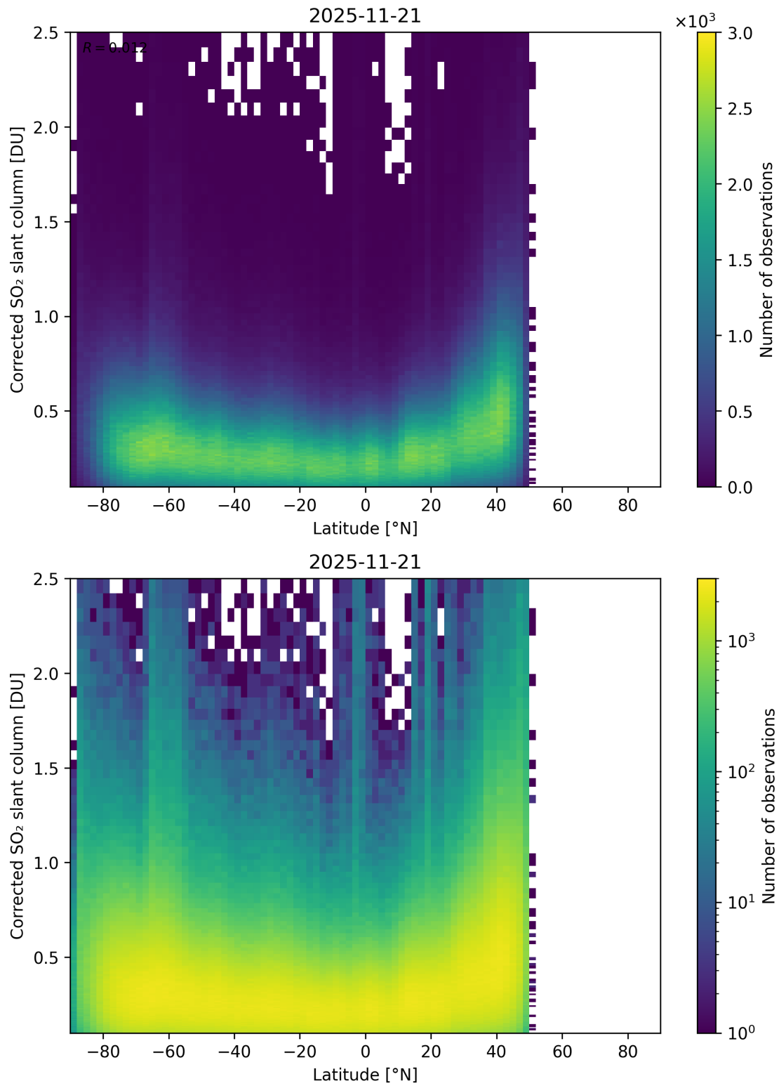
Figure 159: Scatter density plot of “Latitude” against “Corrected SO 2 slant column” for 2025-11-20 to 2025-11-22.
