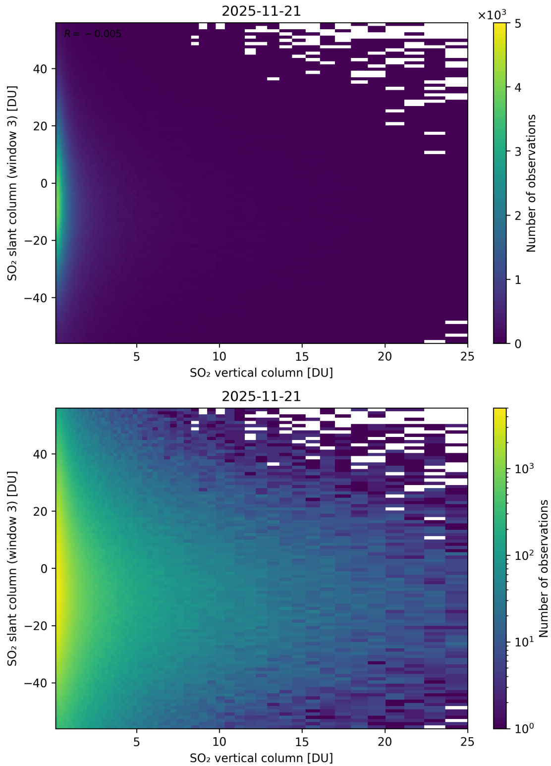
Figure 357: Scatter density plot of “SO 2 vertical column” against “SO 2 slant column (window 3)” for 2025-11-20 to 2025-11-22.
