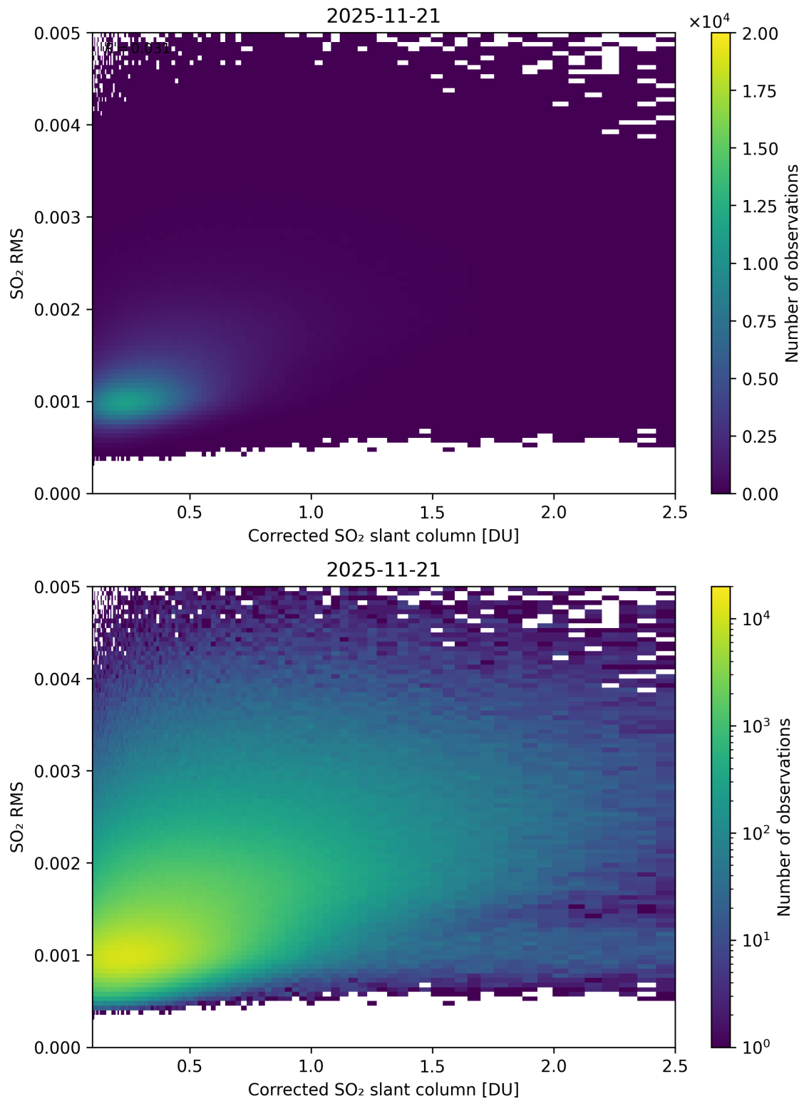
Figure 231: Scatter density plot of “Corrected SO 2 slant column” against “SO 2 RMS” for 2025-11-20 to 2025-11-22.
