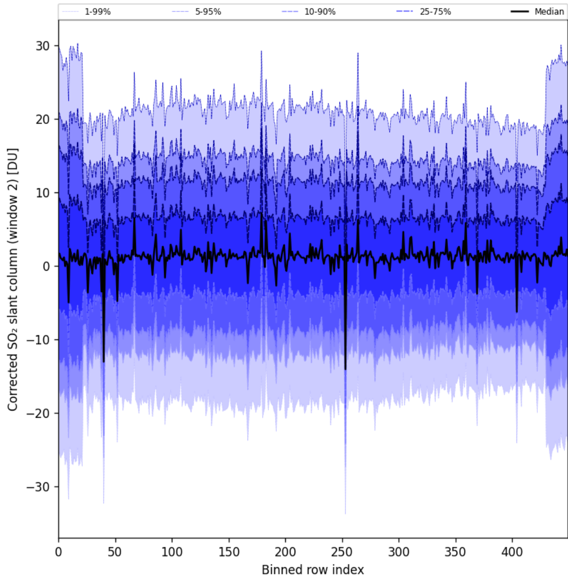
Figure 95: Along track statistics of “Corrected SO 2 slant column (window 2)” for 2025-11-20 to 2025-11-22
