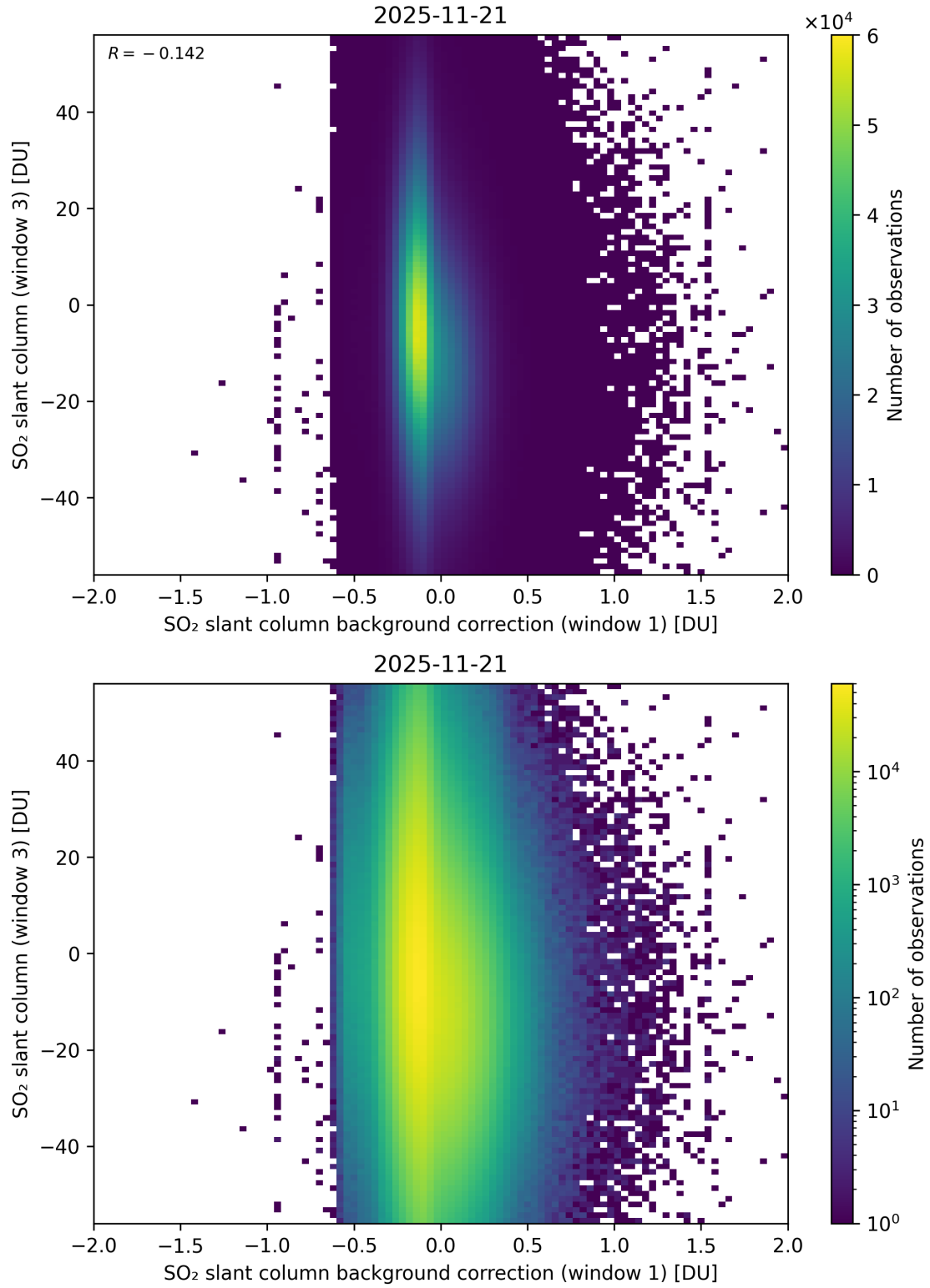
Figure 118: Scatter density plot of “SO 2 slant column background correction (window 1)” against “SO 2 slant column (window 3)” for 2025-11-20 to 2025-11-22.
