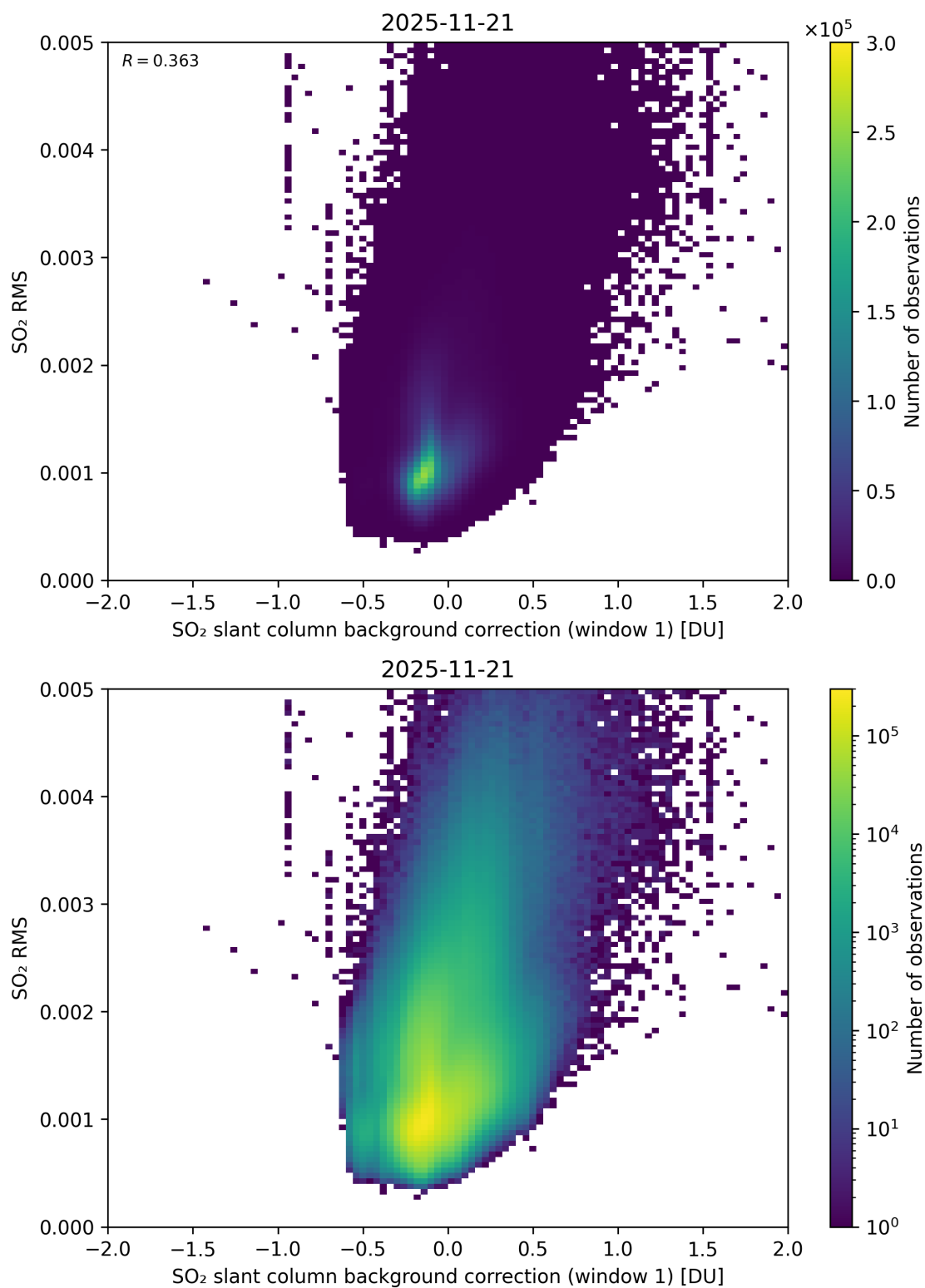
Figure 113: Scatter density plot of “SO 2 slant column background correction (window 1)” against “SO 2 RMS” for 2025-11-20 to 2025-11-22.
