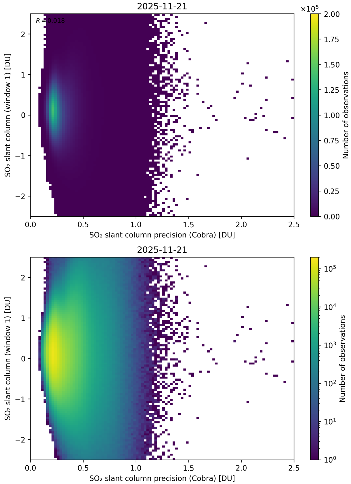
Figure 208: Scatter density plot of “SO 2 slant column precision (Cobra)” against “SO 2 slant column (window 1)” for 2025-11-20 to 2025-11-22.
