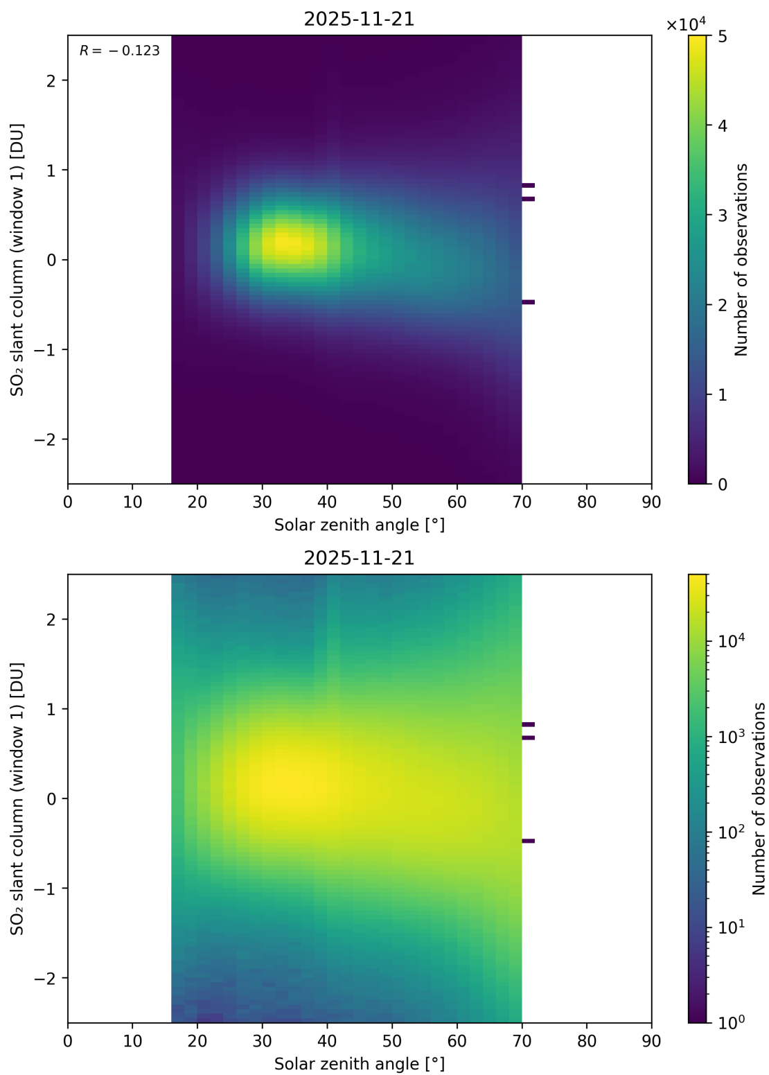
Figure 184: Scatter density plot of “Solar zenith angle” against “SO 2 slant column (window 1)” for 2025-11-20 to 2025-11-22.
