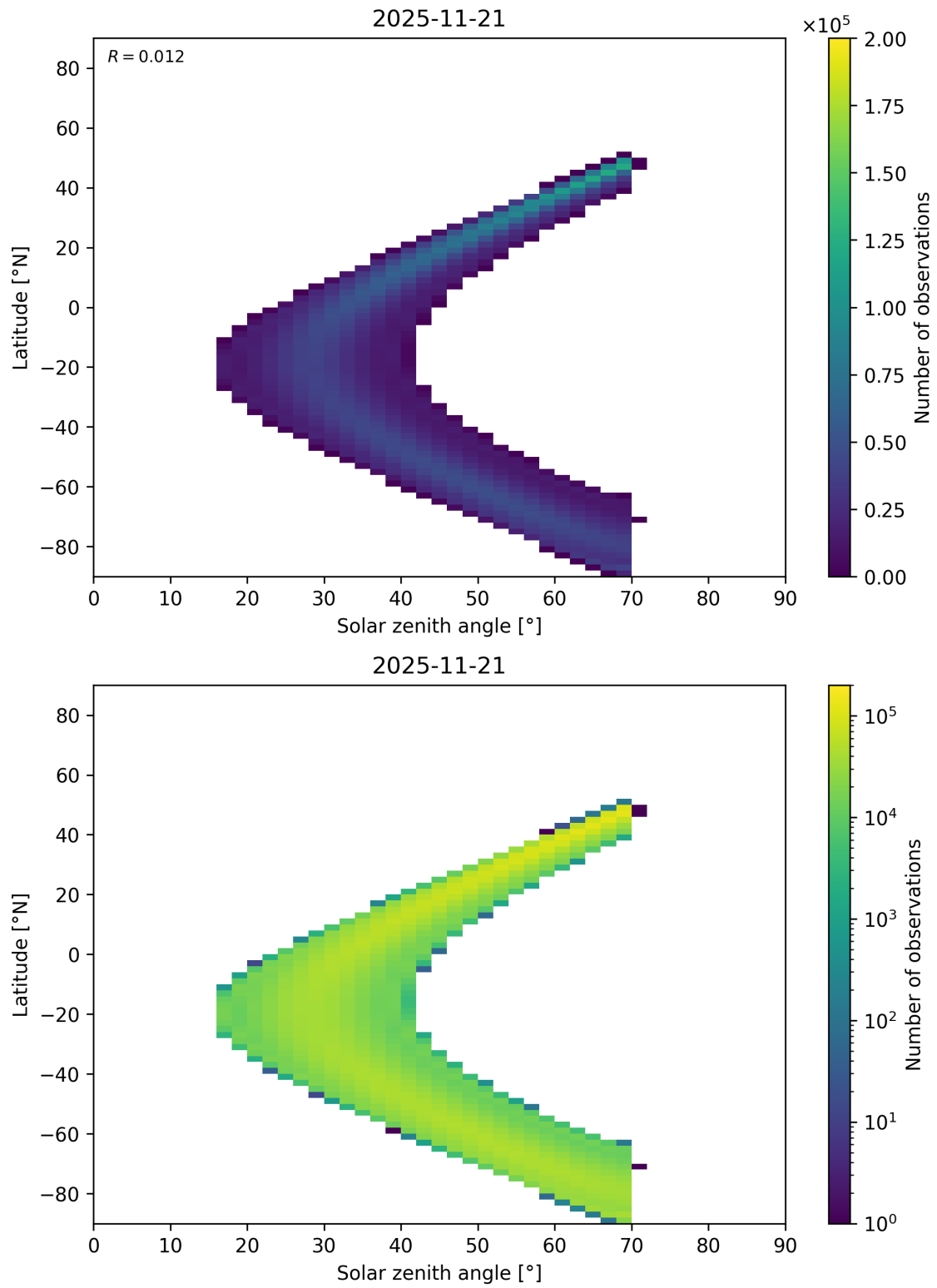
Figure 177: Scatter density plot of “Solar zenith angle” against “Latitude” for 2025-11-20 to 2025-11-22.
