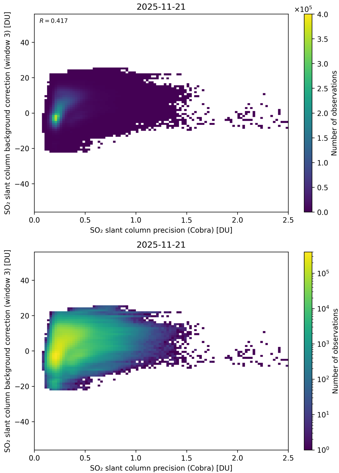
Figure 201: Scatter density plot of “SO 2 slant column precision (Cobra)” against “SO 2 slant column background correction (window 3)” for 2025-11-20 to 2025-11-22.
