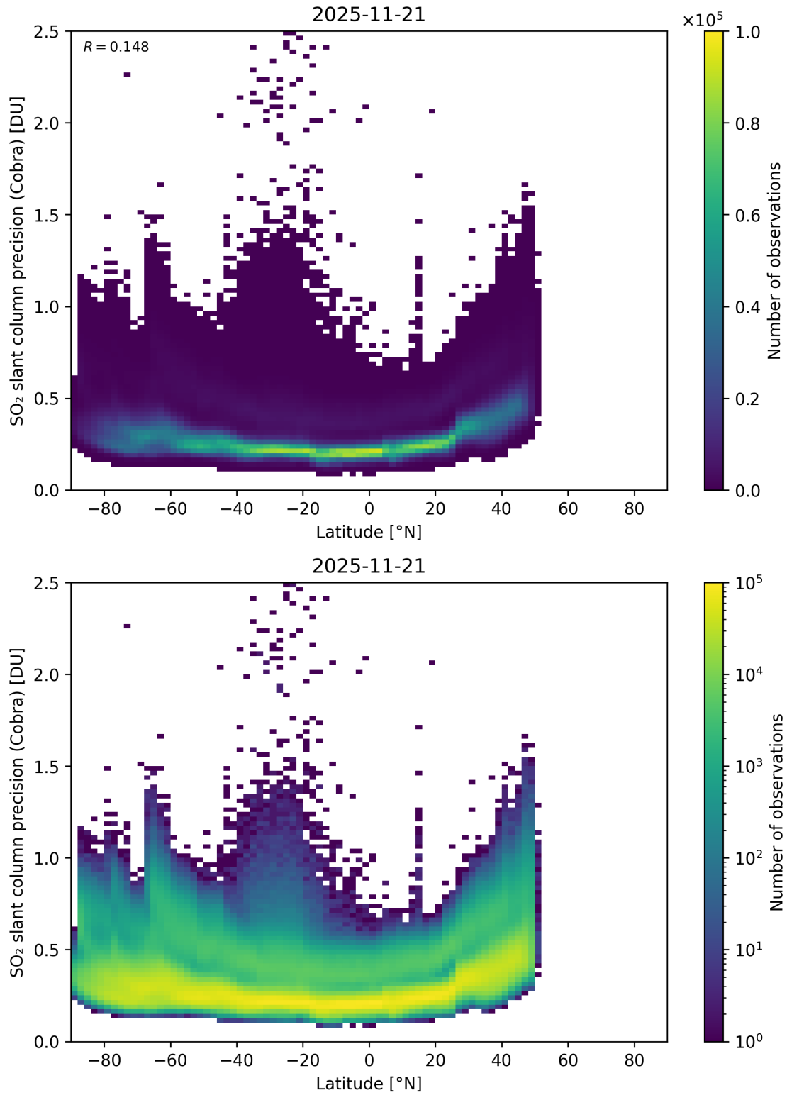
Figure 158: Scatter density plot of “Latitude” against “SO 2 slant column precision (Cobra)” for 2025-11-20 to 2025-11-22.
