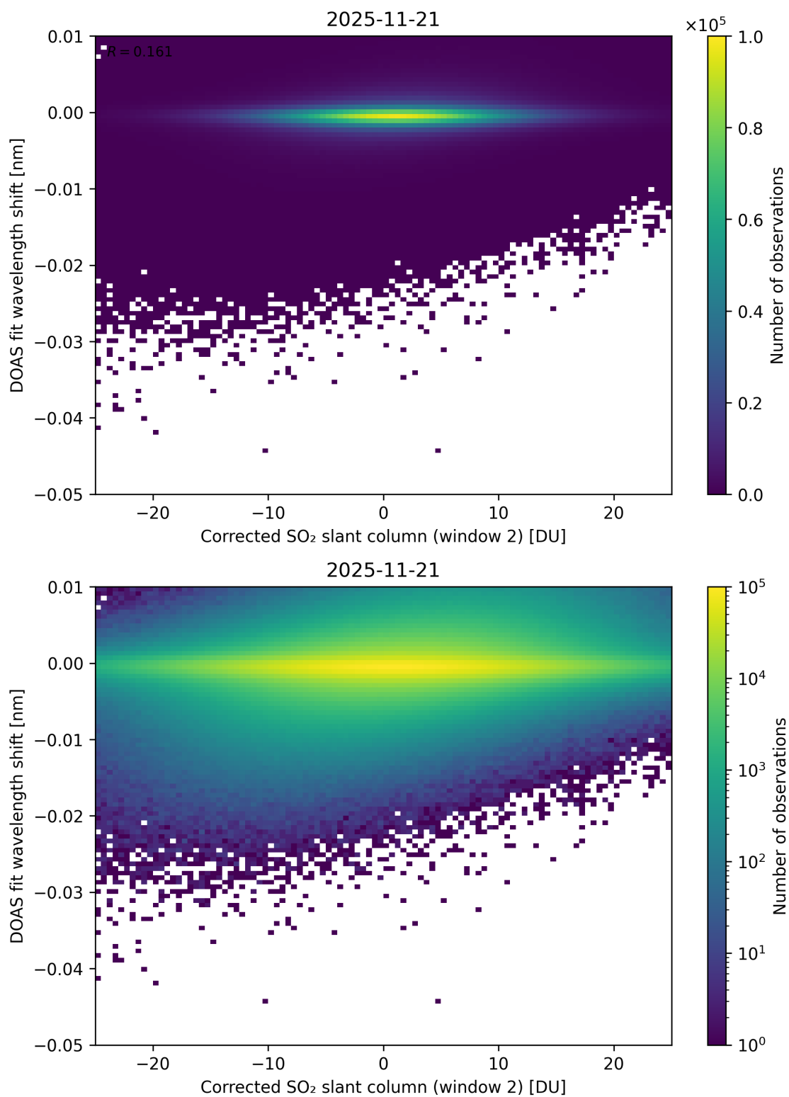
Figure 246: Scatter density plot of “Corrected SO 2 slant column (window 2)” against “DOAS fit wavelength shift” for 2025-11-20 to 2025-11-22.
