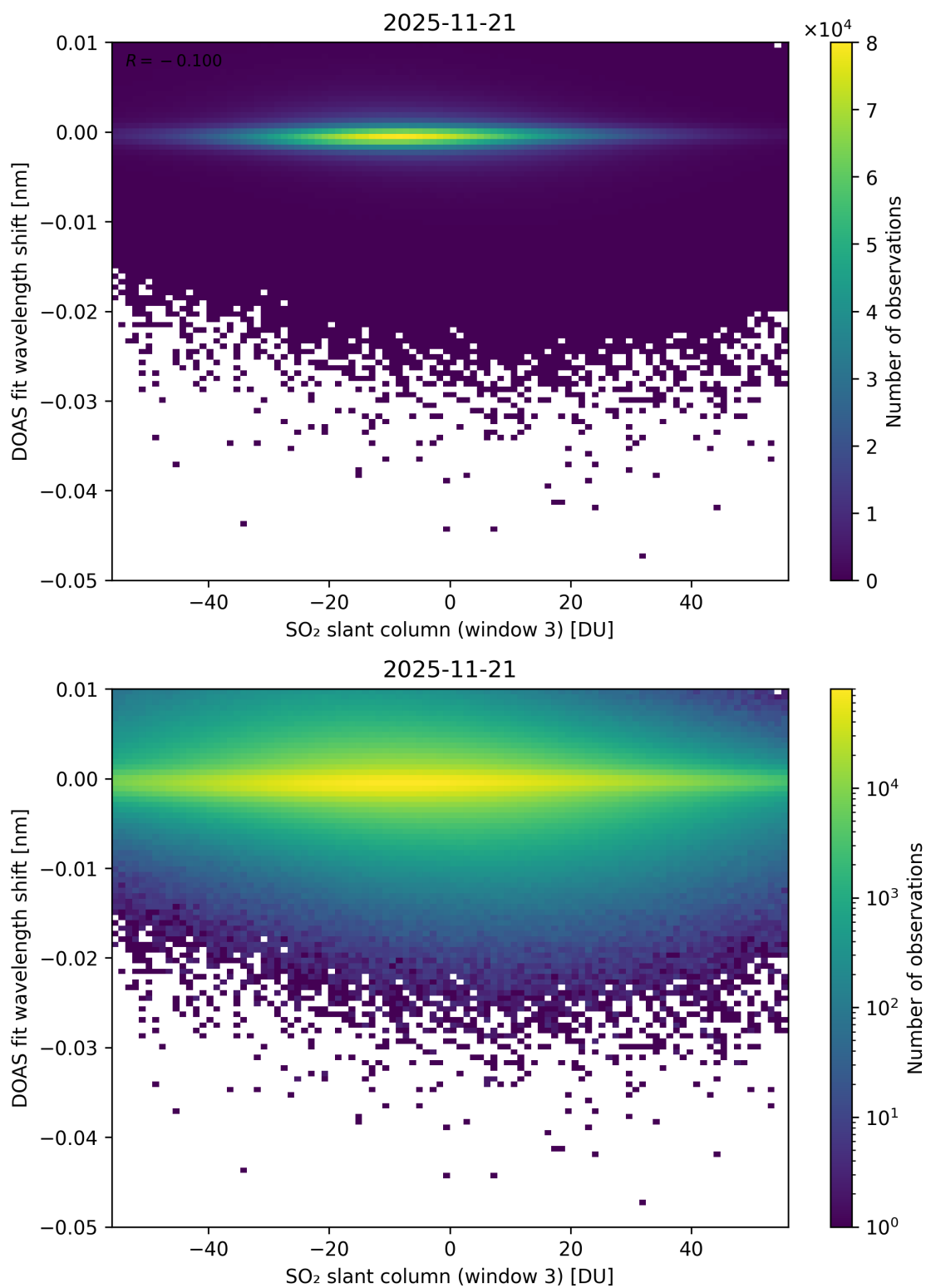
Figure 304: Scatter density plot of “SO 2 slant column (window 3)” against “DOAS fit wavelength shift” for 2025-11-20 to 2025-11-22.
