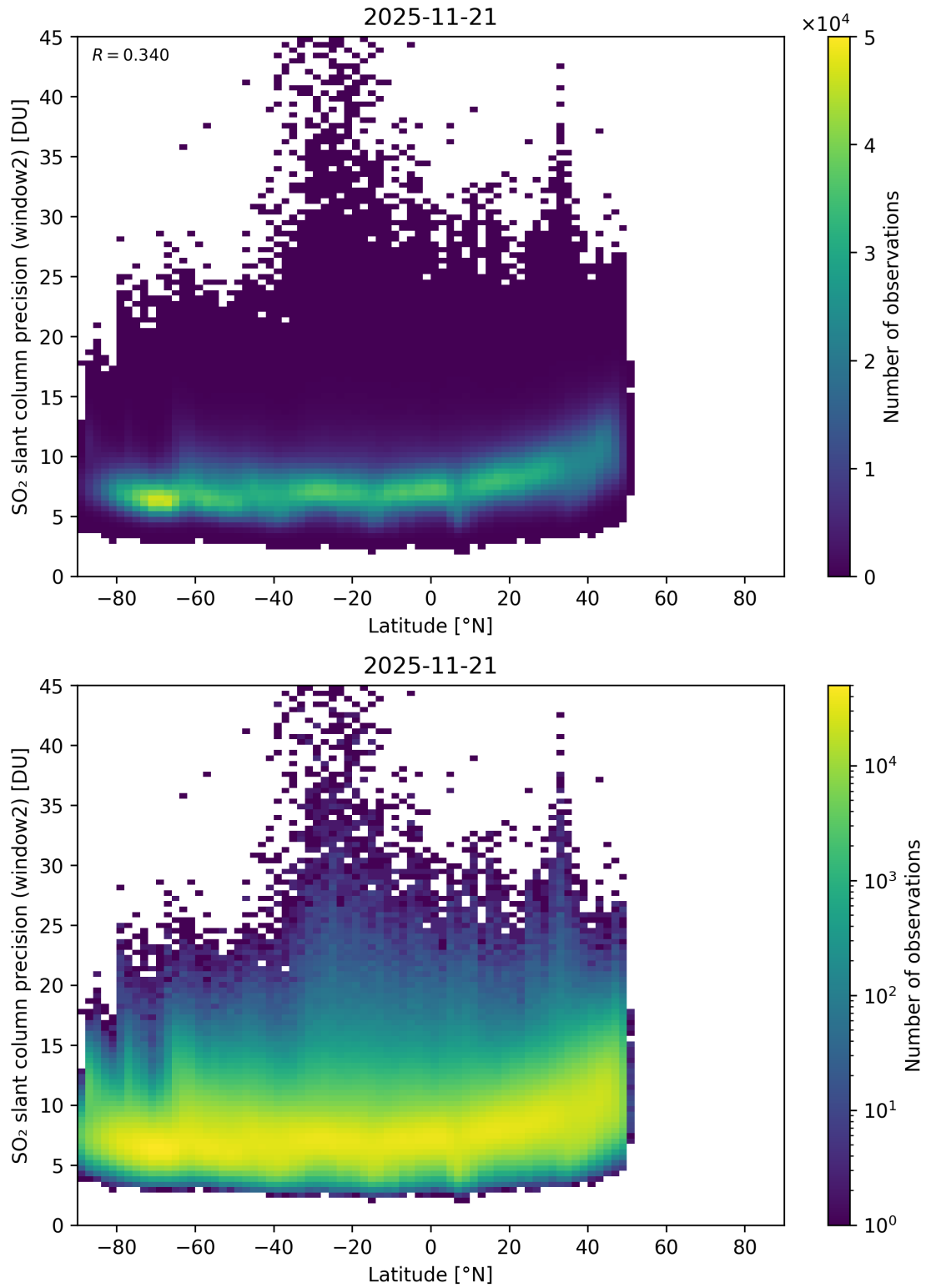
Figure 164: Scatter density plot of “Latitude” against “SO 2 slant column precision (window2)” for 2025-11-20 to 2025-11-22.
