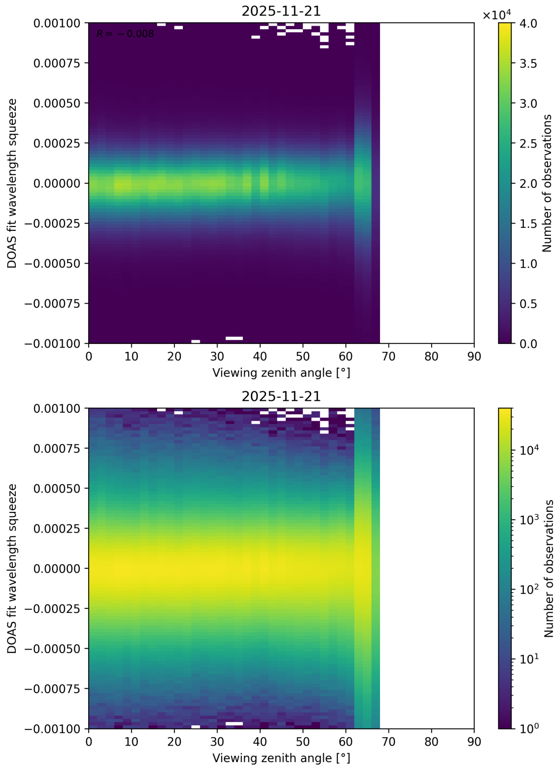
Figure 366: Scatter density plot of “Viewing zenith angle” against “DOAS fit wavelength squeeze” for 2025-11-20 to 2025-11-22.
