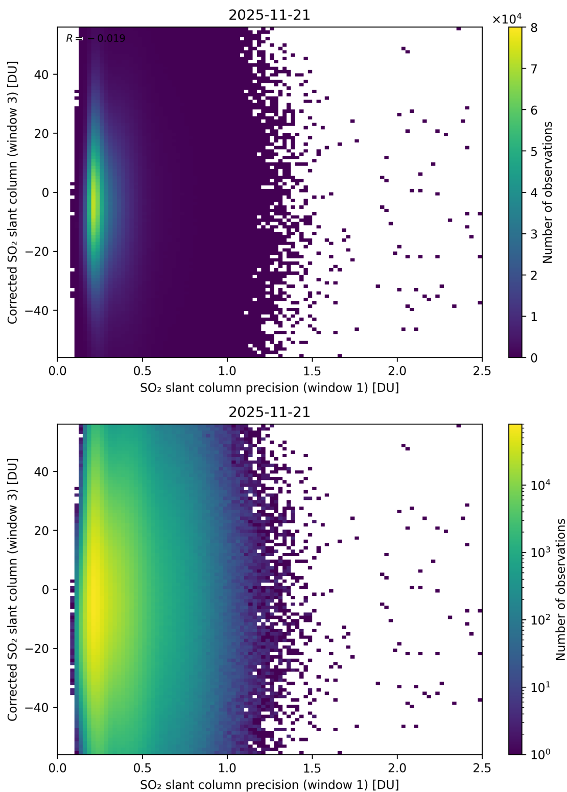
Figure 276: Scatter density plot of “SO 2 slant column precision (window 1)” against “Corrected SO 2 slant column (window 3)” for 2025-11-20 to 2025-11-22.
