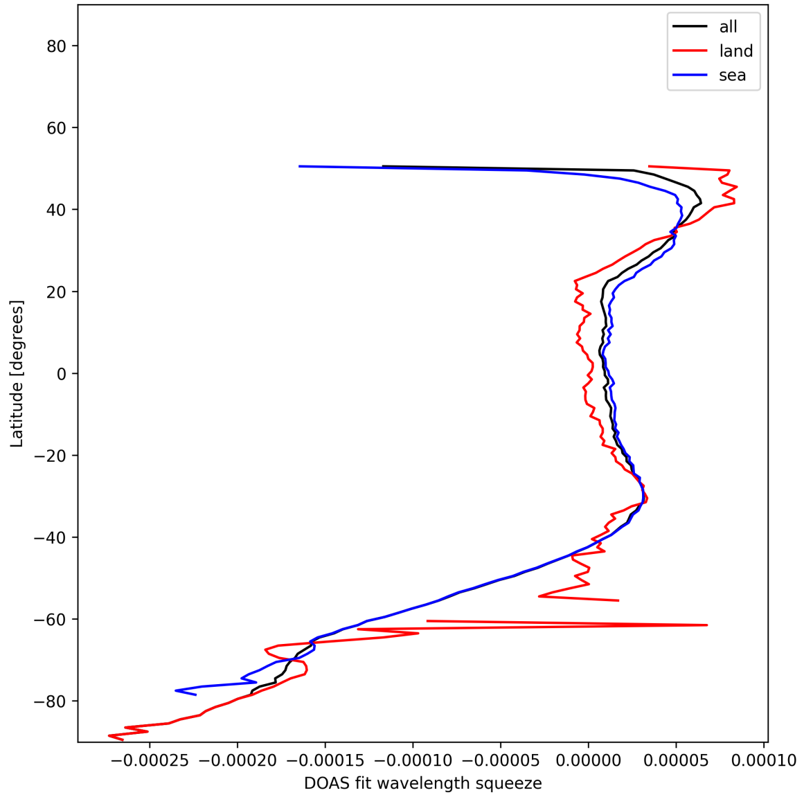
Figure 51: Zonal average of “DOAS fit wavelength squeeze” for 2025-11-20 to 2025-11-22.
