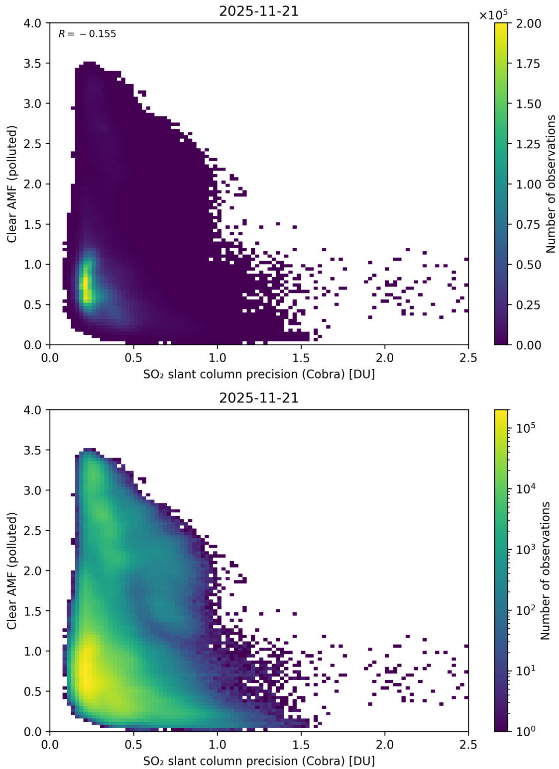
Figure 205: Scatter density plot of “SO 2 slant column precision (Cobra)” against “Clear AMF (polluted)” for 2025-11-20 to 2025-11-22.
