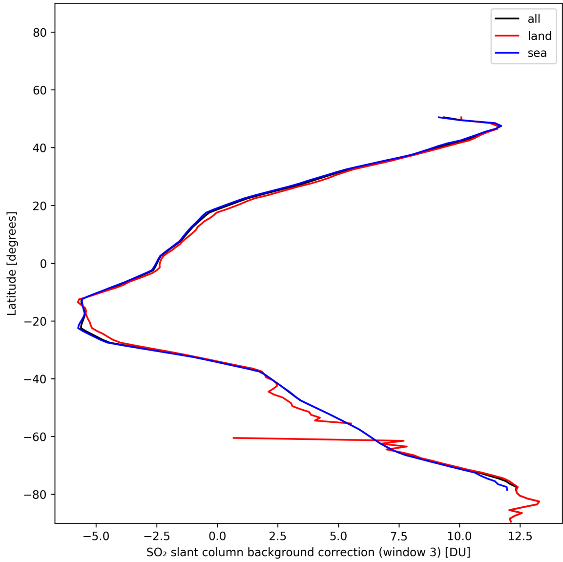
Figure 48: Zonal average of “SO 2 slant column background correction (window 3)” for 2025-11-20 to 2025-11-22.
