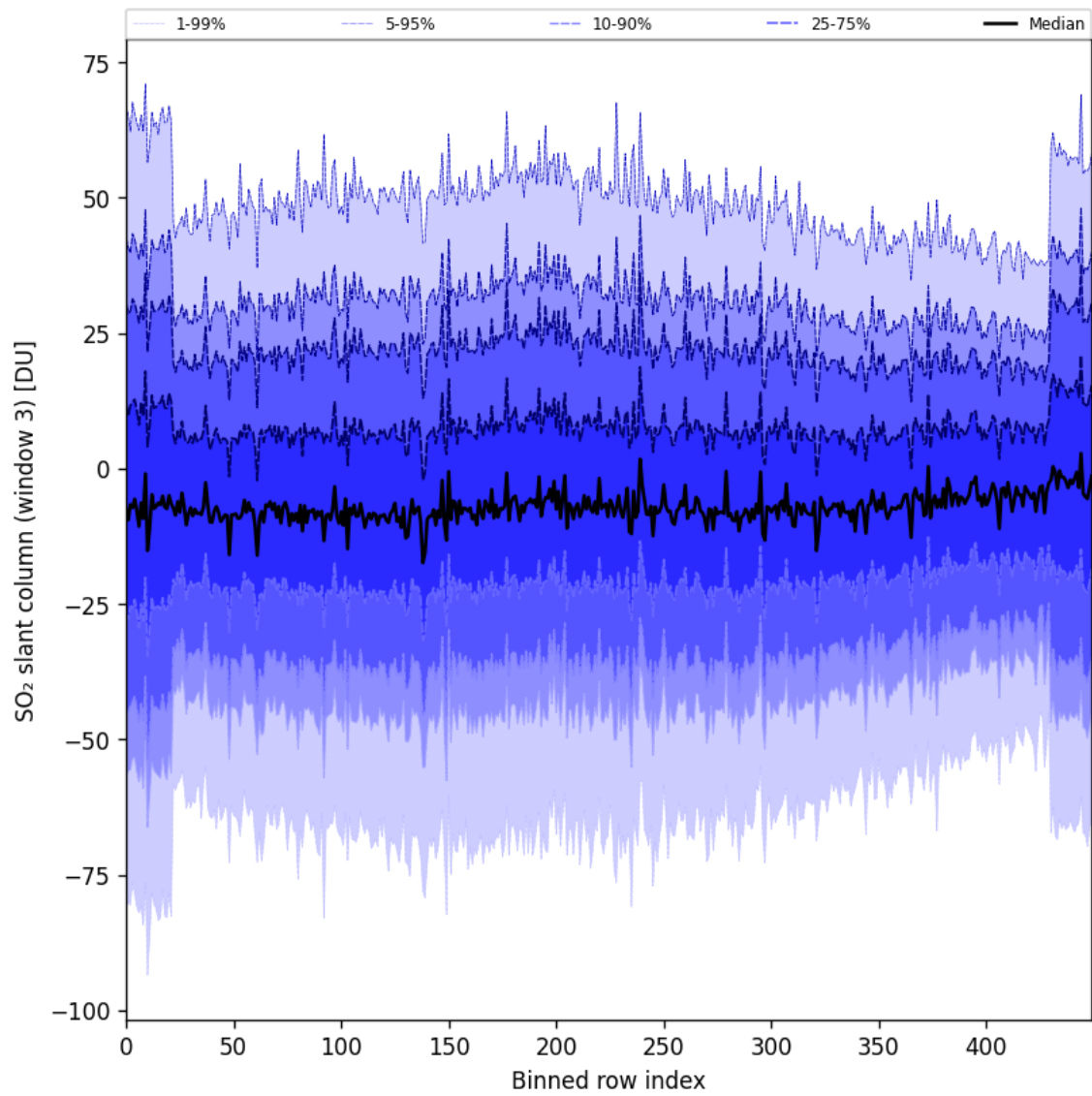
Figure 97: Along track statistics of “SO 2 slant column (window 3)” for 2025-11-20 to 2025-11-22
