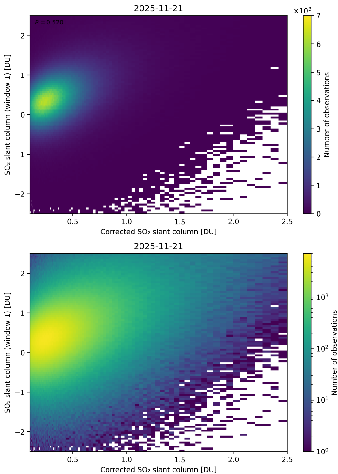
Figure 237: Scatter density plot of “Corrected SO 2 slant column” against “SO 2 slant column (window 1)” for 2025-11-20 to 2025-11-22.
