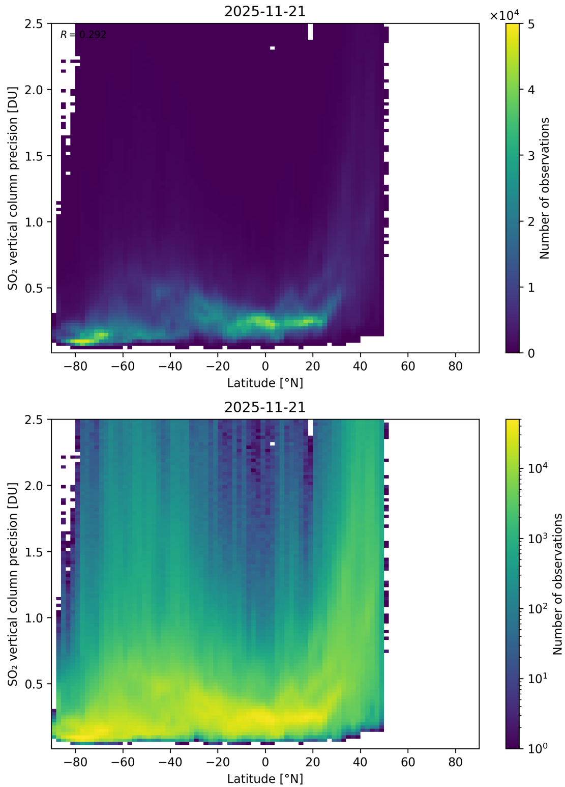
Figure 170: Scatter density plot of “Latitude” against “SO 2 vertical column precision” for 2025-11-20 to 2025-11-22.
