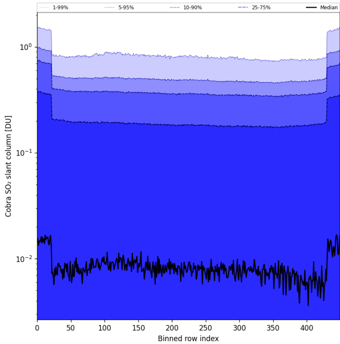
Figure 87: Along track statistics of “Cobra SO 2 slant column” for 2025-11-20 to 2025-11-22
