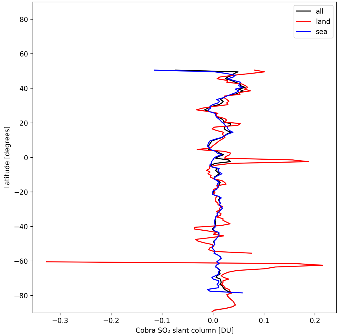
Figure 35: Zonal average of “Cobra SO 2 slant column” for 2025-11-20 to 2025-11-22.
