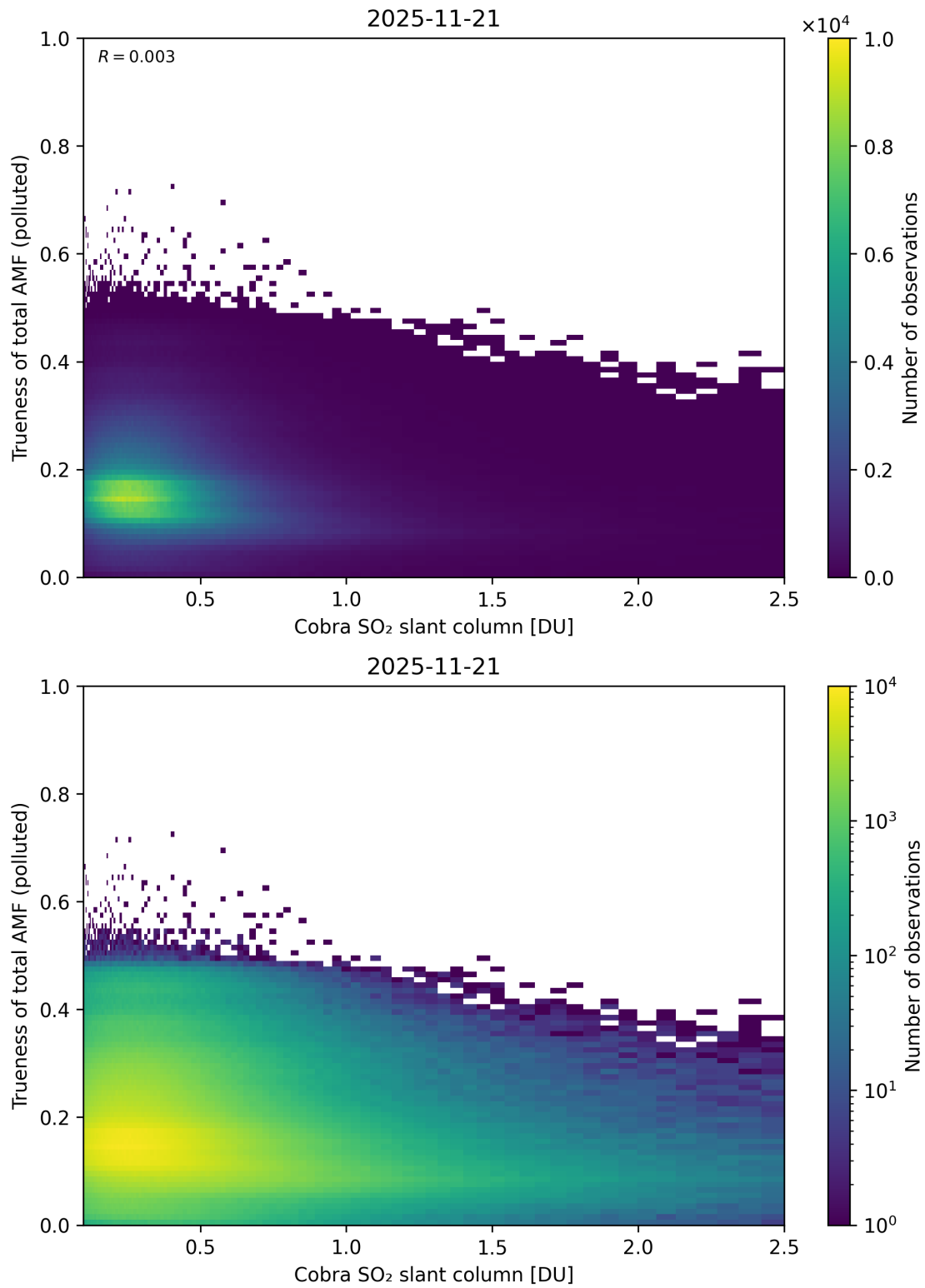
Figure 225: Scatter density plot of “Cobra SO 2 slant column” against “Trueness of total AMF (polluted)” for 2025-11-20 to 2025-11-22.
