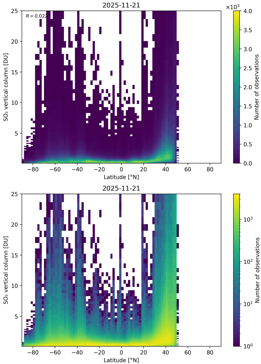
Figure 169: Scatter density plot of “Latitude” against “SO 2 vertical column” for 2025-11-20 to 2025-11-22.
