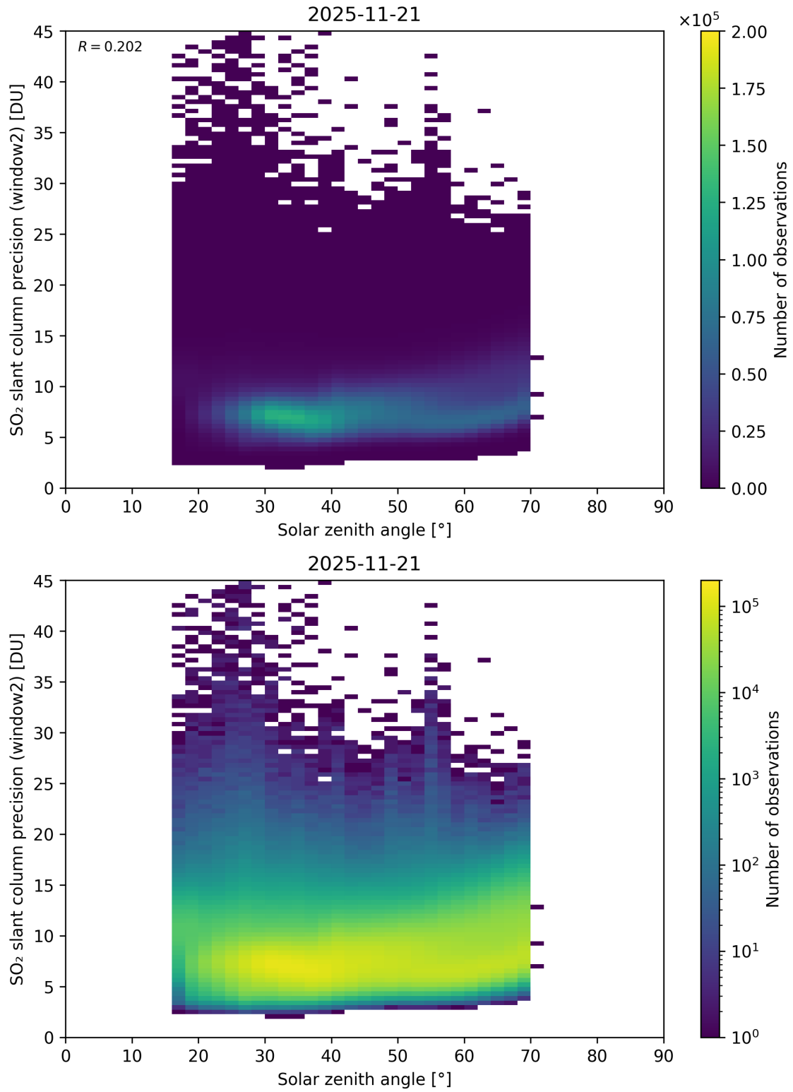
Figure 186: Scatter density plot of “Solar zenith angle” against “SO 2 slant column precision (window2)” for 2025-11-20 to 2025-11-22.
