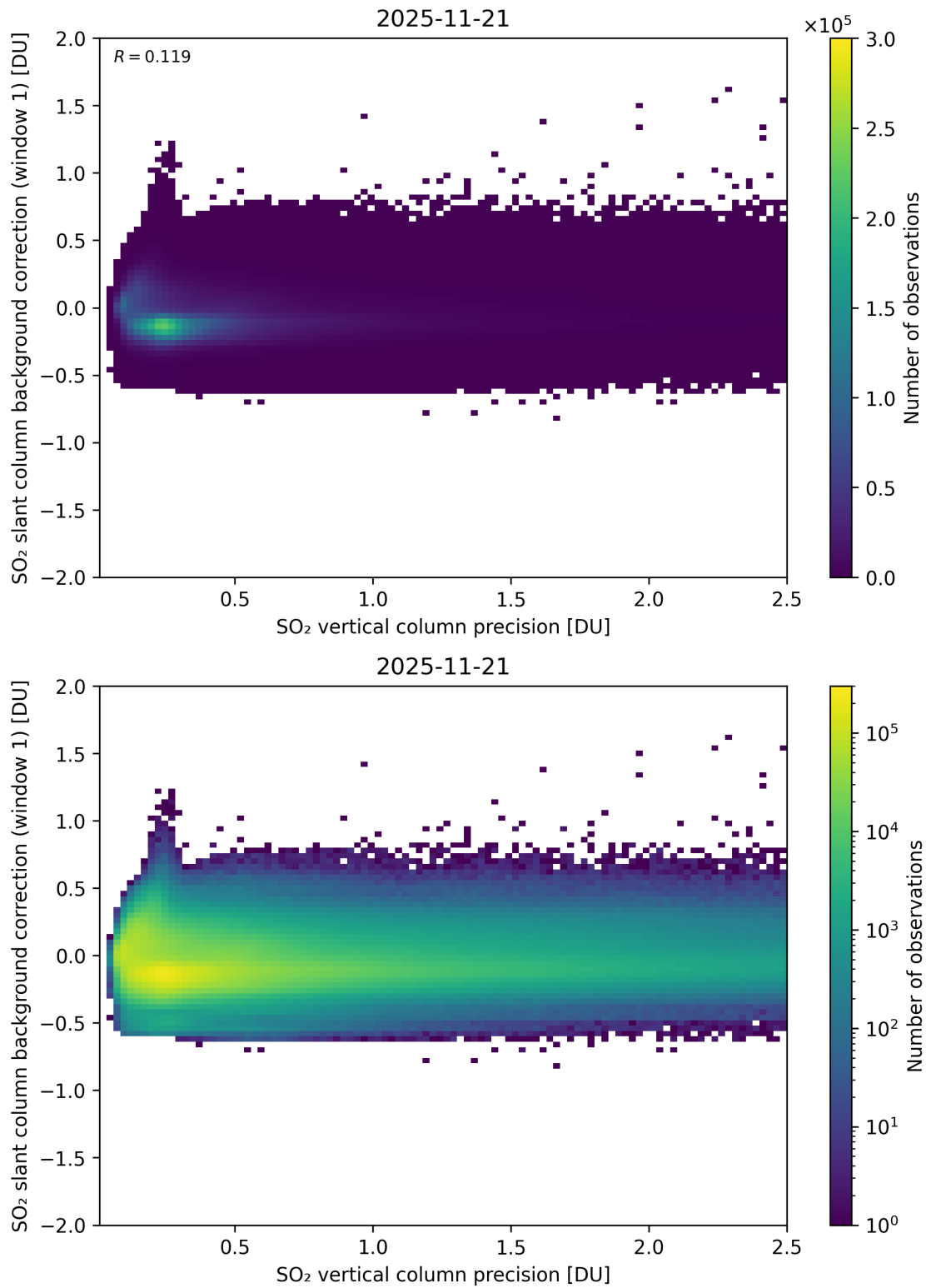
Figure 329: Scatter density plot of “SO 2 vertical column precision” against “SO 2 slant column background correction (window 1)” for 2025-11-20 to 2025-11-22.
