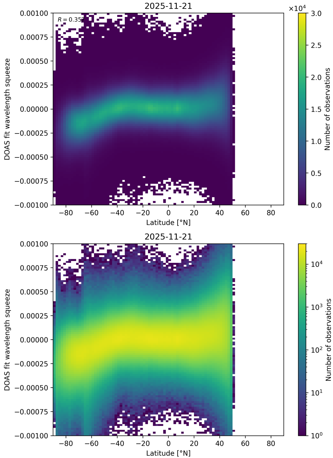
Figure 154: Scatter density plot of “Latitude” against “DOAS fit wavelength squeeze” for 2025-11-20 to 2025-11-22.
