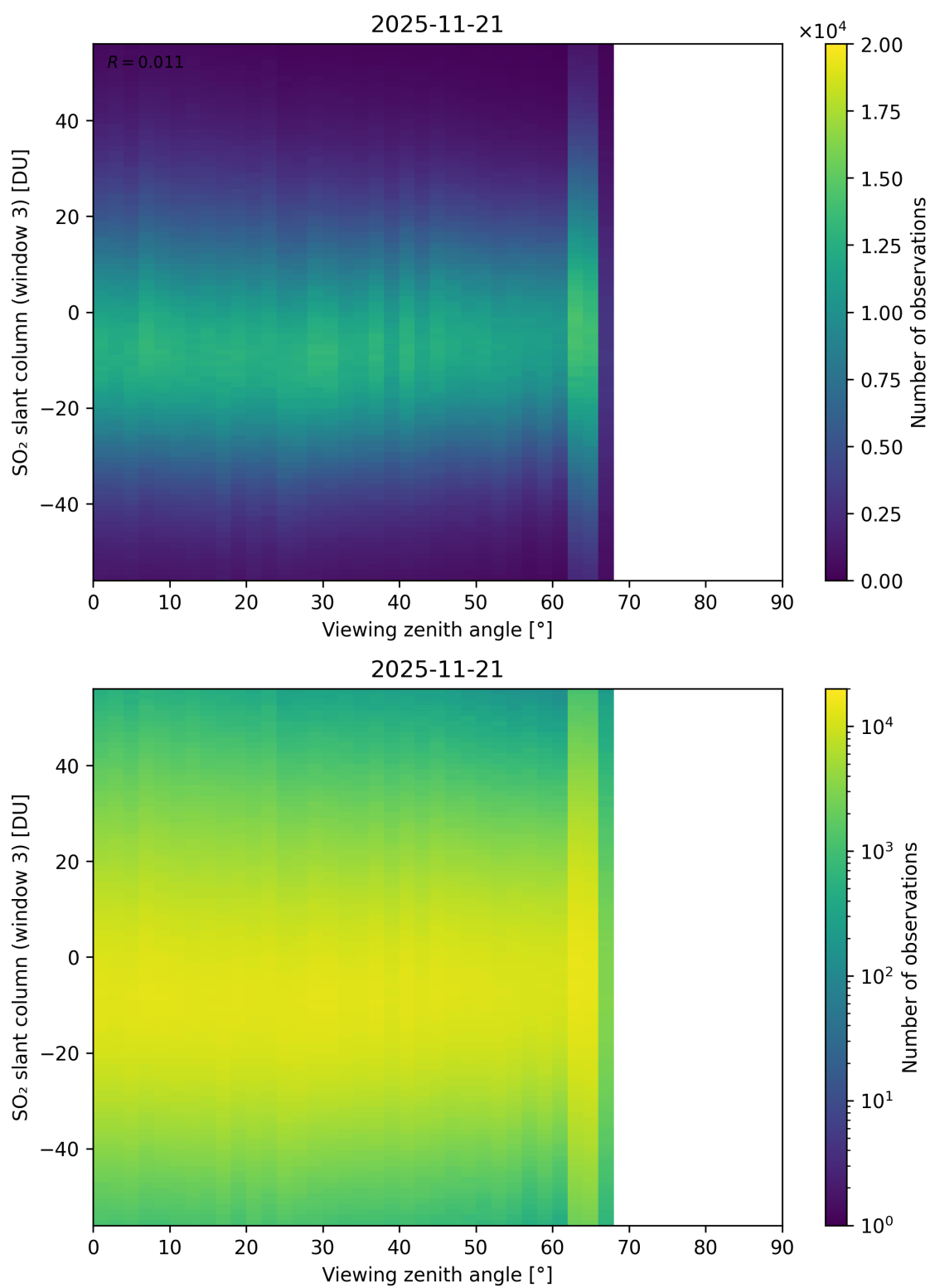
Figure 379: Scatter density plot of “Viewing zenith angle” against “SO 2 slant column (window 3)” for 2025-11-20 to 2025-11-22.
