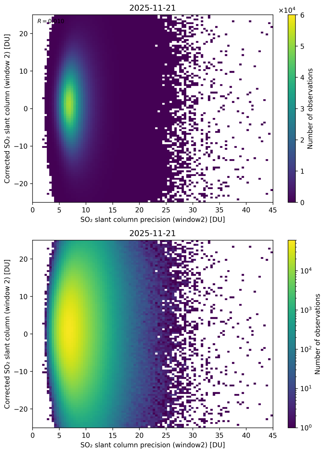
Figure 297: Scatter density plot of “SO 2 slant column precision (window2)” against “Corrected SO 2 slant column (window 2)” for 2025-11-20 to 2025-11-22.
