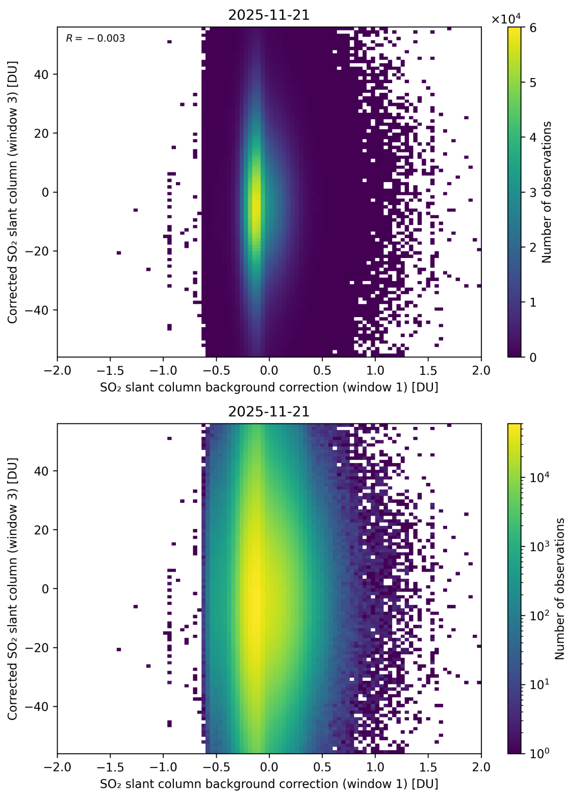
Figure 116: Scatter density plot of “SO 2 slant column background correction (window 1)” against “Corrected SO 2 slant column (window 3)” for 2025-11-20 to 2025-11-22.
