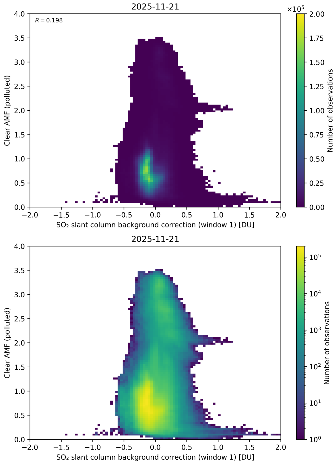
Figure 114: Scatter density plot of “SO 2 slant column background correction (window 1)” against “Clear AMF (polluted)” for 2025-11-20 to 2025-11-22.
