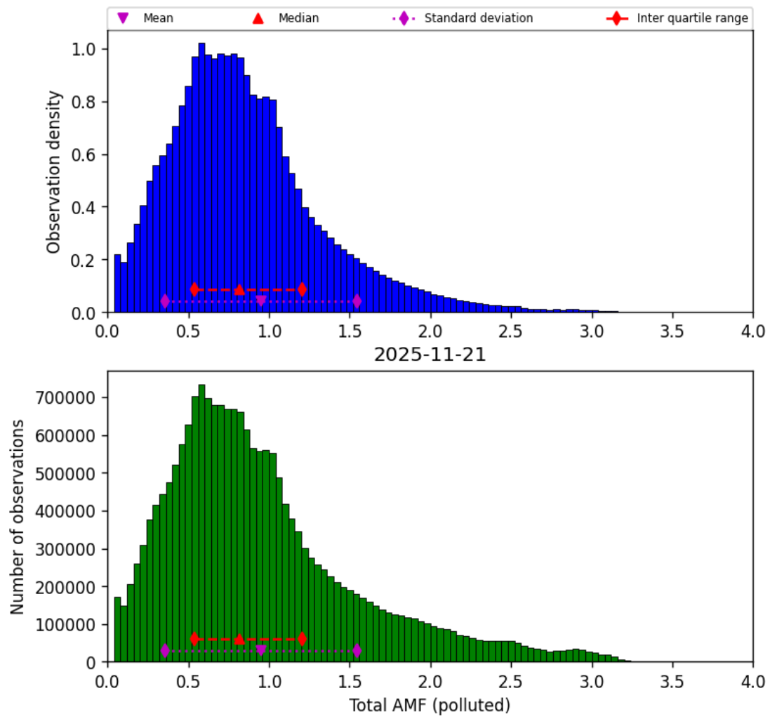
Figure 79: Histogram of “Total AMF (polluted)” for 2025-11-20 to 2025-11-22
