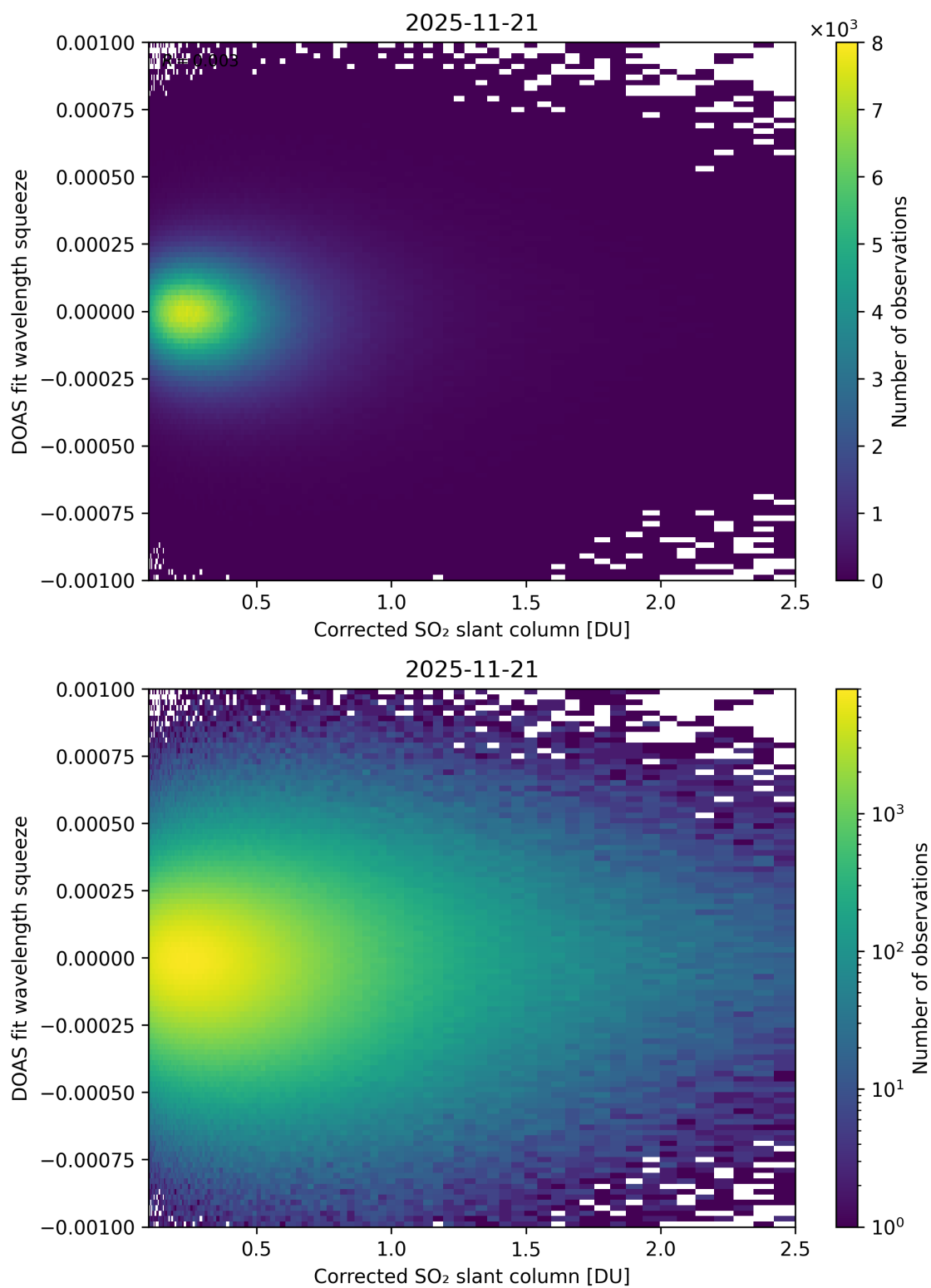
Figure 230: Scatter density plot of "Corrected SO 2 slant column" against "DOAS fit wavelength squeeze" for 2025-11-20 to 2025-11-22.
