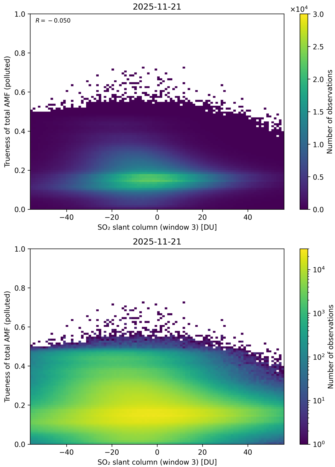
Figure 319: Scatter density plot of “SO 2 slant column (window 3)” against “Trueness of total AMF (polluted)” for 2025-11-20 to 2025-11-22.
