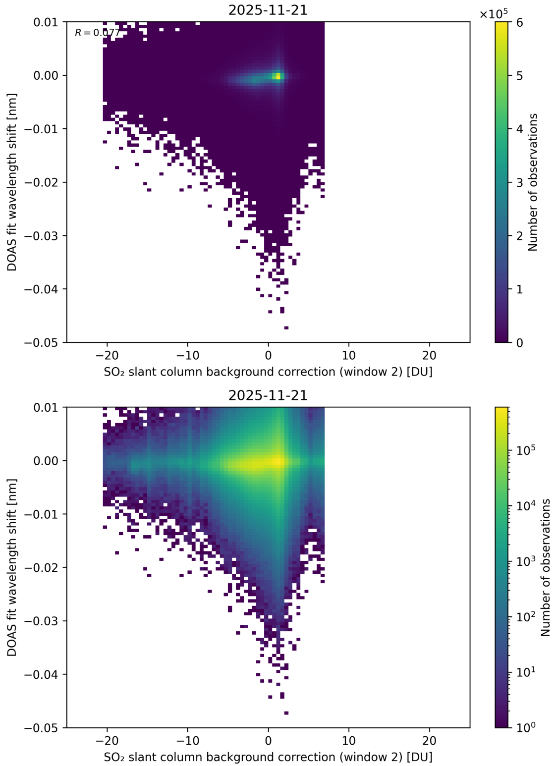
Figure 123: Scatter density plot of “SO 2 slant column background correction (window 2)” against “DOAS fit wavelength shift” for 2025-11-20 to 2025-11-22.
