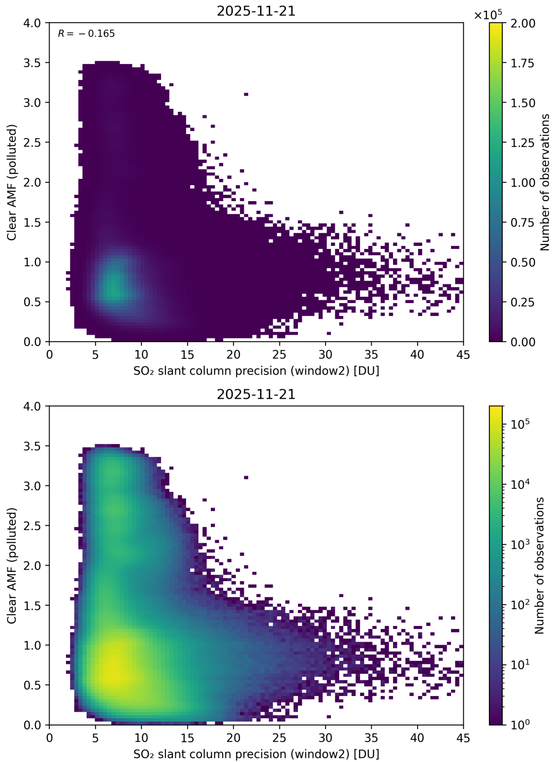
Figure 296: Scatter density plot of “SO 2 slant column precision (window2)” against “Clear AMF (polluted)” for 2025-11-20 to 2025-11-22.
