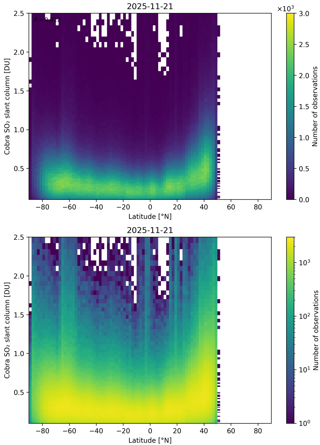
Figure 157: Scatter density plot of “Latitude” against “Cobra SO 2 slant column” for 2025-11-20 to 2025-11-22.
