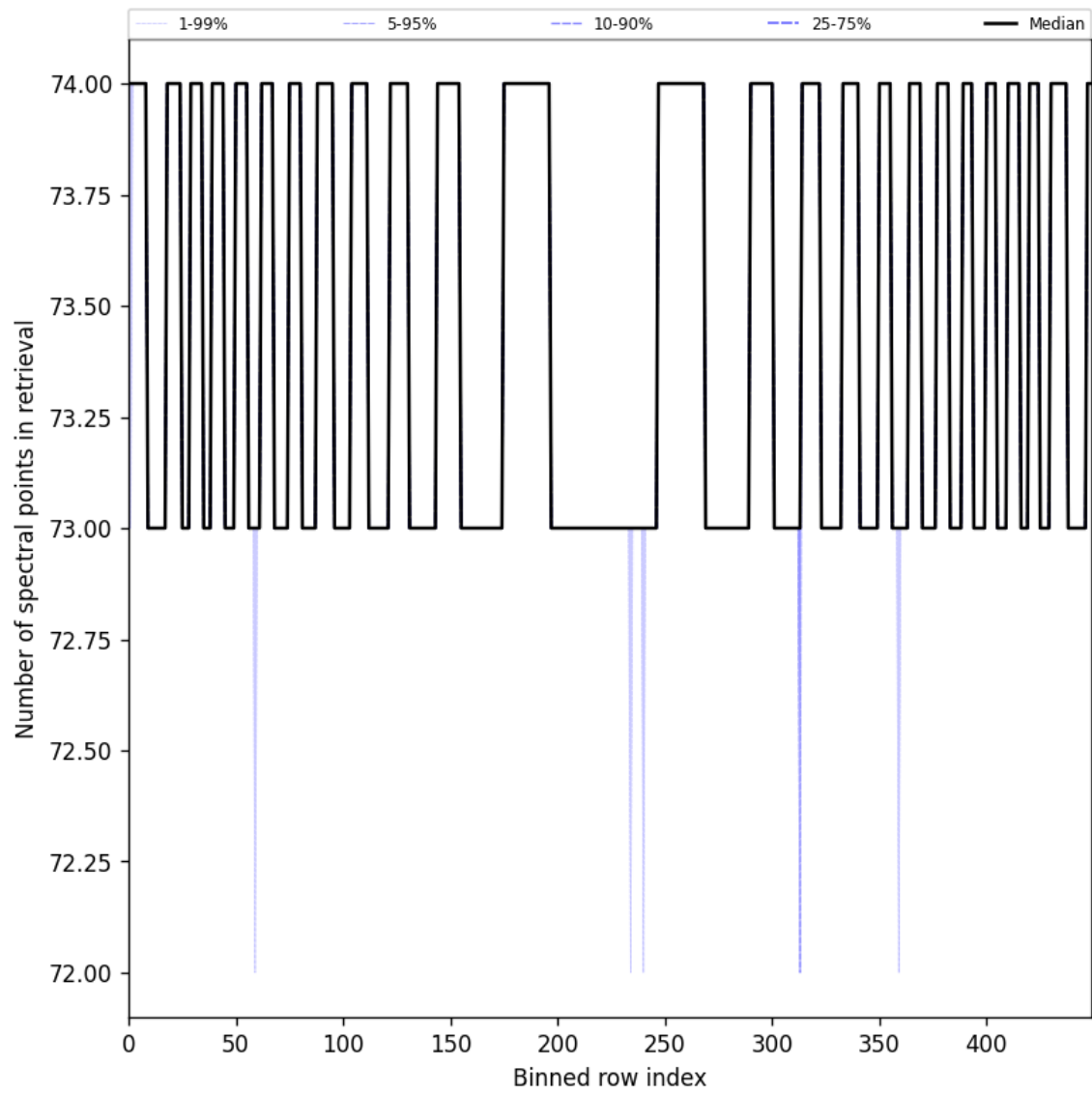
Figure 108: Along track statistics of “Number of spectral points in retrieval” for 2025-11-20 to 2025-11-22
