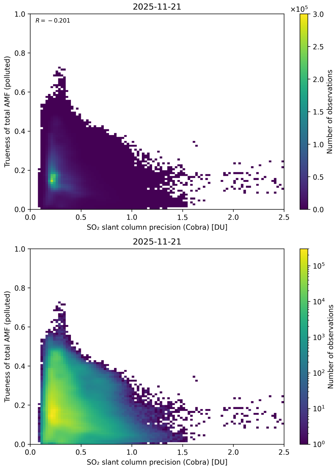
Figure 214: Scatter density plot of “SO 2 slant column precision (Cobra)” against “Trueness of total AMF (polluted)” for 2025-11-20 to 2025-11-22.
