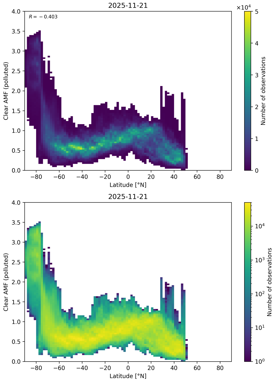
Figure 156: Scatter density plot of “Latitude” against “Clear AMF (polluted)” for 2025-11-20 to 2025-11-22.
