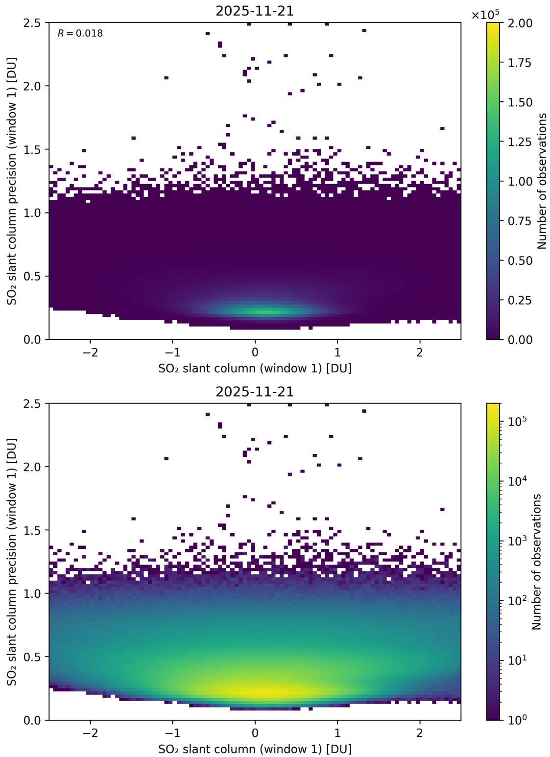
Figure 285: Scatter density plot of “SO 2 slant column (window 1)” against “SO 2 slant column precision (window 1)” for 2025-11-20 to 2025-11-22.
