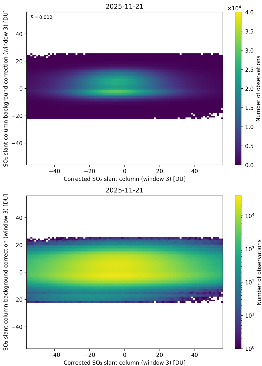
Figure 255: Scatter density plot of “Corrected SO 2 slant column (window 3)” against “SO 2 slant column background correction (window 3)” for 2025-11-20 to 2025-11-22.
