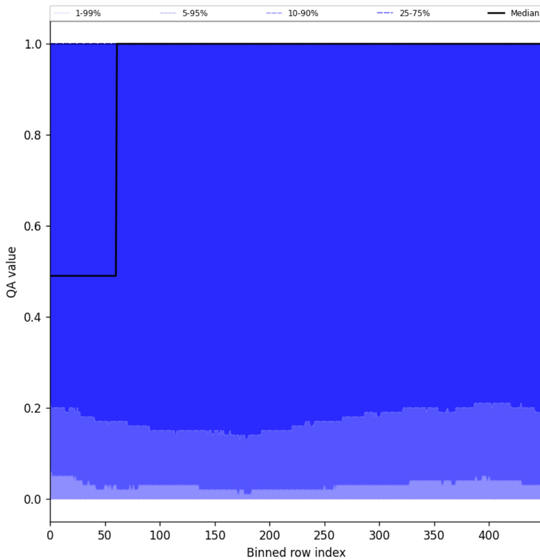
Figure 83: Along track statistics of “QA value” for 2025-11-20 to 2025-11-22
