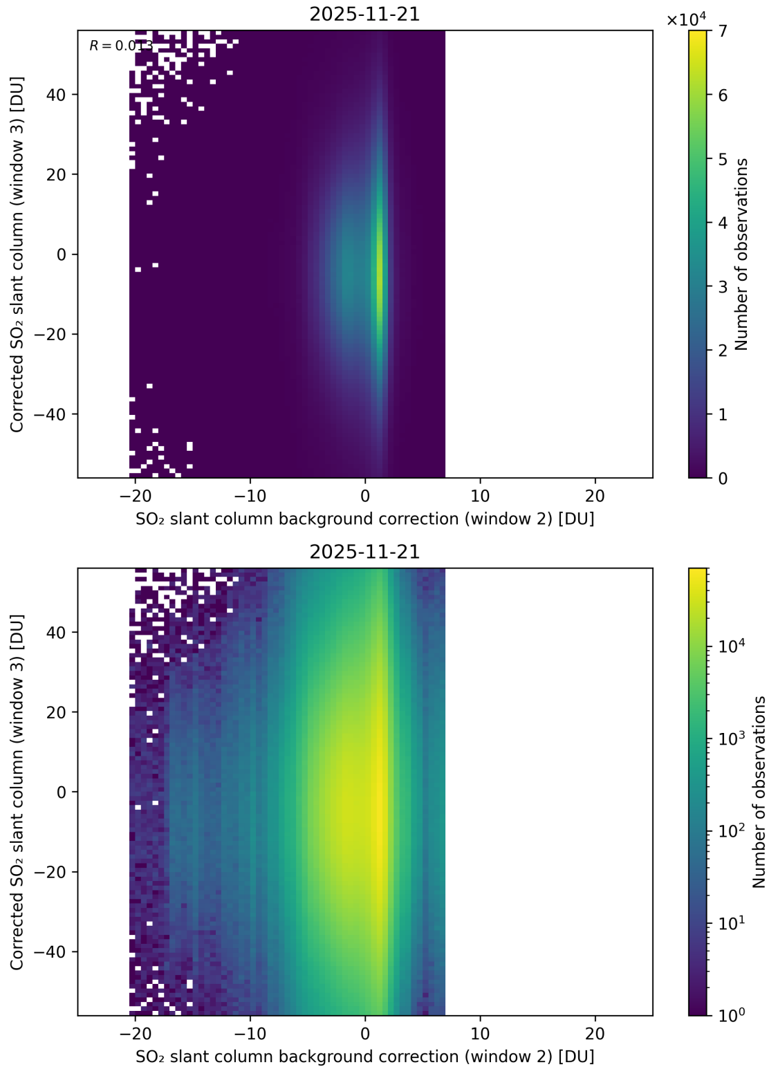
Figure 127: Scatter density plot of “SO 2 slant column background correction (window 2)” against “Corrected SO 2 slant column (window 3)” for 2025-11-20 to 2025-11-22.
