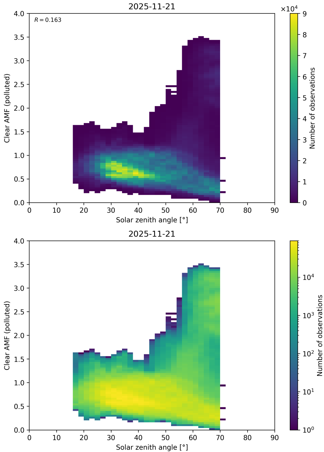
Figure 178: Scatter density plot of “Solar zenith angle” against “Clear AMF (polluted)” for 2025-11-20 to 2025-11-22.
