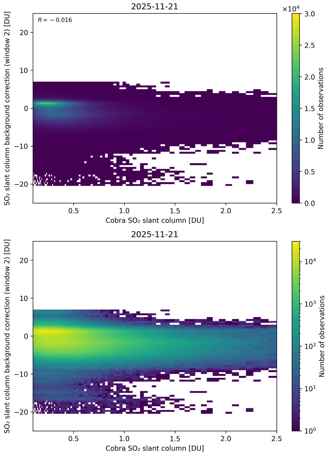
Figure 194: Scatter density plot of “Cobra SO 2 slant column” against “SO 2 slant column background correction (window 2)” for 2025-11-20 to 2025-11-22.
