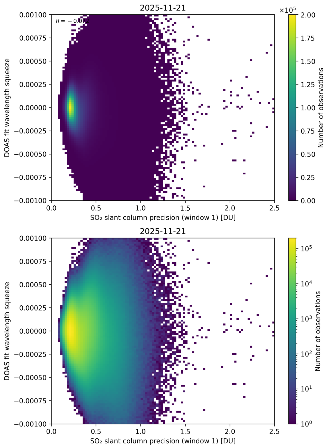
Figure 272: Scatter density plot of “SO 2 slant column precision (window 1)” against “DOAS fit wavelength squeeze” for 2025-11-20 to 2025-11-22.
