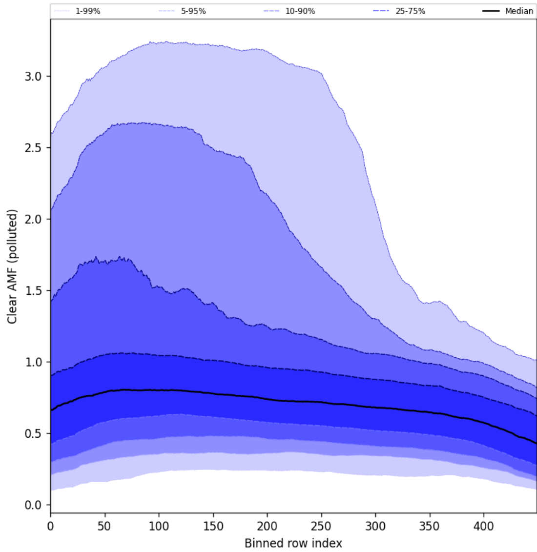
Figure 107: Along track statistics of “Clear AMF (polluted)” for 2025-11-20 to 2025-11-22
