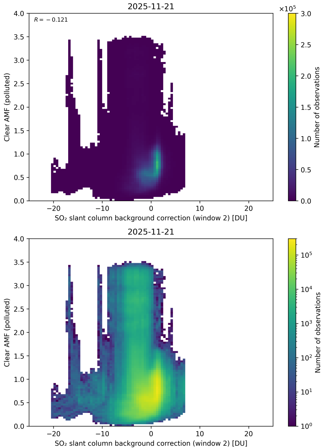
Figure 126: Scatter density plot of “SO 2 slant column background correction (window 2)” against “Clear AMF (polluted)” for 2025-11-20 to 2025-11-22.
