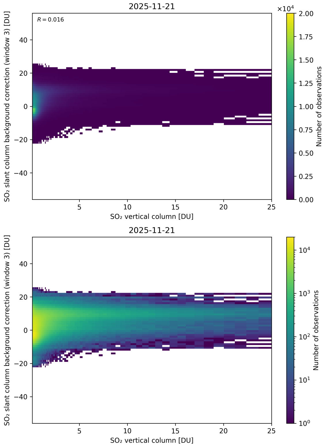
Figure 325: Scatter density plot of “SO 2 vertical column” against “SO 2 slant column background correction (window 3)” for 2025-11-20 to 2025-11-22.
