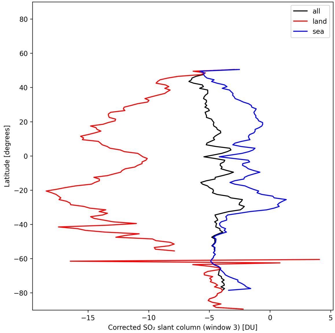
Figure 47: Zonal average of “Corrected SO 2 slant column (window 3)” for 2025-11-20 to 2025-11-22.
