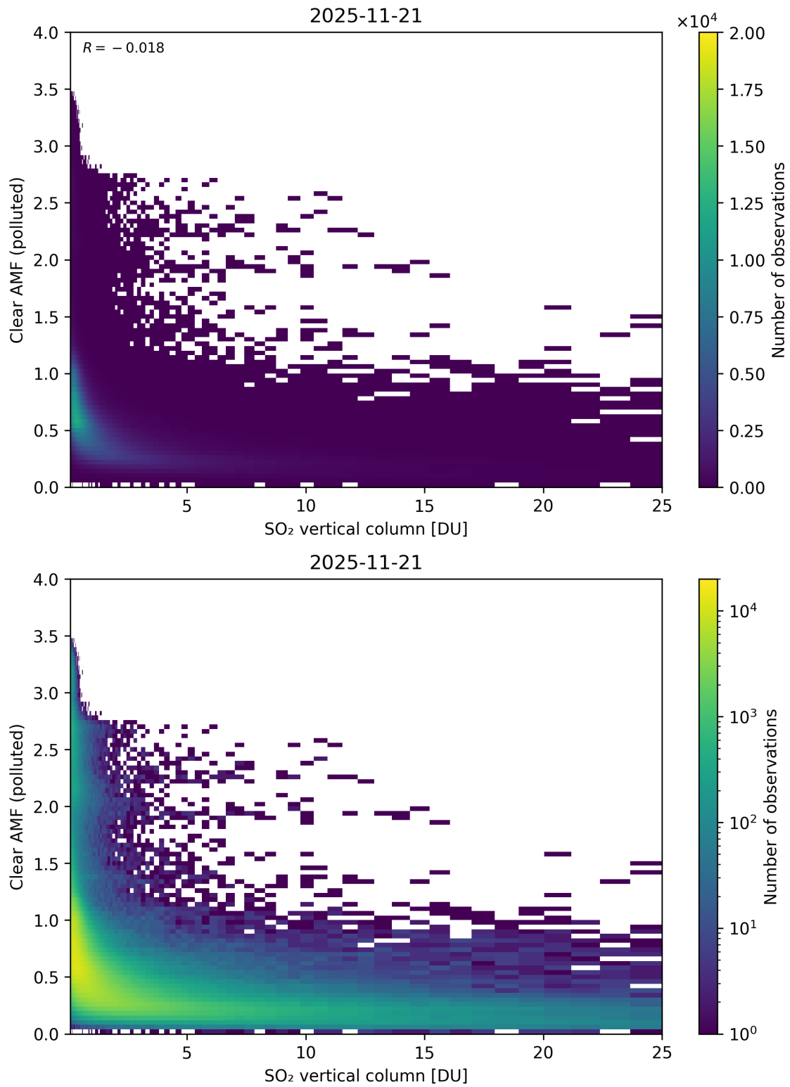
Figure 348: Scatter density plot of “SO 2 vertical column” against “Clear AMF (polluted)” for 2025-11-20 to 2025-11-22.
