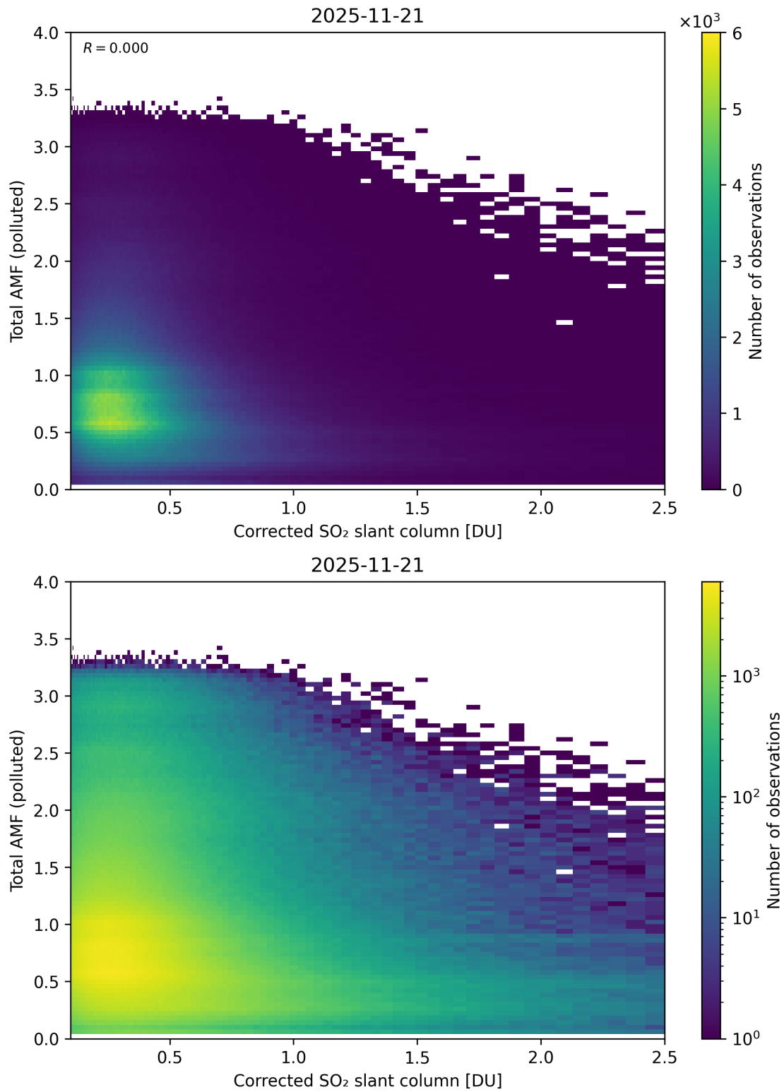
Figure 242: Scatter density plot of “Corrected SO 2 slant column” against “Total AMF (polluted)” for 2025-11-20 to 2025-11-22.
