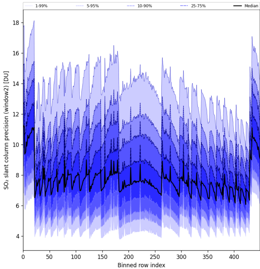
Figure 94: Along track statistics of “SO 2 slant column precision (window2)” for 2025-11-20 to 2025-11-22
