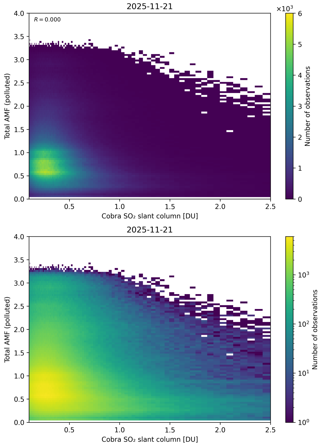
Figure 224: Scatter density plot of “Cobra SO 2 slant column” against “Total AMF (polluted)” for 2025-11-20 to 2025-11-22.
