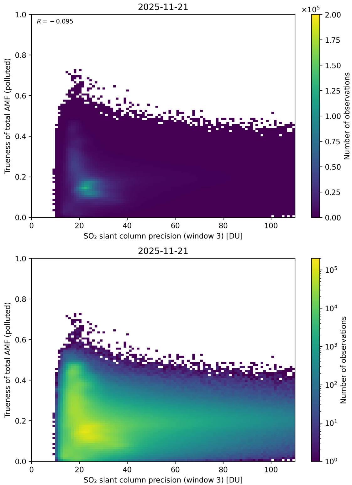
Figure 314: Scatter density plot of “SO 2 slant column precision (window 3)” against “Trueness of total AMF (polluted)” for 2025-11-20 to 2025-11-22.
