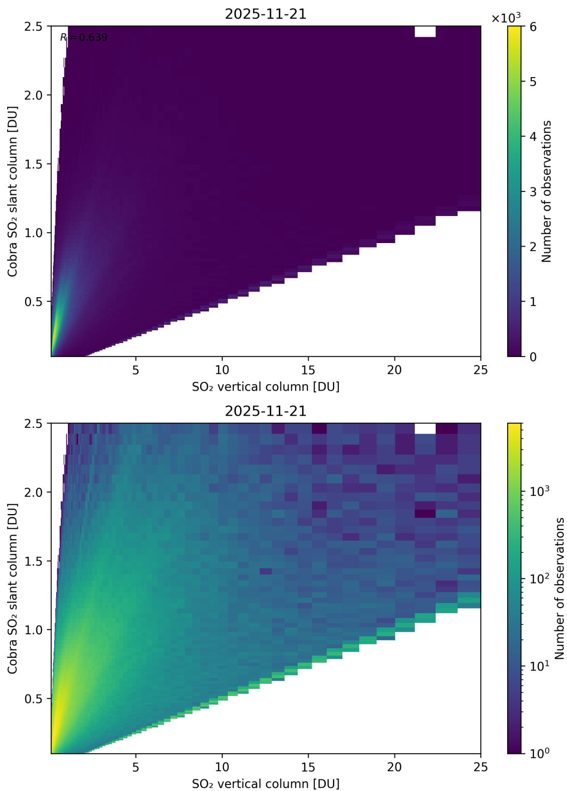
Figure 349: Scatter density plot of “SO 2 vertical column” against “Cobra SO 2 slant column” for 2025-11-20 to 2025-11-22.
