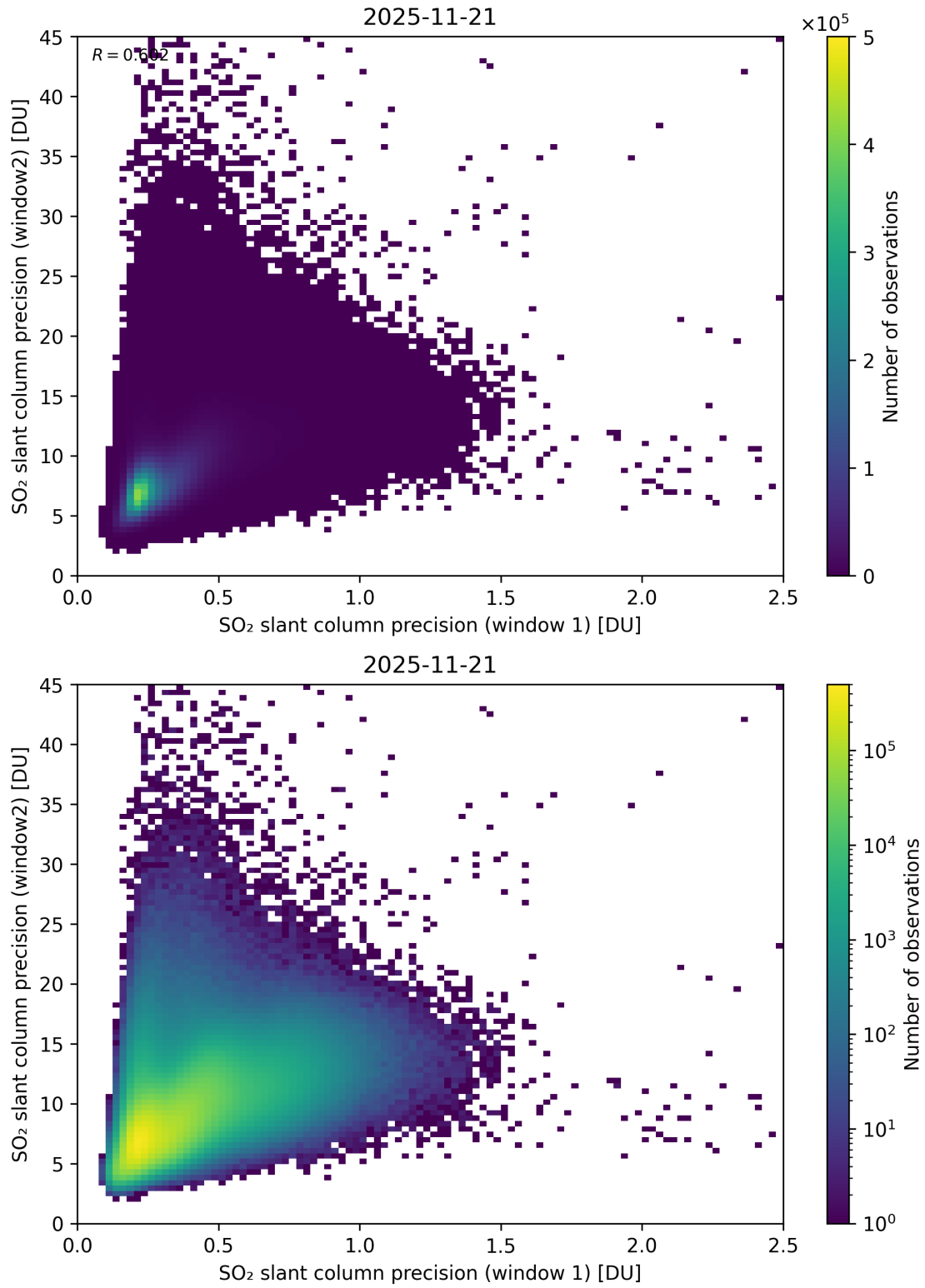
Figure 277: Scatter density plot of “SO 2 slant column precision (window 1)” against “SO 2 slant column precision (window2)” for 2025-11-20 to 2025-11-22.
