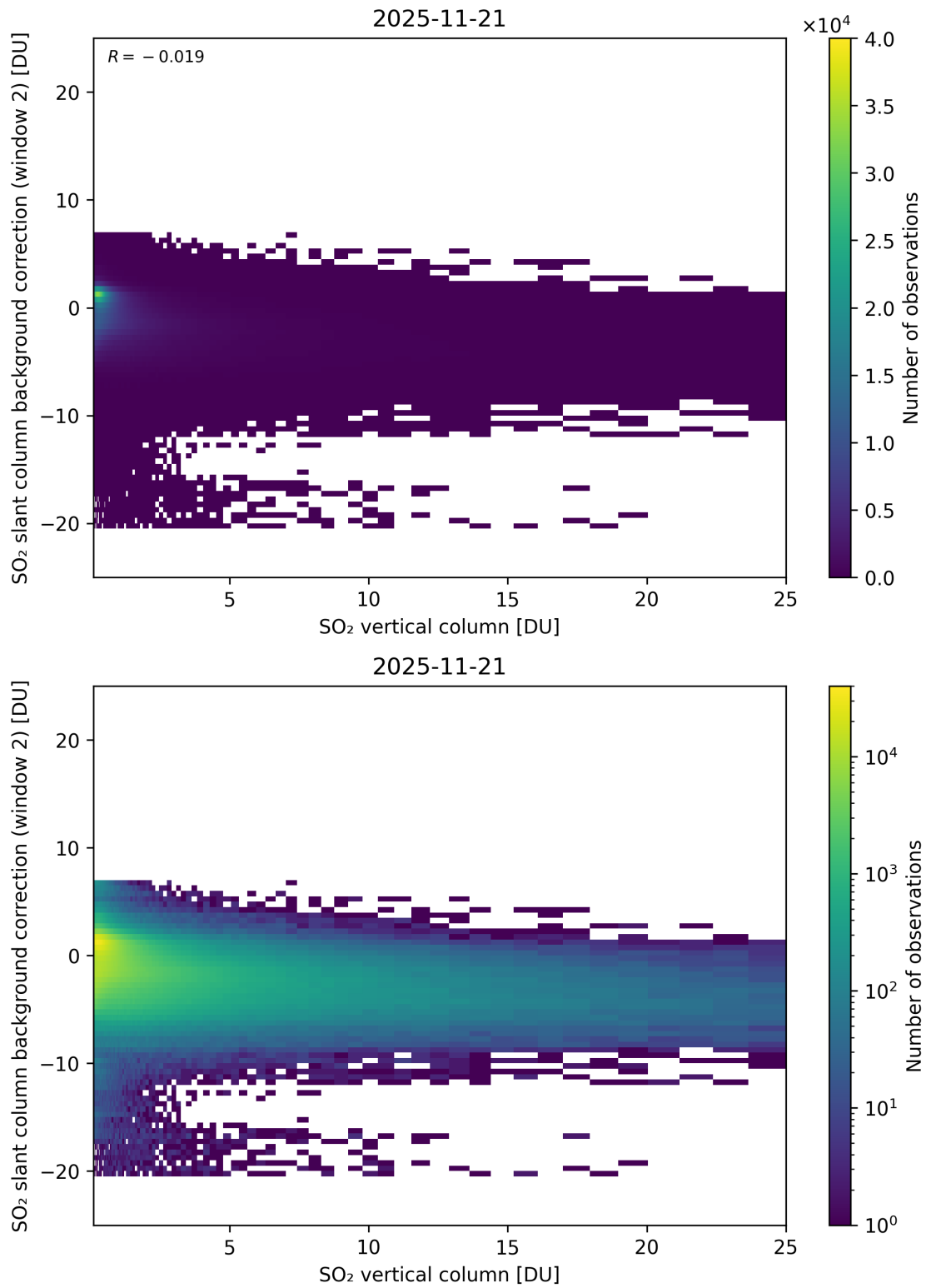
Figure 324: Scatter density plot of “SO 2 vertical column” against “SO 2 slant column background correction (window 2)” for 2025-11-20 to 2025-11-22.
