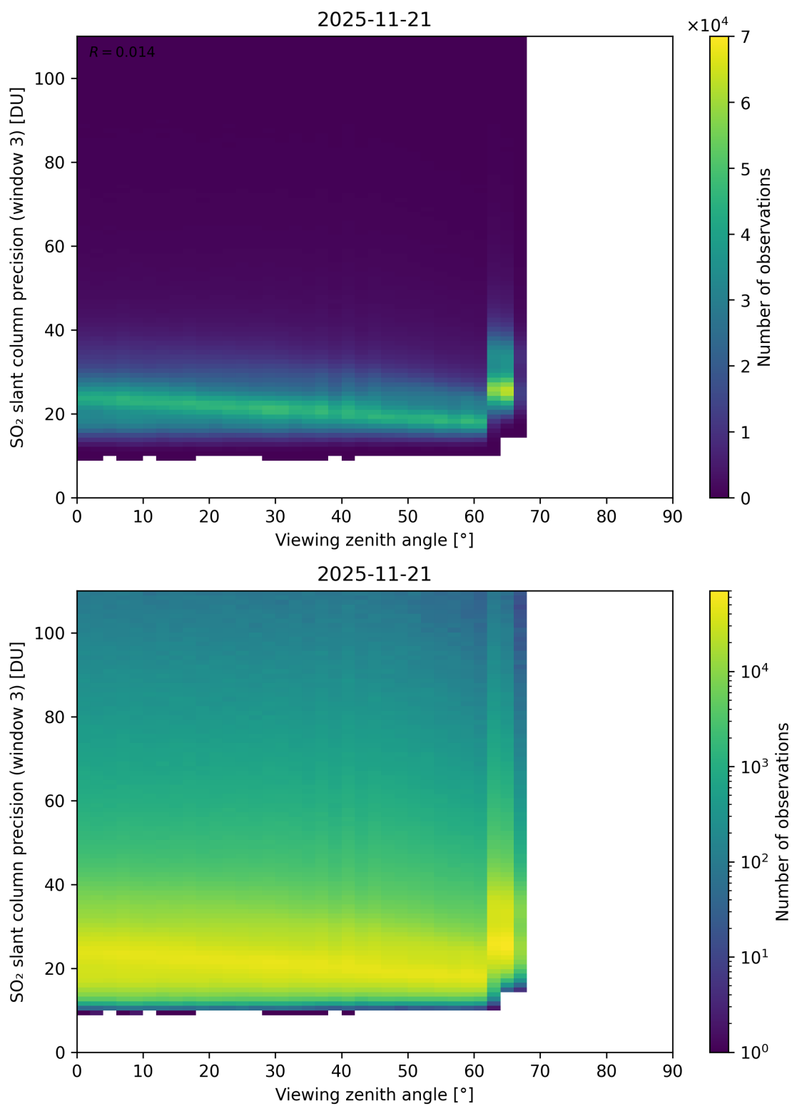
Figure 380: Scatter density plot of “Viewing zenith angle” against “SO 2 slant column precision (window 3)” for 2025-11-20 to 2025-11-22.
