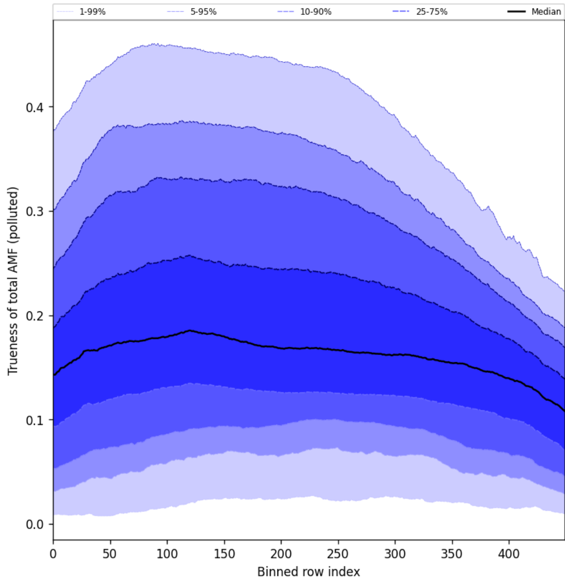
Figure 106: Along track statistics of “Trueness of total AMF (polluted)” for 2025-11-20 to 2025-11-22
