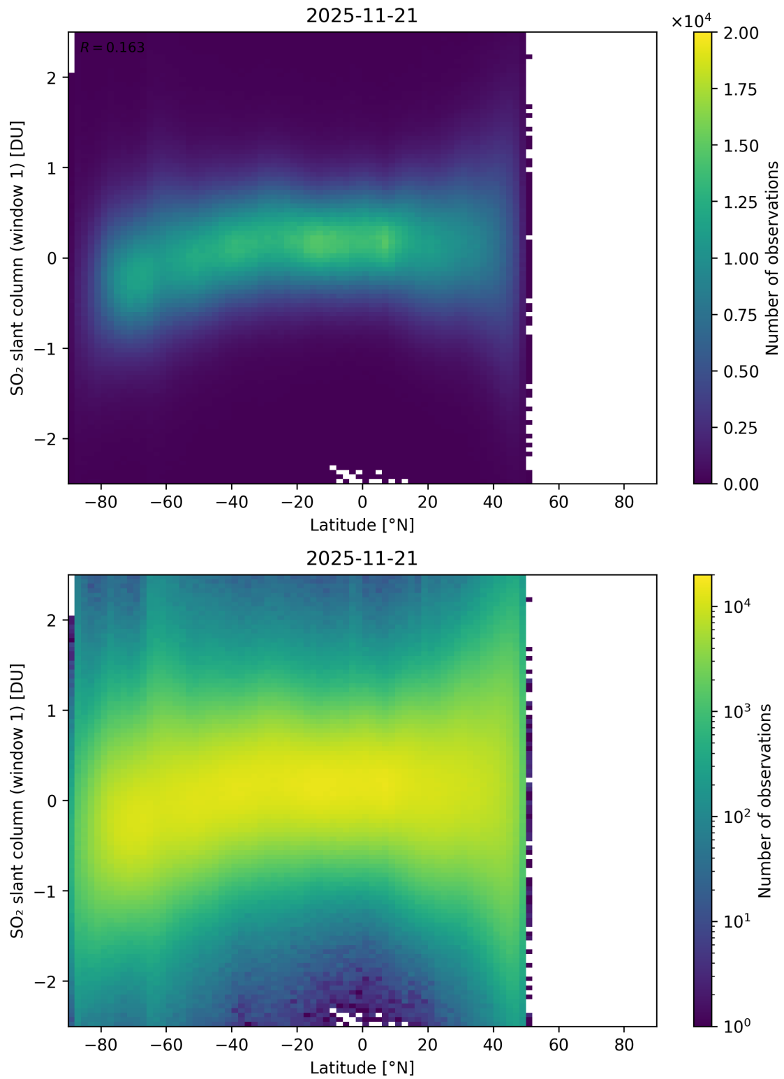
Figure 162: Scatter density plot of “Latitude” against “SO 2 slant column (window 1)” for 2025-11-20 to 2025-11-22.
