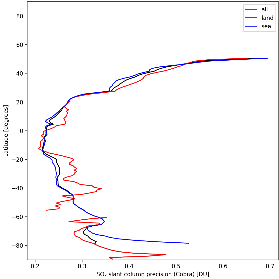
Figure 36: Zonal average of “SO 2 slant column precision (Cobra)” for 2025-11-20 to 2025-11-22.
