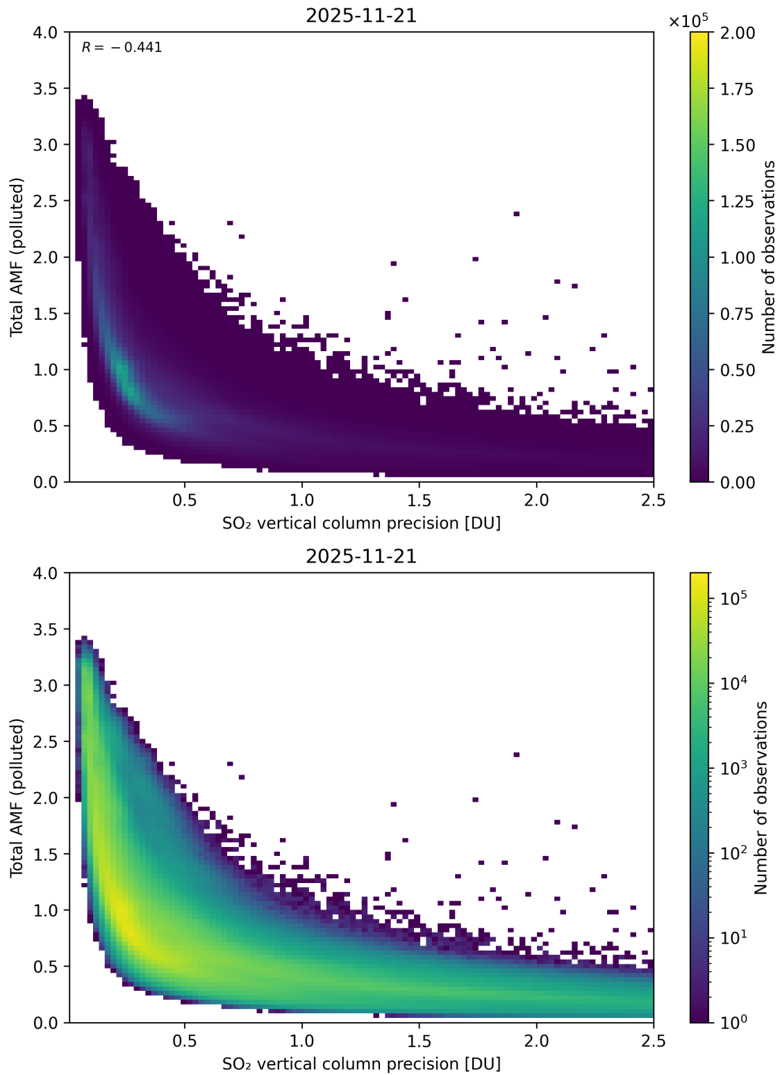
Figure 346: Scatter density plot of “SO 2 vertical column precision” against “Total AMF (polluted)” for 2025-11-20 to 2025-11-22.
