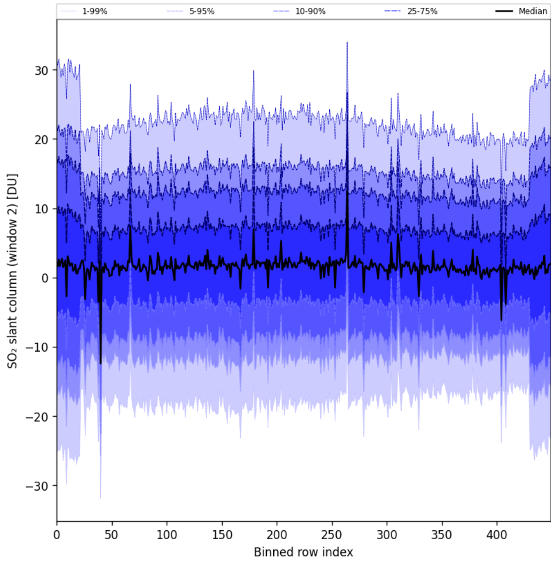
Figure 93: Along track statistics of “SO 2 slant column (window 2)” for 2025-11-20 to 2025-11-22
