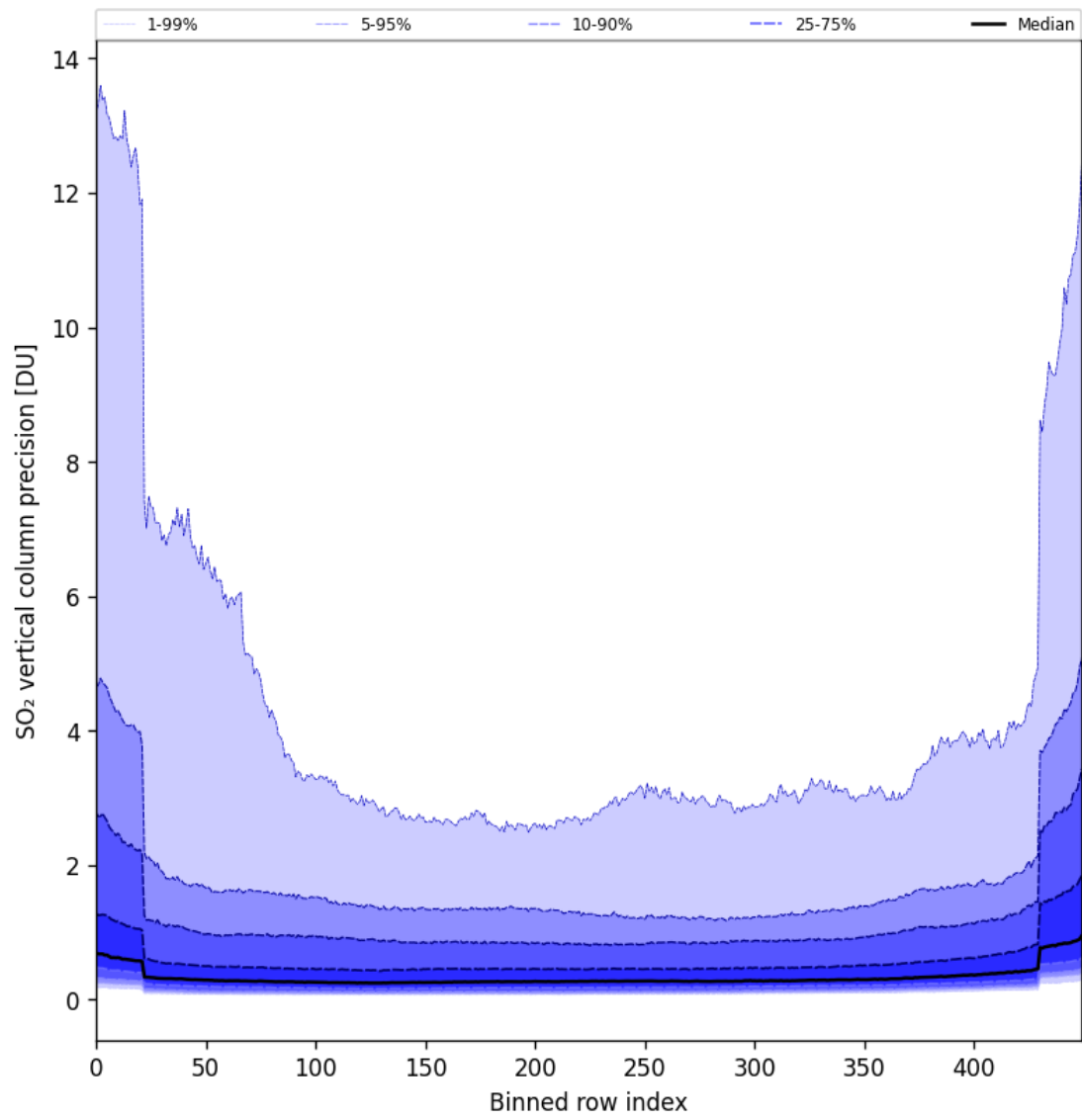
Figure 85: Along track statistics of “SO 2 vertical column precision” for 2025-11-20 to 2025-11-22
