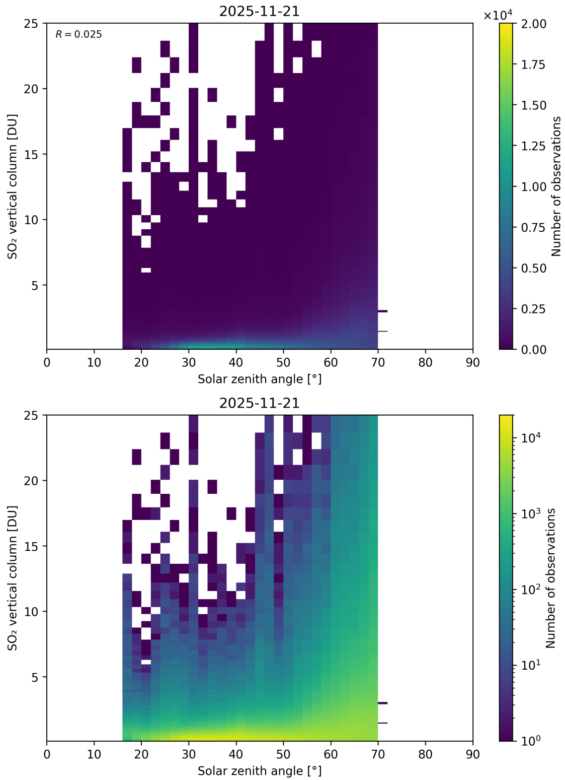
Figure 191: Scatter density plot of “Solar zenith angle” against “SO 2 vertical column” for 2025-11-20 to 2025-11-22.
