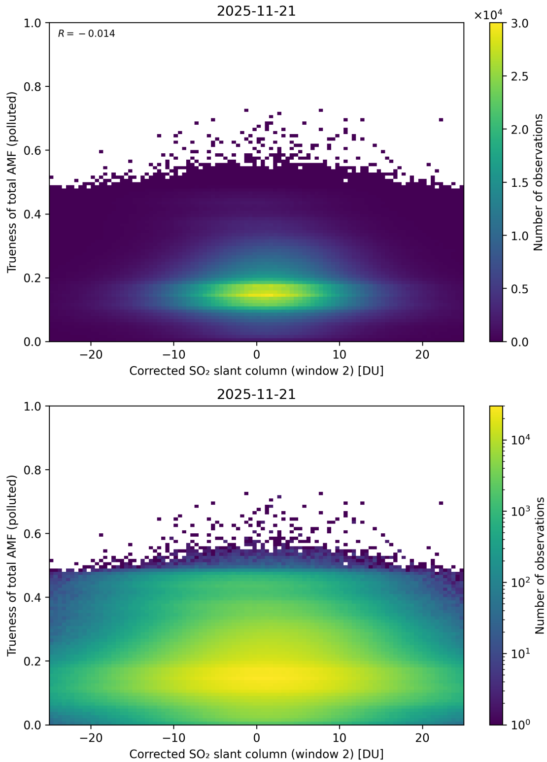
Figure 254: Scatter density plot of “Corrected SO 2 slant column (window 2)” against “Trueness of total AMF (polluted)” for 2025-11-20 to 2025-11-22.
