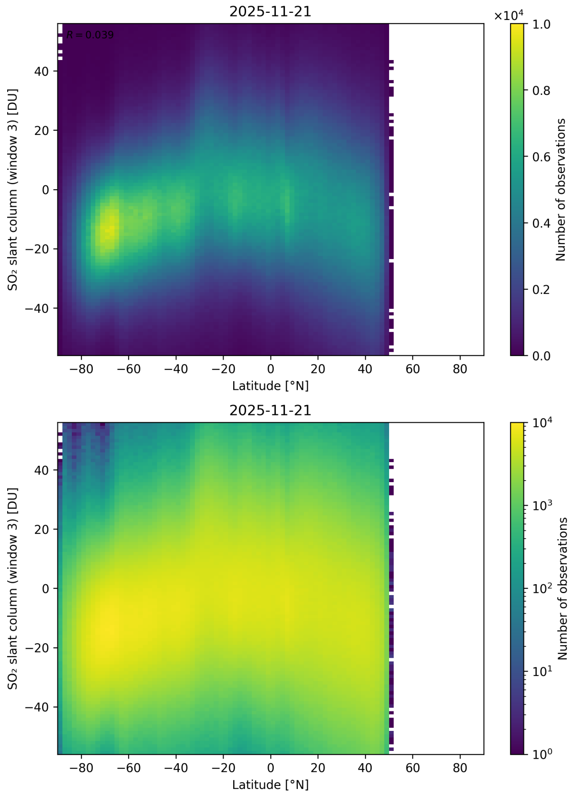
Figure 165: Scatter density plot of “Latitude” against “SO 2 slant column (window 3)” for 2025-11-20 to 2025-11-22.
