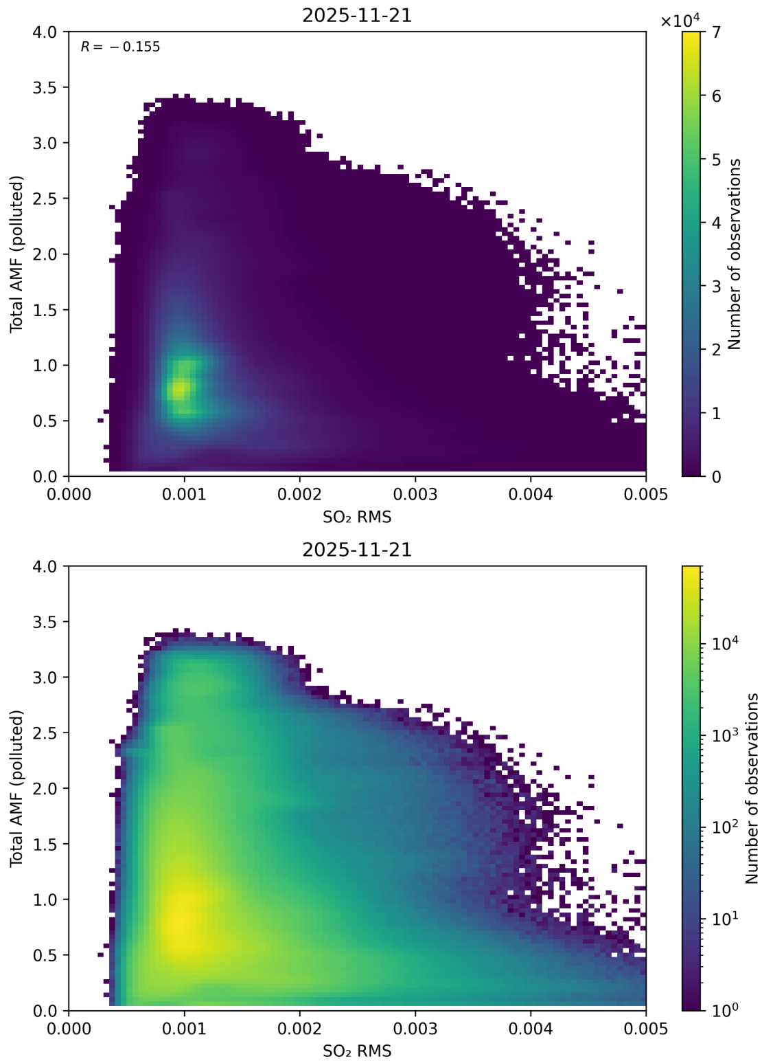
Figure 148: Scatter density plot of “SO 2 RMS” against “Total AMF (polluted)” for 2025-11-20 to 2025-11-22.
