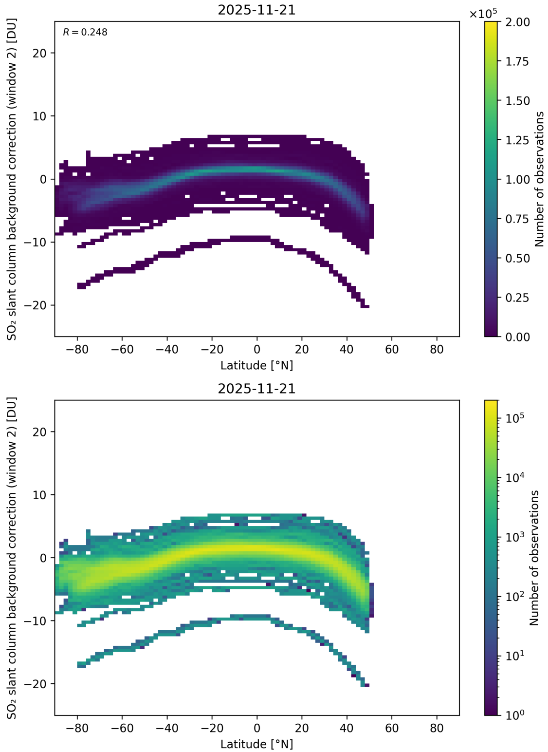
Figure 151: Scatter density plot of “Latitude” against “SO 2 slant column background correction (window 2)” for 2025-11-20 to 2025-11-22.
