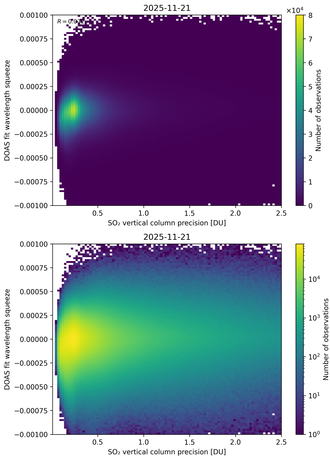
Figure 333: Scatter density plot of “SO 2 vertical column precision” against “DOAS fit wavelength squeeze” for 2025-11-20 to 2025-11-22.
