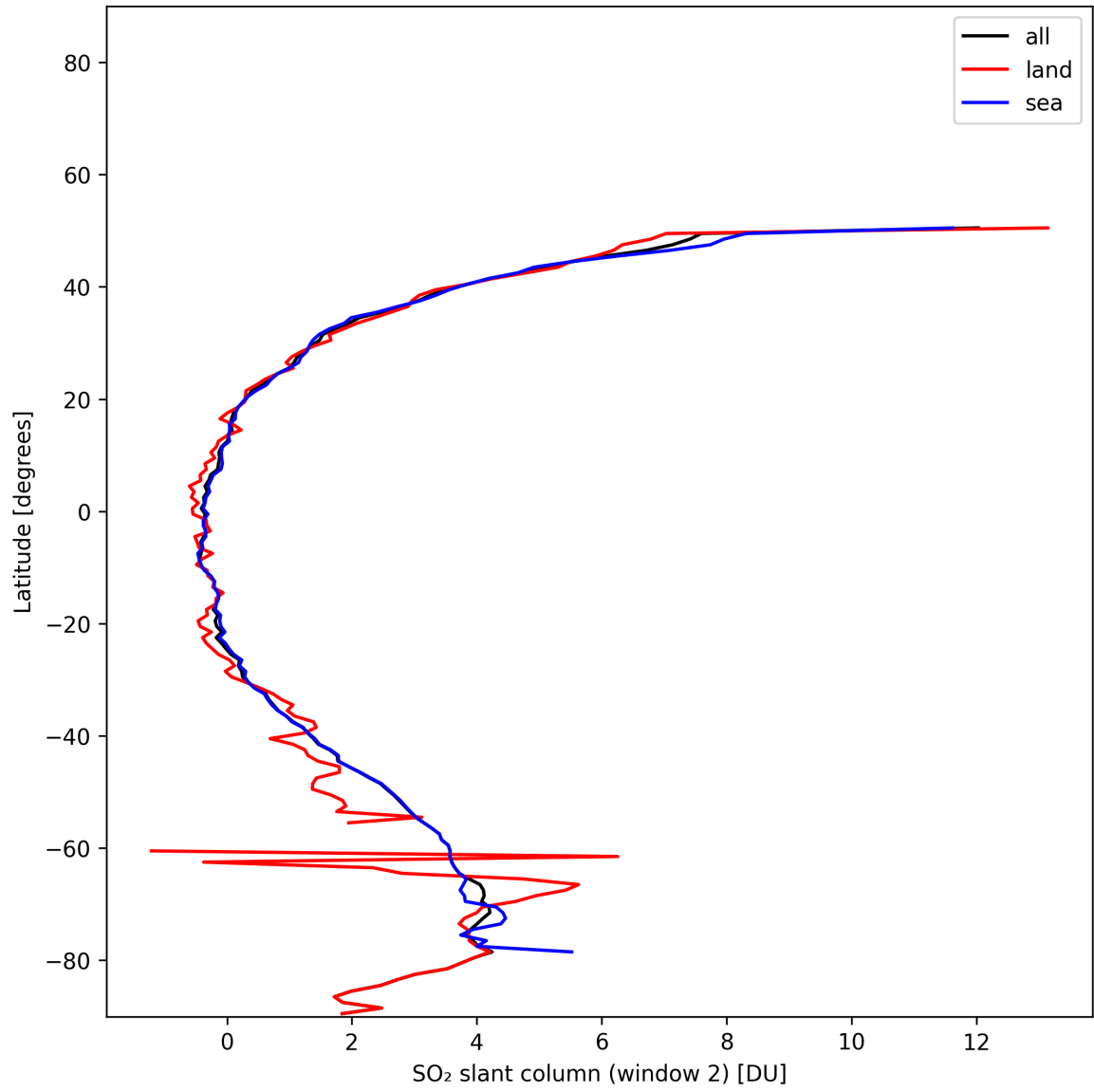
Figure 41: Zonal average of “SO 2 slant column (window 2)” for 2025-11-20 to 2025-11-22.
