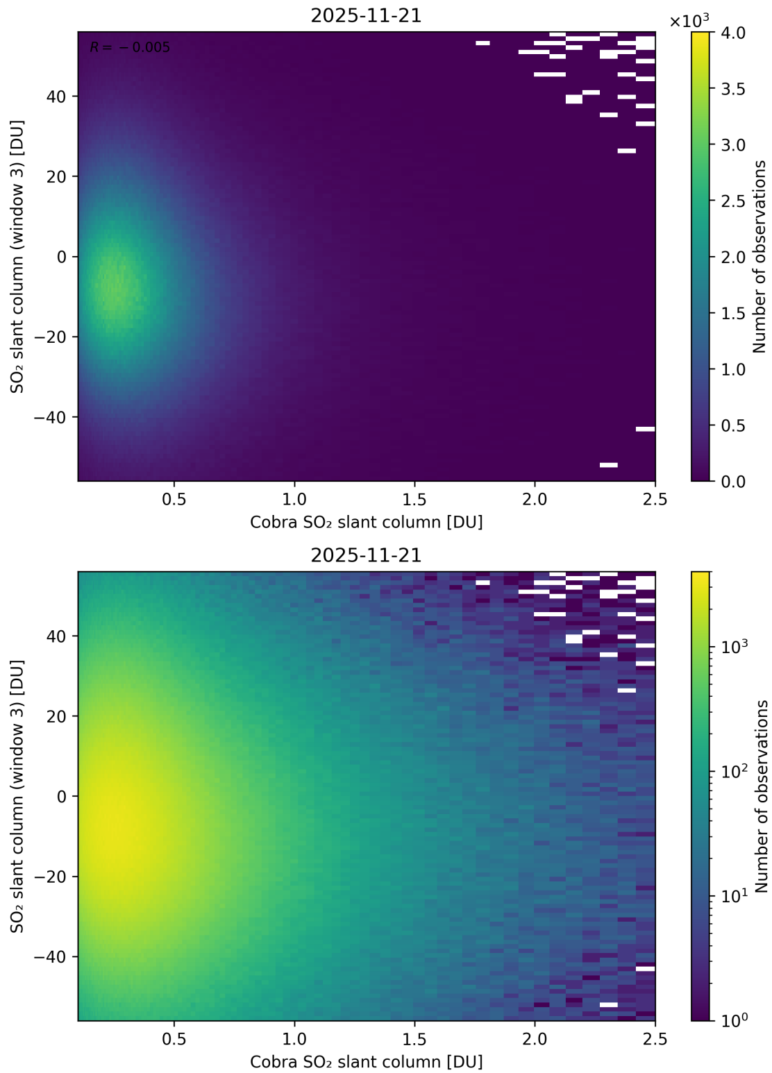
Figure 222: Scatter density plot of “Cobra SO 2 slant column” against “SO 2 slant column (window 3)” for 2025-11-20 to 2025-11-22.
