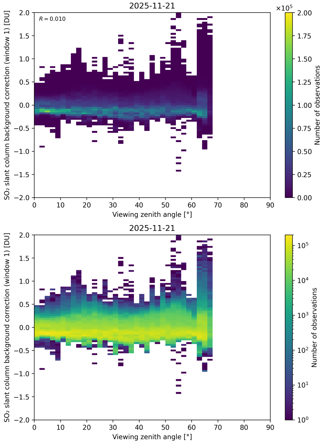
Figure 362: Scatter density plot of “Viewing zenith angle” against “SO 2 slant column background correction (window 1)” for 2025-11-20 to 2025-11-22.
