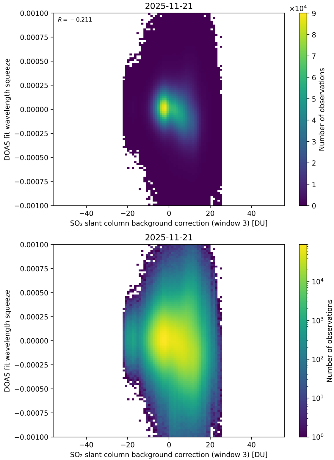
Figure 133: Scatter density plot of “SO 2 slant column background correction (window 3)” against “DOAS fit wavelength squeeze” for 2025-11-20 to 2025-11-22.
