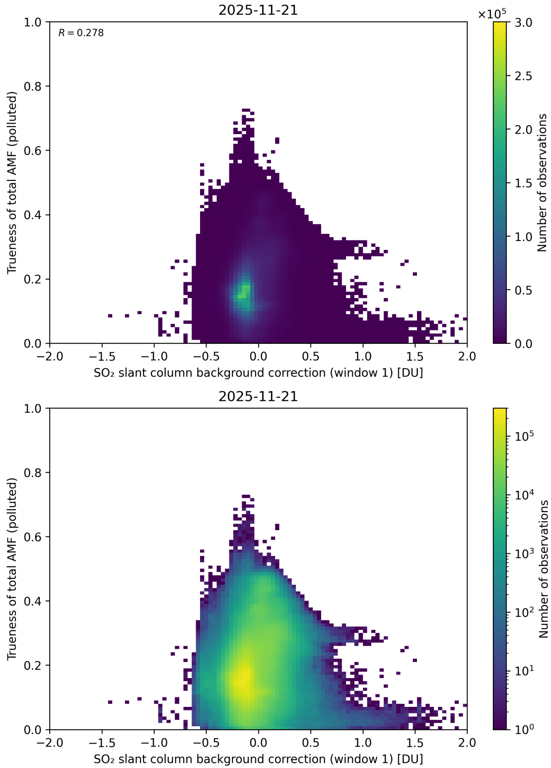
Figure 121: Scatter density plot of “SO 2 slant column background correction (window 1)” against “Trueness of total AMF (polluted)” for 2025-11-20 to 2025-11-22.
