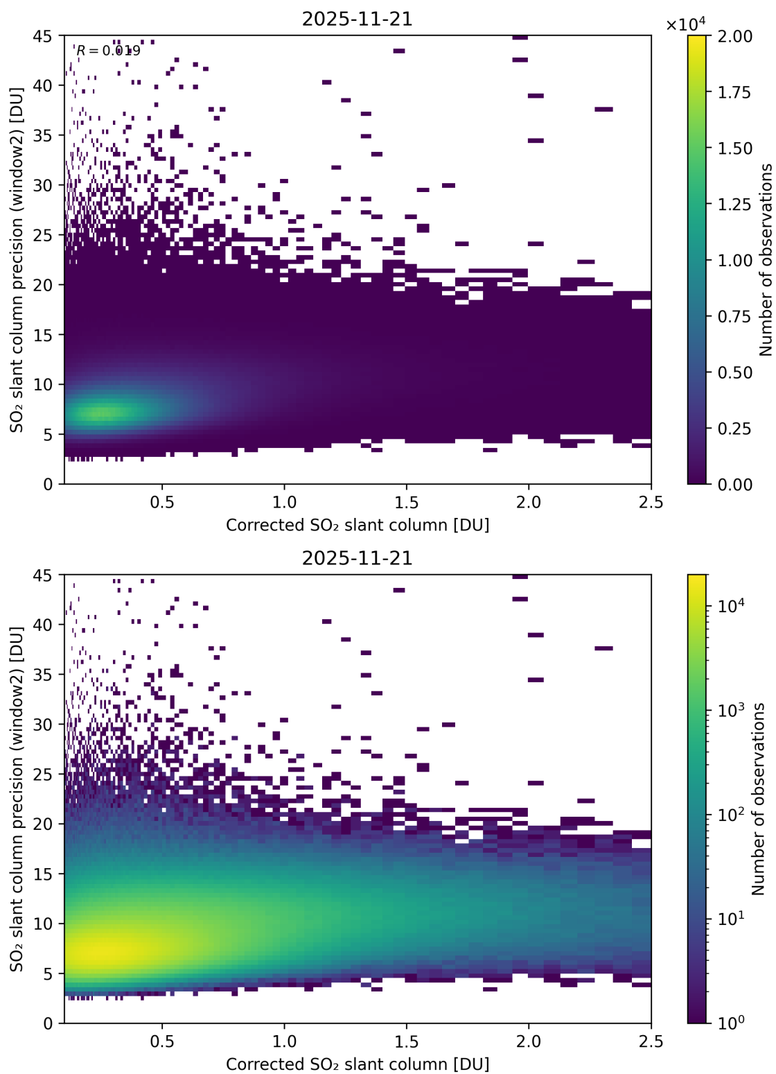
Figure 239: Scatter density plot of “Corrected SO 2 slant column” against “SO 2 slant column precision (window2)” for 2025-11-20 to 2025-11-22.
