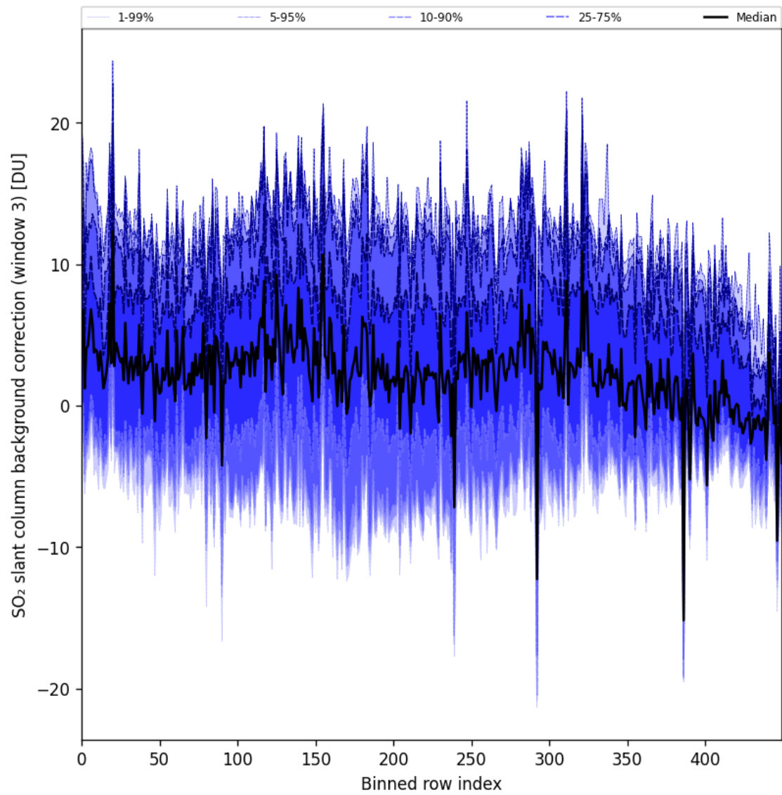
Figure 100: Along track statistics of “SO 2 slant column background correction (window 3)” for 2025-11-20 to 2025-11-22
