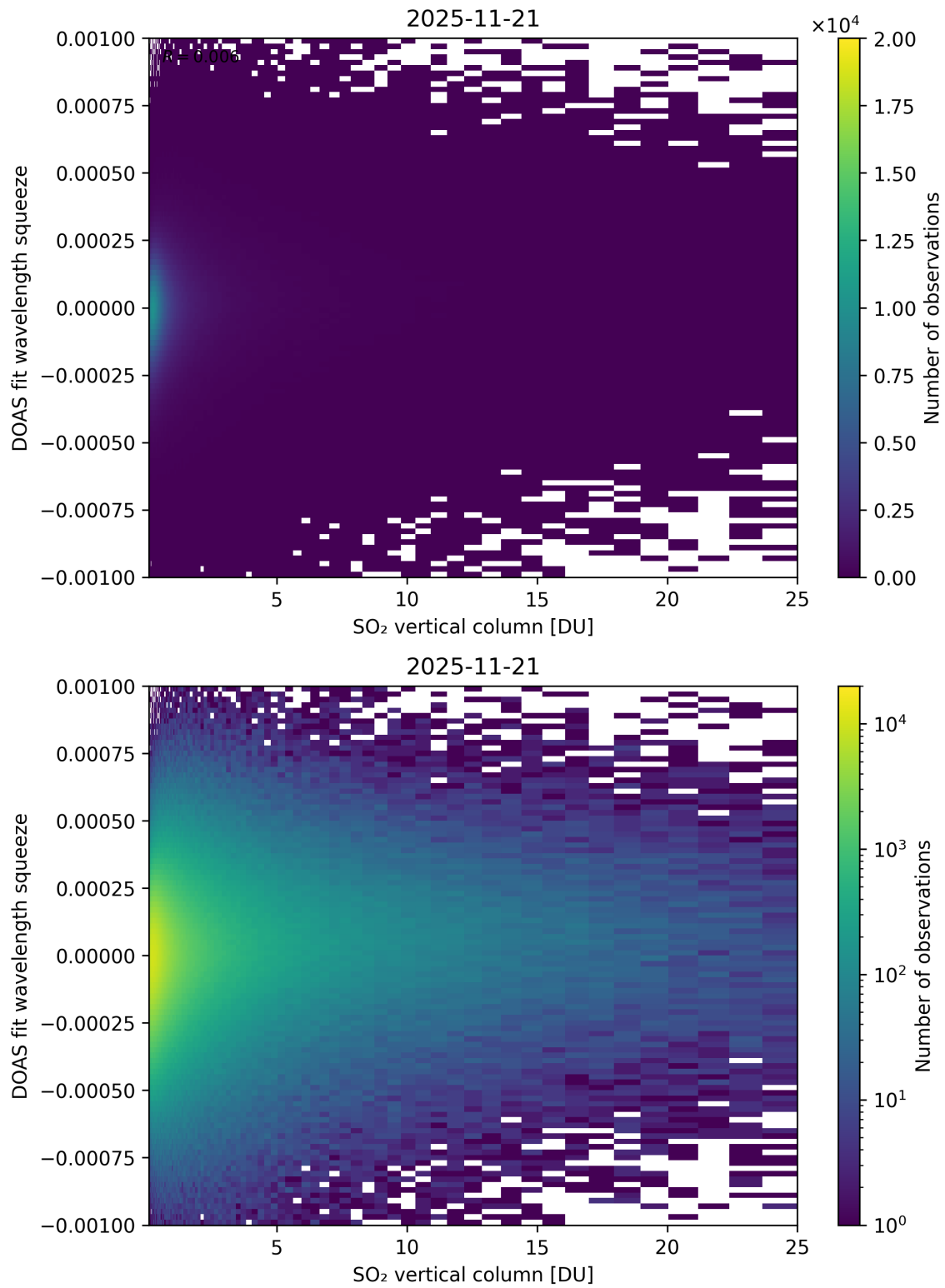
Figure 327: Scatter density plot of “SO 2 vertical column” against “DOAS fit wavelength squeeze” for 2025-11-20 to 2025-11-22.
