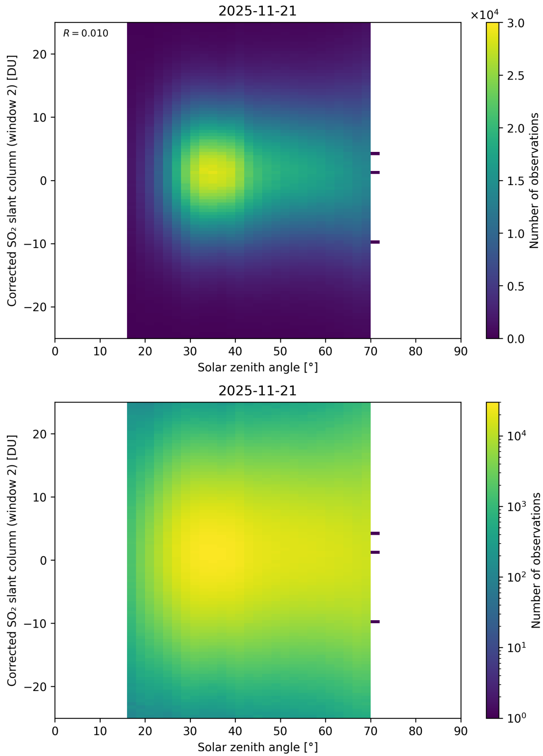
Figure 182: Scatter density plot of “Solar zenith angle” against “Corrected SO 2 slant column (window 2)” for 2025-11-20 to 2025-11-22.
