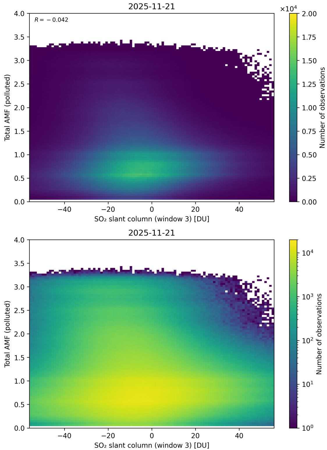
Figure 318: Scatter density plot of “SO 2 slant column (window 3)” against “Total AMF (polluted)” for 2025-11-20 to 2025-11-22.
