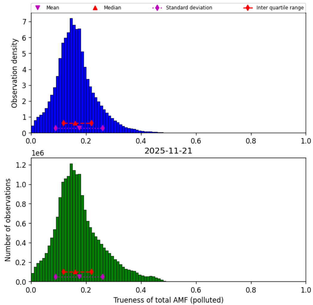
Figure 80: Histogram of “Trueness of total AMF (polluted)” for 2025-11-20 to 2025-11-22
