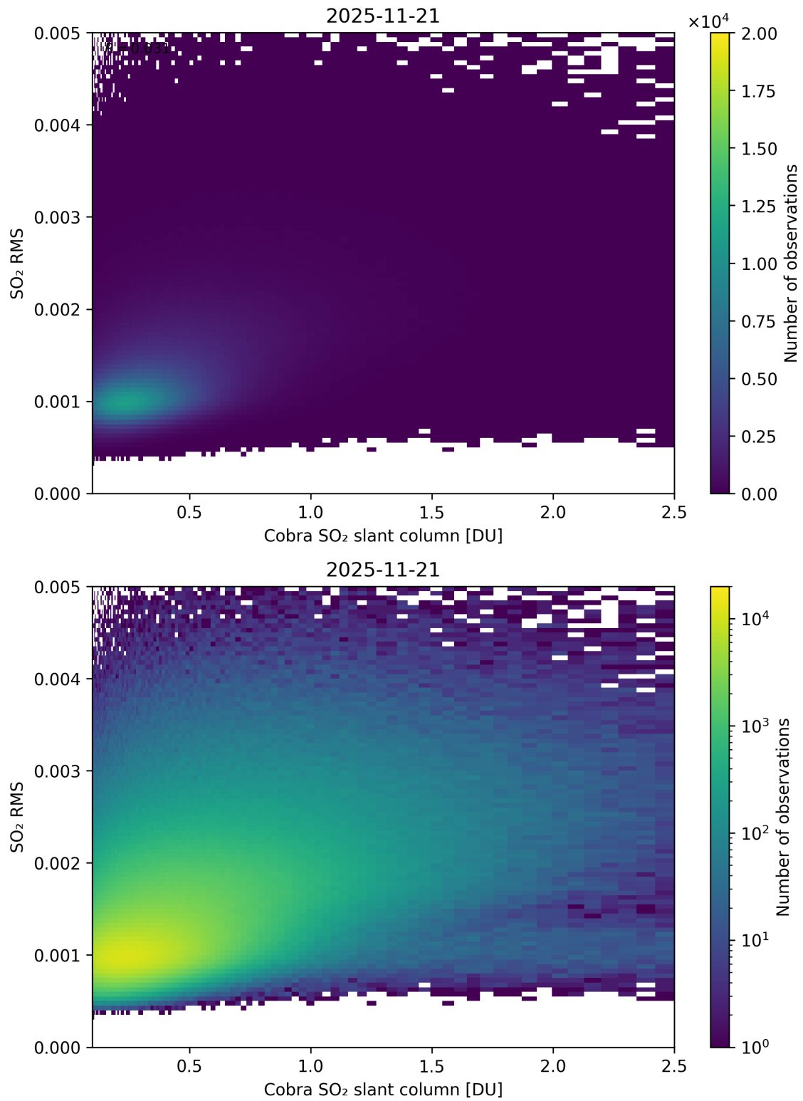
Figure 198: Scatter density plot of “Cobra SO 2 slant column” against “SO 2 RMS” for 2025-11-20 to 2025-11-22.
