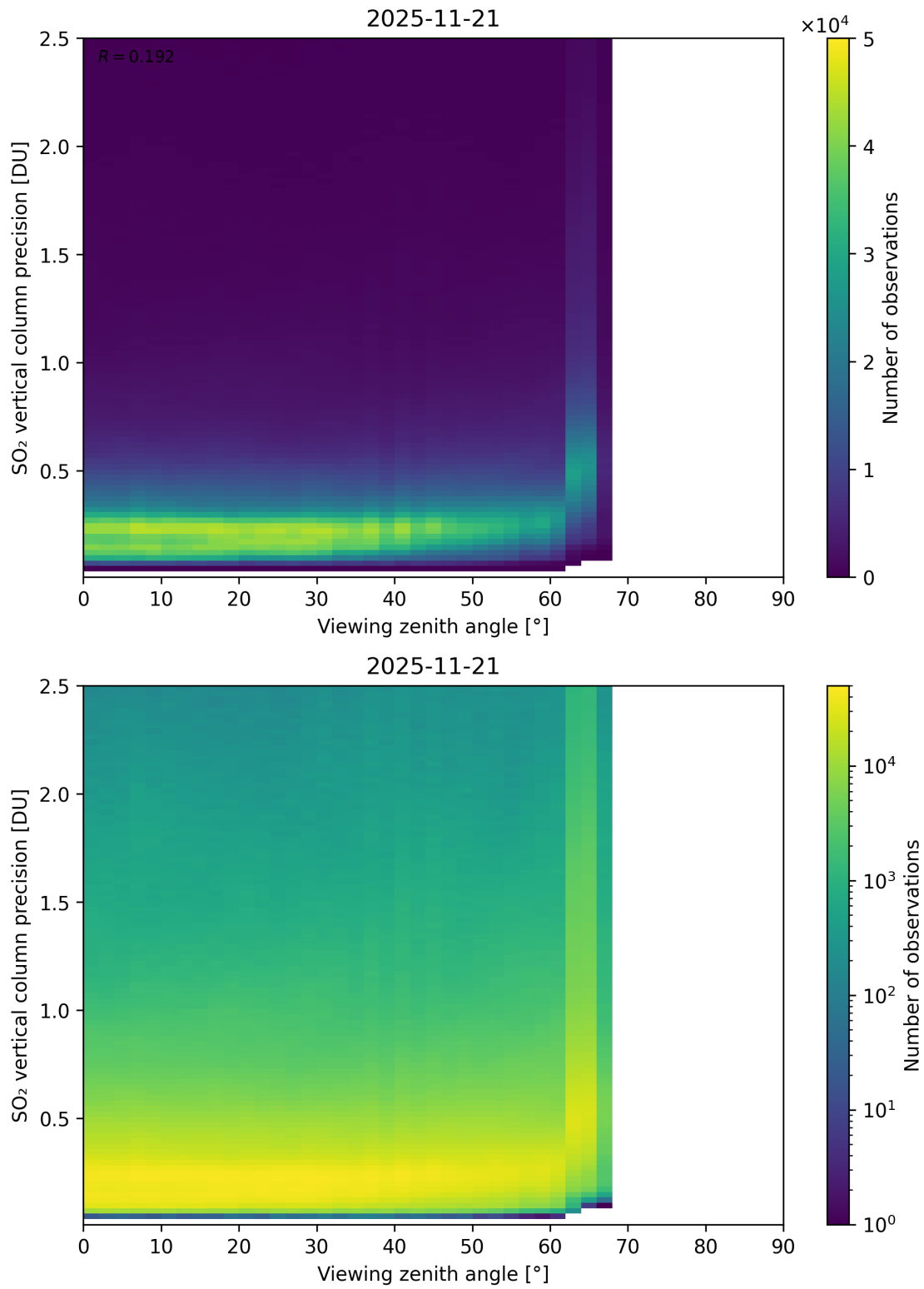
Figure 384: Scatter density plot of “Viewing zenith angle” against “SO 2 vertical column precision” for 2025-11-20 to 2025-11-22.
