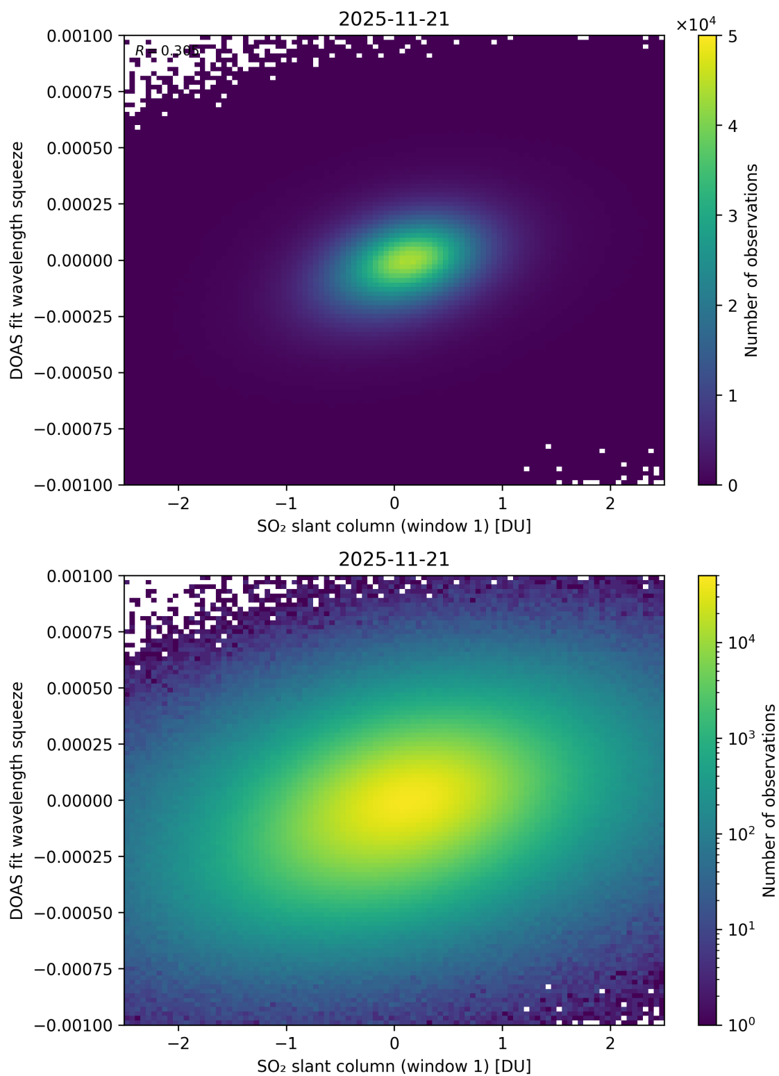
Figure 266: Scatter density plot of “SO 2 slant column (window 1)” against “DOAS fit wavelength squeeze” for 2025-11-20 to 2025-11-22.
