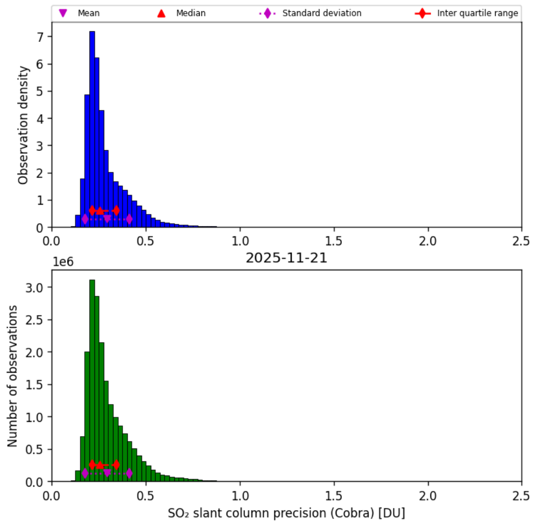
Figure 62: Histogram of “SO 2 slant column precision (Cobra)” for 2025-11-20 to 2025-11-22
