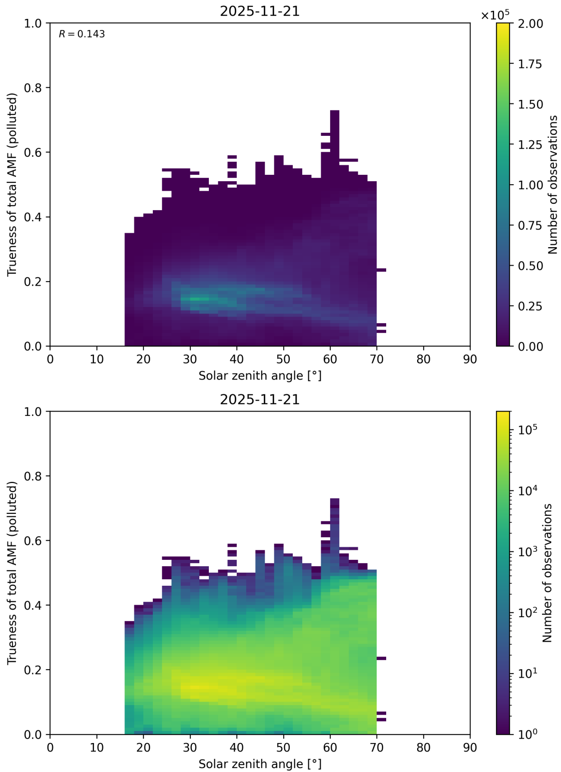
Figure 190: Scatter density plot of “Solar zenith angle” against “Trueness of total AMF (polluted)” for 2025-11-20 to 2025-11-22.
