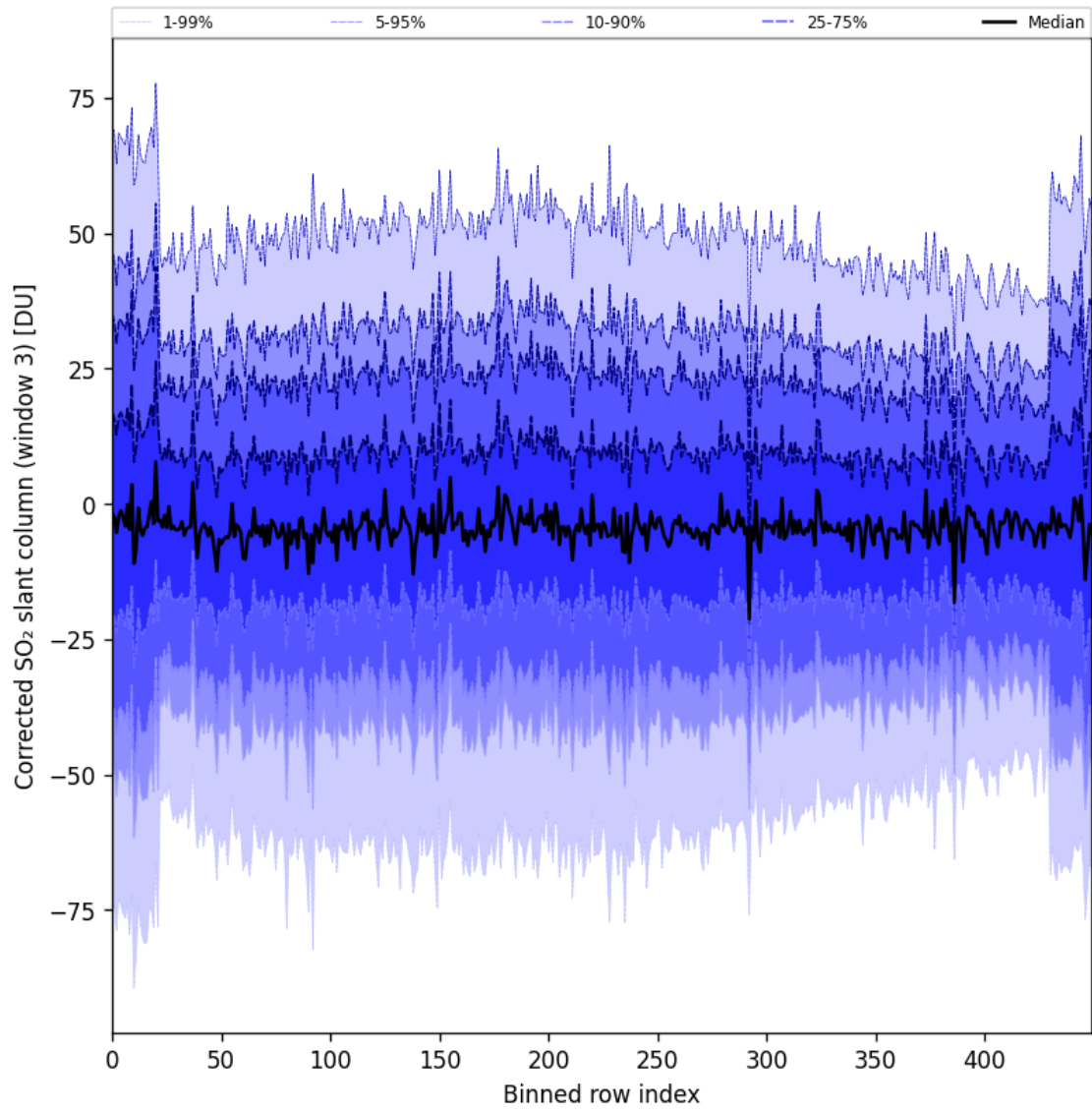
Figure 99: Along track statistics of “Corrected SO 2 slant column (window 3)” for 2025-11-20 to 2025-11-22
