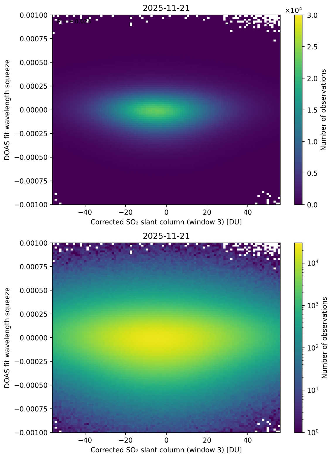
Figure 257: Scatter density plot of “Corrected SO 2 slant column (window 3)” against “DOAS fit wavelength squeeze” for 2025-11-20 to 2025-11-22.
