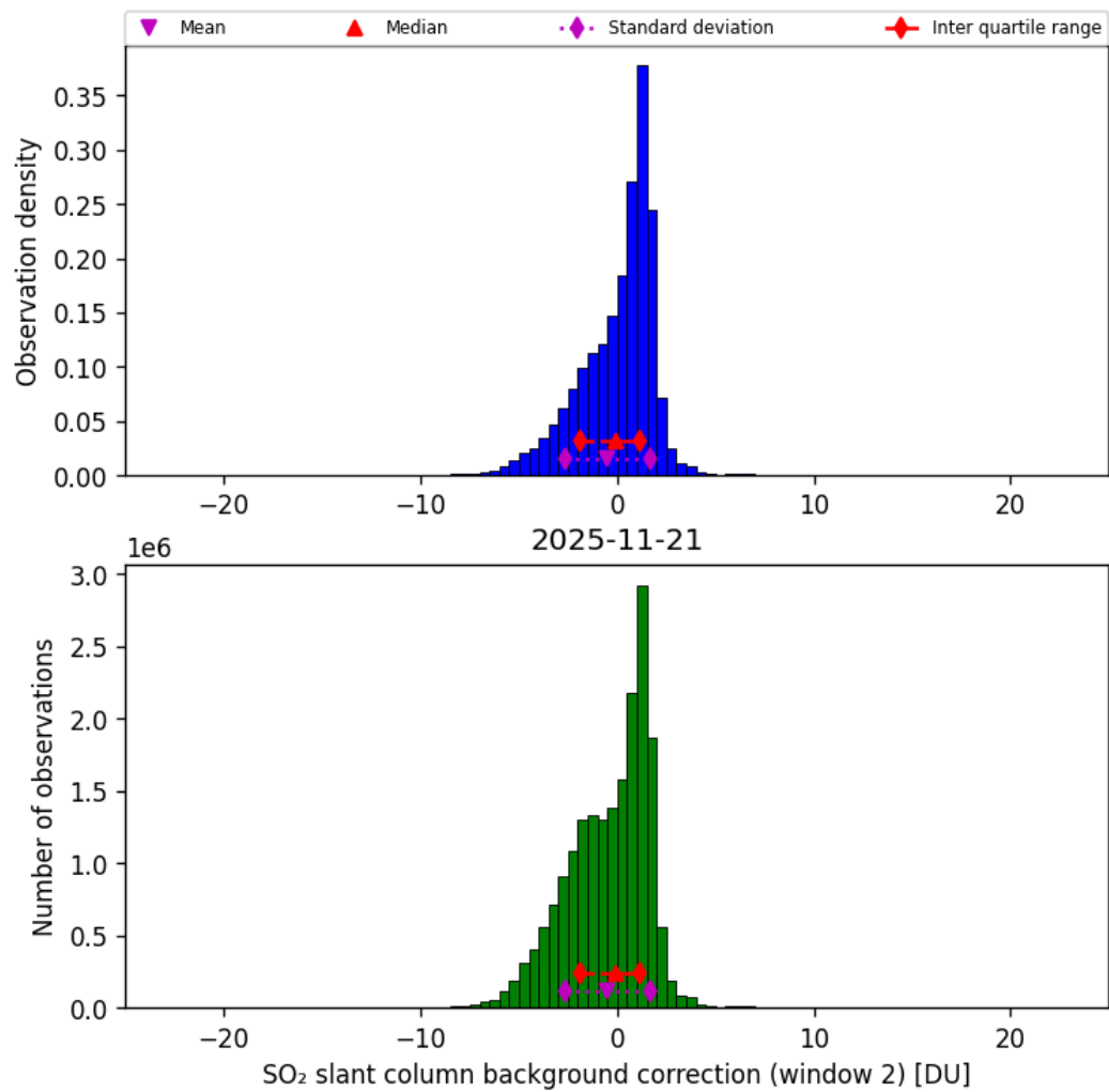
Figure 70: Histogram of “SO 2 slant column background correction (window 2)” for 2025-11-20 to 2025-11-22
