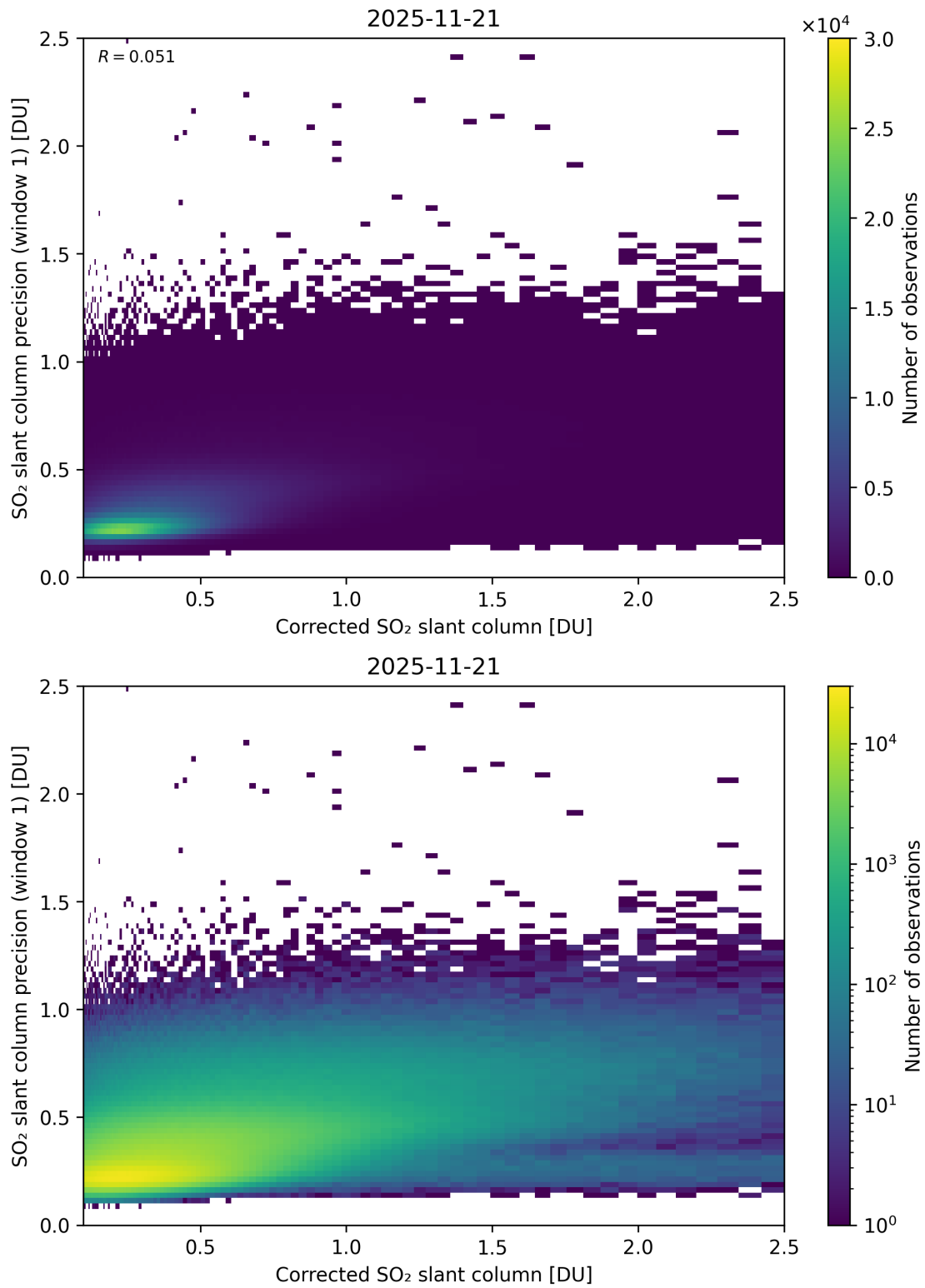
Figure 238: Scatter density plot of “Corrected SO 2 slant column” against “SO 2 slant column precision (window 1)” for 2025-11-20 to 2025-11-22.
