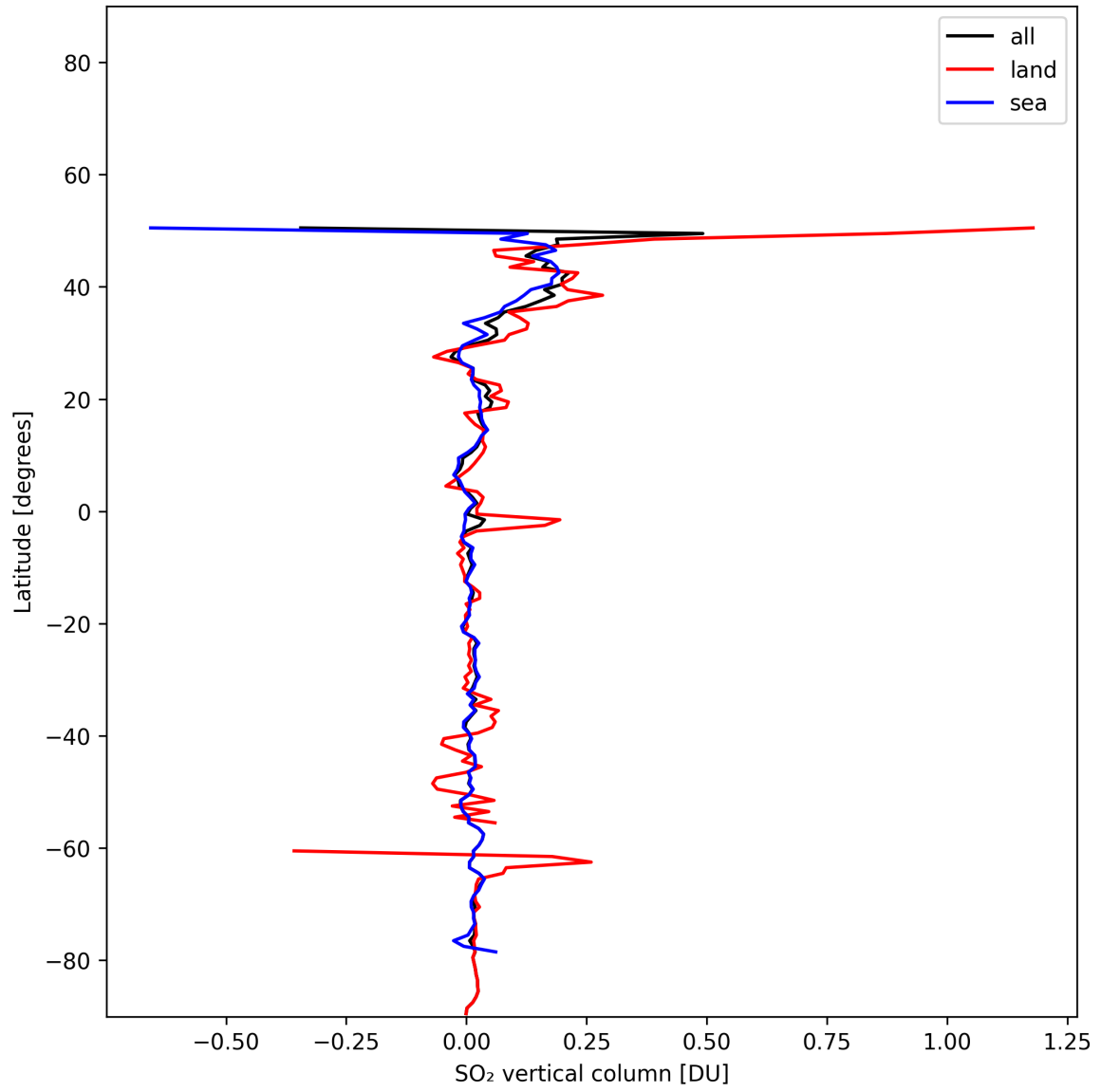
Figure 32: Zonal average of “SO 2 vertical column” for 2025-11-20 to 2025-11-22.
