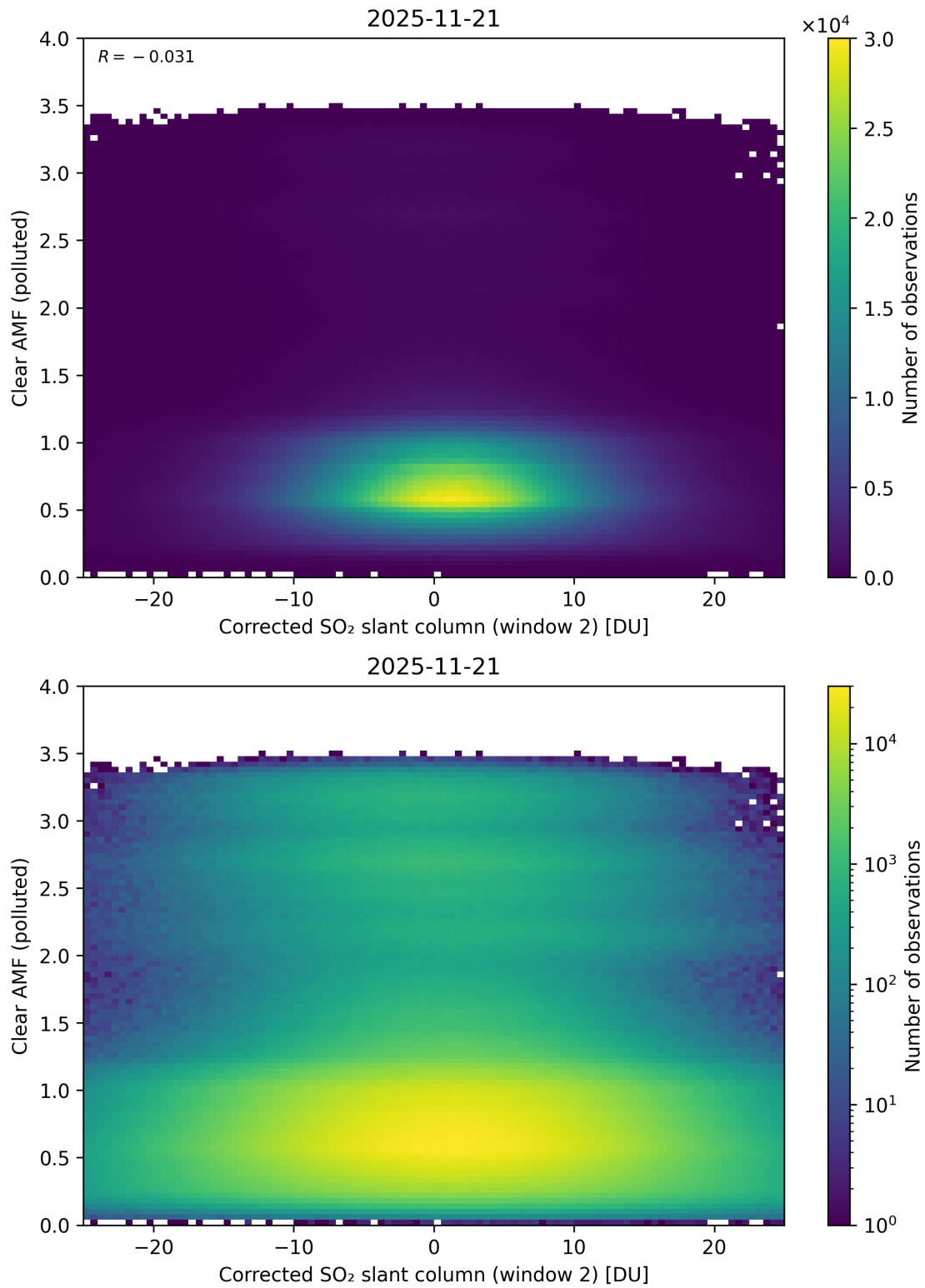
Figure 249: Scatter density plot of “Corrected SO 2 slant column (window 2)” against “Clear AMF (polluted)” for 2025-11-20 to 2025-11-22.
