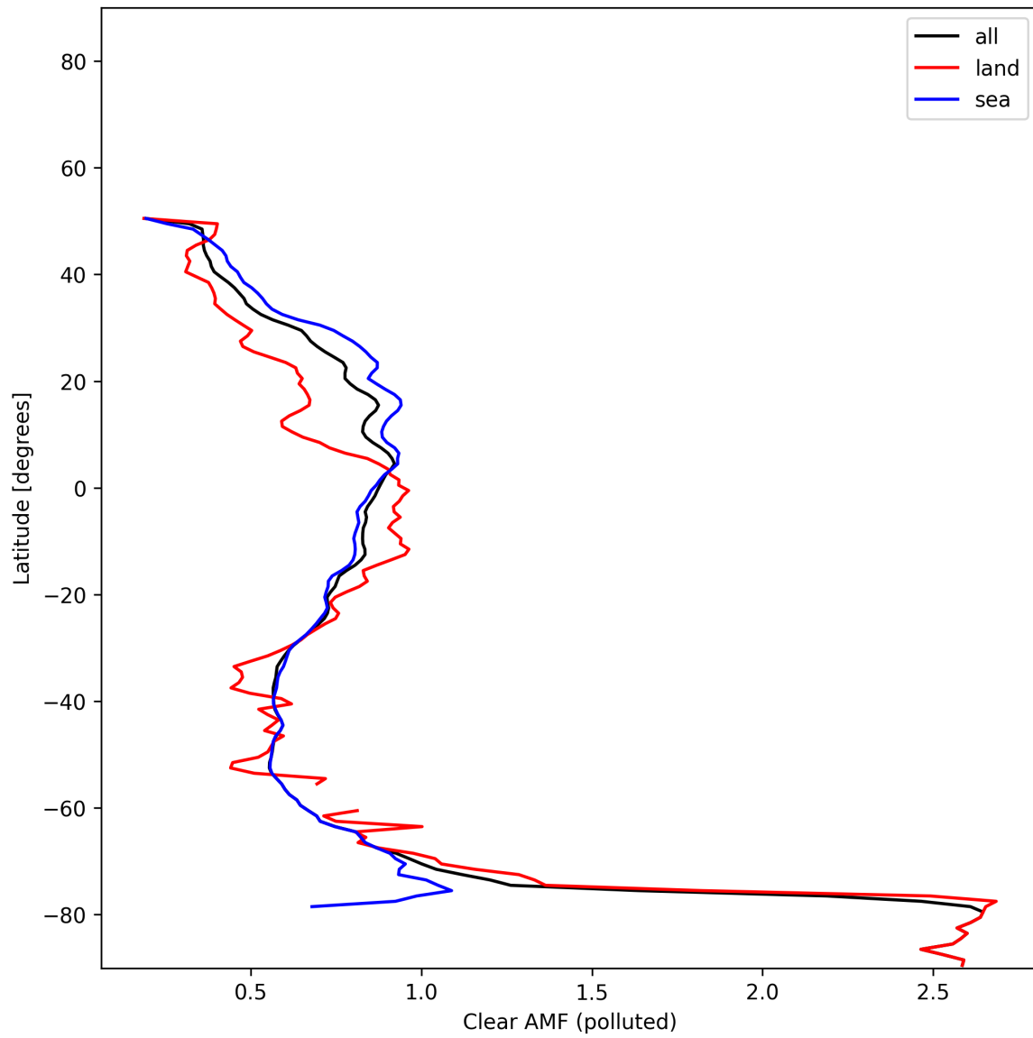
Figure 55: Zonal average of “Clear AMF (polluted)” for 2025-11-20 to 2025-11-22.
