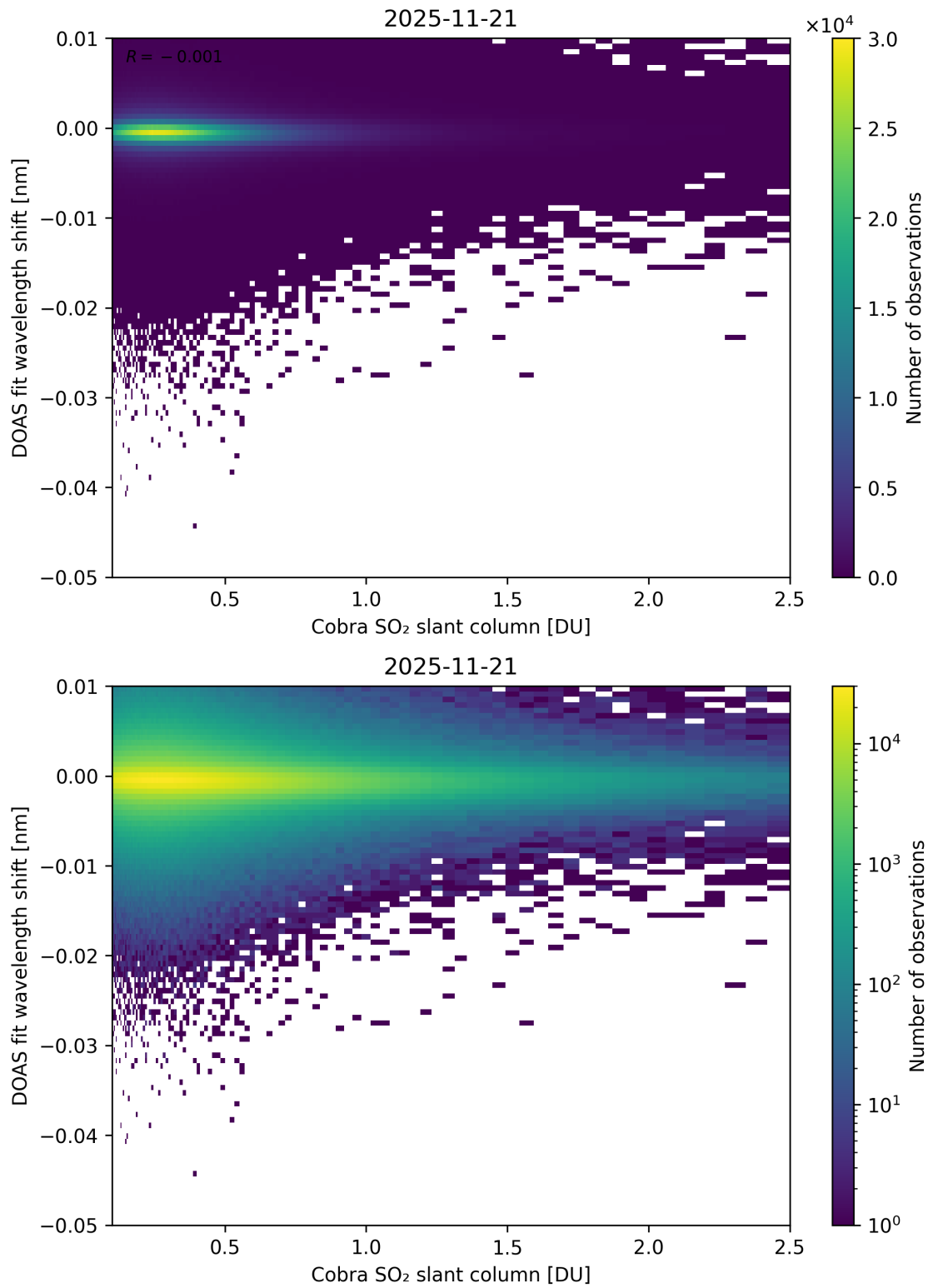
Figure 196: Scatter density plot of “Cobra SO 2 slant column” against “DOAS fit wavelength shift” for 2025-11-20 to 2025-11-22.
