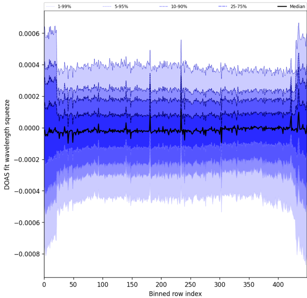
Figure 103: Along track statistics of “DOAS fit wavelength squeeze” for 2025-11-20 to 2025-11-22
