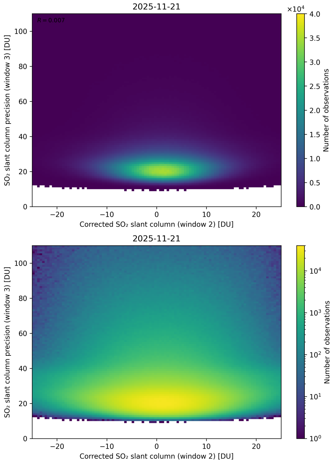
Figure 252: Scatter density plot of “Corrected SO 2 slant column (window 2)” against “SO 2 slant column precision (window 3)” for 2025-11-20 to 2025-11-22.
