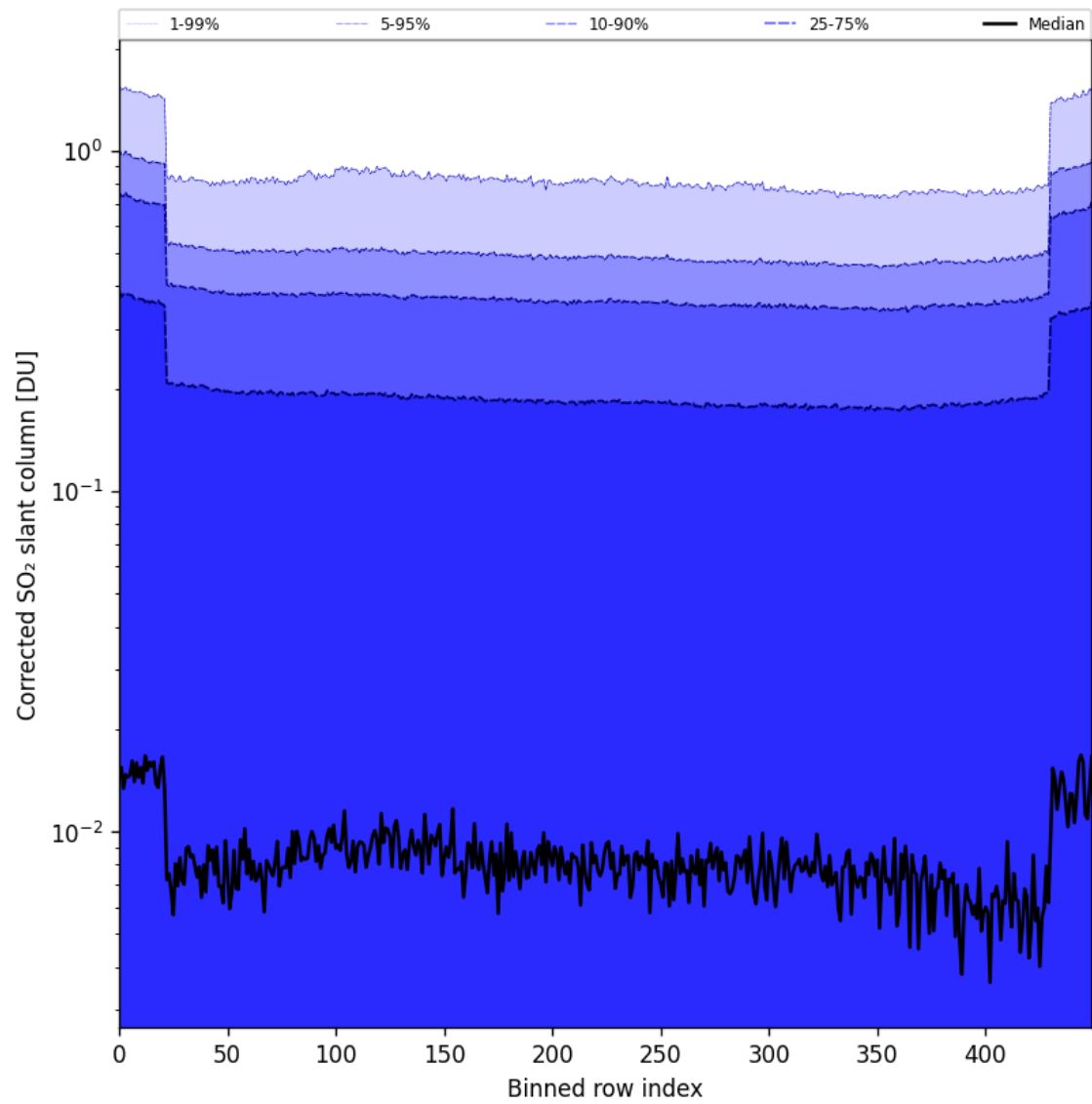
Figure 86: Along track statistics of “Corrected SO 2 slant column” for 2025-11-20 to 2025-11-22
