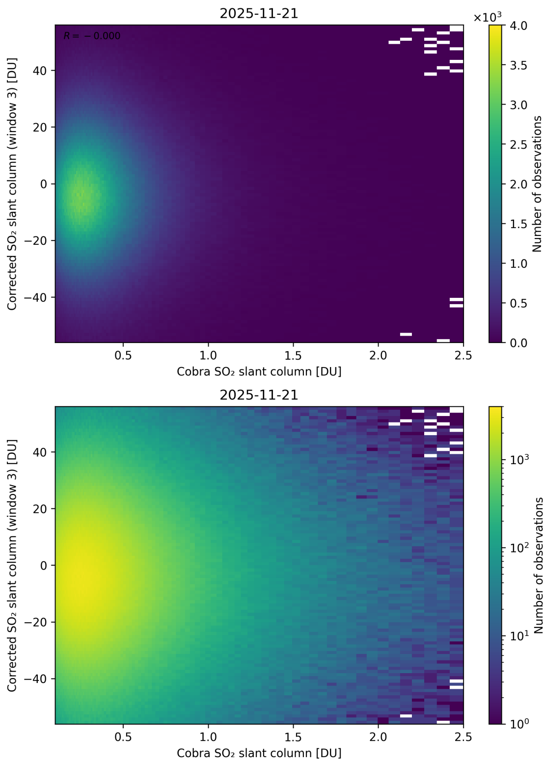
Figure 218: Scatter density plot of “Cobra SO 2 slant column” against “Corrected SO 2 slant column (window 3)” for 2025-11-20 to 2025-11-22.
