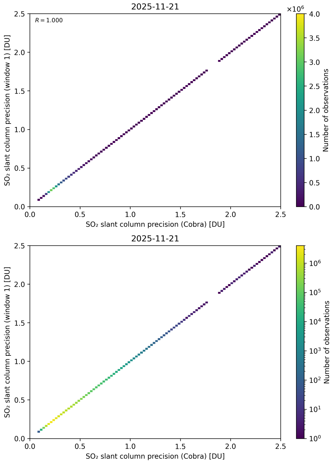
Figure 209: Scatter density plot of “SO 2 slant column precision (Cobra)” against “SO 2 slant column precision (window 1)” for 2025-11-20 to 2025-11-22.
