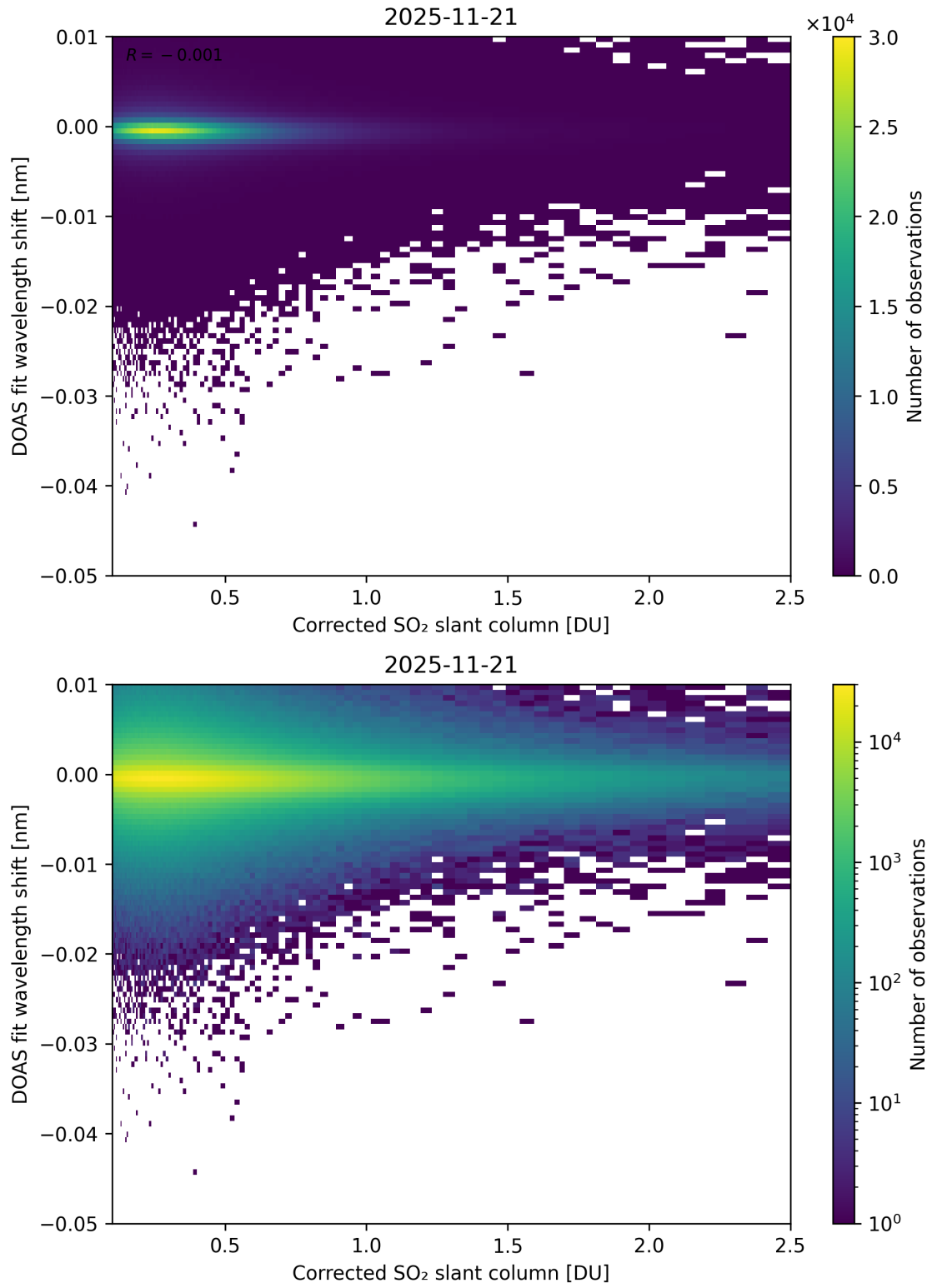
Figure 229: Scatter density plot of “Corrected SO 2 slant column” against “DOAS fit wavelength shift” for 2025-11-20 to 2025-11-22.
