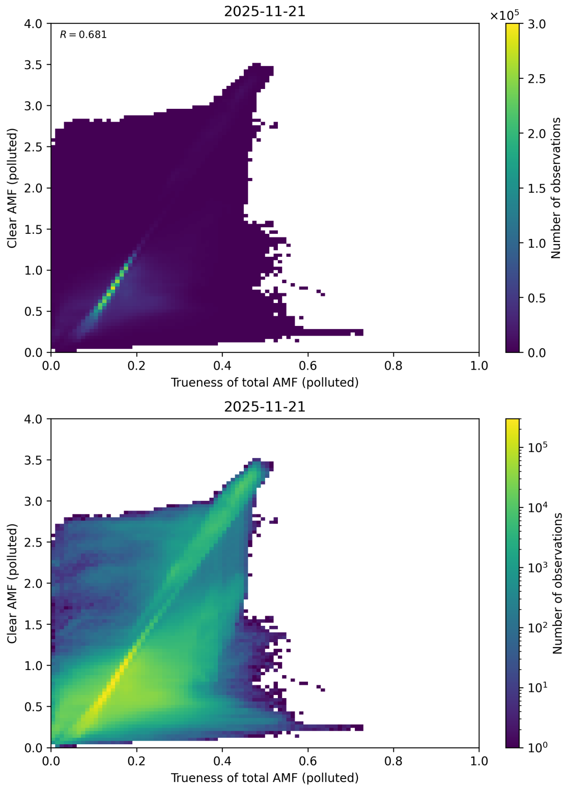
Figure 322: Scatter density plot of “Trueness of total AMF (polluted)” against “Clear AMF (polluted)” for 2025-11-20 to 2025-11-22.
