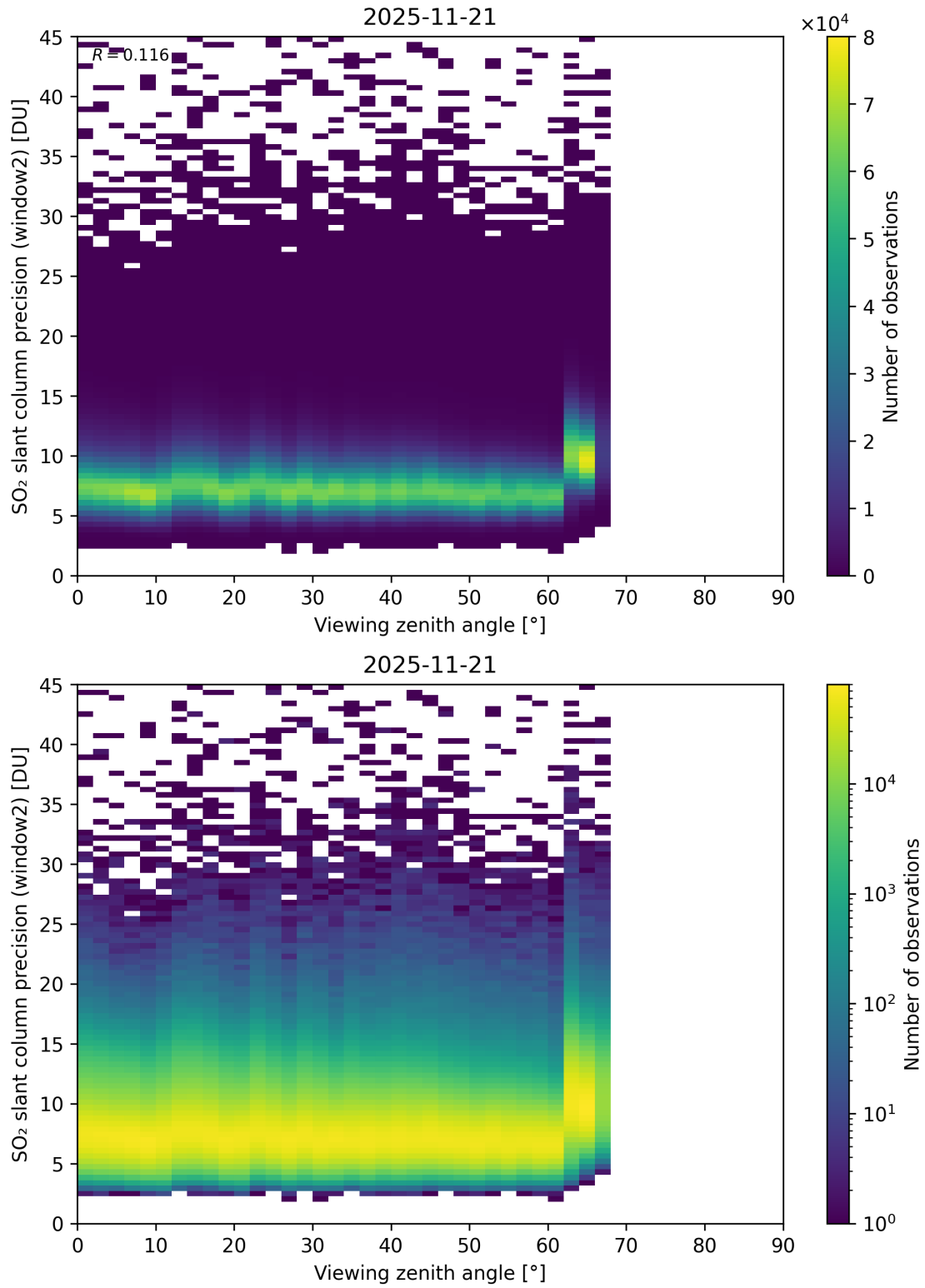
Figure 378: Scatter density plot of “Viewing zenith angle” against “SO 2 slant column precision (window2)” for 2025-11-20 to 2025-11-22.
