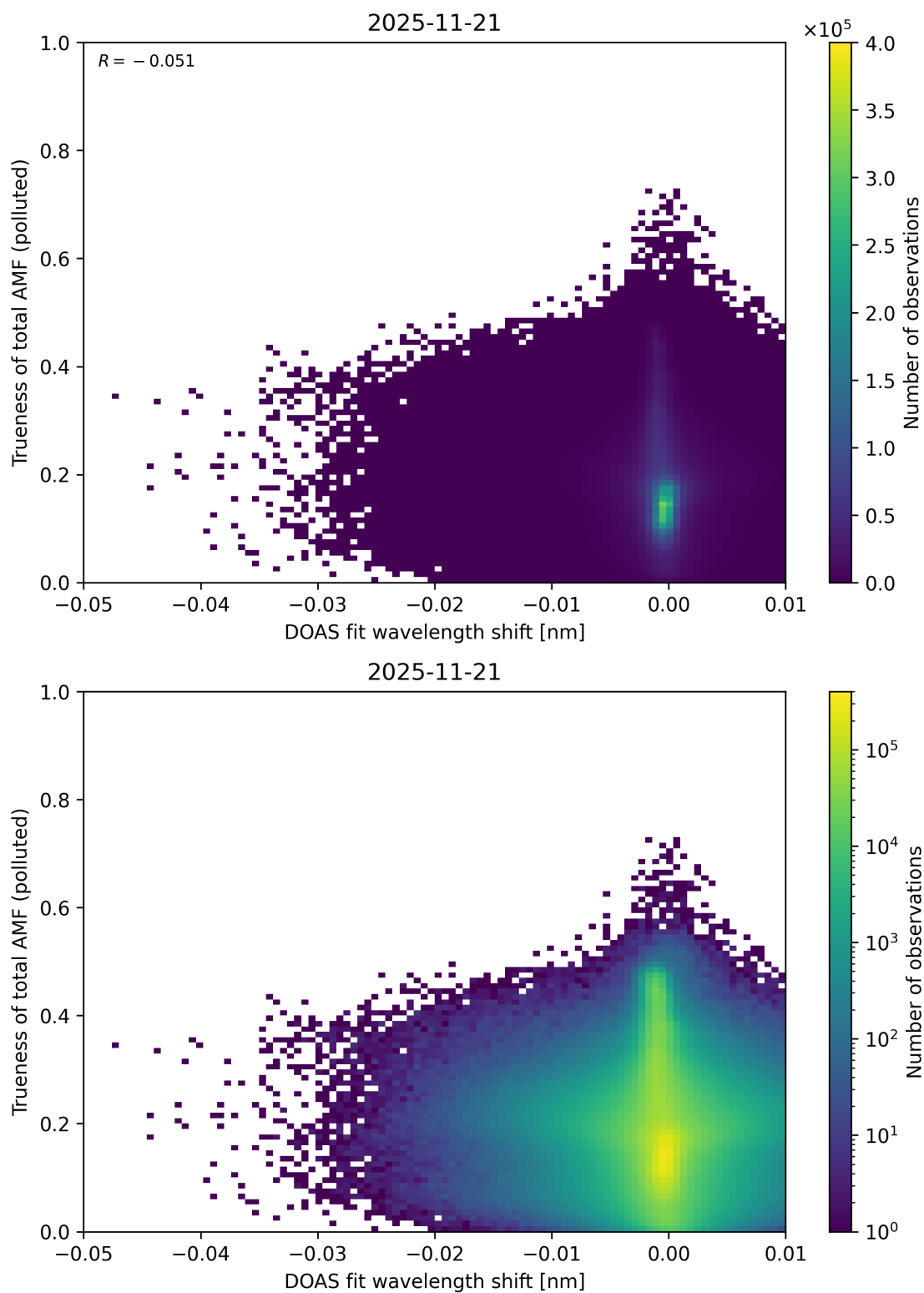
Figure 142: Scatter density plot of “DOAS fit wavelength shift” against “Trueness of total AMF (polluted)” for 2025-11-20 to 2025-11-22.
