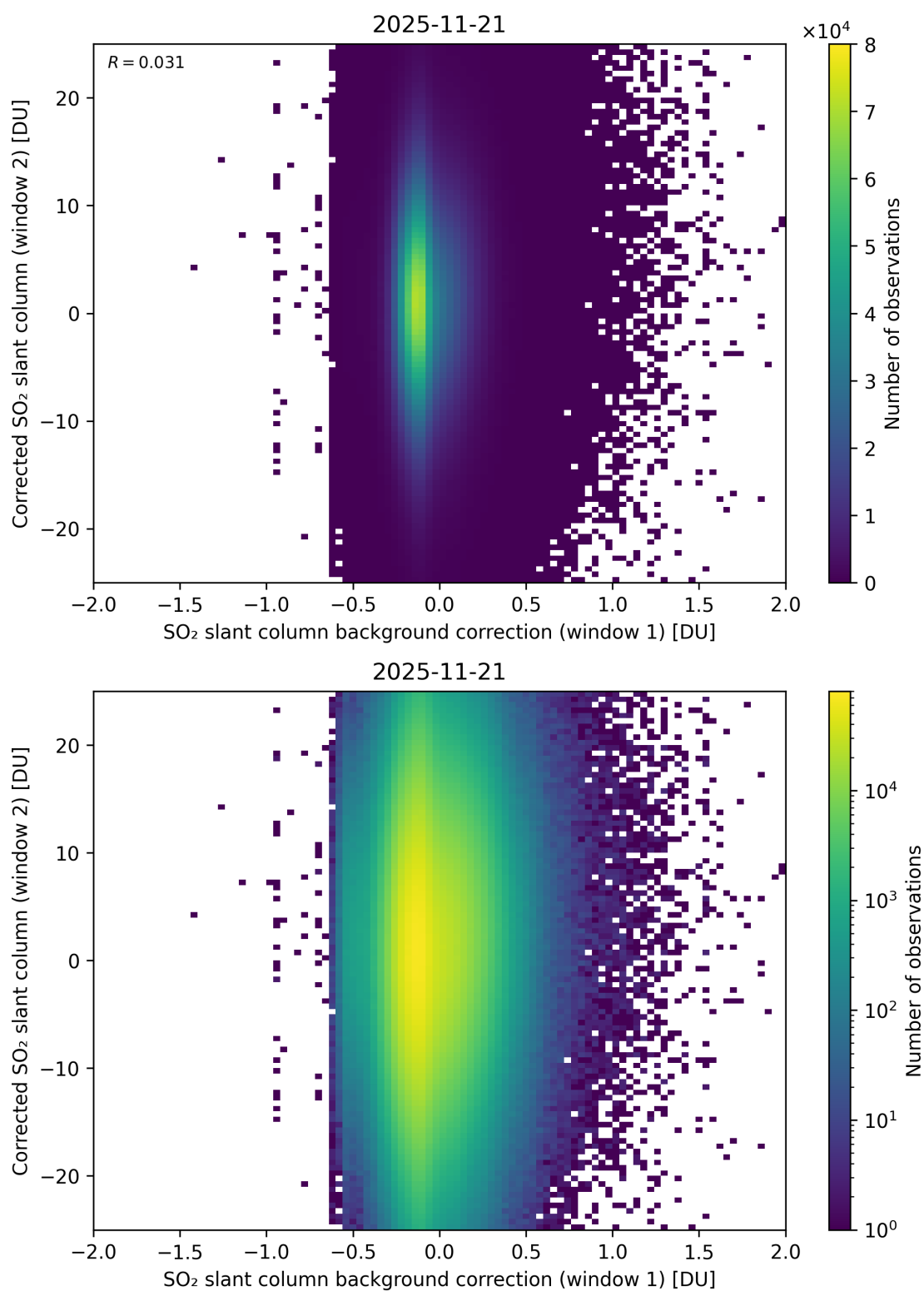
Figure 115: Scatter density plot of “SO 2 slant column background correction (window 1)” against “Corrected SO 2 slant column (window 2)” for 2025-11-20 to 2025-11-22.
