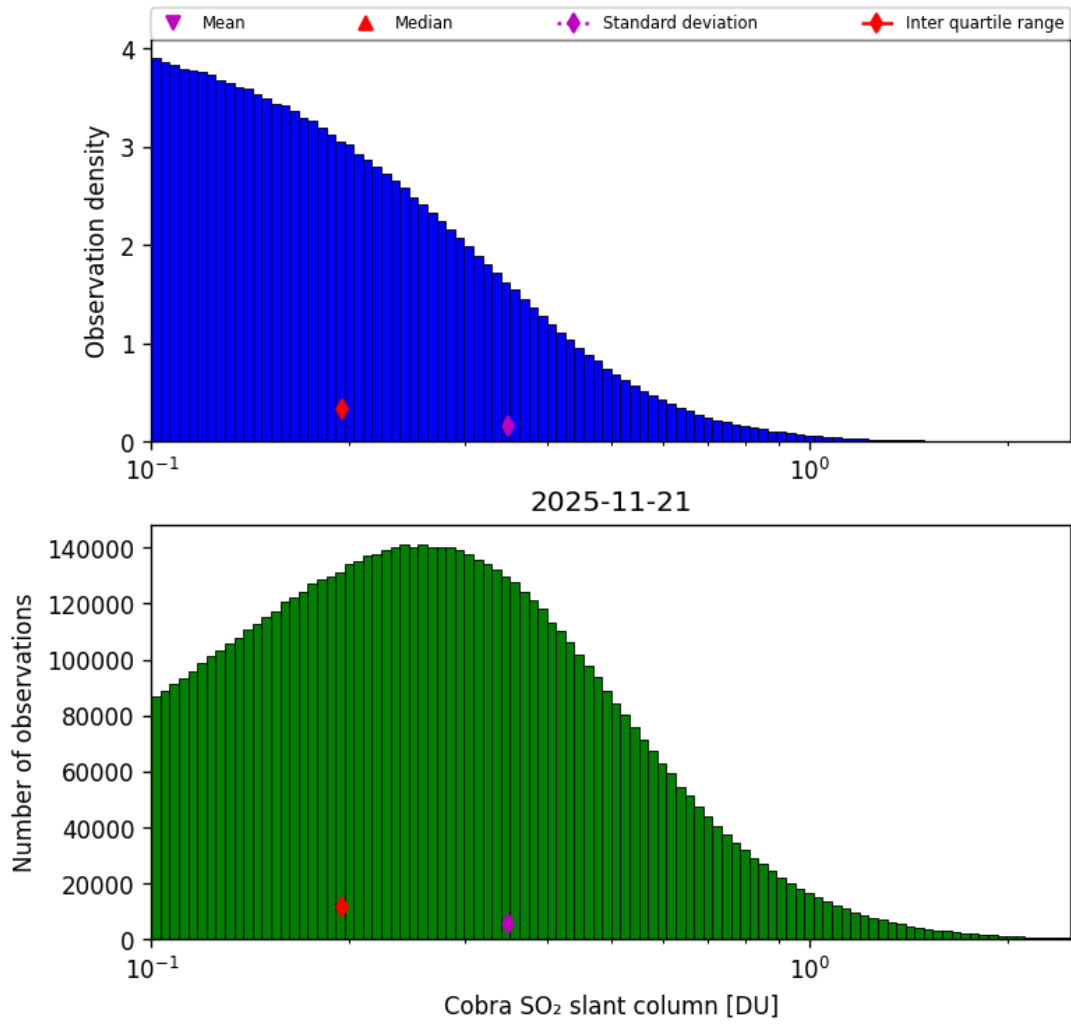
Figure 61: Histogram of “Cobra SO 2 slant column” for 2025-11-20 to 2025-11-22
