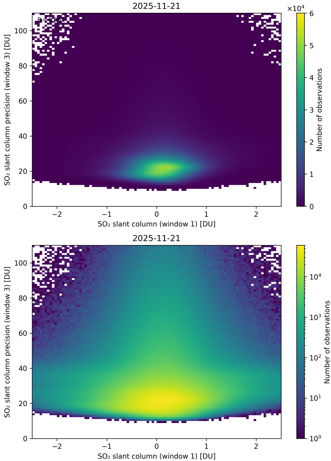
Figure 288: Scatter density plot of “SO 2 slant column (window 1)” against “SO 2 slant column precision (window 3)” for 2025-11-20 to 2025-11-22.
