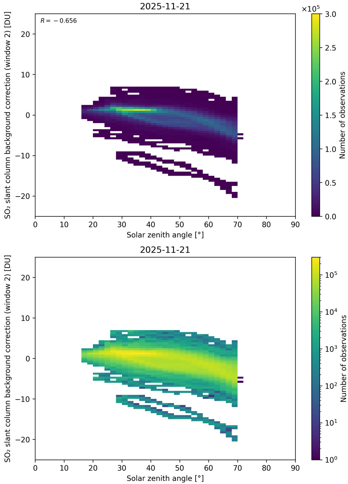
Figure 172: Scatter density plot of “Solar zenith angle” against “SO 2 slant column background correction (window 2)” for 2025-11-20 to 2025-11-22.
