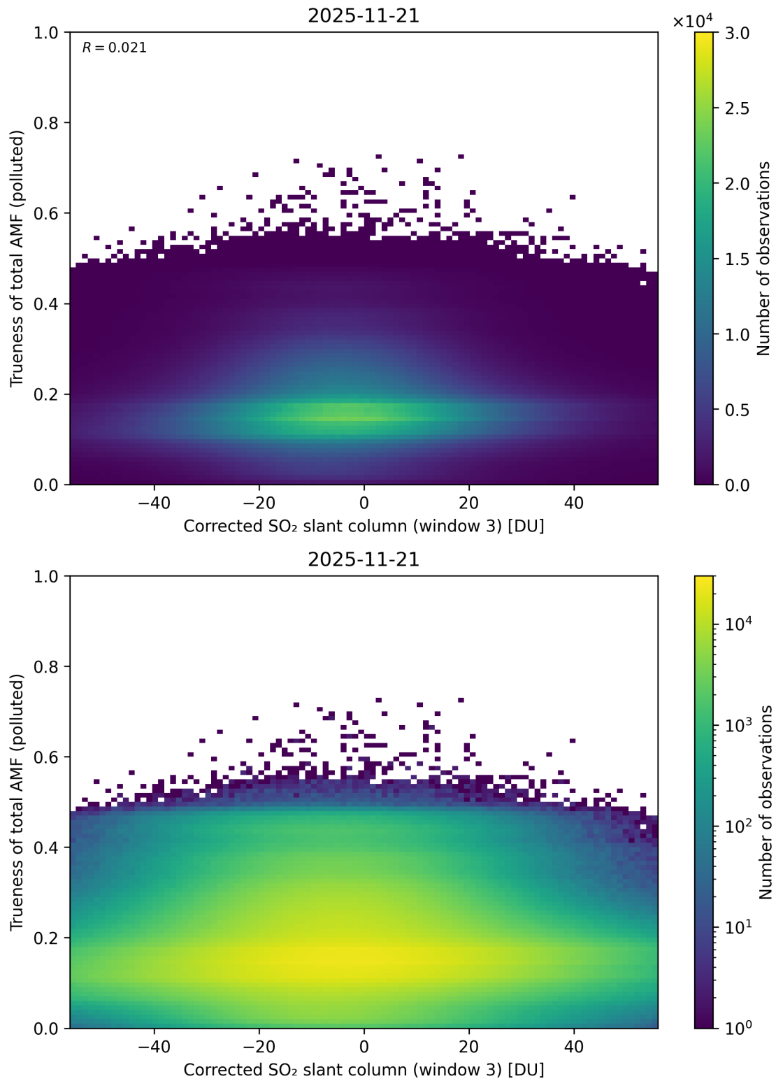
Figure 261: Scatter density plot of “Corrected SO 2 slant column (window 3)” against “Trueness of total AMF (polluted)” for 2025-11-20 to 2025-11-22.
