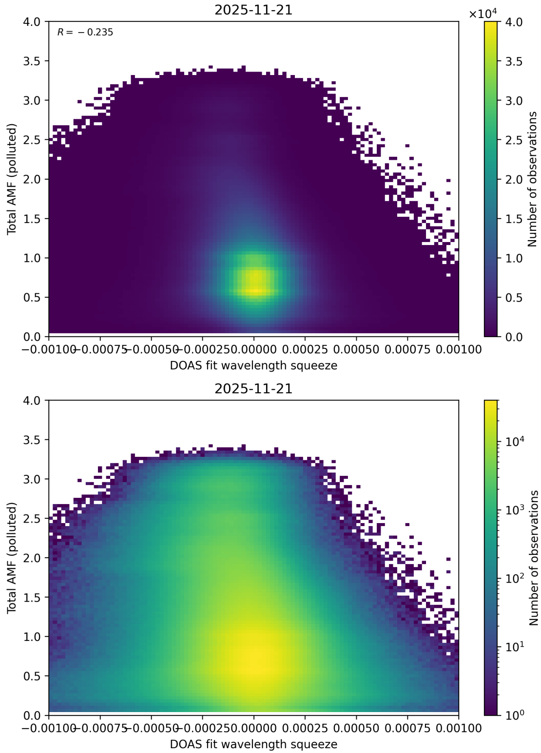
Figure 145: Scatter density plot of “DOAS fit wavelength squeeze” against “Total AMF (polluted)” for 2025-11-20 to 2025-11-22.
