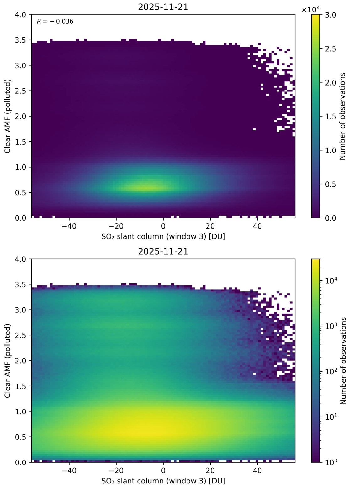
Figure 315: Scatter density plot of “SO 2 slant column (window 3)” against “Clear AMF (polluted)” for 2025-11-20 to 2025-11-22.
