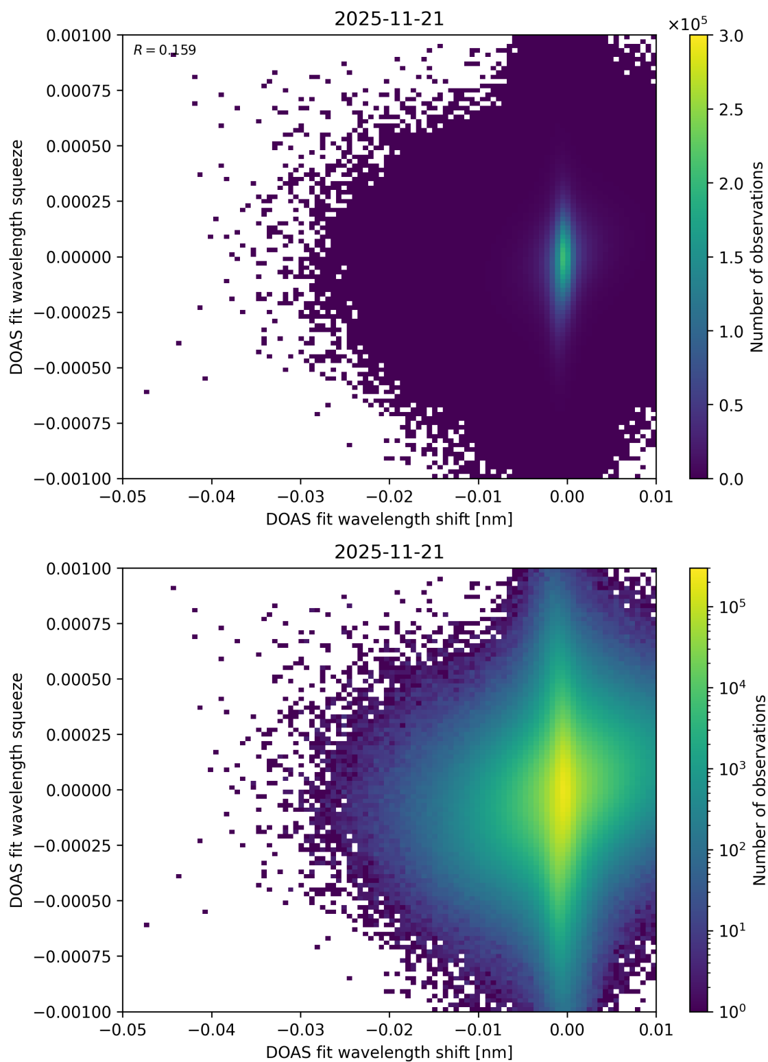
Figure 138: Scatter density plot of “DOAS fit wavelength shift” against “DOAS fit wavelength squeeze” for 2025-11-20 to 2025-11-22.
