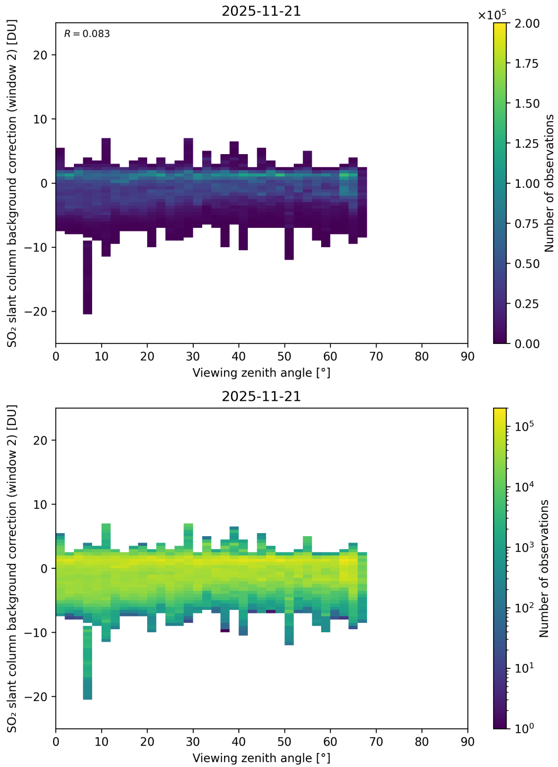
Figure 363: Scatter density plot of “Viewing zenith angle” against “SO 2 slant column background correction (window 2)” for 2025-11-20 to 2025-11-22.
