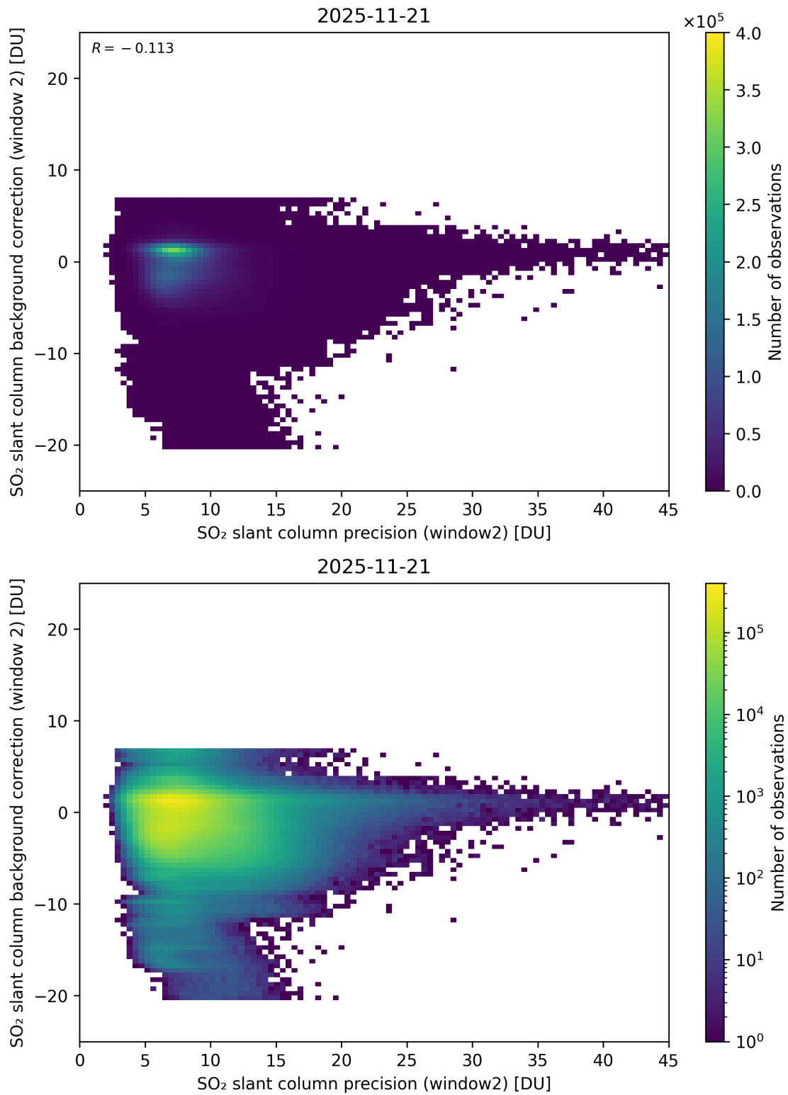
Figure 291: Scatter density plot of “SO 2 slant column precision (window2)” against “SO 2 slant column background correction (window 2)” for 2025-11-20 to 2025-11-22.
