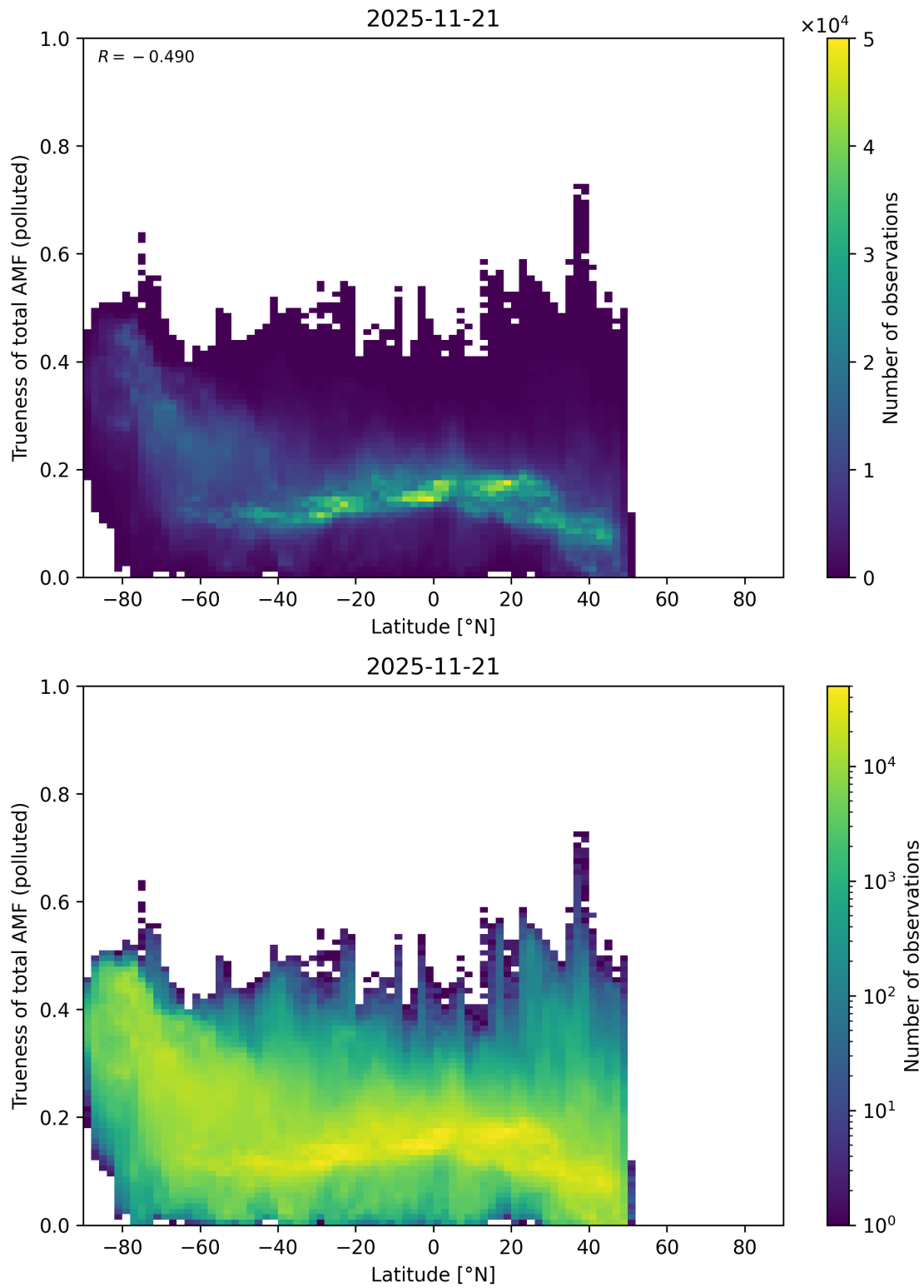
Figure 168: Scatter density plot of “Latitude” against “Trueness of total AMF (polluted)” for 2025-11-20 to 2025-11-22.
