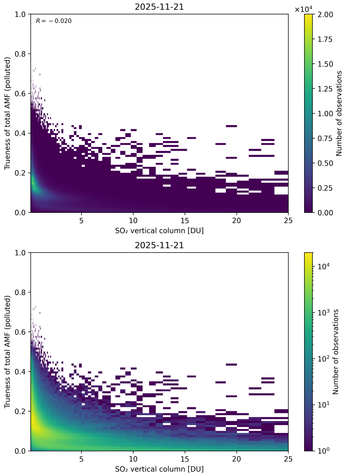
Figure 360: Scatter density plot of “SO 2 vertical column” against “Trueness of total AMF (polluted)” for 2025-11-20 to 2025-11-22.
