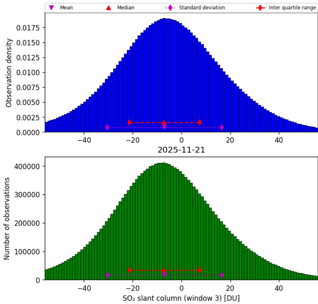
Figure 71: Histogram of “SO 2 slant column (window 3)” for 2025-11-20 to 2025-11-22
