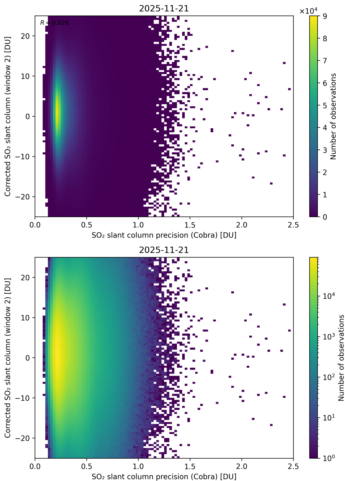
Figure 206: Scatter density plot of “SO 2 slant column precision (Cobra)” against “Corrected SO 2 slant column (window 2)” for 2025-11-20 to 2025-11-22.
