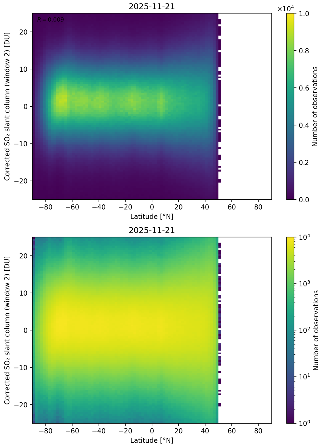
Figure 160: Scatter density plot of “Latitude” against “Corrected SO 2 slant column (window 2)” for 2025-11-20 to 2025-11-22.
