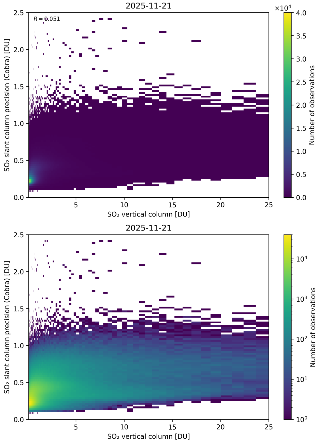
Figure 350: Scatter density plot of “SO 2 vertical column” against “SO 2 slant column precision (Cobra)” for 2025-11-20 to 2025-11-22.
