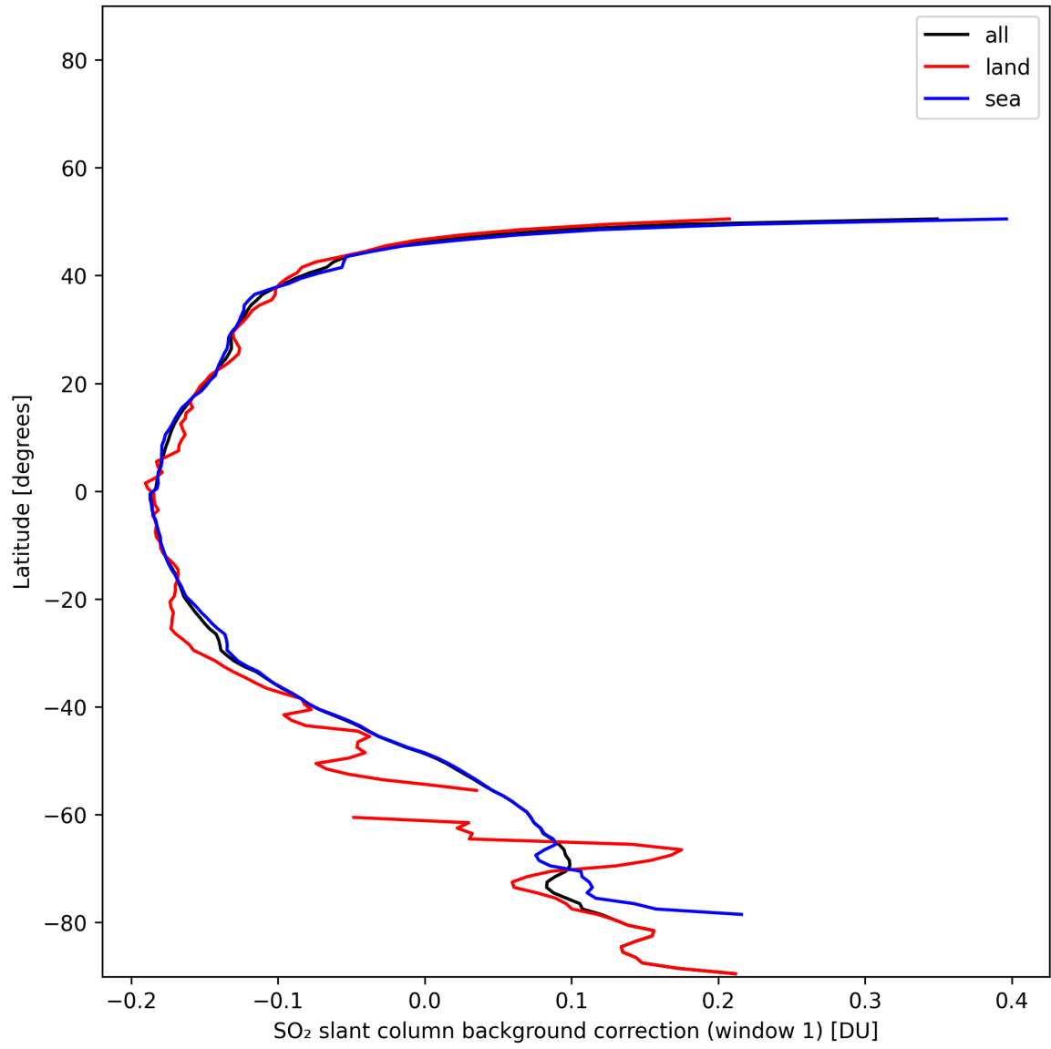
Figure 40: Zonal average of “SO 2 slant column background correction (window 1)” for 2025-11-20 to 2025-11-22.
