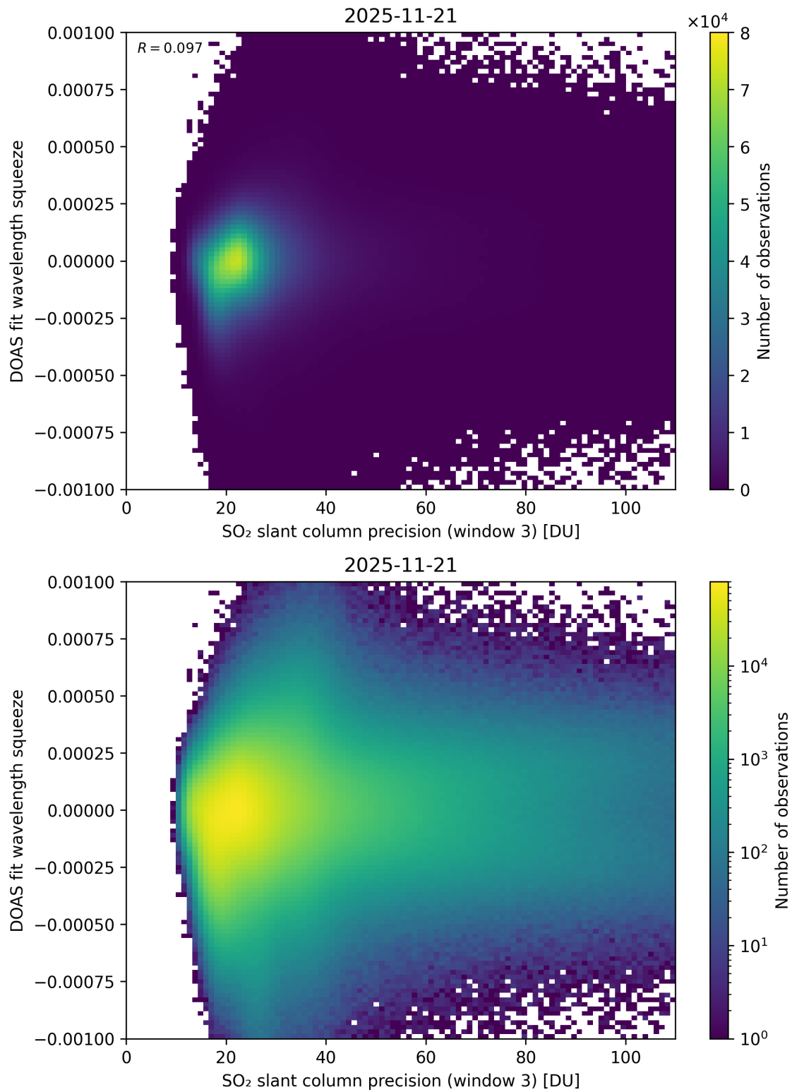
Figure 309: Scatter density plot of “SO 2 slant column precision (window 3)” against “DOAS fit wavelength squeeze” for 2025-11-20 to 2025-11-22.
