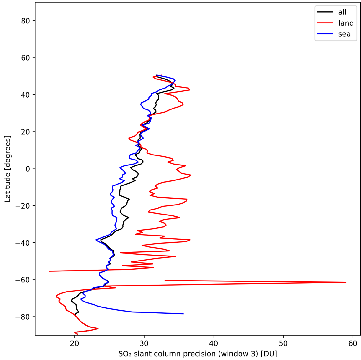
Figure 46: Zonal average of “SO 2 slant column precision (window 3)” for 2025-11-20 to 2025-11-22.
