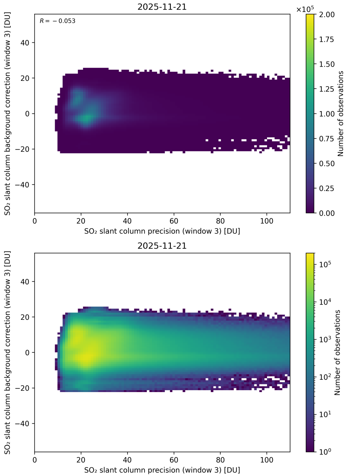
Figure 307: Scatter density plot of “SO 2 slant column precision (window 3)” against “SO 2 slant column background correction (window 3)” for 2025-11-20 to 2025-11-22.
