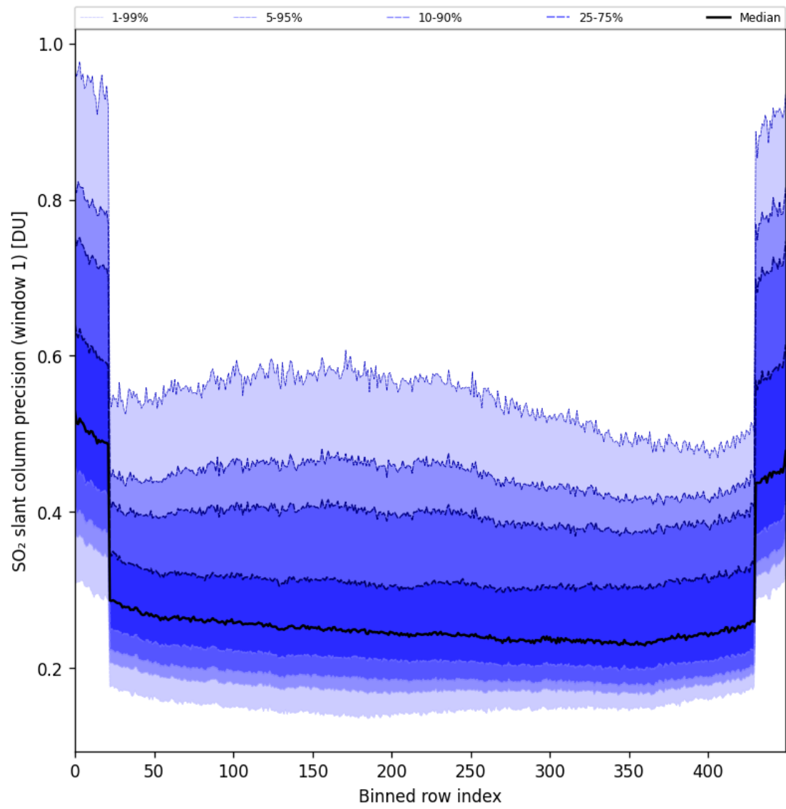
Figure 90: Along track statistics of “SO 2 slant column precision (window 1)” for 2025-11-20 to 2025-11-22
