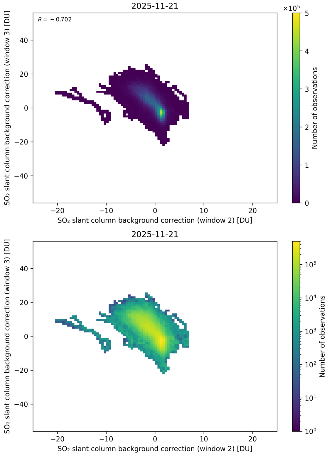
Figure 122: Scatter density plot of “SO 2 slant column background correction (window 2)” against “SO 2 slant column background correction (window 3)” for 2025-11-20 to 2025-11-22.
