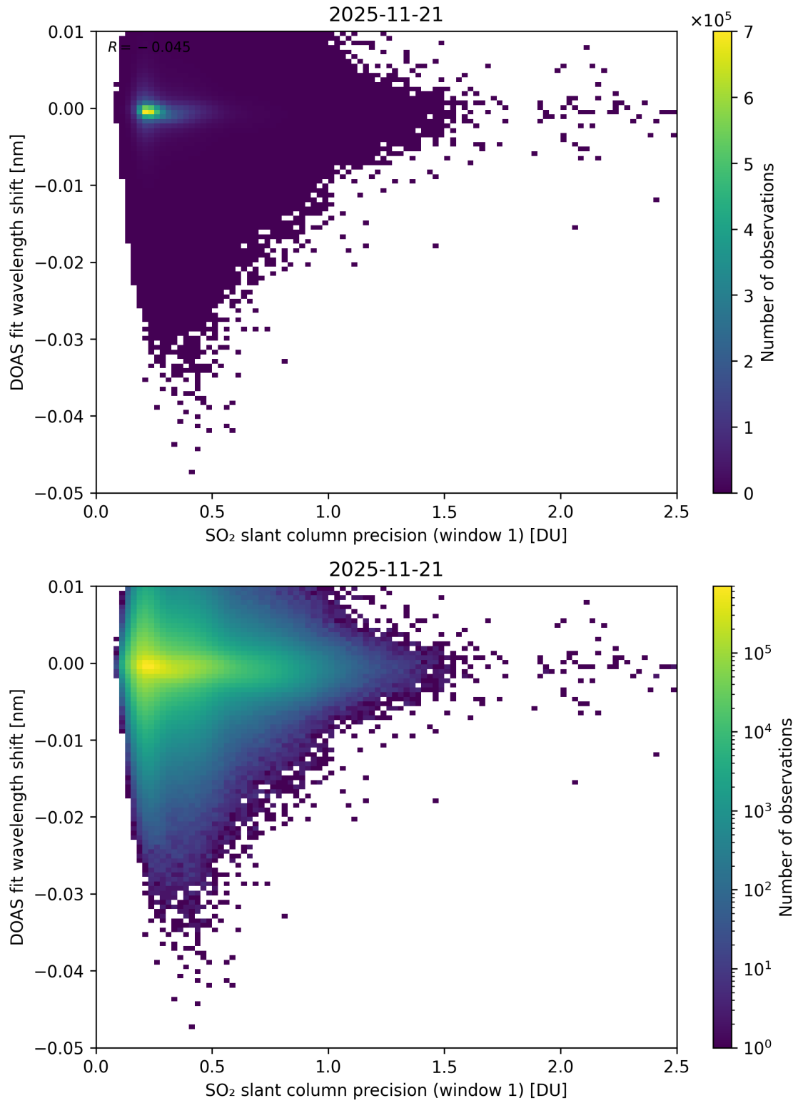
Figure 271: Scatter density plot of “SO 2 slant column precision (window 1)” against “DOAS fit wavelength shift” for 2025-11-20 to 2025-11-22.
