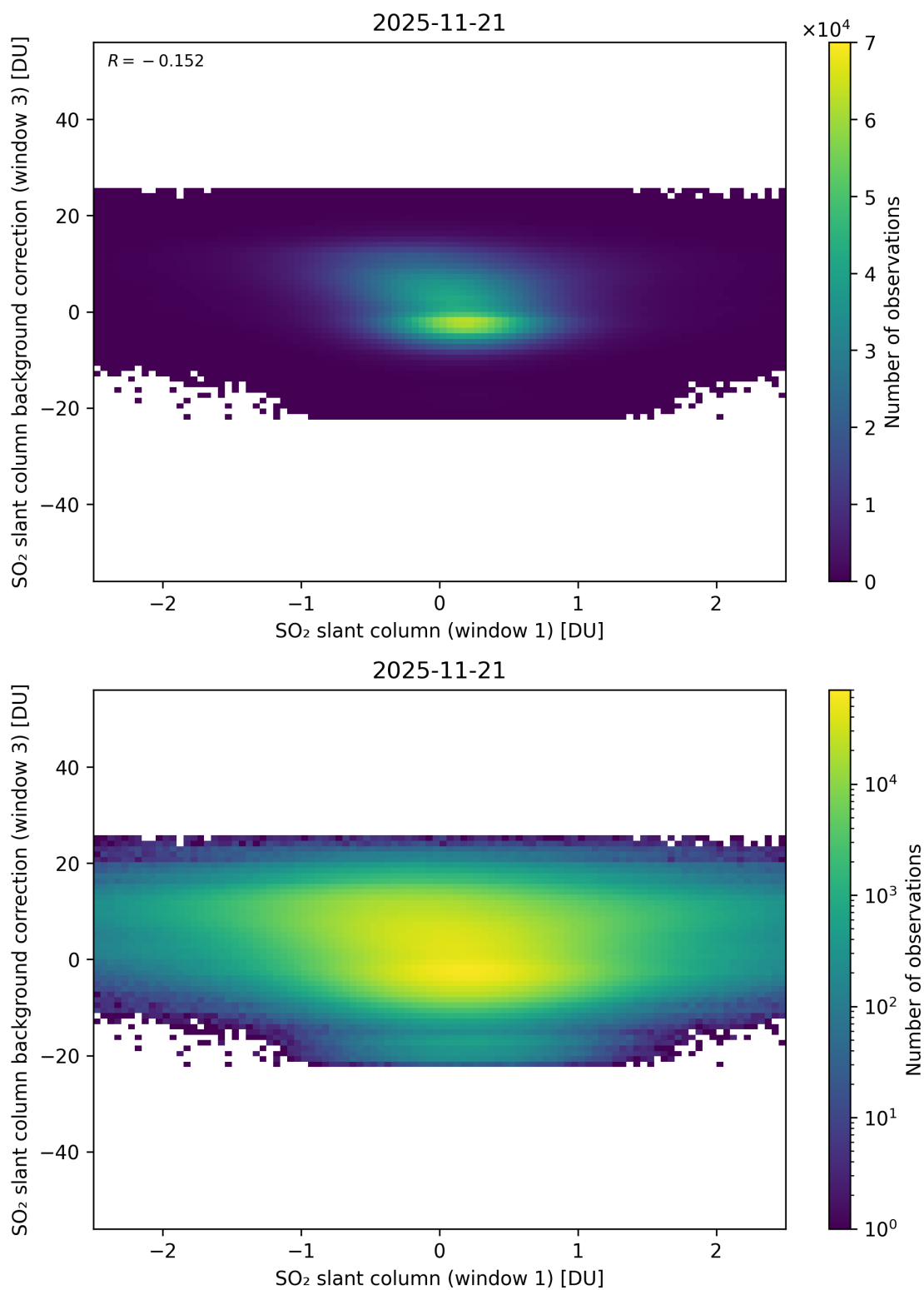
Figure 264: Scatter density plot of “SO 2 slant column (window 1)” against “SO 2 slant column background correction (window 3)” for 2025-11-20 to 2025-11-22.
