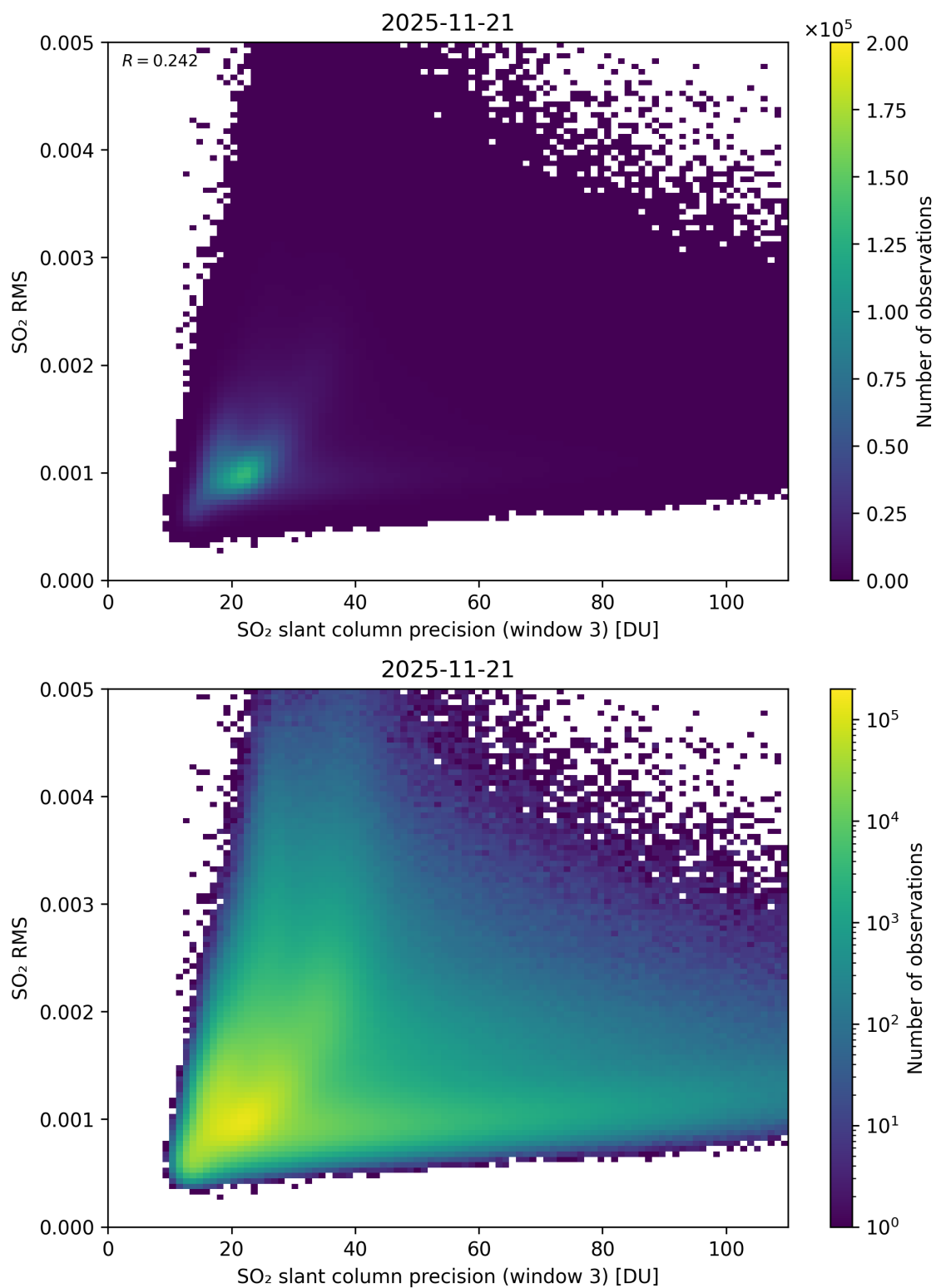
Figure 310: Scatter density plot of “SO 2 slant column precision (window 3)” against “SO 2 RMS” for 2025-11-20 to 2025-11-22.
