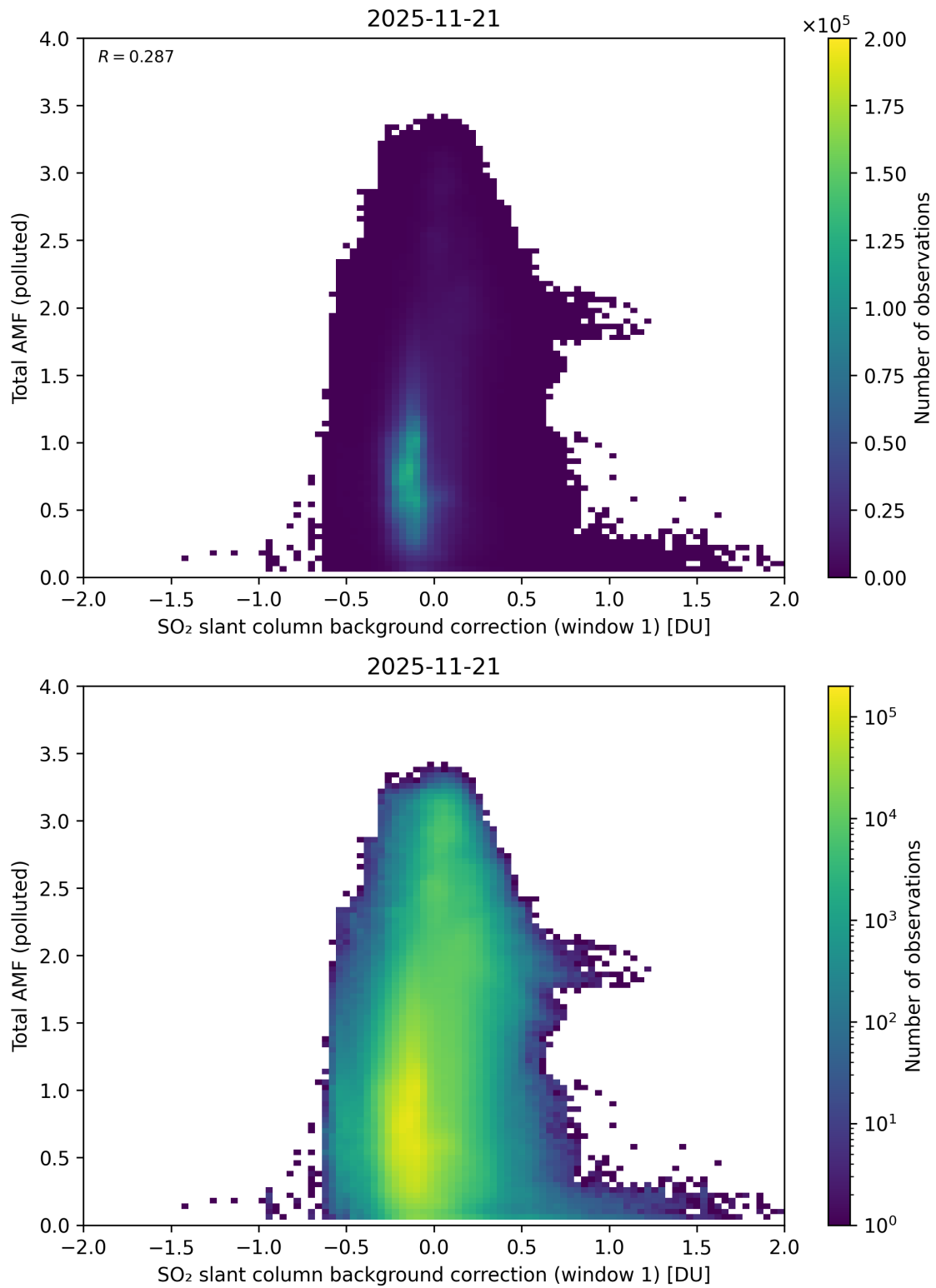
Figure 120: Scatter density plot of “SO 2 slant column background correction (window 1)” against “Total AMF (polluted)” for 2025-11-20 to 2025-11-22.
