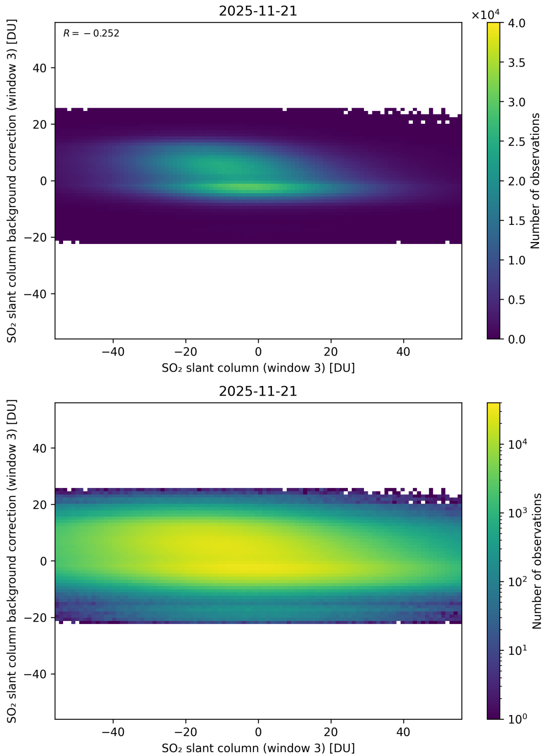
Figure 303: Scatter density plot of “SO 2 slant column (window 3)” against “SO 2 slant column background correction (window 3)” for 2025-11-20 to 2025-11-22.
