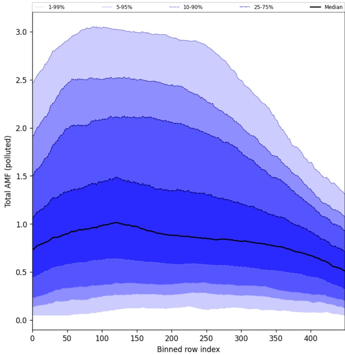
Figure 105: Along track statistics of “Total AMF (polluted)” for 2025-11-20 to 2025-11-22
