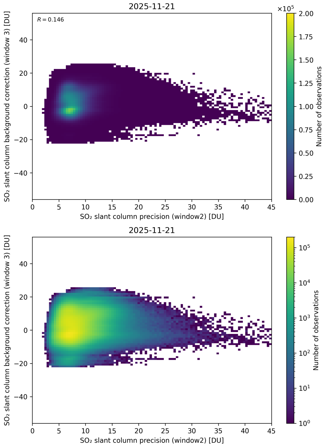
Figure 292: Scatter density plot of “SO 2 slant column precision (window2)” against “SO 2 slant column background correction (window 3)” for 2025-11-20 to 2025-11-22.
