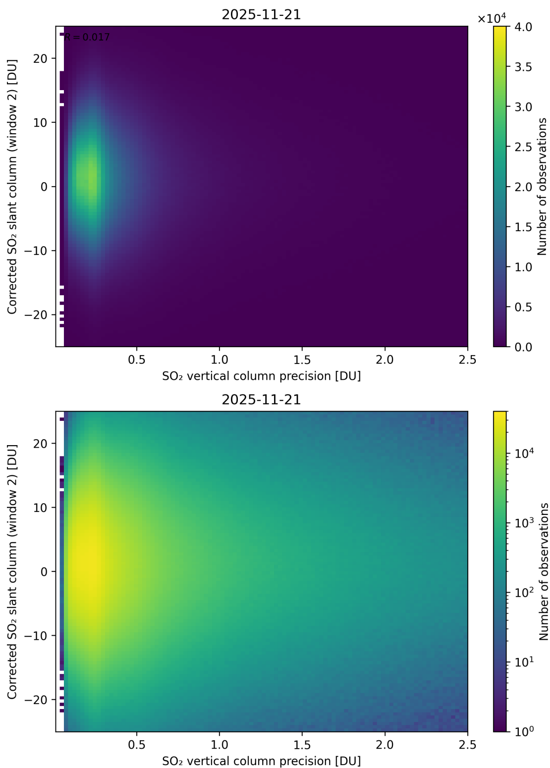
Figure 339: Scatter density plot of “SO 2 vertical column precision” against “Corrected SO 2 slant column (window 2)” for 2025-11-20 to 2025-11-22.
