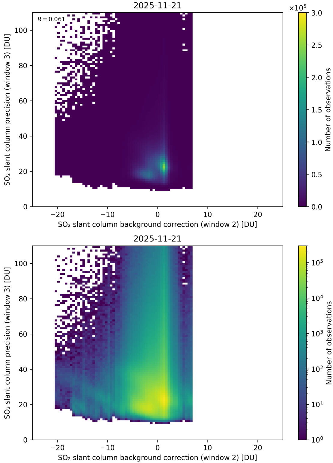
Figure 129: Scatter density plot of “SO 2 slant column background correction (window 2)” against “SO 2 slant column precision (window 3)” for 2025-11-20 to 2025-11-22.
