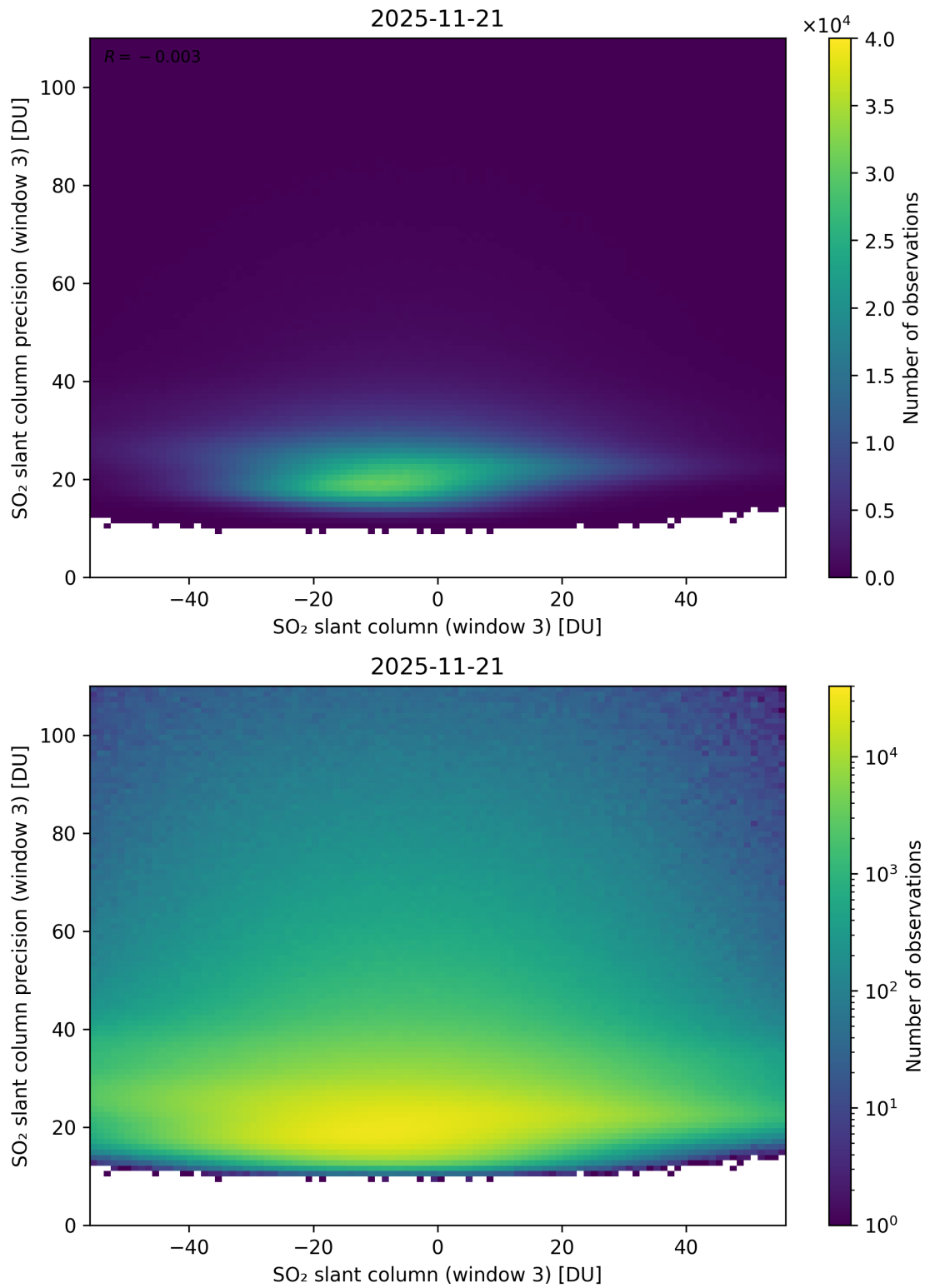
Figure 317: Scatter density plot of “SO 2 slant column (window 3)” against “SO 2 slant column precision (window 3)” for 2025-11-20 to 2025-11-22.
