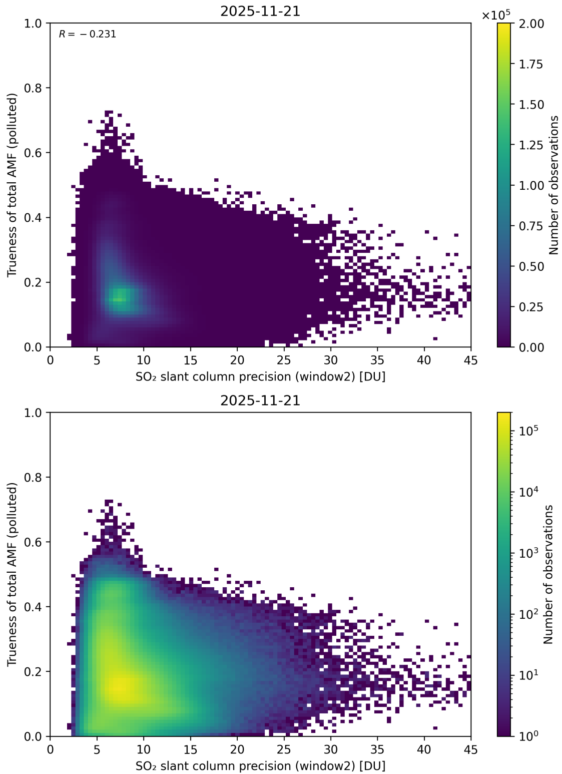
Figure 302: Scatter density plot of “SO 2 slant column precision (window2)” against “Trueness of total AMF (polluted)” for 2025-11-20 to 2025-11-22.
