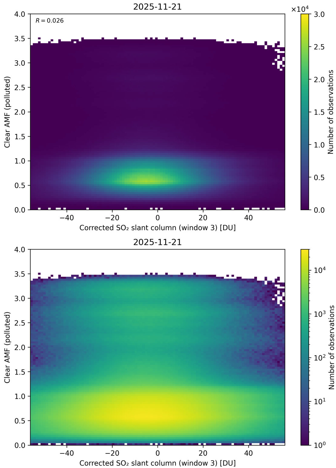
Figure 259: Scatter density plot of “Corrected SO 2 slant column (window 3)” against “Clear AMF (polluted)” for 2025-11-20 to 2025-11-22.
