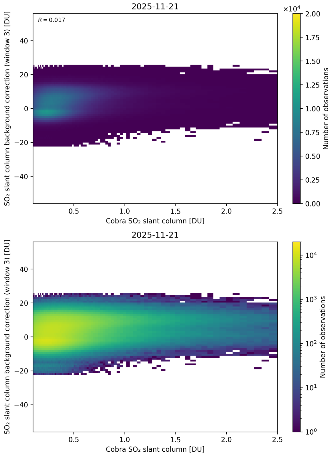
Figure 195: Scatter density plot of “Cobra SO 2 slant column” against “SO 2 slant column background correction (window 3)” for 2025-11-20 to 2025-11-22.
