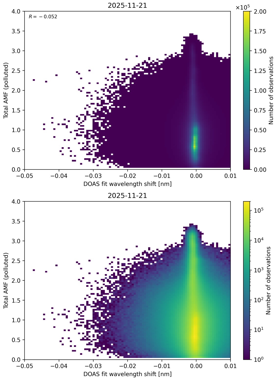
Figure 141: Scatter density plot of “DOAS fit wavelength shift” against “Total AMF (polluted)” for 2025-11-20 to 2025-11-22.
