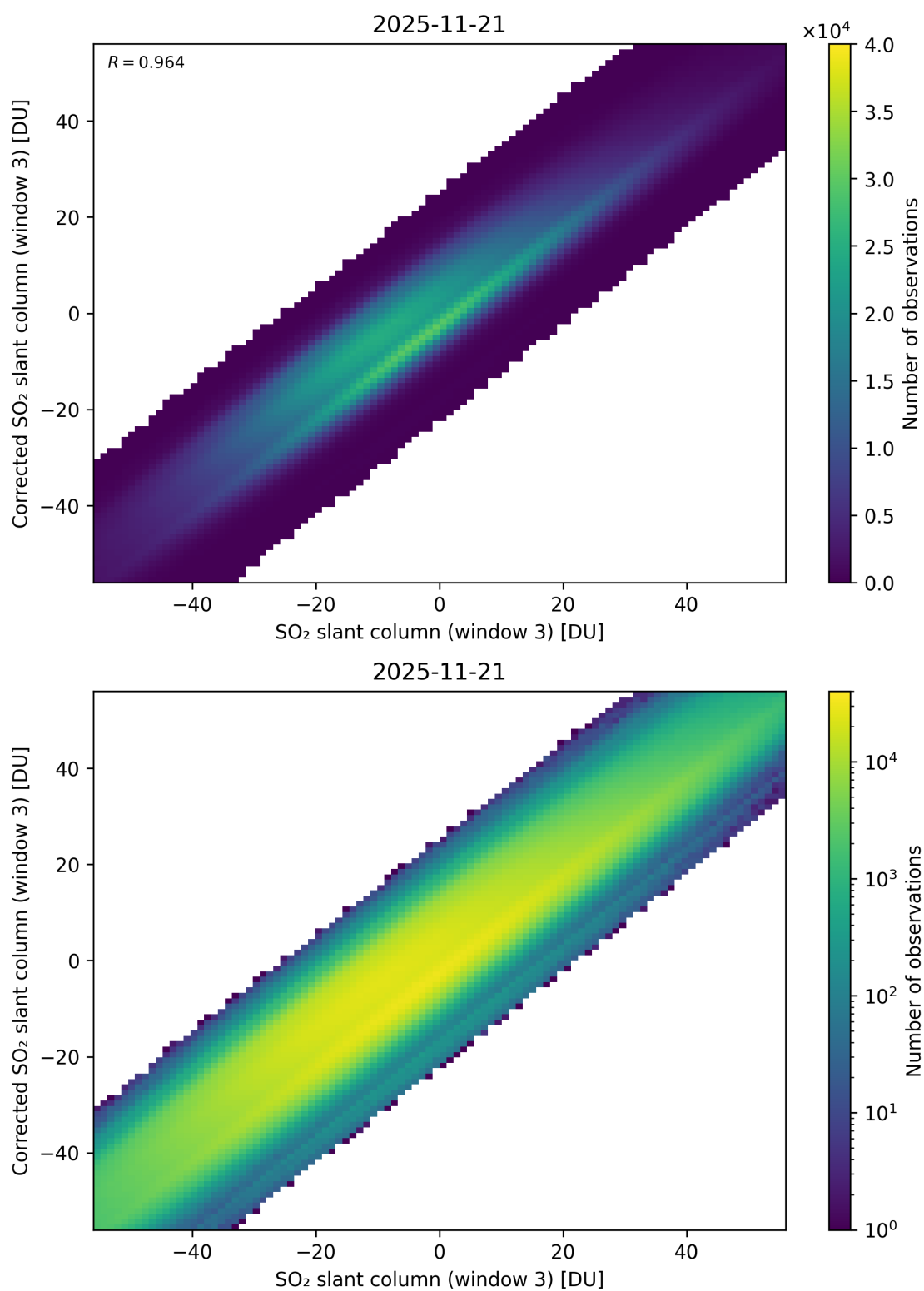
Figure 316: Scatter density plot of “SO 2 slant column (window 3)” against “Corrected SO 2 slant column (window 3)” for 2025-11-20 to 2025-11-22.
