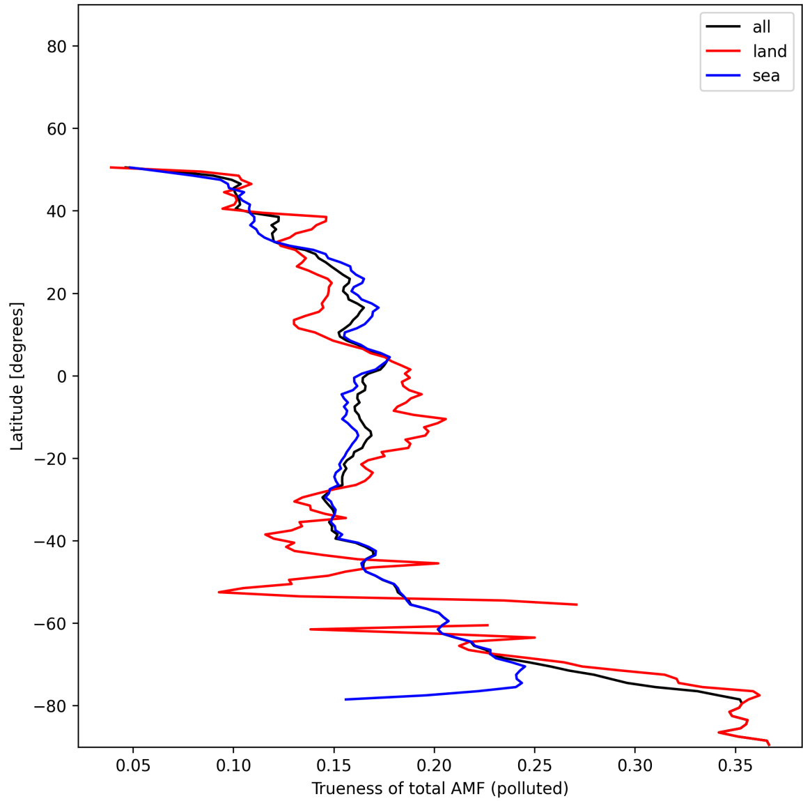
Figure 54: Zonal average of “Trueness of total AMF (polluted)” for 2025-11-20 to 2025-11-22.
