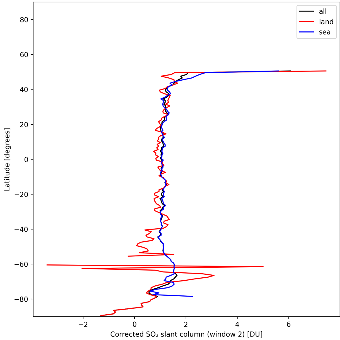
Figure 43: Zonal average of “Corrected SO 2 slant column (window 2)” for 2025-11-20 to 2025-11-22.
