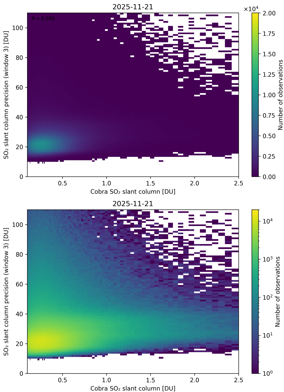
Figure 223: Scatter density plot of “Cobra SO 2 slant column” against “SO 2 slant column precision (window 3)” for 2025-11-20 to 2025-11-22.
