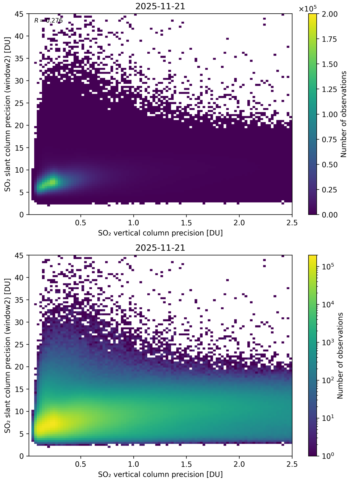
Figure 343: Scatter density plot of “SO 2 vertical column precision” against “SO 2 slant column precision (window2)” for 2025-11-20 to 2025-11-22.
