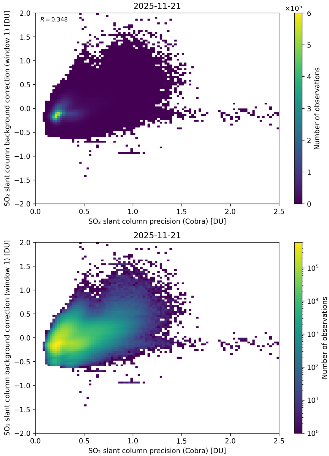
Figure 199: Scatter density plot of “SO 2 slant column precision (Cobra)” against “SO 2 slant column background correction (window 1)” for 2025-11-20 to 2025-11-22.
