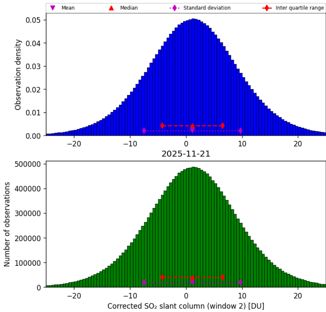
Figure 69: Histogram of “Corrected SO 2 slant column (window 2)” for 2025-11-20 to 2025-11-22
