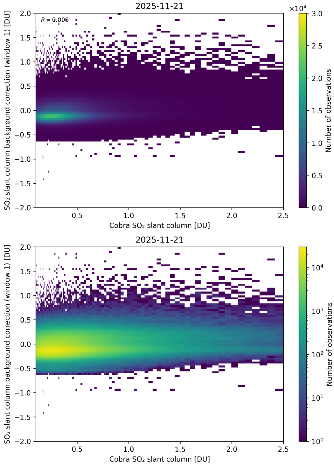
Figure 193: Scatter density plot of “Cobra SO 2 slant column” against “SO 2 slant column background correction (window 1)” for 2025-11-20 to 2025-11-22.
