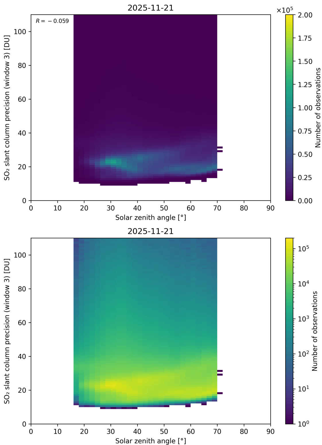
Figure 188: Scatter density plot of “Solar zenith angle” against “SO 2 slant column precision (window 3)” for 2025-11-20 to 2025-11-22.
