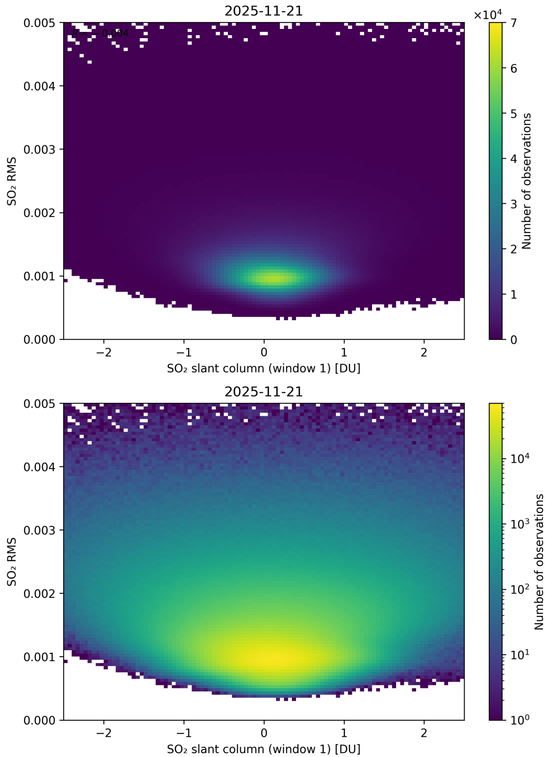
Figure 267: Scatter density plot of “SO 2 slant column (window 1)” against “SO 2 RMS” for 2025-11-20 to 2025-11-22.
