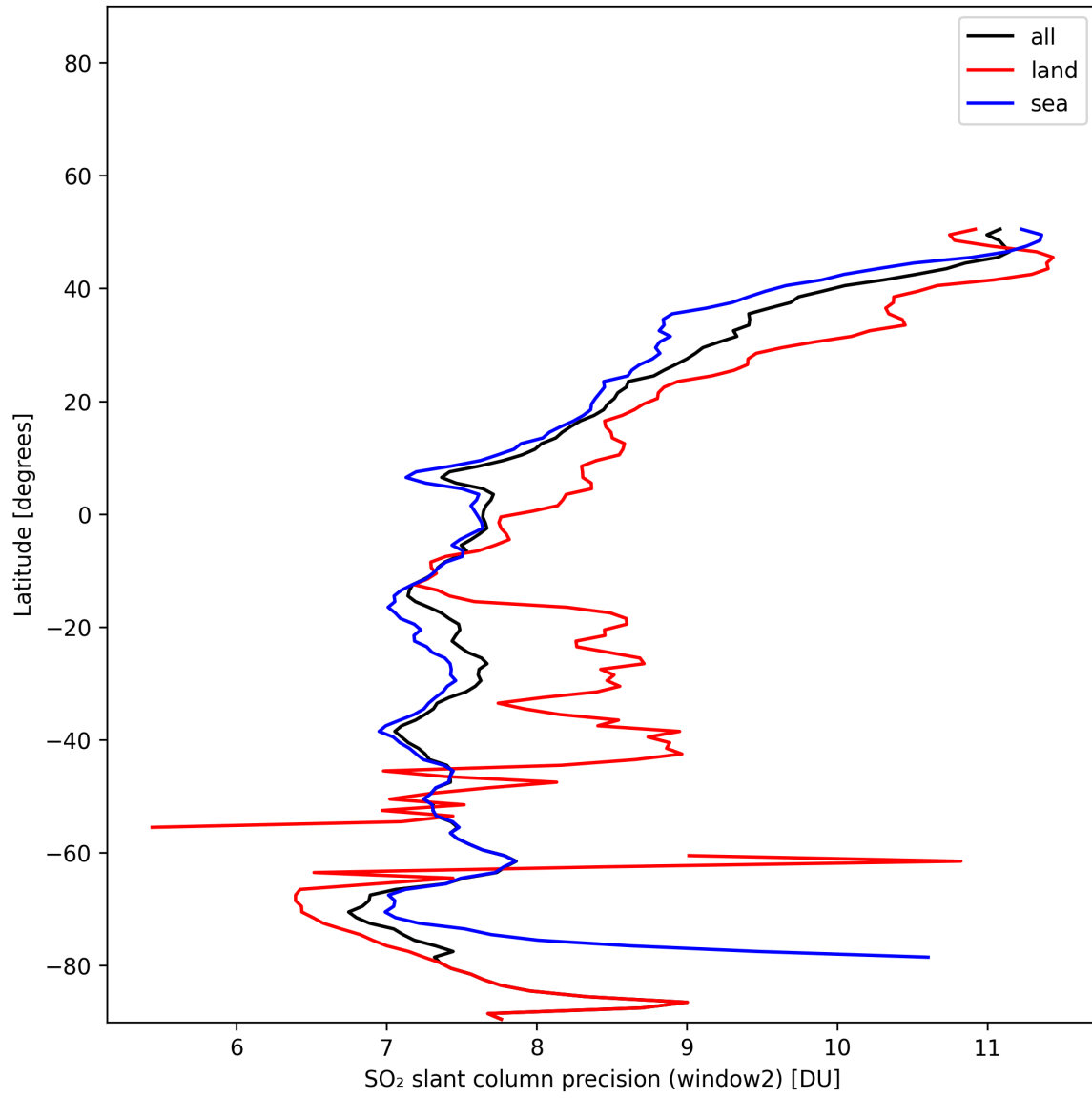
Figure 42: Zonal average of “SO 2 slant column precision (window2)” for 2025-11-20 to 2025-11-22.
