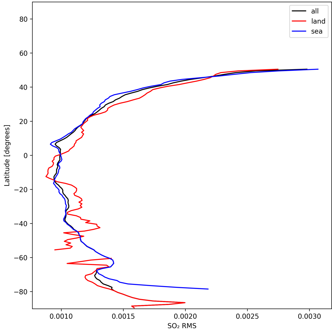
Figure 52: Zonal average of “SO 2 RMS” for 2025-11-20 to 2025-11-22.
