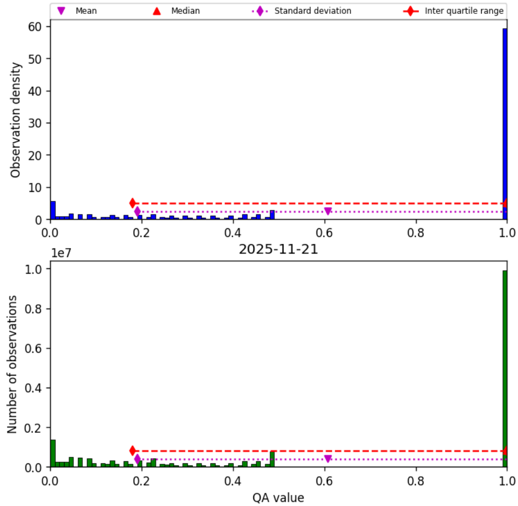
Figure 57: Histogram of “QA value” for 2025-11-20 to 2025-11-22
