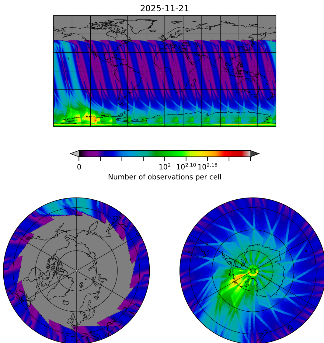
Figure 30: Map of the number of observations for 2025-11-20 to 2025-11-22
