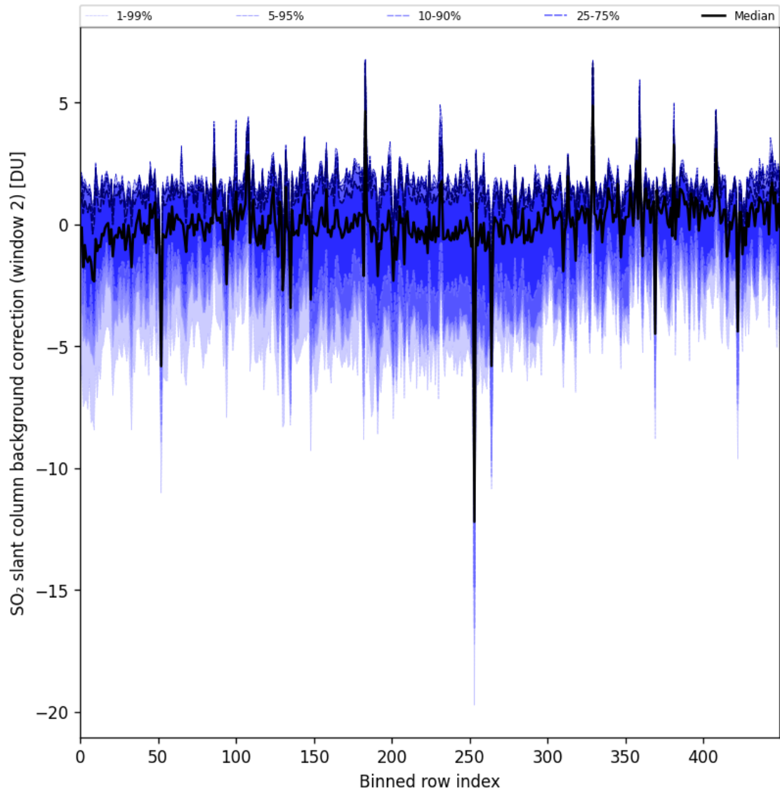
Figure 96: Along track statistics of “SO 2 slant column background correction (window 2)” for 2025-11-20 to 2025-11-22
