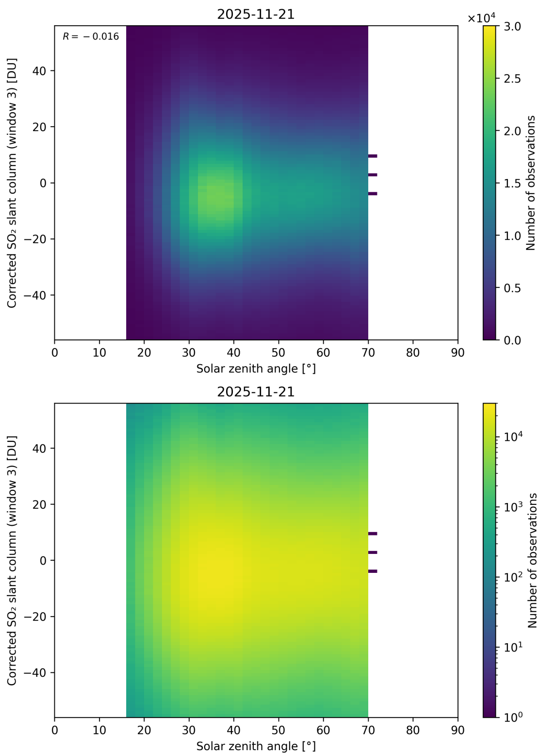
Figure 183: Scatter density plot of “Solar zenith angle” against “Corrected SO 2 slant column (window 3)” for 2025-11-20 to 2025-11-22.
