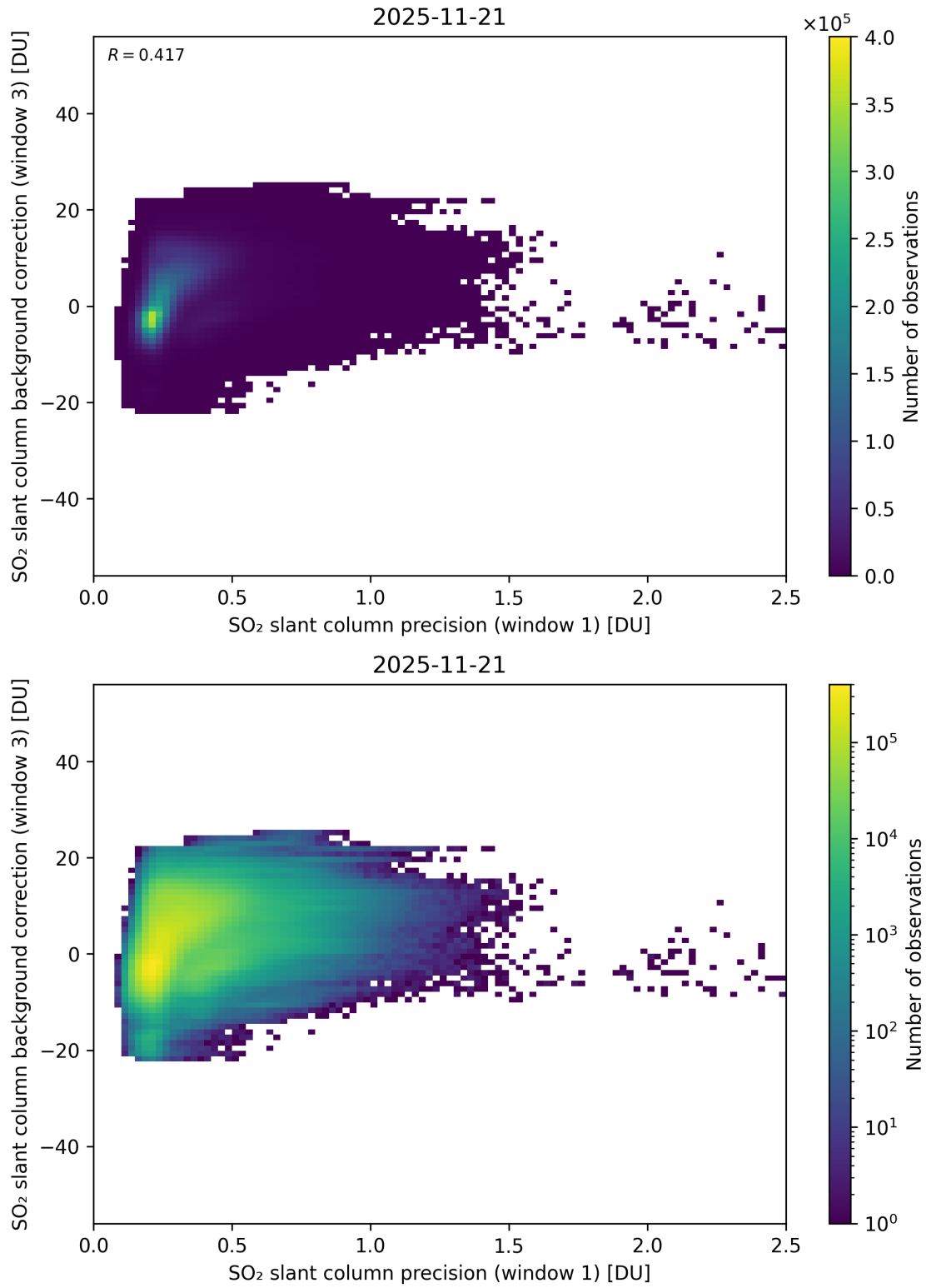
Figure 270: Scatter density plot of “SO 2 slant column precision (window 1)” against “SO 2 slant column background correction (window 3)” for 2025-11-20 to 2025-11-22.
