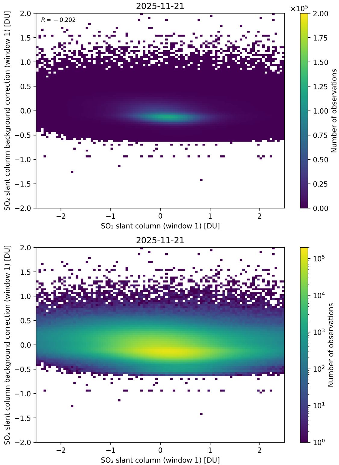
Figure 262: Scatter density plot of “SO 2 slant column (window 1)” against “SO 2 slant column background correction (window 1)” for 2025-11-20 to 2025-11-22.
