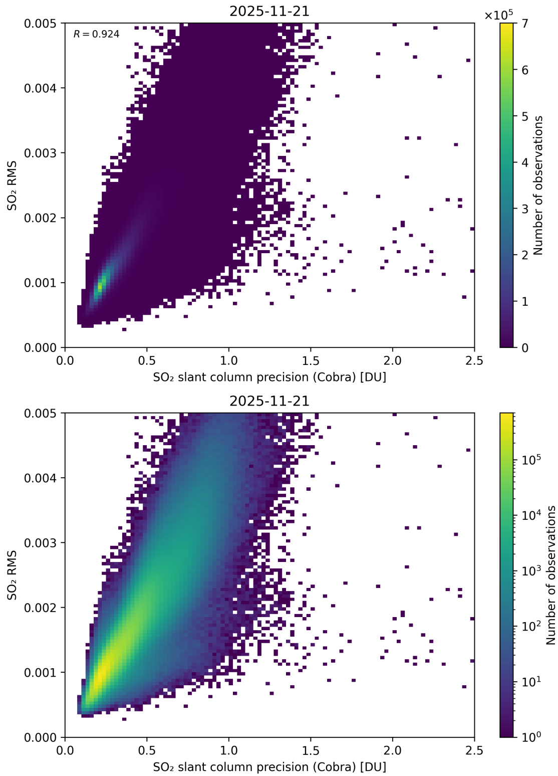
Figure 204: Scatter density plot of “SO 2 slant column precision (Cobra)” against “SO 2 RMS” for 2025-11-20 to 2025-11-22.
