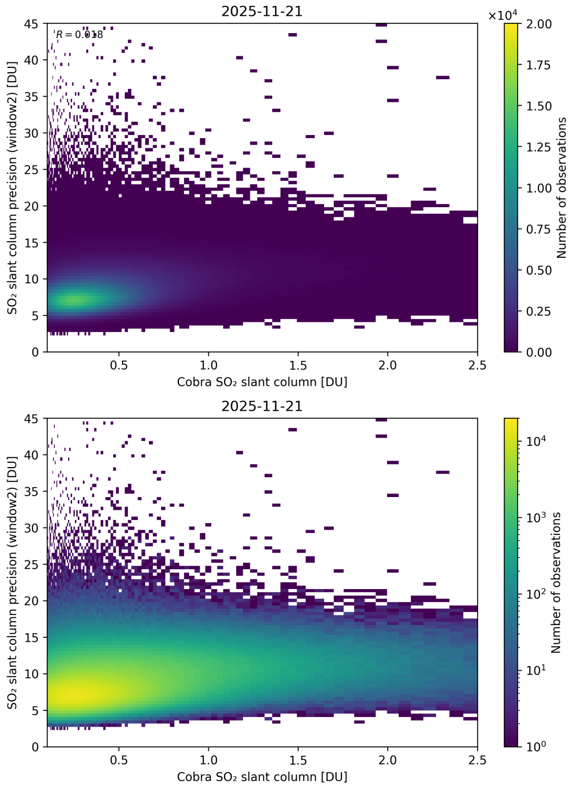
Figure 221: Scatter density plot of “Cobra SO 2 slant column” against “SO 2 slant column precision (window2)” for 2025-11-20 to 2025-11-22.
