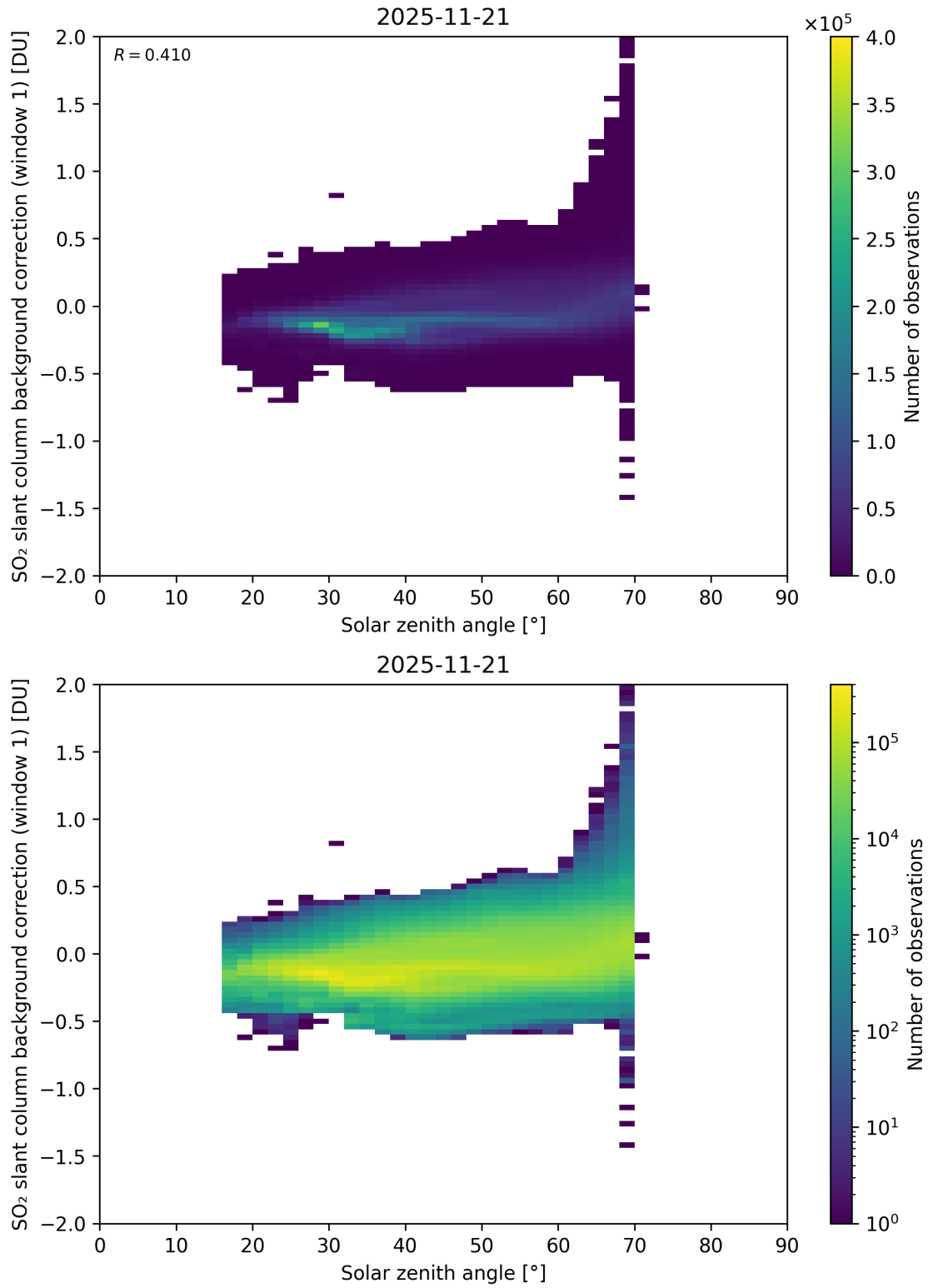
Figure 171: Scatter density plot of “Solar zenith angle” against “SO 2 slant column background correction (window 1)” for 2025-11-20 to 2025-11-22.
