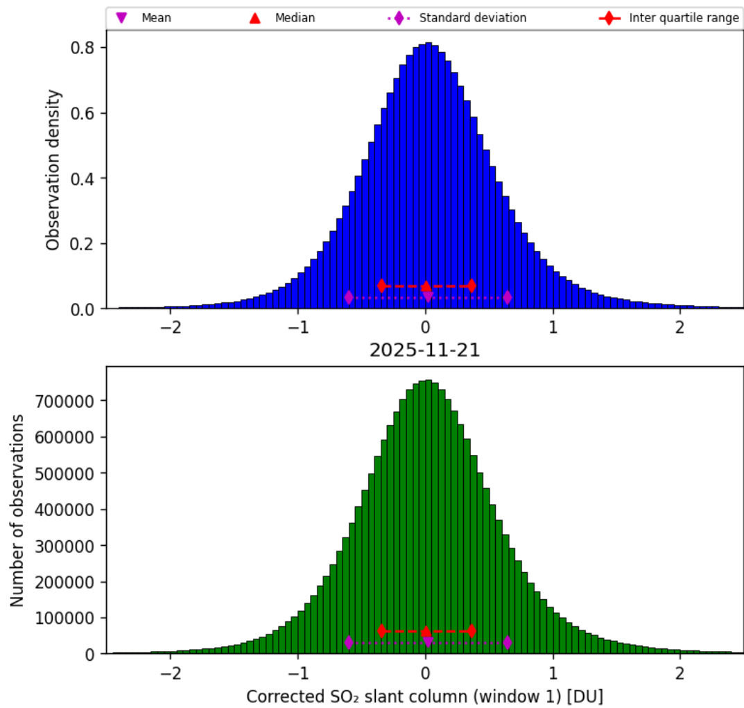
Figure 65: Histogram of “Corrected SO 2 slant column (window 1)” for 2025-11-20 to 2025-11-22
