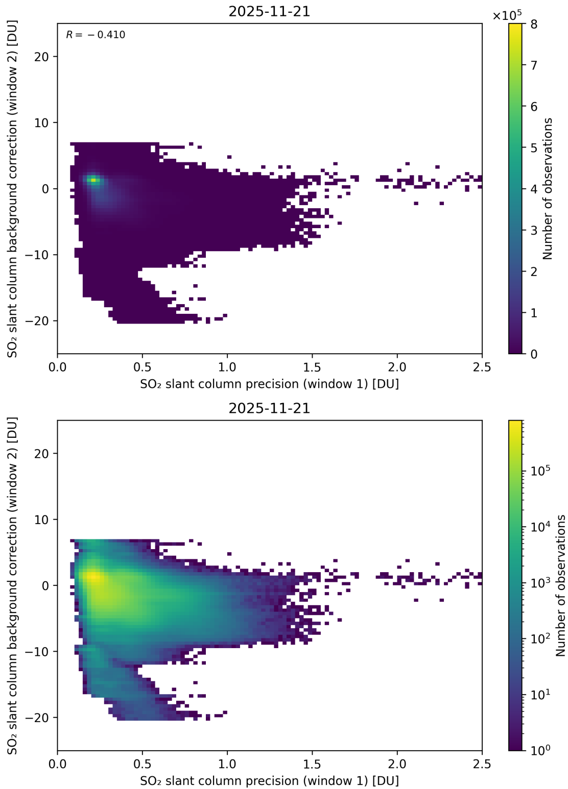
Figure 269: Scatter density plot of “SO 2 slant column precision (window 1)” against “SO 2 slant column background correction (window 2)” for 2025-11-20 to 2025-11-22.
