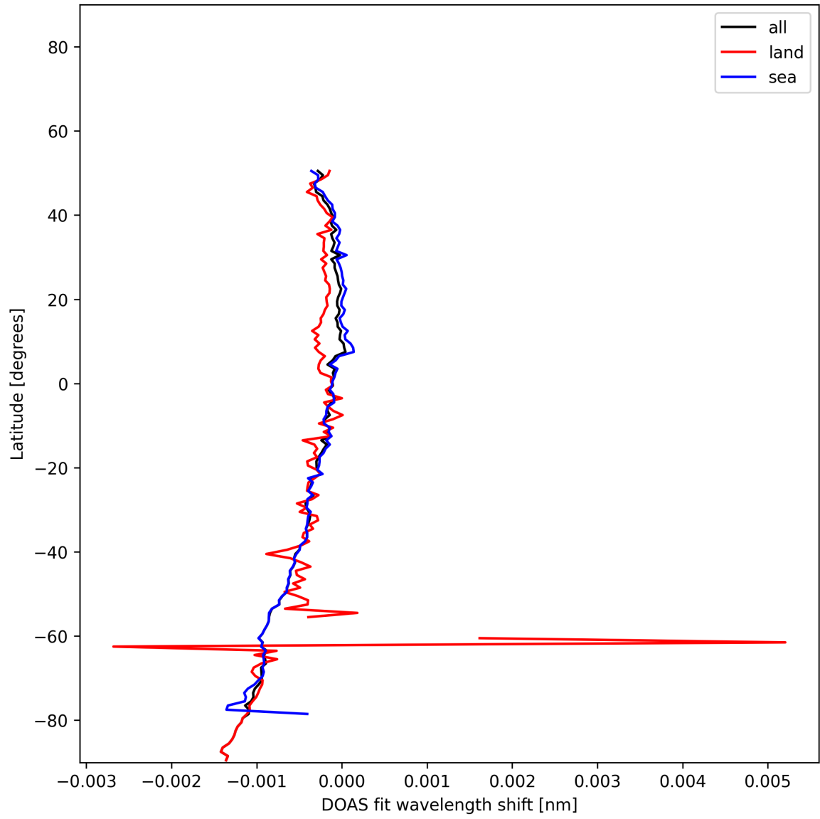
Figure 50: Zonal average of “DOAS fit wavelength shift” for 2025-11-20 to 2025-11-22.
