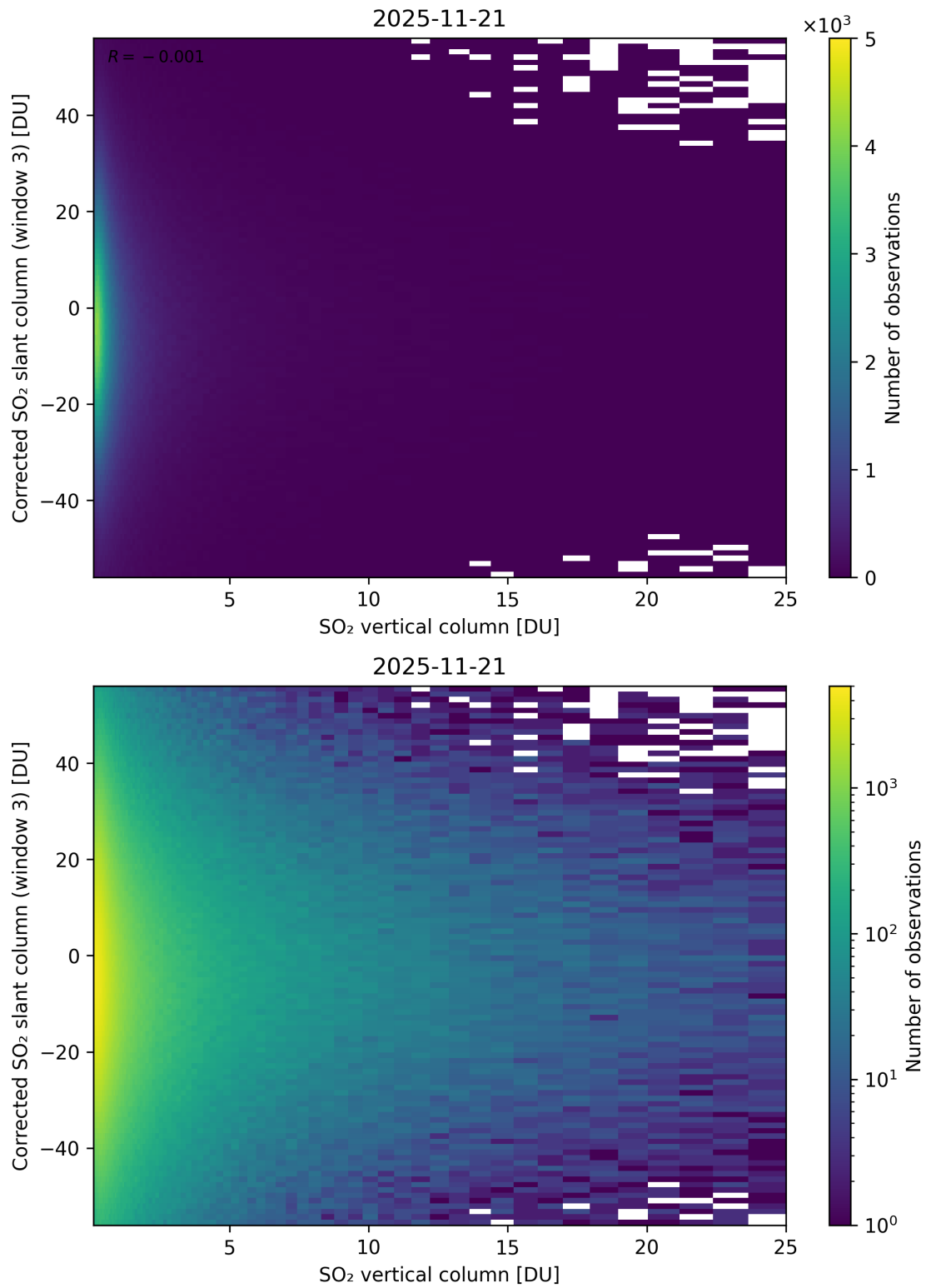
Figure 353: Scatter density plot of “SO 2 vertical column” against “Corrected SO 2 slant column (window 3)” for 2025-11-20 to 2025-11-22.
