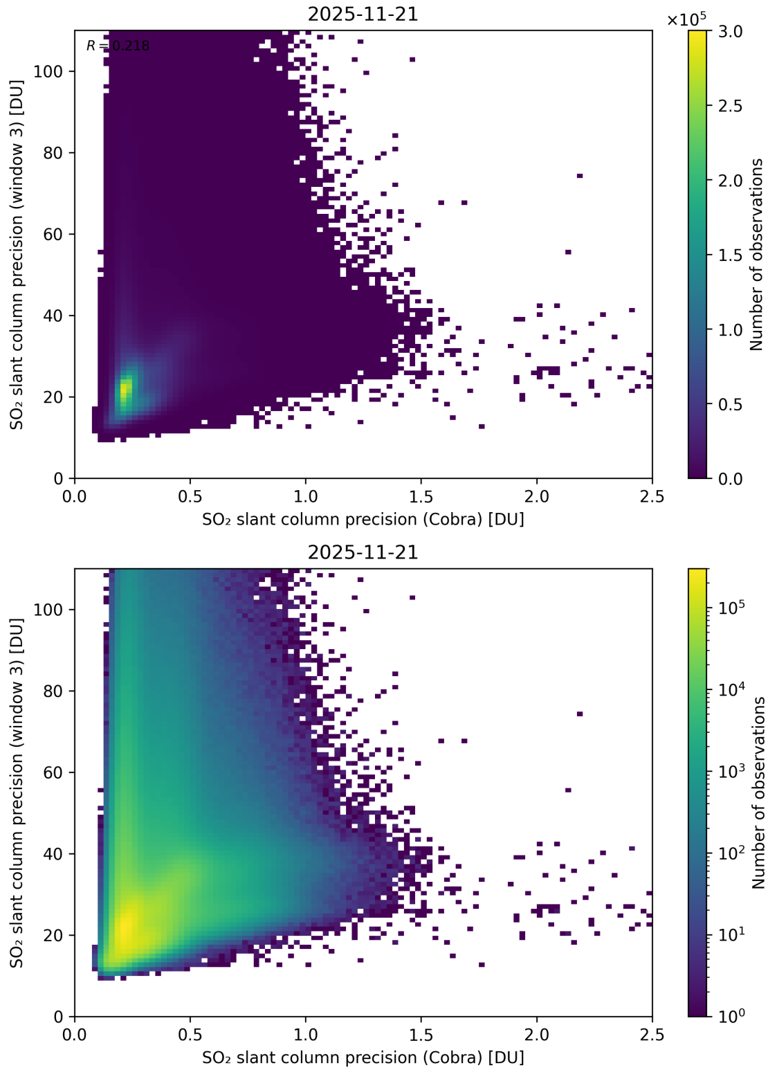
Figure 212: Scatter density plot of “SO 2 slant column precision (Cobra)” against “SO 2 slant column precision (window 3)” for 2025-11-20 to 2025-11-22.
