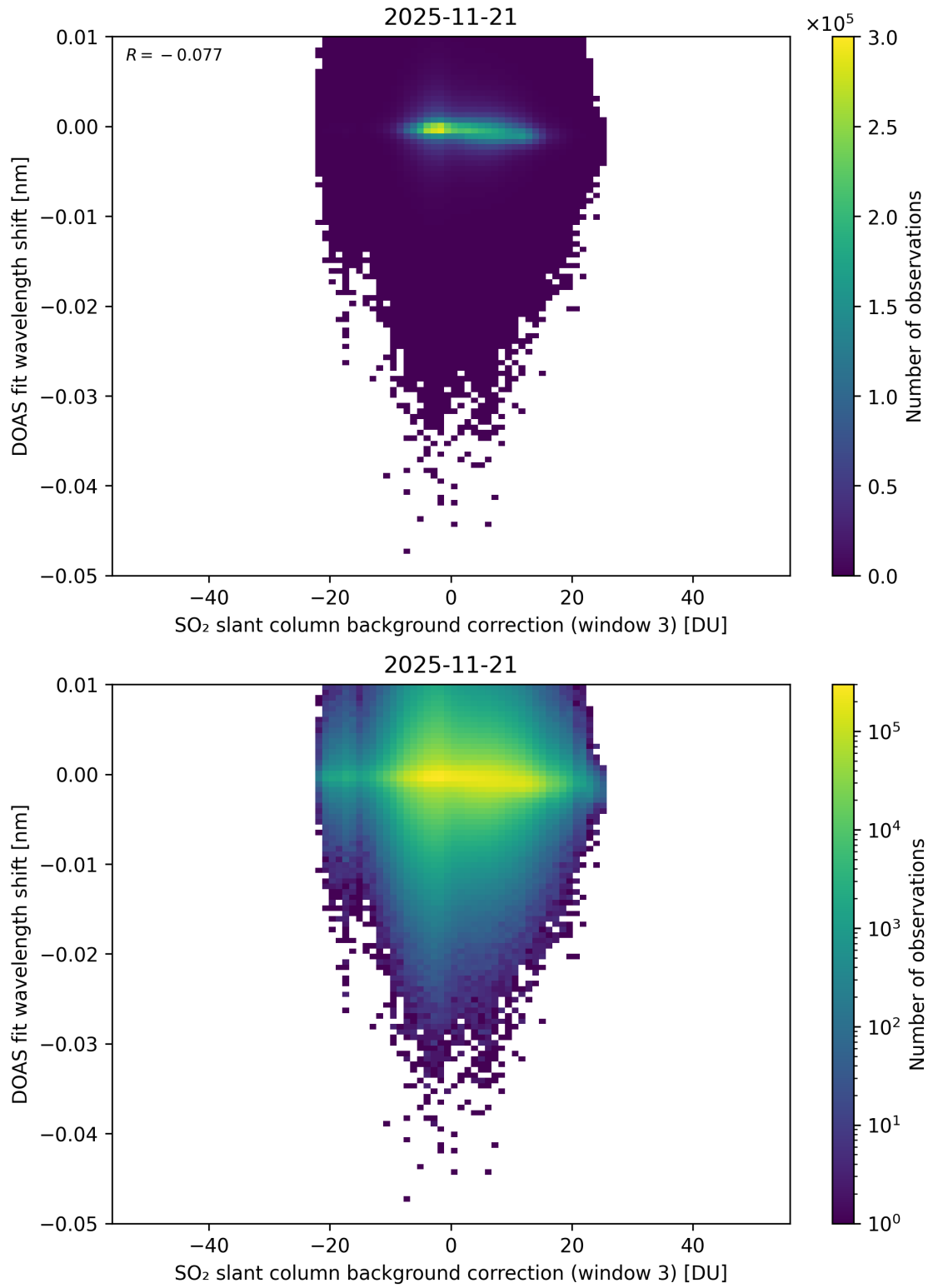
Figure 132: Scatter density plot of “SO 2 slant column background correction (window 3)” against “DOAS fit wavelength shift” for 2025-11-20 to 2025-11-22.
