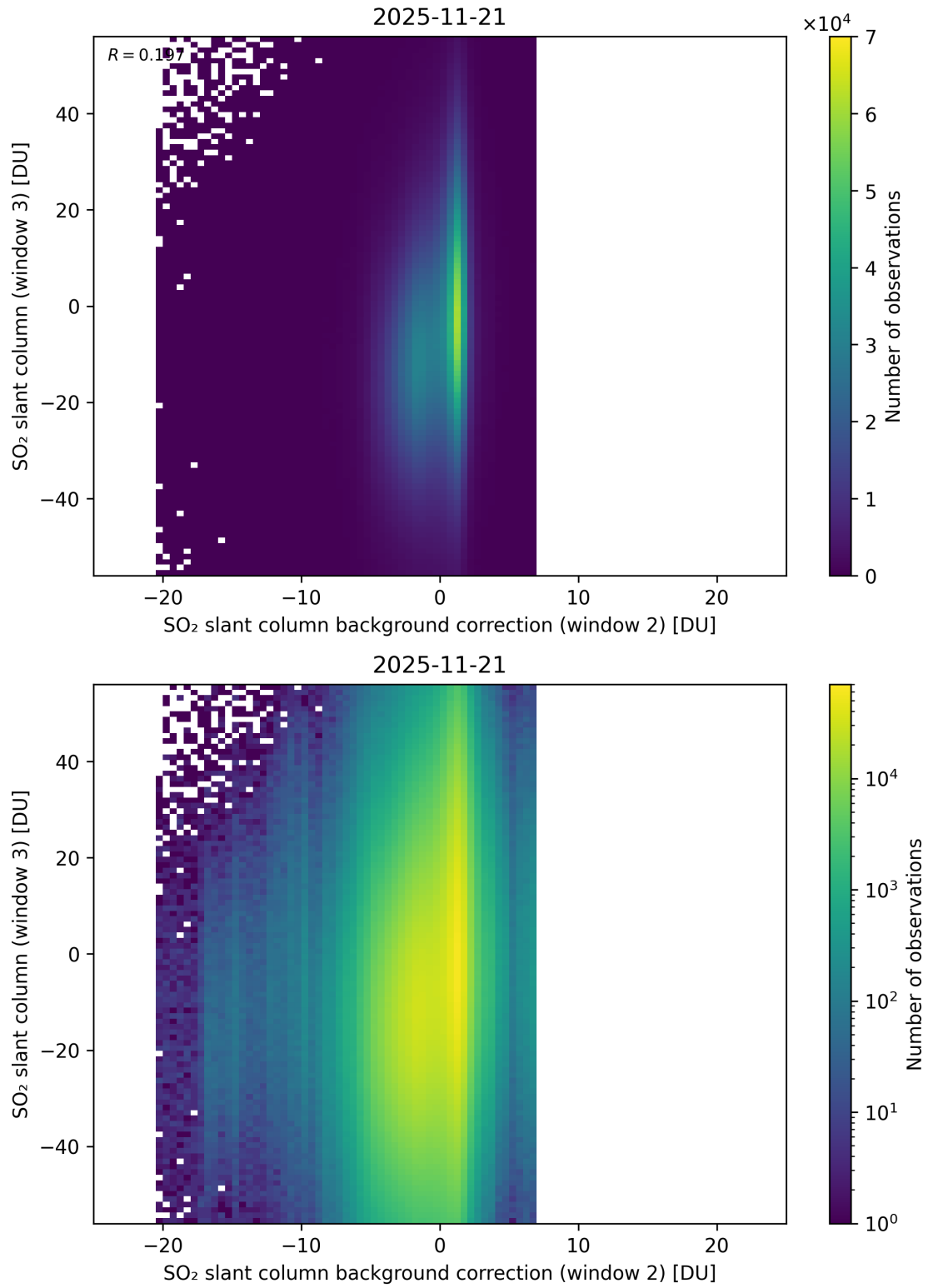
Figure 128: Scatter density plot of “SO 2 slant column background correction (window 2)” against “SO 2 slant column (window 3)” for 2025-11-20 to 2025-11-22.
