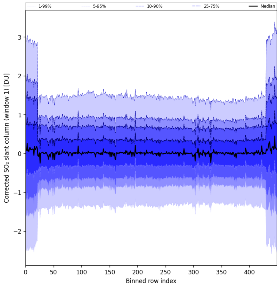
Figure 91: Along track statistics of “Corrected SO 2 slant column (window 1)” for 2025-11-20 to 2025-11-22
