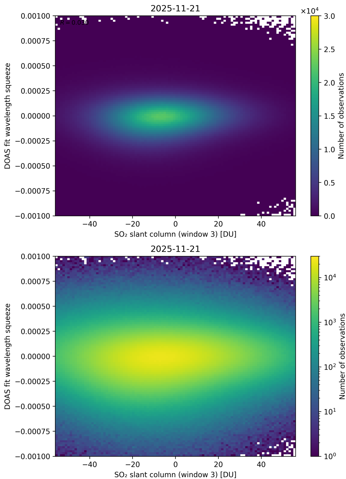
Figure 305: Scatter density plot of “SO 2 slant column (window 3)” against “DOAS fit wavelength squeeze” for 2025-11-20 to 2025-11-22.
