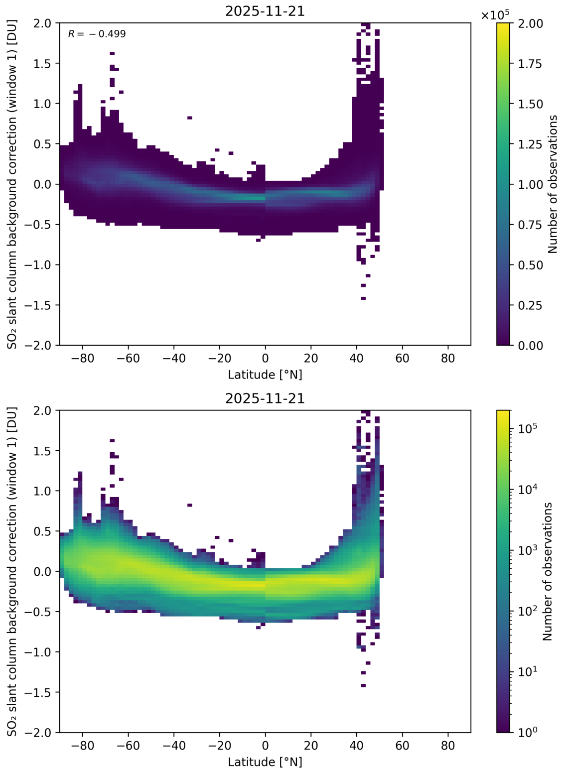
Figure 150: Scatter density plot of “Latitude” against “SO 2 slant column background correction (window 1)” for 2025-11-20 to 2025-11-22.
