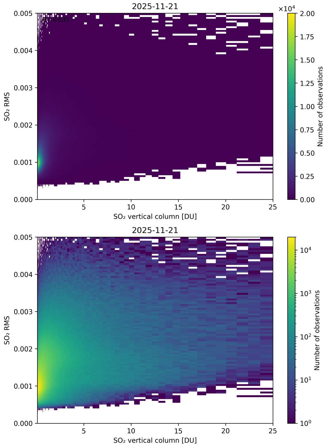
Figure 328: Scatter density plot of “SO 2 vertical column” against “SO 2 RMS” for 2025-11-20 to 2025-11-22.
