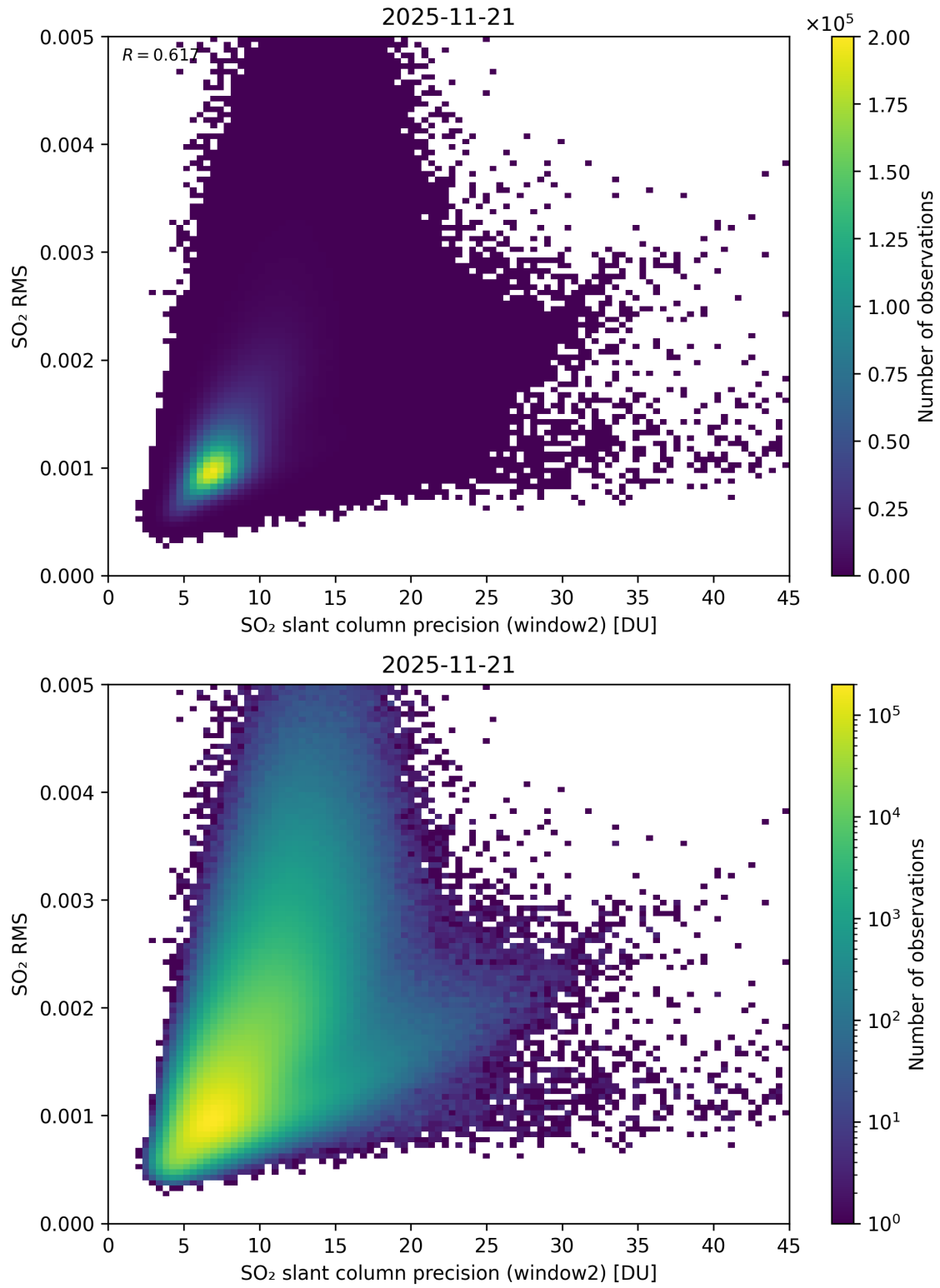
Figure 295: Scatter density plot of “SO 2 slant column precision (window2)” against “SO 2 RMS” for 2025-11-20 to 2025-11-22.
