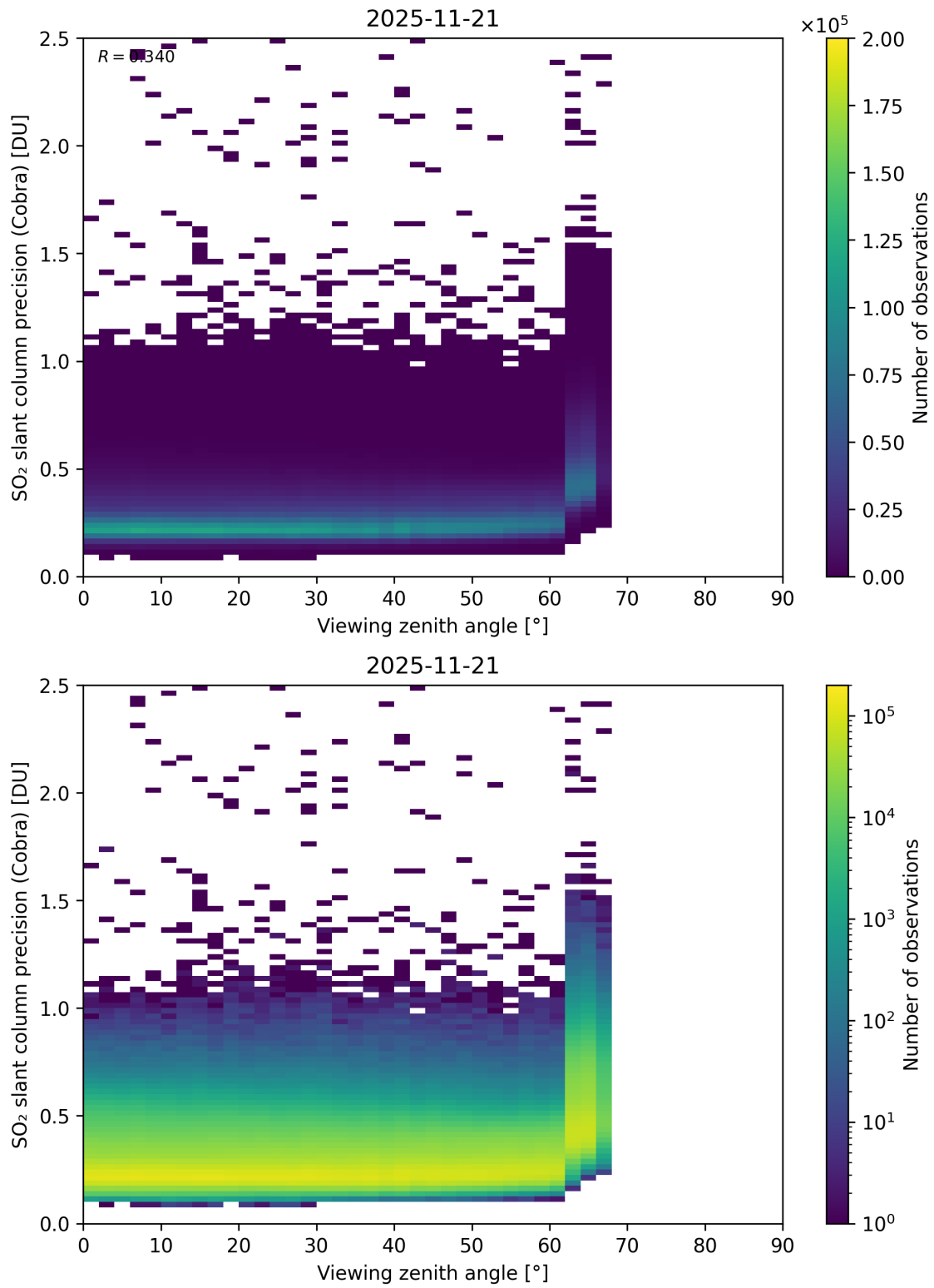
Figure 372: Scatter density plot of “Viewing zenith angle” against “SO 2 slant column precision (Cobra)” for 2025-11-20 to 2025-11-22.
