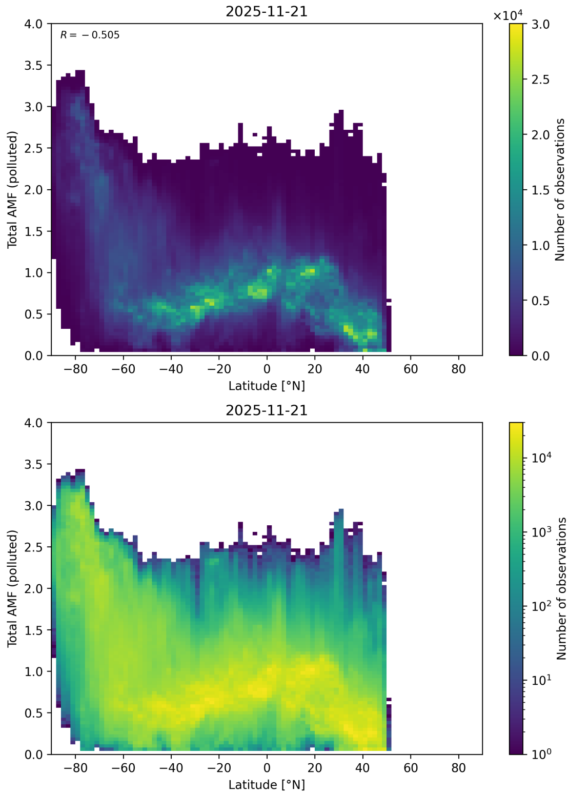
Figure 167: Scatter density plot of “Latitude” against “Total AMF (polluted)” for 2025-11-20 to 2025-11-22.
