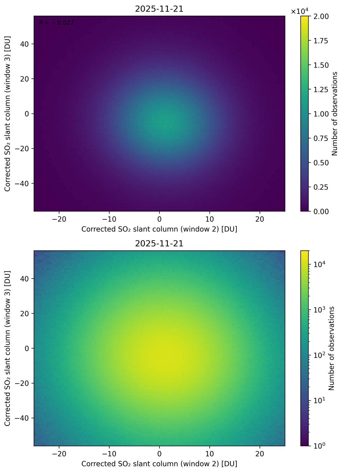
Figure 250: Scatter density plot of “Corrected SO 2 slant column (window 2)” against “Corrected SO 2 slant column (window 3)” for 2025-11-20 to 2025-11-22.
