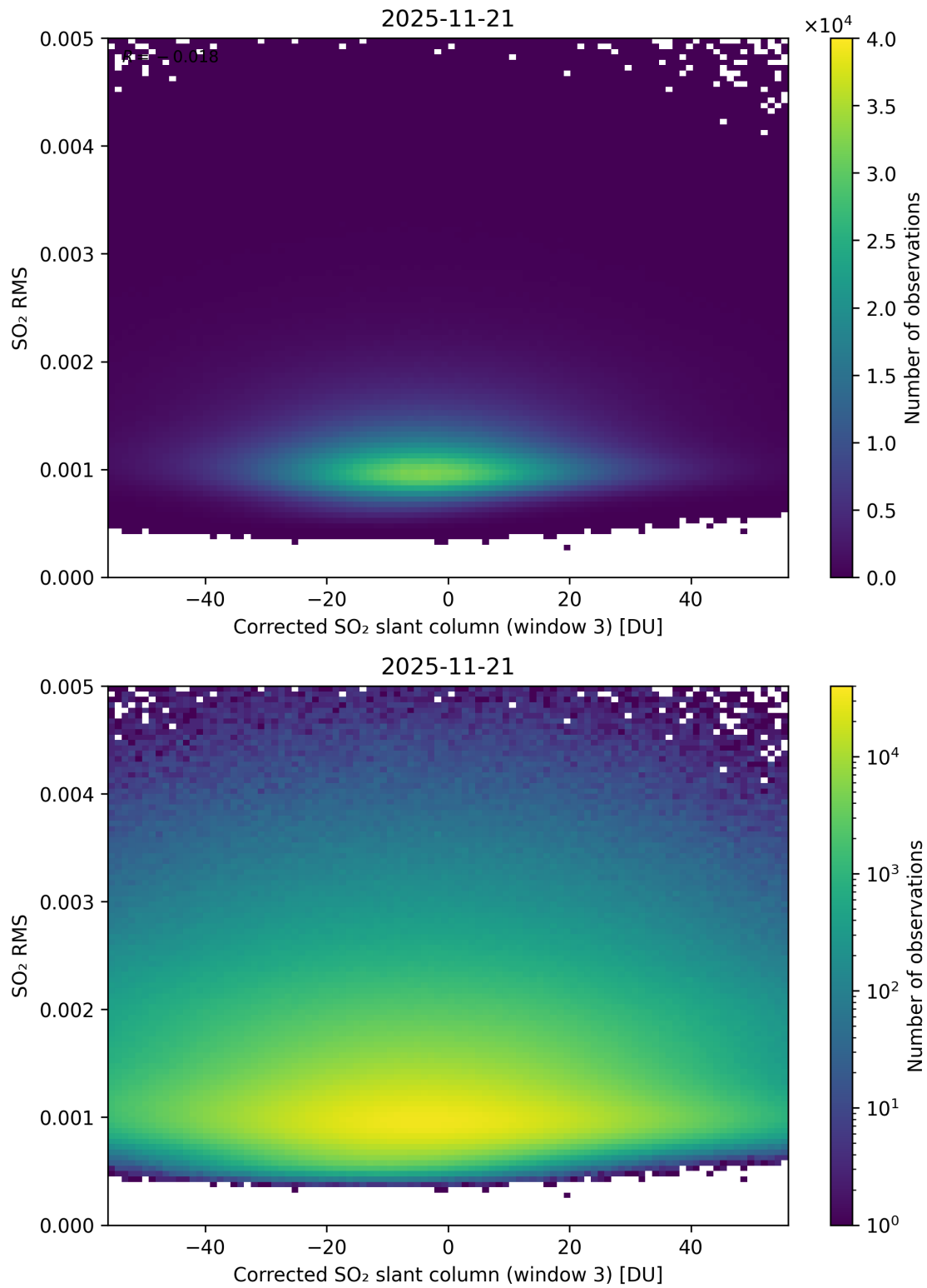
Figure 258: Scatter density plot of “Corrected SO 2 slant column (window 3)” against “SO 2 RMS” for 2025-11-20 to 2025-11-22.
