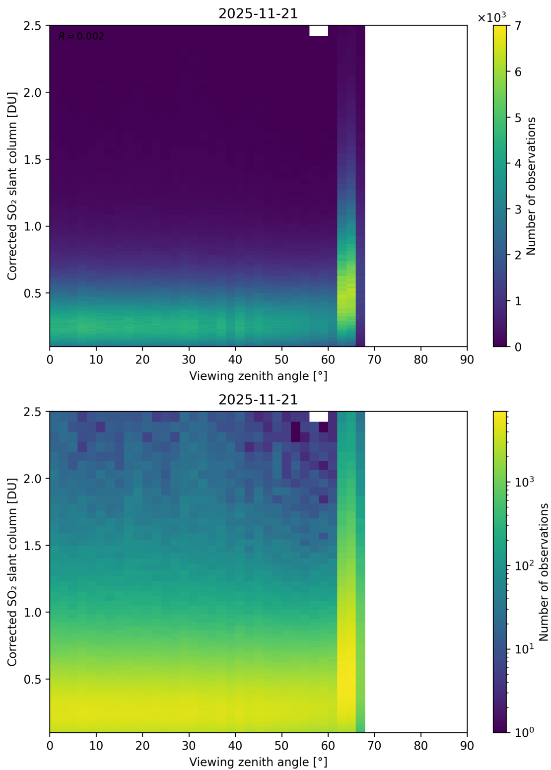
Figure 373: Scatter density plot of “Viewing zenith angle” against “Corrected SO 2 slant column” for 2025-11-20 to 2025-11-22.
