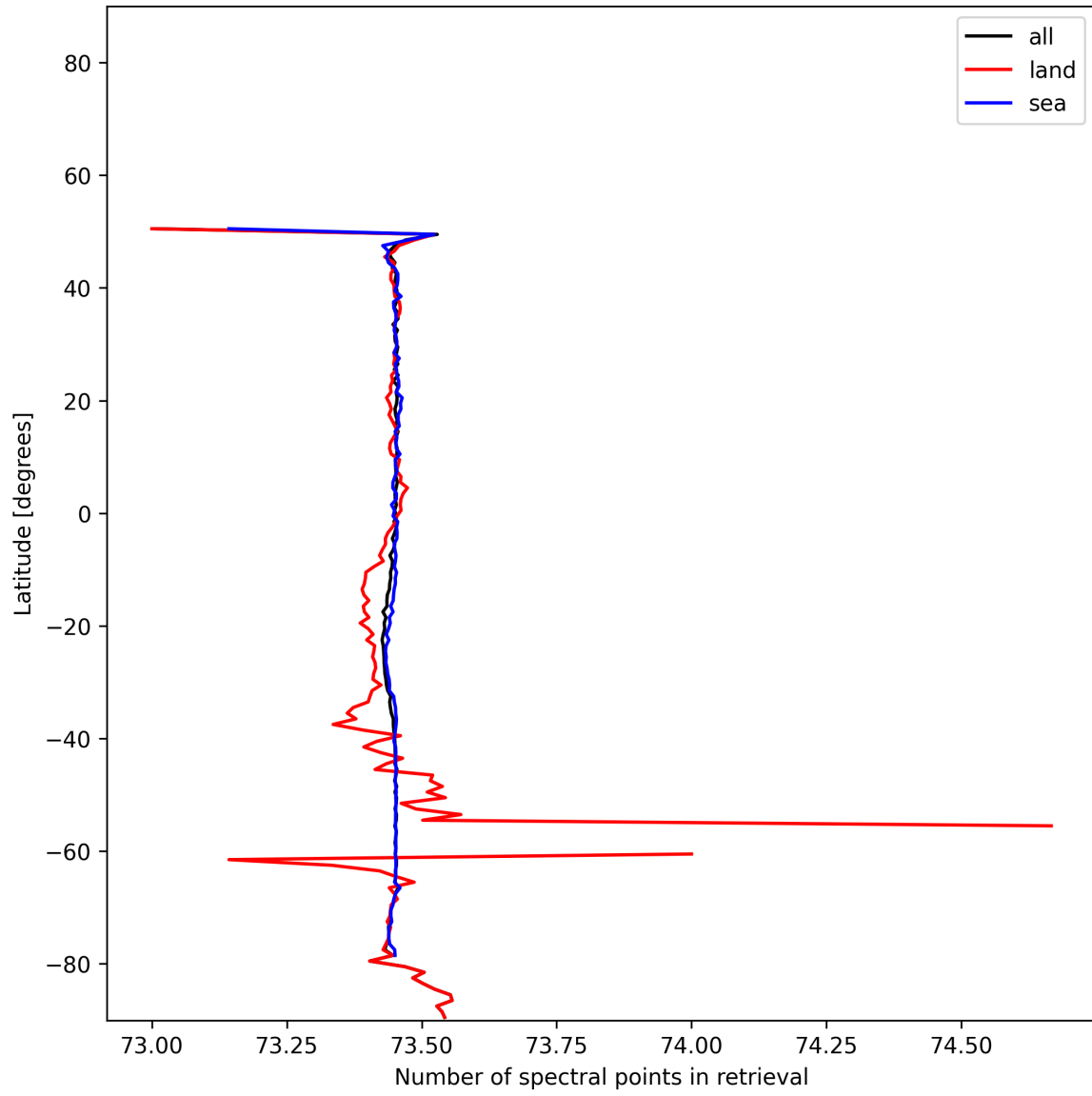
Figure 56: Zonal average of “Number of spectral points in retrieval” for 2025-11-20 to 2025-11-22.
