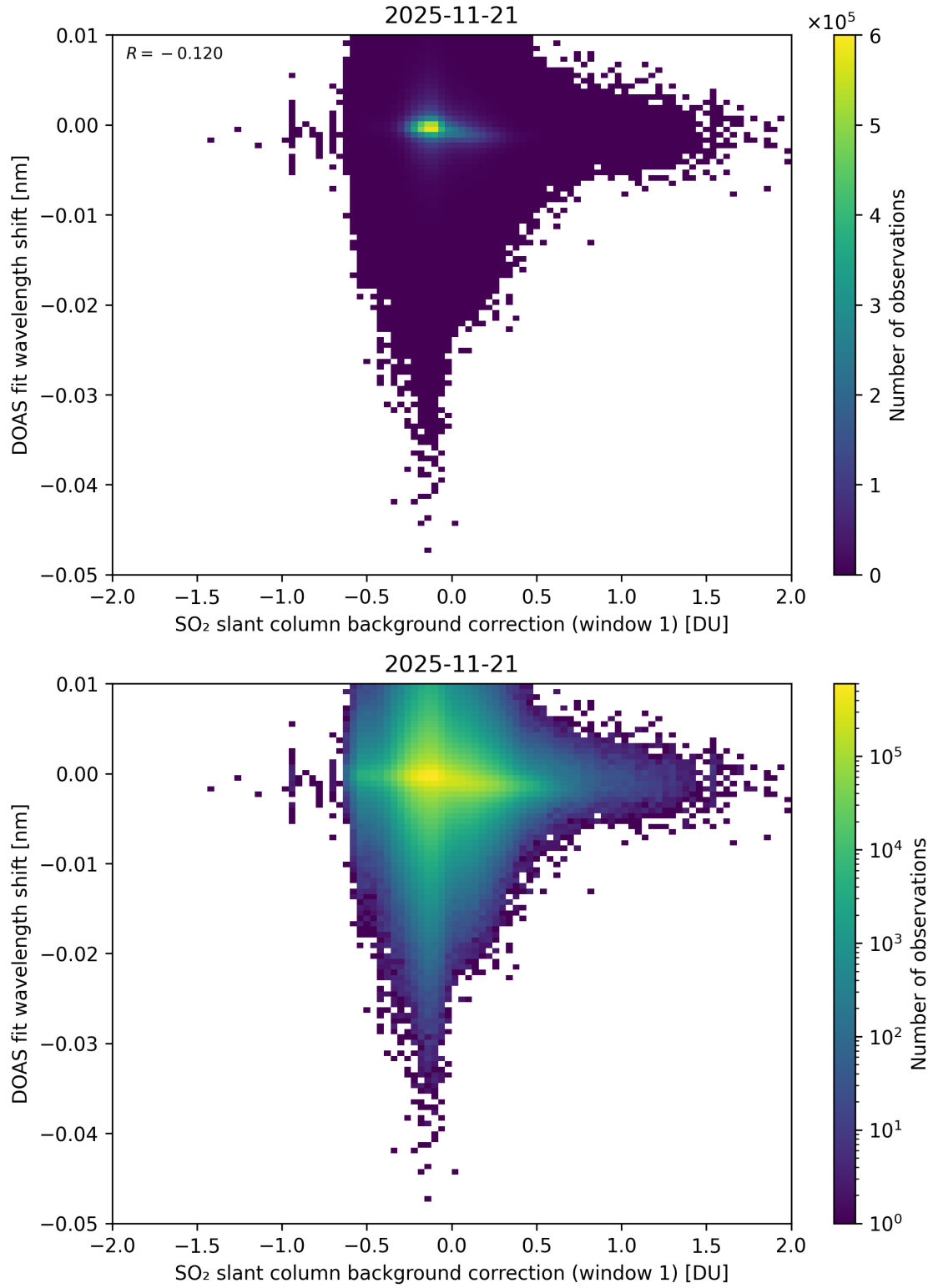
Figure 111: Scatter density plot of “SO 2 slant column background correction (window 1)” against “DOAS fit wavelength shift” for 2025-11-20 to 2025-11-22.
