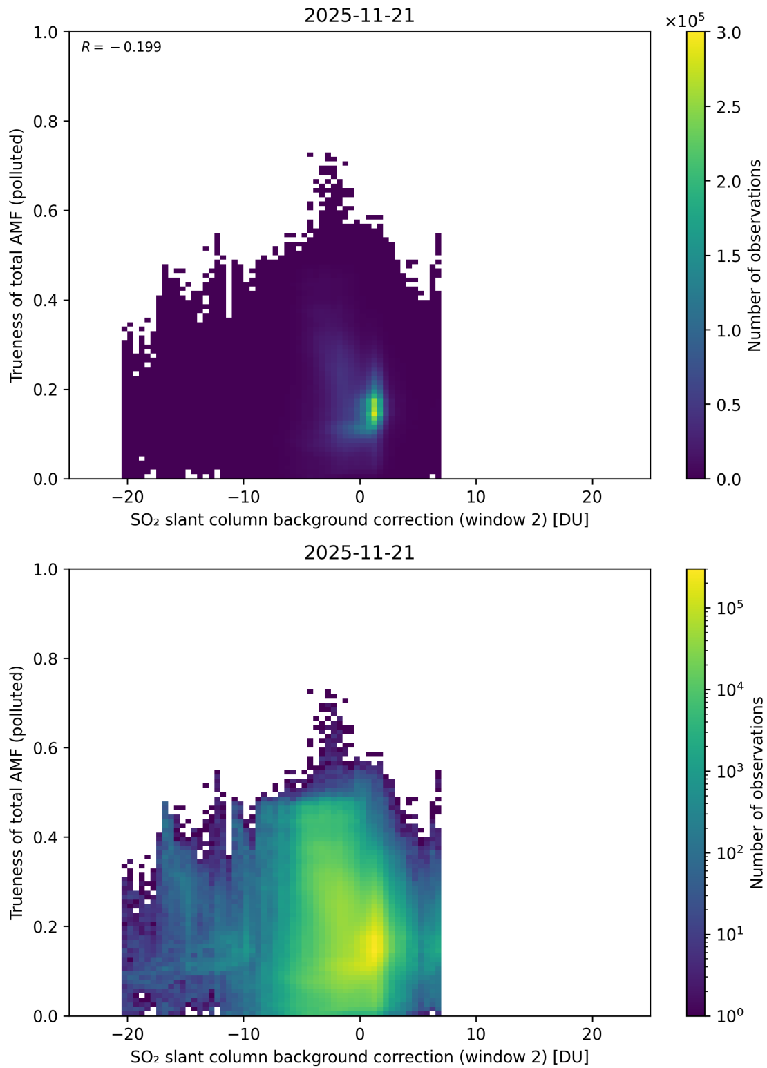
Figure 131: Scatter density plot of “SO 2 slant column background correction (window 2)” against “Trueness of total AMF (polluted)” for 2025-11-20 to 2025-11-22.
