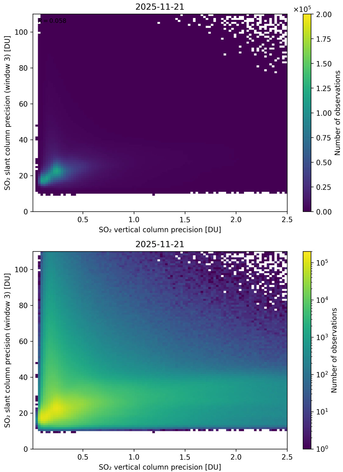
Figure 345: Scatter density plot of “SO 2 vertical column precision” against “SO 2 slant column precision (window 3)” for 2025-11-20 to 2025-11-22.
