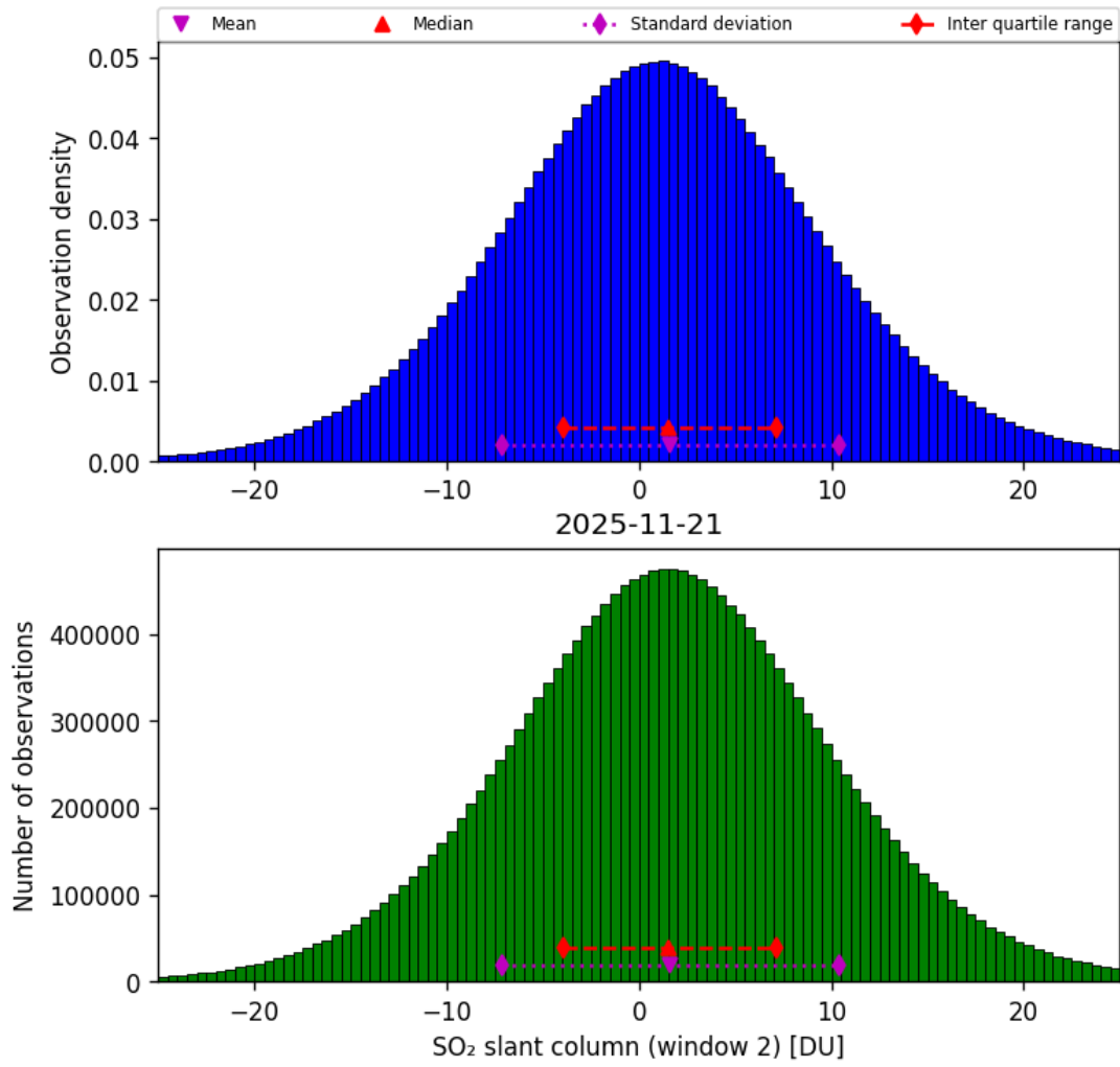
Figure 67: Histogram of “SO 2 slant column (window 2)” for 2025-11-20 to 2025-11-22
