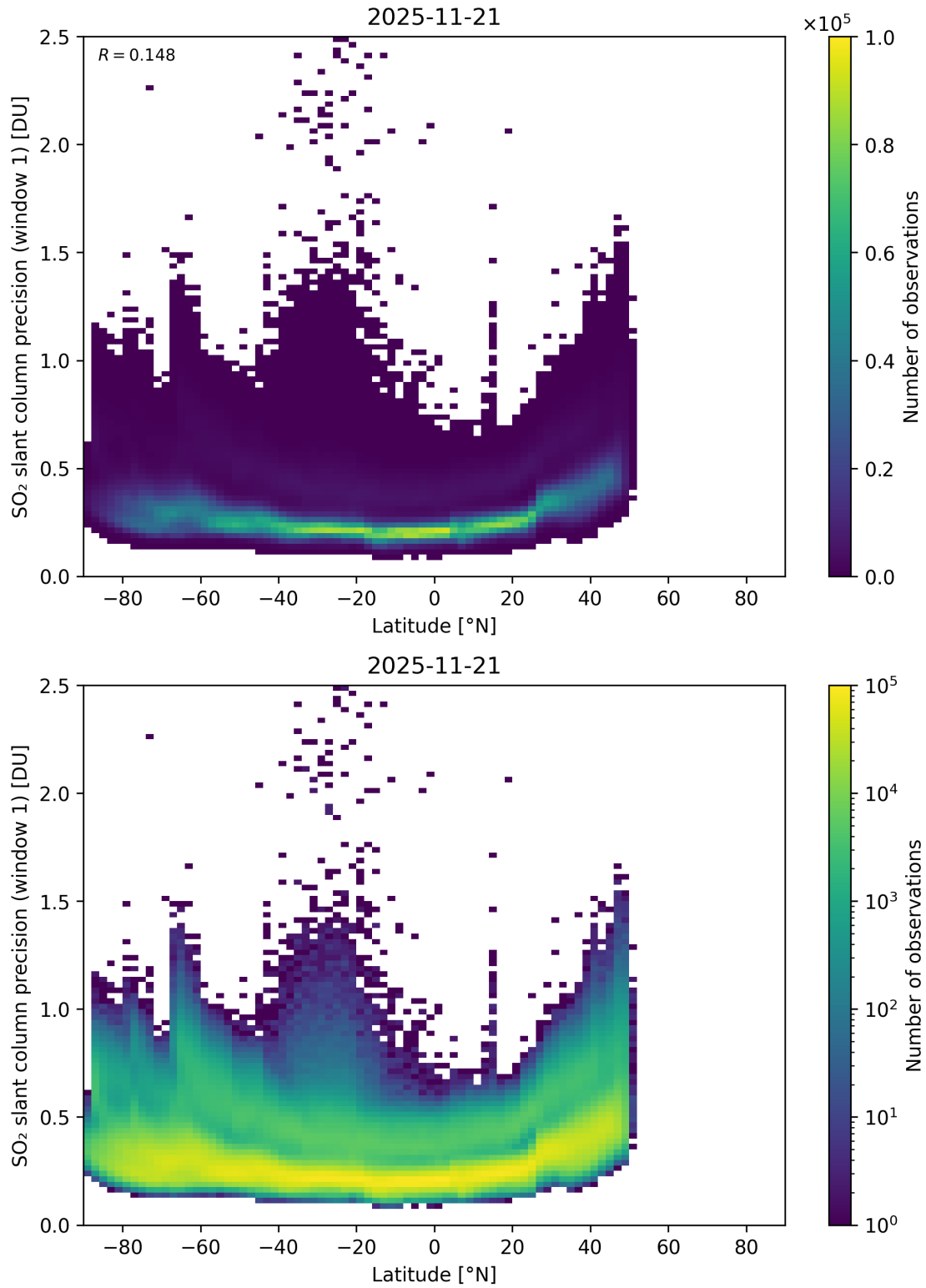
Figure 163: Scatter density plot of “Latitude” against “SO 2 slant column precision (window 1)” for 2025-11-20 to 2025-11-22.
