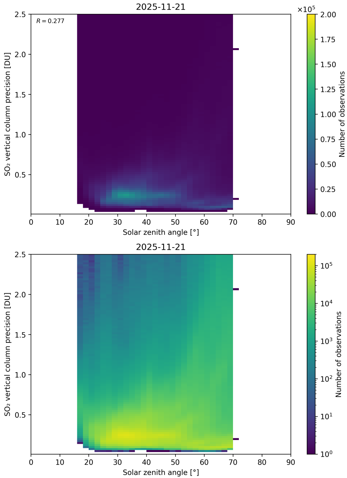
Figure 192: Scatter density plot of “Solar zenith angle” against “SO 2 vertical column precision” for 2025-11-20 to 2025-11-22.
