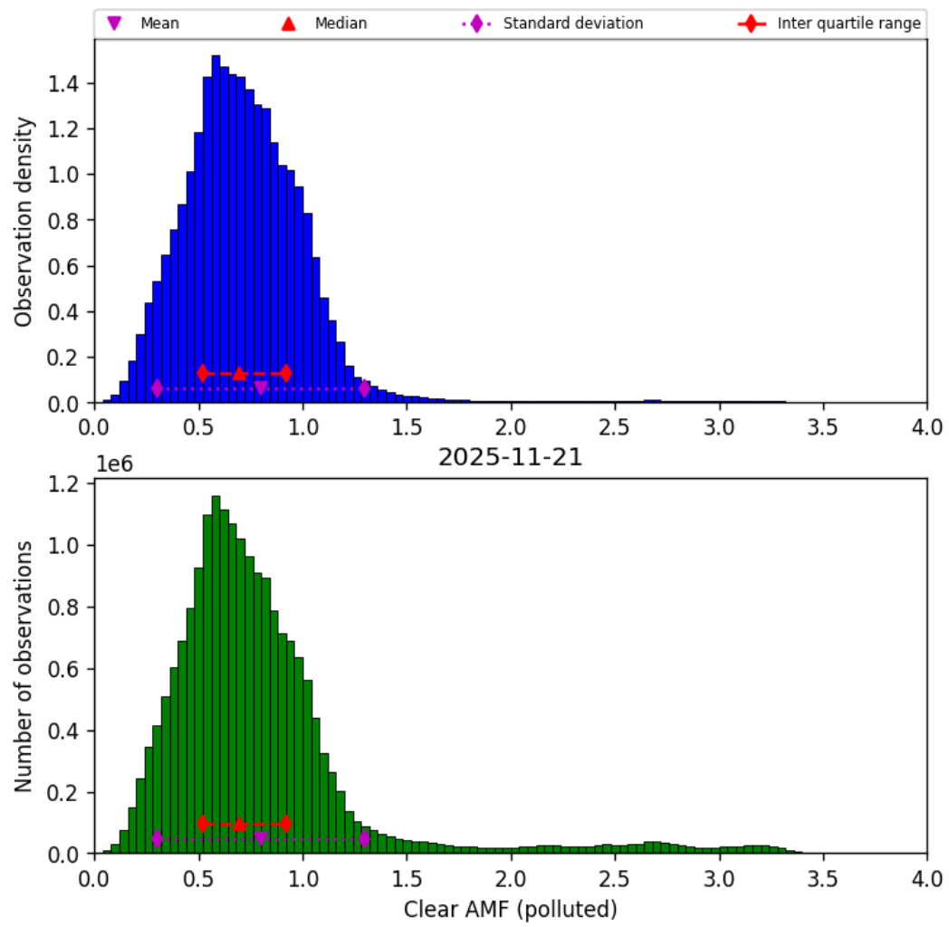
Figure 81: Histogram of “Clear AMF (polluted)” for 2025-11-20 to 2025-11-22
