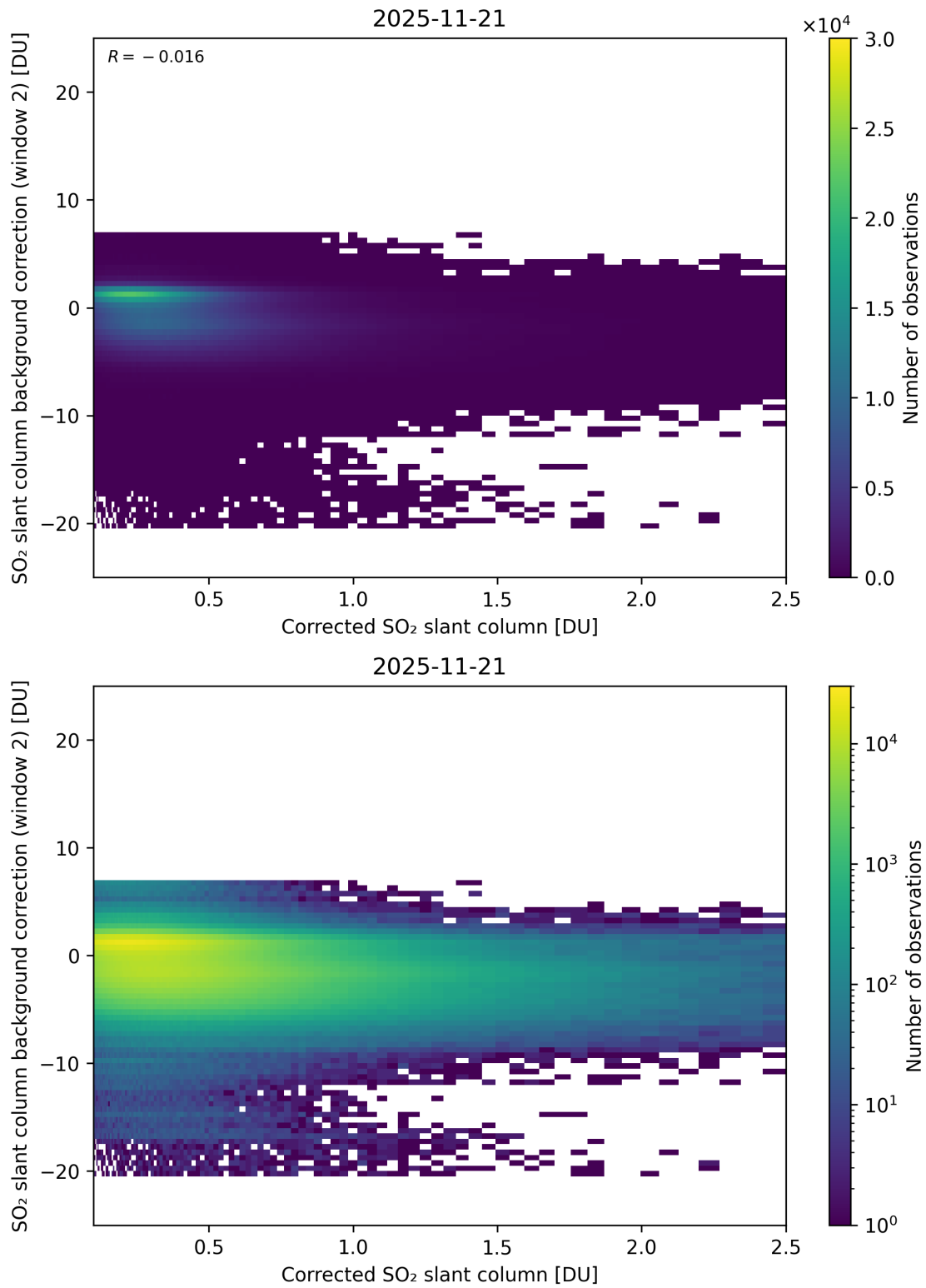
Figure 227: Scatter density plot of “Corrected SO 2 slant column” against “SO 2 slant column background correction (window 2)” for 2025-11-20 to 2025-11-22.
