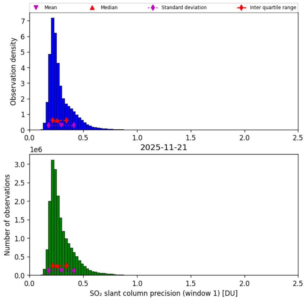
Figure 64: Histogram of “SO 2 slant column precision (window 1)” for 2025-11-20 to 2025-11-22
