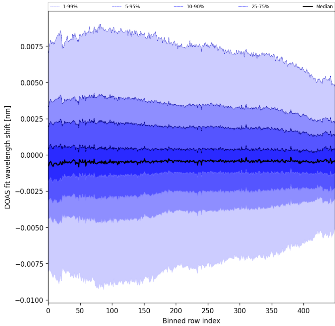
Figure 102: Along track statistics of “DOAS fit wavelength shift” for 2025-11-20 to 2025-11-22
