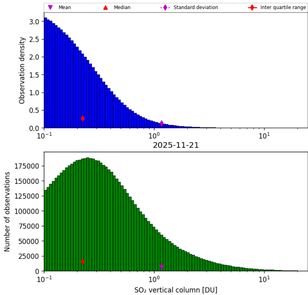
Figure 58: Histogram of “SO 2 vertical column” for 2025-11-20 to 2025-11-22
