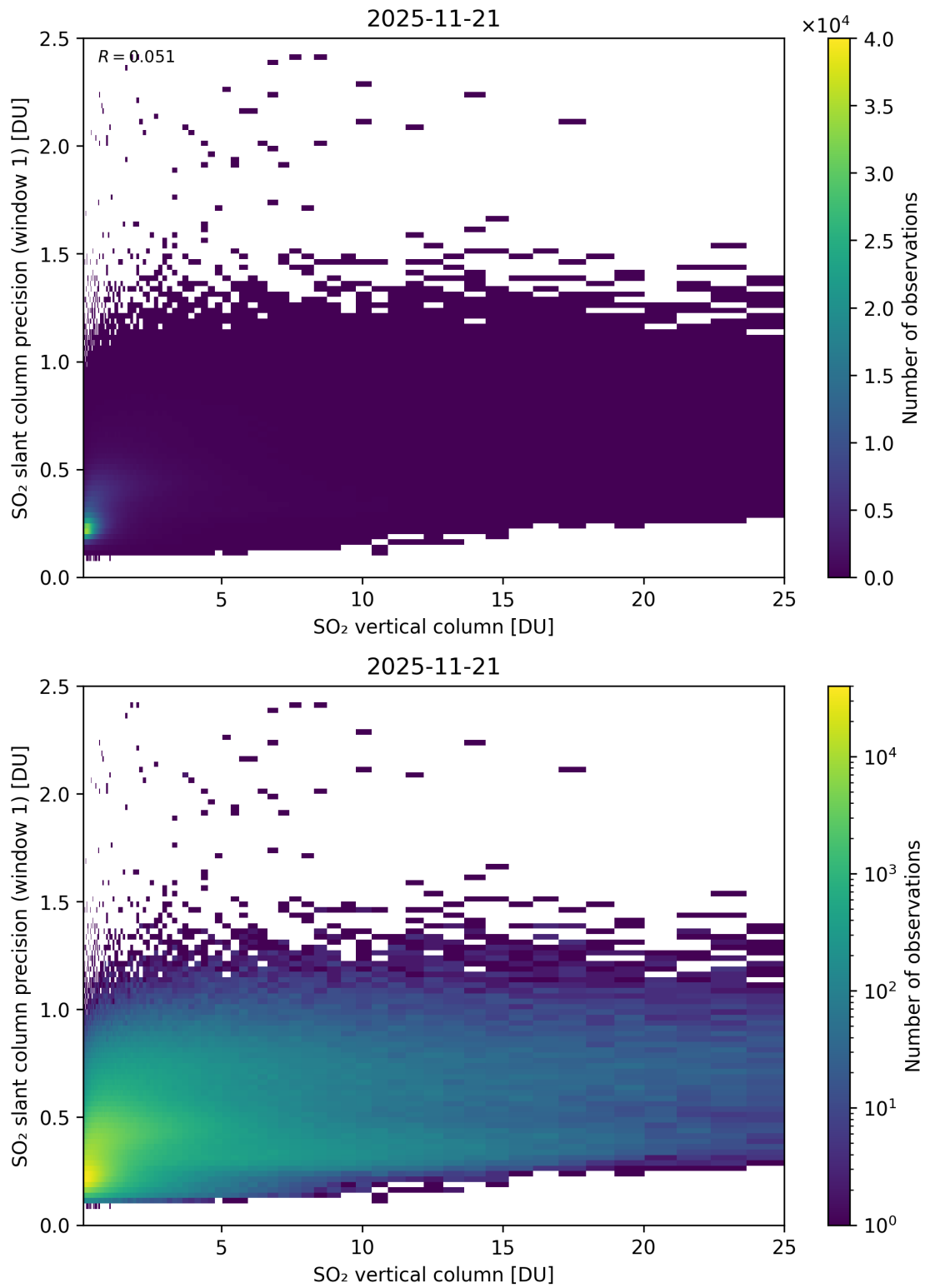
Figure 355: Scatter density plot of “SO 2 vertical column” against “SO 2 slant column precision (window 1)” for 2025-11-20 to 2025-11-22.
