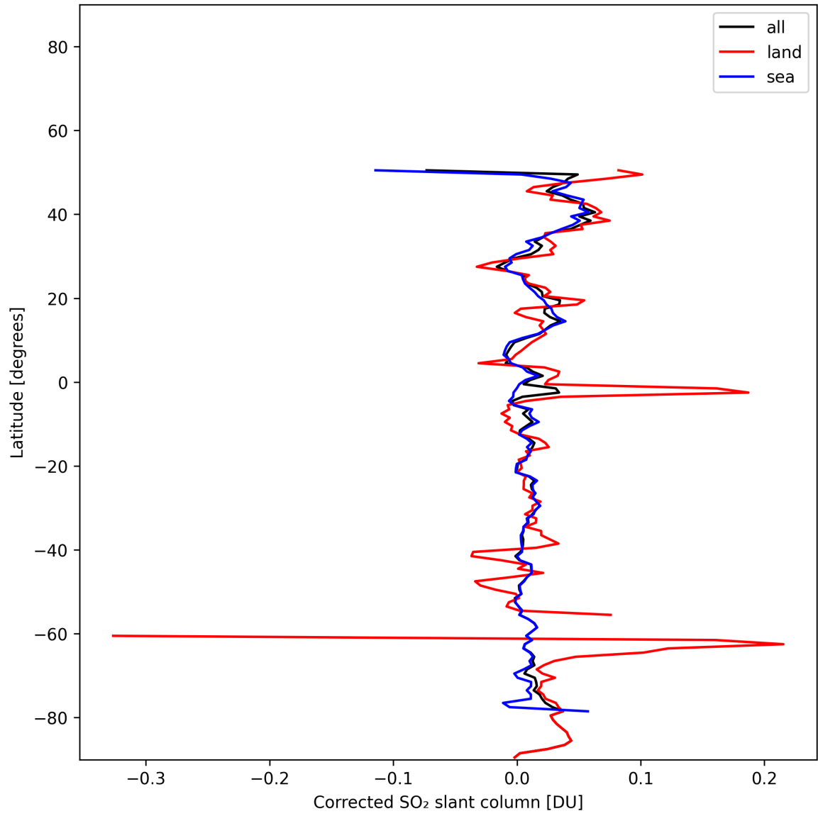
Figure 34: Zonal average of "Corrected SO 2 slant column" for 2025-11-20 to 2025-11-22.
