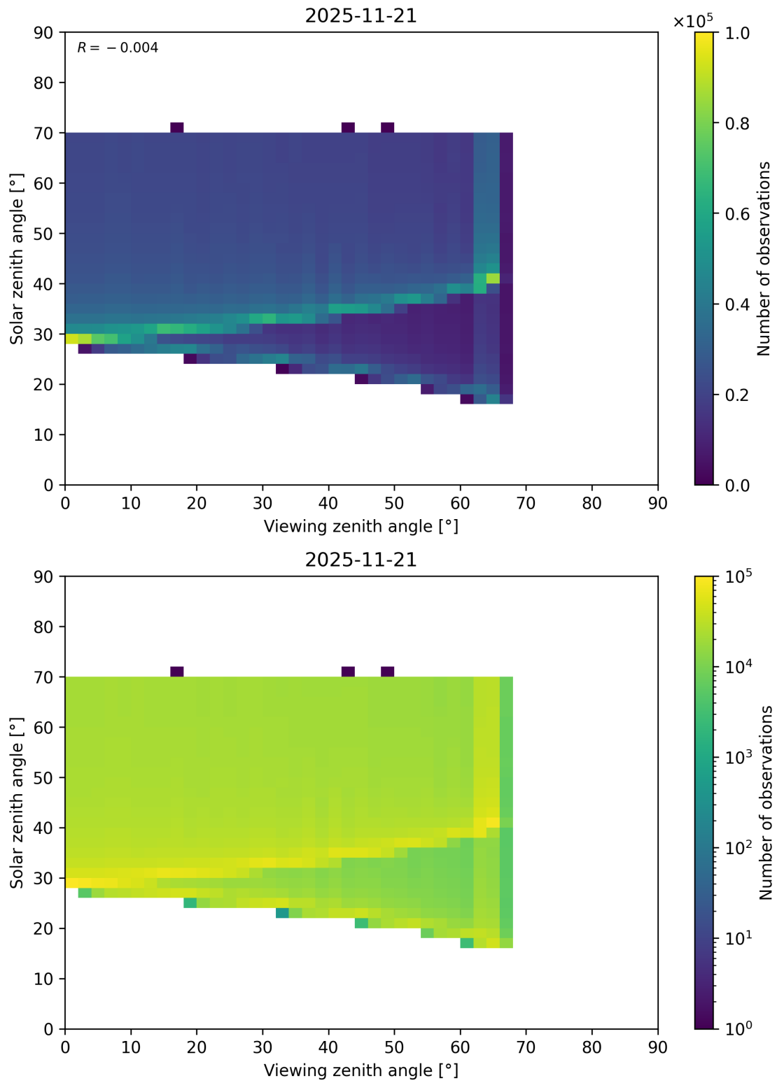
Figure 369: Scatter density plot of “Viewing zenith angle” against “Solar zenith angle” for 2025-11-20 to 2025-11-22.
