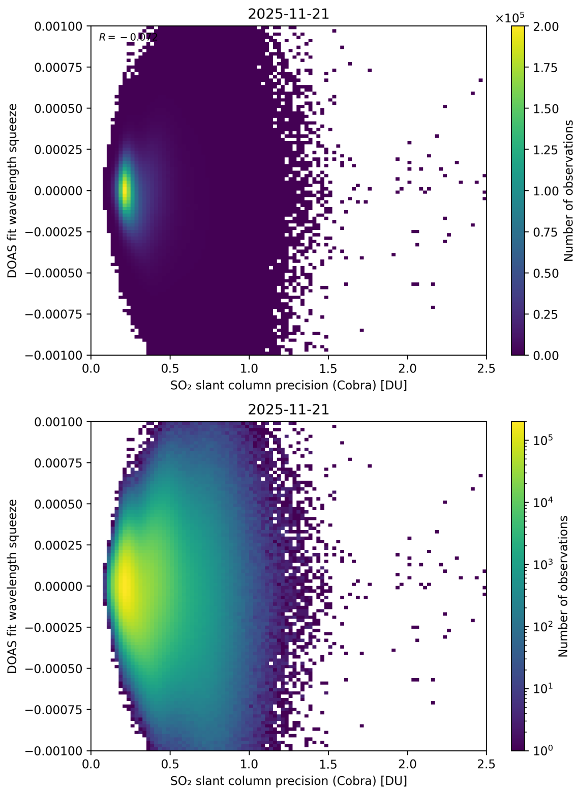
Figure 203: Scatter density plot of “SO 2 slant column precision (Cobra)” against “DOAS fit wavelength squeeze” for 2025-11-20 to 2025-11-22.
