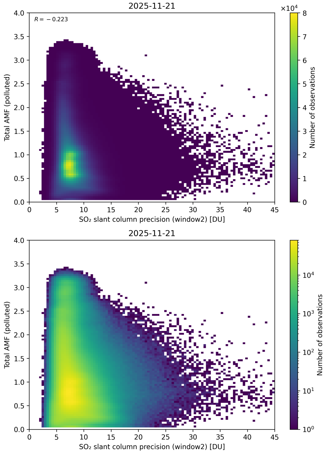
Figure 301: Scatter density plot of “SO 2 slant column precision (window2)” against “Total AMF (polluted)” for 2025-11-20 to 2025-11-22.
