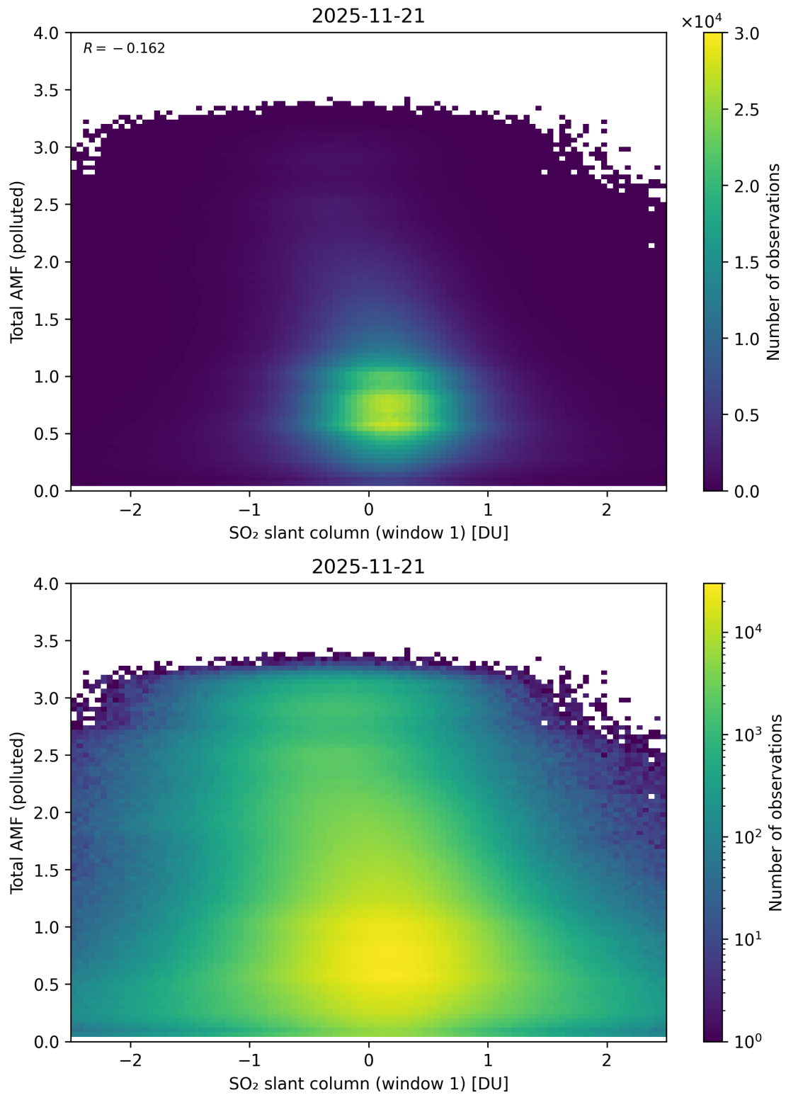
Figure 289: Scatter density plot of “SO 2 slant column (window 1)” against “Total AMF (polluted)” for 2025-11-20 to 2025-11-22.
