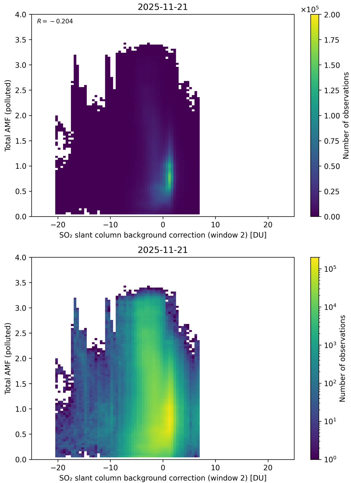
Figure 130: Scatter density plot of “SO 2 slant column background correction (window 2)” against “Total AMF (polluted)” for 2025-11-20 to 2025-11-22.
