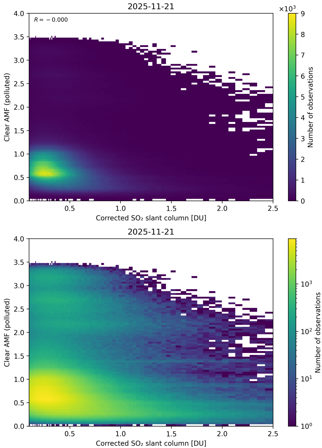
Figure 232: Scatter density plot of “Corrected SO 2 slant column” against “Clear AMF (polluted)” for 2025-11-20 to 2025-11-22.
