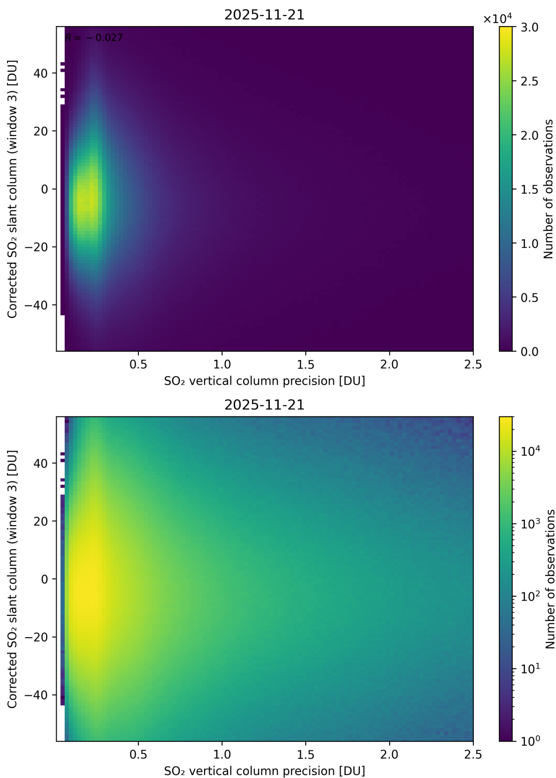
Figure 340: Scatter density plot of “SO 2 vertical column precision” against “Corrected SO 2 slant column (window 3)” for 2025-11-20 to 2025-11-22.
