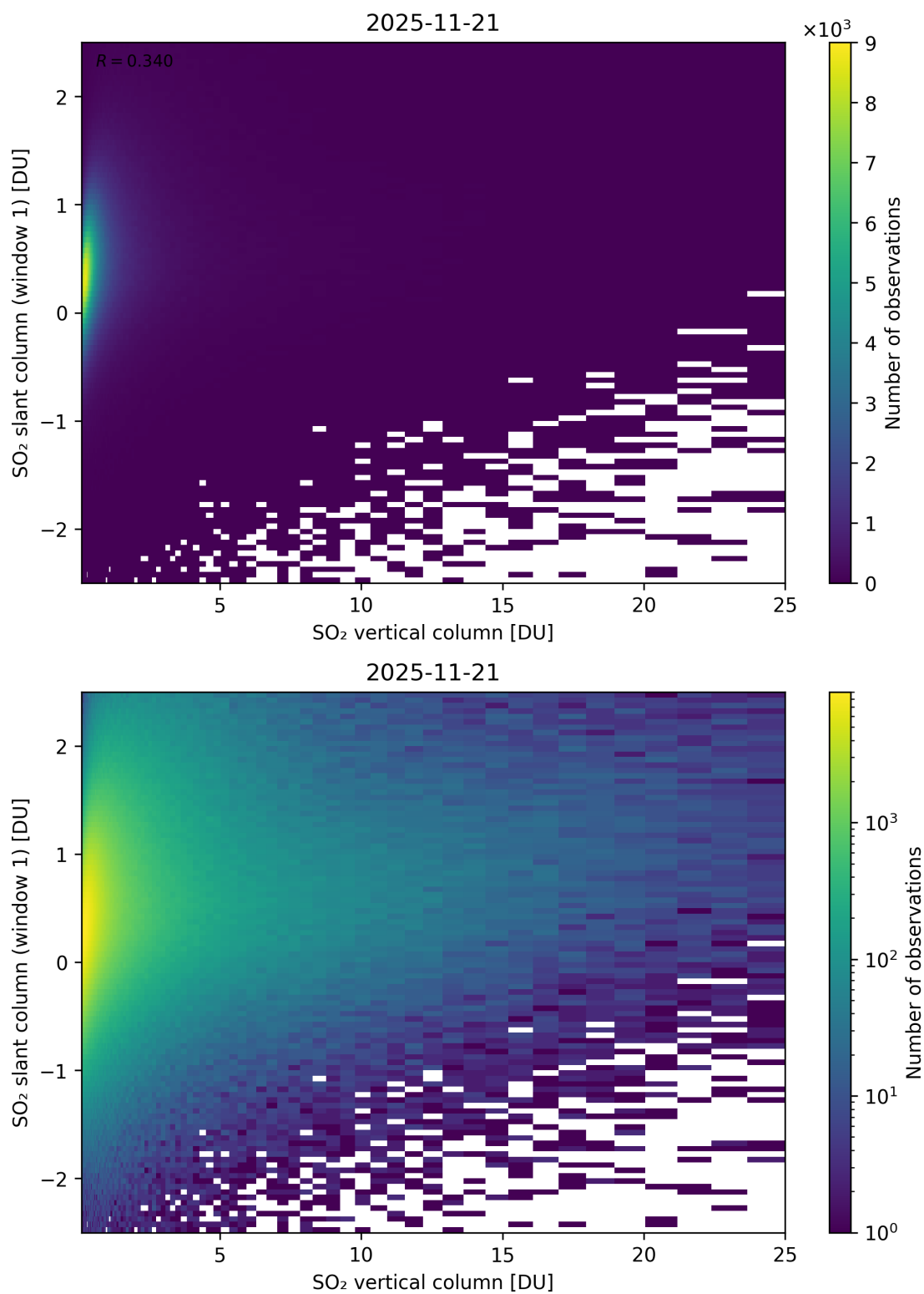
Figure 354: Scatter density plot of “SO 2 vertical column” against “SO 2 slant column (window 1)” for 2025-11-20 to 2025-11-22.
