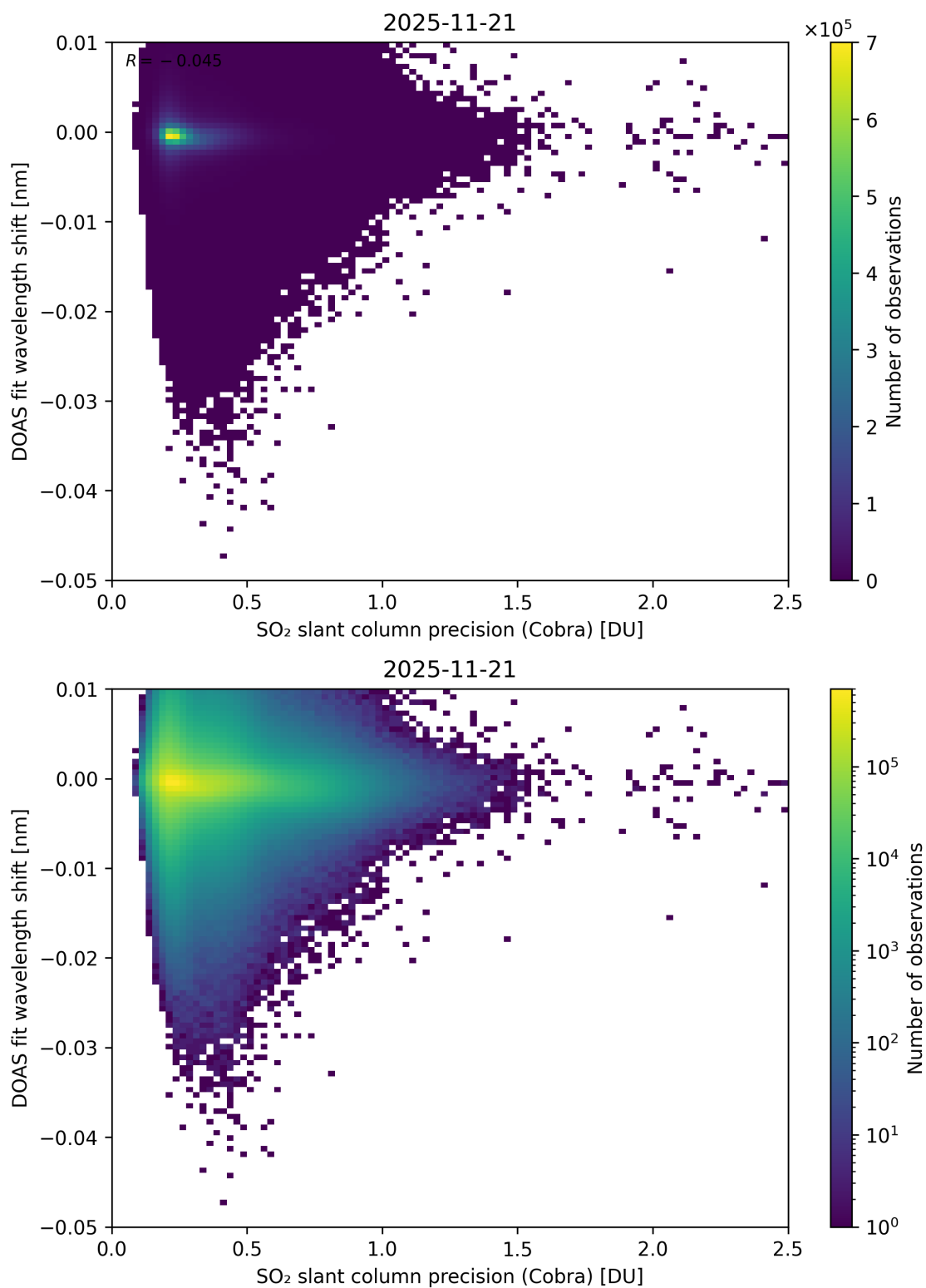
Figure 202: Scatter density plot of “SO 2 slant column precision (Cobra)” against “DOAS fit wavelength shift” for 2025-11-20 to 2025-11-22.
