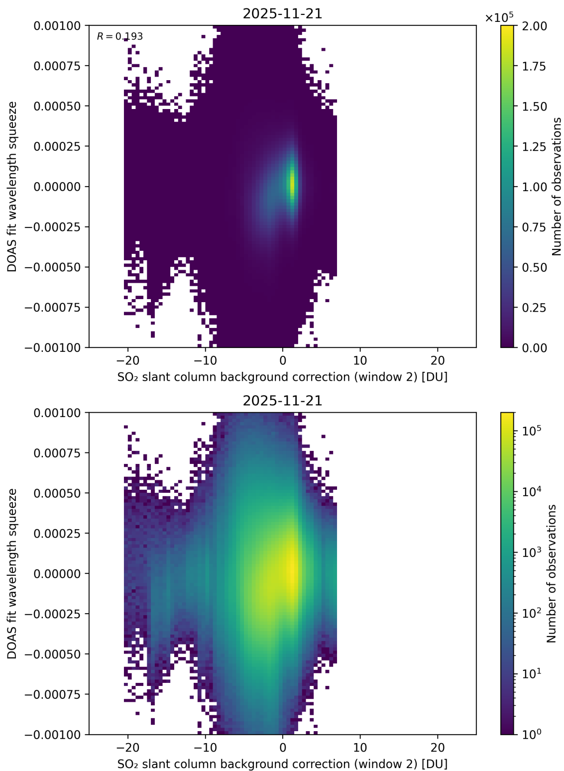
Figure 124: Scatter density plot of “SO 2 slant column background correction (window 2)” against “DOAS fit wavelength squeeze” for 2025-11-20 to 2025-11-22.
