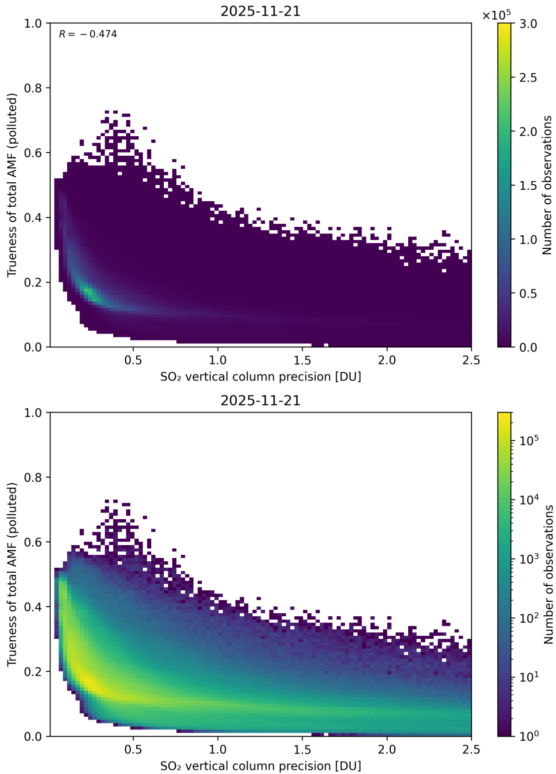
Figure 347: Scatter density plot of “SO 2 vertical column precision” against “Trueness of total AMF (polluted)” for 2025-11-20 to 2025-11-22.
