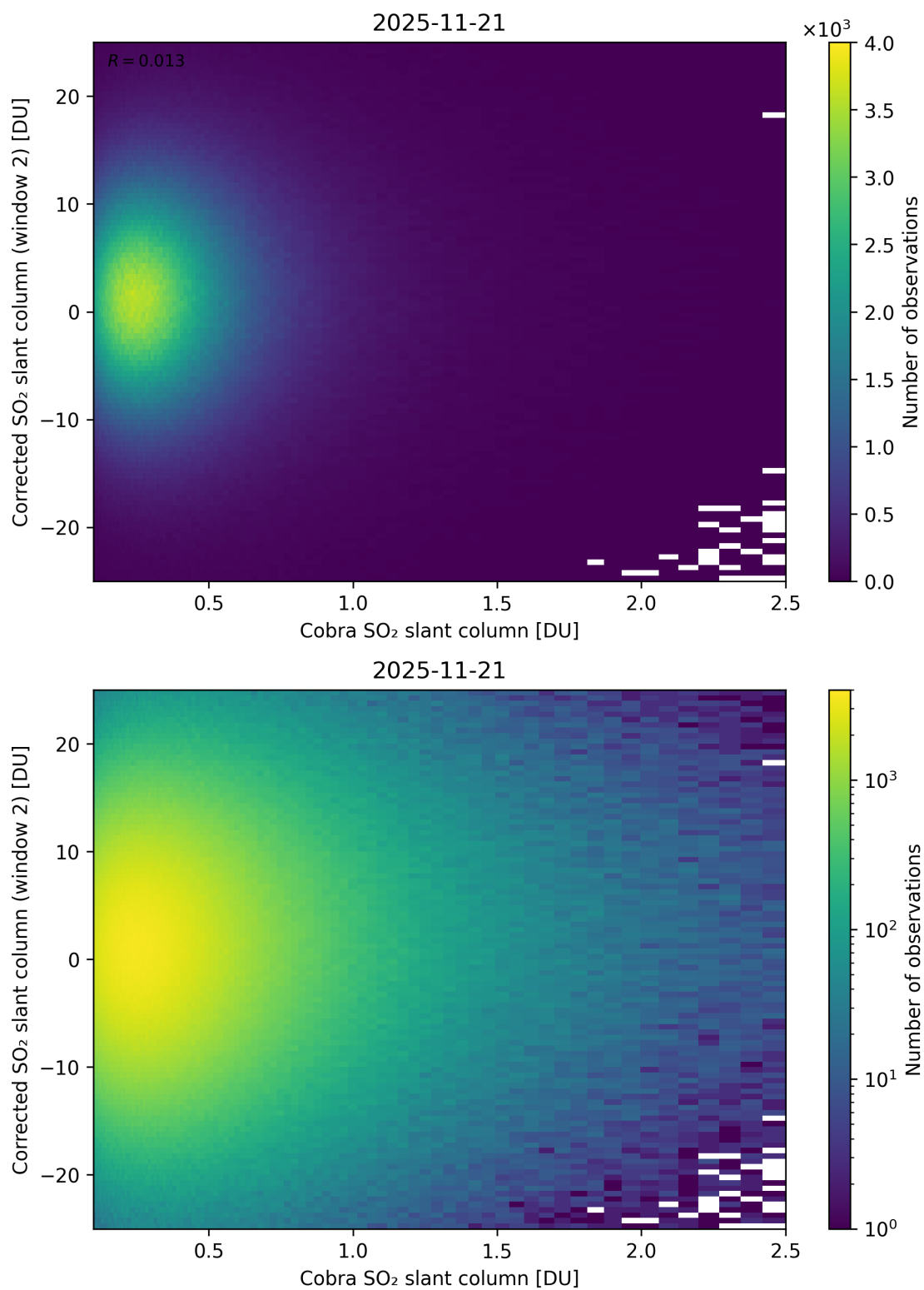
Figure 217: Scatter density plot of “Cobra SO 2 slant column” against “Corrected SO 2 slant column (window 2)” for 2025-11-20 to 2025-11-22.
