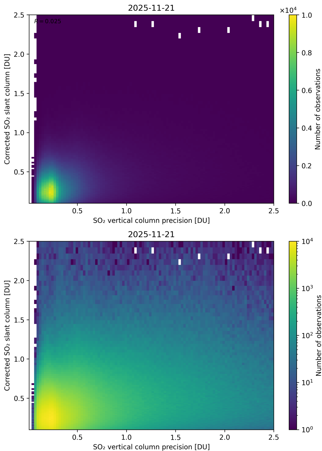
Figure 338: Scatter density plot of “SO 2 vertical column precision” against “Corrected SO 2 slant column” for 2025-11-20 to 2025-11-22.
