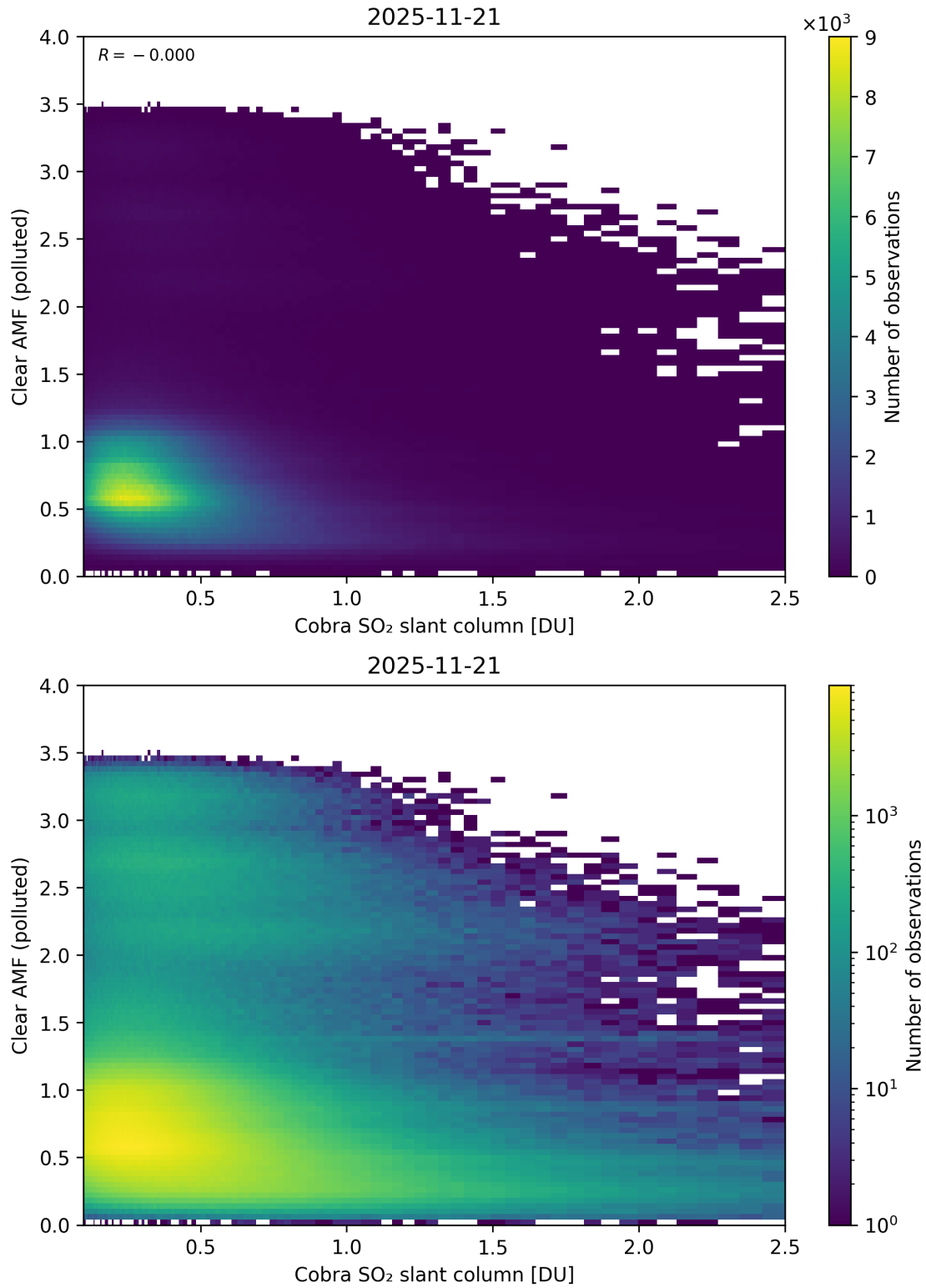
Figure 215: Scatter density plot of “Cobra SO 2 slant column” against “Clear AMF (polluted)” for 2025-11-20 to 2025-11-22.
