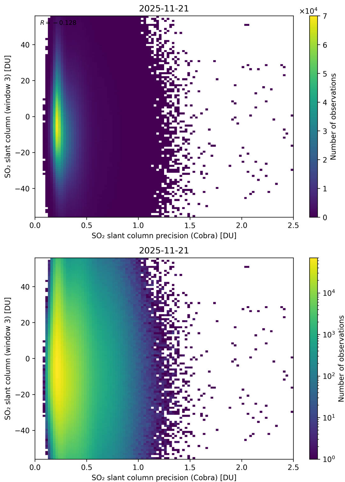
Figure 211: Scatter density plot of “SO 2 slant column precision (Cobra)” against “SO 2 slant column (window 3)” for 2025-11-20 to 2025-11-22.
