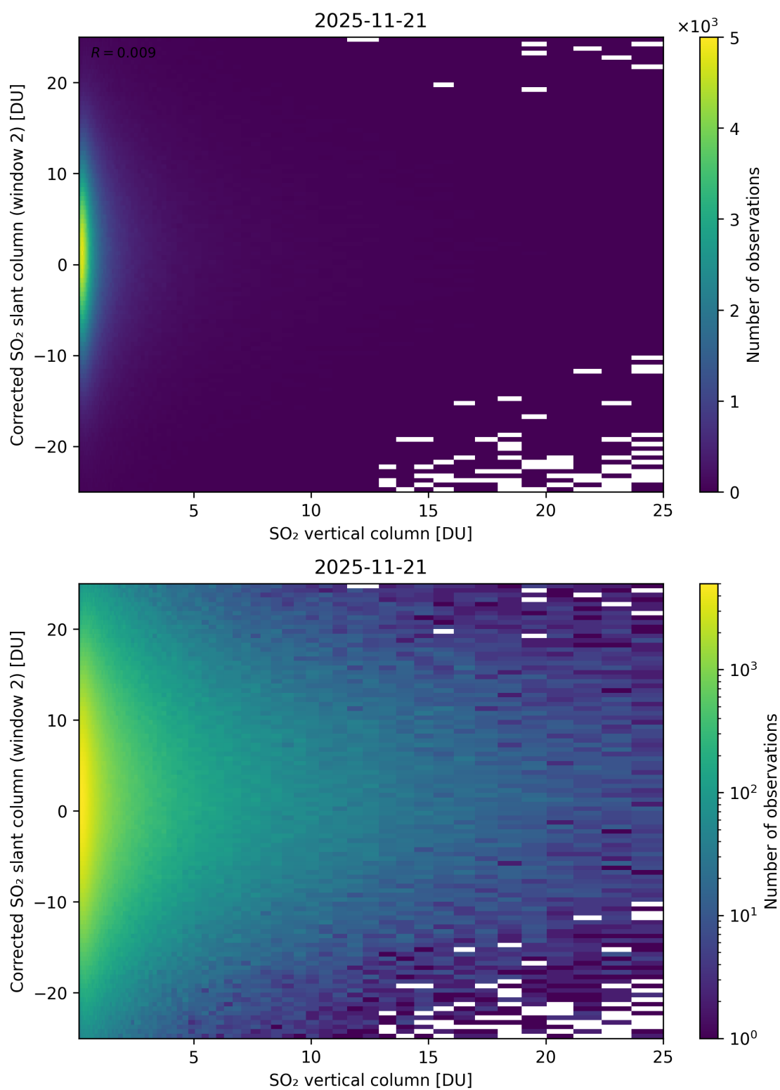
Figure 352: Scatter density plot of “SO 2 vertical column” against “Corrected SO 2 slant column (window 2)” for 2025-11-20 to 2025-11-22.
