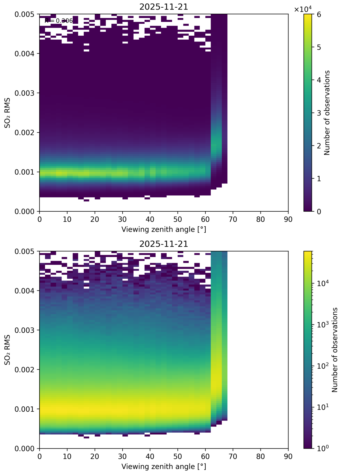
Figure 367: Scatter density plot of “Viewing zenith angle” against “SO 2 RMS” for 2025-11-20 to 2025-11-22.
