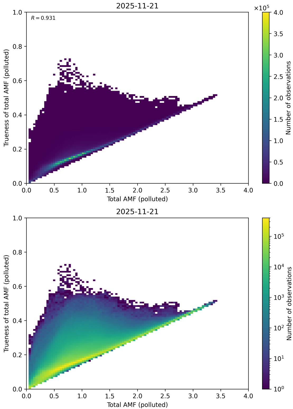
Figure 321: Scatter density plot of “Total AMF (polluted)” against “Trueness of total AMF (polluted)” for 2025-11-20 to 2025-11-22.
