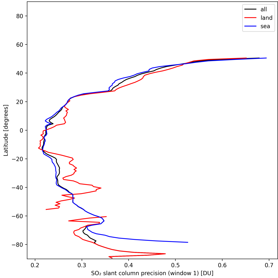
Figure 38: Zonal average of “SO 2 slant column precision (window 1)” for 2025-11-20 to 2025-11-22.
