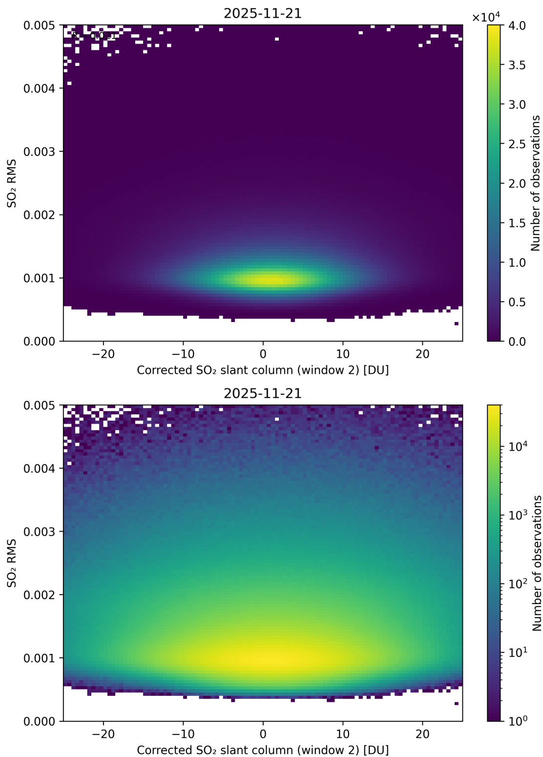
Figure 248: Scatter density plot of “Corrected SO 2 slant column (window 2)” against “SO 2 RMS” for 2025-11-20 to 2025-11-22.
