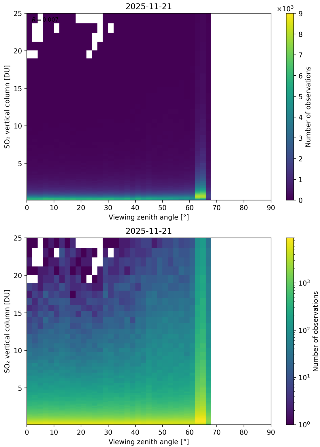
Figure 383: Scatter density plot of “Viewing zenith angle” against “SO 2 vertical column” for 2025-11-20 to 2025-11-22.
