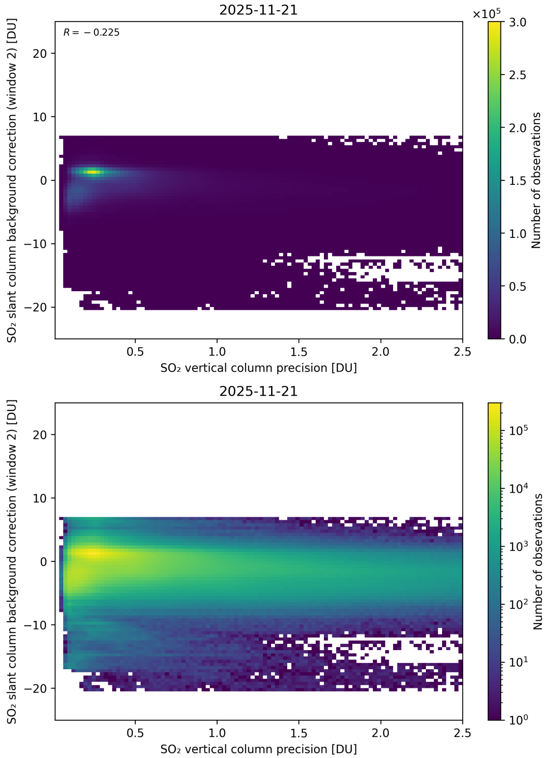
Figure 330: Scatter density plot of “SO 2 vertical column precision” against “SO 2 slant column background correction (window 2)” for 2025-11-20 to 2025-11-22.
