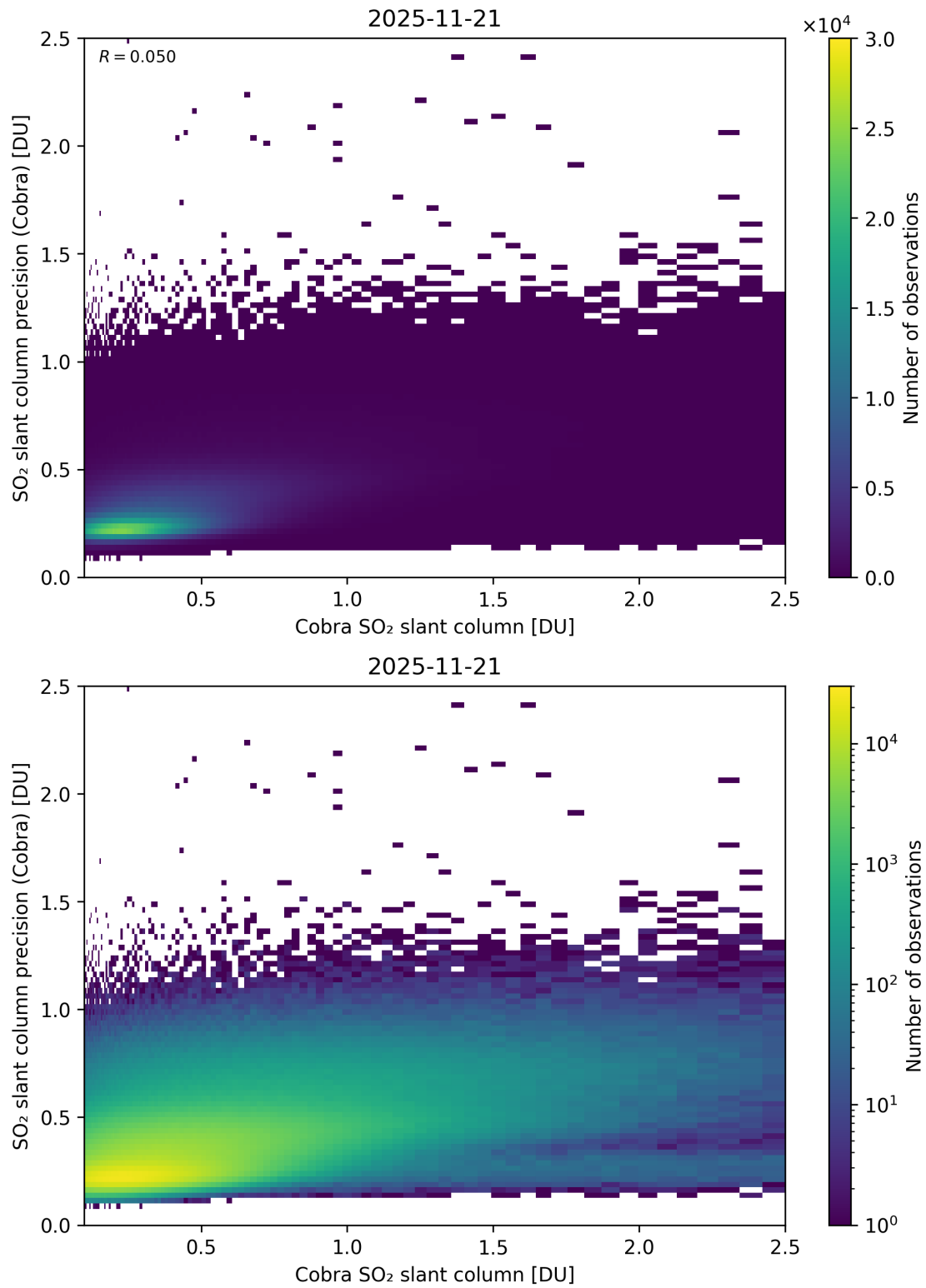
Figure 216: Scatter density plot of “Cobra SO 2 slant column” against “SO 2 slant column precision (Cobra)” for 2025-11-20 to 2025-11-22.
