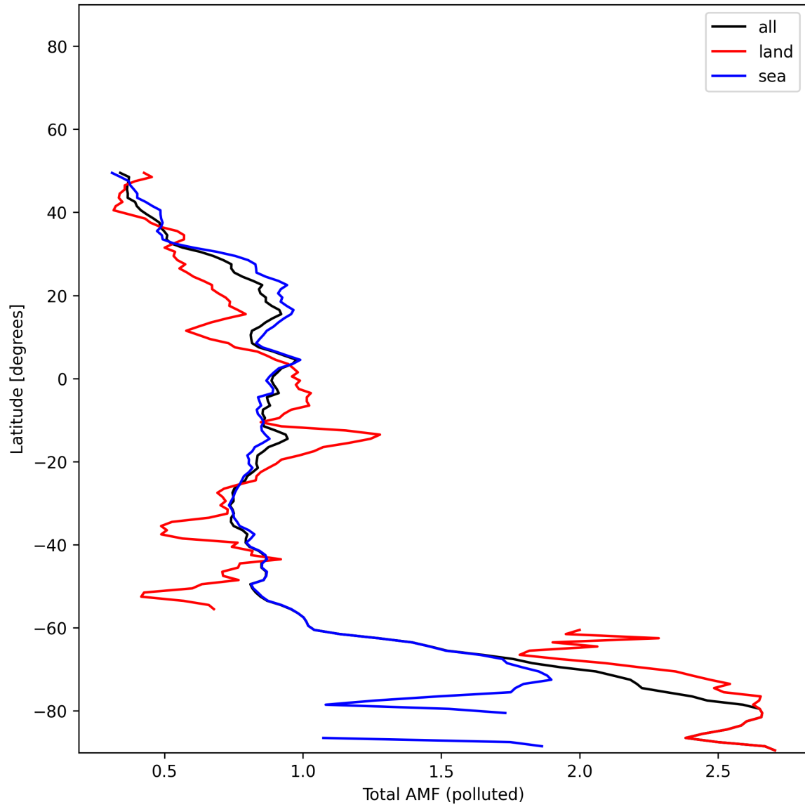
Figure 53: Zonal average of “Total AMF (polluted)” for 2025-11-21 to 2025-11-23.
