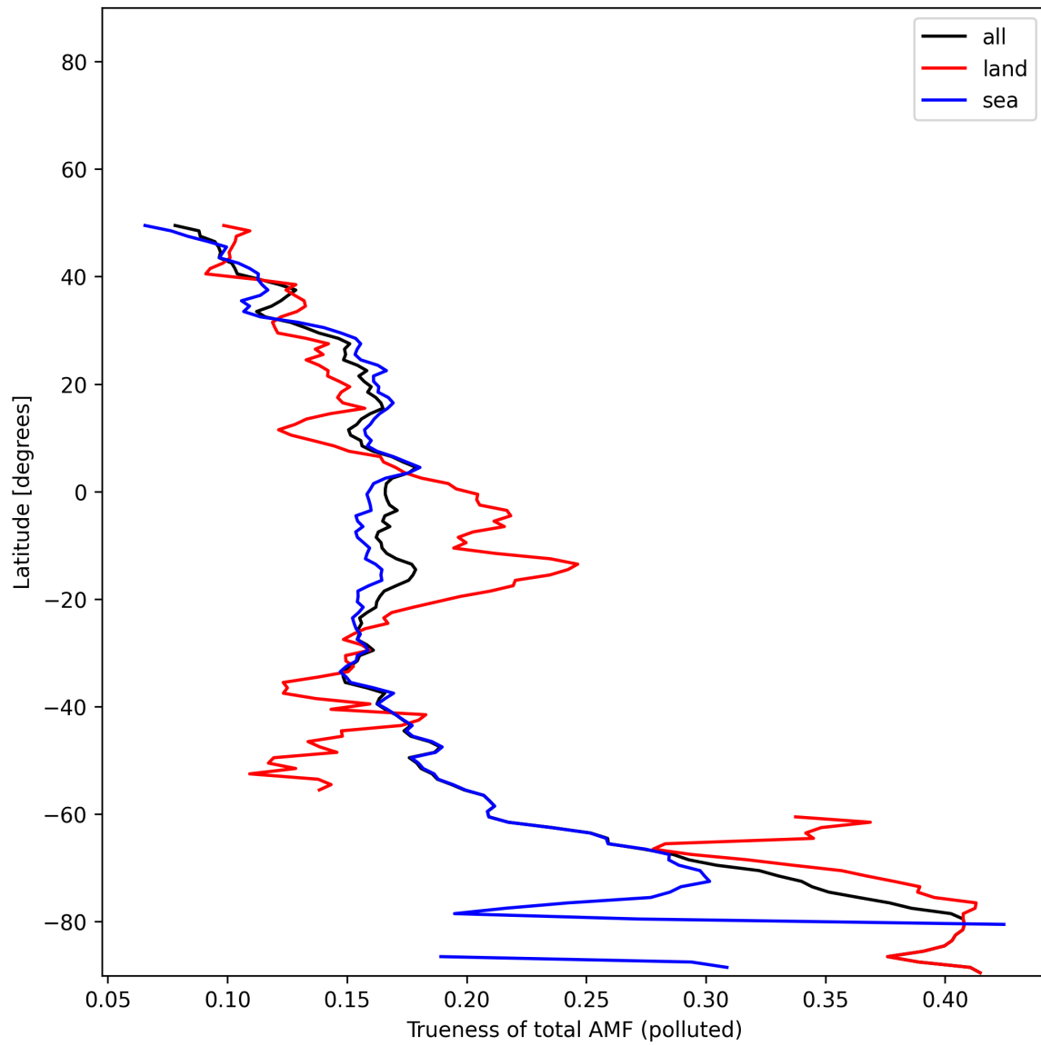
Figure 54: Zonal average of “Trueness of total AMF (polluted)” for 2025-11-21 to 2025-11-23.
