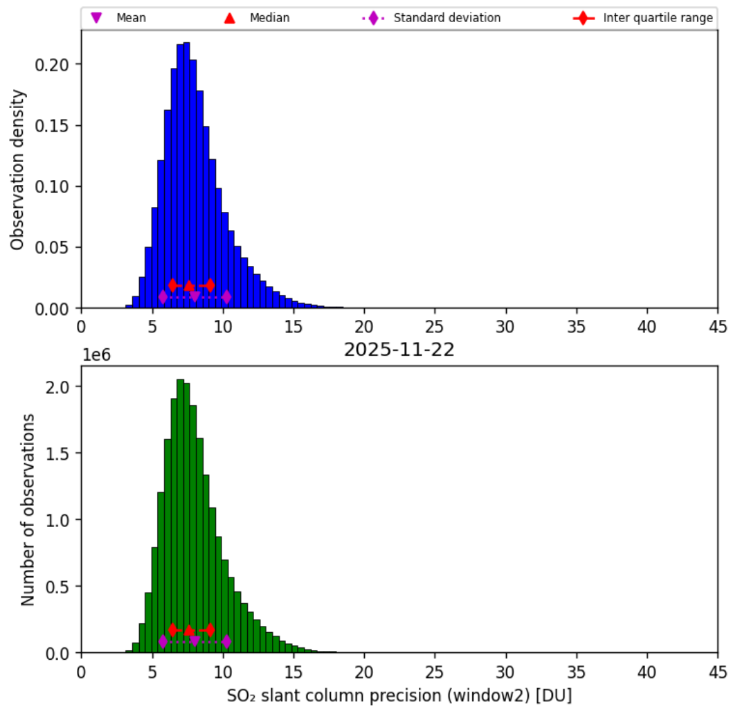
Figure 68: Histogram of “SO 2 slant column precision (window2)” for 2025-11-21 to 2025-11-23
