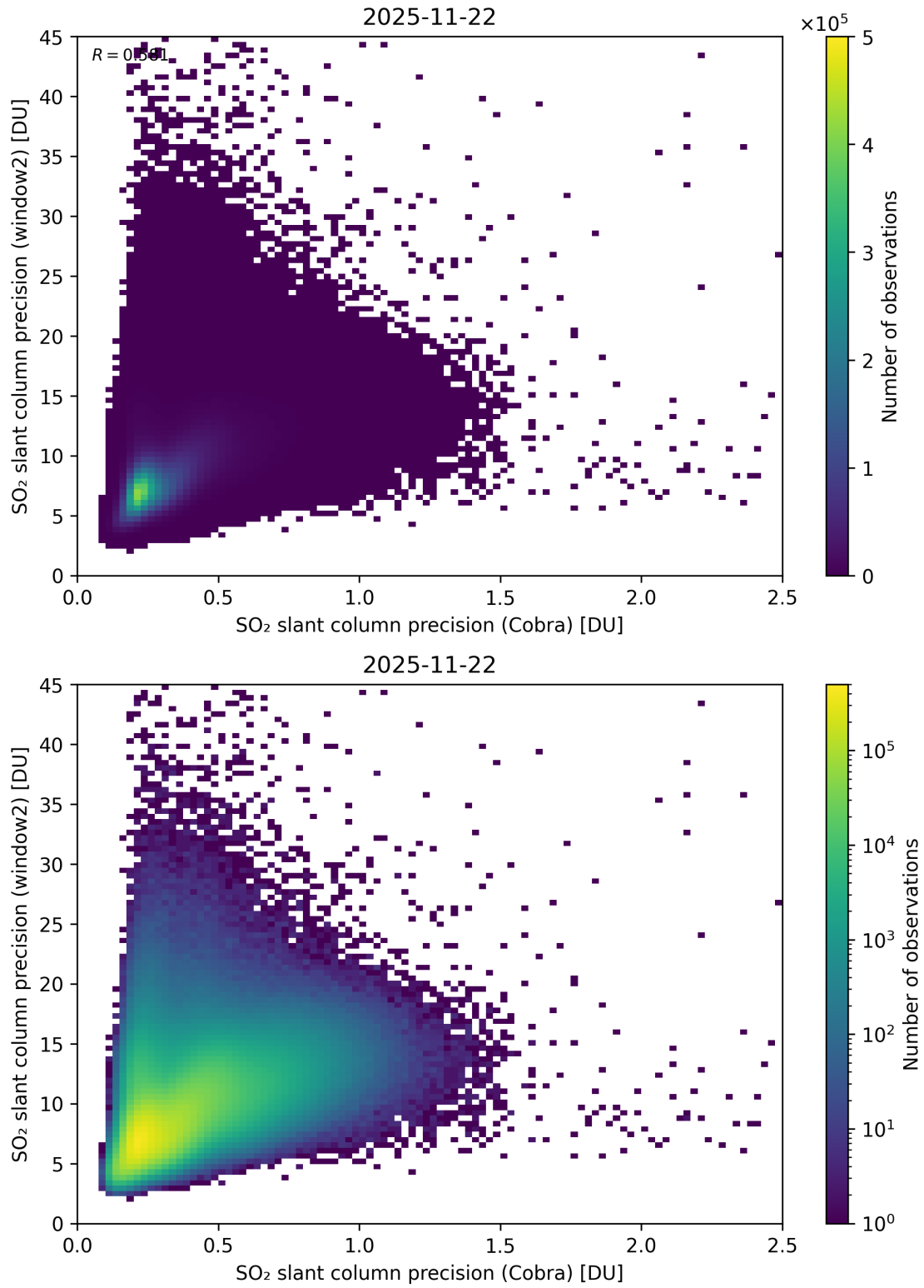
Figure 210: Scatter density plot of “SO 2 slant column precision (Cobra)” against “SO 2 slant column precision (window2)” for 2025-11-21 to 2025-11-23.
