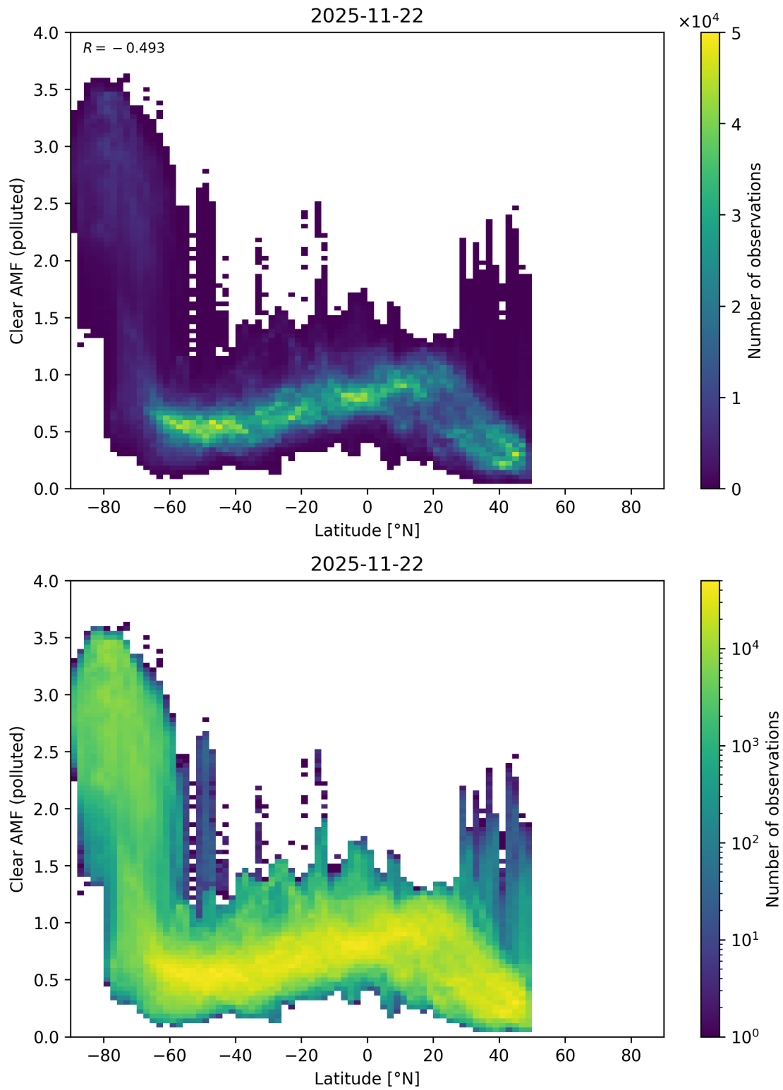
Figure 156: Scatter density plot of “Latitude” against “Clear AMF (polluted)” for 2025-11-21 to 2025-11-23.
