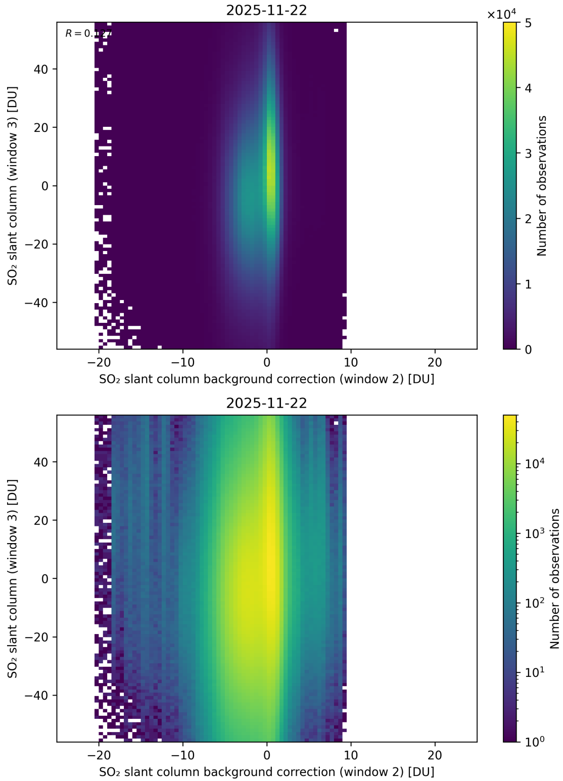
Figure 128: Scatter density plot of “SO 2 slant column background correction (window 2)” against “SO 2 slant column (window 3)” for 2025-11-21 to 2025-11-23.
