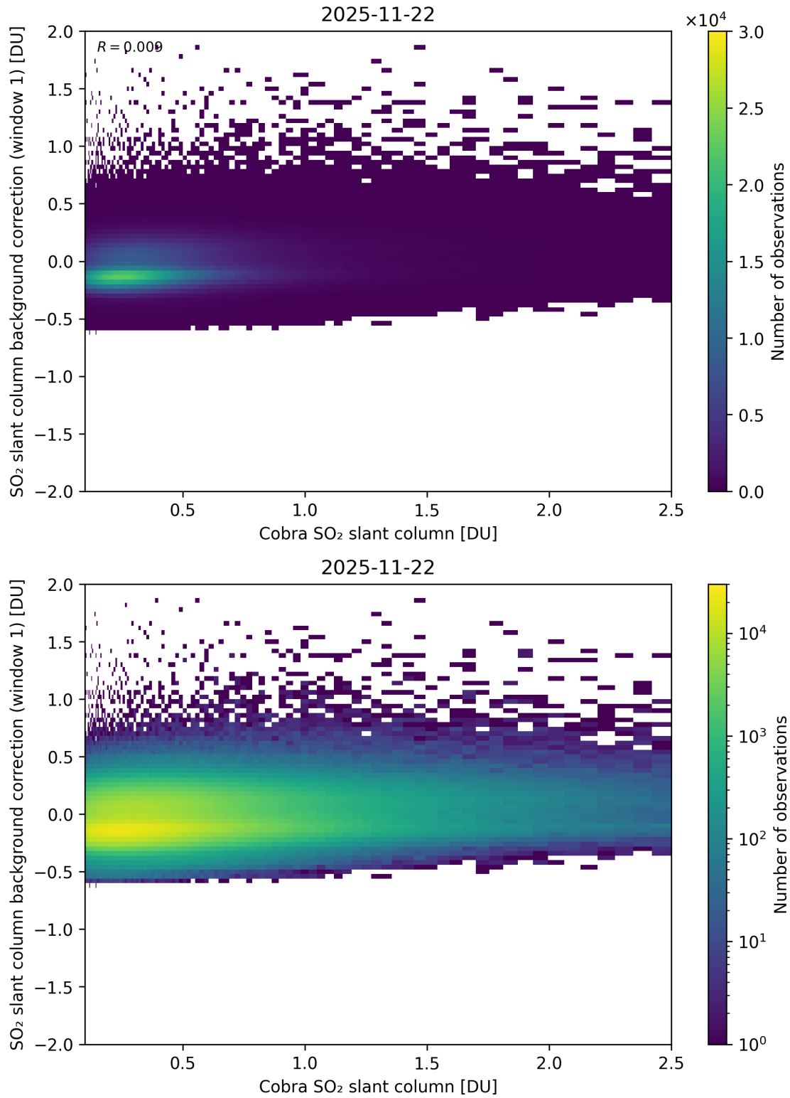
Figure 193: Scatter density plot of “Cobra SO 2 slant column” against “SO 2 slant column background correction (window 1)” for 2025-11-21 to 2025-11-23.
