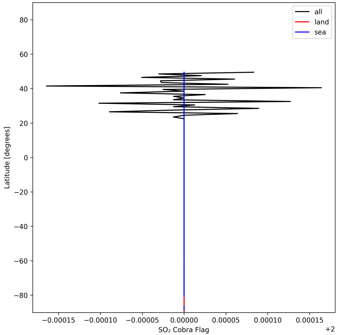
Figure 49: Zonal average of “SO 2 Cobra Flag” for 2025-11-21 to 2025-11-23.
