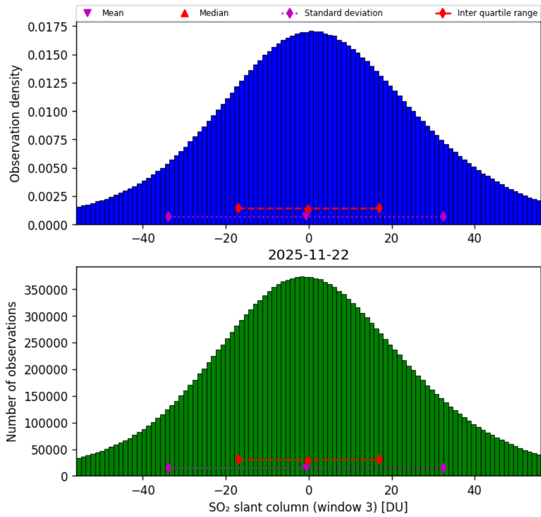
Figure 71: Histogram of “SO 2 slant column (window 3)” for 2025-11-21 to 2025-11-23
