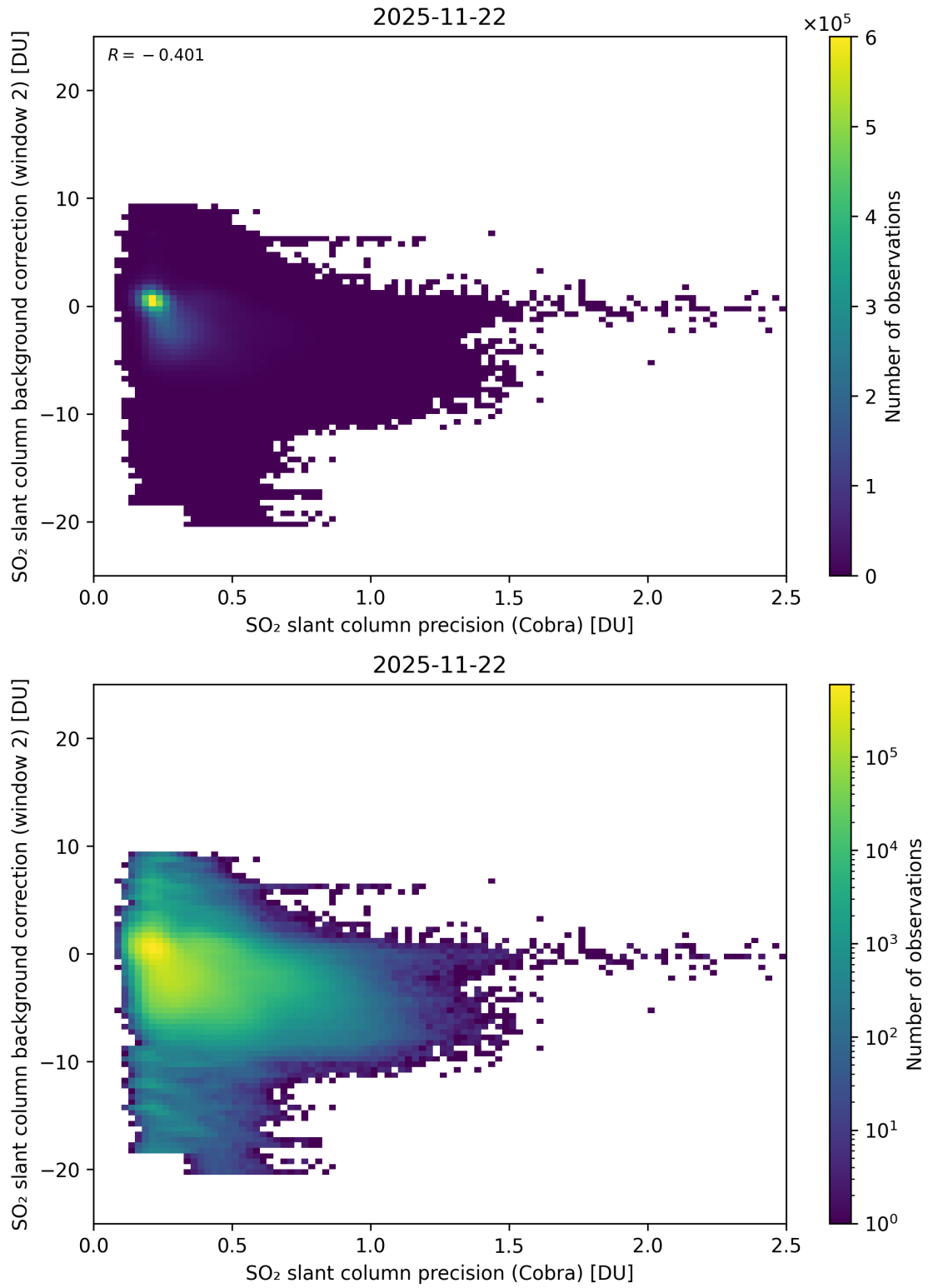
Figure 200: Scatter density plot of “SO 2 slant column precision (Cobra)” against “SO 2 slant column background correction (window 2)” for 2025-11-21 to 2025-11-23.
