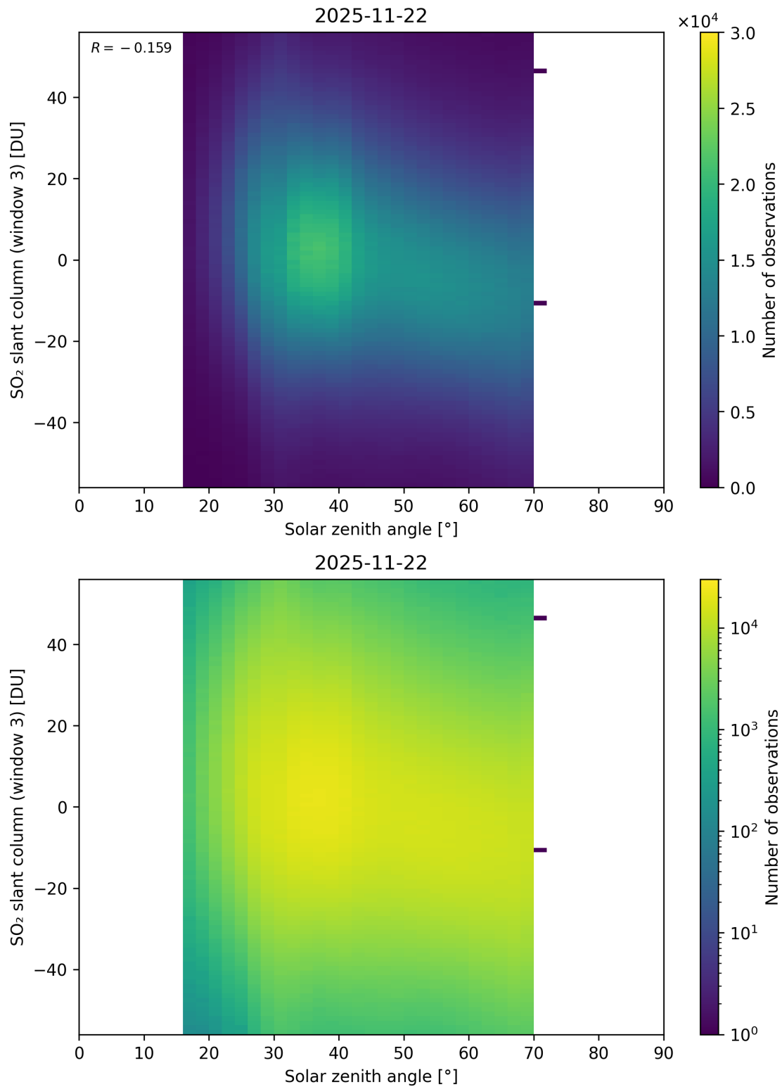
Figure 187: Scatter density plot of “Solar zenith angle” against “SO 2 slant column (window 3)” for 2025-11-21 to 2025-11-23.
