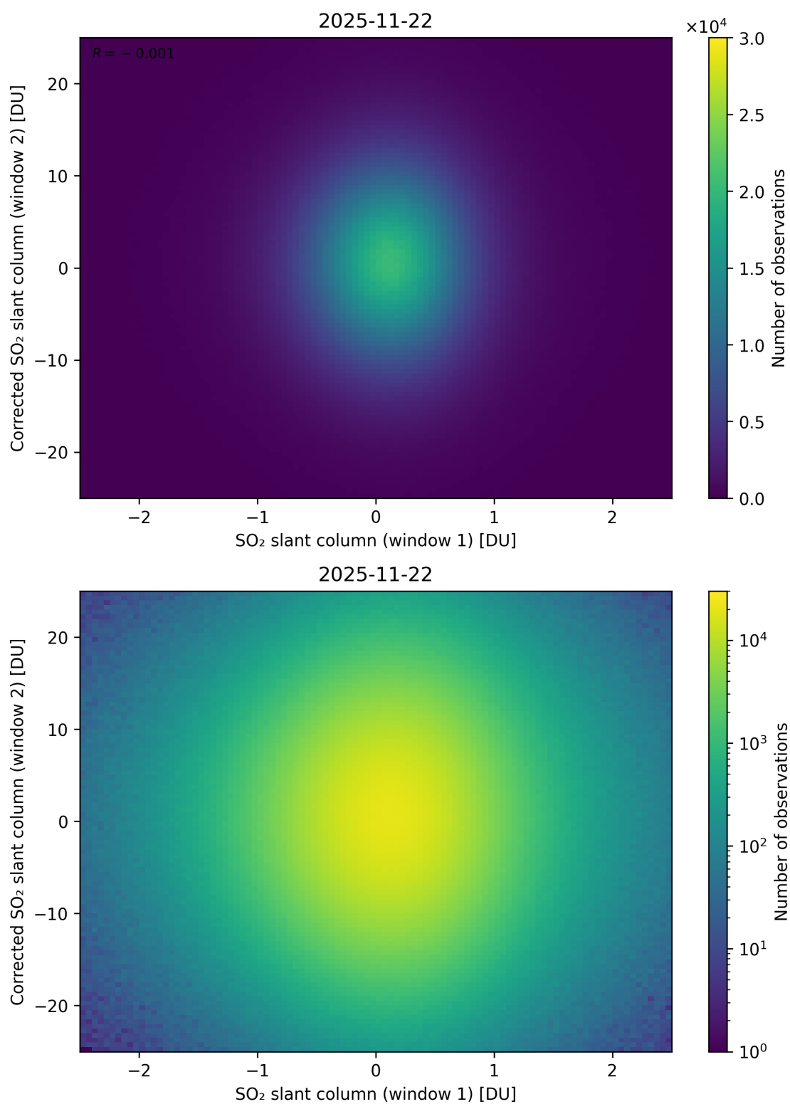
Figure 283: Scatter density plot of “SO 2 slant column (window 1)” against “Corrected SO 2 slant column (window 2)” for 2025-11-21 to 2025-11-23.
