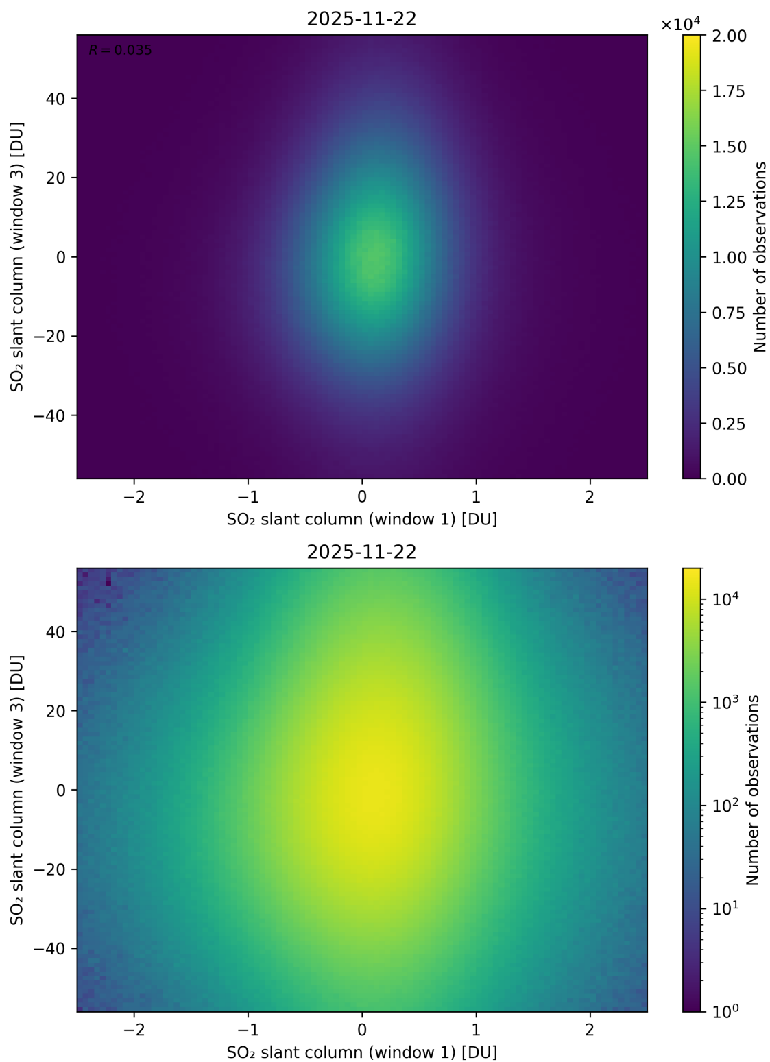
Figure 287: Scatter density plot of “SO 2 slant column (window 1)” against “SO 2 slant column (window 3)” for 2025-11-21 to 2025-11-23.
