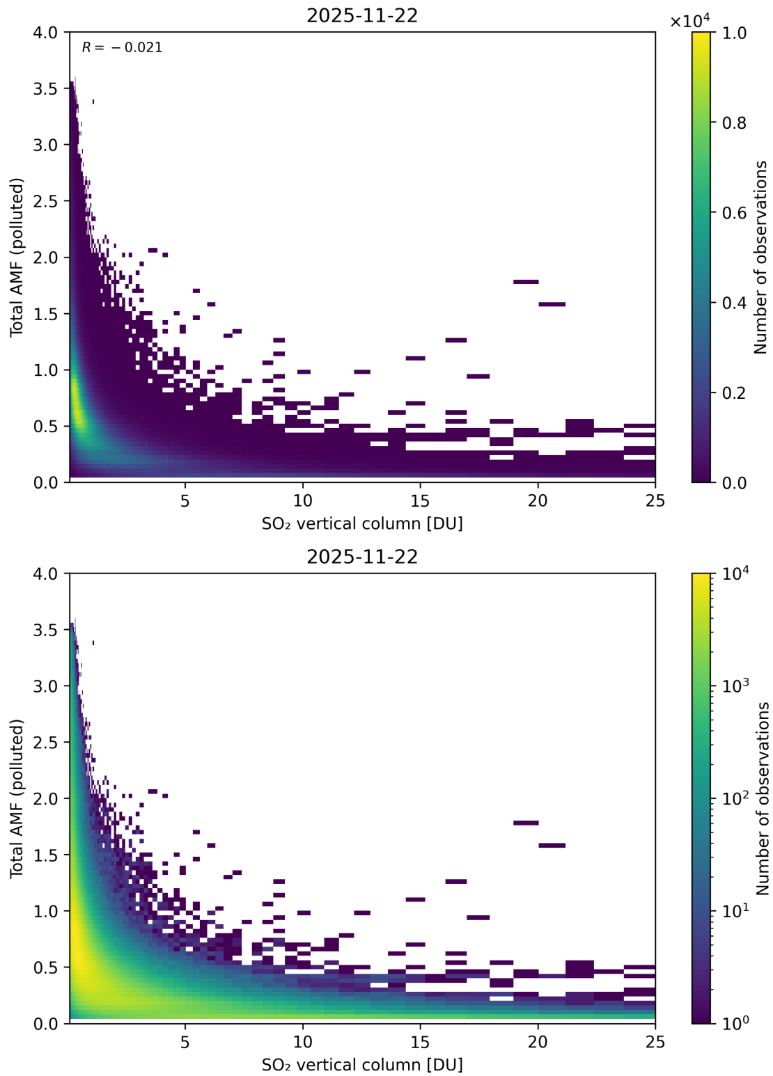
Figure 359: Scatter density plot of “SO 2 vertical column” against “Total AMF (polluted)” for 2025-11-21 to 2025-11-23.
