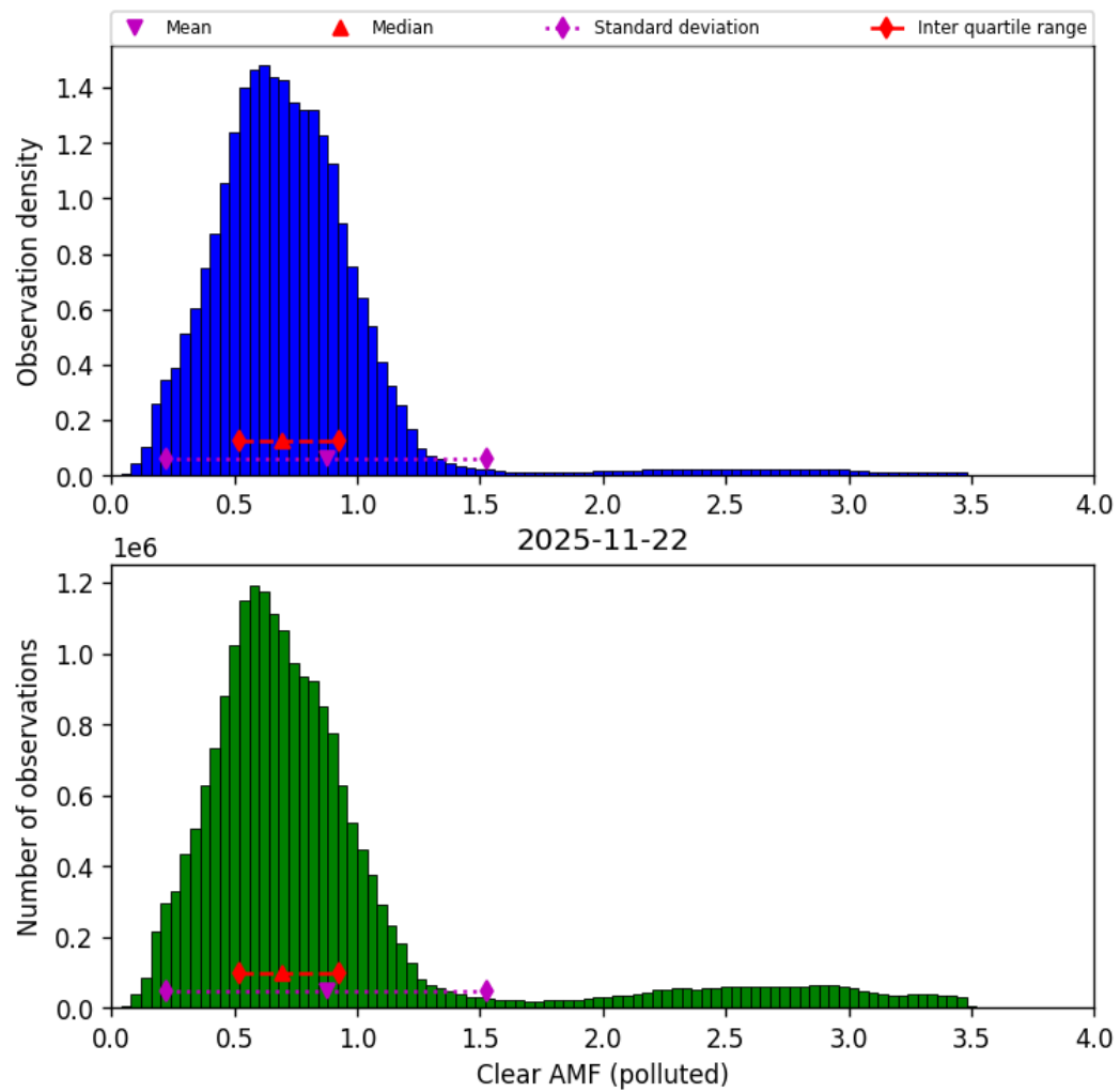
Figure 81: Histogram of “Clear AMF (polluted)” for 2025-11-21 to 2025-11-23
