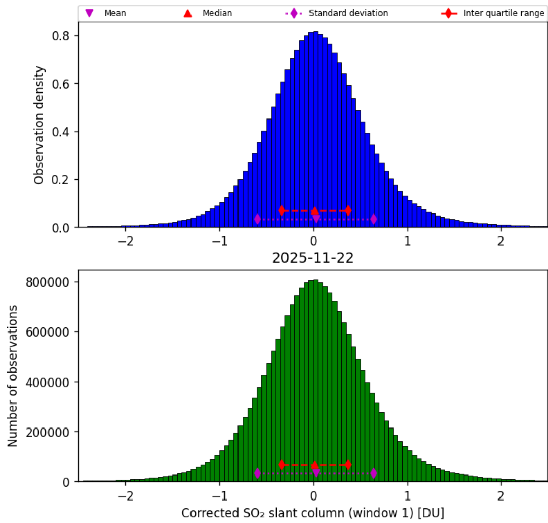
Figure 65: Histogram of “Corrected SO 2 slant column (window 1)” for 2025-11-21 to 2025-11-23
