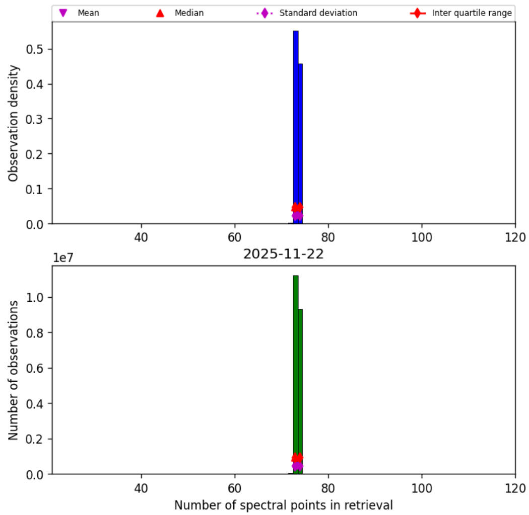
Figure 82: Histogram of “Number of spectral points in retrieval” for 2025-11-21 to 2025-11-23
