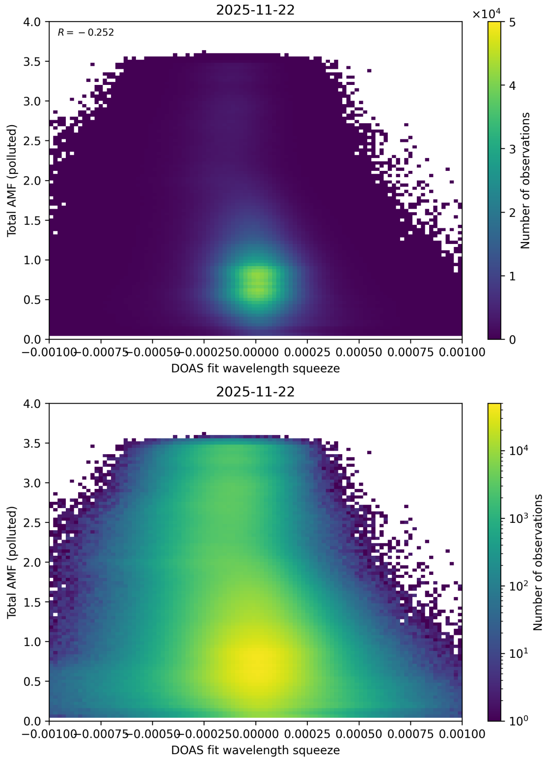
Figure 145: Scatter density plot of “DOAS fit wavelength squeeze” against “Total AMF (polluted)” for 2025-11-21 to 2025-11-23.
