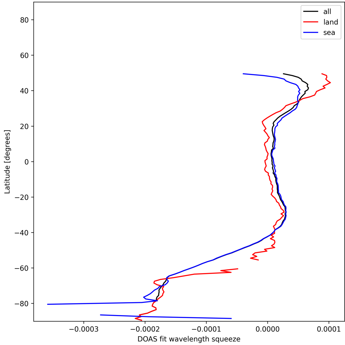
Figure 51: Zonal average of “DOAS fit wavelength squeeze” for 2025-11-21 to 2025-11-23.
