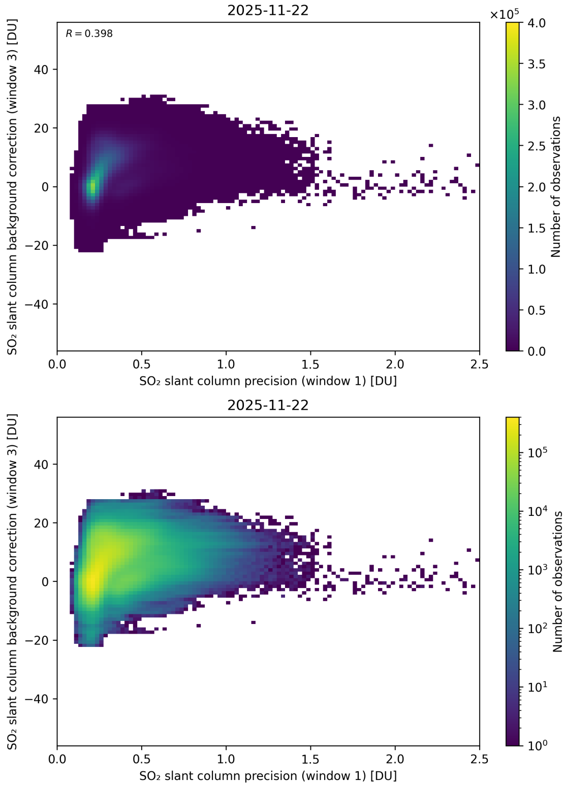
Figure 270: Scatter density plot of “SO 2 slant column precision (window 1)” against “SO 2 slant column background correction (window 3)” for 2025-11-21 to 2025-11-23.
