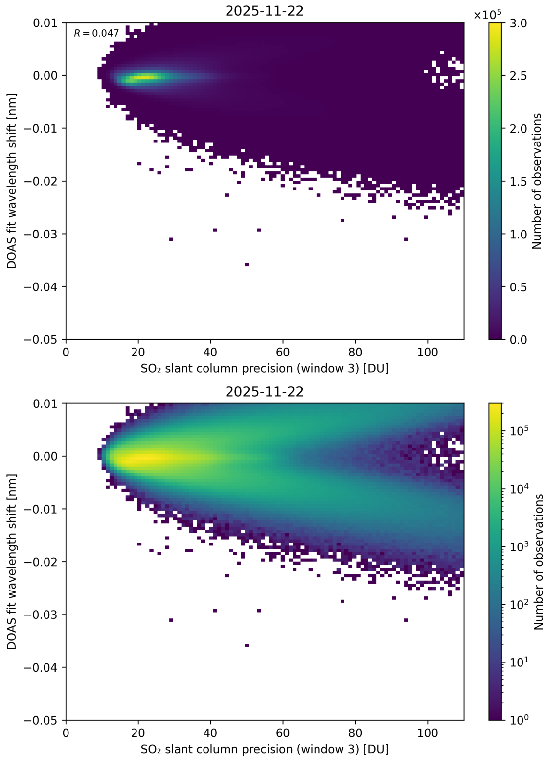
Figure 308: Scatter density plot of “SO 2 slant column precision (window 3)” against “DOAS fit wavelength shift” for 2025-11-21 to 2025-11-23.
