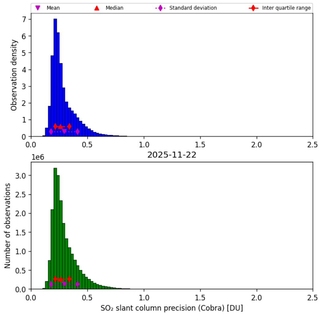
Figure 62: Histogram of “SO 2 slant column precision (Cobra)” for 2025-11-21 to 2025-11-23
