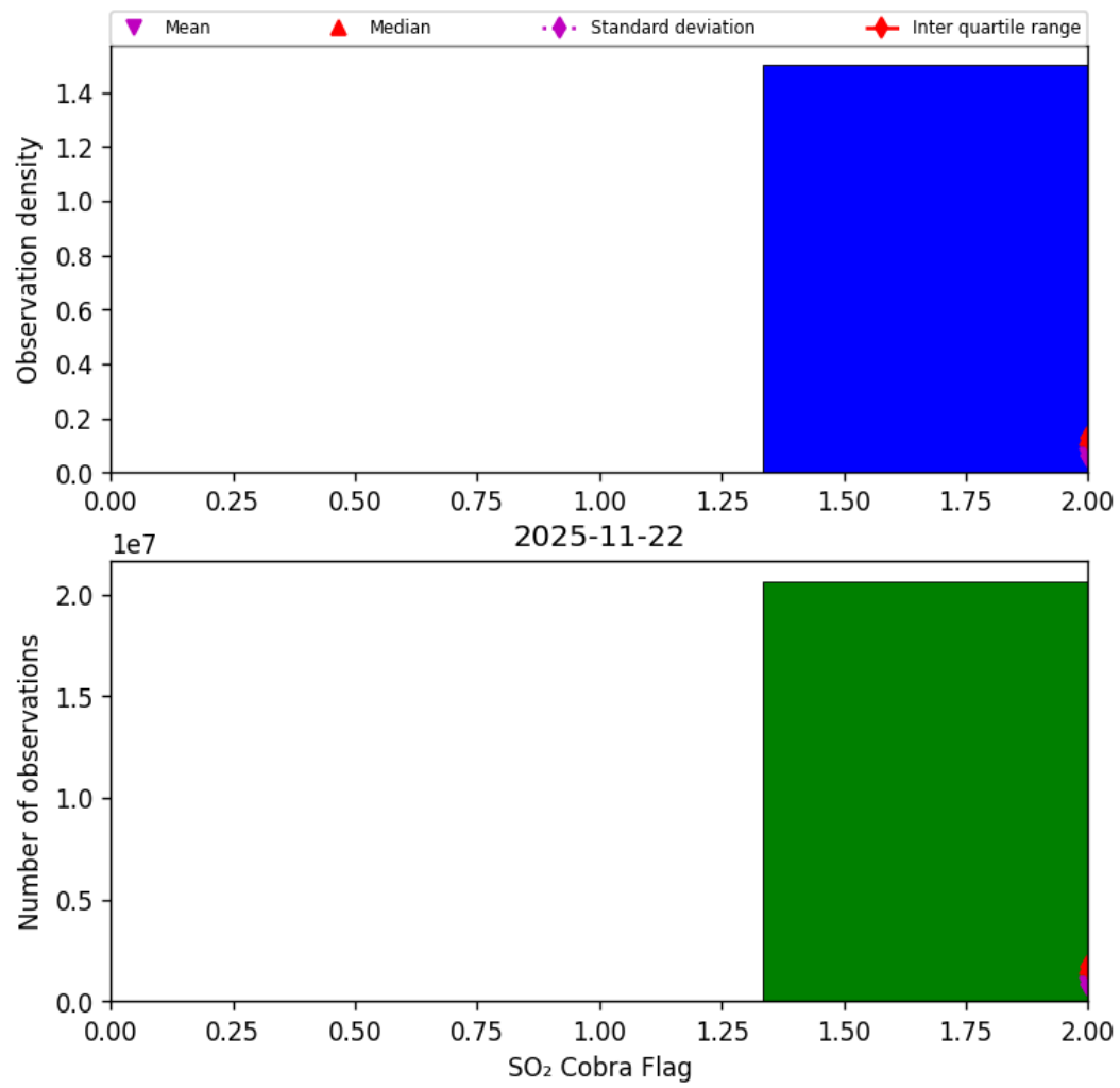
Figure 75: Histogram of “SO 2 Cobra Flag” for 2025-11-21 to 2025-11-23
