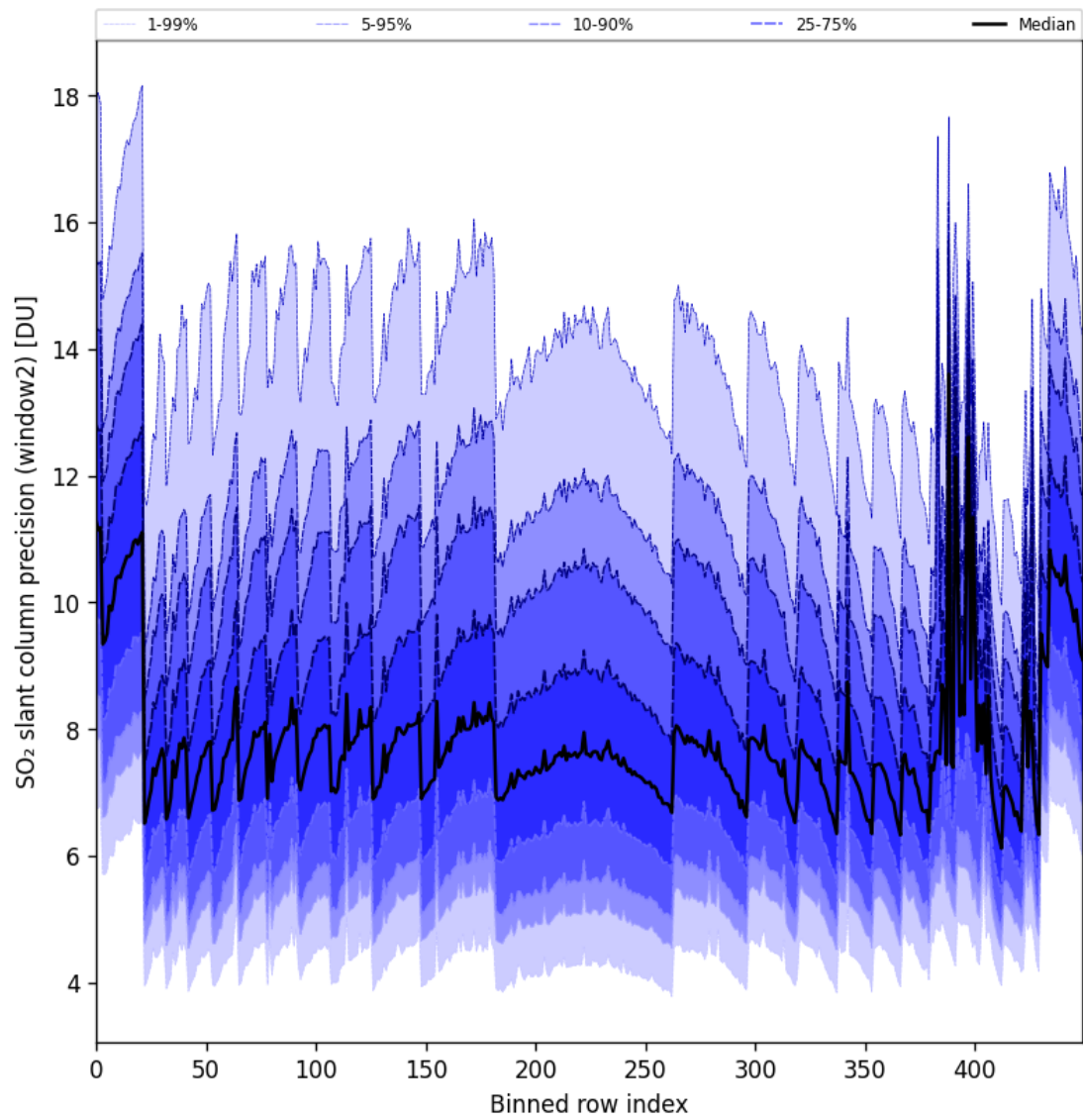
Figure 94: Along track statistics of “SO 2 slant column precision (window2)” for 2025-11-21 to 2025-11-23
