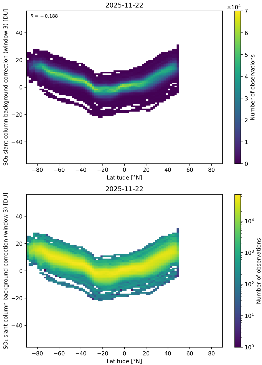
Figure 152: Scatter density plot of “Latitude” against “SO 2 slant column background correction (window 3)” for 2025-11-21 to 2025-11-23.
