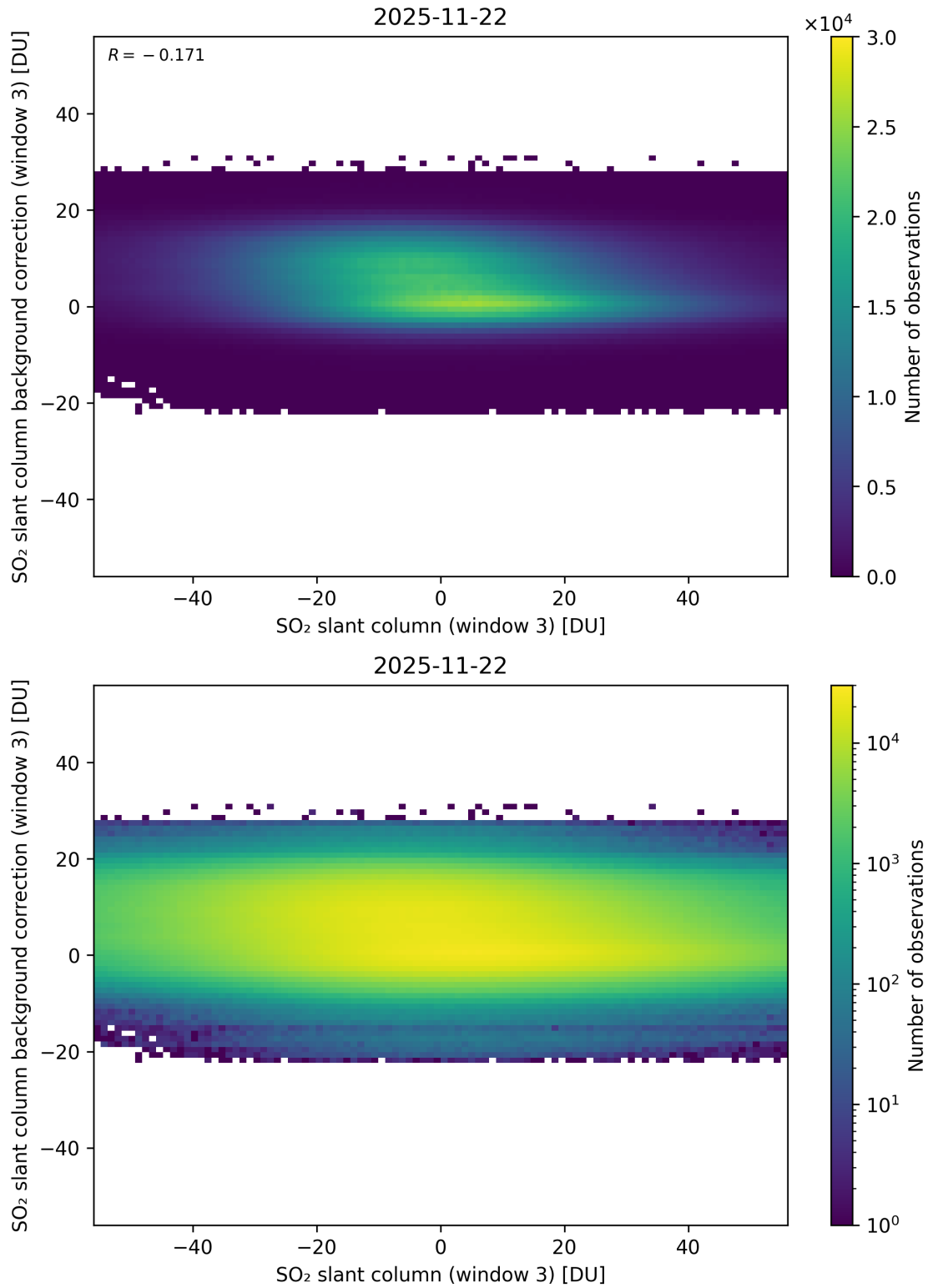
Figure 303: Scatter density plot of “SO 2 slant column (window 3)” against “SO 2 slant column background correction (window 3)” for 2025-11-21 to 2025-11-23.
