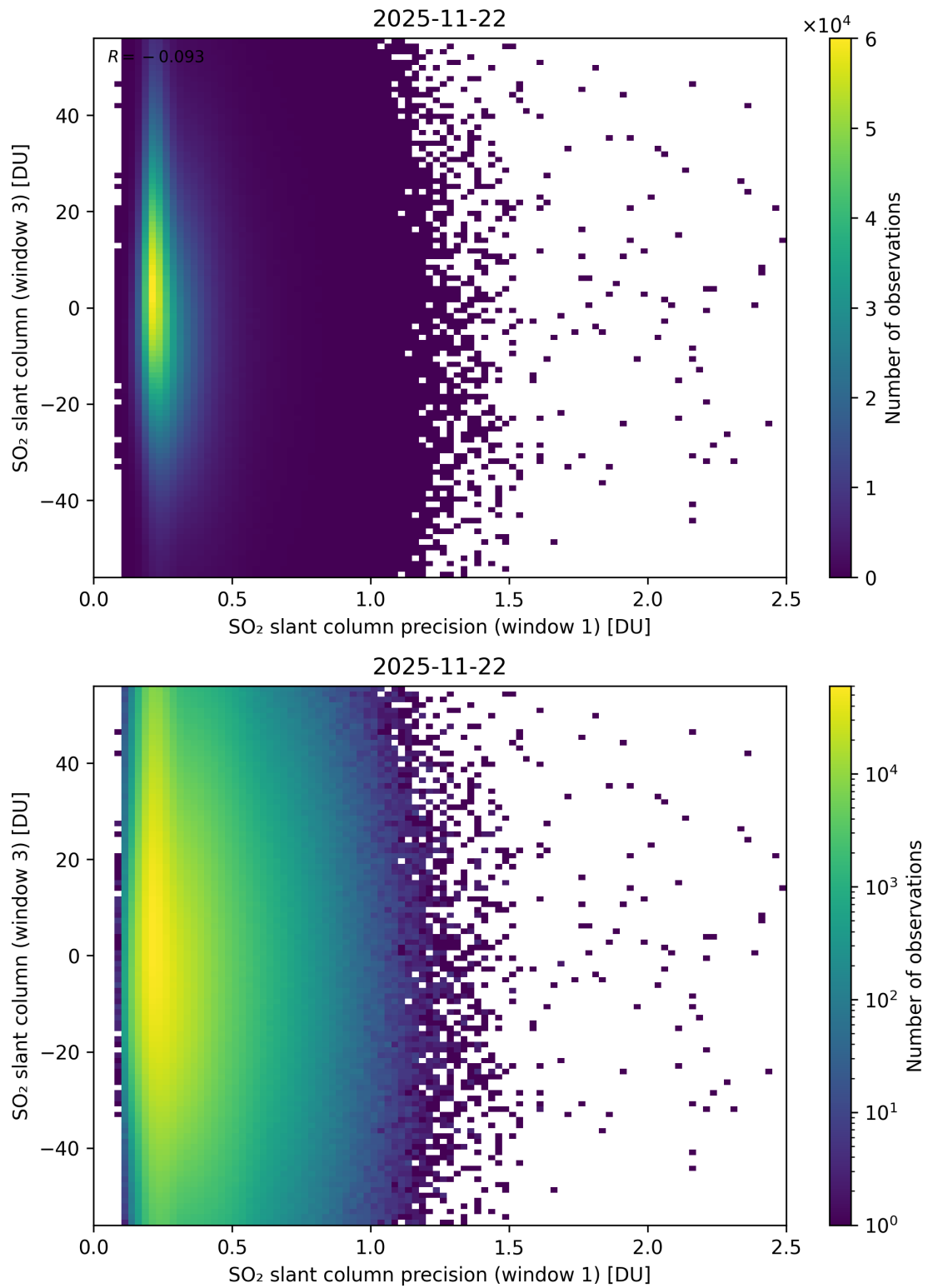
Figure 278: Scatter density plot of “SO 2 slant column precision (window 1)” against “SO 2 slant column (window 3)” for 2025-11-21 to 2025-11-23.
