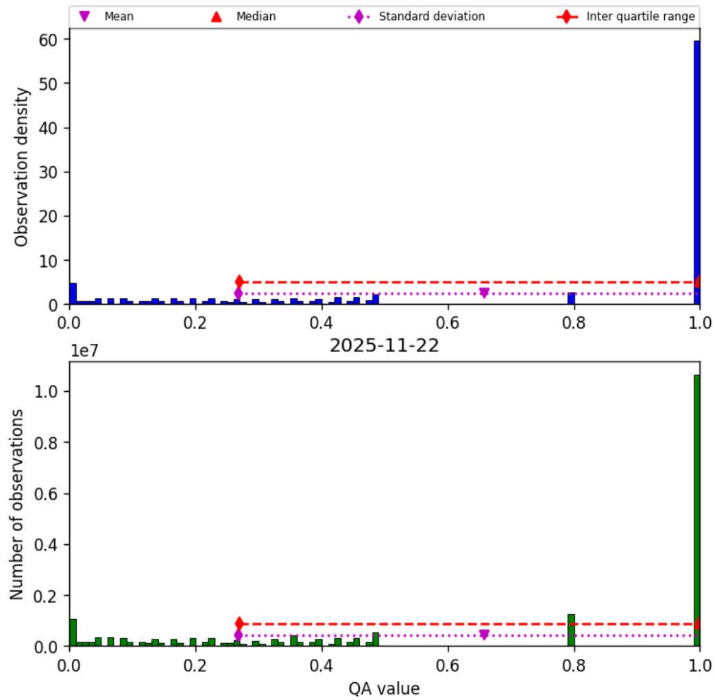
Figure 57: Histogram of “QA value” for 2025-11-21 to 2025-11-23
