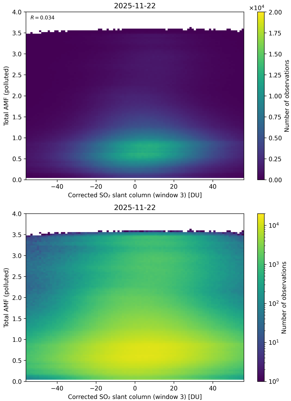
Figure 260: Scatter density plot of “Corrected SO 2 slant column (window 3)” against “Total AMF (polluted)” for 2025-11-21 to 2025-11-23.
