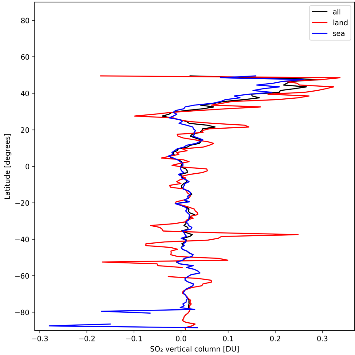
Figure 32: Zonal average of “SO 2 vertical column” for 2025-11-21 to 2025-11-23.
