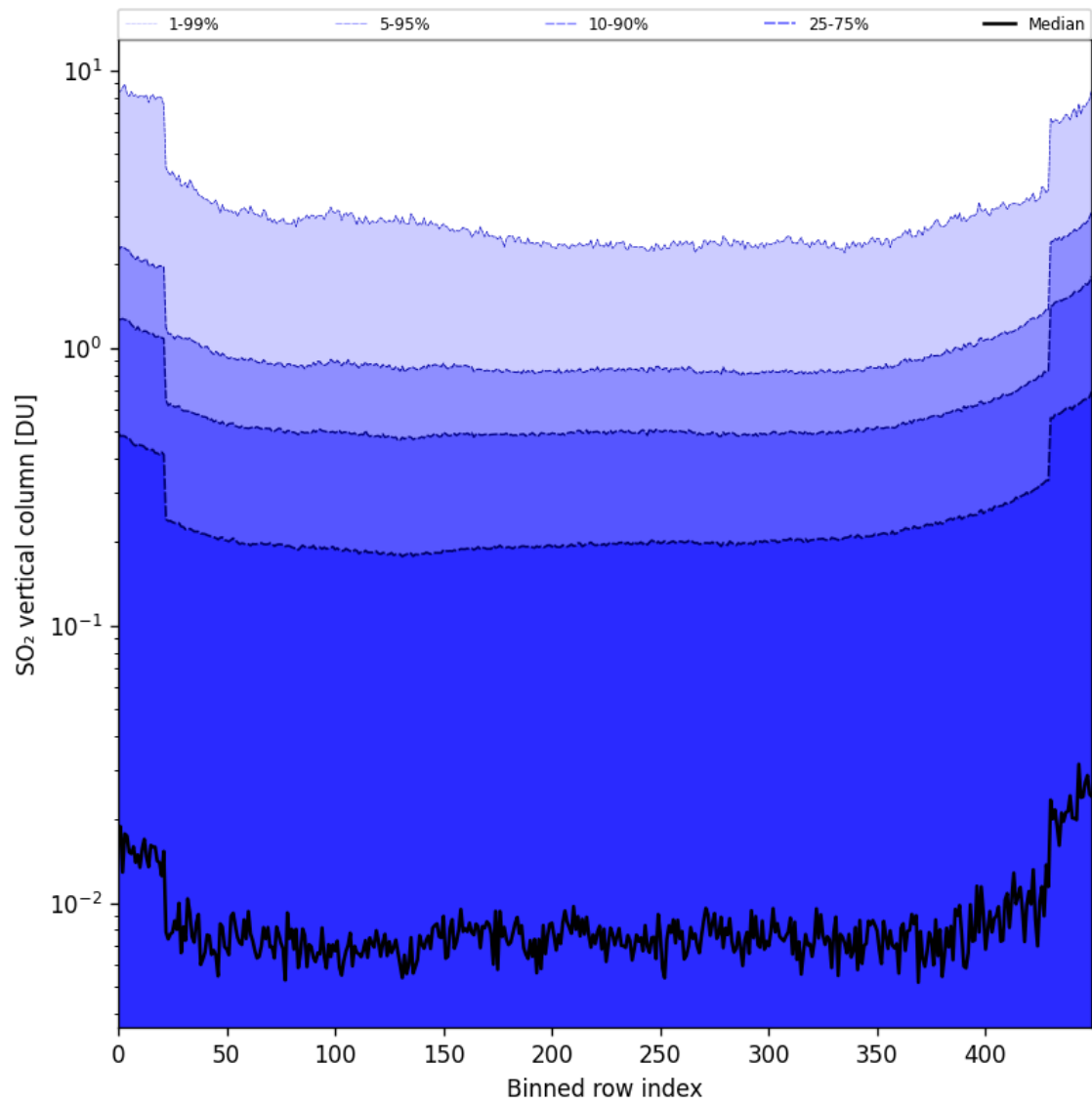
Figure 84: Along track statistics of “SO 2 vertical column” for 2025-11-21 to 2025-11-23
