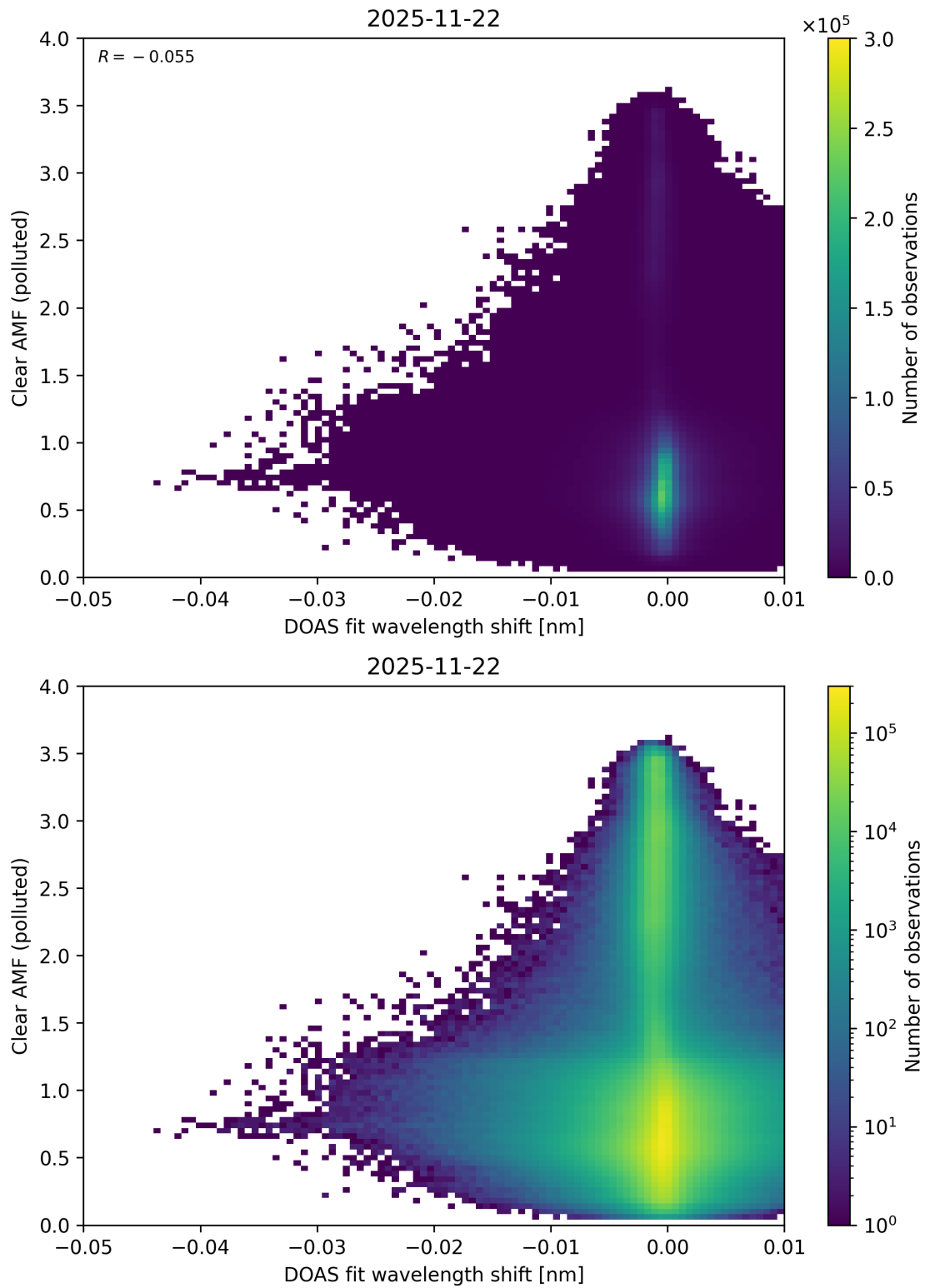
Figure 140: Scatter density plot of “DOAS fit wavelength shift” against “Clear AMF (polluted)” for 2025-11-21 to 2025-11-23.
