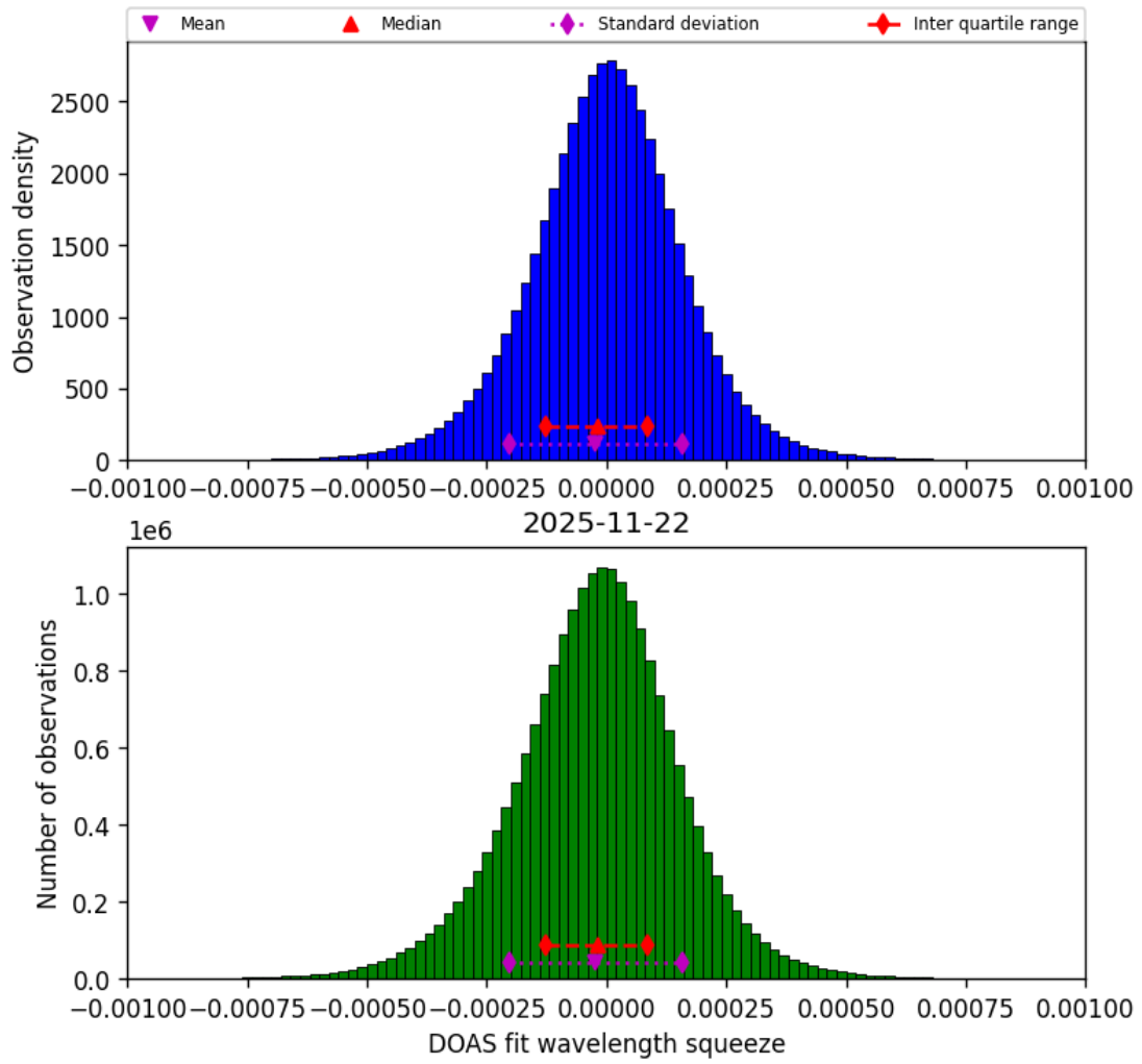
Figure 77: Histogram of “DOAS fit wavelength squeeze” for 2025-11-21 to 2025-11-23
