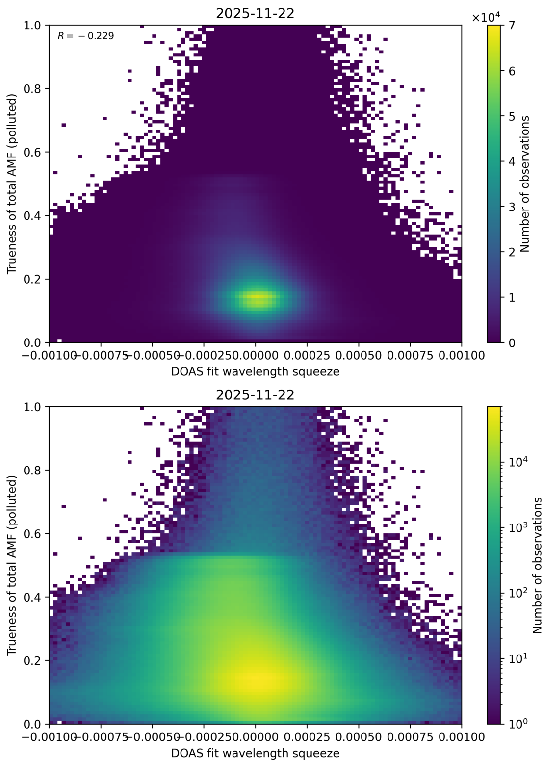
Figure 146: Scatter density plot of “DOAS fit wavelength squeeze” against “Trueness of total AMF (polluted)” for 2025-11-21 to 2025-11-23.
