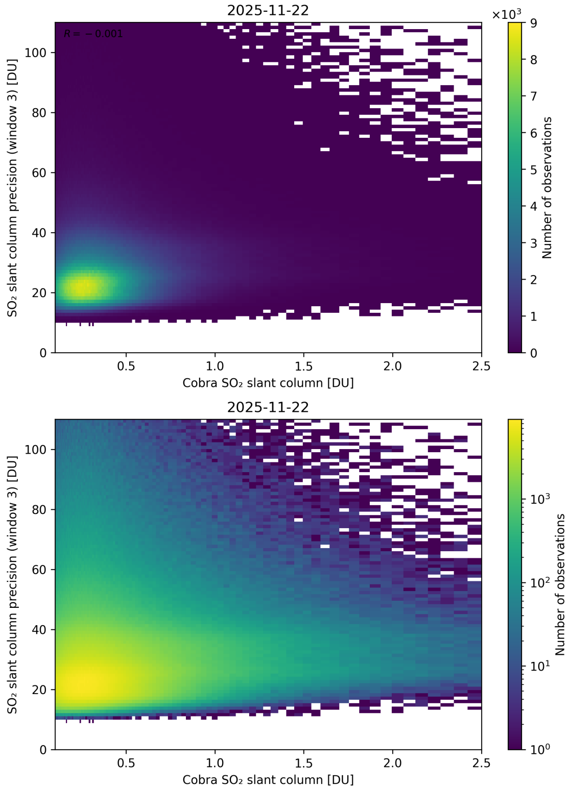
Figure 223: Scatter density plot of “Cobra SO 2 slant column” against “SO 2 slant column precision (window 3)” for 2025-11-21 to 2025-11-23.
