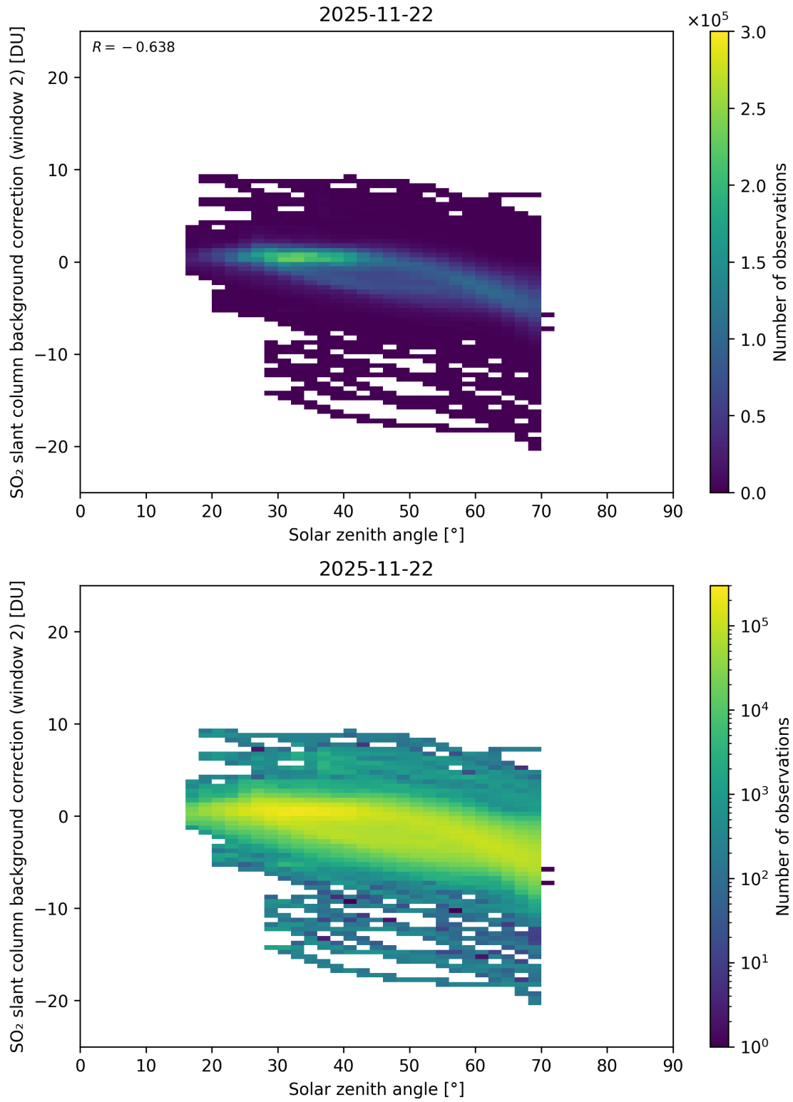
Figure 172: Scatter density plot of “Solar zenith angle” against “SO 2 slant column background correction (window 2)” for 2025-11-21 to 2025-11-23.
