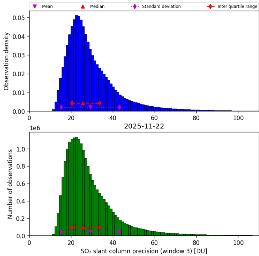
Figure 72: Histogram of “SO 2 slant column precision (window 3)” for 2025-11-21 to 2025-11-23
