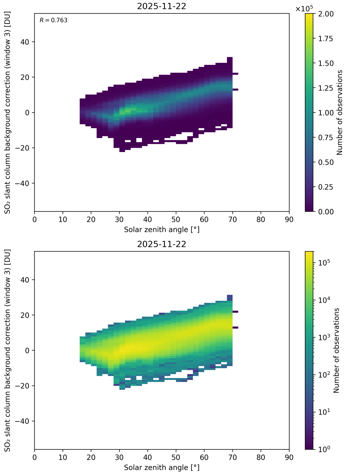
Figure 173: Scatter density plot of “Solar zenith angle” against “SO 2 slant column background correction (window 3)” for 2025-11-21 to 2025-11-23.
