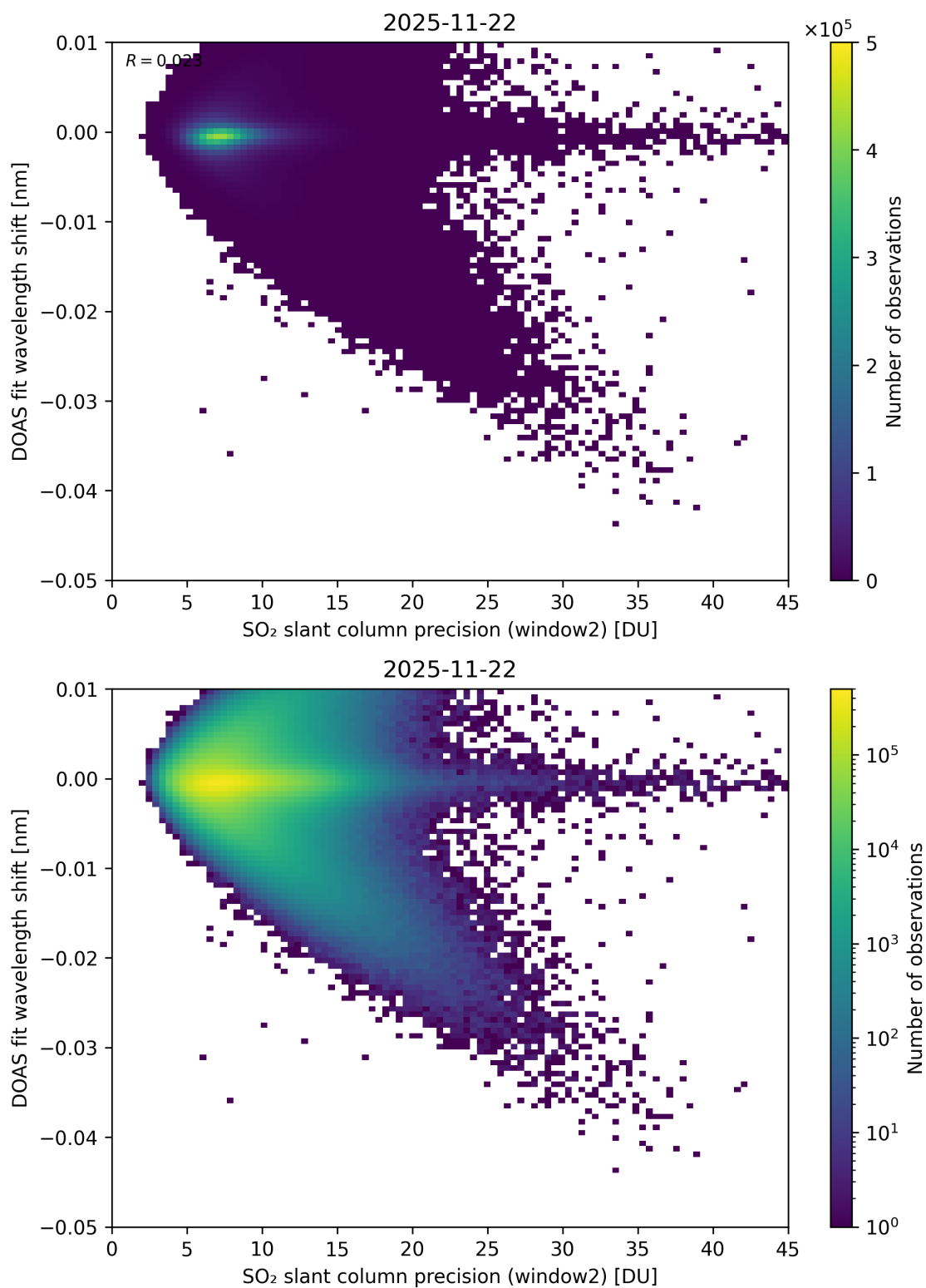
Figure 293: Scatter density plot of “SO 2 slant column precision (window2)” against “DOAS fit wavelength shift” for 2025-11-21 to 2025-11-23.
