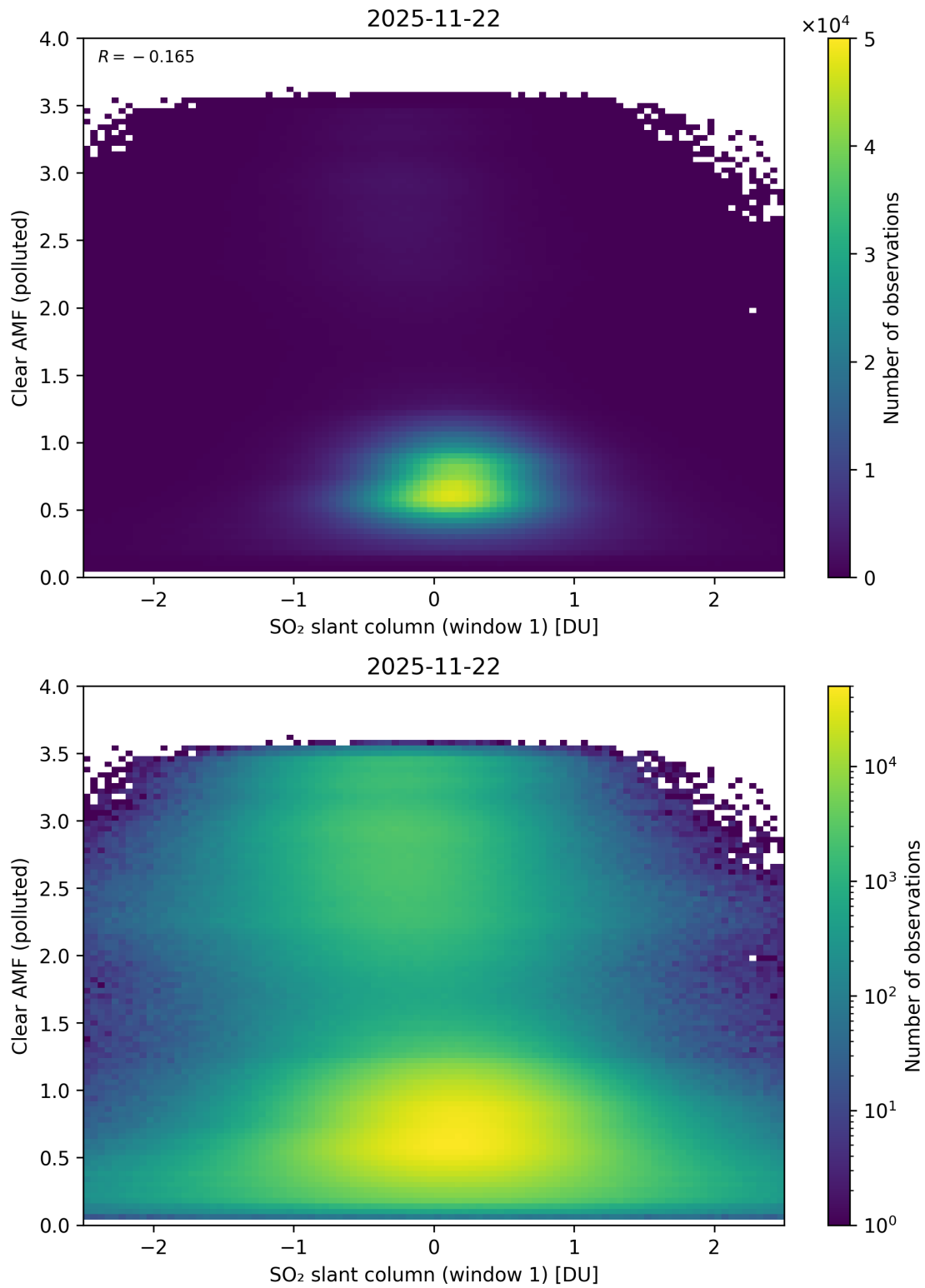
Figure 282: Scatter density plot of “SO 2 slant column (window 1)” against “Clear AMF (polluted)” for 2025-11-21 to 2025-11-23.
