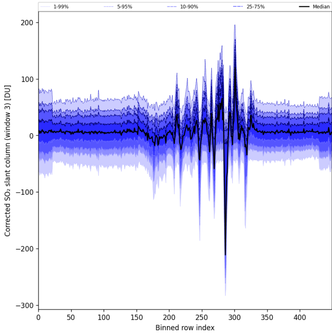
Figure 99: Along track statistics of “Corrected SO 2 slant column (window 3)” for 2025-11-21 to 2025-11-23
