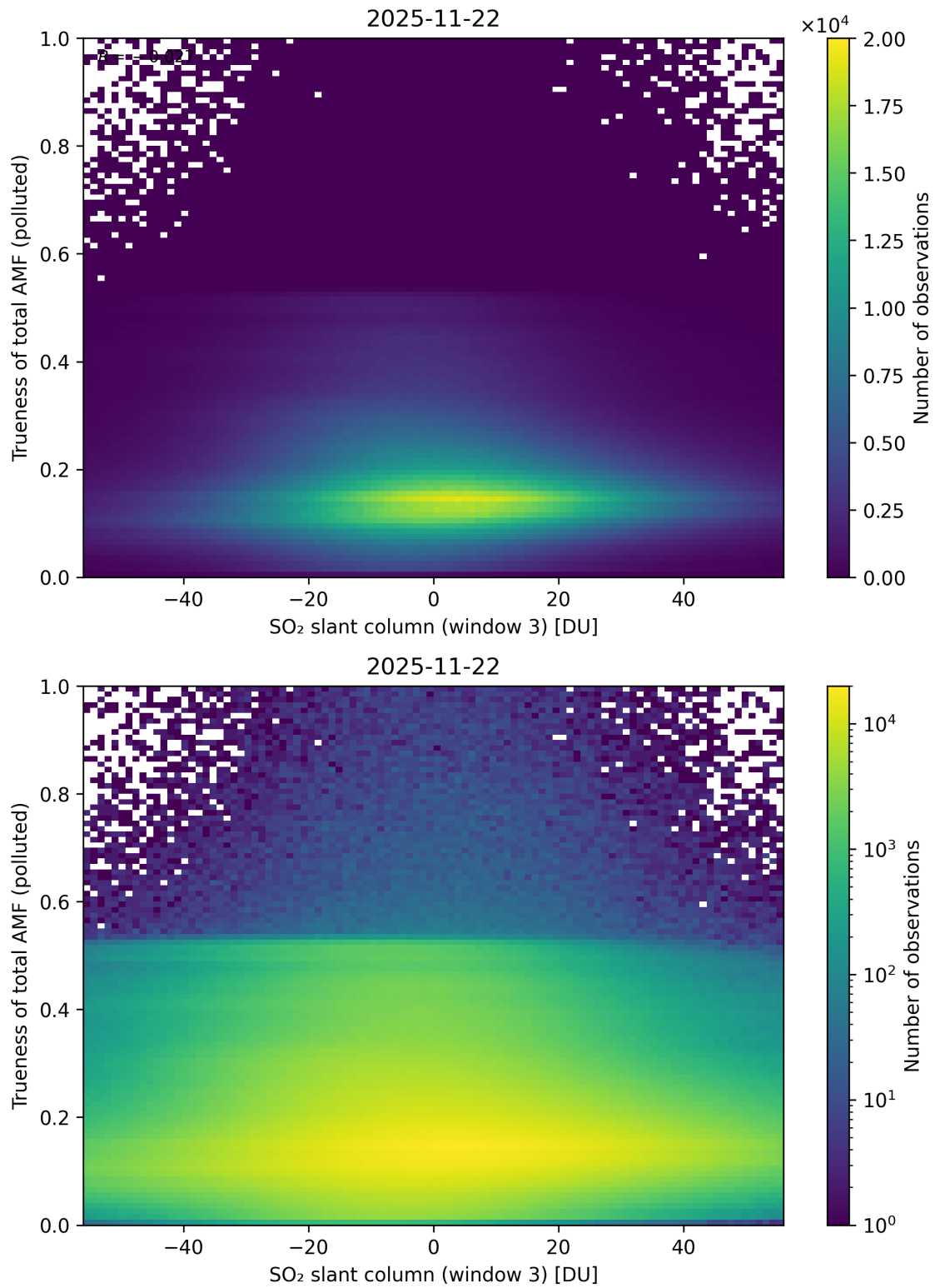
Figure 319: Scatter density plot of “SO 2 slant column (window 3)” against “Trueness of total AMF (polluted)” for 2025-11-21 to 2025-11-23.
