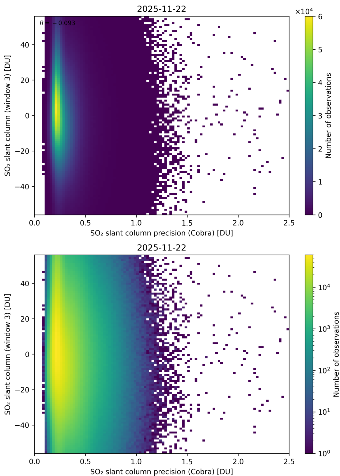
Figure 211: Scatter density plot of “SO 2 slant column precision (Cobra)” against “SO 2 slant column (window 3)” for 2025-11-21 to 2025-11-23.
