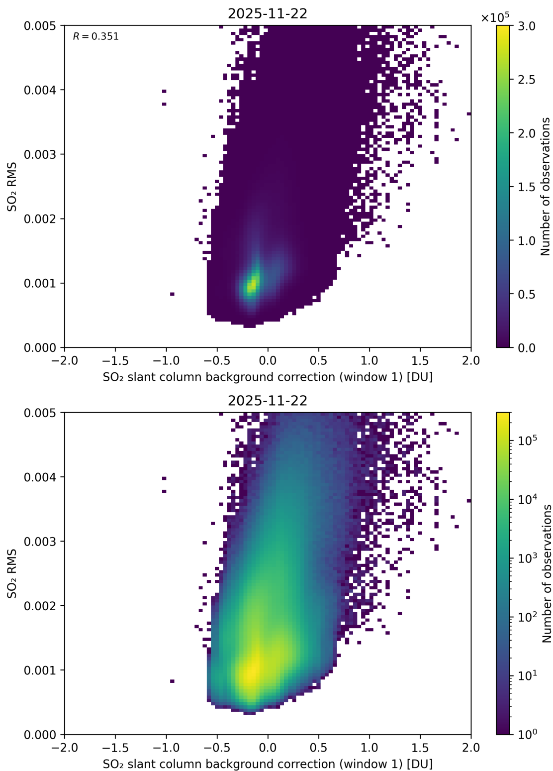
Figure 113: Scatter density plot of “SO 2 slant column background correction (window 1)” against “SO 2 RMS” for 2025-11-21 to 2025-11-23.
