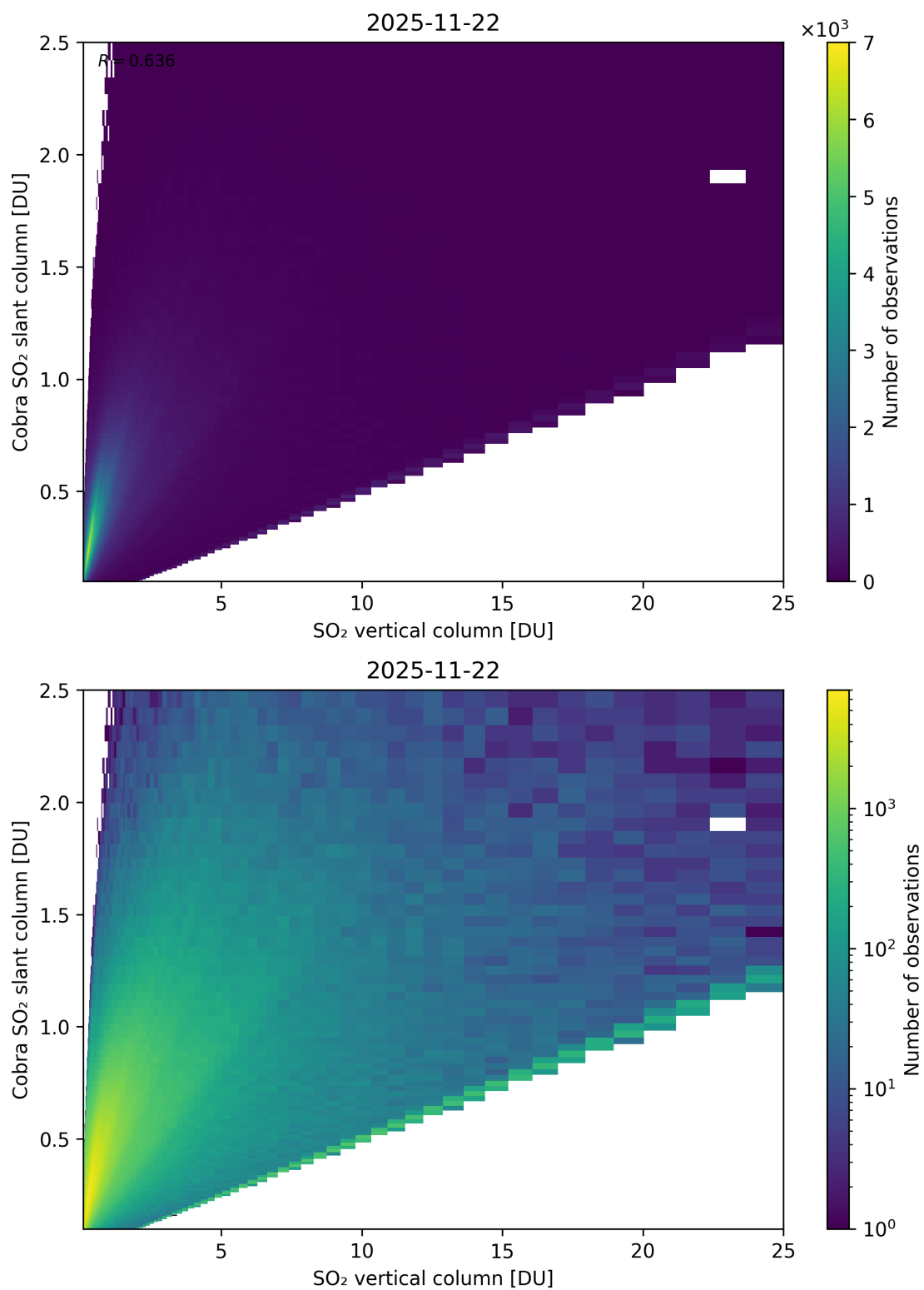
Figure 349: Scatter density plot of “SO 2 vertical column” against “Cobra SO 2 slant column” for 2025-11-21 to 2025-11-23.
