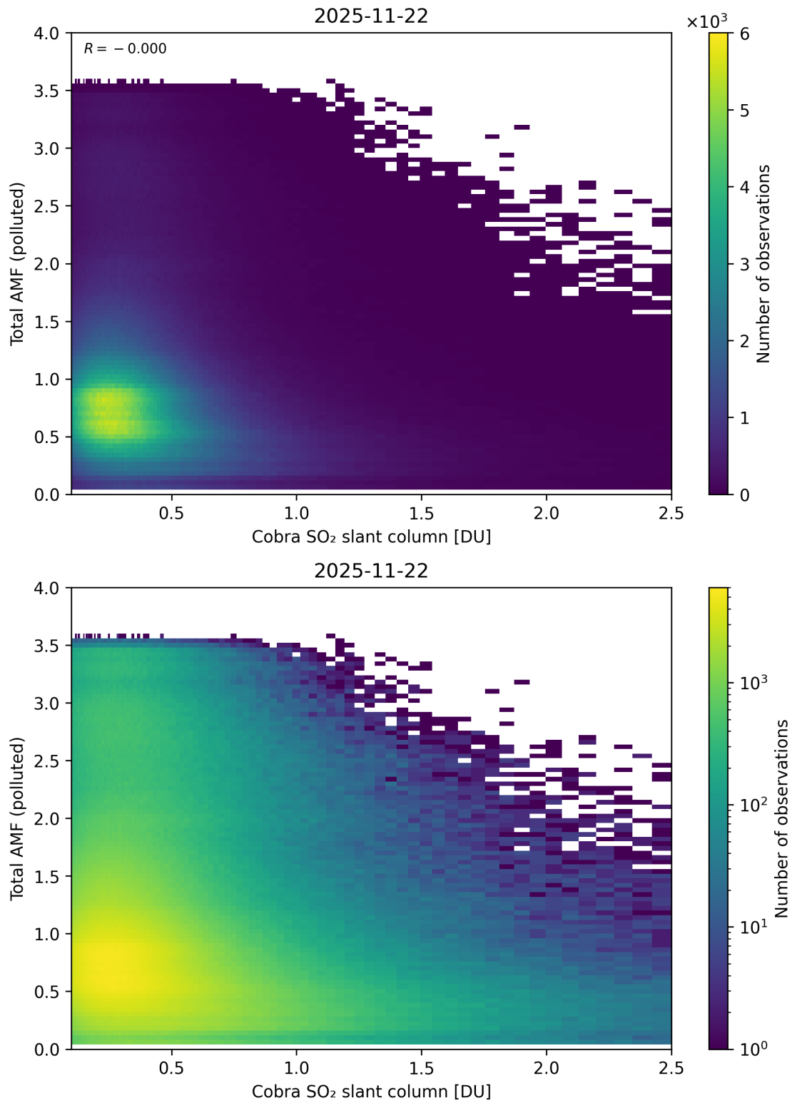
Figure 224: Scatter density plot of “Cobra SO 2 slant column” against “Total AMF (polluted)” for 2025-11-21 to 2025-11-23.
