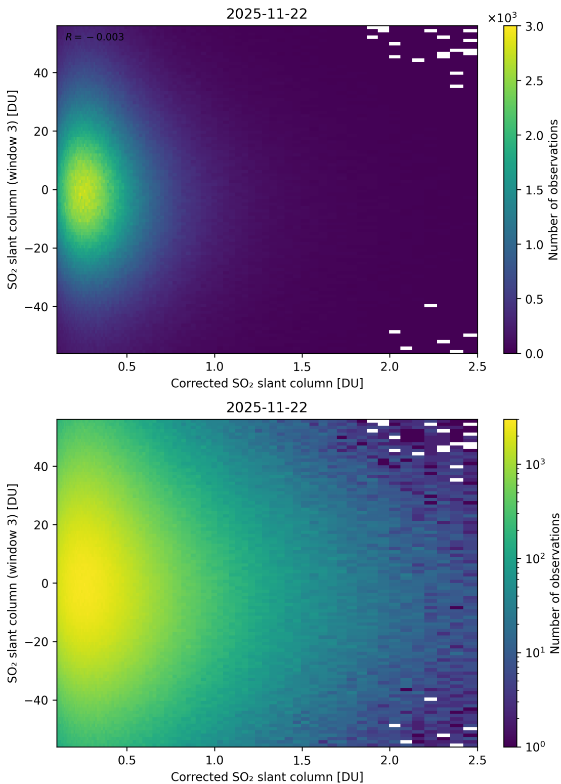
Figure 240: Scatter density plot of “Corrected SO 2 slant column” against “SO 2 slant column (window 3)” for 2025-11-21 to 2025-11-23.
