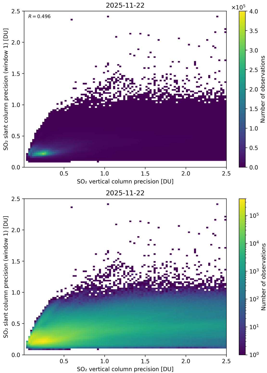
Figure 342: Scatter density plot of “SO 2 vertical column precision” against “SO 2 slant column precision (window 1)” for 2025-11-21 to 2025-11-23.
