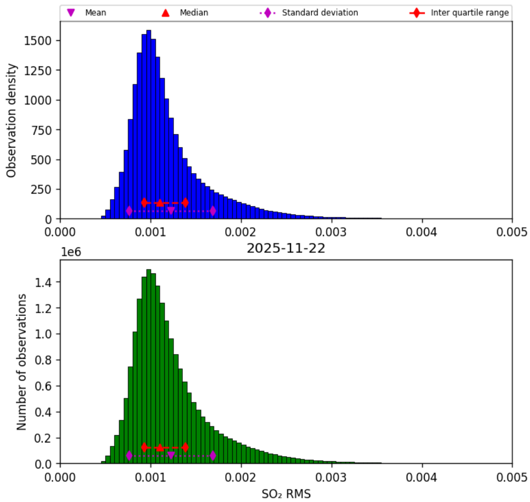
Figure 78: Histogram of “SO 2 RMS” for 2025-11-21 to 2025-11-23
