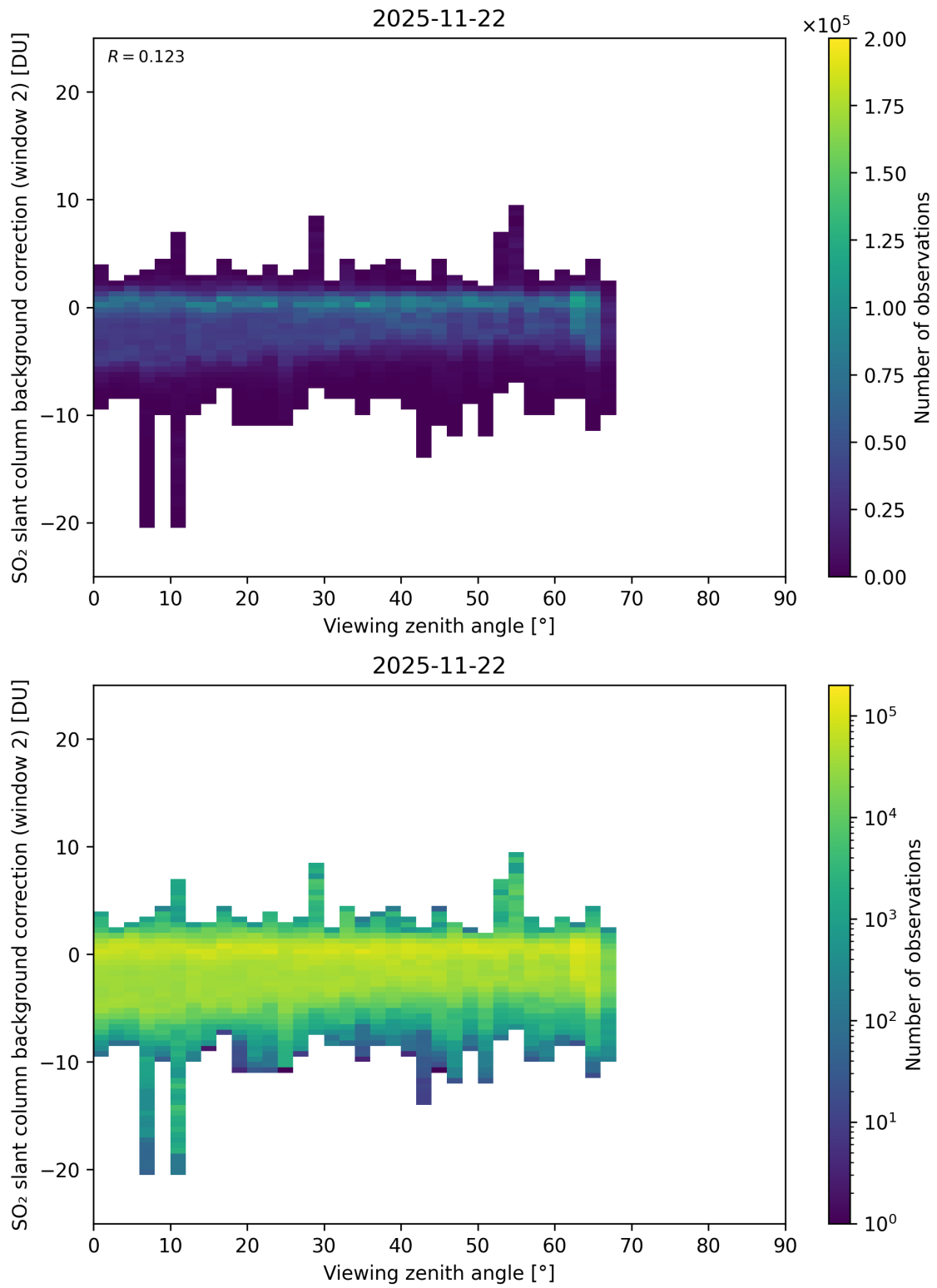
Figure 363: Scatter density plot of “Viewing zenith angle” against “SO 2 slant column background correction (window 2)” for 2025-11-21 to 2025-11-23.
