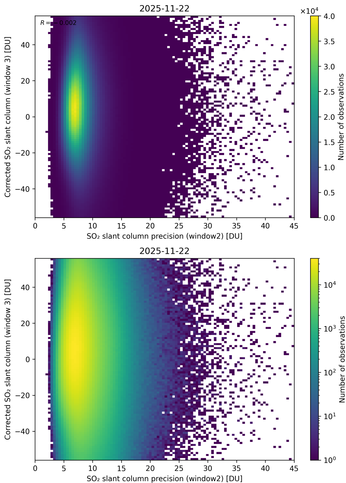
Figure 298: Scatter density plot of “SO 2 slant column precision (window2)” against “Corrected SO 2 slant column (window 3)” for 2025-11-21 to 2025-11-23.
