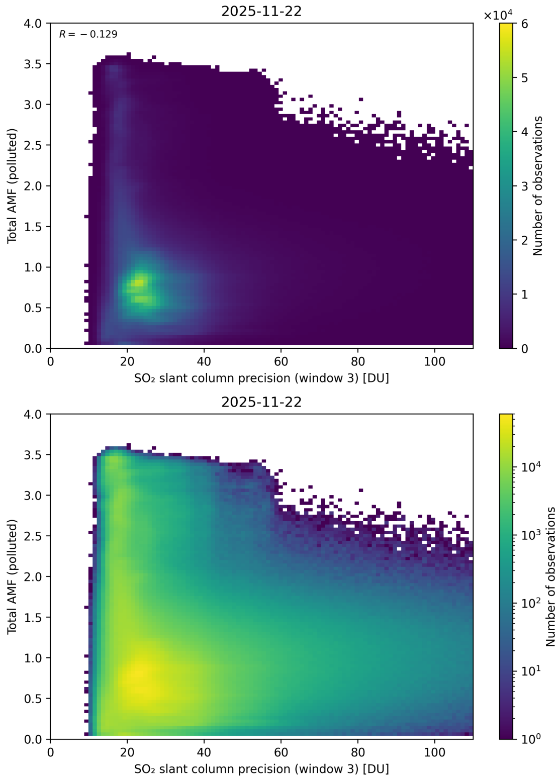
Figure 313: Scatter density plot of “SO 2 slant column precision (window 3)” against “Total AMF (polluted)” for 2025-11-21 to 2025-11-23.
