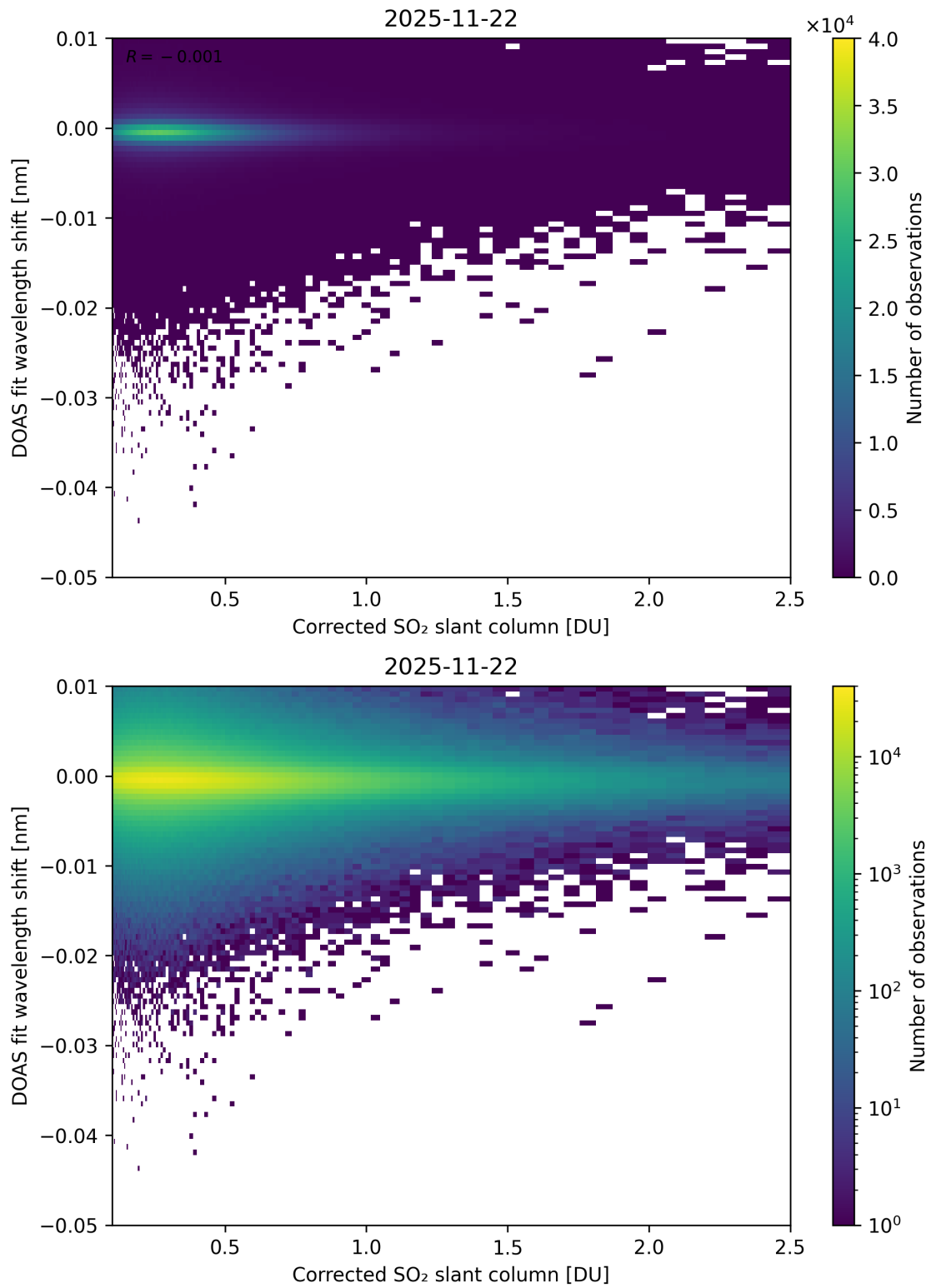
Figure 229: Scatter density plot of “Corrected SO 2 slant column” against “DOAS fit wavelength shift” for 2025-11-21 to 2025-11-23.
