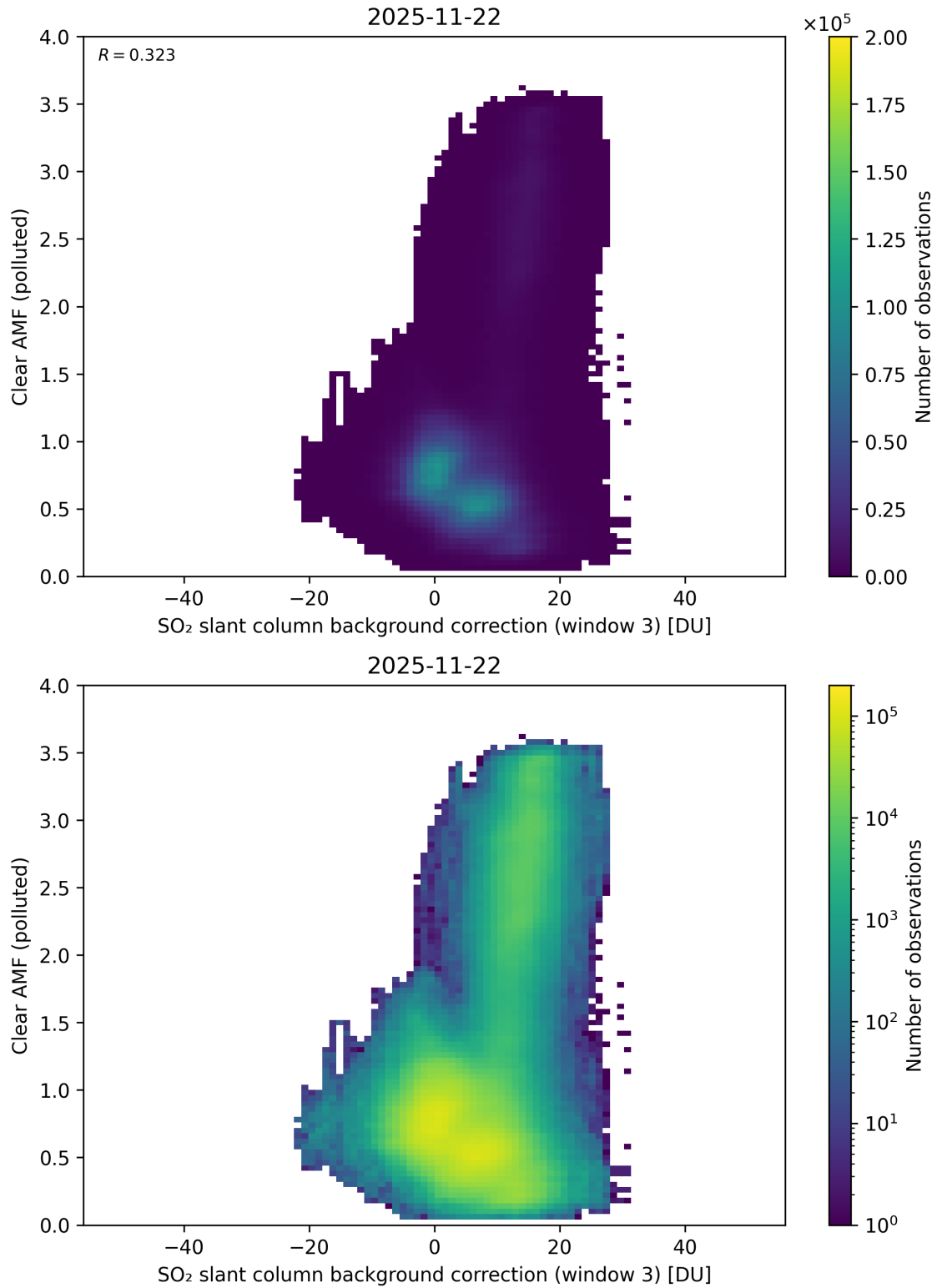
Figure 135: Scatter density plot of “SO 2 slant column background correction (window 3)” against “Clear AMF (polluted)” for 2025-11-21 to 2025-11-23.
