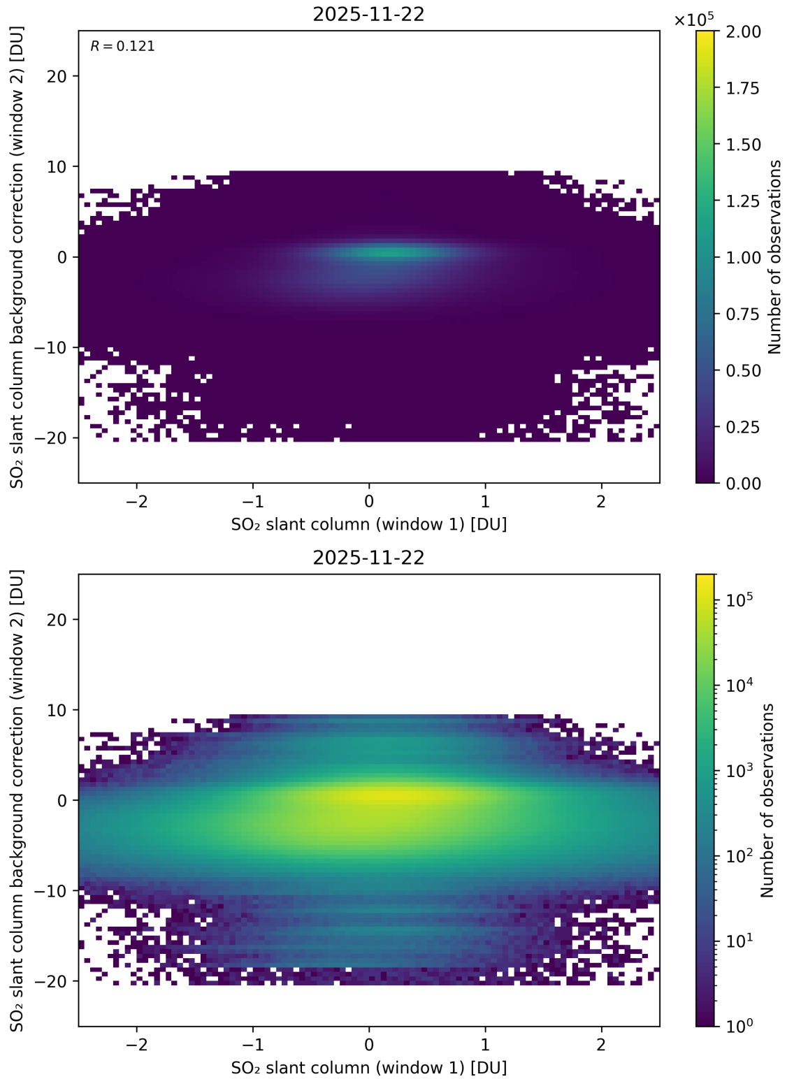
Figure 263: Scatter density plot of “SO 2 slant column (window 1)” against “SO 2 slant column background correction (window 2)” for 2025-11-21 to 2025-11-23.
