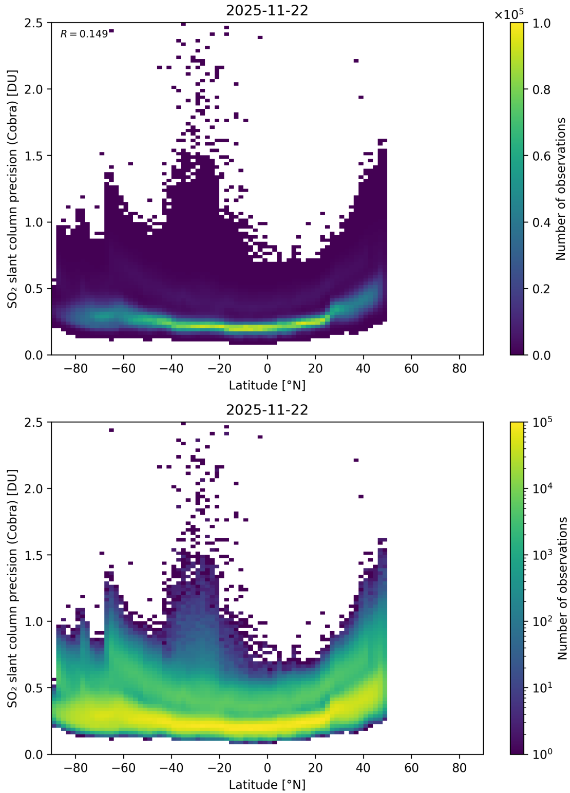
Figure 158: Scatter density plot of “Latitude” against “SO 2 slant column precision (Cobra)” for 2025-11-21 to 2025-11-23.
