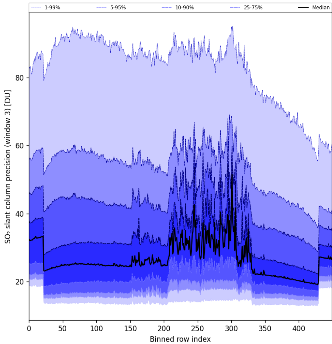
Figure 98: Along track statistics of “SO 2 slant column precision (window 3)” for 2025-11-21 to 2025-11-23
