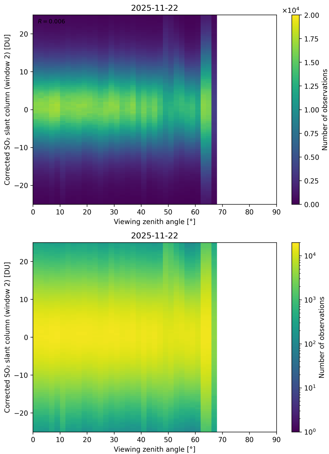
Figure 374: Scatter density plot of “Viewing zenith angle” against “Corrected SO 2 slant column (window 2)” for 2025-11-21 to 2025-11-23.
