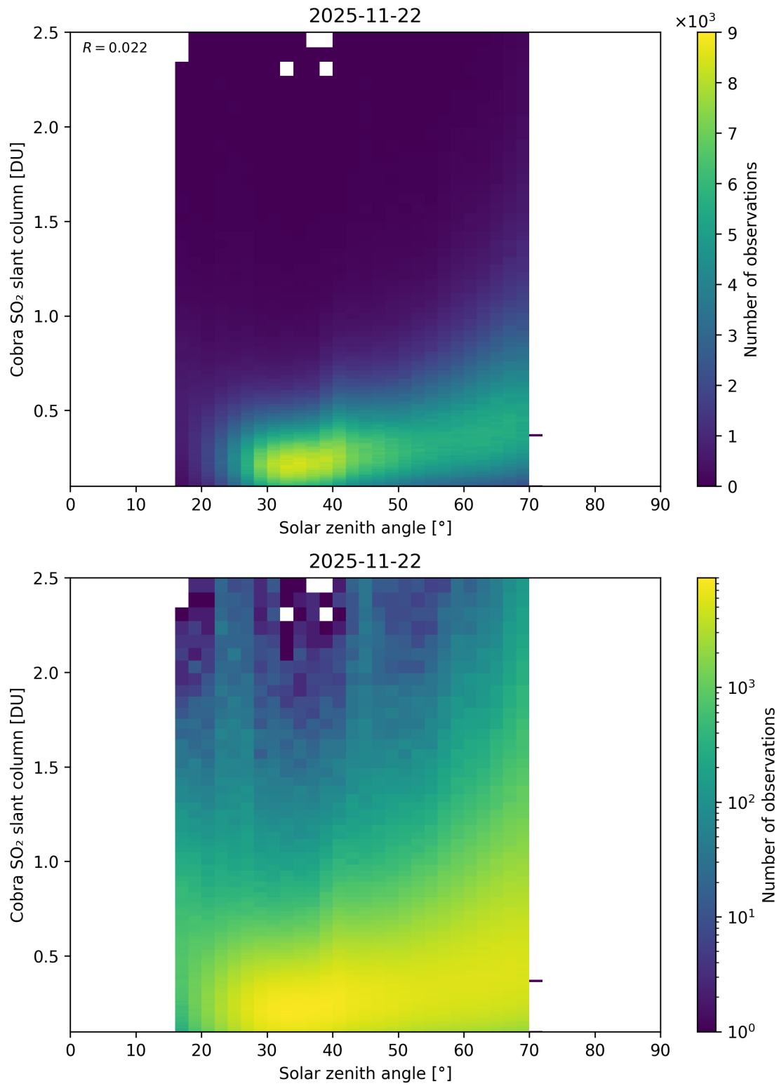
Figure 179: Scatter density plot of “Solar zenith angle” against “Cobra SO 2 slant column” for 2025-11-21 to 2025-11-23.
