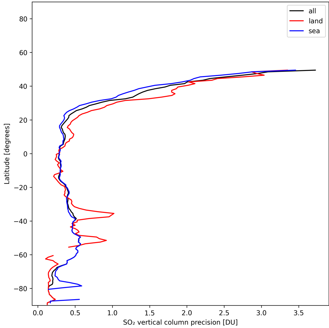
Figure 33: Zonal average of “SO 2 vertical column precision” for 2025-11-21 to 2025-11-23.
