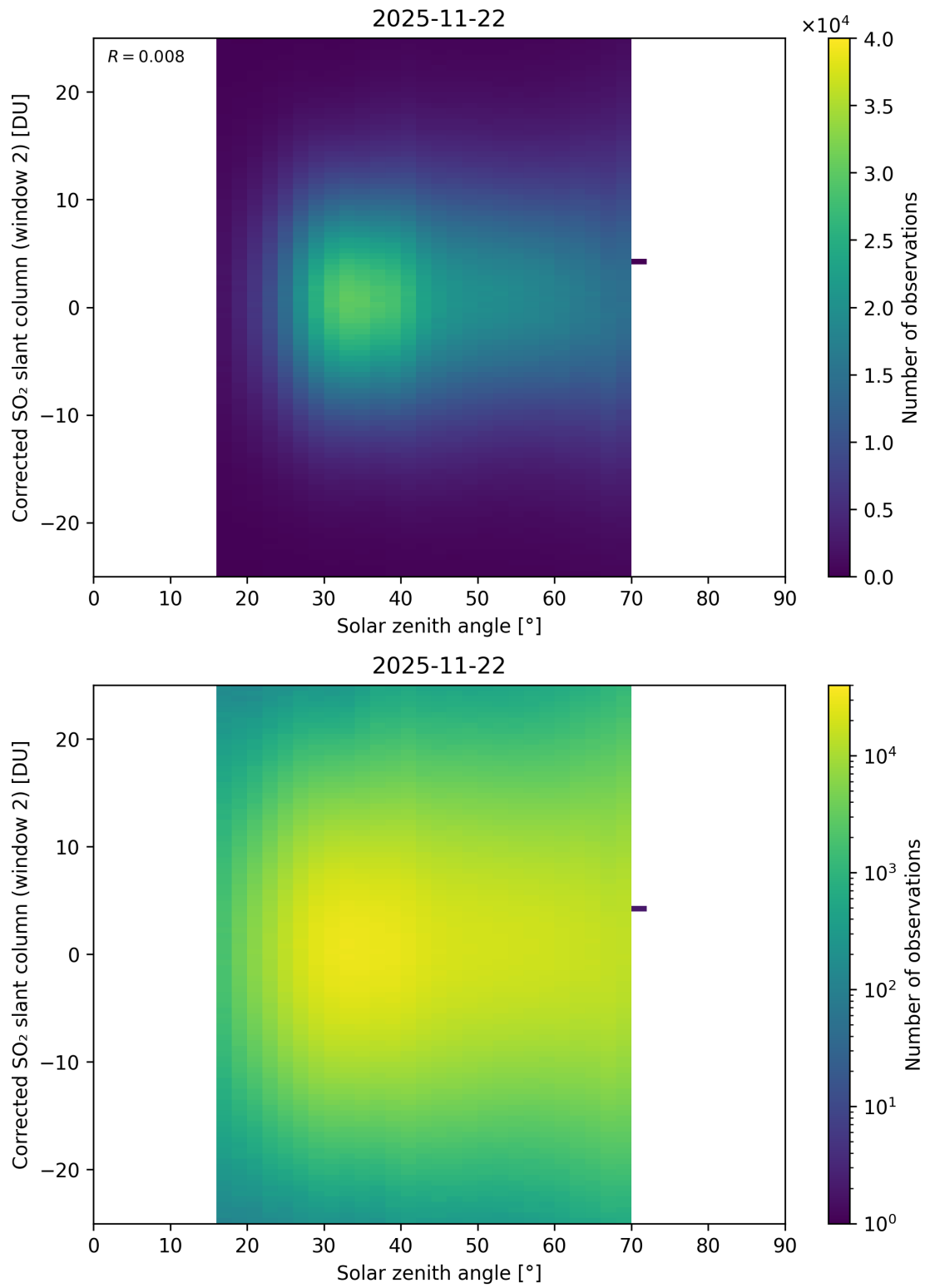
Figure 182: Scatter density plot of “Solar zenith angle” against “Corrected SO 2 slant column (window 2)” for 2025-11-21 to 2025-11-23.
