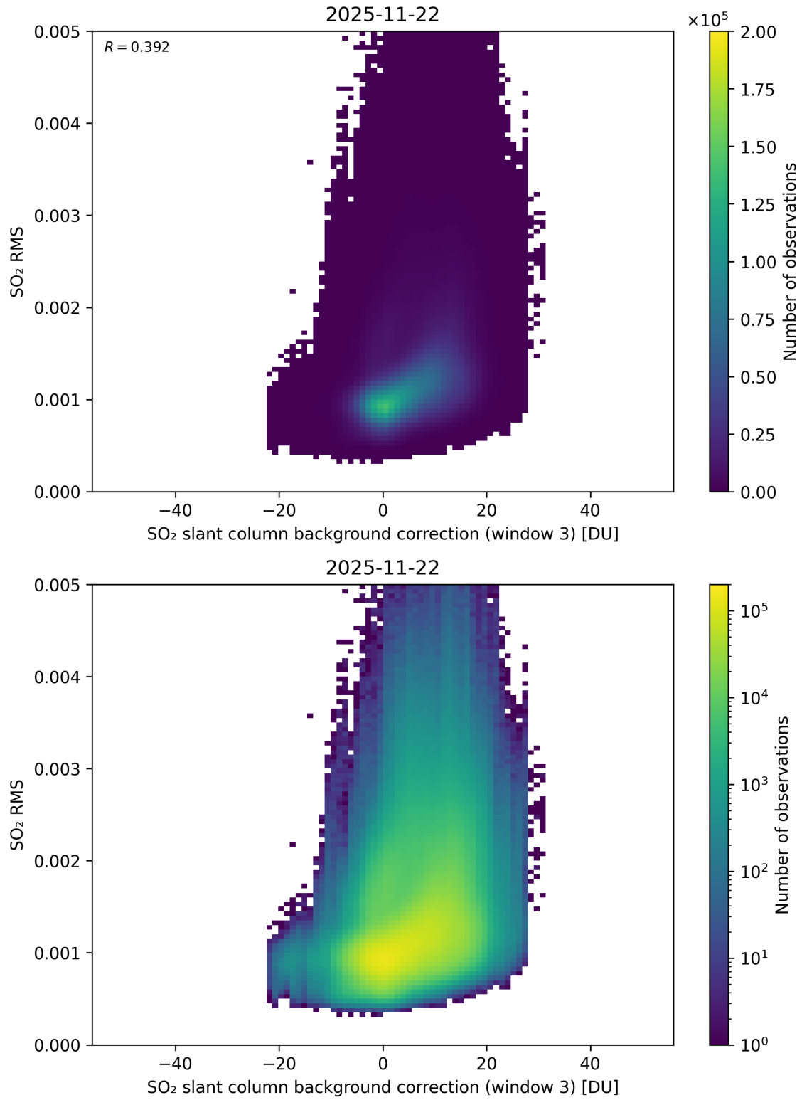
Figure 134: Scatter density plot of “SO 2 slant column background correction (window 3)” against “SO 2 RMS” for 2025-11-21 to 2025-11-23.
