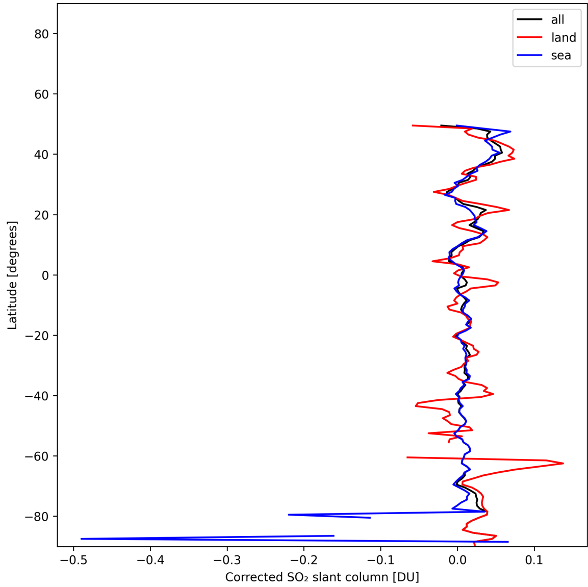
Figure 34: Zonal average of “Corrected SO 2 slant column” for 2025-11-21 to 2025-11-23.
