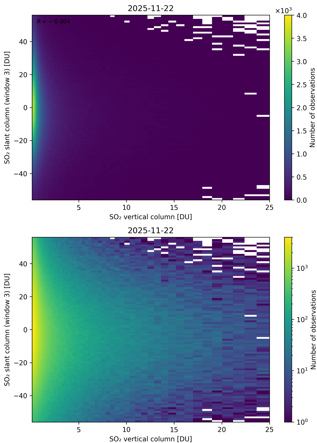
Figure 357: Scatter density plot of “SO 2 vertical column” against “SO 2 slant column (window 3)” for 2025-11-21 to 2025-11-23.
