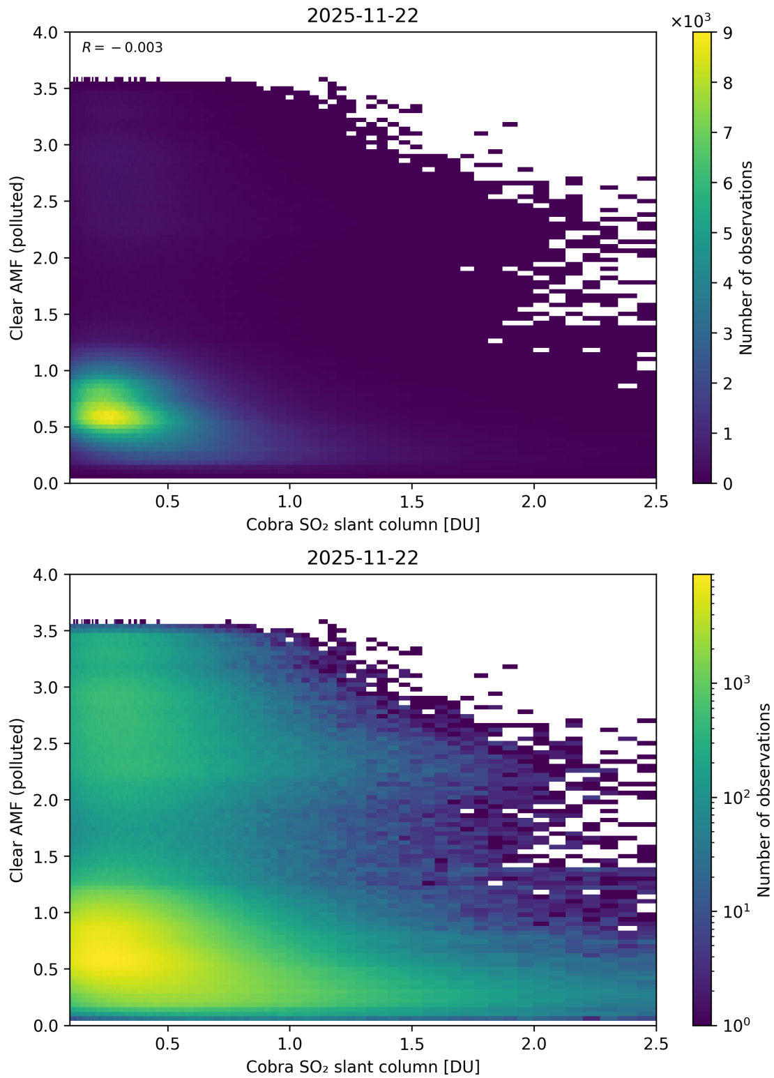
Figure 215: Scatter density plot of “Cobra SO 2 slant column” against “Clear AMF (polluted)” for 2025-11-21 to 2025-11-23.
