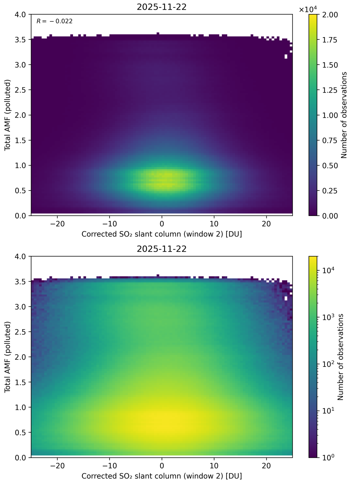
Figure 253: Scatter density plot of “Corrected SO 2 slant column (window 2)” against “Total AMF (polluted)” for 2025-11-21 to 2025-11-23.
