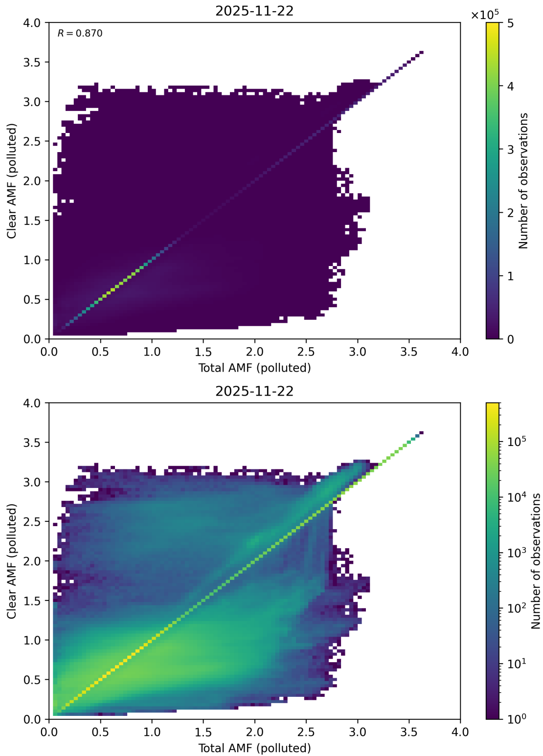
Figure 320: Scatter density plot of “Total AMF (polluted)” against “Clear AMF (polluted)” for 2025-11-21 to 2025-11-23.
