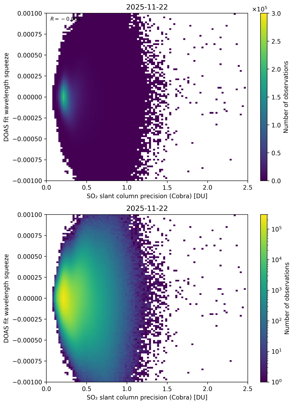
Figure 203: Scatter density plot of “SO 2 slant column precision (Cobra)” against “DOAS fit wavelength squeeze” for 2025-11-21 to 2025-11-23.
