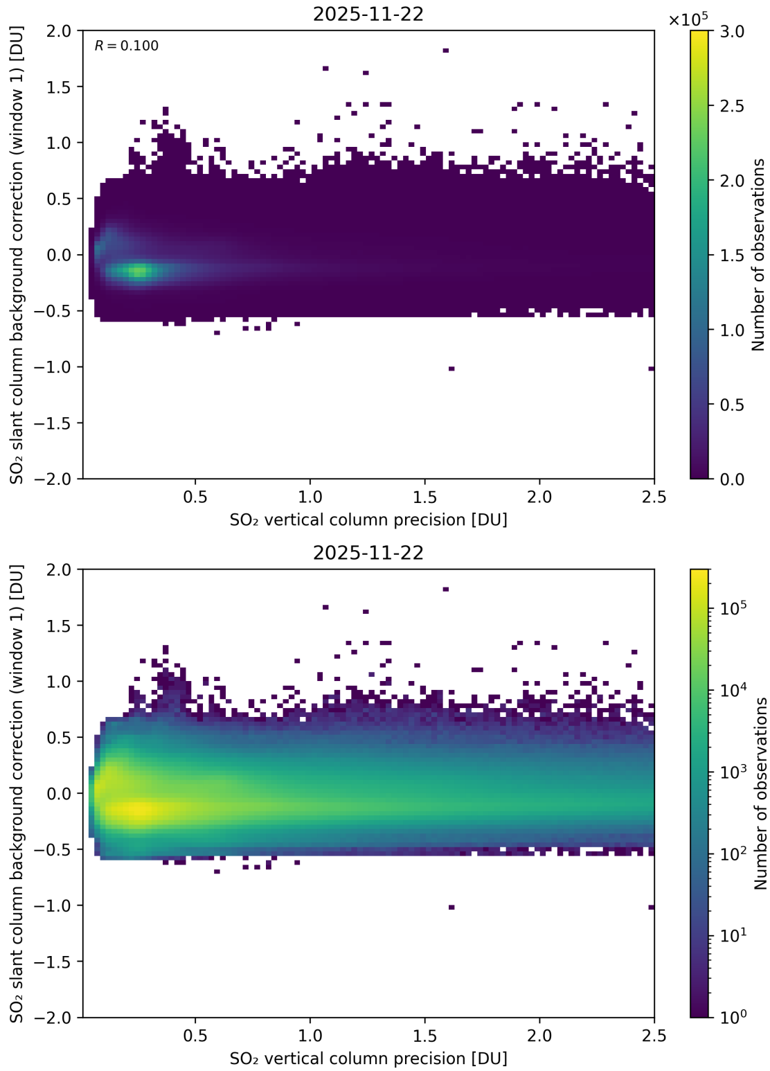
Figure 329: Scatter density plot of “SO 2 vertical column precision” against “SO 2 slant column background correction (window 1)” for 2025-11-21 to 2025-11-23.
