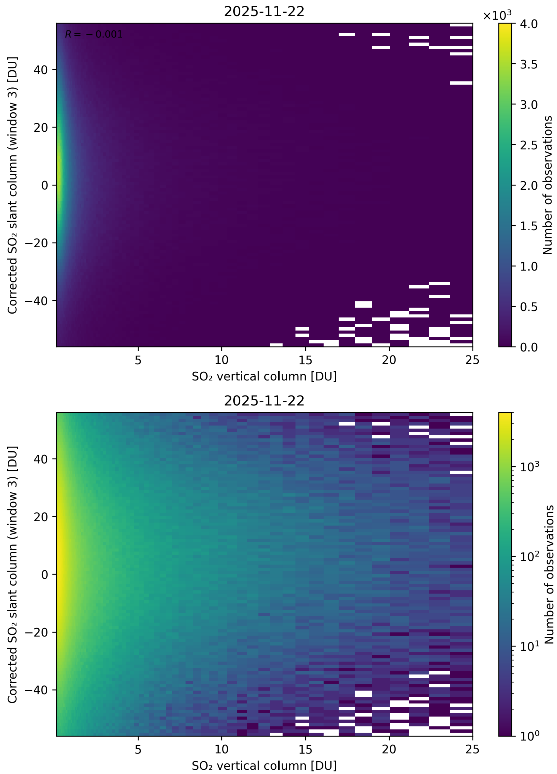
Figure 353: Scatter density plot of “SO 2 vertical column” against “Corrected SO 2 slant column (window 3)” for 2025-11-21 to 2025-11-23.
