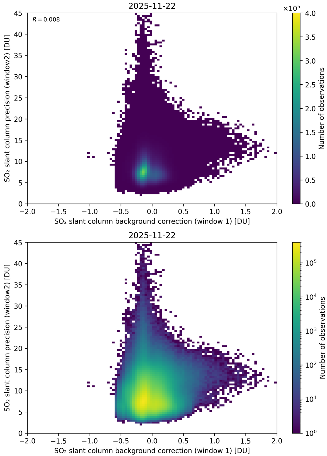
Figure 117: Scatter density plot of “SO 2 slant column background correction (window 1)” against “SO 2 slant column precision (window2)” for 2025-11-21 to 2025-11-23.
