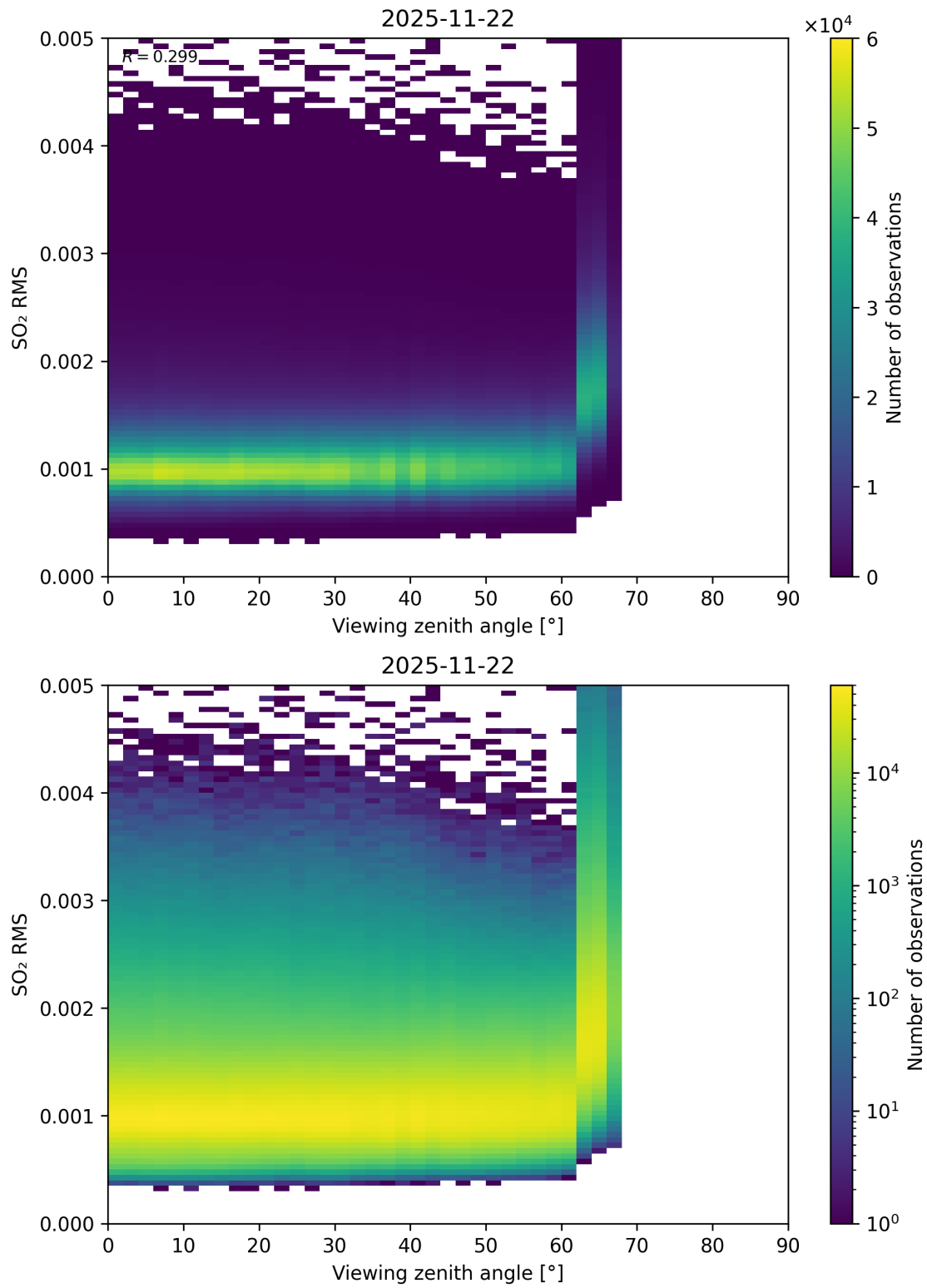
Figure 367: Scatter density plot of “Viewing zenith angle” against “SO 2 RMS” for 2025-11-21 to 2025-11-23.
