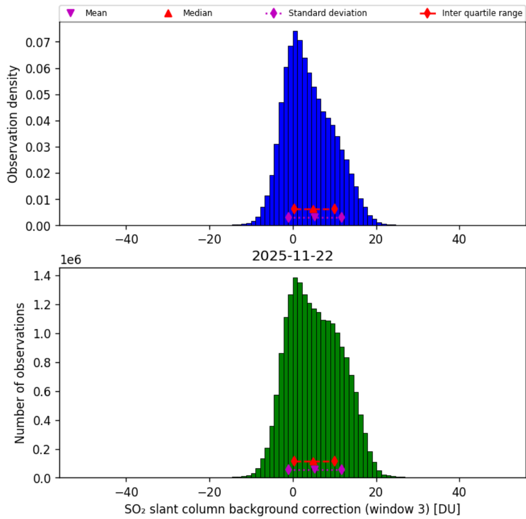
Figure 74: Histogram of “SO 2 slant column background correction (window 3)” for 2025-11-21 to 2025-11-23
