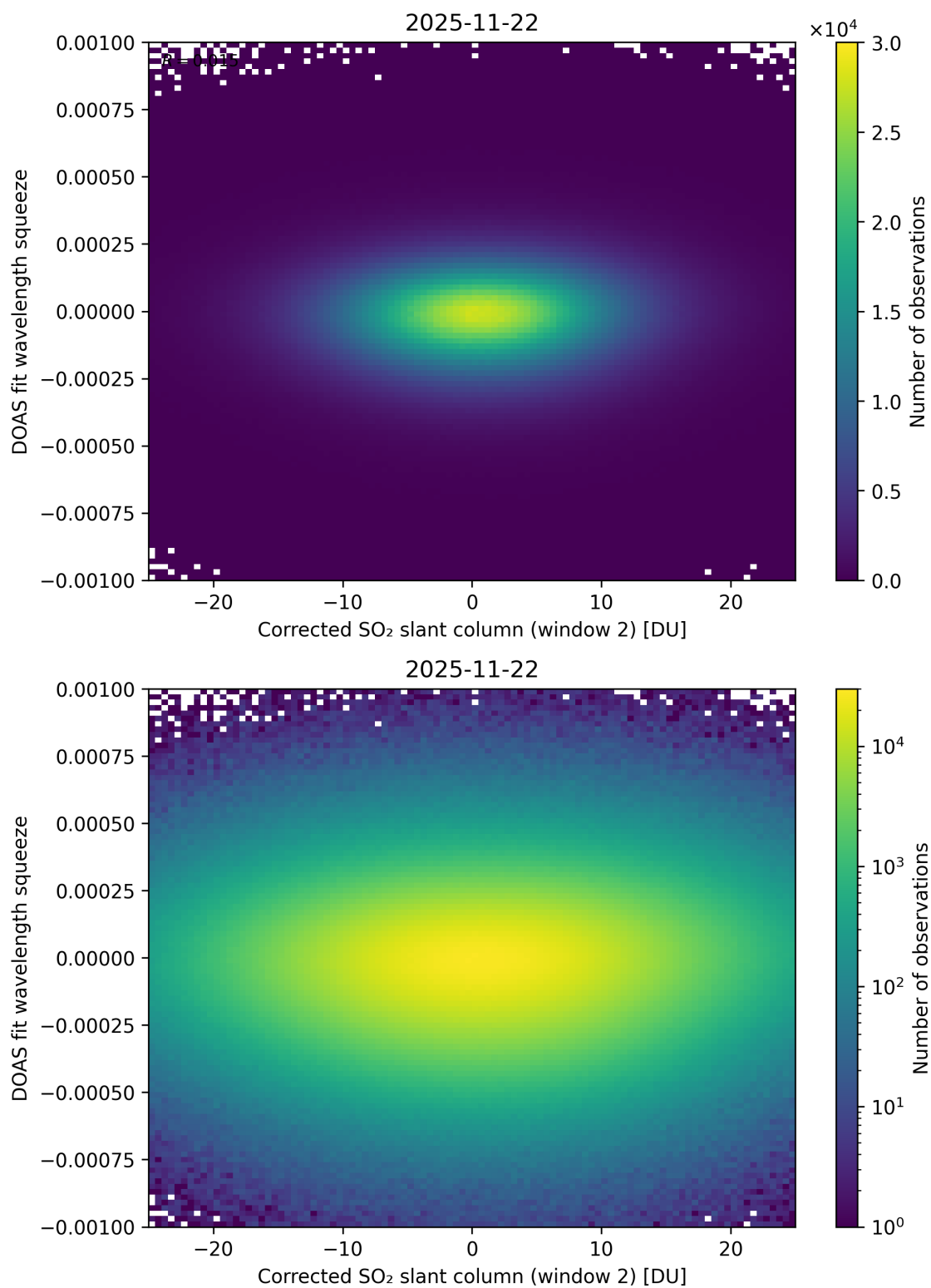
Figure 247: Scatter density plot of “Corrected SO 2 slant column (window 2)” against “DOAS fit wavelength squeeze” for 2025-11-21 to 2025-11-23.
