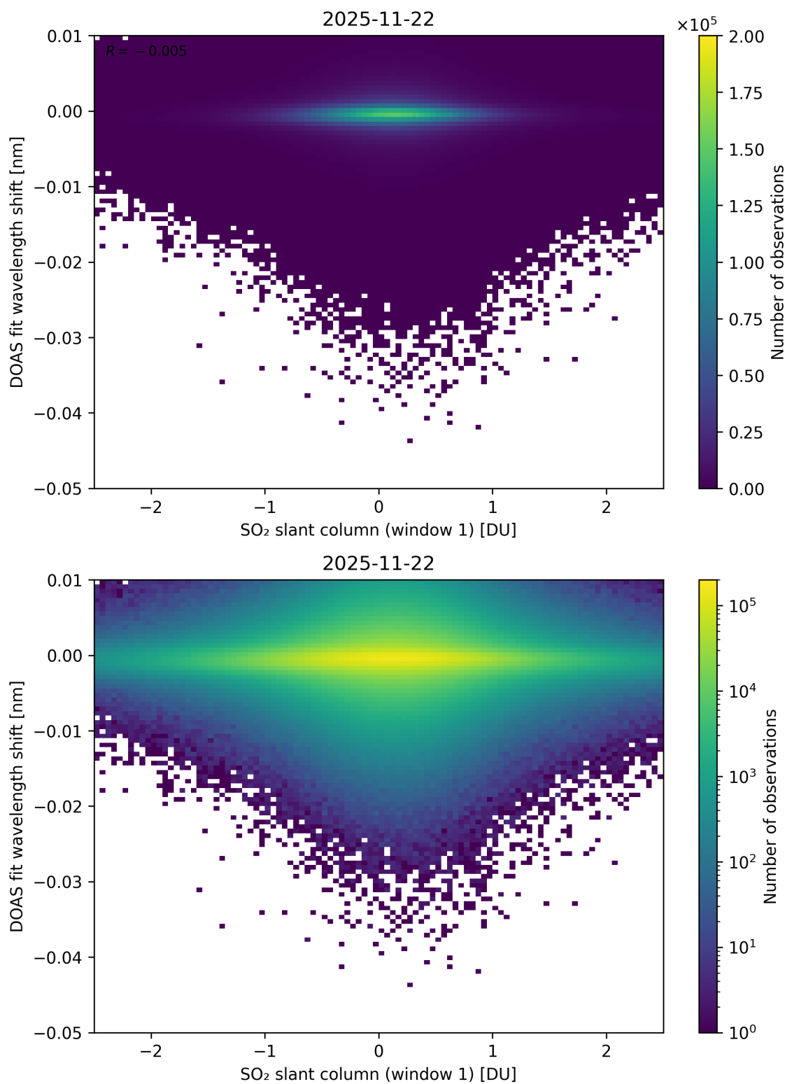
Figure 265: Scatter density plot of “SO 2 slant column (window 1)” against “DOAS fit wavelength shift” for 2025-11-21 to 2025-11-23.
