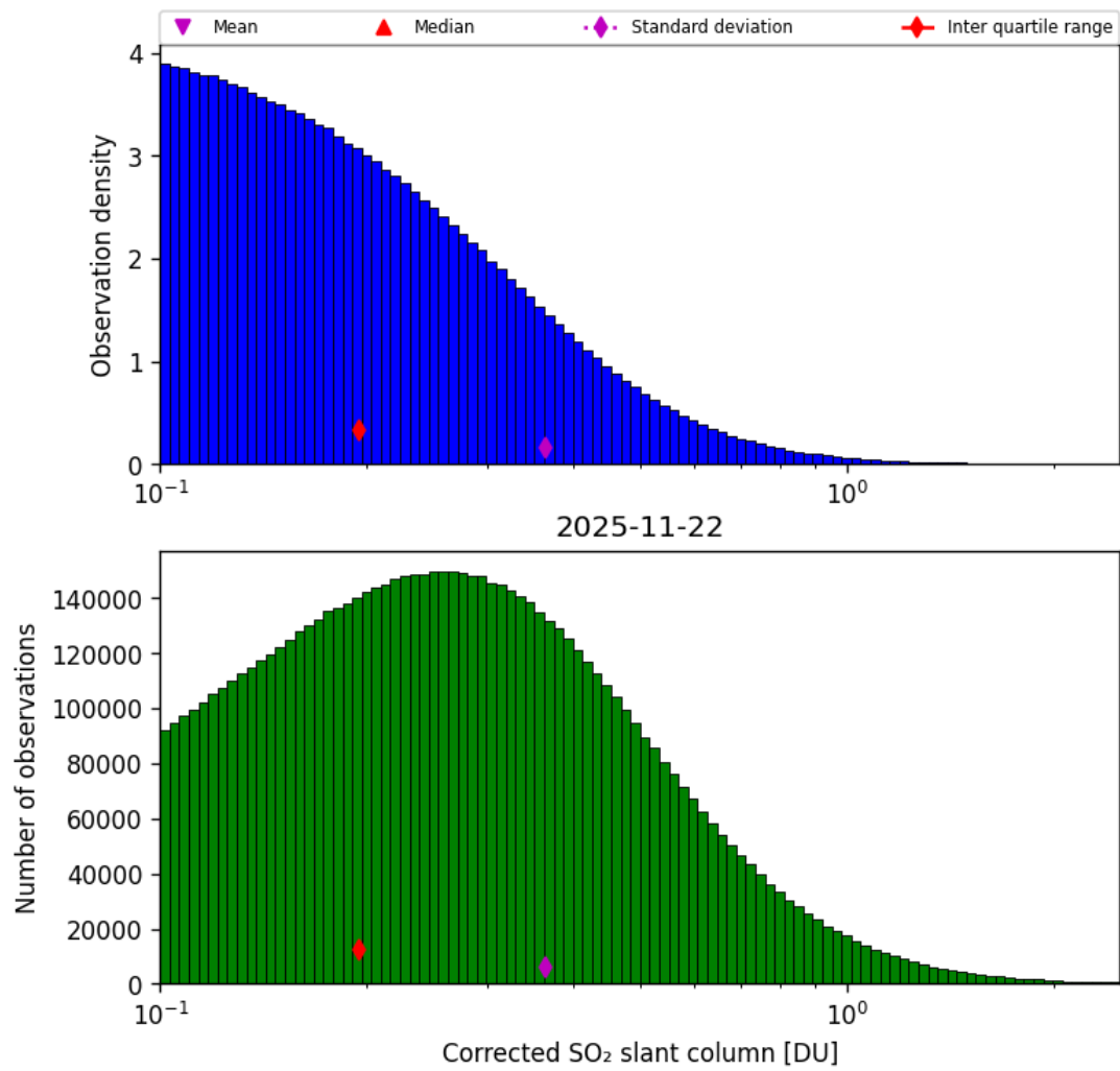
Figure 60: Histogram of “Corrected SO 2 slant column” for 2025-11-21 to 2025-11-23
