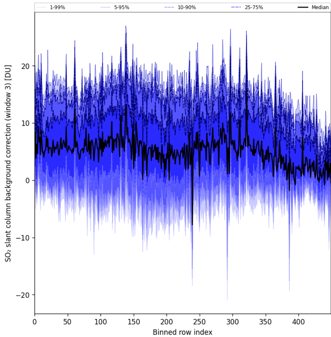
Figure 100: Along track statistics of “SO 2 slant column background correction (window 3)” for 2025-11-21 to 2025-11-23
