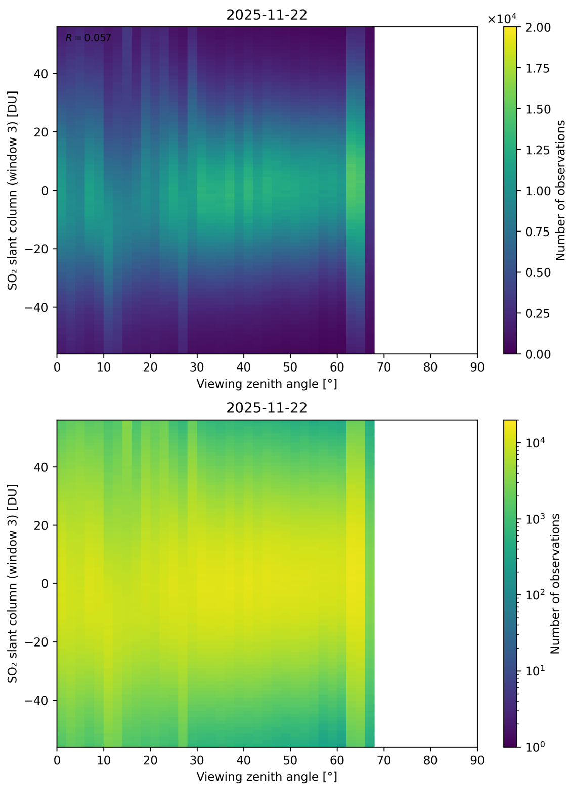
Figure 379: Scatter density plot of “Viewing zenith angle” against “SO 2 slant column (window 3)” for 2025-11-21 to 2025-11-23.
