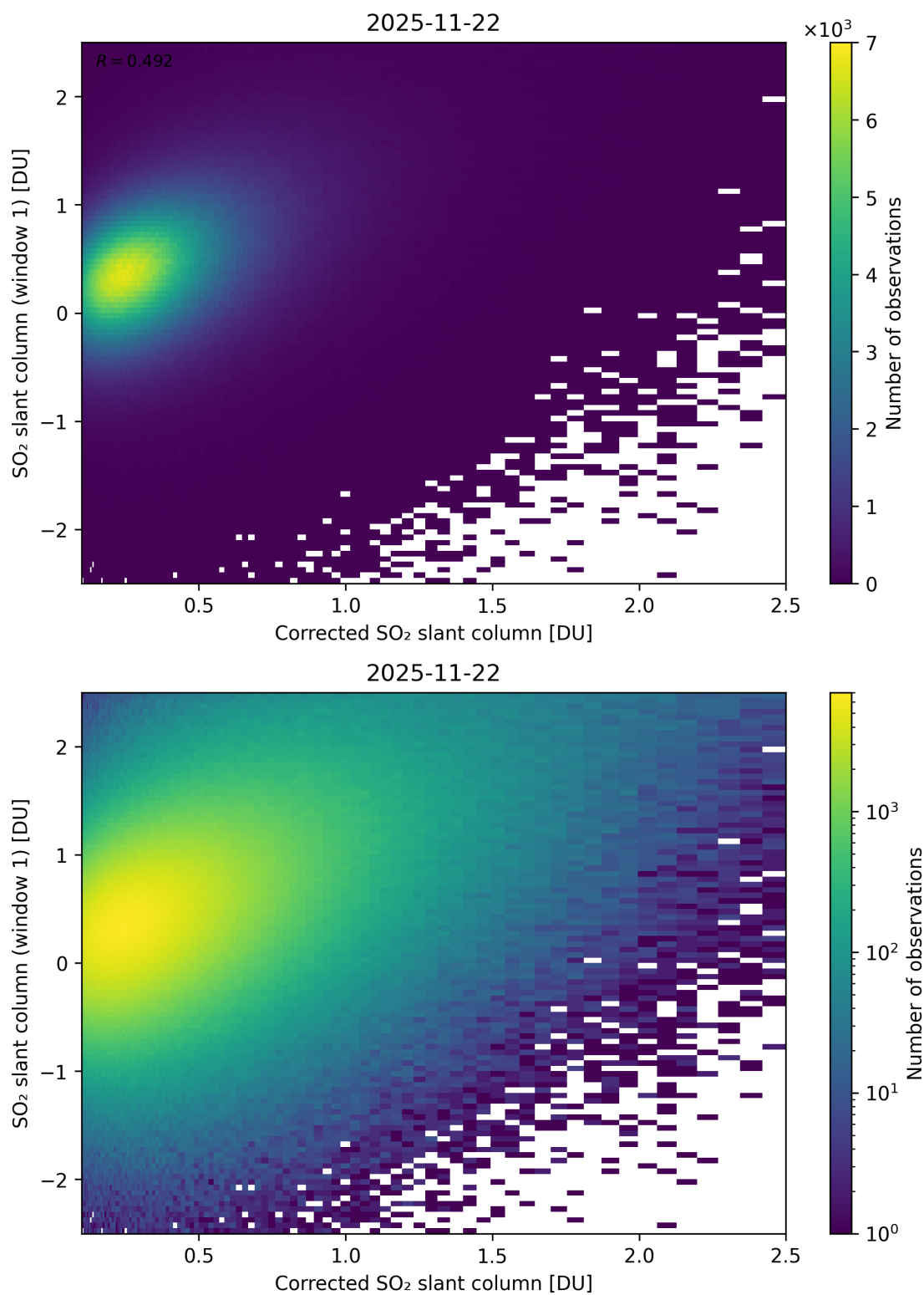
Figure 237: Scatter density plot of “Corrected SO 2 slant column” against “SO 2 slant column (window 1)” for 2025-11-21 to 2025-11-23.
