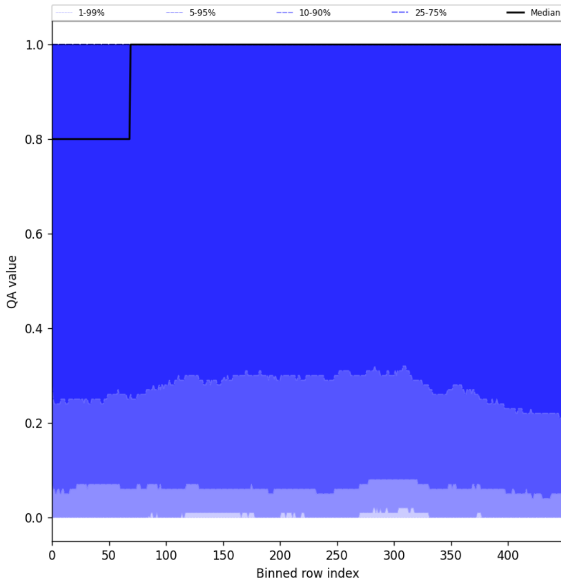
Figure 83: Along track statistics of “QA value” for 2025-11-21 to 2025-11-23
