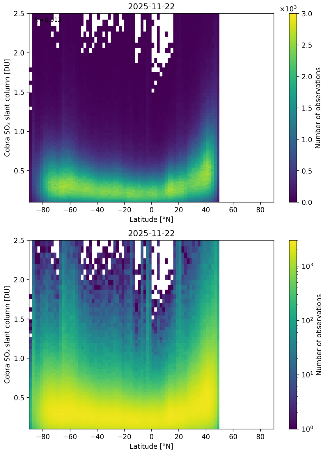
Figure 157: Scatter density plot of “Latitude” against “Cobra SO 2 slant column” for 2025-11-21 to 2025-11-23.
