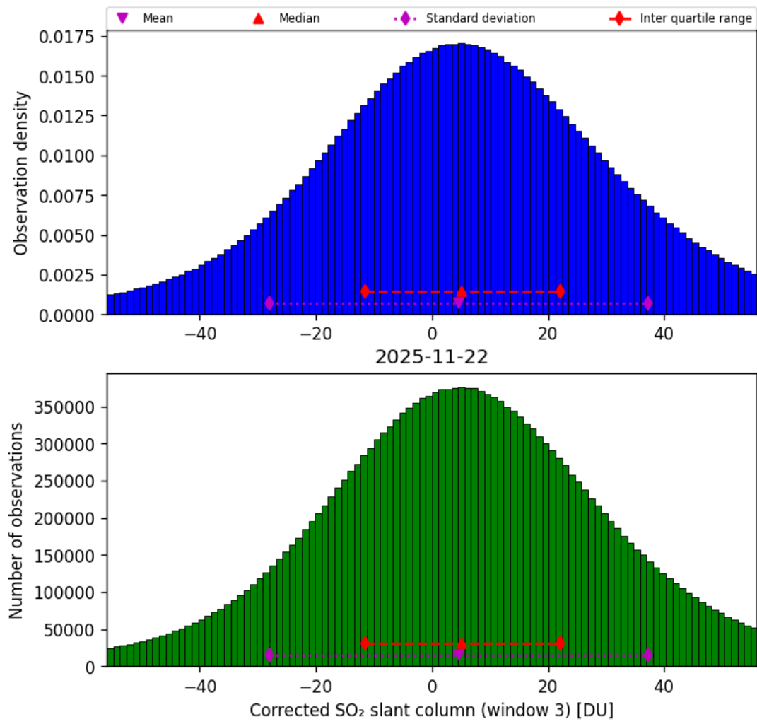
Figure 73: Histogram of “Corrected SO 2 slant column (window 3)” for 2025-11-21 to 2025-11-23
