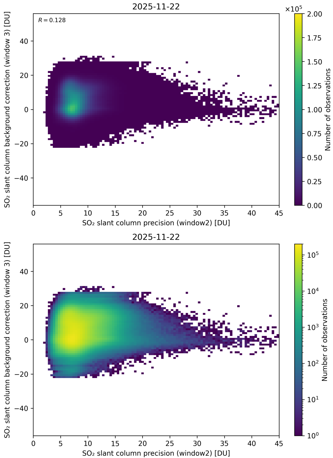
Figure 292: Scatter density plot of “SO 2 slant column precision (window2)” against “SO 2 slant column background correction (window 3)” for 2025-11-21 to 2025-11-23.
