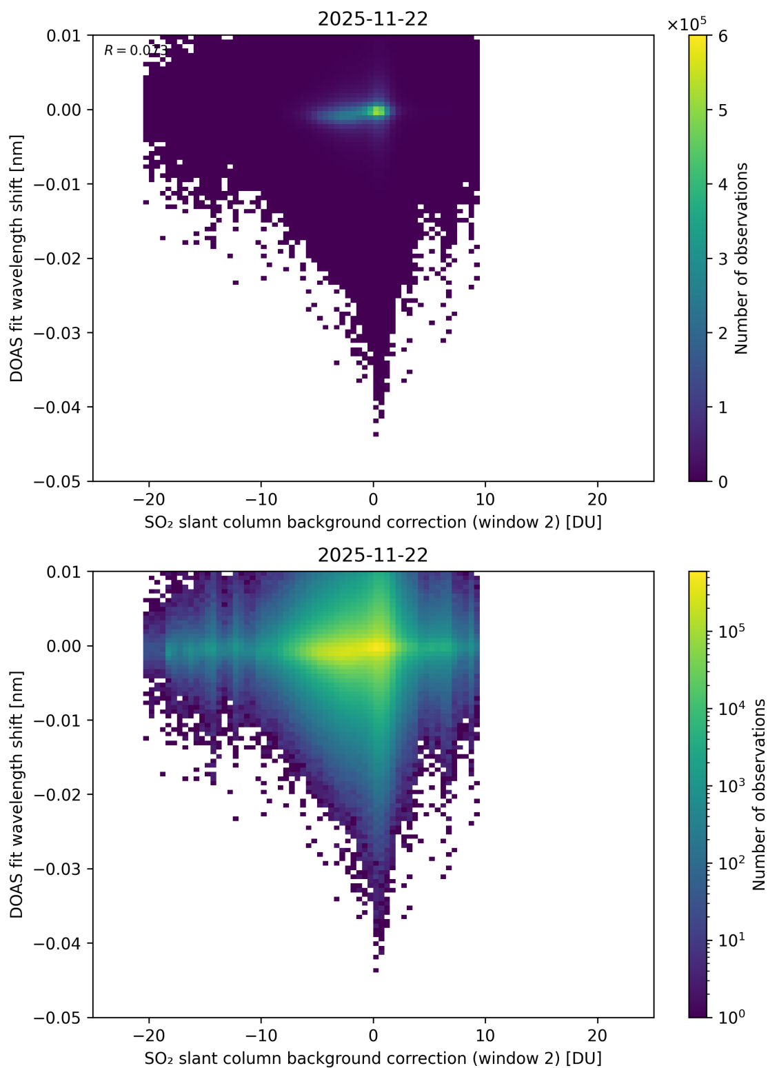
Figure 123: Scatter density plot of “SO 2 slant column background correction (window 2)” against “DOAS fit wavelength shift” for 2025-11-21 to 2025-11-23.
