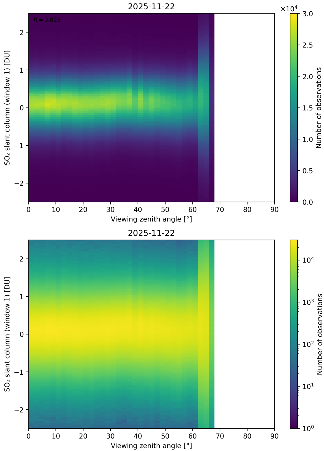
Figure 376: Scatter density plot of “Viewing zenith angle” against “SO 2 slant column (window 1)” for 2025-11-21 to 2025-11-23.
