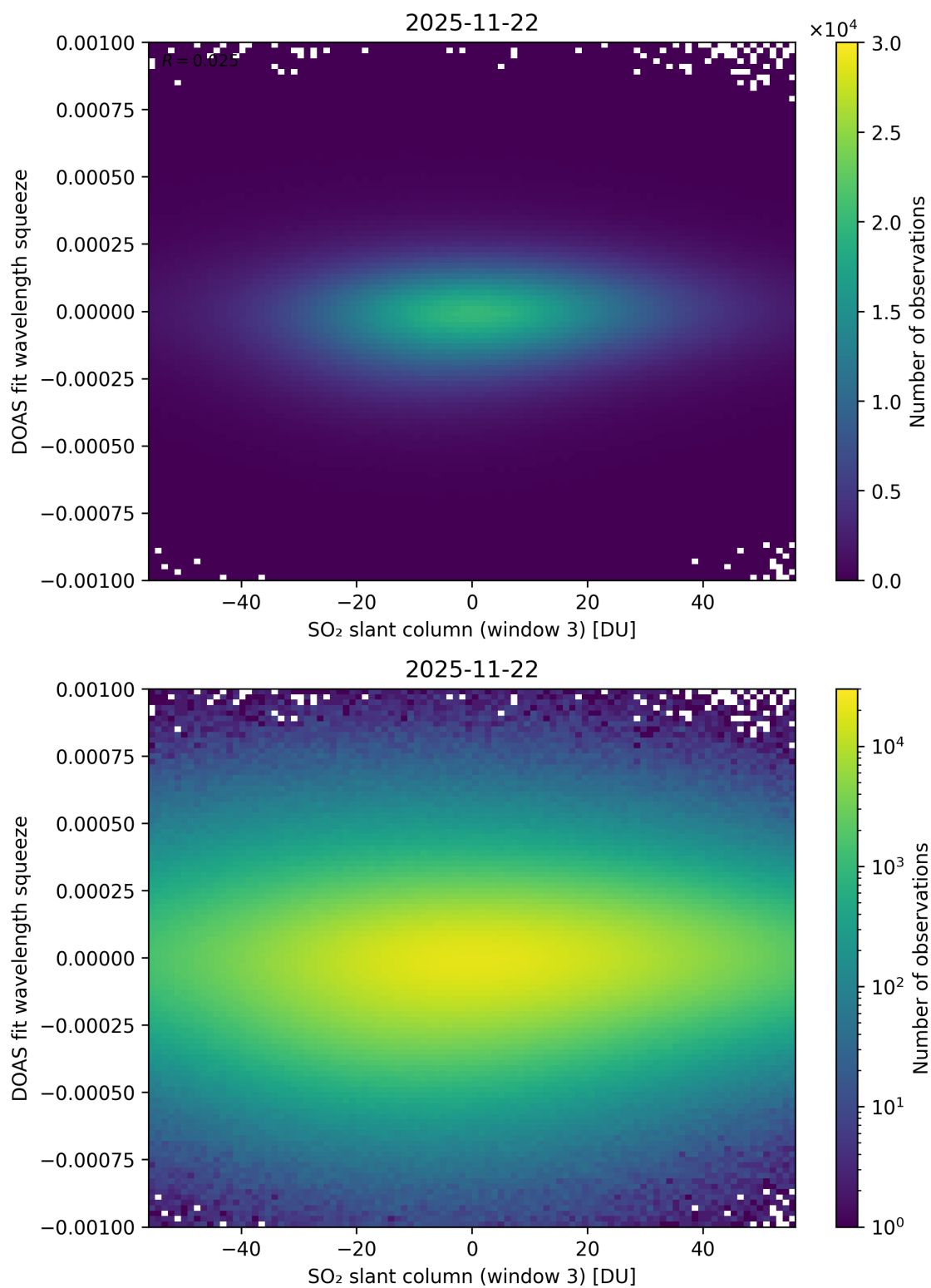
Figure 305: Scatter density plot of “SO 2 slant column (window 3)” against “DOAS fit wavelength squeeze” for 2025-11-21 to 2025-11-23.
