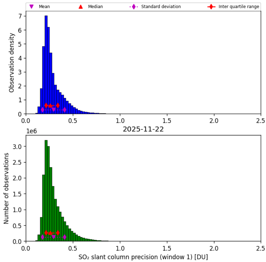
Figure 64: Histogram of “SO 2 slant column precision (window 1)” for 2025-11-21 to 2025-11-23
