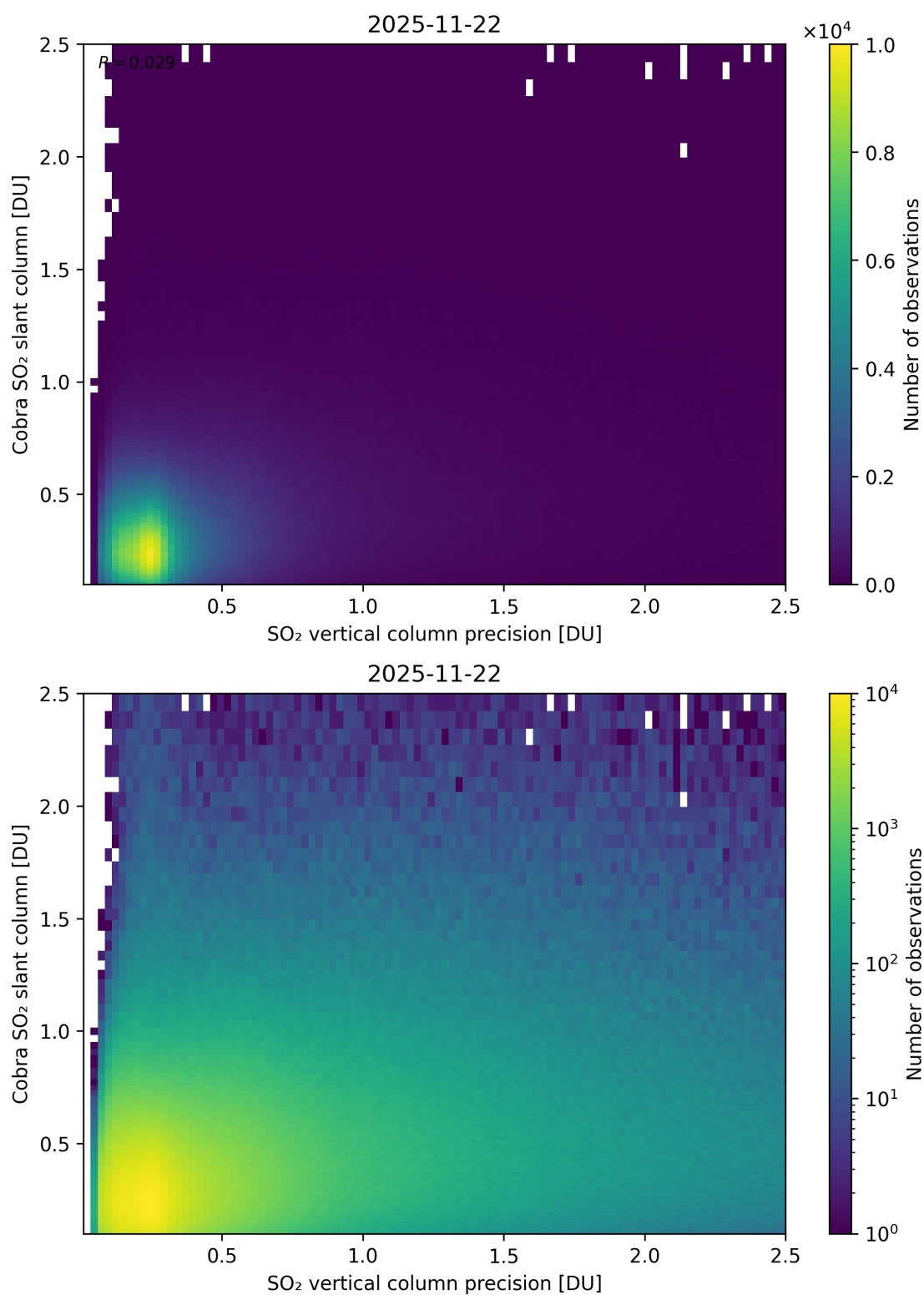
Figure 336: Scatter density plot of “SO 2 vertical column precision” against “Cobra SO 2 slant column” for 2025-11-21 to 2025-11-23.
