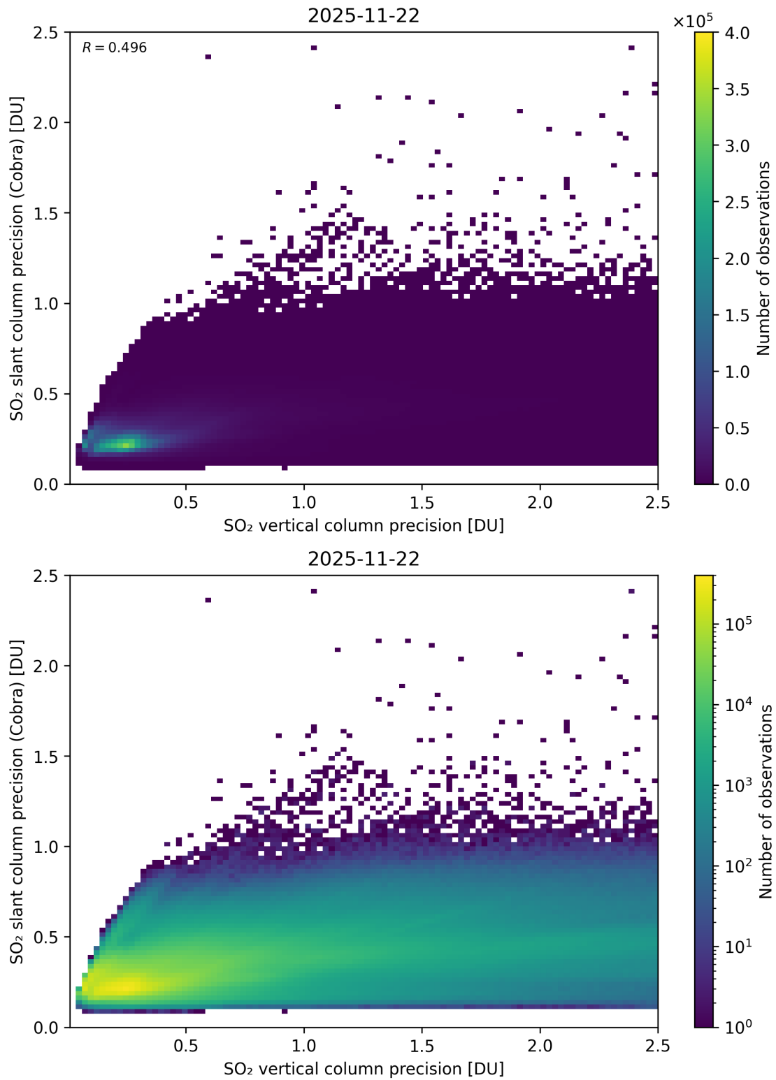
Figure 337: Scatter density plot of “SO 2 vertical column precision” against “SO 2 slant column precision (Cobra)” for 2025-11-21 to 2025-11-23.
