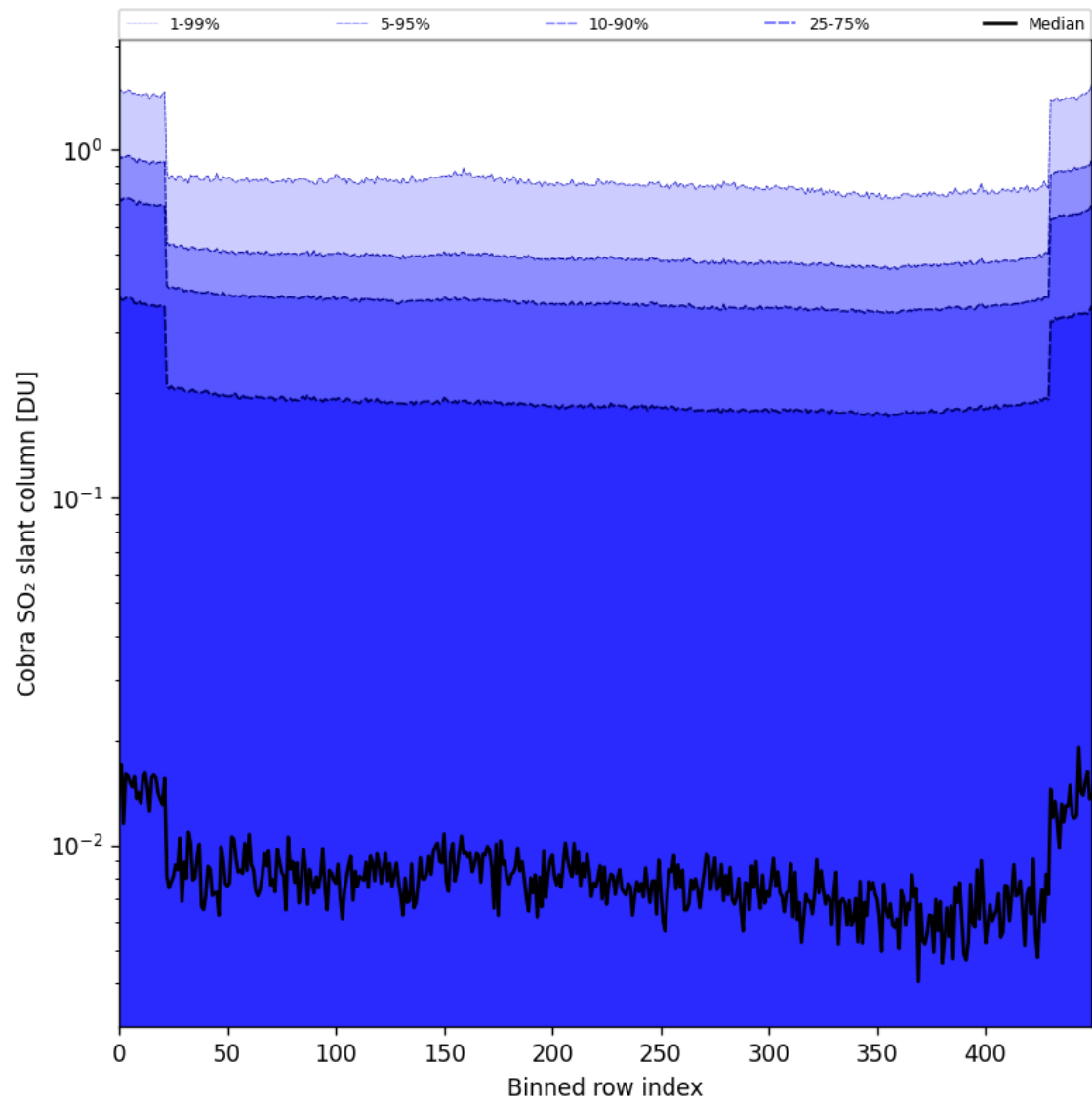
Figure 87: Along track statistics of "Cobra SO 2 slant column" for 2025-11-21 to 2025-11-23
