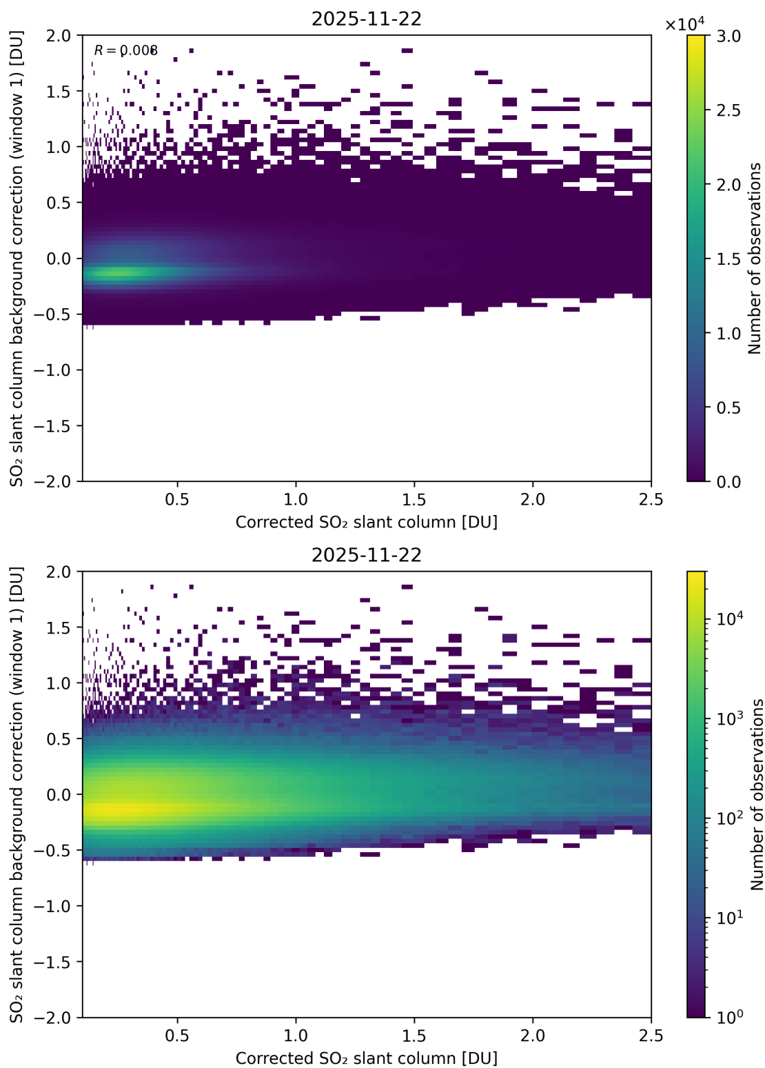
Figure 226: Scatter density plot of “Corrected SO 2 slant column” against “SO 2 slant column background correction (window 1)” for 2025-11-21 to 2025-11-23.
