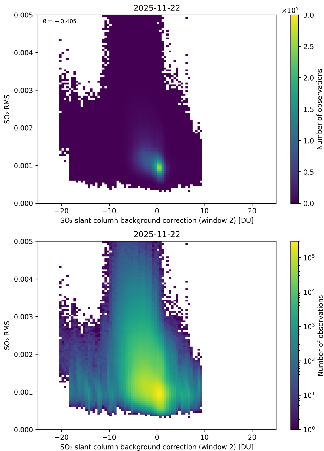
Figure 125: Scatter density plot of “SO 2 slant column background correction (window 2)” against “SO 2 RMS” for 2025-11-21 to 2025-11-23.
