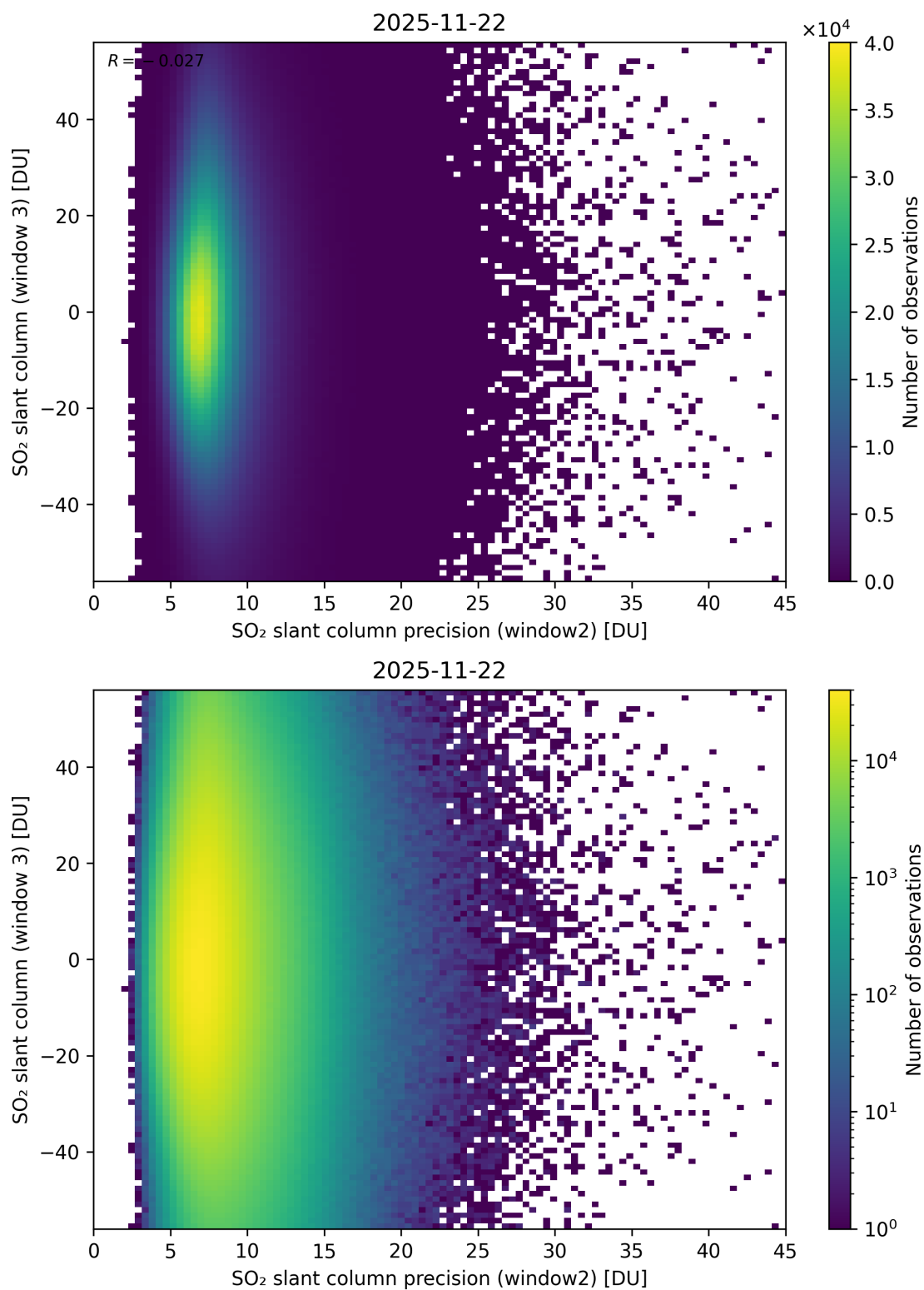
Figure 299: Scatter density plot of “SO 2 slant column precision (window2)” against “SO 2 slant column (window 3)” for 2025-11-21 to 2025-11-23.
