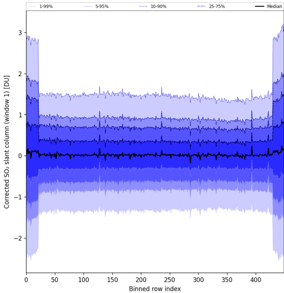
Figure 91: Along track statistics of “Corrected SO 2 slant column (window 1)” for 2025-11-21 to 2025-11-23
