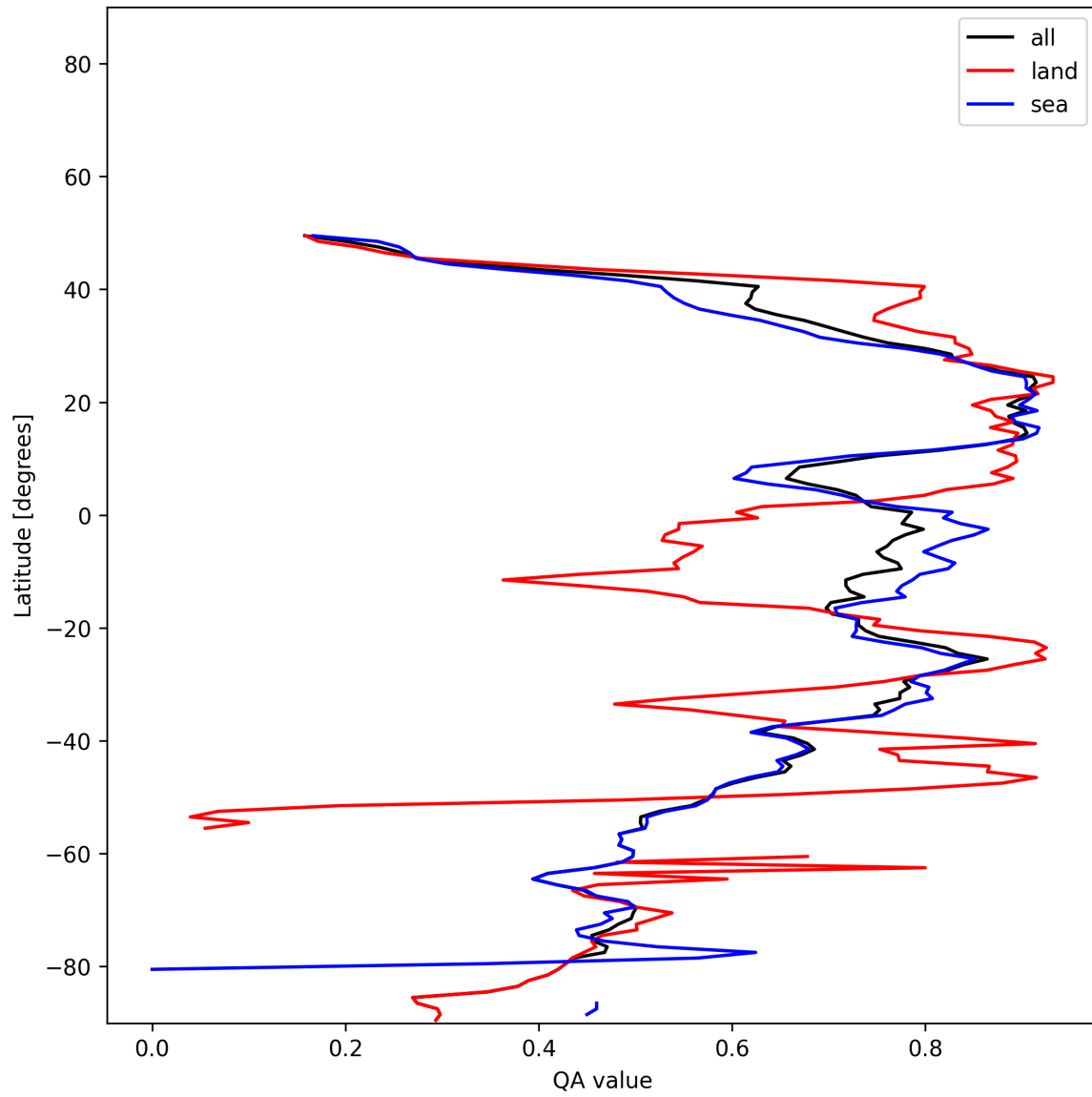
Figure 31: Zonal average of “QA value” for 2025-11-21 to 2025-11-23.
