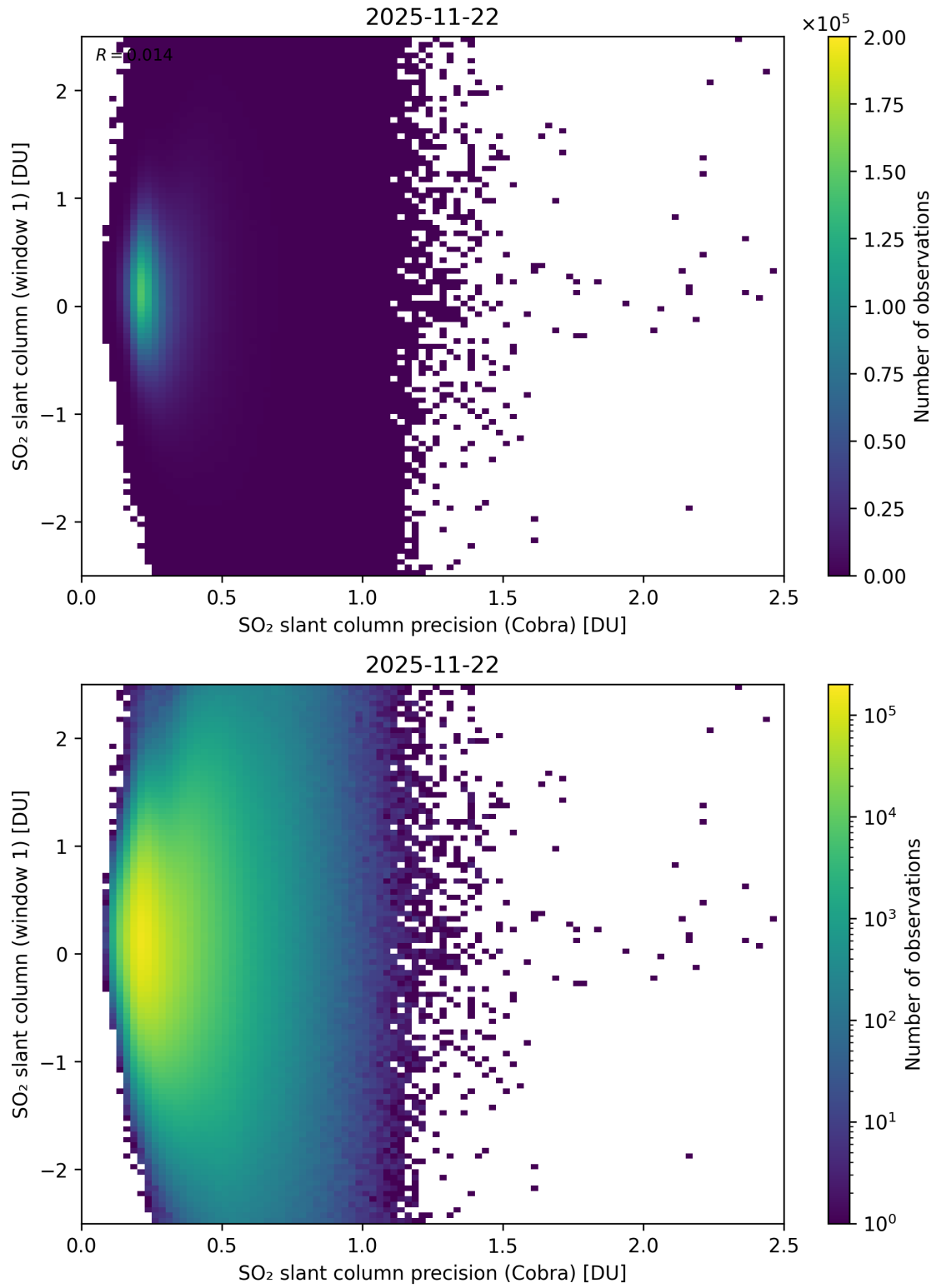
Figure 208: Scatter density plot of “SO 2 slant column precision (Cobra)” against “SO 2 slant column (window 1)” for 2025-11-21 to 2025-11-23.
