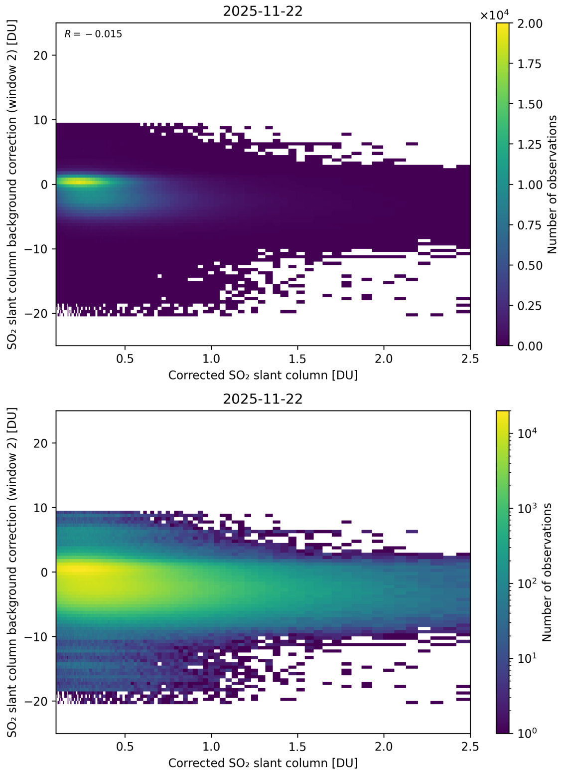
Figure 227: Scatter density plot of “Corrected SO 2 slant column” against “SO 2 slant column background correction (window 2)” for 2025-11-21 to 2025-11-23.
