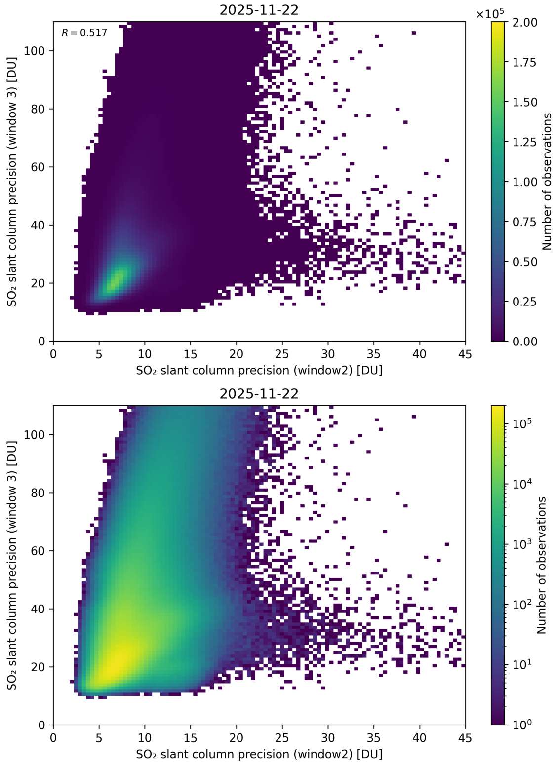
Figure 300: Scatter density plot of “SO 2 slant column precision (window2)” against “SO 2 slant column precision (window 3)” for 2025-11-21 to 2025-11-23.
