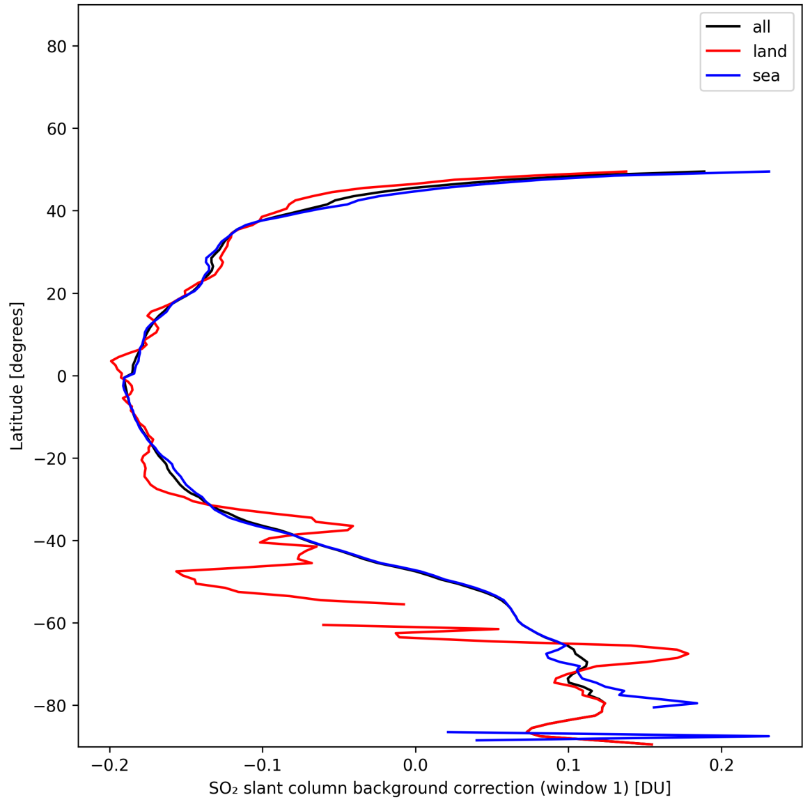
Figure 40: Zonal average of “SO 2 slant column background correction (window 1)” for 2025-11-21 to 2025-11-23.
