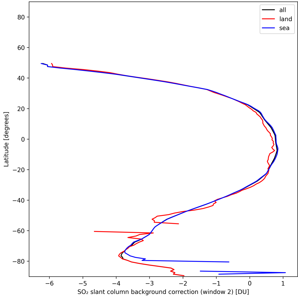
Figure 44: Zonal average of “SO 2 slant column background correction (window 2)” for 2025-11-21 to 2025-11-23.
