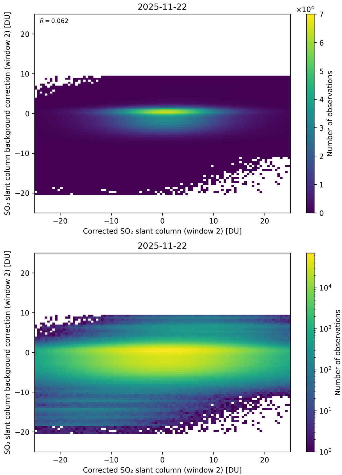
Figure 244: Scatter density plot of “Corrected SO 2 slant column (window 2)” against “SO 2 slant column background correction (window 2)” for 2025-11-21 to 2025-11-23.
