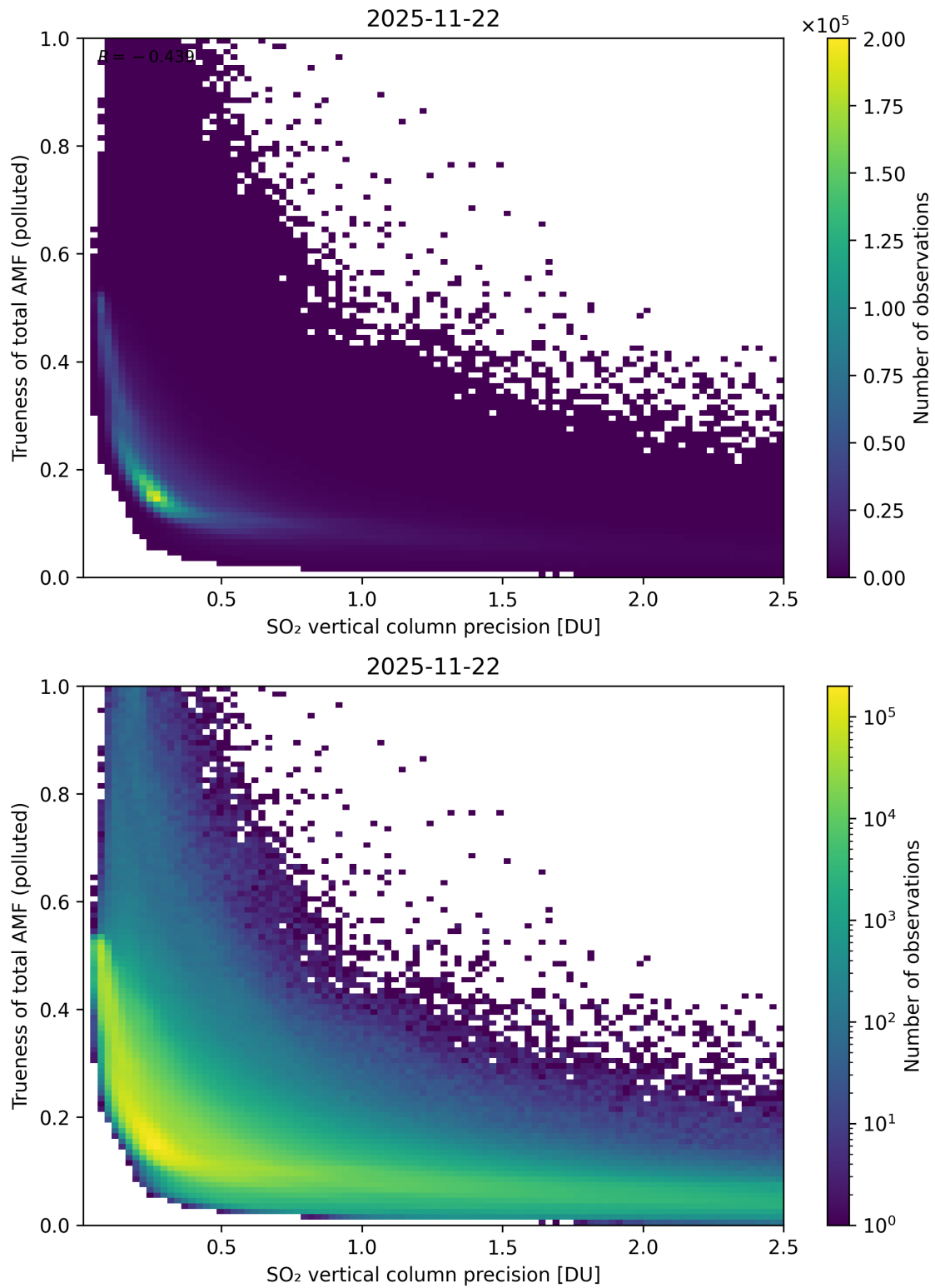
Figure 347: Scatter density plot of “SO 2 vertical column precision” against “Trueness of total AMF (polluted)” for 2025-11-21 to 2025-11-23.
