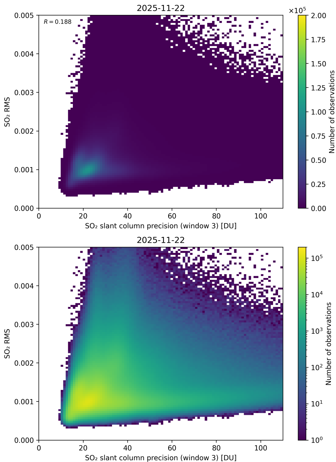
Figure 310: Scatter density plot of “SO 2 slant column precision (window 3)” against “SO 2 RMS” for 2025-11-21 to 2025-11-23.
