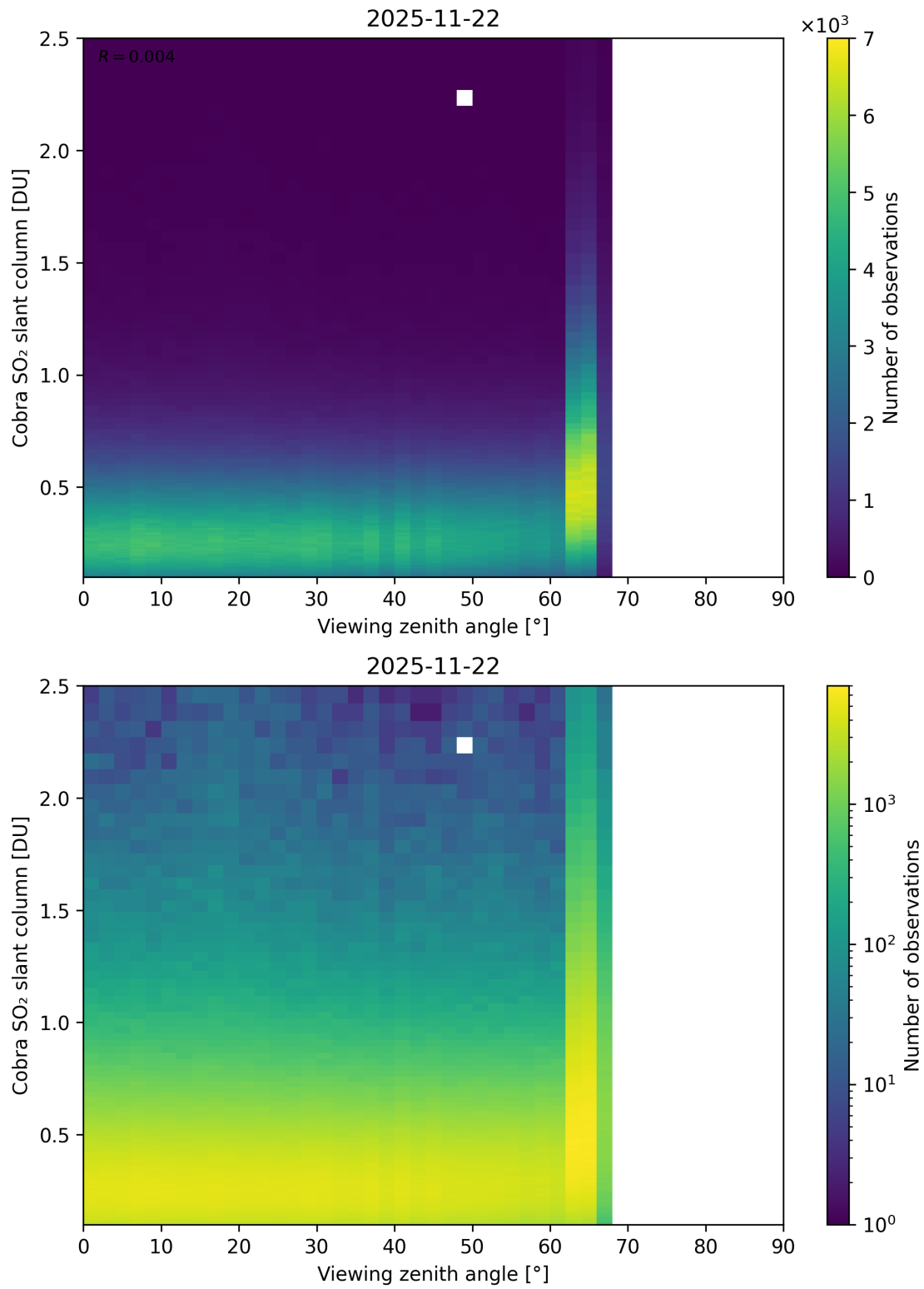
Figure 371: Scatter density plot of “Viewing zenith angle” against “Cobra SO 2 slant column” for 2025-11-21 to 2025-11-23.
