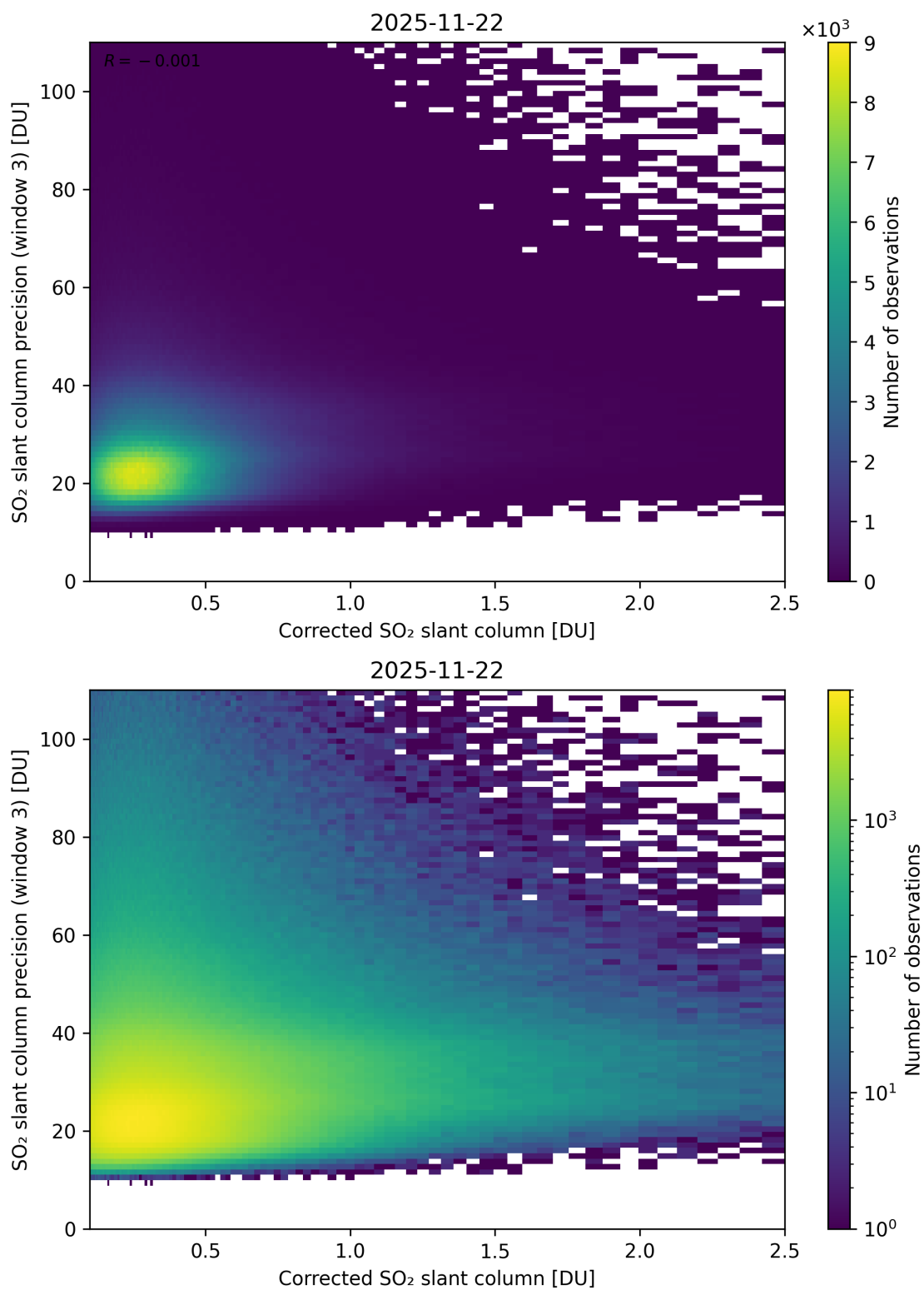
Figure 241: Scatter density plot of “Corrected SO 2 slant column” against “SO 2 slant column precision (window 3)” for 2025-11-21 to 2025-11-23.
