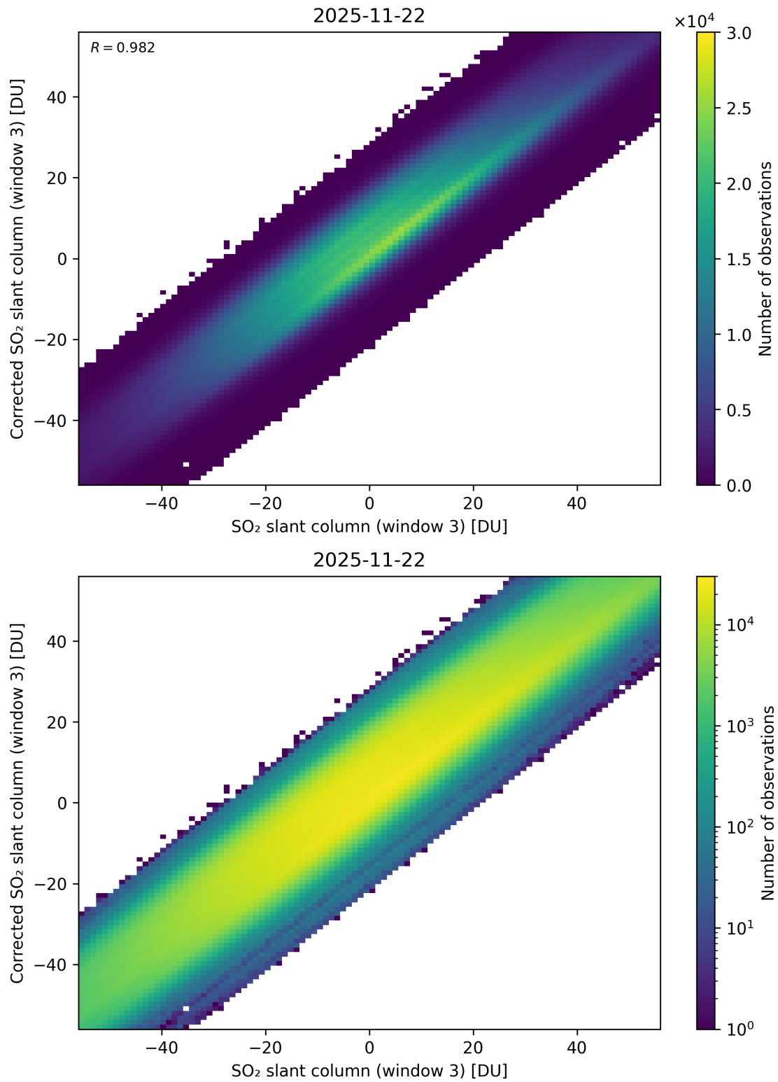
Figure 316: Scatter density plot of “SO 2 slant column (window 3)” against “Corrected SO 2 slant column (window 3)” for 2025-11-21 to 2025-11-23.
