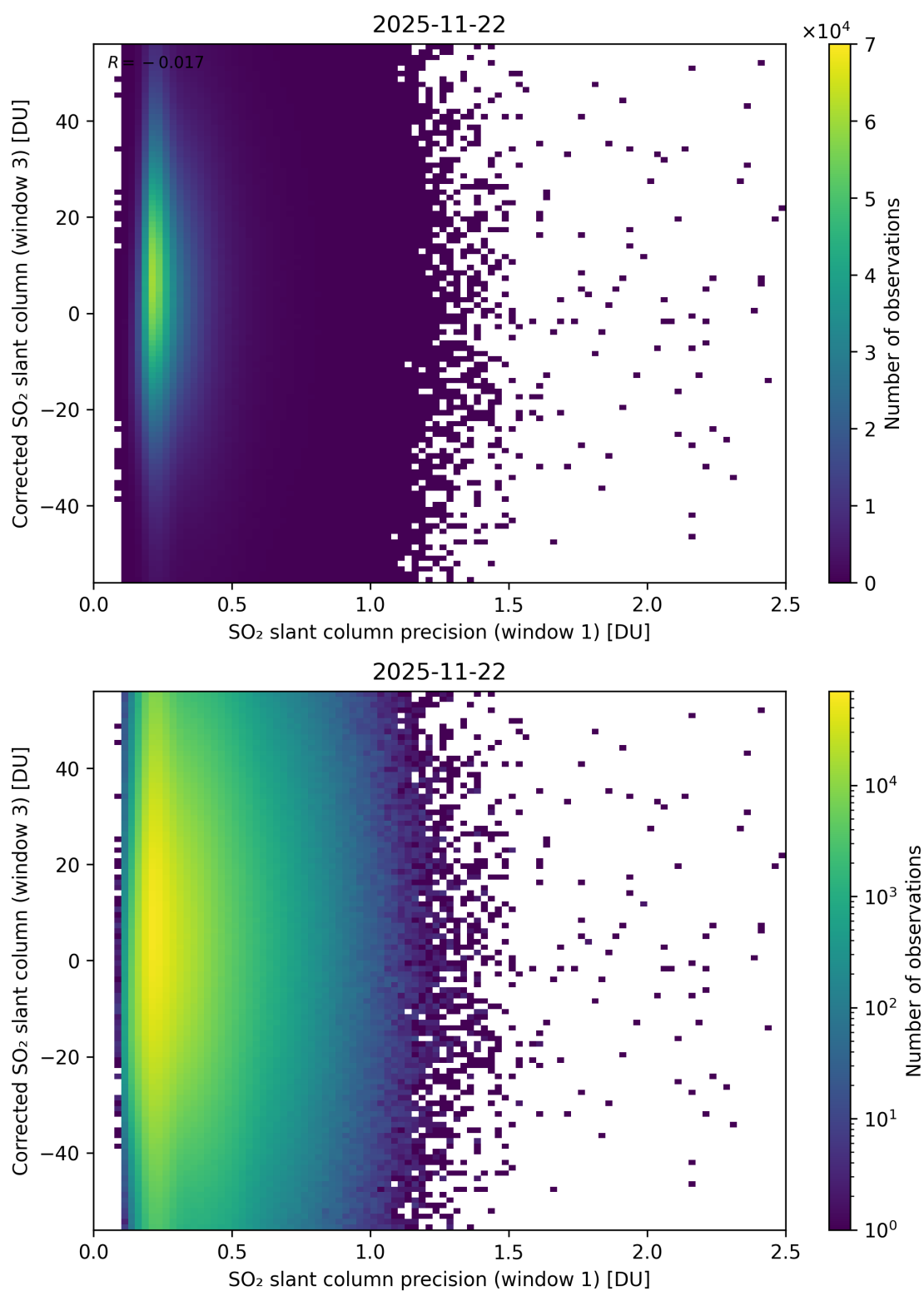
Figure 276: Scatter density plot of “SO 2 slant column precision (window 1)” against “Corrected SO 2 slant column (window 3)” for 2025-11-21 to 2025-11-23.
