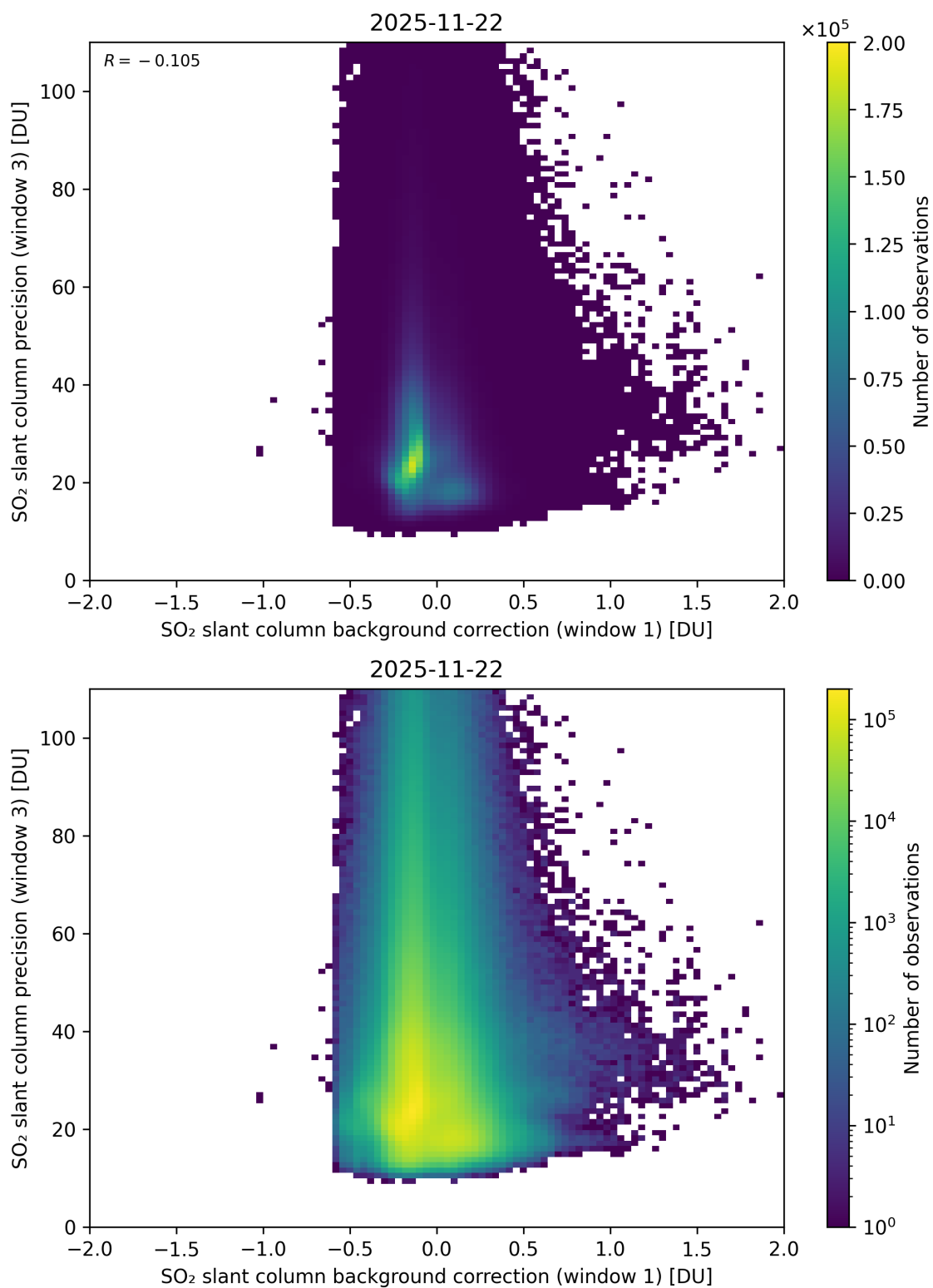
Figure 119: Scatter density plot of “SO 2 slant column background correction (window 1)” against “SO 2 slant column precision (window 3)” for 2025-11-21 to 2025-11-23.
