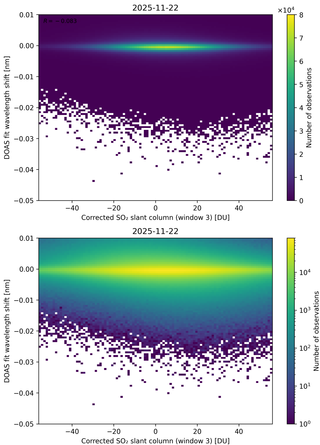
Figure 256: Scatter density plot of “Corrected SO 2 slant column (window 3)” against “DOAS fit wavelength shift” for 2025-11-21 to 2025-11-23.
