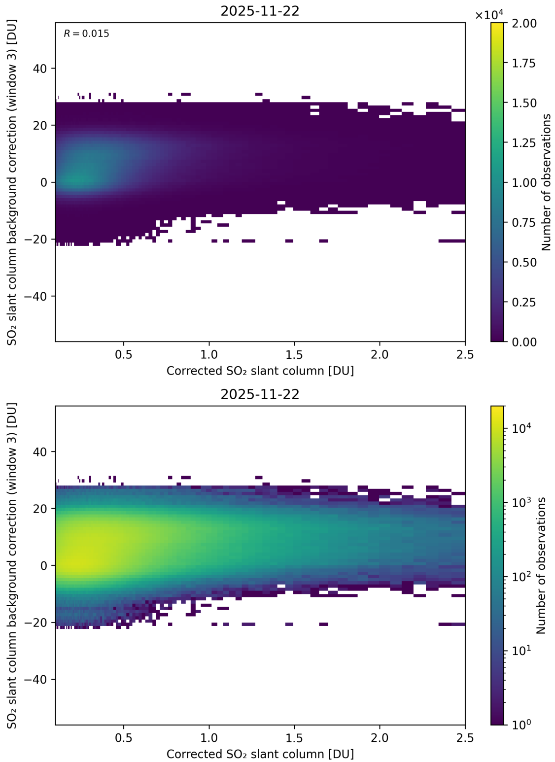
Figure 228: Scatter density plot of “Corrected SO 2 slant column” against “SO 2 slant column background correction (window 3)” for 2025-11-21 to 2025-11-23.
