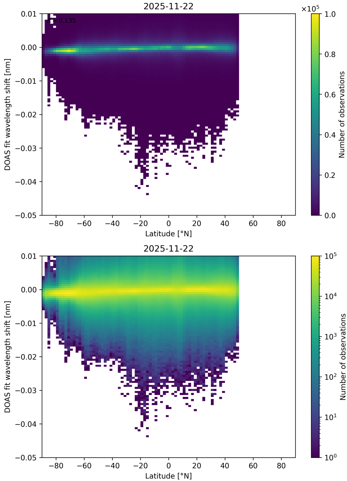
Figure 153: Scatter density plot of “Latitude” against “DOAS fit wavelength shift” for 2025-11-21 to 2025-11-23.
