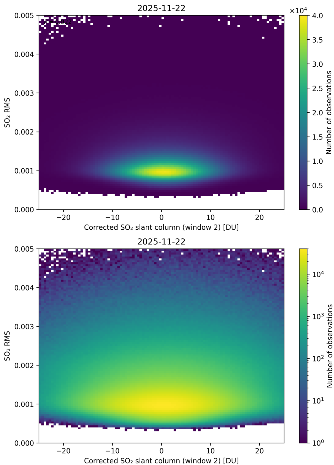
Figure 248: Scatter density plot of “Corrected SO 2 slant column (window 2)” against “SO 2 RMS” for 2025-11-21 to 2025-11-23.
