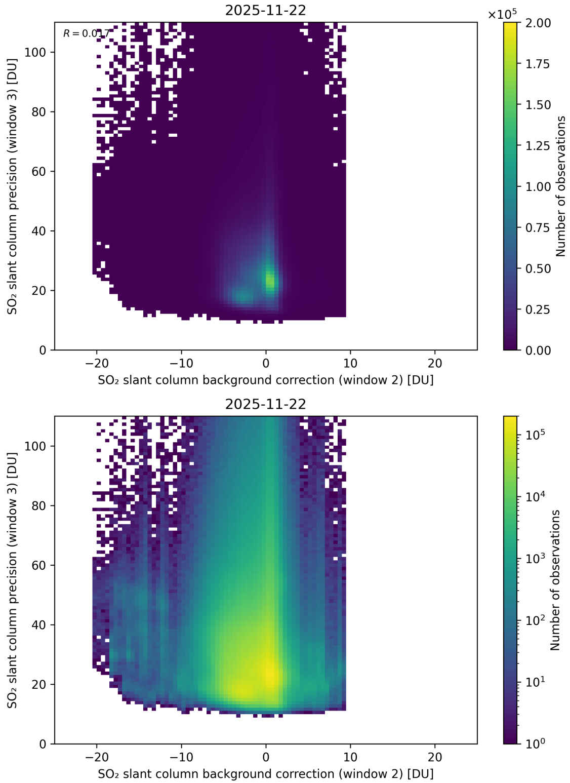
Figure 129: Scatter density plot of “SO 2 slant column background correction (window 2)” against “SO 2 slant column precision (window 3)” for 2025-11-21 to 2025-11-23.
