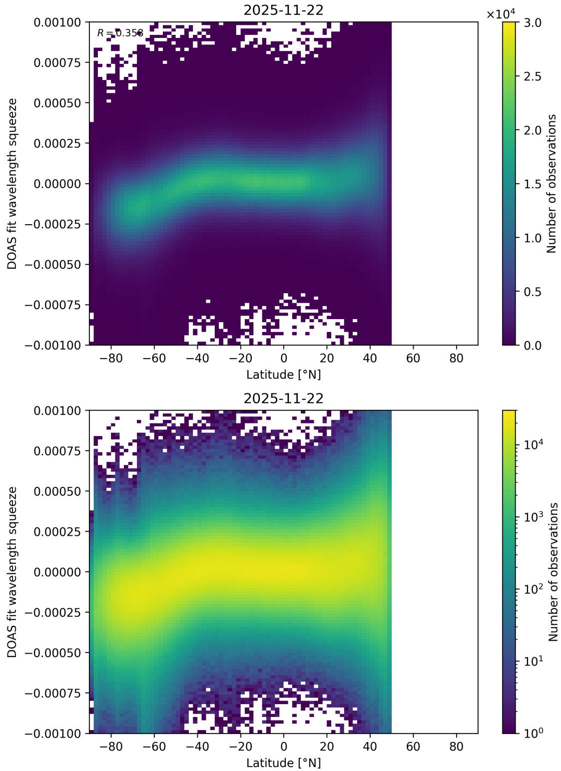
Figure 154: Scatter density plot of “Latitude” against “DOAS fit wavelength squeeze” for 2025-11-21 to 2025-11-23.
