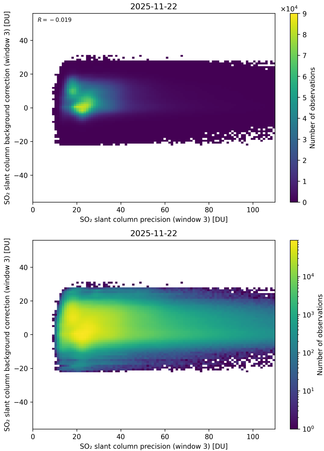
Figure 307: Scatter density plot of “SO 2 slant column precision (window 3)” against “SO 2 slant column background correction (window 3)” for 2025-11-21 to 2025-11-23.
