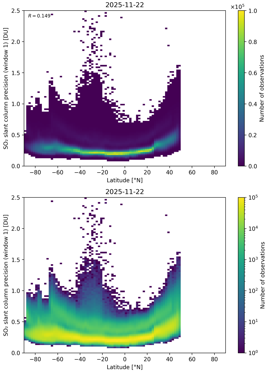
Figure 163: Scatter density plot of “Latitude” against “SO 2 slant column precision (window 1)” for 2025-11-21 to 2025-11-23.
