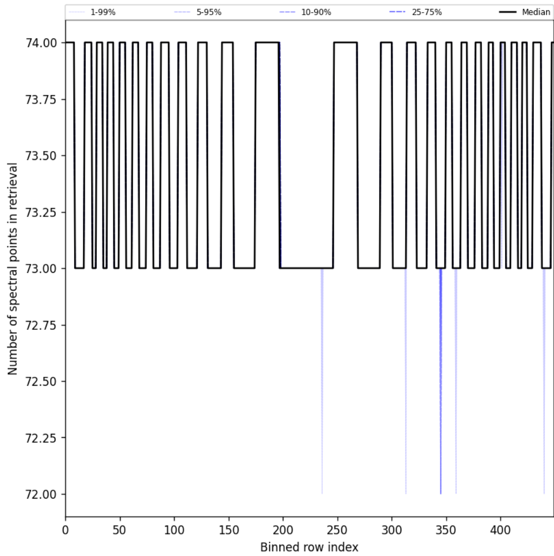
Figure 108: Along track statistics of “Number of spectral points in retrieval” for 2025-11-21 to 2025-11-23
