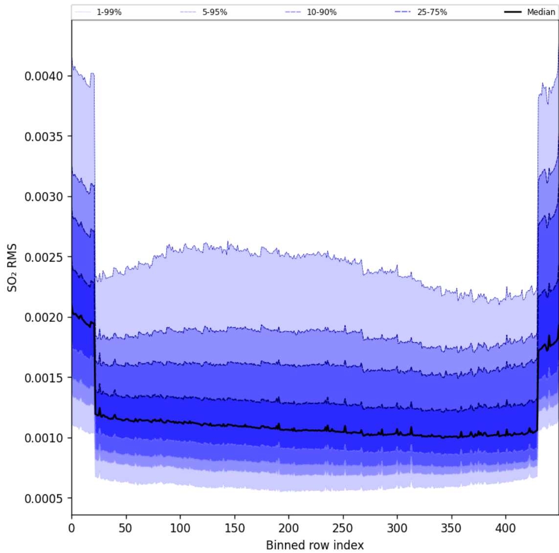
Figure 104: Along track statistics of “SO 2 RMS” for 2025-11-21 to 2025-11-23
