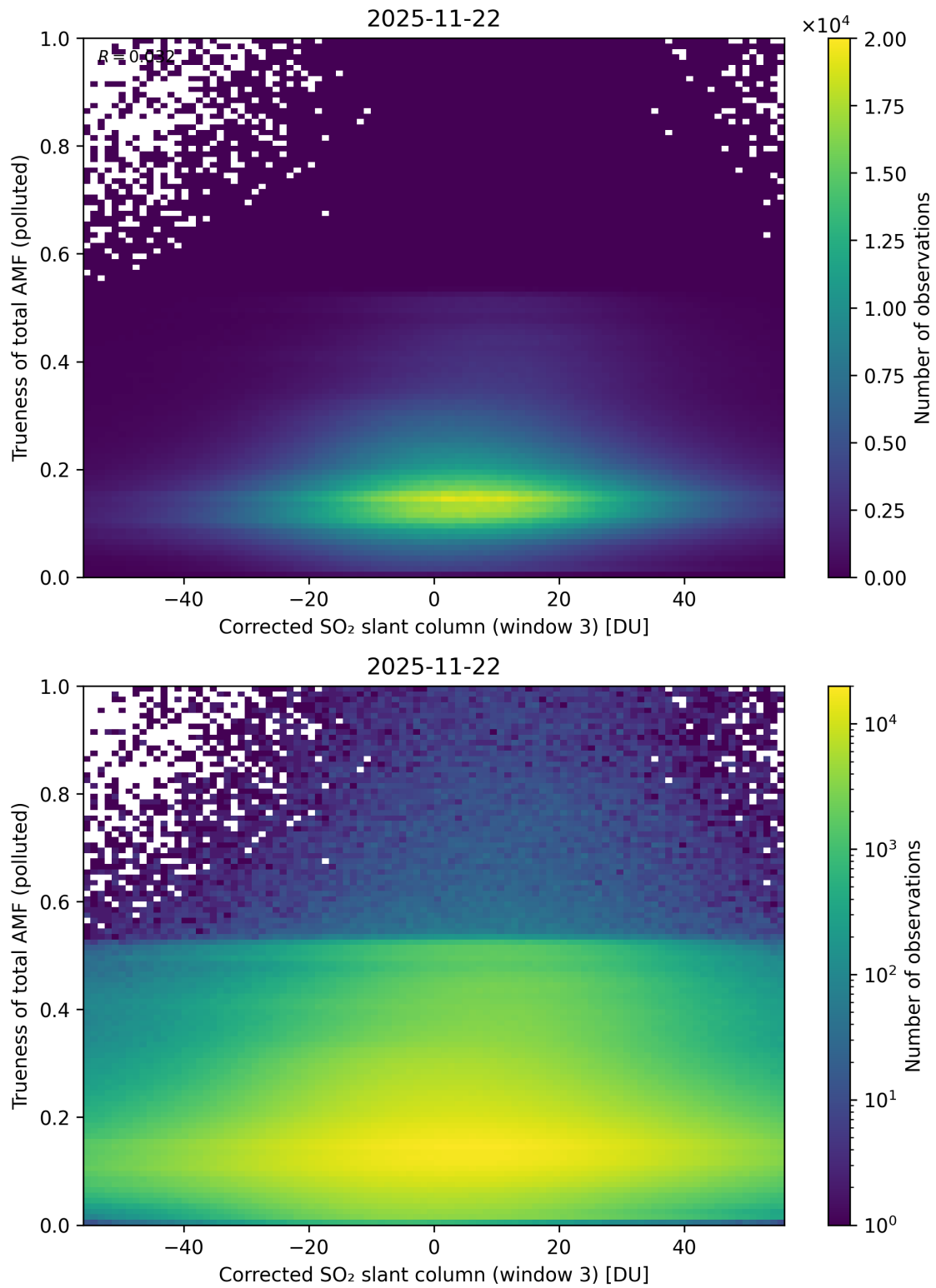
Figure 261: Scatter density plot of “Corrected SO 2 slant column (window 3)” against “Trueness of total AMF (polluted)” for 2025-11-21 to 2025-11-23.
