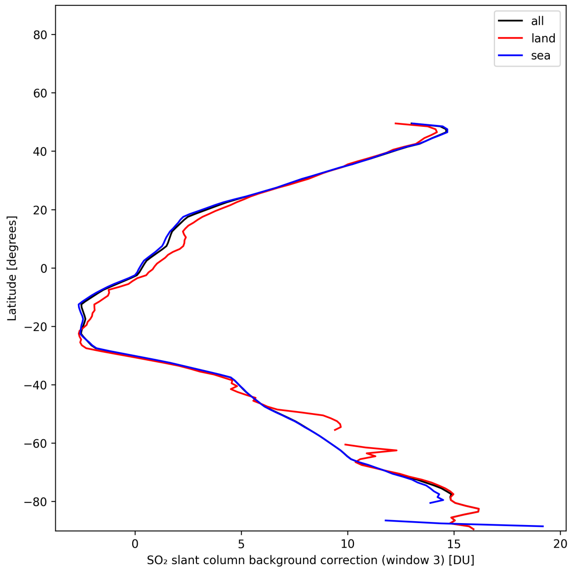
Figure 48: Zonal average of “SO 2 slant column background correction (window 3)” for 2025-11-21 to 2025-11-23.
