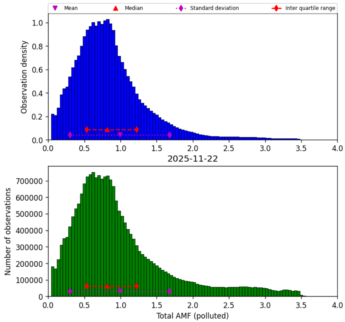
Figure 79: Histogram of “Total AMF (polluted)” for 2025-11-21 to 2025-11-23
