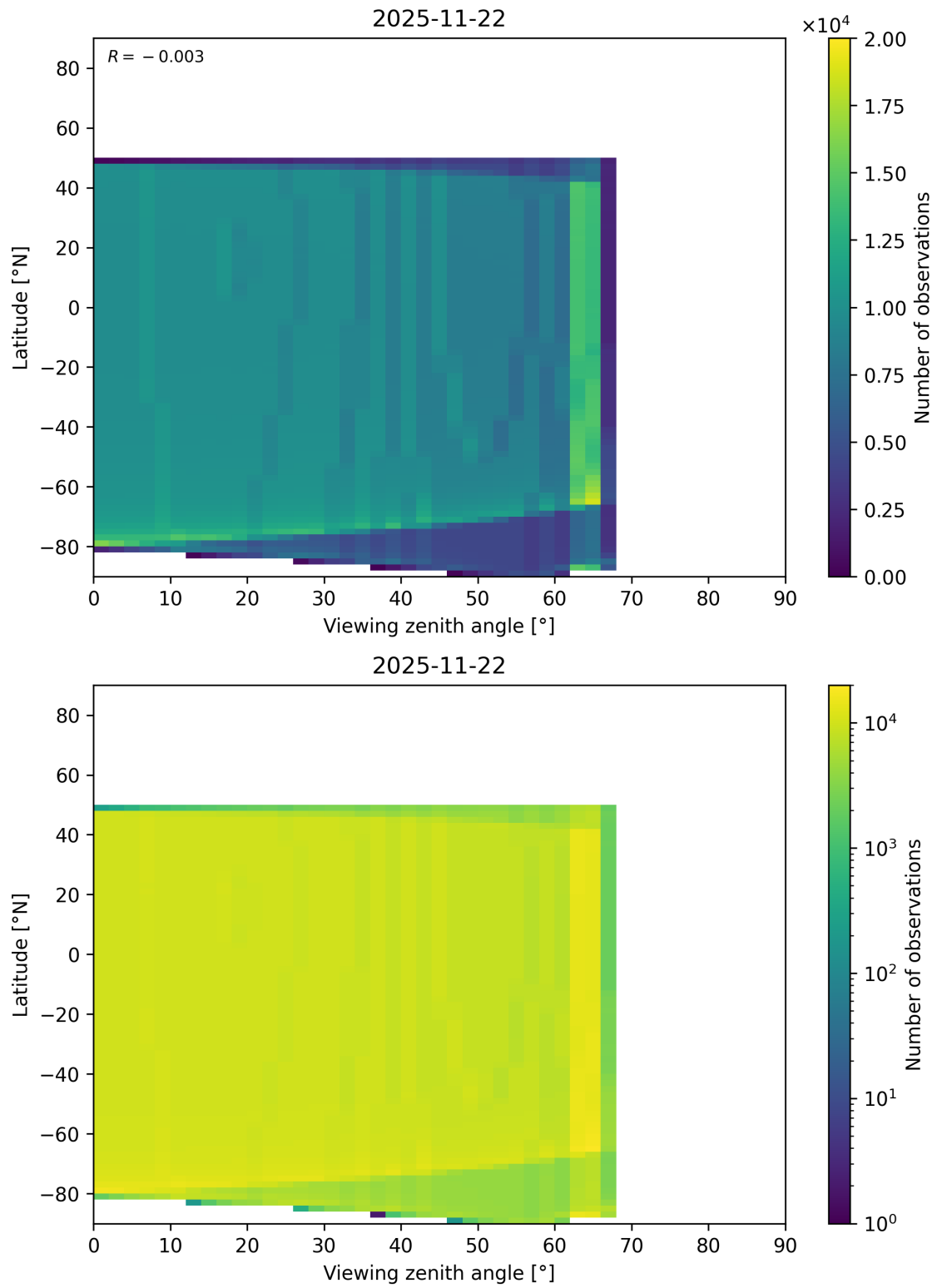
Figure 368: Scatter density plot of “Viewing zenith angle” against “Latitude” for 2025-11-21 to 2025-11-23.
