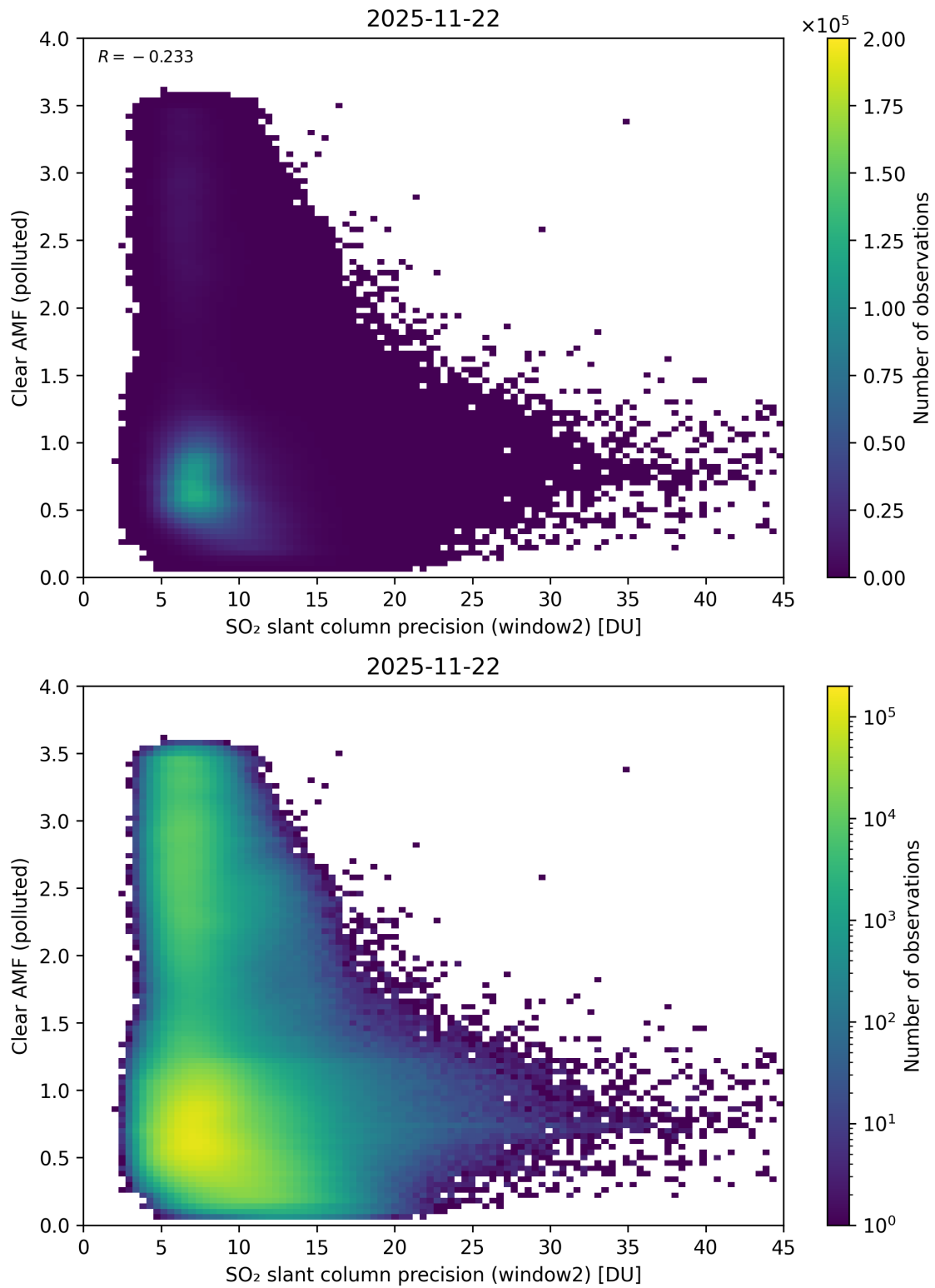
Figure 296: Scatter density plot of “SO 2 slant column precision (window2)” against “Clear AMF (polluted)” for 2025-11-21 to 2025-11-23.
