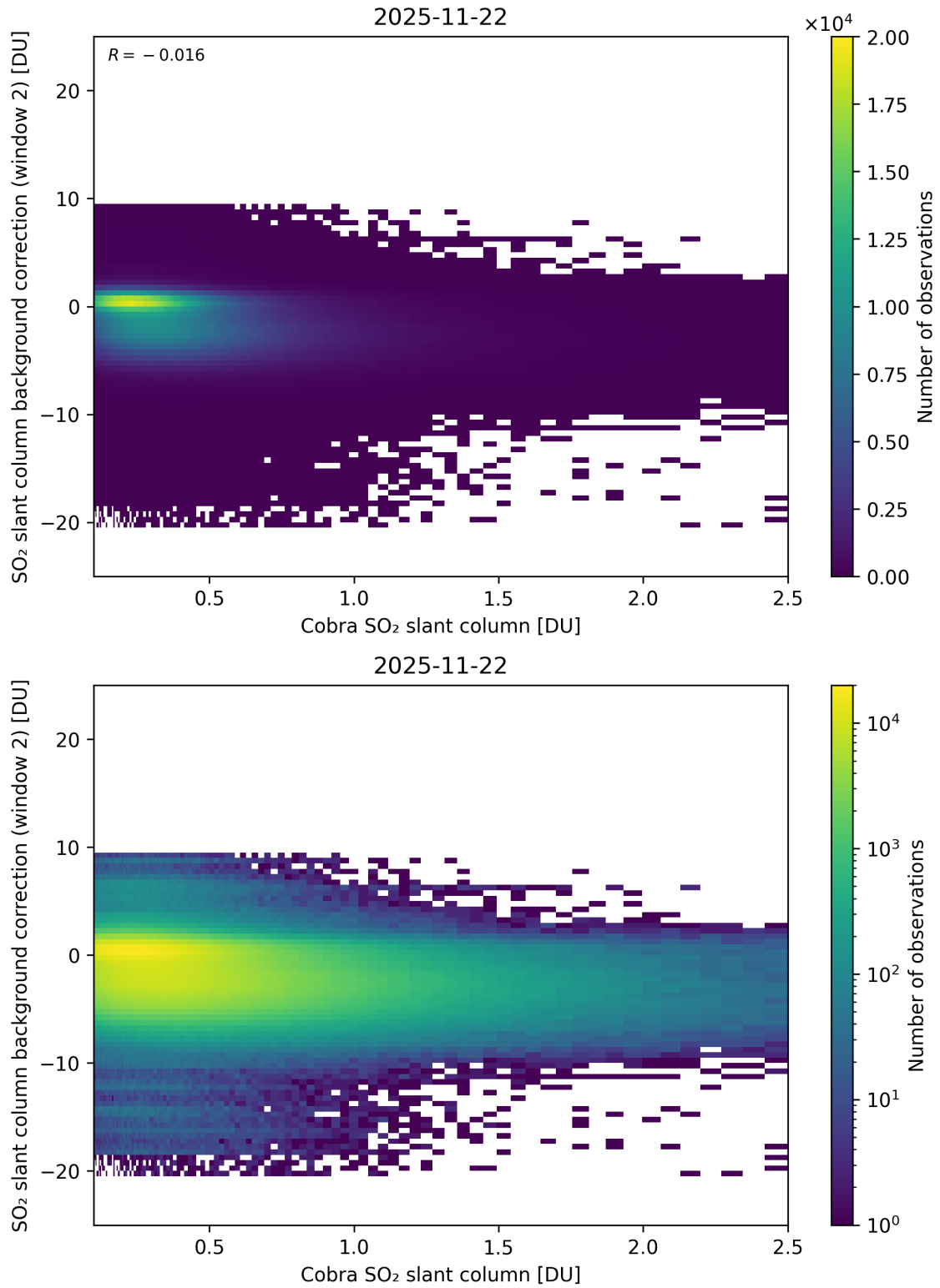
Figure 194: Scatter density plot of “Cobra SO 2 slant column” against “SO 2 slant column background correction (window 2)” for 2025-11-21 to 2025-11-23.
