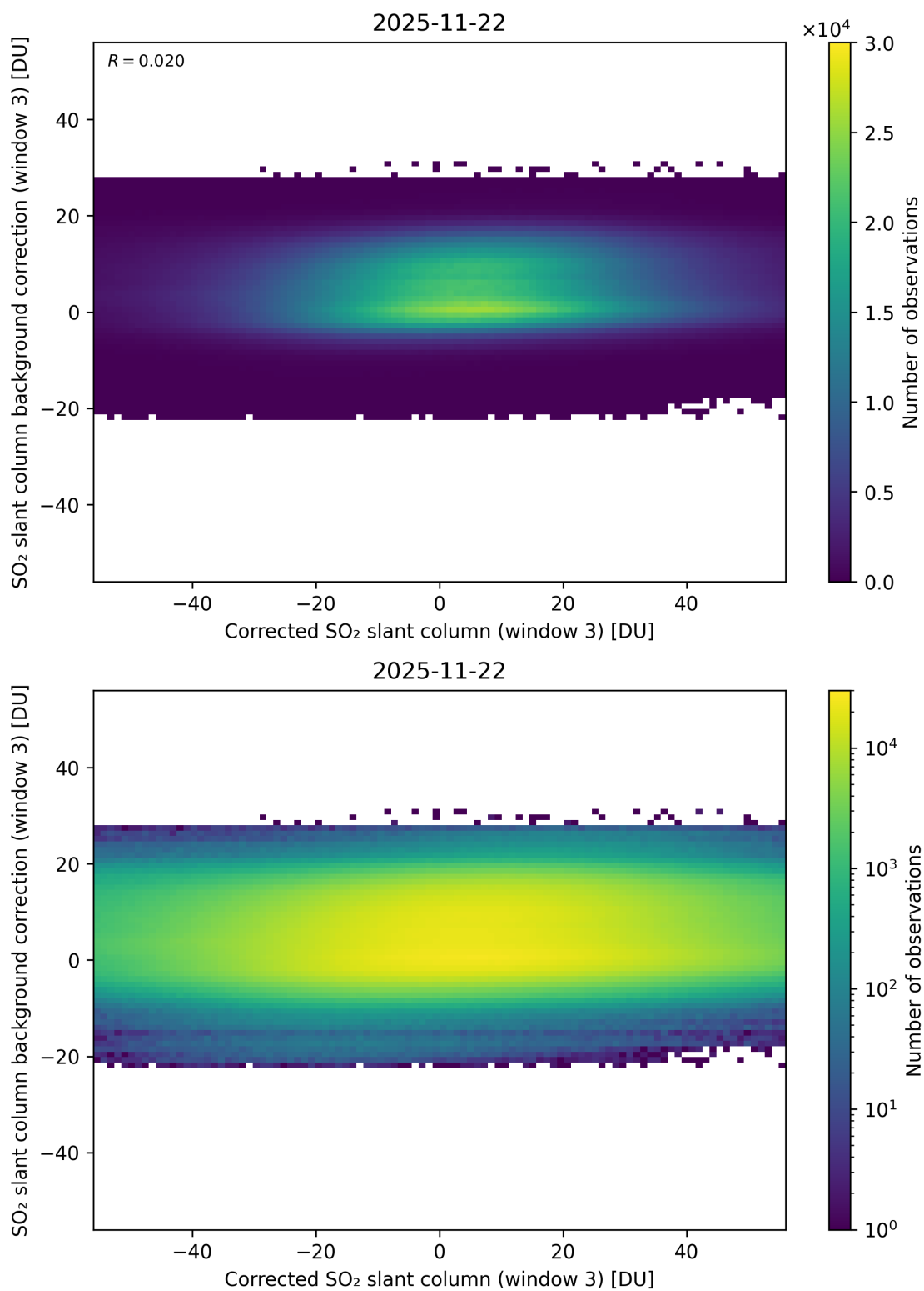
Figure 255: Scatter density plot of “Corrected SO 2 slant column (window 3)” against “SO 2 slant column background correction (window 3)” for 2025-11-21 to 2025-11-23.
