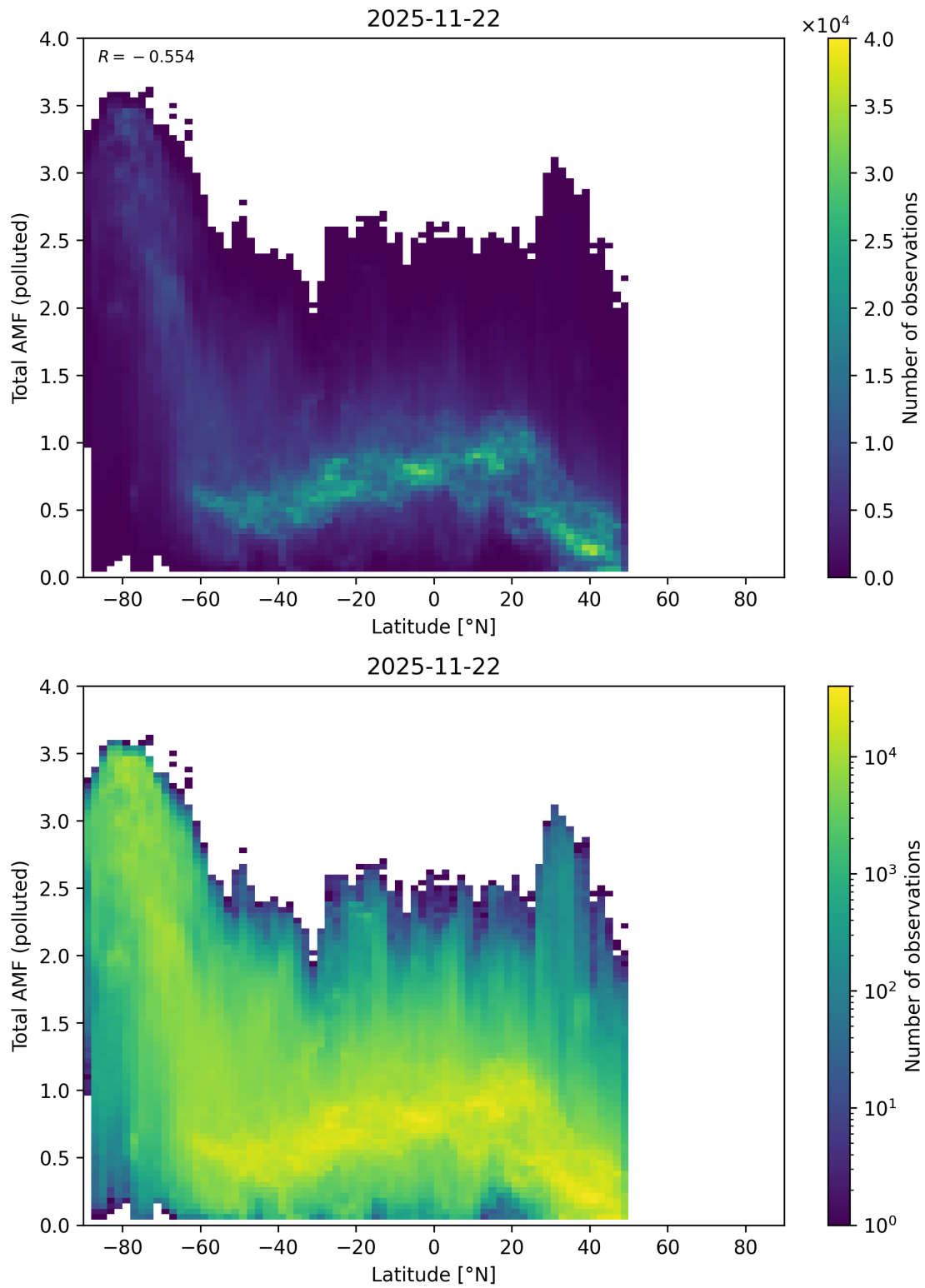
Figure 167: Scatter density plot of “Latitude” against “Total AMF (polluted)” for 2025-11-21 to 2025-11-23.
