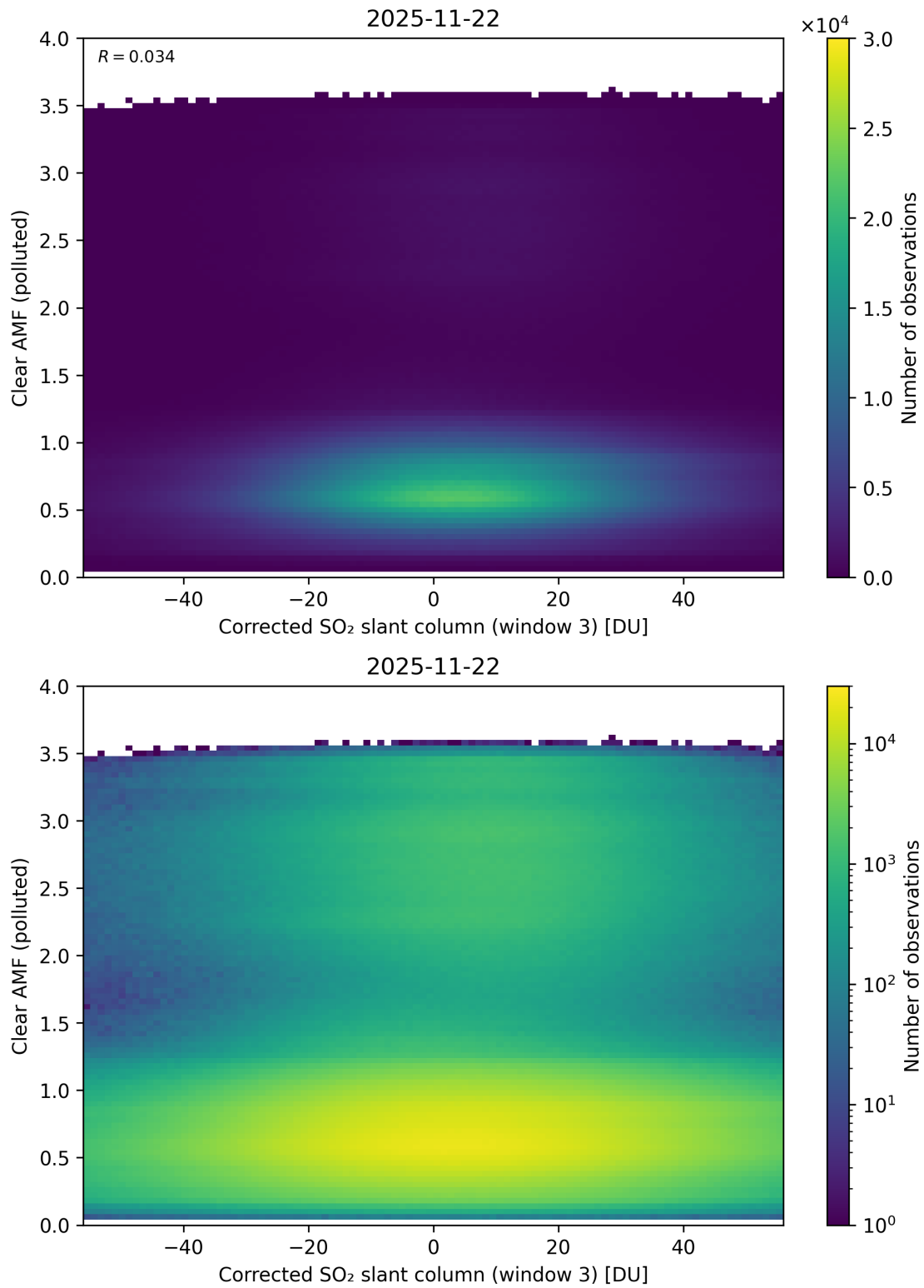
Figure 259: Scatter density plot of “Corrected SO 2 slant column (window 3)” against “Clear AMF (polluted)” for 2025-11-21 to 2025-11-23.
