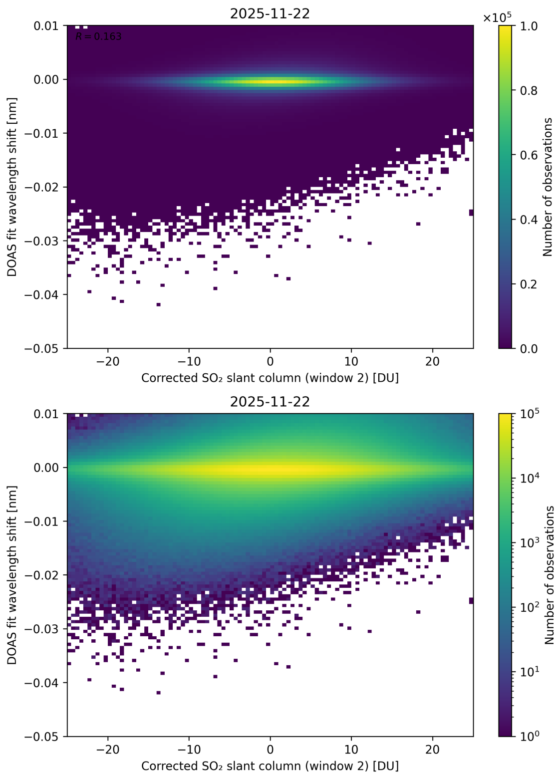
Figure 246: Scatter density plot of “Corrected SO 2 slant column (window 2)” against “DOAS fit wavelength shift” for 2025-11-21 to 2025-11-23.
