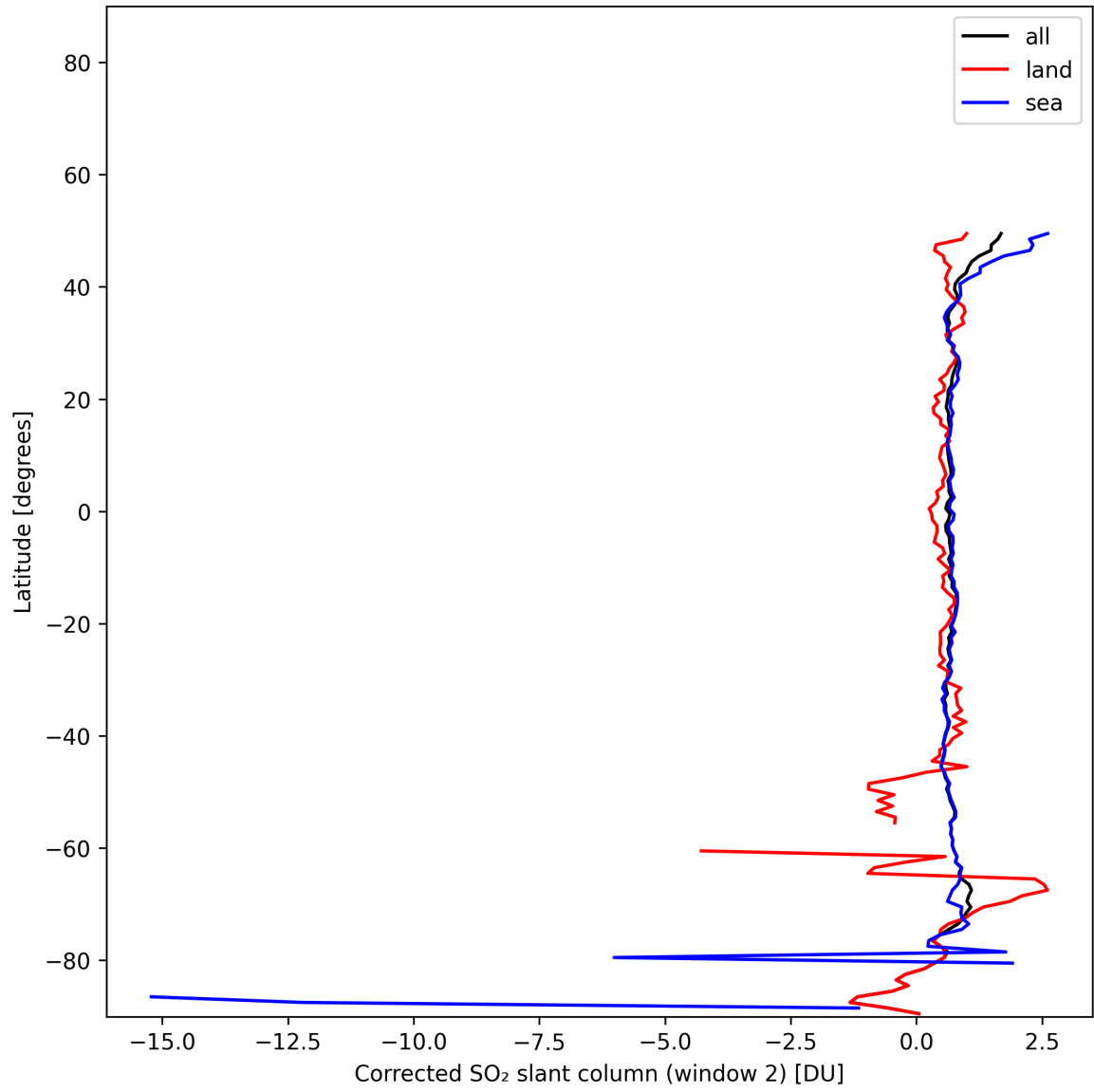
Figure 43: Zonal average of “Corrected SO 2 slant column (window 2)” for 2025-11-21 to 2025-11-23.
