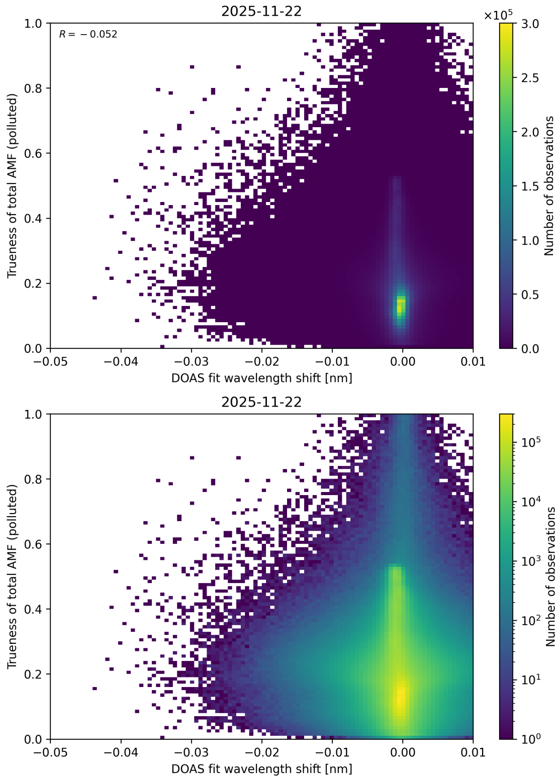
Figure 142: Scatter density plot of “DOAS fit wavelength shift” against “Trueness of total AMF (polluted)” for 2025-11-21 to 2025-11-23.
