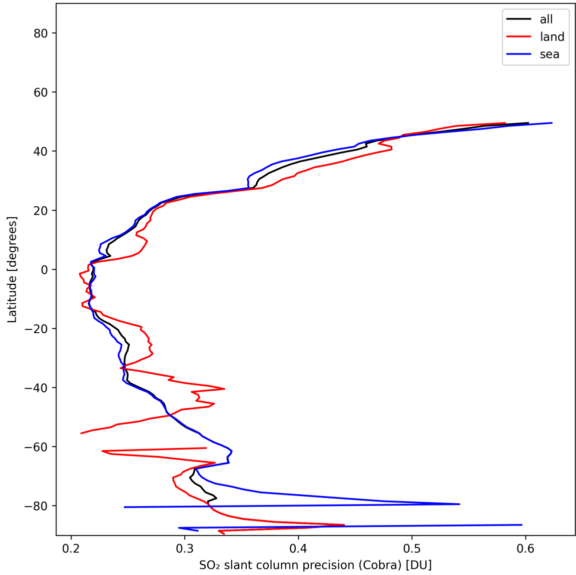
Figure 36: Zonal average of “SO 2 slant column precision (Cobra)” for 2025-11-21 to 2025-11-23.
