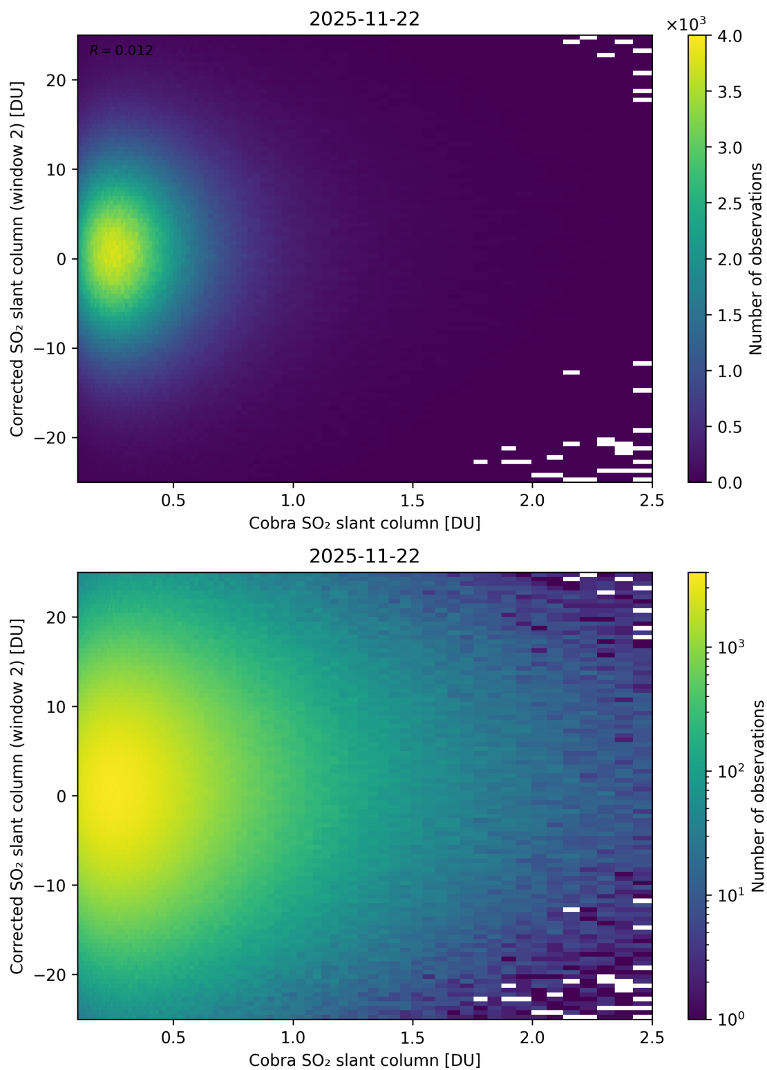
Figure 217: Scatter density plot of “Cobra SO 2 slant column” against “Corrected SO 2 slant column (window 2)” for 2025-11-21 to 2025-11-23.
