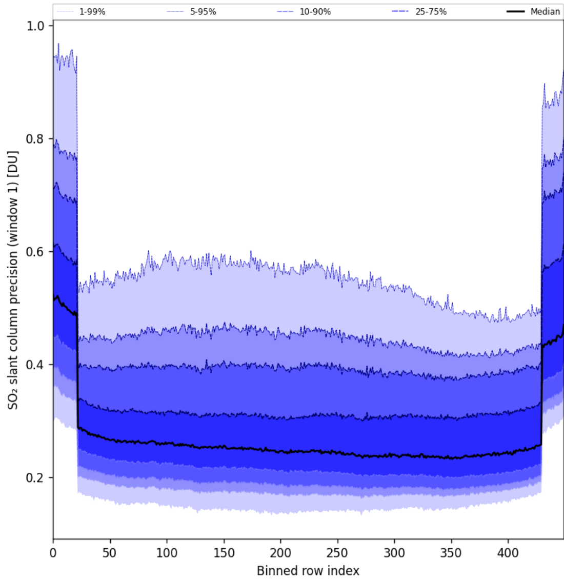
Figure 90: Along track statistics of “SO 2 slant column precision (window 1)” for 2025-11-21 to 2025-11-23
