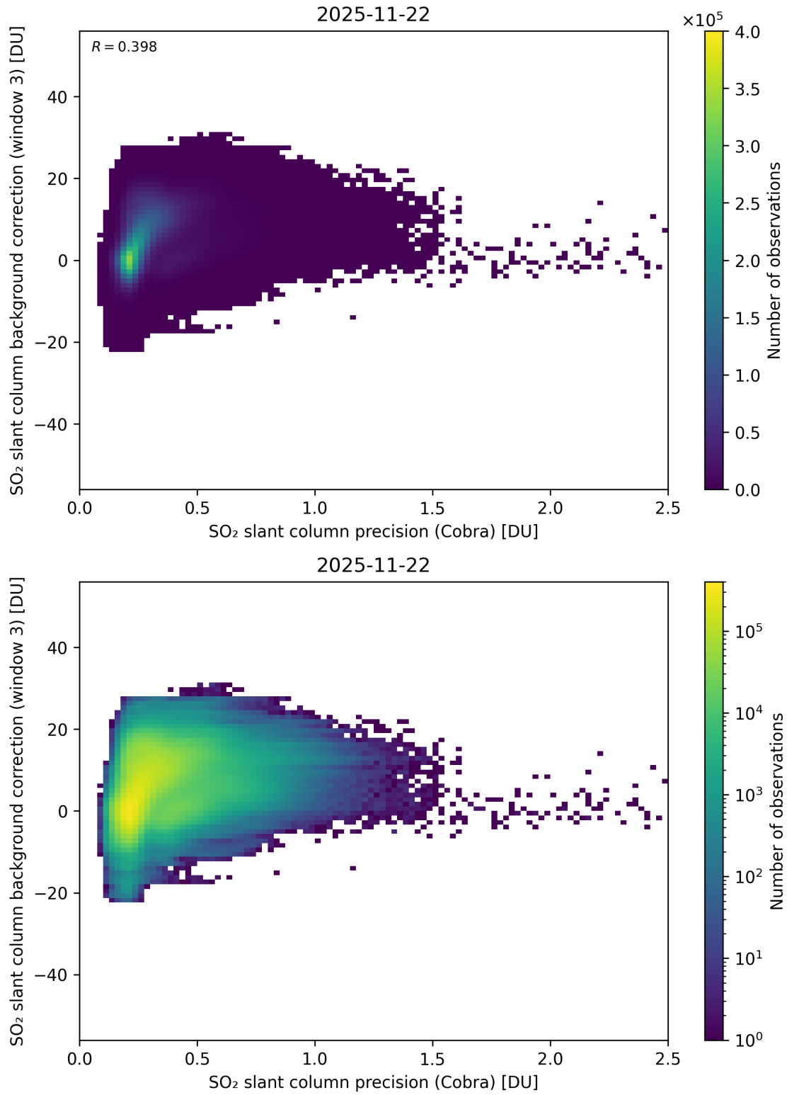
Figure 201: Scatter density plot of “SO 2 slant column precision (Cobra)” against “SO 2 slant column background correction (window 3)” for 2025-11-21 to 2025-11-23.
