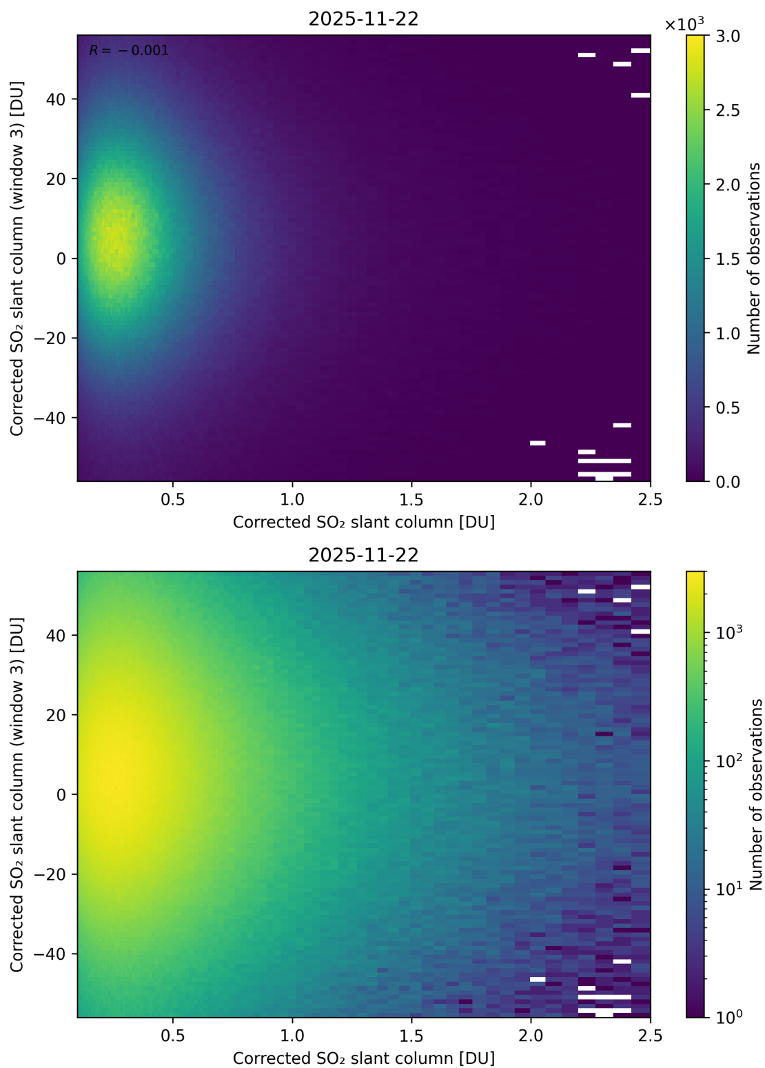
Figure 236: Scatter density plot of “Corrected SO 2 slant column” against “Corrected SO 2 slant column (window 3)” for 2025-11-21 to 2025-11-23.
