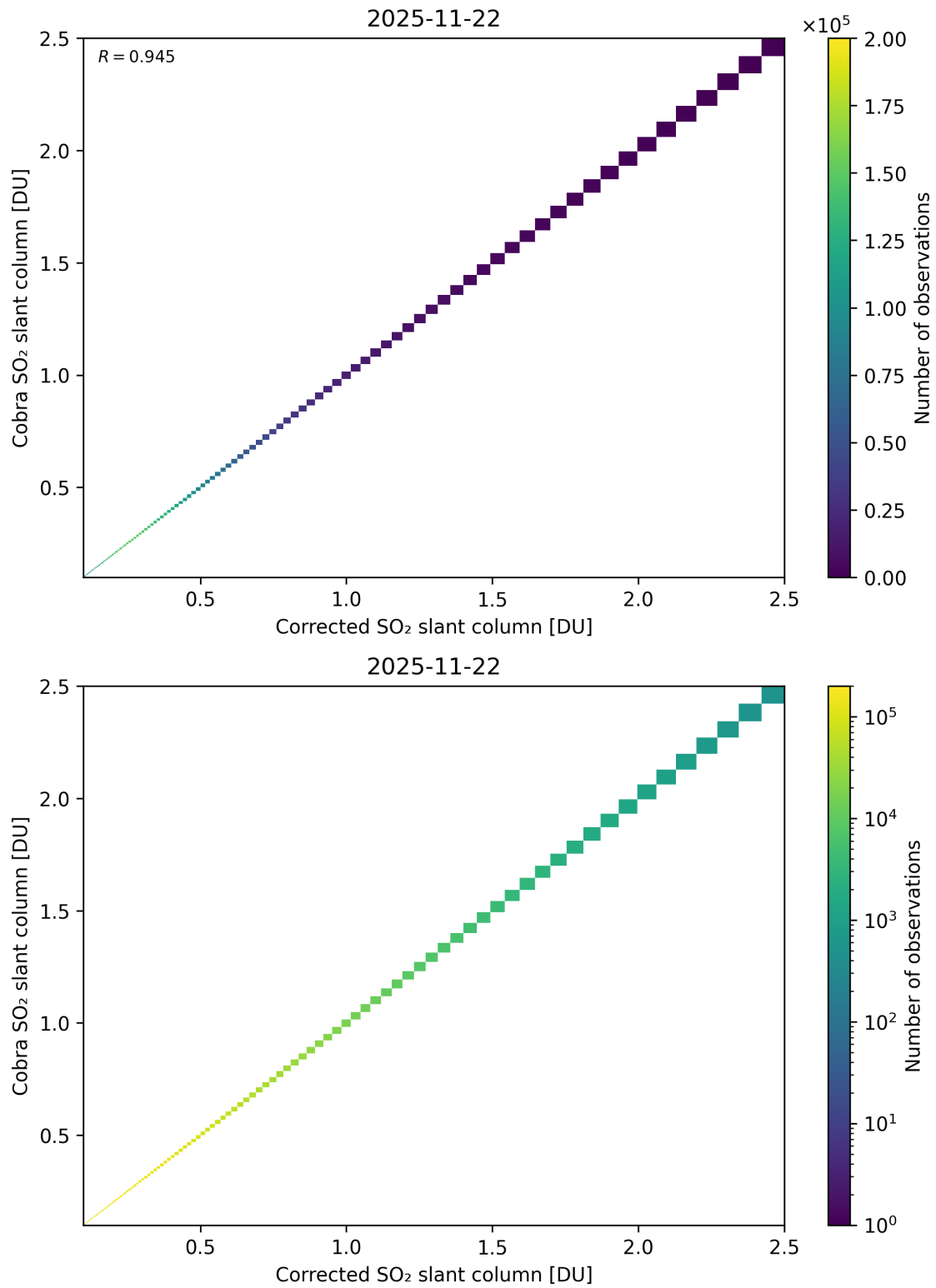
Figure 233: Scatter density plot of “Corrected SO 2 slant column” against “Cobra SO 2 slant column” for 2025-11-21 to 2025-11-23.
