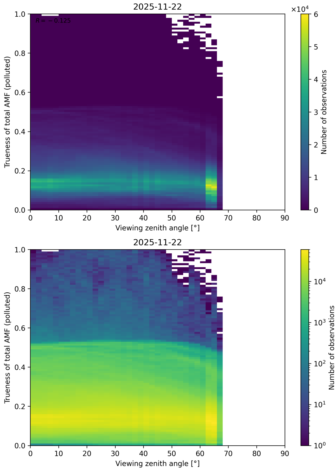
Figure 382: Scatter density plot of “Viewing zenith angle” against “Trueness of total AMF (polluted)” for 2025-11-21 to 2025-11-23.
