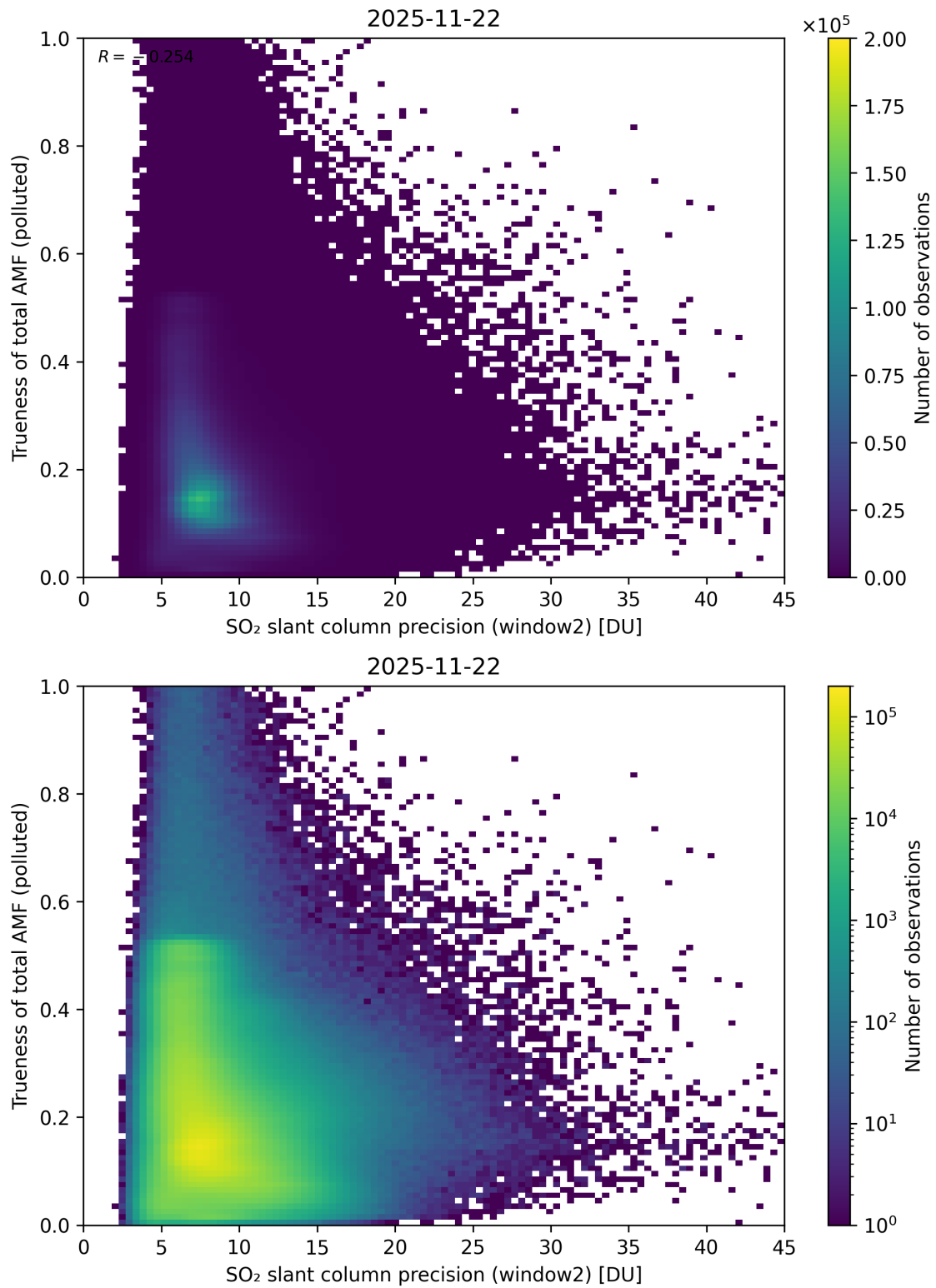
Figure 302: Scatter density plot of “SO 2 slant column precision (window2)” against “Trueness of total AMF (polluted)” for 2025-11-21 to 2025-11-23.
