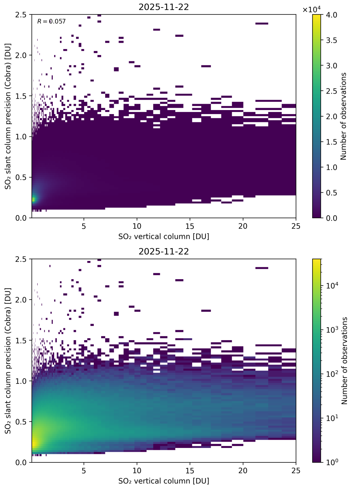
Figure 350: Scatter density plot of “SO 2 vertical column” against “SO 2 slant column precision (Cobra)” for 2025-11-21 to 2025-11-23.
