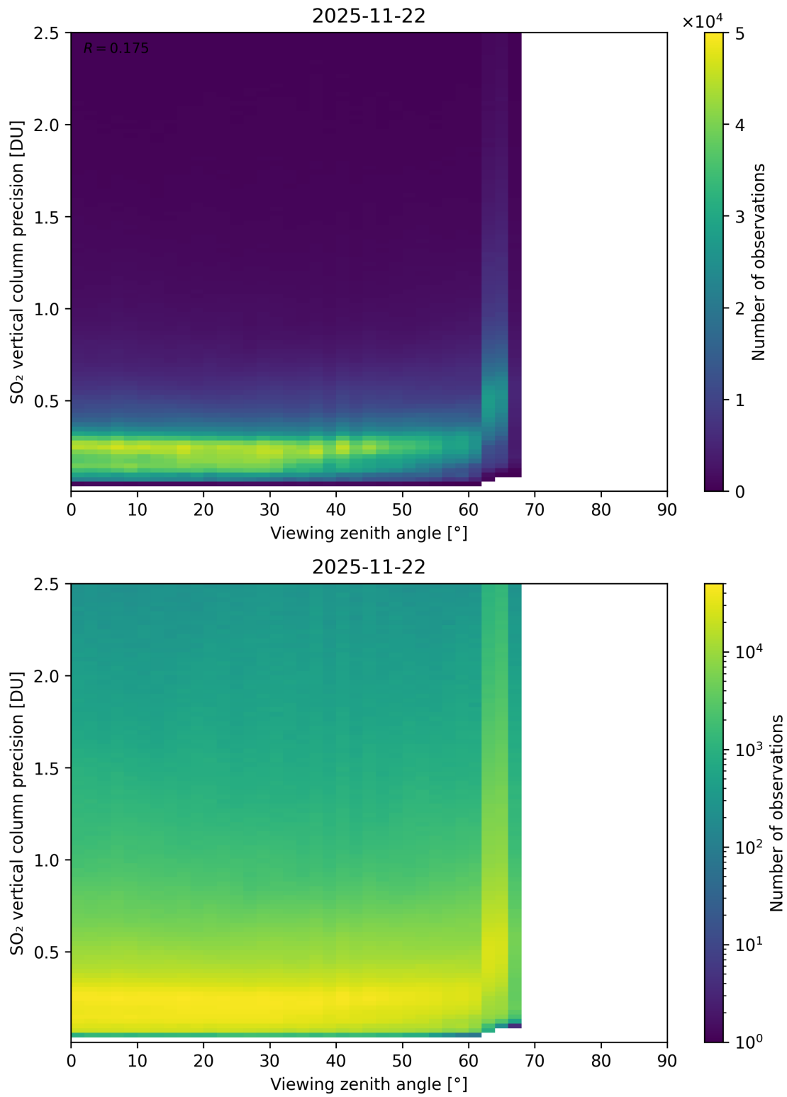
Figure 384: Scatter density plot of “Viewing zenith angle” against “SO 2 vertical column precision” for 2025-11-21 to 2025-11-23.
