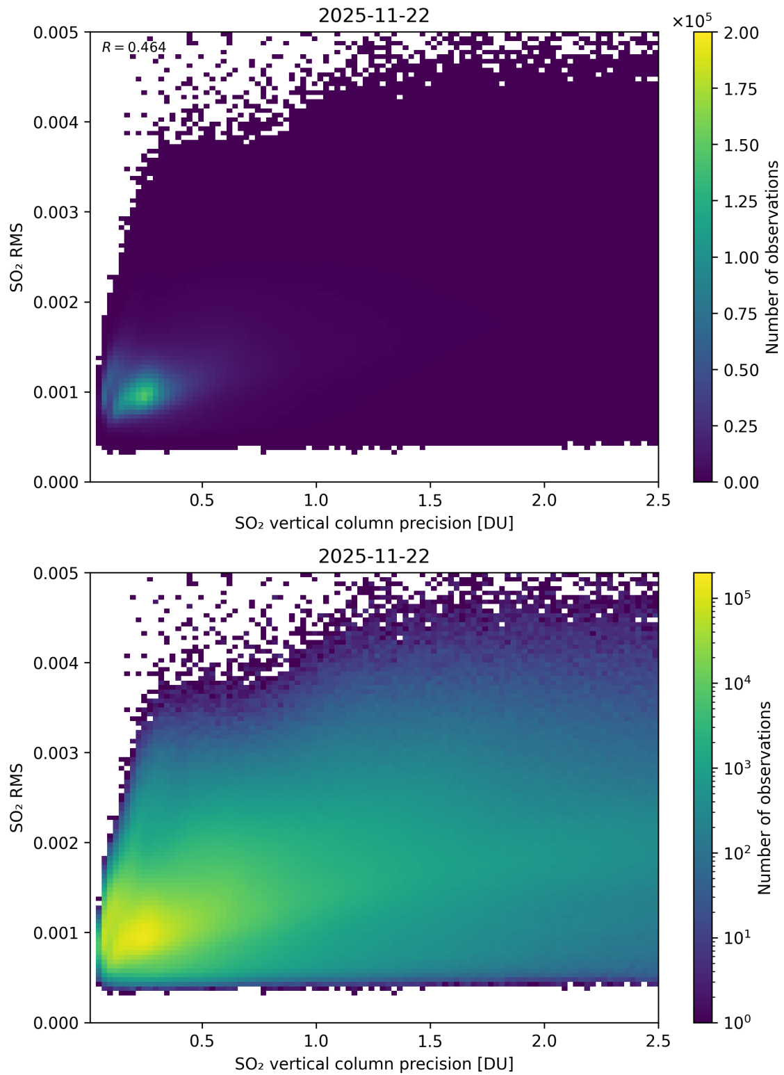
Figure 334: Scatter density plot of “SO 2 vertical column precision” against “SO 2 RMS” for 2025-11-21 to 2025-11-23.
