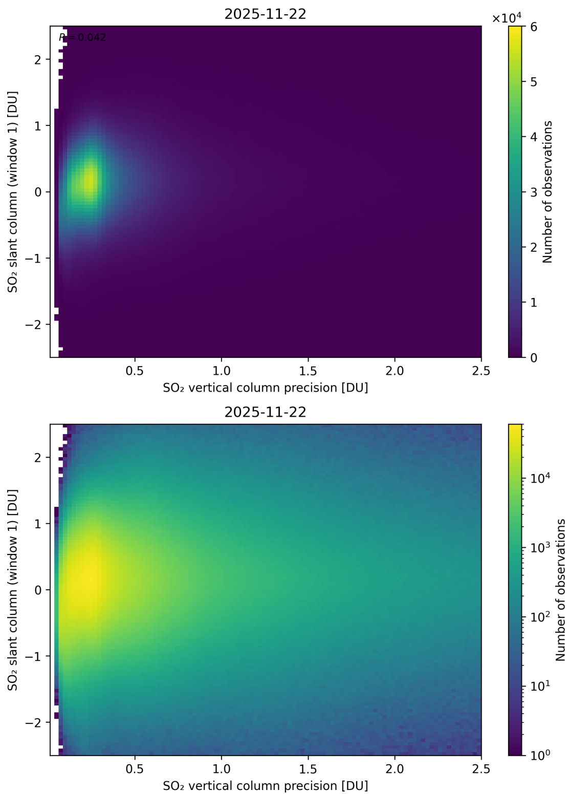
Figure 341: Scatter density plot of “SO 2 vertical column precision” against “SO 2 slant column (window 1)” for 2025-11-21 to 2025-11-23.
