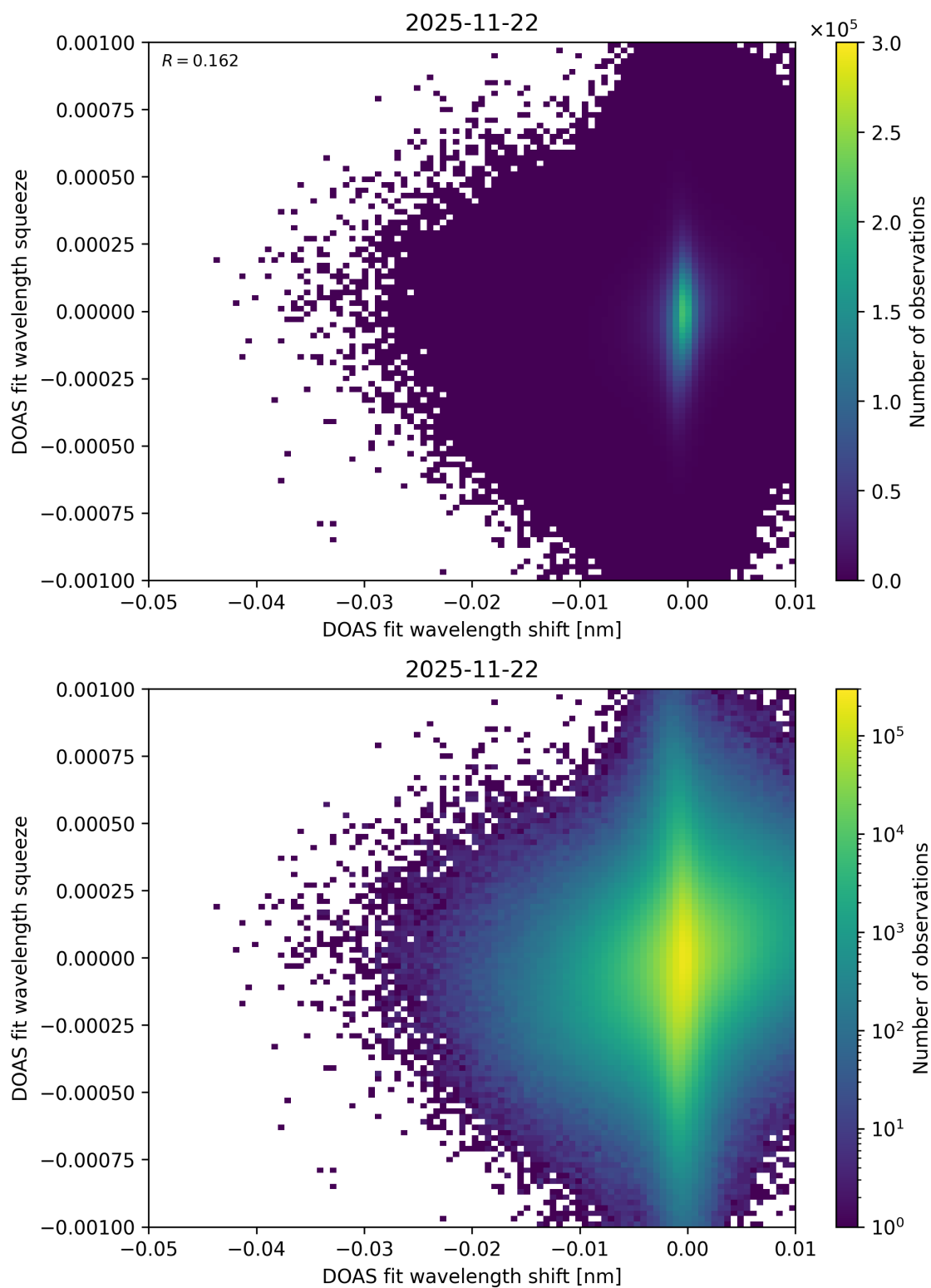
Figure 138: Scatter density plot of “DOAS fit wavelength shift” against “DOAS fit wavelength squeeze” for 2025-11-21 to 2025-11-23.
