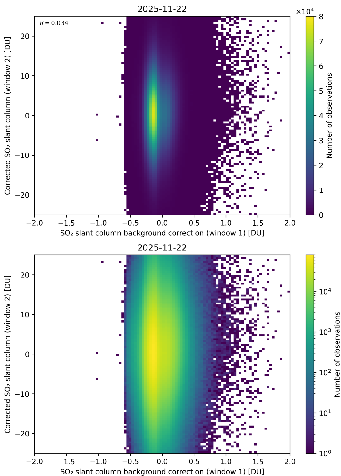
Figure 115: Scatter density plot of “SO 2 slant column background correction (window 1)” against “Corrected SO 2 slant column (window 2)” for 2025-11-21 to 2025-11-23.
