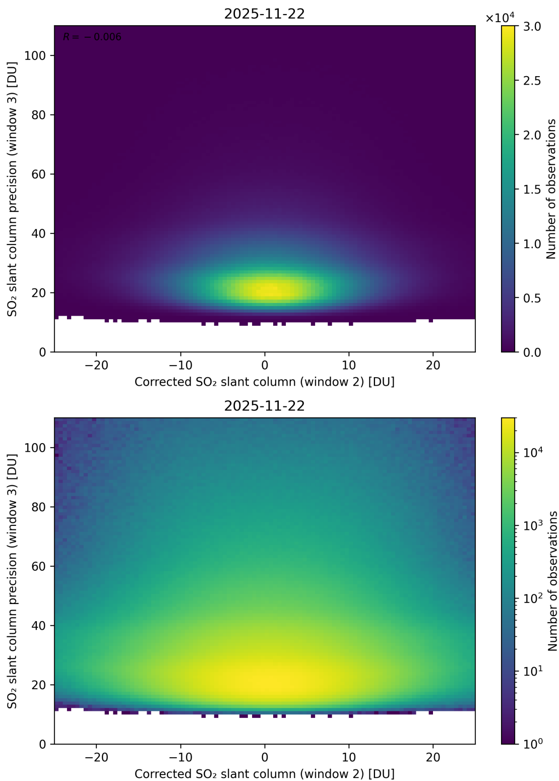
Figure 252: Scatter density plot of “Corrected SO 2 slant column (window 2)” against “SO 2 slant column precision (window 3)” for 2025-11-21 to 2025-11-23.
