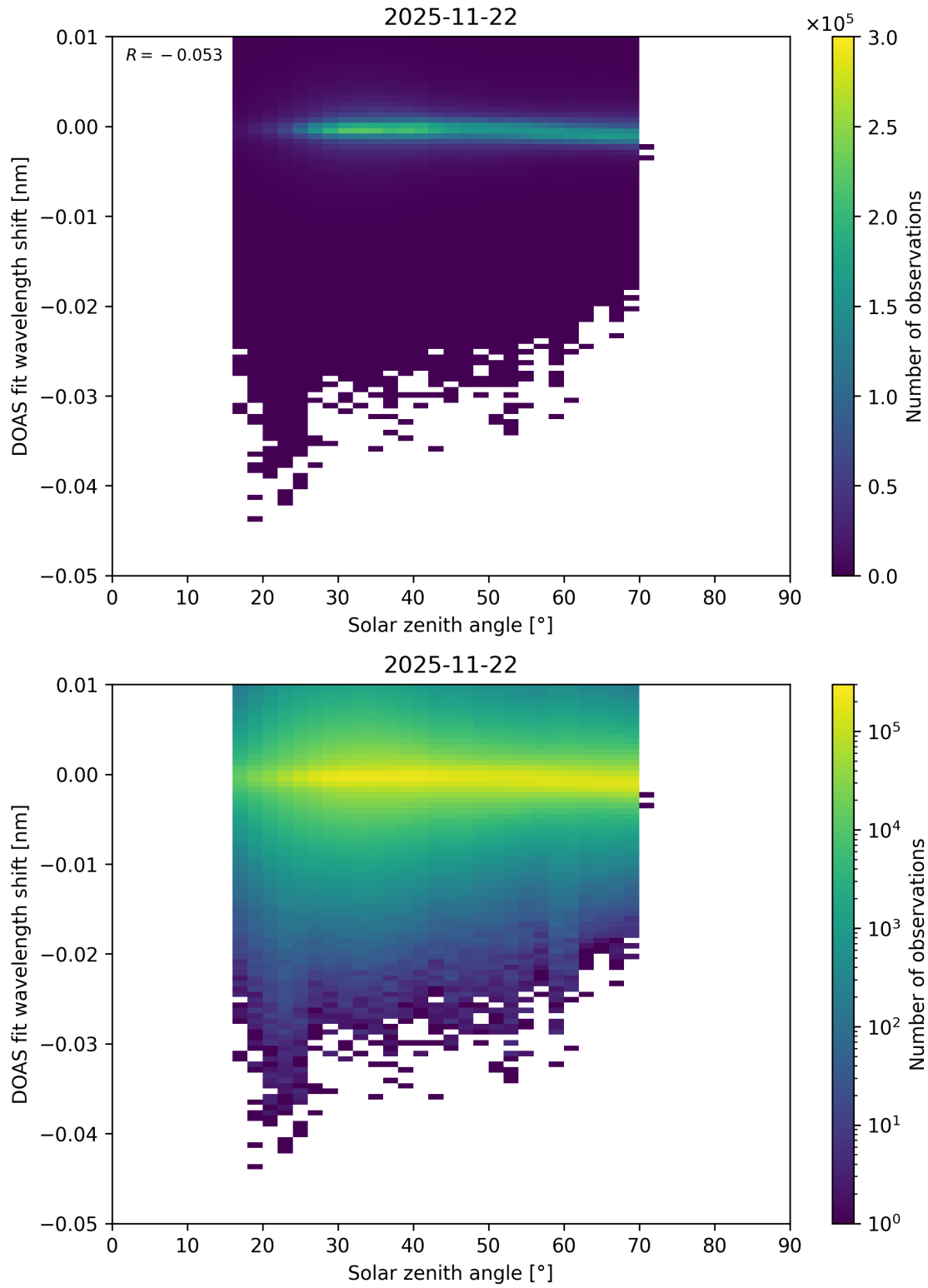
Figure 174: Scatter density plot of “Solar zenith angle” against “DOAS fit wavelength shift” for 2025-11-21 to 2025-11-23.
