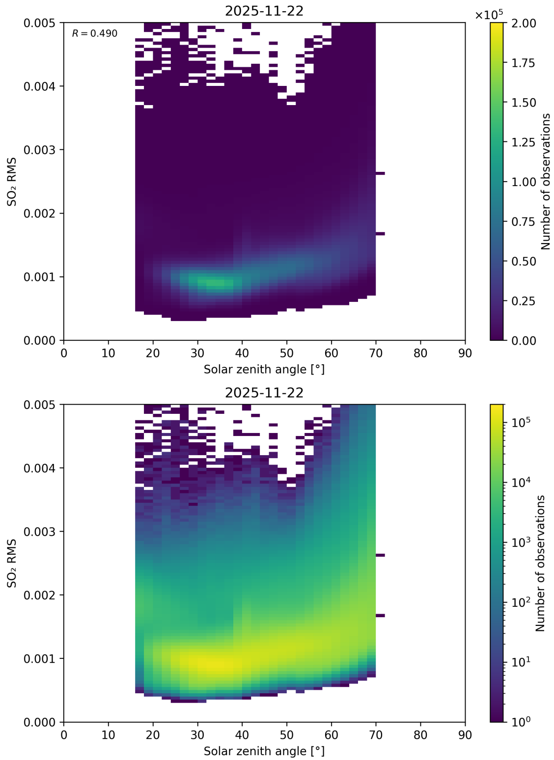
Figure 176: Scatter density plot of “Solar zenith angle” against “SO 2 RMS” for 2025-11-21 to 2025-11-23.
