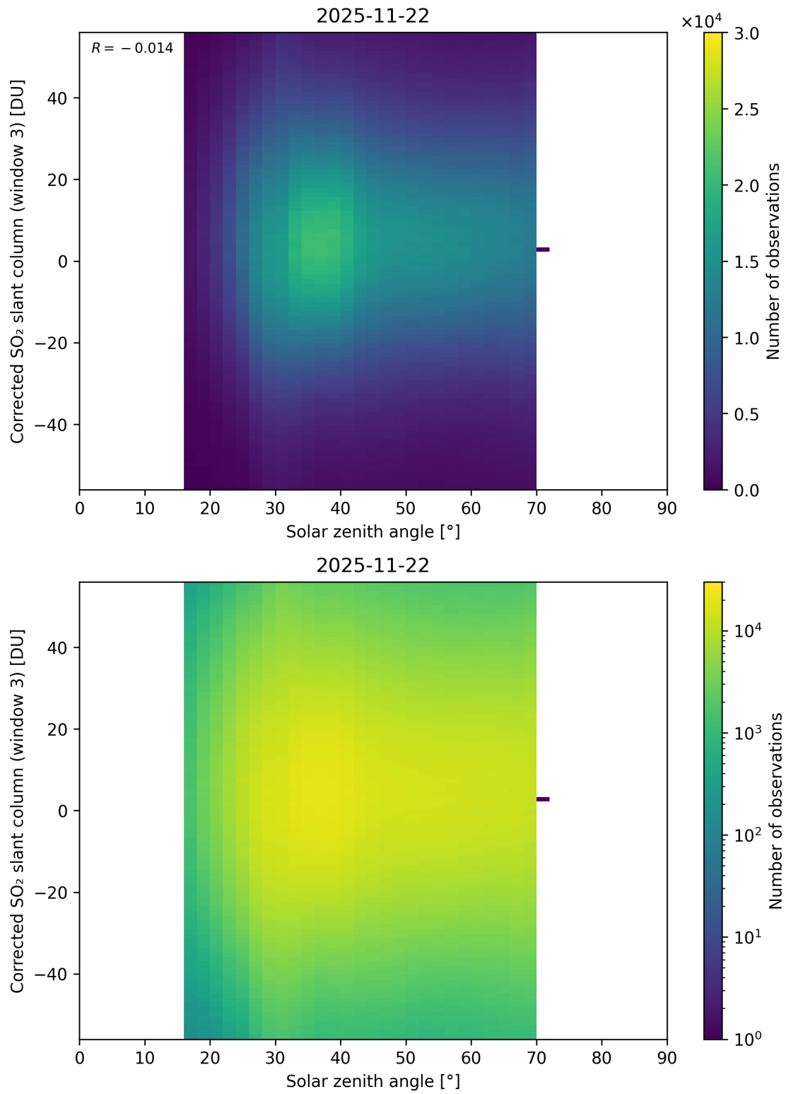
Figure 183: Scatter density plot of “Solar zenith angle” against “Corrected SO 2 slant column (window 3)” for 2025-11-21 to 2025-11-23.
