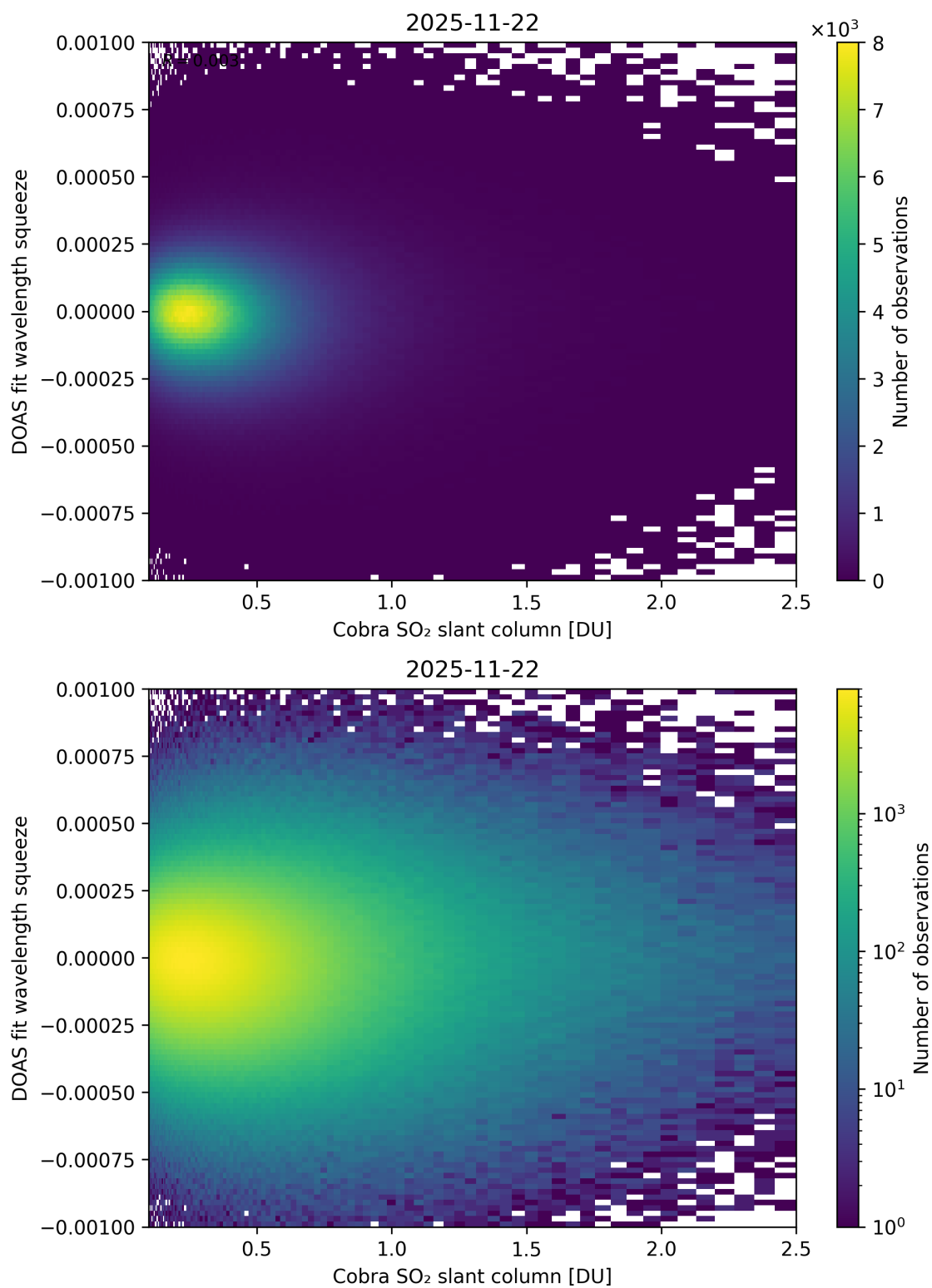
Figure 197: Scatter density plot of “Cobra SO 2 slant column” against “DOAS fit wavelength squeeze” for 2025-11-21 to 2025-11-23.
