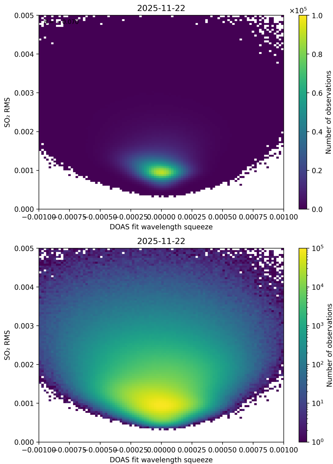
Figure 143: Scatter density plot of “DOAS fit wavelength squeeze” against “SO 2 RMS” for 2025-11-21 to 2025-11-23.
