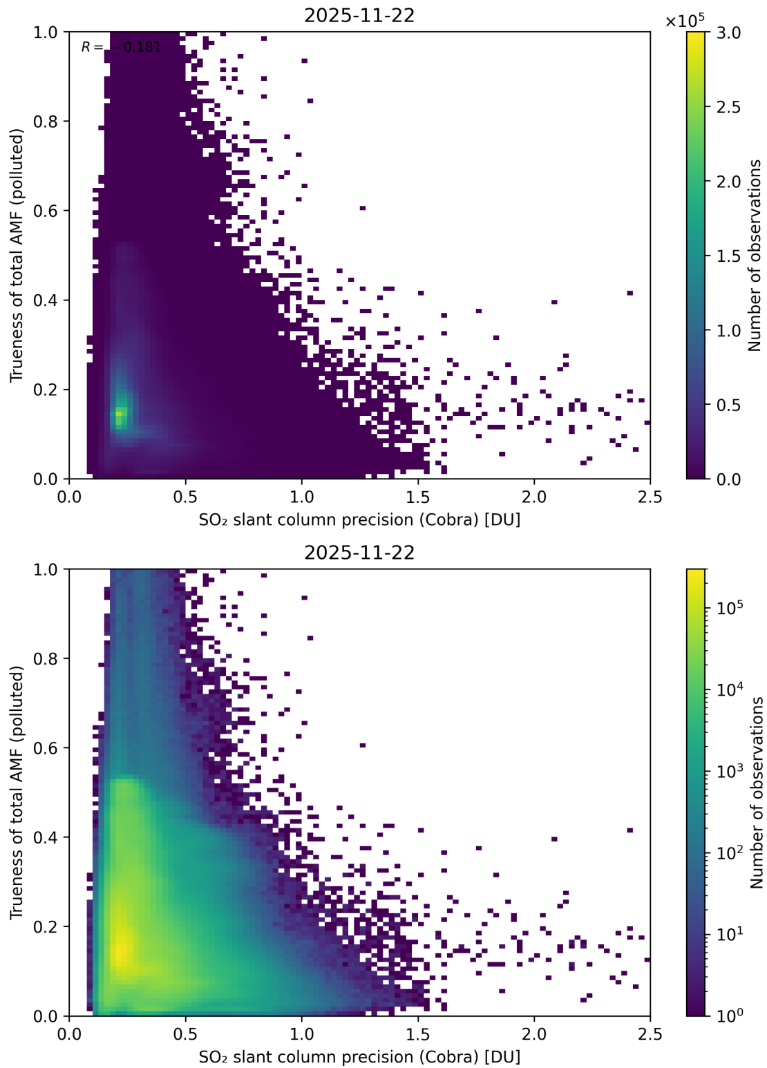
Figure 214: Scatter density plot of “SO 2 slant column precision (Cobra)” against “Trueness of total AMF (polluted)” for 2025-11-21 to 2025-11-23.
