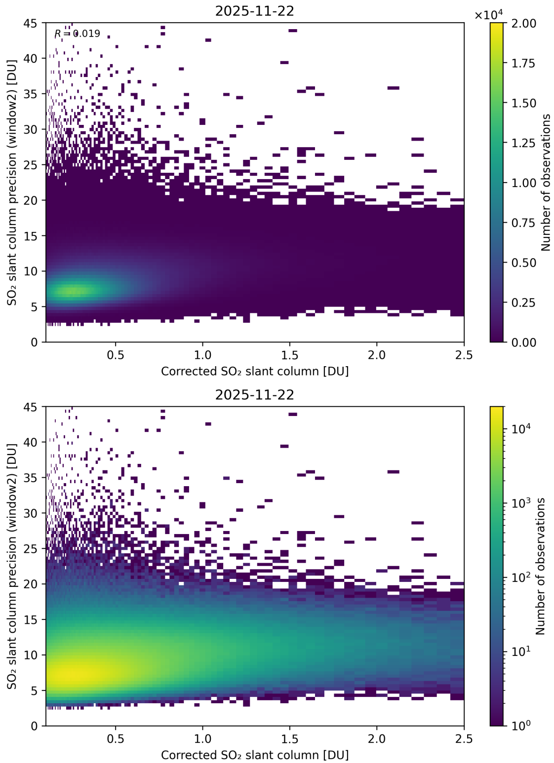
Figure 239: Scatter density plot of “Corrected SO 2 slant column” against “SO 2 slant column precision (window2)” for 2025-11-21 to 2025-11-23.
