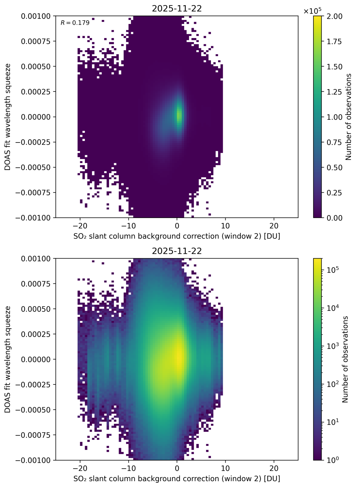
Figure 124: Scatter density plot of “SO 2 slant column background correction (window 2)” against “DOAS fit wavelength squeeze” for 2025-11-21 to 2025-11-23.
