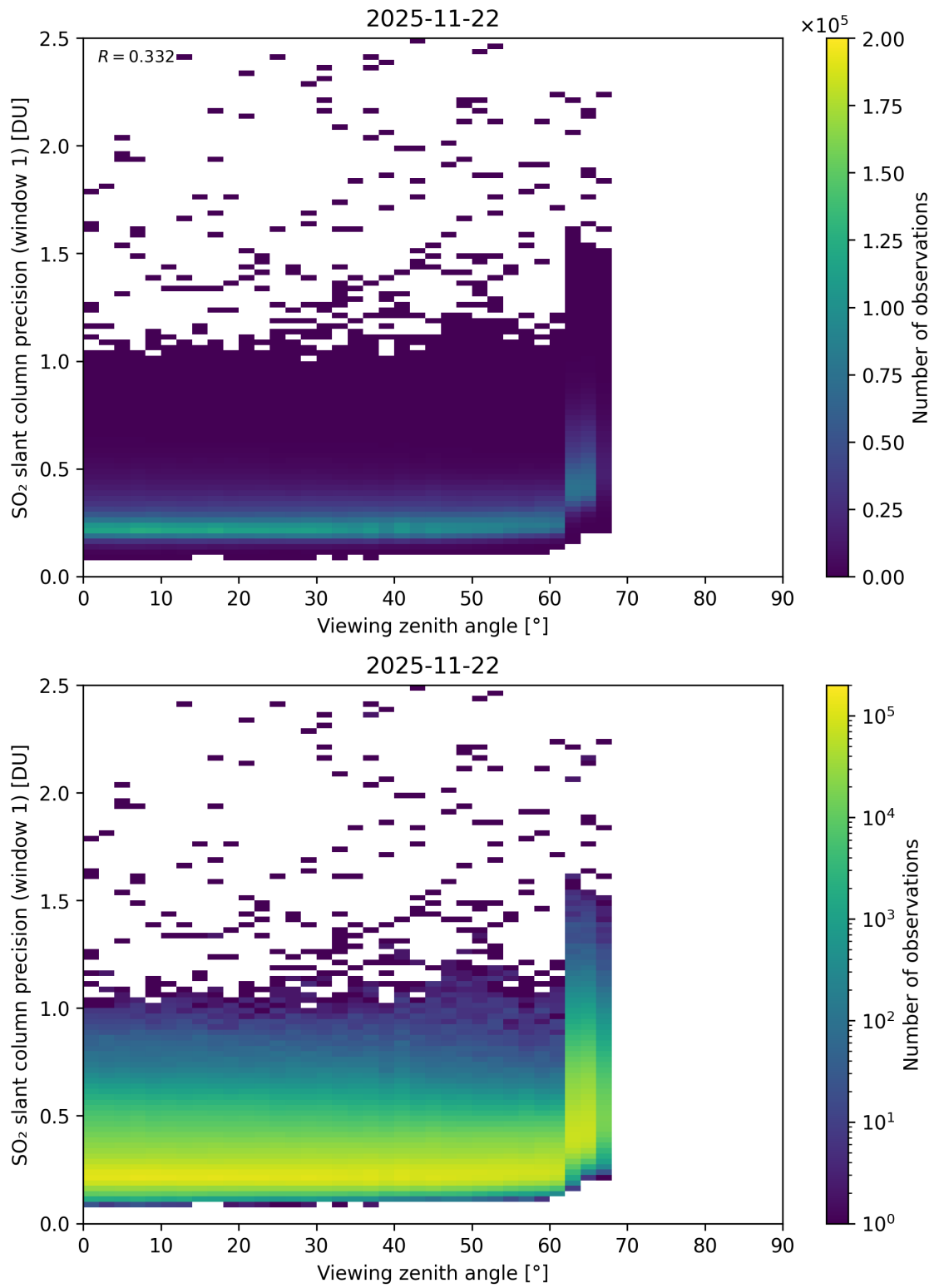
Figure 377: Scatter density plot of “Viewing zenith angle” against “SO 2 slant column precision (window 1)” for 2025-11-21 to 2025-11-23.
