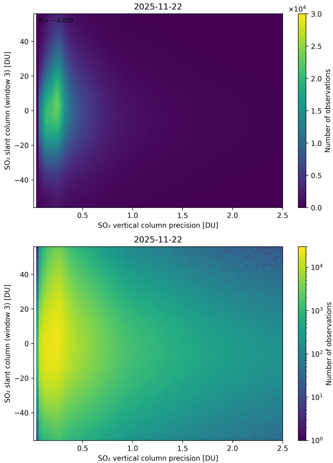
Figure 344: Scatter density plot of “SO 2 vertical column precision” against “SO 2 slant column (window 3)” for 2025-11-21 to 2025-11-23.
