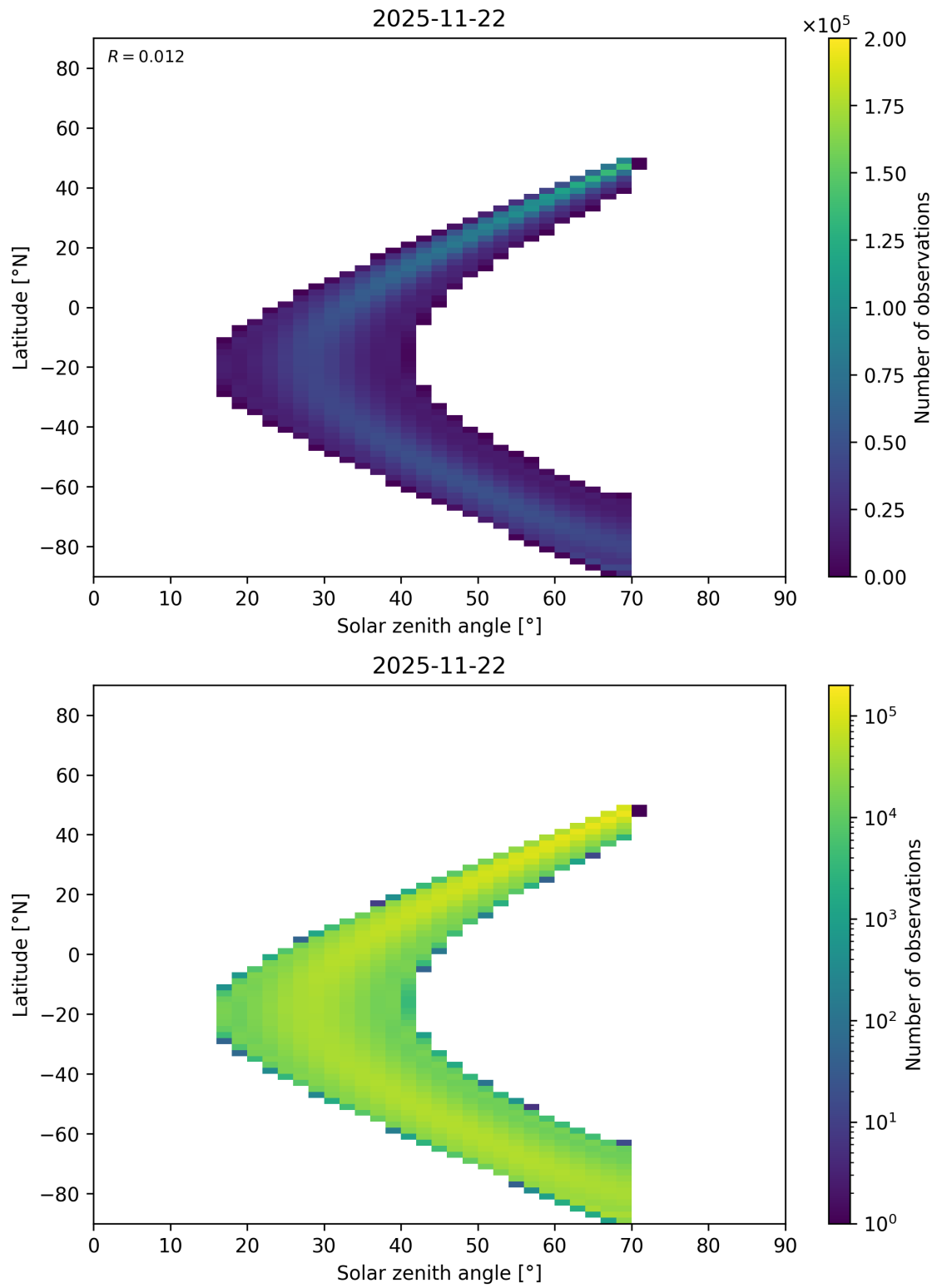
Figure 177: Scatter density plot of “Solar zenith angle” against “Latitude” for 2025-11-21 to 2025-11-23.
