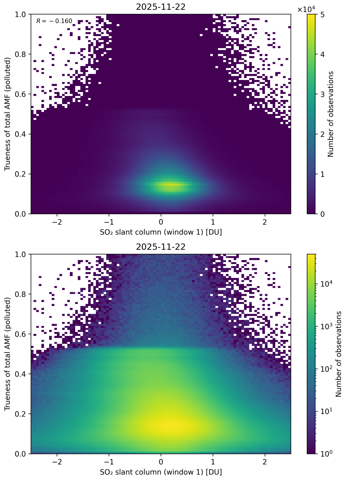
Figure 290: Scatter density plot of “SO 2 slant column (window 1)” against “Trueness of total AMF (polluted)” for 2025-11-21 to 2025-11-23.
