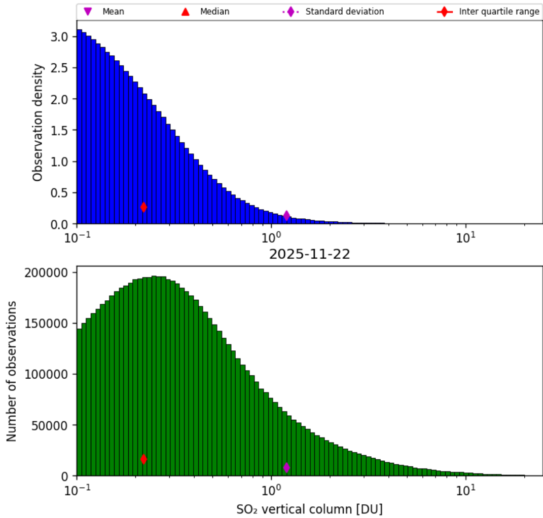
Figure 58: Histogram of “SO 2 vertical column” for 2025-11-21 to 2025-11-23
