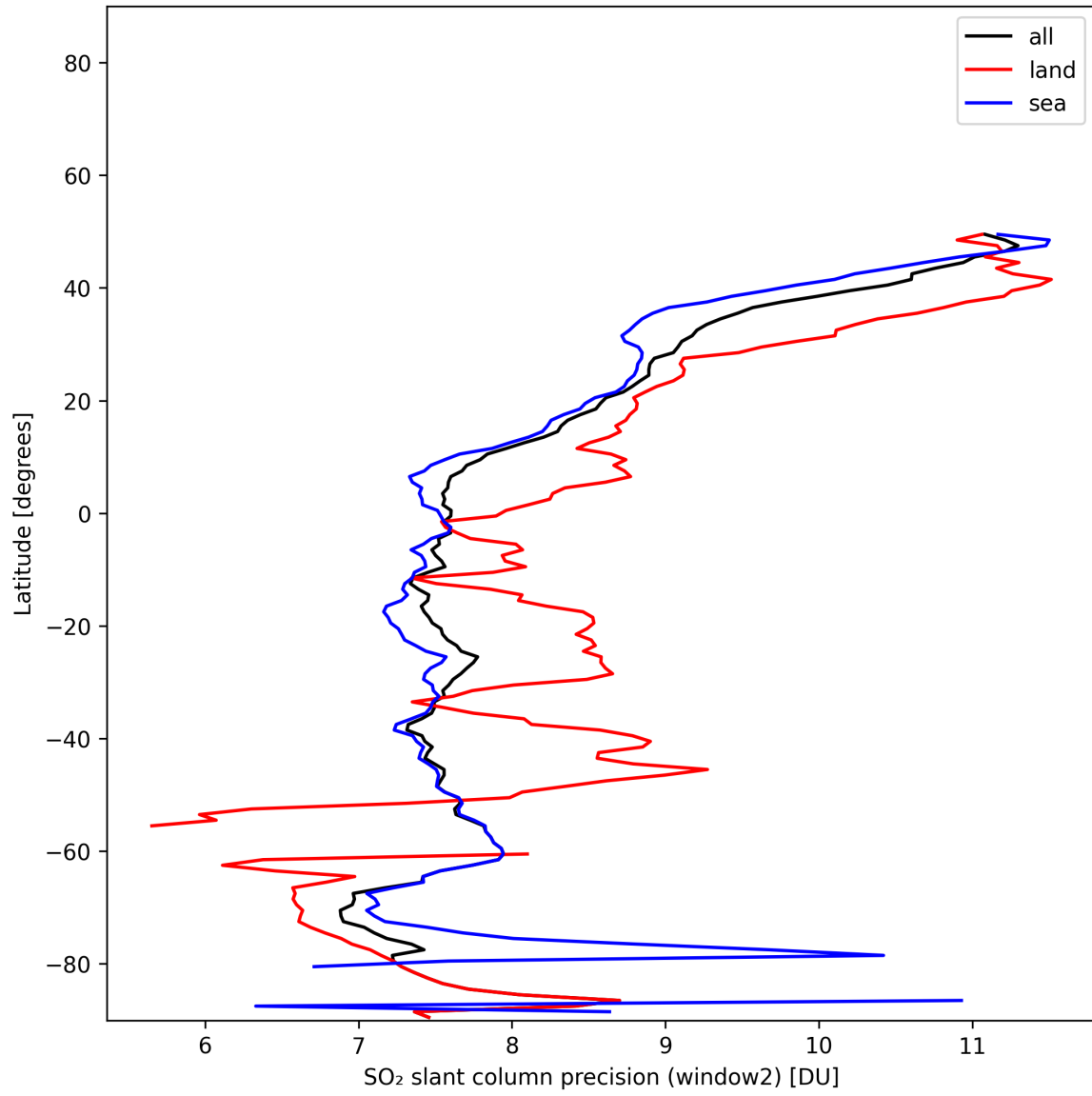
Figure 42: Zonal average of “SO 2 slant column precision (window2)” for 2025-11-21 to 2025-11-23.
