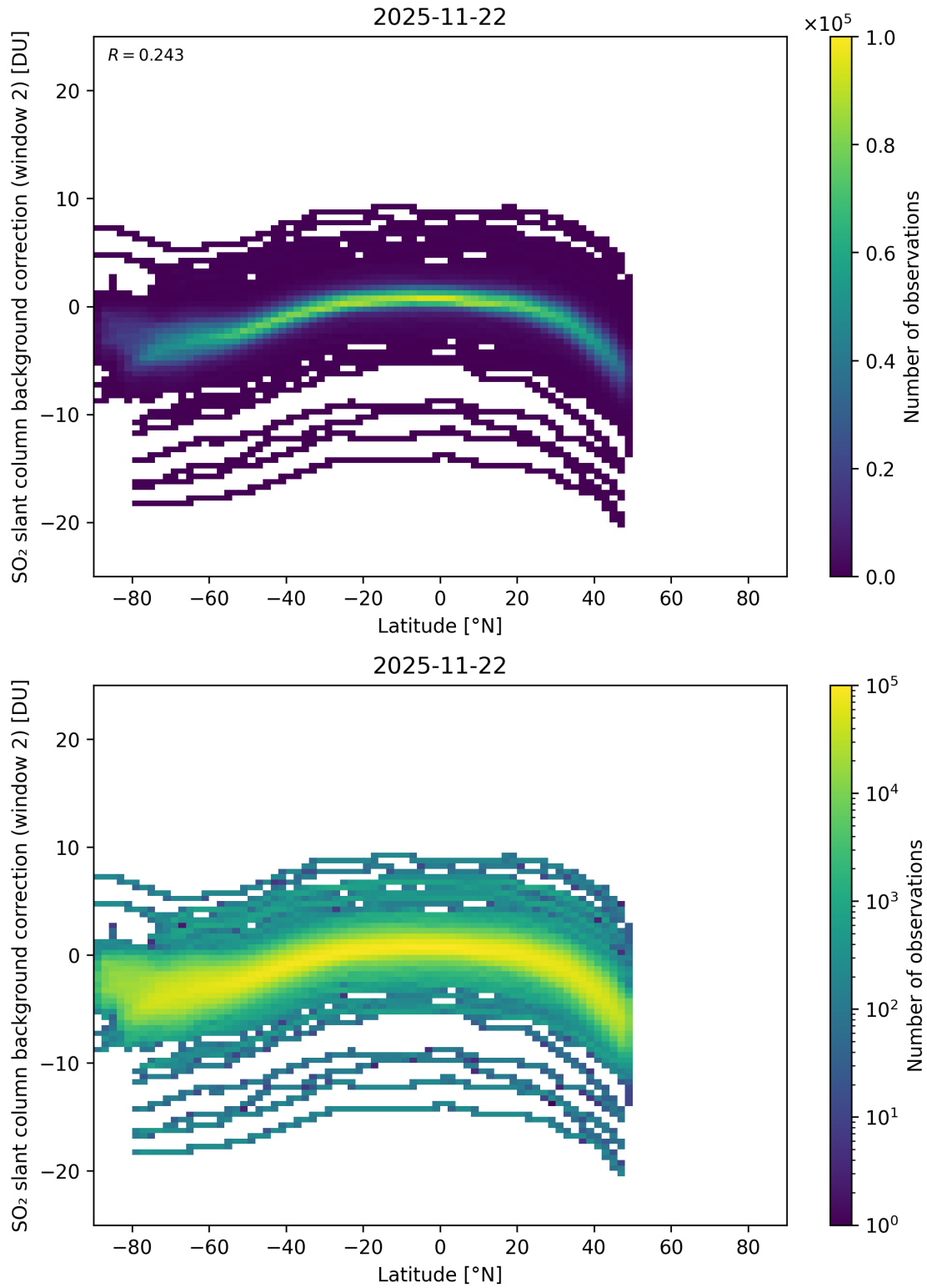
Figure 151: Scatter density plot of “Latitude” against “SO 2 slant column background correction (window 2)” for 2025-11-21 to 2025-11-23.
