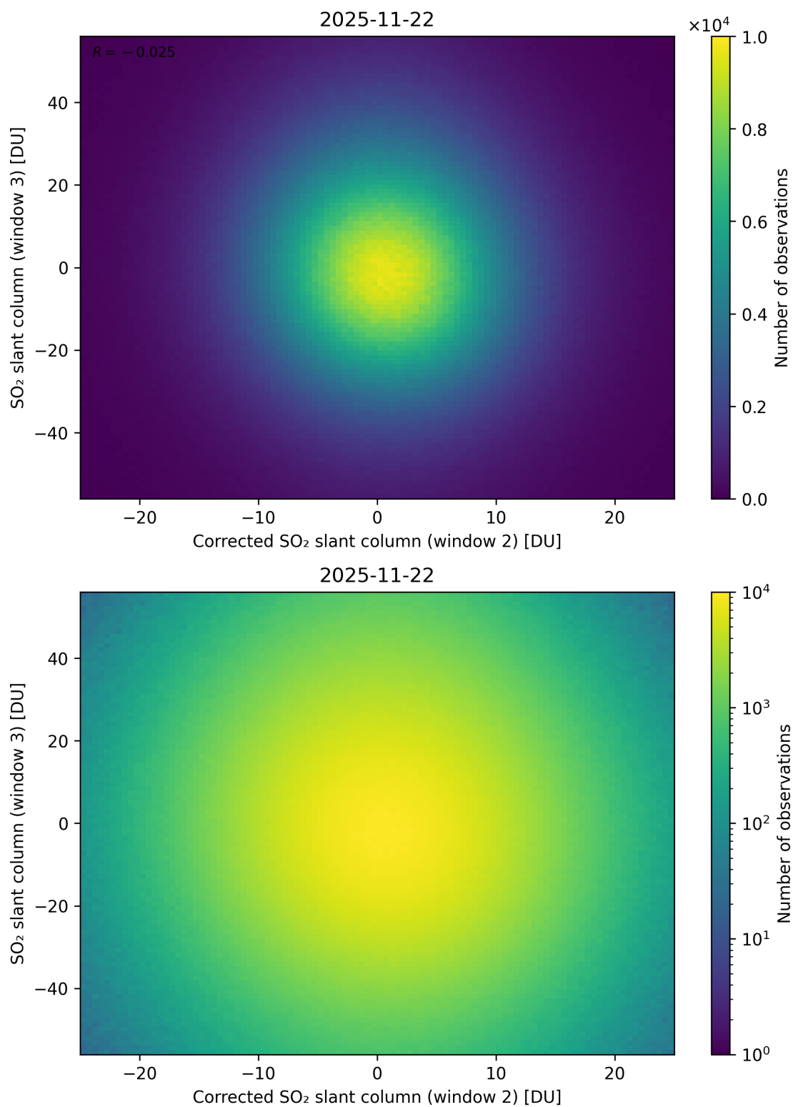
Figure 251: Scatter density plot of “Corrected SO 2 slant column (window 2)” against “SO 2 slant column (window 3)” for 2025-11-21 to 2025-11-23.
