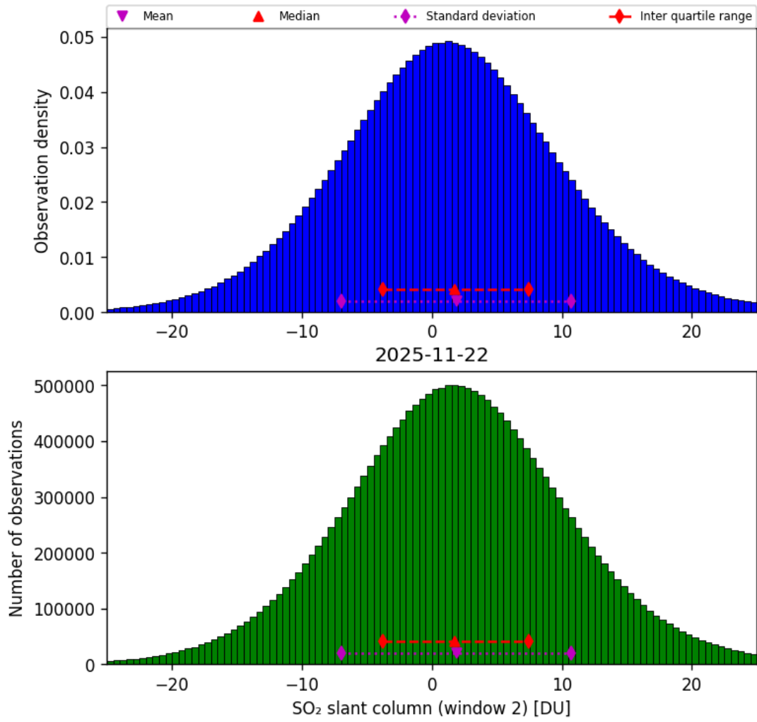
Figure 67: Histogram of “SO 2 slant column (window 2)” for 2025-11-21 to 2025-11-23
