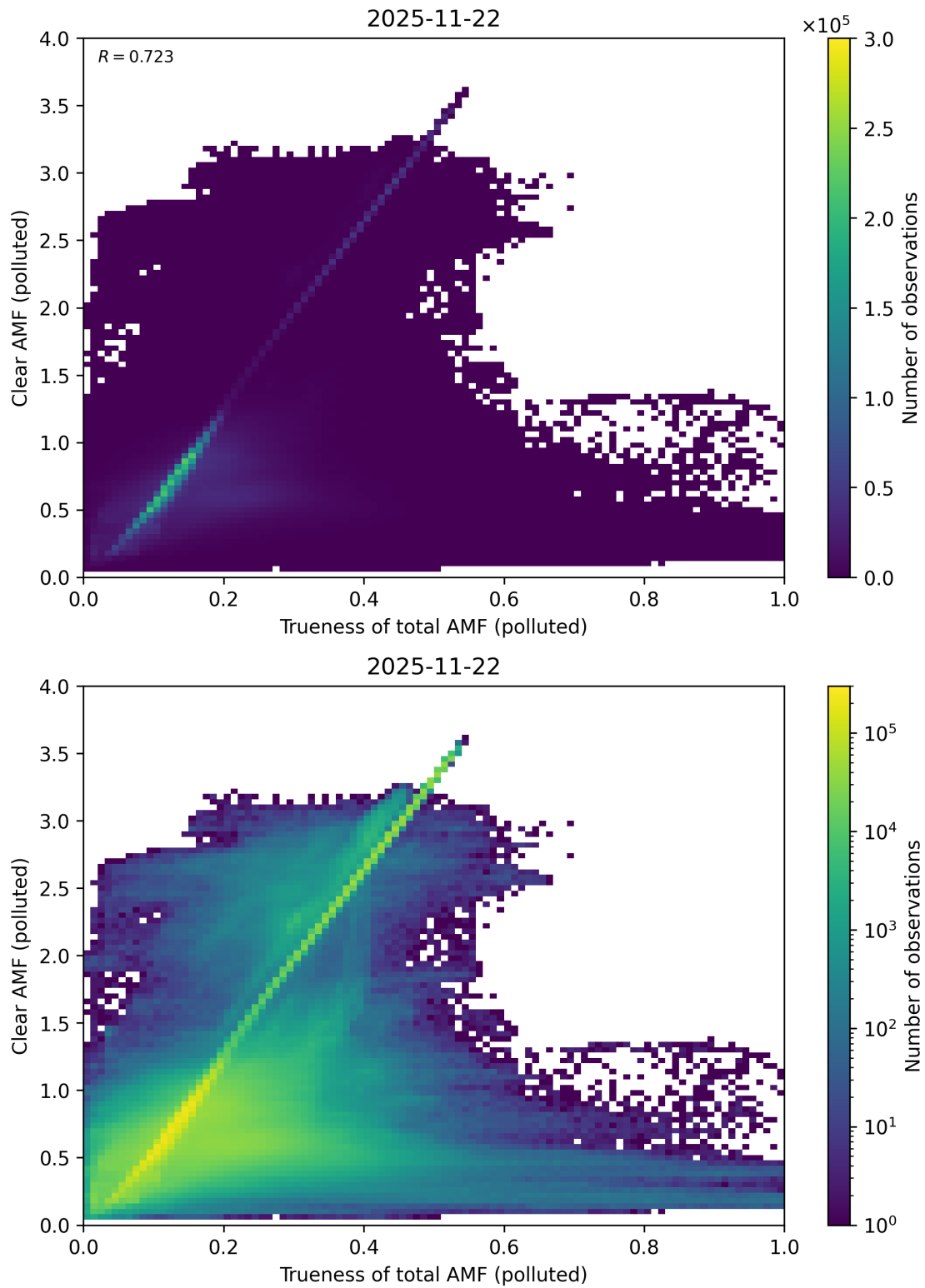
Figure 322: Scatter density plot of “Trueness of total AMF (polluted)” against “Clear AMF (polluted)” for 2025-11-21 to 2025-11-23.
