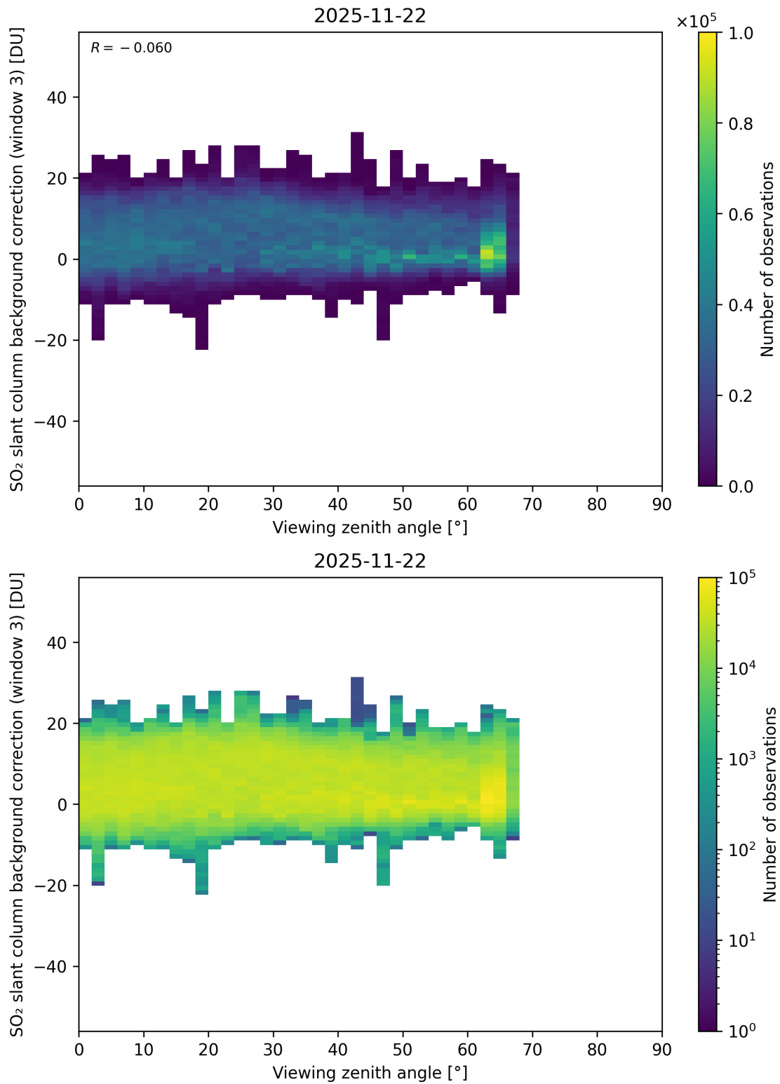
Figure 364: Scatter density plot of “Viewing zenith angle” against “SO 2 slant column background correction (window 3)” for 2025-11-21 to 2025-11-23.
