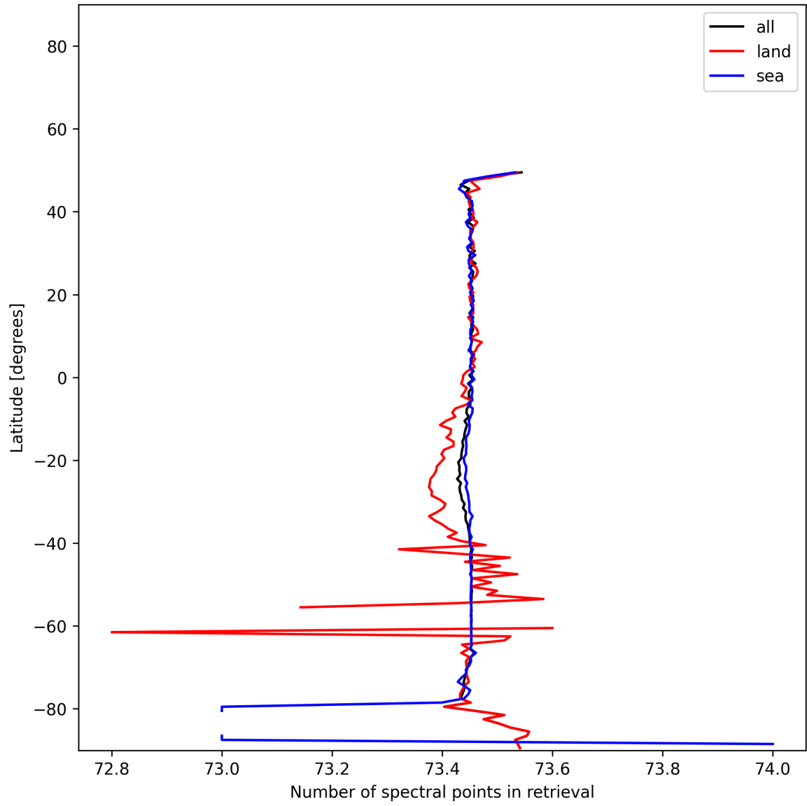
Figure 56: Zonal average of “Number of spectral points in retrieval” for 2025-11-21 to 2025-11-23.
