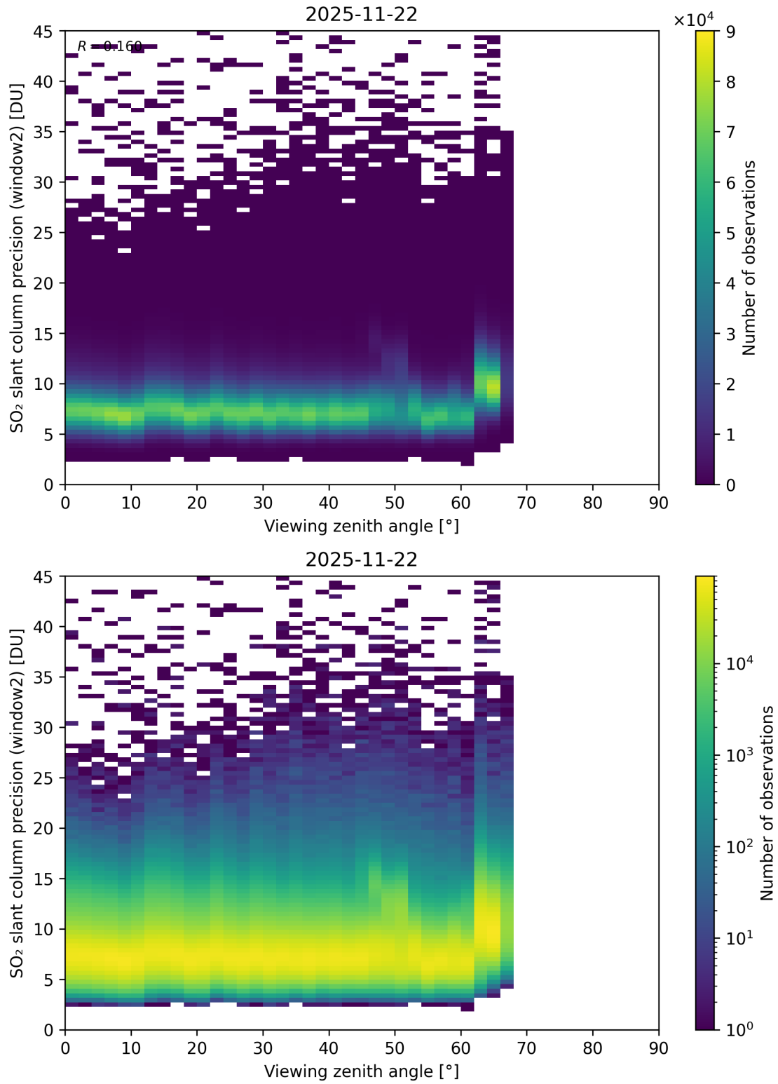
Figure 378: Scatter density plot of “Viewing zenith angle” against “SO 2 slant column precision (window2)” for 2025-11-21 to 2025-11-23.
