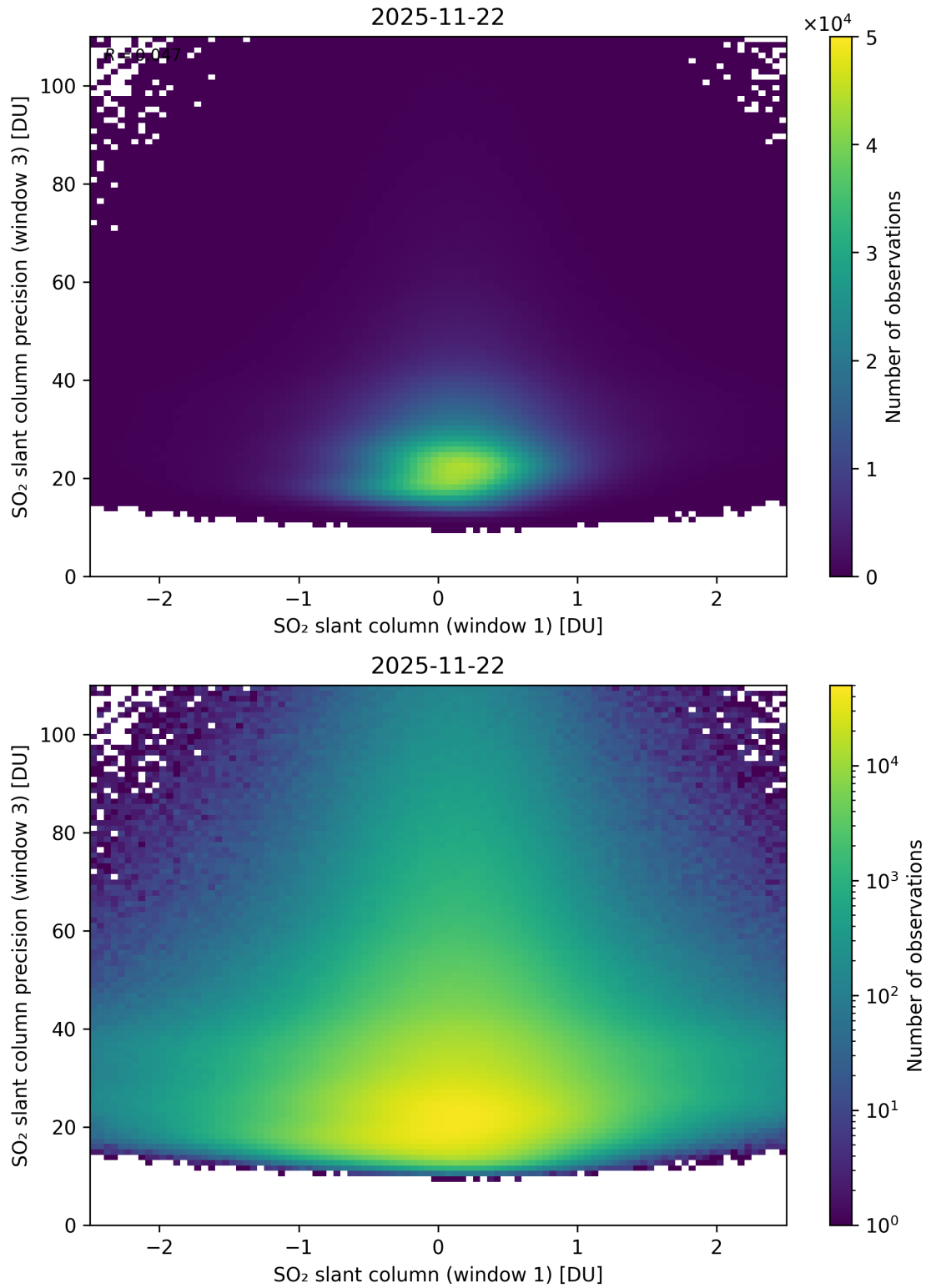
Figure 288: Scatter density plot of “SO 2 slant column (window 1)” against “SO 2 slant column precision (window 3)” for 2025-11-21 to 2025-11-23.
