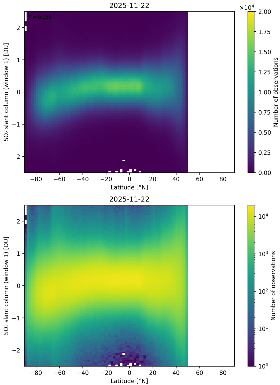
Figure 162: Scatter density plot of “Latitude” against “SO 2 slant column (window 1)” for 2025-11-21 to 2025-11-23.
