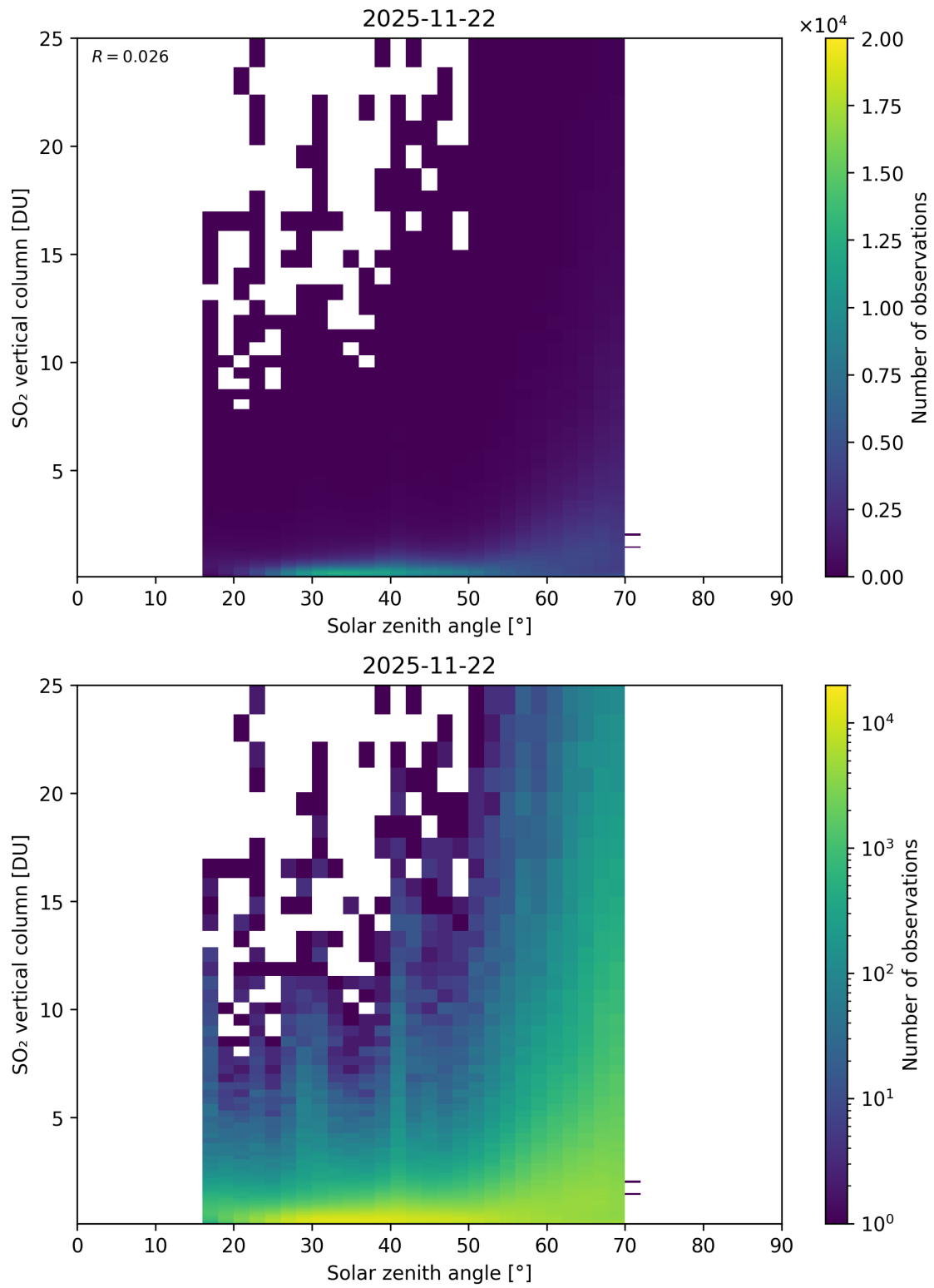
Figure 191: Scatter density plot of “Solar zenith angle” against “SO 2 vertical column” for 2025-11-21 to 2025-11-23.
