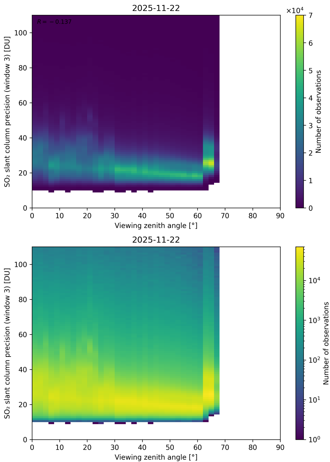
Figure 380: Scatter density plot of “Viewing zenith angle” against “SO 2 slant column precision (window 3)” for 2025-11-21 to 2025-11-23.
