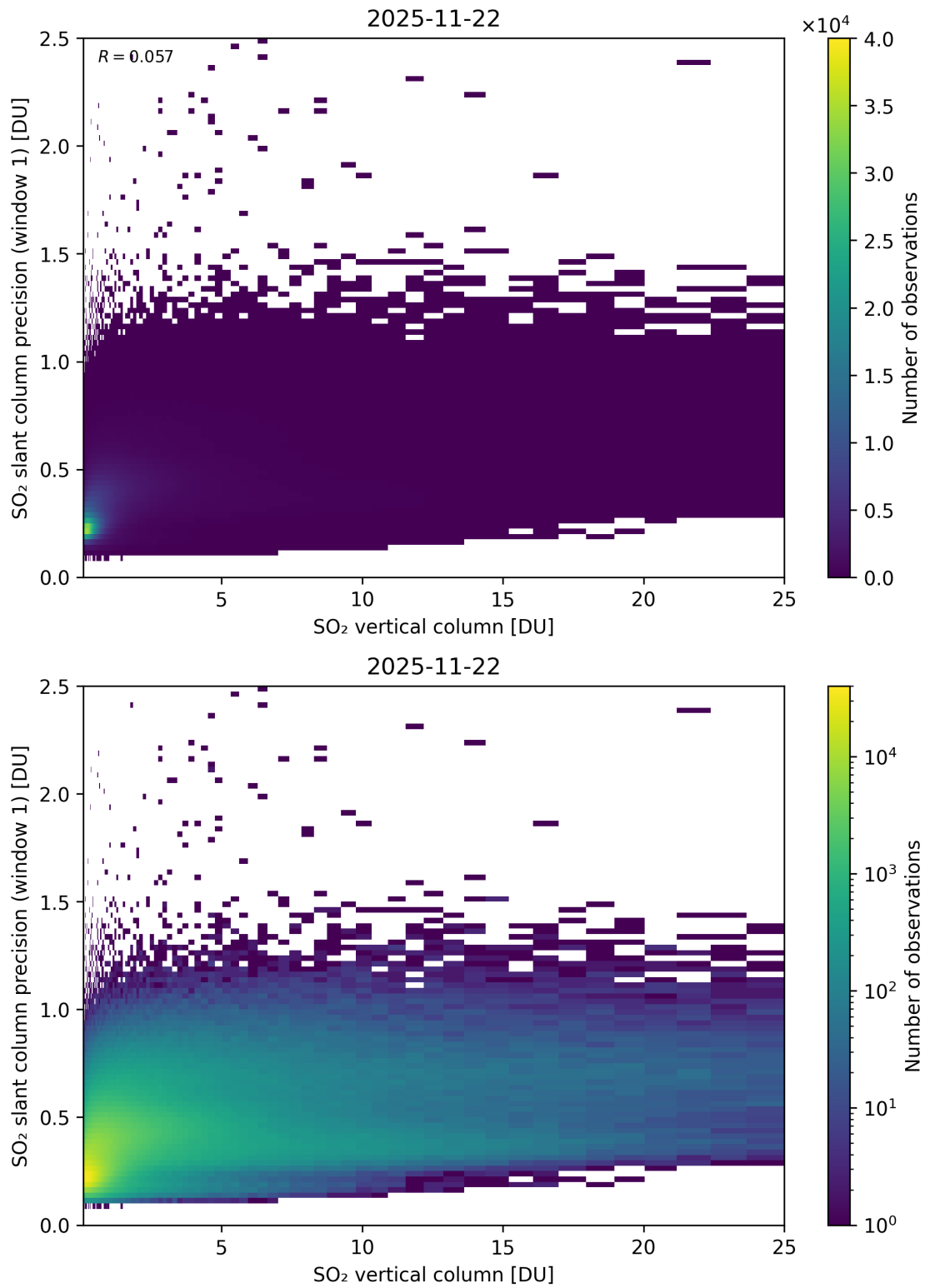
Figure 355: Scatter density plot of “SO 2 vertical column” against “SO 2 slant column precision (window 1)” for 2025-11-21 to 2025-11-23.
