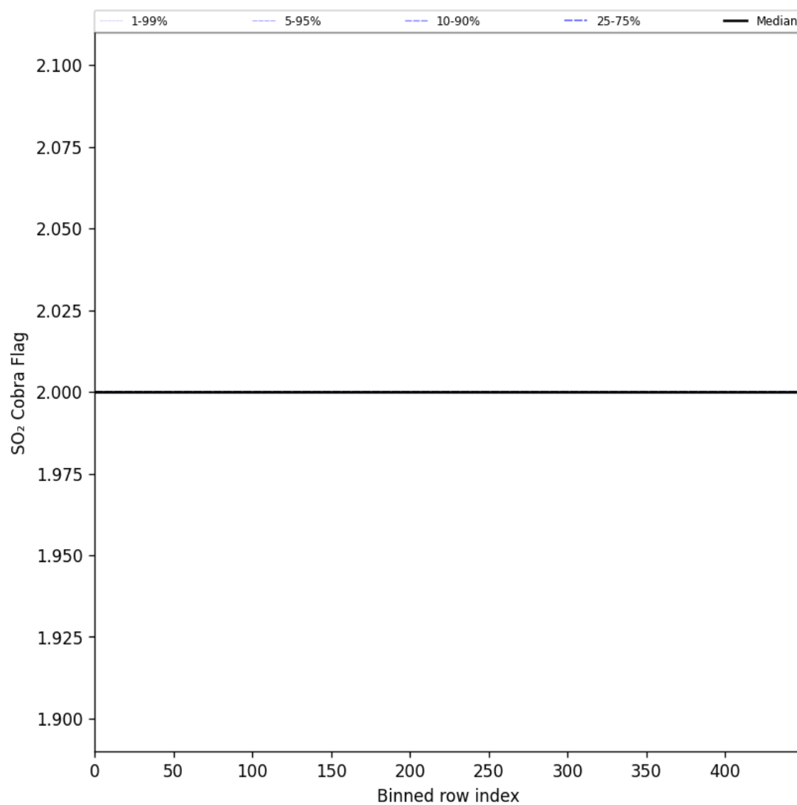
Figure 101: Along track statistics of “SO 2 Cobra Flag” for 2025-11-21 to 2025-11-23
