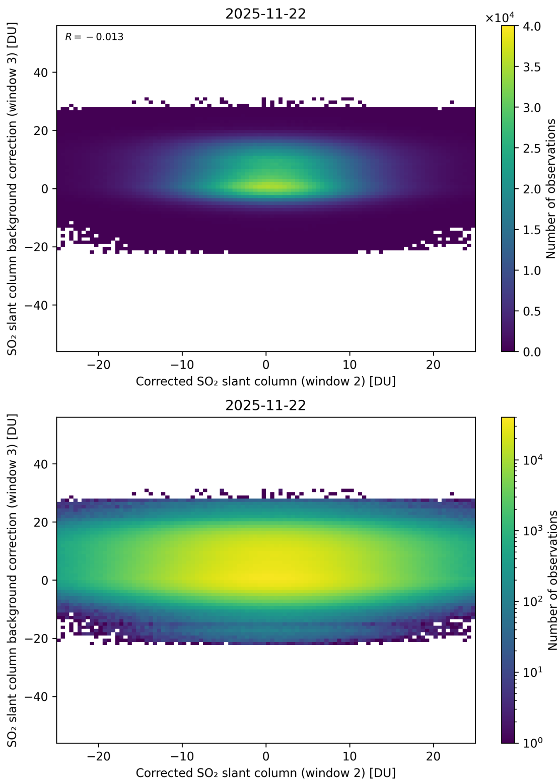
Figure 245: Scatter density plot of “Corrected SO 2 slant column (window 2)” against “SO 2 slant column background correction (window 3)” for 2025-11-21 to 2025-11-23.
