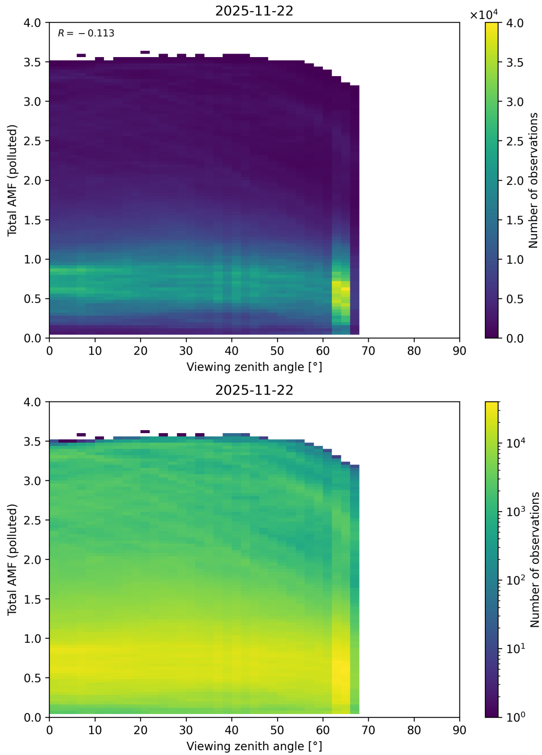
Figure 381: Scatter density plot of “Viewing zenith angle” against “Total AMF (polluted)” for 2025-11-21 to 2025-11-23.
