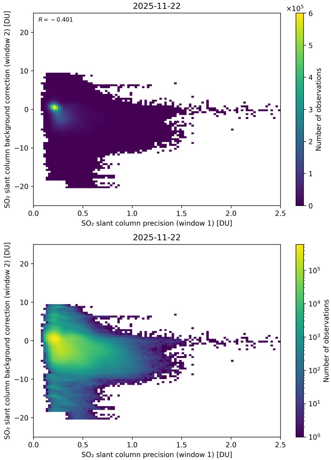
Figure 269: Scatter density plot of “SO 2 slant column precision (window 1)” against “SO 2 slant column background correction (window 2)” for 2025-11-21 to 2025-11-23.
