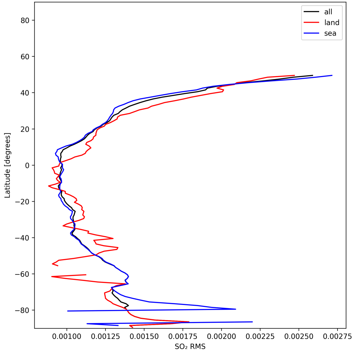
Figure 52: Zonal average of “SO 2 RMS” for 2025-11-21 to 2025-11-23.
