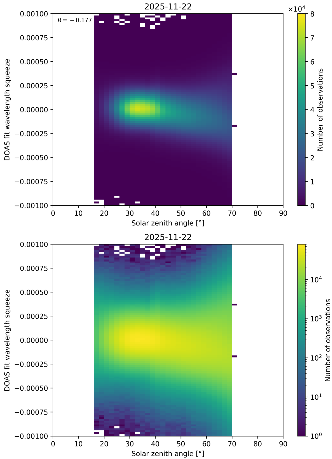
Figure 175: Scatter density plot of “Solar zenith angle” against “DOAS fit wavelength squeeze” for 2025-11-21 to 2025-11-23.
