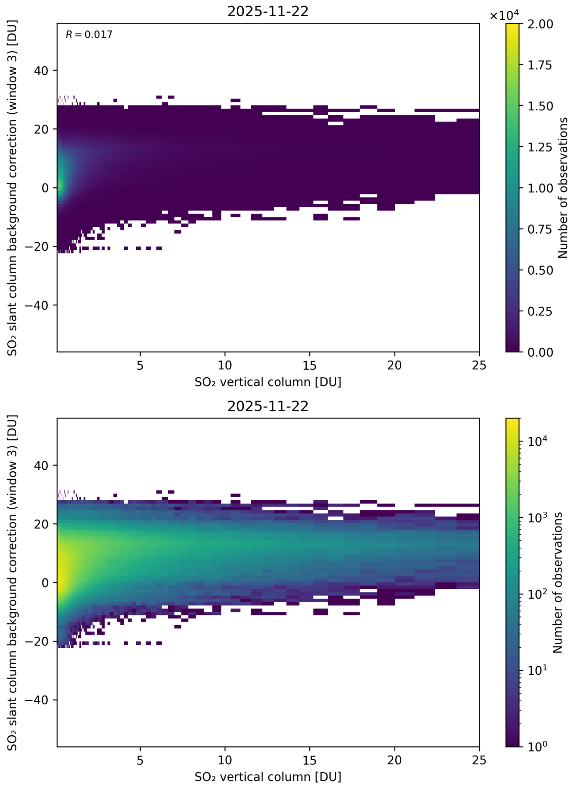
Figure 325: Scatter density plot of “SO 2 vertical column” against “SO 2 slant column background correction (window 3)” for 2025-11-21 to 2025-11-23.
