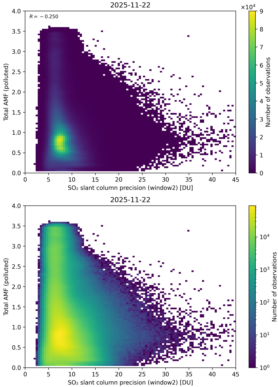
Figure 301: Scatter density plot of “SO 2 slant column precision (window2)” against “Total AMF (polluted)” for 2025-11-21 to 2025-11-23.
