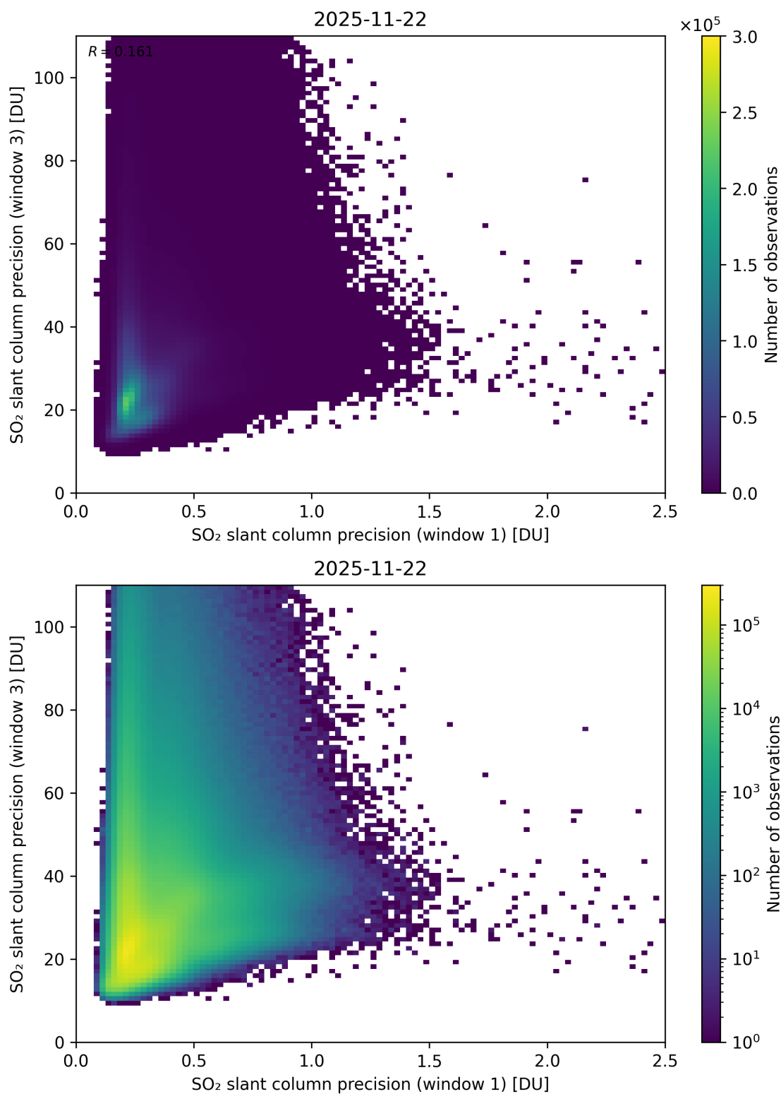
Figure 279: Scatter density plot of “SO 2 slant column precision (window 1)” against “SO 2 slant column precision (window 3)” for 2025-11-21 to 2025-11-23.
