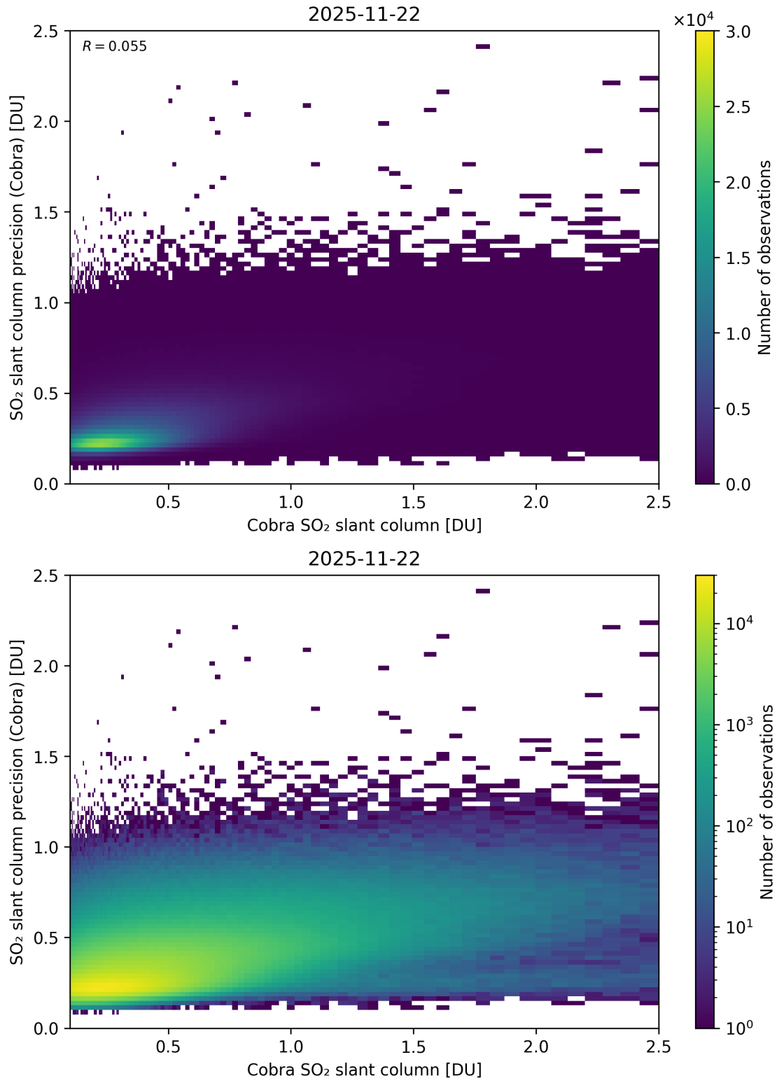
Figure 216: Scatter density plot of “Cobra SO 2 slant column” against “SO 2 slant column precision (Cobra)” for 2025-11-21 to 2025-11-23.
