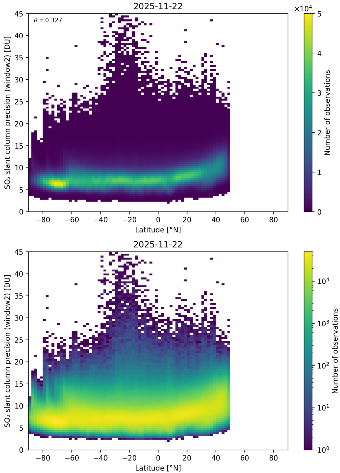
Figure 164: Scatter density plot of “Latitude” against “SO 2 slant column precision (window2)” for 2025-11-21 to 2025-11-23.
