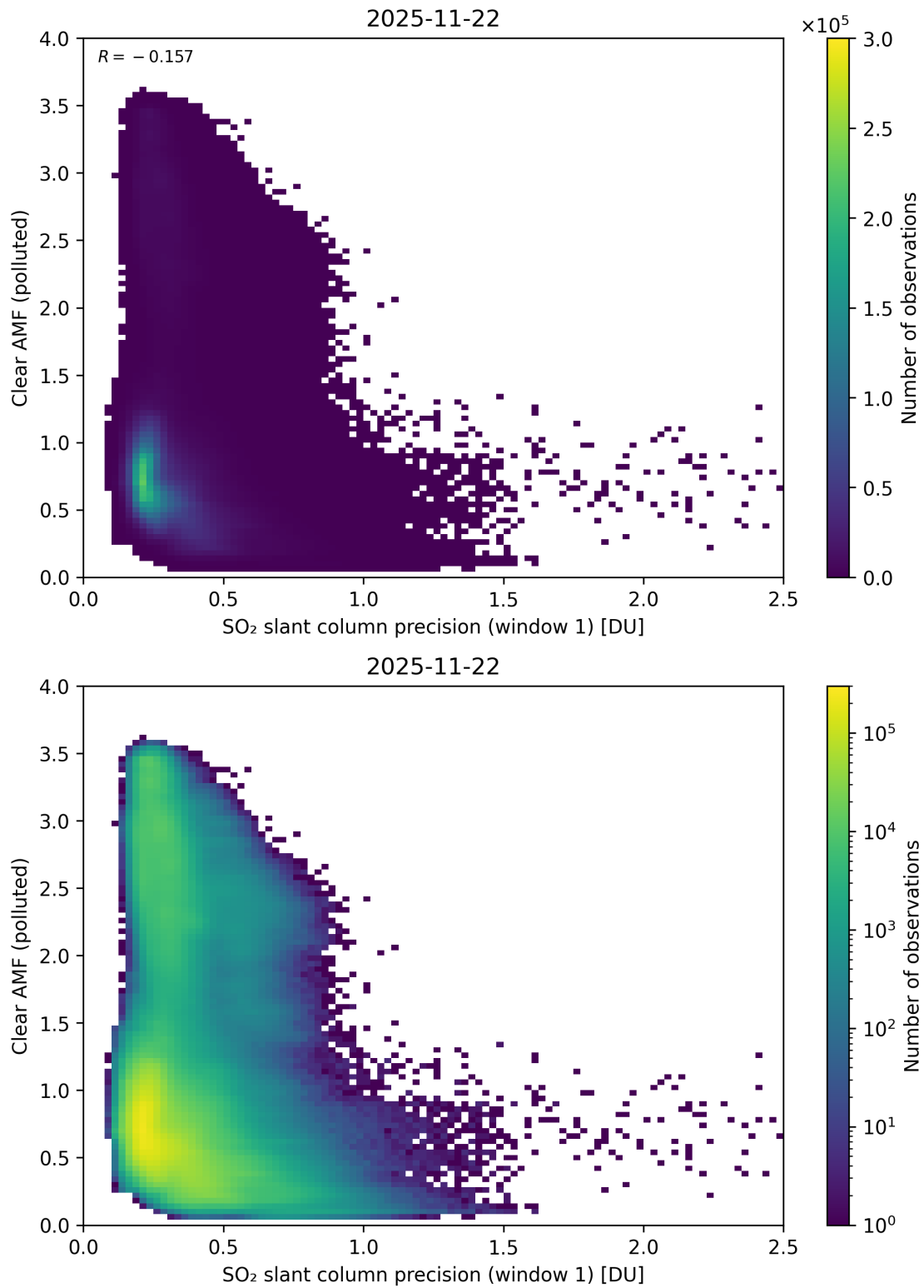
Figure 274: Scatter density plot of “SO 2 slant column precision (window 1)” against “Clear AMF (polluted)” for 2025-11-21 to 2025-11-23.
