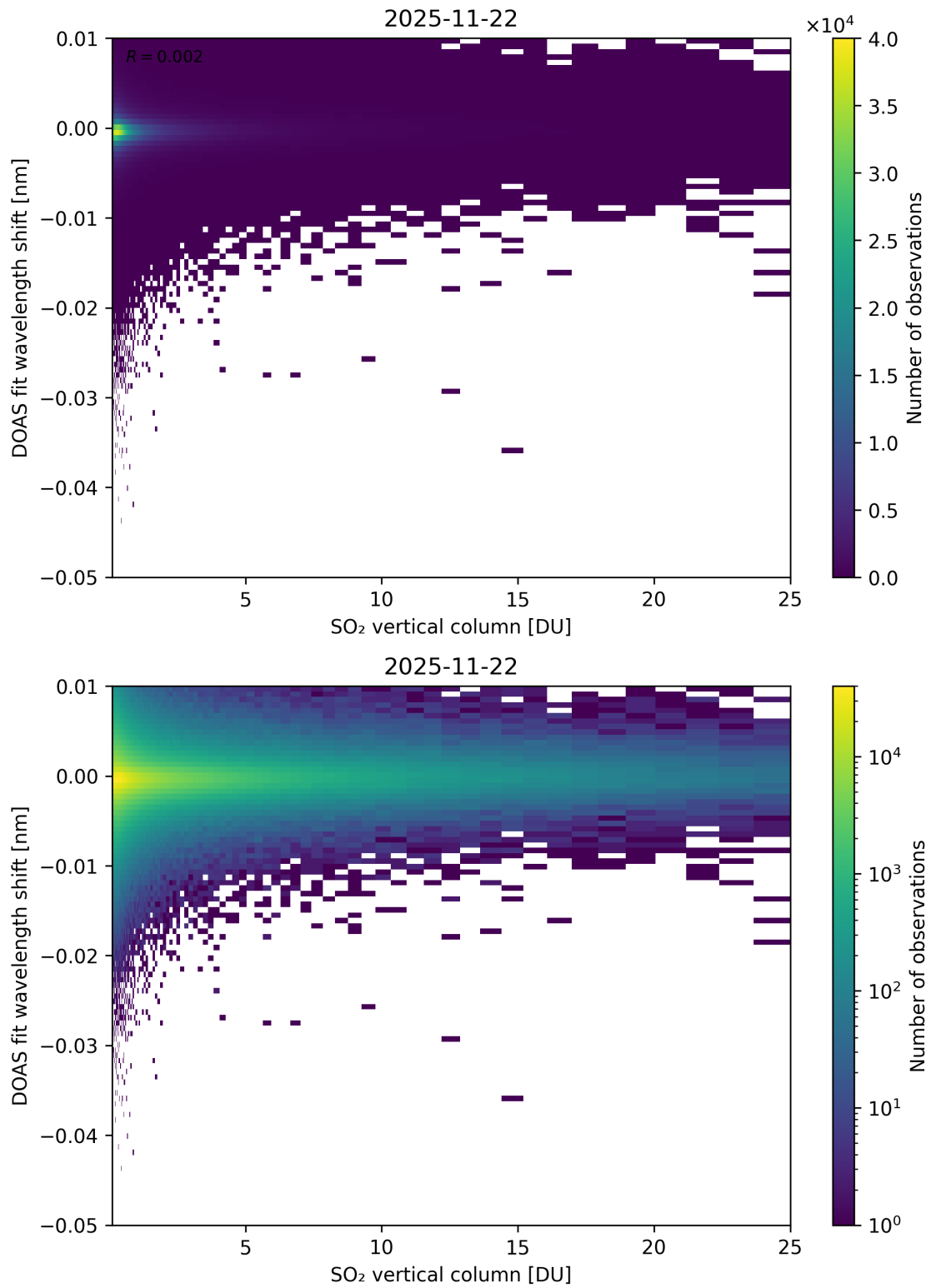
Figure 326: Scatter density plot of “SO 2 vertical column” against “DOAS fit wavelength shift” for 2025-11-21 to 2025-11-23.
