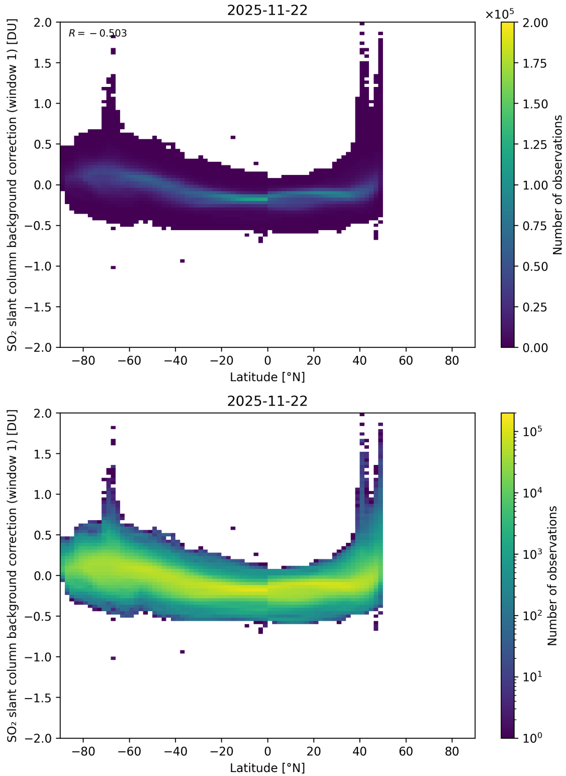
Figure 150: Scatter density plot of “Latitude” against “SO 2 slant column background correction (window 1)” for 2025-11-21 to 2025-11-23.
