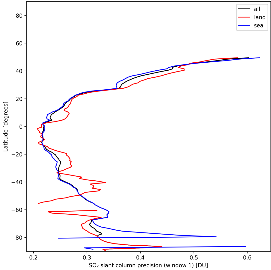
Figure 38: Zonal average of “SO 2 slant column precision (window 1)” for 2025-11-21 to 2025-11-23.
