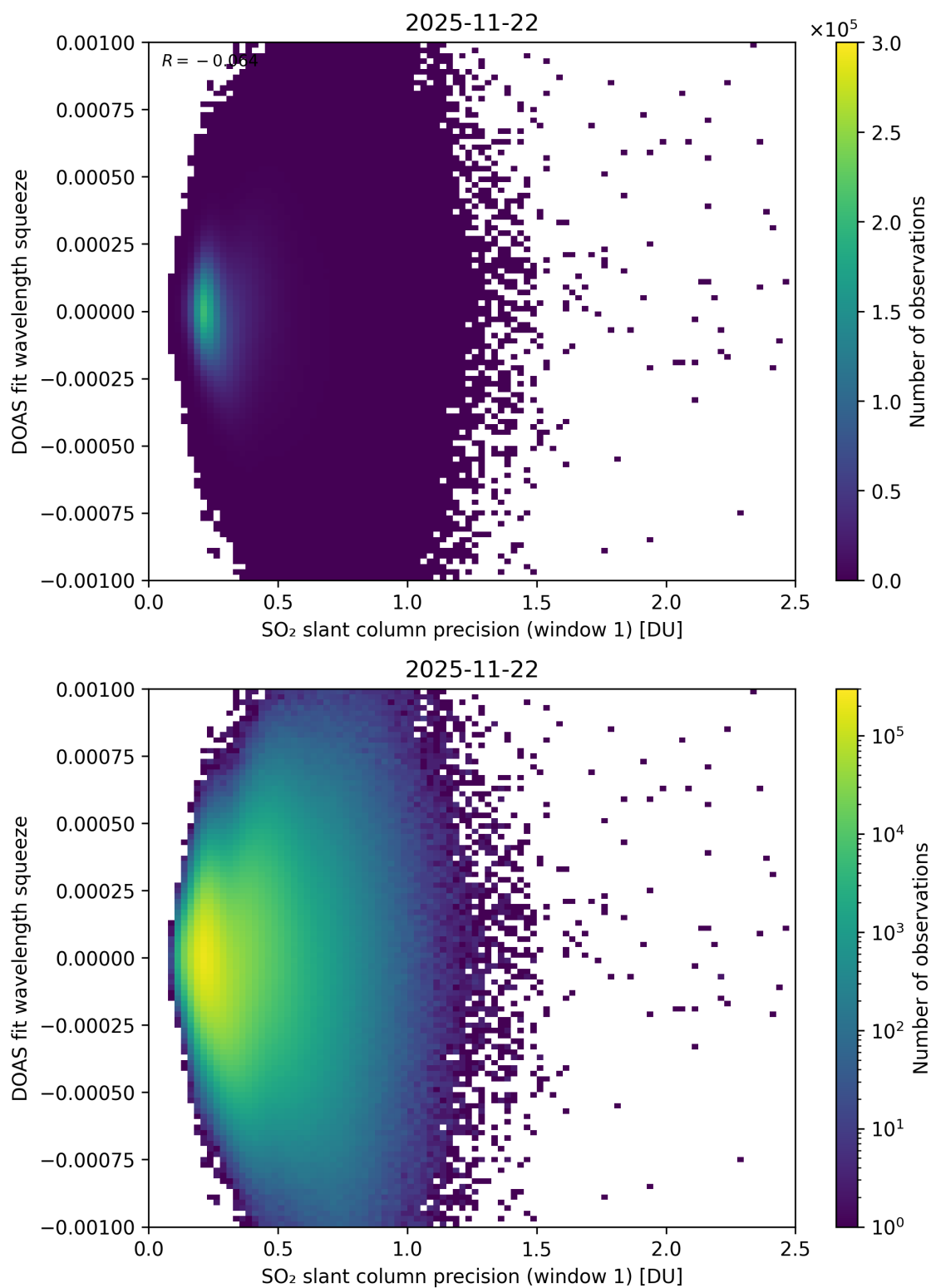
Figure 272: Scatter density plot of “SO 2 slant column precision (window 1)” against “DOAS fit wavelength squeeze” for 2025-11-21 to 2025-11-23.
