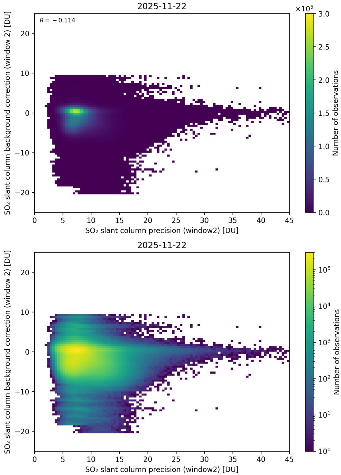
Figure 291: Scatter density plot of “SO 2 slant column precision (window2)” against “SO 2 slant column background correction (window 2)” for 2025-11-21 to 2025-11-23.
