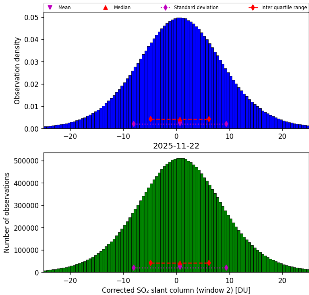
Figure 69: Histogram of “Corrected SO 2 slant column (window 2)” for 2025-11-21 to 2025-11-23
