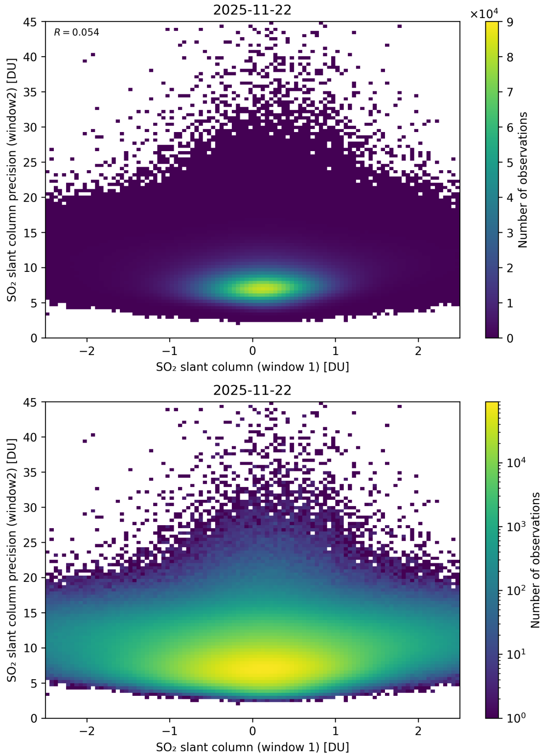
Figure 286: Scatter density plot of “SO 2 slant column (window 1)” against “SO 2 slant column precision (window2)” for 2025-11-21 to 2025-11-23.
