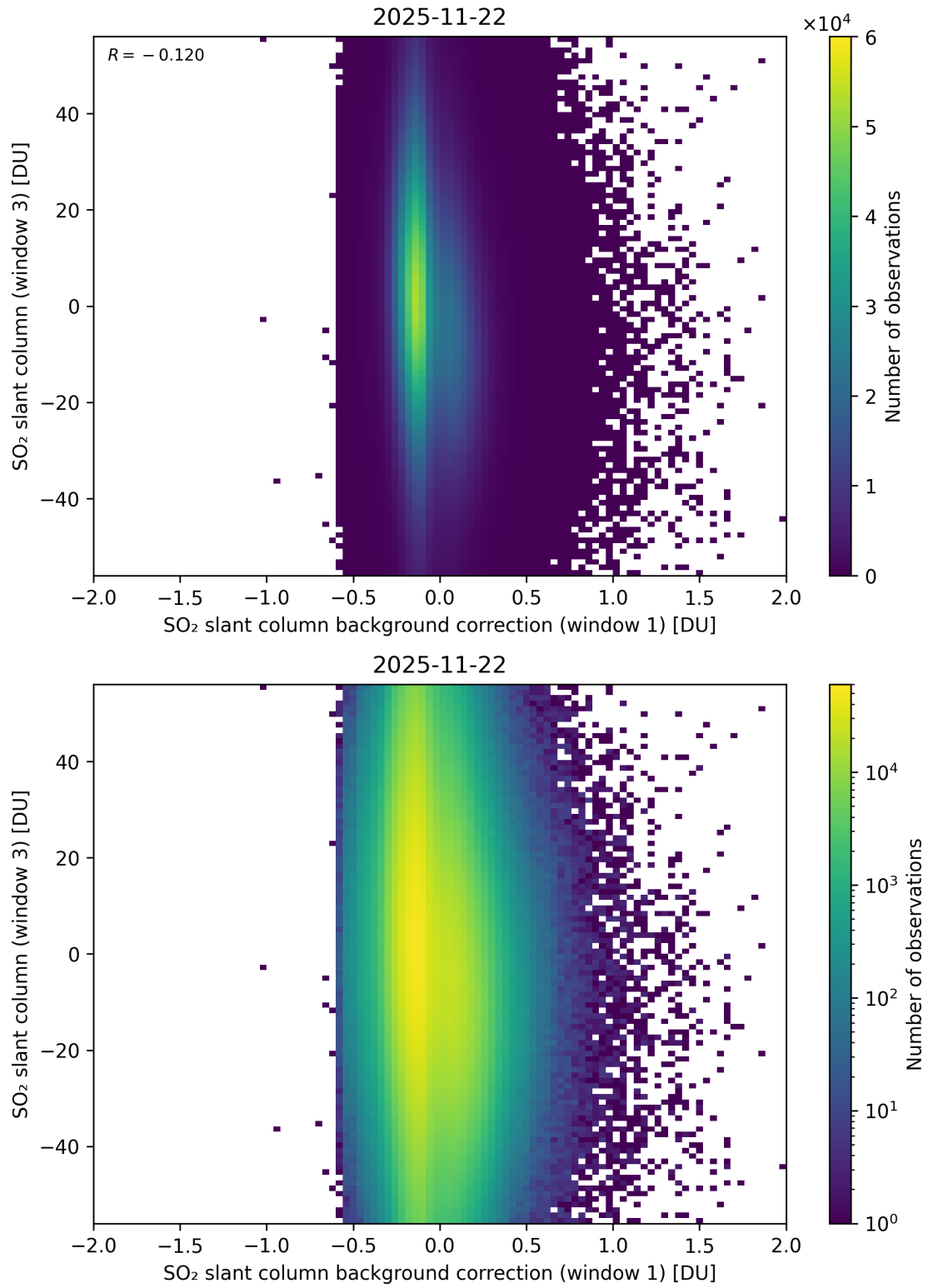
Figure 118: Scatter density plot of “SO 2 slant column background correction (window 1)” against “SO 2 slant column (window 3)” for 2025-11-21 to 2025-11-23.
