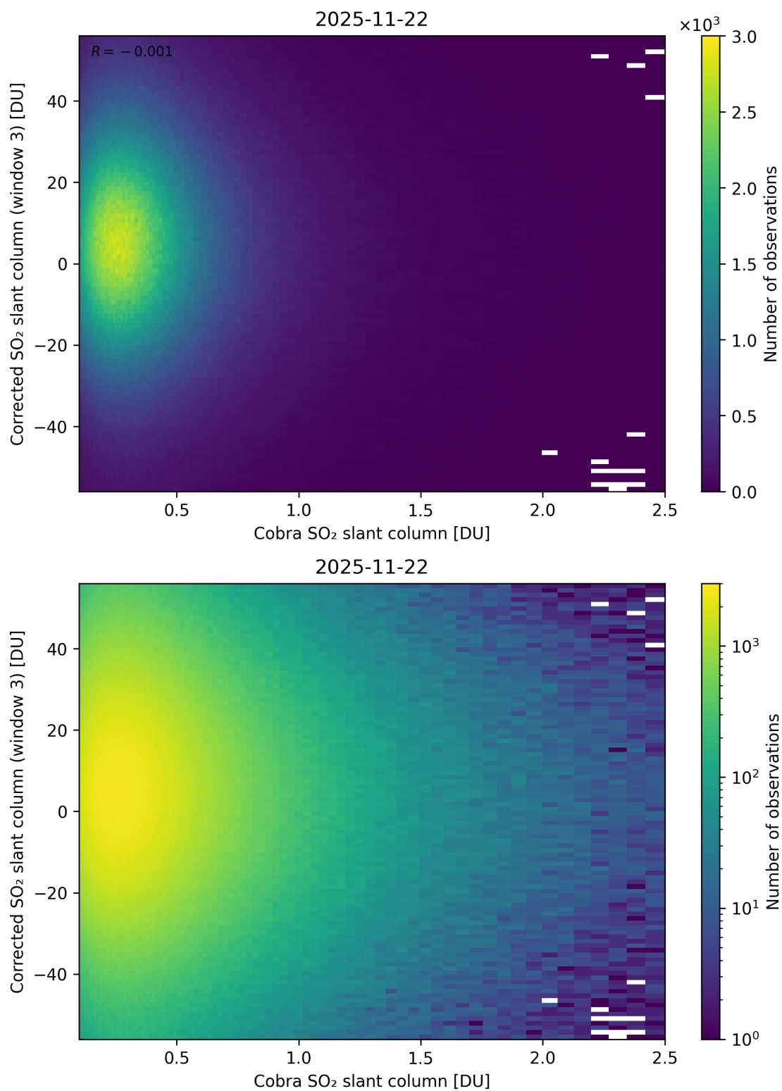
Figure 218: Scatter density plot of “Cobra SO 2 slant column” against “Corrected SO 2 slant column (window 3)” for 2025-11-21 to 2025-11-23.
