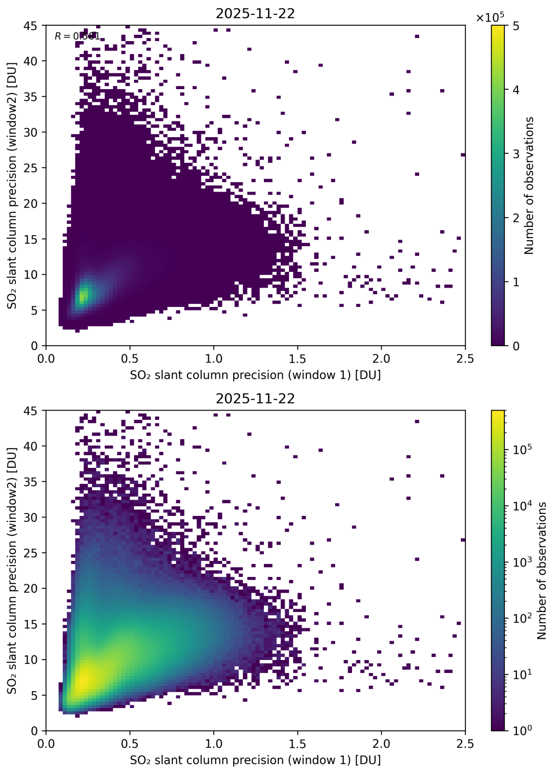
Figure 277: Scatter density plot of “SO 2 slant column precision (window 1)” against “SO 2 slant column precision (window2)” for 2025-11-21 to 2025-11-23.
