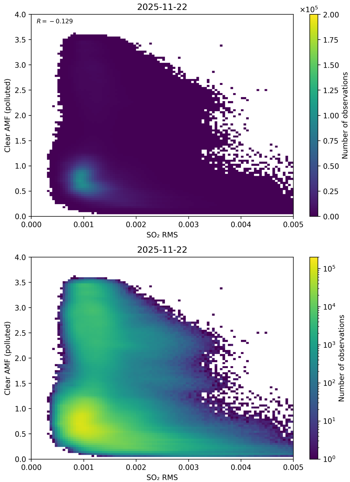
Figure 147: Scatter density plot of “SO 2 RMS” against “Clear AMF (polluted)” for 2025-11-21 to 2025-11-23.
