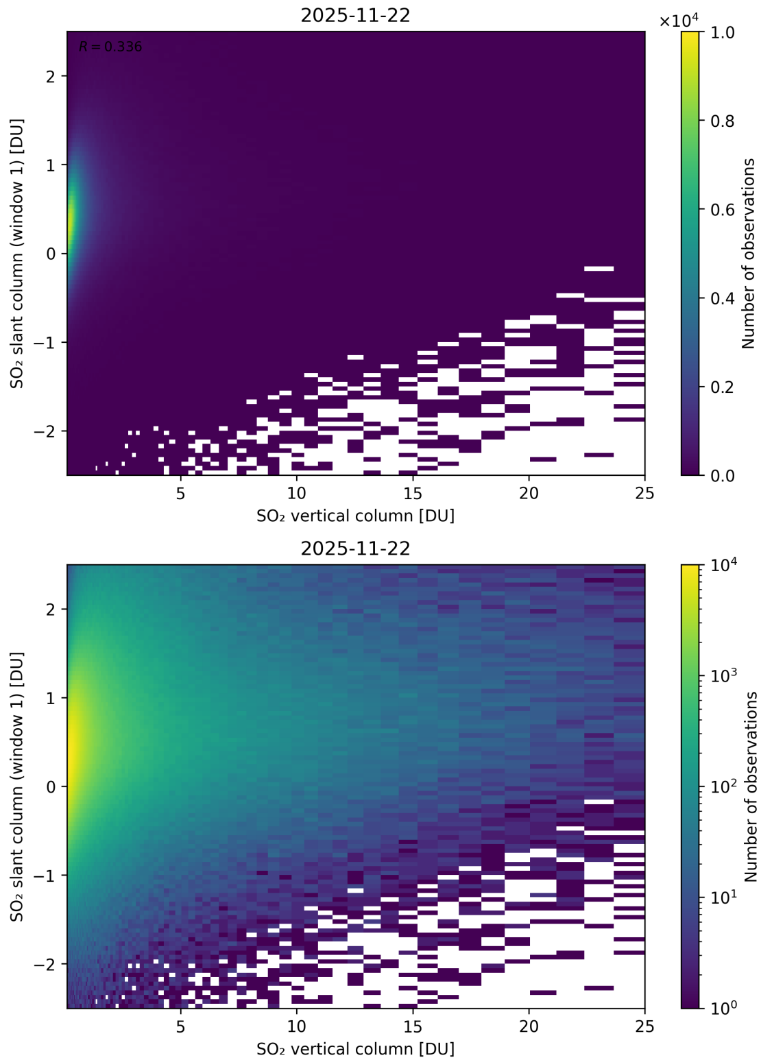
Figure 354: Scatter density plot of “SO 2 vertical column” against “SO 2 slant column (window 1)” for 2025-11-21 to 2025-11-23.
