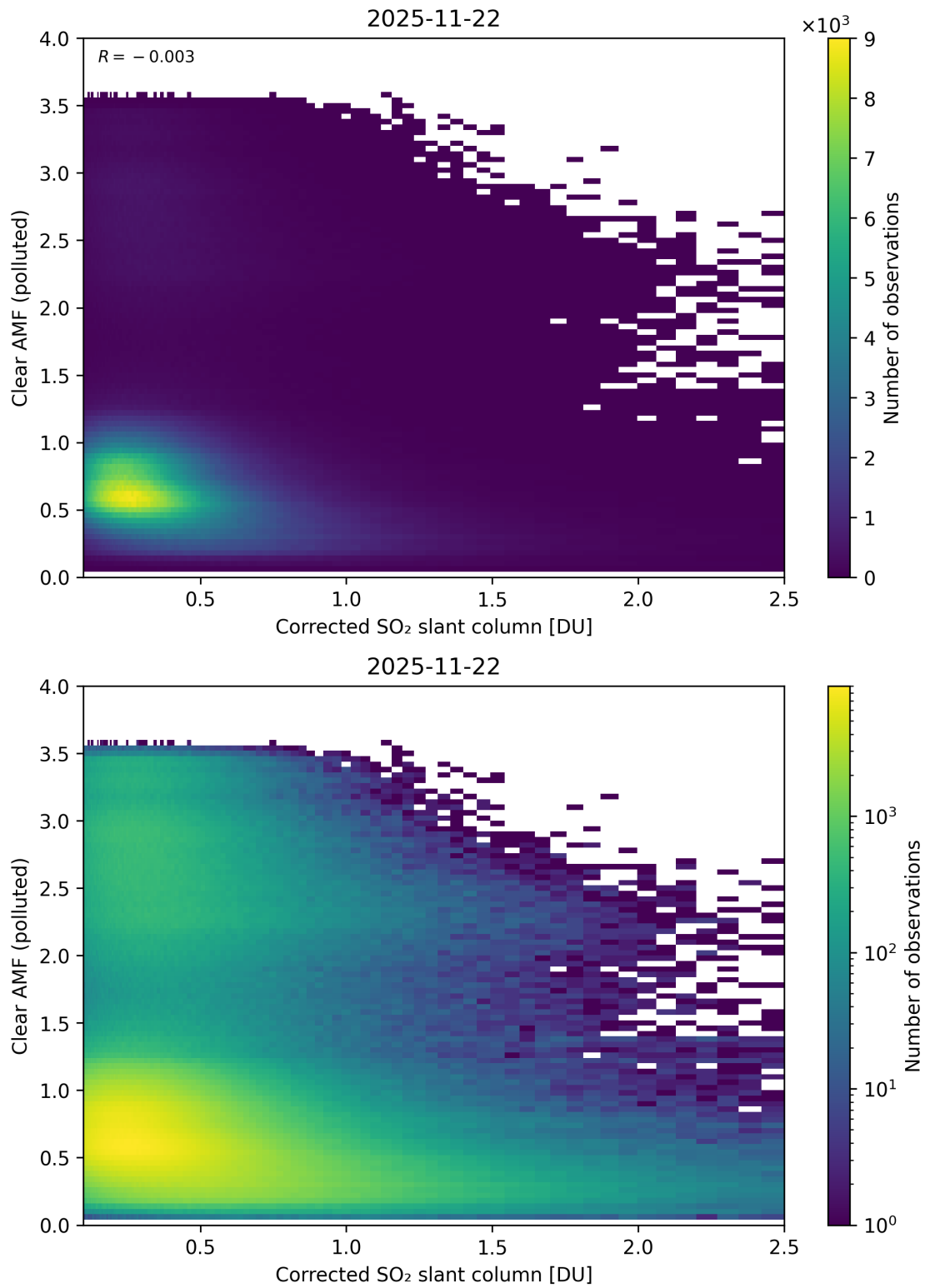
Figure 232: Scatter density plot of “Corrected SO 2 slant column” against “Clear AMF (polluted)” for 2025-11-21 to 2025-11-23.
