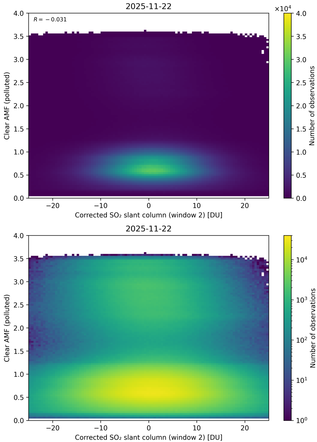
Figure 249: Scatter density plot of “Corrected SO 2 slant column (window 2)” against “Clear AMF (polluted)” for 2025-11-21 to 2025-11-23.
