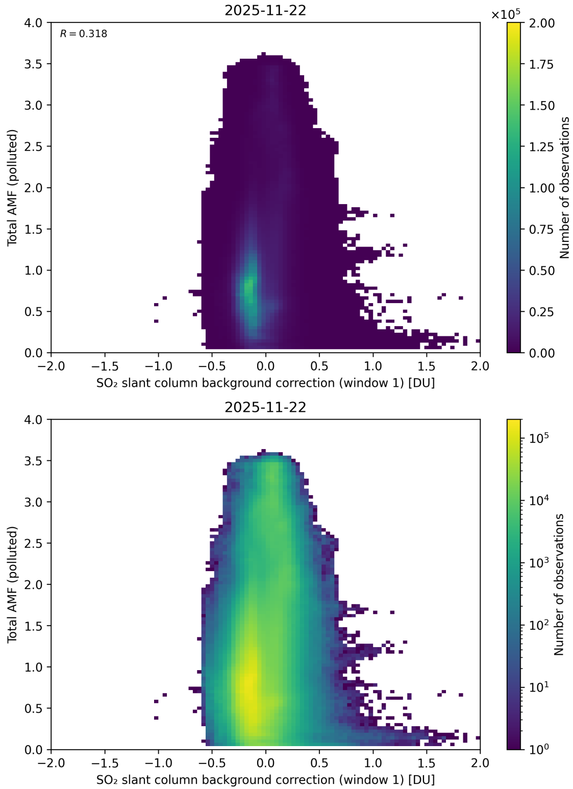
Figure 120: Scatter density plot of “SO 2 slant column background correction (window 1)” against “Total AMF (polluted)” for 2025-11-21 to 2025-11-23.
