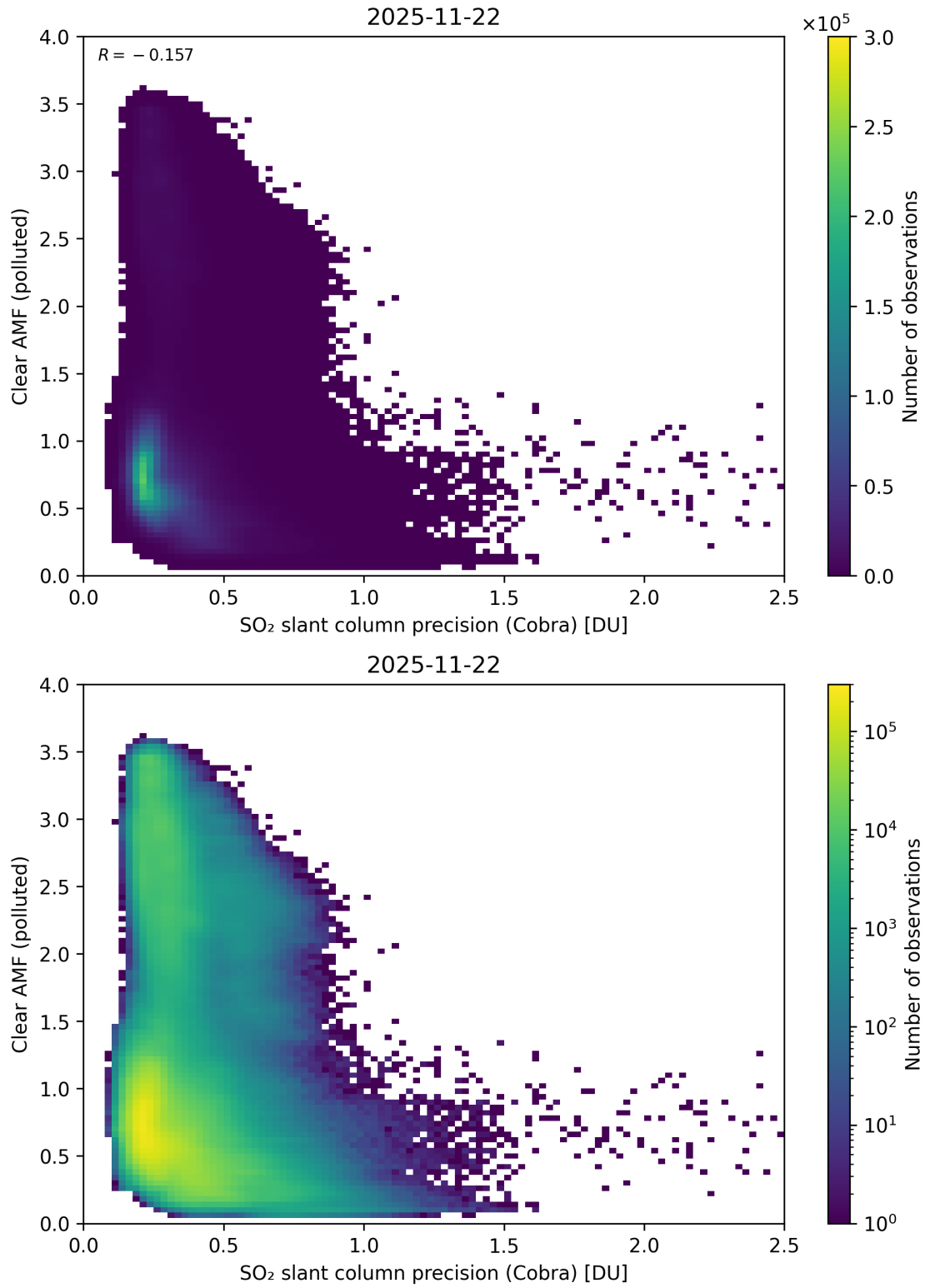
Figure 205: Scatter density plot of “SO 2 slant column precision (Cobra)” against “Clear AMF (polluted)” for 2025-11-21 to 2025-11-23.
