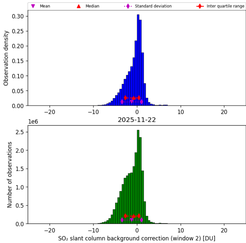
Figure 70: Histogram of “SO 2 slant column background correction (window 2)” for 2025-11-21 to 2025-11-23
