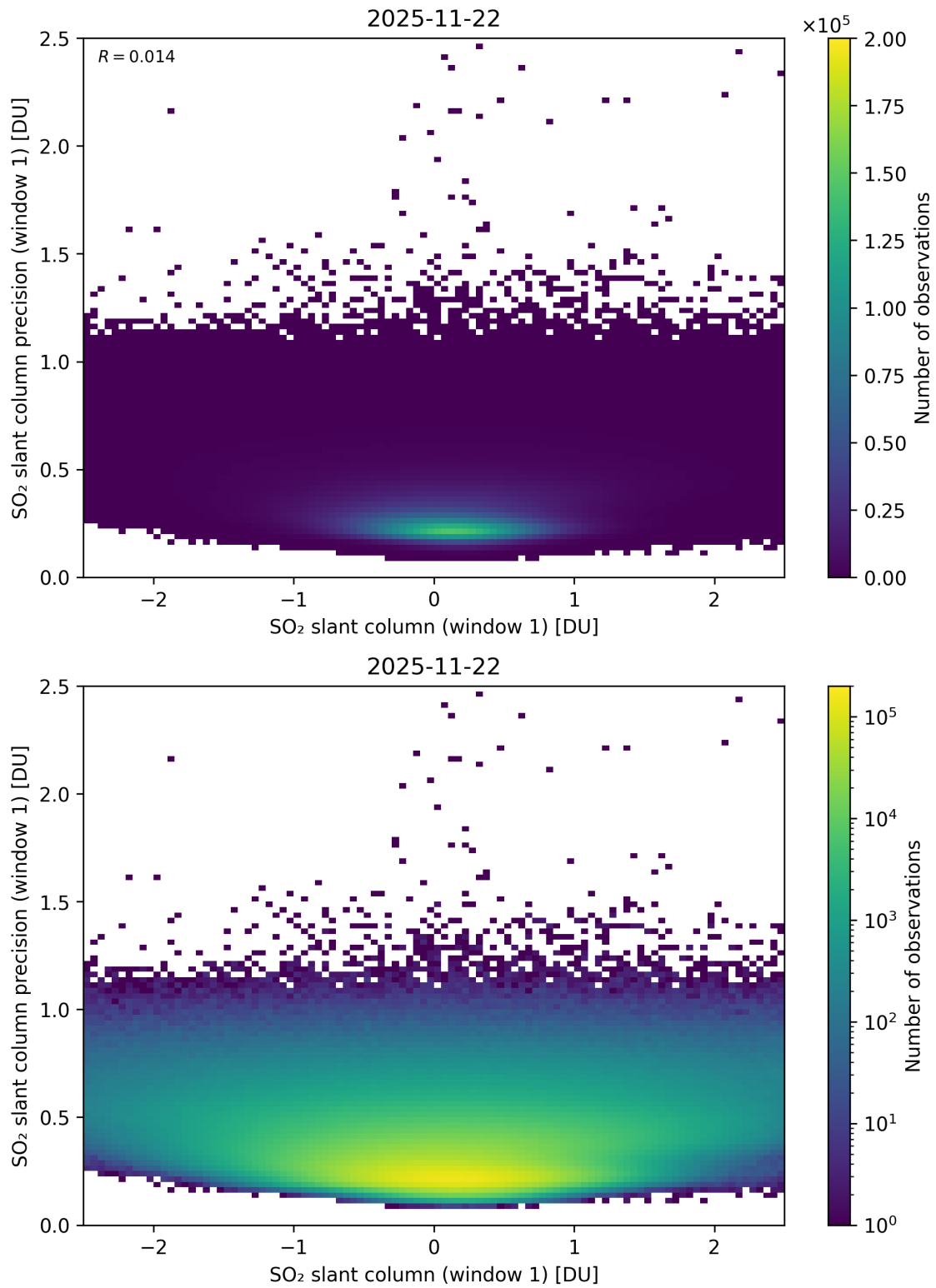
Figure 285: Scatter density plot of “SO 2 slant column (window 1)” against “SO 2 slant column precision (window 1)” for 2025-11-21 to 2025-11-23.
