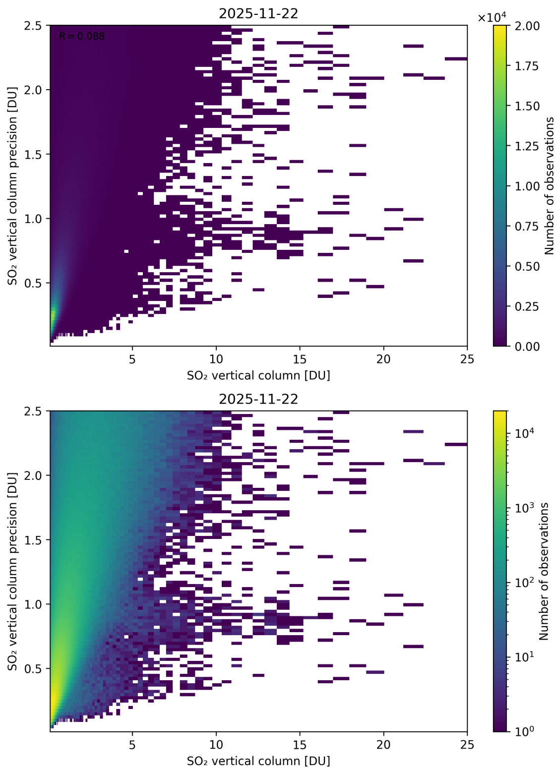
Figure 361: Scatter density plot of “SO 2 vertical column” against “SO 2 vertical column precision” for 2025-11-21 to 2025-11-23.
