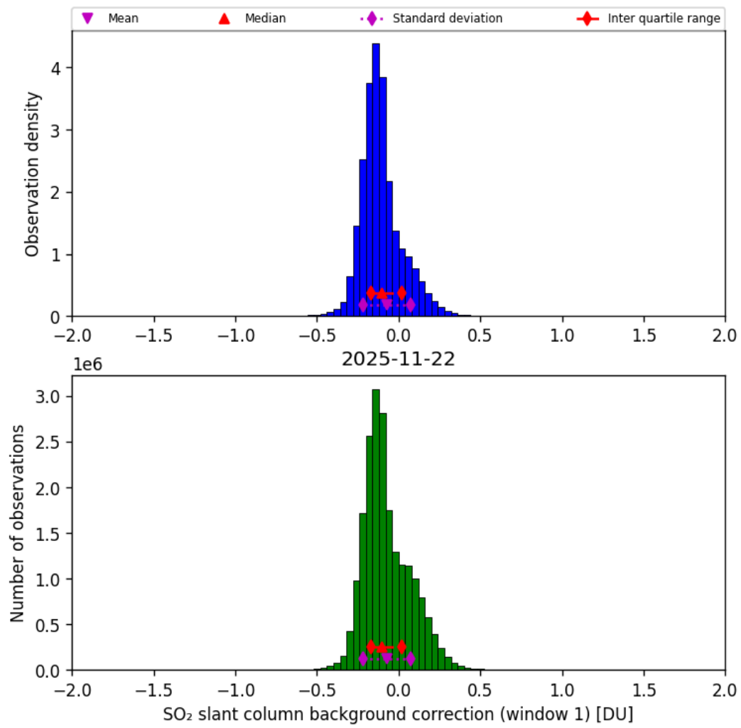
Figure 66: Histogram of “SO 2 slant column background correction (window 1)” for 2025-11-21 to 2025-11-23
