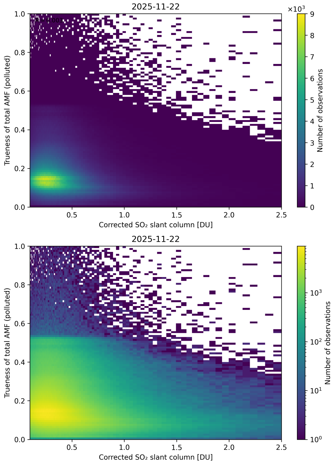
Figure 243: Scatter density plot of “Corrected SO 2 slant column” against “Trueness of total AMF (polluted)” for 2025-11-21 to 2025-11-23.
