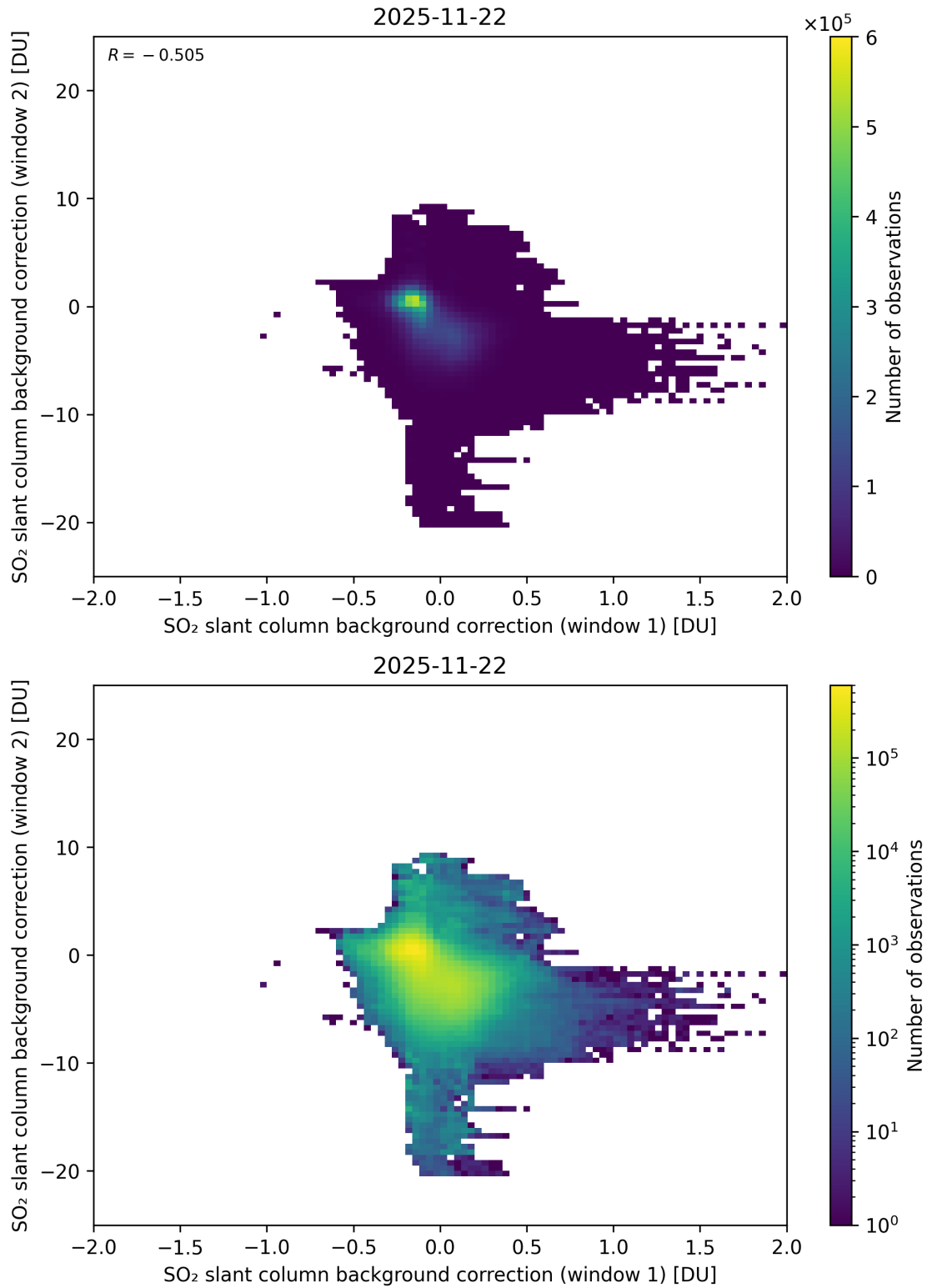
Figure 109: Scatter density plot of “SO 2 slant column background correction (window 1)” against “SO 2 slant column background correction (window 2)” for 2025-11-21 to 2025-11-23.
