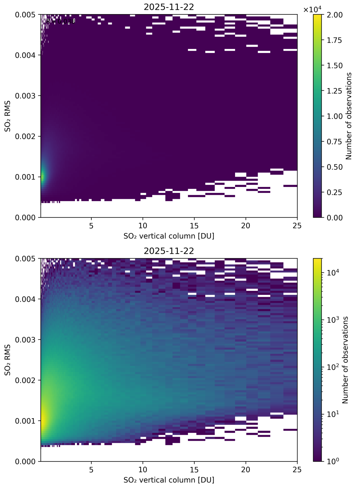
Figure 328: Scatter density plot of “SO 2 vertical column” against “SO 2 RMS” for 2025-11-21 to 2025-11-23.
