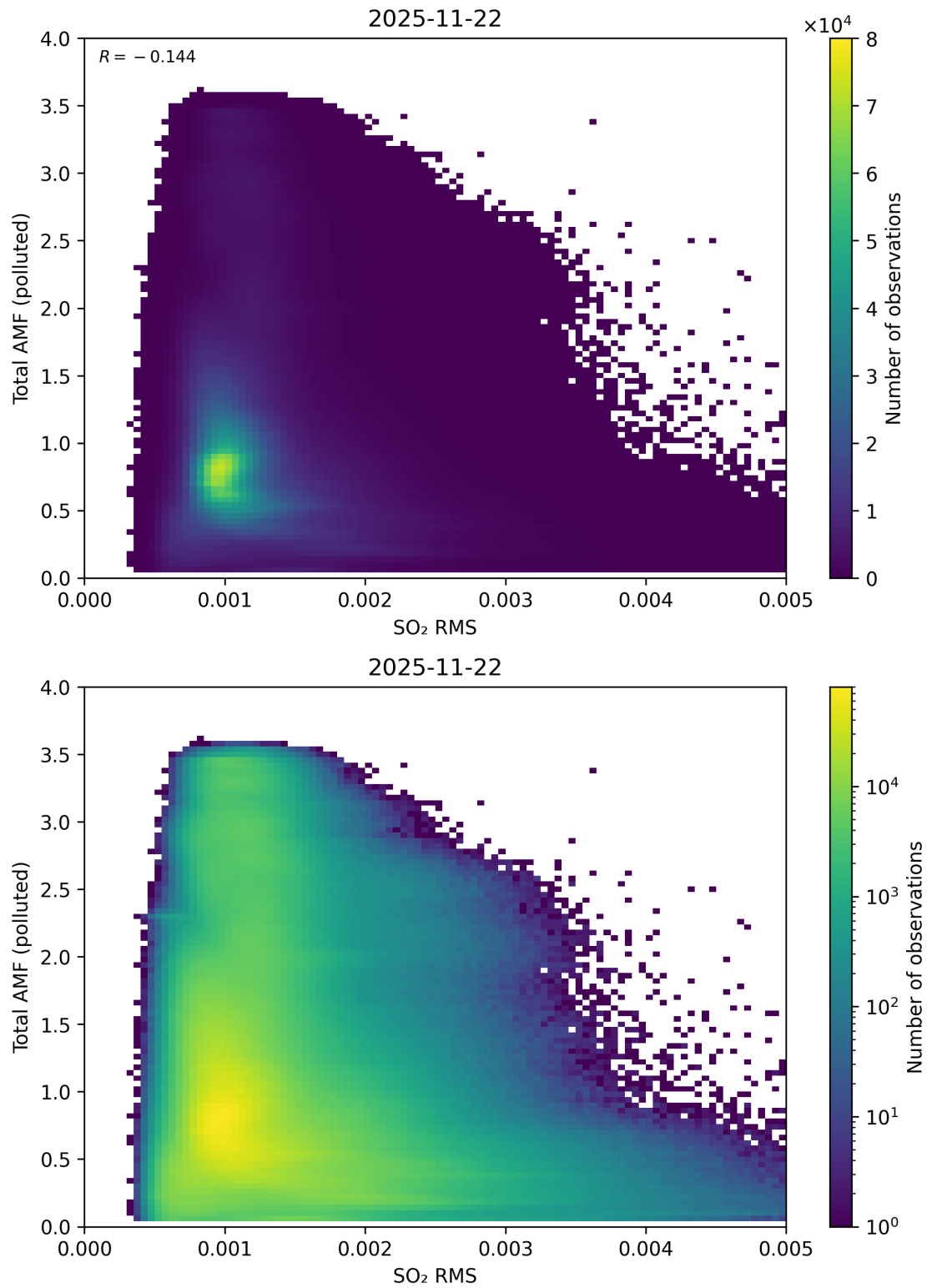
Figure 148: Scatter density plot of “SO 2 RMS” against “Total AMF (polluted)” for 2025-11-21 to 2025-11-23.
