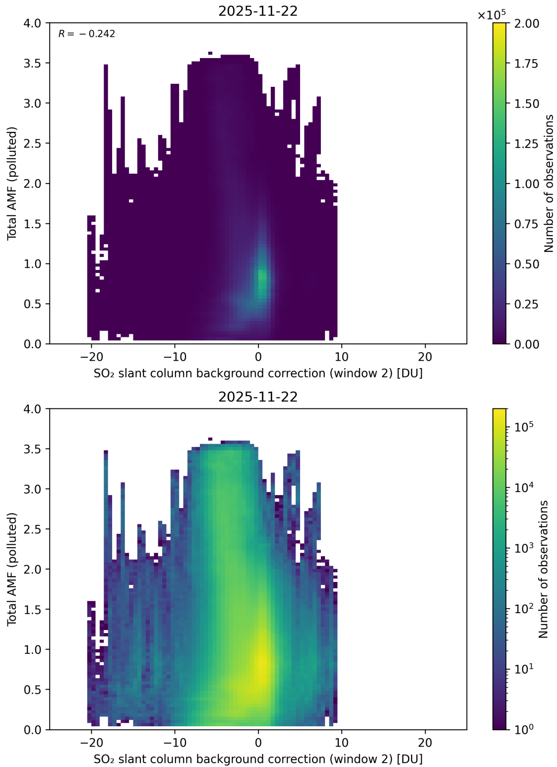
Figure 130: Scatter density plot of “SO 2 slant column background correction (window 2)” against “Total AMF (polluted)” for 2025-11-21 to 2025-11-23.
