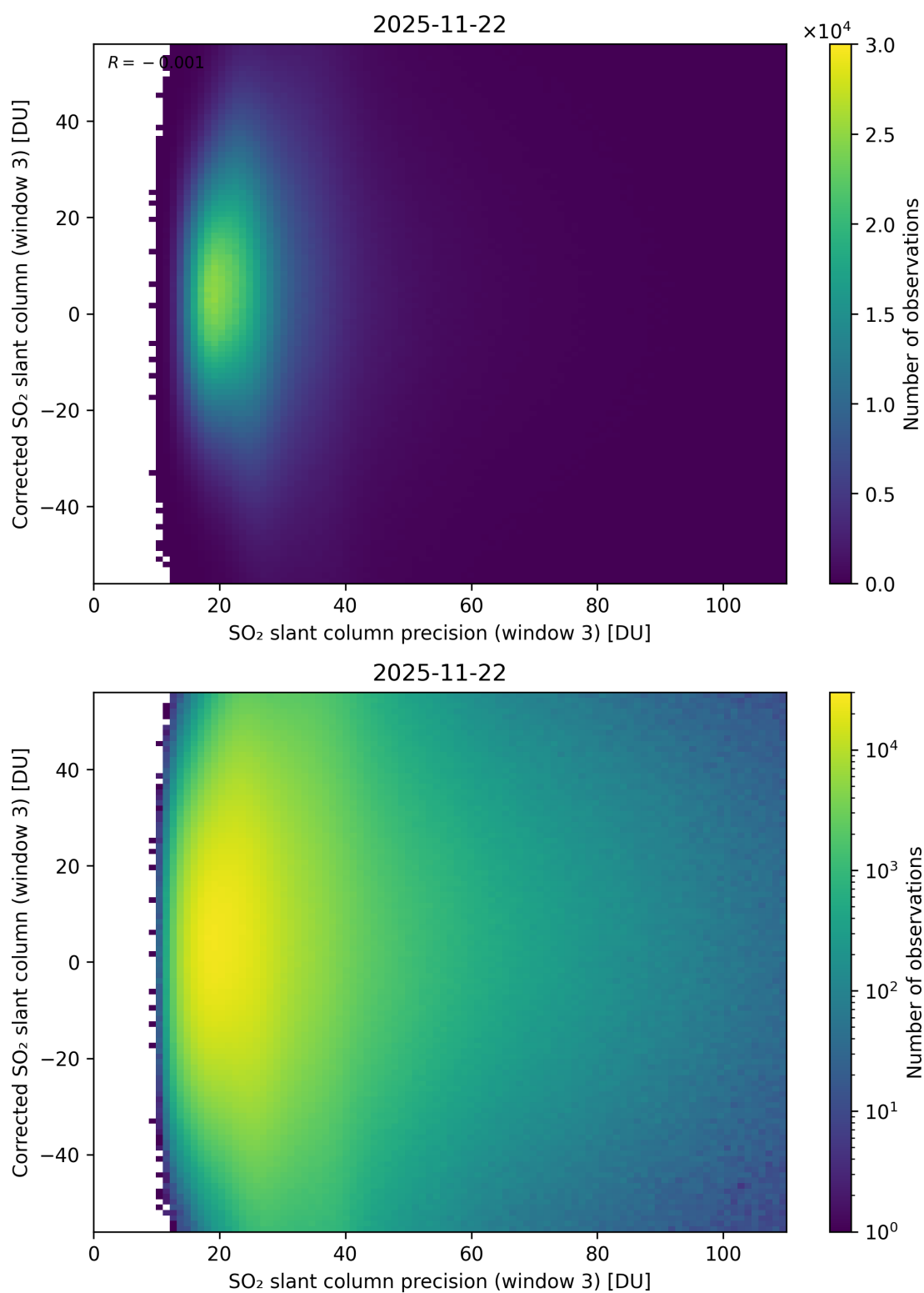
Figure 312: Scatter density plot of “SO 2 slant column precision (window 3)” against “Corrected SO 2 slant column (window 3)” for 2025-11-21 to 2025-11-23.
