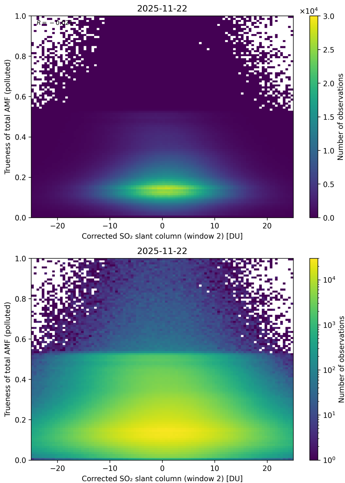
Figure 254: Scatter density plot of “Corrected SO 2 slant column (window 2)” against “Trueness of total AMF (polluted)” for 2025-11-21 to 2025-11-23.
