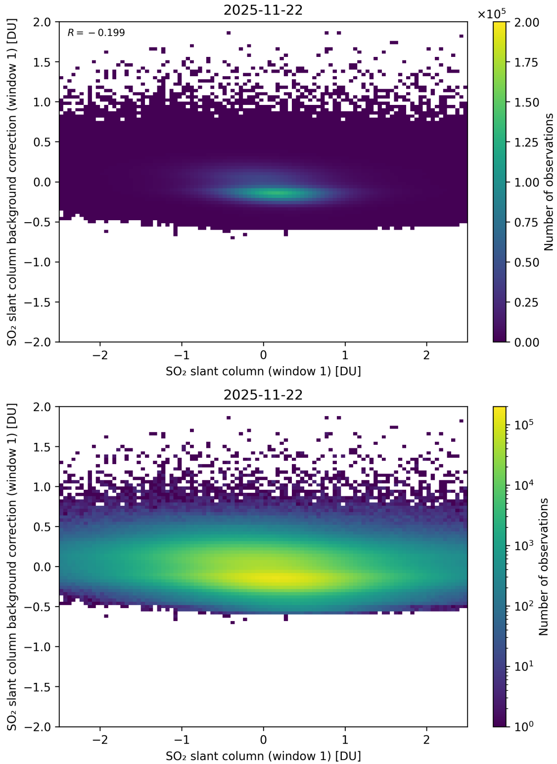
Figure 262: Scatter density plot of “SO 2 slant column (window 1)” against “SO 2 slant column background correction (window 1)” for 2025-11-21 to 2025-11-23.
