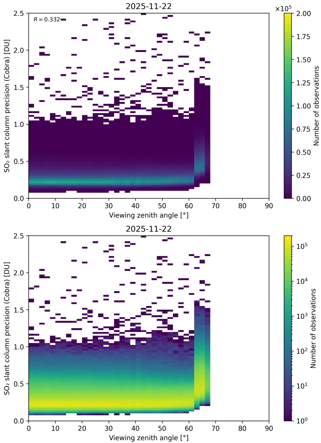
Figure 372: Scatter density plot of “Viewing zenith angle” against “SO 2 slant column precision (Cobra)” for 2025-11-21 to 2025-11-23.
