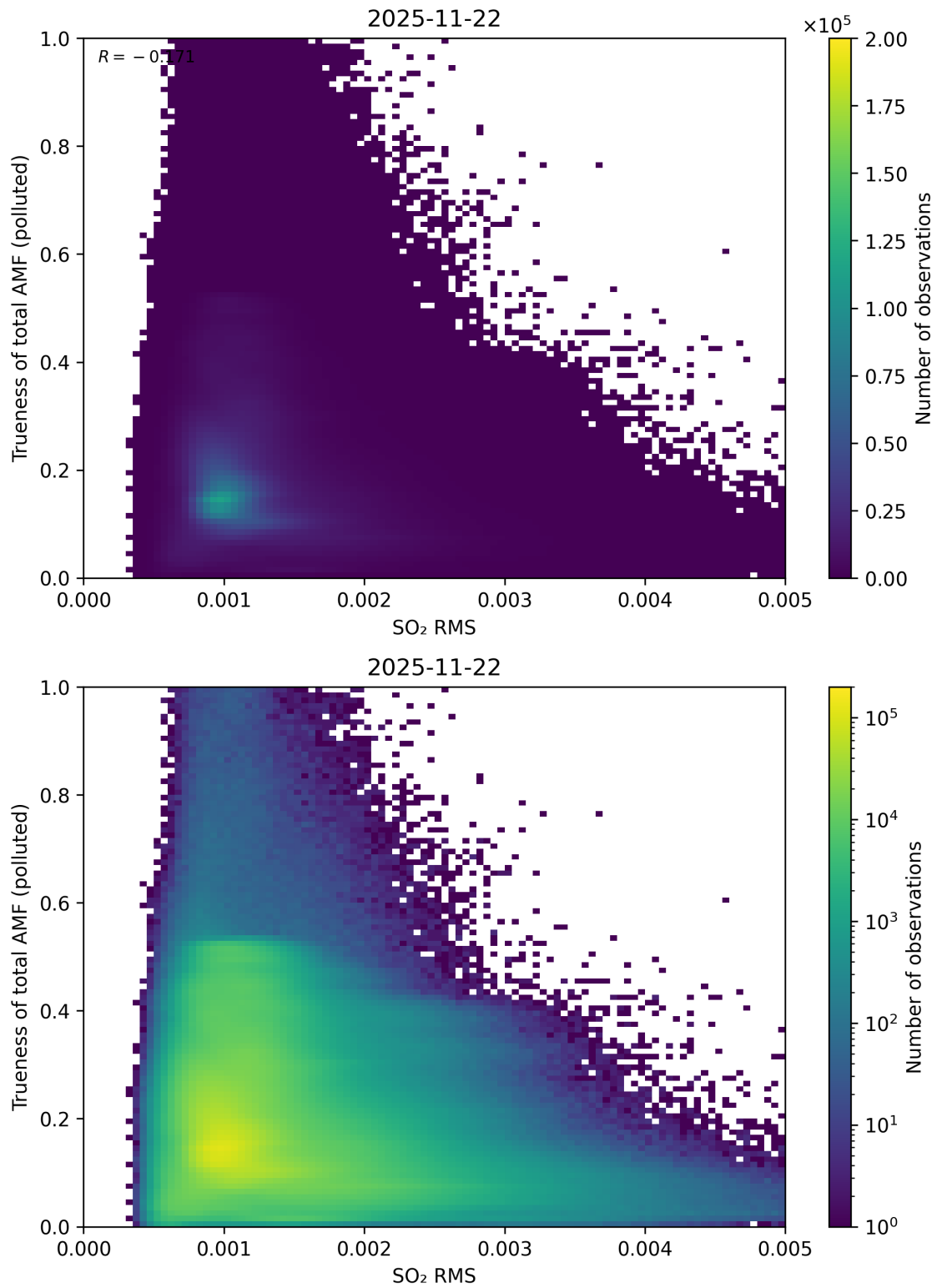
Figure 149: Scatter density plot of “SO 2 RMS” against “Trueness of total AMF (polluted)” for 2025-11-21 to 2025-11-23.
