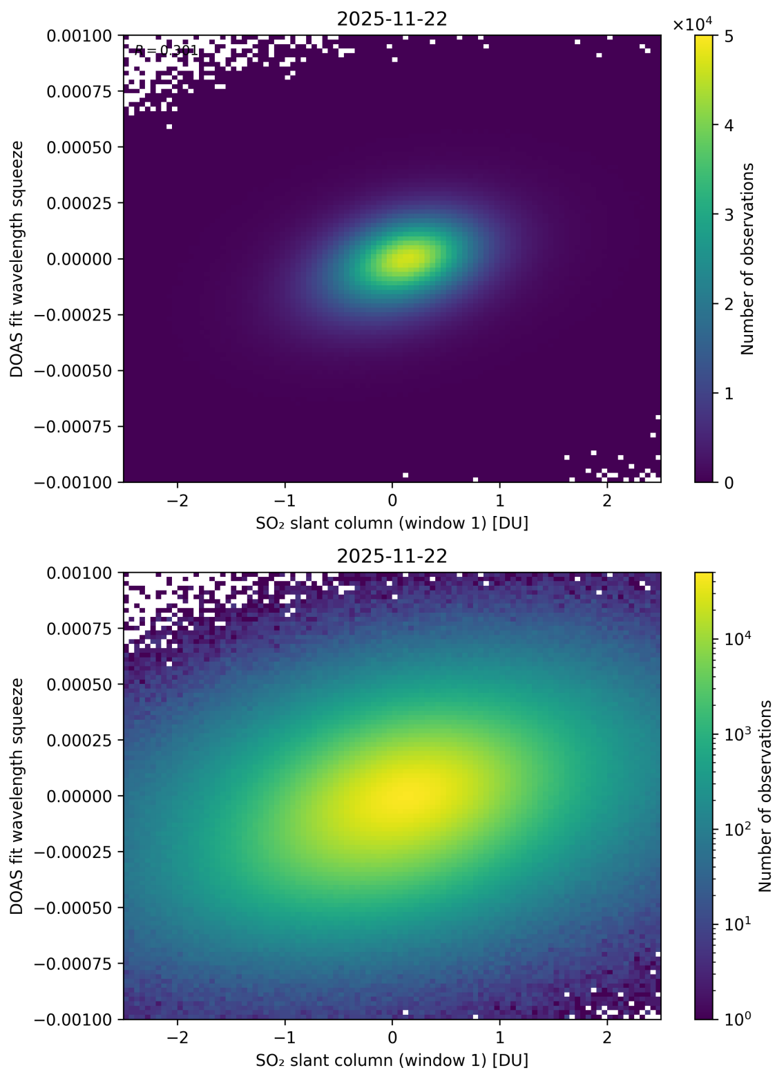
Figure 266: Scatter density plot of “SO 2 slant column (window 1)” against “DOAS fit wavelength squeeze” for 2025-11-21 to 2025-11-23.
