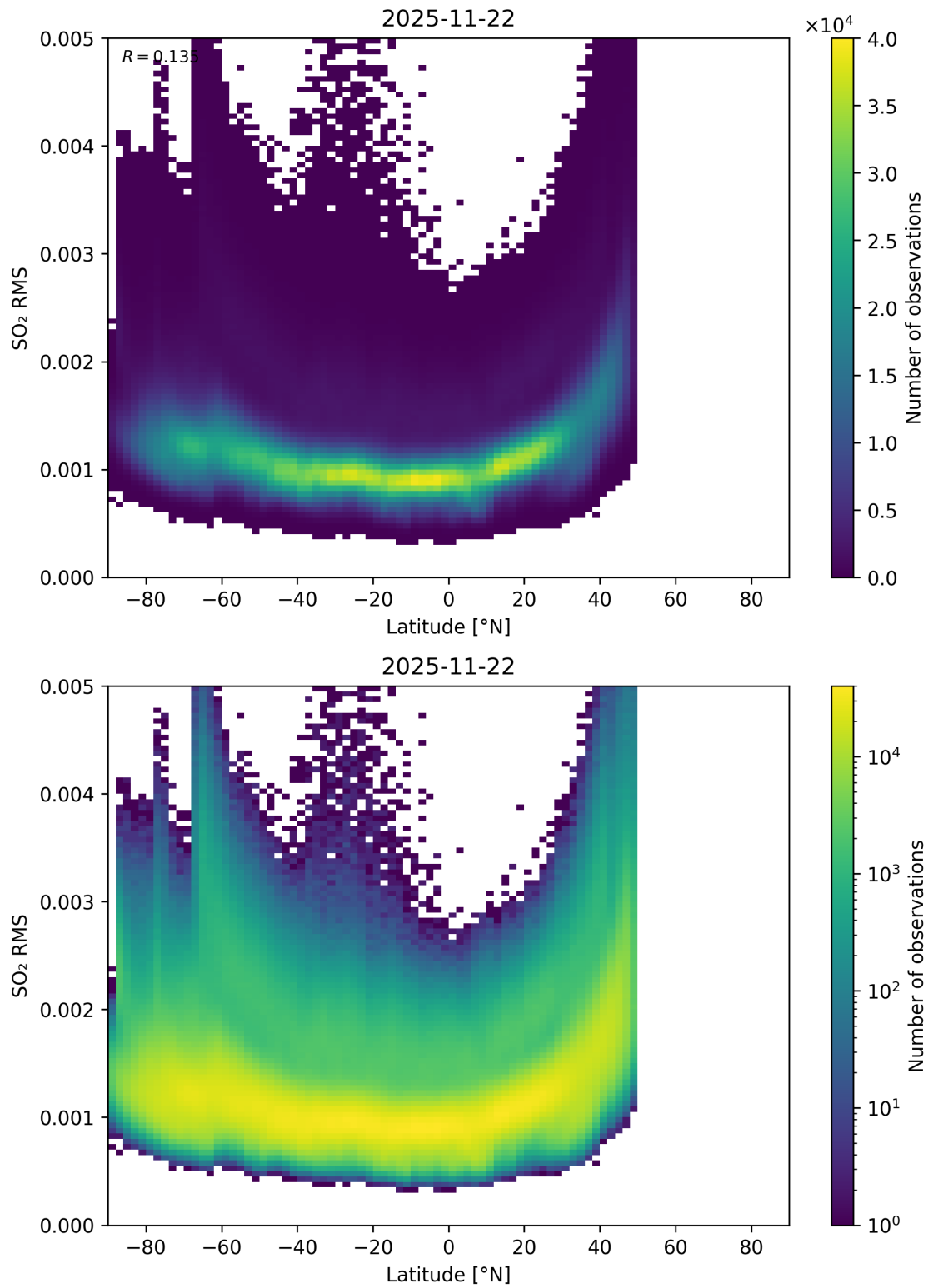
Figure 155: Scatter density plot of “Latitude” against “SO 2 RMS” for 2025-11-21 to 2025-11-23.
