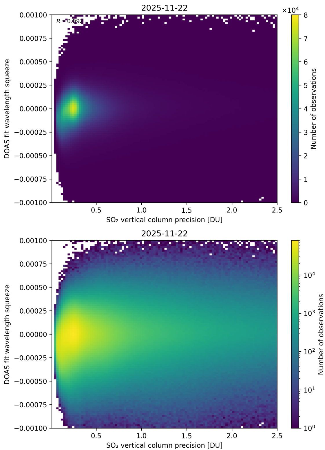
Figure 333: Scatter density plot of “SO 2 vertical column precision” against “DOAS fit wavelength squeeze” for 2025-11-21 to 2025-11-23.
