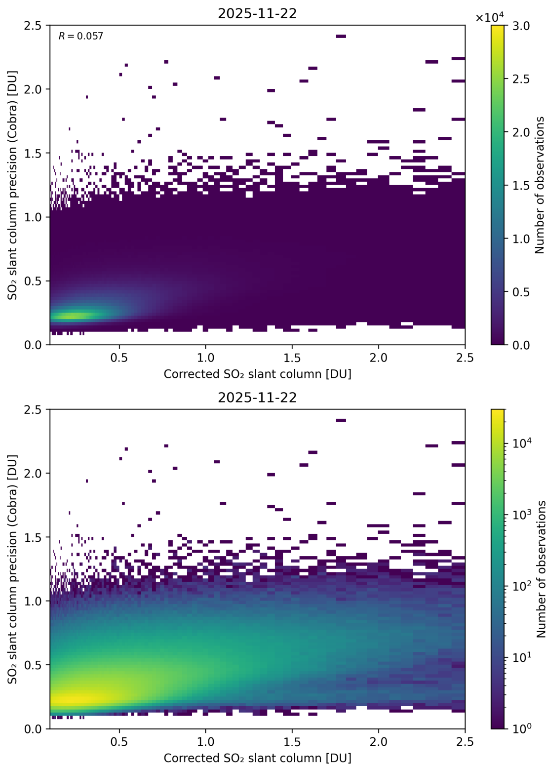
Figure 234: Scatter density plot of “Corrected SO 2 slant column” against “SO 2 slant column precision (Cobra)” for 2025-11-21 to 2025-11-23.
