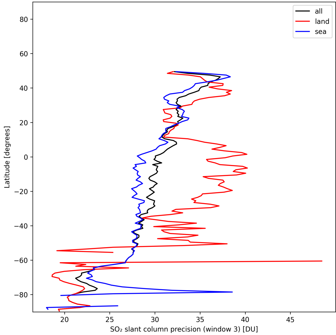
Figure 46: Zonal average of “SO 2 slant column precision (window 3)” for 2025-11-21 to 2025-11-23.
