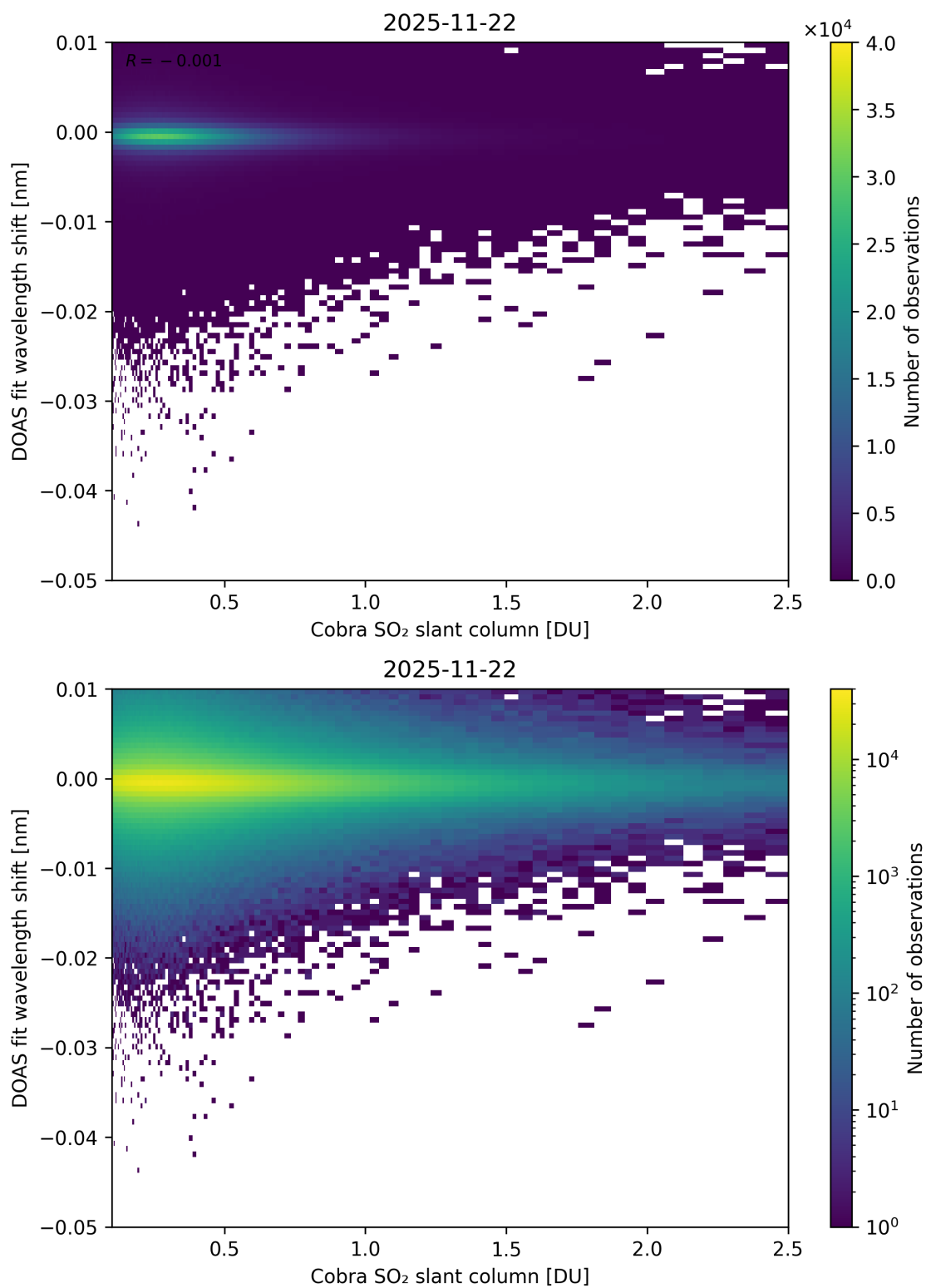
Figure 196: Scatter density plot of “Cobra SO 2 slant column” against “DOAS fit wavelength shift” for 2025-11-21 to 2025-11-23.
