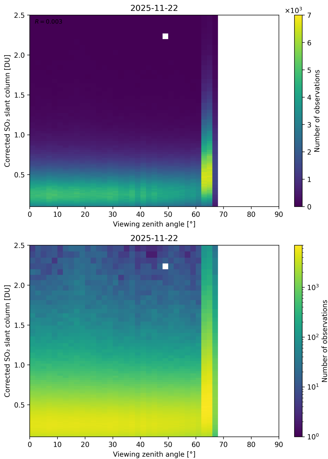
Figure 373: Scatter density plot of “Viewing zenith angle” against “Corrected SO 2 slant column” for 2025-11-21 to 2025-11-23.
