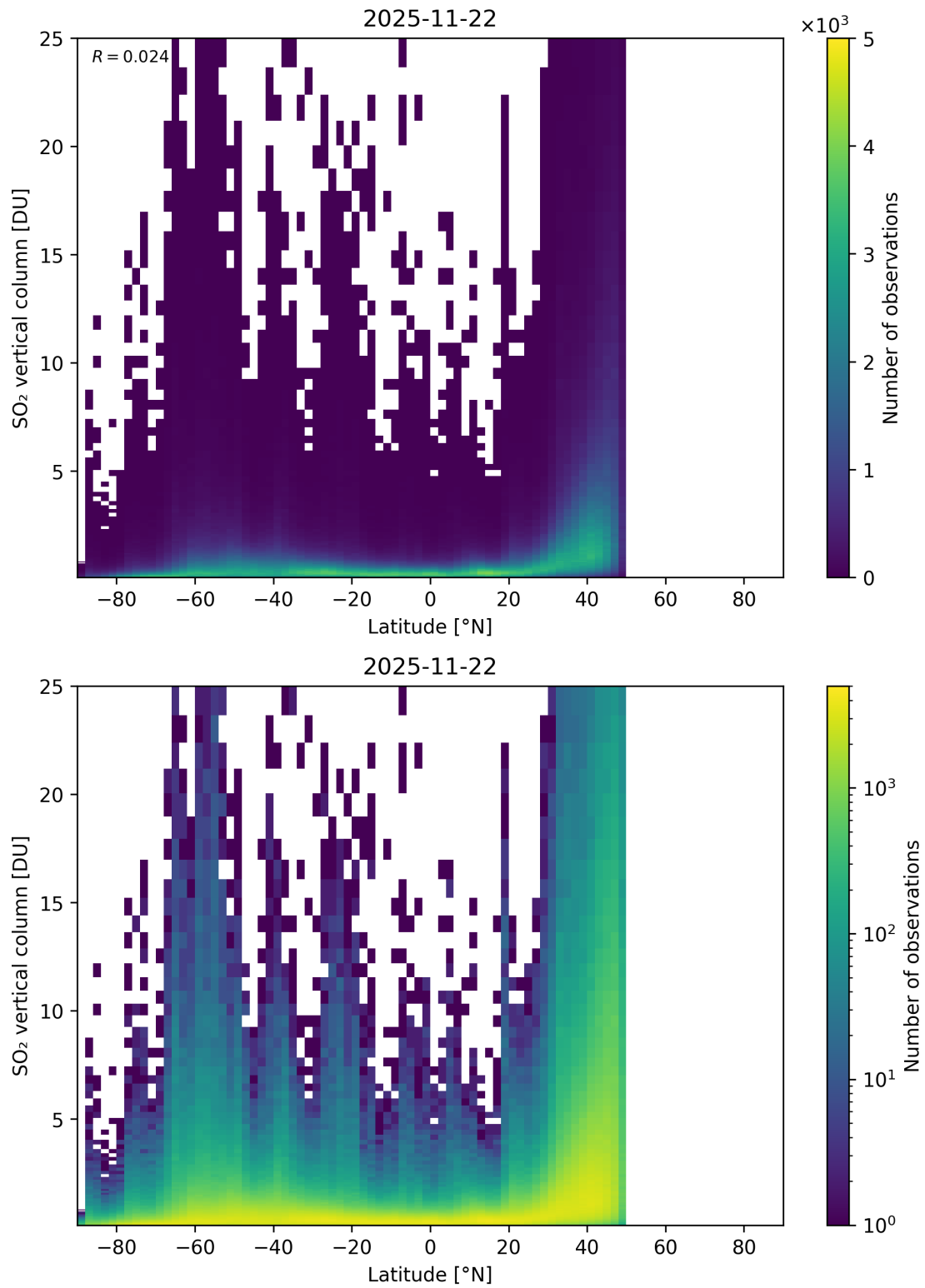
Figure 169: Scatter density plot of “Latitude” against “SO 2 vertical column” for 2025-11-21 to 2025-11-23.
