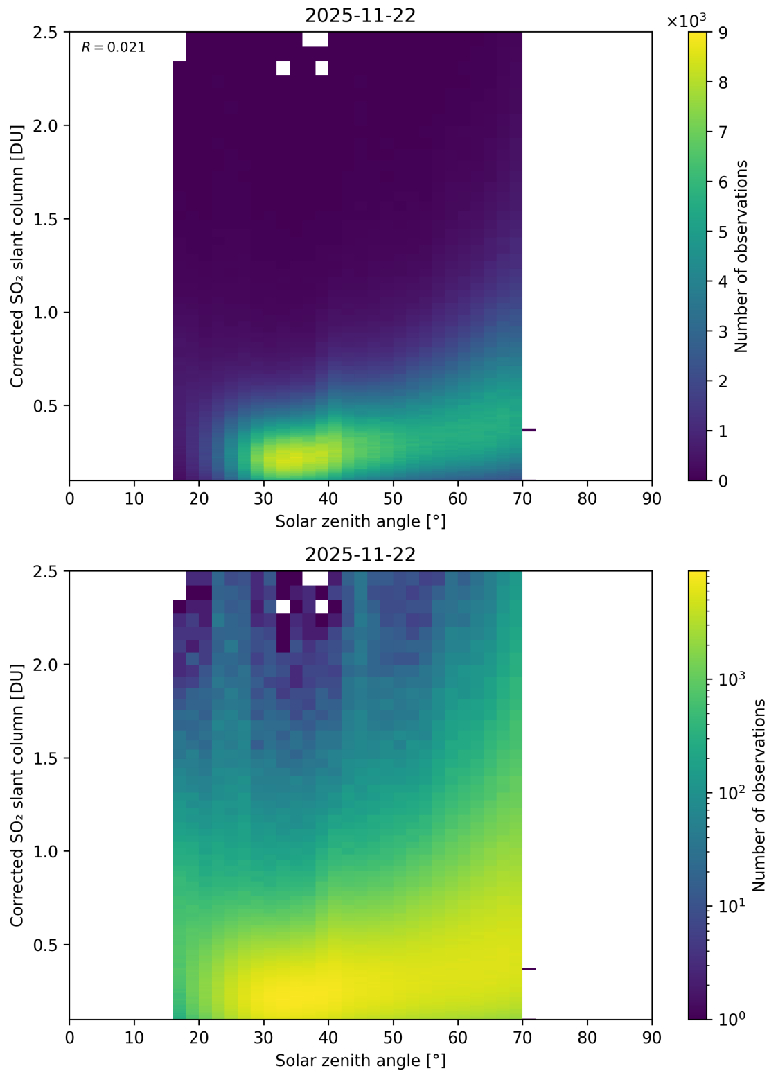
Figure 181: Scatter density plot of “Solar zenith angle” against “Corrected SO 2 slant column” for 2025-11-21 to 2025-11-23.
