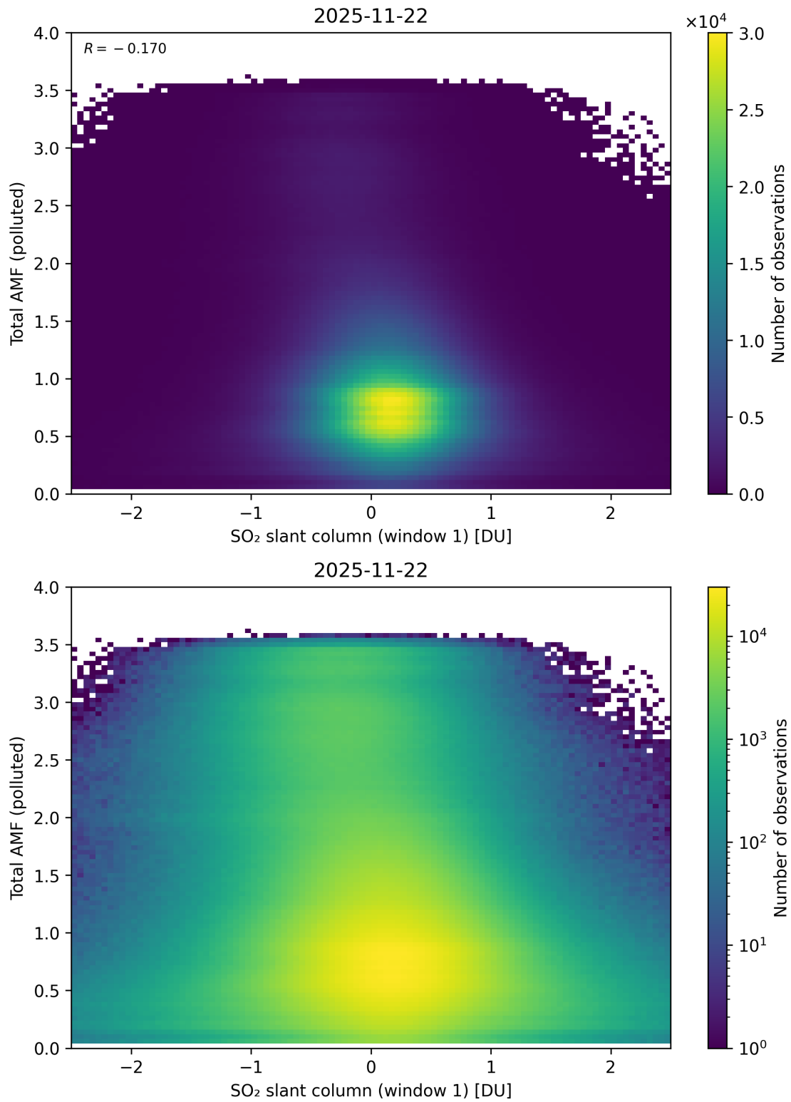
Figure 289: Scatter density plot of “SO 2 slant column (window 1)” against “Total AMF (polluted)” for 2025-11-21 to 2025-11-23.
