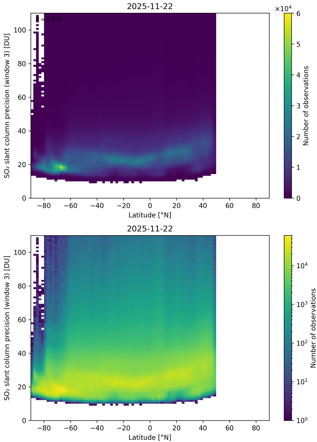
Figure 166: Scatter density plot of “Latitude” against “SO 2 slant column precision (window 3)” for 2025-11-21 to 2025-11-23.
