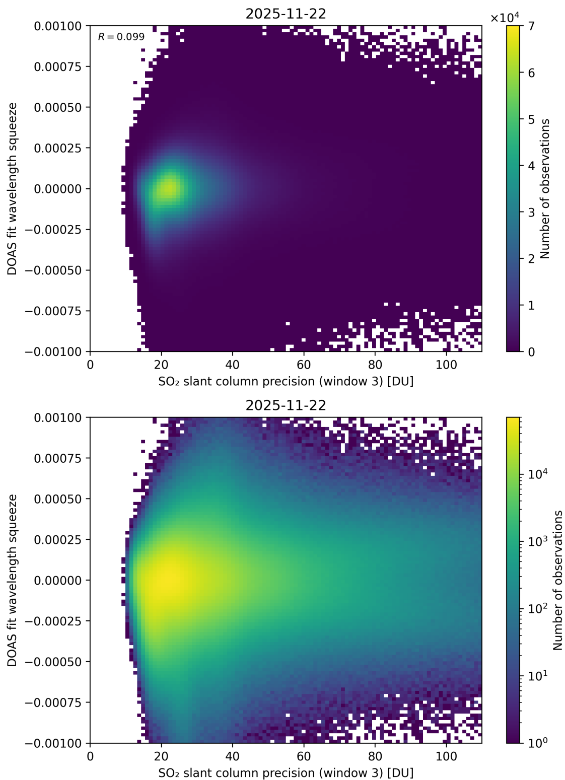
Figure 309: Scatter density plot of “SO 2 slant column precision (window 3)” against “DOAS fit wavelength squeeze” for 2025-11-21 to 2025-11-23.
