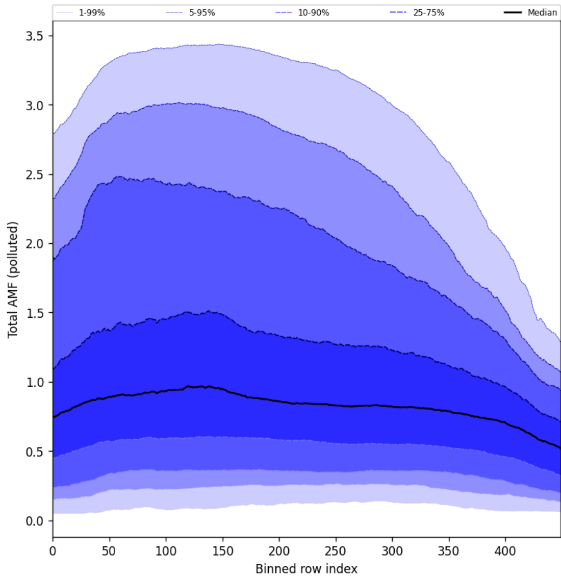
Figure 105: Along track statistics of “Total AMF (polluted)” for 2025-11-21 to 2025-11-23
