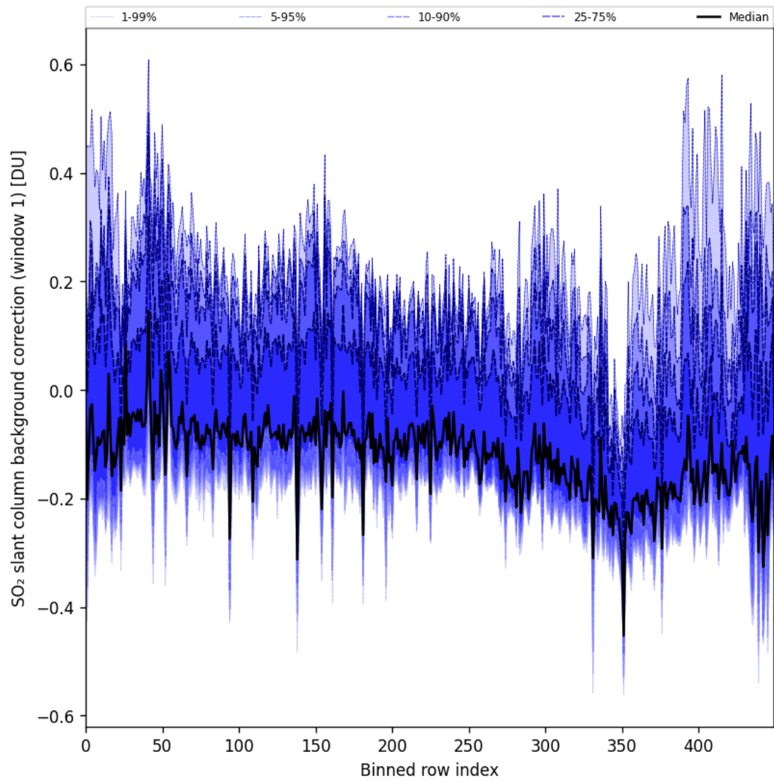
Figure 92: Along track statistics of “SO 2 slant column background correction (window 1)” for 2025-11-21 to 2025-11-23
