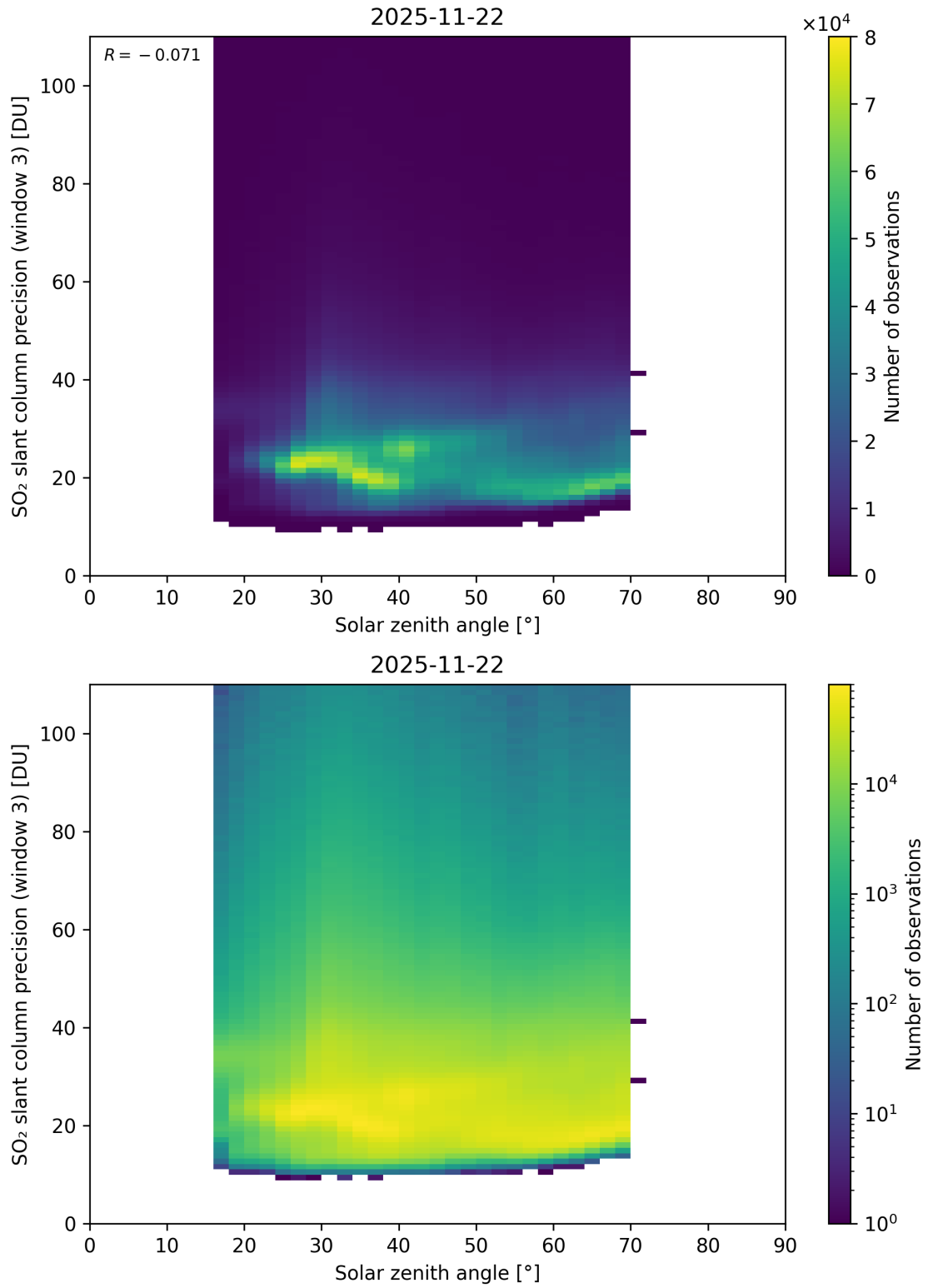
Figure 188: Scatter density plot of “Solar zenith angle” against “SO 2 slant column precision (window 3)” for 2025-11-21 to 2025-11-23.
