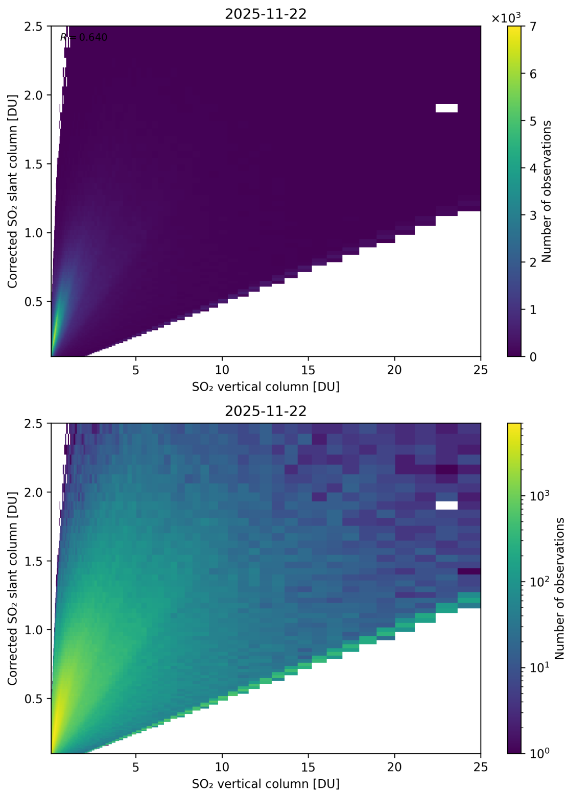
Figure 351: Scatter density plot of “SO 2 vertical column” against “Corrected SO 2 slant column” for 2025-11-21 to 2025-11-23.
