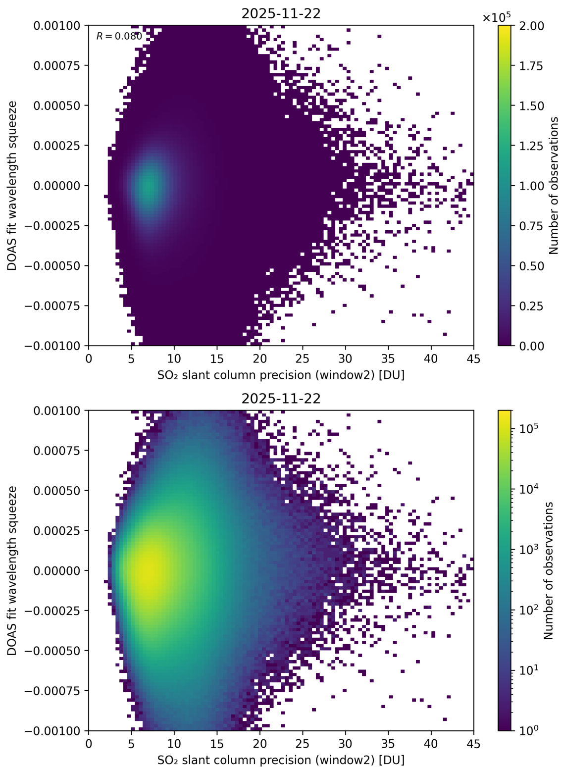
Figure 294: Scatter density plot of “SO 2 slant column precision (window2)” against “DOAS fit wavelength squeeze” for 2025-11-21 to 2025-11-23.
