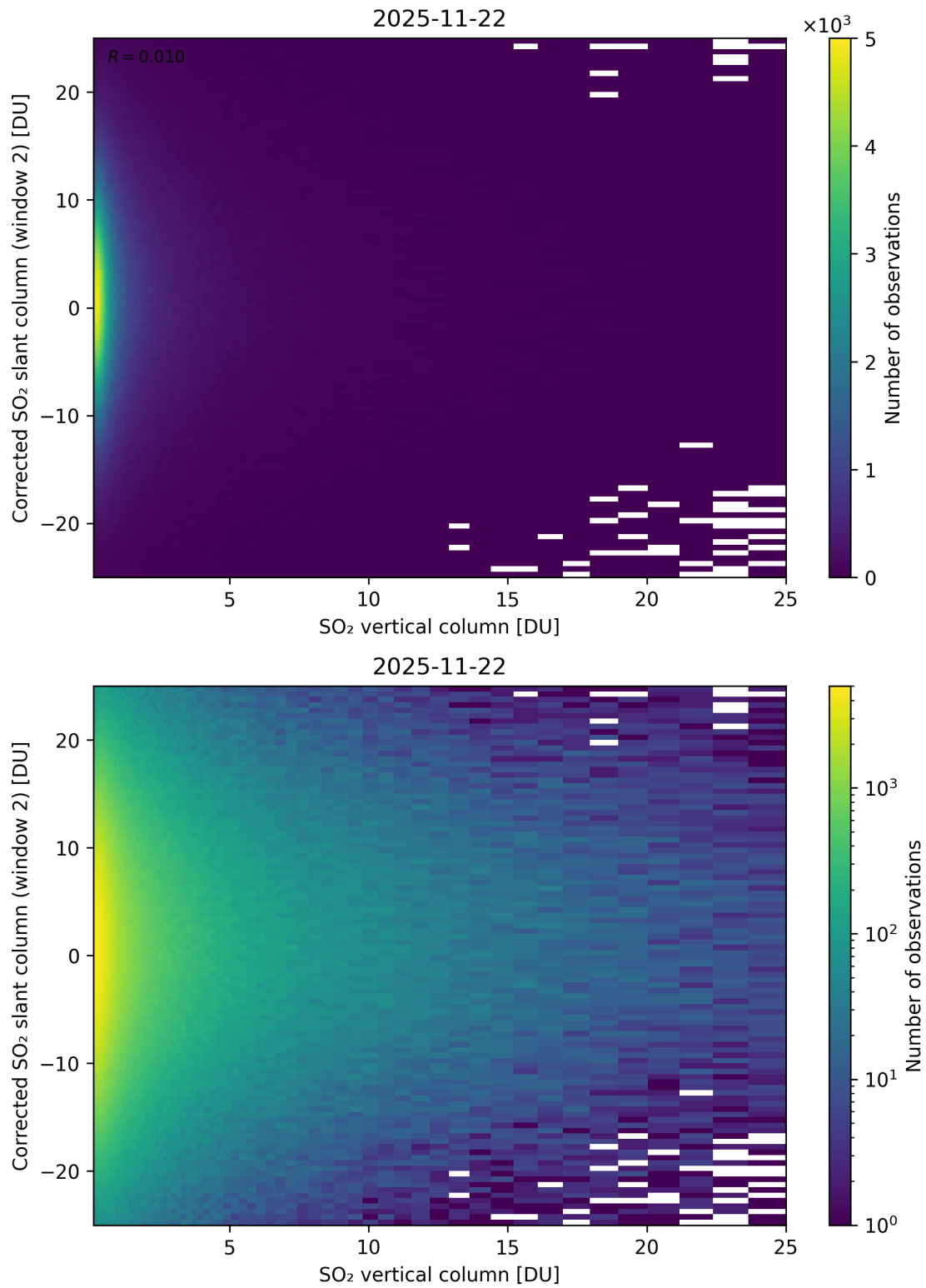
Figure 352: Scatter density plot of “SO 2 vertical column” against “Corrected SO 2 slant column (window 2)” for 2025-11-21 to 2025-11-23.
