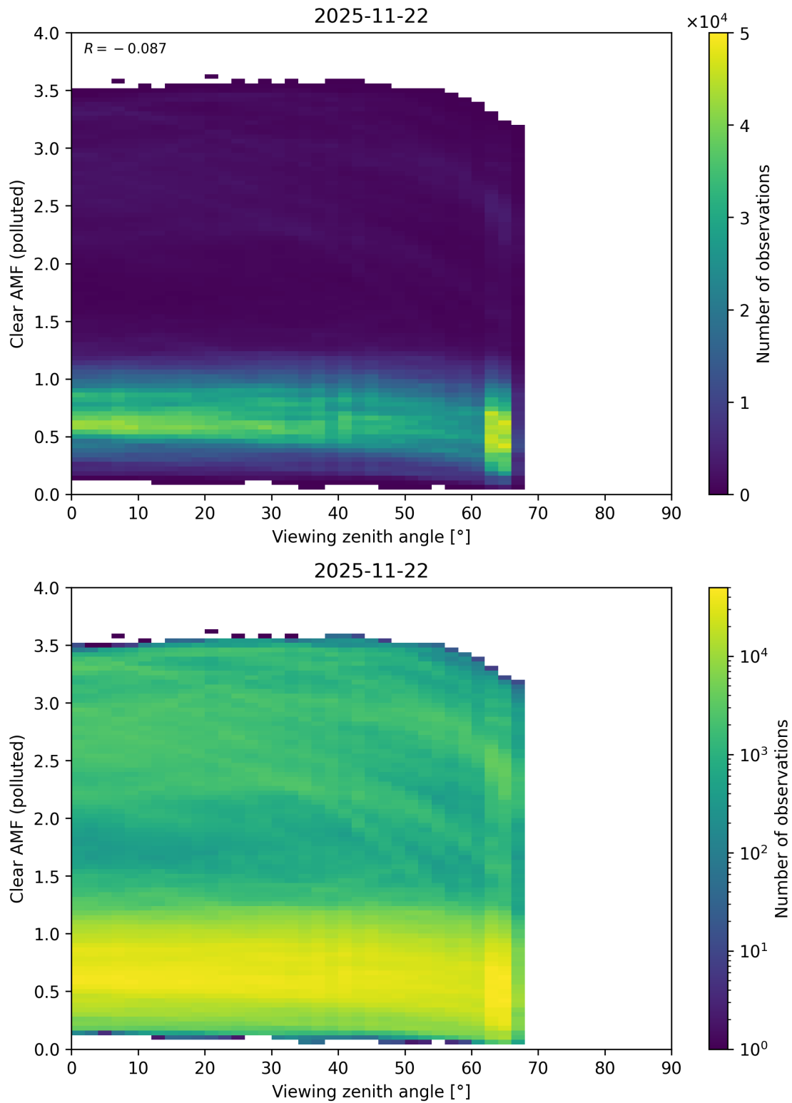
Figure 370: Scatter density plot of “Viewing zenith angle” against “Clear AMF (polluted)” for 2025-11-21 to 2025-11-23.
