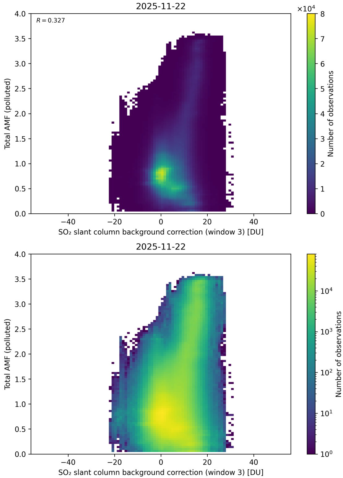
Figure 136: Scatter density plot of “SO 2 slant column background correction (window 3)” against “Total AMF (polluted)” for 2025-11-21 to 2025-11-23.
