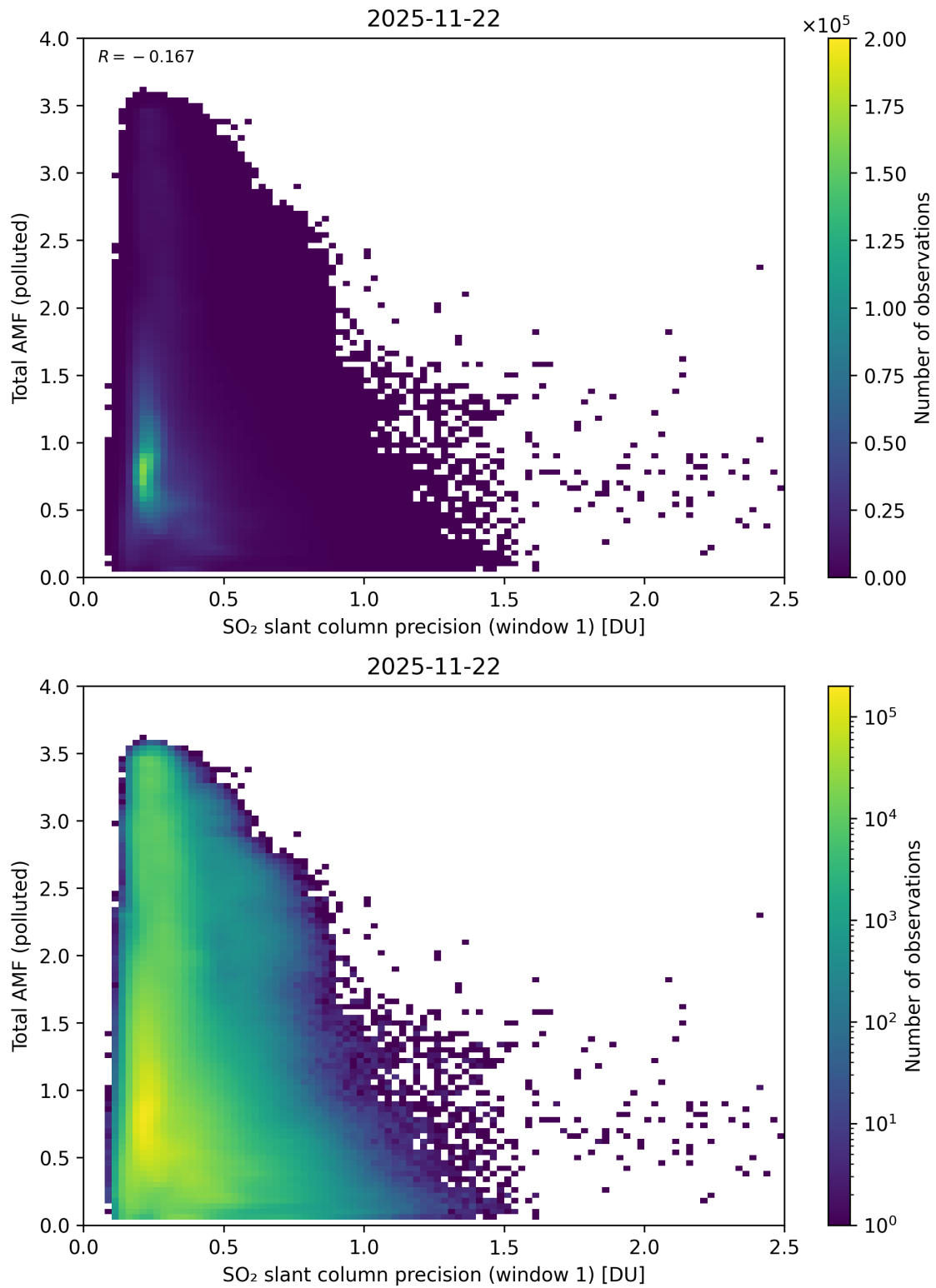
Figure 280: Scatter density plot of “SO 2 slant column precision (window 1)” against “Total AMF (polluted)” for 2025-11-21 to 2025-11-23.
