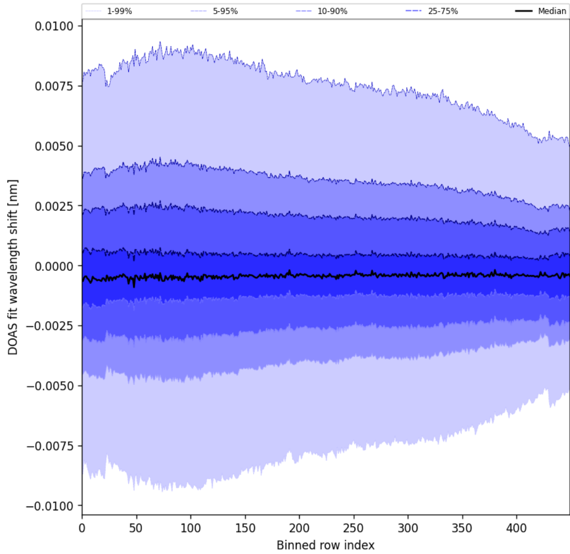
Figure 102: Along track statistics of “DOAS fit wavelength shift” for 2025-11-21 to 2025-11-23
