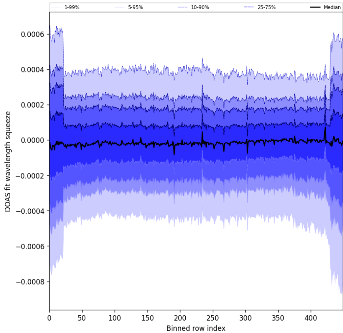
Figure 103: Along track statistics of “DOAS fit wavelength squeeze” for 2025-11-21 to 2025-11-23
