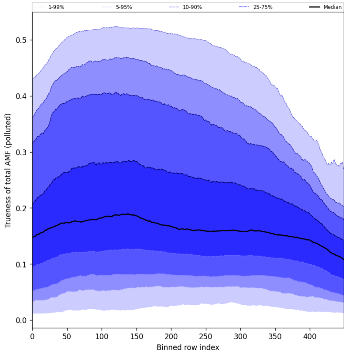
Figure 106: Along track statistics of “Trueness of total AMF (polluted)” for 2025-11-21 to 2025-11-23
