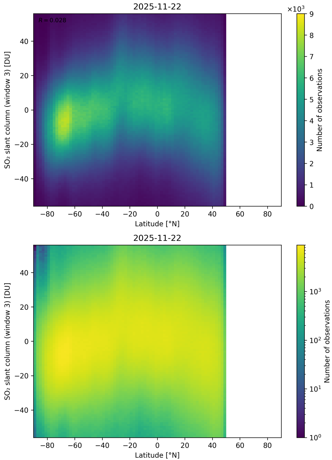
Figure 165: Scatter density plot of “Latitude” against “SO 2 slant column (window 3)” for 2025-11-21 to 2025-11-23.
