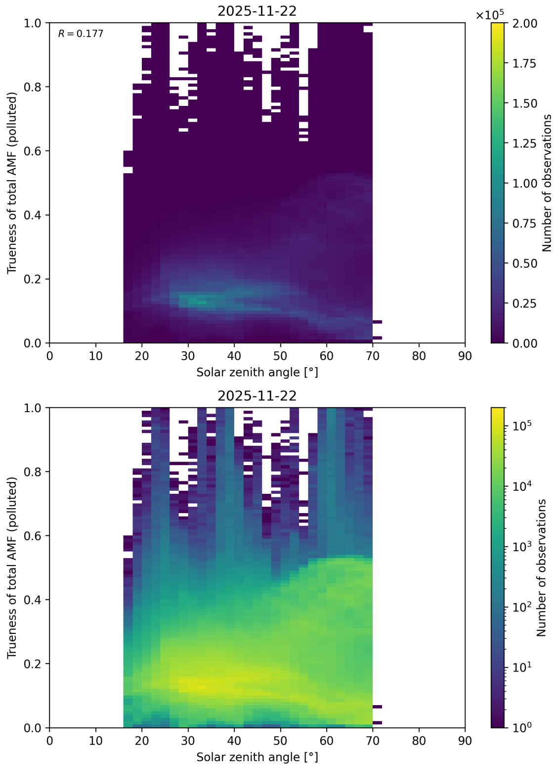
Figure 190: Scatter density plot of “Solar zenith angle” against “Trueness of total AMF (polluted)” for 2025-11-21 to 2025-11-23.
