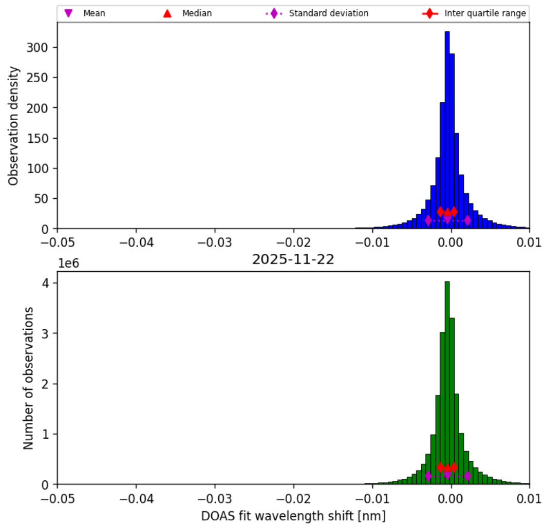
Figure 76: Histogram of “DOAS fit wavelength shift” for 2025-11-21 to 2025-11-23
