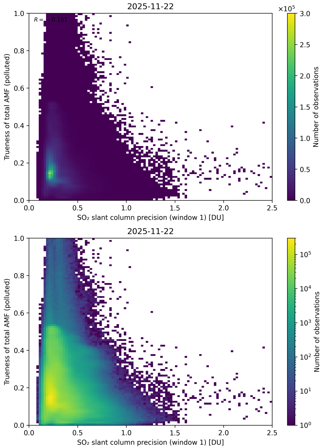
Figure 281: Scatter density plot of “SO 2 slant column precision (window 1)” against “Trueness of total AMF (polluted)” for 2025-11-21 to 2025-11-23.
