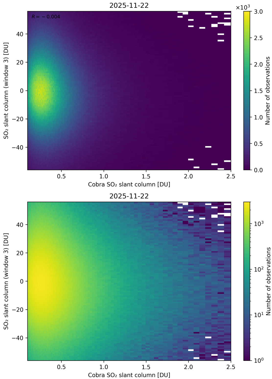
Figure 222: Scatter density plot of “Cobra SO 2 slant column” against “SO 2 slant column (window 3)” for 2025-11-21 to 2025-11-23.
