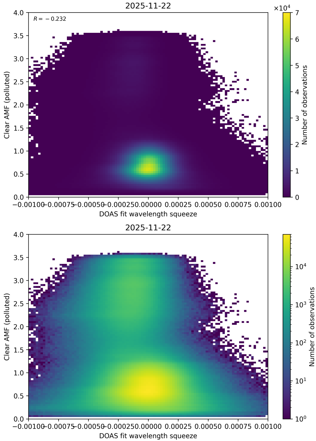
Figure 144: Scatter density plot of “DOAS fit wavelength squeeze” against “Clear AMF (polluted)” for 2025-11-21 to 2025-11-23.
