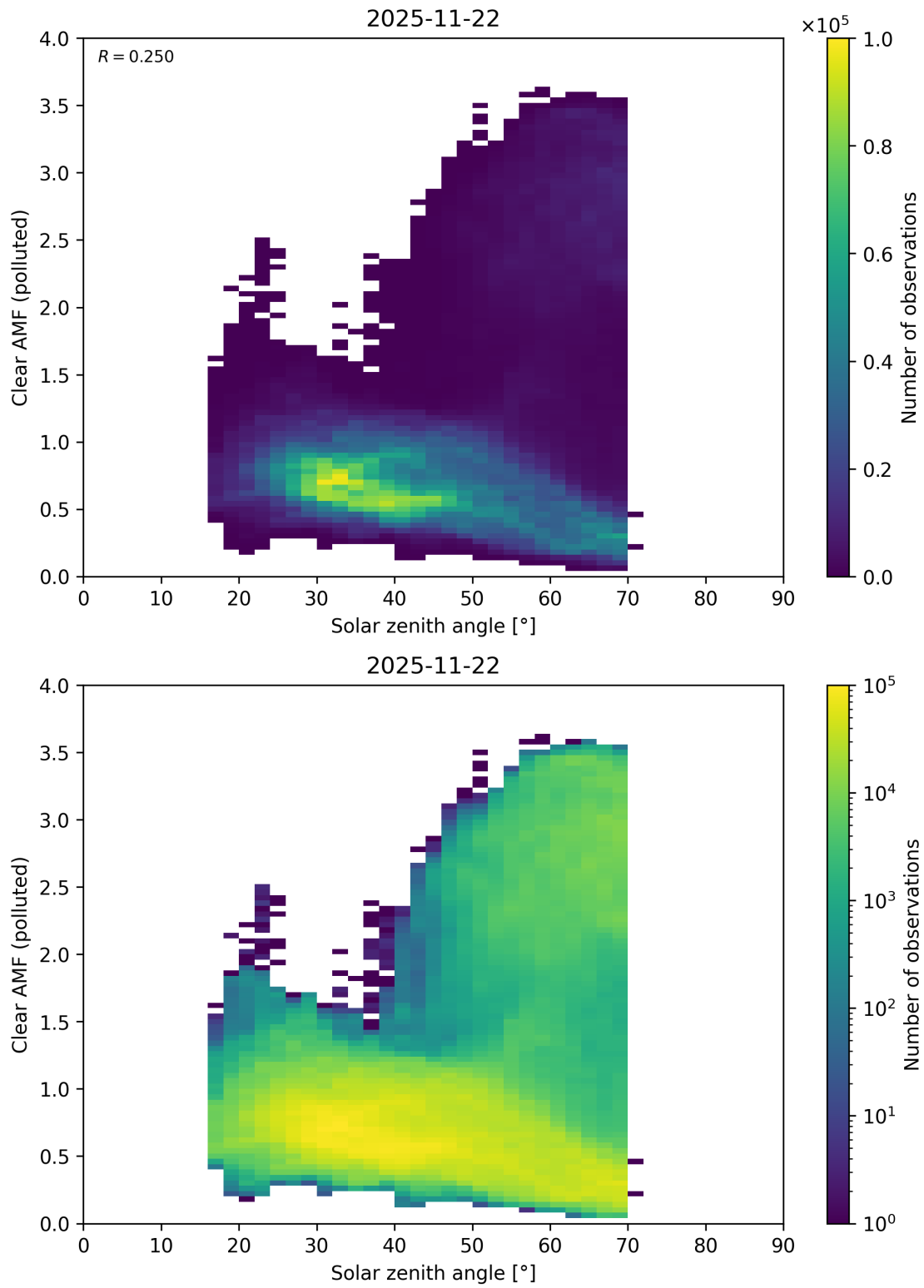
Figure 178: Scatter density plot of “Solar zenith angle” against “Clear AMF (polluted)” for 2025-11-21 to 2025-11-23.
