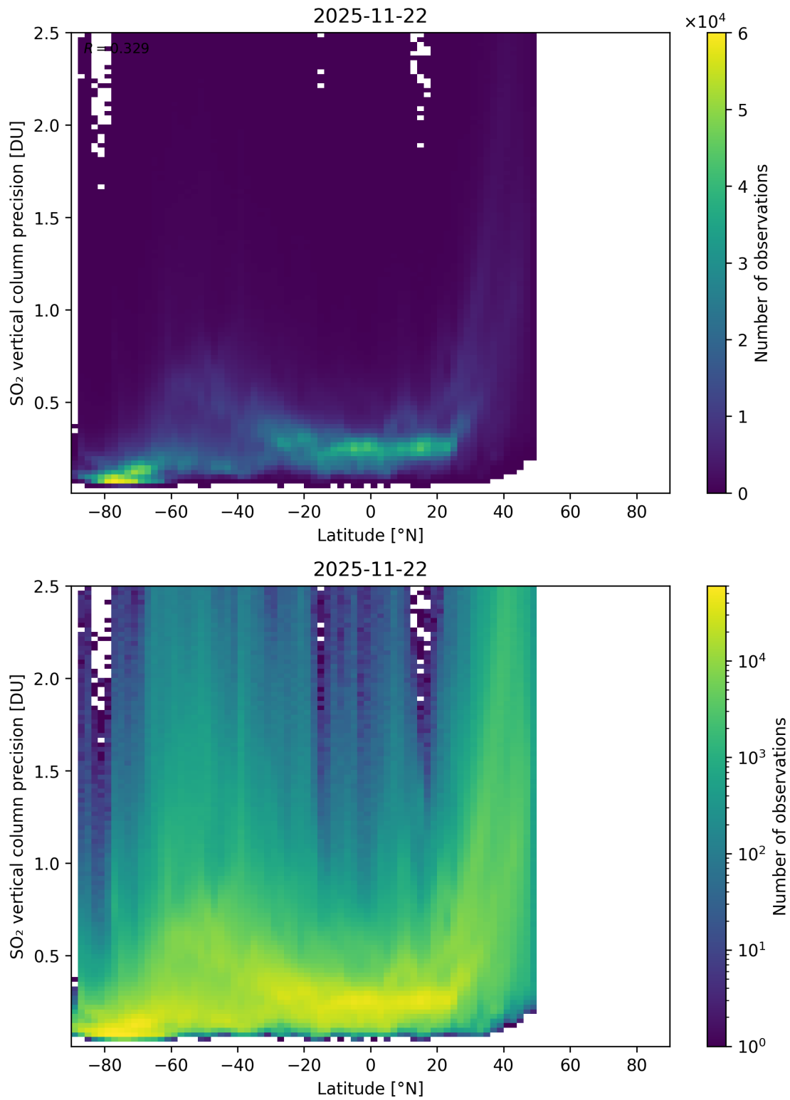
Figure 170: Scatter density plot of “Latitude” against “SO 2 vertical column precision” for 2025-11-21 to 2025-11-23.
