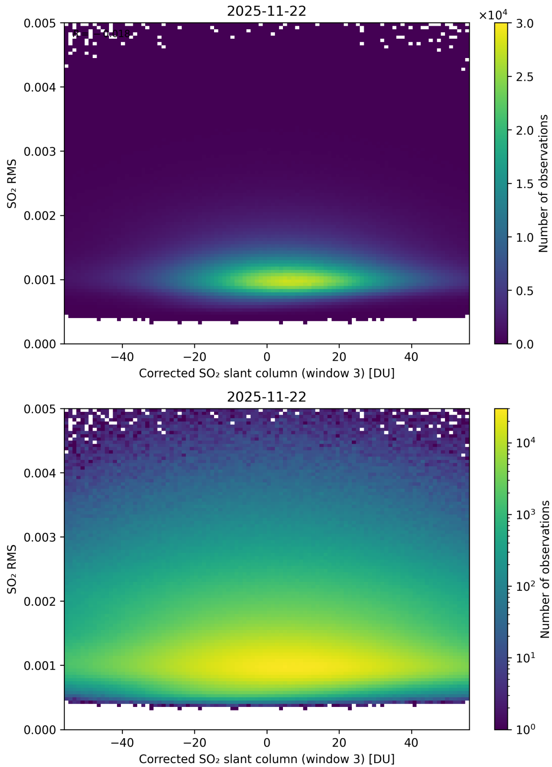
Figure 258: Scatter density plot of “Corrected SO 2 slant column (window 3)” against “SO 2 RMS” for 2025-11-21 to 2025-11-23.
