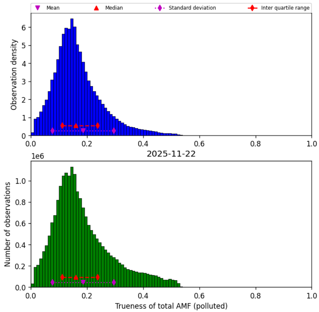
Figure 80: Histogram of “Trueness of total AMF (polluted)” for 2025-11-21 to 2025-11-23
