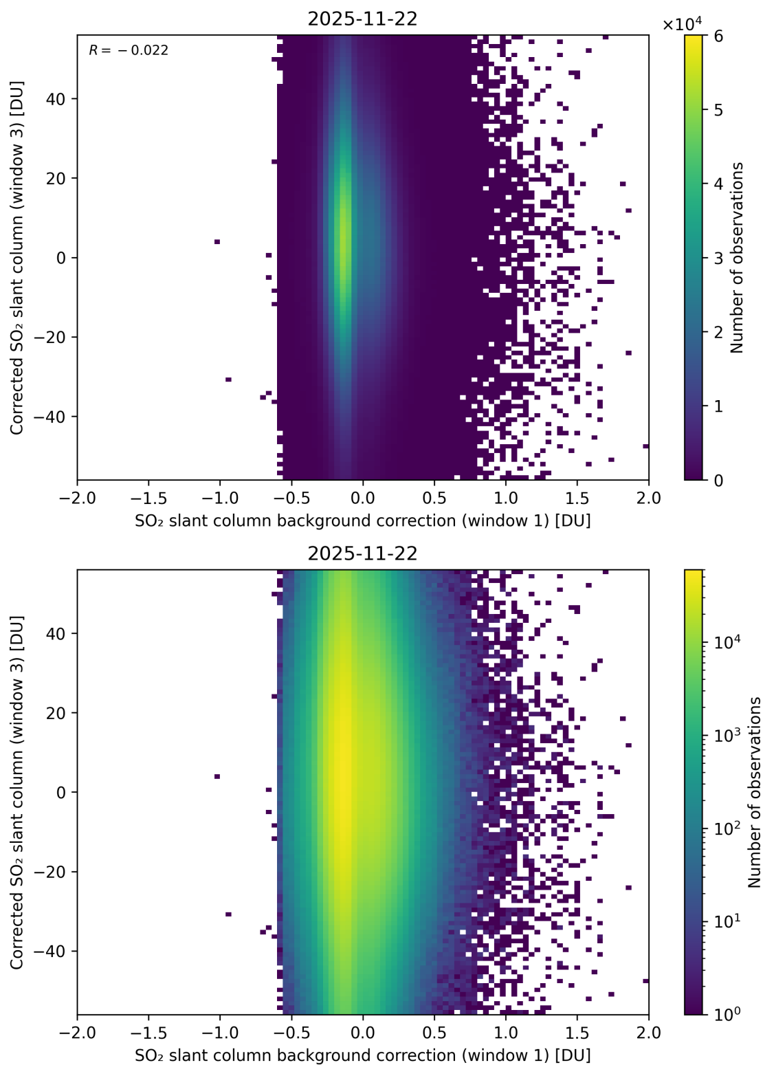
Figure 116: Scatter density plot of “SO 2 slant column background correction (window 1)” against “Corrected SO 2 slant column (window 3)” for 2025-11-21 to 2025-11-23.
