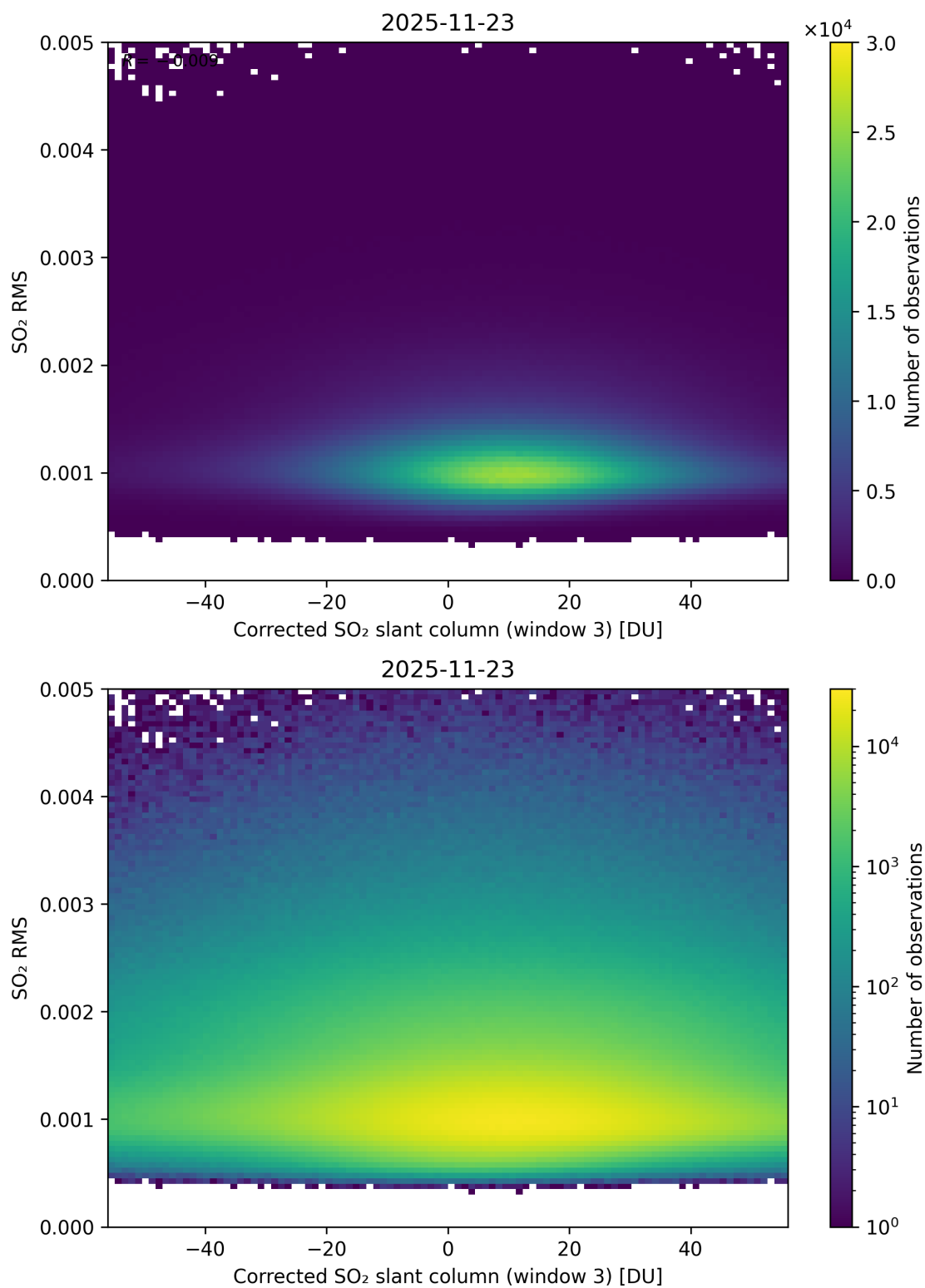
Figure 258: Scatter density plot of “Corrected SO 2 slant column (window 3)” against “SO 2 RMS” for 2025-11-23 to 2025-11-24.
