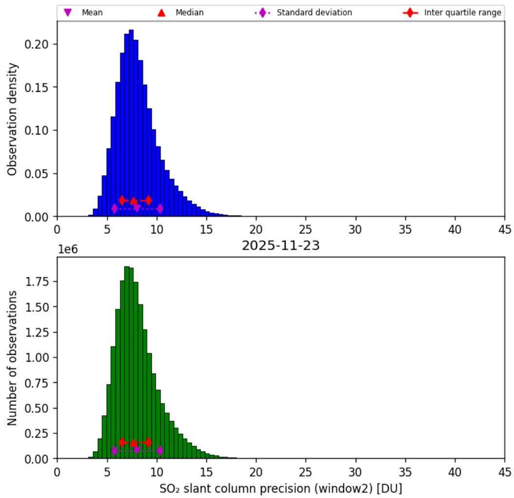
Figure 68: Histogram of “SO 2 slant column precision (window2)” for 2025-11-23 to 2025-11-24
