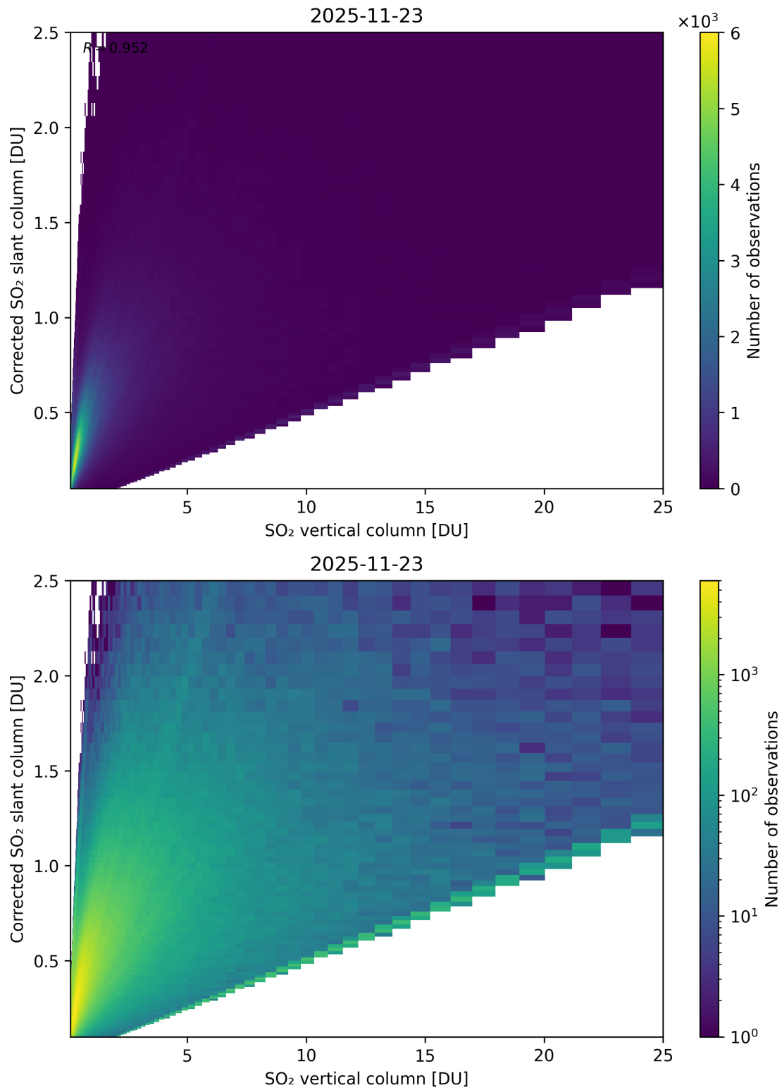
Figure 351: Scatter density plot of “SO 2 vertical column” against “Corrected SO 2 slant column” for 2025-11-23 to 2025-11-24.
