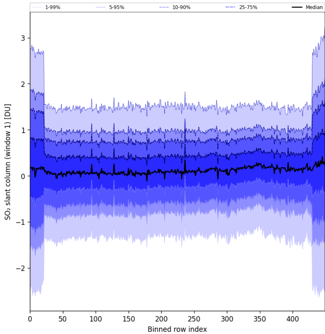
Figure 89: Along track statistics of “SO 2 slant column (window 1)” for 2025-11-23 to 2025-11-24
