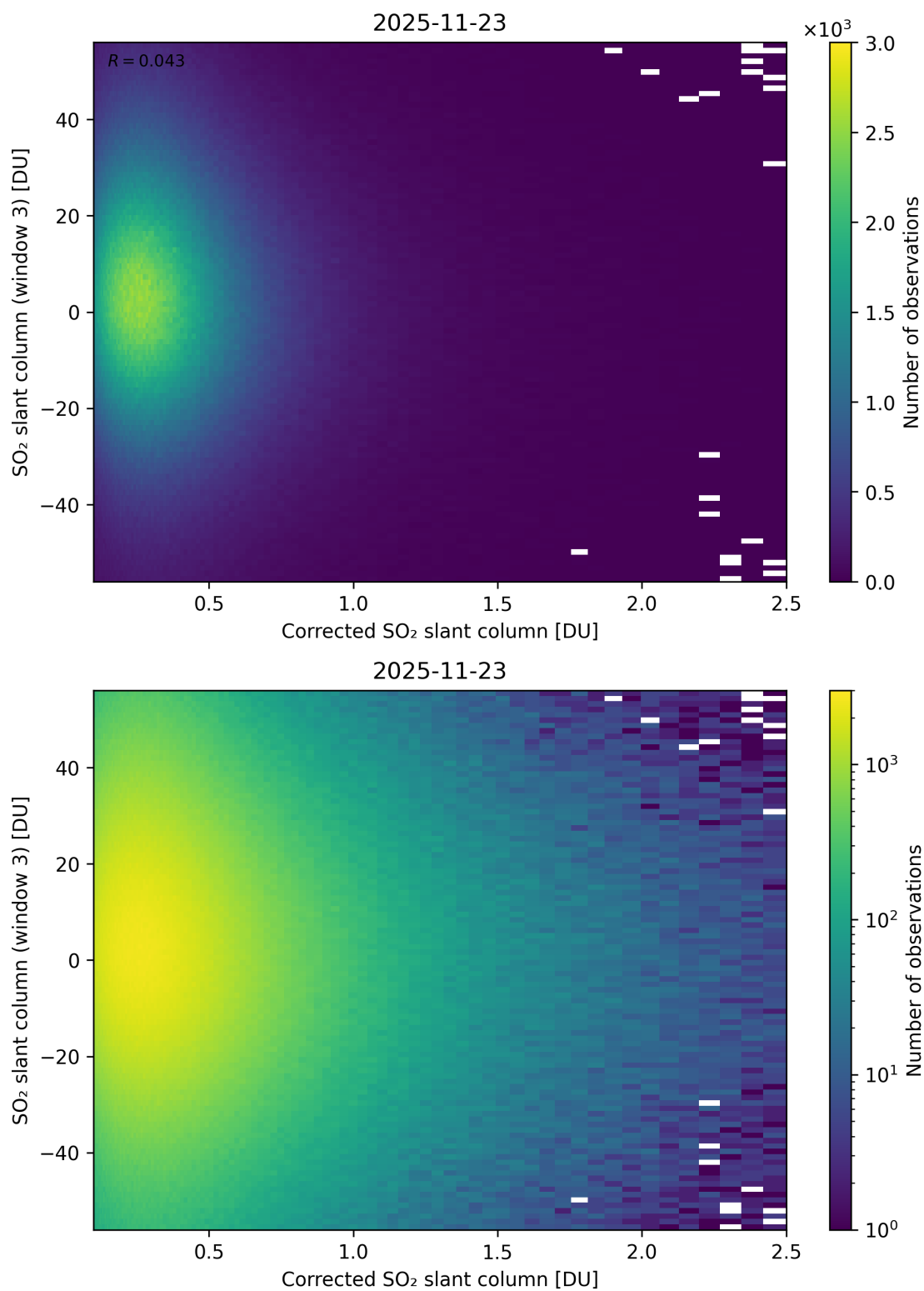
Figure 240: Scatter density plot of “Corrected SO 2 slant column” against “SO 2 slant column (window 3)” for 2025-11-23 to 2025-11-24.
