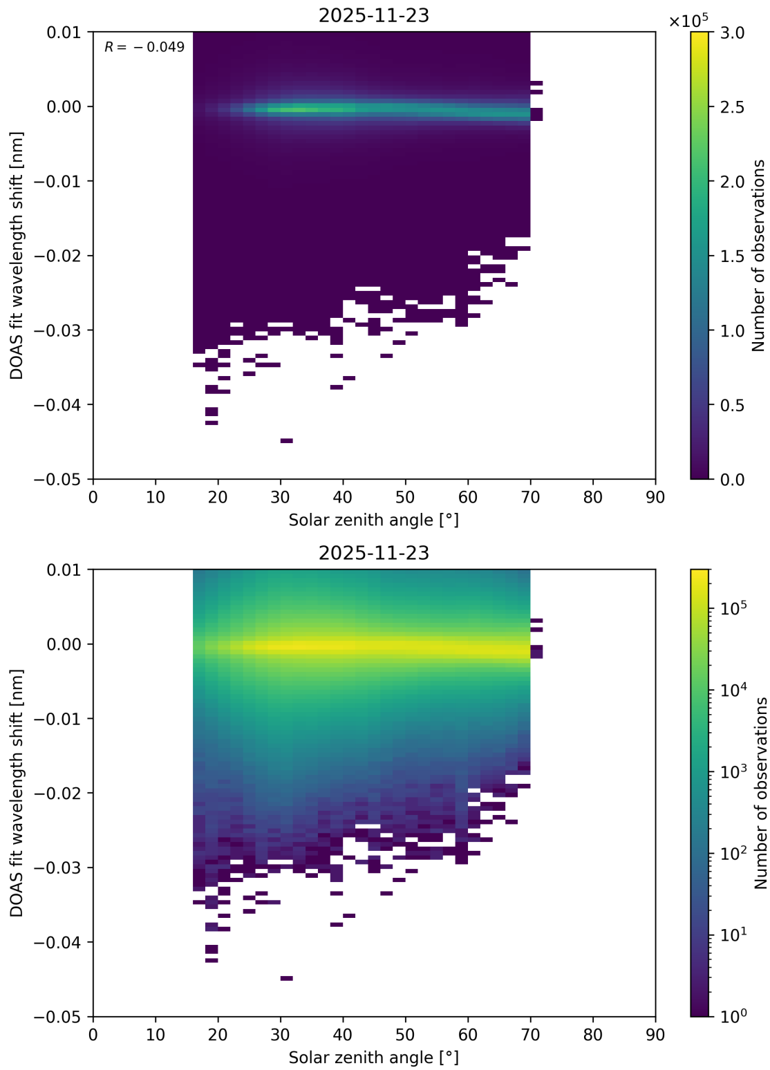
Figure 174: Scatter density plot of “Solar zenith angle” against “DOAS fit wavelength shift” for 2025-11-23 to 2025-11-24.
