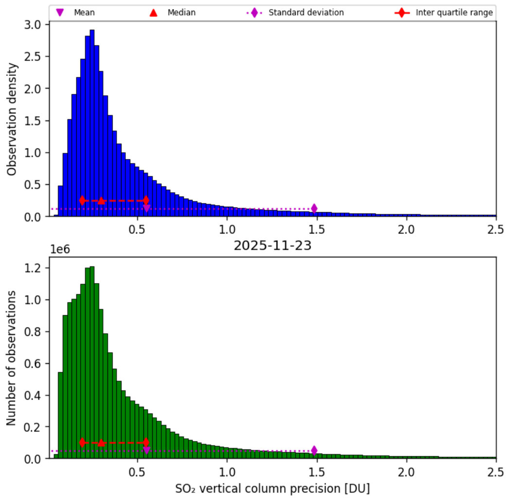
Figure 59: Histogram of “SO 2 vertical column precision” for 2025-11-23 to 2025-11-24
