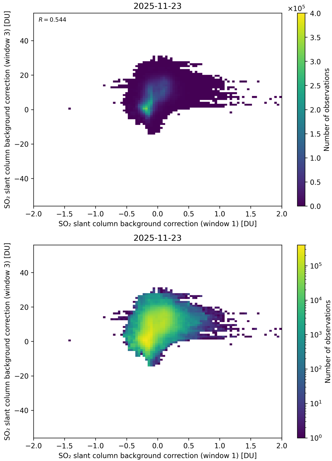
Figure 110: Scatter density plot of “SO 2 slant column background correction (window 1)” against “SO 2 slant column background correction (window 3)” for 2025-11-23 to 2025-11-24.
