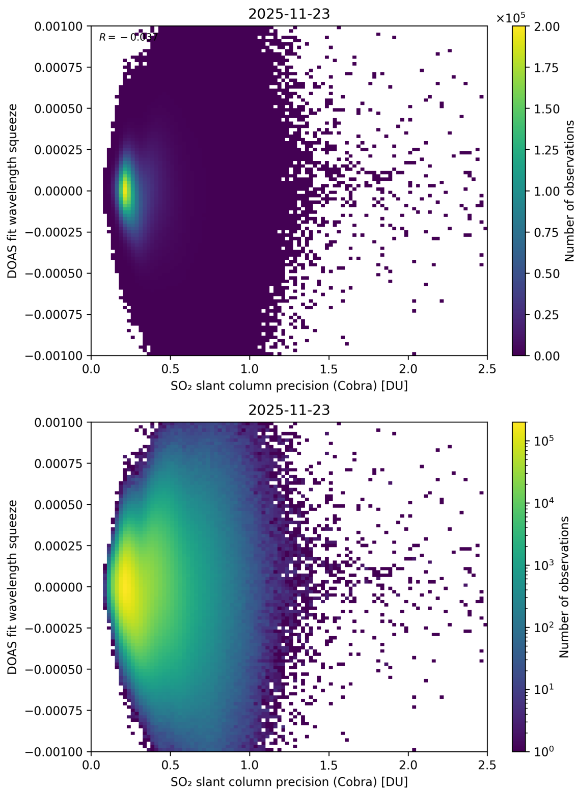
Figure 203: Scatter density plot of “SO 2 slant column precision (Cobra)” against “DOAS fit wavelength squeeze” for 2025-11-23 to 2025-11-24.
