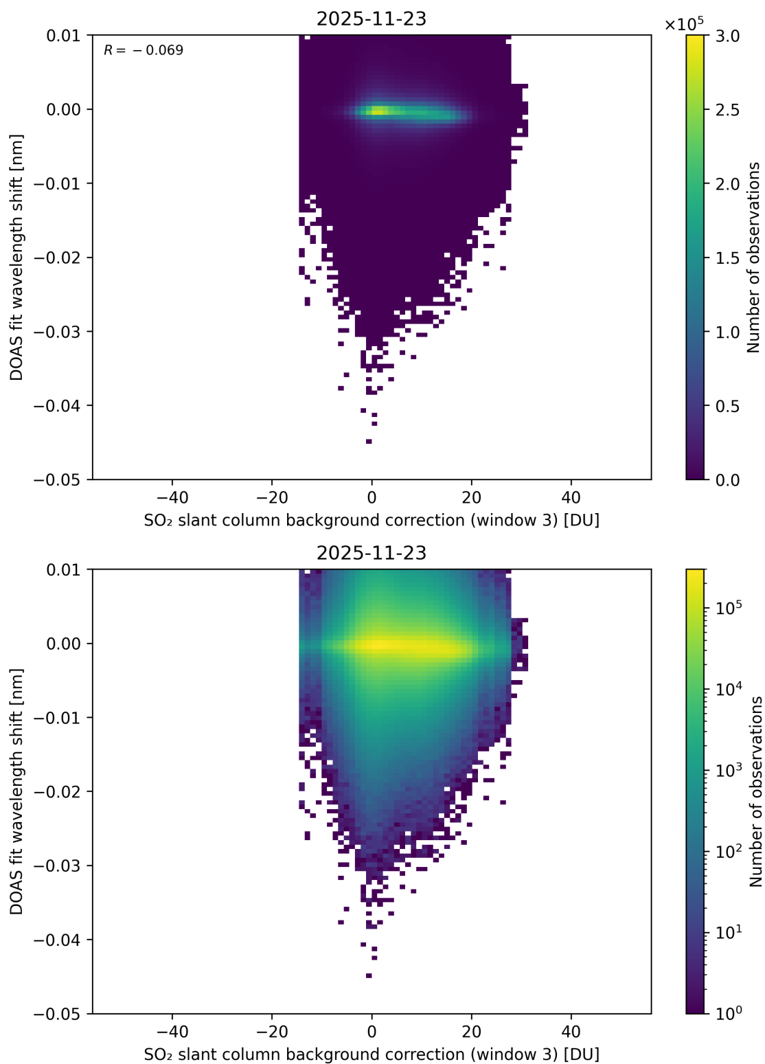
Figure 132: Scatter density plot of “SO 2 slant column background correction (window 3)” against “DOAS fit wavelength shift” for 2025-11-23 to 2025-11-24.
