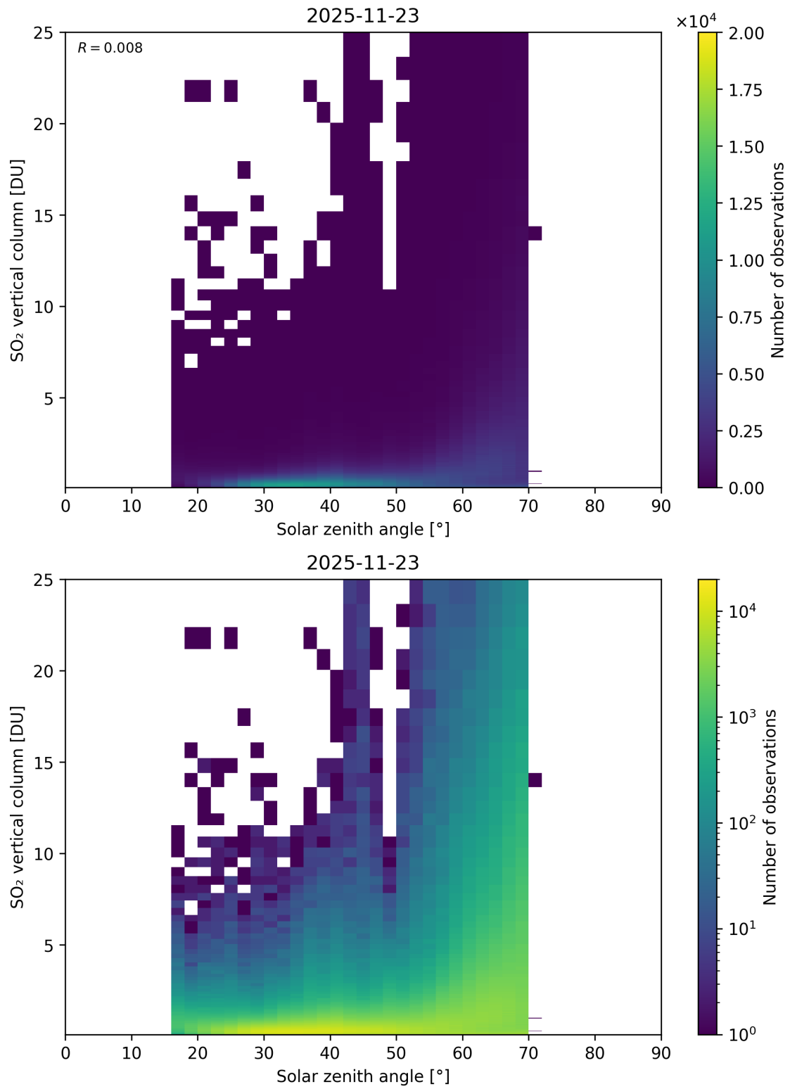
Figure 191: Scatter density plot of “Solar zenith angle” against “SO 2 vertical column” for 2025-11-23 to 2025-11-24.
