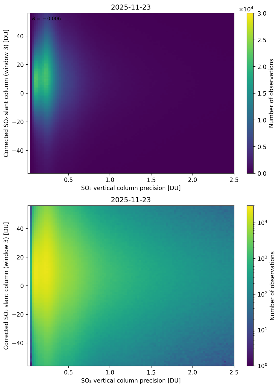
Figure 340: Scatter density plot of “SO 2 vertical column precision” against “Corrected SO 2 slant column (window 3)” for 2025-11-23 to 2025-11-24.
