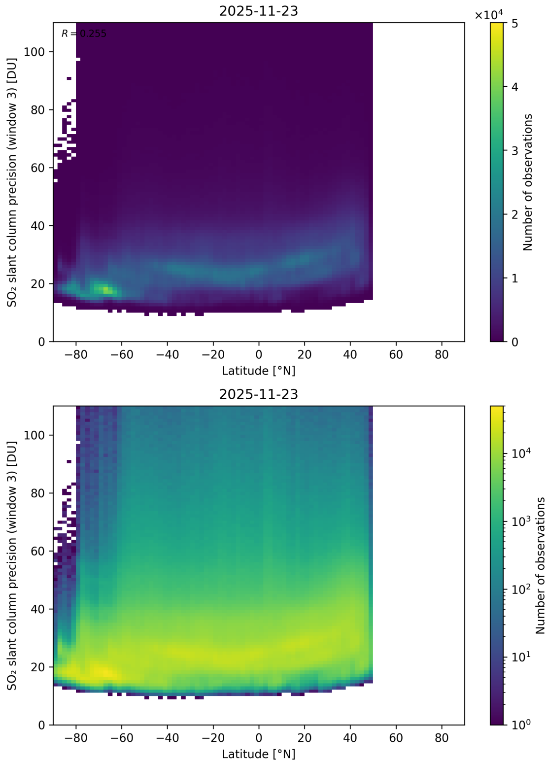
Figure 166: Scatter density plot of “Latitude” against “SO 2 slant column precision (window 3)” for 2025-11-23 to 2025-11-24.
