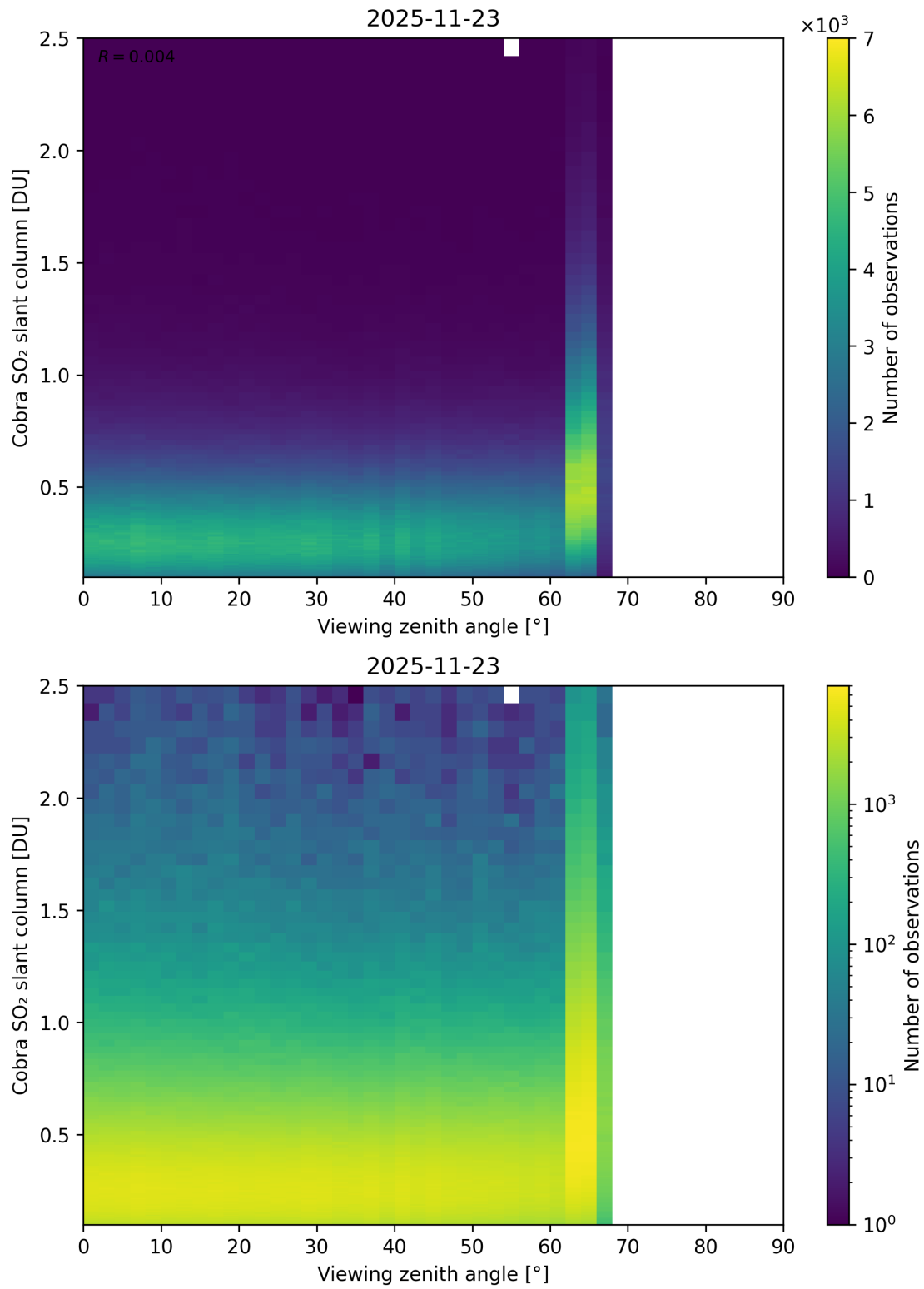
Figure 371: Scatter density plot of “Viewing zenith angle” against “Cobra SO 2 slant column” for 2025-11-23 to 2025-11-24.
