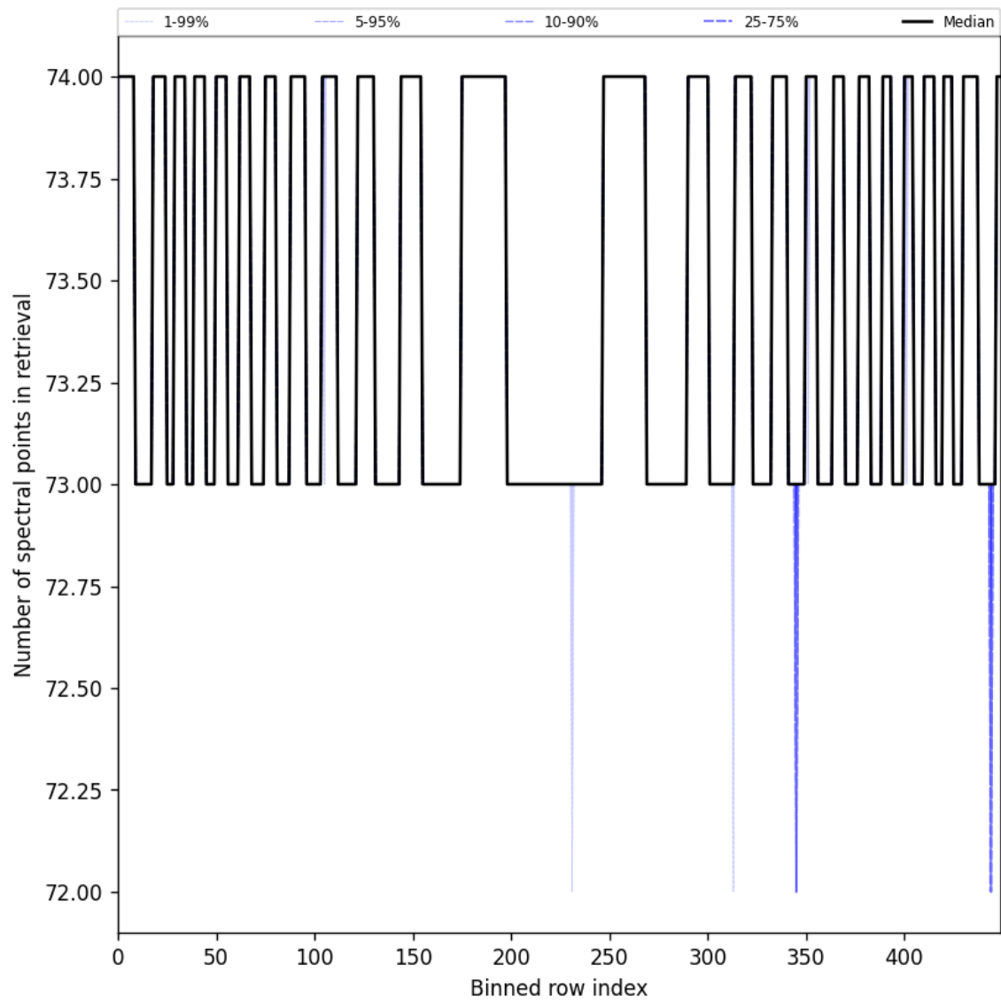
Figure 108: Along track statistics of “Number of spectral points in retrieval” for 2025-11-23 to 2025-11-24
