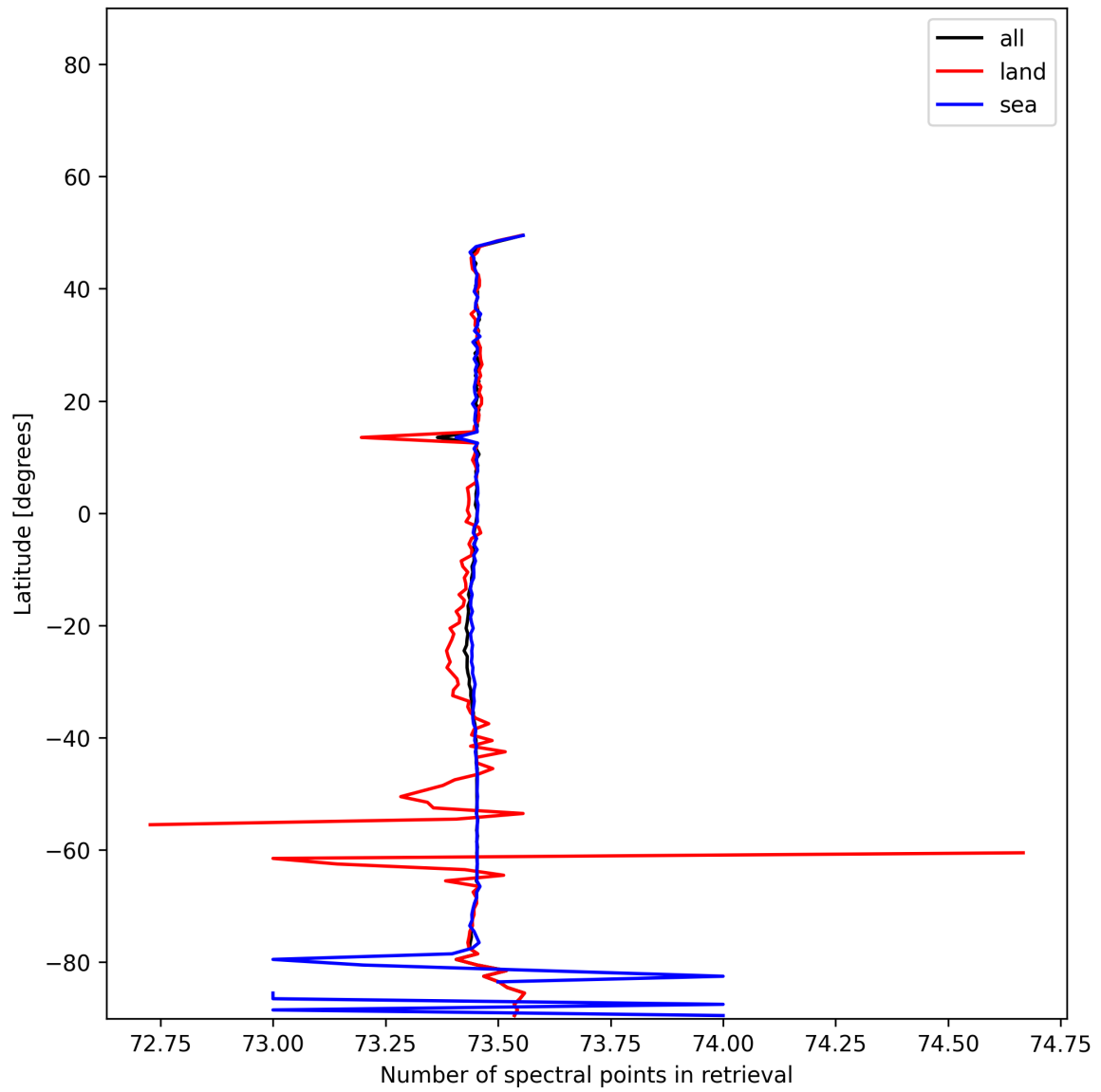
Figure 56: Zonal average of “Number of spectral points in retrieval” for 2025-11-23 to 2025-11-24.
