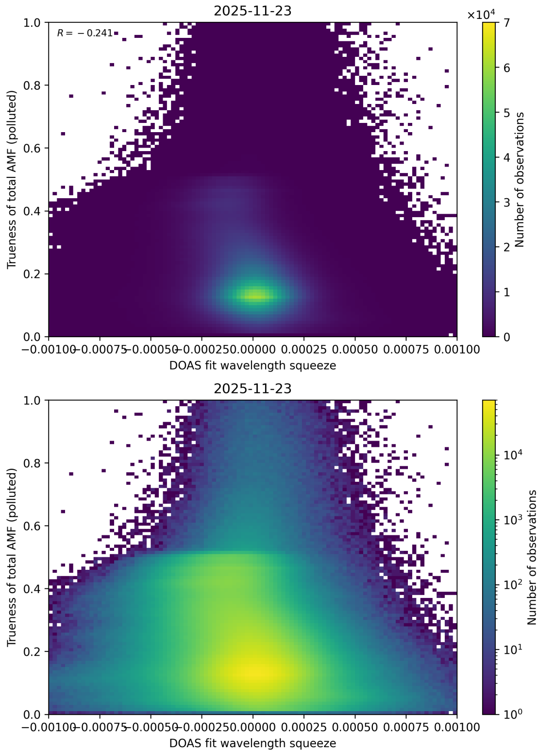
Figure 146: Scatter density plot of “DOAS fit wavelength squeeze” against “Trueness of total AMF (polluted)” for 2025-11-23 to 2025-11-24.
