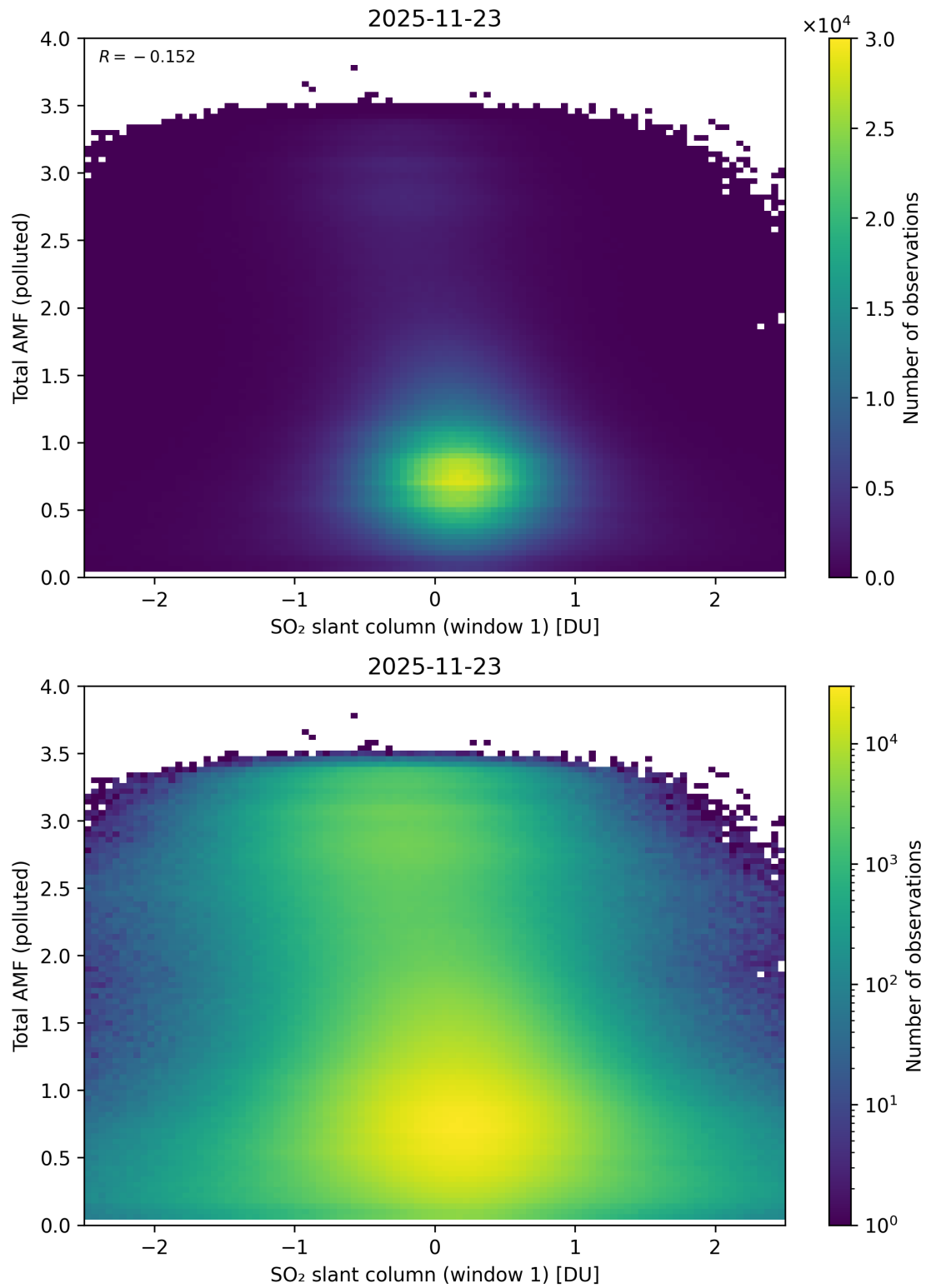
Figure 289: Scatter density plot of “SO 2 slant column (window 1)” against “Total AMF (polluted)” for 2025-11-23 to 2025-11-24.
