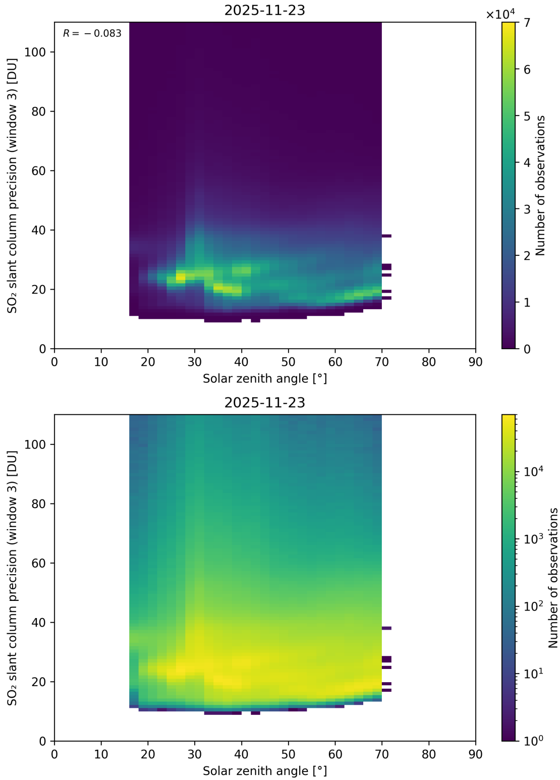
Figure 188: Scatter density plot of “Solar zenith angle” against “SO 2 slant column precision (window 3)” for 2025-11-23 to 2025-11-24.
