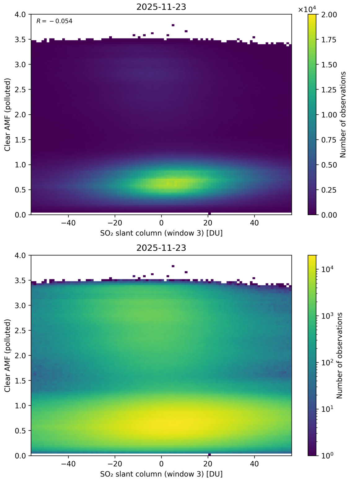
Figure 315: Scatter density plot of “SO 2 slant column (window 3)” against “Clear AMF (polluted)” for 2025-11-23 to 2025-11-24.
