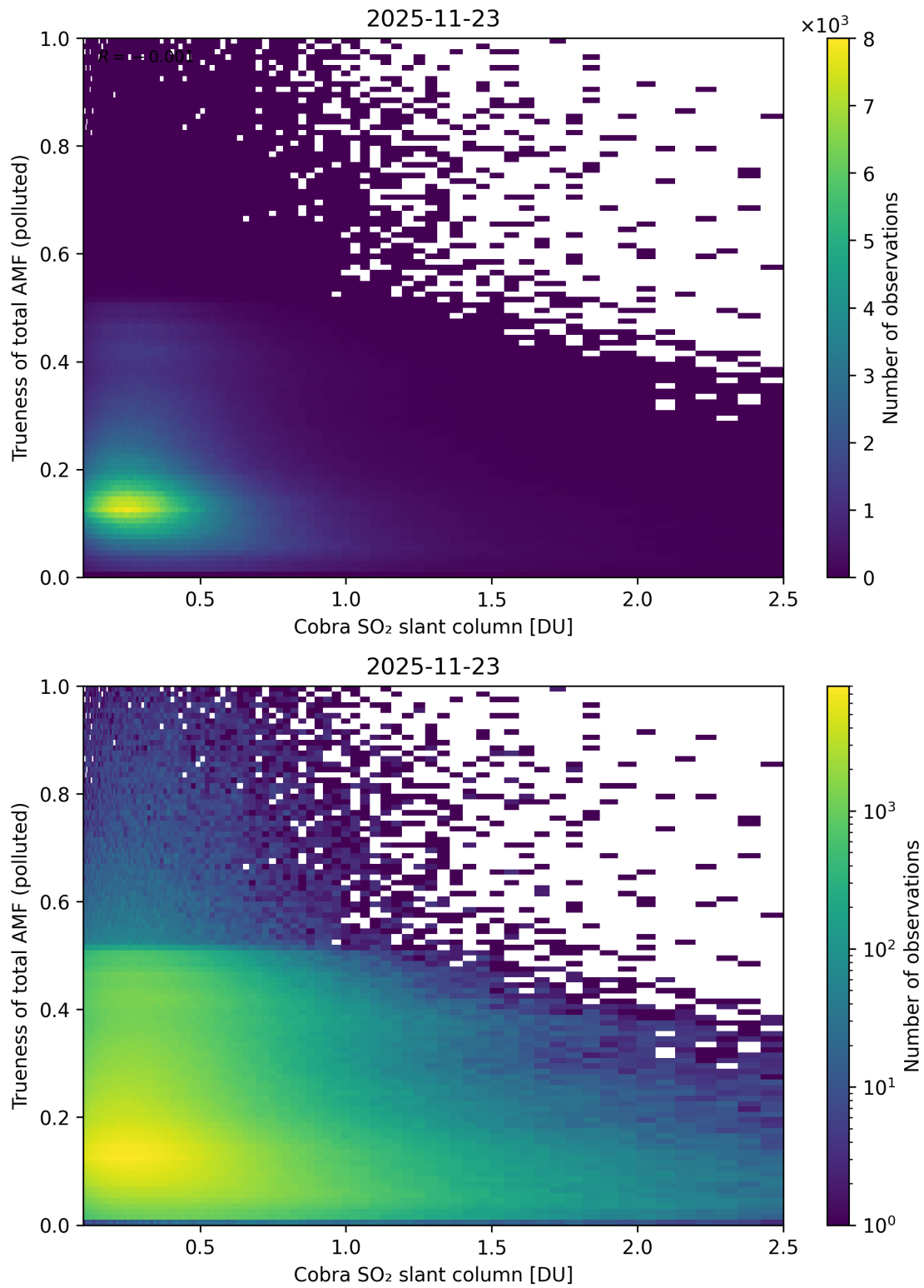
Figure 225: Scatter density plot of “Cobra SO 2 slant column” against “Trueness of total AMF (polluted)” for 2025-11-23 to 2025-11-24.
