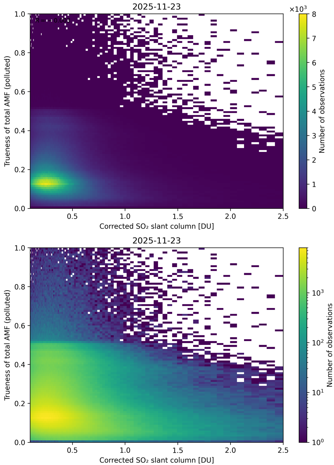
Figure 243: Scatter density plot of “Corrected SO 2 slant column” against “Trueness of total AMF (polluted)” for 2025-11-23 to 2025-11-24.
