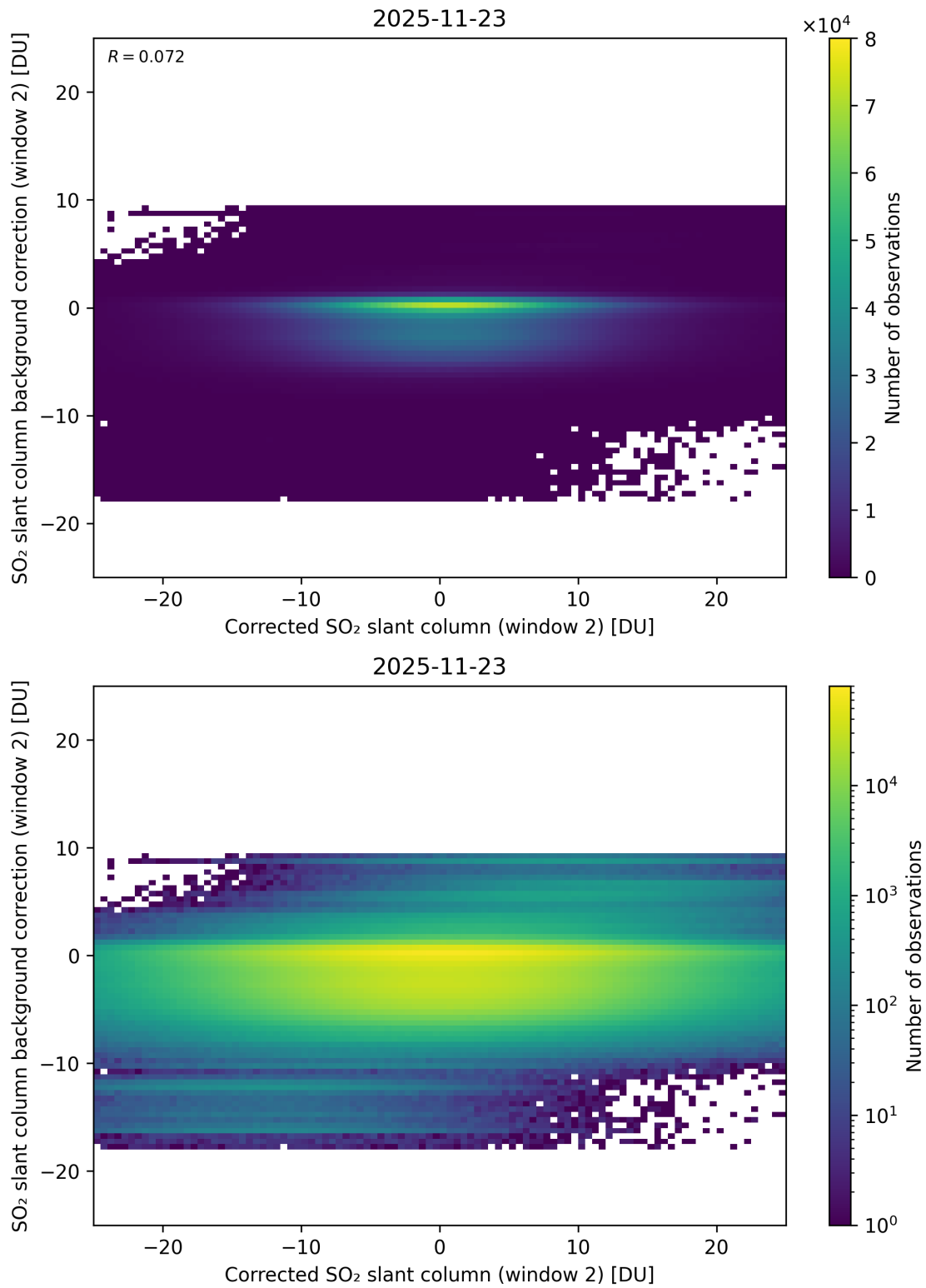
Figure 244: Scatter density plot of “Corrected SO 2 slant column (window 2)” against “SO 2 slant column background correction (window 2)” for 2025-11-23 to 2025-11-24.
