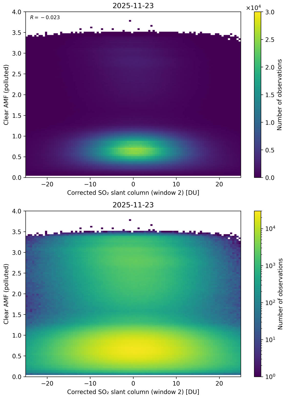
Figure 249: Scatter density plot of “Corrected SO 2 slant column (window 2)” against “Clear AMF (polluted)” for 2025-11-23 to 2025-11-24.
