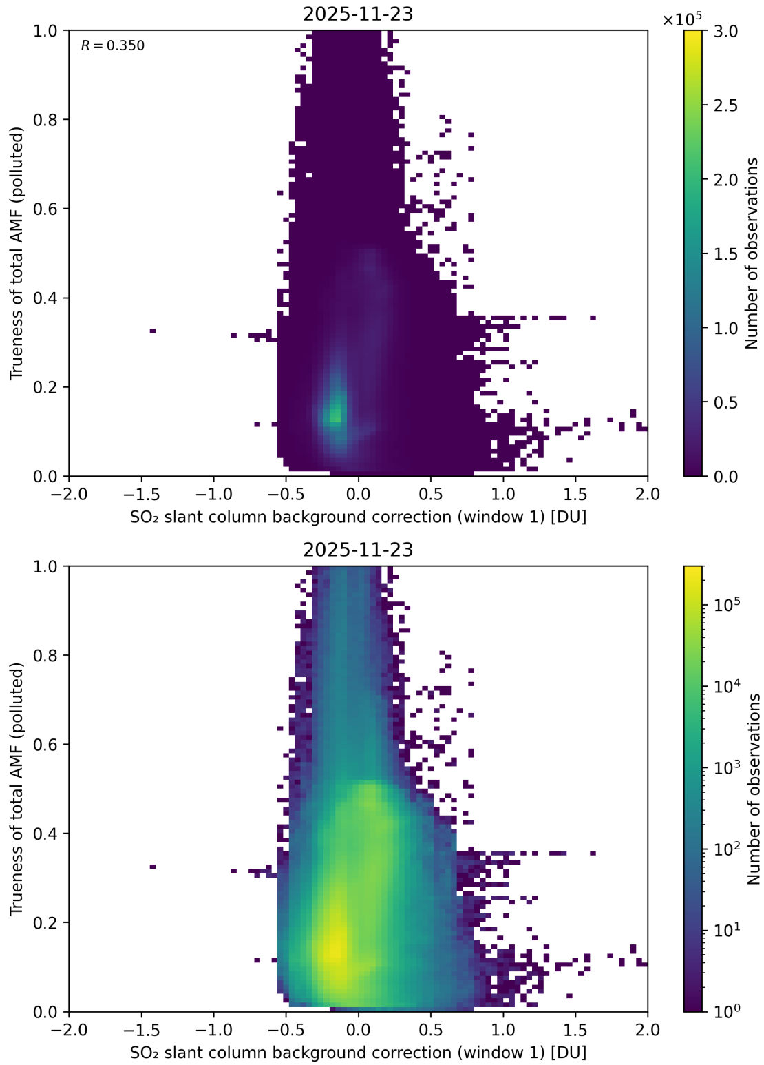
Figure 121: Scatter density plot of “SO 2 slant column background correction (window 1)” against “Trueness of total AMF (polluted)” for 2025-11-23 to 2025-11-24.
