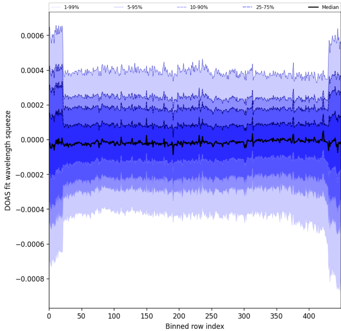
Figure 103: Along track statistics of “DOAS fit wavelength squeeze” for 2025-11-23 to 2025-11-24
