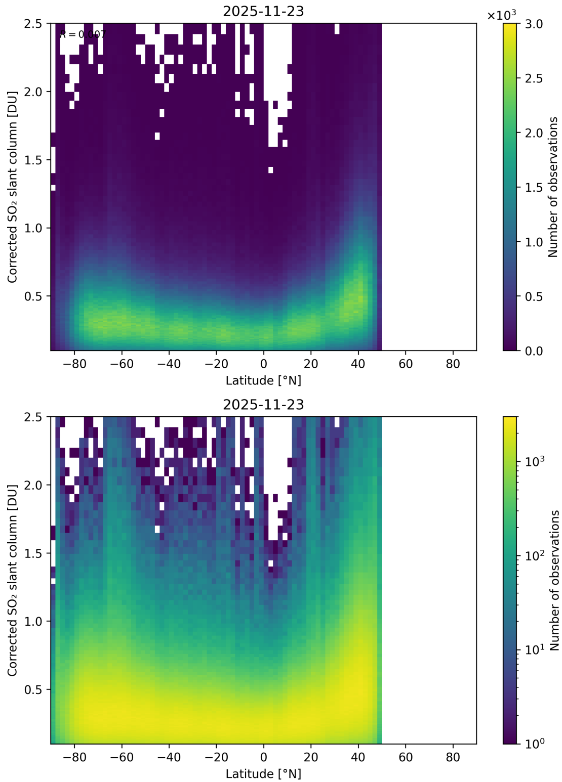
Figure 159: Scatter density plot of “Latitude” against “Corrected SO 2 slant column” for 2025-11-23 to 2025-11-24.
