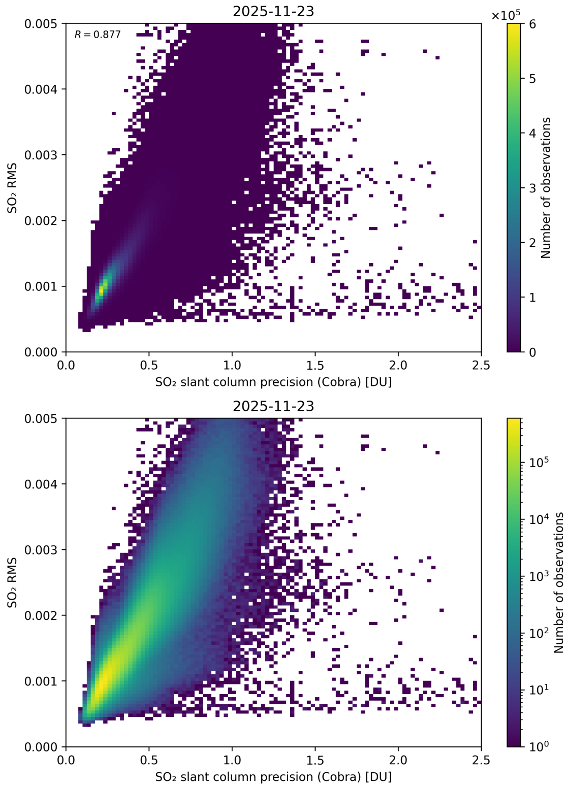
Figure 204: Scatter density plot of “SO 2 slant column precision (Cobra)” against “SO 2 RMS” for 2025-11-23 to 2025-11-24.
