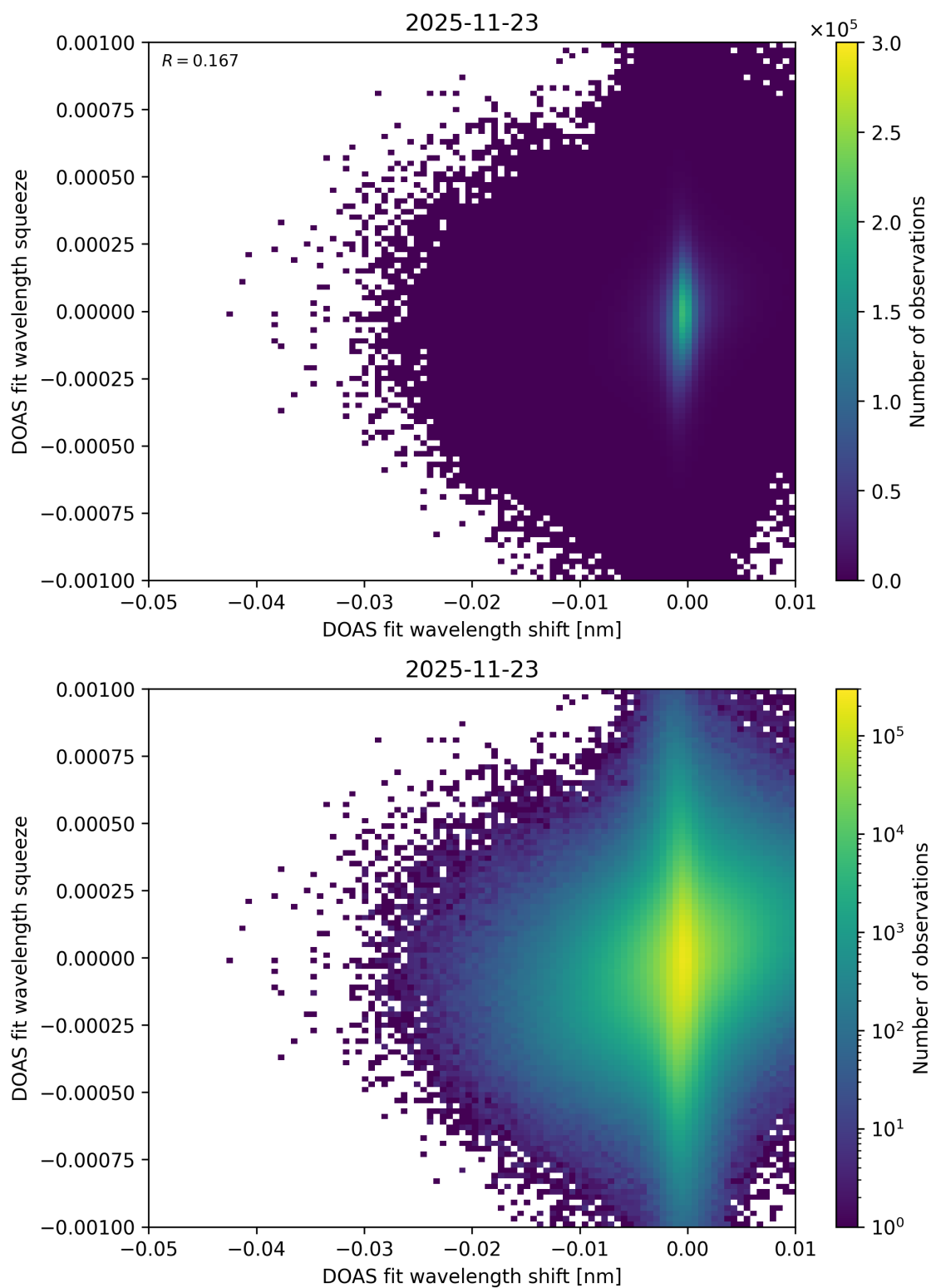
Figure 138: Scatter density plot of “DOAS fit wavelength shift” against “DOAS fit wavelength squeeze” for 2025-11-23 to 2025-11-24.
