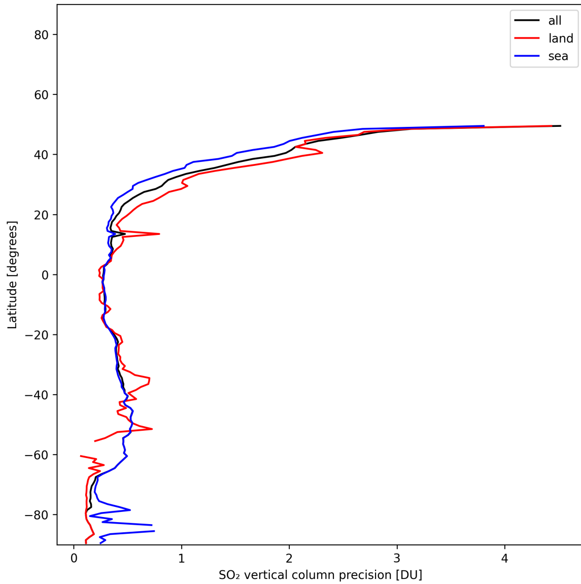
Figure 33: Zonal average of “SO 2 vertical column precision” for 2025-11-23 to 2025-11-24.
