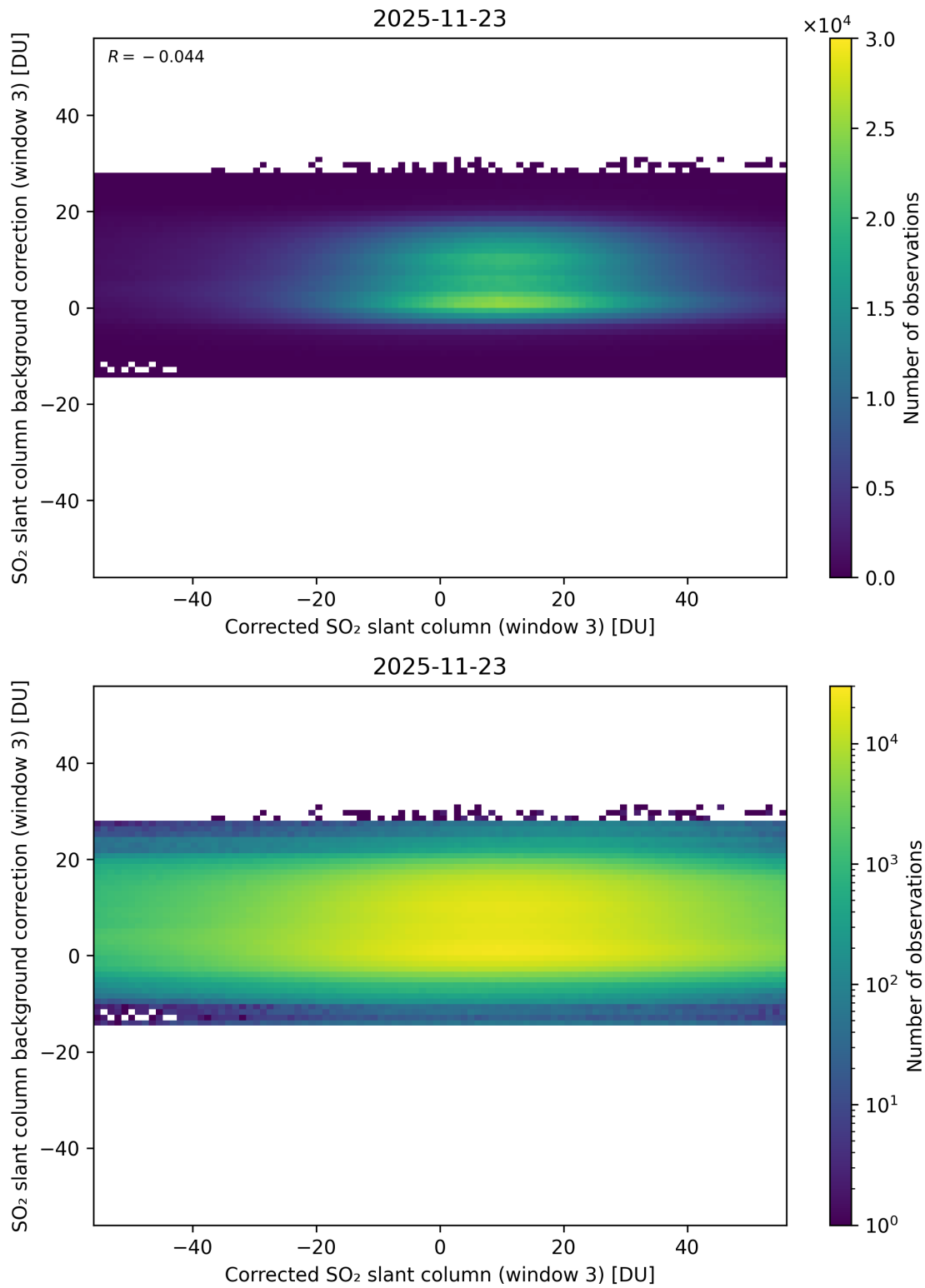
Figure 255: Scatter density plot of “Corrected SO 2 slant column (window 3)” against “SO 2 slant column background correction (window 3)” for 2025-11-23 to 2025-11-24.
