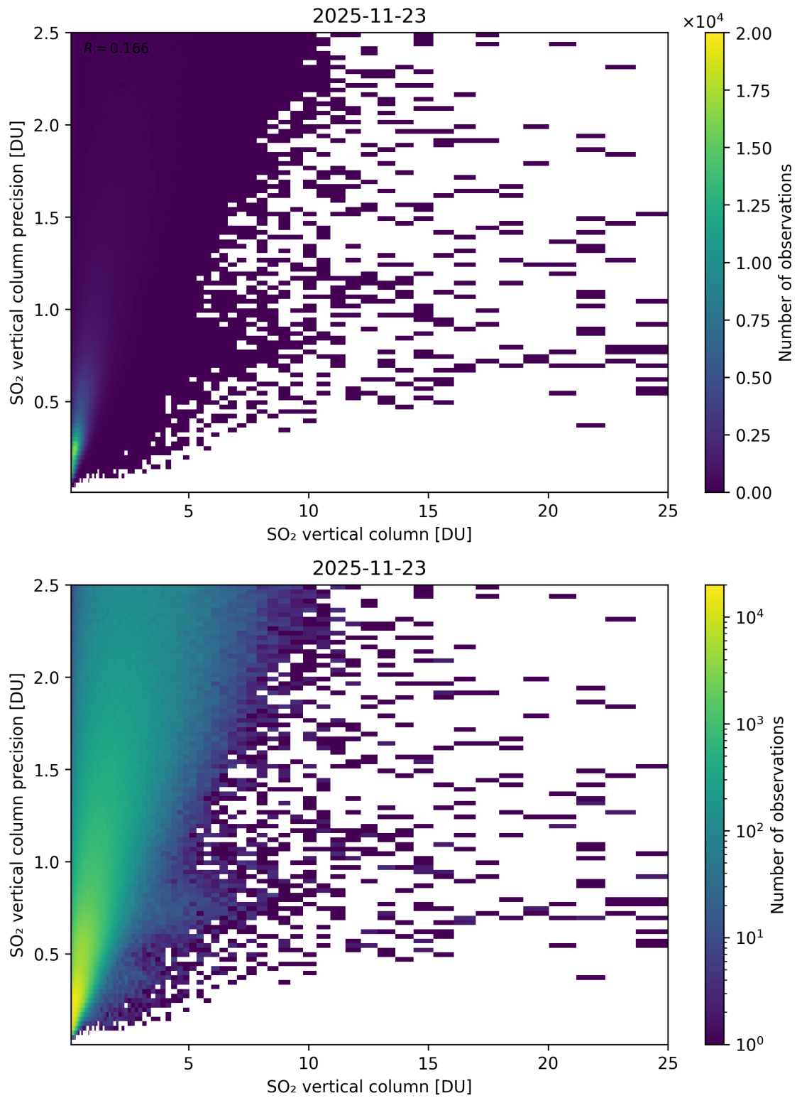
Figure 361: Scatter density plot of “SO 2 vertical column” against “SO 2 vertical column precision” for 2025-11-23 to 2025-11-24.
