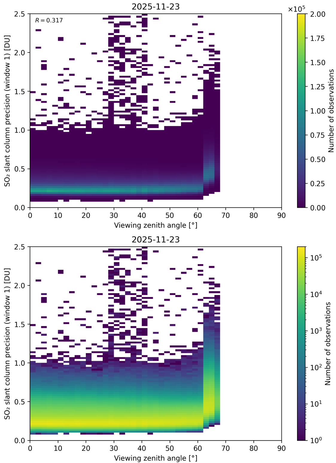
Figure 377: Scatter density plot of “Viewing zenith angle” against “SO 2 slant column precision (window 1)” for 2025-11-23 to 2025-11-24.
