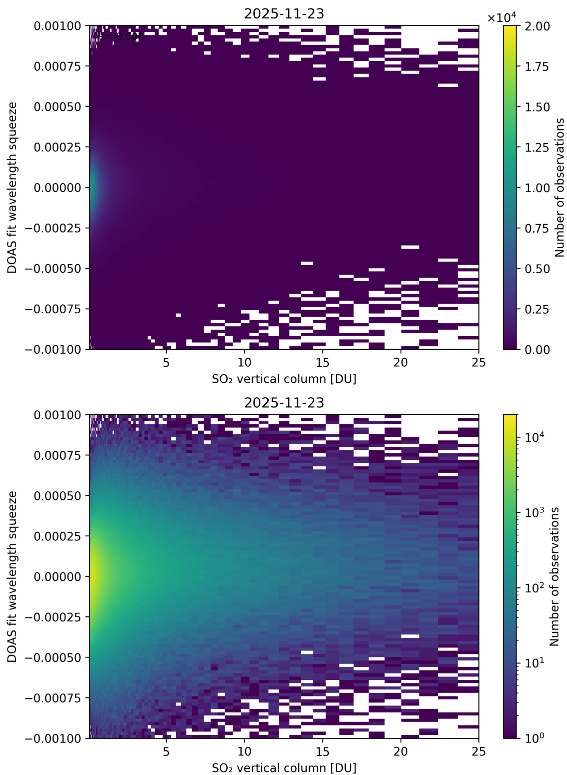
Figure 327: Scatter density plot of “SO 2 vertical column” against “DOAS fit wavelength squeeze” for 2025-11-23 to 2025-11-24.
