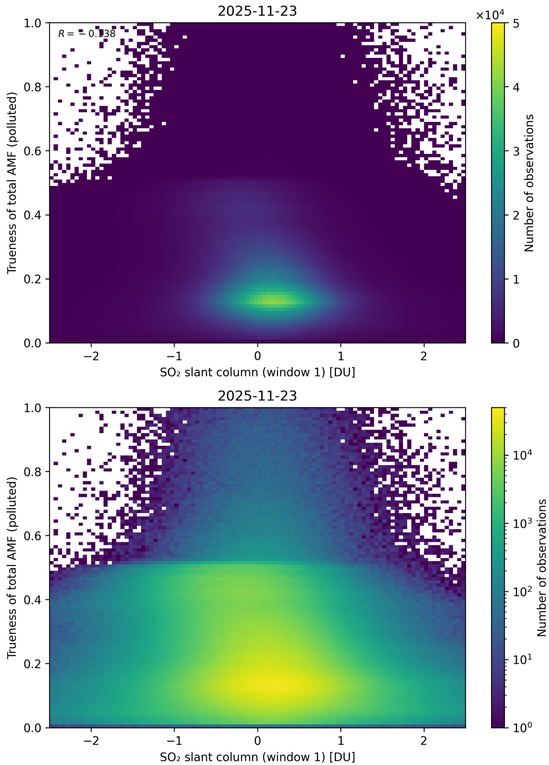
Figure 290: Scatter density plot of “SO 2 slant column (window 1)” against “Trueness of total AMF (polluted)” for 2025-11-23 to 2025-11-24.
