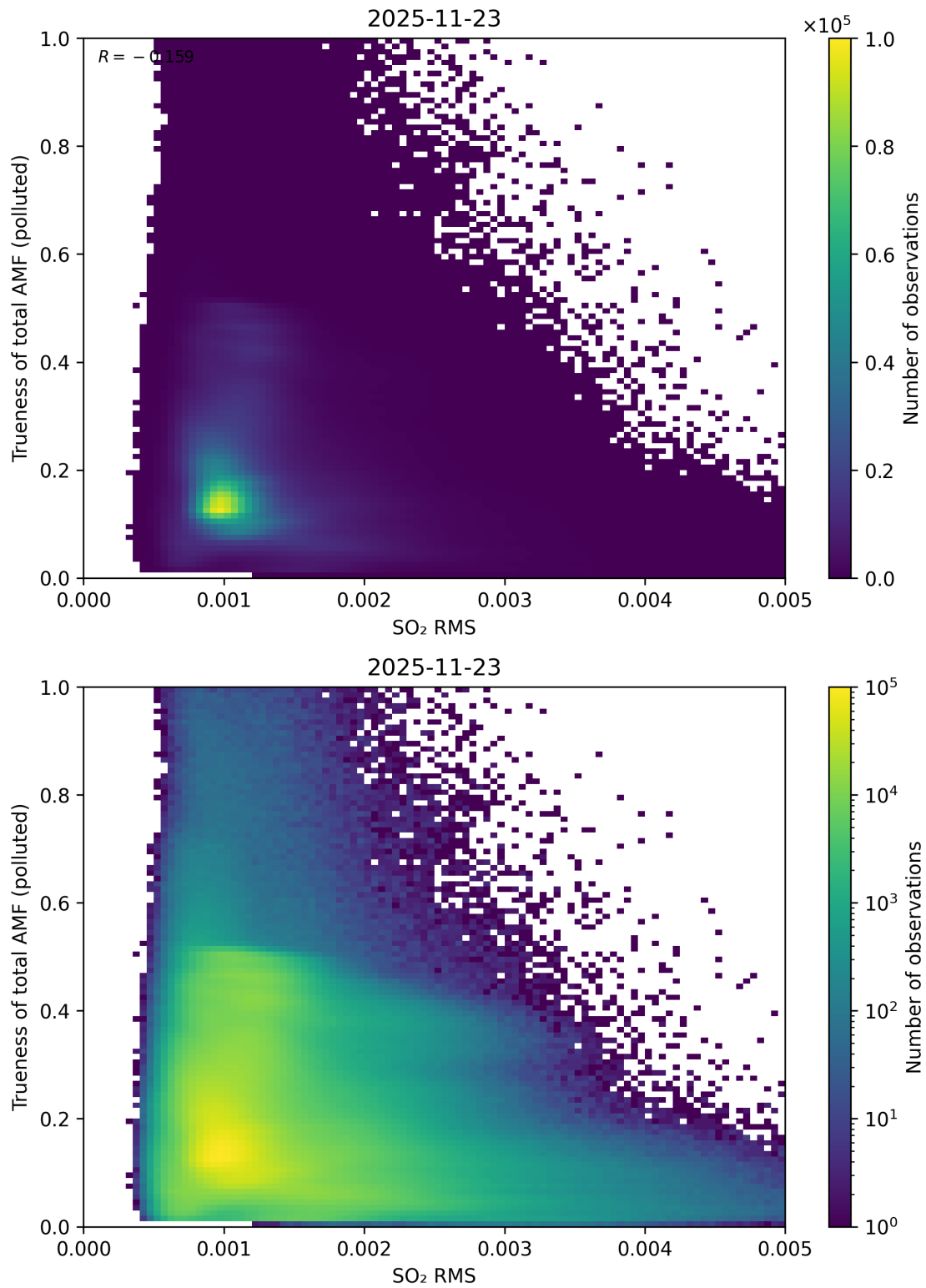
Figure 149: Scatter density plot of “SO 2 RMS” against “Trueness of total AMF (polluted)” for 2025-11-23 to 2025-11-24.
