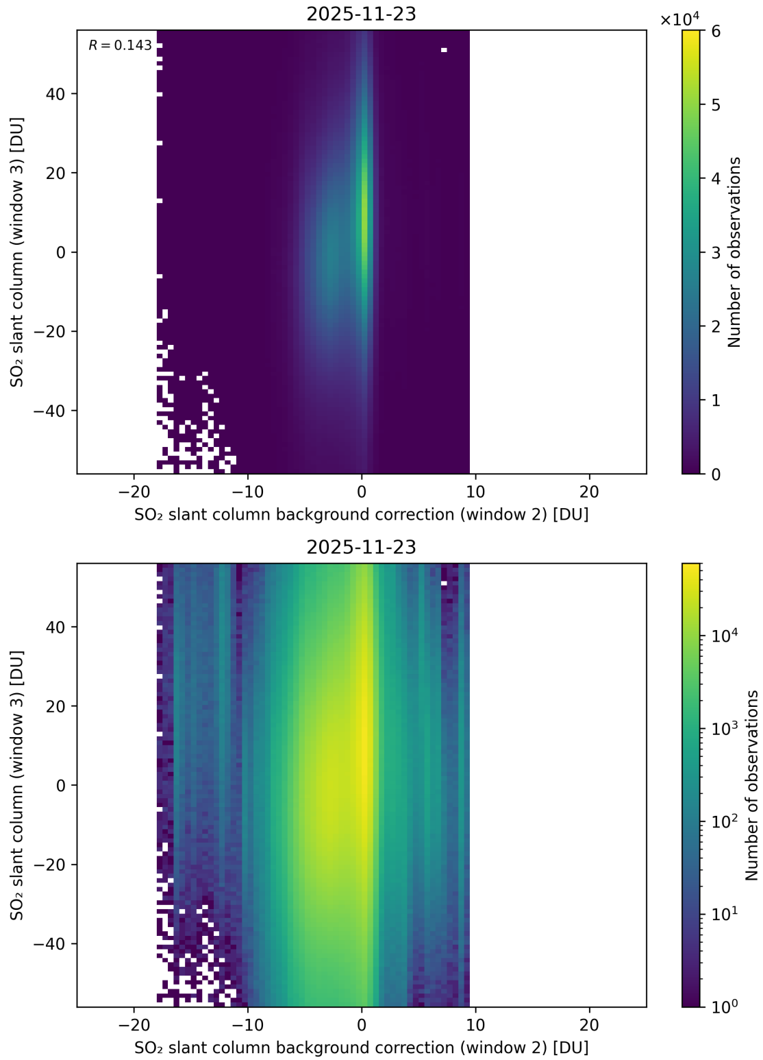
Figure 128: Scatter density plot of “SO 2 slant column background correction (window 2)” against “SO 2 slant column (window 3)” for 2025-11-23 to 2025-11-24.
