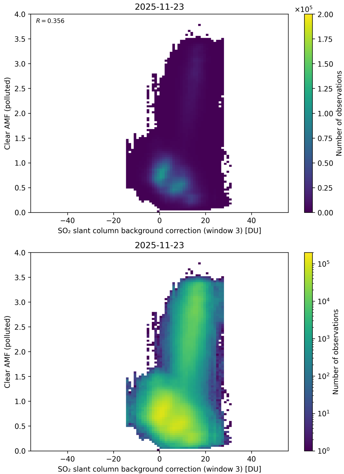
Figure 135: Scatter density plot of “SO 2 slant column background correction (window 3)” against “Clear AMF (polluted)” for 2025-11-23 to 2025-11-24.
