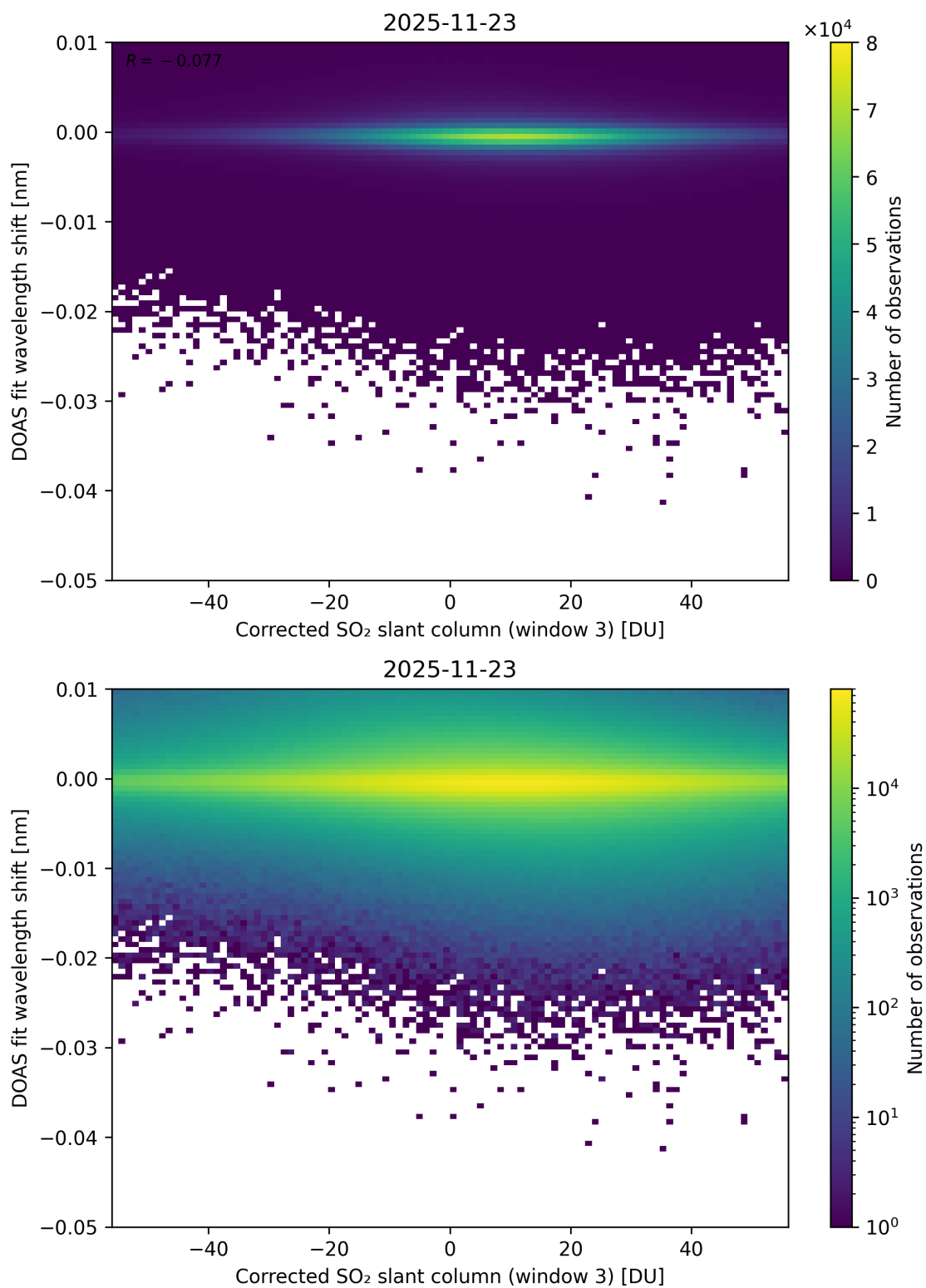
Figure 256: Scatter density plot of “Corrected SO 2 slant column (window 3)” against “DOAS fit wavelength shift” for 2025-11-23 to 2025-11-24.
