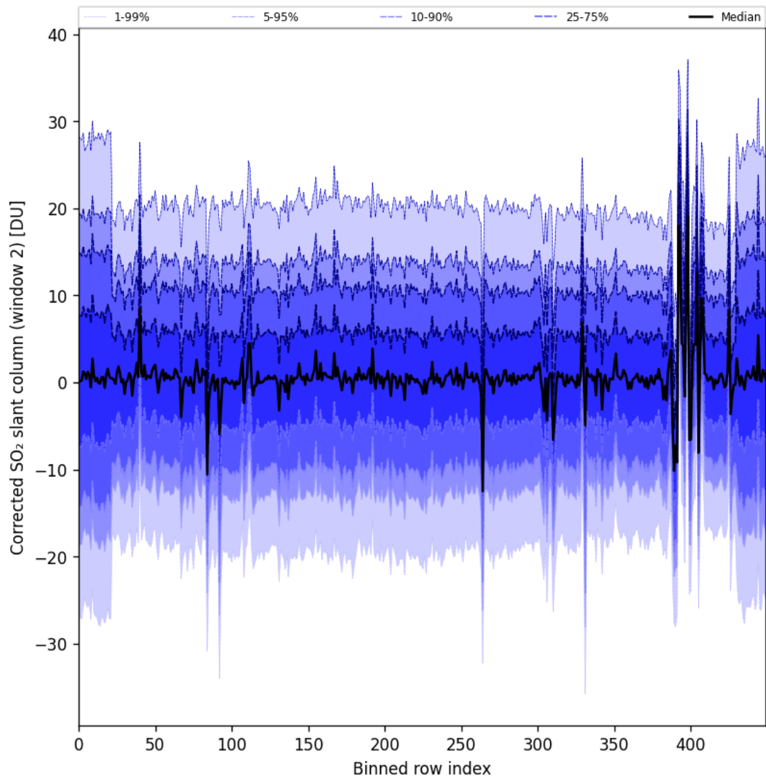
Figure 95: Along track statistics of “Corrected SO 2 slant column (window 2)” for 2025-11-23 to 2025-11-24
