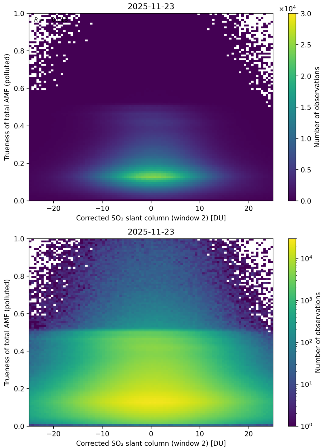
Figure 254: Scatter density plot of “Corrected SO 2 slant column (window 2)” against “Trueness of total AMF (polluted)” for 2025-11-23 to 2025-11-24.
