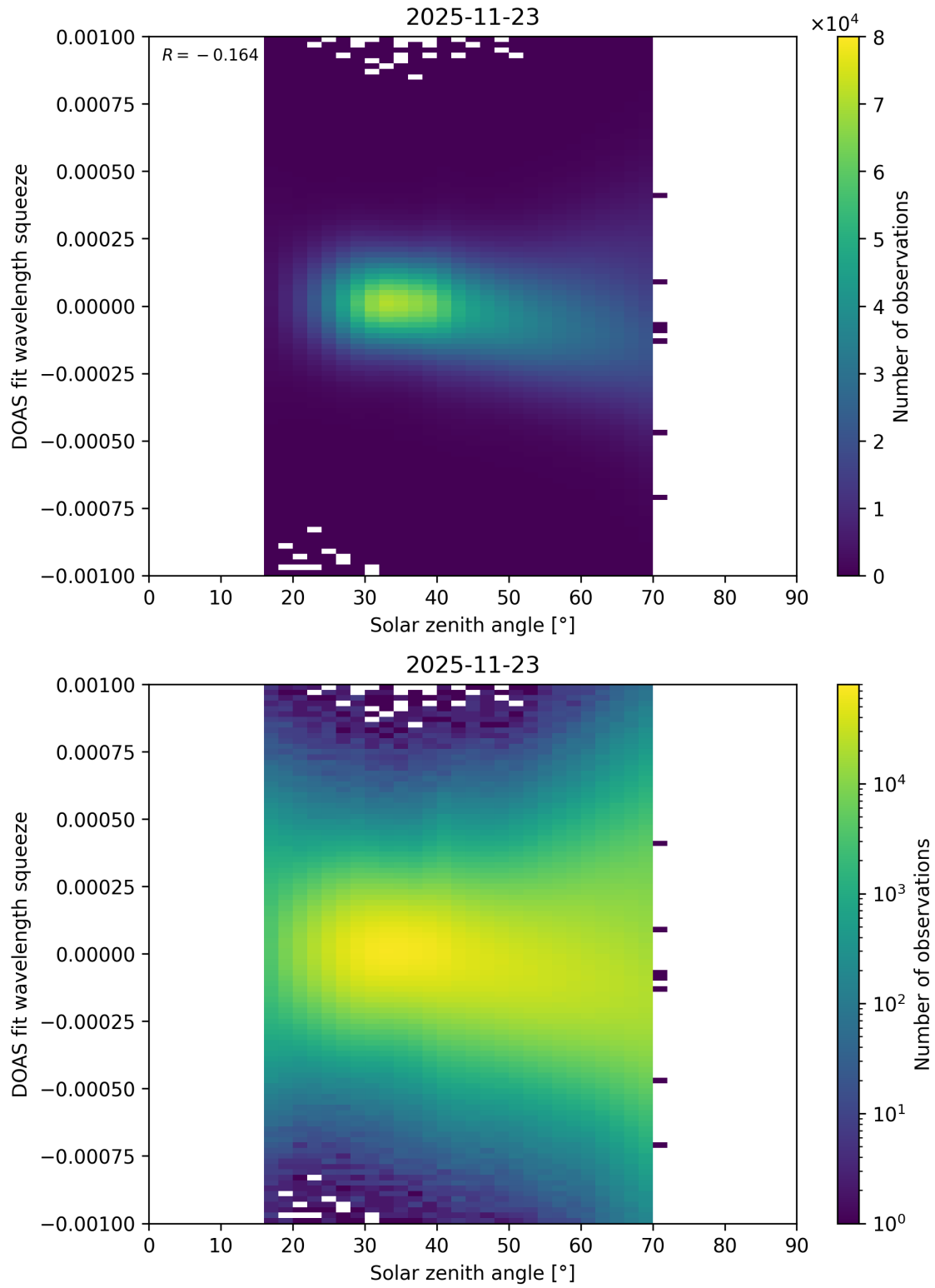
Figure 175: Scatter density plot of “Solar zenith angle” against “DOAS fit wavelength squeeze” for 2025-11-23 to 2025-11-24.
