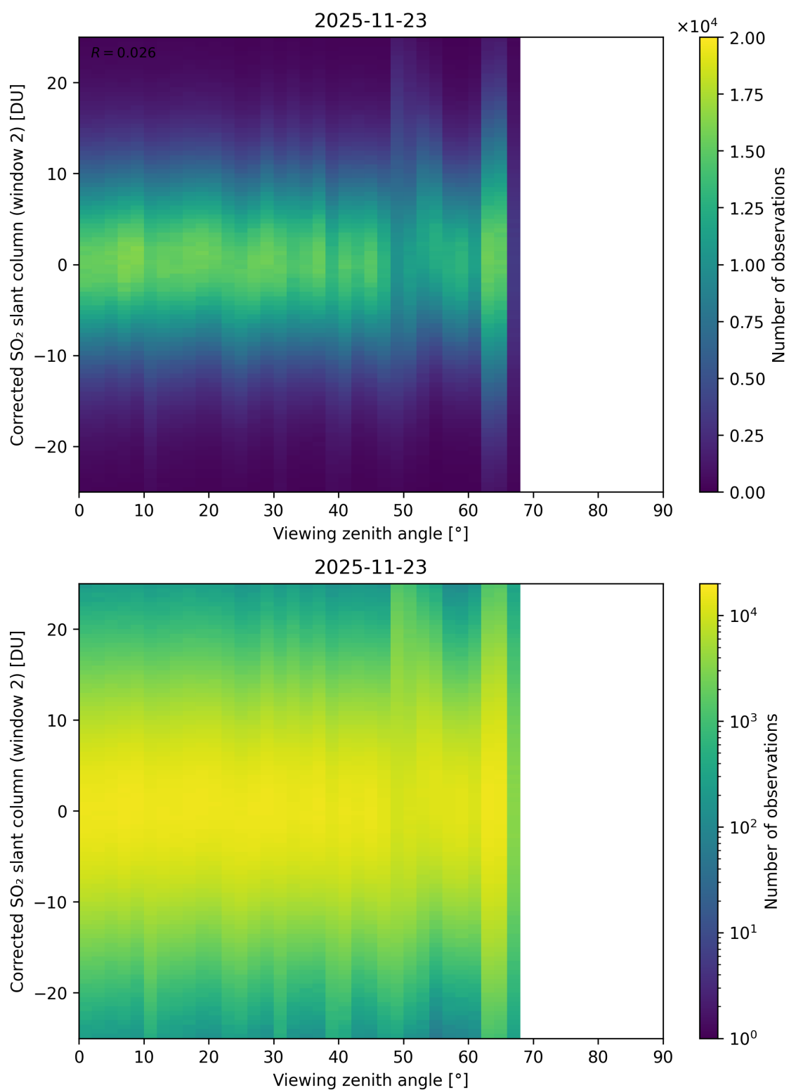
Figure 374: Scatter density plot of “Viewing zenith angle” against “Corrected SO 2 slant column (window 2)” for 2025-11-23 to 2025-11-24.
