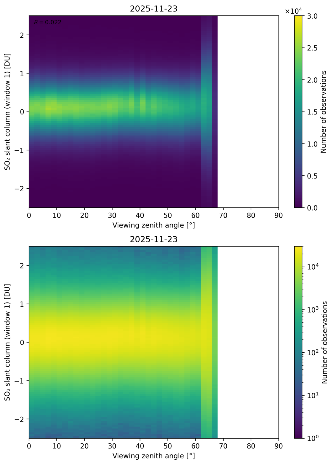
Figure 376: Scatter density plot of “Viewing zenith angle” against “SO 2 slant column (window 1)” for 2025-11-23 to 2025-11-24.
