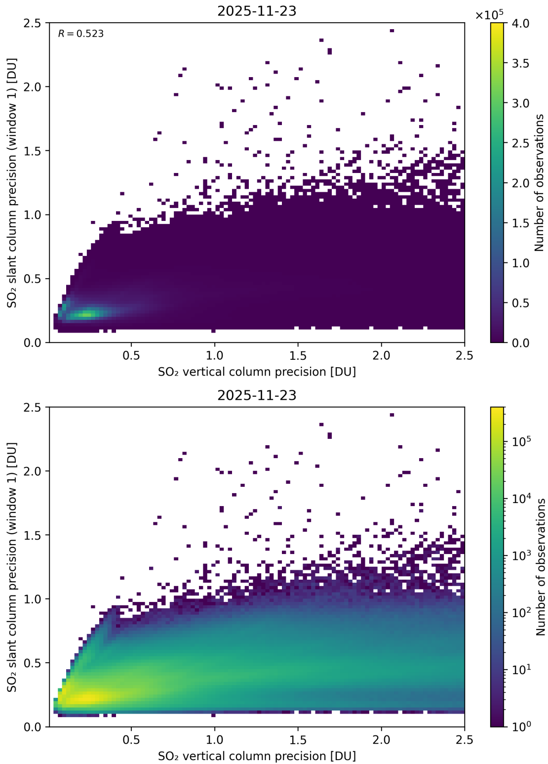
Figure 342: Scatter density plot of “SO 2 vertical column precision” against “SO 2 slant column precision (window 1)” for 2025-11-23 to 2025-11-24.
