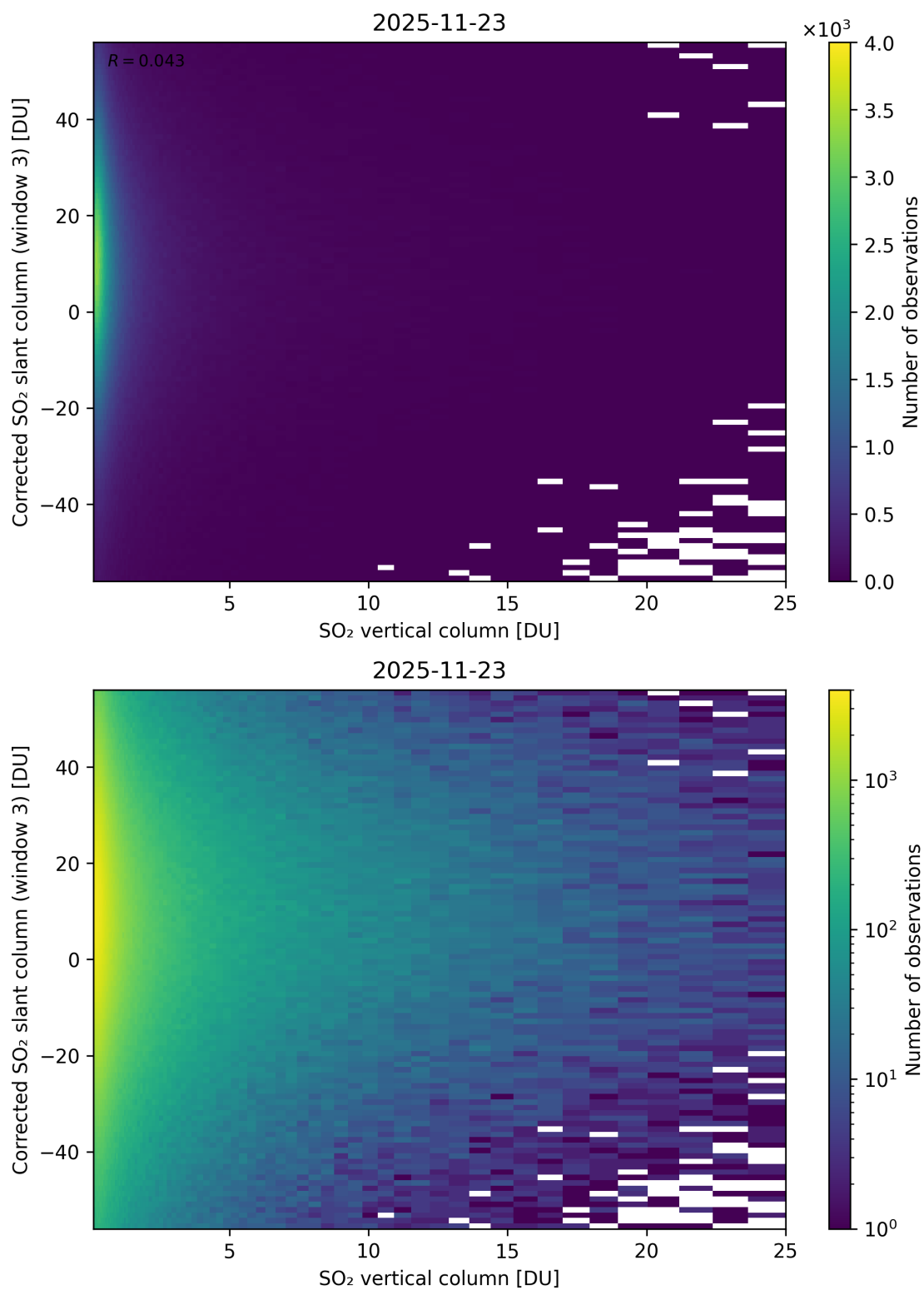
Figure 353: Scatter density plot of “SO 2 vertical column” against “Corrected SO 2 slant column (window 3)” for 2025-11-23 to 2025-11-24.
