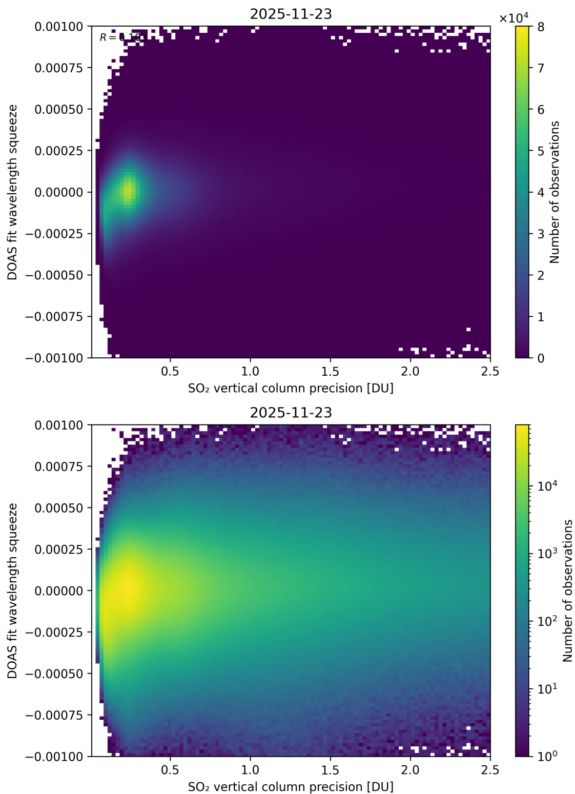
Figure 333: Scatter density plot of “SO 2 vertical column precision” against “DOAS fit wavelength squeeze” for 2025-11-23 to 2025-11-24.
