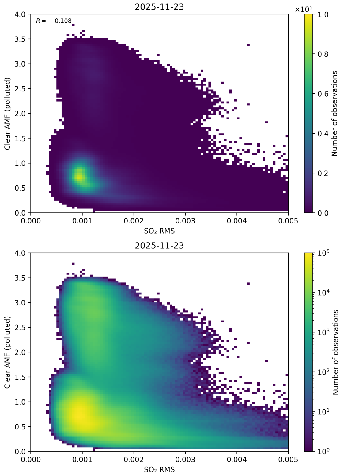
Figure 147: Scatter density plot of “SO 2 RMS” against “Clear AMF (polluted)” for 2025-11-23 to 2025-11-24.
