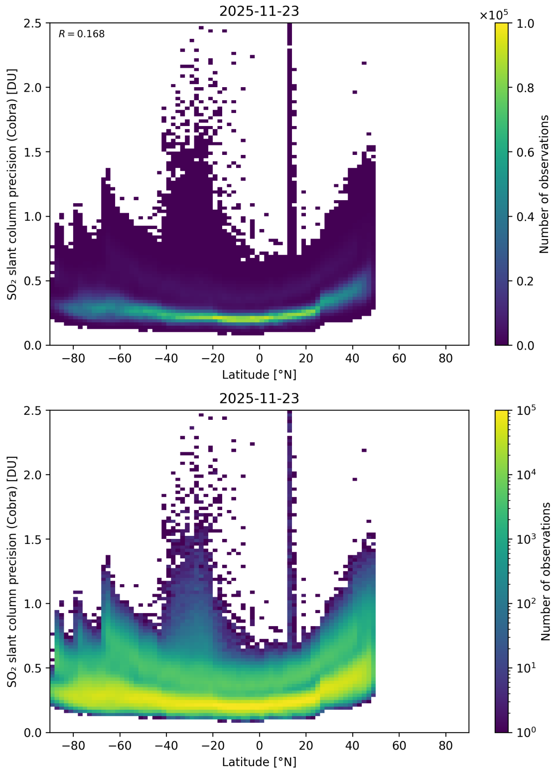
Figure 158: Scatter density plot of “Latitude” against “SO 2 slant column precision (Cobra)” for 2025-11-23 to 2025-11-24.
