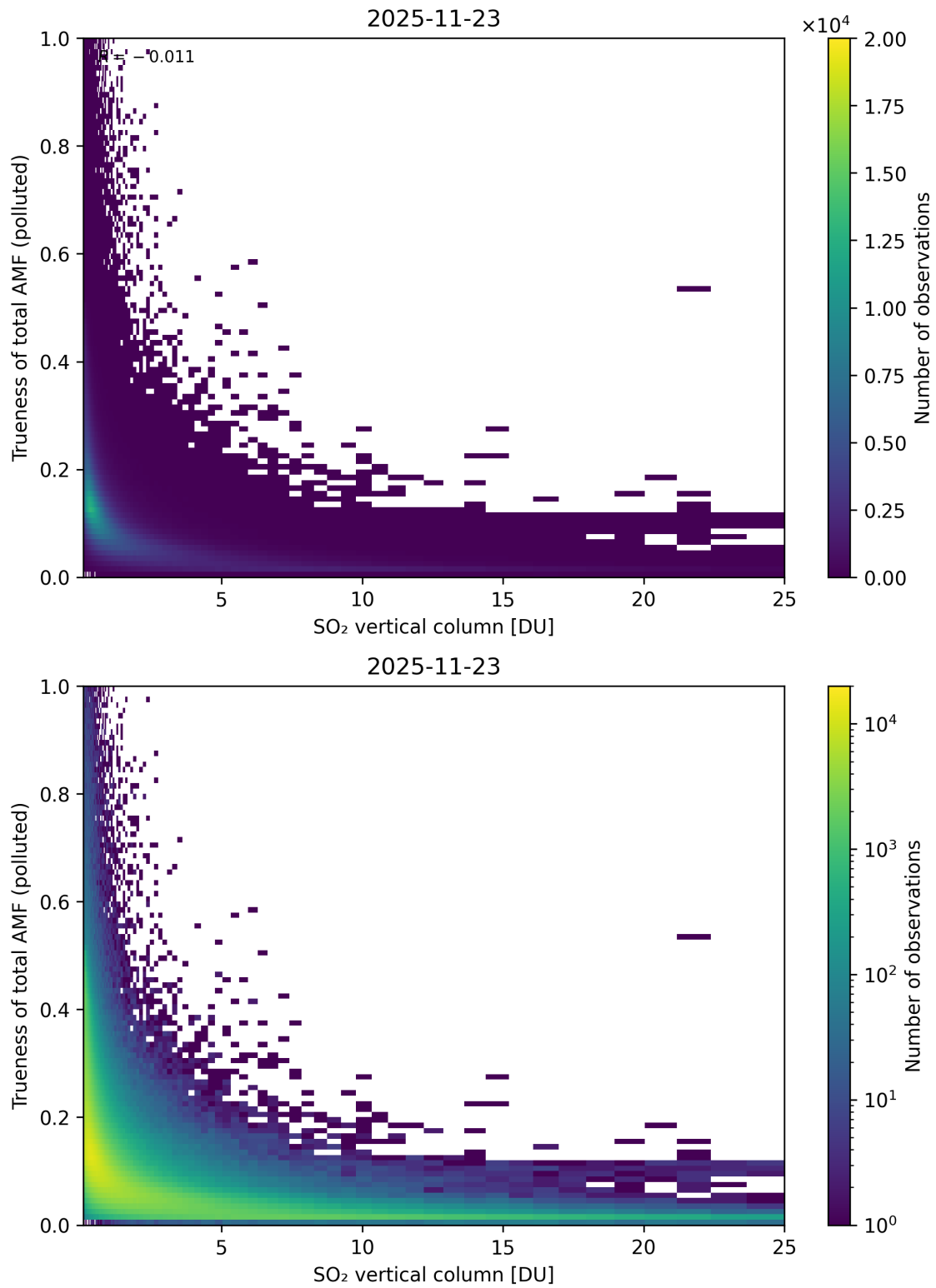
Figure 360: Scatter density plot of “SO 2 vertical column” against “Truthness of total AMF (polluted)” for 2025-11-23 to 2025-11-24.
