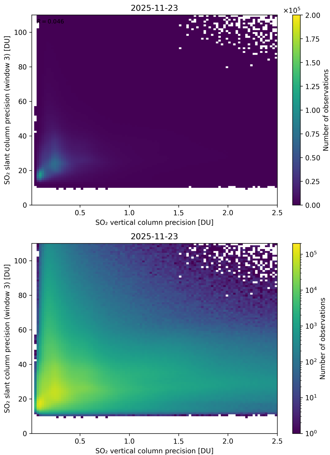
Figure 345: Scatter density plot of “SO 2 vertical column precision” against “SO 2 slant column precision (window 3)” for 2025-11-23 to 2025-11-24.
