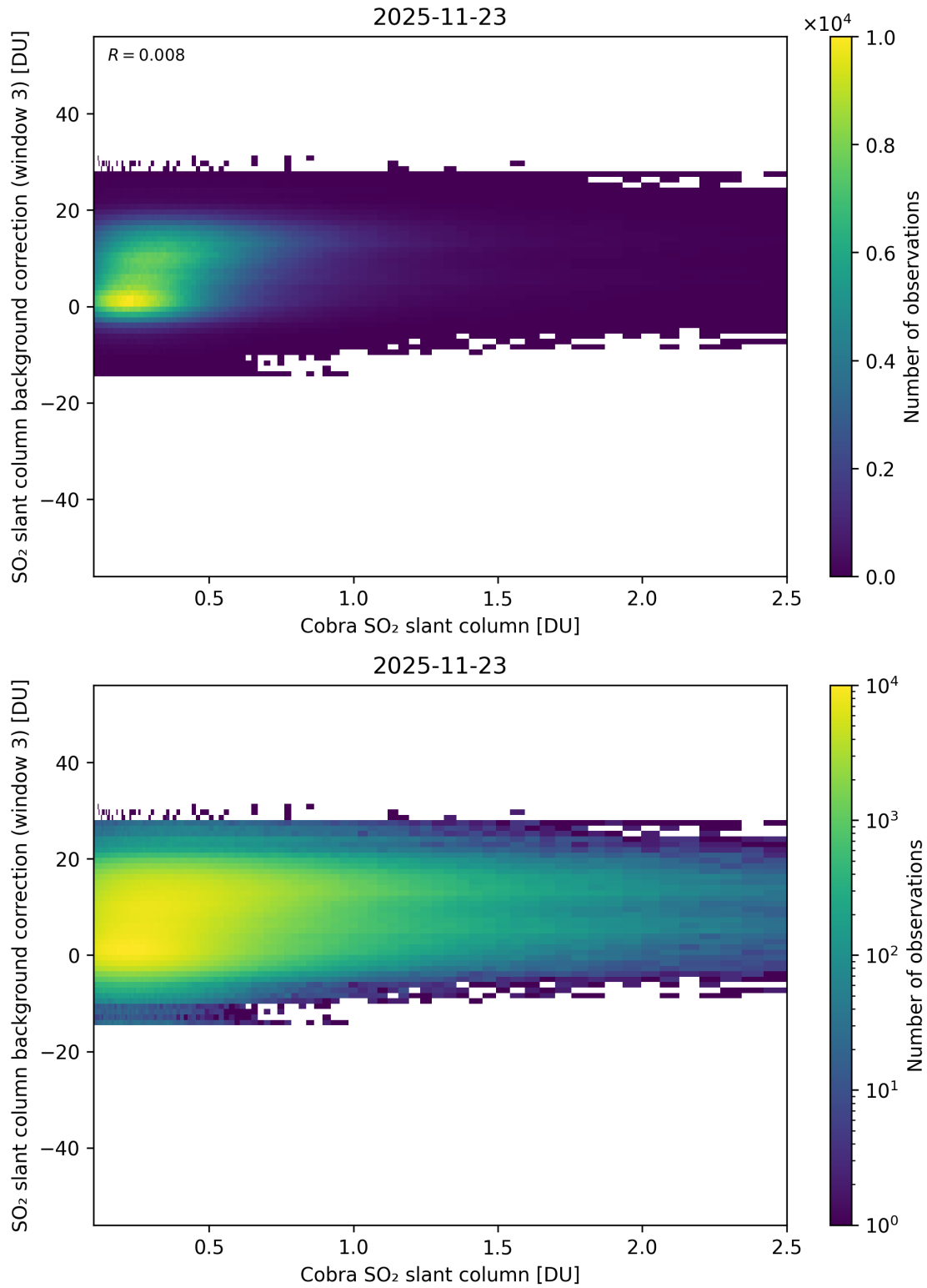
Figure 195: Scatter density plot of “Cobra SO 2 slant column” against “SO 2 slant column background correction (window 3)” for 2025-11-23 to 2025-11-24.
