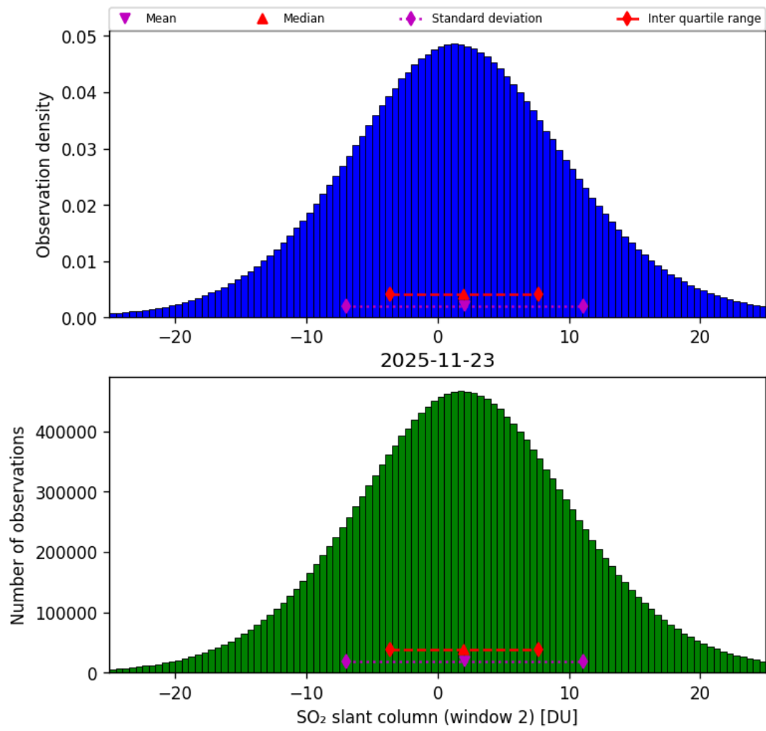
Figure 67: Histogram of “SO 2 slant column (window 2)” for 2025-11-23 to 2025-11-24
