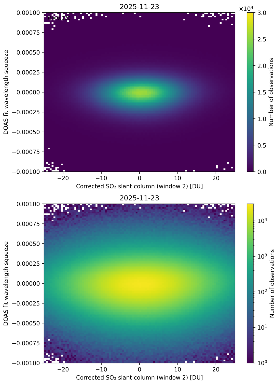
Figure 247: Scatter density plot of “Corrected SO 2 slant column (window 2)” against “DOAS fit wavelength squeeze” for 2025-11-23 to 2025-11-24.
