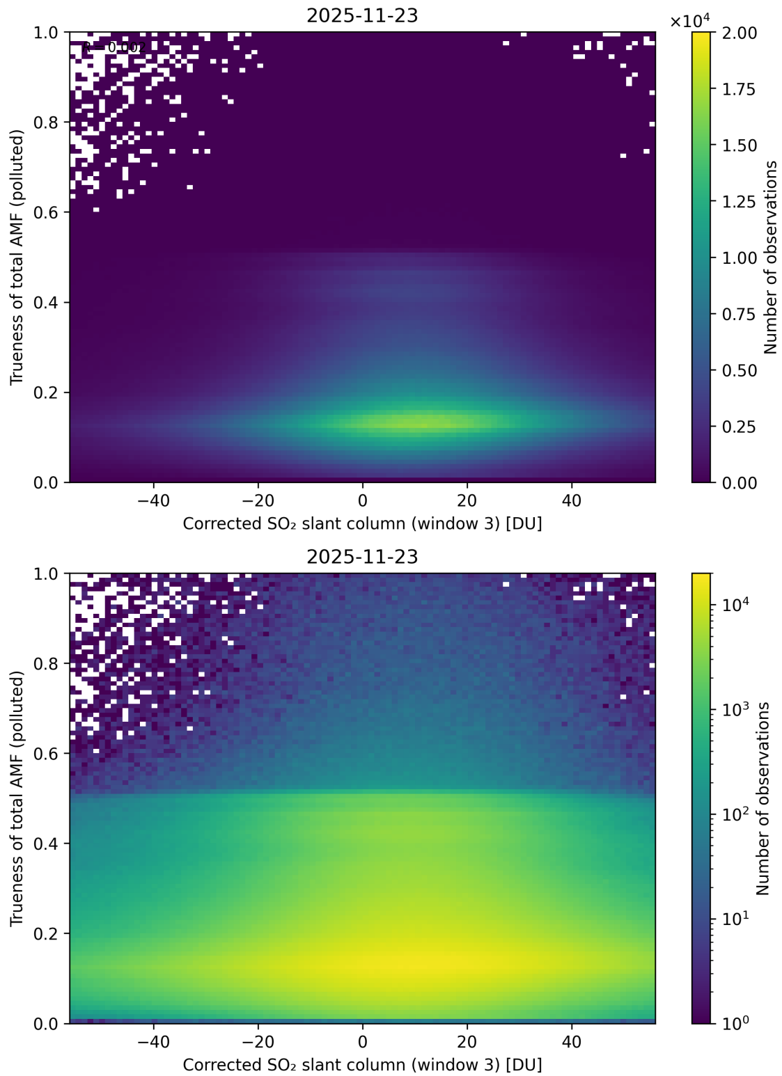
Figure 261: Scatter density plot of “Corrected SO 2 slant column (window 3)” against “Trueness of total AMF (polluted)” for 2025-11-23 to 2025-11-24.
