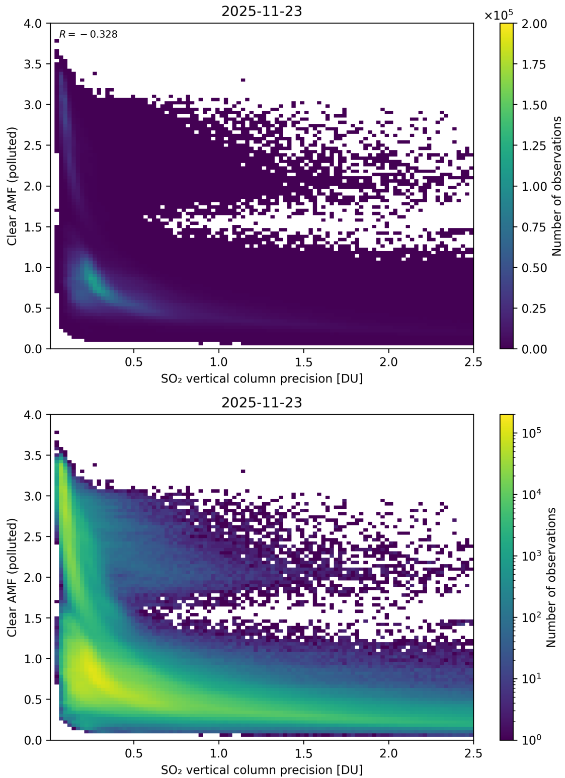
Figure 335: Scatter density plot of “SO 2 vertical column precision” against “Clear AMF (polluted)” for 2025-11-23 to 2025-11-24.
