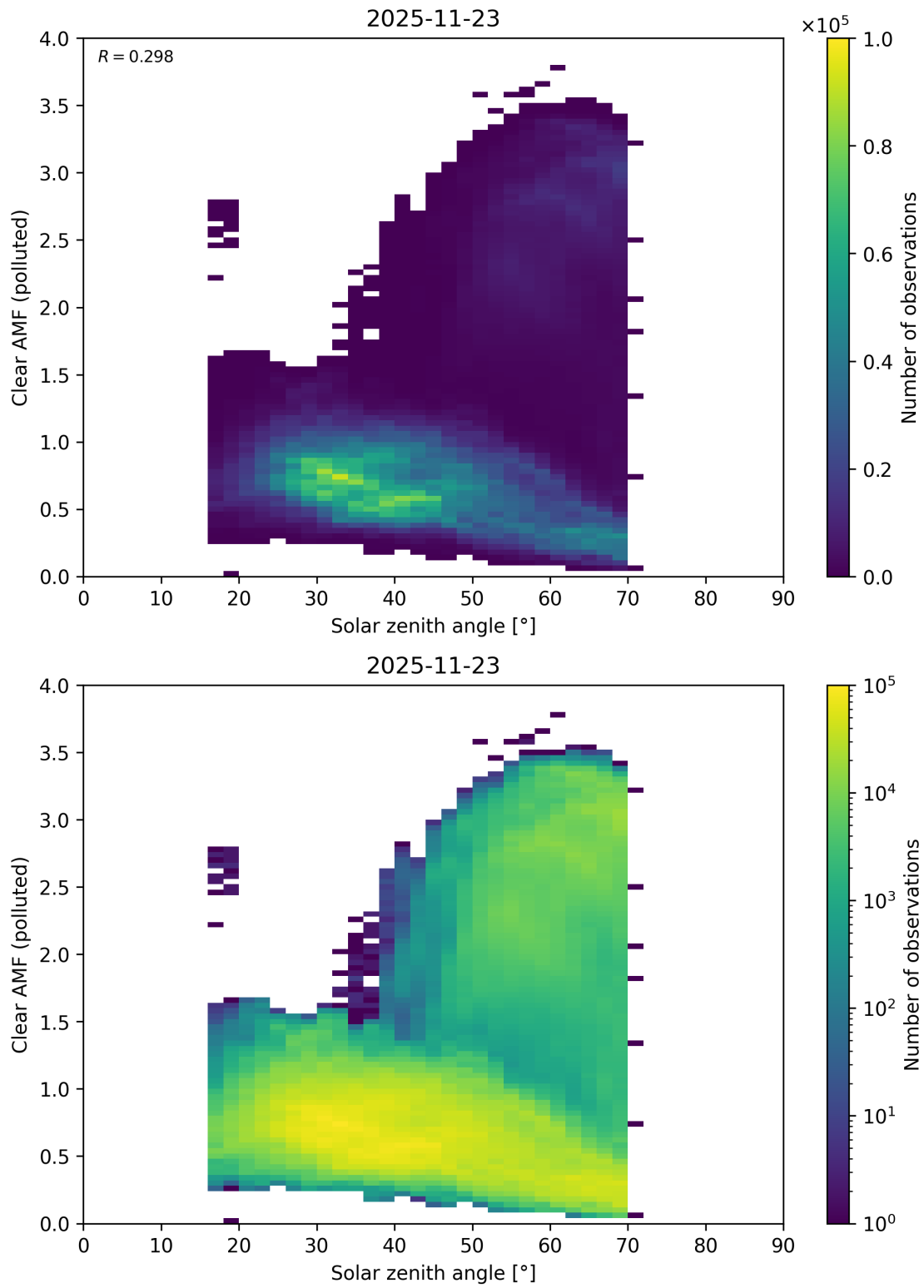
Figure 178: Scatter density plot of “Solar zenith angle” against “Clear AMF (polluted)” for 2025-11-23 to 2025-11-24.
