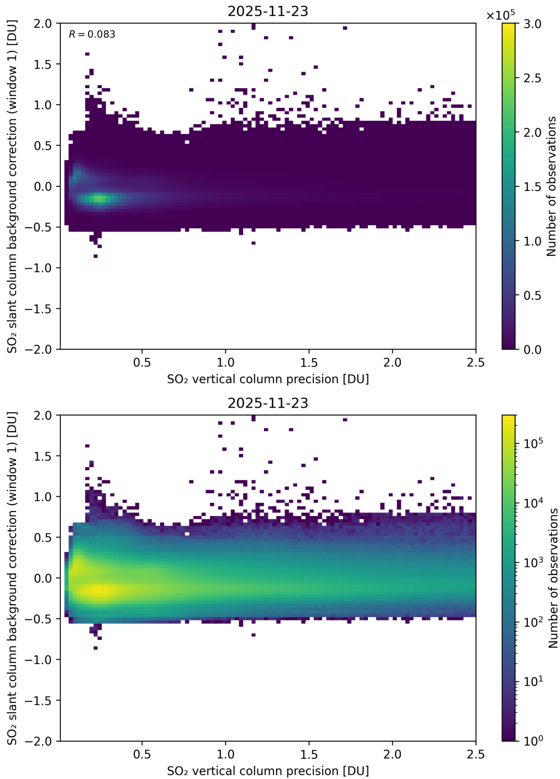
Figure 329: Scatter density plot of “SO 2 vertical column precision” against “SO 2 slant column background correction (window 1)” for 2025-11-23 to 2025-11-24.
