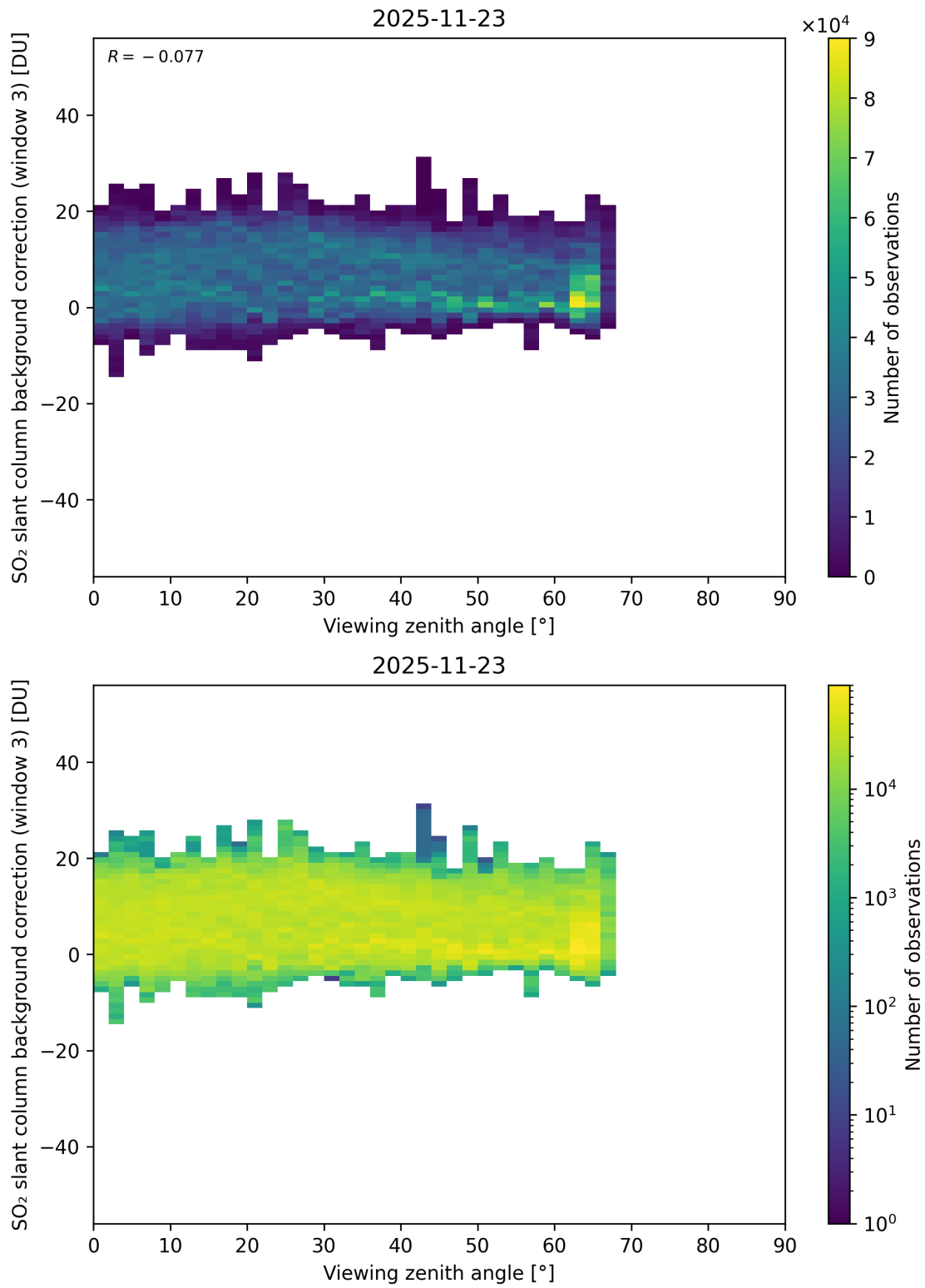
Figure 364: Scatter density plot of “Viewing zenith angle” against “SO 2 slant column background correction (window 3)” for 2025-11-23 to 2025-11-24.
