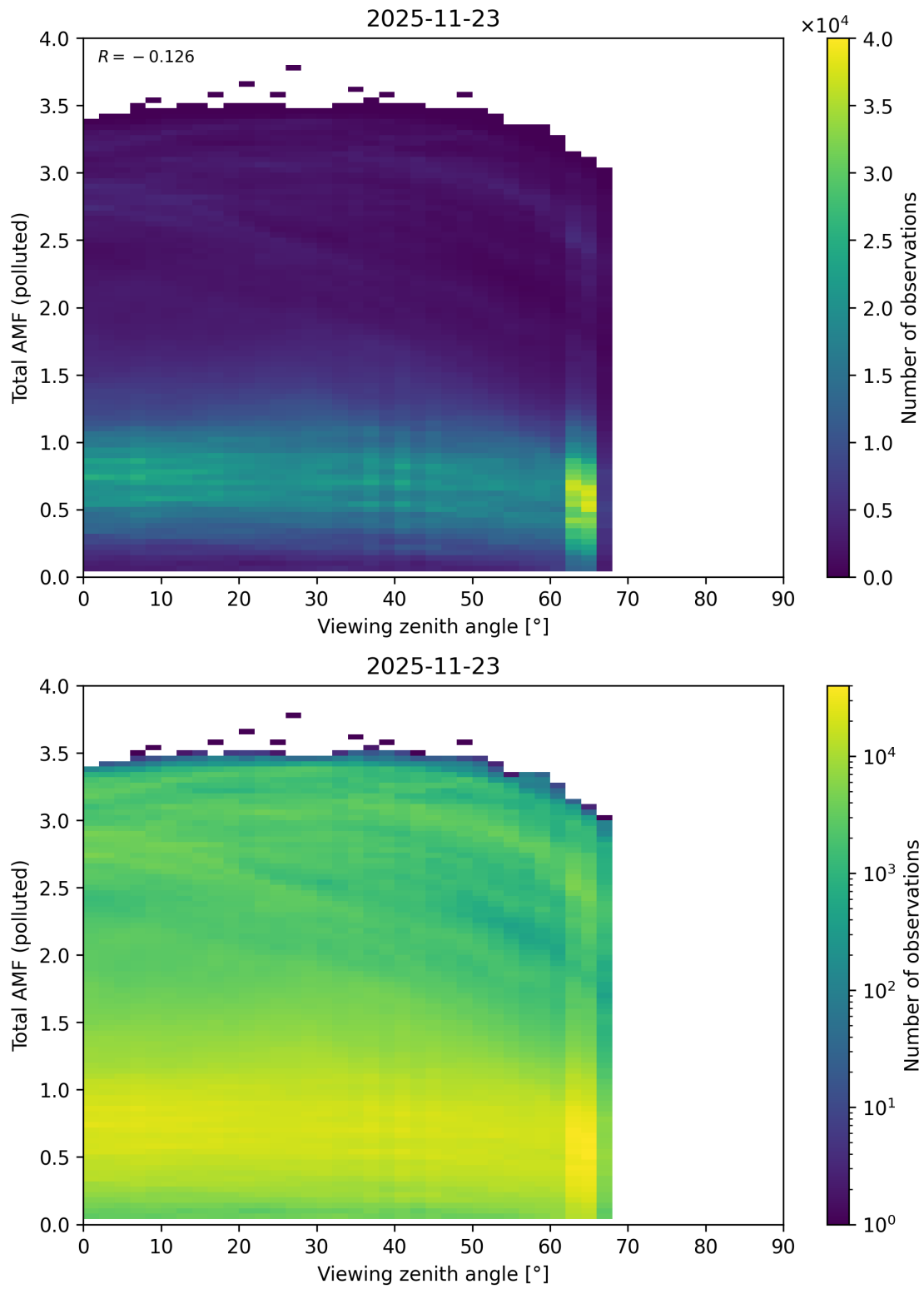
Figure 381: Scatter density plot of “Viewing zenith angle” against “Total AMF (polluted)” for 2025-11-23 to 2025-11-24.
