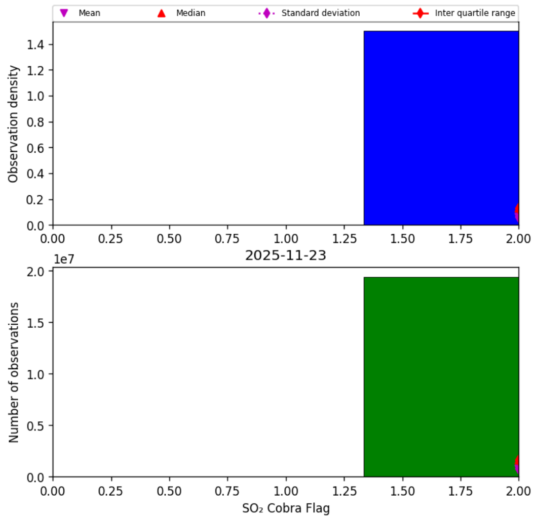
Figure 75: Histogram of "SO 2 Cobra Flag" for 2025-11-23 to 2025-11-24
