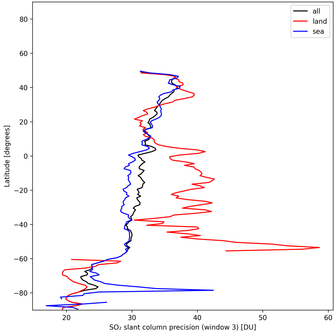
Figure 46: Zonal average of “SO 2 slant column precision (window 3)” for 2025-11-23 to 2025-11-24.
