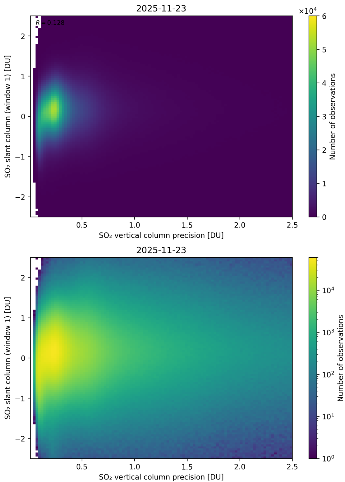
Figure 341: Scatter density plot of “SO 2 vertical column precision” against “SO 2 slant column (window 1)” for 2025-11-23 to 2025-11-24.
