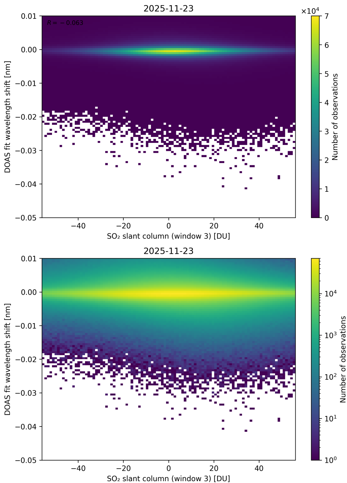
Figure 304: Scatter density plot of “SO 2 slant column (window 3)” against “DOAS fit wavelength shift” for 2025-11-23 to 2025-11-24.
