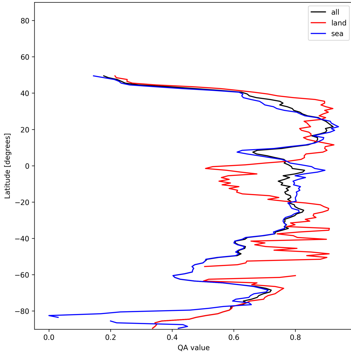
Figure 31: Zonal average of “QA value” for 2025-11-23 to 2025-11-24.
