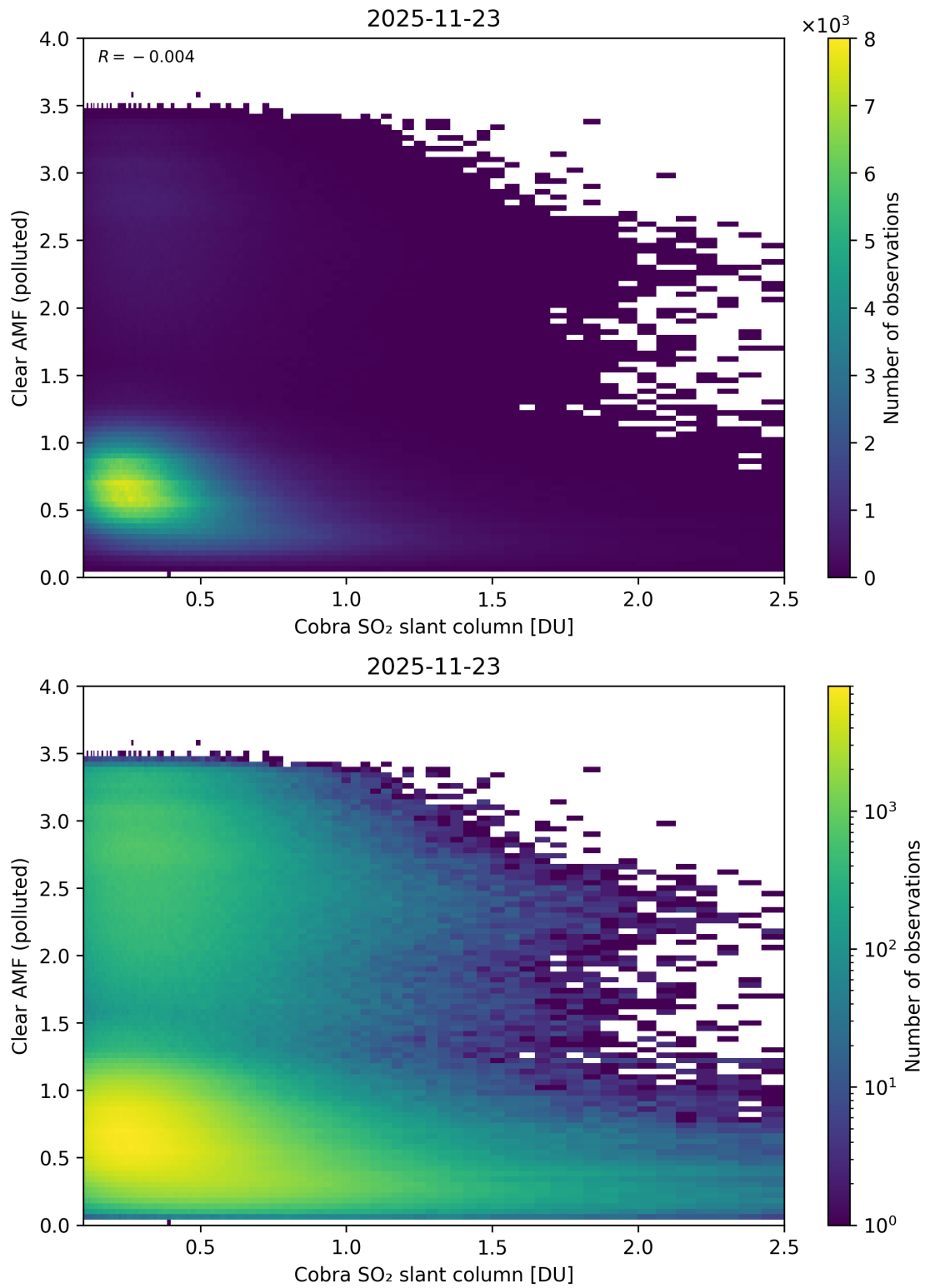
Figure 215: Scatter density plot of “Cobra SO 2 slant column” against “Clear AMF (polluted)” for 2025-11-23 to 2025-11-24.
