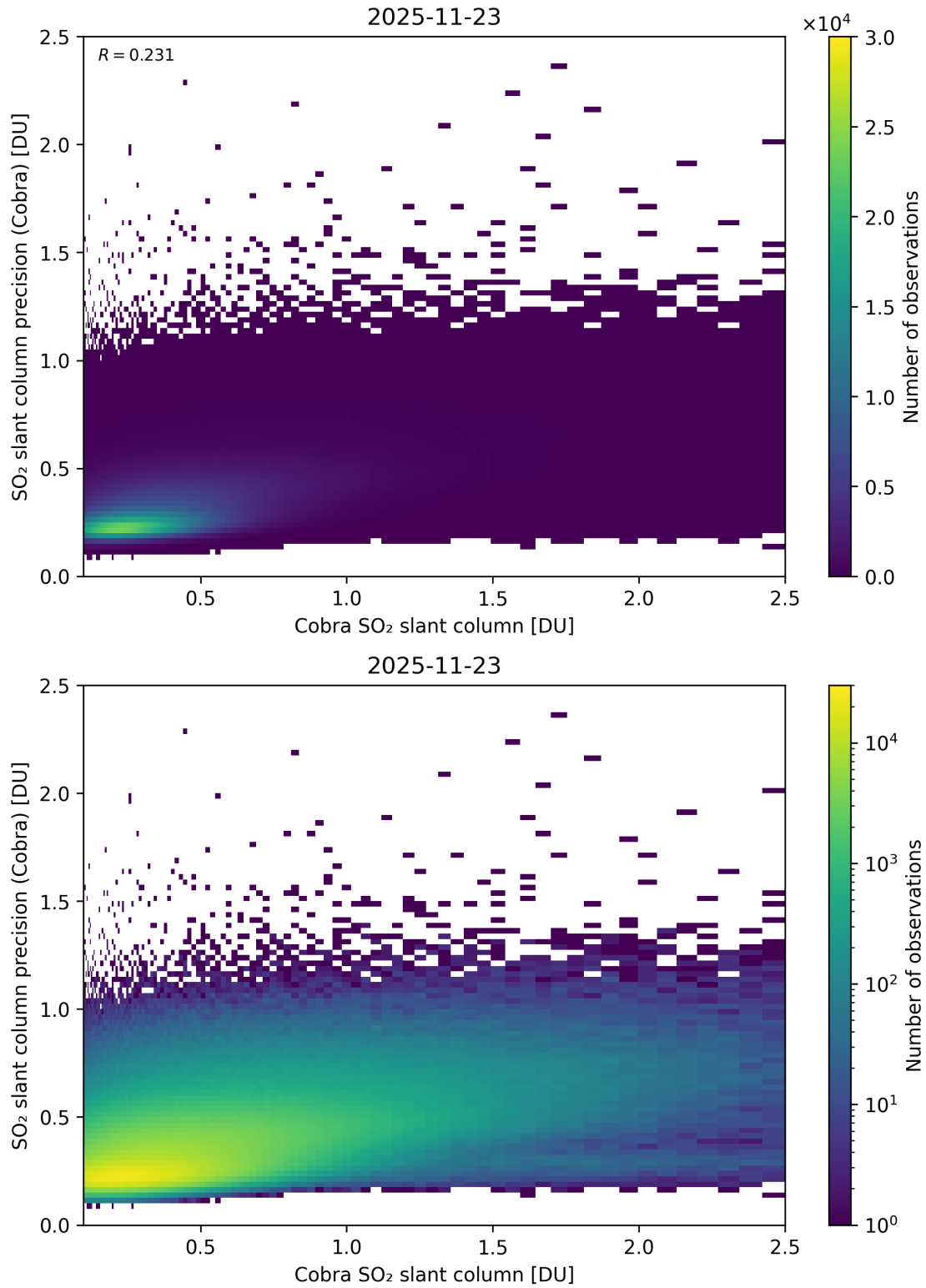
Figure 216: Scatter density plot of “Cobra SO 2 slant column” against “SO 2 slant column precision (Cobra)” for 2025-11-23 to 2025-11-24.
