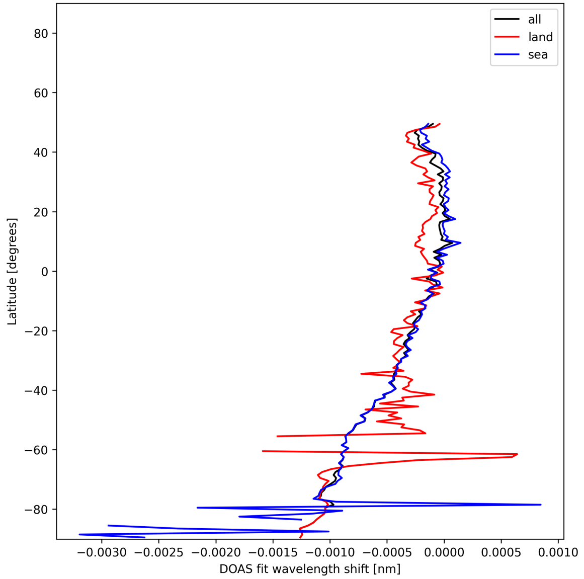
Figure 50: Zonal average of “DOAS fit wavelength shift” for 2025-11-23 to 2025-11-24.
