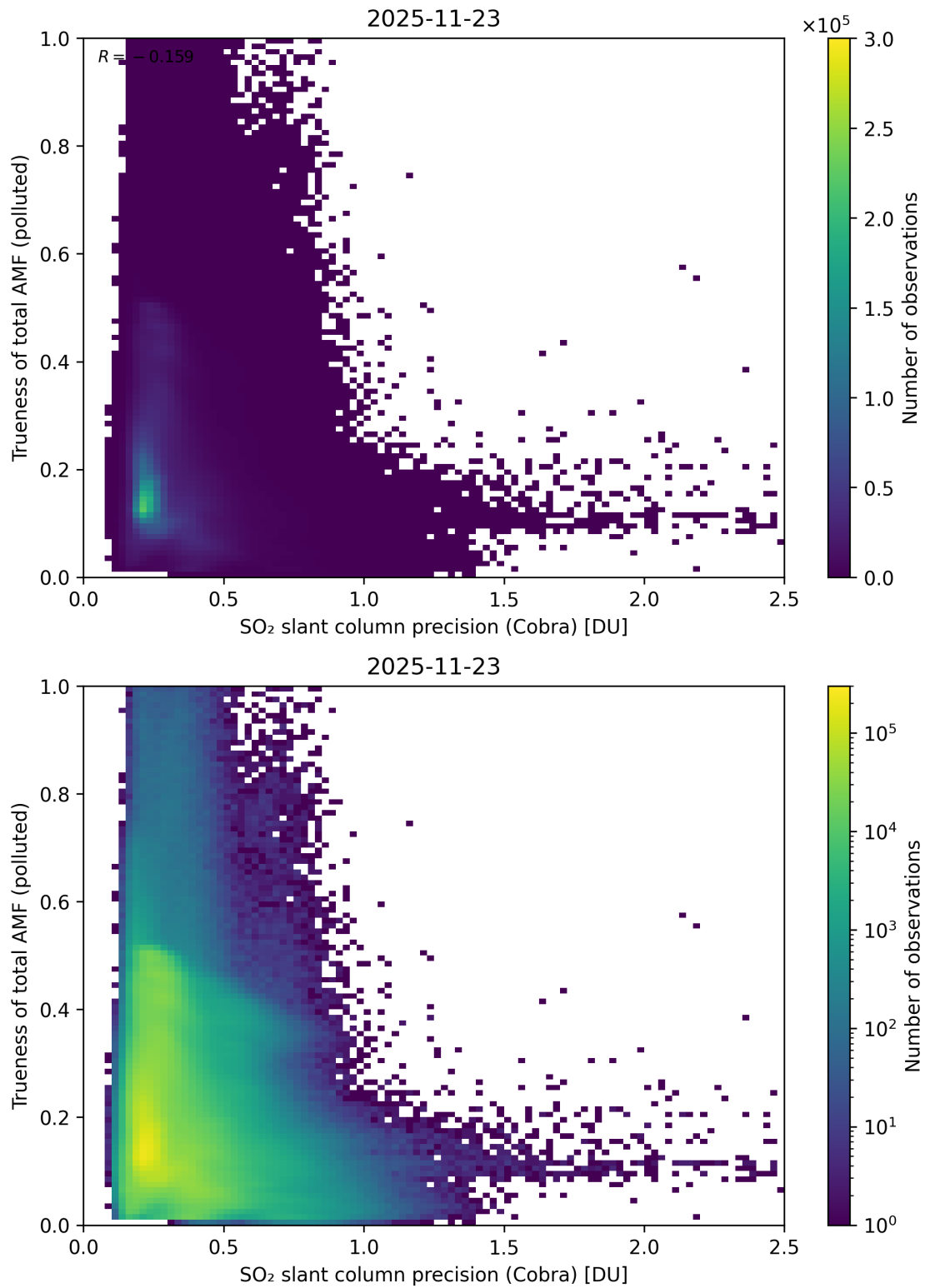
Figure 214: Scatter density plot of “SO 2 slant column precision (Cobra)” against “Trueness of total AMF (polluted)” for 2025-11-23 to 2025-11-24.
