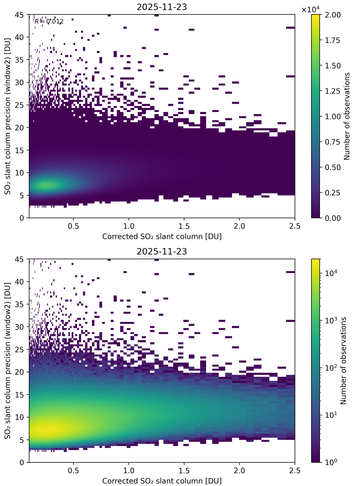
Figure 239: Scatter density plot of “Corrected SO 2 slant column” against “SO 2 slant column precision (window2)” for 2025-11-23 to 2025-11-24.
