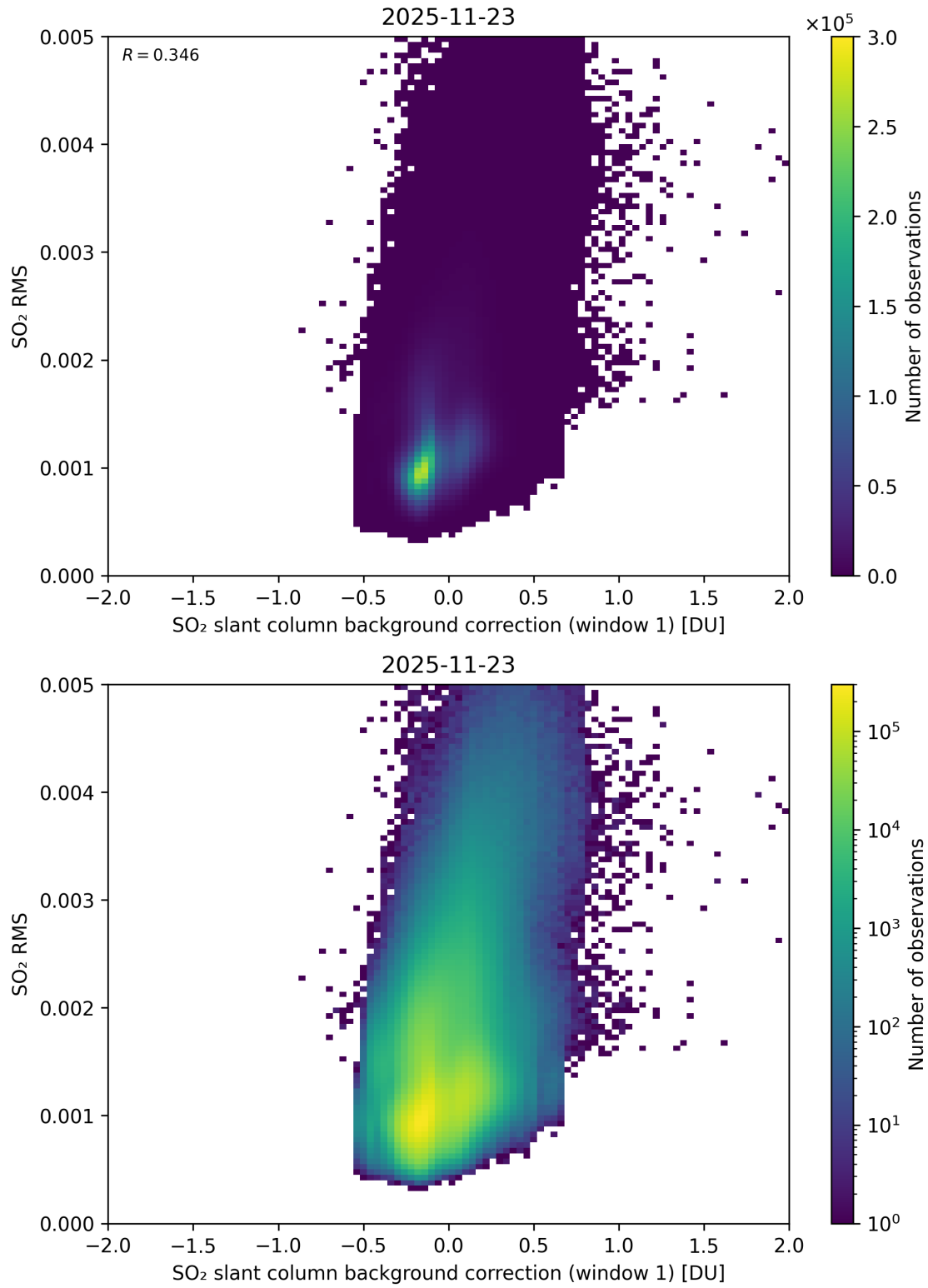
Figure 113: Scatter density plot of “SO 2 slant column background correction (window 1)” against “SO 2 RMS” for 2025-11-23 to 2025-11-24.
