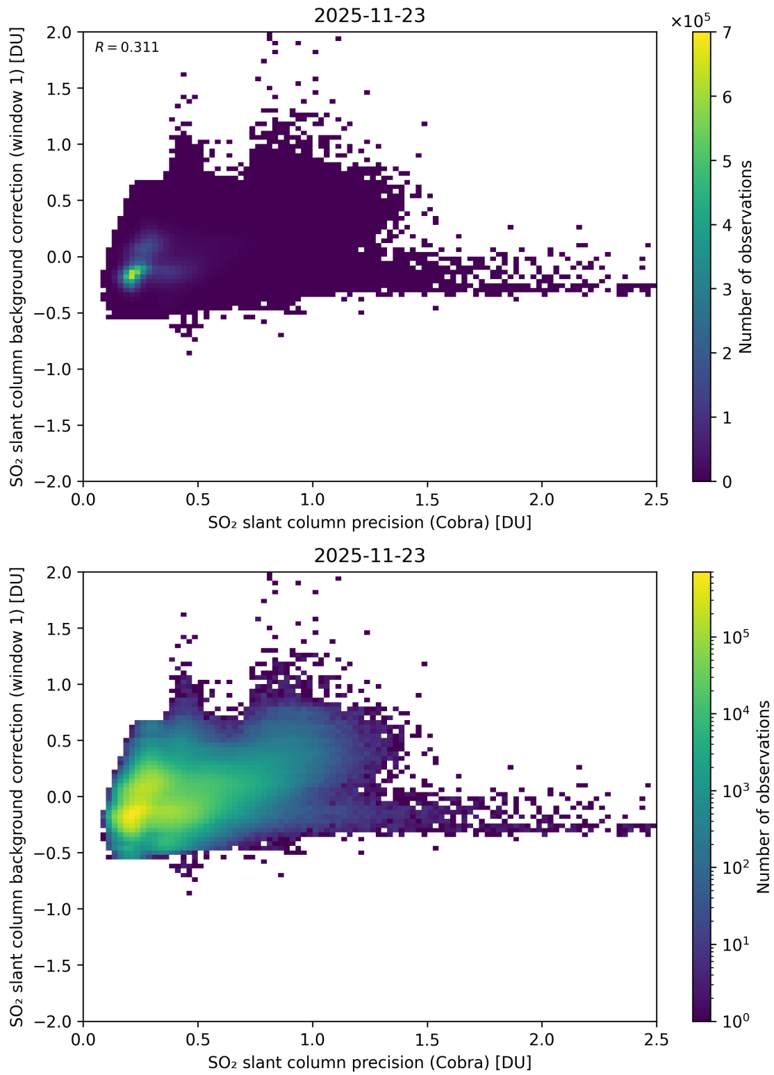
Figure 199: Scatter density plot of “SO 2 slant column precision (Cobra)” against “SO 2 slant column background correction (window 1)” for 2025-11-23 to 2025-11-24.
