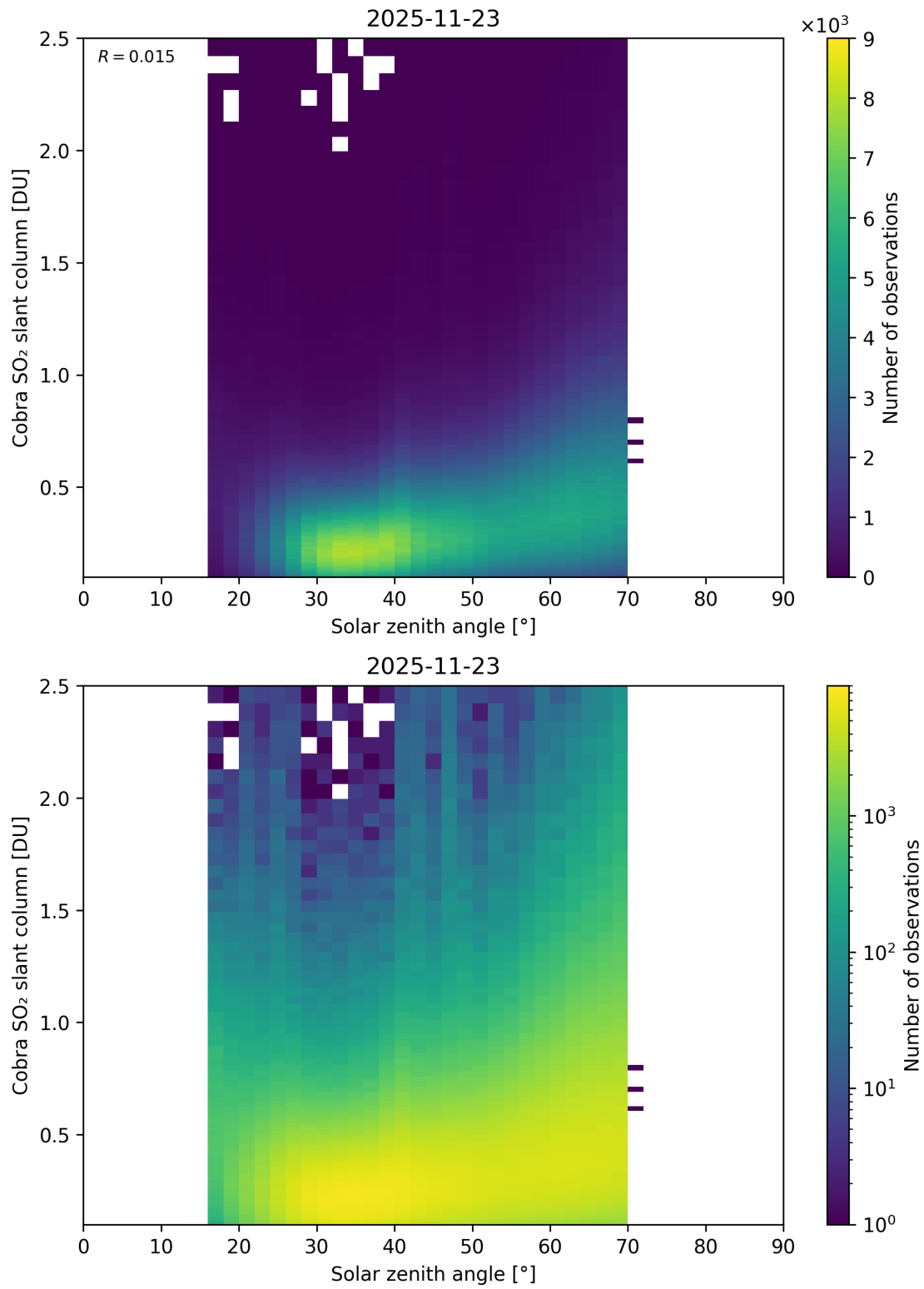
Figure 179: Scatter density plot of “Solar zenith angle” against “Cobra SO 2 slant column” for 2025-11-23 to 2025-11-24.
