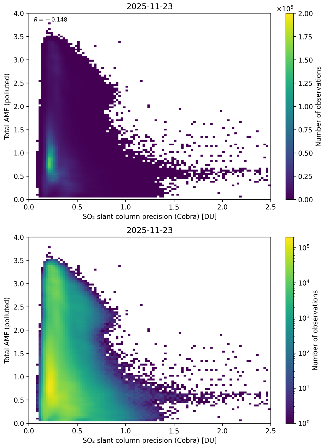
Figure 213: Scatter density plot of “SO 2 slant column precision (Cobra)” against “Total AMF (polluted)” for 2025-11-23 to 2025-11-24.
