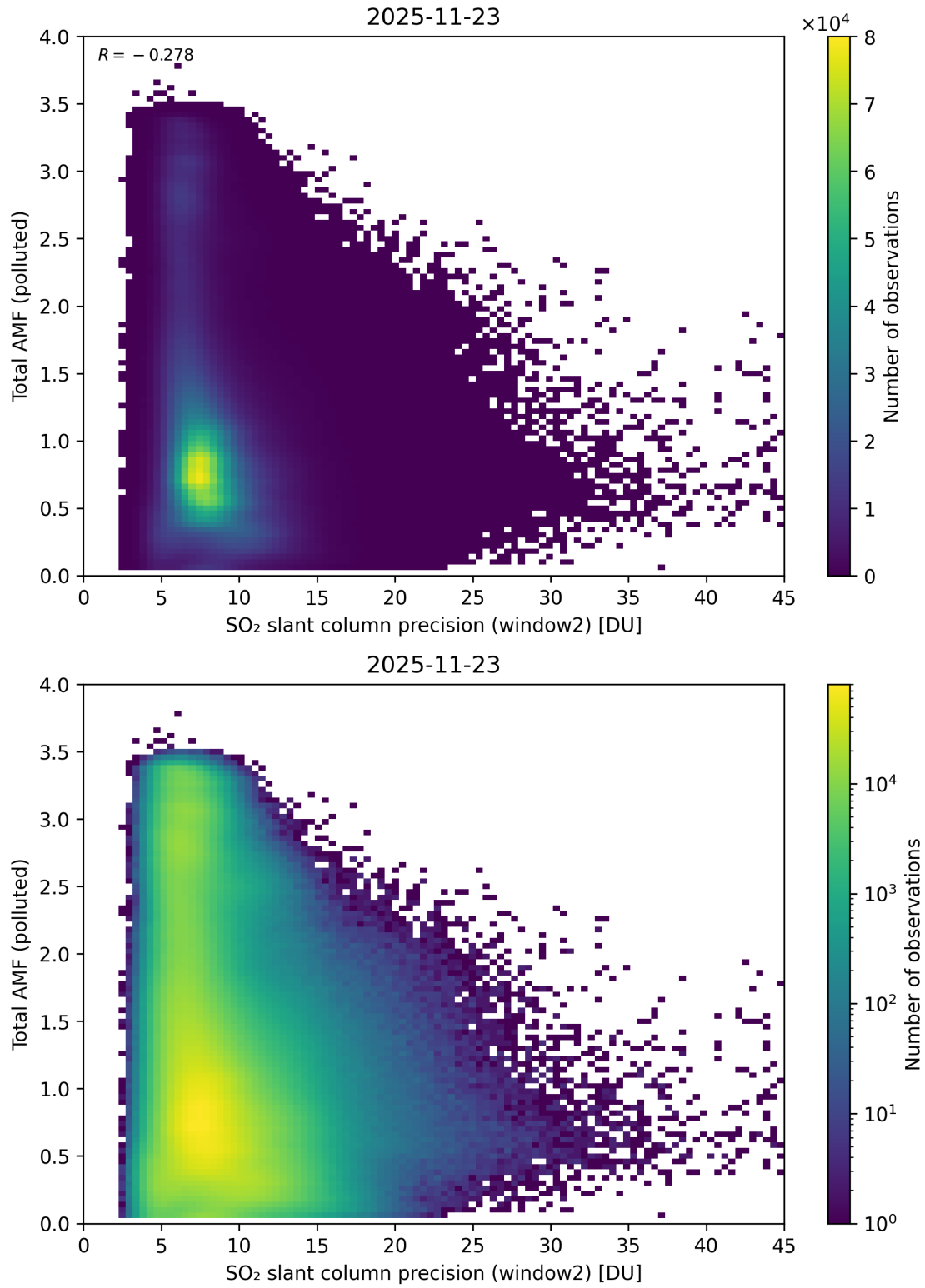
Figure 301: Scatter density plot of “SO 2 slant column precision (window2)” against “Total AMF (polluted)” for 2025-11-23 to 2025-11-24.
