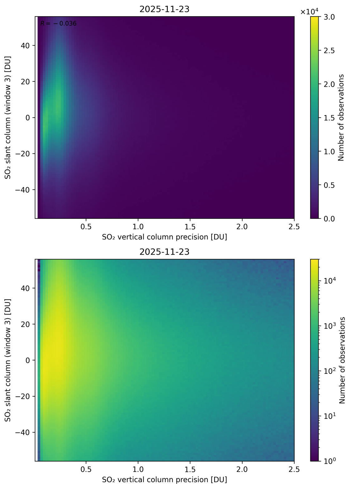
Figure 344: Scatter density plot of “SO 2 vertical column precision” against “SO 2 slant column (window 3)” for 2025-11-23 to 2025-11-24.
