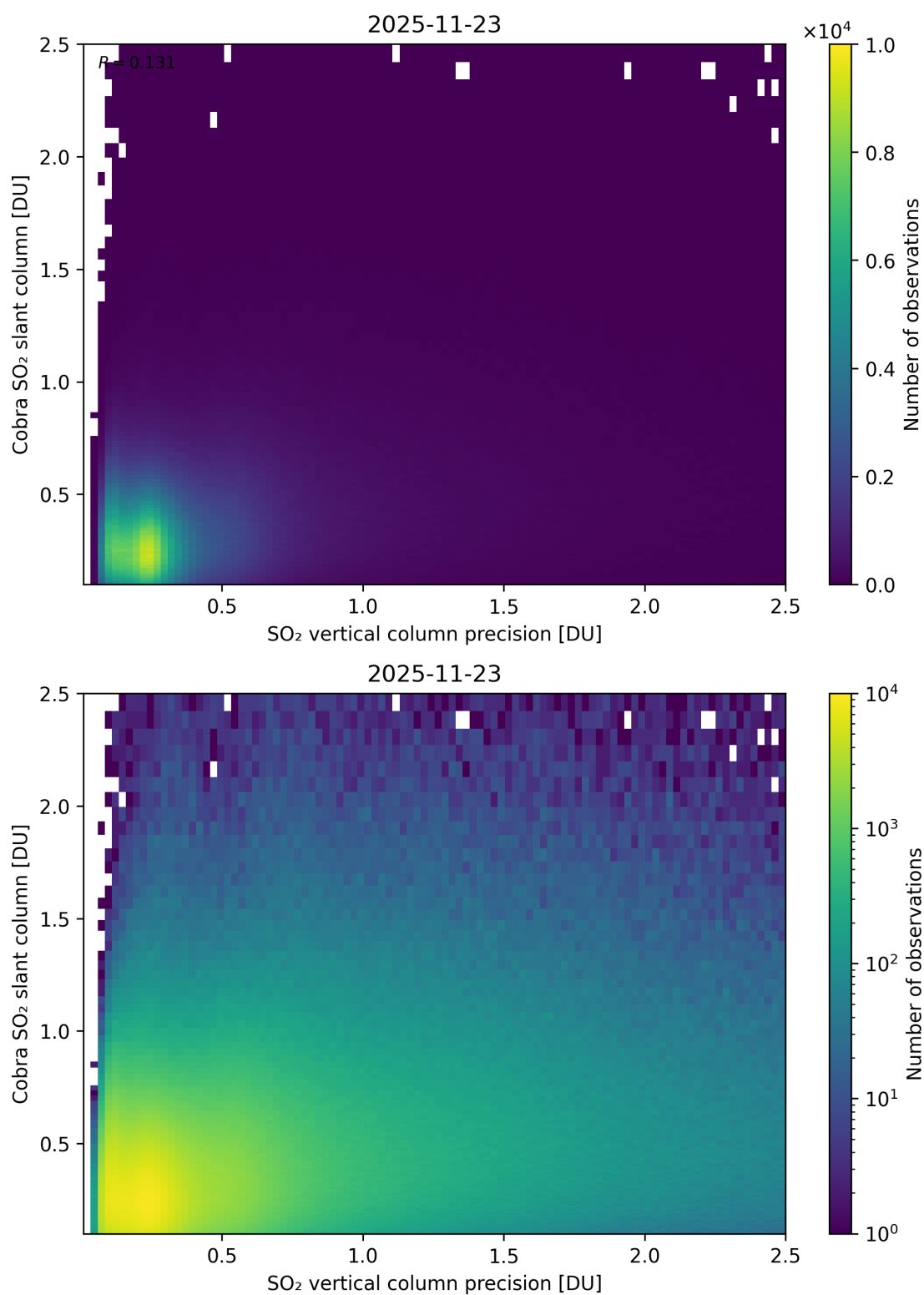
Figure 336: Scatter density plot of “SO 2 vertical column precision” against “Cobra SO 2 slant column” for 2025-11-23 to 2025-11-24.
