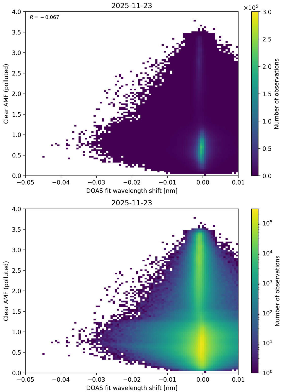
Figure 140: Scatter density plot of “DOAS fit wavelength shift” against “Clear AMF (polluted)” for 2025-11-23 to 2025-11-24.
