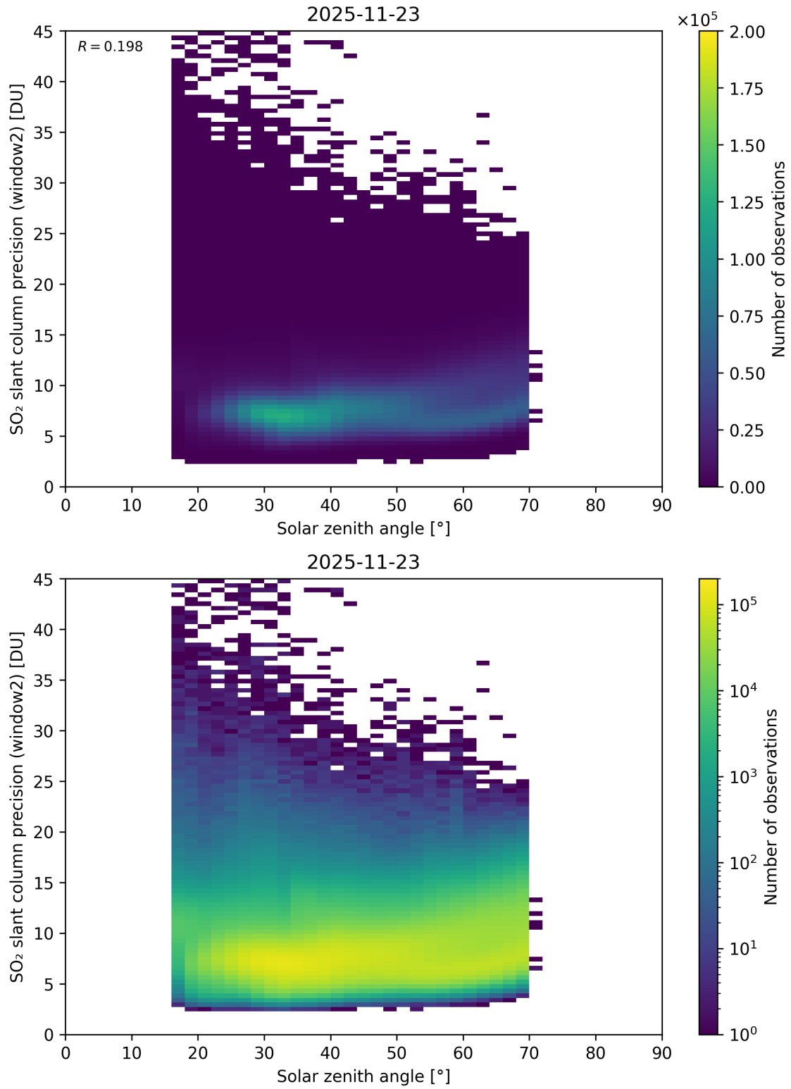
Figure 186: Scatter density plot of “Solar zenith angle” against “SO 2 slant column precision (window2)” for 2025-11-23 to 2025-11-24.
