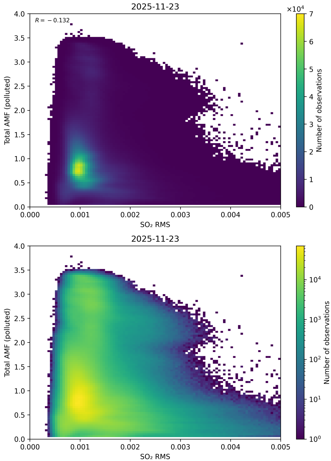
Figure 148: Scatter density plot of “SO 2 RMS” against “Total AMF (polluted)” for 2025-11-23 to 2025-11-24.
