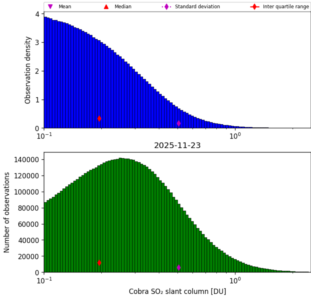
Figure 61: Histogram of “Cobra SO 2 slant column” for 2025-11-23 to 2025-11-24
