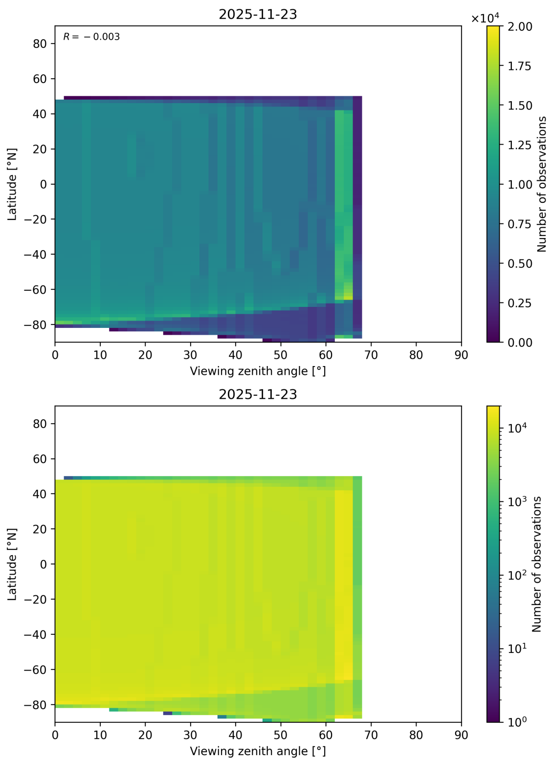
Figure 368: Scatter density plot of “Viewing zenith angle” against “Latitude” for 2025-11-23 to 2025-11-24.
