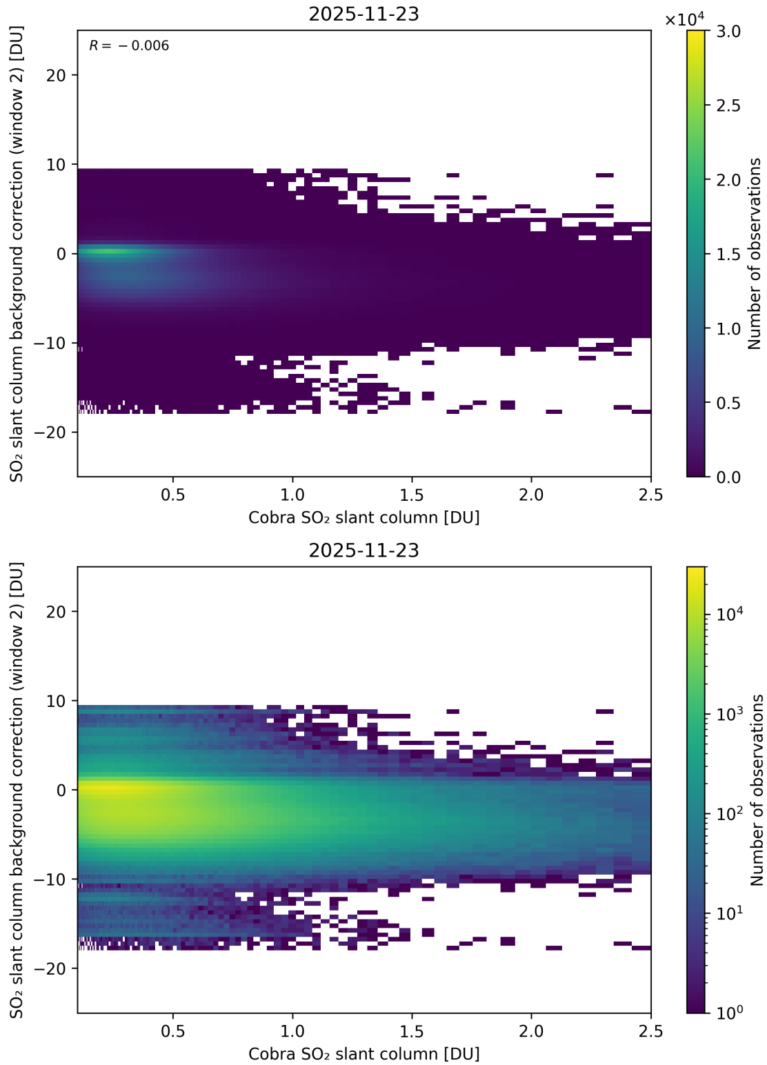
Figure 194: Scatter density plot of “Cobra SO 2 slant column” against “SO 2 slant column background correction (window 2)” for 2025-11-23 to 2025-11-24.
