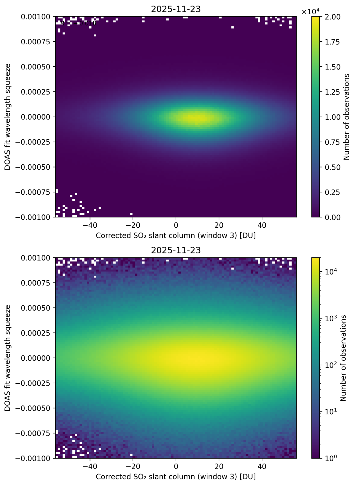
Figure 257: Scatter density plot of “Corrected SO 2 slant column (window 3)” against “DOAS fit wavelength squeeze” for 2025-11-23 to 2025-11-24.
