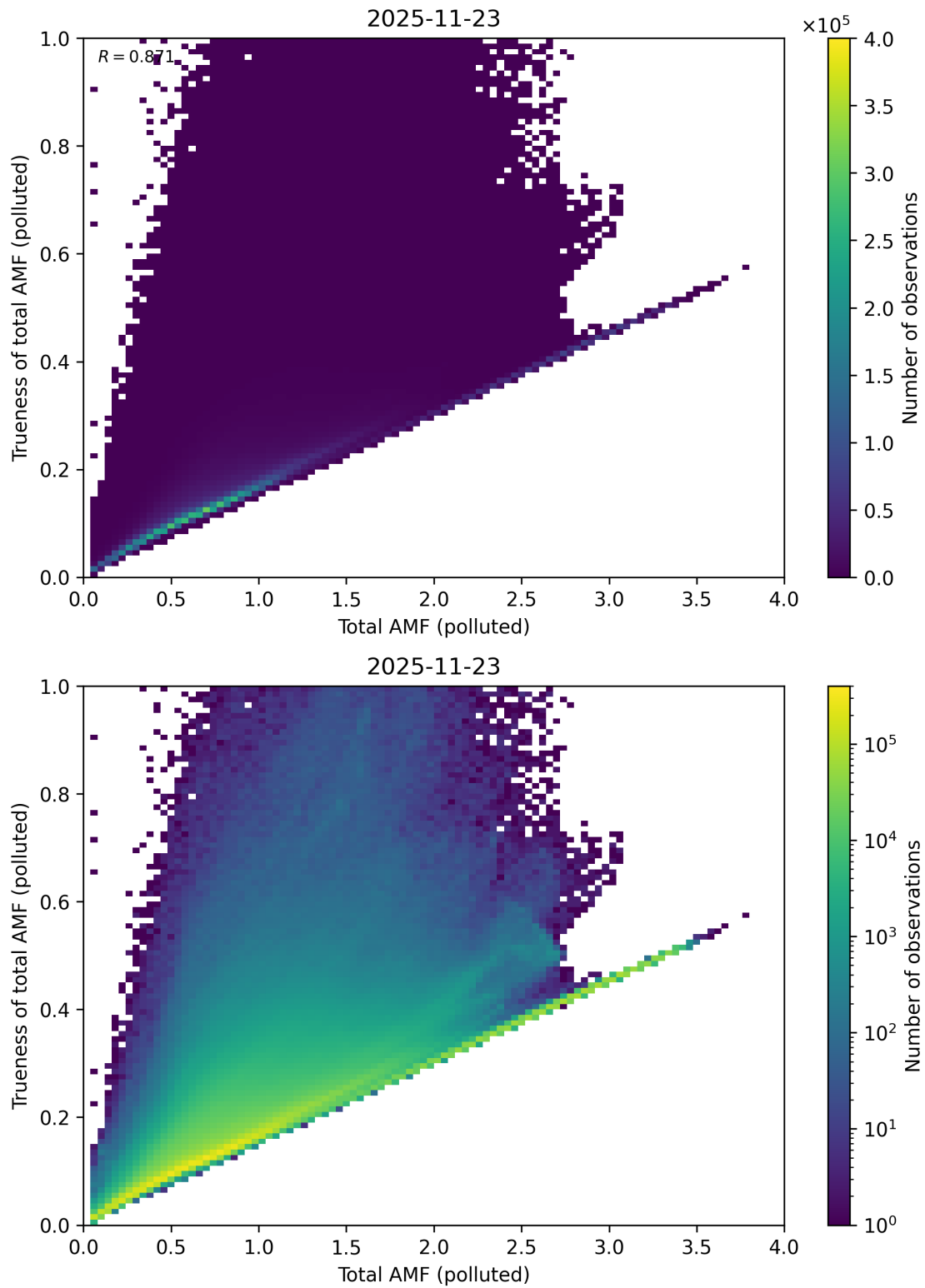
Figure 321: Scatter density plot of “Total AMF (polluted)” against “Trueness of total AMF (polluted)” for 2025-11-23 to 2025-11-24.
