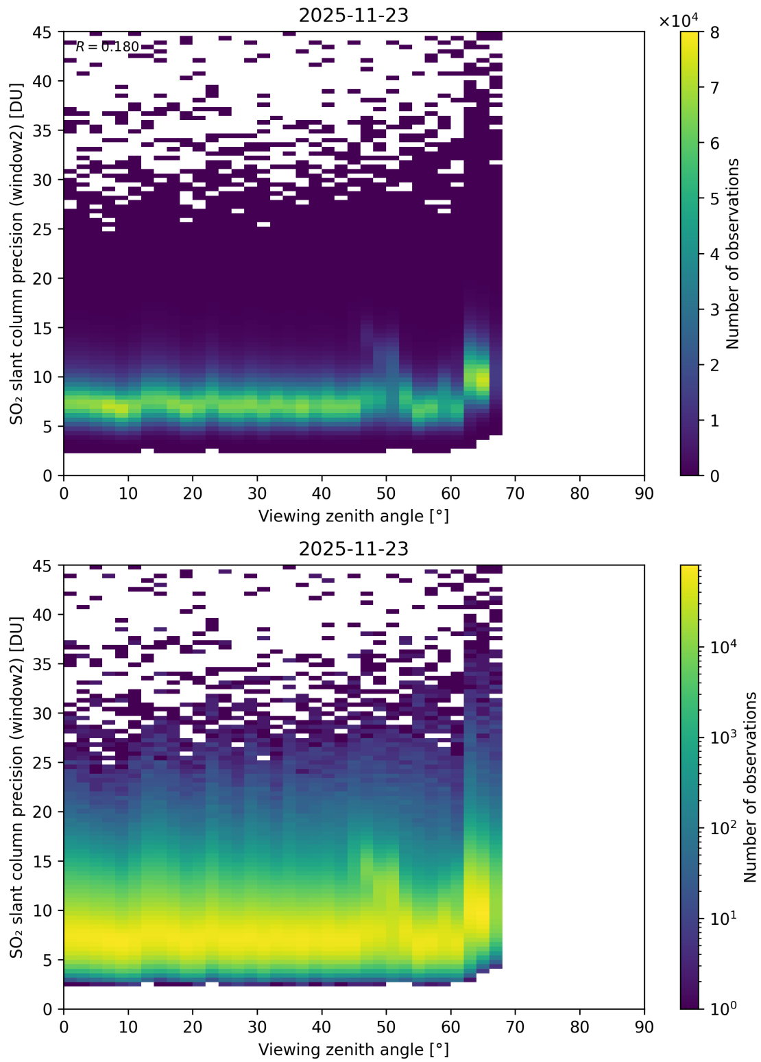
Figure 378: Scatter density plot of “Viewing zenith angle” against “SO 2 slant column precision (window2)” for 2025-11-23 to 2025-11-24.
