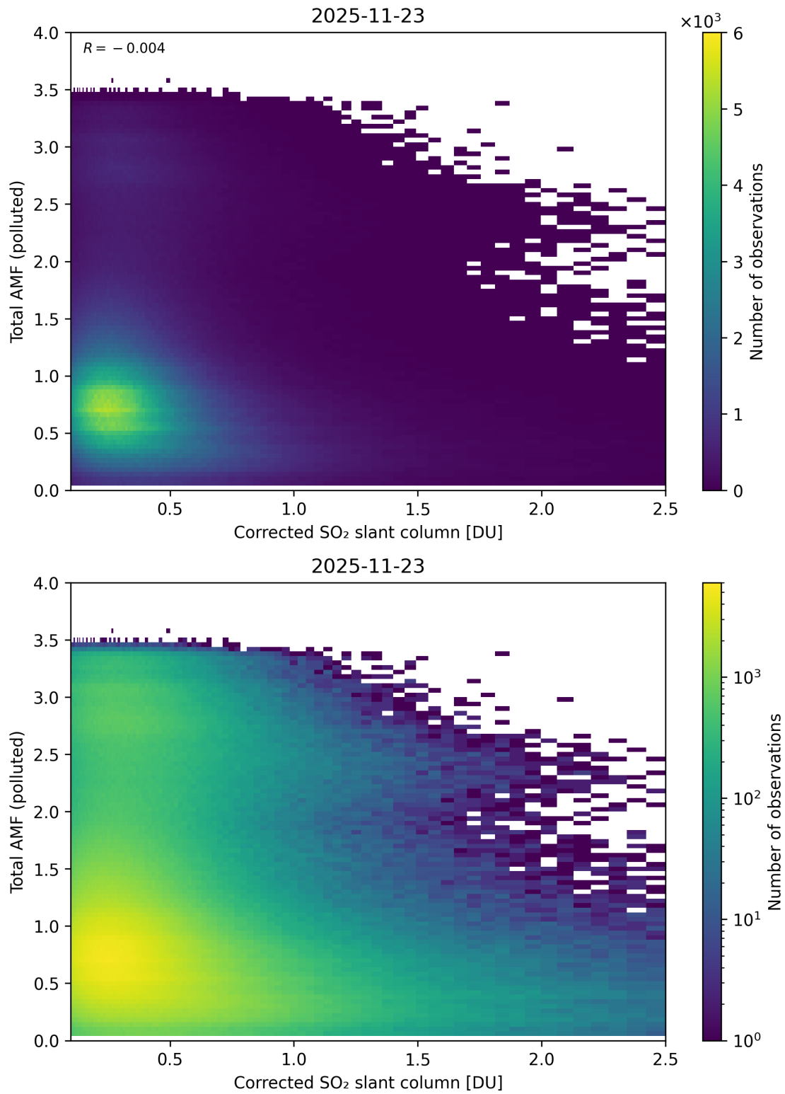
Figure 242: Scatter density plot of “Corrected SO 2 slant column” against “Total AMF (polluted)” for 2025-11-23 to 2025-11-24.
