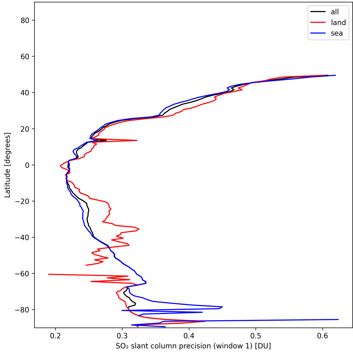
Figure 38: Zonal average of “SO 2 slant column precision (window 1)” for 2025-11-23 to 2025-11-24.
