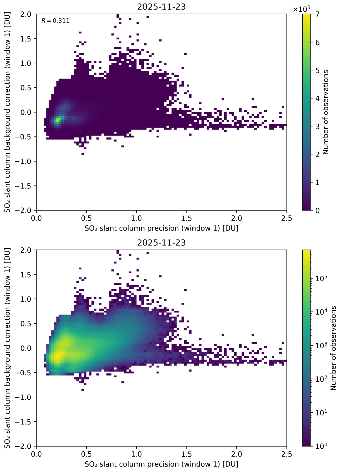
Figure 268: Scatter density plot of “SO 2 slant column precision (window 1)” against “SO 2 slant column background correction (window 1)” for 2025-11-23 to 2025-11-24.
