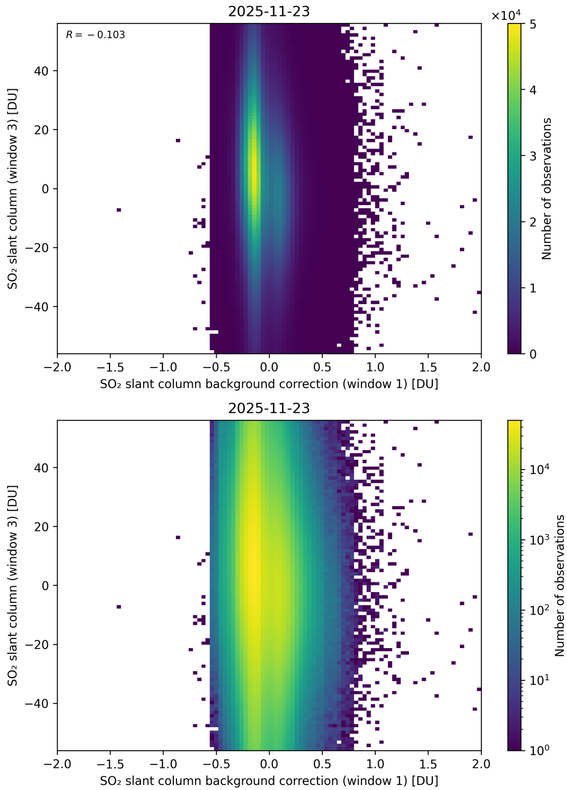
Figure 118: Scatter density plot of “SO 2 slant column background correction (window 1)” against “SO 2 slant column (window 3)” for 2025-11-23 to 2025-11-24.
