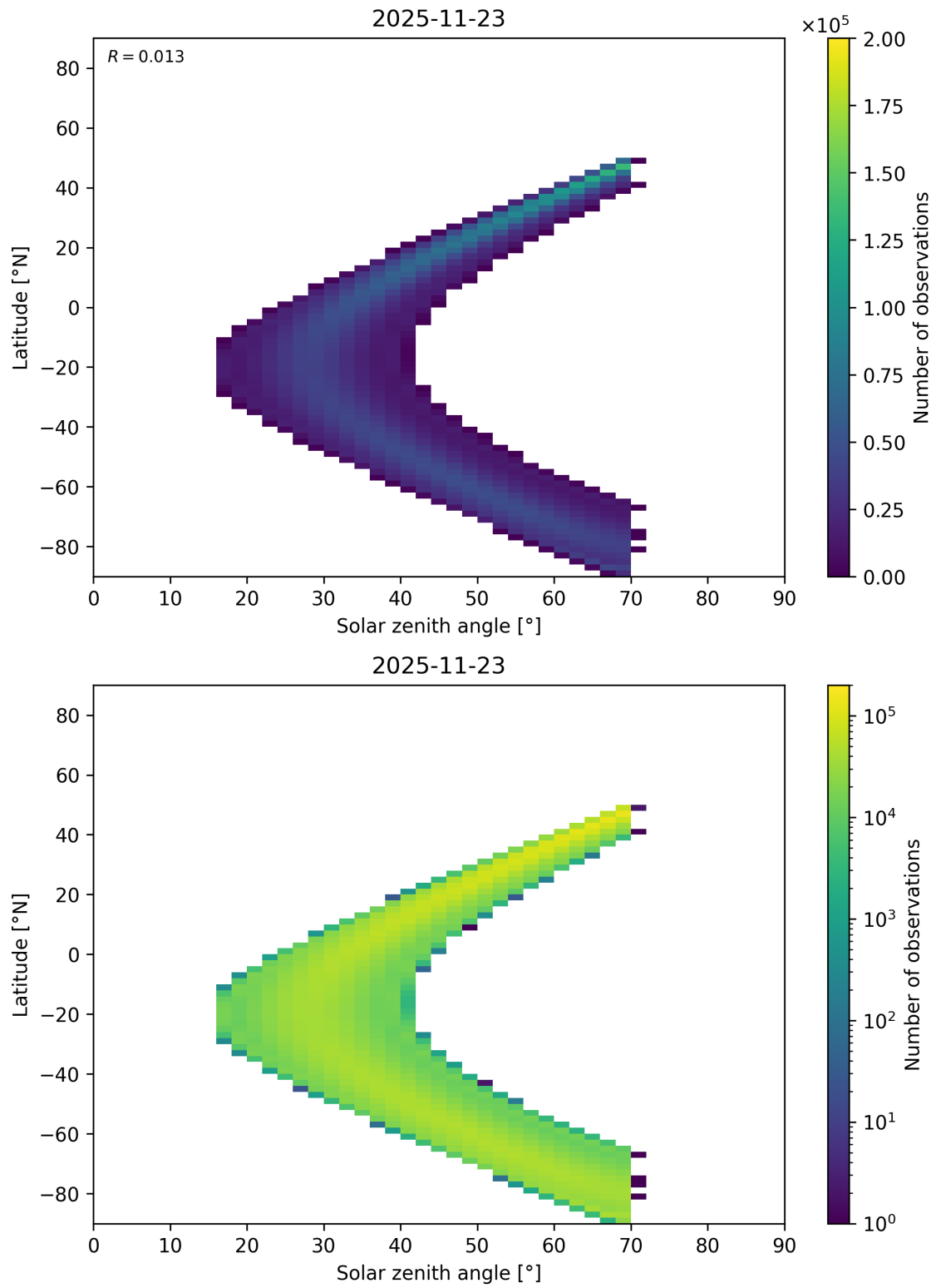
Figure 177: Scatter density plot of “Solar zenith angle” against “Latitude” for 2025-11-23 to 2025-11-24.
