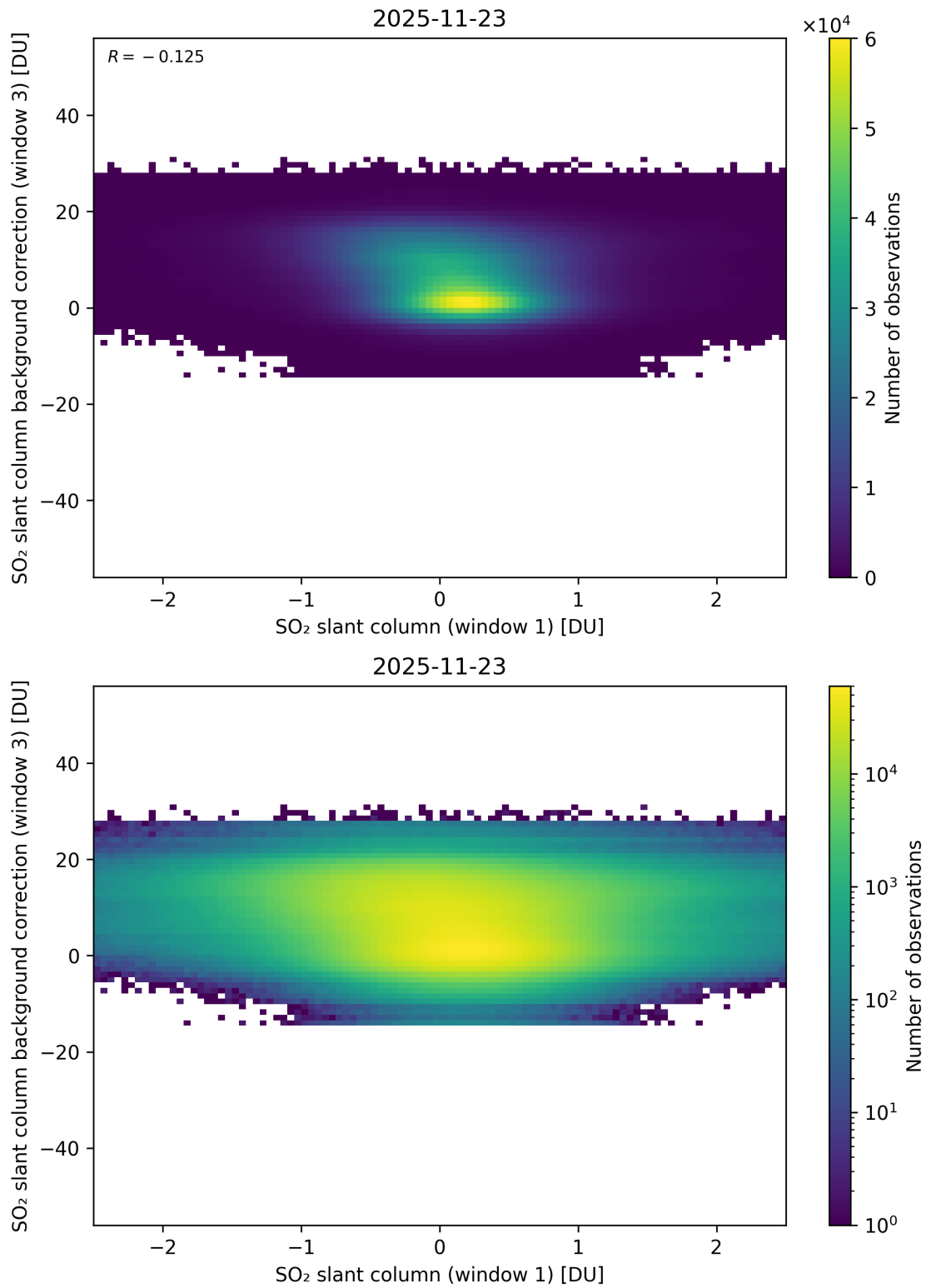
Figure 264: Scatter density plot of “SO 2 slant column (window 1)” against “SO 2 slant column background correction (window 3)” for 2025-11-23 to 2025-11-24.
