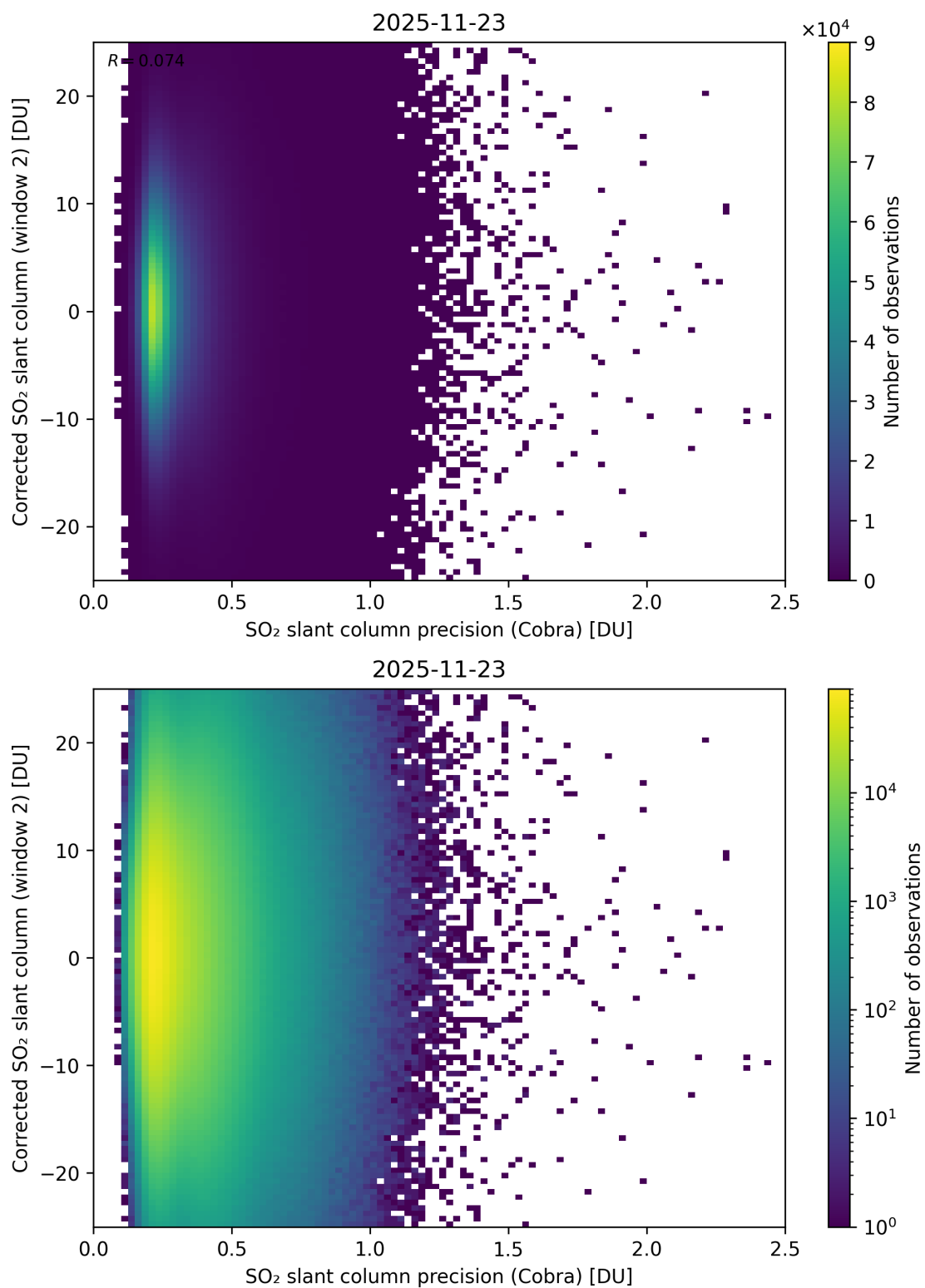
Figure 206: Scatter density plot of “SO 2 slant column precision (Cobra)” against “Corrected SO 2 slant column (window 2)” for 2025-11-23 to 2025-11-24.
