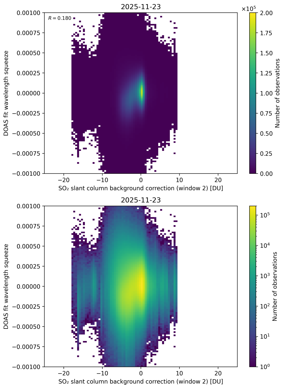
Figure 124: Scatter density plot of “SO 2 slant column background correction (window 2)” against “DOAS fit wavelength squeeze” for 2025-11-23 to 2025-11-24.
