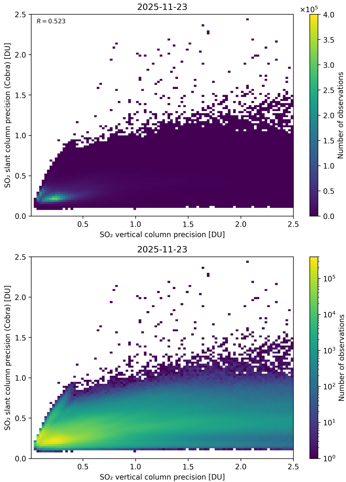
Figure 337: Scatter density plot of “SO 2 vertical column precision” against “SO 2 slant column precision (Cobra)” for 2025-11-23 to 2025-11-24.
