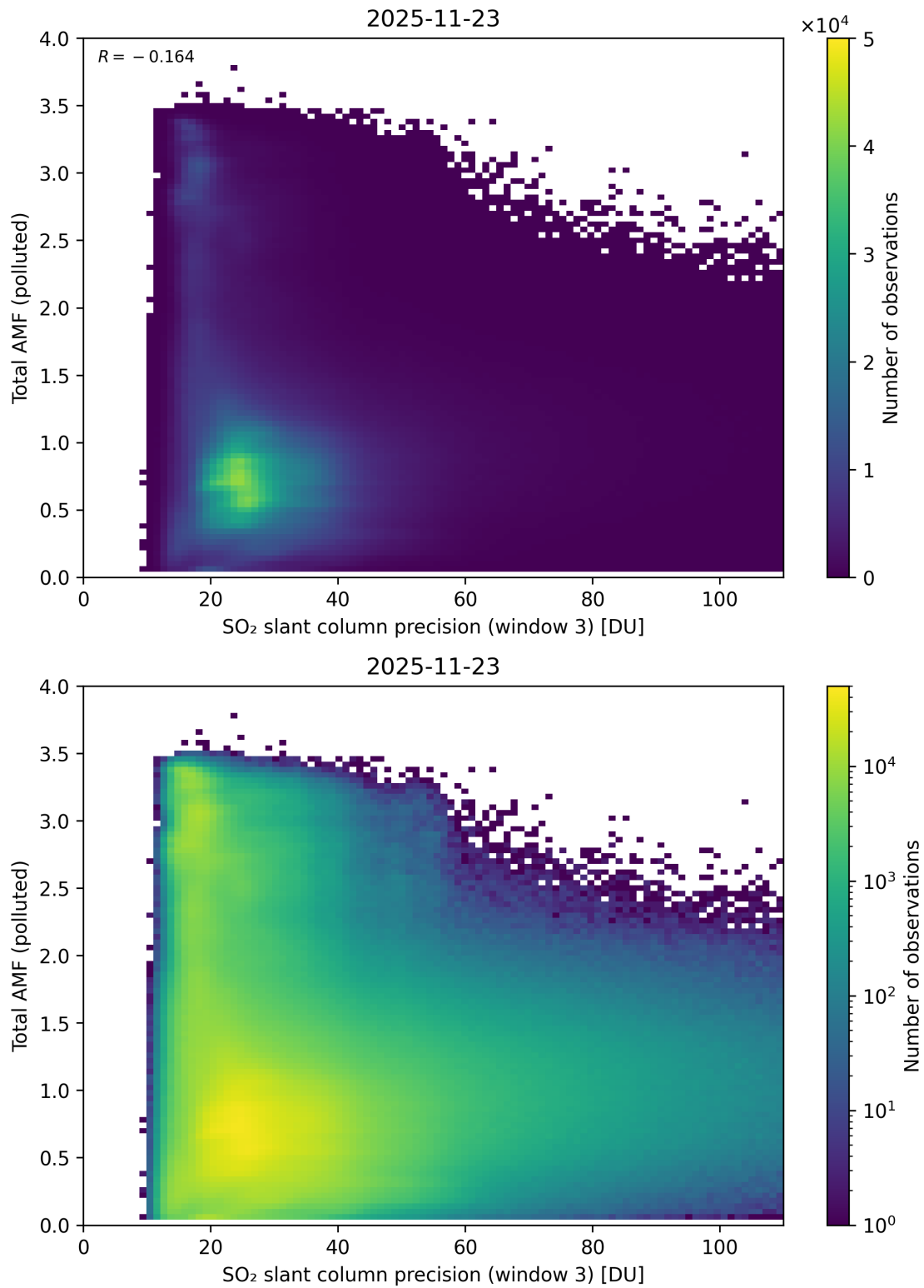
Figure 313: Scatter density plot of “SO 2 slant column precision (window 3)” against “Total AMF (polluted)” for 2025-11-23 to 2025-11-24.
