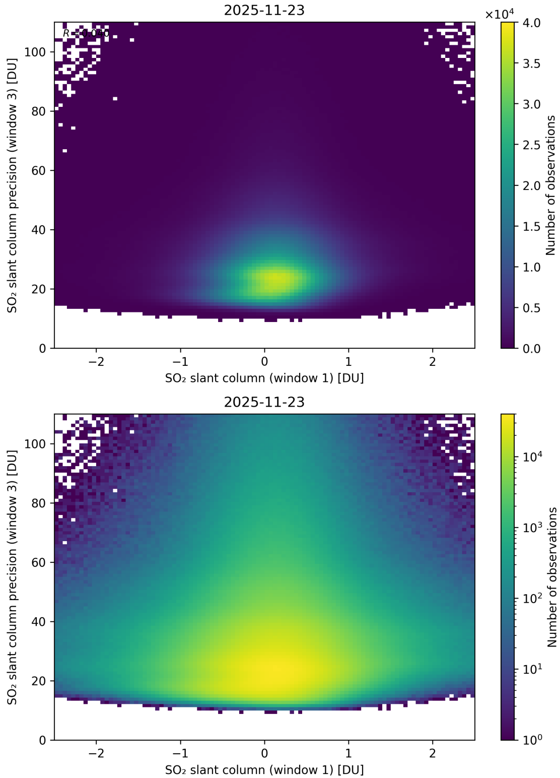
Figure 288: Scatter density plot of “SO 2 slant column (window 1)” against “SO 2 slant column precision (window 3)” for 2025-11-23 to 2025-11-24.
