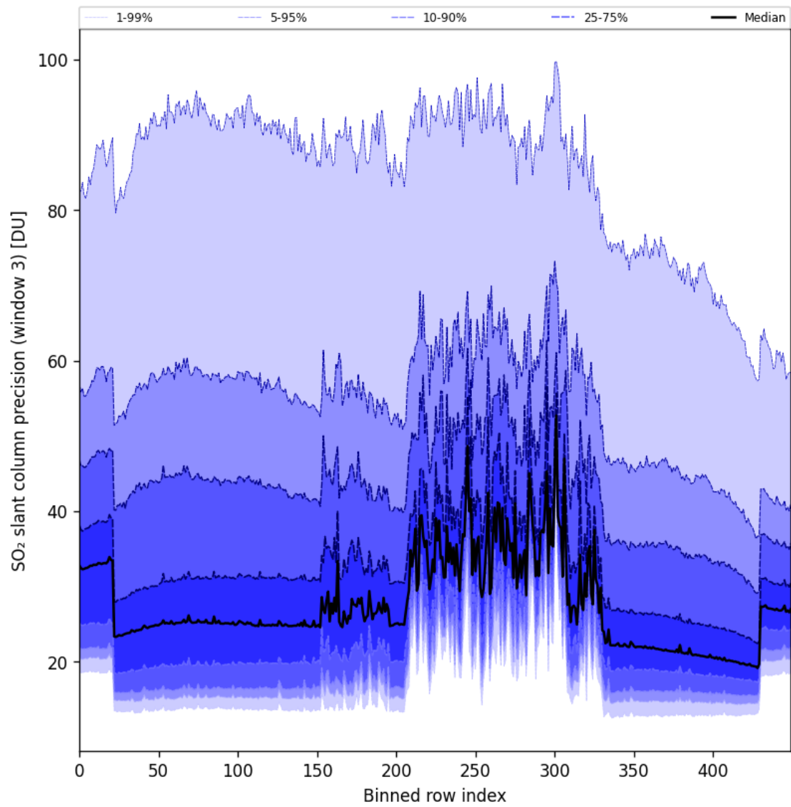
Figure 98: Along track statistics of “SO 2 slant column precision (window 3)” for 2025-11-23 to 2025-11-24
