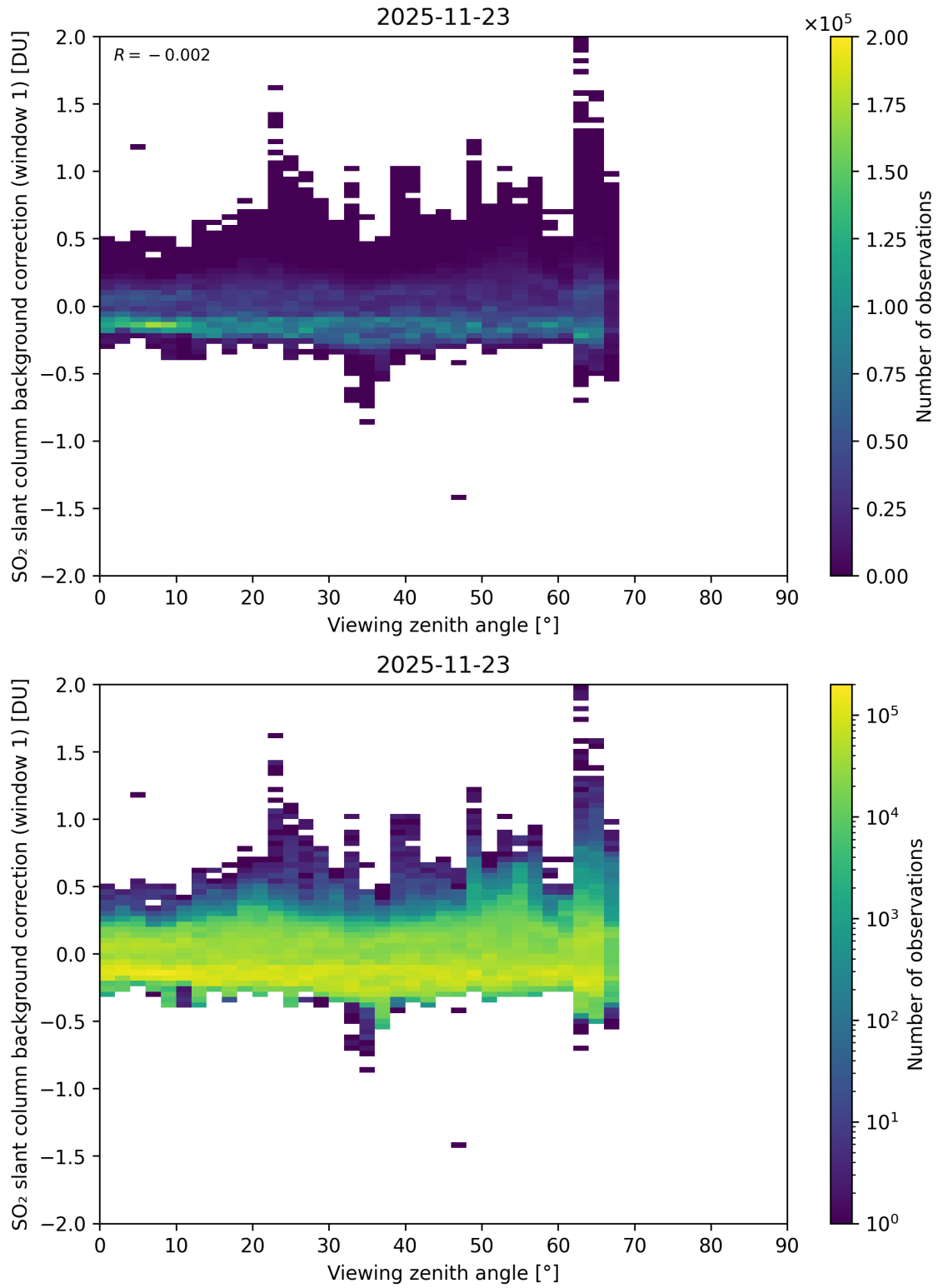
Figure 362: Scatter density plot of “Viewing zenith angle” against “SO 2 slant column background correction (window 1)” for 2025-11-23 to 2025-11-24.
