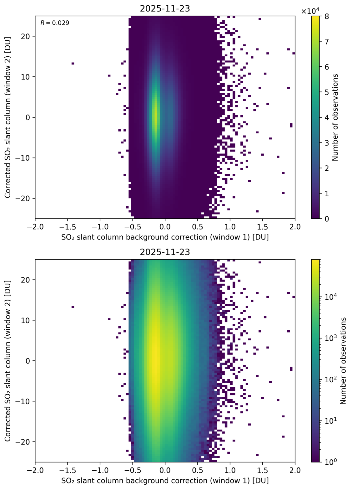
Figure 115: Scatter density plot of “SO 2 slant column background correction (window 1)” against “Corrected SO 2 slant column (window 2)” for 2025-11-23 to 2025-11-24.
