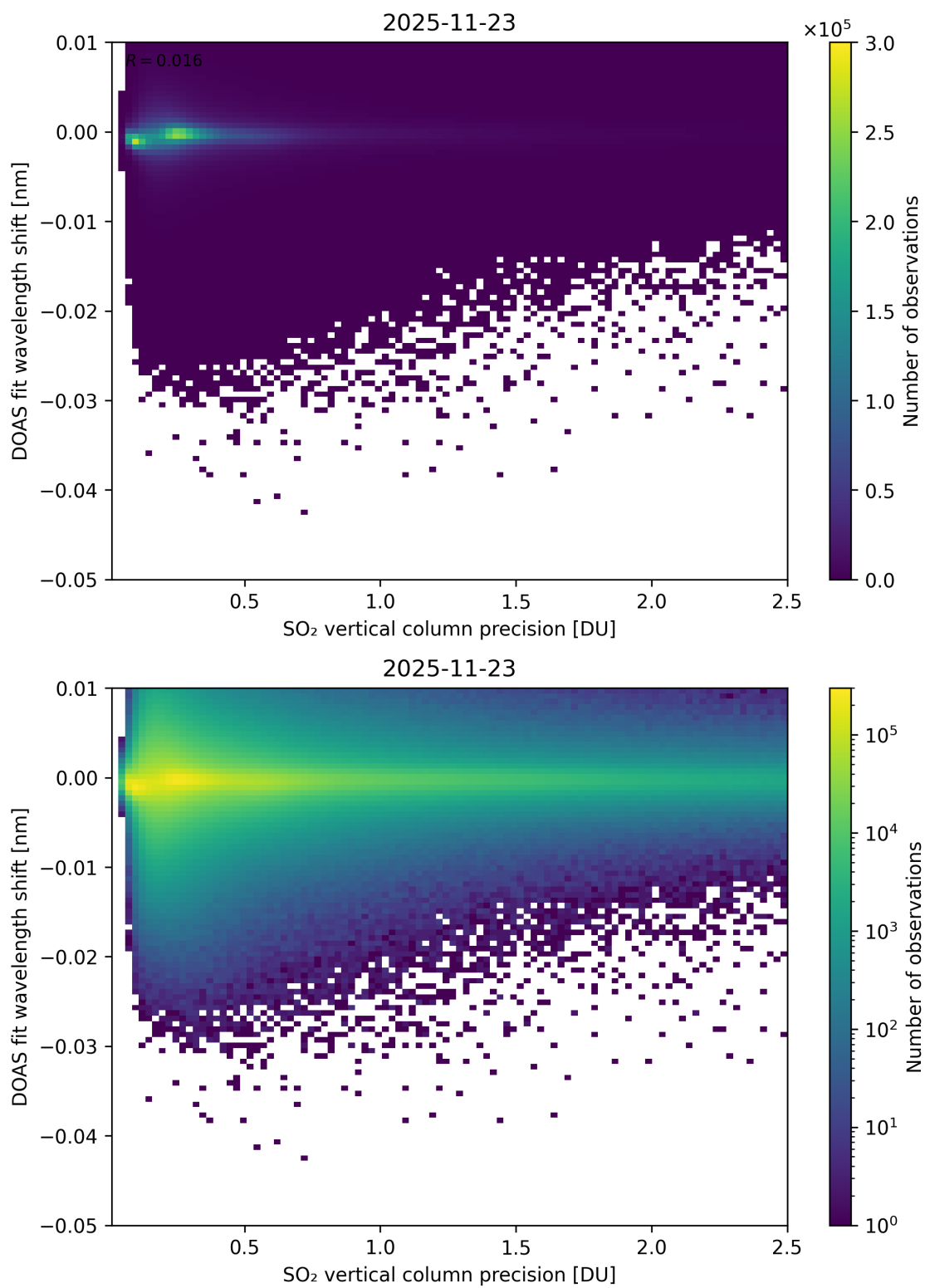
Figure 332: Scatter density plot of “SO 2 vertical column precision” against “DOAS fit wavelength shift” for 2025-11-23 to 2025-11-24.
