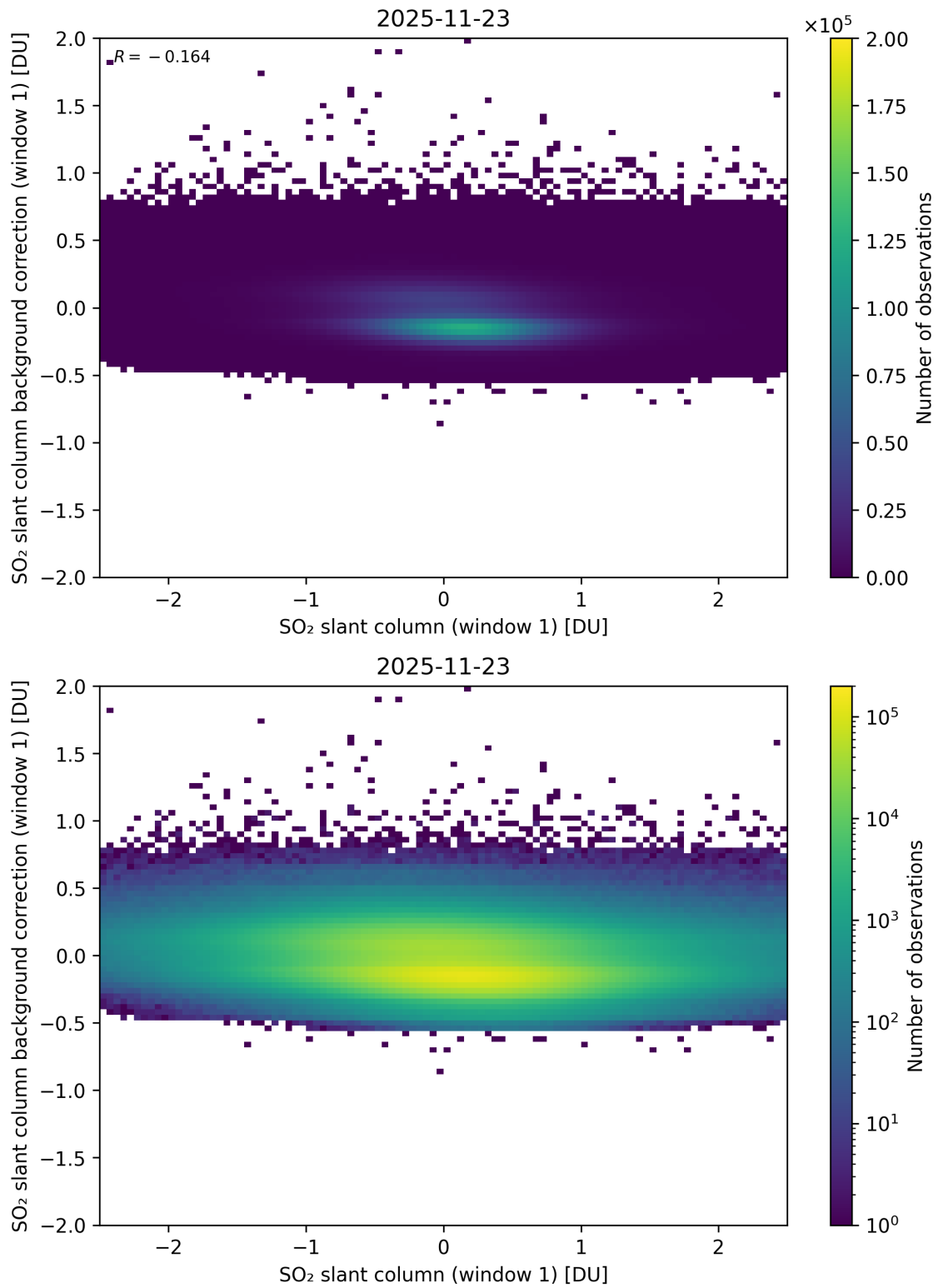
Figure 262: Scatter density plot of “SO 2 slant column (window 1)” against “SO 2 slant column background correction (window 1)” for 2025-11-23 to 2025-11-24.
