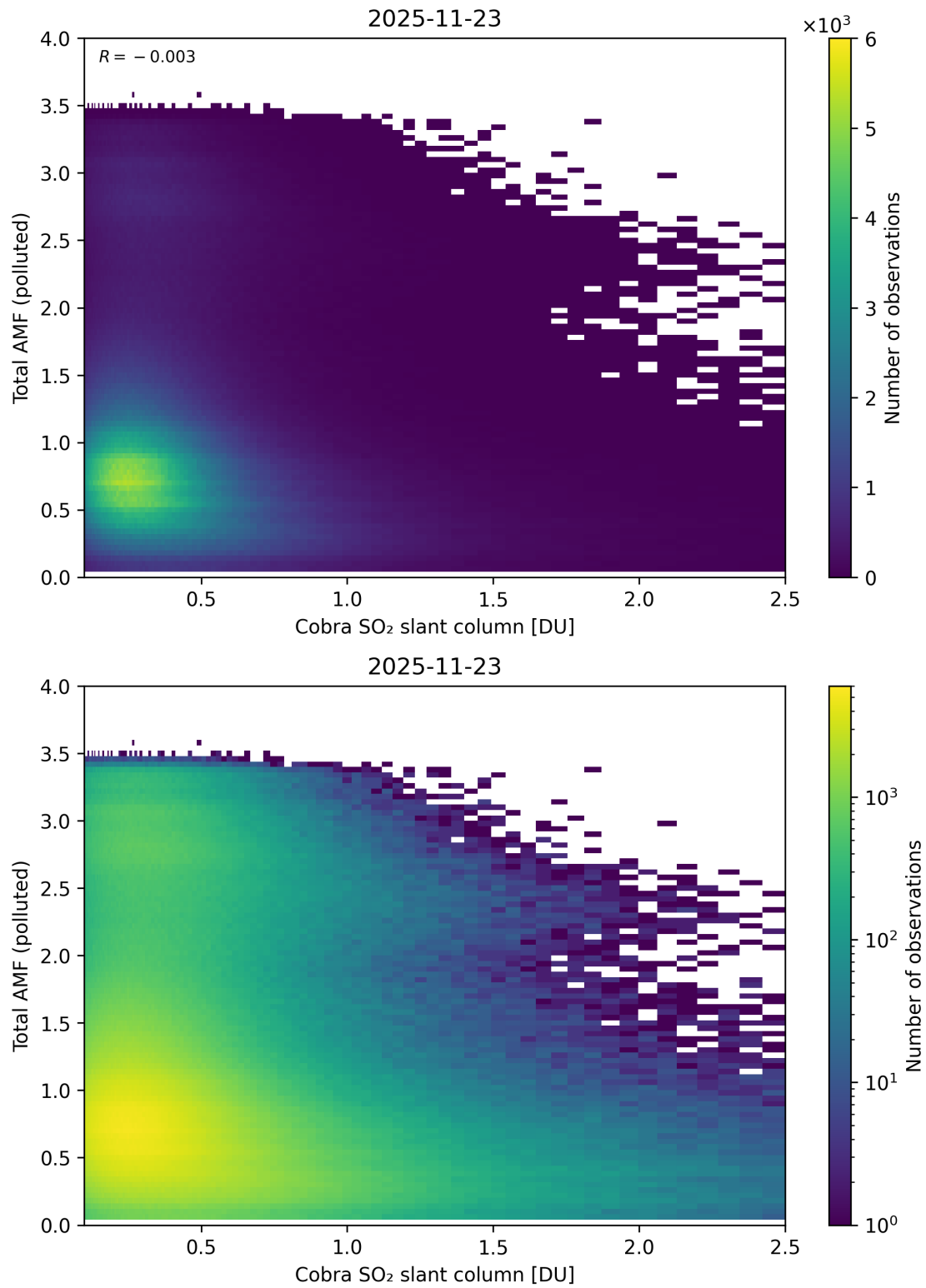
Figure 224: Scatter density plot of “Cobra SO 2 slant column” against “Total AMF (polluted)” for 2025-11-23 to 2025-11-24.
