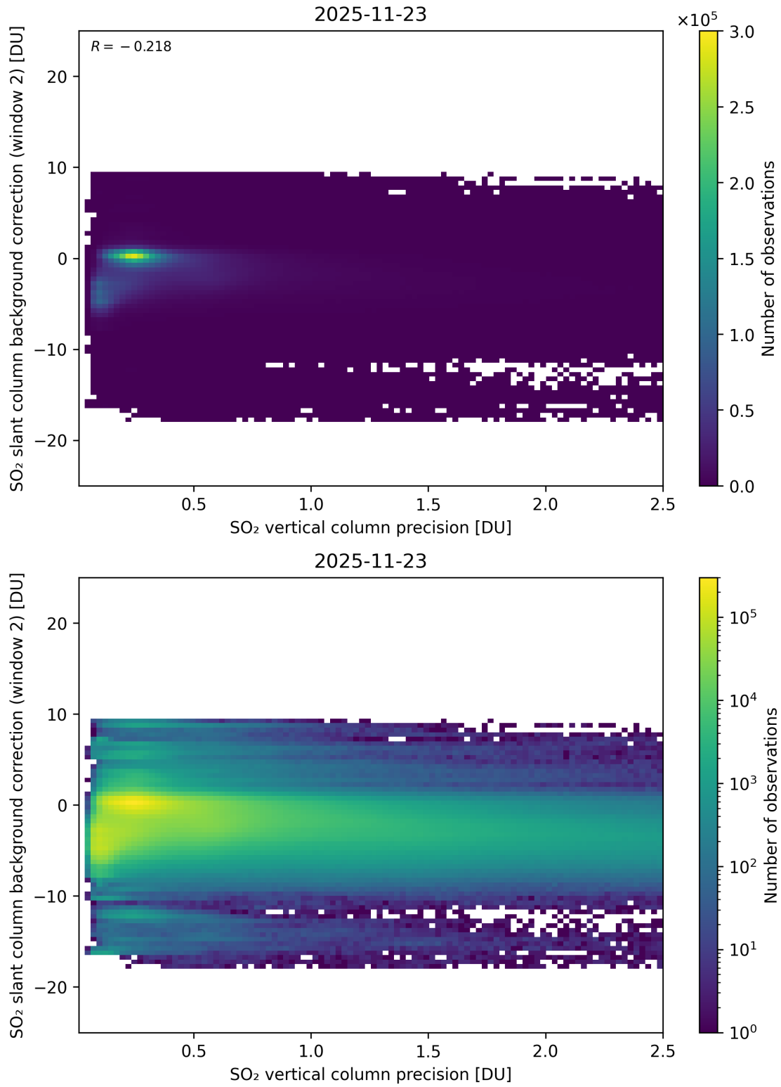
Figure 330: Scatter density plot of “SO 2 vertical column precision” against “SO 2 slant column background correction (window 2)” for 2025-11-23 to 2025-11-24.
