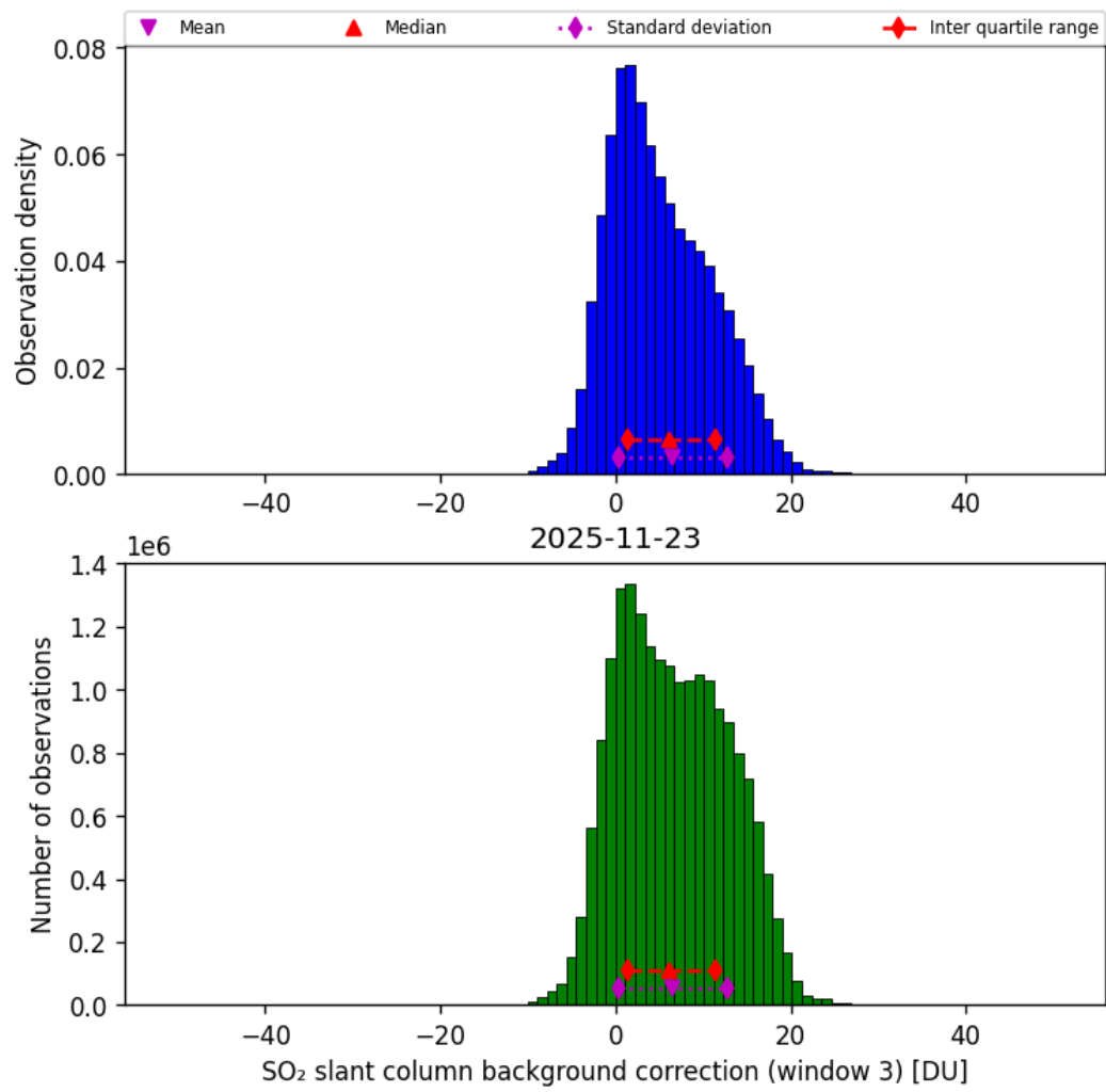
Figure 74: Histogram of “SO 2 slant column background correction (window 3)” for 2025-11-23 to 2025-11-24
