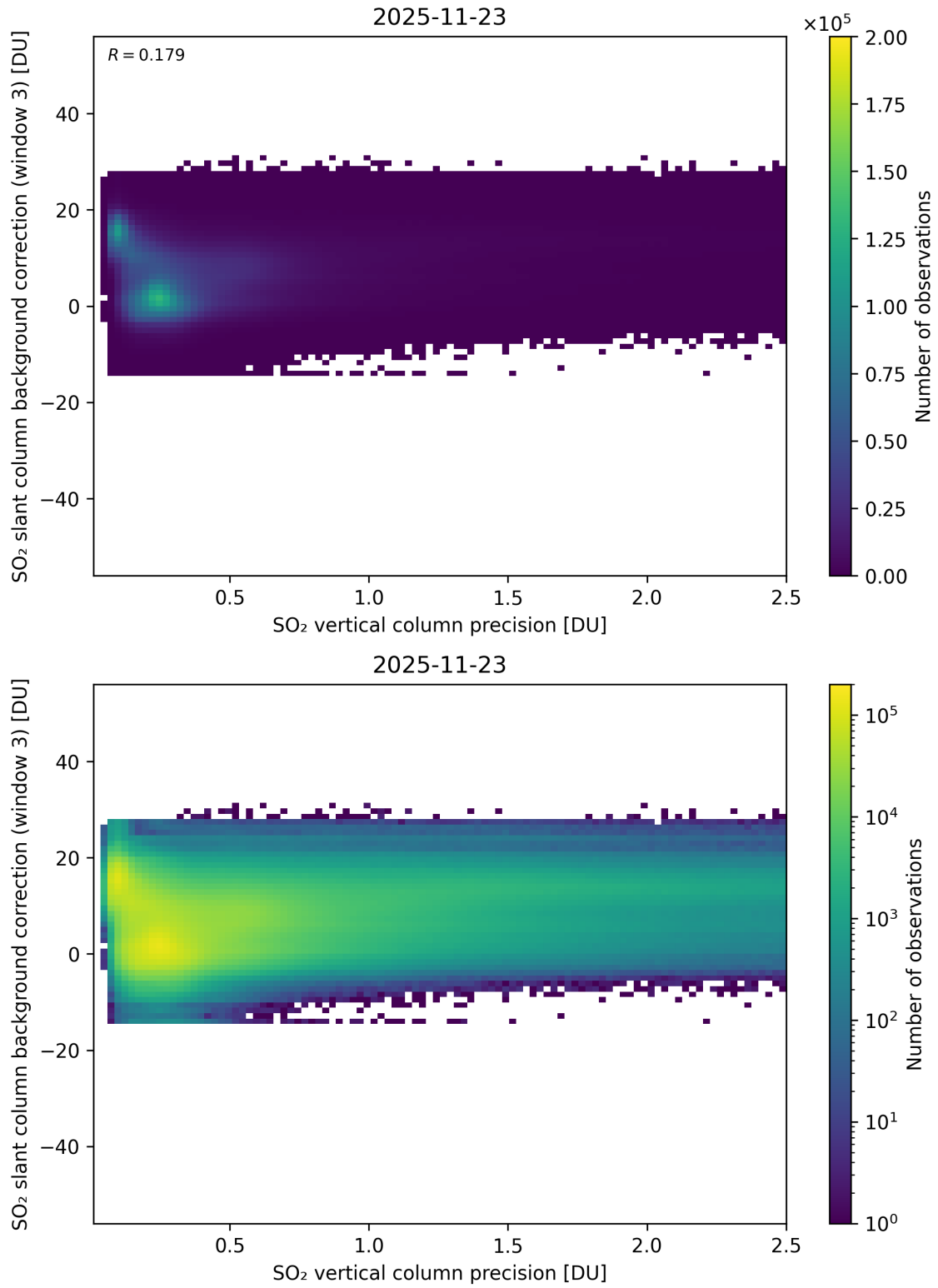
Figure 331: Scatter density plot of “SO 2 vertical column precision” against “SO 2 slant column background correction (window 3)” for 2025-11-23 to 2025-11-24.
