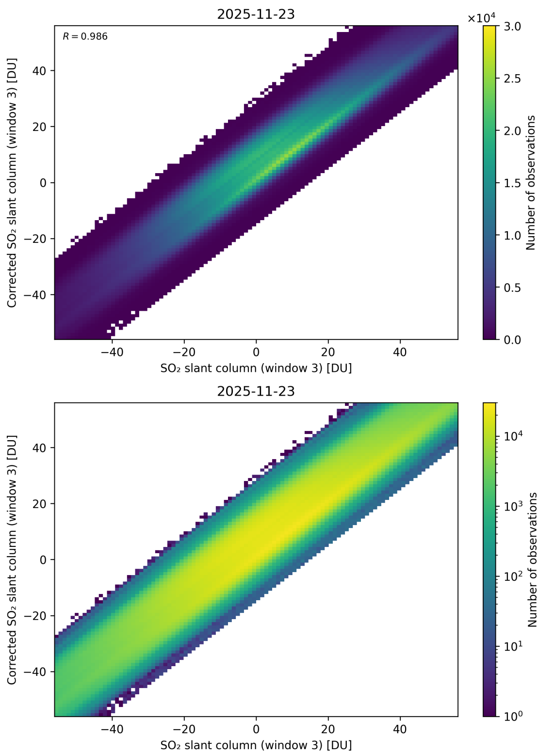
Figure 316: Scatter density plot of “SO 2 slant column (window 3)” against “Corrected SO 2 slant column (window 3)” for 2025-11-23 to 2025-11-24.
