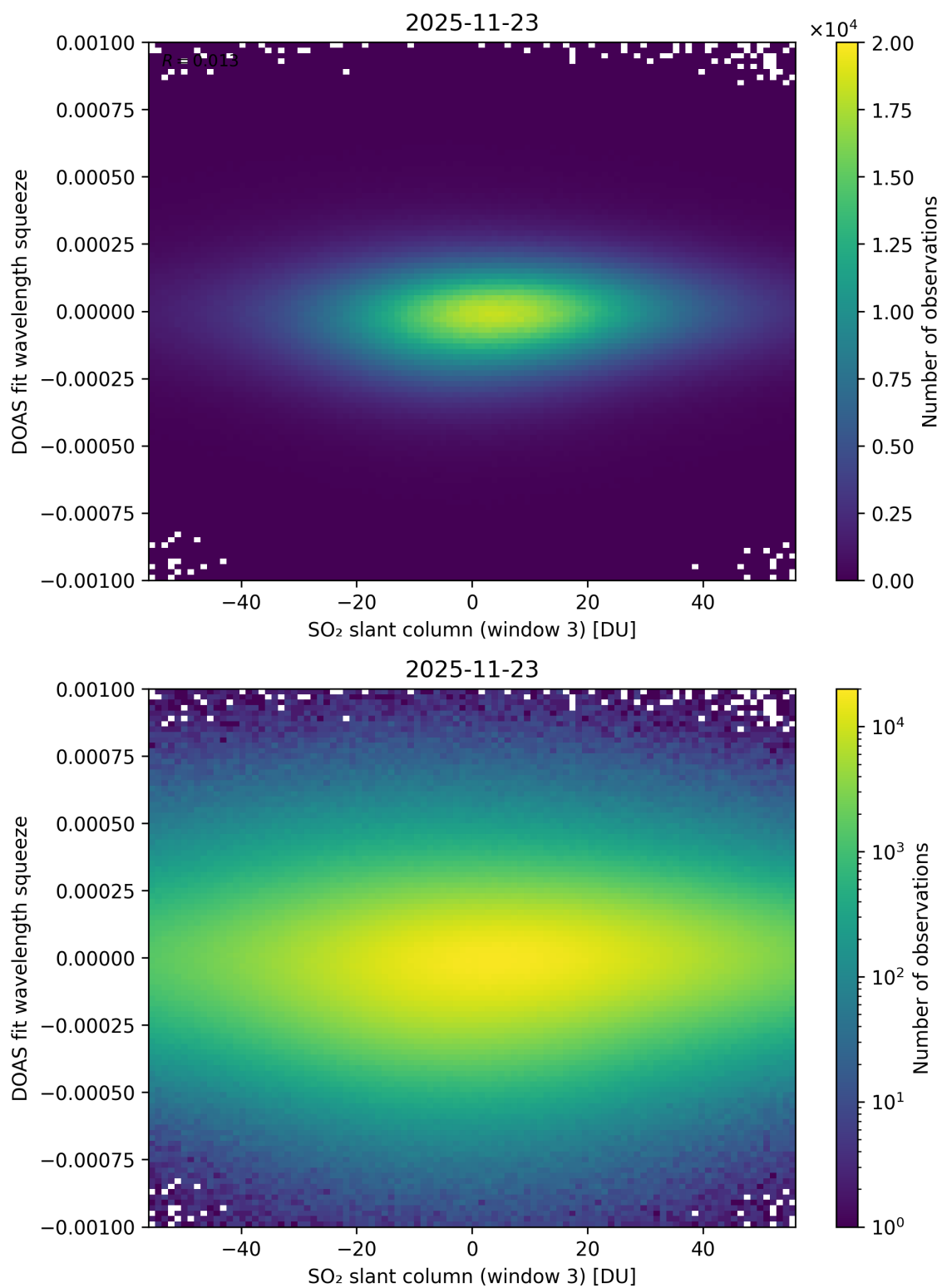
Figure 305: Scatter density plot of “SO 2 slant column (window 3)” against “DOAS fit wavelength squeeze” for 2025-11-23 to 2025-11-24.
