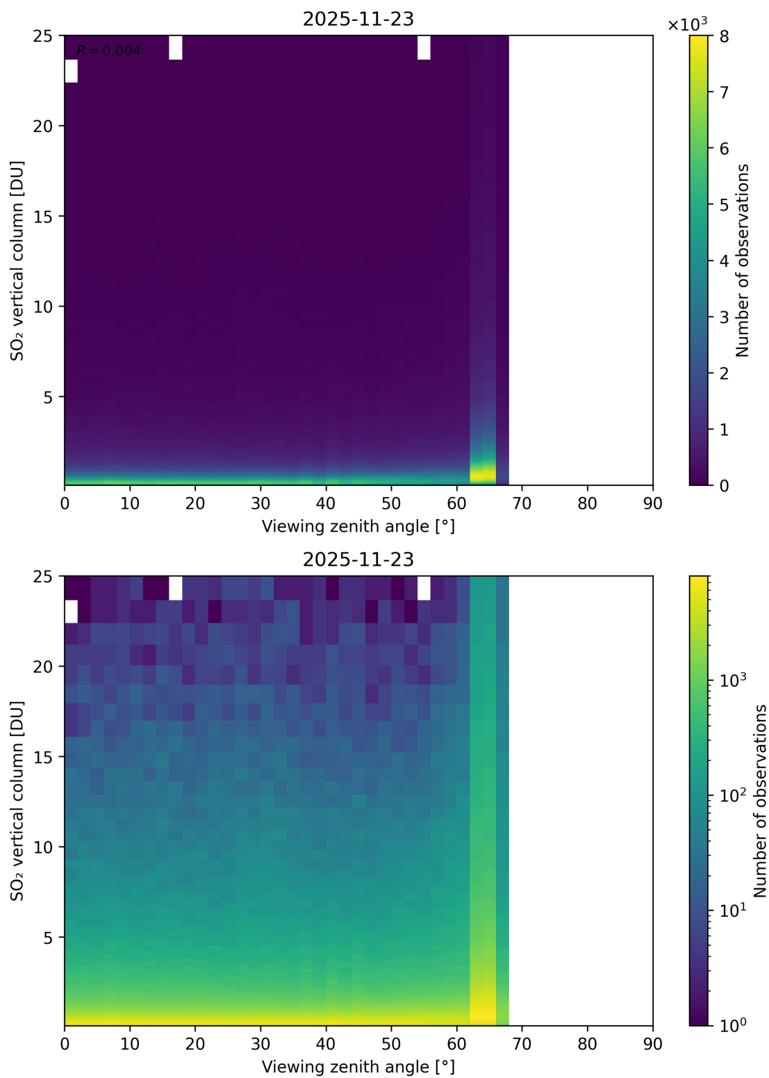
Figure 383: Scatter density plot of “Viewing zenith angle” against “SO 2 vertical column” for 2025-11-23 to 2025-11-24.
