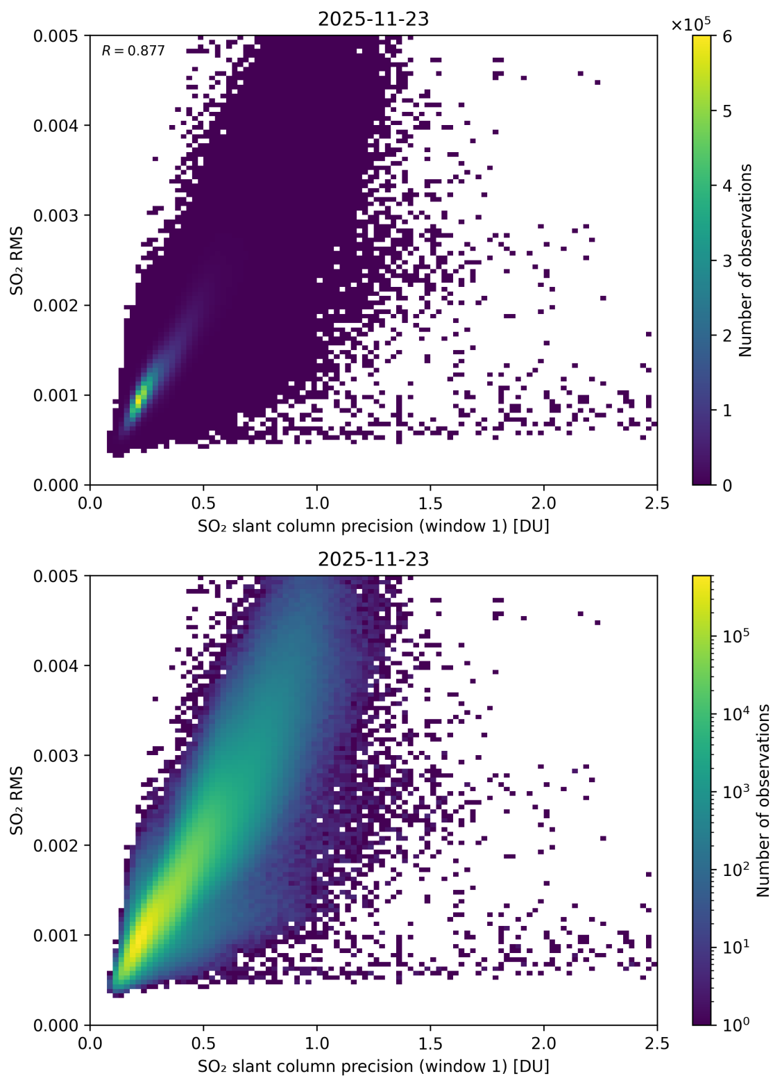
Figure 273: Scatter density plot of “SO 2 slant column precision (window 1)” against “SO 2 RMS” for 2025-11-23 to 2025-11-24.
