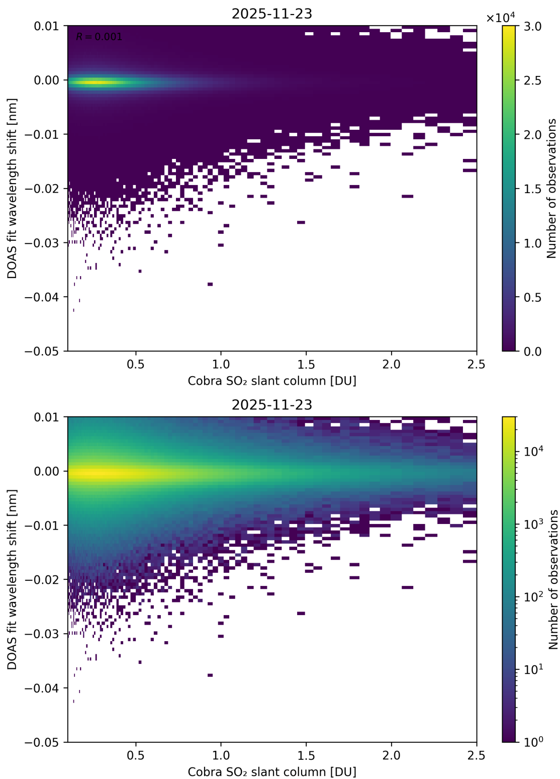
Figure 196: Scatter density plot of “Cobra SO 2 slant column” against “DOAS fit wavelength shift” for 2025-11-23 to 2025-11-24.
