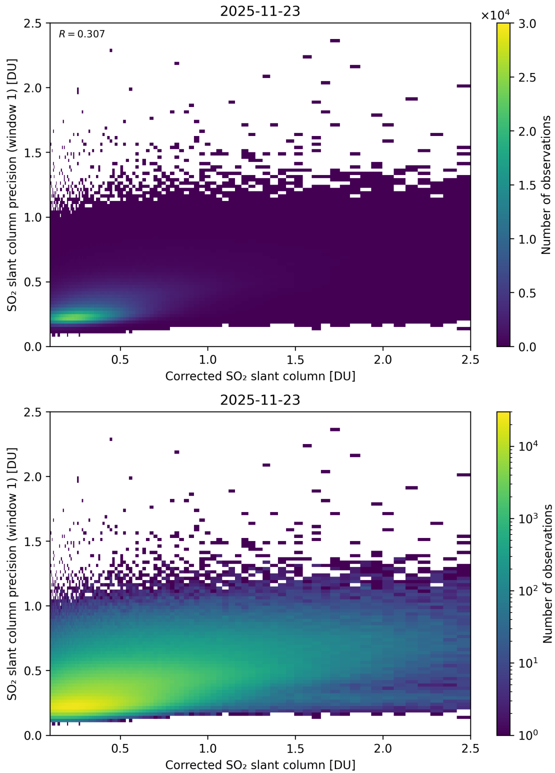
Figure 238: Scatter density plot of “Corrected SO 2 slant column” against “SO 2 slant column precision (window 1)” for 2025-11-23 to 2025-11-24.
