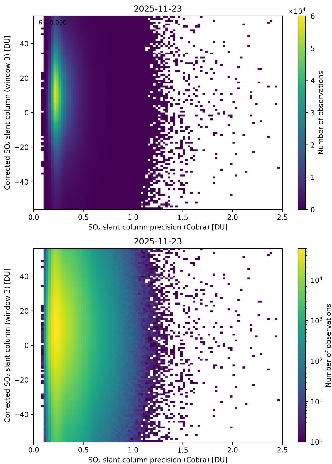
Figure 207: Scatter density plot of “SO 2 slant column precision (Cobra)” against “Corrected SO 2 slant column (window 3)” for 2025-11-23 to 2025-11-24.
