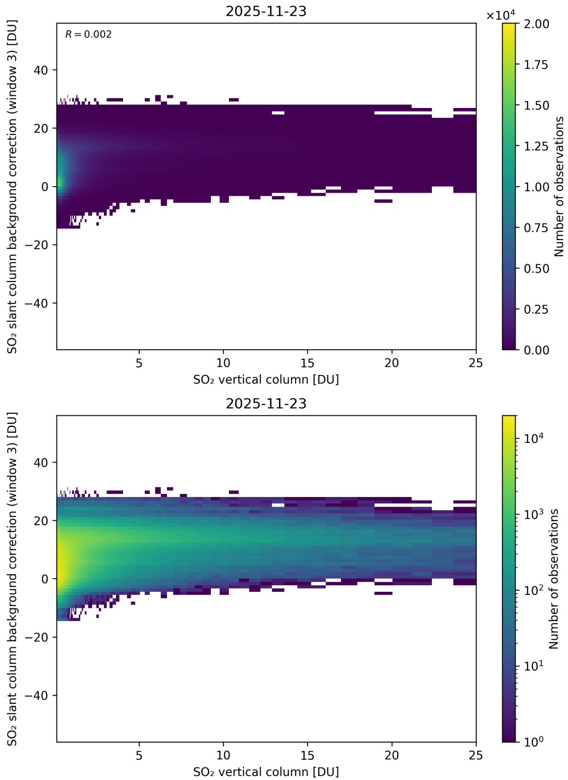
Figure 325: Scatter density plot of “SO 2 vertical column” against “SO 2 slant column background correction (window 3)” for 2025-11-23 to 2025-11-24.
