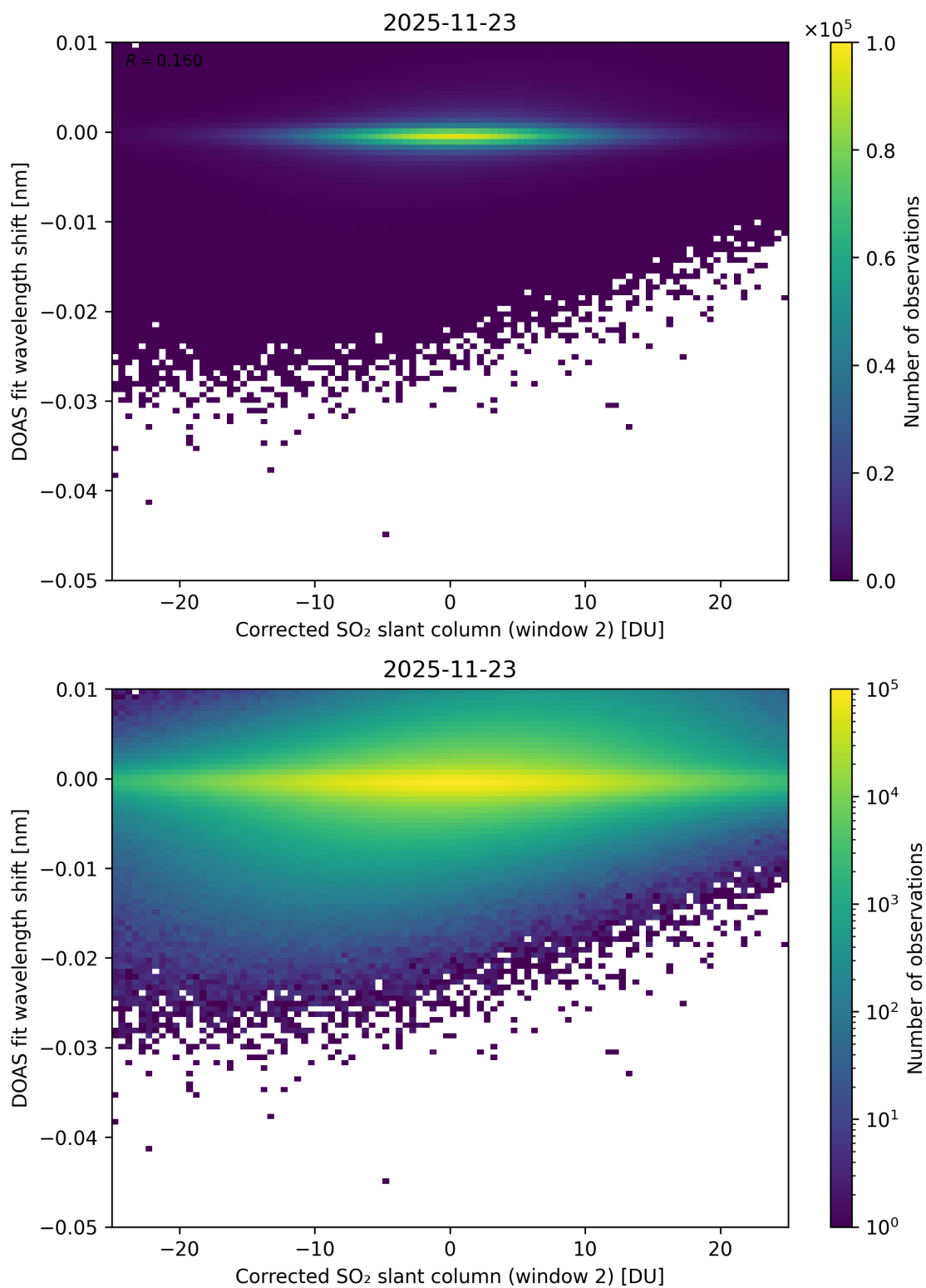
Figure 246: Scatter density plot of “Corrected SO 2 slant column (window 2)” against “DOAS fit wavelength shift” for 2025-11-23 to 2025-11-24.
