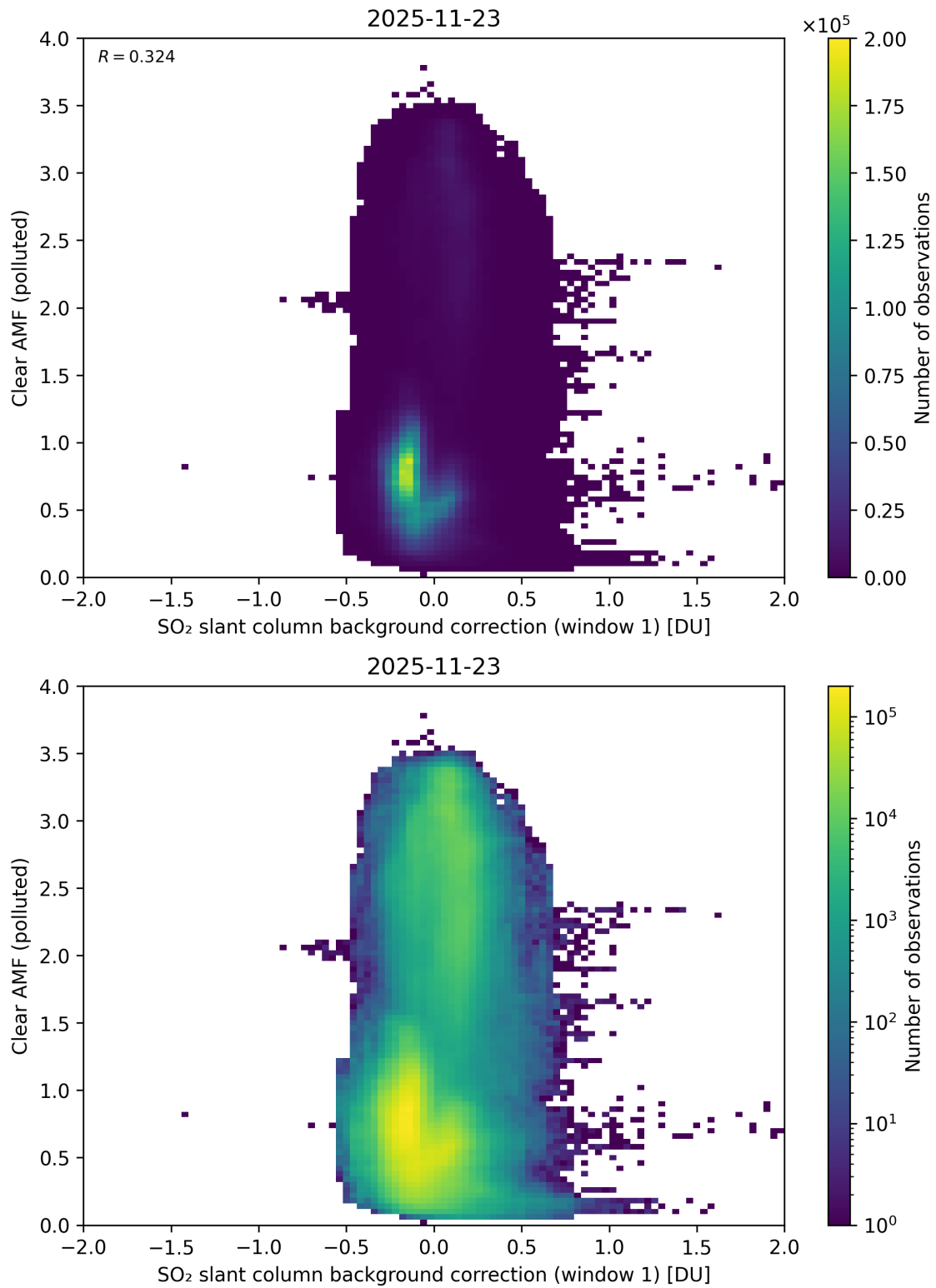
Figure 114: Scatter density plot of “SO 2 slant column background correction (window 1)” against “Clear AMF (polluted)” for 2025-11-23 to 2025-11-24.
