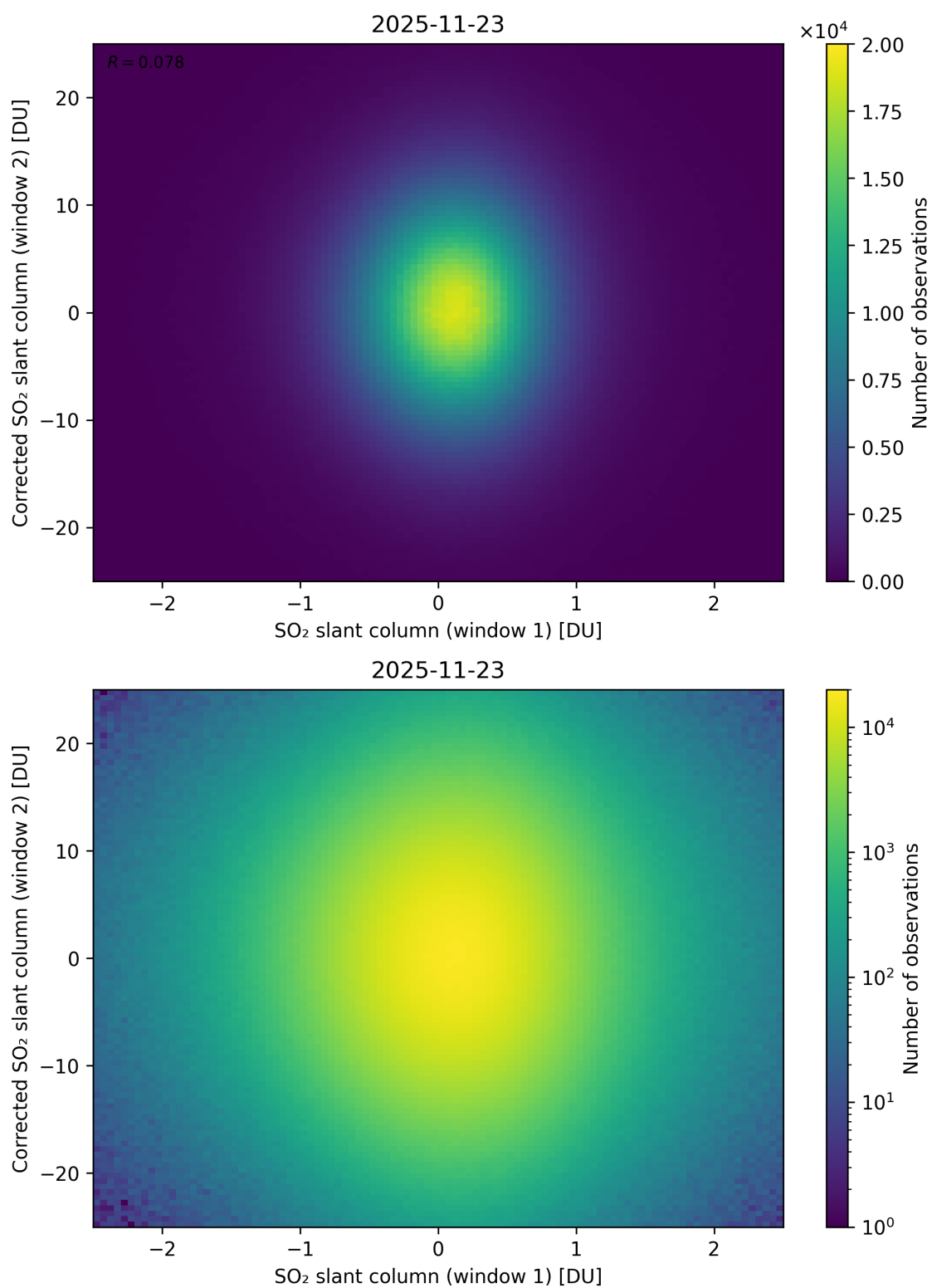
Figure 283: Scatter density plot of “SO 2 slant column (window 1)” against “Corrected SO 2 slant column (window 2)” for 2025-11-23 to 2025-11-24.
