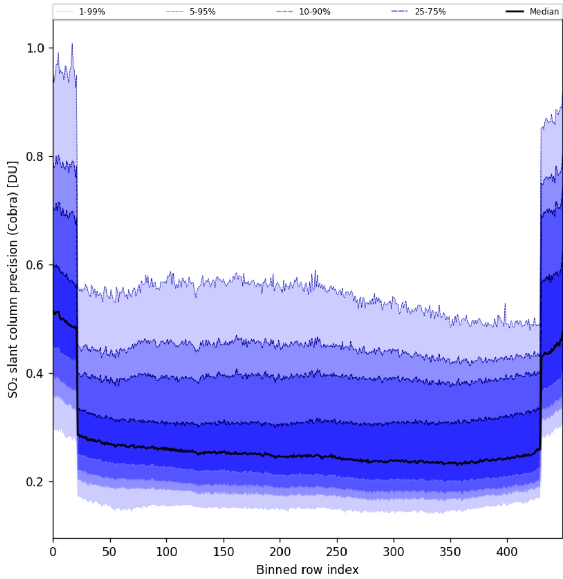
Figure 88: Along track statistics of “SO 2 slant column precision (Cobra)” for 2025-11-23 to 2025-11-24
