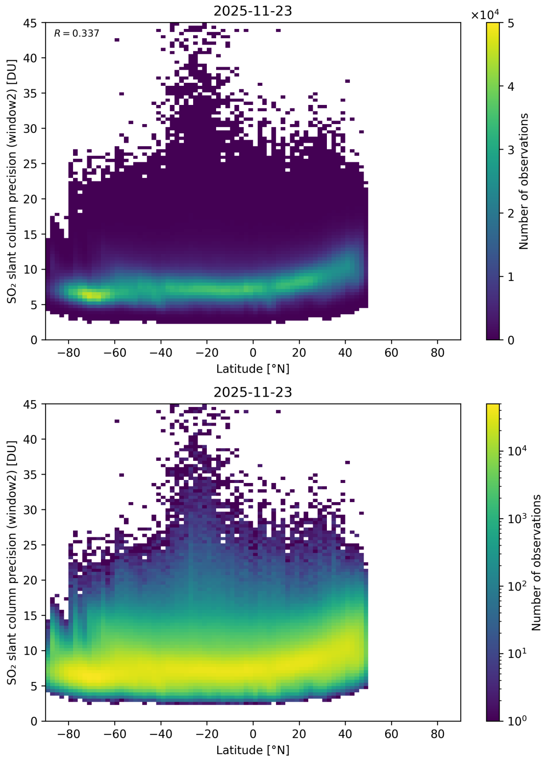
Figure 164: Scatter density plot of “Latitude” against “SO 2 slant column precision (window2)” for 2025-11-23 to 2025-11-24.
