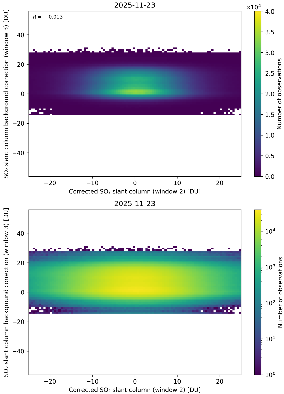
Figure 245: Scatter density plot of “Corrected SO 2 slant column (window 2)” against “SO 2 slant column background correction (window 3)” for 2025-11-23 to 2025-11-24.
