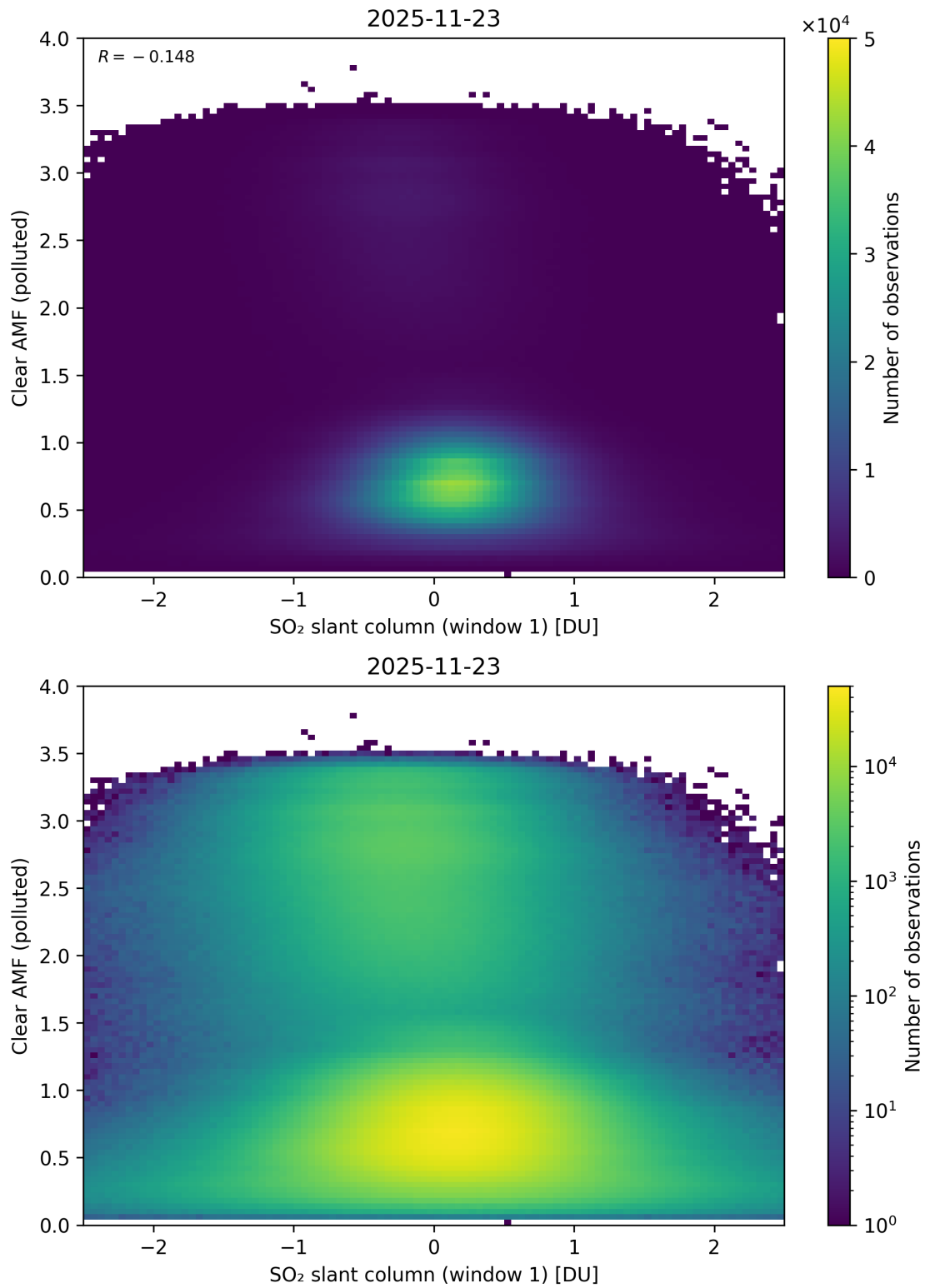
Figure 282: Scatter density plot of “SO 2 slant column (window 1)” against “Clear AMF (polluted)” for 2025-11-23 to 2025-11-24.
