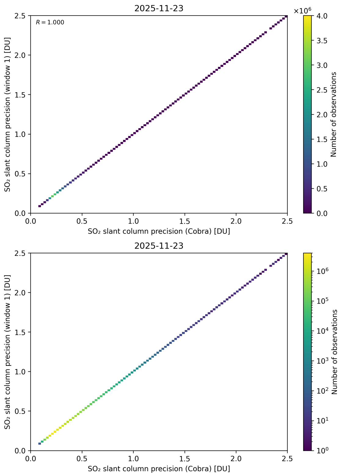
Figure 209: Scatter density plot of “SO 2 slant column precision (Cobra)” against “SO 2 slant column precision (window 1)” for 2025-11-23 to 2025-11-24.
