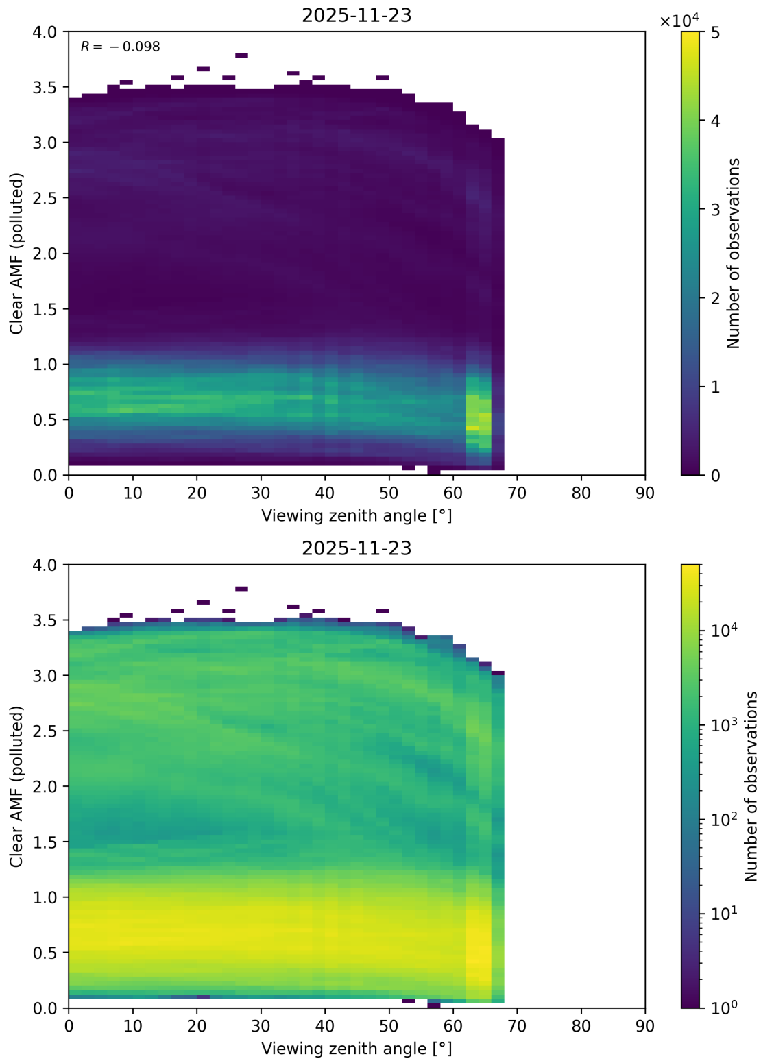
Figure 370: Scatter density plot of “Viewing zenith angle” against “Clear AMF (polluted)” for 2025-11-23 to 2025-11-24.
