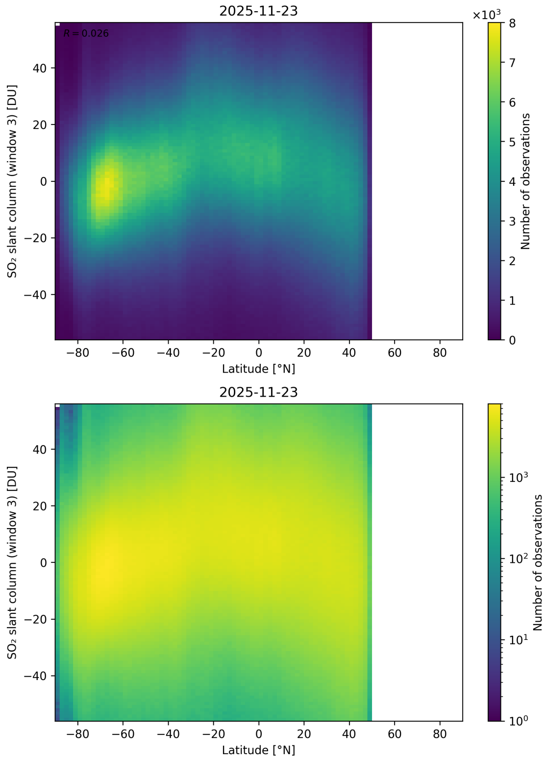
Figure 165: Scatter density plot of “Latitude” against “SO 2 slant column (window 3)” for 2025-11-23 to 2025-11-24.
