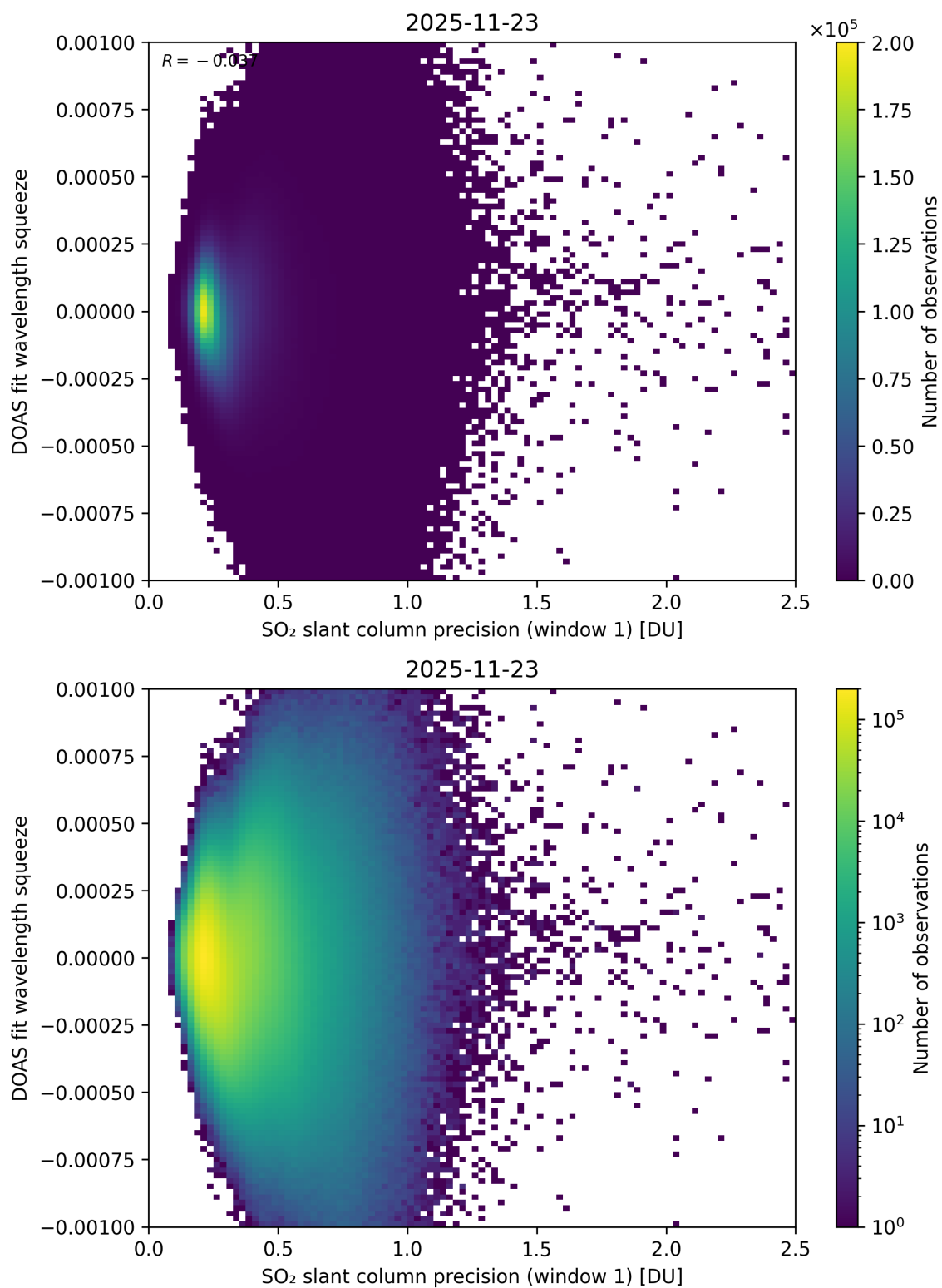
Figure 272: Scatter density plot of “SO 2 slant column precision (window 1)” against “DOAS fit wavelength squeeze” for 2025-11-23 to 2025-11-24.
