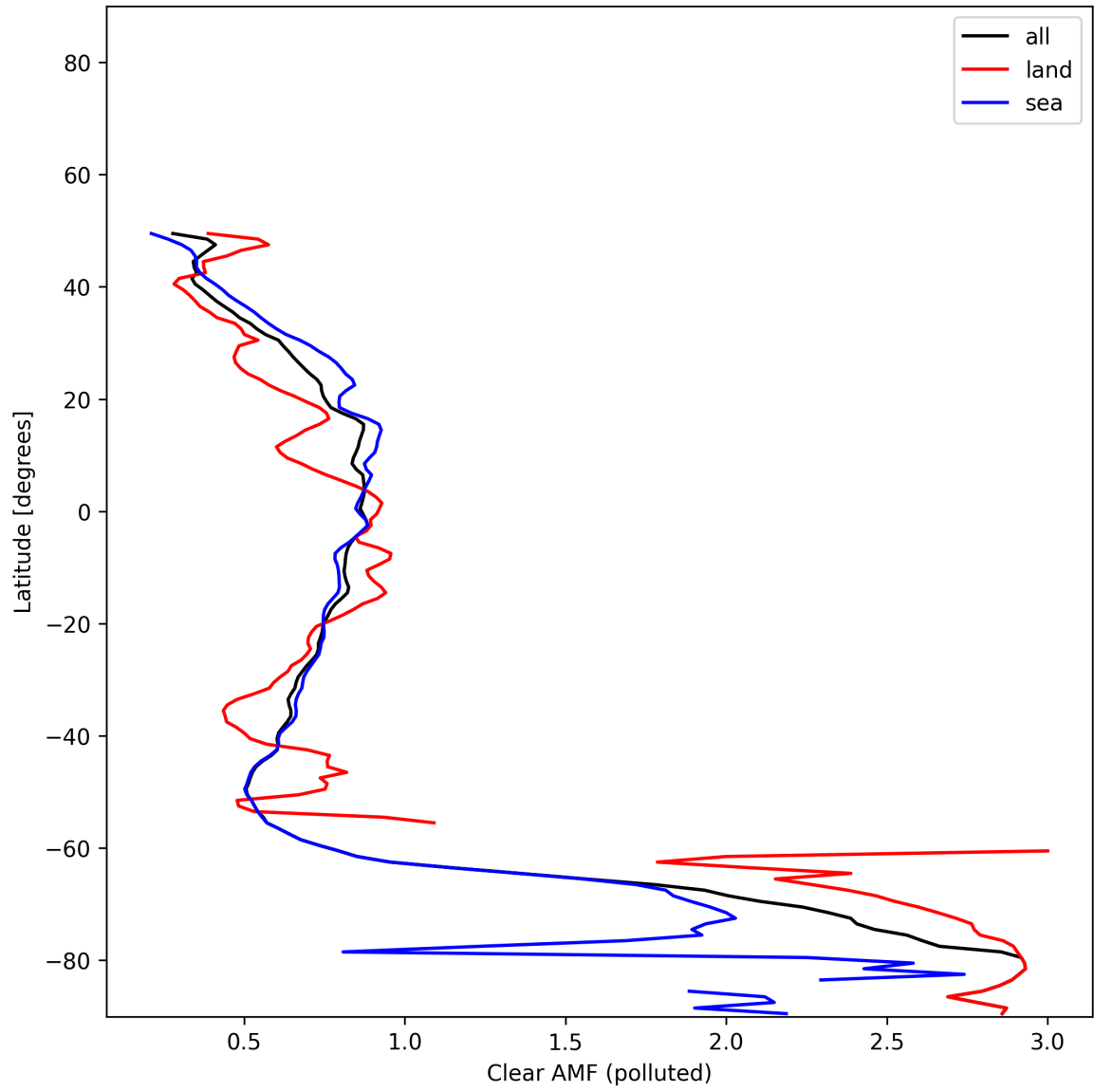
Figure 55: Zonal average of “Clear AMF (polluted)” for 2025-11-23 to 2025-11-24.
