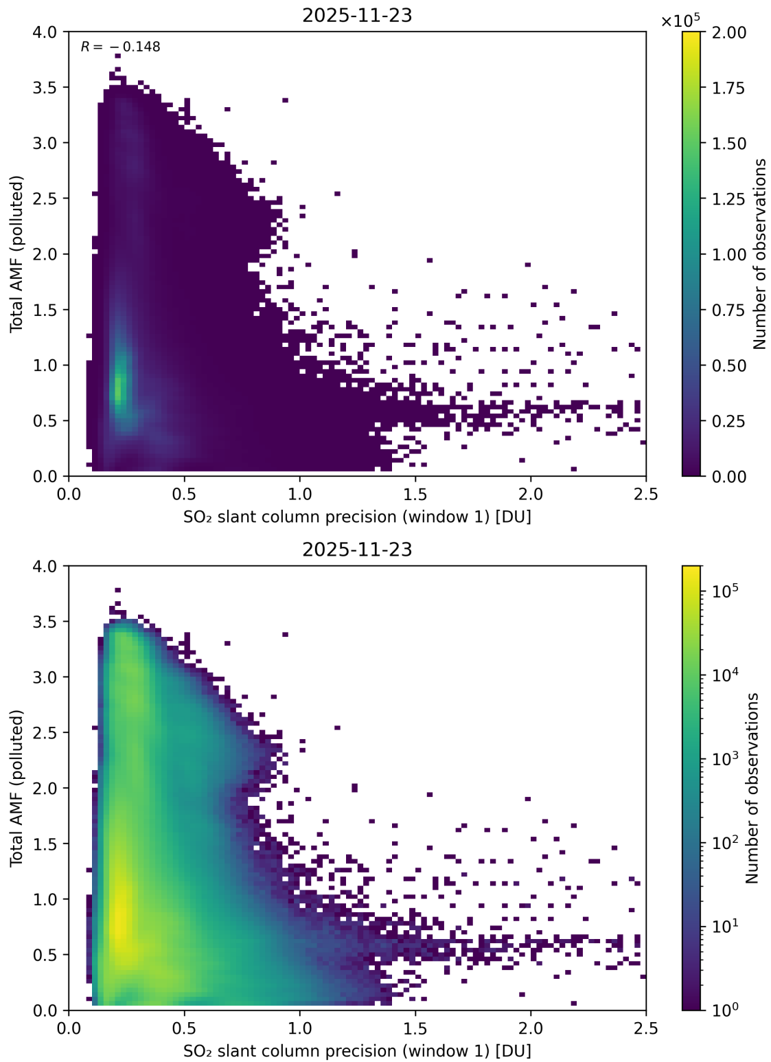
Figure 280: Scatter density plot of “SO 2 slant column precision (window 1)” against “Total AMF (polluted)” for 2025-11-23 to 2025-11-24.
