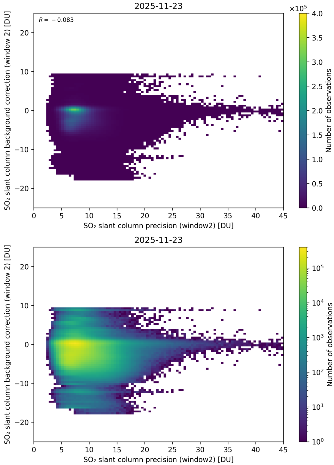
Figure 291: Scatter density plot of “SO 2 slant column precision (window2)” against “SO 2 slant column background correction (window 2)” for 2025-11-23 to 2025-11-24.
