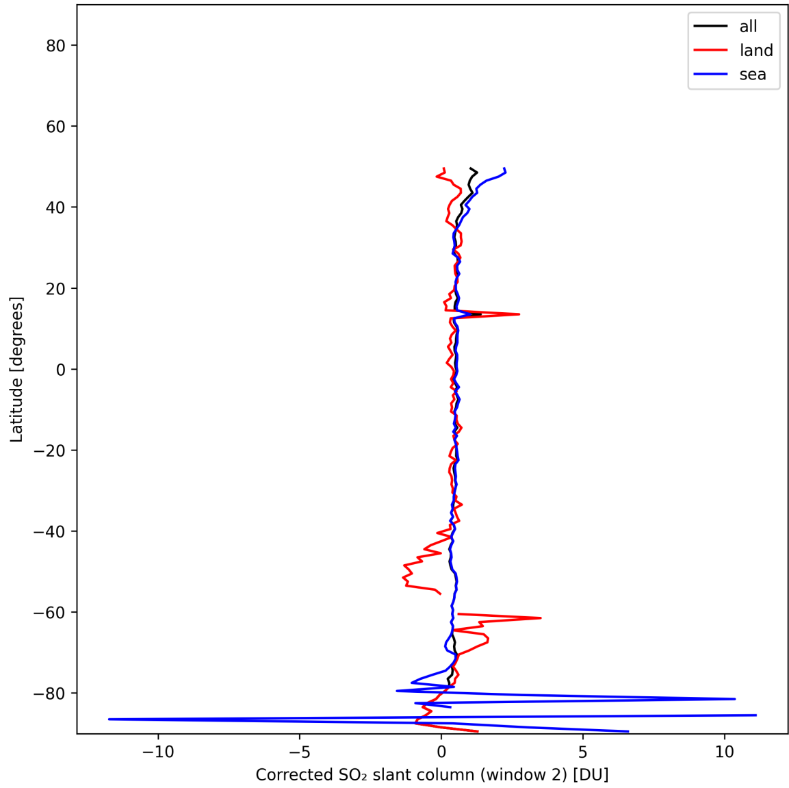
Figure 43: Zonal average of “Corrected SO 2 slant column (window 2)” for 2025-11-23 to 2025-11-24.
