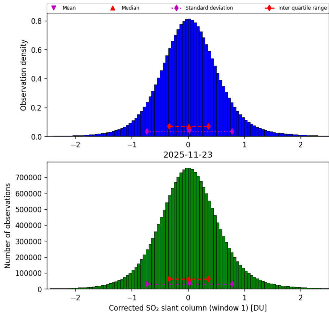
Figure 65: Histogram of “Corrected SO 2 slant column (window 1)” for 2025-11-23 to 2025-11-24
