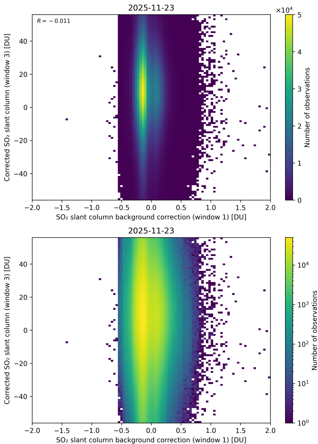
Figure 116: Scatter density plot of “SO 2 slant column background correction (window 1)” against “Corrected SO 2 slant column (window 3)” for 2025-11-23 to 2025-11-24.
