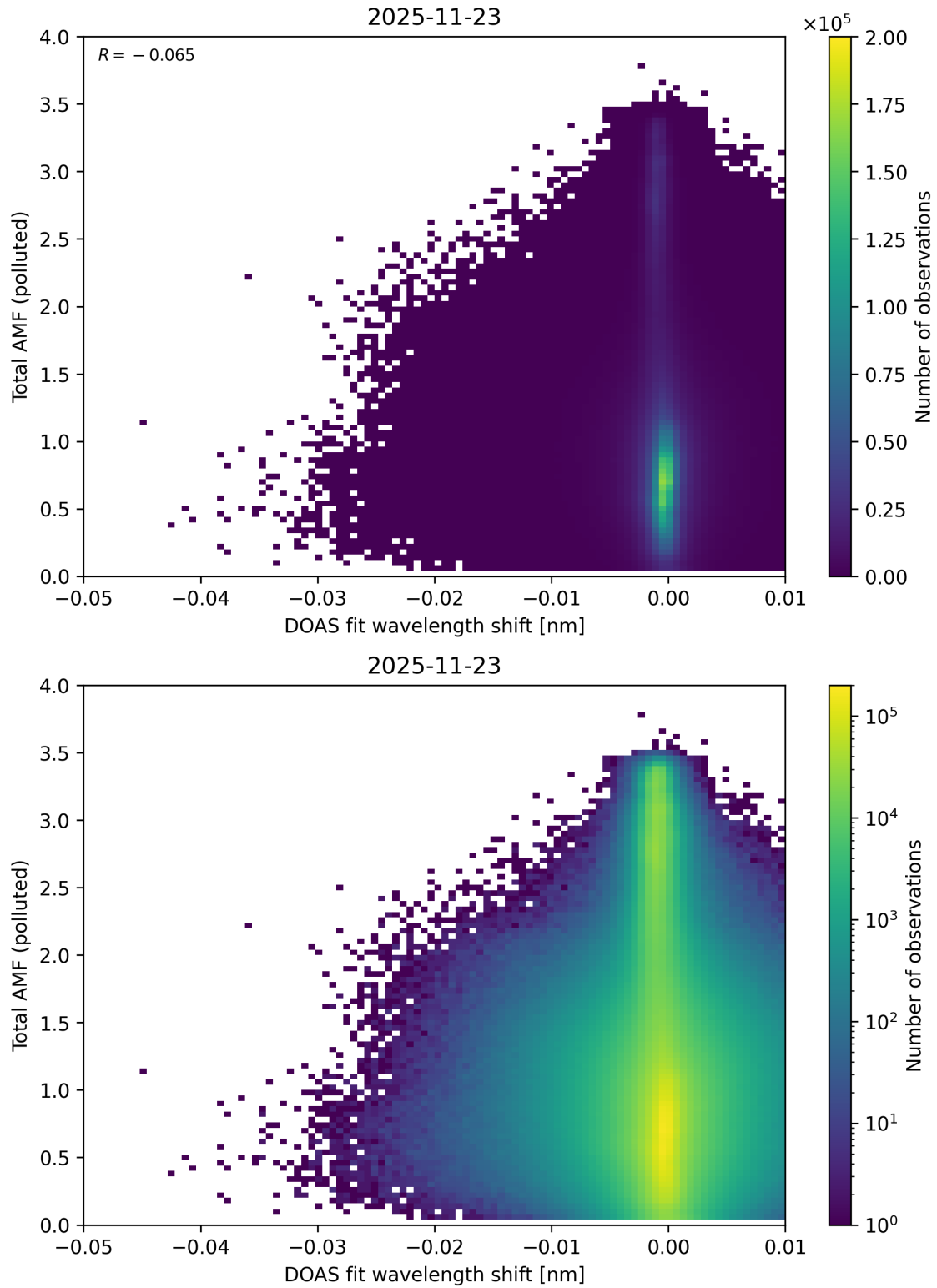
Figure 141: Scatter density plot of “DOAS fit wavelength shift” against “Total AMF (polluted)” for 2025-11-23 to 2025-11-24.
