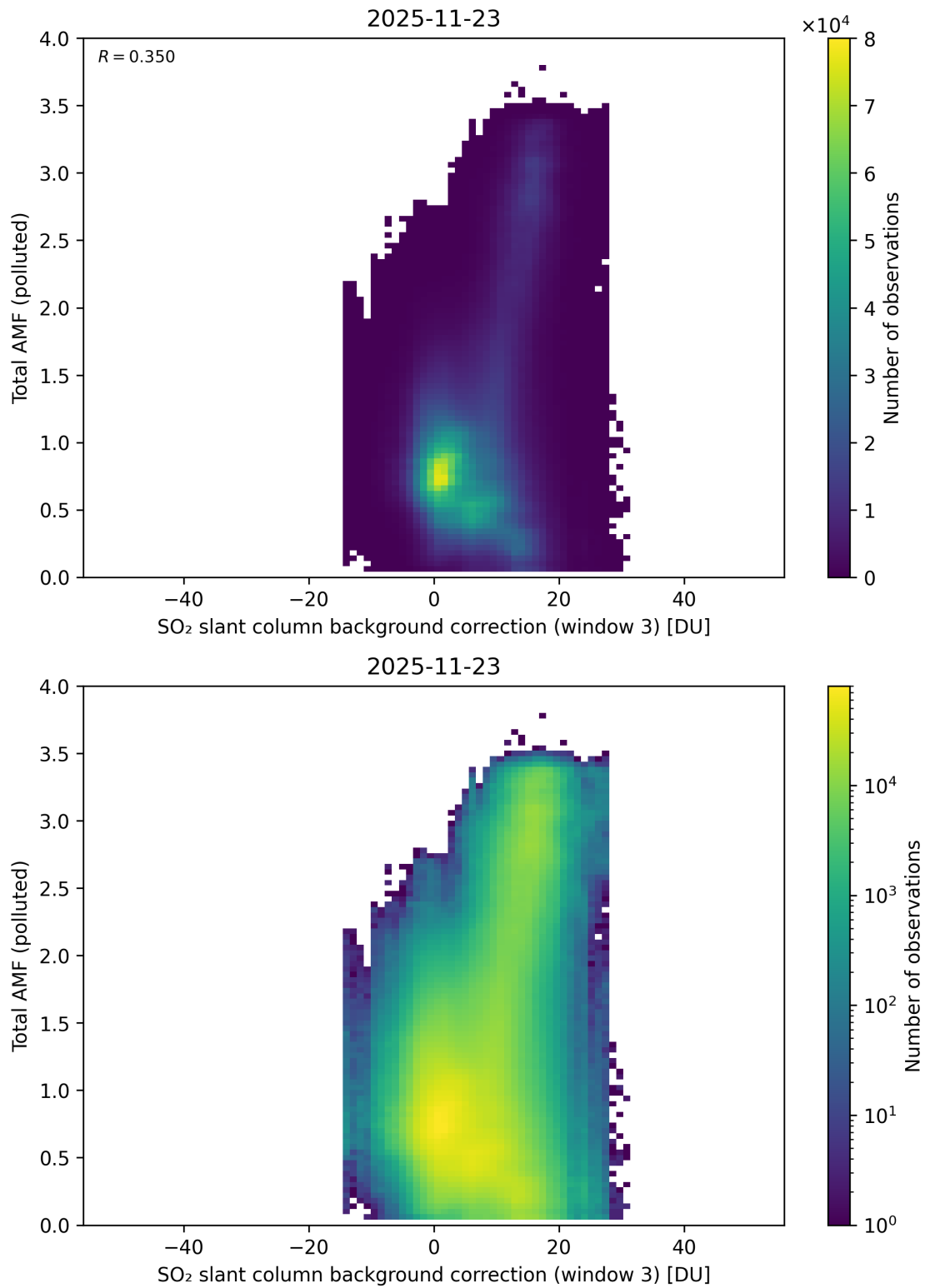
Figure 136: Scatter density plot of “SO 2 slant column background correction (window 3)” against “Total AMF (polluted)” for 2025-11-23 to 2025-11-24.
