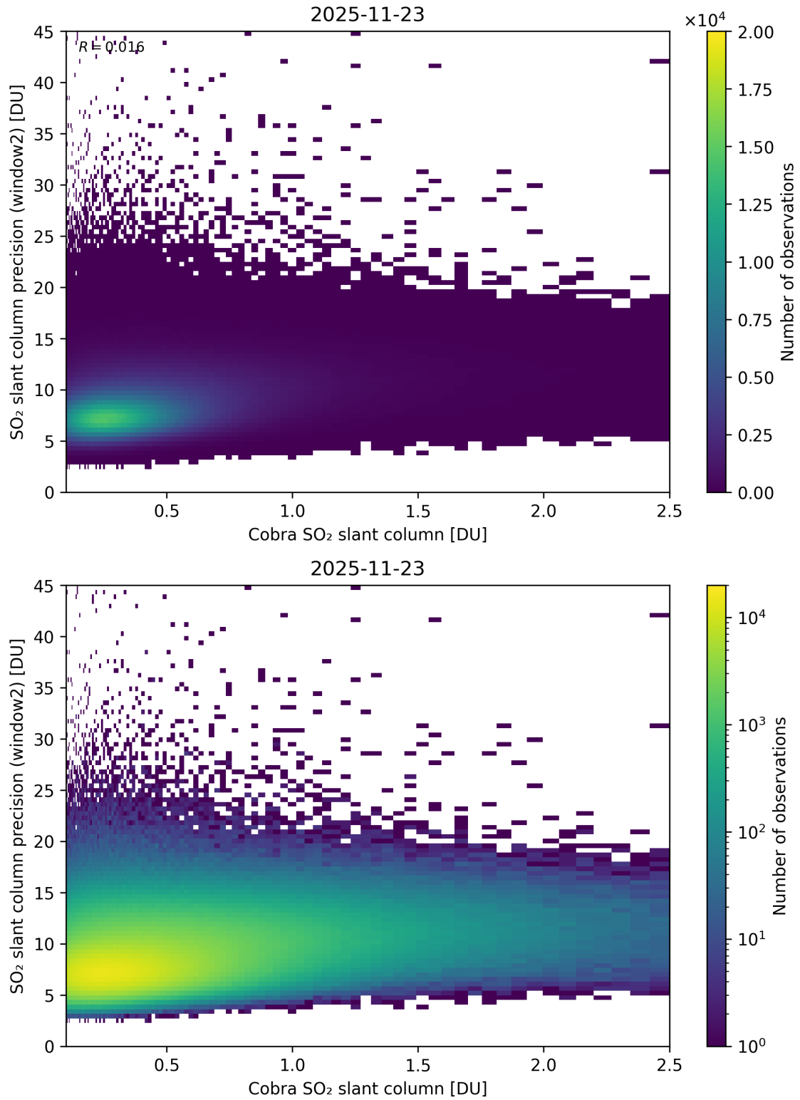
Figure 221: Scatter density plot of “Cobra SO 2 slant column” against “SO 2 slant column precision (window2)” for 2025-11-23 to 2025-11-24.
