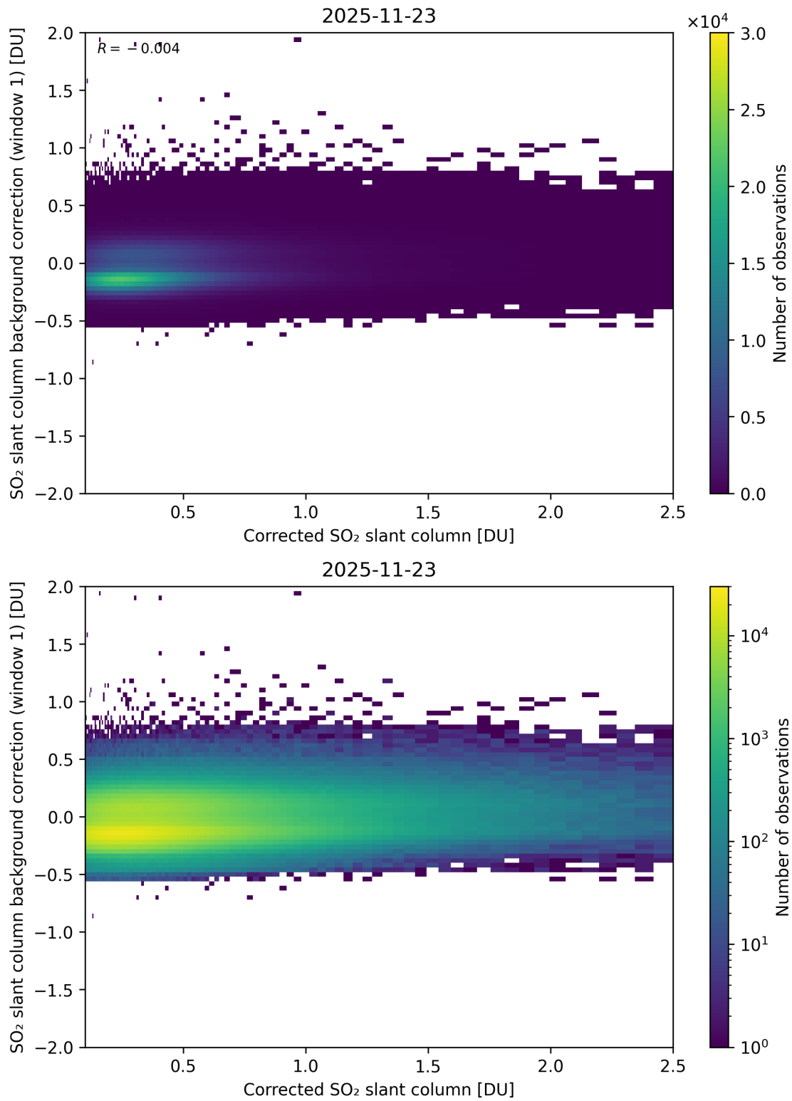
Figure 226: Scatter density plot of “Corrected SO 2 slant column” against “SO 2 slant column background correction (window 1)” for 2025-11-23 to 2025-11-24.
