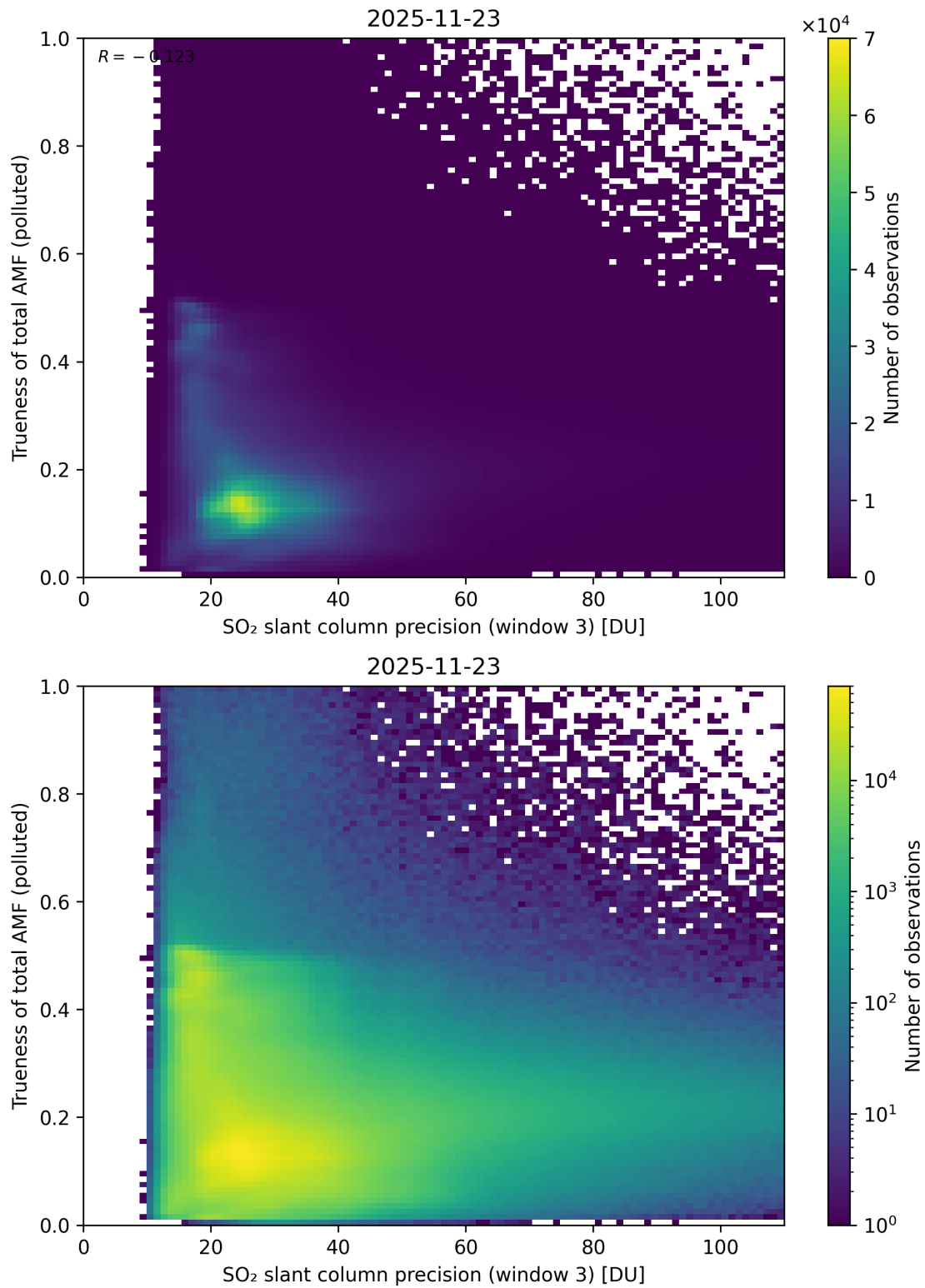
Figure 314: Scatter density plot of “SO 2 slant column precision (window 3)” against “Trueness of total AMF (polluted)” for 2025-11-23 to 2025-11-24.
