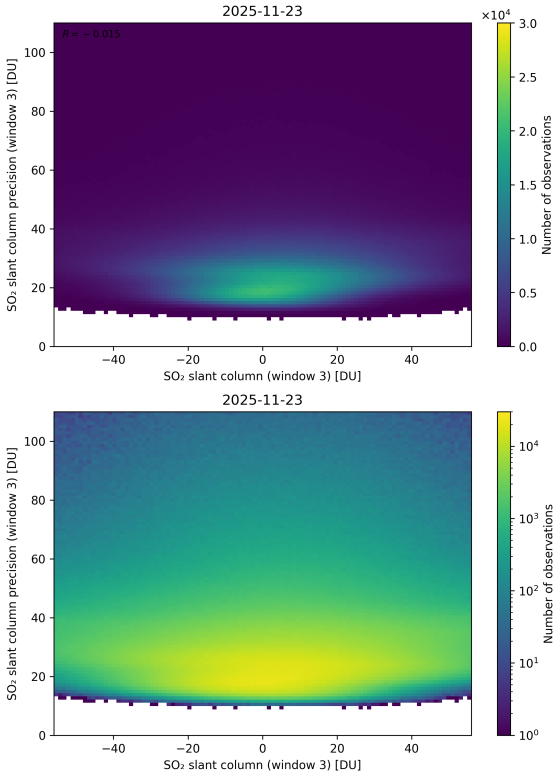
Figure 317: Scatter density plot of “SO 2 slant column (window 3)” against “SO 2 slant column precision (window 3)” for 2025-11-23 to 2025-11-24.
