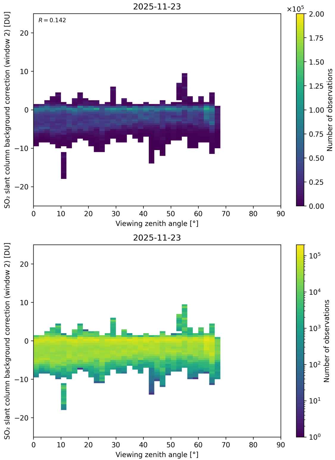
Figure 363: Scatter density plot of “Viewing zenith angle” against “SO 2 slant column background correction (window 2)” for 2025-11-23 to 2025-11-24.
