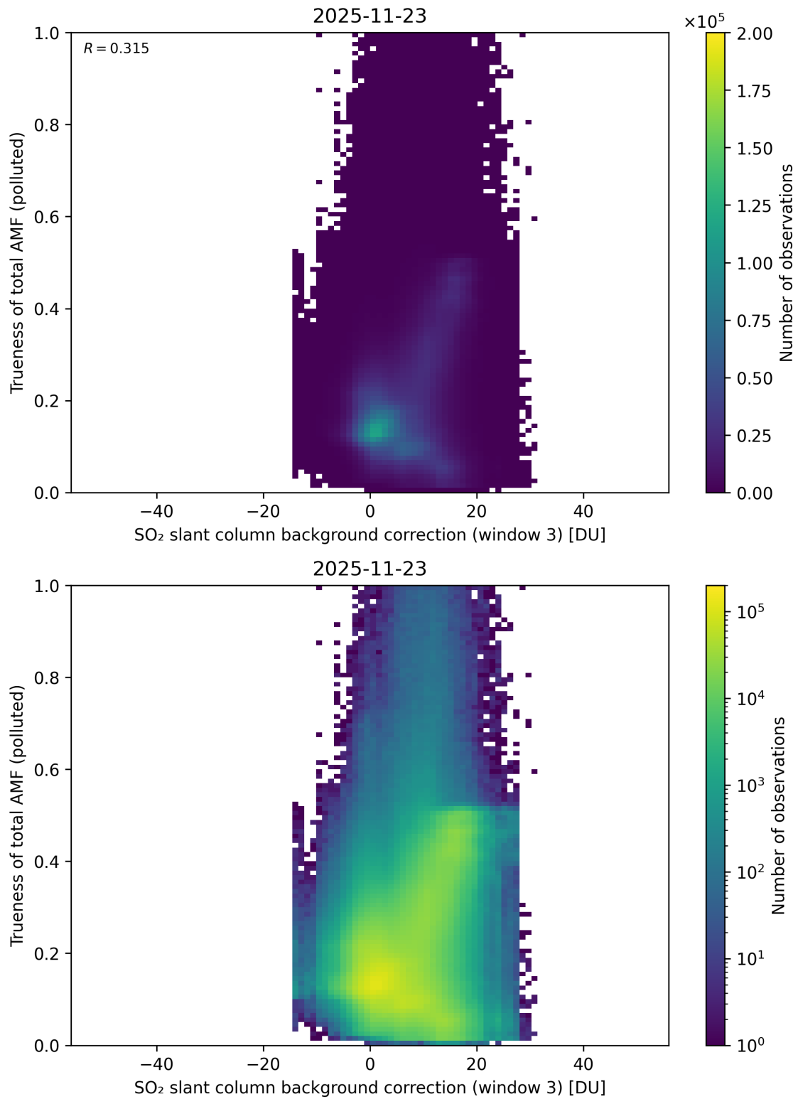
Figure 137: Scatter density plot of “SO 2 slant column background correction (window 3)” against “Trueness of total AMF (polluted)” for 2025-11-23 to 2025-11-24.
