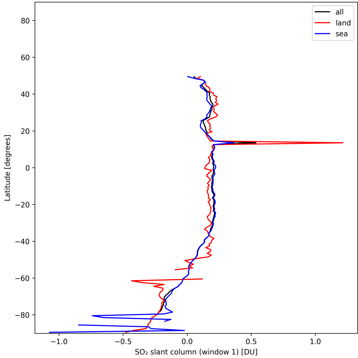
Figure 37: Zonal average of “SO 2 slant column (window 1)” for 2025-11-23 to 2025-11-24.
