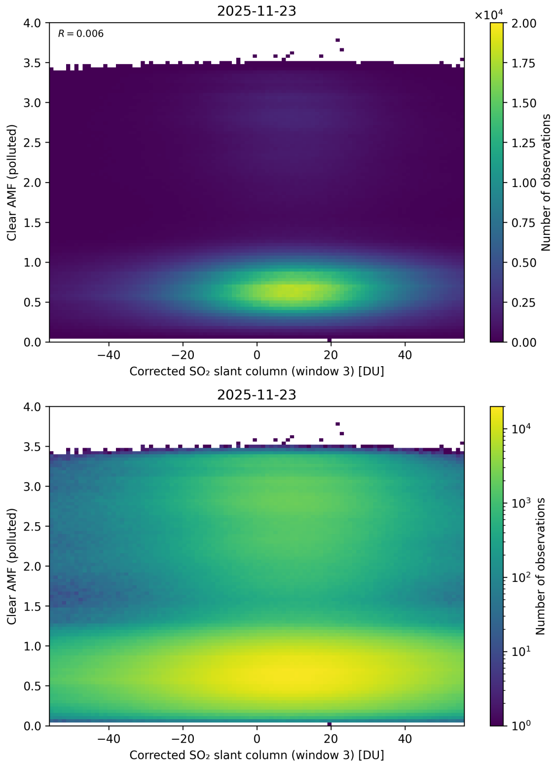
Figure 259: Scatter density plot of “Corrected SO 2 slant column (window 3)” against “Clear AMF (polluted)” for 2025-11-23 to 2025-11-24.
