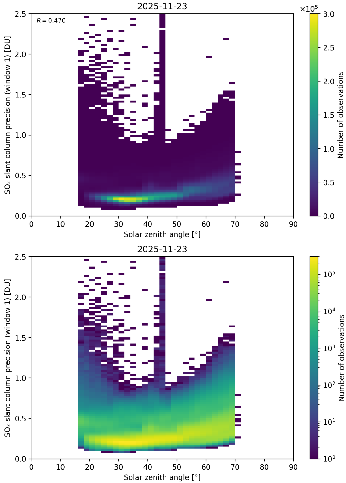
Figure 185: Scatter density plot of “Solar zenith angle” against “SO 2 slant column precision (window 1)” for 2025-11-23 to 2025-11-24.
