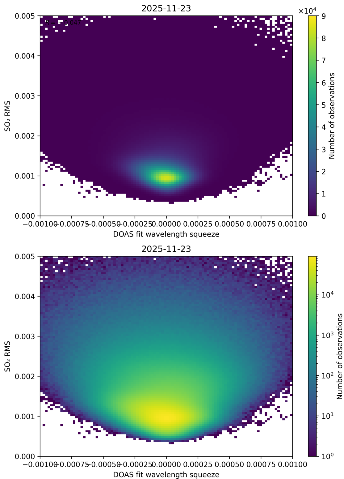
Figure 143: Scatter density plot of “DOAS fit wavelength squeeze” against “SO 2 RMS” for 2025-11-23 to 2025-11-24.
