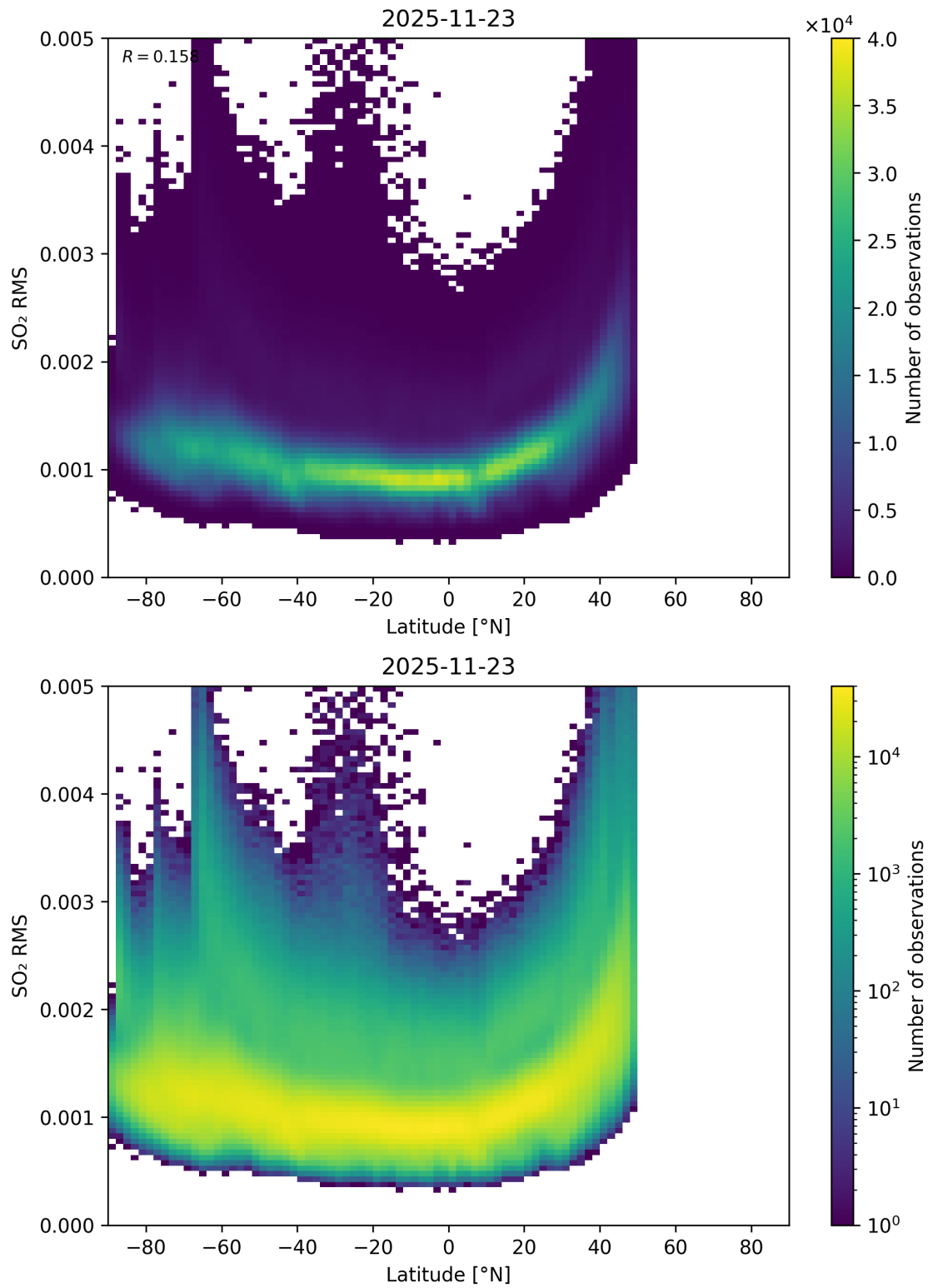
Figure 155: Scatter density plot of “Latitude” against “SO 2 RMS” for 2025-11-23 to 2025-11-24.
