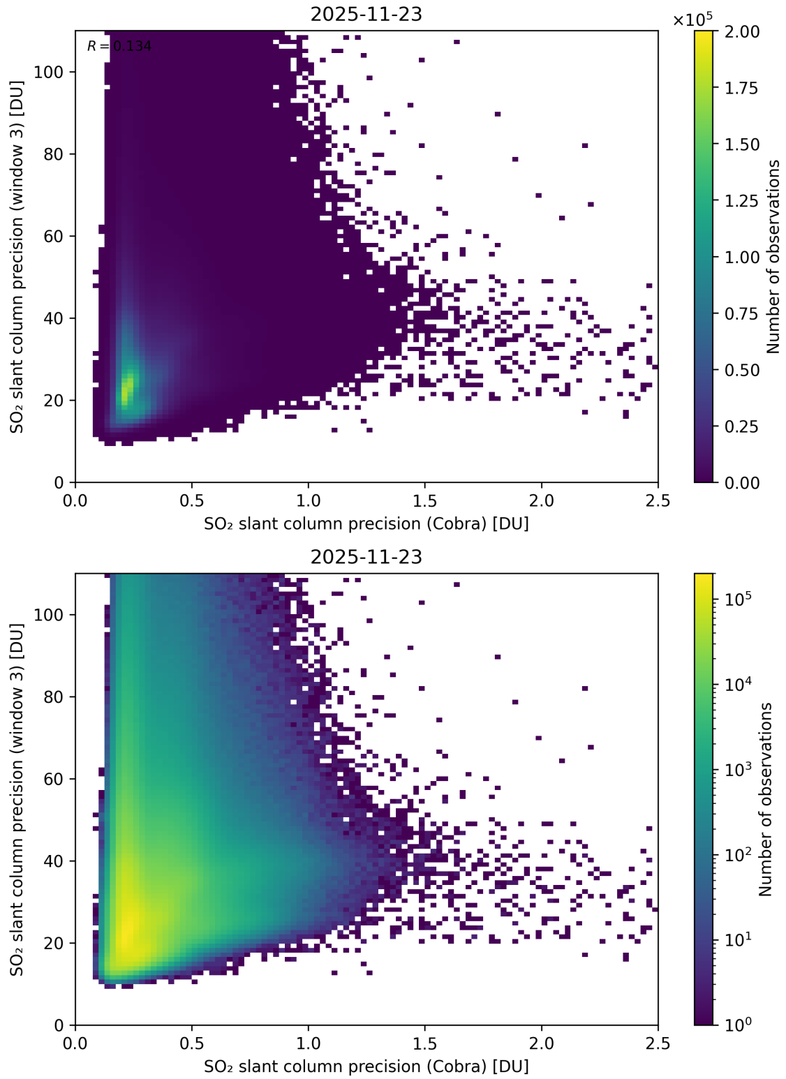
Figure 212: Scatter density plot of “SO 2 slant column precision (Cobra)” against “SO 2 slant column precision (window 3)” for 2025-11-23 to 2025-11-24.
