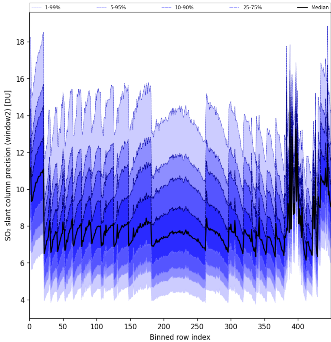
Figure 94: Along track statistics of “SO 2 slant column precision (window2)” for 2025-11-23 to 2025-11-24
