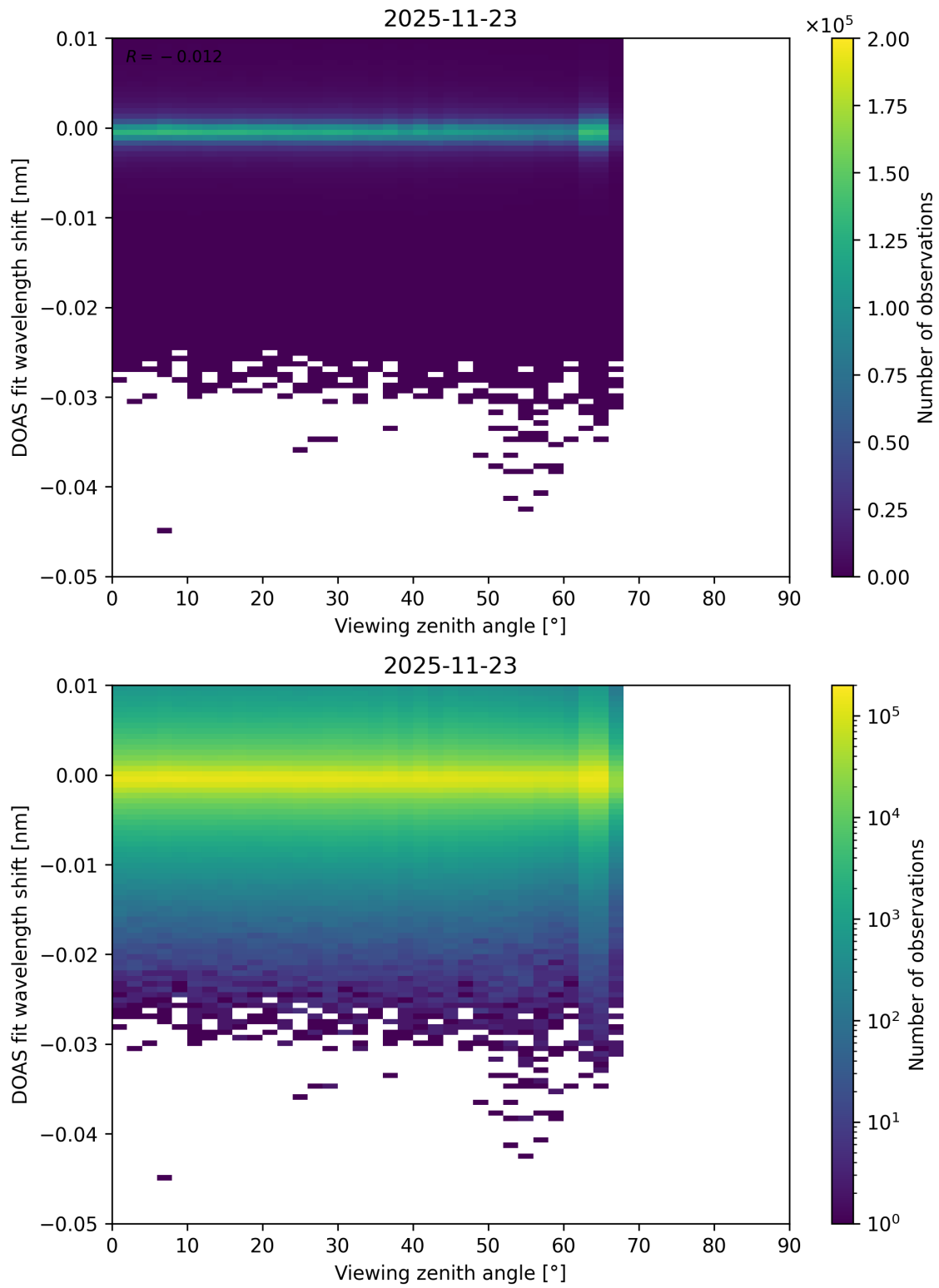
Figure 365: Scatter density plot of “Viewing zenith angle” against “DOAS fit wavelength shift” for 2025-11-23 to 2025-11-24.
