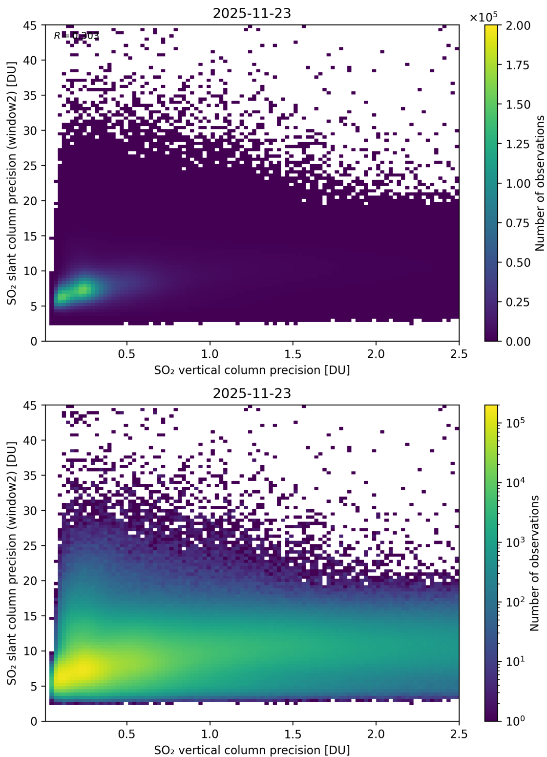
Figure 343: Scatter density plot of “SO 2 vertical column precision” against “SO 2 slant column precision (window2)” for 2025-11-23 to 2025-11-24.
