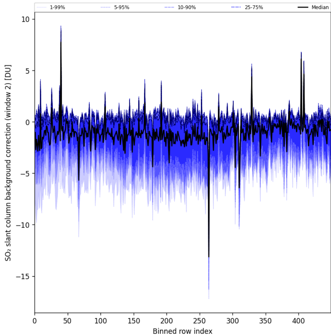
Figure 96: Along track statistics of “SO 2 slant column background correction (window 2)” for 2025-11-23 to 2025-11-24
