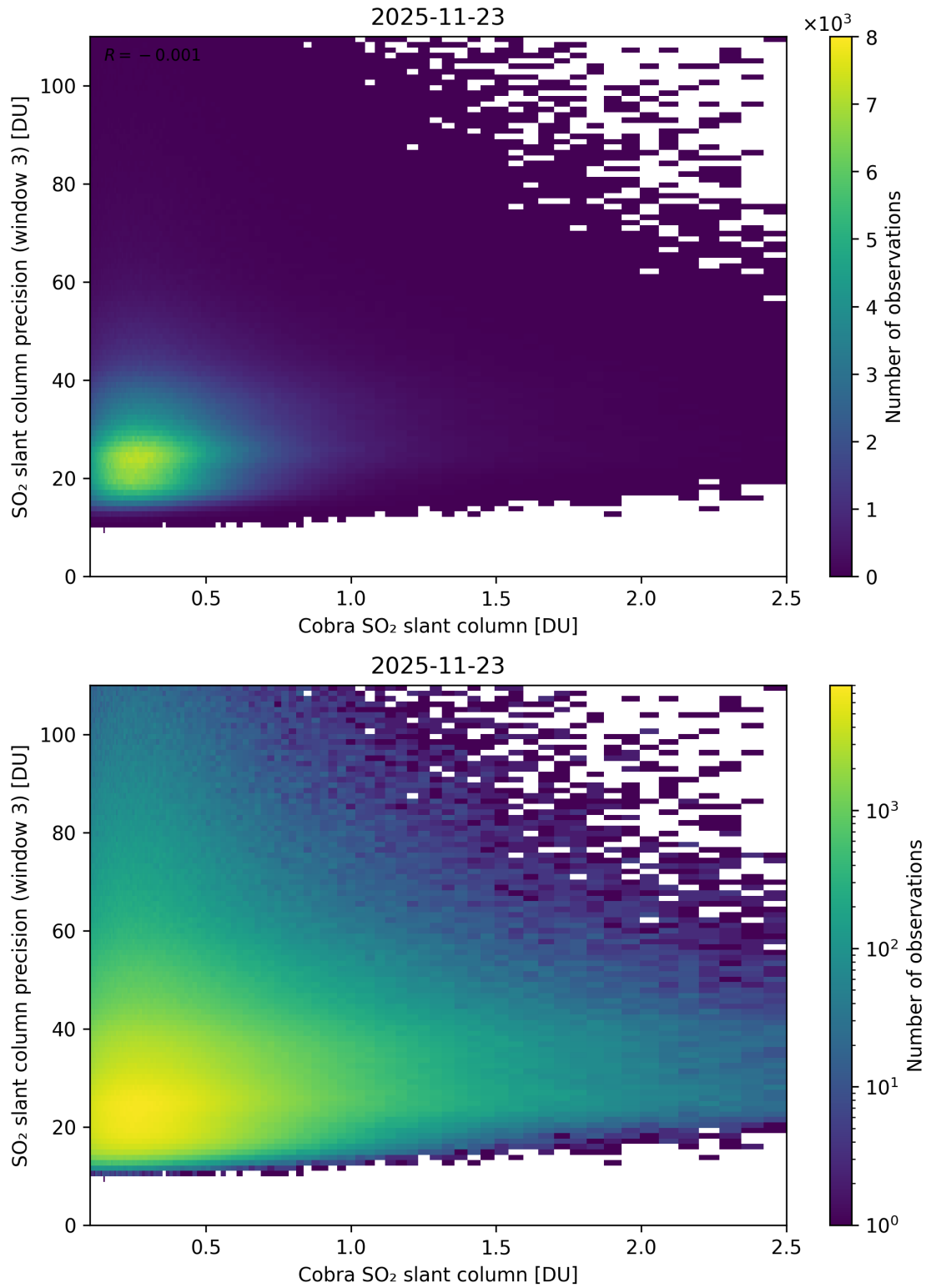
Figure 223: Scatter density plot of “Cobra SO 2 slant column” against “SO 2 slant column precision (window 3)” for 2025-11-23 to 2025-11-24.
