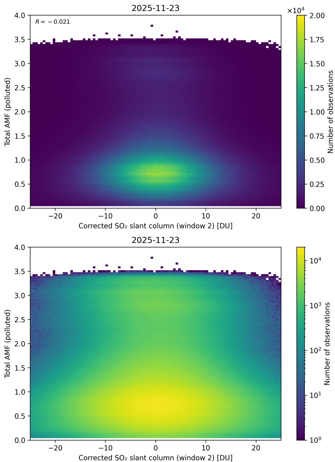
Figure 253: Scatter density plot of “Corrected SO 2 slant column (window 2)” against “Total AMF (polluted)” for 2025-11-23 to 2025-11-24.
