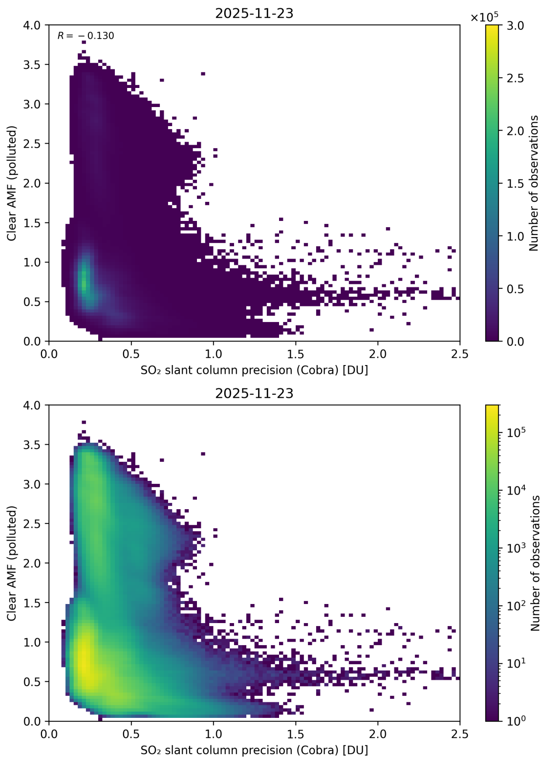
Figure 205: Scatter density plot of “SO 2 slant column precision (Cobra)” against “Clear AMF (polluted)” for 2025-11-23 to 2025-11-24.
