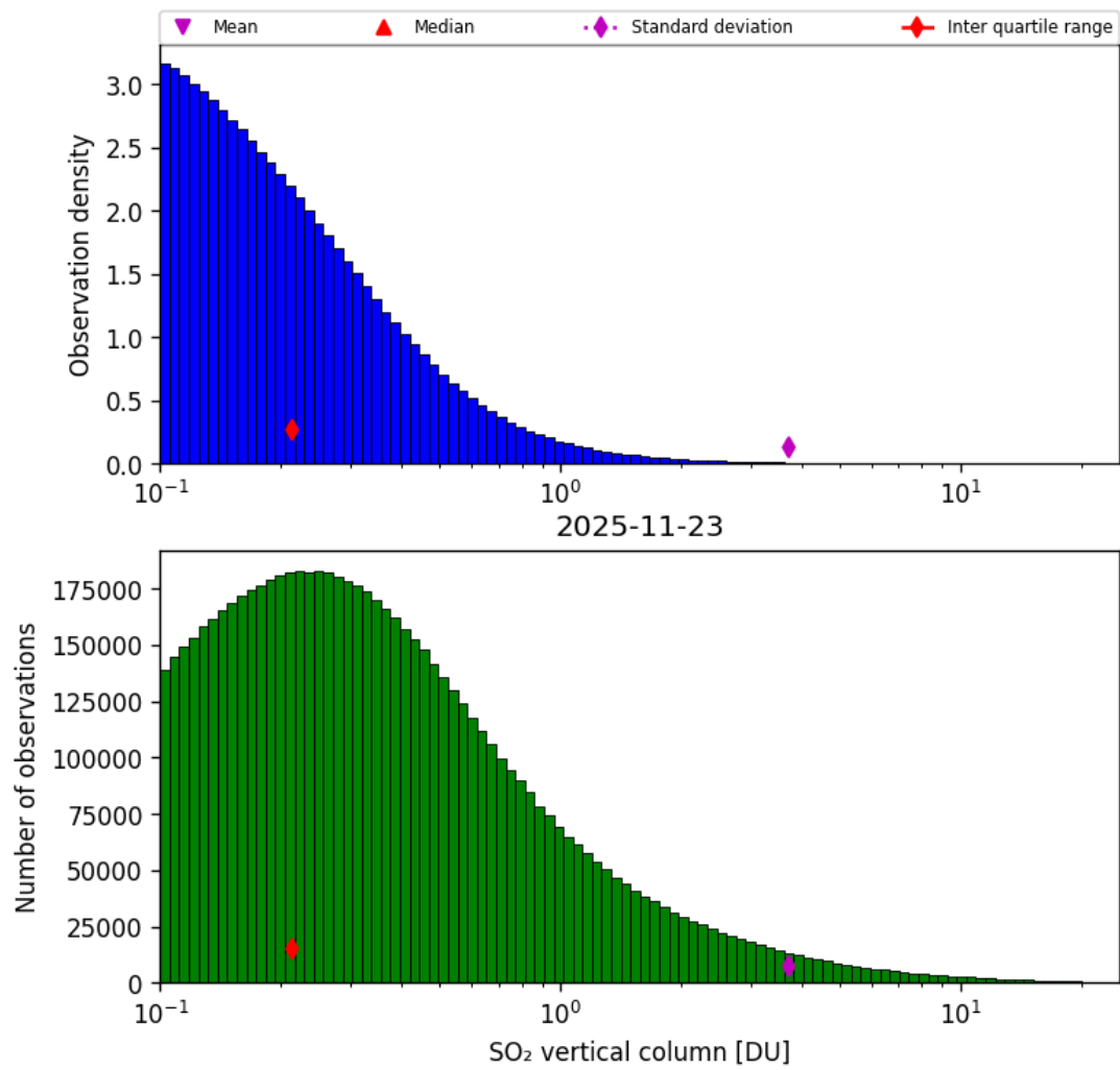
Figure 58: Histogram of “SO 2 vertical column” for 2025-11-23 to 2025-11-24
