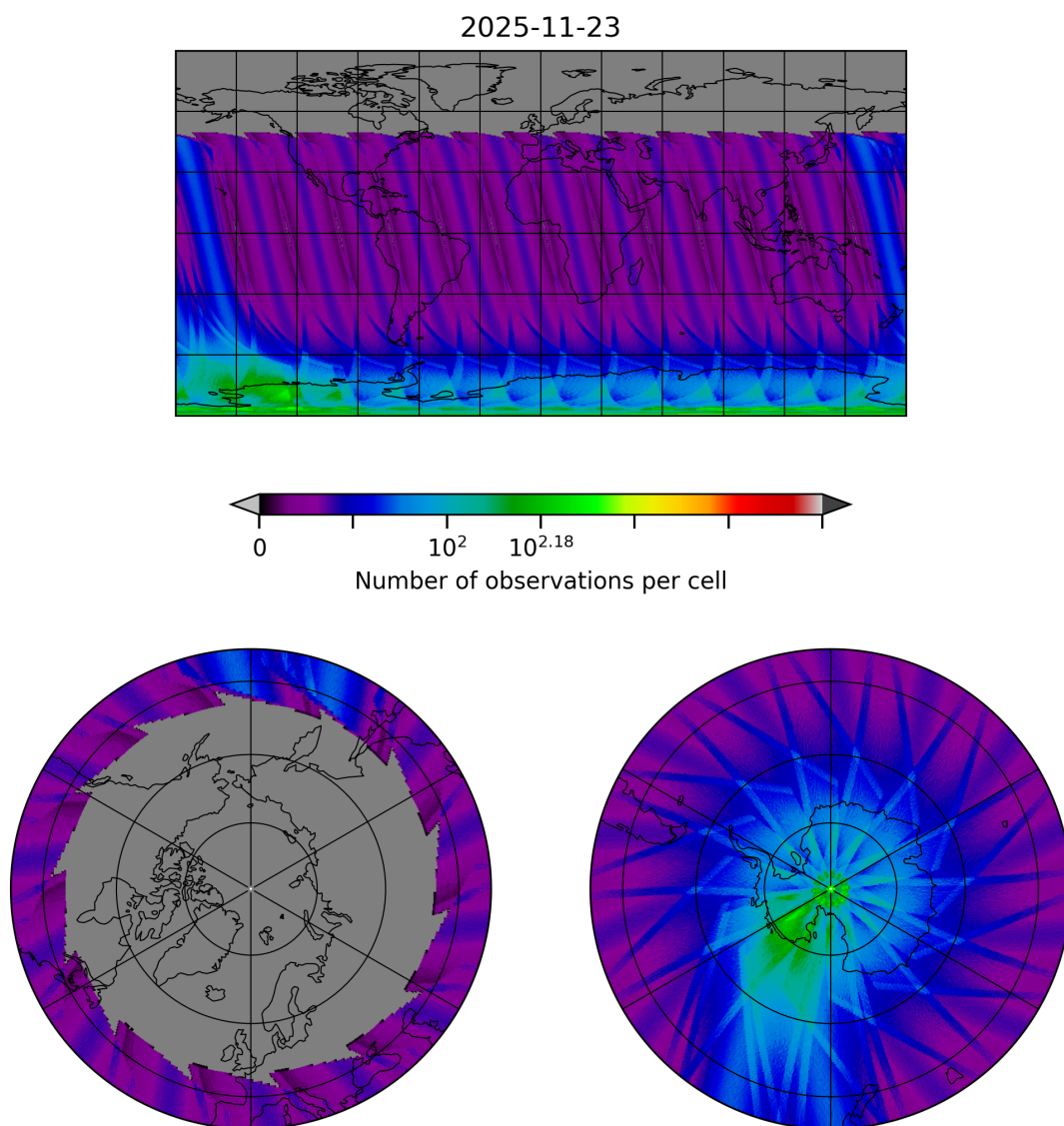
Figure 30: Map of the number of observations for 2025-11-23 to 2025-11-24
