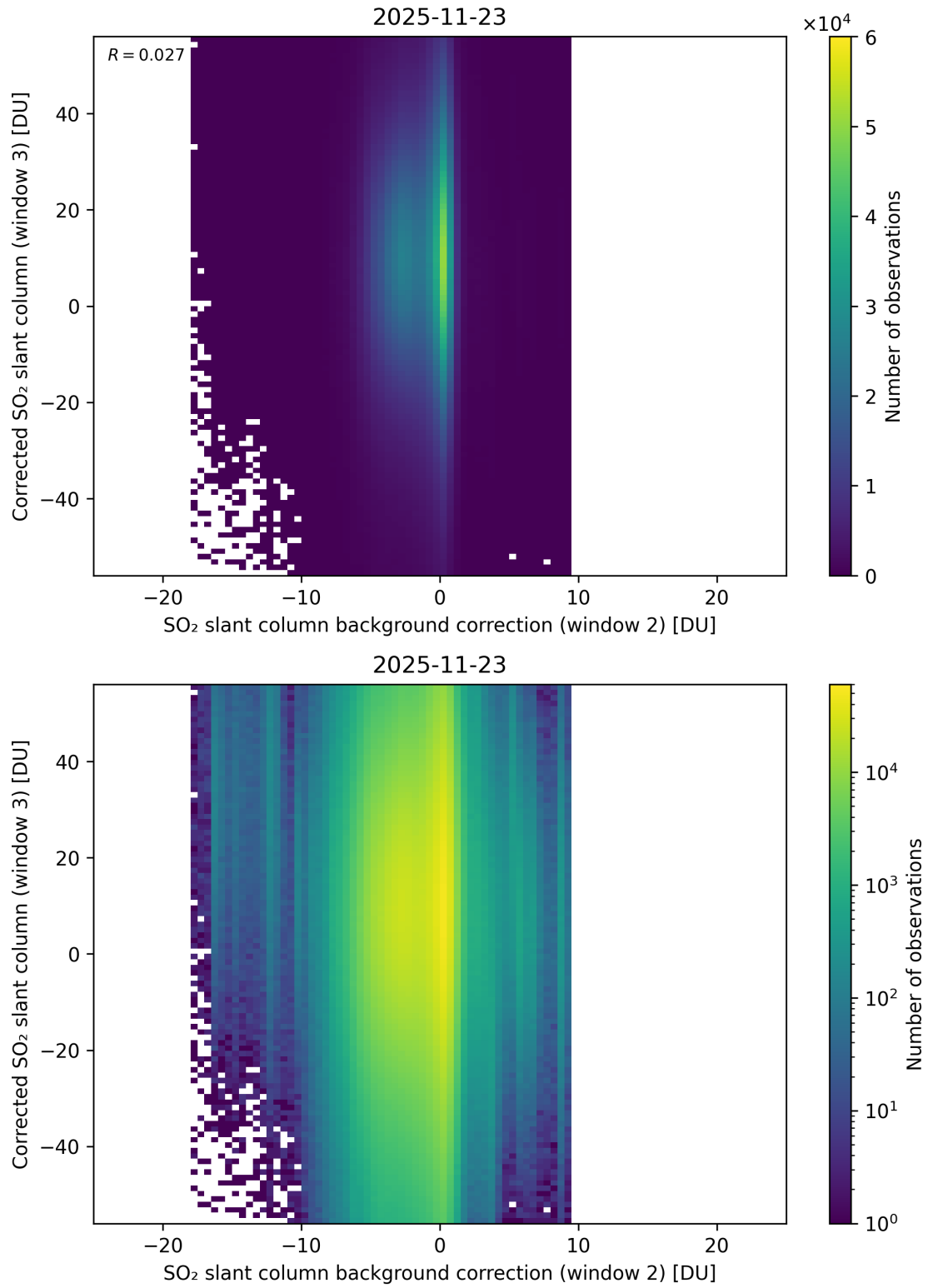
Figure 127: Scatter density plot of “SO 2 slant column background correction (window 2)” against “Corrected SO 2 slant column (window 3)” for 2025-11-23 to 2025-11-24.
