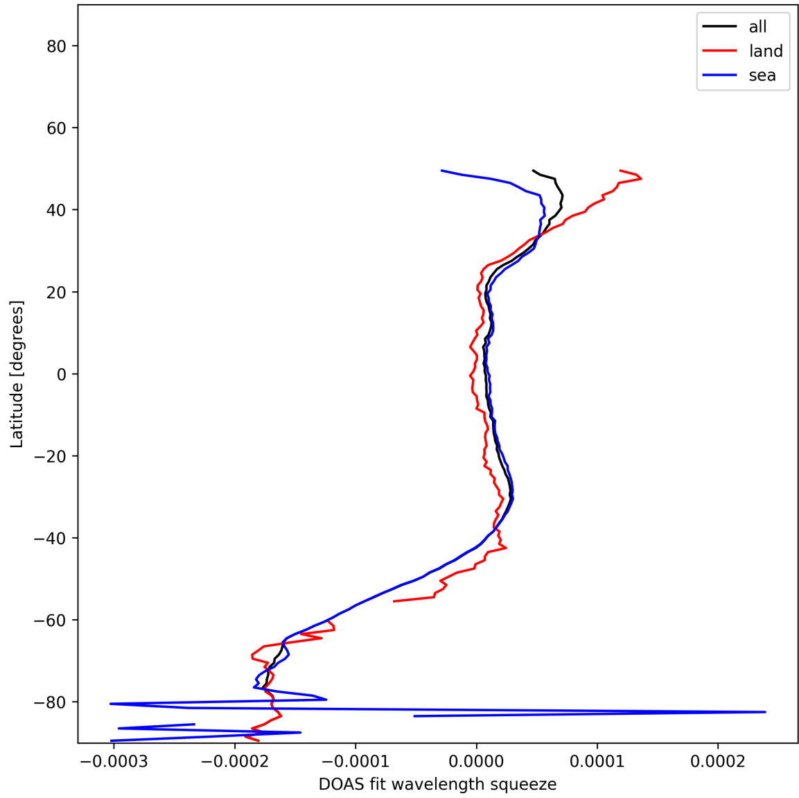
Figure 51: Zonal average of “DOAS fit wavelength squeeze” for 2025-11-23 to 2025-11-24.
