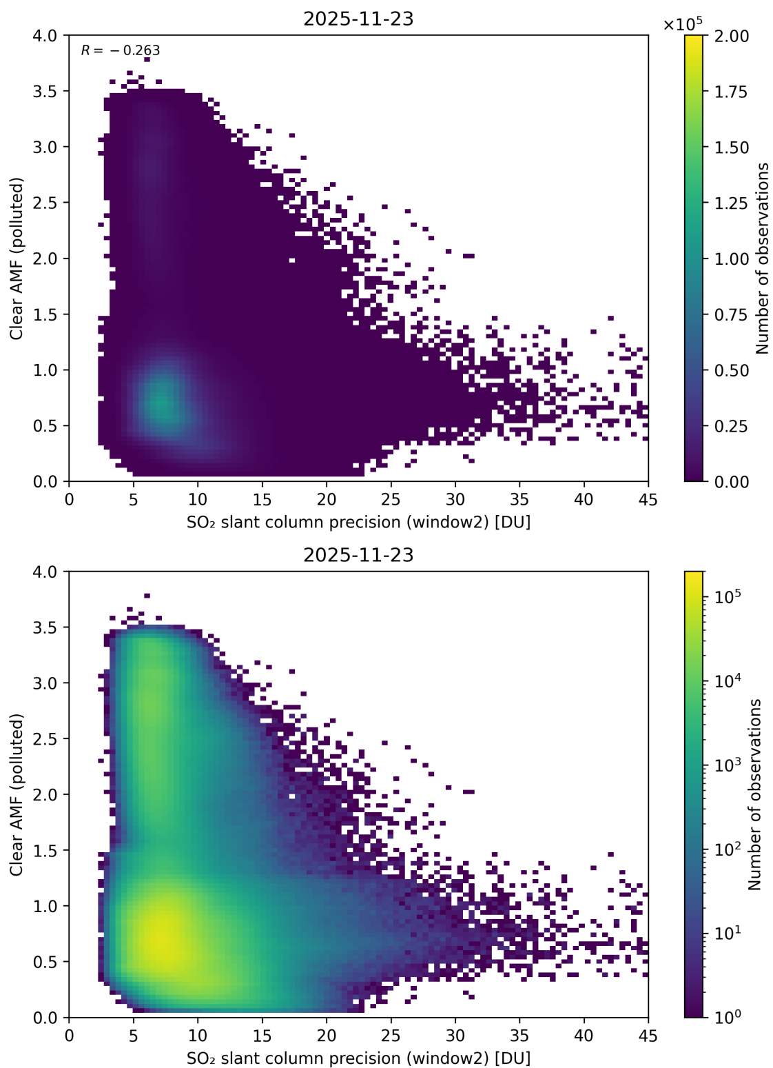
Figure 296: Scatter density plot of “SO 2 slant column precision (window2)” against “Clear AMF (polluted)” for 2025-11-23 to 2025-11-24.
