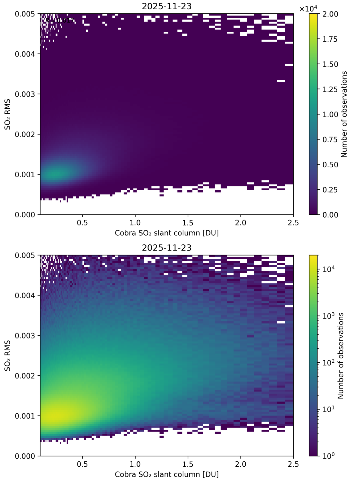
Figure 198: Scatter density plot of “Cobra SO 2 slant column” against “SO 2 RMS” for 2025-11-23 to 2025-11-24.
