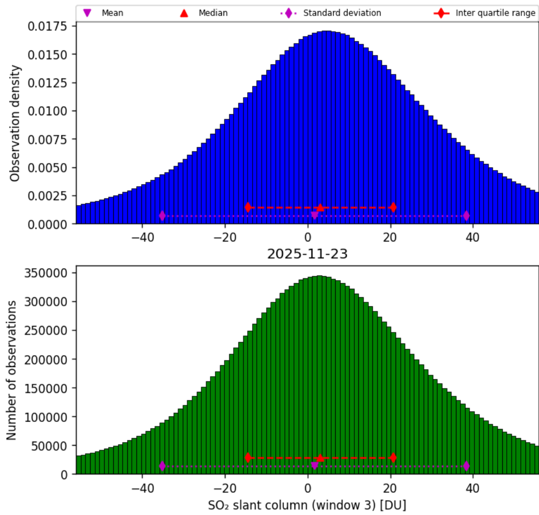
Figure 71: Histogram of “SO 2 slant column (window 3)” for 2025-11-23 to 2025-11-24
