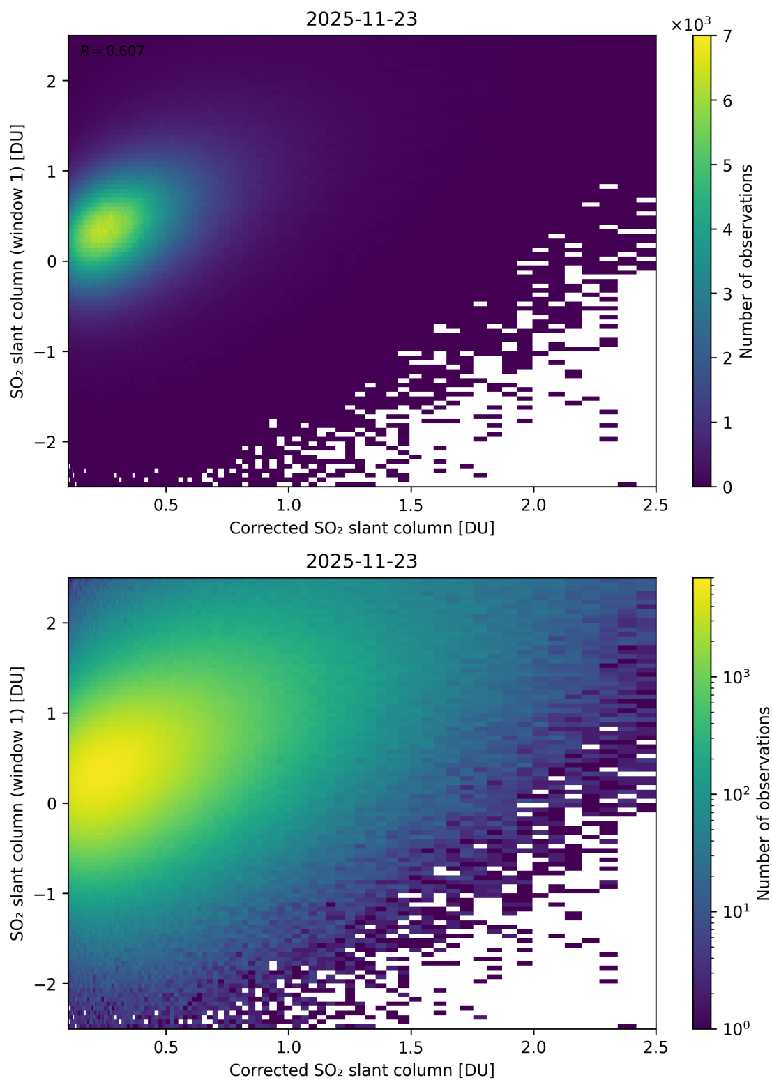
Figure 237: Scatter density plot of “Corrected SO 2 slant column” against “SO 2 slant column (window 1)” for 2025-11-23 to 2025-11-24.
