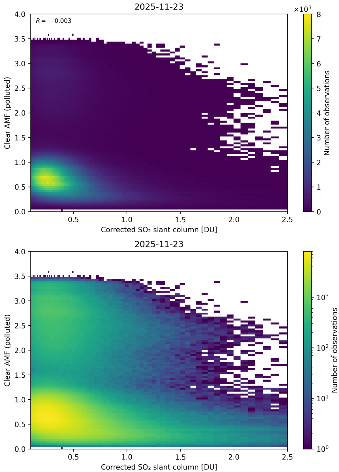
Figure 232: Scatter density plot of “Corrected SO 2 slant column” against “Clear AMF (polluted)” for 2025-11-23 to 2025-11-24.
