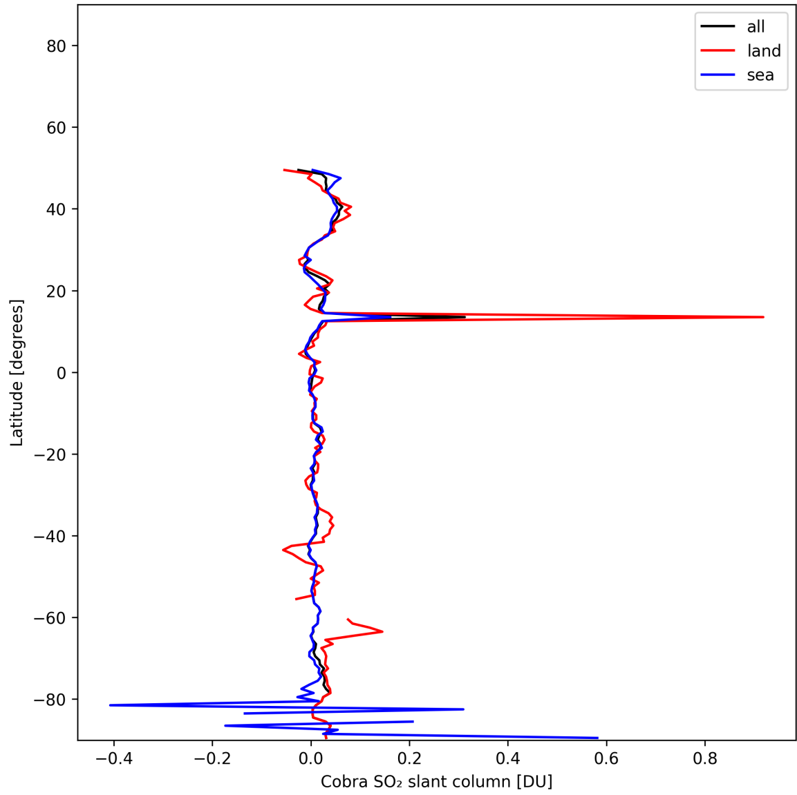
Figure 35: Zonal average of “Cobra SO 2 slant column” for 2025-11-23 to 2025-11-24.
