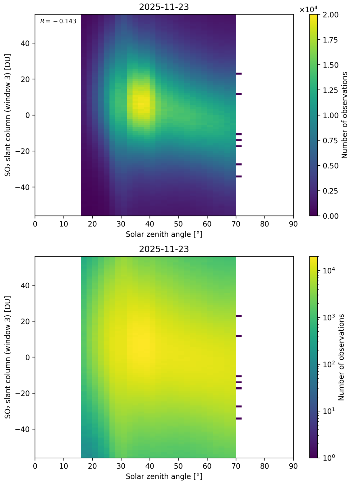
Figure 187: Scatter density plot of “Solar zenith angle” against “SO 2 slant column (window 3)” for 2025-11-23 to 2025-11-24.
