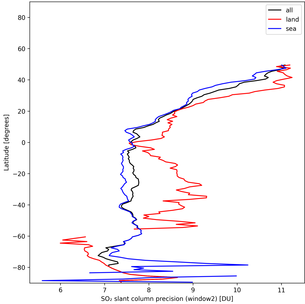
Figure 42: Zonal average of “SO 2 slant column precision (window2)” for 2025-11-23 to 2025-11-24.
