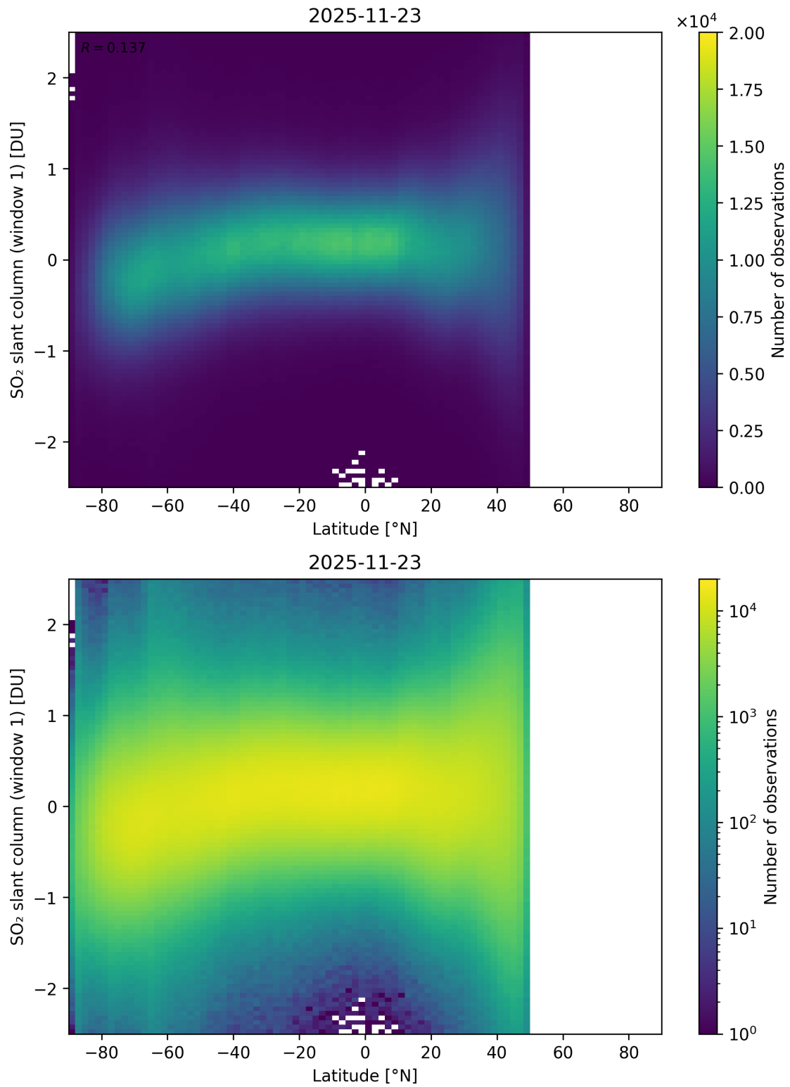
Figure 162: Scatter density plot of “Latitude” against “SO 2 slant column (window 1)” for 2025-11-23 to 2025-11-24.
