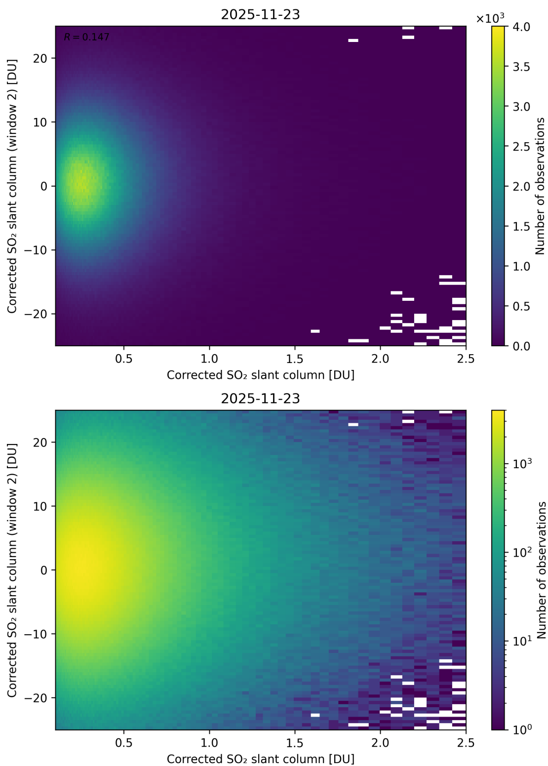
Figure 235: Scatter density plot of “Corrected SO 2 slant column” against “Corrected SO 2 slant column (window 2)” for 2025-11-23 to 2025-11-24.
