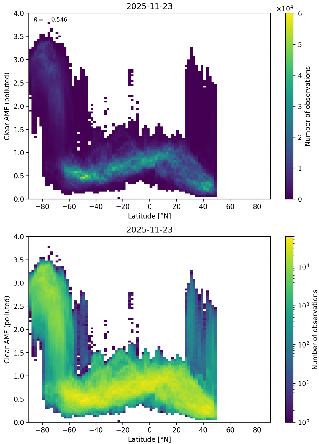
Figure 156: Scatter density plot of “Latitude” against “Clear AMF (polluted)” for 2025-11-23 to 2025-11-24.
