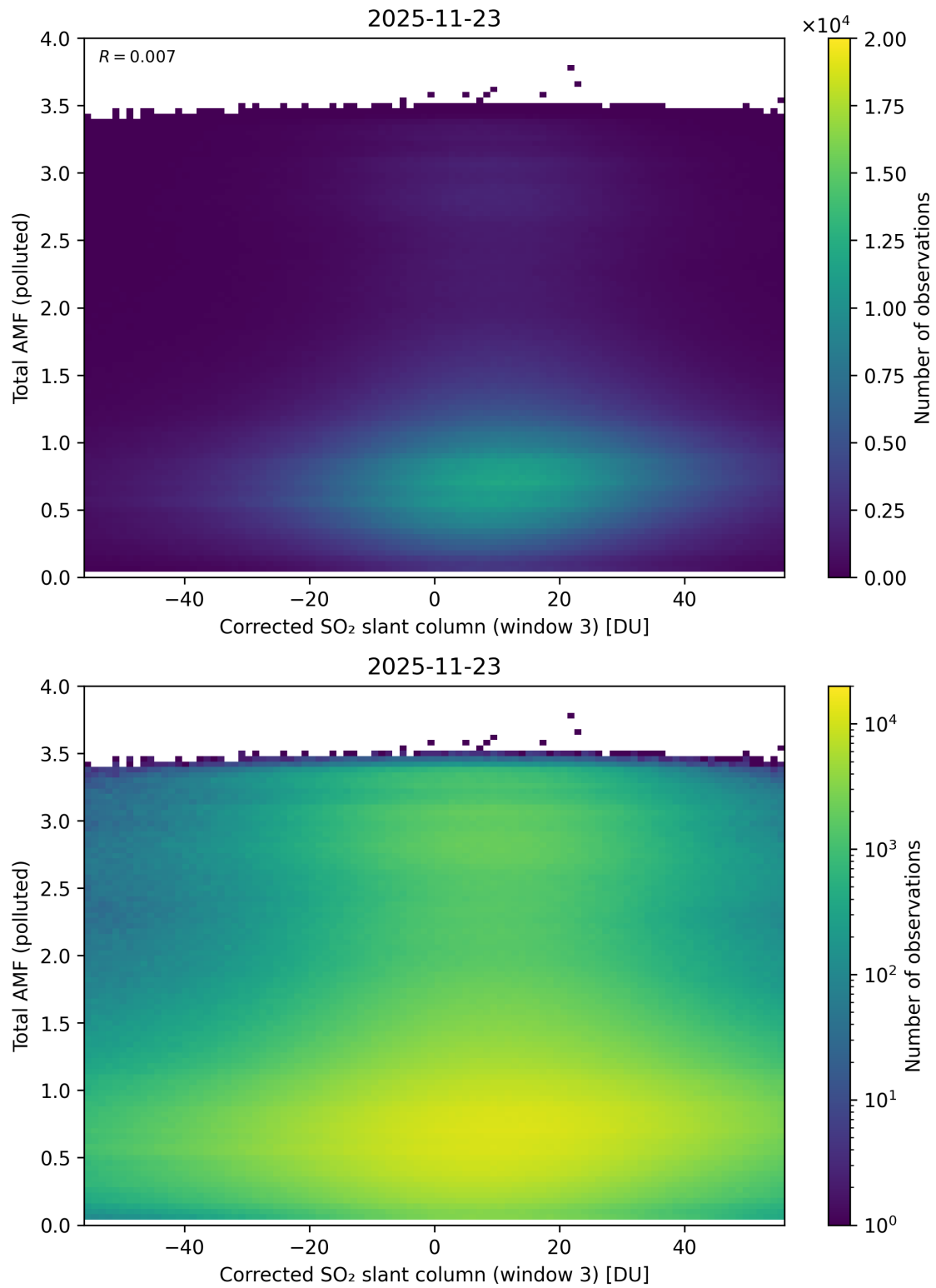
Figure 260: Scatter density plot of “Corrected SO 2 slant column (window 3)” against “Total AMF (polluted)” for 2025-11-23 to 2025-11-24.
