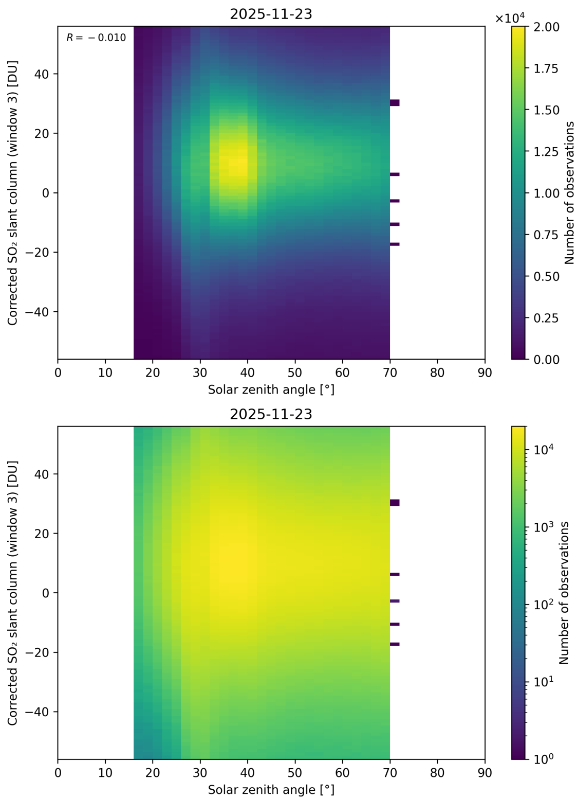
Figure 183: Scatter density plot of “Solar zenith angle” against “Corrected SO 2 slant column (window 3)” for 2025-11-23 to 2025-11-24.
