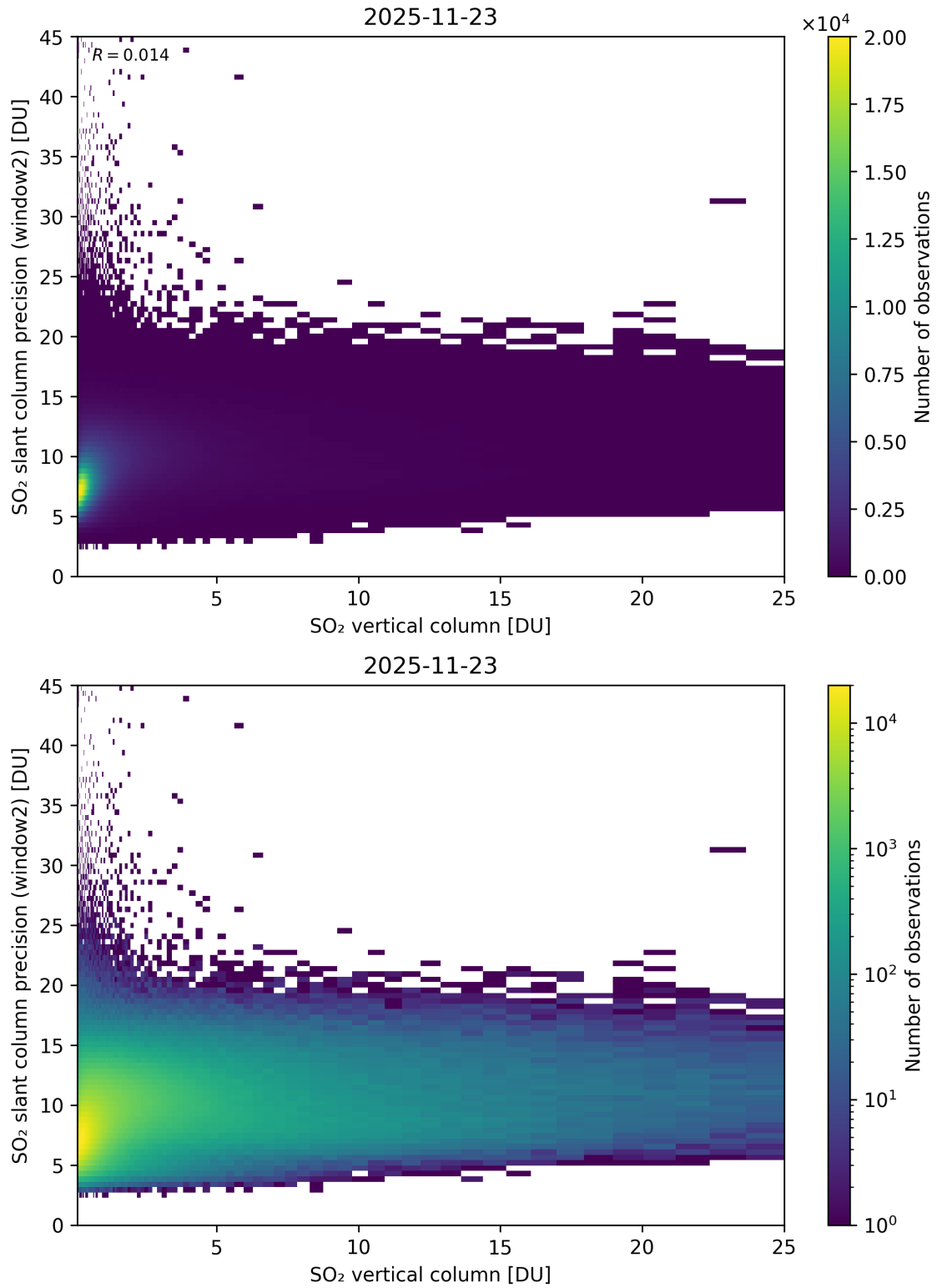
Figure 356: Scatter density plot of “SO 2 vertical column” against “SO 2 slant column precision (window2)” for 2025-11-23 to 2025-11-24.
