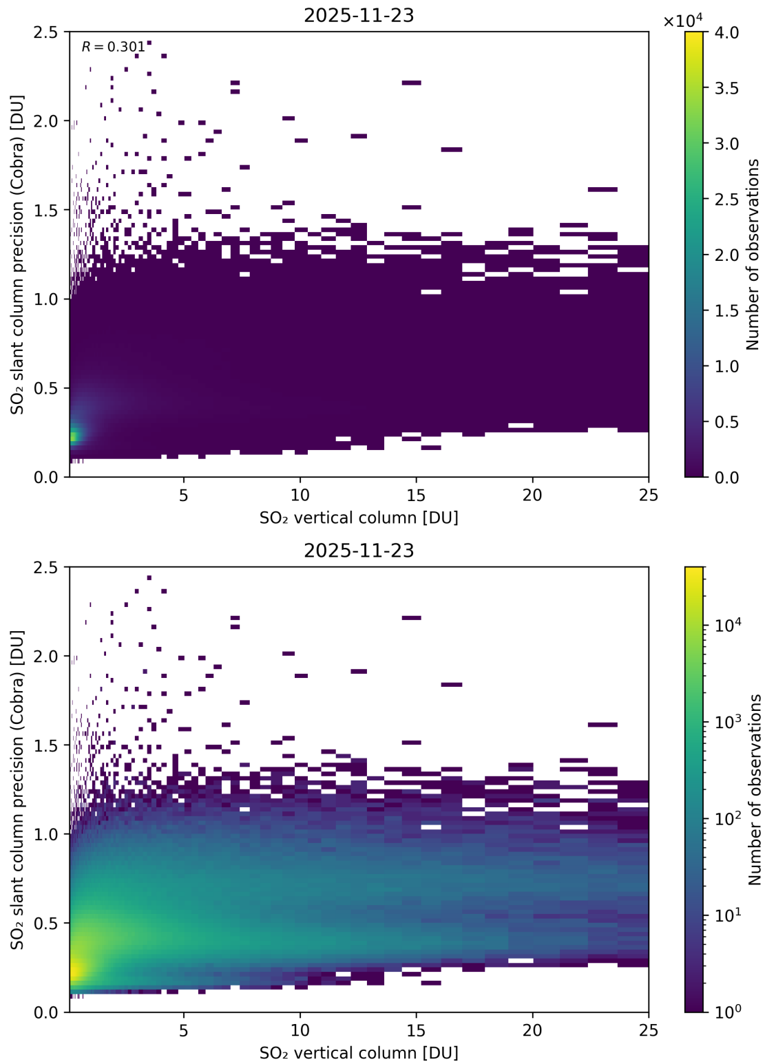
Figure 350: Scatter density plot of “SO 2 vertical column” against “SO 2 slant column precision (Cobra)” for 2025-11-23 to 2025-11-24.
