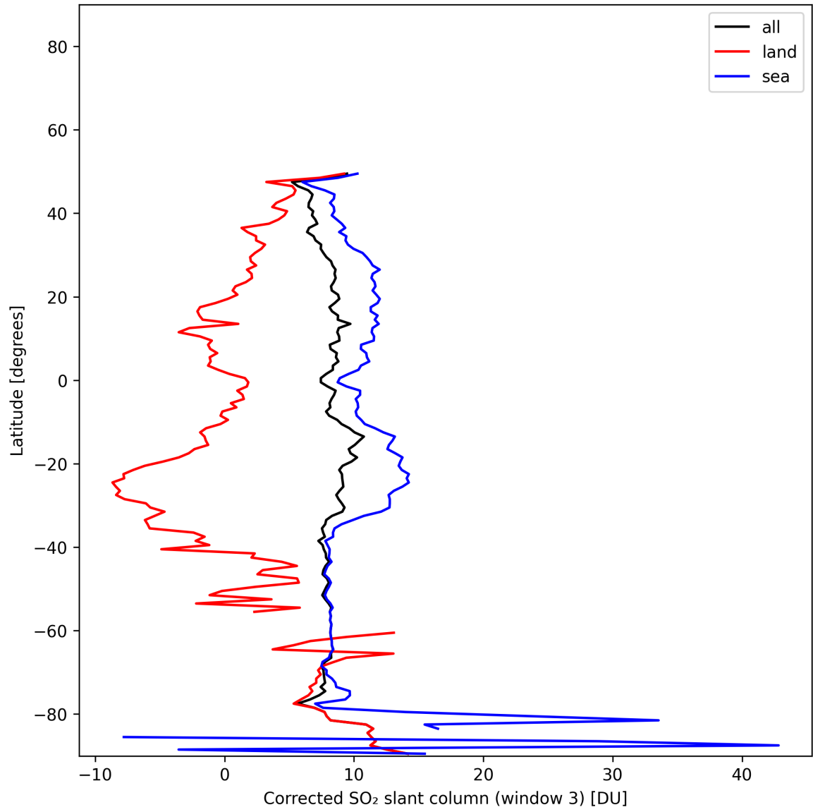
Figure 47: Zonal average of “Corrected SO 2 slant column (window 3)” for 2025-11-23 to 2025-11-24.
