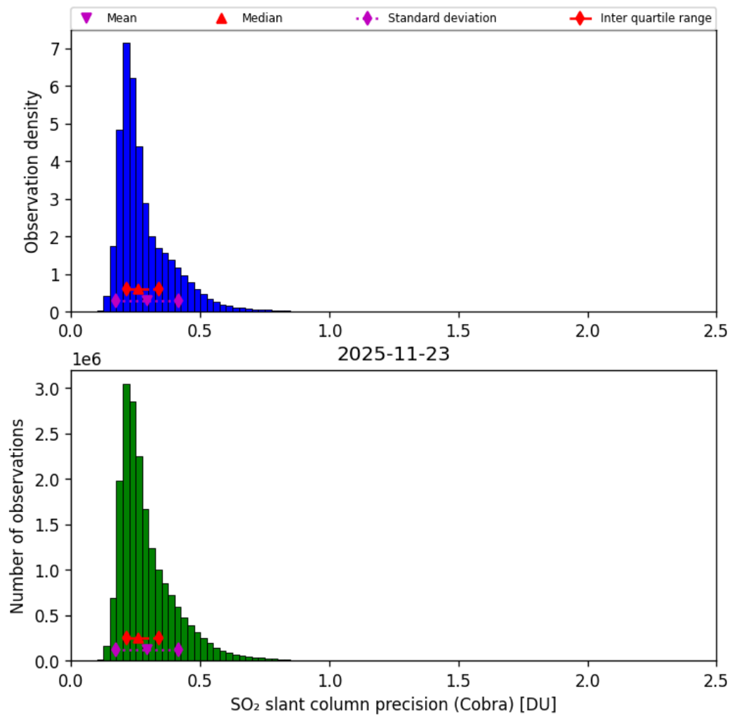
Figure 62: Histogram of “SO 2 slant column precision (Cobra)” for 2025-11-23 to 2025-11-24
