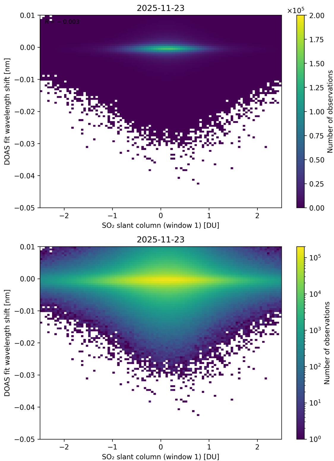
Figure 265: Scatter density plot of “SO 2 slant column (window 1)” against “DOAS fit wavelength shift” for 2025-11-23 to 2025-11-24.
