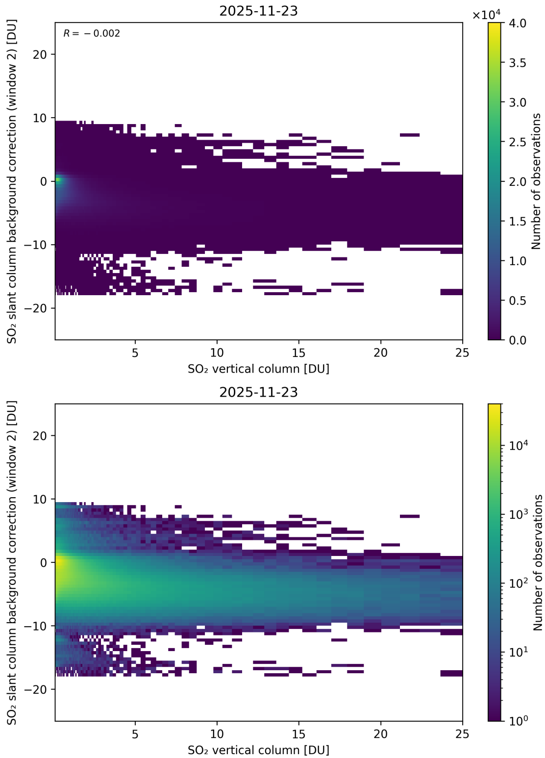
Figure 324: Scatter density plot of “SO 2 vertical column” against “SO 2 slant column background correction (window 2)” for 2025-11-23 to 2025-11-24.
