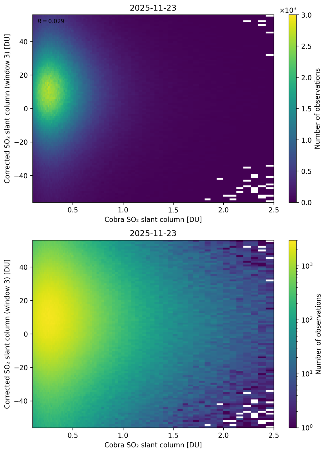
Figure 218: Scatter density plot of “Cobra SO 2 slant column” against “Corrected SO 2 slant column (window 3)” for 2025-11-23 to 2025-11-24.
