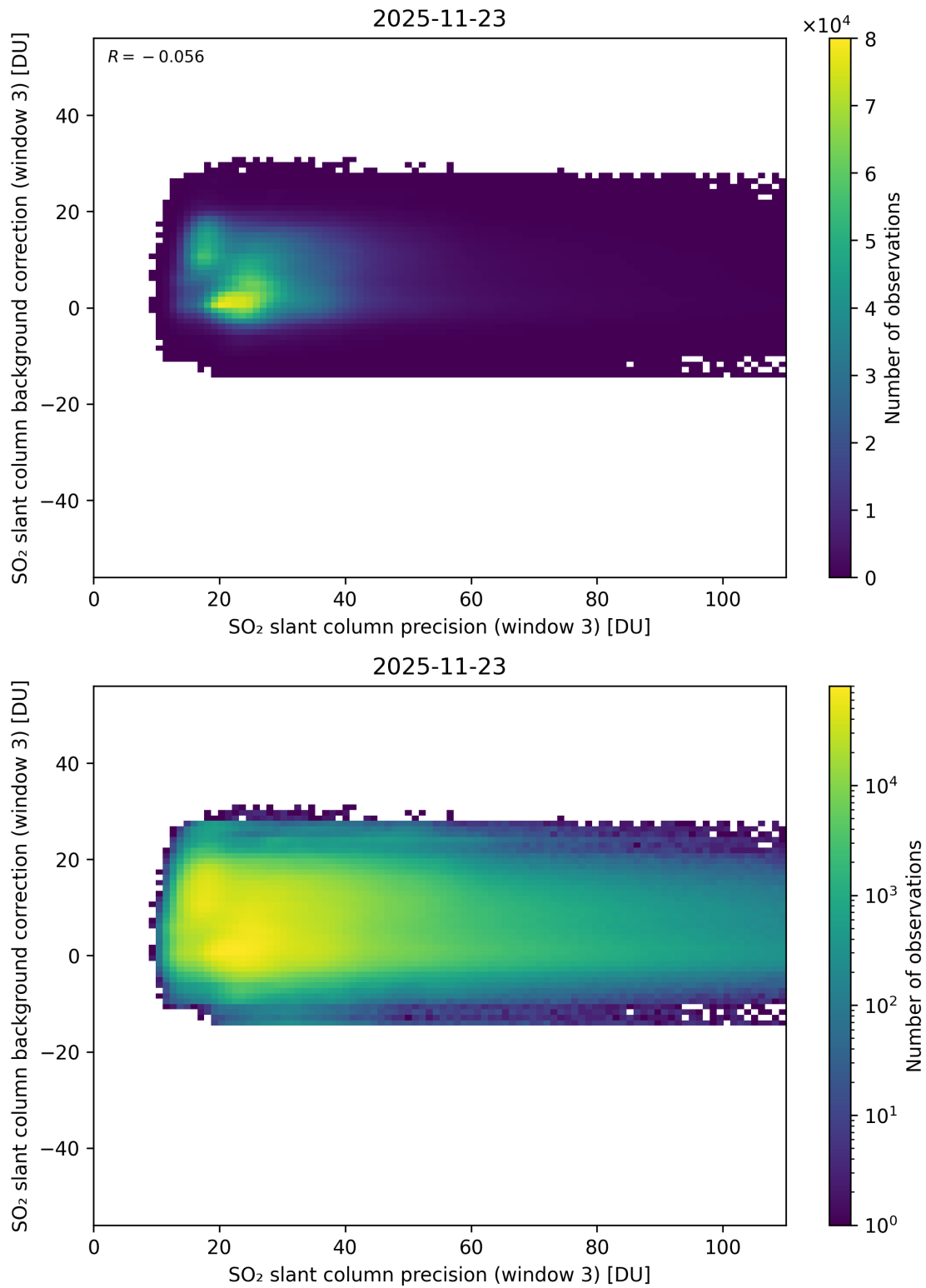
Figure 307: Scatter density plot of “SO 2 slant column precision (window 3)” against “SO 2 slant column background correction (window 3)” for 2025-11-23 to 2025-11-24.
