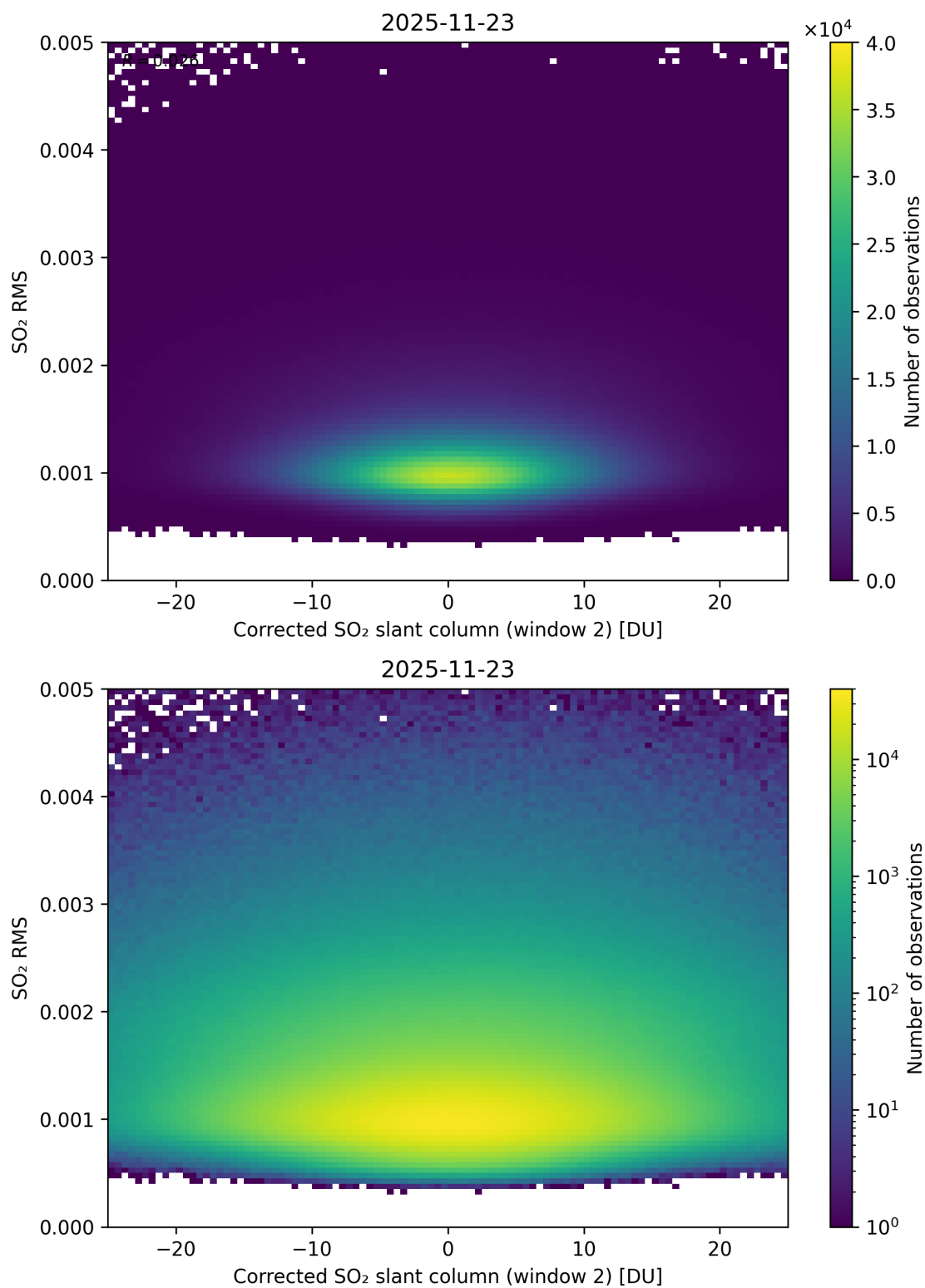
Figure 248: Scatter density plot of “Corrected SO 2 slant column (window 2)” against “SO 2 RMS” for 2025-11-23 to 2025-11-24.
