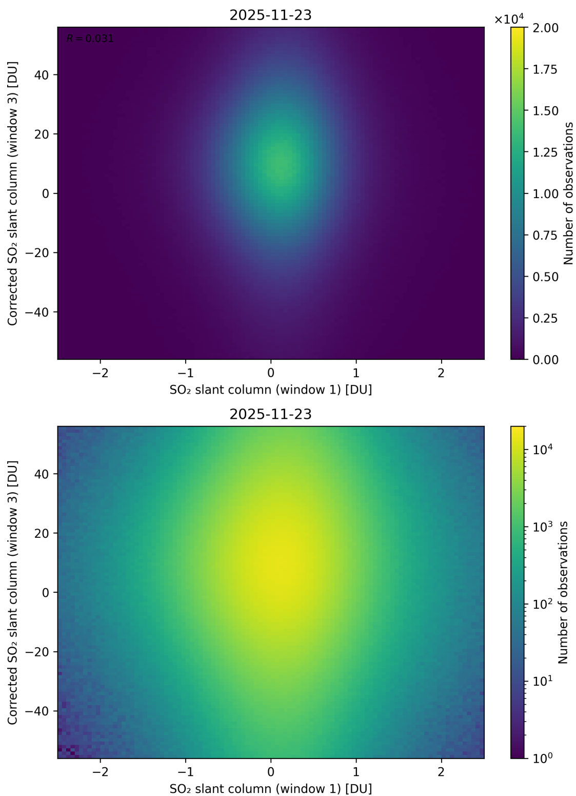
Figure 284: Scatter density plot of “SO 2 slant column (window 1)” against “Corrected SO 2 slant column (window 3)” for 2025-11-23 to 2025-11-24.
