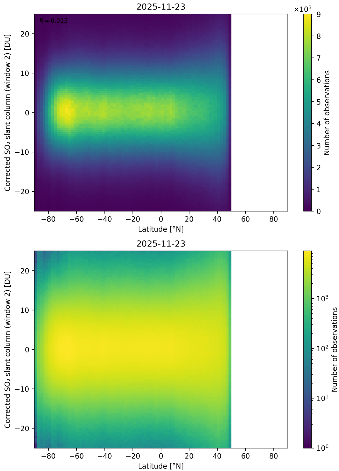
Figure 160: Scatter density plot of “Latitude” against “Corrected SO 2 slant column (window 2)” for 2025-11-23 to 2025-11-24.
