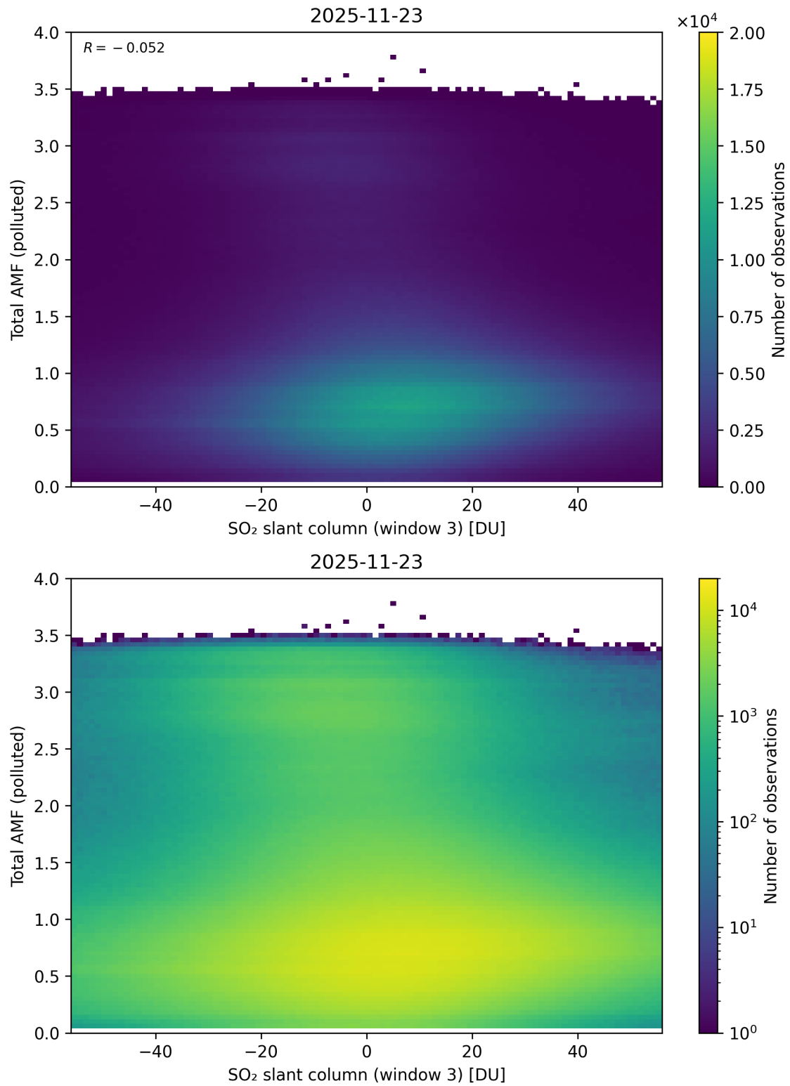
Figure 318: Scatter density plot of “SO 2 slant column (window 3)” against “Total AMF (polluted)” for 2025-11-23 to 2025-11-24.
