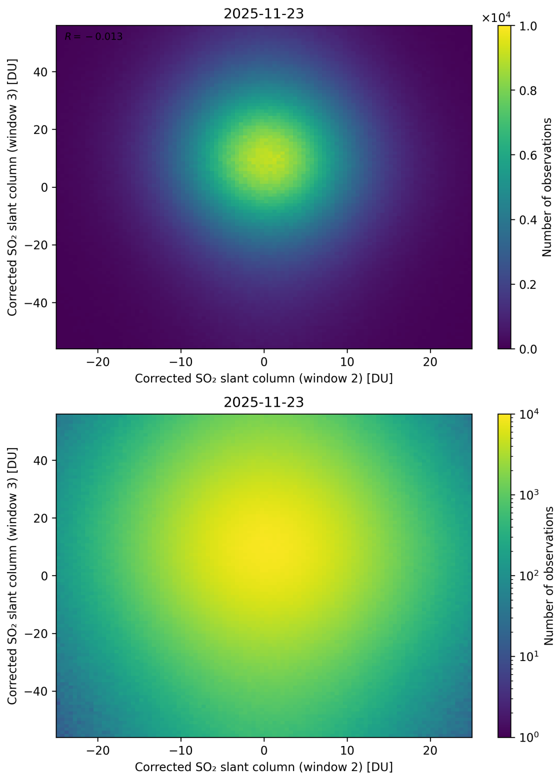
Figure 250: Scatter density plot of “Corrected SO 2 slant column (window 2)” against “Corrected SO 2 slant column (window 3)” for 2025-11-23 to 2025-11-24.
