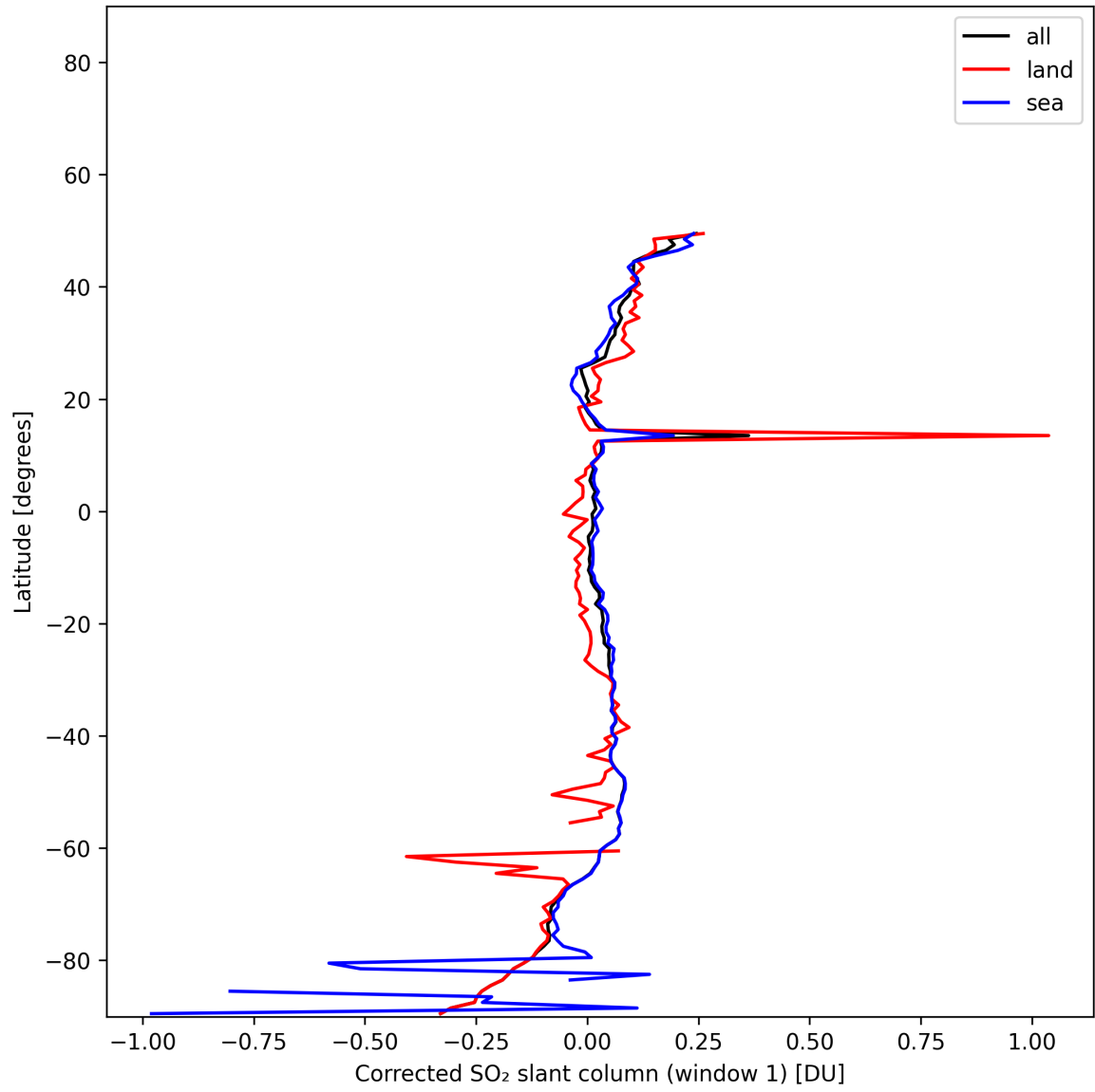
Figure 39: Zonal average of “Corrected SO 2 slant column (window 1)” for 2025-11-23 to 2025-11-24.
