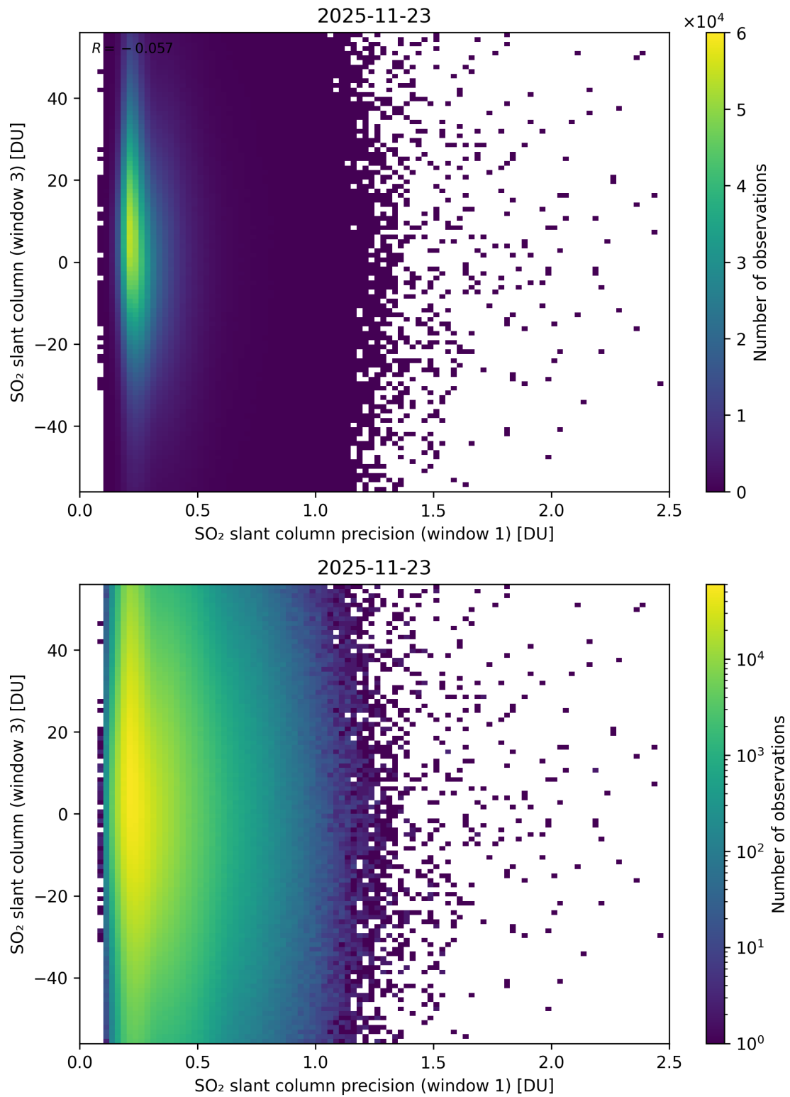
Figure 278: Scatter density plot of “SO 2 slant column precision (window 1)” against “SO 2 slant column (window 3)” for 2025-11-23 to 2025-11-24.
