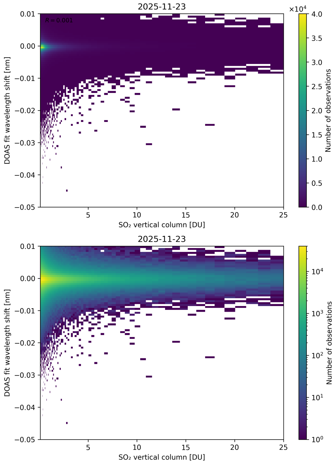
Figure 326: Scatter density plot of “SO 2 vertical column” against “DOAS fit wavelength shift” for 2025-11-23 to 2025-11-24.
