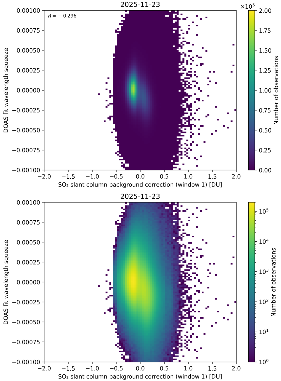
Figure 112: Scatter density plot of “SO 2 slant column background correction (window 1)” against “DOAS fit wavelength squeeze” for 2025-11-23 to 2025-11-24.
