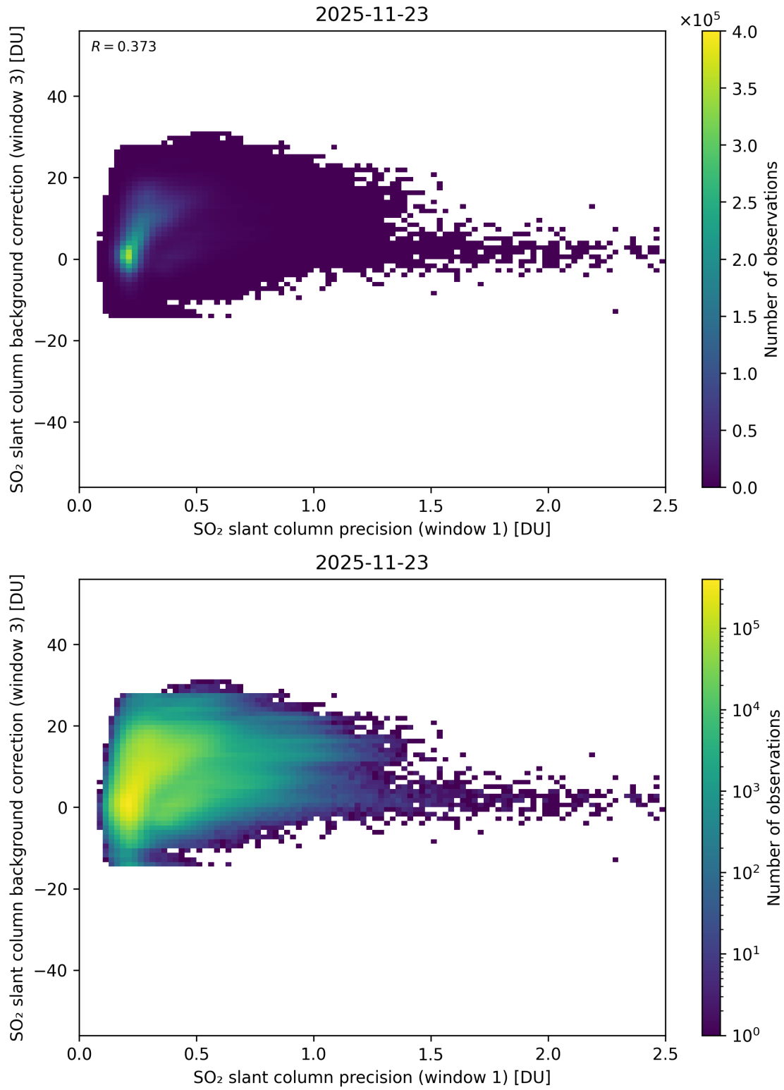
Figure 270: Scatter density plot of “SO 2 slant column precision (window 1)” against “SO 2 slant column background correction (window 3)” for 2025-11-23 to 2025-11-24.
