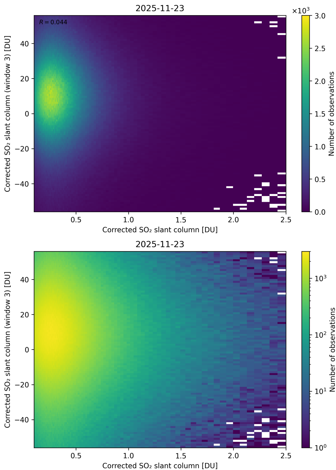
Figure 236: Scatter density plot of “Corrected SO 2 slant column” against “Corrected SO 2 slant column (window 3)” for 2025-11-23 to 2025-11-24.
