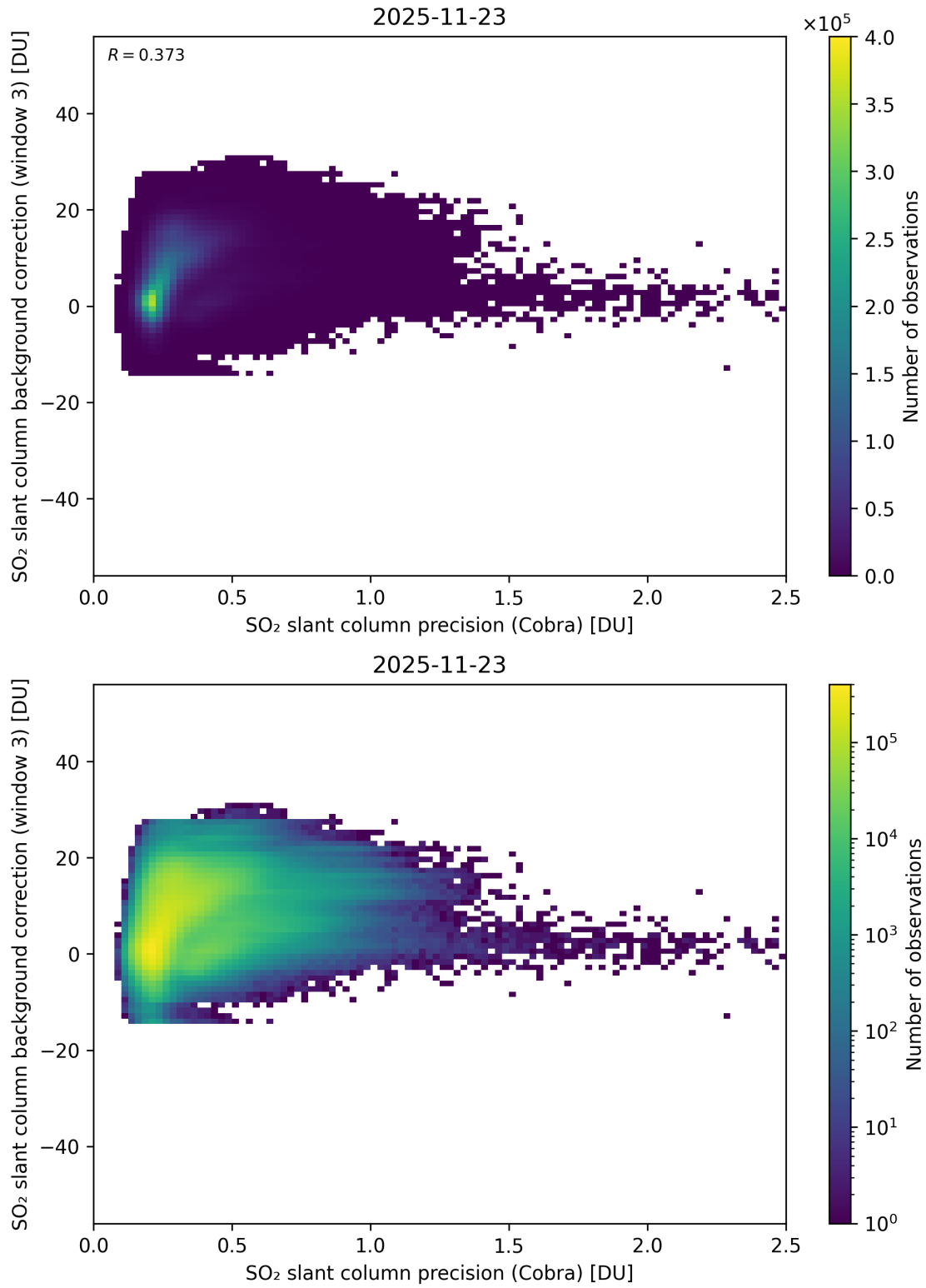
Figure 201: Scatter density plot of “SO 2 slant column precision (Cobra)” against “SO 2 slant column background correction (window 3)” for 2025-11-23 to 2025-11-24.
