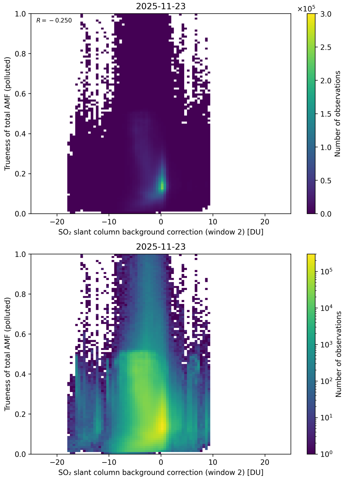
Figure 131: Scatter density plot of “SO 2 slant column background correction (window 2)” against “Trueness of total AMF (polluted)” for 2025-11-23 to 2025-11-24.
