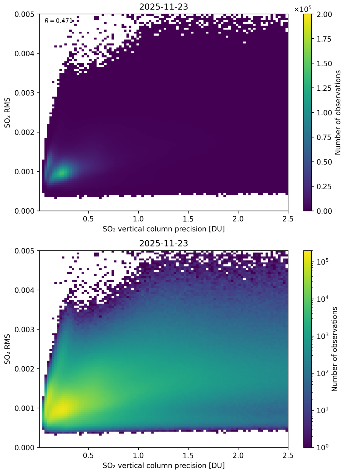
Figure 334: Scatter density plot of “SO 2 vertical column precision” against “SO 2 RMS” for 2025-11-23 to 2025-11-24.
