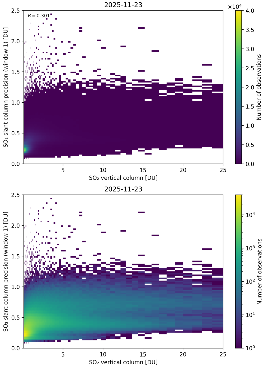
Figure 355: Scatter density plot of “SO 2 vertical column” against “SO 2 slant column precision (window 1)” for 2025-11-23 to 2025-11-24.
