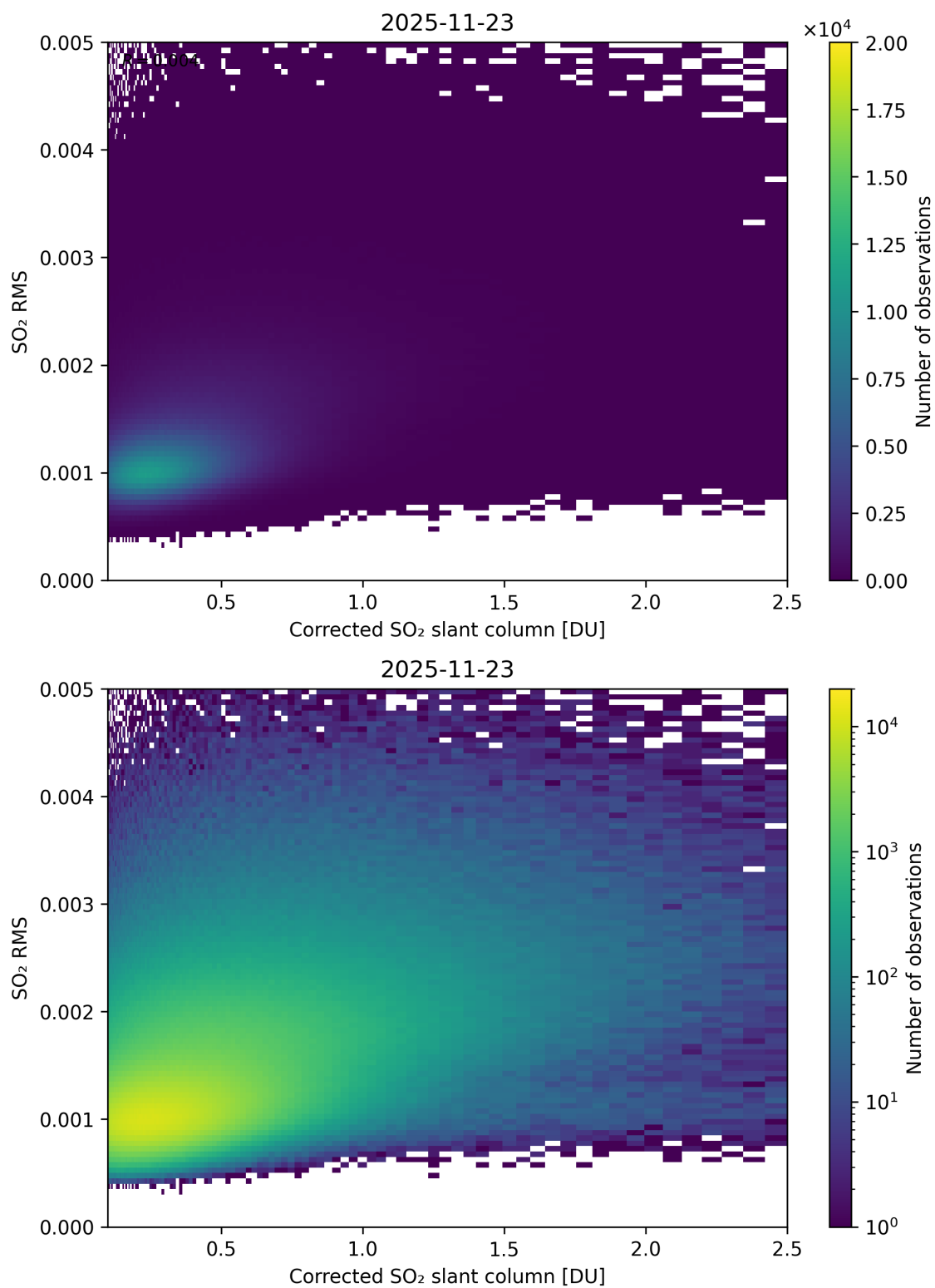
Figure 231: Scatter density plot of “Corrected SO 2 slant column” against “SO 2 RMS” for 2025-11-23 to 2025-11-24.
