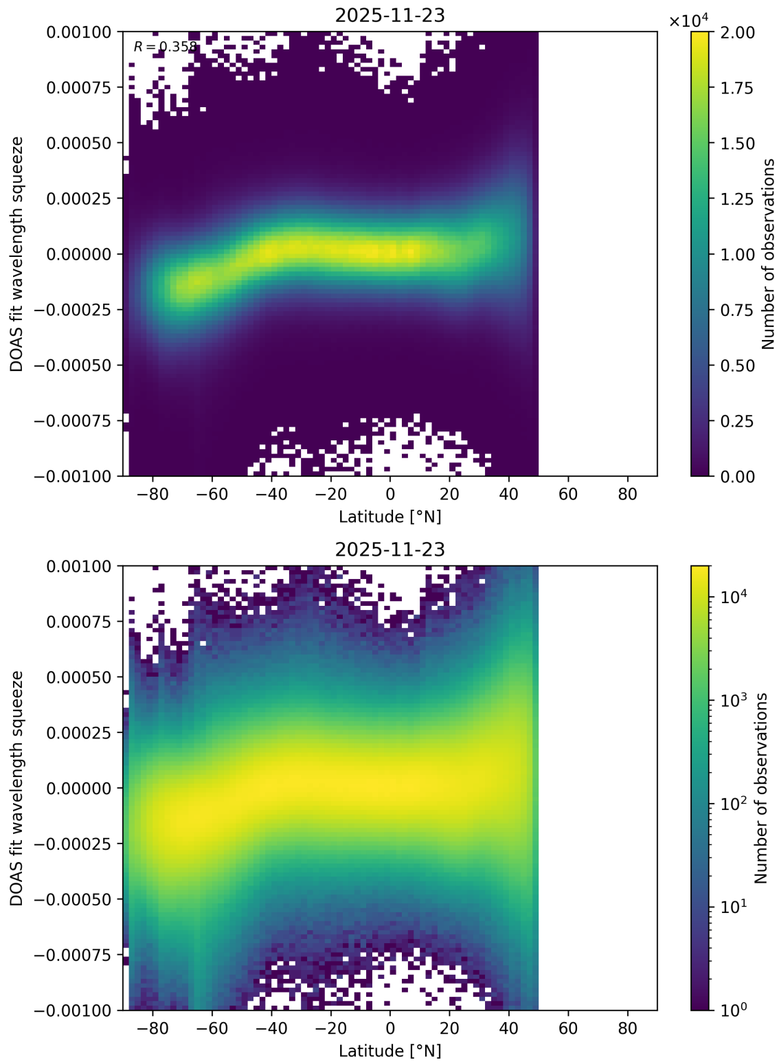
Figure 154: Scatter density plot of “Latitude” against “DOAS fit wavelength squeeze” for 2025-11-23 to 2025-11-24.
