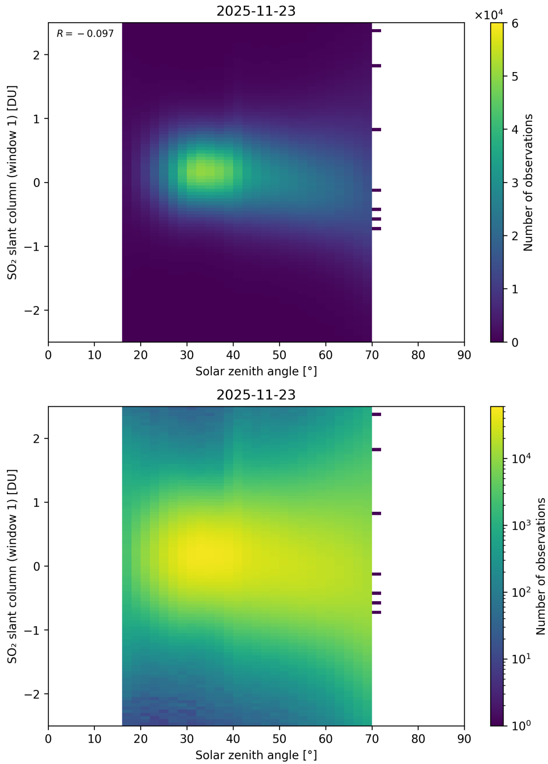
Figure 184: Scatter density plot of “Solar zenith angle” against “SO 2 slant column (window 1)” for 2025-11-23 to 2025-11-24.
