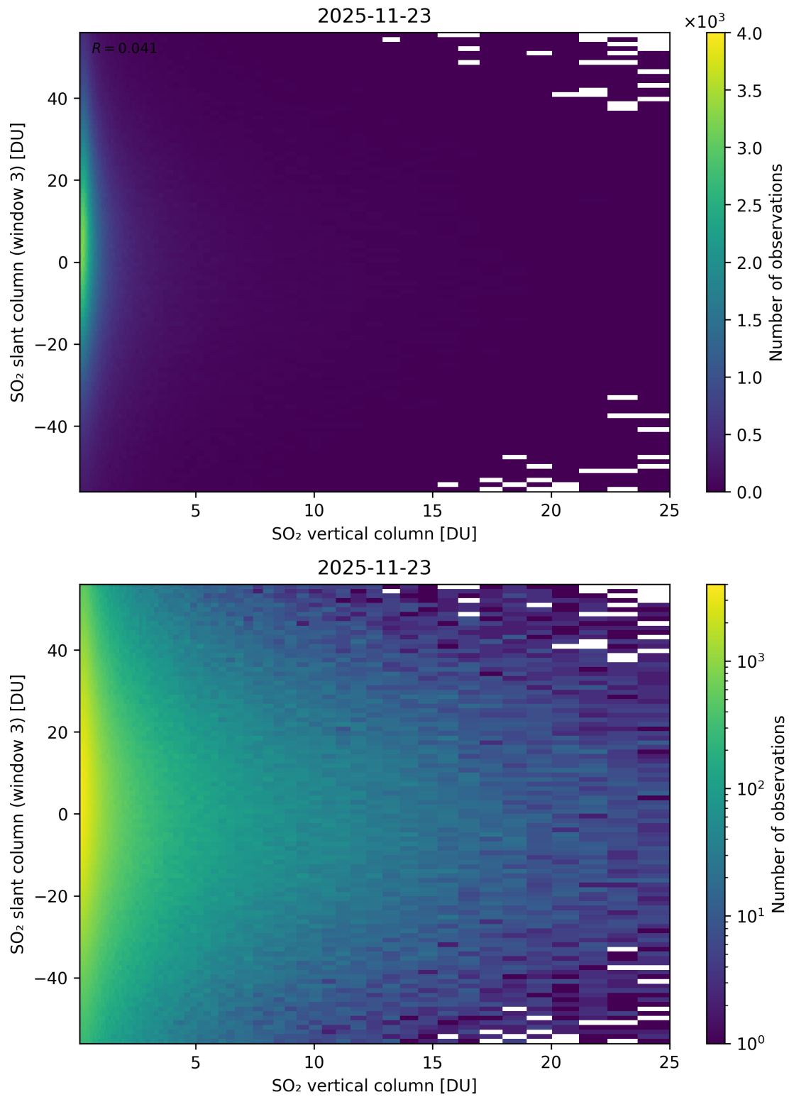
Figure 357: Scatter density plot of “SO 2 vertical column” against “SO 2 slant column (window 3)” for 2025-11-23 to 2025-11-24.
