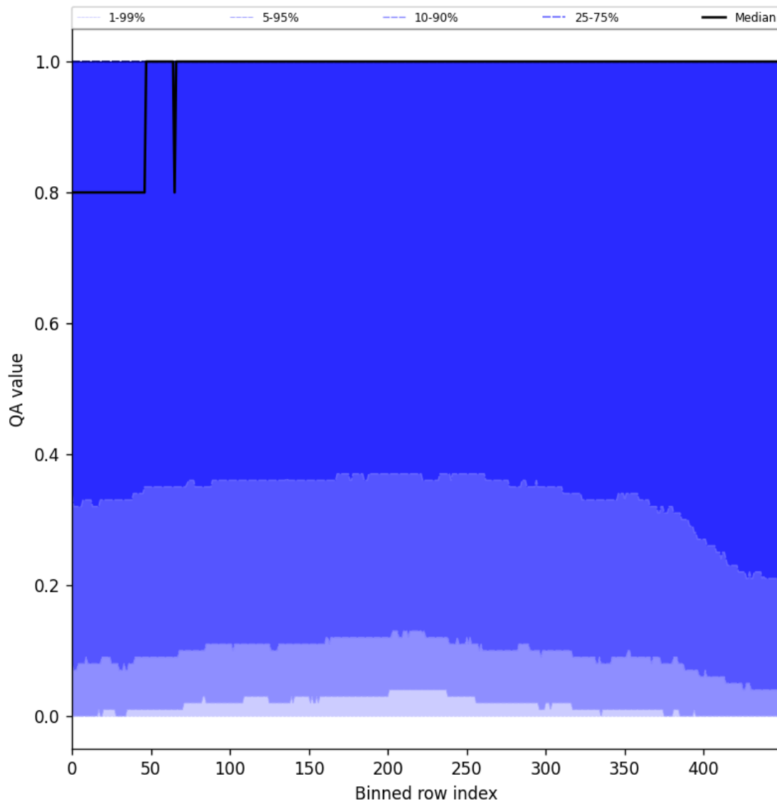
Figure 83: Along track statistics of “QA value” for 2025-11-23 to 2025-11-24
