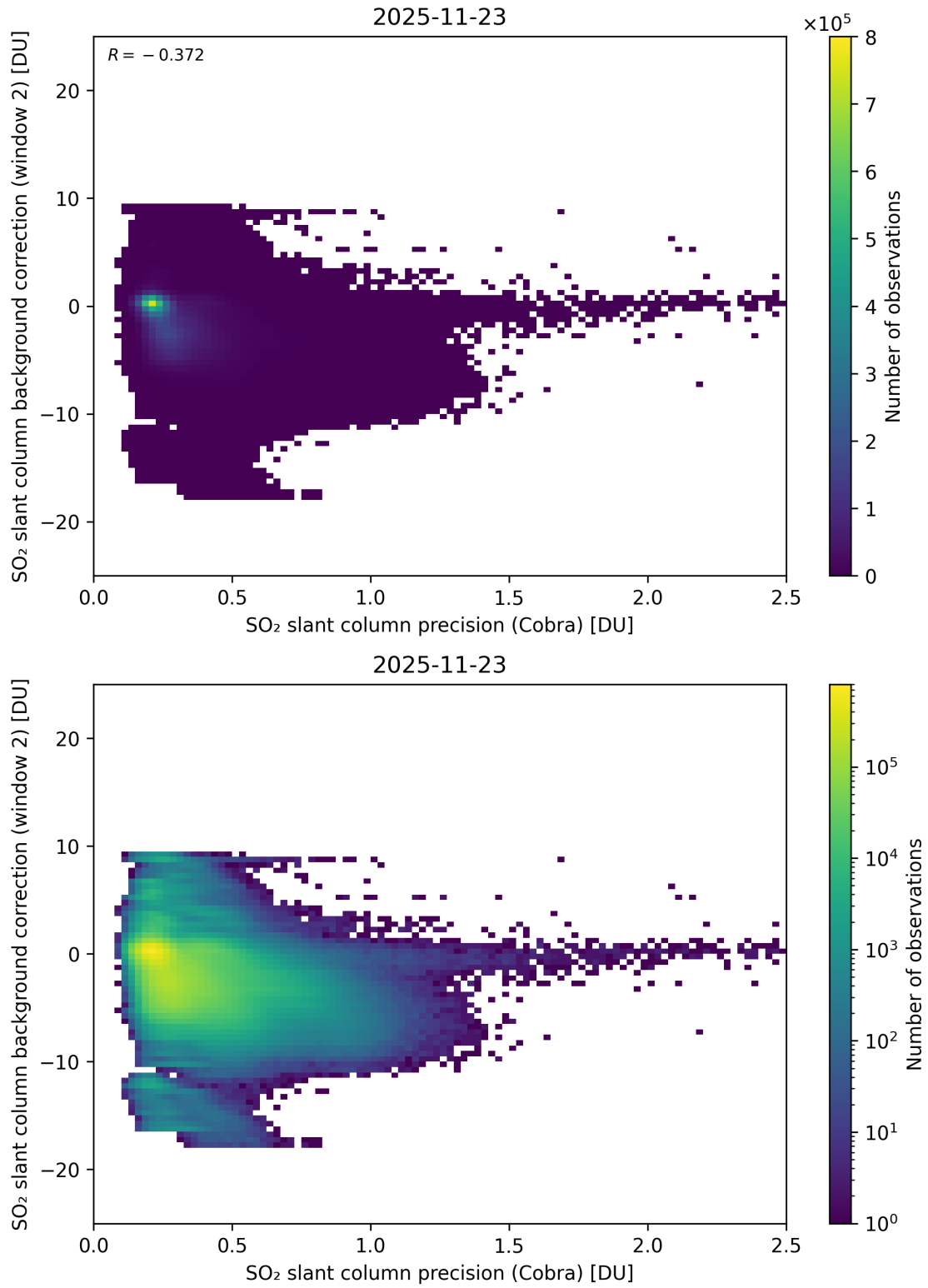
Figure 200: Scatter density plot of “SO 2 slant column precision (Cobra)” against “SO 2 slant column background correction (window 2)” for 2025-11-23 to 2025-11-24.
