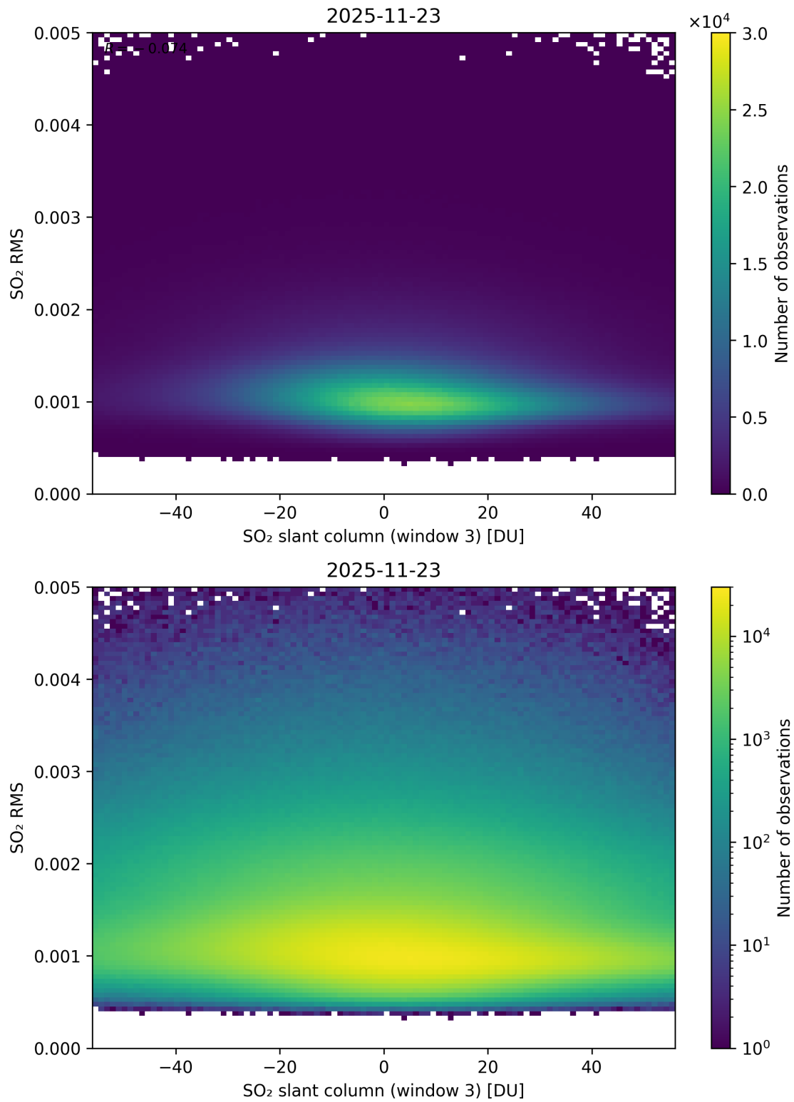
Figure 306: Scatter density plot of “SO 2 slant column (window 3)” against “SO 2 RMS” for 2025-11-23 to 2025-11-24.
