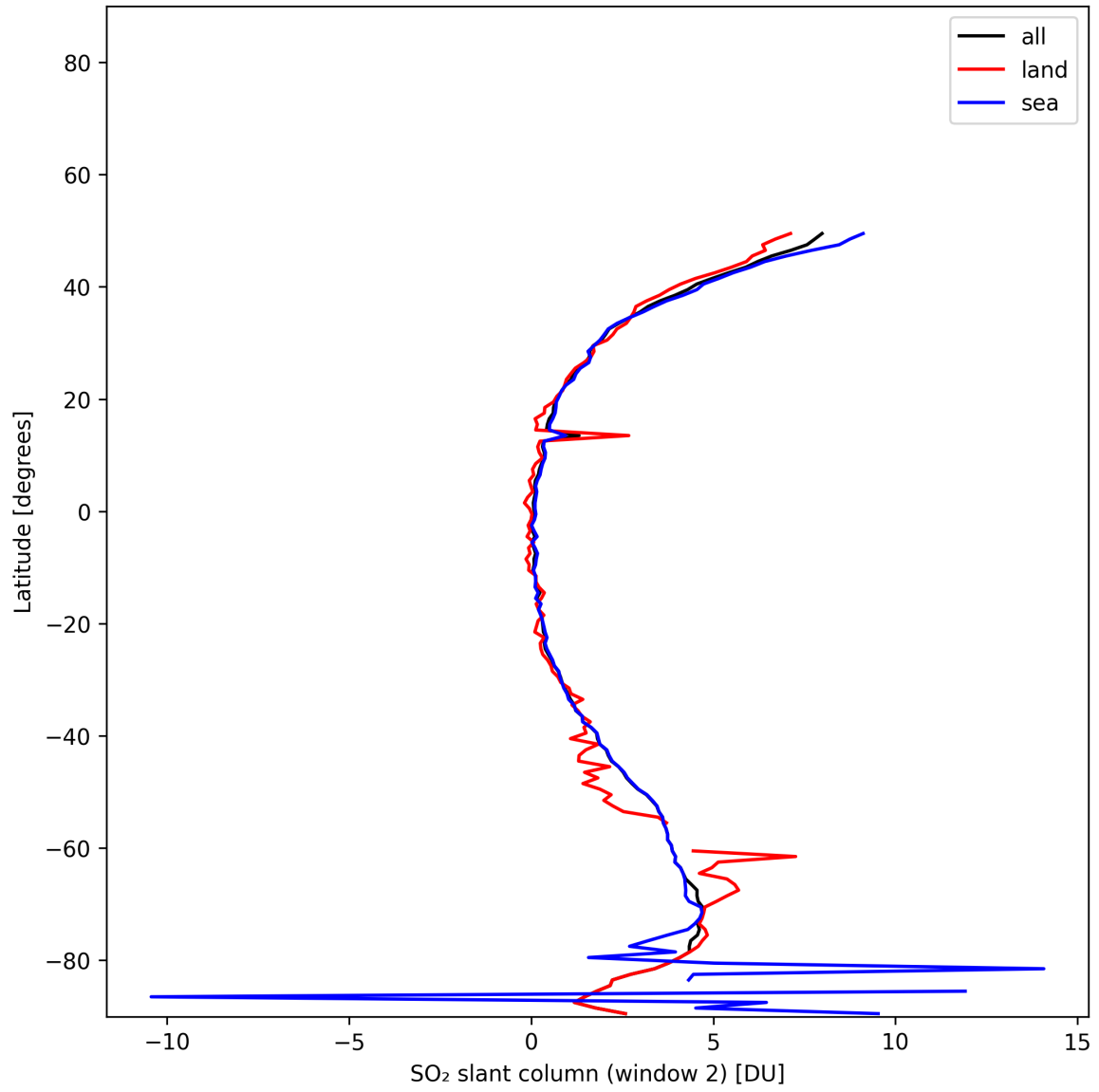
Figure 41: Zonal average of “SO 2 slant column (window 2)” for 2025-11-23 to 2025-11-24.
