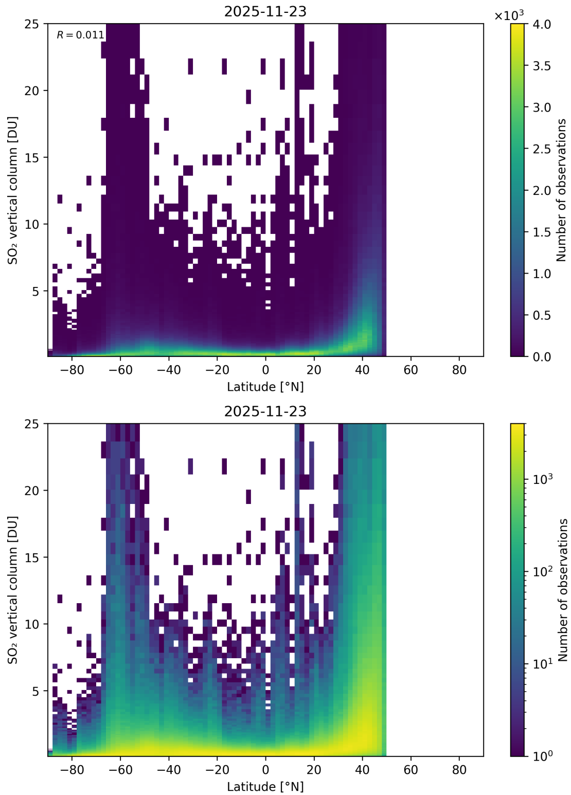
Figure 169: Scatter density plot of “Latitude” against “SO 2 vertical column” for 2025-11-23 to 2025-11-24.
