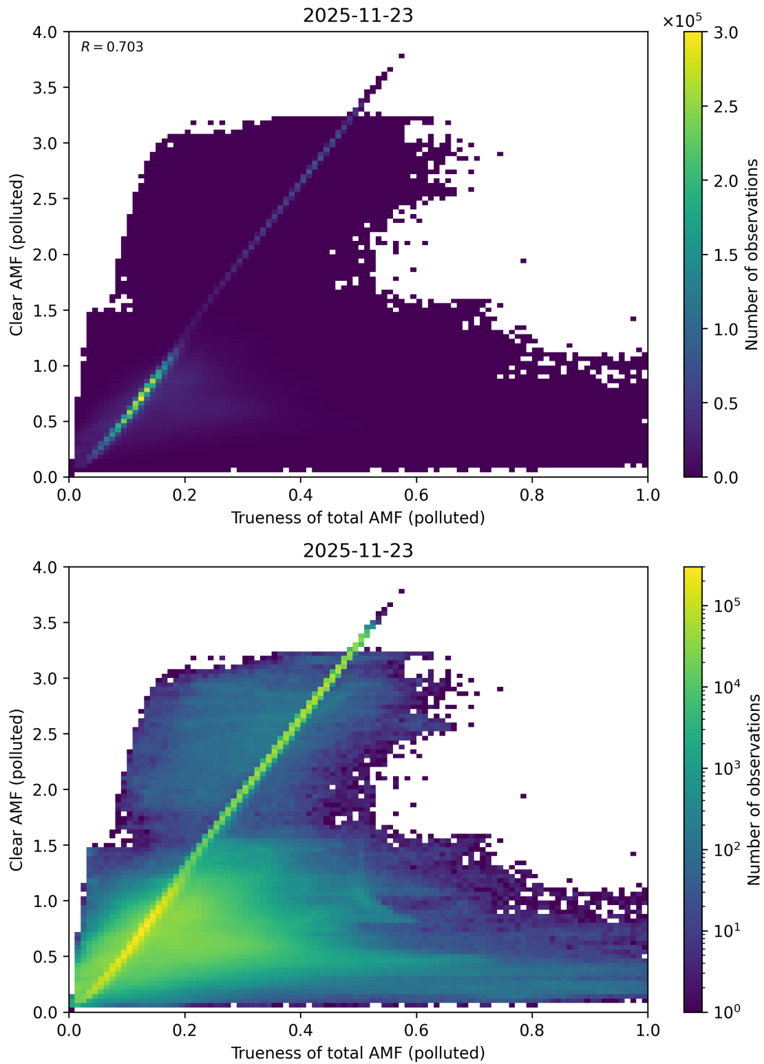
Figure 322: Scatter density plot of “Trueness of total AMF (polluted)” against “Clear AMF (polluted)” for 2025-11-23 to 2025-11-24.
