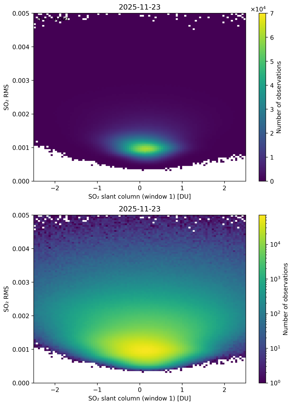
Figure 267: Scatter density plot of “SO 2 slant column (window 1)” against “SO 2 RMS” for 2025-11-23 to 2025-11-24.
