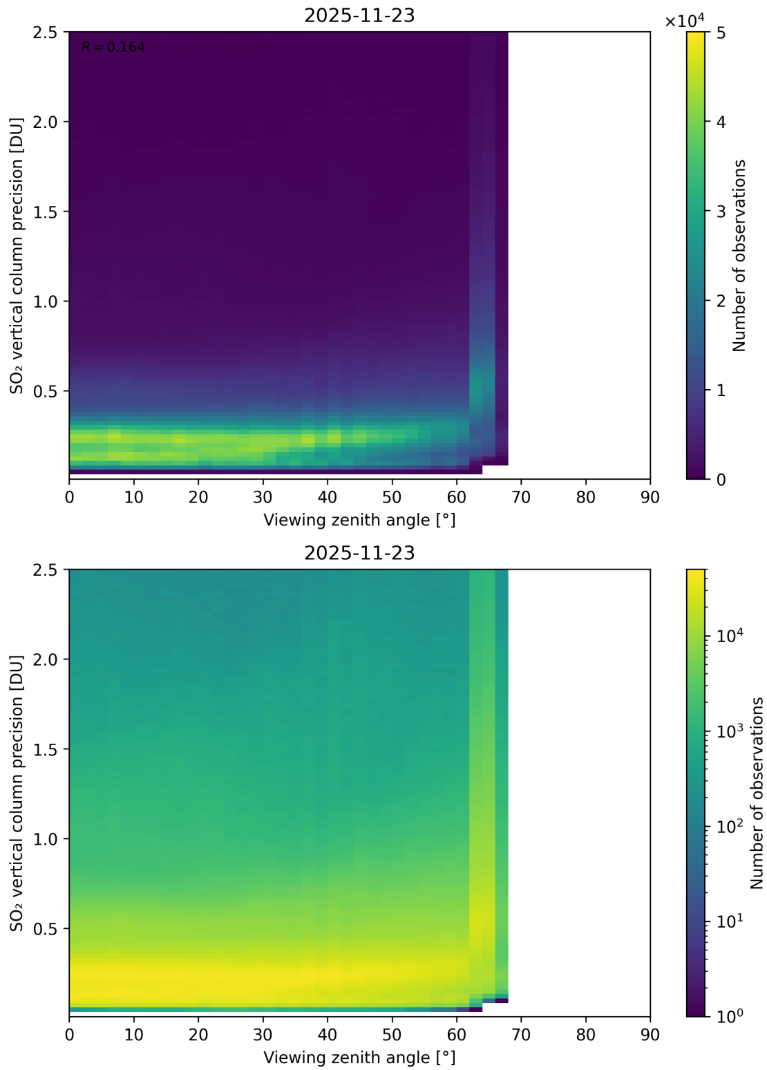
Figure 384: Scatter density plot of “Viewing zenith angle” against “SO 2 vertical column precision” for 2025-11-23 to 2025-11-24.
