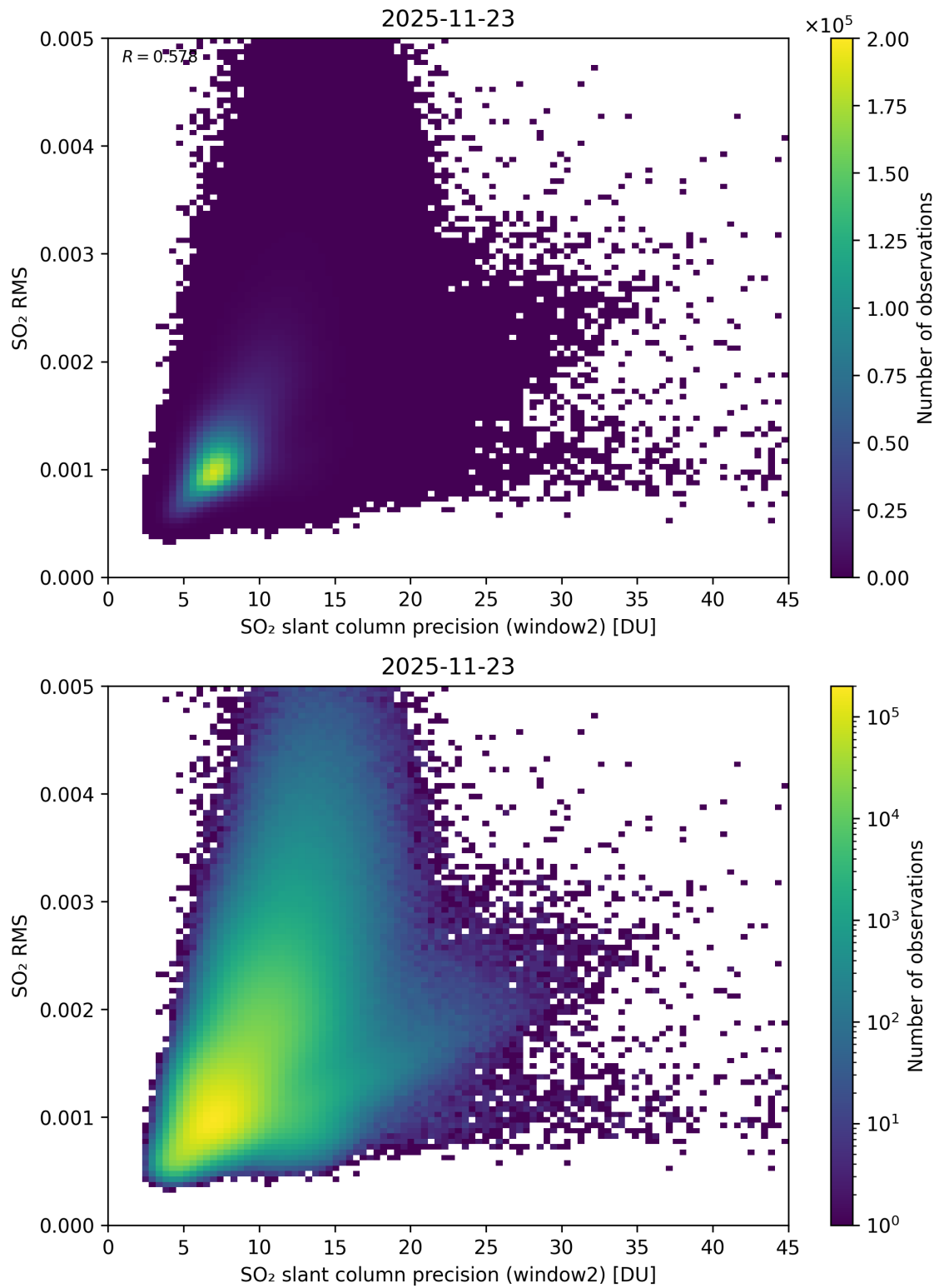
Figure 295: Scatter density plot of “SO 2 slant column precision (window2)” against “SO 2 RMS” for 2025-11-23 to 2025-11-24.
