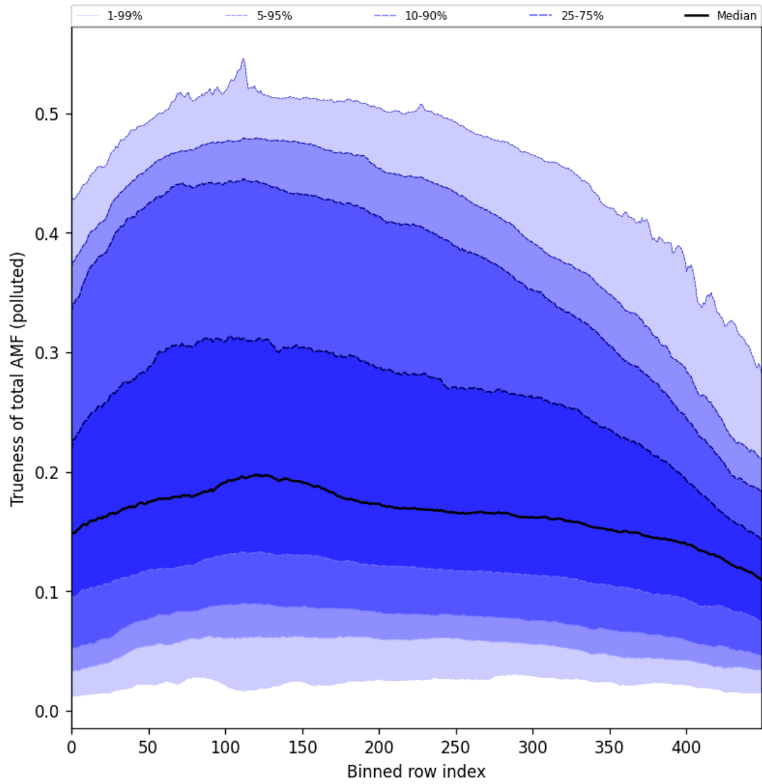
Figure 106: Along track statistics of “Trueness of total AMF (polluted)” for 2025-11-23 to 2025-11-24
