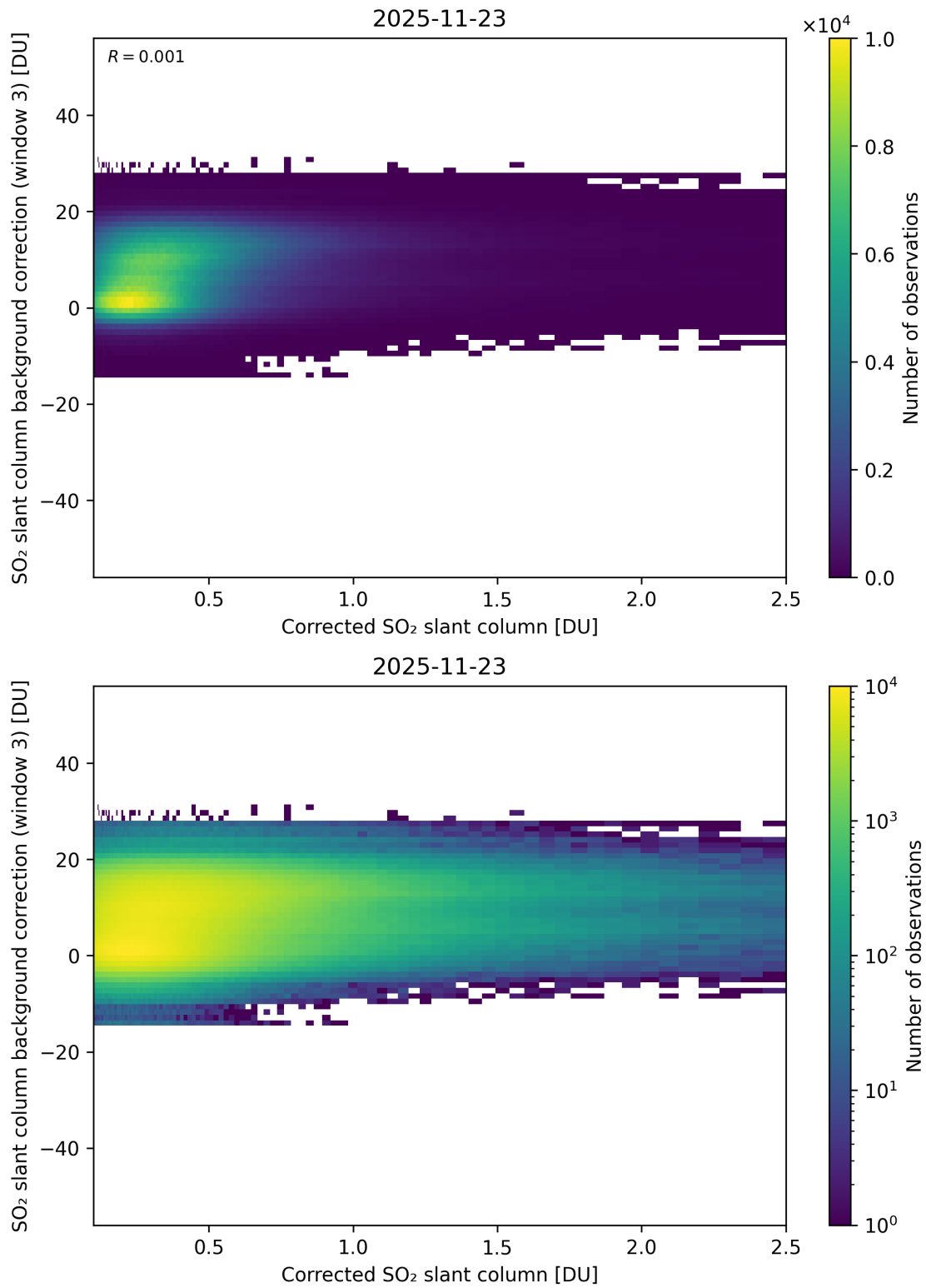
Figure 228: Scatter density plot of “Corrected SO 2 slant column” against “SO 2 slant column background correction (window 3)” for 2025-11-23 to 2025-11-24.
