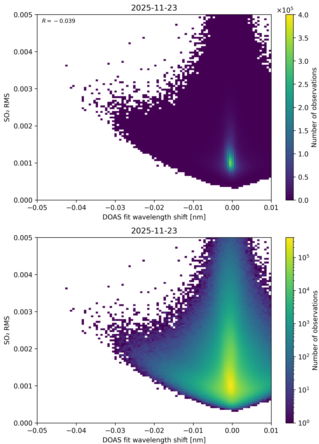
Figure 139: Scatter density plot of “DOAS fit wavelength shift” against “SO 2 RMS” for 2025-11-23 to 2025-11-24.
