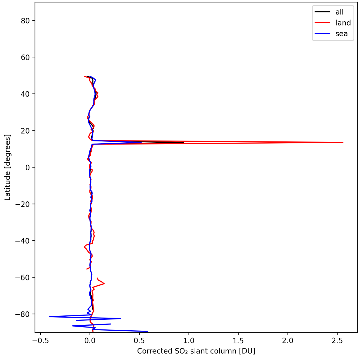
Figure 34: Zonal average of "Corrected SO 2 slant column" for 2025-11-23 to 2025-11-24.
