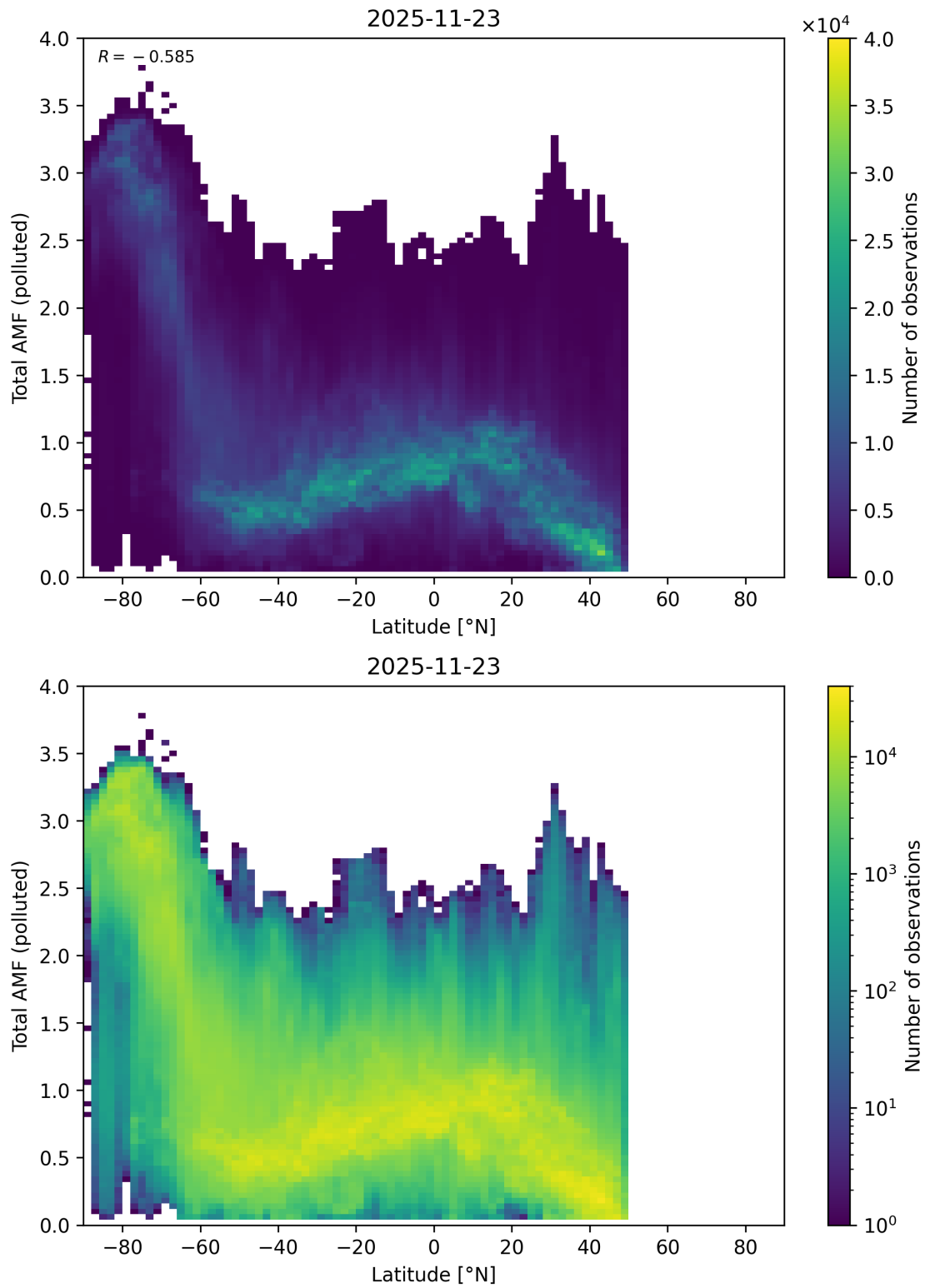
Figure 167: Scatter density plot of “Latitude” against “Total AMF (polluted)” for 2025-11-23 to 2025-11-24.
