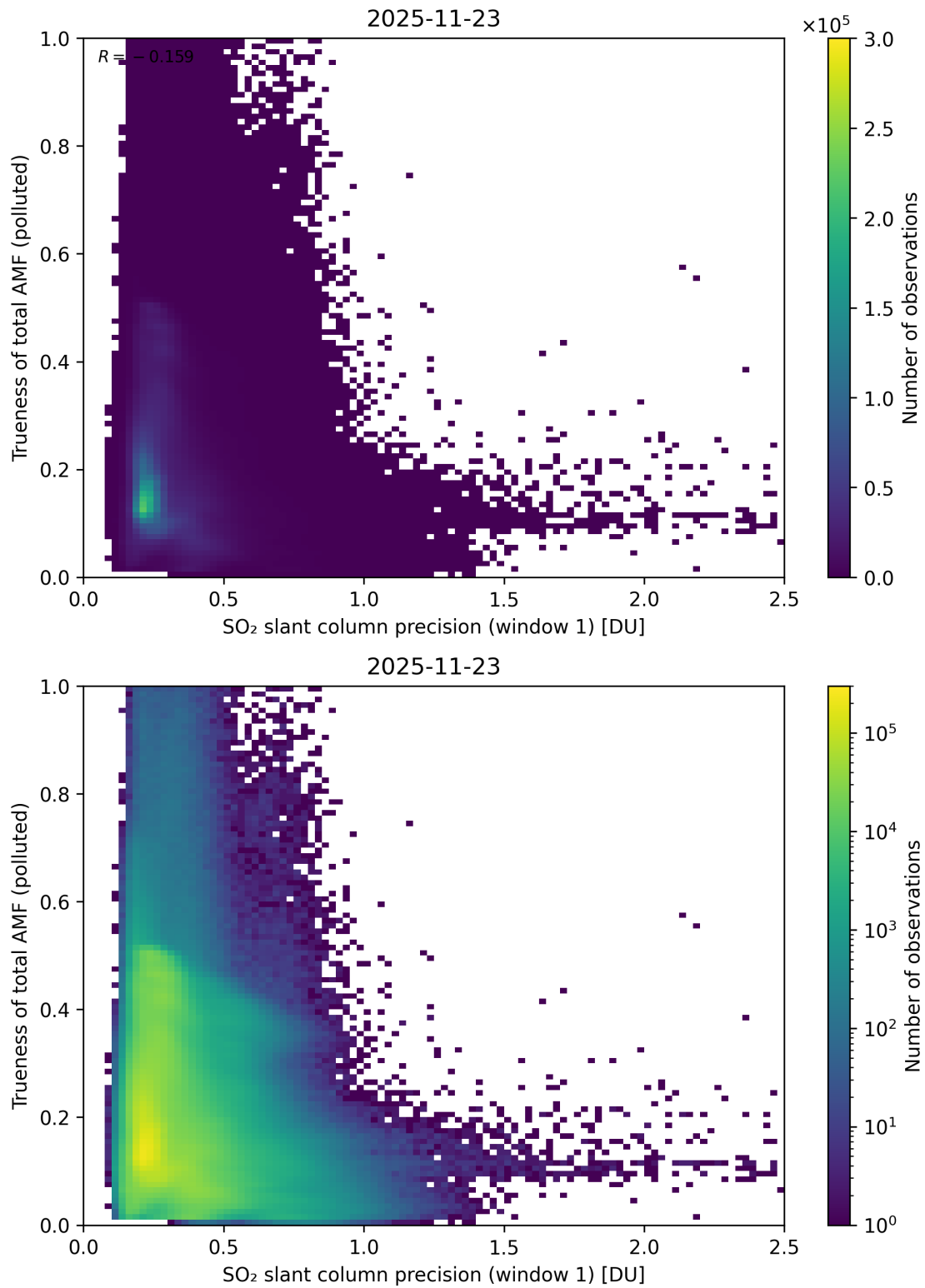
Figure 281: Scatter density plot of “SO 2 slant column precision (window 1)” against “Trueness of total AMF (polluted)” for 2025-11-23 to 2025-11-24.
