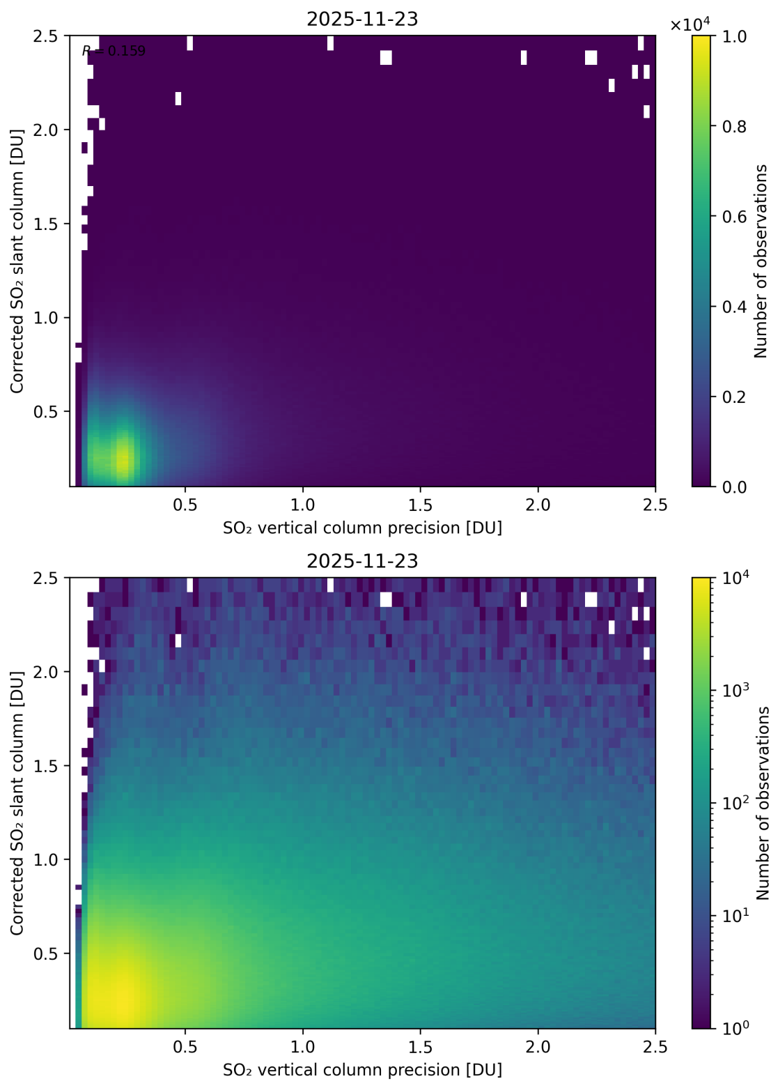
Figure 338: Scatter density plot of “SO 2 vertical column precision” against “Corrected SO 2 slant column” for 2025-11-23 to 2025-11-24.
