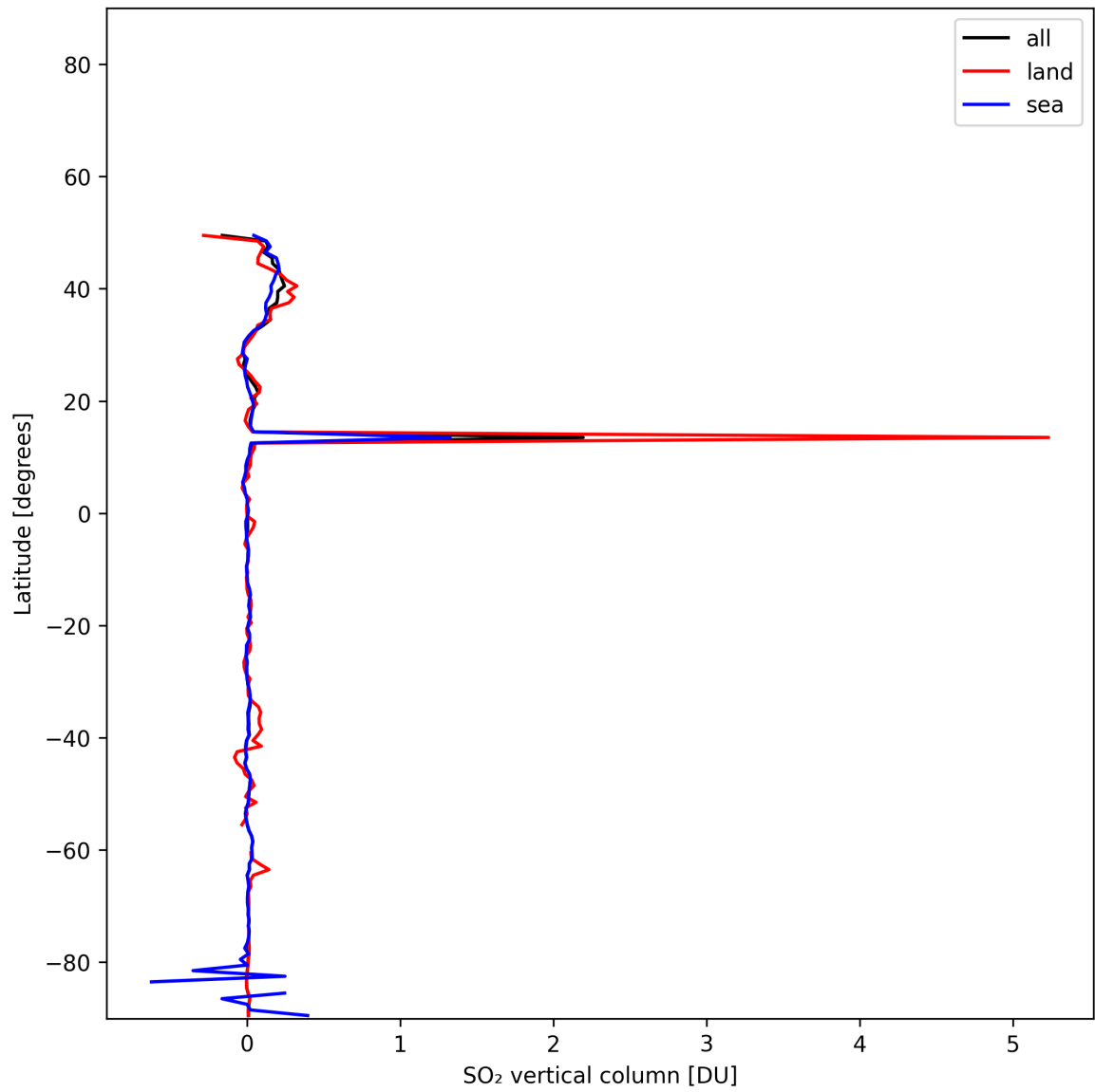
Figure 32: Zonal average of “SO 2 vertical column” for 2025-11-23 to 2025-11-24.
