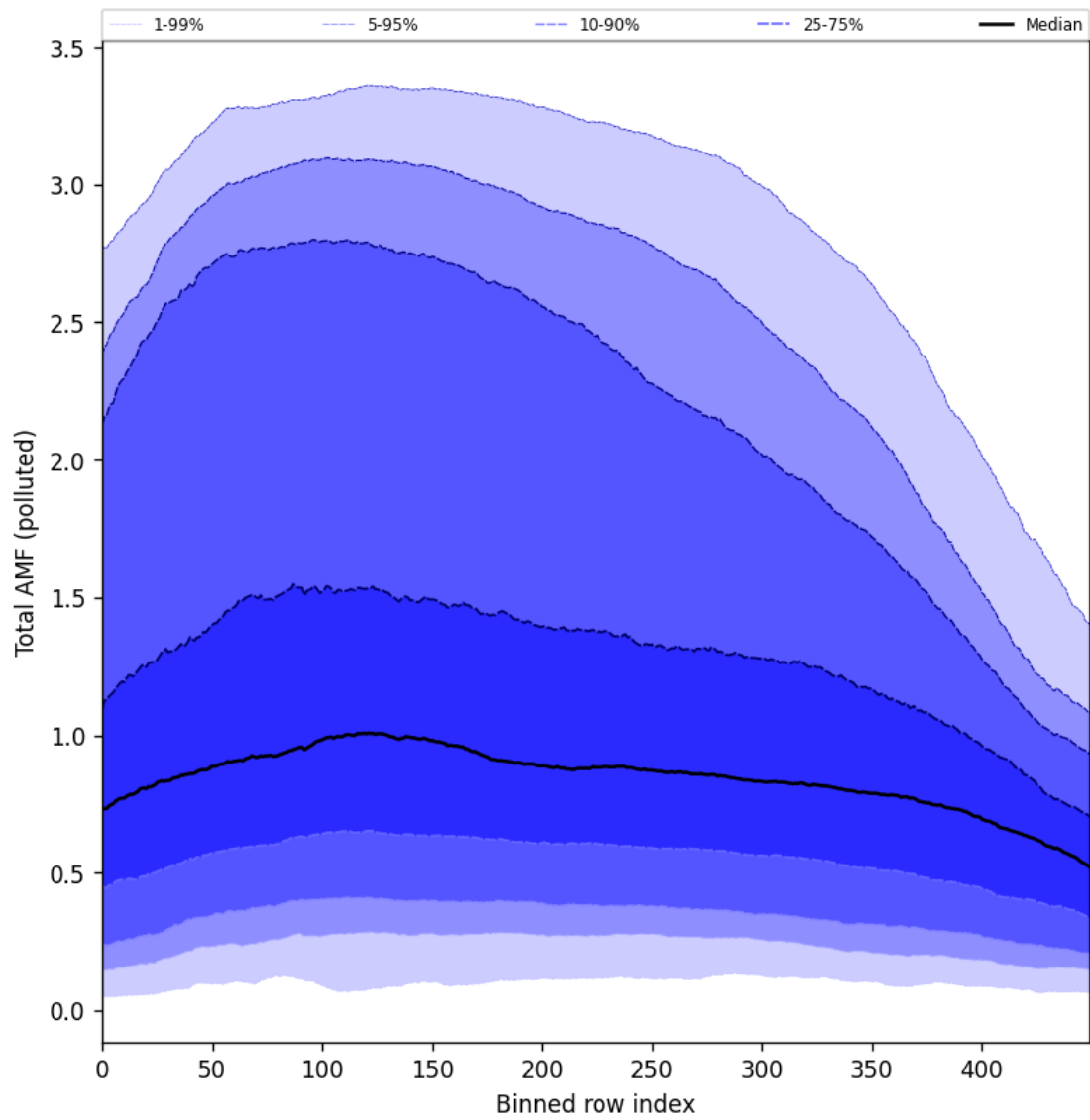
Figure 105: Along track statistics of “Total AMF (polluted)” for 2025-11-23 to 2025-11-24
