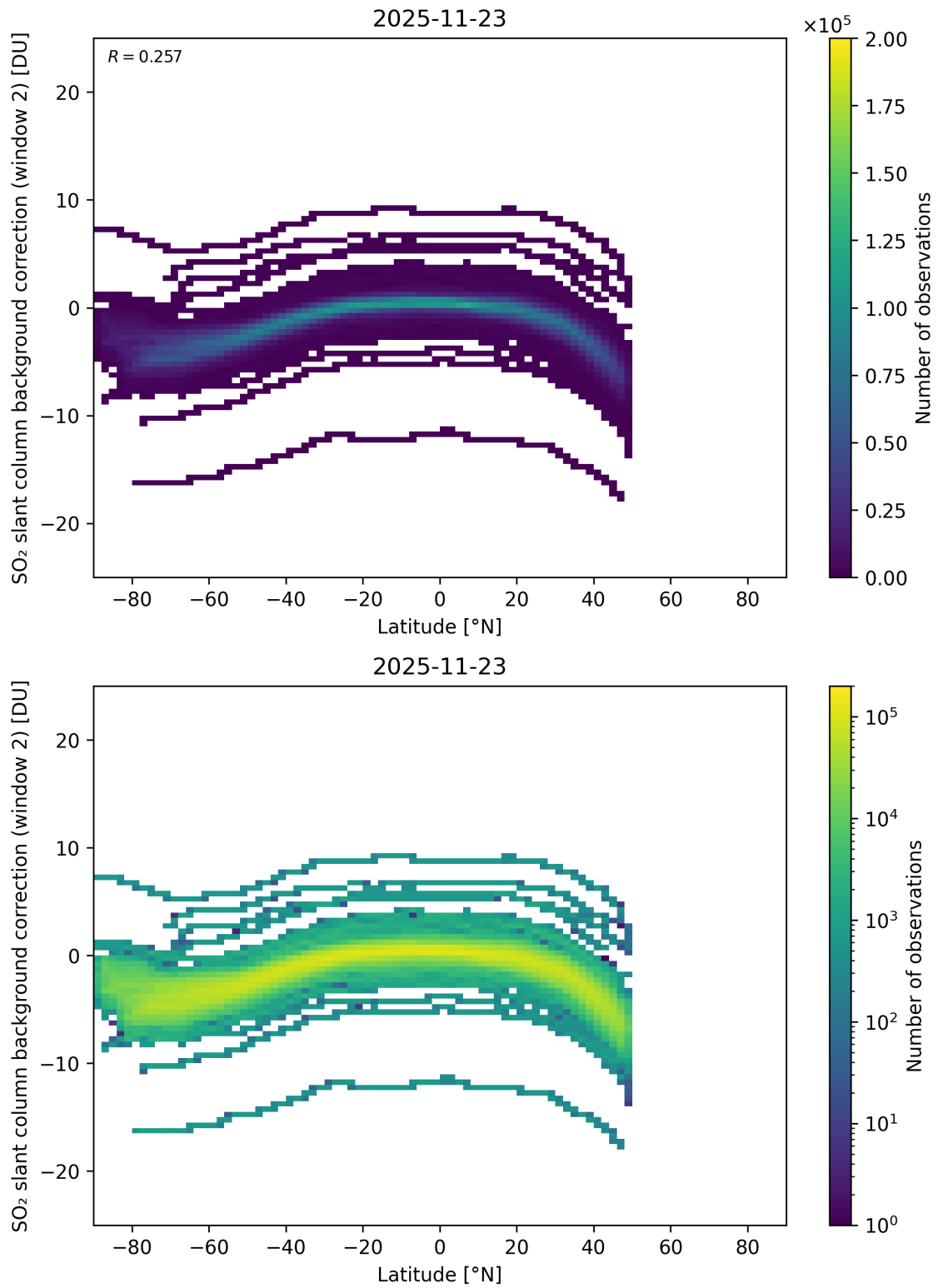
Figure 151: Scatter density plot of “Latitude” against “SO 2 slant column background correction (window 2)” for 2025-11-23 to 2025-11-24.
