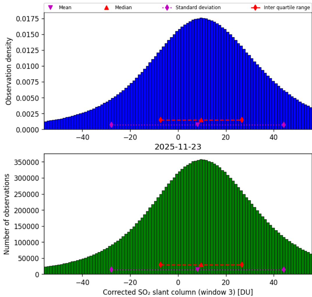
Figure 73: Histogram of "Corrected SO 2 slant column (window 3)" for 2025-11-23 to 2025-11-24
