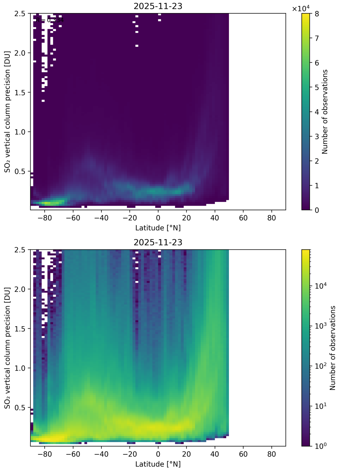
Figure 170: Scatter density plot of “Latitude” against “SO 2 vertical column precision” for 2025-11-23 to 2025-11-24.
