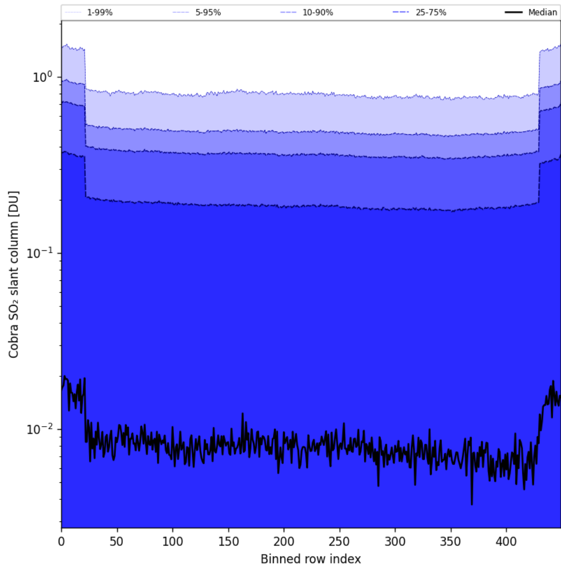
Figure 87: Along track statistics of “Cobra SO 2 slant column” for 2025-11-23 to 2025-11-24
