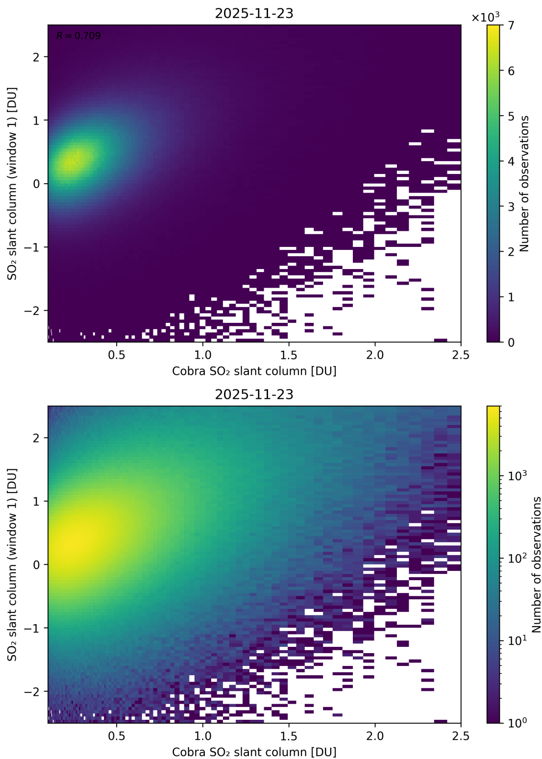
Figure 219: Scatter density plot of “Cobra SO 2 slant column” against “SO 2 slant column (window 1)” for 2025-11-23 to 2025-11-24.
