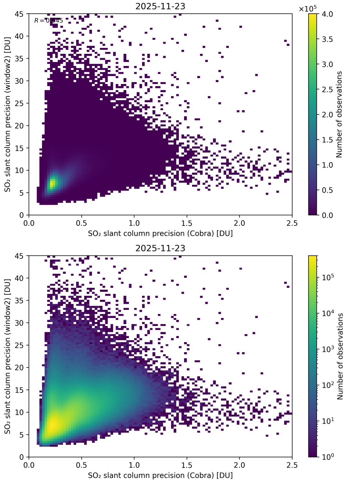
Figure 210: Scatter density plot of “SO 2 slant column precision (Cobra)” against “SO 2 slant column precision (window2)” for 2025-11-23 to 2025-11-24.
