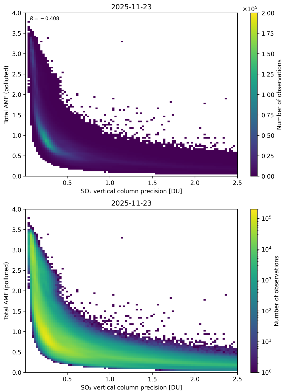
Figure 346: Scatter density plot of “SO 2 vertical column precision” against “Total AMF (polluted)” for 2025-11-23 to 2025-11-24.
