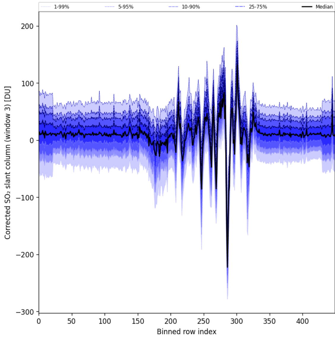
Figure 99: Along track statistics of “Corrected SO 2 slant column (window 3)” for 2025-11-23 to 2025-11-24
