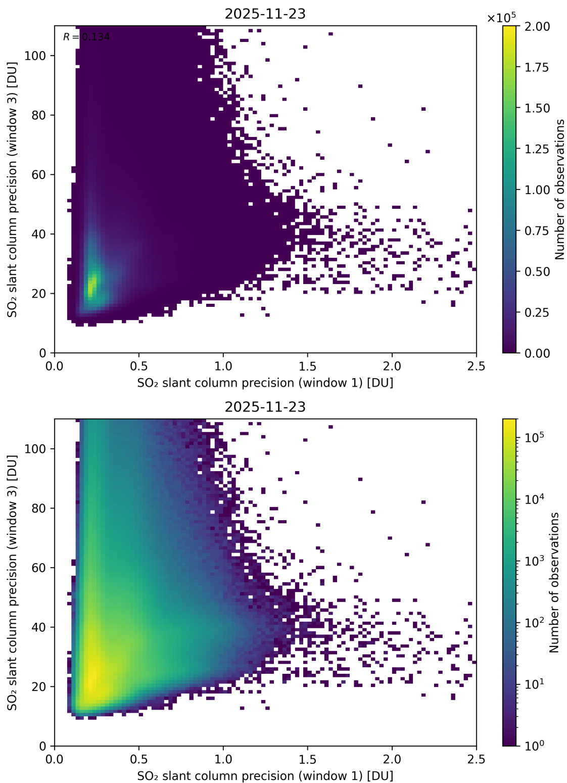
Figure 279: Scatter density plot of “SO 2 slant column precision (window 1)” against “SO 2 slant column precision (window 3)” for 2025-11-23 to 2025-11-24.
