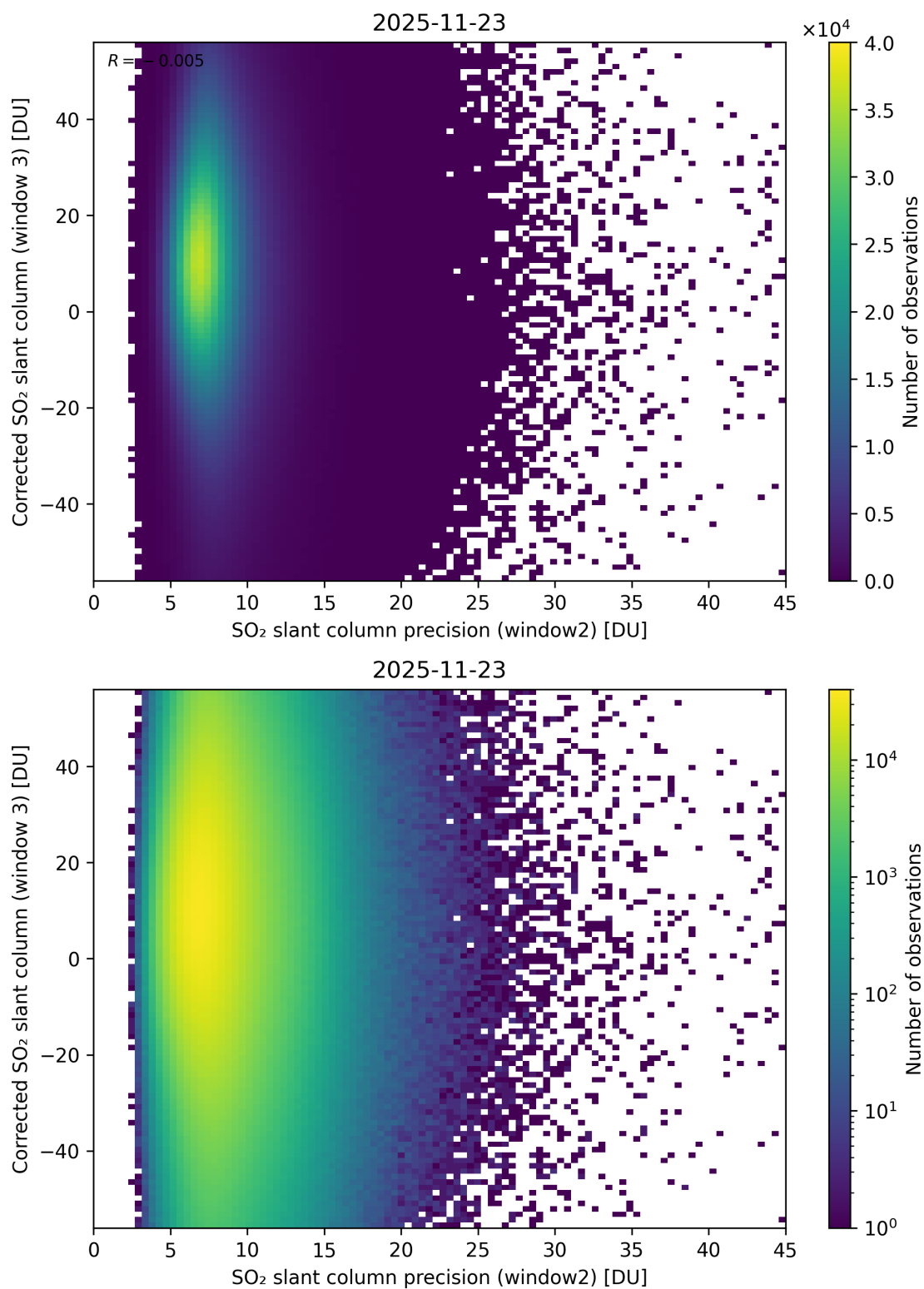
Figure 298: Scatter density plot of “SO 2 slant column precision (window2)” against “Corrected SO 2 slant column (window 3)” for 2025-11-23 to 2025-11-24.
