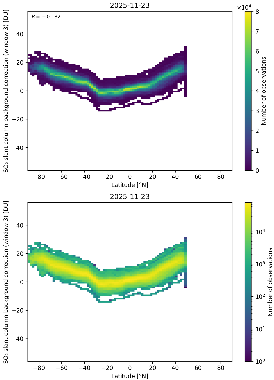
Figure 152: Scatter density plot of “Latitude” against “SO 2 slant column background correction (window 3)” for 2025-11-23 to 2025-11-24.
