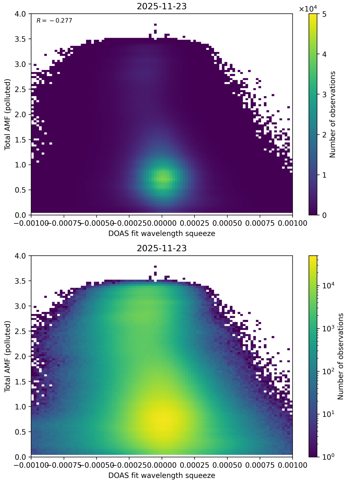
Figure 145: Scatter density plot of “DOAS fit wavelength squeeze” against “Total AMF (polluted)” for 2025-11-23 to 2025-11-24.
