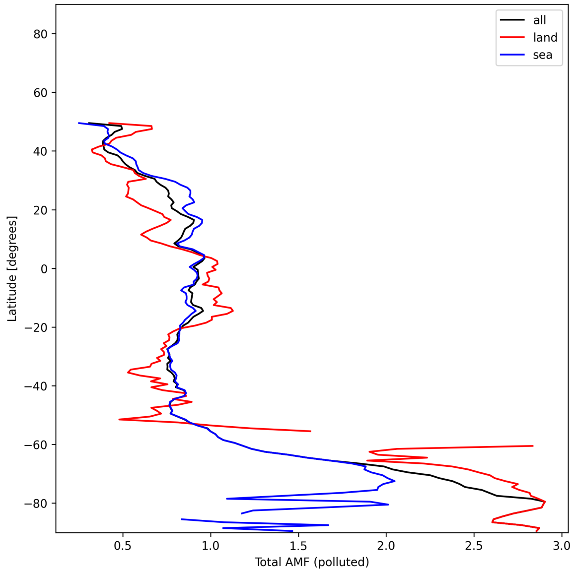
Figure 53: Zonal average of “Total AMF (polluted)” for 2025-11-23 to 2025-11-24.
