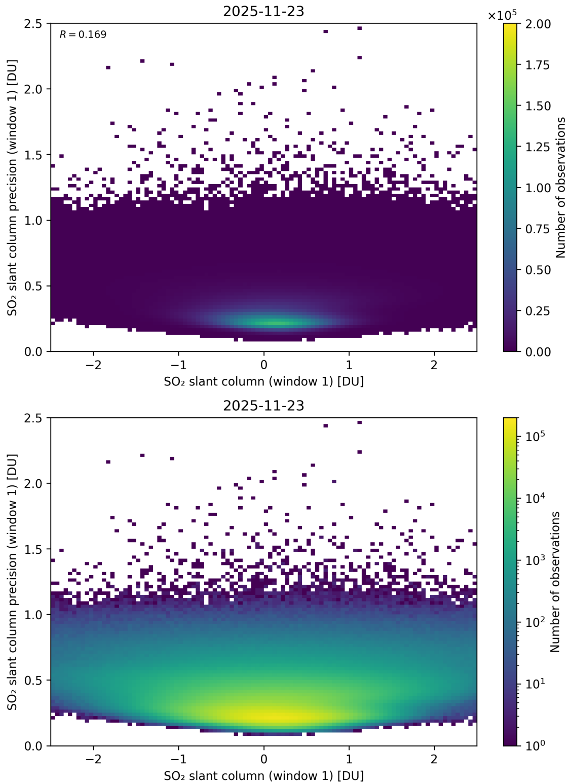
Figure 285: Scatter density plot of “SO 2 slant column (window 1)” against “SO 2 slant column precision (window 1)” for 2025-11-23 to 2025-11-24.
