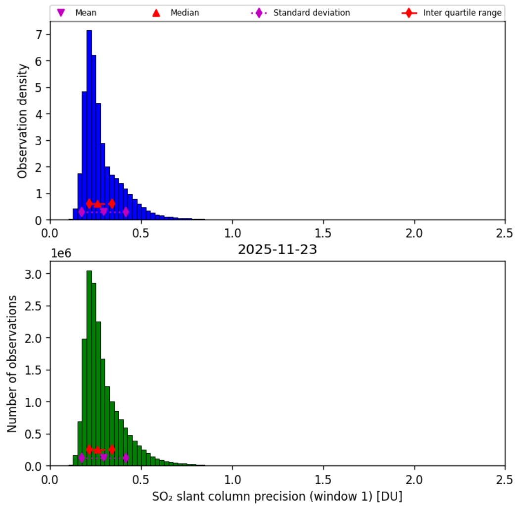
Figure 64: Histogram of “SO 2 slant column precision (window 1)” for 2025-11-23 to 2025-11-24
