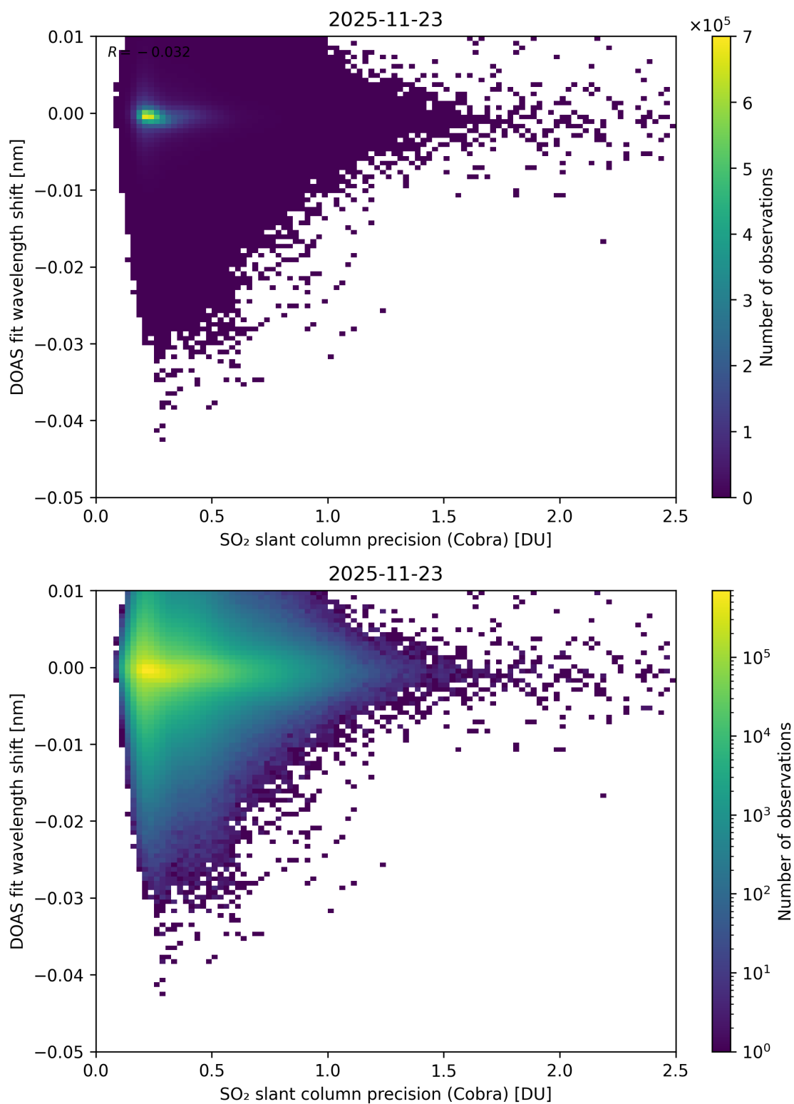
Figure 202: Scatter density plot of “SO 2 slant column precision (Cobra)” against “DOAS fit wavelength shift” for 2025-11-23 to 2025-11-24.
