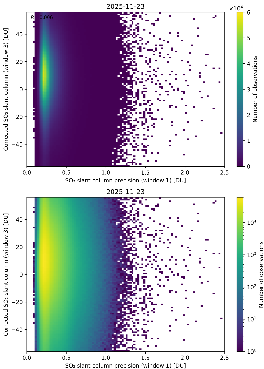
Figure 276: Scatter density plot of “SO 2 slant column precision (window 1)” against “Corrected SO 2 slant column (window 3)” for 2025-11-23 to 2025-11-24.
