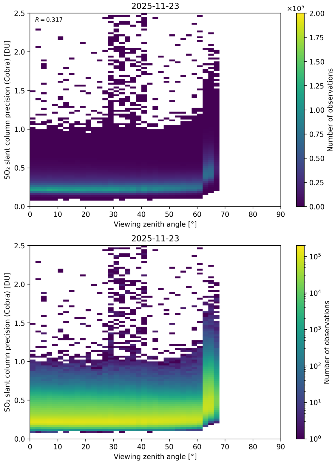
Figure 372: Scatter density plot of “Viewing zenith angle” against “SO 2 slant column precision (Cobra)” for 2025-11-23 to 2025-11-24.
