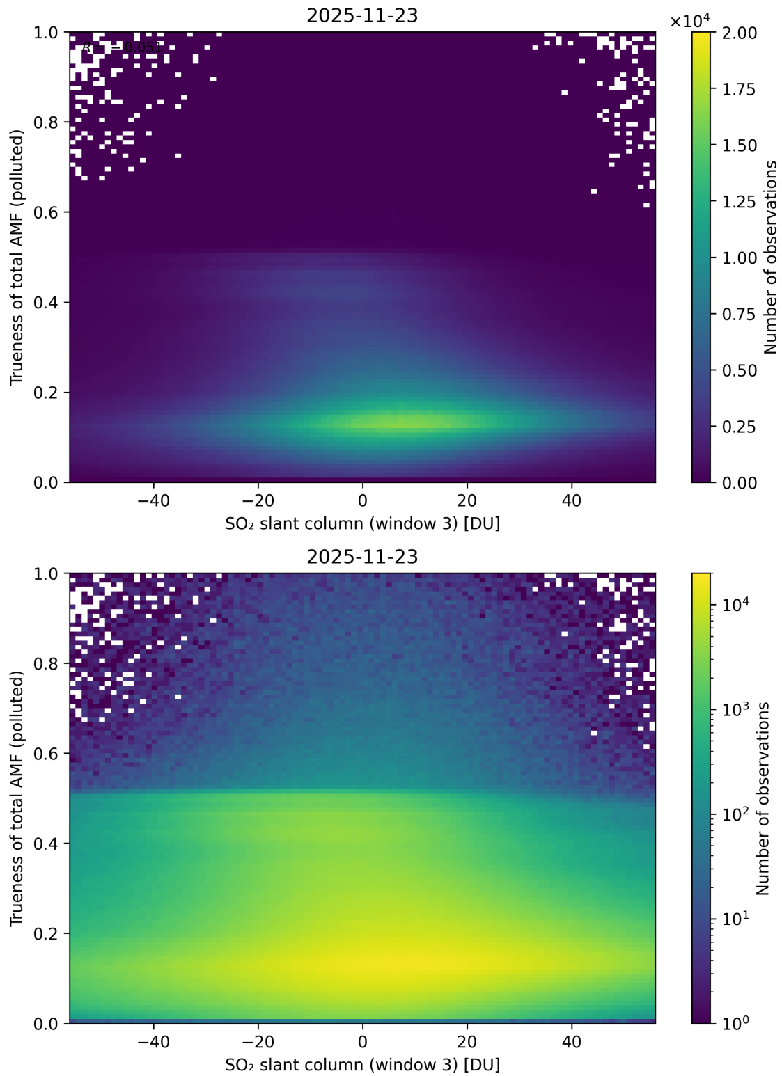
Figure 319: Scatter density plot of “SO 2 slant column (window 3)” against “Trueness of total AMF (polluted)” for 2025-11-23 to 2025-11-24.
