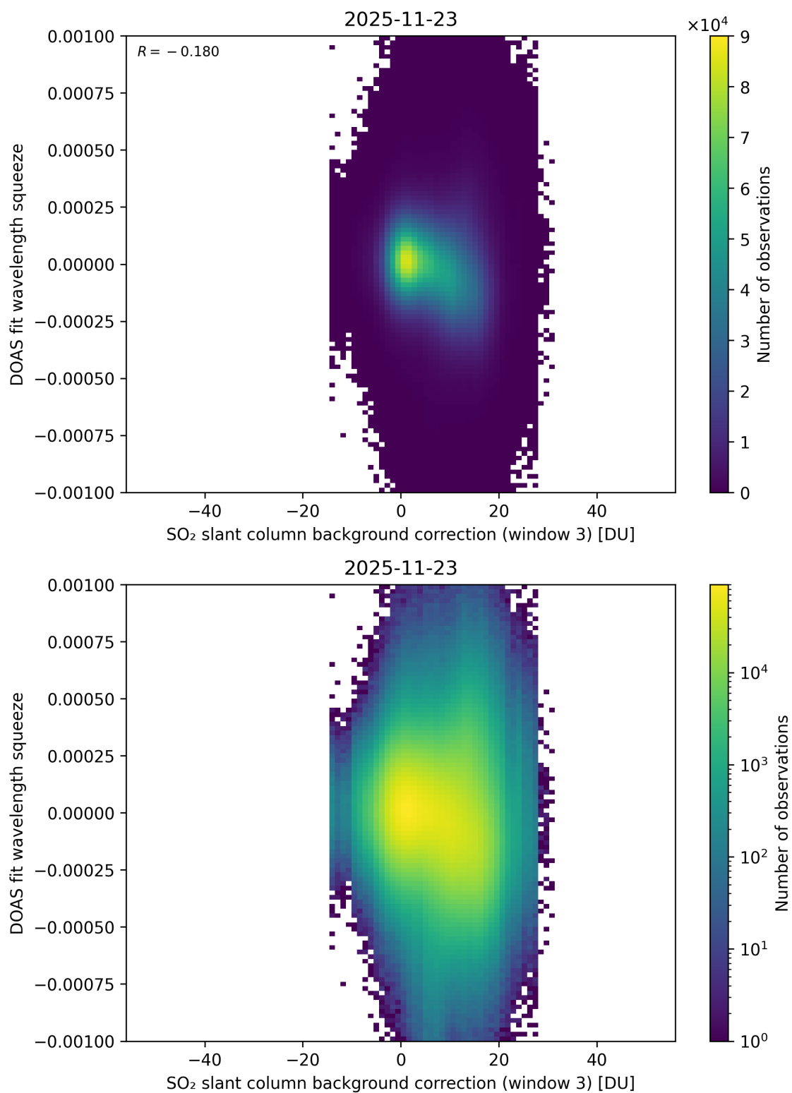
Figure 133: Scatter density plot of “SO 2 slant column background correction (window 3)” against “DOAS fit wavelength squeeze” for 2025-11-23 to 2025-11-24.
