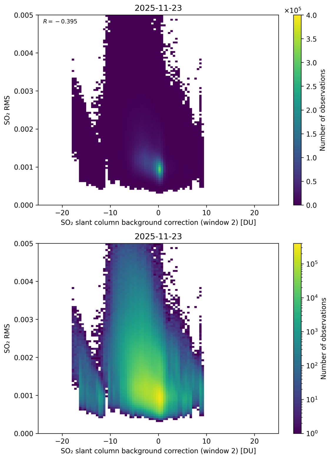
Figure 125: Scatter density plot of “SO 2 slant column background correction (window 2)” against “SO 2 RMS” for 2025-11-23 to 2025-11-24.
