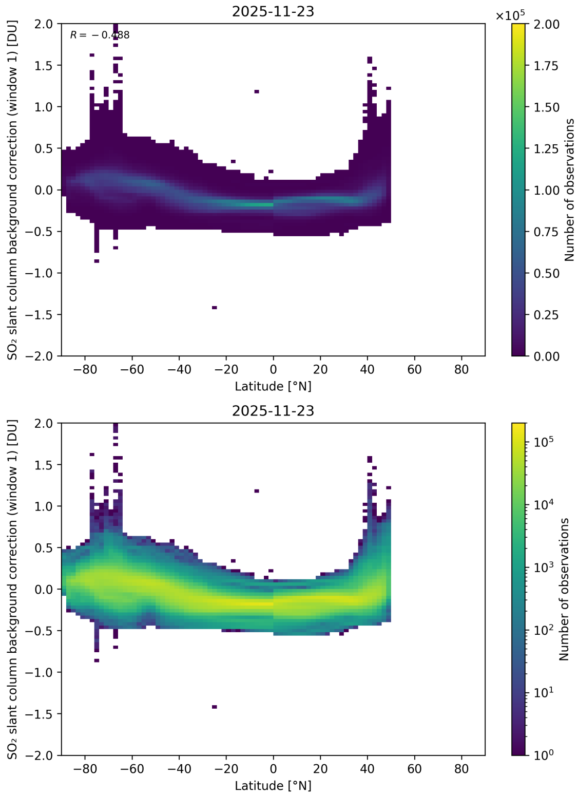
Figure 150: Scatter density plot of “Latitude” against “SO 2 slant column background correction (window 1)” for 2025-11-23 to 2025-11-24.
