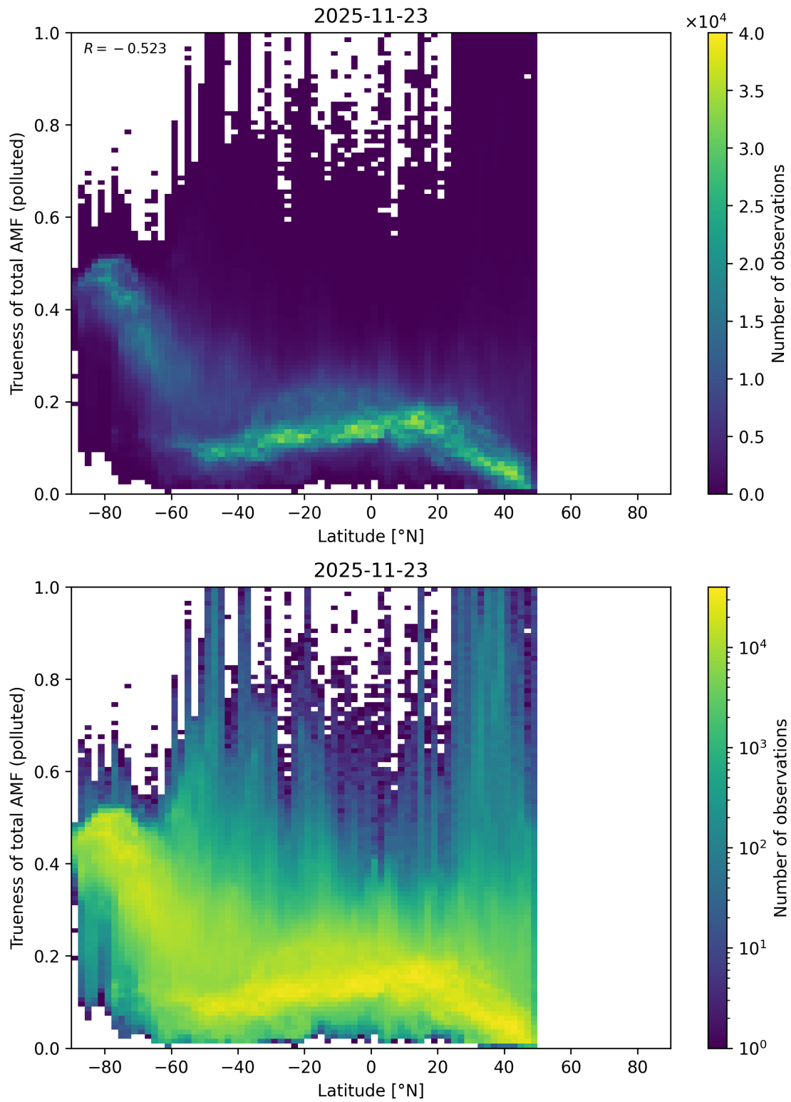
Figure 168: Scatter density plot of “Latitude” against “Trueness of total AMF (polluted)” for 2025-11-23 to 2025-11-24.
