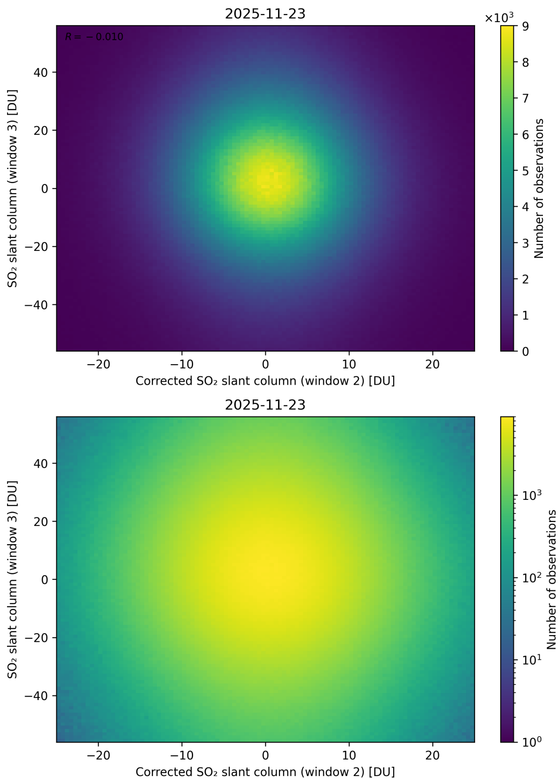
Figure 251: Scatter density plot of “Corrected SO 2 slant column (window 2)” against “SO 2 slant column (window 3)” for 2025-11-23 to 2025-11-24.
