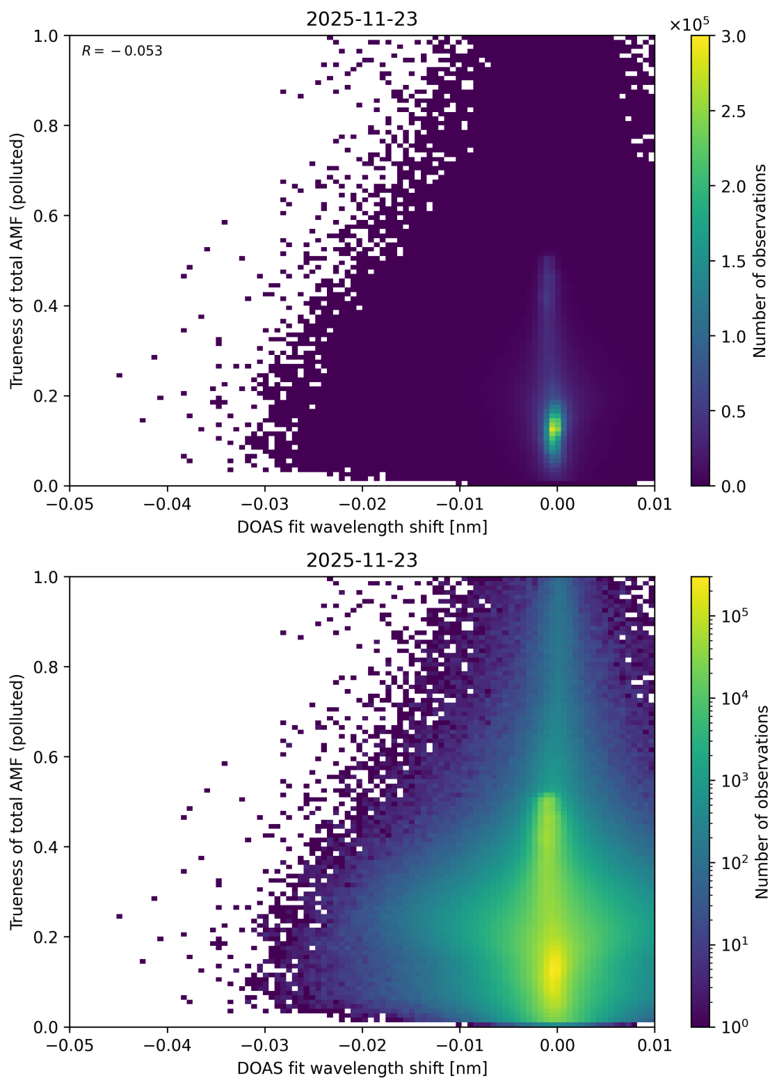
Figure 142: Scatter density plot of “DOAS fit wavelength shift” against “Trueness of total AMF (polluted)” for 2025-11-23 to 2025-11-24.
