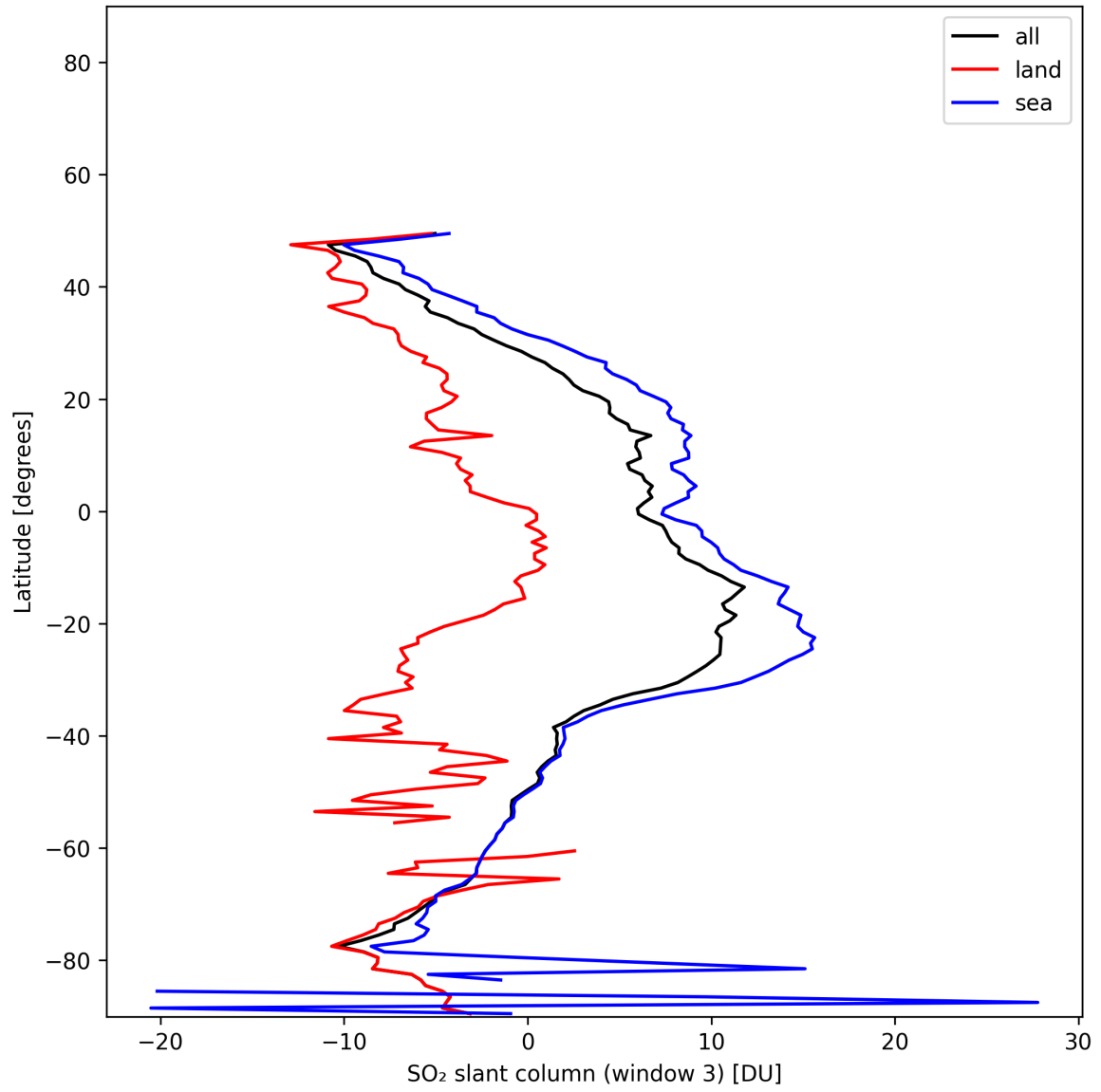
Figure 45: Zonal average of “SO 2 slant column (window 3)” for 2025-11-23 to 2025-11-24.
