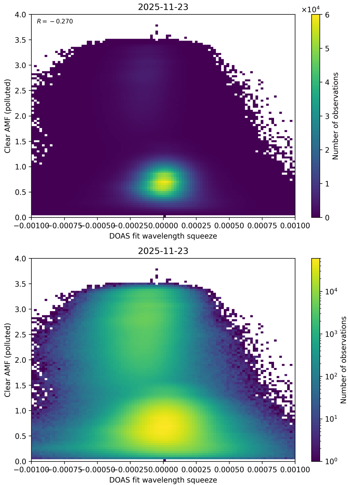
Figure 144: Scatter density plot of “DOAS fit wavelength squeeze” against “Clear AMF (polluted)” for 2025-11-23 to 2025-11-24.
