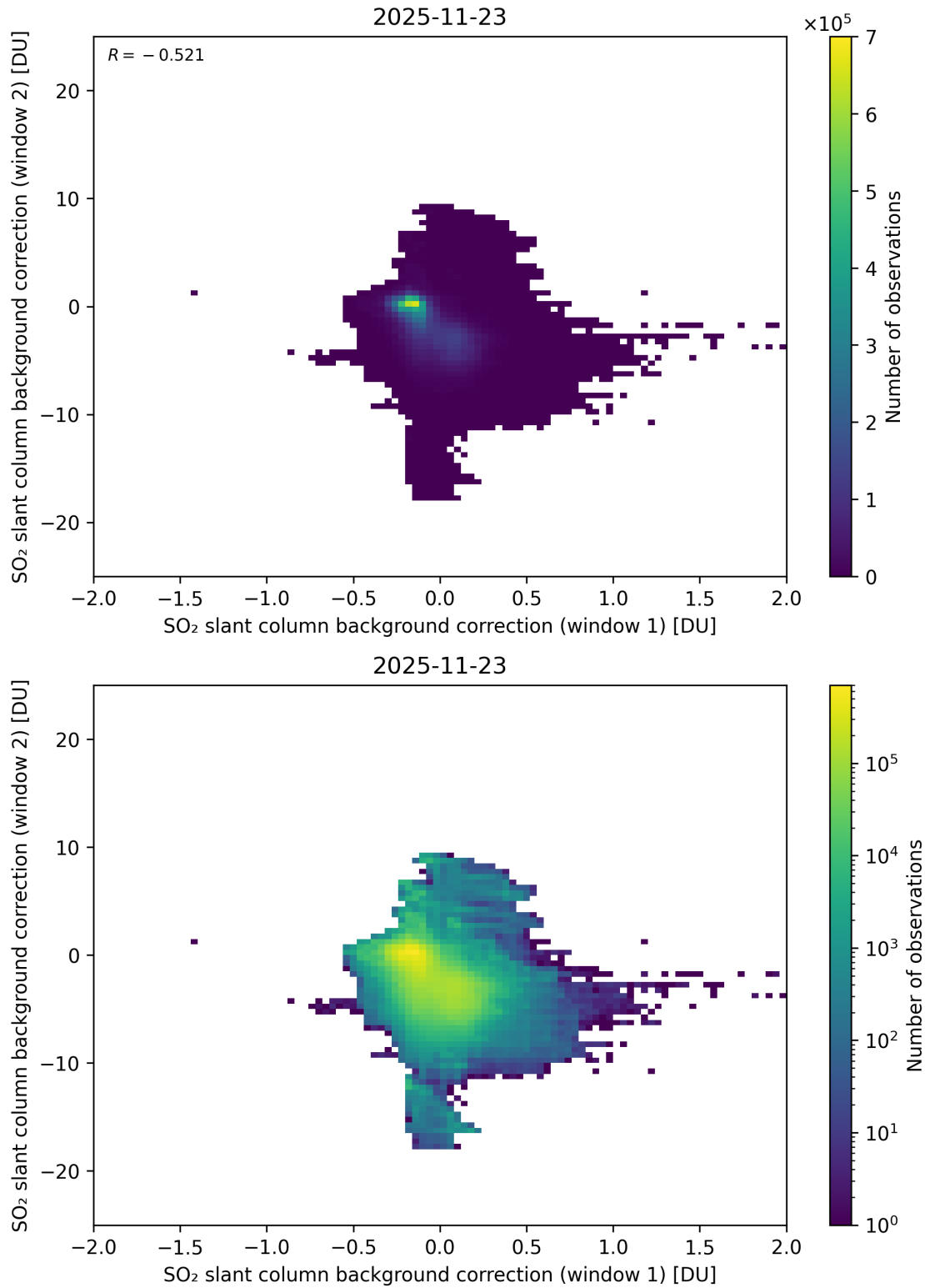
Figure 109: Scatter density plot of “SO 2 slant column background correction (window 1)” against “SO 2 slant column background correction (window 2)” for 2025-11-23 to 2025-11-24.
