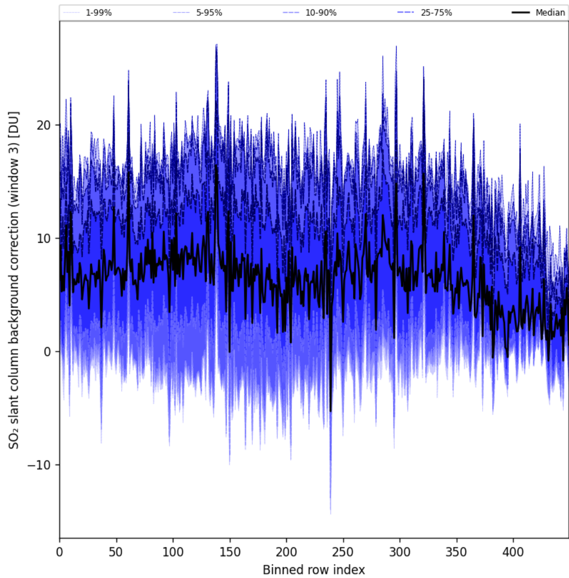
Figure 100: Along track statistics of “SO 2 slant column background correction (window 3)” for 2025-11-23 to 2025-11-24
