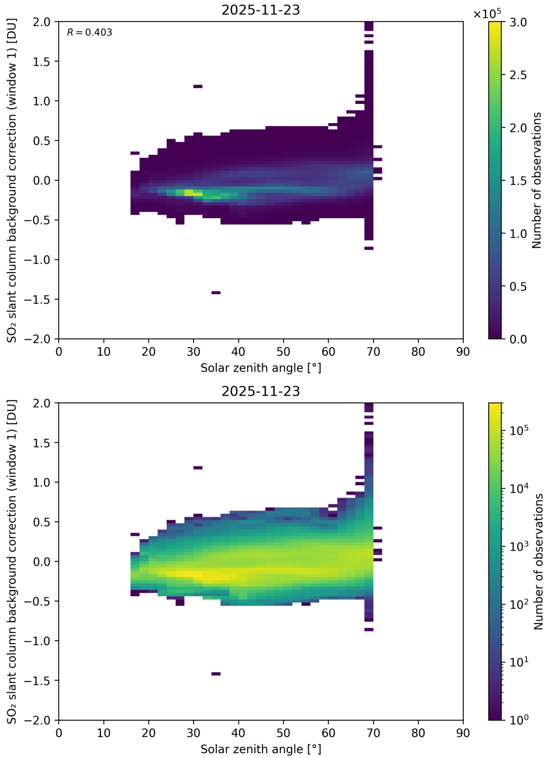
Figure 171: Scatter density plot of “Solar zenith angle” against “SO 2 slant column background correction (window 1)” for 2025-11-23 to 2025-11-24.
