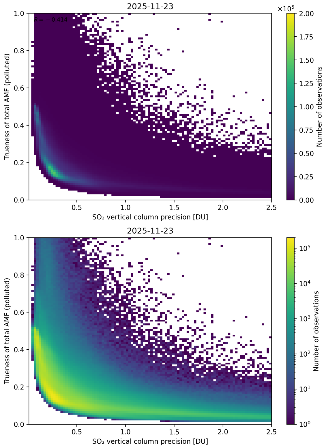
Figure 347: Scatter density plot of “SO 2 vertical column precision” against “Trueness of total AMF (polluted)” for 2025-11-23 to 2025-11-24.
