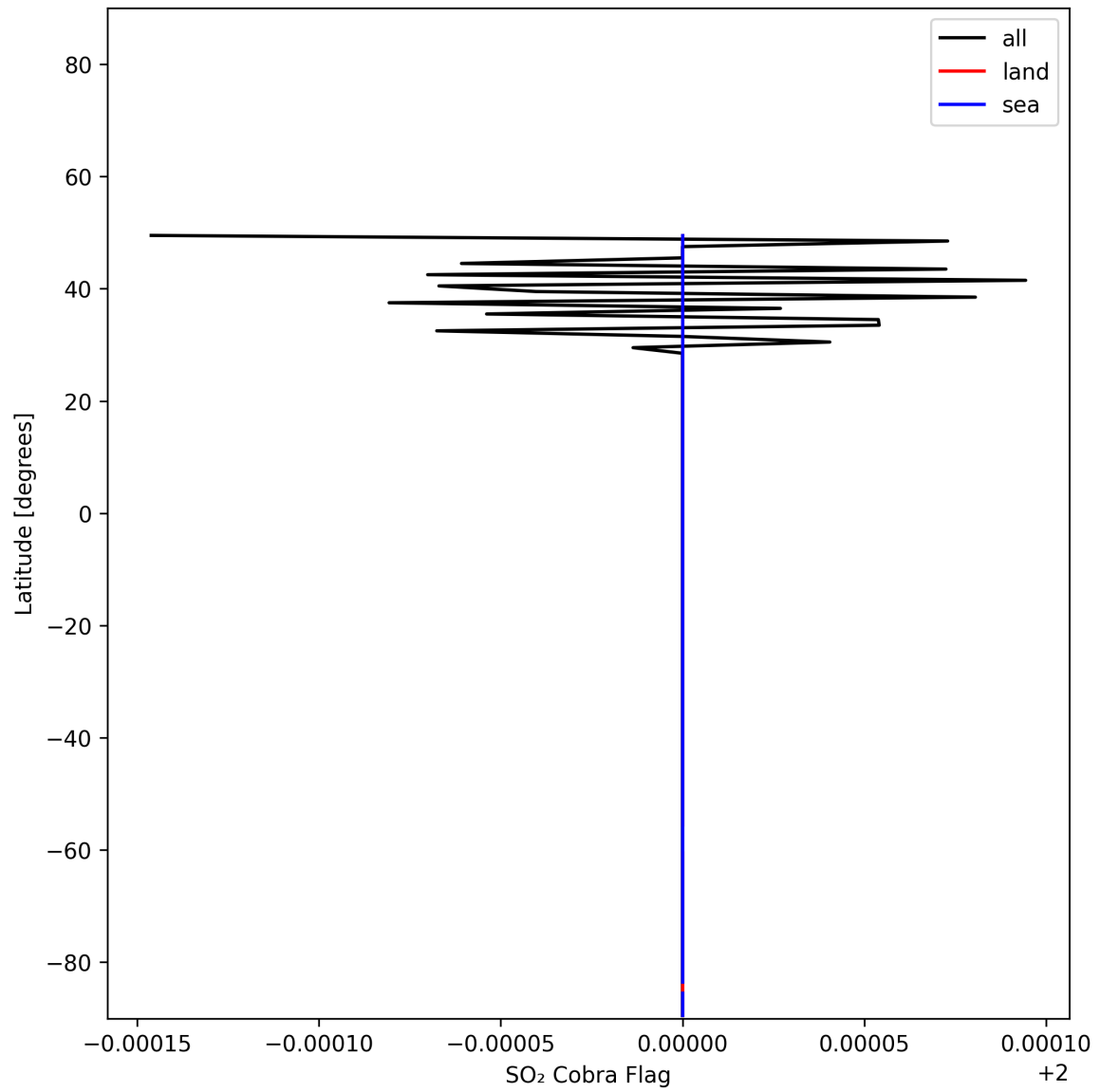
Figure 49: Zonal average of "SO 2 Cobra Flag" for 2025-11-23 to 2025-11-24.
