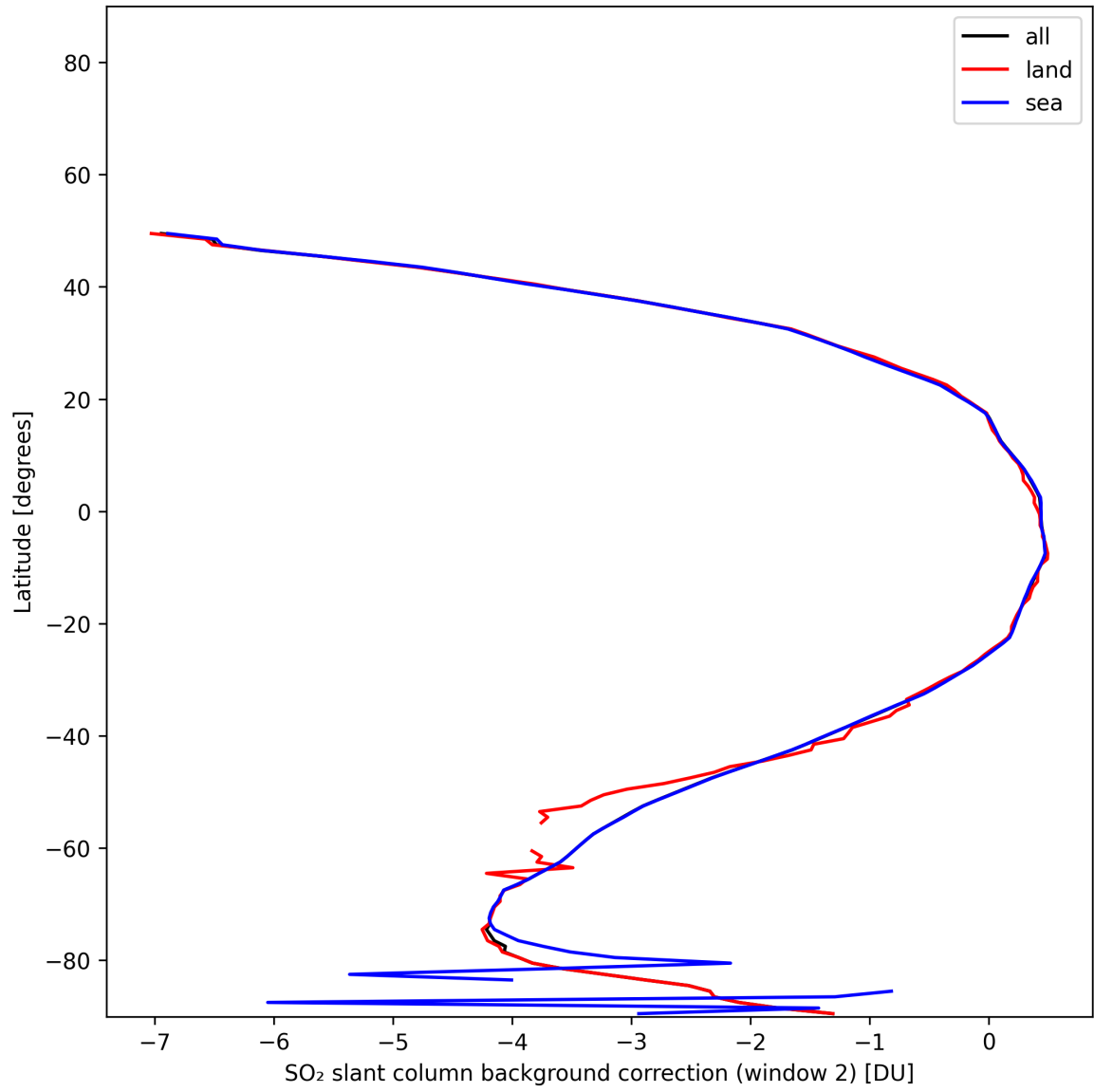
Figure 44: Zonal average of “SO 2 slant column background correction (window 2)” for 2025-11-23 to 2025-11-24.
