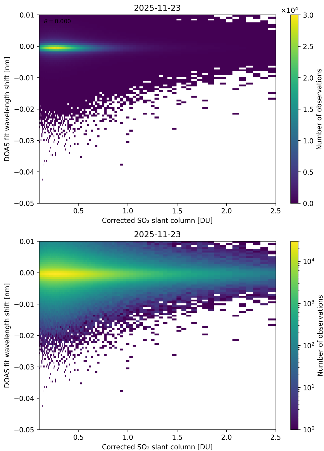
Figure 229: Scatter density plot of “Corrected SO 2 slant column” against “DOAS fit wavelength shift” for 2025-11-23 to 2025-11-24.
