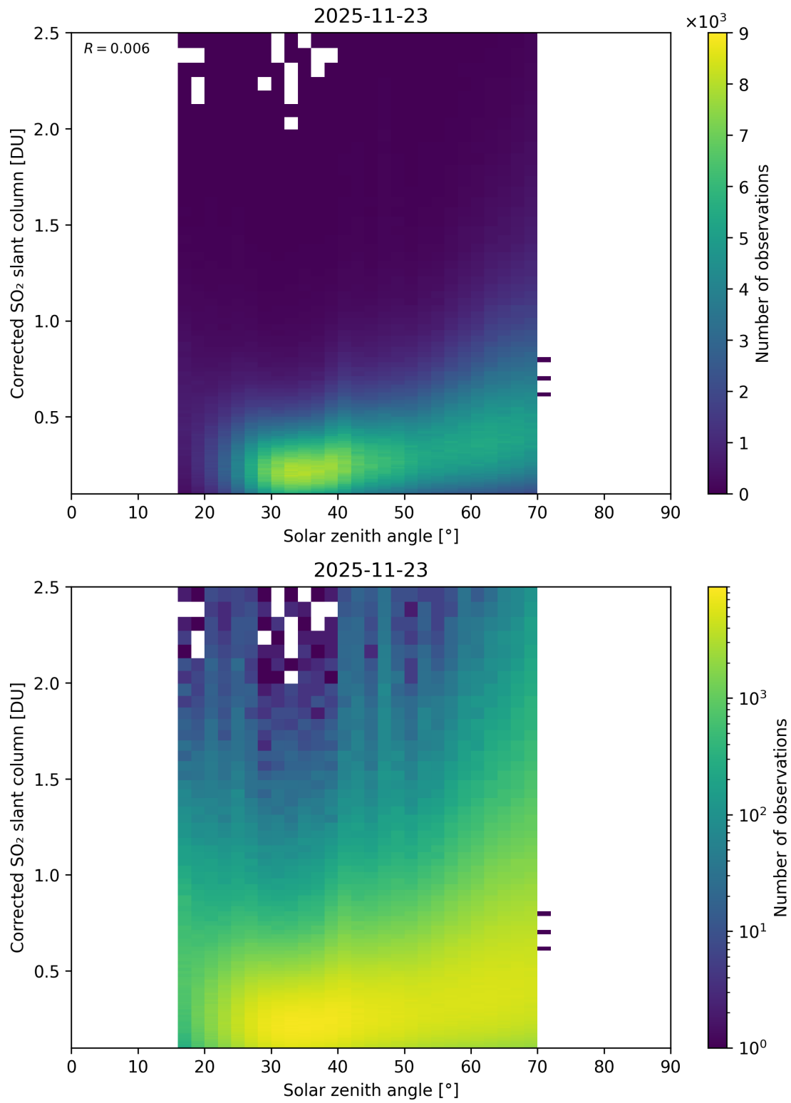
Figure 181: Scatter density plot of “Solar zenith angle” against “Corrected SO 2 slant column” for 2025-11-23 to 2025-11-24.
