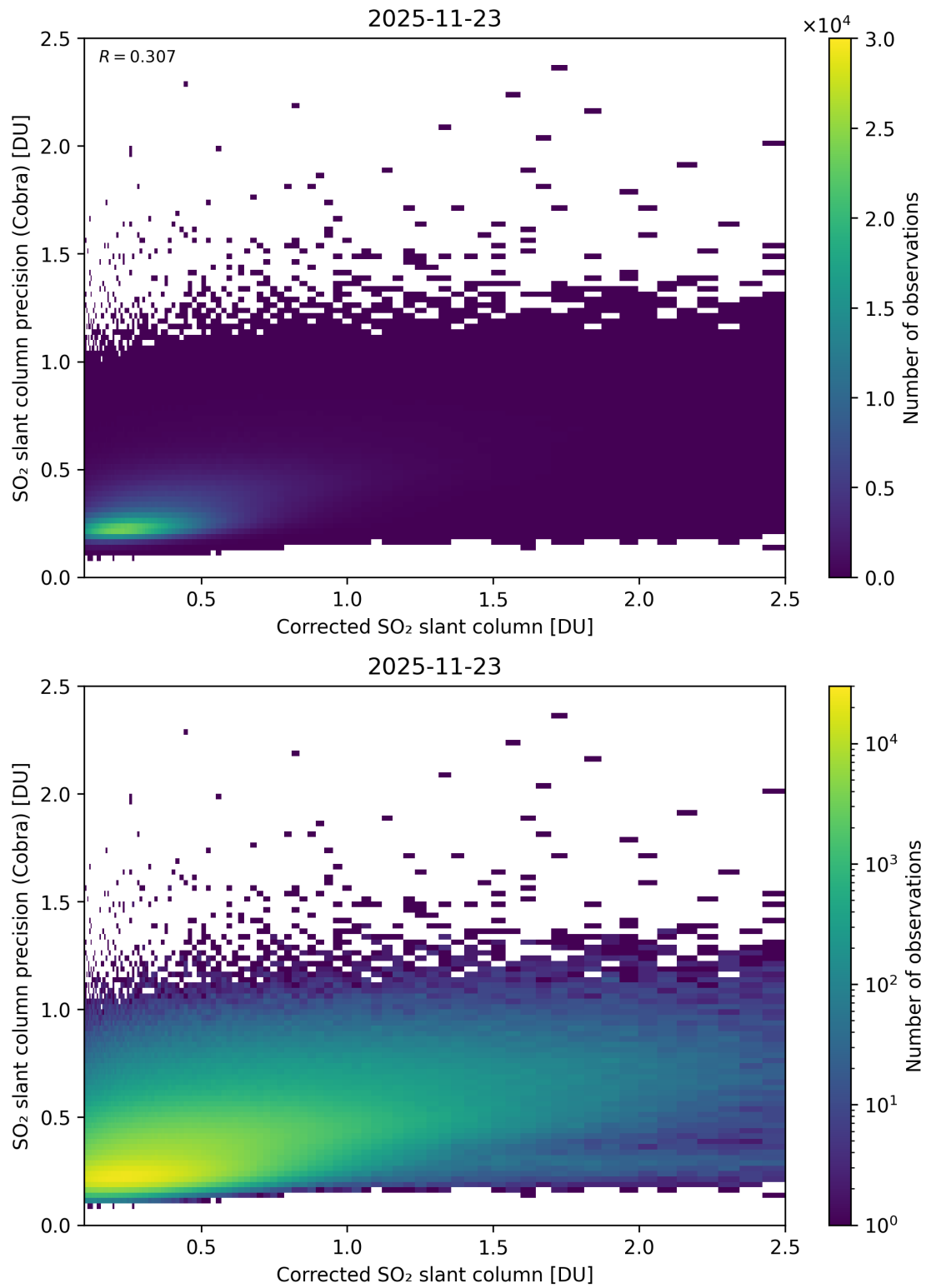
Figure 234: Scatter density plot of “Corrected SO 2 slant column” against “SO 2 slant column precision (Cobra)” for 2025-11-23 to 2025-11-24.
