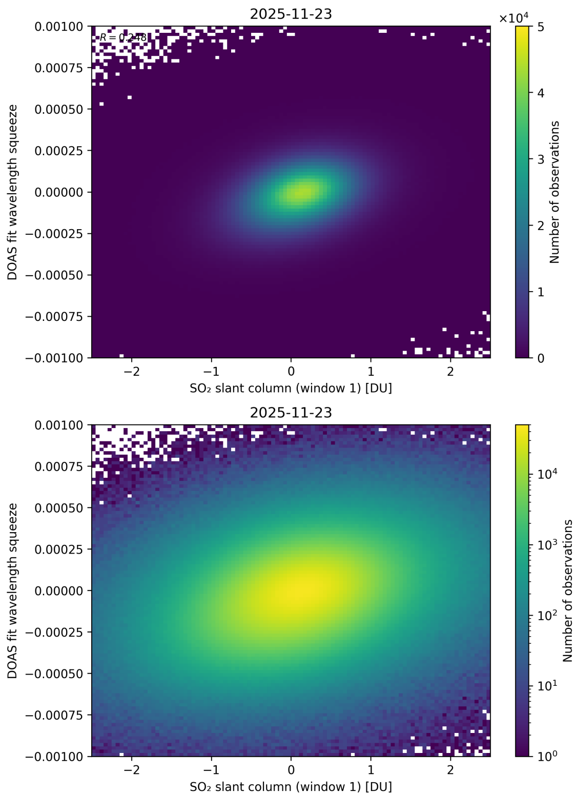
Figure 266: Scatter density plot of “SO 2 slant column (window 1)” against “DOAS fit wavelength squeeze” for 2025-11-23 to 2025-11-24.
