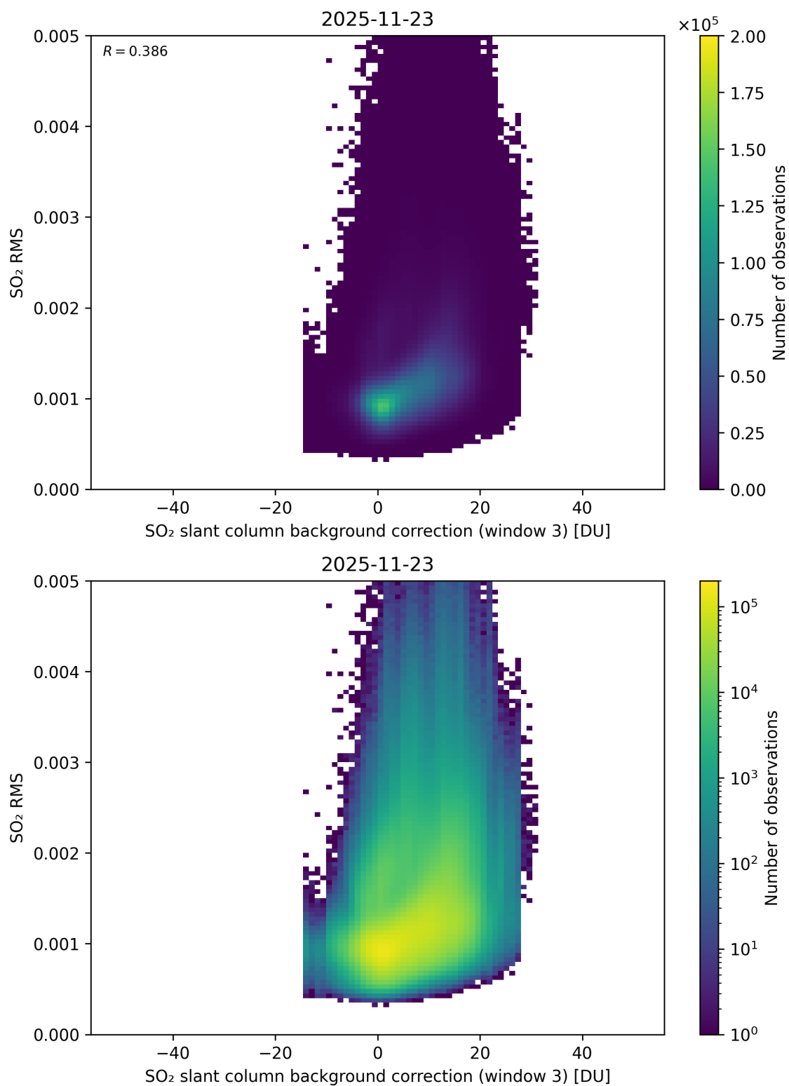
Figure 134: Scatter density plot of “SO 2 slant column background correction (window 3)” against “SO 2 RMS” for 2025-11-23 to 2025-11-24.
