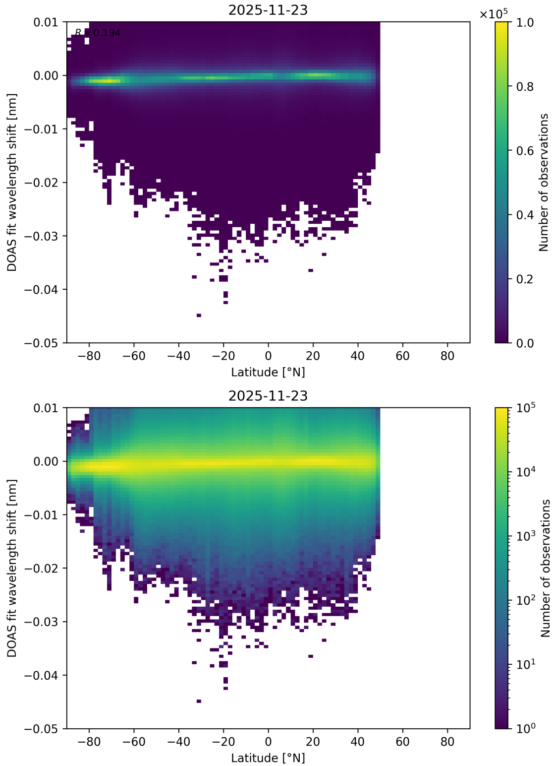
Figure 153: Scatter density plot of “Latitude” against “DOAS fit wavelength shift” for 2025-11-23 to 2025-11-24.
