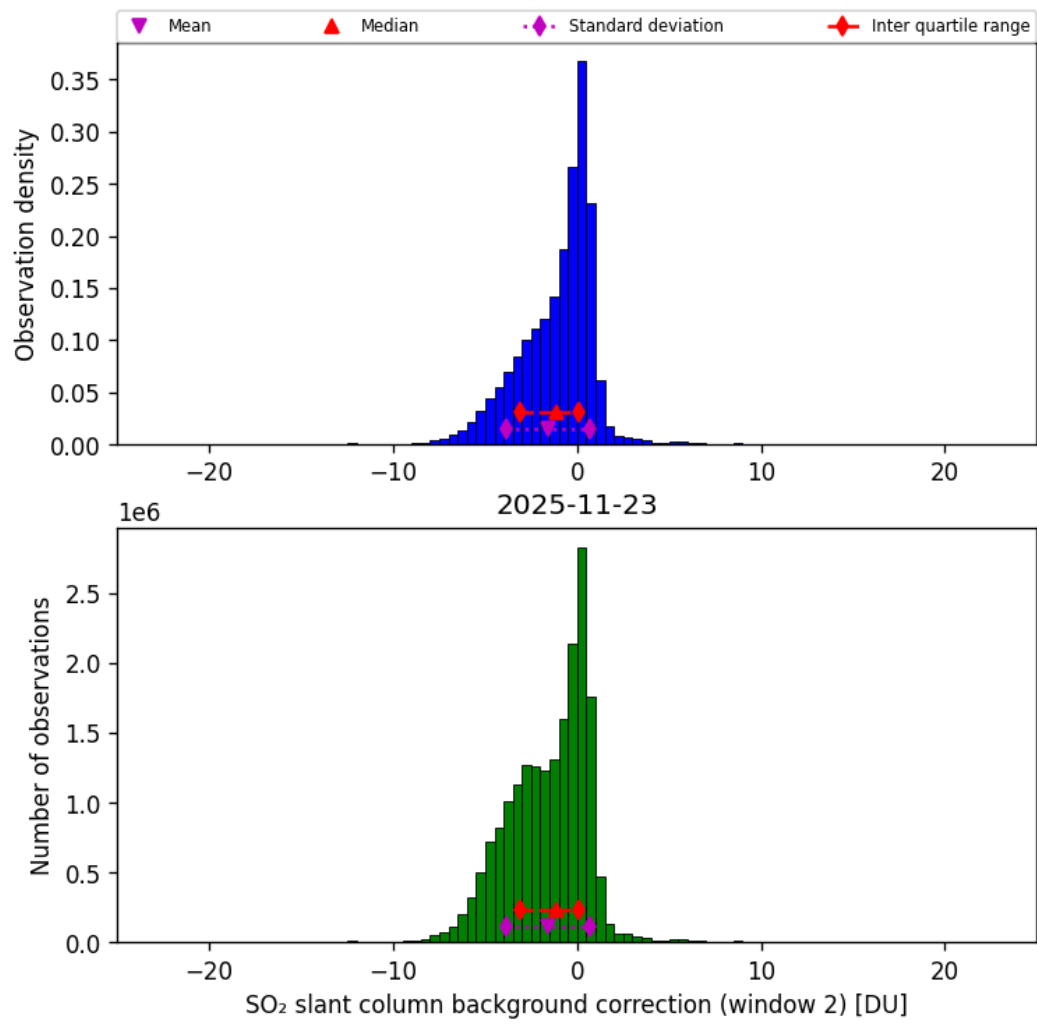
Figure 70: Histogram of “SO 2 slant column background correction (window 2)” for 2025-11-23 to 2025-11-24
