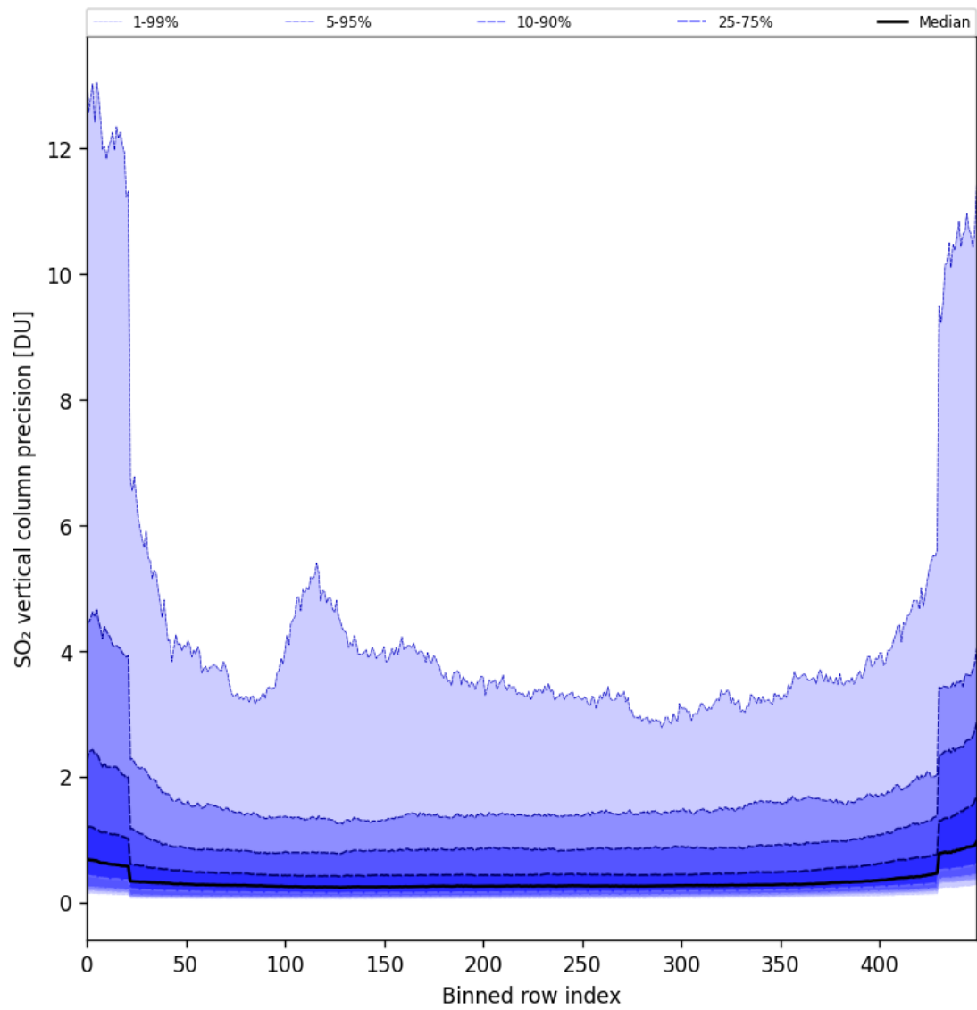
Figure 85: Along track statistics of “SO 2 vertical column precision” for 2025-11-23 to 2025-11-24
