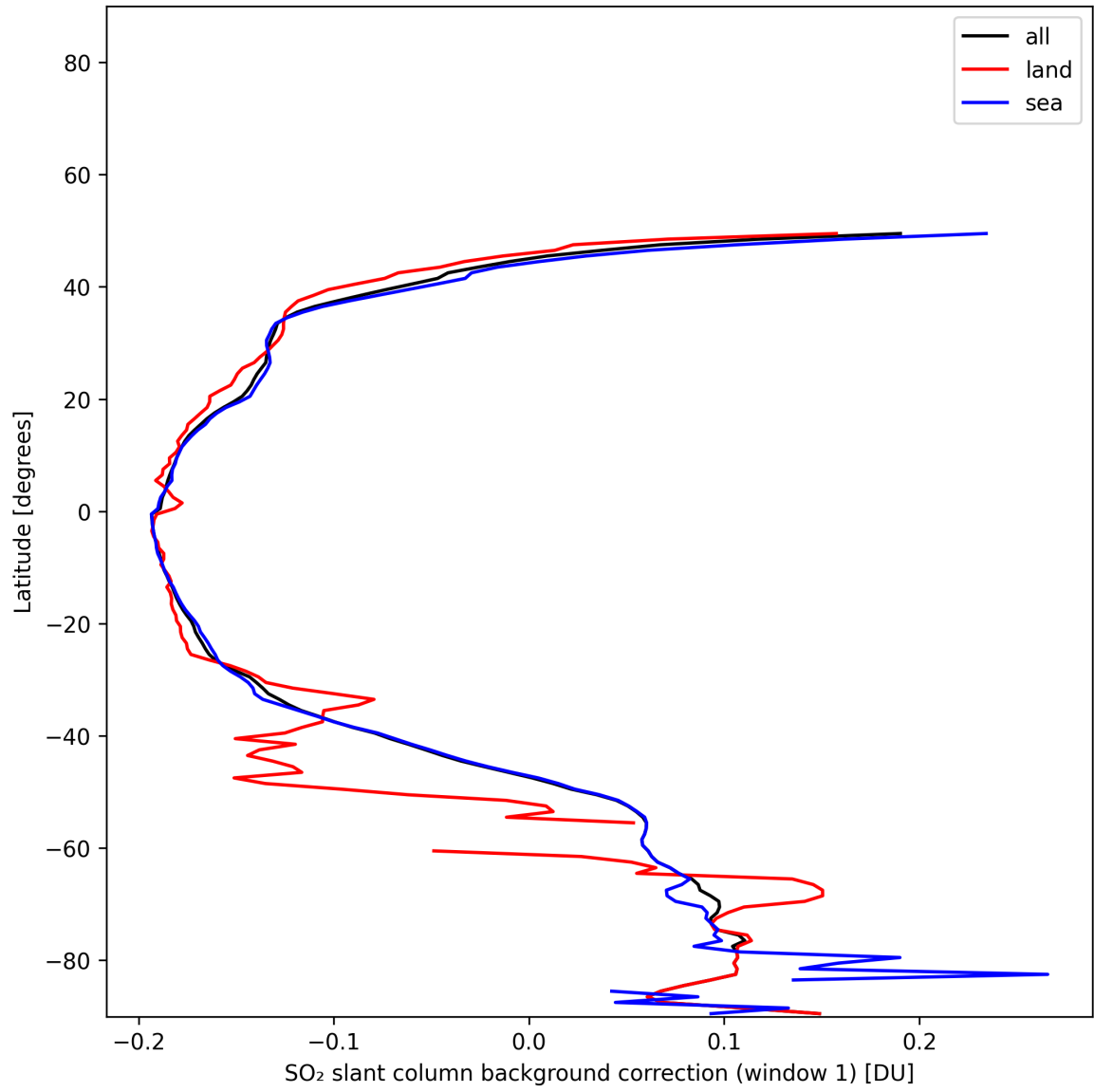
Figure 40: Zonal average of “SO 2 slant column background correction (window 1)” for 2025-11-23 to 2025-11-24.
