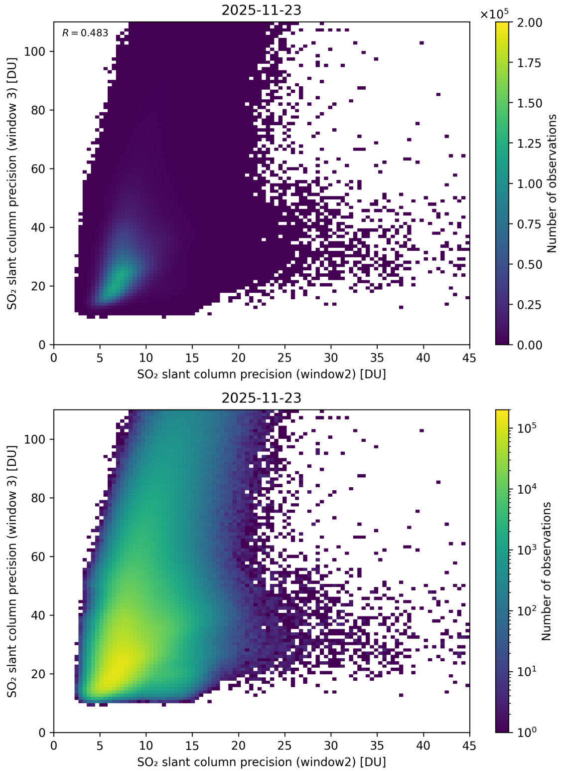
Figure 300: Scatter density plot of “SO 2 slant column precision (window2)” against “SO 2 slant column precision (window 3)” for 2025-11-23 to 2025-11-24.
