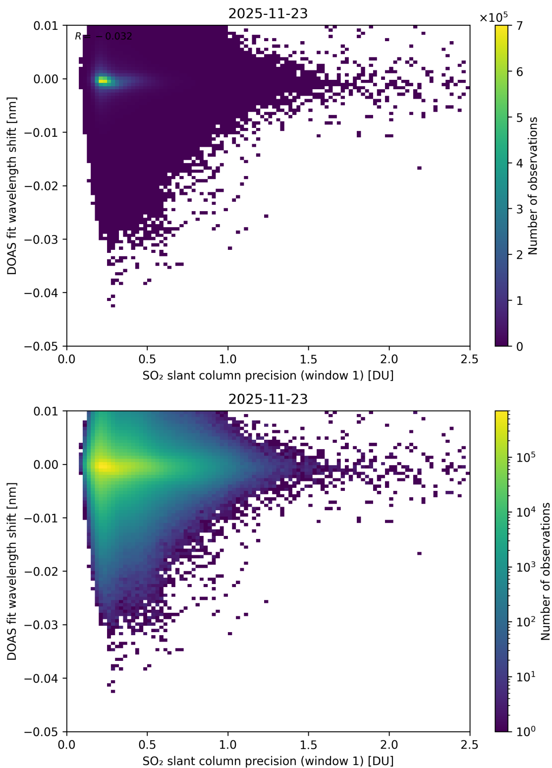
Figure 271: Scatter density plot of “SO 2 slant column precision (window 1)” against “DOAS fit wavelength shift” for 2025-11-23 to 2025-11-24.
