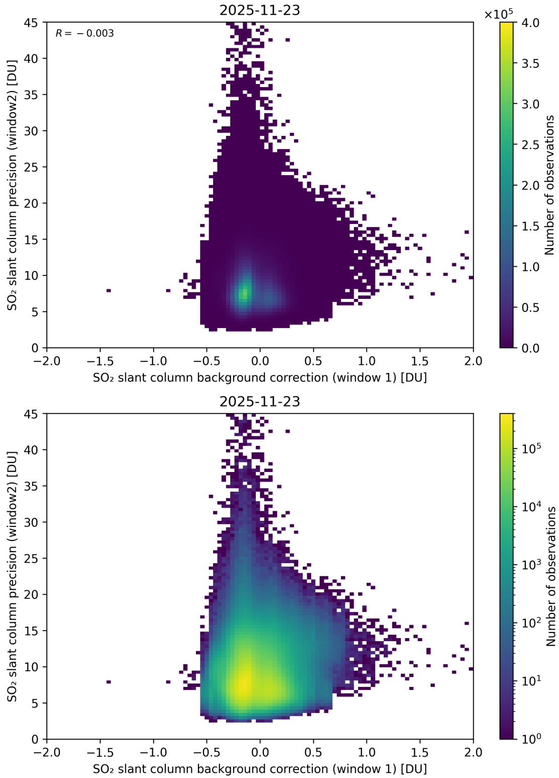
Figure 117: Scatter density plot of “SO 2 slant column background correction (window 1)” against “SO 2 slant column precision (window2)” for 2025-11-23 to 2025-11-24.
