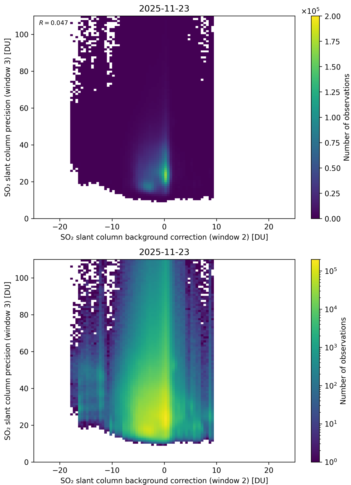
Figure 129: Scatter density plot of “SO 2 slant column background correction (window 2)” against “SO 2 slant column precision (window 3)” for 2025-11-23 to 2025-11-24.
