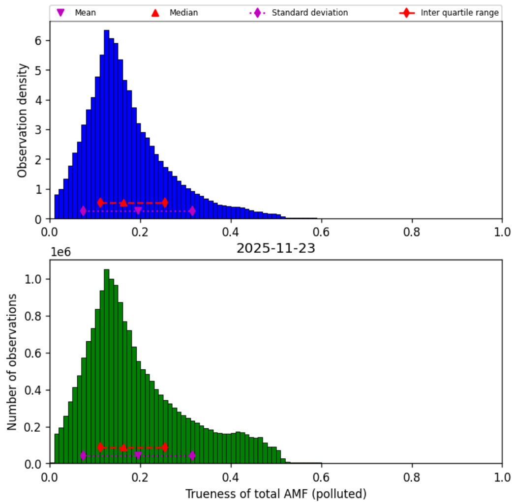
Figure 80: Histogram of “Trueness of total AMF (polluted)” for 2025-11-23 to 2025-11-24
