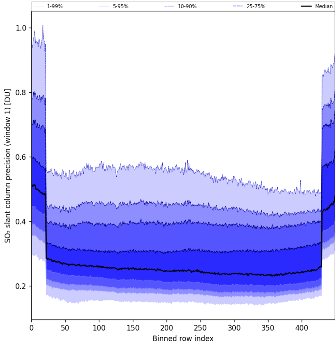
Figure 90: Along track statistics of “SO 2 slant column precision (window 1)” for 2025-11-23 to 2025-11-24
