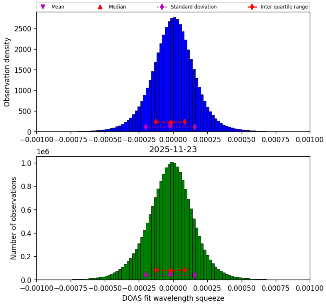
Figure 77: Histogram of “DOAS fit wavelength squeeze” for 2025-11-23 to 2025-11-24
