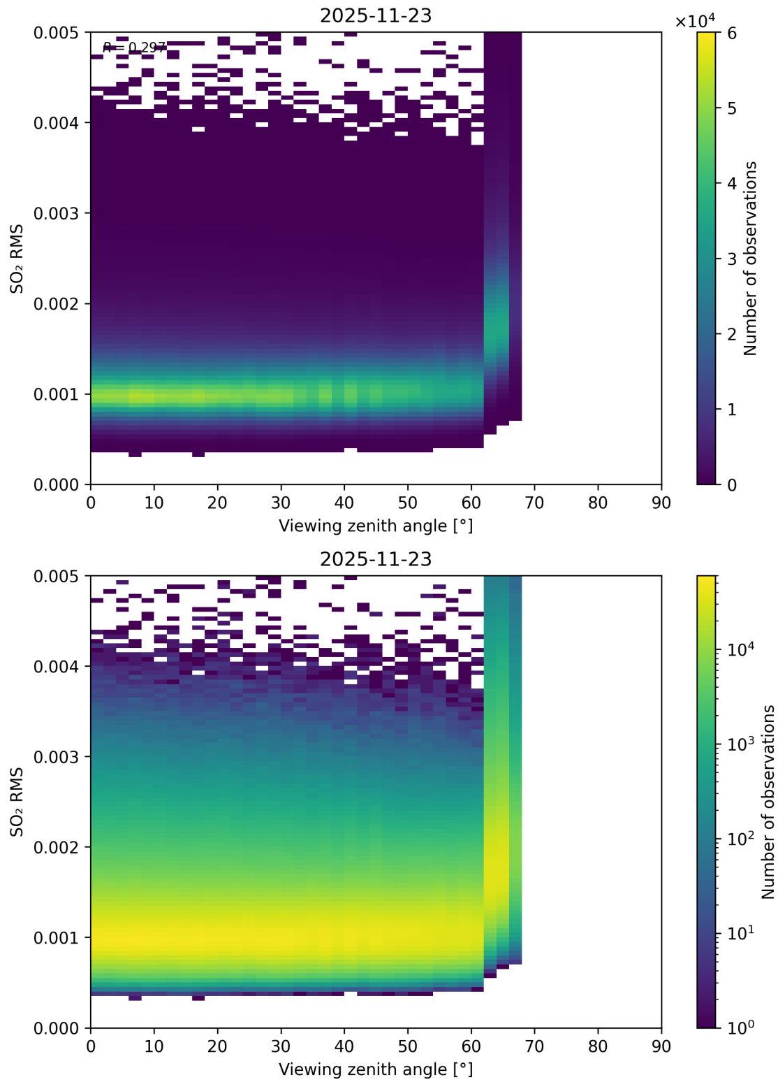
Figure 367: Scatter density plot of “Viewing zenith angle” against “SO 2 RMS” for 2025-11-23 to 2025-11-24.
