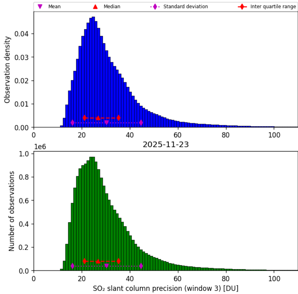
Figure 72: Histogram of “SO 2 slant column precision (window 3)” for 2025-11-23 to 2025-11-24
