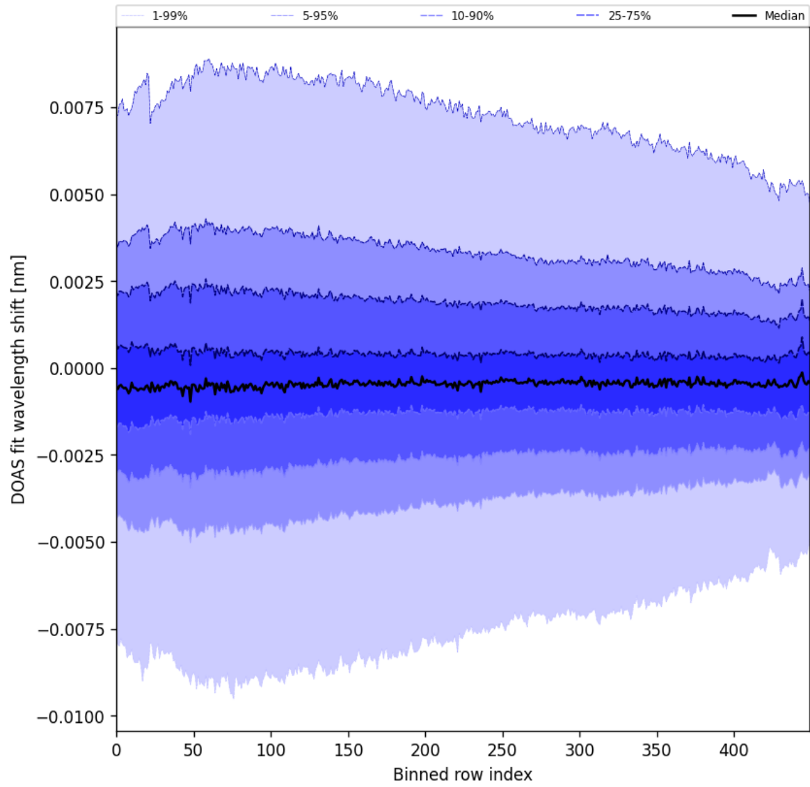
Figure 102: Along track statistics of “DOAS fit wavelength shift” for 2025-11-23 to 2025-11-25
