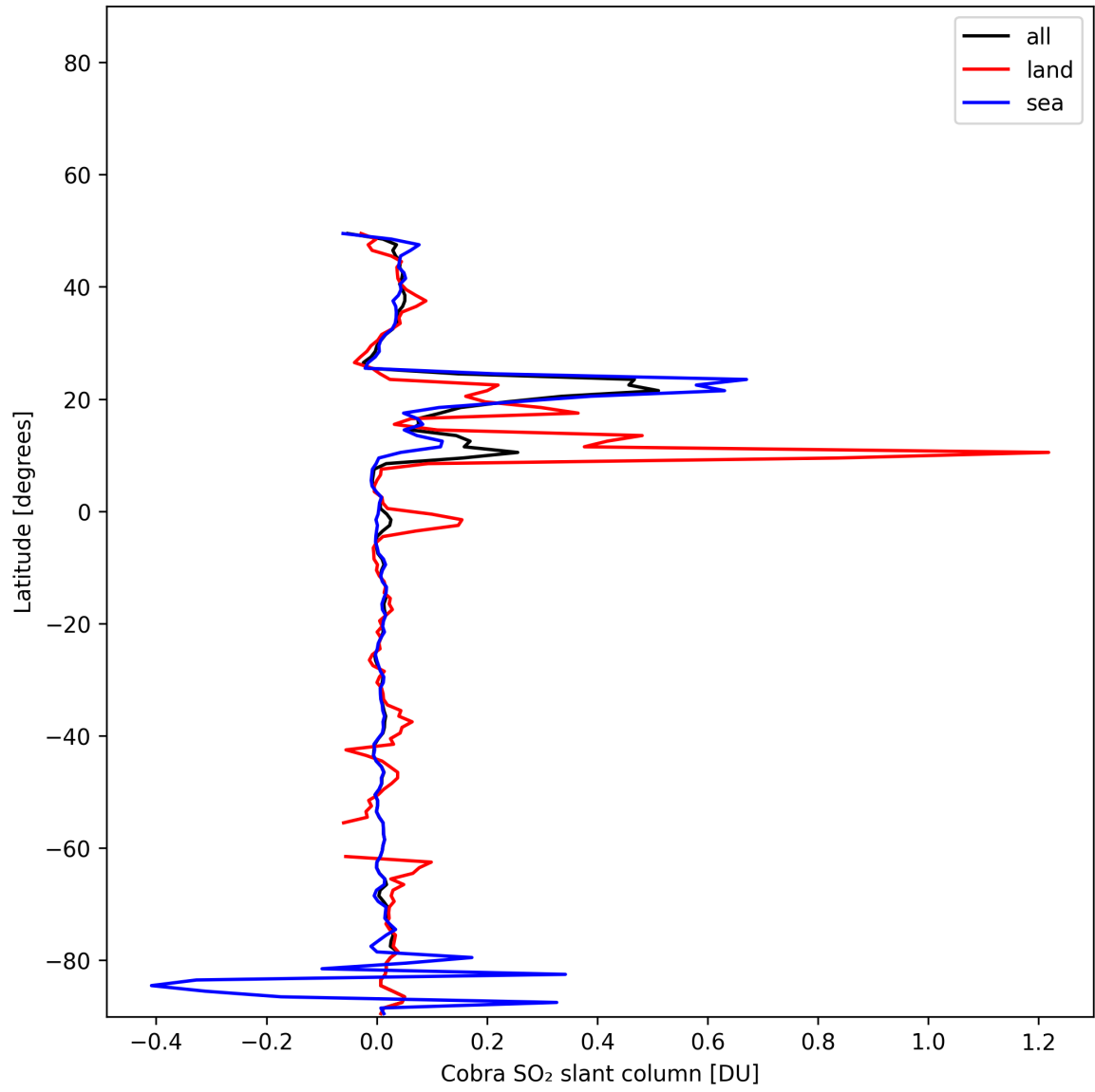
Figure 35: Zonal average of “Cobra SO 2 slant column” for 2025-11-23 to 2025-11-25.
