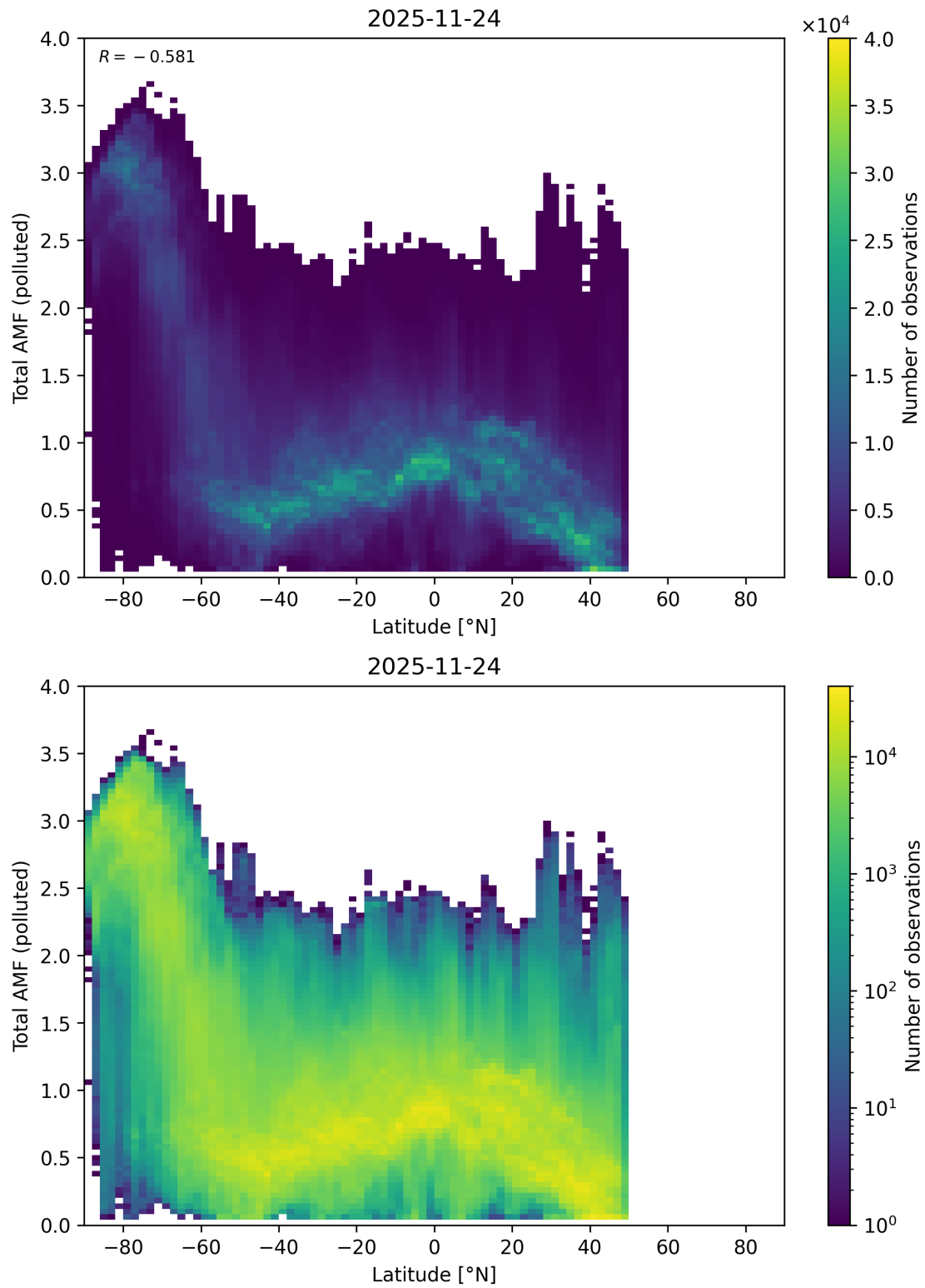
Figure 167: Scatter density plot of “Latitude” against “Total AMF (polluted)” for 2025-11-23 to 2025-11-25.
