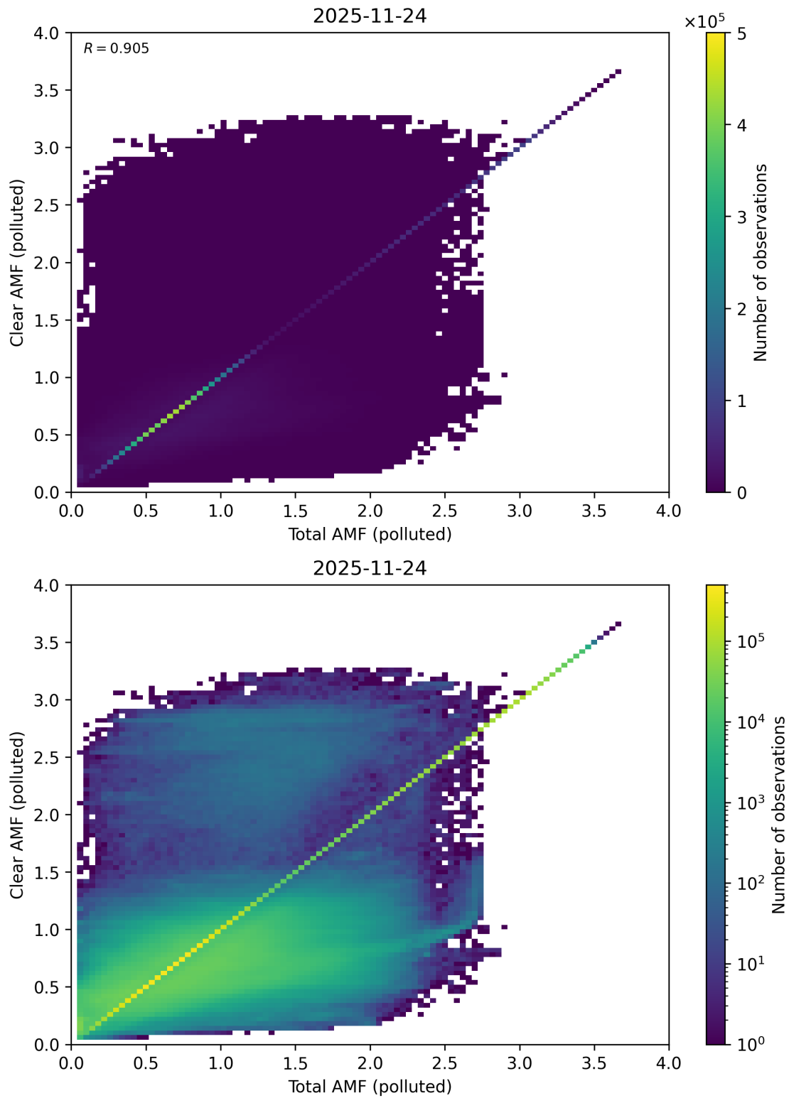
Figure 320: Scatter density plot of “Total AMF (polluted)” against “Clear AMF (polluted)” for 2025-11-23 to 2025-11-25.
