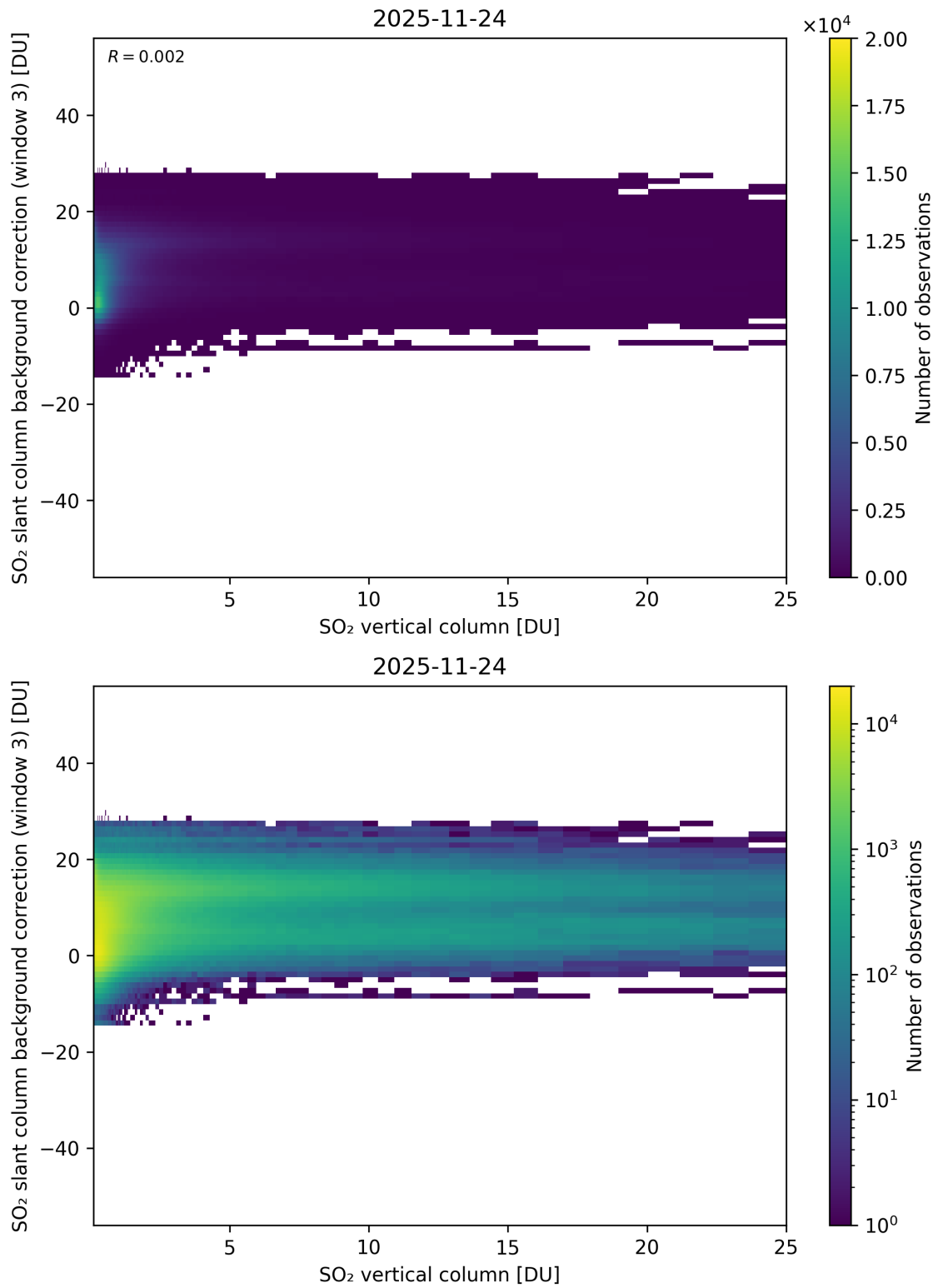
Figure 325: Scatter density plot of “SO 2 vertical column” against “SO 2 slant column background correction (window 3)” for 2025-11-23 to 2025-11-25.
