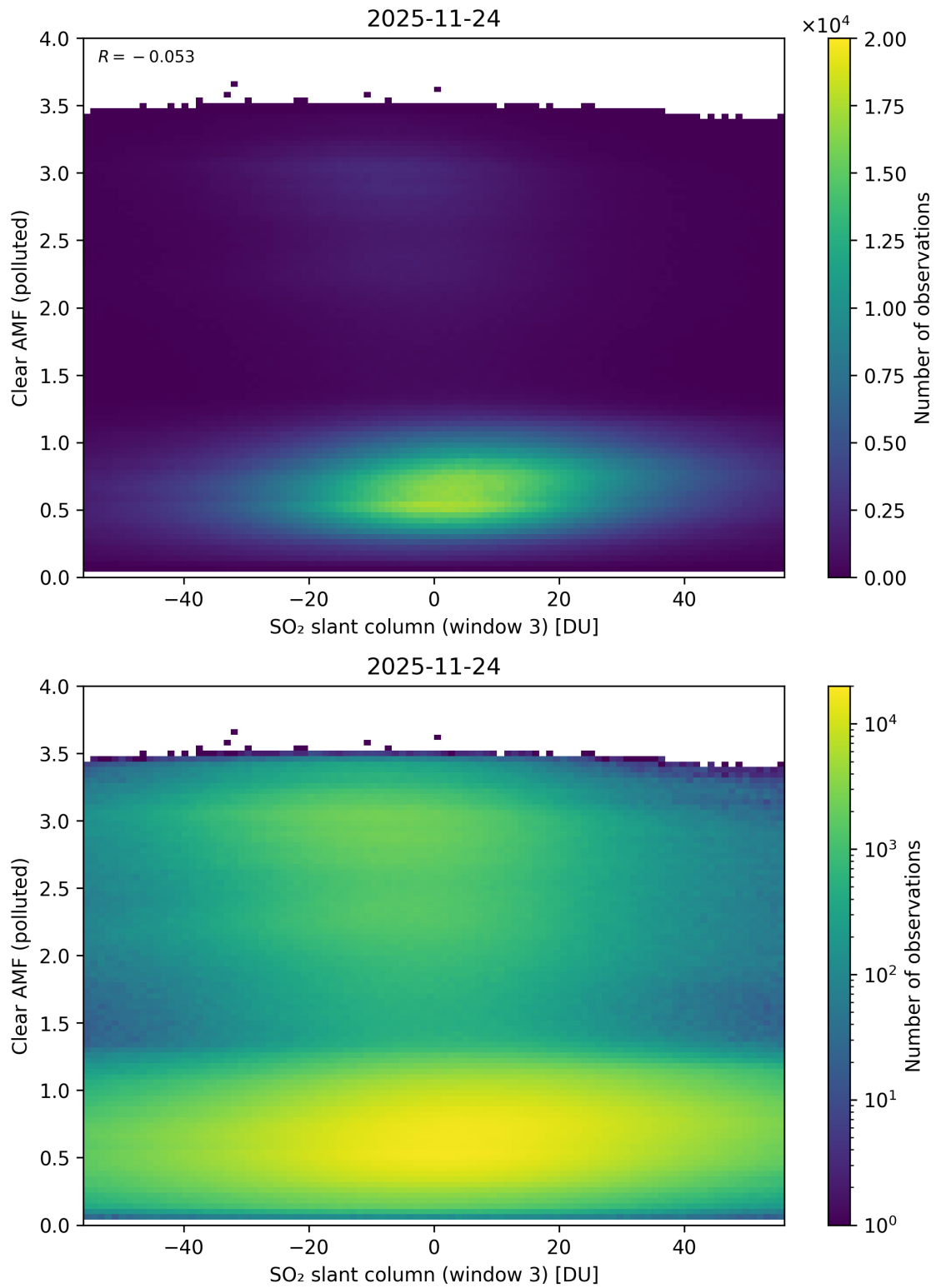
Figure 315: Scatter density plot of “SO 2 slant column (window 3)” against “Clear AMF (polluted)” for 2025-11-23 to 2025-11-25.
