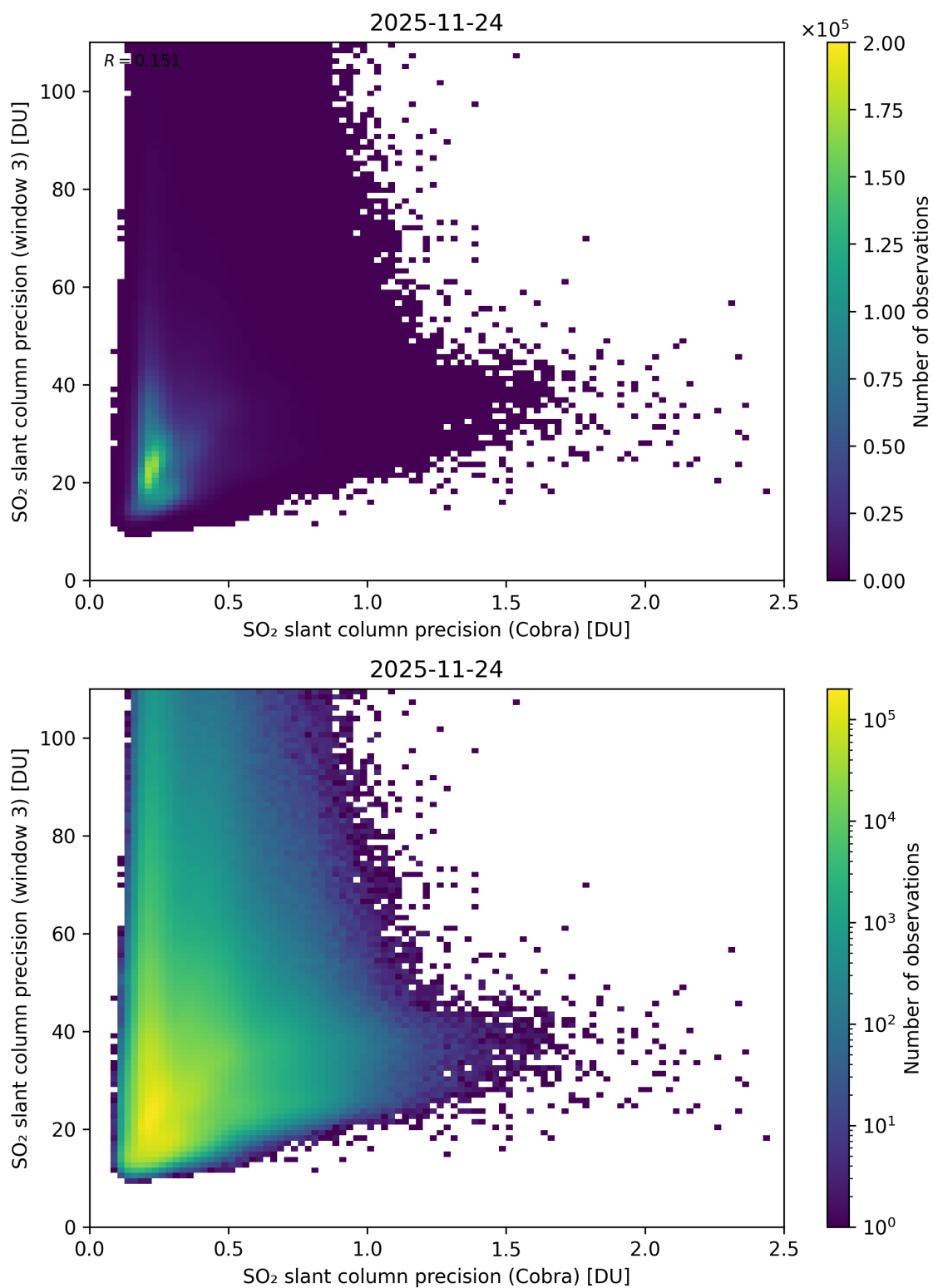
Figure 212: Scatter density plot of “SO 2 slant column precision (Cobra)” against “SO 2 slant column precision (window 3)” for 2025-11-23 to 2025-11-25.
