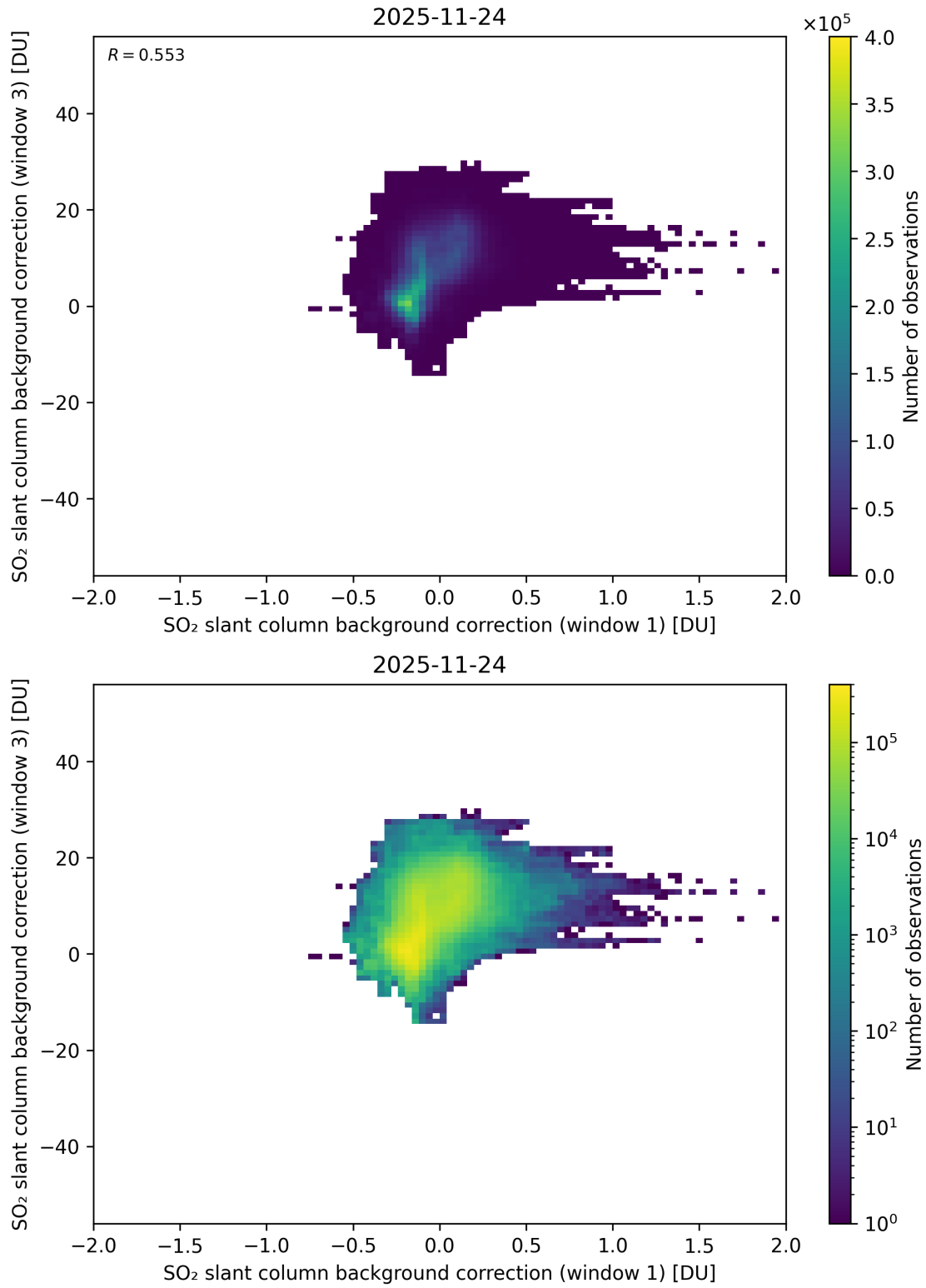
Figure 110: Scatter density plot of “SO 2 slant column background correction (window 1)” against “SO 2 slant column background correction (window 3)” for 2025-11-23 to 2025-11-25.
