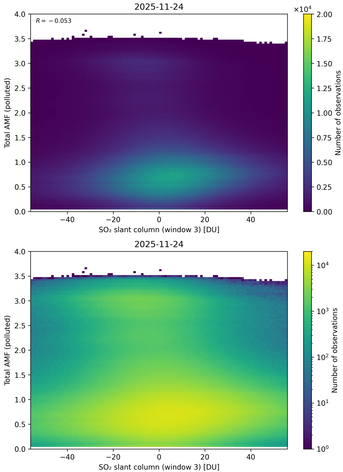
Figure 318: Scatter density plot of “SO 2 slant column (window 3)” against “Total AMF (polluted)” for 2025-11-23 to 2025-11-25.
