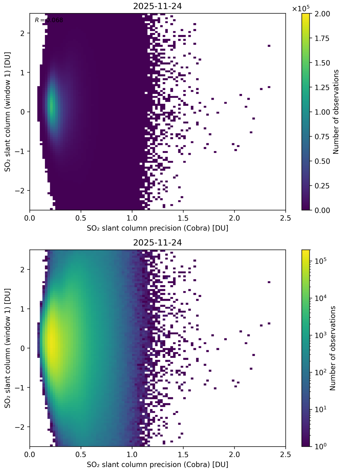
Figure 208: Scatter density plot of “SO 2 slant column precision (Cobra)” against “SO 2 slant column (window 1)” for 2025-11-23 to 2025-11-25.
