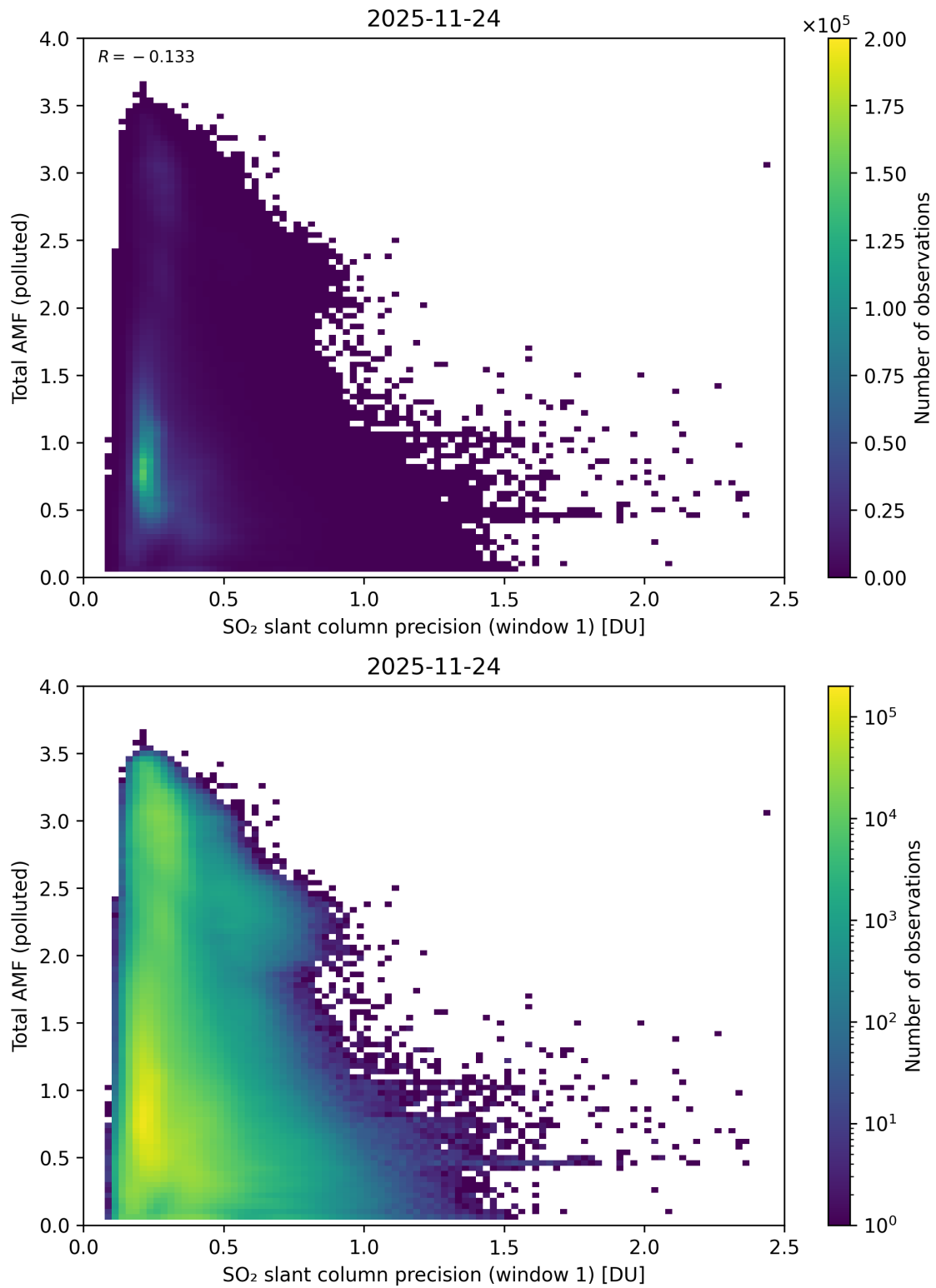
Figure 280: Scatter density plot of “SO 2 slant column precision (window 1)” against “Total AMF (polluted)” for 2025-11-23 to 2025-11-25.
