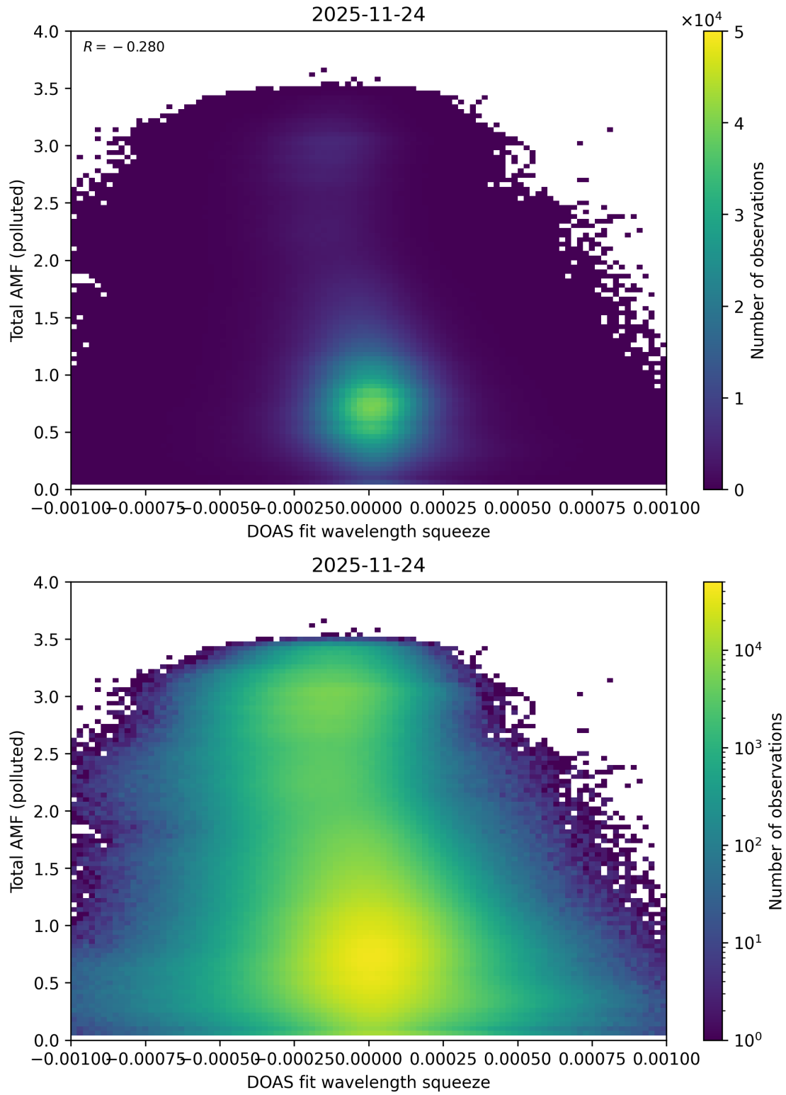
Figure 145: Scatter density plot of “DOAS fit wavelength squeeze” against “Total AMF (polluted)” for 2025-11-23 to 2025-11-25.
