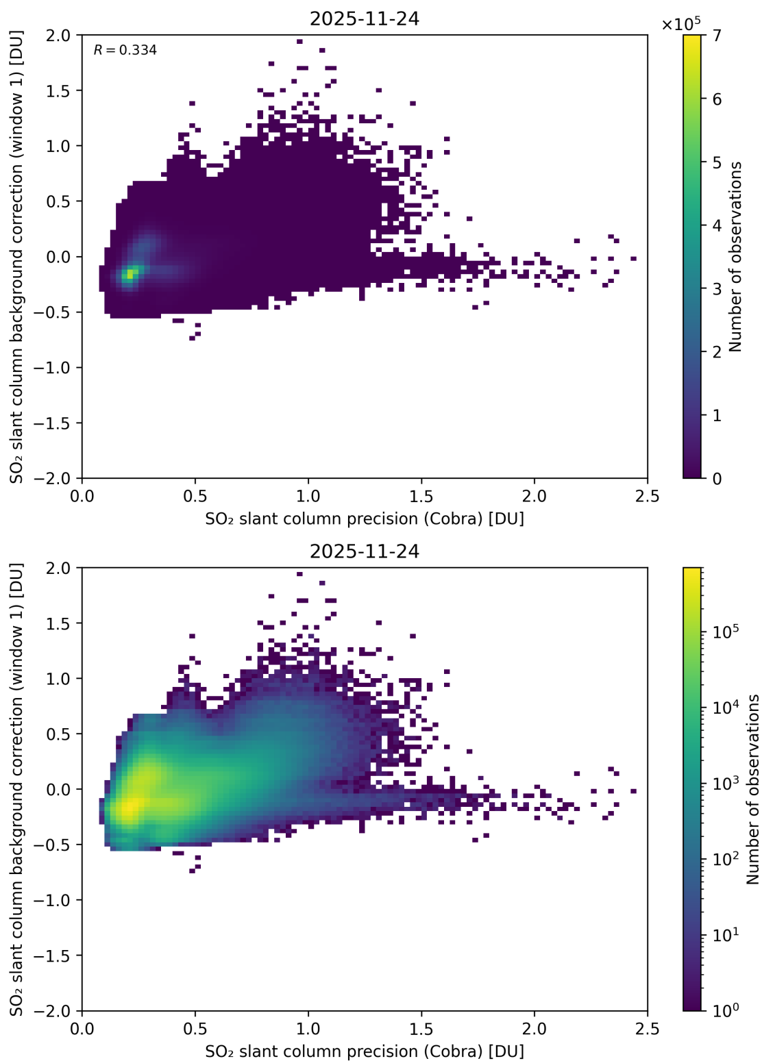
Figure 199: Scatter density plot of “SO 2 slant column precision (Cobra)” against “SO 2 slant column background correction (window 1)” for 2025-11-23 to 2025-11-25.
