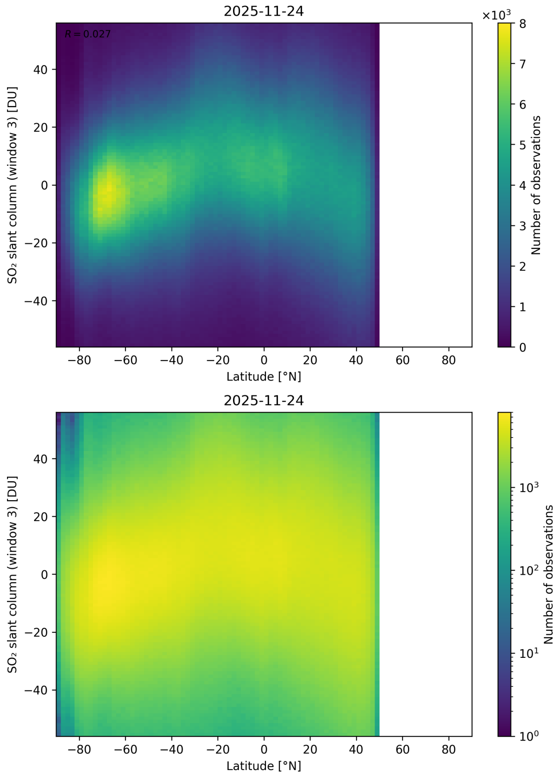
Figure 165: Scatter density plot of “Latitude” against “SO 2 slant column (window 3)” for 2025-11-23 to 2025-11-25.
