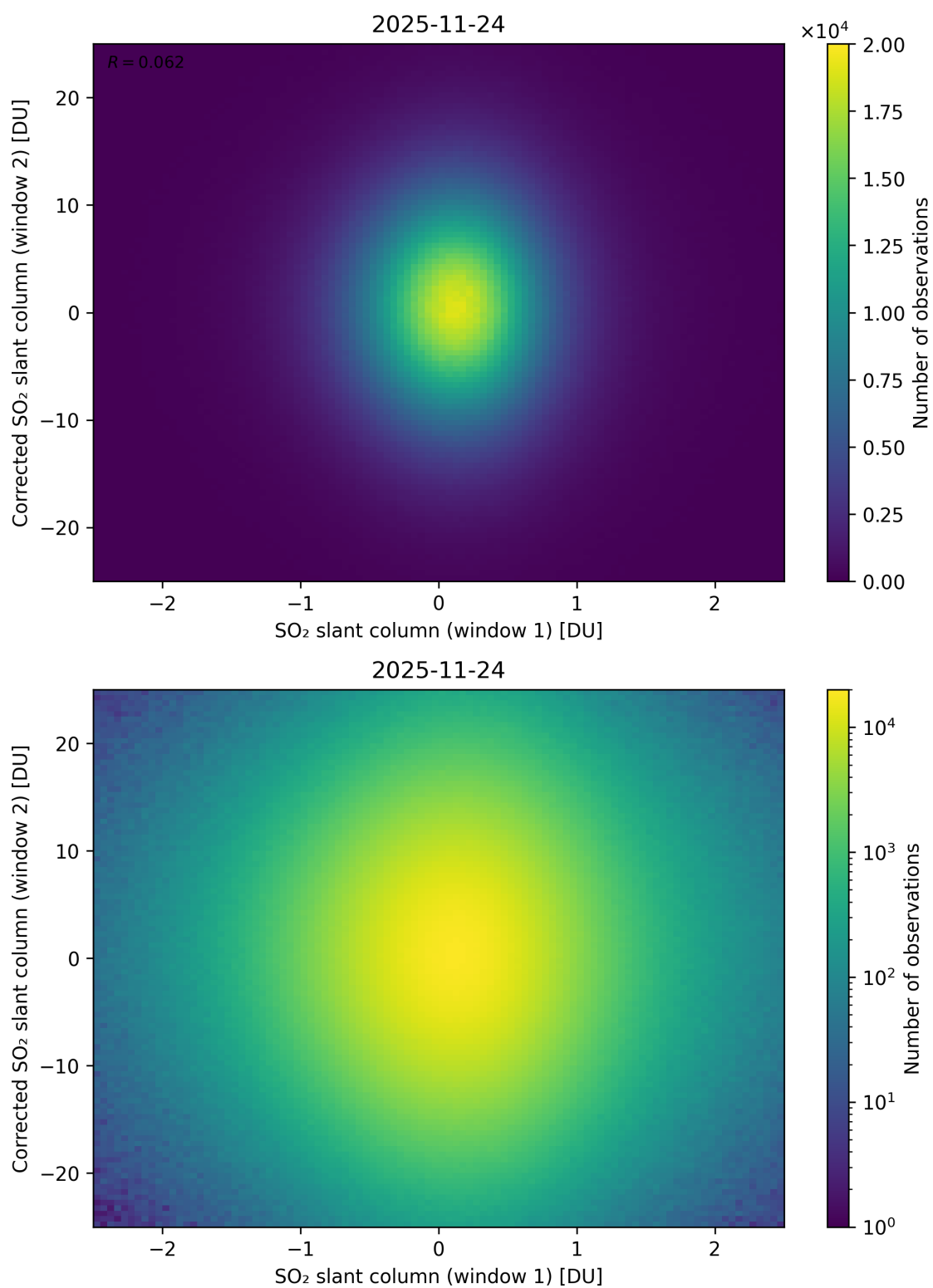
Figure 283: Scatter density plot of “SO 2 slant column (window 1)” against “Corrected SO 2 slant column (window 2)” for 2025-11-23 to 2025-11-25.
