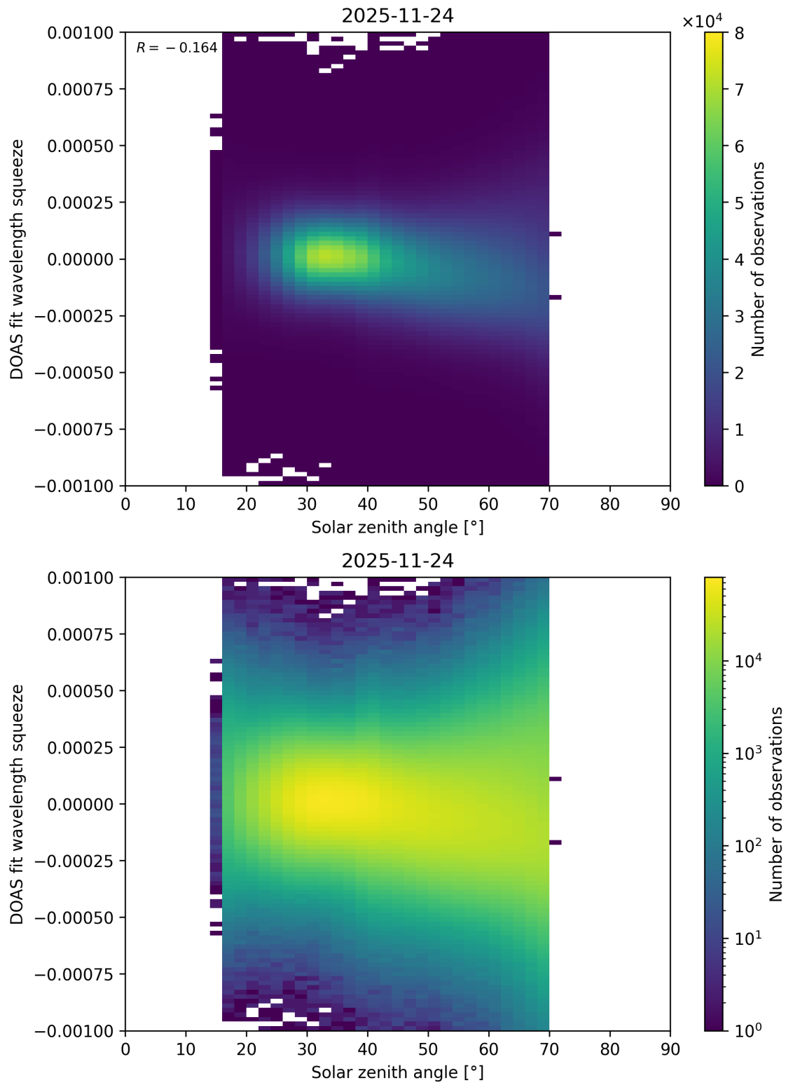
Figure 175: Scatter density plot of “Solar zenith angle” against “DOAS fit wavelength squeeze” for 2025-11-23 to 2025-11-25.
