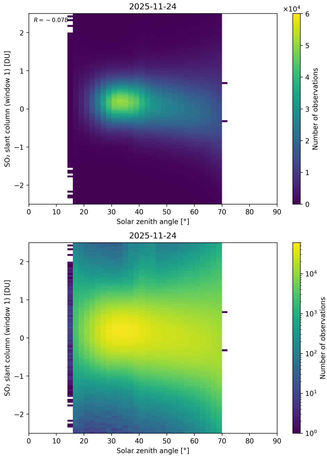
Figure 184: Scatter density plot of “Solar zenith angle” against “SO 2 slant column (window 1)” for 2025-11-23 to 2025-11-25.
