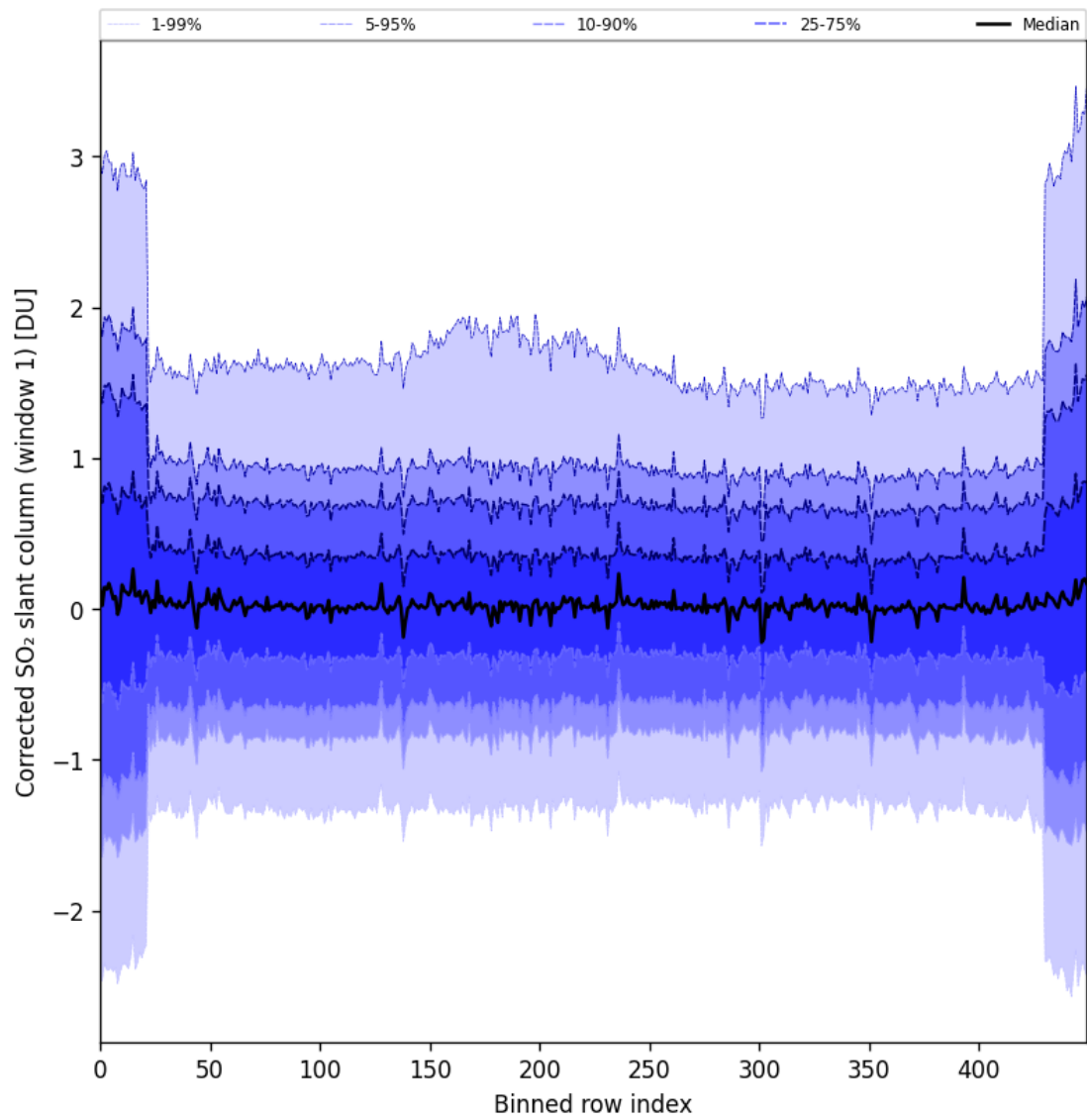
Figure 91: Along track statistics of “Corrected SO 2 slant column (window 1)” for 2025-11-23 to 2025-11-25
