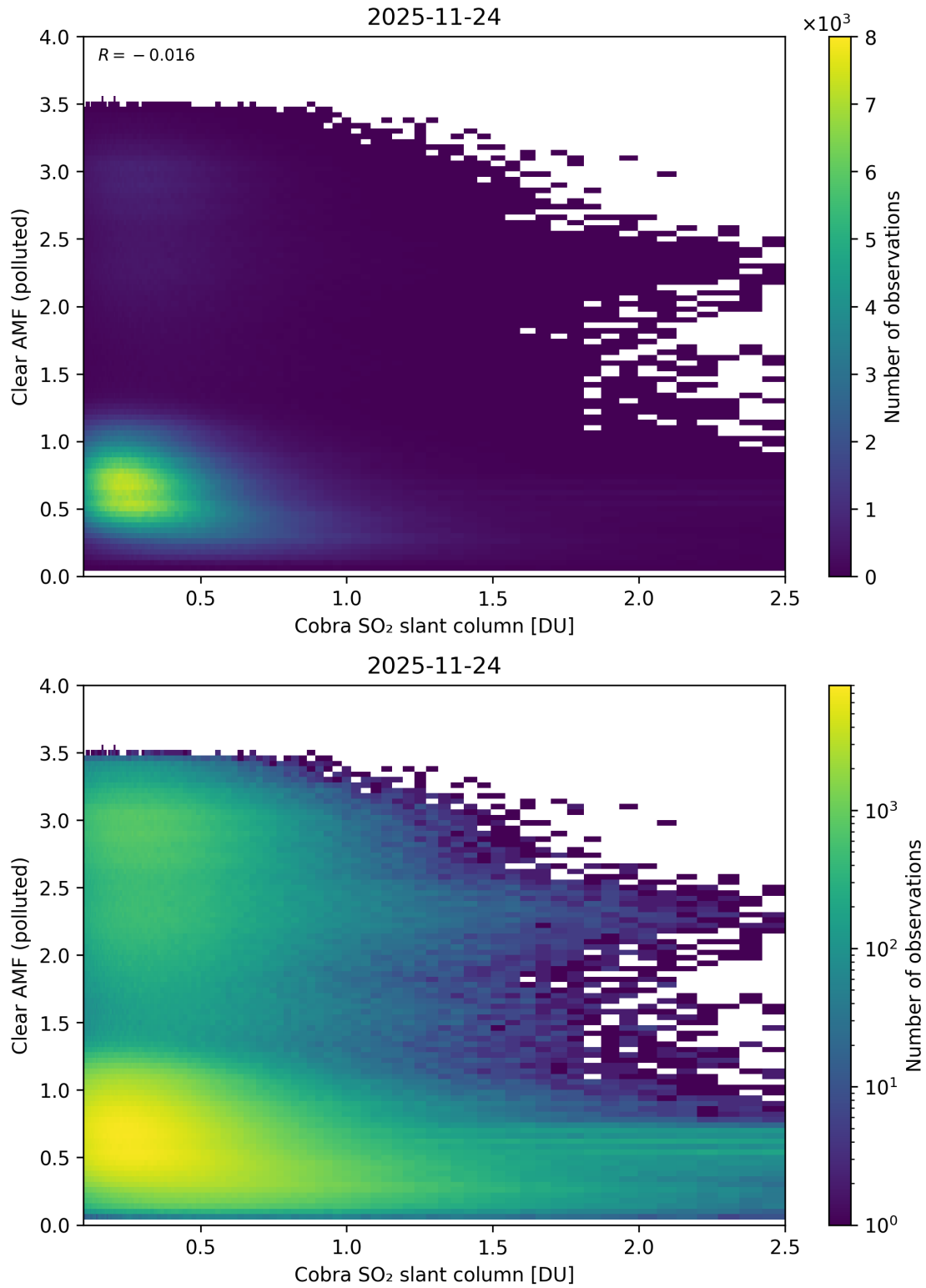
Figure 215: Scatter density plot of “Cobra SO 2 slant column” against “Clear AMF (polluted)” for 2025-11-23 to 2025-11-25.
