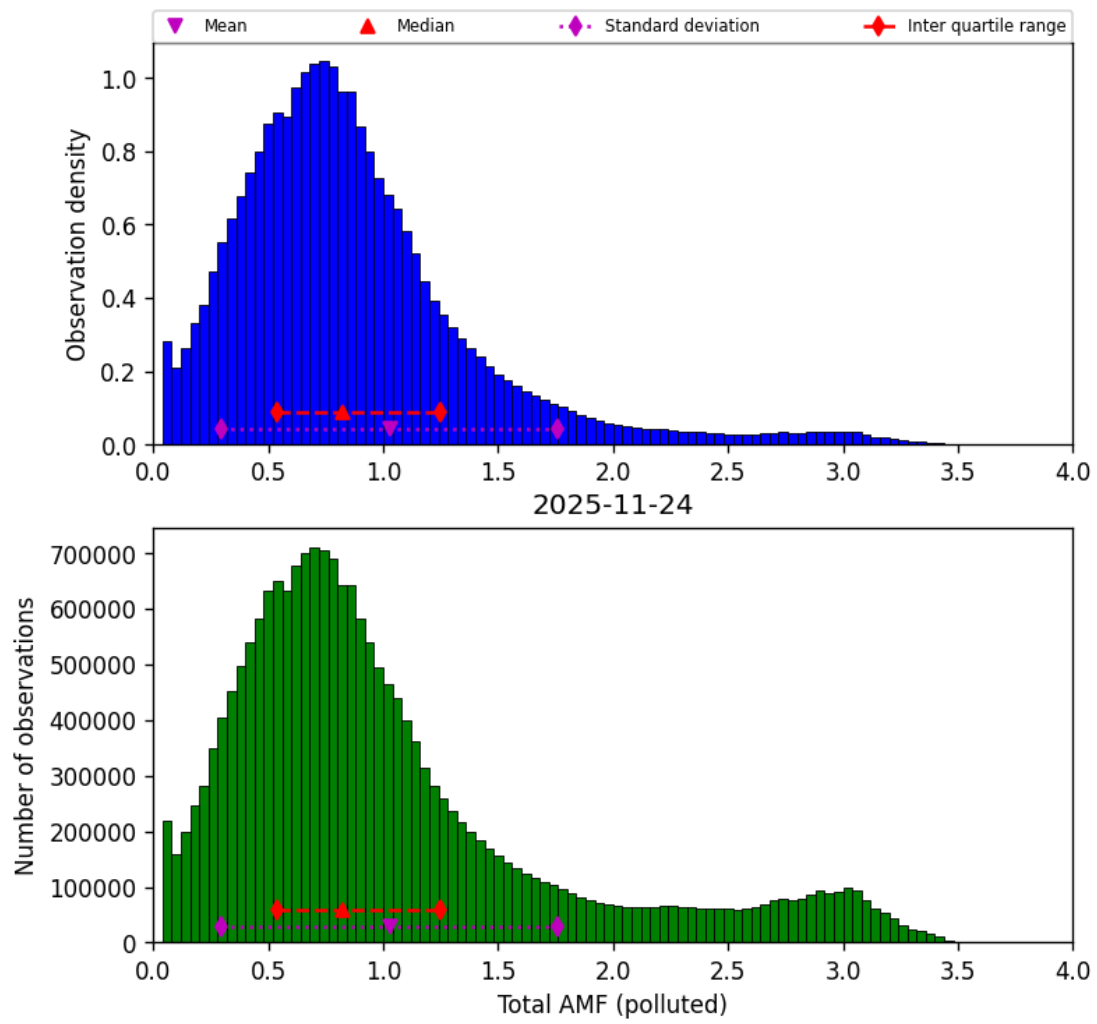
Figure 79: Histogram of “Total AMF (polluted)” for 2025-11-23 to 2025-11-25
