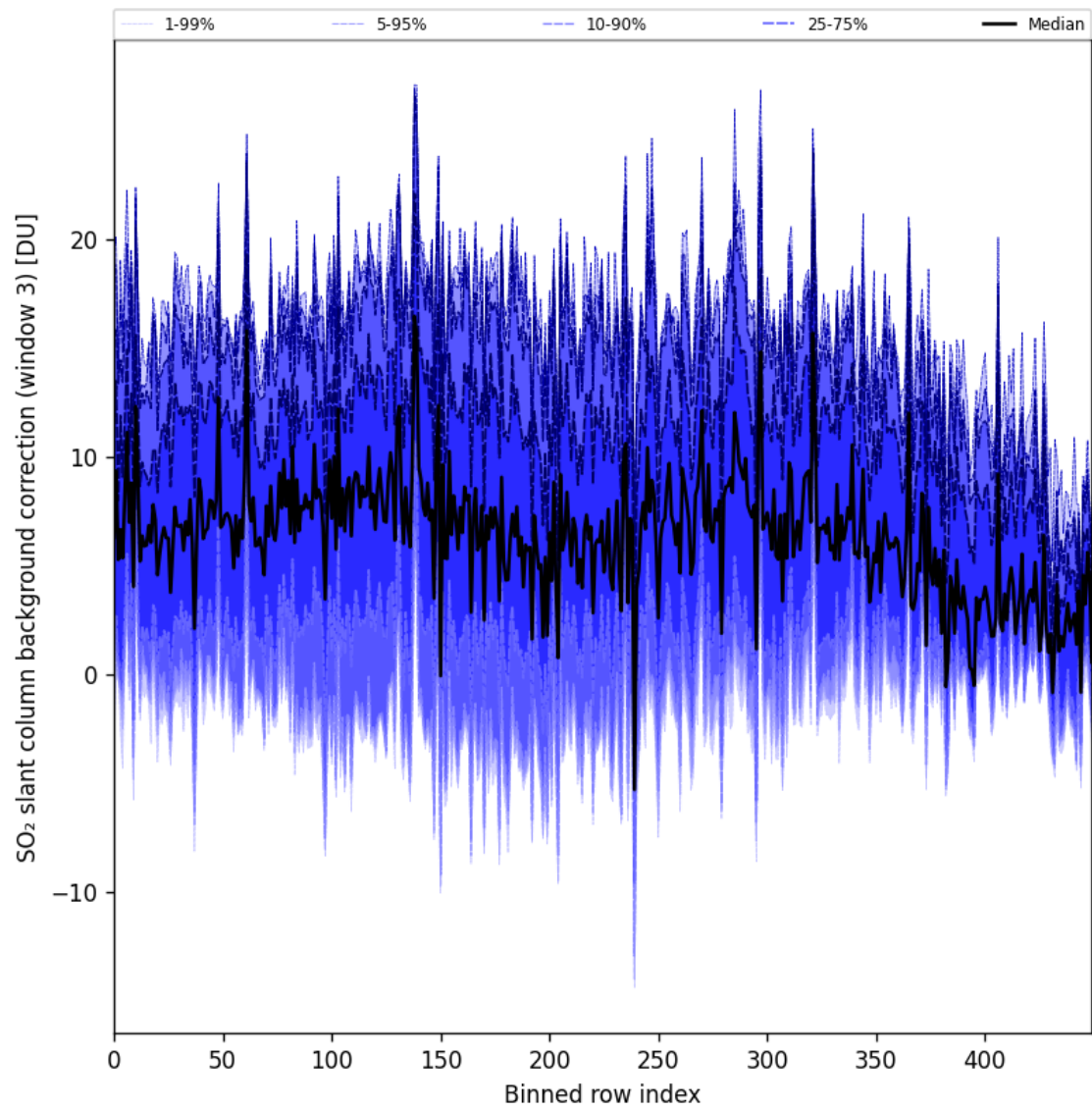
Figure 100: Along track statistics of “SO 2 slant column background correction (window 3)” for 2025-11-23 to 2025-11-25
