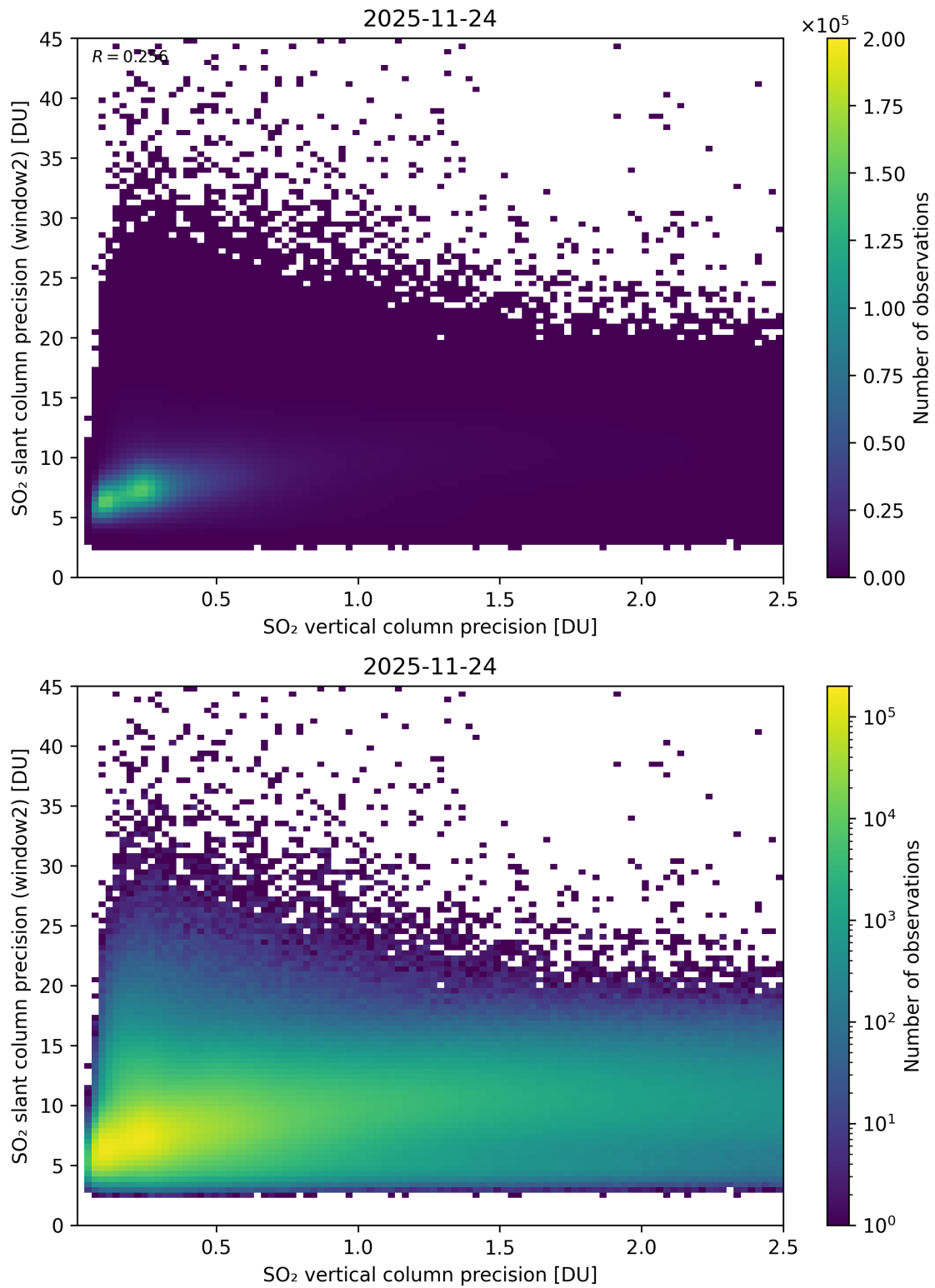
Figure 343: Scatter density plot of “SO 2 vertical column precision” against “SO 2 slant column precision (window2)” for 2025-11-23 to 2025-11-25.
