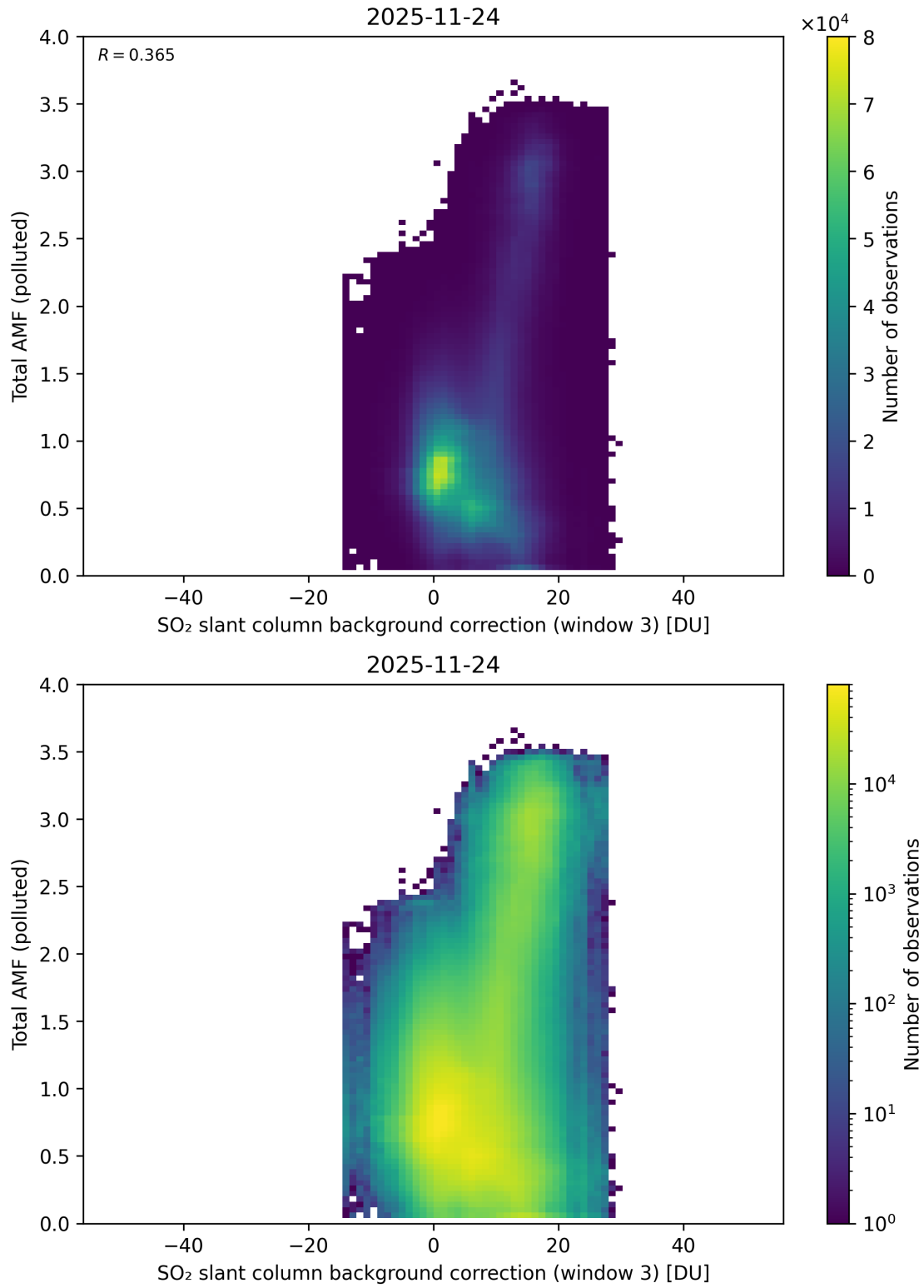
Figure 136: Scatter density plot of “SO 2 slant column background correction (window 3)” against “Total AMF (polluted)” for 2025-11-23 to 2025-11-25.
