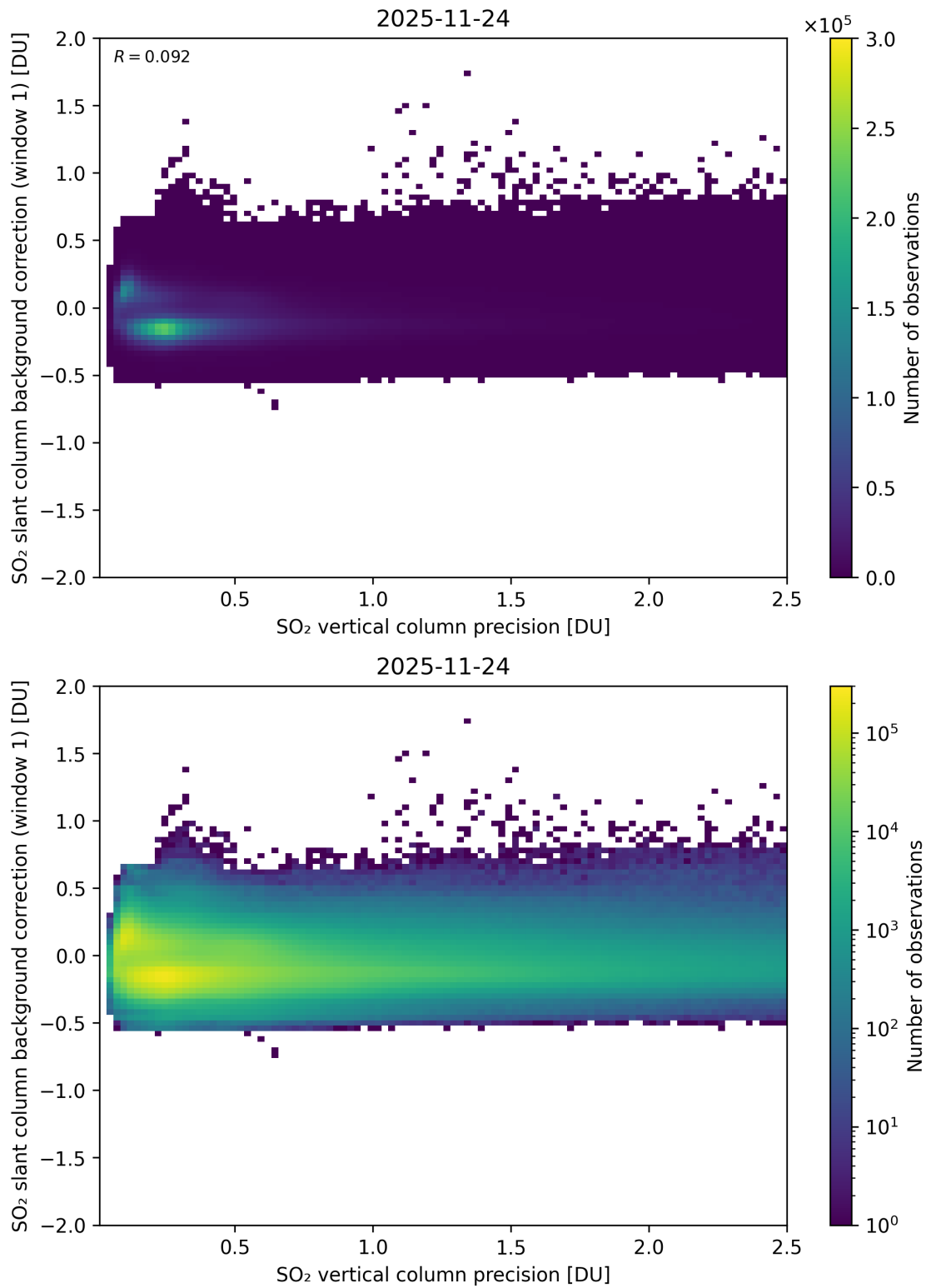
Figure 329: Scatter density plot of “SO 2 vertical column precision” against “SO 2 slant column background correction (window 1)” for 2025-11-23 to 2025-11-25.
