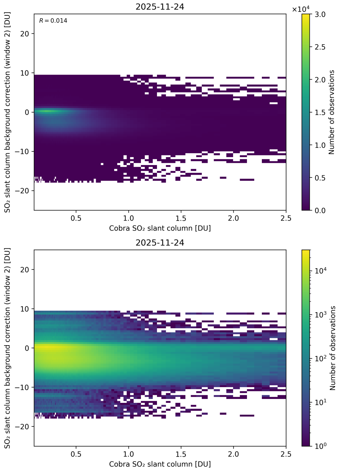
Figure 194: Scatter density plot of “Cobra SO 2 slant column” against “SO 2 slant column background correction (window 2)” for 2025-11-23 to 2025-11-25.
