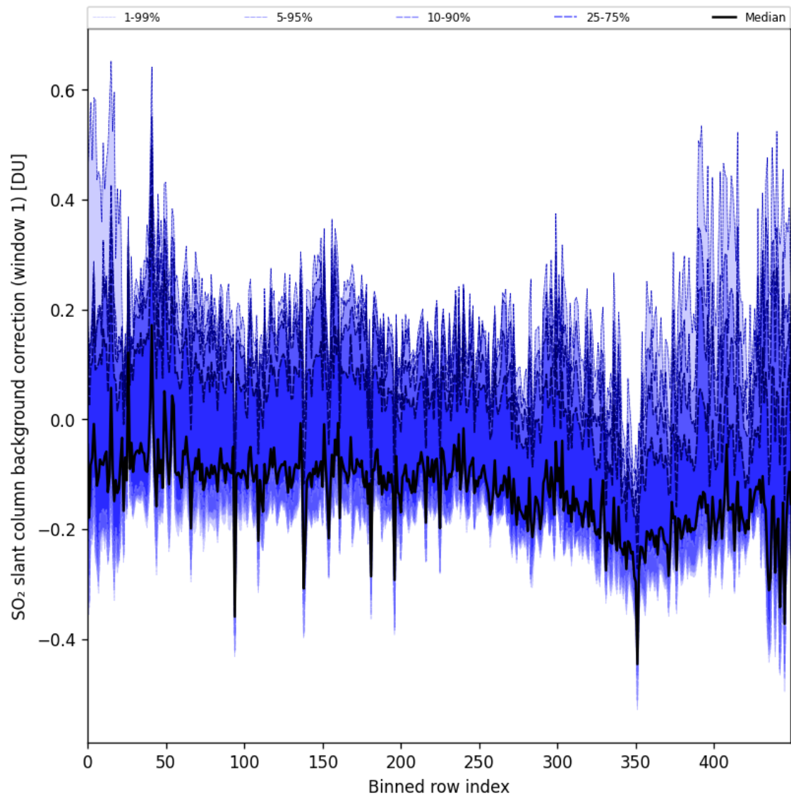
Figure 92: Along track statistics of “SO 2 slant column background correction (window 1)” for 2025-11-23 to 2025-11-25
