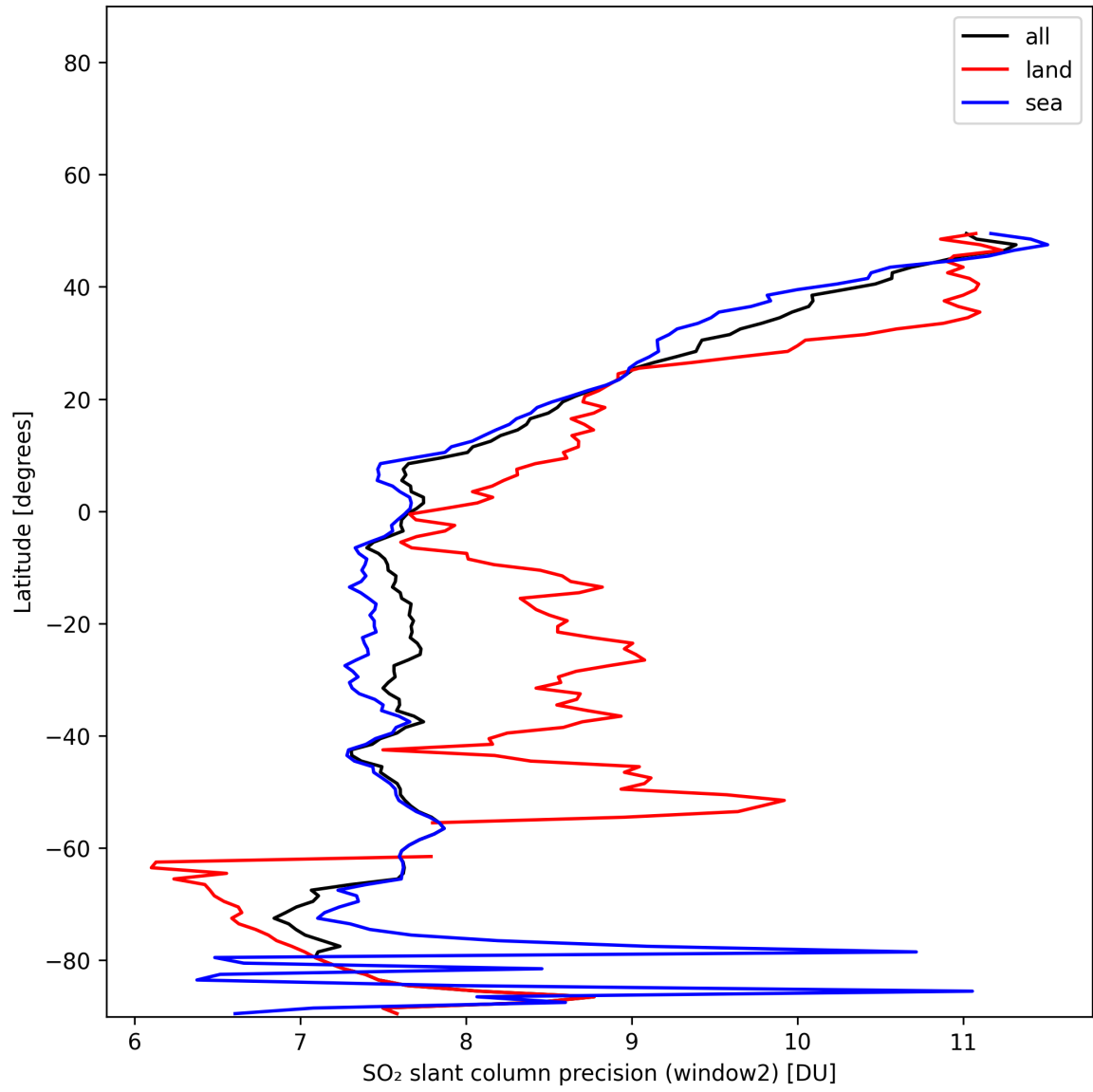
Figure 42: Zonal average of “SO 2 slant column precision (window2)” for 2025-11-23 to 2025-11-25.
