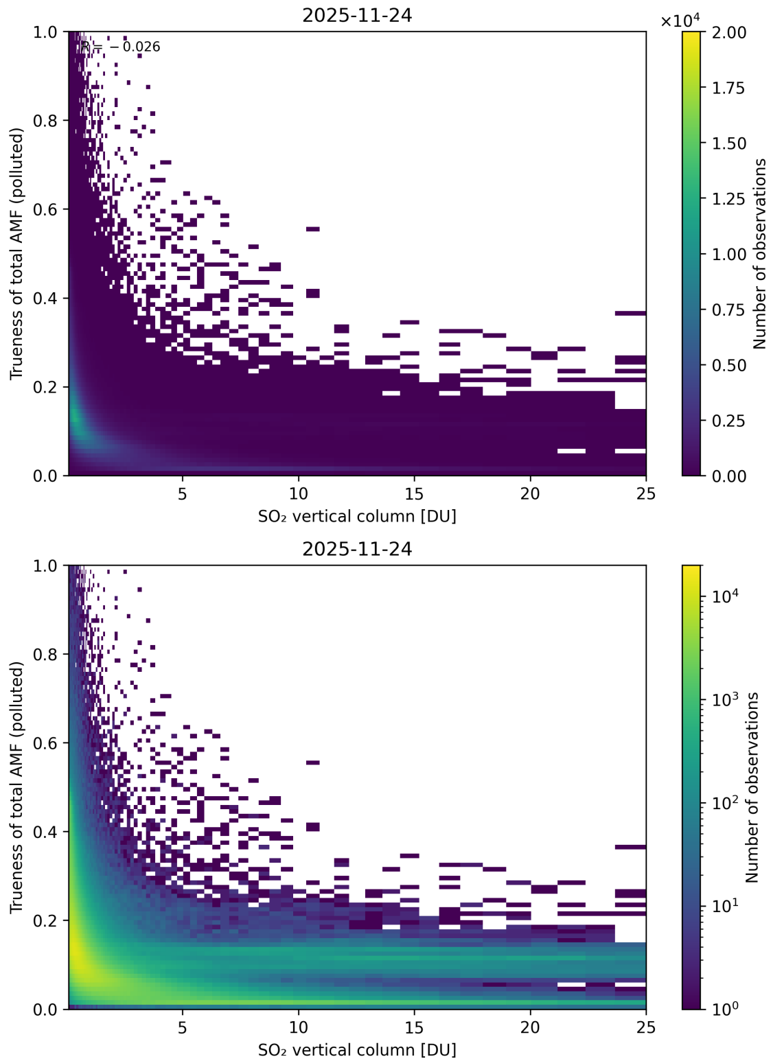
Figure 360: Scatter density plot of “SO 2 vertical column” against “Trueness of total AMF (polluted)” for 2025-11-23 to 2025-11-25.
