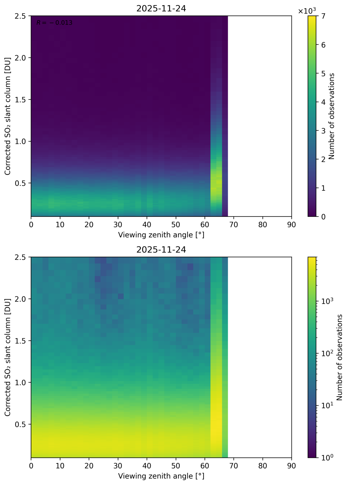
Figure 373: Scatter density plot of “Viewing zenith angle” against “Corrected SO 2 slant column” for 2025-11-23 to 2025-11-25.
