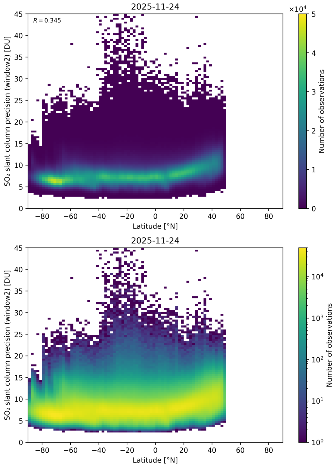
Figure 164: Scatter density plot of “Latitude” against “SO 2 slant column precision (window2)” for 2025-11-23 to 2025-11-25.
