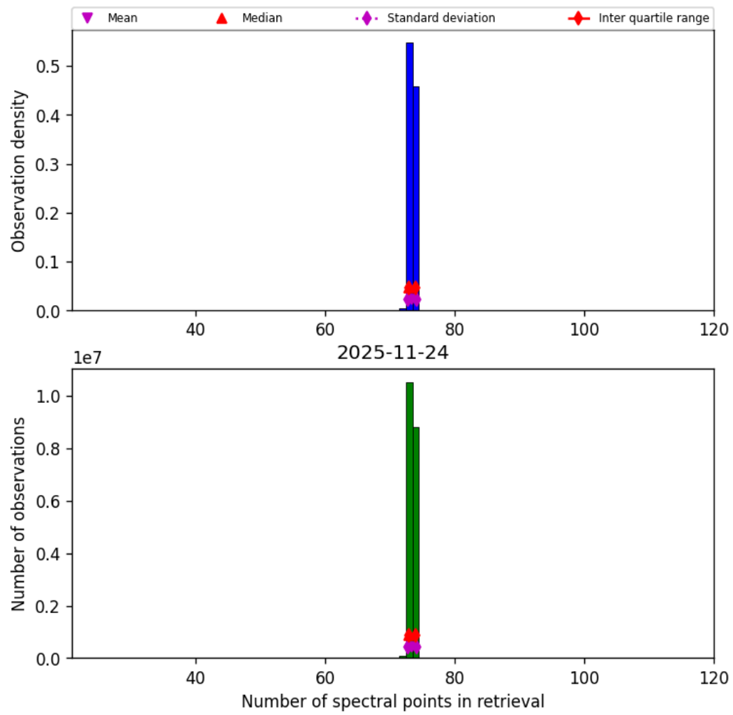
Figure 82: Histogram of “Number of spectral points in retrieval” for 2025-11-23 to 2025-11-25
