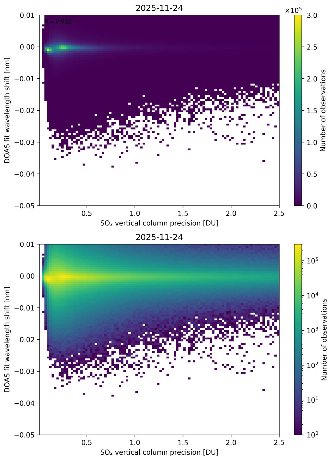
Figure 332: Scatter density plot of “SO 2 vertical column precision” against “DOAS fit wavelength shift” for 2025-11-23 to 2025-11-25.
