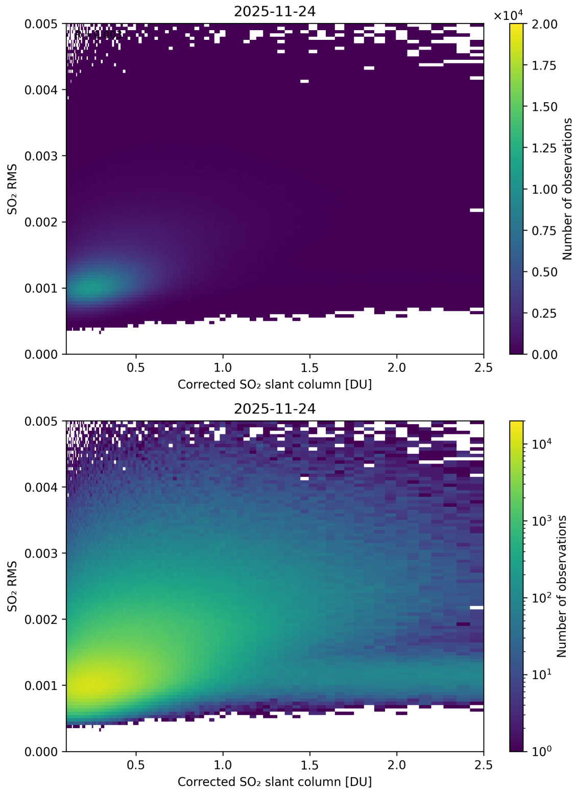
Figure 231: Scatter density plot of “Corrected SO 2 slant column” against “SO 2 RMS” for 2025-11-23 to 2025-11-25.
