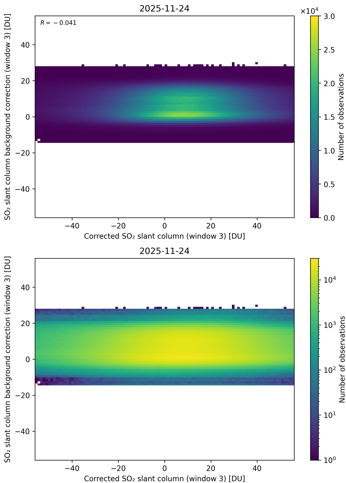
Figure 255: Scatter density plot of “Corrected SO 2 slant column (window 3)” against “SO 2 slant column background correction (window 3)” for 2025-11-23 to 2025-11-25.
