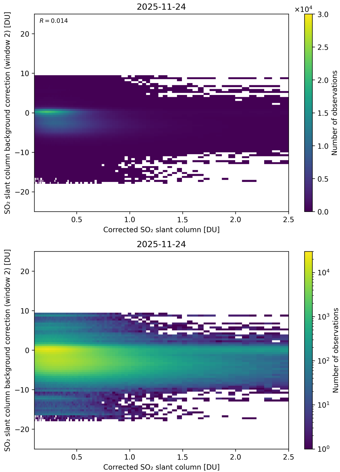
Figure 227: Scatter density plot of “Corrected SO 2 slant column” against “SO 2 slant column background correction (window 2)” for 2025-11-23 to 2025-11-25.
