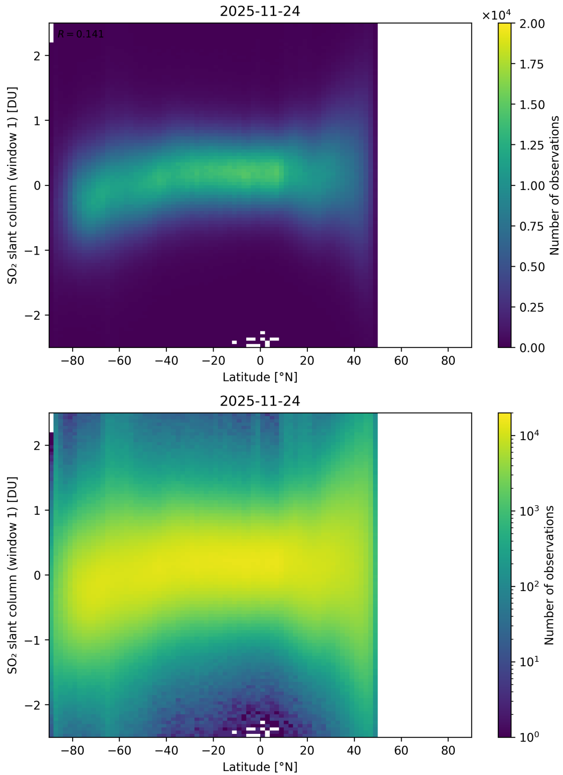
Figure 162: Scatter density plot of “Latitude” against “SO 2 slant column (window 1)” for 2025-11-23 to 2025-11-25.
