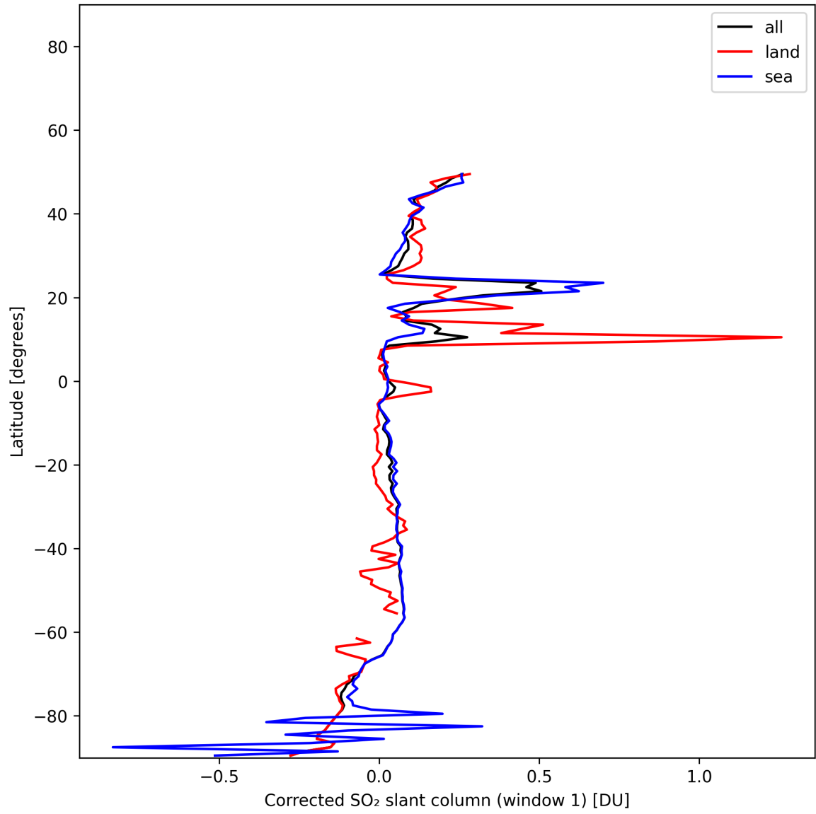
Figure 39: Zonal average of “Corrected SO 2 slant column (window 1)” for 2025-11-23 to 2025-11-25.
