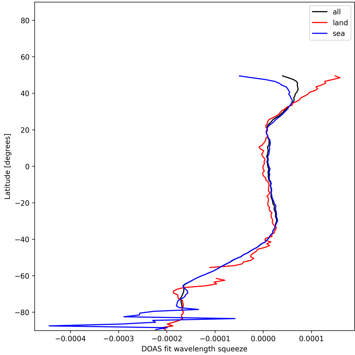
Figure 51: Zonal average of “DOAS fit wavelength squeeze” for 2025-11-23 to 2025-11-25.
