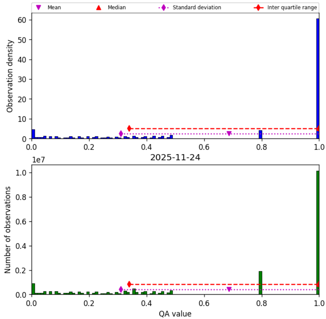
Figure 57: Histogram of “QA value” for 2025-11-23 to 2025-11-25
