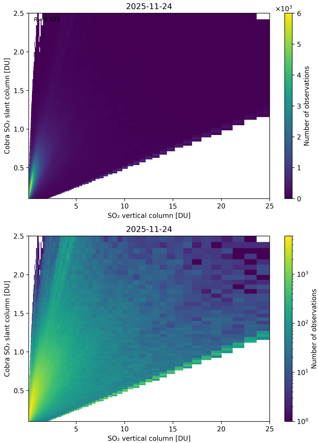
Figure 349: Scatter density plot of “SO 2 vertical column” against “Cobra SO 2 slant column” for 2025-11-23 to 2025-11-25.
