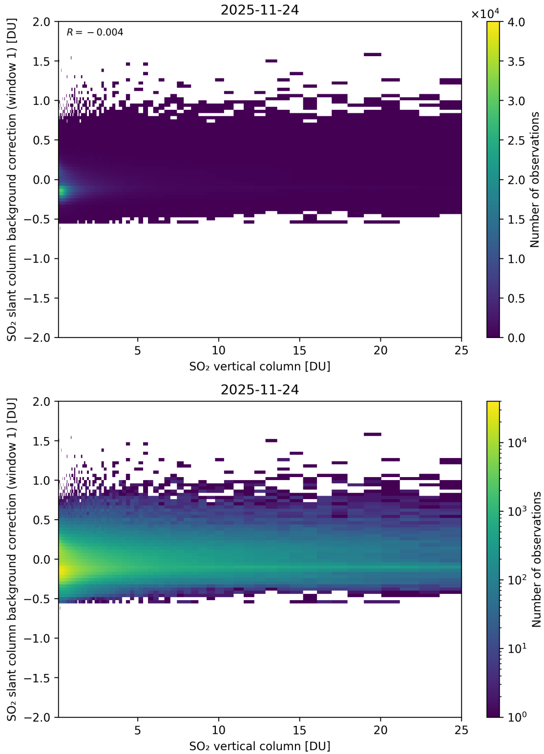
Figure 323: Scatter density plot of “SO 2 vertical column” against “SO 2 slant column background correction (window 1)” for 2025-11-23 to 2025-11-25.
