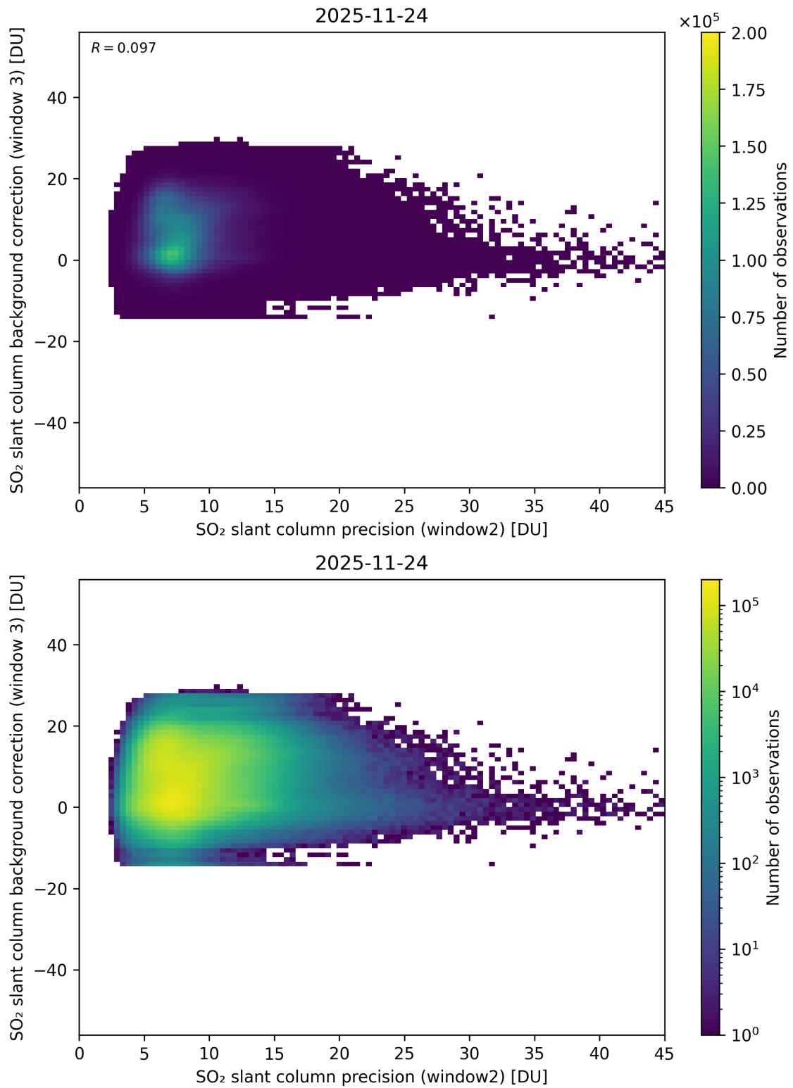
Figure 292: Scatter density plot of “SO 2 slant column precision (window2)” against “SO 2 slant column background correction (window 3)” for 2025-11-23 to 2025-11-25.
