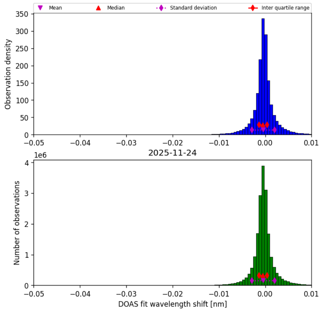
Figure 76: Histogram of “DOAS fit wavelength shift” for 2025-11-23 to 2025-11-25
