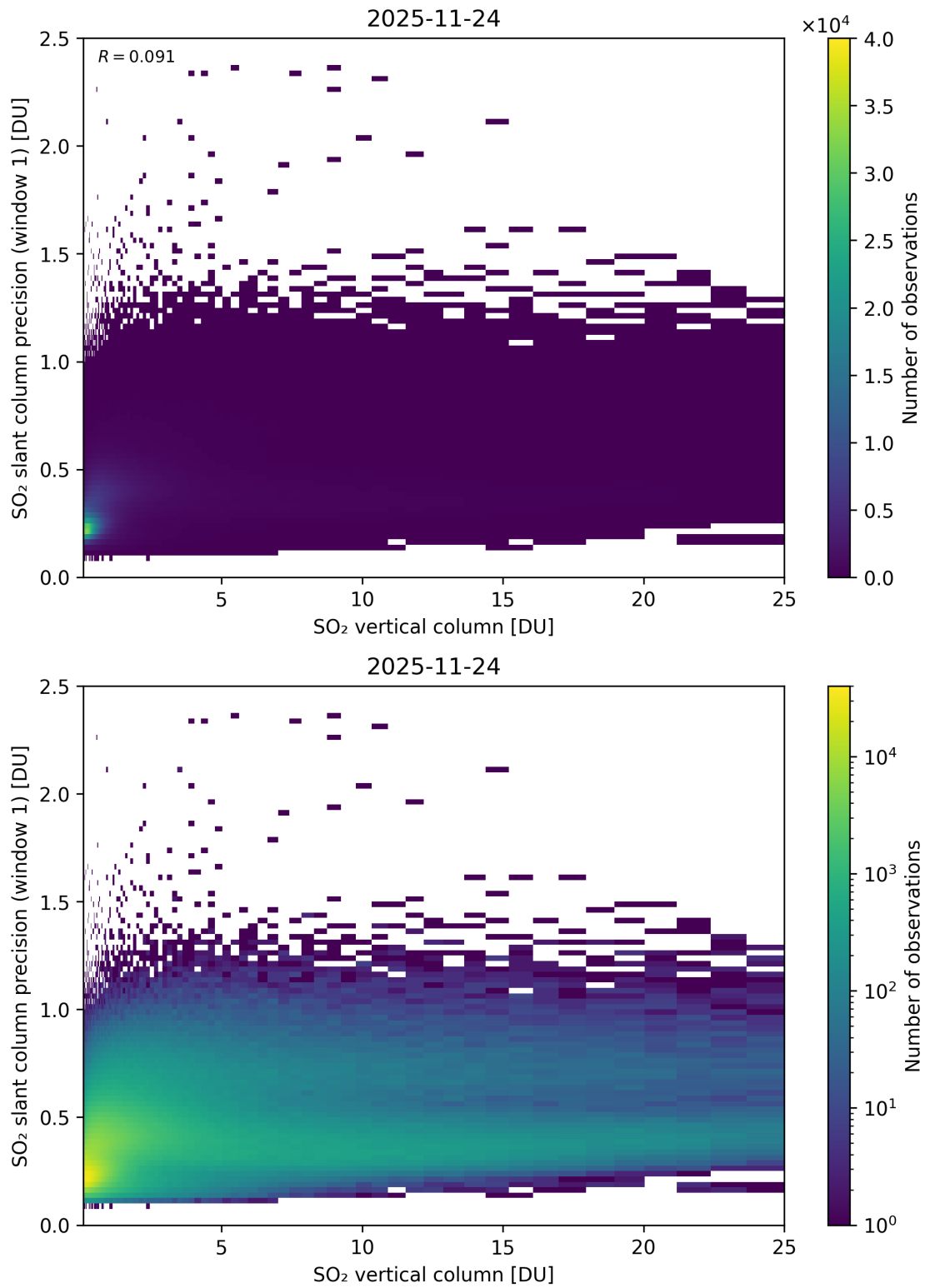
Figure 355: Scatter density plot of “SO 2 vertical column” against “SO 2 slant column precision (window 1)” for 2025-11-23 to 2025-11-25.
