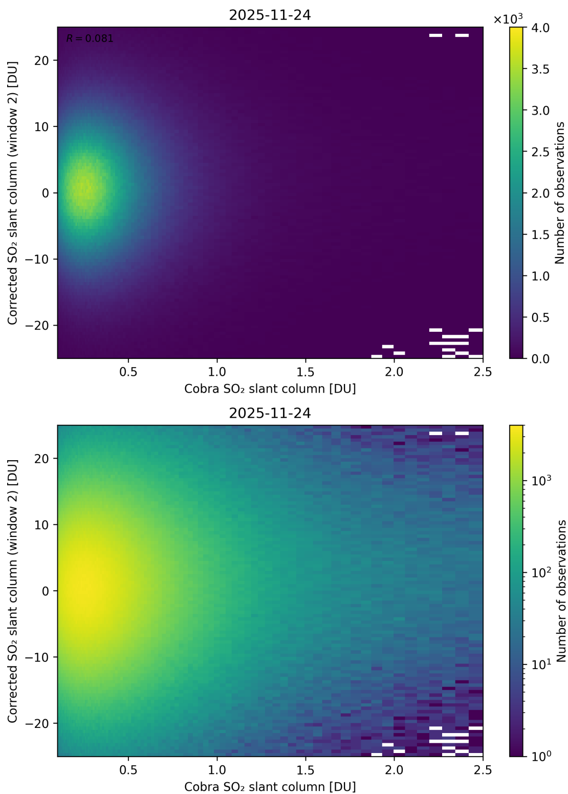
Figure 217: Scatter density plot of “Cobra SO 2 slant column” against “Corrected SO 2 slant column (window 2)” for 2025-11-23 to 2025-11-25.
