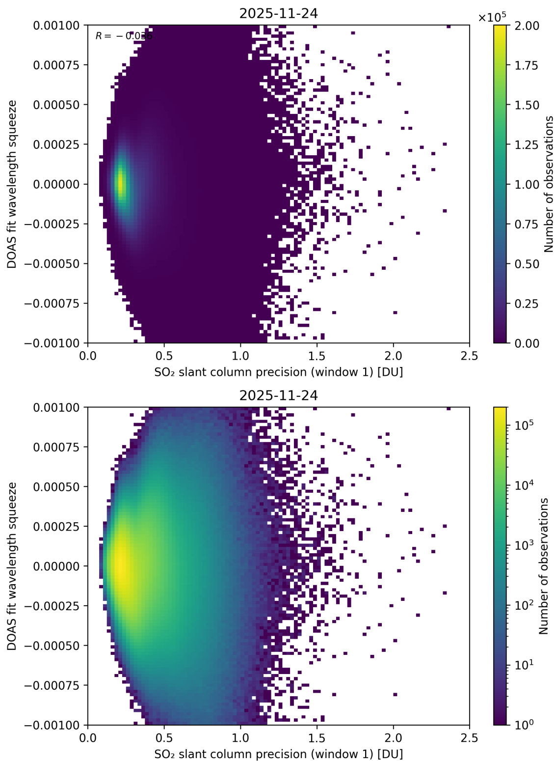
Figure 272: Scatter density plot of “SO 2 slant column precision (window 1)” against “DOAS fit wavelength squeeze” for 2025-11-23 to 2025-11-25.
