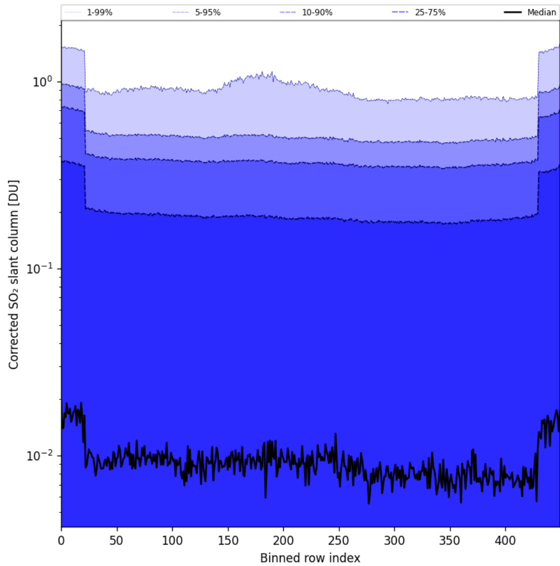
Figure 86: Along track statistics of “Corrected SO 2 slant column” for 2025-11-23 to 2025-11-25
