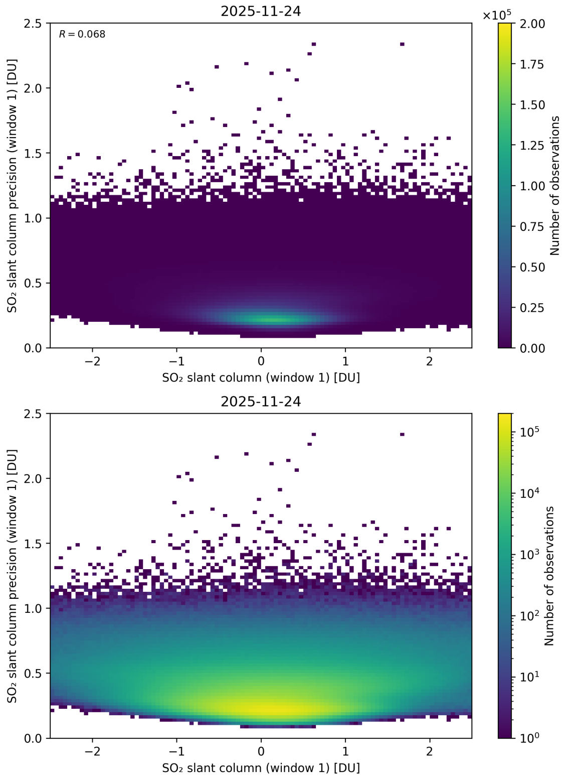
Figure 285: Scatter density plot of “SO 2 slant column (window 1)” against “SO 2 slant column precision (window 1)” for 2025-11-23 to 2025-11-25.
