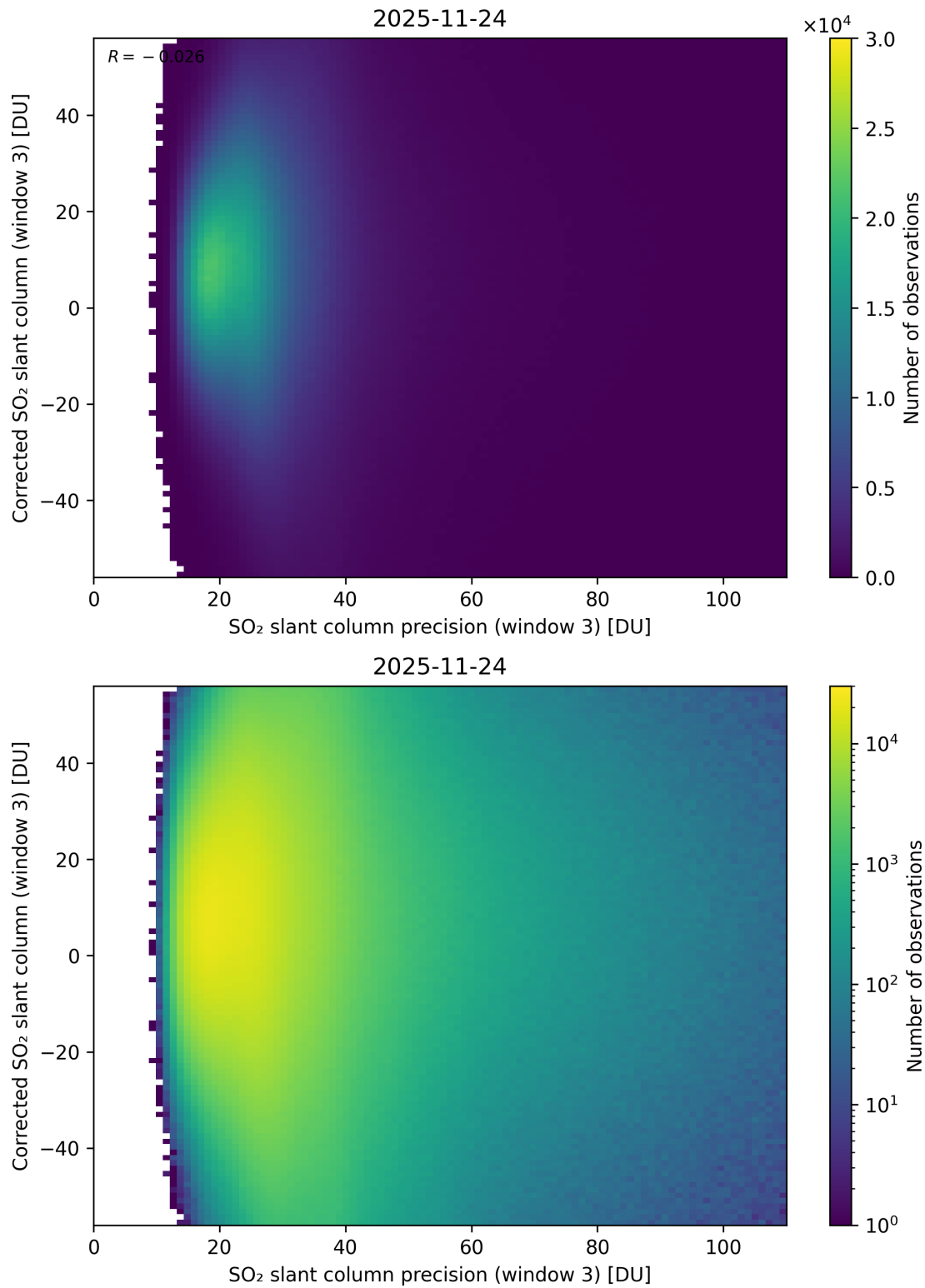
Figure 312: Scatter density plot of “SO 2 slant column precision (window 3)” against “Corrected SO 2 slant column (window 3)” for 2025-11-23 to 2025-11-25.
