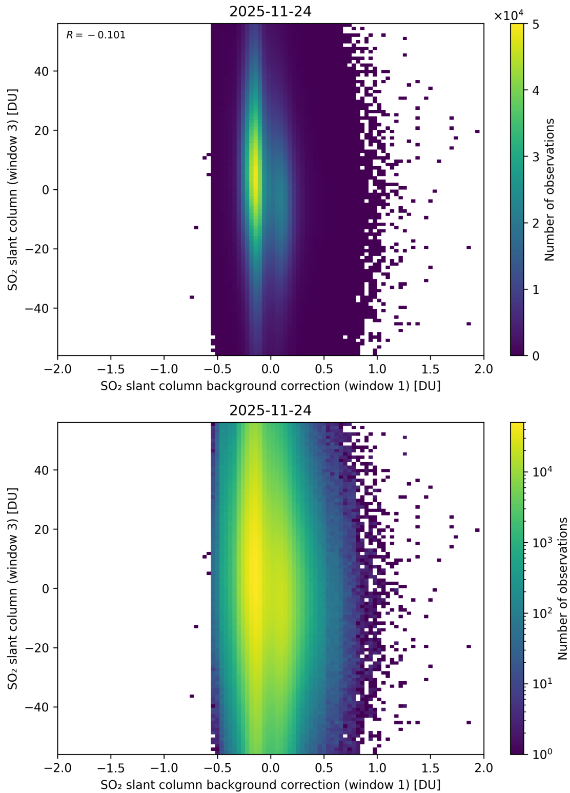
Figure 118: Scatter density plot of “SO 2 slant column background correction (window 1)” against “SO 2 slant column (window 3)” for 2025-11-23 to 2025-11-25.
