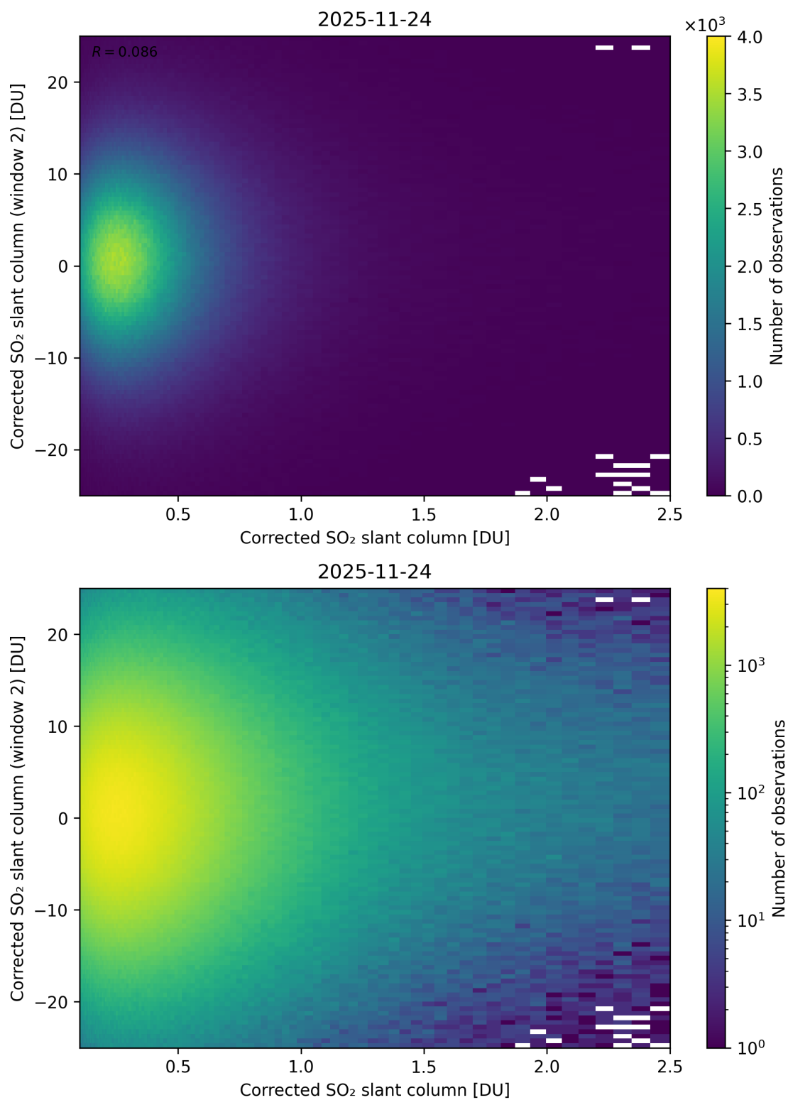
Figure 235: Scatter density plot of “Corrected SO 2 slant column” against “Corrected SO 2 slant column (window 2)” for 2025-11-23 to 2025-11-25.
