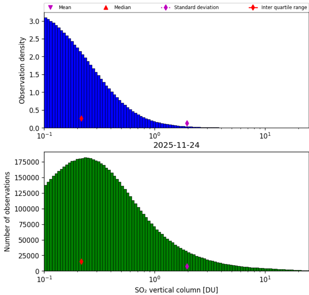
Figure 58: Histogram of “SO 2 vertical column” for 2025-11-23 to 2025-11-25
