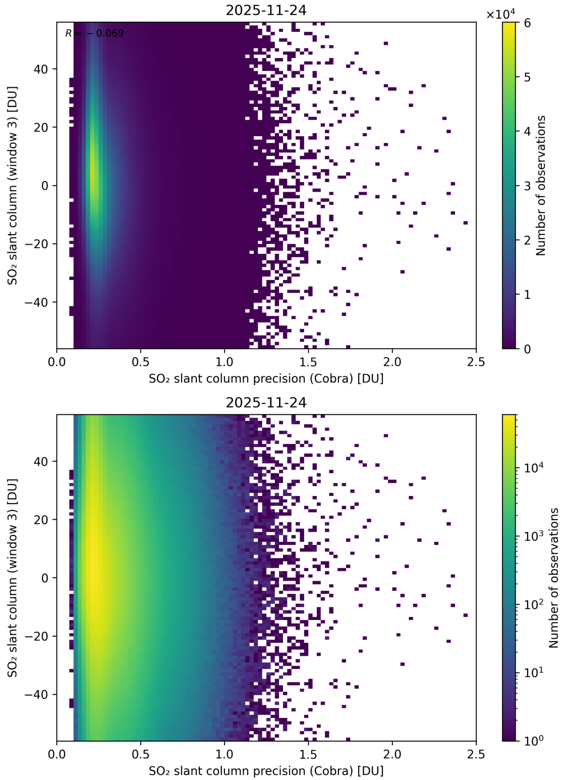
Figure 211: Scatter density plot of “SO 2 slant column precision (Cobra)” against “SO 2 slant column (window 3)” for 2025-11-23 to 2025-11-25.
