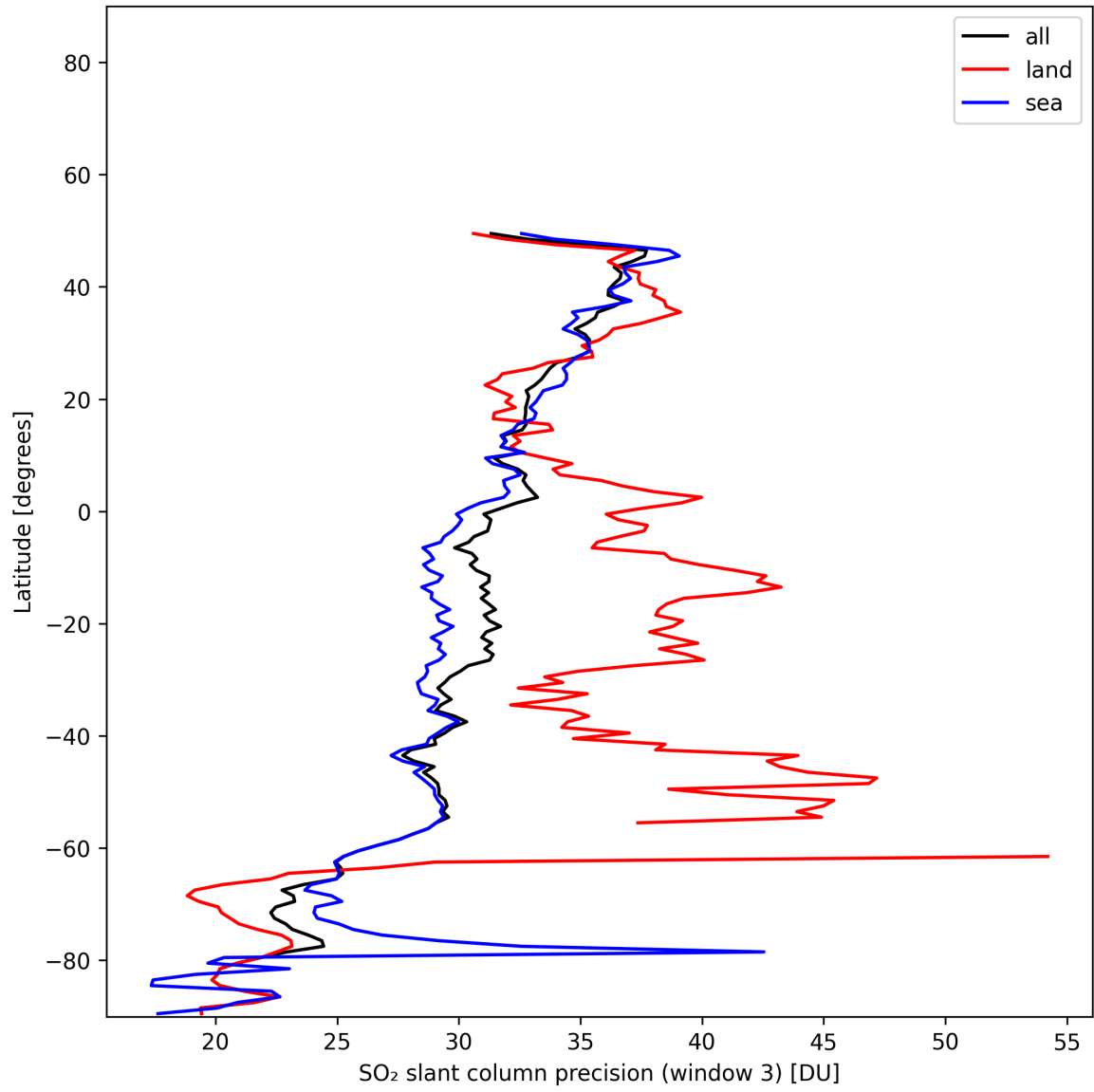
Figure 46: Zonal average of “SO 2 slant column precision (window 3)” for 2025-11-23 to 2025-11-25.
