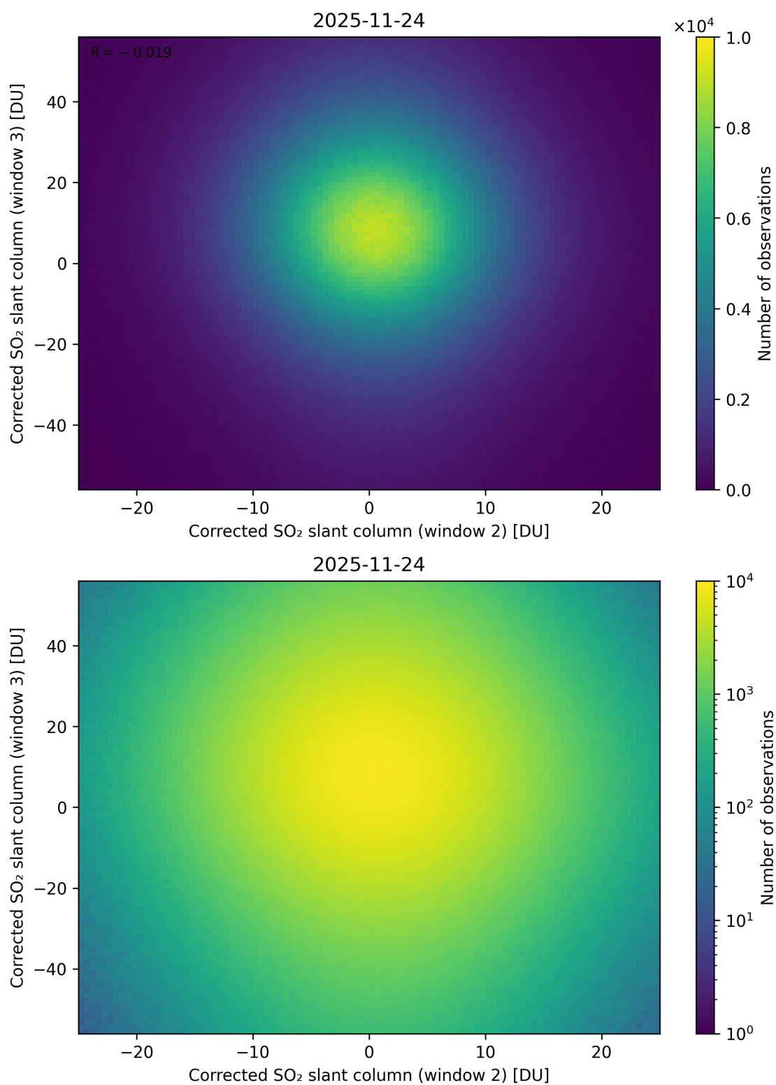
Figure 250: Scatter density plot of “Corrected SO 2 slant column (window 2)” against “Corrected SO 2 slant column (window 3)” for 2025-11-23 to 2025-11-25.
