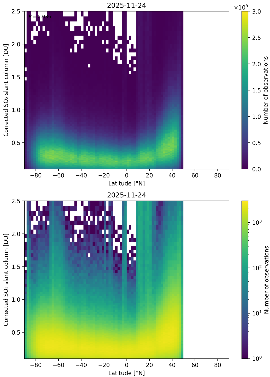
Figure 159: Scatter density plot of “Latitude” against “Corrected SO 2 slant column” for 2025-11-23 to 2025-11-25.
