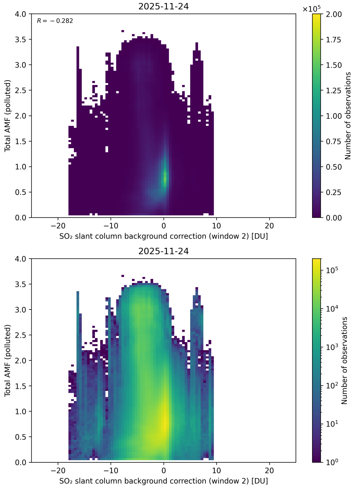
Figure 130: Scatter density plot of “SO 2 slant column background correction (window 2)” against “Total AMF (polluted)” for 2025-11-23 to 2025-11-25.
