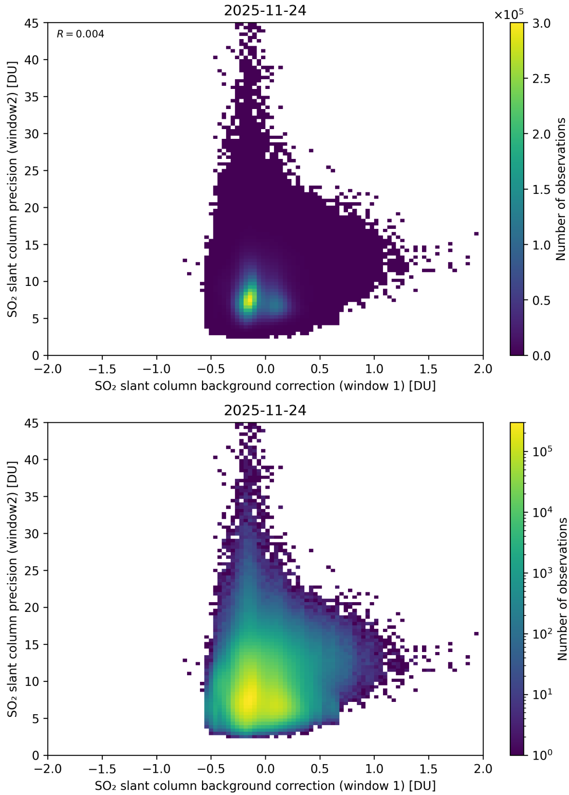
Figure 117: Scatter density plot of “SO 2 slant column background correction (window 1)” against “SO 2 slant column precision (window2)” for 2025-11-23 to 2025-11-25.
