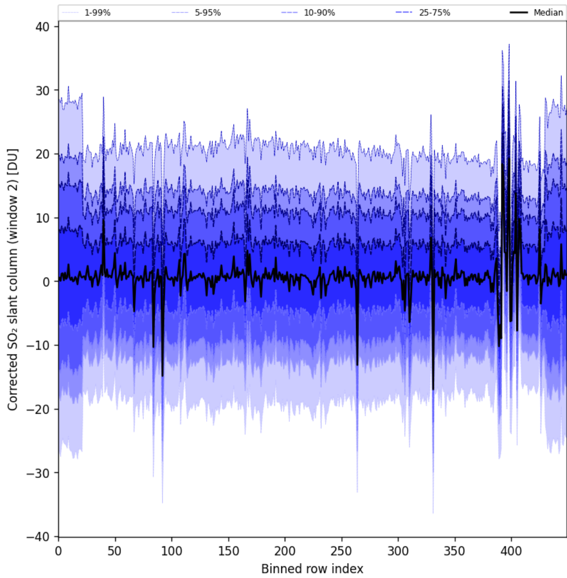
Figure 95: Along track statistics of “Corrected SO 2 slant column (window 2)” for 2025-11-23 to 2025-11-25
