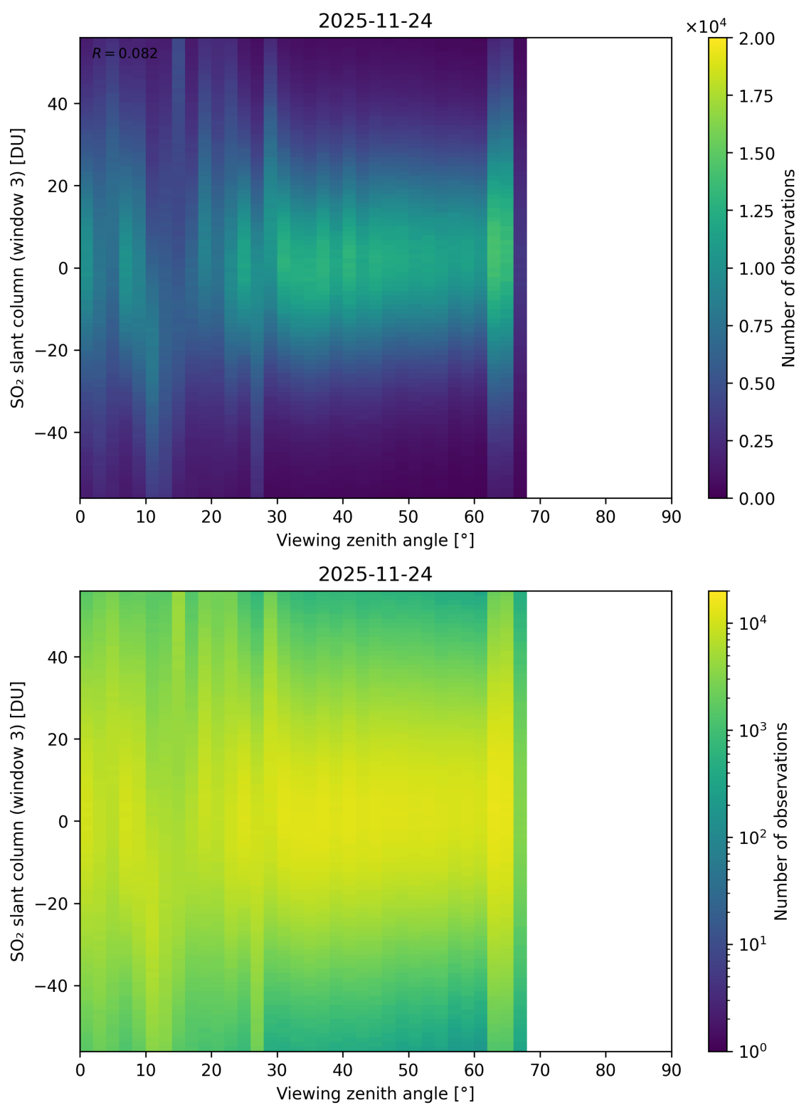
Figure 379: Scatter density plot of “Viewing zenith angle” against “SO 2 slant column (window 3)” for 2025-11-23 to 2025-11-25.
