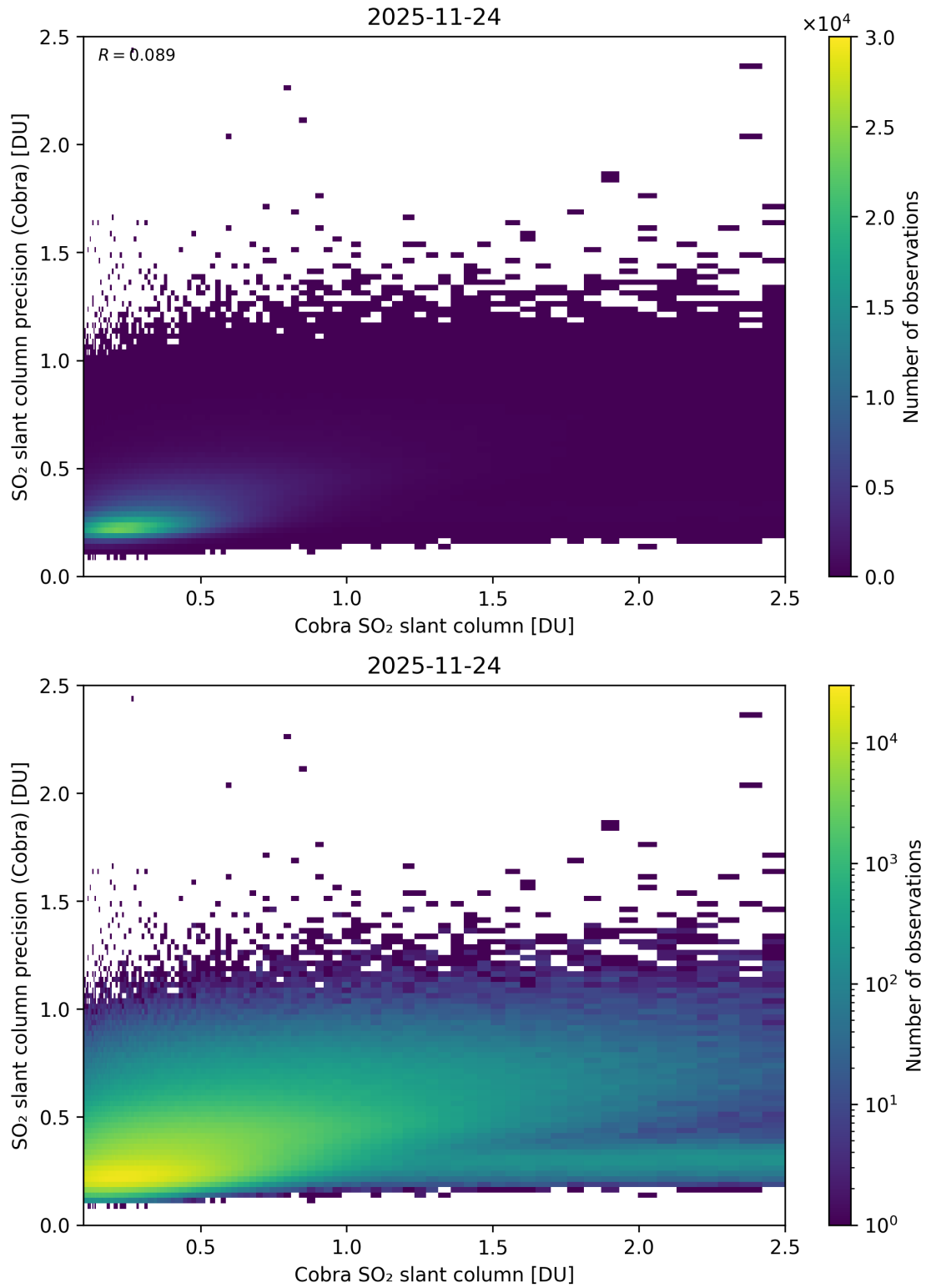
Figure 216: Scatter density plot of “Cobra SO 2 slant column” against “SO 2 slant column precision (Cobra)” for 2025-11-23 to 2025-11-25.
