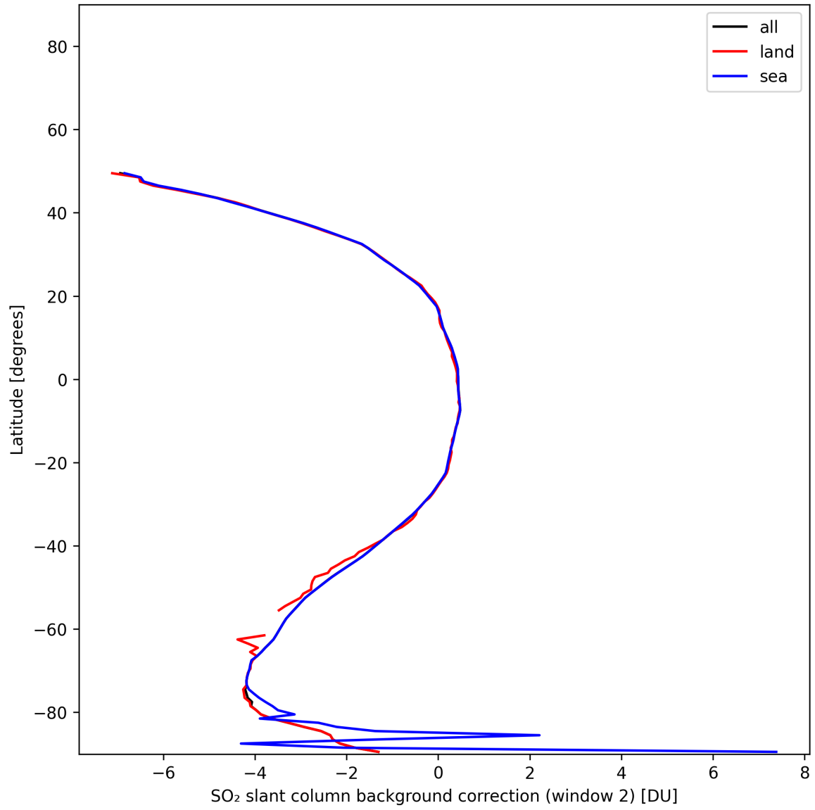
Figure 44: Zonal average of “SO 2 slant column background correction (window 2)” for 2025-11-23 to 2025-11-25.
