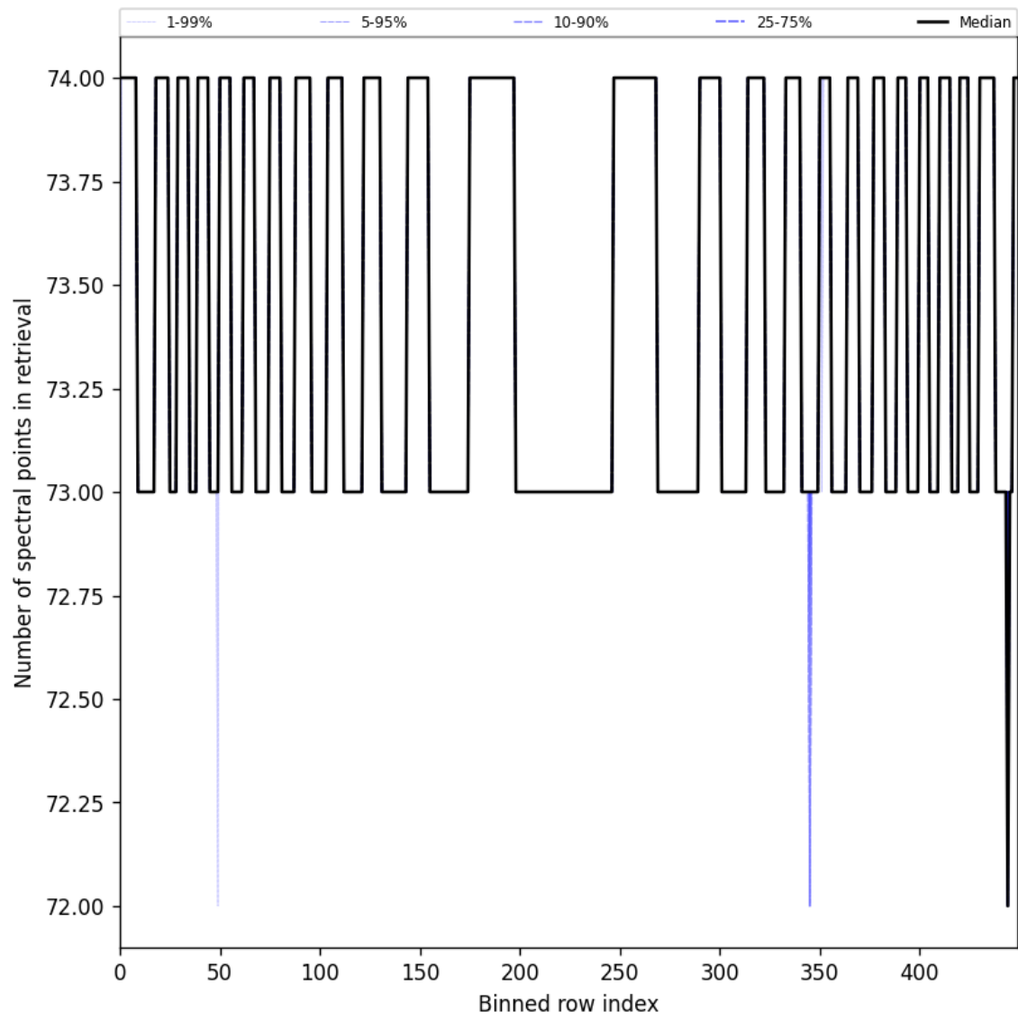
Figure 108: Along track statistics of “Number of spectral points in retrieval” for 2025-11-23 to 2025-11-25
