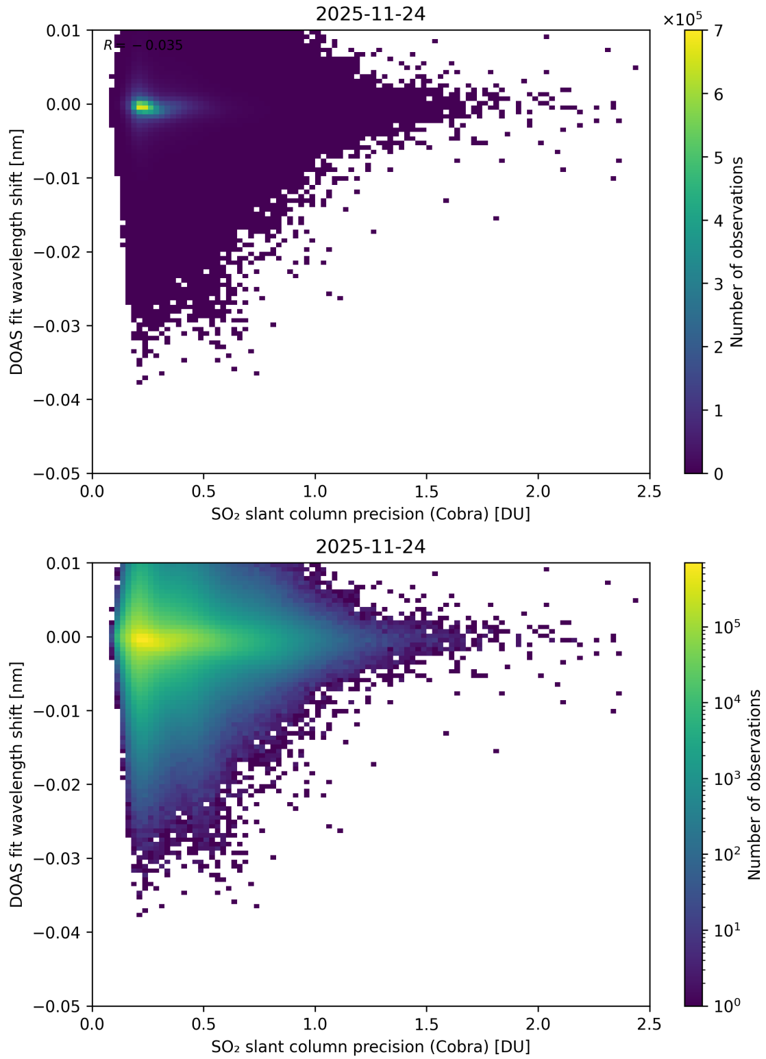
Figure 202: Scatter density plot of “SO 2 slant column precision (Cobra)” against “DOAS fit wavelength shift” for 2025-11-23 to 2025-11-25.
