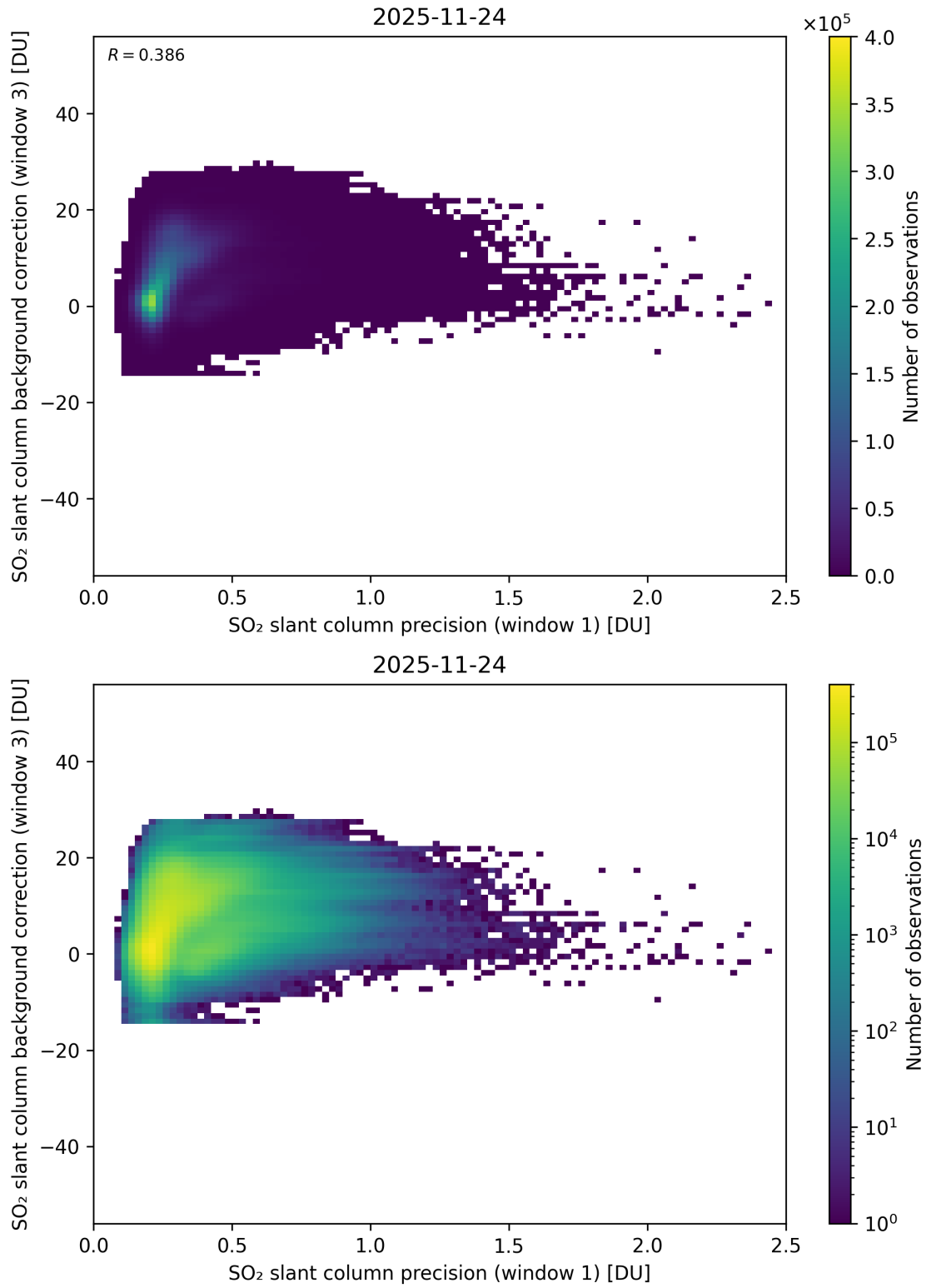
Figure 270: Scatter density plot of “SO 2 slant column precision (window 1)” against “SO 2 slant column background correction (window 3)” for 2025-11-23 to 2025-11-25.
