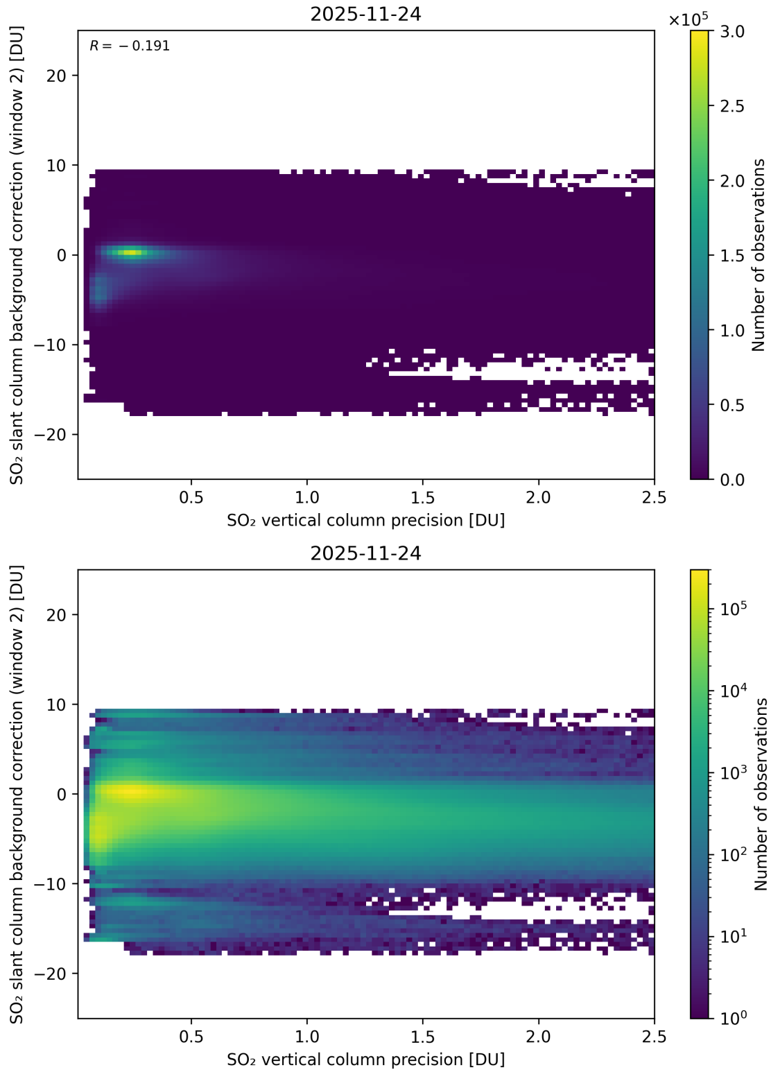
Figure 330: Scatter density plot of “SO 2 vertical column precision” against “SO 2 slant column background correction (window 2)” for 2025-11-23 to 2025-11-25.
