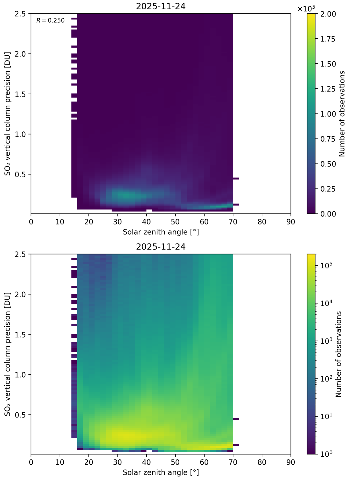
Figure 192: Scatter density plot of “Solar zenith angle” against “SO 2 vertical column precision” for 2025-11-23 to 2025-11-25.
