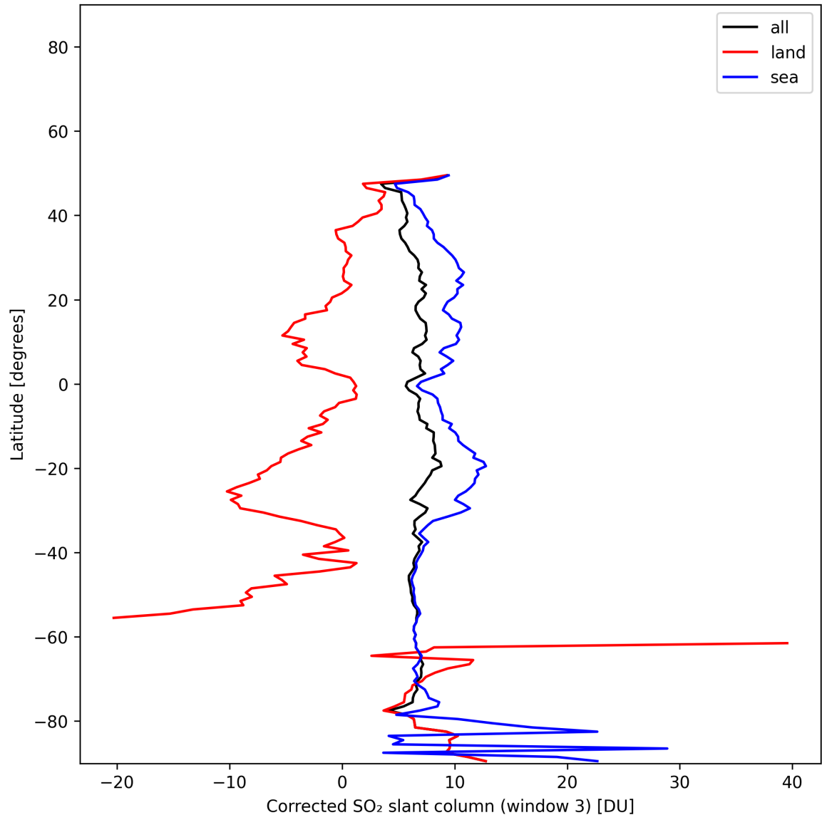
Figure 47: Zonal average of “Corrected SO 2 slant column (window 3)” for 2025-11-23 to 2025-11-25.
