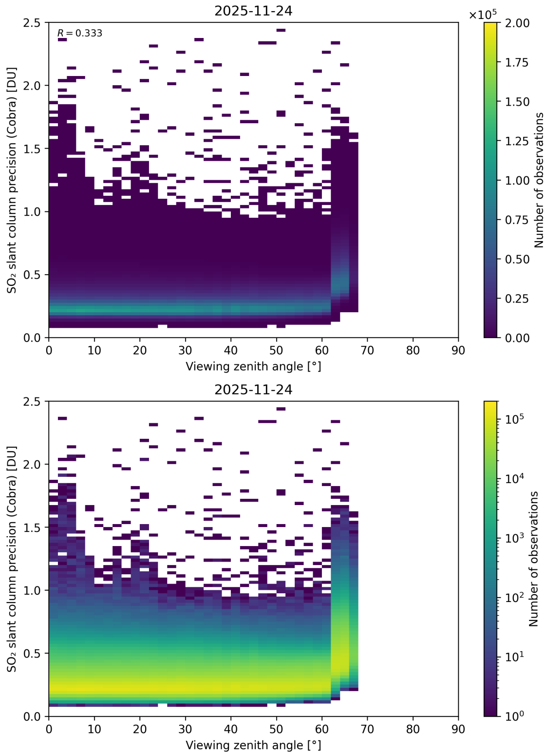
Figure 372: Scatter density plot of “Viewing zenith angle” against “SO 2 slant column precision (Cobra)” for 2025-11-23 to 2025-11-25.
