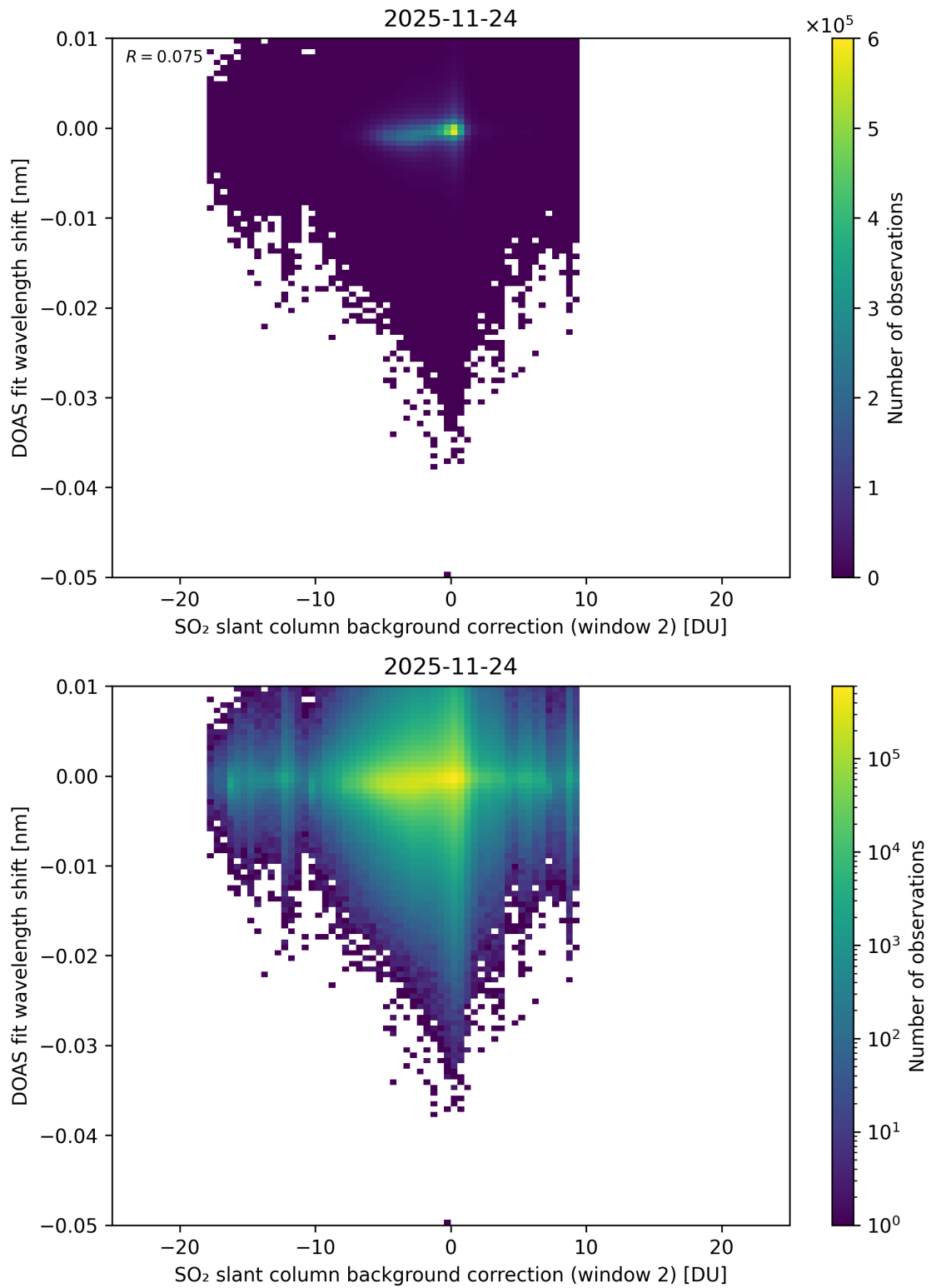
Figure 123: Scatter density plot of “SO 2 slant column background correction (window 2)” against “DOAS fit wavelength shift” for 2025-11-23 to 2025-11-25.
