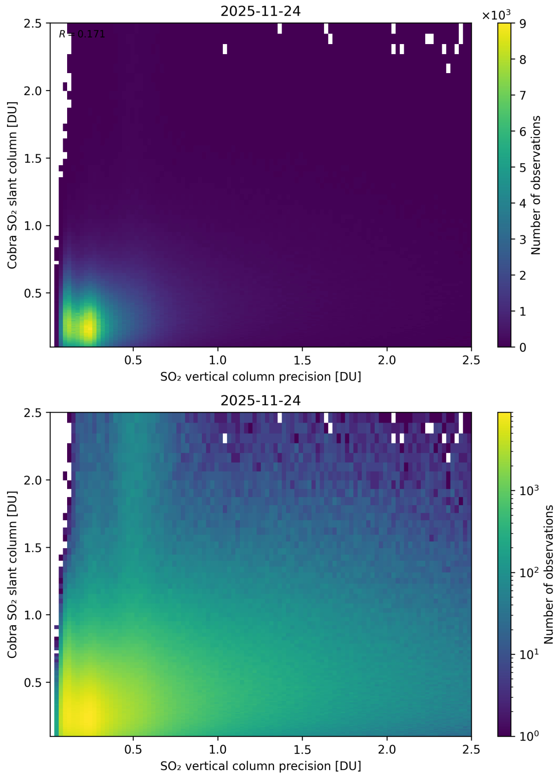
Figure 336: Scatter density plot of “SO 2 vertical column precision” against “Cobra SO 2 slant column” for 2025-11-23 to 2025-11-25.
