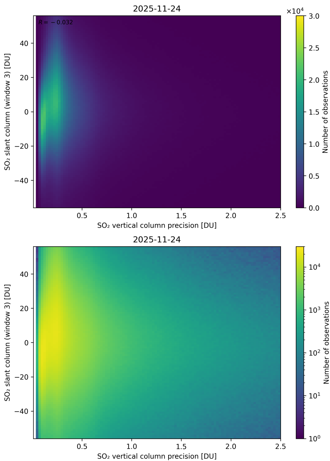
Figure 344: Scatter density plot of “SO 2 vertical column precision” against “SO 2 slant column (window 3)” for 2025-11-23 to 2025-11-25.
