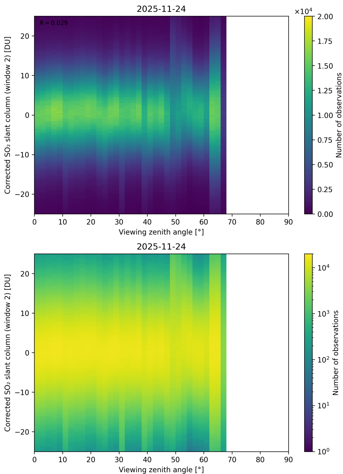
Figure 374: Scatter density plot of “Viewing zenith angle” against “Corrected SO 2 slant column (window 2)” for 2025-11-23 to 2025-11-25.
