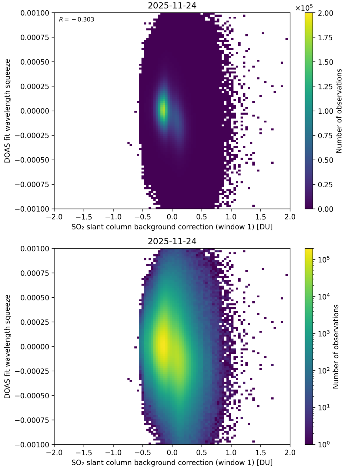
Figure 112: Scatter density plot of “SO 2 slant column background correction (window 1)” against “DOAS fit wavelength squeeze” for 2025-11-23 to 2025-11-25.
