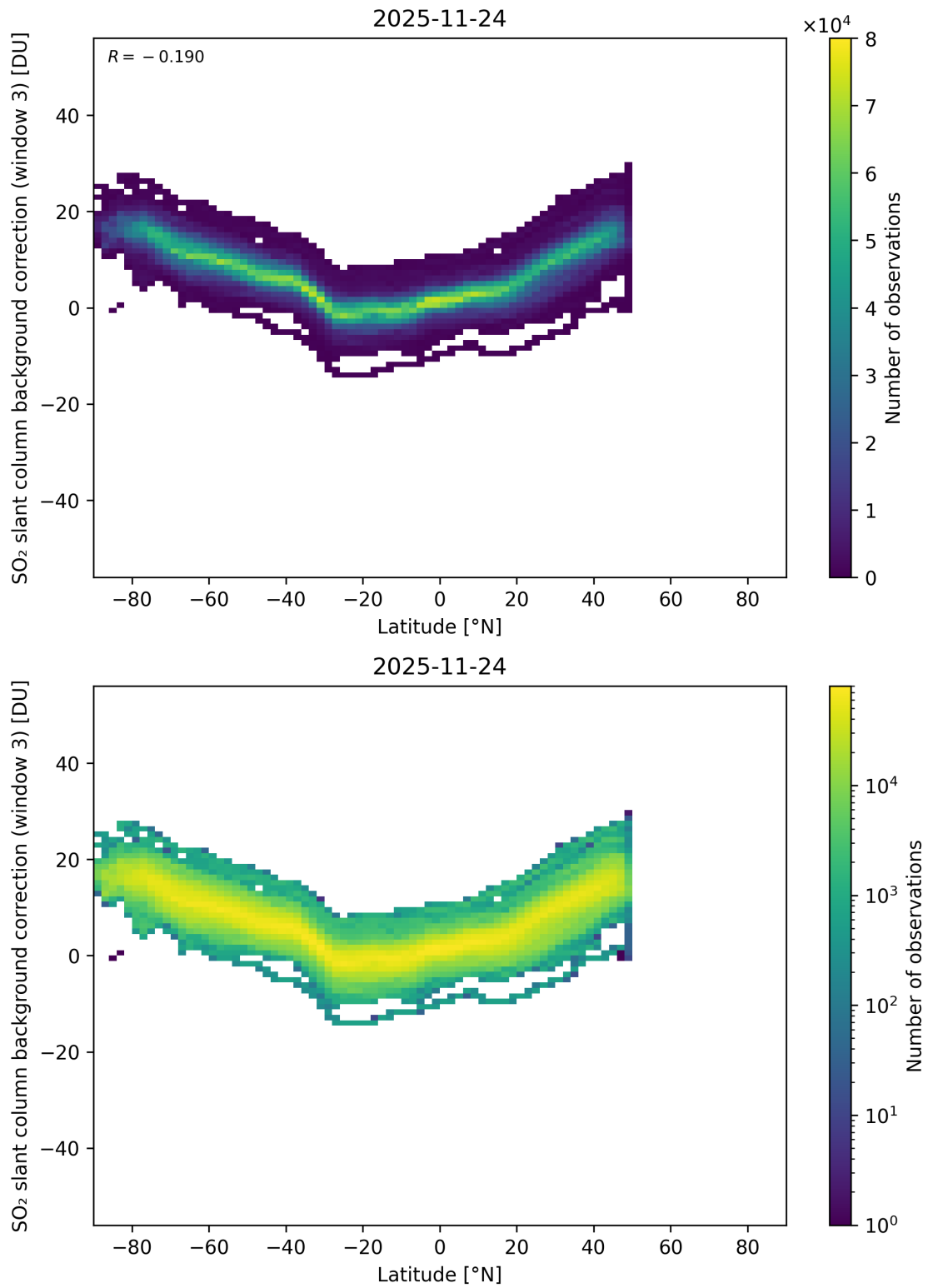
Figure 152: Scatter density plot of “Latitude” against “SO 2 slant column background correction (window 3)” for 2025-11-23 to 2025-11-25.
