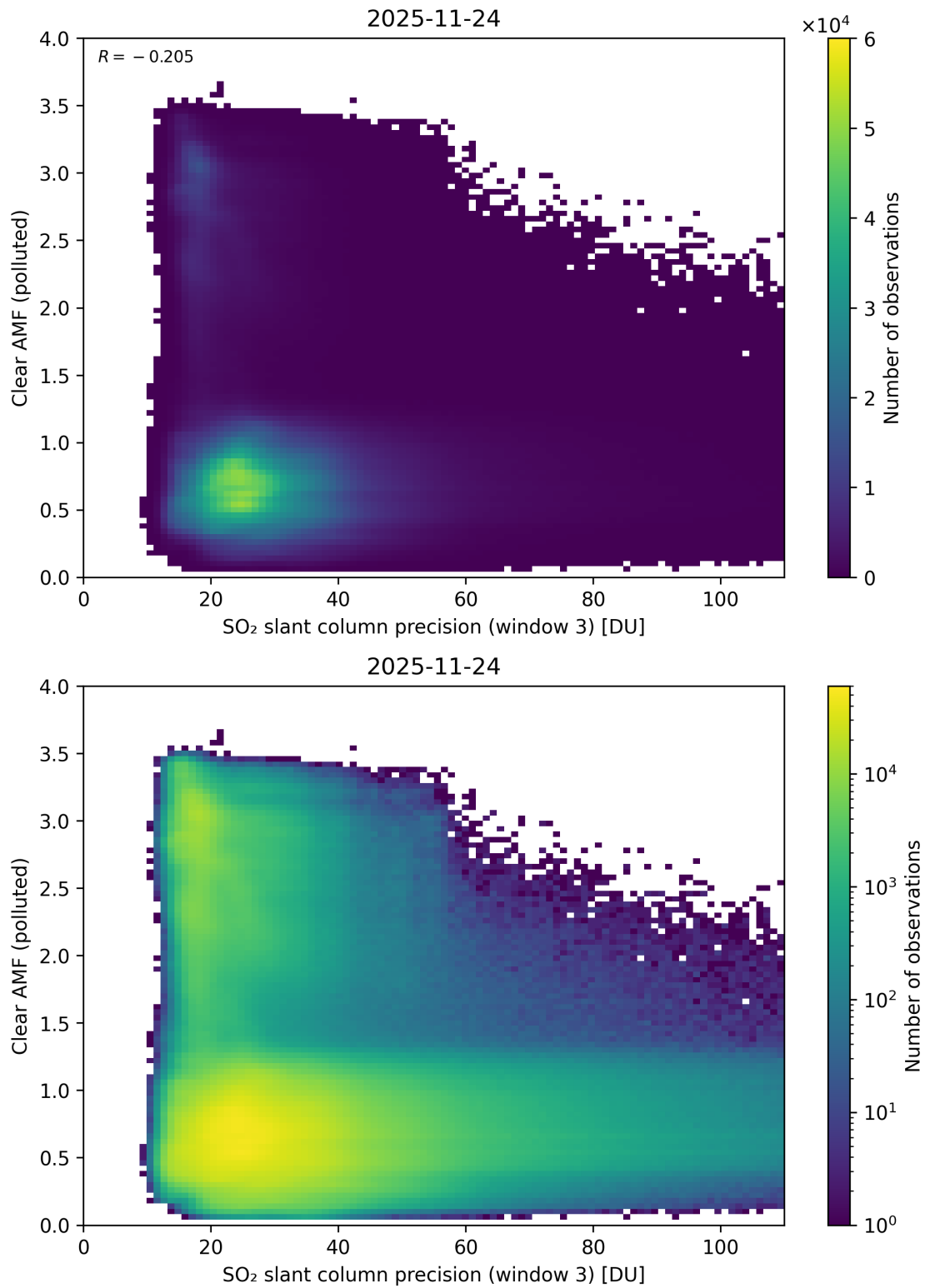
Figure 311: Scatter density plot of “SO 2 slant column precision (window 3)” against “Clear AMF (polluted)” for 2025-11-23 to 2025-11-25.
