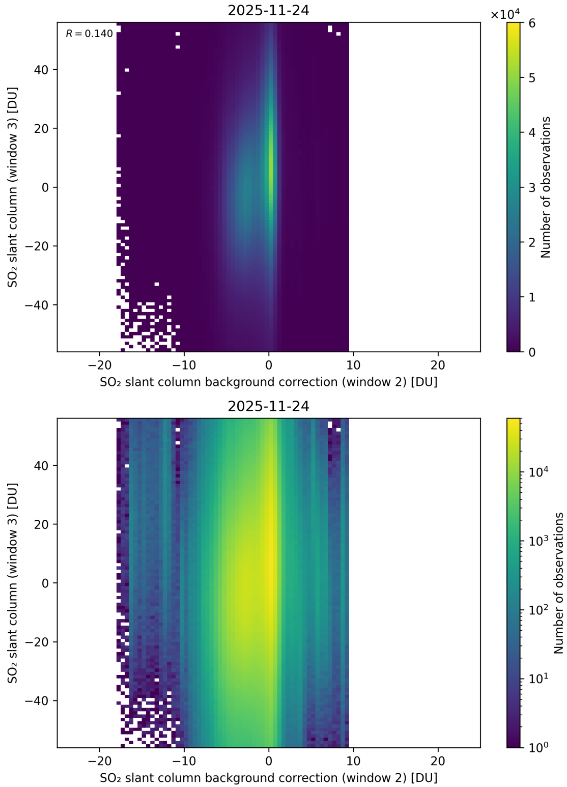
Figure 128: Scatter density plot of “SO 2 slant column background correction (window 2)” against “SO 2 slant column (window 3)” for 2025-11-23 to 2025-11-25.
