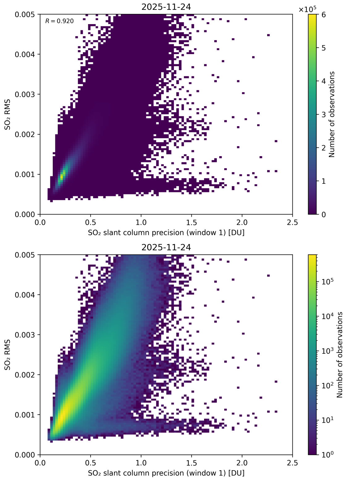
Figure 273: Scatter density plot of “SO 2 slant column precision (window 1)” against “SO 2 RMS” for 2025-11-23 to 2025-11-25.
