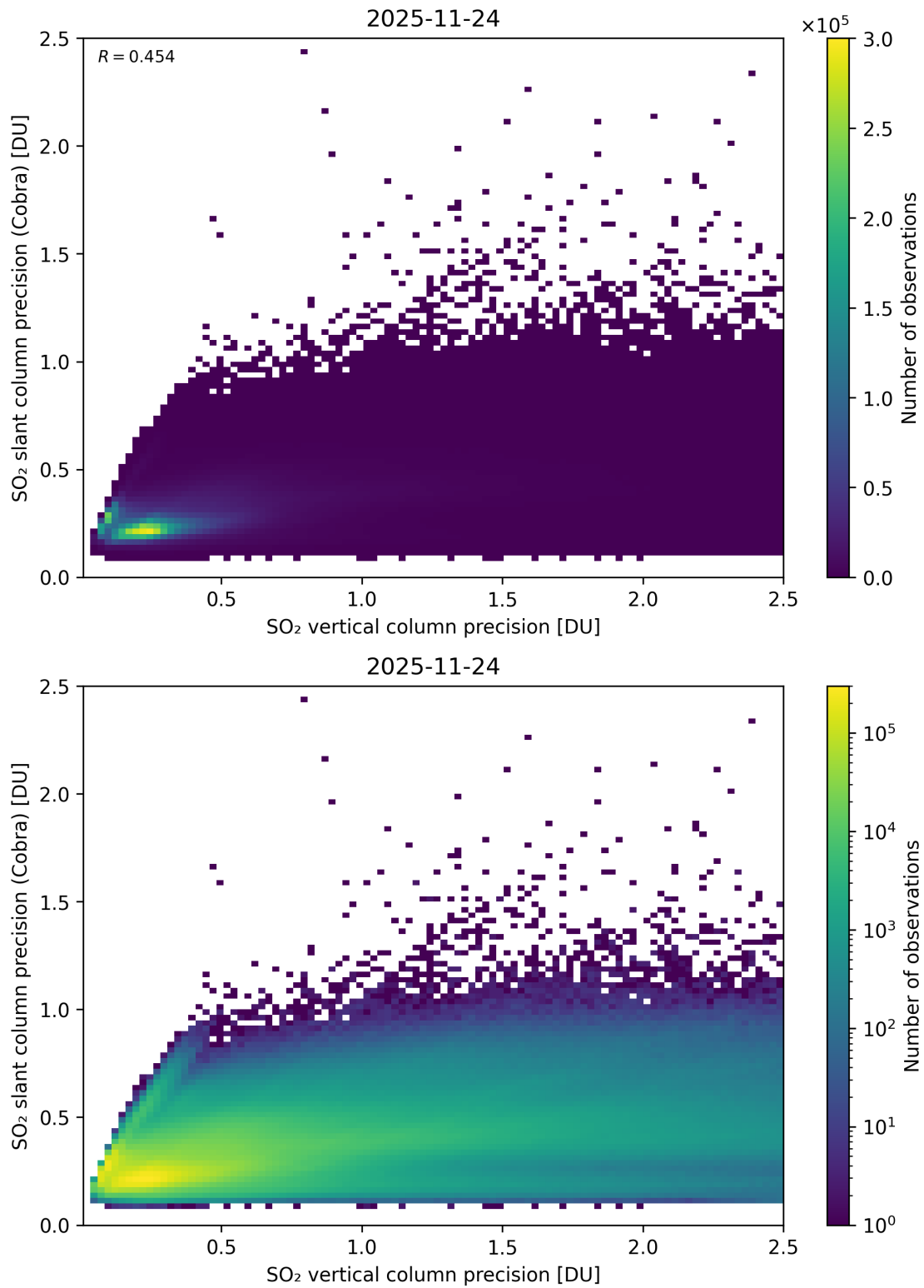
Figure 337: Scatter density plot of “SO 2 vertical column precision” against “SO 2 slant column precision (Cobra)” for 2025-11-23 to 2025-11-25.
