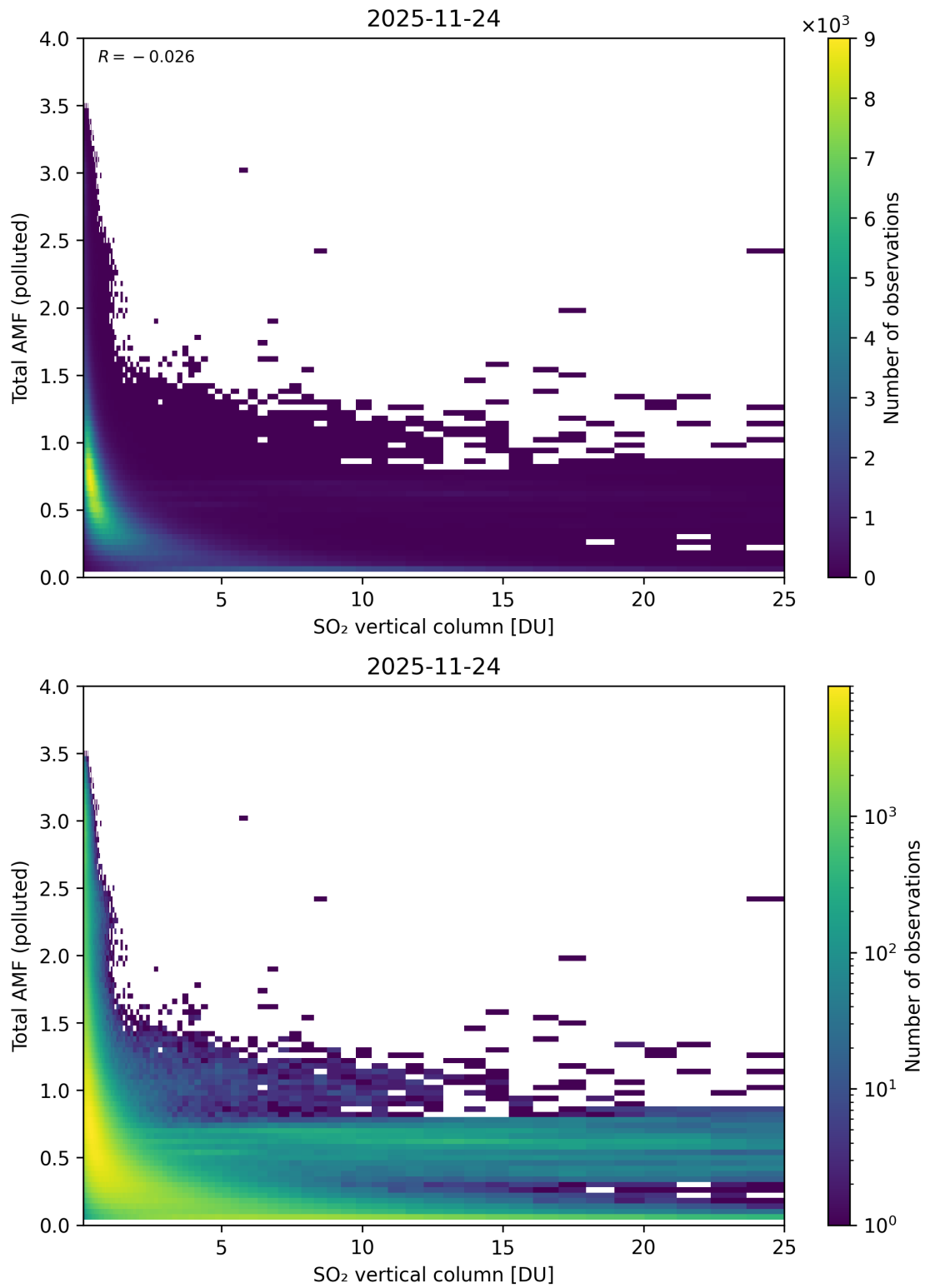
Figure 359: Scatter density plot of “SO 2 vertical column” against “Total AMF (polluted)” for 2025-11-23 to 2025-11-25.
