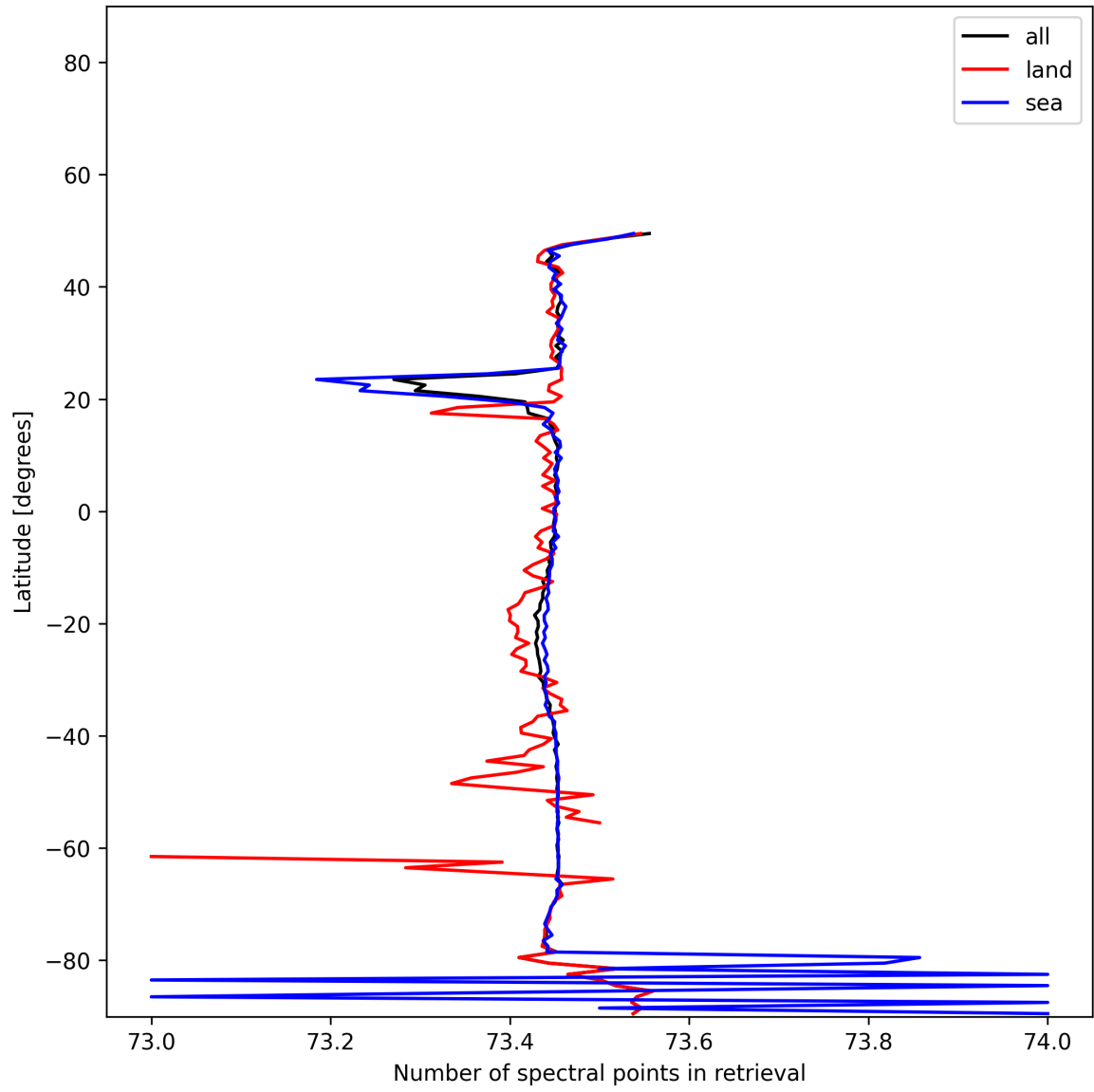
Figure 56: Zonal average of “Number of spectral points in retrieval” for 2025-11-23 to 2025-11-25.
