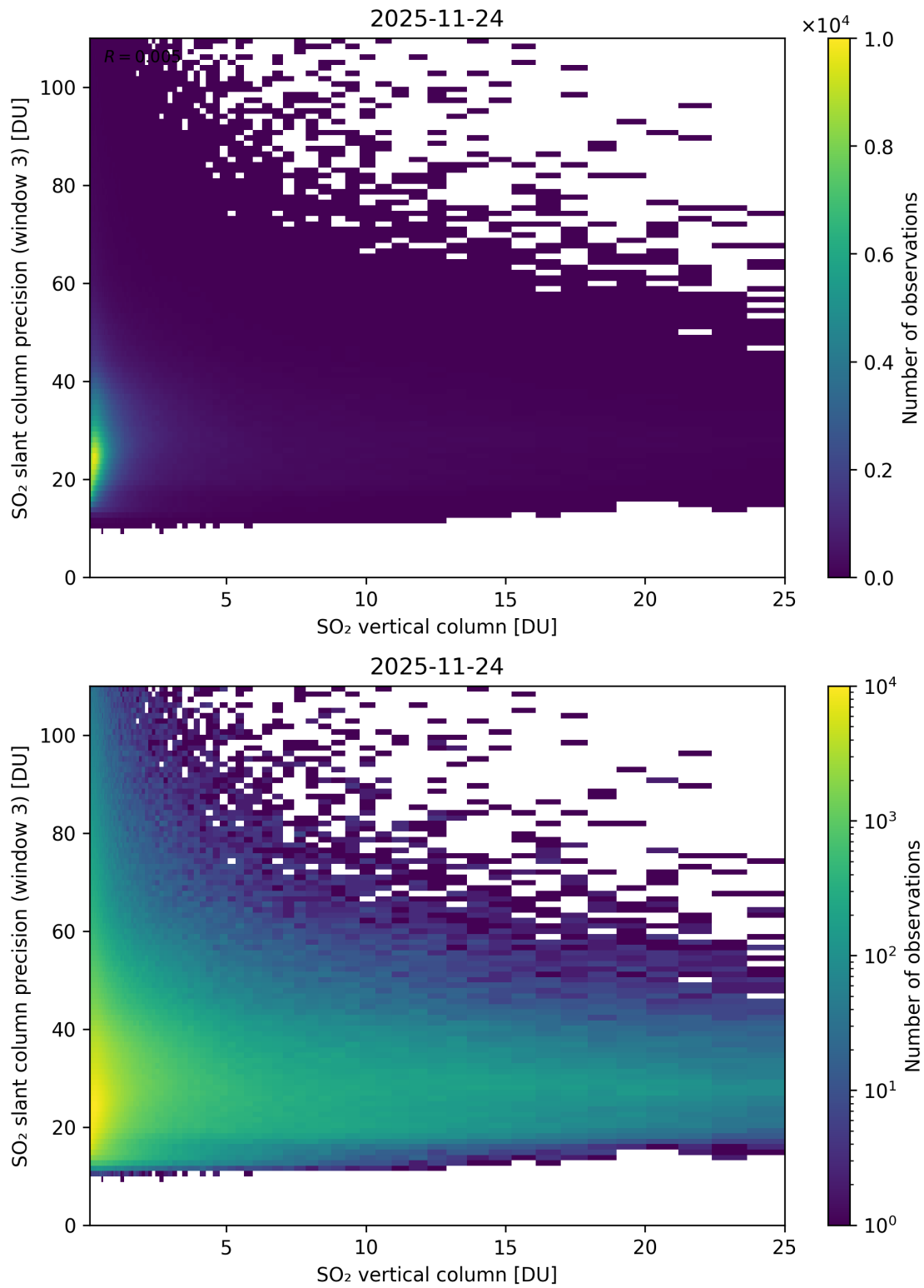
Figure 358: Scatter density plot of “SO 2 vertical column” against “SO 2 slant column precision (window 3)” for 2025-11-23 to 2025-11-25.
