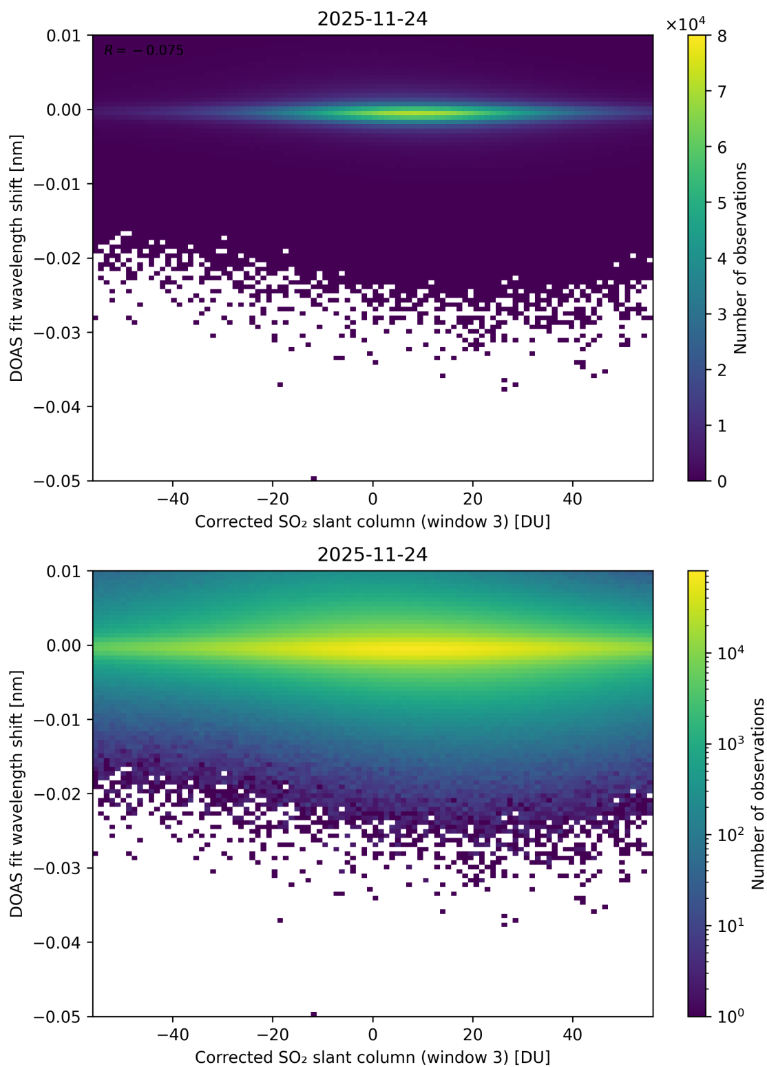
Figure 256: Scatter density plot of “Corrected SO 2 slant column (window 3)” against “DOAS fit wavelength shift” for 2025-11-23 to 2025-11-25.
