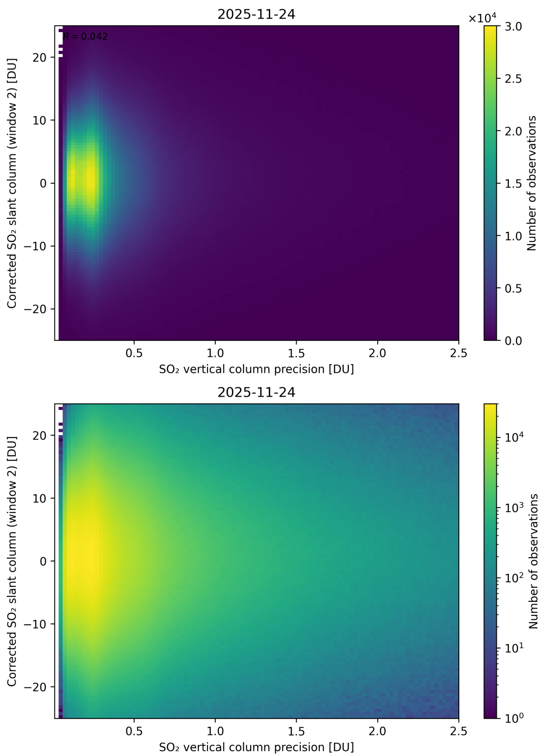
Figure 339: Scatter density plot of “SO 2 vertical column precision” against “Corrected SO 2 slant column (window 2)” for 2025-11-23 to 2025-11-25.
