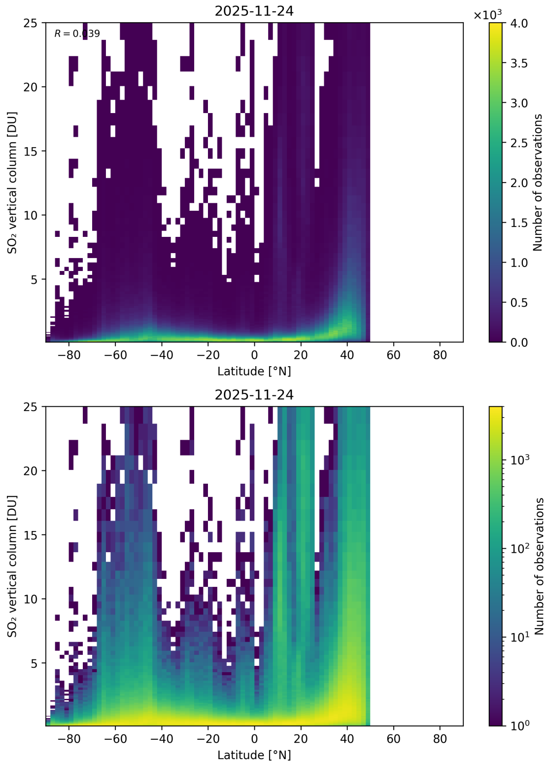
Figure 169: Scatter density plot of “Latitude” against “SO 2 vertical column” for 2025-11-23 to 2025-11-25.
