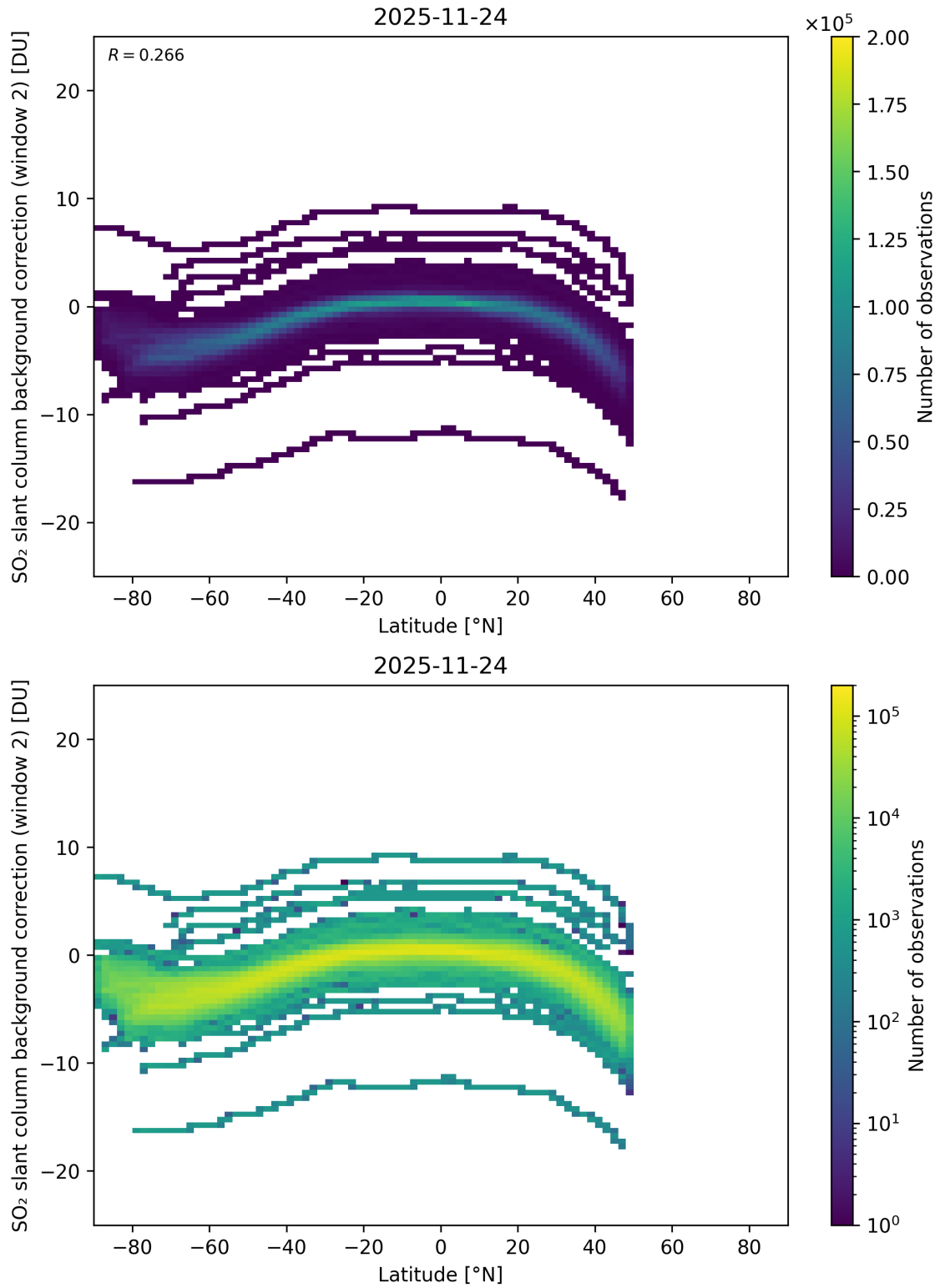
Figure 151: Scatter density plot of “Latitude” against “SO 2 slant column background correction (window 2)” for 2025-11-23 to 2025-11-25.
