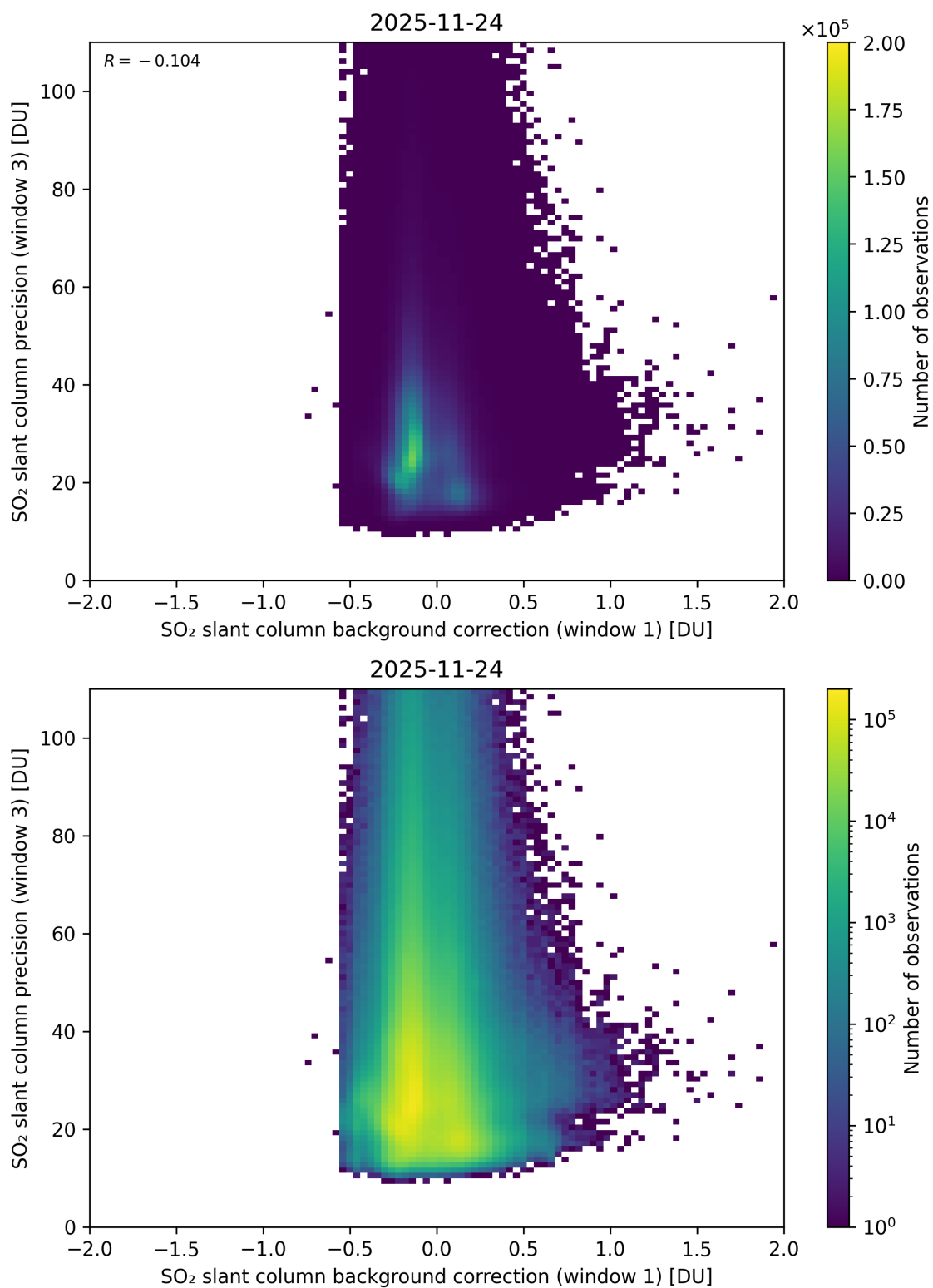
Figure 119: Scatter density plot of “SO 2 slant column background correction (window 1)” against “SO 2 slant column precision (window 3)” for 2025-11-23 to 2025-11-25.
