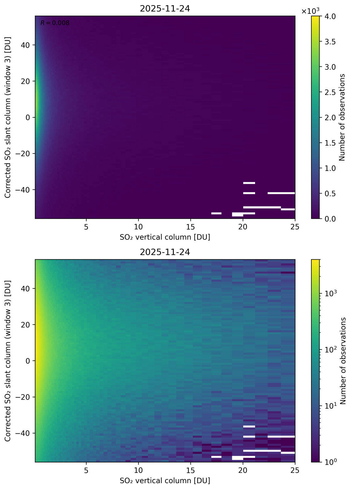
Figure 353: Scatter density plot of “SO 2 vertical column” against “Corrected SO 2 slant column (window 3)” for 2025-11-23 to 2025-11-25.
