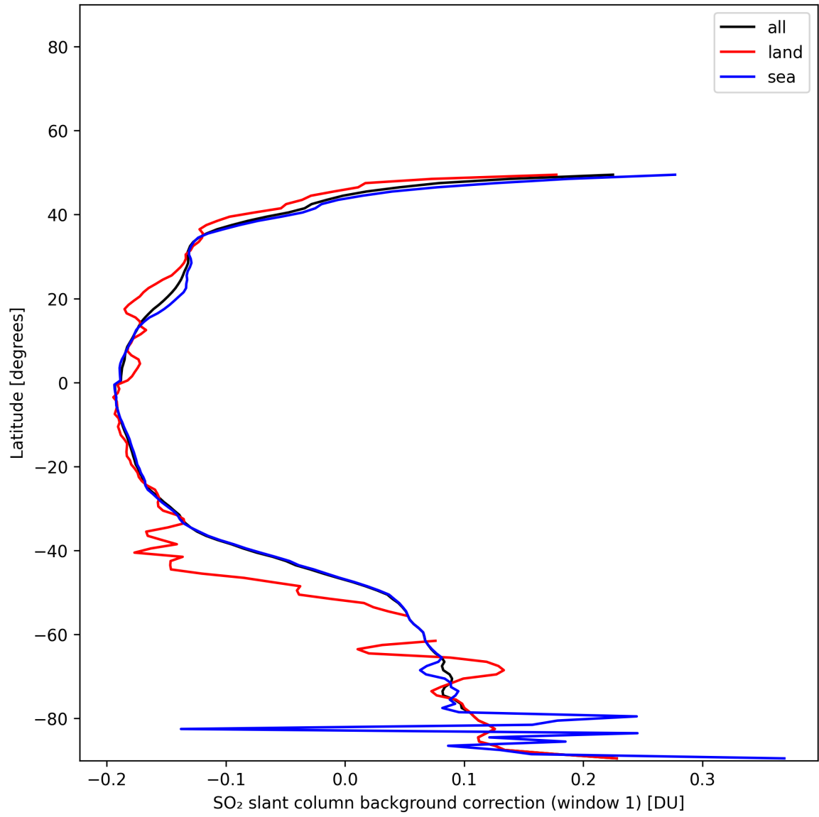
Figure 40: Zonal average of “SO 2 slant column background correction (window 1)” for 2025-11-23 to 2025-11-25.
