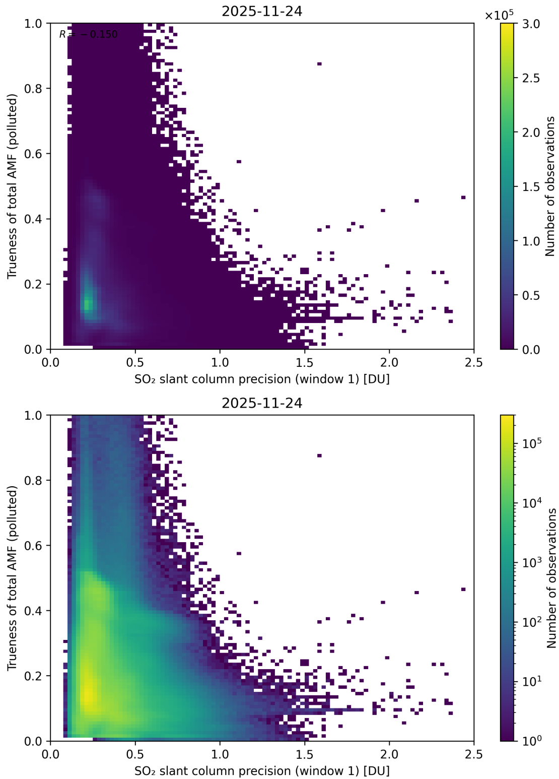
Figure 281: Scatter density plot of “SO 2 slant column precision (window 1)” against “Trueness of total AMF (polluted)” for 2025-11-23 to 2025-11-25.
