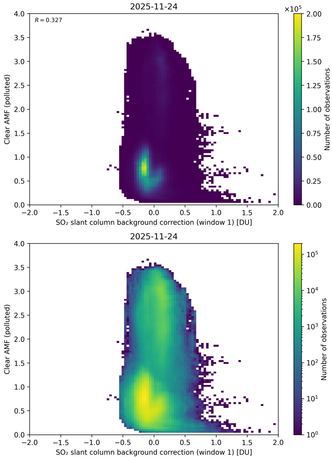
Figure 114: Scatter density plot of “SO 2 slant column background correction (window 1)” against “Clear AMF (polluted)” for 2025-11-23 to 2025-11-25.
