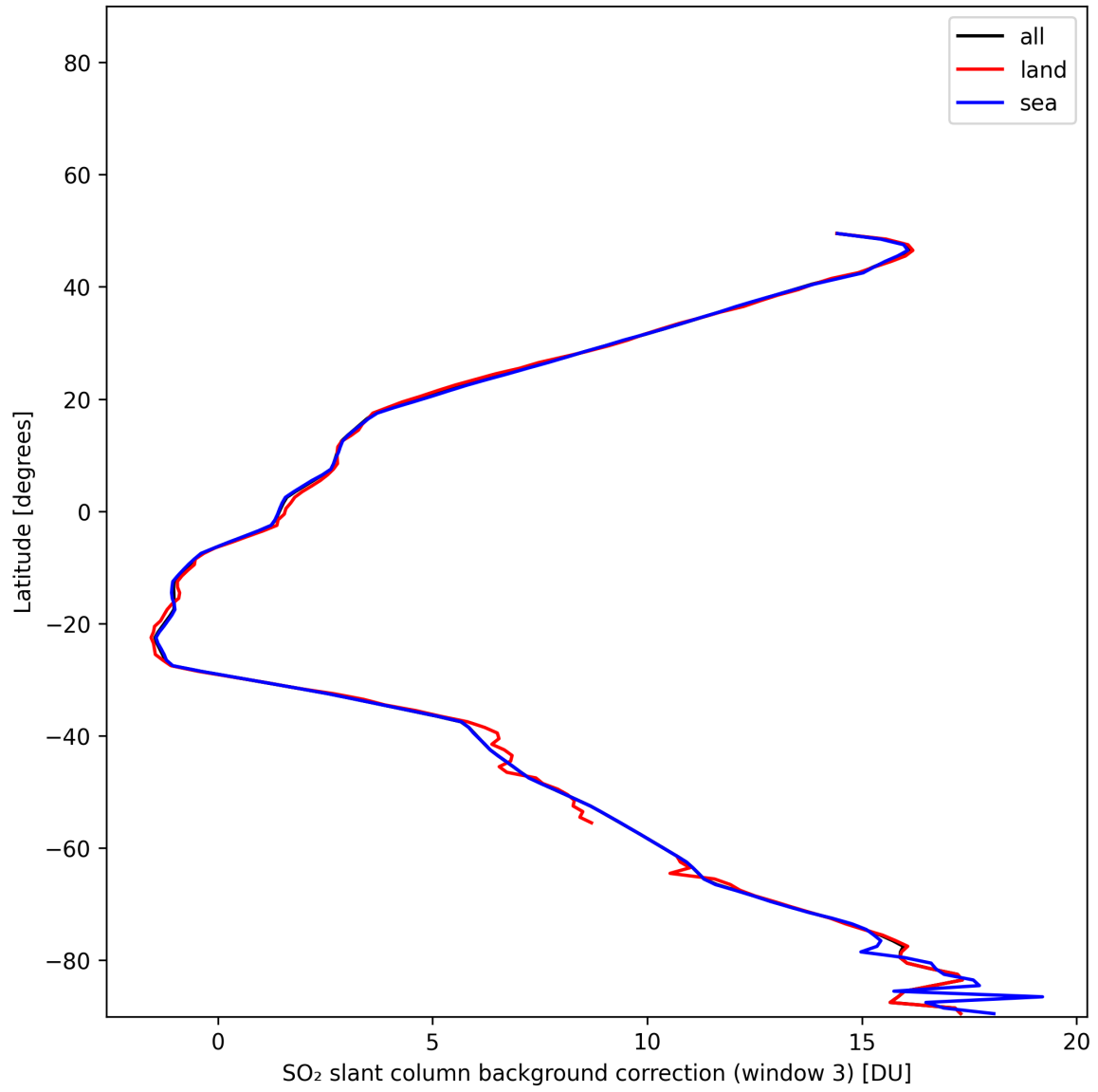
Figure 48: Zonal average of “SO 2 slant column background correction (window 3)” for 2025-11-23 to 2025-11-25.
