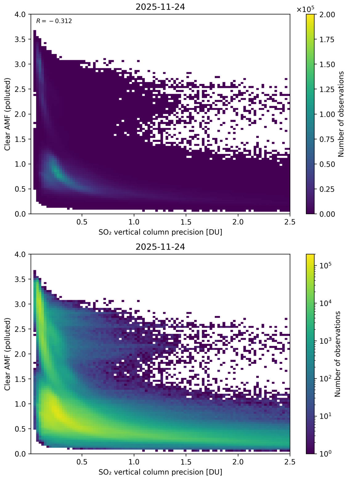
Figure 335: Scatter density plot of “SO 2 vertical column precision” against “Clear AMF (polluted)” for 2025-11-23 to 2025-11-25.
