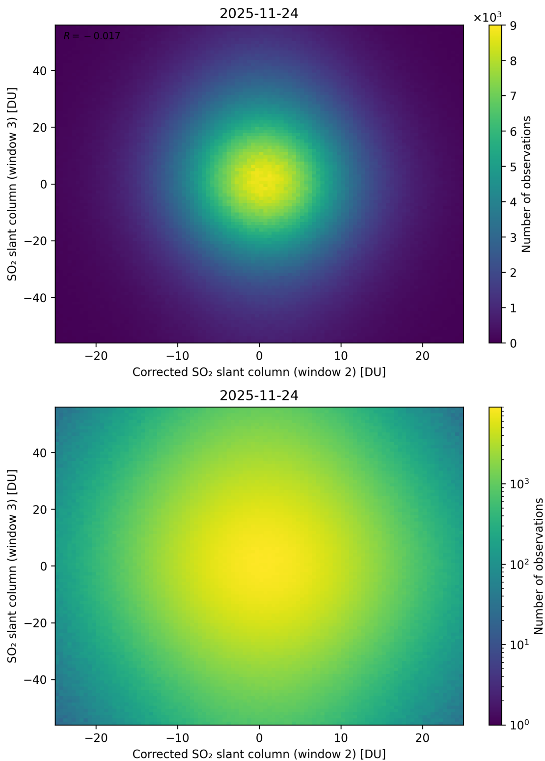
Figure 251: Scatter density plot of “Corrected SO 2 slant column (window 2)” against “SO 2 slant column (window 3)” for 2025-11-23 to 2025-11-25.
