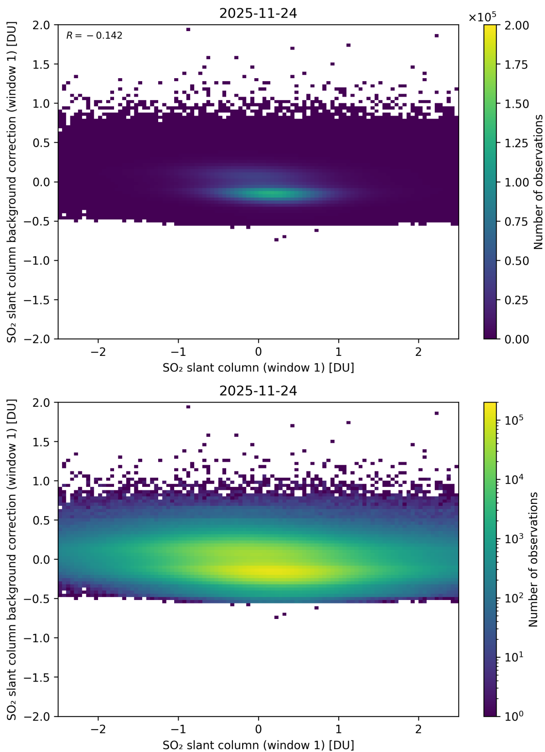
Figure 262: Scatter density plot of “SO 2 slant column (window 1)” against “SO 2 slant column background correction (window 1)” for 2025-11-23 to 2025-11-25.
