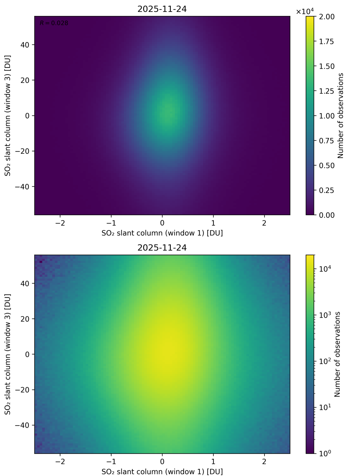
Figure 287: Scatter density plot of “SO 2 slant column (window 1)” against “SO 2 slant column (window 3)” for 2025-11-23 to 2025-11-25.
