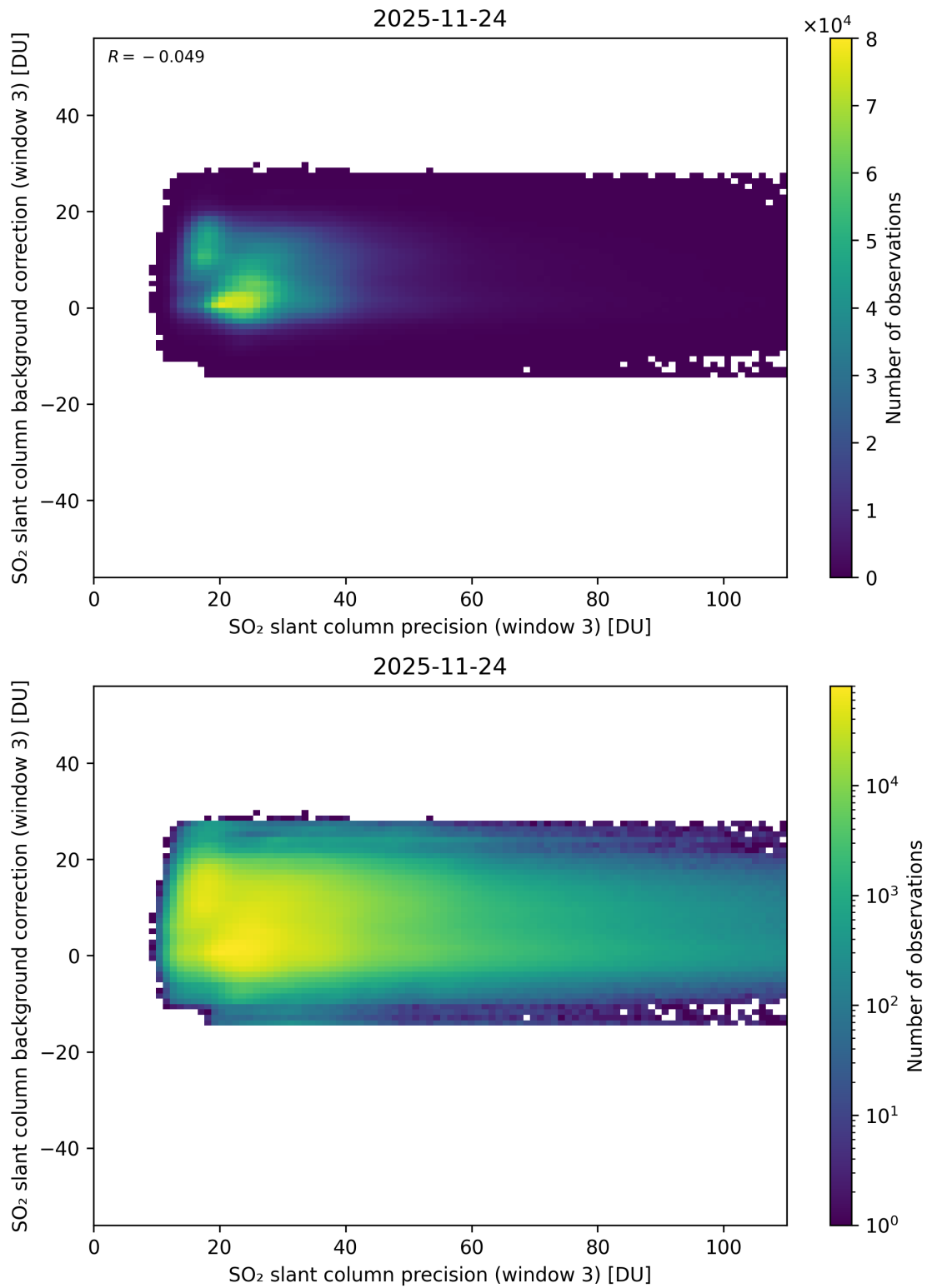
Figure 307: Scatter density plot of “SO 2 slant column precision (window 3)” against “SO 2 slant column background correction (window 3)” for 2025-11-23 to 2025-11-25.
