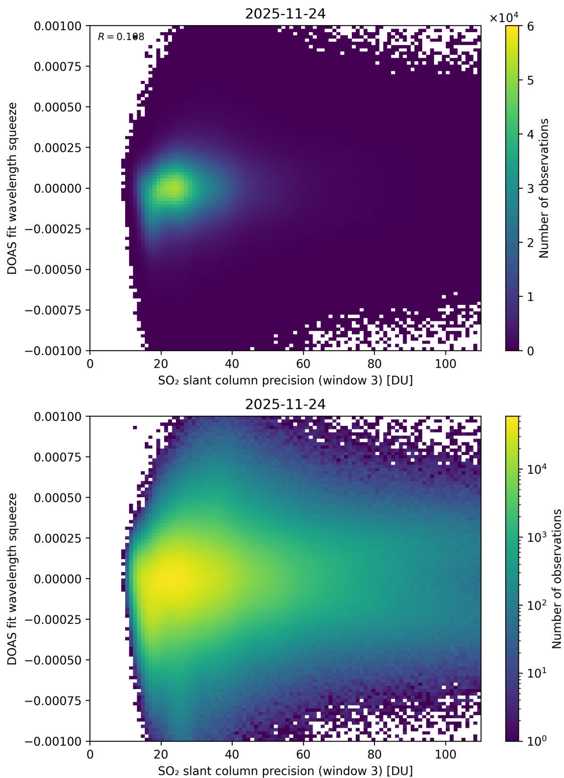
Figure 309: Scatter density plot of “SO 2 slant column precision (window 3)” against “DOAS fit wavelength squeeze” for 2025-11-23 to 2025-11-25.
