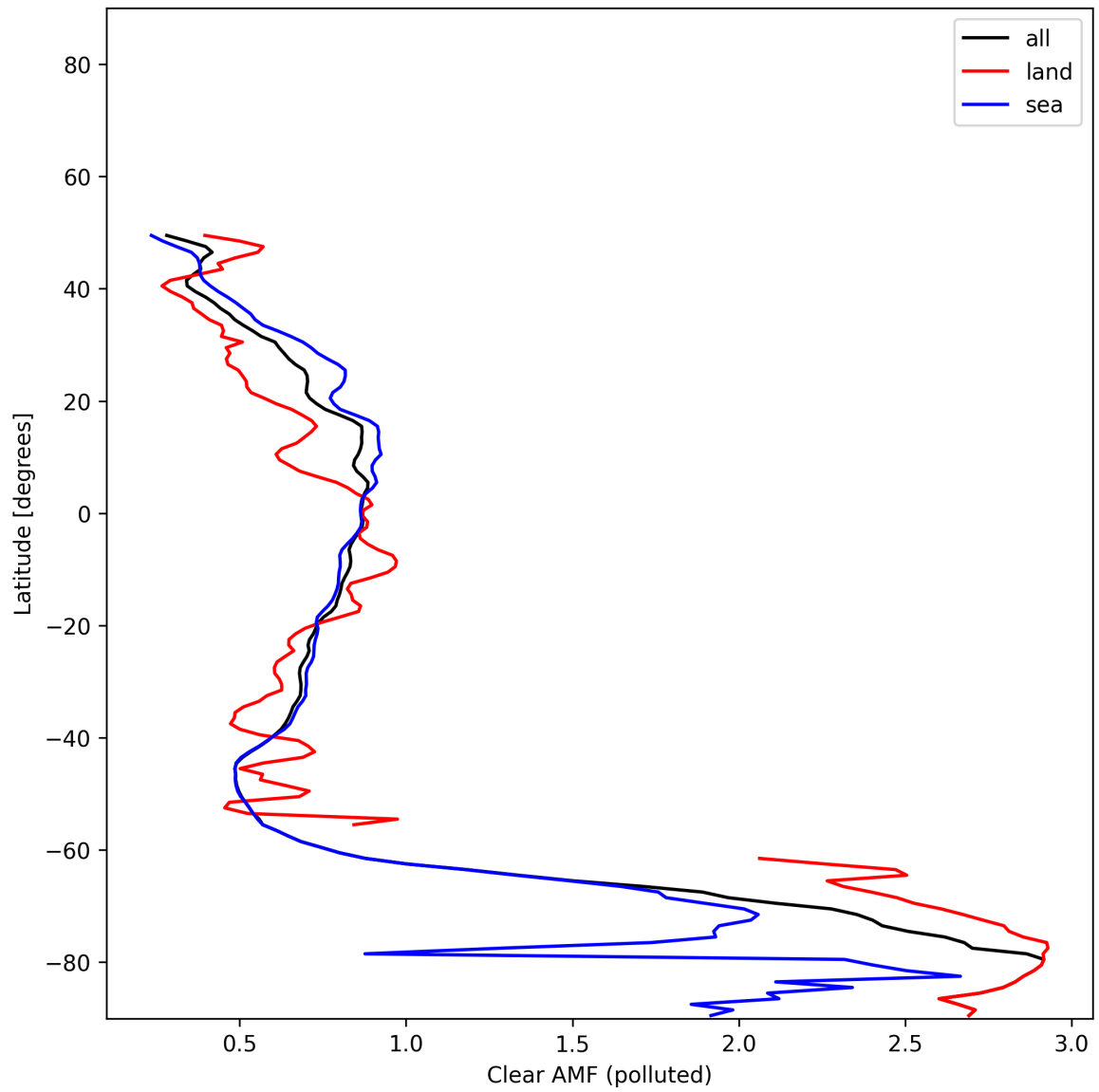
Figure 55: Zonal average of “Clear AMF (polluted)” for 2025-11-23 to 2025-11-25.
