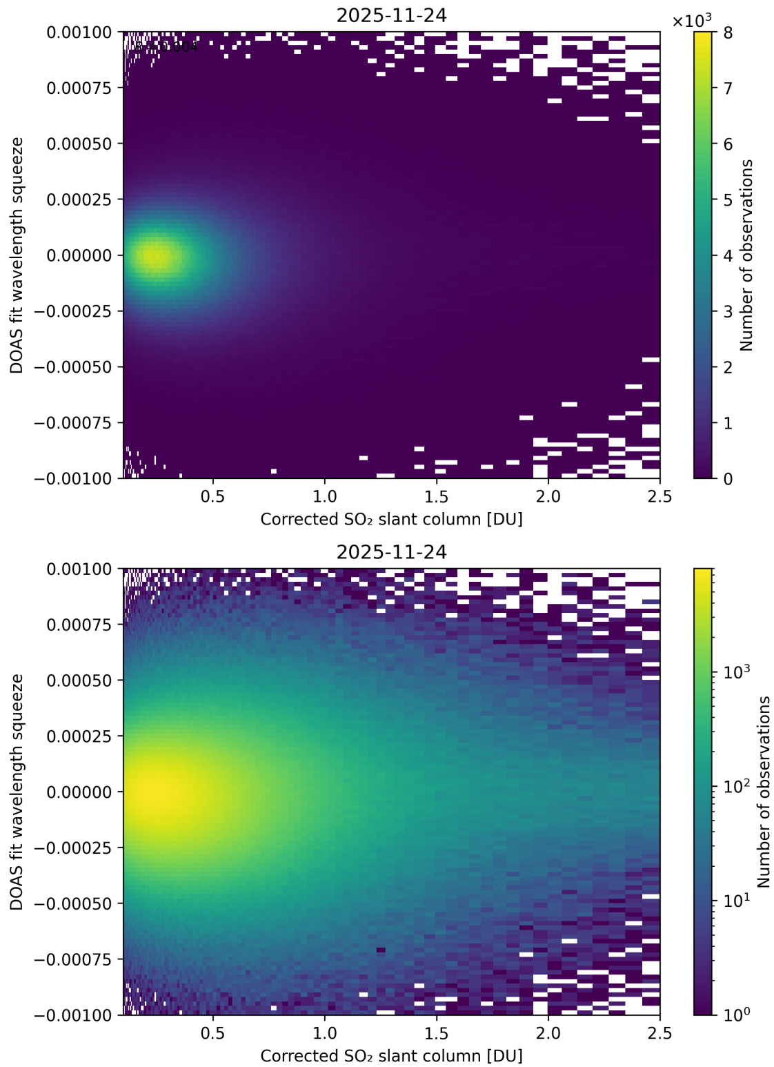
Figure 230: Scatter density plot of “Corrected SO 2 slant column” against “DOAS fit wavelength squeeze” for 2025-11-23 to 2025-11-25.
