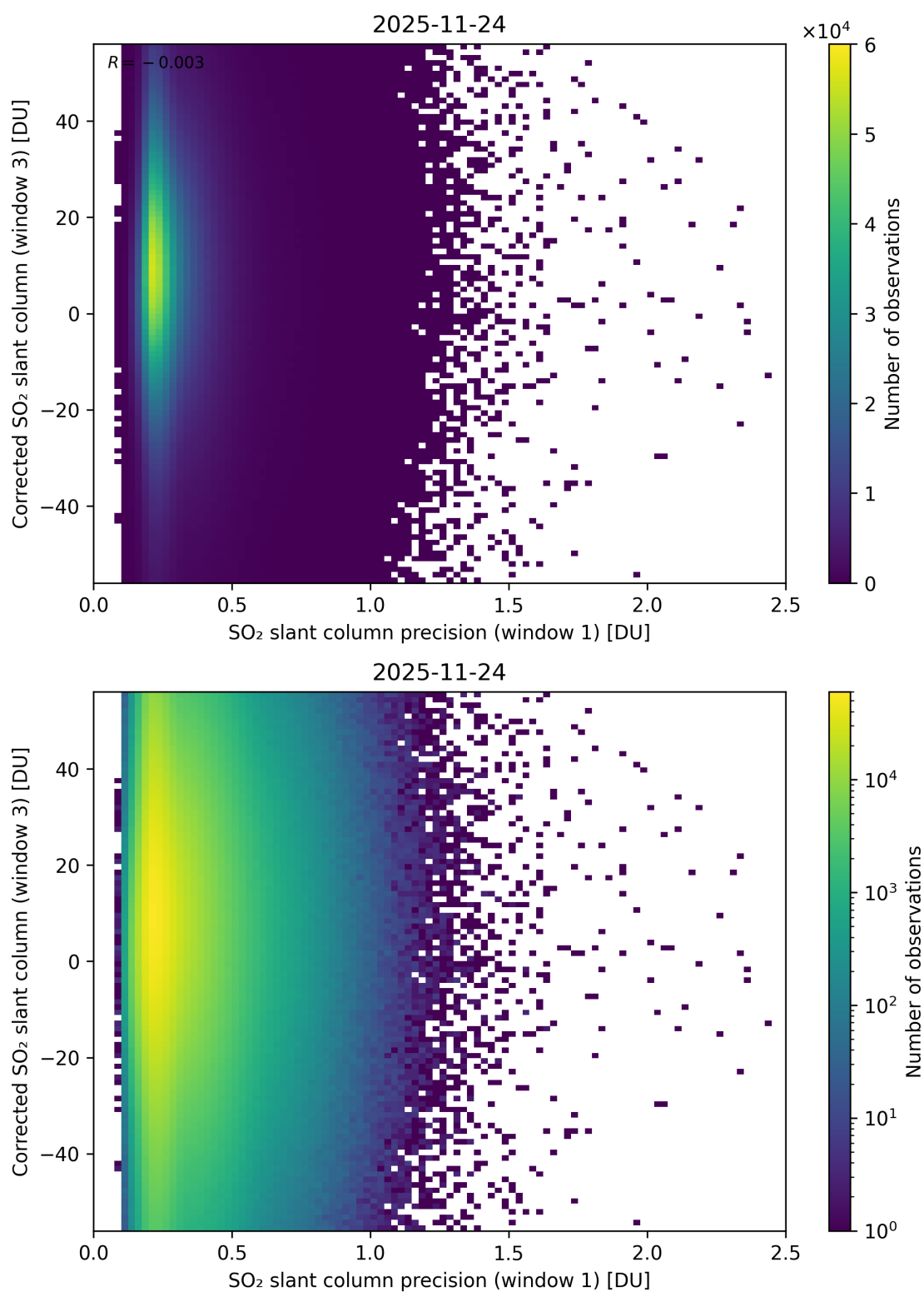
Figure 276: Scatter density plot of “SO 2 slant column precision (window 1)” against “Corrected SO 2 slant column (window 3)” for 2025-11-23 to 2025-11-25.
