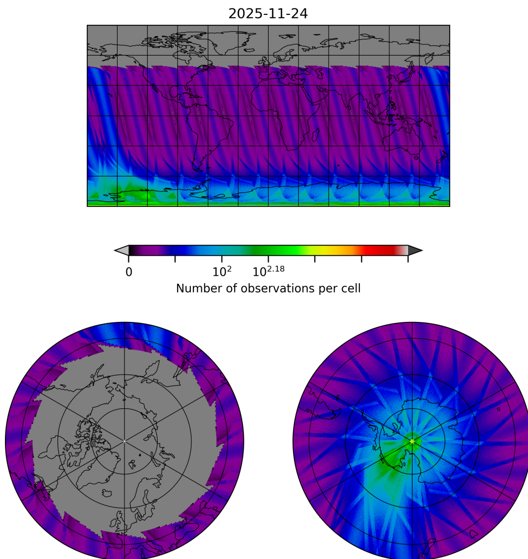
Figure 30: Map of the number of observations for 2025-11-23 to 2025-11-25
