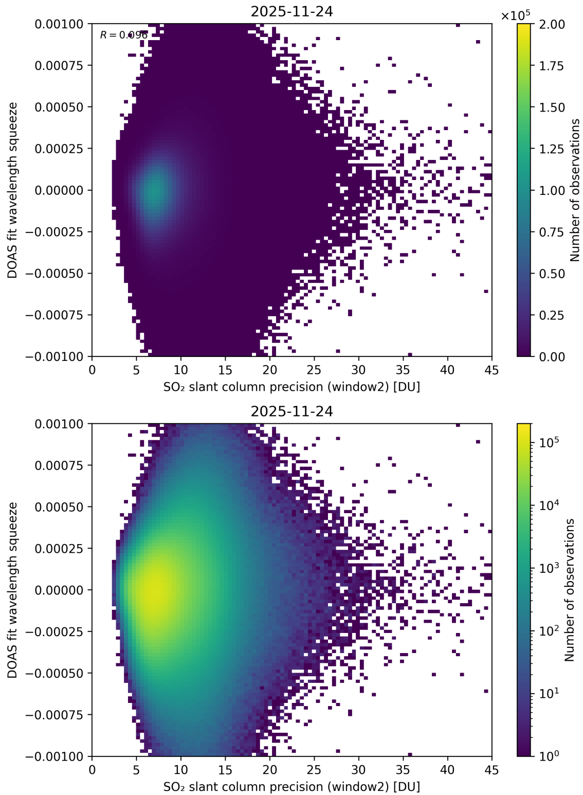
Figure 294: Scatter density plot of “SO 2 slant column precision (window2)” against “DOAS fit wavelength squeeze” for 2025-11-23 to 2025-11-25.
