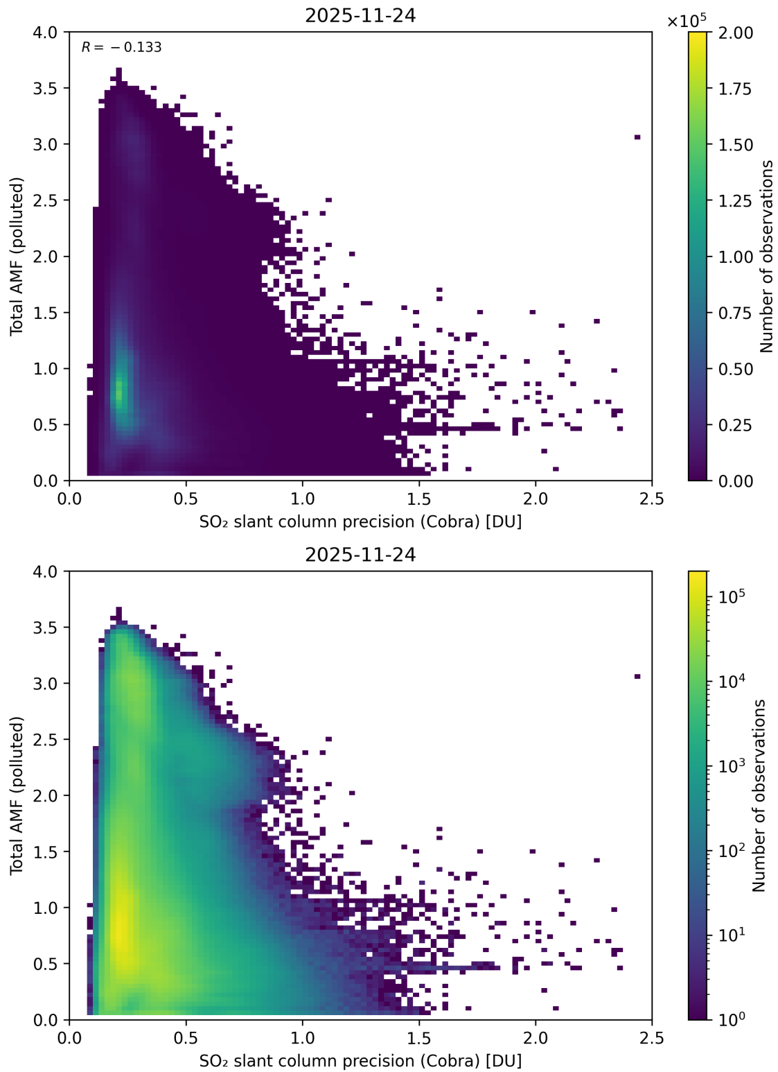
Figure 213: Scatter density plot of “SO 2 slant column precision (Cobra)” against “Total AMF (polluted)” for 2025-11-23 to 2025-11-25.
