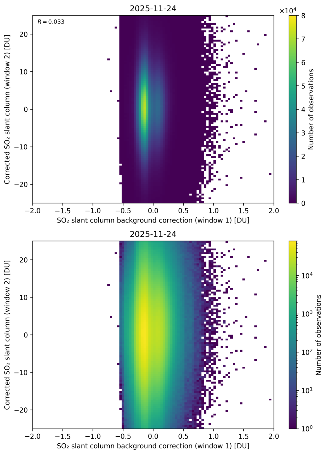
Figure 115: Scatter density plot of “SO 2 slant column background correction (window 1)” against “Corrected SO 2 slant column (window 2)” for 2025-11-23 to 2025-11-25.
