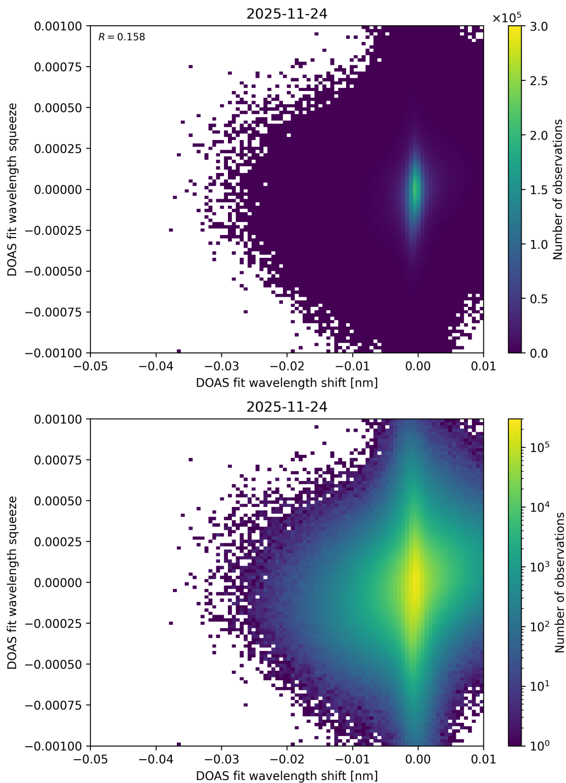
Figure 138: Scatter density plot of “DOAS fit wavelength shift” against “DOAS fit wavelength squeeze” for 2025-11-23 to 2025-11-25.
