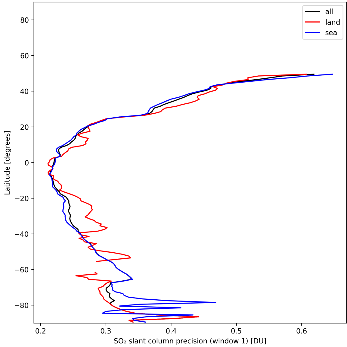
Figure 38: Zonal average of “SO 2 slant column precision (window 1)” for 2025-11-23 to 2025-11-25.
