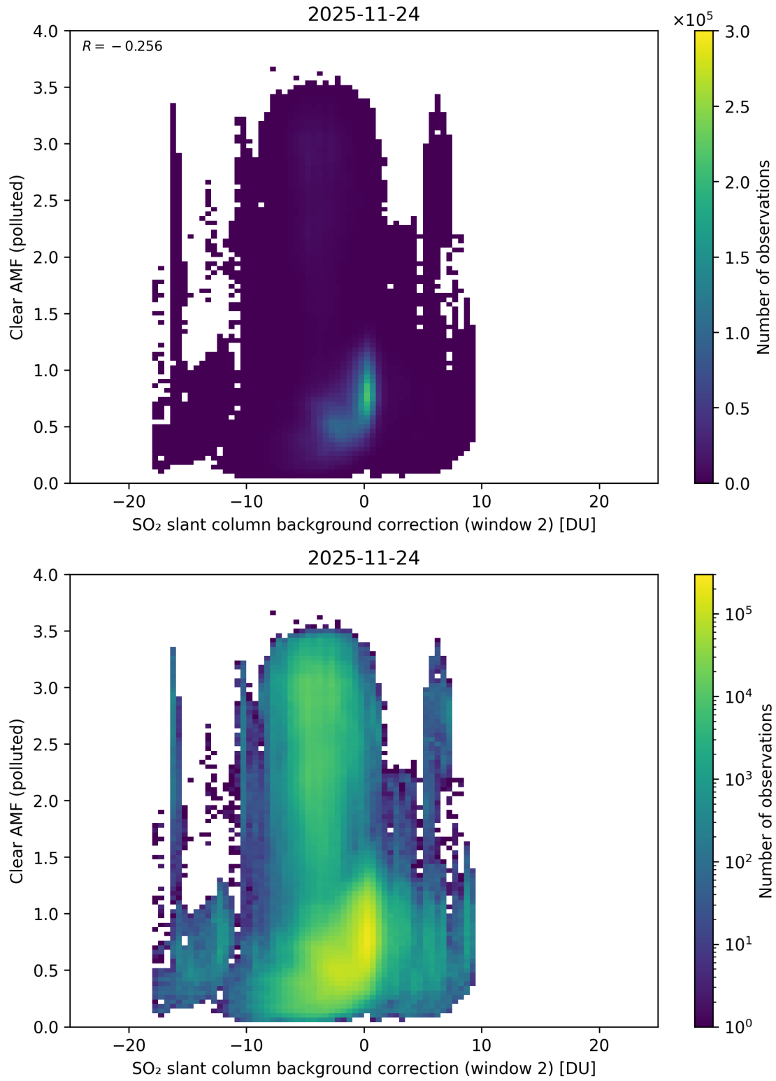
Figure 126: Scatter density plot of “SO 2 slant column background correction (window 2)” against “Clear AMF (polluted)” for 2025-11-23 to 2025-11-25.
