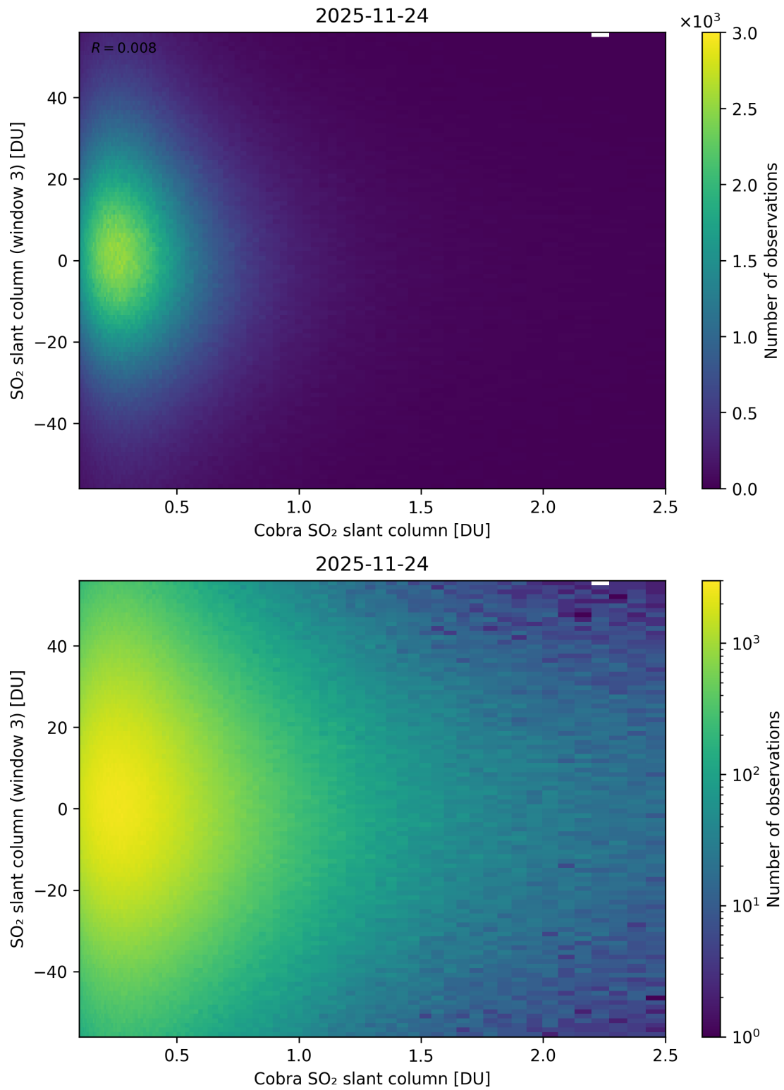
Figure 222: Scatter density plot of “Cobra SO 2 slant column” against “SO 2 slant column (window 3)” for 2025-11-23 to 2025-11-25.
