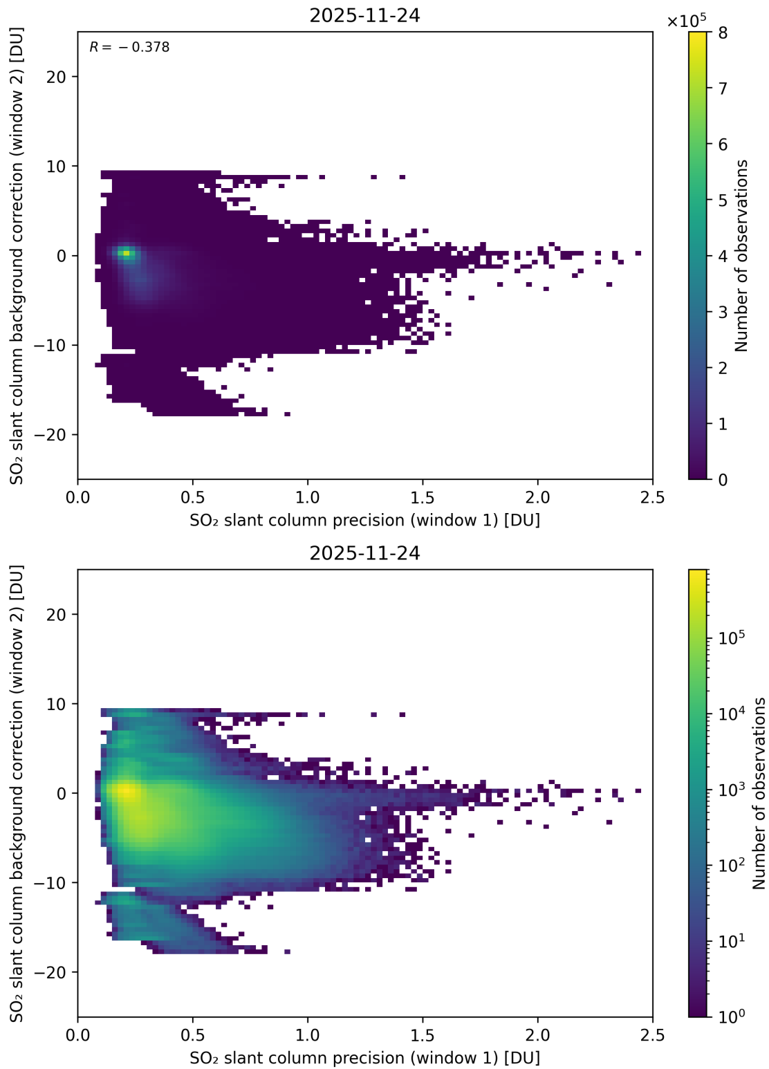
Figure 269: Scatter density plot of “SO 2 slant column precision (window 1)” against “SO 2 slant column background correction (window 2)” for 2025-11-23 to 2025-11-25.
