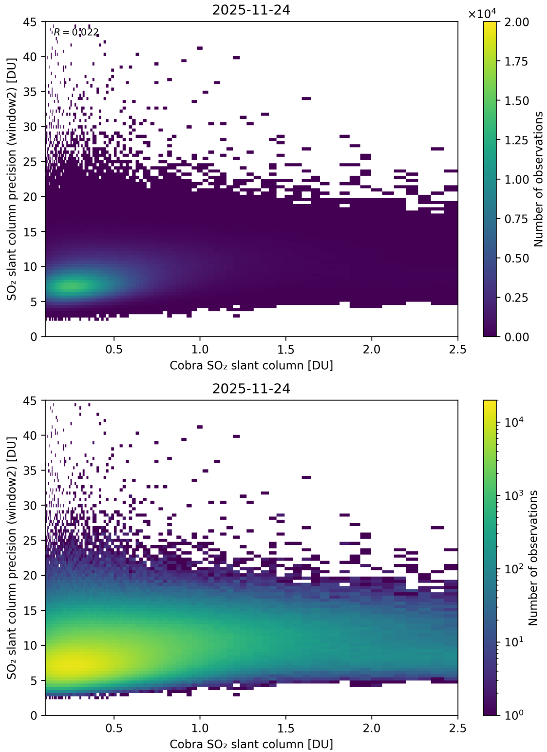
Figure 221: Scatter density plot of “Cobra SO 2 slant column” against “SO 2 slant column precision (window2)” for 2025-11-23 to 2025-11-25.
