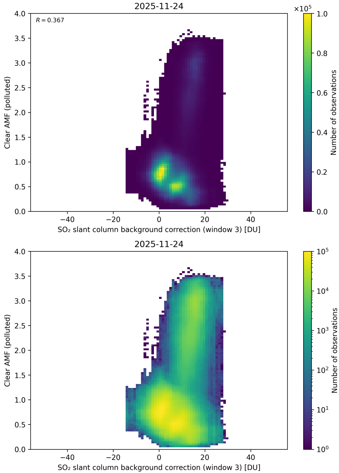
Figure 135: Scatter density plot of “SO 2 slant column background correction (window 3)” against “Clear AMF (polluted)” for 2025-11-23 to 2025-11-25.
