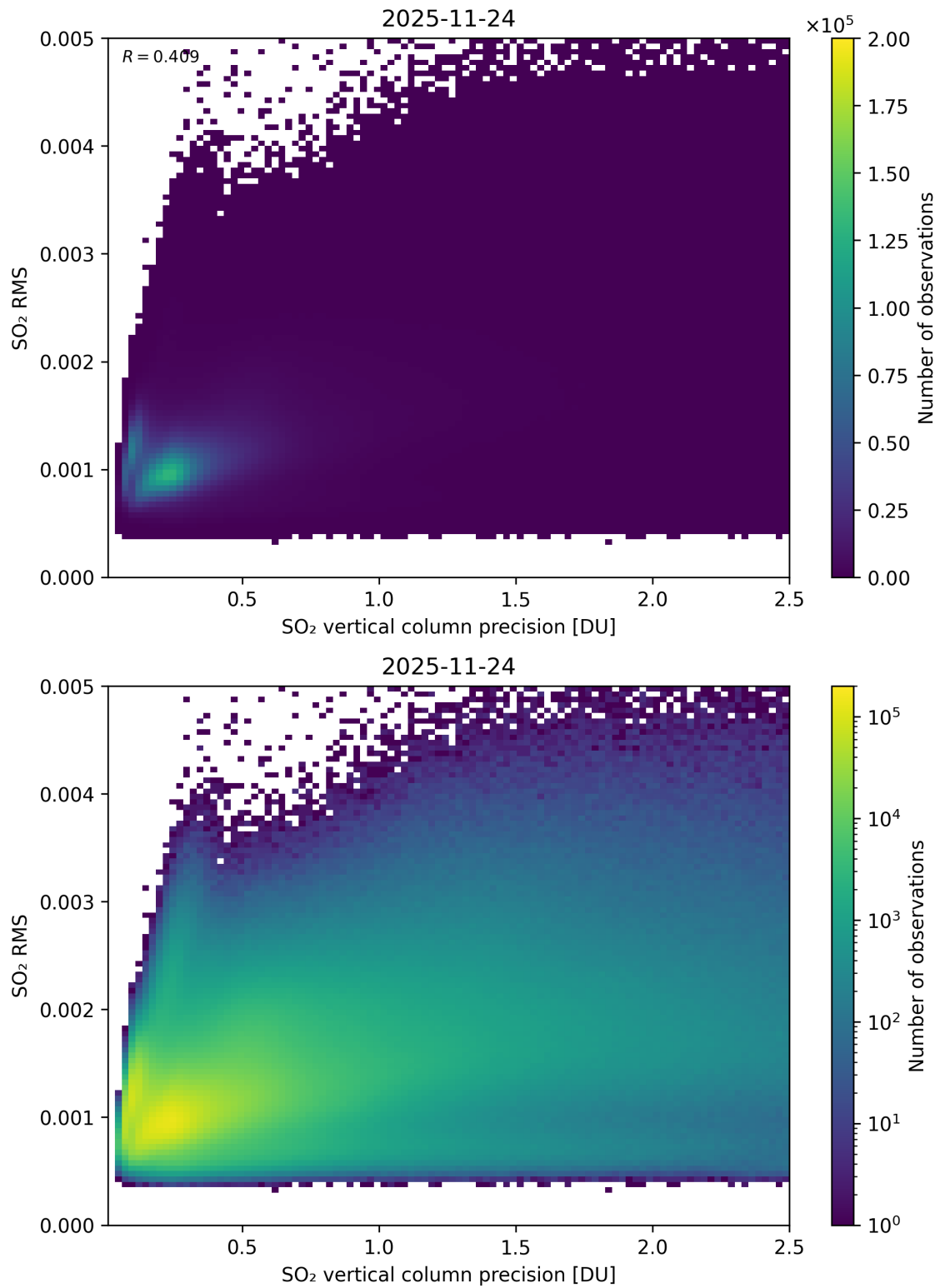
Figure 334: Scatter density plot of “SO 2 vertical column precision” against “SO 2 RMS” for 2025-11-23 to 2025-11-25.
