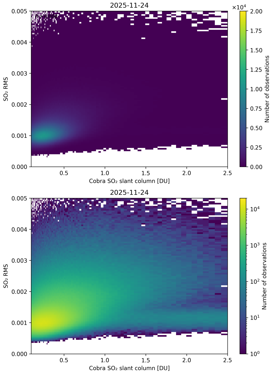
Figure 198: Scatter density plot of “Cobra SO 2 slant column” against “SO 2 RMS” for 2025-11-23 to 2025-11-25.
