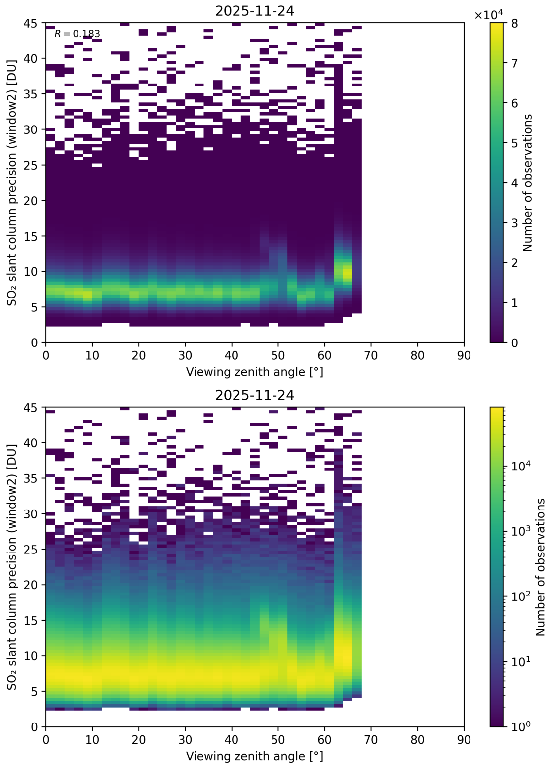
Figure 378: Scatter density plot of “Viewing zenith angle” against “SO 2 slant column precision (window2)” for 2025-11-23 to 2025-11-25.
