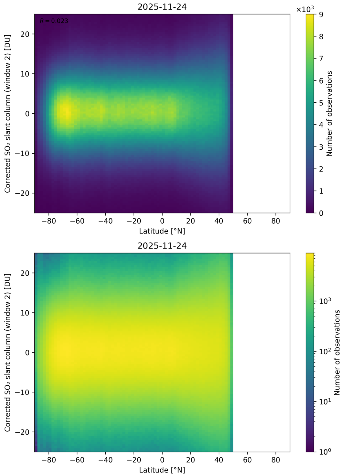
Figure 160: Scatter density plot of “Latitude” against “Corrected SO 2 slant column (window 2)” for 2025-11-23 to 2025-11-25.
