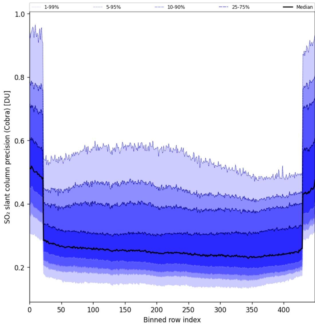
Figure 88: Along track statistics of “SO 2 slant column precision (Cobra)” for 2025-11-23 to 2025-11-25
