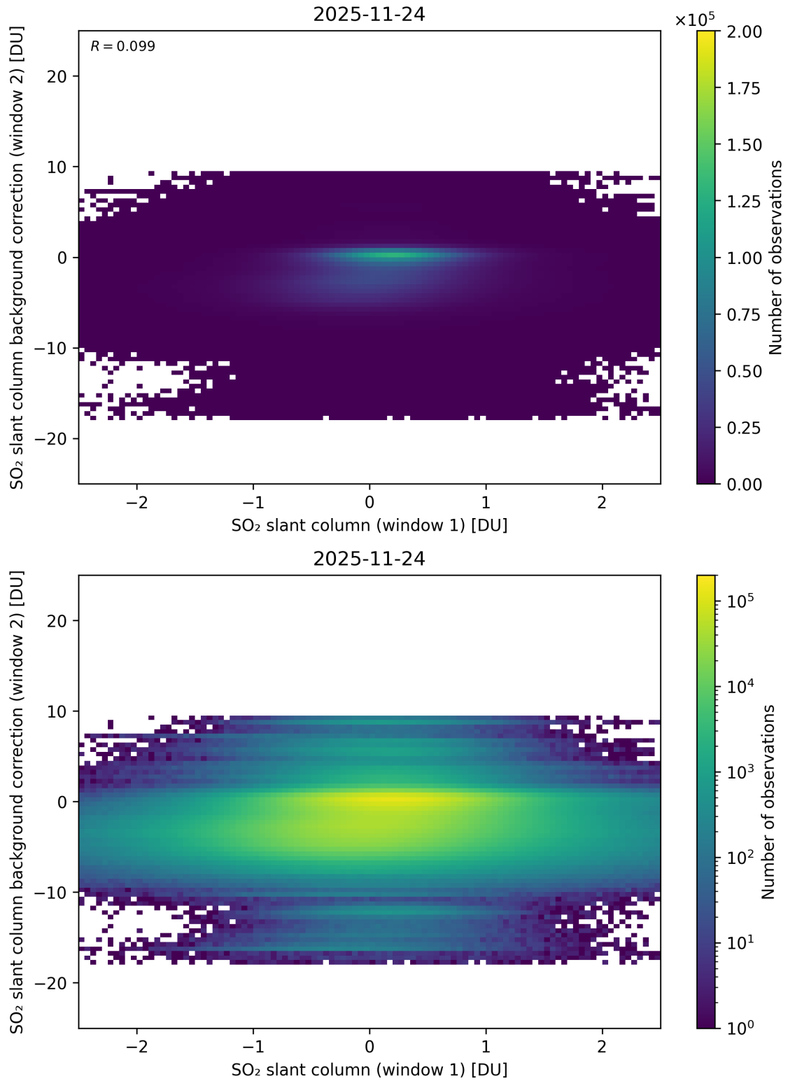
Figure 263: Scatter density plot of “SO 2 slant column (window 1)” against “SO 2 slant column background correction (window 2)” for 2025-11-23 to 2025-11-25.
