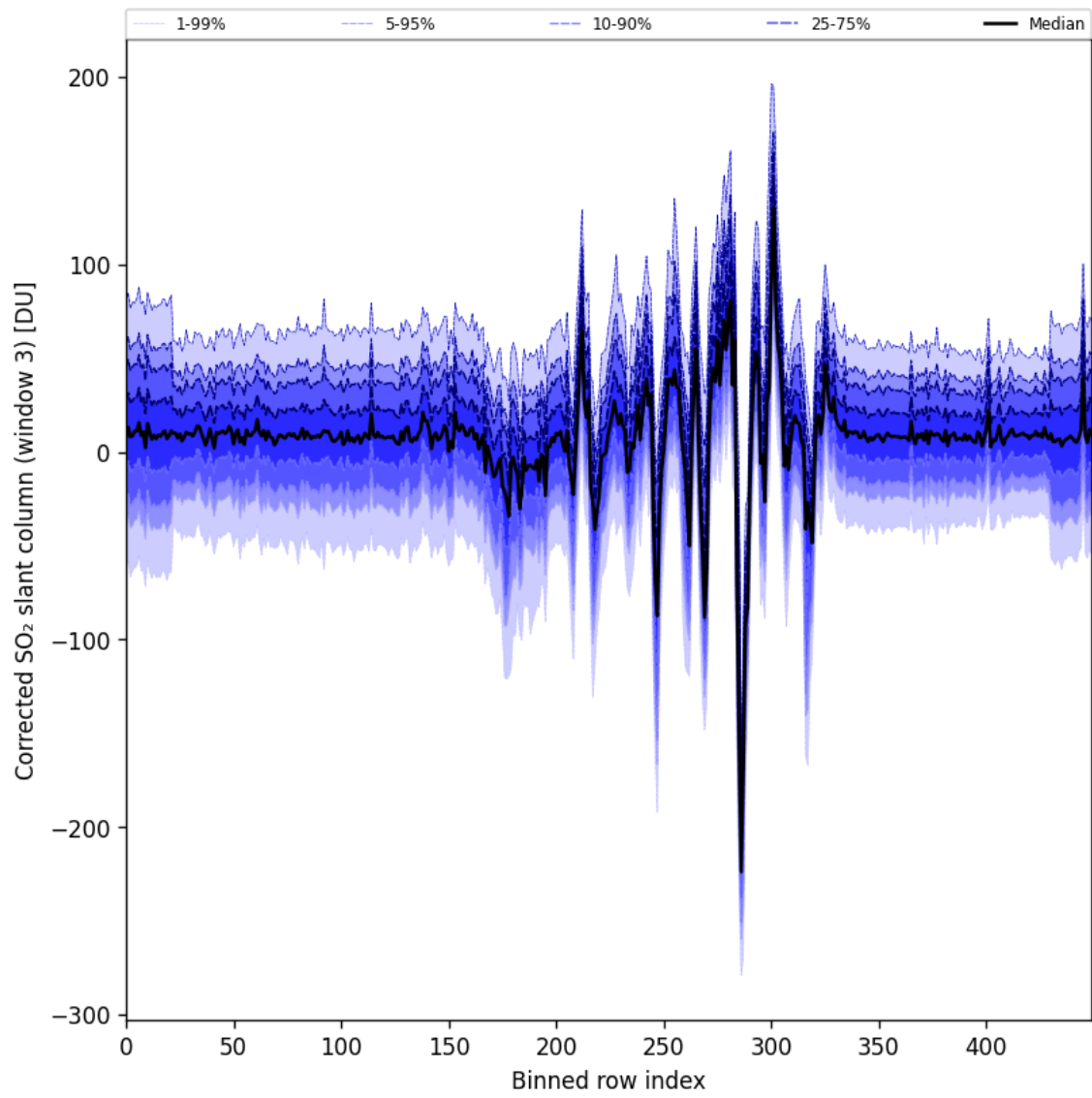
Figure 99: Along track statistics of “Corrected SO 2 slant column (window 3)” for 2025-11-23 to 2025-11-25
