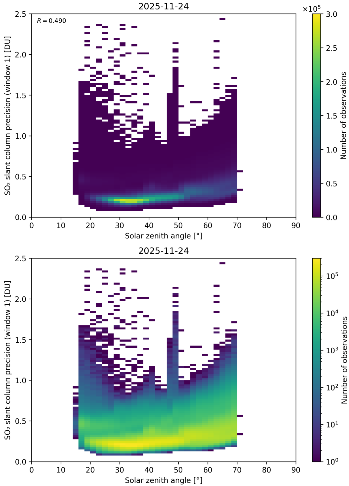
Figure 185: Scatter density plot of “Solar zenith angle” against “SO 2 slant column precision (window 1)” for 2025-11-23 to 2025-11-25.
