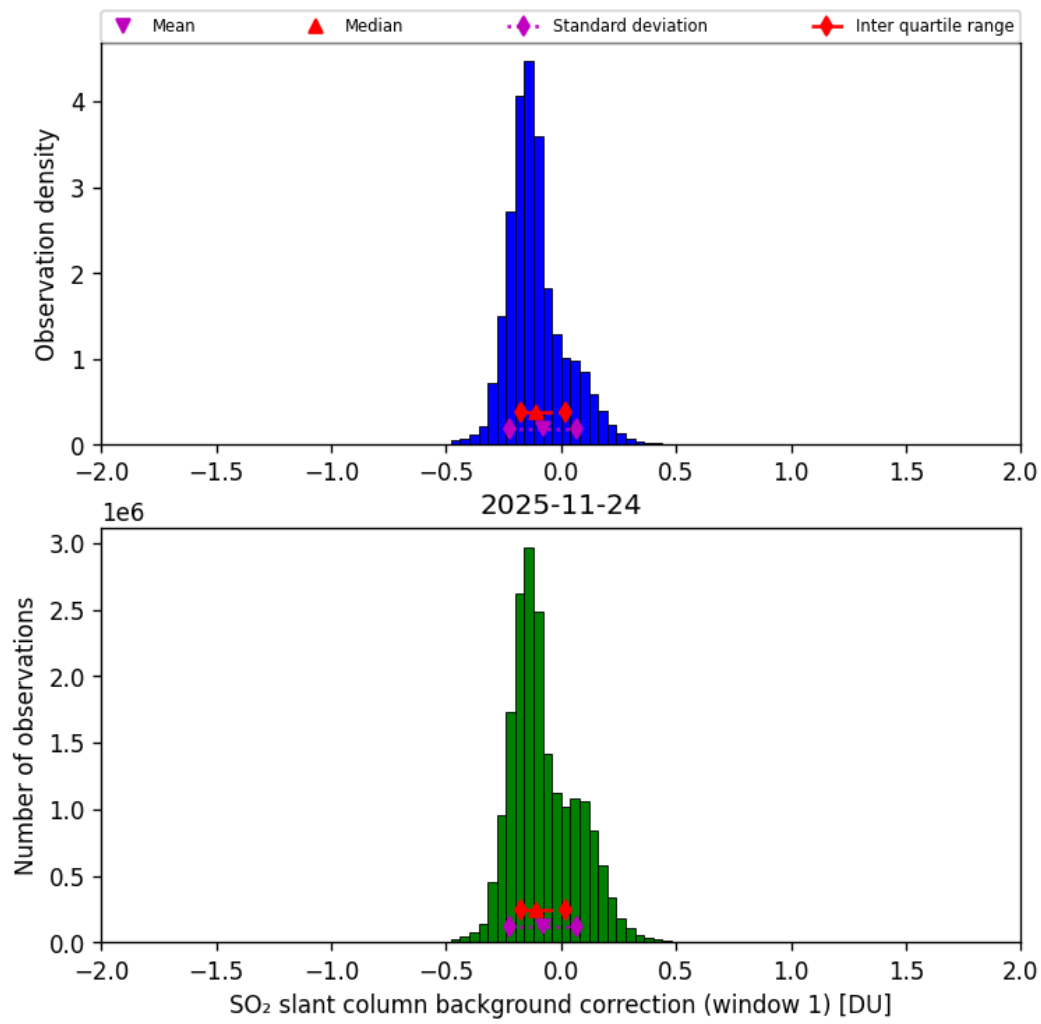
Figure 66: Histogram of “SO 2 slant column background correction (window 1)” for 2025-11-23 to 2025-11-25
