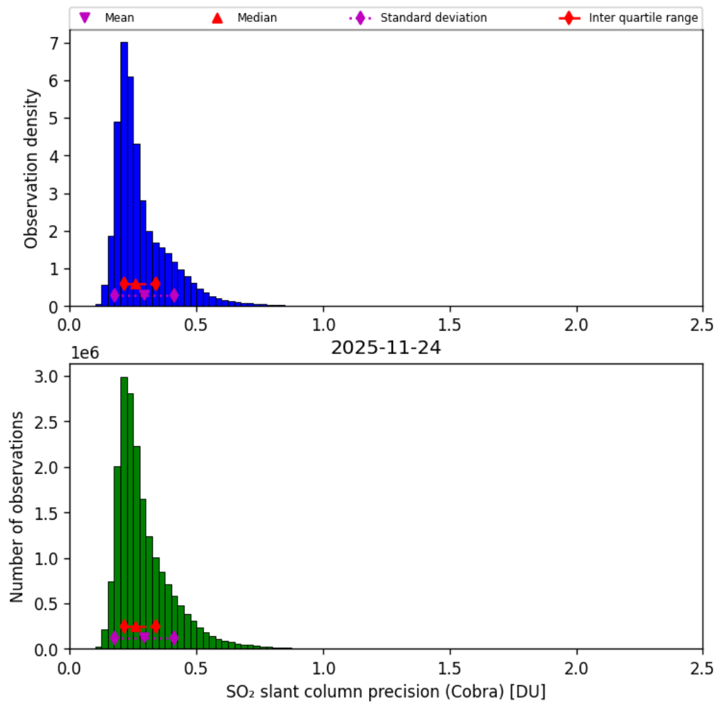
Figure 62: Histogram of “SO 2 slant column precision (Cobra)” for 2025-11-23 to 2025-11-25
