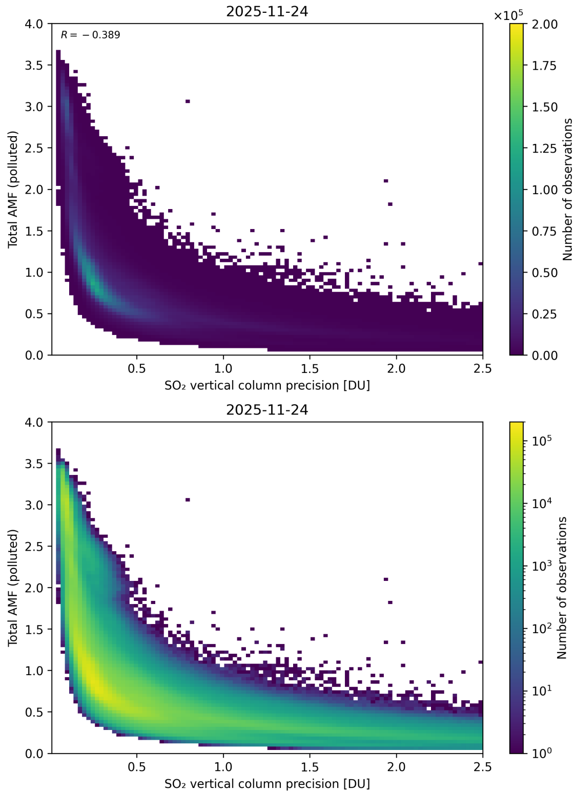
Figure 346: Scatter density plot of “SO 2 vertical column precision” against “Total AMF (polluted)” for 2025-11-23 to 2025-11-25.
