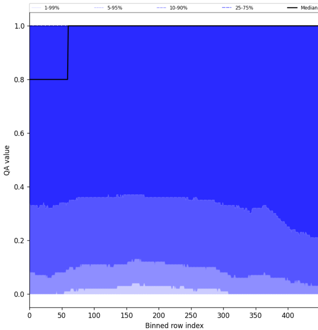
Figure 83: Along track statistics of “QA value” for 2025-11-23 to 2025-11-25
