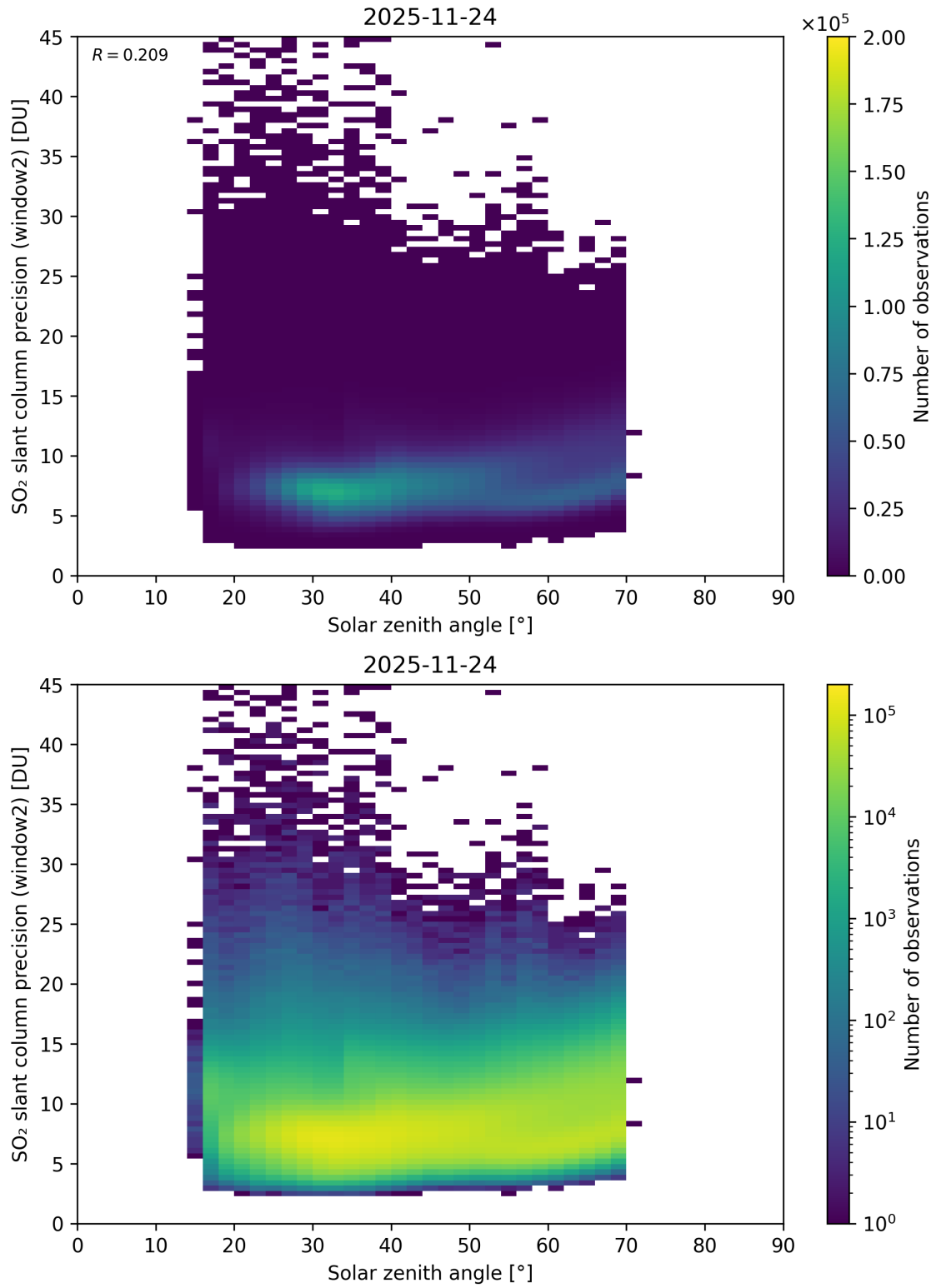
Figure 186: Scatter density plot of “Solar zenith angle” against “SO 2 slant column precision (window2)” for 2025-11-23 to 2025-11-25.
