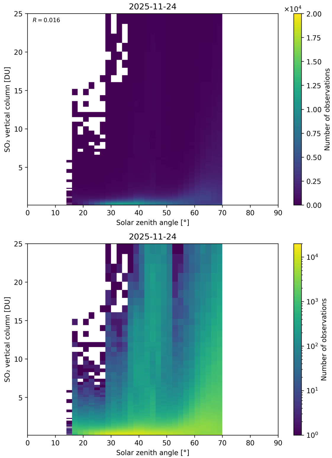
Figure 191: Scatter density plot of “Solar zenith angle” against “SO 2 vertical column” for 2025-11-23 to 2025-11-25.
