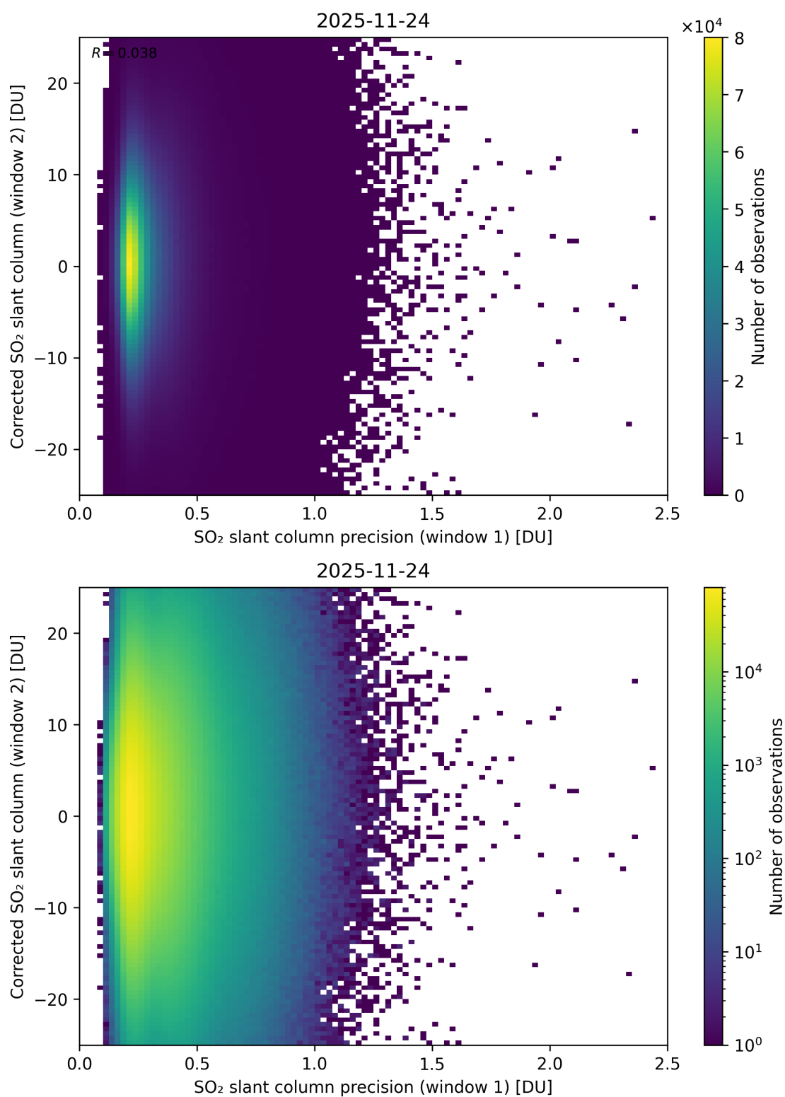
Figure 275: Scatter density plot of “SO 2 slant column precision (window 1)” against “Corrected SO 2 slant column (window 2)” for 2025-11-23 to 2025-11-25.
