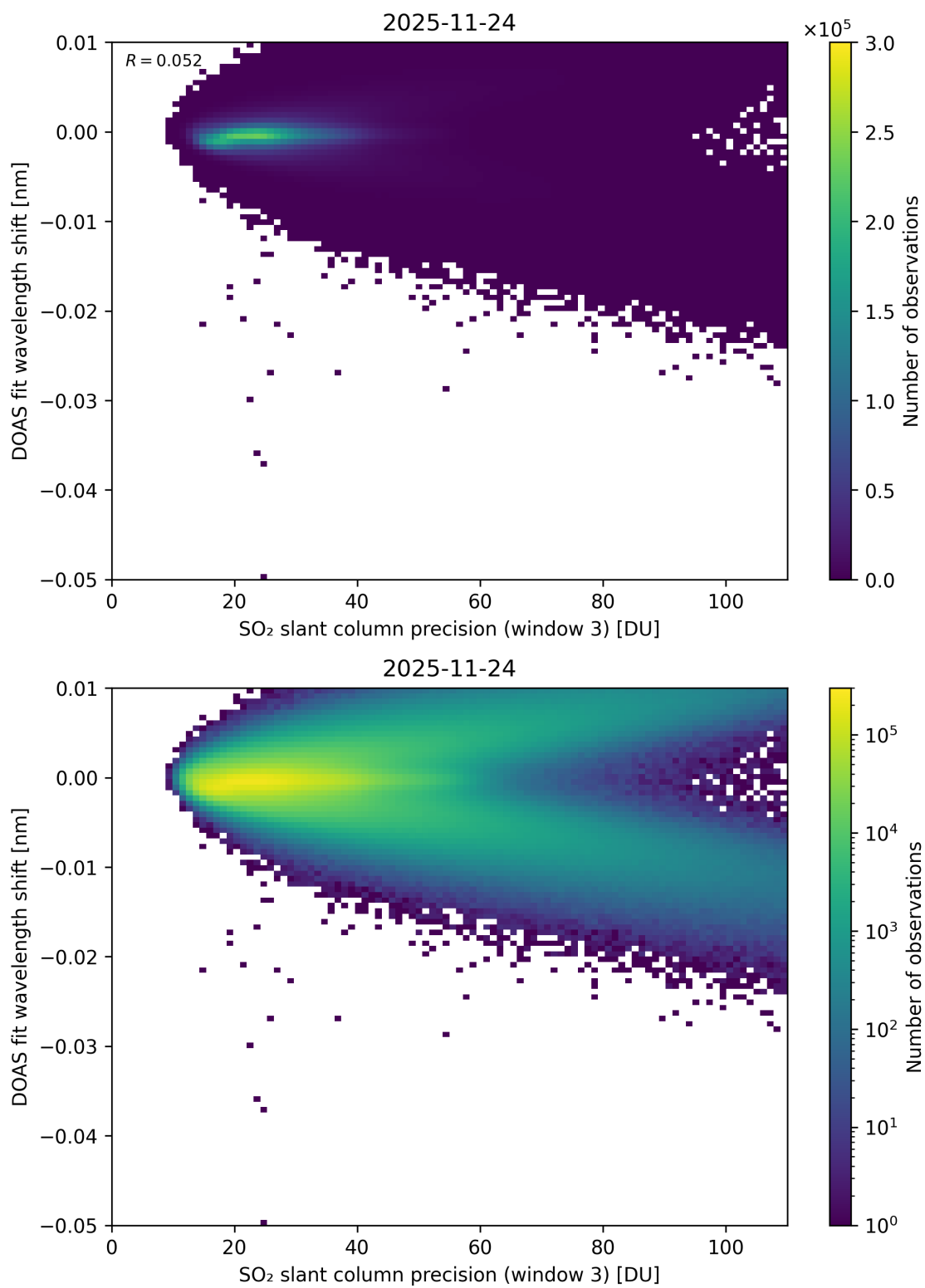
Figure 308: Scatter density plot of “SO 2 slant column precision (window 3)” against “DOAS fit wavelength shift” for 2025-11-23 to 2025-11-25.
