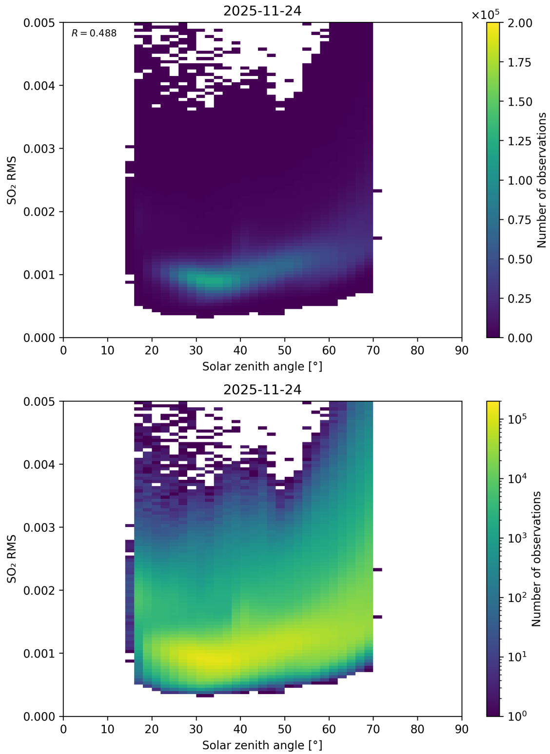
Figure 176: Scatter density plot of “Solar zenith angle” against “SO 2 RMS” for 2025-11-23 to 2025-11-25.
