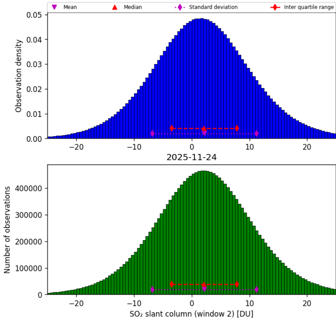
Figure 67: Histogram of “SO 2 slant column (window 2)” for 2025-11-23 to 2025-11-25
