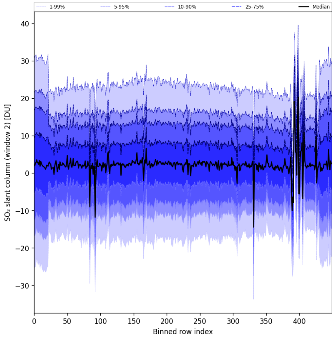
Figure 93: Along track statistics of “SO 2 slant column (window 2)” for 2025-11-23 to 2025-11-25
