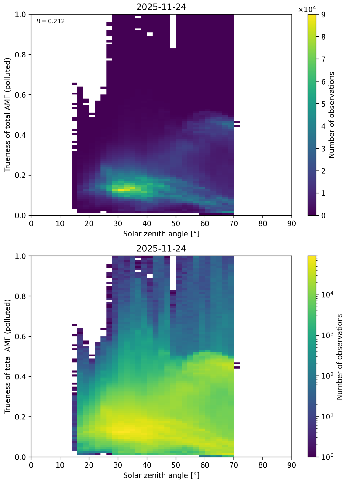
Figure 190: Scatter density plot of “Solar zenith angle” against “Trueness of total AMF (polluted)” for 2025-11-23 to 2025-11-25.
