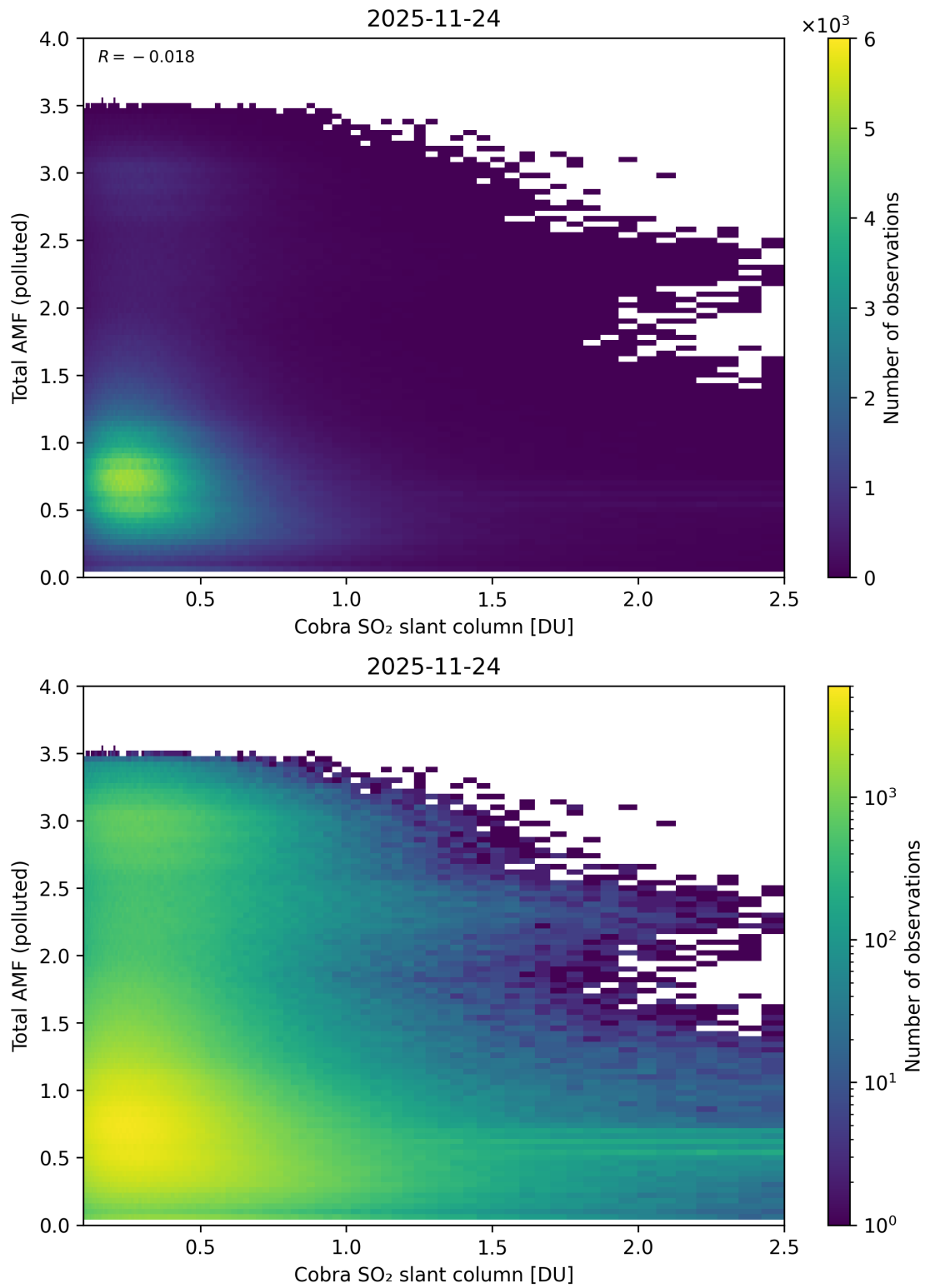
Figure 224: Scatter density plot of “Cobra SO 2 slant column” against “Total AMF (polluted)” for 2025-11-23 to 2025-11-25.
