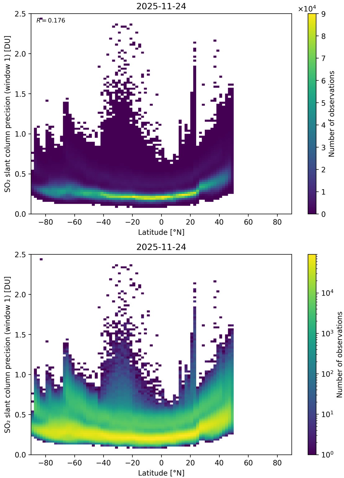
Figure 163: Scatter density plot of “Latitude” against “SO 2 slant column precision (window 1)” for 2025-11-23 to 2025-11-25.
