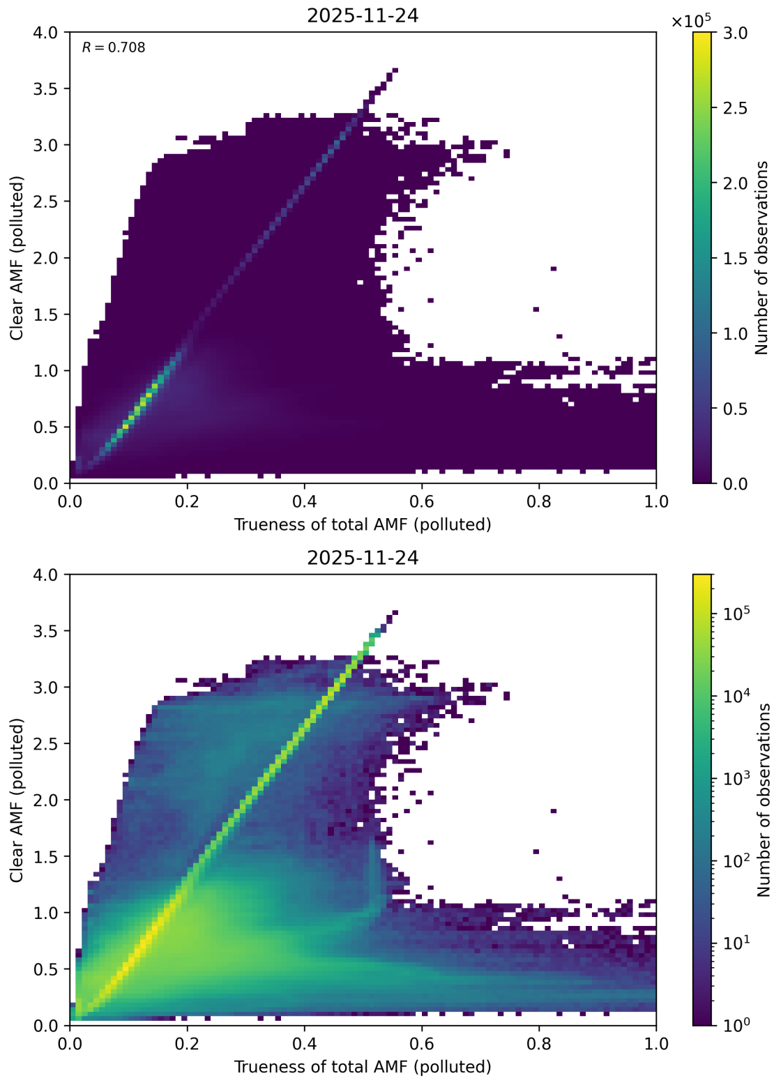
Figure 322: Scatter density plot of “Trueness of total AMF (polluted)” against “Clear AMF (polluted)” for 2025-11-23 to 2025-11-25.
