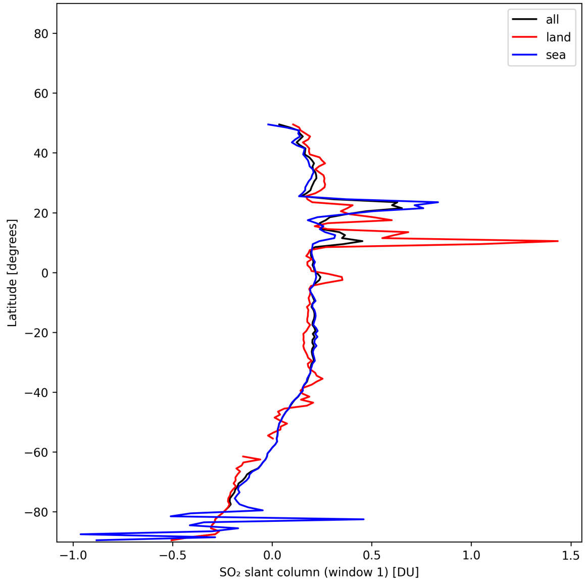
Figure 37: Zonal average of “SO 2 slant column (window 1)” for 2025-11-23 to 2025-11-25.
