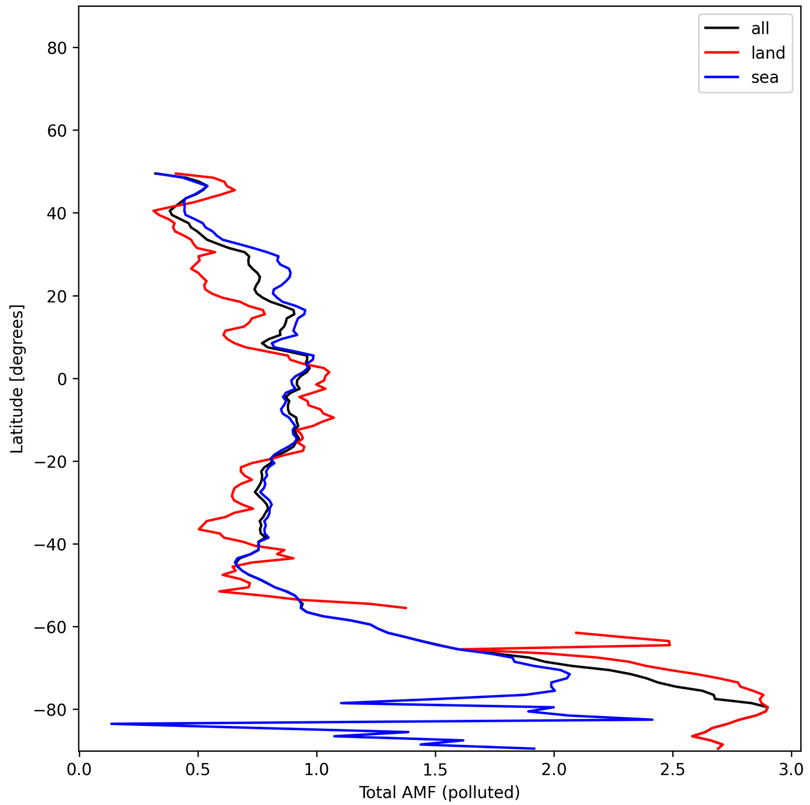
Figure 53: Zonal average of “Total AMF (polluted)” for 2025-11-23 to 2025-11-25.
