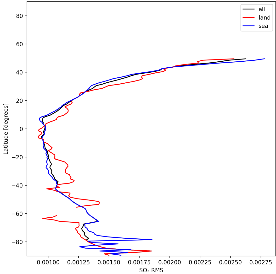
Figure 52: Zonal average of “SO 2 RMS” for 2025-11-23 to 2025-11-25.
