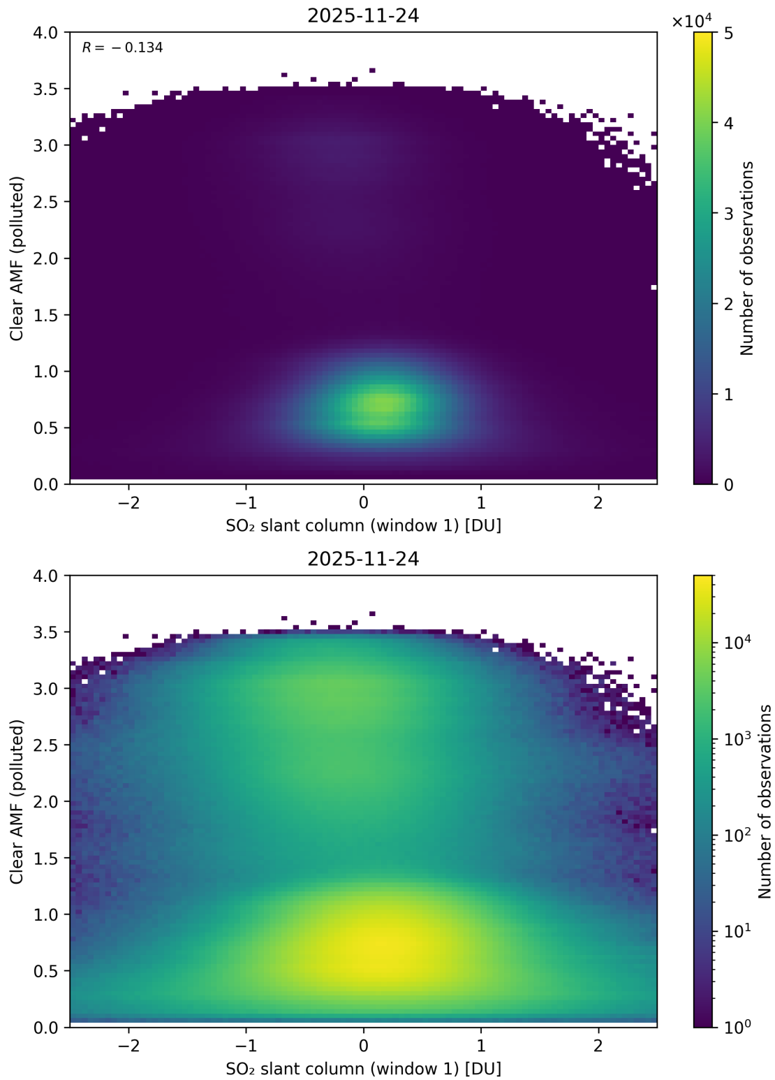
Figure 282: Scatter density plot of “SO 2 slant column (window 1)” against “Clear AMF (polluted)” for 2025-11-23 to 2025-11-25.
