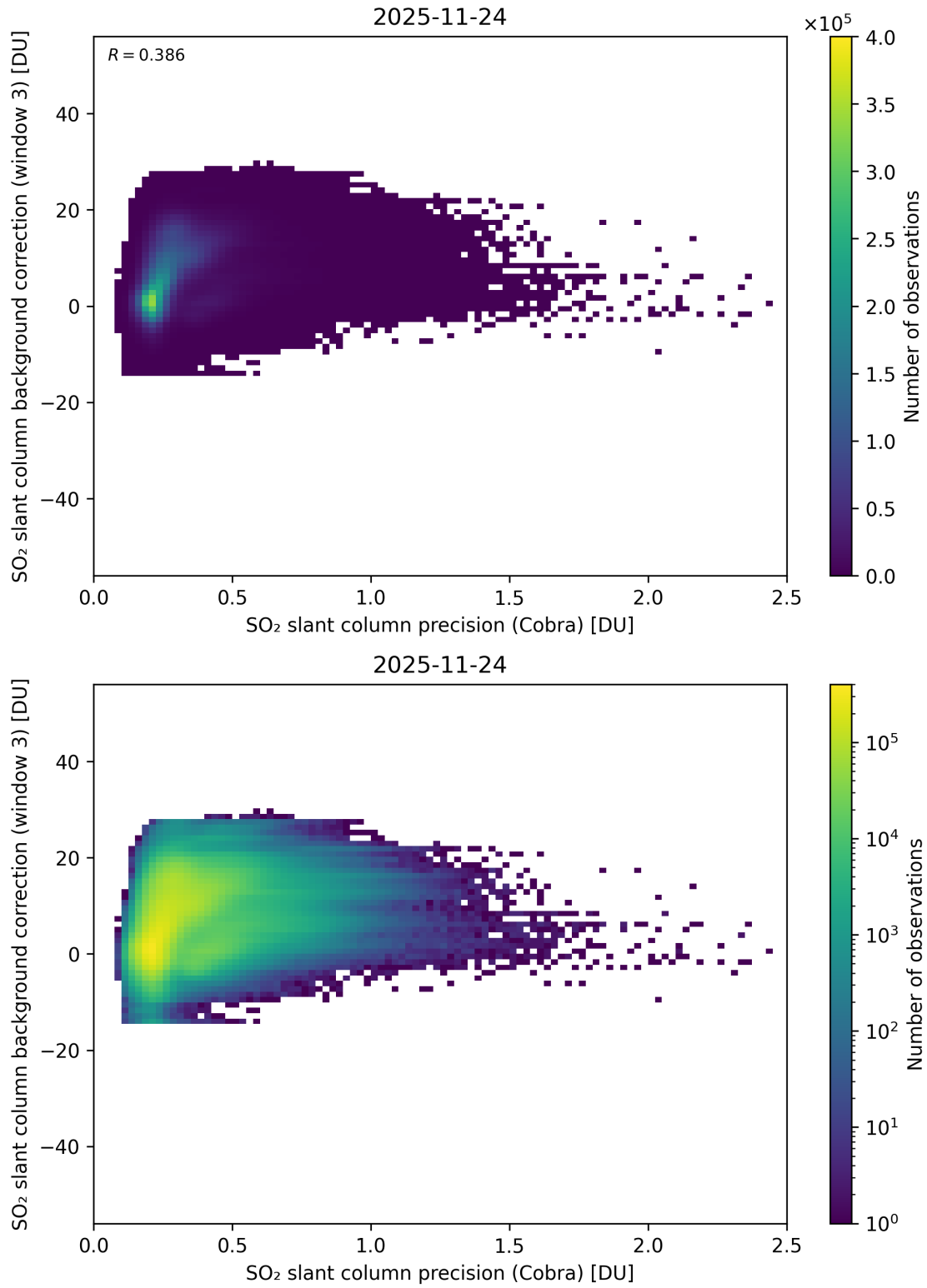
Figure 201: Scatter density plot of “SO 2 slant column precision (Cobra)” against “SO 2 slant column background correction (window 3)” for 2025-11-23 to 2025-11-25.
