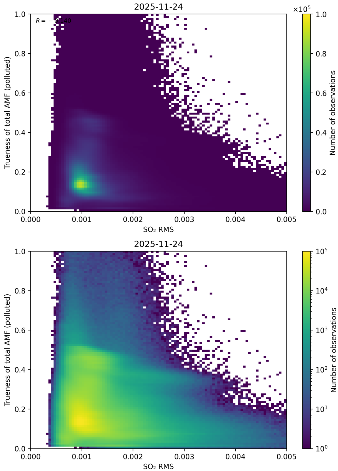
Figure 149: Scatter density plot of “SO 2 RMS” against “Trueness of total AMF (polluted)” for 2025-11-23 to 2025-11-25.
