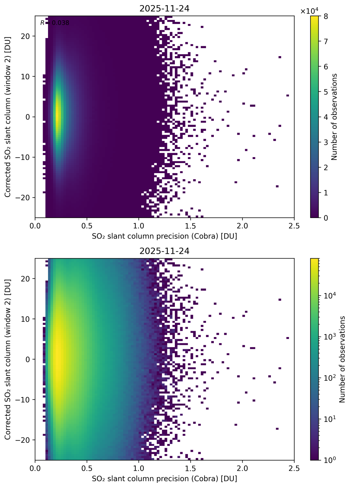
Figure 206: Scatter density plot of “SO 2 slant column precision (Cobra)” against “Corrected SO 2 slant column (window 2)” for 2025-11-23 to 2025-11-25.
