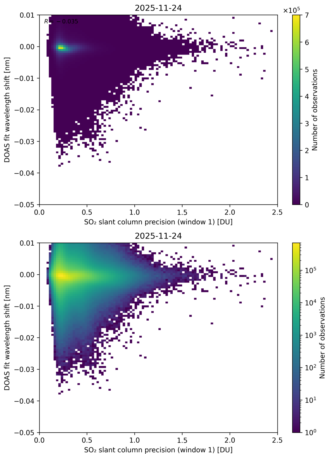
Figure 271: Scatter density plot of “SO 2 slant column precision (window 1)” against “DOAS fit wavelength shift” for 2025-11-23 to 2025-11-25.
