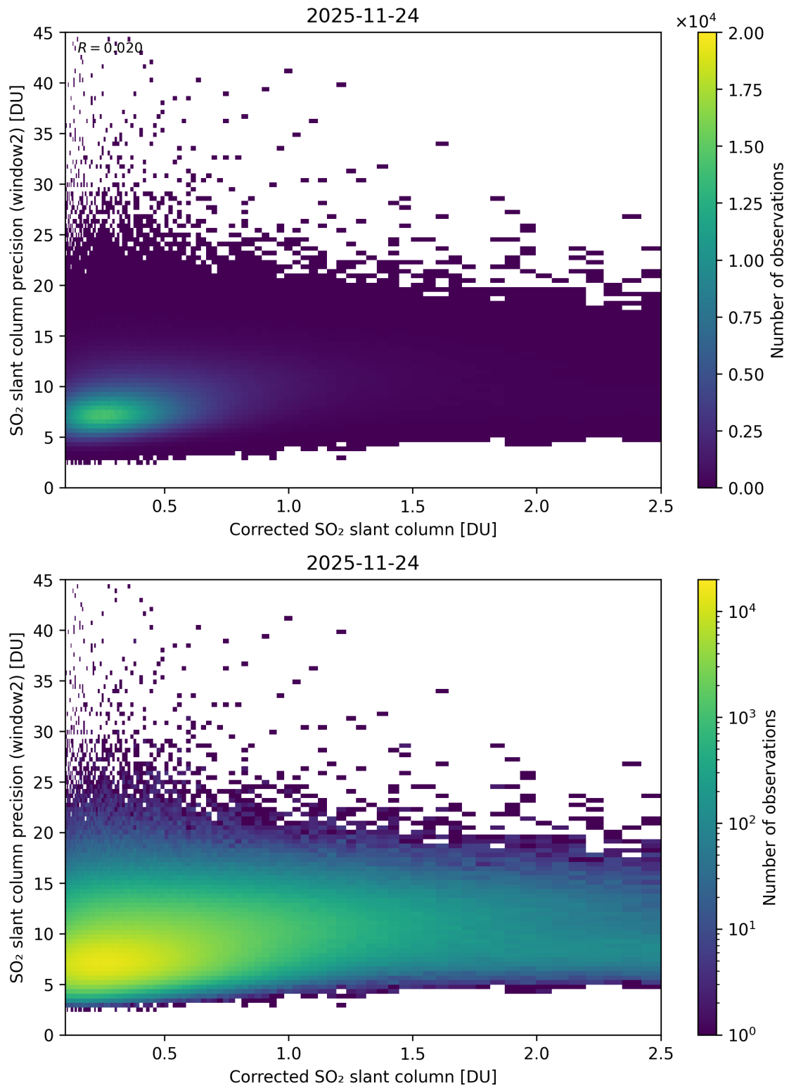
Figure 239: Scatter density plot of “Corrected SO 2 slant column” against “SO 2 slant column precision (window2)” for 2025-11-23 to 2025-11-25.
