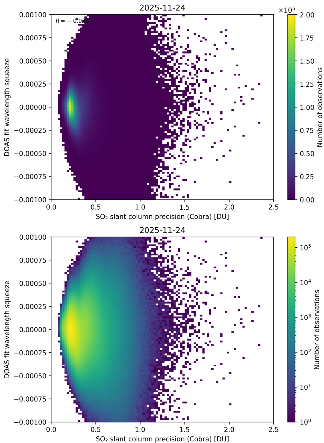
Figure 203: Scatter density plot of “SO 2 slant column precision (Cobra)” against “DOAS fit wavelength squeeze” for 2025-11-23 to 2025-11-25.
