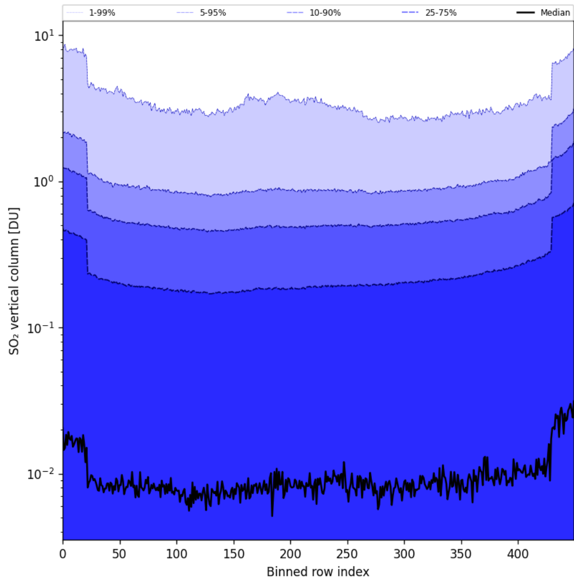
Figure 84: Along track statistics of “SO 2 vertical column” for 2025-11-23 to 2025-11-25
