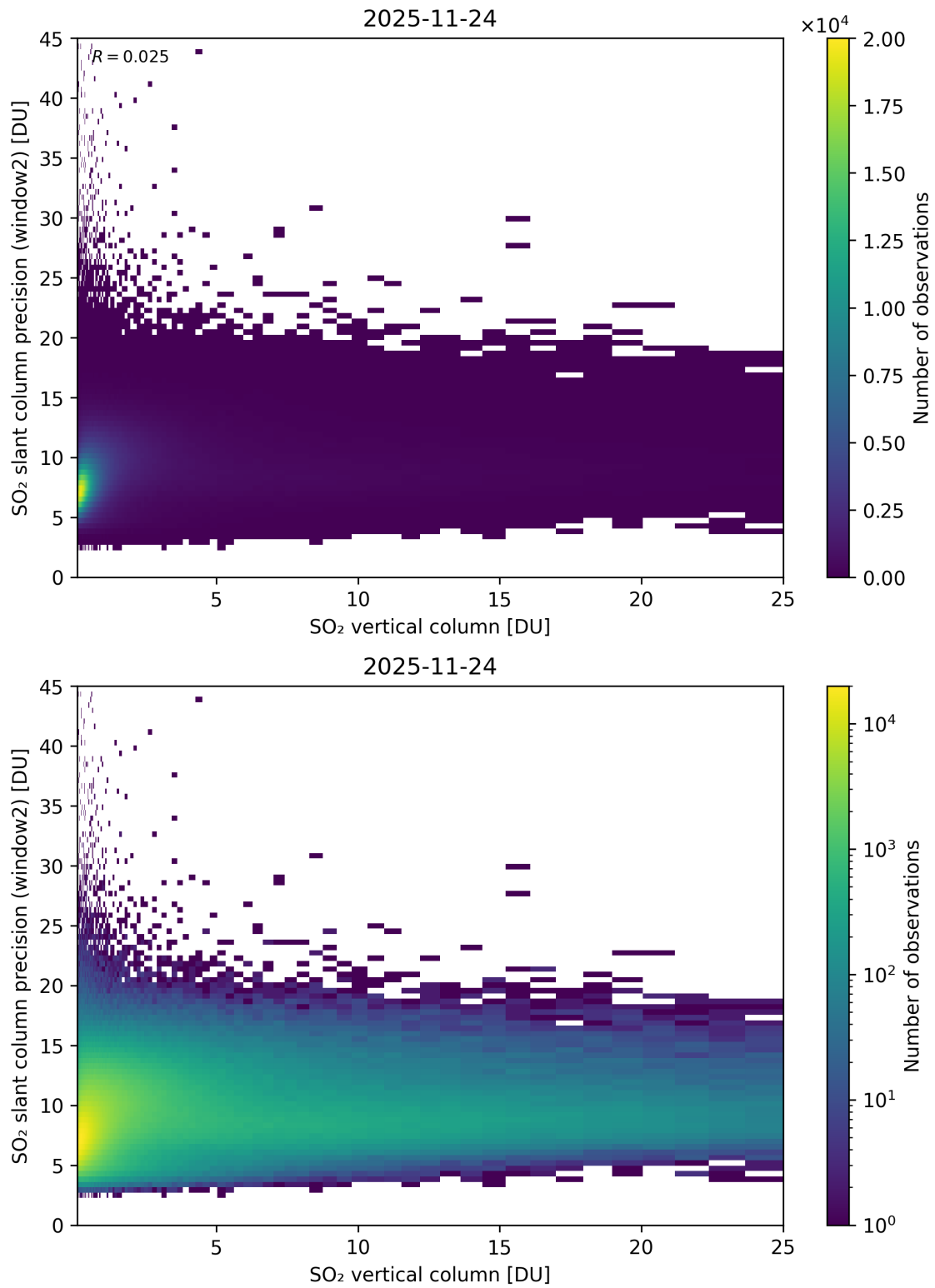
Figure 356: Scatter density plot of “SO 2 vertical column” against “SO 2 slant column precision (window2)” for 2025-11-23 to 2025-11-25.
