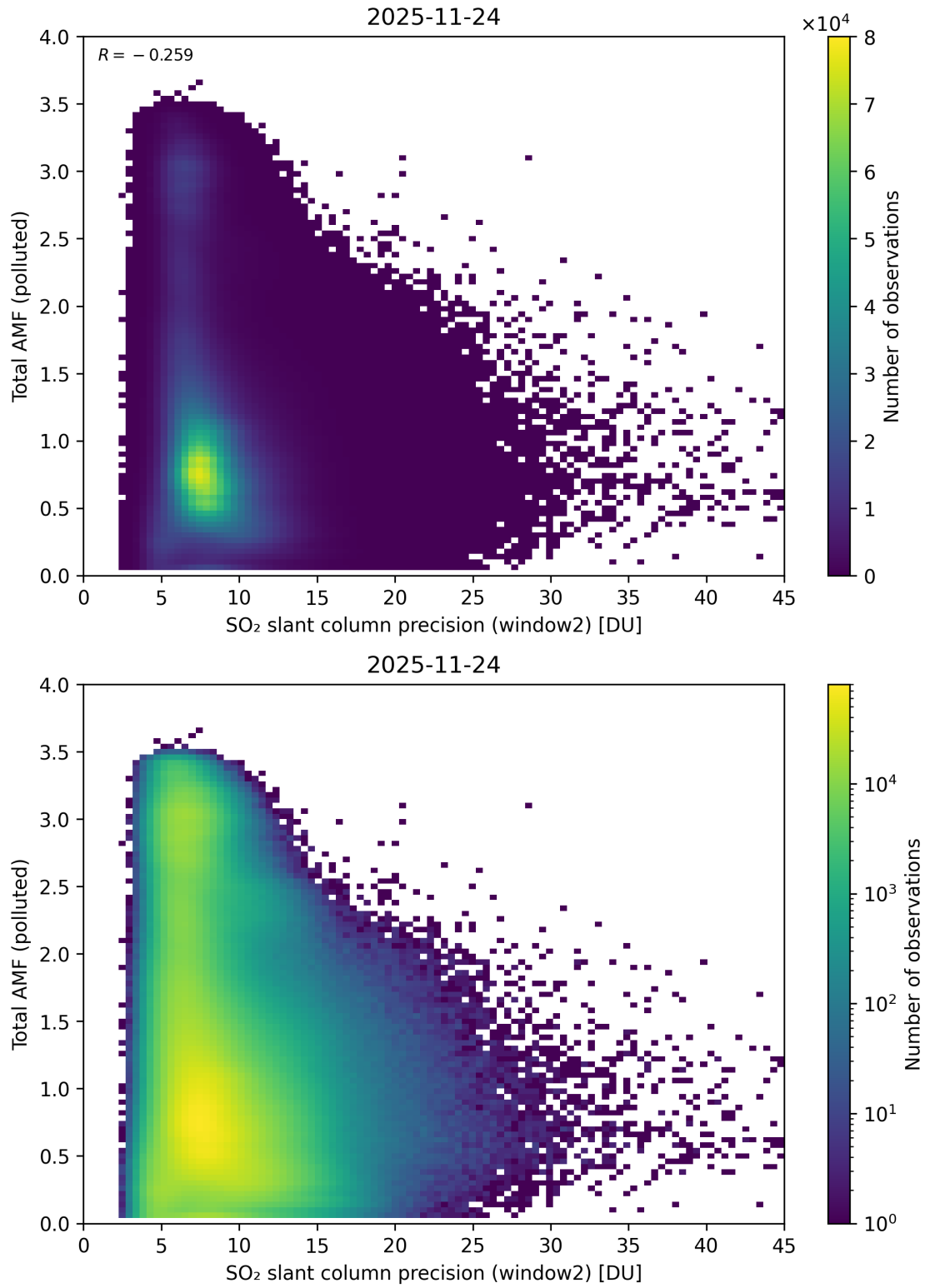
Figure 301: Scatter density plot of “SO 2 slant column precision (window2)” against “Total AMF (polluted)” for 2025-11-23 to 2025-11-25.
