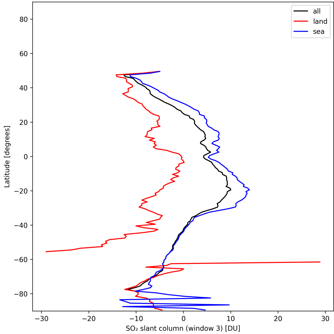
Figure 45: Zonal average of “SO 2 slant column (window 3)” for 2025-11-23 to 2025-11-25.
