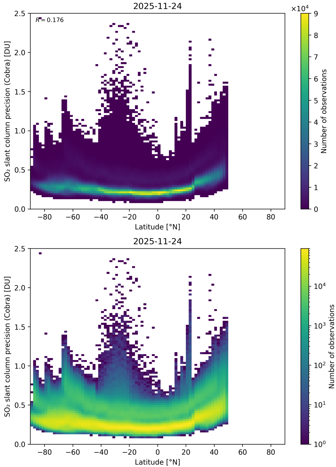
Figure 158: Scatter density plot of “Latitude” against “SO 2 slant column precision (Cobra)” for 2025-11-23 to 2025-11-25.
