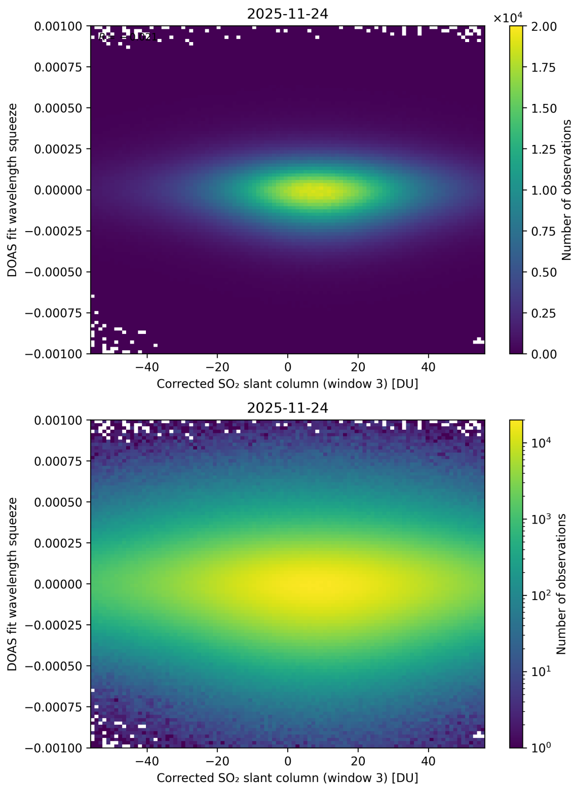
Figure 257: Scatter density plot of “Corrected SO 2 slant column (window 3)” against “DOAS fit wavelength squeeze” for 2025-11-23 to 2025-11-25.
