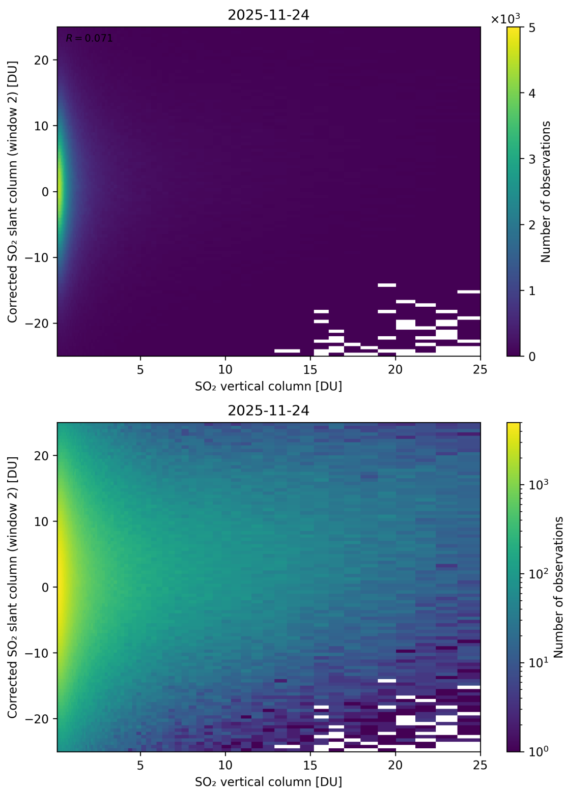
Figure 352: Scatter density plot of “SO 2 vertical column” against “Corrected SO 2 slant column (window 2)” for 2025-11-23 to 2025-11-25.
