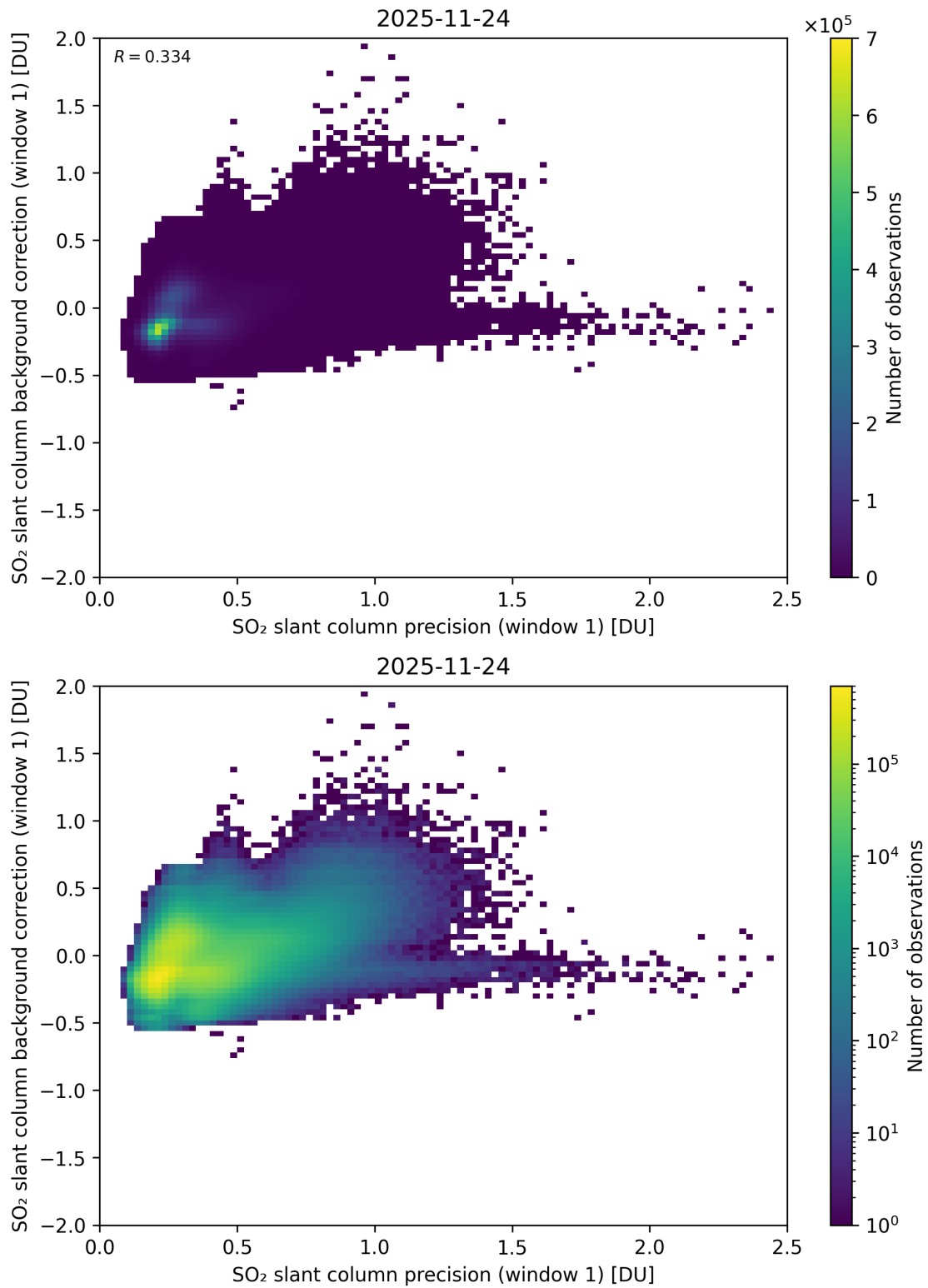
Figure 268: Scatter density plot of “SO 2 slant column precision (window 1)” against “SO 2 slant column background correction (window 1)” for 2025-11-23 to 2025-11-25.
