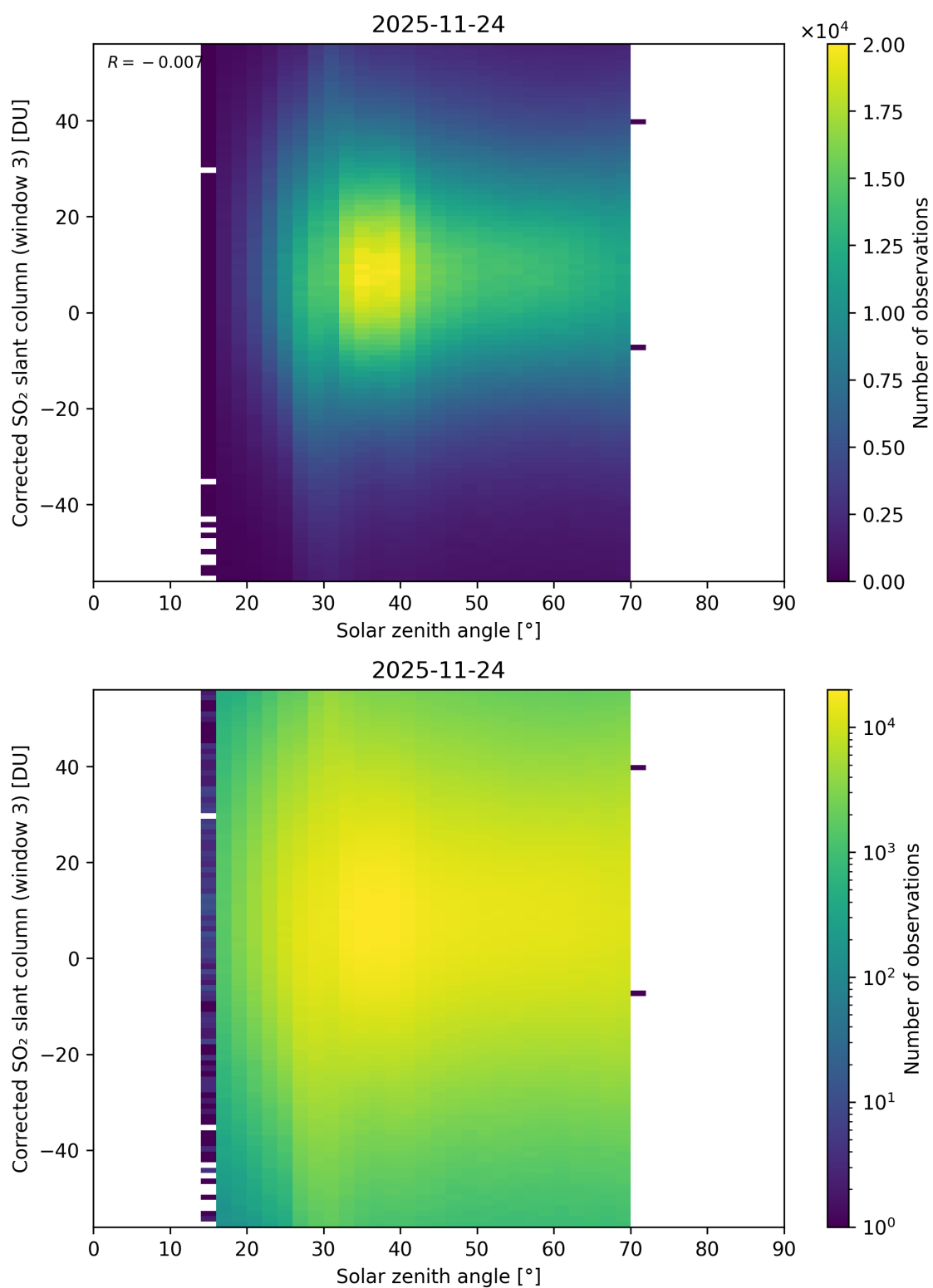
Figure 183: Scatter density plot of “Solar zenith angle” against “Corrected SO 2 slant column (window 3)” for 2025-11-23 to 2025-11-25.
