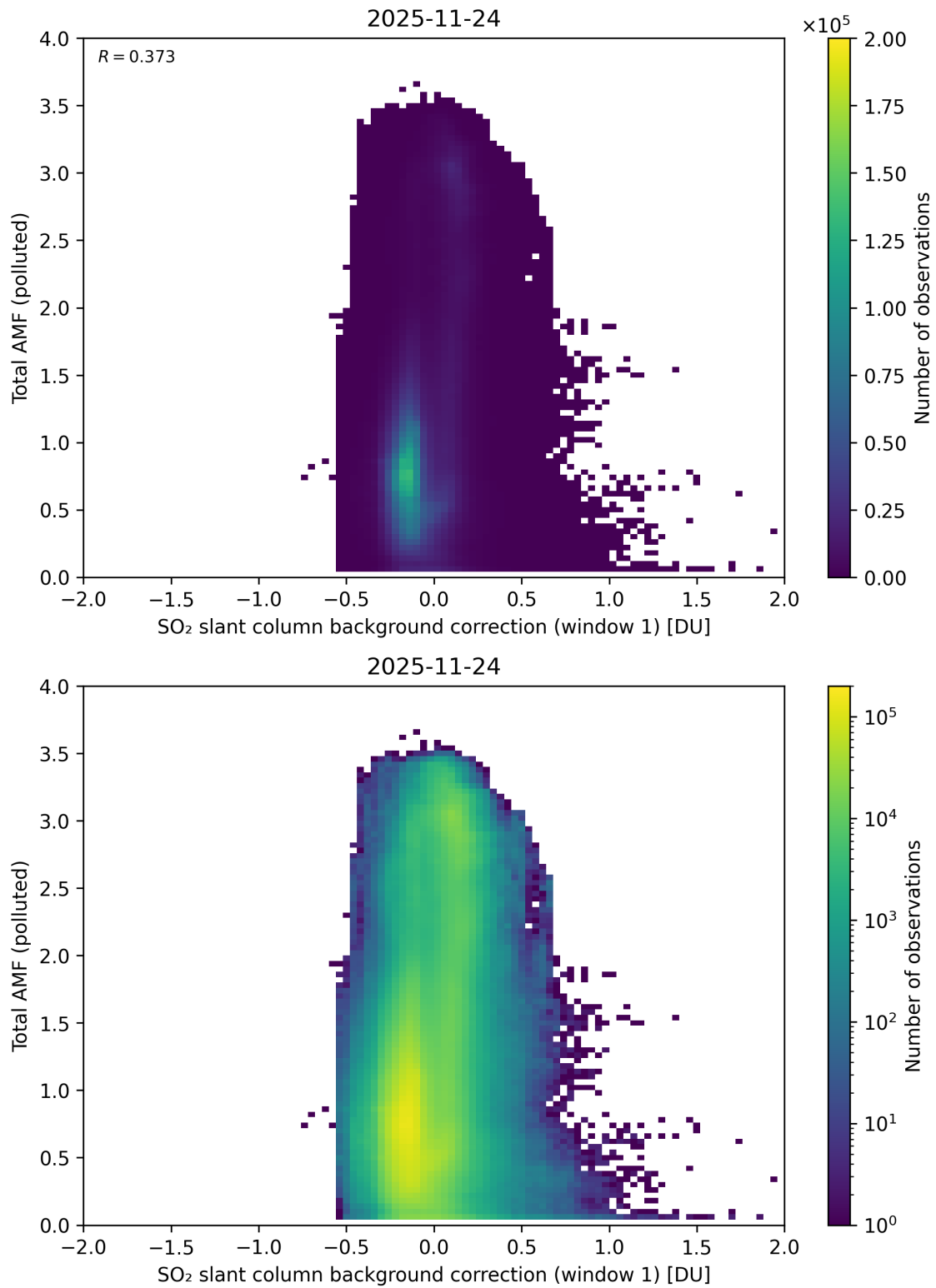
Figure 120: Scatter density plot of “SO 2 slant column background correction (window 1)” against “Total AMF (polluted)” for 2025-11-23 to 2025-11-25.
