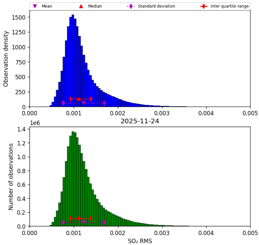
Figure 78: Histogram of “SO 2 RMS” for 2025-11-23 to 2025-11-25
