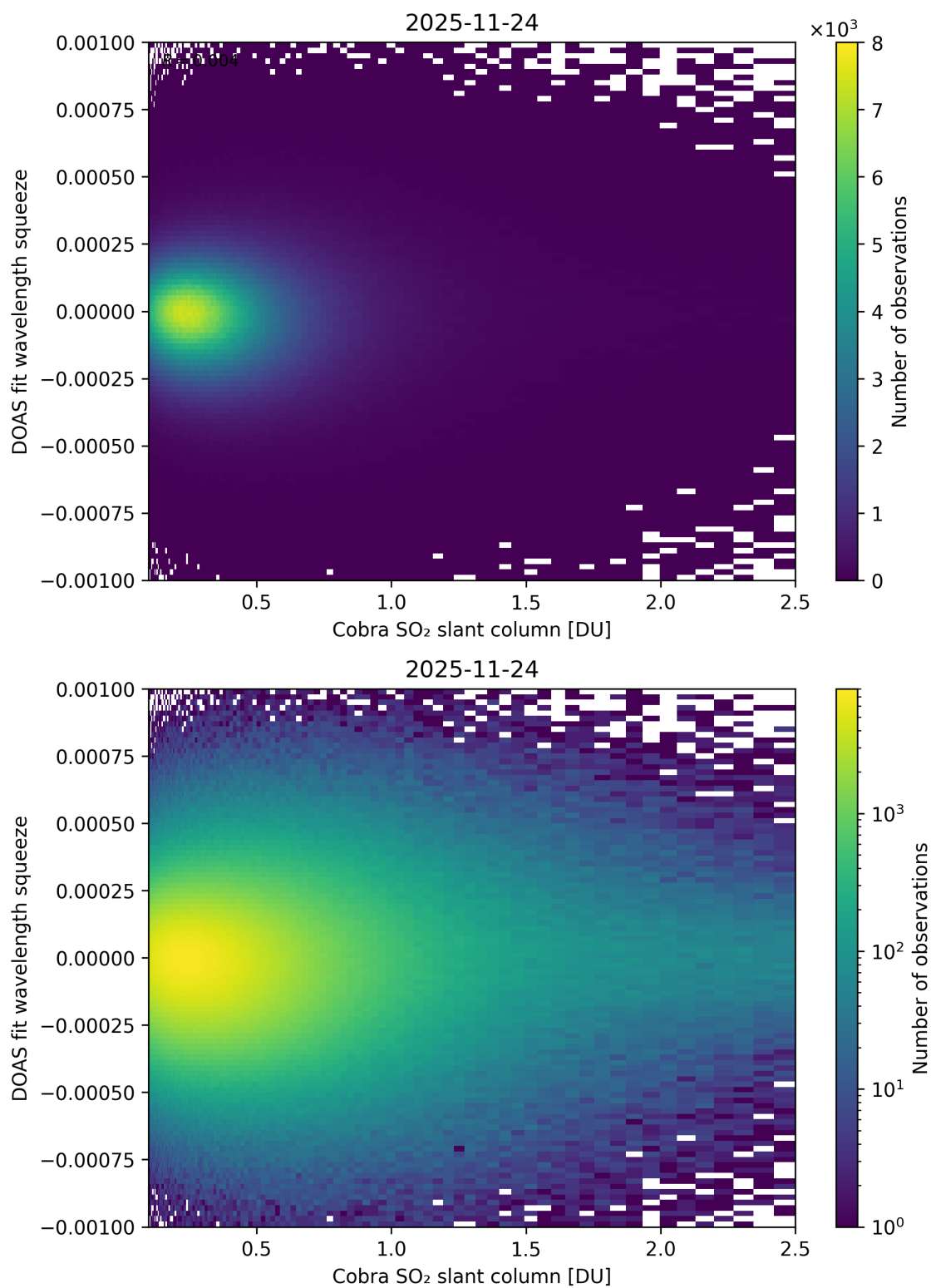
Figure 197: Scatter density plot of “Cobra SO 2 slant column” against “DOAS fit wavelength squeeze” for 2025-11-23 to 2025-11-25.
