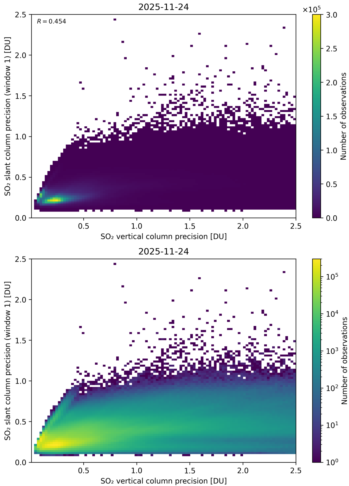
Figure 342: Scatter density plot of “SO 2 vertical column precision” against “SO 2 slant column precision (window 1)” for 2025-11-23 to 2025-11-25.
