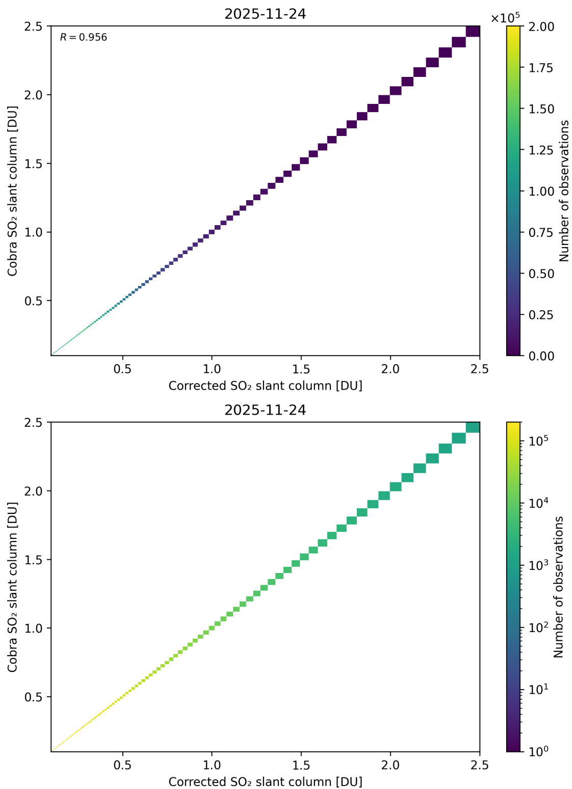
Figure 233: Scatter density plot of “Corrected SO 2 slant column” against “Cobra SO 2 slant column” for 2025-11-23 to 2025-11-25.
