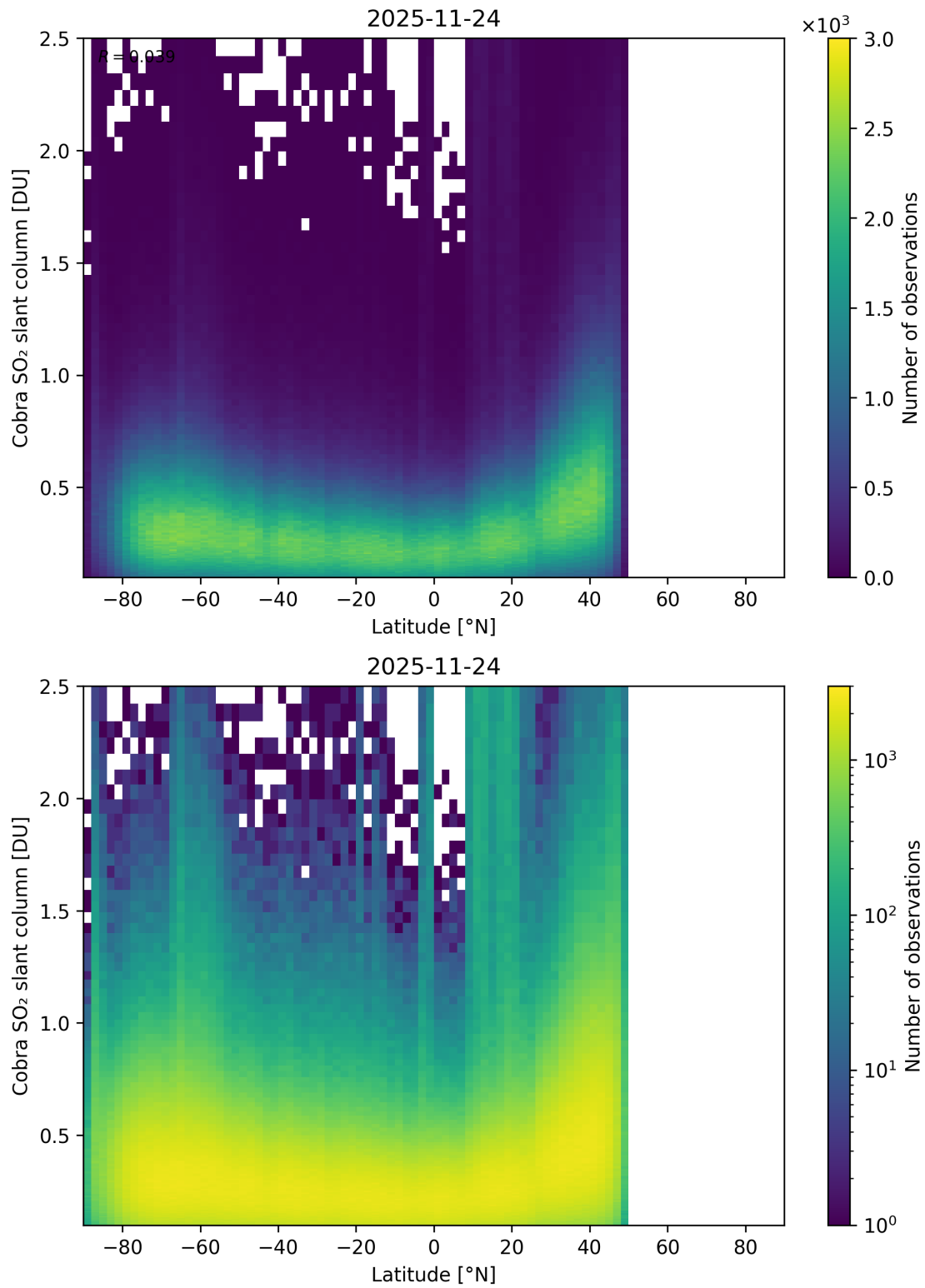
Figure 157: Scatter density plot of “Latitude” against “Cobra SO 2 slant column” for 2025-11-23 to 2025-11-25.
