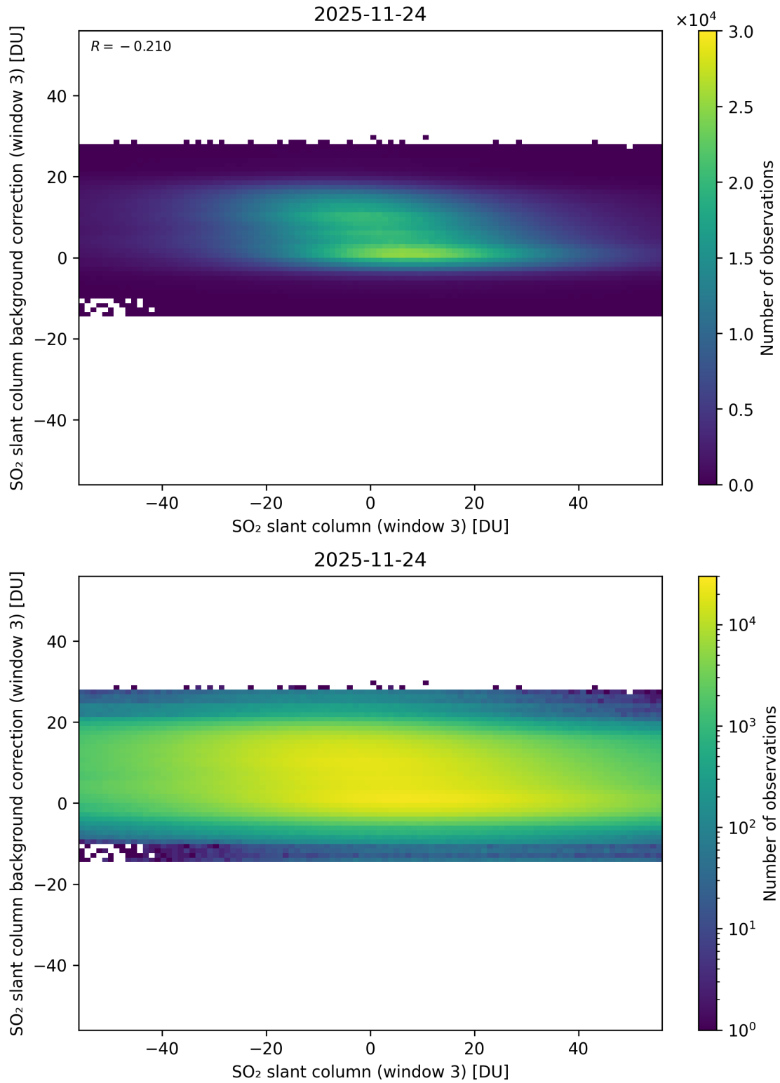
Figure 303: Scatter density plot of “SO 2 slant column (window 3)” against “SO 2 slant column background correction (window 3)” for 2025-11-23 to 2025-11-25.
