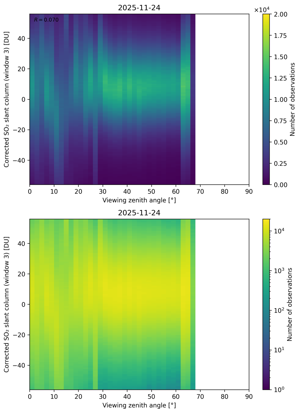
Figure 375: Scatter density plot of “Viewing zenith angle” against “Corrected SO 2 slant column (window 3)” for 2025-11-23 to 2025-11-25.
