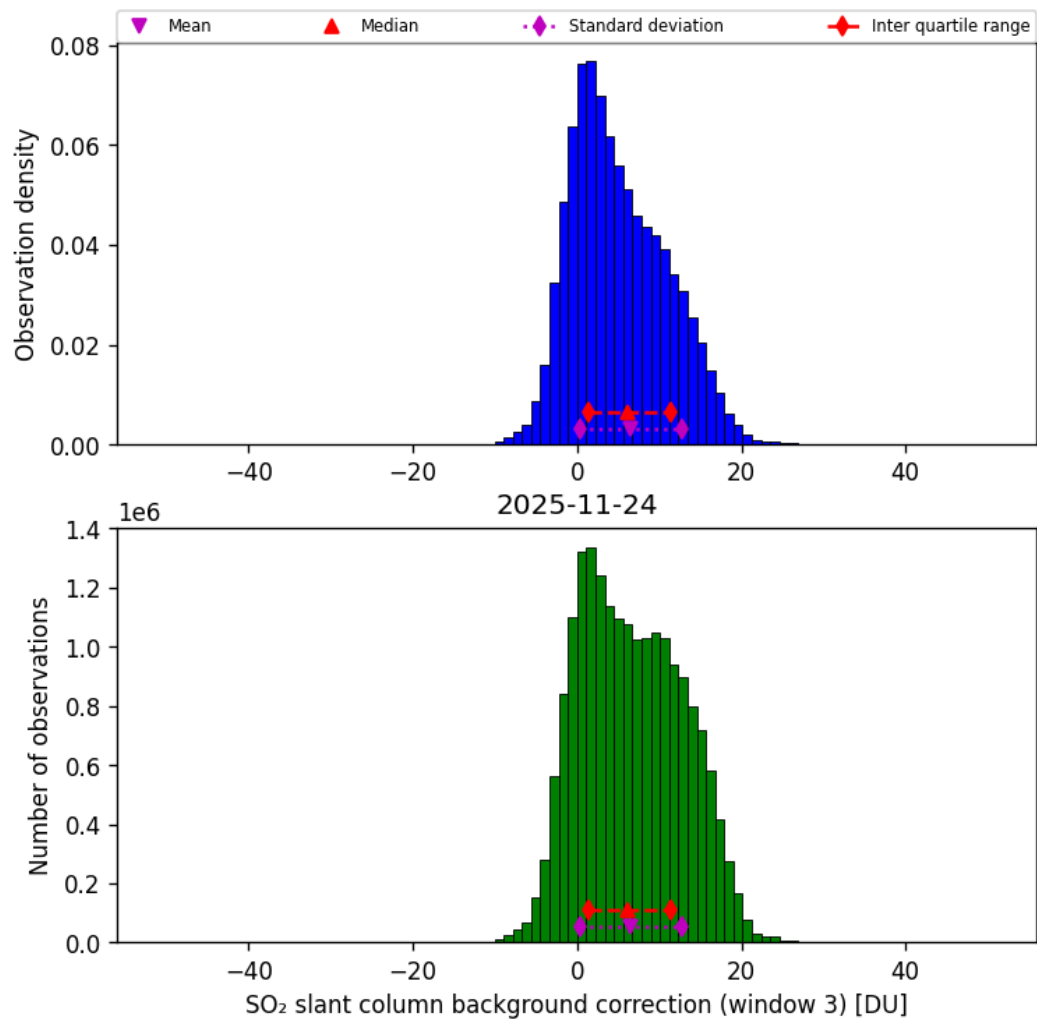
Figure 74: Histogram of “SO 2 slant column background correction (window 3)” for 2025-11-23 to 2025-11-25
