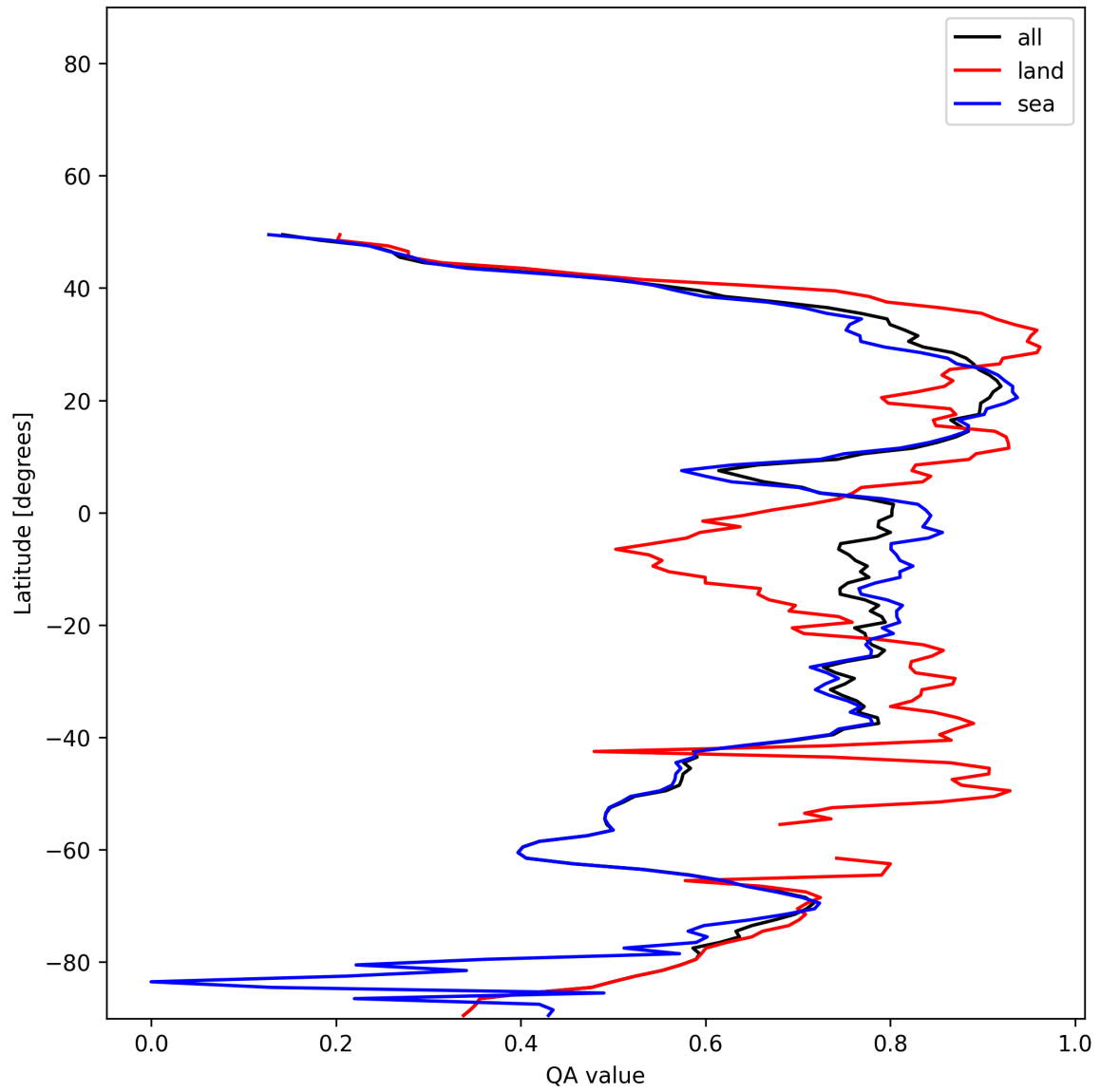
Figure 31: Zonal average of “QA value” for 2025-11-23 to 2025-11-25.
