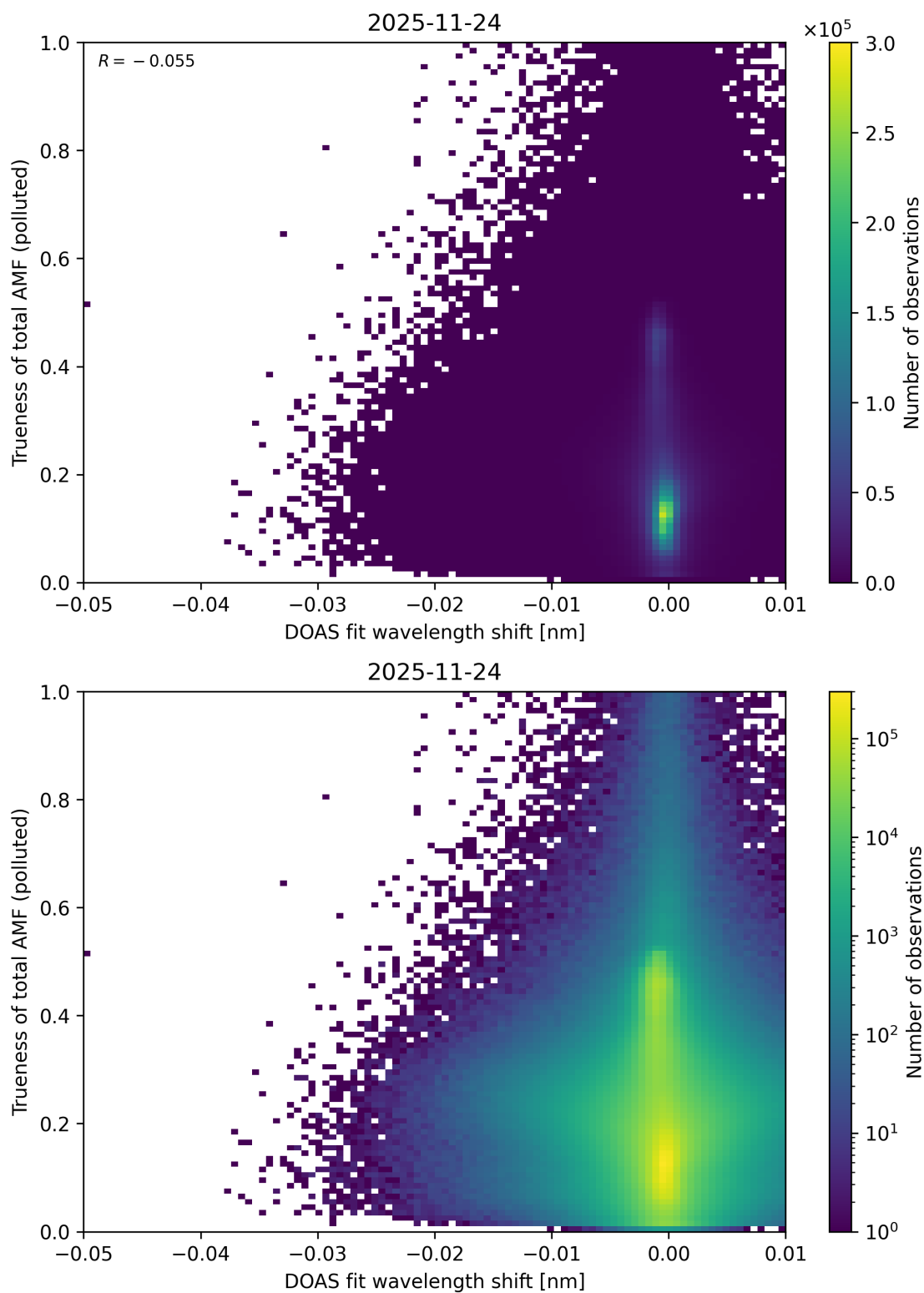
Figure 142: Scatter density plot of “DOAS fit wavelength shift” against “Trueness of total AMF (polluted)” for 2025-11-23 to 2025-11-25.
