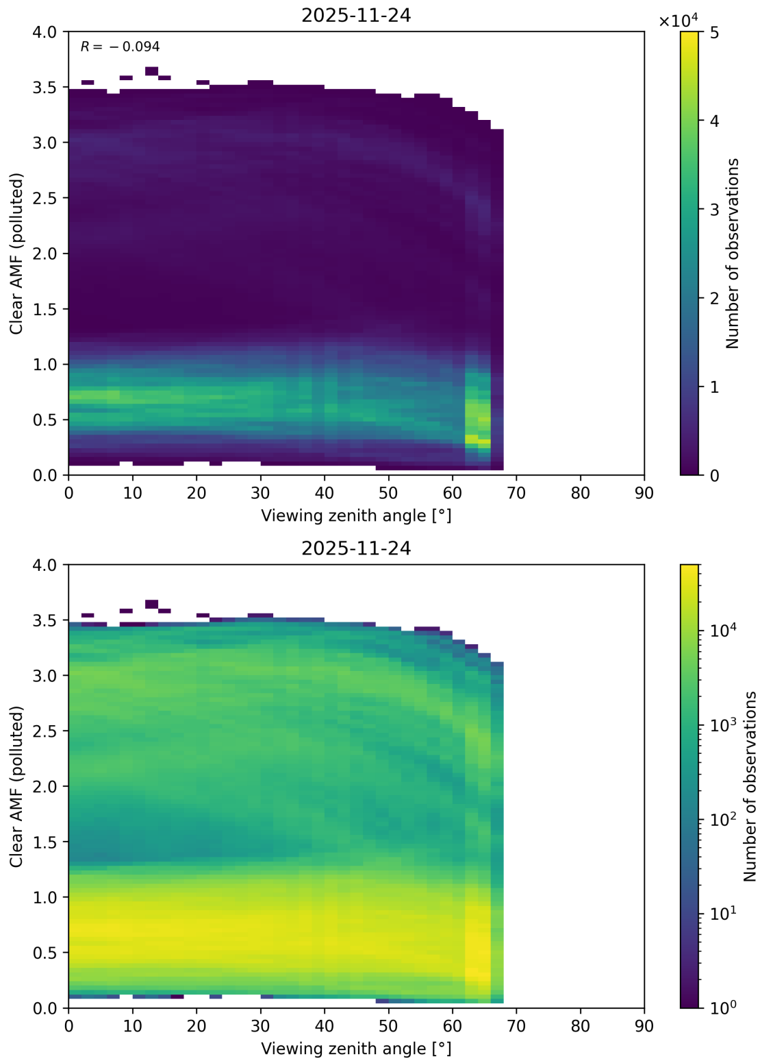
Figure 370: Scatter density plot of “Viewing zenith angle” against “Clear AMF (polluted)” for 2025-11-23 to 2025-11-25.
