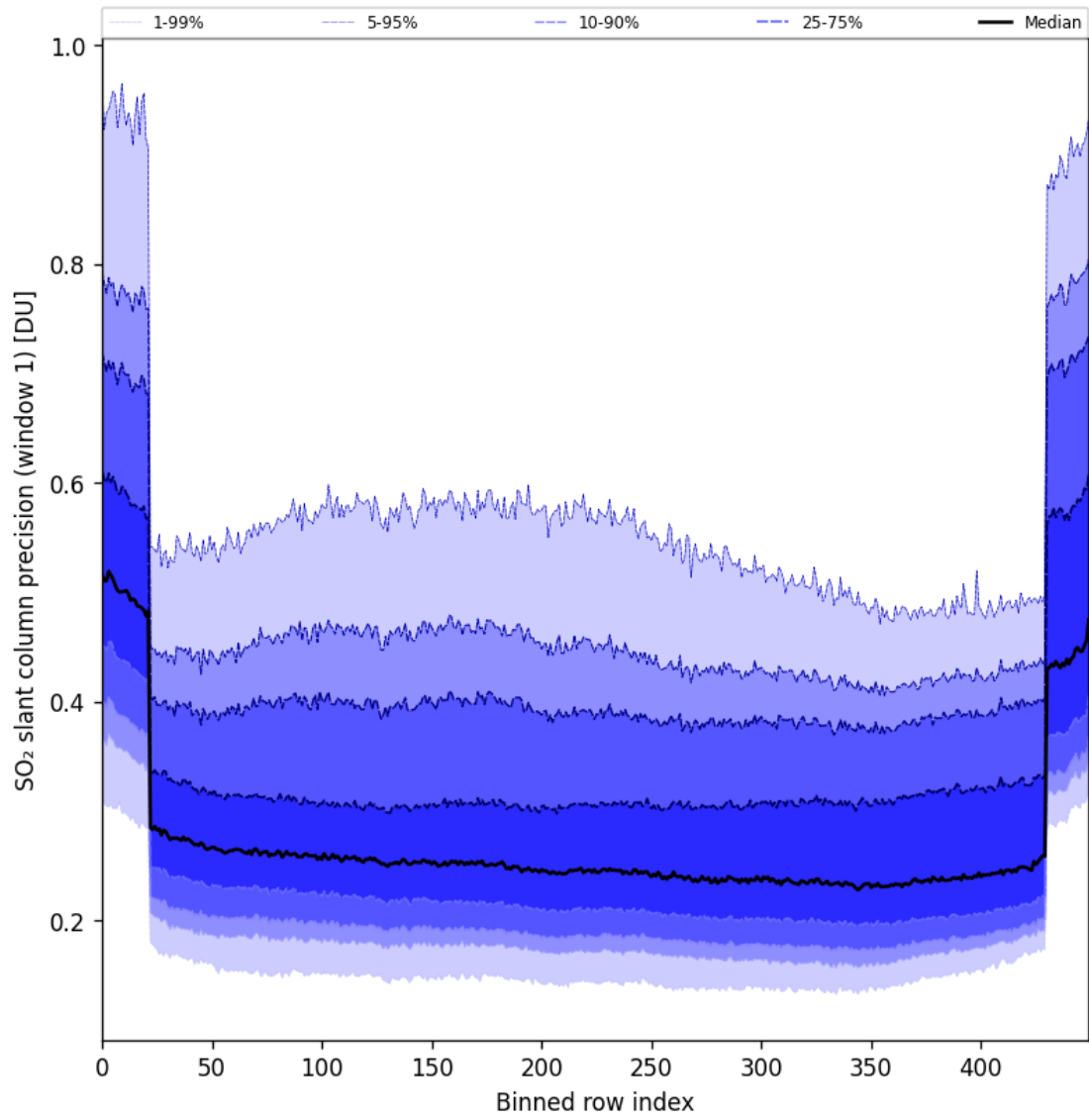
Figure 90: Along track statistics of “SO 2 slant column precision (window 1)” for 2025-11-23 to 2025-11-25
