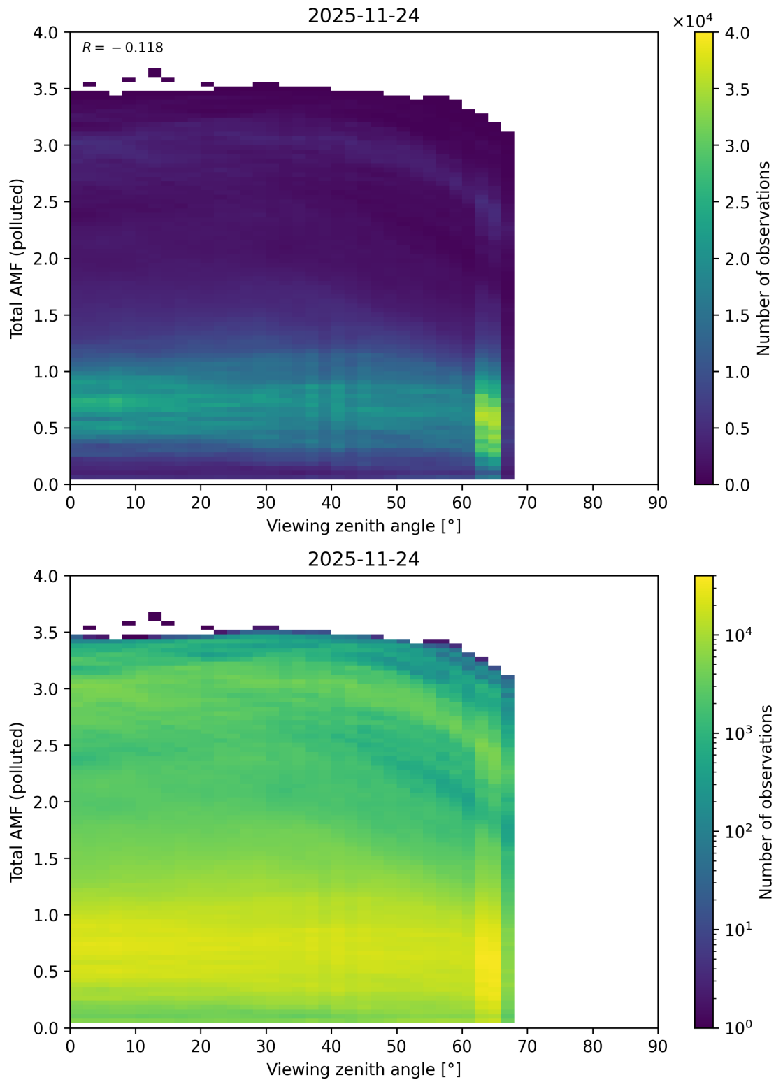
Figure 381: Scatter density plot of “Viewing zenith angle” against “Total AMF (polluted)” for 2025-11-23 to 2025-11-25.
