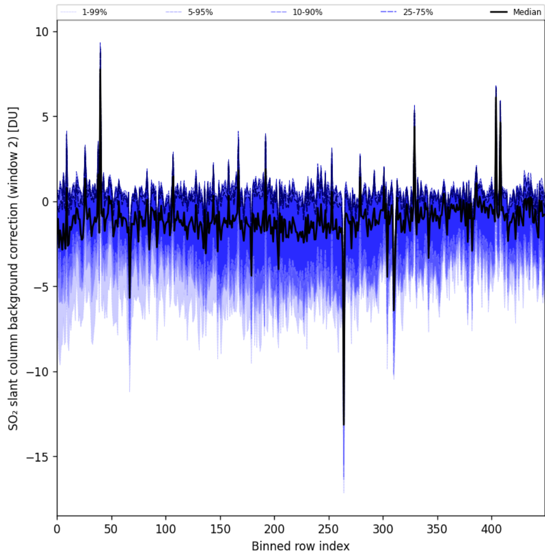
Figure 96: Along track statistics of “SO 2 slant column background correction (window 2)” for 2025-11-23 to 2025-11-25
