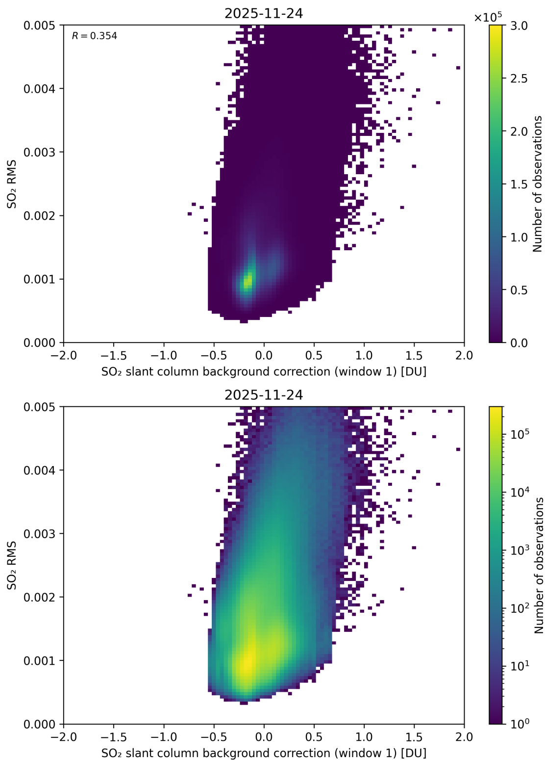
Figure 113: Scatter density plot of “SO 2 slant column background correction (window 1)” against “SO 2 RMS” for 2025-11-23 to 2025-11-25.
