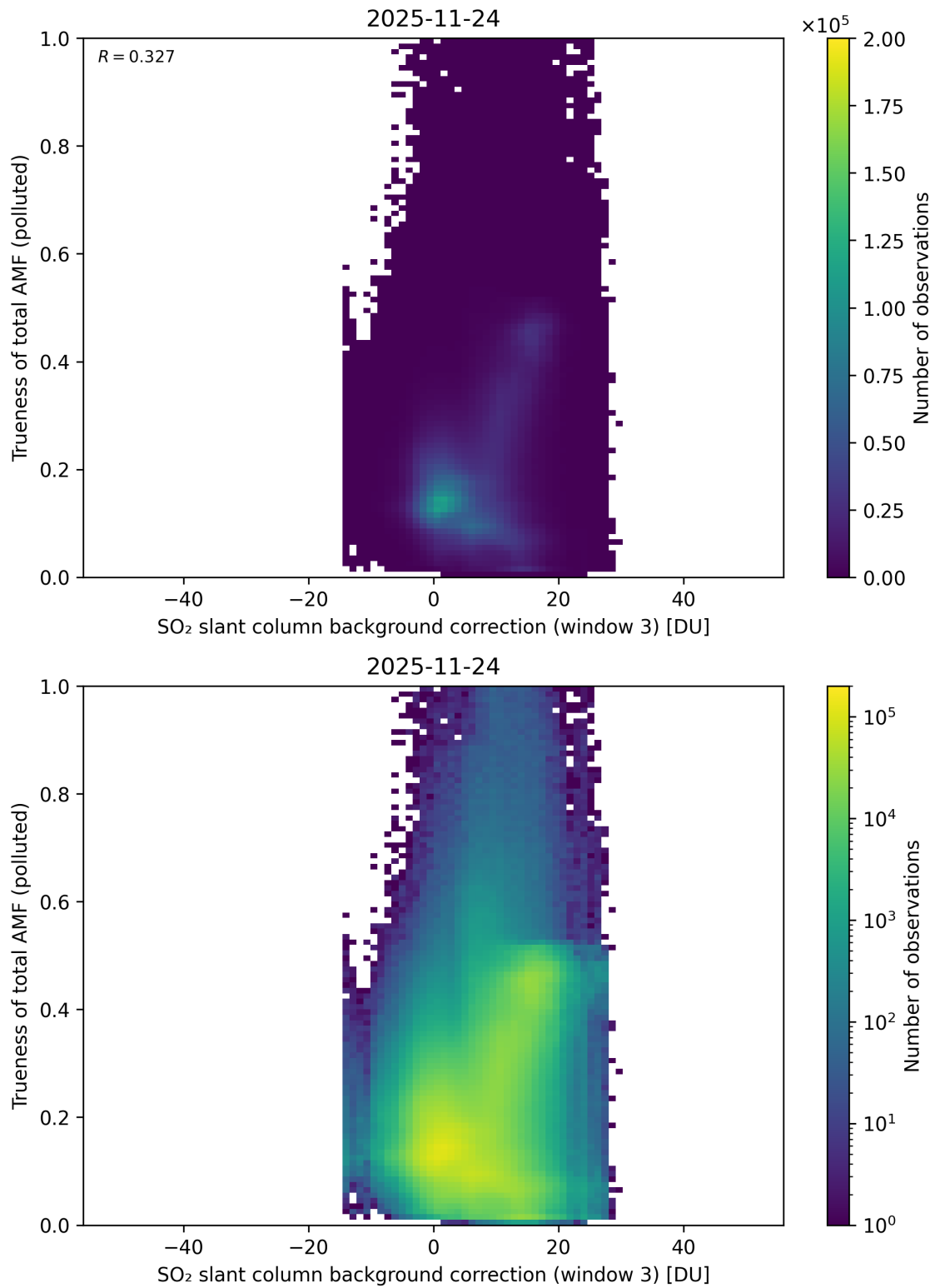
Figure 137: Scatter density plot of “SO 2 slant column background correction (window 3)” against “Trueness of total AMF (polluted)” for 2025-11-23 to 2025-11-25.
