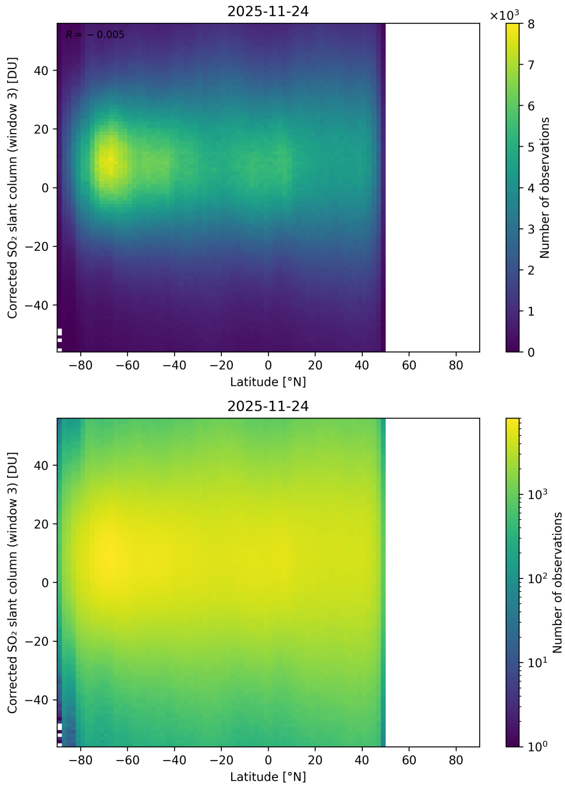
Figure 161: Scatter density plot of “Latitude” against “Corrected SO 2 slant column (window 3)” for 2025-11-23 to 2025-11-25.
