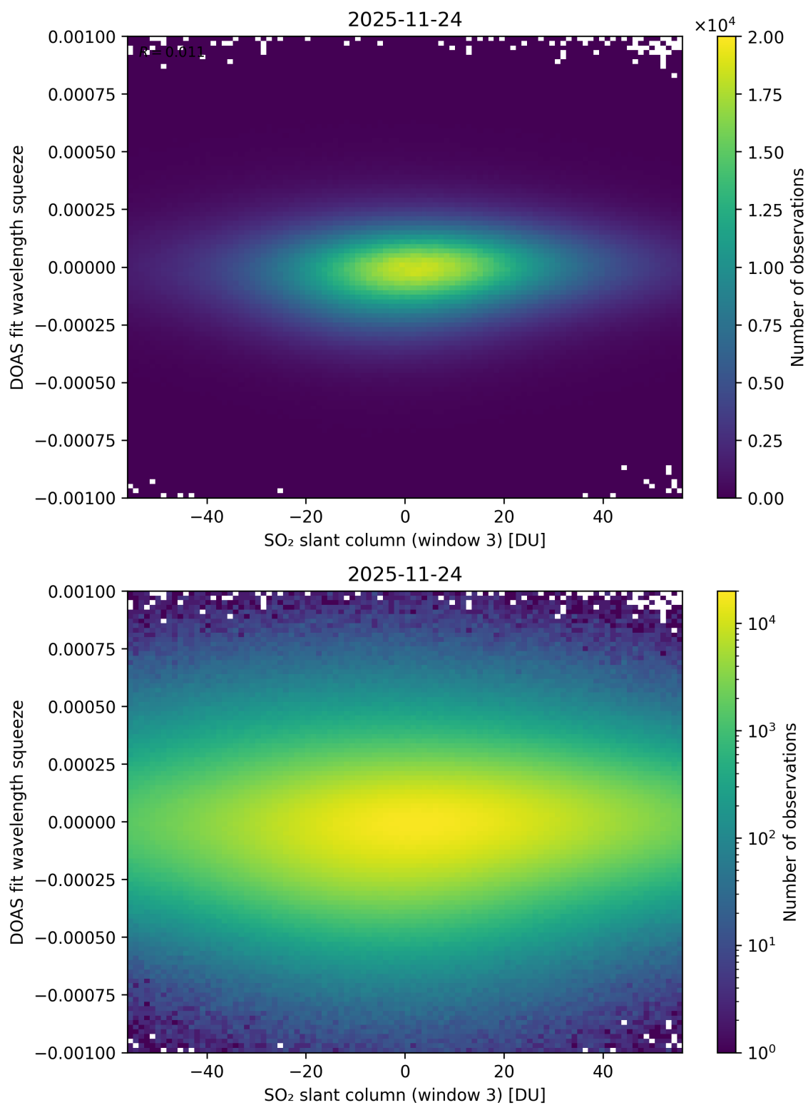
Figure 305: Scatter density plot of “SO 2 slant column (window 3)” against “DOAS fit wavelength squeeze” for 2025-11-23 to 2025-11-25.
