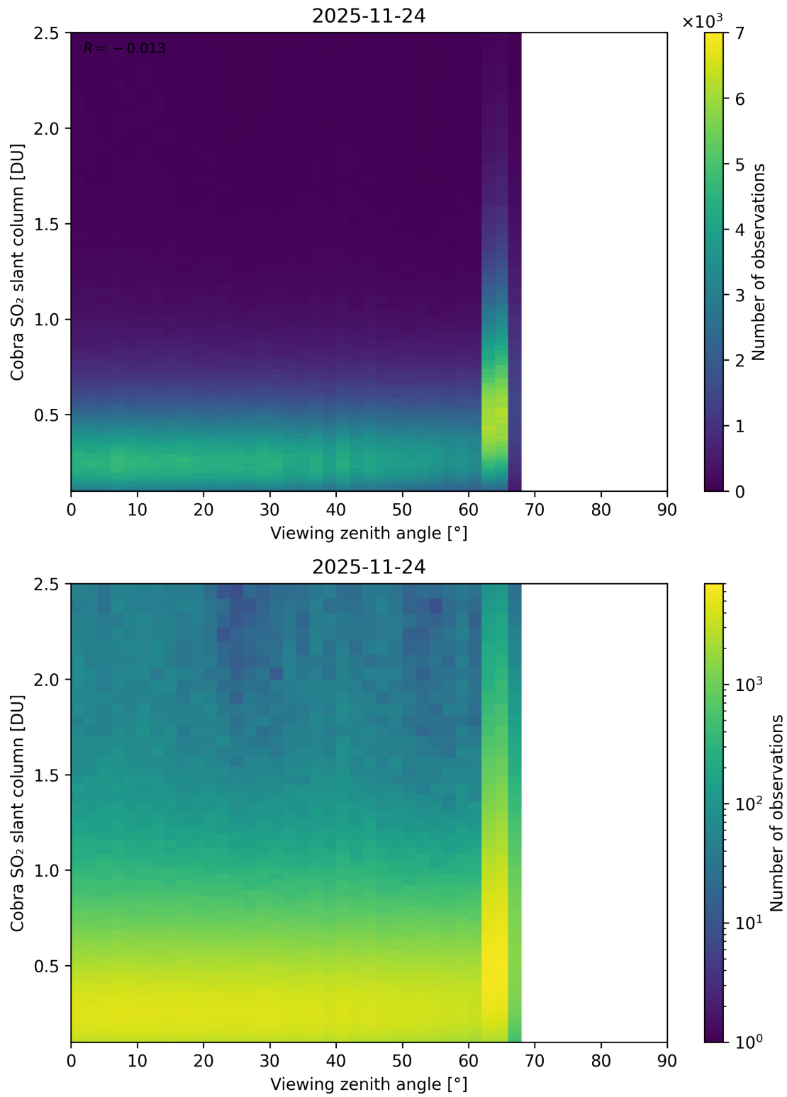
Figure 371: Scatter density plot of “Viewing zenith angle” against “Cobra SO 2 slant column” for 2025-11-23 to 2025-11-25.
