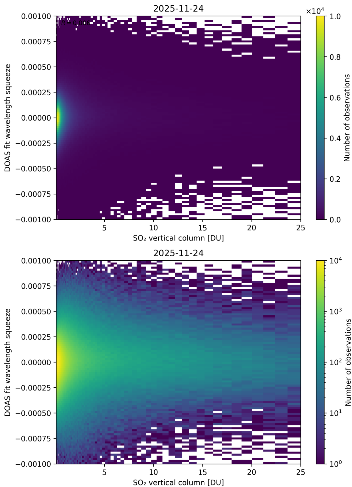
Figure 327: Scatter density plot of “SO 2 vertical column” against “DOAS fit wavelength squeeze” for 2025-11-23 to 2025-11-25.
