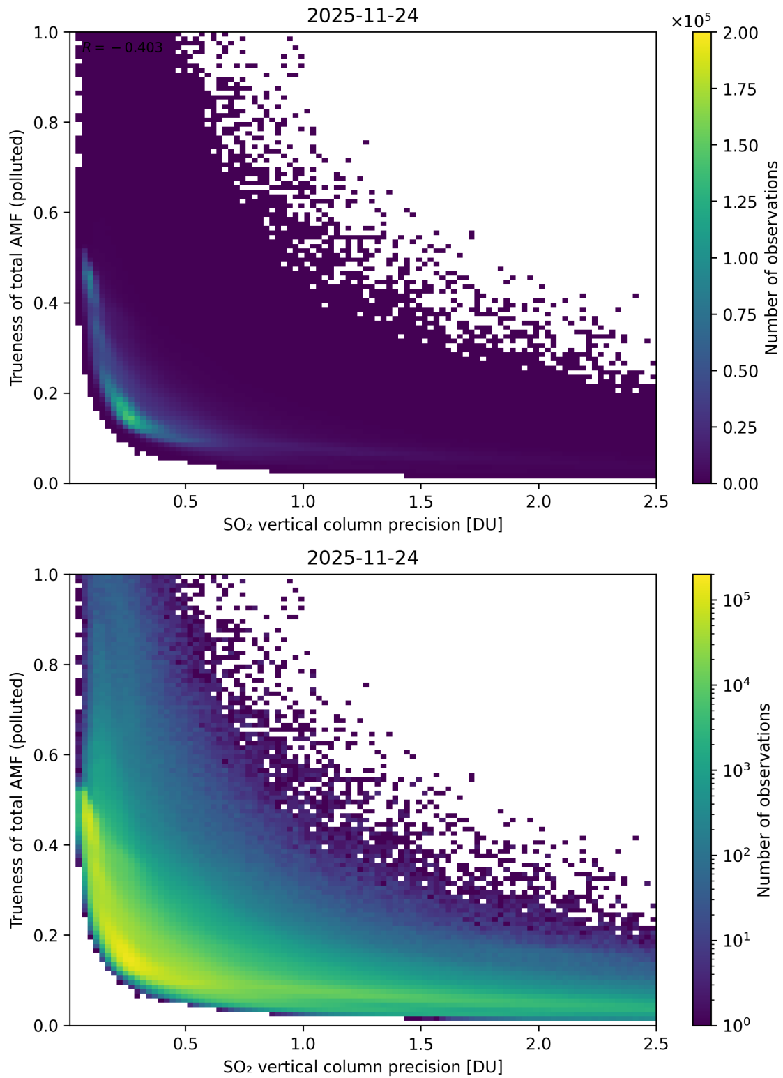
Figure 347: Scatter density plot of “SO 2 vertical column precision” against “Trueness of total AMF (polluted)” for 2025-11-23 to 2025-11-25.
