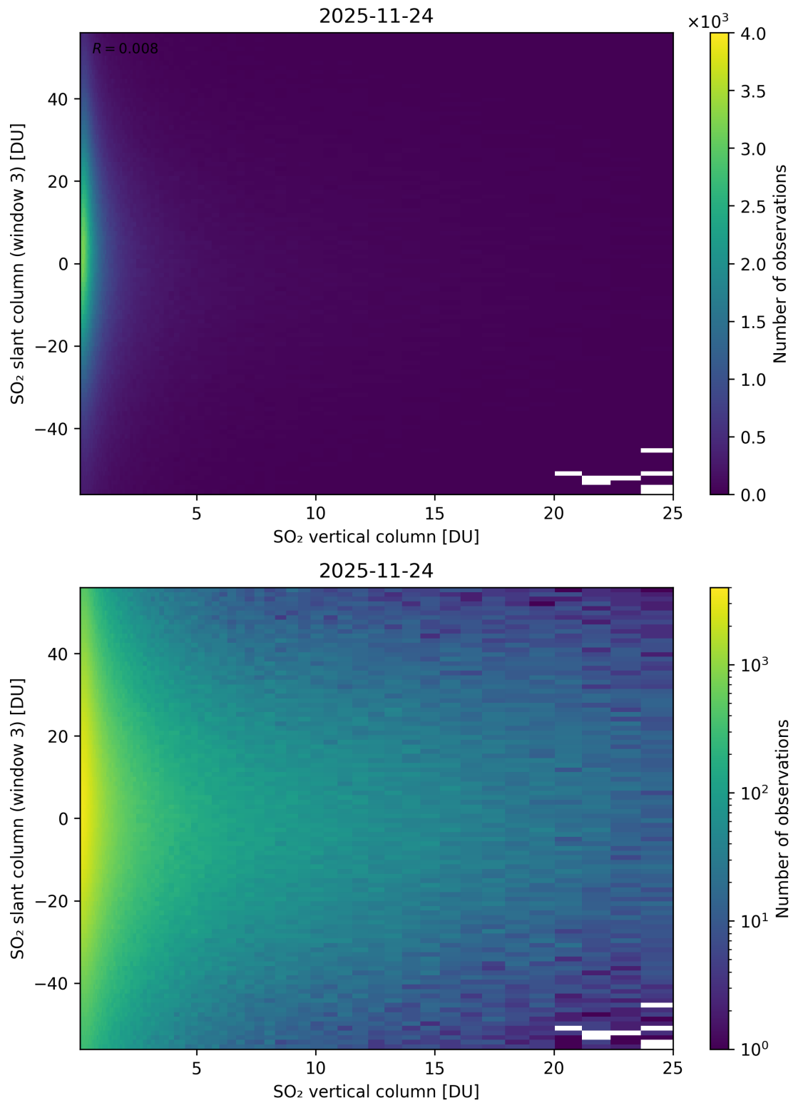
Figure 357: Scatter density plot of “SO 2 vertical column” against “SO 2 slant column (window 3)” for 2025-11-23 to 2025-11-25.
