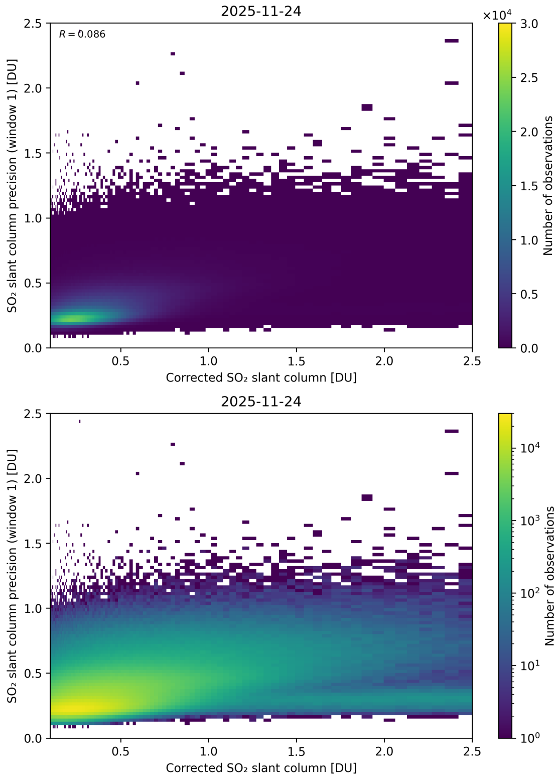
Figure 238: Scatter density plot of “Corrected SO 2 slant column” against “SO 2 slant column precision (window 1)” for 2025-11-23 to 2025-11-25.
