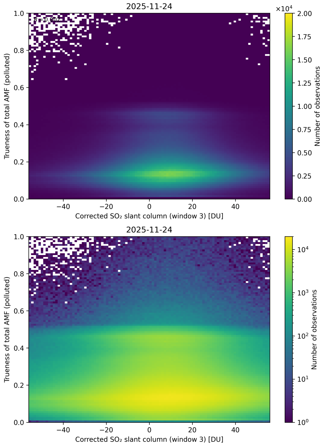
Figure 261: Scatter density plot of “Corrected SO 2 slant column (window 3)” against “Trueness of total AMF (polluted)” for 2025-11-23 to 2025-11-25.
