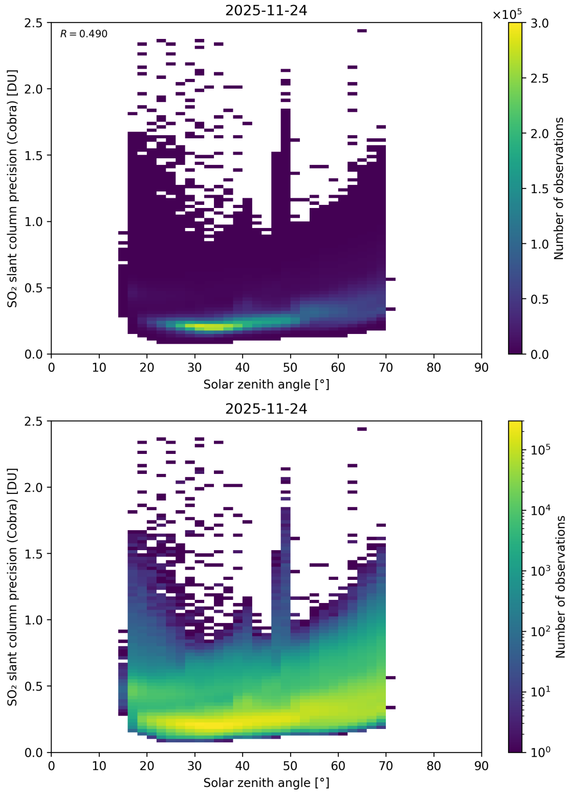
Figure 180: Scatter density plot of “Solar zenith angle” against “SO 2 slant column precision (Cobra)” for 2025-11-23 to 2025-11-25.
