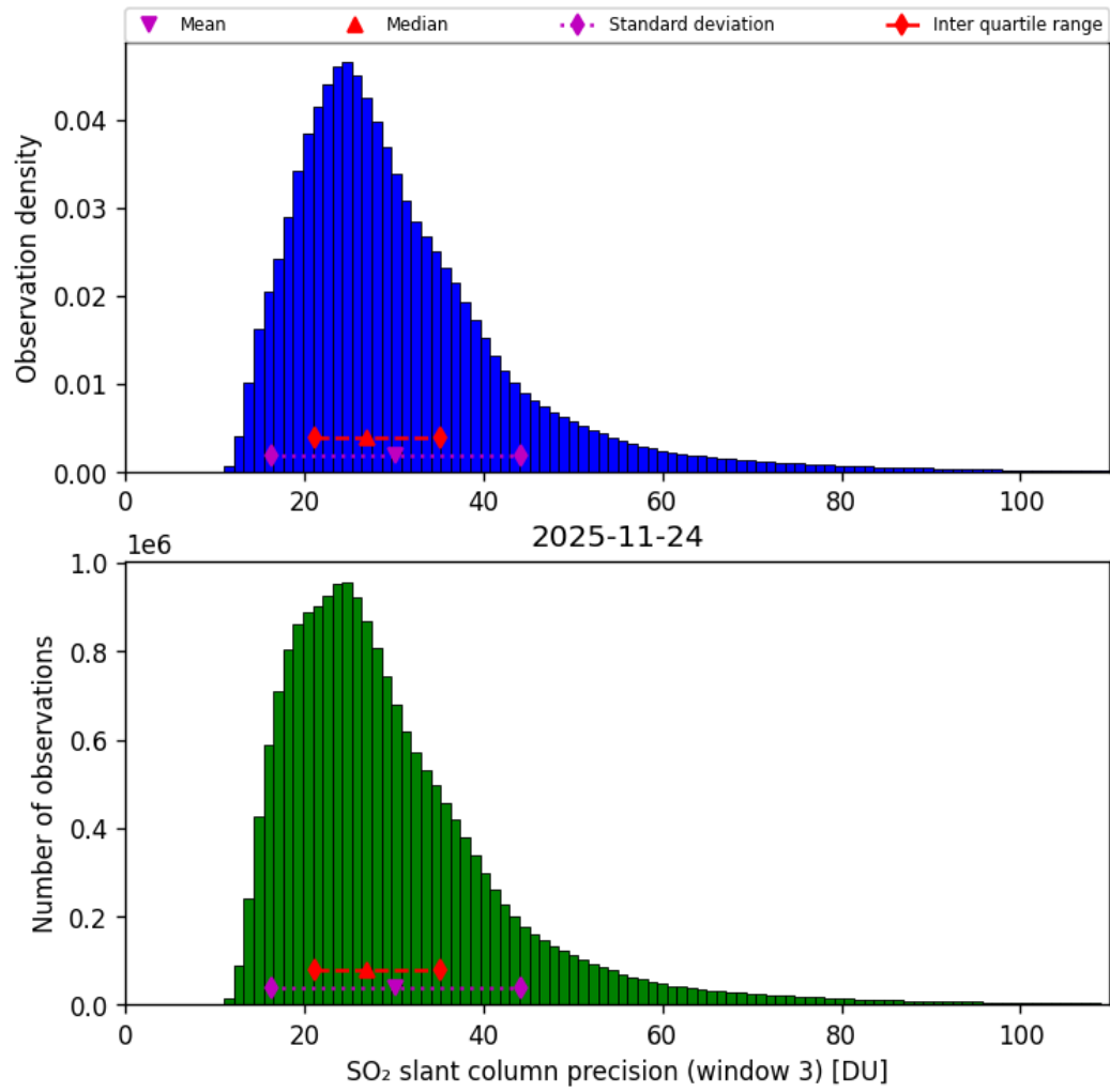
Figure 72: Histogram of “SO 2 slant column precision (window 3)” for 2025-11-23 to 2025-11-25
