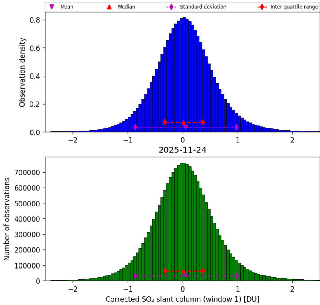
Figure 65: Histogram of “Corrected SO 2 slant column (window 1)” for 2025-11-23 to 2025-11-25
