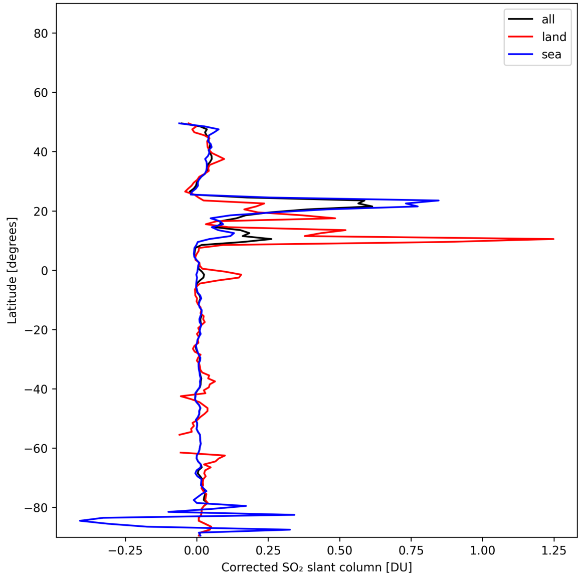
Figure 34: Zonal average of “Corrected SO 2 slant column” for 2025-11-23 to 2025-11-25.
