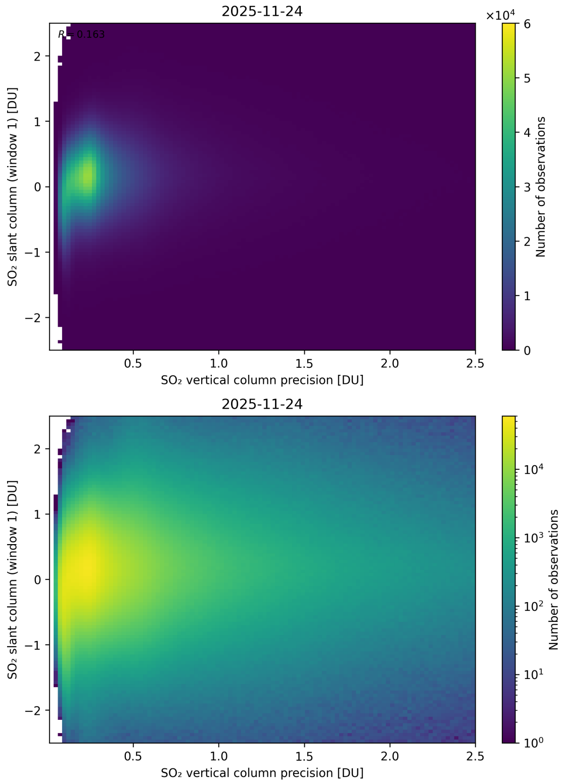
Figure 341: Scatter density plot of “SO 2 vertical column precision” against “SO 2 slant column (window 1)” for 2025-11-23 to 2025-11-25.
