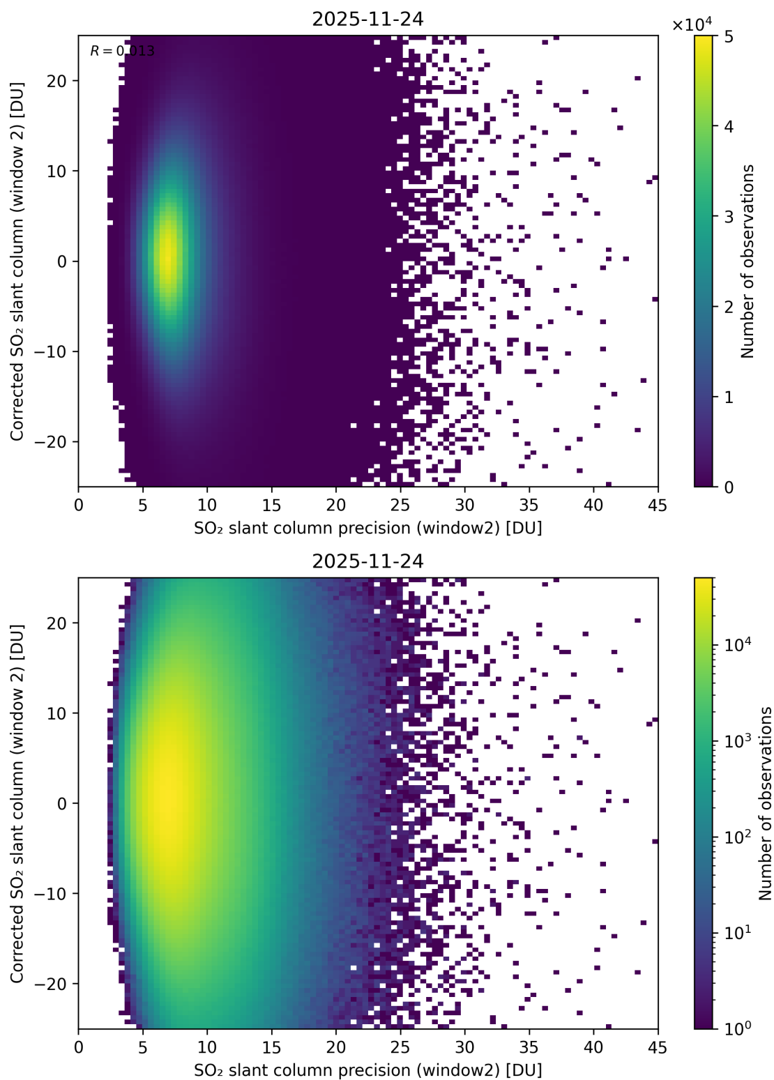
Figure 297: Scatter density plot of “SO 2 slant column precision (window2)” against “Corrected SO 2 slant column (window 2)” for 2025-11-23 to 2025-11-25.
