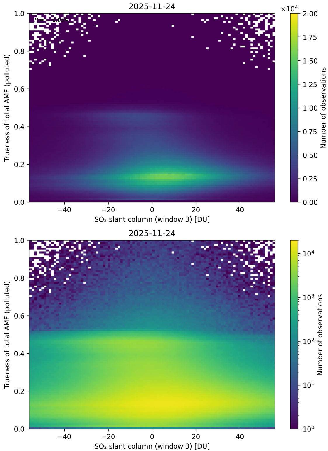
Figure 319: Scatter density plot of “SO 2 slant column (window 3)” against “Trueness of total AMF (polluted)” for 2025-11-23 to 2025-11-25.
