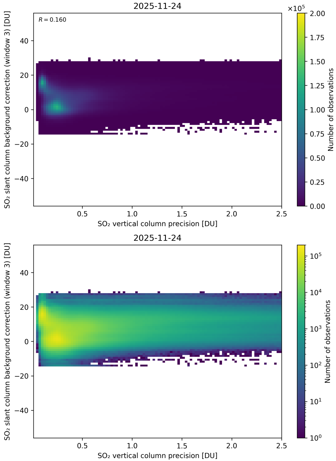
Figure 331: Scatter density plot of “SO 2 vertical column precision” against “SO 2 slant column background correction (window 3)” for 2025-11-23 to 2025-11-25.
