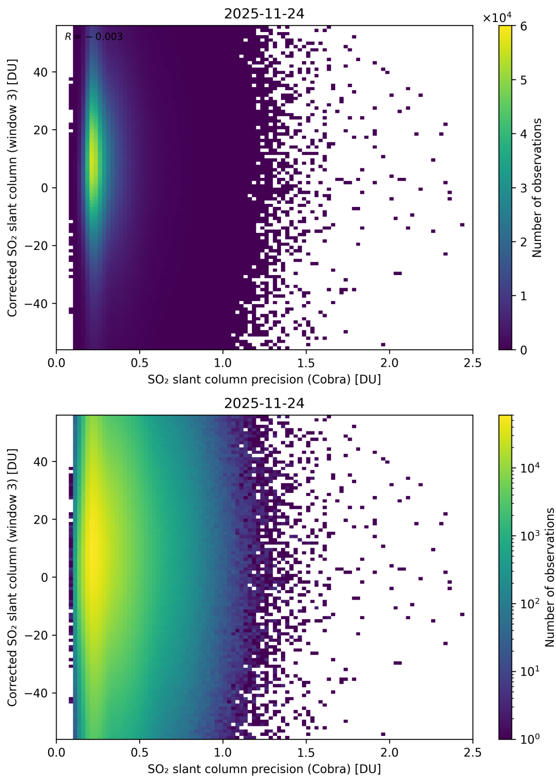
Figure 207: Scatter density plot of “SO 2 slant column precision (Cobra)” against “Corrected SO 2 slant column (window 3)” for 2025-11-23 to 2025-11-25.
