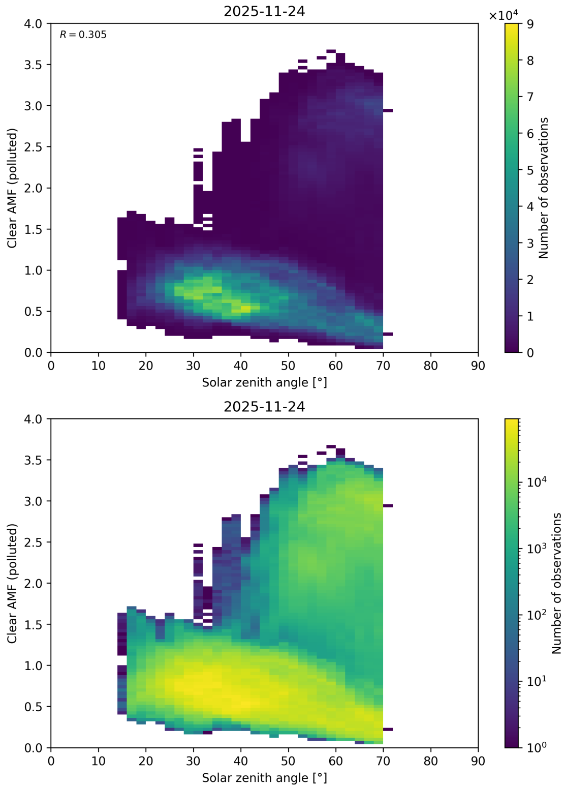
Figure 178: Scatter density plot of “Solar zenith angle” against “Clear AMF (polluted)” for 2025-11-23 to 2025-11-25.
