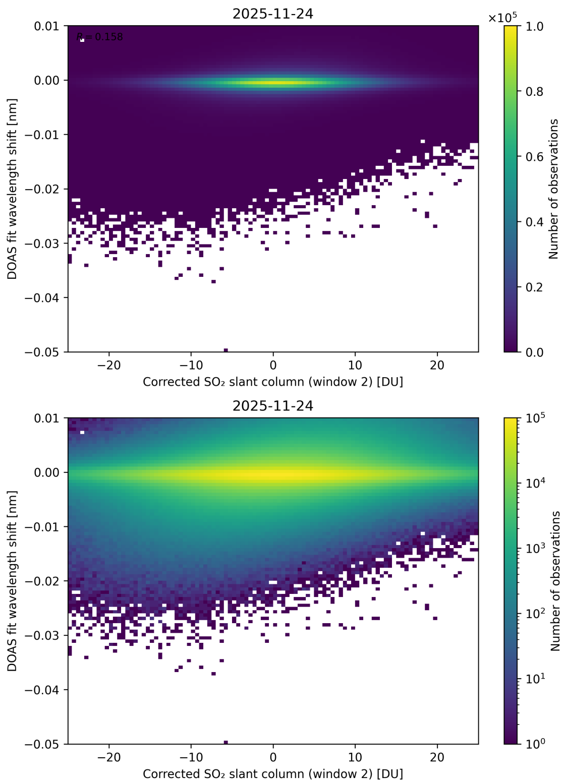
Figure 246: Scatter density plot of “Corrected SO 2 slant column (window 2)” against “DOAS fit wavelength shift” for 2025-11-23 to 2025-11-25.
