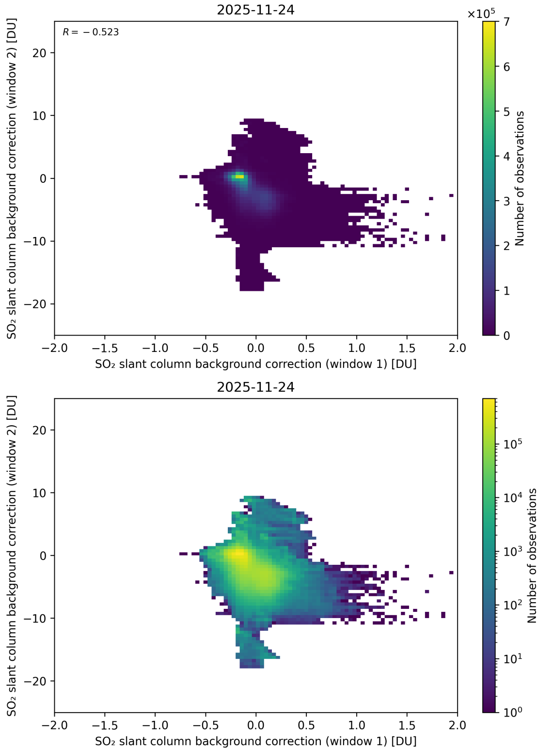
Figure 109: Scatter density plot of “SO 2 slant column background correction (window 1)” against “SO 2 slant column background correction (window 2)” for 2025-11-23 to 2025-11-25.
