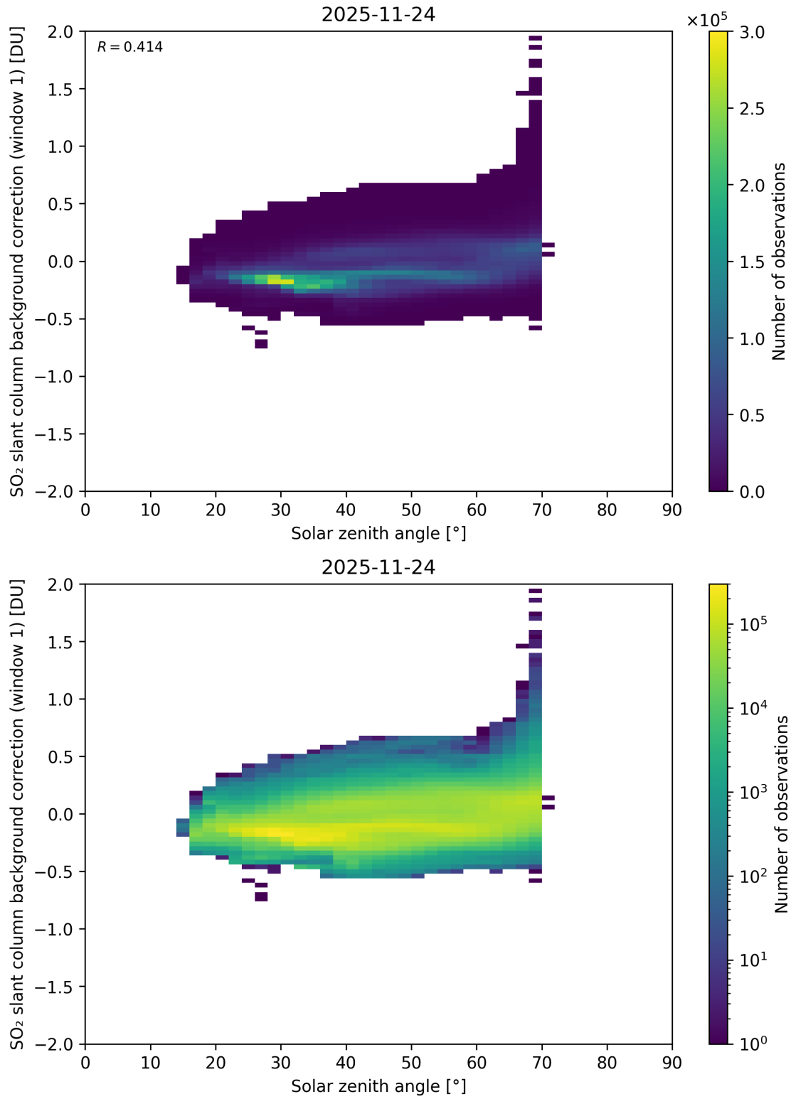
Figure 171: Scatter density plot of “Solar zenith angle” against “SO 2 slant column background correction (window 1)” for 2025-11-23 to 2025-11-25.
