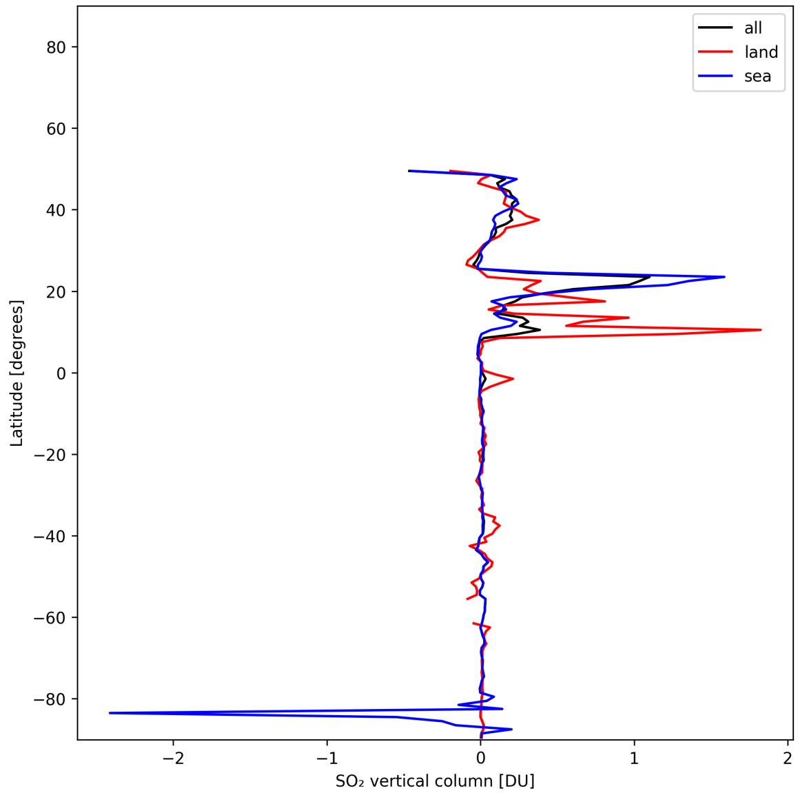
Figure 32: Zonal average of “SO 2 vertical column” for 2025-11-23 to 2025-11-25.
