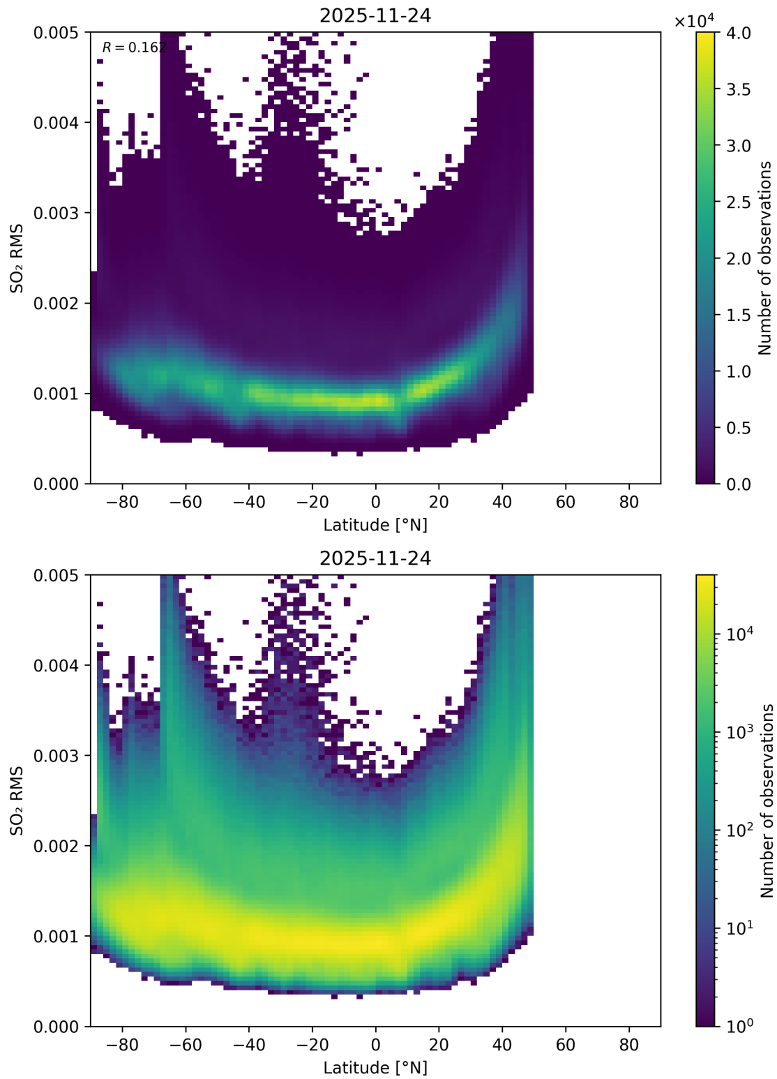
Figure 155: Scatter density plot of “Latitude” against “SO 2 RMS” for 2025-11-23 to 2025-11-25.
