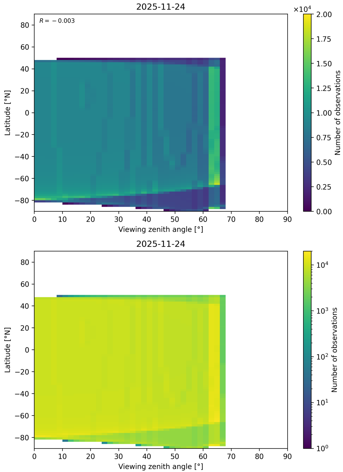
Figure 368: Scatter density plot of “Viewing zenith angle” against “Latitude” for 2025-11-23 to 2025-11-25.
