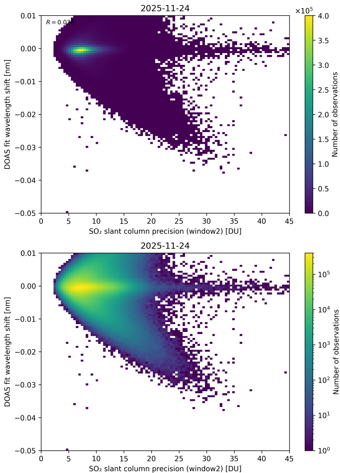
Figure 293: Scatter density plot of “SO 2 slant column precision (window2)” against “DOAS fit wavelength shift” for 2025-11-23 to 2025-11-25.
