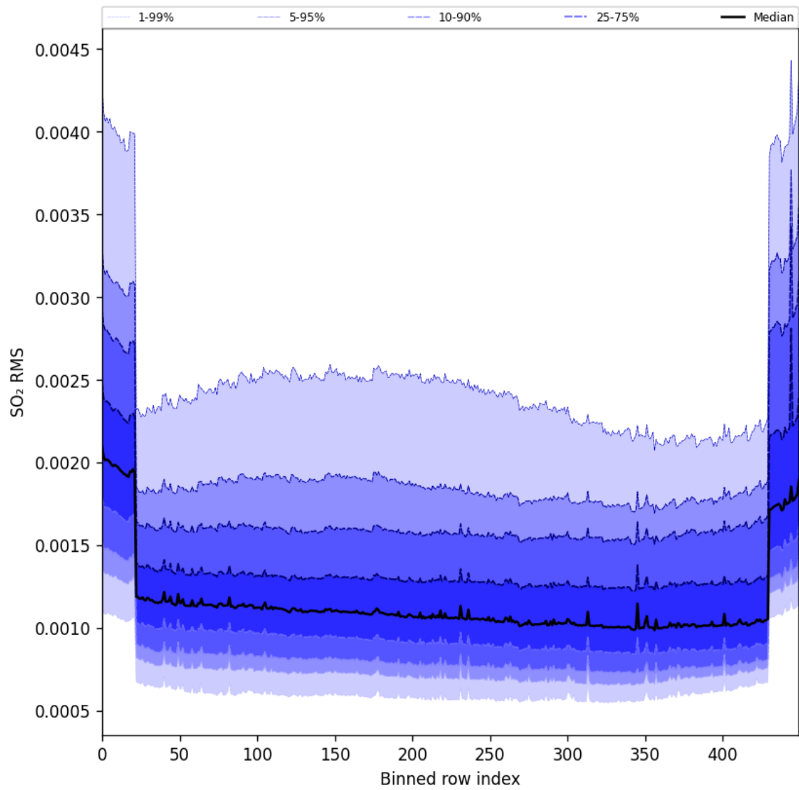
Figure 104: Along track statistics of “SO 2 RMS” for 2025-11-23 to 2025-11-25
