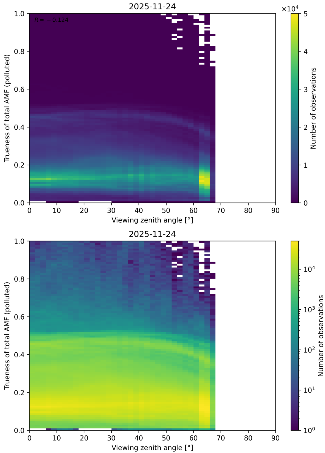
Figure 382: Scatter density plot of “Viewing zenith angle” against “Trueness of total AMF (polluted)” for 2025-11-23 to 2025-11-25.
