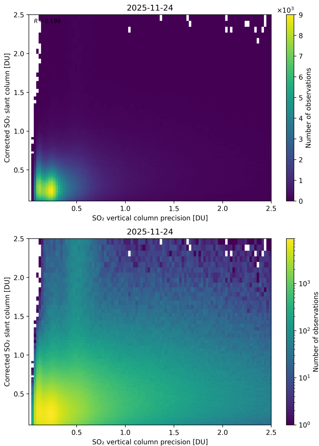
Figure 338: Scatter density plot of “SO 2 vertical column precision” against “Corrected SO 2 slant column” for 2025-11-23 to 2025-11-25.
