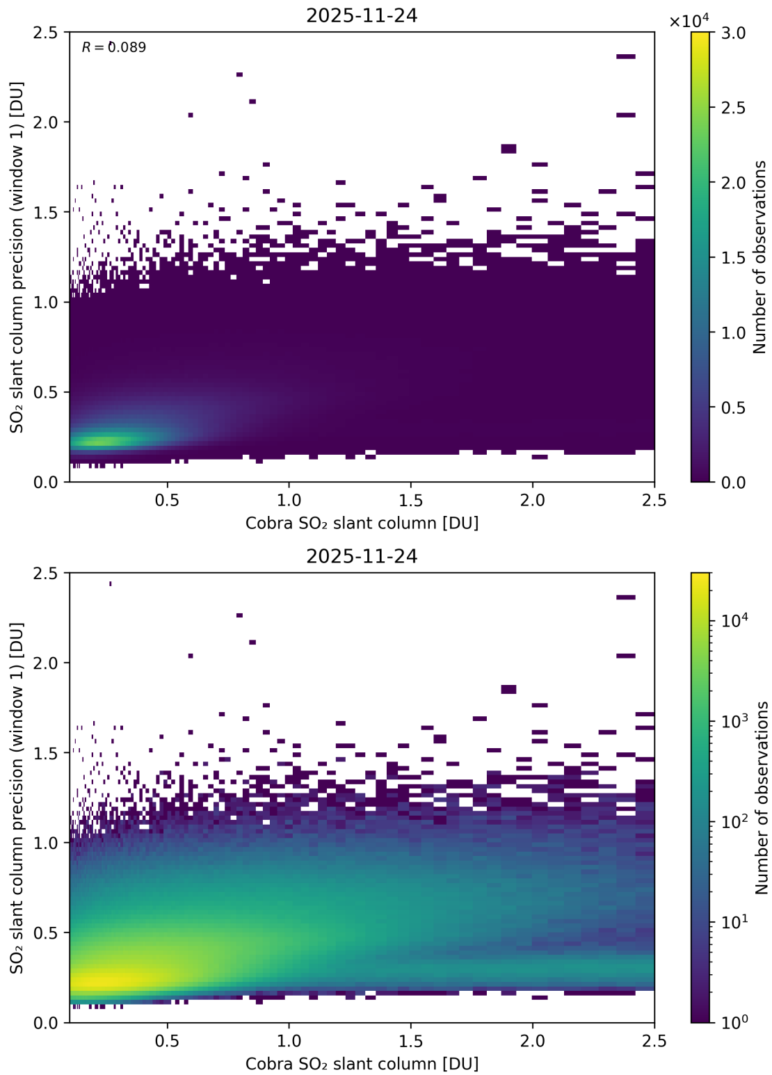
Figure 220: Scatter density plot of “Cobra SO 2 slant column” against “SO 2 slant column precision (window 1)” for 2025-11-23 to 2025-11-25.
