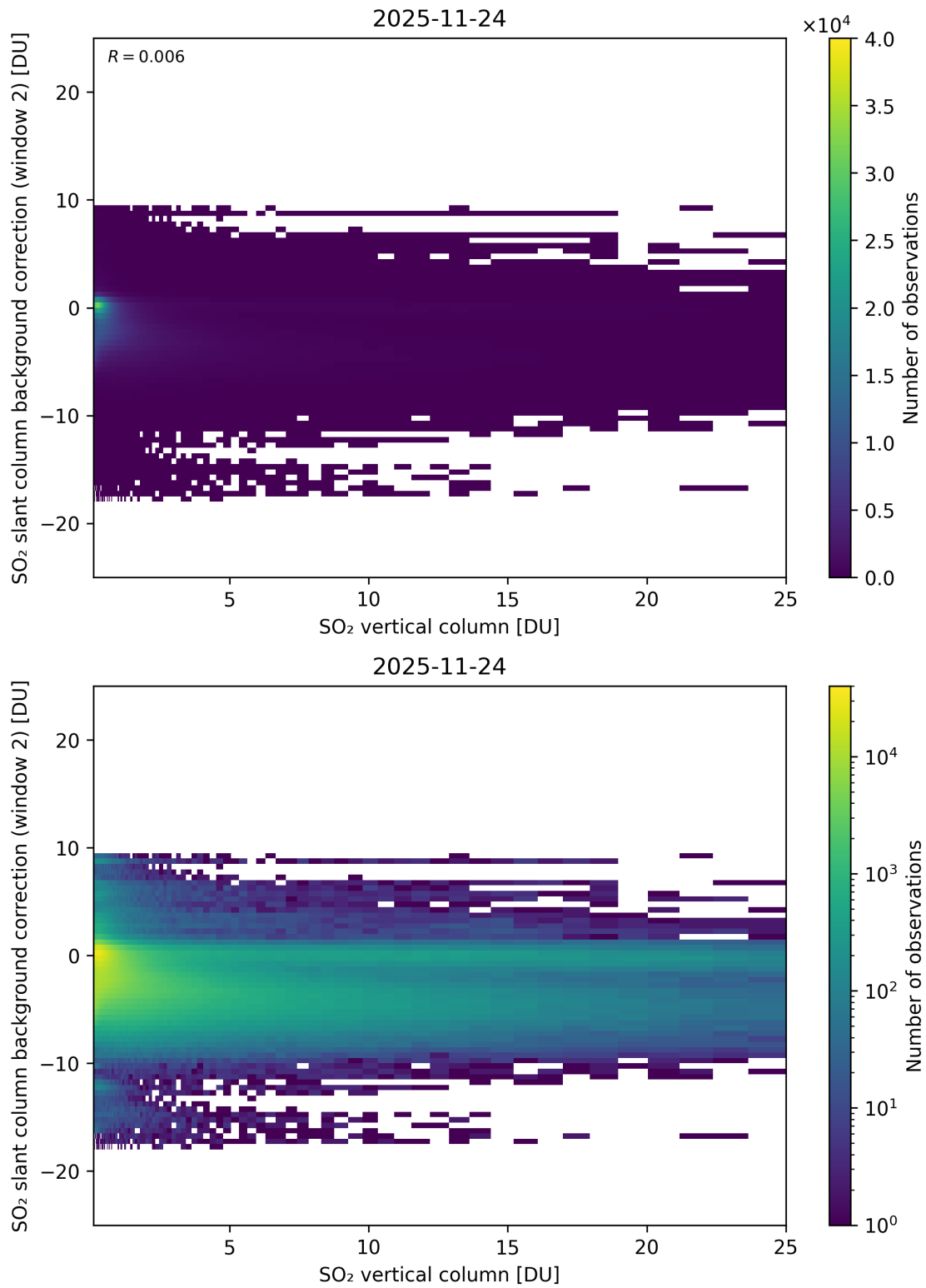
Figure 324: Scatter density plot of “SO 2 vertical column” against “SO 2 slant column background correction (window 2)” for 2025-11-23 to 2025-11-25.
