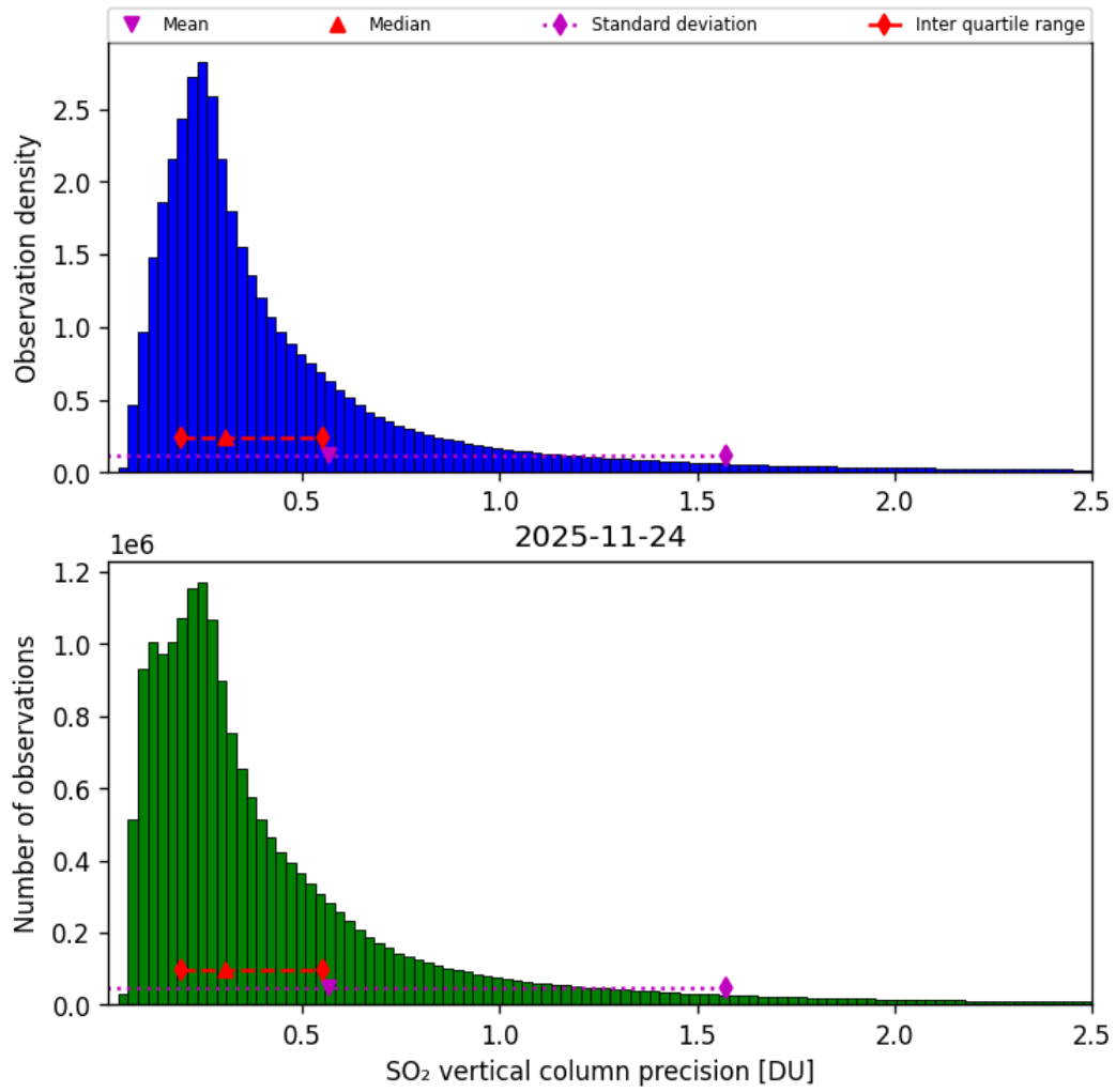
Figure 59: Histogram of “SO 2 vertical column precision” for 2025-11-23 to 2025-11-25
