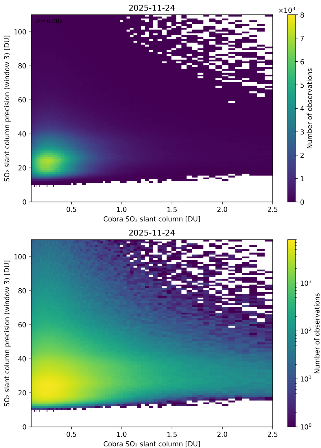
Figure 223: Scatter density plot of “Cobra SO 2 slant column” against “SO 2 slant column precision (window 3)” for 2025-11-23 to 2025-11-25.
