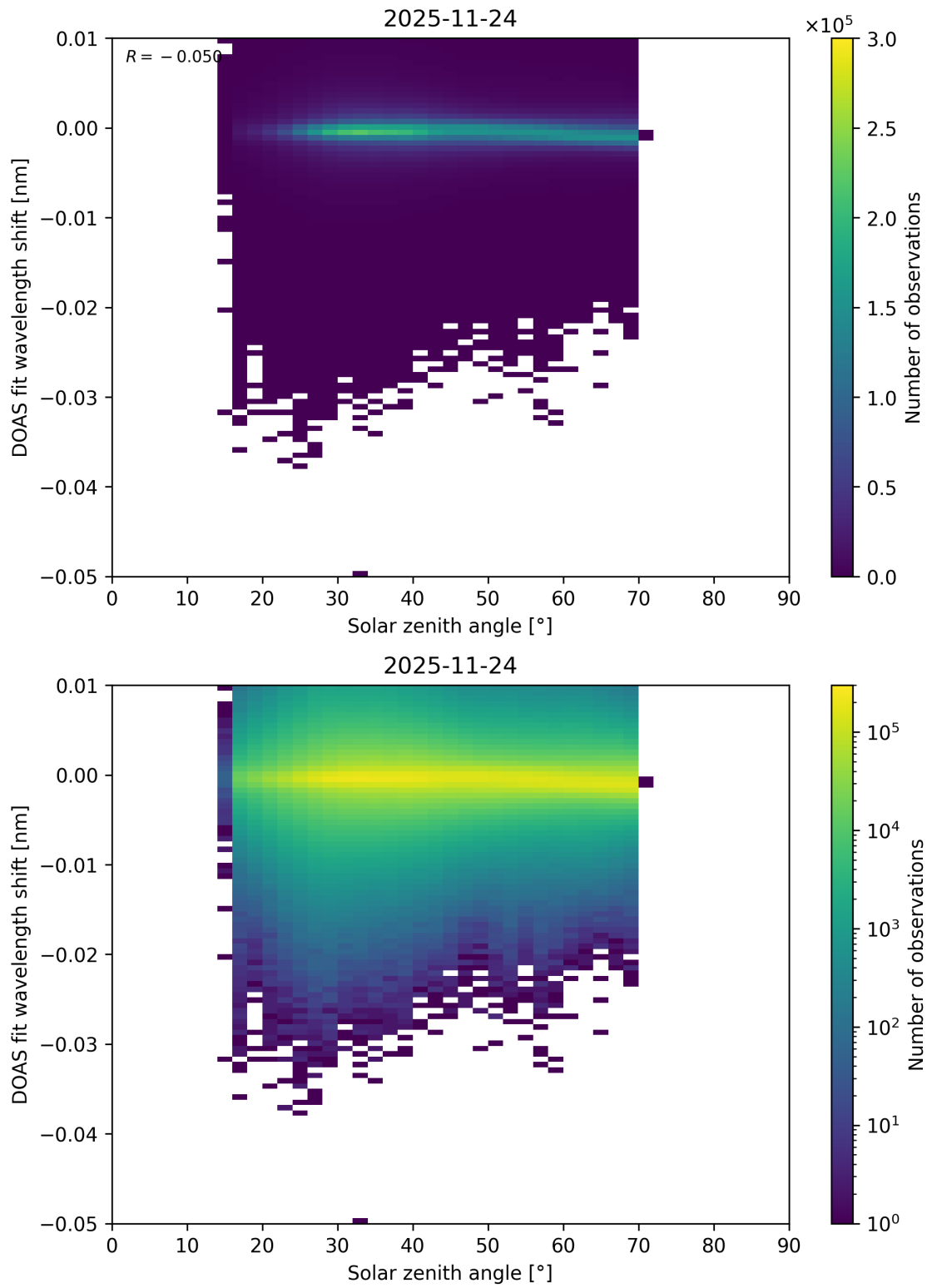
Figure 174: Scatter density plot of “Solar zenith angle” against “DOAS fit wavelength shift” for 2025-11-23 to 2025-11-25.
