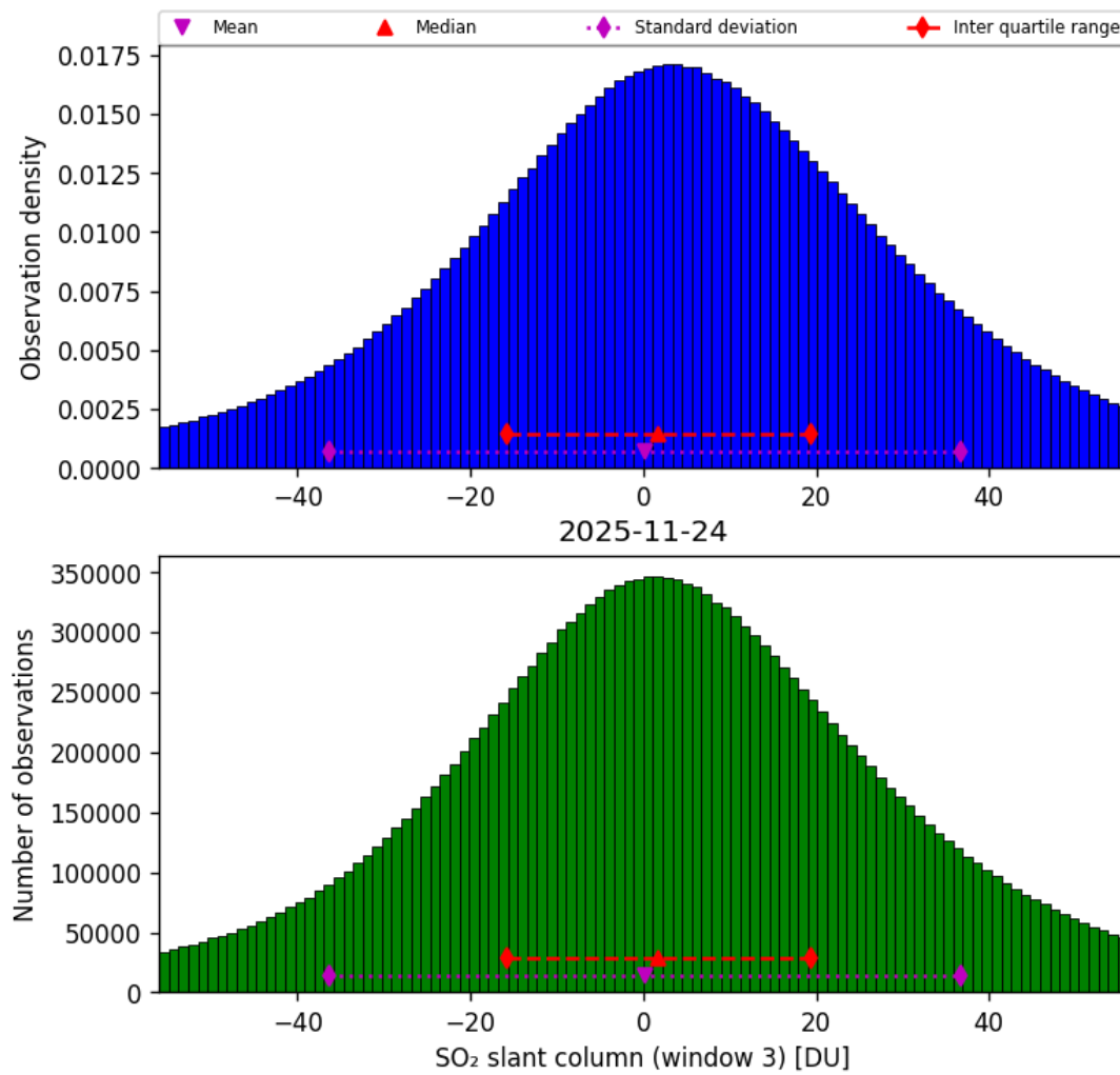
Figure 71: Histogram of “SO 2 slant column (window 3)” for 2025-11-23 to 2025-11-25
