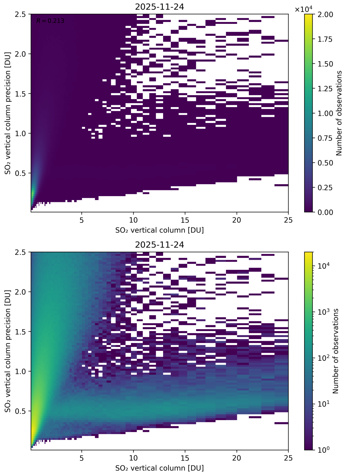
Figure 361: Scatter density plot of “SO 2 vertical column” against “SO 2 vertical column precision” for 2025-11-23 to 2025-11-25.
