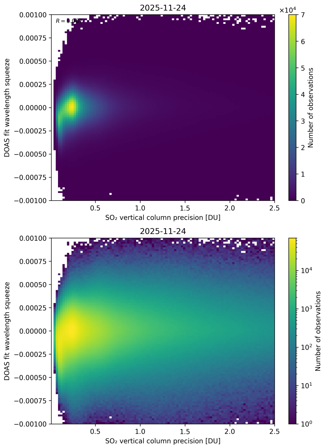
Figure 333: Scatter density plot of “SO 2 vertical column precision” against “DOAS fit wavelength squeeze” for 2025-11-23 to 2025-11-25.
