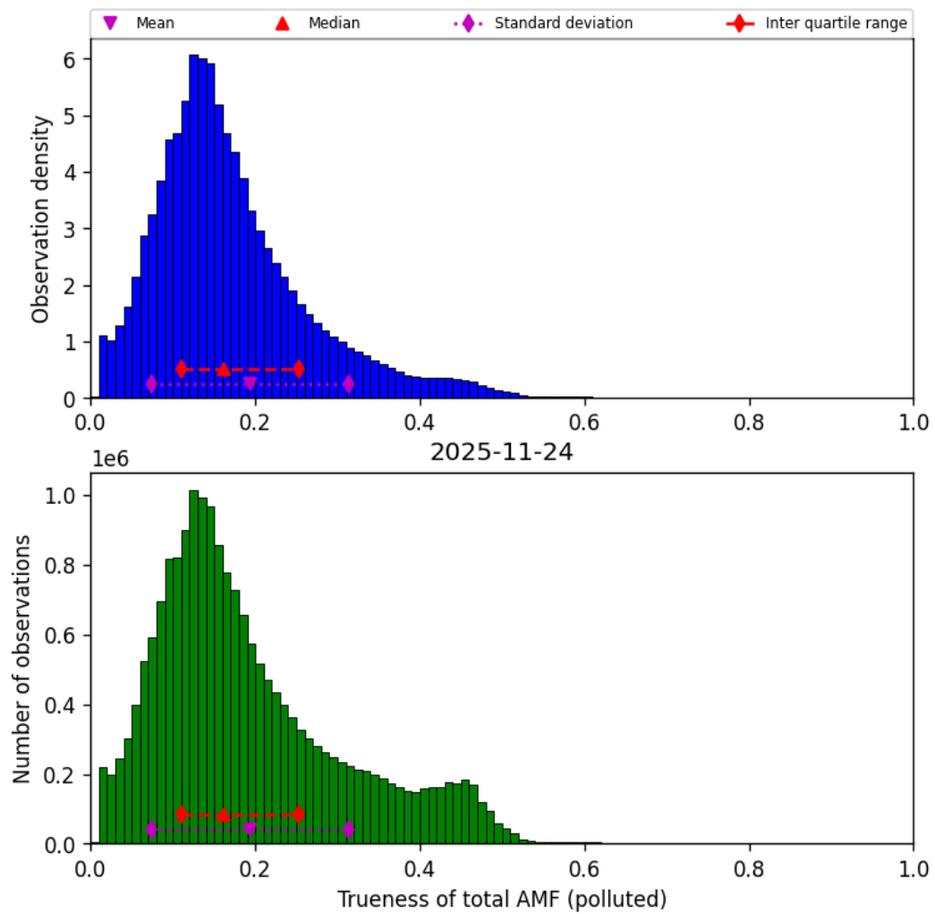
Figure 80: Histogram of “Trueness of total AMF (polluted)” for 2025-11-23 to 2025-11-25
