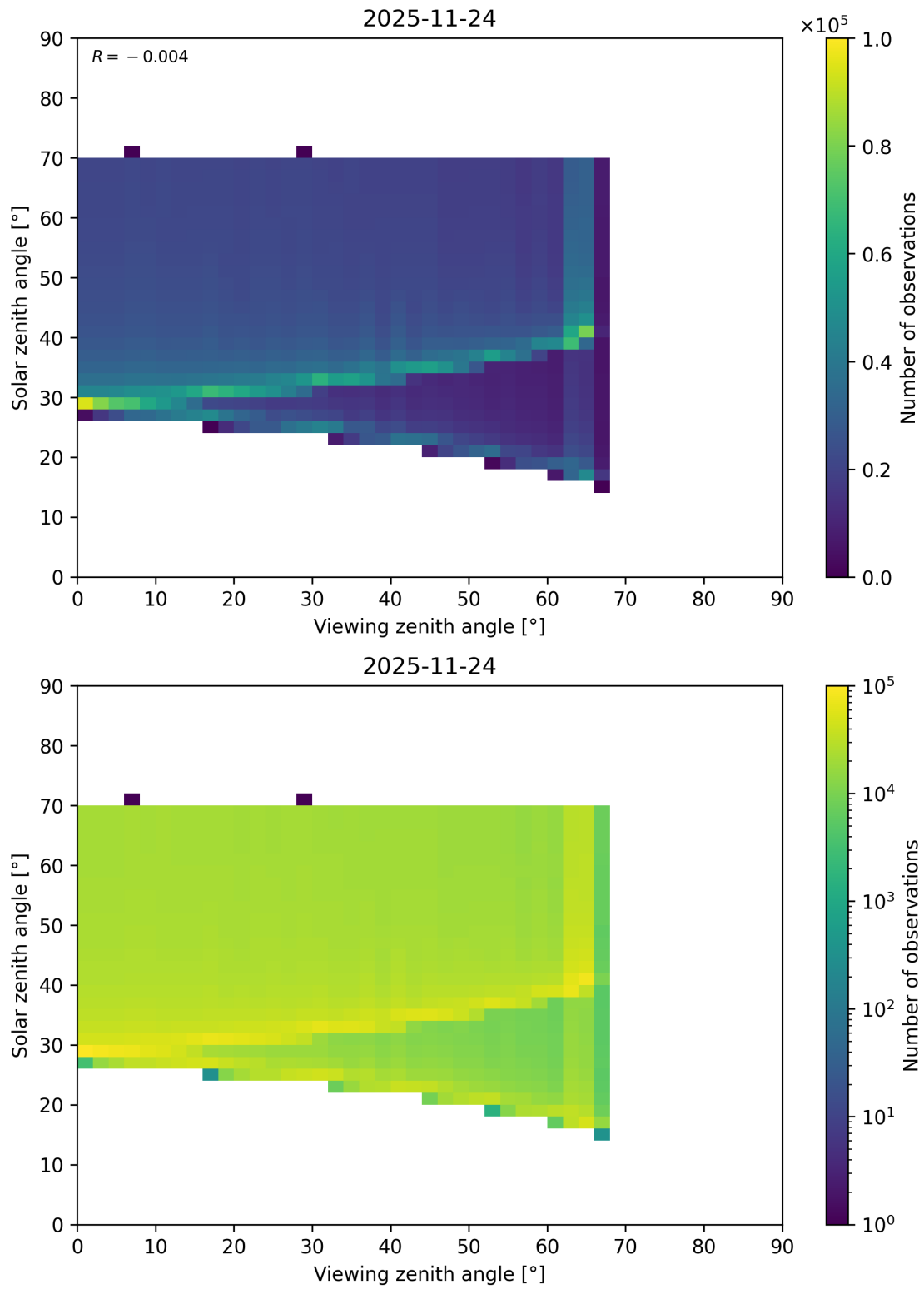
Figure 369: Scatter density plot of “Viewing zenith angle” against “Solar zenith angle” for 2025-11-23 to 2025-11-25.
