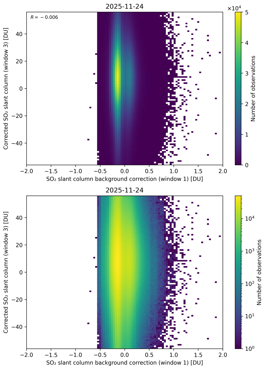
Figure 116: Scatter density plot of “SO 2 slant column background correction (window 1)” against “Corrected SO 2 slant column (window 3)” for 2025-11-23 to 2025-11-25.
