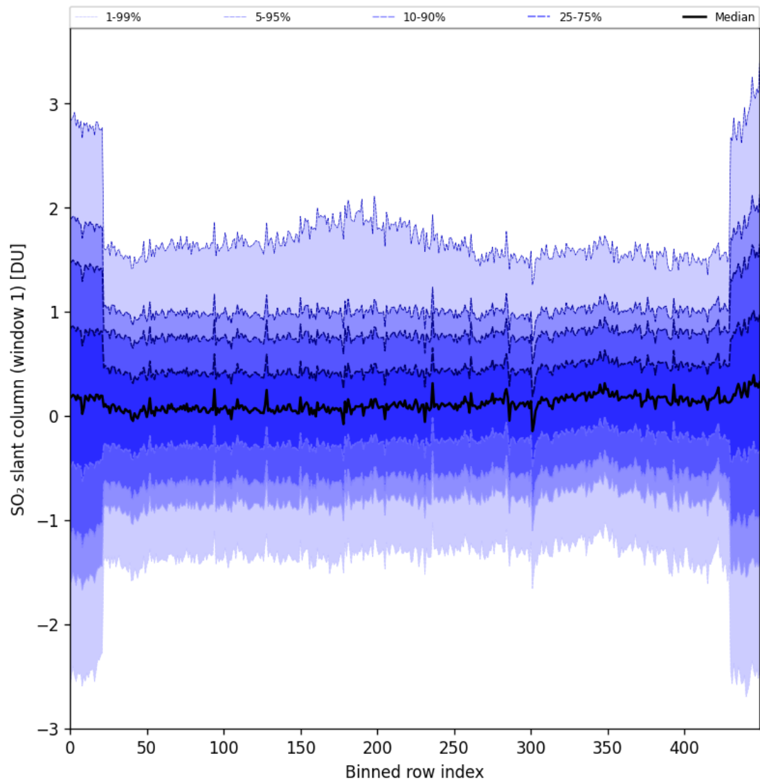
Figure 89: Along track statistics of "SO 2 slant column (window 1)" for 2025-11-23 to 2025-11-25
