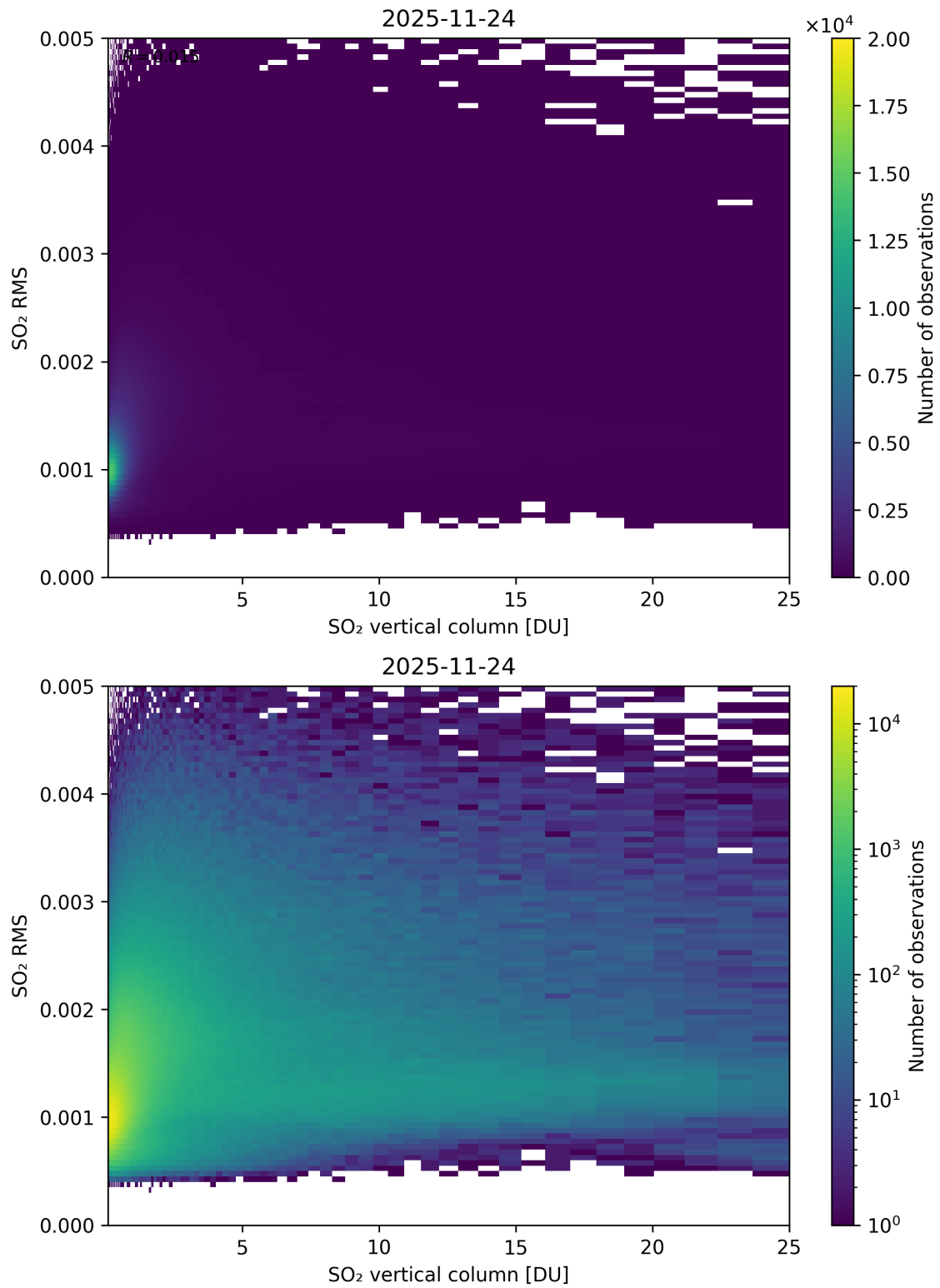
Figure 328: Scatter density plot of “SO 2 vertical column” against “SO 2 RMS” for 2025-11-23 to 2025-11-25.
