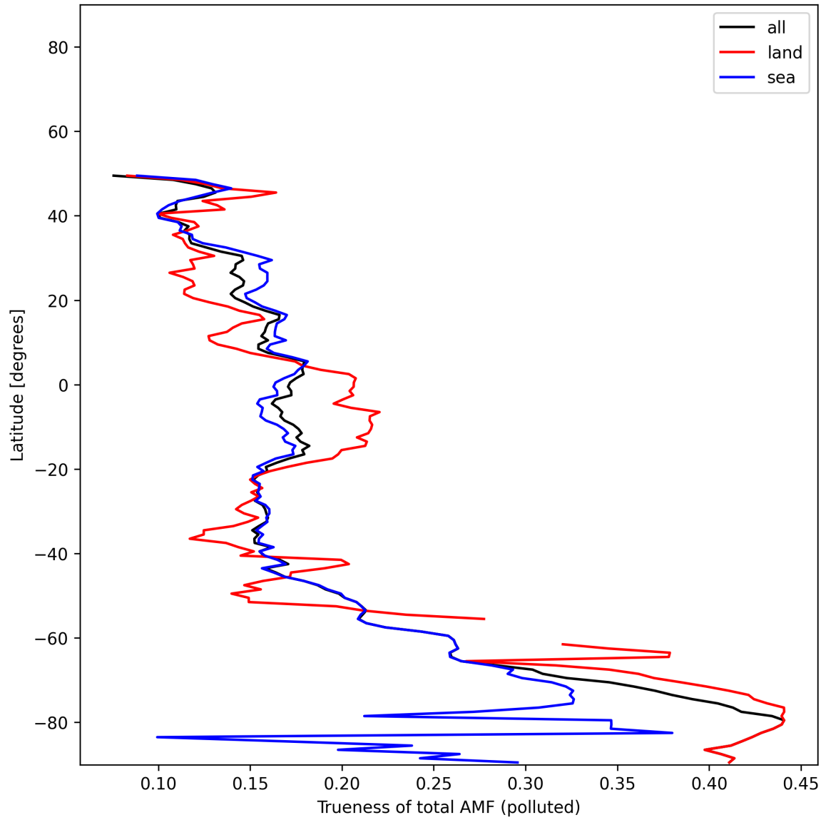
Figure 54: Zonal average of “Trueness of total AMF (polluted)” for 2025-11-23 to 2025-11-25.
