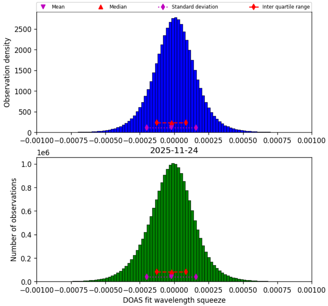
Figure 77: Histogram of “DOAS fit wavelength squeeze” for 2025-11-23 to 2025-11-25
