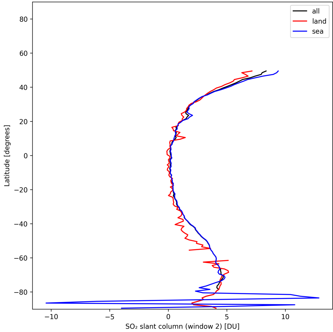
Figure 41: Zonal average of “SO 2 slant column (window 2)” for 2025-11-23 to 2025-11-25.
