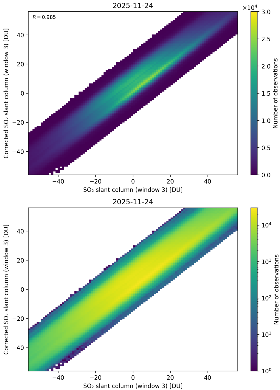
Figure 316: Scatter density plot of “SO 2 slant column (window 3)” against “Corrected SO 2 slant column (window 3)” for 2025-11-23 to 2025-11-25.
