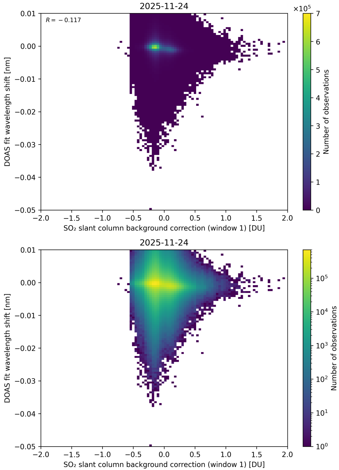
Figure 111: Scatter density plot of “SO 2 slant column background correction (window 1)” against “DOAS fit wavelength shift” for 2025-11-23 to 2025-11-25.
