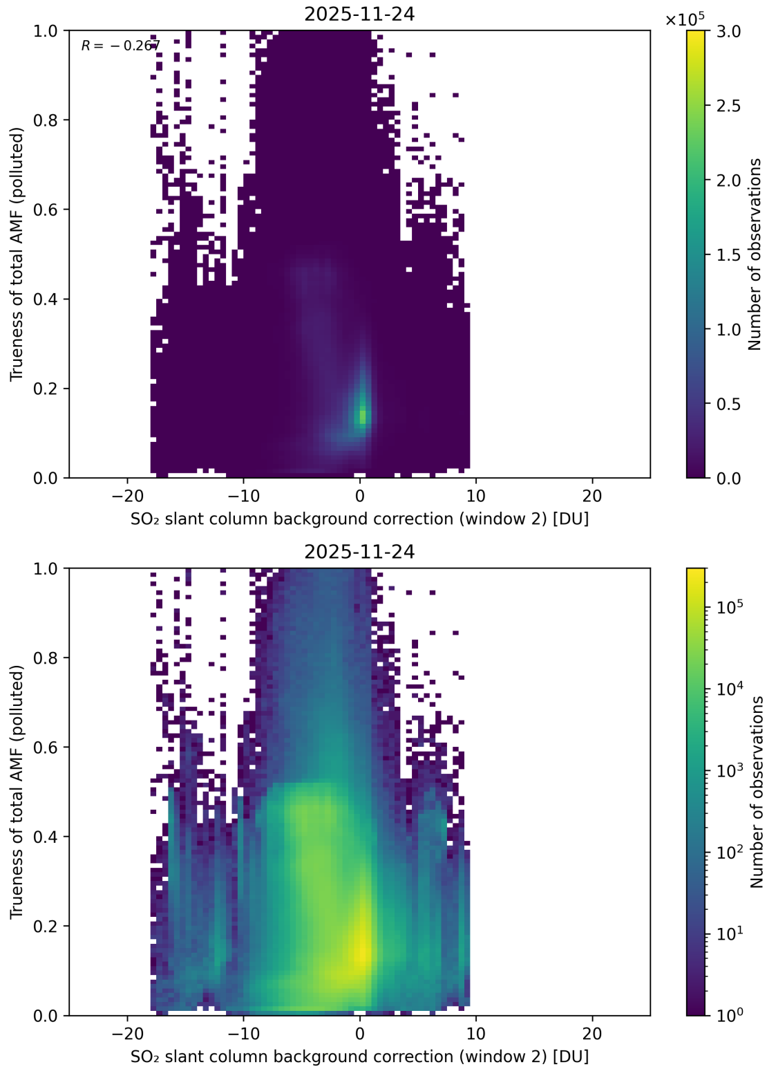
Figure 131: Scatter density plot of “SO 2 slant column background correction (window 2)” against “Trueness of total AMF (polluted)” for 2025-11-23 to 2025-11-25.
