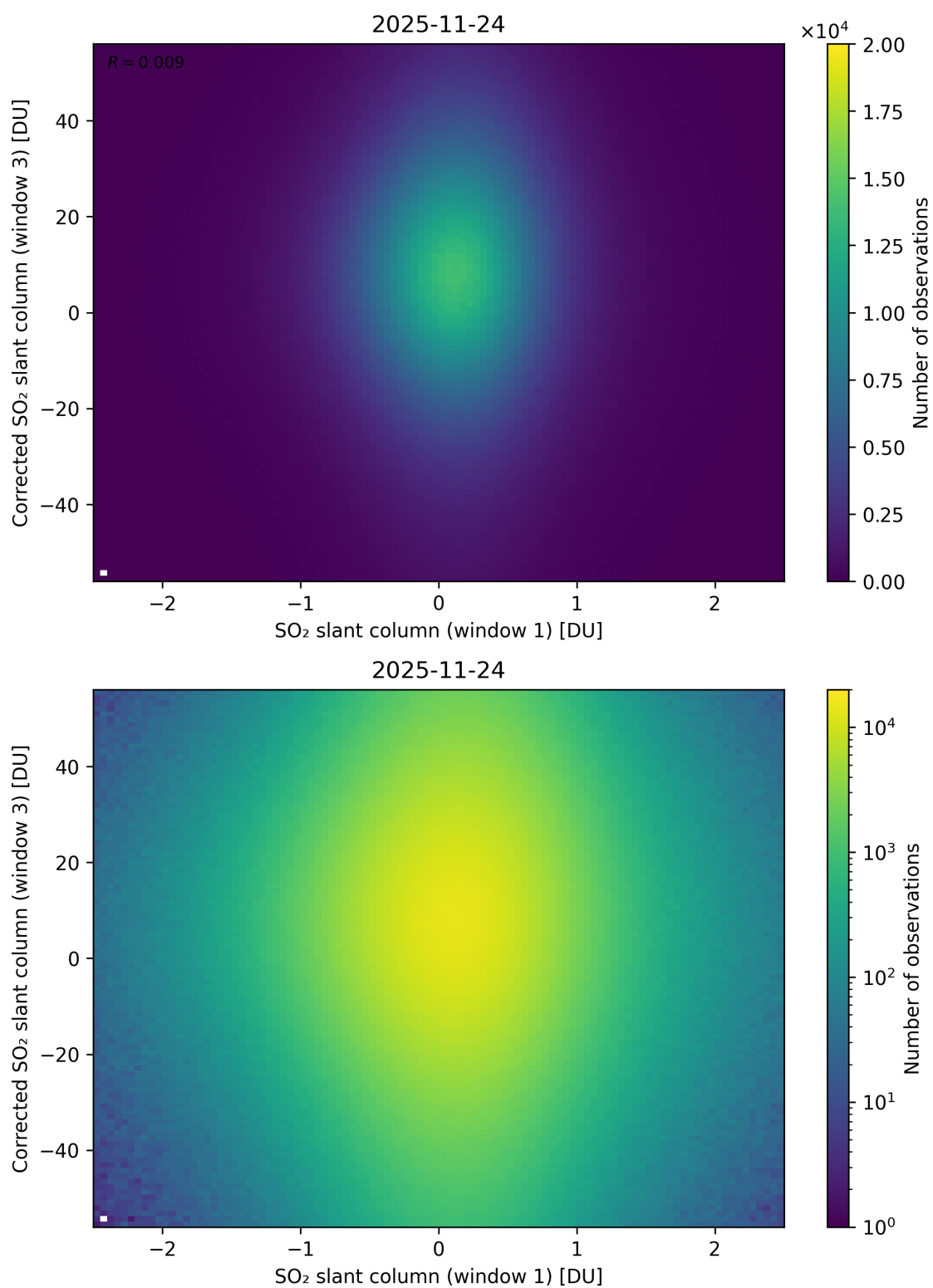
Figure 284: Scatter density plot of “SO 2 slant column (window 1)” against “Corrected SO 2 slant column (window 3)” for 2025-11-23 to 2025-11-25.
