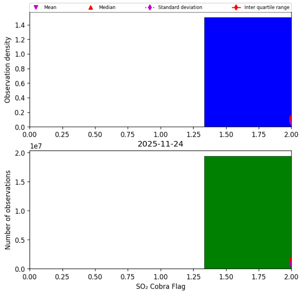
Figure 75: Histogram of “SO 2 Cobra Flag” for 2025-11-23 to 2025-11-25
