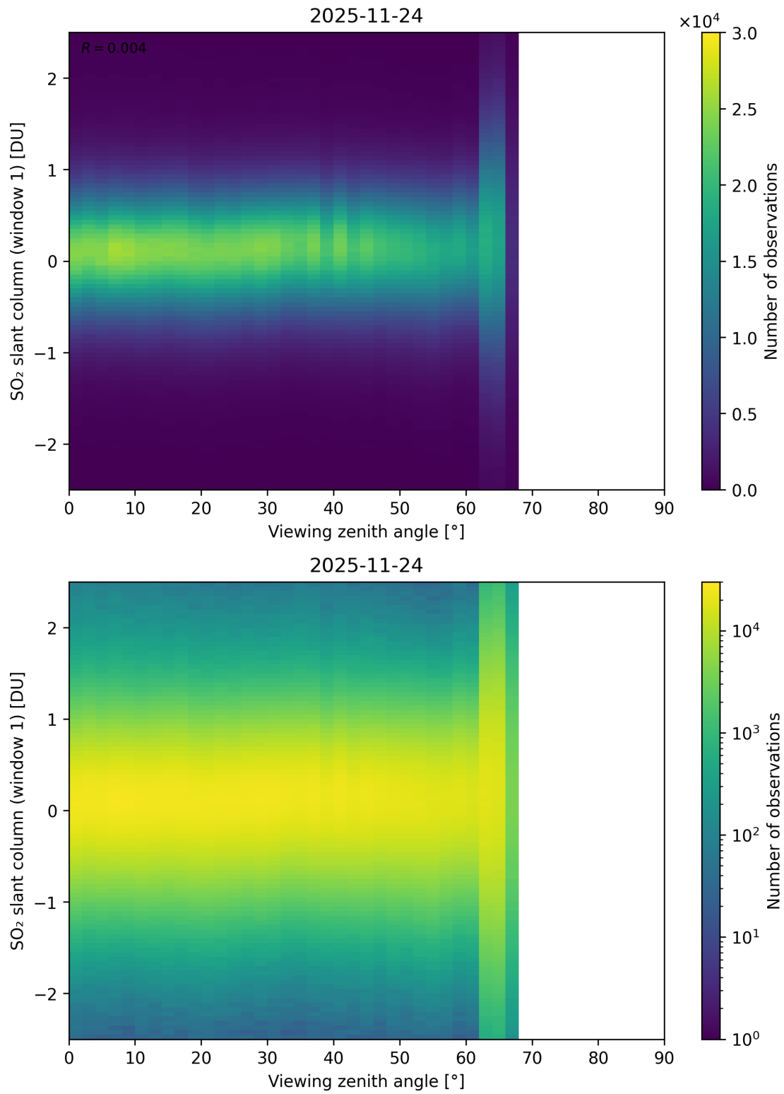
Figure 376: Scatter density plot of “Viewing zenith angle” against “SO 2 slant column (window 1)” for 2025-11-23 to 2025-11-25.
