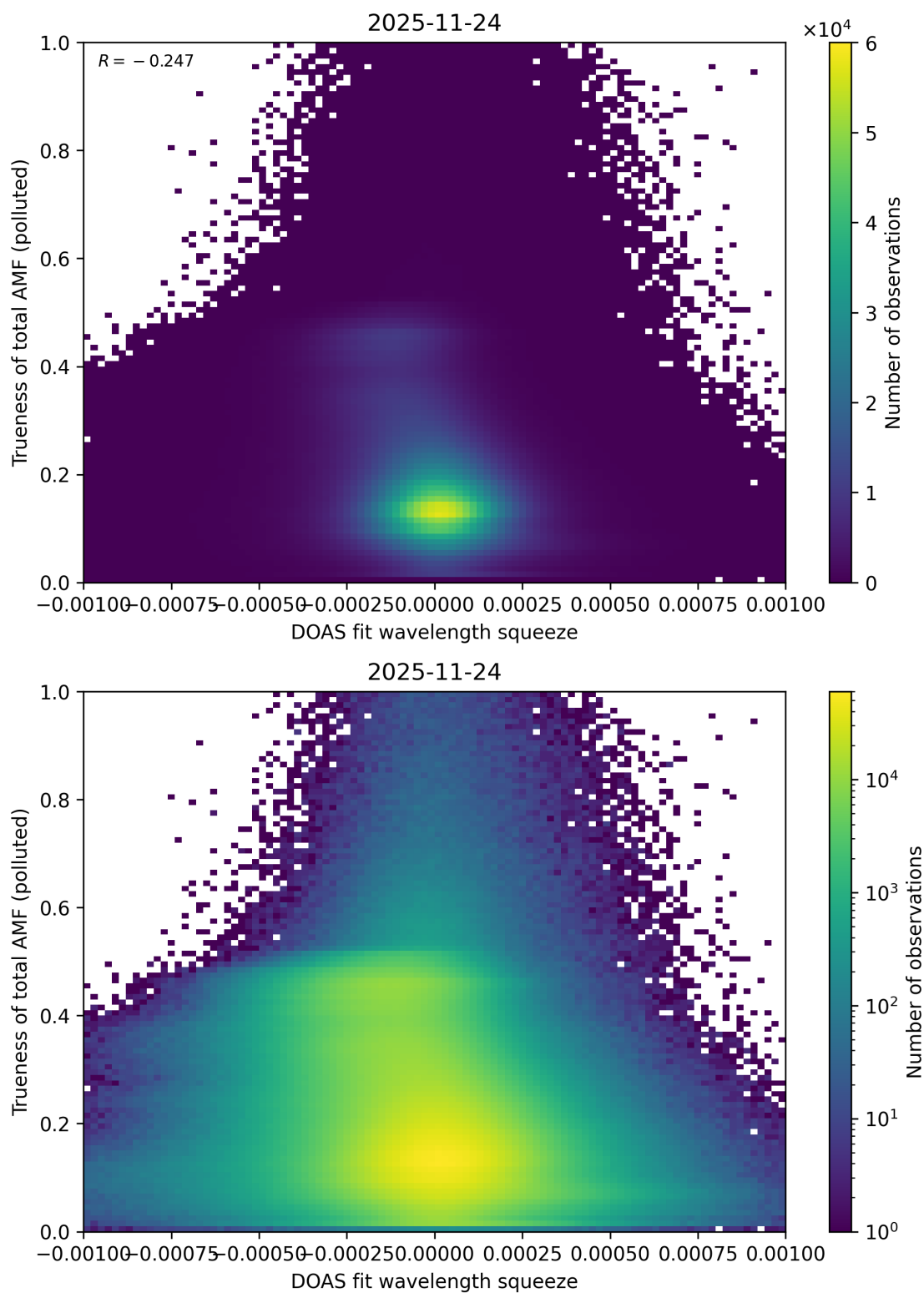
Figure 146: Scatter density plot of “DOAS fit wavelength squeeze” against “Trueness of total AMF (polluted)” for 2025-11-23 to 2025-11-25.
