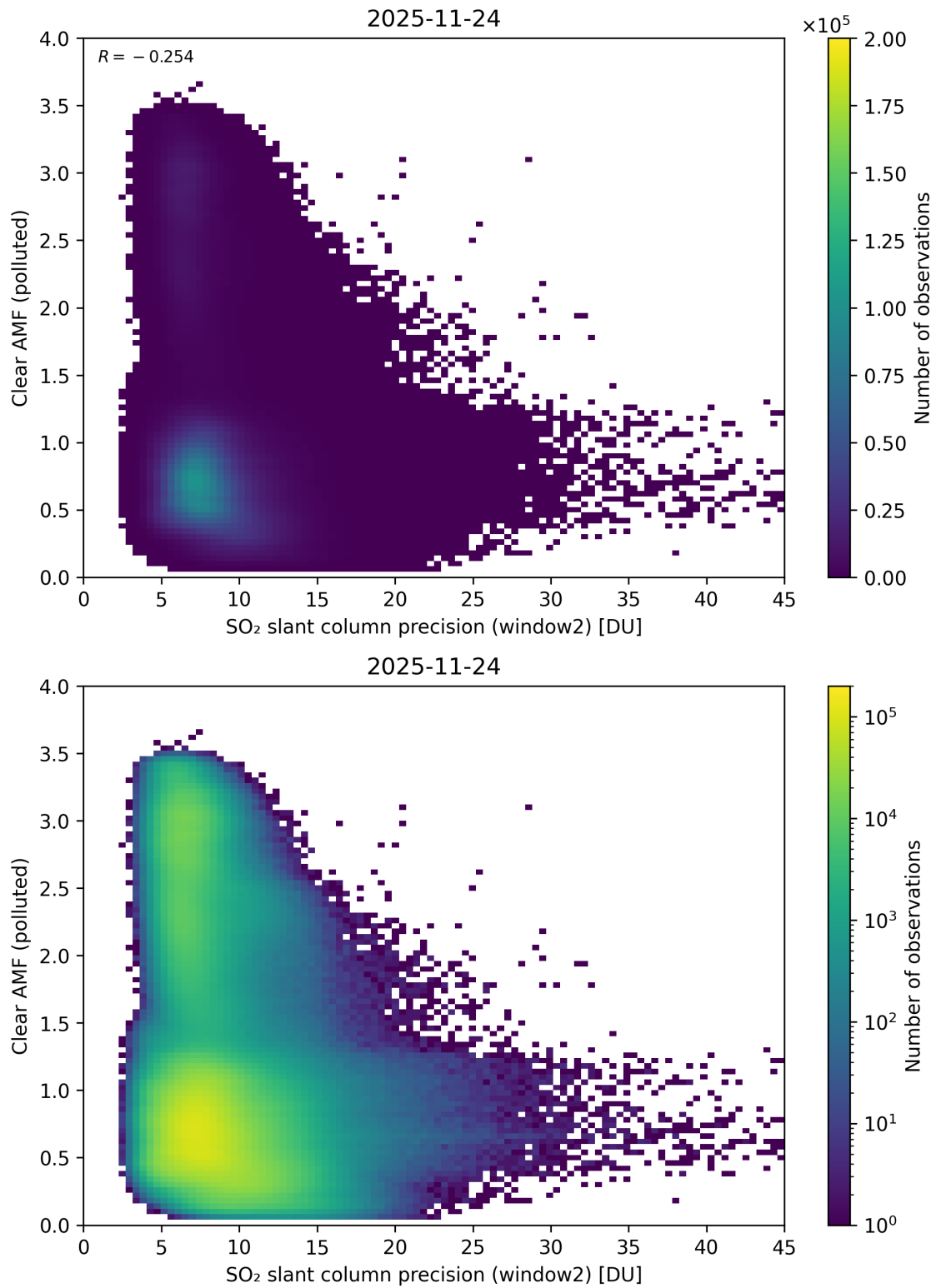
Figure 296: Scatter density plot of “SO 2 slant column precision (window2)” against “Clear AMF (polluted)” for 2025-11-23 to 2025-11-25.
