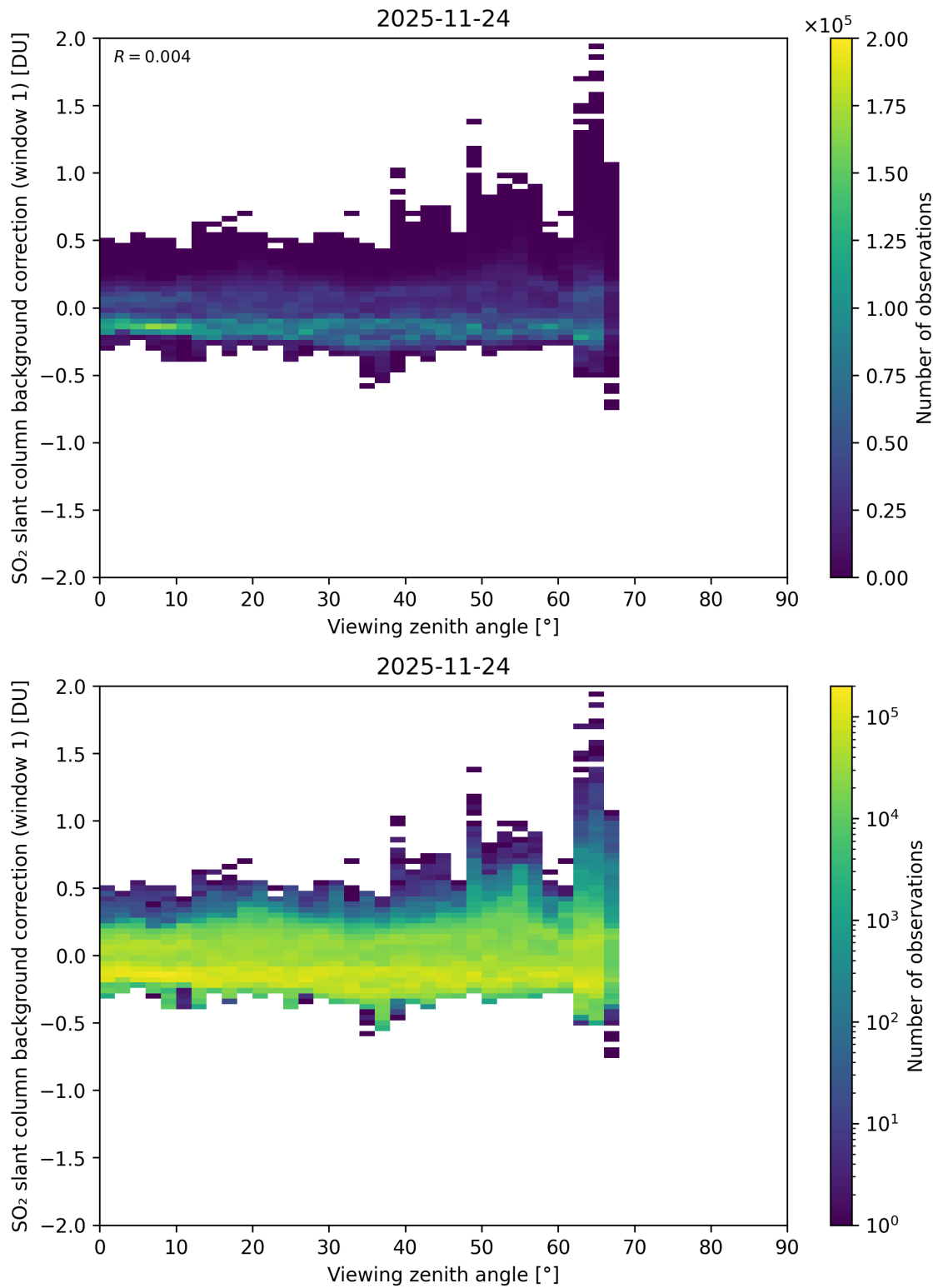
Figure 362: Scatter density plot of “Viewing zenith angle” against “SO 2 slant column background correction (window 1)” for 2025-11-23 to 2025-11-25.
