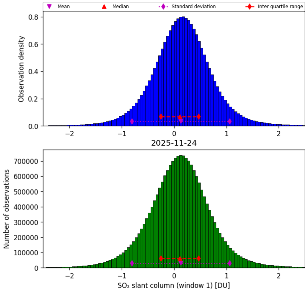
Figure 63: Histogram of “SO 2 slant column (window 1)” for 2025-11-23 to 2025-11-25
