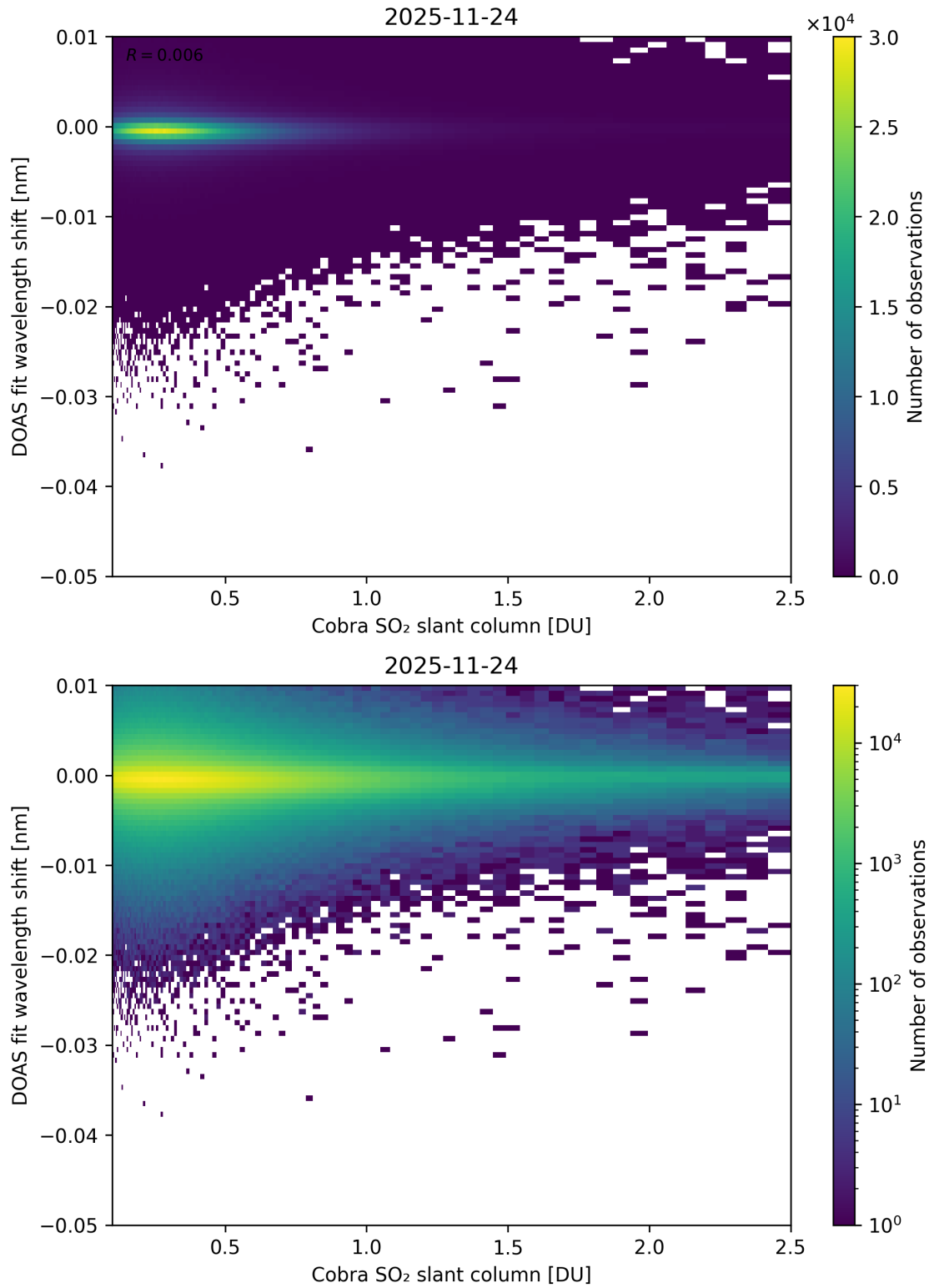
Figure 196: Scatter density plot of “Cobra SO 2 slant column” against “DOAS fit wavelength shift” for 2025-11-23 to 2025-11-25.
