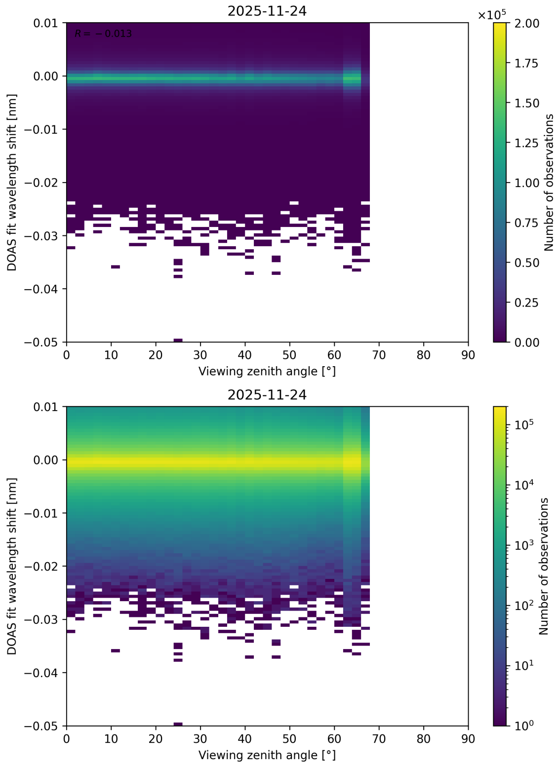
Figure 365: Scatter density plot of “Viewing zenith angle” against “DOAS fit wavelength shift” for 2025-11-23 to 2025-11-25.
