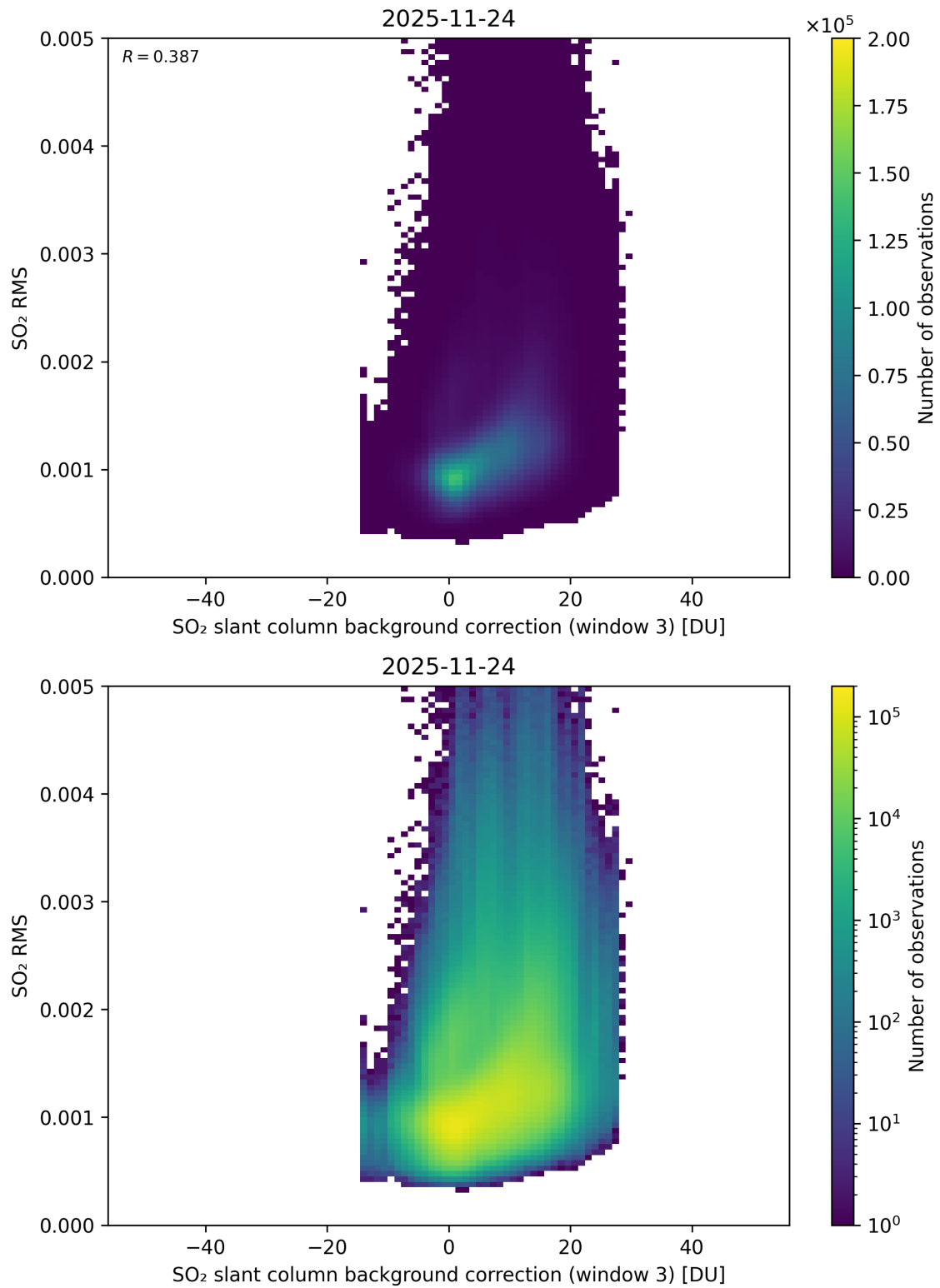
Figure 134: Scatter density plot of “SO 2 slant column background correction (window 3)” against “SO 2 RMS” for 2025-11-23 to 2025-11-25.
