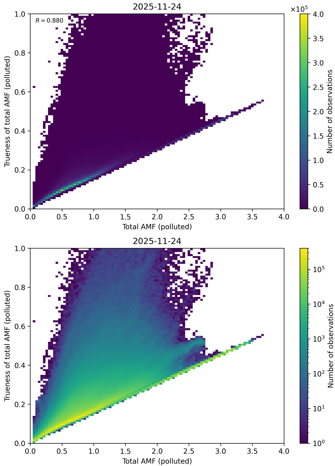
Figure 321: Scatter density plot of “Total AMF (polluted)” against “Trueness of total AMF (polluted)” for 2025-11-23 to 2025-11-25.
