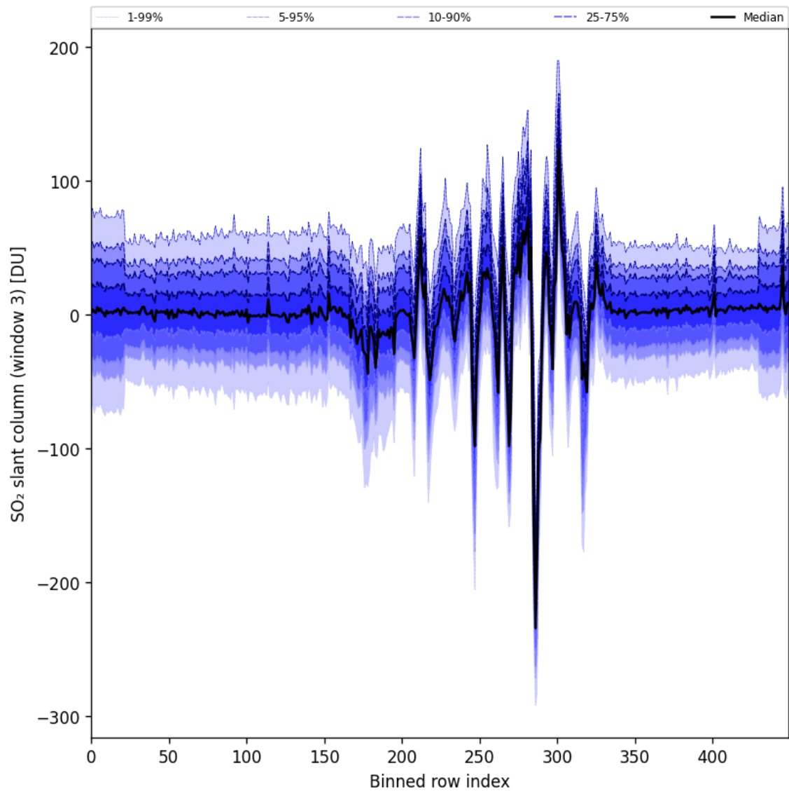
Figure 97: Along track statistics of “SO 2 slant column (window 3)” for 2025-11-23 to 2025-11-25
