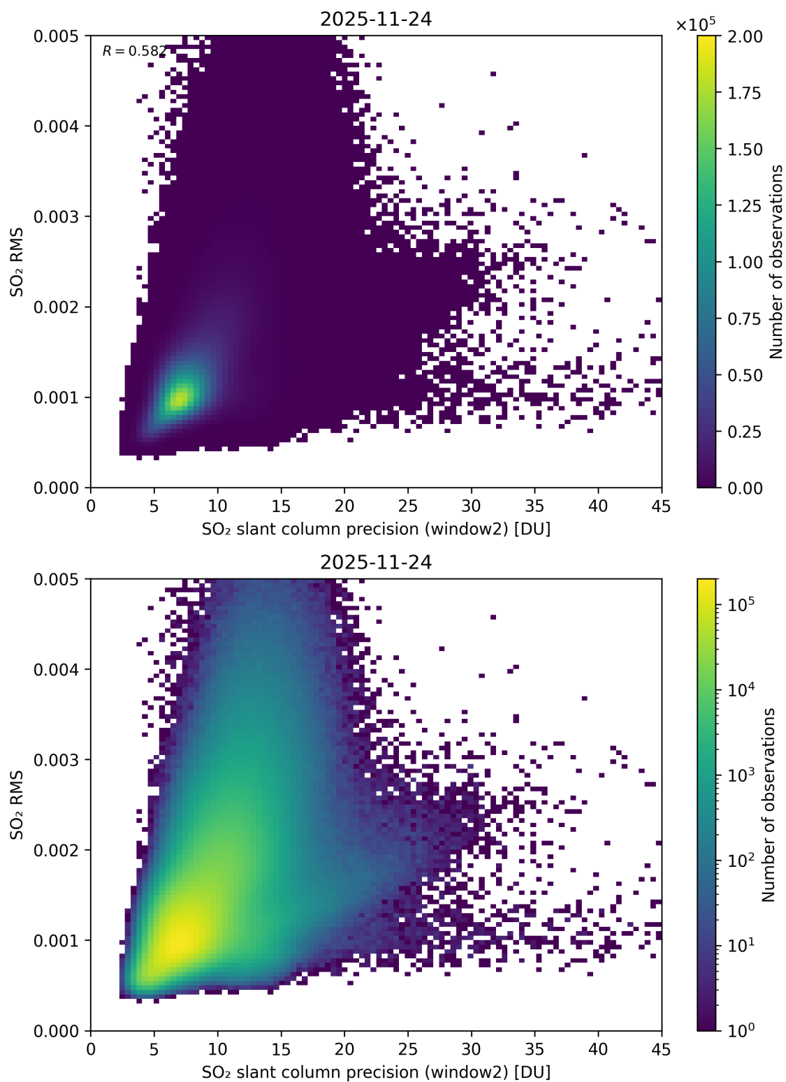
Figure 295: Scatter density plot of “SO 2 slant column precision (window2)” against “SO 2 RMS” for 2025-11-23 to 2025-11-25.
