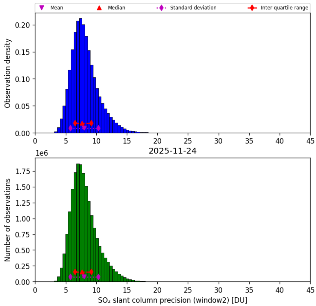
Figure 68: Histogram of “SO 2 slant column precision (window2)” for 2025-11-23 to 2025-11-25
