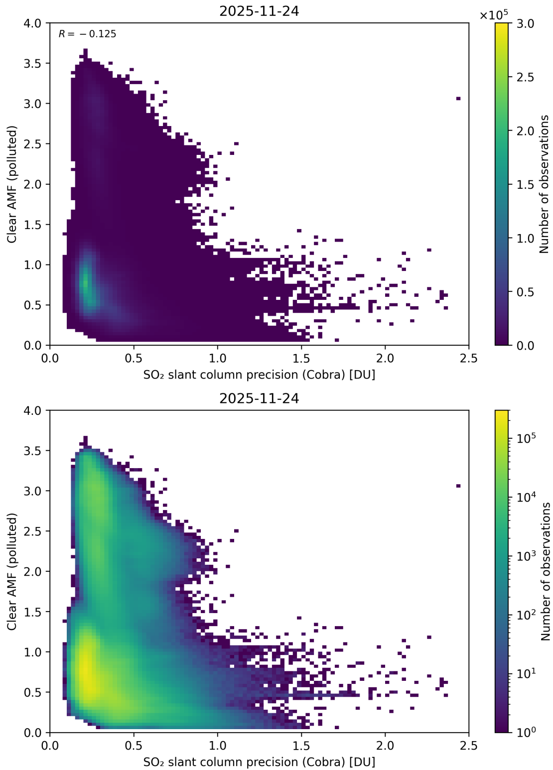
Figure 205: Scatter density plot of “SO 2 slant column precision (Cobra)” against “Clear AMF (polluted)” for 2025-11-23 to 2025-11-25.
