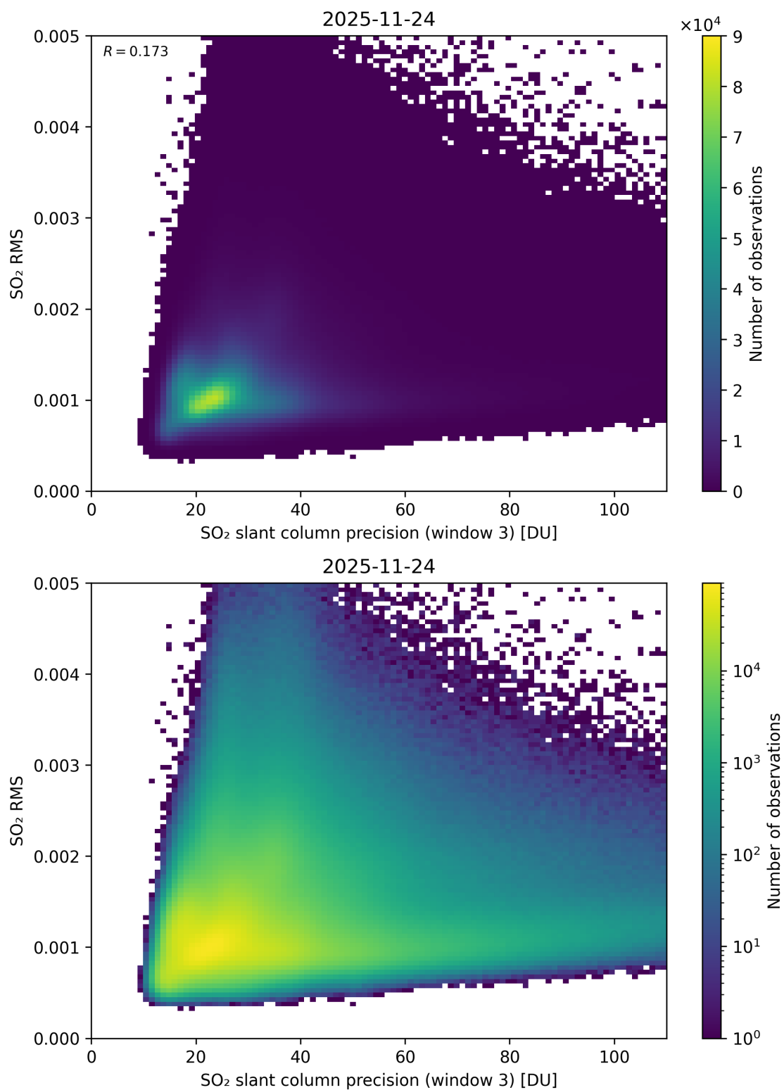
Figure 310: Scatter density plot of “SO 2 slant column precision (window 3)” against “SO 2 RMS” for 2025-11-23 to 2025-11-25.
