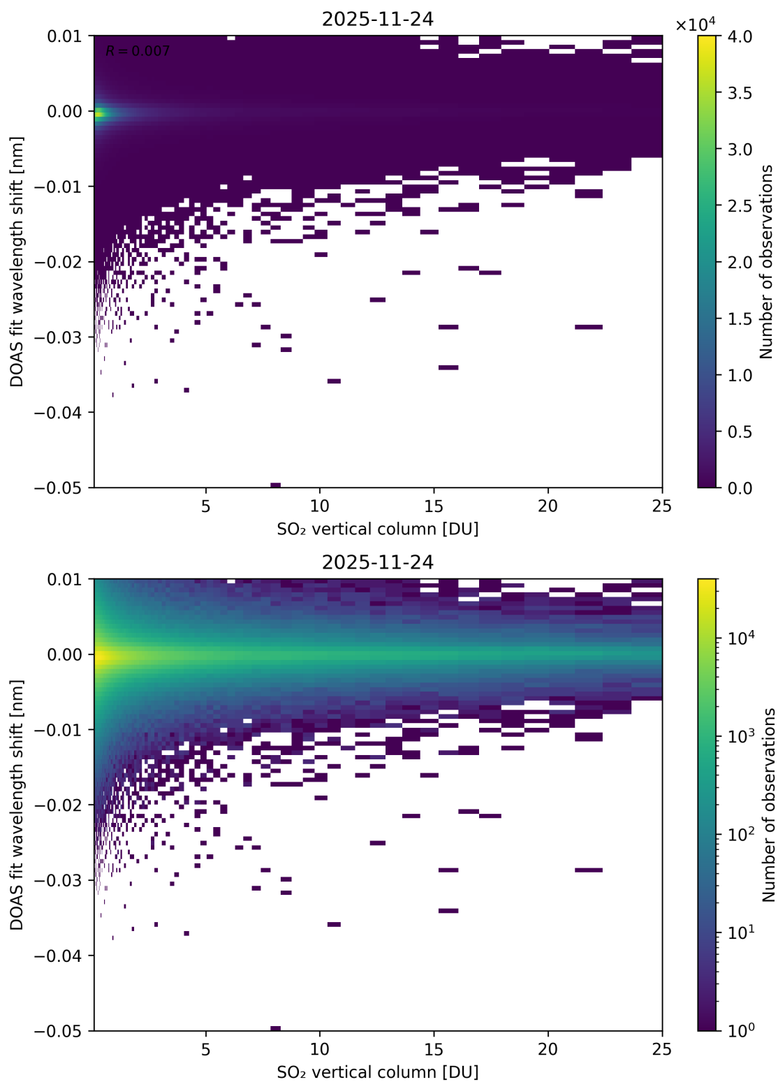
Figure 326: Scatter density plot of “SO 2 vertical column” against “DOAS fit wavelength shift” for 2025-11-23 to 2025-11-25.
