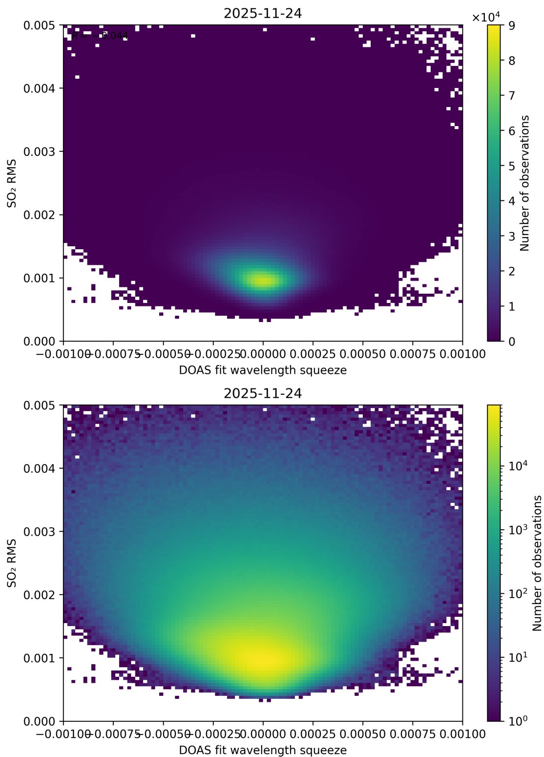
Figure 143: Scatter density plot of “DOAS fit wavelength squeeze” against “SO 2 RMS” for 2025-11-23 to 2025-11-25.
