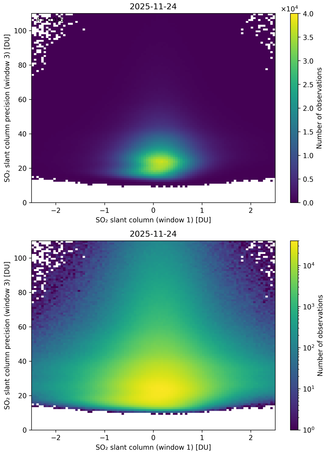
Figure 288: Scatter density plot of “SO 2 slant column (window 1)” against “SO 2 slant column precision (window 3)” for 2025-11-23 to 2025-11-25.
