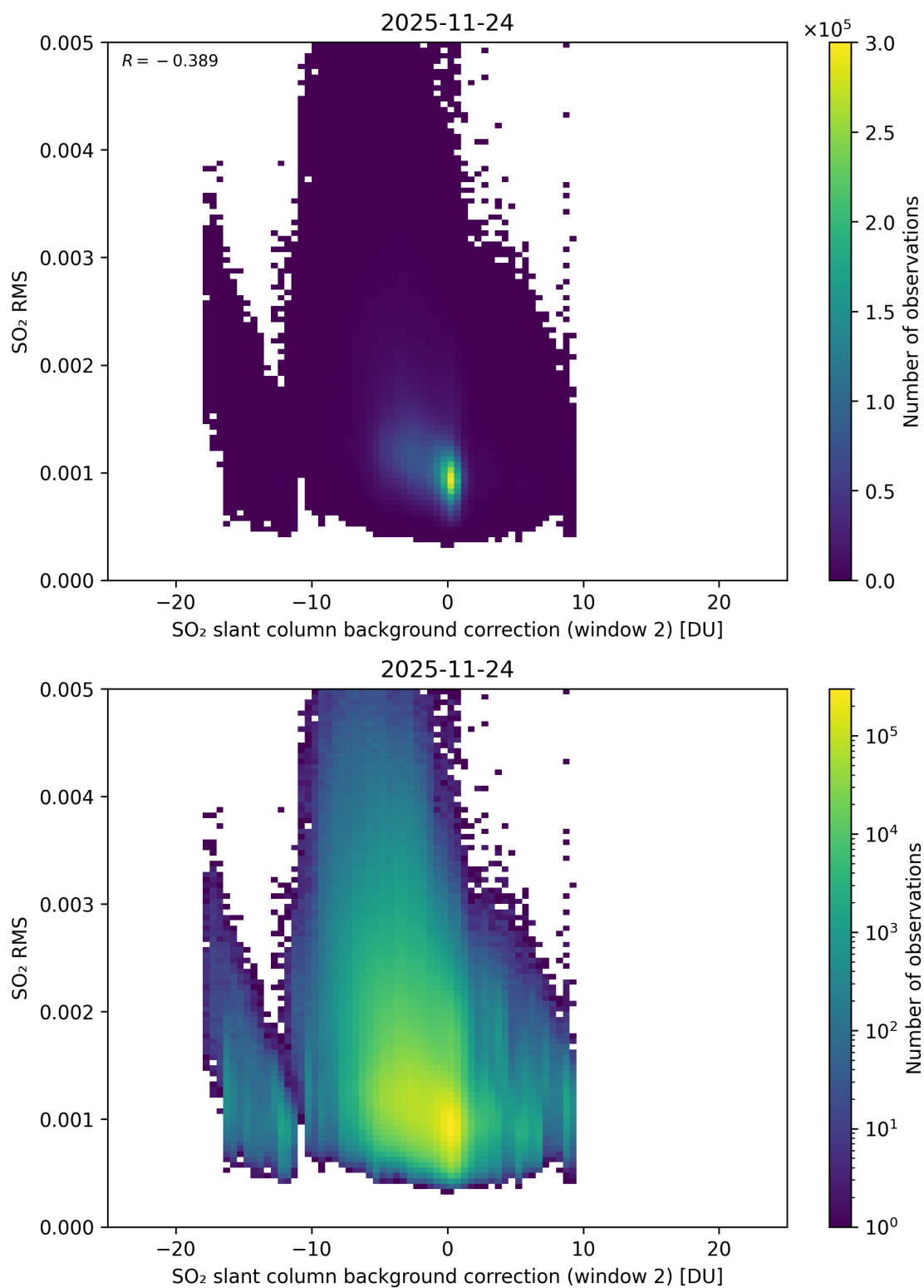
Figure 125: Scatter density plot of “SO 2 slant column background correction (window 2)” against “SO 2 RMS” for 2025-11-23 to 2025-11-25.
