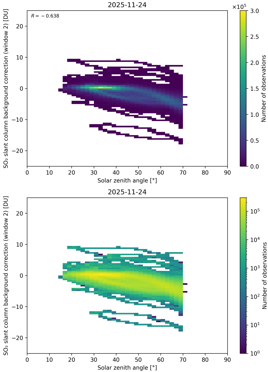
Figure 172: Scatter density plot of “Solar zenith angle” against “SO 2 slant column background correction (window 2)” for 2025-11-23 to 2025-11-25.
