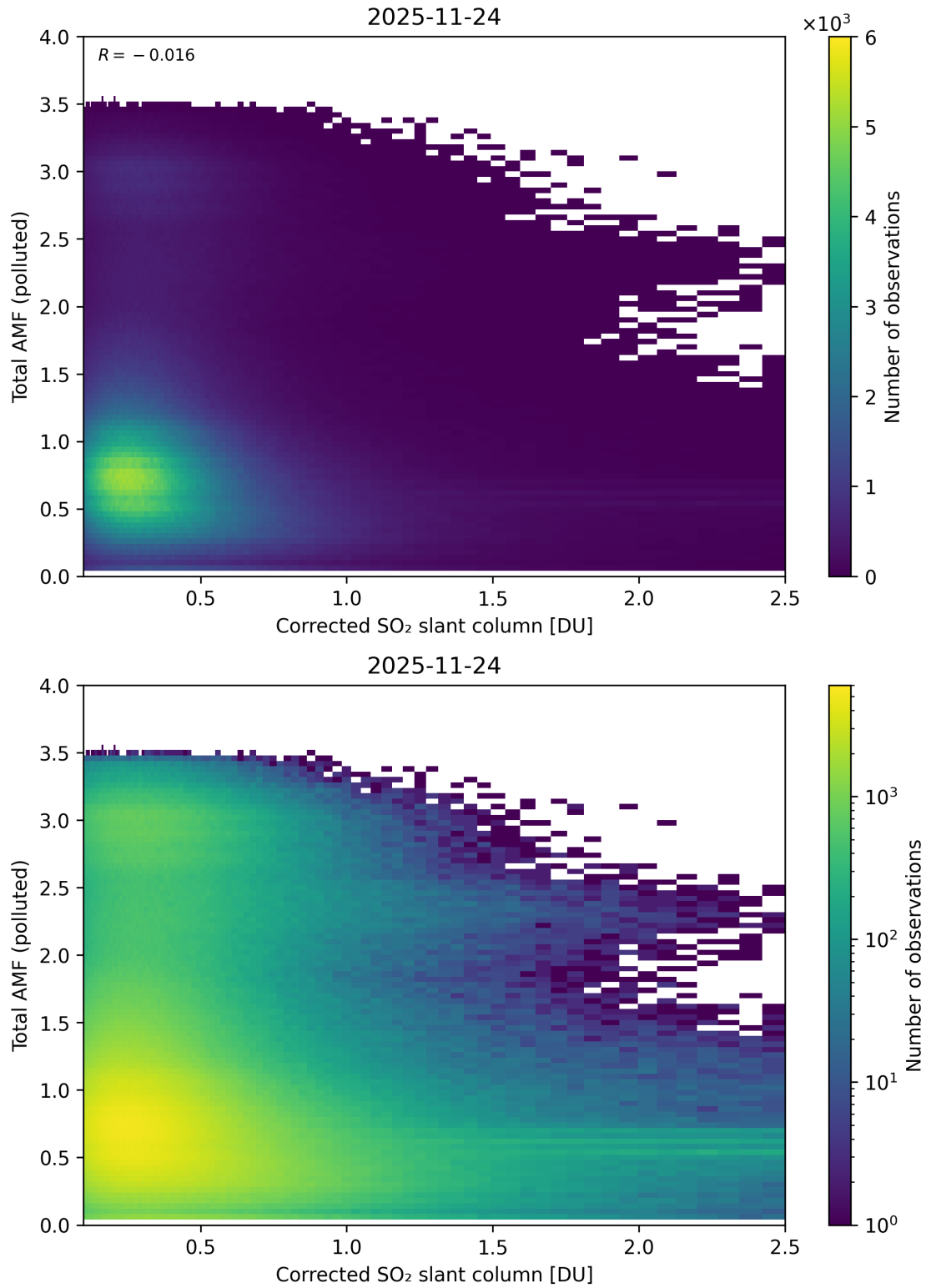
Figure 242: Scatter density plot of “Corrected SO 2 slant column” against “Total AMF (polluted)” for 2025-11-23 to 2025-11-25.
