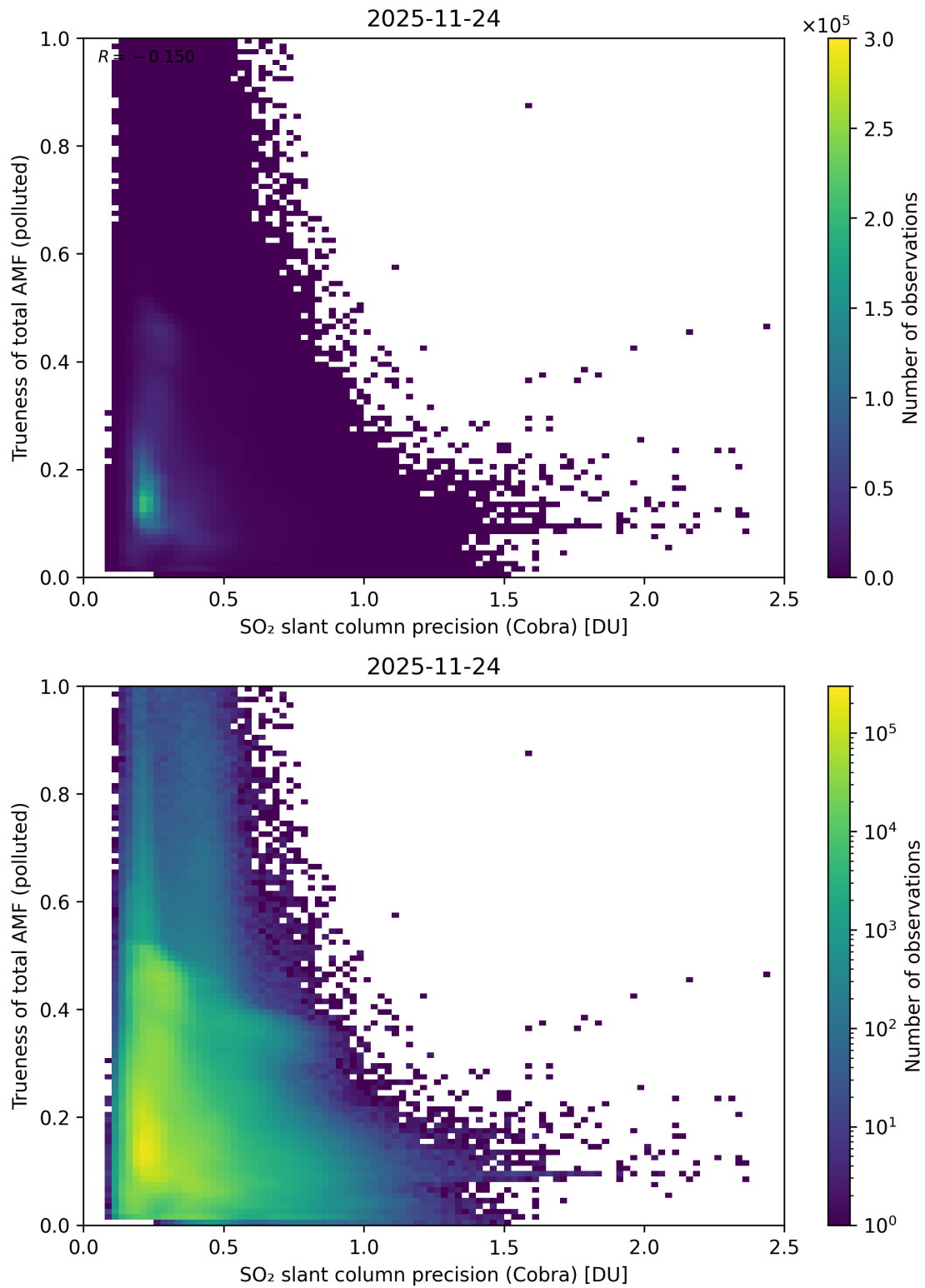
Figure 214: Scatter density plot of “SO 2 slant column precision (Cobra)” against “Trueness of total AMF (polluted)” for 2025-11-23 to 2025-11-25.
