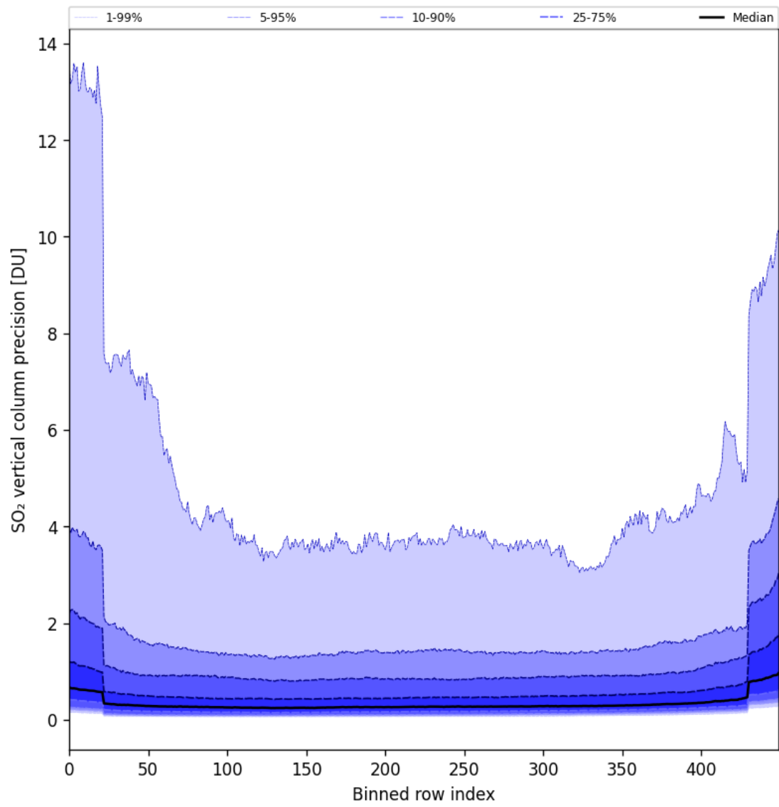
Figure 85: Along track statistics of “SO 2 vertical column precision” for 2025-11-23 to 2025-11-25
