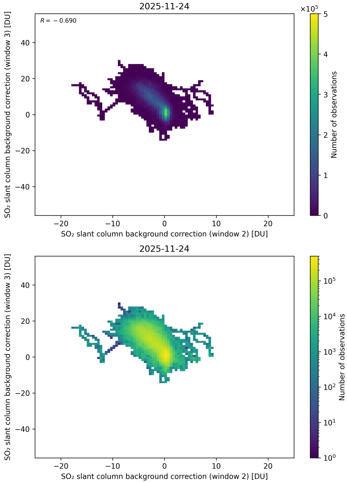
Figure 122: Scatter density plot of “SO 2 slant column background correction (window 2)” against “SO 2 slant column background correction (window 3)” for 2025-11-23 to 2025-11-25.
