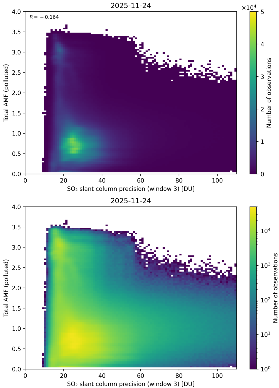
Figure 313: Scatter density plot of “SO 2 slant column precision (window 3)” against “Total AMF (polluted)” for 2025-11-23 to 2025-11-25.
