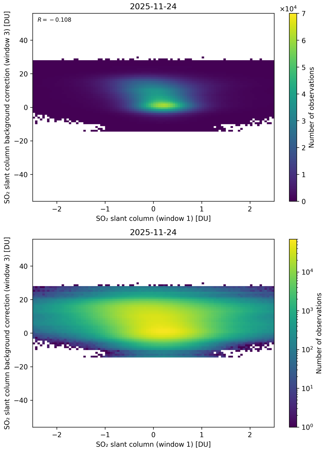
Figure 264: Scatter density plot of “SO 2 slant column (window 1)” against “SO 2 slant column background correction (window 3)” for 2025-11-23 to 2025-11-25.
