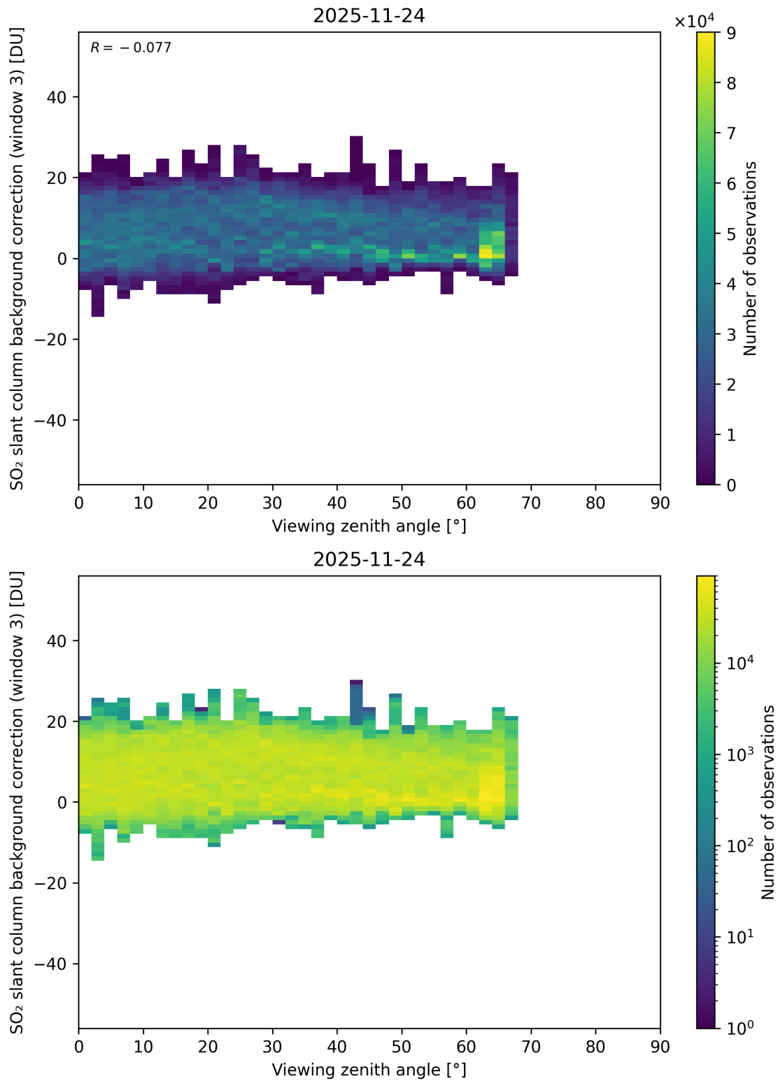
Figure 364: Scatter density plot of “Viewing zenith angle” against “SO 2 slant column background correction (window 3)” for 2025-11-23 to 2025-11-25.
