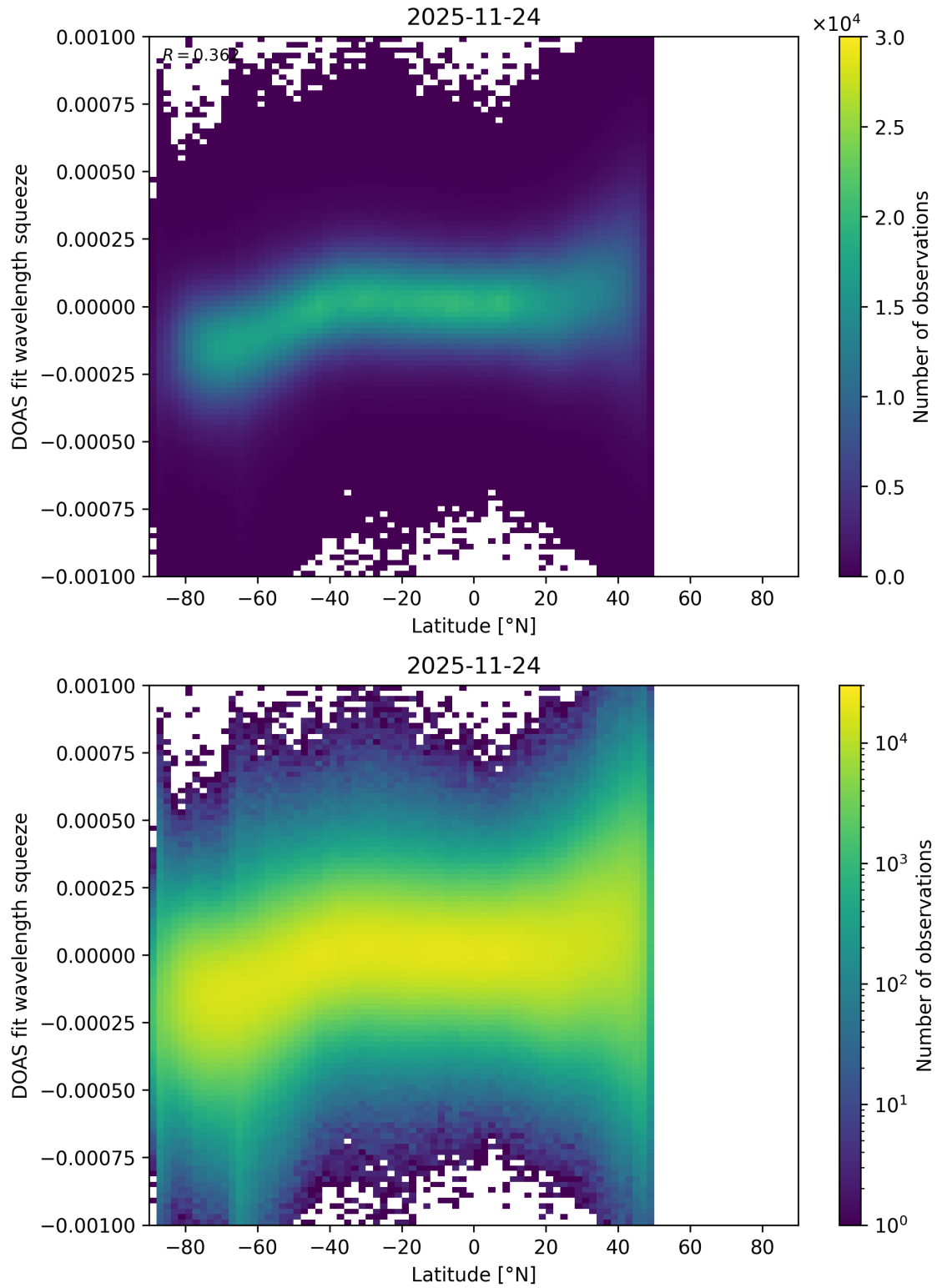
Figure 154: Scatter density plot of “Latitude” against “DOAS fit wavelength squeeze” for 2025-11-23 to 2025-11-25.
