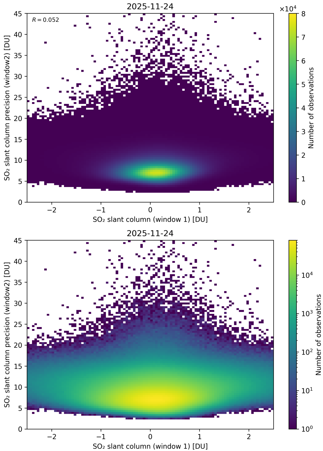
Figure 286: Scatter density plot of “SO 2 slant column (window 1)” against “SO 2 slant column precision (window2)” for 2025-11-23 to 2025-11-25.
