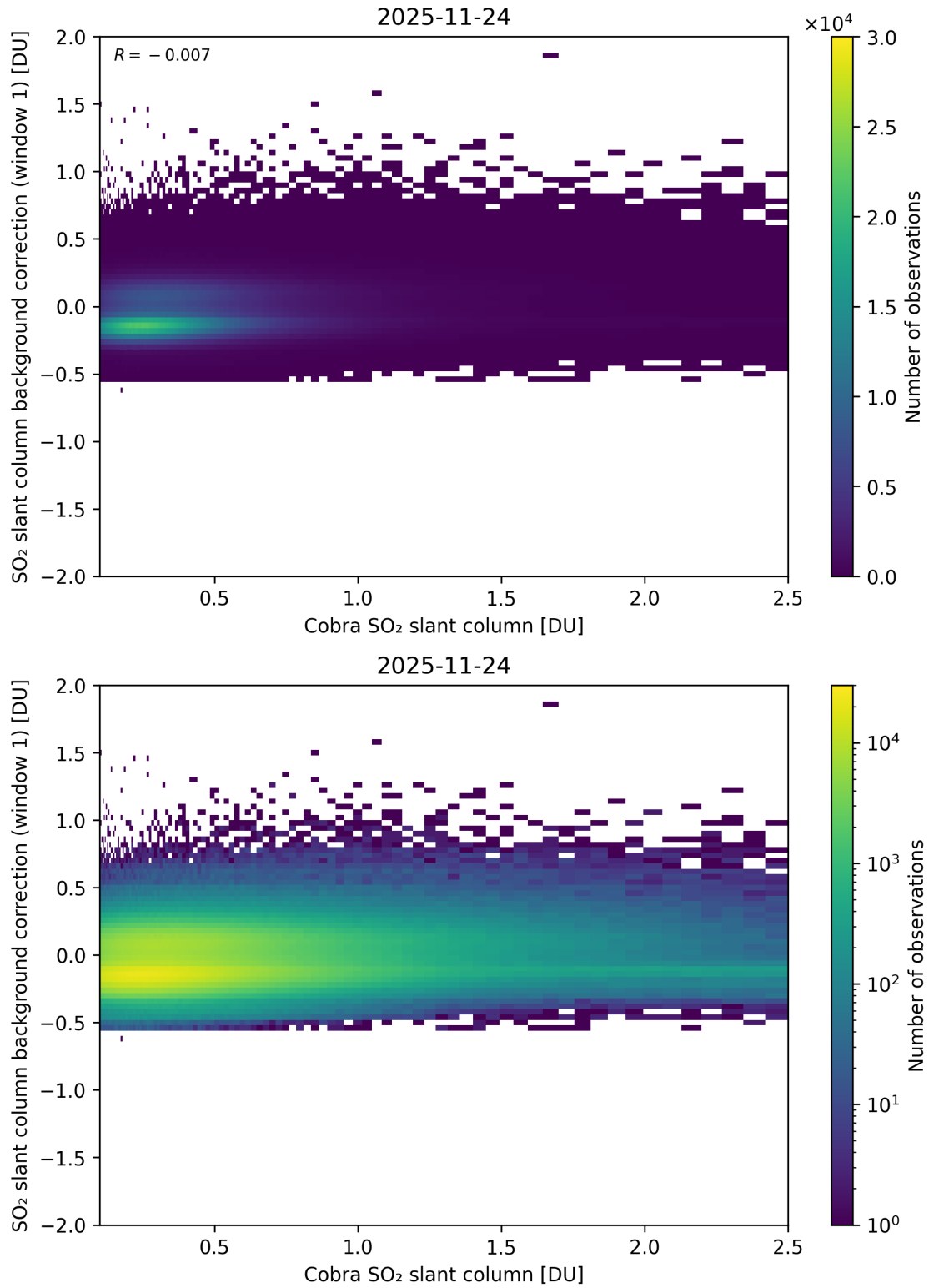
Figure 193: Scatter density plot of “Cobra SO 2 slant column” against “SO 2 slant column background correction (window 1)” for 2025-11-23 to 2025-11-25.
