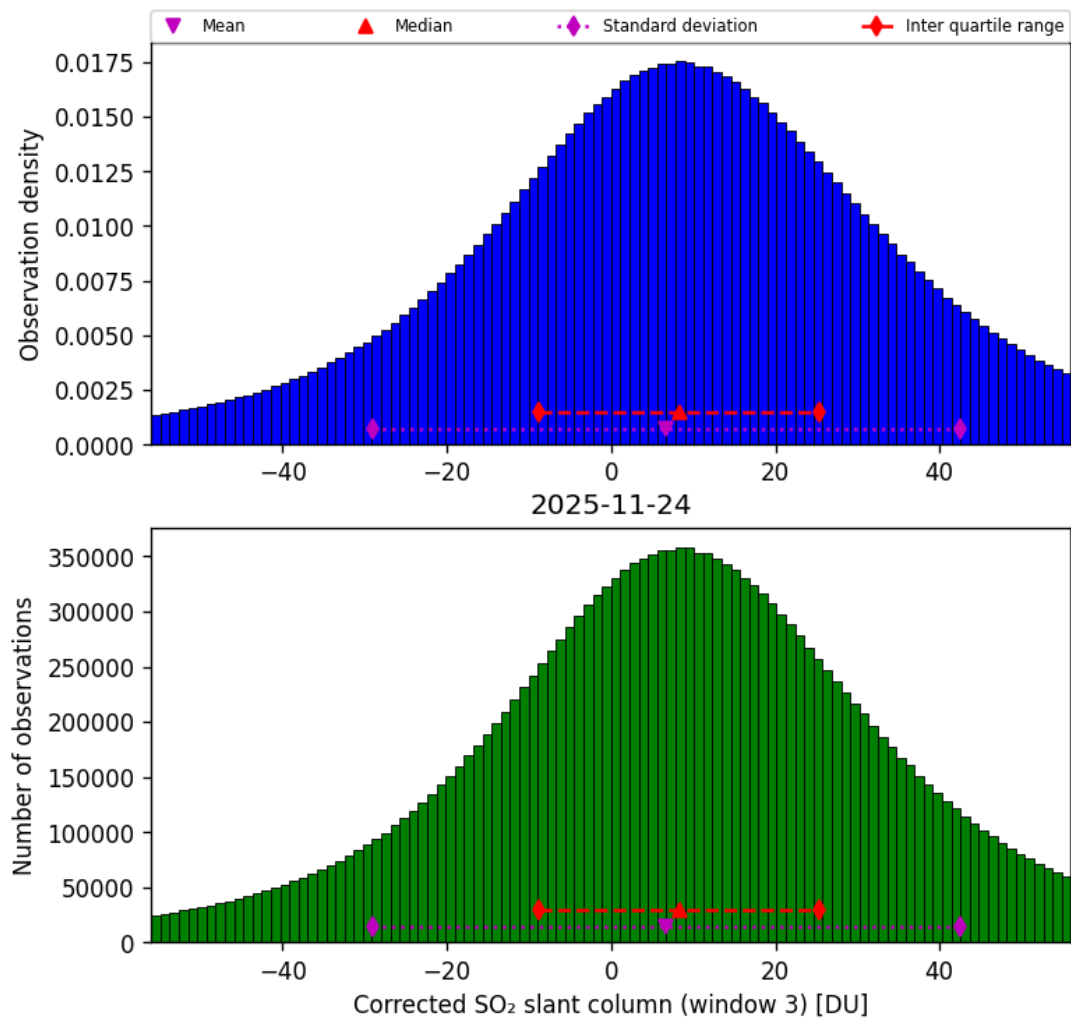
Figure 73: Histogram of “Corrected SO 2 slant column (window 3)” for 2025-11-23 to 2025-11-25
