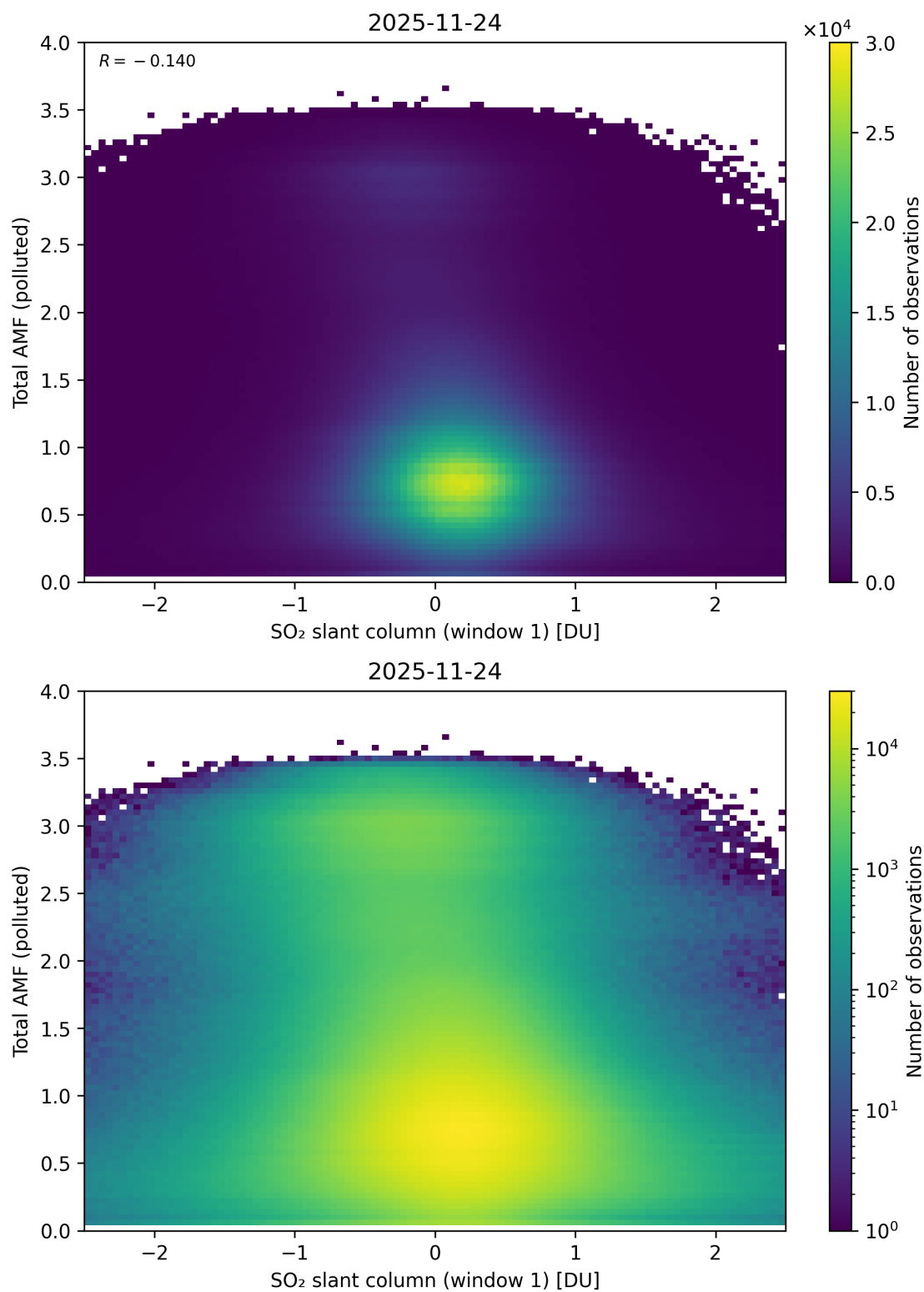
Figure 289: Scatter density plot of “SO 2 slant column (window 1)” against “Total AMF (polluted)” for 2025-11-23 to 2025-11-25.
