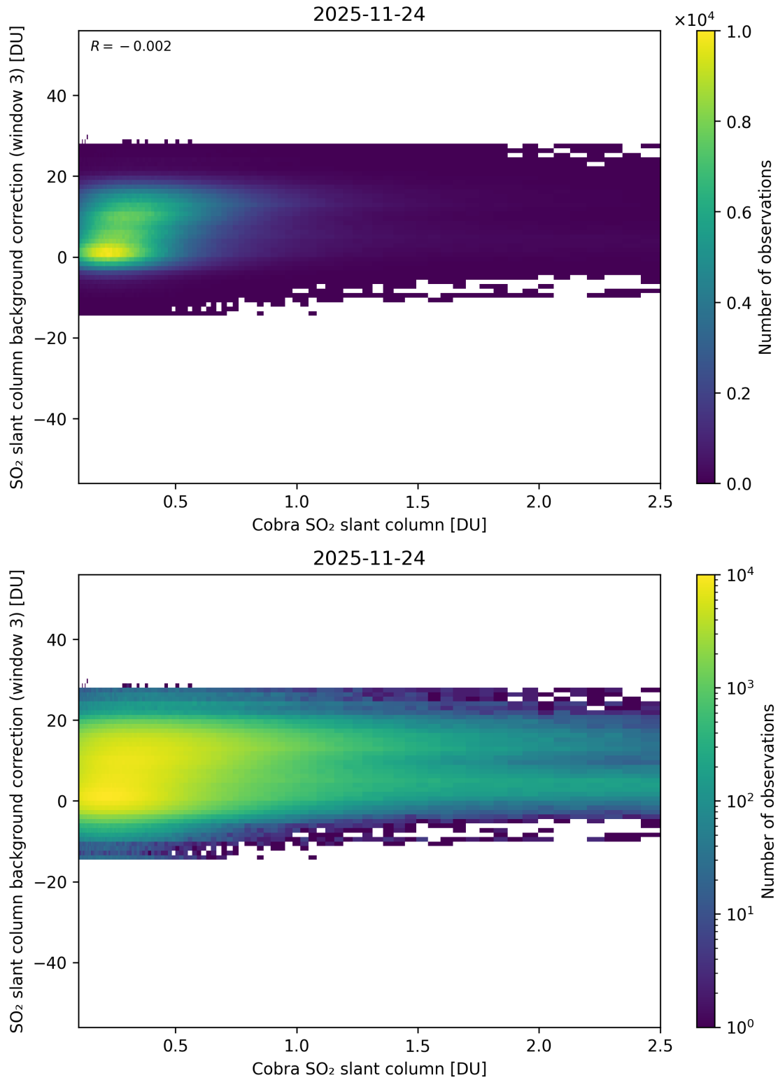
Figure 195: Scatter density plot of “Cobra SO 2 slant column” against “SO 2 slant column background correction (window 3)” for 2025-11-23 to 2025-11-25.
