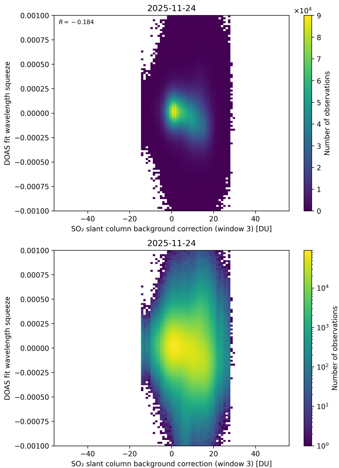
Figure 133: Scatter density plot of “SO 2 slant column background correction (window 3)” against “DOAS fit wavelength squeeze” for 2025-11-23 to 2025-11-25.
