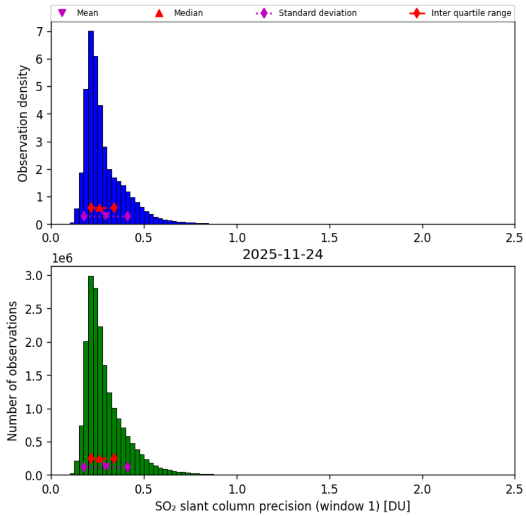
Figure 64: Histogram of “SO 2 slant column precision (window 1)” for 2025-11-23 to 2025-11-25
