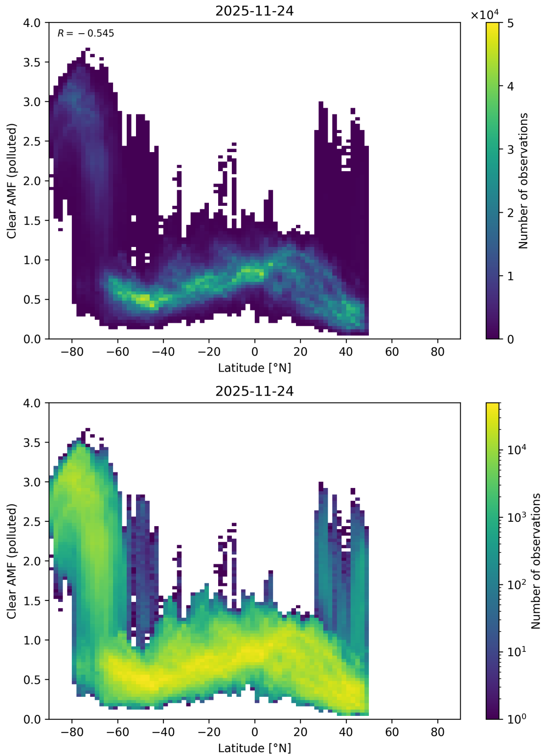
Figure 156: Scatter density plot of “Latitude” against “Clear AMF (polluted)” for 2025-11-23 to 2025-11-25.
