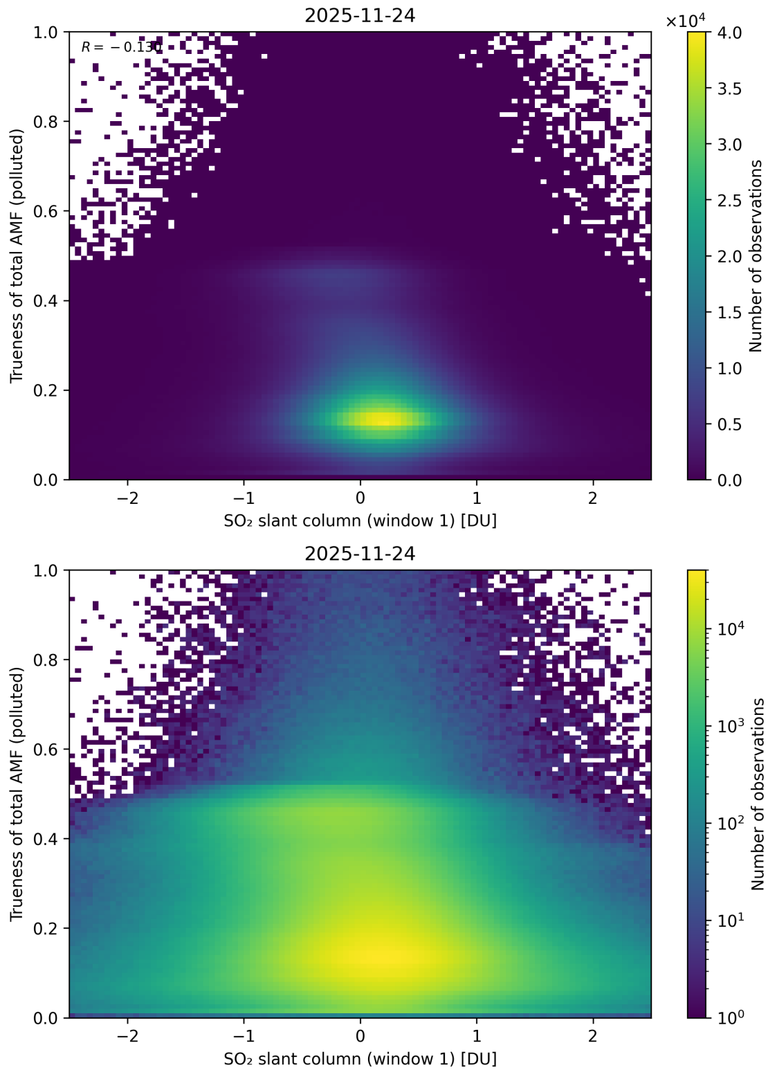
Figure 290: Scatter density plot of “SO 2 slant column (window 1)” against “Trueness of total AMF (polluted)” for 2025-11-23 to 2025-11-25.
