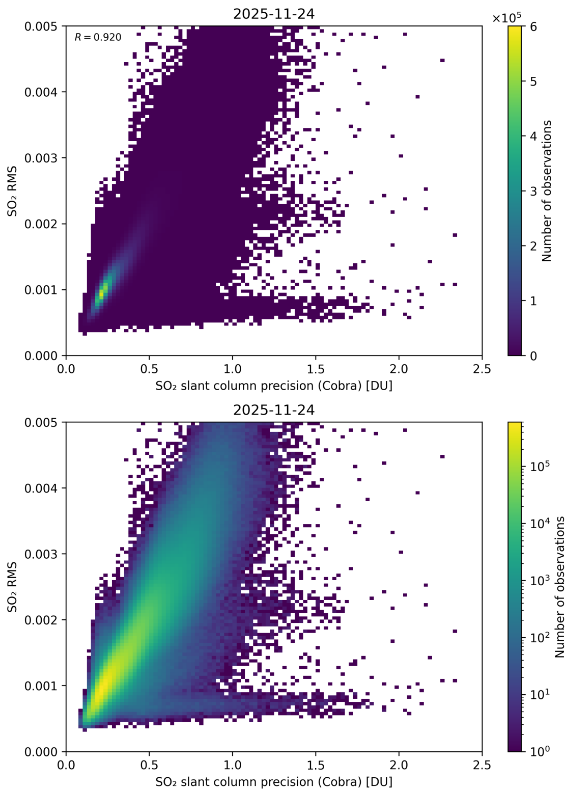
Figure 204: Scatter density plot of “SO 2 slant column precision (Cobra)” against “SO 2 RMS” for 2025-11-23 to 2025-11-25.
