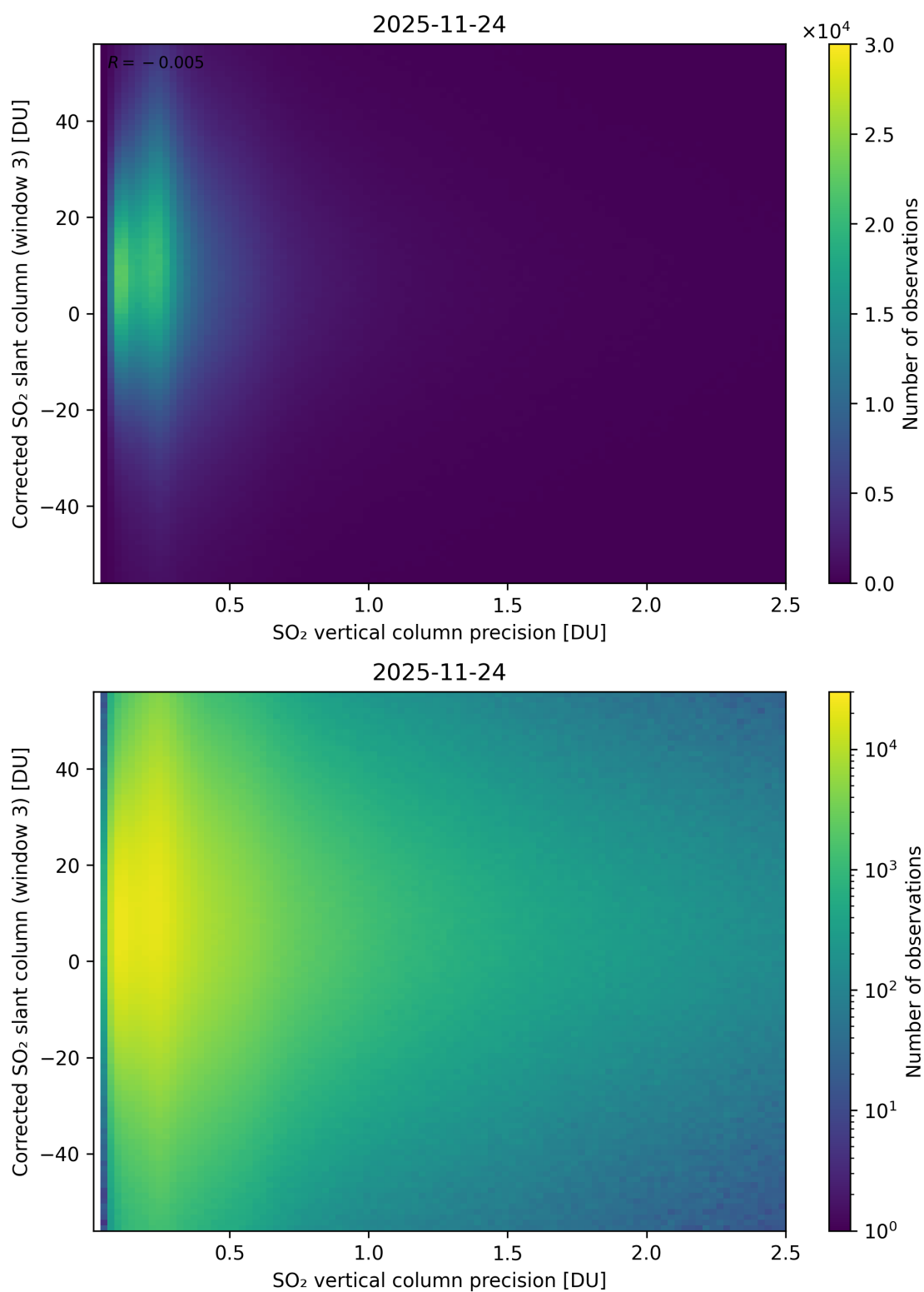
Figure 340: Scatter density plot of “SO 2 vertical column precision” against “Corrected SO 2 slant column (window 3)” for 2025-11-23 to 2025-11-25.
