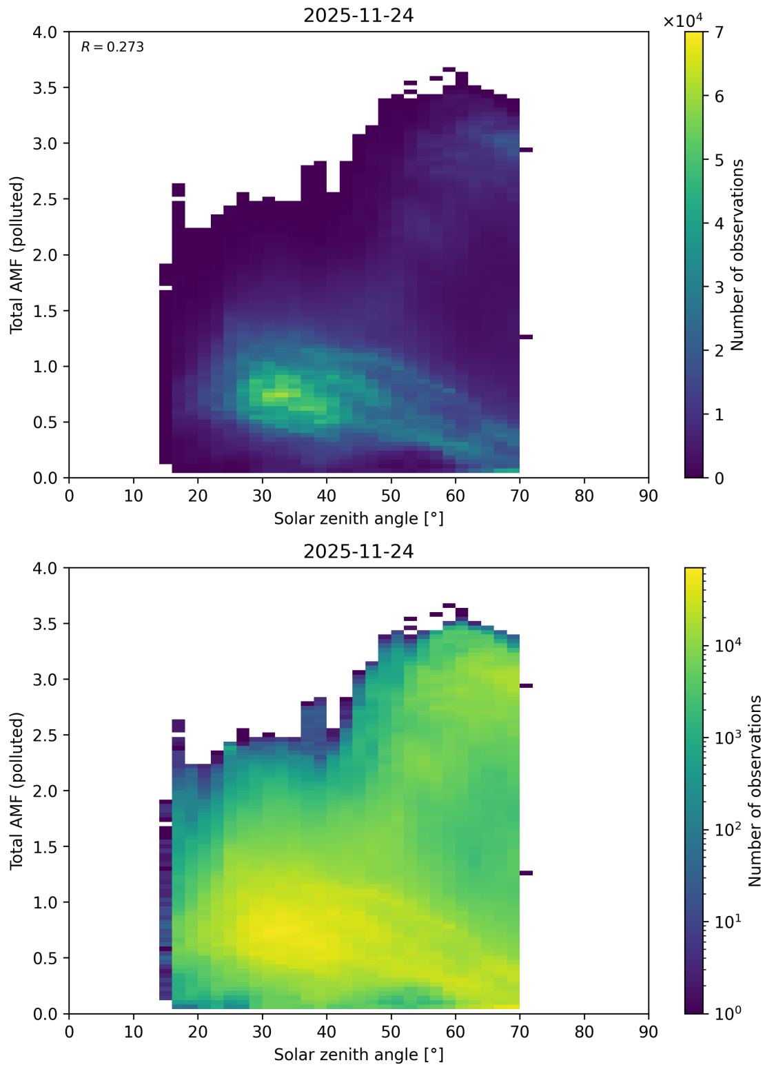
Figure 189: Scatter density plot of “Solar zenith angle” against “Total AMF (polluted)” for 2025-11-23 to 2025-11-25.
