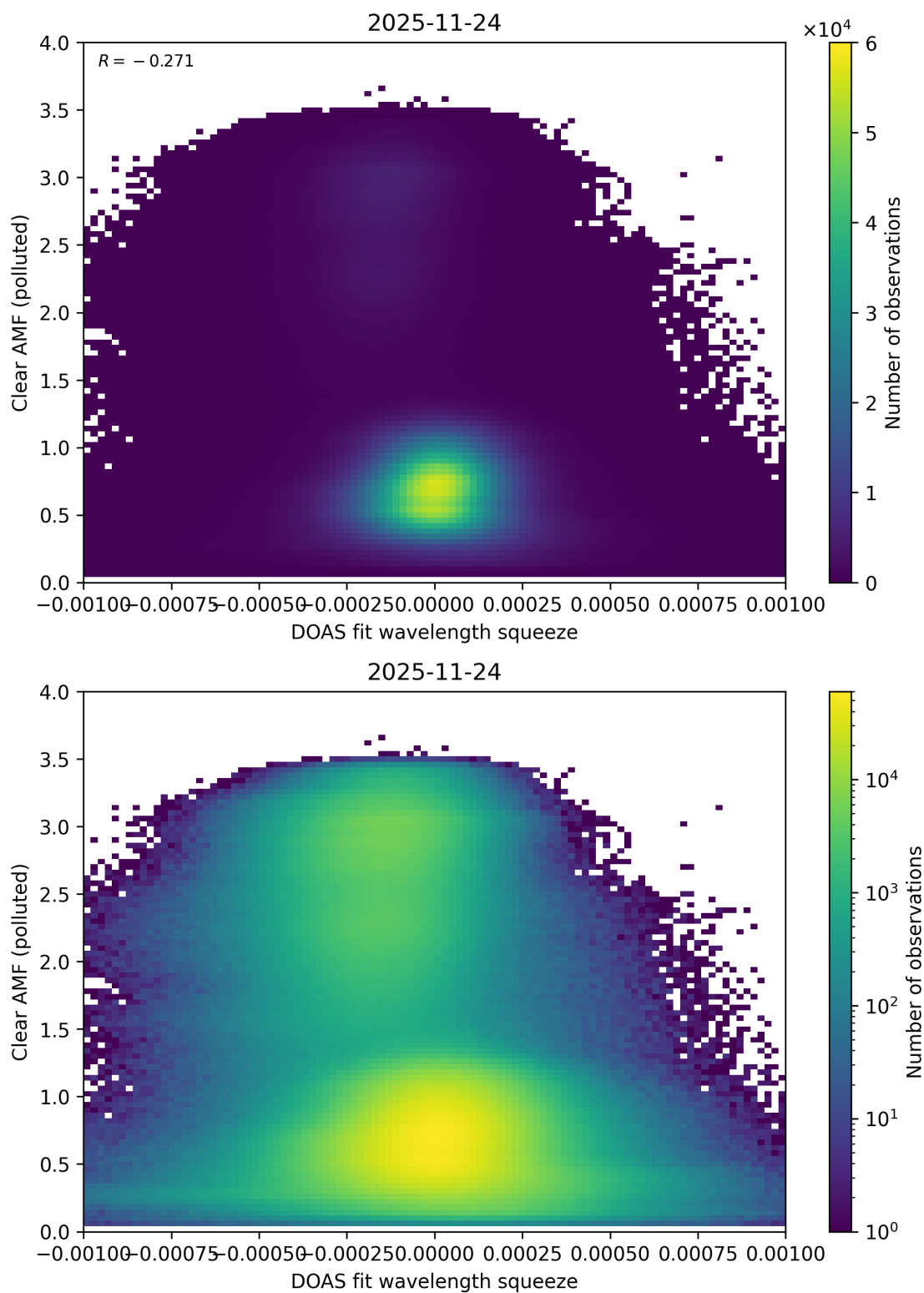
Figure 144: Scatter density plot of “DOAS fit wavelength squeeze” against “Clear AMF (polluted)” for 2025-11-23 to 2025-11-25.
