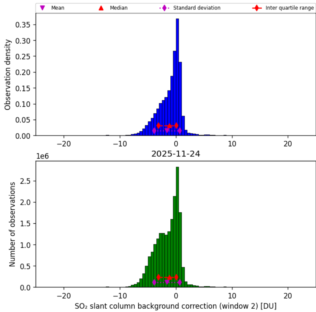
Figure 70: Histogram of “SO 2 slant column background correction (window 2)” for 2025-11-23 to 2025-11-25
