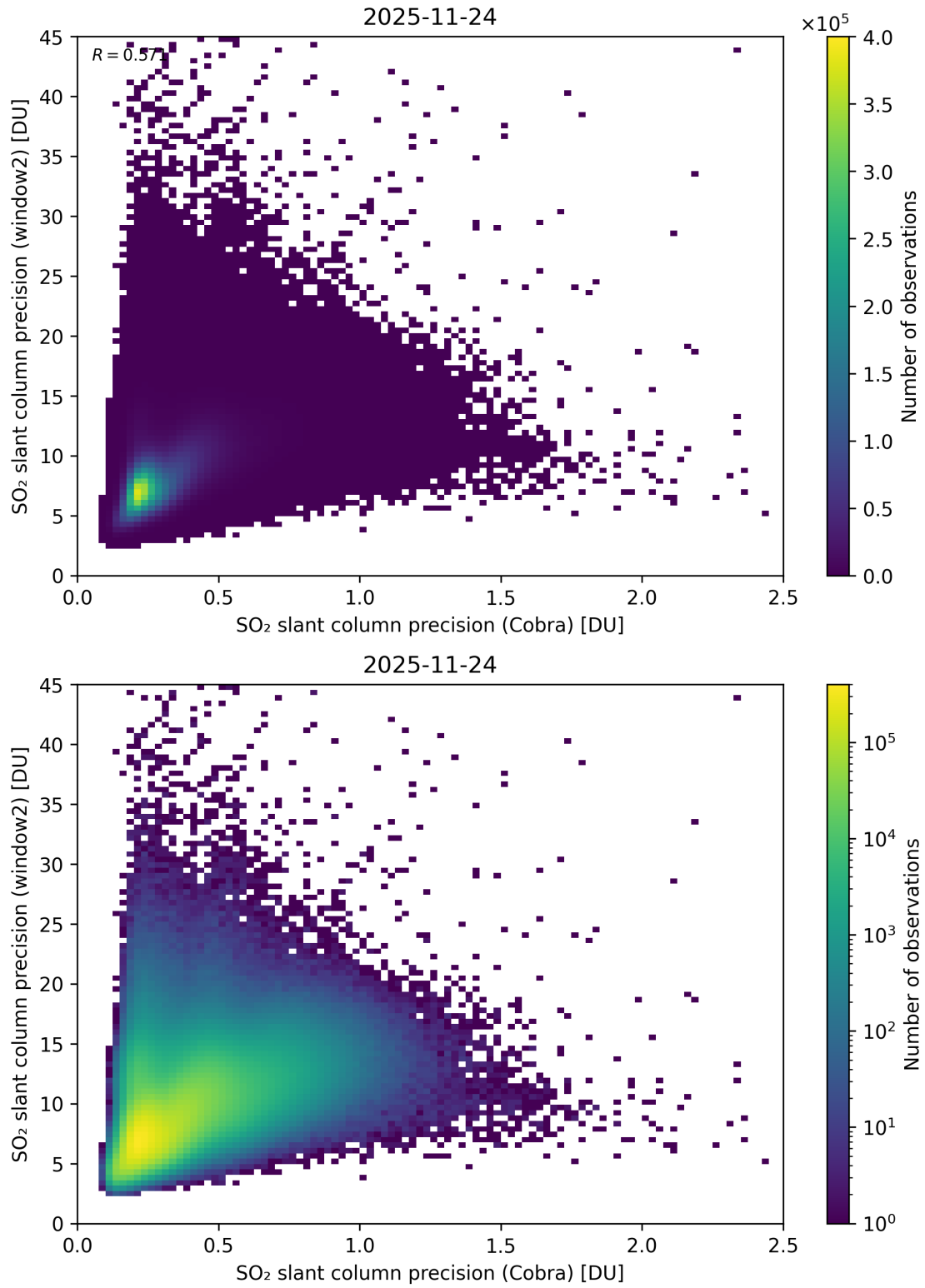
Figure 210: Scatter density plot of “SO 2 slant column precision (Cobra)” against “SO 2 slant column precision (window2)” for 2025-11-23 to 2025-11-25.
