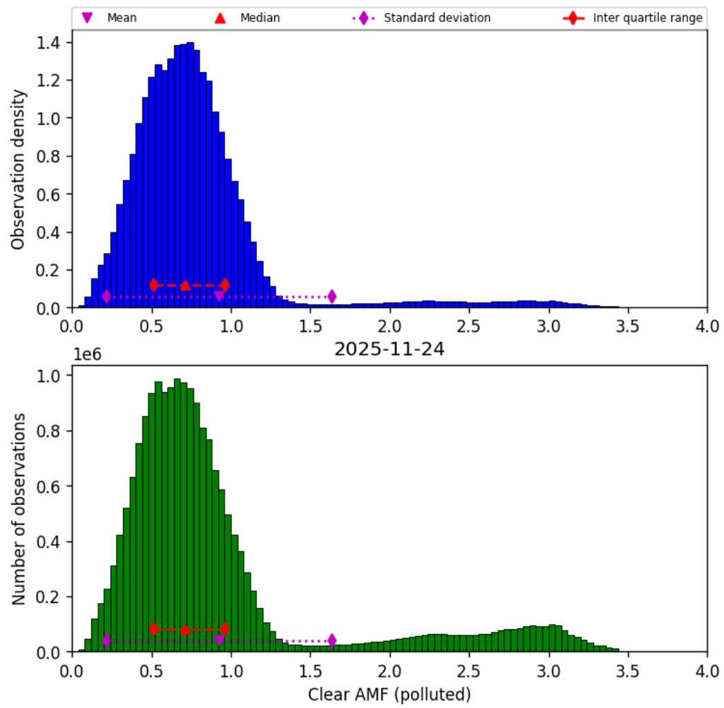
Figure 81: Histogram of “Clear AMF (polluted)” for 2025-11-23 to 2025-11-25
