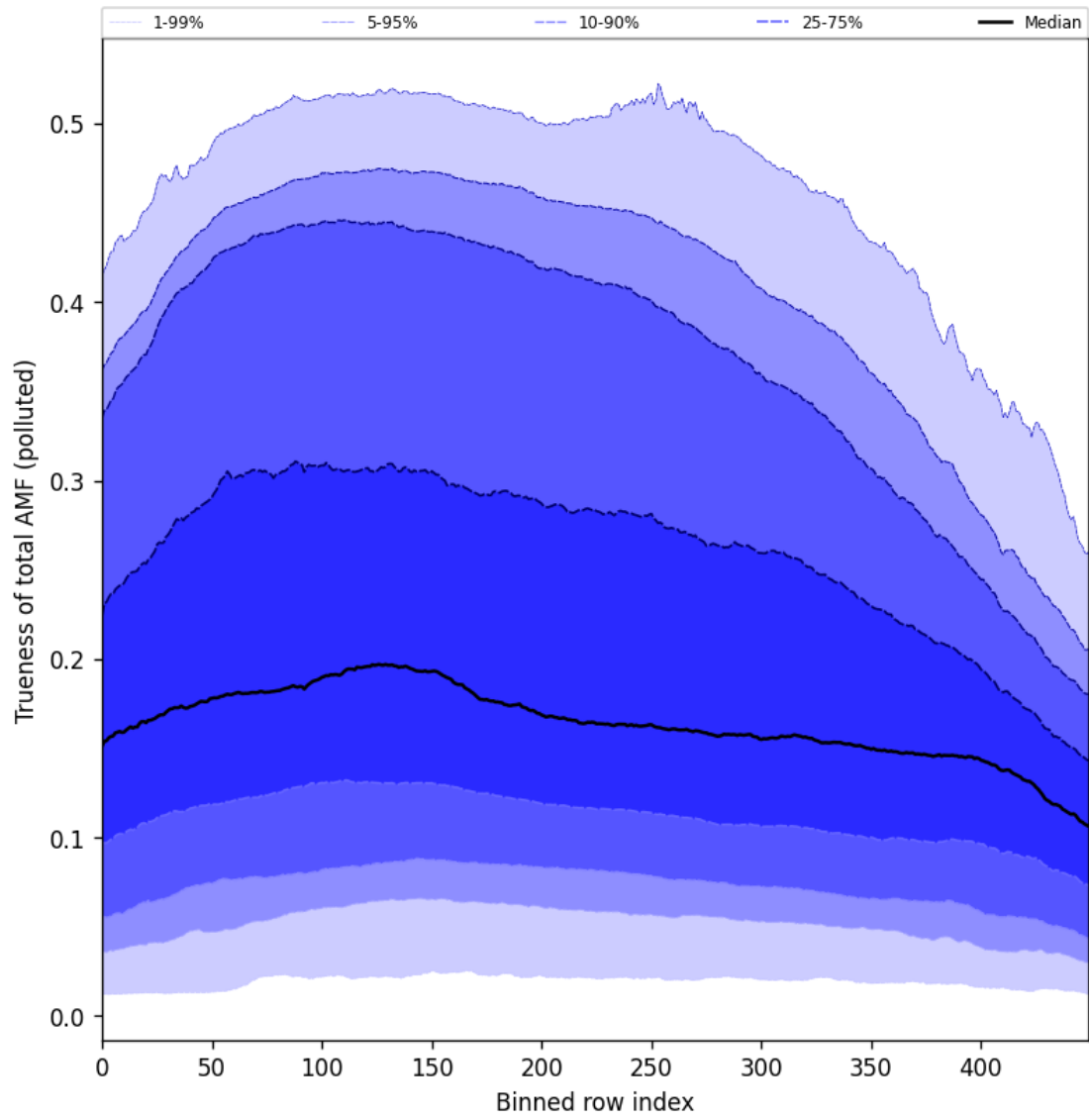
Figure 106: Along track statistics of “Trueness of total AMF (polluted)” for 2025-11-23 to 2025-11-25
