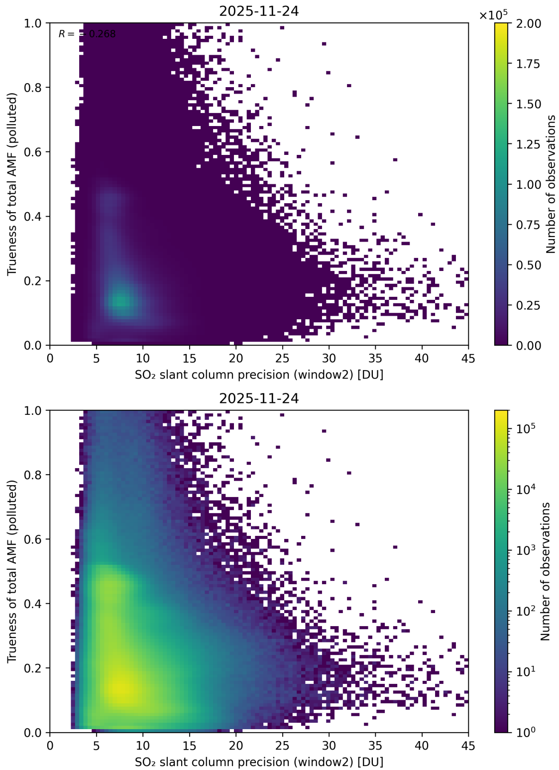
Figure 302: Scatter density plot of “SO 2 slant column precision (window2)” against “Trueness of total AMF (polluted)” for 2025-11-23 to 2025-11-25.
