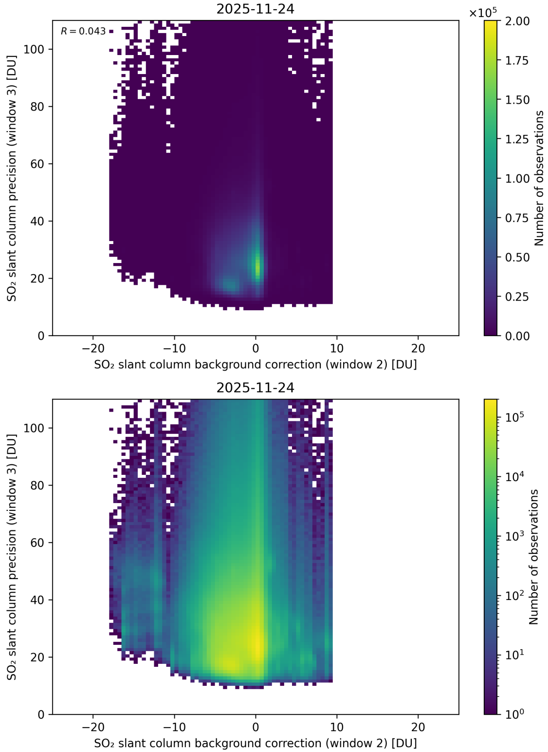
Figure 129: Scatter density plot of “SO 2 slant column background correction (window 2)” against “SO 2 slant column precision (window 3)” for 2025-11-23 to 2025-11-25.
