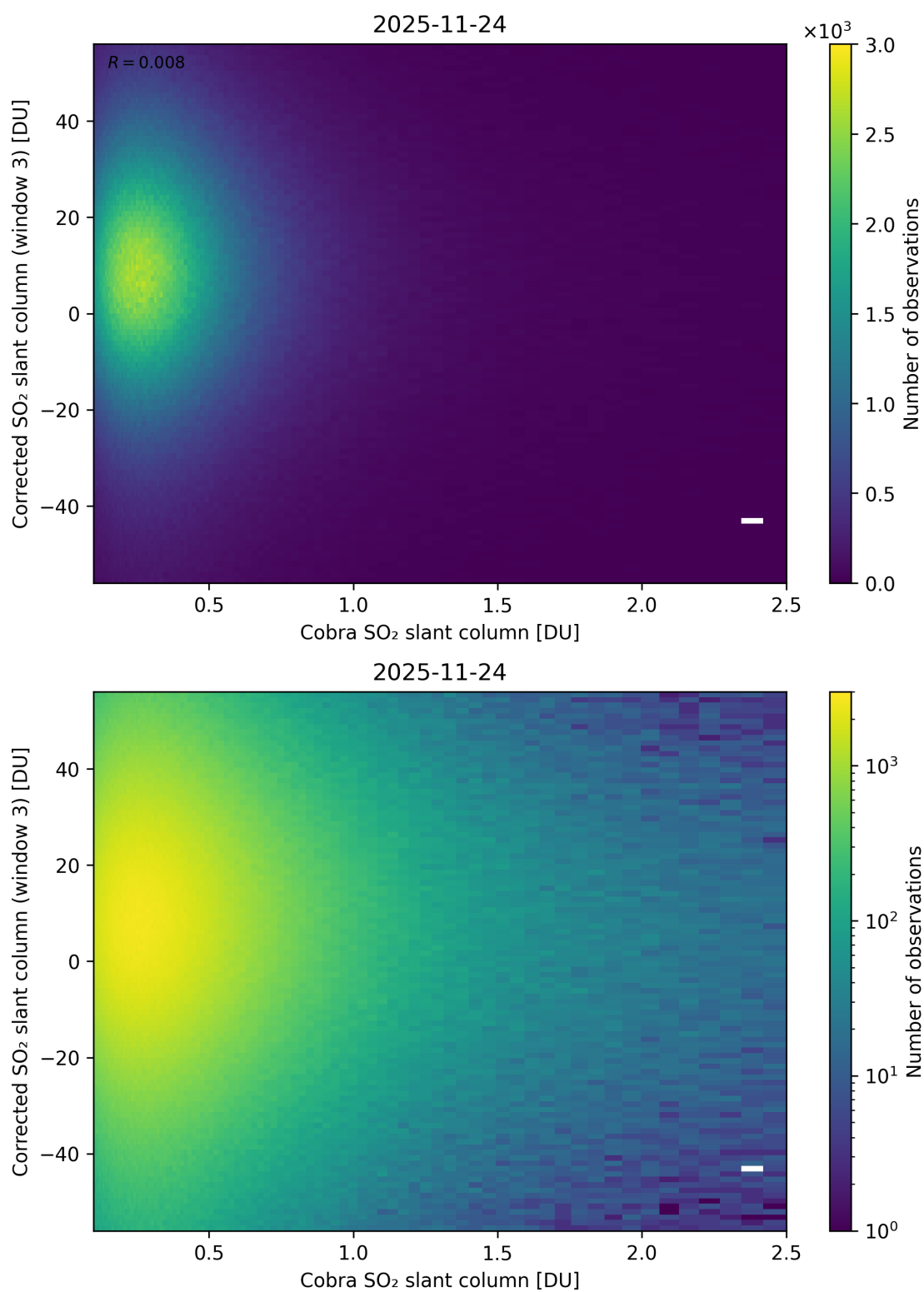
Figure 218: Scatter density plot of “Cobra SO 2 slant column” against “Corrected SO 2 slant column (window 3)” for 2025-11-23 to 2025-11-25.
