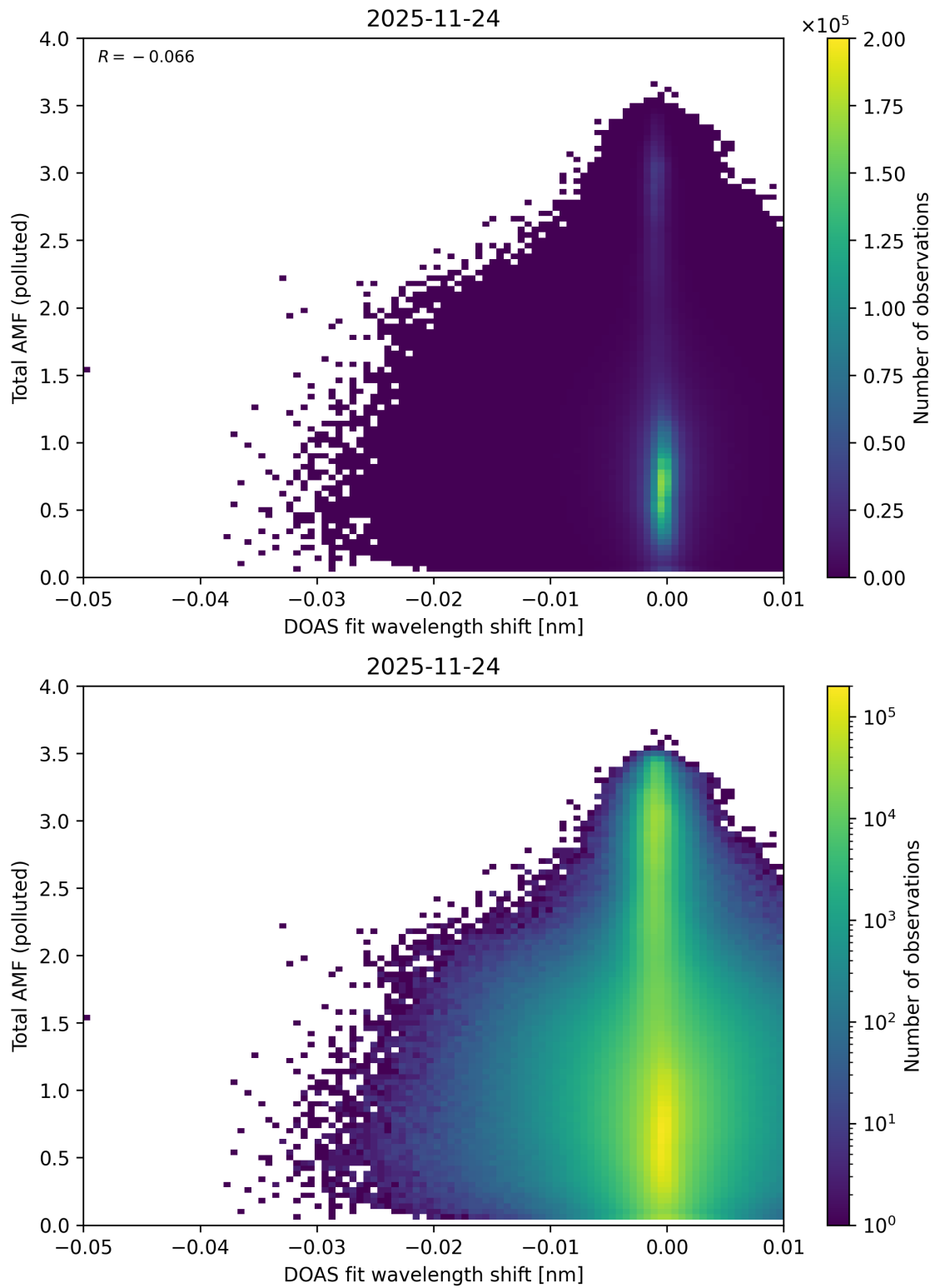
Figure 141: Scatter density plot of “DOAS fit wavelength shift” against “Total AMF (polluted)” for 2025-11-23 to 2025-11-25.
