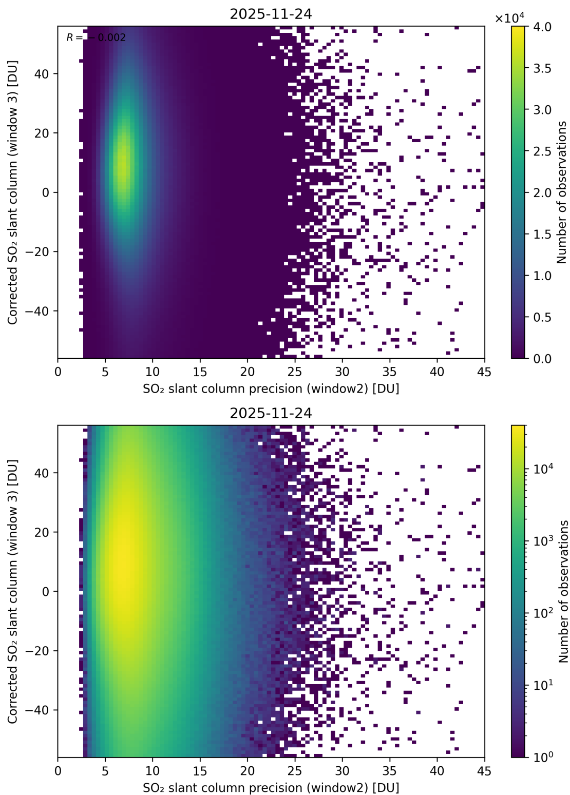
Figure 298: Scatter density plot of “SO 2 slant column precision (window2)” against “Corrected SO 2 slant column (window 3)” for 2025-11-23 to 2025-11-25.
