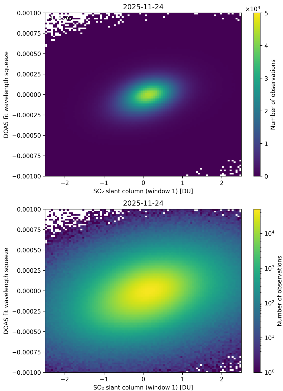
Figure 266: Scatter density plot of “SO 2 slant column (window 1)” against “DOAS fit wavelength squeeze” for 2025-11-23 to 2025-11-25.
