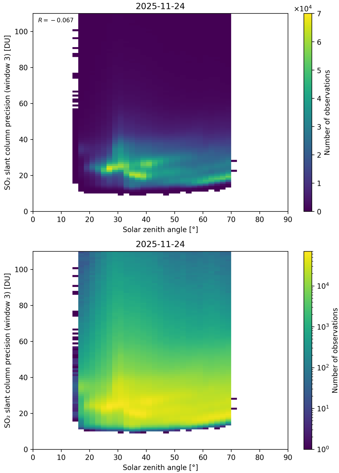
Figure 188: Scatter density plot of “Solar zenith angle” against “SO 2 slant column precision (window 3)” for 2025-11-23 to 2025-11-25.
