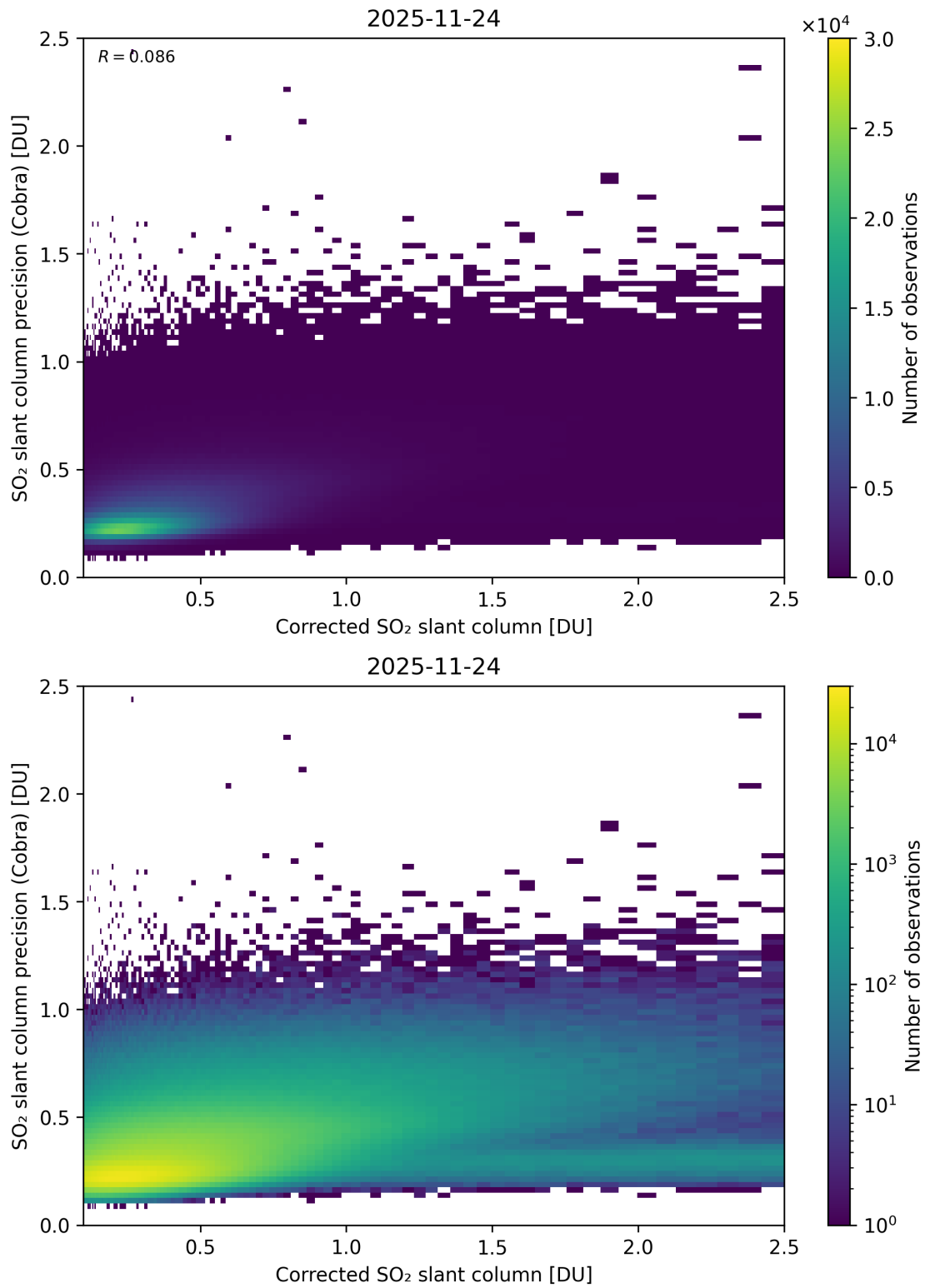
Figure 234: Scatter density plot of “Corrected SO 2 slant column” against “SO 2 slant column precision (Cobra)” for 2025-11-23 to 2025-11-25.
