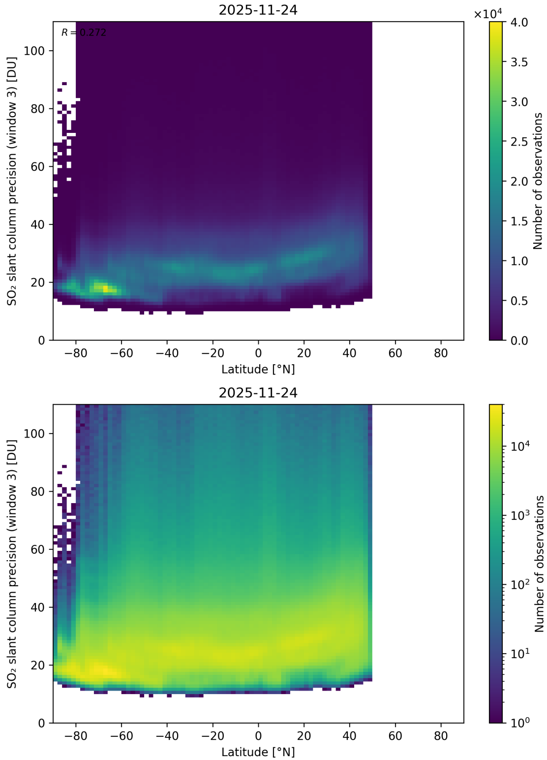
Figure 166: Scatter density plot of “Latitude” against “SO 2 slant column precision (window 3)” for 2025-11-23 to 2025-11-25.
