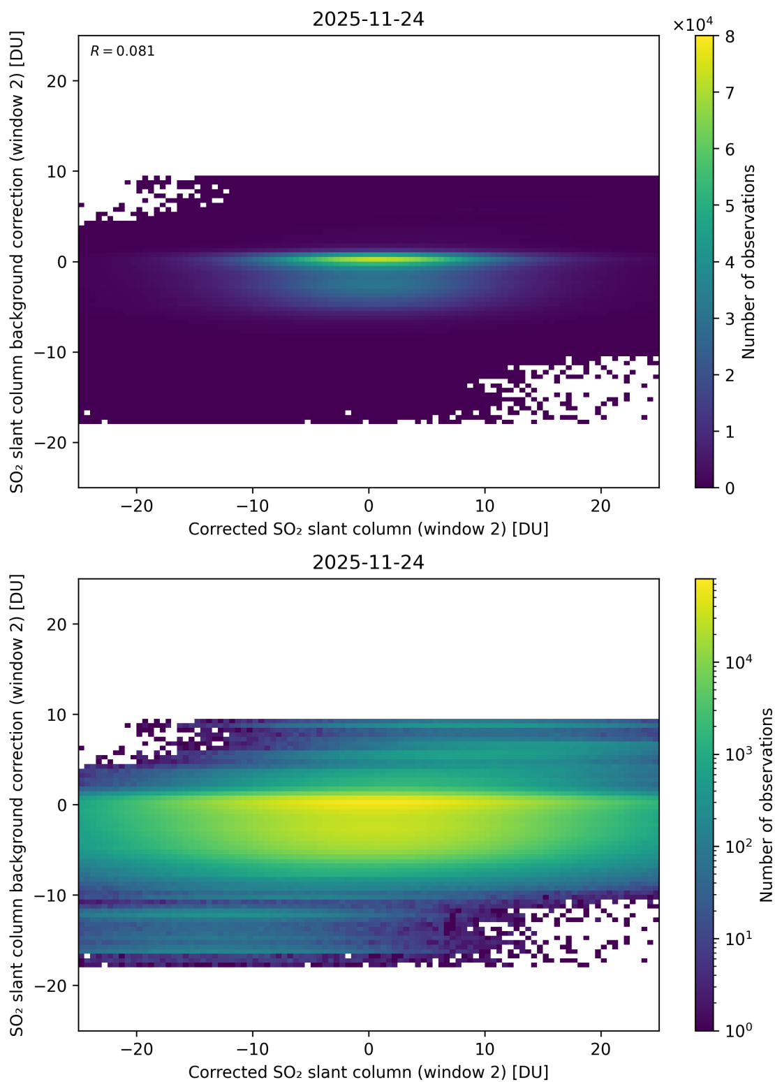
Figure 244: Scatter density plot of “Corrected SO 2 slant column (window 2)” against “SO 2 slant column background correction (window 2)” for 2025-11-23 to 2025-11-25.
