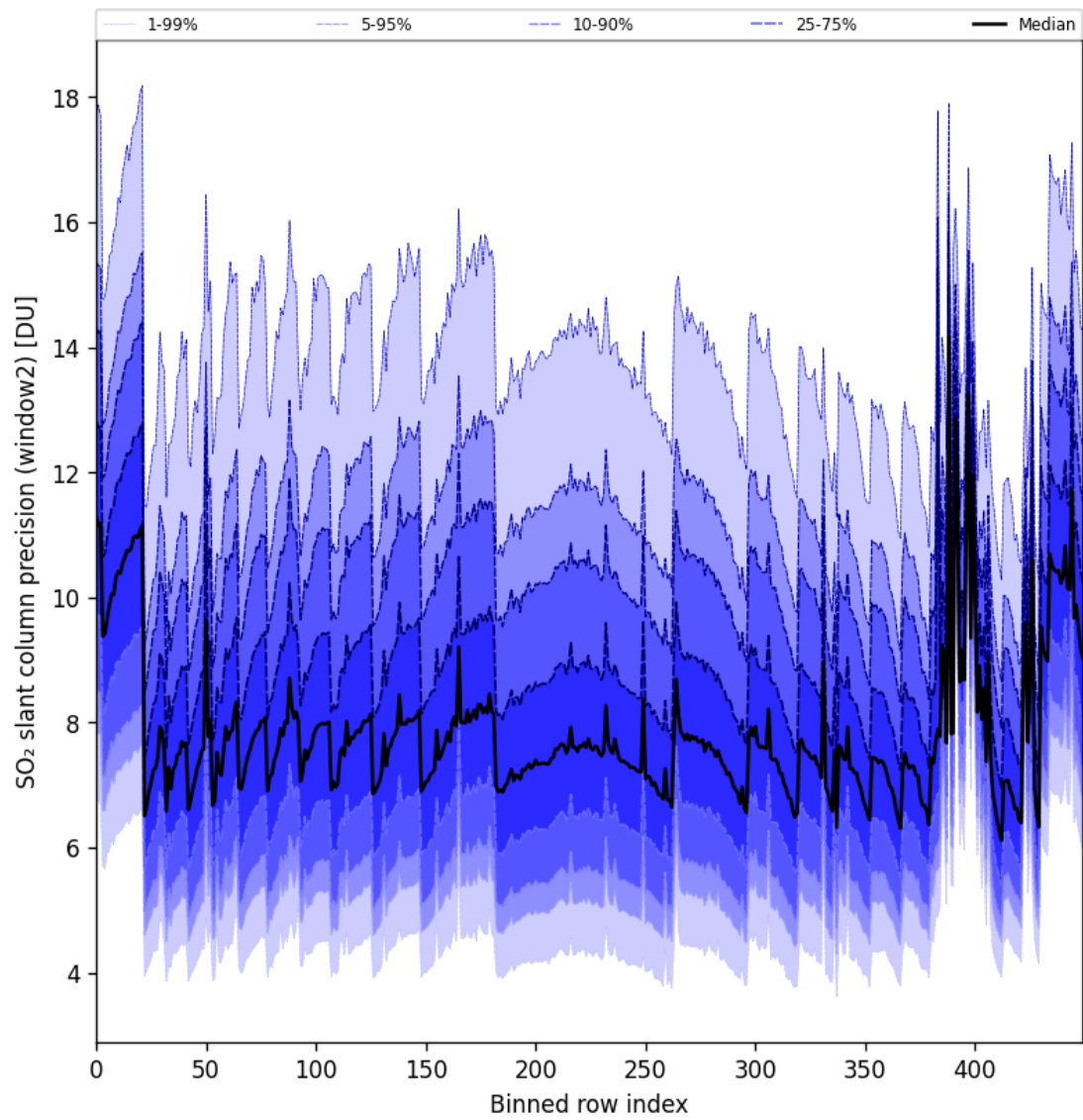
Figure 94: Along track statistics of “SO 2 slant column precision (window2)” for 2025-11-23 to 2025-11-25
