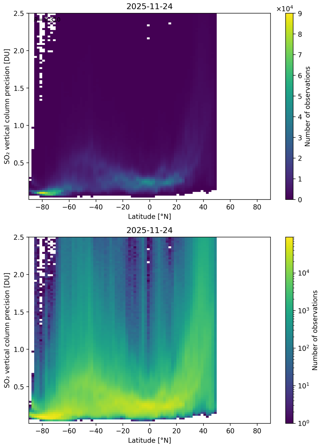
Figure 170: Scatter density plot of “Latitude” against “SO 2 vertical column precision” for 2025-11-23 to 2025-11-25.
