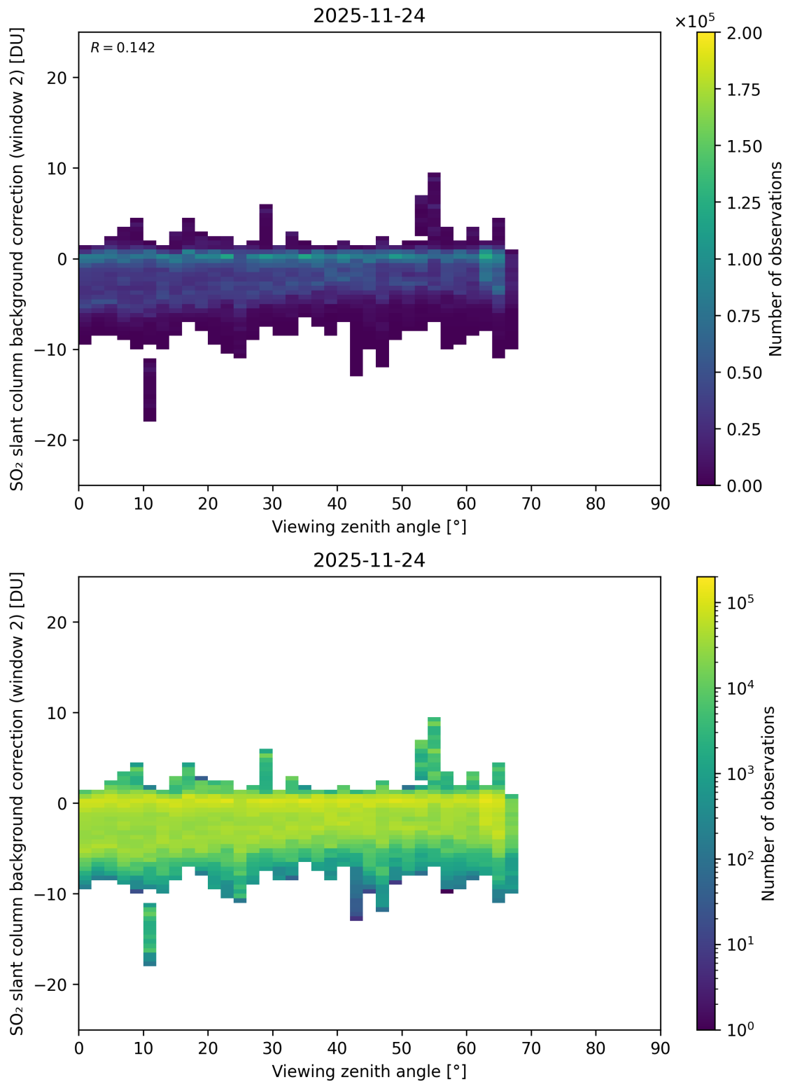
Figure 363: Scatter density plot of “Viewing zenith angle” against “SO 2 slant column background correction (window 2)” for 2025-11-23 to 2025-11-25.
