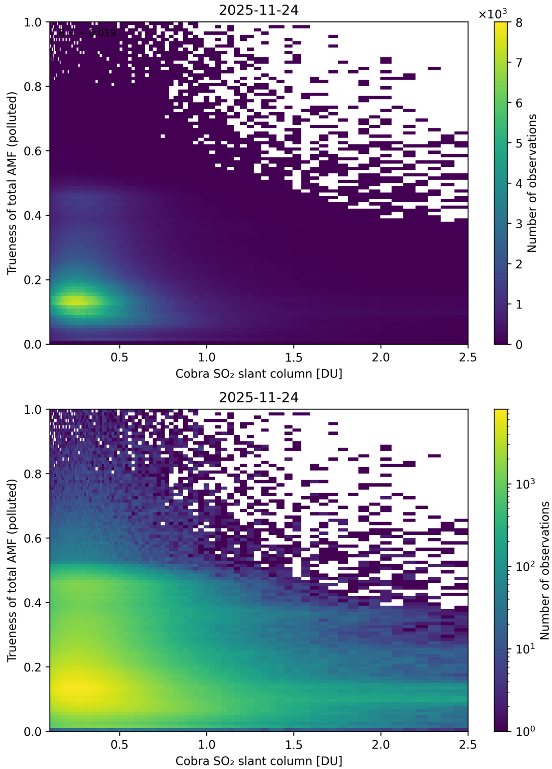
Figure 225: Scatter density plot of “Cobra SO 2 slant column” against “Trueness of total AMF (polluted)” for 2025-11-23 to 2025-11-25.
