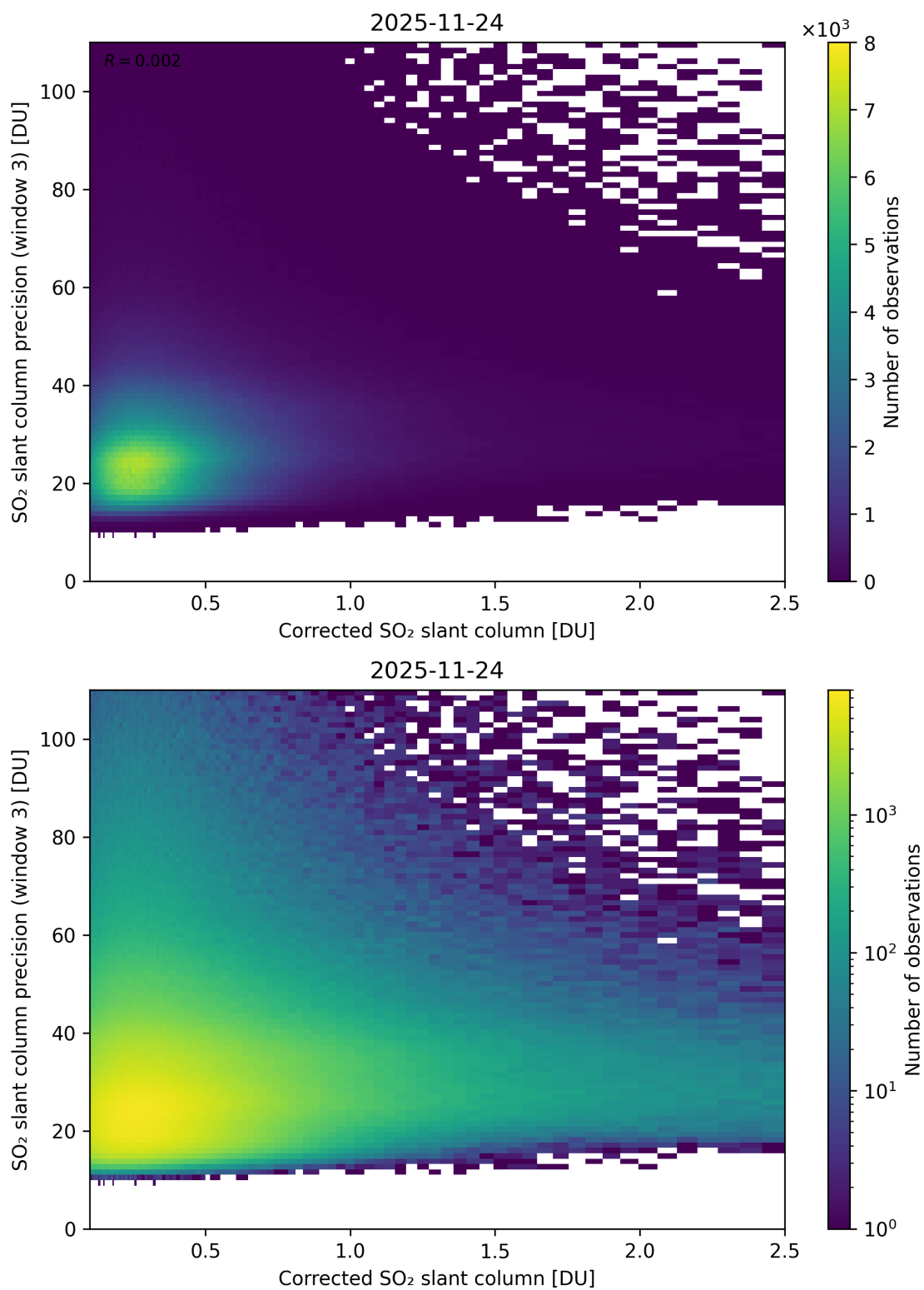
Figure 241: Scatter density plot of “Corrected SO 2 slant column” against “SO 2 slant column precision (window 3)” for 2025-11-23 to 2025-11-25.
