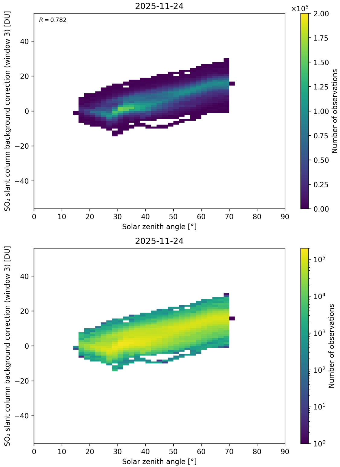
Figure 173: Scatter density plot of “Solar zenith angle” against “SO 2 slant column background correction (window 3)” for 2025-11-23 to 2025-11-25.
