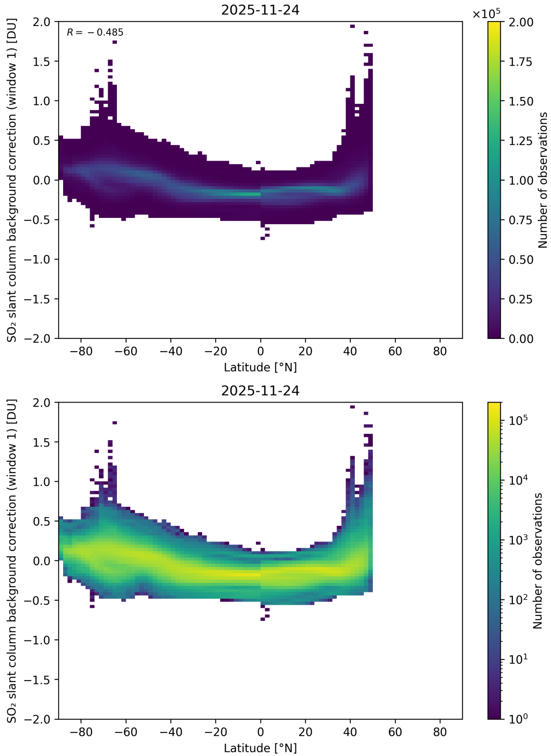
Figure 150: Scatter density plot of “Latitude” against “SO 2 slant column background correction (window 1)” for 2025-11-23 to 2025-11-25.
