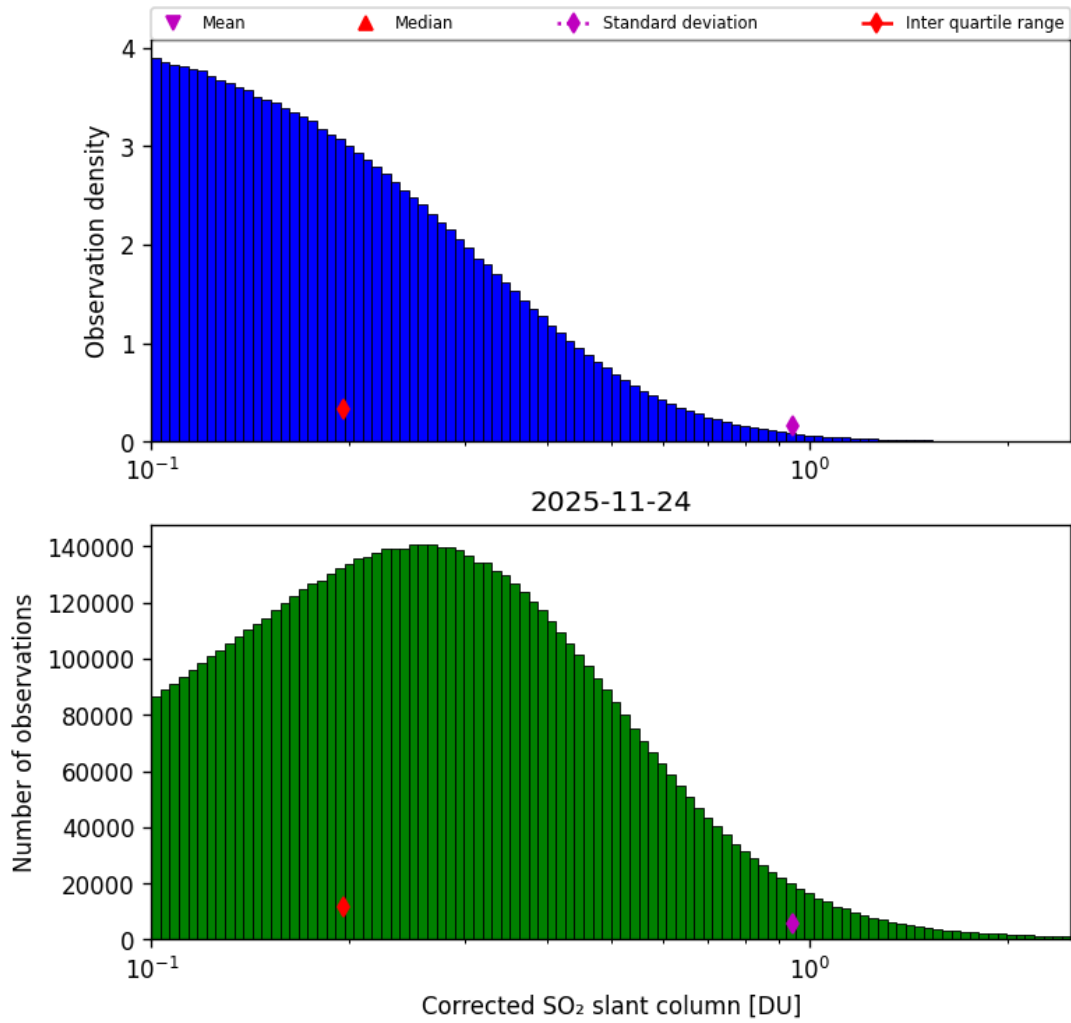
Figure 60: Histogram of "Corrected SO 2 slant column" for 2025-11-23 to 2025-11-25
