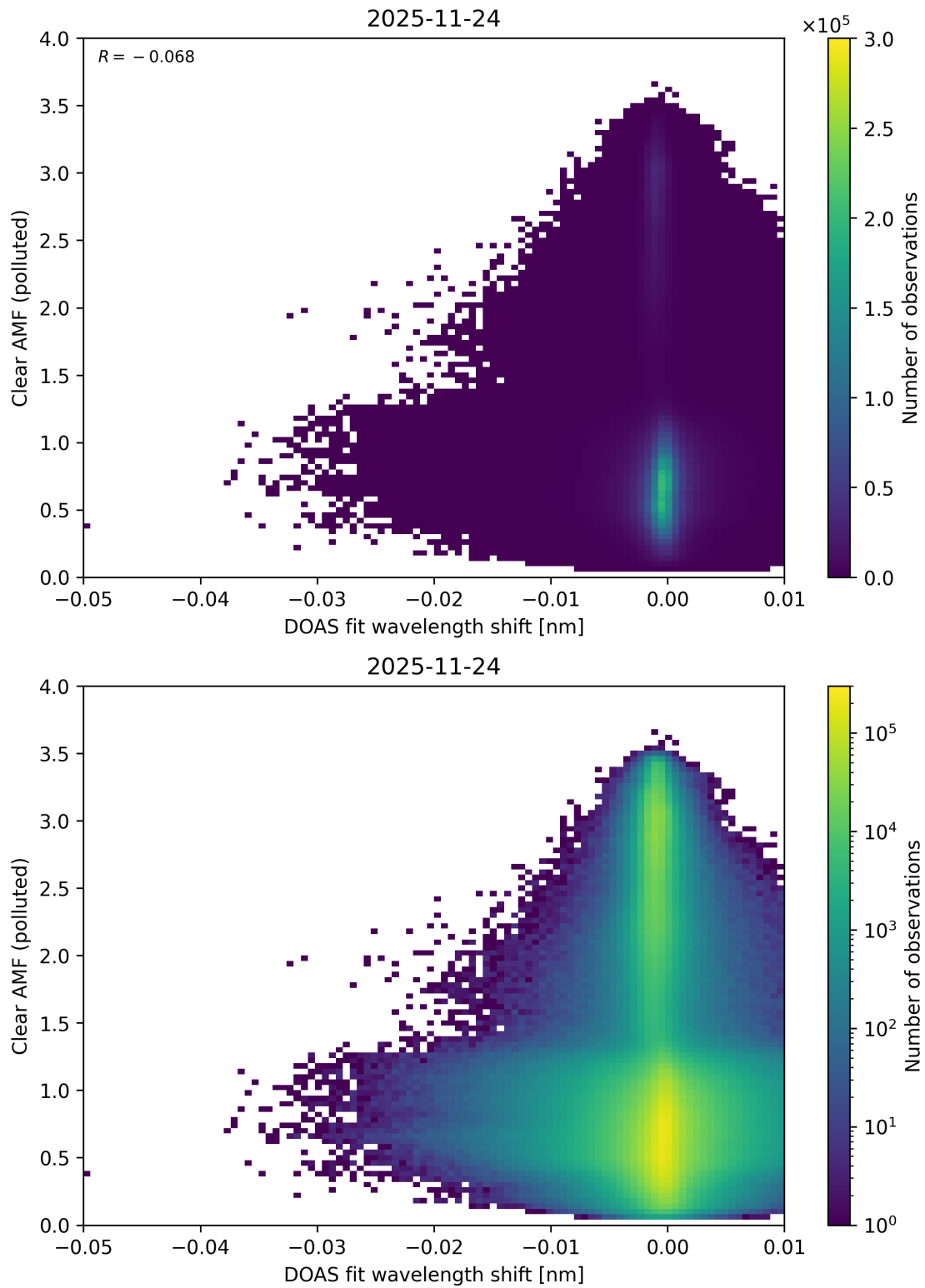
Figure 140: Scatter density plot of “DOAS fit wavelength shift” against “Clear AMF (polluted)” for 2025-11-23 to 2025-11-25.
