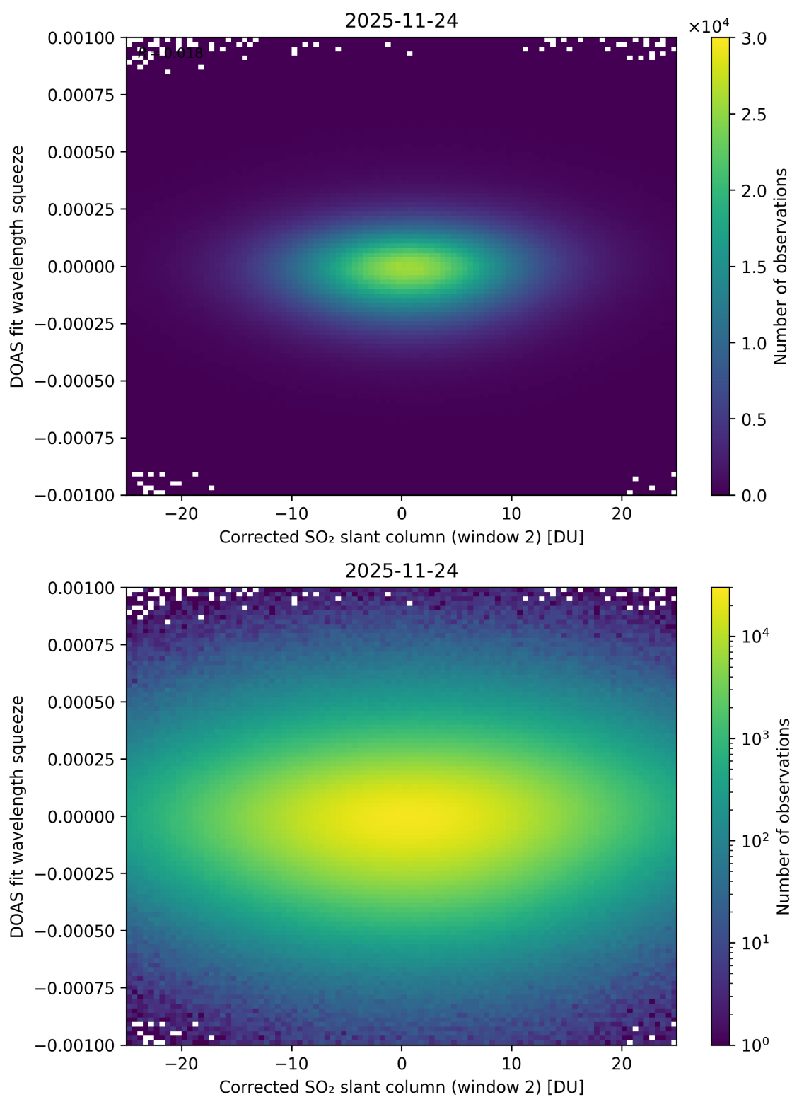
Figure 247: Scatter density plot of “Corrected SO 2 slant column (window 2)” against “DOAS fit wavelength squeeze” for 2025-11-23 to 2025-11-25.
