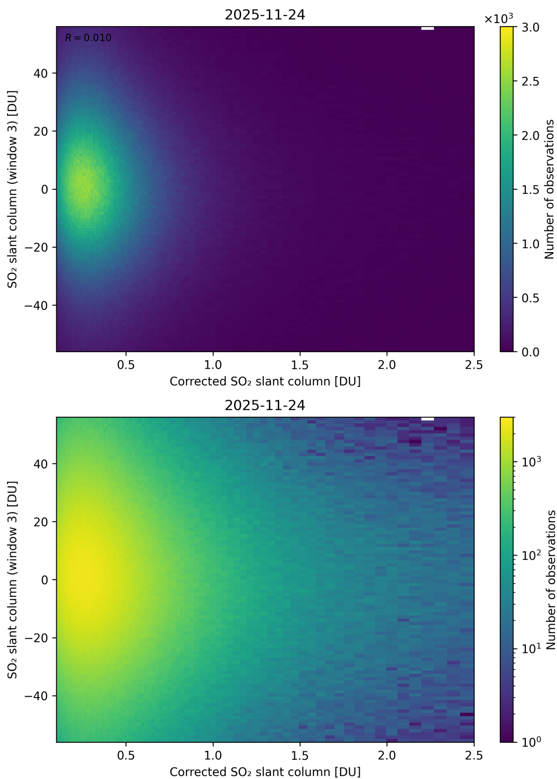
Figure 240: Scatter density plot of “Corrected SO 2 slant column” against “SO 2 slant column (window 3)” for 2025-11-23 to 2025-11-25.
