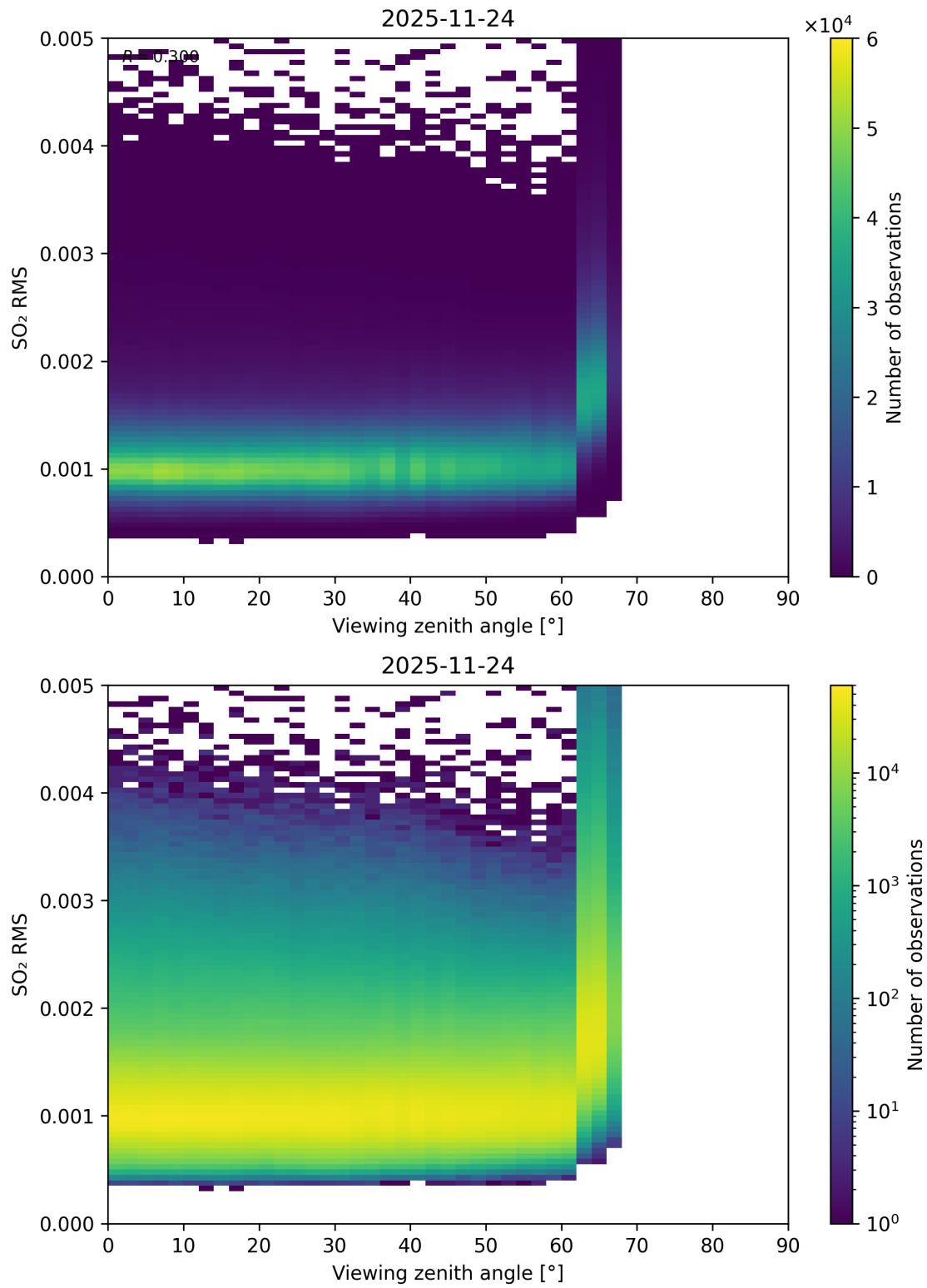
Figure 367: Scatter density plot of “Viewing zenith angle” against “SO 2 RMS” for 2025-11-23 to 2025-11-25.
