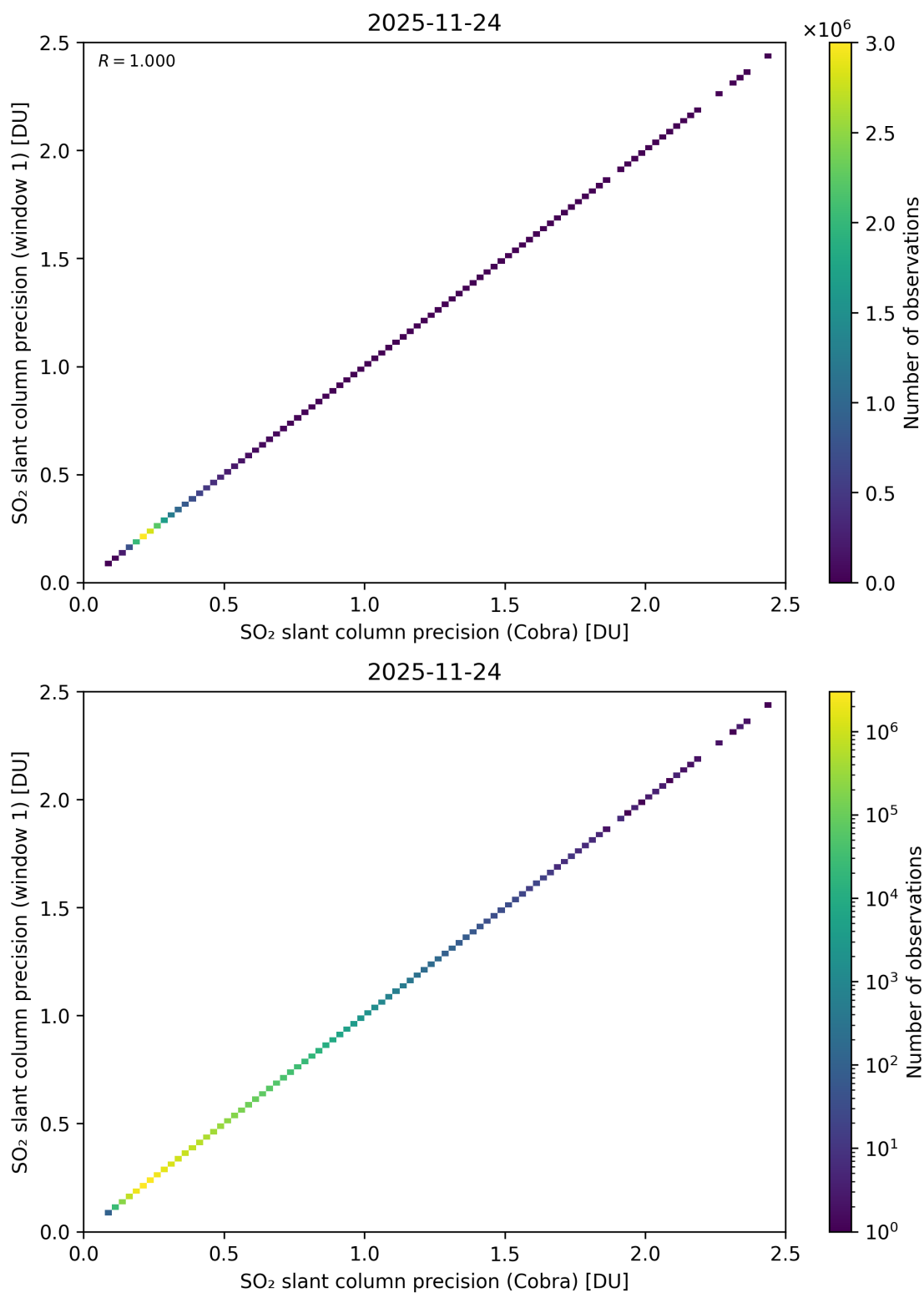
Figure 209: Scatter density plot of “SO 2 slant column precision (Cobra)” against “SO 2 slant column precision (window 1)” for 2025-11-23 to 2025-11-25.
