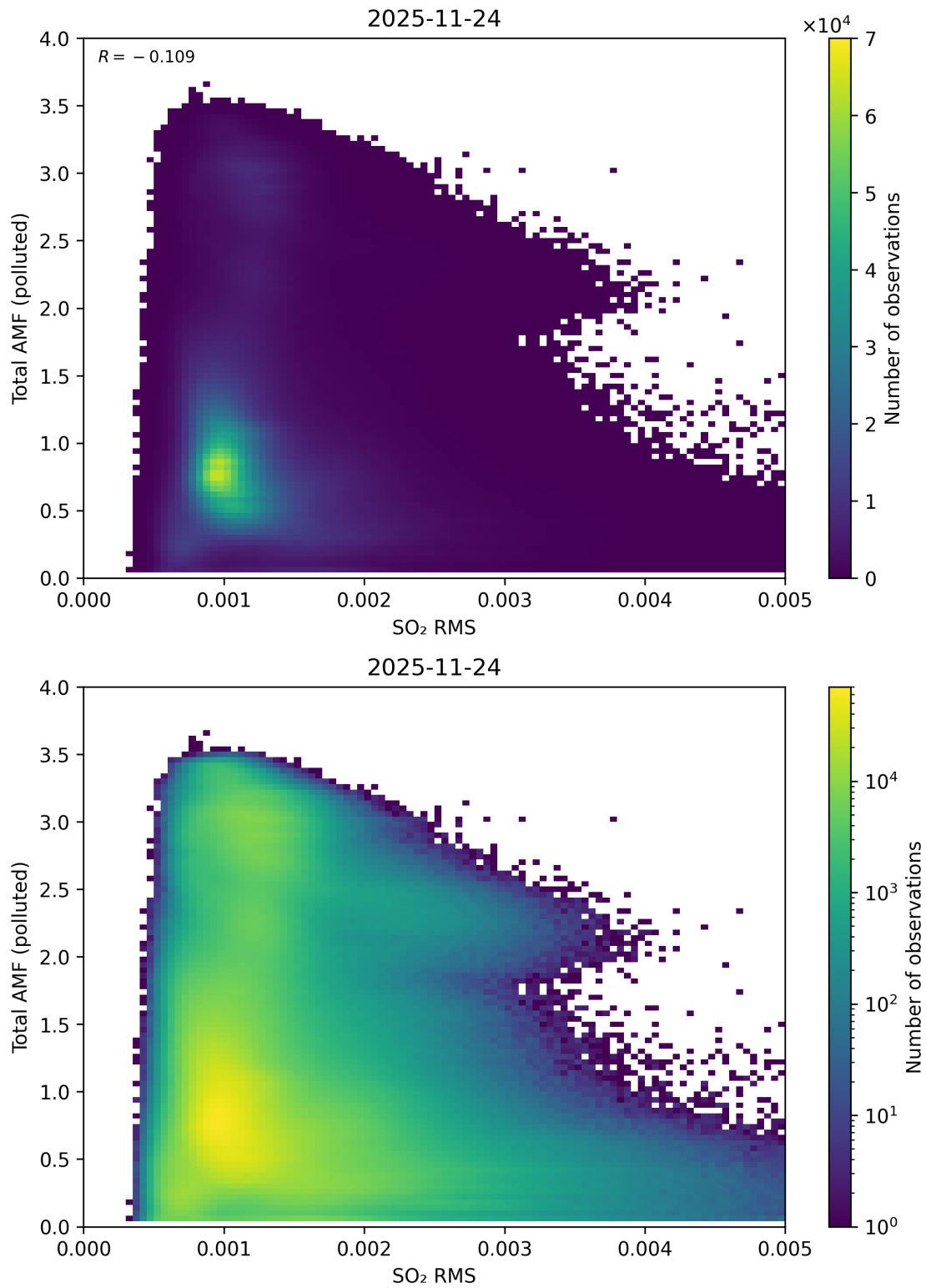
Figure 148: Scatter density plot of “SO 2 RMS” against “Total AMF (polluted)” for 2025-11-23 to 2025-11-25.
