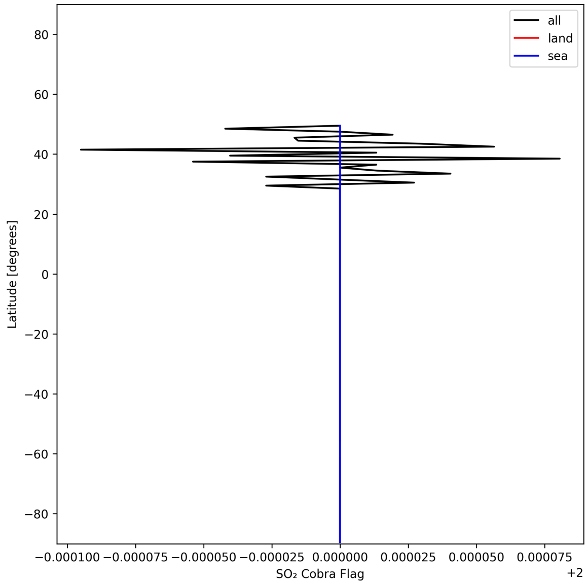
Figure 49: Zonal average of “SO 2 Cobra Flag” for 2025-11-23 to 2025-11-25.
