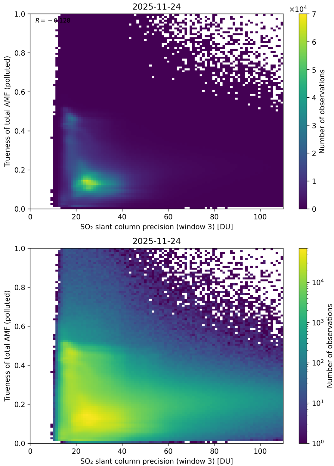
Figure 314: Scatter density plot of “SO 2 slant column precision (window 3)” against “Trueness of total AMF (polluted)” for 2025-11-23 to 2025-11-25.
