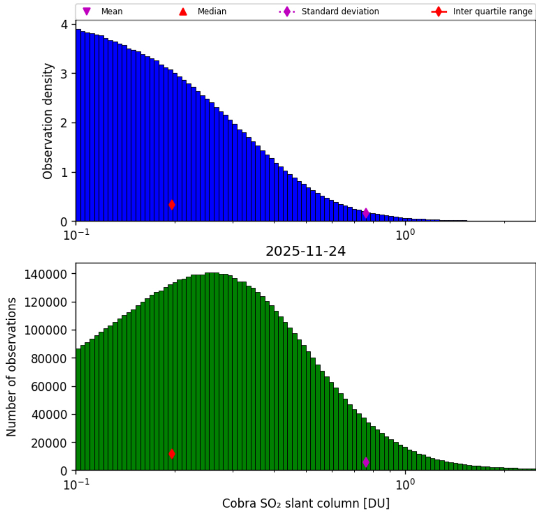
Figure 61: Histogram of “Cobra SO 2 slant column” for 2025-11-23 to 2025-11-25
