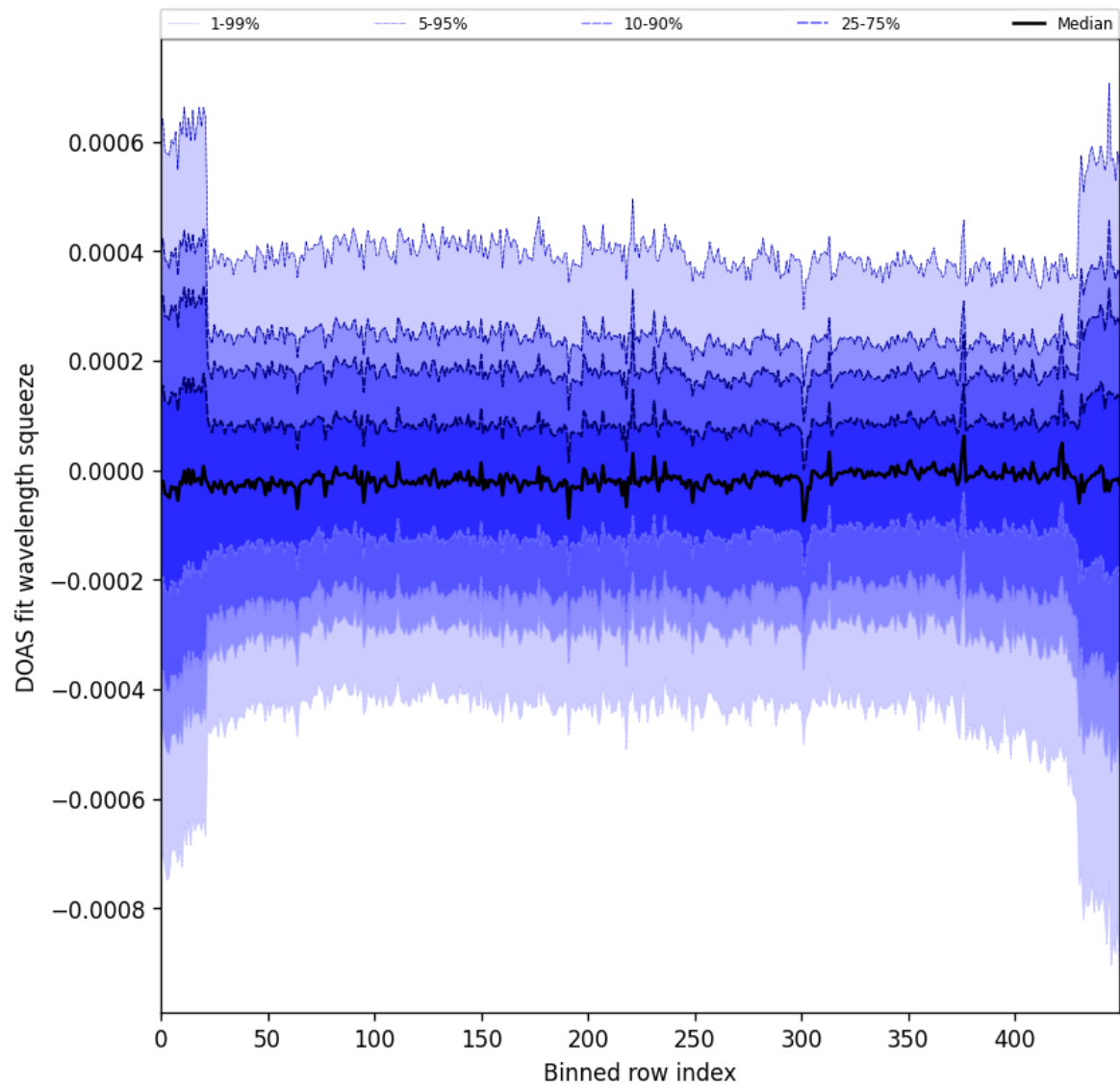
Figure 103: Along track statistics of “DOAS fit wavelength squeeze” for 2025-11-23 to 2025-11-25
