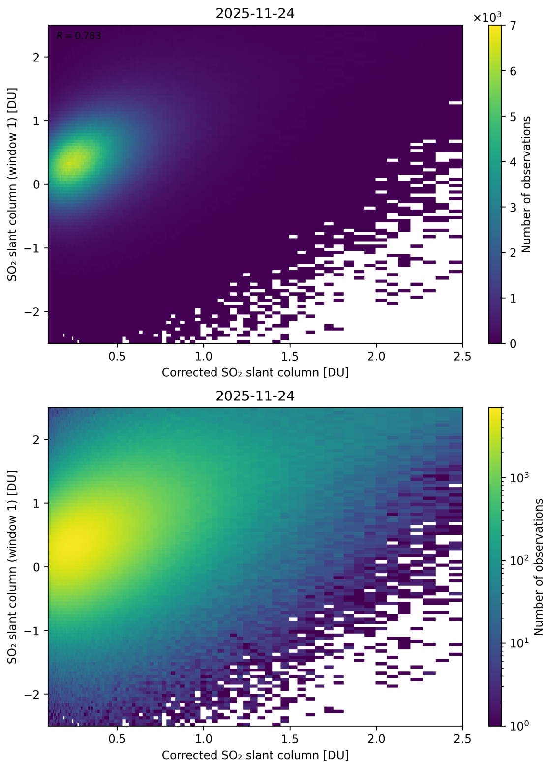
Figure 237: Scatter density plot of “Corrected SO 2 slant column” against “SO 2 slant column (window 1)” for 2025-11-23 to 2025-11-25.
