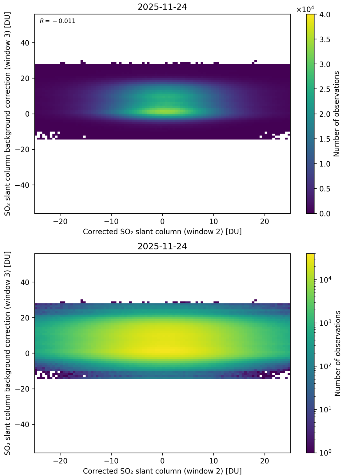
Figure 245: Scatter density plot of “Corrected SO 2 slant column (window 2)” against “SO 2 slant column background correction (window 3)” for 2025-11-23 to 2025-11-25.
