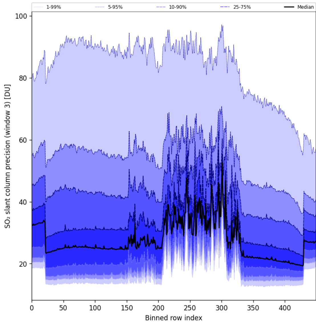
Figure 98: Along track statistics of “SO 2 slant column precision (window 3)” for 2025-11-23 to 2025-11-25
