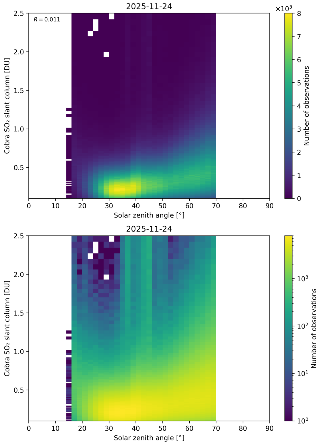
Figure 179: Scatter density plot of “Solar zenith angle” against “Cobra SO 2 slant column” for 2025-11-23 to 2025-11-25.
