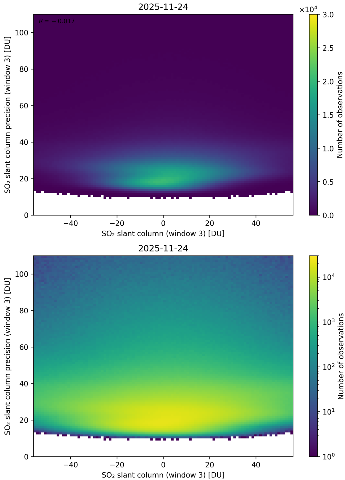
Figure 317: Scatter density plot of “SO 2 slant column (window 3)” against “SO 2 slant column precision (window 3)” for 2025-11-23 to 2025-11-25.
