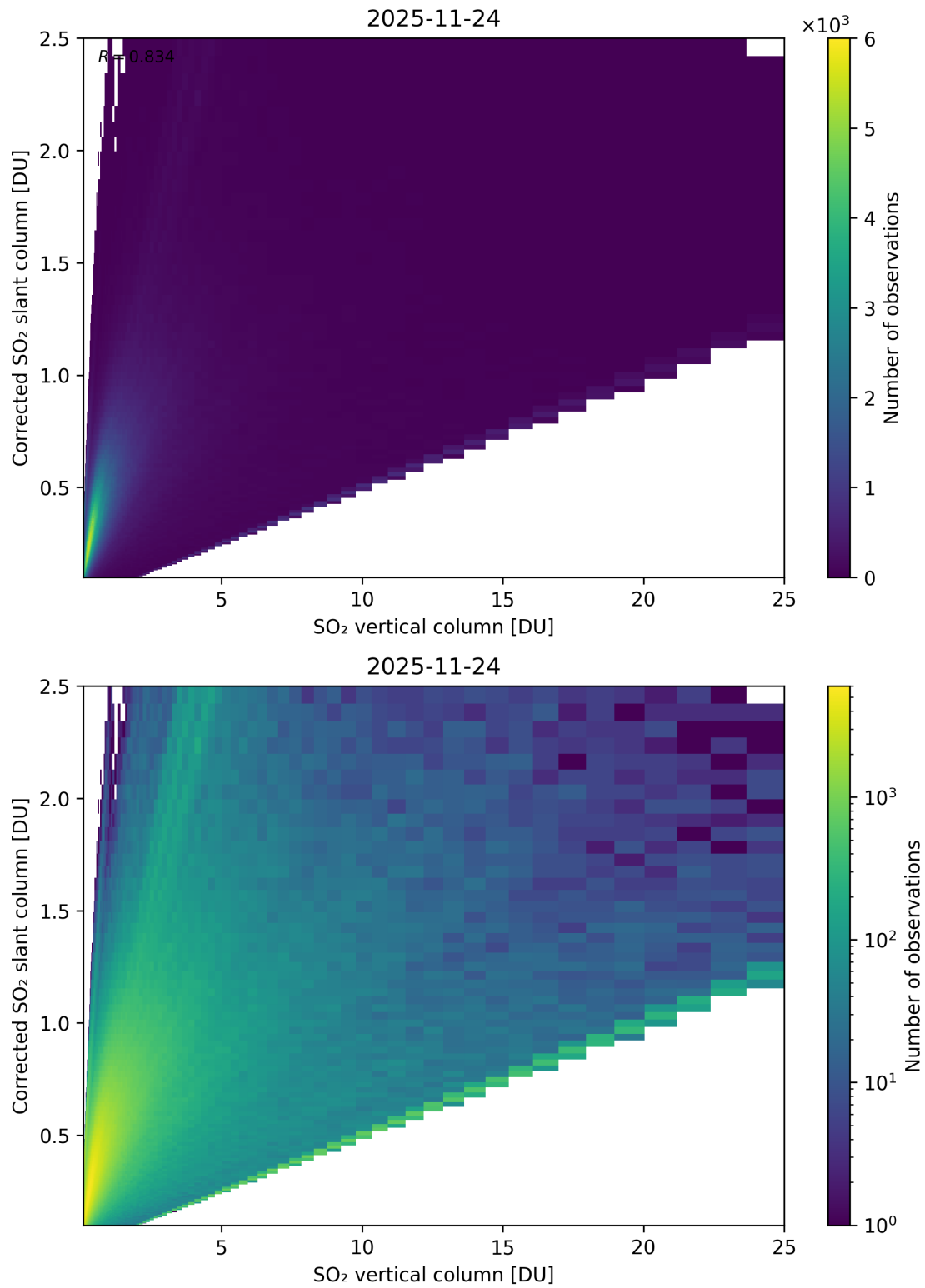
Figure 351: Scatter density plot of “SO 2 vertical column” against “Corrected SO 2 slant column” for 2025-11-23 to 2025-11-25.
