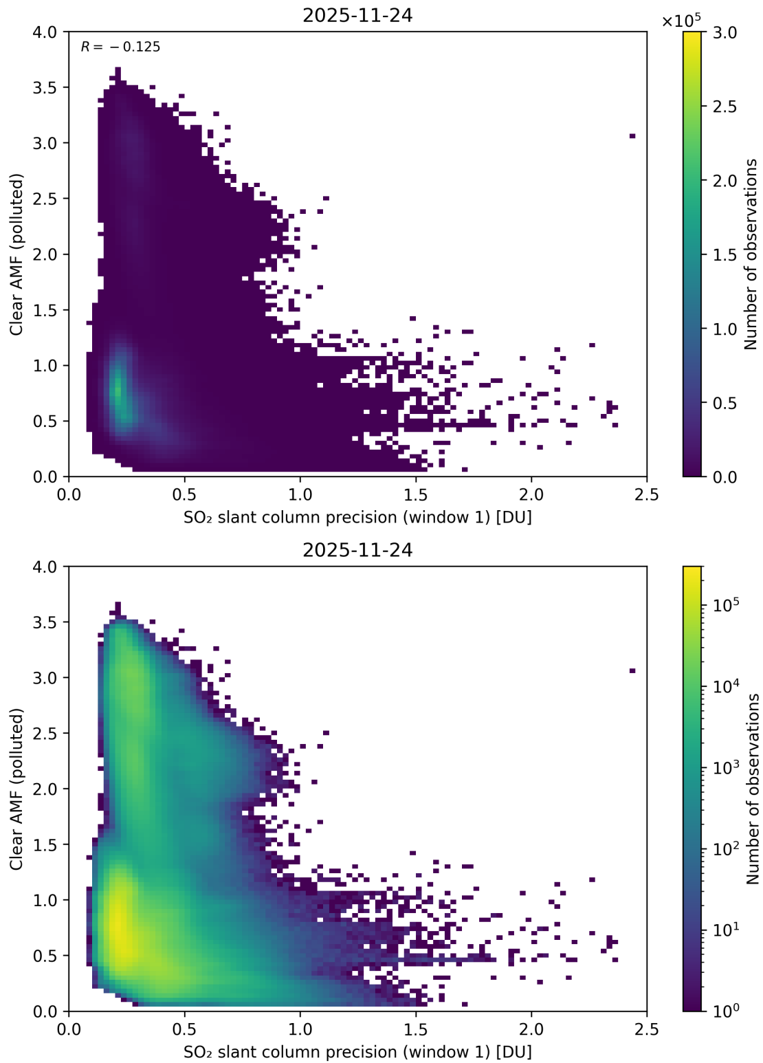
Figure 274: Scatter density plot of “SO 2 slant column precision (window 1)” against “Clear AMF (polluted)” for 2025-11-23 to 2025-11-25.
