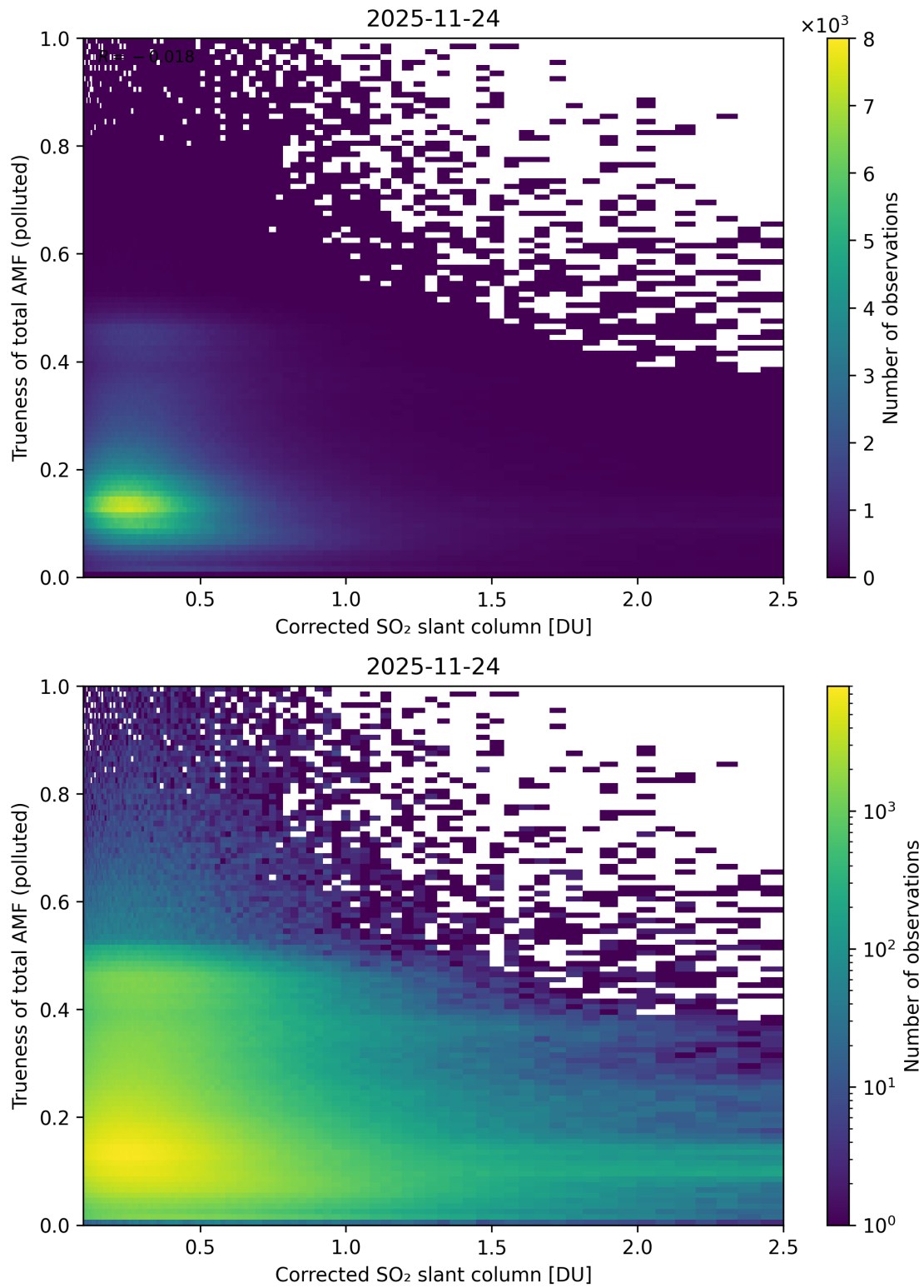
Figure 243: Scatter density plot of “Corrected SO 2 slant column” against “Trueness of total AMF (polluted)” for 2025-11-23 to 2025-11-25.
