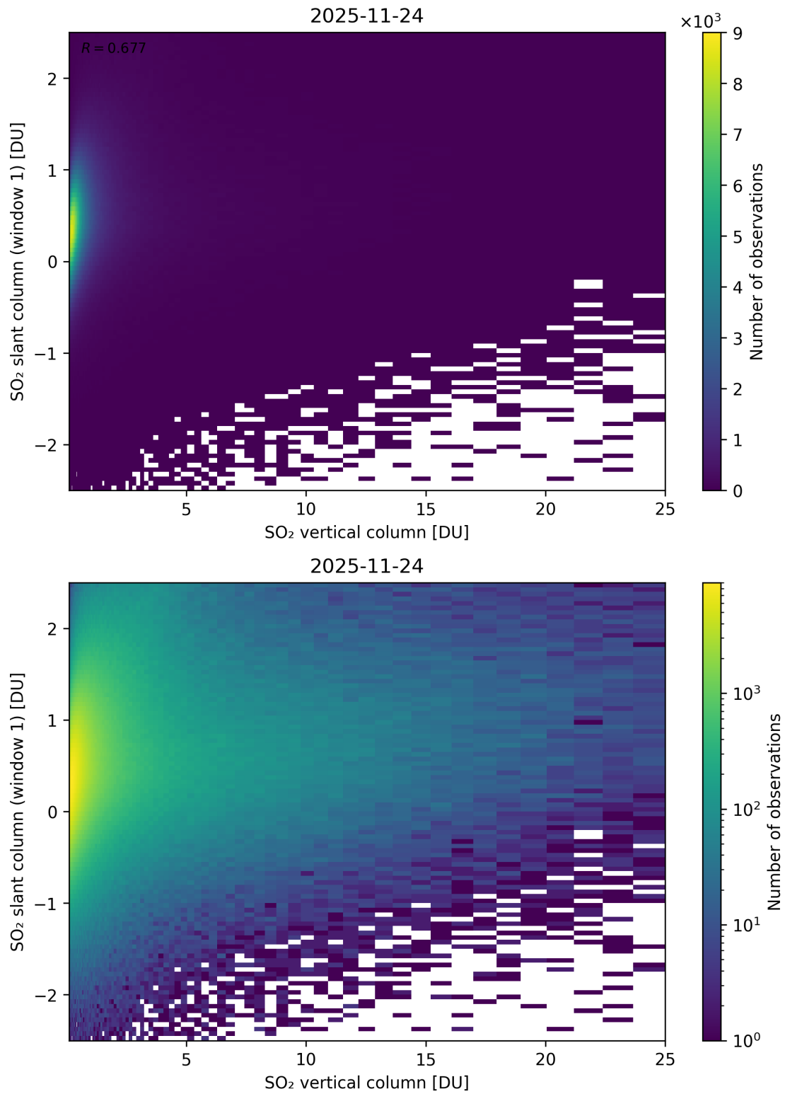
Figure 354: Scatter density plot of “SO 2 vertical column” against “SO 2 slant column (window 1)” for 2025-11-23 to 2025-11-25.
