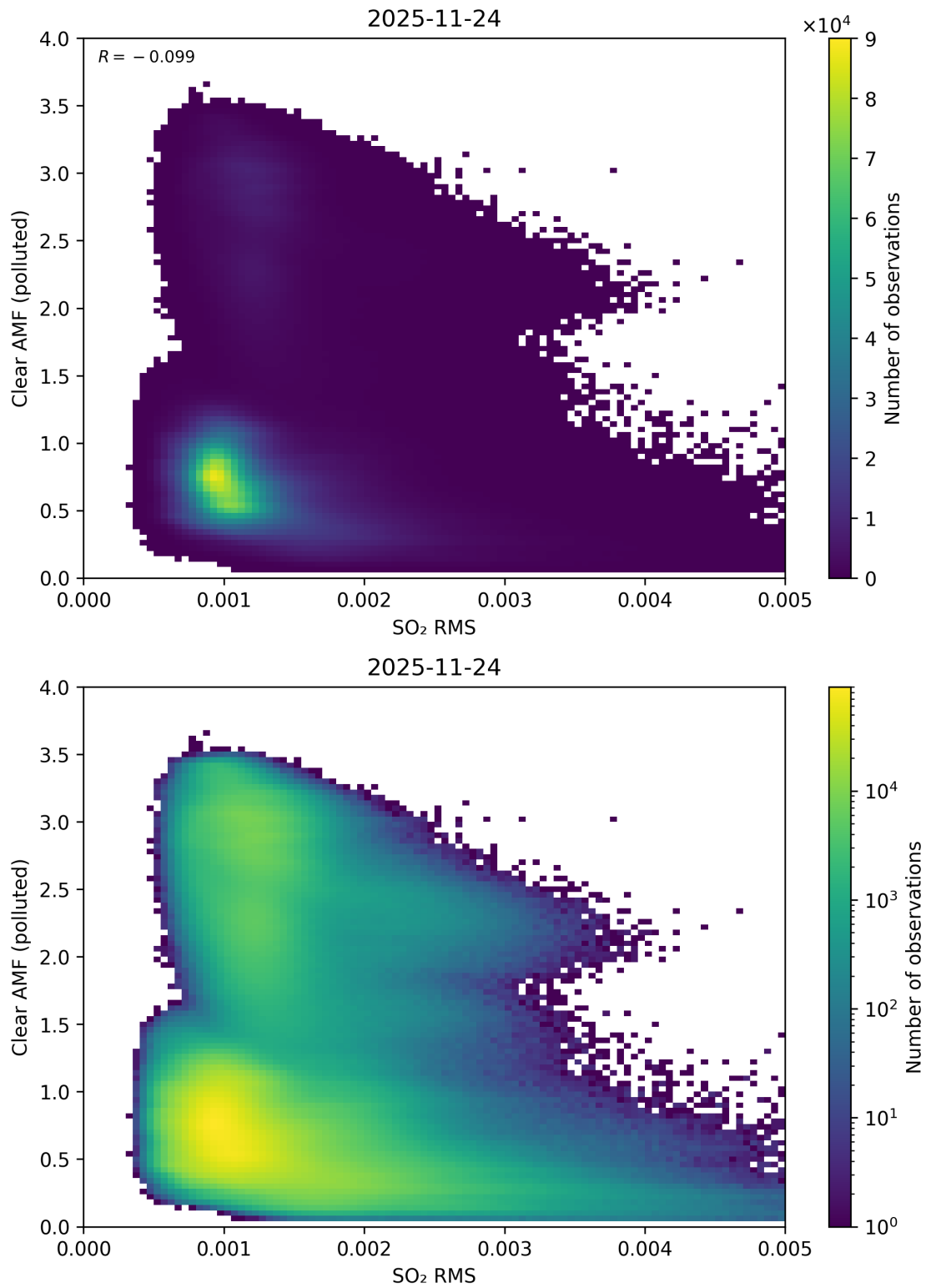
Figure 147: Scatter density plot of “SO 2 RMS” against “Clear AMF (polluted)” for 2025-11-23 to 2025-11-25.
