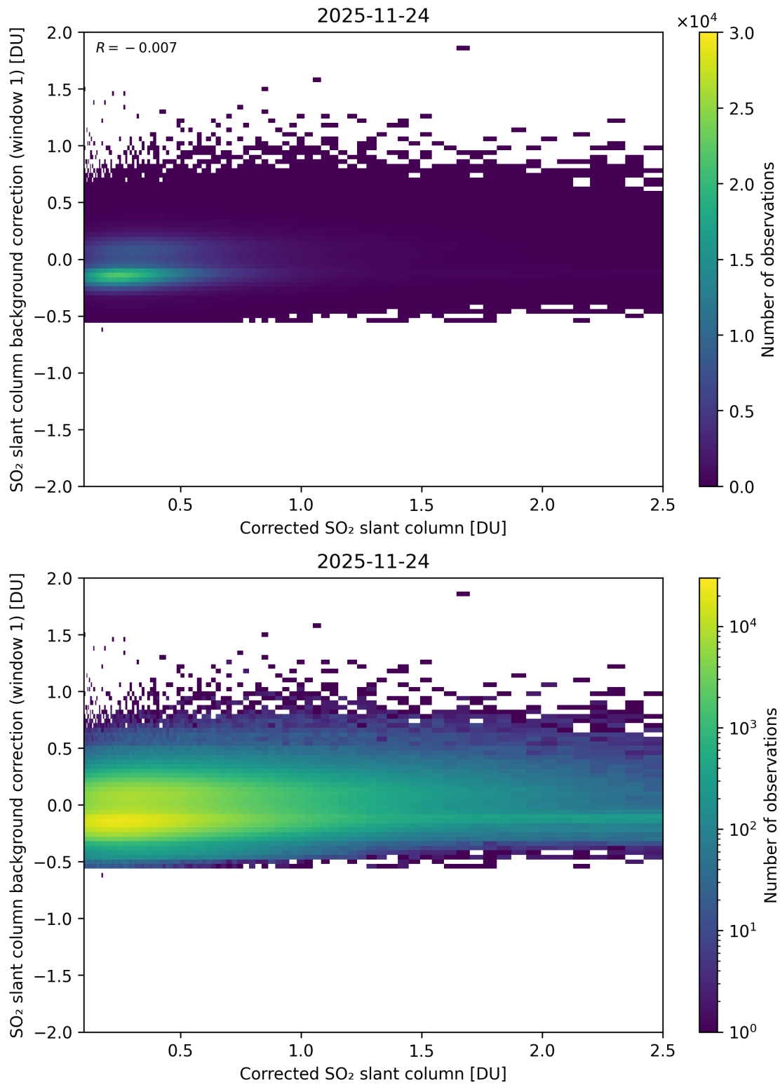
Figure 226: Scatter density plot of “Corrected SO 2 slant column” against “SO 2 slant column background correction (window 1)” for 2025-11-23 to 2025-11-25.
