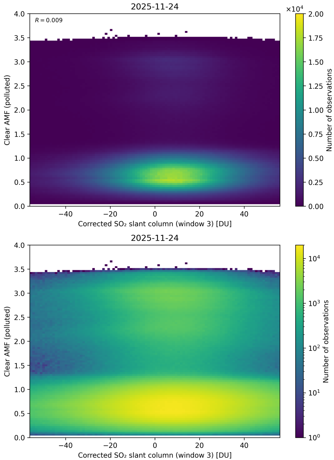
Figure 259: Scatter density plot of “Corrected SO 2 slant column (window 3)” against “Clear AMF (polluted)” for 2025-11-23 to 2025-11-25.
