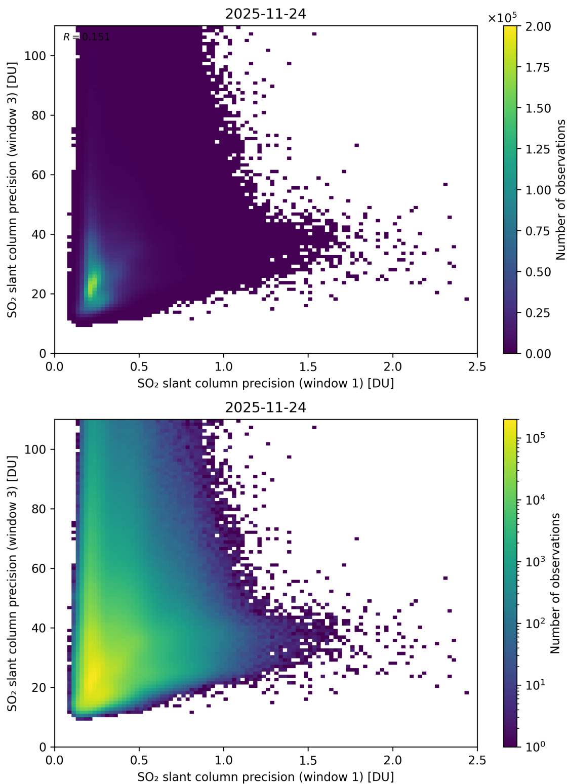
Figure 279: Scatter density plot of “SO 2 slant column precision (window 1)” against “SO 2 slant column precision (window 3)” for 2025-11-23 to 2025-11-25.
