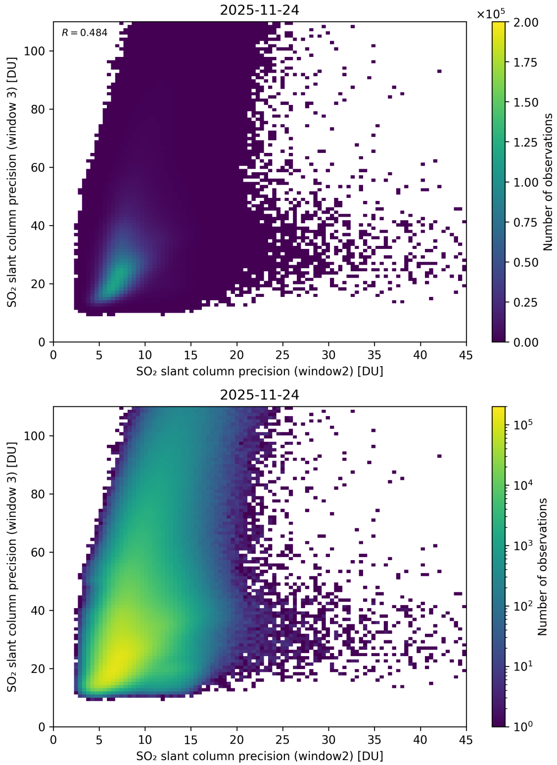
Figure 300: Scatter density plot of “SO 2 slant column precision (window2)” against “SO 2 slant column precision (window 3)” for 2025-11-23 to 2025-11-25.
