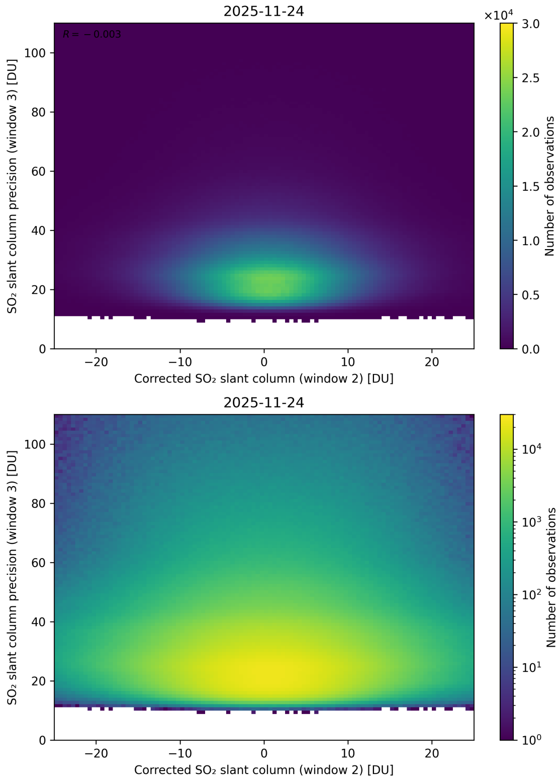
Figure 252: Scatter density plot of “Corrected SO 2 slant column (window 2)” against “SO 2 slant column precision (window 3)” for 2025-11-23 to 2025-11-25.
