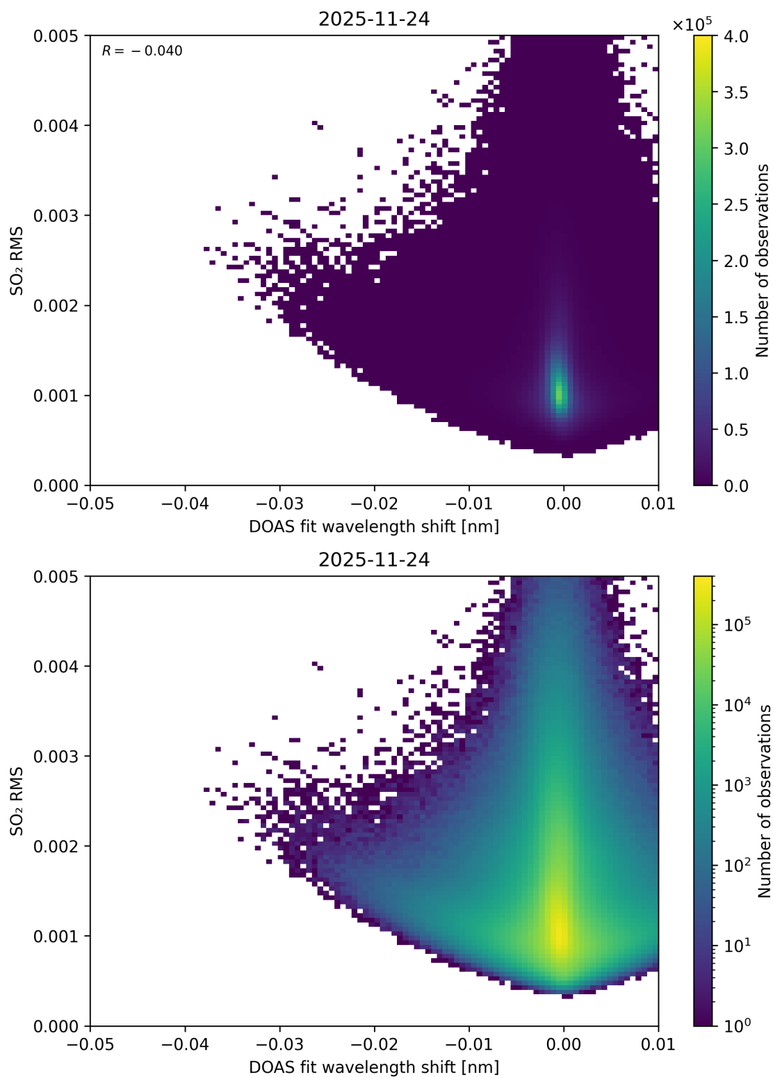
Figure 139: Scatter density plot of “DOAS fit wavelength shift” against “SO 2 RMS” for 2025-11-23 to 2025-11-25.
