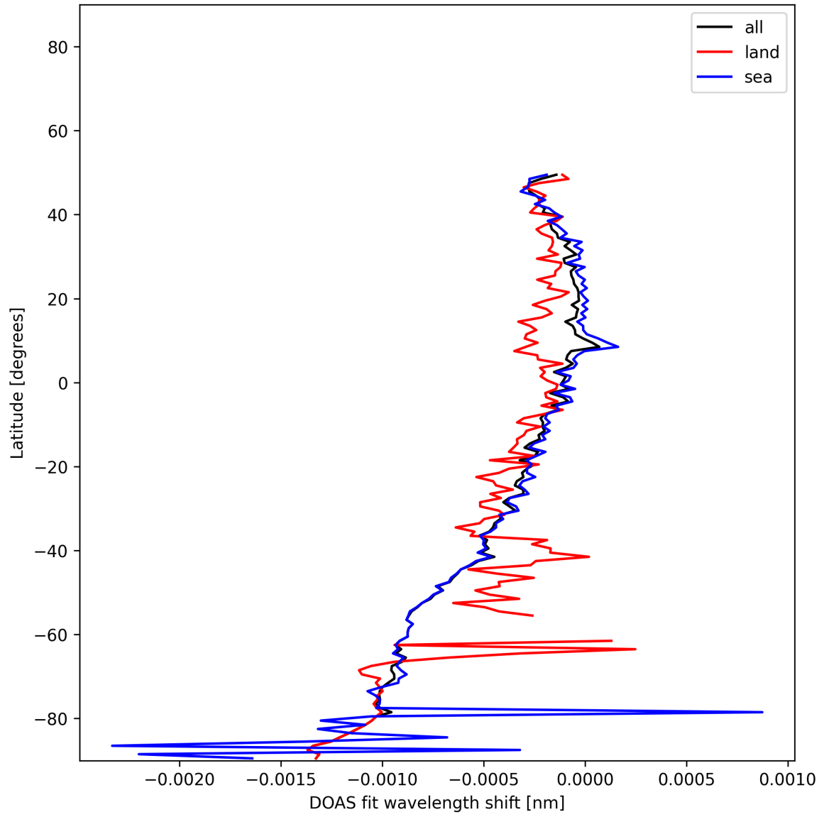
Figure 50: Zonal average of “DOAS fit wavelength shift” for 2025-11-23 to 2025-11-25.
