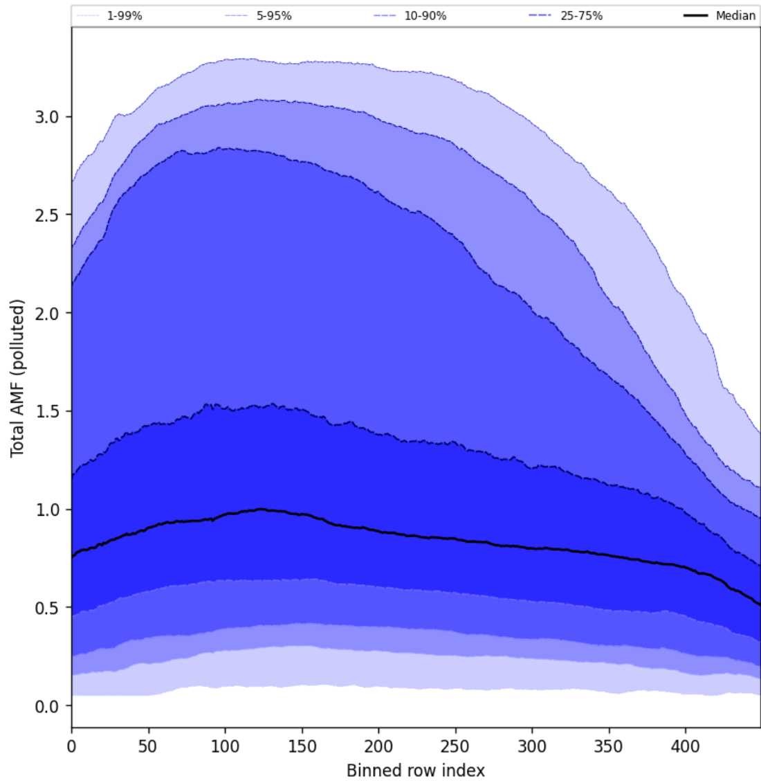
Figure 105: Along track statistics of “Total AMF (polluted)” for 2025-11-23 to 2025-11-25
