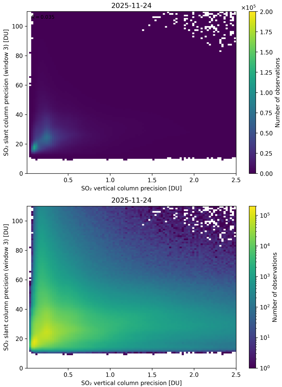
Figure 345: Scatter density plot of “SO 2 vertical column precision” against “SO 2 slant column precision (window 3)” for 2025-11-23 to 2025-11-25.
