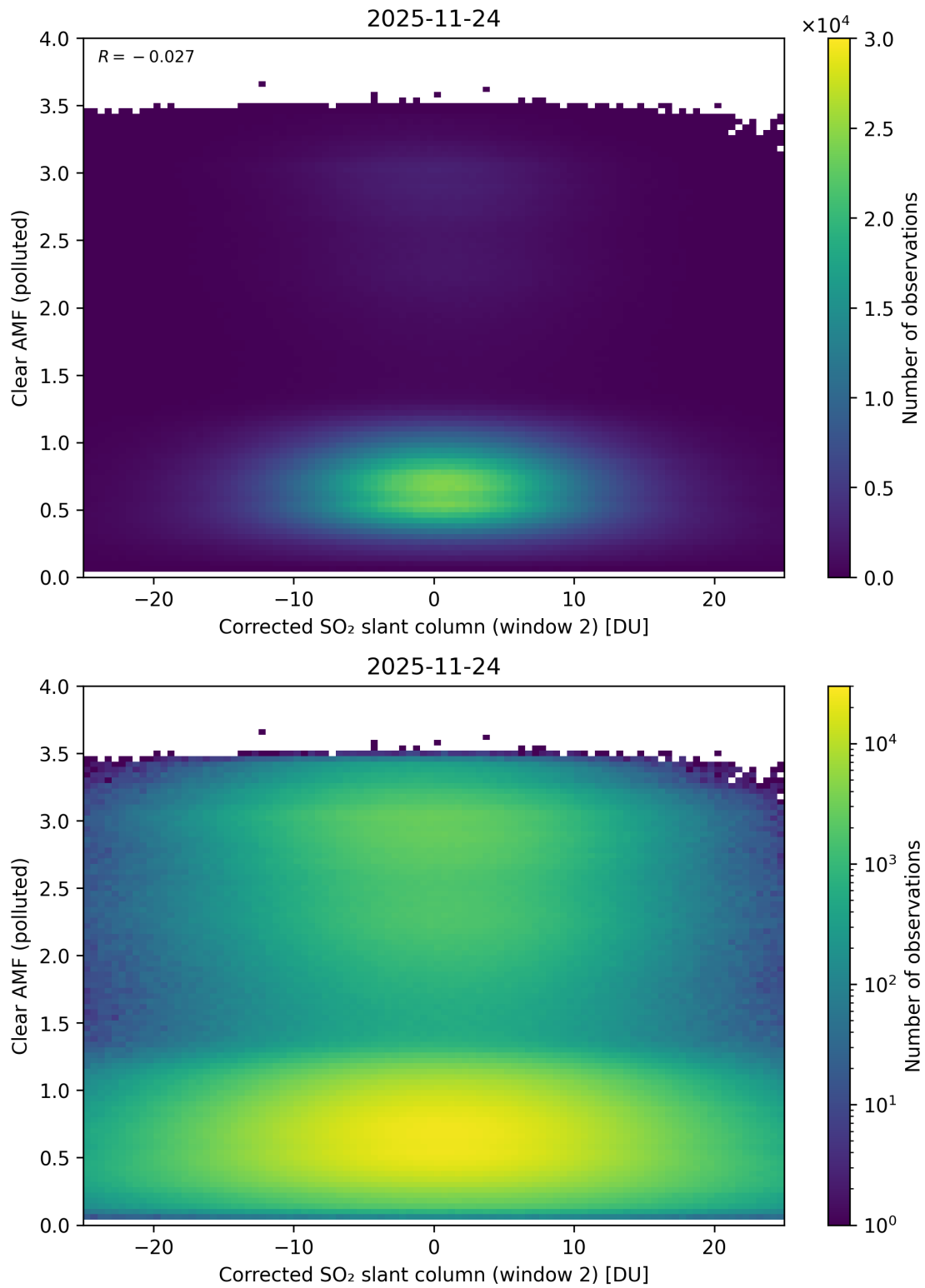
Figure 249: Scatter density plot of “Corrected SO 2 slant column (window 2)” against “Clear AMF (polluted)” for 2025-11-23 to 2025-11-25.
