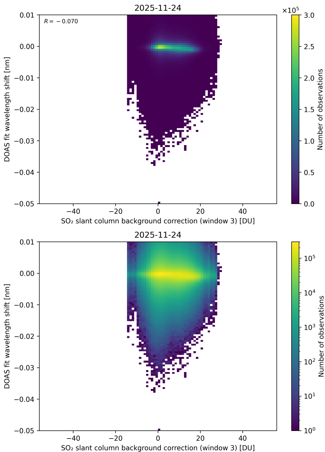
Figure 132: Scatter density plot of “SO 2 slant column background correction (window 3)” against “DOAS fit wavelength shift” for 2025-11-23 to 2025-11-25.
