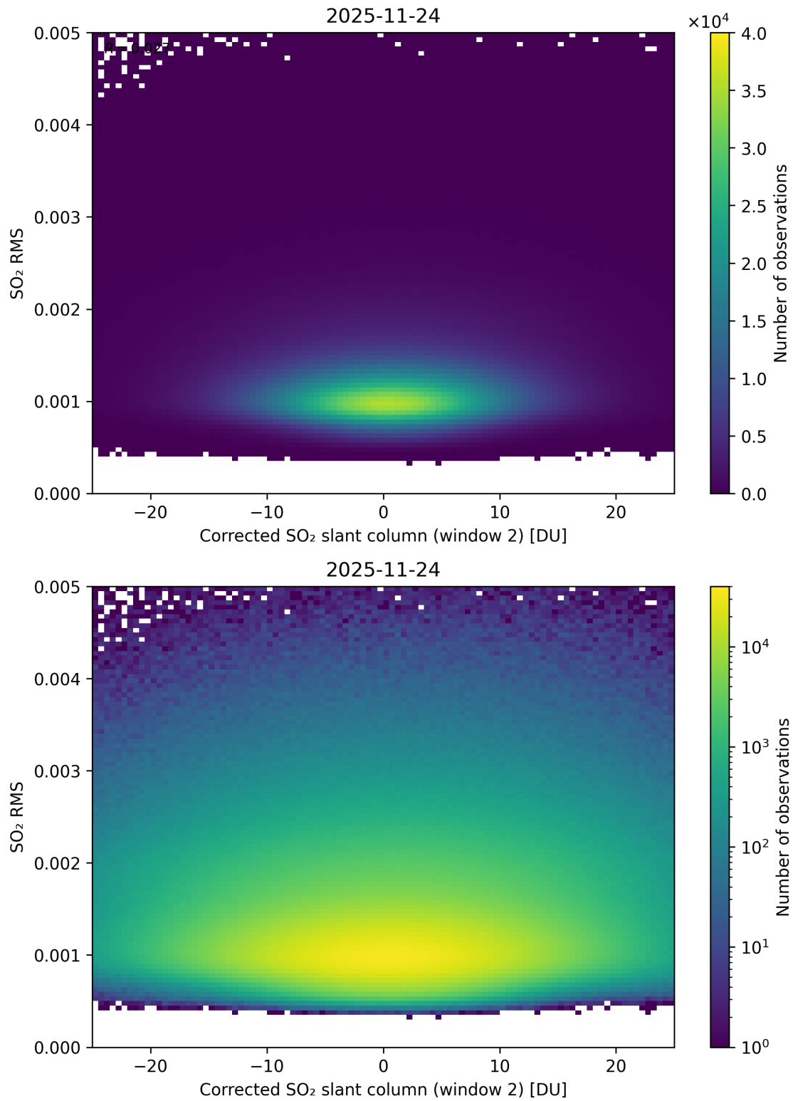
Figure 248: Scatter density plot of “Corrected SO 2 slant column (window 2)” against “SO 2 RMS” for 2025-11-23 to 2025-11-25.
