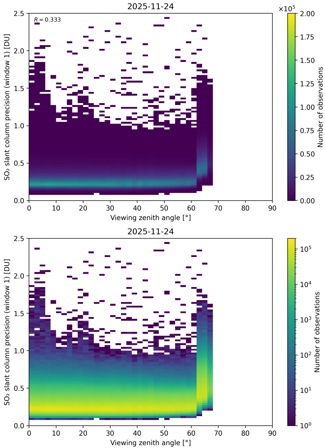
Figure 377: Scatter density plot of “Viewing zenith angle” against “SO 2 slant column precision (window 1)” for 2025-11-23 to 2025-11-25.
