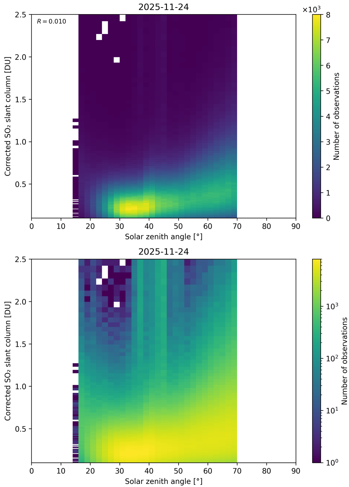
Figure 181: Scatter density plot of “Solar zenith angle” against “Corrected SO 2 slant column” for 2025-11-23 to 2025-11-25.
