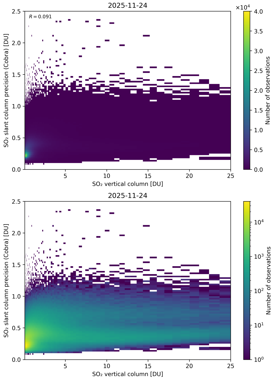
Figure 350: Scatter density plot of “SO 2 vertical column” against “SO 2 slant column precision (Cobra)” for 2025-11-23 to 2025-11-25.
