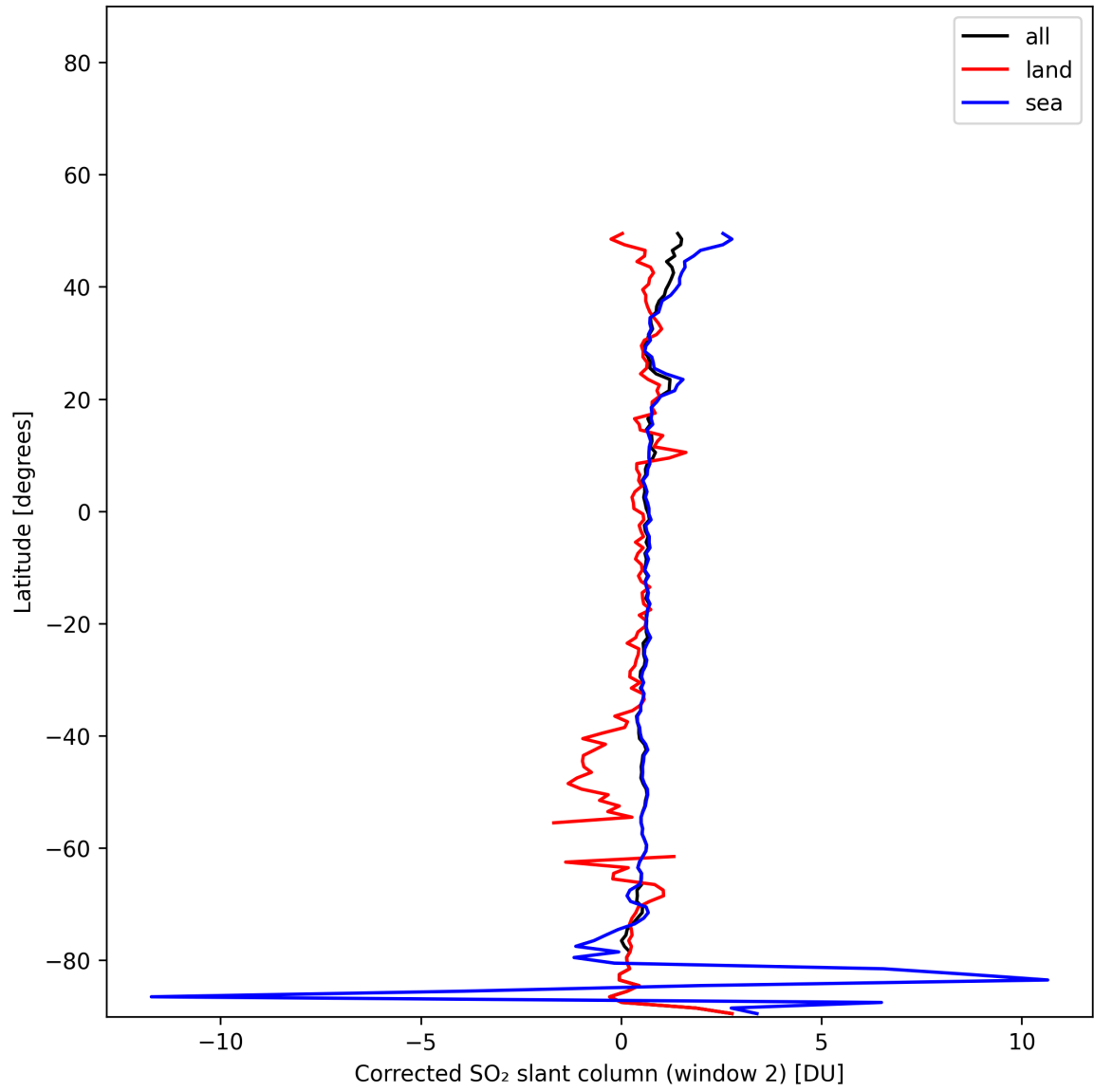
Figure 43: Zonal average of “Corrected SO 2 slant column (window 2)” for 2025-11-23 to 2025-11-25.
