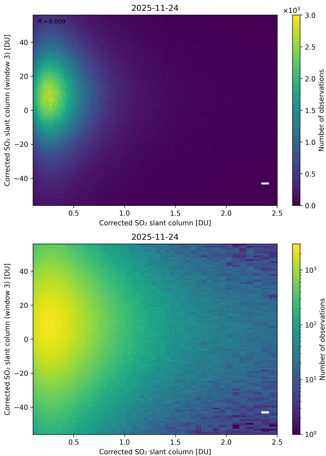
Figure 236: Scatter density plot of “Corrected SO 2 slant column” against “Corrected SO 2 slant column (window 3)” for 2025-11-23 to 2025-11-25.
