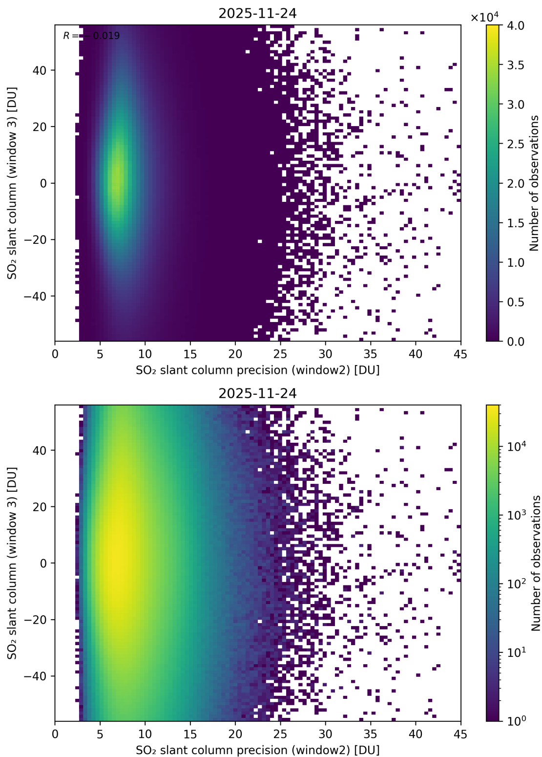
Figure 299: Scatter density plot of “SO 2 slant column precision (window2)” against “SO 2 slant column (window 3)” for 2025-11-23 to 2025-11-25.
