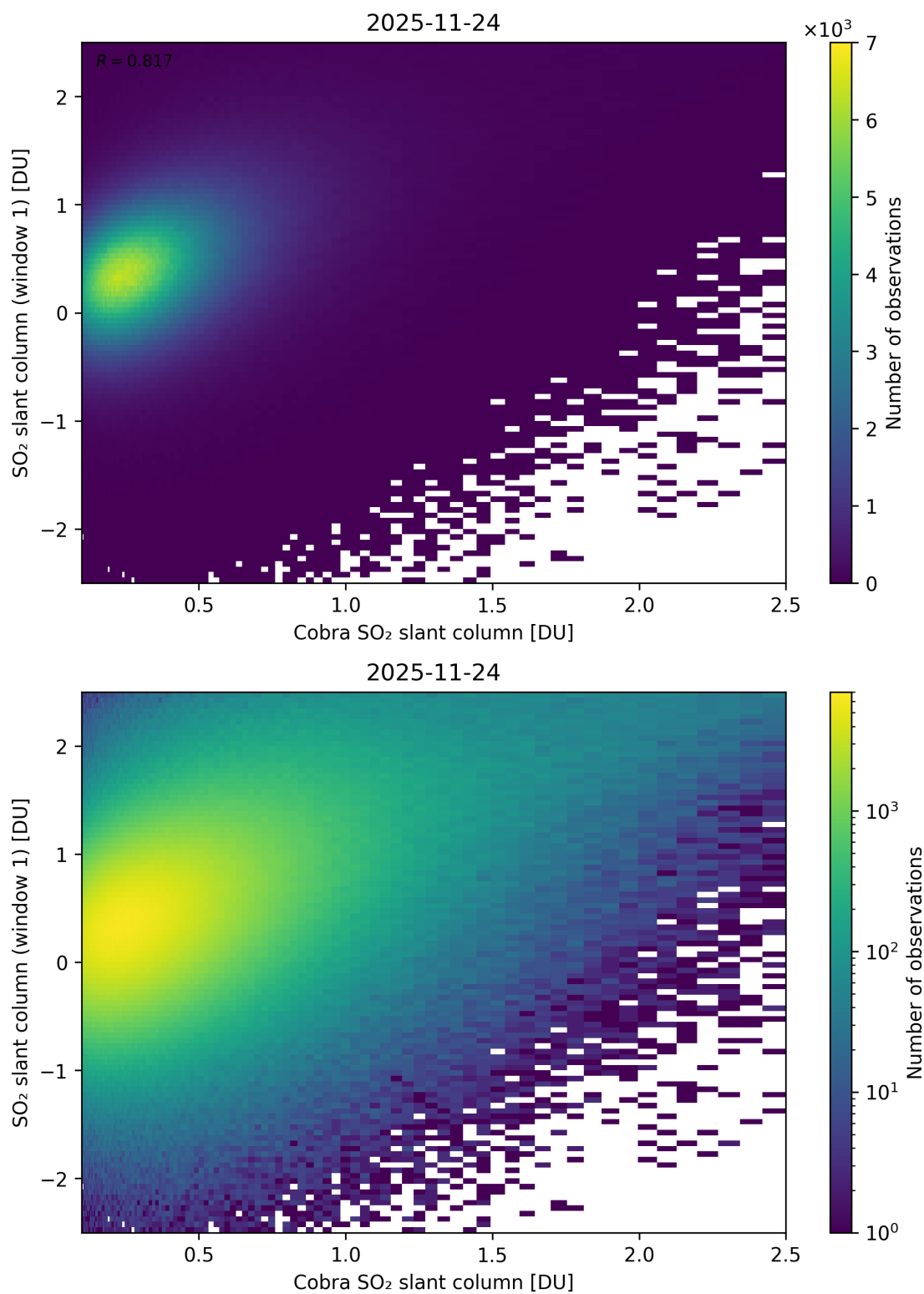
Figure 219: Scatter density plot of “Cobra SO 2 slant column” against “SO 2 slant column (window 1)” for 2025-11-23 to 2025-11-25.
