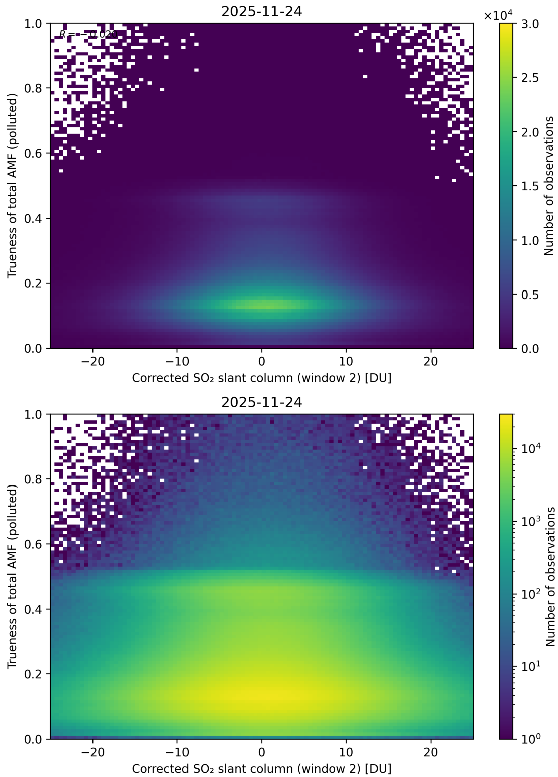
Figure 254: Scatter density plot of “Corrected SO 2 slant column (window 2)” against “Trueness of total AMF (polluted)” for 2025-11-23 to 2025-11-25.
