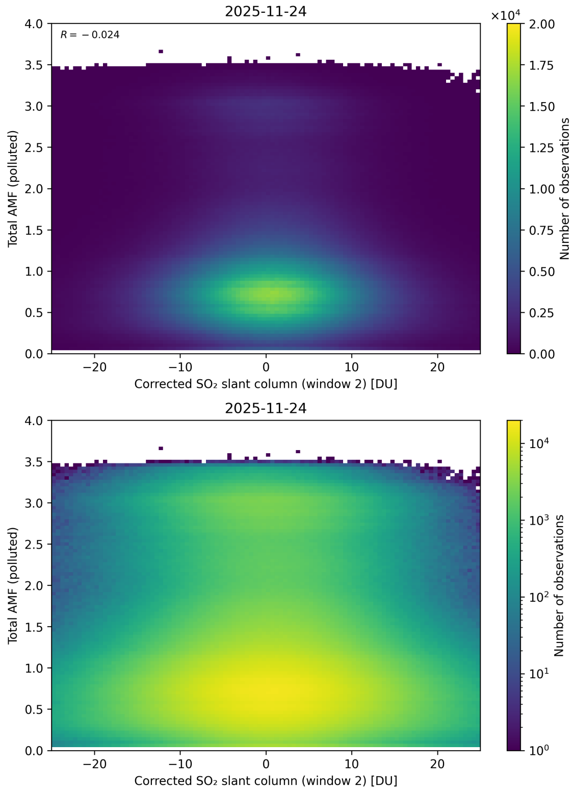
Figure 253: Scatter density plot of “Corrected SO 2 slant column (window 2)” against “Total AMF (polluted)” for 2025-11-23 to 2025-11-25.
