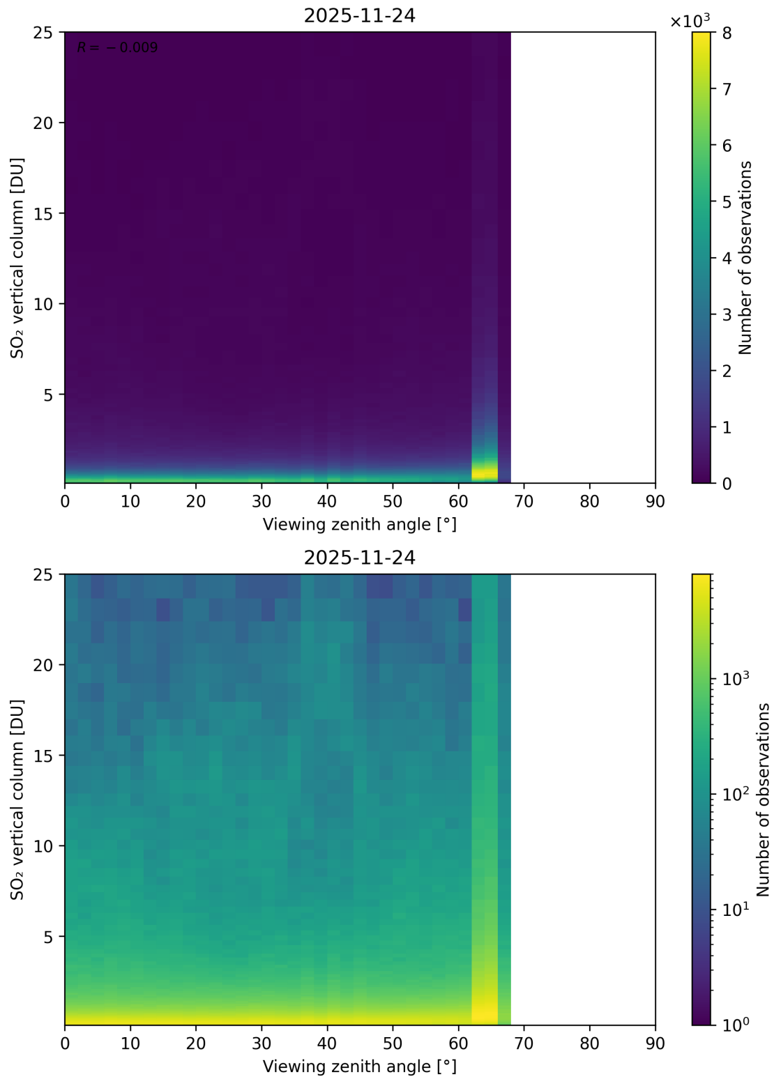
Figure 383: Scatter density plot of “Viewing zenith angle” against “SO 2 vertical column” for 2025-11-23 to 2025-11-25.
