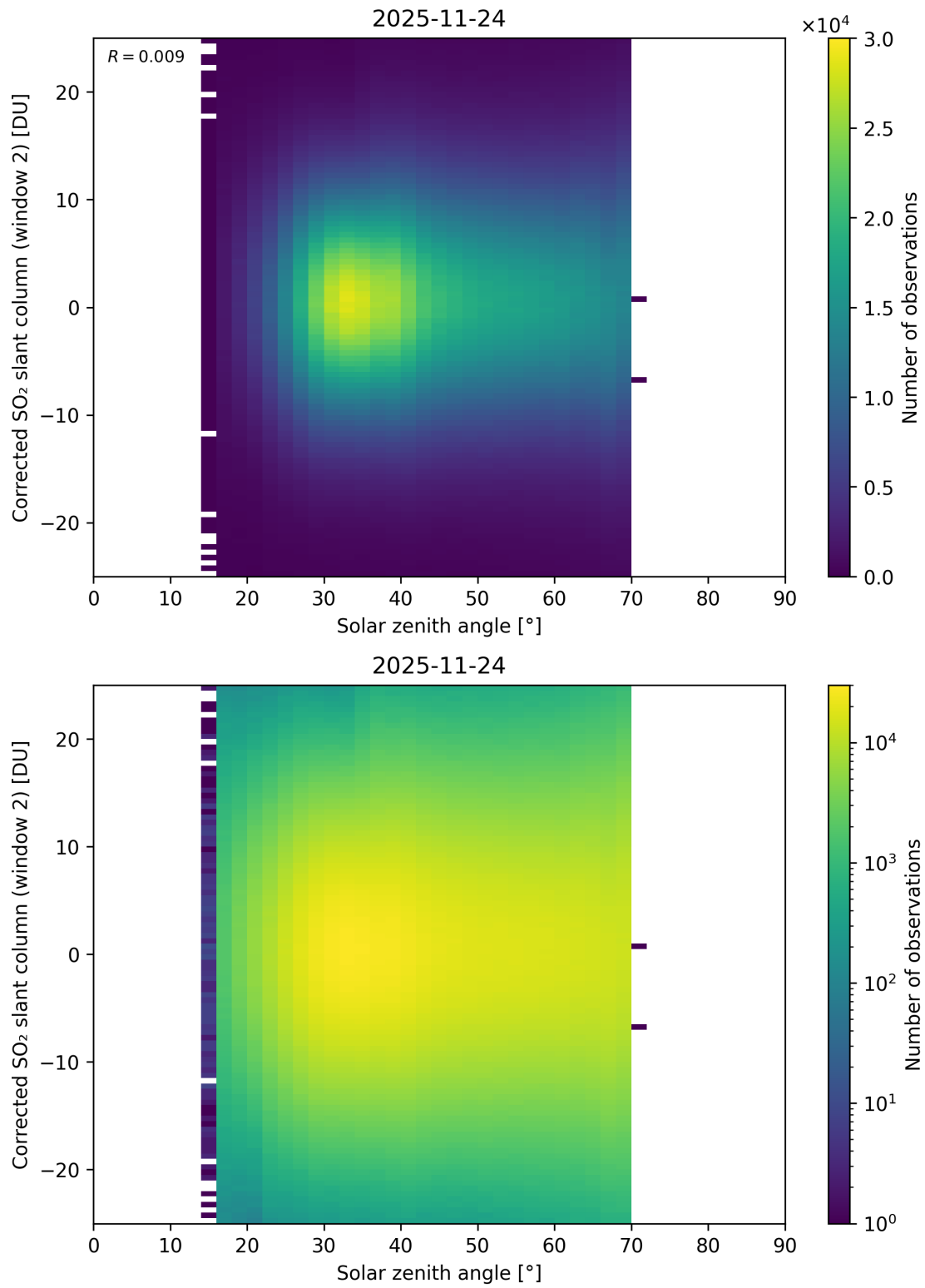
Figure 182: Scatter density plot of “Solar zenith angle” against “Corrected SO 2 slant column (window 2)” for 2025-11-23 to 2025-11-25.
