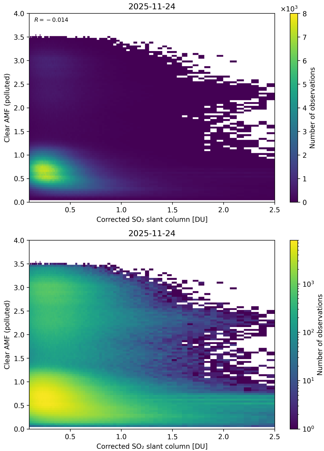
Figure 232: Scatter density plot of “Corrected SO 2 slant column” against “Clear AMF (polluted)” for 2025-11-23 to 2025-11-25.
