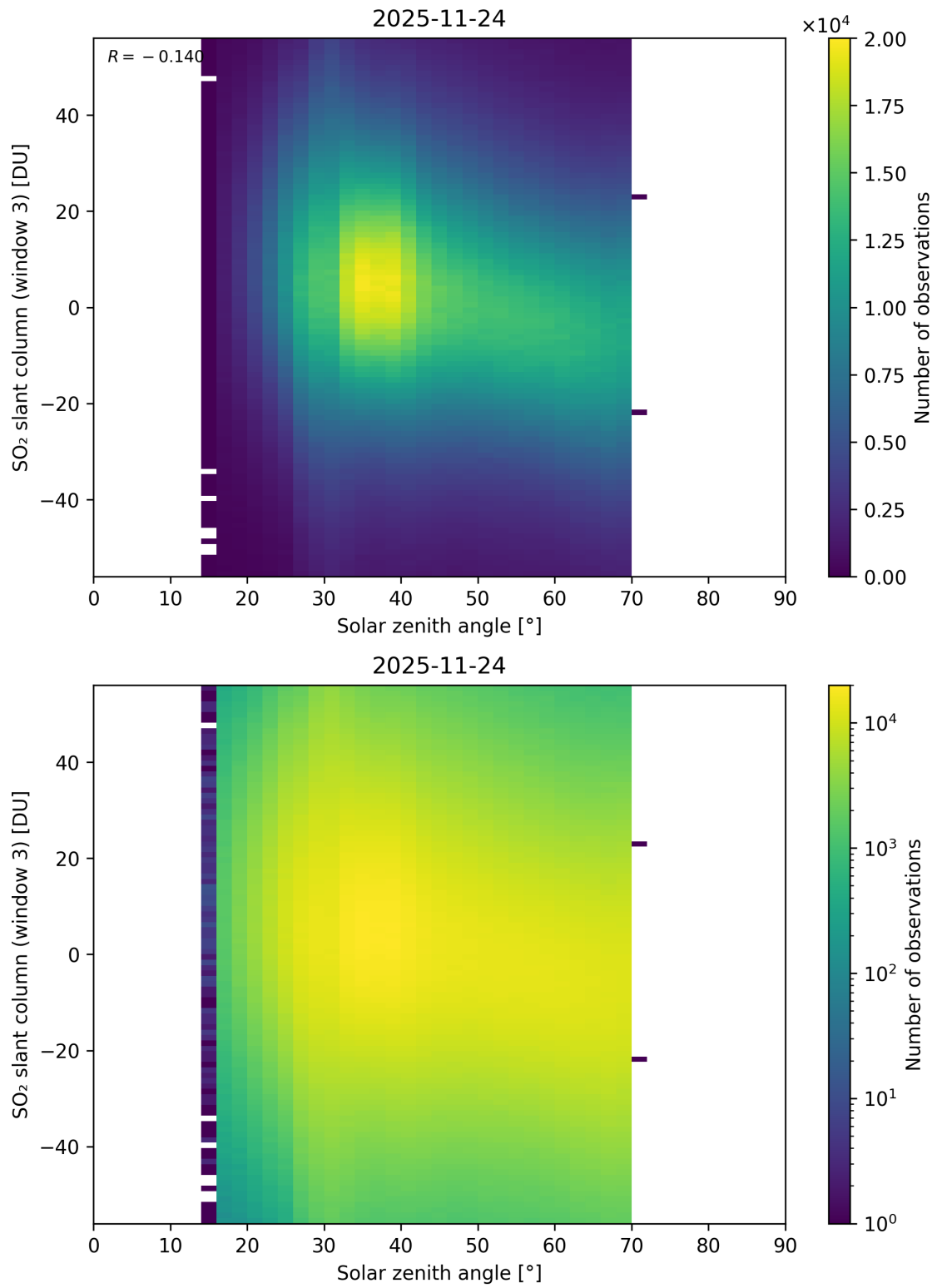
Figure 187: Scatter density plot of “Solar zenith angle” against “SO 2 slant column (window 3)” for 2025-11-23 to 2025-11-25.
