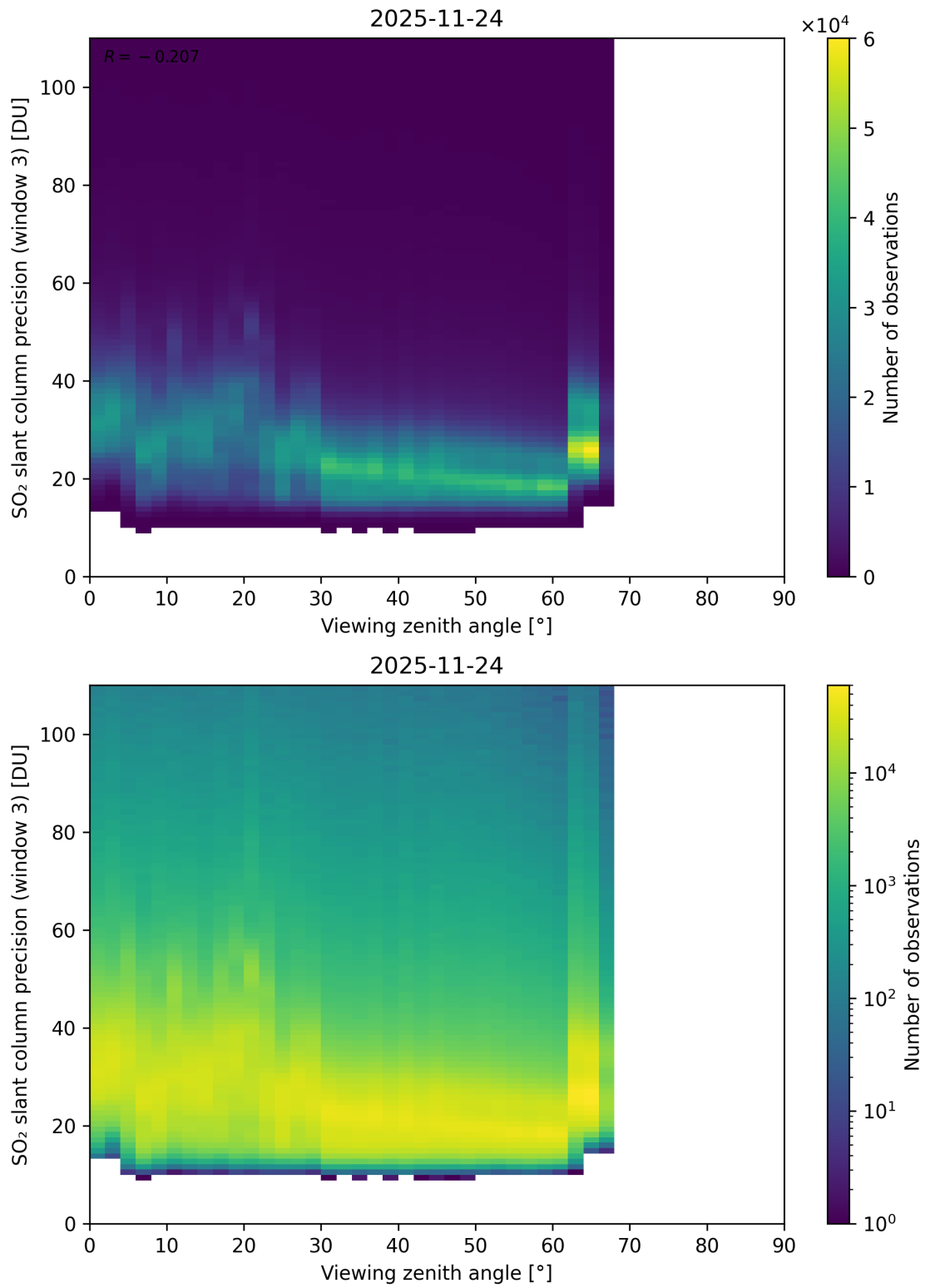
Figure 380: Scatter density plot of “Viewing zenith angle” against “SO 2 slant column precision (window 3)” for 2025-11-23 to 2025-11-25.
