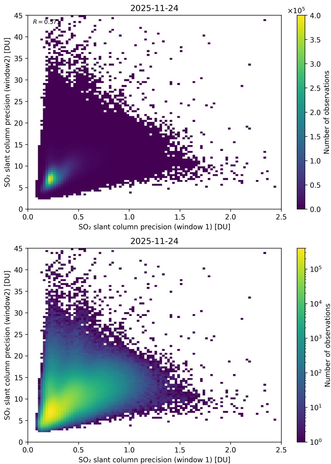
Figure 277: Scatter density plot of “SO 2 slant column precision (window 1)” against “SO 2 slant column precision (window2)” for 2025-11-23 to 2025-11-25.
