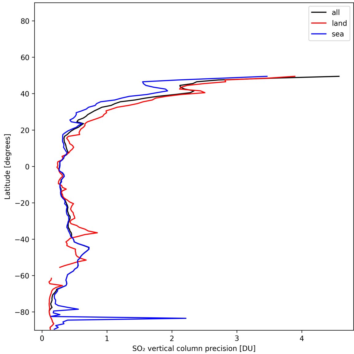
Figure 33: Zonal average of “SO 2 vertical column precision” for 2025-11-23 to 2025-11-25.
