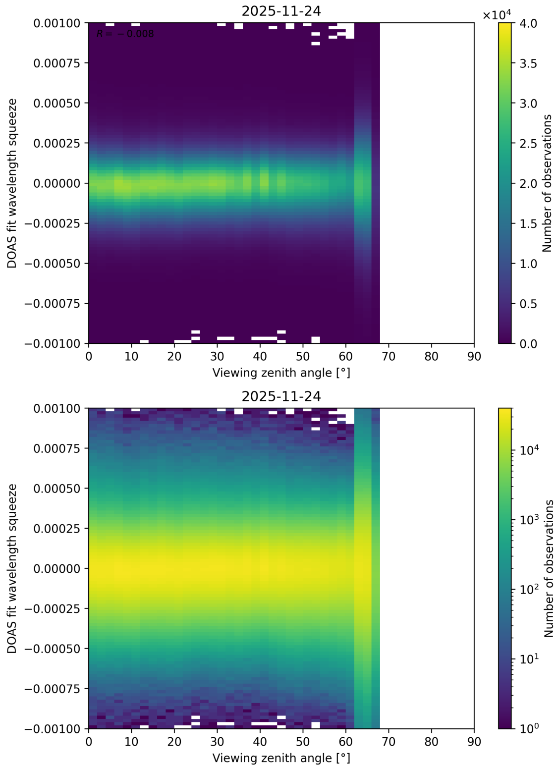
Figure 366: Scatter density plot of “Viewing zenith angle” against “DOAS fit wavelength squeeze” for 2025-11-23 to 2025-11-25.
