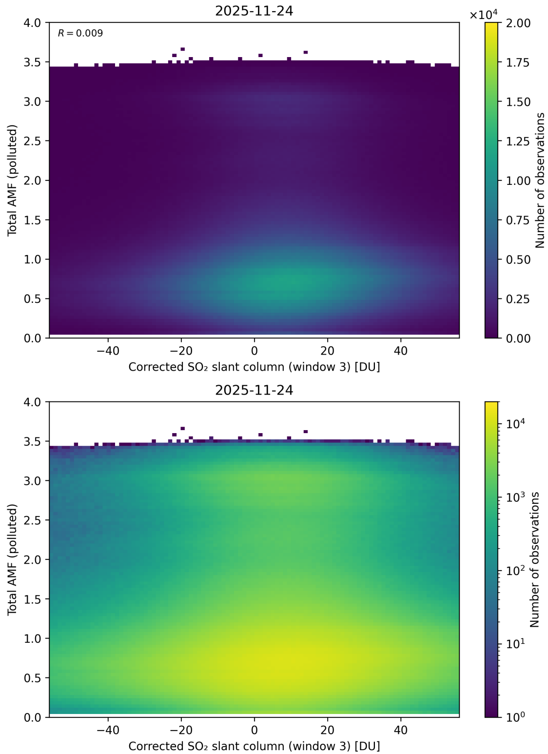
Figure 260: Scatter density plot of “Corrected SO 2 slant column (window 3)” against “Total AMF (polluted)” for 2025-11-23 to 2025-11-25.
