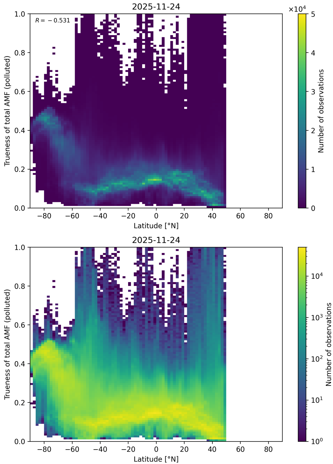
Figure 168: Scatter density plot of “Latitude” against “Trueness of total AMF (polluted)” for 2025-11-23 to 2025-11-25.
