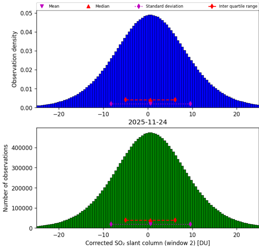
Figure 69: Histogram of “Corrected SO 2 slant column (window 2)” for 2025-11-23 to 2025-11-25
