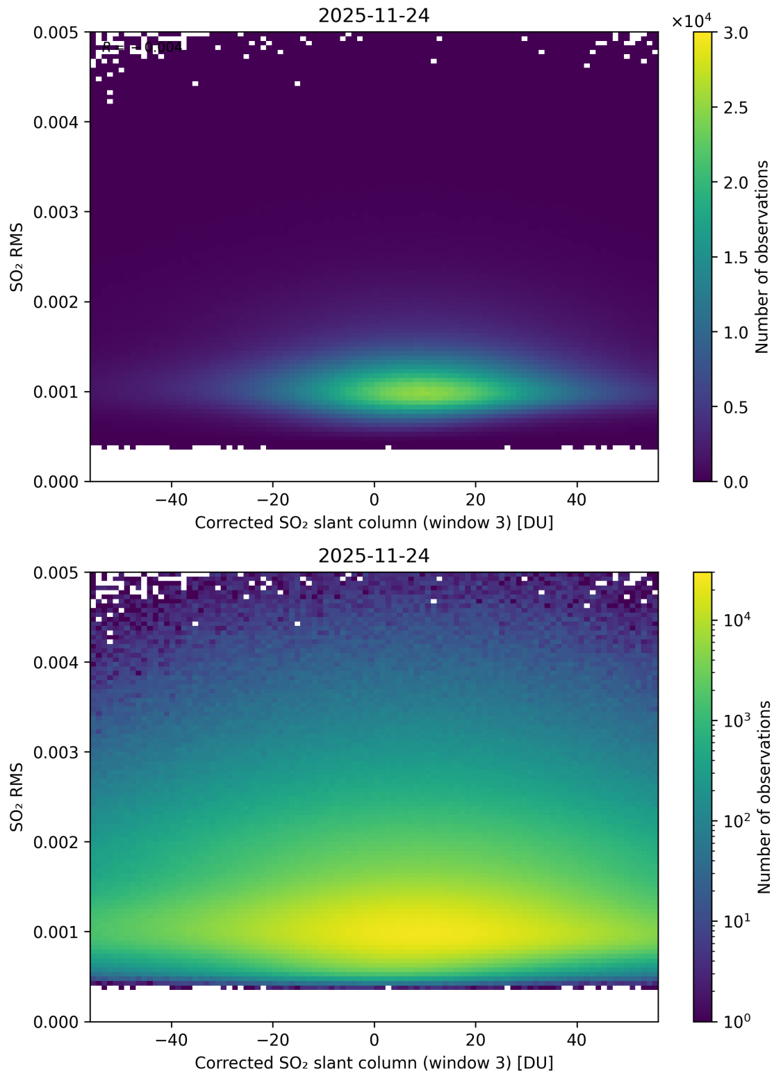
Figure 258: Scatter density plot of “Corrected SO 2 slant column (window 3)” against “SO 2 RMS” for 2025-11-23 to 2025-11-25.
