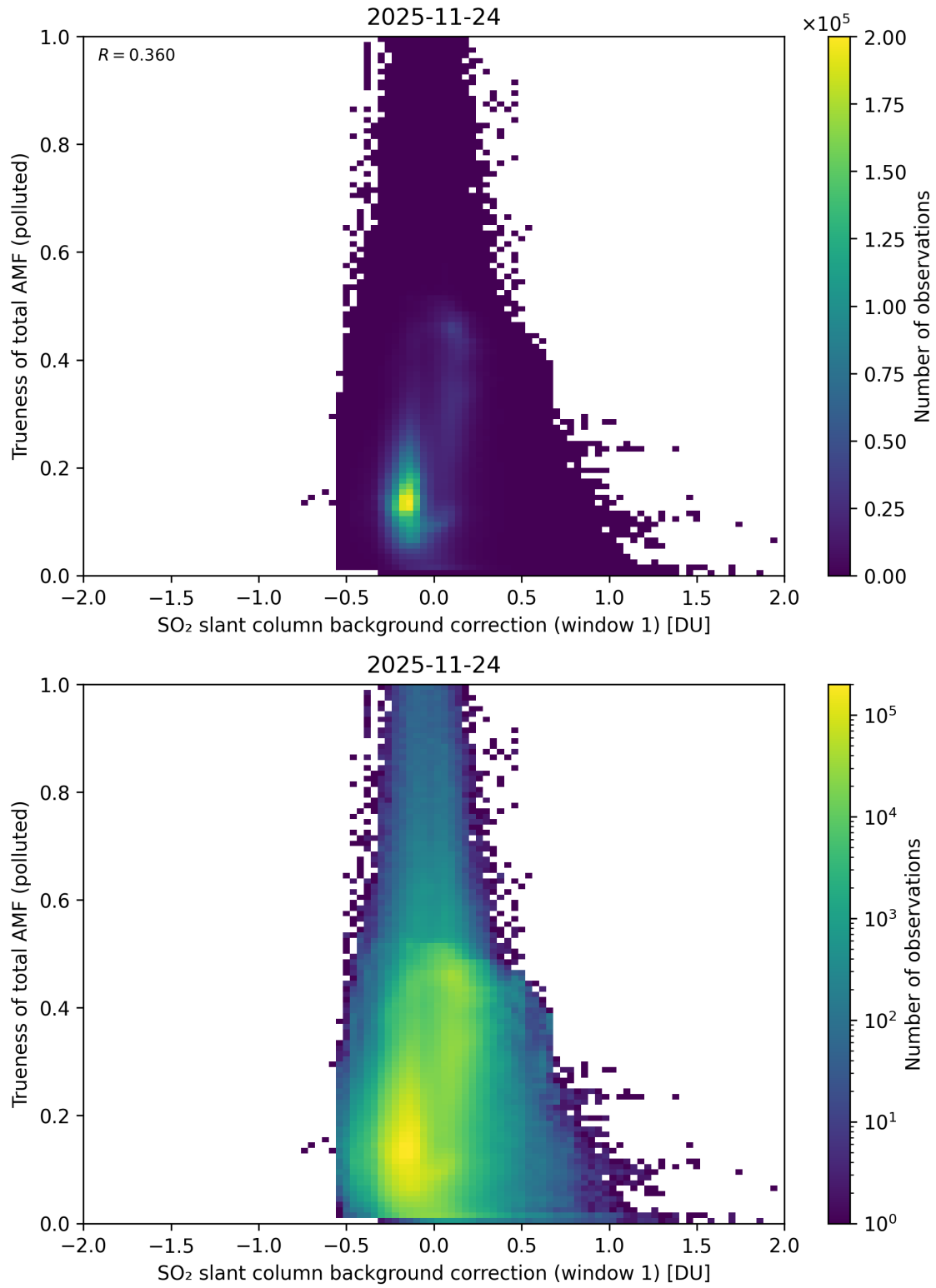
Figure 121: Scatter density plot of “SO 2 slant column background correction (window 1)” against “Trueness of total AMF (polluted)” for 2025-11-23 to 2025-11-25.
