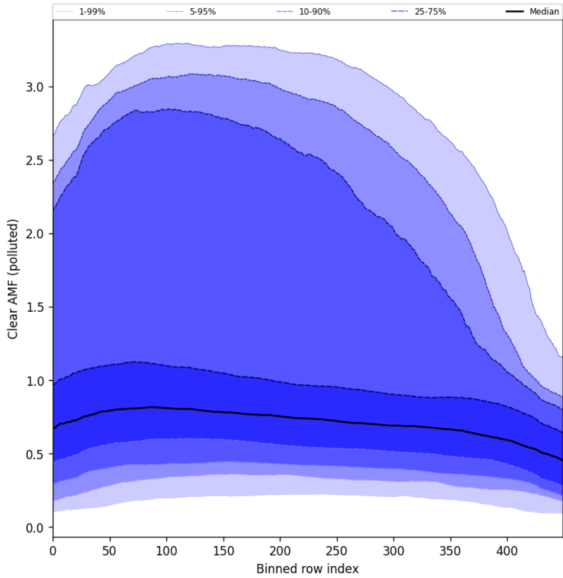
Figure 107: Along track statistics of “Clear AMF (polluted)” for 2025-11-23 to 2025-11-25
