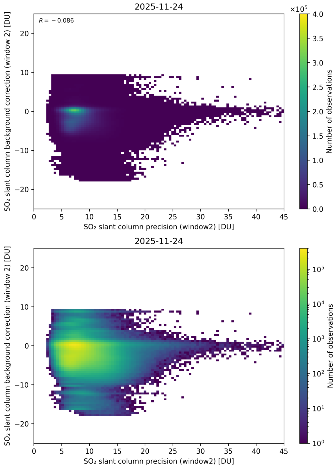
Figure 291: Scatter density plot of “SO 2 slant column precision (window2)” against “SO 2 slant column background correction (window 2)” for 2025-11-23 to 2025-11-25.
