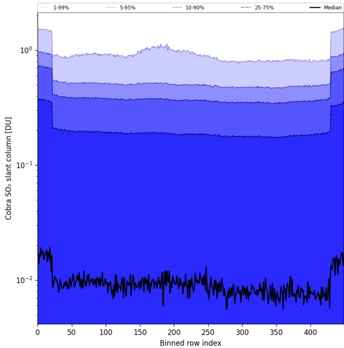
Figure 87: Along track statistics of “Cobra SO 2 slant column” for 2025-11-23 to 2025-11-25
