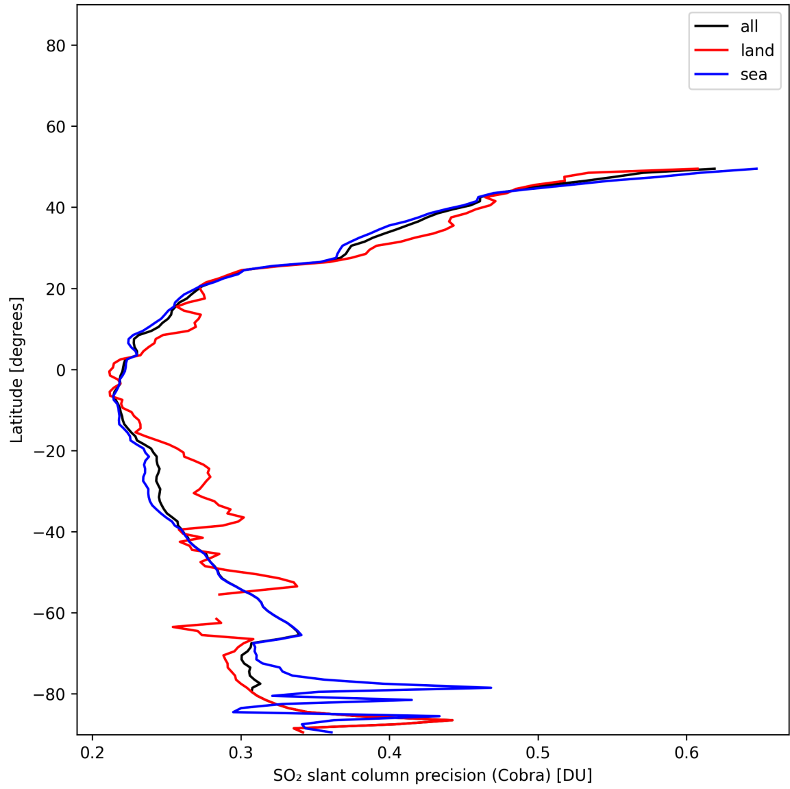
Figure 36: Zonal average of “SO 2 slant column precision (Cobra)” for 2025-11-23 to 2025-11-25.
