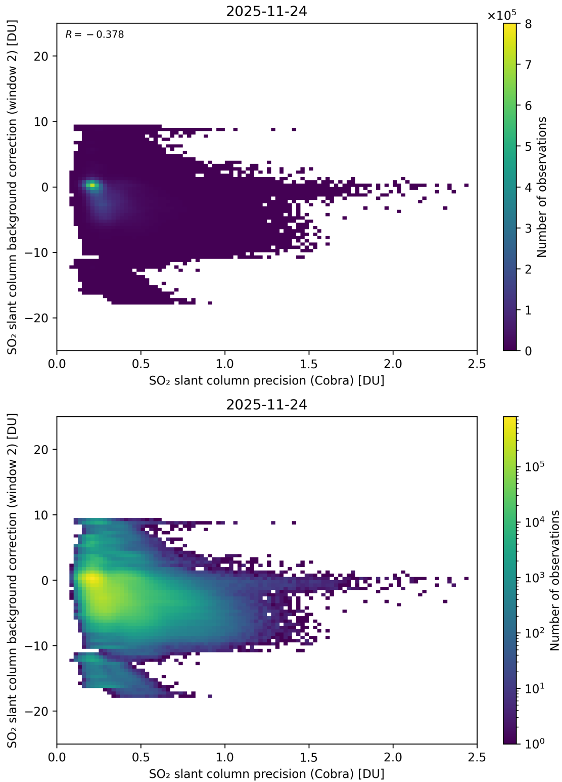
Figure 200: Scatter density plot of “SO 2 slant column precision (Cobra)” against “SO 2 slant column background correction (window 2)” for 2025-11-23 to 2025-11-25.
