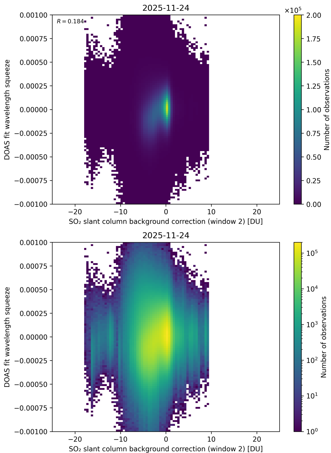
Figure 124: Scatter density plot of “SO 2 slant column background correction (window 2)” against “DOAS fit wavelength squeeze” for 2025-11-23 to 2025-11-25.
