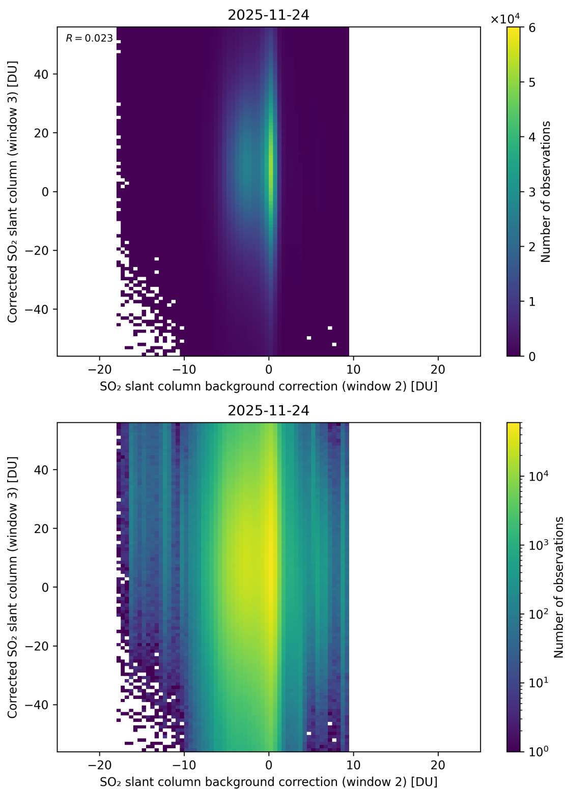
Figure 127: Scatter density plot of “SO 2 slant column background correction (window 2)” against “Corrected SO 2 slant column (window 3)” for 2025-11-23 to 2025-11-25.
