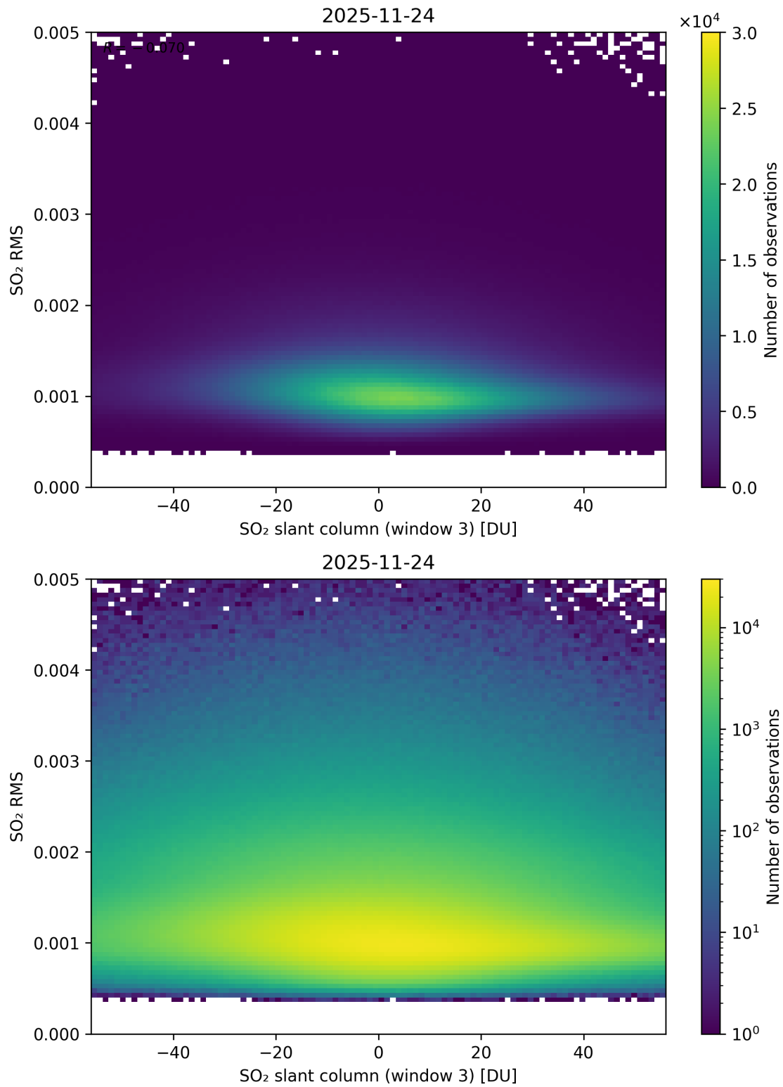
Figure 306: Scatter density plot of “SO 2 slant column (window 3)” against “SO 2 RMS” for 2025-11-23 to 2025-11-25.
