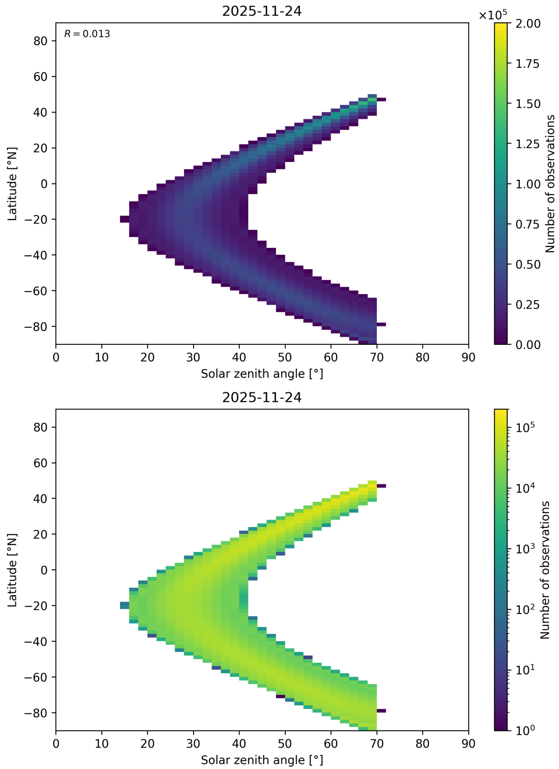
Figure 177: Scatter density plot of “Solar zenith angle” against “Latitude” for 2025-11-23 to 2025-11-25.
