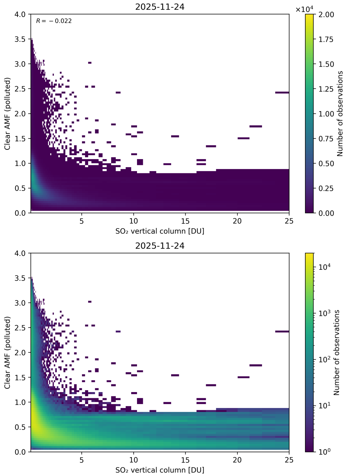
Figure 348: Scatter density plot of “SO 2 vertical column” against “Clear AMF (polluted)” for 2025-11-23 to 2025-11-25.
