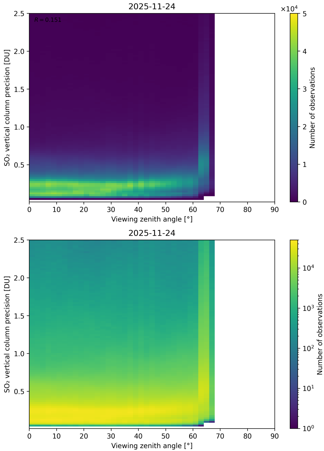
Figure 384: Scatter density plot of “Viewing zenith angle” against “SO 2 vertical column precision” for 2025-11-23 to 2025-11-25.
