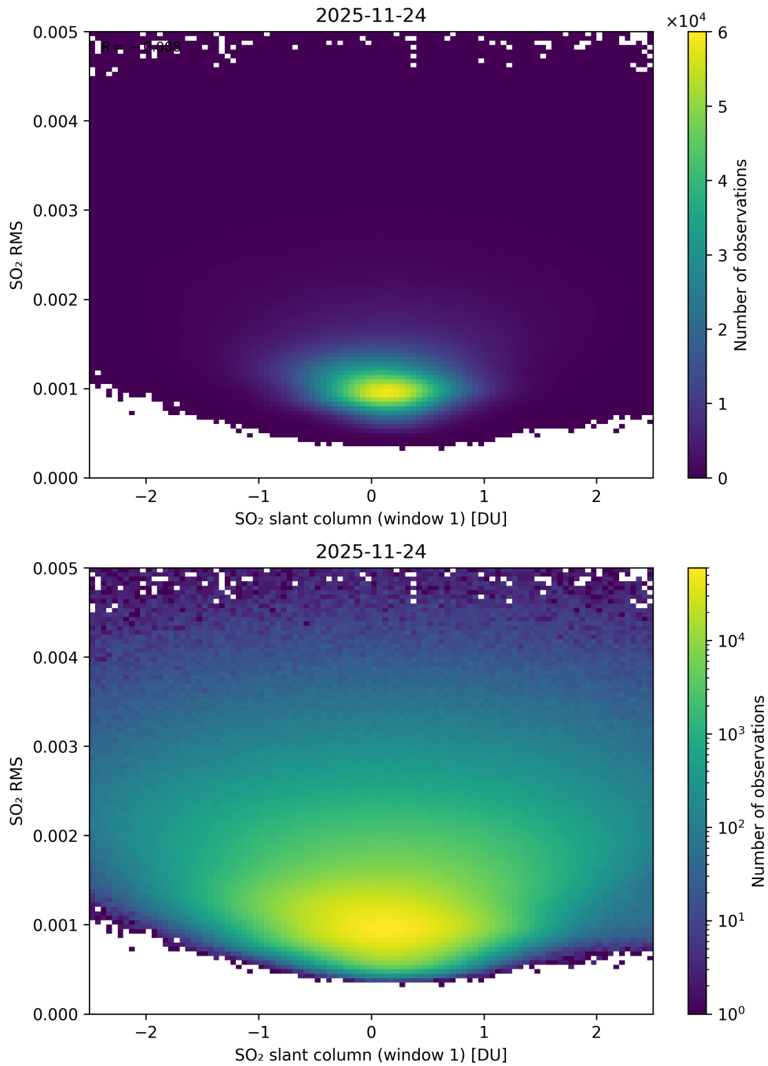
Figure 267: Scatter density plot of “SO 2 slant column (window 1)” against “SO 2 RMS” for 2025-11-23 to 2025-11-25.
