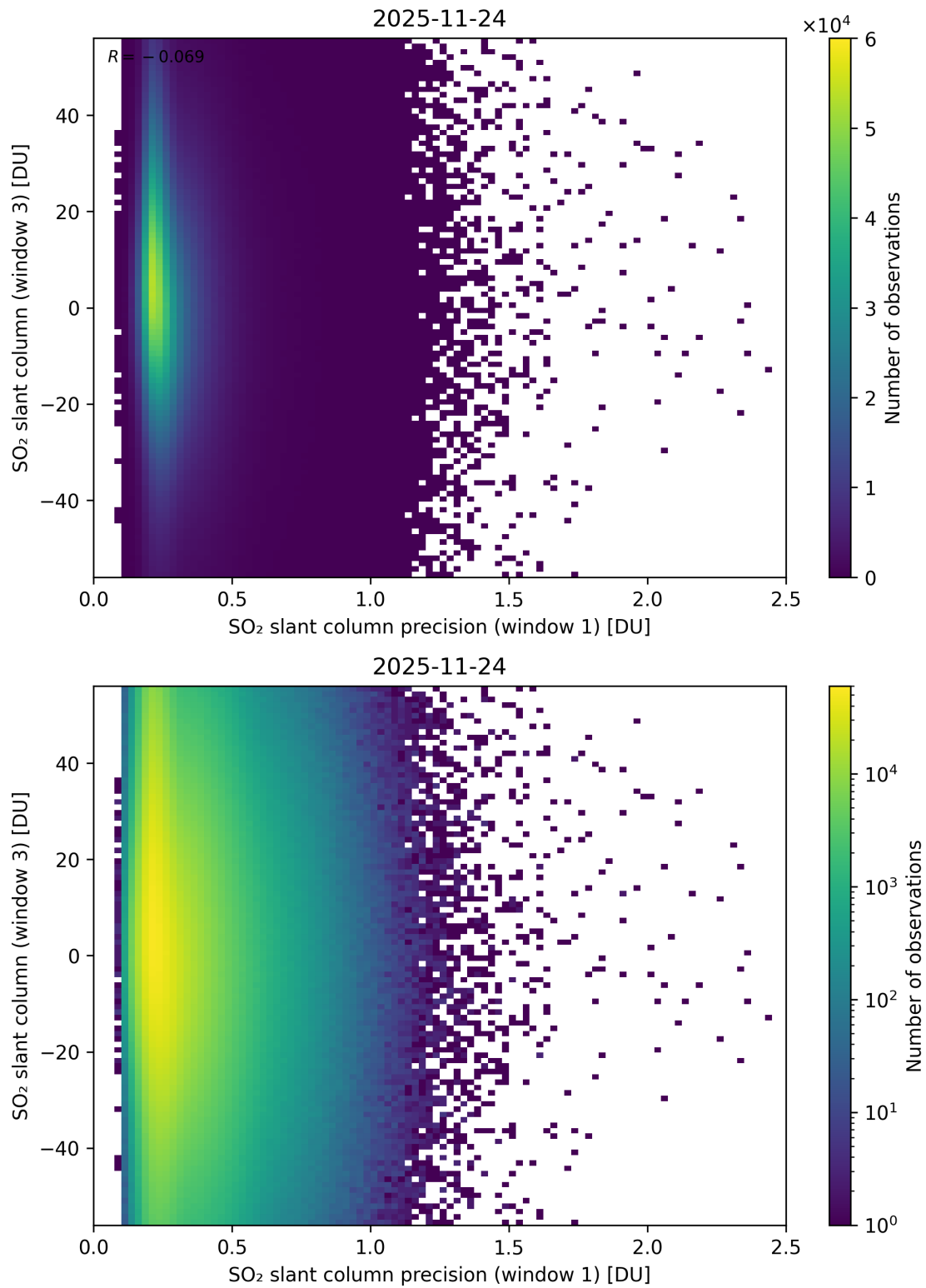
Figure 278: Scatter density plot of “SO 2 slant column precision (window 1)” against “SO 2 slant column (window 3)” for 2025-11-23 to 2025-11-25.
