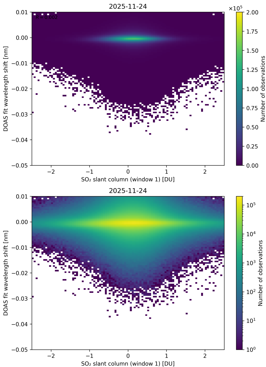
Figure 265: Scatter density plot of “SO 2 slant column (window 1)” against “DOAS fit wavelength shift” for 2025-11-23 to 2025-11-25.
