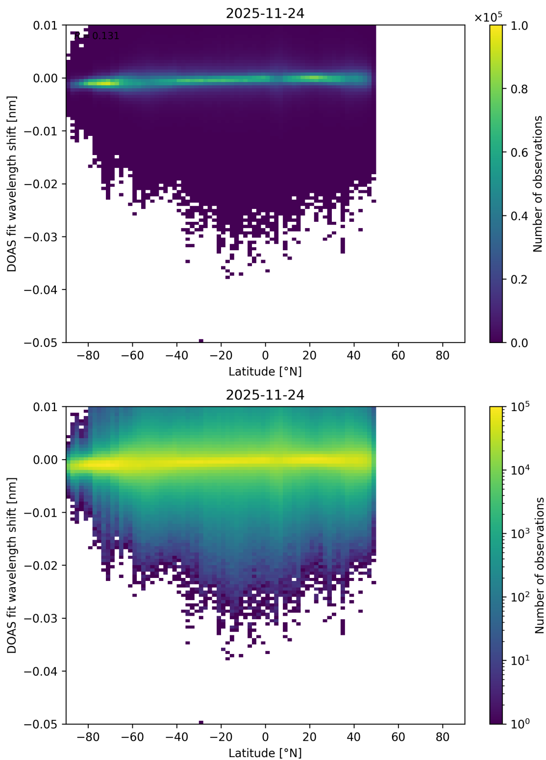
Figure 153: Scatter density plot of “Latitude” against “DOAS fit wavelength shift” for 2025-11-23 to 2025-11-25.
