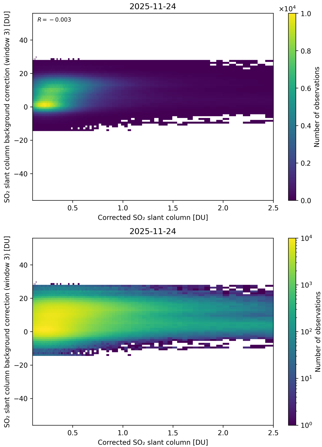
Figure 228: Scatter density plot of “Corrected SO 2 slant column” against “SO 2 slant column background correction (window 3)” for 2025-11-23 to 2025-11-25.
