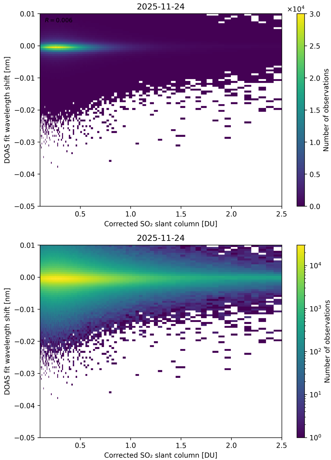
Figure 229: Scatter density plot of “Corrected SO 2 slant column” against “DOAS fit wavelength shift” for 2025-11-23 to 2025-11-25.
