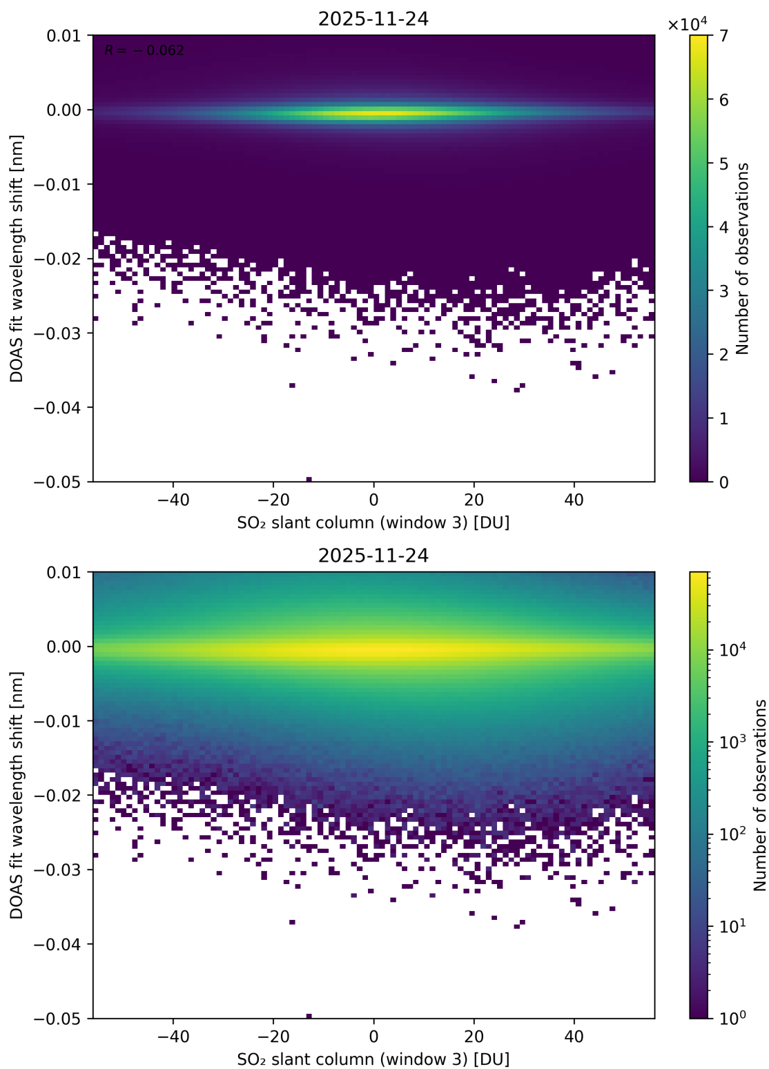
Figure 304: Scatter density plot of “SO 2 slant column (window 3)” against “DOAS fit wavelength shift” for 2025-11-23 to 2025-11-25.
