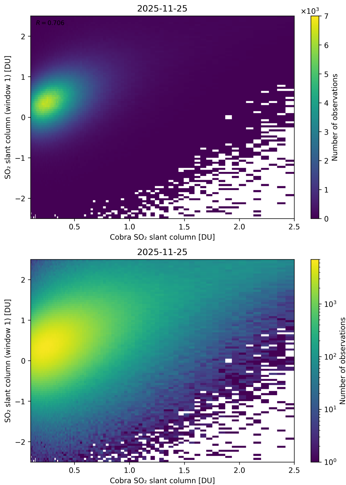
Figure 219: Scatter density plot of “Cobra SO 2 slant column” against “SO 2 slant column (window 1)” for 2025-11-24 to 2025-11-26.
