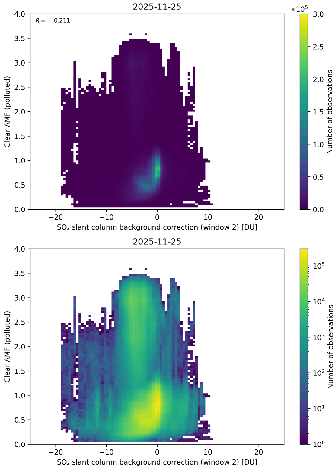
Figure 126: Scatter density plot of “SO 2 slant column background correction (window 2)” against “Clear AMF (polluted)” for 2025-11-24 to 2025-11-26.
