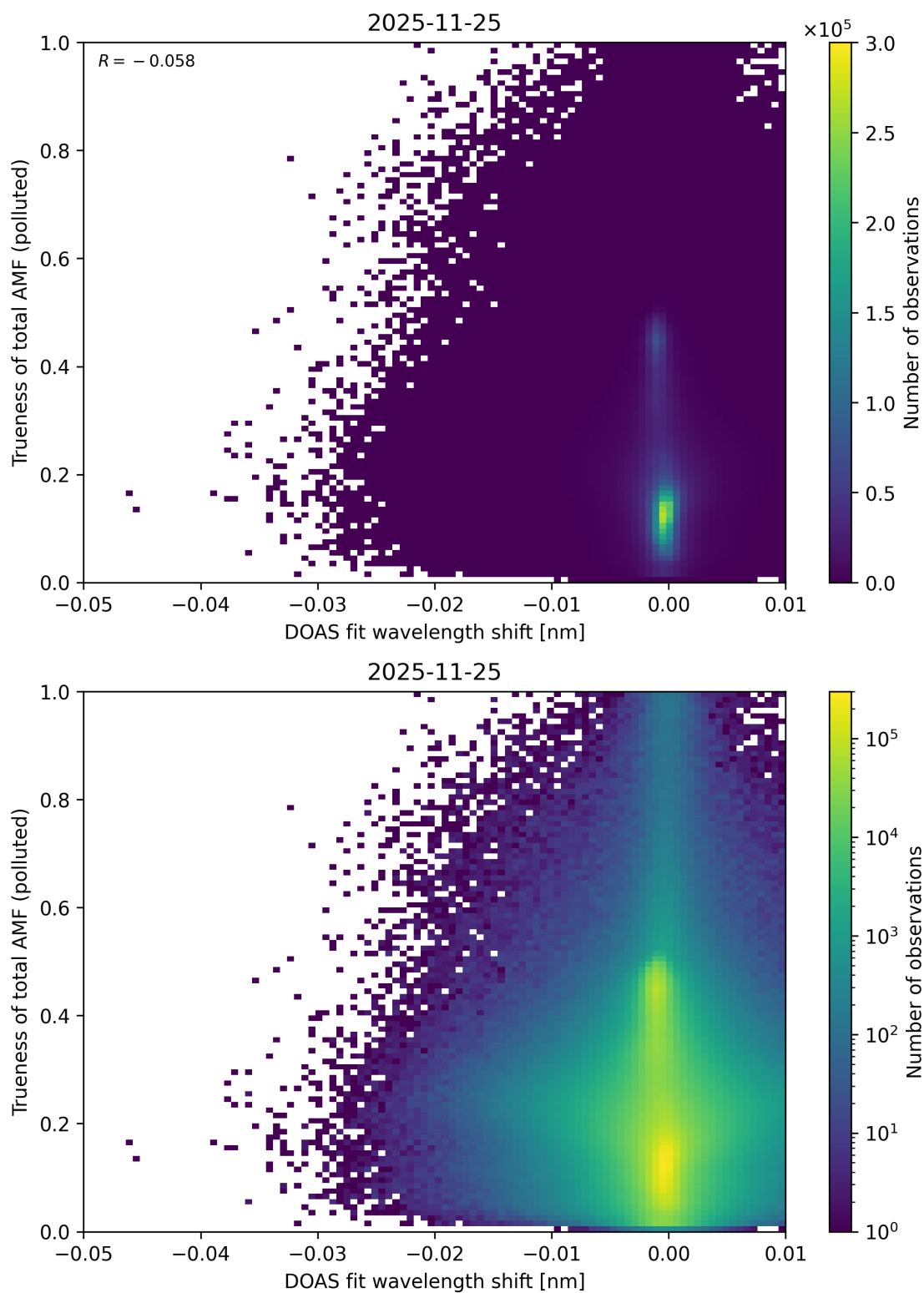
Figure 142: Scatter density plot of “DOAS fit wavelength shift” against “Trueness of total AMF (polluted)” for 2025-11-24 to 2025-11-26.
