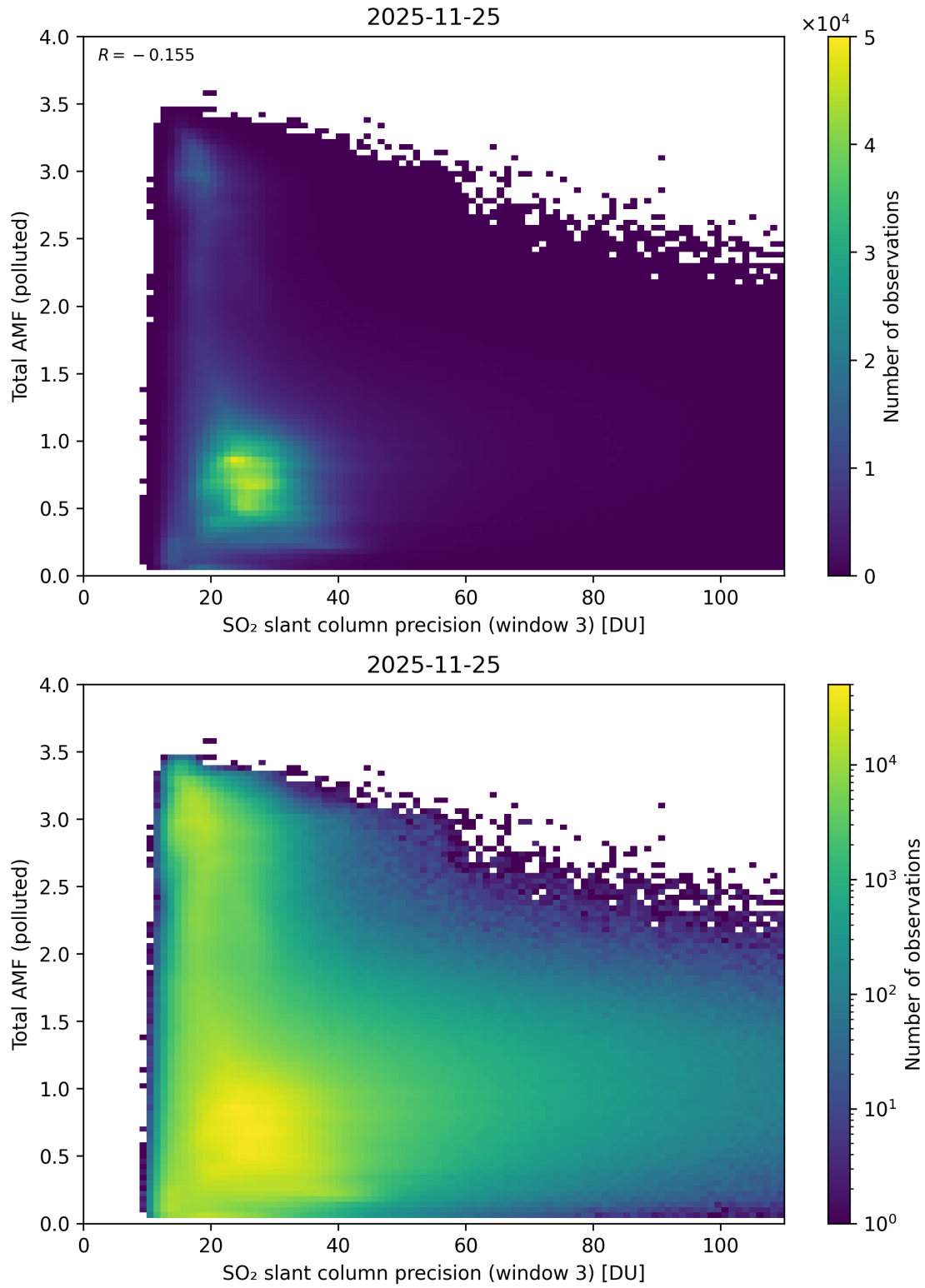
Figure 313: Scatter density plot of “SO 2 slant column precision (window 3)” against “Total AMF (polluted)” for 2025-11-24 to 2025-11-26.
