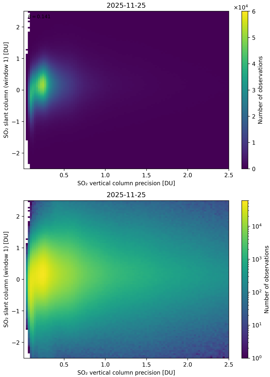
Figure 341: Scatter density plot of “SO 2 vertical column precision” against “SO 2 slant column (window 1)” for 2025-11-24 to 2025-11-26.
