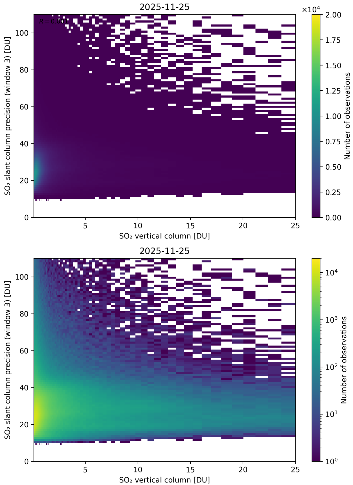
Figure 358: Scatter density plot of “SO 2 vertical column” against “SO 2 slant column precision (window 3)” for 2025-11-24 to 2025-11-26.
