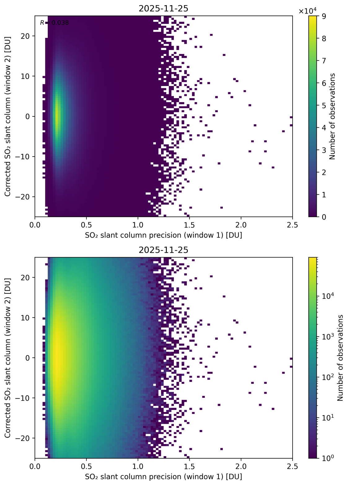
Figure 275: Scatter density plot of “SO 2 slant column precision (window 1)” against “Corrected SO 2 slant column (window 2)” for 2025-11-24 to 2025-11-26.
