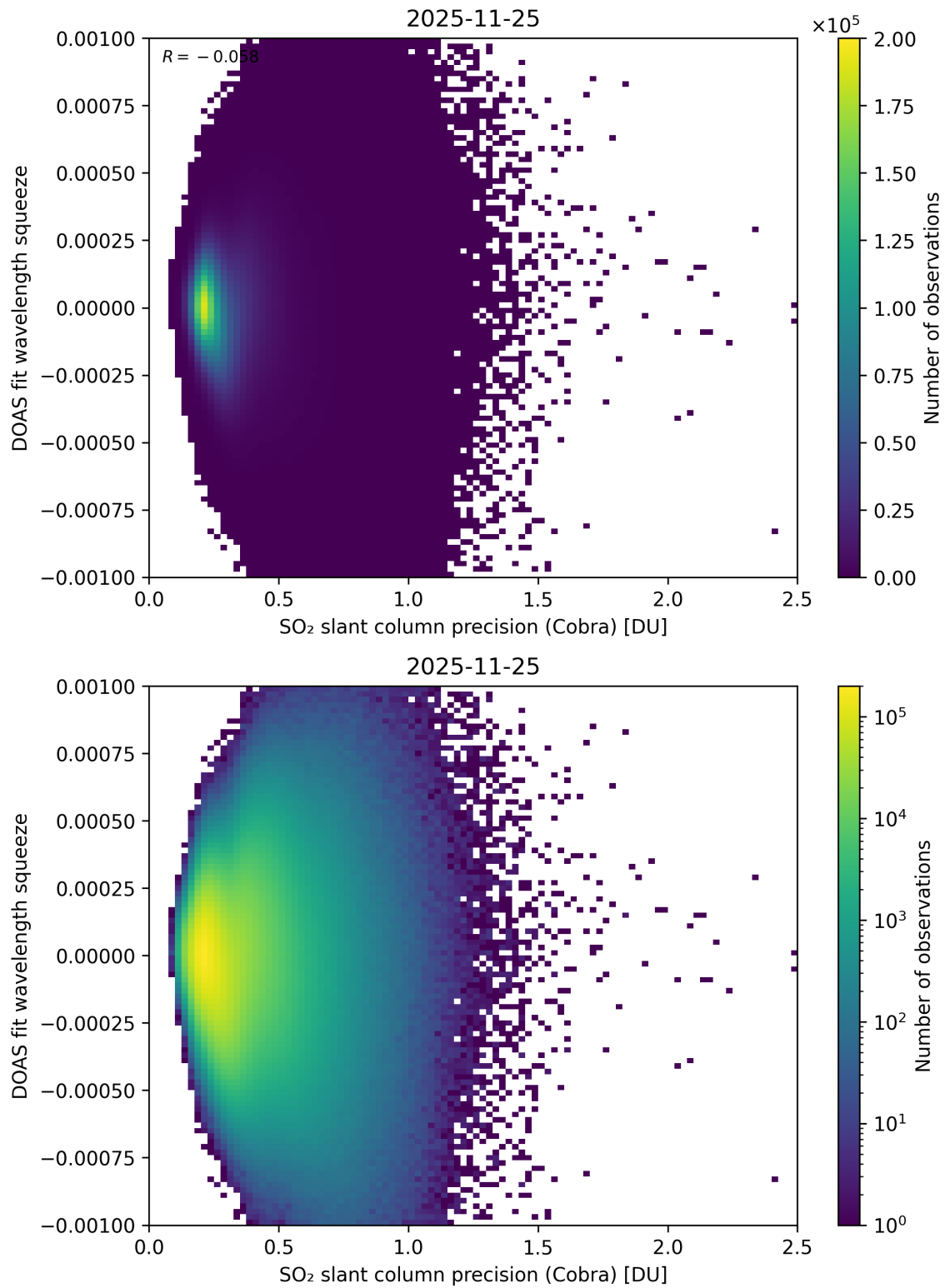
Figure 203: Scatter density plot of “SO 2 slant column precision (Cobra)” against “DOAS fit wavelength squeeze” for 2025-11-24 to 2025-11-26.
