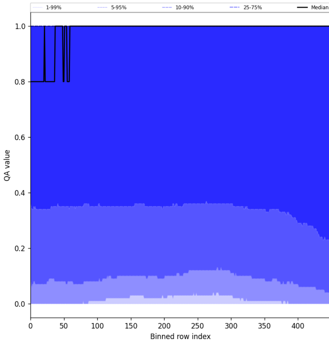
Figure 83: Along track statistics of “QA value” for 2025-11-24 to 2025-11-26
