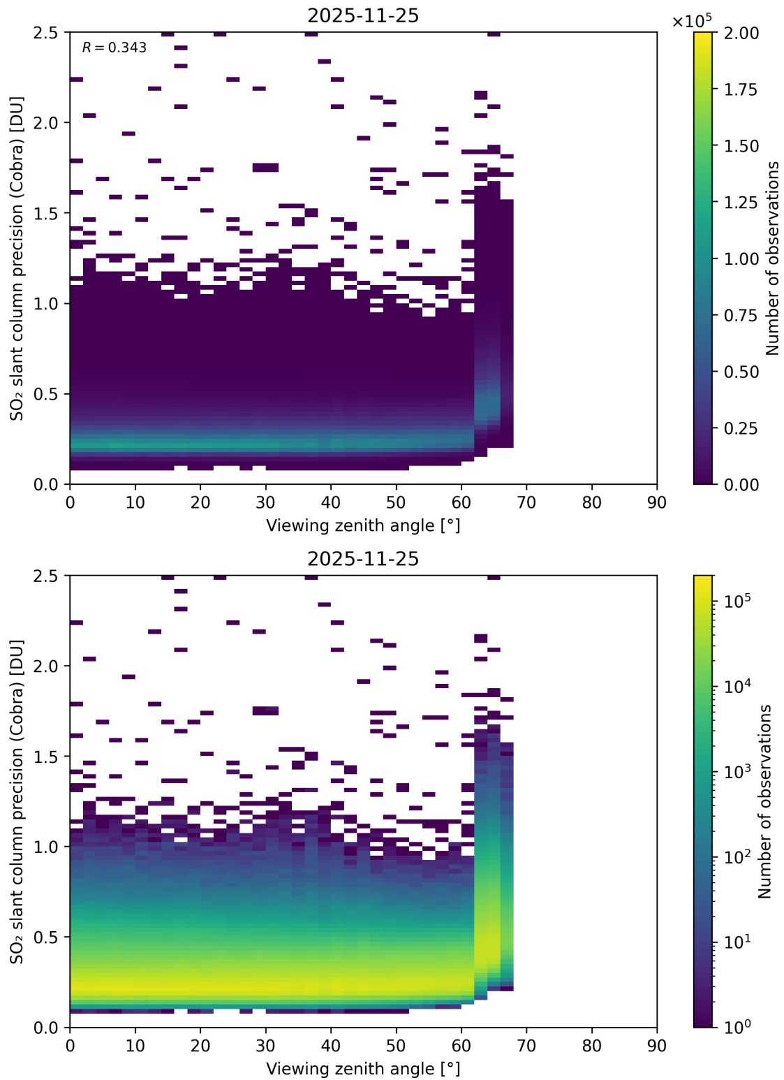
Figure 372: Scatter density plot of “Viewing zenith angle” against “SO 2 slant column precision (Cobra)” for 2025-11-24 to 2025-11-26.
