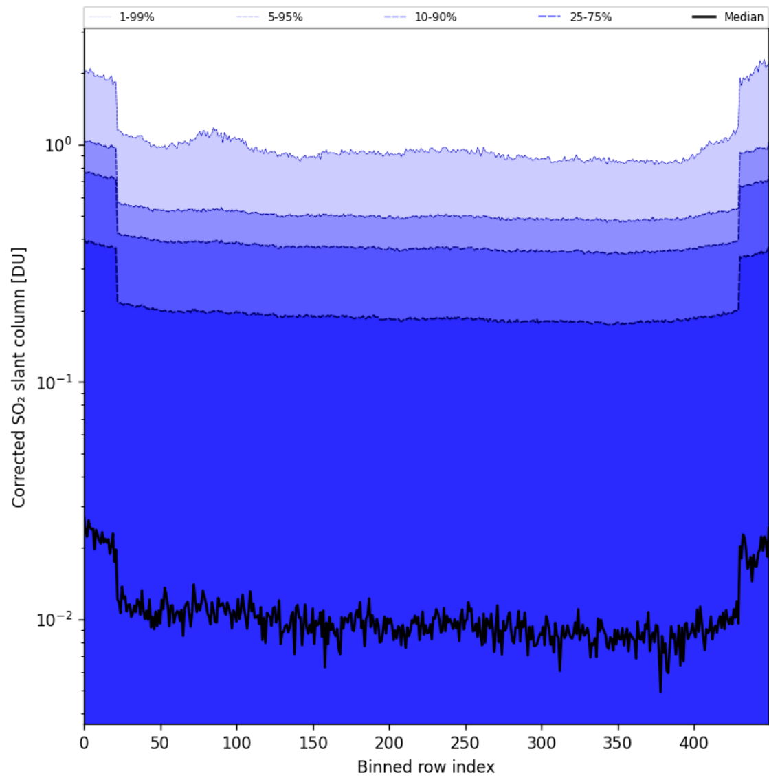
Figure 86: Along track statistics of “Corrected SO 2 slant column” for 2025-11-24 to 2025-11-26
