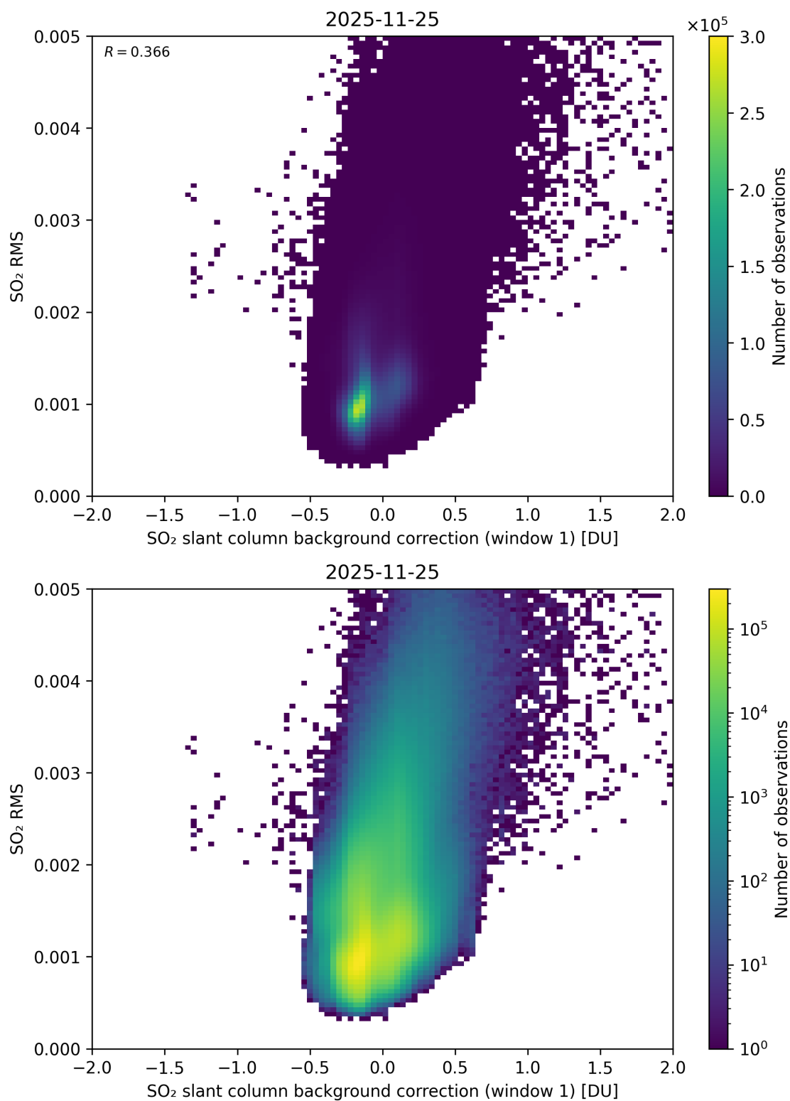
Figure 113: Scatter density plot of “SO 2 slant column background correction (window 1)” against “SO 2 RMS” for 2025-11-24 to 2025-11-26.
