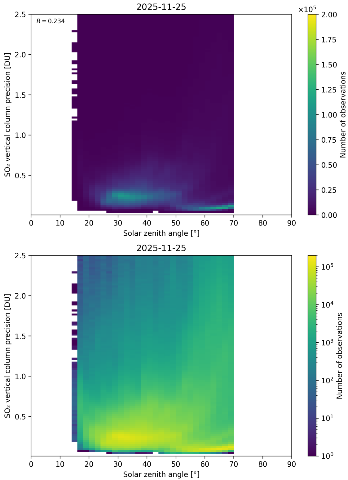
Figure 192: Scatter density plot of “Solar zenith angle” against “SO 2 vertical column precision” for 2025-11-24 to 2025-11-26.
