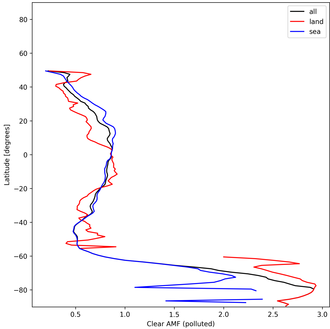
Figure 55: Zonal average of “Clear AMF (polluted)” for 2025-11-24 to 2025-11-26.
