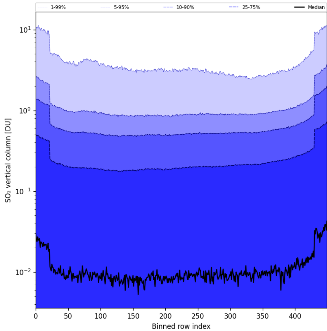
Figure 84: Along track statistics of “SO 2 vertical column” for 2025-11-24 to 2025-11-26
