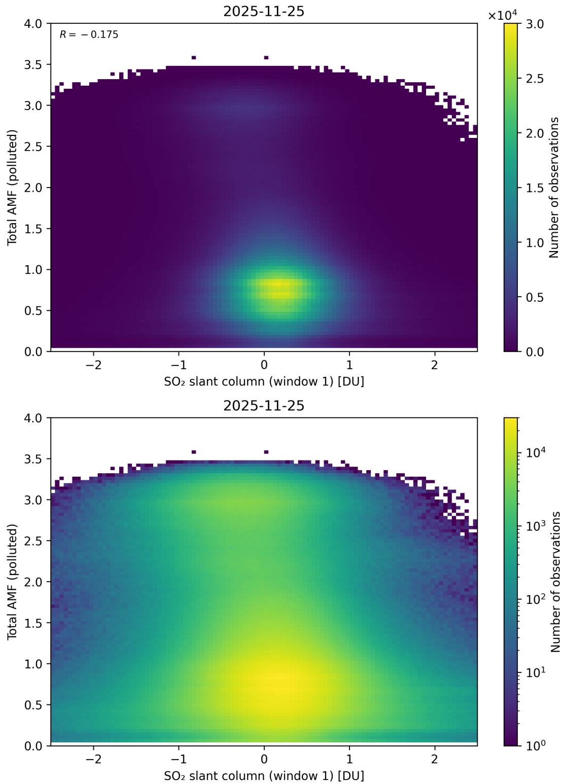
Figure 289: Scatter density plot of “SO 2 slant column (window 1)” against “Total AMF (polluted)” for 2025-11-24 to 2025-11-26.
