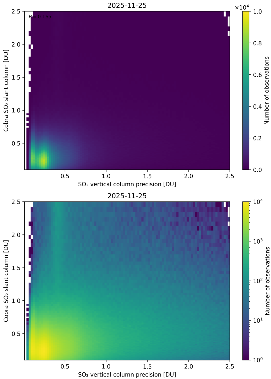
Figure 336: Scatter density plot of “SO 2 vertical column precision” against “Cobra SO 2 slant column” for 2025-11-24 to 2025-11-26.
