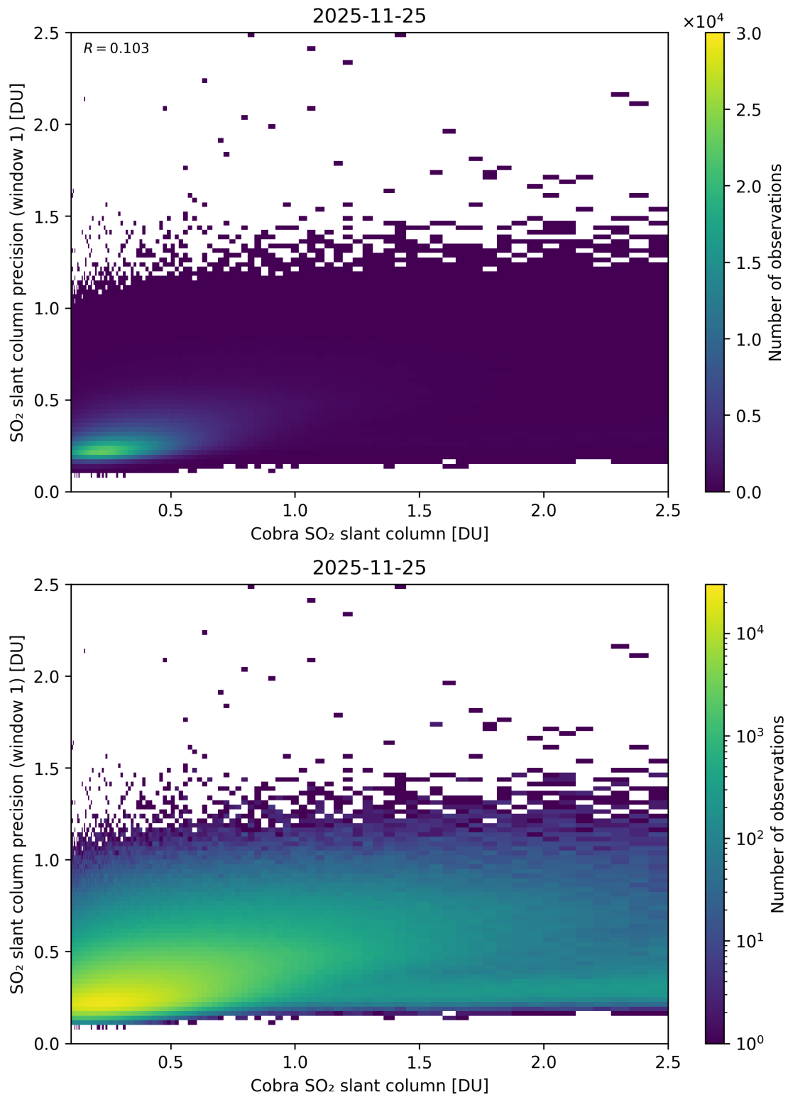
Figure 220: Scatter density plot of “Cobra SO 2 slant column” against “SO 2 slant column precision (window 1)” for 2025-11-24 to 2025-11-26.
