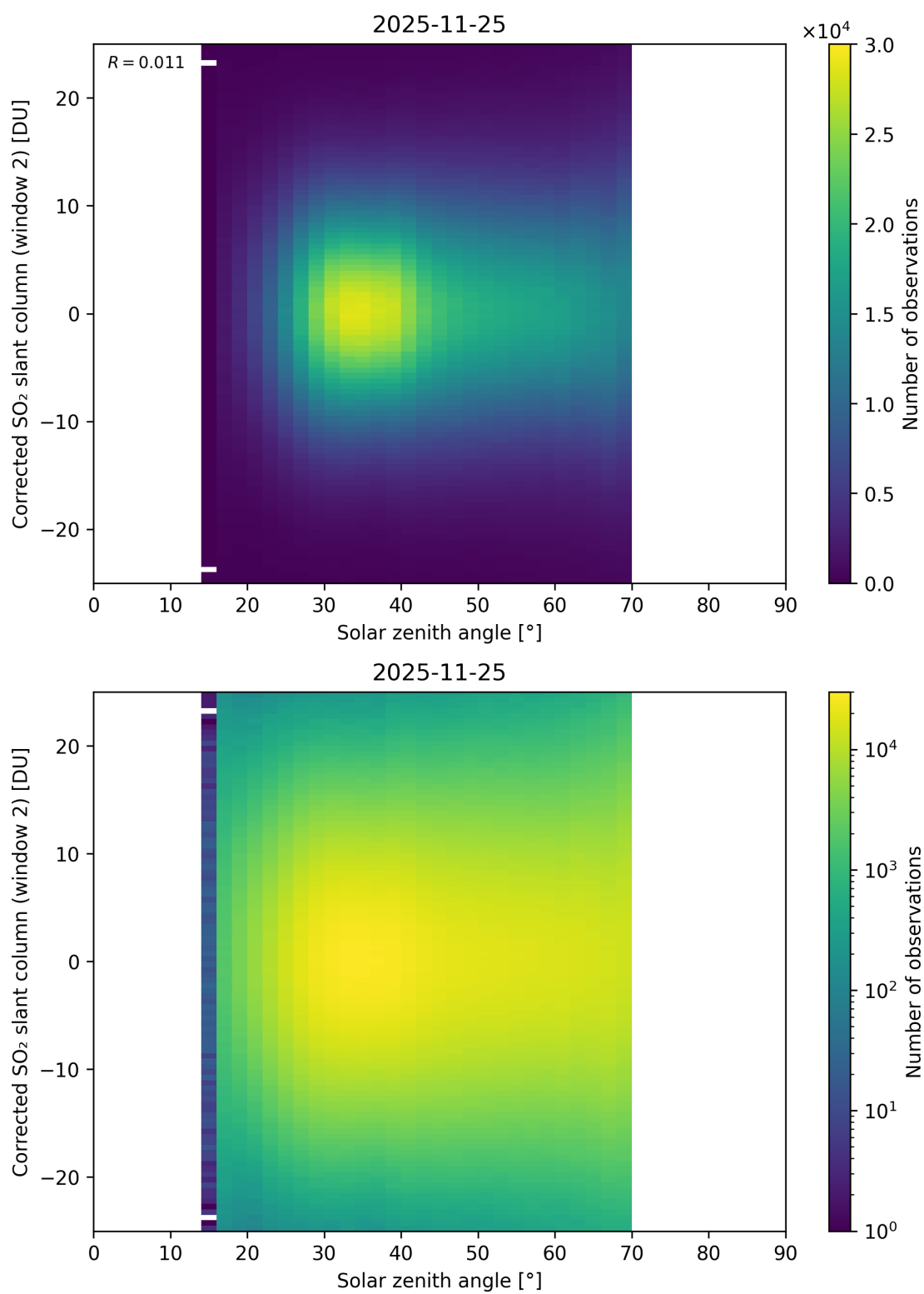
Figure 182: Scatter density plot of “Solar zenith angle” against “Corrected SO 2 slant column (window 2)” for 2025-11-24 to 2025-11-26.
