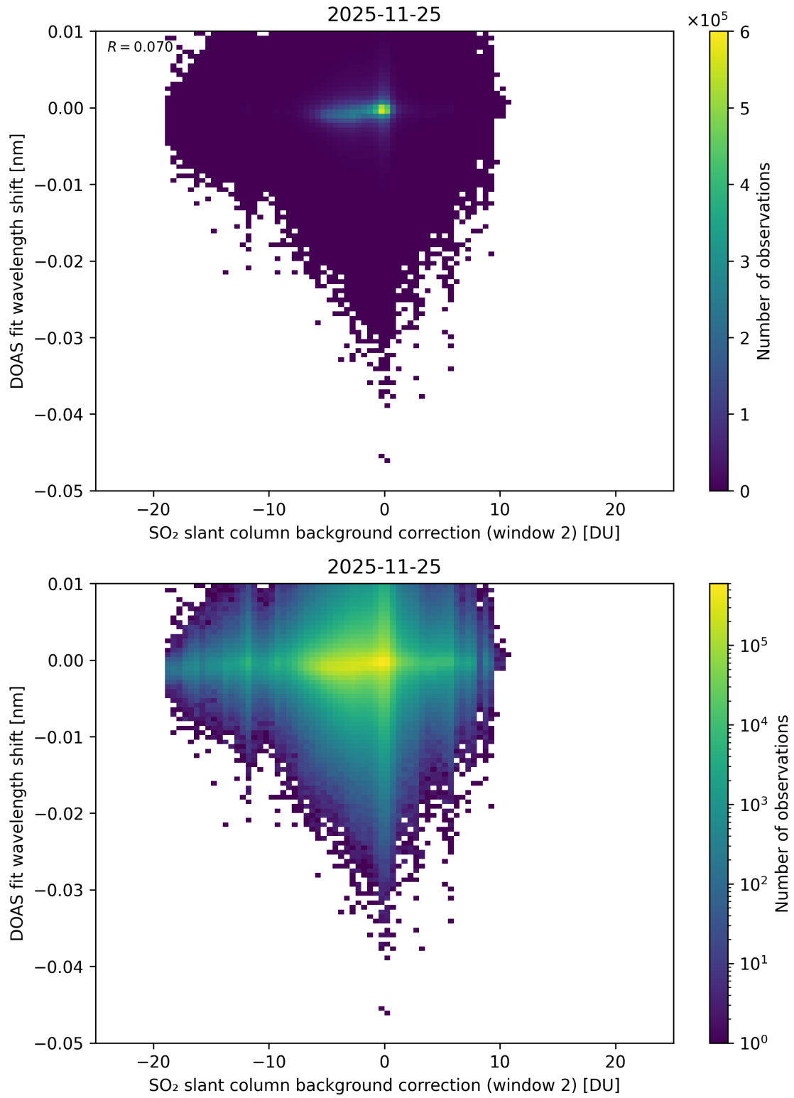
Figure 123: Scatter density plot of “SO 2 slant column background correction (window 2)” against “DOAS fit wavelength shift” for 2025-11-24 to 2025-11-26.
