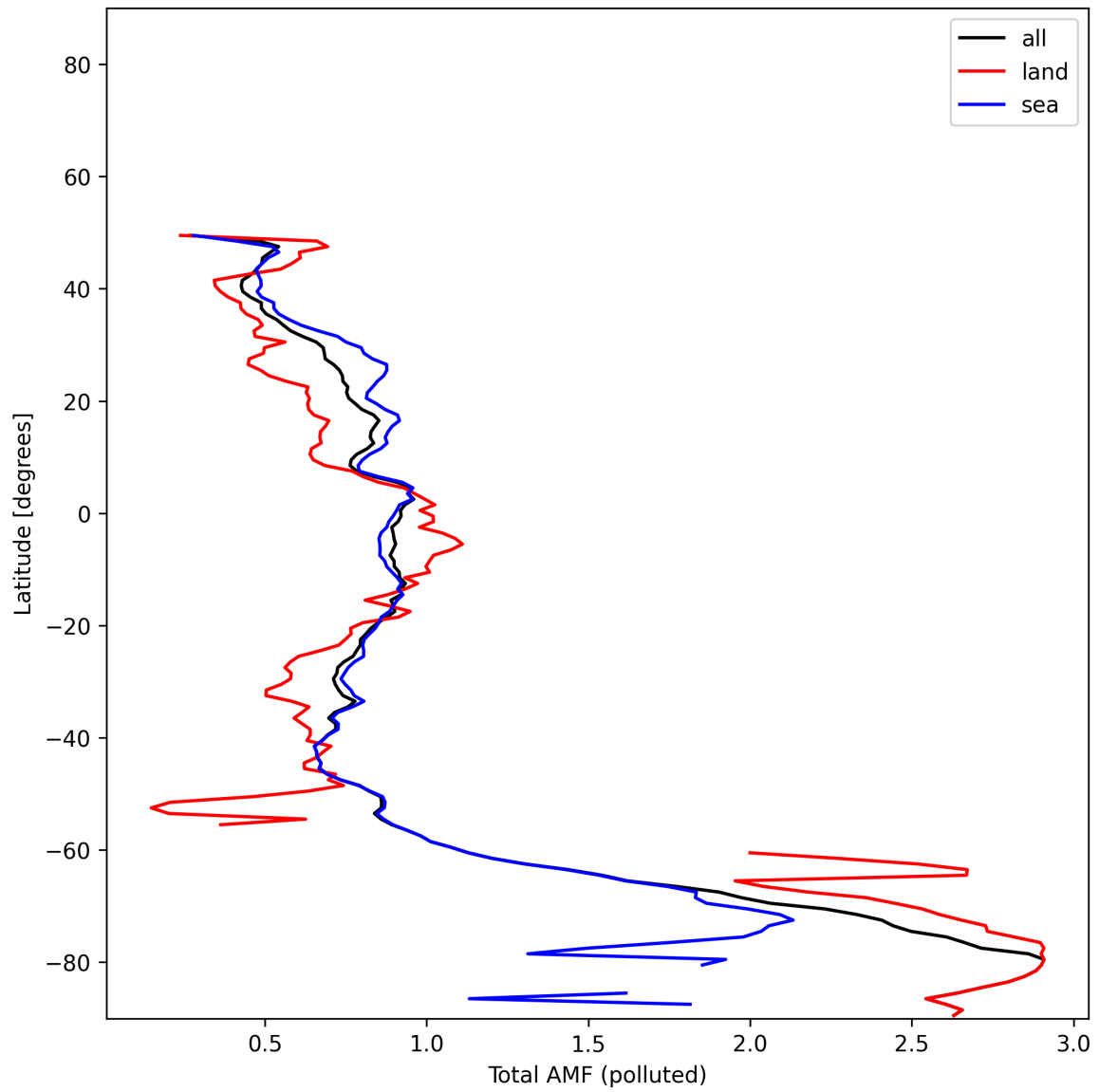
Figure 53: Zonal average of “Total AMF (polluted)” for 2025-11-24 to 2025-11-26.
