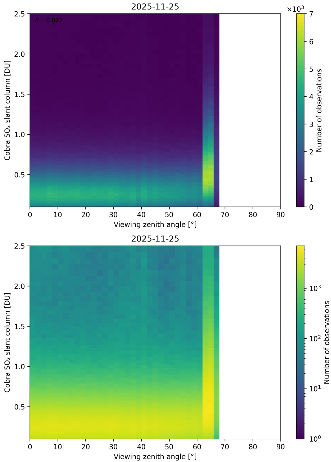
Figure 371: Scatter density plot of “Viewing zenith angle” against “Cobra SO 2 slant column” for 2025-11-24 to 2025-11-26.
