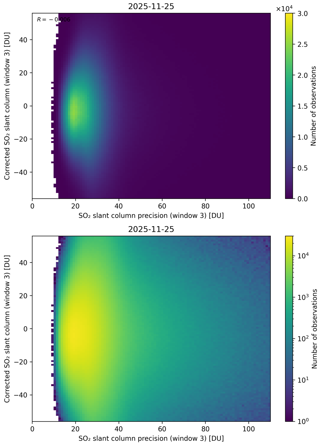
Figure 312: Scatter density plot of “SO 2 slant column precision (window 3)” against “Corrected SO 2 slant column (window 3)” for 2025-11-24 to 2025-11-26.
