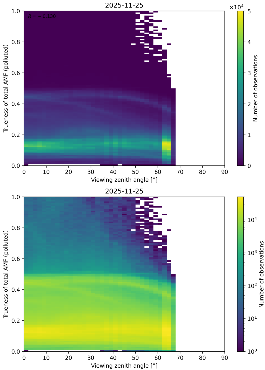
Figure 382: Scatter density plot of “Viewing zenith angle” against “Trueness of total AMF (polluted)” for 2025-11-24 to 2025-11-26.
