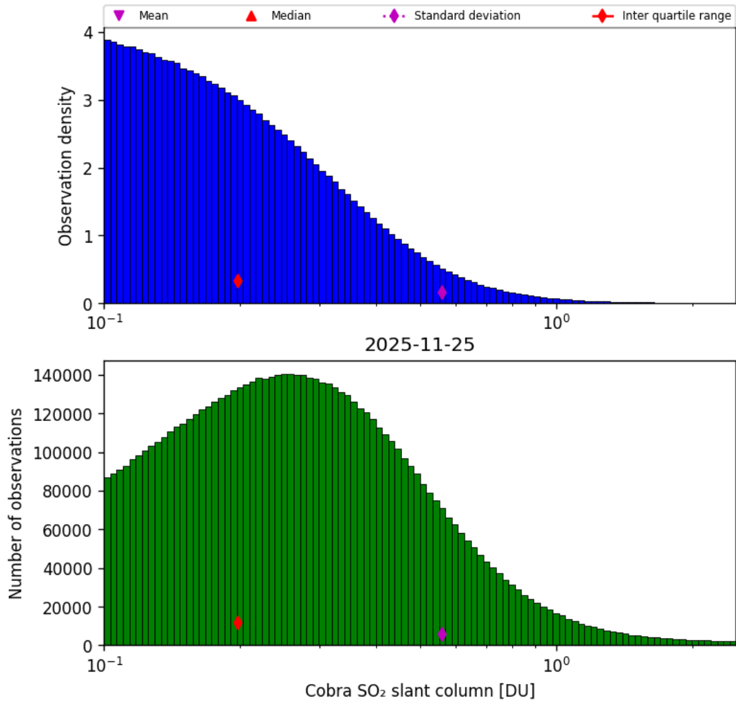
Figure 61: Histogram of “Cobra SO 2 slant column” for 2025-11-24 to 2025-11-26
