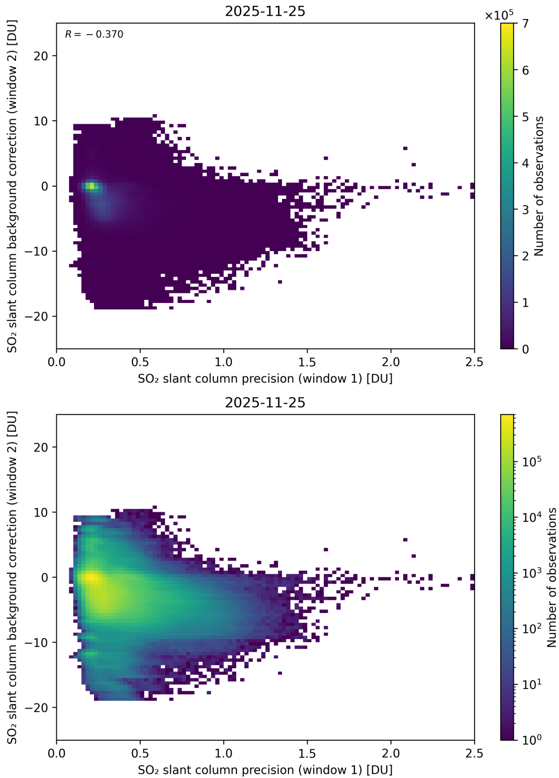
Figure 269: Scatter density plot of “SO 2 slant column precision (window 1)” against “SO 2 slant column background correction (window 2)” for 2025-11-24 to 2025-11-26.
