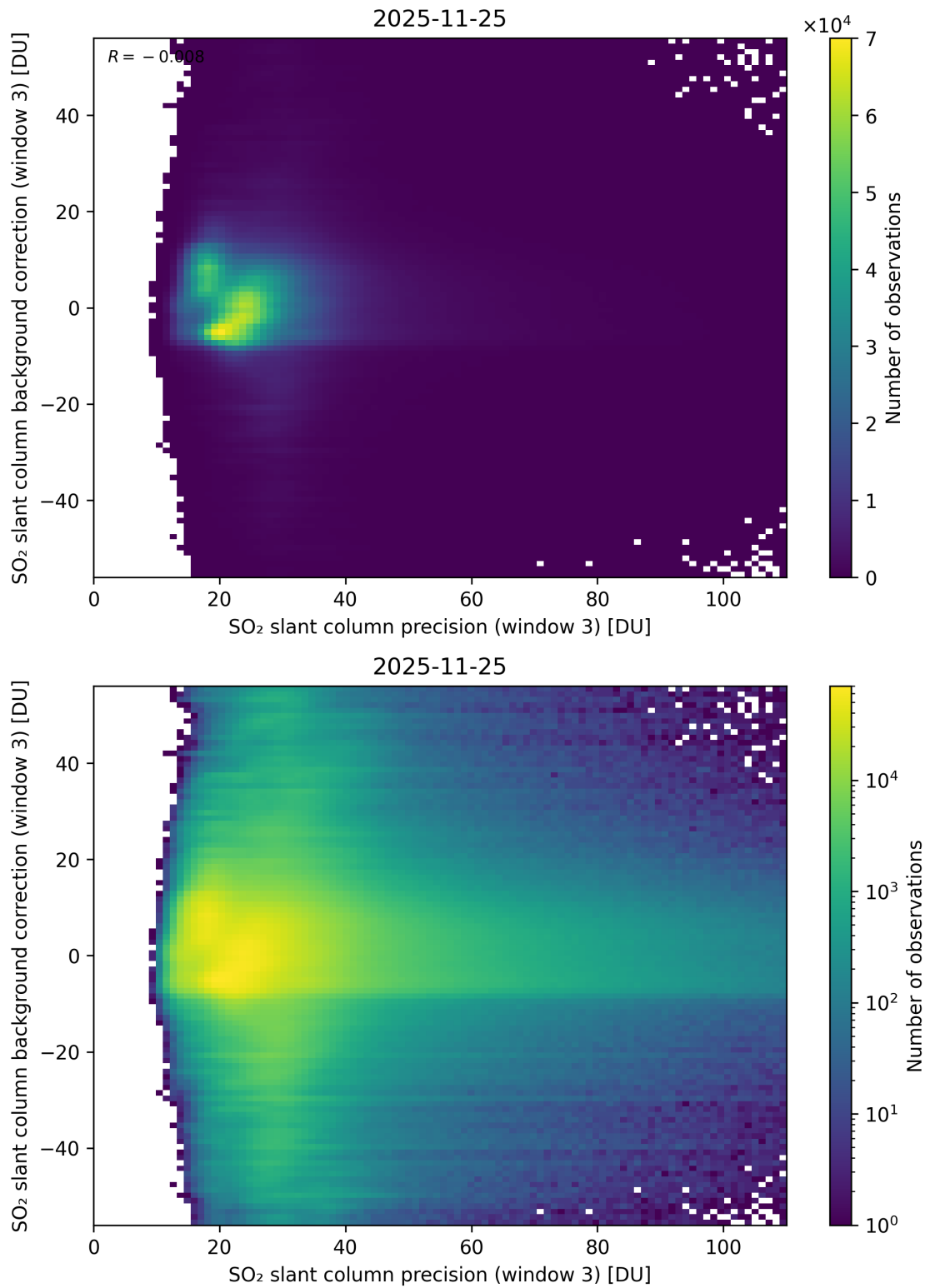
Figure 307: Scatter density plot of “SO 2 slant column precision (window 3)” against “SO 2 slant column background correction (window 3)” for 2025-11-24 to 2025-11-26.
