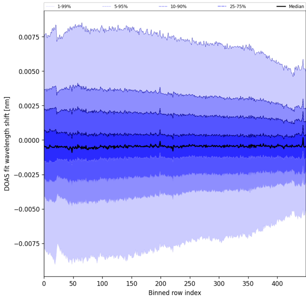
Figure 102: Along track statistics of “DOAS fit wavelength shift” for 2025-11-24 to 2025-11-26
