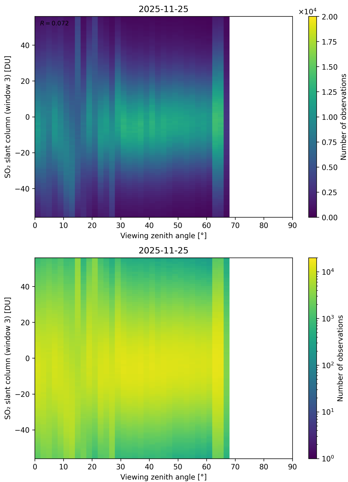
Figure 379: Scatter density plot of “Viewing zenith angle” against “SO 2 slant column (window 3)” for 2025-11-24 to 2025-11-26.
