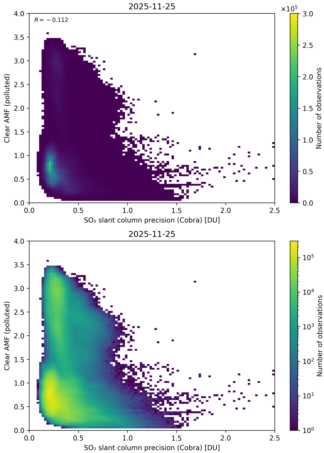
Figure 205: Scatter density plot of “SO 2 slant column precision (Cobra)” against “Clear AMF (polluted)” for 2025-11-24 to 2025-11-26.
