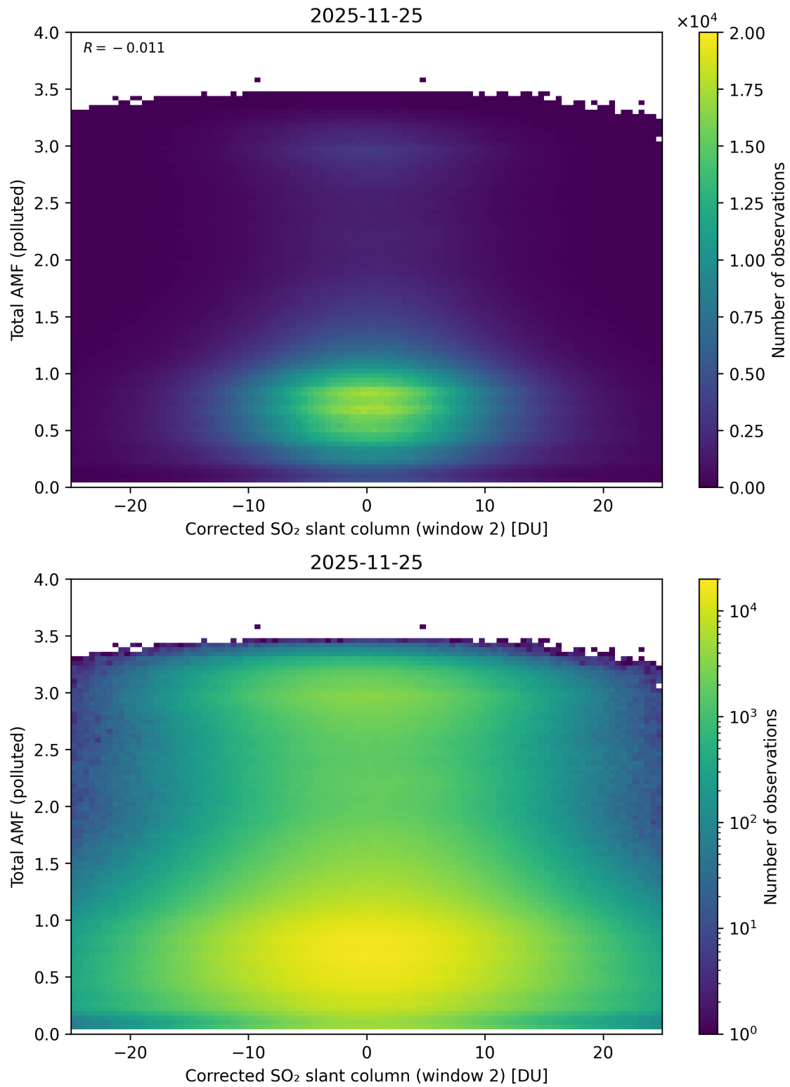
Figure 253: Scatter density plot of “Corrected SO 2 slant column (window 2)” against “Total AMF (polluted)” for 2025-11-24 to 2025-11-26.
