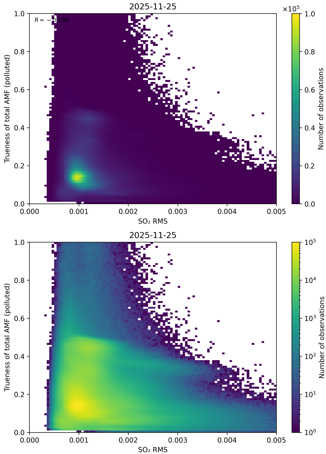
Figure 149: Scatter density plot of “SO 2 RMS” against “Trueness of total AMF (polluted)” for 2025-11-24 to 2025-11-26.
