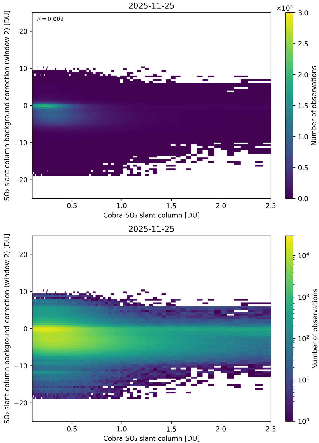
Figure 194: Scatter density plot of “Cobra SO 2 slant column” against “SO 2 slant column background correction (window 2)” for 2025-11-24 to 2025-11-26.
