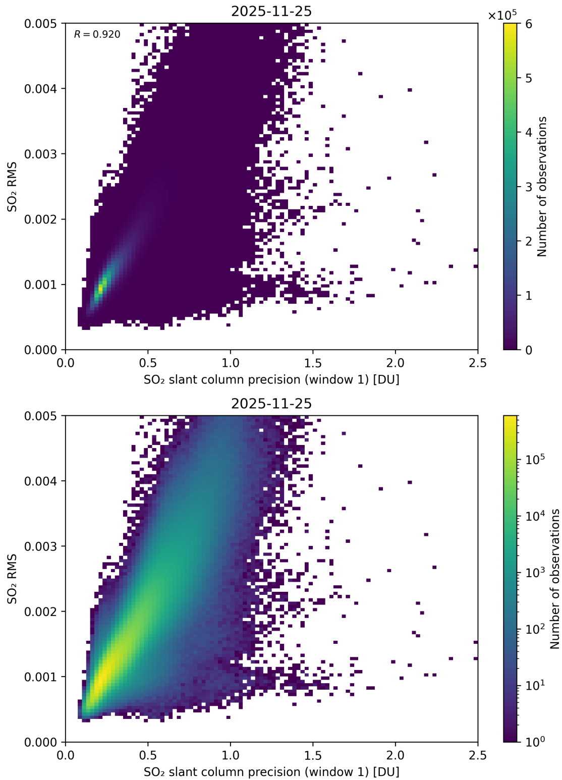
Figure 273: Scatter density plot of “SO 2 slant column precision (window 1)” against “SO 2 RMS” for 2025-11-24 to 2025-11-26.
