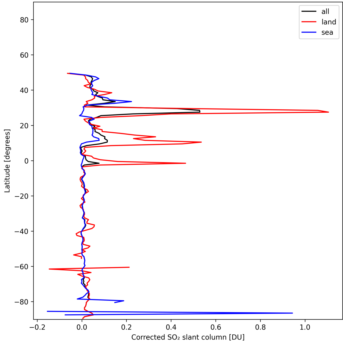
Figure 34: Zonal average of “Corrected SO 2 slant column” for 2025-11-24 to 2025-11-26.
