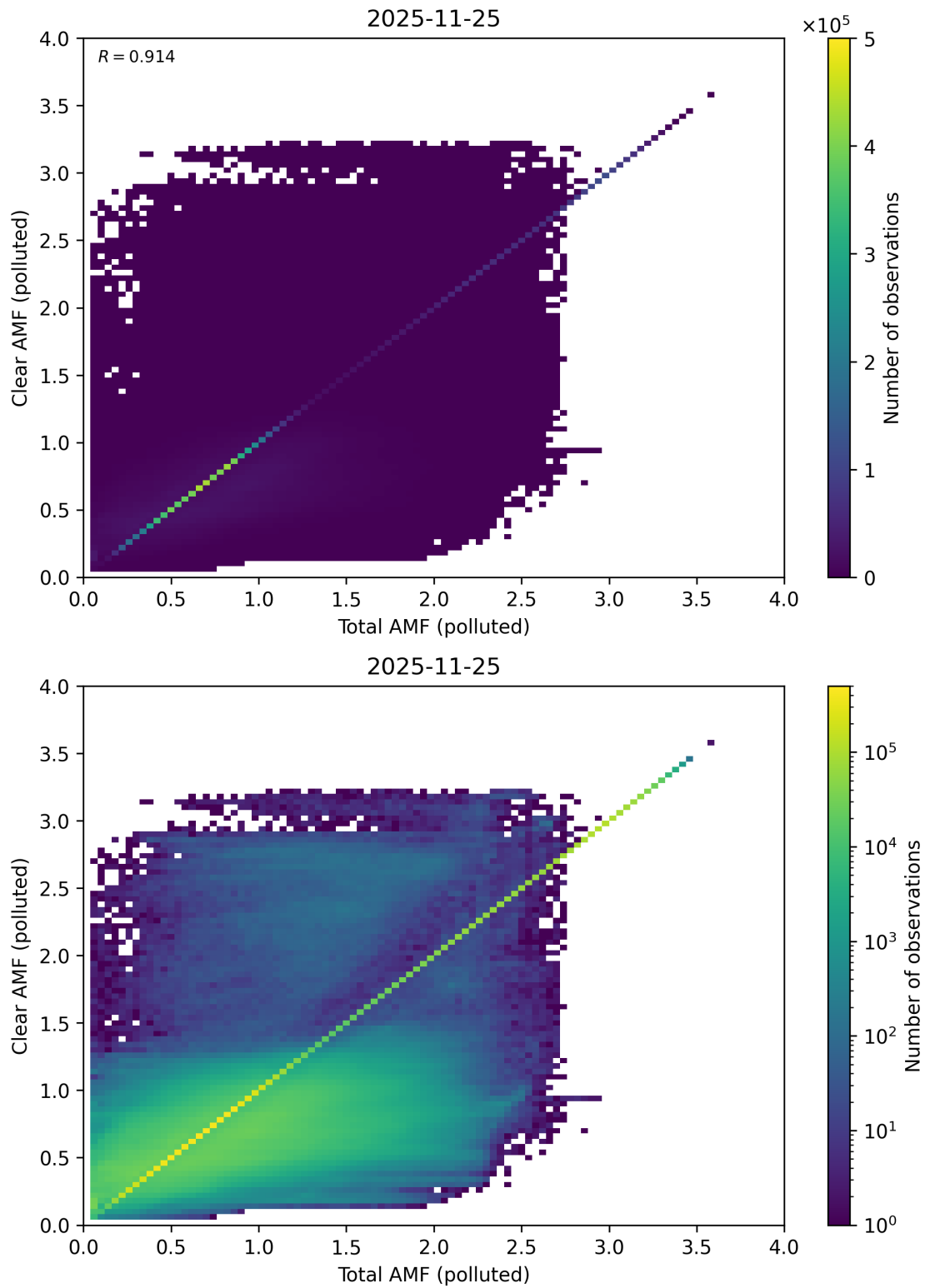
Figure 320: Scatter density plot of “Total AMF (polluted)” against “Clear AMF (polluted)” for 2025-11-24 to 2025-11-26.
