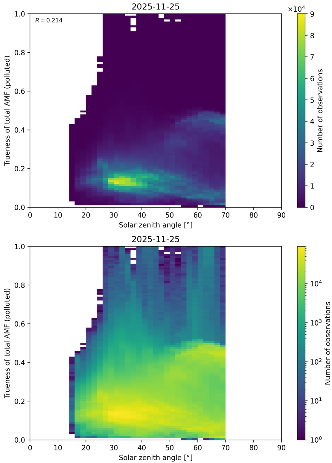
Figure 190: Scatter density plot of “Solar zenith angle” against “Trueness of total AMF (polluted)” for 2025-11-24 to 2025-11-26.
