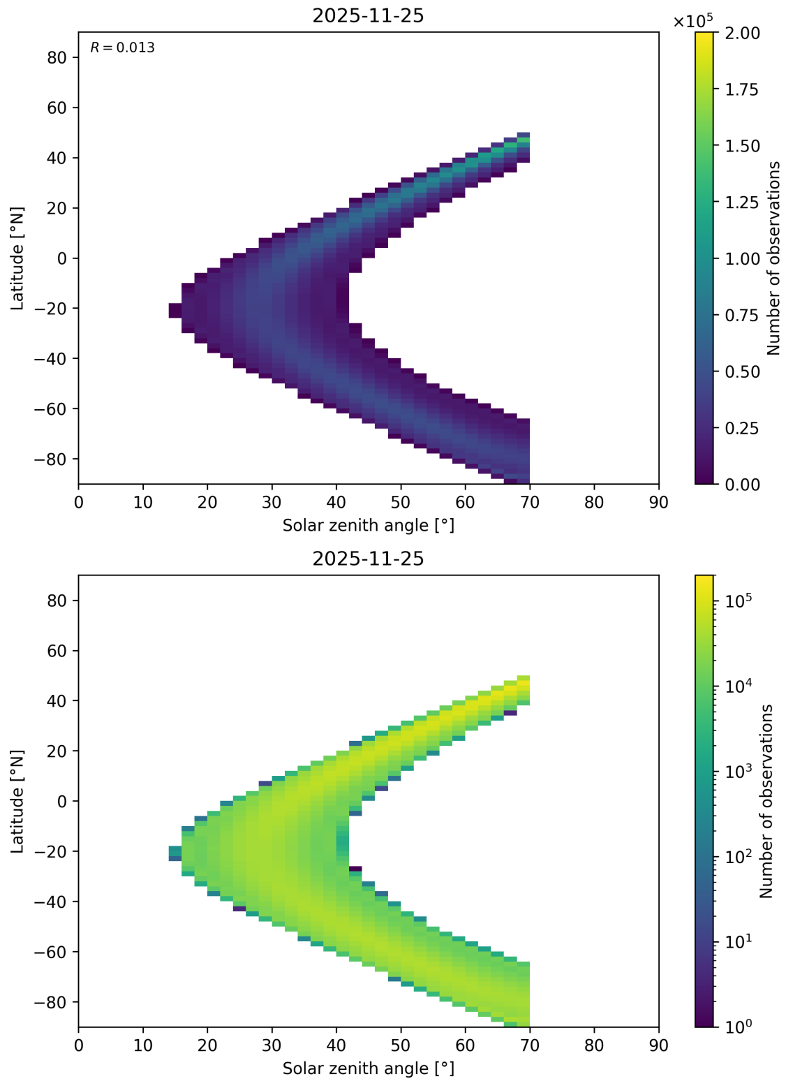
Figure 177: Scatter density plot of “Solar zenith angle” against “Latitude” for 2025-11-24 to 2025-11-26.
