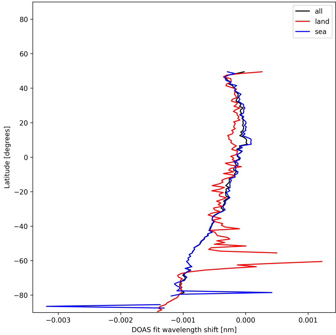
Figure 50: Zonal average of “DOAS fit wavelength shift” for 2025-11-24 to 2025-11-26.
