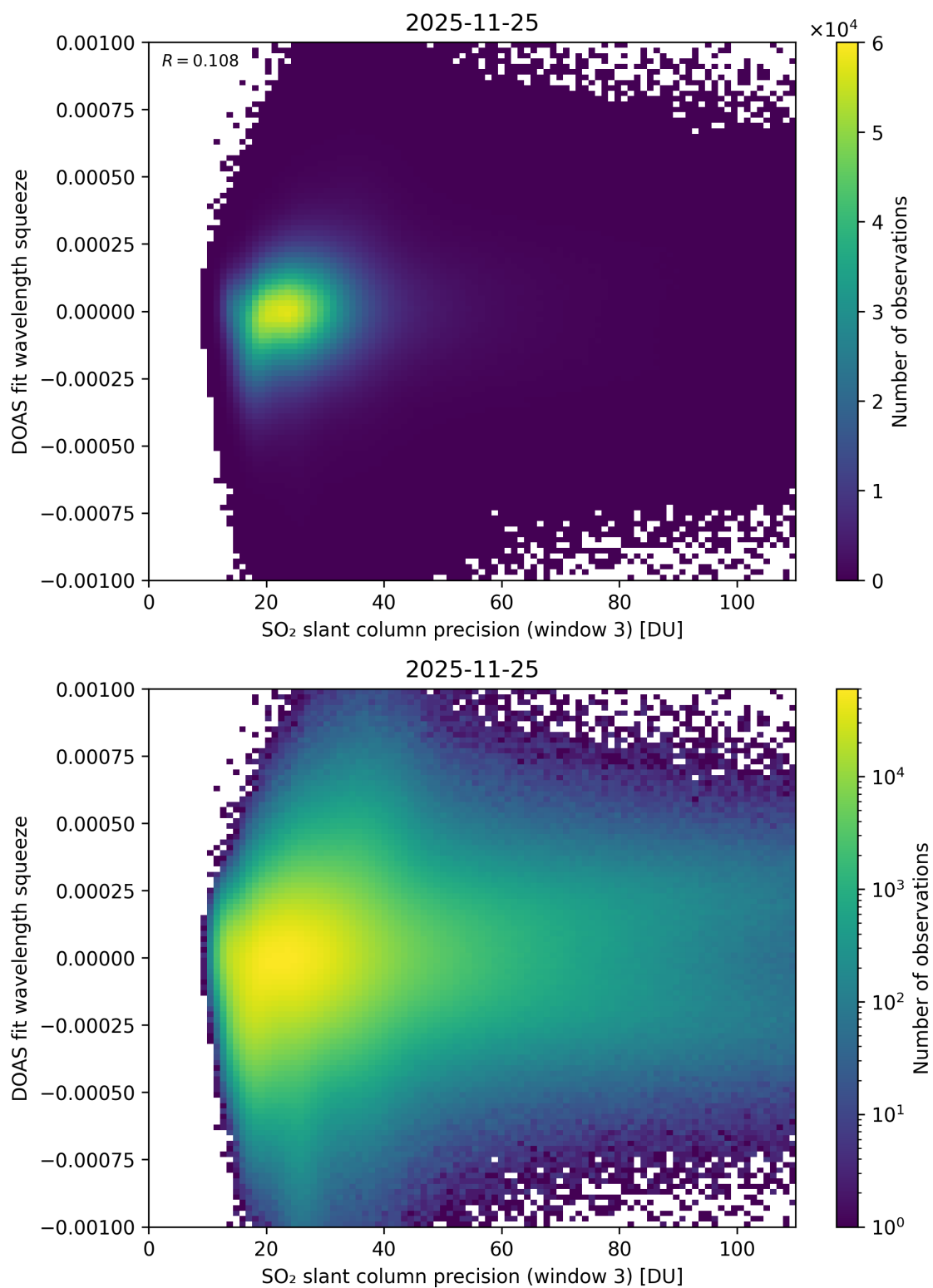
Figure 309: Scatter density plot of “SO 2 slant column precision (window 3)” against “DOAS fit wavelength squeeze” for 2025-11-24 to 2025-11-26.
