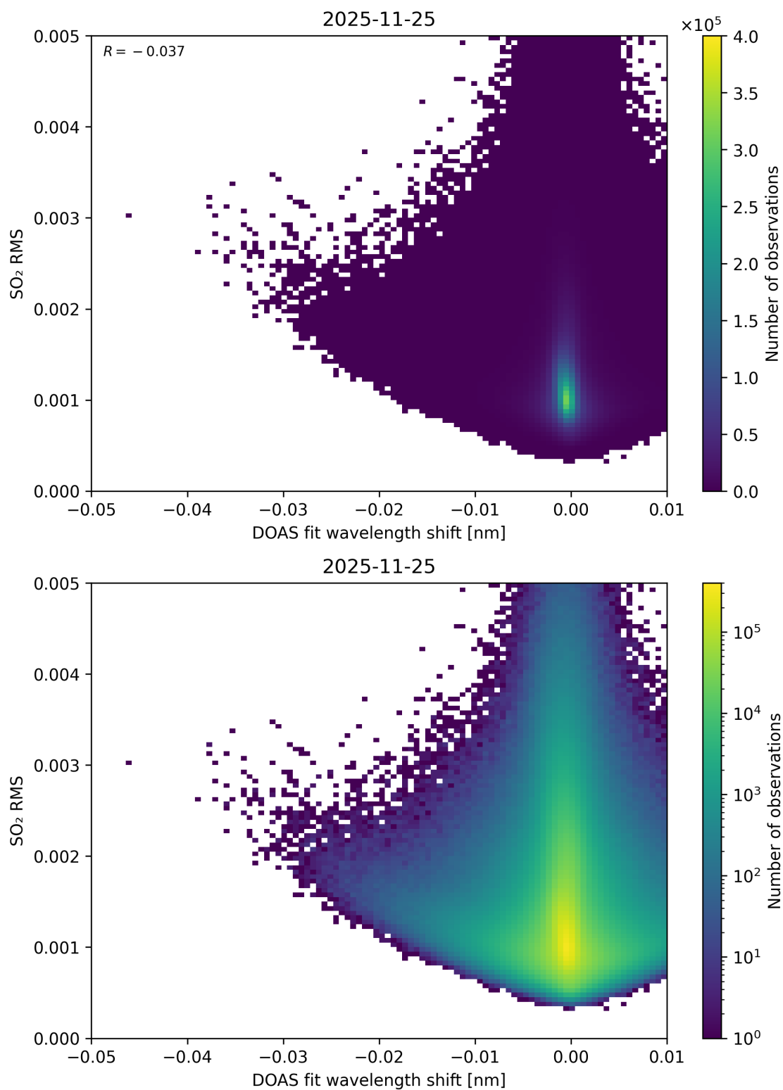
Figure 139: Scatter density plot of “DOAS fit wavelength shift” against “SO 2 RMS” for 2025-11-24 to 2025-11-26.
