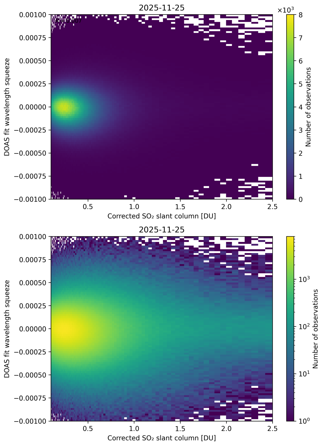
Figure 230: Scatter density plot of "Corrected SO 2 slant column" against "DOAS fit wavelength squeeze" for 2025-11-24 to 2025-11-26.
