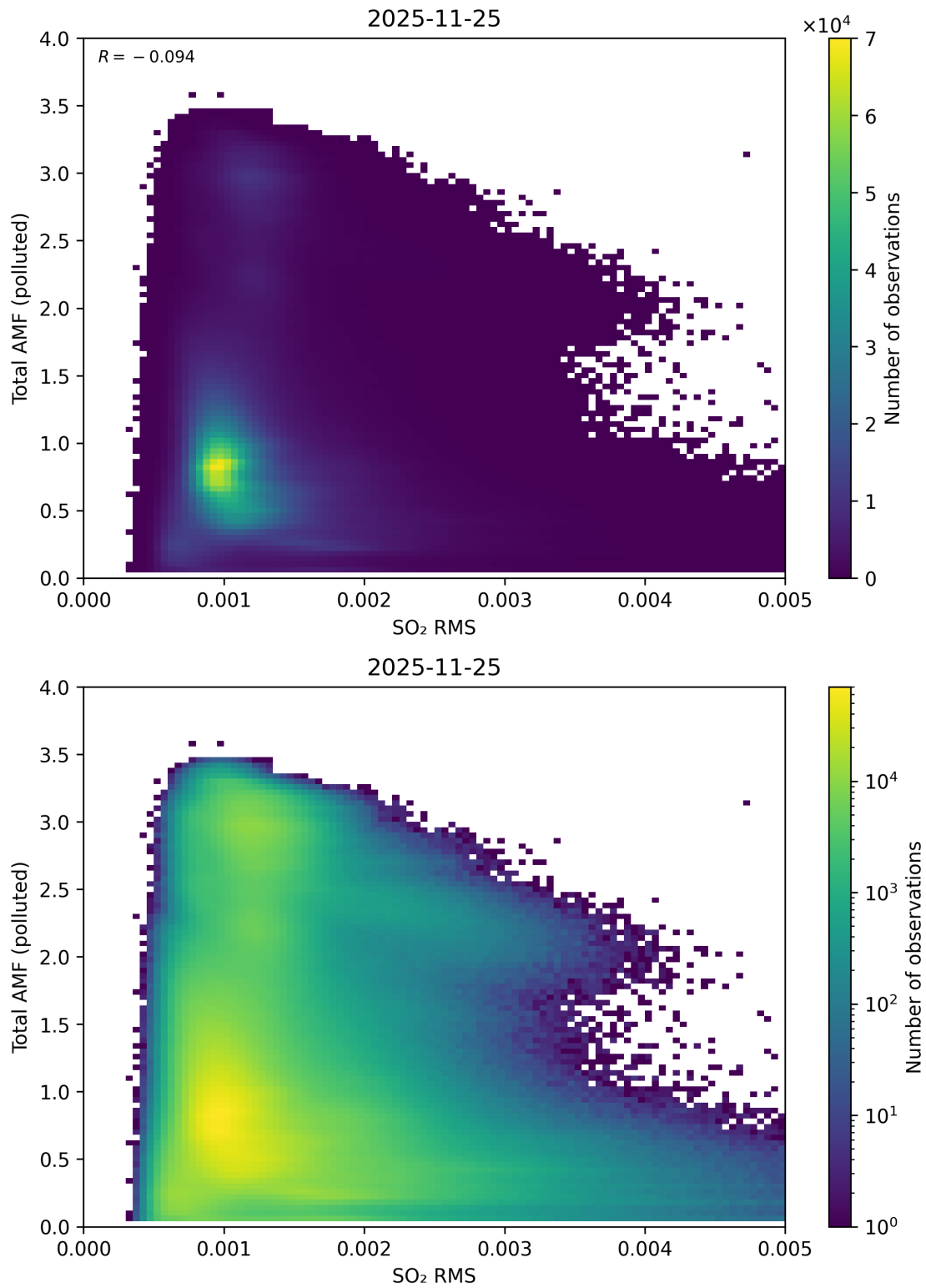
Figure 148: Scatter density plot of “SO 2 RMS” against “Total AMF (polluted)” for 2025-11-24 to 2025-11-26.
