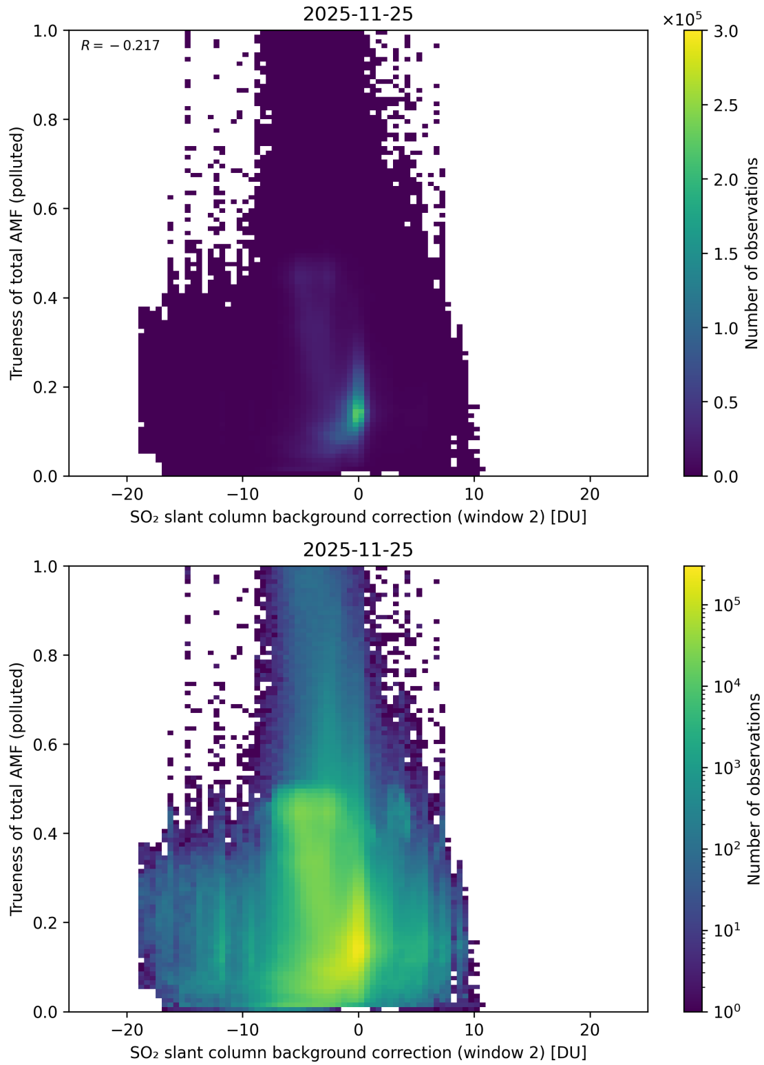
Figure 131: Scatter density plot of “SO 2 slant column background correction (window 2)” against “Trueness of total AMF (polluted)” for 2025-11-24 to 2025-11-26.
