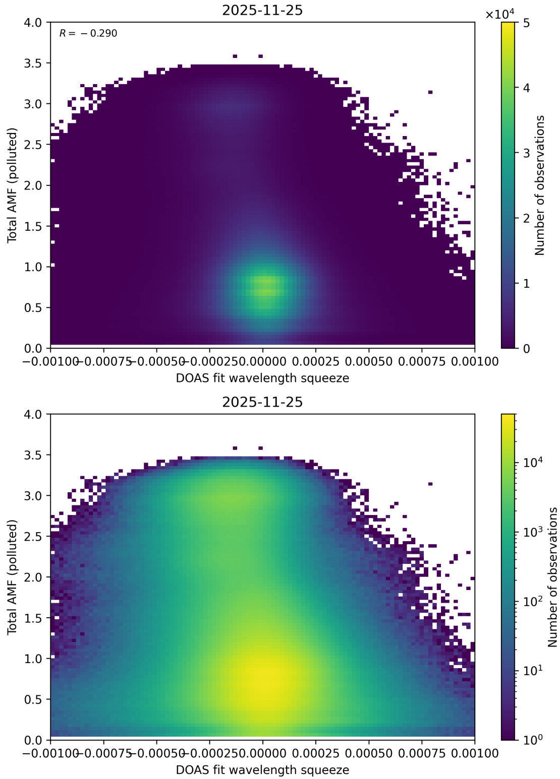
Figure 145: Scatter density plot of “DOAS fit wavelength squeeze” against “Total AMF (polluted)” for 2025-11-24 to 2025-11-26.
