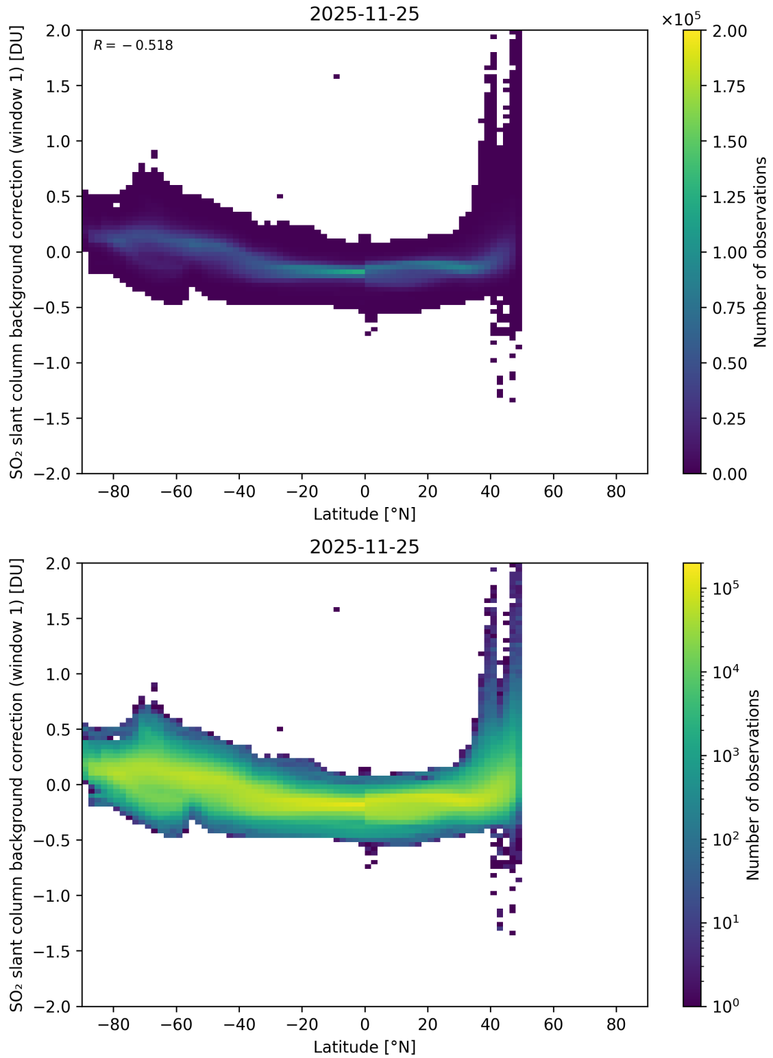
Figure 150: Scatter density plot of “Latitude” against “SO 2 slant column background correction (window 1)” for 2025-11-24 to 2025-11-26.
