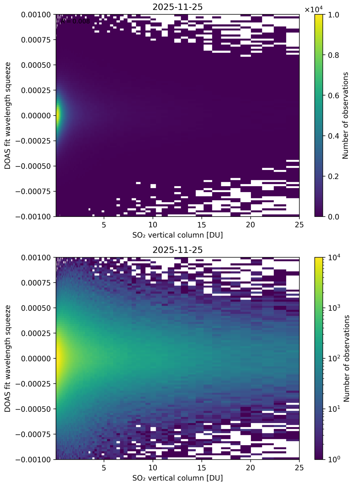
Figure 327: Scatter density plot of “SO 2 vertical column” against “DOAS fit wavelength squeeze” for 2025-11-24 to 2025-11-26.
