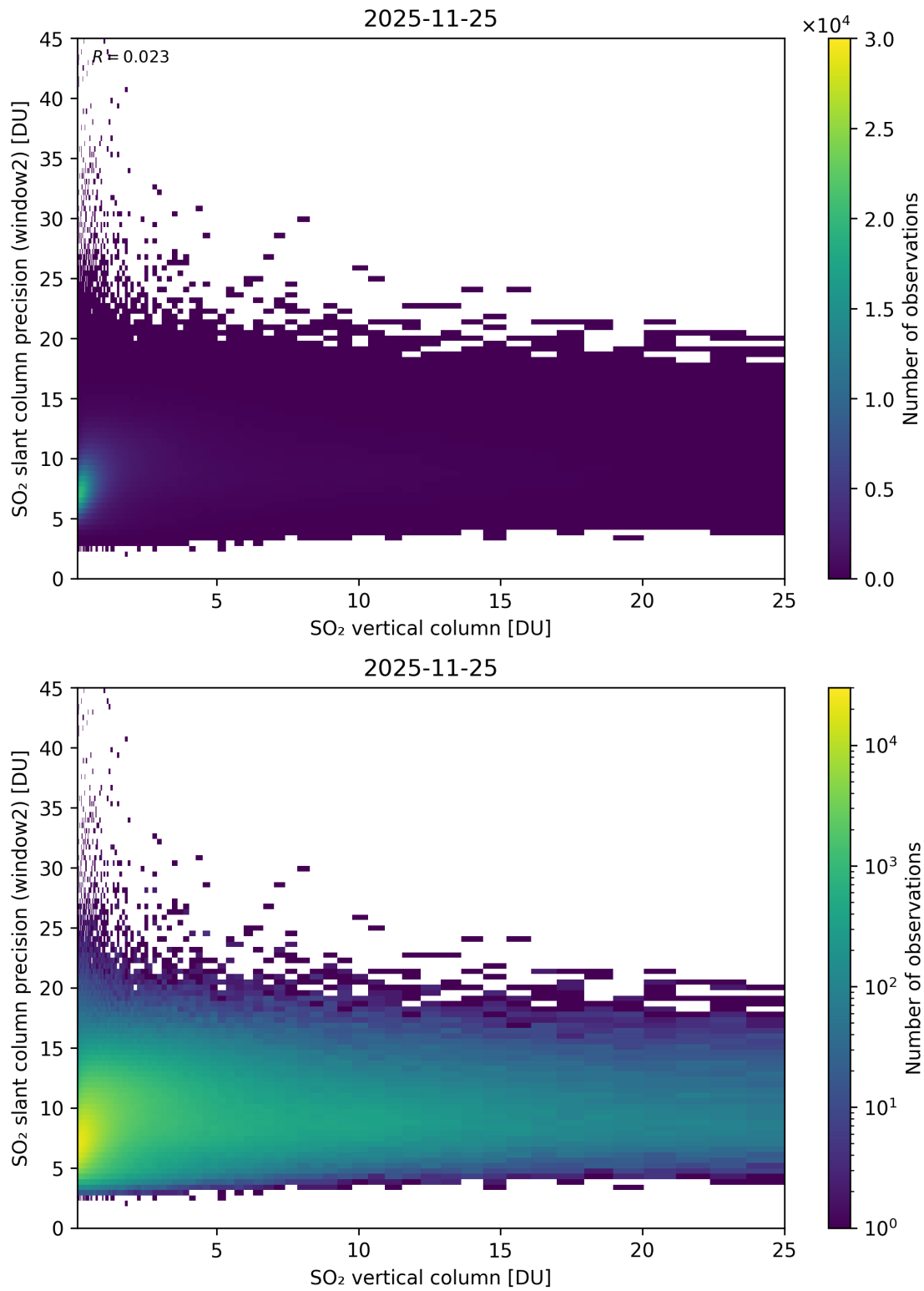
Figure 356: Scatter density plot of “SO 2 vertical column” against “SO 2 slant column precision (window2)” for 2025-11-24 to 2025-11-26.
