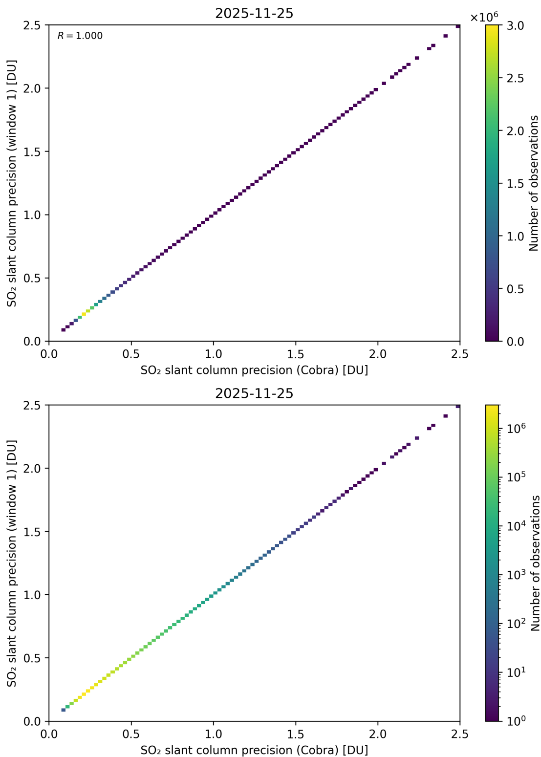
Figure 209: Scatter density plot of “SO 2 slant column precision (Cobra)” against “SO 2 slant column precision (window 1)” for 2025-11-24 to 2025-11-26.
