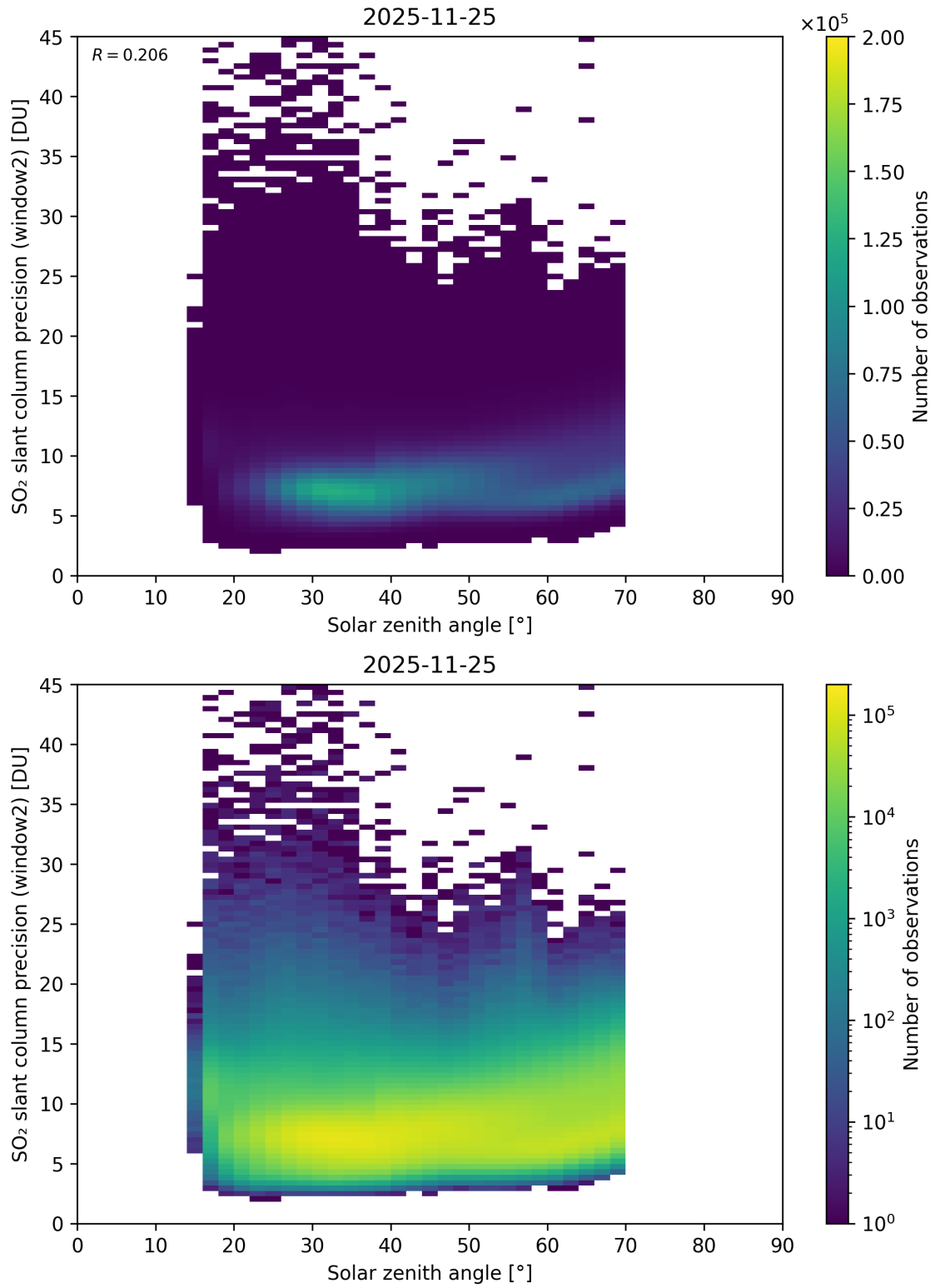
Figure 186: Scatter density plot of “Solar zenith angle” against “SO 2 slant column precision (window2)” for 2025-11-24 to 2025-11-26.
