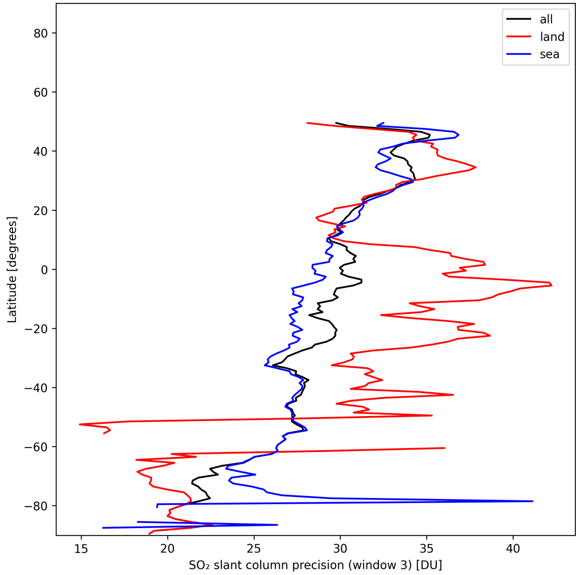
Figure 46: Zonal average of “SO 2 slant column precision (window 3)” for 2025-11-24 to 2025-11-26.
