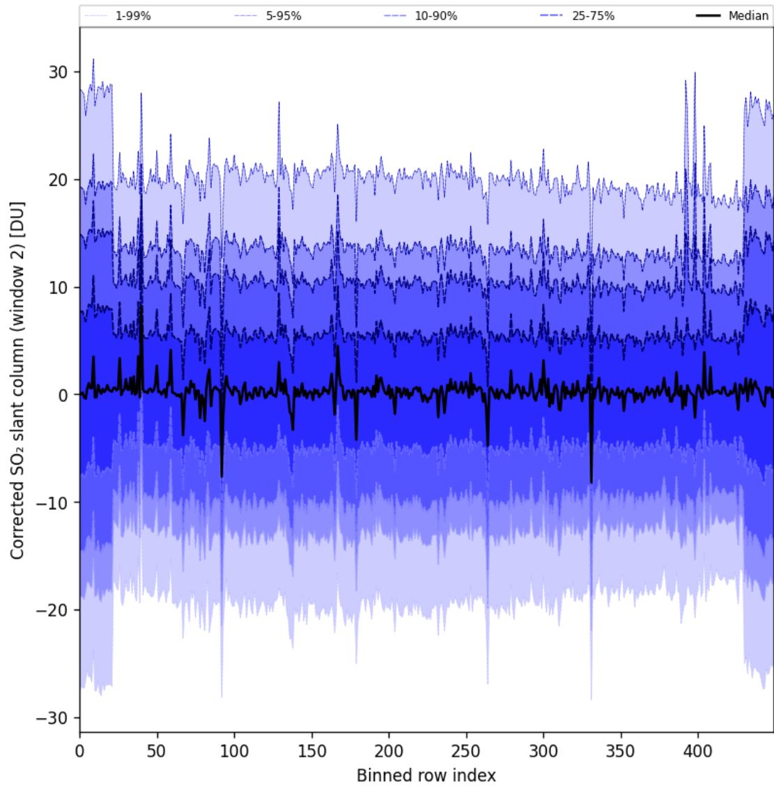
Figure 95: Along track statistics of “Corrected SO 2 slant column (window 2)” for 2025-11-24 to 2025-11-26
