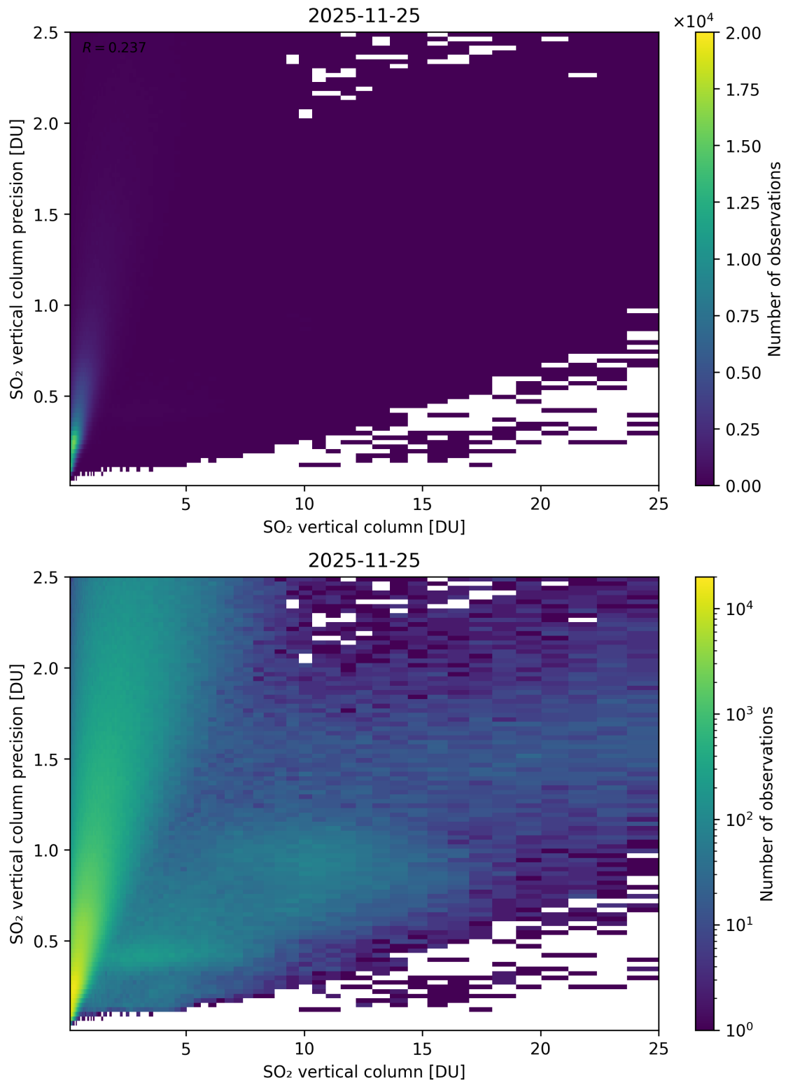
Figure 361: Scatter density plot of “SO 2 vertical column” against “SO 2 vertical column precision” for 2025-11-24 to 2025-11-26.
