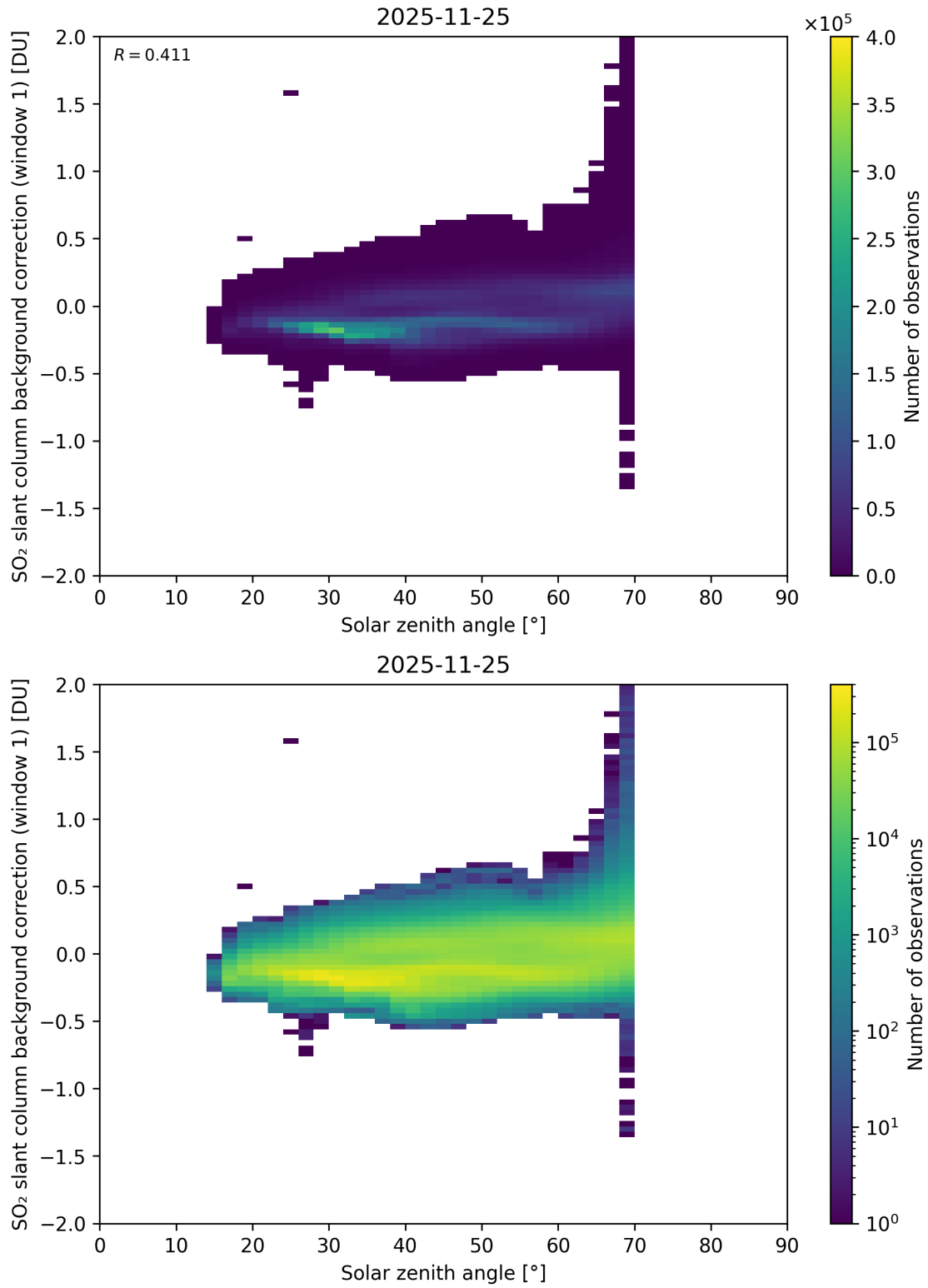
Figure 171: Scatter density plot of “Solar zenith angle” against “SO 2 slant column background correction (window 1)” for 2025-11-24 to 2025-11-26.
