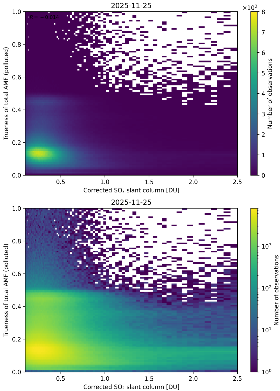
Figure 243: Scatter density plot of “Corrected SO 2 slant column” against “Trueness of total AMF (polluted)” for 2025-11-24 to 2025-11-26.
