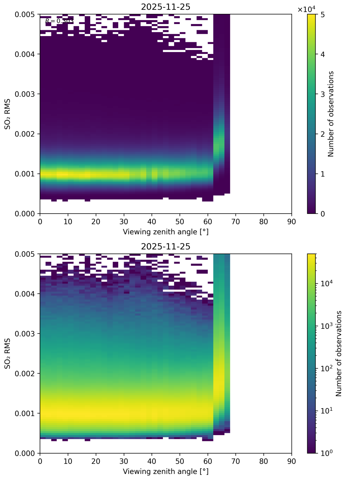
Figure 367: Scatter density plot of “Viewing zenith angle” against “SO 2 RMS” for 2025-11-24 to 2025-11-26.
