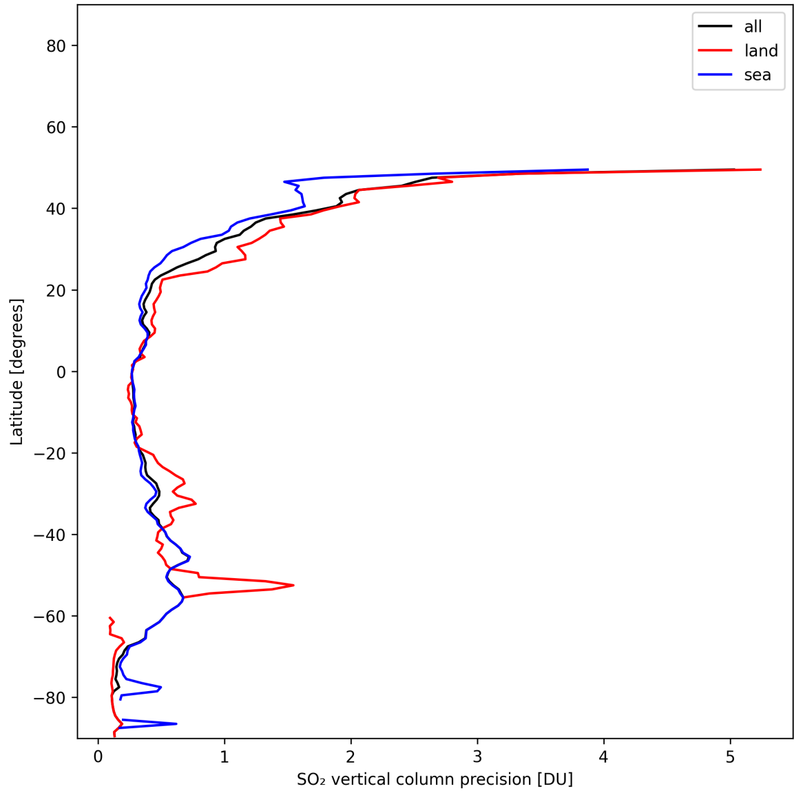
Figure 33: Zonal average of “SO 2 vertical column precision” for 2025-11-24 to 2025-11-26.
