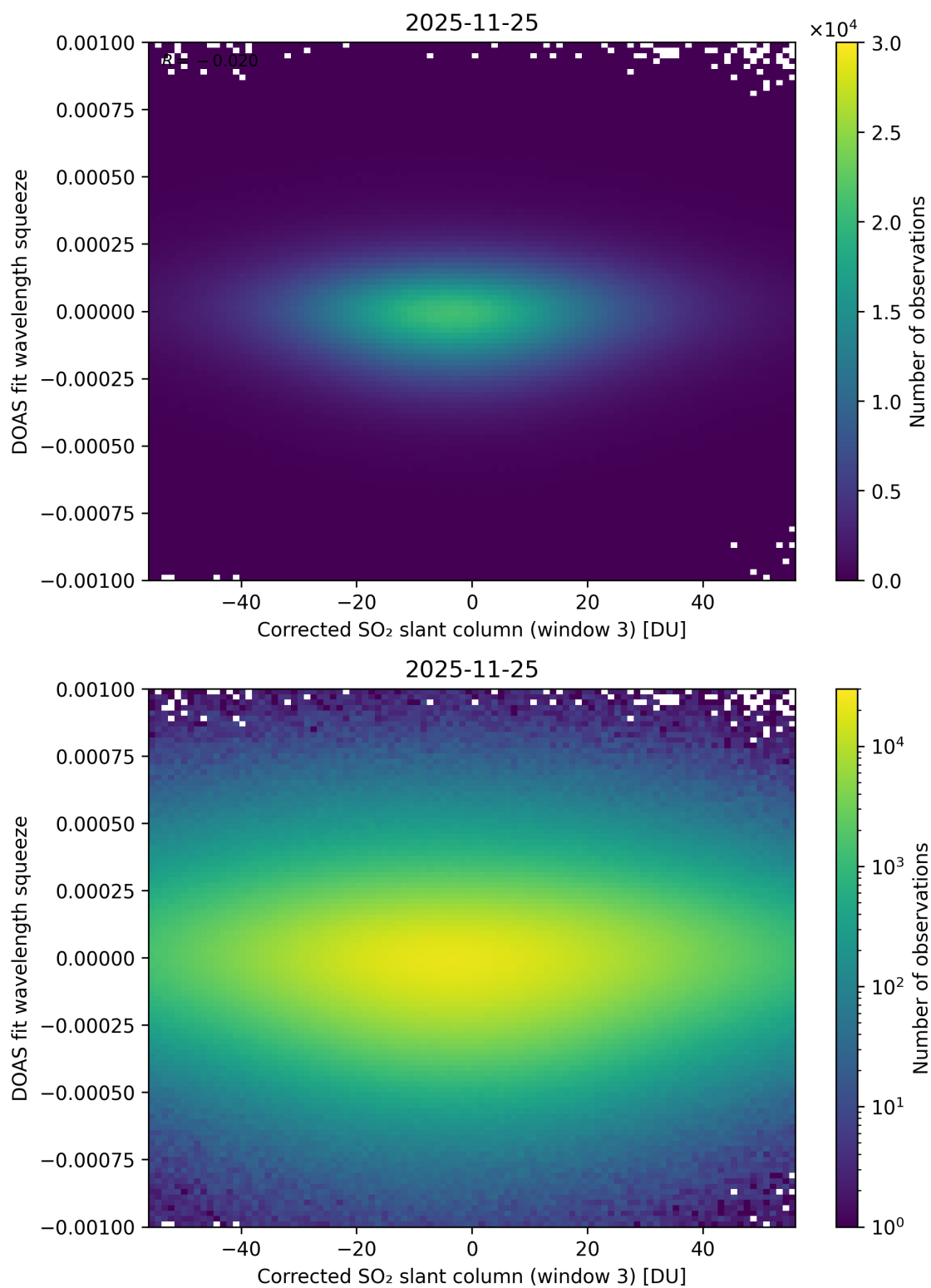
Figure 257: Scatter density plot of “Corrected SO 2 slant column (window 3)” against “DOAS fit wavelength squeeze” for 2025-11-24 to 2025-11-26.
