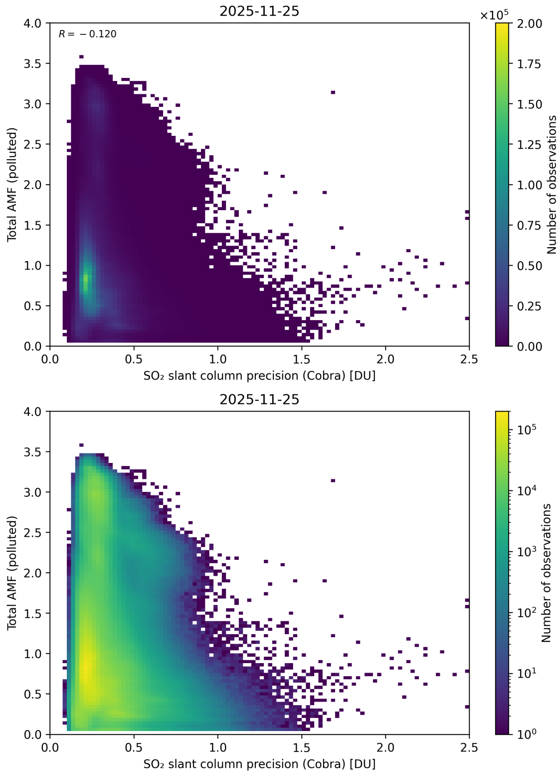
Figure 213: Scatter density plot of “SO 2 slant column precision (Cobra)” against “Total AMF (polluted)” for 2025-11-24 to 2025-11-26.
