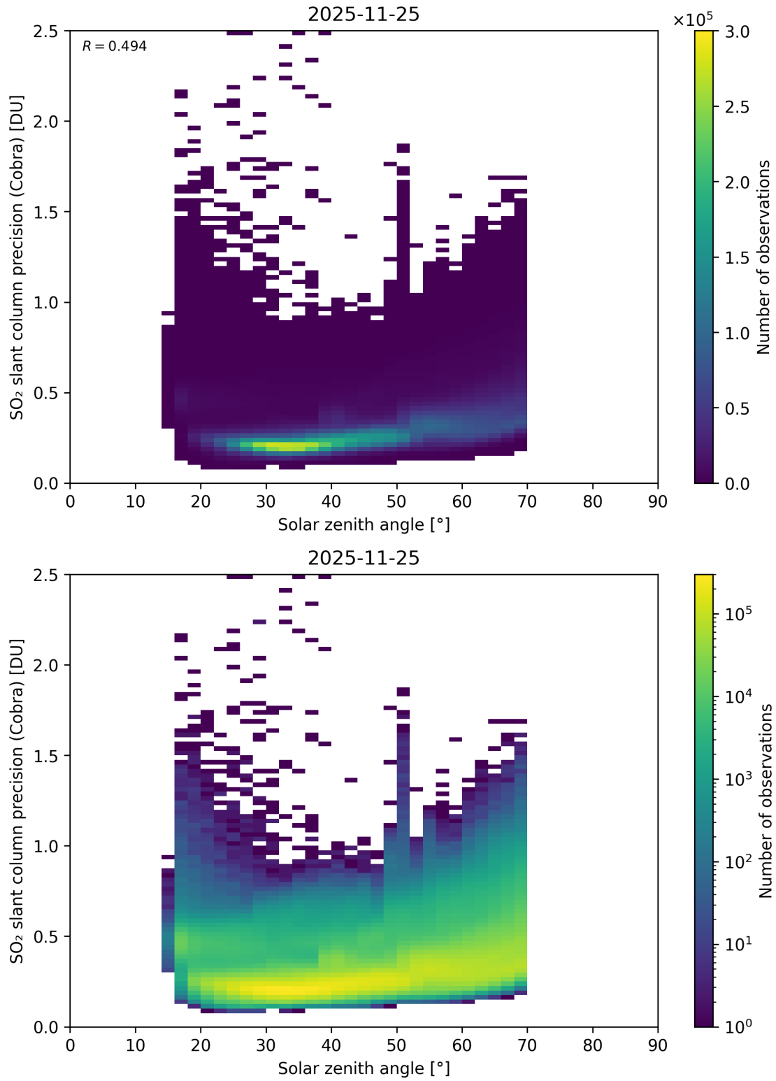
Figure 180: Scatter density plot of “Solar zenith angle” against “SO 2 slant column precision (Cobra)” for 2025-11-24 to 2025-11-26.
