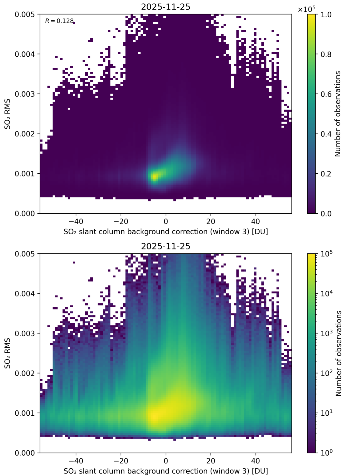
Figure 134: Scatter density plot of “SO 2 slant column background correction (window 3)” against “SO 2 RMS” for 2025-11-24 to 2025-11-26.
