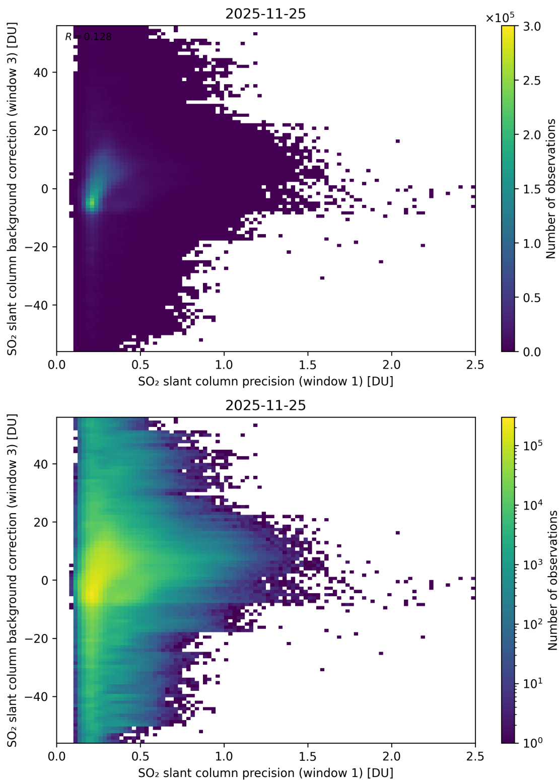
Figure 270: Scatter density plot of “SO 2 slant column precision (window 1)” against “SO 2 slant column background correction (window 3)” for 2025-11-24 to 2025-11-26.
