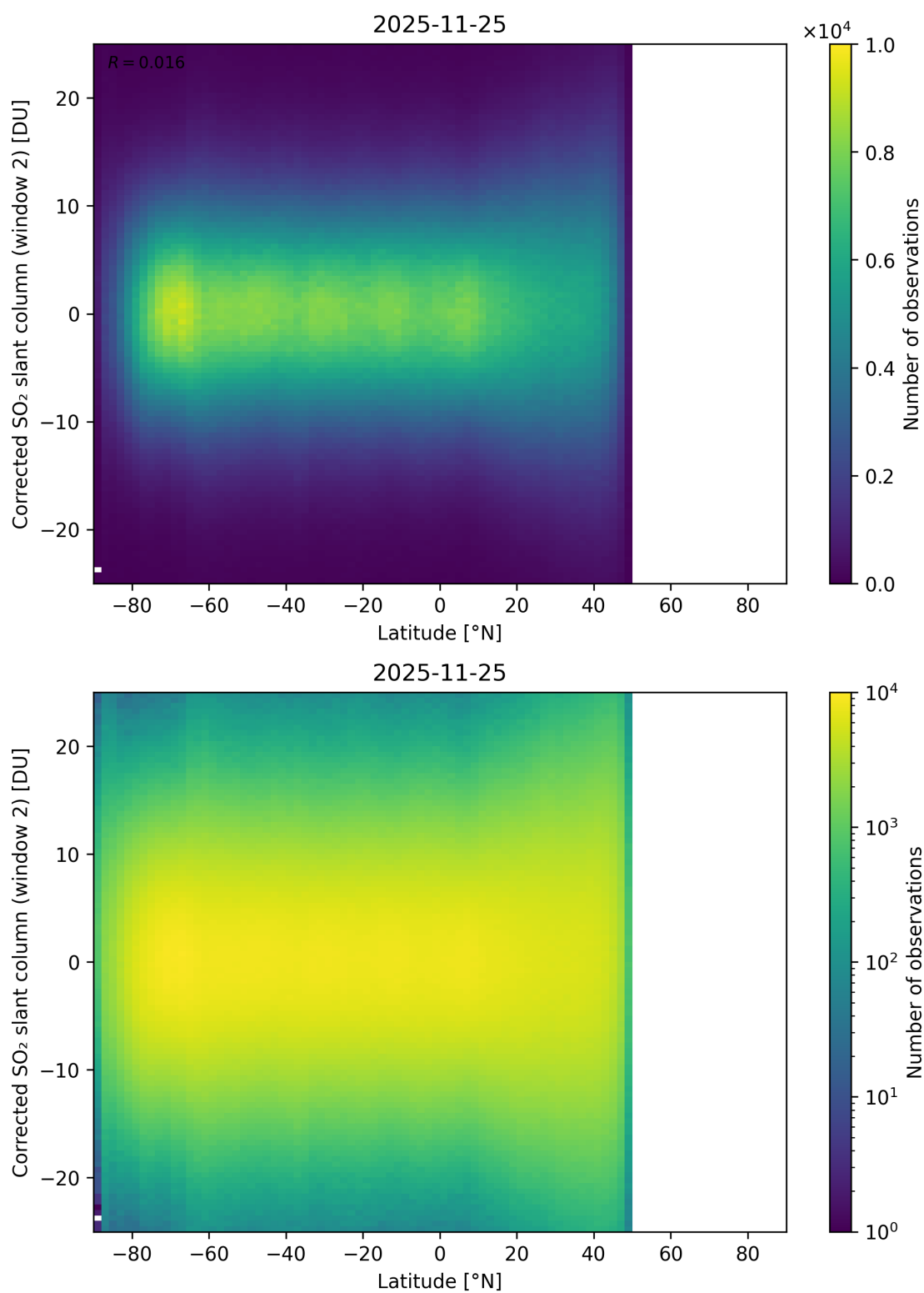
Figure 160: Scatter density plot of “Latitude” against “Corrected SO 2 slant column (window 2)” for 2025-11-24 to 2025-11-26.
