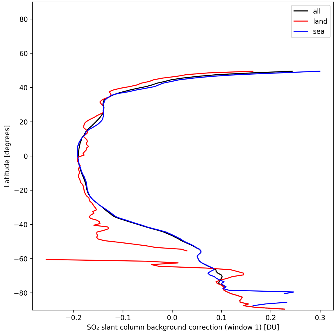
Figure 40: Zonal average of “SO 2 slant column background correction (window 1)” for 2025-11-24 to 2025-11-26.
