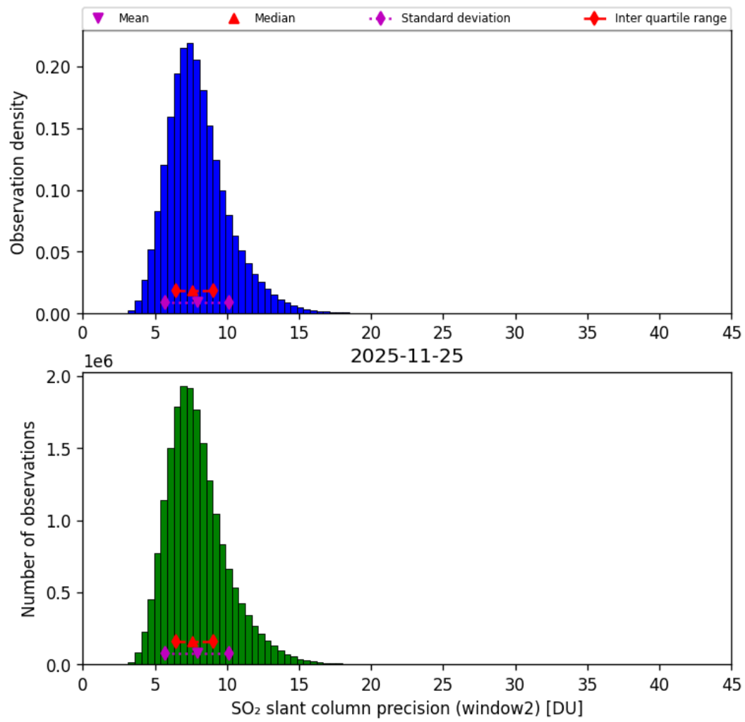
Figure 68: Histogram of “SO 2 slant column precision (window2)” for 2025-11-24 to 2025-11-26
