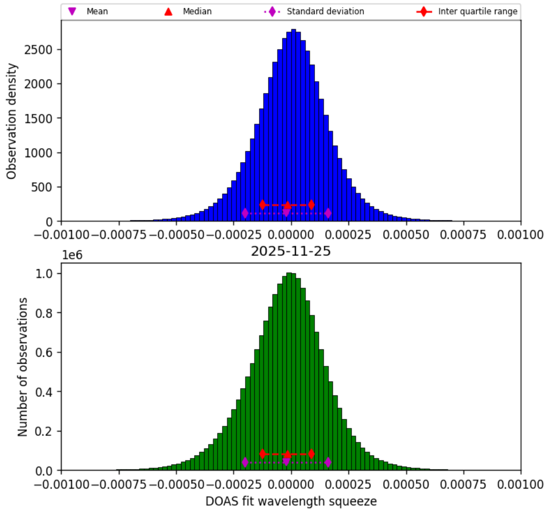
Figure 77: Histogram of “DOAS fit wavelength squeeze” for 2025-11-24 to 2025-11-26
