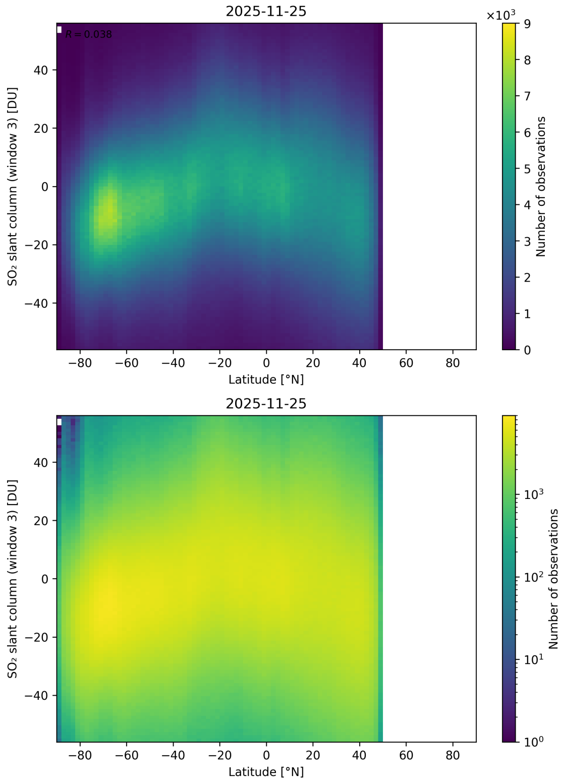
Figure 165: Scatter density plot of “Latitude” against “SO 2 slant column (window 3)” for 2025-11-24 to 2025-11-26.
