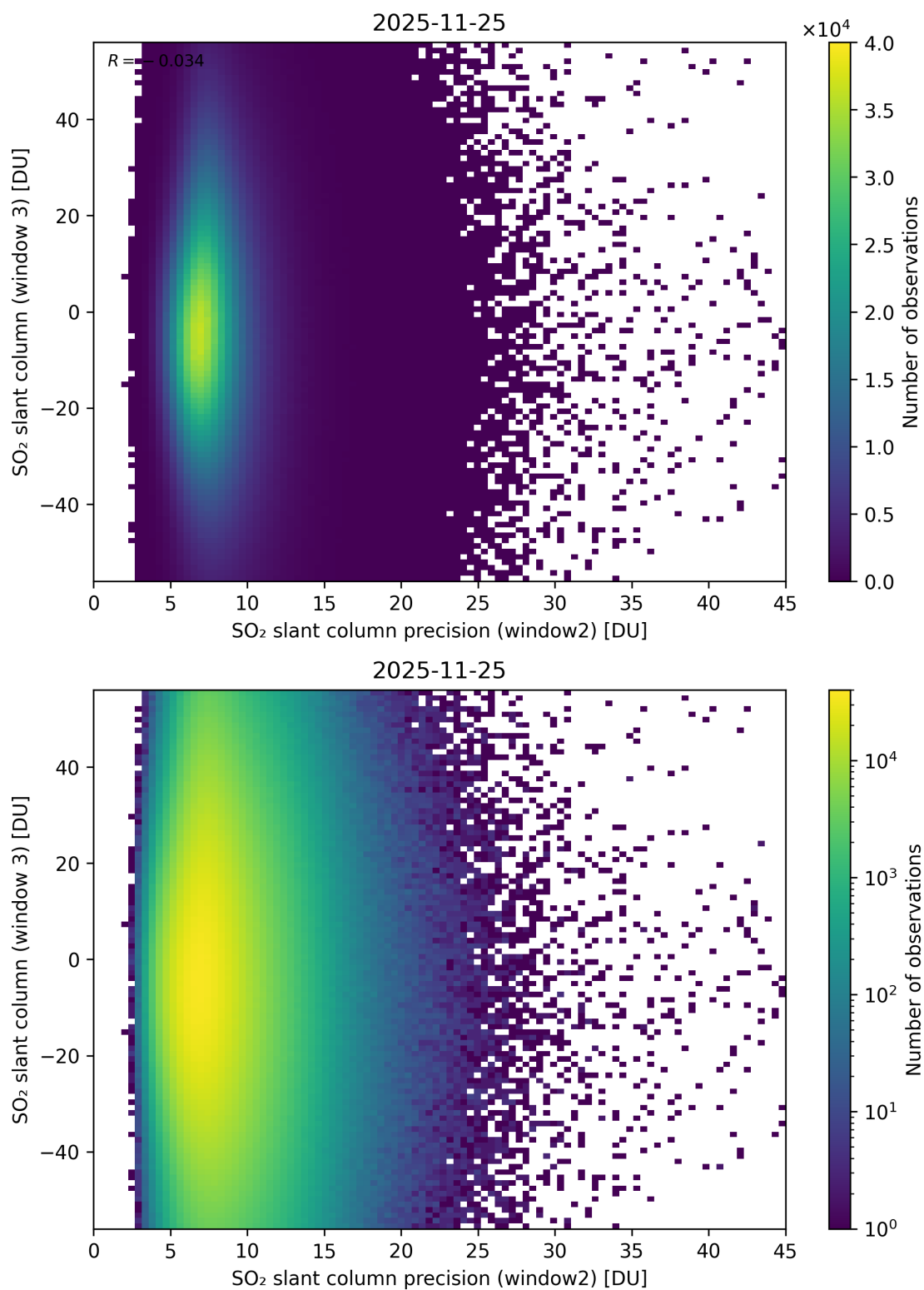
Figure 299: Scatter density plot of “SO 2 slant column precision (window2)” against “SO 2 slant column (window 3)” for 2025-11-24 to 2025-11-26.
