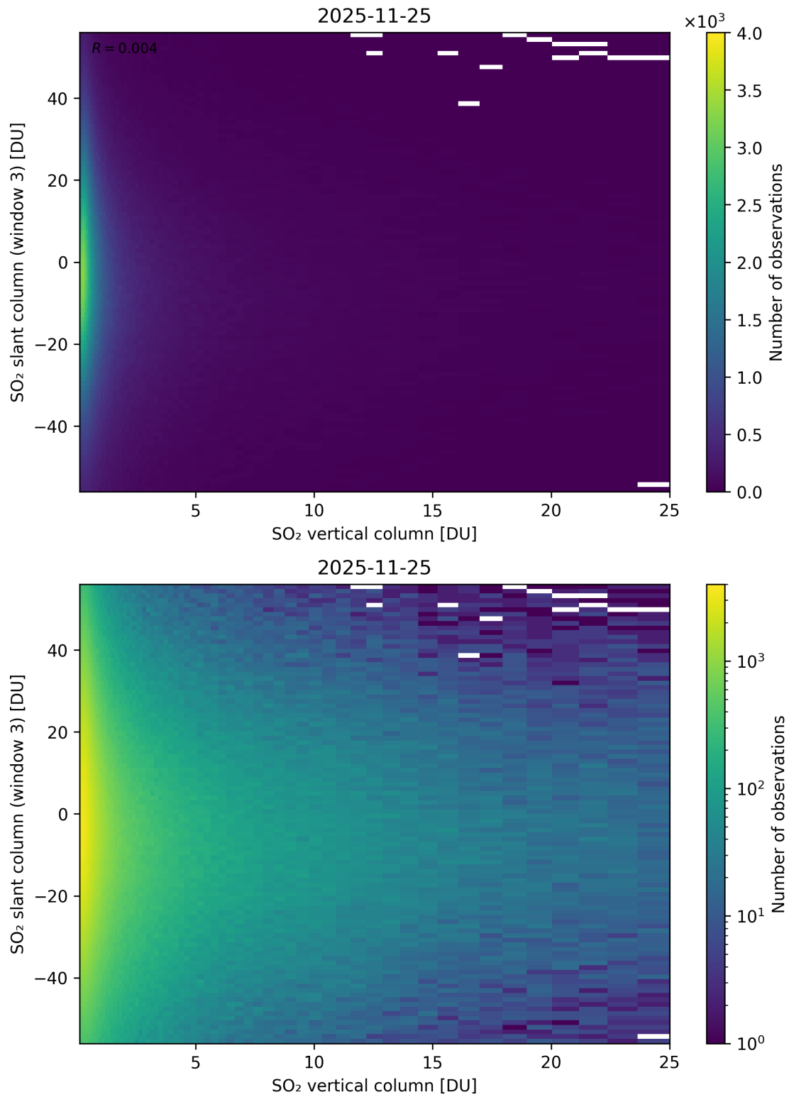
Figure 357: Scatter density plot of “SO 2 vertical column” against “SO 2 slant column (window 3)” for 2025-11-24 to 2025-11-26.
