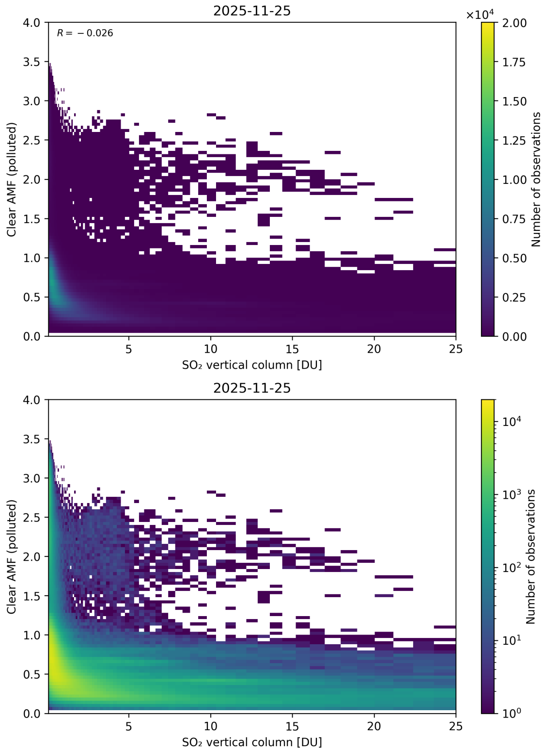
Figure 348: Scatter density plot of “SO 2 vertical column” against “Clear AMF (polluted)” for 2025-11-24 to 2025-11-26.
