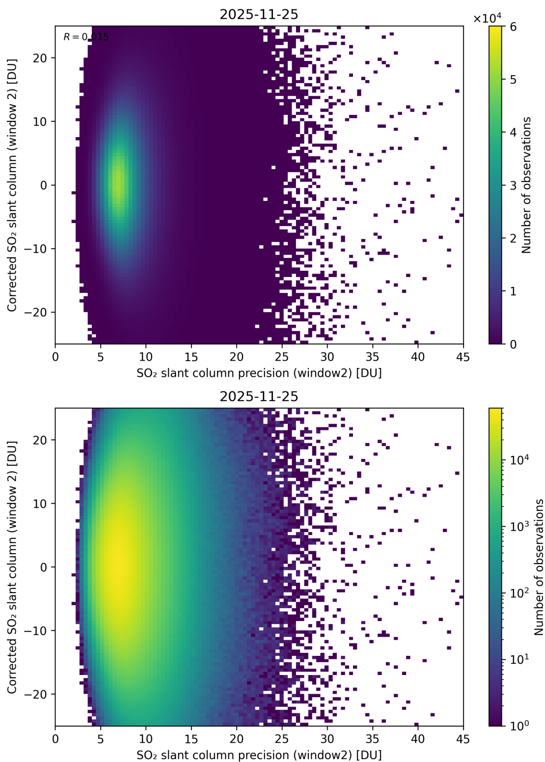
Figure 297: Scatter density plot of “SO 2 slant column precision (window2)” against “Corrected SO 2 slant column (window 2)” for 2025-11-24 to 2025-11-26.
