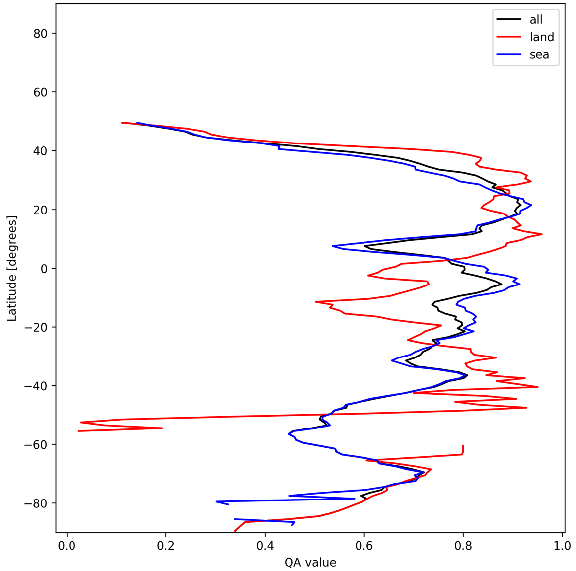
Figure 31: Zonal average of “QA value” for 2025-11-24 to 2025-11-26.
