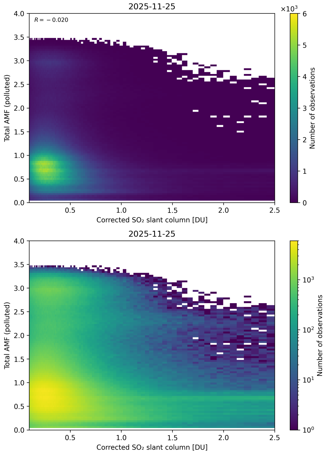
Figure 242: Scatter density plot of “Corrected SO 2 slant column” against “Total AMF (polluted)” for 2025-11-24 to 2025-11-26.
