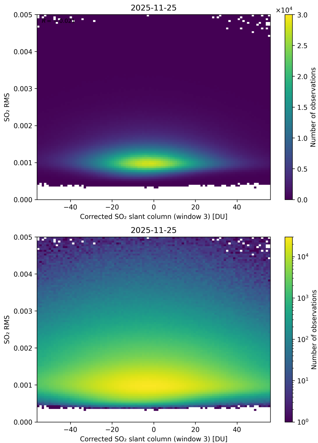
Figure 258: Scatter density plot of “Corrected SO 2 slant column (window 3)” against “SO 2 RMS” for 2025-11-24 to 2025-11-26.
