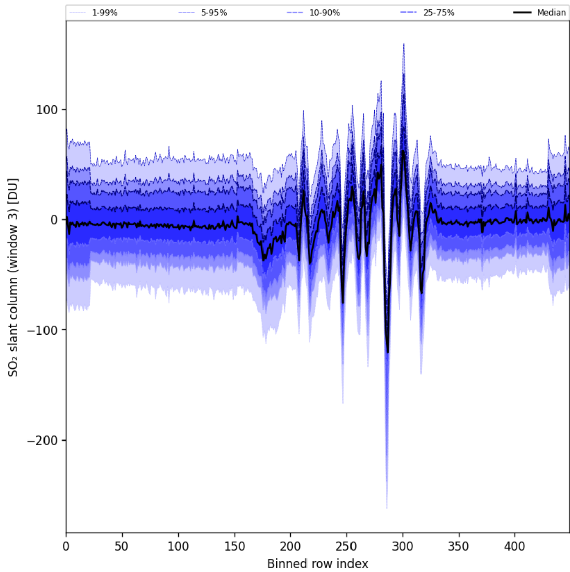
Figure 97: Along track statistics of “SO 2 slant column (window 3)” for 2025-11-24 to 2025-11-26
