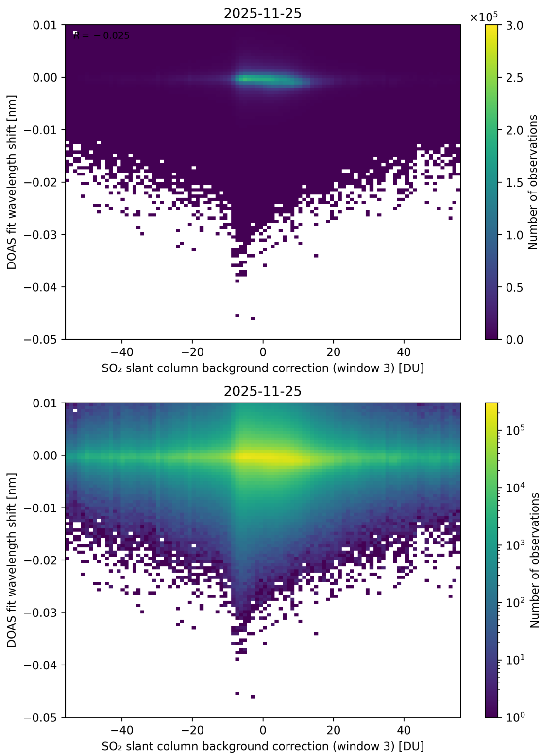
Figure 132: Scatter density plot of “SO 2 slant column background correction (window 3)” against “DOAS fit wavelength shift” for 2025-11-24 to 2025-11-26.
