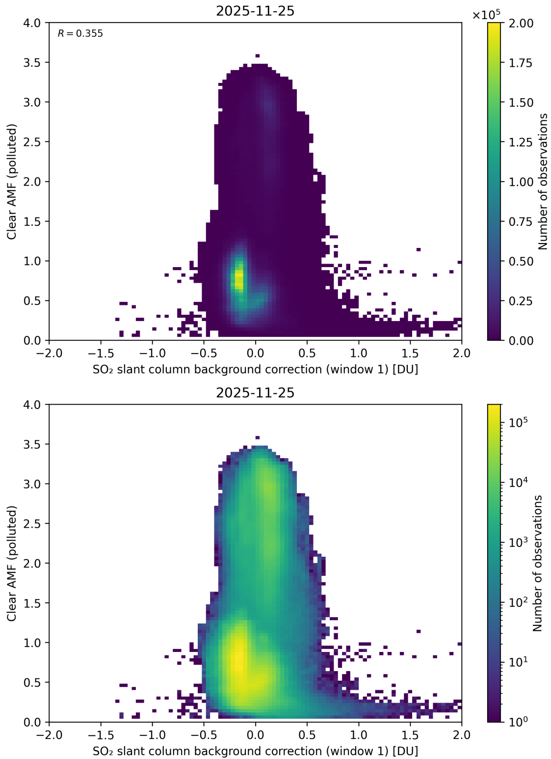
Figure 114: Scatter density plot of “SO 2 slant column background correction (window 1)” against “Clear AMF (polluted)” for 2025-11-24 to 2025-11-26.
