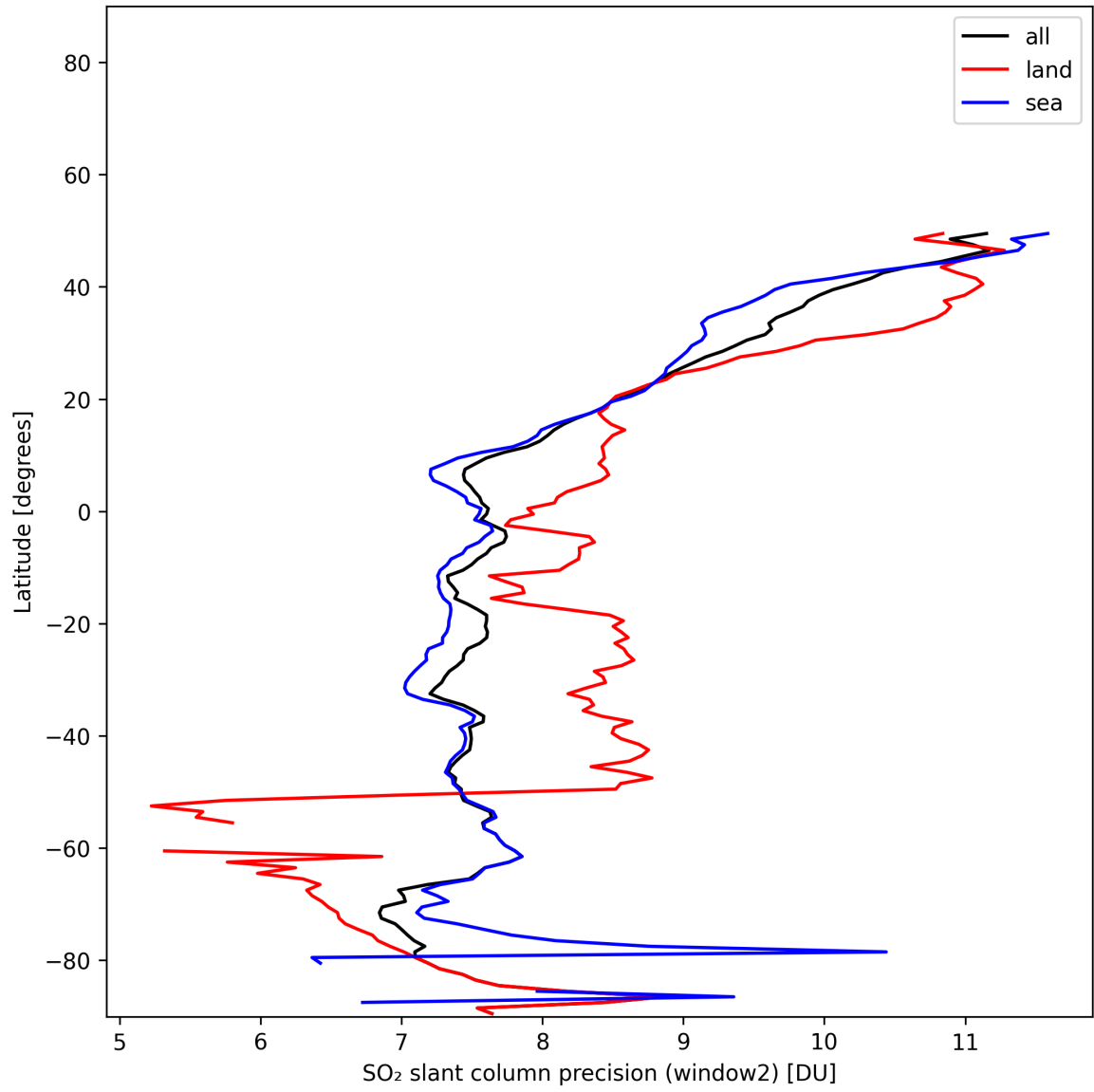
Figure 42: Zonal average of “SO 2 slant column precision (window2)” for 2025-11-24 to 2025-11-26.
