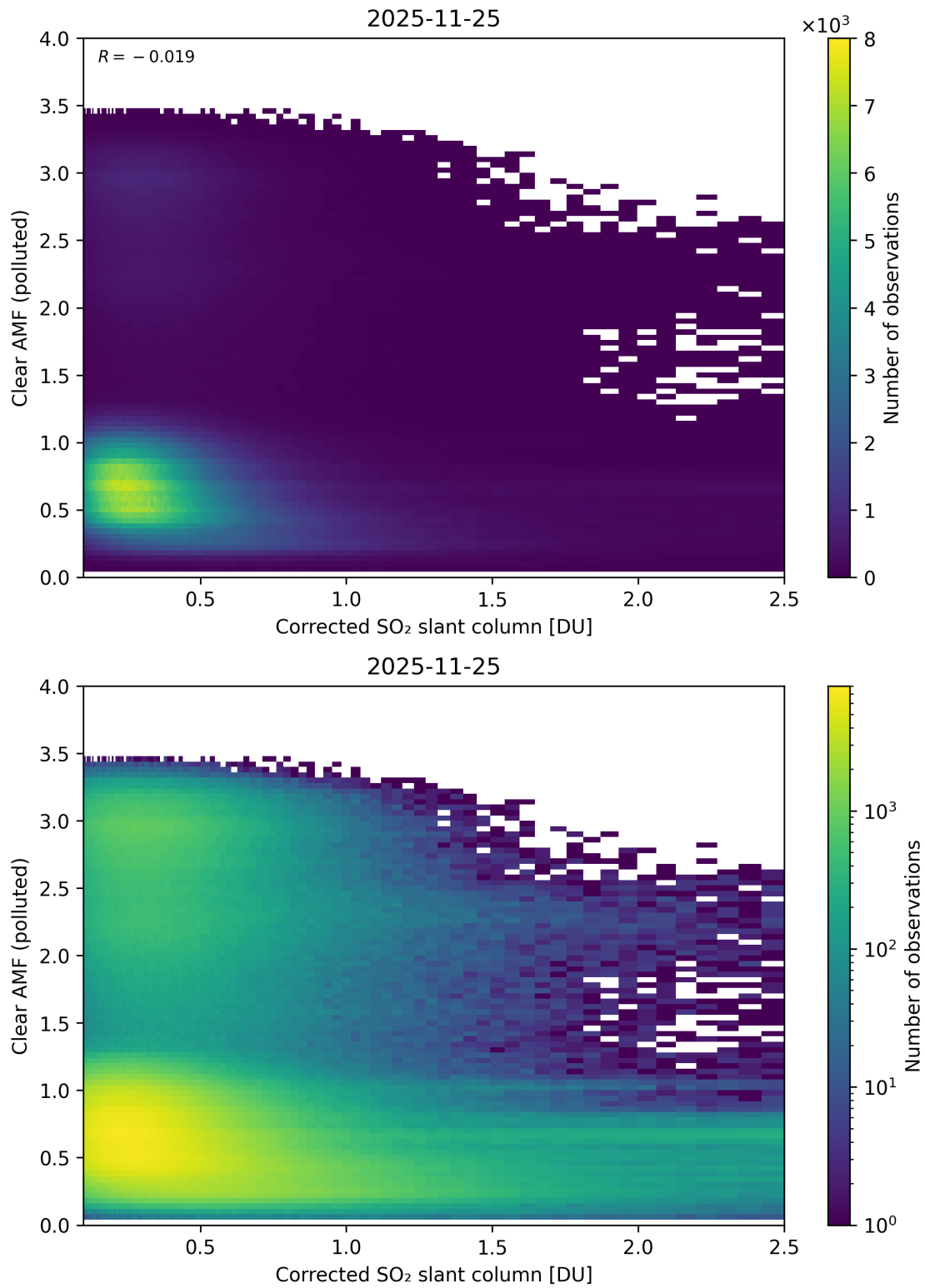
Figure 232: Scatter density plot of “Corrected SO 2 slant column” against “Clear AMF (polluted)” for 2025-11-24 to 2025-11-26.
