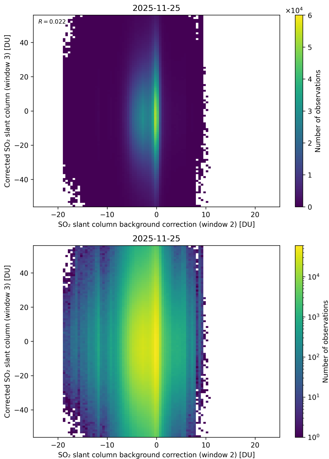
Figure 127: Scatter density plot of “SO 2 slant column background correction (window 2)” against “Corrected SO 2 slant column (window 3)” for 2025-11-24 to 2025-11-26.
