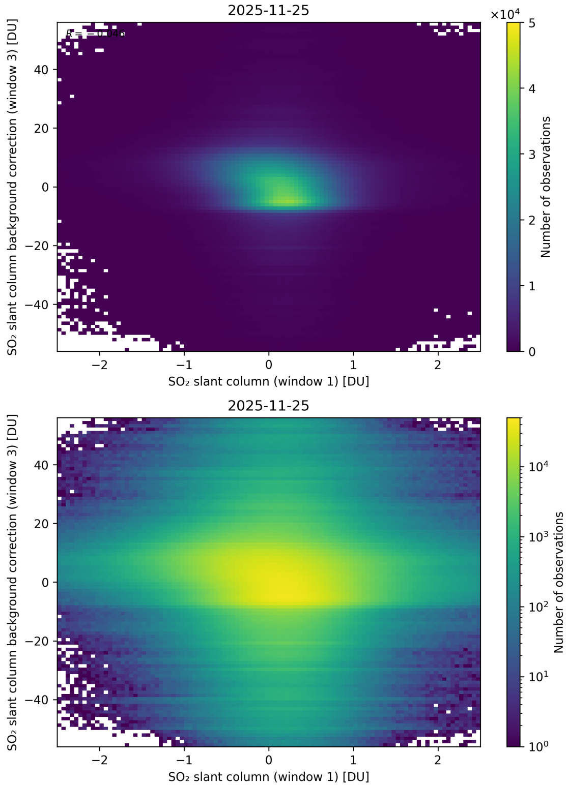
Figure 264: Scatter density plot of “SO 2 slant column (window 1)” against “SO 2 slant column background correction (window 3)” for 2025-11-24 to 2025-11-26.
