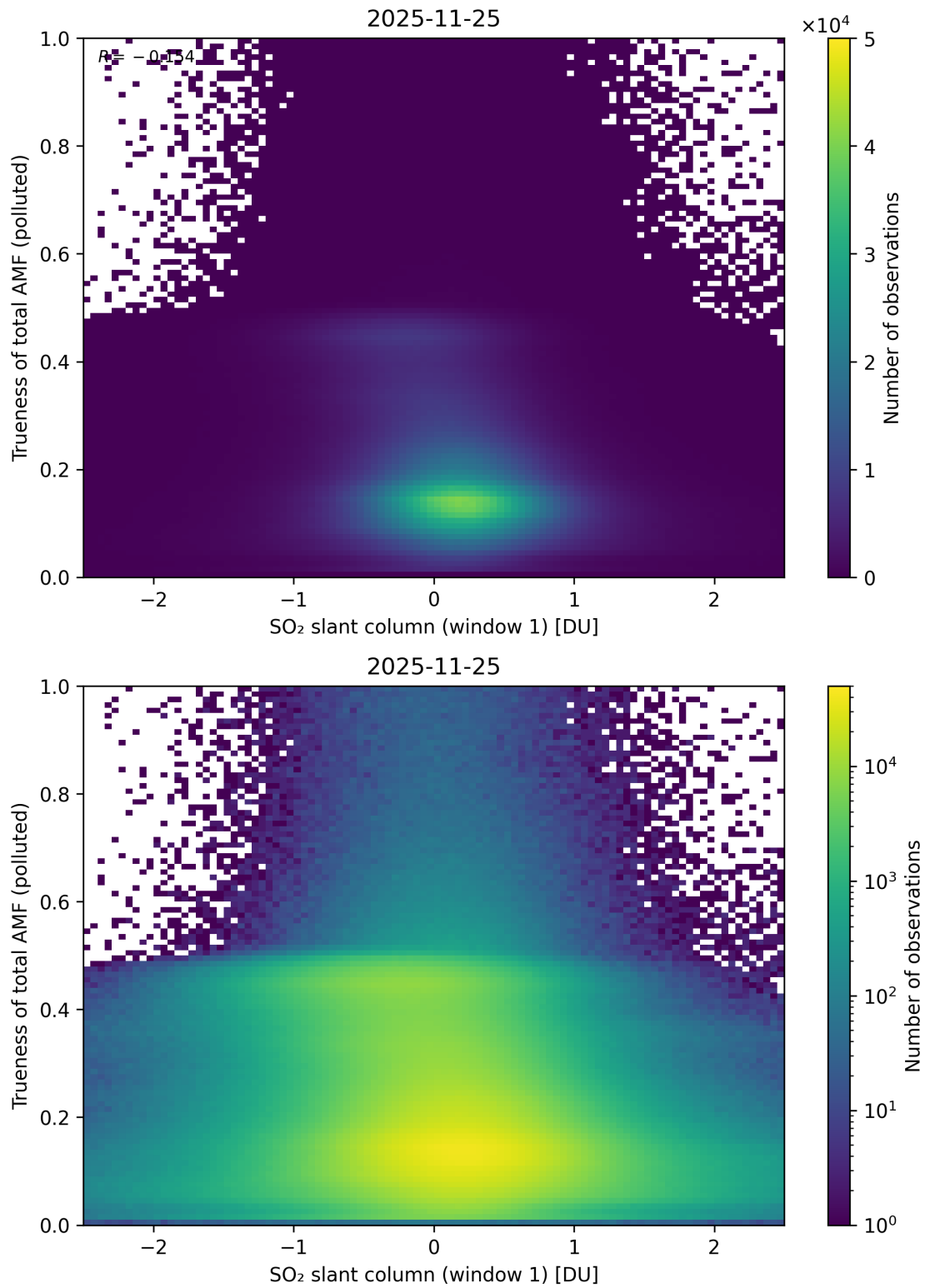
Figure 290: Scatter density plot of “SO 2 slant column (window 1)” against “Trueness of total AMF (polluted)” for 2025-11-24 to 2025-11-26.
