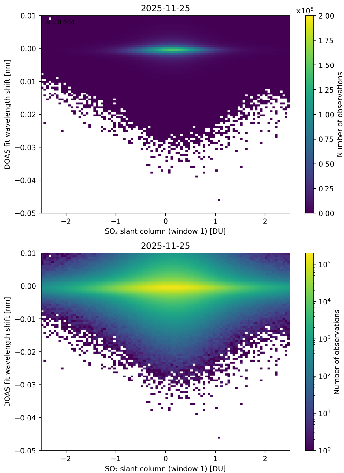
Figure 265: Scatter density plot of “SO 2 slant column (window 1)” against “DOAS fit wavelength shift” for 2025-11-24 to 2025-11-26.
