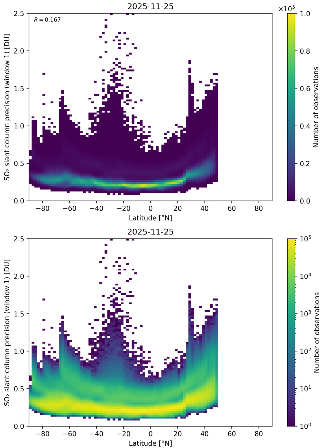
Figure 163: Scatter density plot of “Latitude” against “SO 2 slant column precision (window 1)” for 2025-11-24 to 2025-11-26.
