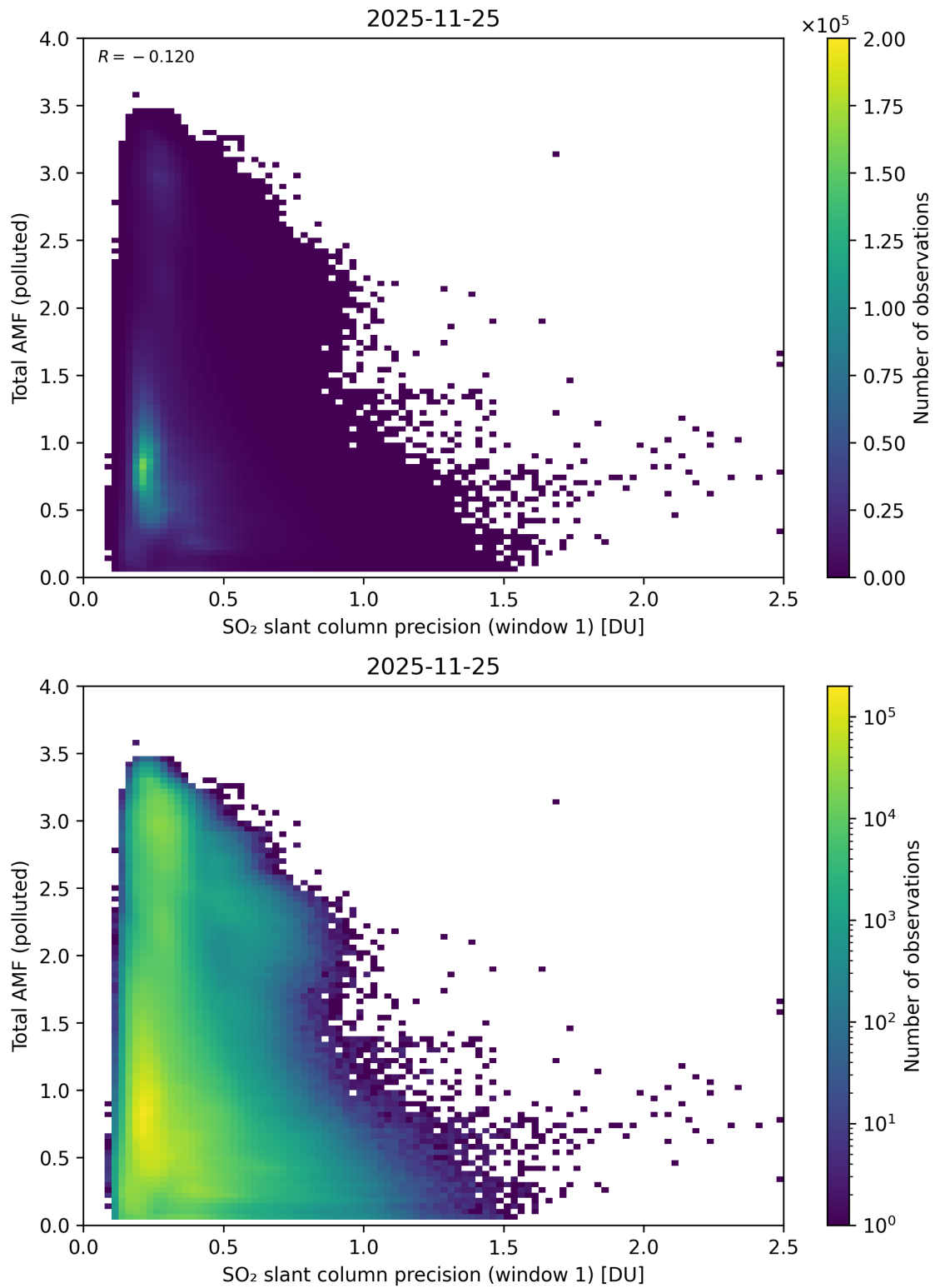
Figure 280: Scatter density plot of “SO 2 slant column precision (window 1)” against “Total AMF (polluted)” for 2025-11-24 to 2025-11-26.
