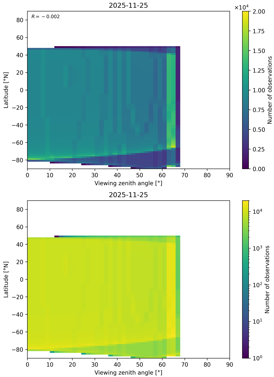
Figure 368: Scatter density plot of “Viewing zenith angle” against “Latitude” for 2025-11-24 to 2025-11-26.
