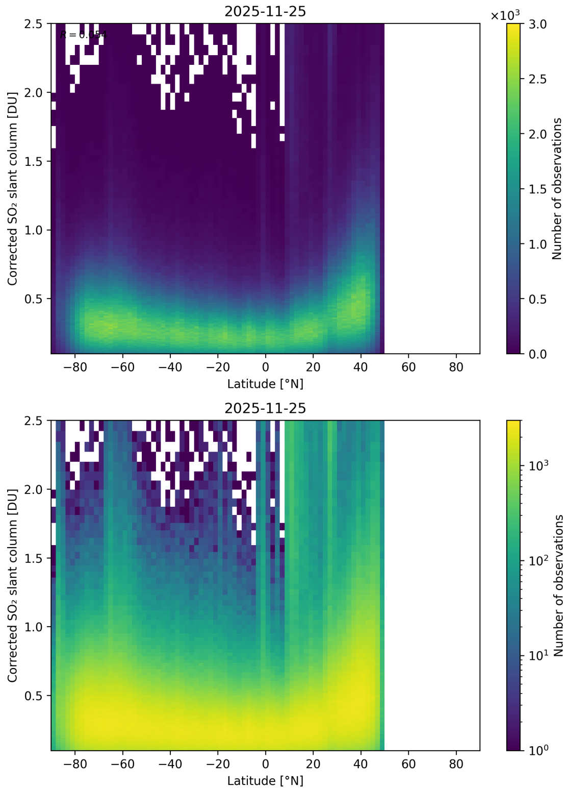
Figure 159: Scatter density plot of “Latitude” against “Corrected SO 2 slant column” for 2025-11-24 to 2025-11-26.
