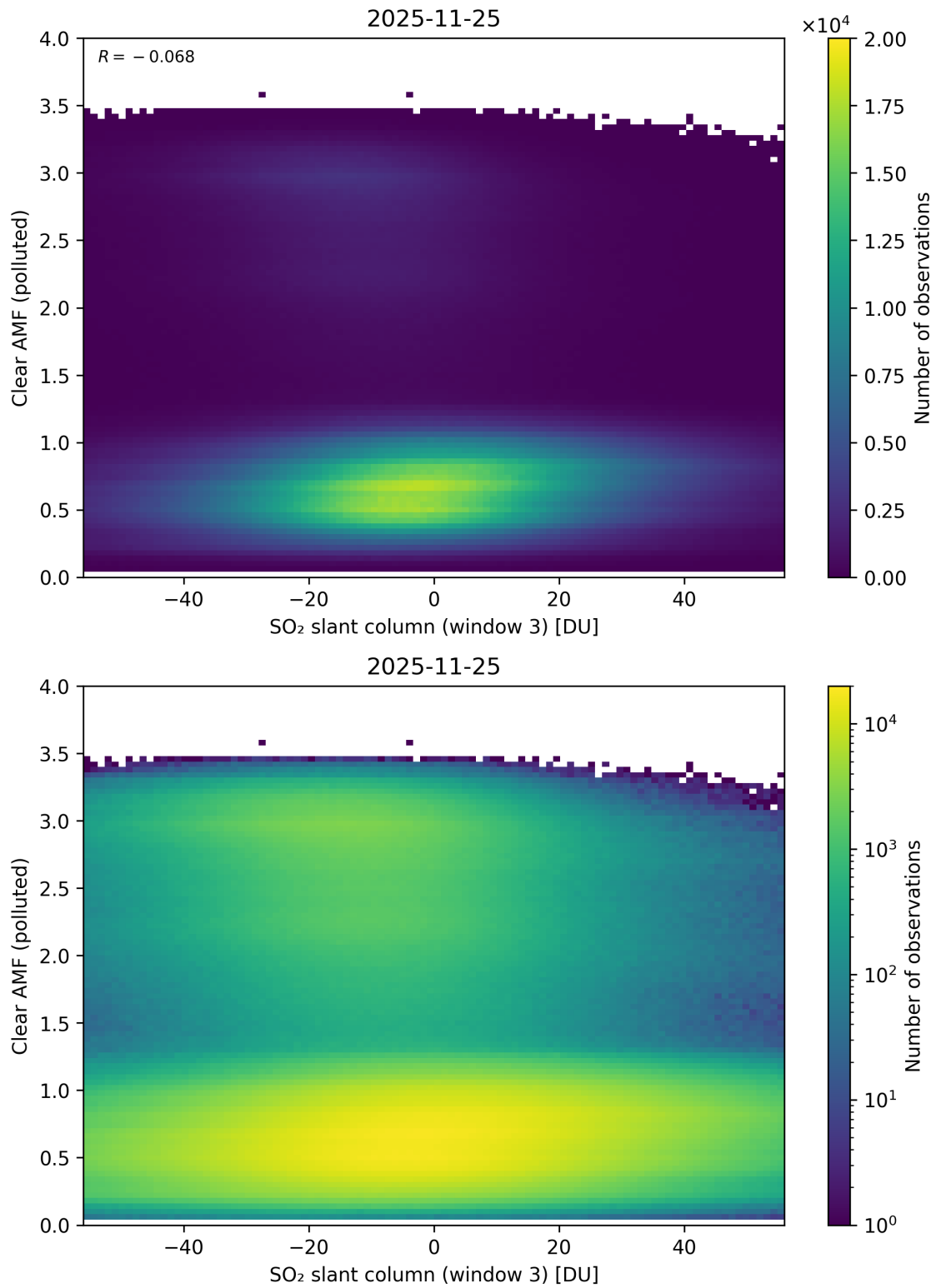
Figure 315: Scatter density plot of “SO 2 slant column (window 3)” against “Clear AMF (polluted)” for 2025-11-24 to 2025-11-26.
