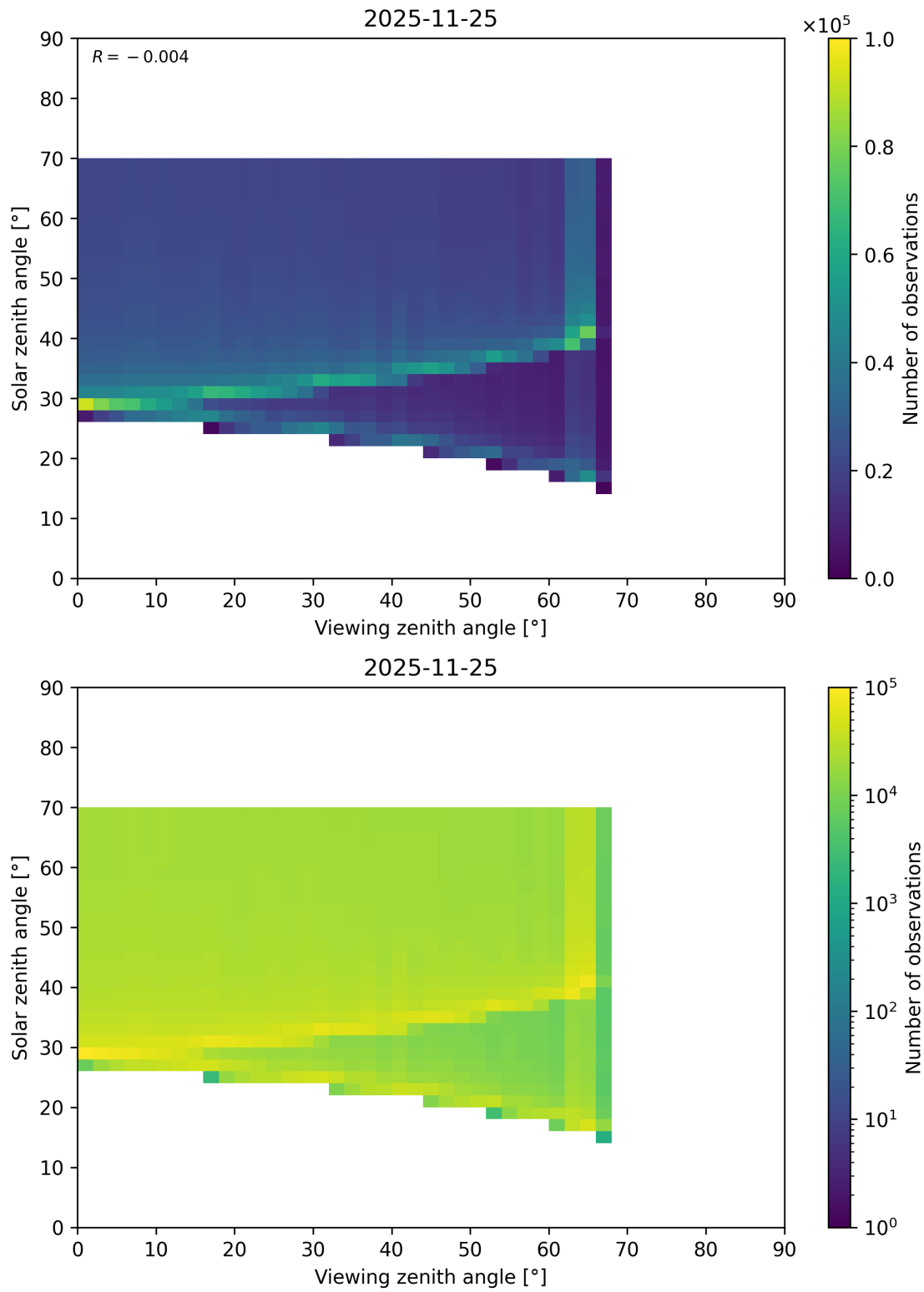
Figure 369: Scatter density plot of “Viewing zenith angle” against “Solar zenith angle” for 2025-11-24 to 2025-11-26.
