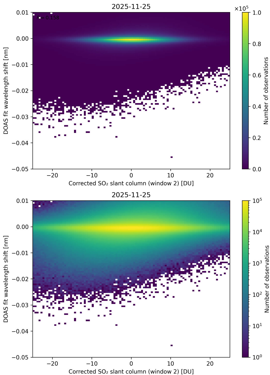
Figure 246: Scatter density plot of “Corrected SO 2 slant column (window 2)” against “DOAS fit wavelength shift” for 2025-11-24 to 2025-11-26.
