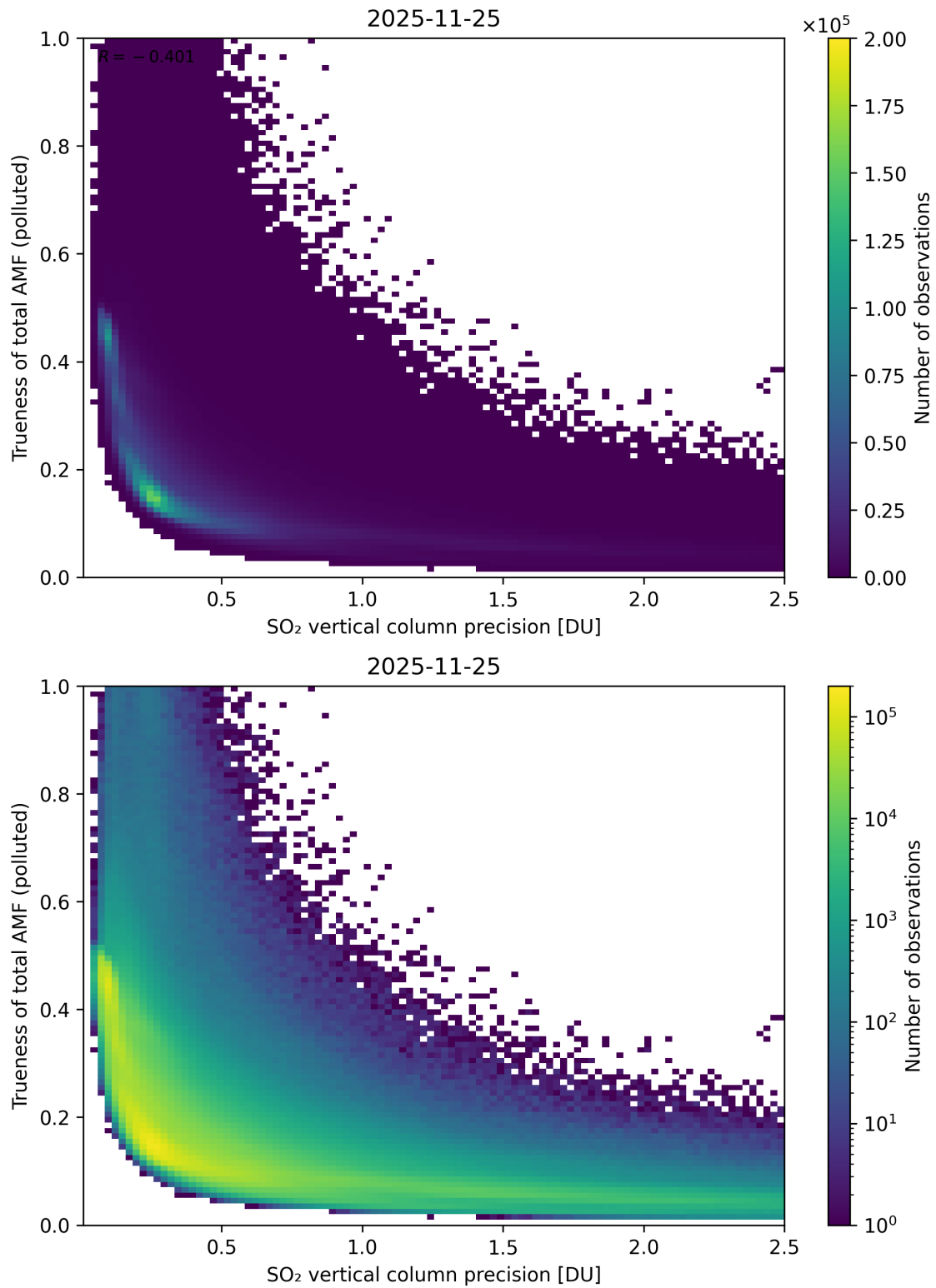
Figure 347: Scatter density plot of “SO 2 vertical column precision” against “Trueness of total AMF (polluted)” for 2025-11-24 to 2025-11-26.
