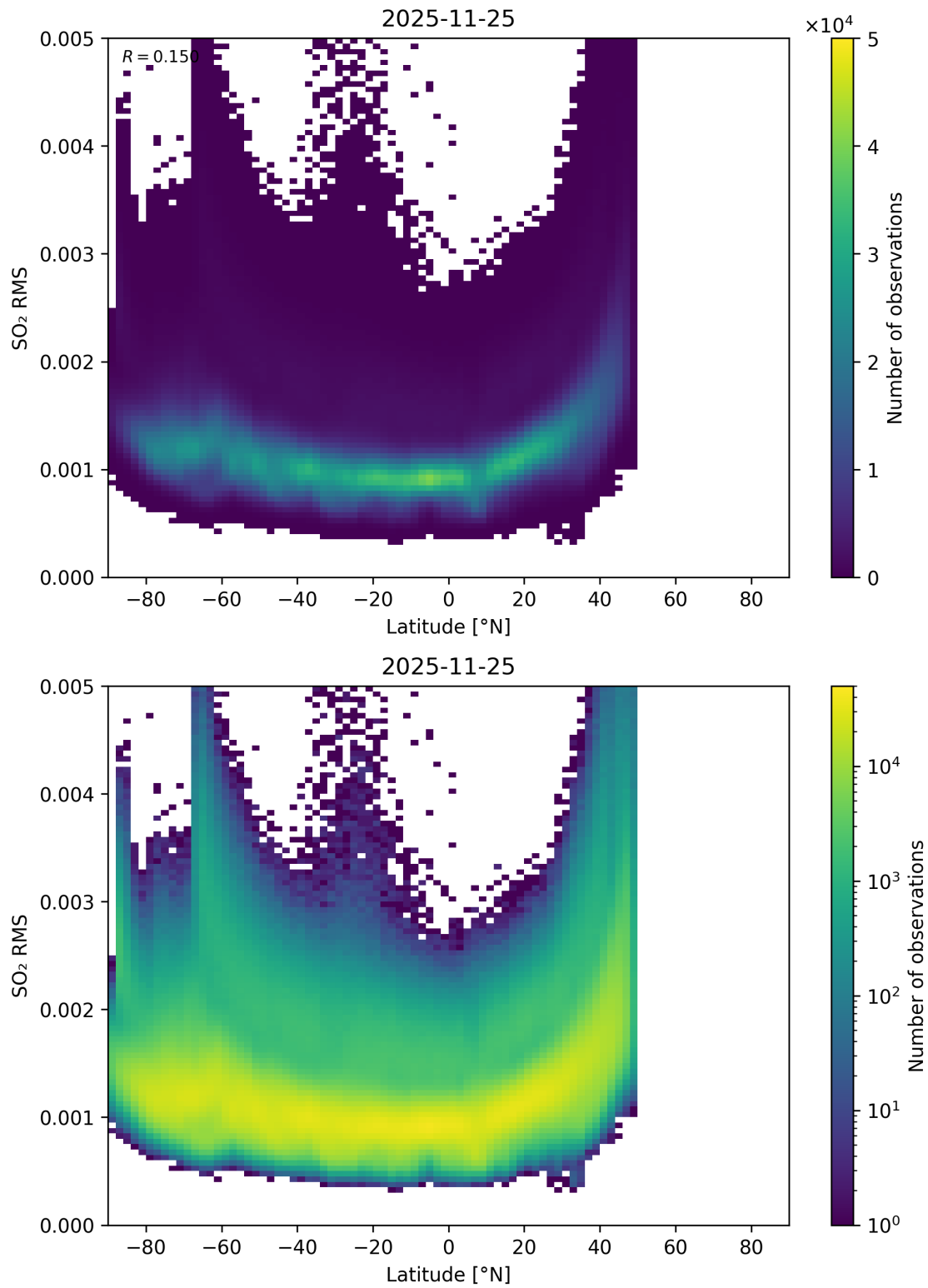
Figure 155: Scatter density plot of “Latitude” against “SO 2 RMS” for 2025-11-24 to 2025-11-26.
