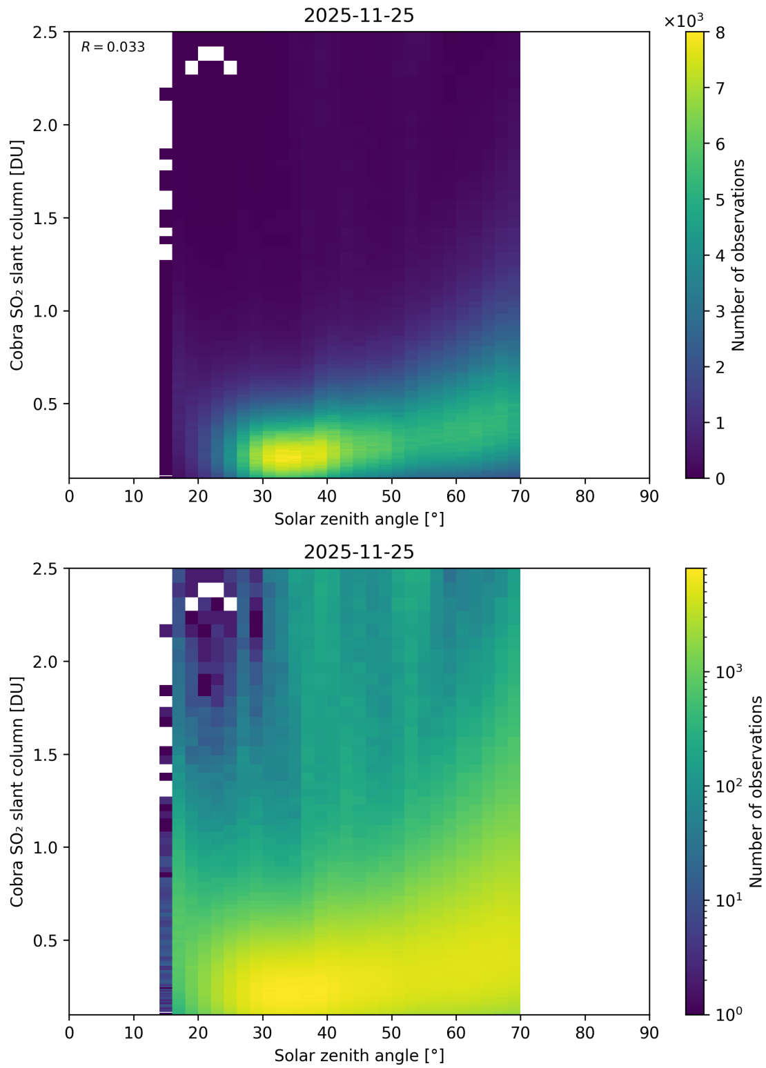
Figure 179: Scatter density plot of “Solar zenith angle” against “Cobra SO 2 slant column” for 2025-11-24 to 2025-11-26.
