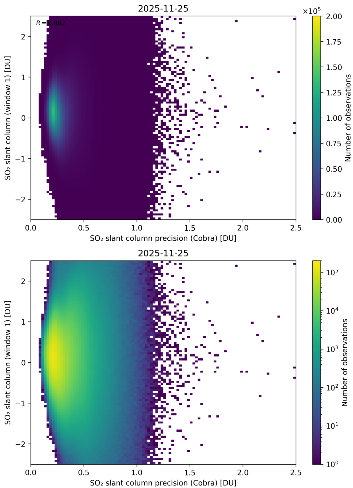
Figure 208: Scatter density plot of “SO 2 slant column precision (Cobra)” against “SO 2 slant column (window 1)” for 2025-11-24 to 2025-11-26.
