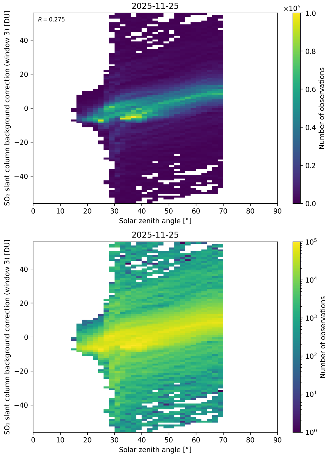
Figure 173: Scatter density plot of “Solar zenith angle” against “SO 2 slant column background correction (window 3)” for 2025-11-24 to 2025-11-26.
