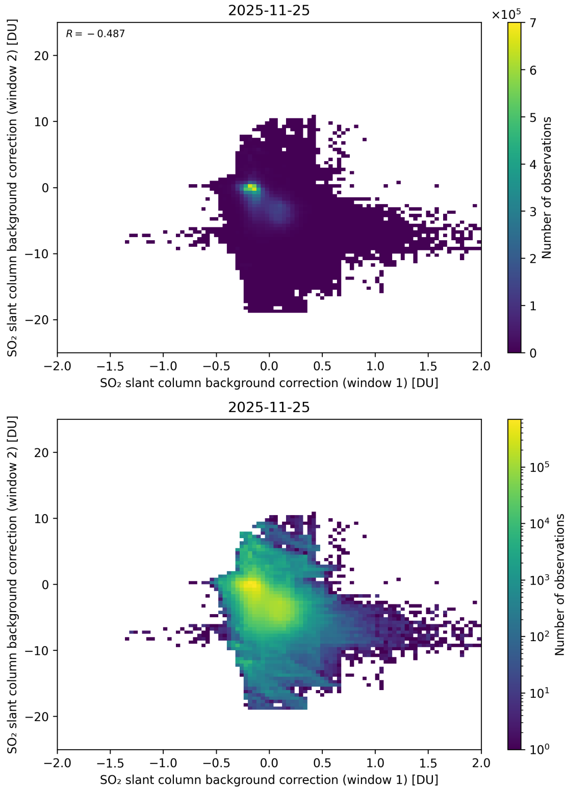
Figure 109: Scatter density plot of “SO 2 slant column background correction (window 1)” against “SO 2 slant column background correction (window 2)” for 2025-11-24 to 2025-11-26.
