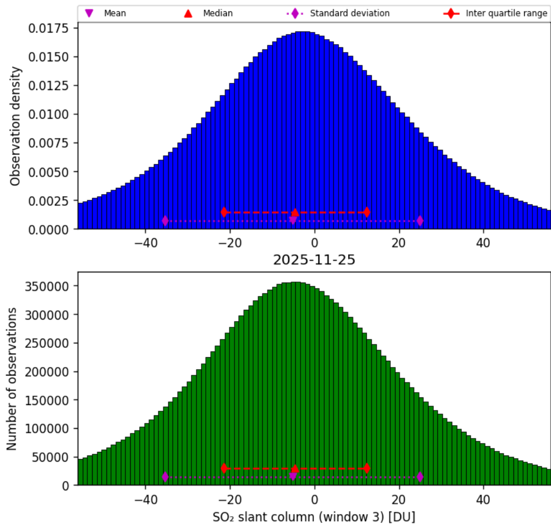
Figure 71: Histogram of “SO 2 slant column (window 3)” for 2025-11-24 to 2025-11-26
