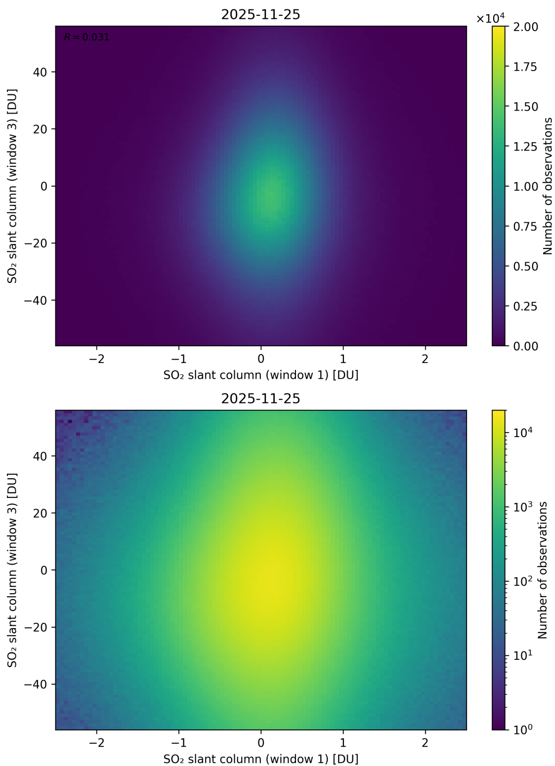
Figure 287: Scatter density plot of “SO 2 slant column (window 1)” against “SO 2 slant column (window 3)” for 2025-11-24 to 2025-11-26.
