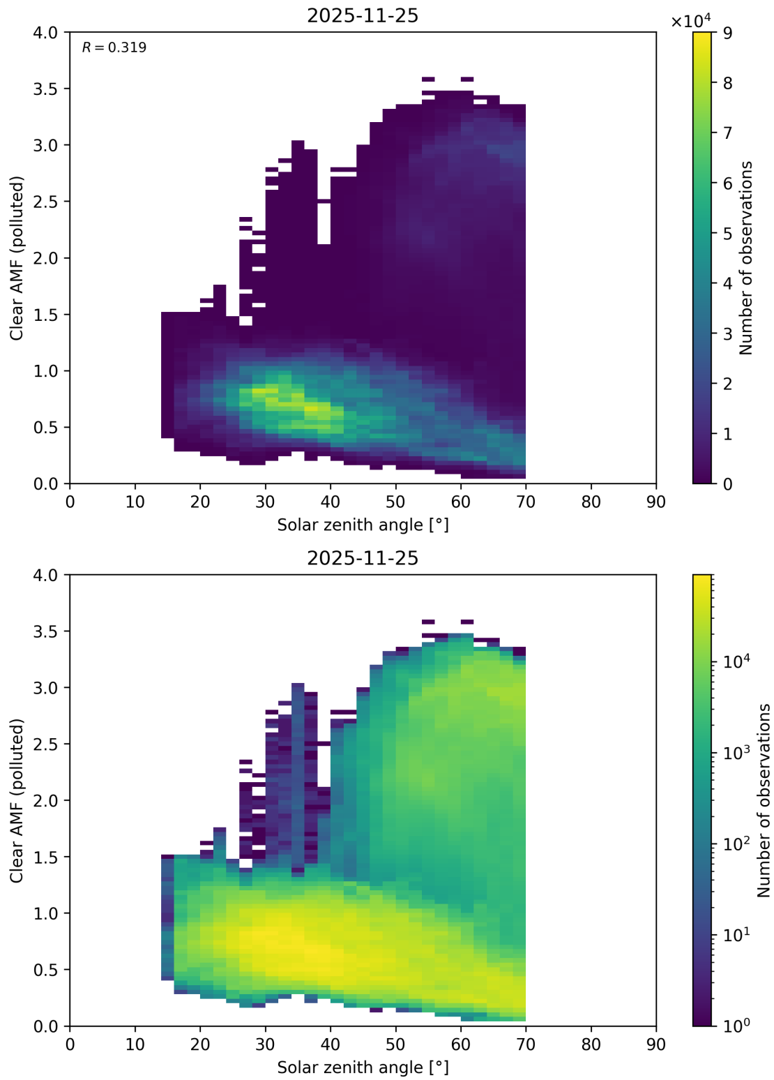
Figure 178: Scatter density plot of “Solar zenith angle” against “Clear AMF (polluted)” for 2025-11-24 to 2025-11-26.
