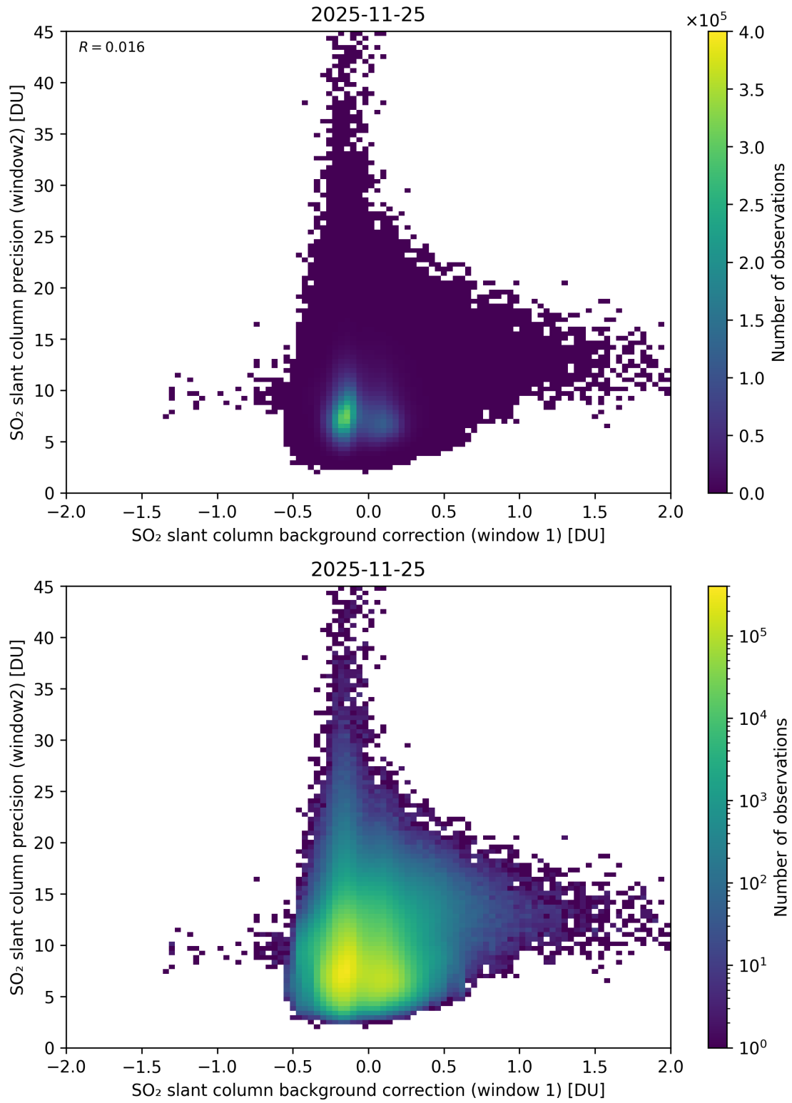
Figure 117: Scatter density plot of “SO 2 slant column background correction (window 1)” against “SO 2 slant column precision (window2)” for 2025-11-24 to 2025-11-26.
