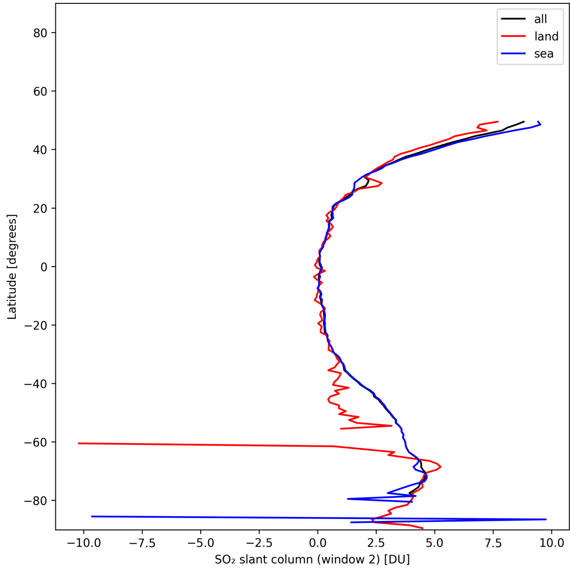
Figure 41: Zonal average of “SO 2 slant column (window 2)” for 2025-11-24 to 2025-11-26.
