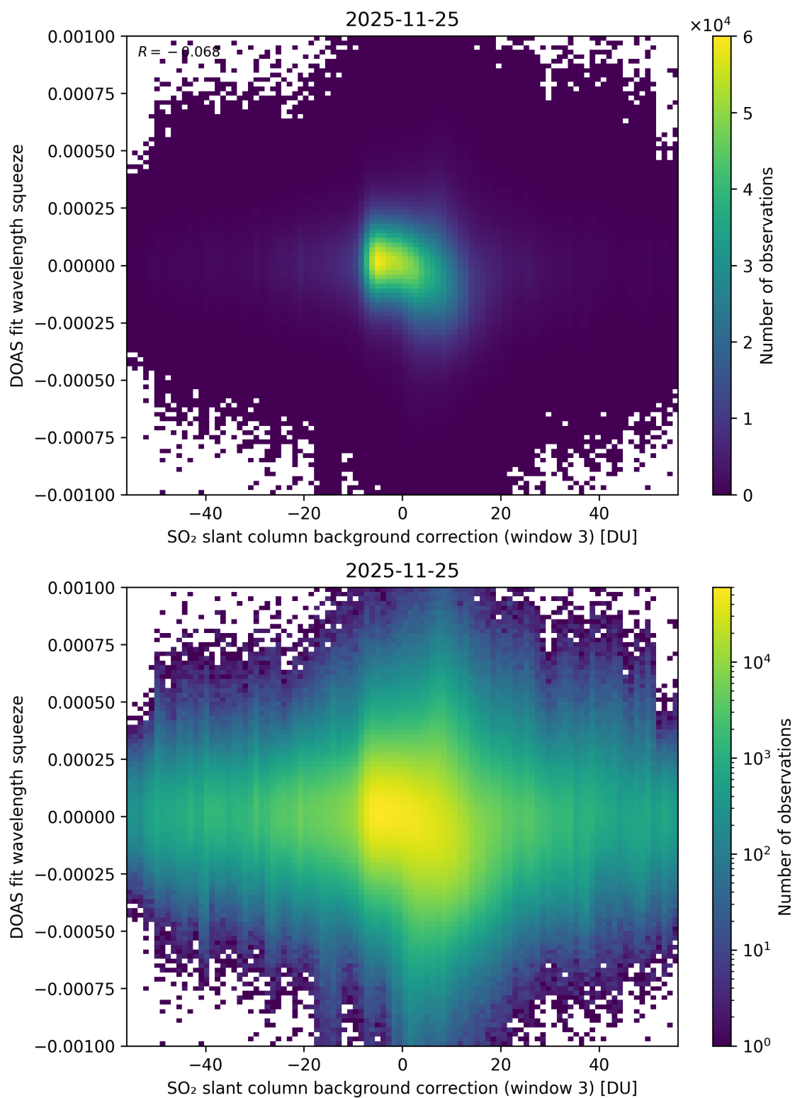
Figure 133: Scatter density plot of “SO 2 slant column background correction (window 3)” against “DOAS fit wavelength squeeze” for 2025-11-24 to 2025-11-26.
