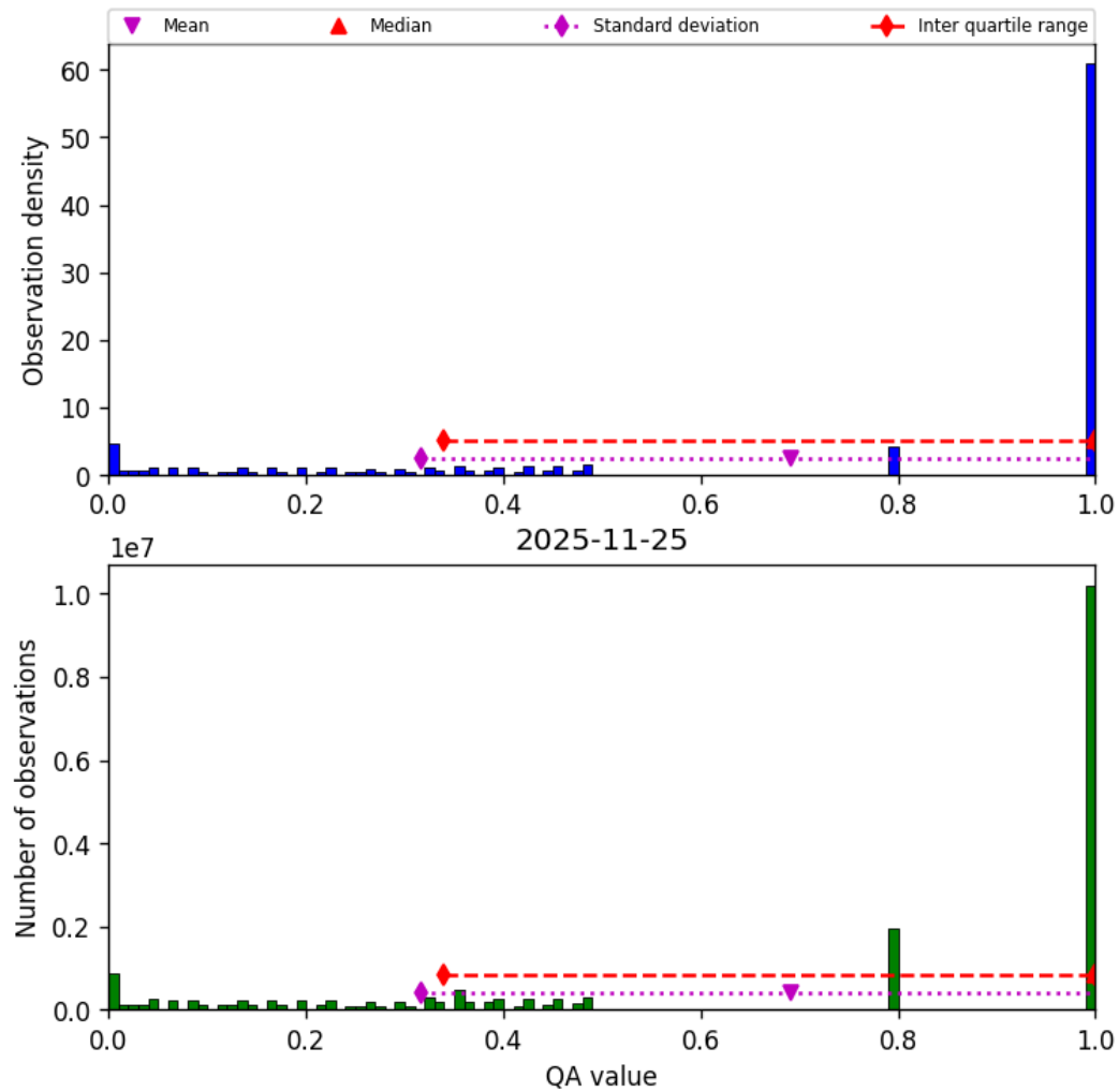
Figure 57: Histogram of “QA value” for 2025-11-24 to 2025-11-26
