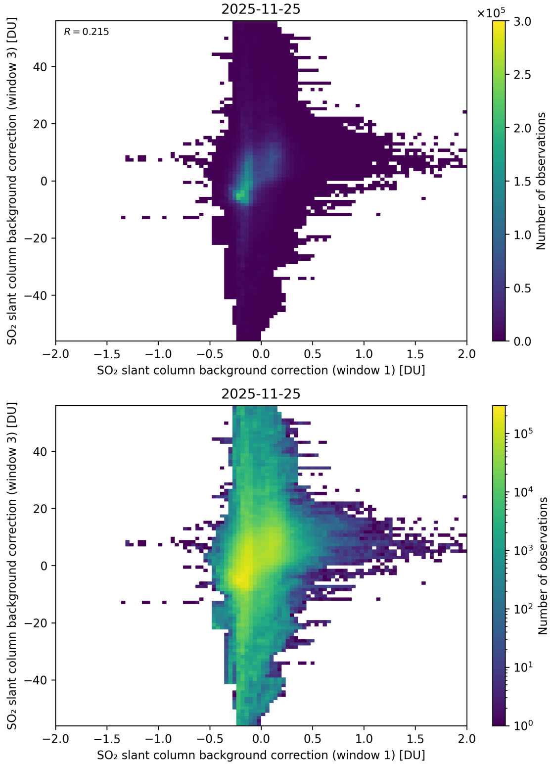
Figure 110: Scatter density plot of “SO 2 slant column background correction (window 1)” against “SO 2 slant column background correction (window 3)” for 2025-11-24 to 2025-11-26.
