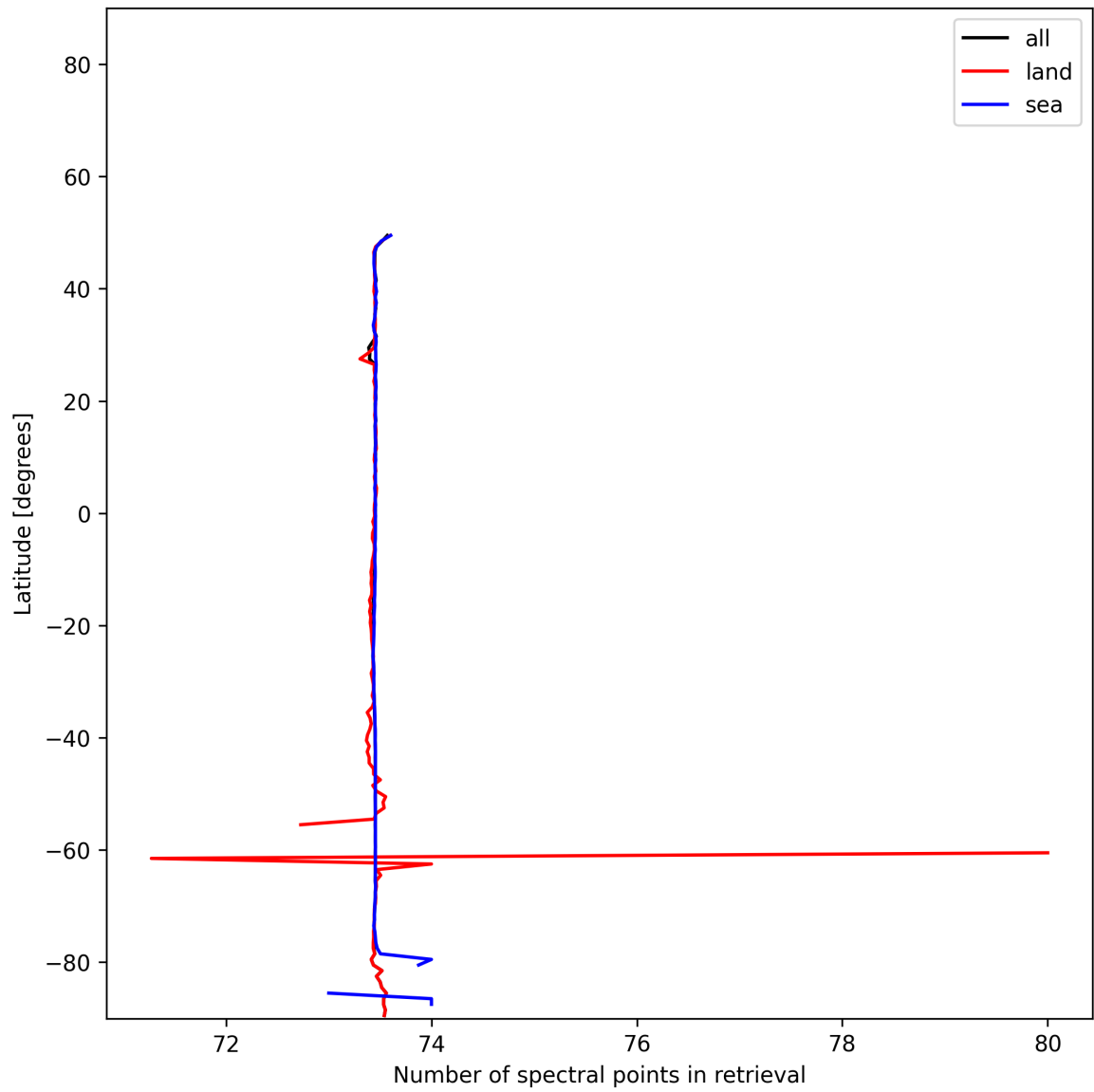
Figure 56: Zonal average of “Number of spectral points in retrieval” for 2025-11-24 to 2025-11-26.
