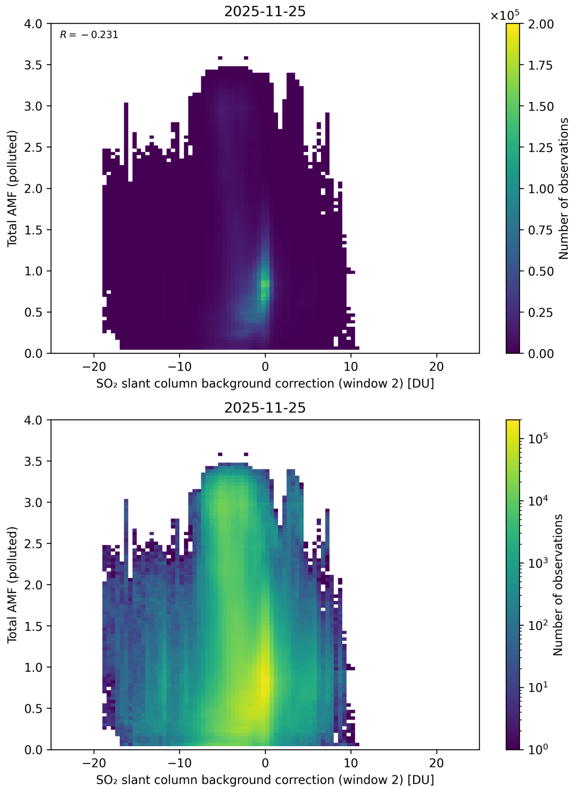
Figure 130: Scatter density plot of “SO 2 slant column background correction (window 2)” against “Total AMF (polluted)” for 2025-11-24 to 2025-11-26.
