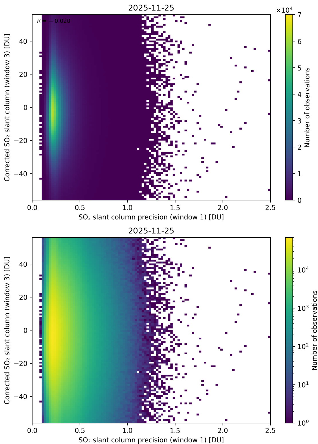
Figure 276: Scatter density plot of “SO 2 slant column precision (window 1)” against “Corrected SO 2 slant column (window 3)” for 2025-11-24 to 2025-11-26.
