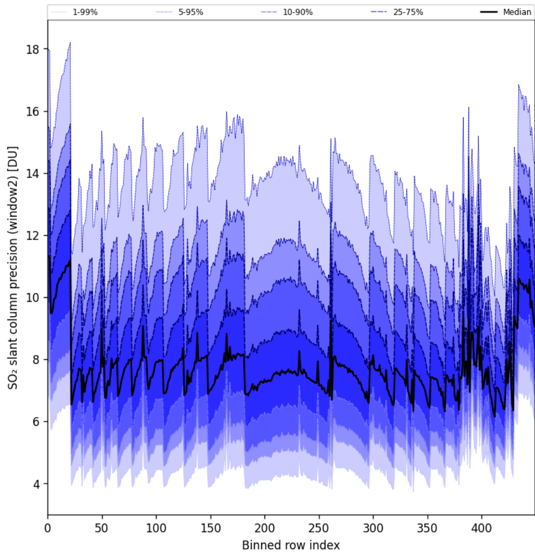
Figure 94: Along track statistics of “SO 2 slant column precision (window2)” for 2025-11-24 to 2025-11-26
