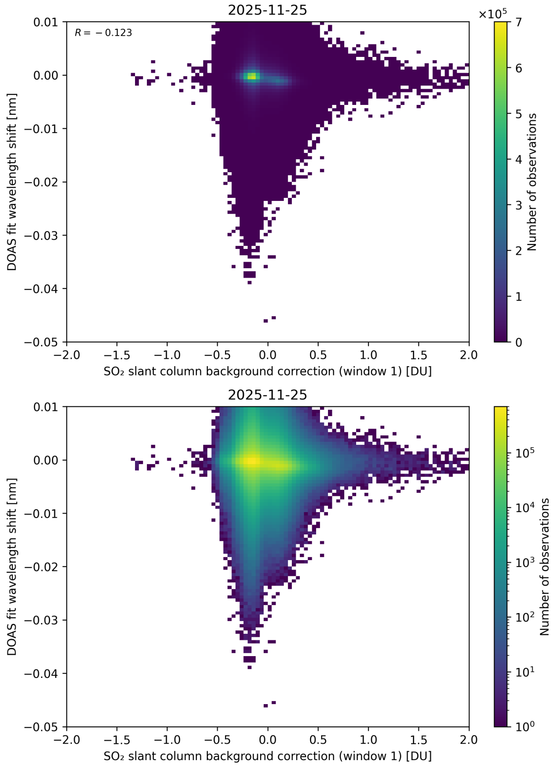
Figure 111: Scatter density plot of “SO 2 slant column background correction (window 1)” against “DOAS fit wavelength shift” for 2025-11-24 to 2025-11-26.
