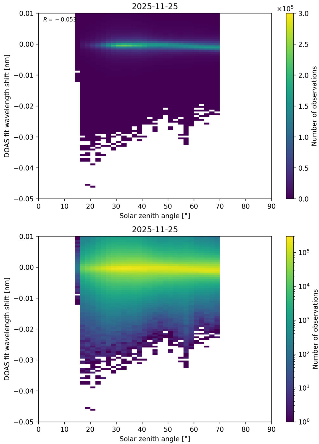
Figure 174: Scatter density plot of “Solar zenith angle” against “DOAS fit wavelength shift” for 2025-11-24 to 2025-11-26.
