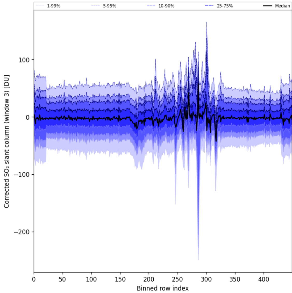
Figure 99: Along track statistics of "Corrected SO 2 slant column (window 3)" for 2025-11-24 to 2025-11-26
