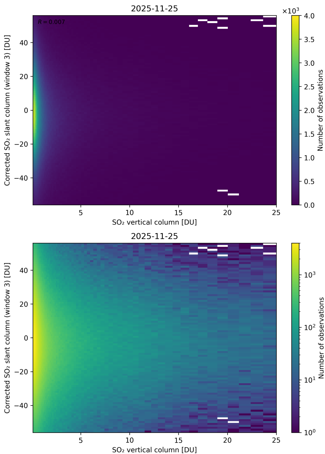
Figure 353: Scatter density plot of “SO 2 vertical column” against “Corrected SO 2 slant column (window 3)” for 2025-11-24 to 2025-11-26.
