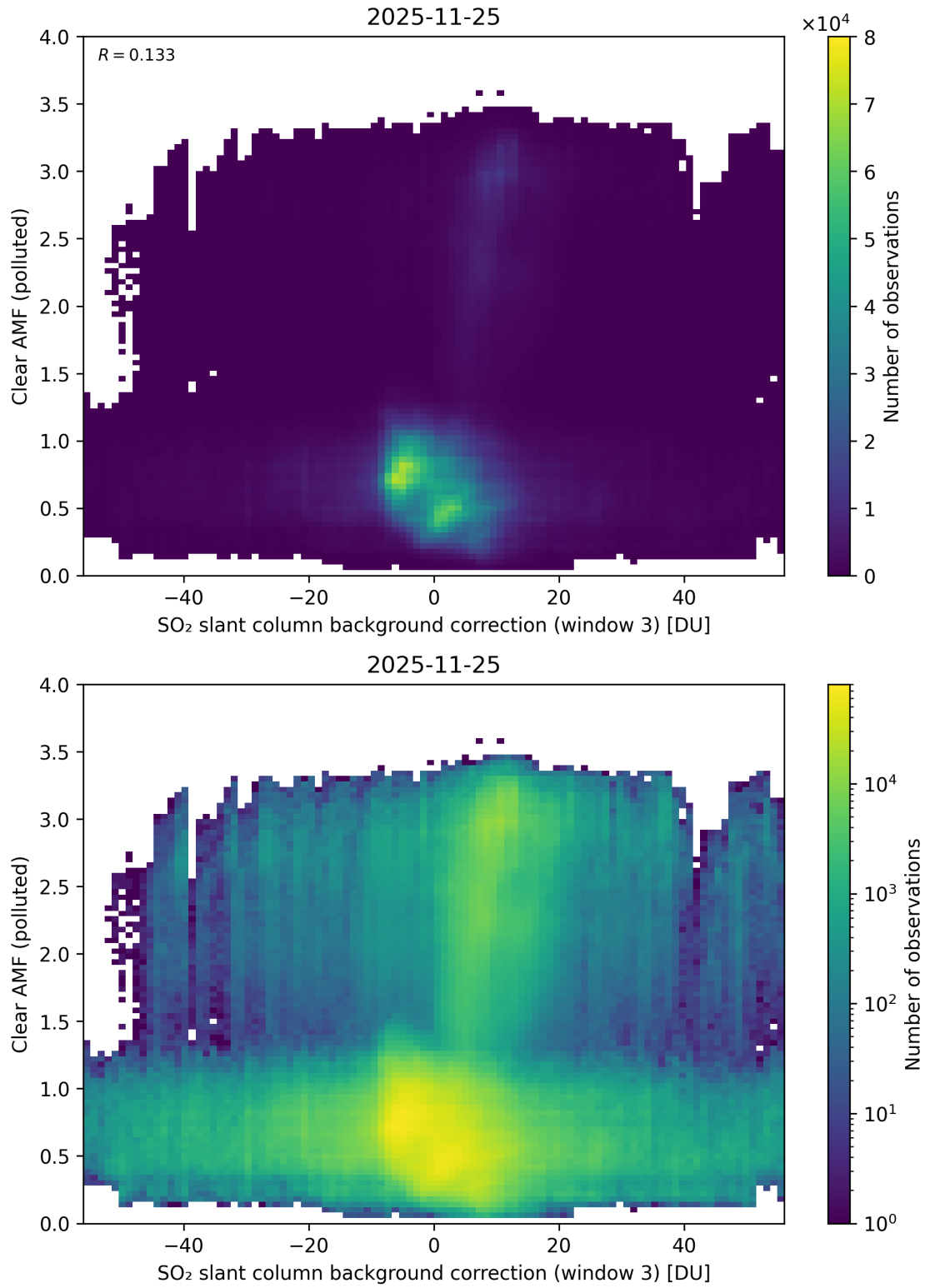
Figure 135: Scatter density plot of “SO 2 slant column background correction (window 3)” against “Clear AMF (polluted)” for 2025-11-24 to 2025-11-26.
