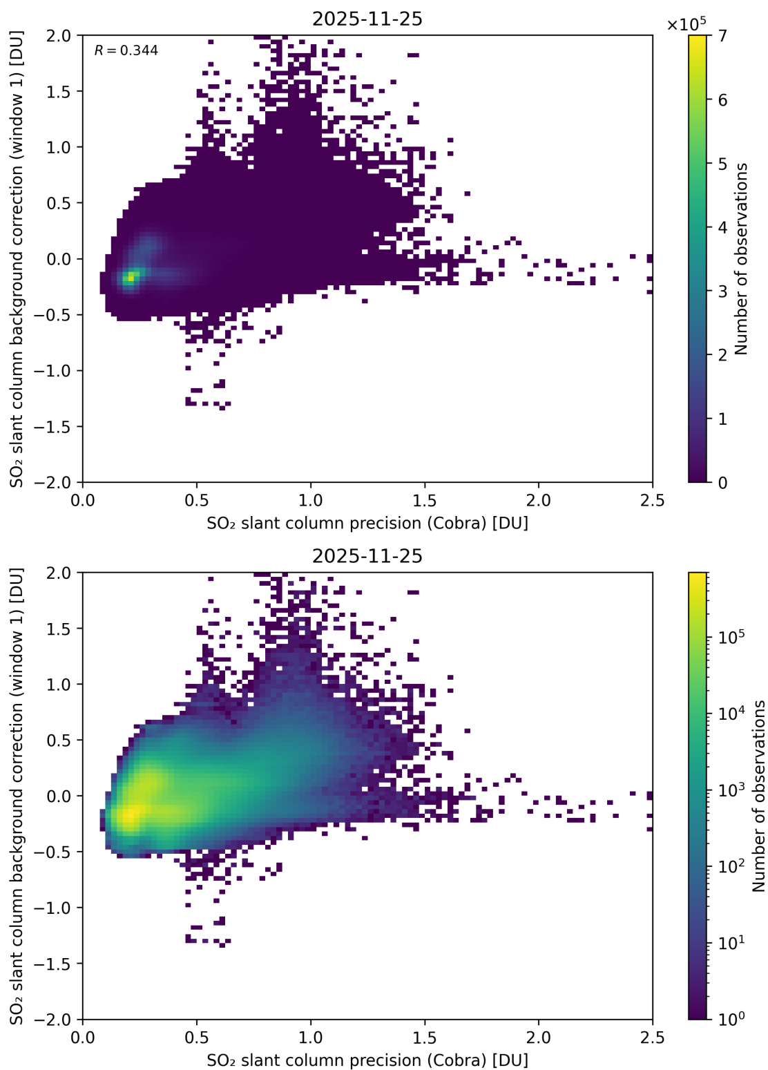
Figure 199: Scatter density plot of “SO 2 slant column precision (Cobra)” against “SO 2 slant column background correction (window 1)” for 2025-11-24 to 2025-11-26.
