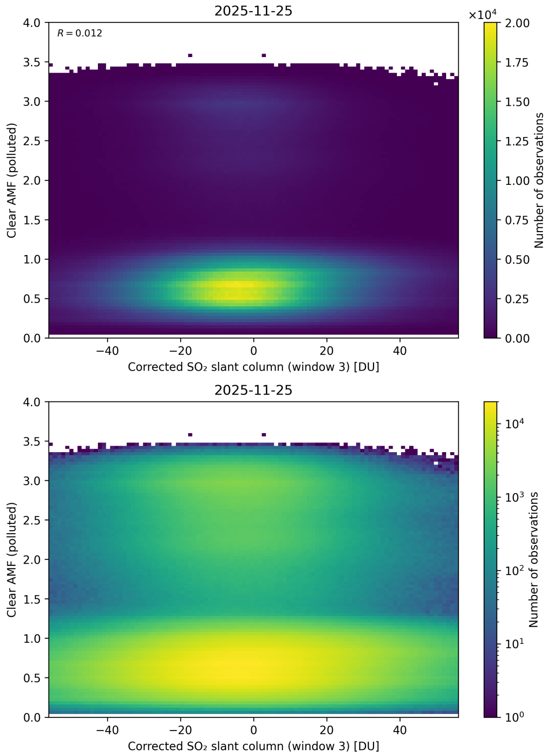
Figure 259: Scatter density plot of “Corrected SO 2 slant column (window 3)” against “Clear AMF (polluted)” for 2025-11-24 to 2025-11-26.
