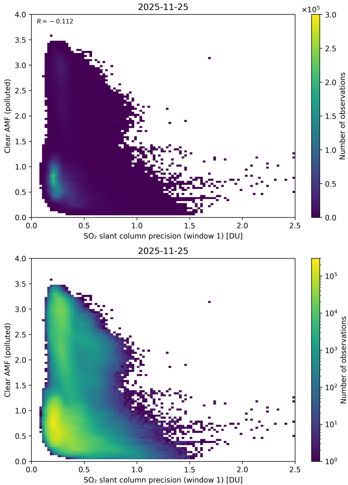
Figure 274: Scatter density plot of “SO 2 slant column precision (window 1)” against “Clear AMF (polluted)” for 2025-11-24 to 2025-11-26.
