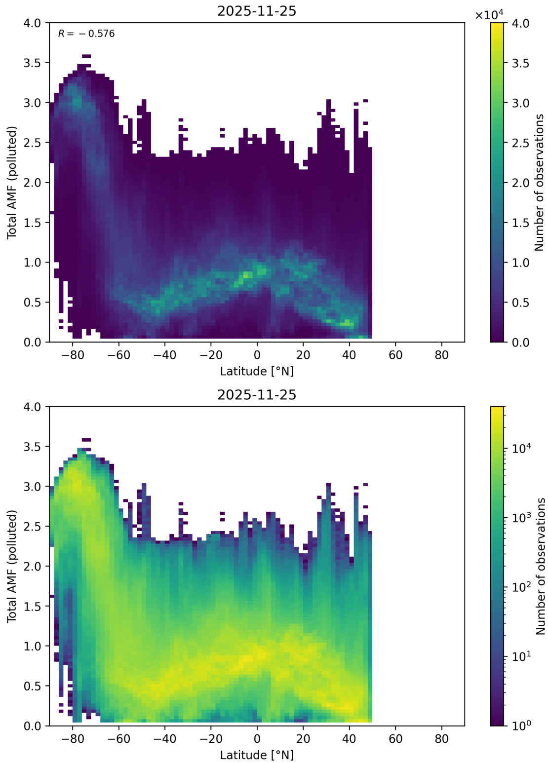
Figure 167: Scatter density plot of “Latitude” against “Total AMF (polluted)” for 2025-11-24 to 2025-11-26.
