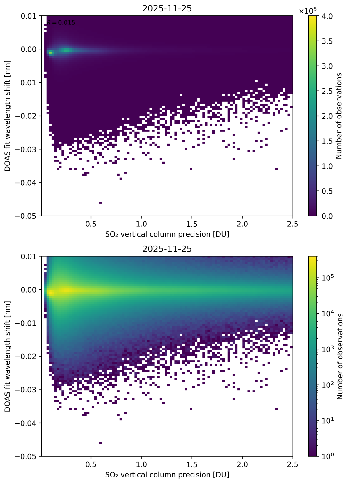
Figure 332: Scatter density plot of “SO 2 vertical column precision” against “DOAS fit wavelength shift” for 2025-11-24 to 2025-11-26.
