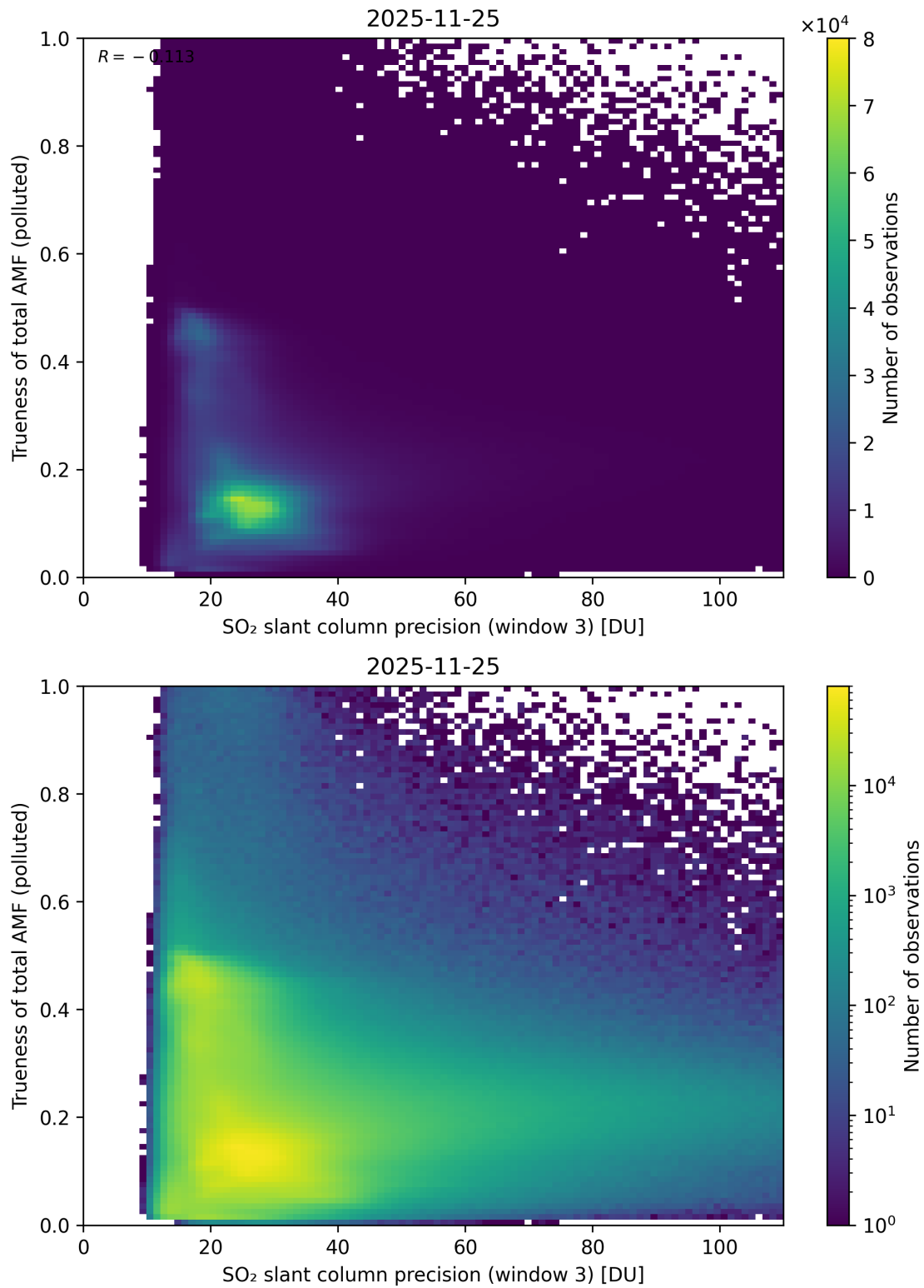
Figure 314: Scatter density plot of “SO 2 slant column precision (window 3)” against “Trueness of total AMF (polluted)” for 2025-11-24 to 2025-11-26.
