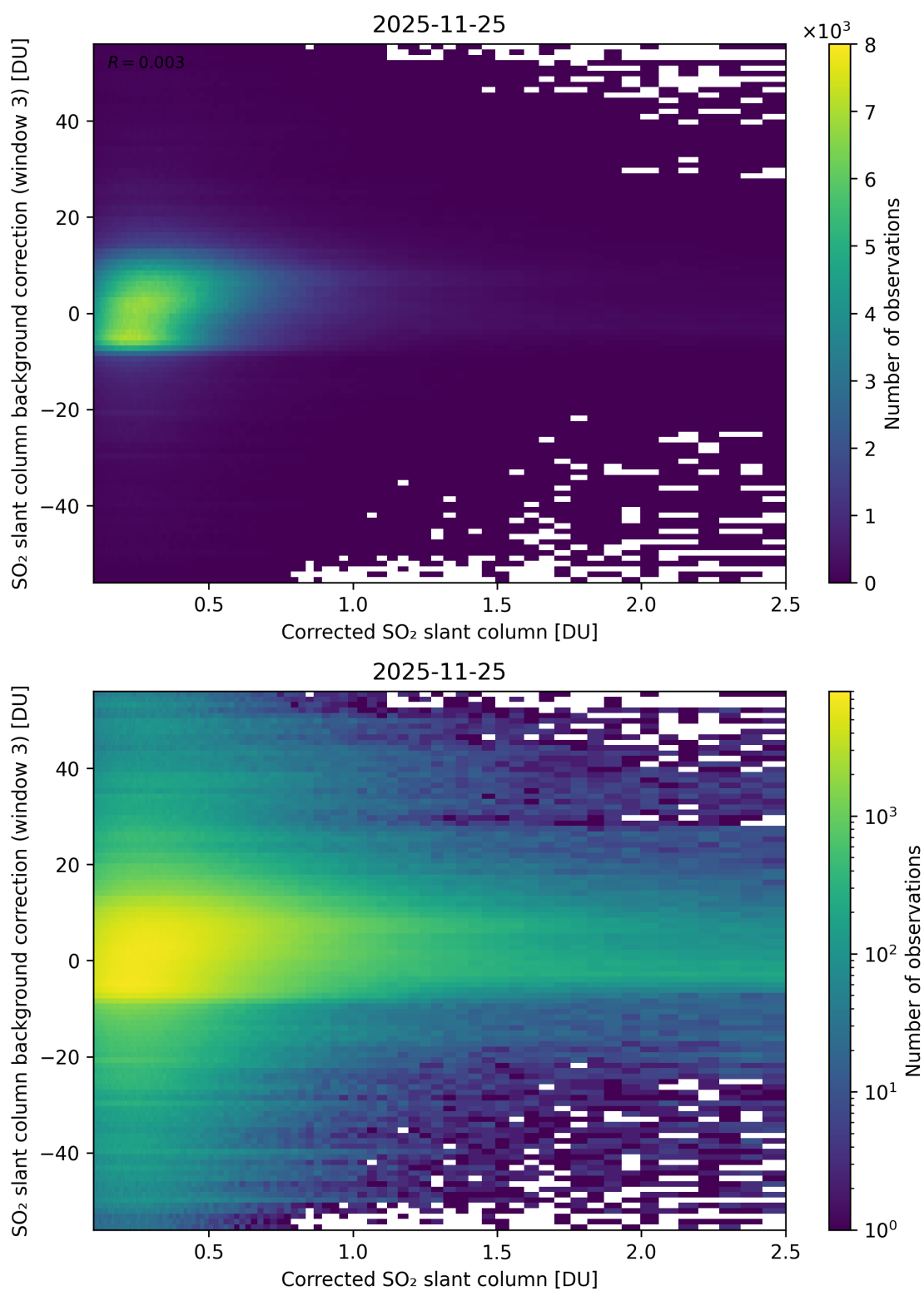
Figure 228: Scatter density plot of “Corrected SO 2 slant column” against “SO 2 slant column background correction (window 3)” for 2025-11-24 to 2025-11-26.
