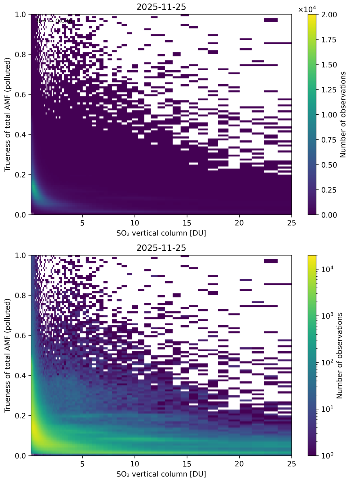
Figure 360: Scatter density plot of “SO 2 vertical column” against “Trueness of total AMF (polluted)” for 2025-11-24 to 2025-11-26.
