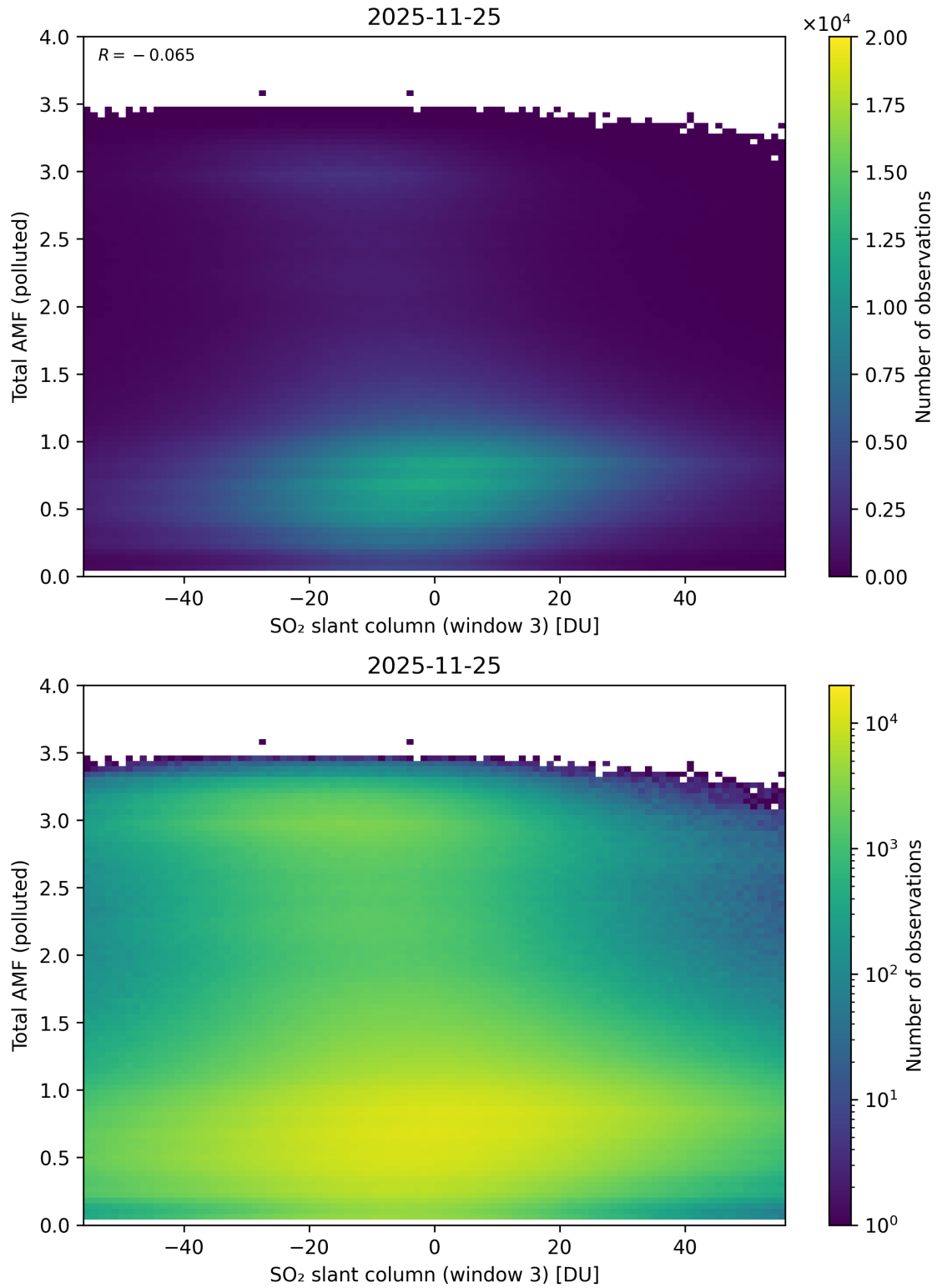
Figure 318: Scatter density plot of “SO 2 slant column (window 3)” against “Total AMF (polluted)” for 2025-11-24 to 2025-11-26.
