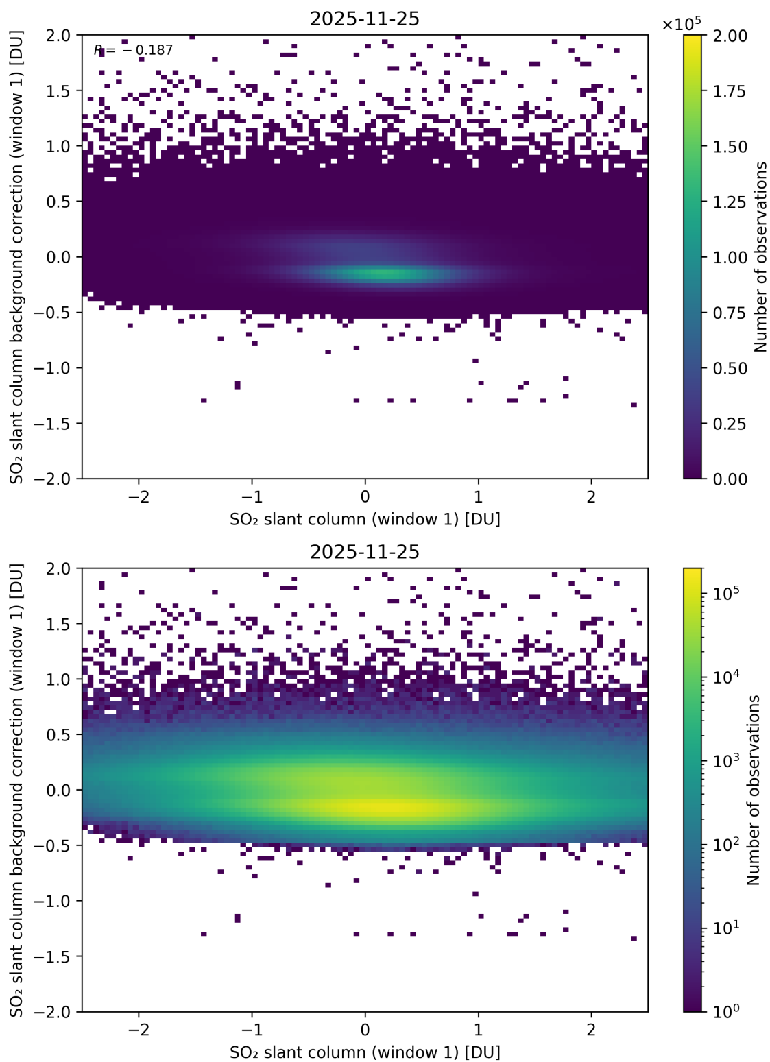
Figure 262: Scatter density plot of “SO 2 slant column (window 1)” against “SO 2 slant column background correction (window 1)” for 2025-11-24 to 2025-11-26.
