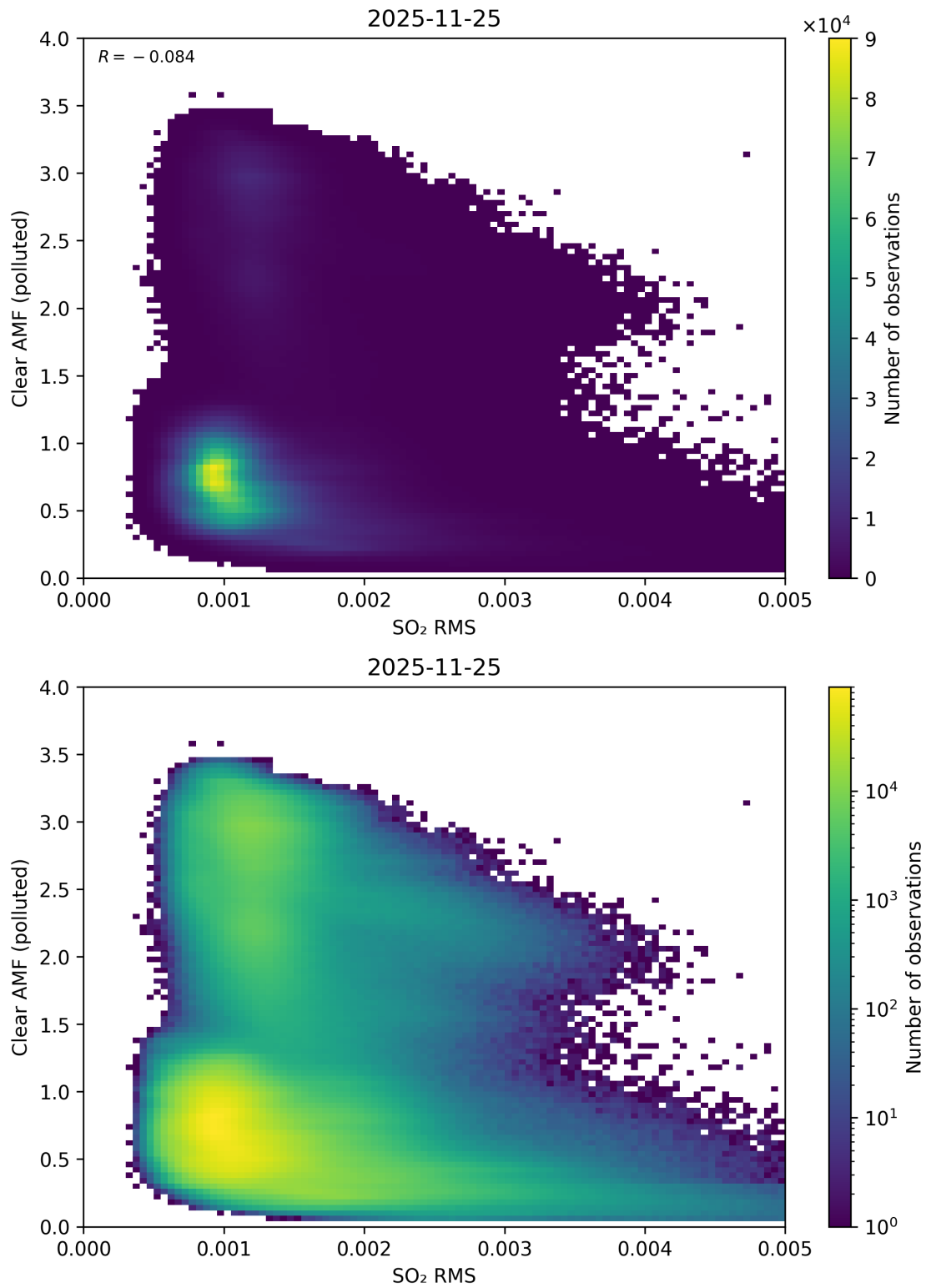
Figure 147: Scatter density plot of “SO 2 RMS” against “Clear AMF (polluted)” for 2025-11-24 to 2025-11-26.
