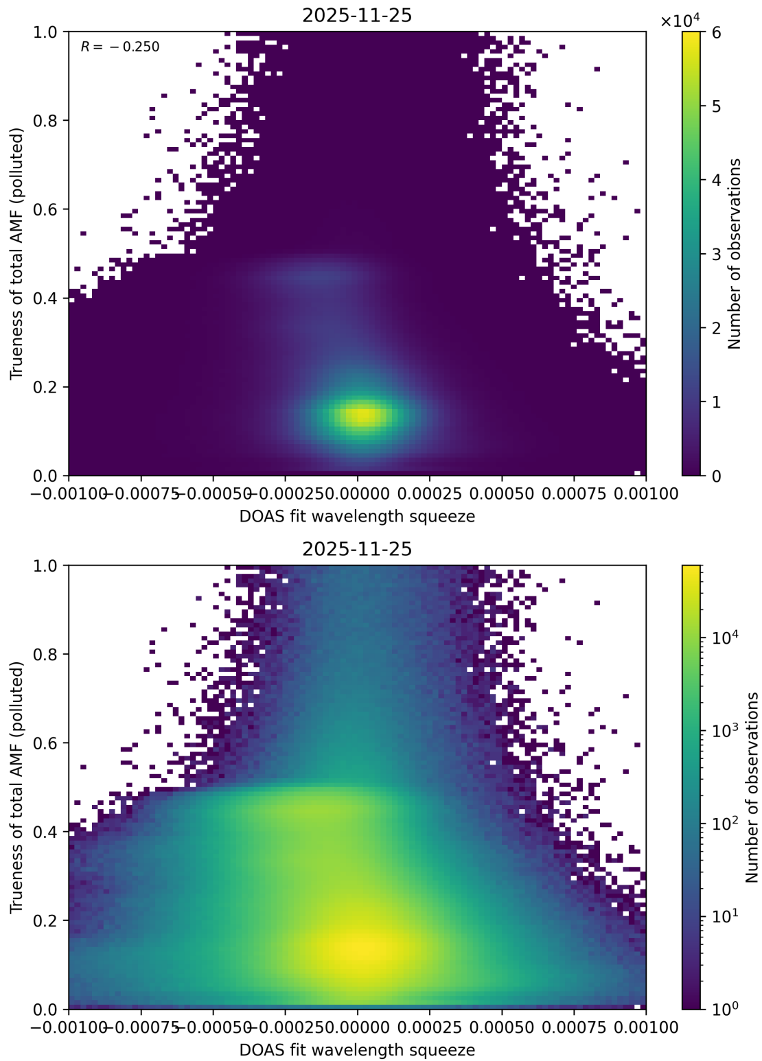
Figure 146: Scatter density plot of “DOAS fit wavelength squeeze” against “Trueness of total AMF (polluted)” for 2025-11-24 to 2025-11-26.
