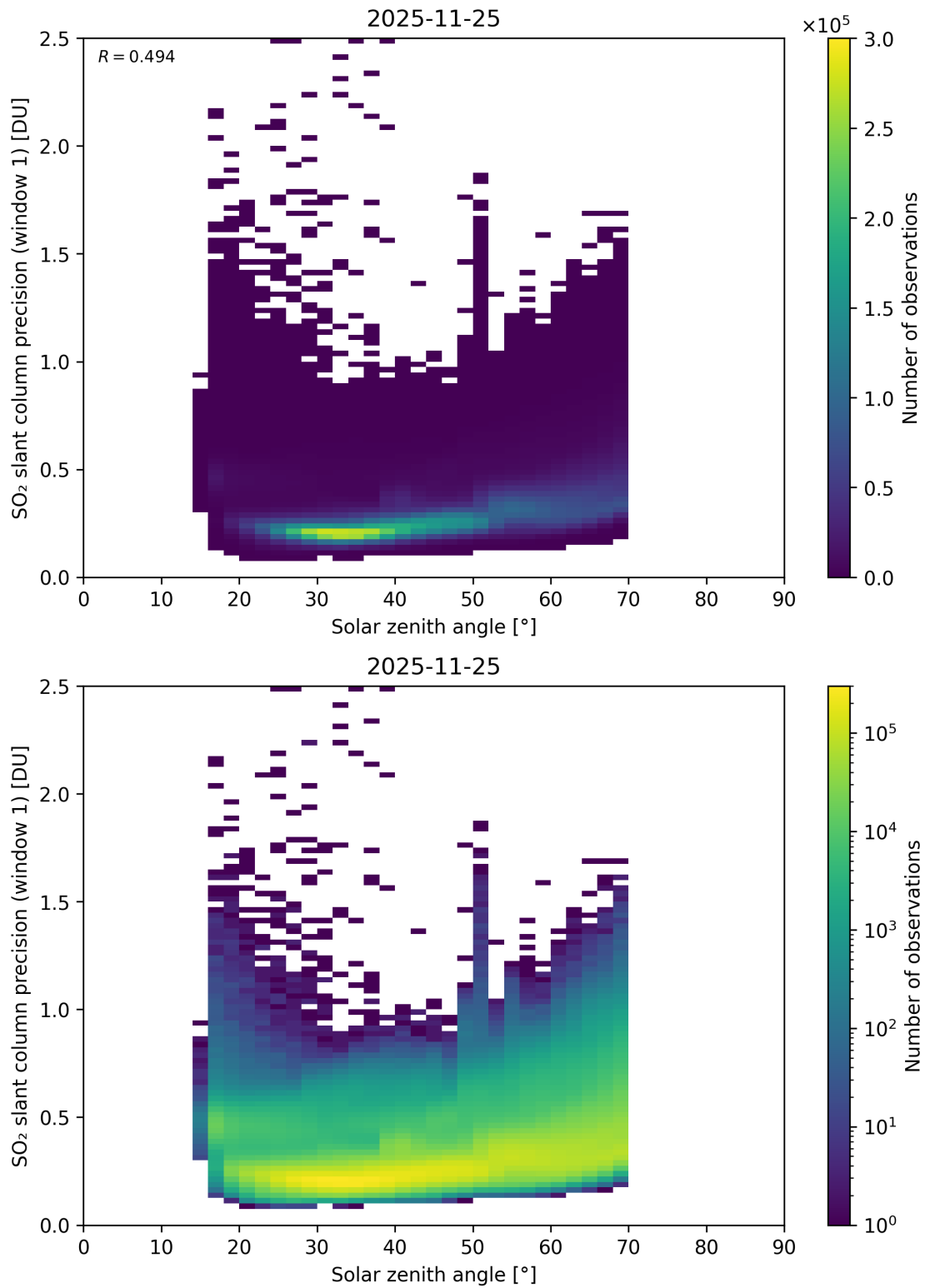
Figure 185: Scatter density plot of “Solar zenith angle” against “SO 2 slant column precision (window 1)” for 2025-11-24 to 2025-11-26.
