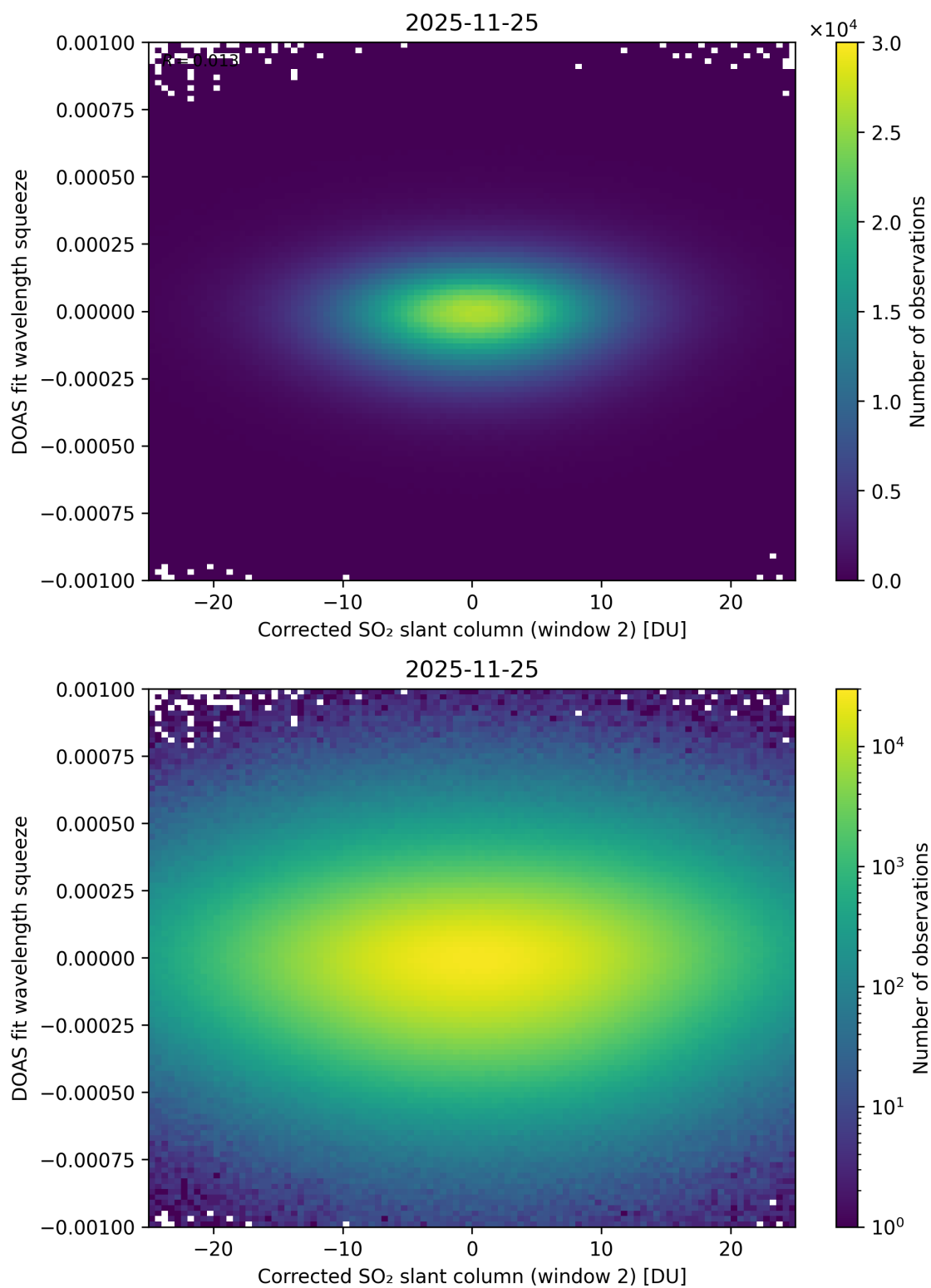
Figure 247: Scatter density plot of “Corrected SO 2 slant column (window 2)” against “DOAS fit wavelength squeeze” for 2025-11-24 to 2025-11-26.
