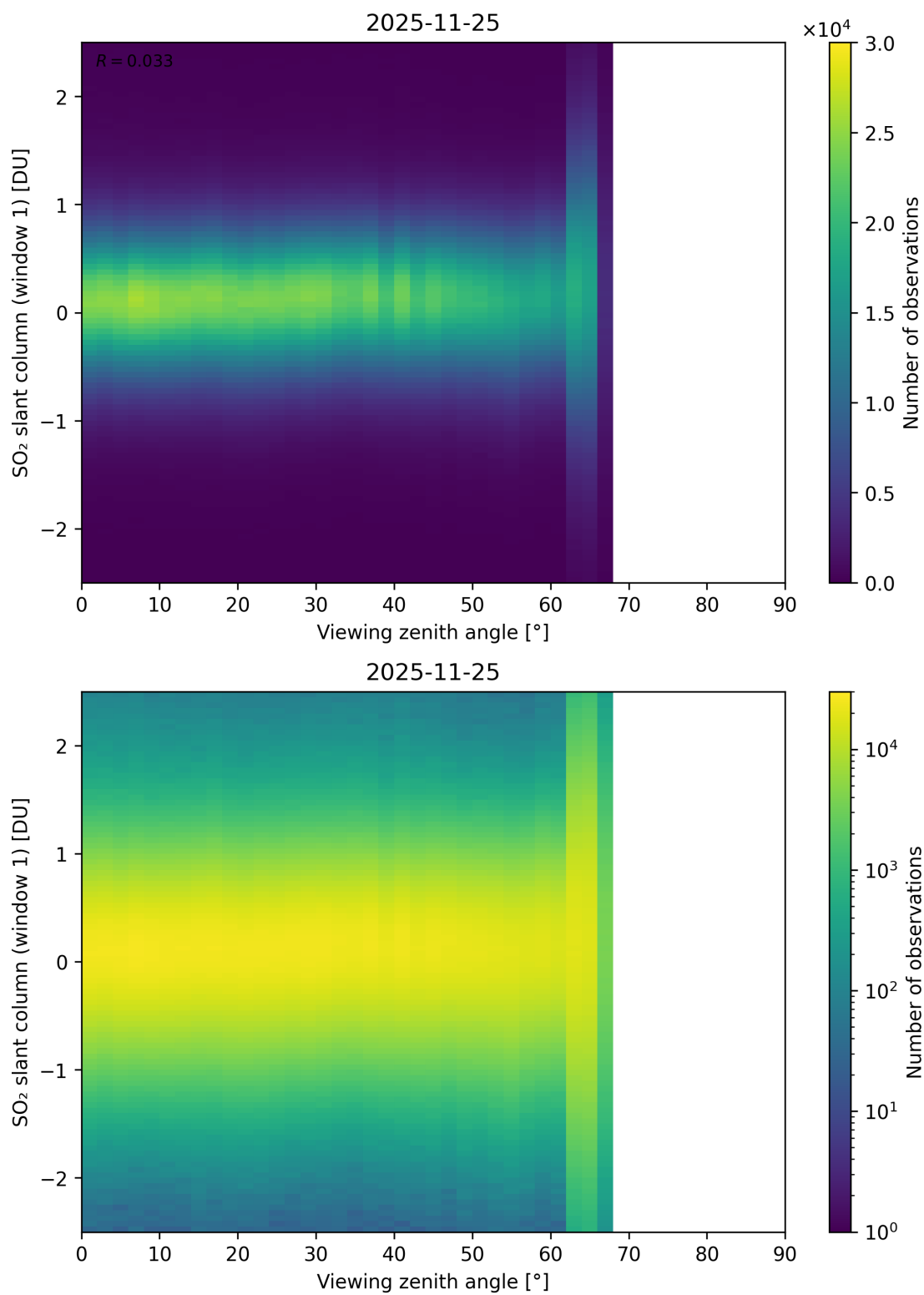
Figure 376: Scatter density plot of “Viewing zenith angle” against “SO 2 slant column (window 1)” for 2025-11-24 to 2025-11-26.
