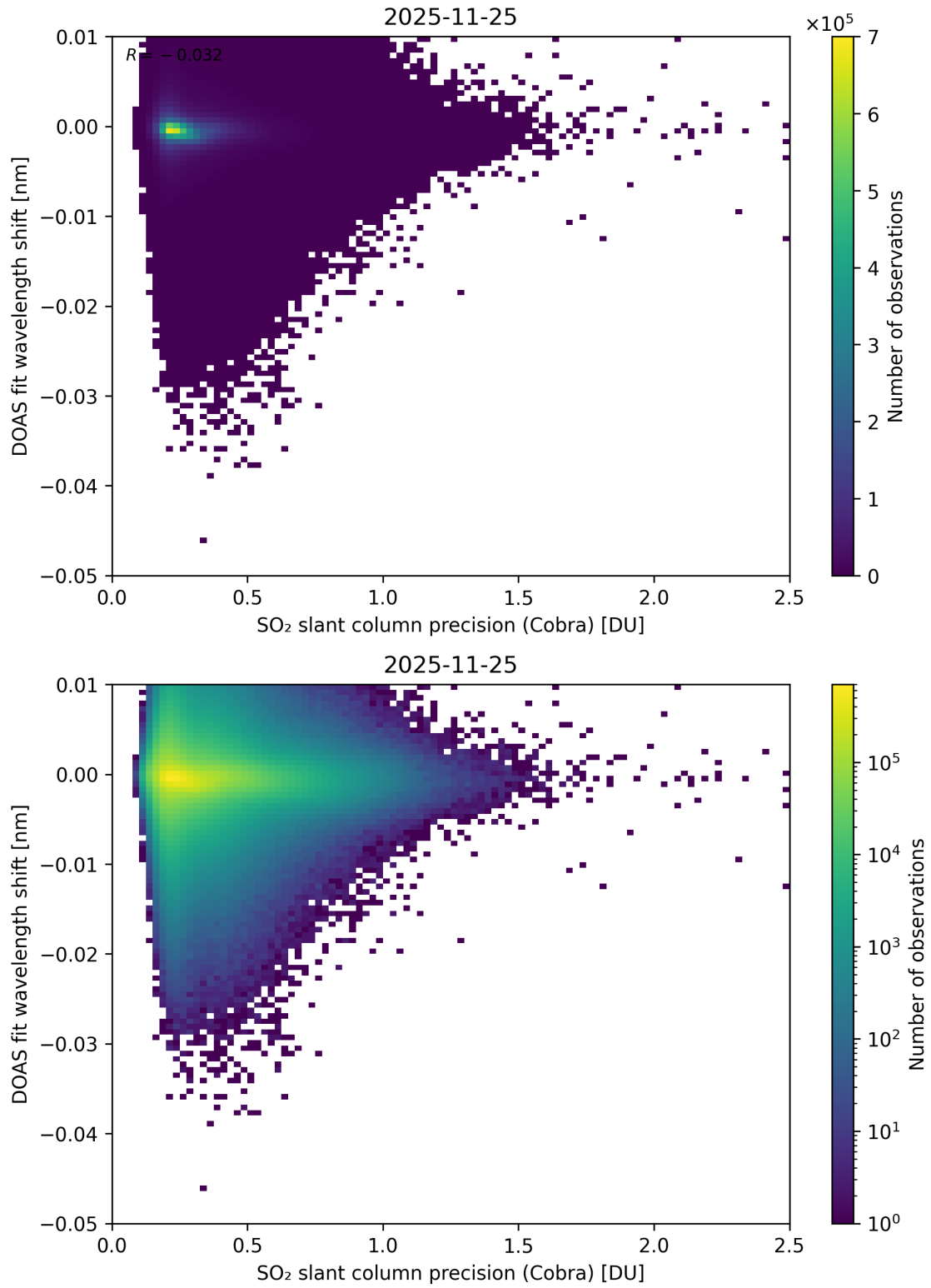
Figure 202: Scatter density plot of “SO 2 slant column precision (Cobra)” against “DOAS fit wavelength shift” for 2025-11-24 to 2025-11-26.
