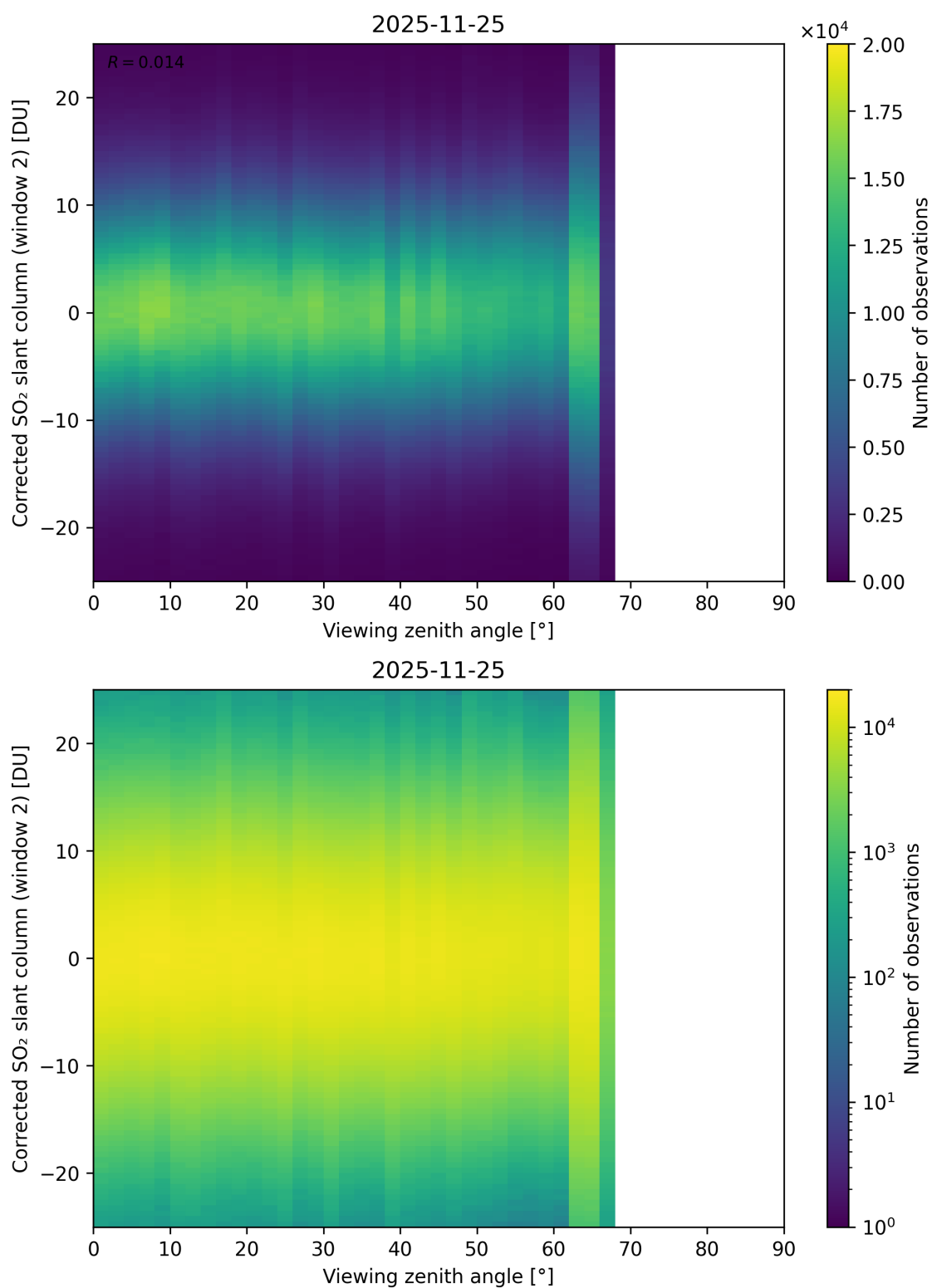
Figure 374: Scatter density plot of “Viewing zenith angle” against “Corrected SO 2 slant column (window 2)” for 2025-11-24 to 2025-11-26.
