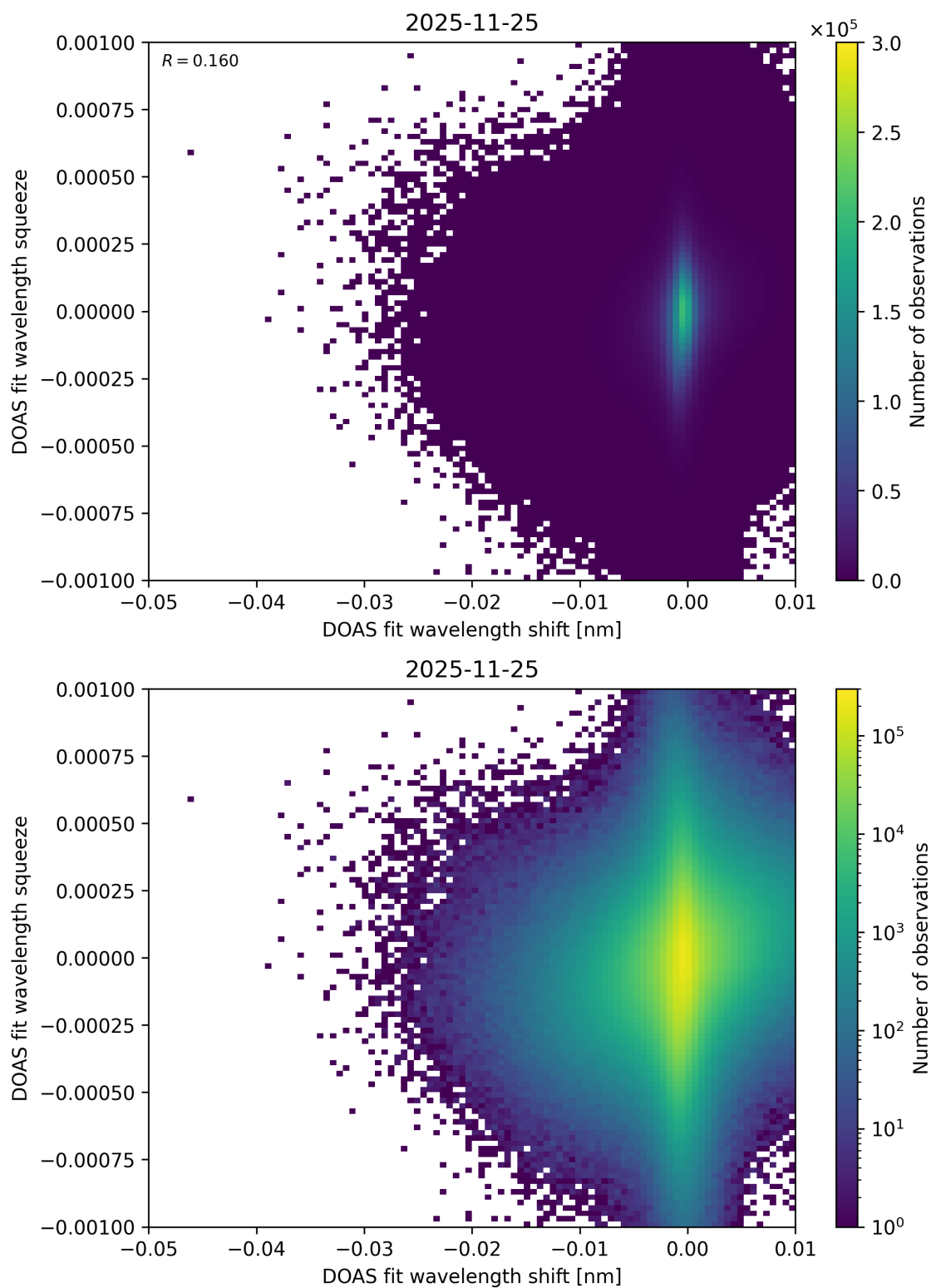
Figure 138: Scatter density plot of “DOAS fit wavelength shift” against “DOAS fit wavelength squeeze” for 2025-11-24 to 2025-11-26.
