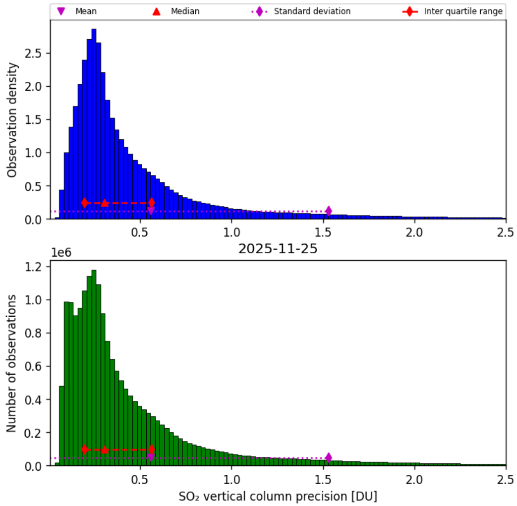
Figure 59: Histogram of “SO 2 vertical column precision” for 2025-11-24 to 2025-11-26
