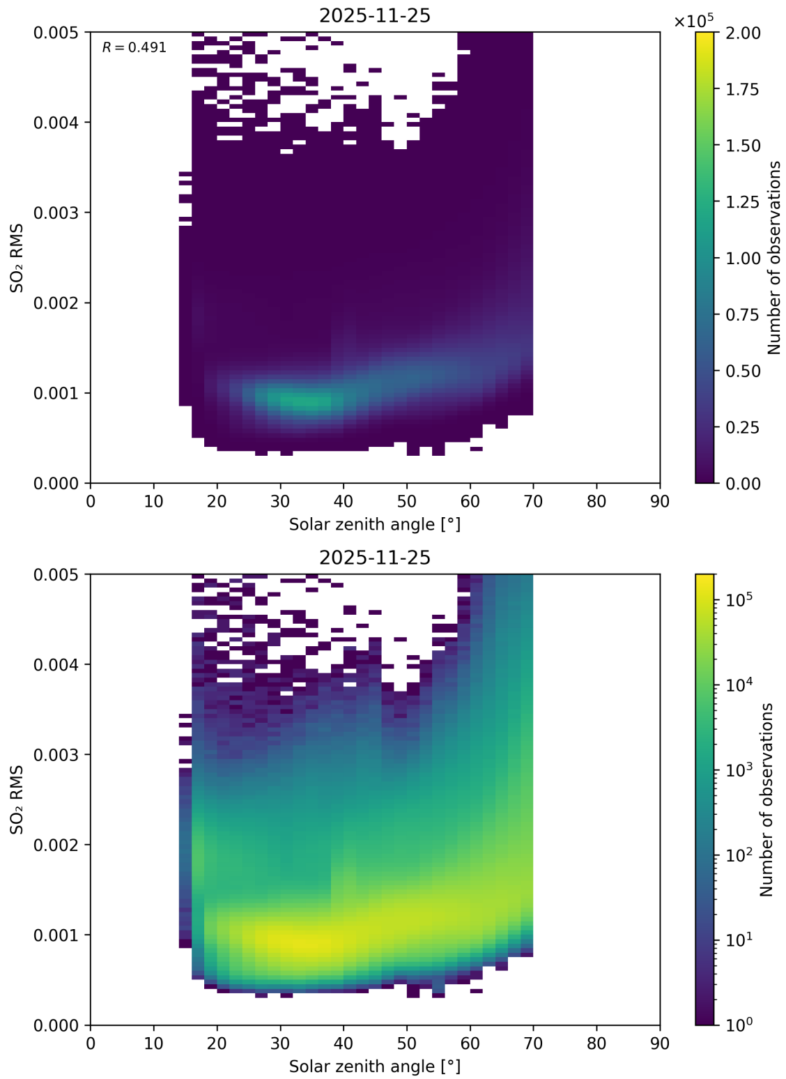
Figure 176: Scatter density plot of “Solar zenith angle” against “SO 2 RMS” for 2025-11-24 to 2025-11-26.
