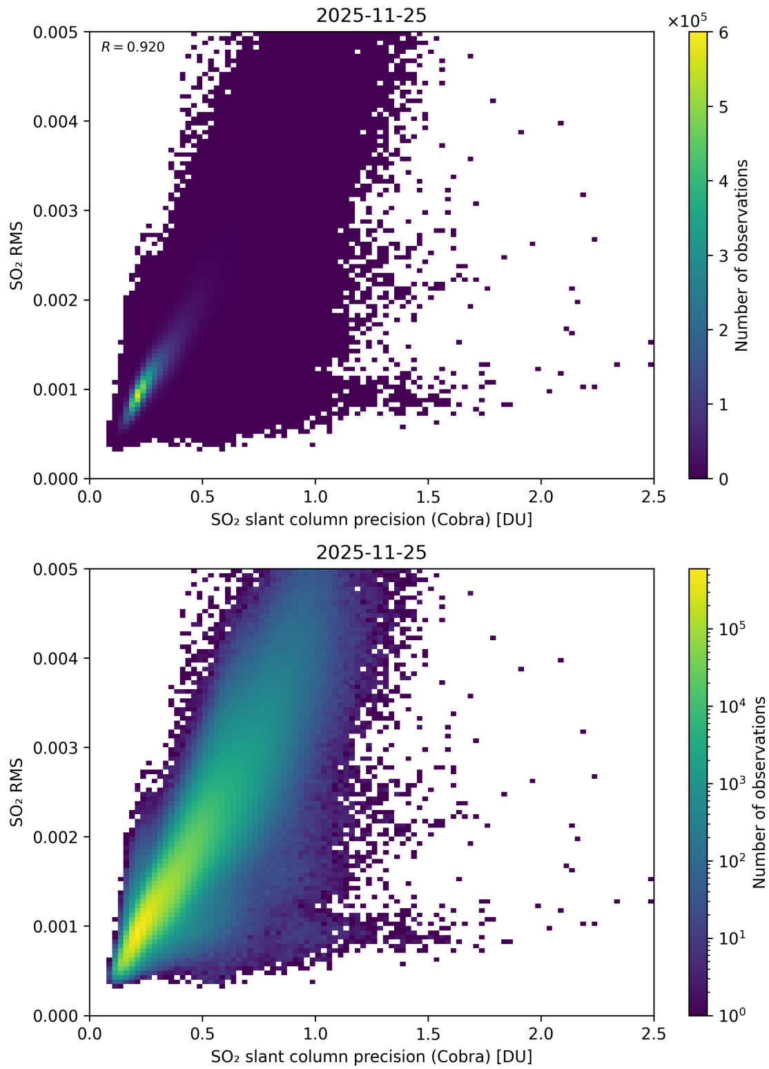
Figure 204: Scatter density plot of “SO 2 slant column precision (Cobra)” against “SO 2 RMS” for 2025-11-24 to 2025-11-26.
