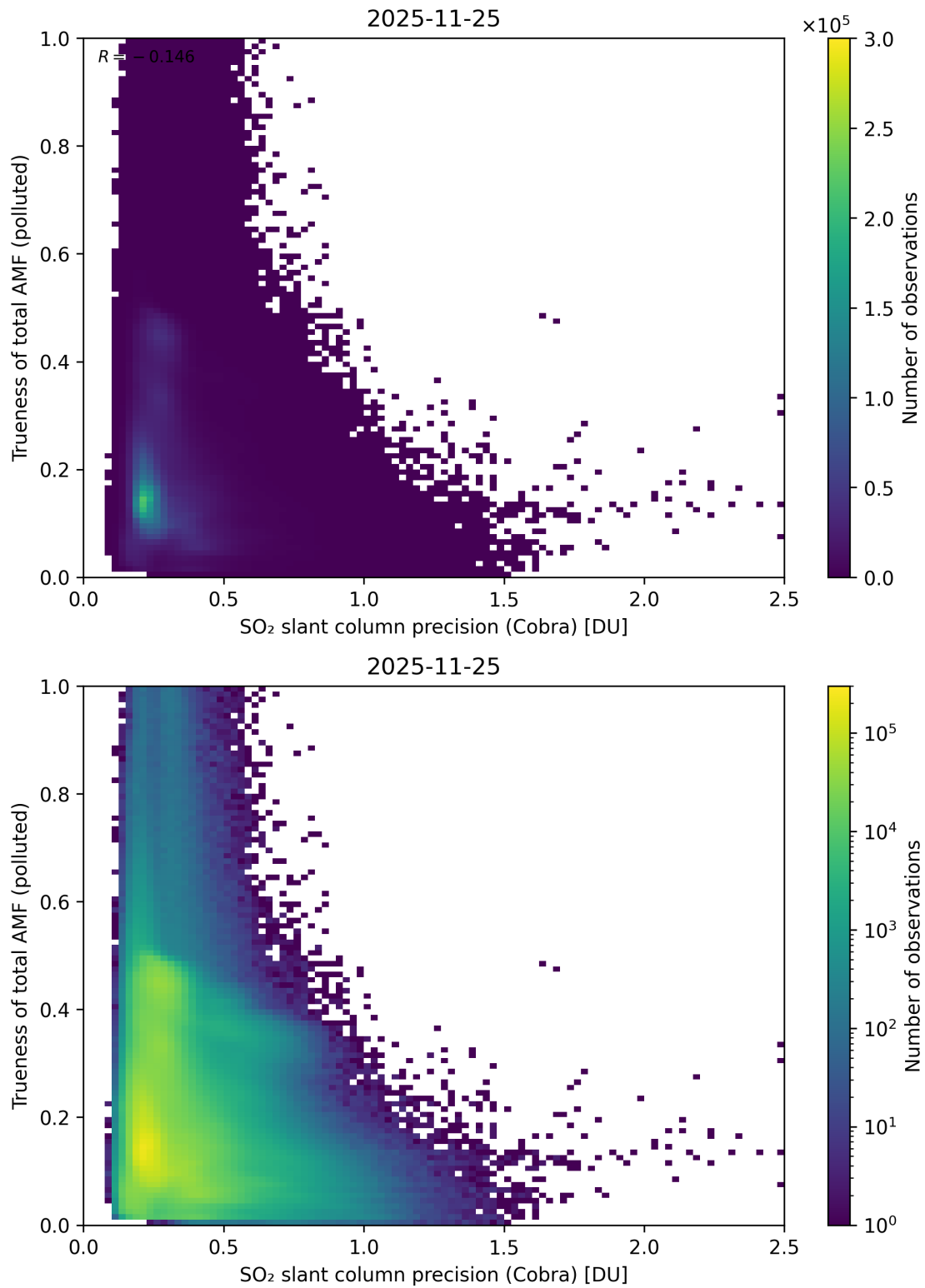
Figure 214: Scatter density plot of “SO 2 slant column precision (Cobra)” against “Trueness of total AMF (polluted)” for 2025-11-24 to 2025-11-26.
