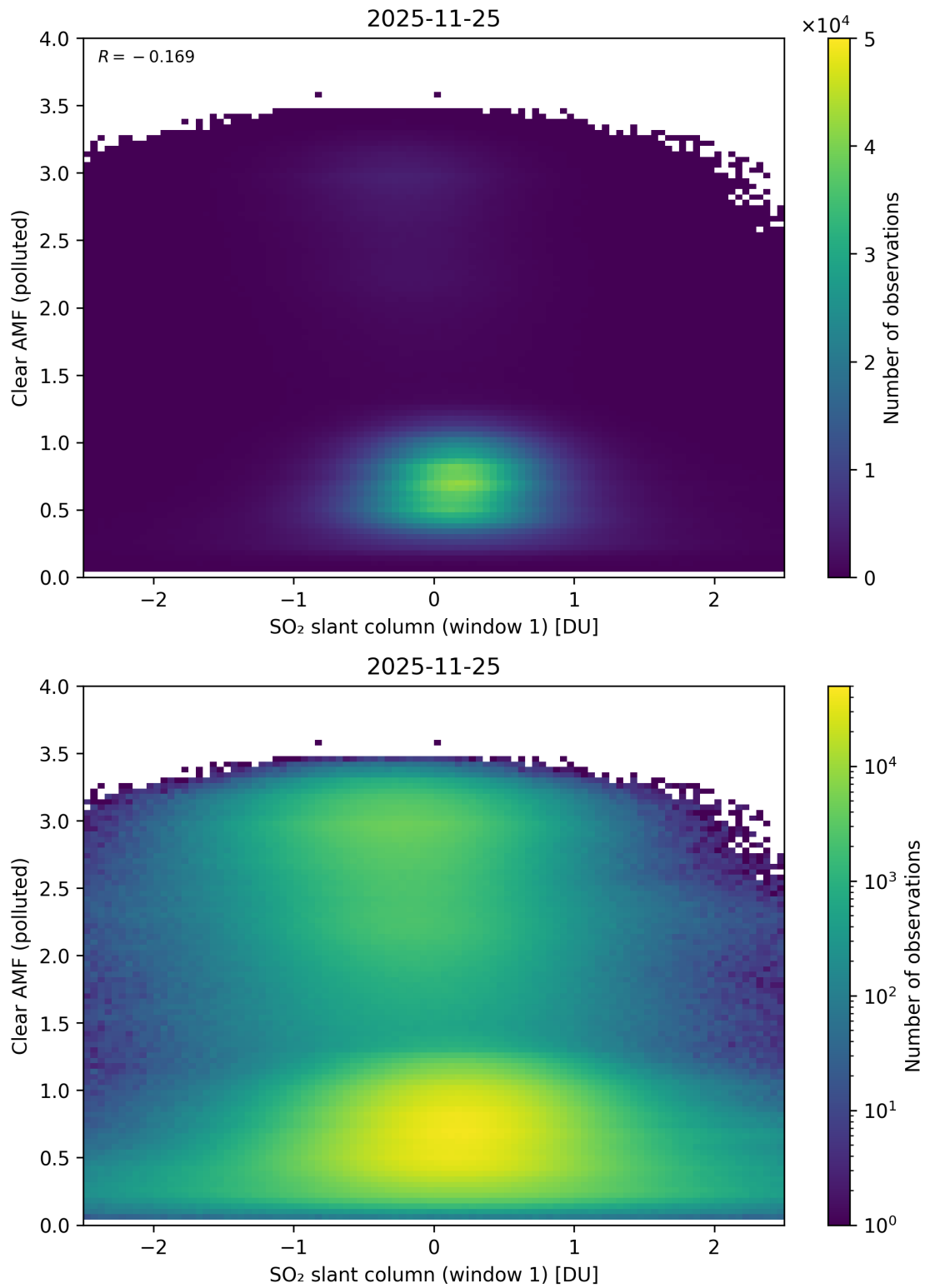
Figure 282: Scatter density plot of “SO 2 slant column (window 1)” against “Clear AMF (polluted)” for 2025-11-24 to 2025-11-26.
