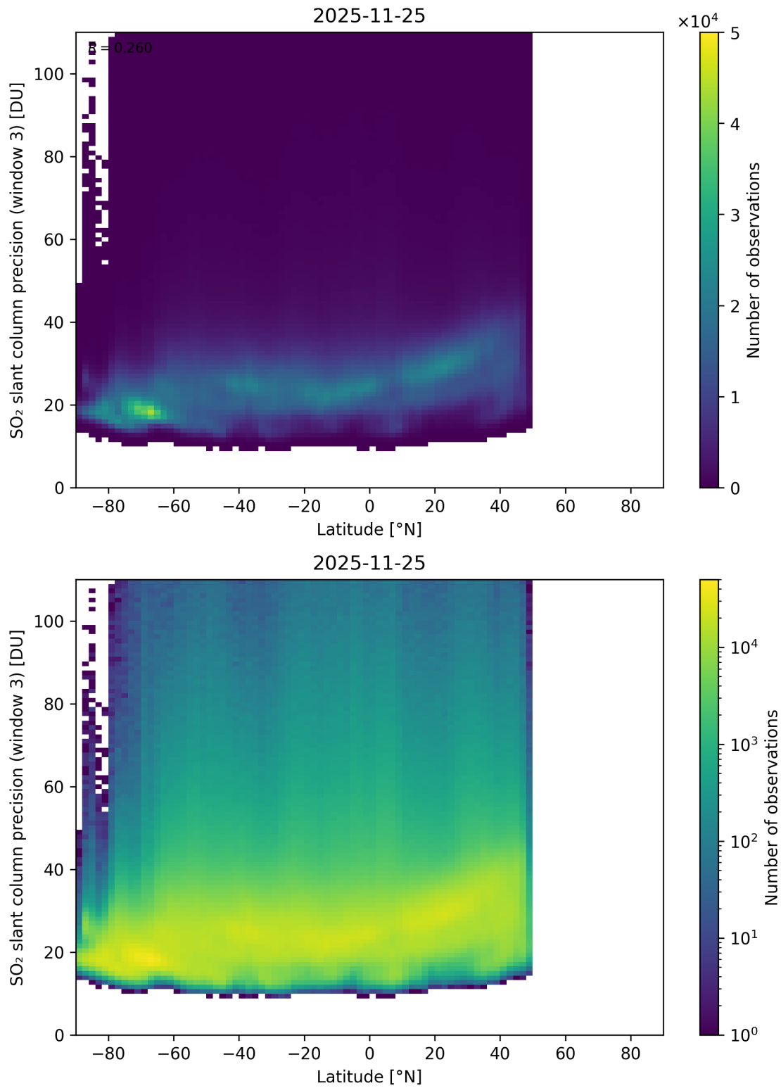
Figure 166: Scatter density plot of “Latitude” against “SO 2 slant column precision (window 3)” for 2025-11-24 to 2025-11-26.
