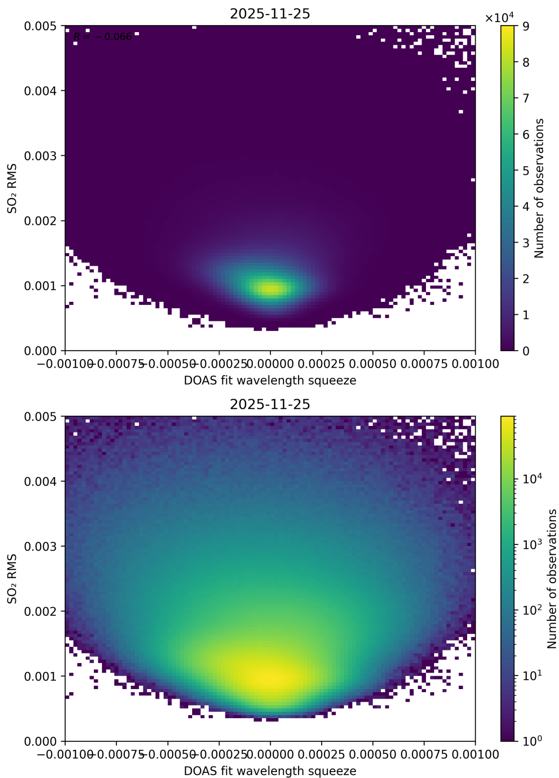
Figure 143: Scatter density plot of “DOAS fit wavelength squeeze” against “SO 2 RMS” for 2025-11-24 to 2025-11-26.
