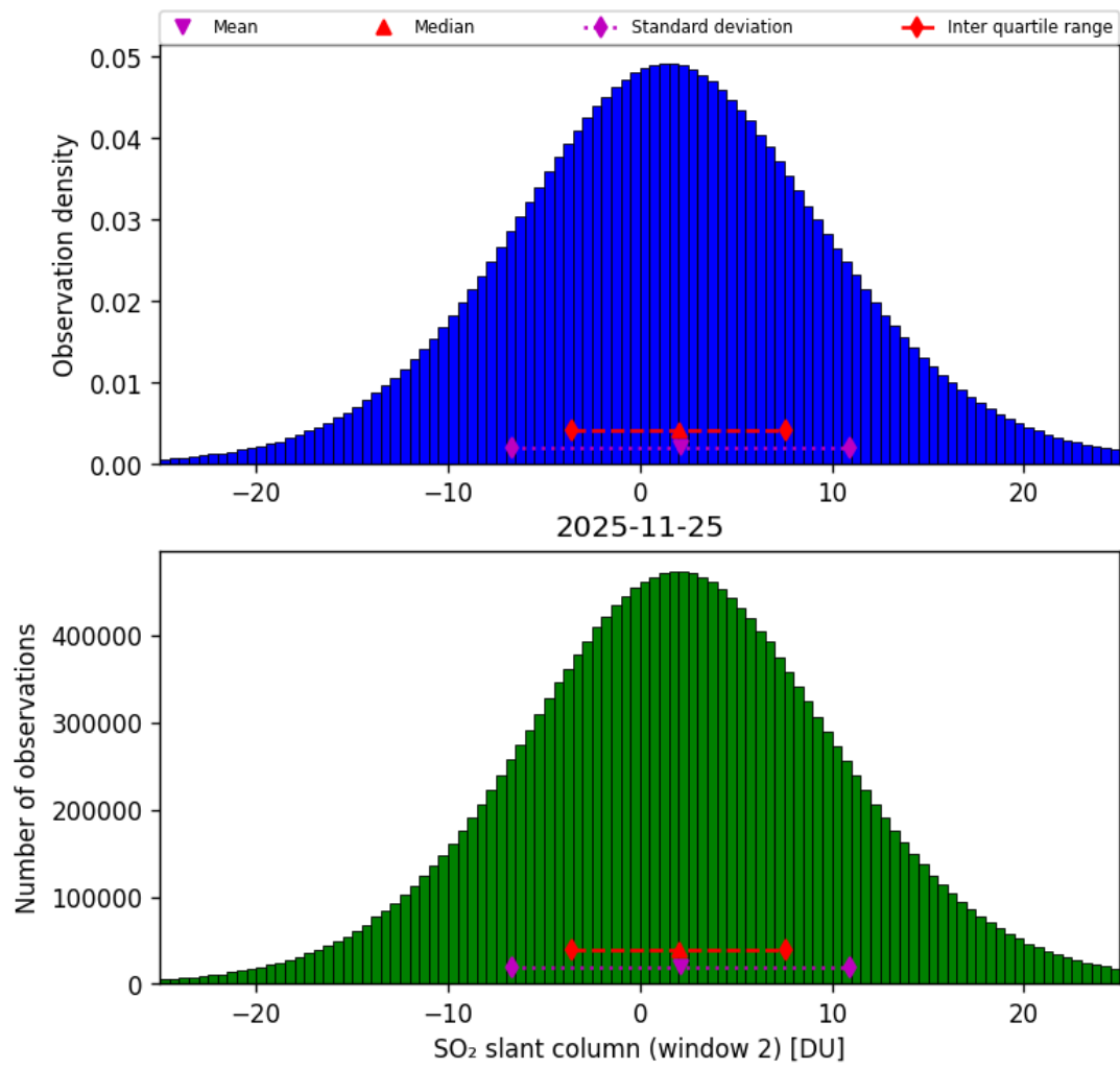
Figure 67: Histogram of “SO 2 slant column (window 2)” for 2025-11-24 to 2025-11-26
