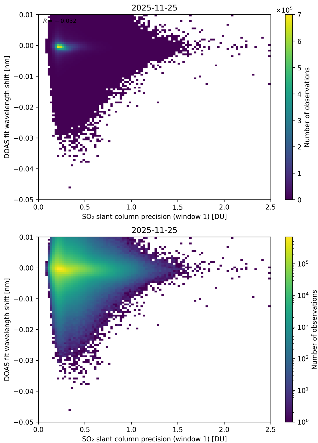
Figure 271: Scatter density plot of “SO 2 slant column precision (window 1)” against “DOAS fit wavelength shift” for 2025-11-24 to 2025-11-26.
