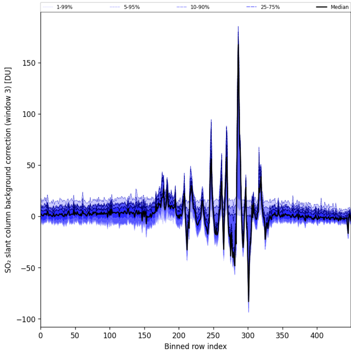
Figure 100: Along track statistics of “SO 2 slant column background correction (window 3)” for 2025-11-24 to 2025-11-26
