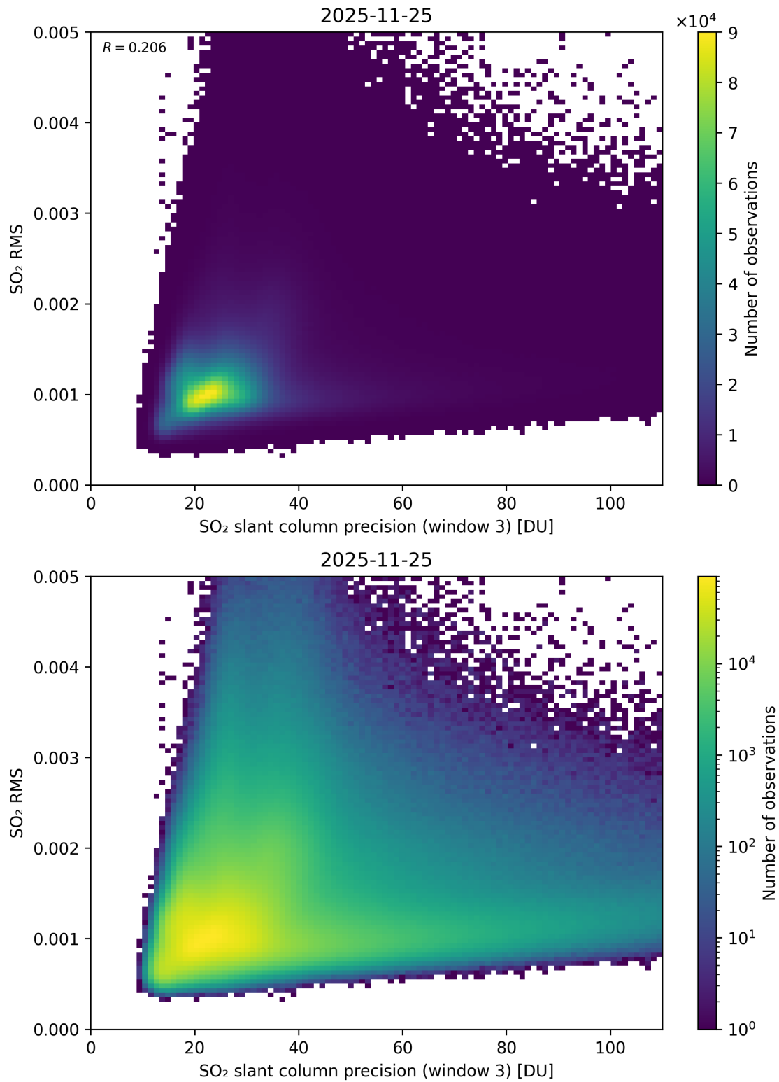
Figure 310: Scatter density plot of “SO 2 slant column precision (window 3)” against “SO 2 RMS” for 2025-11-24 to 2025-11-26.
