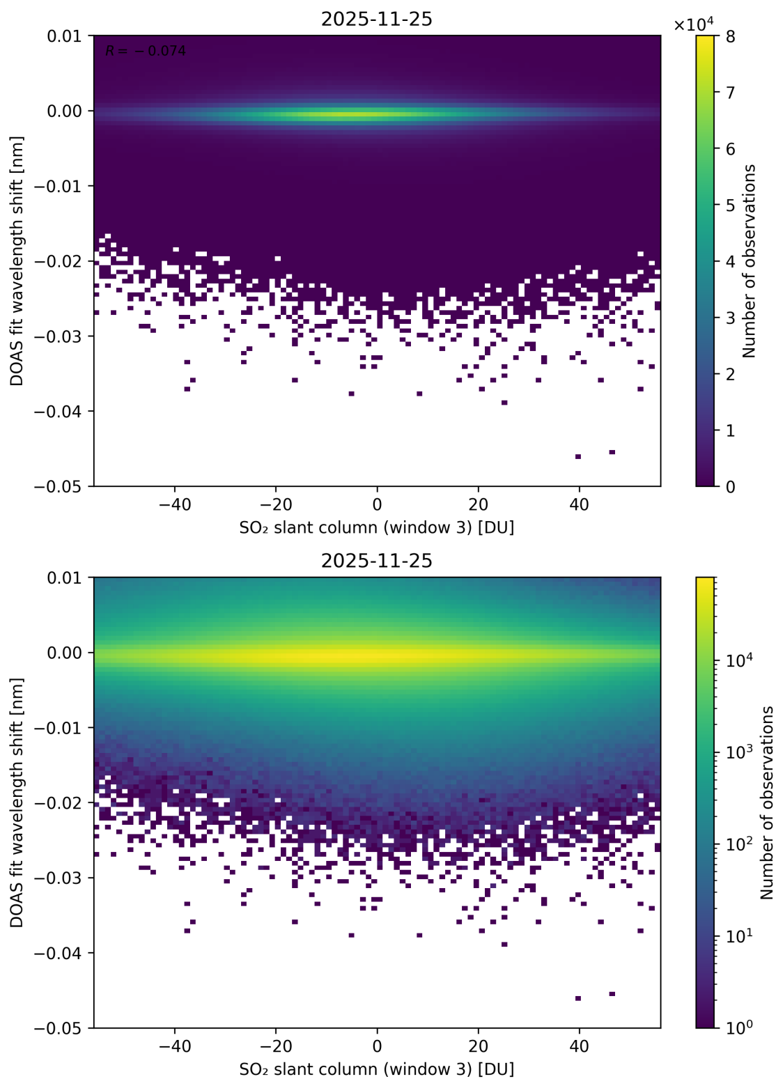
Figure 304: Scatter density plot of “SO 2 slant column (window 3)” against “DOAS fit wavelength shift” for 2025-11-24 to 2025-11-26.
