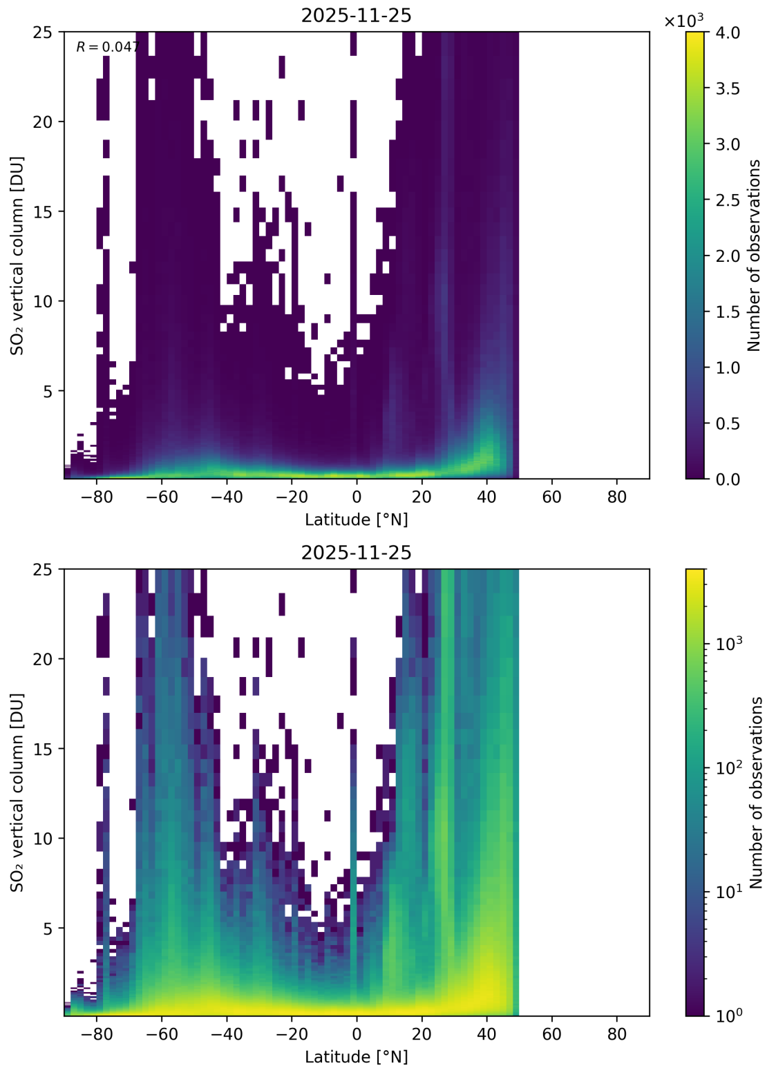
Figure 169: Scatter density plot of “Latitude” against “SO 2 vertical column” for 2025-11-24 to 2025-11-26.
