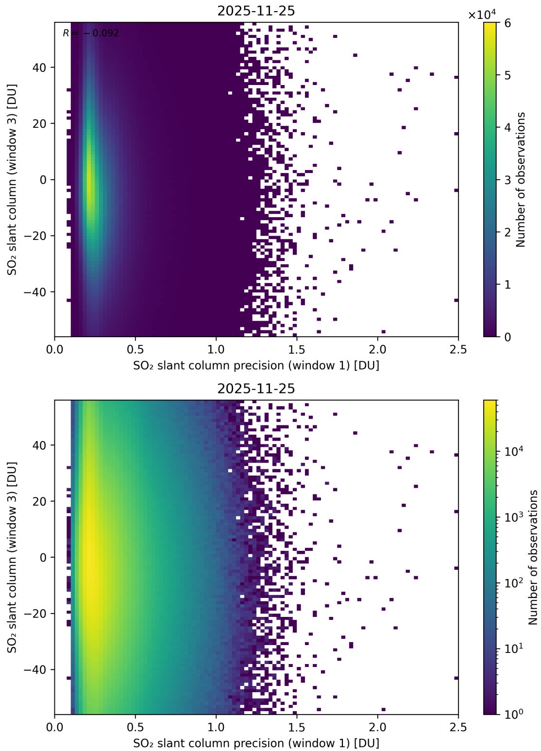
Figure 278: Scatter density plot of “SO 2 slant column precision (window 1)” against “SO 2 slant column (window 3)” for 2025-11-24 to 2025-11-26.
