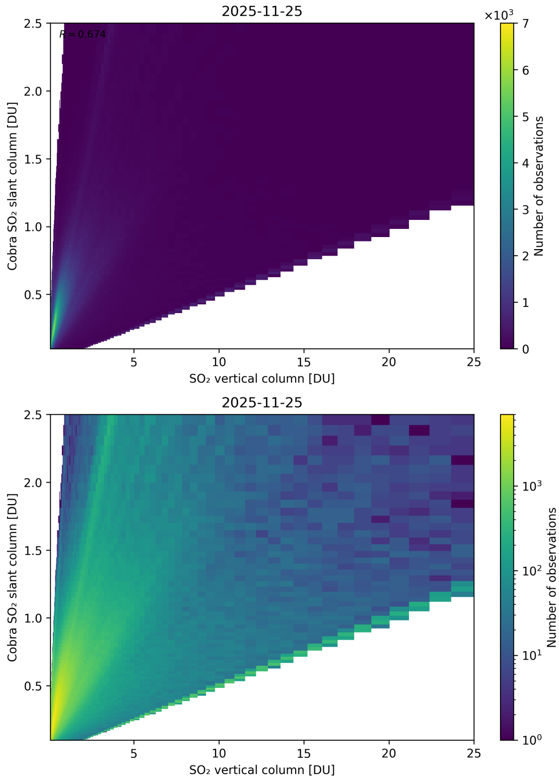
Figure 349: Scatter density plot of “SO 2 vertical column” against “Cobra SO 2 slant column” for 2025-11-24 to 2025-11-26.
