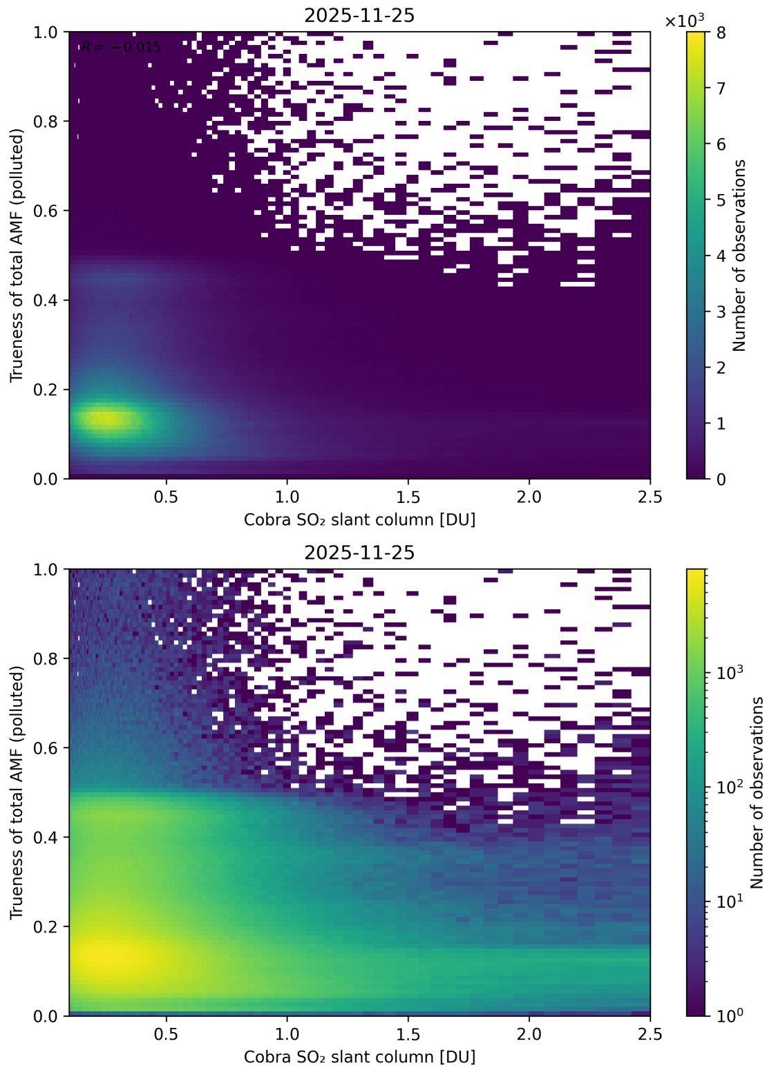
Figure 225: Scatter density plot of “Cobra SO 2 slant column” against “Trueness of total AMF (polluted)” for 2025-11-24 to 2025-11-26.
