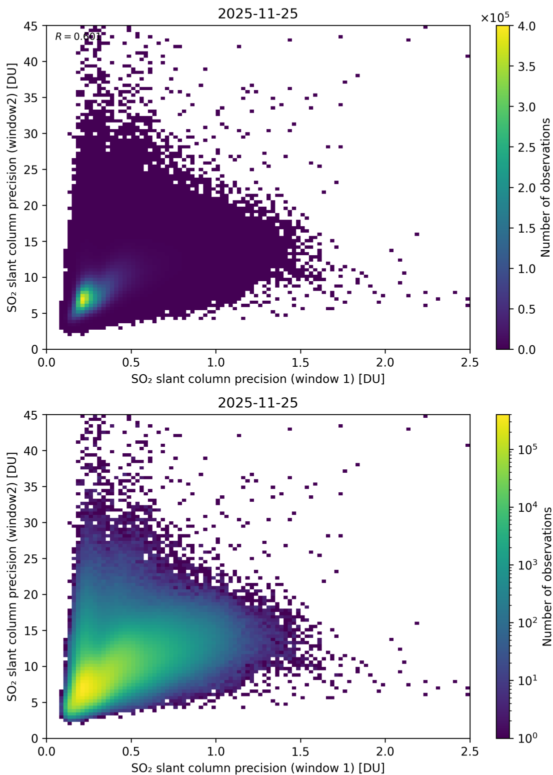
Figure 277: Scatter density plot of “SO 2 slant column precision (window 1)” against “SO 2 slant column precision (window 2)” for 2025-11-24 to 2025-11-26.
