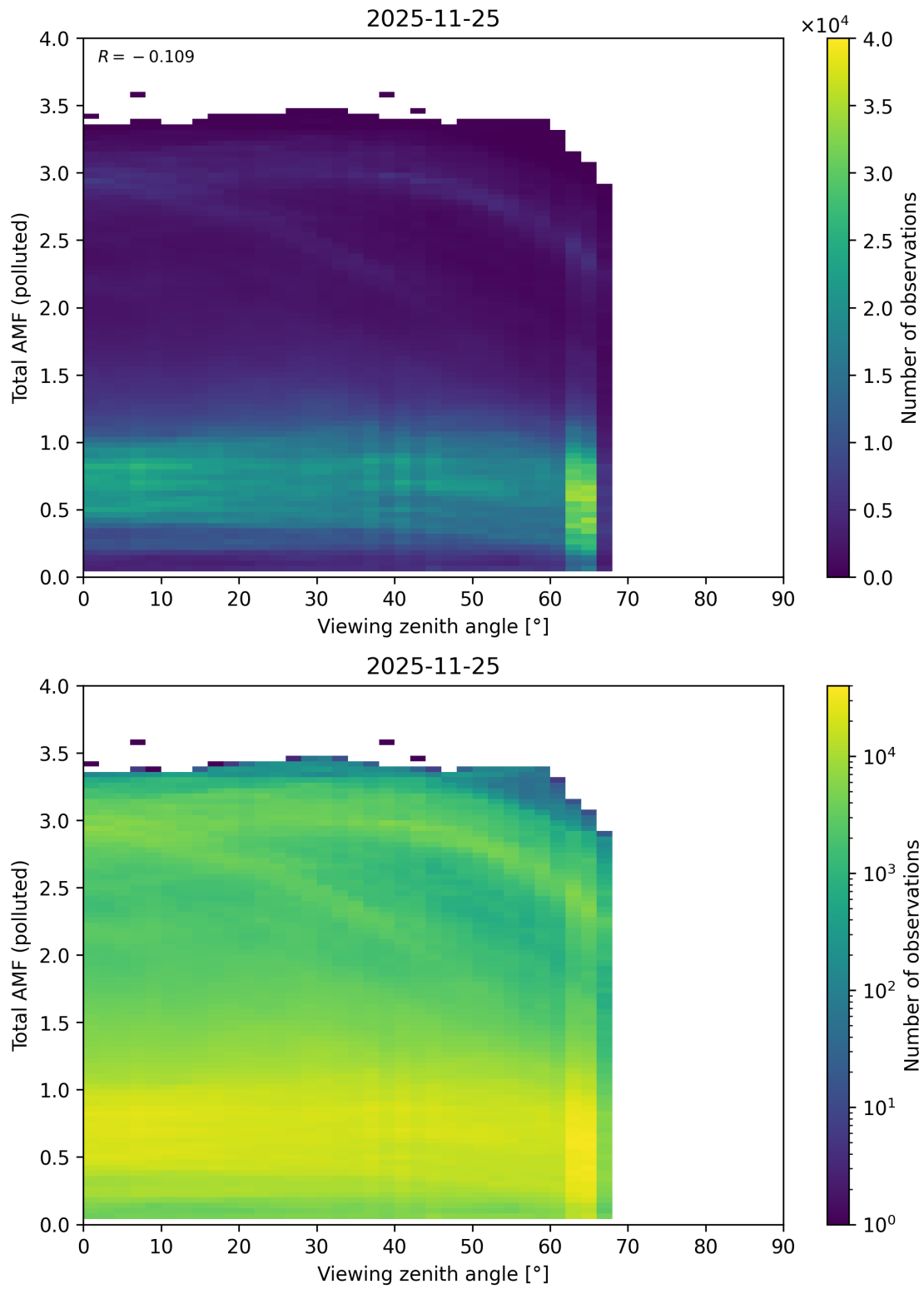
Figure 381: Scatter density plot of “Viewing zenith angle” against “Total AMF (polluted)” for 2025-11-24 to 2025-11-26.
