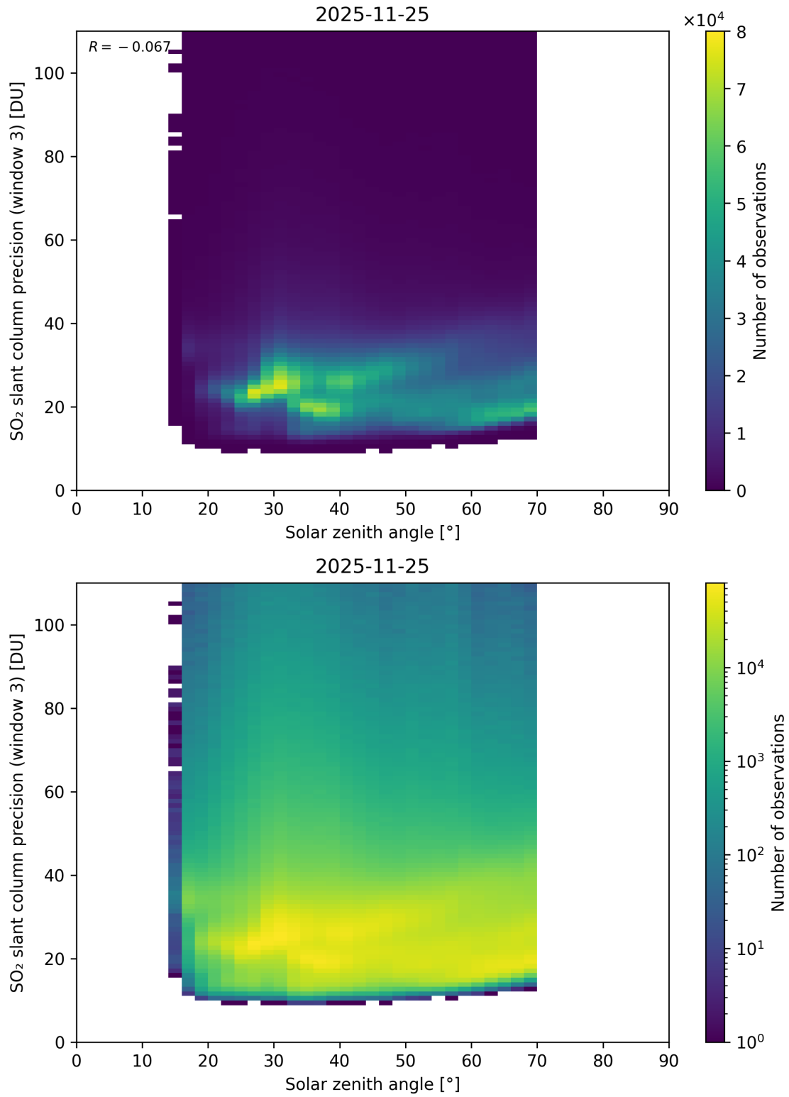
Figure 188: Scatter density plot of “Solar zenith angle” against “SO 2 slant column precision (window 3)” for 2025-11-24 to 2025-11-26.
