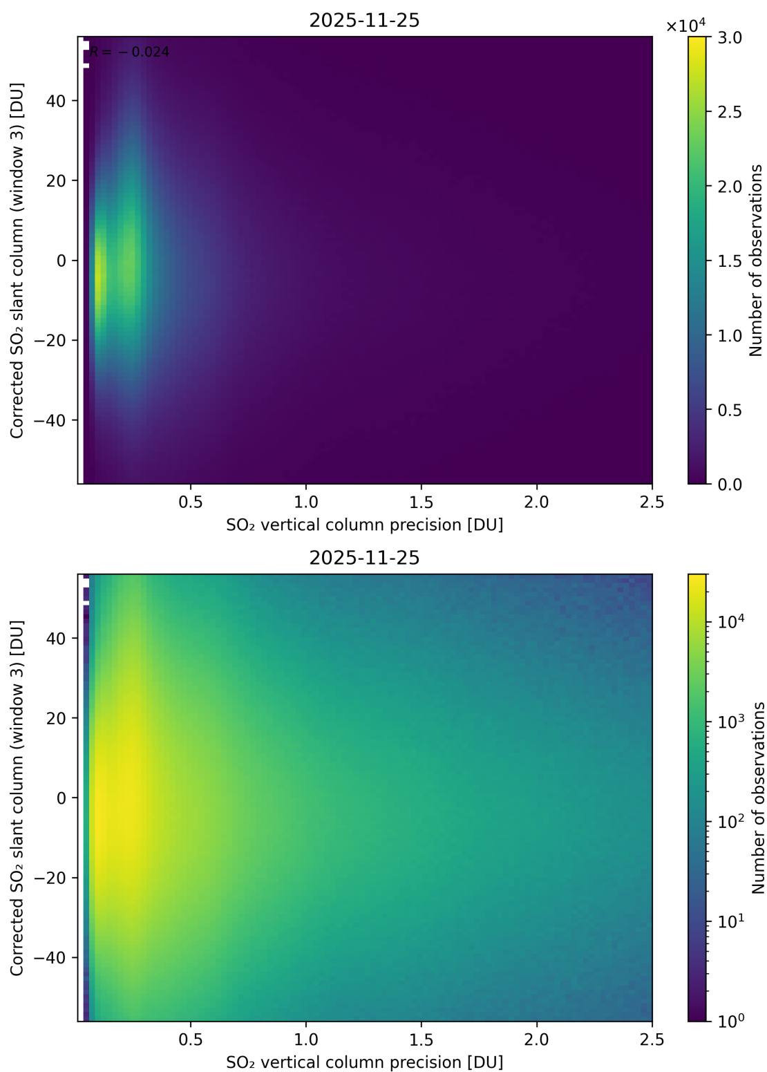
Figure 340: Scatter density plot of “SO 2 vertical column precision” against “Corrected SO 2 slant column (window 3)” for 2025-11-24 to 2025-11-26.
