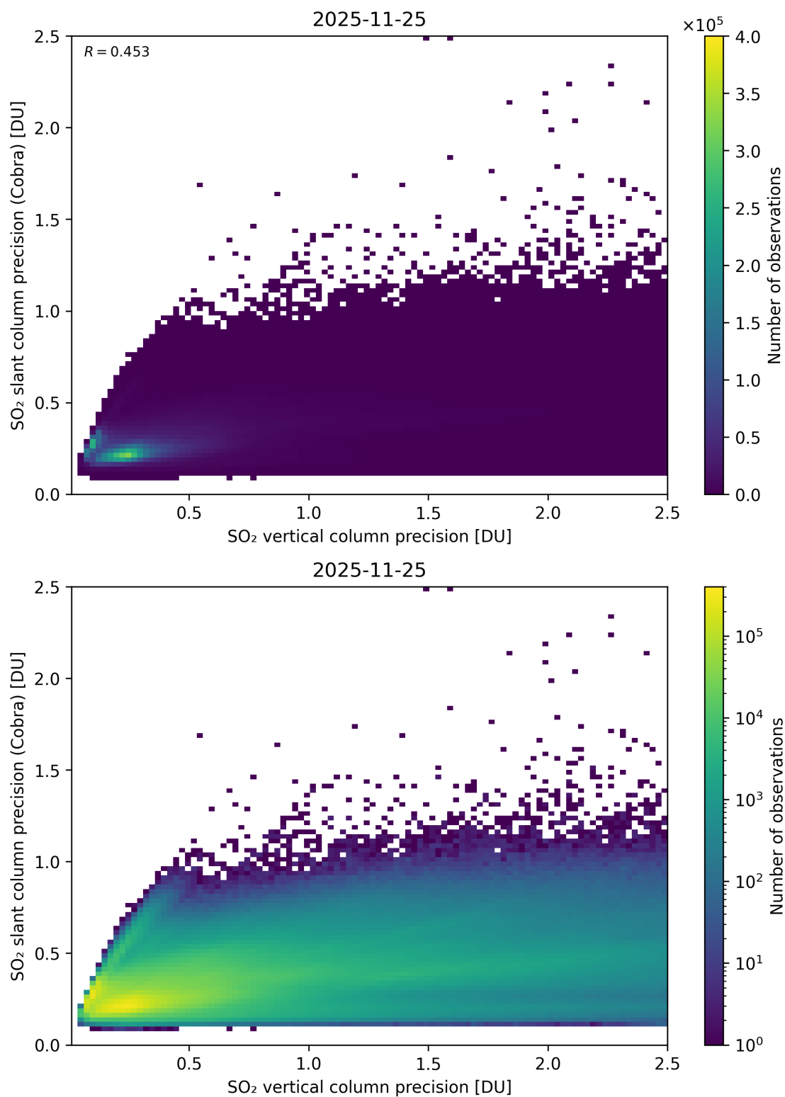
Figure 337: Scatter density plot of “SO 2 vertical column precision” against “SO 2 slant column precision (Cobra)” for 2025-11-24 to 2025-11-26.
