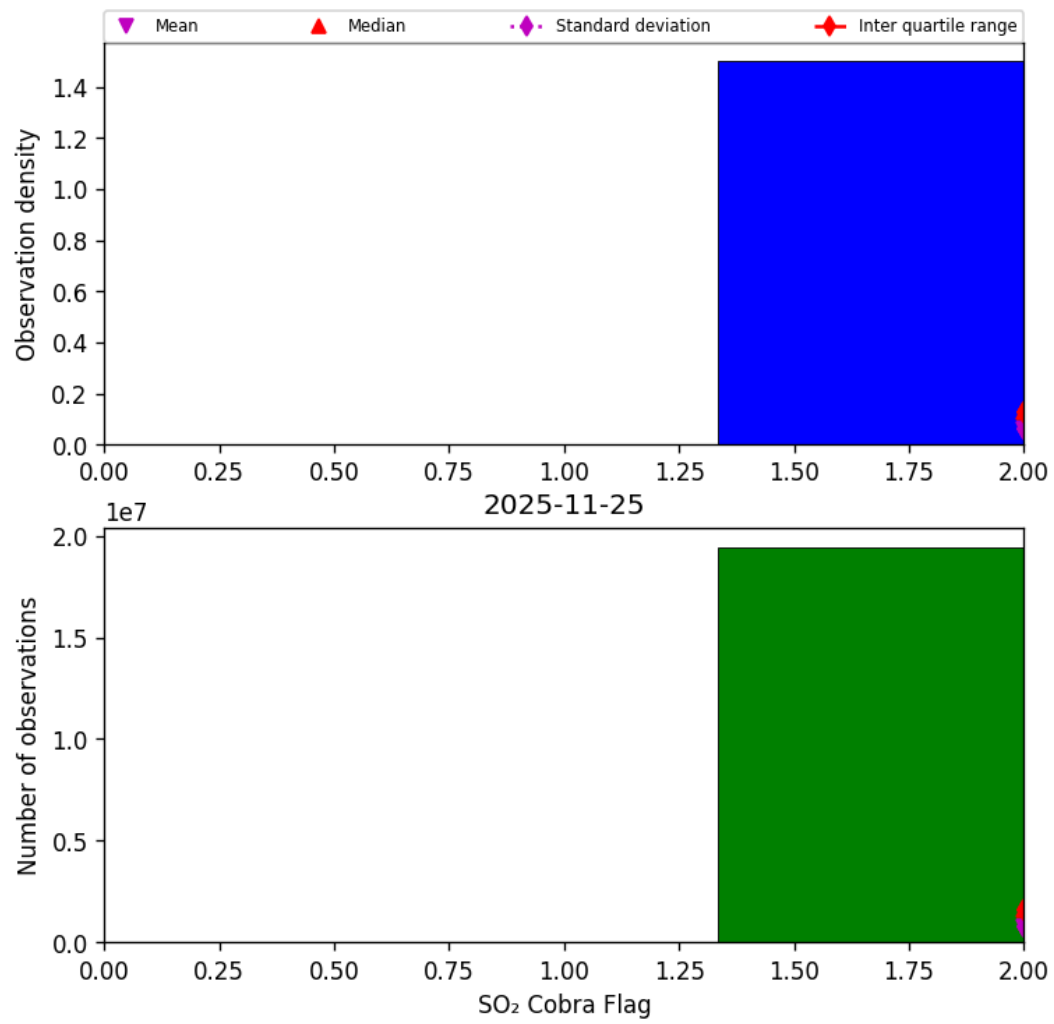
Figure 75: Histogram of “SO 2 Cobra Flag” for 2025-11-24 to 2025-11-26
