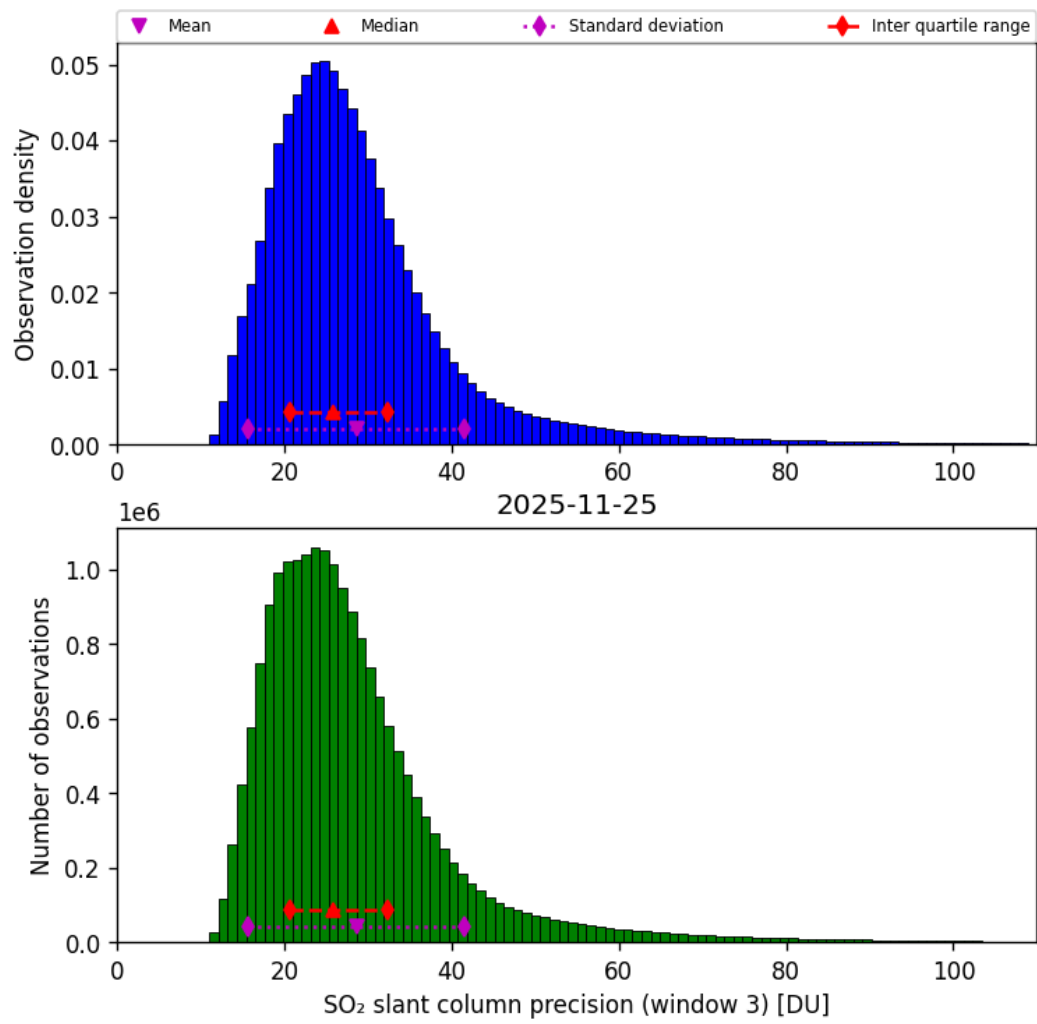
Figure 72: Histogram of “SO 2 slant column precision (window 3)” for 2025-11-24 to 2025-11-26
