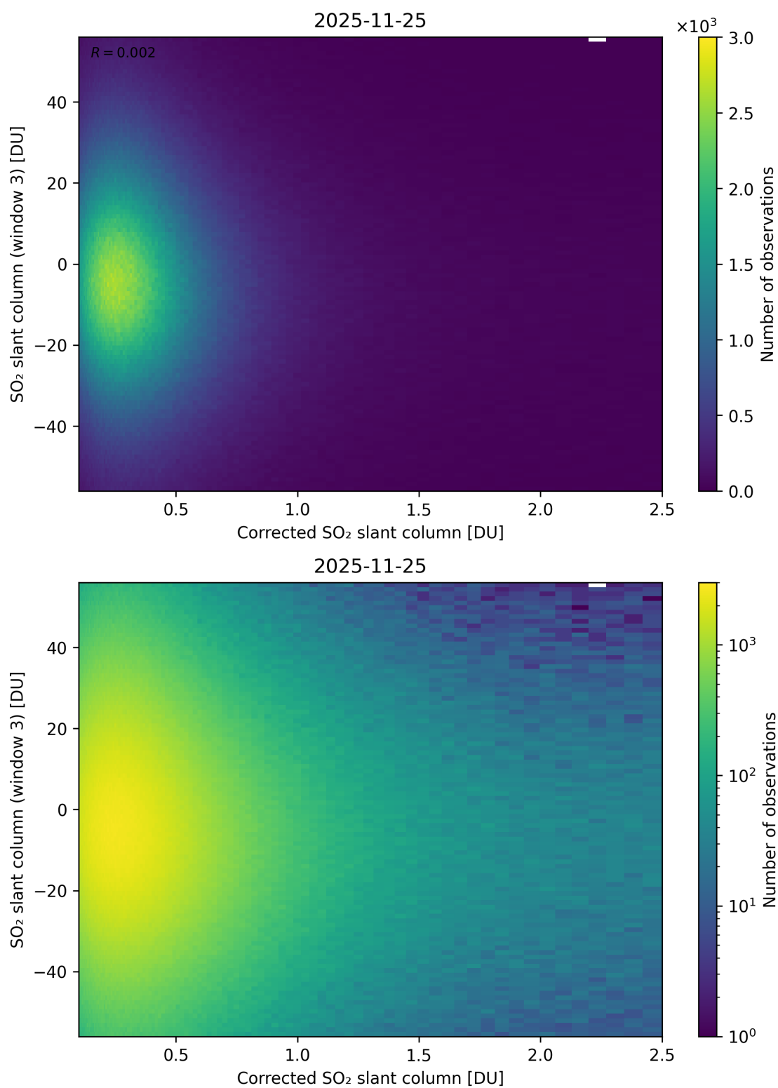
Figure 240: Scatter density plot of “Corrected SO 2 slant column” against “SO 2 slant column (window 3)” for 2025-11-24 to 2025-11-26.
