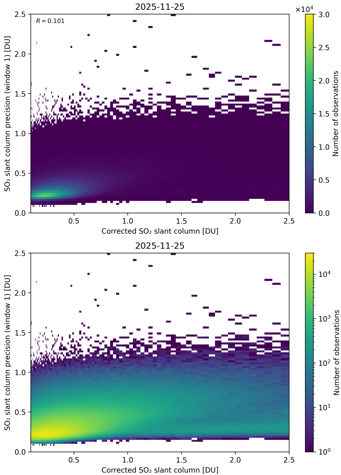
Figure 238: Scatter density plot of “Corrected SO 2 slant column” against “SO 2 slant column precision (window 1)” for 2025-11-24 to 2025-11-26.
