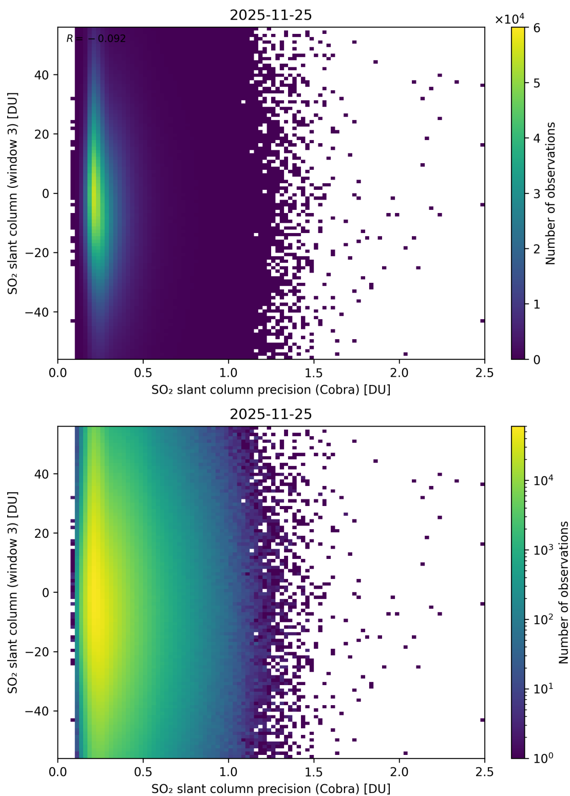
Figure 211: Scatter density plot of “SO 2 slant column precision (Cobra)” against “SO 2 slant column (window 3)” for 2025-11-24 to 2025-11-26.
