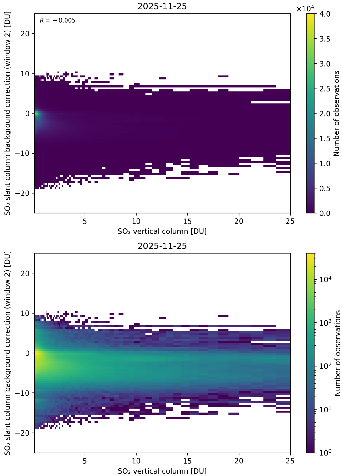
Figure 324: Scatter density plot of “SO 2 vertical column” against “SO 2 slant column background correction (window 2)” for 2025-11-24 to 2025-11-26.
