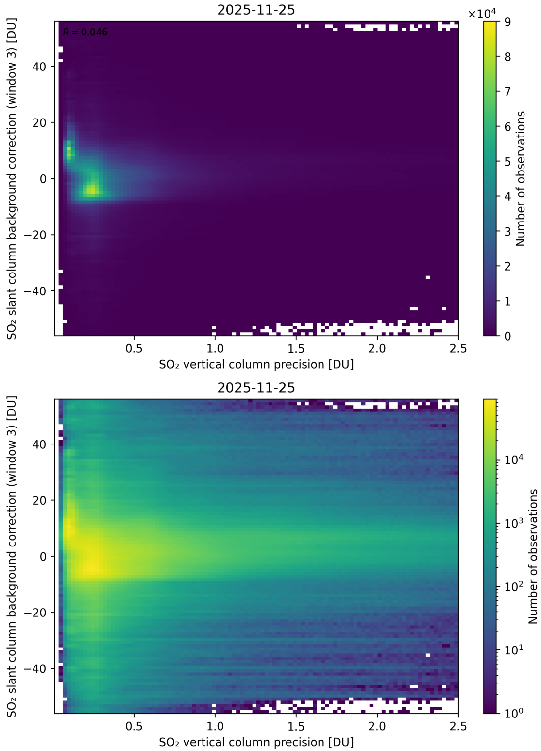
Figure 331: Scatter density plot of “SO 2 vertical column precision” against “SO 2 slant column background correction (window 3)” for 2025-11-24 to 2025-11-26.
