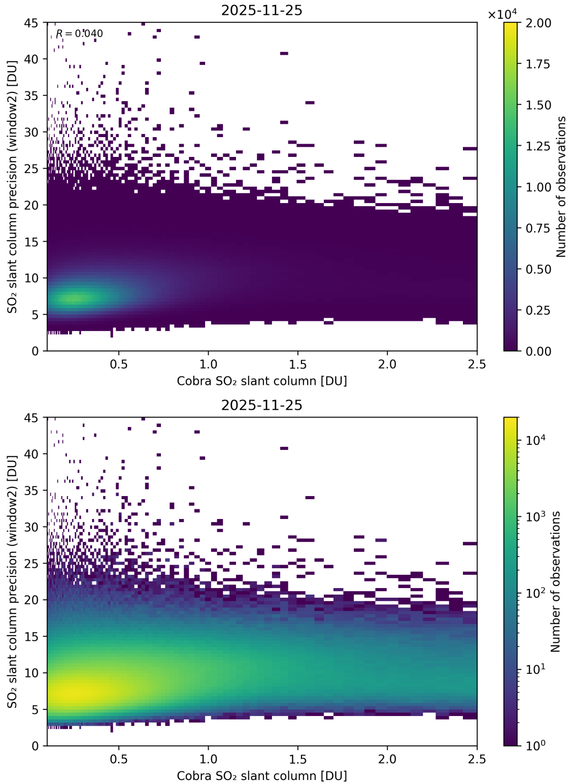
Figure 221: Scatter density plot of “Cobra SO 2 slant column” against “SO 2 slant column precision (window2)” for 2025-11-24 to 2025-11-26.
