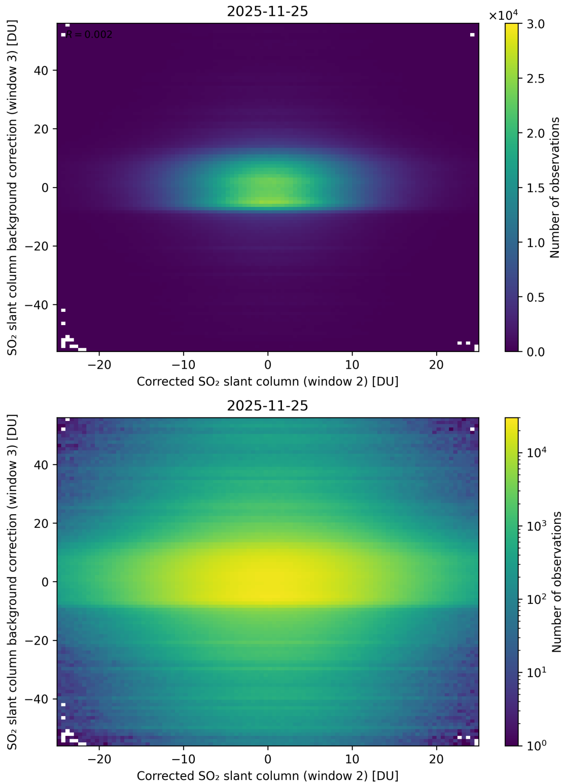
Figure 245: Scatter density plot of “Corrected SO 2 slant column (window 2)” against “SO 2 slant column background correction (window 3)” for 2025-11-24 to 2025-11-26.
