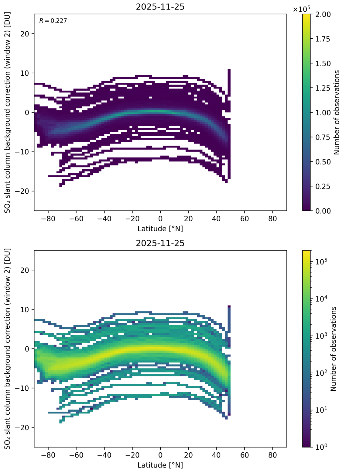
Figure 151: Scatter density plot of “Latitude” against “SO 2 slant column background correction (window 2)” for 2025-11-24 to 2025-11-26.
