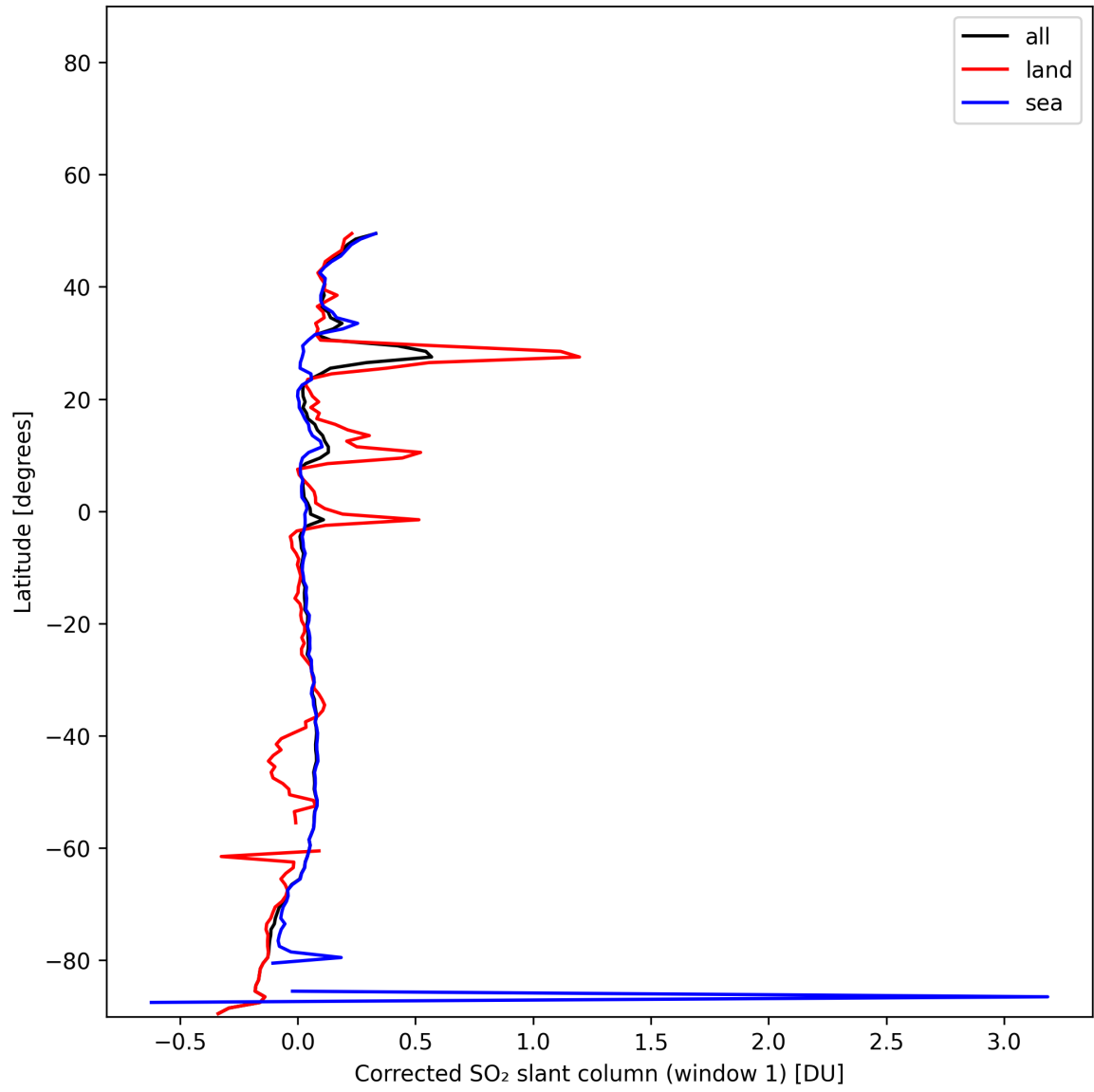
Figure 39: Zonal average of “Corrected SO 2 slant column (window 1)” for 2025-11-24 to 2025-11-26.
