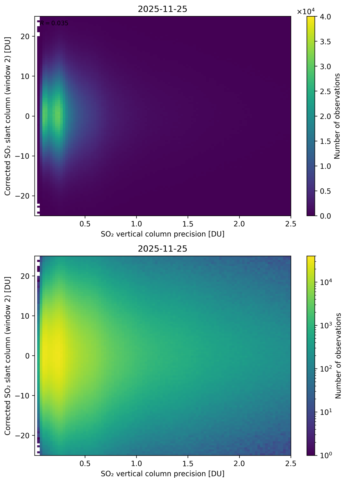
Figure 339: Scatter density plot of “SO 2 vertical column precision” against “Corrected SO 2 slant column (window 2)” for 2025-11-24 to 2025-11-26.
