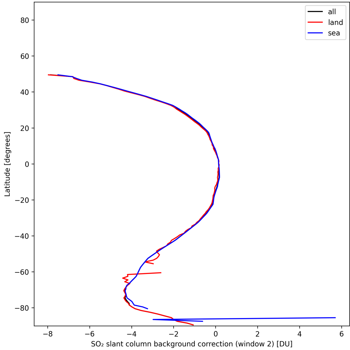
Figure 44: Zonal average of “SO 2 slant column background correction (window 2)” for 2025-11-24 to 2025-11-26.
