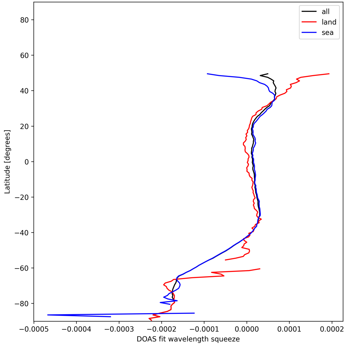
Figure 51: Zonal average of “DOAS fit wavelength squeeze” for 2025-11-24 to 2025-11-26.
