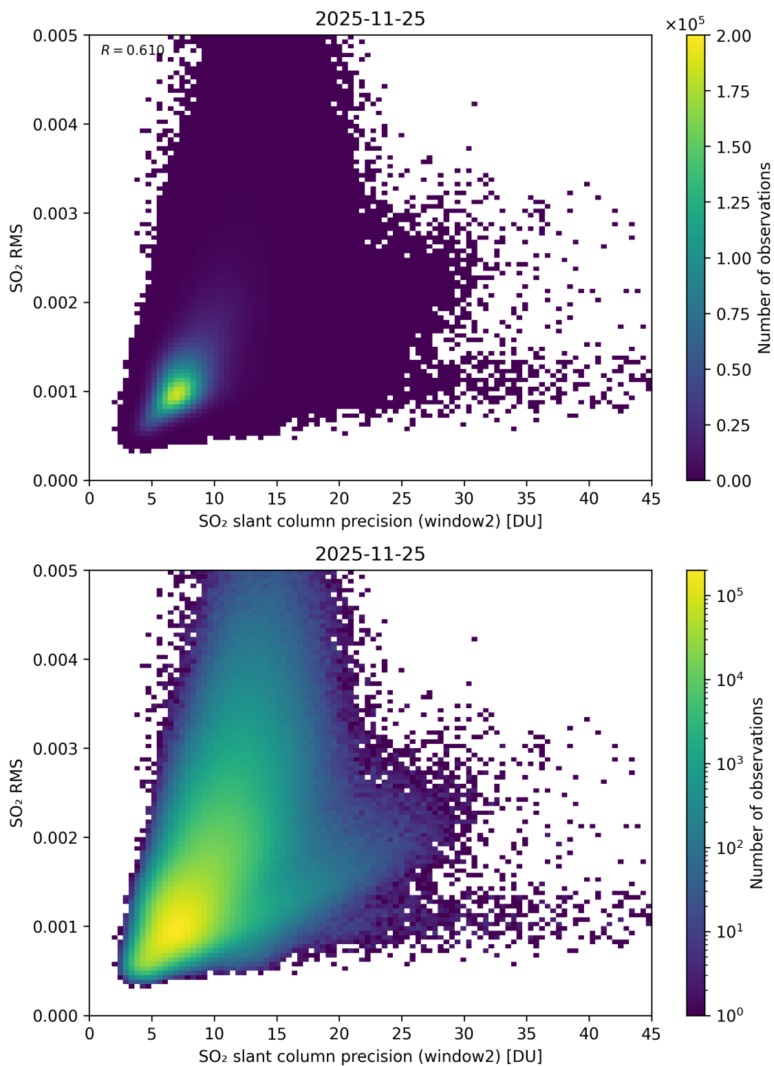
Figure 295: Scatter density plot of “SO 2 slant column precision (window2)” against “SO 2 RMS” for 2025-11-24 to 2025-11-26.
