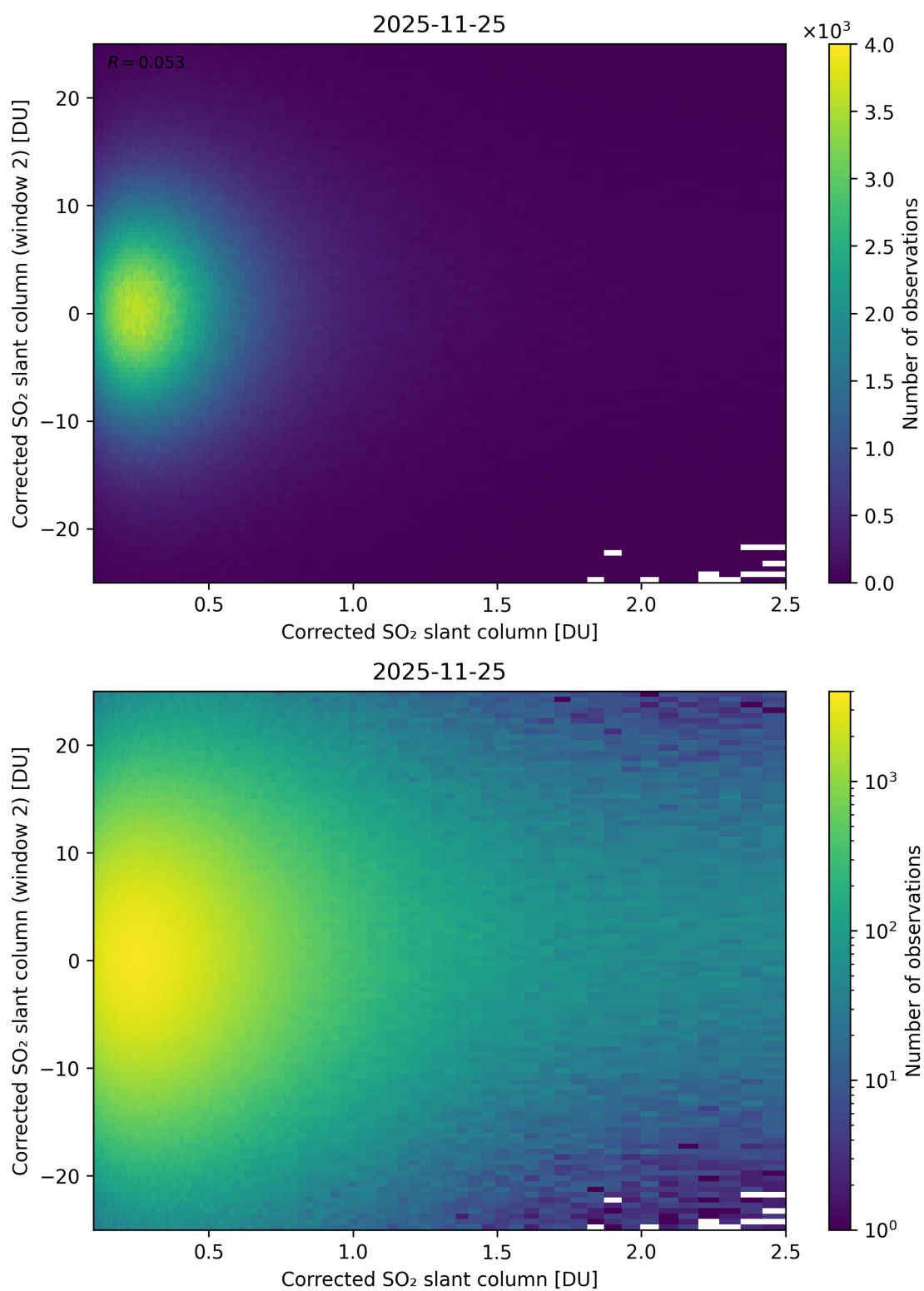
Figure 235: Scatter density plot of “Corrected SO 2 slant column” against “Corrected SO 2 slant column (window 2)” for 2025-11-24 to 2025-11-26.
