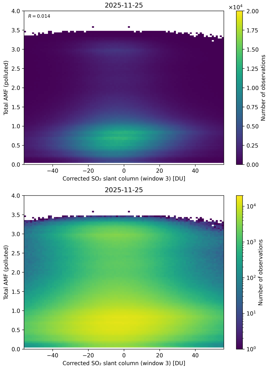
Figure 260: Scatter density plot of “Corrected SO 2 slant column (window 3)” against “Total AMF (polluted)” for 2025-11-24 to 2025-11-26.
