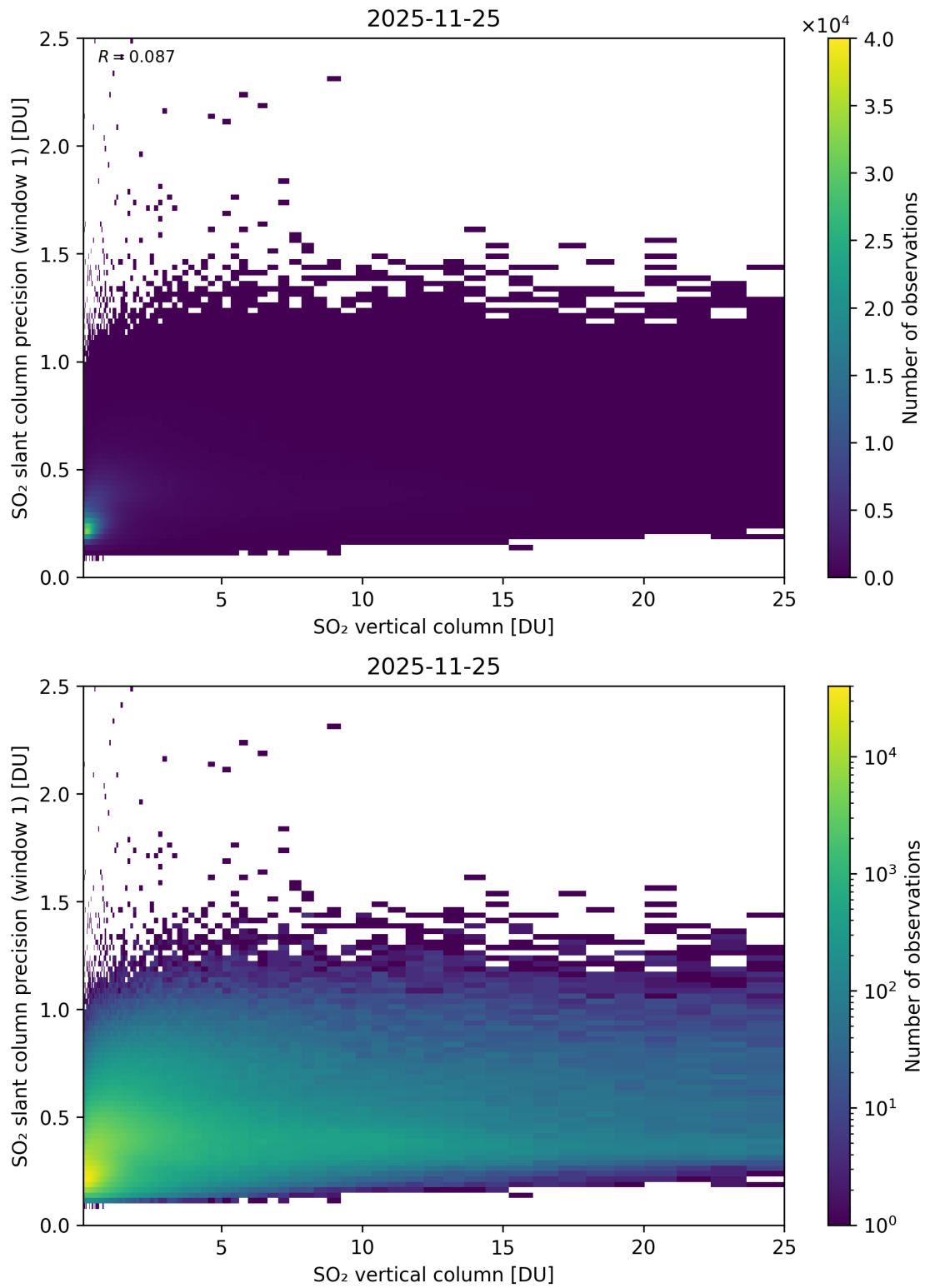
Figure 355: Scatter density plot of “SO 2 vertical column” against “SO 2 slant column precision (window 1)” for 2025-11-24 to 2025-11-26.
