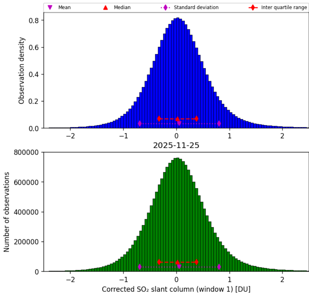
Figure 65: Histogram of “Corrected SO 2 slant column (window 1)” for 2025-11-24 to 2025-11-26
