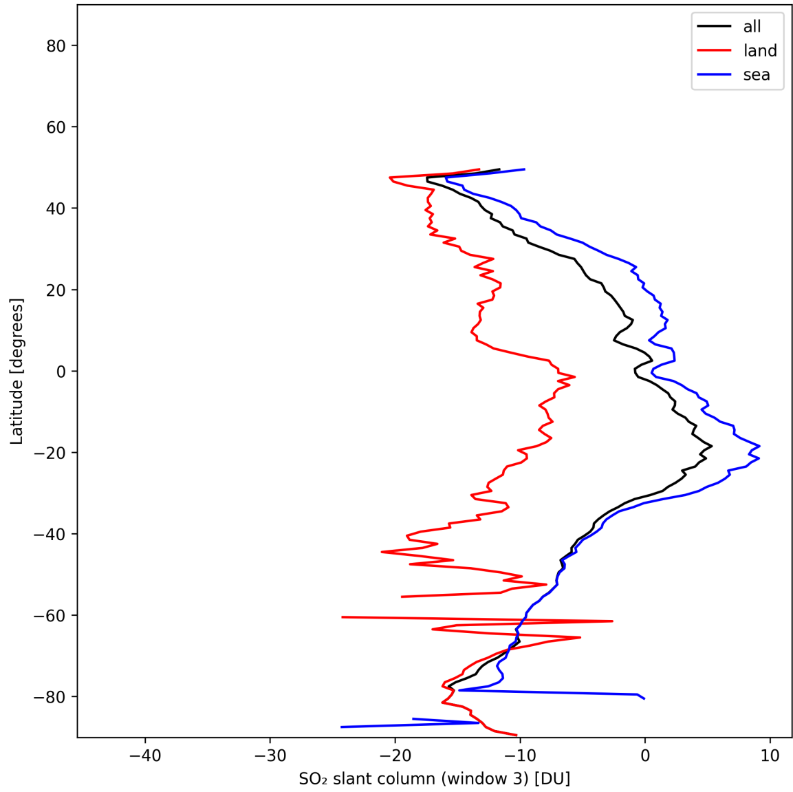
Figure 45: Zonal average of “SO 2 slant column (window 3)” for 2025-11-24 to 2025-11-26.
