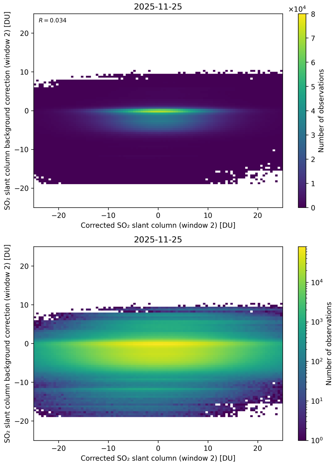
Figure 244: Scatter density plot of “Corrected SO 2 slant column (window 2)” against “SO 2 slant column background correction (window 2)” for 2025-11-24 to 2025-11-26.
