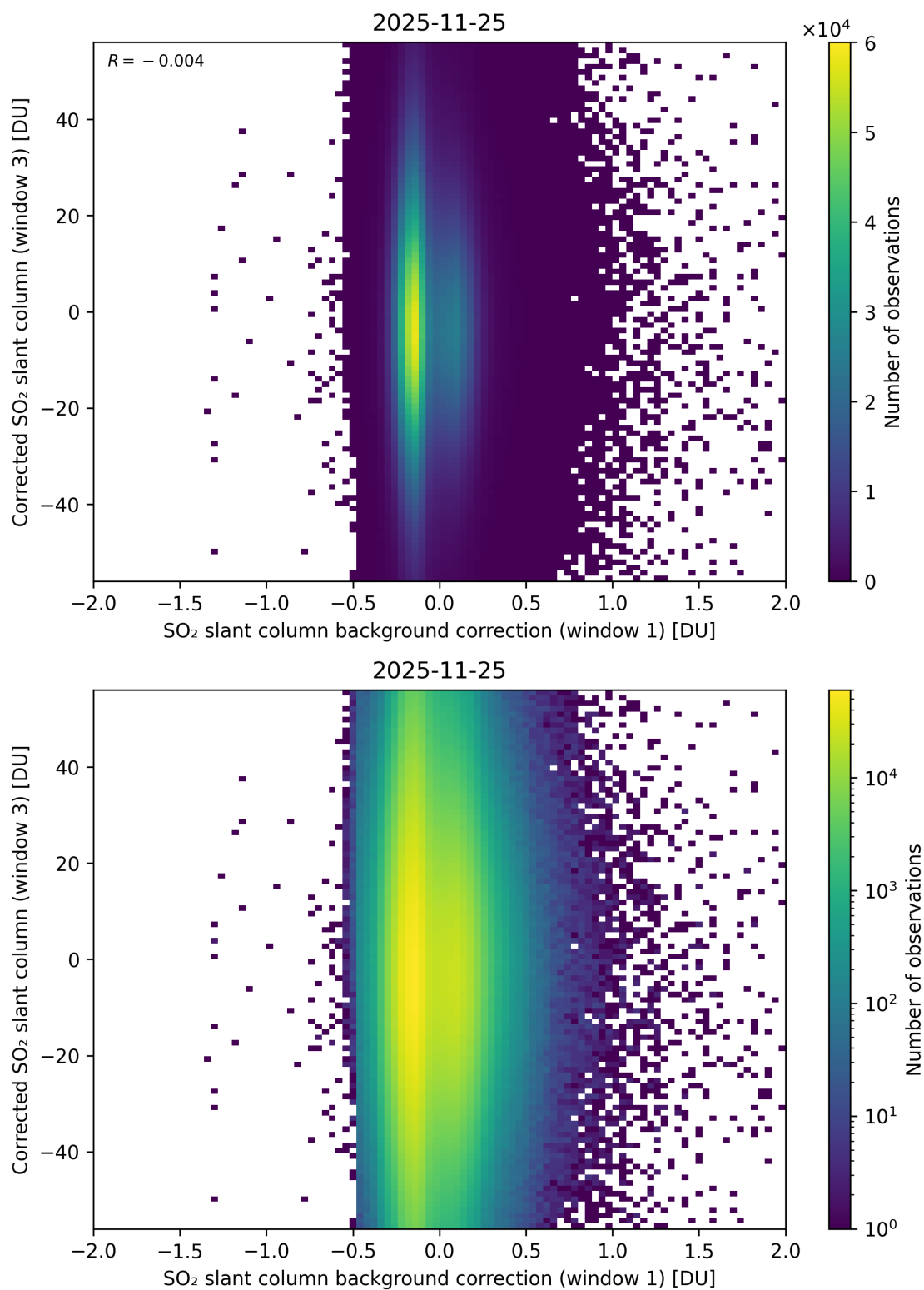
Figure 116: Scatter density plot of “SO 2 slant column background correction (window 1)” against “Corrected SO 2 slant column (window 3)” for 2025-11-24 to 2025-11-26.
