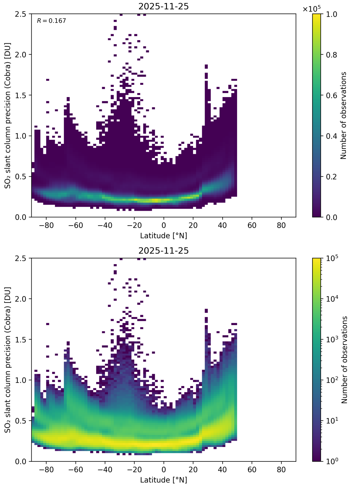
Figure 158: Scatter density plot of “Latitude” against “SO 2 slant column precision (Cobra)” for 2025-11-24 to 2025-11-26.
