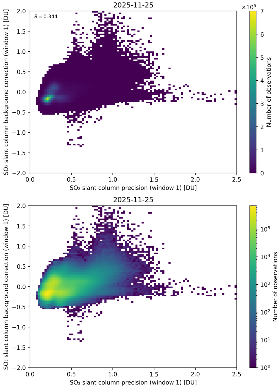
Figure 268: Scatter density plot of “SO 2 slant column precision (window 1)” against “SO 2 slant column background correction (window 1)” for 2025-11-24 to 2025-11-26.
