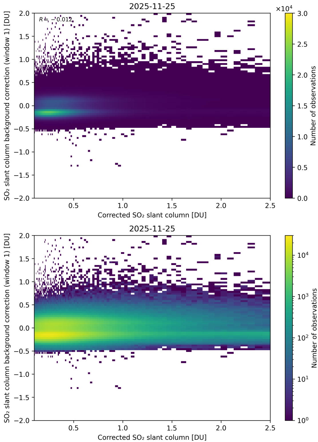
Figure 226: Scatter density plot of “Corrected SO 2 slant column” against “SO 2 slant column background correction (window 1)” for 2025-11-24 to 2025-11-26.
