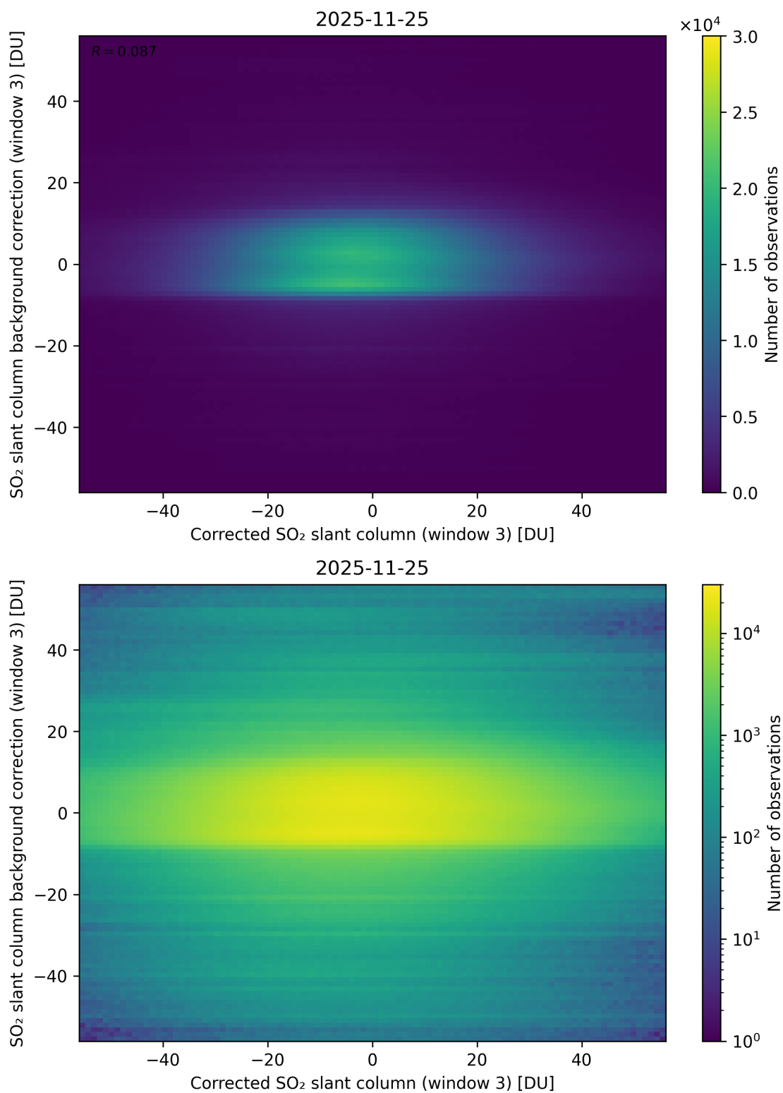
Figure 255: Scatter density plot of “Corrected SO 2 slant column (window 3)” against “SO 2 slant column background correction (window 3)” for 2025-11-24 to 2025-11-26.
