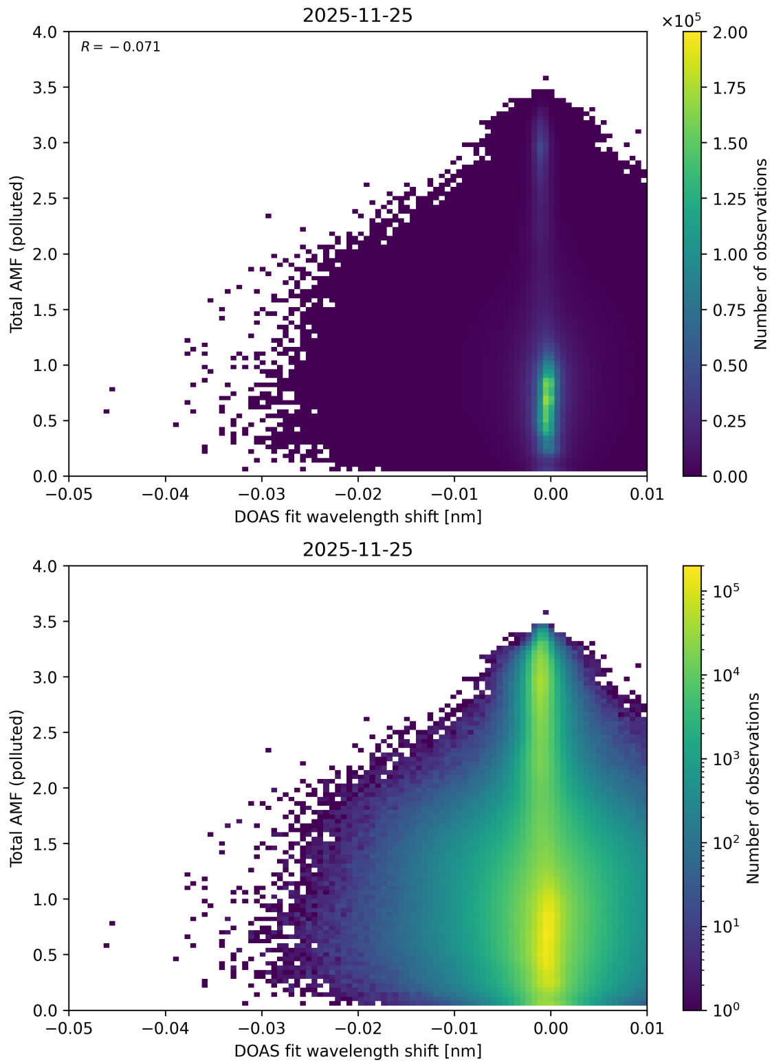
Figure 141: Scatter density plot of “DOAS fit wavelength shift” against “Total AMF (polluted)” for 2025-11-24 to 2025-11-26.
