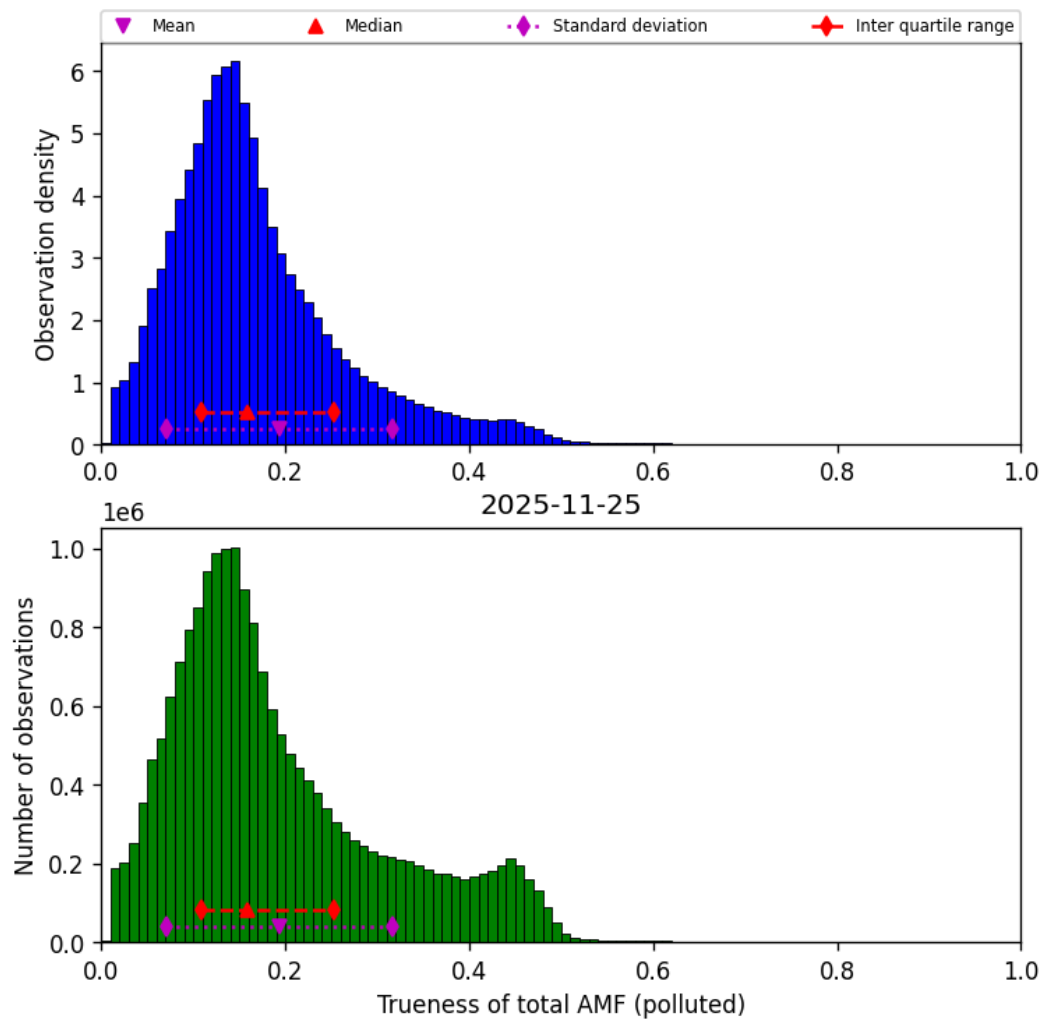
Figure 80: Histogram of “Trueness of total AMF (polluted)” for 2025-11-24 to 2025-11-26
