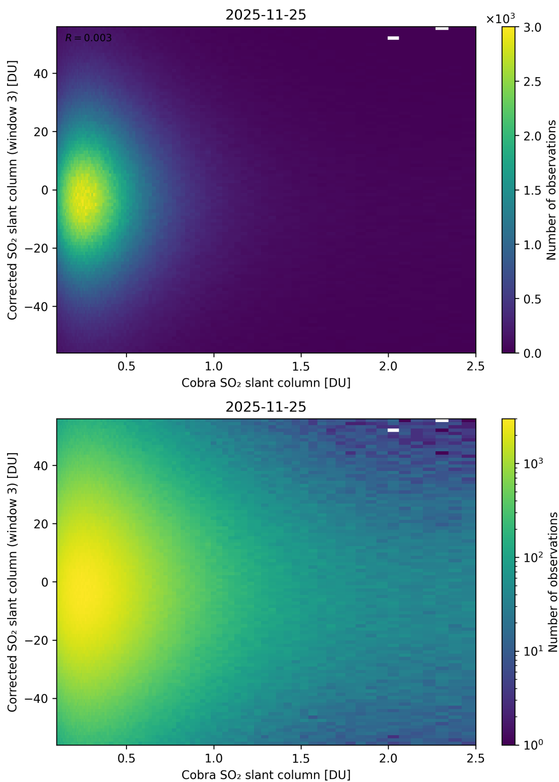
Figure 218: Scatter density plot of “Cobra SO 2 slant column” against “Corrected SO 2 slant column (window 3)” for 2025-11-24 to 2025-11-26.
