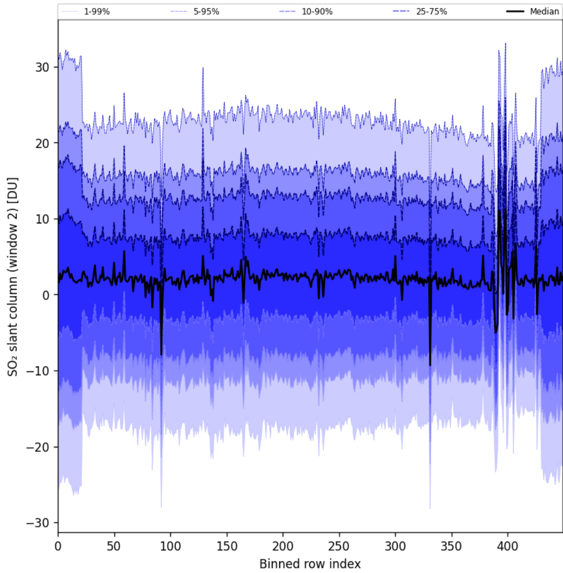
Figure 93: Along track statistics of “SO 2 slant column (window 2)” for 2025-11-24 to 2025-11-26
