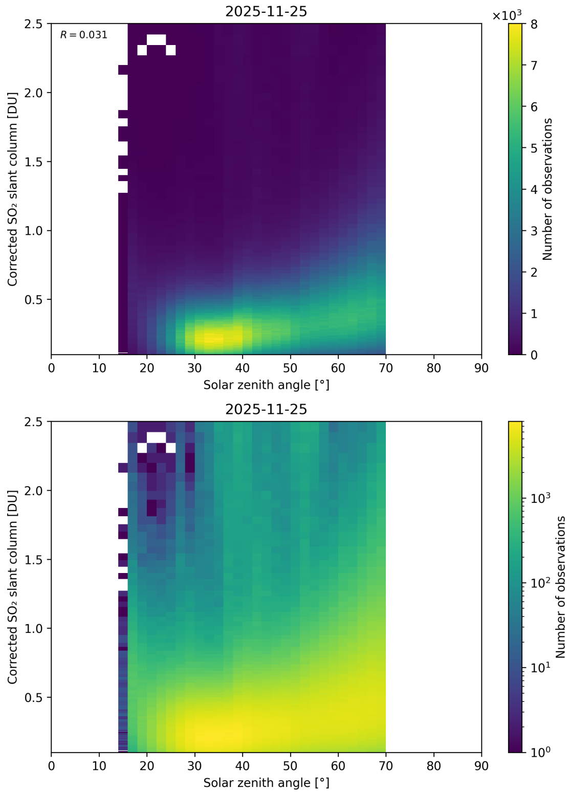
Figure 181: Scatter density plot of “Solar zenith angle” against “Corrected SO 2 slant column” for 2025-11-24 to 2025-11-26.
