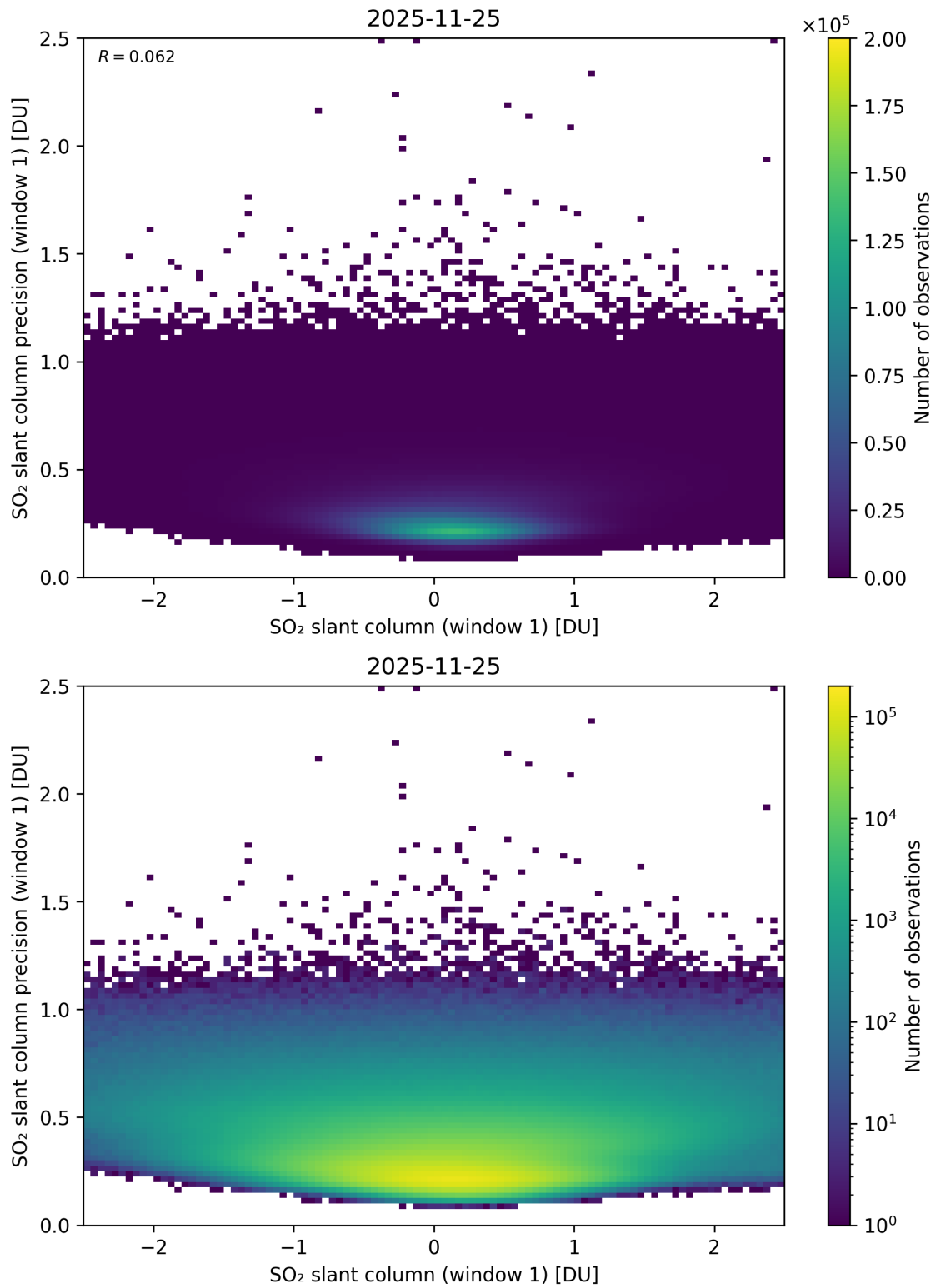
Figure 285: Scatter density plot of “SO 2 slant column (window 1)” against “SO 2 slant column precision (window 1)” for 2025-11-24 to 2025-11-26.
