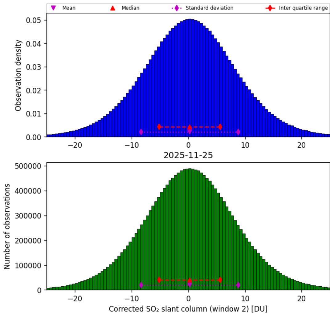
Figure 69: Histogram of “Corrected SO 2 slant column (window 2)” for 2025-11-24 to 2025-11-26
