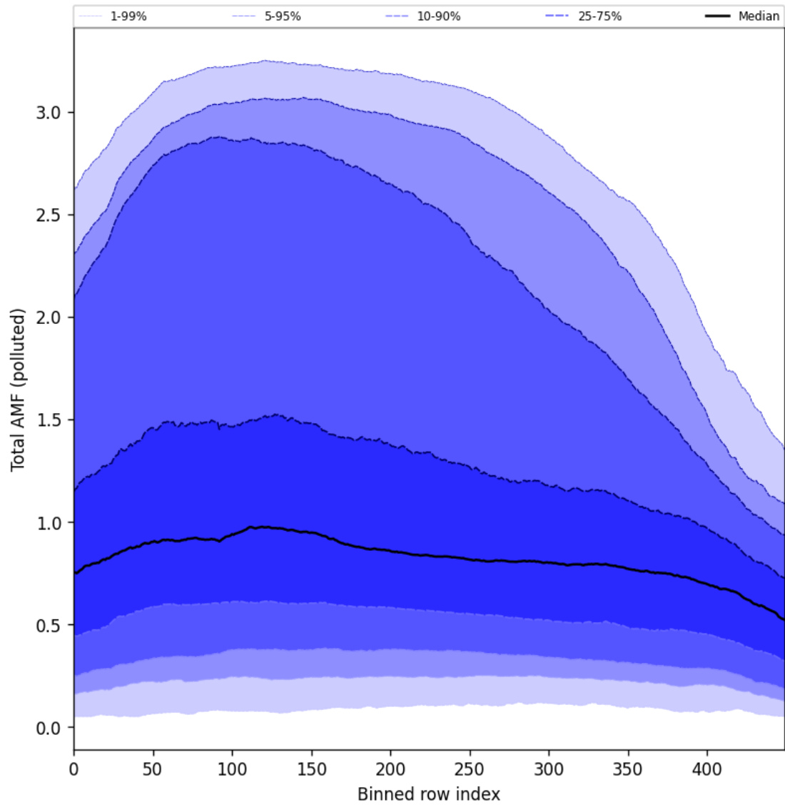
Figure 105: Along track statistics of “Total AMF (polluted)” for 2025-11-24 to 2025-11-26
