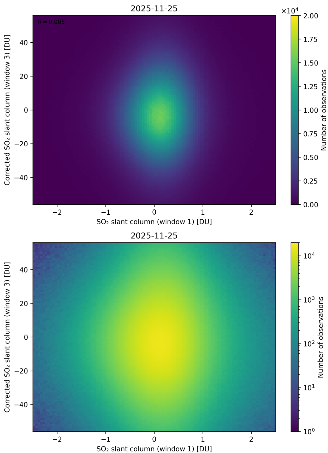
Figure 284: Scatter density plot of “SO 2 slant column (window 1)” against “Corrected SO 2 slant column (window 3)” for 2025-11-24 to 2025-11-26.
