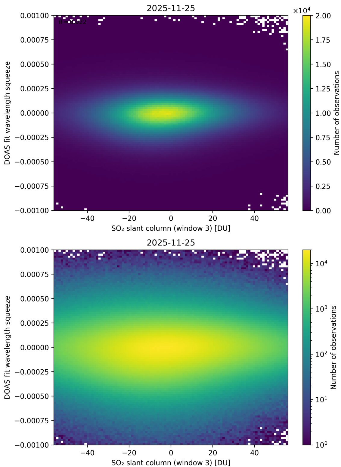
Figure 305: Scatter density plot of “SO 2 slant column (window 3)” against “DOAS fit wavelength squeeze” for 2025-11-24 to 2025-11-26.
