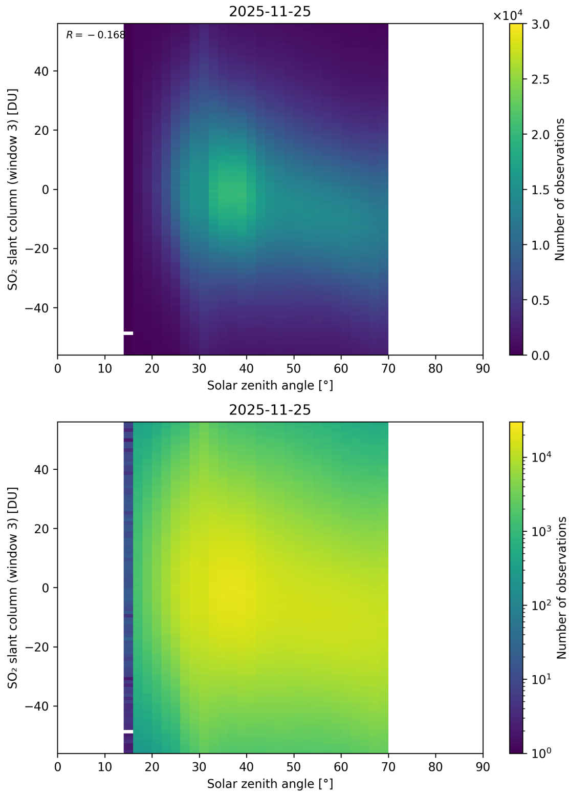
Figure 187: Scatter density plot of “Solar zenith angle” against “SO 2 slant column (window 3)” for 2025-11-24 to 2025-11-26.
