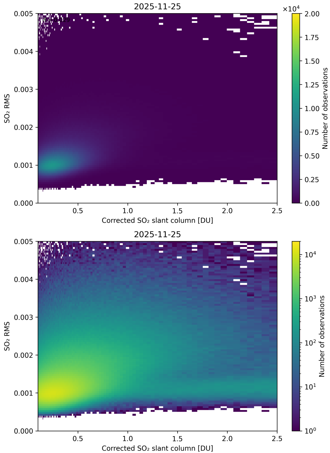
Figure 231: Scatter density plot of “Corrected SO 2 slant column” against “SO 2 RMS” for 2025-11-24 to 2025-11-26.
