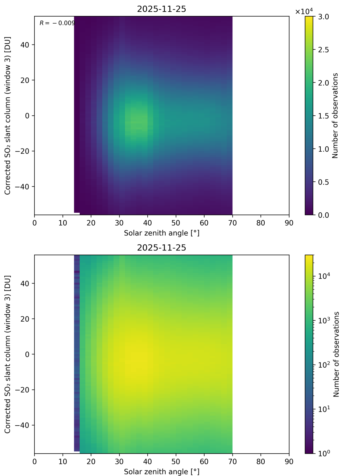
Figure 183: Scatter density plot of “Solar zenith angle” against “Corrected SO 2 slant column (window 3)” for 2025-11-24 to 2025-11-26.
