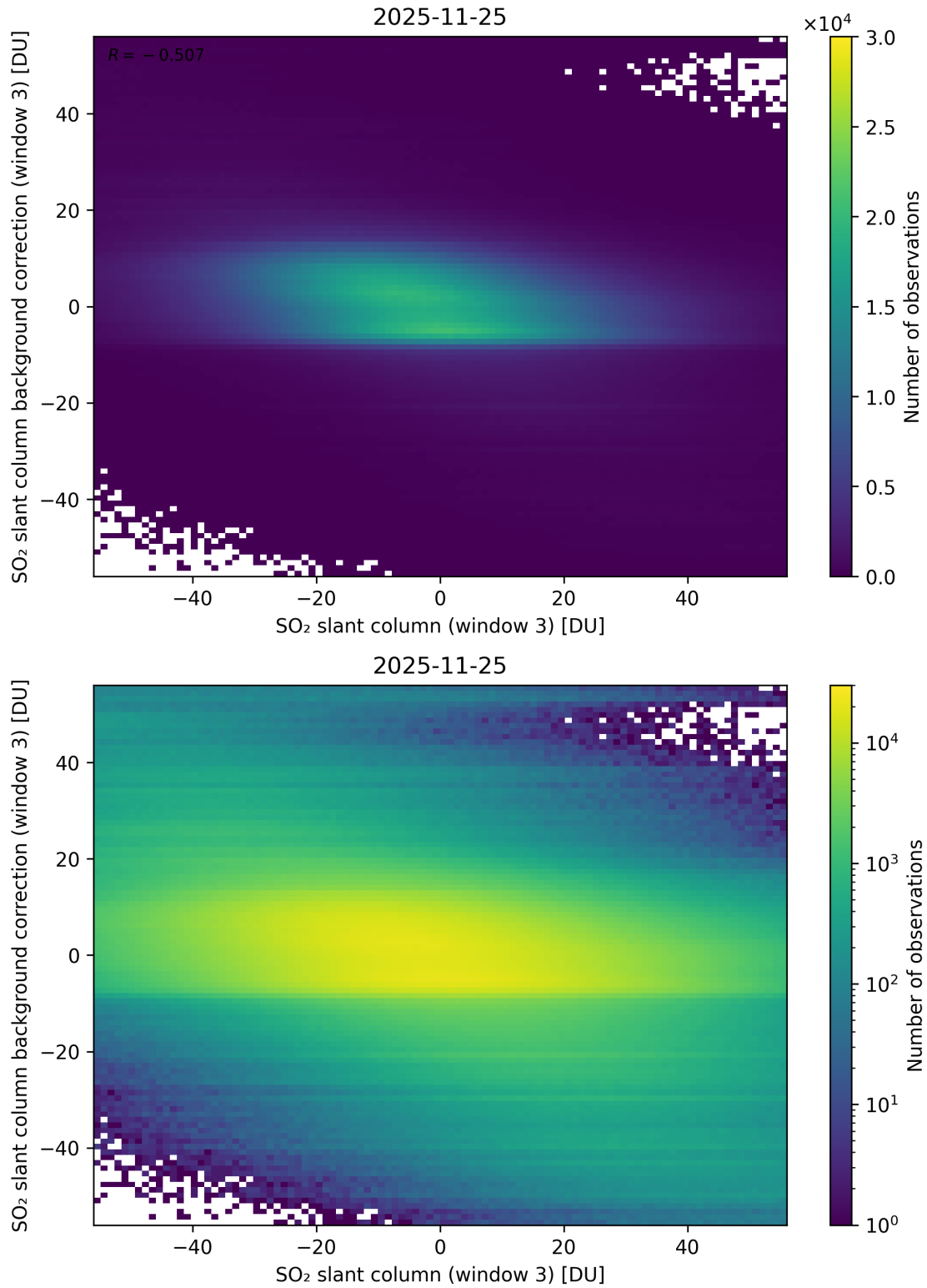
Figure 303: Scatter density plot of “SO 2 slant column (window 3)” against “SO 2 slant column background correction (window 3)” for 2025-11-24 to 2025-11-26.
