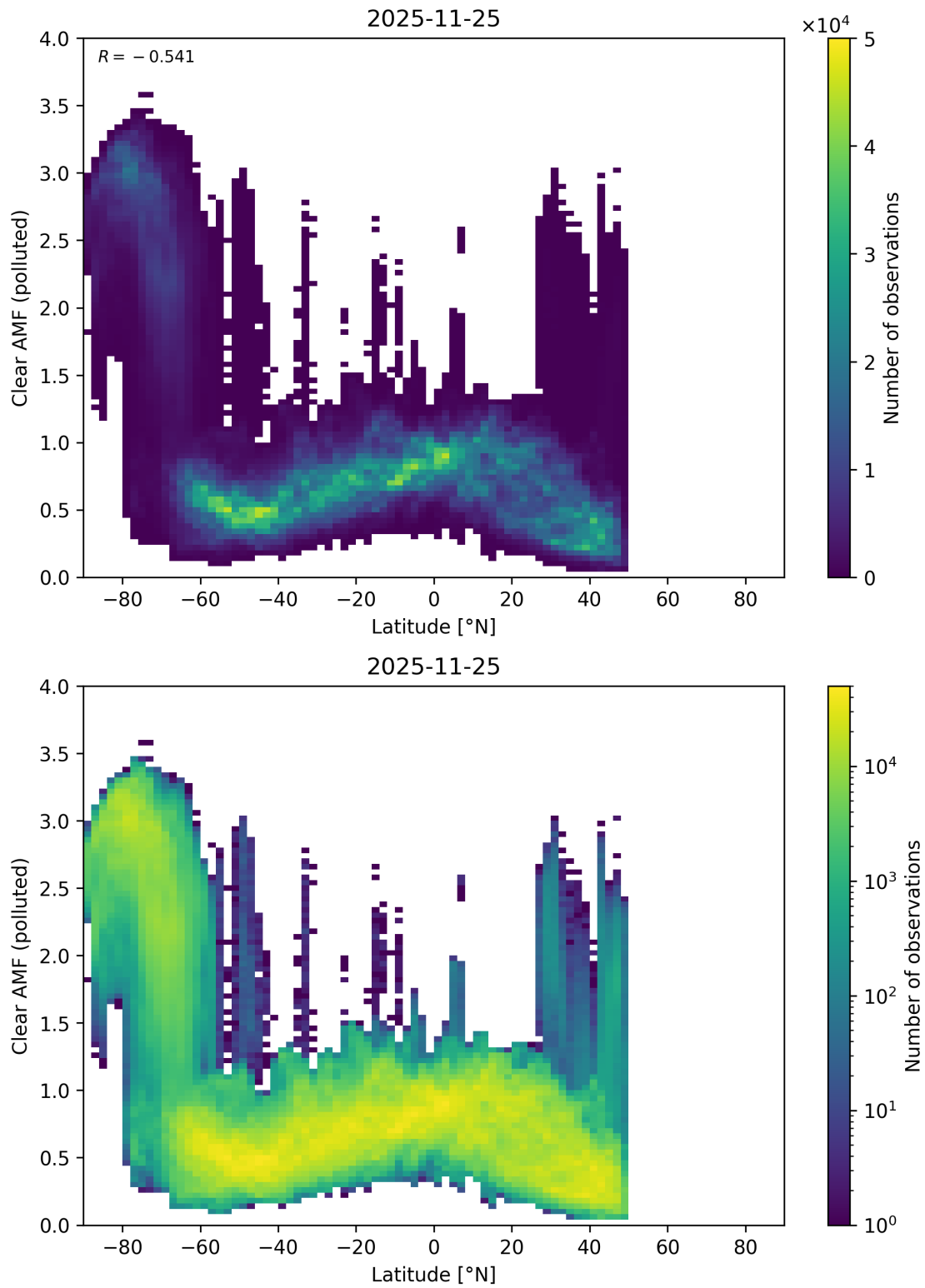
Figure 156: Scatter density plot of “Latitude” against “Clear AMF (polluted)” for 2025-11-24 to 2025-11-26.
