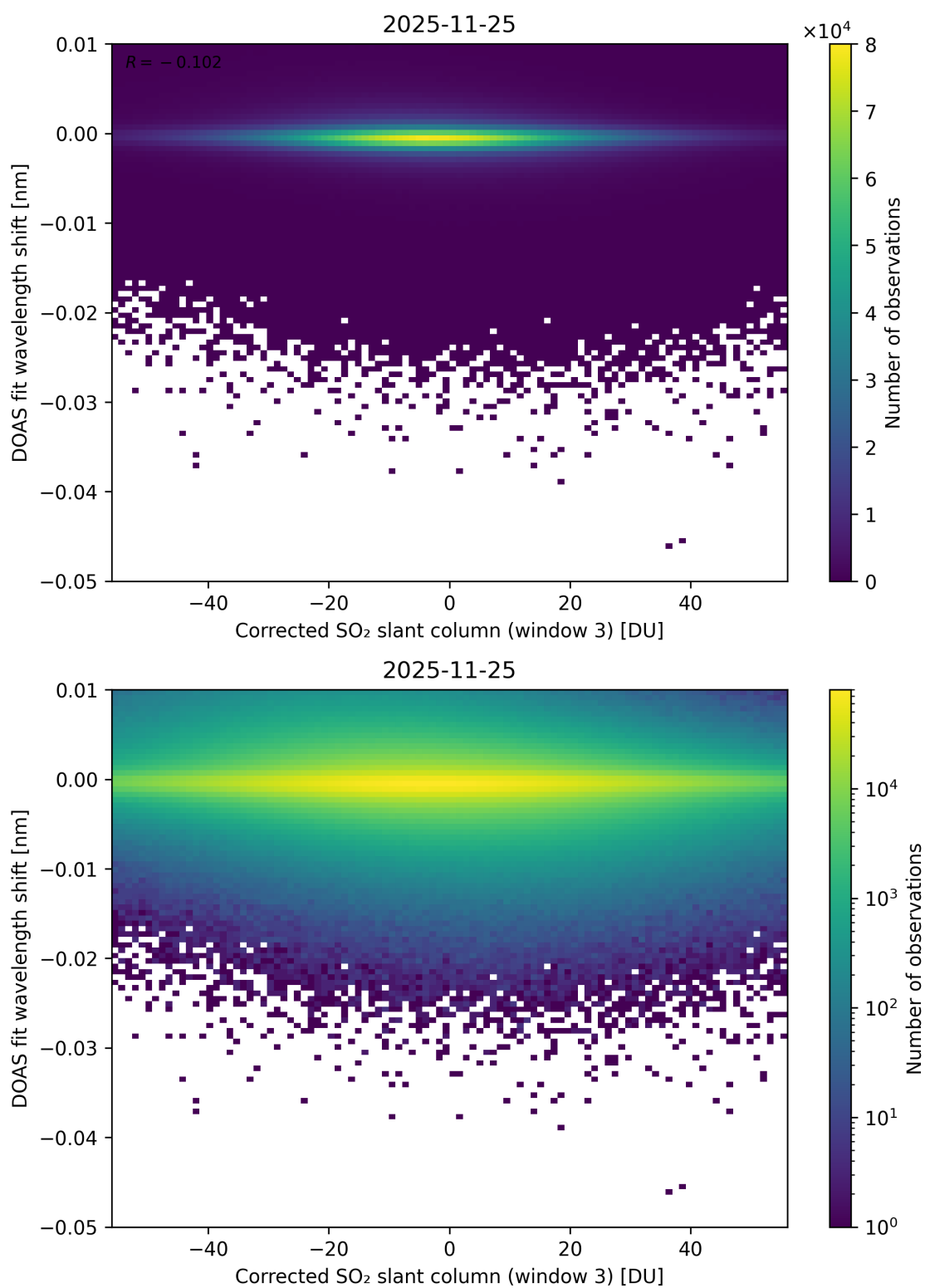
Figure 256: Scatter density plot of “Corrected SO 2 slant column (window 3)” against “DOAS fit wavelength shift” for 2025-11-24 to 2025-11-26.
