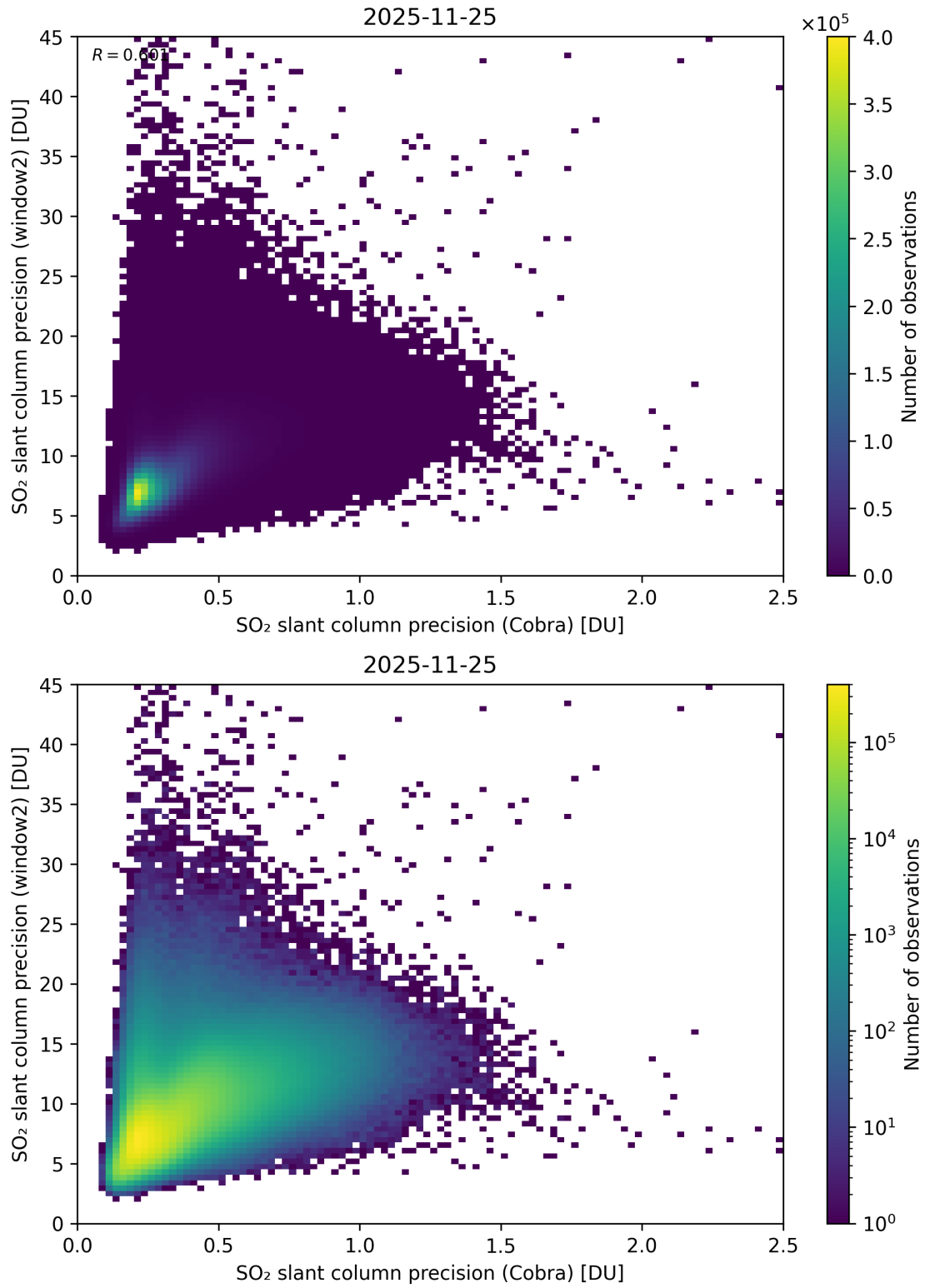
Figure 210: Scatter density plot of “SO 2 slant column precision (Cobra)” against “SO 2 slant column precision (window2)” for 2025-11-24 to 2025-11-26.
