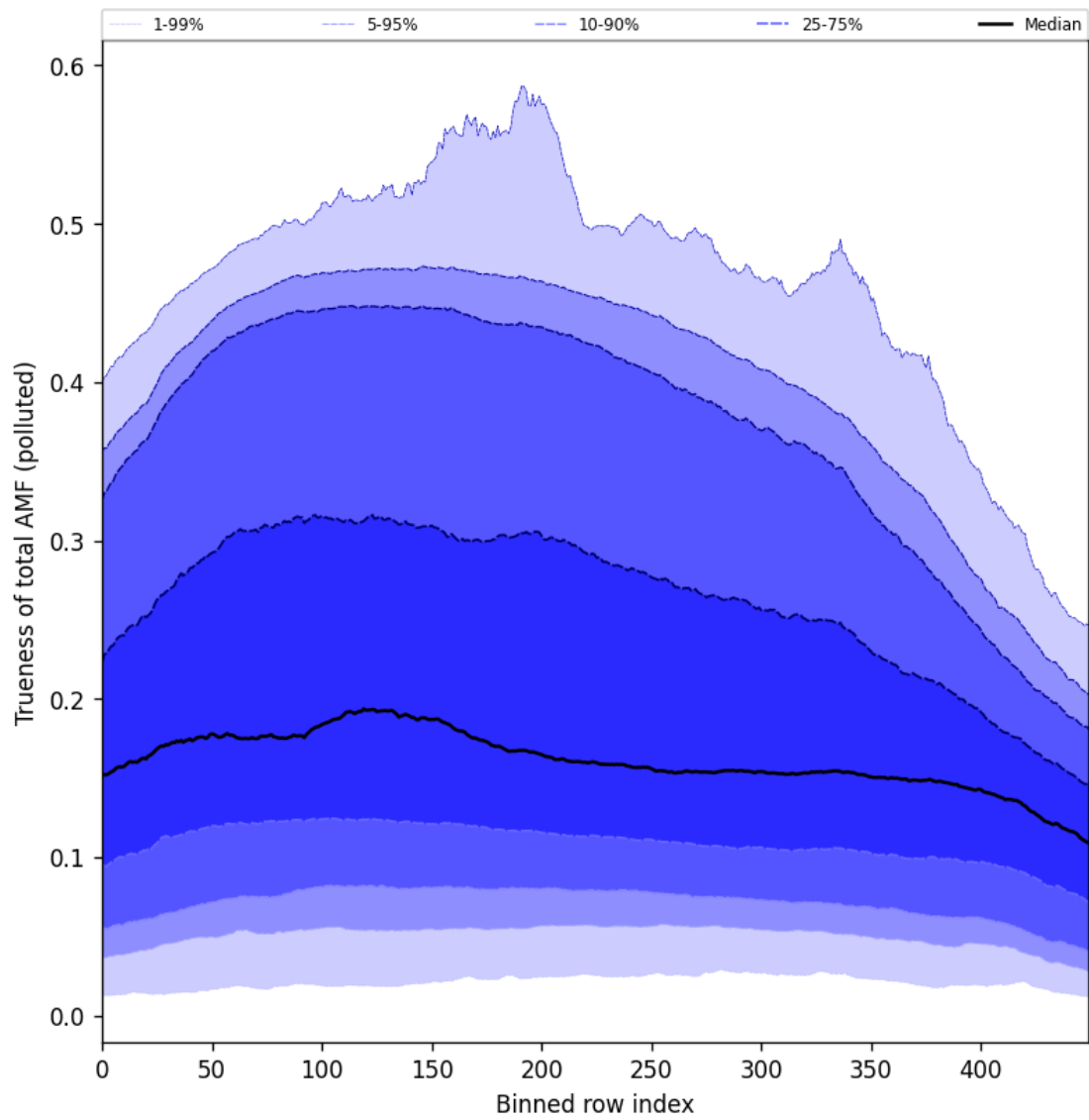
Figure 106: Along track statistics of “Trueness of total AMF (polluted)” for 2025-11-24 to 2025-11-26
