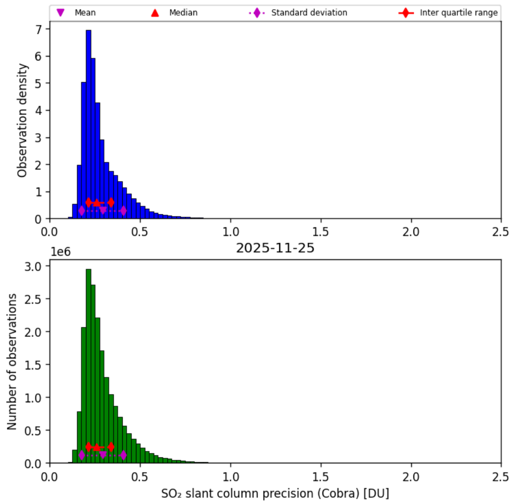
Figure 62: Histogram of “SO 2 slant column precision (Cobra)” for 2025-11-24 to 2025-11-26
