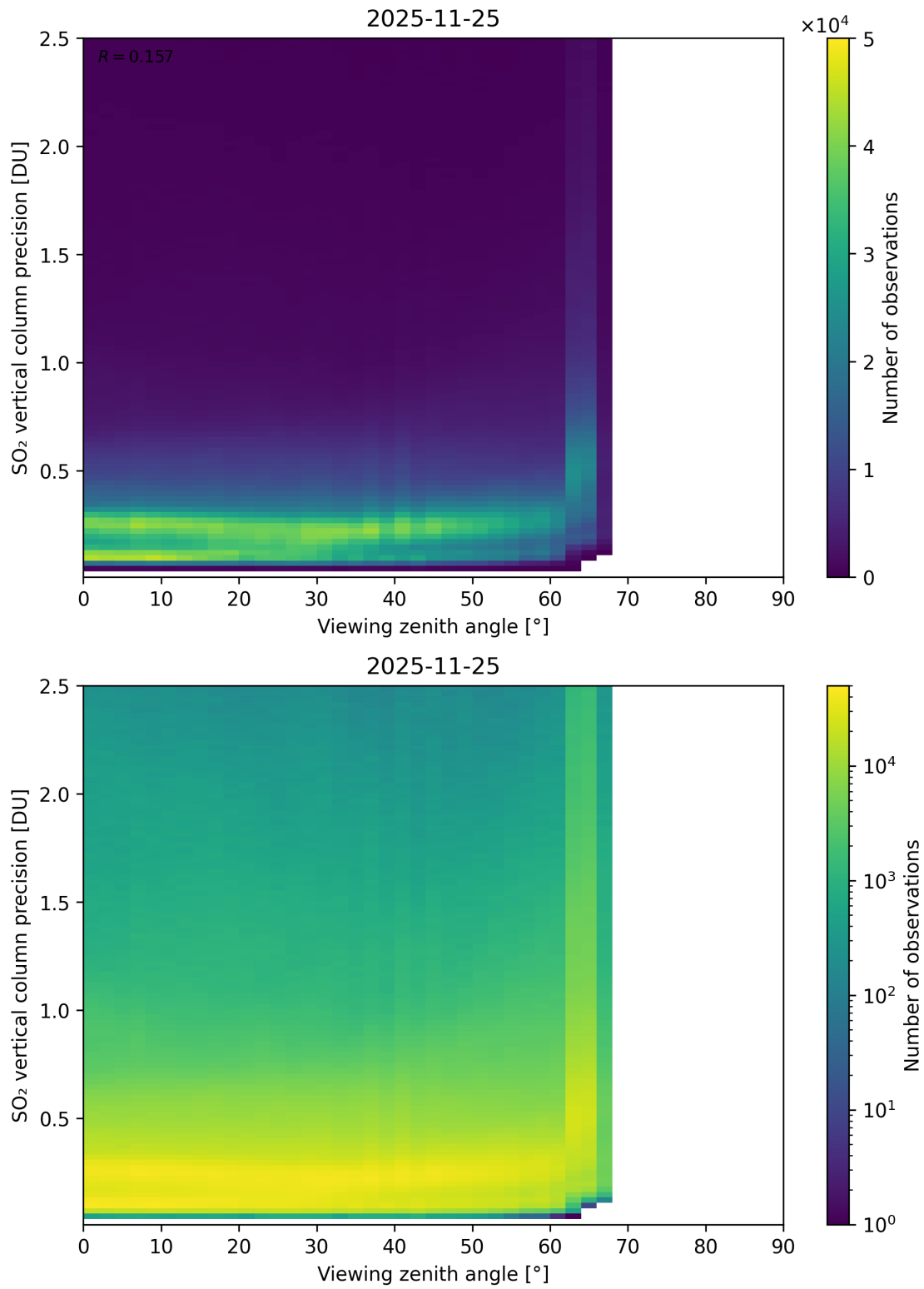
Figure 384: Scatter density plot of “Viewing zenith angle” against “SO 2 vertical column precision” for 2025-11-24 to 2025-11-26.
