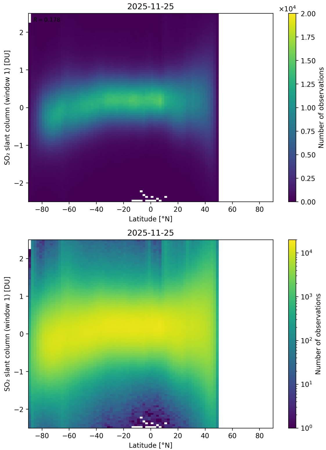
Figure 162: Scatter density plot of “Latitude” against “SO 2 slant column (window 1)” for 2025-11-24 to 2025-11-26.
