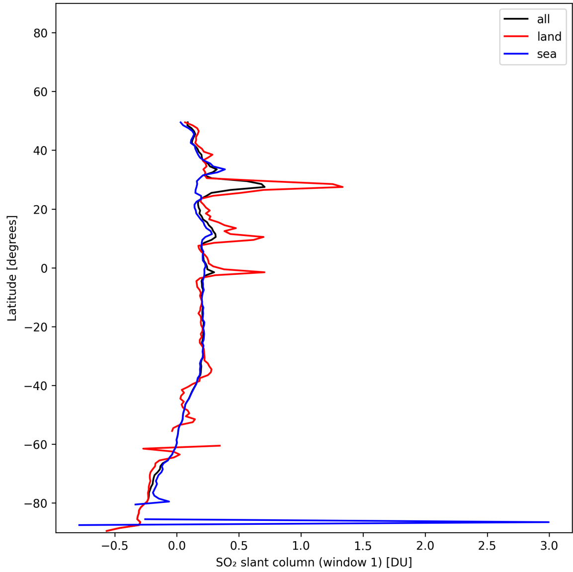
Figure 37: Zonal average of “SO 2 slant column (window 1)” for 2025-11-24 to 2025-11-26.
