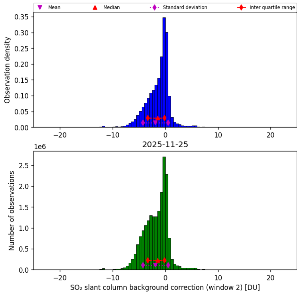
Figure 70: Histogram of “SO 2 slant column background correction (window 2)” for 2025-11-24 to 2025-11-26
