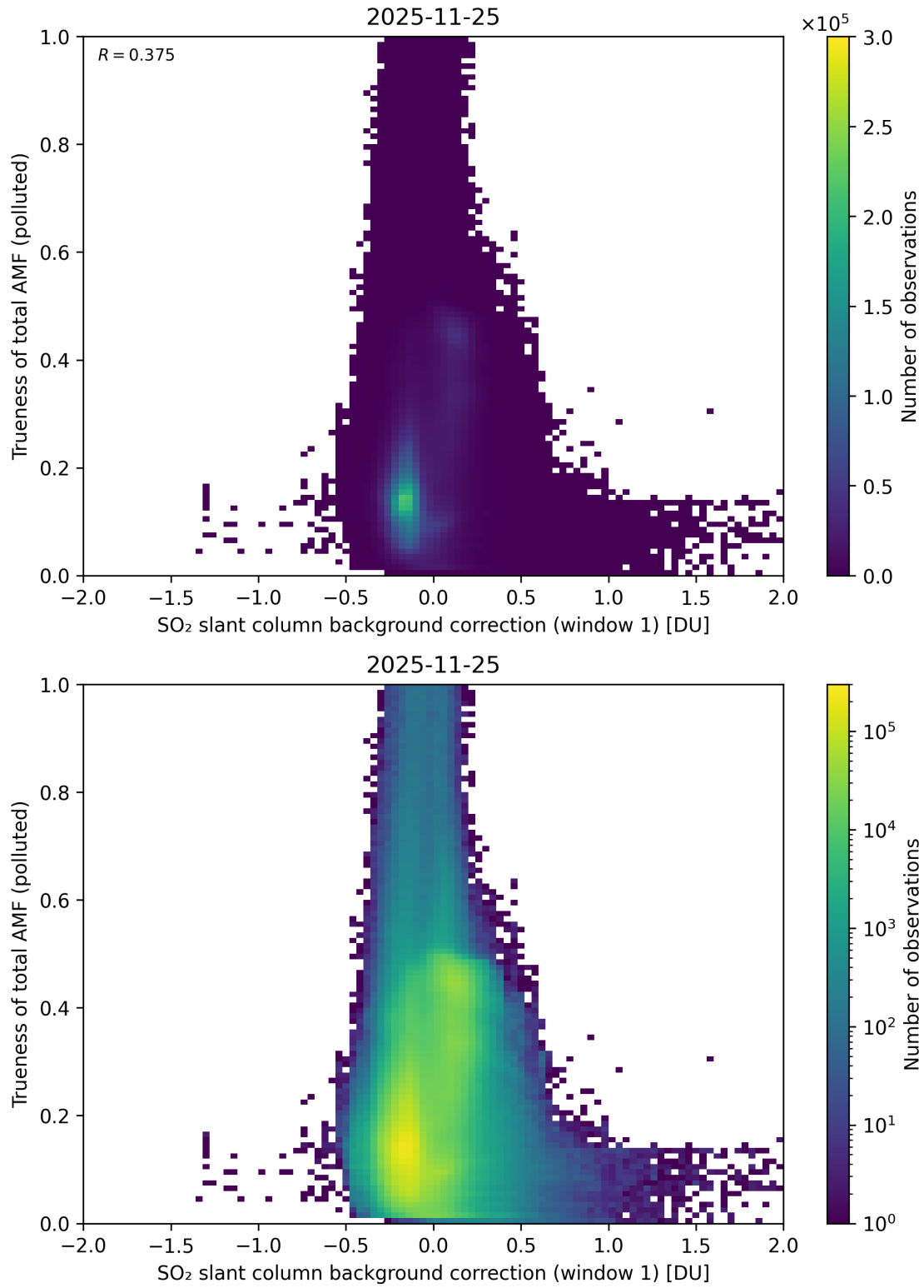
Figure 121: Scatter density plot of “SO 2 slant column background correction (window 1)” against “Trueness of total AMF (polluted)” for 2025-11-24 to 2025-11-26.
