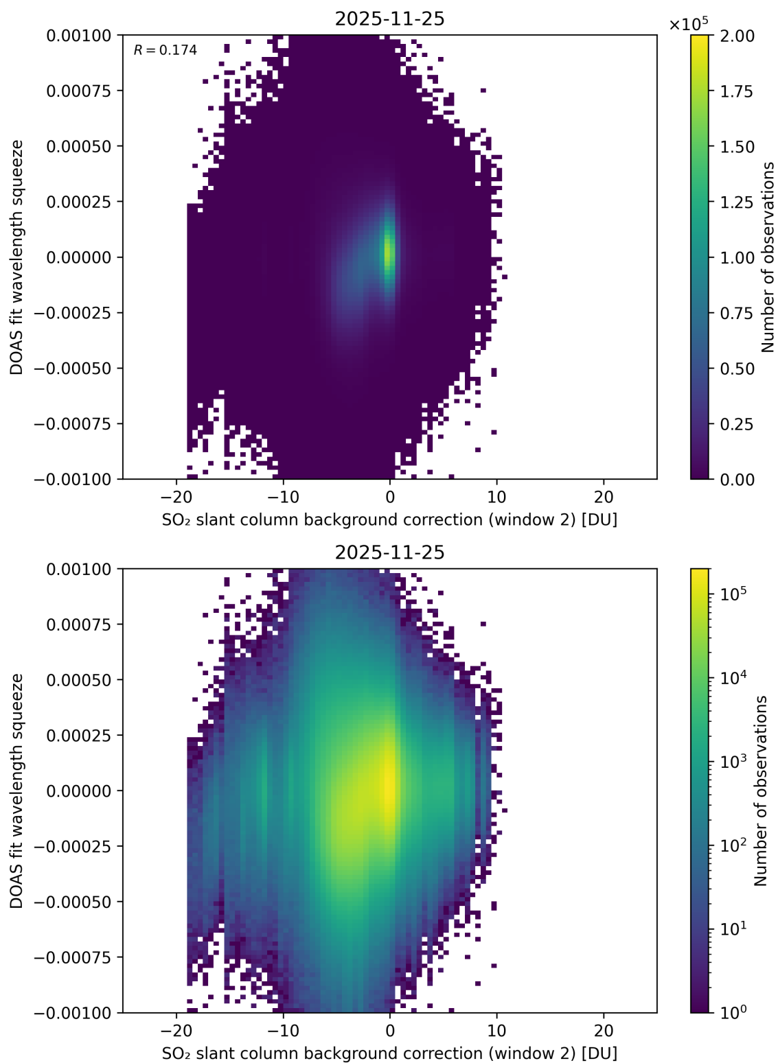
Figure 124: Scatter density plot of “SO 2 slant column background correction (window 2)” against “DOAS fit wavelength squeeze” for 2025-11-24 to 2025-11-26.
