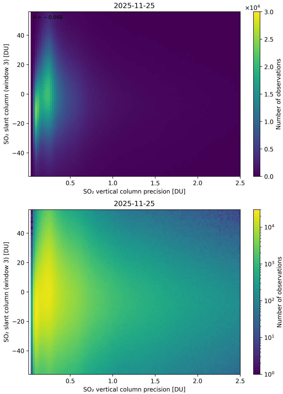
Figure 344: Scatter density plot of “SO 2 vertical column precision” against “SO 2 slant column (window 3)” for 2025-11-24 to 2025-11-26.
