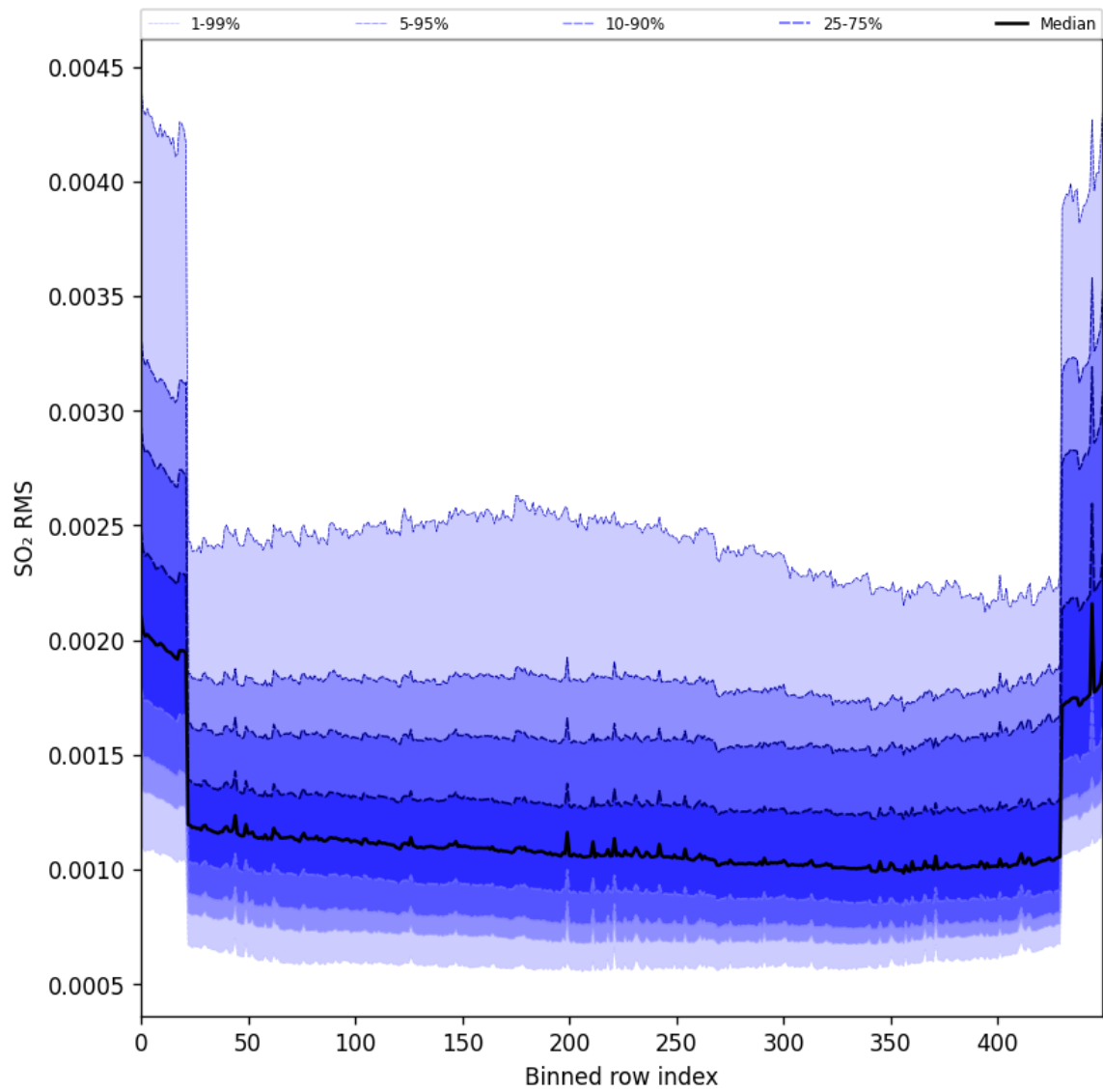
Figure 104: Along track statistics of “SO 2 RMS” for 2025-11-24 to 2025-11-26
