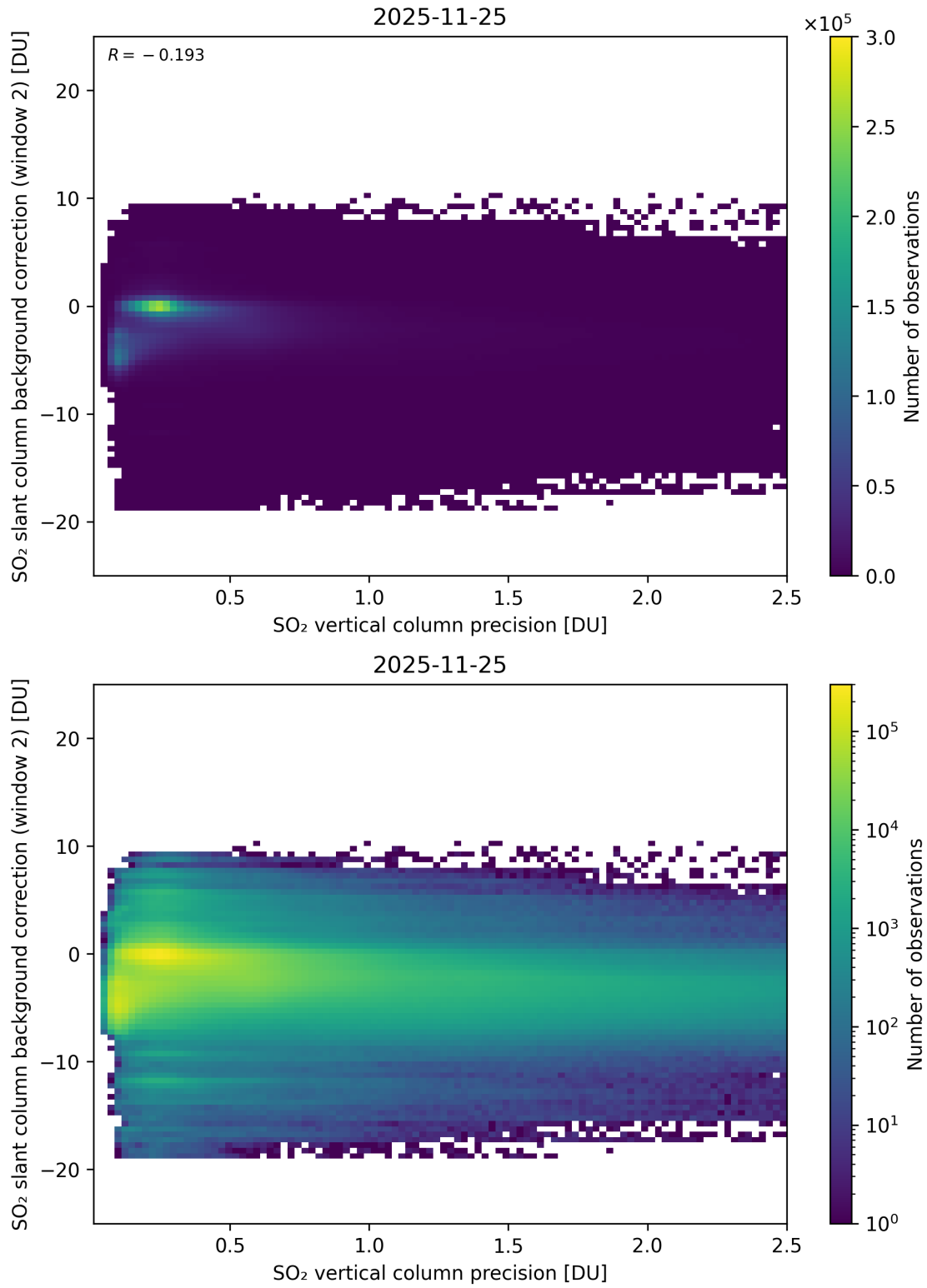
Figure 330: Scatter density plot of “SO 2 vertical column precision” against “SO 2 slant column background correction (window 2)” for 2025-11-24 to 2025-11-26.
