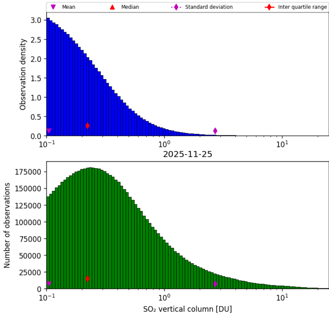
Figure 58: Histogram of "SO 2 vertical column" for 2025-11-24 to 2025-11-26
