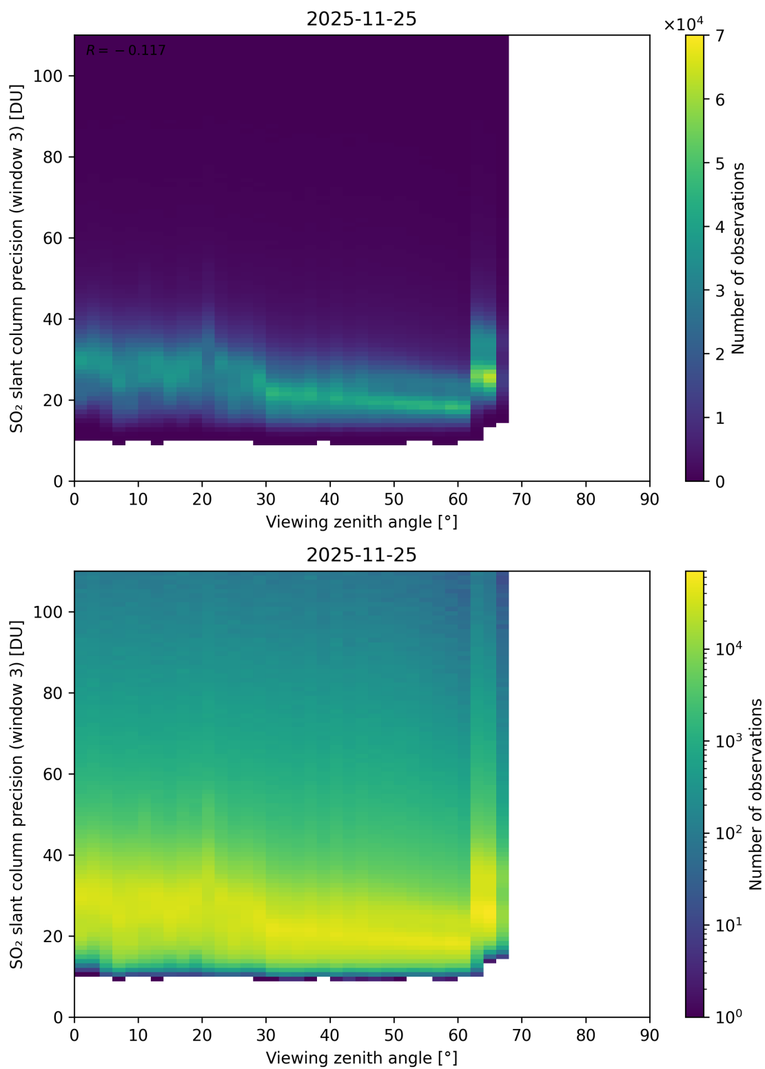
Figure 380: Scatter density plot of “Viewing zenith angle” against “SO 2 slant column precision (window 3)” for 2025-11-24 to 2025-11-26.
