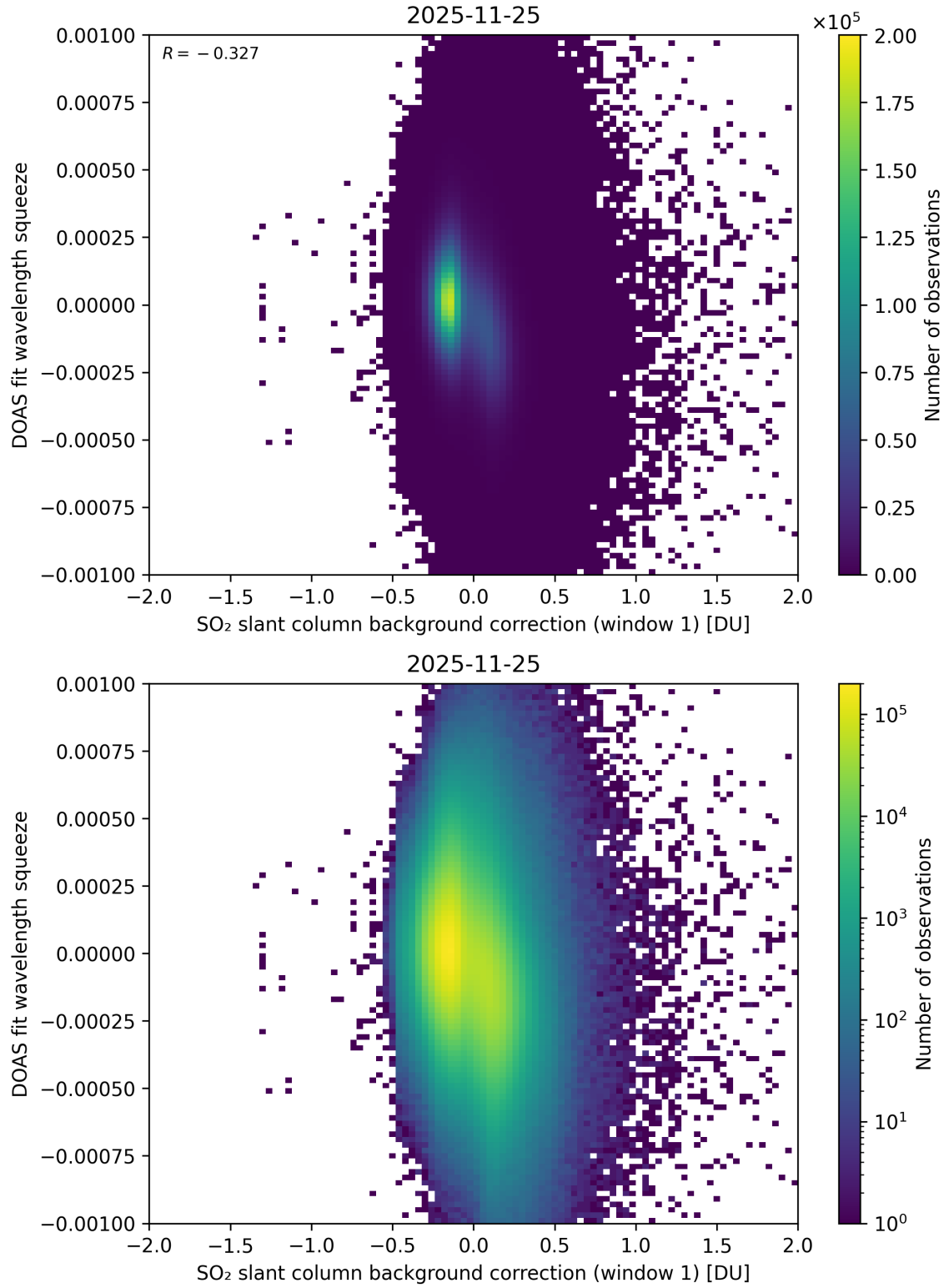
Figure 112: Scatter density plot of “SO 2 slant column background correction (window 1)” against “DOAS fit wavelength squeeze” for 2025-11-24 to 2025-11-26.
