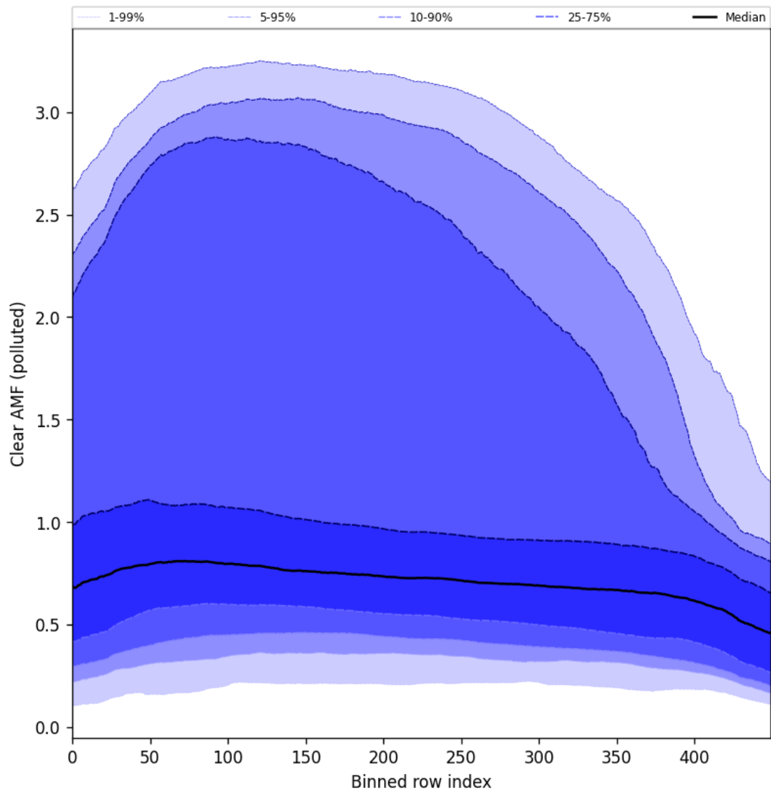
Figure 107: Along track statistics of “Clear AMF (polluted)” for 2025-11-24 to 2025-11-26
