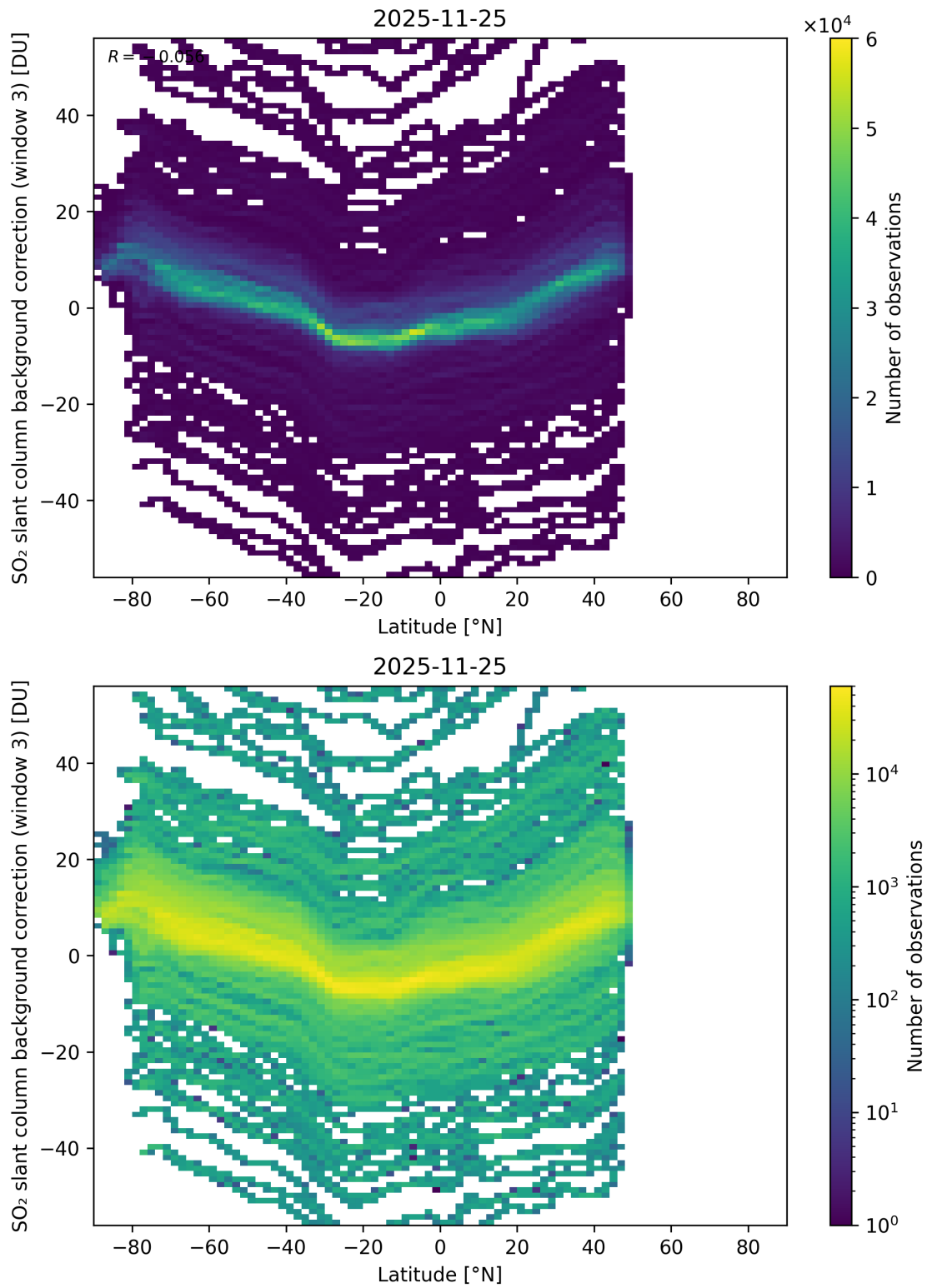
Figure 152: Scatter density plot of “Latitude” against “SO 2 slant column background correction (window 3)” for 2025-11-24 to 2025-11-26.
