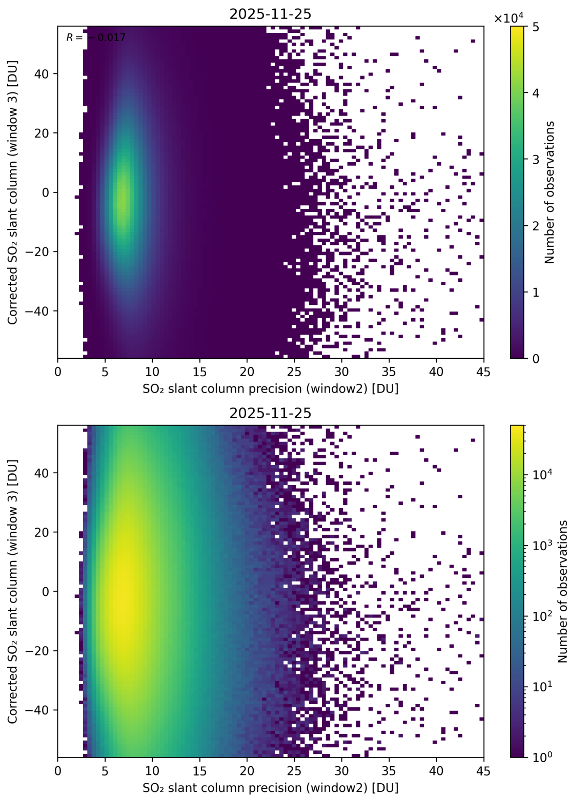
Figure 298: Scatter density plot of “SO 2 slant column precision (window2)” against “Corrected SO 2 slant column (window 3)” for 2025-11-24 to 2025-11-26.
