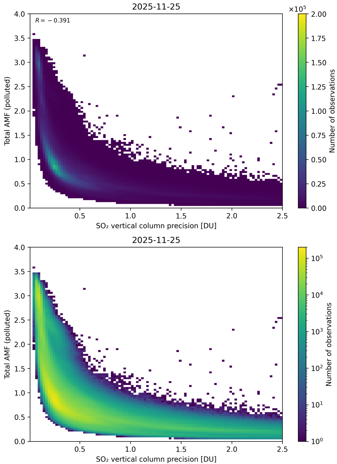
Figure 346: Scatter density plot of “SO 2 vertical column precision” against “Total AMF (polluted)” for 2025-11-24 to 2025-11-26.
