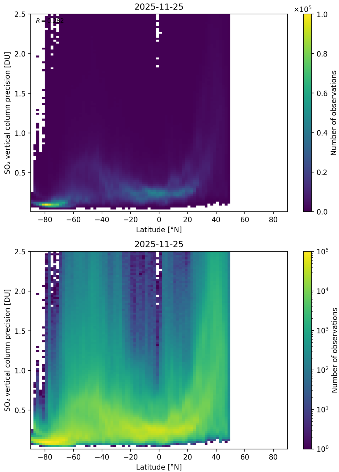
Figure 170: Scatter density plot of “Latitude” against “SO 2 vertical column precision” for 2025-11-24 to 2025-11-26.
