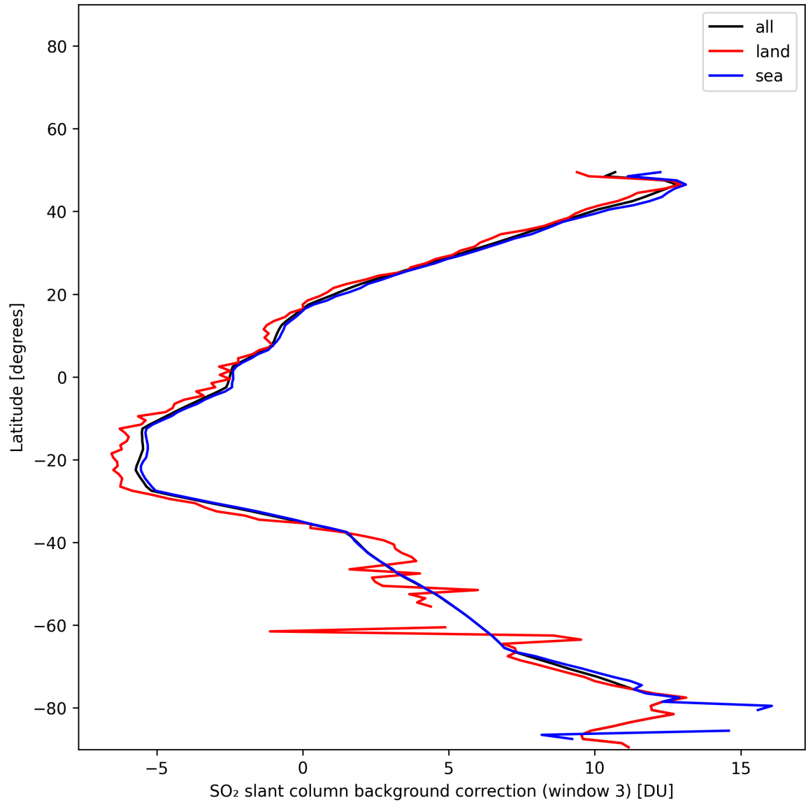
Figure 48: Zonal average of “SO 2 slant column background correction (window 3)” for 2025-11-24 to 2025-11-26.
