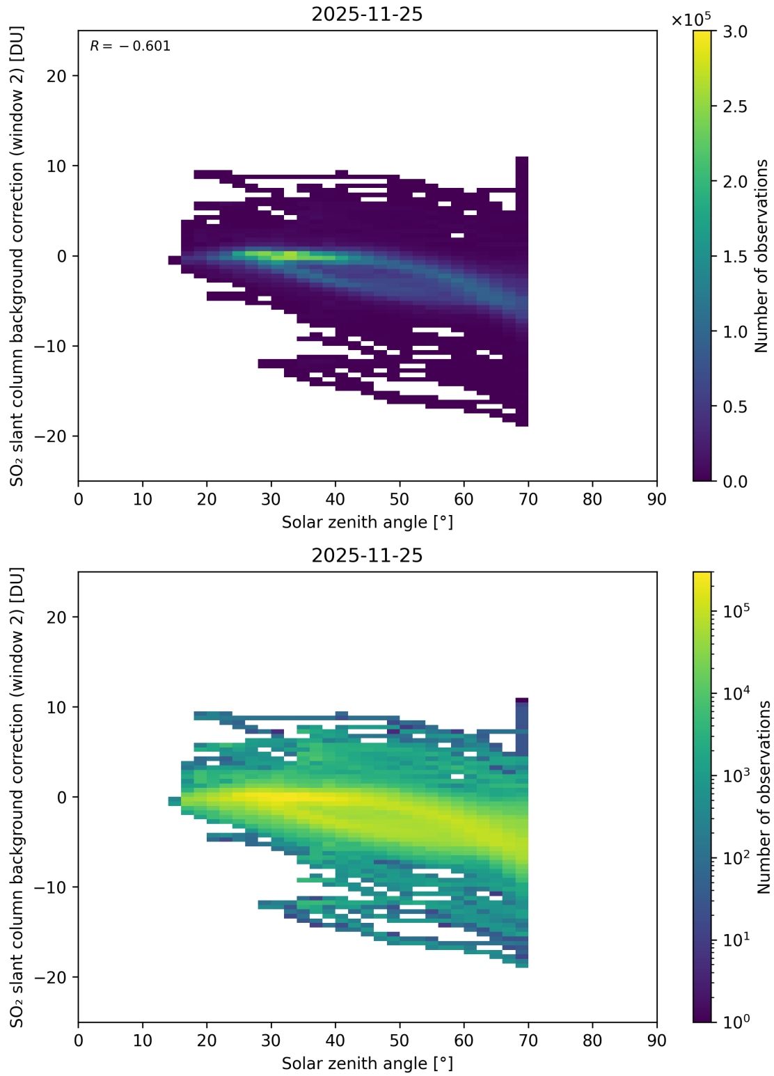
Figure 172: Scatter density plot of “Solar zenith angle” against “SO 2 slant column background correction (window 2)” for 2025-11-24 to 2025-11-26.
