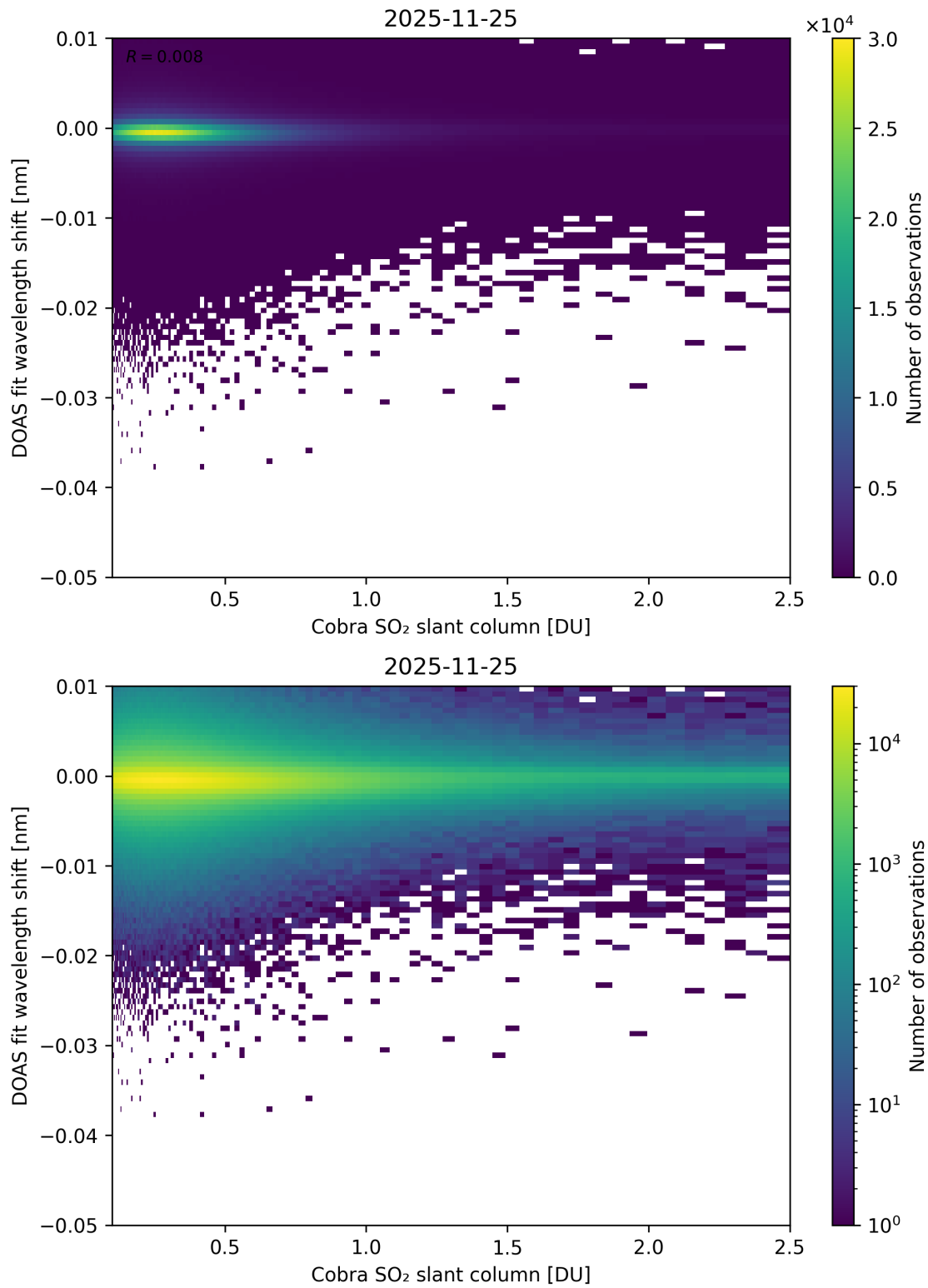
Figure 196: Scatter density plot of “Cobra SO 2 slant column” against “DOAS fit wavelength shift” for 2025-11-24 to 2025-11-26.
