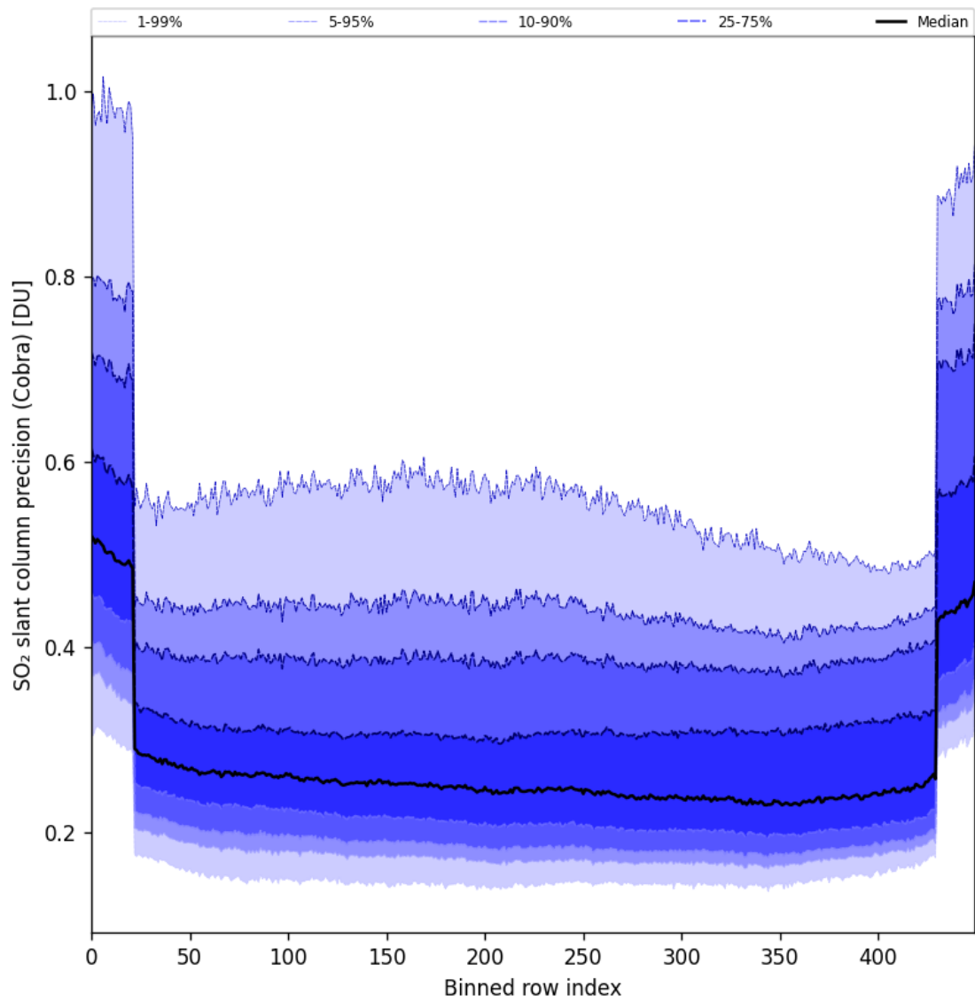
Figure 88: Along track statistics of “SO 2 slant column precision (Cobra)” for 2025-11-24 to 2025-11-26
