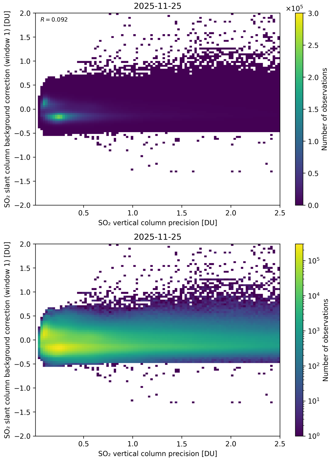
Figure 329: Scatter density plot of “SO 2 vertical column precision” against “SO 2 slant column background correction (window 1)” for 2025-11-24 to 2025-11-26.
