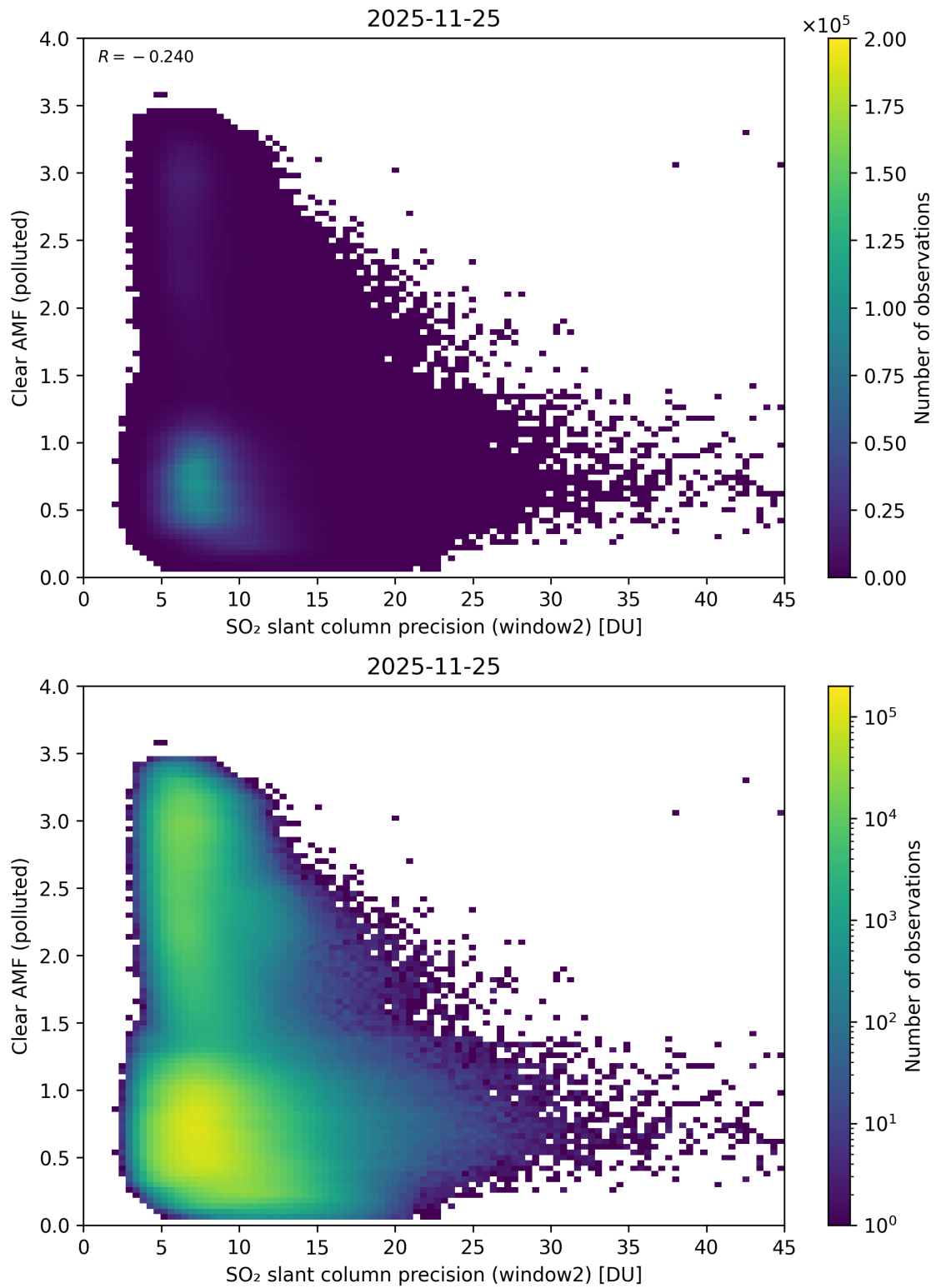
Figure 296: Scatter density plot of “SO 2 slant column precision (window2)” against “Clear AMF (polluted)” for 2025-11-24 to 2025-11-26.
