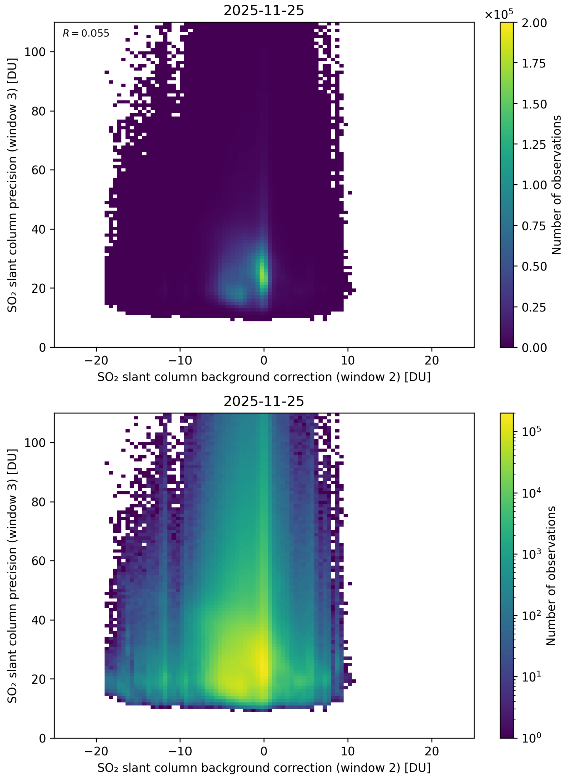
Figure 129: Scatter density plot of “SO 2 slant column background correction (window 2)” against “SO 2 slant column precision (window 3)” for 2025-11-24 to 2025-11-26.
