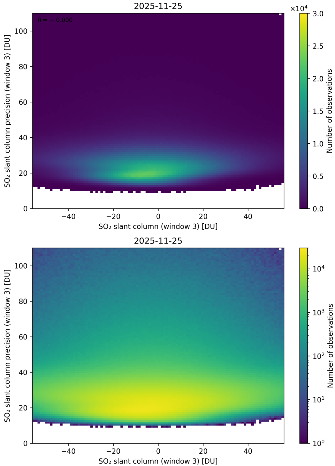
Figure 317: Scatter density plot of “SO 2 slant column (window 3)” against “SO 2 slant column precision (window 3)” for 2025-11-24 to 2025-11-26.
