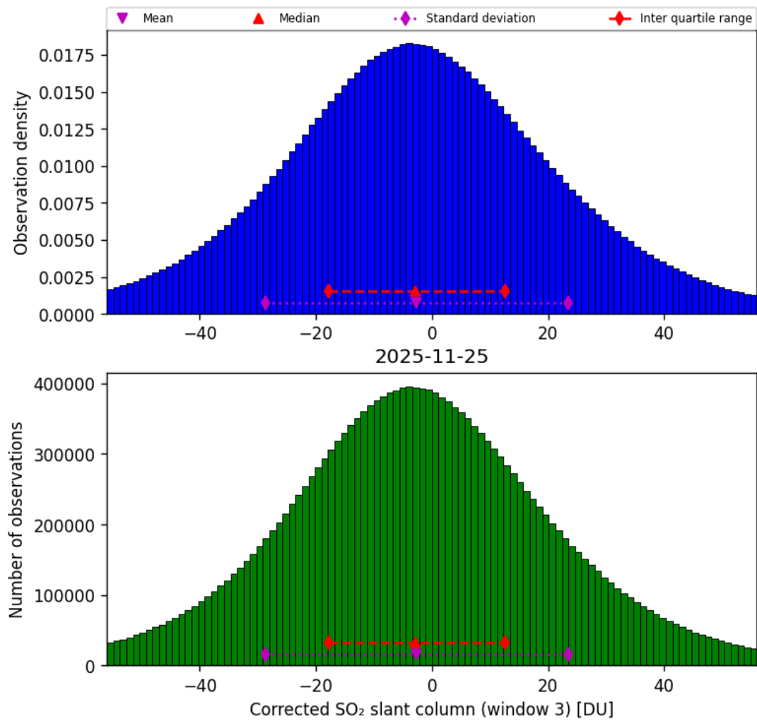
Figure 73: Histogram of “Corrected SO 2 slant column (window 3)” for 2025-11-24 to 2025-11-26
