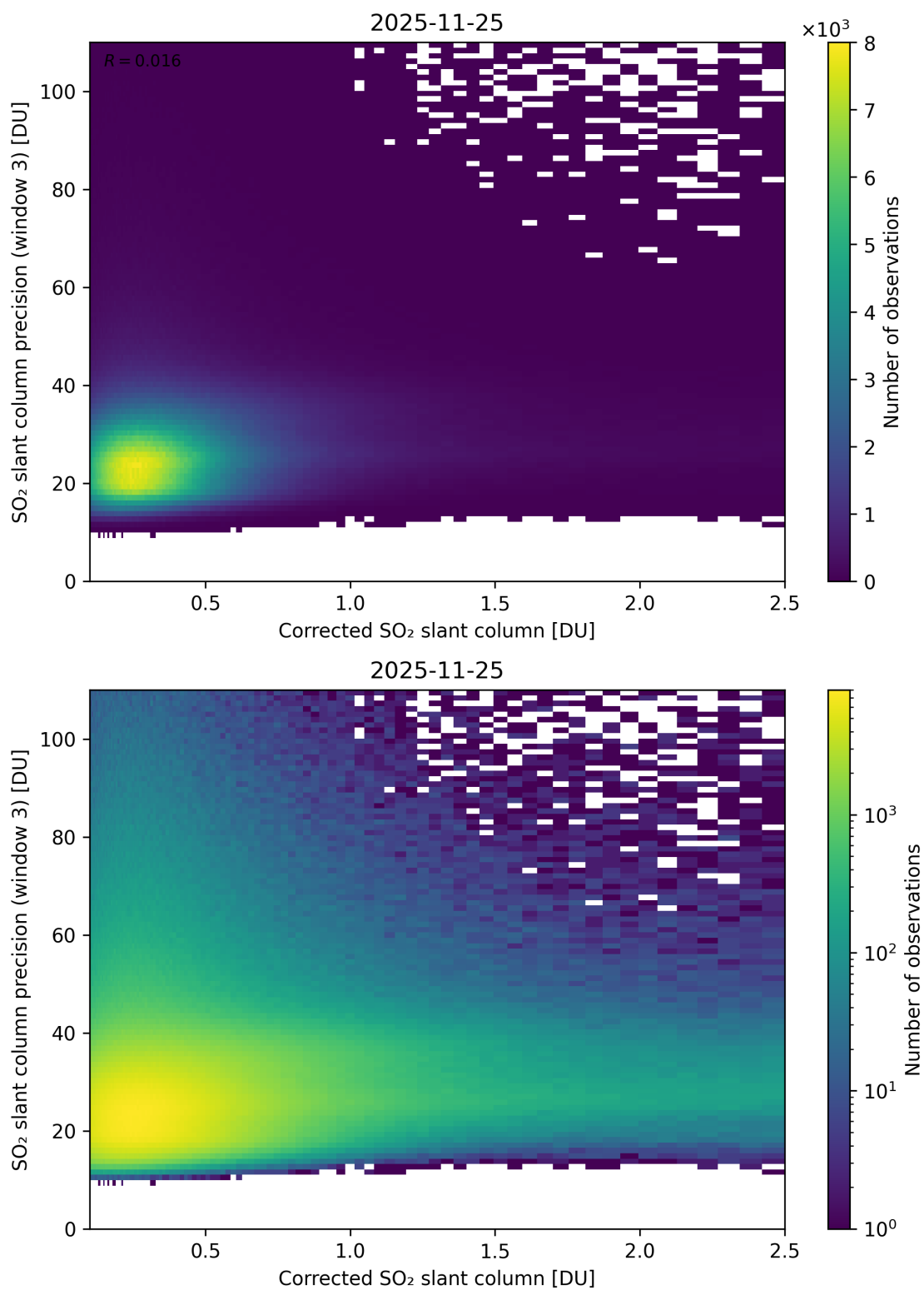
Figure 241: Scatter density plot of “Corrected SO 2 slant column” against “SO 2 slant column precision (window 3)” for 2025-11-24 to 2025-11-26.
