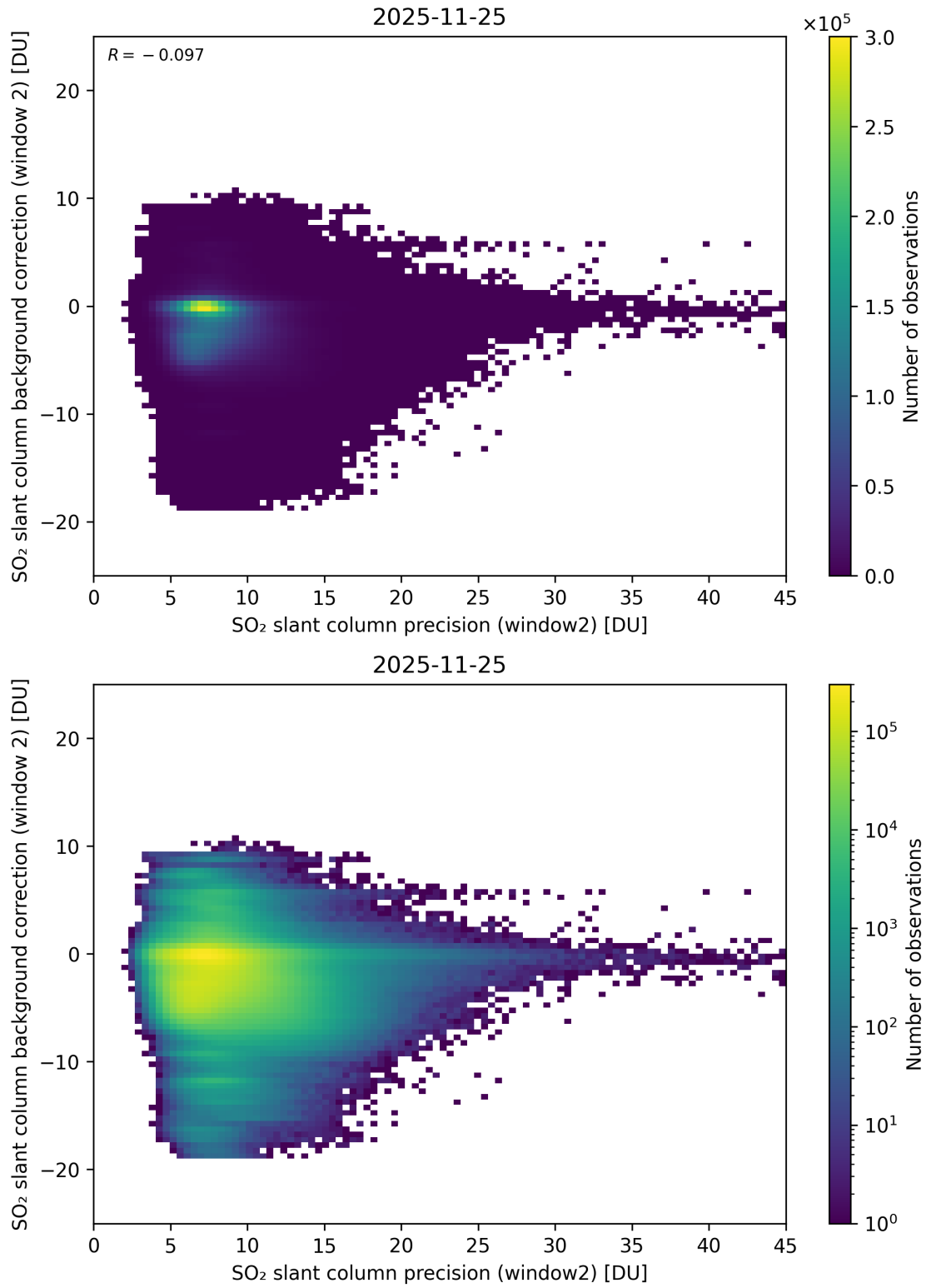
Figure 291: Scatter density plot of “SO 2 slant column precision (window2)” against “SO 2 slant column background correction (window 2)” for 2025-11-24 to 2025-11-26.
