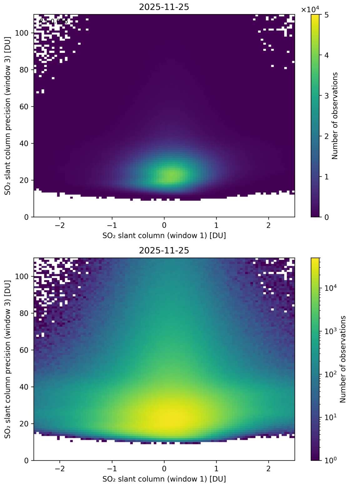
Figure 288: Scatter density plot of “SO 2 slant column (window 1)” against “SO 2 slant column precision (window 3)” for 2025-11-24 to 2025-11-26.
