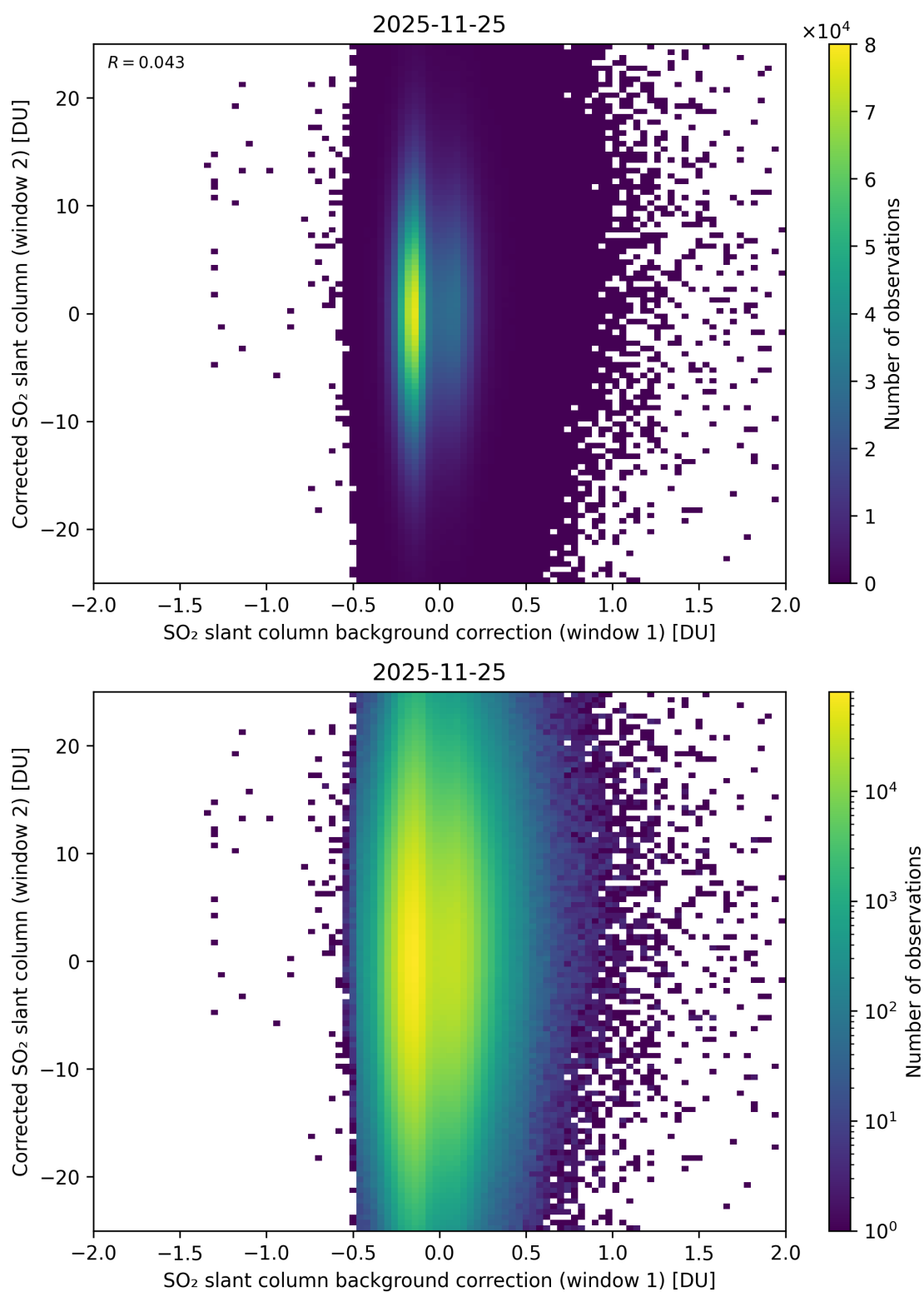
Figure 115: Scatter density plot of “SO 2 slant column background correction (window 1)” against “Corrected SO 2 slant column (window 2)” for 2025-11-24 to 2025-11-26.
