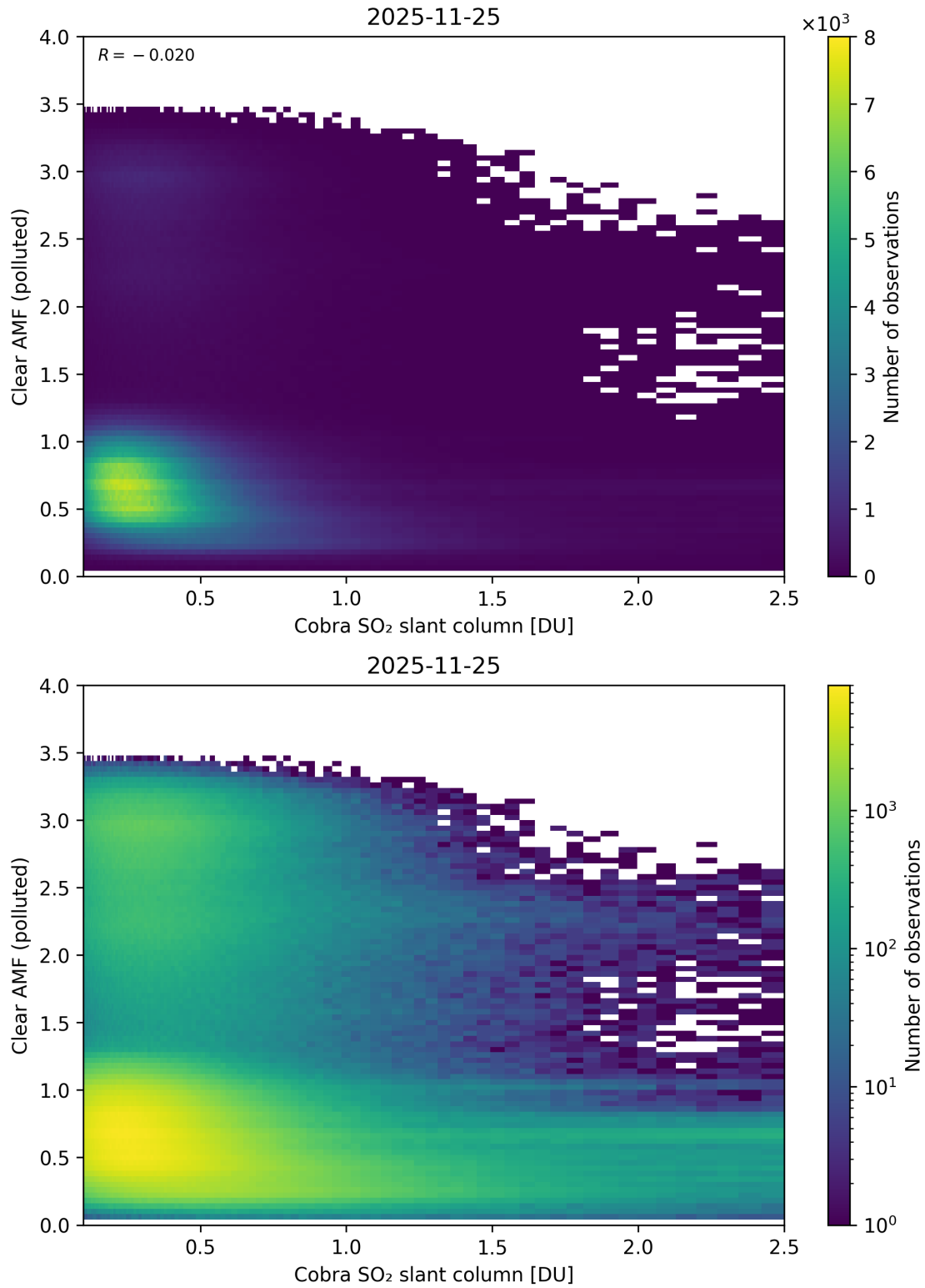
Figure 215: Scatter density plot of “Cobra SO 2 slant column” against “Clear AMF (polluted)” for 2025-11-24 to 2025-11-26.
