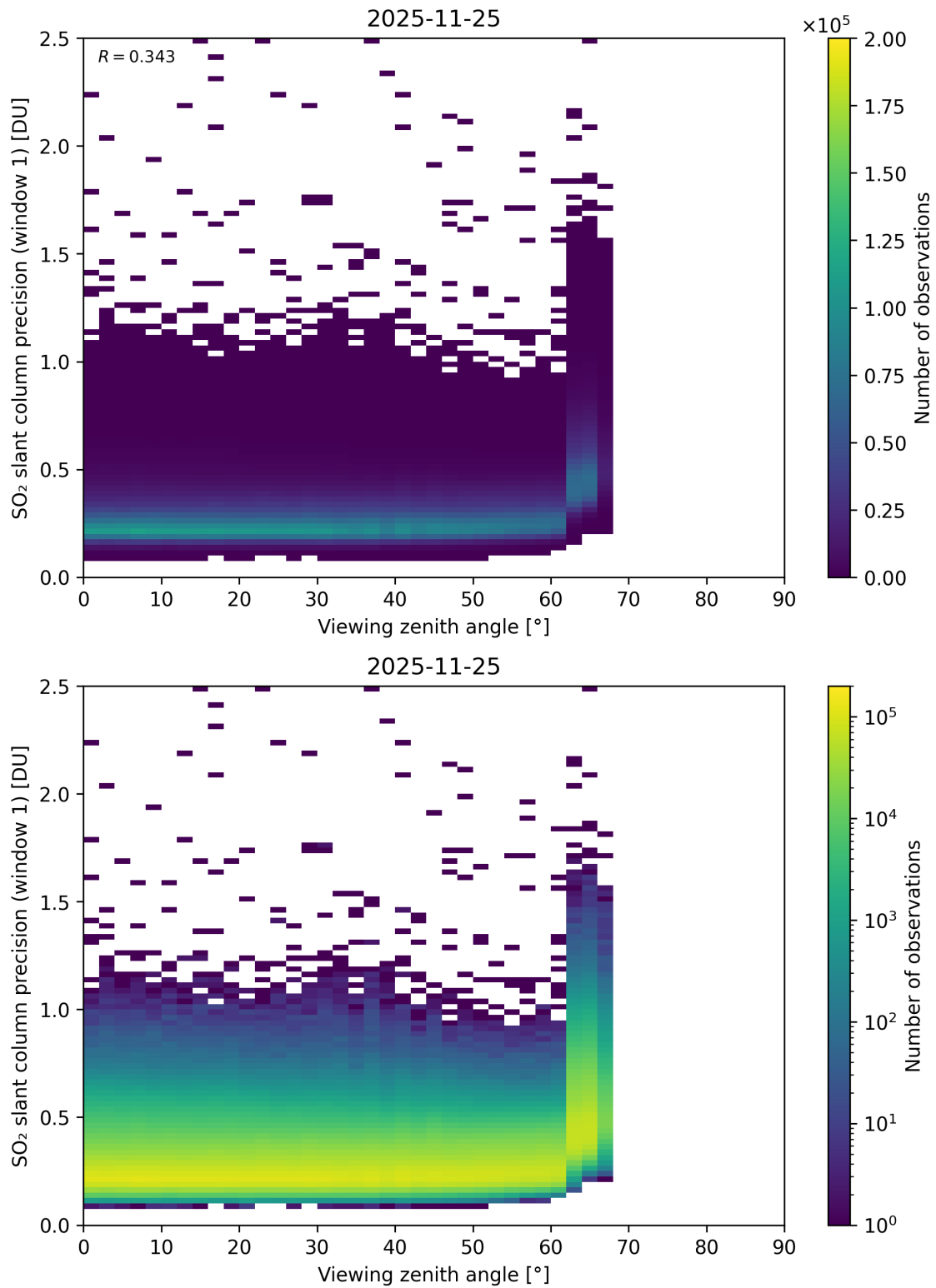
Figure 377: Scatter density plot of “Viewing zenith angle” against “SO 2 slant column precision (window 1)” for 2025-11-24 to 2025-11-26.
