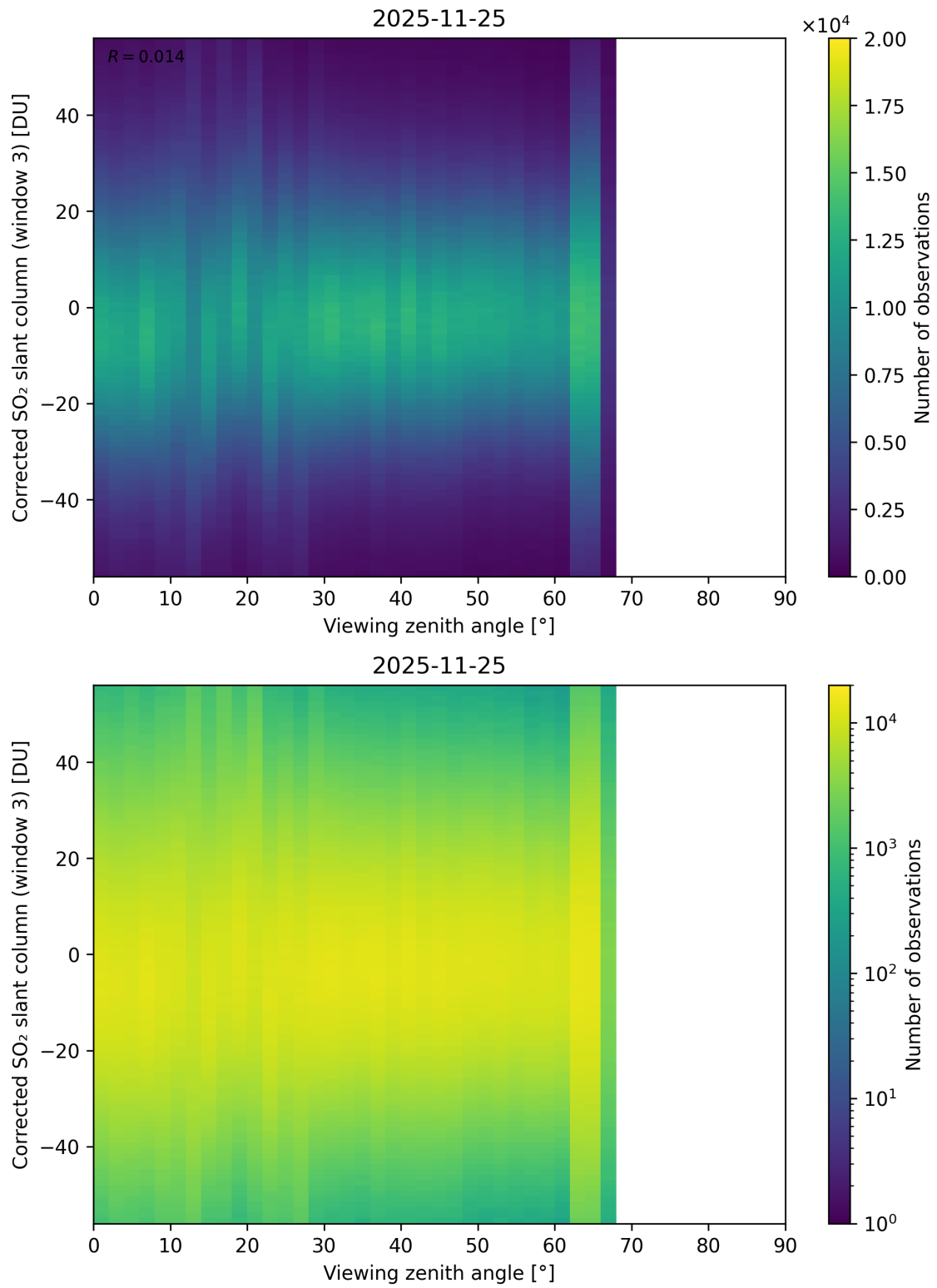
Figure 375: Scatter density plot of “Viewing zenith angle” against “Corrected SO 2 slant column (window 3)” for 2025-11-24 to 2025-11-26.
