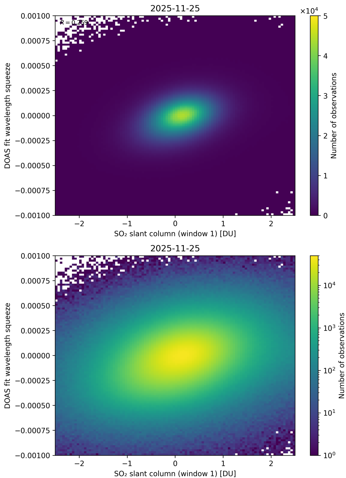
Figure 266: Scatter density plot of “SO 2 slant column (window 1)” against “DOAS fit wavelength squeeze” for 2025-11-24 to 2025-11-26.
