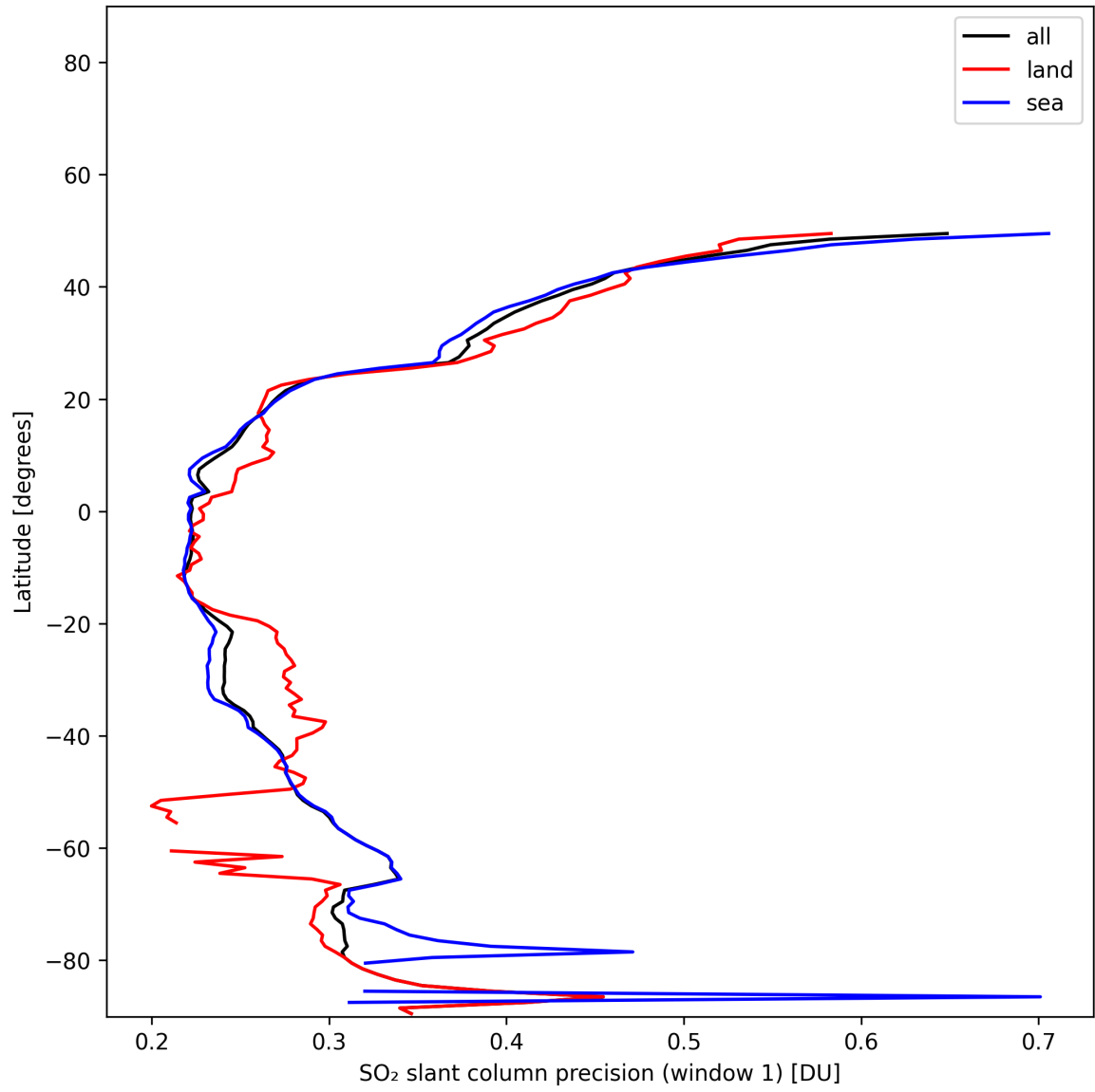
Figure 38: Zonal average of “SO 2 slant column precision (window 1)” for 2025-11-24 to 2025-11-26.
