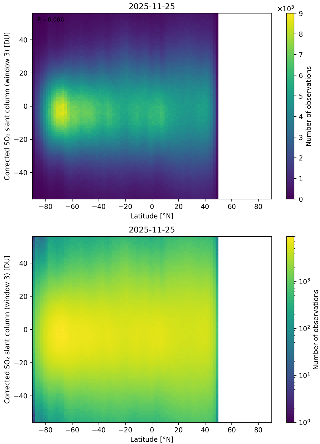
Figure 161: Scatter density plot of “Latitude” against “Corrected SO 2 slant column (window 3)” for 2025-11-24 to 2025-11-26.
