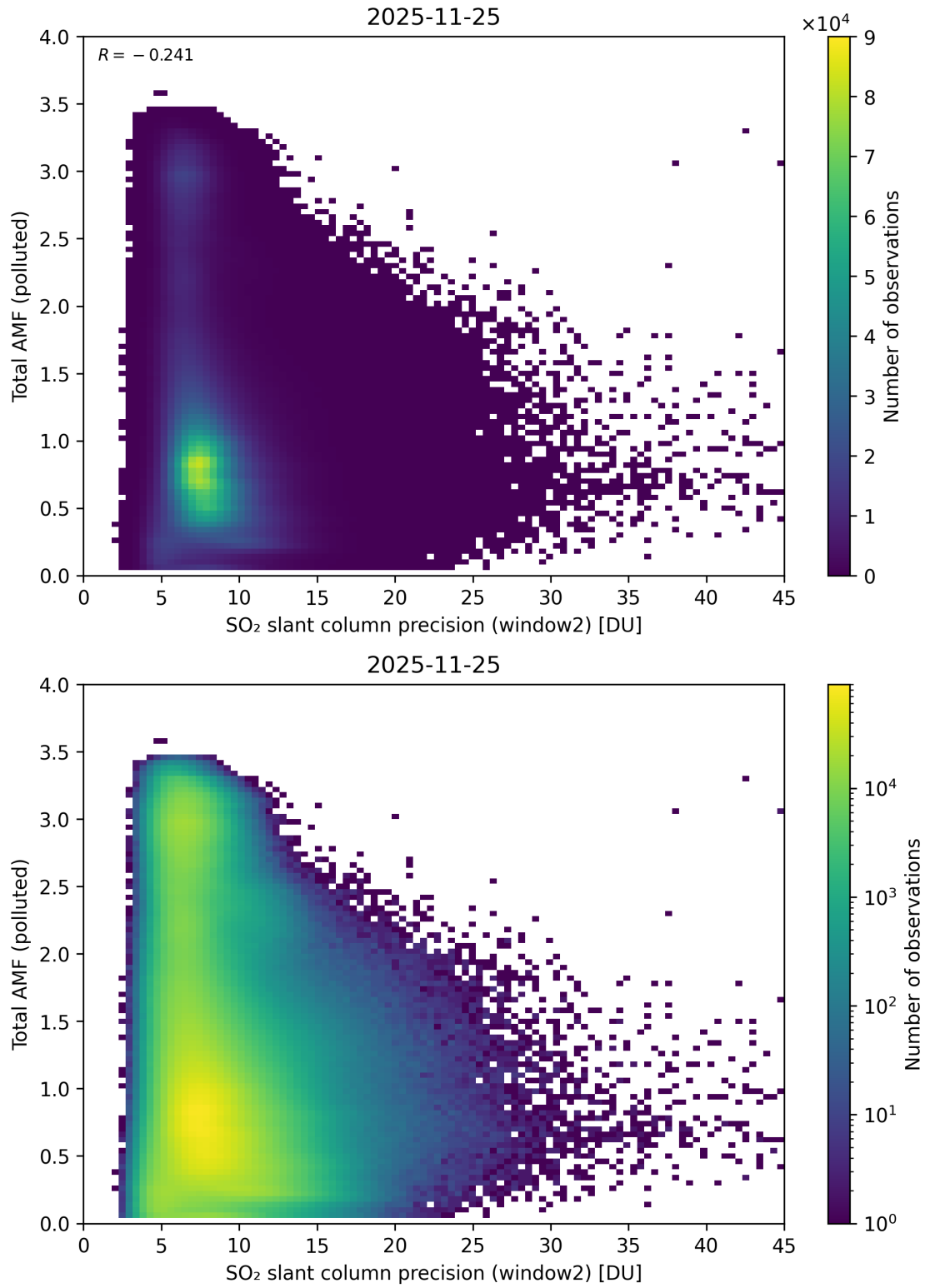
Figure 301: Scatter density plot of “SO 2 slant column precision (window2)” against “Total AMF (polluted)” for 2025-11-24 to 2025-11-26.
