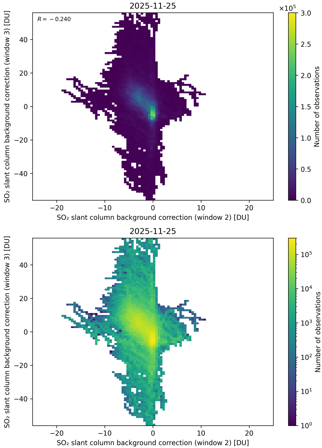
Figure 122: Scatter density plot of “SO 2 slant column background correction (window 2)” against “SO 2 slant column background correction (window 3)” for 2025-11-24 to 2025-11-26.
