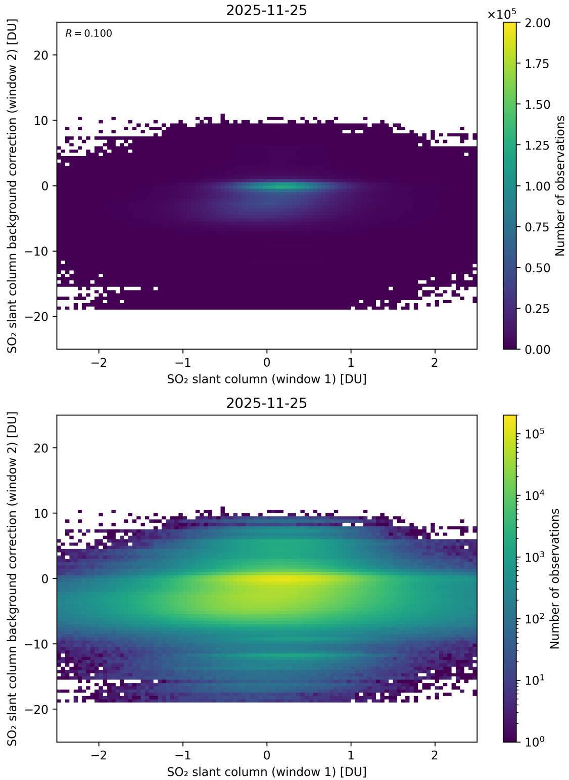
Figure 263: Scatter density plot of “SO 2 slant column (window 1)” against “SO 2 slant column background correction (window 2)” for 2025-11-24 to 2025-11-26.
