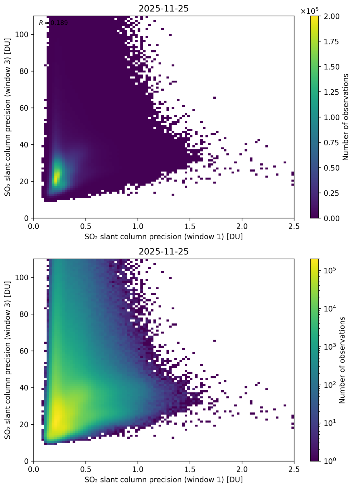
Figure 279: Scatter density plot of “SO 2 slant column precision (window 1)” against “SO 2 slant column precision (window 3)” for 2025-11-24 to 2025-11-26.
