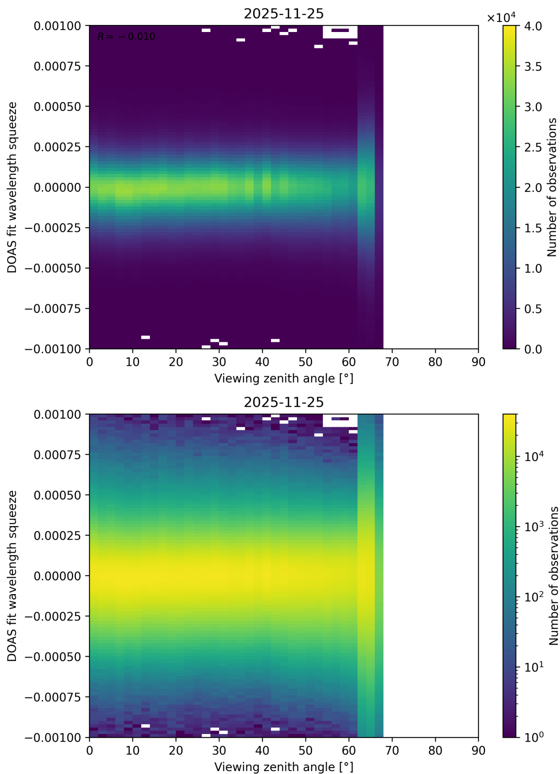
Figure 366: Scatter density plot of “Viewing zenith angle” against “DOAS fit wavelength squeeze” for 2025-11-24 to 2025-11-26.
