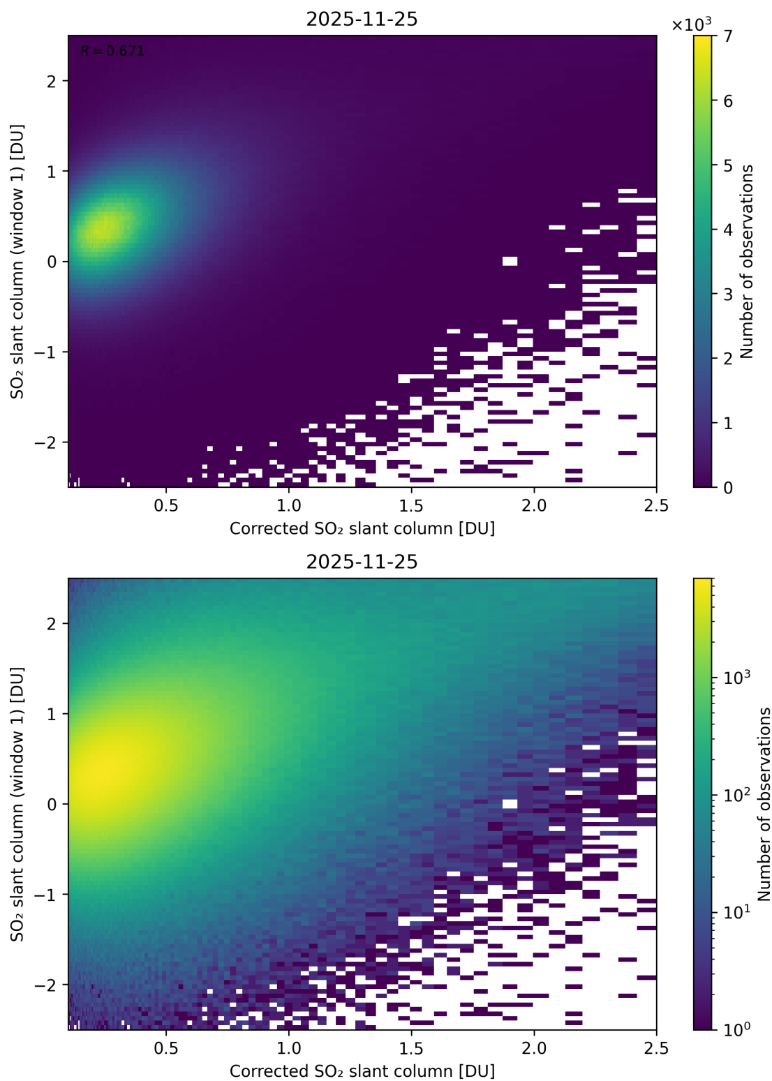
Figure 237: Scatter density plot of “Corrected SO 2 slant column” against “SO 2 slant column (window 1)” for 2025-11-24 to 2025-11-26.
