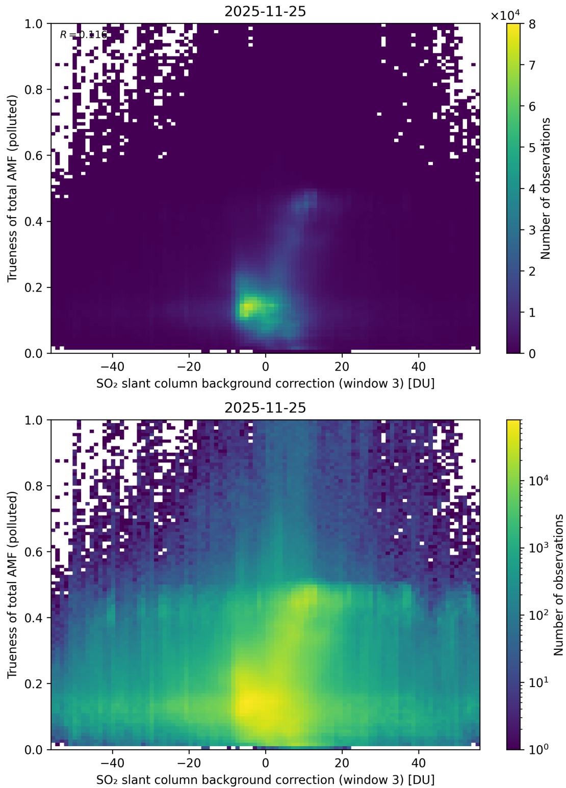
Figure 137: Scatter density plot of “SO 2 slant column background correction (window 3)” against “Trueness of total AMF (polluted)” for 2025-11-24 to 2025-11-26.
