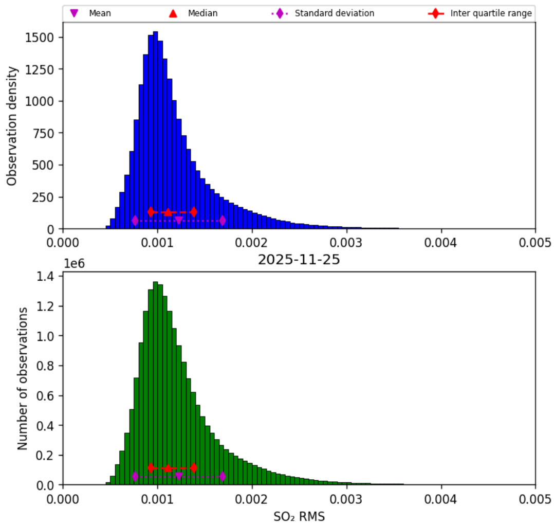
Figure 78: Histogram of "SO 2 RMS" for 2025-11-24 to 2025-11-26
