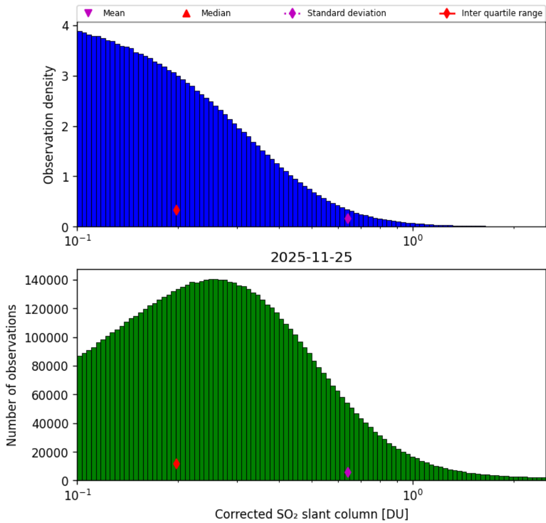
Figure 60: Histogram of “Corrected SO 2 slant column” for 2025-11-24 to 2025-11-26
