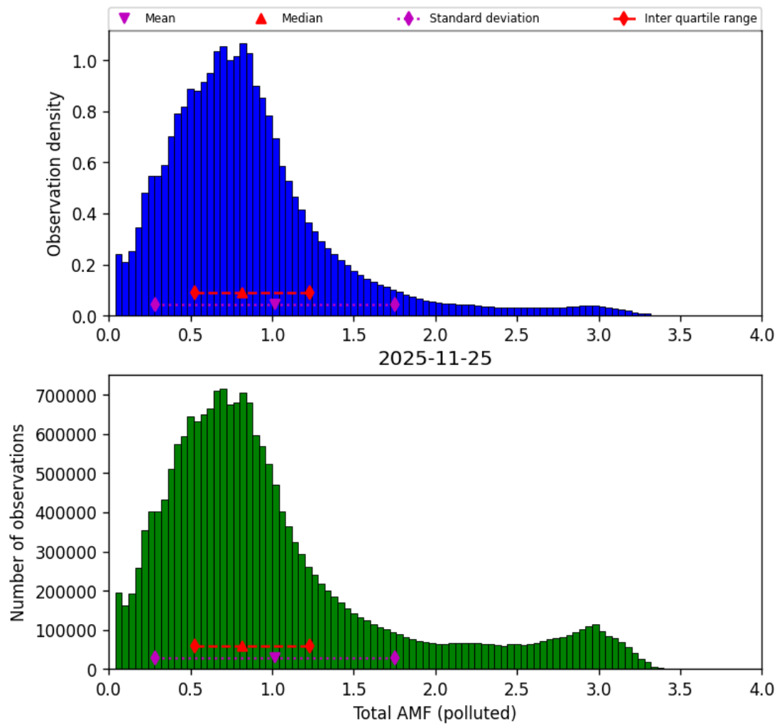
Figure 79: Histogram of “Total AMF (polluted)” for 2025-11-24 to 2025-11-26
