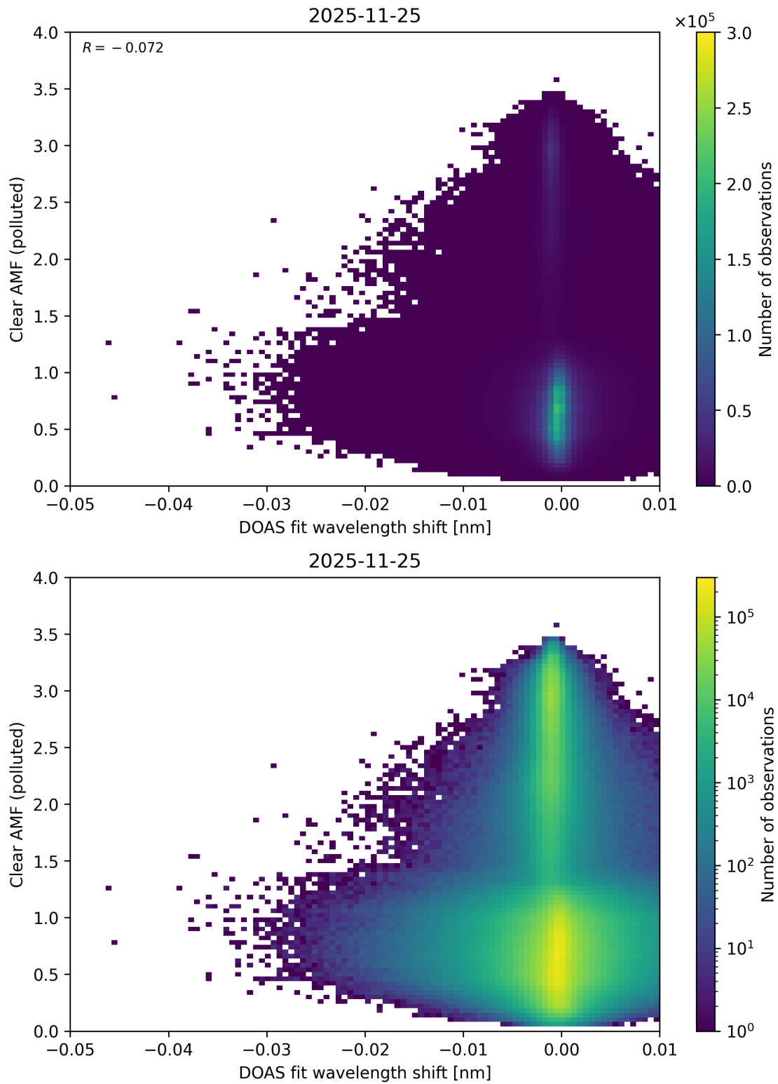
Figure 140: Scatter density plot of “DOAS fit wavelength shift” against “Clear AMF (polluted)” for 2025-11-24 to 2025-11-26.
