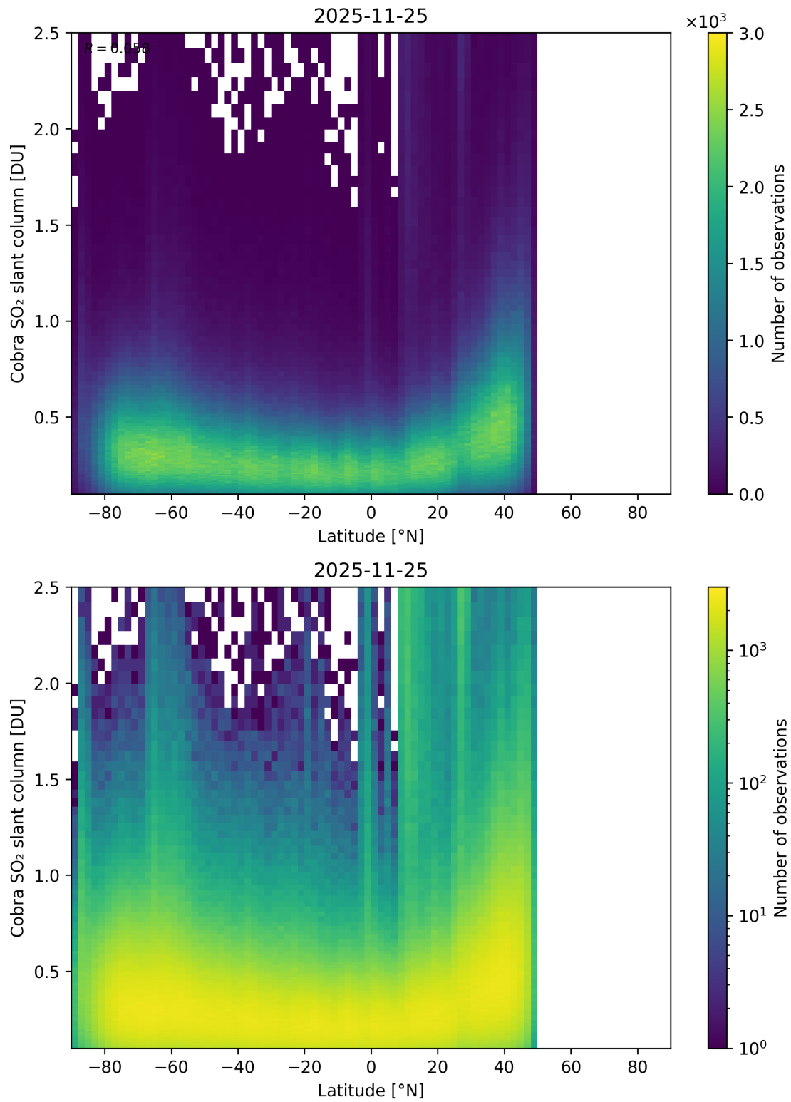
Figure 157: Scatter density plot of “Latitude” against “Cobra SO 2 slant column” for 2025-11-24 to 2025-11-26.
