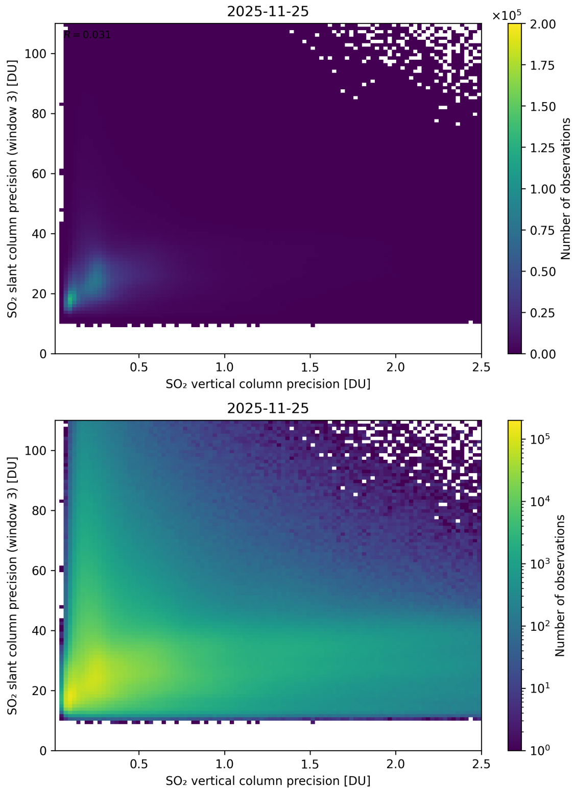
Figure 345: Scatter density plot of “SO 2 vertical column precision” against “SO 2 slant column precision (window 3)” for 2025-11-24 to 2025-11-26.
