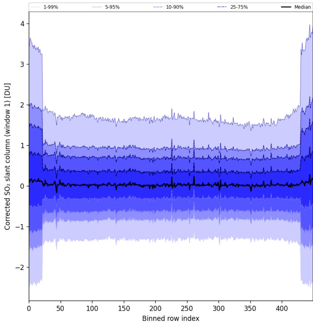
Figure 91: Along track statistics of “Corrected SO 2 slant column (window 1)” for 2025-11-24 to 2025-11-26
