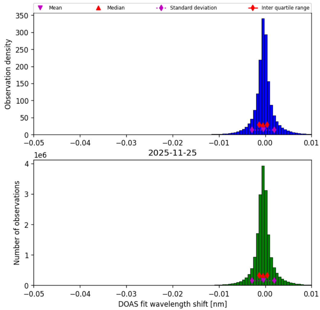
Figure 76: Histogram of “DOAS fit wavelength shift” for 2025-11-24 to 2025-11-26
