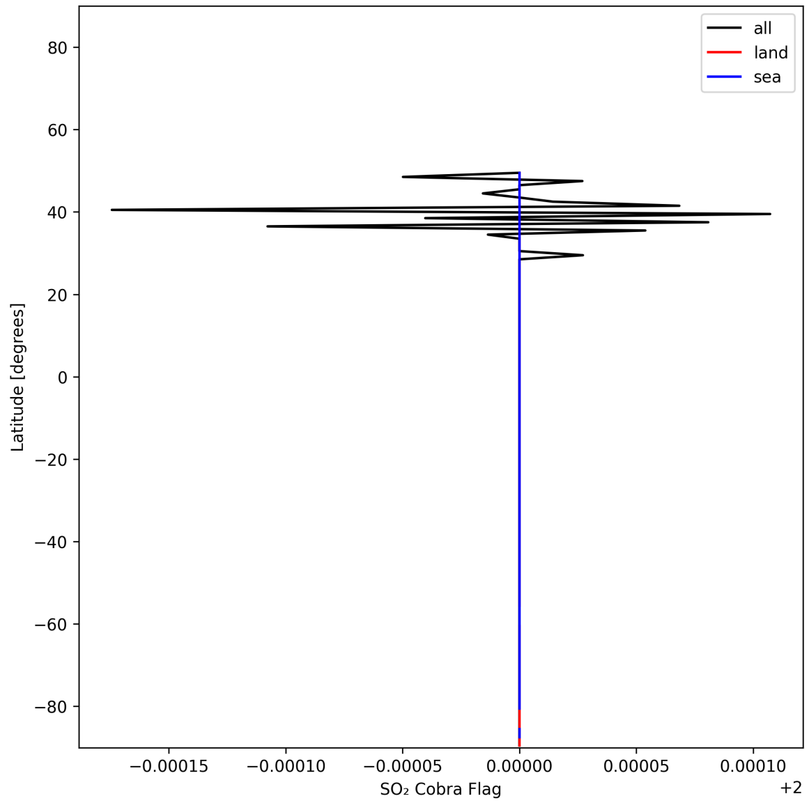
Figure 49: Zonal average of "SO 2 Cobra Flag" for 2025-11-24 to 2025-11-26.
