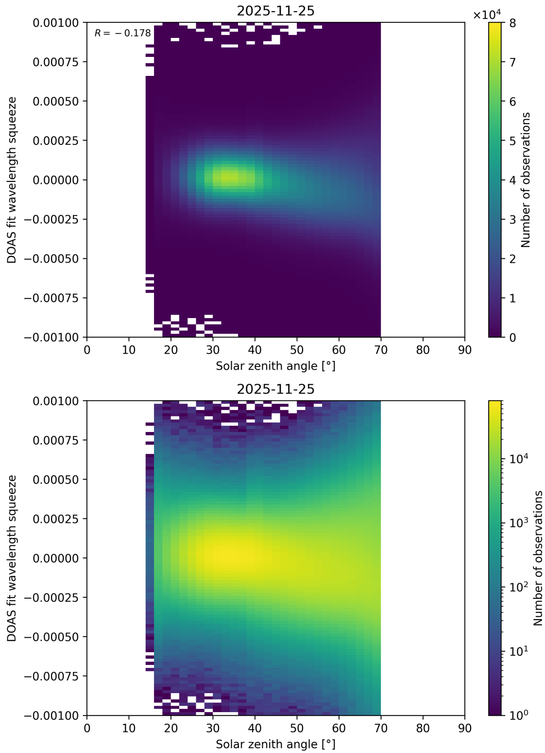
Figure 175: Scatter density plot of “Solar zenith angle” against “DOAS fit wavelength squeeze” for 2025-11-24 to 2025-11-26.
