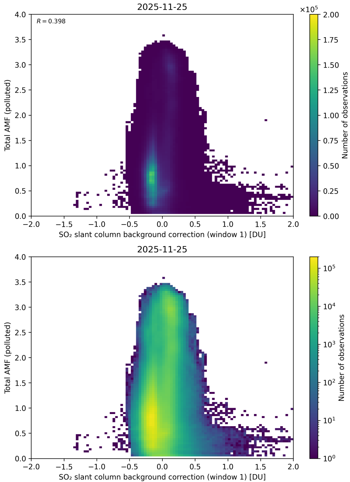
Figure 120: Scatter density plot of “SO 2 slant column background correction (window 1)” against “Total AMF (polluted)” for 2025-11-24 to 2025-11-26.
