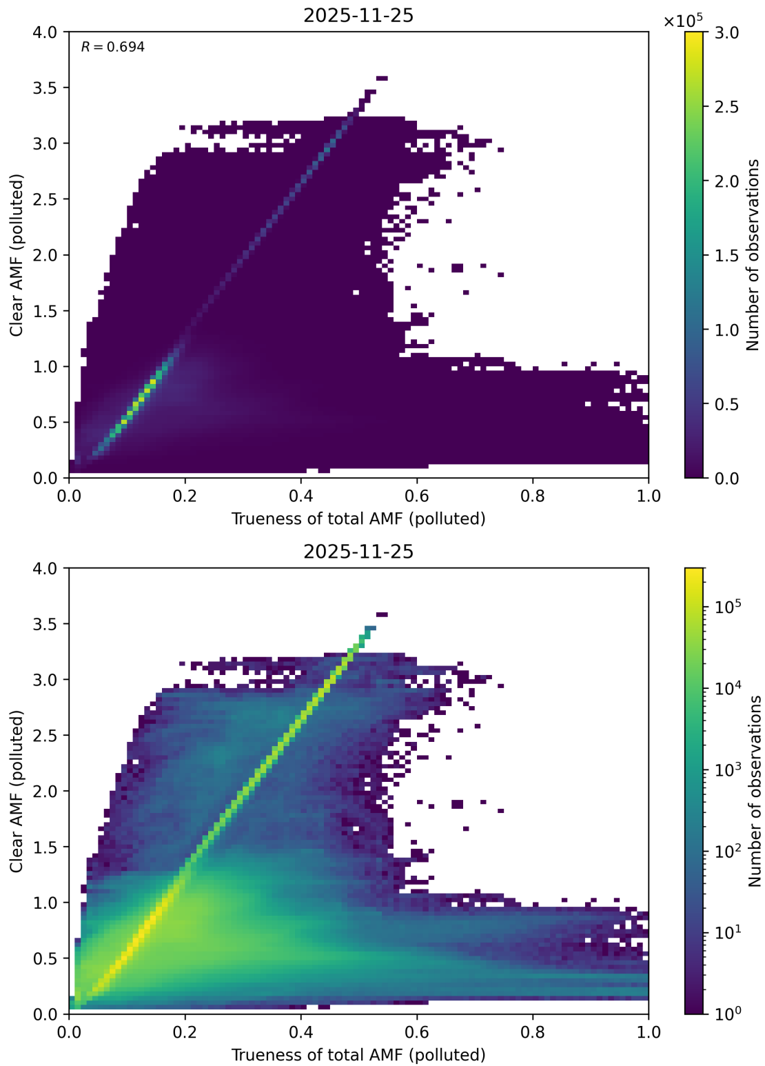
Figure 322: Scatter density plot of “Trueness of total AMF (polluted)” against “Clear AMF (polluted)” for 2025-11-24 to 2025-11-26.
