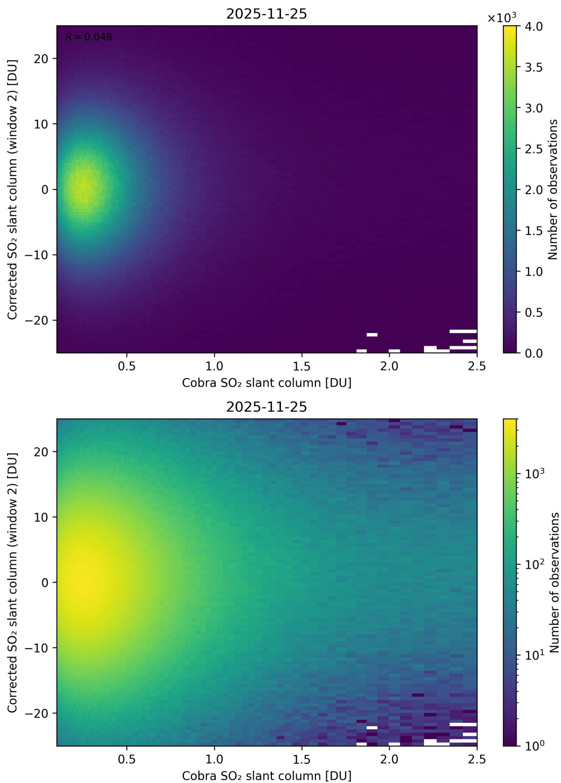
Figure 217: Scatter density plot of “Cobra SO 2 slant column” against “Corrected SO 2 slant column (window 2)” for 2025-11-24 to 2025-11-26.
