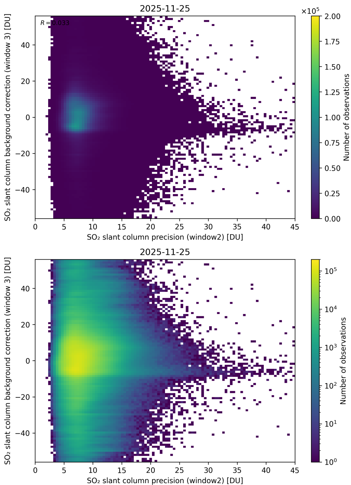
Figure 292: Scatter density plot of “SO 2 slant column precision (window2)” against “SO 2 slant column background correction (window 3)” for 2025-11-24 to 2025-11-26.
