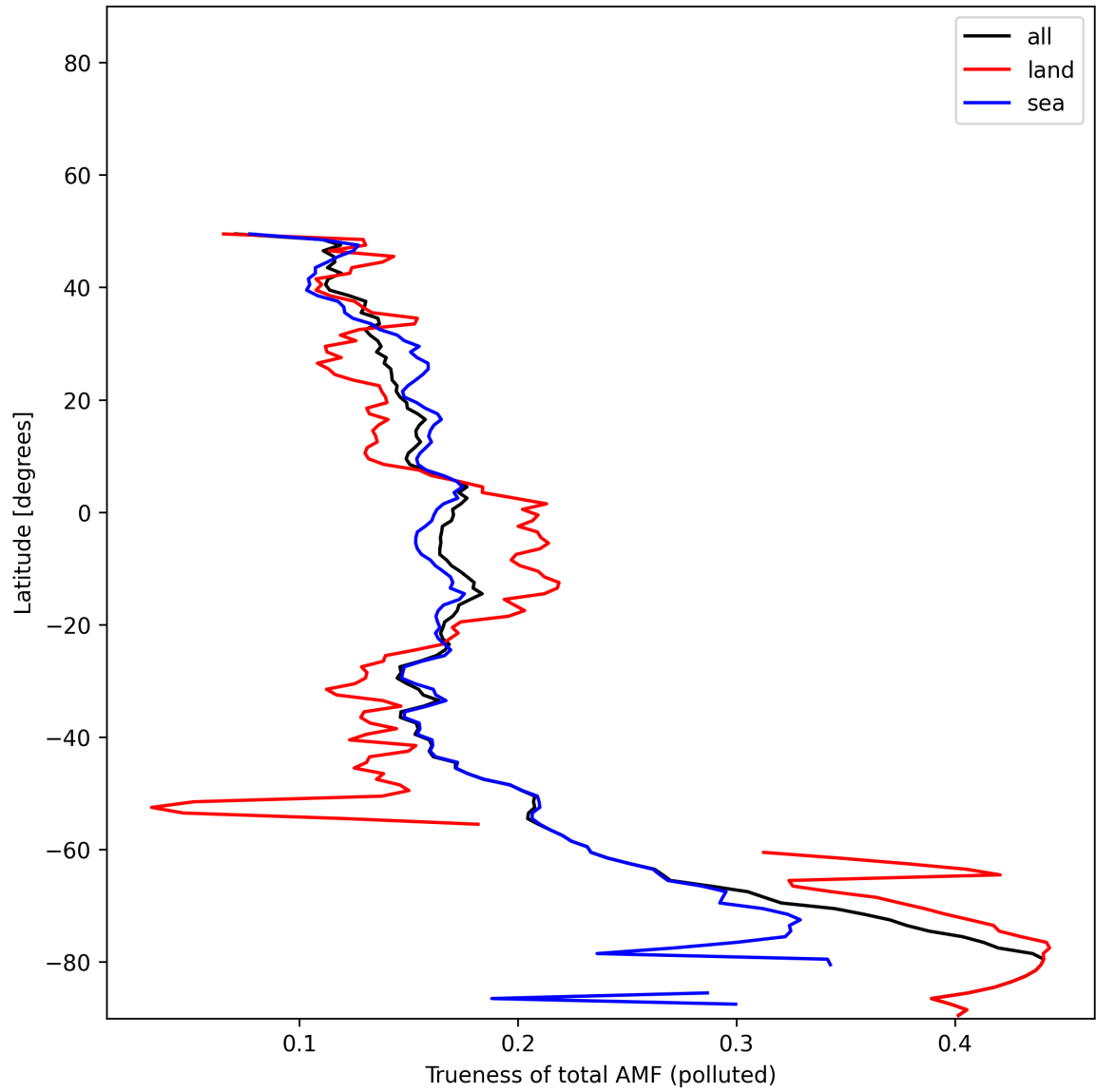
Figure 54: Zonal average of “Trueness of total AMF (polluted)” for 2025-11-24 to 2025-11-26.
