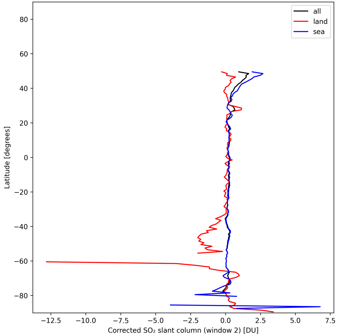
Figure 43: Zonal average of “Corrected SO 2 slant column (window 2)” for 2025-11-24 to 2025-11-26.
