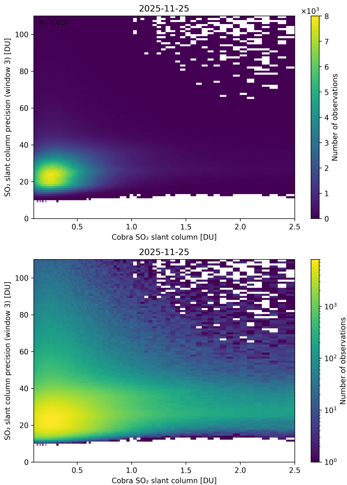
Figure 223: Scatter density plot of “Cobra SO 2 slant column” against “SO 2 slant column precision (window 3)” for 2025-11-24 to 2025-11-26.
