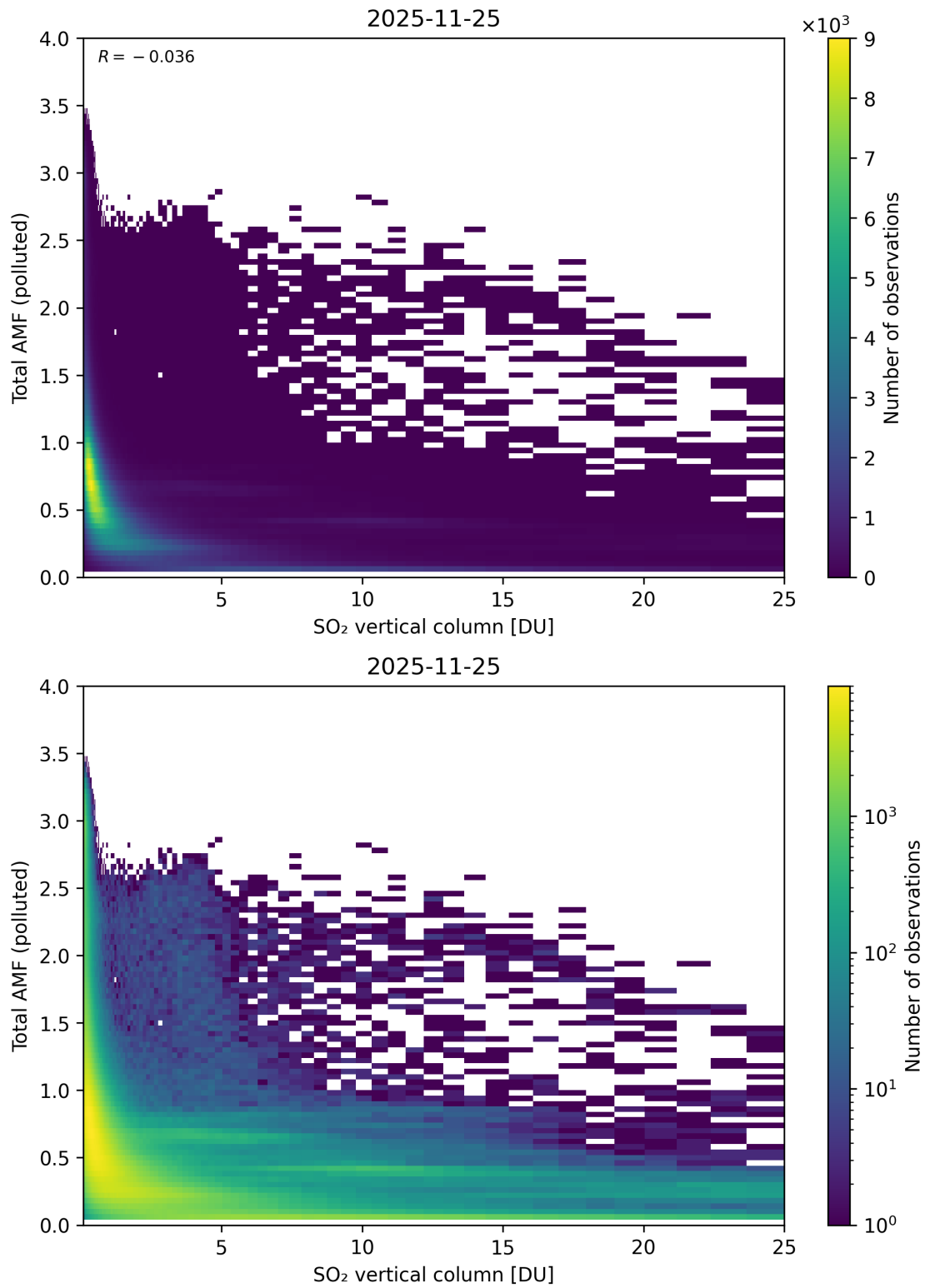
Figure 359: Scatter density plot of “SO 2 vertical column” against “Total AMF (polluted)” for 2025-11-24 to 2025-11-26.
