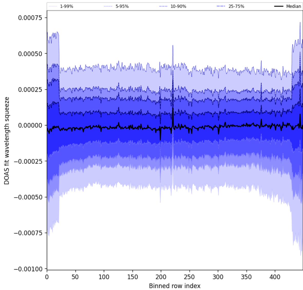
Figure 103: Along track statistics of “DOAS fit wavelength squeeze” for 2025-11-24 to 2025-11-26
