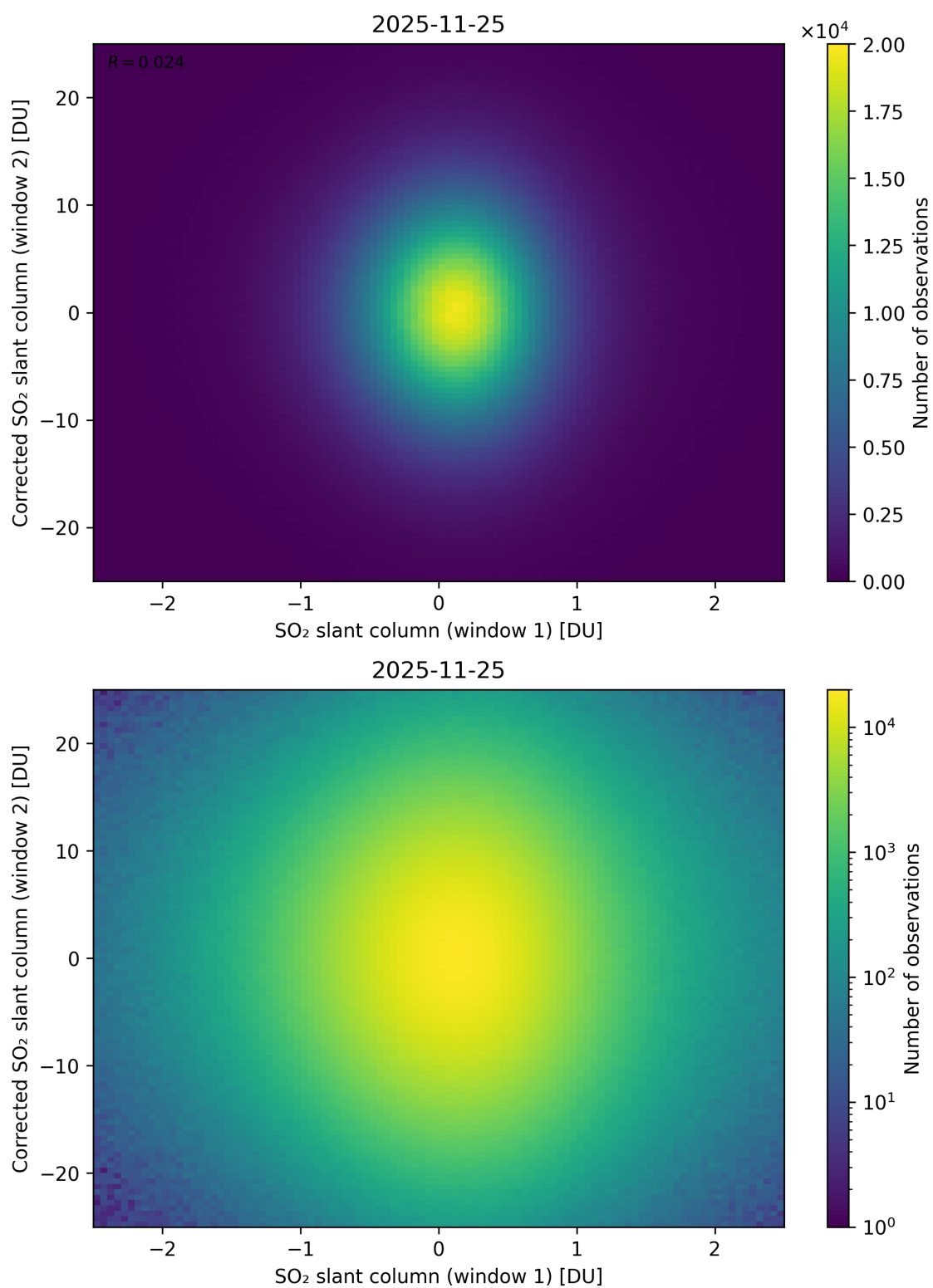
Figure 283: Scatter density plot of “SO 2 slant column (window 1)” against “Corrected SO 2 slant column (window 2)” for 2025-11-24 to 2025-11-26.
