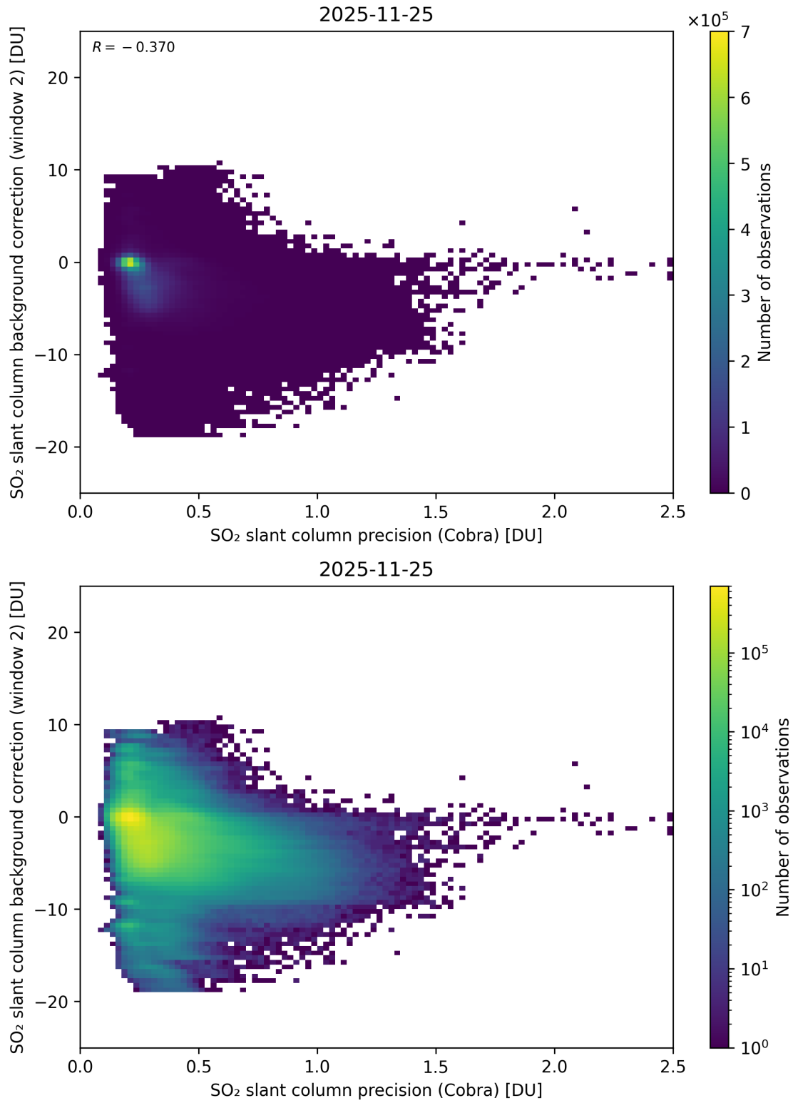
Figure 200: Scatter density plot of “SO 2 slant column precision (Cobra)” against “SO 2 slant column background correction (window 2)” for 2025-11-24 to 2025-11-26.
