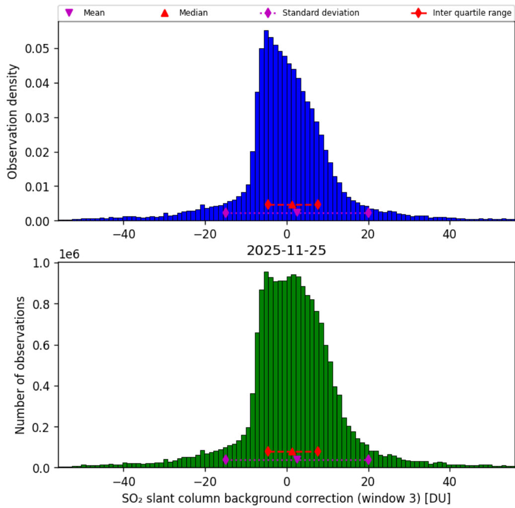
Figure 74: Histogram of “SO 2 slant column background correction (window 3)” for 2025-11-24 to 2025-11-26
