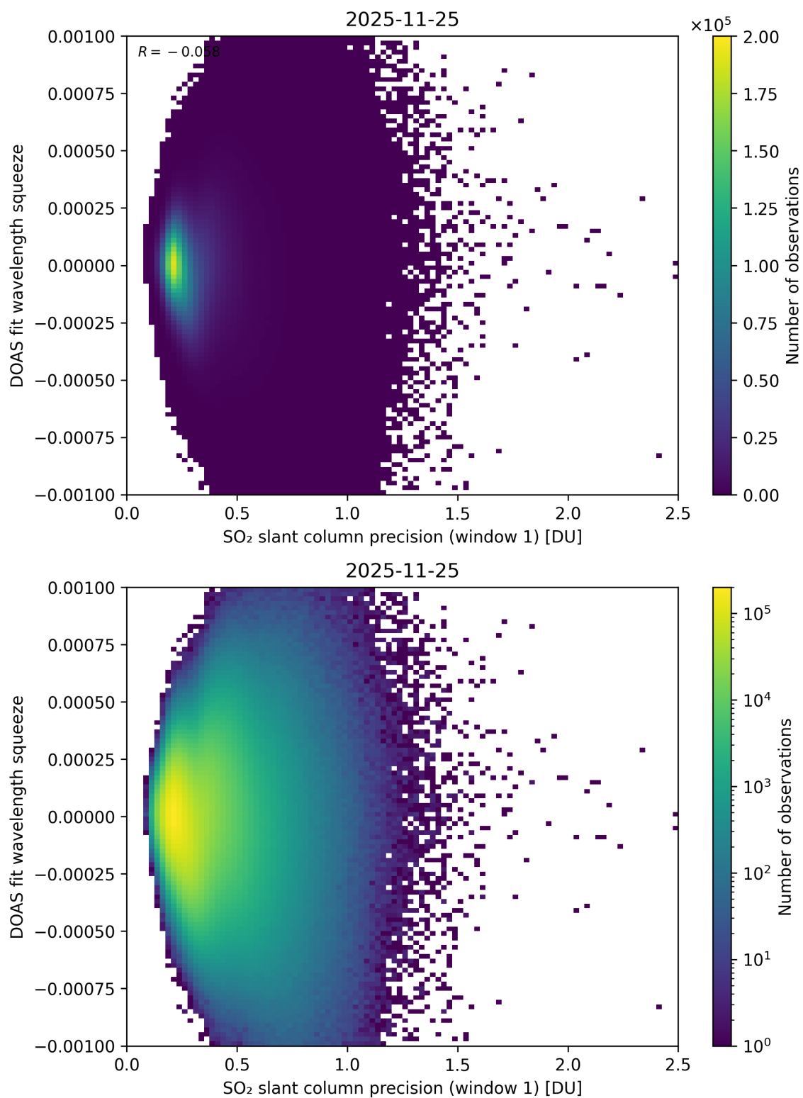
Figure 272: Scatter density plot of “SO 2 slant column precision (window 1)” against “DOAS fit wavelength squeeze” for 2025-11-24 to 2025-11-26.
