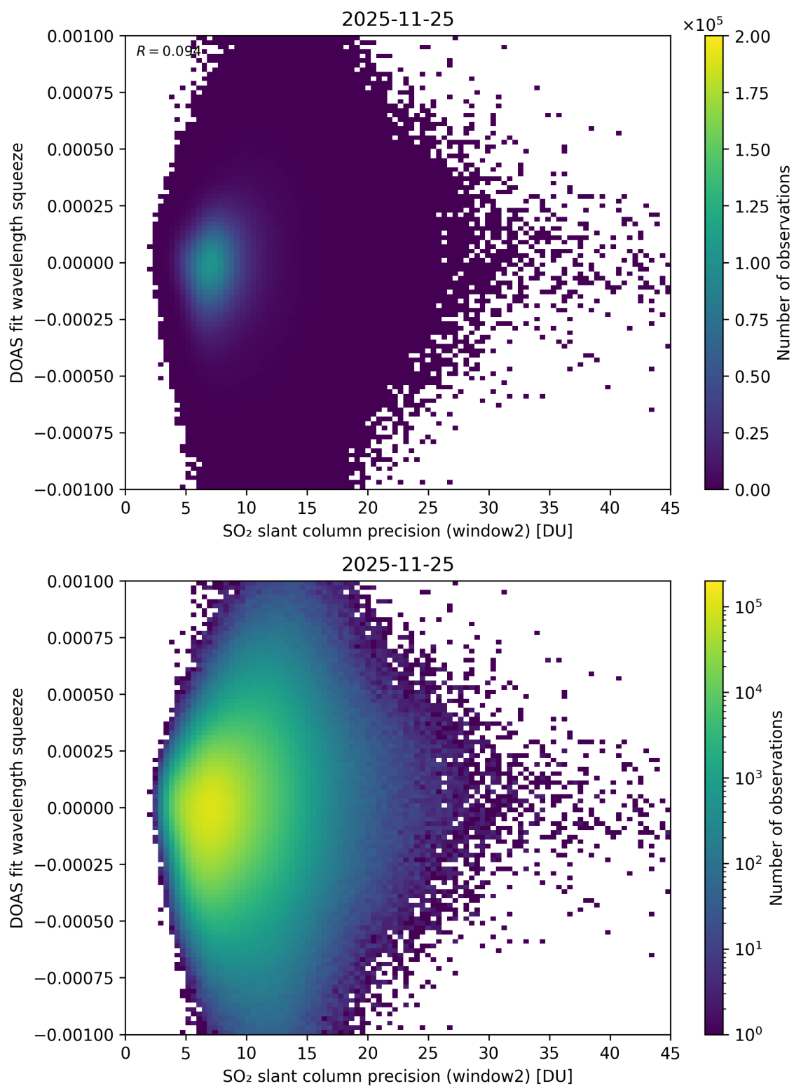
Figure 294: Scatter density plot of “SO 2 slant column precision (window2)” against “DOAS fit wavelength squeeze” for 2025-11-24 to 2025-11-26.
