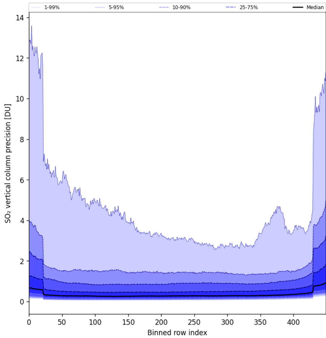
Figure 85: Along track statistics of “SO 2 vertical column precision” for 2025-11-24 to 2025-11-26
