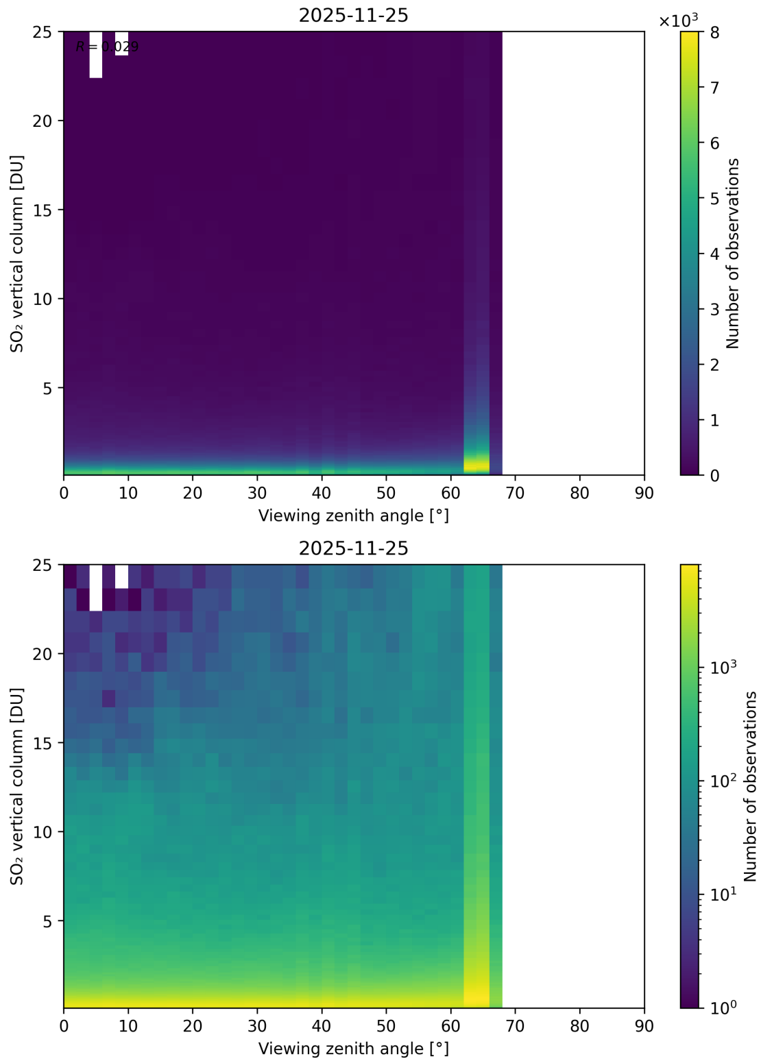
Figure 383: Scatter density plot of “Viewing zenith angle” against “SO 2 vertical column” for 2025-11-24 to 2025-11-26.
