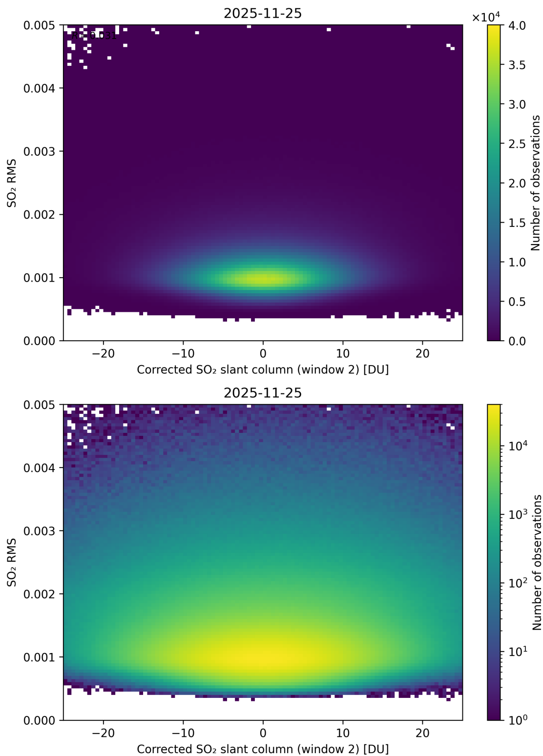
Figure 248: Scatter density plot of “Corrected SO 2 slant column (window 2)” against “SO 2 RMS” for 2025-11-24 to 2025-11-26.
