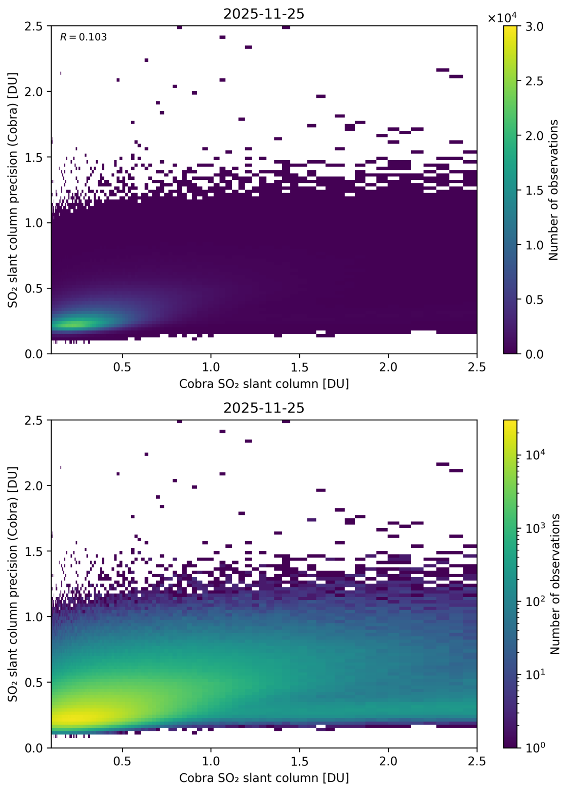
Figure 216: Scatter density plot of “Cobra SO 2 slant column” against “SO 2 slant column precision (Cobra)” for 2025-11-24 to 2025-11-26.
