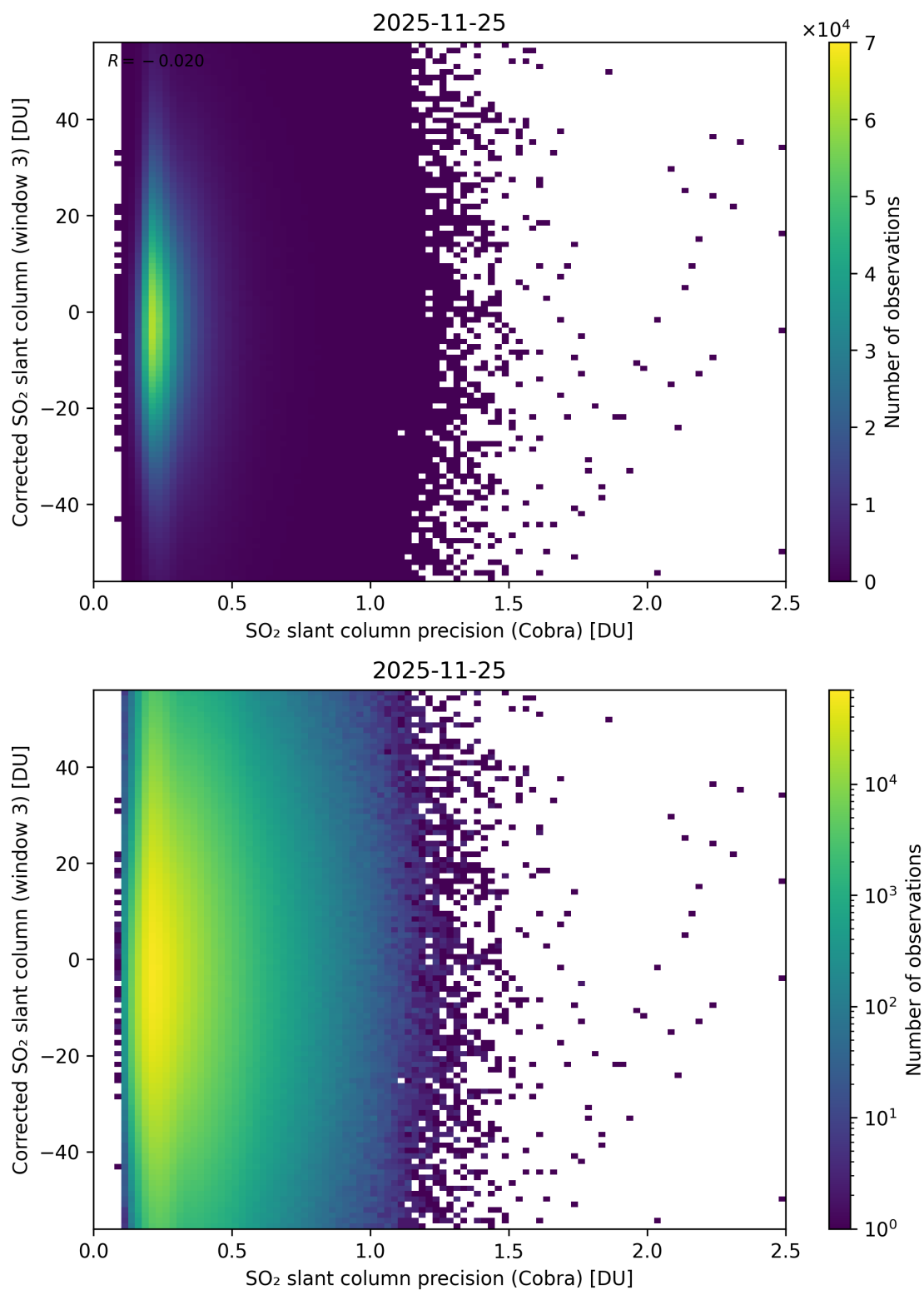
Figure 207: Scatter density plot of “SO 2 slant column precision (Cobra)” against “Corrected SO 2 slant column (window 3)” for 2025-11-24 to 2025-11-26.
