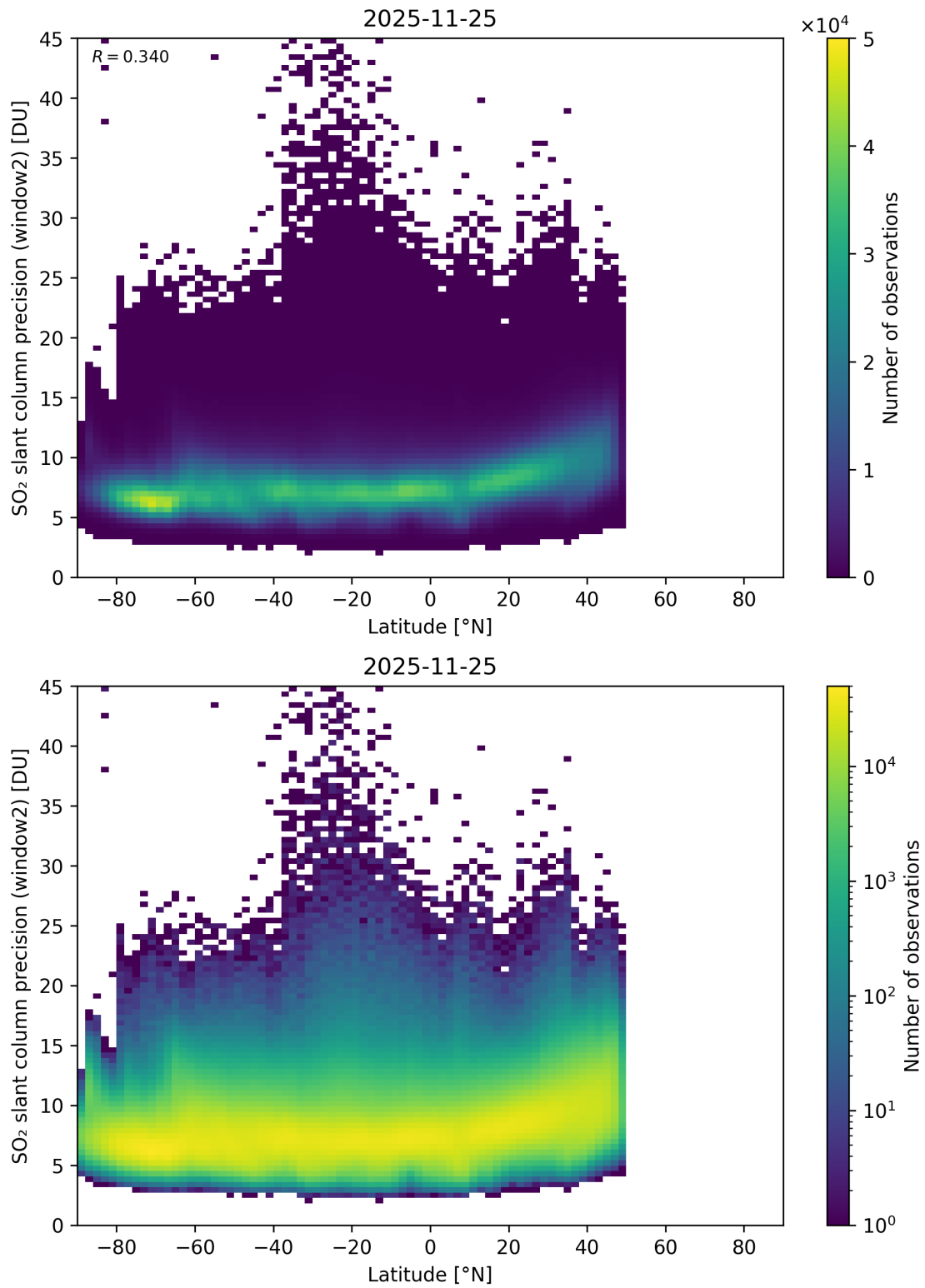
Figure 164: Scatter density plot of “Latitude” against “SO 2 slant column precision (window2)” for 2025-11-24 to 2025-11-26.
