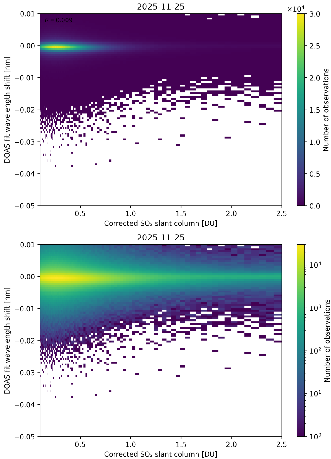
Figure 229: Scatter density plot of “Corrected SO 2 slant column” against “DOAS fit wavelength shift” for 2025-11-24 to 2025-11-26.
