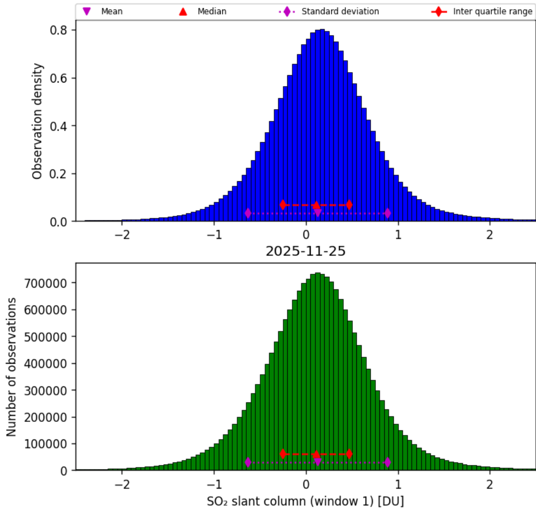
Figure 63: Histogram of “SO 2 slant column (window 1)” for 2025-11-24 to 2025-11-26
