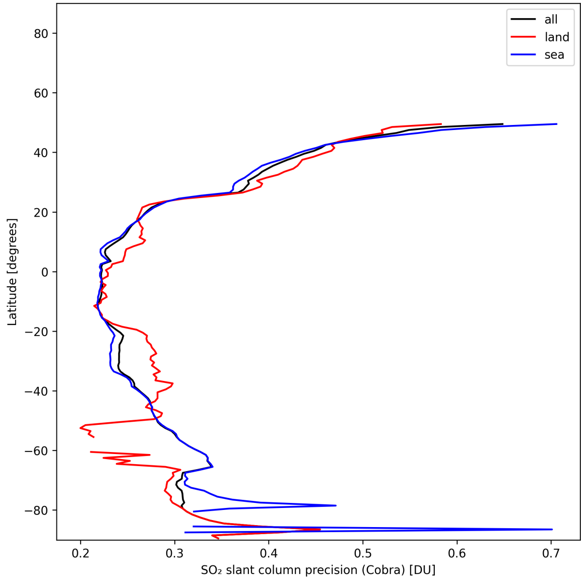
Figure 36: Zonal average of “SO 2 slant column precision (Cobra)” for 2025-11-24 to 2025-11-26.
