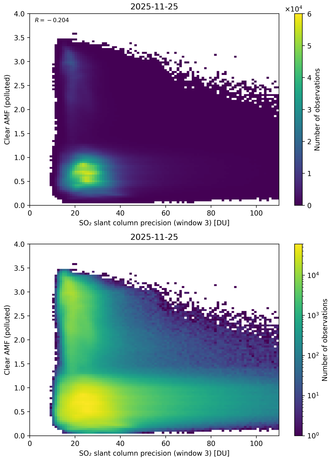
Figure 311: Scatter density plot of “SO 2 slant column precision (window 3)” against “Clear AMF (polluted)” for 2025-11-24 to 2025-11-26.
