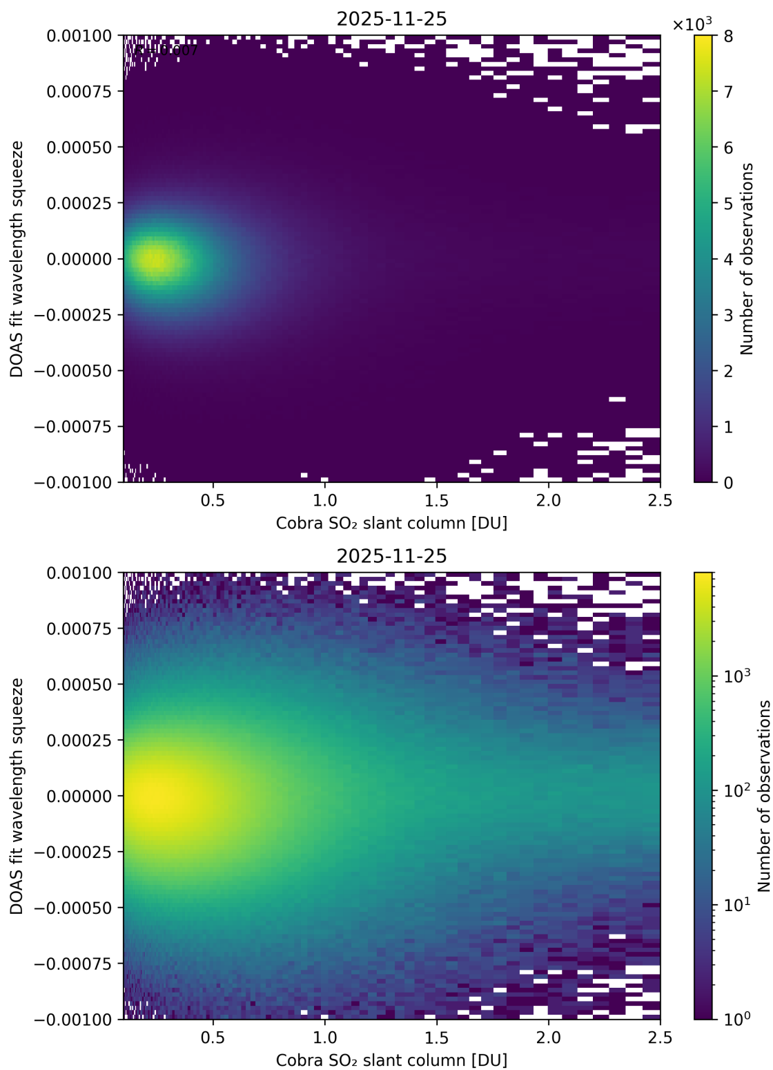
Figure 197: Scatter density plot of “Cobra SO 2 slant column” against “DOAS fit wavelength squeeze” for 2025-11-24 to 2025-11-26.
