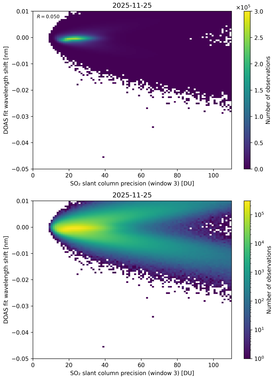
Figure 308: Scatter density plot of “SO 2 slant column precision (window 3)” against “DOAS fit wavelength shift” for 2025-11-24 to 2025-11-26.
