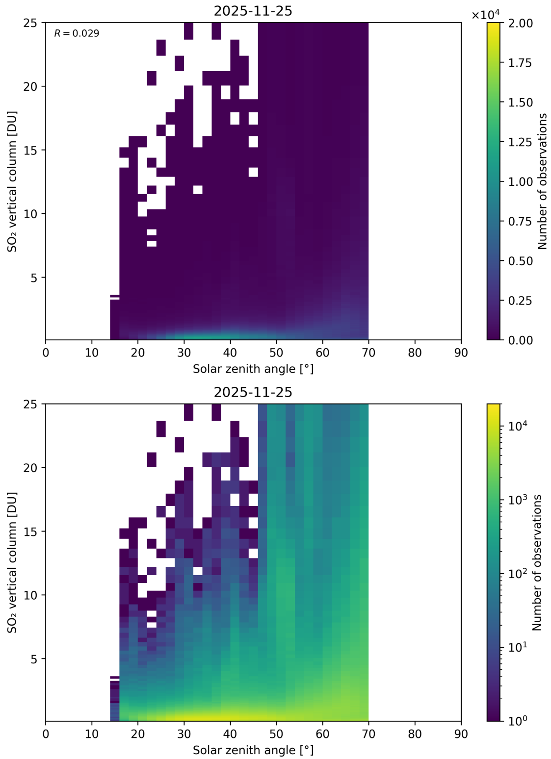
Figure 191: Scatter density plot of “Solar zenith angle” against “SO 2 vertical column” for 2025-11-24 to 2025-11-26.
