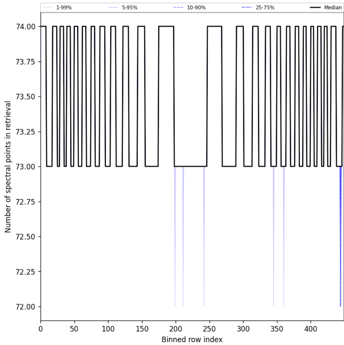
Figure 108: Along track statistics of “Number of spectral points in retrieval” for 2025-11-24 to 2025-11-26
