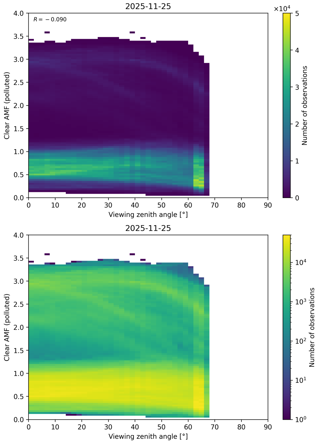
Figure 370: Scatter density plot of “Viewing zenith angle” against “Clear AMF (polluted)” for 2025-11-24 to 2025-11-26.
