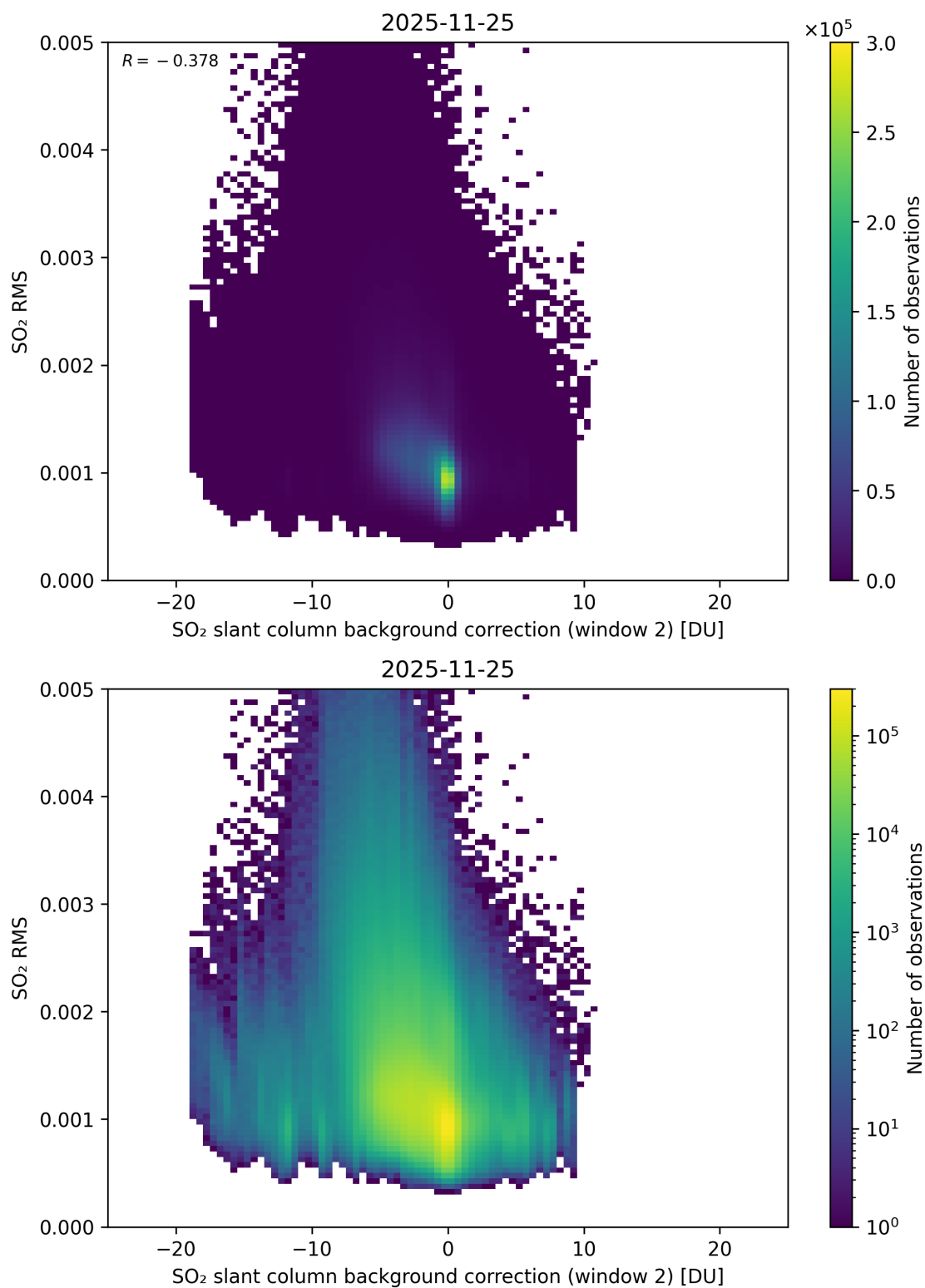
Figure 125: Scatter density plot of “SO 2 slant column background correction (window 2)” against “SO 2 RMS” for 2025-11-24 to 2025-11-26.
