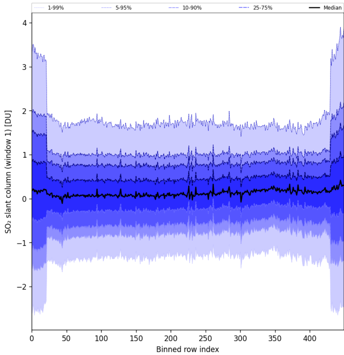
Figure 89: Along track statistics of “SO 2 slant column (window 1)” for 2025-11-24 to 2025-11-26
