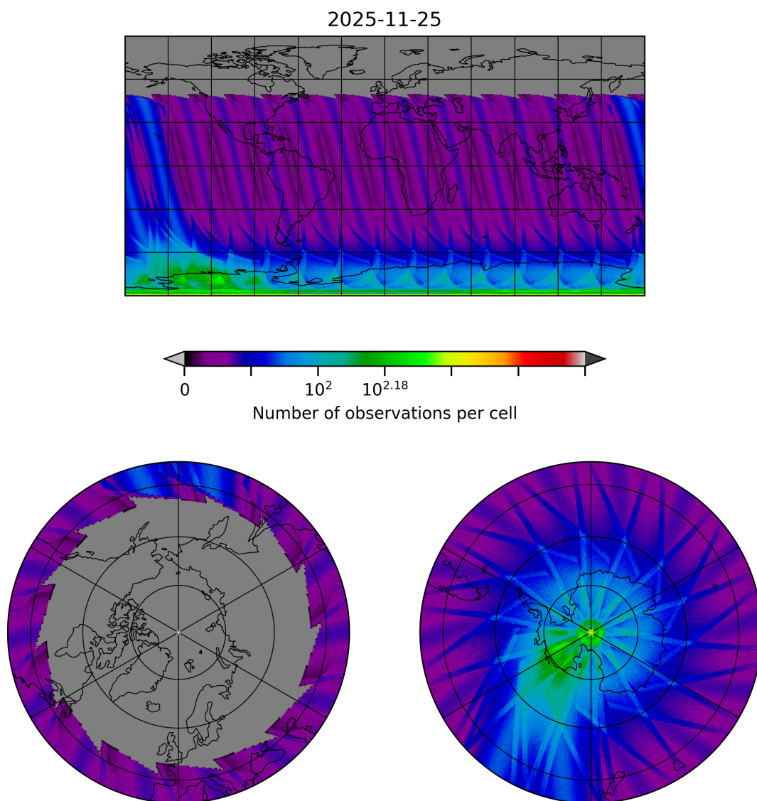
Figure 30: Map of the number of observations for 2025-11-24 to 2025-11-26
