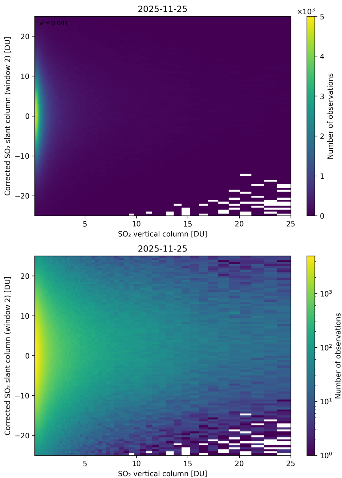
Figure 352: Scatter density plot of “SO 2 vertical column” against “Corrected SO 2 slant column (window 2)” for 2025-11-24 to 2025-11-26.
