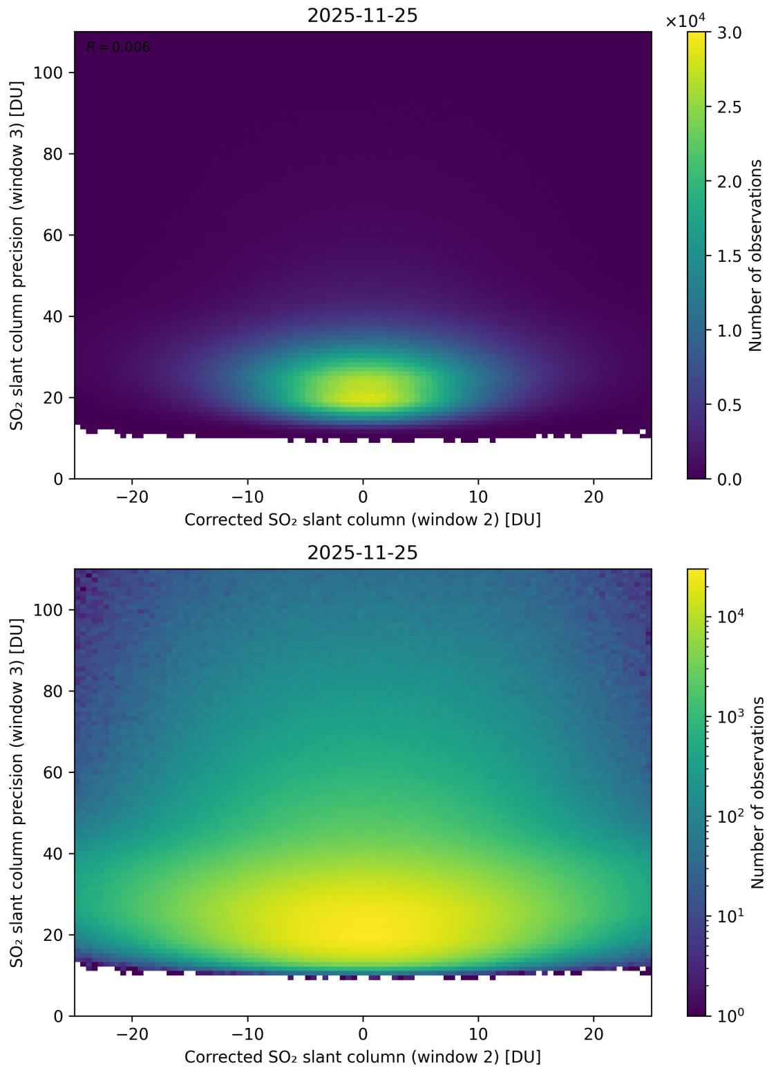
Figure 252: Scatter density plot of “Corrected SO 2 slant column (window 2)” against “SO 2 slant column precision (window 3)” for 2025-11-24 to 2025-11-26.
