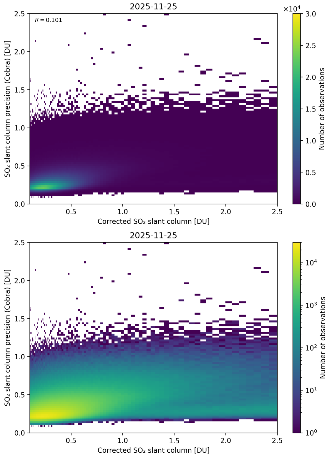
Figure 234: Scatter density plot of “Corrected SO 2 slant column” against “SO 2 slant column precision (Cobra)” for 2025-11-24 to 2025-11-26.
