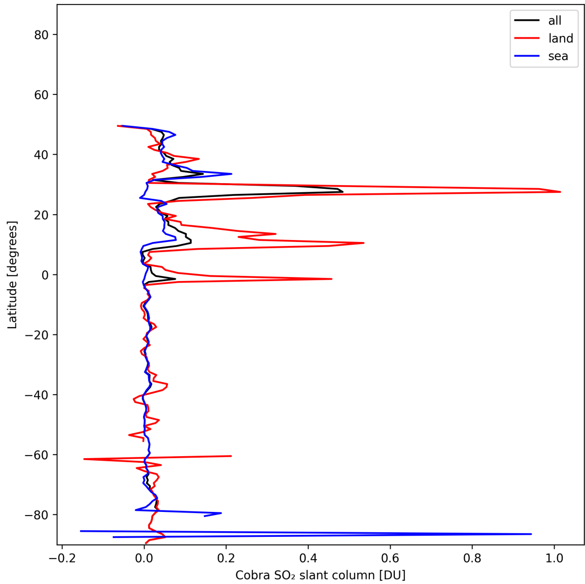
Figure 35: Zonal average of “Cobra SO 2 slant column” for 2025-11-24 to 2025-11-26.
