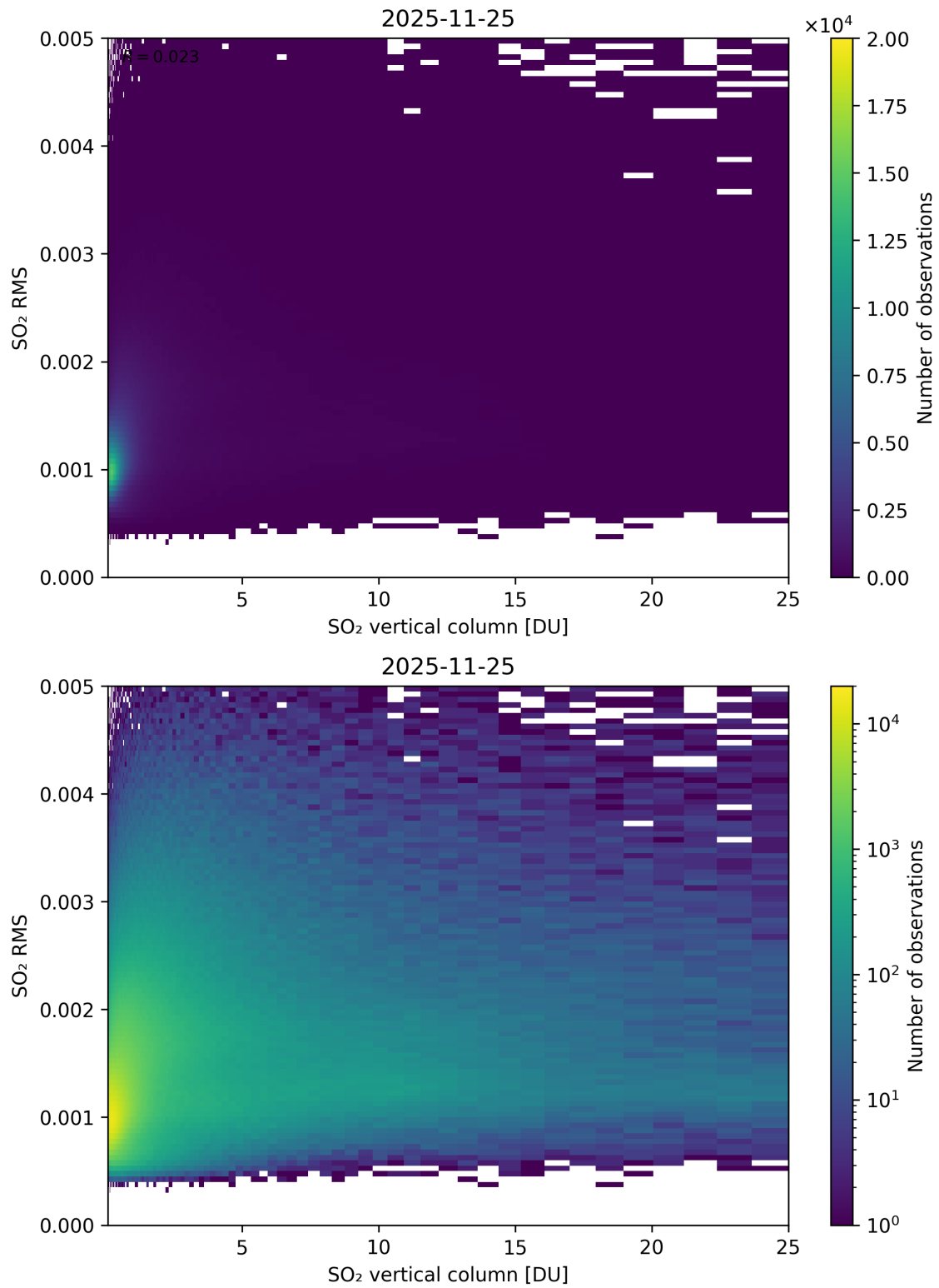
Figure 328: Scatter density plot of “SO 2 vertical column” against “SO 2 RMS” for 2025-11-24 to 2025-11-26.
