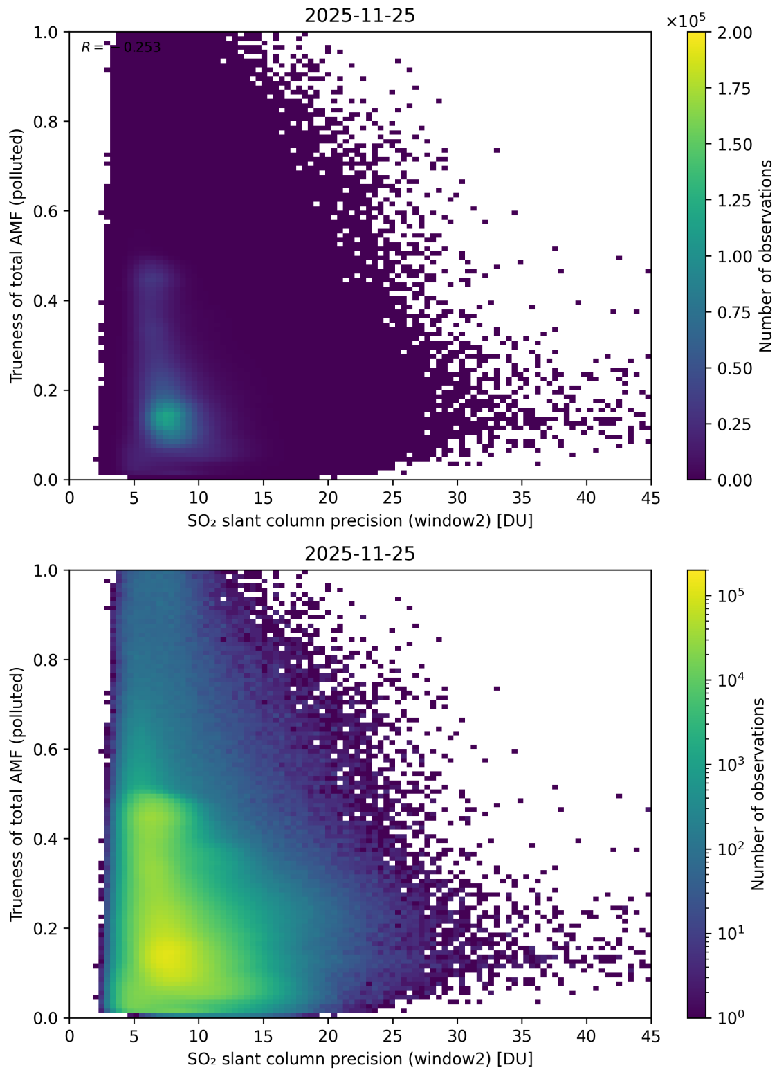
Figure 302: Scatter density plot of “SO 2 slant column precision (window2)” against “Trueness of total AMF (polluted)” for 2025-11-24 to 2025-11-26.
