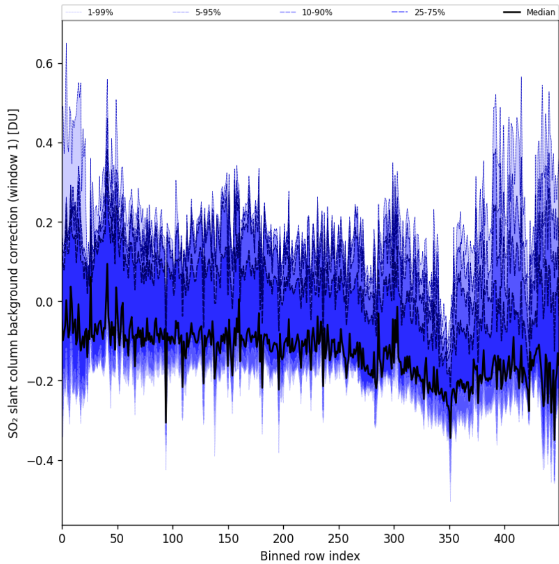
Figure 92: Along track statistics of “SO 2 slant column background correction (window 1)” for 2025-11-24 to 2025-11-26
