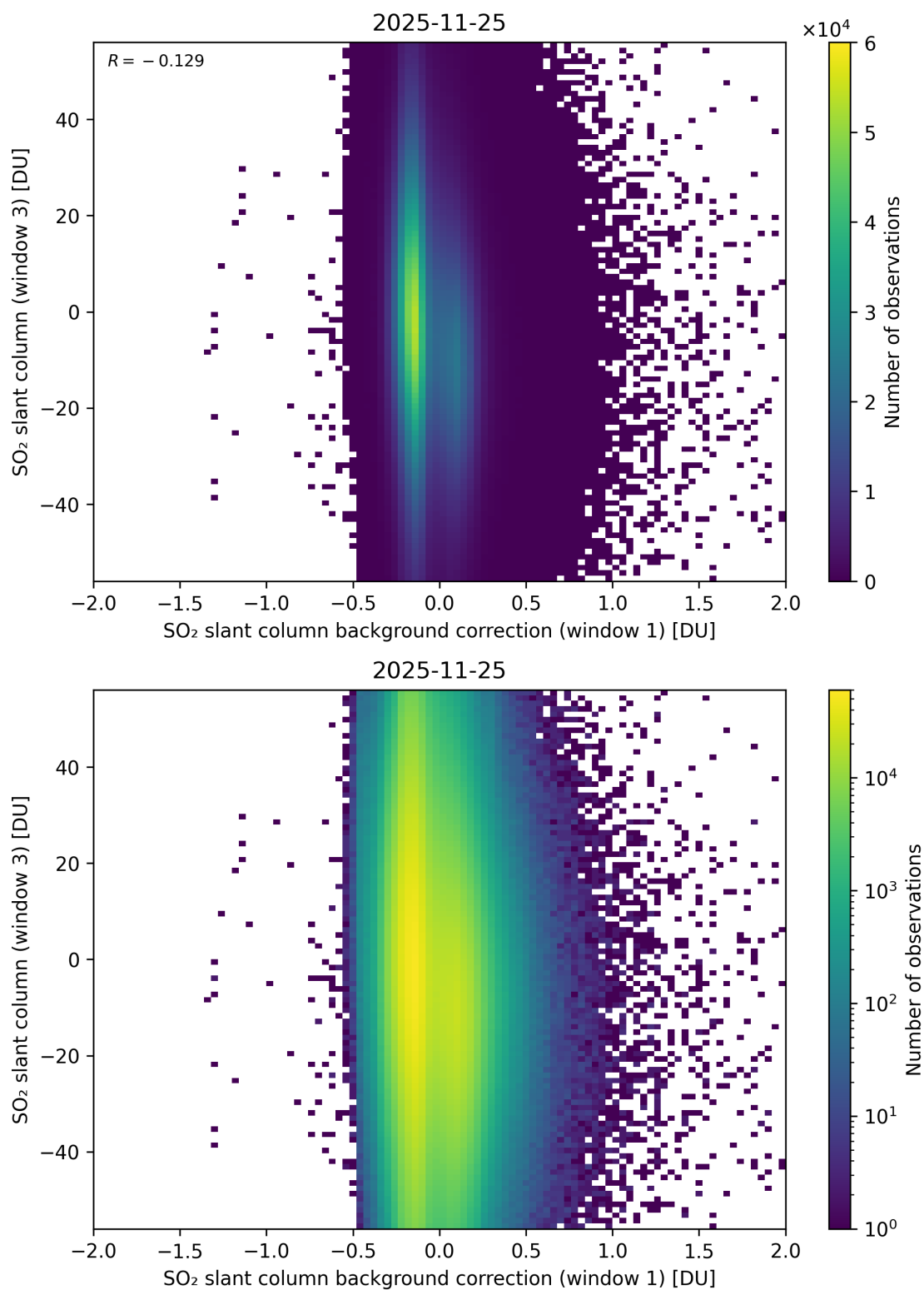
Figure 118: Scatter density plot of “SO 2 slant column background correction (window 1)” against “SO 2 slant column (window 3)” for 2025-11-24 to 2025-11-26.
