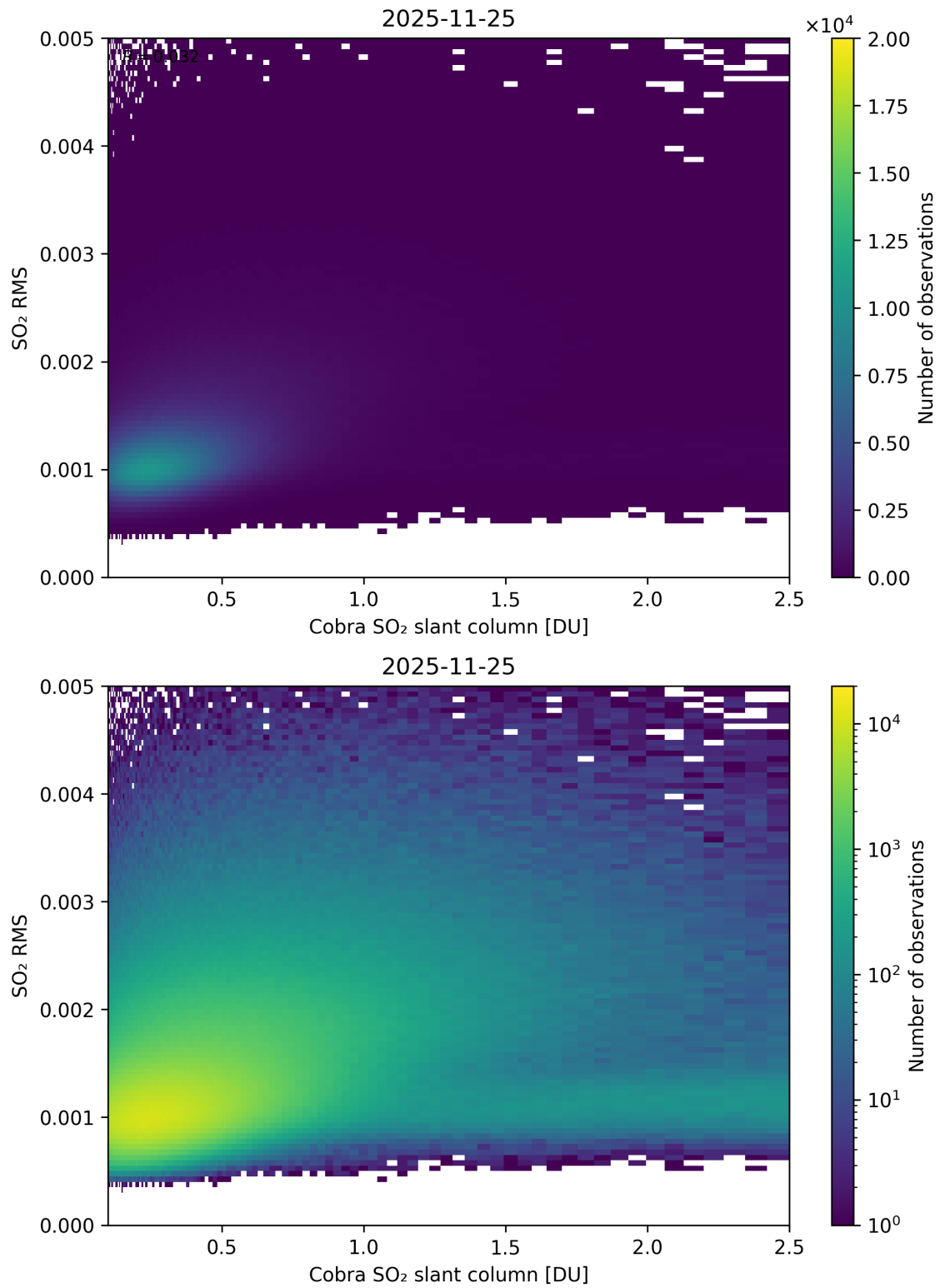
Figure 198: Scatter density plot of “Cobra SO 2 slant column” against “SO 2 RMS” for 2025-11-24 to 2025-11-26.
