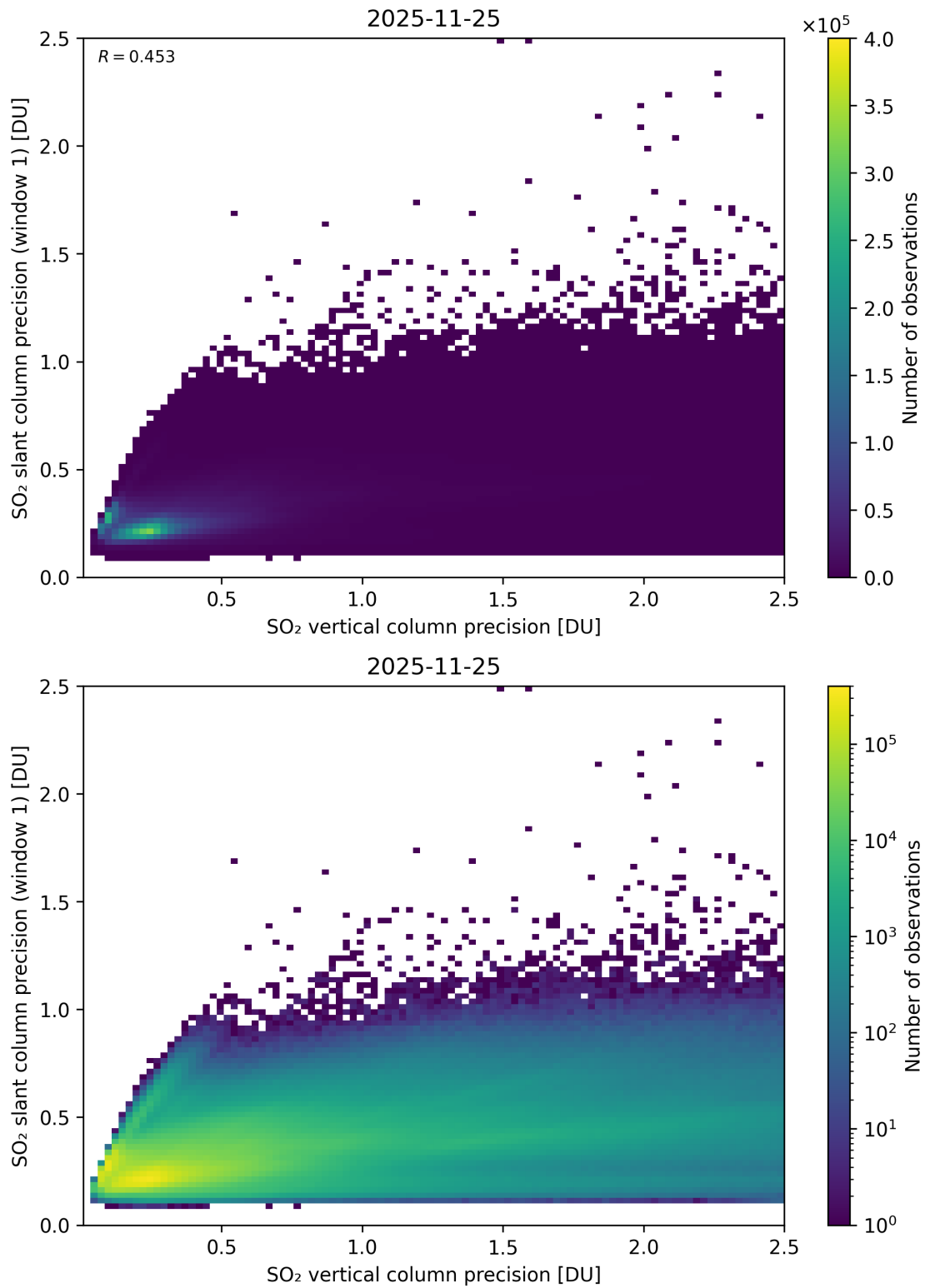
Figure 342: Scatter density plot of “SO 2 vertical column precision” against “SO 2 slant column precision (window 1)” for 2025-11-24 to 2025-11-26.
