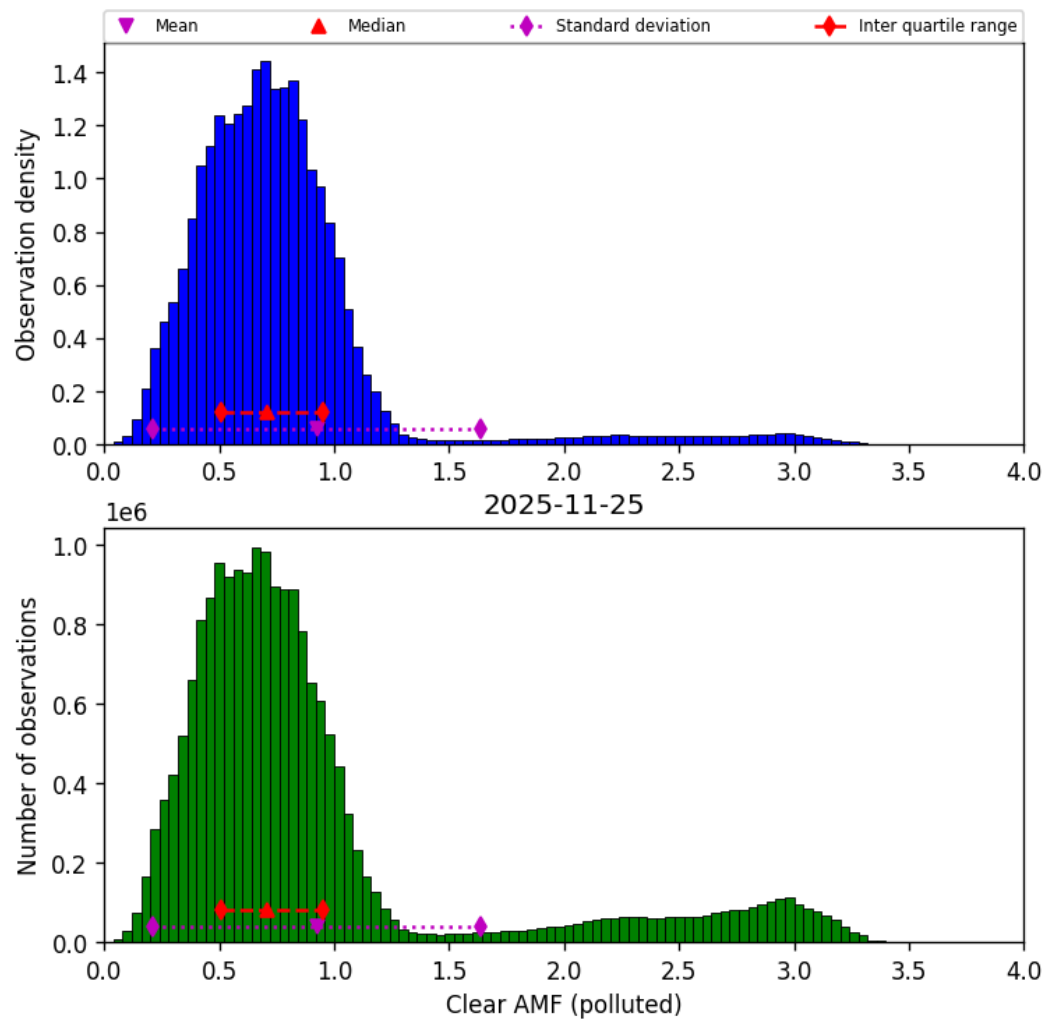
Figure 81: Histogram of “Clear AMF (polluted)” for 2025-11-24 to 2025-11-26
