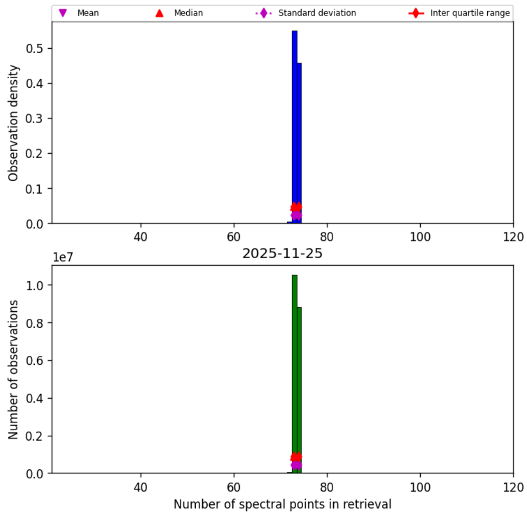
Figure 82: Histogram of “Number of spectral points in retrieval” for 2025-11-24 to 2025-11-26
