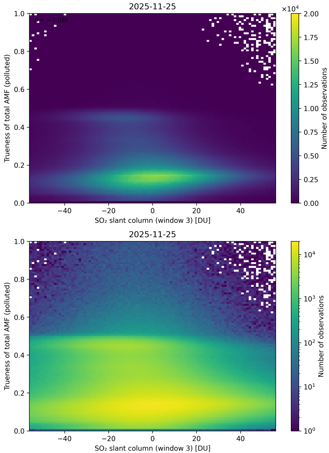
Figure 319: Scatter density plot of “SO 2 slant column (window 3)” against “Trueness of total AMF (polluted)” for 2025-11-24 to 2025-11-26.
