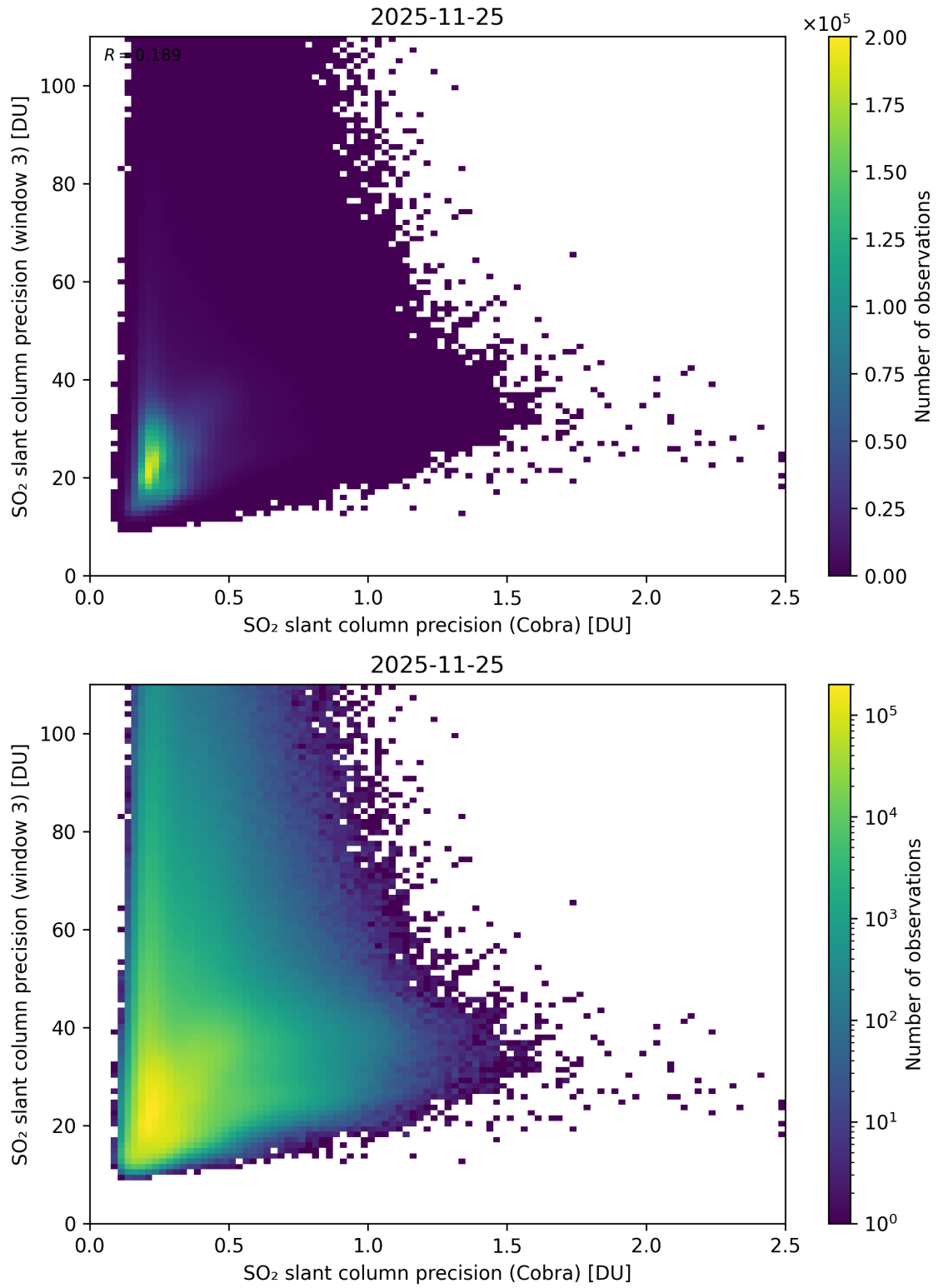
Figure 212: Scatter density plot of “SO 2 slant column precision (Cobra)” against “SO 2 slant column precision (window 3)” for 2025-11-24 to 2025-11-26.
