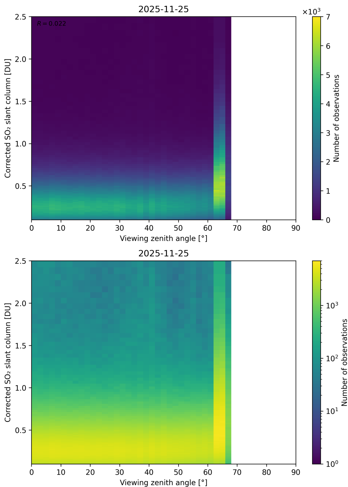
Figure 373: Scatter density plot of “Viewing zenith angle” against “Corrected SO 2 slant column” for 2025-11-24 to 2025-11-26.
