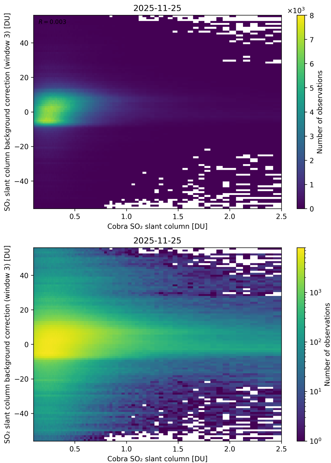
Figure 195: Scatter density plot of “Cobra SO 2 slant column” against “SO 2 slant column background correction (window 3)” for 2025-11-24 to 2025-11-26.
