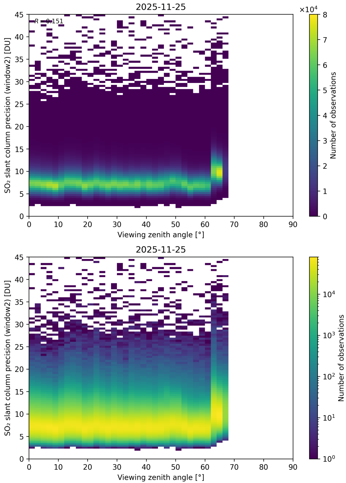
Figure 378: Scatter density plot of “Viewing zenith angle” against “SO 2 slant column precision (window2)” for 2025-11-24 to 2025-11-26.
