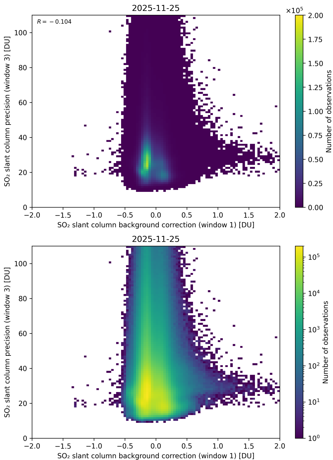
Figure 119: Scatter density plot of “SO 2 slant column background correction (window 1)” against “SO 2 slant column precision (window 3)” for 2025-11-24 to 2025-11-26.
