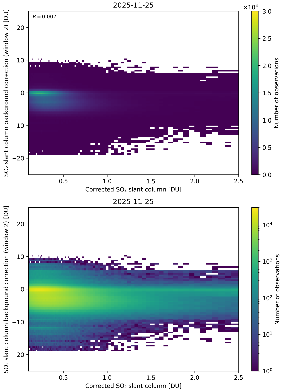
Figure 227: Scatter density plot of “Corrected SO 2 slant column” against “SO 2 slant column background correction (window 2)” for 2025-11-24 to 2025-11-26.
