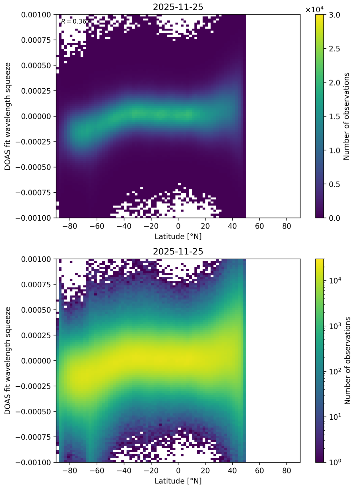
Figure 154: Scatter density plot of “Latitude” against “DOAS fit wavelength squeeze” for 2025-11-24 to 2025-11-26.
