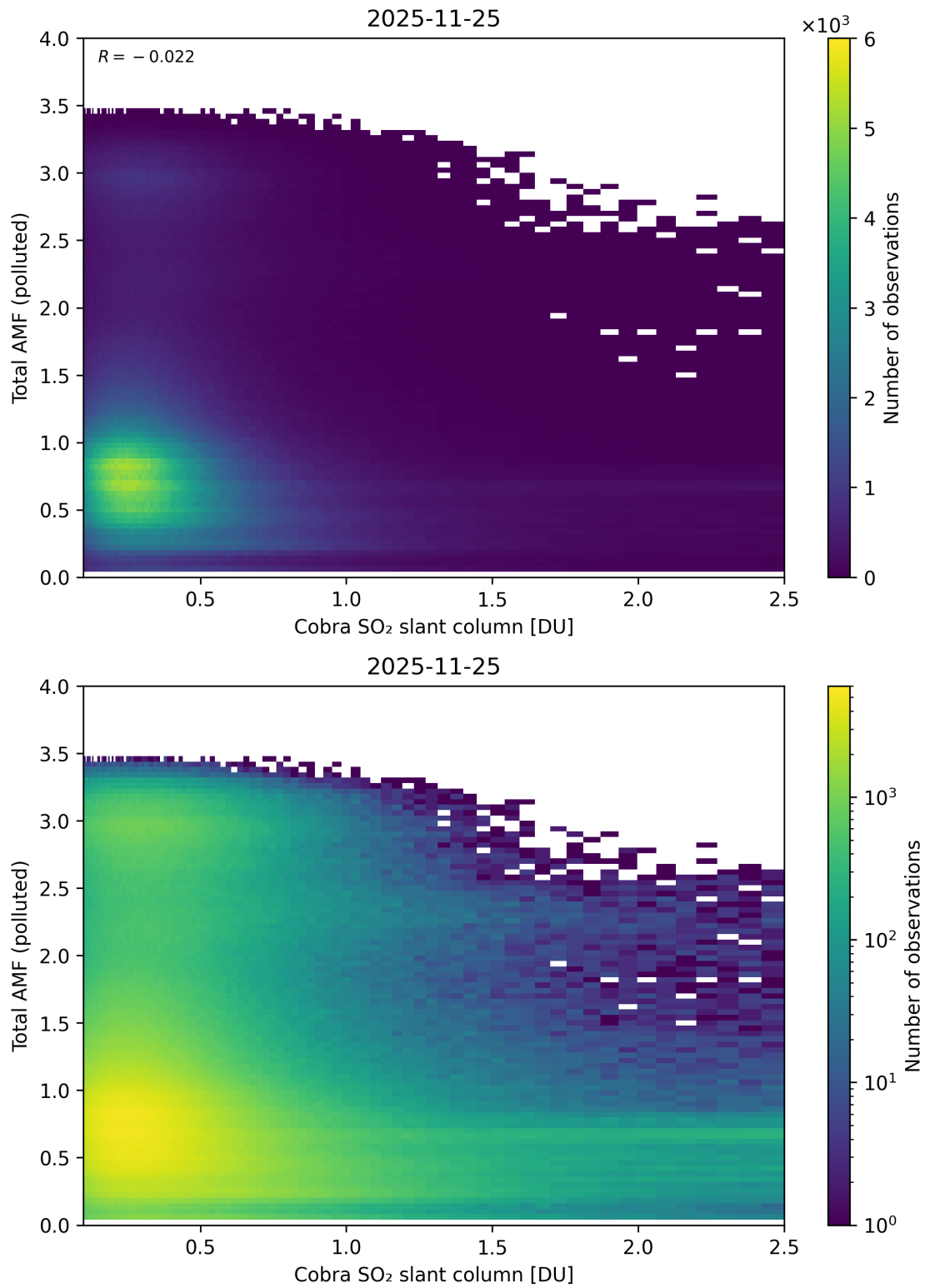
Figure 224: Scatter density plot of “Cobra SO 2 slant column” against “Total AMF (polluted)” for 2025-11-24 to 2025-11-26.
