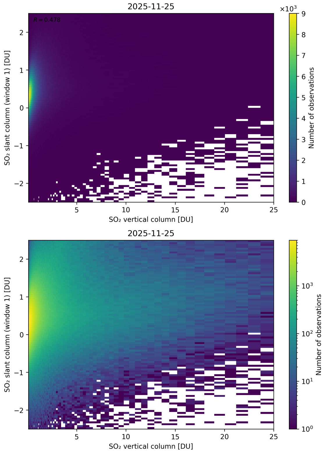
Figure 354: Scatter density plot of “SO 2 vertical column” against “SO 2 slant column (window 1)” for 2025-11-24 to 2025-11-26.
