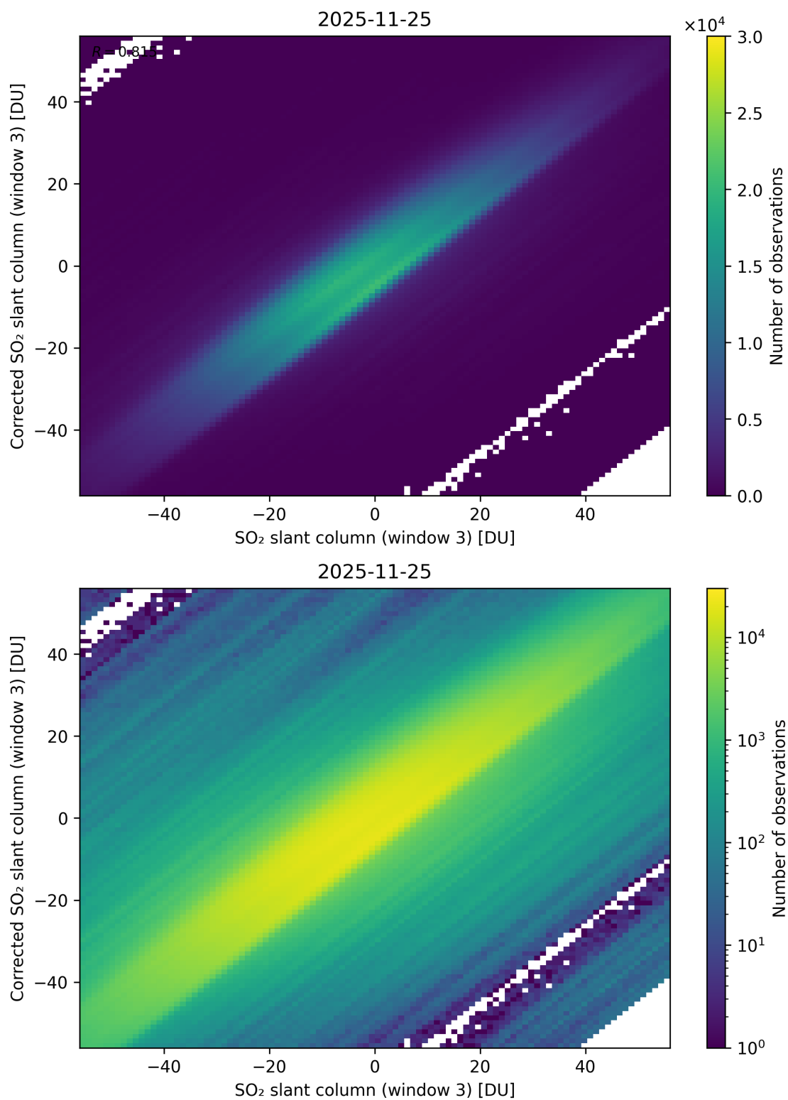
Figure 316: Scatter density plot of “SO 2 slant column (window 3)” against “Corrected SO 2 slant column (window 3)” for 2025-11-24 to 2025-11-26.
