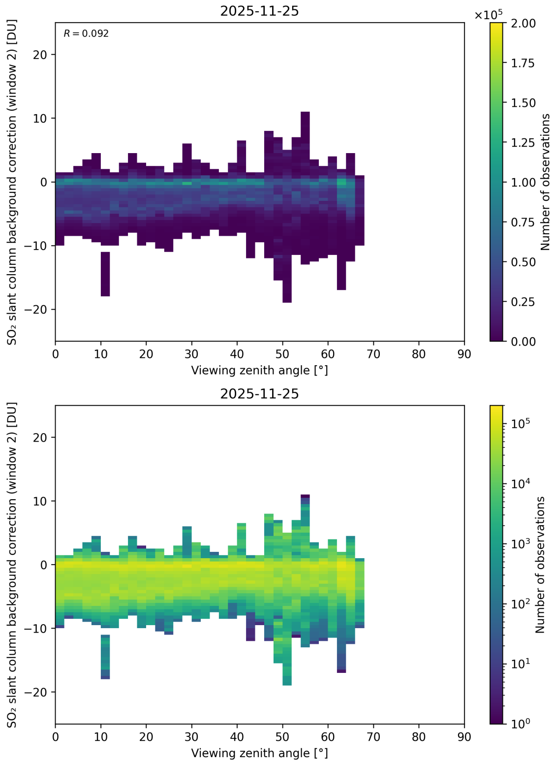
Figure 363: Scatter density plot of “Viewing zenith angle” against “SO 2 slant column background correction (window 2)” for 2025-11-24 to 2025-11-26.
