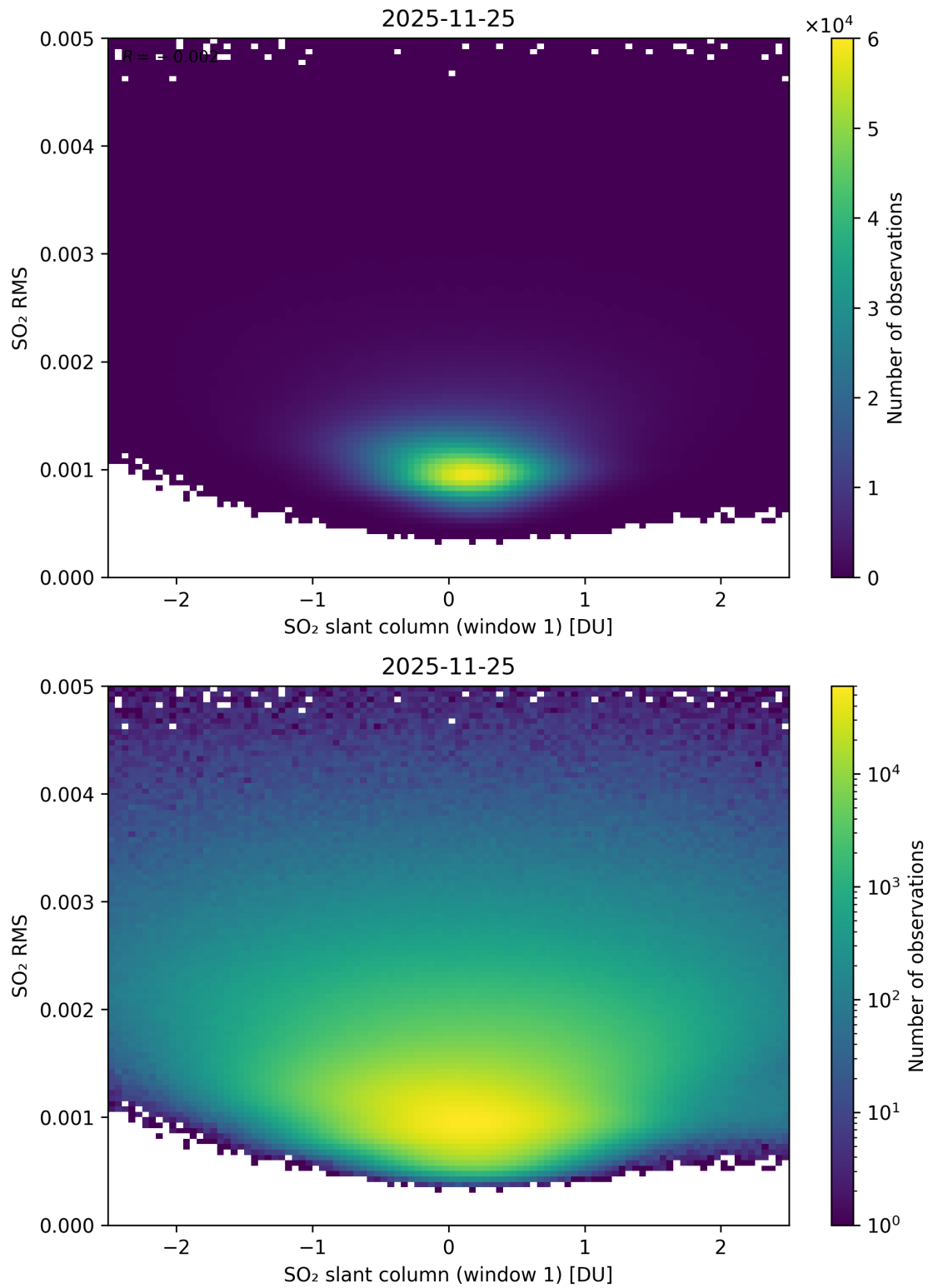
Figure 267: Scatter density plot of “SO 2 slant column (window 1)” against “SO 2 RMS” for 2025-11-24 to 2025-11-26.
