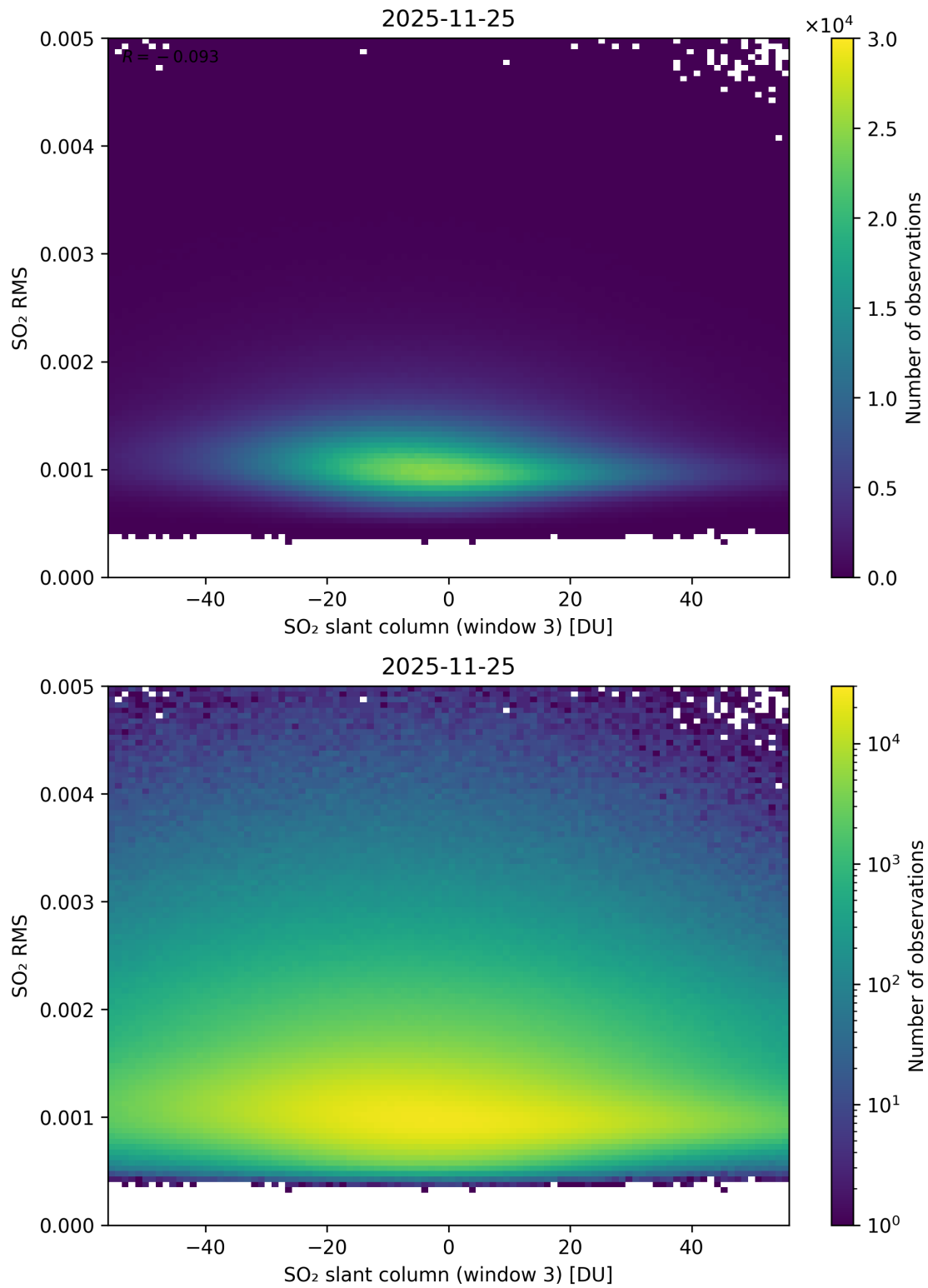
Figure 306: Scatter density plot of “SO 2 slant column (window 3)” against “SO 2 RMS” for 2025-11-24 to 2025-11-26.
