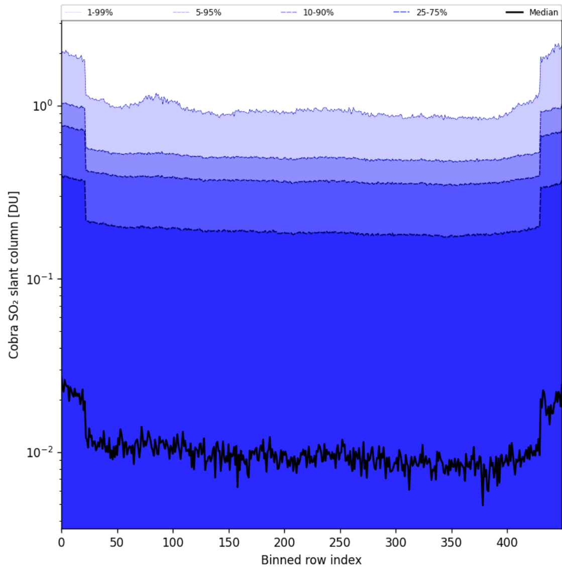
Figure 87: Along track statistics of “Cobra SO 2 slant column” for 2025-11-24 to 2025-11-26
