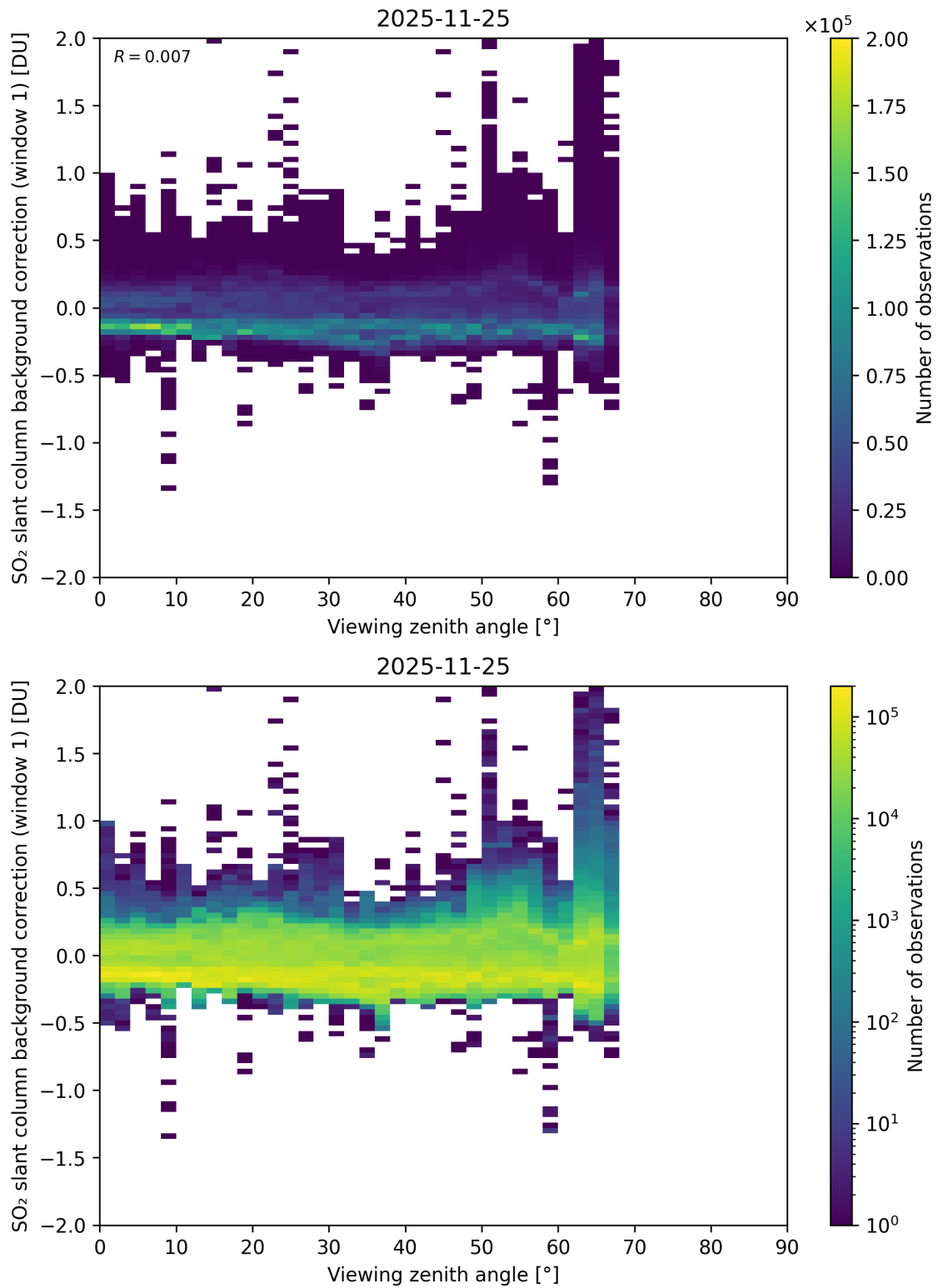
Figure 362: Scatter density plot of “Viewing zenith angle” against “SO 2 slant column background correction (window 1)” for 2025-11-24 to 2025-11-26.
