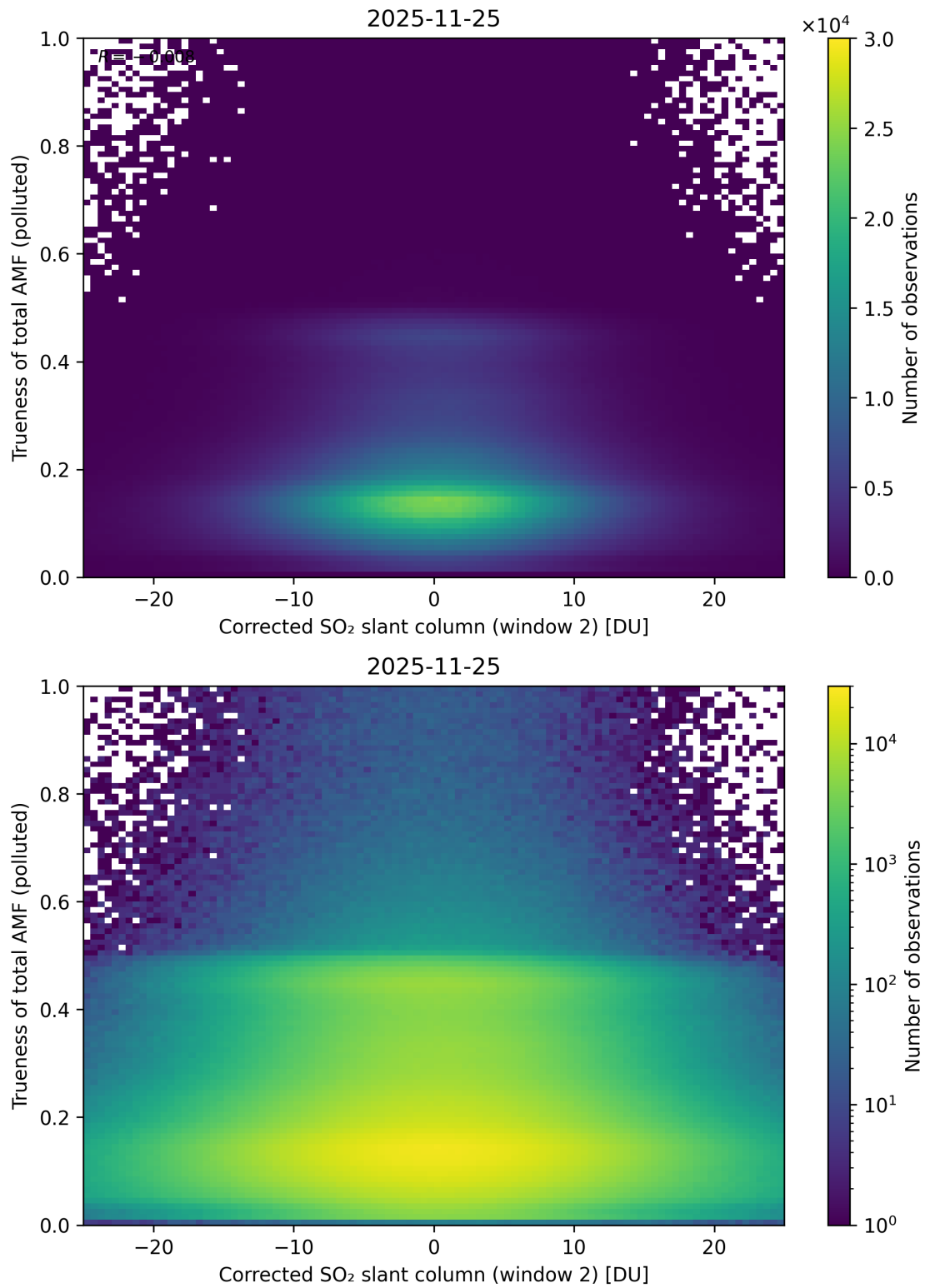
Figure 254: Scatter density plot of “Corrected SO 2 slant column (window 2)” against “Trueness of total AMF (polluted)” for 2025-11-24 to 2025-11-26.
