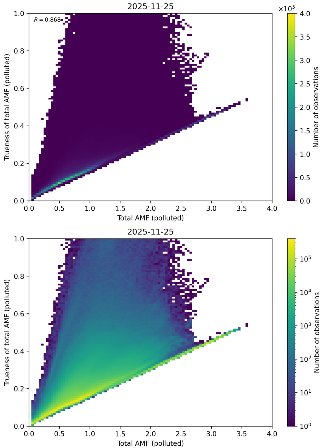
Figure 321: Scatter density plot of “Total AMF (polluted)” against “Trueness of total AMF (polluted)” for 2025-11-24 to 2025-11-26.
