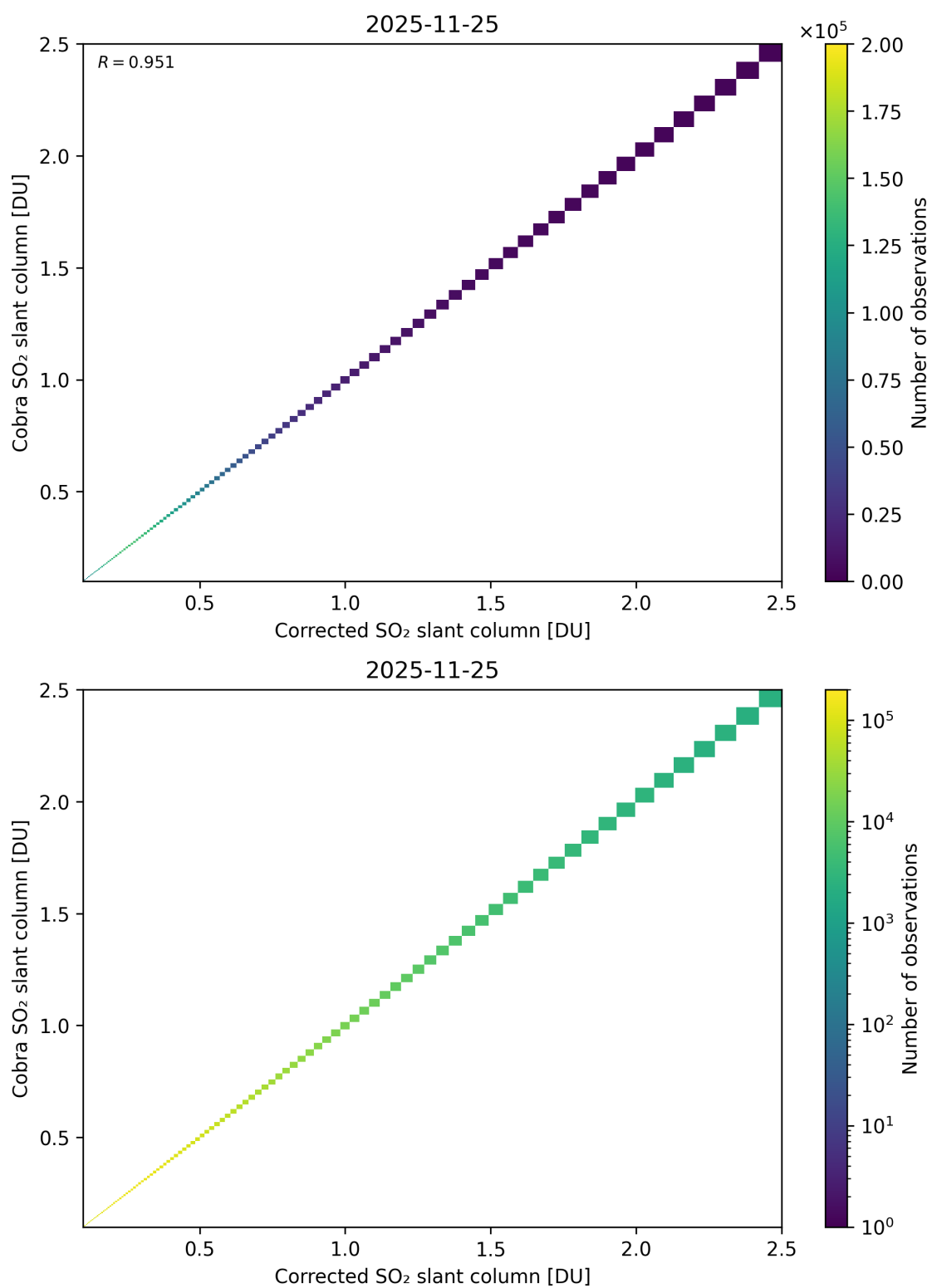
Figure 233: Scatter density plot of “Corrected SO 2 slant column” against “Cobra SO 2 slant column” for 2025-11-24 to 2025-11-26.
