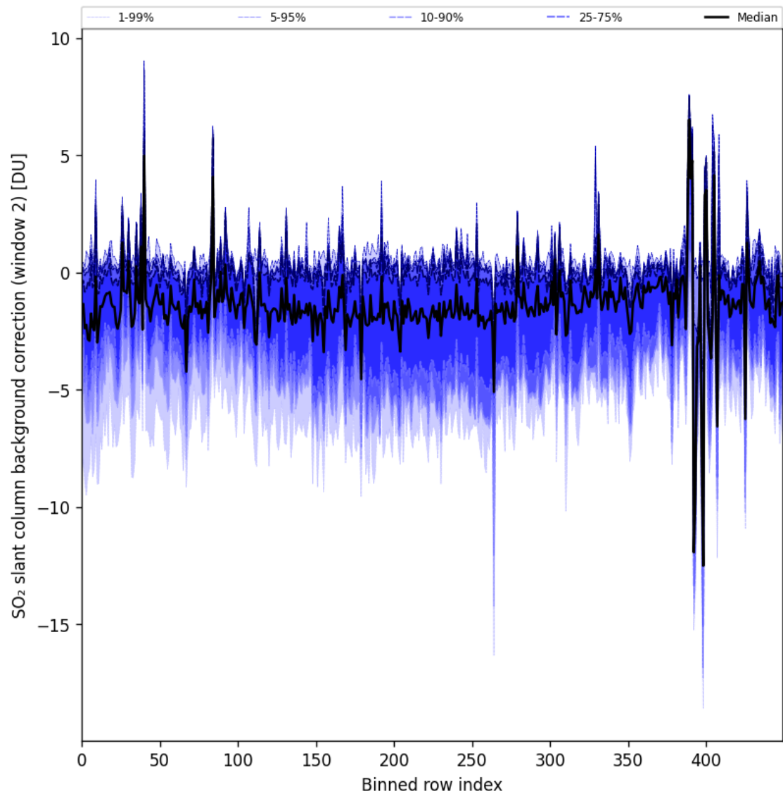
Figure 96: Along track statistics of "SO 2 slant column background correction (window 2)" for 2025-11-24 to 2025-11-26
