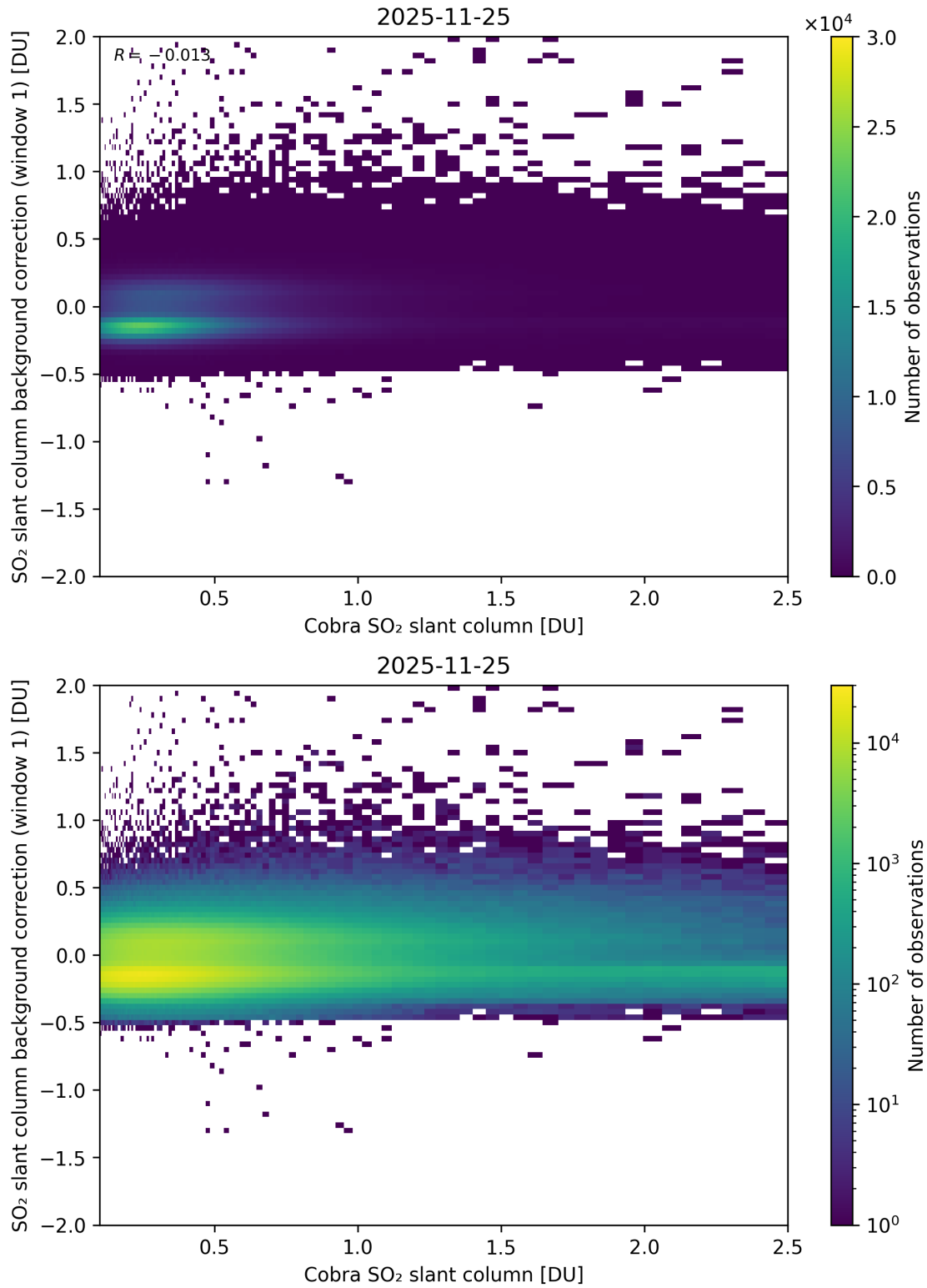
Figure 193: Scatter density plot of “Cobra SO 2 slant column” against “SO 2 slant column background correction (window 1)” for 2025-11-24 to 2025-11-26.
