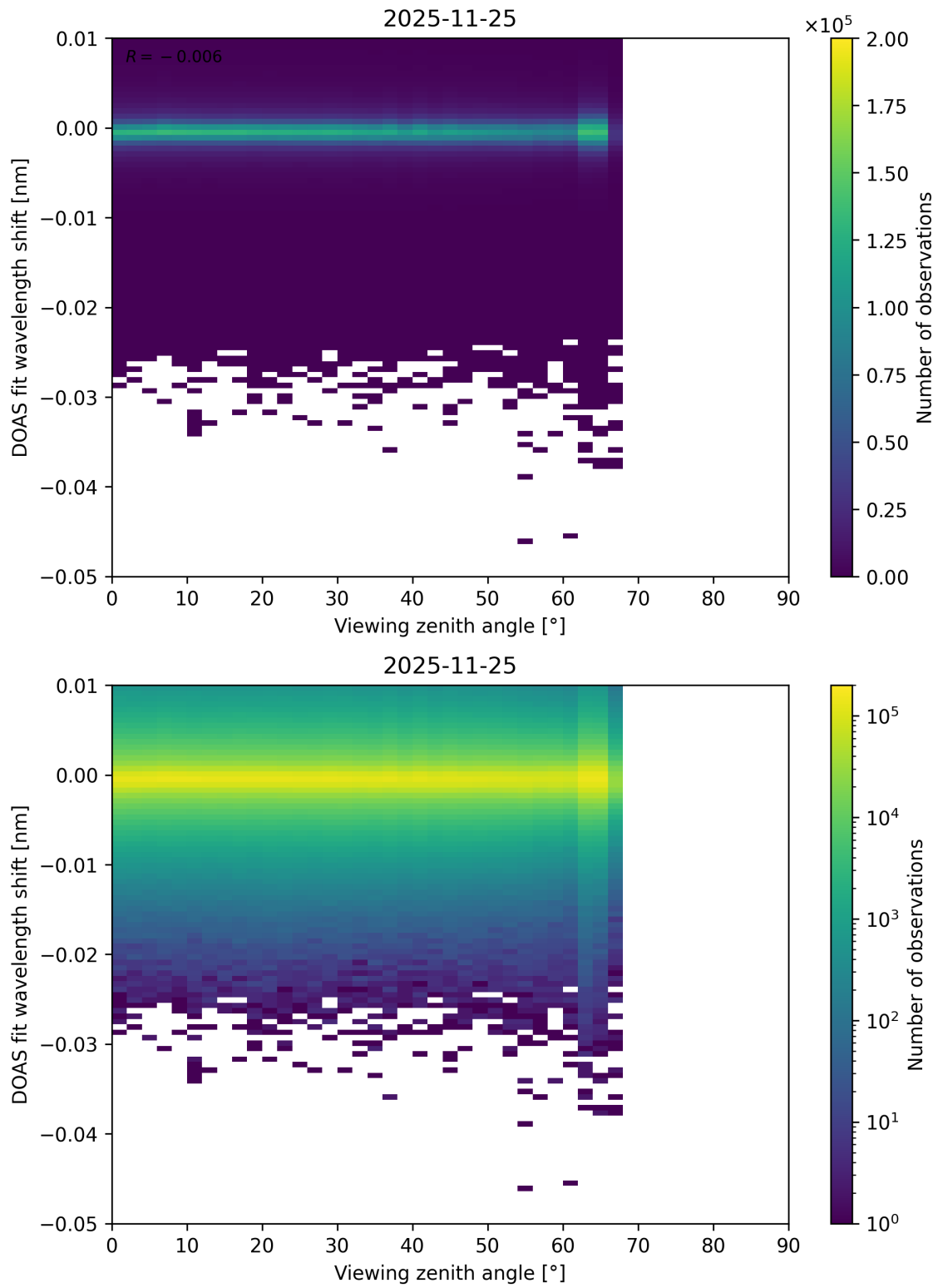
Figure 365: Scatter density plot of “Viewing zenith angle” against “DOAS fit wavelength shift” for 2025-11-24 to 2025-11-26.
