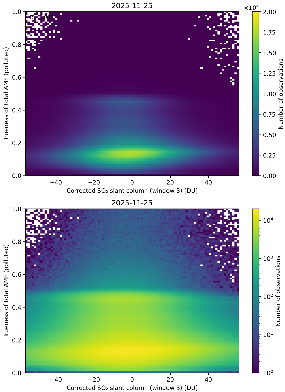
Figure 261: Scatter density plot of “Corrected SO 2 slant column (window 3)” against “Trueness of total AMF (polluted)” for 2025-11-24 to 2025-11-26.
