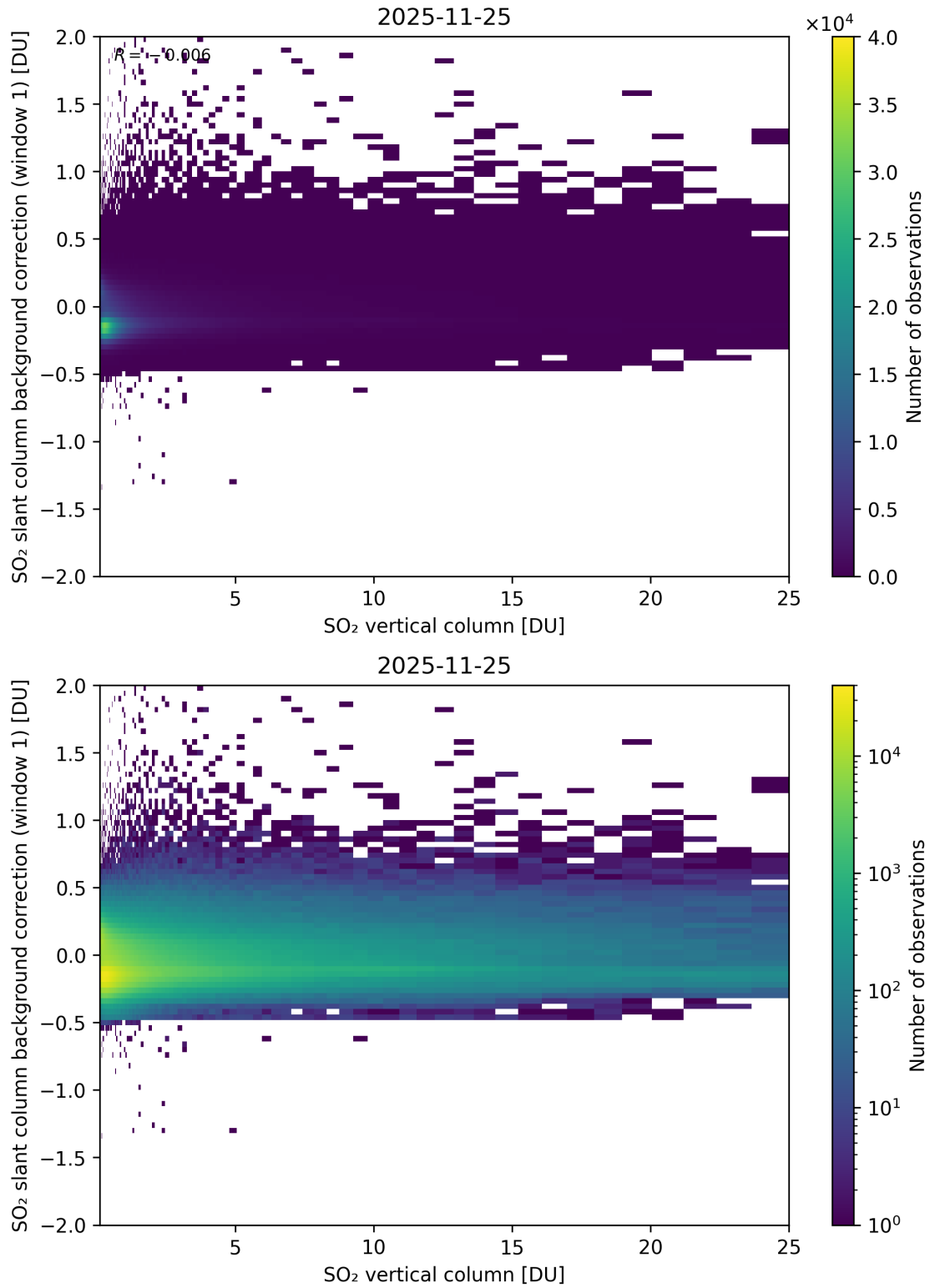
Figure 323: Scatter density plot of “SO 2 vertical column” against “SO 2 slant column background correction (window 1)” for 2025-11-24 to 2025-11-26.
