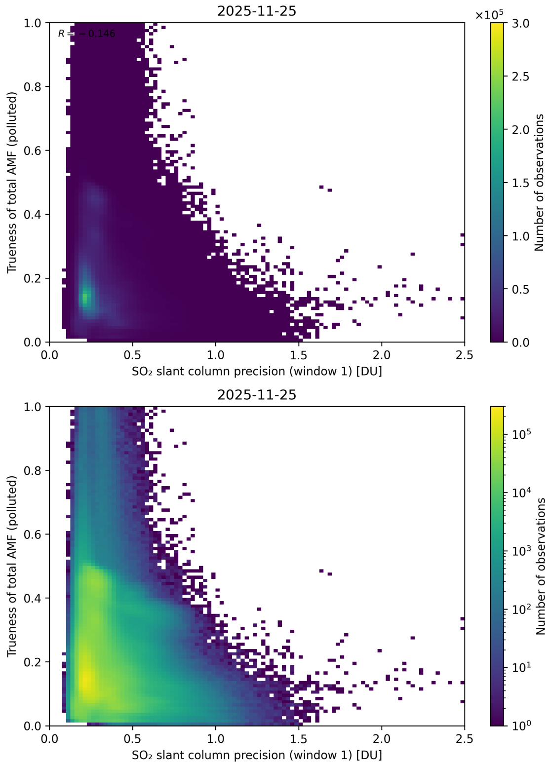
Figure 281: Scatter density plot of “SO 2 slant column precision (window 1)” against “Trueness of total AMF (polluted)” for 2025-11-24 to 2025-11-26.
