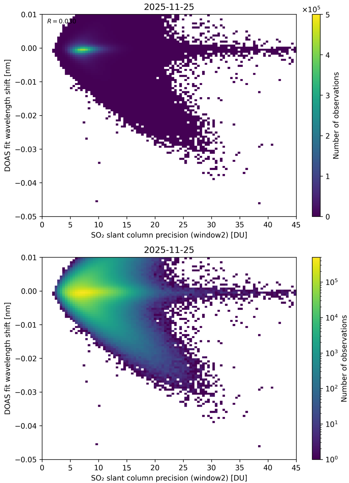
Figure 293: Scatter density plot of “SO 2 slant column precision (window2)” against “DOAS fit wavelength shift” for 2025-11-24 to 2025-11-26.
