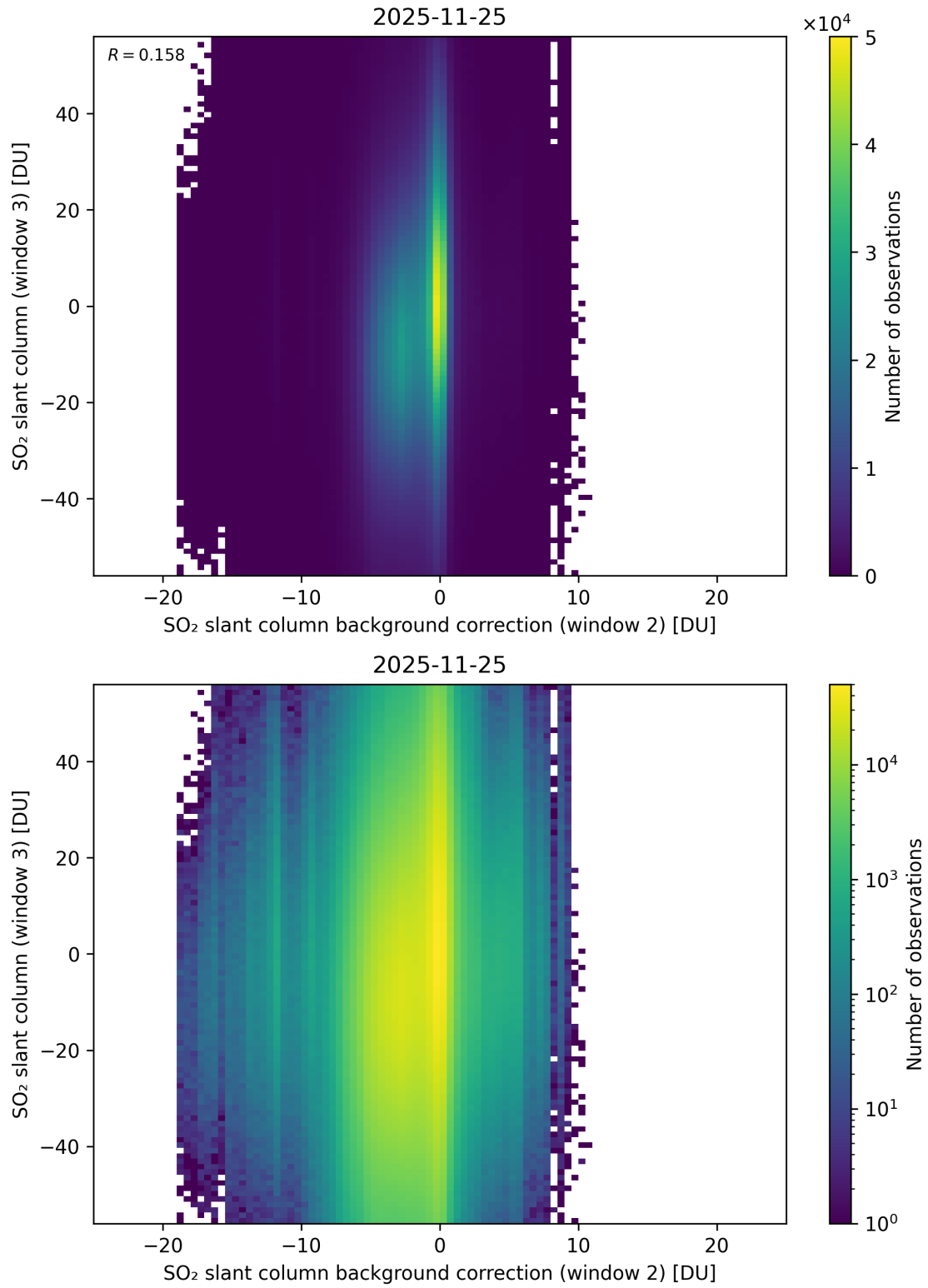
Figure 128: Scatter density plot of “SO 2 slant column background correction (window 2)” against “SO 2 slant column (window 3)” for 2025-11-24 to 2025-11-26.
