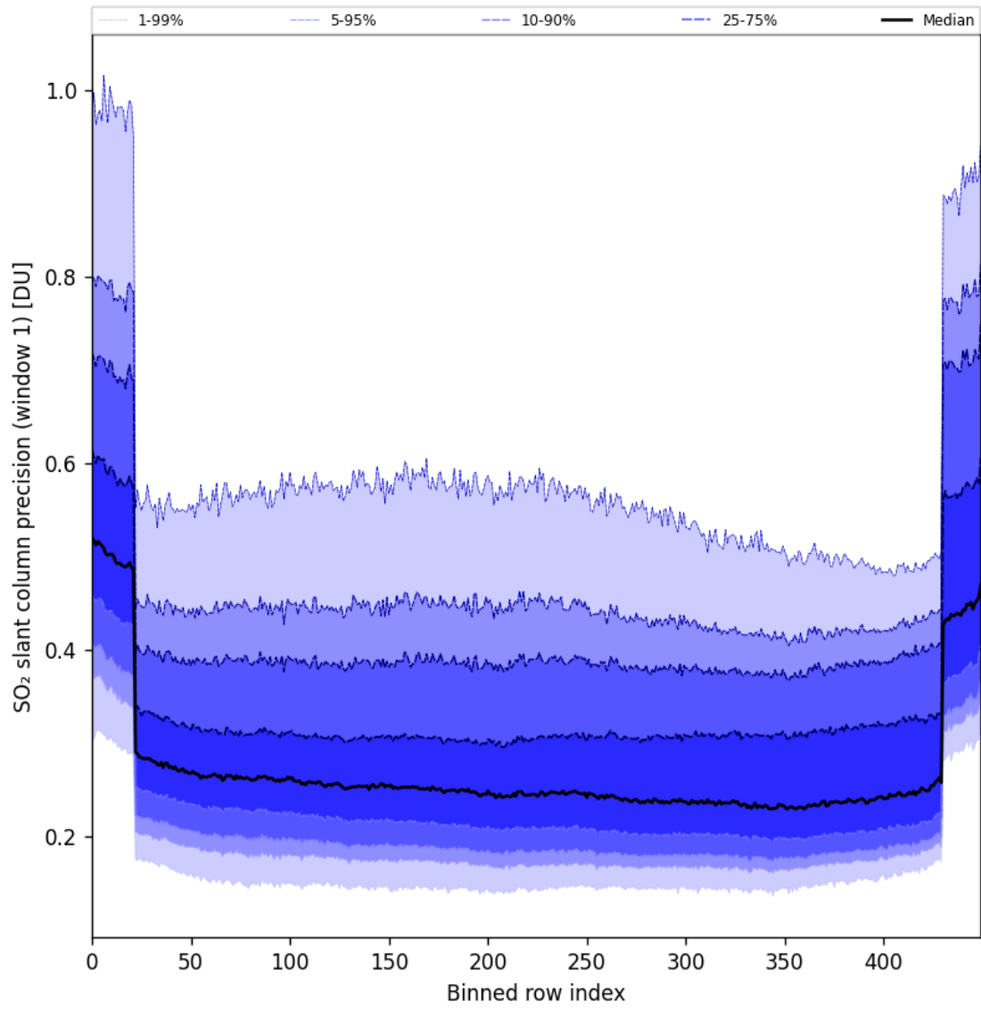
Figure 90: Along track statistics of “SO 2 slant column precision (window 1)” for 2025-11-24 to 2025-11-26
