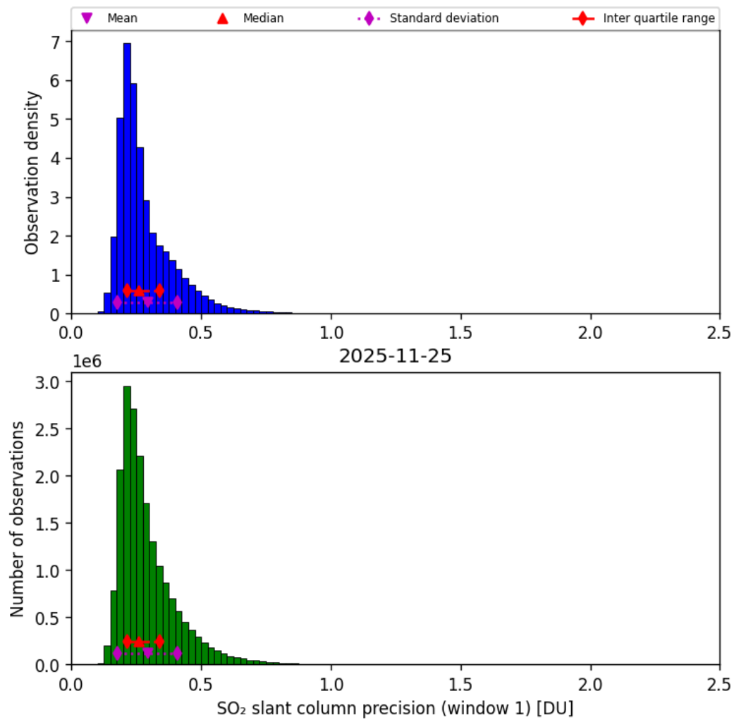
Figure 64: Histogram of “SO 2 slant column precision (window 1)” for 2025-11-24 to 2025-11-26
