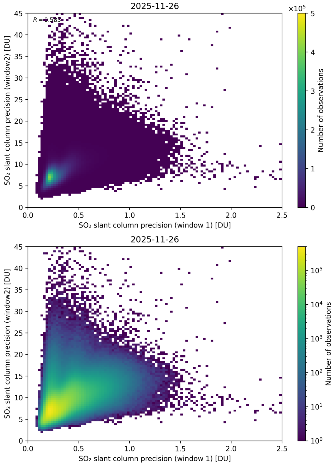
Figure 277: Scatter density plot of “SO 2 slant column precision (window 1)” against “SO 2 slant column precision (window 2)” for 2025-11-25 to 2025-11-27.
