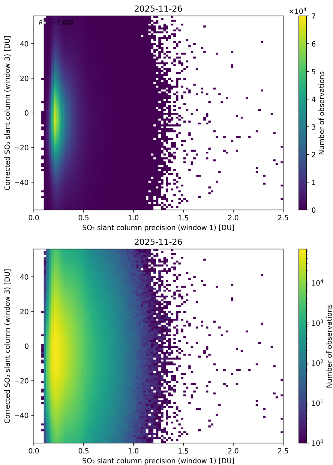
Figure 276: Scatter density plot of “SO 2 slant column precision (window 1)” against “Corrected SO 2 slant column (window 3)” for 2025-11-25 to 2025-11-27.
