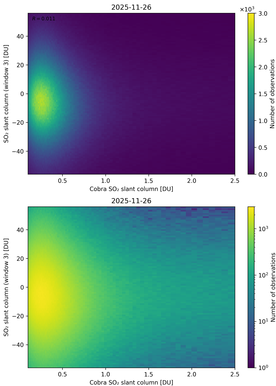
Figure 222: Scatter density plot of “Cobra SO 2 slant column” against “SO 2 slant column (window 3)” for 2025-11-25 to 2025-11-27.
