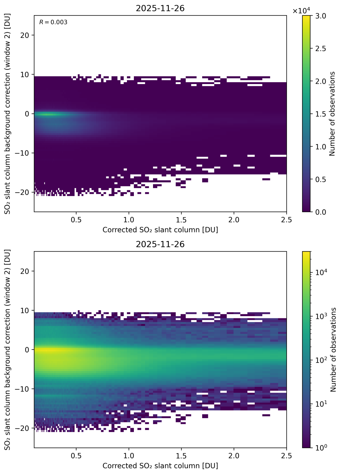
Figure 227: Scatter density plot of “Corrected SO 2 slant column” against “SO 2 slant column background correction (window 2)” for 2025-11-25 to 2025-11-27.
