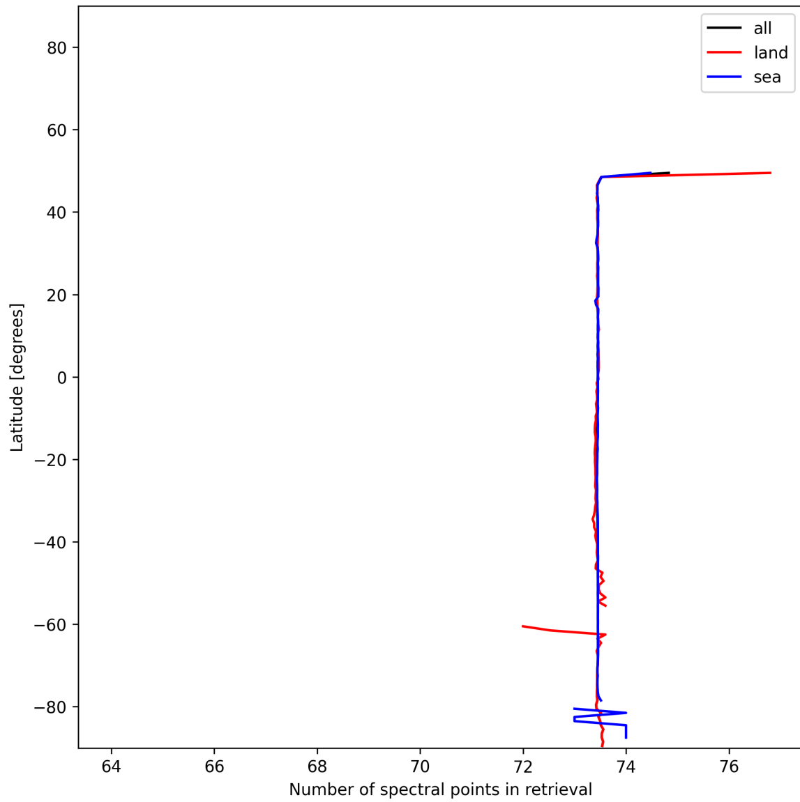
Figure 56: Zonal average of “Number of spectral points in retrieval” for 2025-11-25 to 2025-11-27.
