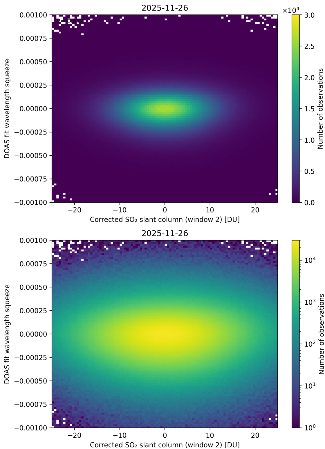
Figure 247: Scatter density plot of “Corrected SO 2 slant column (window 2)” against “DOAS fit wavelength squeeze” for 2025-11-25 to 2025-11-27.
