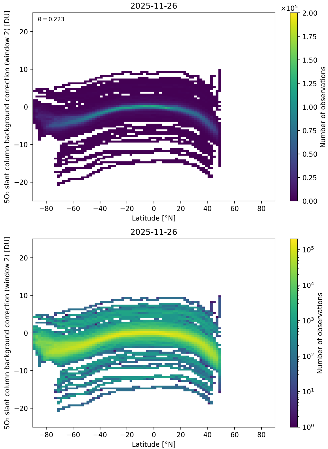
Figure 151: Scatter density plot of “Latitude” against “SO 2 slant column background correction (window 2)” for 2025-11-25 to 2025-11-27.
