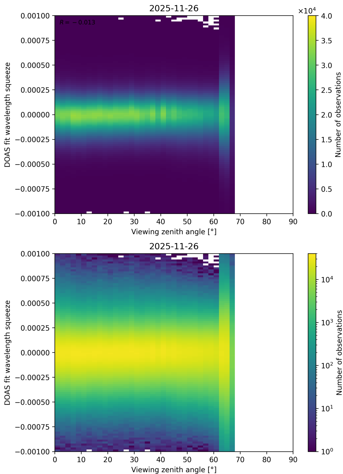
Figure 366: Scatter density plot of “Viewing zenith angle” against “DOAS fit wavelength squeeze” for 2025-11-25 to 2025-11-27.
