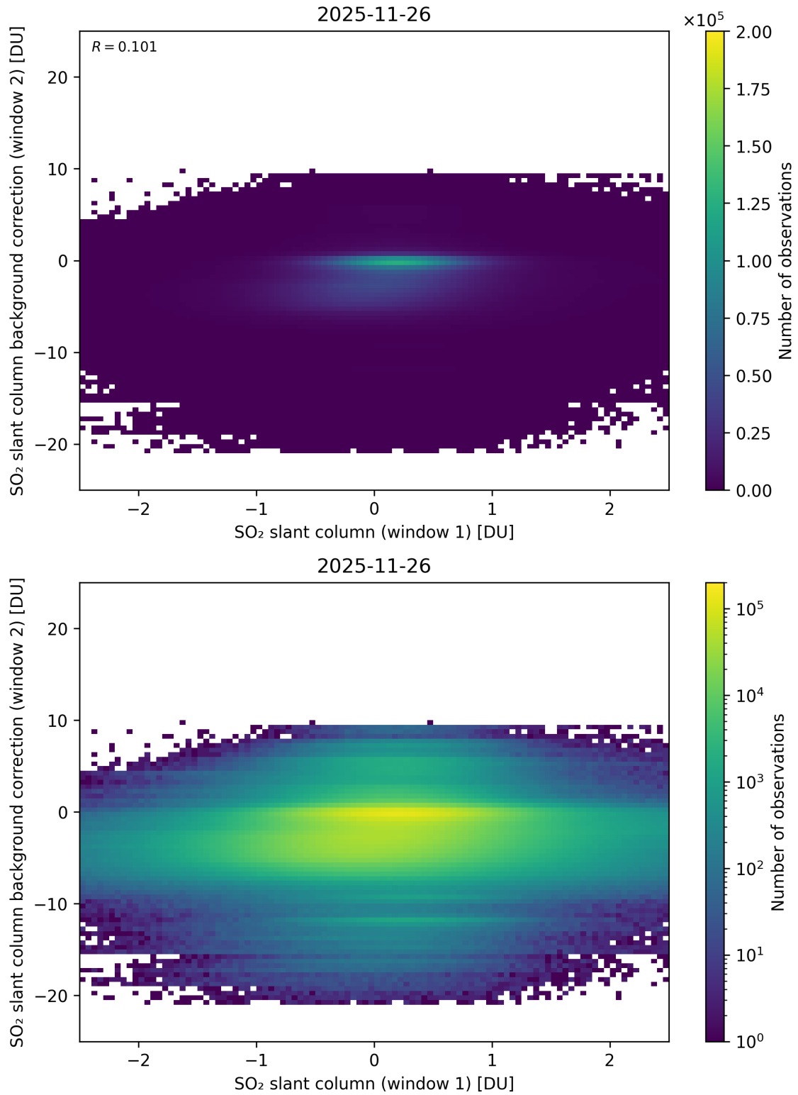
Figure 263: Scatter density plot of “SO 2 slant column (window 1)” against “SO 2 slant column background correction (window 2)” for 2025-11-25 to 2025-11-27.
