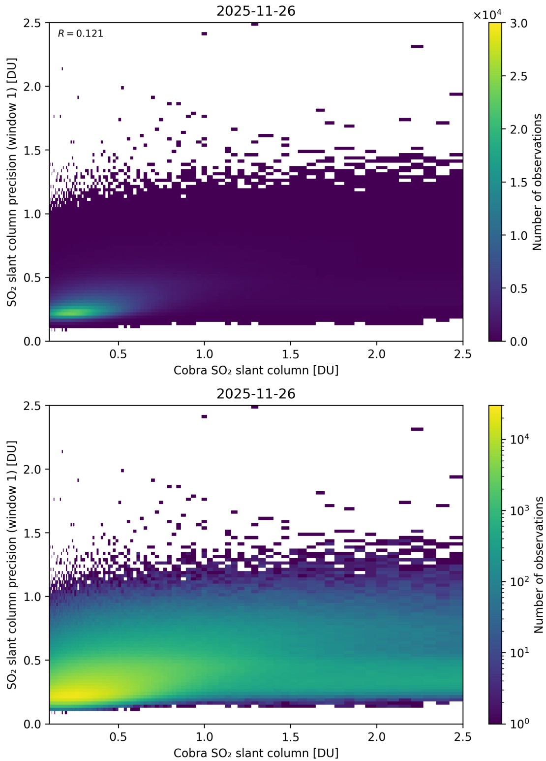
Figure 220: Scatter density plot of “Cobra SO 2 slant column” against “SO 2 slant column precision (window 1)” for 2025-11-25 to 2025-11-27.
