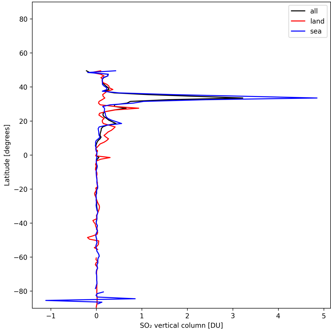
Figure 32: Zonal average of “SO 2 vertical column” for 2025-11-25 to 2025-11-27.
