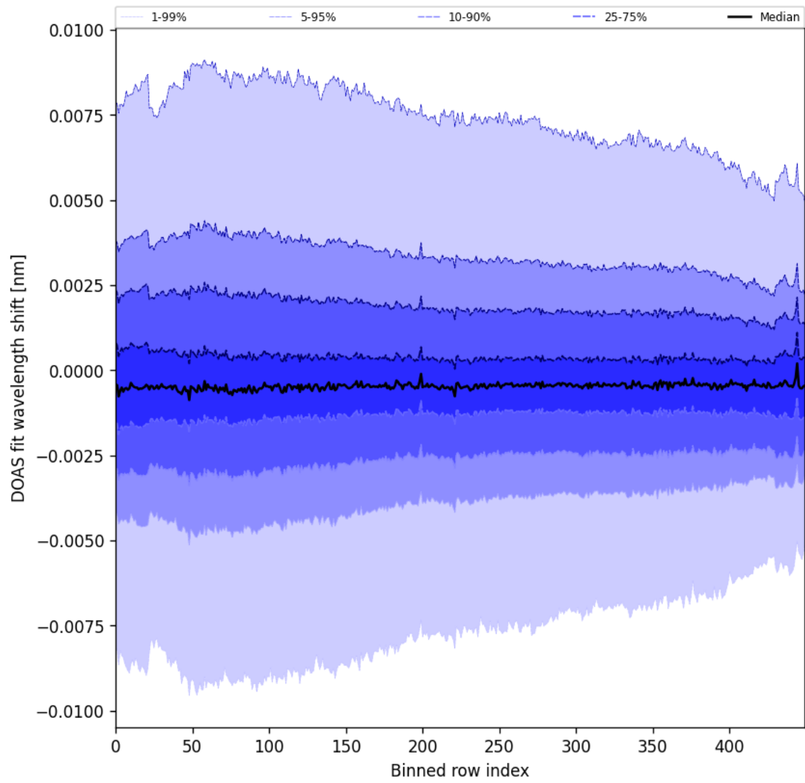
Figure 102: Along track statistics of “DOAS fit wavelength shift” for 2025-11-25 to 2025-11-27
