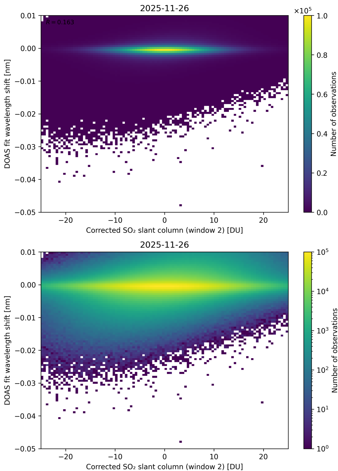
Figure 246: Scatter density plot of “Corrected SO 2 slant column (window 2)” against “DOAS fit wavelength shift” for 2025-11-25 to 2025-11-27.
