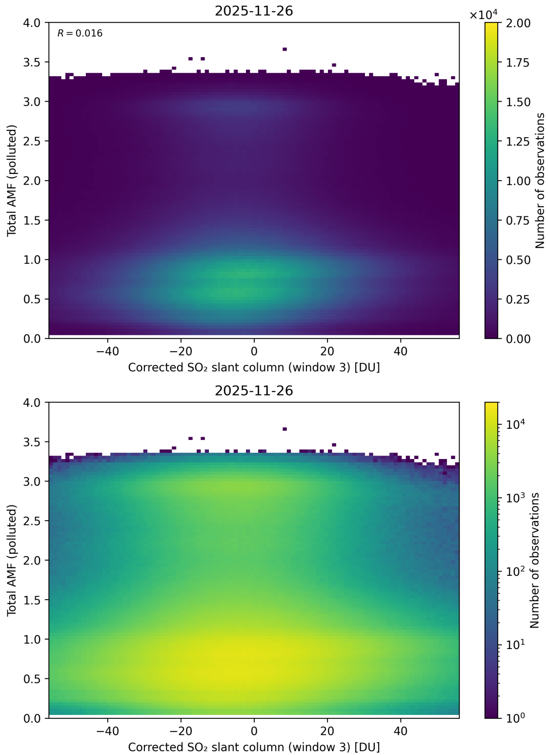
Figure 260: Scatter density plot of “Corrected SO 2 slant column (window 3)” against “Total AMF (polluted)” for 2025-11-25 to 2025-11-27.
