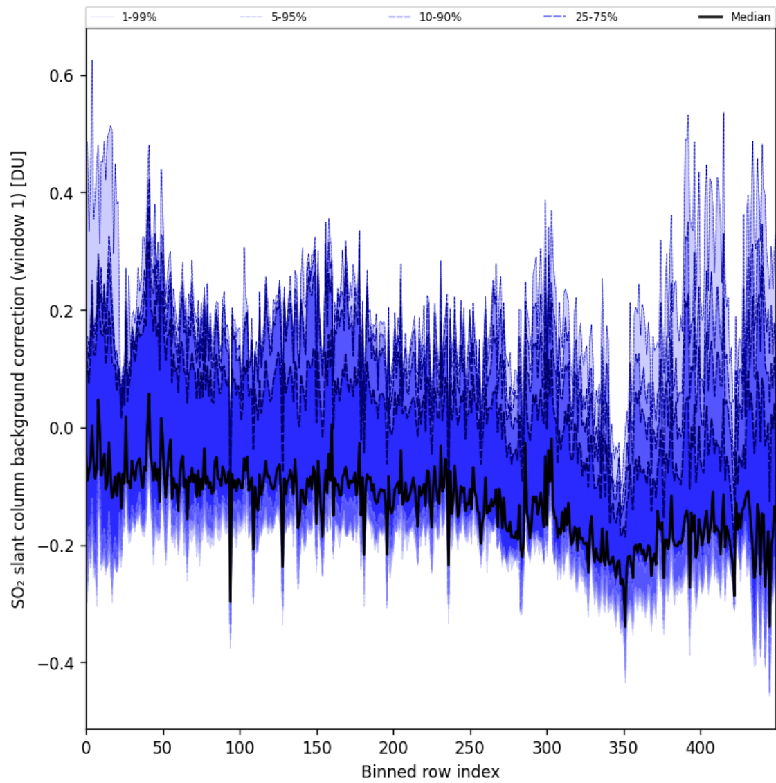
Figure 92: Along track statistics of “SO 2 slant column background correction (window 1)” for 2025-11-25 to 2025-11-27
