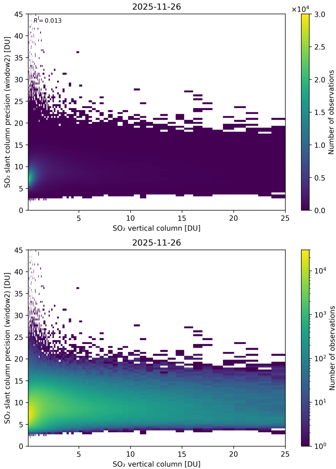
Figure 356: Scatter density plot of “SO 2 vertical column” against “SO 2 slant column precision (window2)” for 2025-11-25 to 2025-11-27.
