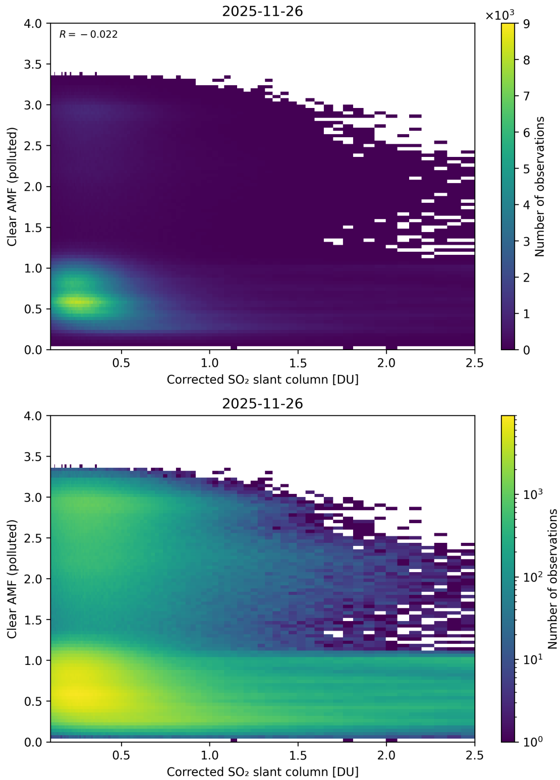
Figure 232: Scatter density plot of “Corrected SO 2 slant column” against “Clear AMF (polluted)” for 2025-11-25 to 2025-11-27.
