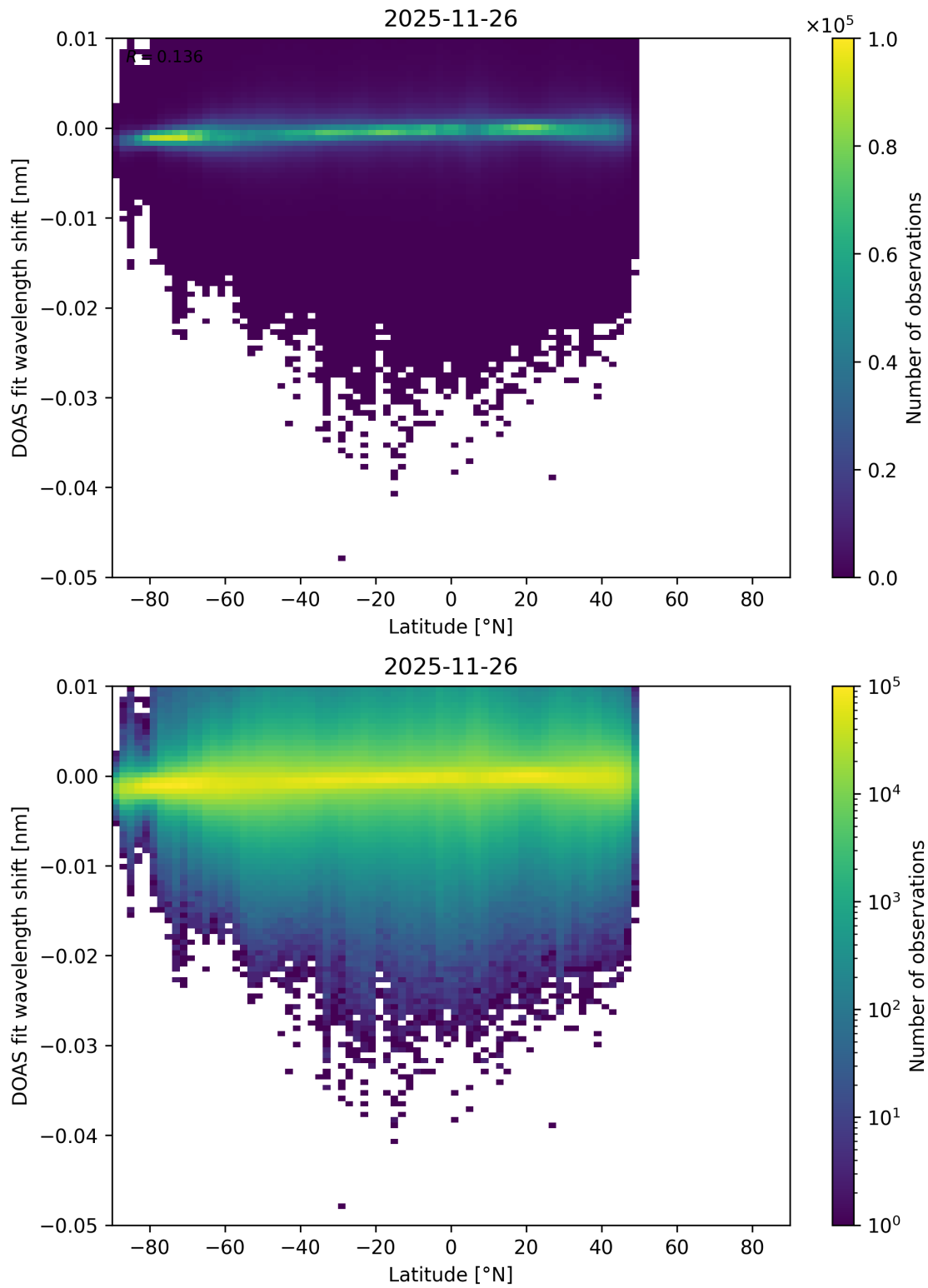
Figure 153: Scatter density plot of “Latitude” against “DOAS fit wavelength shift” for 2025-11-25 to 2025-11-27.
