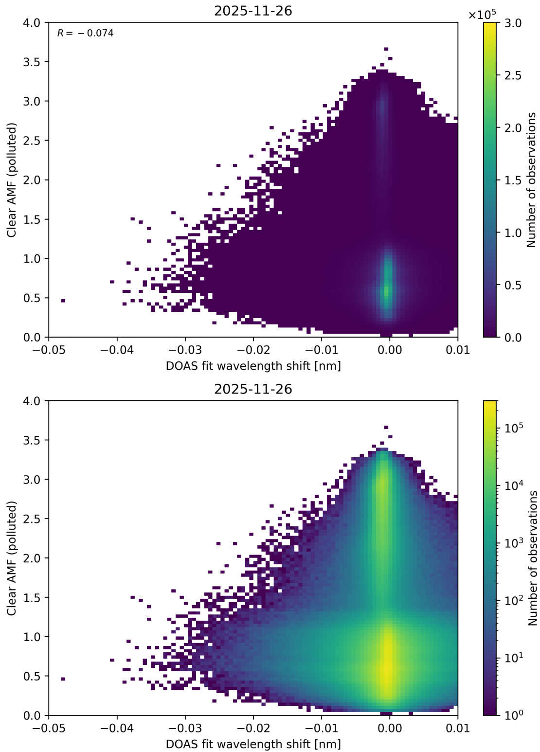
Figure 140: Scatter density plot of “DOAS fit wavelength shift” against “Clear AMF (polluted)” for 2025-11-25 to 2025-11-27.
