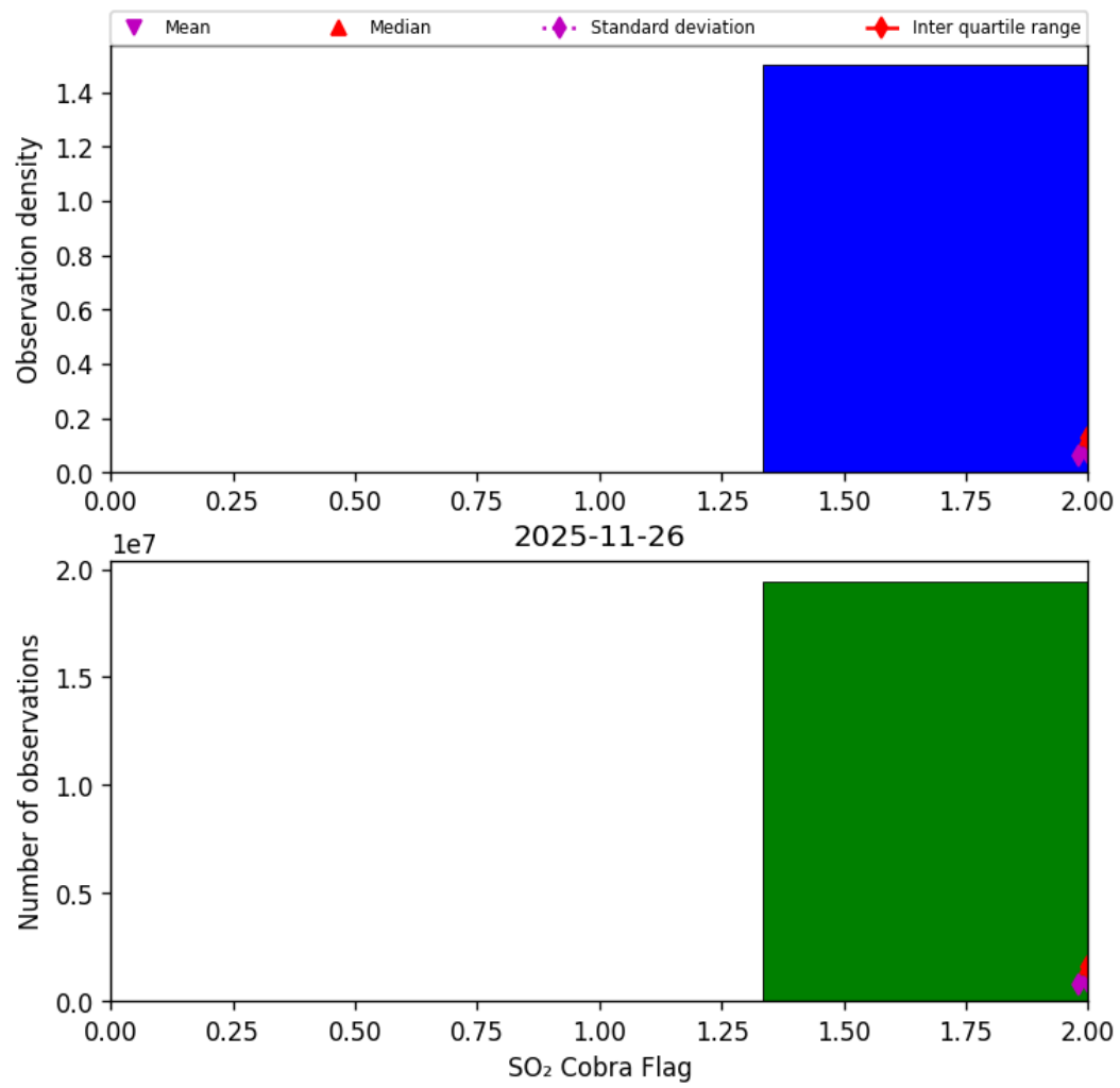
Figure 75: Histogram of “SO 2 Cobra Flag” for 2025-11-25 to 2025-11-27
