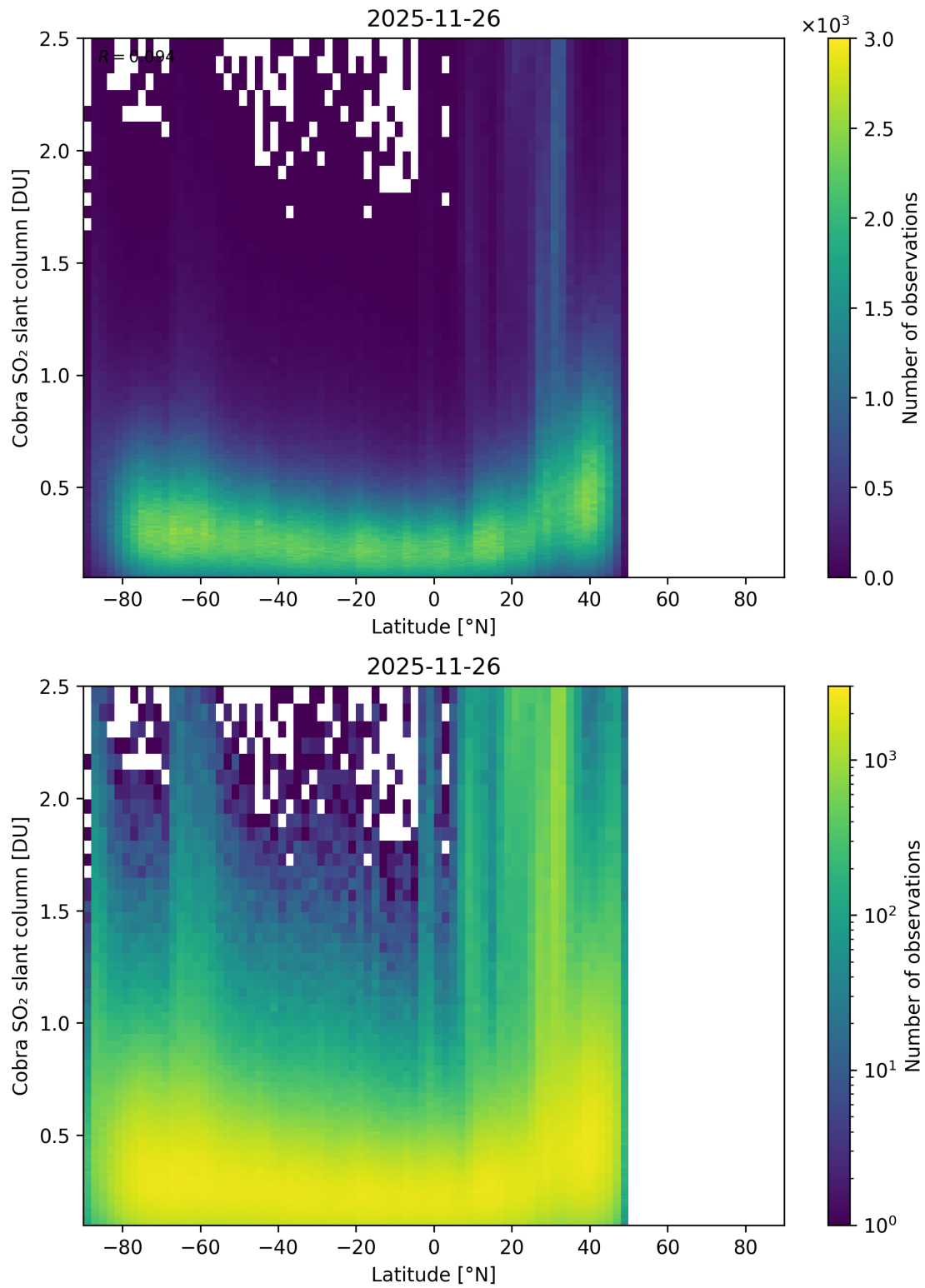
Figure 157: Scatter density plot of “Latitude” against “Cobra SO 2 slant column” for 2025-11-25 to 2025-11-27.
