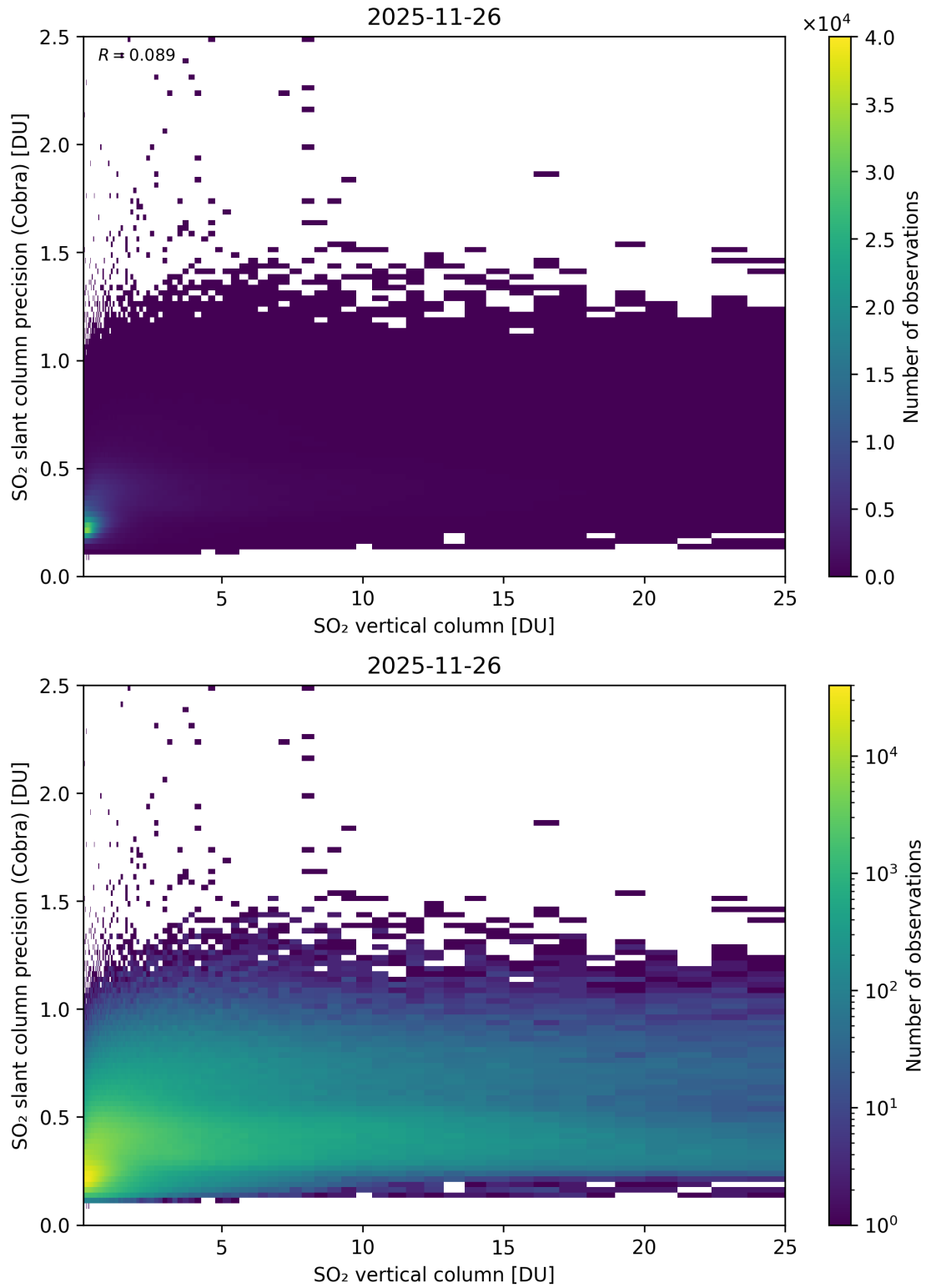
Figure 350: Scatter density plot of “SO 2 vertical column” against “SO 2 slant column precision (Cobra)” for 2025-11-25 to 2025-11-27.
