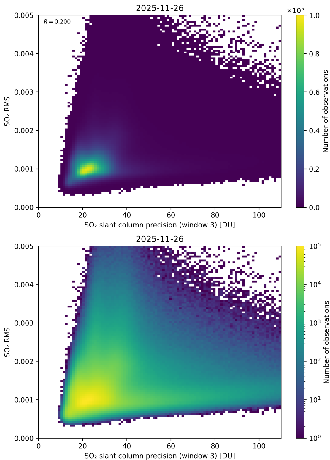
Figure 310: Scatter density plot of “SO 2 slant column precision (window 3)” against “SO 2 RMS” for 2025-11-25 to 2025-11-27.
