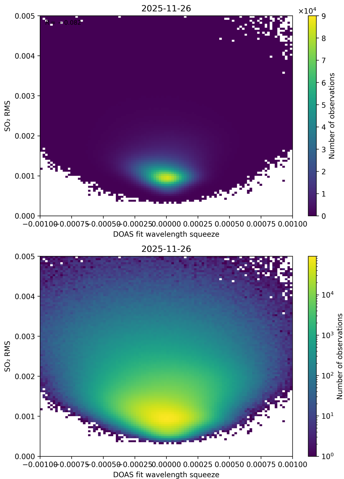
Figure 143: Scatter density plot of “DOAS fit wavelength squeeze” against “SO 2 RMS” for 2025-11-25 to 2025-11-27.
