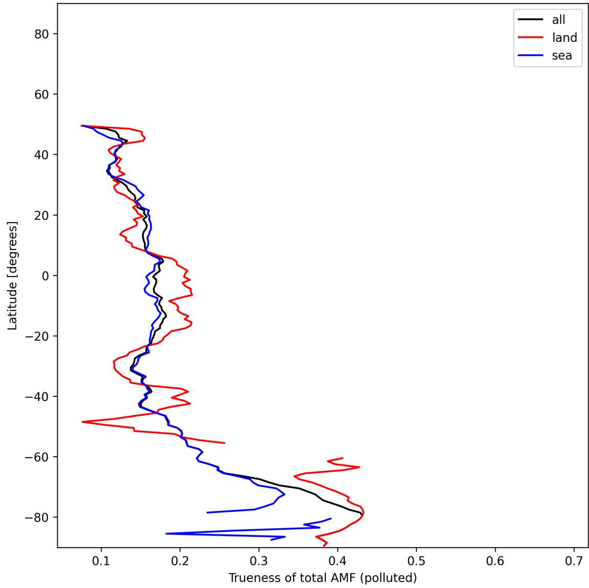
Figure 54: Zonal average of “Trueness of total AMF (polluted)” for 2025-11-25 to 2025-11-27.
