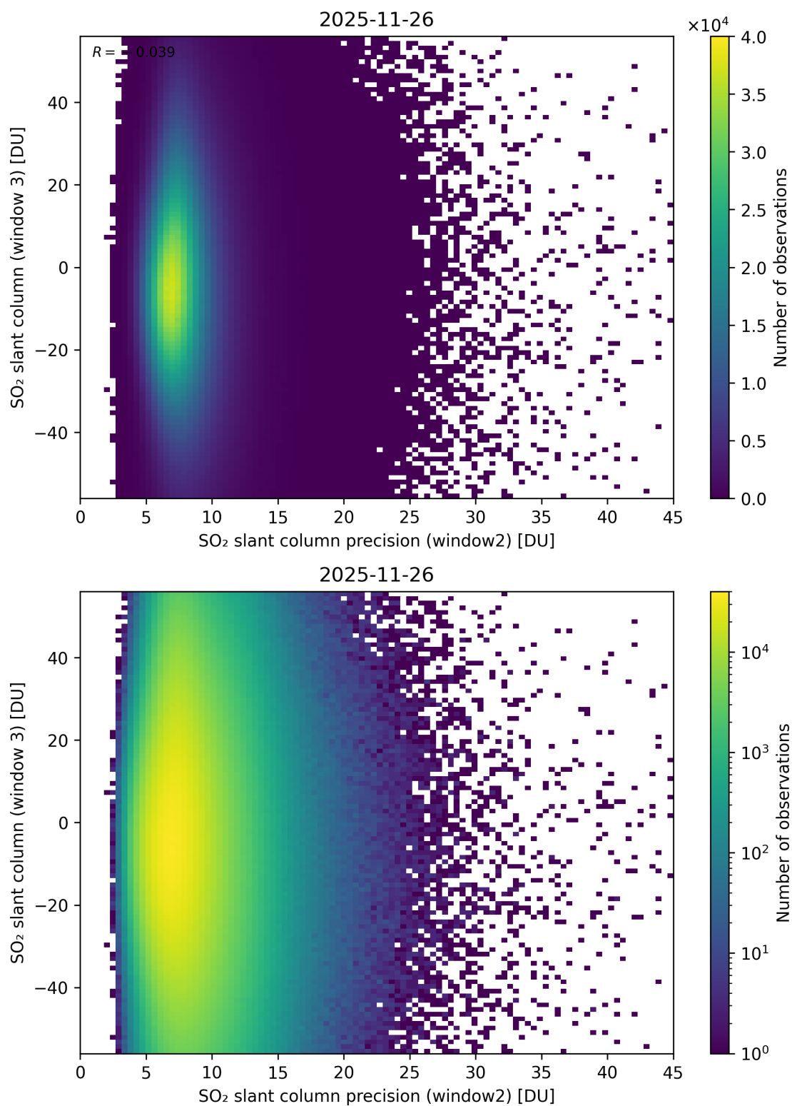
Figure 299: Scatter density plot of “SO 2 slant column precision (window2)” against “SO 2 slant column (window 3)” for 2025-11-25 to 2025-11-27.
