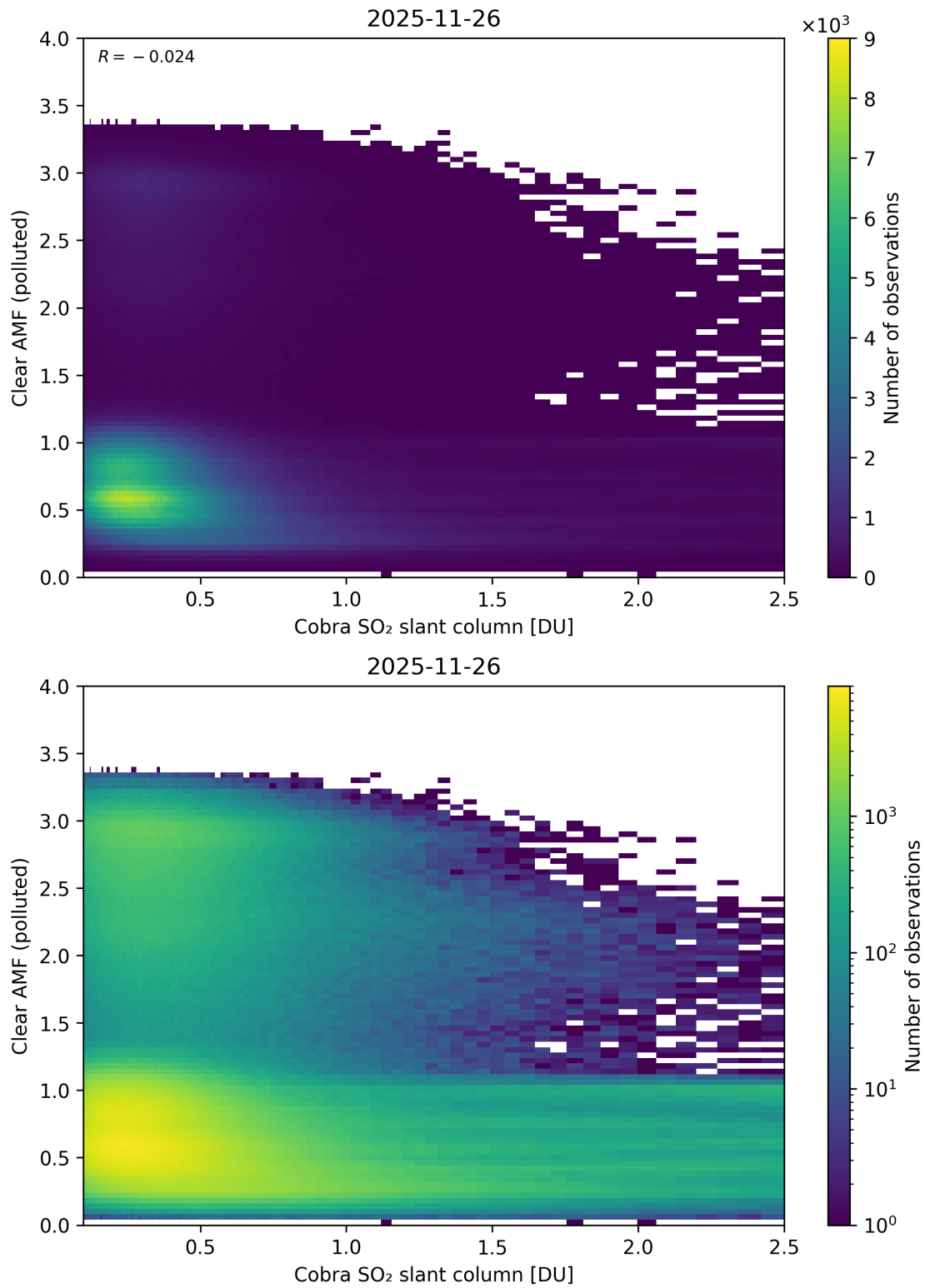
Figure 215: Scatter density plot of “Cobra SO 2 slant column” against “Clear AMF (polluted)” for 2025-11-25 to 2025-11-27.
