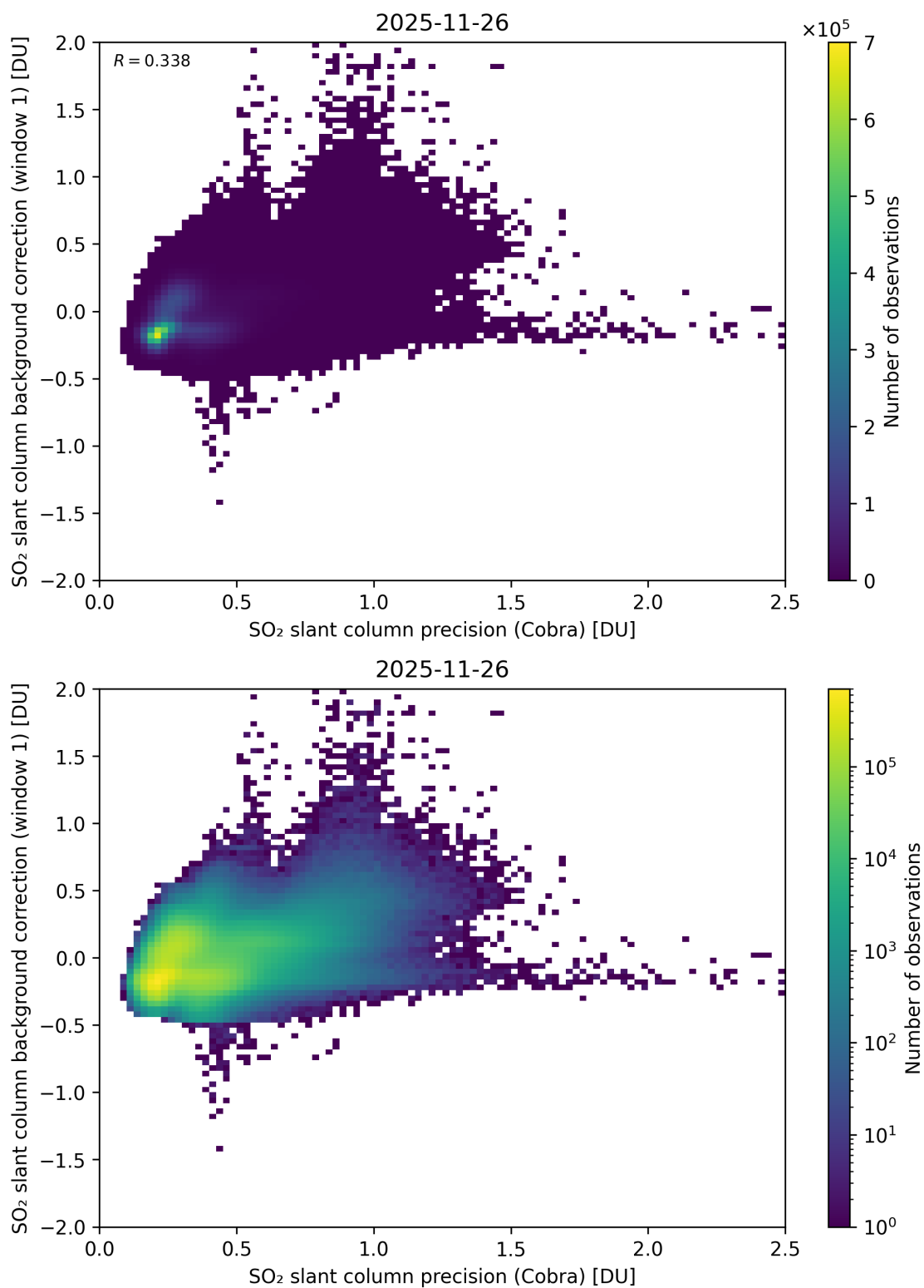
Figure 199: Scatter density plot of “SO 2 slant column precision (Cobra)” against “SO 2 slant column background correction (window 1)” for 2025-11-25 to 2025-11-27.
