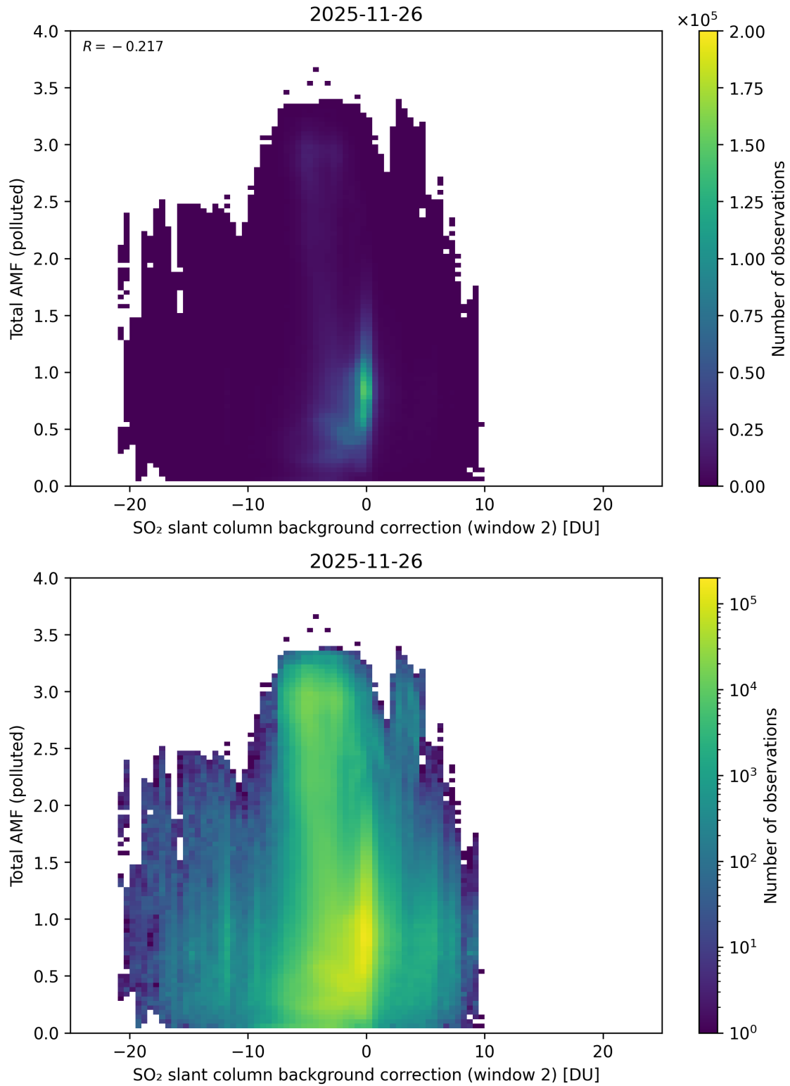
Figure 130: Scatter density plot of “SO 2 slant column background correction (window 2)” against “Total AMF (polluted)” for 2025-11-25 to 2025-11-27.
