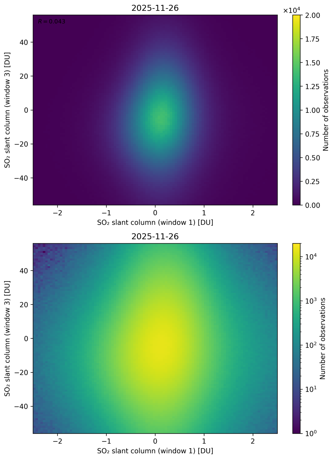
Figure 287: Scatter density plot of “SO 2 slant column (window 1)” against “SO 2 slant column (window 3)” for 2025-11-25 to 2025-11-27.
