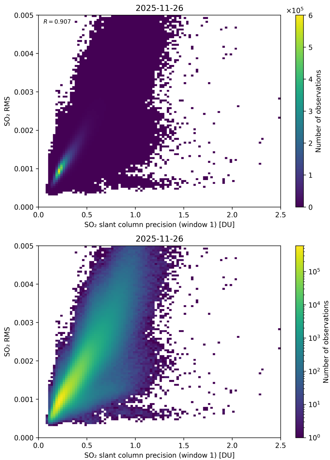
Figure 273: Scatter density plot of “SO 2 slant column precision (window 1)” against “SO 2 RMS” for 2025-11-25 to 2025-11-27.
