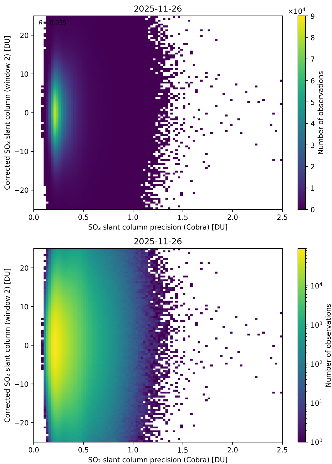
Figure 206: Scatter density plot of “SO 2 slant column precision (Cobra)” against “Corrected SO 2 slant column (window 2)” for 2025-11-25 to 2025-11-27.
