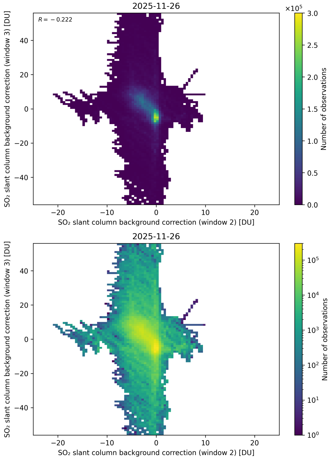
Figure 122: Scatter density plot of “SO 2 slant column background correction (window 2)” against “SO 2 slant column background correction (window 3)” for 2025-11-25 to 2025-11-27.
