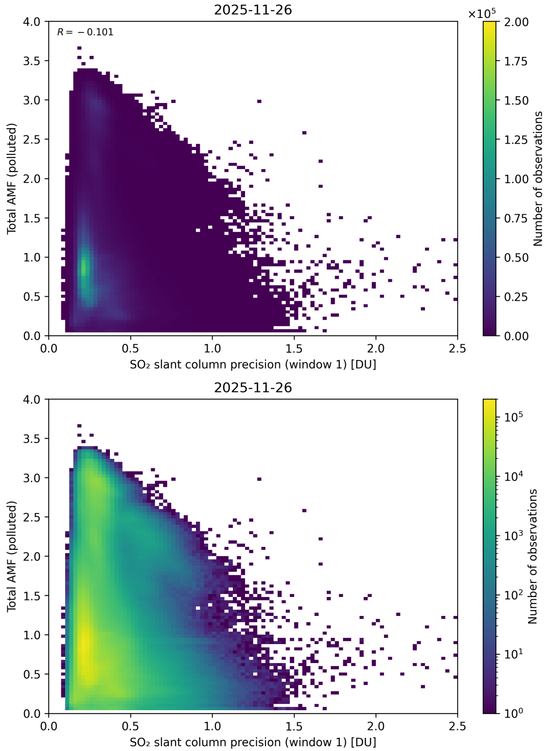
Figure 280: Scatter density plot of “SO 2 slant column precision (window 1)” against “Total AMF (polluted)” for 2025-11-25 to 2025-11-27.
