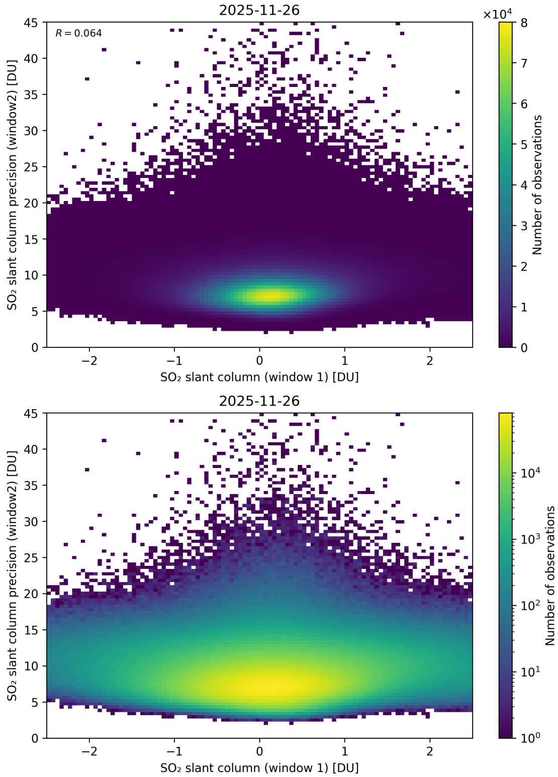
Figure 286: Scatter density plot of “SO 2 slant column (window 1)” against “SO 2 slant column precision (window2)” for 2025-11-25 to 2025-11-27.
