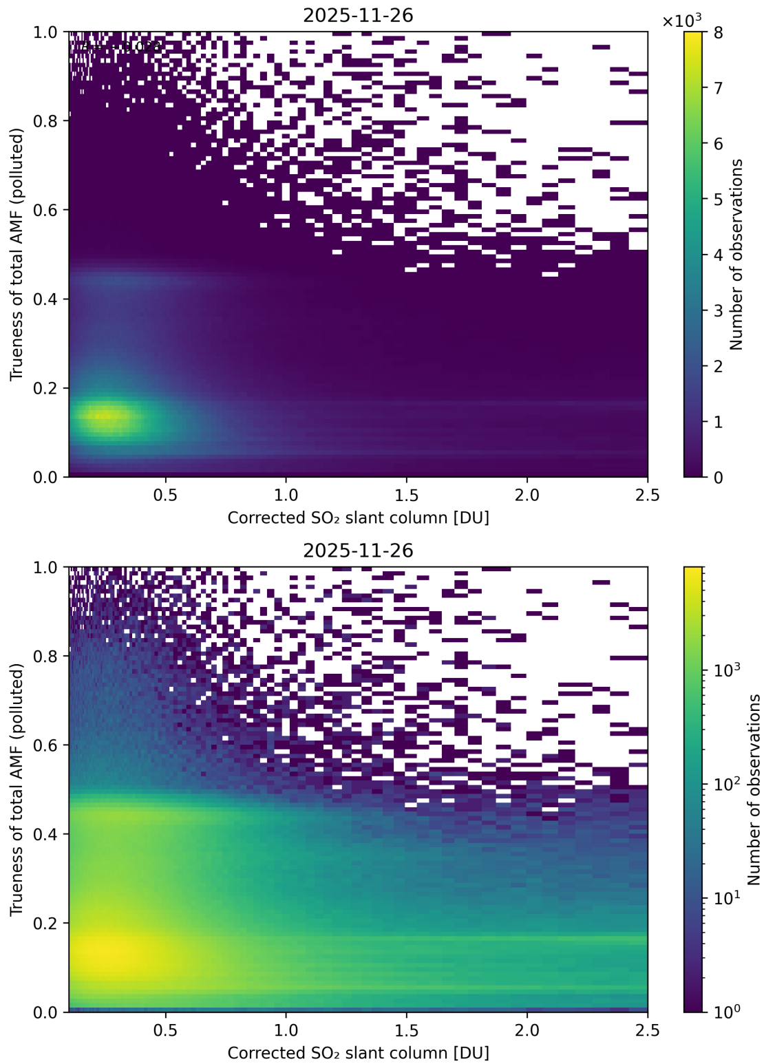
Figure 243: Scatter density plot of “Corrected SO 2 slant column” against “Trueness of total AMF (polluted)” for 2025-11-25 to 2025-11-27.
