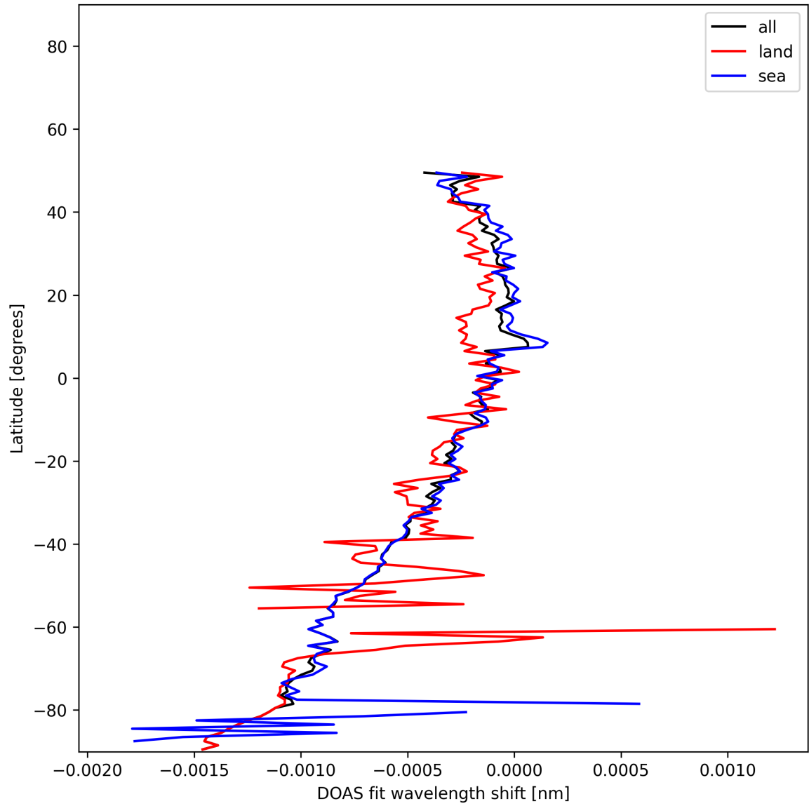
Figure 50: Zonal average of "DOAS fit wavelength shift" for 2025-11-25 to 2025-11-27.
