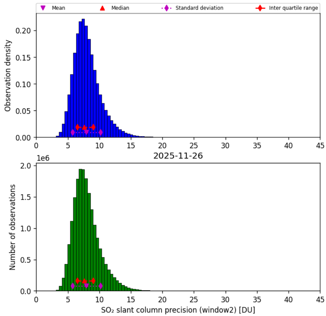
Figure 68: Histogram of “SO 2 slant column precision (window2)” for 2025-11-25 to 2025-11-27
