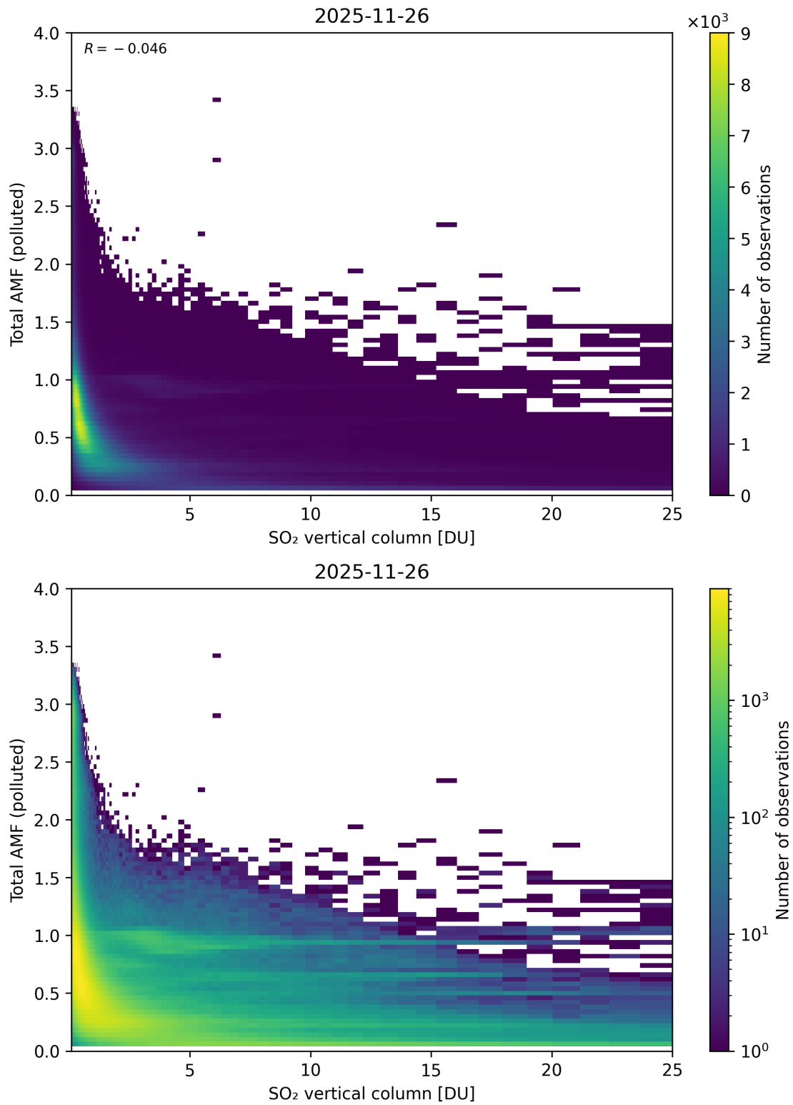
Figure 359: Scatter density plot of “SO 2 vertical column” against “Total AMF (polluted)” for 2025-11-25 to 2025-11-27.
