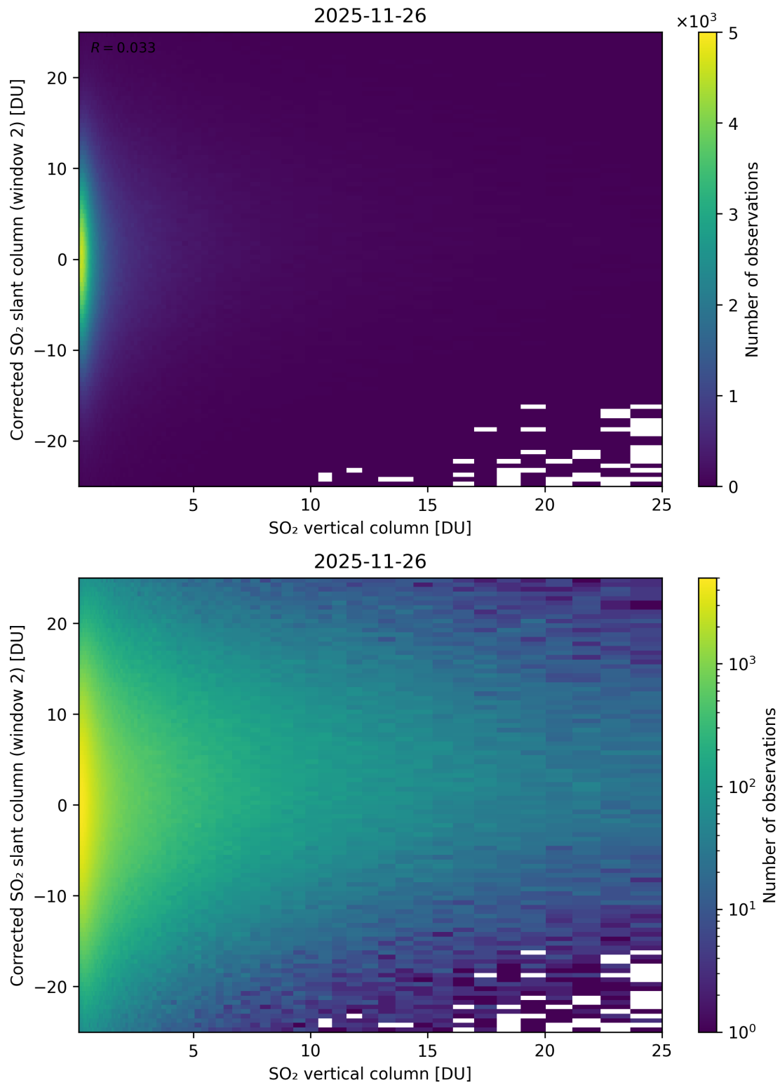
Figure 352: Scatter density plot of “SO 2 vertical column” against “Corrected SO 2 slant column (window 2)” for 2025-11-25 to 2025-11-27.
