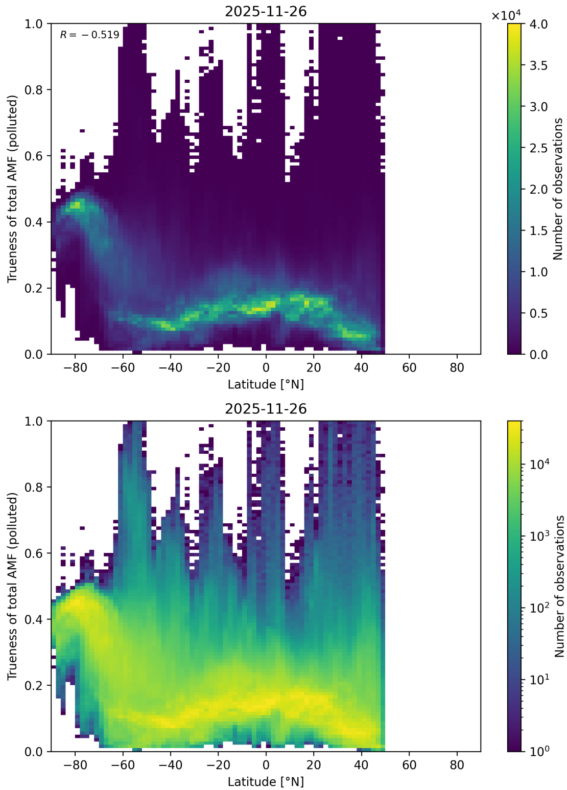
Figure 168: Scatter density plot of “Latitude” against “Trueness of total AMF (polluted)” for 2025-11-25 to 2025-11-27.
