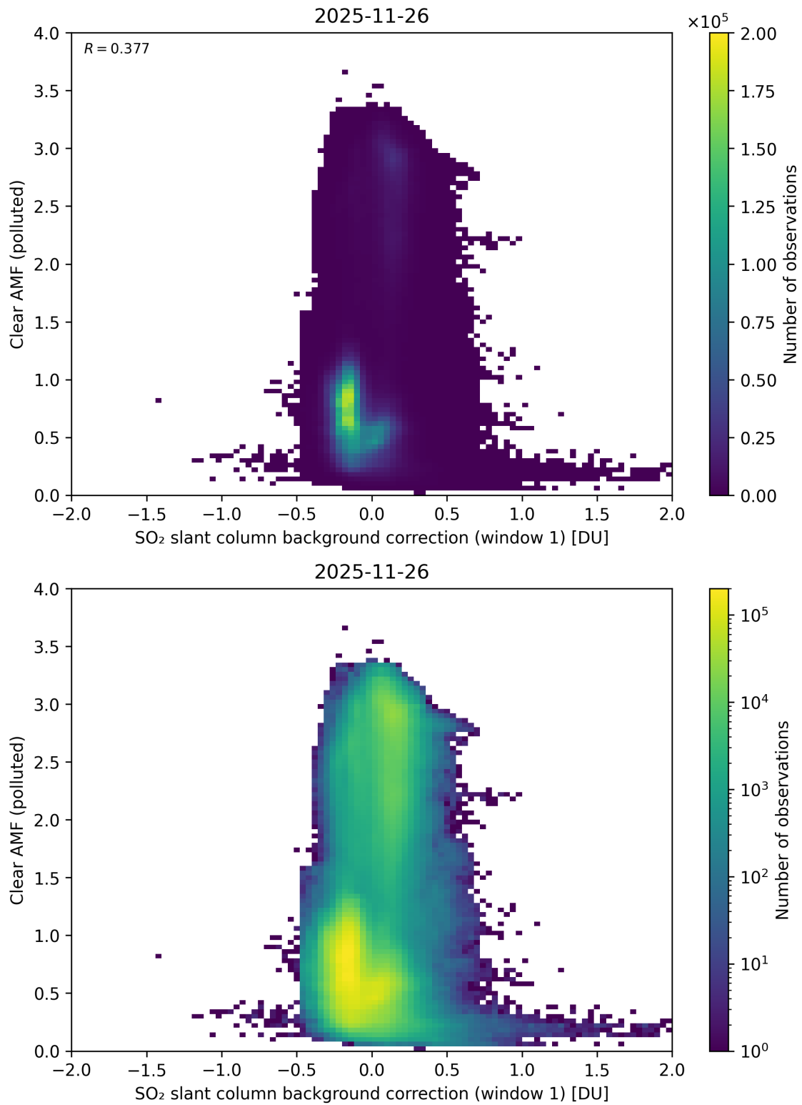
Figure 114: Scatter density plot of “SO 2 slant column background correction (window 1)” against “Clear AMF (polluted)” for 2025-11-25 to 2025-11-27.
