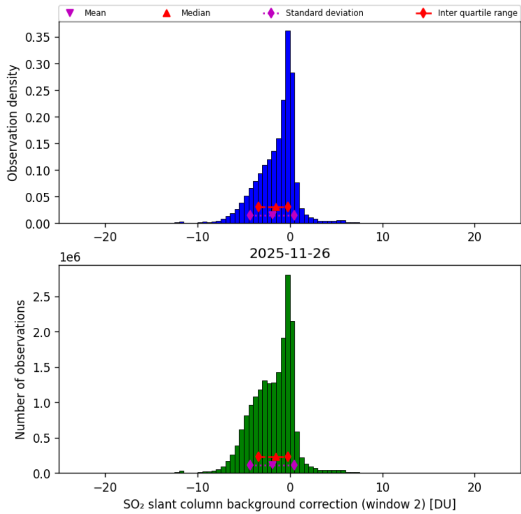
Figure 70: Histogram of “SO 2 slant column background correction (window 2)” for 2025-11-25 to 2025-11-27
