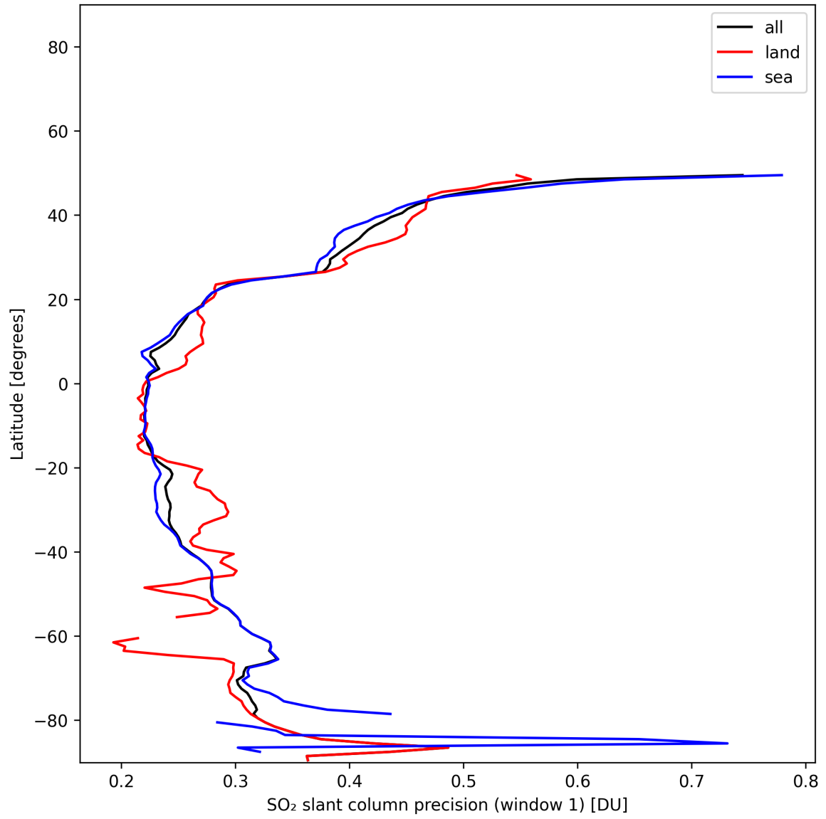
Figure 38: Zonal average of “SO 2 slant column precision (window 1)” for 2025-11-25 to 2025-11-27.
