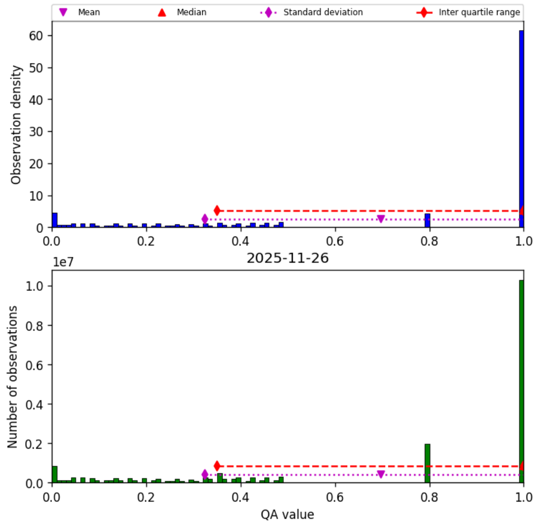
Figure 57: Histogram of “QA value” for 2025-11-25 to 2025-11-27
