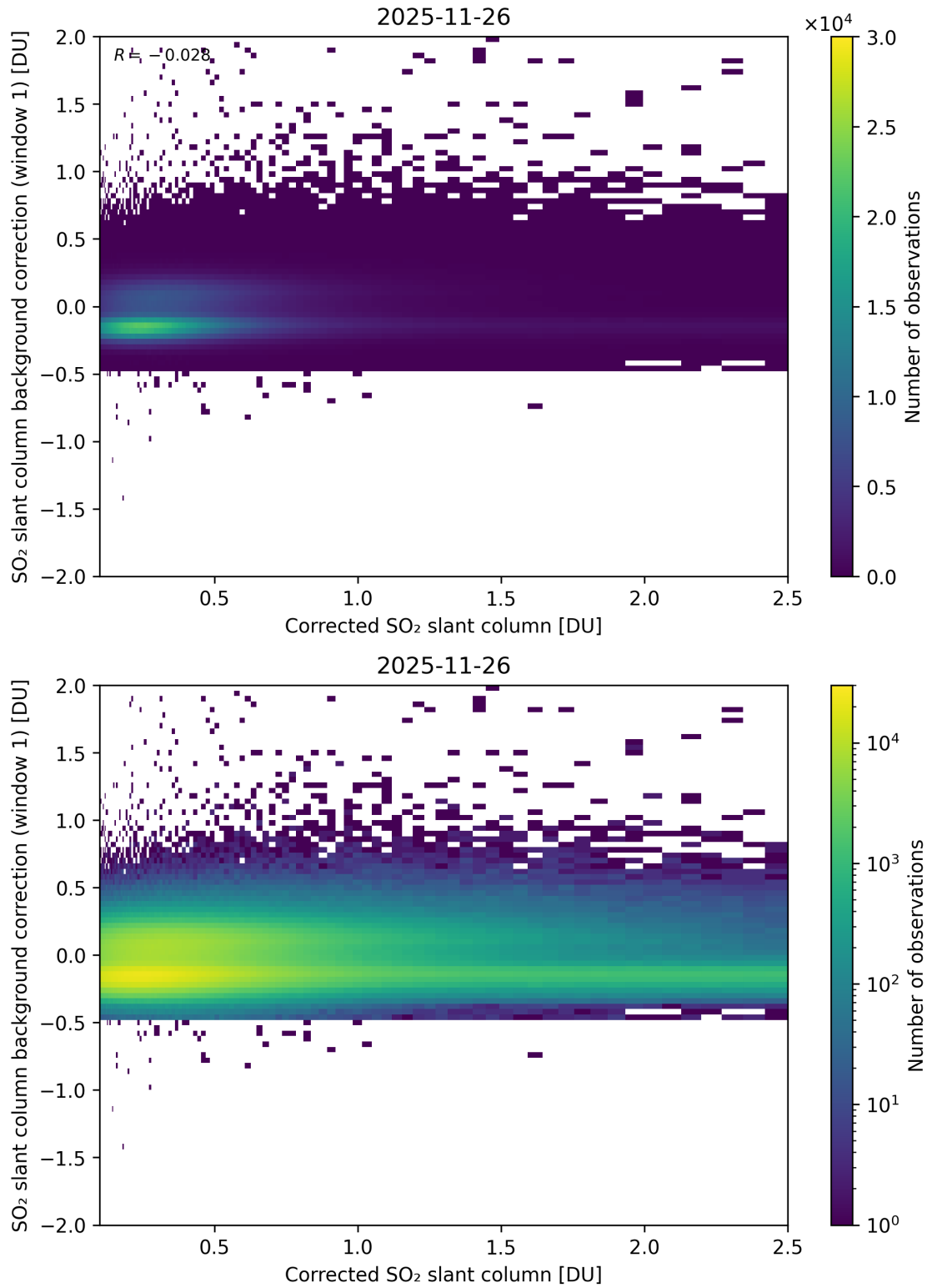
Figure 226: Scatter density plot of “Corrected SO 2 slant column” against “SO 2 slant column background correction (window 1)” for 2025-11-25 to 2025-11-27.
