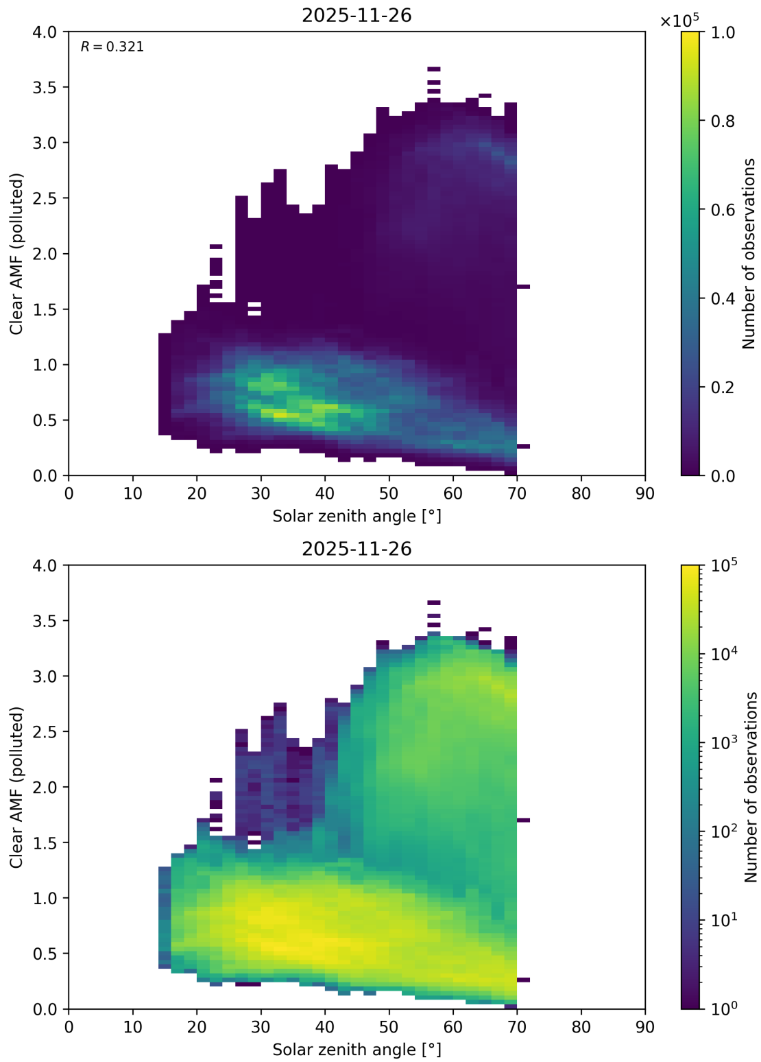
Figure 178: Scatter density plot of “Solar zenith angle” against “Clear AMF (polluted)” for 2025-11-25 to 2025-11-27.
