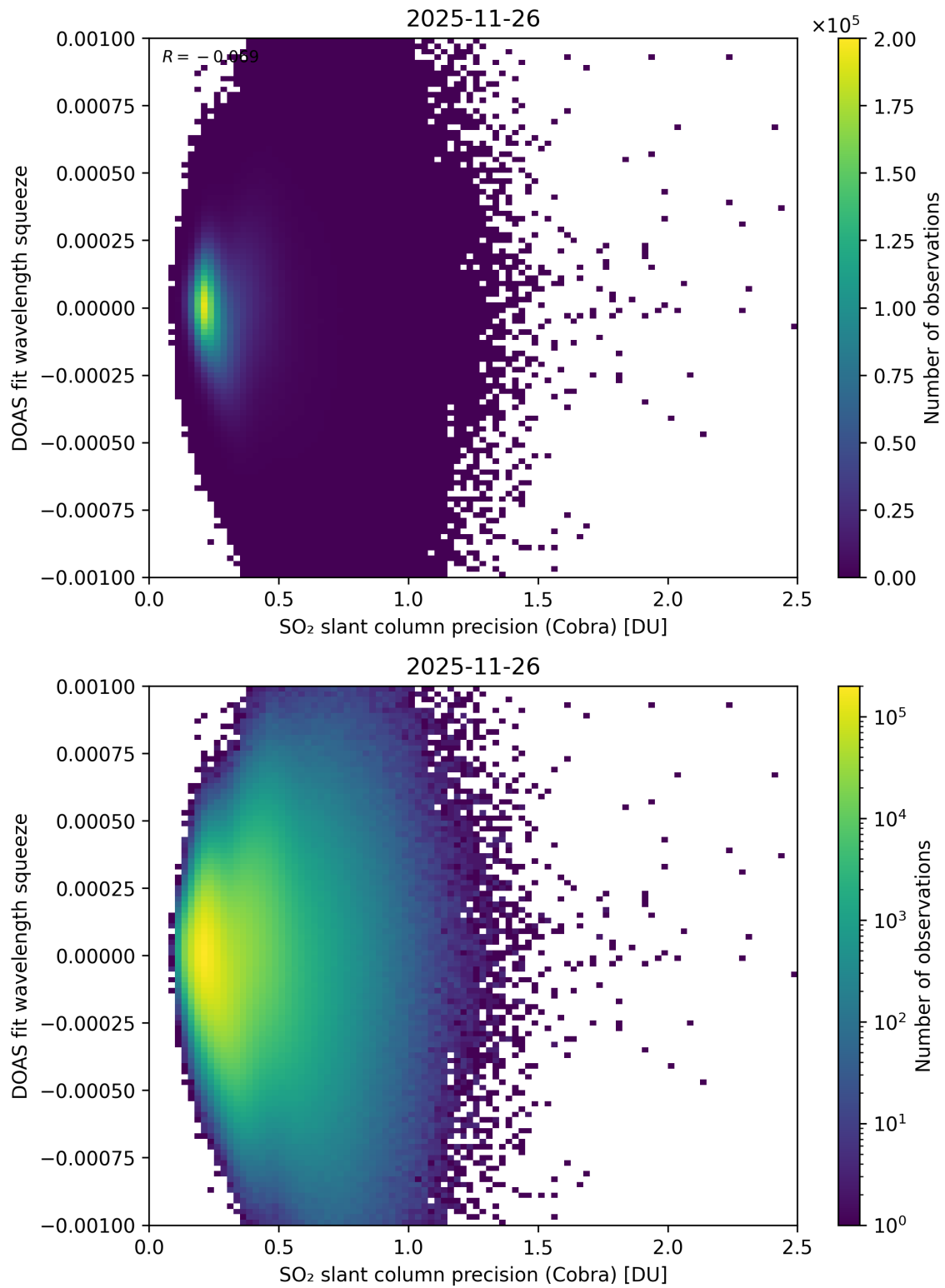
Figure 203: Scatter density plot of “SO 2 slant column precision (Cobra)” against “DOAS fit wavelength squeeze” for 2025-11-25 to 2025-11-27.
