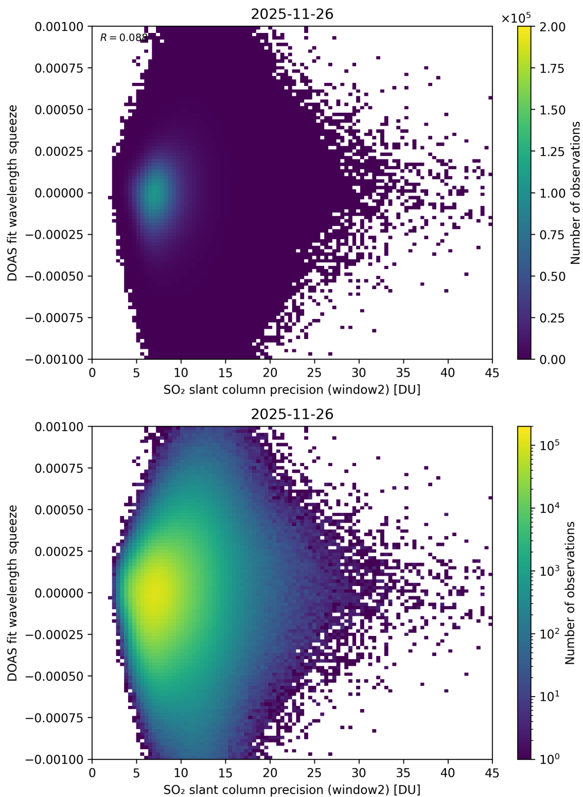
Figure 294: Scatter density plot of “SO 2 slant column precision (window2)” against “DOAS fit wavelength squeeze” for 2025-11-25 to 2025-11-27.
