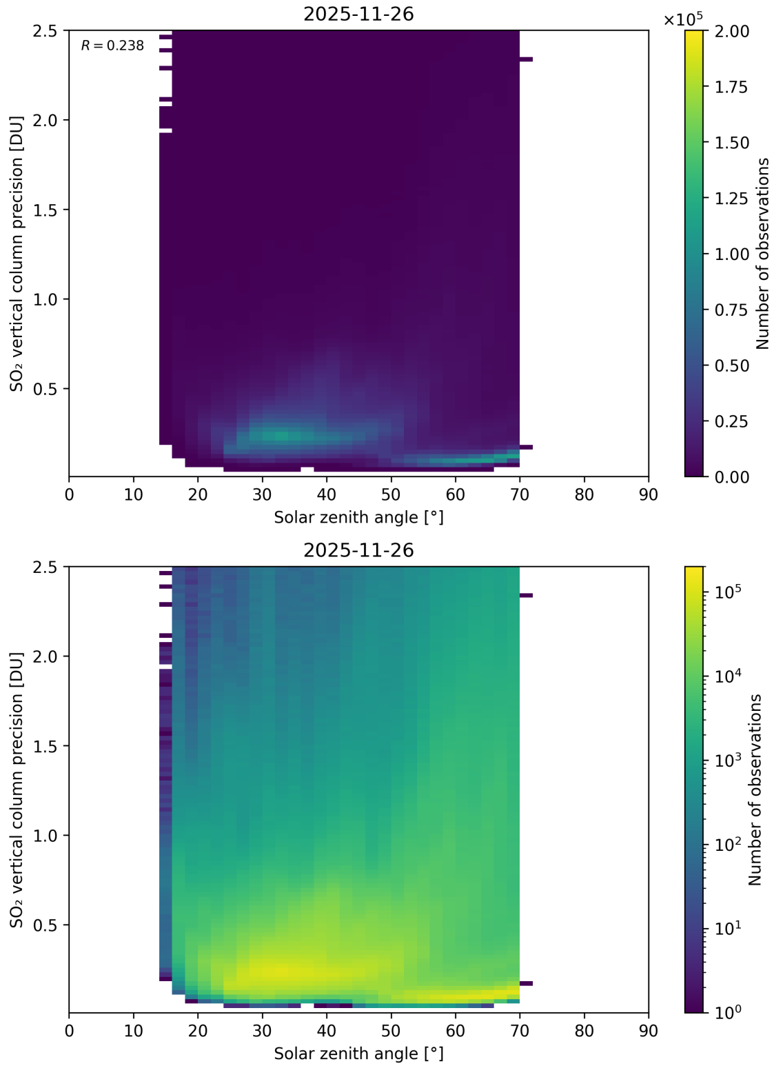
Figure 192: Scatter density plot of “Solar zenith angle” against “SO 2 vertical column precision” for 2025-11-25 to 2025-11-27.
