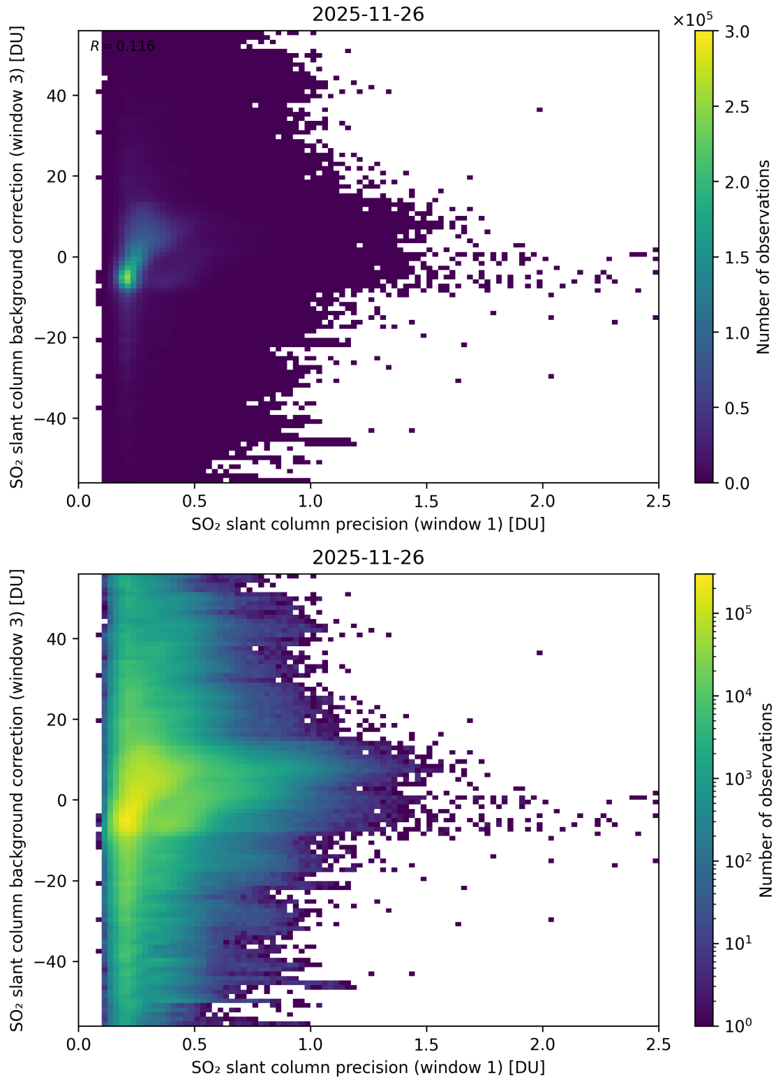
Figure 270: Scatter density plot of “SO 2 slant column precision (window 1)” against “SO 2 slant column background correction (window 3)” for 2025-11-25 to 2025-11-27.
