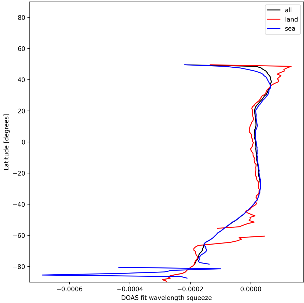
Figure 51: Zonal average of “DOAS fit wavelength squeeze” for 2025-11-25 to 2025-11-27.
