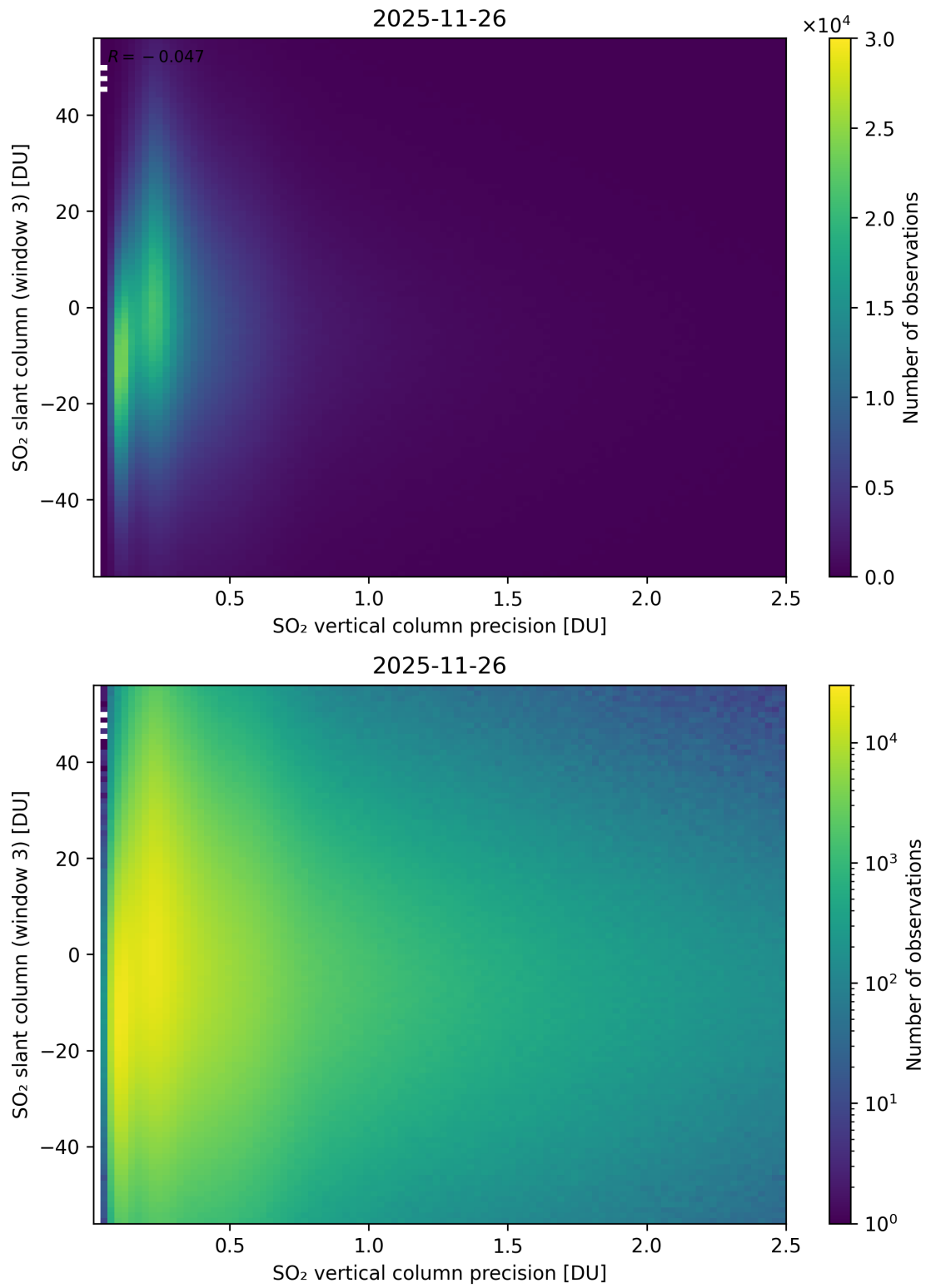
Figure 344: Scatter density plot of “SO 2 vertical column precision” against “SO 2 slant column (window 3)” for 2025-11-25 to 2025-11-27.
