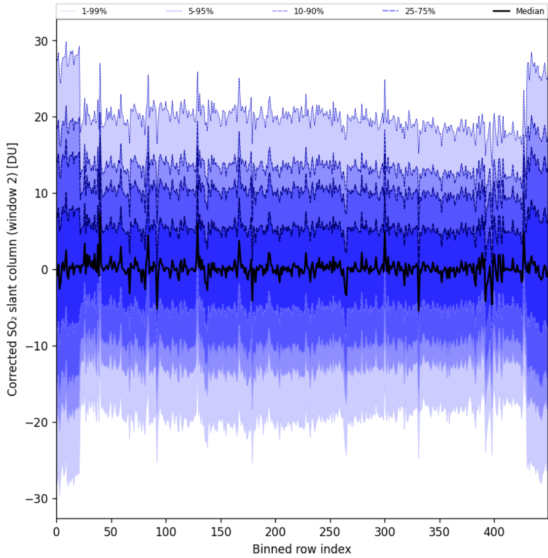
Figure 95: Along track statistics of “Corrected SO 2 slant column (window 2)” for 2025-11-25 to 2025-11-27
