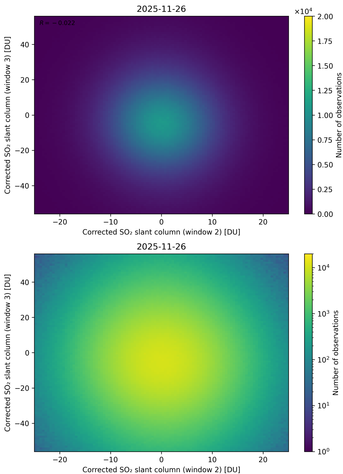
Figure 250: Scatter density plot of “Corrected SO 2 slant column (window 2)” against “Corrected SO 2 slant column (window 3)” for 2025-11-25 to 2025-11-27.
