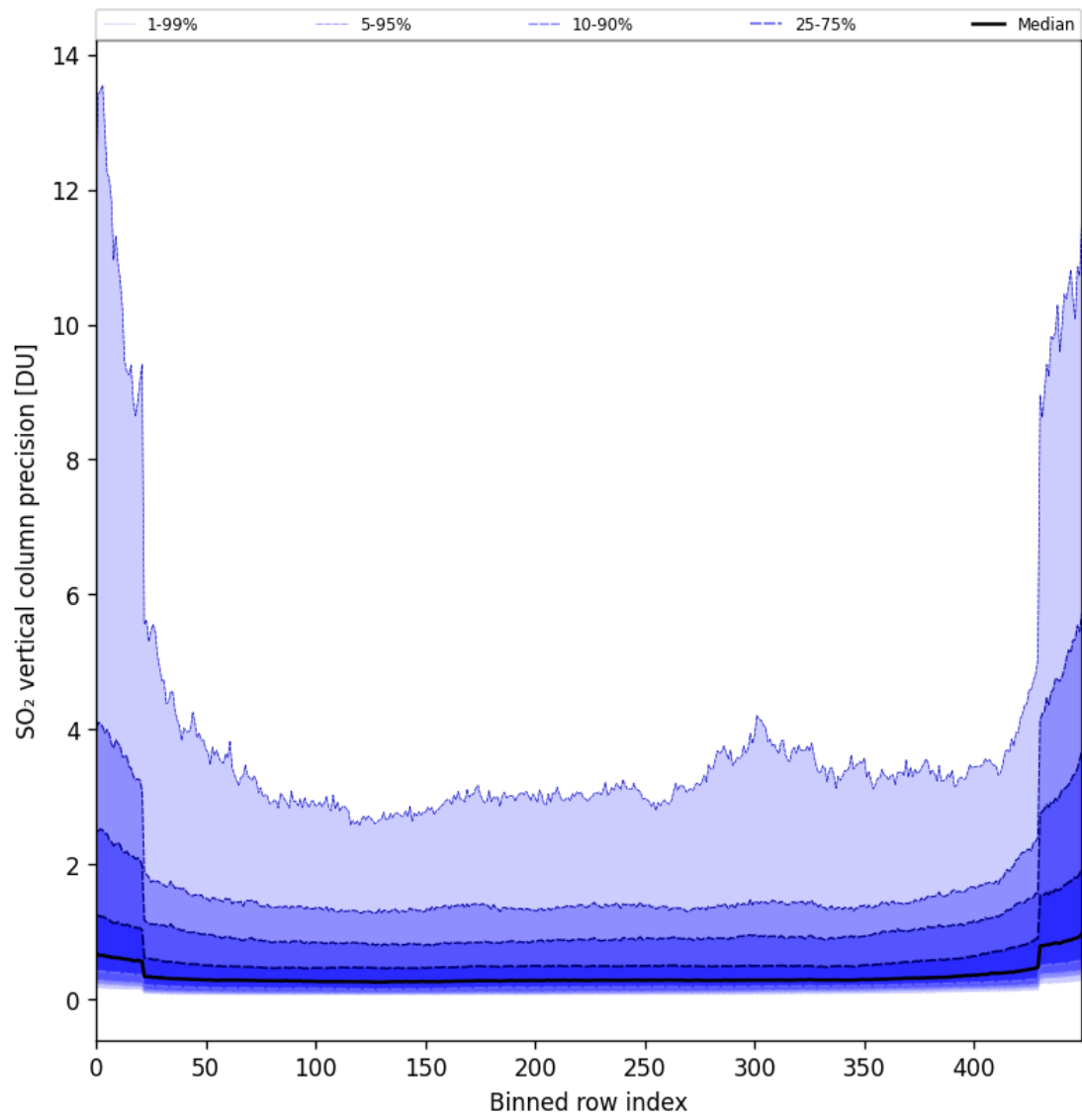
Figure 85: Along track statistics of “SO 2 vertical column precision” for 2025-11-25 to 2025-11-27
