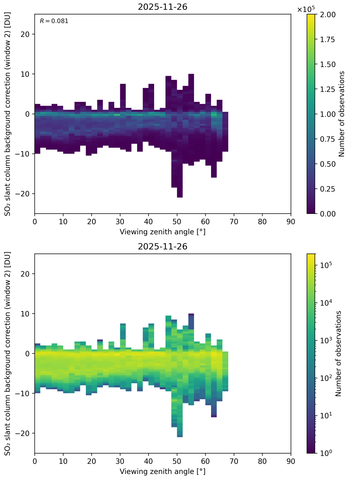
Figure 363: Scatter density plot of “Viewing zenith angle” against “SO 2 slant column background correction (window 2)” for 2025-11-25 to 2025-11-27.
