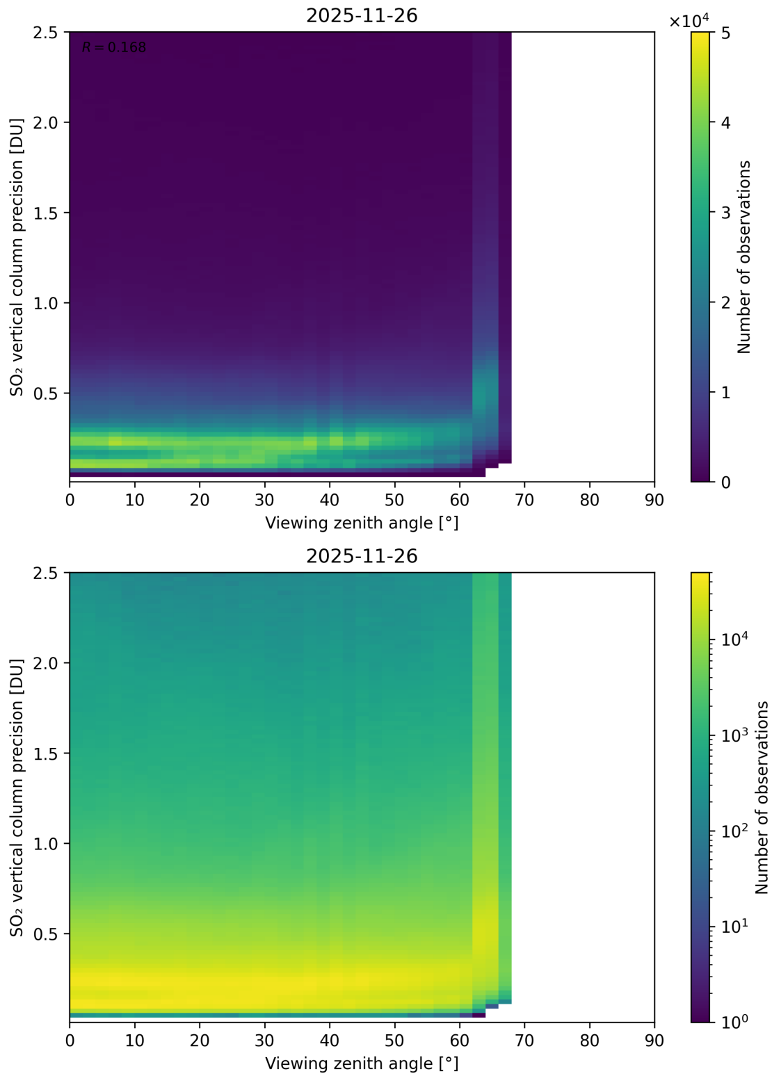
Figure 384: Scatter density plot of “Viewing zenith angle” against “SO 2 vertical column precision” for 2025-11-25 to 2025-11-27.
