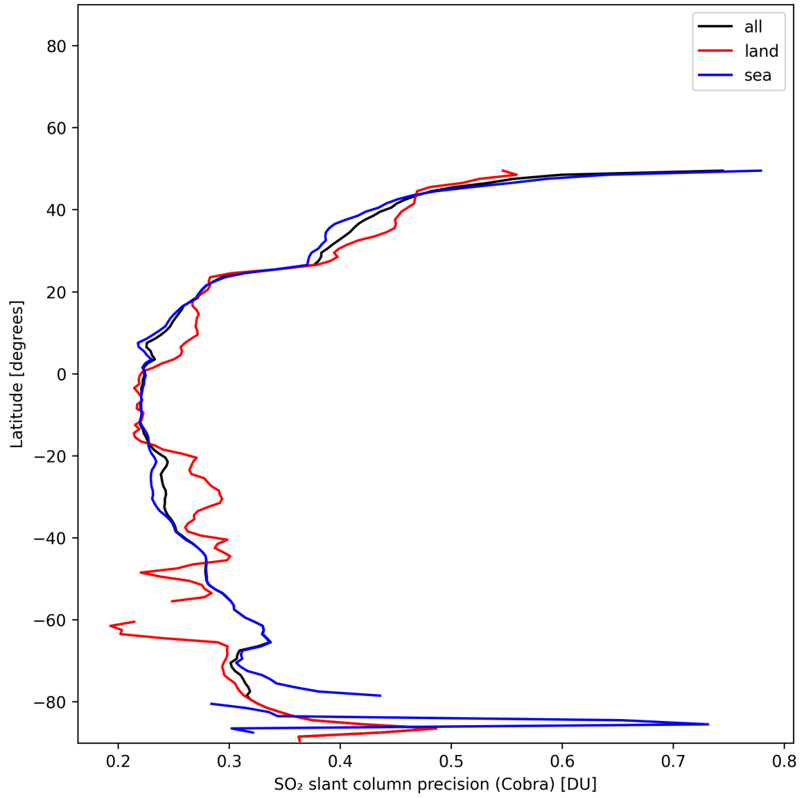
Figure 36: Zonal average of “SO 2 slant column precision (Cobra)” for 2025-11-25 to 2025-11-27.
