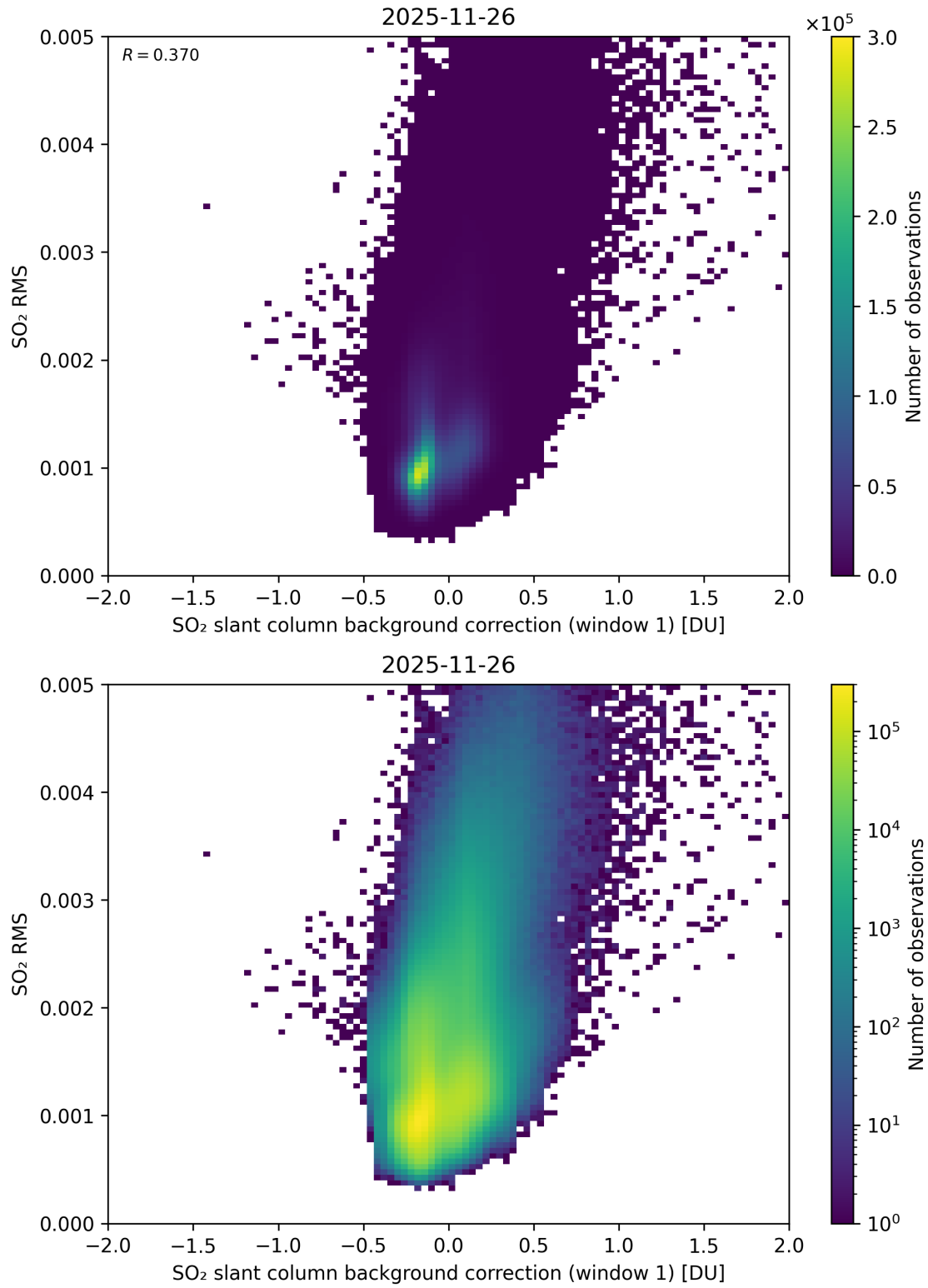
Figure 113: Scatter density plot of “SO 2 slant column background correction (window 1)” against “SO 2 RMS” for 2025-11-25 to 2025-11-27.
