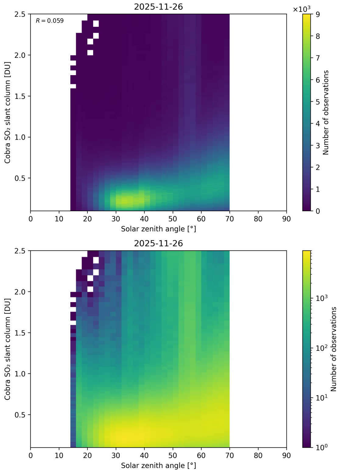
Figure 179: Scatter density plot of “Solar zenith angle” against “Cobra SO 2 slant column” for 2025-11-25 to 2025-11-27.
