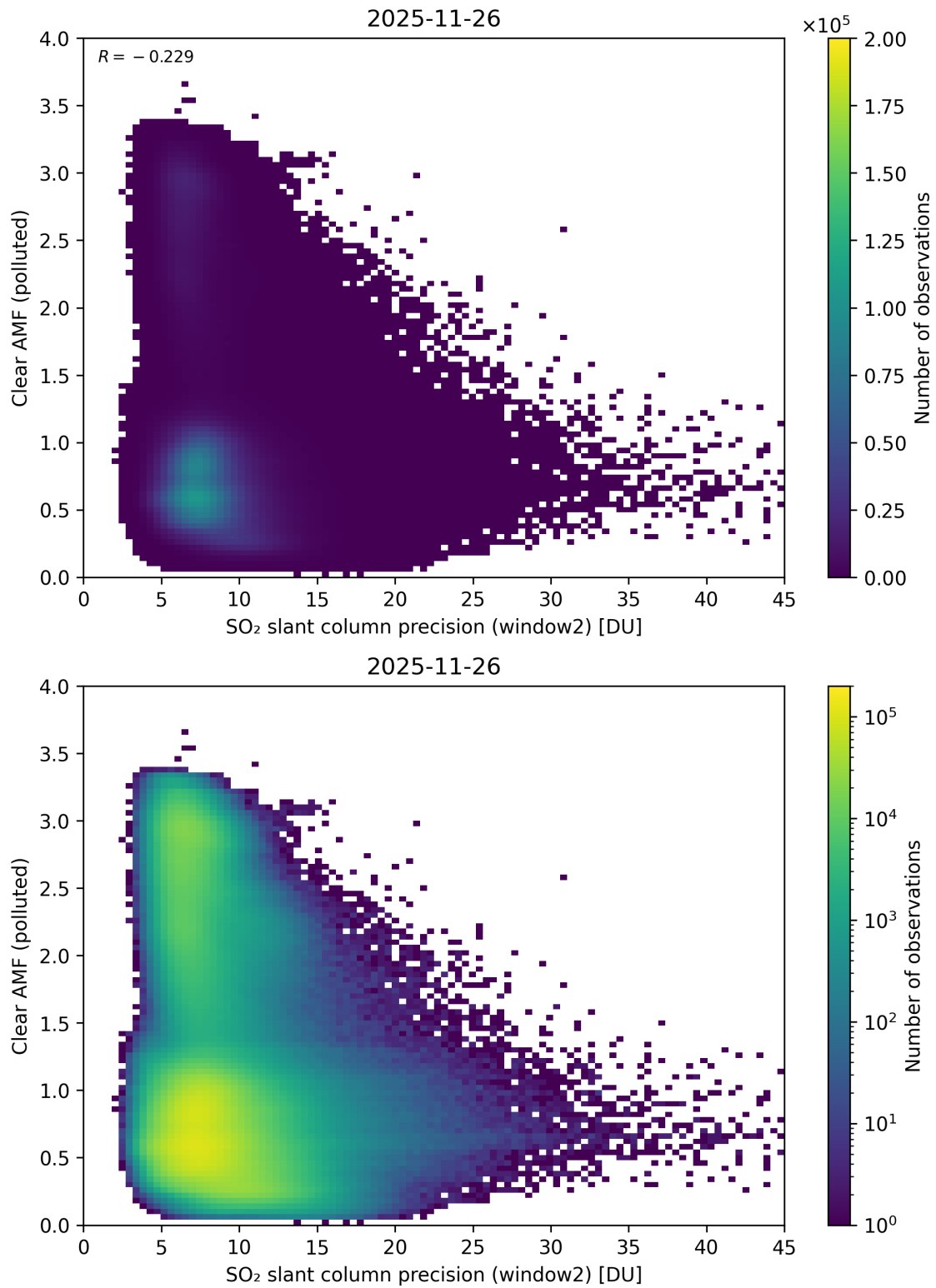
Figure 296: Scatter density plot of “SO 2 slant column precision (window2)” against “Clear AMF (polluted)” for 2025-11-25 to 2025-11-27.
