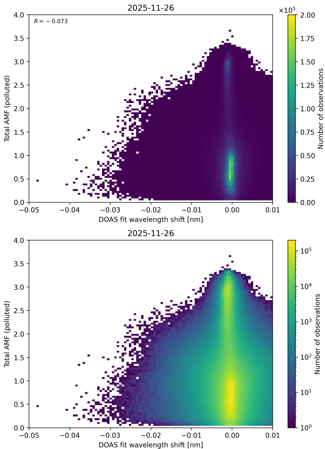
Figure 141: Scatter density plot of “DOAS fit wavelength shift” against “Total AMF (polluted)” for 2025-11-25 to 2025-11-27.
