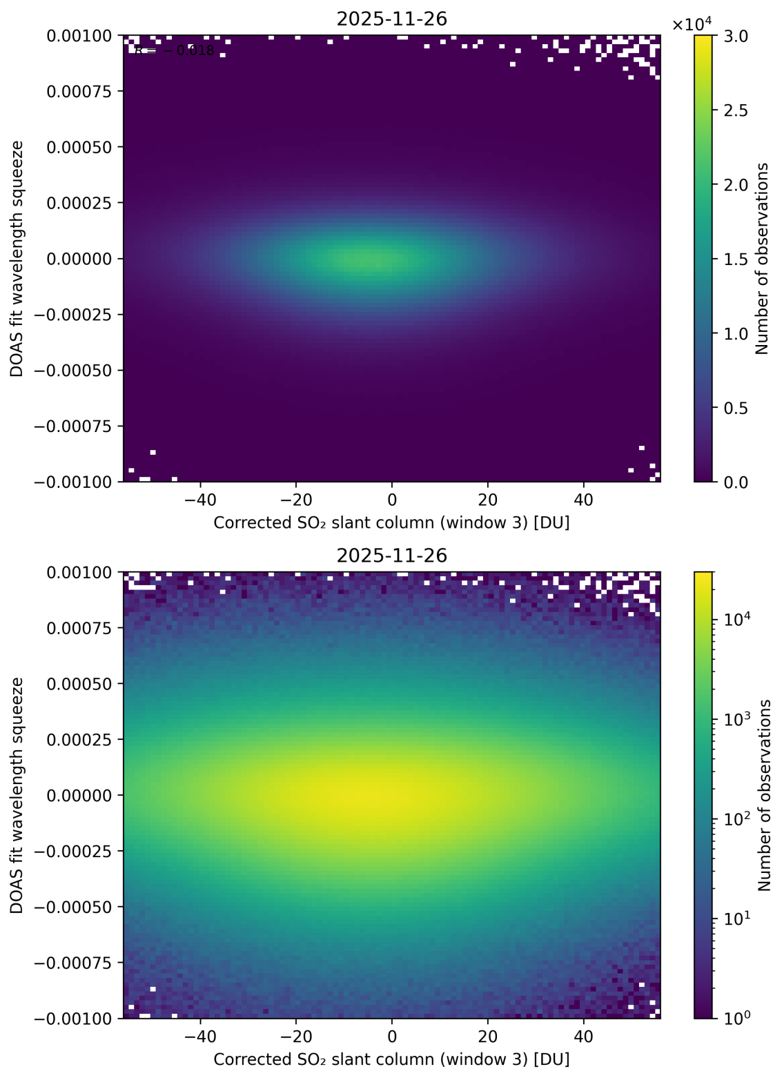
Figure 257: Scatter density plot of “Corrected SO 2 slant column (window 3)” against “DOAS fit wavelength squeeze” for 2025-11-25 to 2025-11-27.
