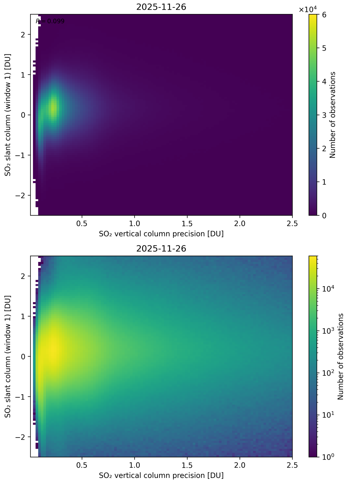
Figure 341: Scatter density plot of “SO 2 vertical column precision” against “SO 2 slant column (window 1)” for 2025-11-25 to 2025-11-27.
