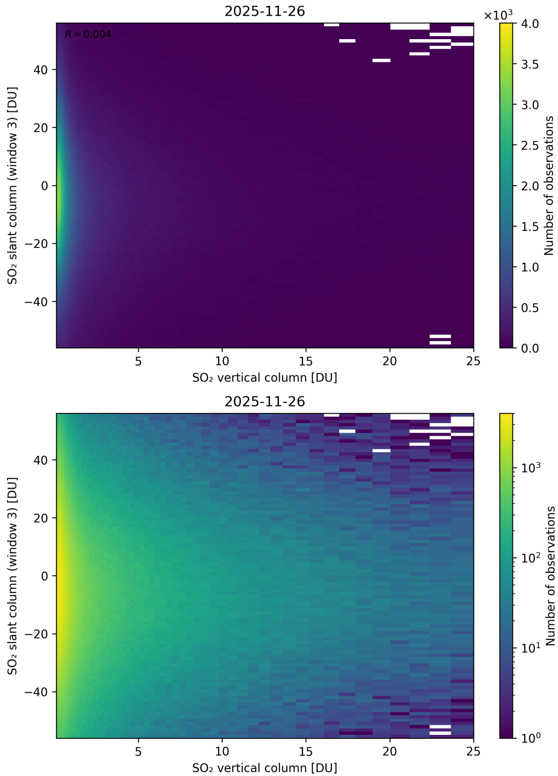
Figure 357: Scatter density plot of “SO 2 vertical column” against “SO 2 slant column (window 3)” for 2025-11-25 to 2025-11-27.
