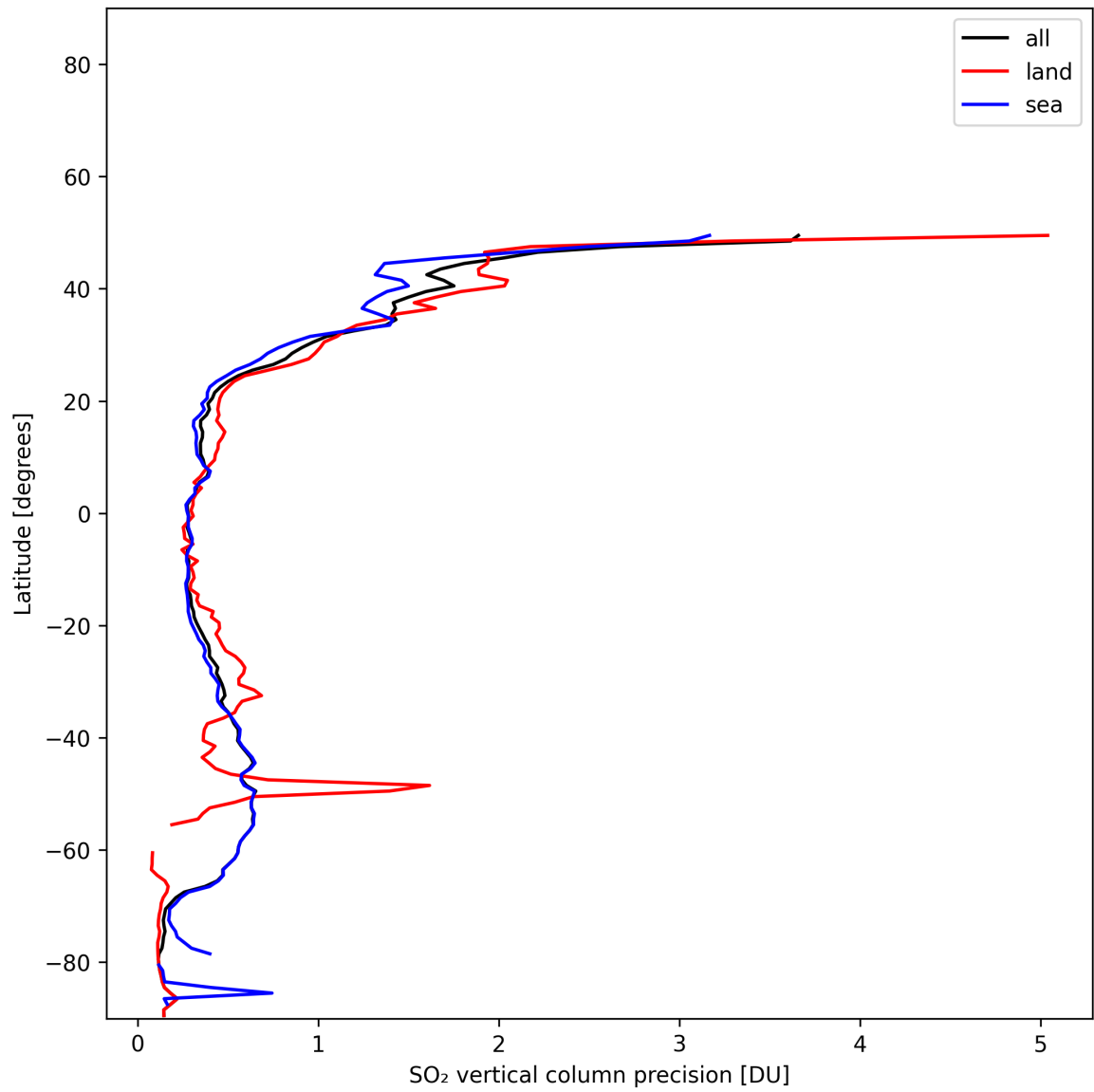
Figure 33: Zonal average of “SO 2 vertical column precision” for 2025-11-25 to 2025-11-27.
