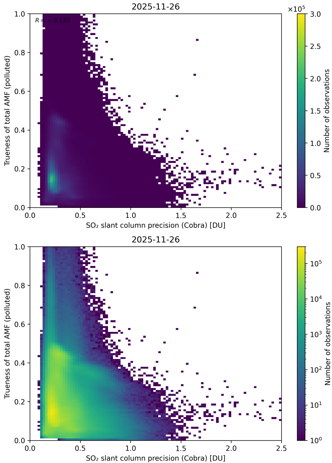
Figure 214: Scatter density plot of “SO 2 slant column precision (Cobra)” against “Trueness of total AMF (polluted)” for 2025-11-25 to 2025-11-27.
