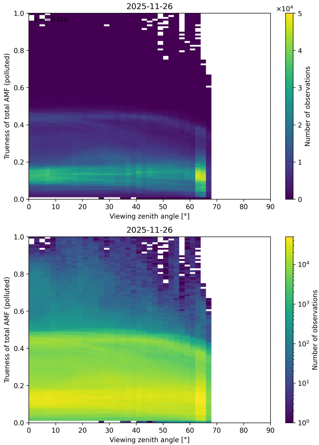
Figure 382: Scatter density plot of “Viewing zenith angle” against “Trueness of total AMF (polluted)” for 2025-11-25 to 2025-11-27.
