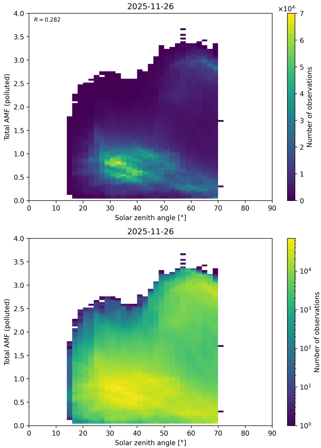
Figure 189: Scatter density plot of “Solar zenith angle” against “Total AMF (polluted)” for 2025-11-25 to 2025-11-27.
