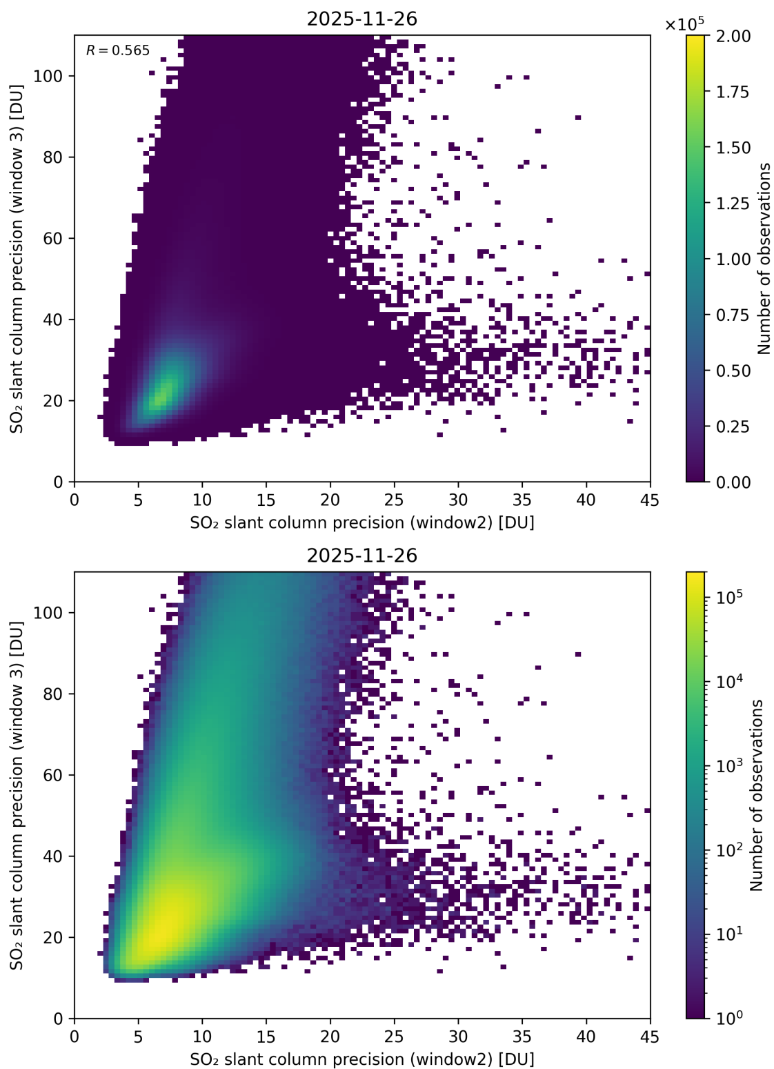
Figure 300: Scatter density plot of “SO 2 slant column precision (window2)” against “SO 2 slant column precision (window 3)” for 2025-11-25 to 2025-11-27.
