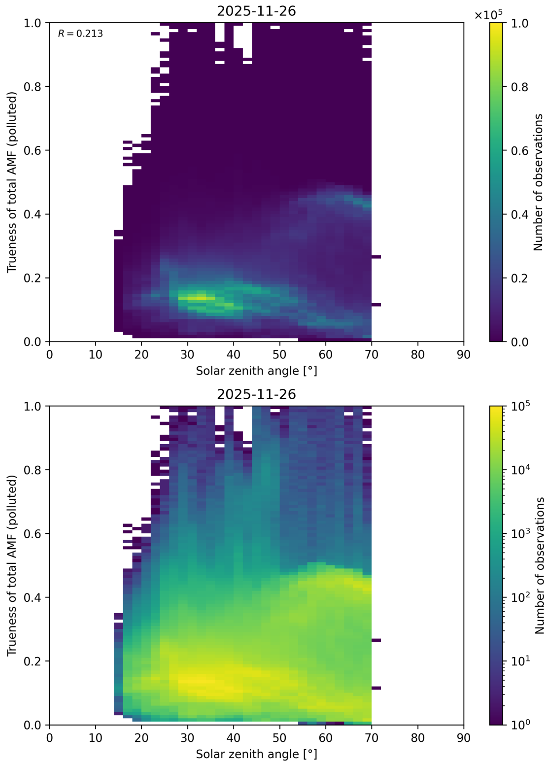
Figure 190: Scatter density plot of “Solar zenith angle” against “Trueness of total AMF (polluted)” for 2025-11-25 to 2025-11-27.
