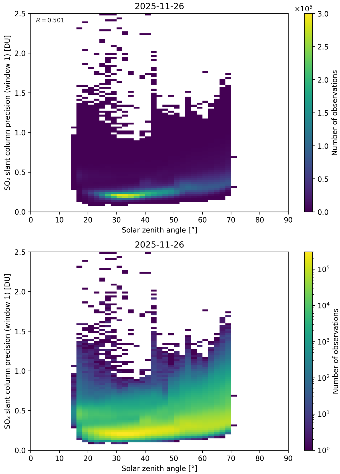
Figure 185: Scatter density plot of “Solar zenith angle” against “SO 2 slant column precision (window 1)” for 2025-11-25 to 2025-11-27.
