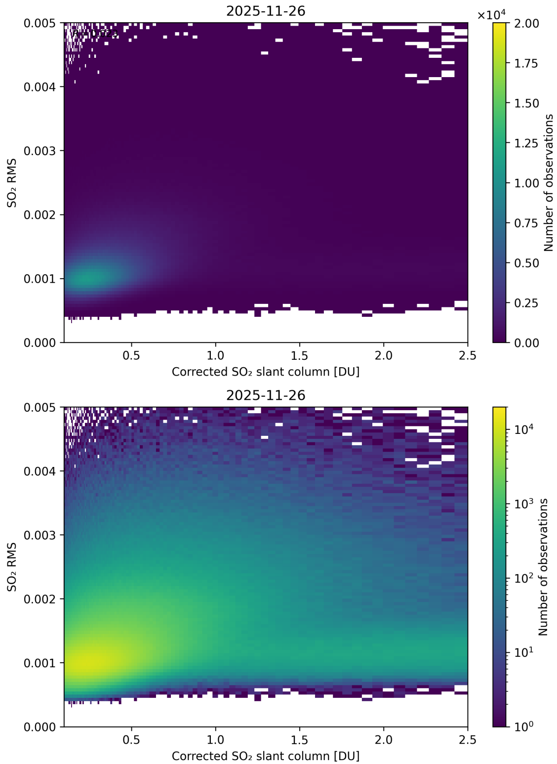
Figure 231: Scatter density plot of “Corrected SO 2 slant column” against “SO 2 RMS” for 2025-11-25 to 2025-11-27.
