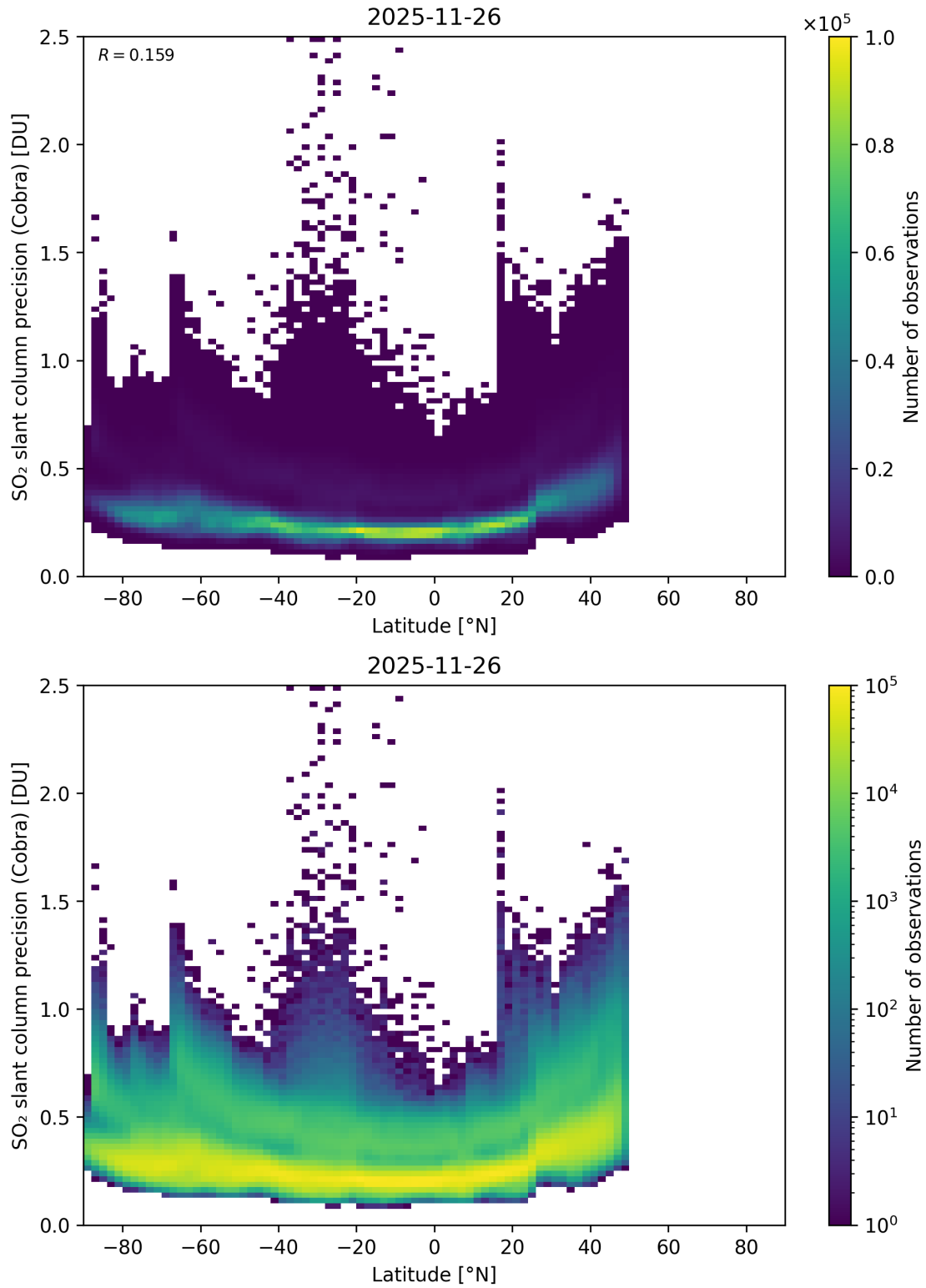
Figure 158: Scatter density plot of “Latitude” against “SO 2 slant column precision (Cobra)” for 2025-11-25 to 2025-11-27.
