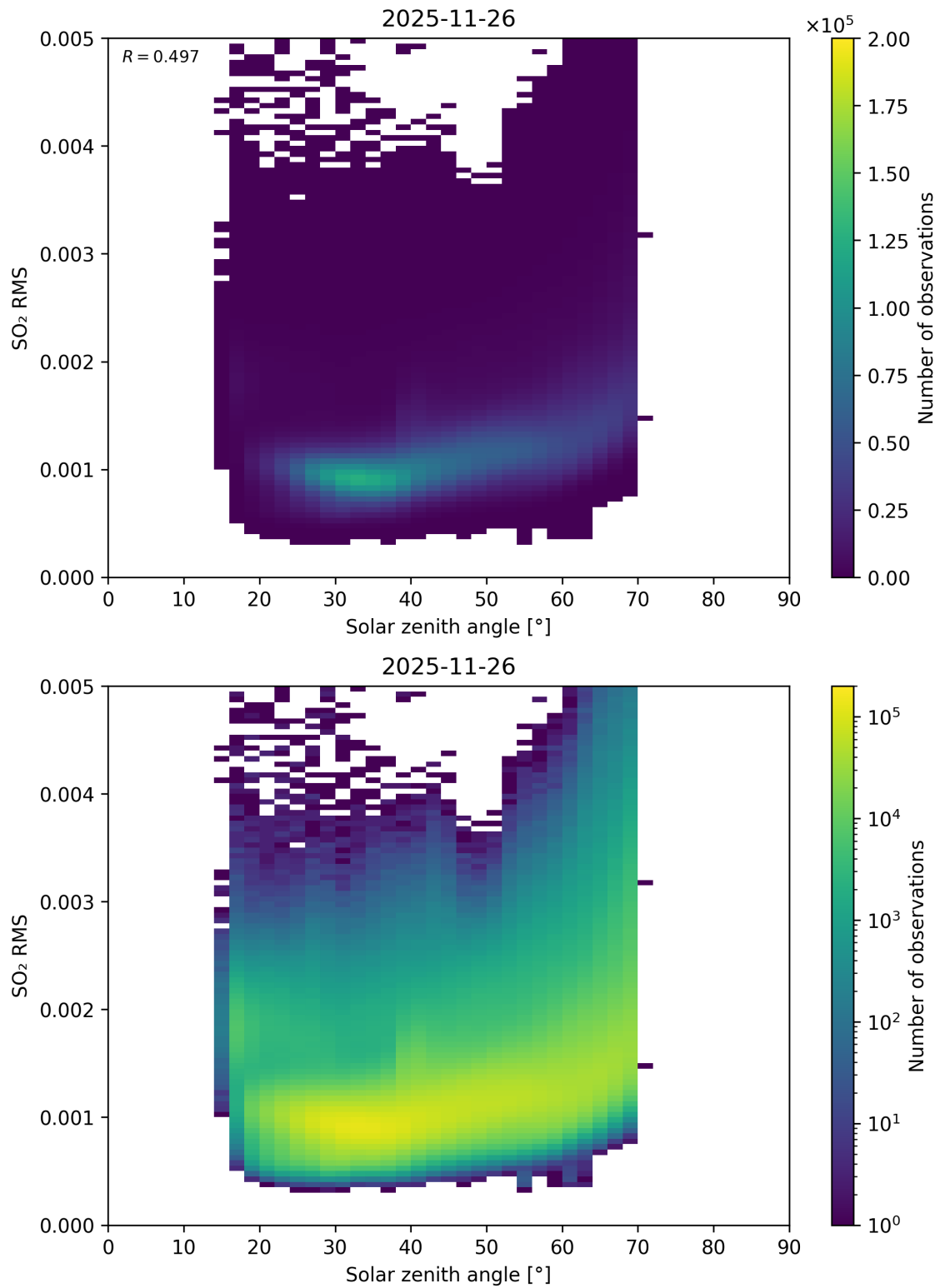
Figure 176: Scatter density plot of “Solar zenith angle” against “SO 2 RMS” for 2025-11-25 to 2025-11-27.
