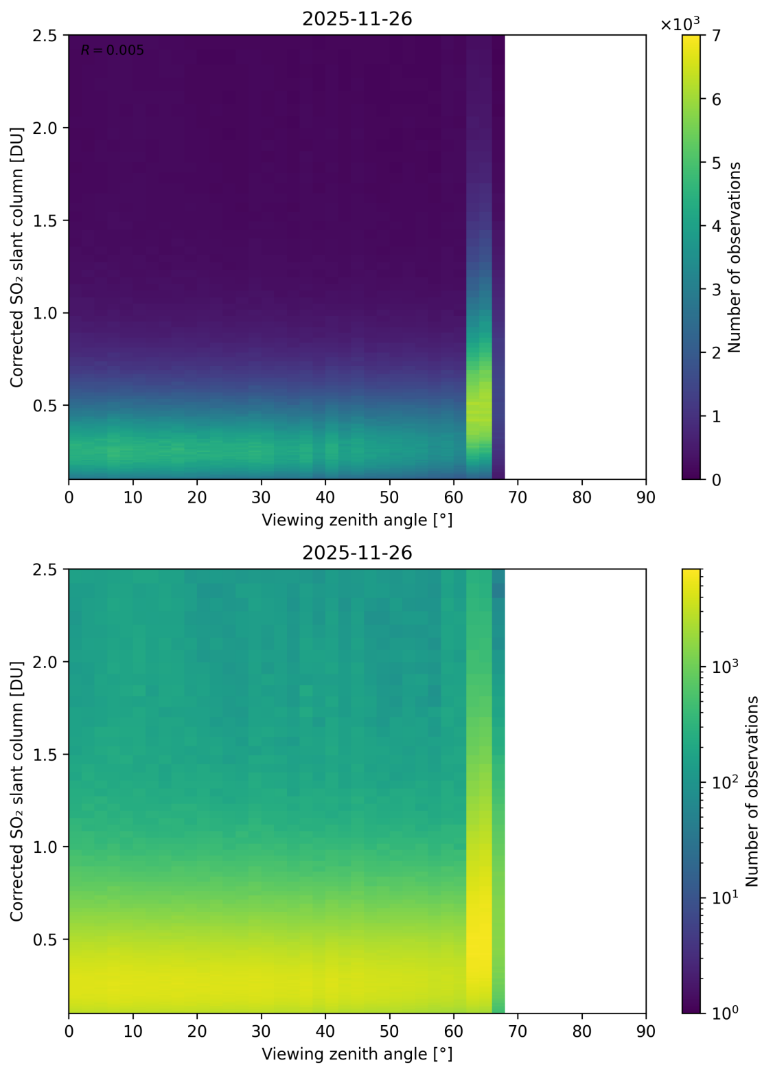
Figure 373: Scatter density plot of “Viewing zenith angle” against “Corrected SO 2 slant column” for 2025-11-25 to 2025-11-27.
