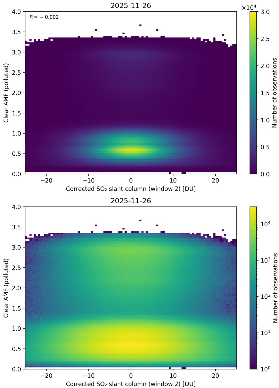
Figure 249: Scatter density plot of “Corrected SO 2 slant column (window 2)” against “Clear AMF (polluted)” for 2025-11-25 to 2025-11-27.
