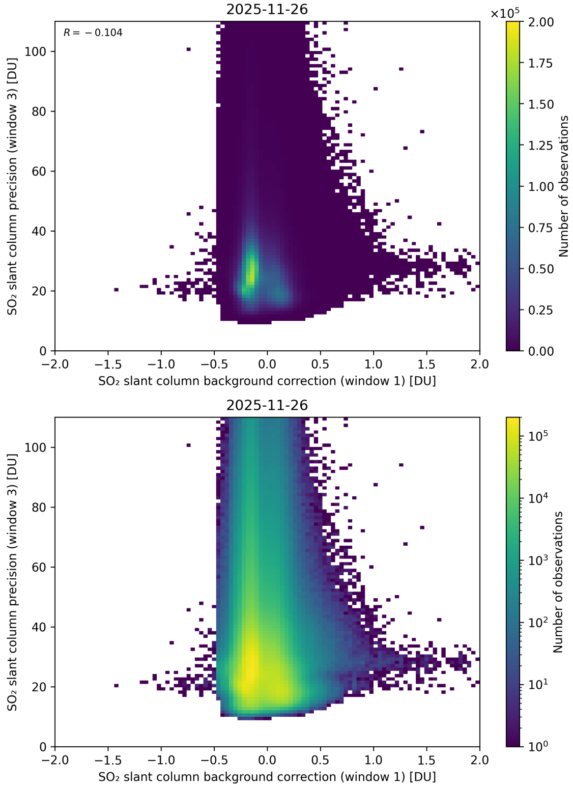
Figure 119: Scatter density plot of “SO 2 slant column background correction (window 1)” against “SO 2 slant column precision (window 3)” for 2025-11-25 to 2025-11-27.
