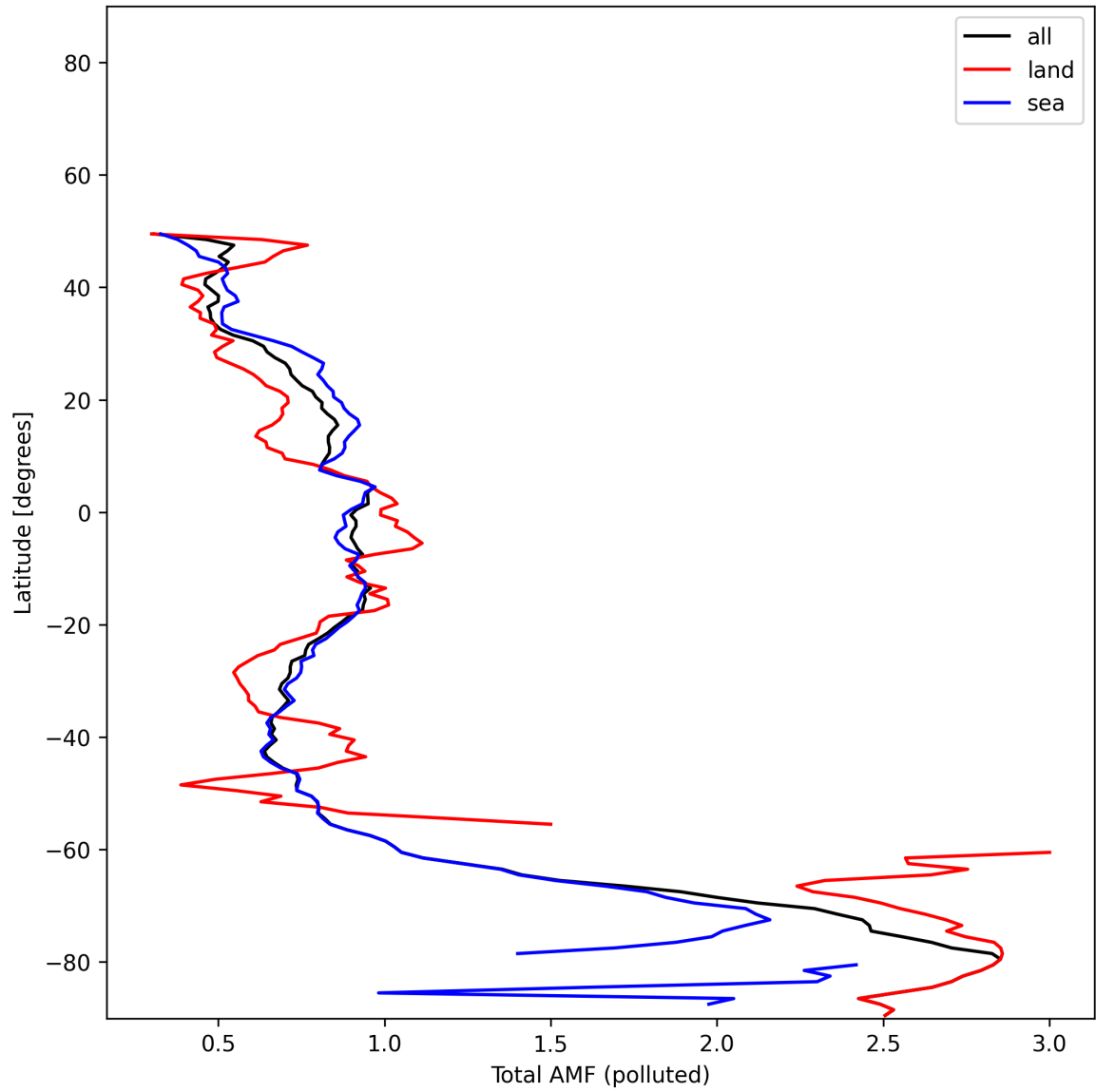
Figure 53: Zonal average of “Total AMF (polluted)” for 2025-11-25 to 2025-11-27.
