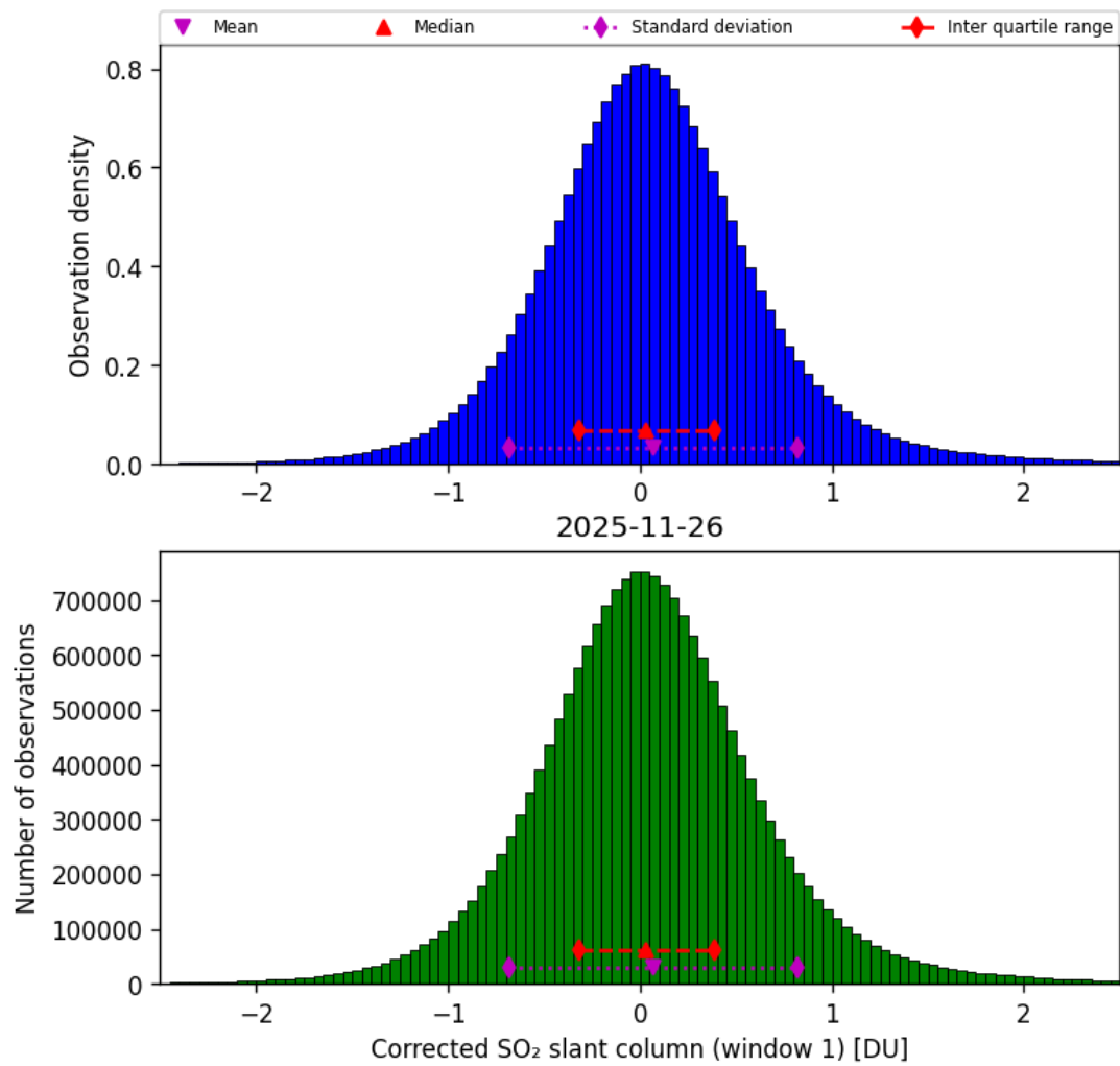
Figure 65: Histogram of “Corrected SO 2 slant column (window 1)” for 2025-11-25 to 2025-11-27
