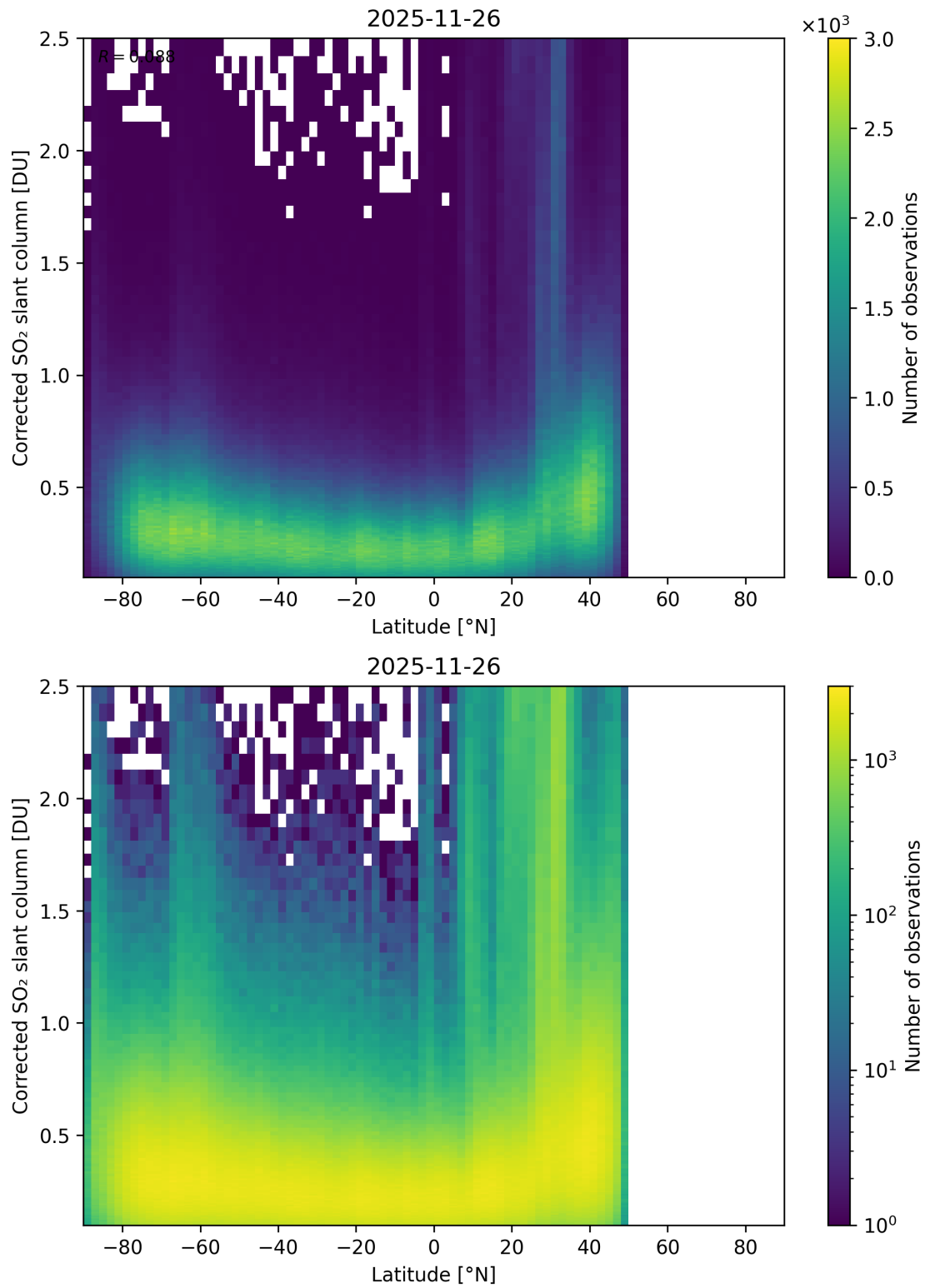
Figure 159: Scatter density plot of “Latitude” against “Corrected SO 2 slant column” for 2025-11-25 to 2025-11-27.
