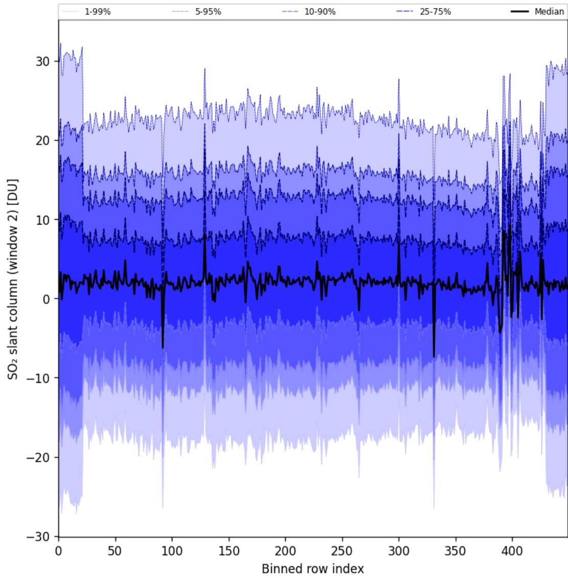
Figure 93: Along track statistics of “SO 2 slant column (window 2)” for 2025-11-25 to 2025-11-27
