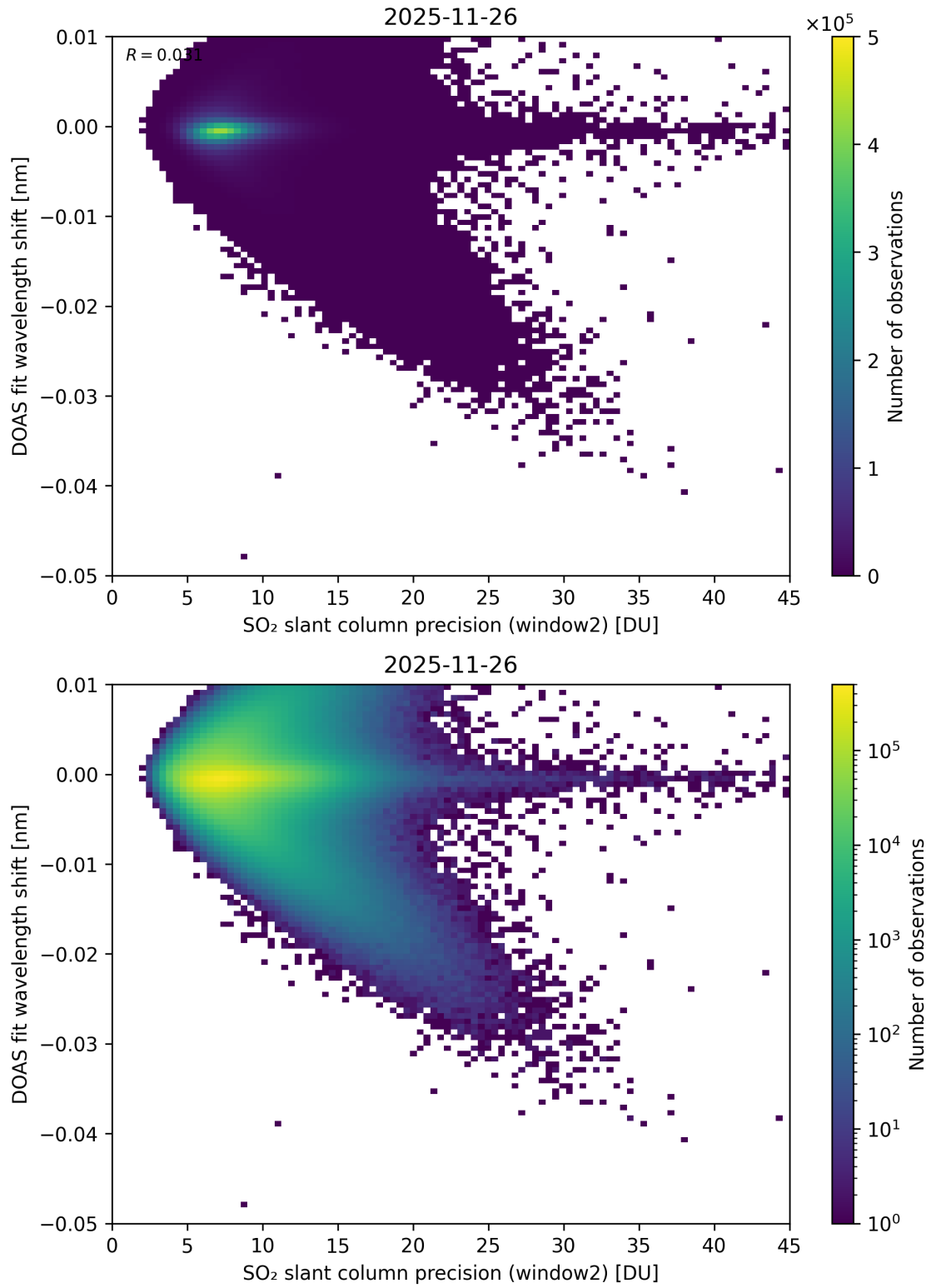
Figure 293: Scatter density plot of “SO 2 slant column precision (window2)” against “DOAS fit wavelength shift” for 2025-11-25 to 2025-11-27.
