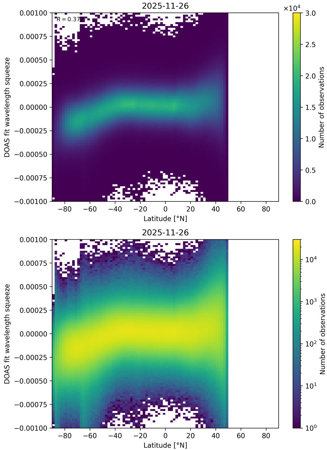
Figure 154: Scatter density plot of “Latitude” against “DOAS fit wavelength squeeze” for 2025-11-25 to 2025-11-27.
