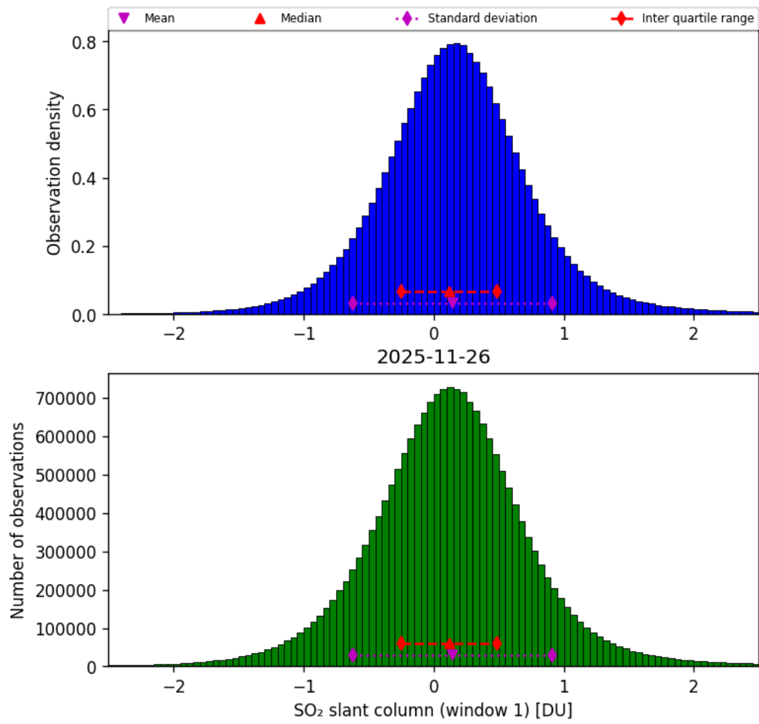
Figure 63: Histogram of “SO 2 slant column (window 1)” for 2025-11-25 to 2025-11-27
