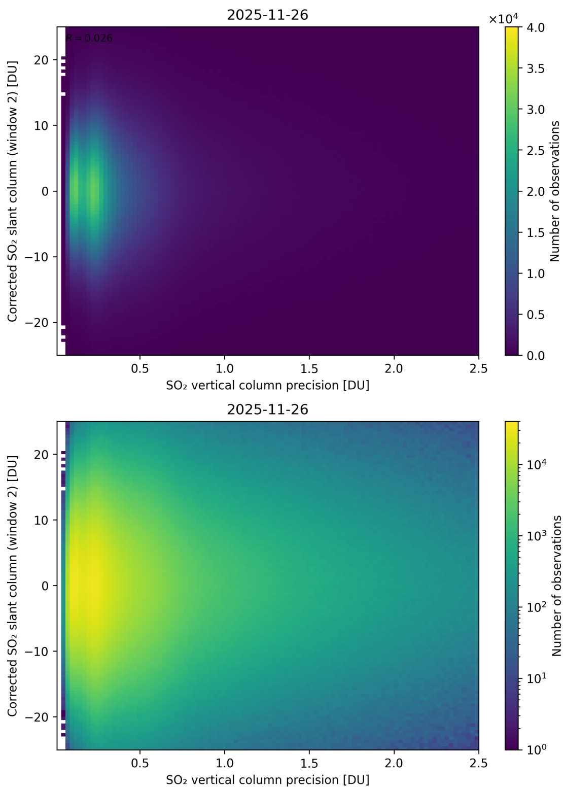
Figure 339: Scatter density plot of “SO 2 vertical column precision” against “Corrected SO 2 slant column (window 2)” for 2025-11-25 to 2025-11-27.
