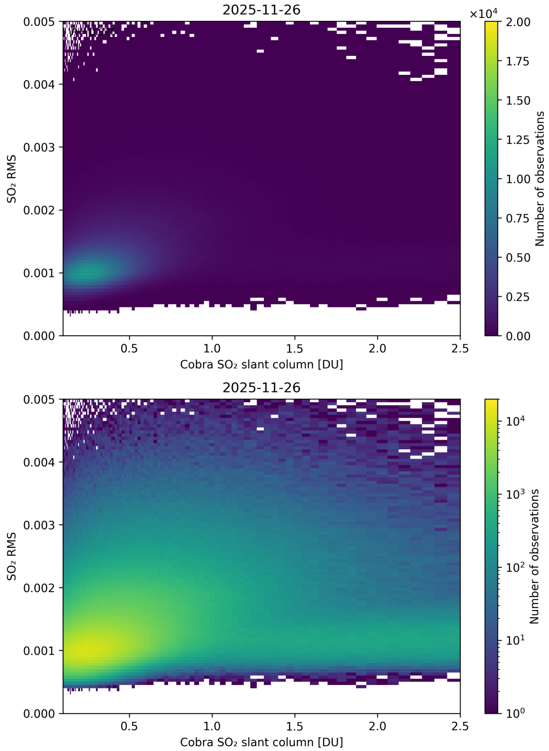
Figure 198: Scatter density plot of “Cobra SO 2 slant column” against “SO 2 RMS” for 2025-11-25 to 2025-11-27.
