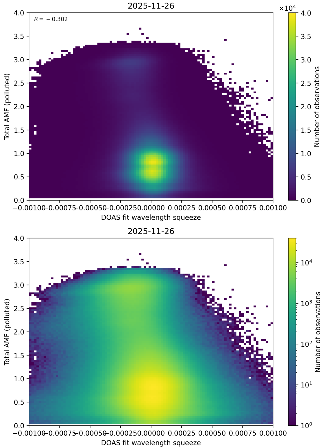
Figure 145: Scatter density plot of “DOAS fit wavelength squeeze” against “Total AMF (polluted)” for 2025-11-25 to 2025-11-27.
