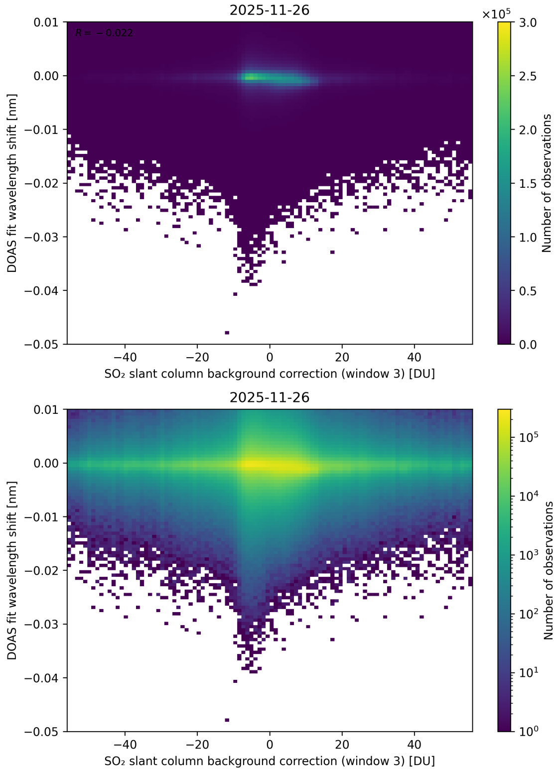
Figure 132: Scatter density plot of “SO 2 slant column background correction (window 3)” against “DOAS fit wavelength shift” for 2025-11-25 to 2025-11-27.
