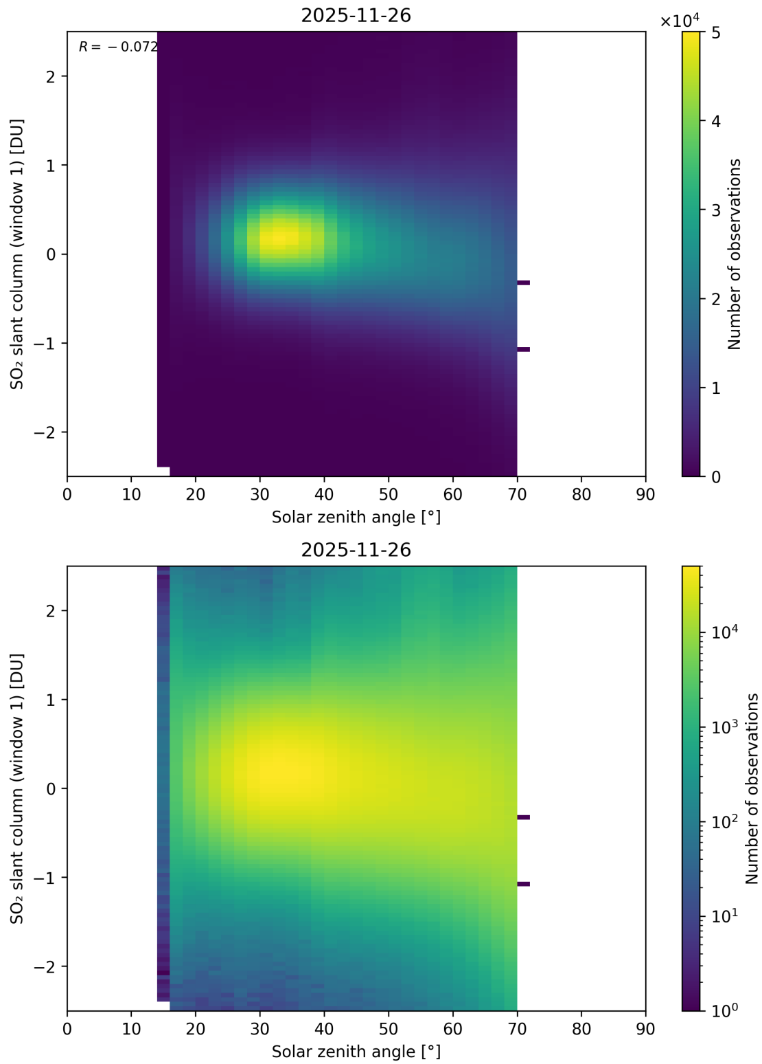
Figure 184: Scatter density plot of “Solar zenith angle” against “SO 2 slant column (window 1)” for 2025-11-25 to 2025-11-27.
