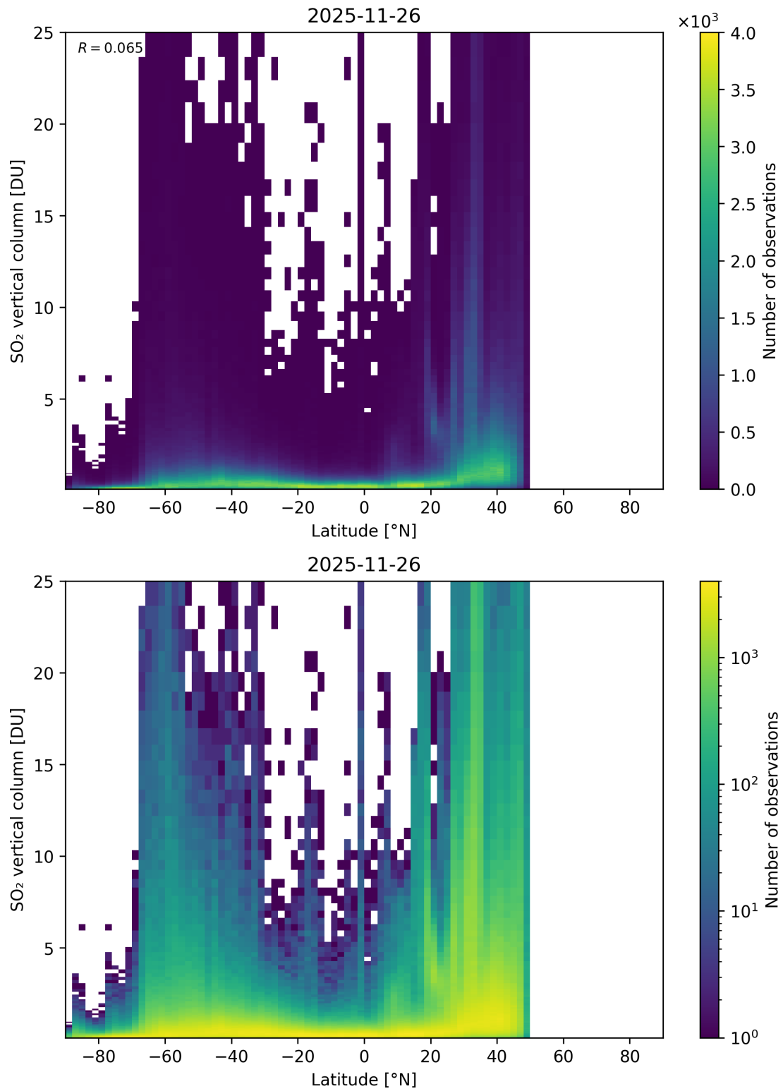
Figure 169: Scatter density plot of “Latitude” against “SO 2 vertical column” for 2025-11-25 to 2025-11-27.
