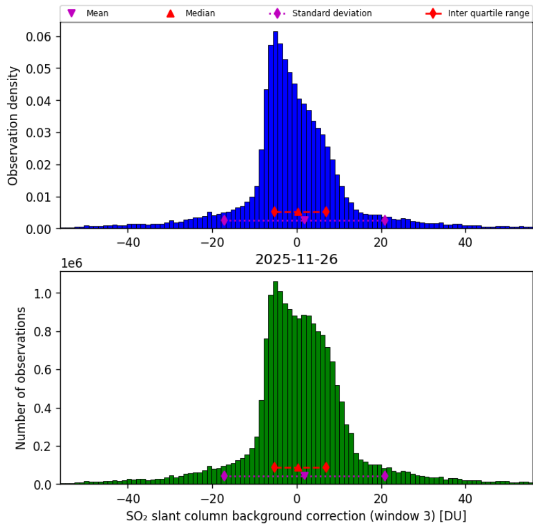
Figure 74: Histogram of “SO 2 slant column background correction (window 3)” for 2025-11-25 to 2025-11-27
