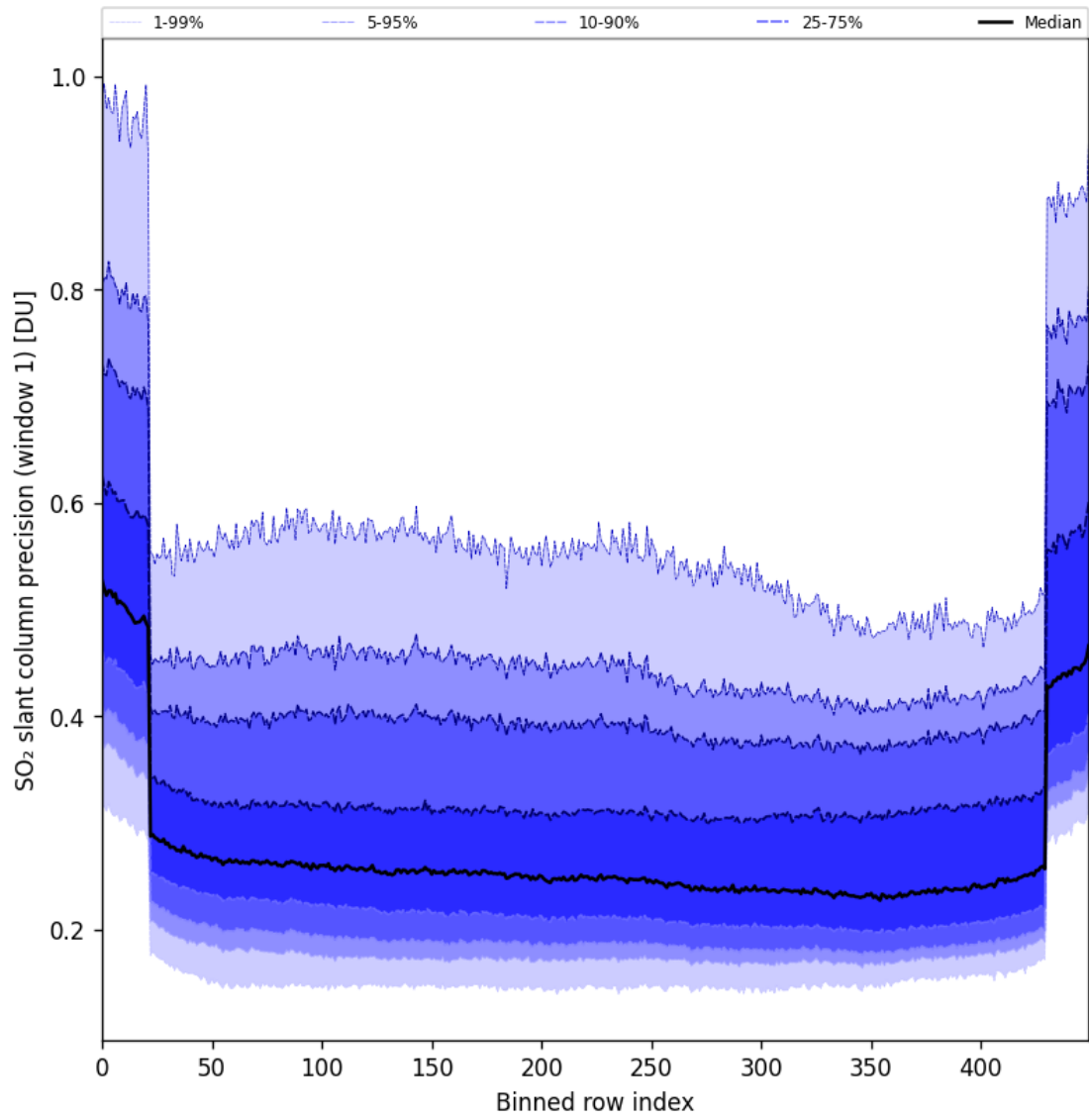
Figure 90: Along track statistics of “SO 2 slant column precision (window 1)” for 2025-11-25 to 2025-11-27
