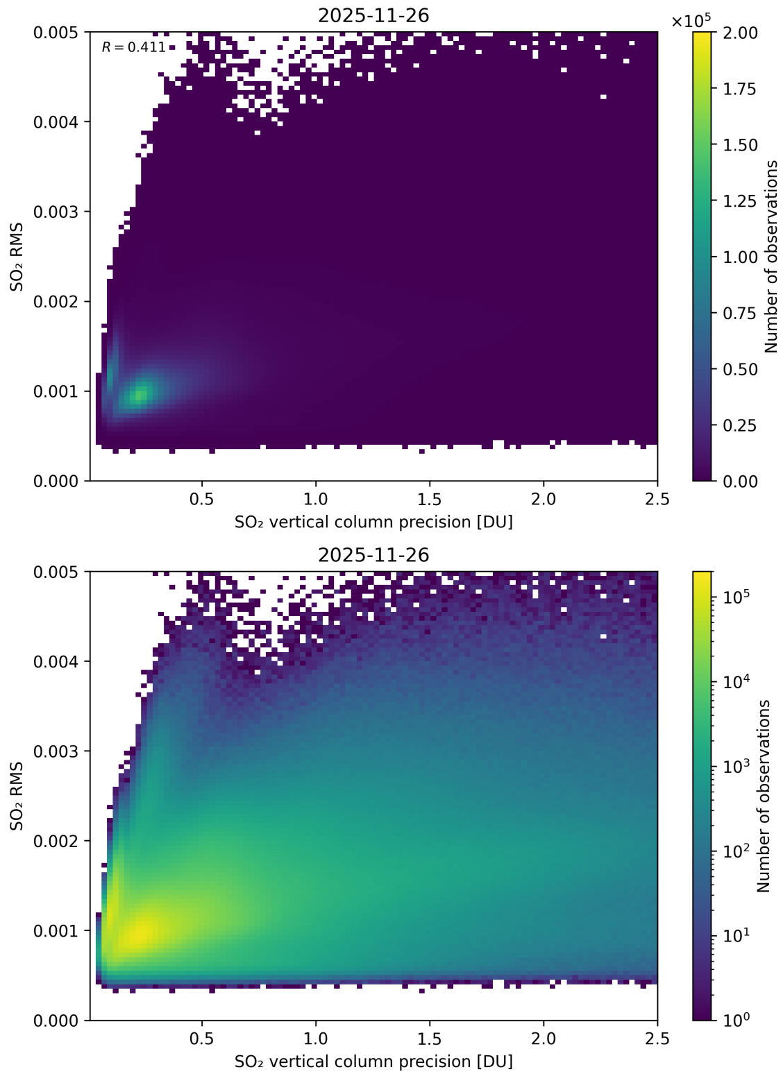
Figure 334: Scatter density plot of “SO 2 vertical column precision” against “SO 2 RMS” for 2025-11-25 to 2025-11-27.
