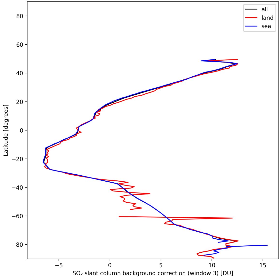
Figure 48: Zonal average of “SO 2 slant column background correction (window 3)” for 2025-11-25 to 2025-11-27.
