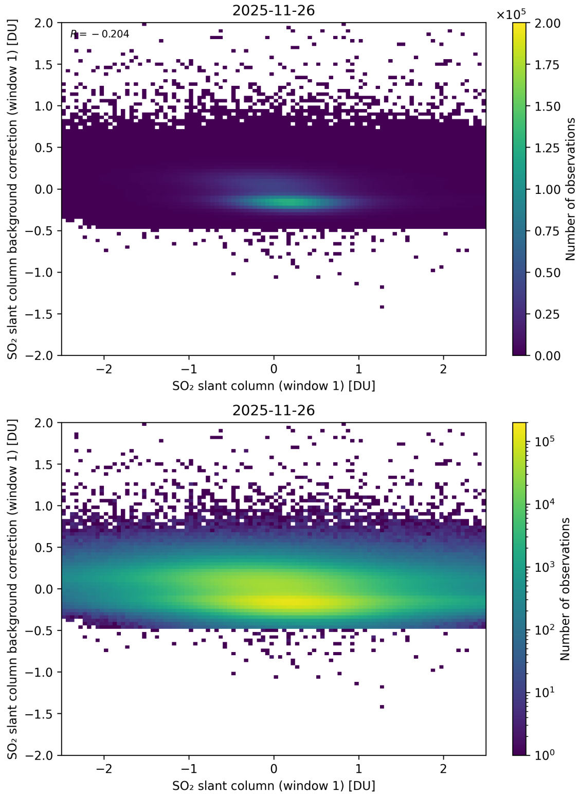
Figure 262: Scatter density plot of “SO 2 slant column (window 1)” against “SO 2 slant column background correction (window 1)” for 2025-11-25 to 2025-11-27.
