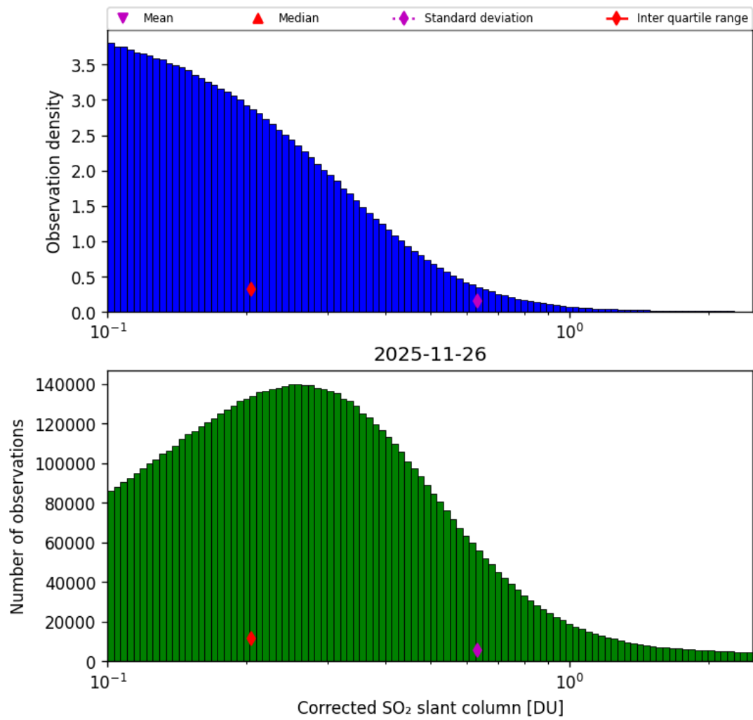
Figure 60: Histogram of “Corrected SO 2 slant column” for 2025-11-25 to 2025-11-27
