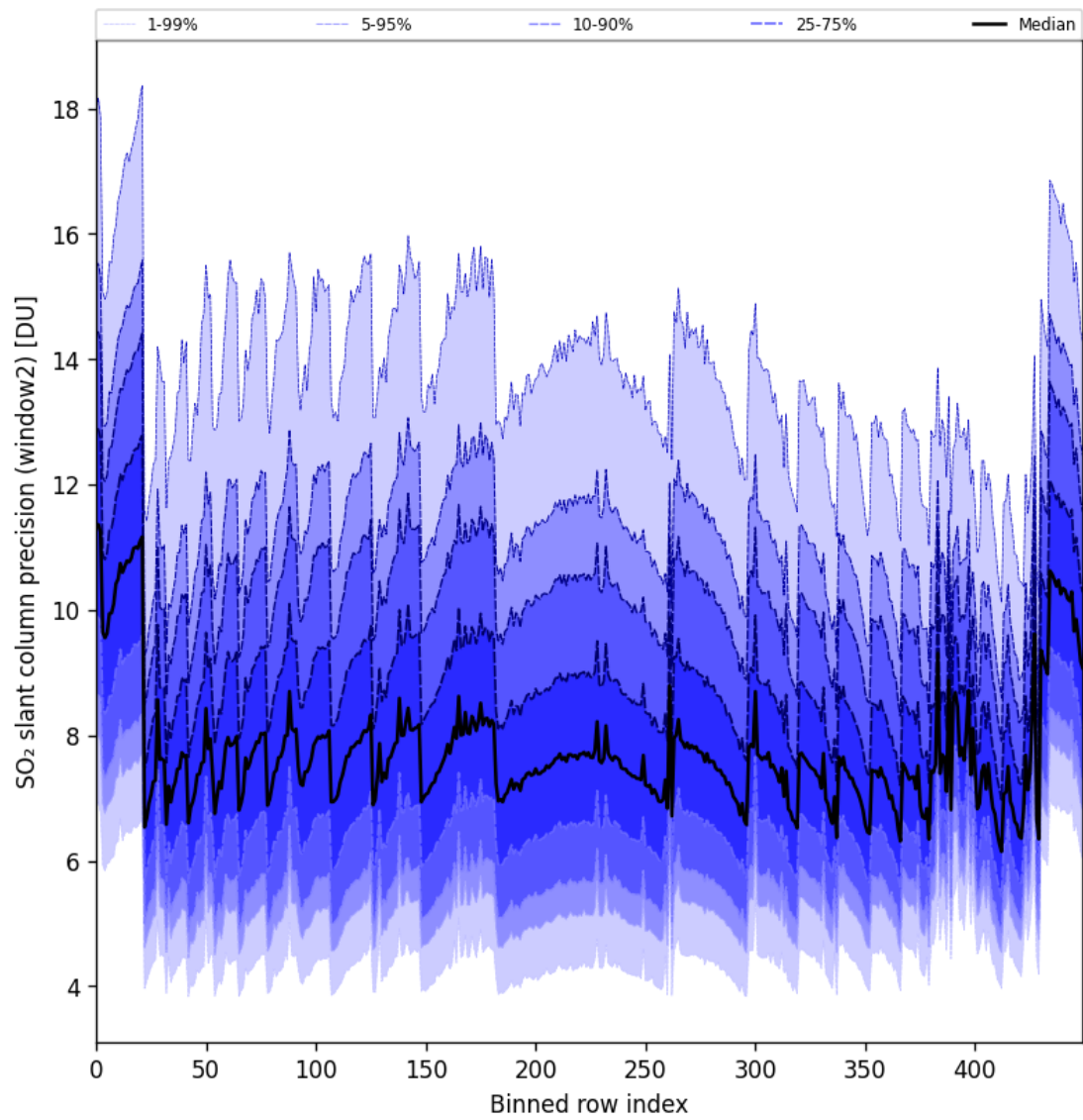
Figure 94: Along track statistics of “SO 2 slant column precision (window2)” for 2025-11-25 to 2025-11-27
