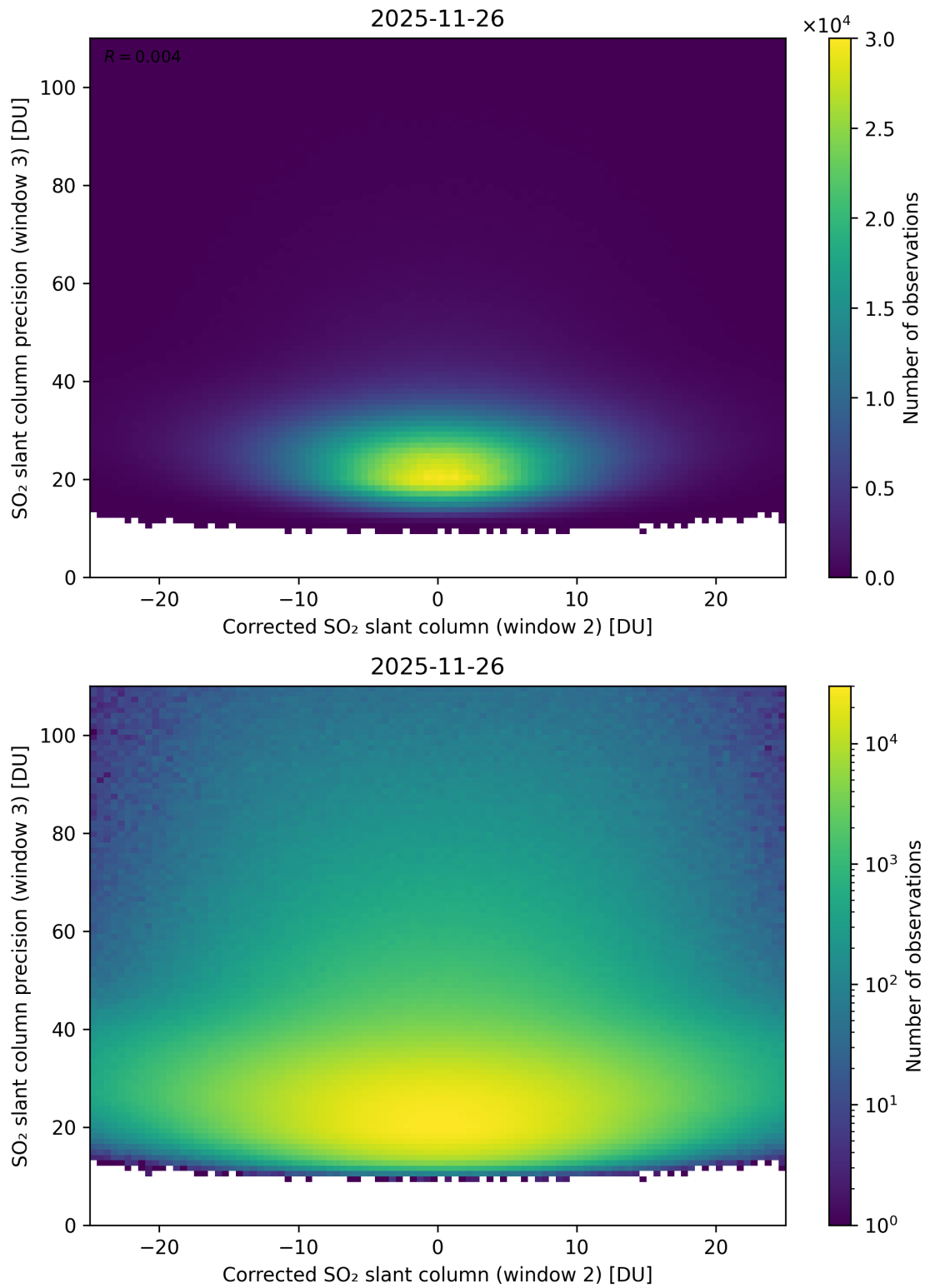
Figure 252: Scatter density plot of “Corrected SO 2 slant column (window 2)” against “SO 2 slant column precision (window 3)” for 2025-11-25 to 2025-11-27.
