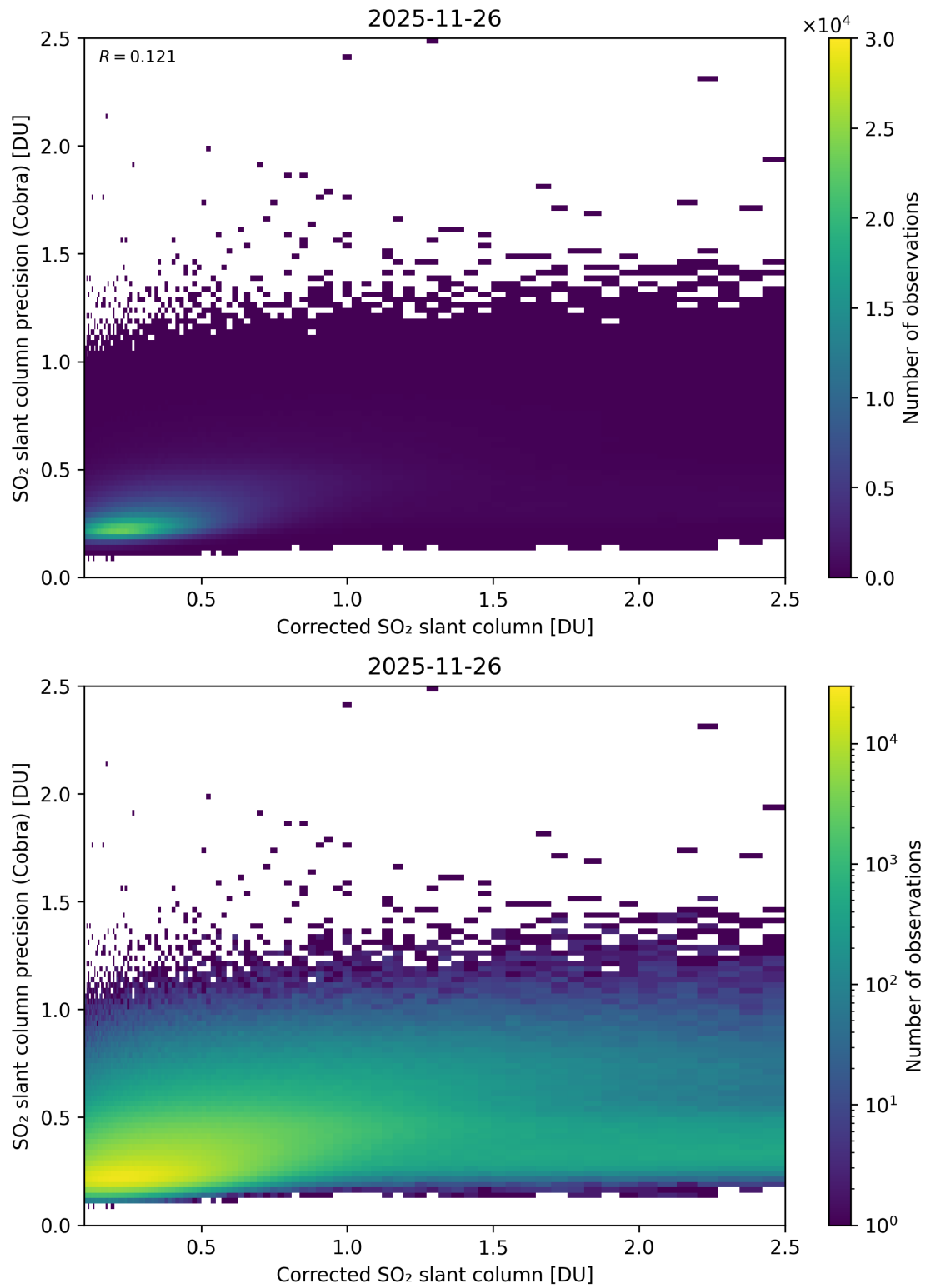
Figure 234: Scatter density plot of “Corrected SO 2 slant column” against “SO 2 slant column precision (Cobra)” for 2025-11-25 to 2025-11-27.
