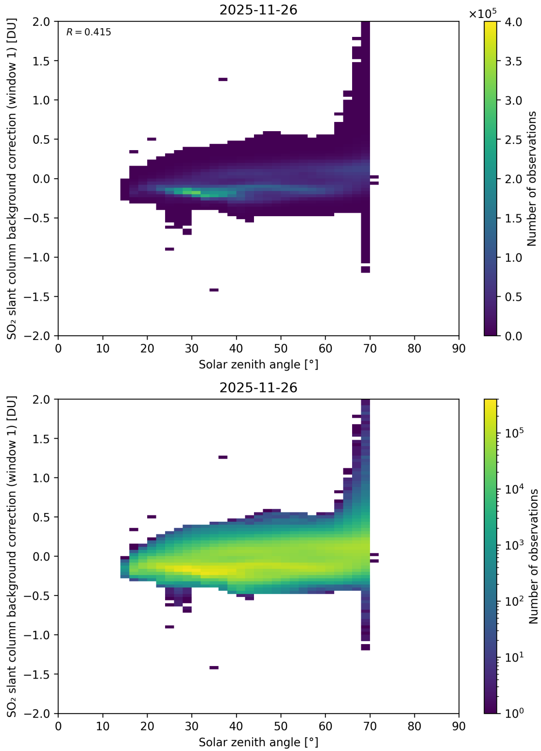
Figure 171: Scatter density plot of “Solar zenith angle” against “SO 2 slant column background correction (window 1)” for 2025-11-25 to 2025-11-27.
