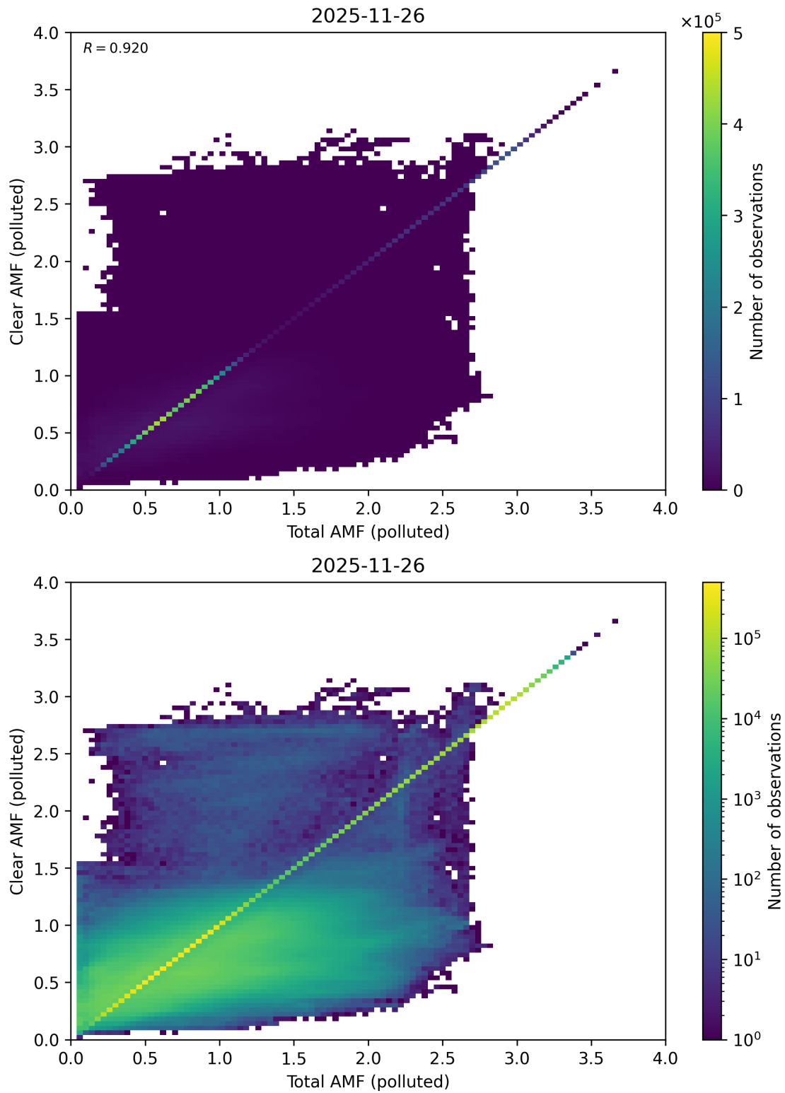
Figure 320: Scatter density plot of “Total AMF (polluted)” against “Clear AMF (polluted)” for 2025-11-25 to 2025-11-27.
