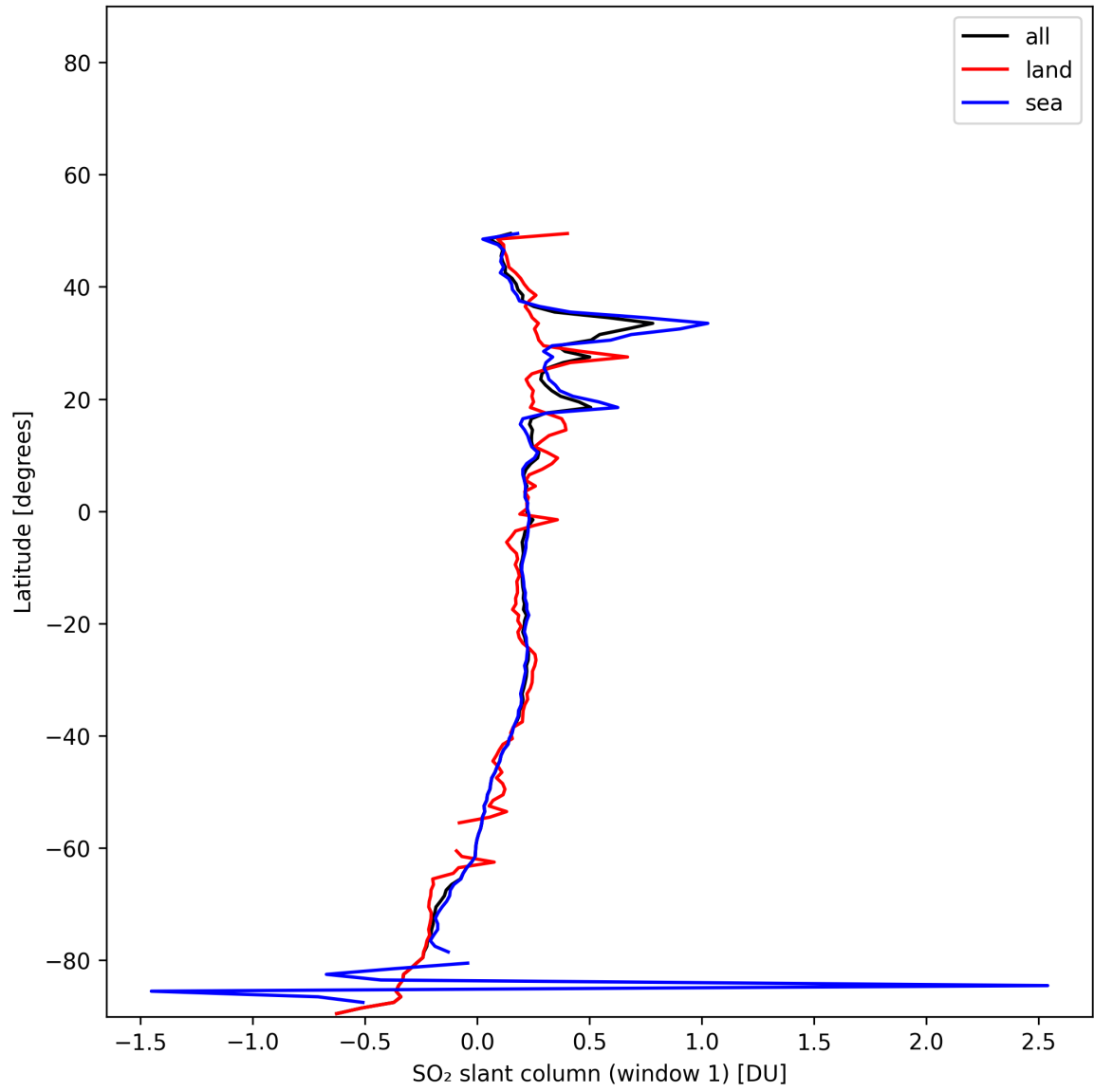
Figure 37: Zonal average of “SO 2 slant column (window 1)” for 2025-11-25 to 2025-11-27.
