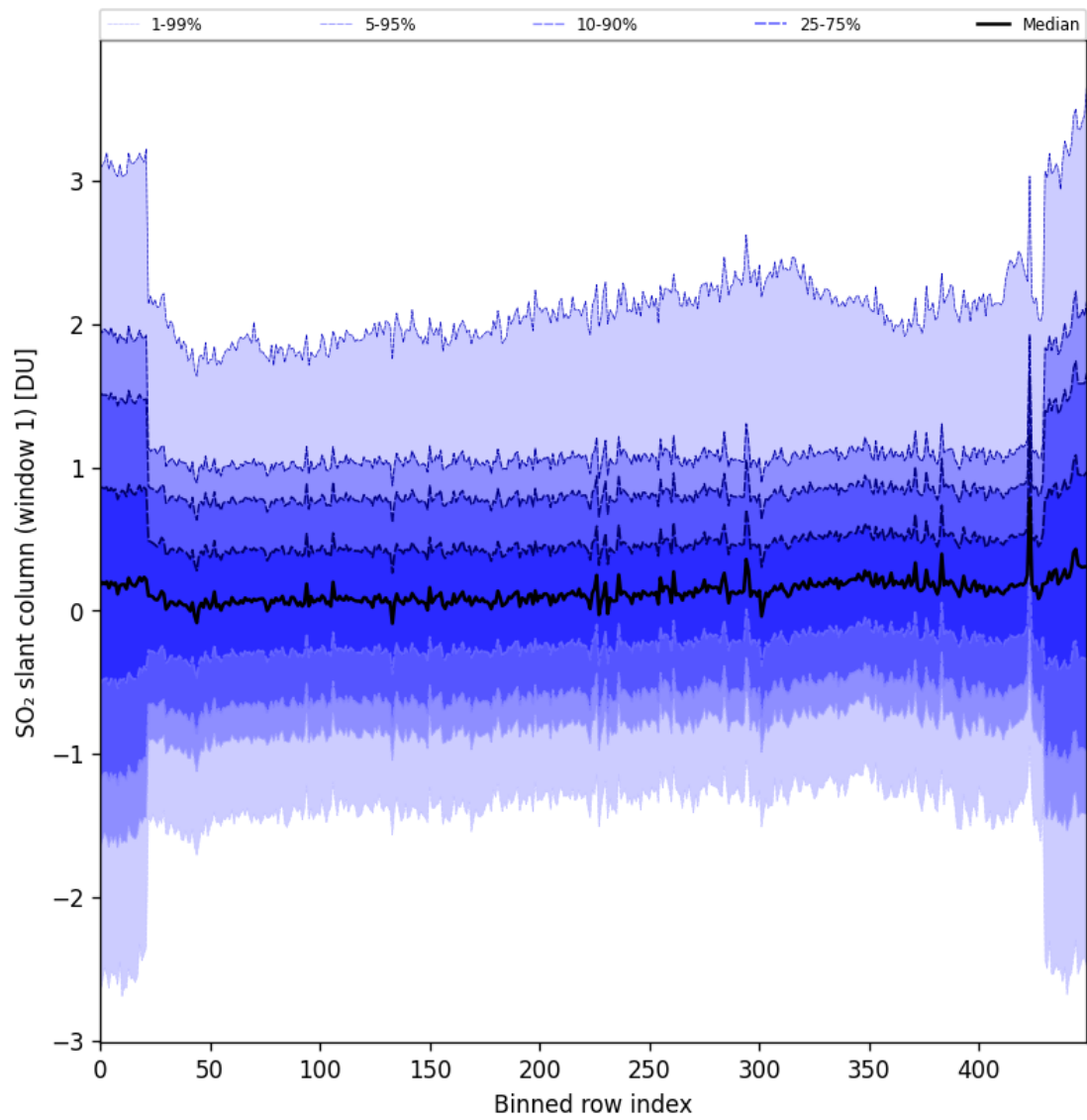
Figure 89: Along track statistics of “SO 2 slant column (window 1)” for 2025-11-25 to 2025-11-27
