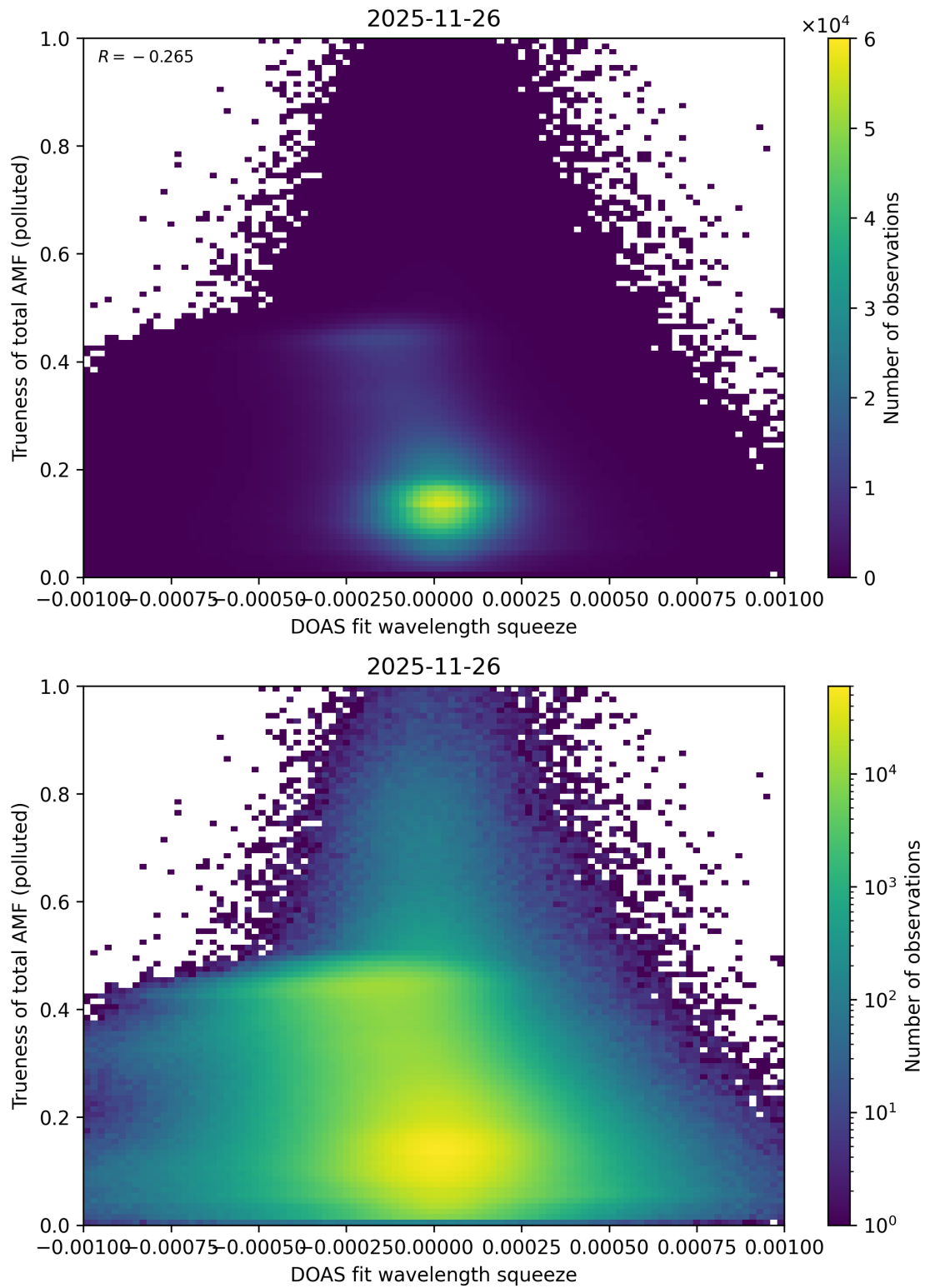
Figure 146: Scatter density plot of “DOAS fit wavelength squeeze” against “Trueness of total AMF (polluted)” for 2025-11-25 to 2025-11-27.
