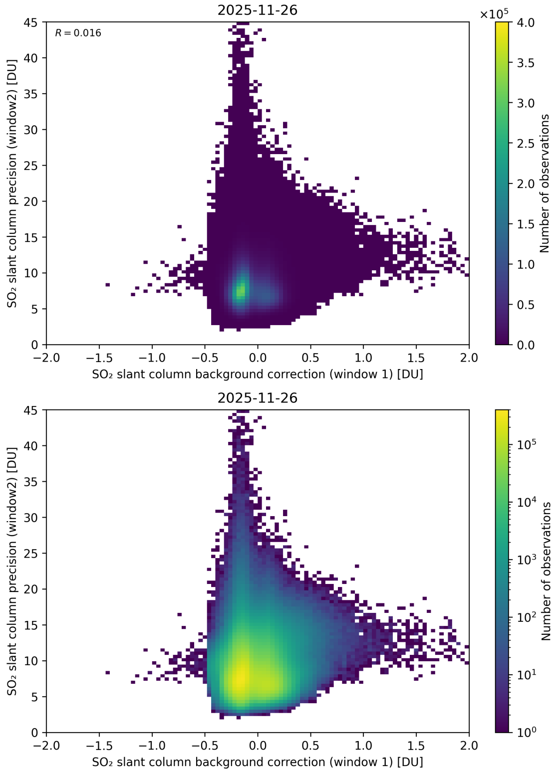
Figure 117: Scatter density plot of “SO 2 slant column background correction (window 1)” against “SO 2 slant column precision (window2)” for 2025-11-25 to 2025-11-27.
