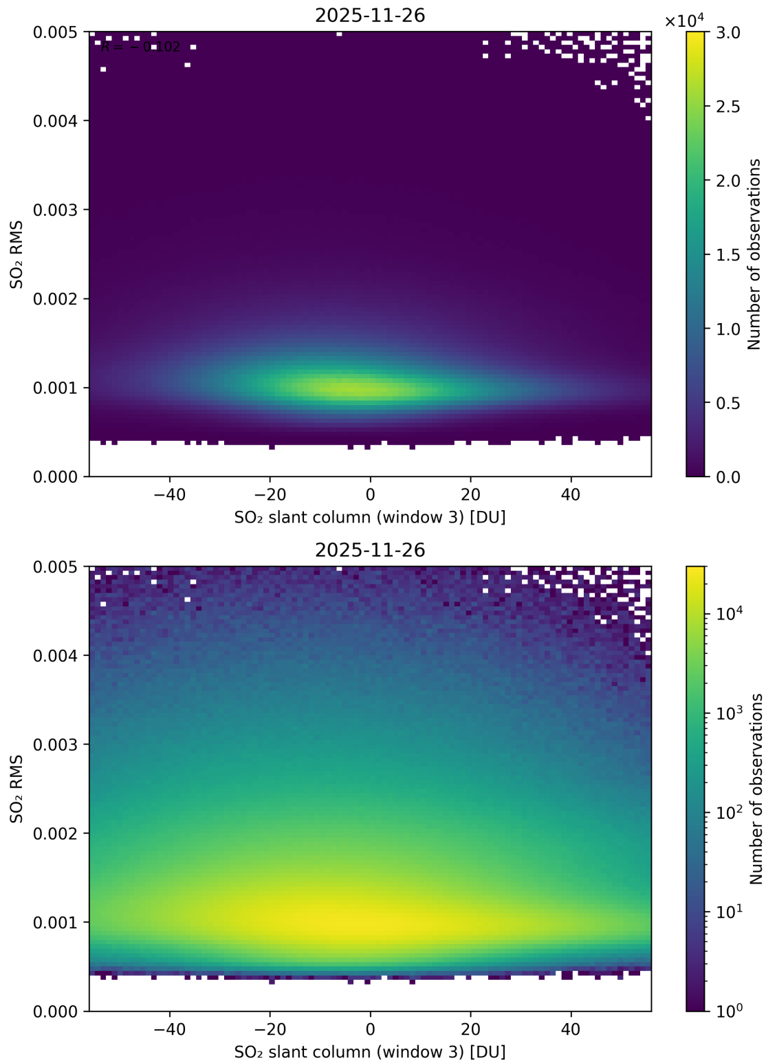
Figure 306: Scatter density plot of “SO 2 slant column (window 3)” against “SO 2 RMS” for 2025-11-25 to 2025-11-27.
