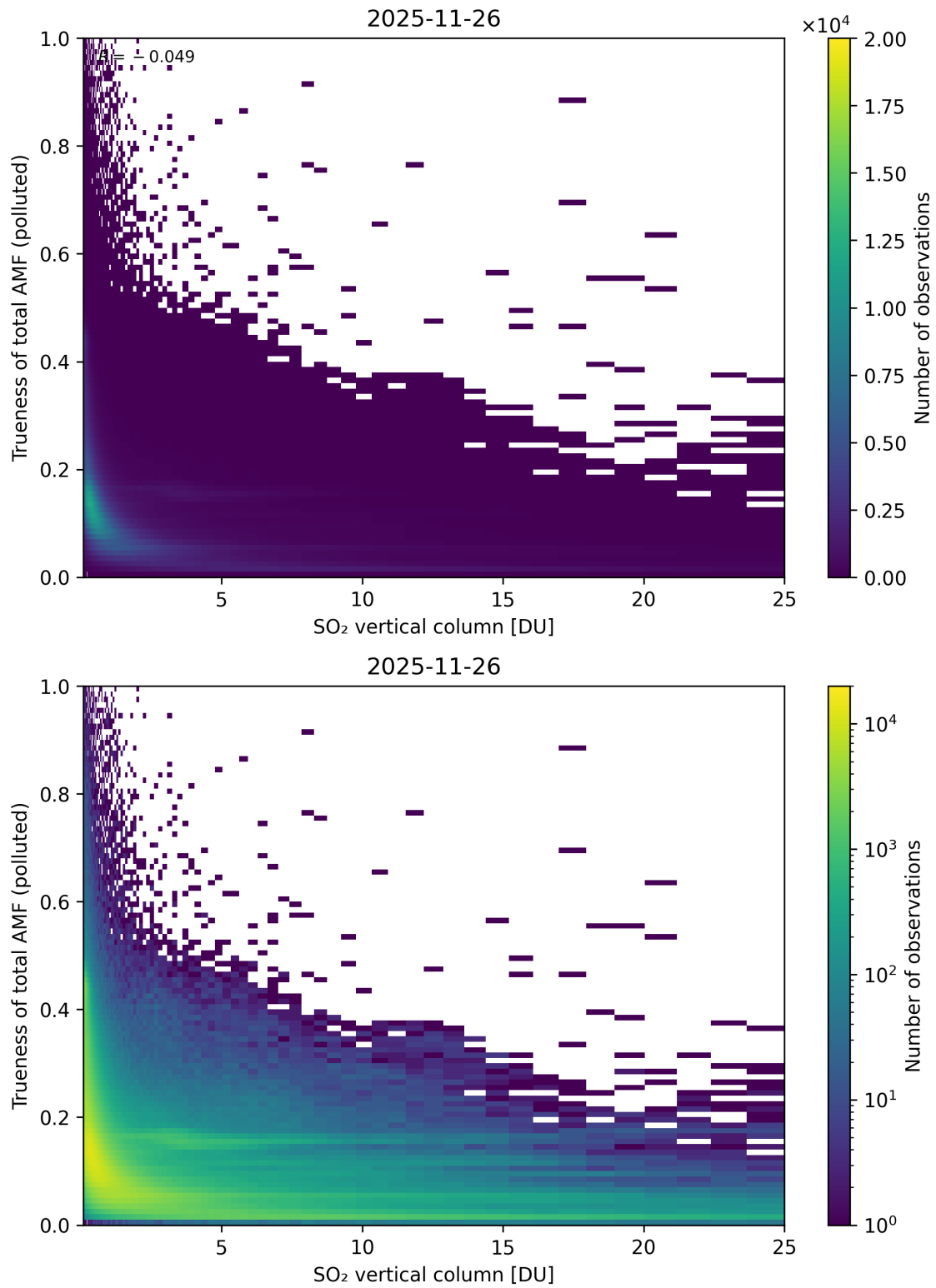
Figure 360: Scatter density plot of “SO 2 vertical column” against “Trueness of total AMF (polluted)” for 2025-11-25 to 2025-11-27.
