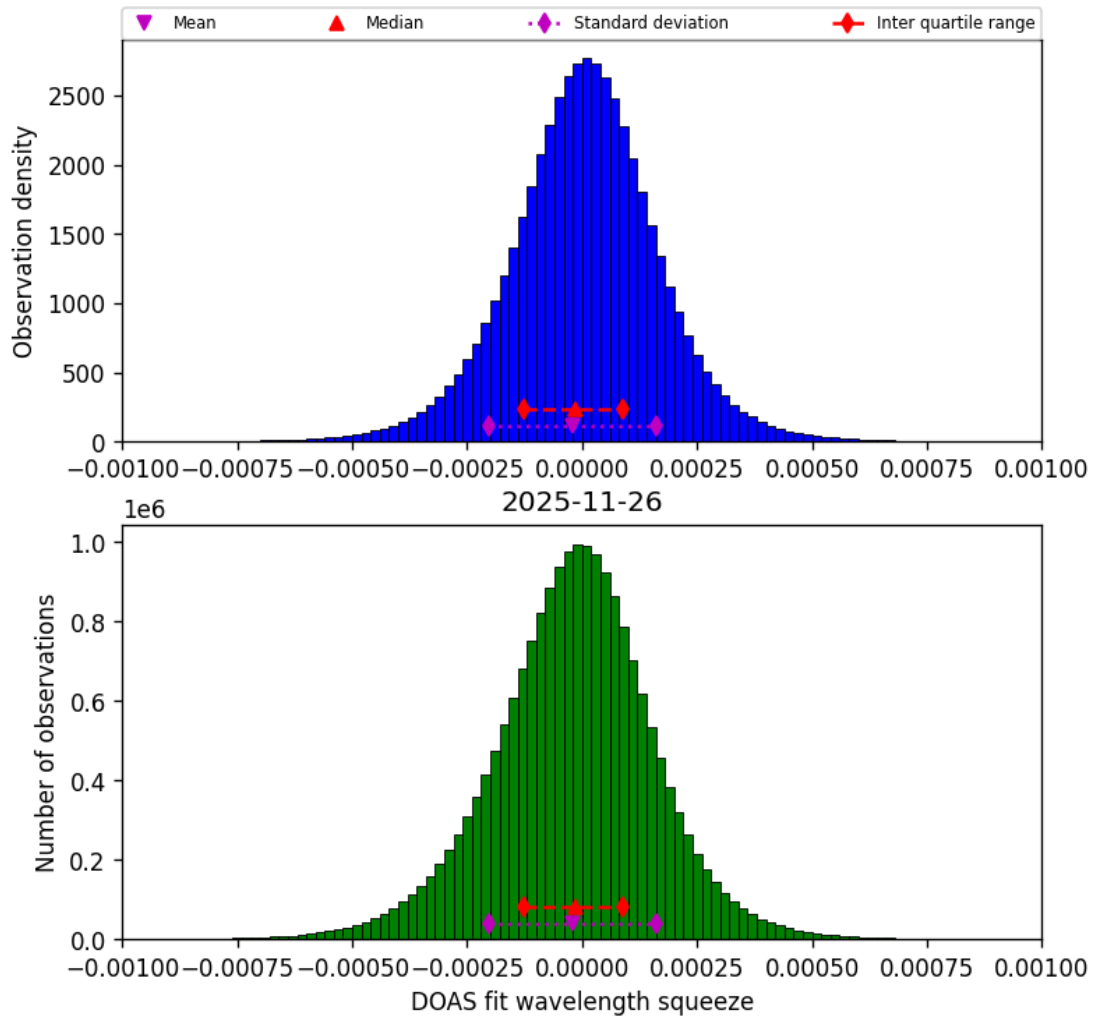
Figure 77: Histogram of “DOAS fit wavelength squeeze” for 2025-11-25 to 2025-11-27
