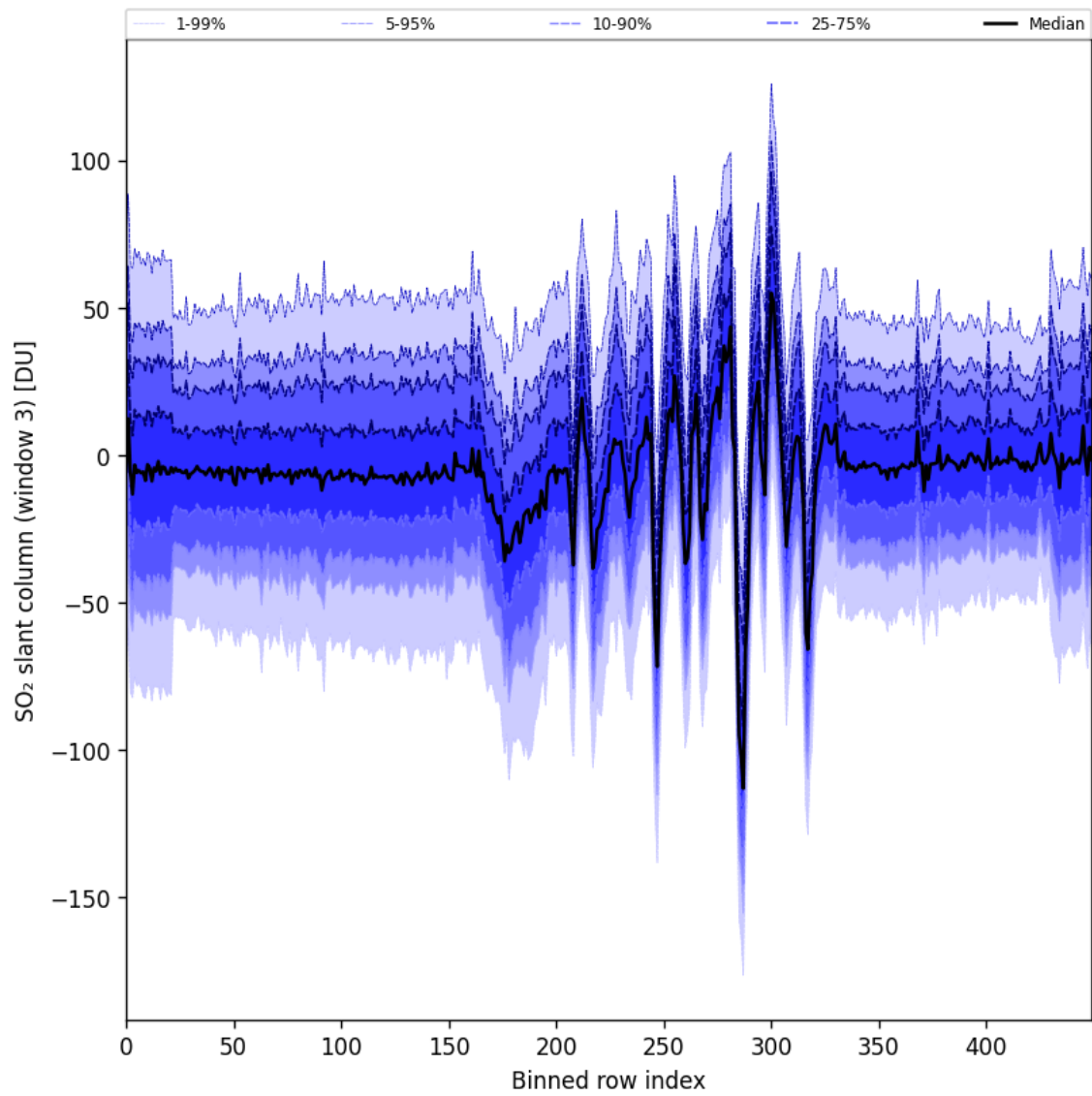
Figure 97: Along track statistics of “SO 2 slant column (window 3)” for 2025-11-25 to 2025-11-27
