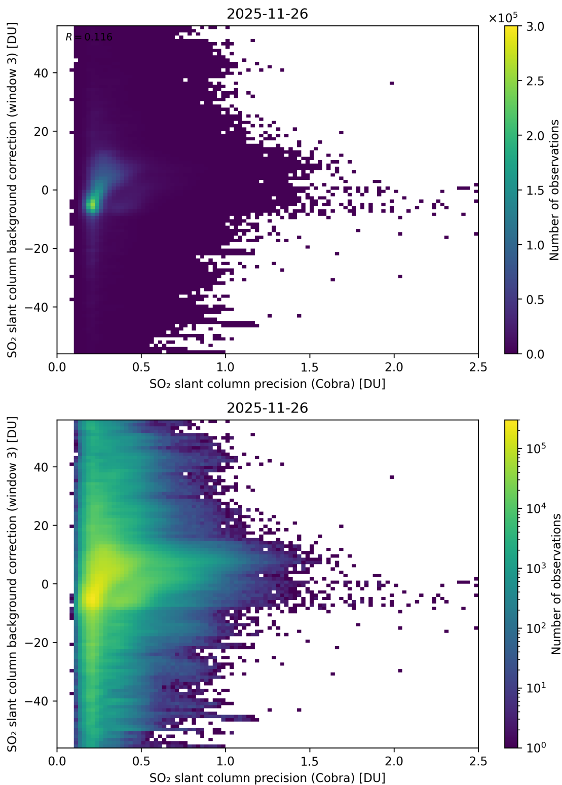
Figure 201: Scatter density plot of “SO 2 slant column precision (Cobra)” against “SO 2 slant column background correction (window 3)” for 2025-11-25 to 2025-11-27.
