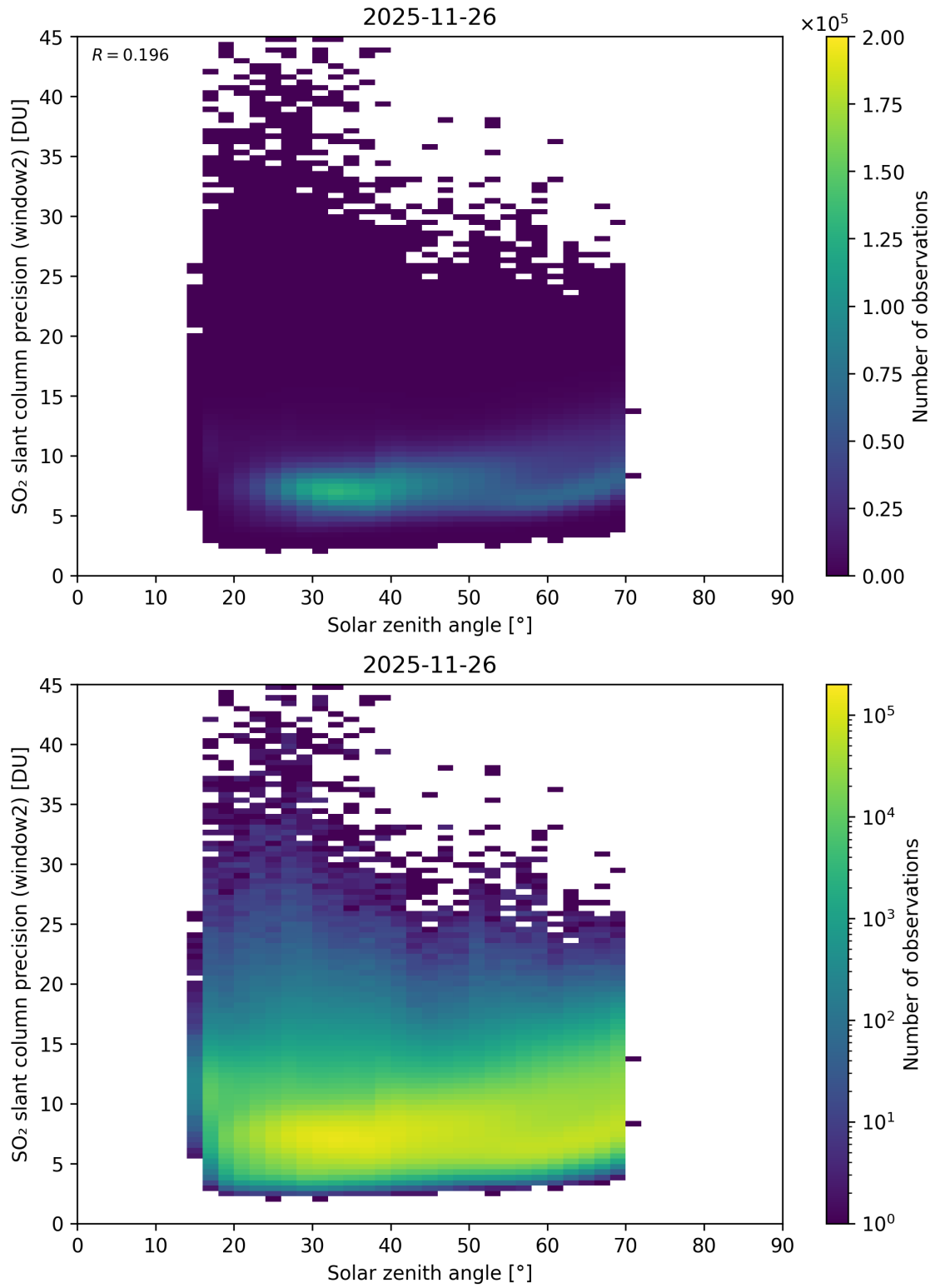
Figure 186: Scatter density plot of “Solar zenith angle” against “SO 2 slant column precision (window2)” for 2025-11-25 to 2025-11-27.
