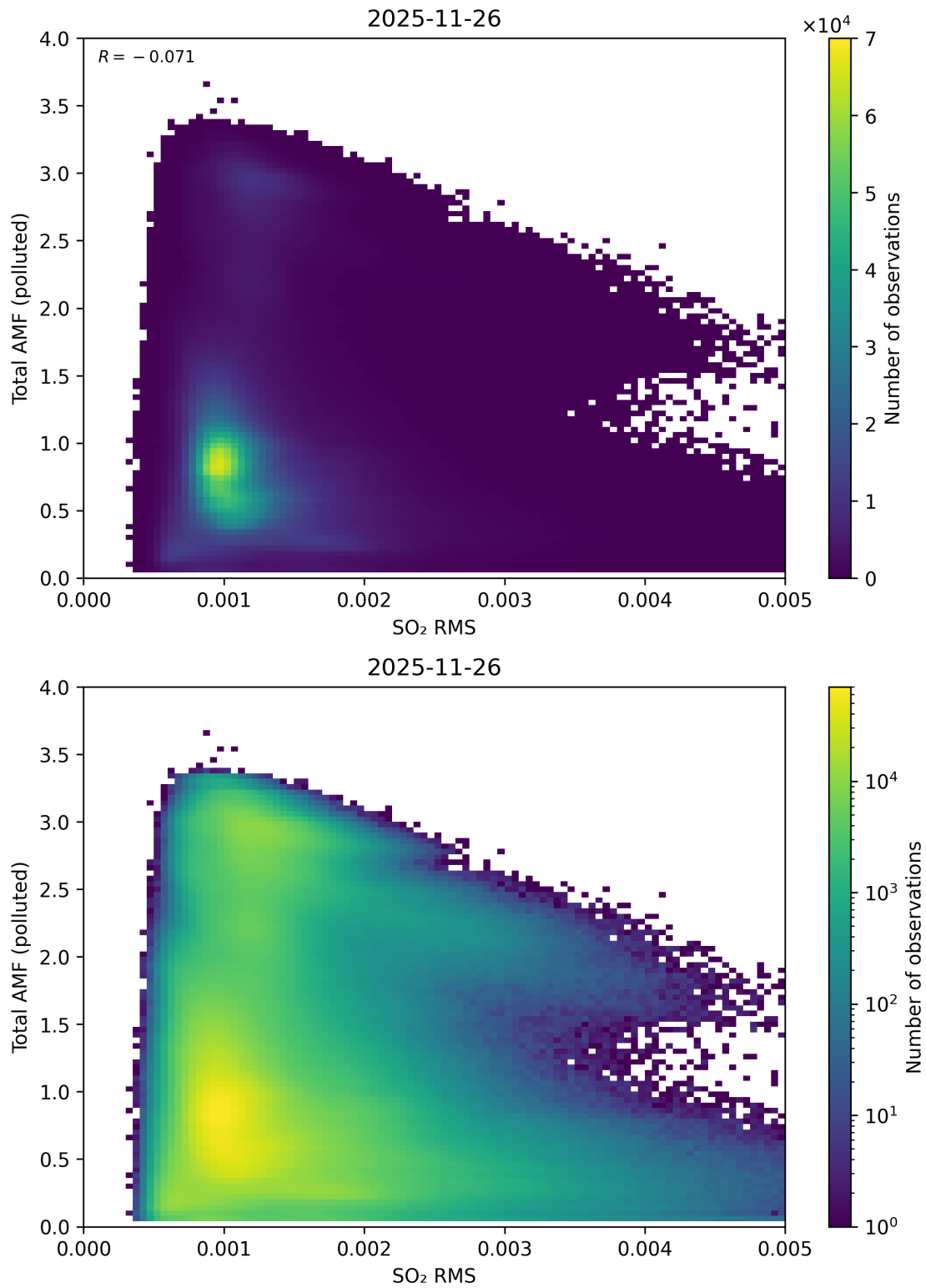
Figure 148: Scatter density plot of “SO 2 RMS” against “Total AMF (polluted)” for 2025-11-25 to 2025-11-27.
