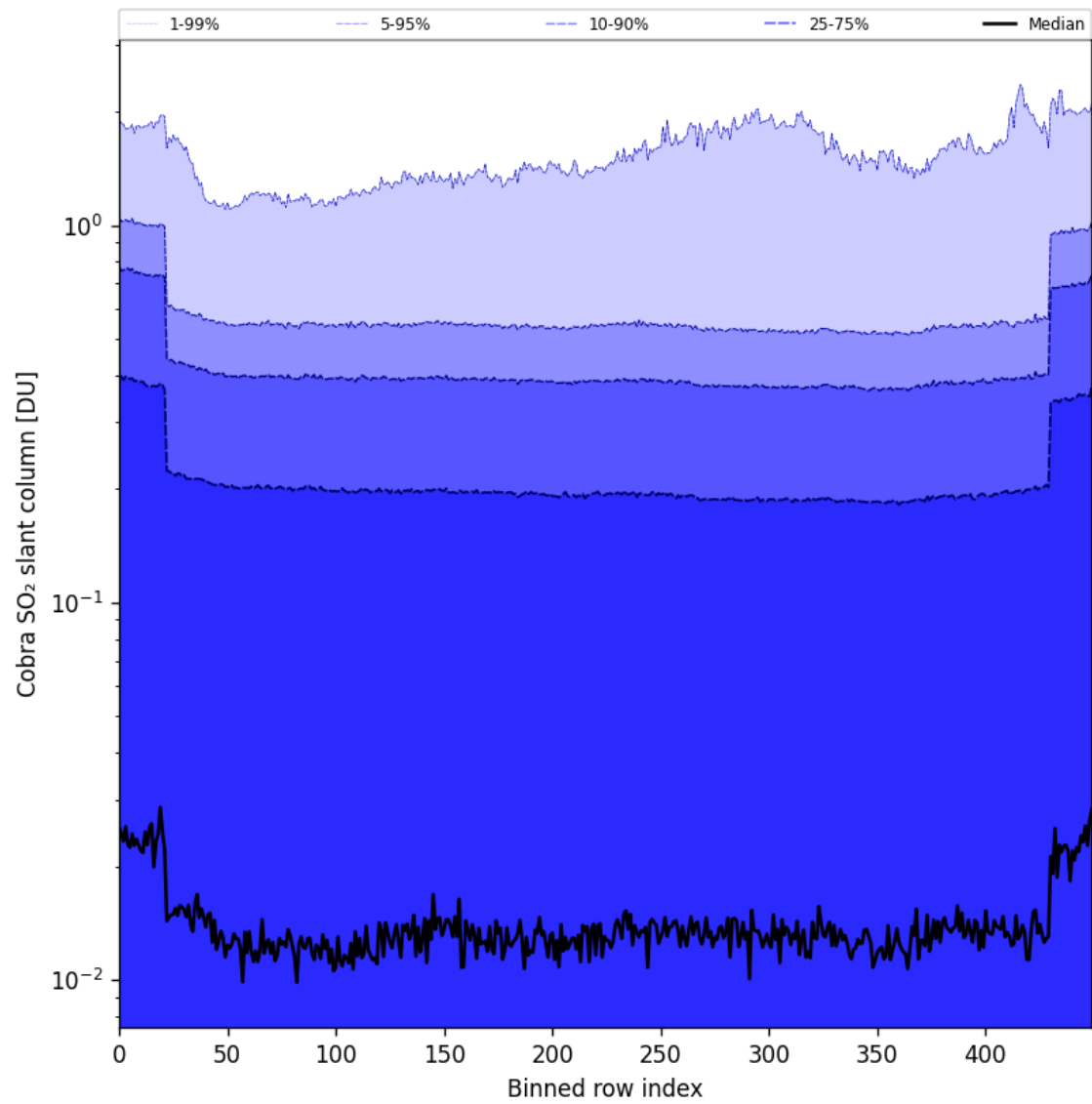
Figure 87: Along track statistics of "Cobra SO 2 slant column" for 2025-11-25 to 2025-11-27
