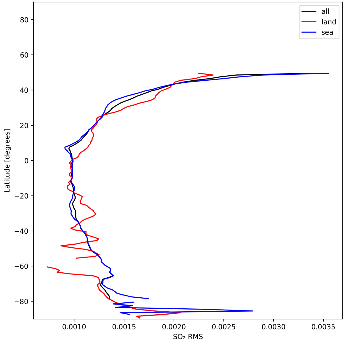
Figure 52: Zonal average of “SO 2 RMS” for 2025-11-25 to 2025-11-27.
