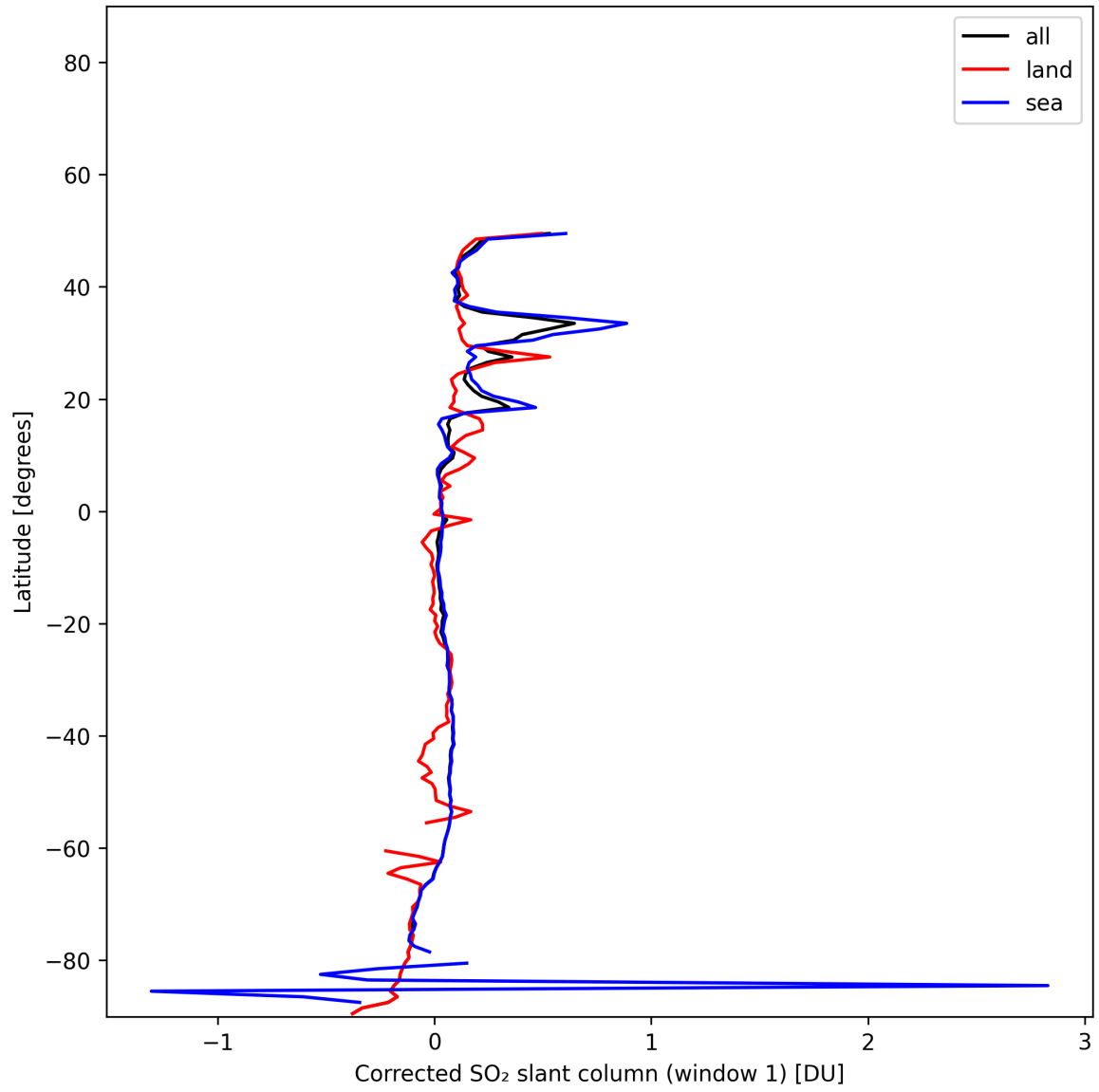
Figure 39: Zonal average of “Corrected SO 2 slant column (window 1)” for 2025-11-25 to 2025-11-27.
