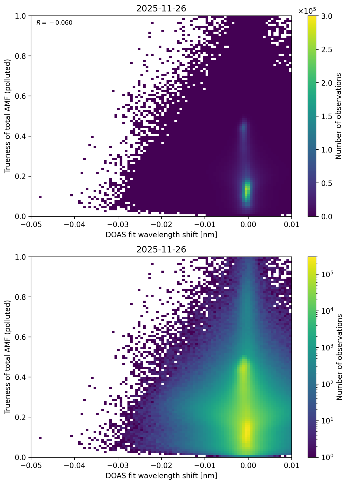
Figure 142: Scatter density plot of “DOAS fit wavelength shift” against “Trueness of total AMF (polluted)” for 2025-11-25 to 2025-11-27.
