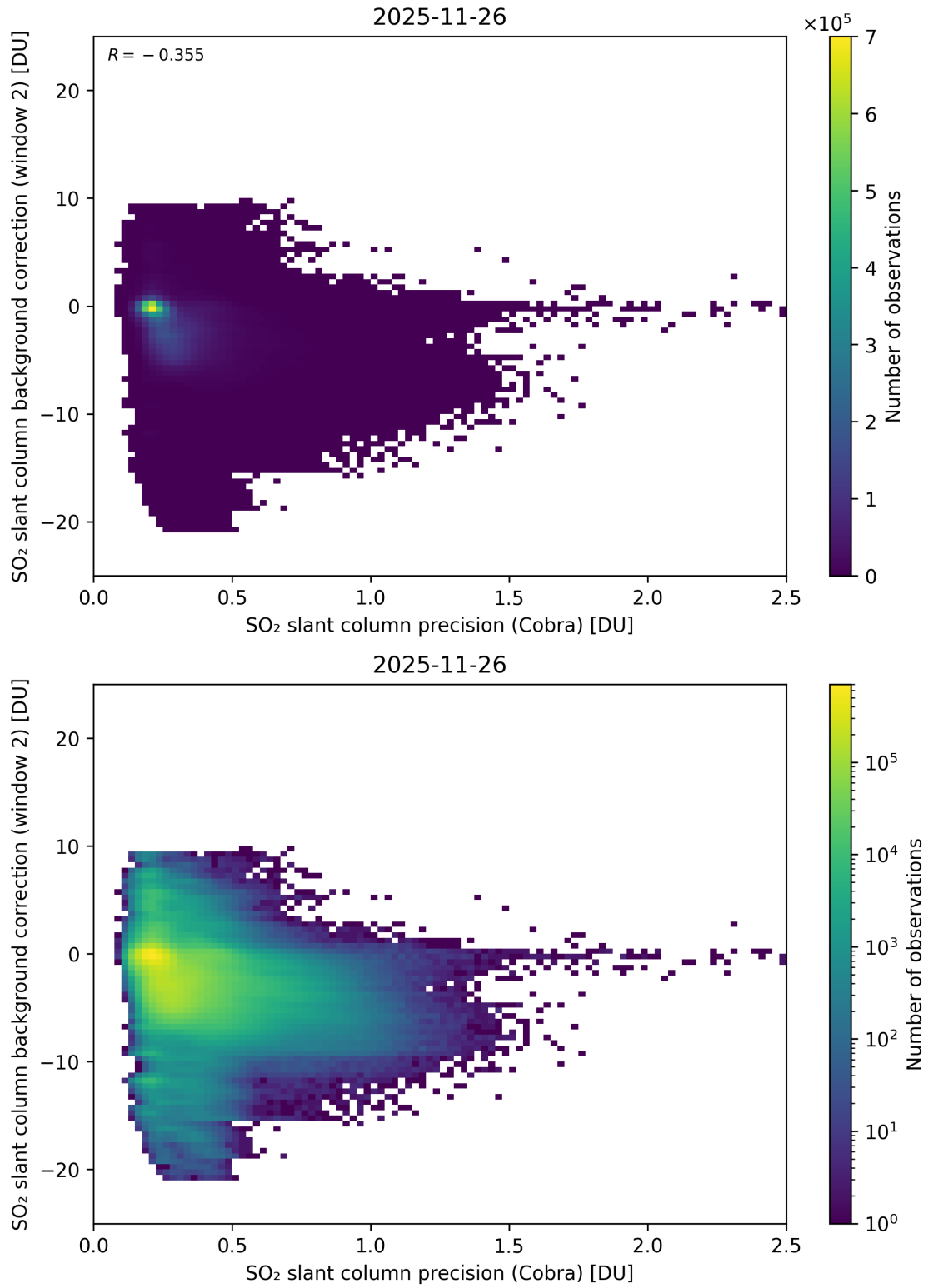
Figure 200: Scatter density plot of “SO 2 slant column precision (Cobra)” against “SO 2 slant column background correction (window 2)” for 2025-11-25 to 2025-11-27.
