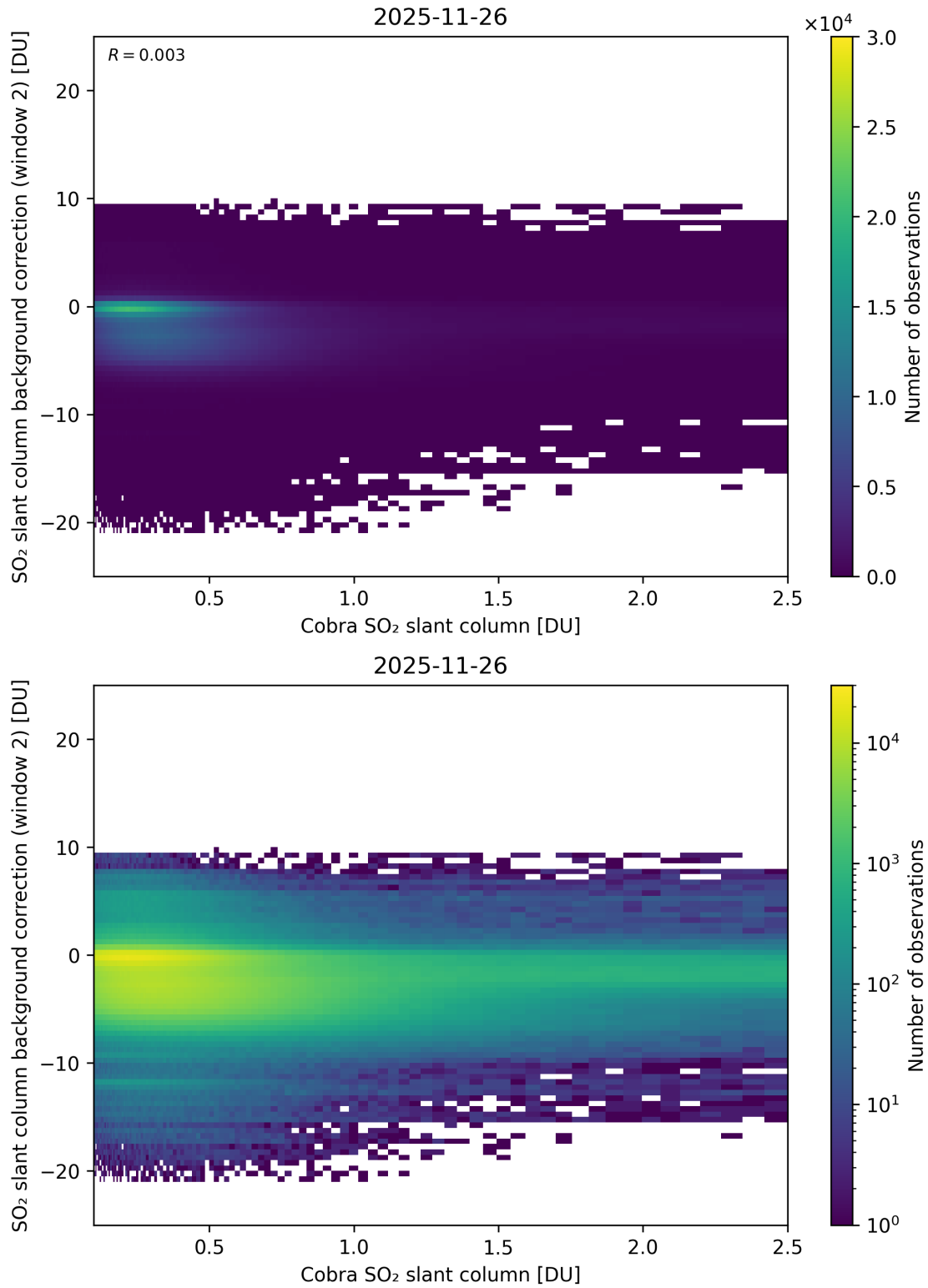
Figure 194: Scatter density plot of “Cobra SO 2 slant column” against “SO 2 slant column background correction (window 2)” for 2025-11-25 to 2025-11-27.
