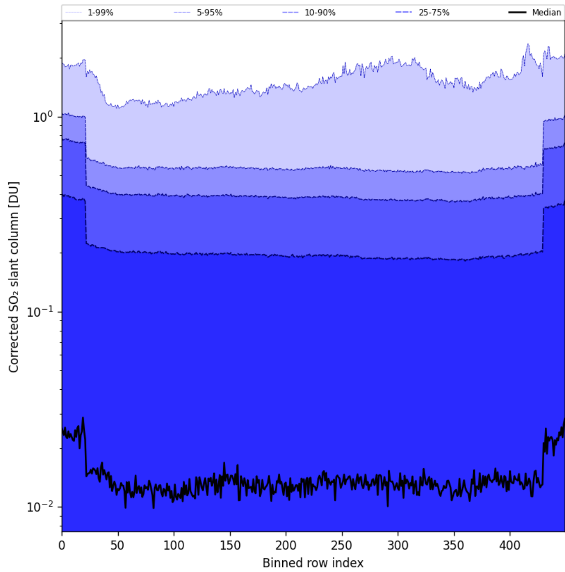
Figure 86: Along track statistics of “Corrected SO 2 slant column” for 2025-11-25 to 2025-11-27
