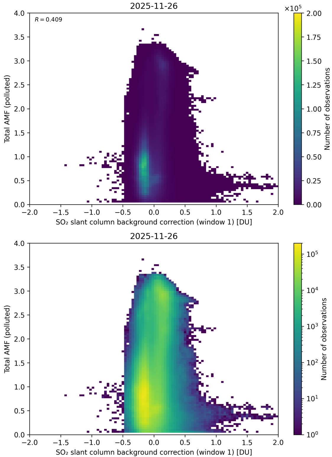
Figure 120: Scatter density plot of “SO 2 slant column background correction (window 1)” against “Total AMF (polluted)” for 2025-11-25 to 2025-11-27.
