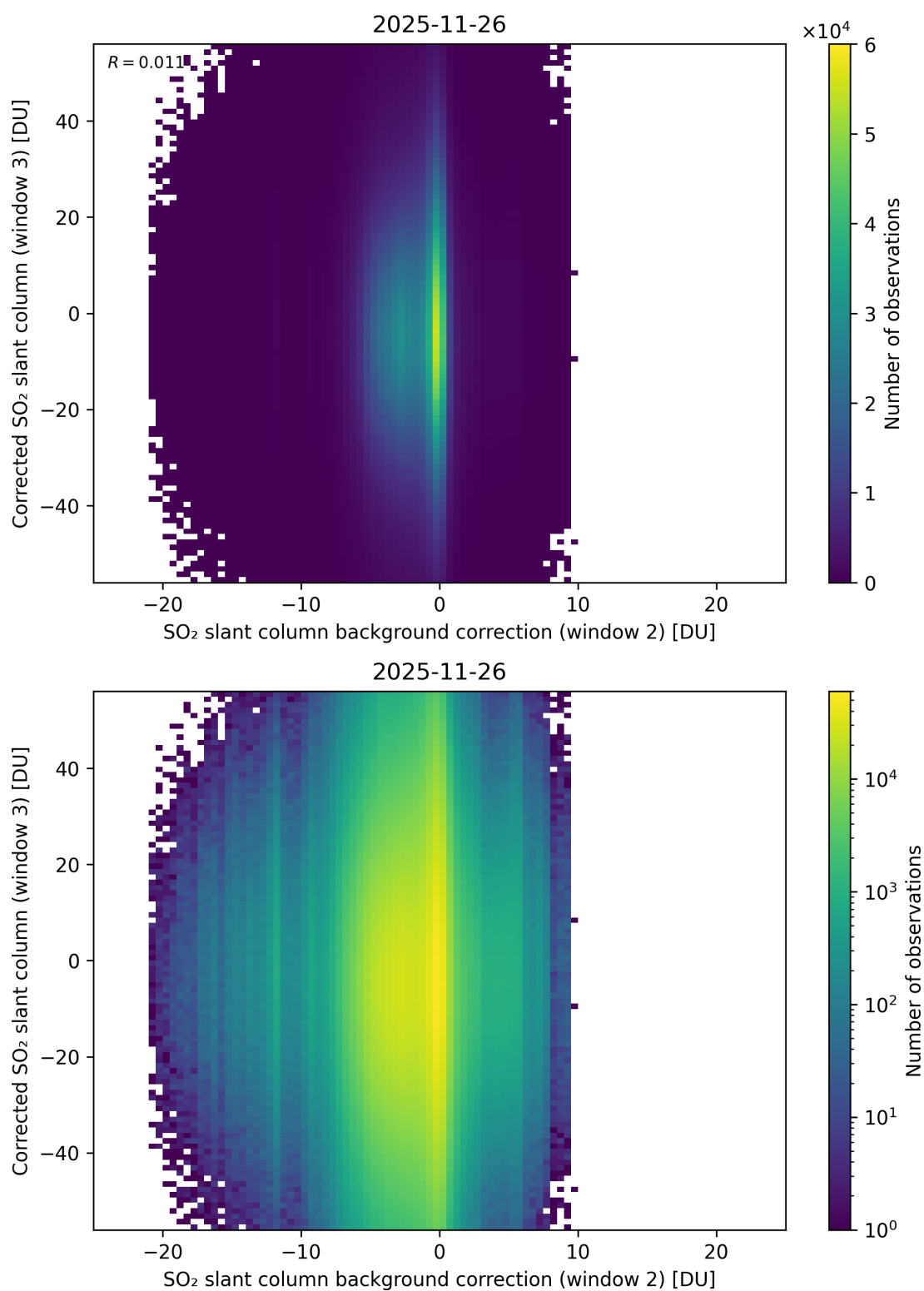
Figure 127: Scatter density plot of “SO 2 slant column background correction (window 2)” against “Corrected SO 2 slant column (window 3)” for 2025-11-25 to 2025-11-27.
