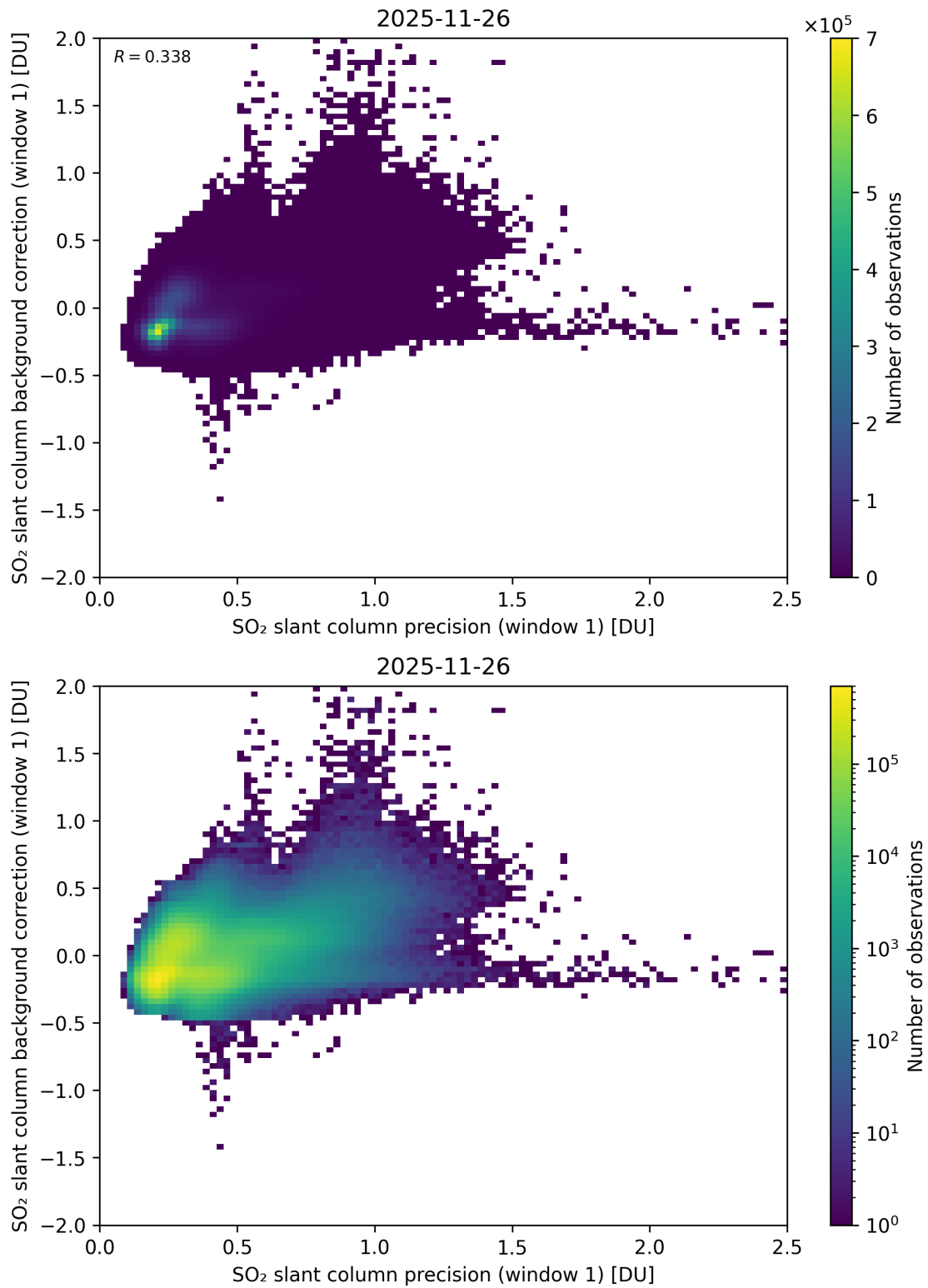
Figure 268: Scatter density plot of “SO 2 slant column precision (window 1)” against “SO 2 slant column background correction (window 1)” for 2025-11-25 to 2025-11-27.
