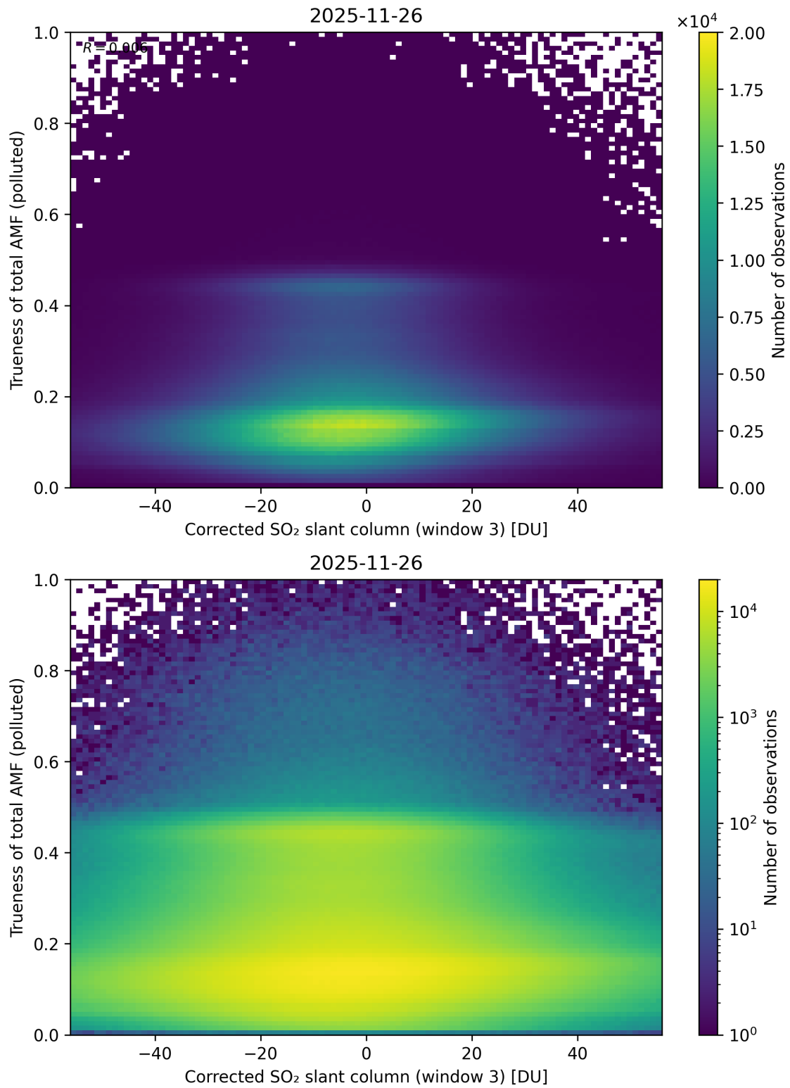
Figure 261: Scatter density plot of “Corrected SO 2 slant column (window 3)” against “Trueness of total AMF (polluted)” for 2025-11-25 to 2025-11-27.
