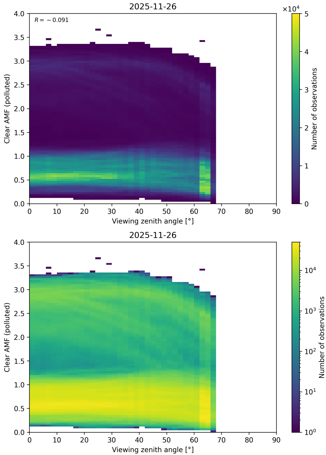
Figure 370: Scatter density plot of “Viewing zenith angle” against “Clear AMF (polluted)” for 2025-11-25 to 2025-11-27.
