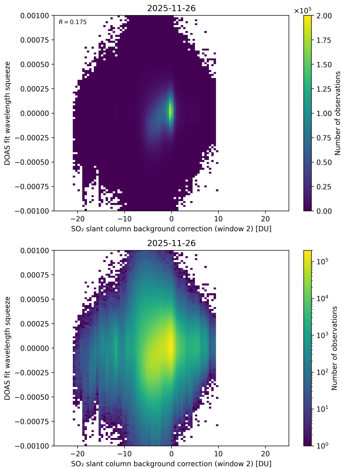
Figure 124: Scatter density plot of “SO 2 slant column background correction (window 2)” against “DOAS fit wavelength squeeze” for 2025-11-25 to 2025-11-27.
