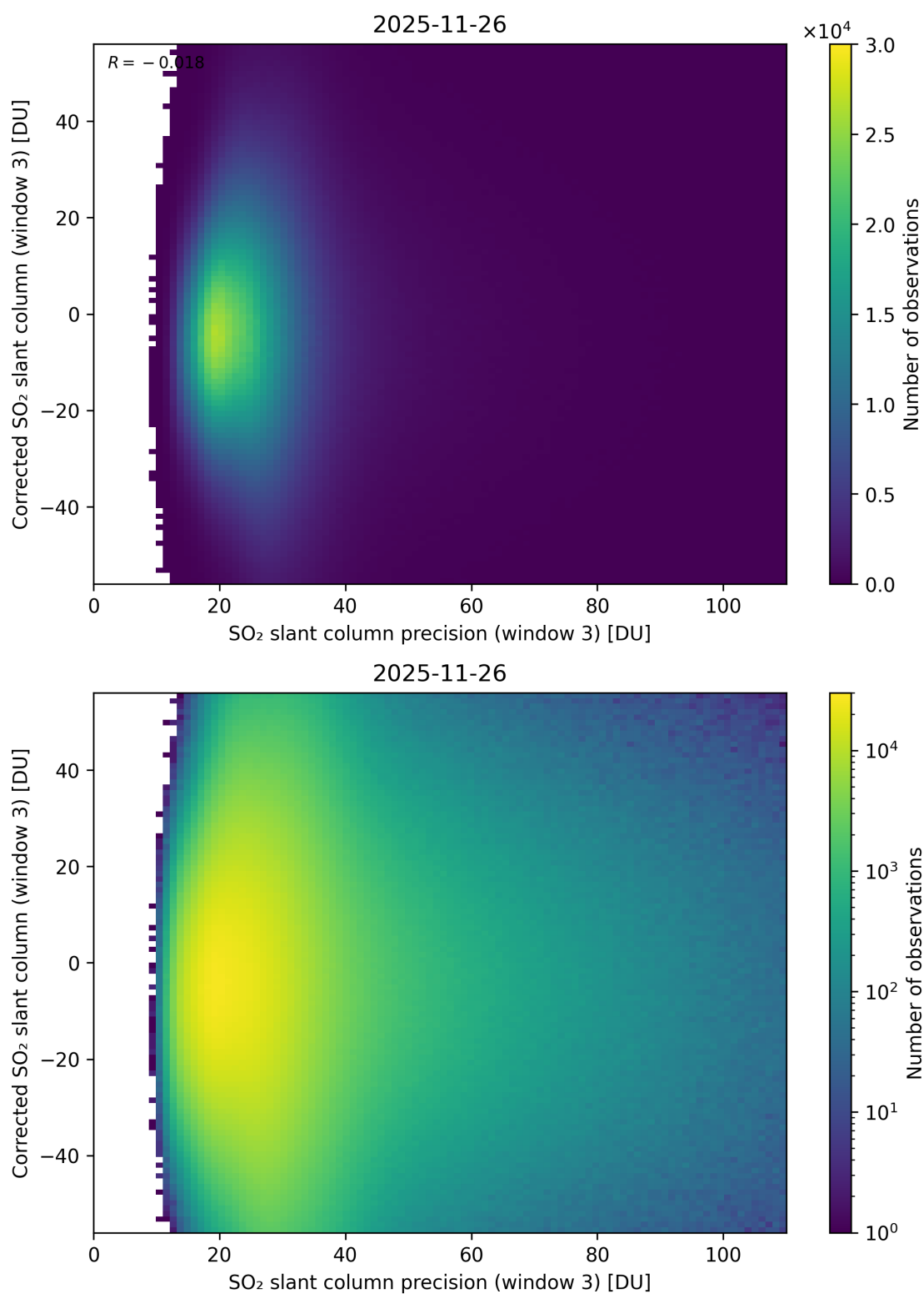
Figure 312: Scatter density plot of “SO 2 slant column precision (window 3)” against “Corrected SO 2 slant column (window 3)” for 2025-11-25 to 2025-11-27.
