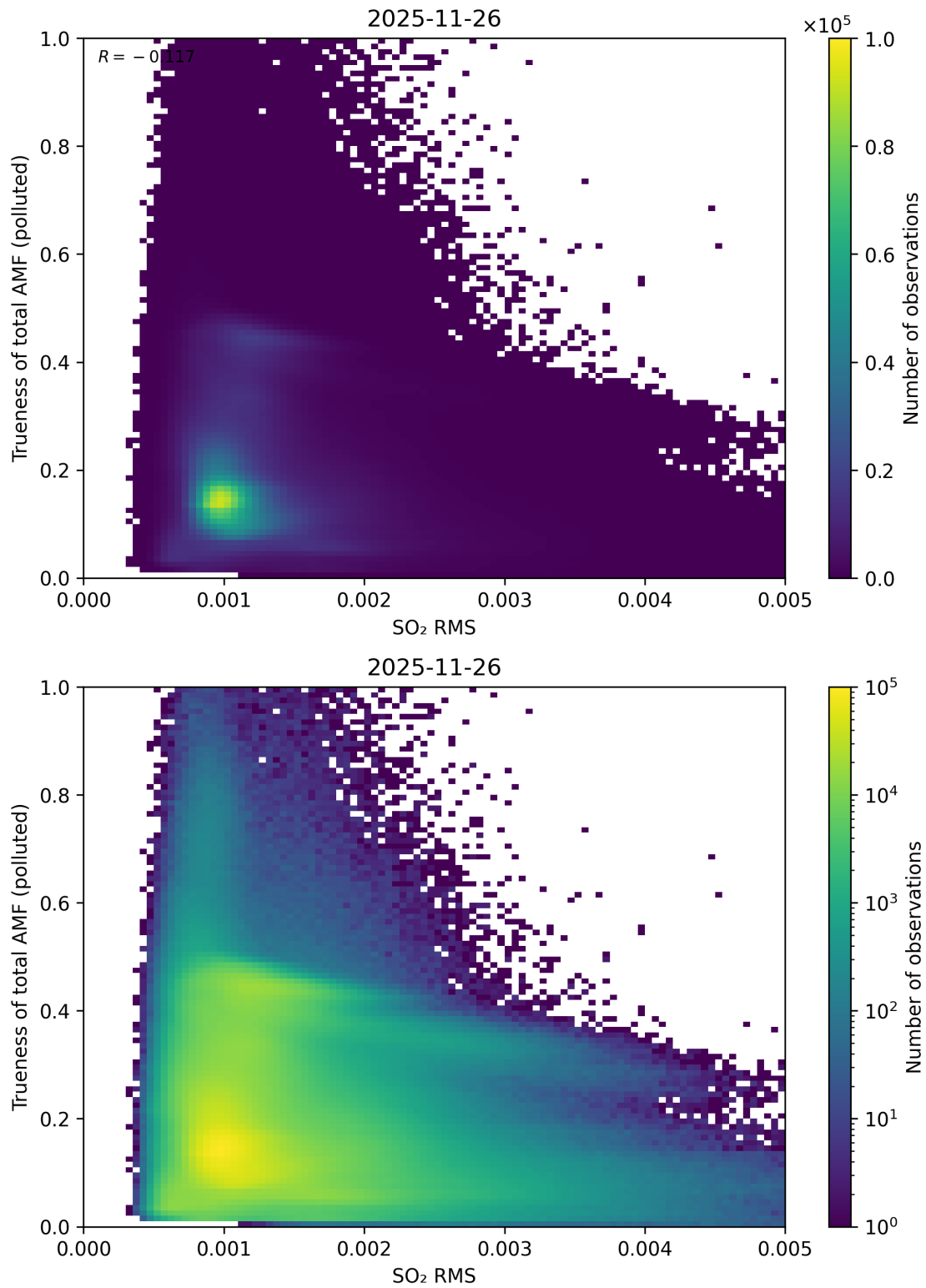
Figure 149: Scatter density plot of “SO 2 RMS” against “Trueness of total AMF (polluted)” for 2025-11-25 to 2025-11-27.
