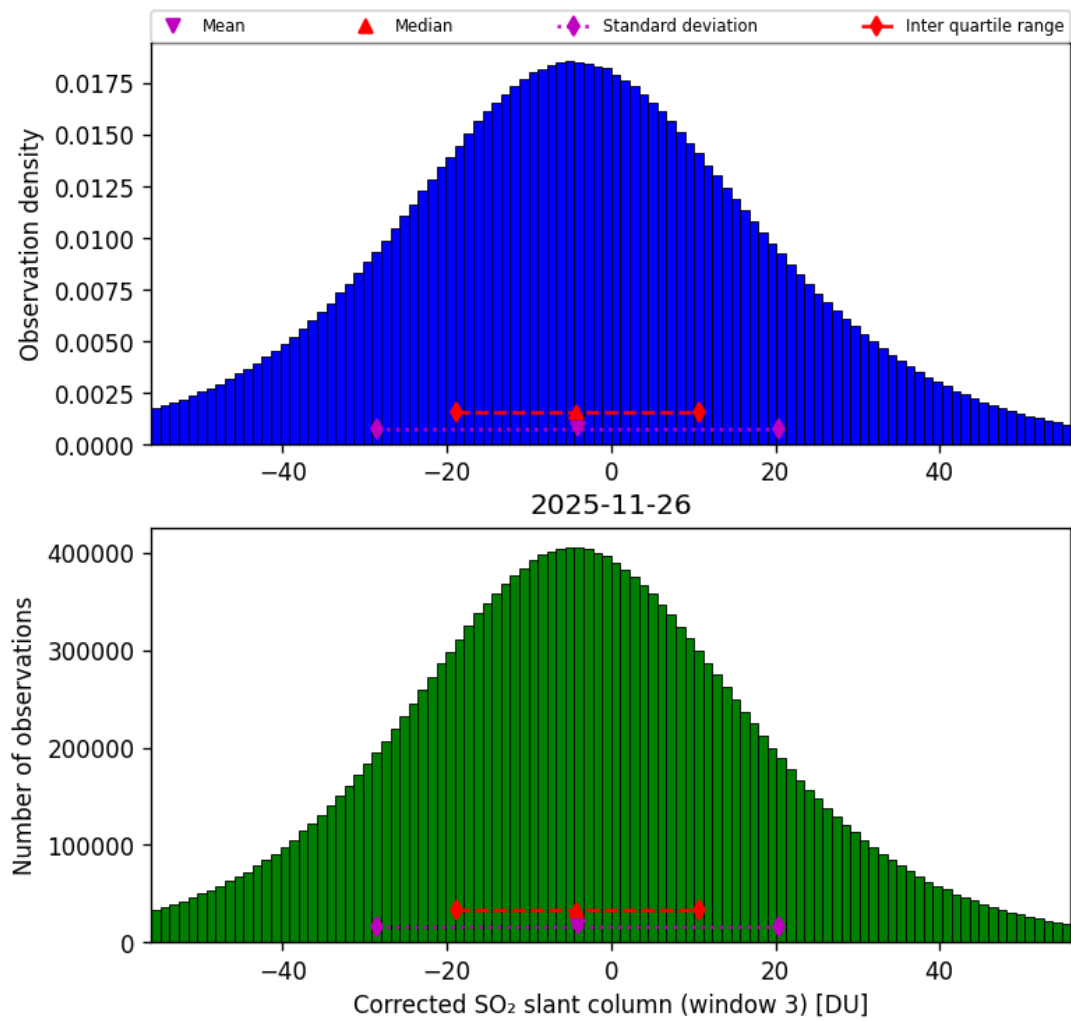
Figure 73: Histogram of “Corrected SO 2 slant column (window 3)” for 2025-11-25 to 2025-11-27
