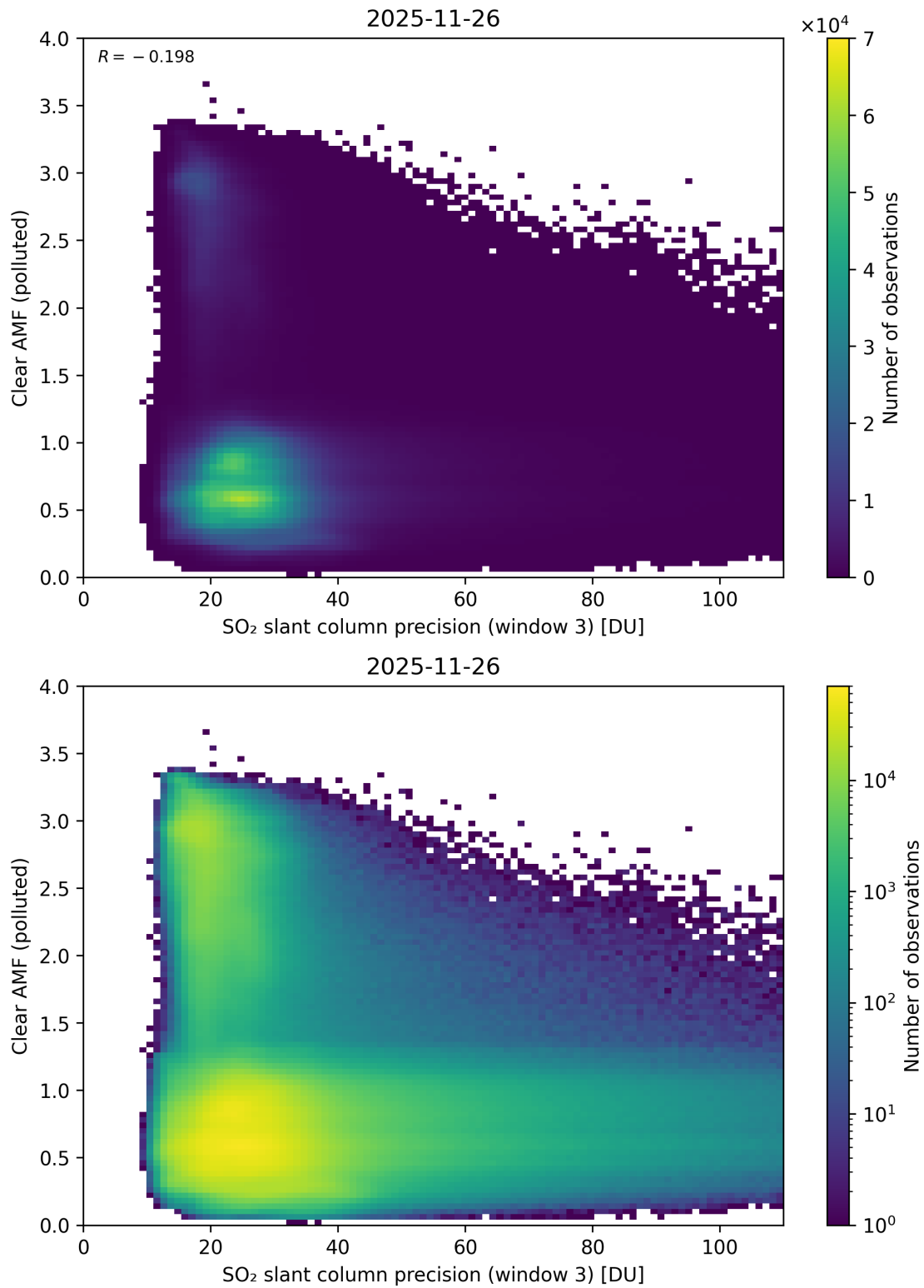
Figure 311: Scatter density plot of “SO 2 slant column precision (window 3)” against “Clear AMF (polluted)” for 2025-11-25 to 2025-11-27.
