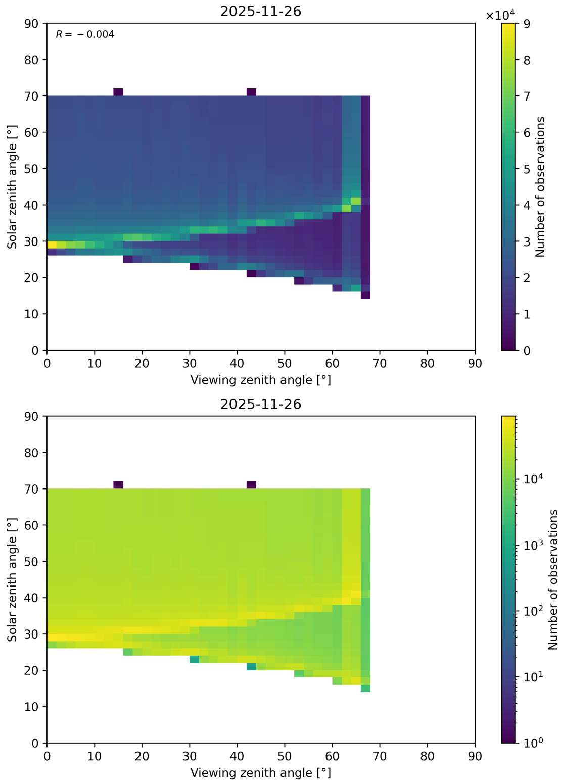
Figure 369: Scatter density plot of “Viewing zenith angle” against “Solar zenith angle” for 2025-11-25 to 2025-11-27.
