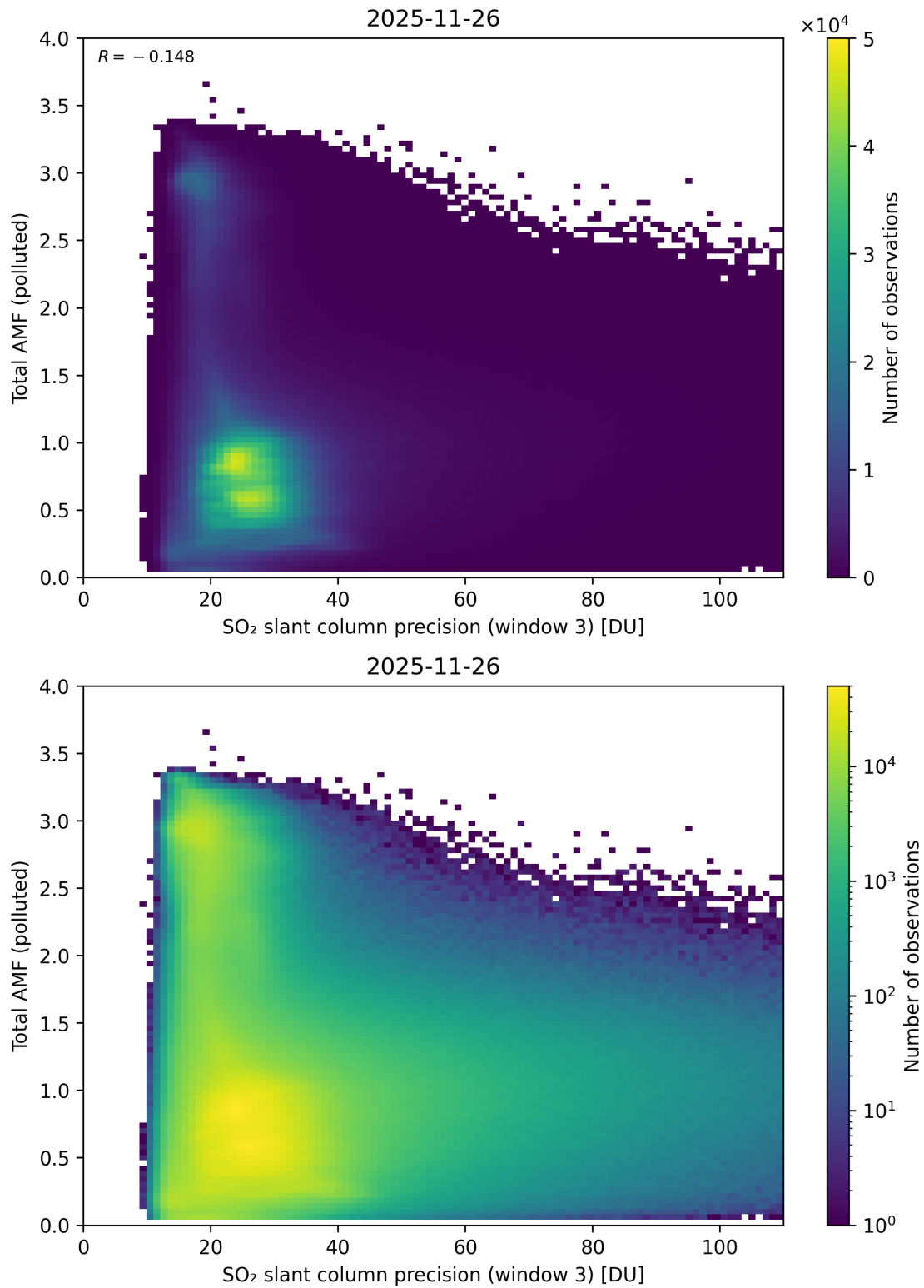
Figure 313: Scatter density plot of “SO 2 slant column precision (window 3)” against “Total AMF (polluted)” for 2025-11-25 to 2025-11-27.
