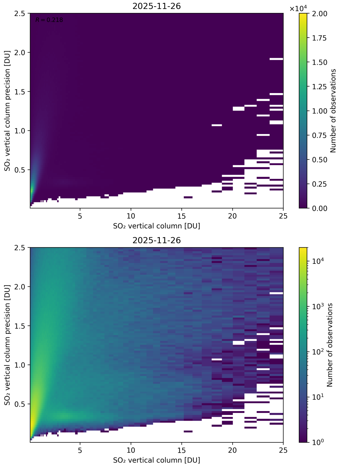
Figure 361: Scatter density plot of “SO 2 vertical column” against “SO 2 vertical column precision” for 2025-11-25 to 2025-11-27.
