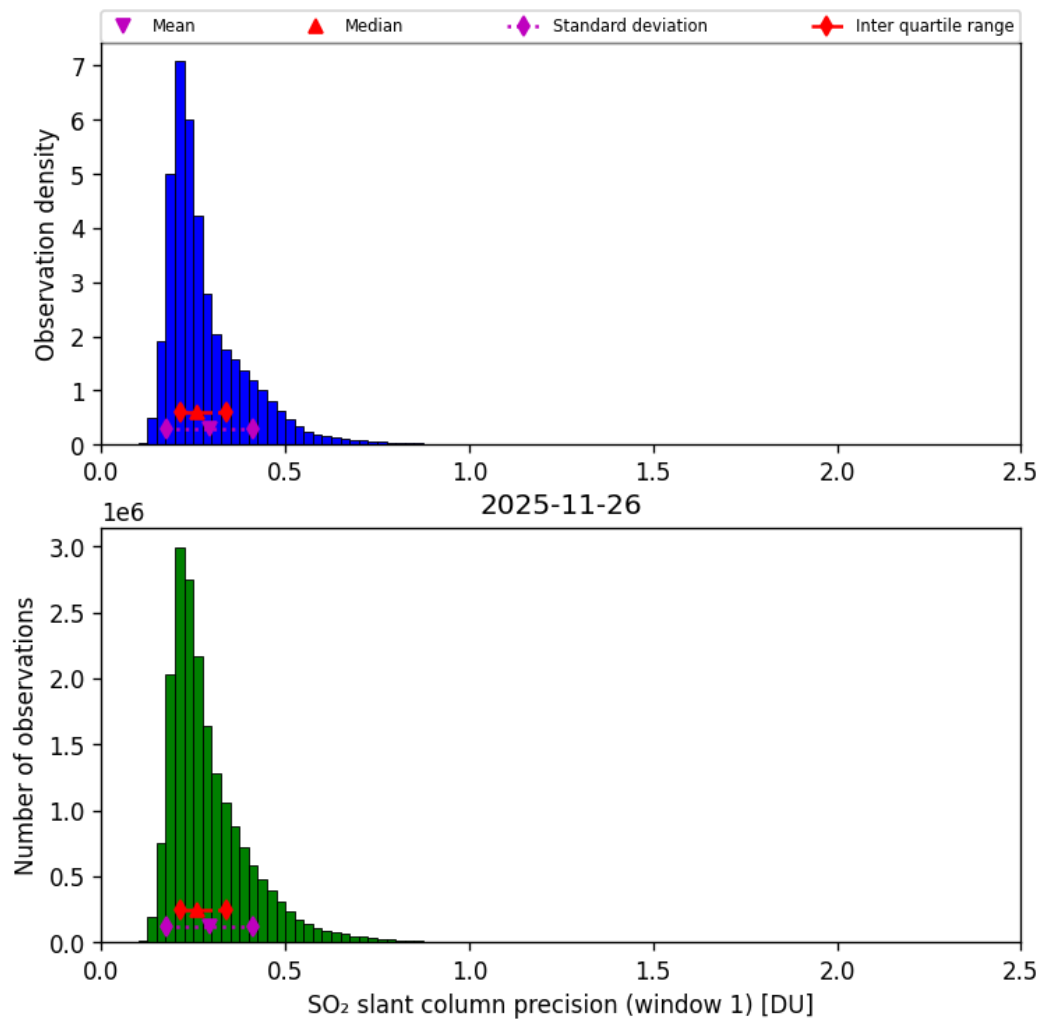
Figure 64: Histogram of “SO 2 slant column precision (window 1)” for 2025-11-25 to 2025-11-27
