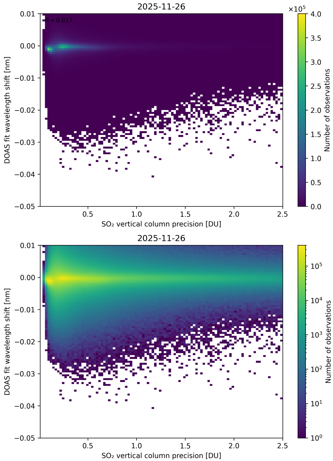
Figure 332: Scatter density plot of “SO 2 vertical column precision” against “DOAS fit wavelength shift” for 2025-11-25 to 2025-11-27.
