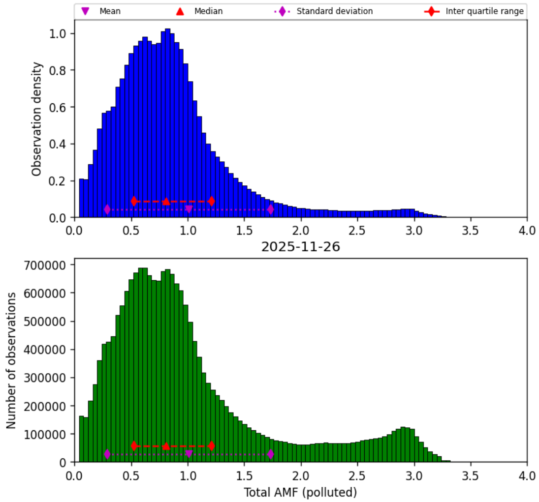
Figure 79: Histogram of “Total AMF (polluted)” for 2025-11-25 to 2025-11-27
