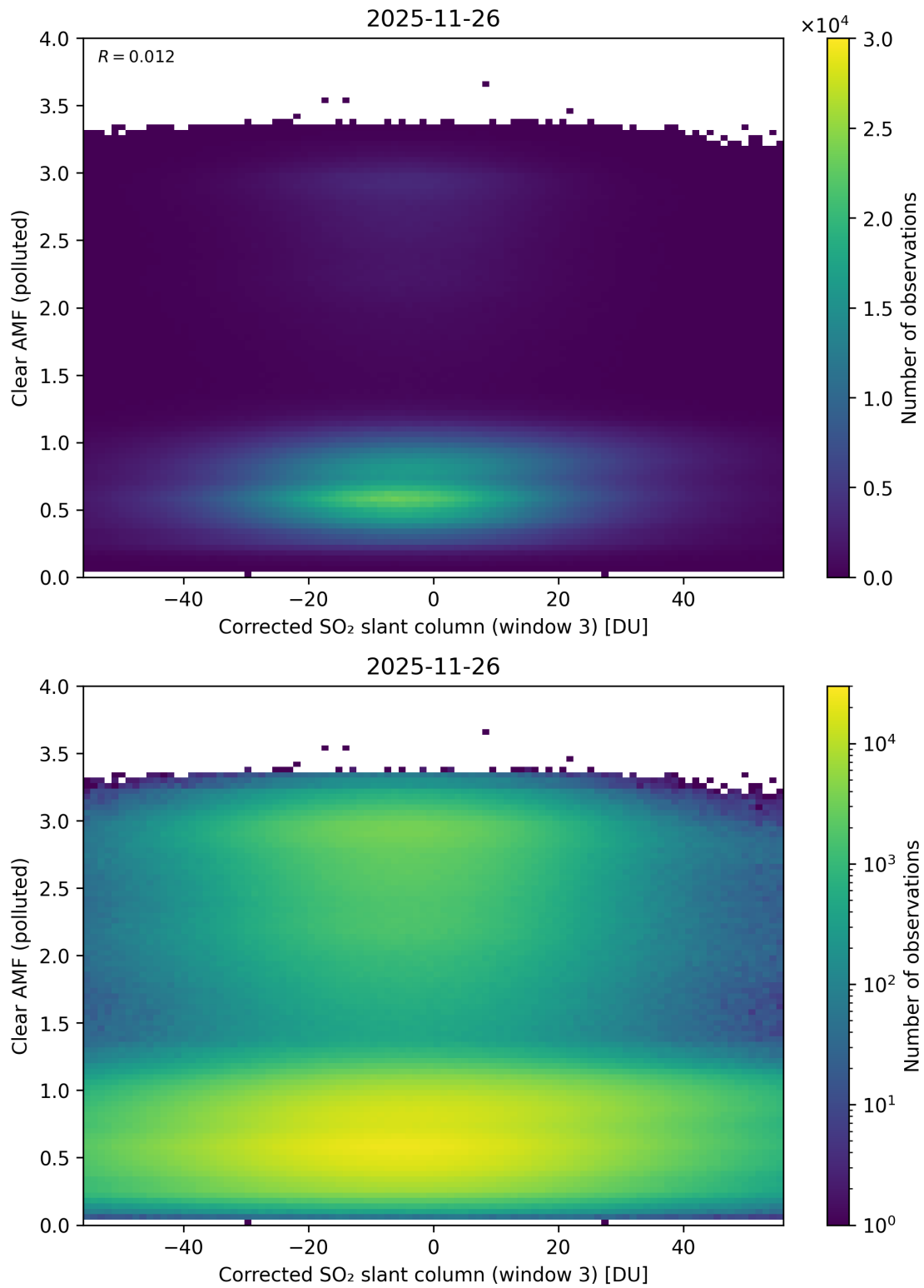
Figure 259: Scatter density plot of “Corrected SO 2 slant column (window 3)” against “Clear AMF (polluted)” for 2025-11-25 to 2025-11-27.
