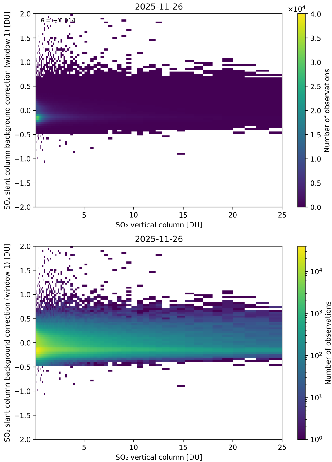
Figure 323: Scatter density plot of “SO 2 vertical column” against “SO 2 slant column background correction (window 1)” for 2025-11-25 to 2025-11-27.
