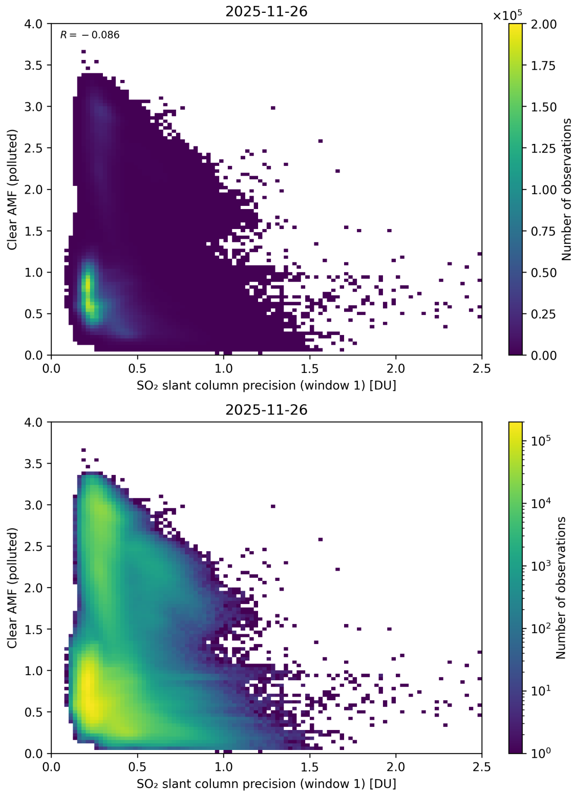
Figure 274: Scatter density plot of “SO 2 slant column precision (window 1)” against “Clear AMF (polluted)” for 2025-11-25 to 2025-11-27.
