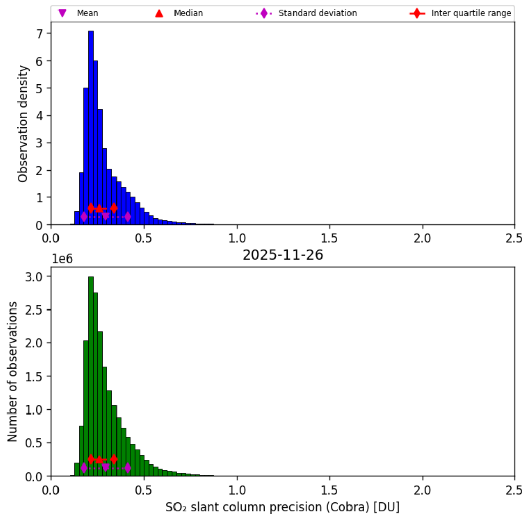
Figure 62: Histogram of “SO 2 slant column precision (Cobra)” for 2025-11-25 to 2025-11-27
