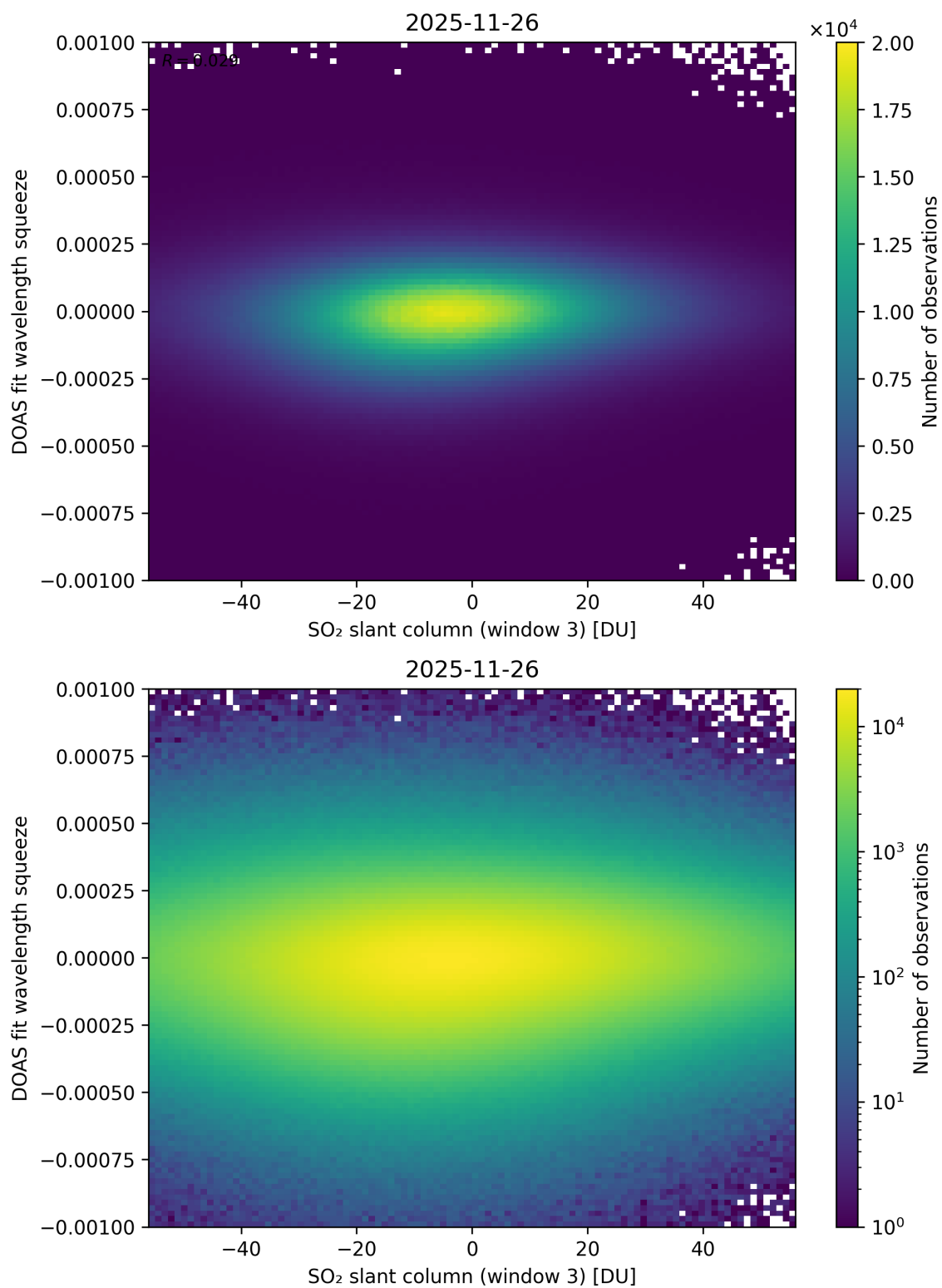
Figure 305: Scatter density plot of “SO 2 slant column (window 3)” against “DOAS fit wavelength squeeze” for 2025-11-25 to 2025-11-27.
