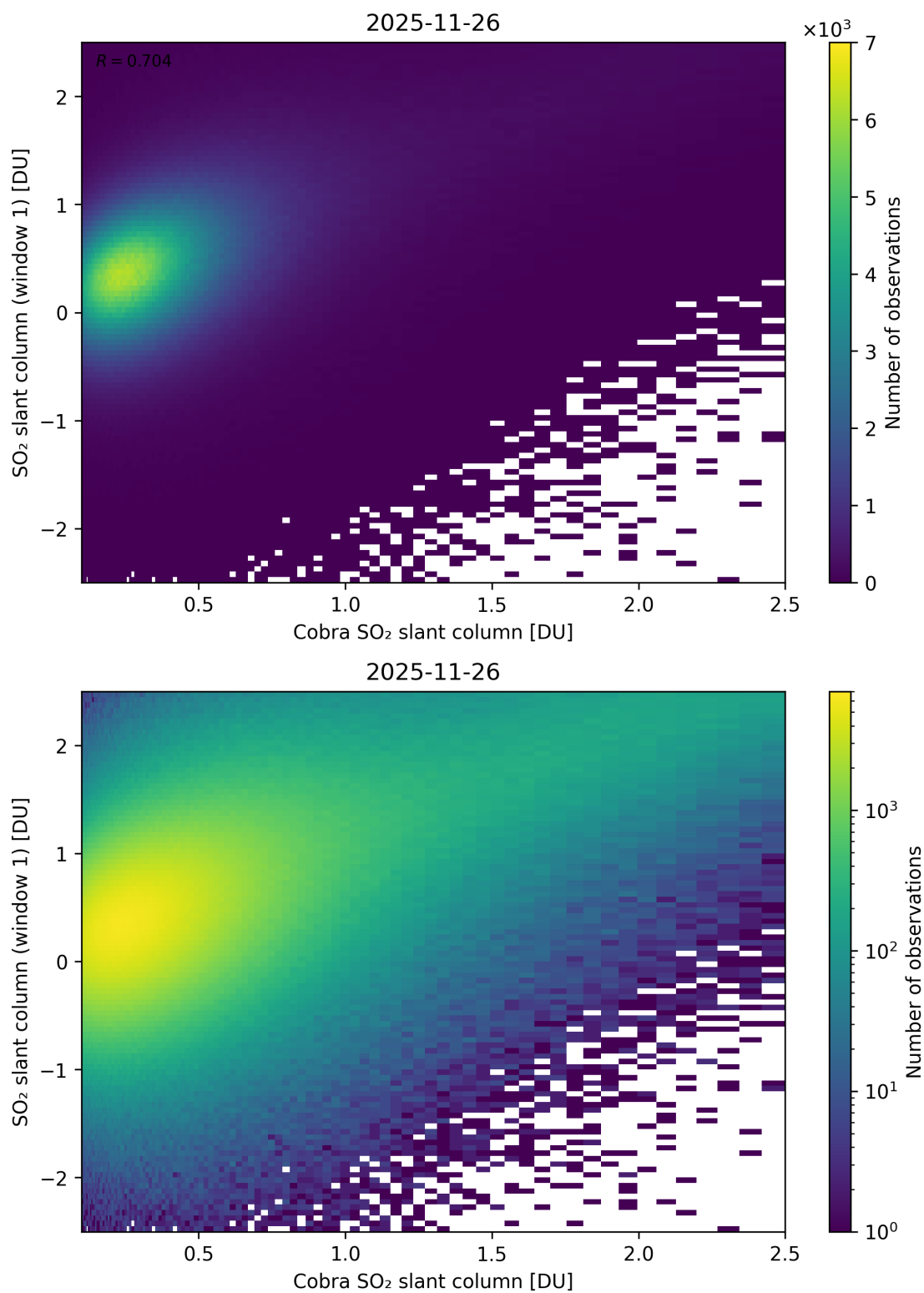
Figure 219: Scatter density plot of “Cobra SO 2 slant column” against “SO 2 slant column (window 1)” for 2025-11-25 to 2025-11-27.
