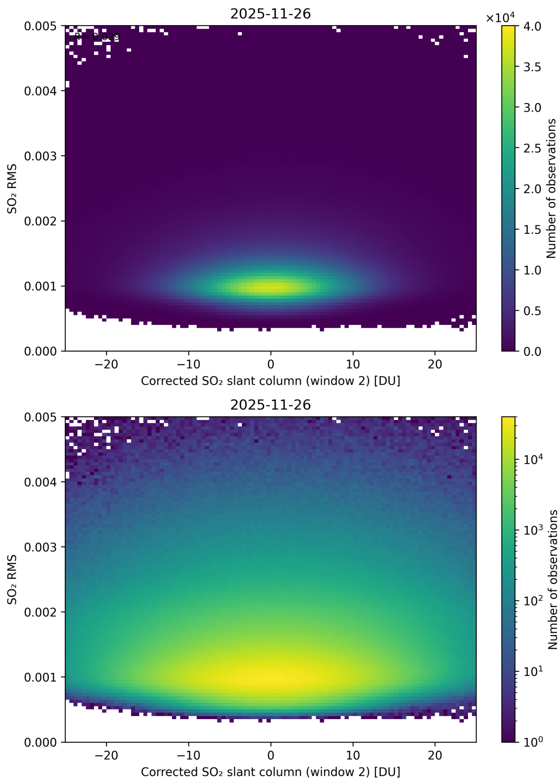
Figure 248: Scatter density plot of “Corrected SO 2 slant column (window 2)” against “SO 2 RMS” for 2025-11-25 to 2025-11-27.
