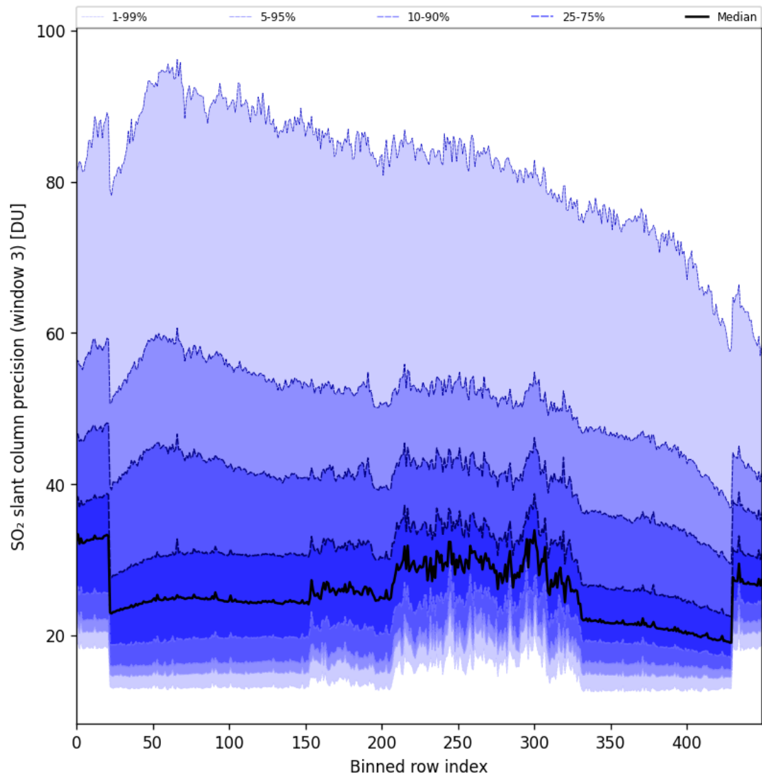
Figure 98: Along track statistics of “SO 2 slant column precision (window 3)” for 2025-11-25 to 2025-11-27
