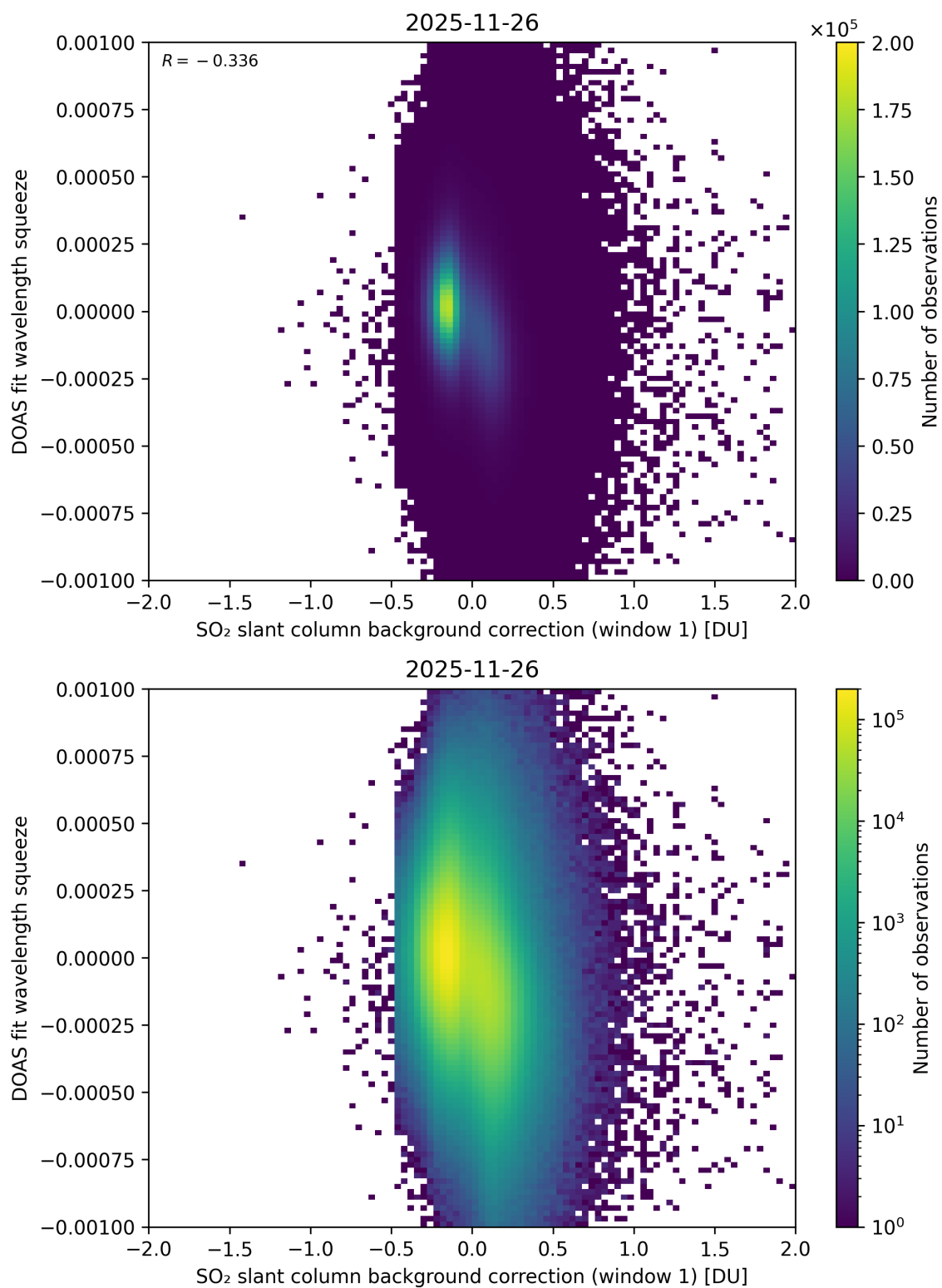
Figure 112: Scatter density plot of “SO 2 slant column background correction (window 1)” against “DOAS fit wavelength squeeze” for 2025-11-25 to 2025-11-27.
