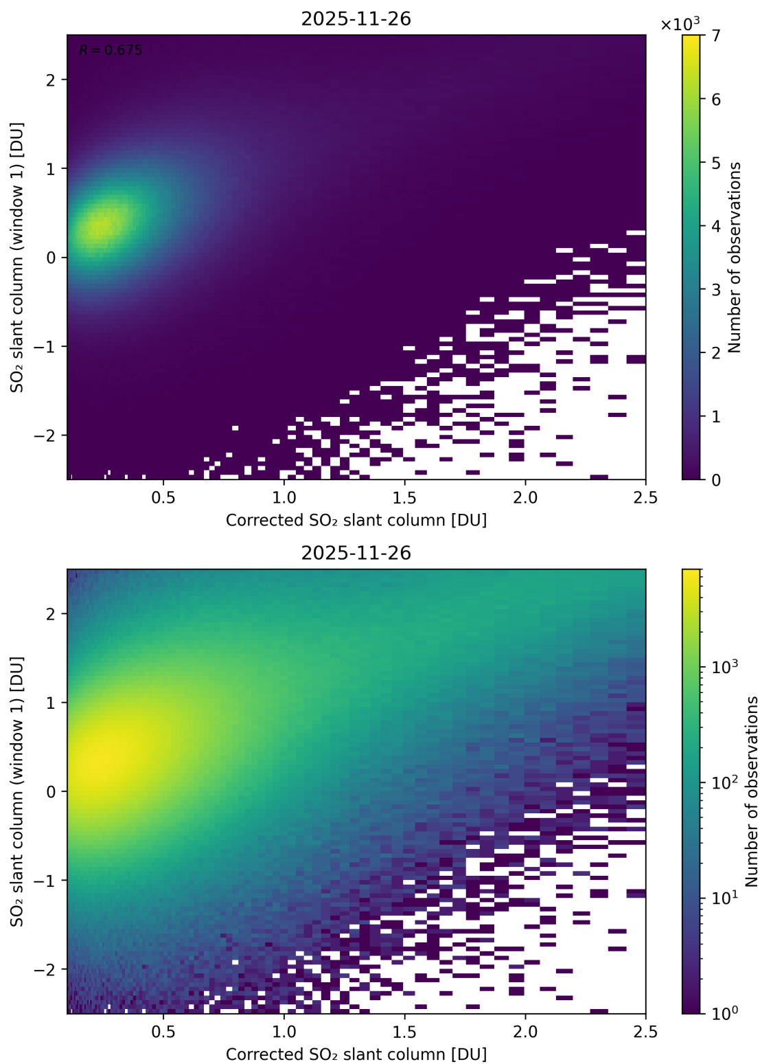
Figure 237: Scatter density plot of “Corrected SO 2 slant column” against “SO 2 slant column (window 1)” for 2025-11-25 to 2025-11-27.
