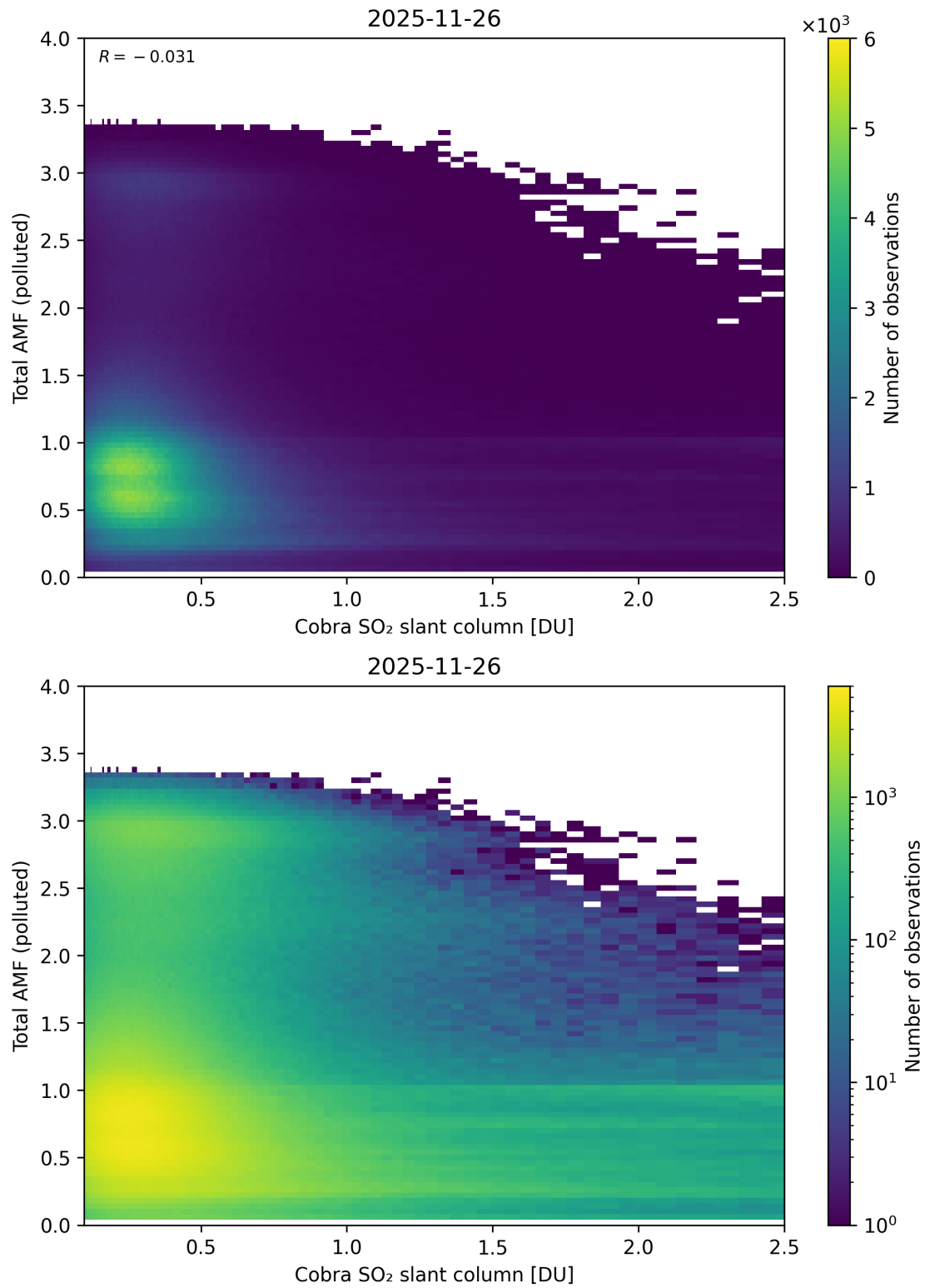
Figure 224: Scatter density plot of “Cobra SO 2 slant column” against “Total AMF (polluted)” for 2025-11-25 to 2025-11-27.
