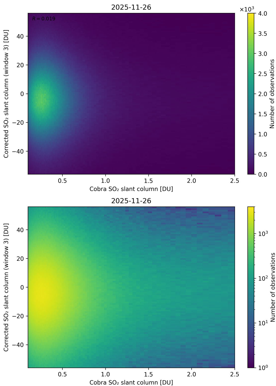
Figure 218: Scatter density plot of “Cobra SO 2 slant column” against “Corrected SO 2 slant column (window 3)” for 2025-11-25 to 2025-11-27.
