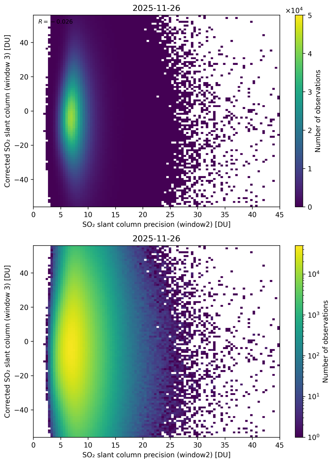
Figure 298: Scatter density plot of “SO 2 slant column precision (window2)” against “Corrected SO 2 slant column (window 3)” for 2025-11-25 to 2025-11-27.
