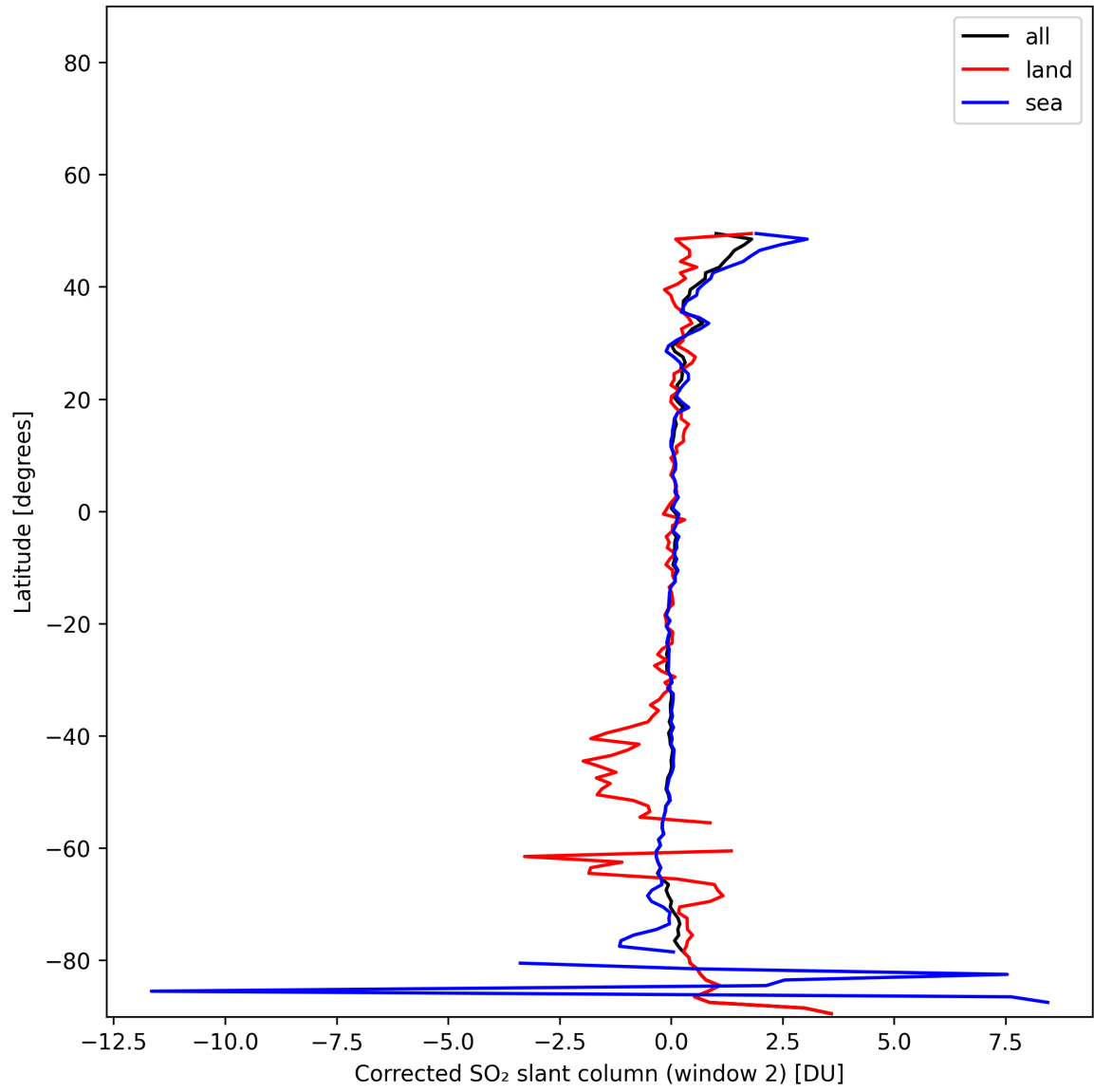
Figure 43: Zonal average of “Corrected SO 2 slant column (window 2)” for 2025-11-25 to 2025-11-27.
