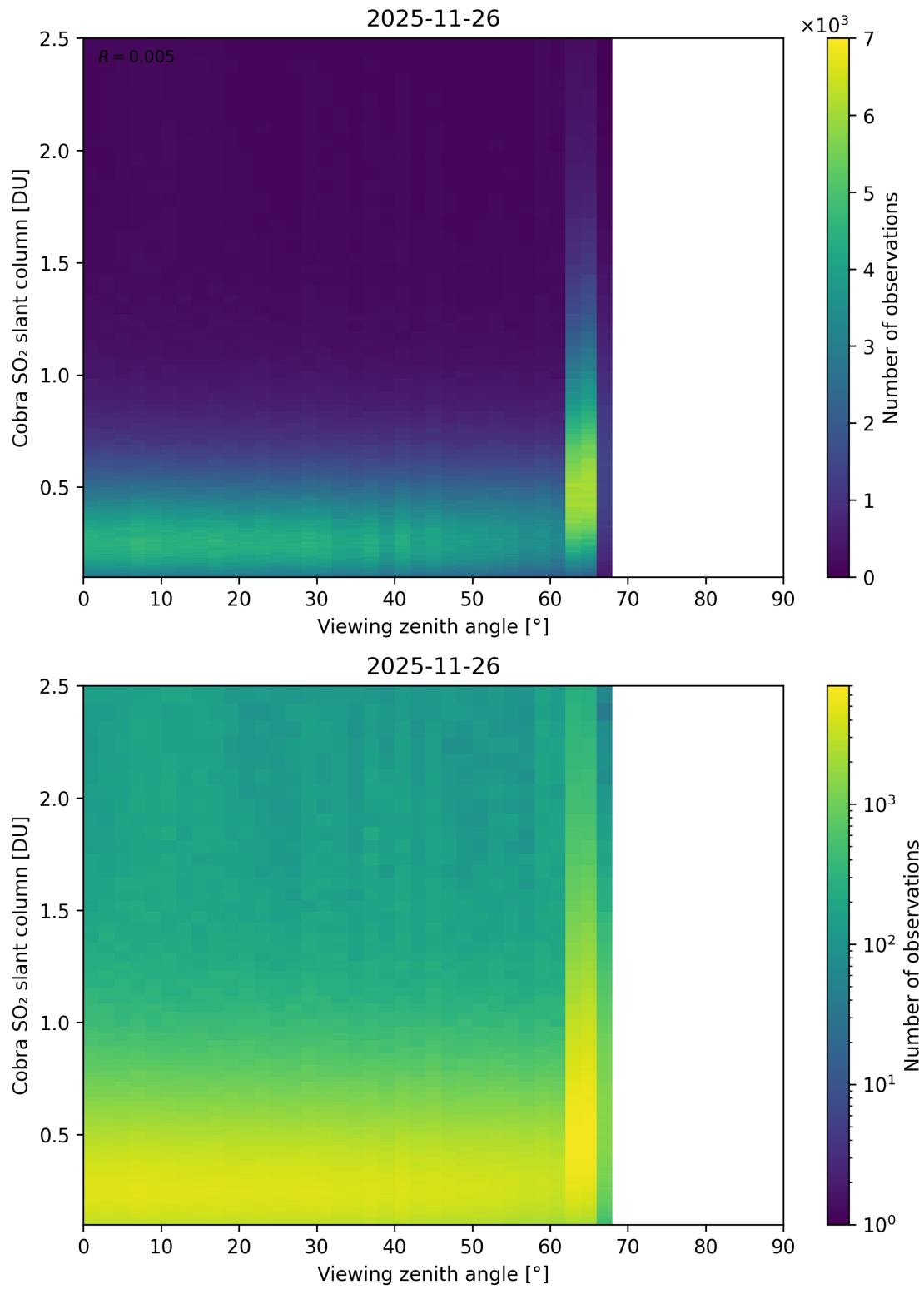
Figure 371: Scatter density plot of “Viewing zenith angle” against “Cobra SO 2 slant column” for 2025-11-25 to 2025-11-27.
