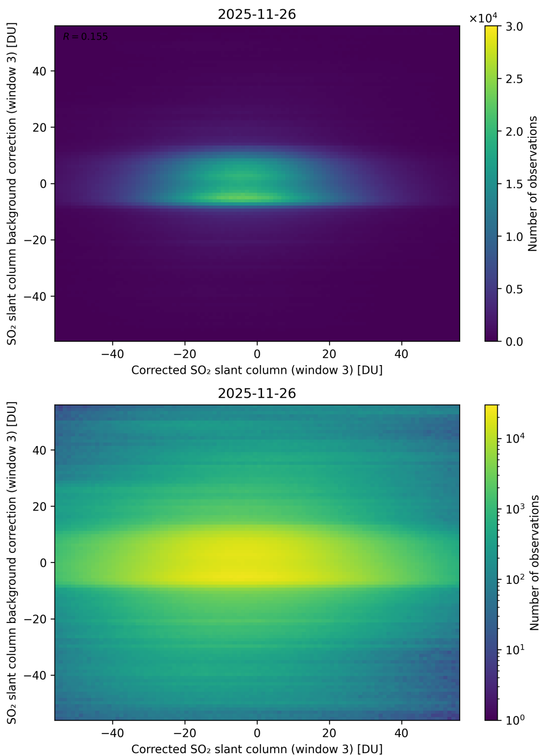
Figure 255: Scatter density plot of “Corrected SO 2 slant column (window 3)” against “SO 2 slant column background correction (window 3)” for 2025-11-25 to 2025-11-27.
