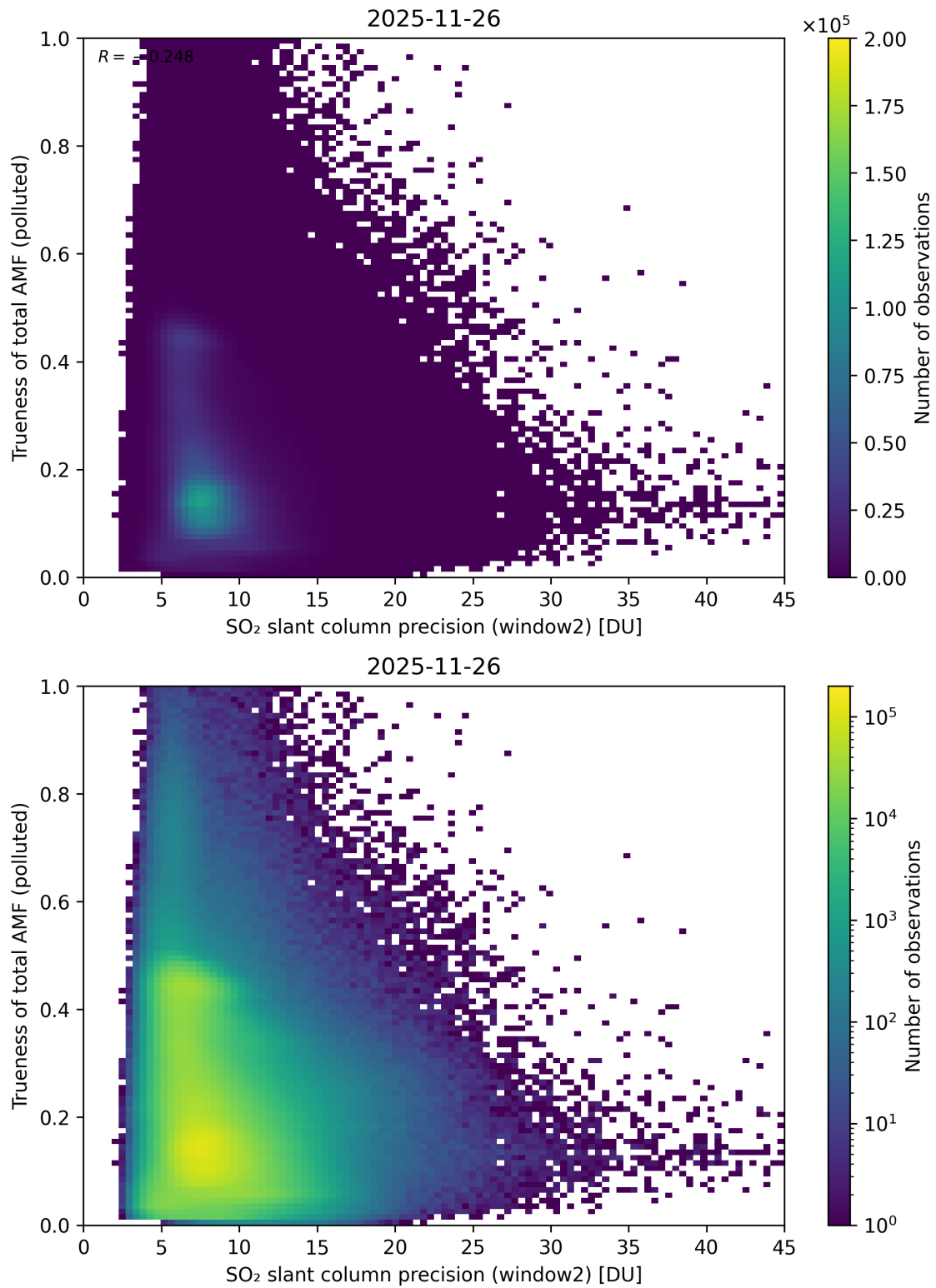
Figure 302: Scatter density plot of “SO 2 slant column precision (window2)” against “Trueness of total AMF (polluted)” for 2025-11-25 to 2025-11-27.
