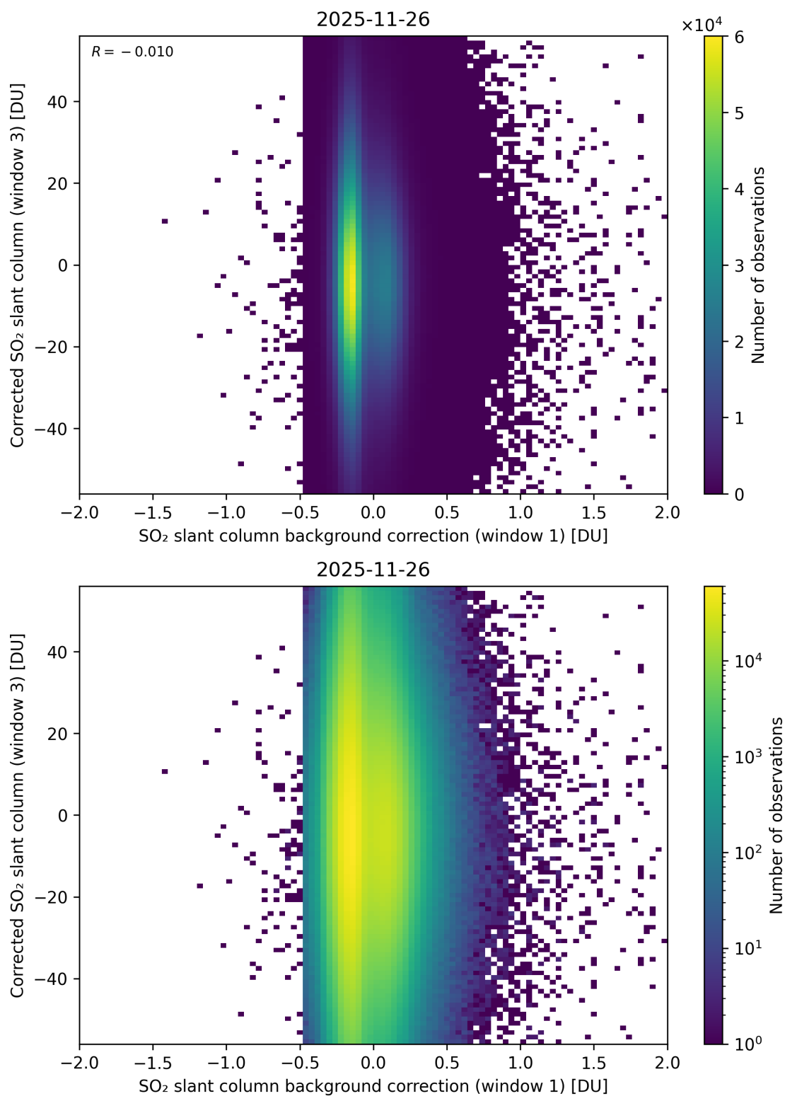
Figure 116: Scatter density plot of “SO 2 slant column background correction (window 1)” against “Corrected SO 2 slant column (window 3)” for 2025-11-25 to 2025-11-27.
