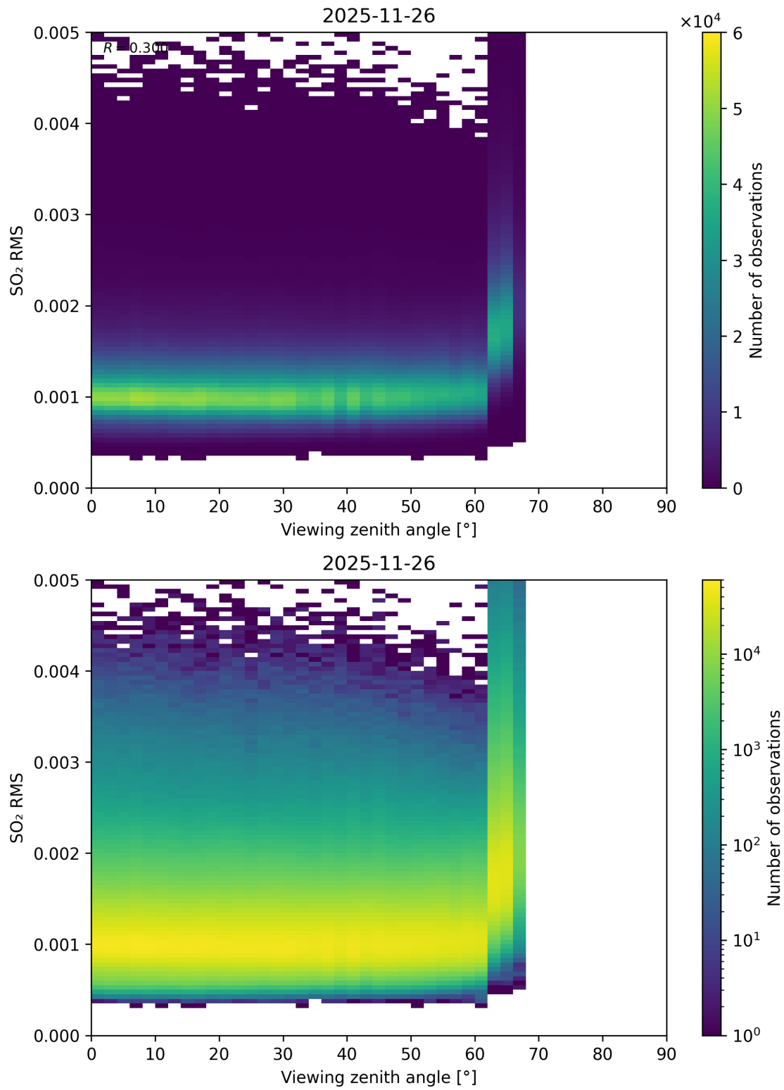
Figure 367: Scatter density plot of “Viewing zenith angle” against “SO 2 RMS” for 2025-11-25 to 2025-11-27.
