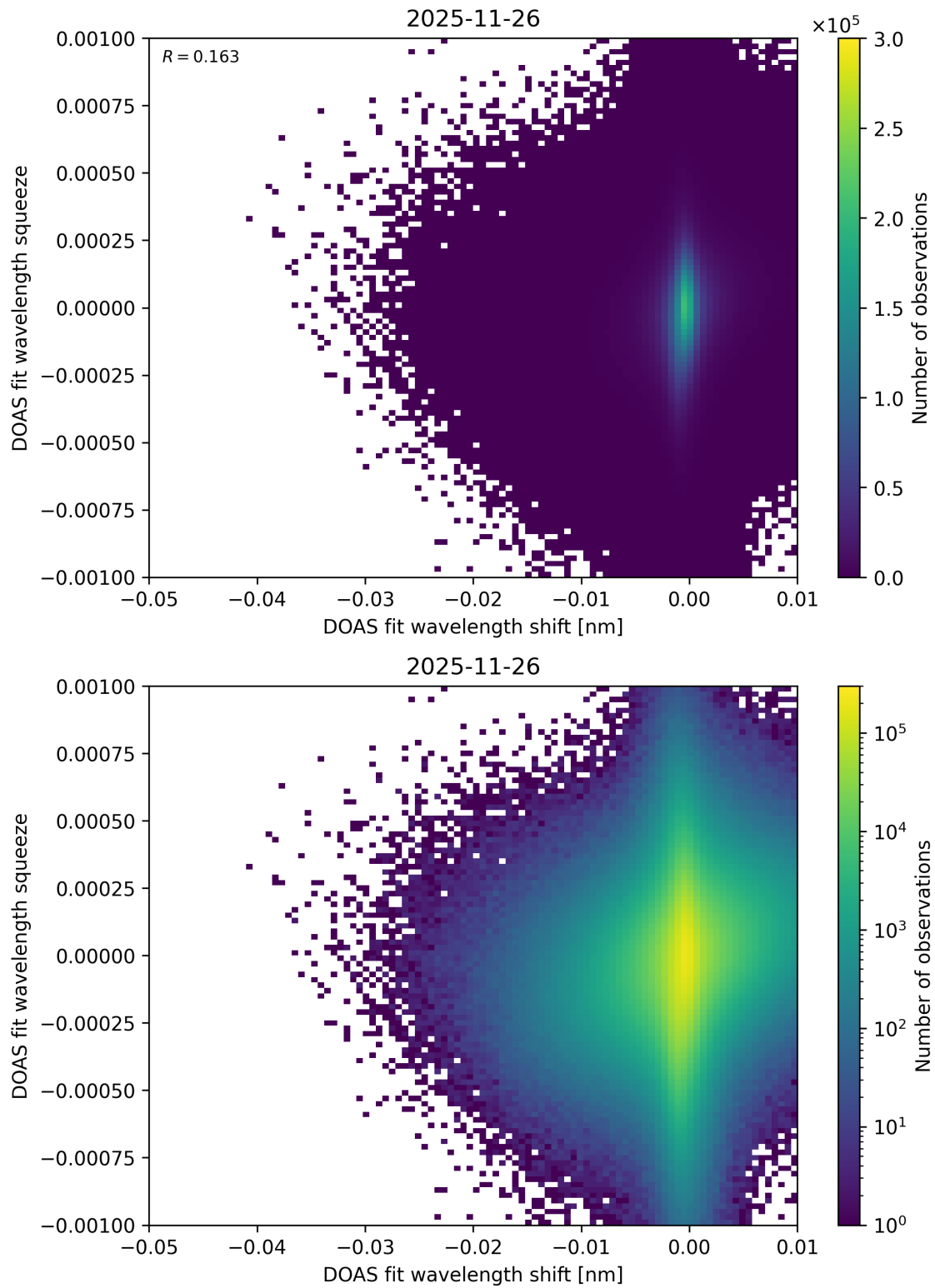
Figure 138: Scatter density plot of “DOAS fit wavelength shift” against “DOAS fit wavelength squeeze” for 2025-11-25 to 2025-11-27.
