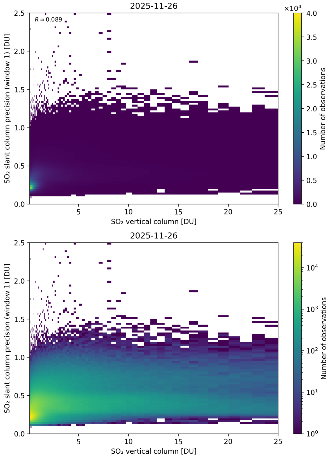
Figure 355: Scatter density plot of “SO 2 vertical column” against “SO 2 slant column precision (window 1)” for 2025-11-25 to 2025-11-27.
