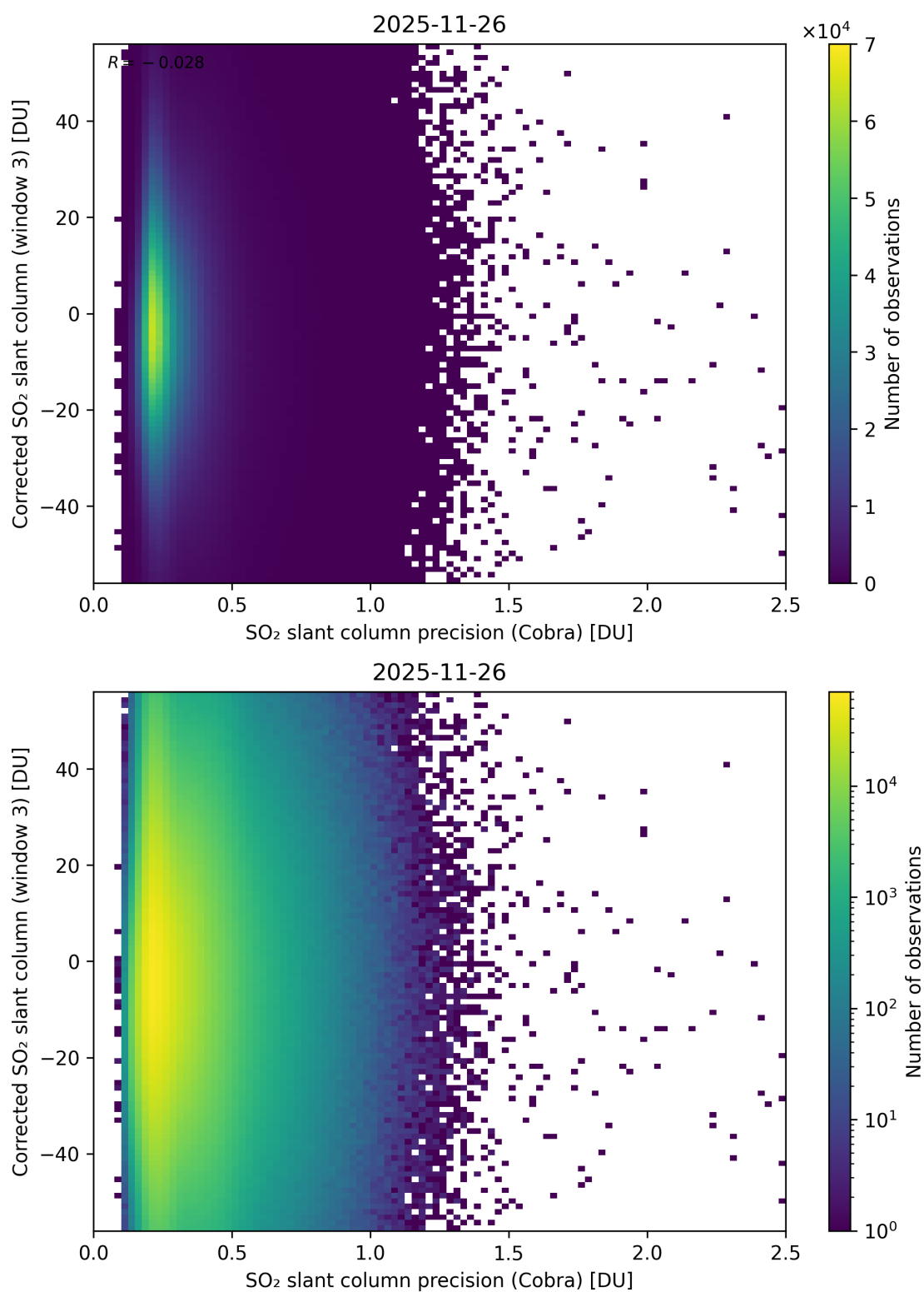
Figure 207: Scatter density plot of “SO 2 slant column precision (Cobra)” against “Corrected SO 2 slant column (window 3)” for 2025-11-25 to 2025-11-27.
