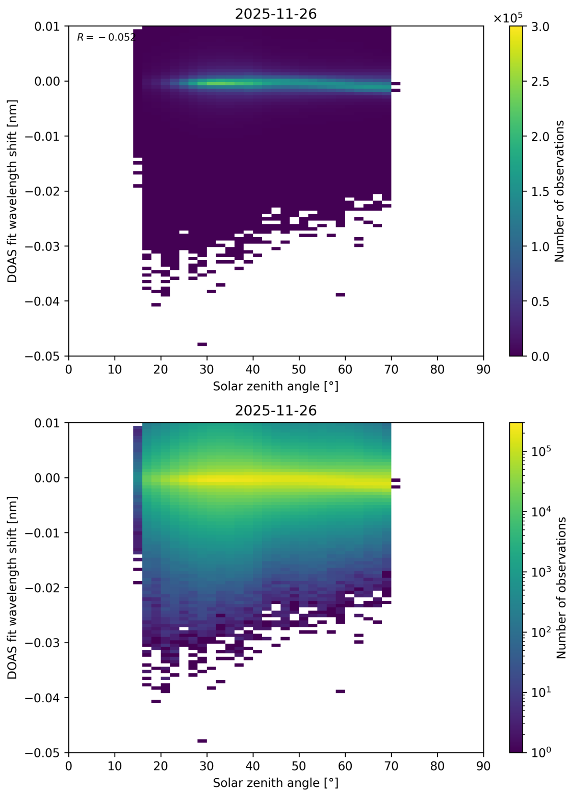
Figure 174: Scatter density plot of “Solar zenith angle” against “DOAS fit wavelength shift” for 2025-11-25 to 2025-11-27.
