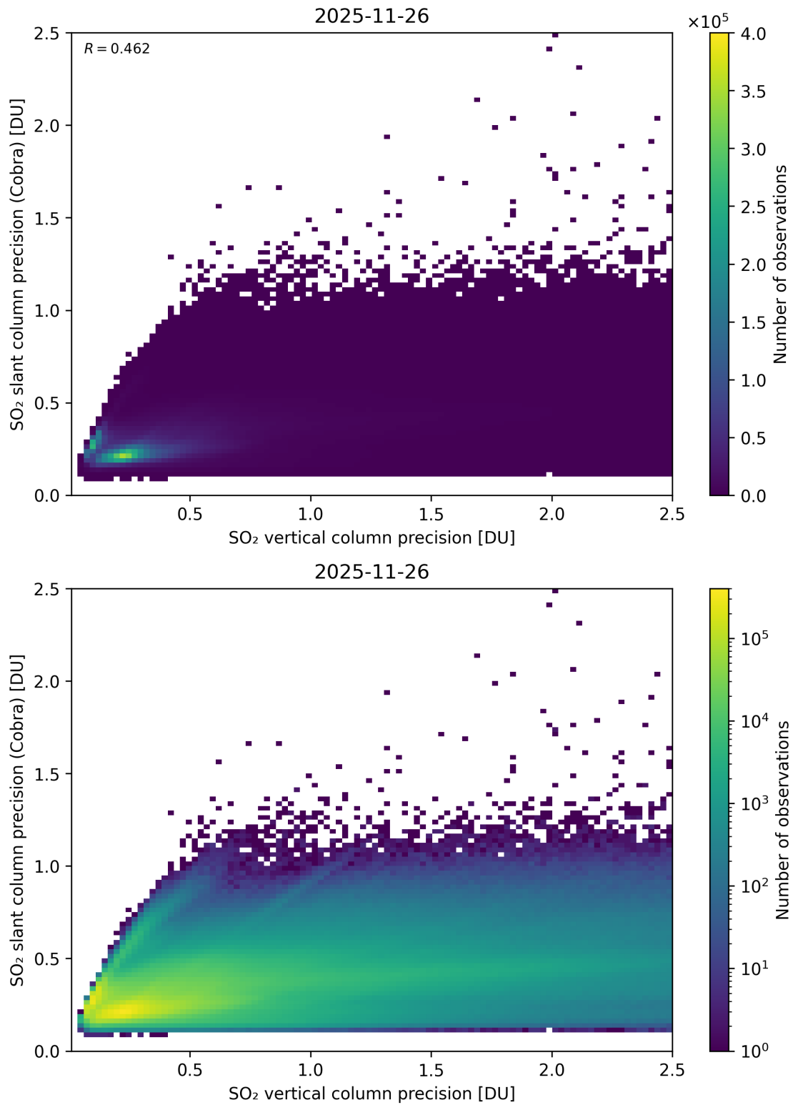
Figure 337: Scatter density plot of “SO 2 vertical column precision” against “SO 2 slant column precision (Cobra)” for 2025-11-25 to 2025-11-27.
