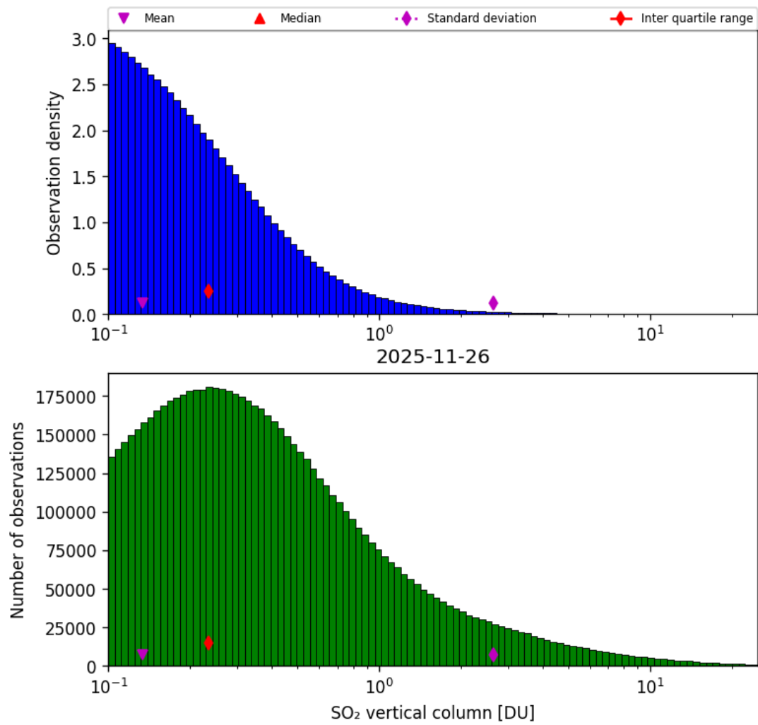
Figure 58: Histogram of “SO 2 vertical column” for 2025-11-25 to 2025-11-27
