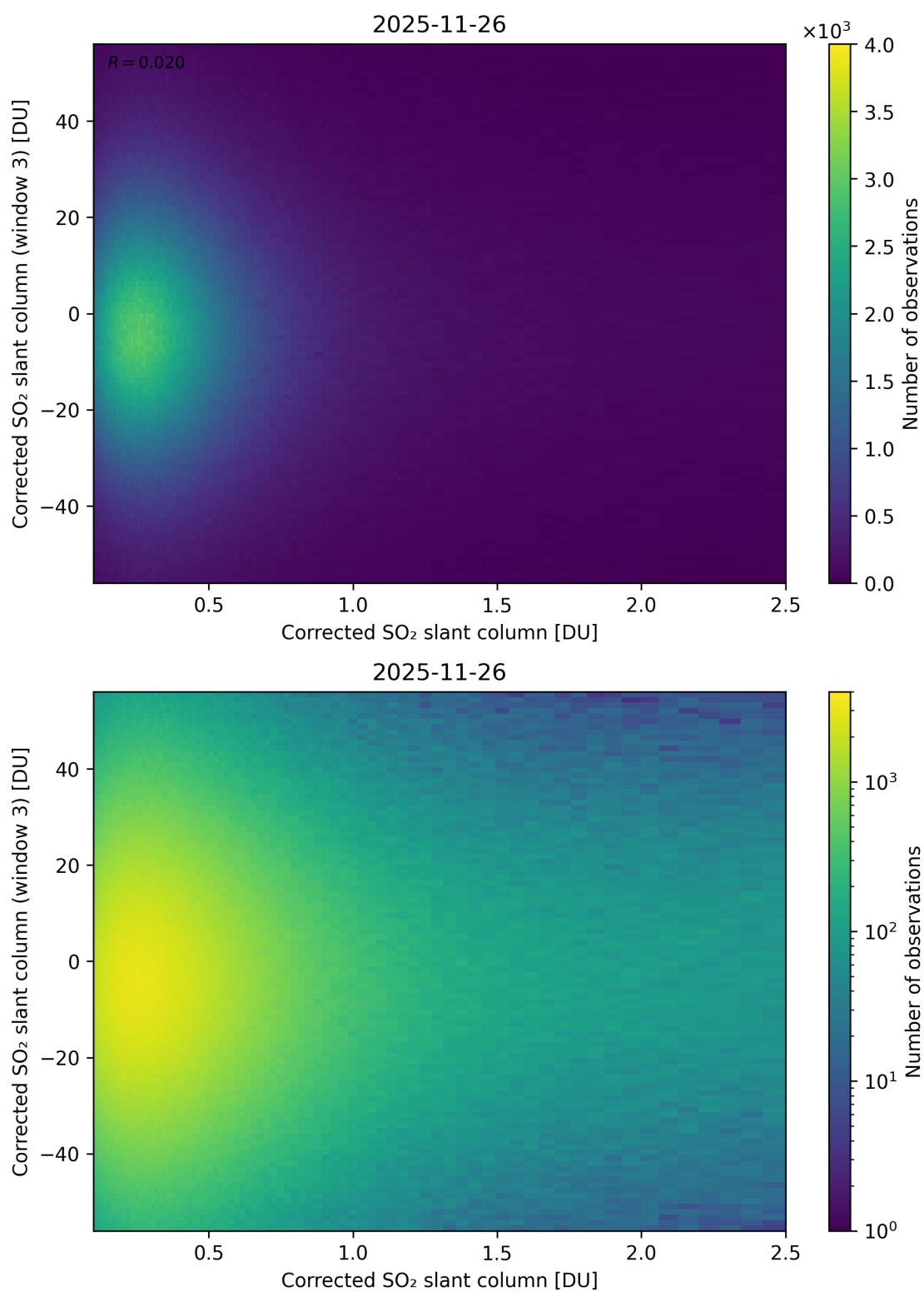
Figure 236: Scatter density plot of “Corrected SO 2 slant column” against “Corrected SO 2 slant column (window 3)” for 2025-11-25 to 2025-11-27.
