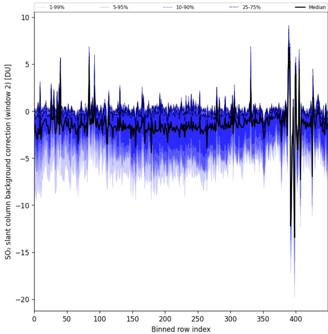
Figure 96: Along track statistics of “SO 2 slant column background correction (window 2)” for 2025-11-25 to 2025-11-27
