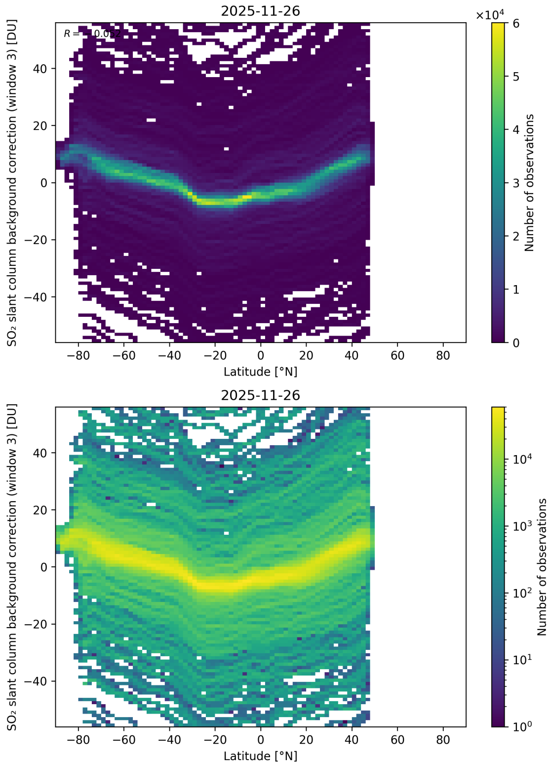
Figure 152: Scatter density plot of “Latitude” against “SO 2 slant column background correction (window 3)” for 2025-11-25 to 2025-11-27.
