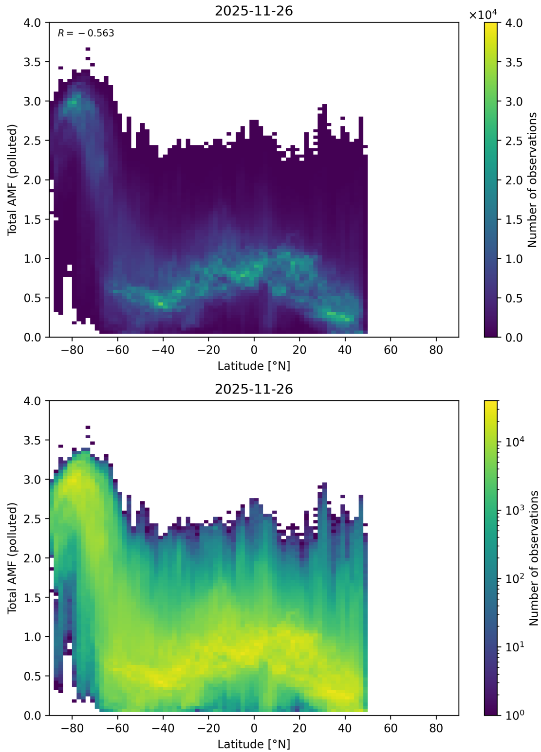
Figure 167: Scatter density plot of “Latitude” against “Total AMF (polluted)” for 2025-11-25 to 2025-11-27.
