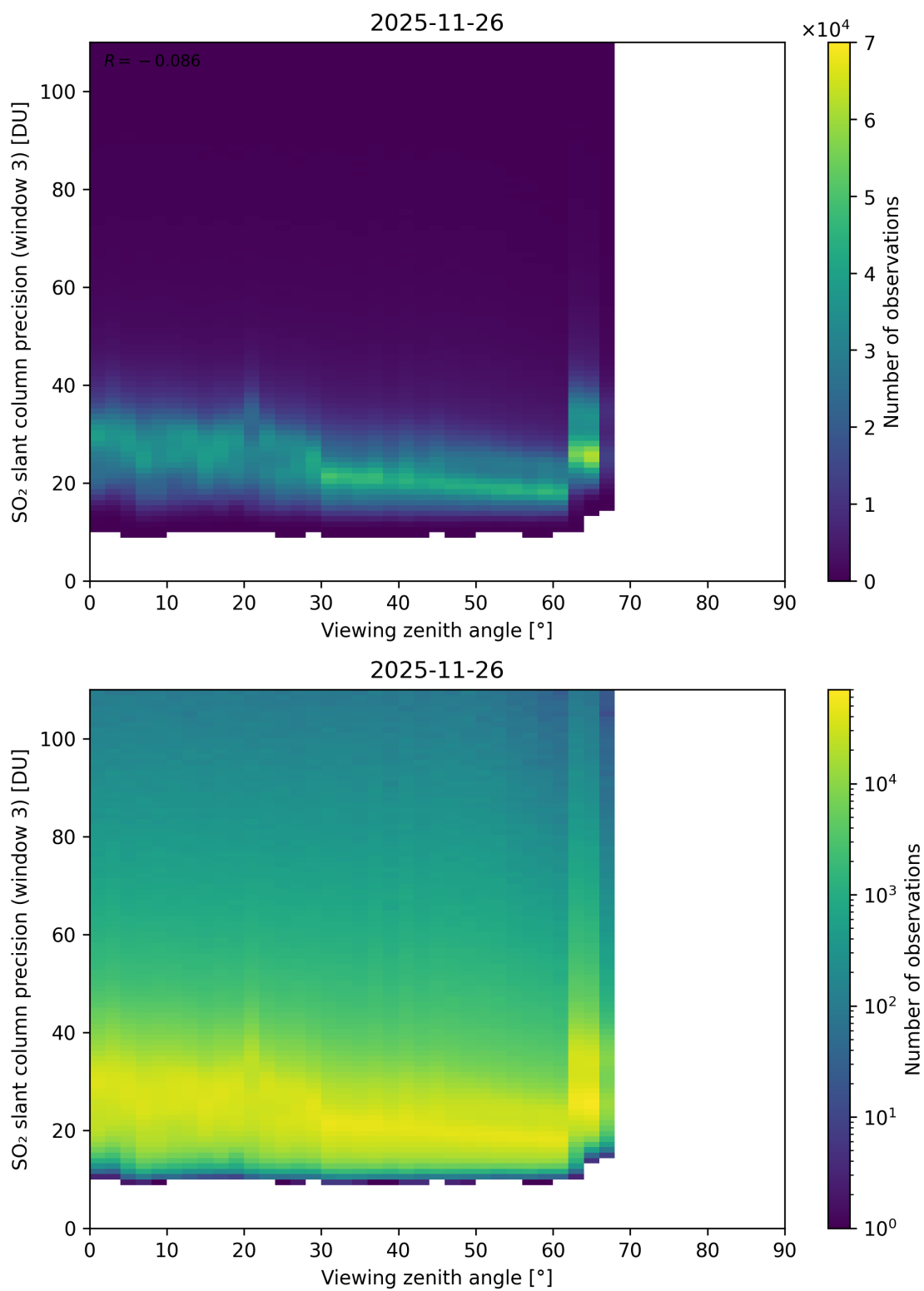
Figure 380: Scatter density plot of “Viewing zenith angle” against “SO 2 slant column precision (window 3)” for 2025-11-25 to 2025-11-27.
