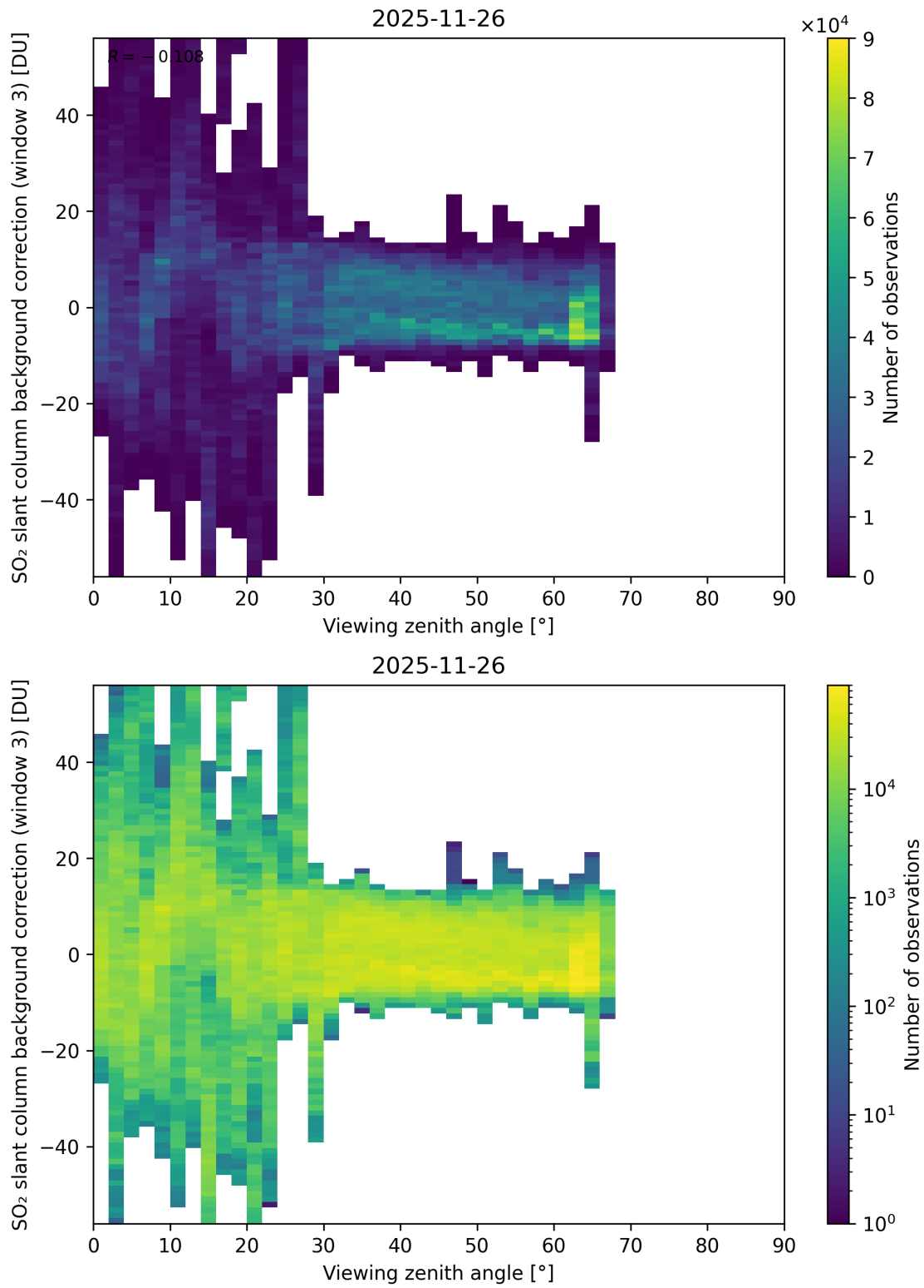
Figure 364: Scatter density plot of “Viewing zenith angle” against “SO 2 slant column background correction (window 3)” for 2025-11-25 to 2025-11-27.
