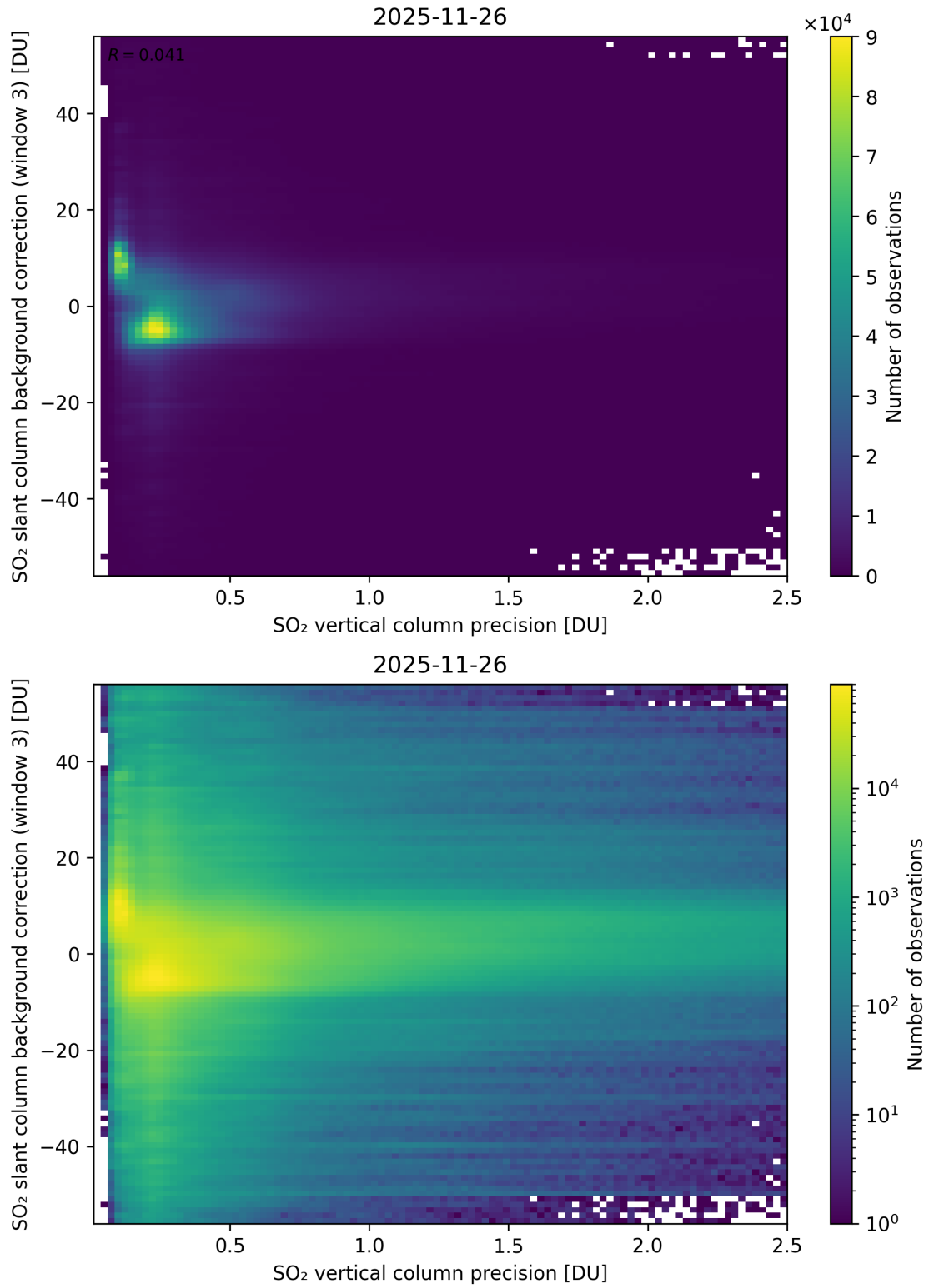
Figure 331: Scatter density plot of “SO 2 vertical column precision” against “SO 2 slant column background correction (window 3)” for 2025-11-25 to 2025-11-27.
