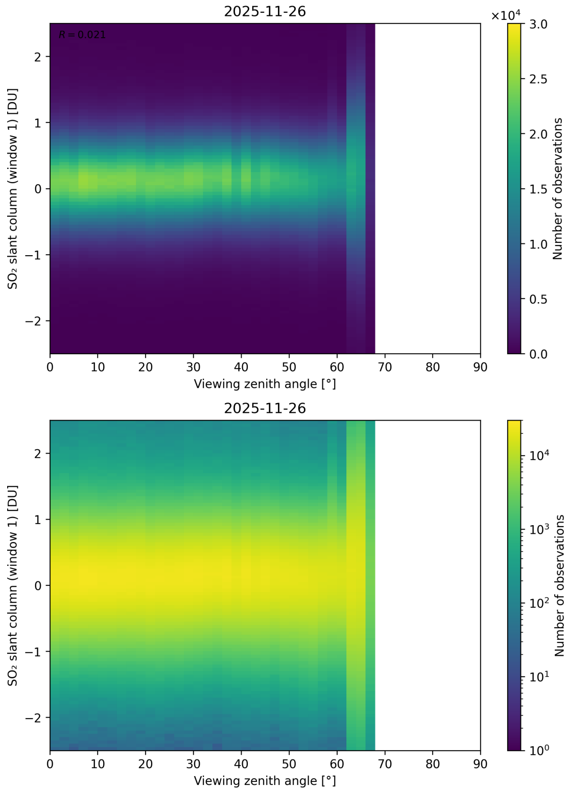
Figure 376: Scatter density plot of “Viewing zenith angle” against “SO 2 slant column (window 1)” for 2025-11-25 to 2025-11-27.
