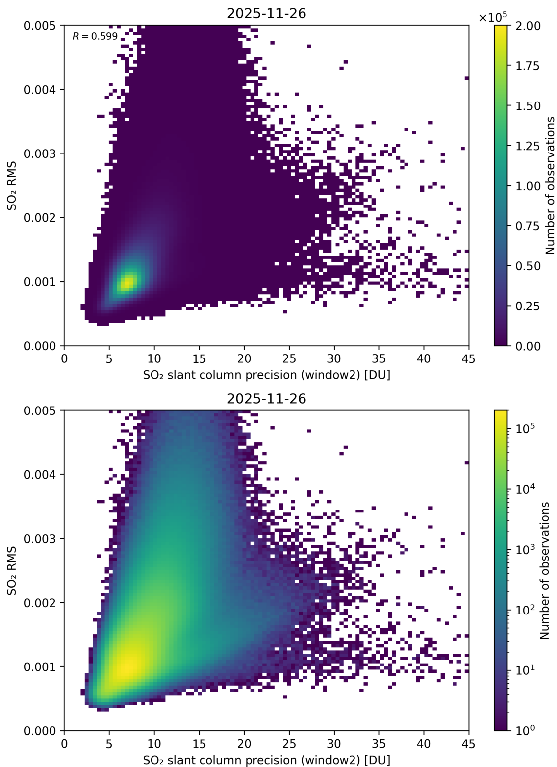
Figure 295: Scatter density plot of “SO 2 slant column precision (window2)” against “SO 2 RMS” for 2025-11-25 to 2025-11-27.
