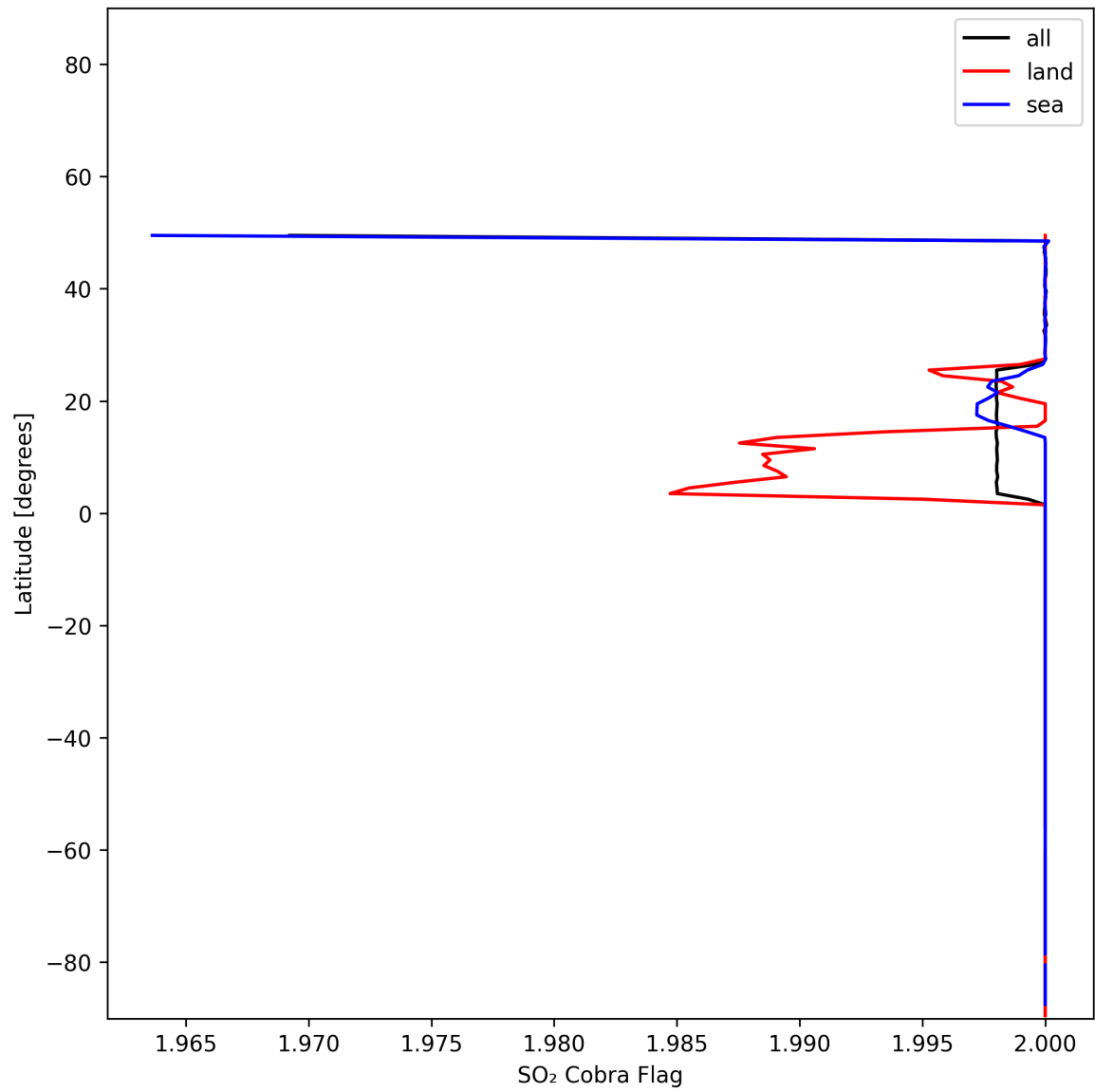
Figure 49: Zonal average of “SO 2 Cobra Flag” for 2025-11-25 to 2025-11-27.
