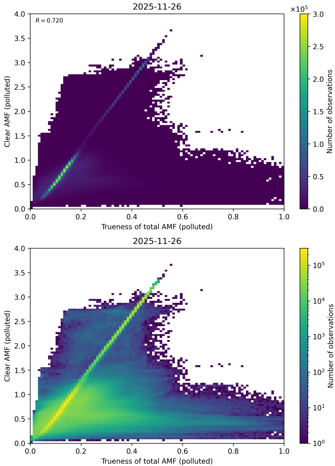
Figure 322: Scatter density plot of “Trueness of total AMF (polluted)” against “Clear AMF (polluted)” for 2025-11-25 to 2025-11-27.
