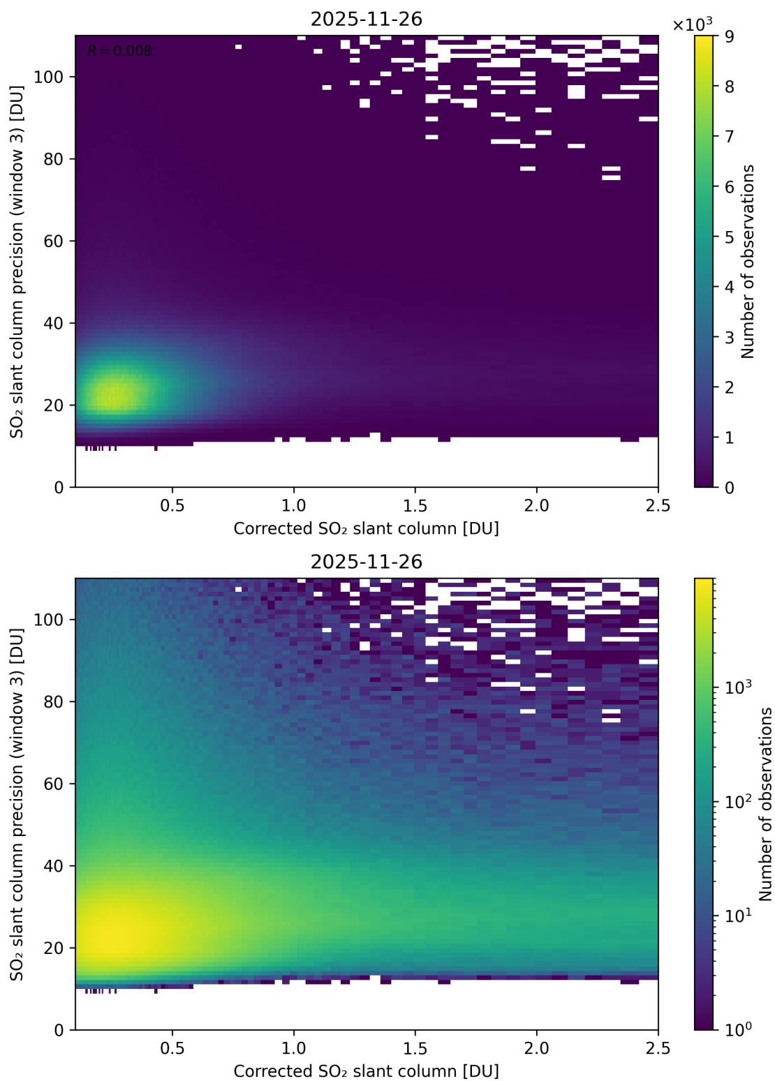
Figure 241: Scatter density plot of “Corrected SO 2 slant column” against “SO 2 slant column precision (window 3)” for 2025-11-25 to 2025-11-27.
