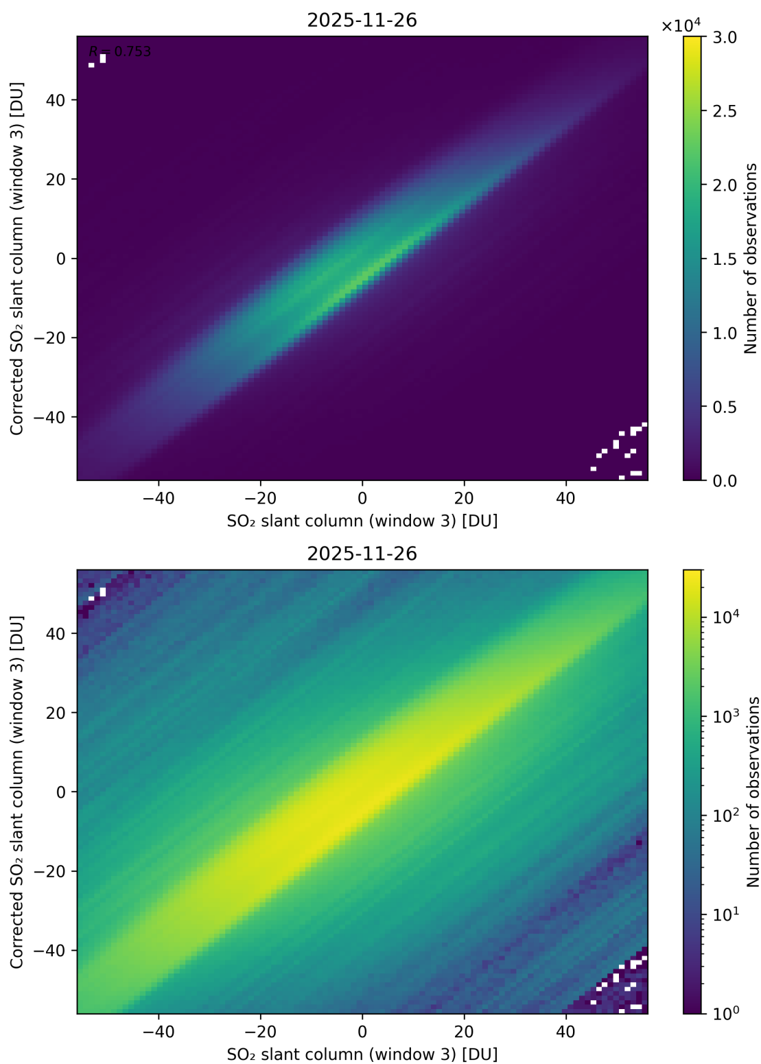
Figure 316: Scatter density plot of “SO 2 slant column (window 3)” against “Corrected SO 2 slant column (window 3)” for 2025-11-25 to 2025-11-27.
