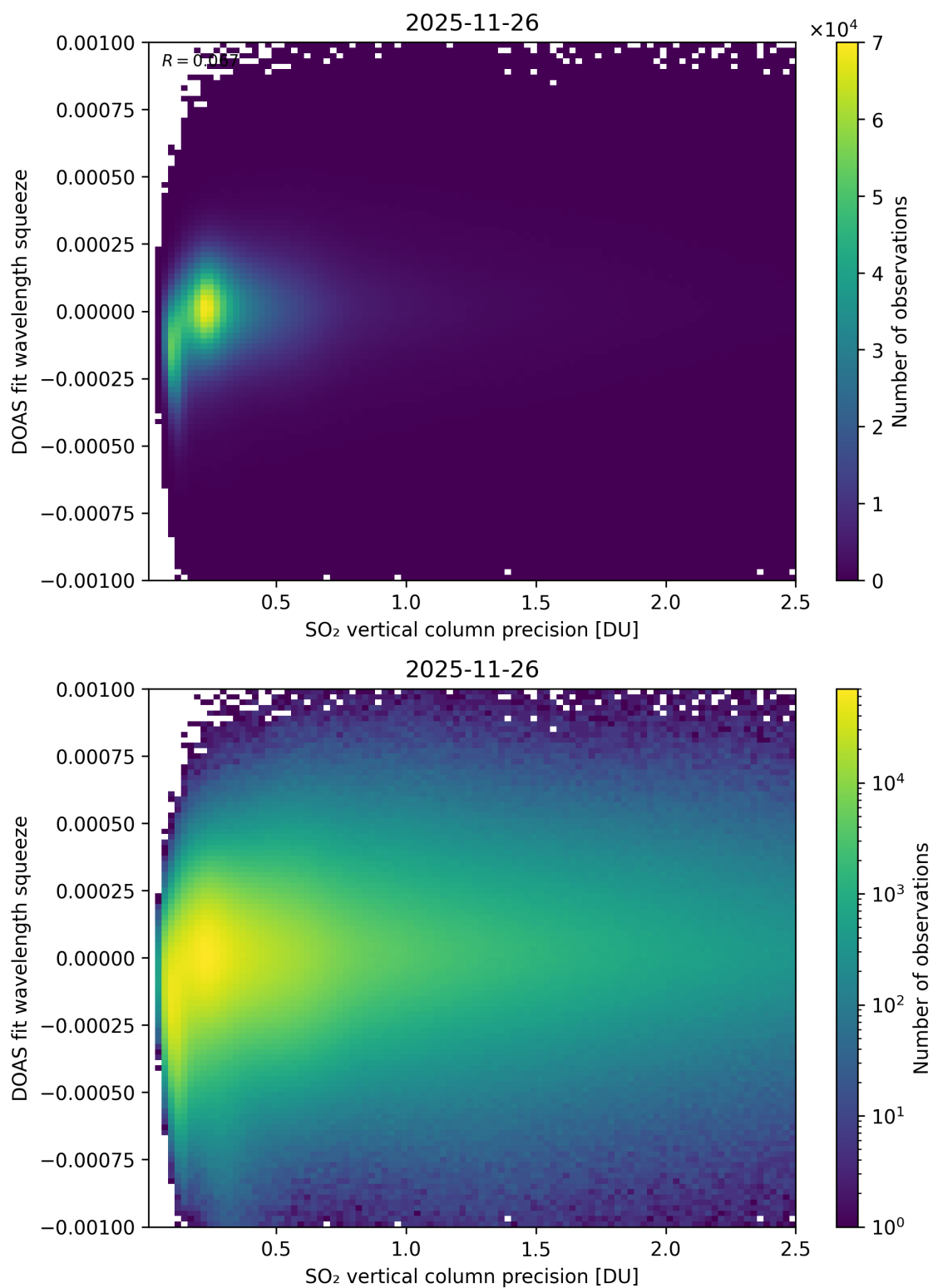
Figure 333: Scatter density plot of “SO 2 vertical column precision” against “DOAS fit wavelength squeeze” for 2025-11-25 to 2025-11-27.
