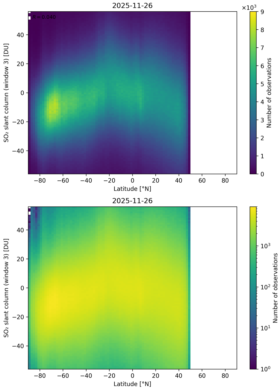
Figure 165: Scatter density plot of “Latitude” against “SO 2 slant column (window 3)” for 2025-11-25 to 2025-11-27.
