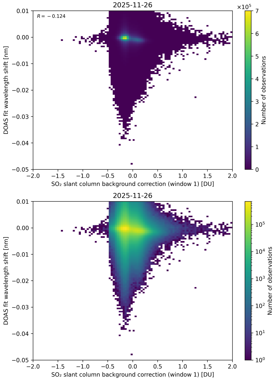
Figure 111: Scatter density plot of “SO 2 slant column background correction (window 1)” against “DOAS fit wavelength shift” for 2025-11-25 to 2025-11-27.
