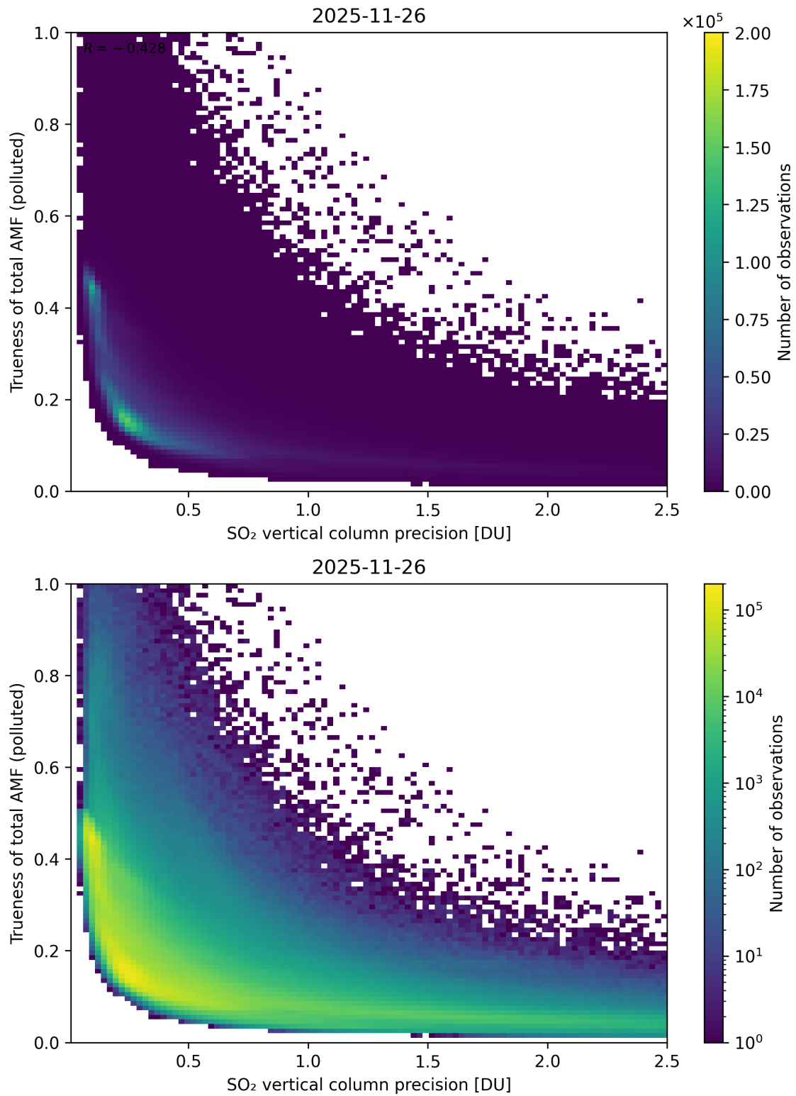
Figure 347: Scatter density plot of “SO 2 vertical column precision” against “Trueness of total AMF (polluted)” for 2025-11-25 to 2025-11-27.
