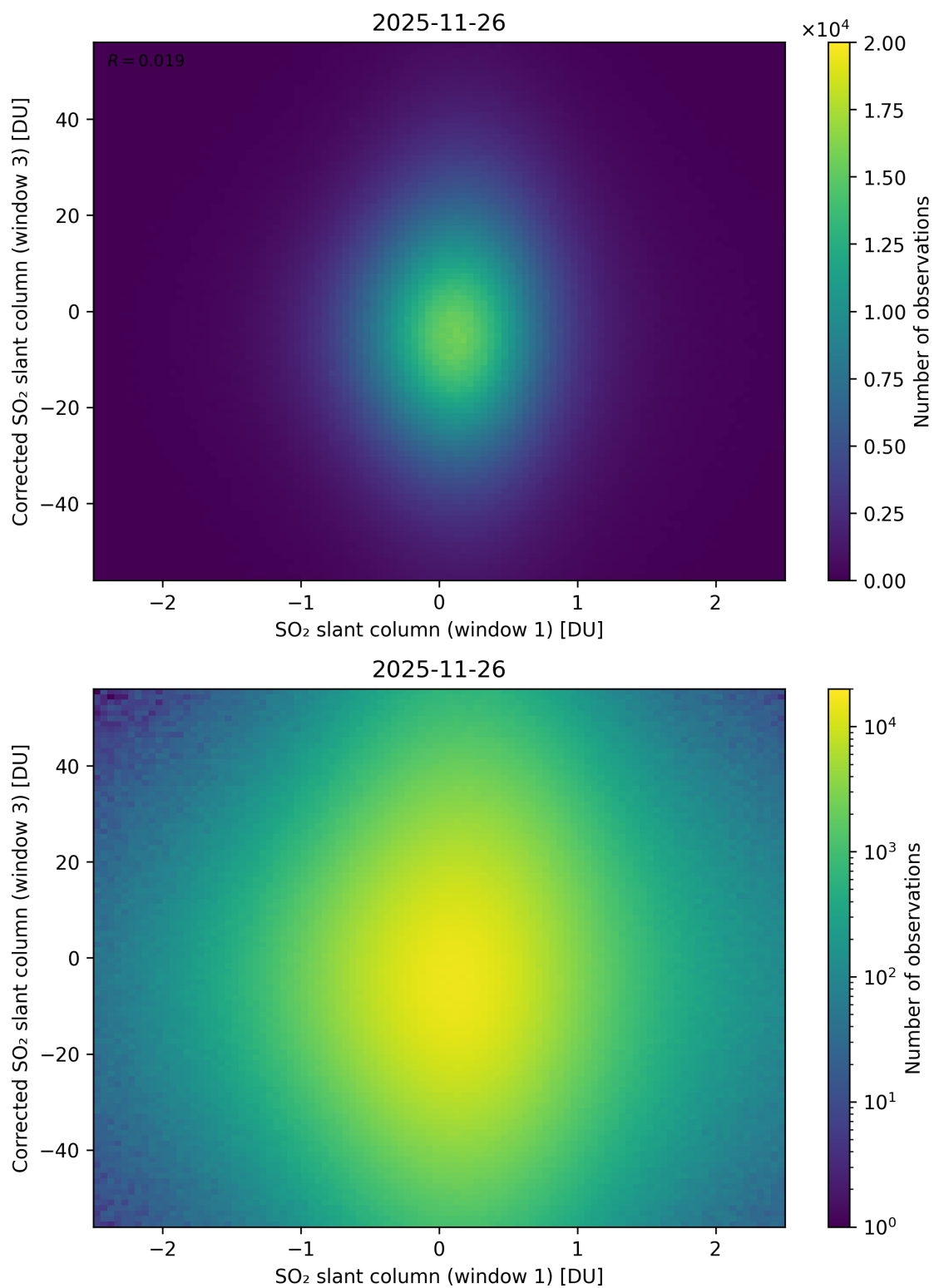
Figure 284: Scatter density plot of “SO 2 slant column (window 1)” against “Corrected SO 2 slant column (window 3)” for 2025-11-25 to 2025-11-27.
