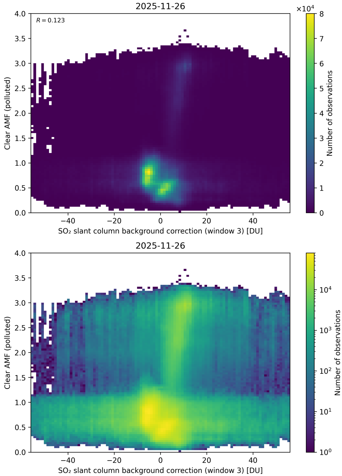
Figure 135: Scatter density plot of “SO 2 slant column background correction (window 3)” against “Clear AMF (polluted)” for 2025-11-25 to 2025-11-27.
