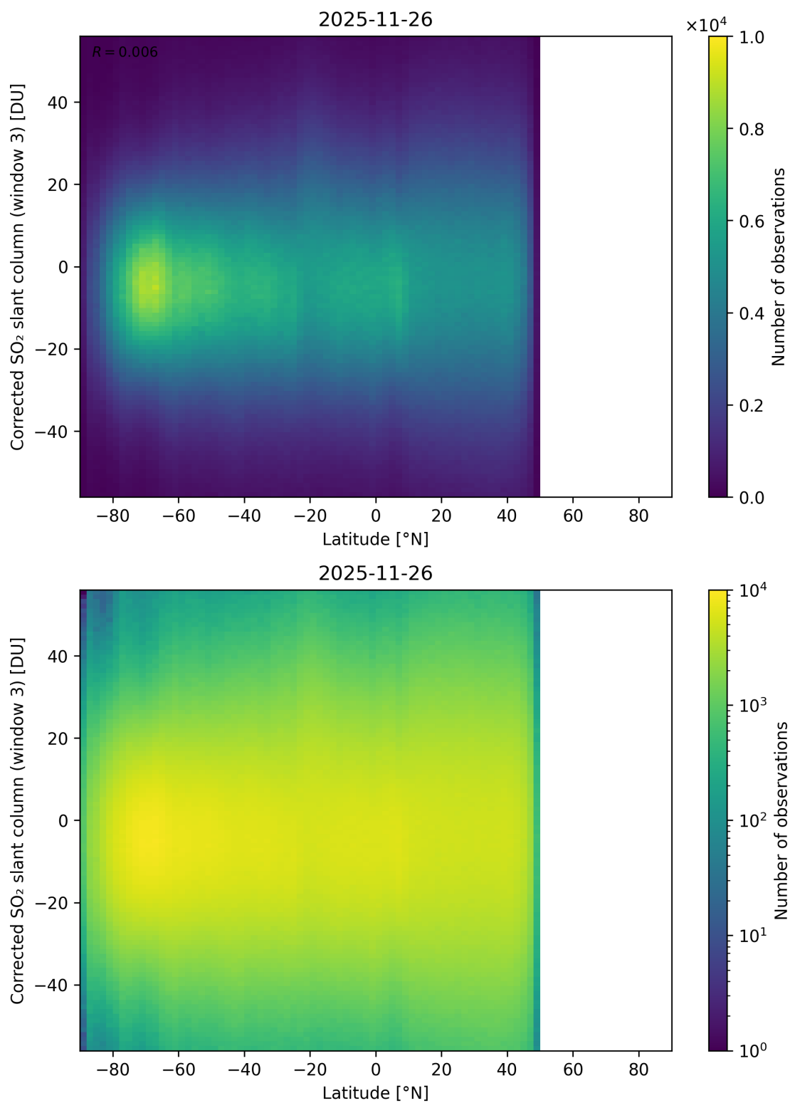
Figure 161: Scatter density plot of “Latitude” against “Corrected SO 2 slant column (window 3)” for 2025-11-25 to 2025-11-27.
