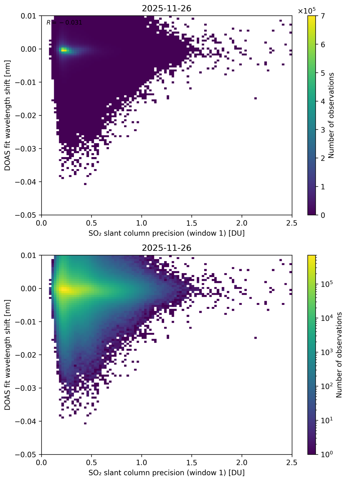
Figure 271: Scatter density plot of “SO 2 slant column precision (window 1)” against “DOAS fit wavelength shift” for 2025-11-25 to 2025-11-27.
