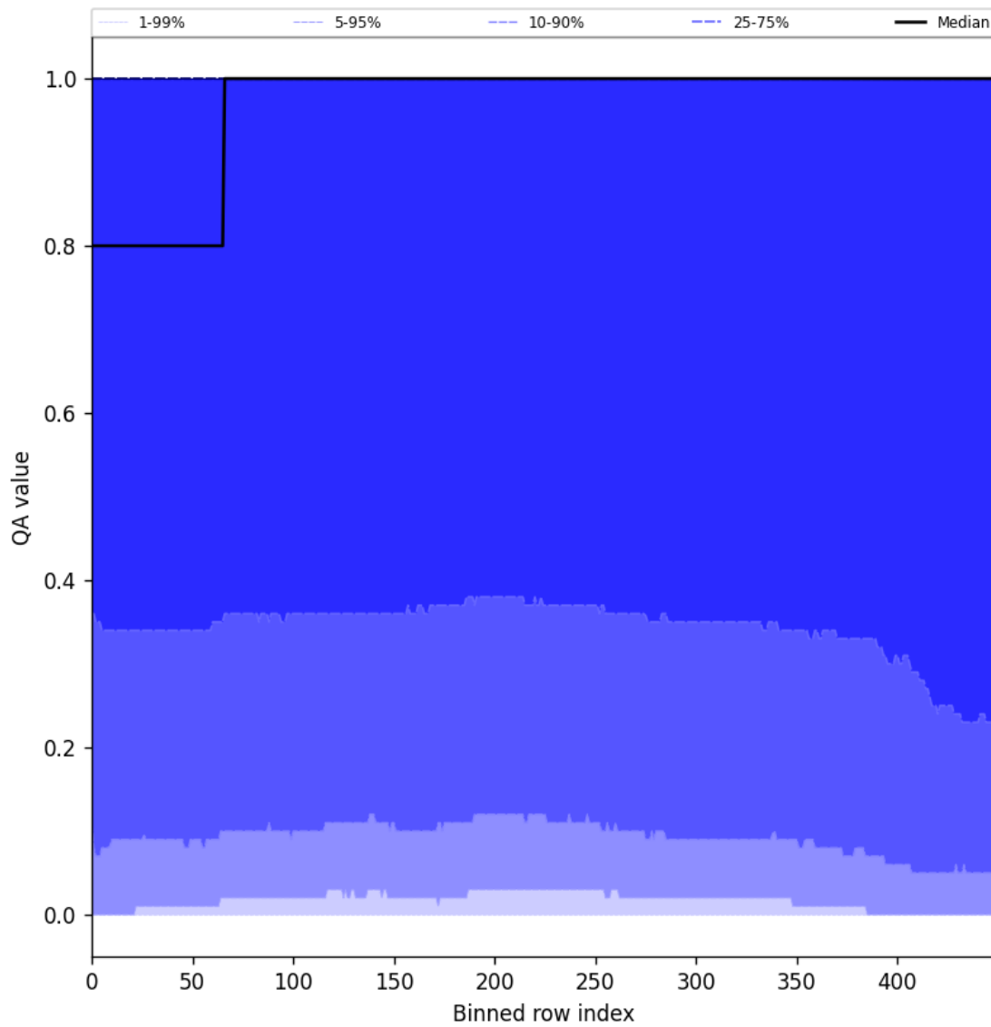
Figure 83: Along track statistics of “QA value” for 2025-11-25 to 2025-11-27
