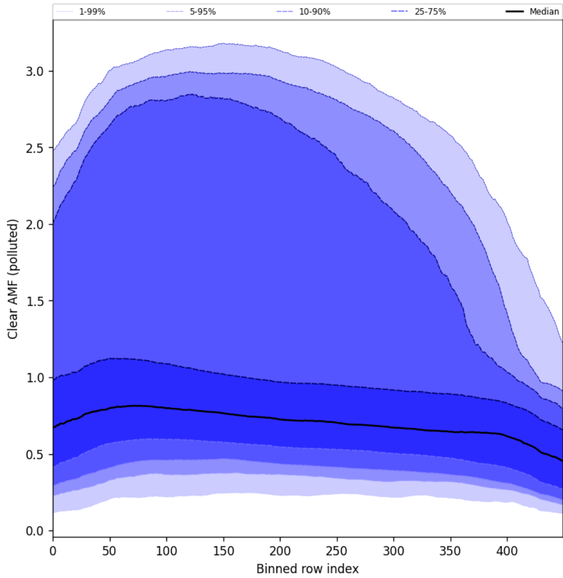
Figure 107: Along track statistics of “Clear AMF (polluted)” for 2025-11-25 to 2025-11-27
