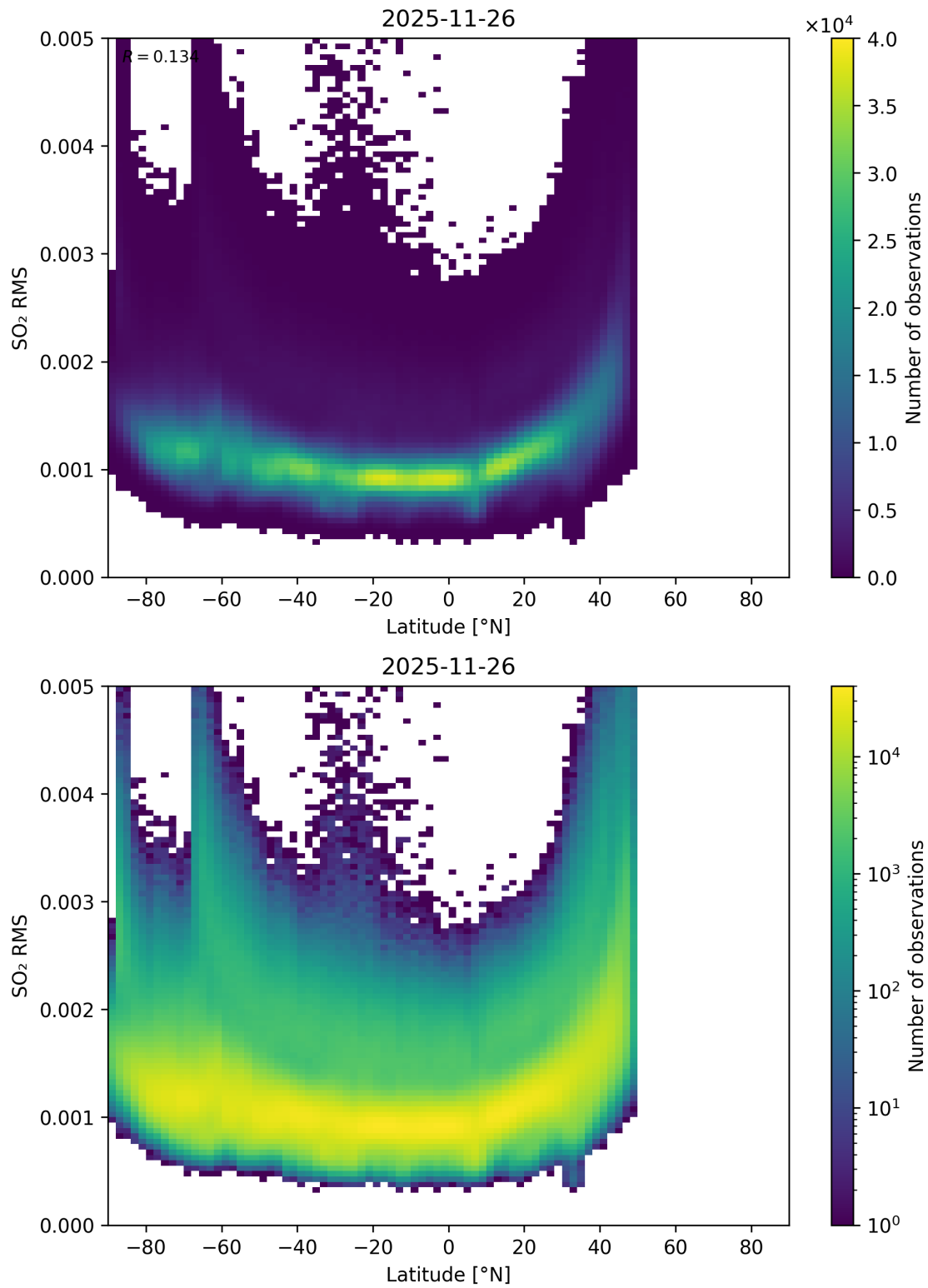
Figure 155: Scatter density plot of “Latitude” against “SO 2 RMS” for 2025-11-25 to 2025-11-27.
