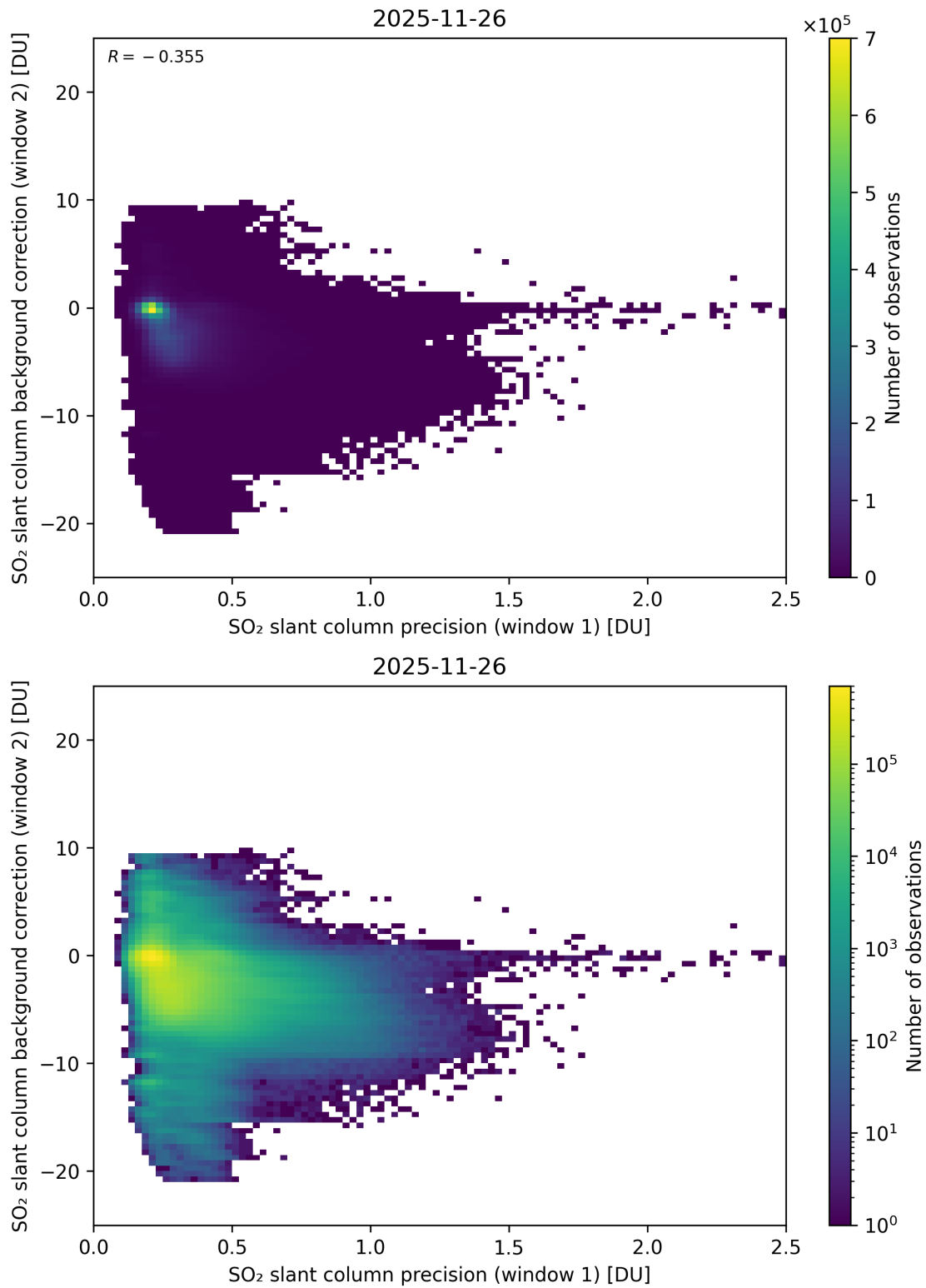
Figure 269: Scatter density plot of “SO 2 slant column precision (window 1)” against “SO 2 slant column background correction (window 2)” for 2025-11-25 to 2025-11-27.
