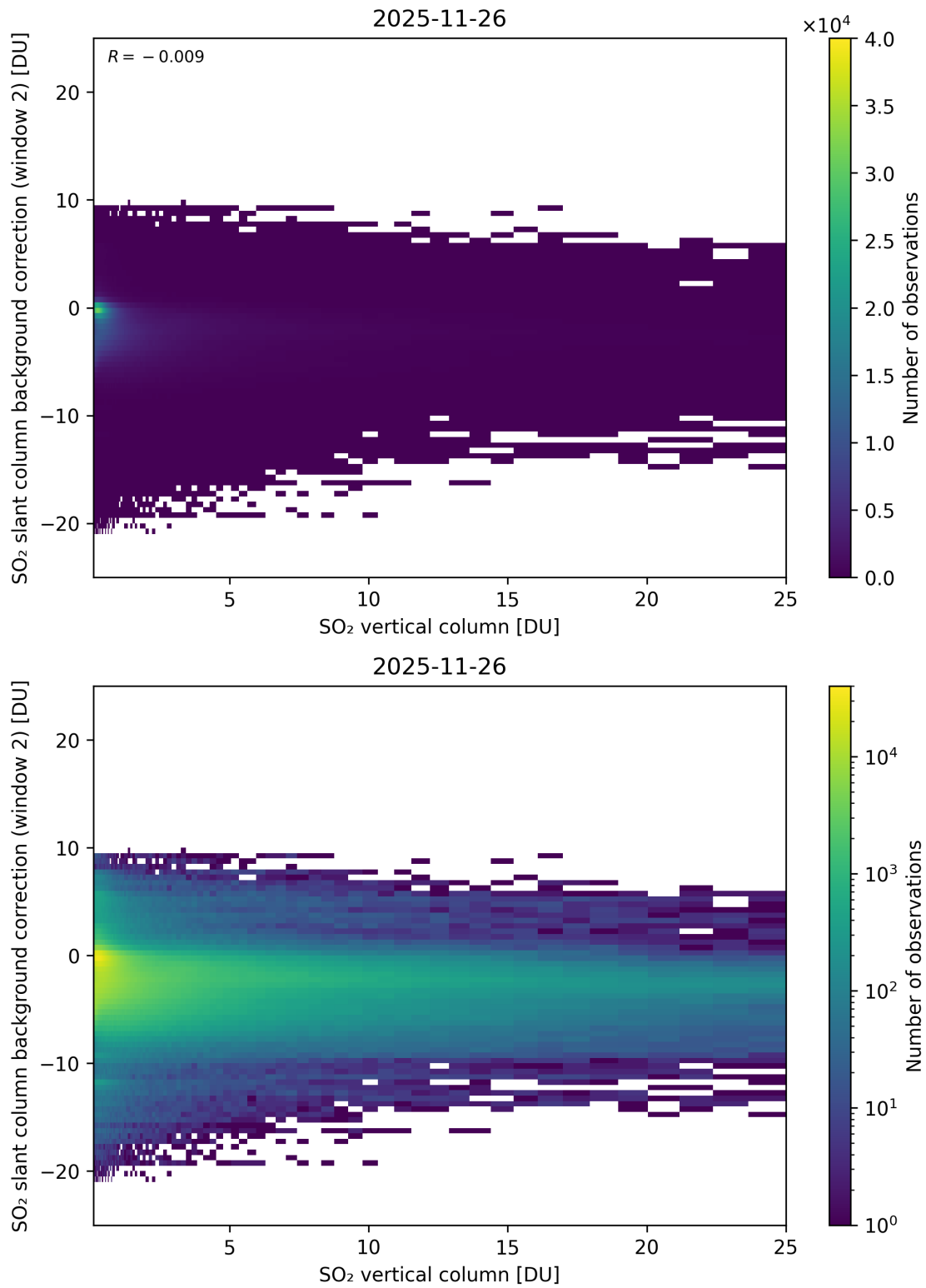
Figure 324: Scatter density plot of “SO 2 vertical column” against “SO 2 slant column background correction (window 2)” for 2025-11-25 to 2025-11-27.
