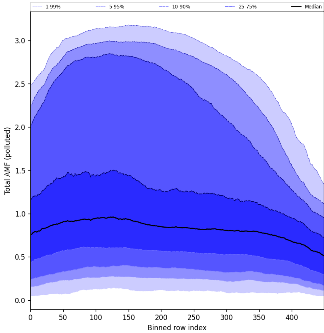
Figure 105: Along track statistics of “Total AMF (polluted)” for 2025-11-25 to 2025-11-27
