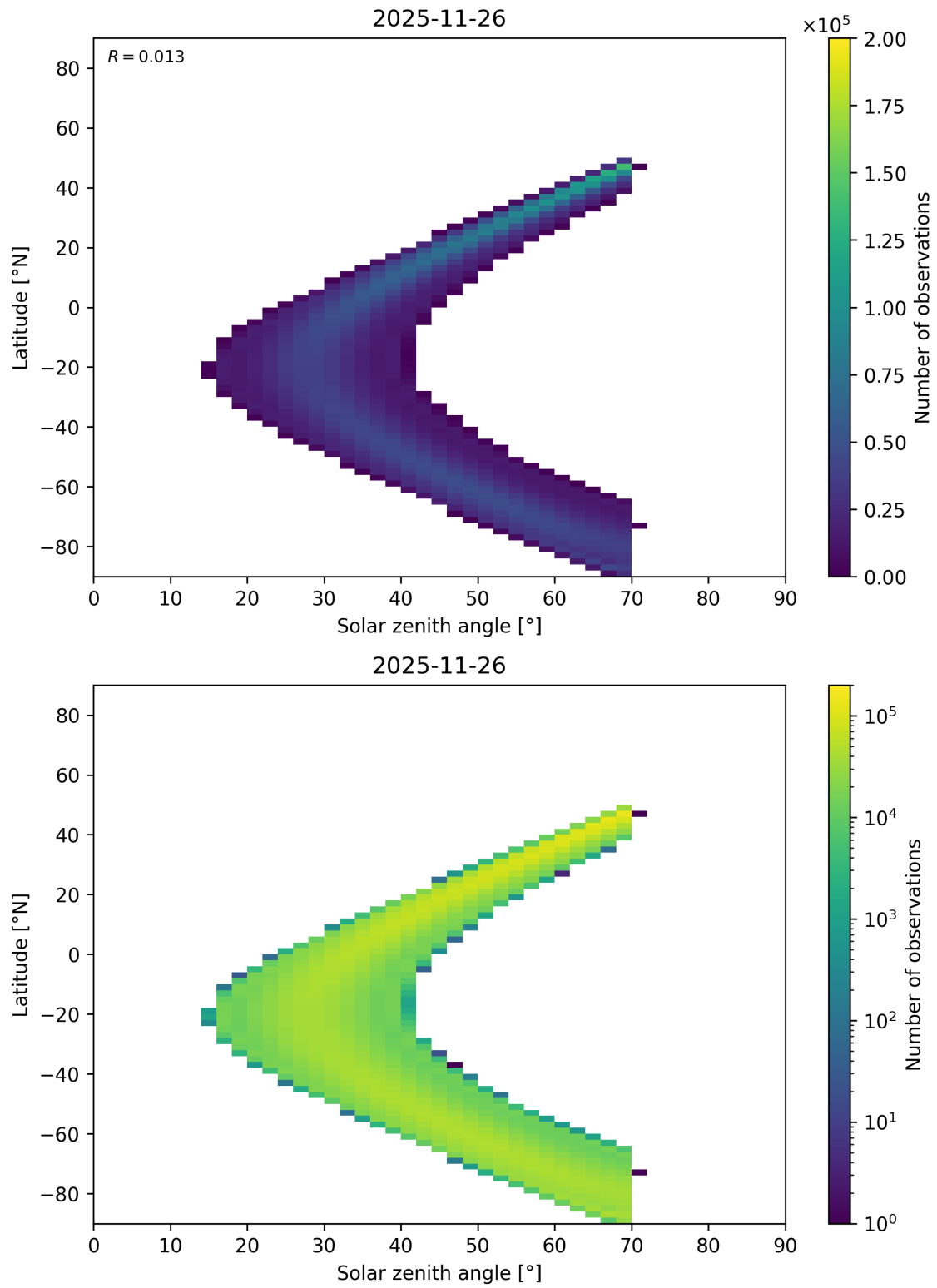
Figure 177: Scatter density plot of “Solar zenith angle” against “Latitude” for 2025-11-25 to 2025-11-27.
