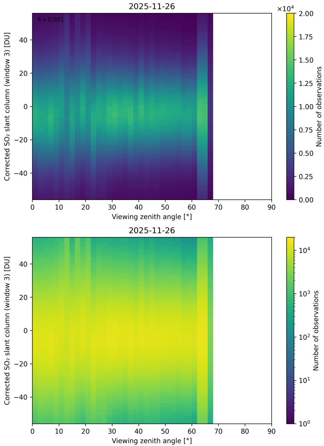
Figure 375: Scatter density plot of “Viewing zenith angle” against “Corrected SO 2 slant column (window 3)” for 2025-11-25 to 2025-11-27.
