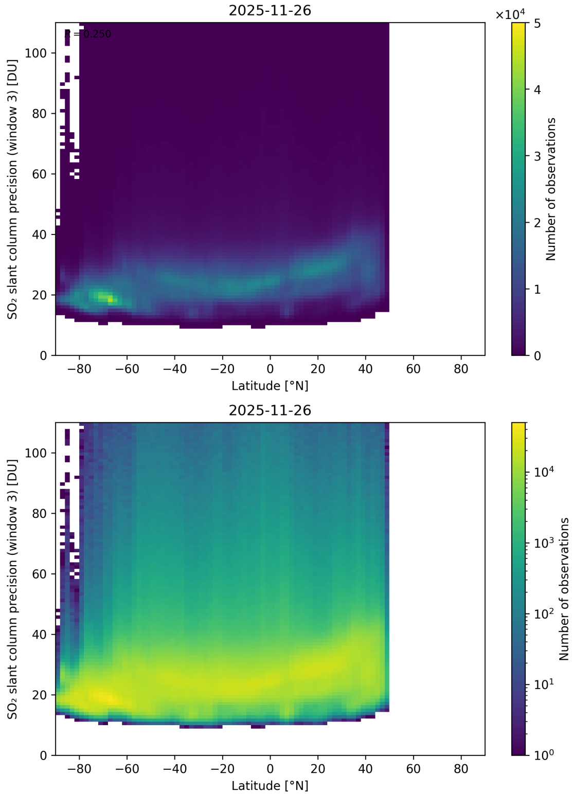
Figure 166: Scatter density plot of “Latitude” against “SO 2 slant column precision (window 3)” for 2025-11-25 to 2025-11-27.
