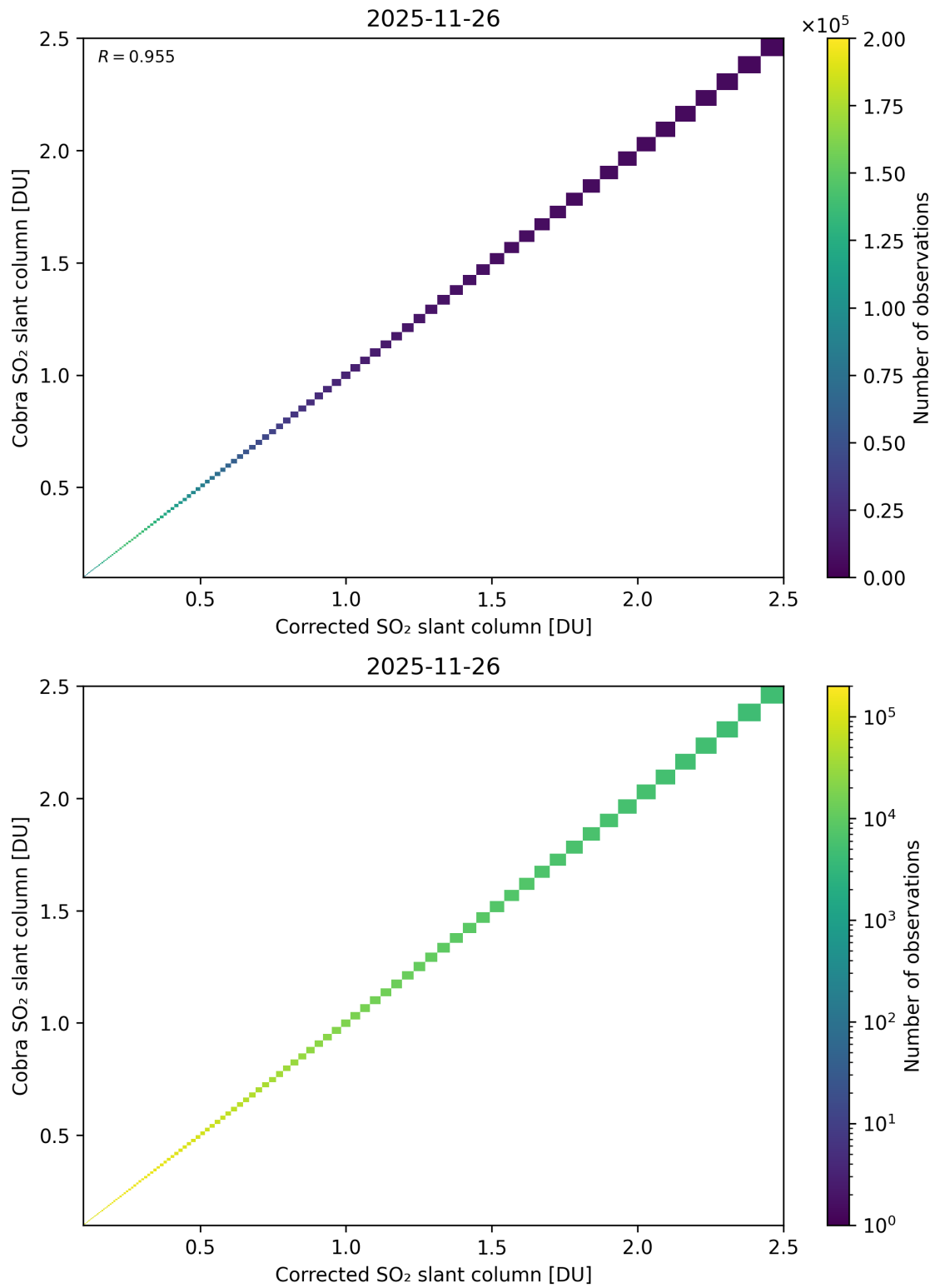
Figure 233: Scatter density plot of “Corrected SO 2 slant column” against “Cobra SO 2 slant column” for 2025-11-25 to 2025-11-27.
