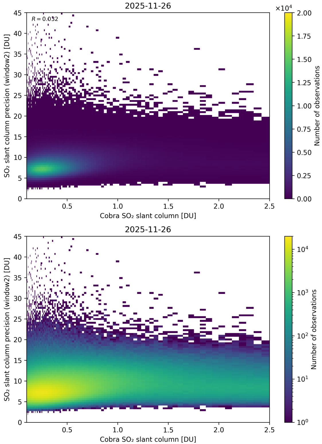
Figure 221: Scatter density plot of “Cobra SO 2 slant column” against “SO 2 slant column precision (window2)” for 2025-11-25 to 2025-11-27.
