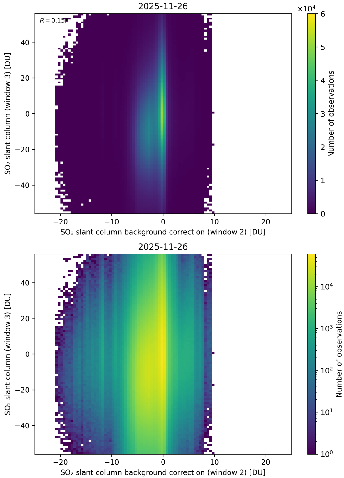
Figure 128: Scatter density plot of “SO 2 slant column background correction (window 2)” against “SO 2 slant column (window 3)” for 2025-11-25 to 2025-11-27.
