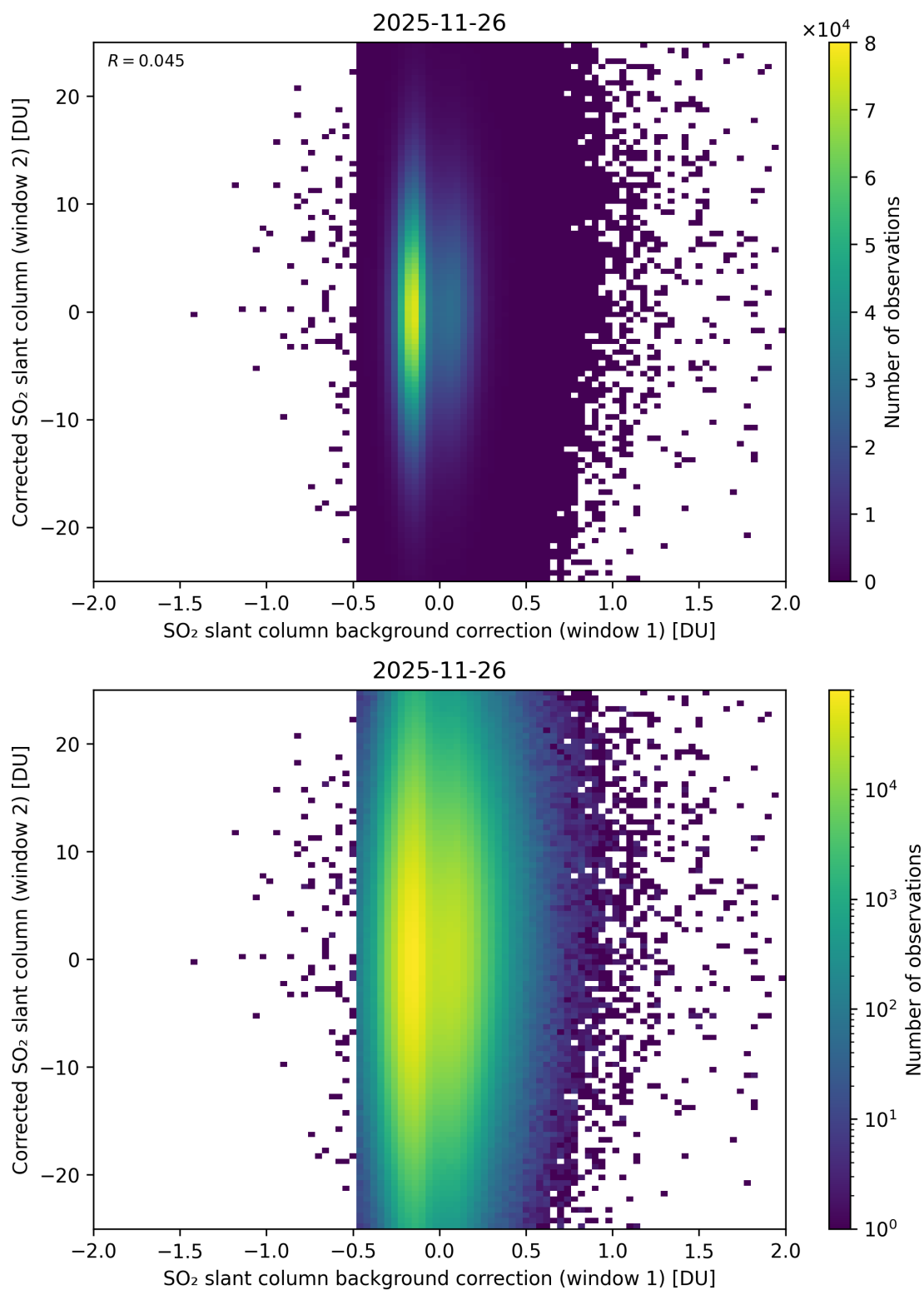
Figure 115: Scatter density plot of “SO 2 slant column background correction (window 1)” against “Corrected SO 2 slant column (window 2)” for 2025-11-25 to 2025-11-27.
