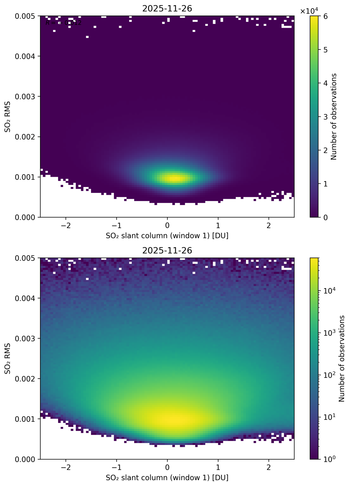
Figure 267: Scatter density plot of “SO 2 slant column (window 1)” against “SO 2 RMS” for 2025-11-25 to 2025-11-27.
