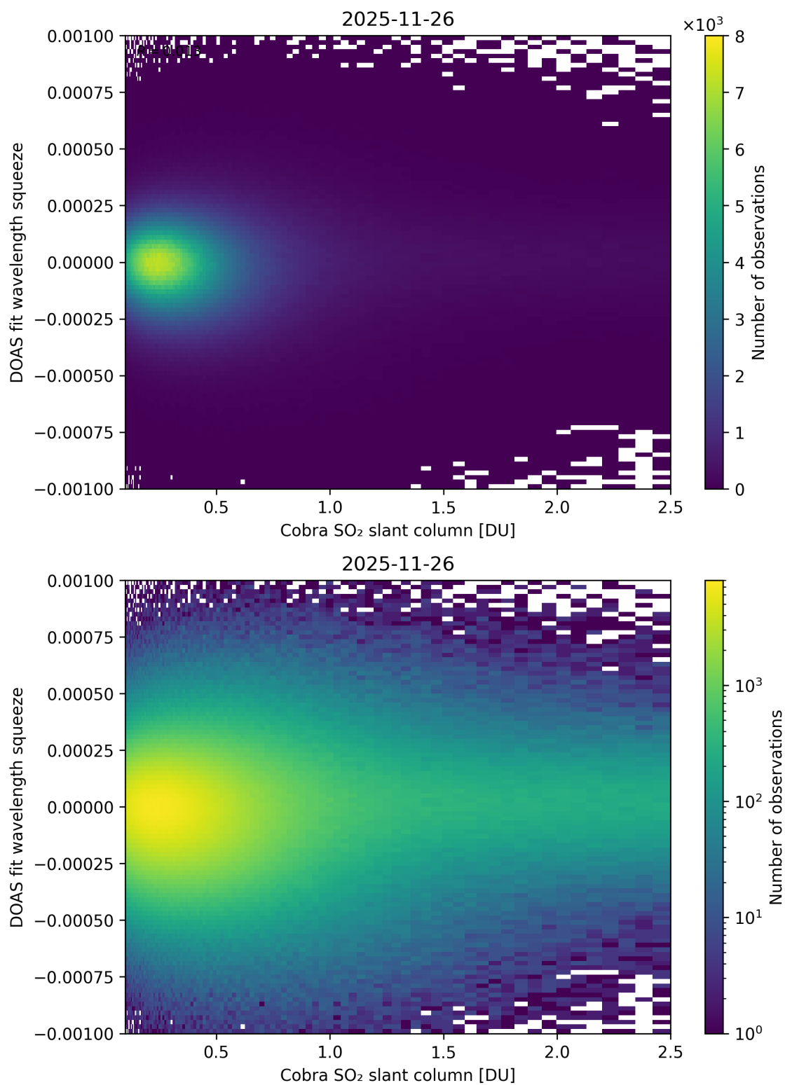
Figure 197: Scatter density plot of “Cobra SO 2 slant column” against “DOAS fit wavelength squeeze” for 2025-11-25 to 2025-11-27.
