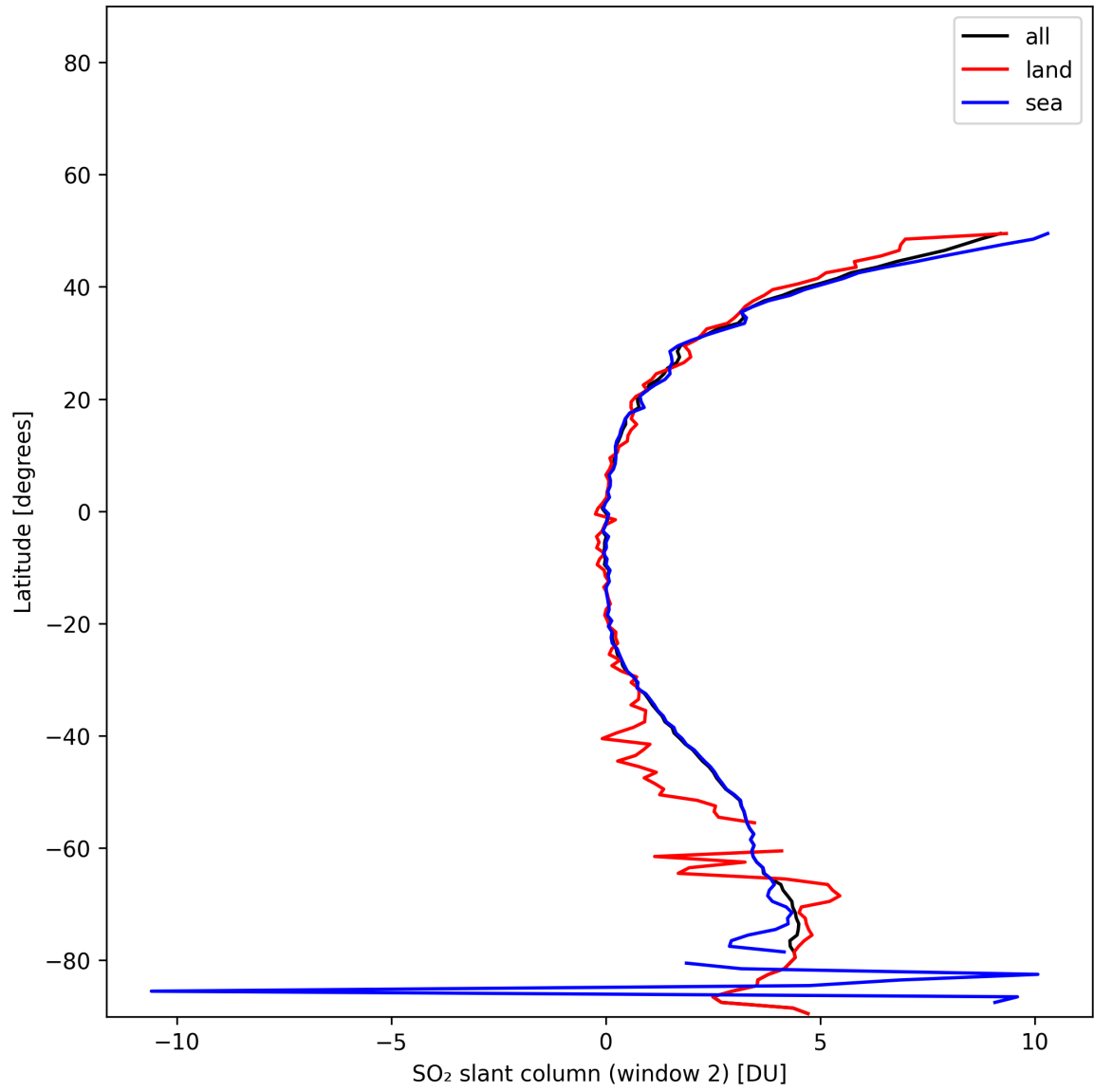
Figure 41: Zonal average of “SO 2 slant column (window 2)” for 2025-11-25 to 2025-11-27.
