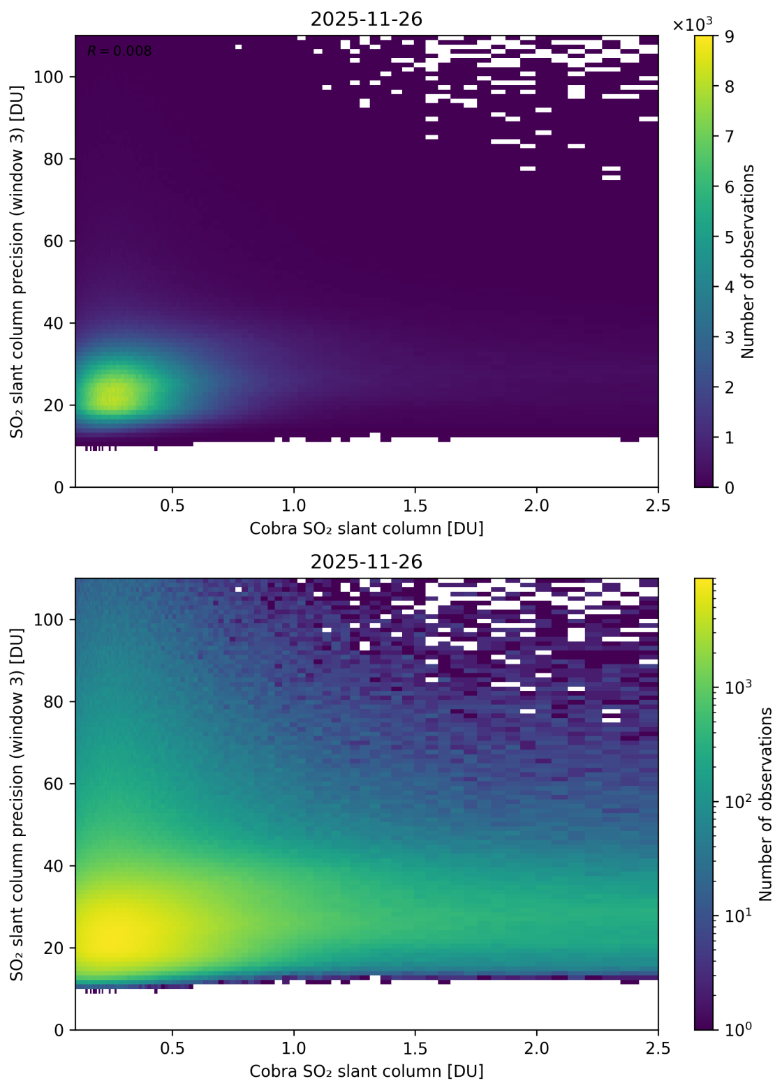
Figure 223: Scatter density plot of “Cobra SO 2 slant column” against “SO 2 slant column precision (window 3)” for 2025-11-25 to 2025-11-27.
