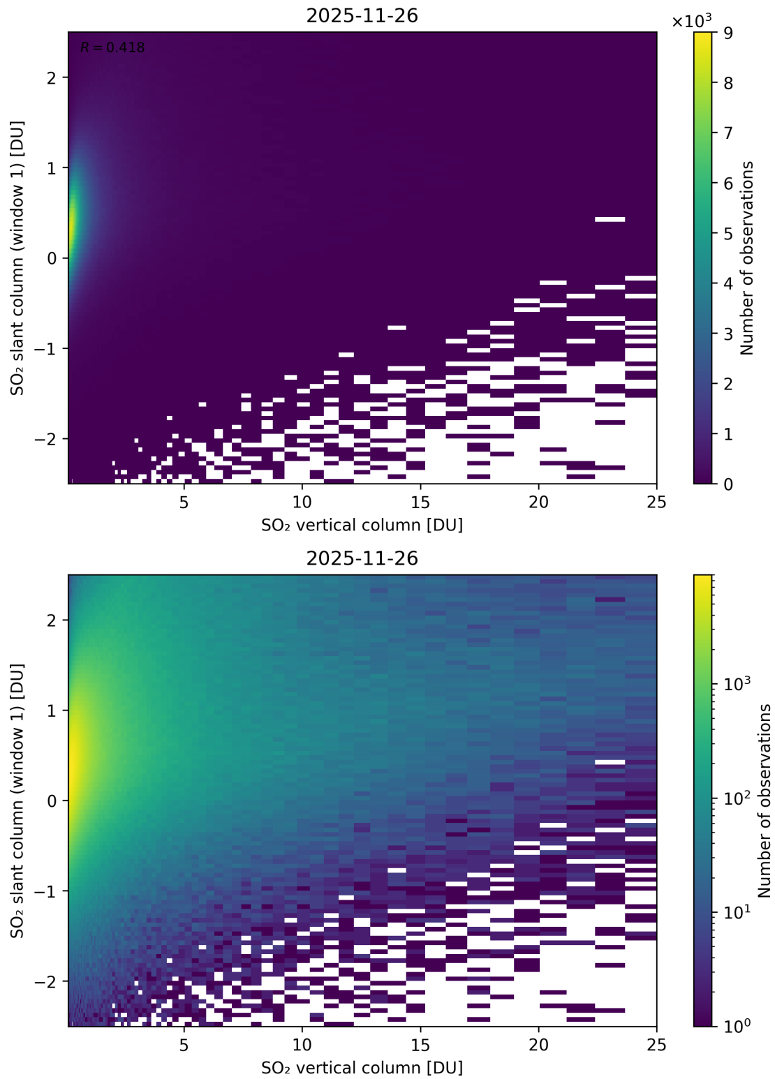
Figure 354: Scatter density plot of “SO 2 vertical column” against “SO 2 slant column (window 1)” for 2025-11-25 to 2025-11-27.
