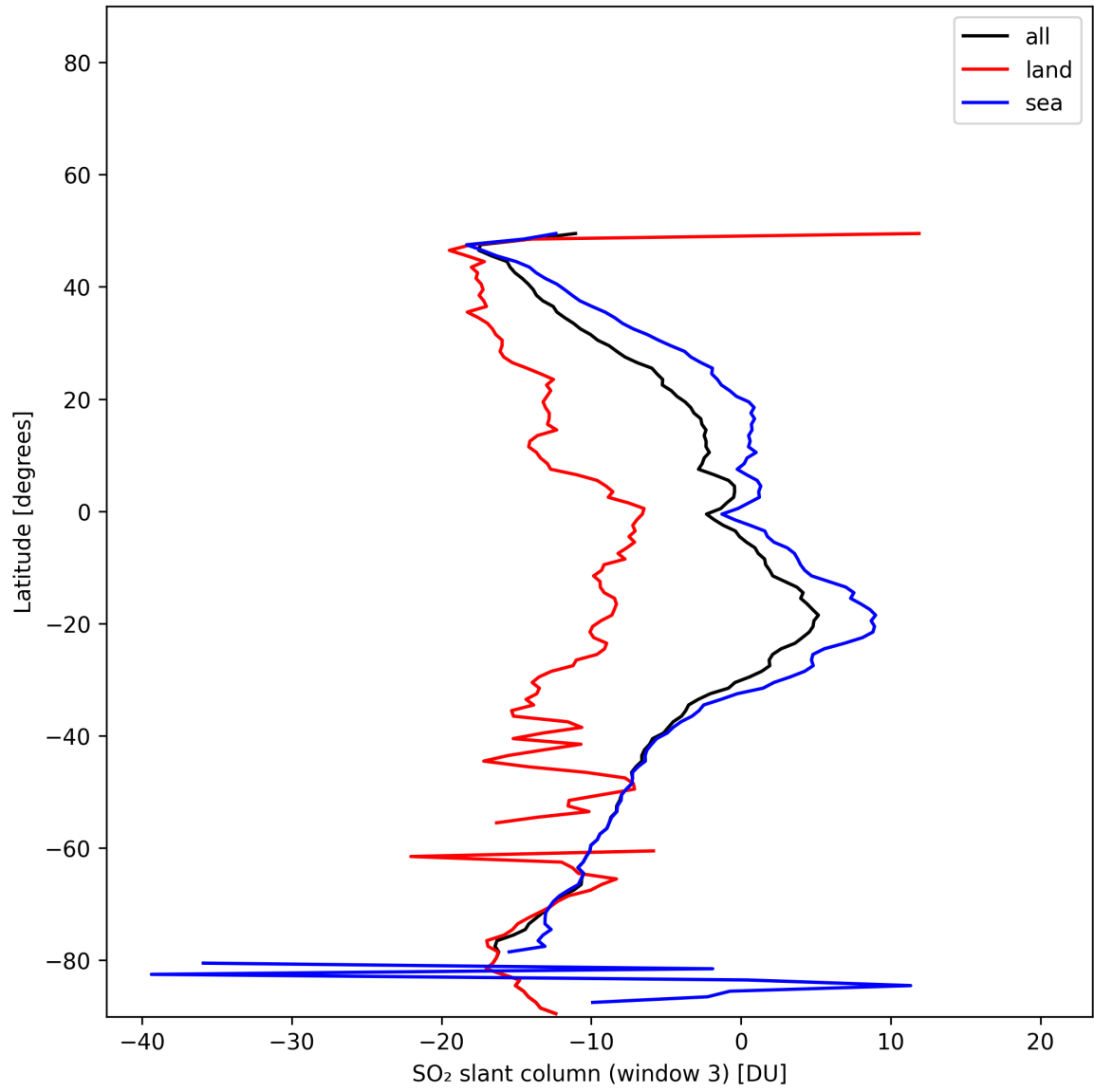
Figure 45: Zonal average of “SO 2 slant column (window 3)” for 2025-11-25 to 2025-11-27.
