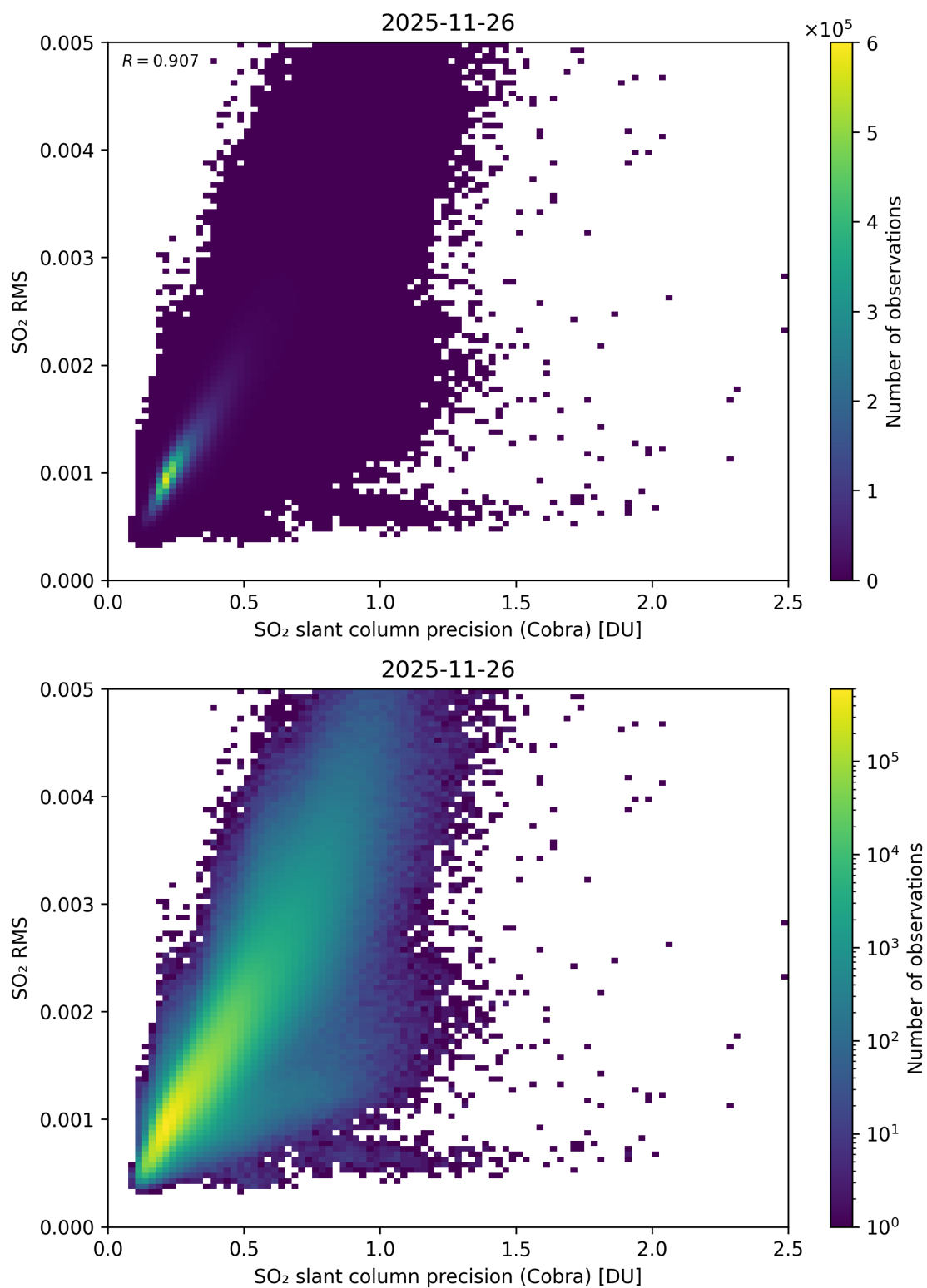
Figure 204: Scatter density plot of “SO 2 slant column precision (Cobra)” against “SO 2 RMS” for 2025-11-25 to 2025-11-27.
