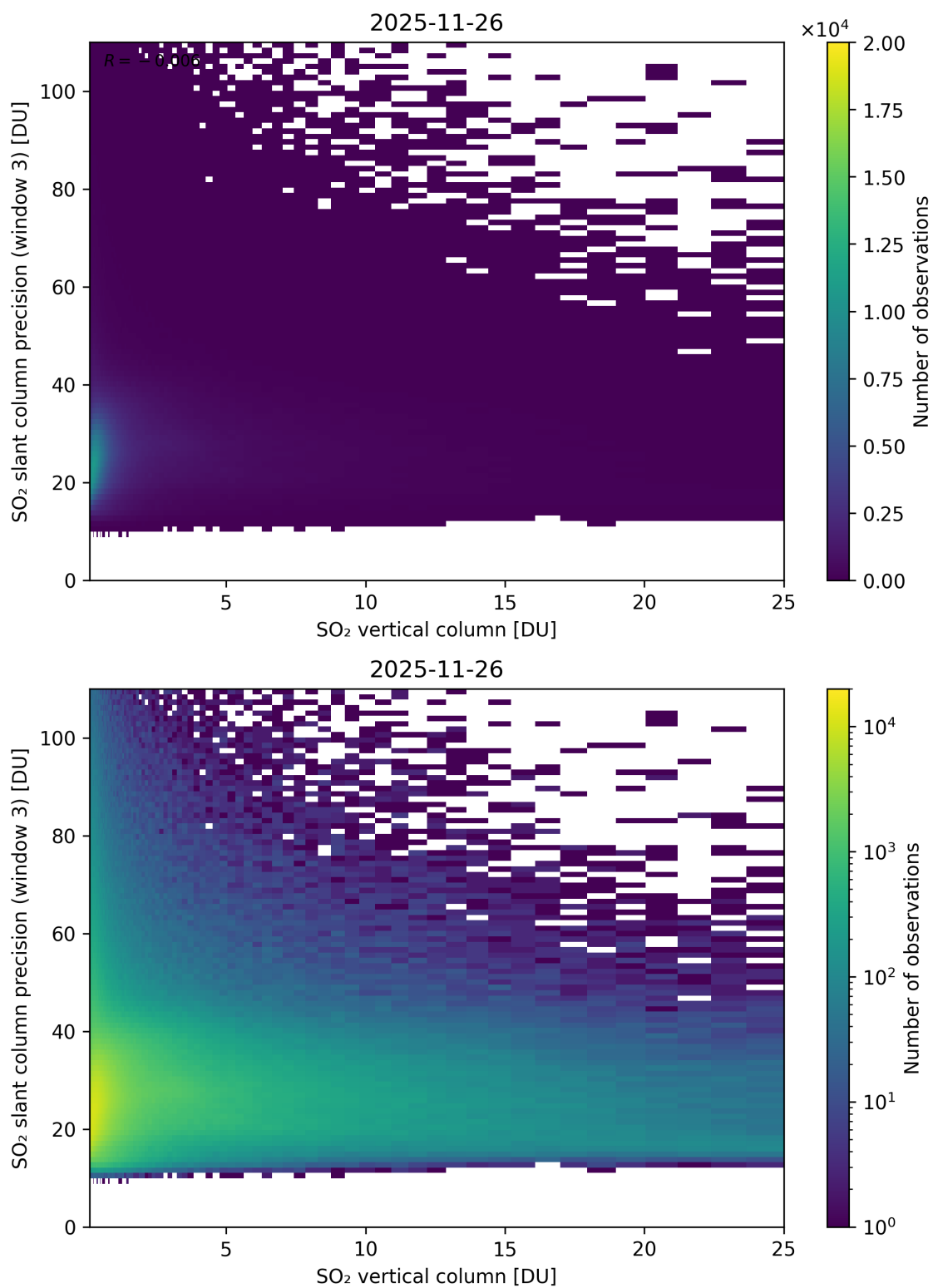
Figure 358: Scatter density plot of “SO 2 vertical column” against “SO 2 slant column precision (window 3)” for 2025-11-25 to 2025-11-27.
