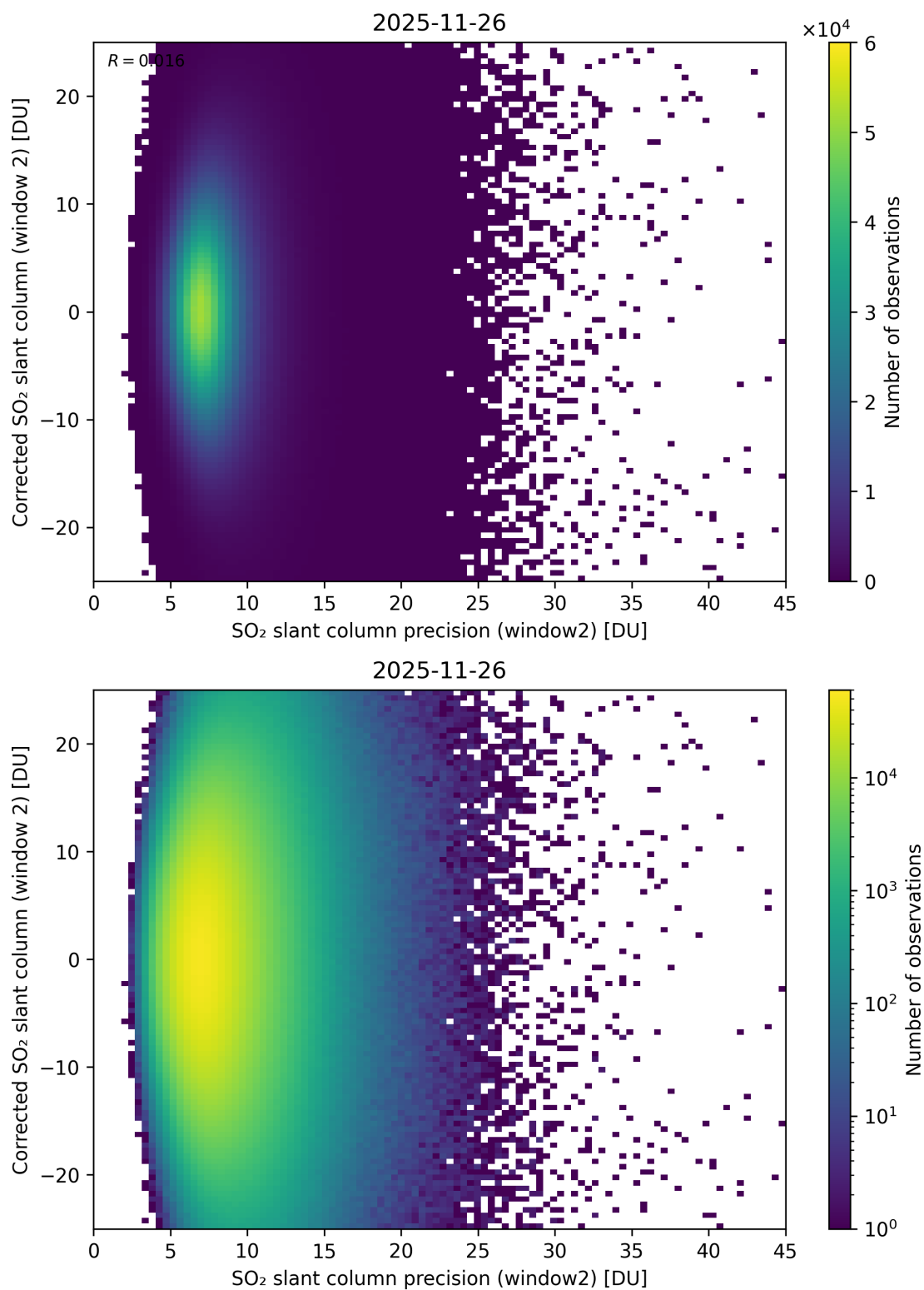
Figure 297: Scatter density plot of “SO 2 slant column precision (window2)” against “Corrected SO 2 slant column (window 2)” for 2025-11-25 to 2025-11-27.
