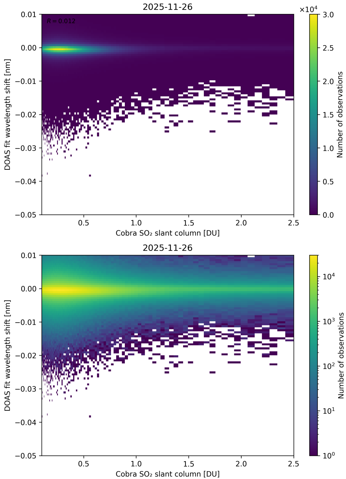
Figure 196: Scatter density plot of “Cobra SO 2 slant column” against “DOAS fit wavelength shift” for 2025-11-25 to 2025-11-27.
