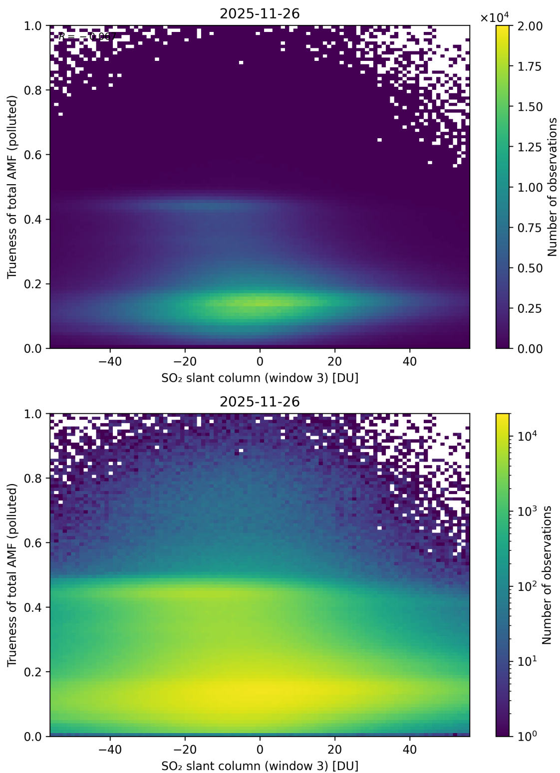
Figure 319: Scatter density plot of “SO 2 slant column (window 3)” against “Trueness of total AMF (polluted)” for 2025-11-25 to 2025-11-27.
