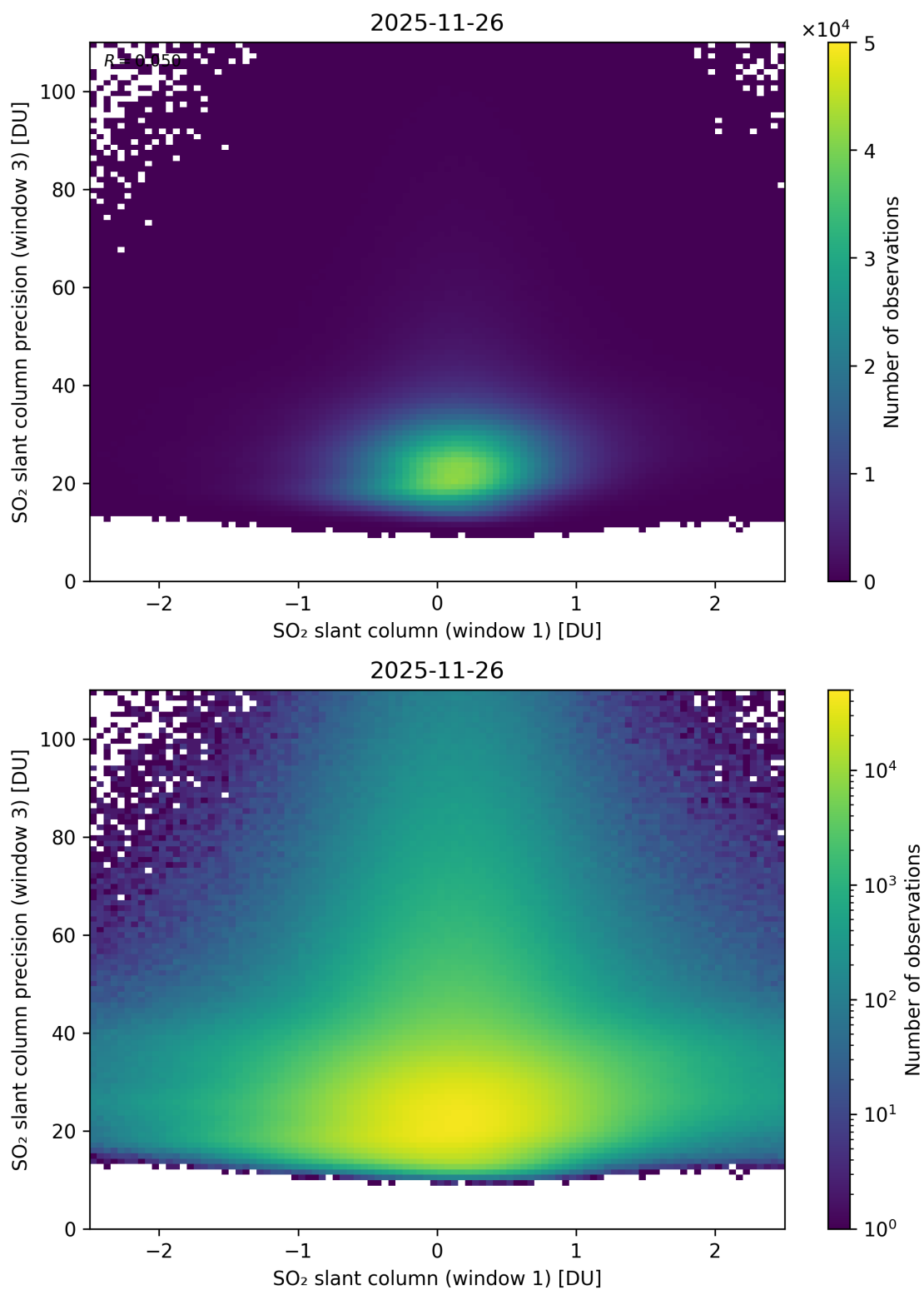
Figure 288: Scatter density plot of “SO 2 slant column (window 1)” against “SO 2 slant column precision (window 3)” for 2025-11-25 to 2025-11-27.
