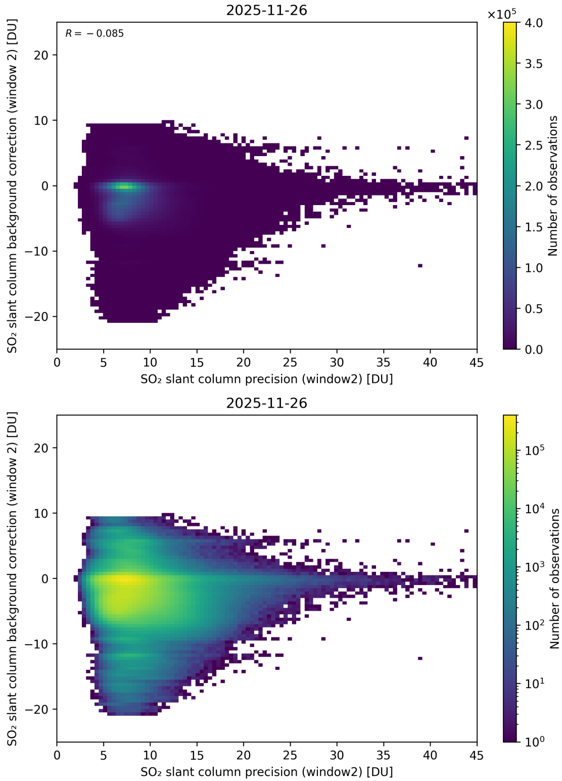
Figure 291: Scatter density plot of “SO 2 slant column precision (window2)” against “SO 2 slant column background correction (window 2)” for 2025-11-25 to 2025-11-27.
