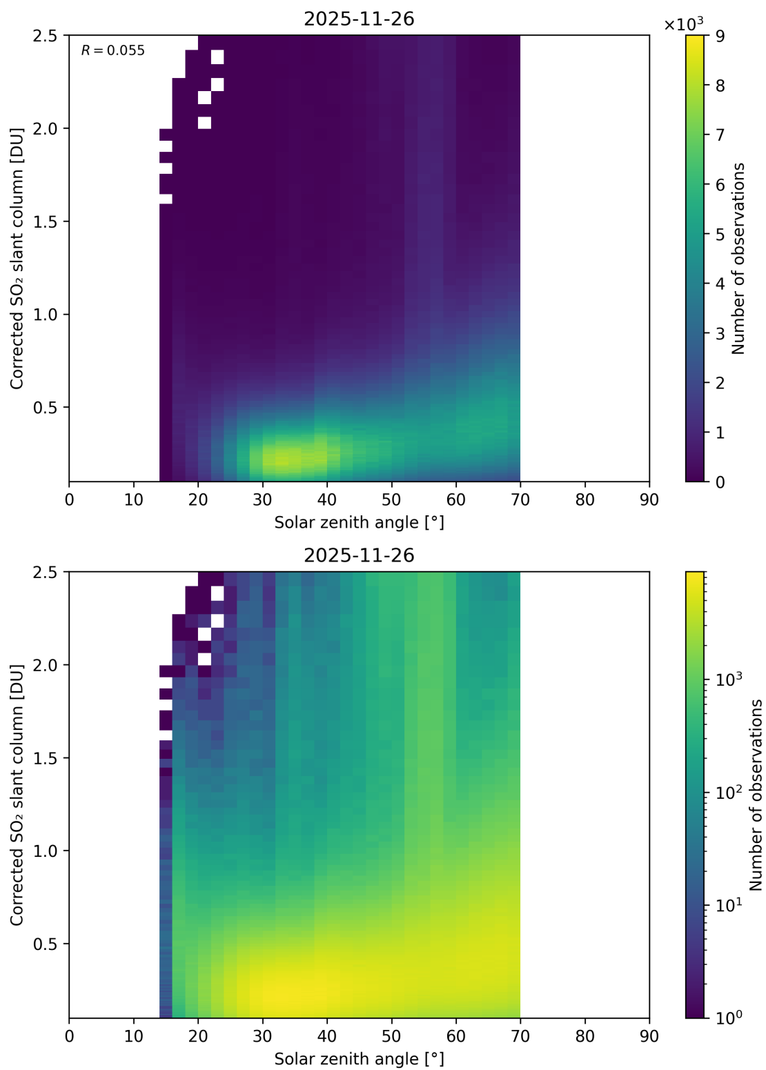
Figure 181: Scatter density plot of “Solar zenith angle” against “Corrected SO 2 slant column” for 2025-11-25 to 2025-11-27.
