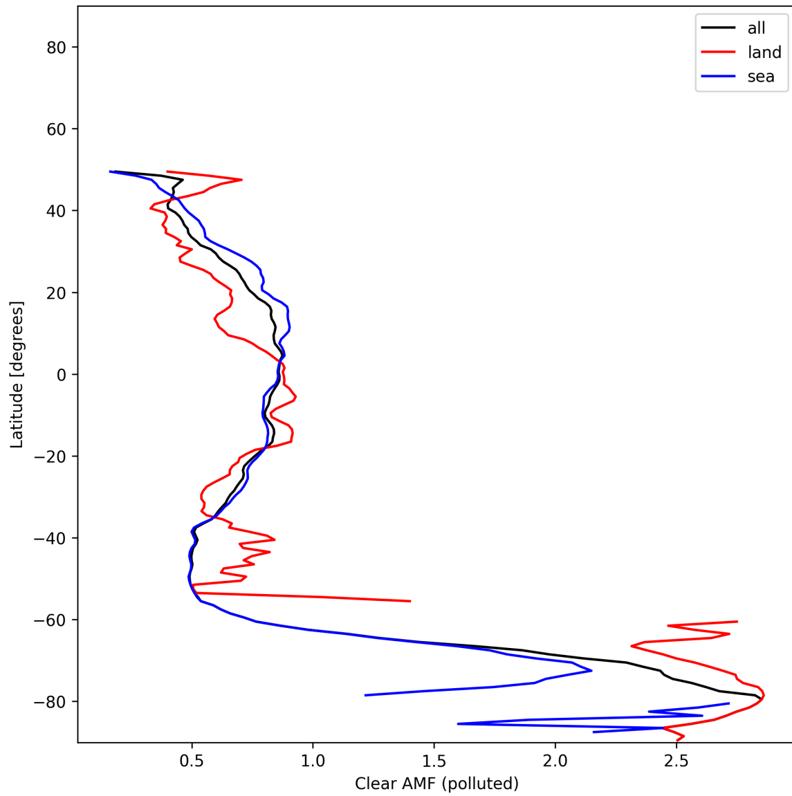
Figure 55: Zonal average of “Clear AMF (polluted)” for 2025-11-25 to 2025-11-27.
