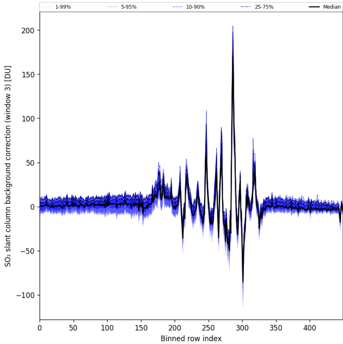
Figure 100: Along track statistics of “SO 2 slant column background correction (window 3)” for 2025-11-25 to 2025-11-27
