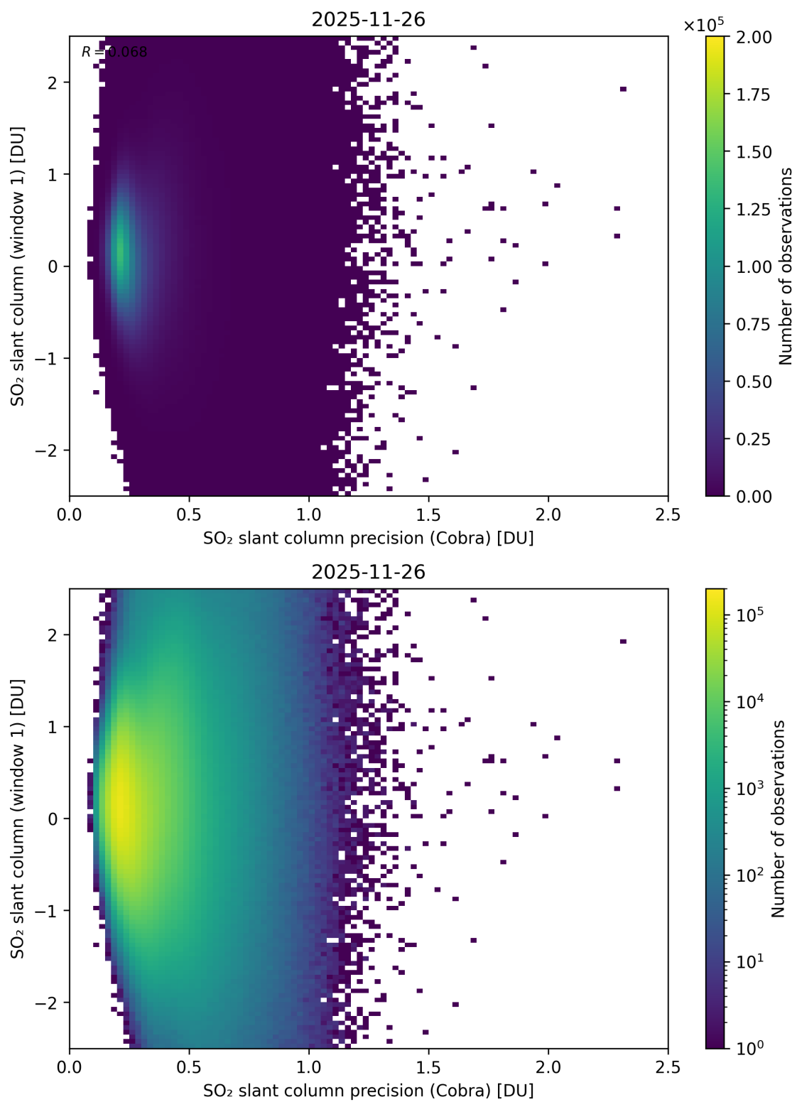
Figure 208: Scatter density plot of “SO 2 slant column precision (Cobra)” against “SO 2 slant column (window 1)” for 2025-11-25 to 2025-11-27.
