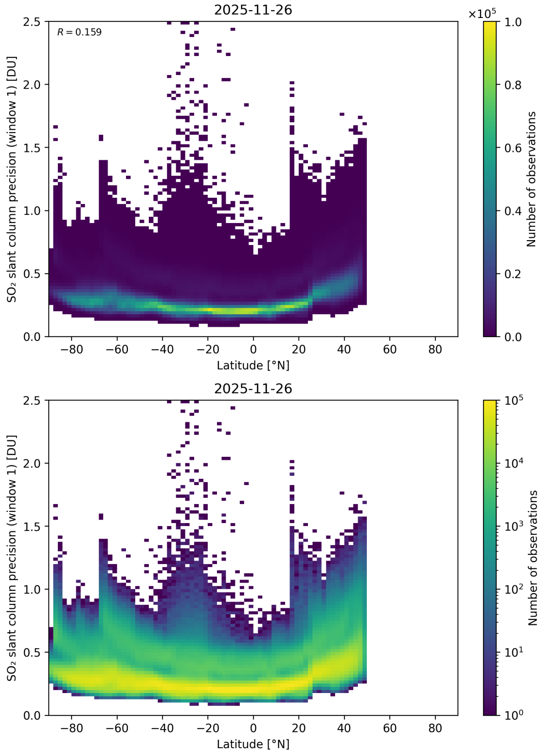
Figure 163: Scatter density plot of “Latitude” against “SO 2 slant column precision (window 1)” for 2025-11-25 to 2025-11-27.
