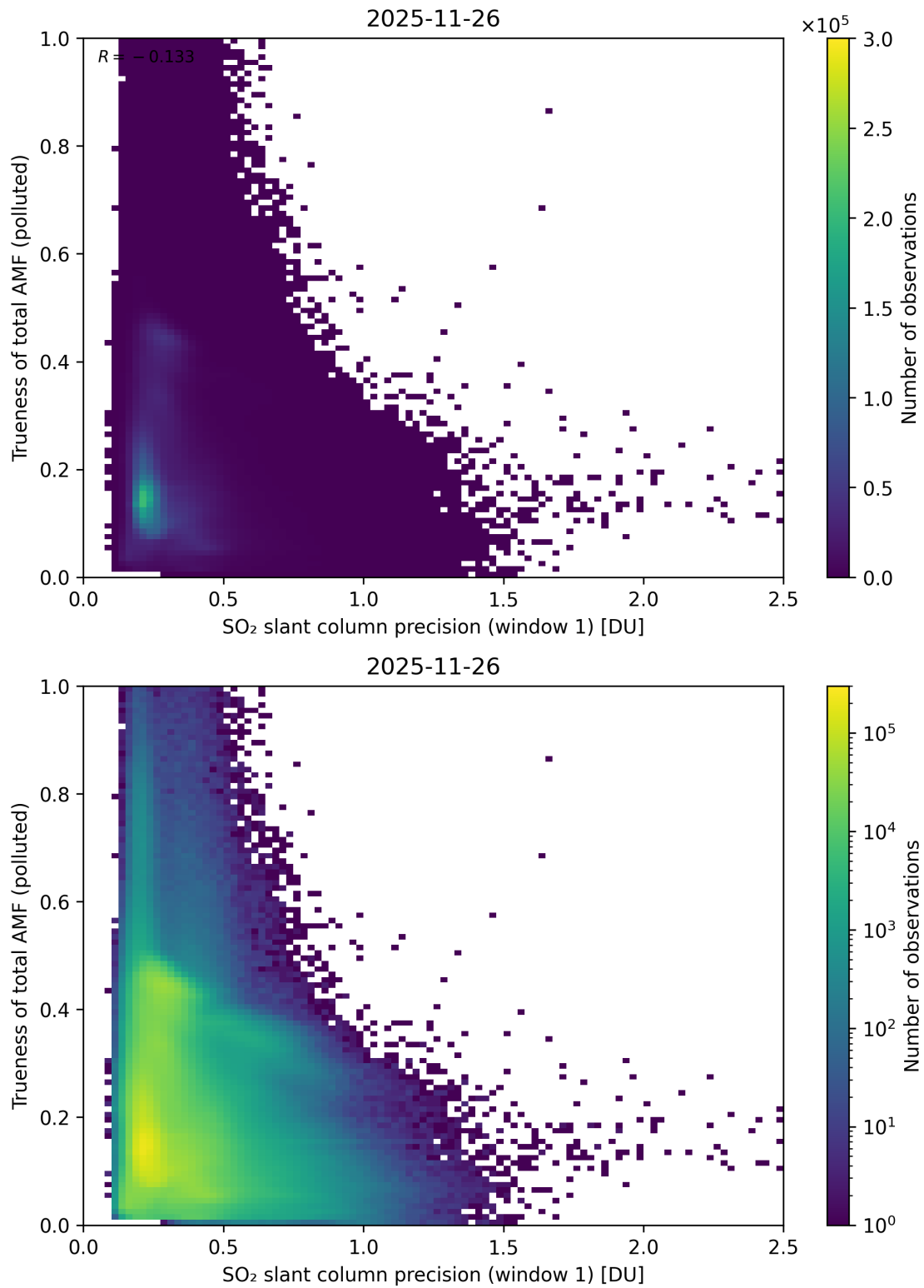
Figure 281: Scatter density plot of “SO 2 slant column precision (window 1)” against “Trueness of total AMF (polluted)” for 2025-11-25 to 2025-11-27.
