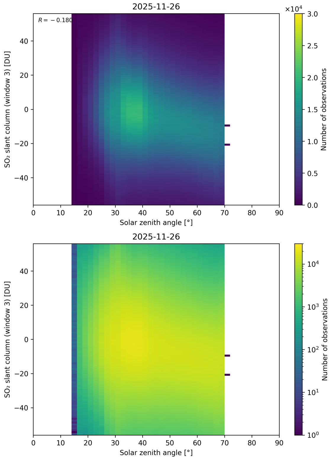
Figure 187: Scatter density plot of “Solar zenith angle” against “SO 2 slant column (window 3)” for 2025-11-25 to 2025-11-27.
