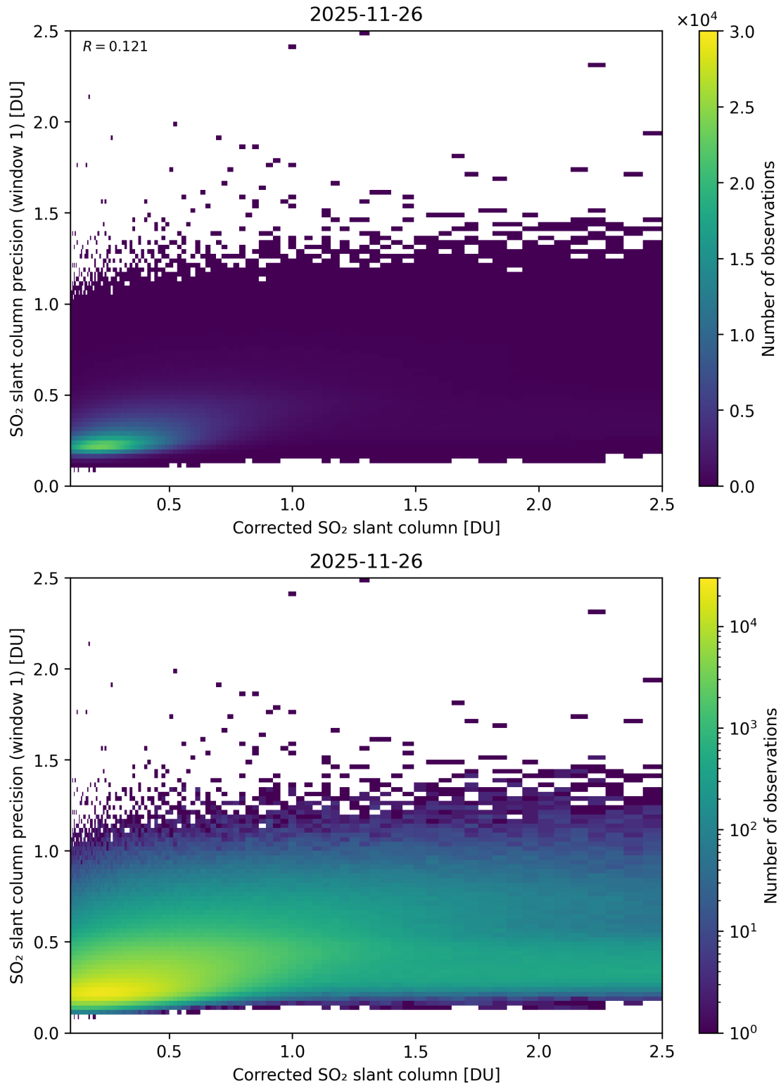
Figure 238: Scatter density plot of “Corrected SO 2 slant column” against “SO 2 slant column precision (window 1)” for 2025-11-25 to 2025-11-27.
