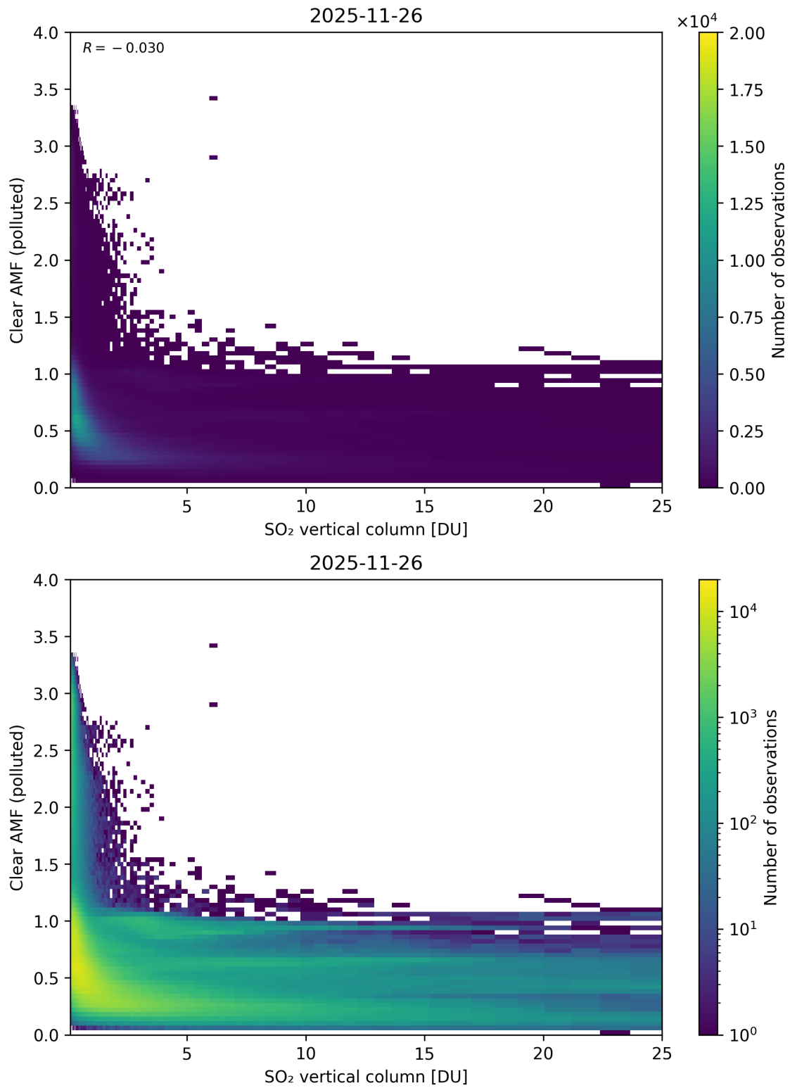
Figure 348: Scatter density plot of “SO 2 vertical column” against “Clear AMF (polluted)” for 2025-11-25 to 2025-11-27.
