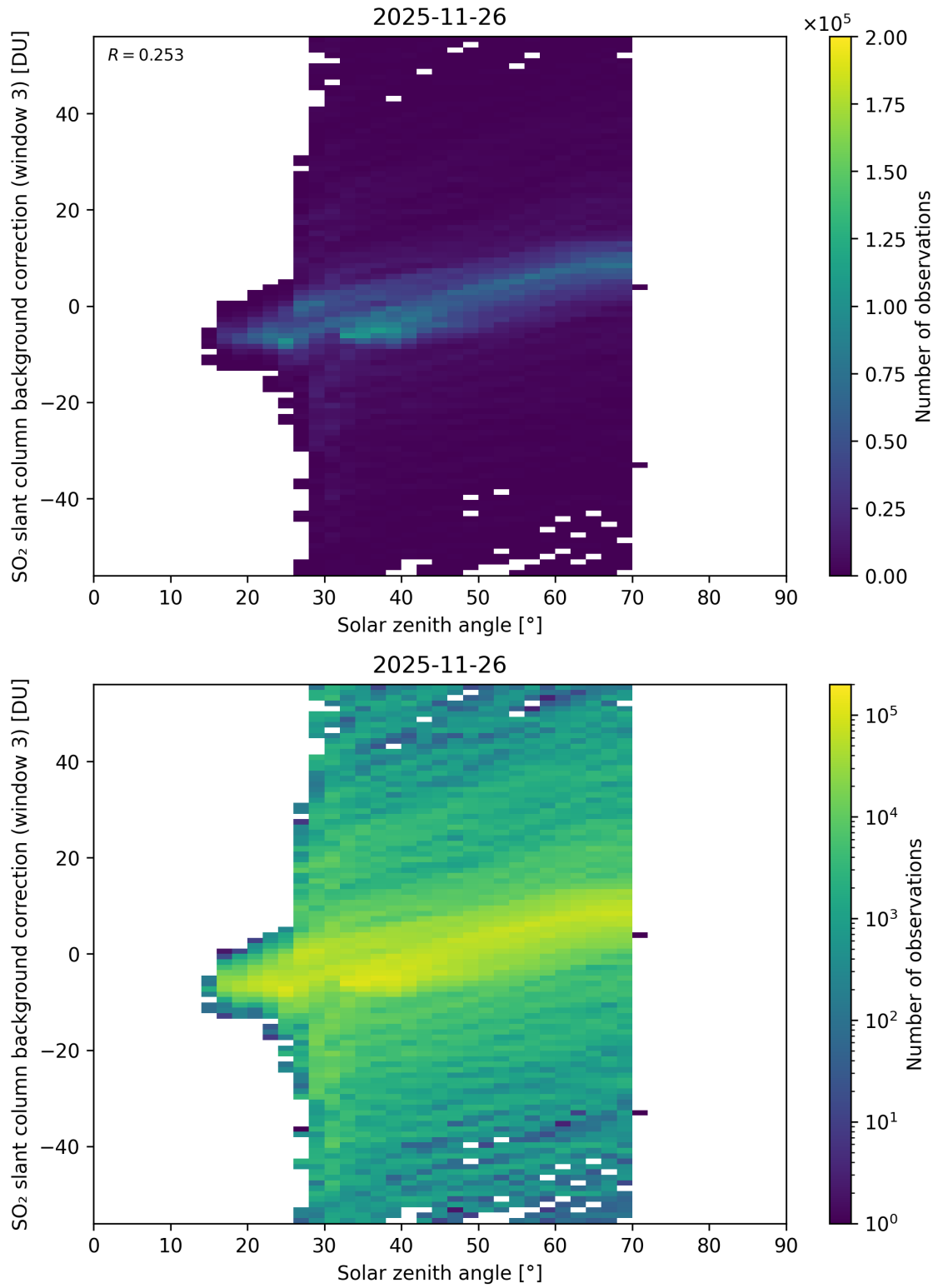
Figure 173: Scatter density plot of “Solar zenith angle” against “SO 2 slant column background correction (window 3)” for 2025-11-25 to 2025-11-27.
