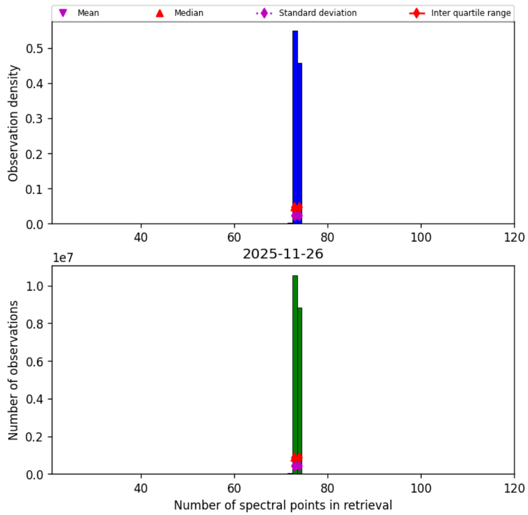
Figure 82: Histogram of “Number of spectral points in retrieval” for 2025-11-25 to 2025-11-27
