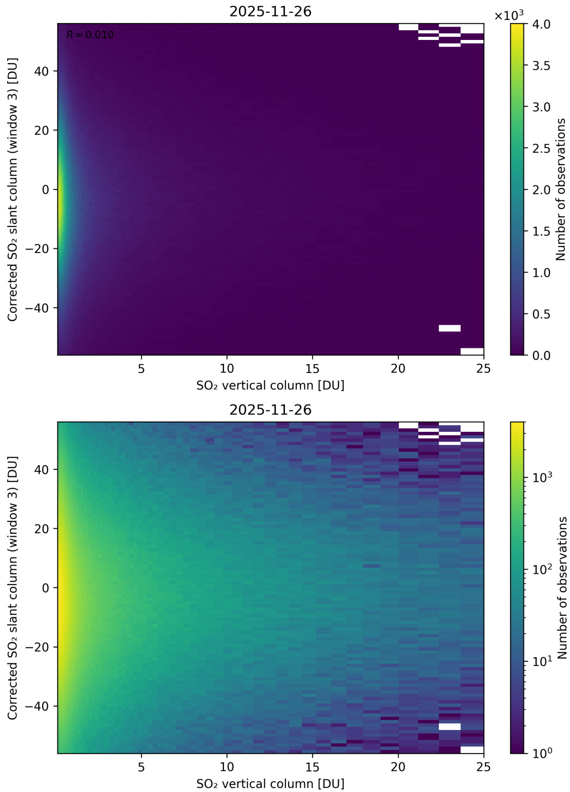
Figure 353: Scatter density plot of “SO 2 vertical column” against “Corrected SO 2 slant column (window 3)” for 2025-11-25 to 2025-11-27.
