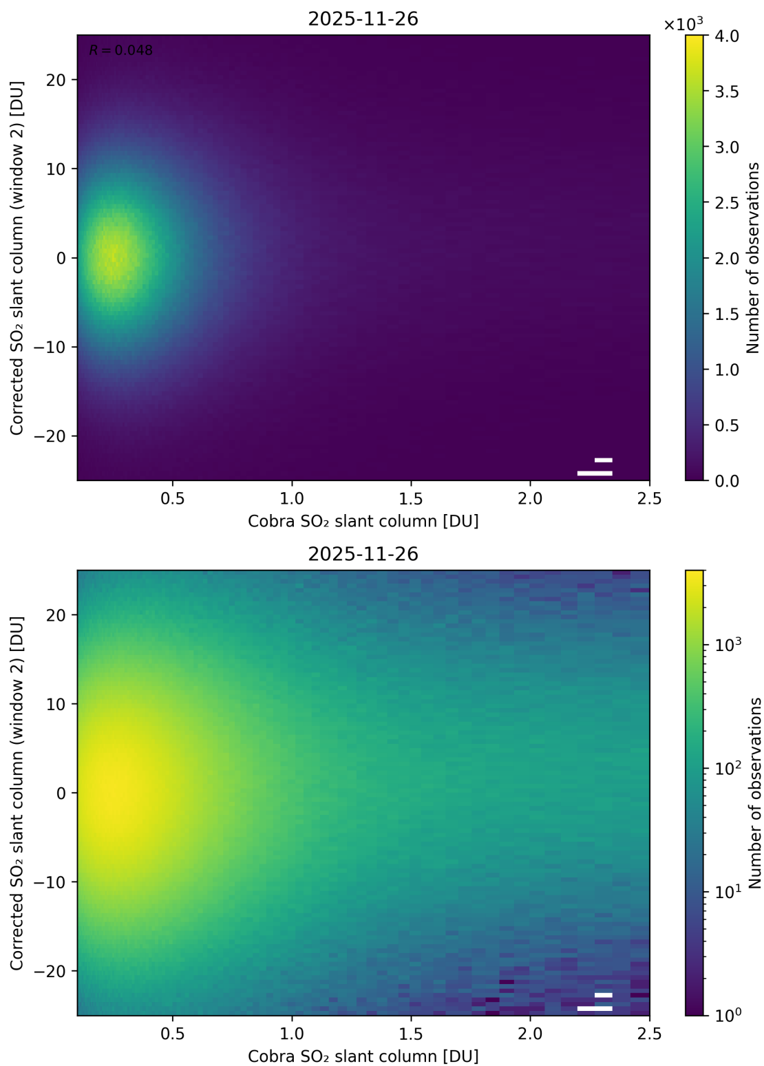
Figure 217: Scatter density plot of “Cobra SO 2 slant column” against “Corrected SO 2 slant column (window 2)” for 2025-11-25 to 2025-11-27.
