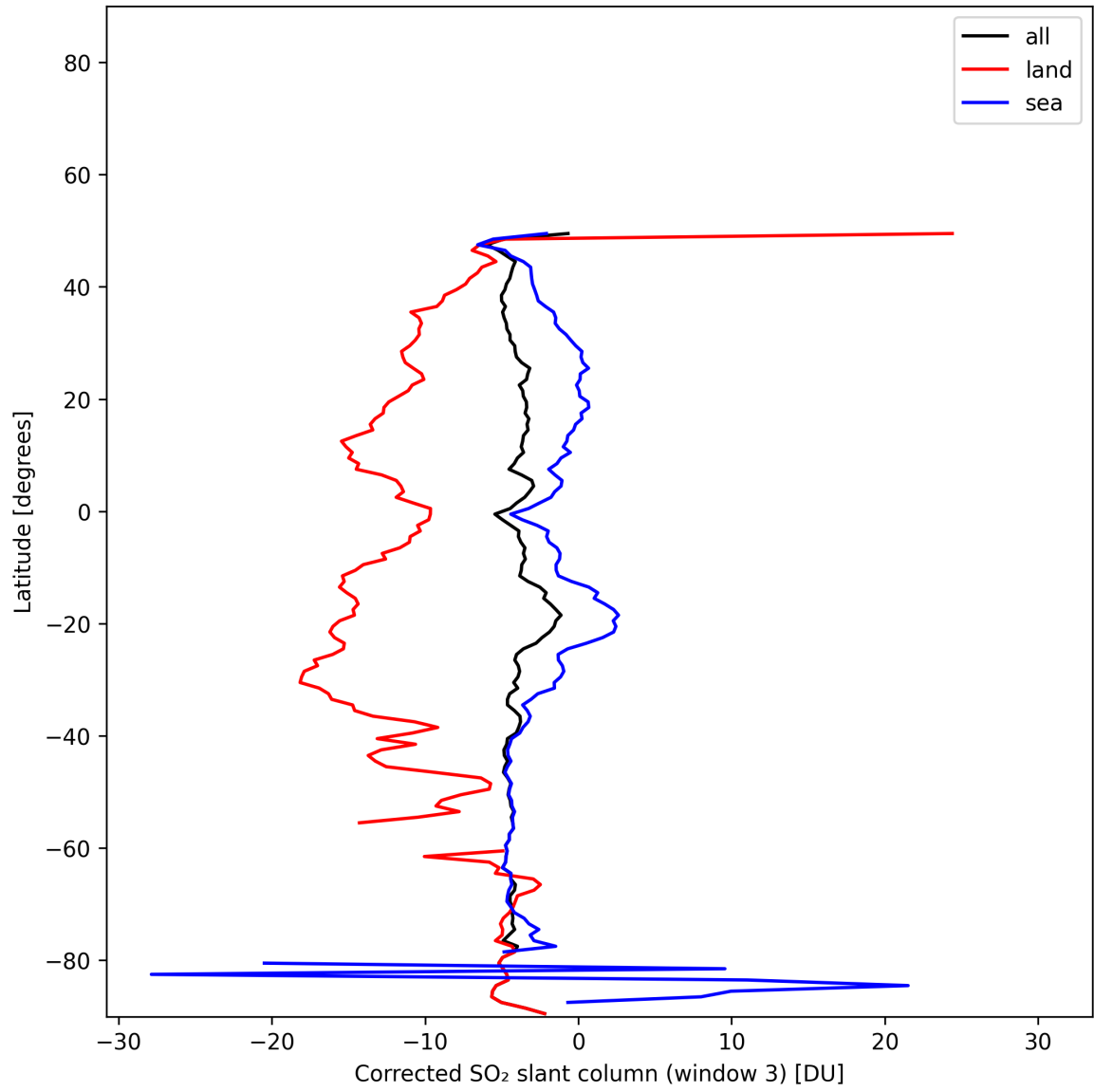
Figure 47: Zonal average of “Corrected SO 2 slant column (window 3)” for 2025-11-25 to 2025-11-27.
