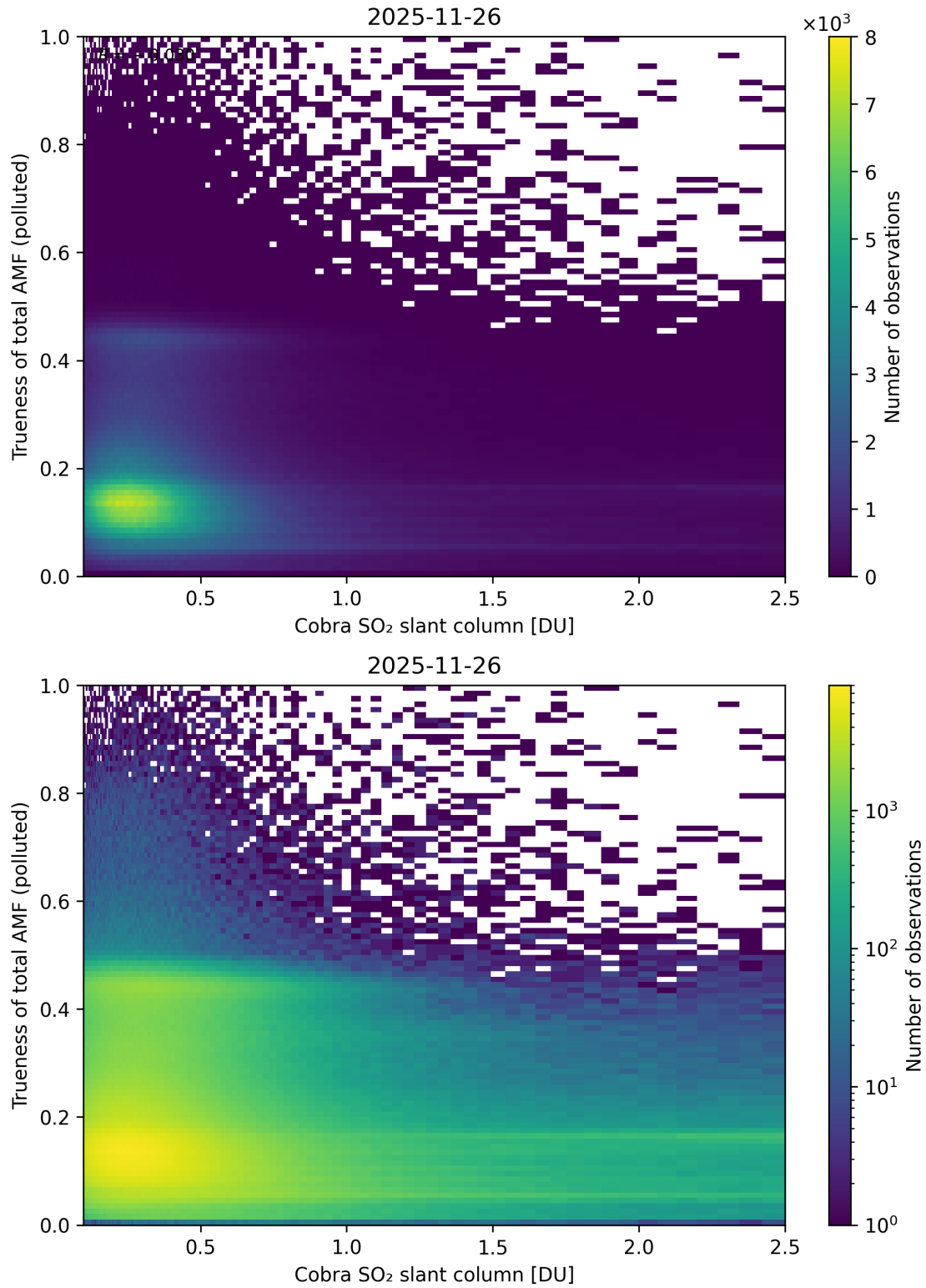
Figure 225: Scatter density plot of “Cobra SO 2 slant column” against “Trueness of total AMF (polluted)” for 2025-11-25 to 2025-11-27.
