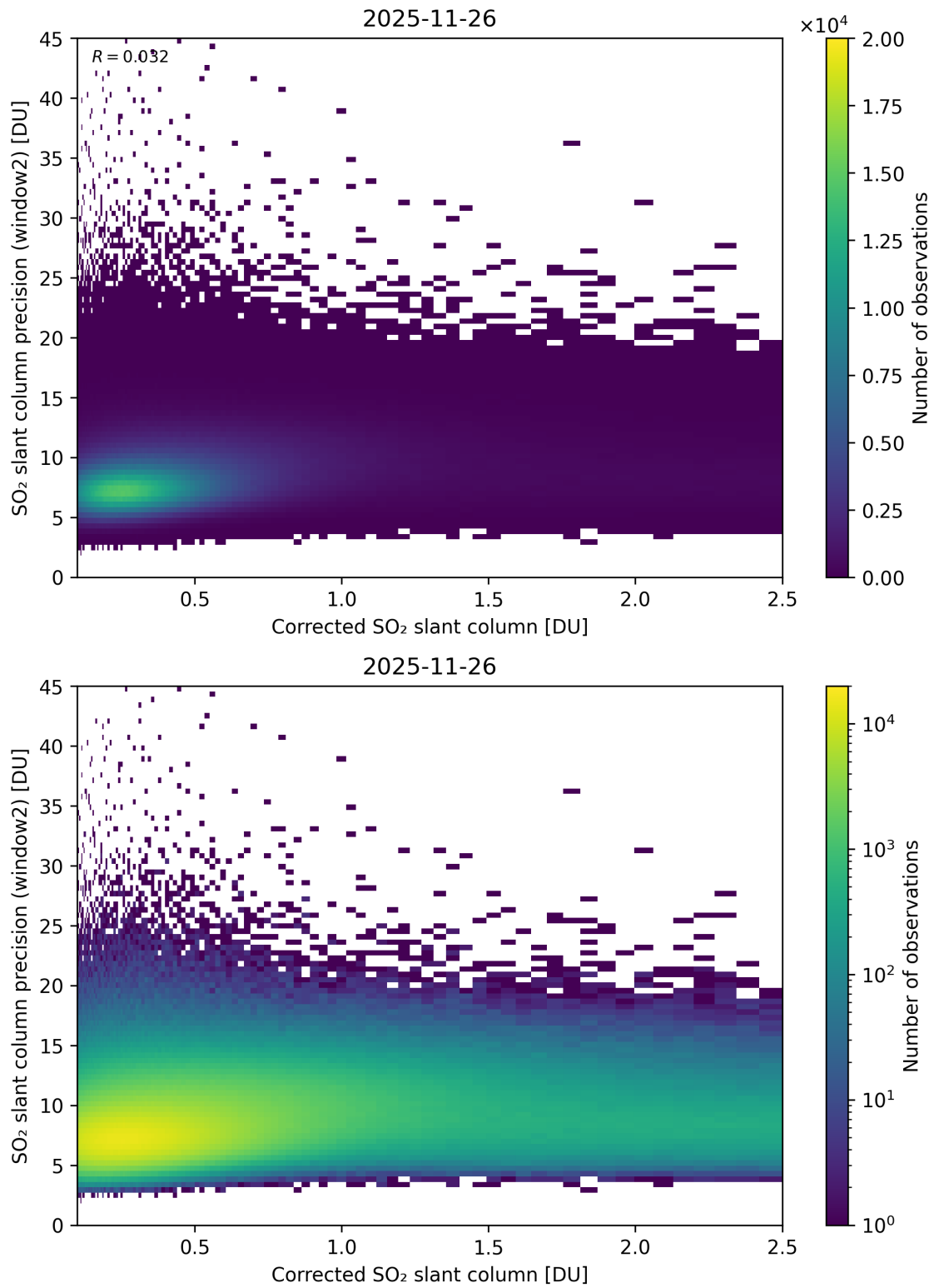
Figure 239: Scatter density plot of “Corrected SO 2 slant column” against “SO 2 slant column precision (window2)” for 2025-11-25 to 2025-11-27.
