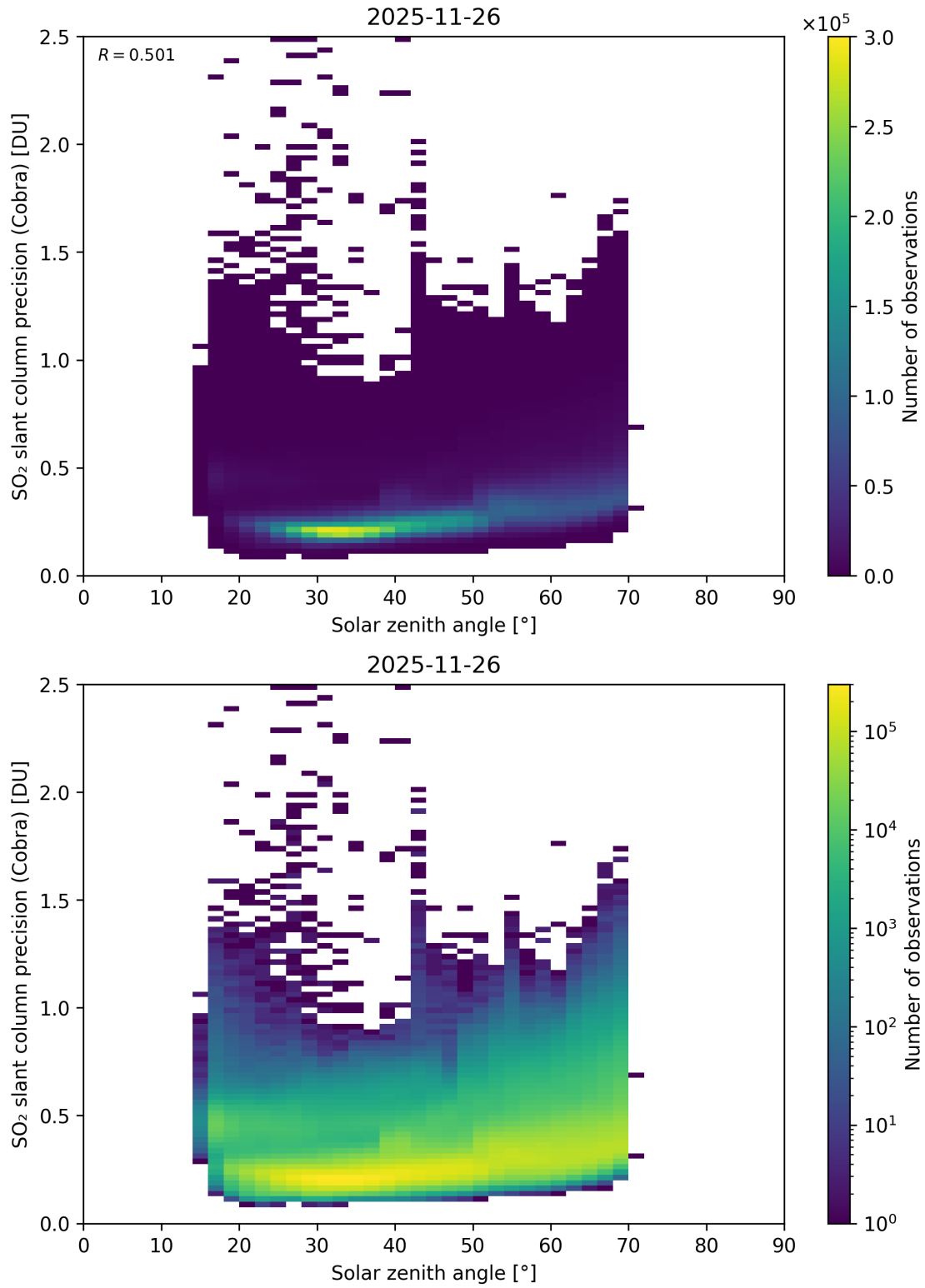
Figure 180: Scatter density plot of “Solar zenith angle” against “SO 2 slant column precision (Cobra)” for 2025-11-25 to 2025-11-27.
