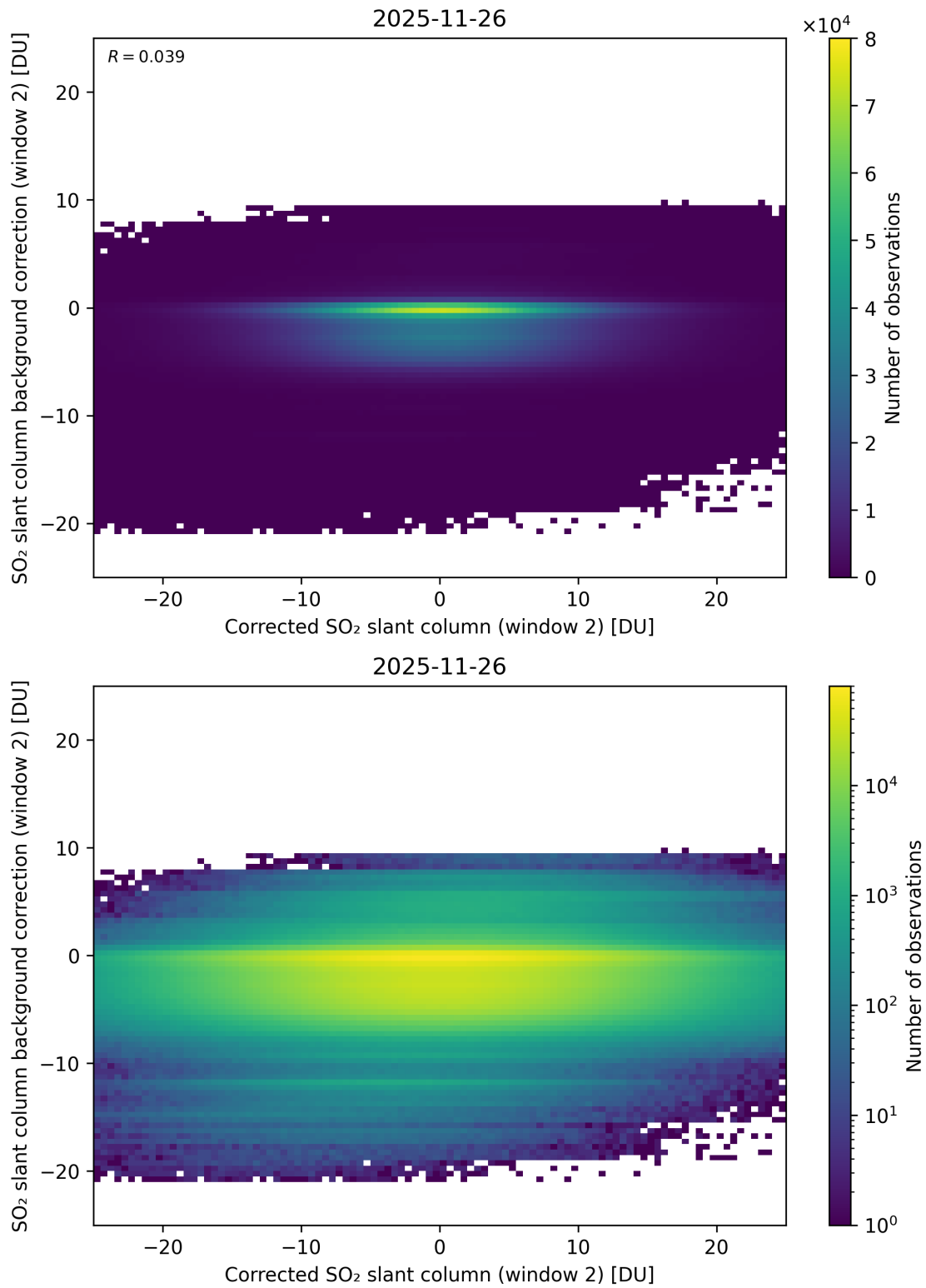
Figure 244: Scatter density plot of “Corrected SO 2 slant column (window 2)” against “SO 2 slant column background correction (window 2)” for 2025-11-25 to 2025-11-27.
