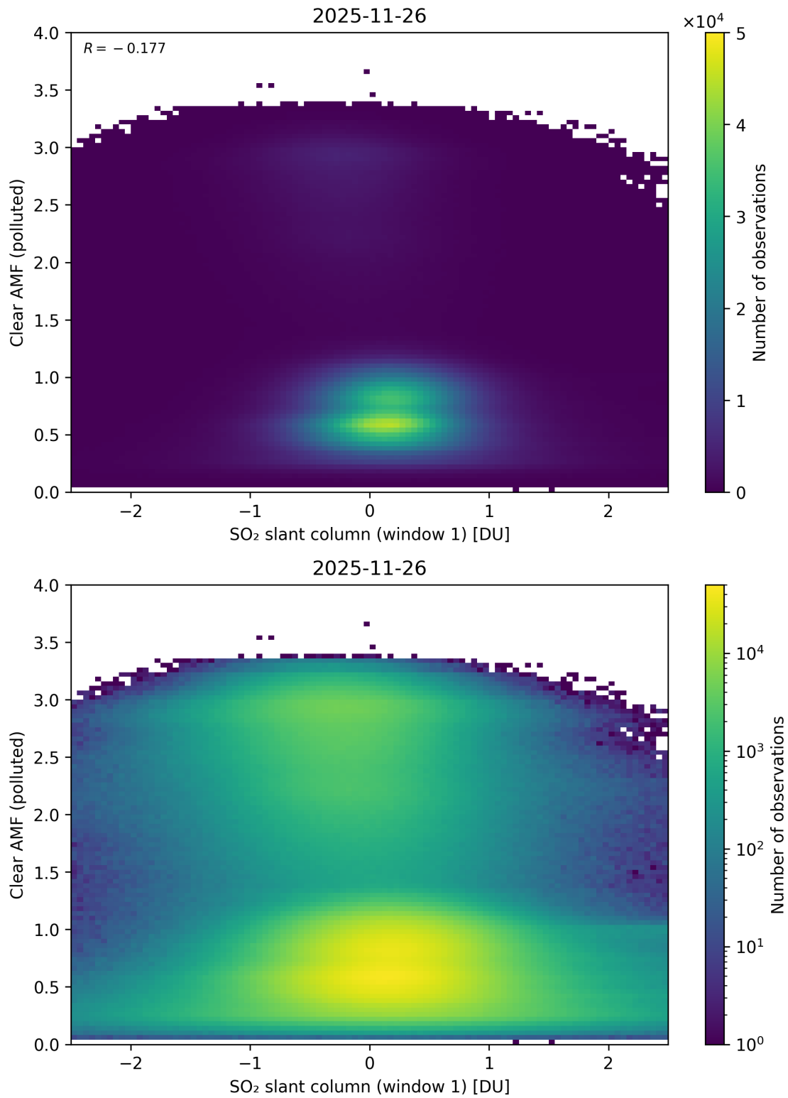
Figure 282: Scatter density plot of “SO 2 slant column (window 1)” against “Clear AMF (polluted)” for 2025-11-25 to 2025-11-27.
