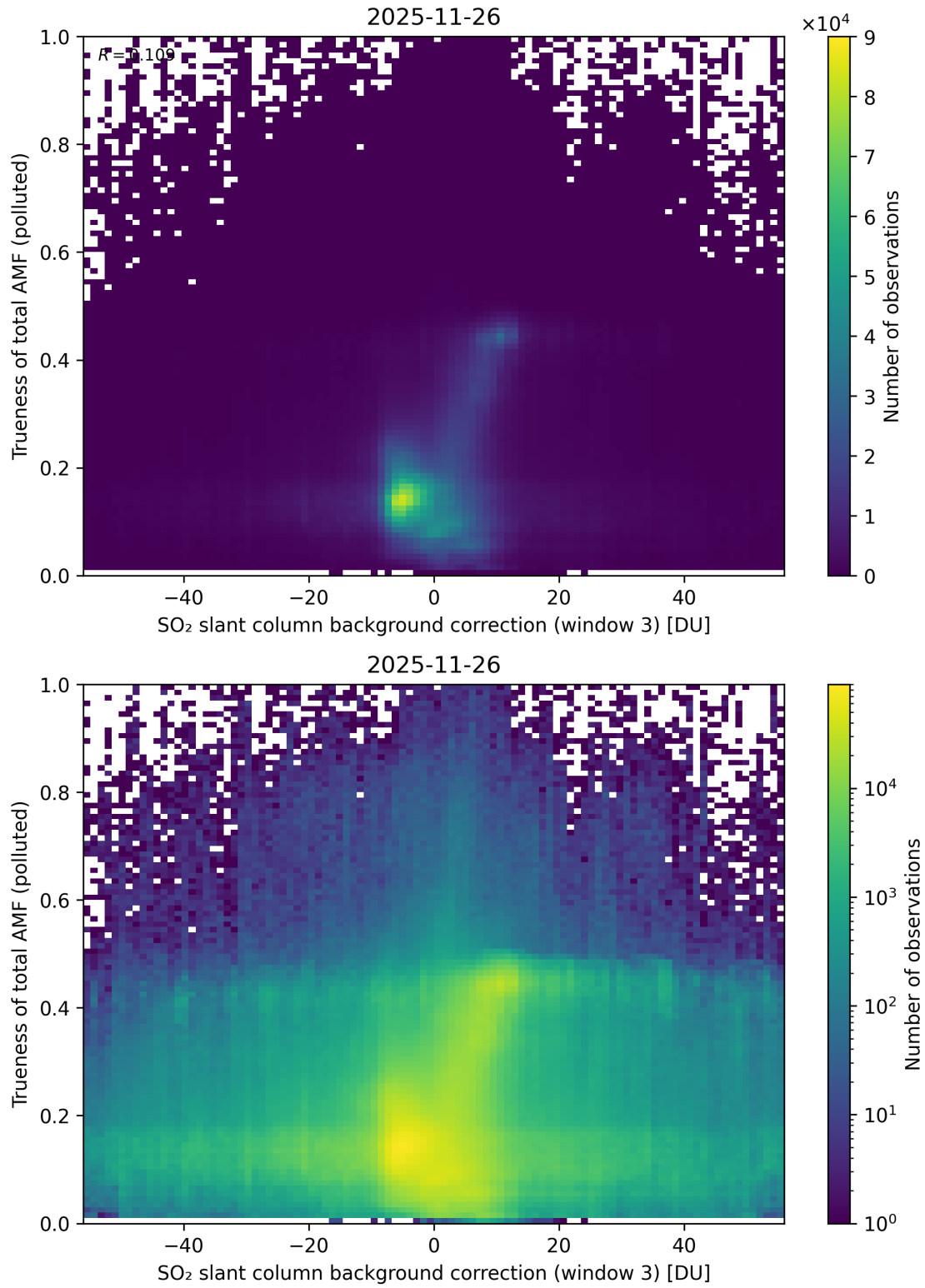
Figure 137: Scatter density plot of “SO 2 slant column background correction (window 3)” against “Trueness of total AMF (polluted)” for 2025-11-25 to 2025-11-27.
