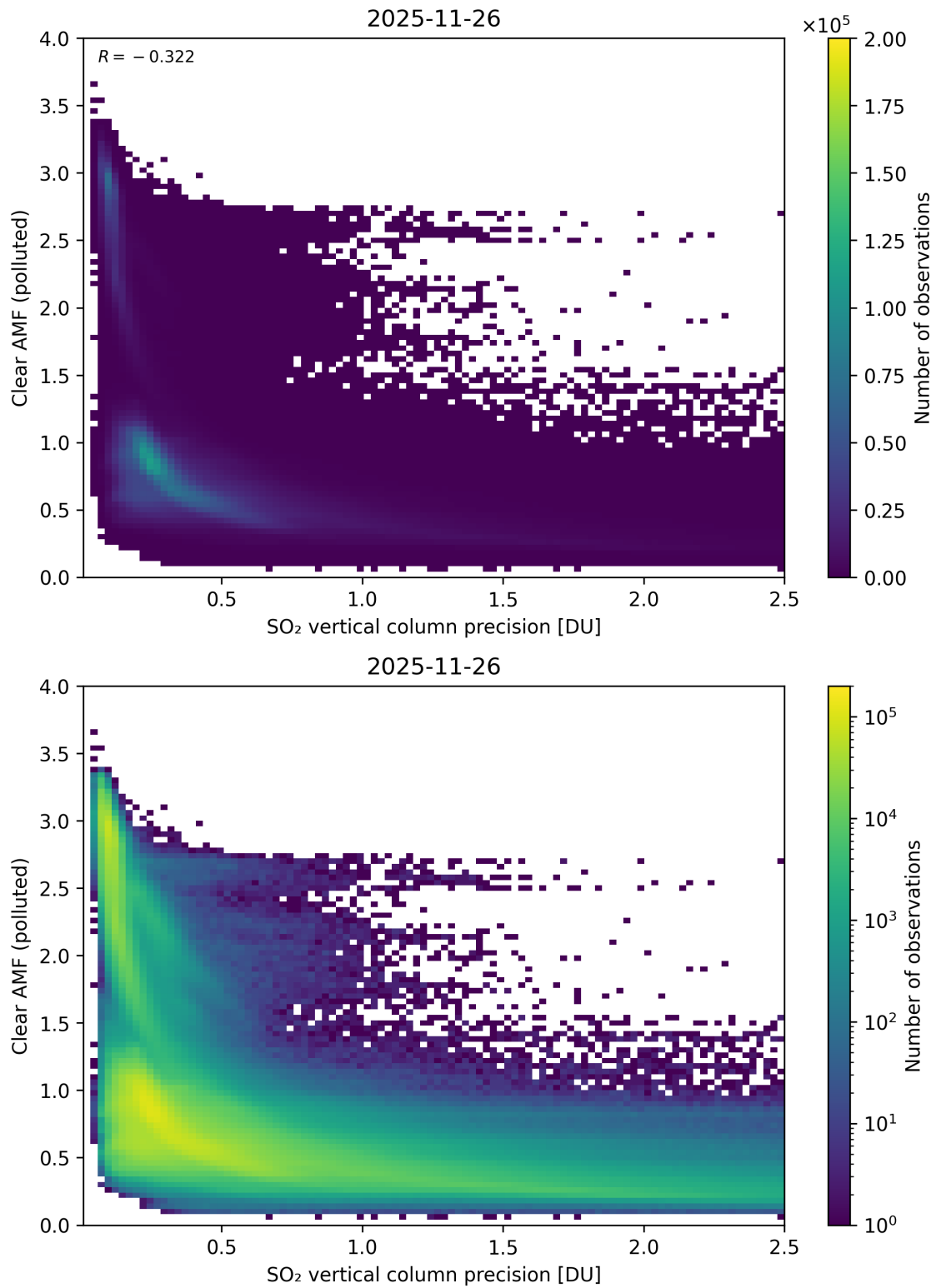
Figure 335: Scatter density plot of “SO 2 vertical column precision” against “Clear AMF (polluted)” for 2025-11-25 to 2025-11-27.
