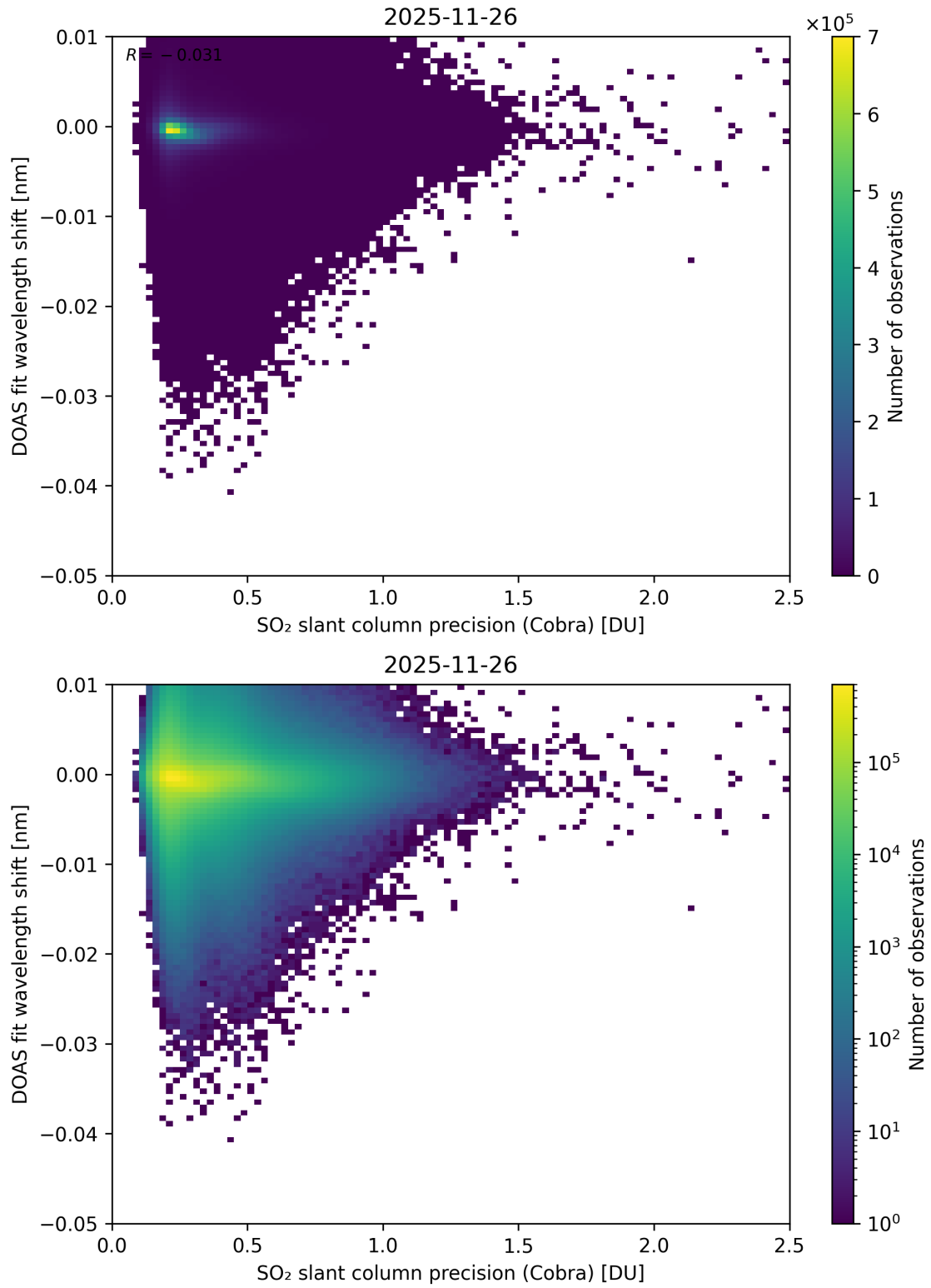
Figure 202: Scatter density plot of “SO 2 slant column precision (Cobra)” against “DOAS fit wavelength shift” for 2025-11-25 to 2025-11-27.
