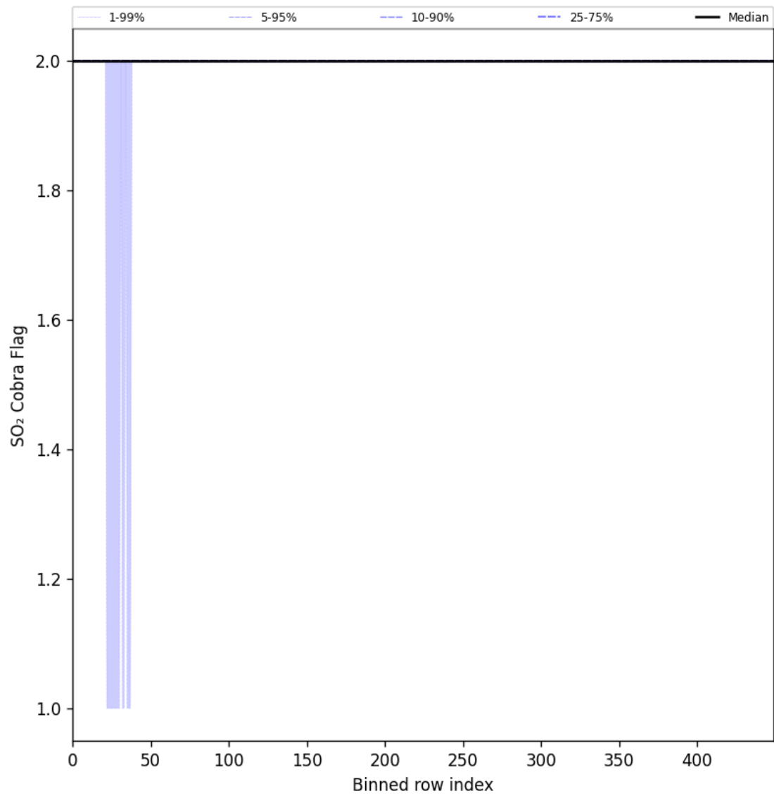
Figure 101: Along track statistics of “SO 2 Cobra Flag” for 2025-11-25 to 2025-11-27
