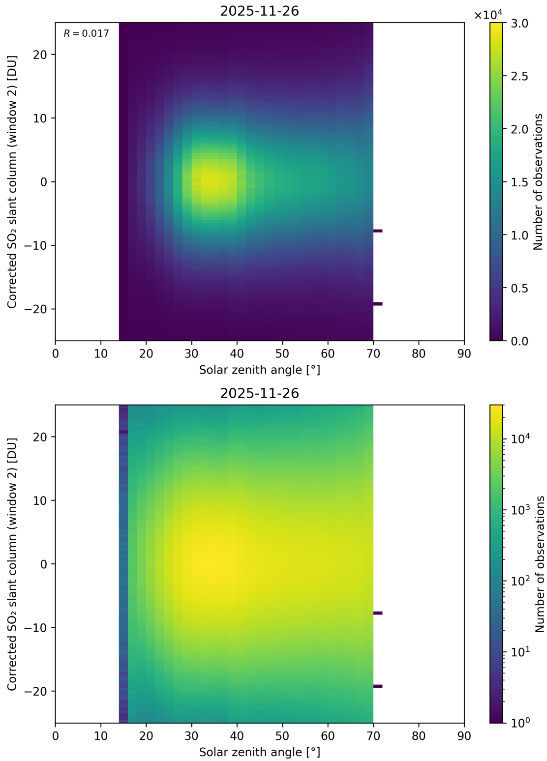
Figure 182: Scatter density plot of “Solar zenith angle” against “Corrected SO 2 slant column (window 2)” for 2025-11-25 to 2025-11-27.
