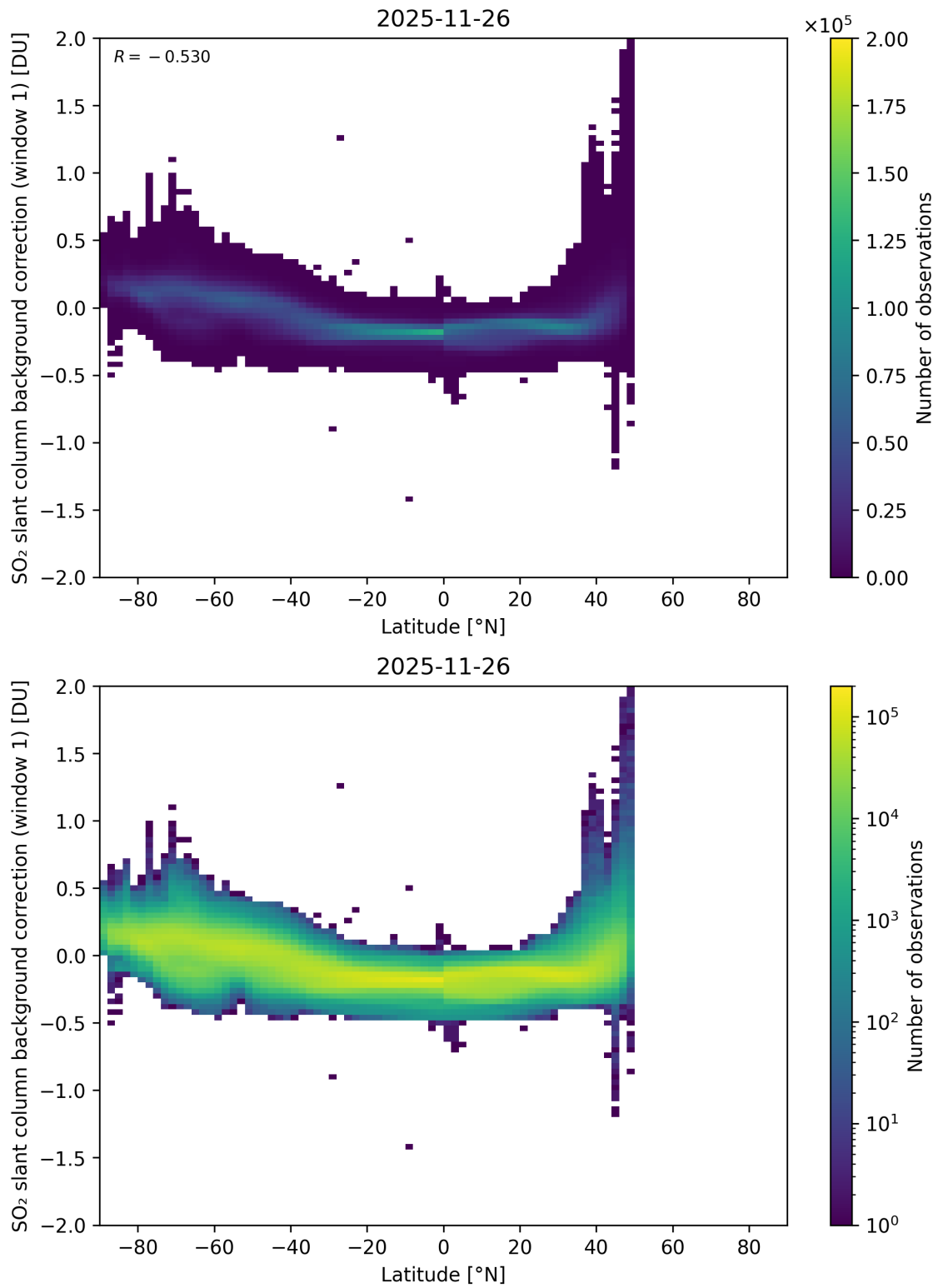
Figure 150: Scatter density plot of “Latitude” against “SO 2 slant column background correction (window 1)” for 2025-11-25 to 2025-11-27.
