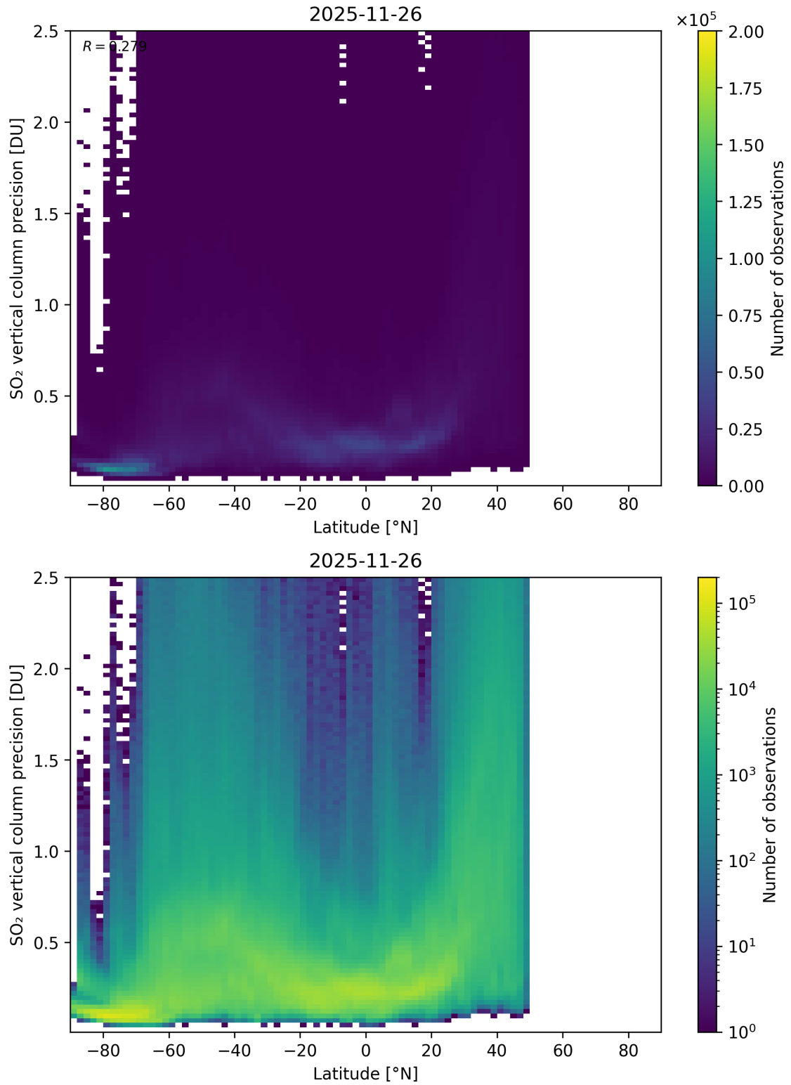
Figure 170: Scatter density plot of “Latitude” against “SO 2 vertical column precision” for 2025-11-25 to 2025-11-27.
