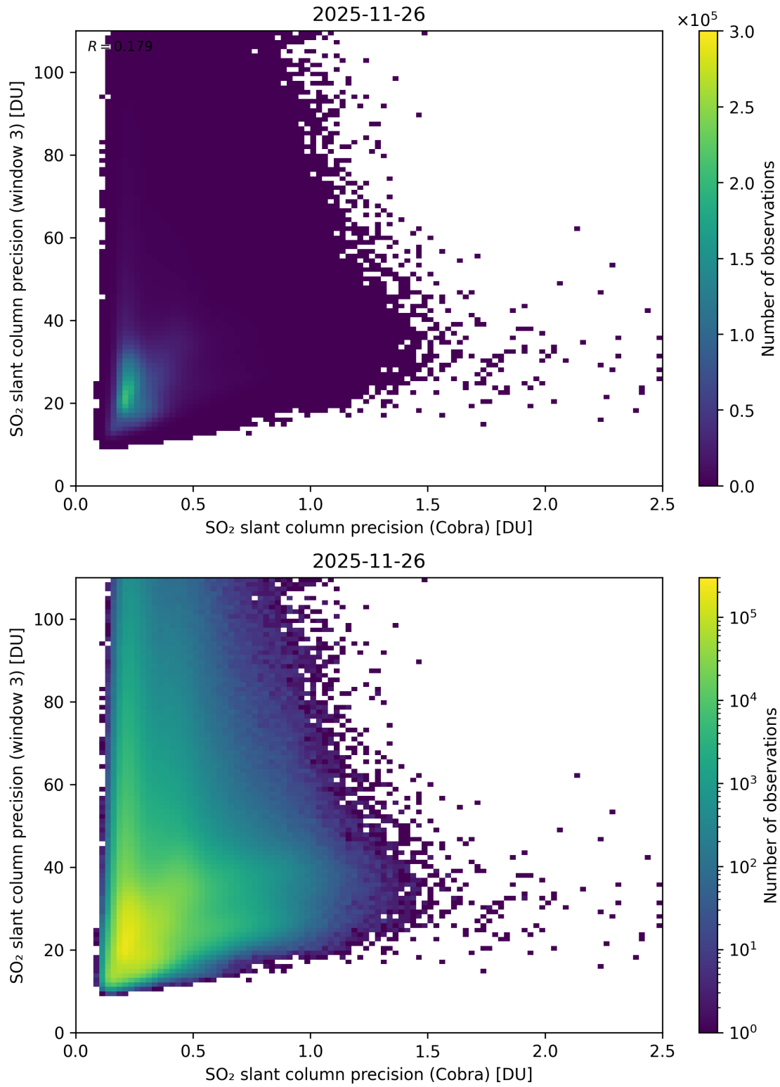
Figure 212: Scatter density plot of “SO 2 slant column precision (Cobra)” against “SO 2 slant column precision (window 3)” for 2025-11-25 to 2025-11-27.
