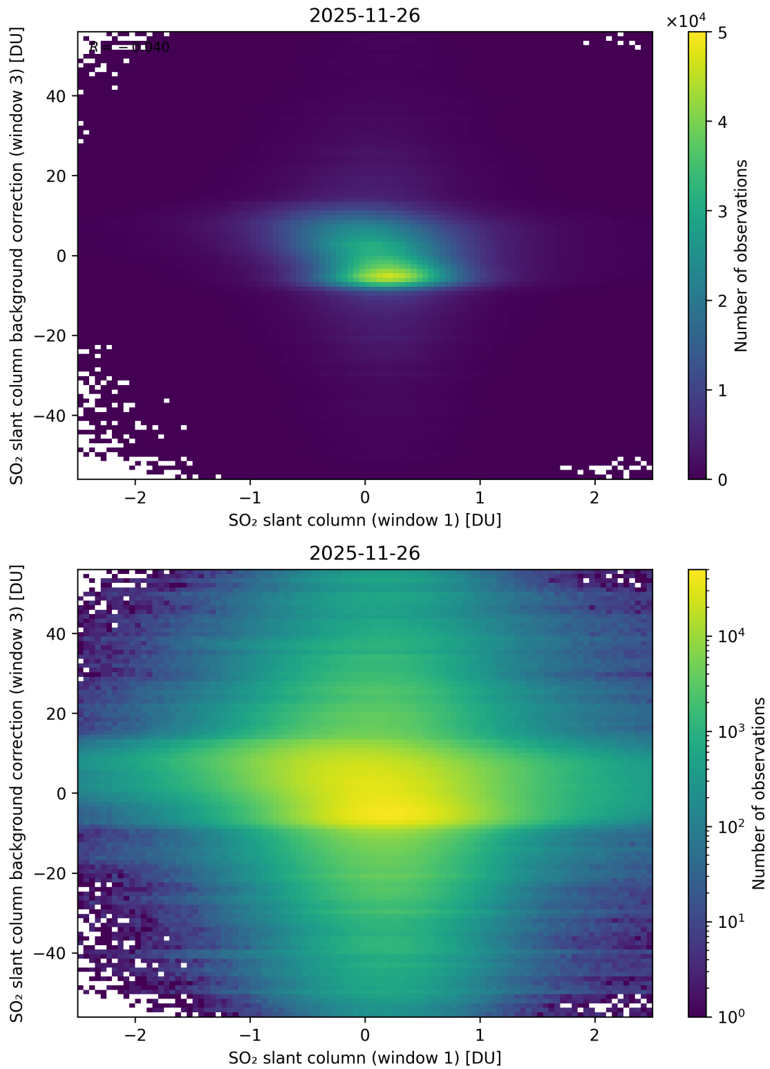
Figure 264: Scatter density plot of “SO 2 slant column (window 1)” against “SO 2 slant column background correction (window 3)” for 2025-11-25 to 2025-11-27.
