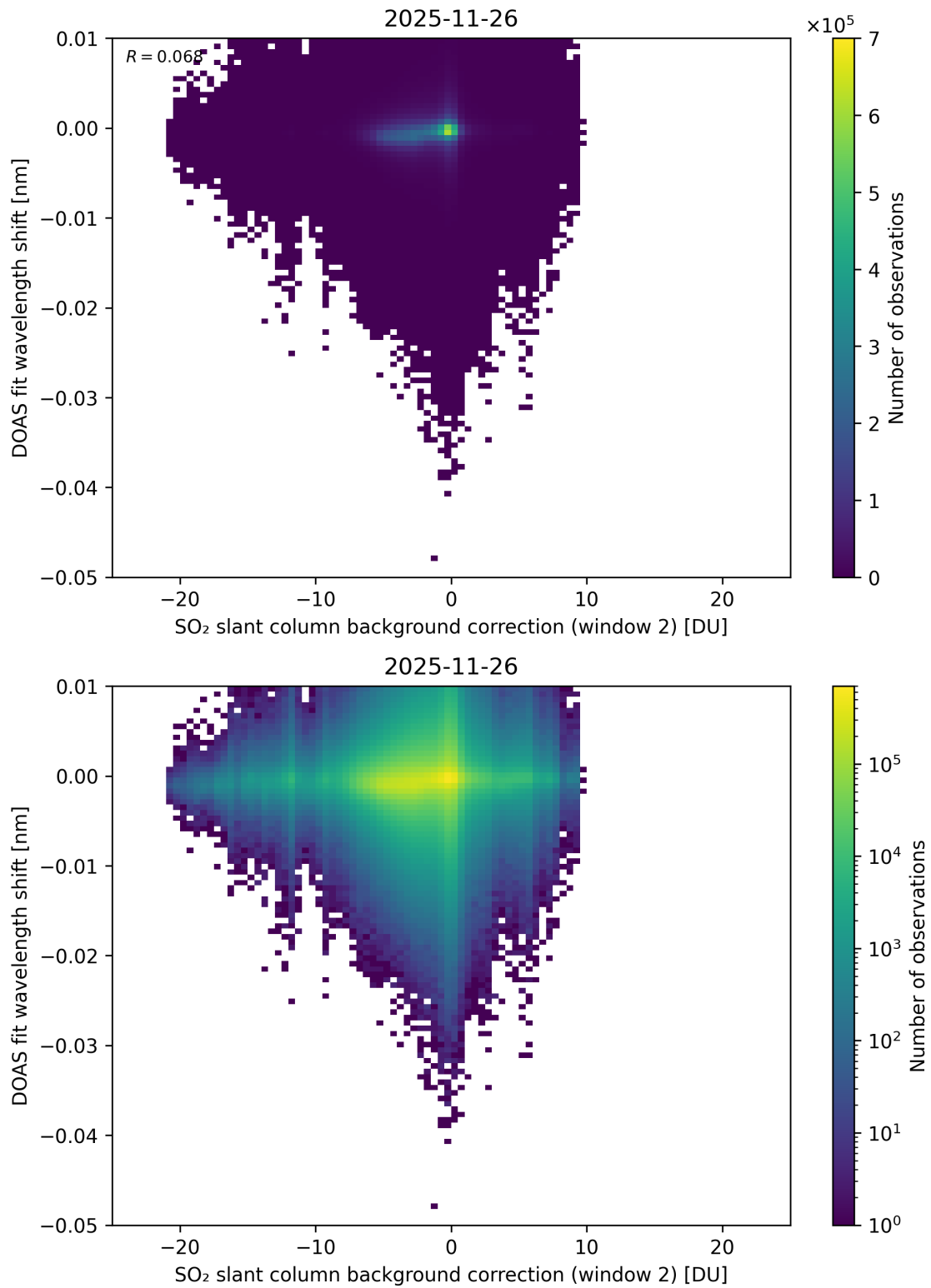
Figure 123: Scatter density plot of “SO 2 slant column background correction (window 2)” against “DOAS fit wavelength shift” for 2025-11-25 to 2025-11-27.
