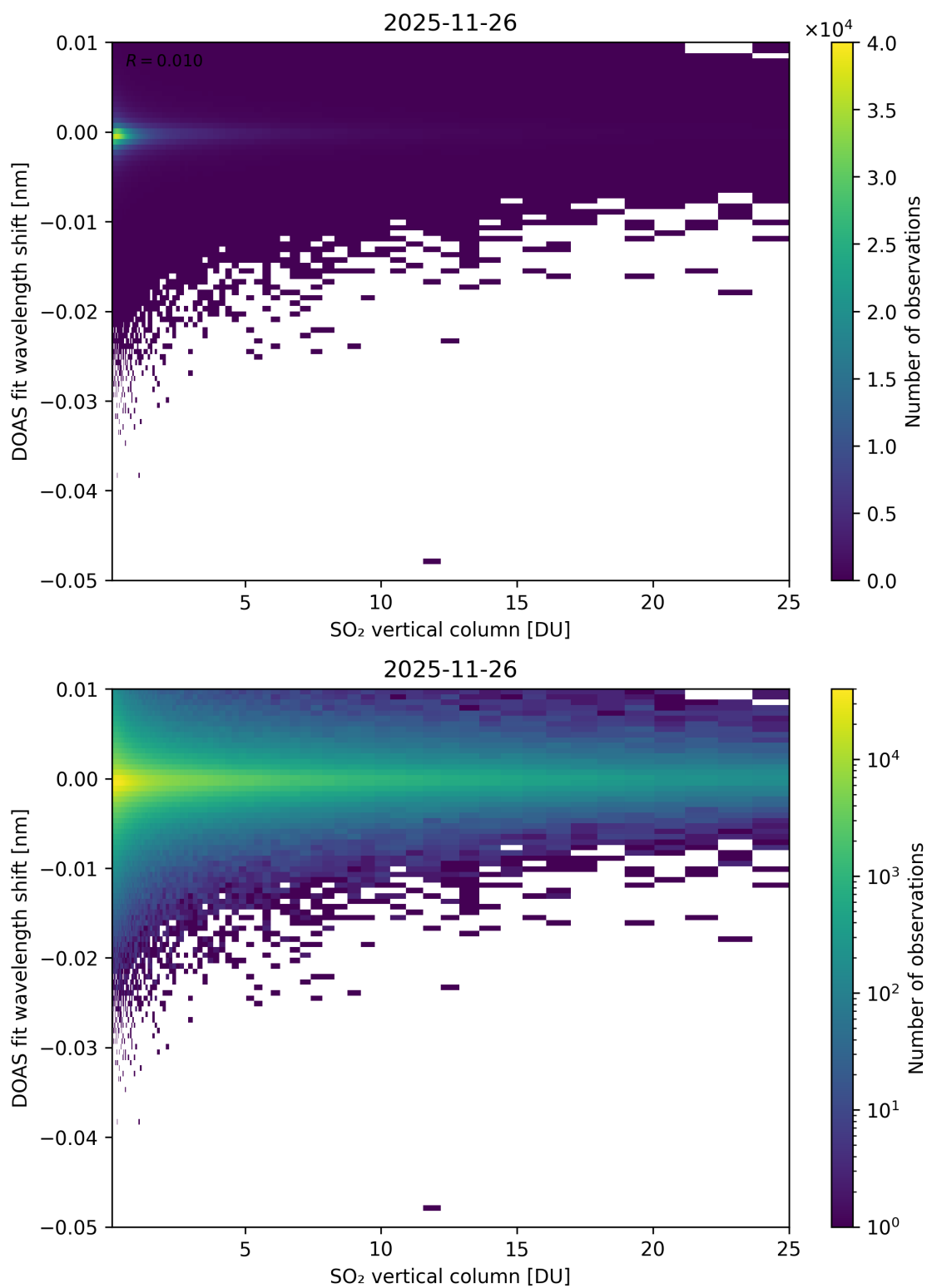
Figure 326: Scatter density plot of “SO 2 vertical column” against “DOAS fit wavelength shift” for 2025-11-25 to 2025-11-27.
