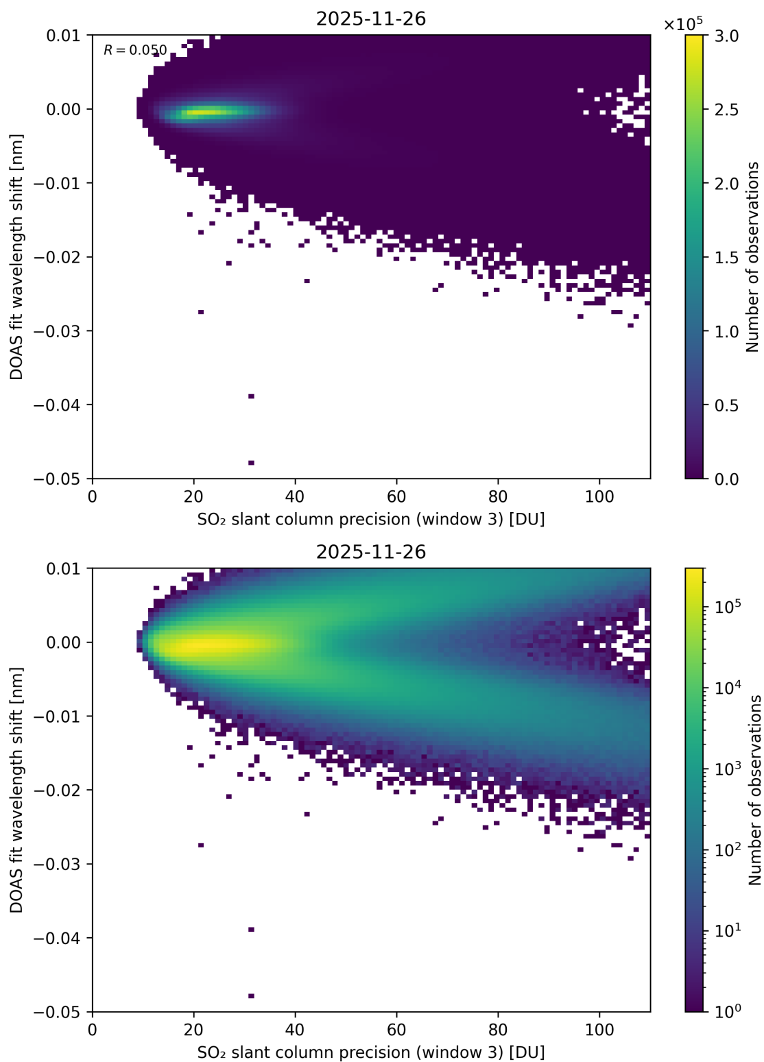
Figure 308: Scatter density plot of “SO 2 slant column precision (window 3)” against “DOAS fit wavelength shift” for 2025-11-25 to 2025-11-27.
