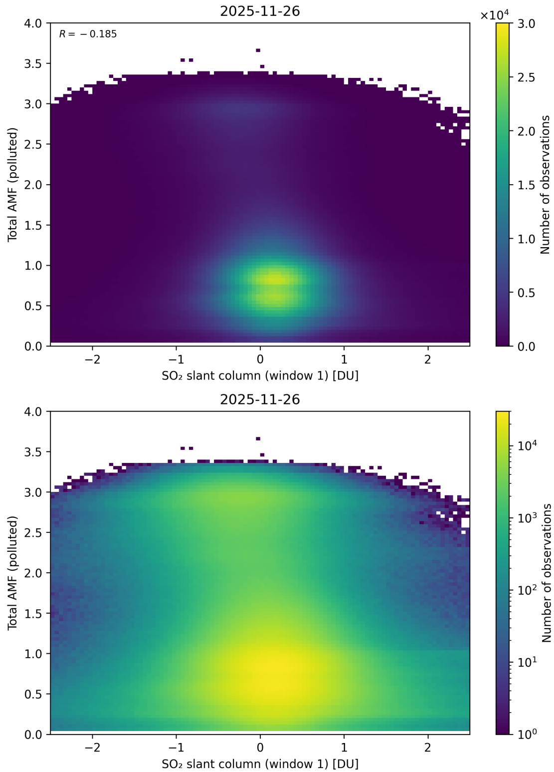
Figure 289: Scatter density plot of “SO 2 slant column (window 1)” against “Total AMF (polluted)” for 2025-11-25 to 2025-11-27.
