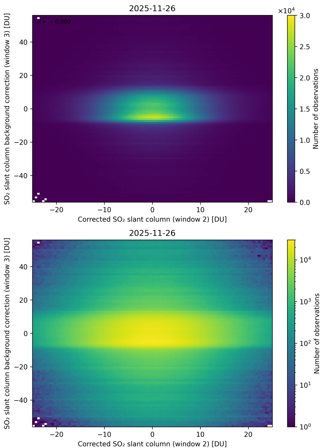
Figure 245: Scatter density plot of “Corrected SO 2 slant column (window 2)” against “SO 2 slant column background correction (window 3)” for 2025-11-25 to 2025-11-27.
