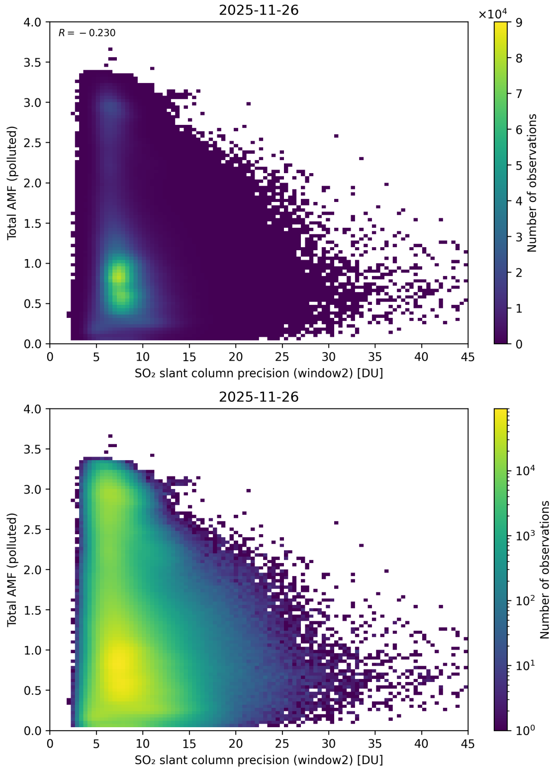
Figure 301: Scatter density plot of “SO 2 slant column precision (window2)” against “Total AMF (polluted)” for 2025-11-25 to 2025-11-27.
