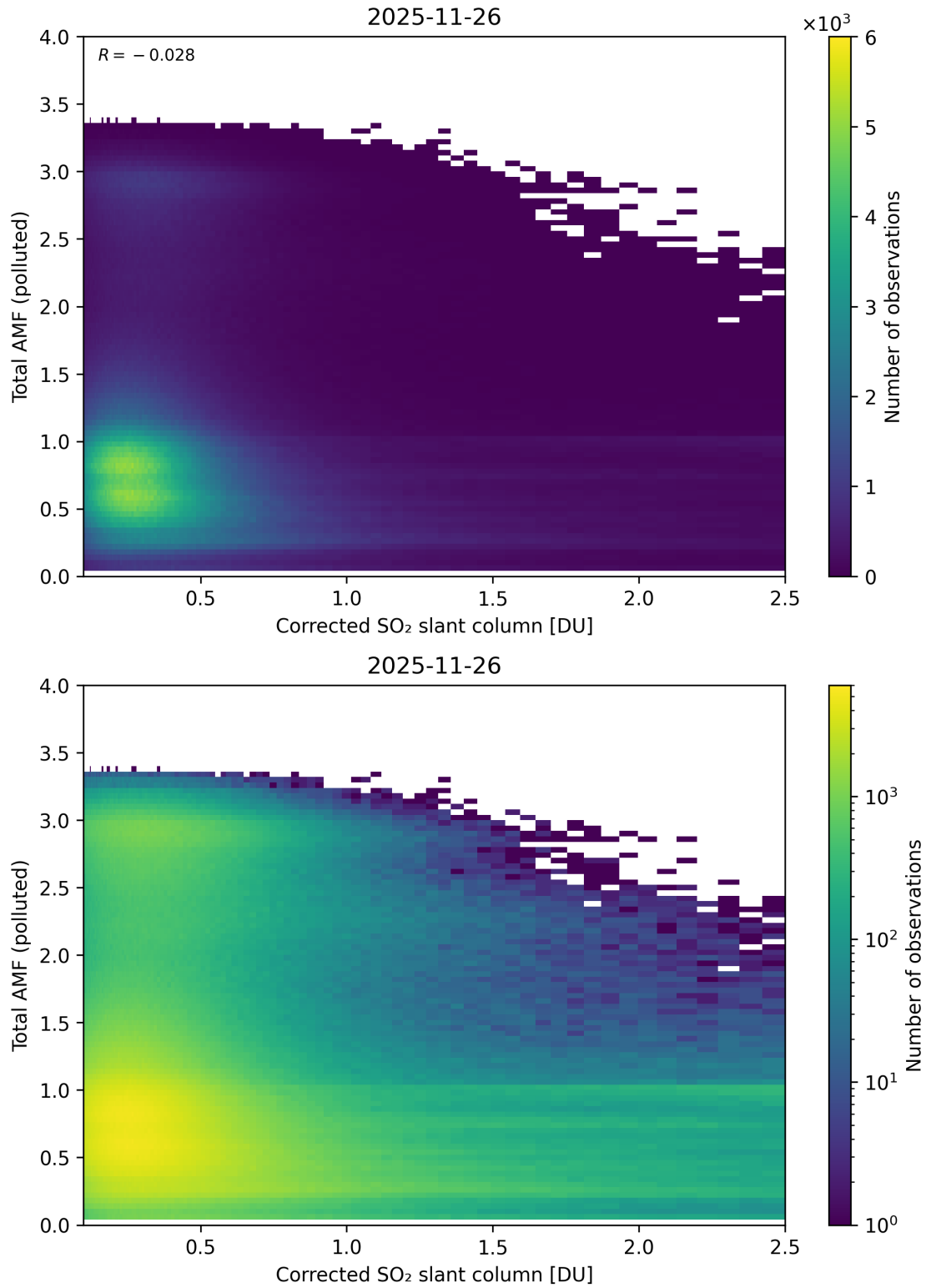
Figure 242: Scatter density plot of “Corrected SO 2 slant column” against “Total AMF (polluted)” for 2025-11-25 to 2025-11-27.
