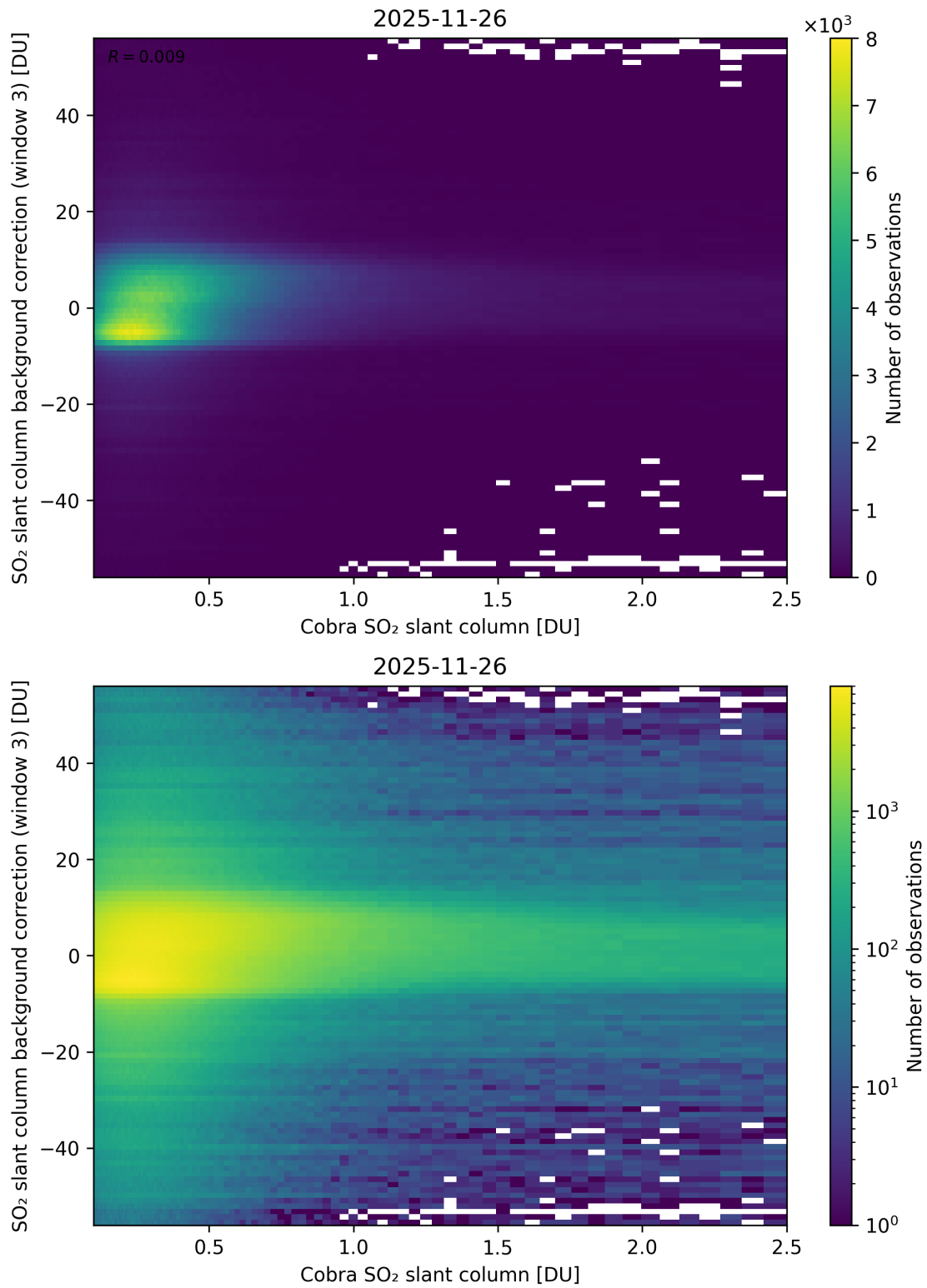
Figure 195: Scatter density plot of “Cobra SO 2 slant column” against “SO 2 slant column background correction (window 3)” for 2025-11-25 to 2025-11-27.
