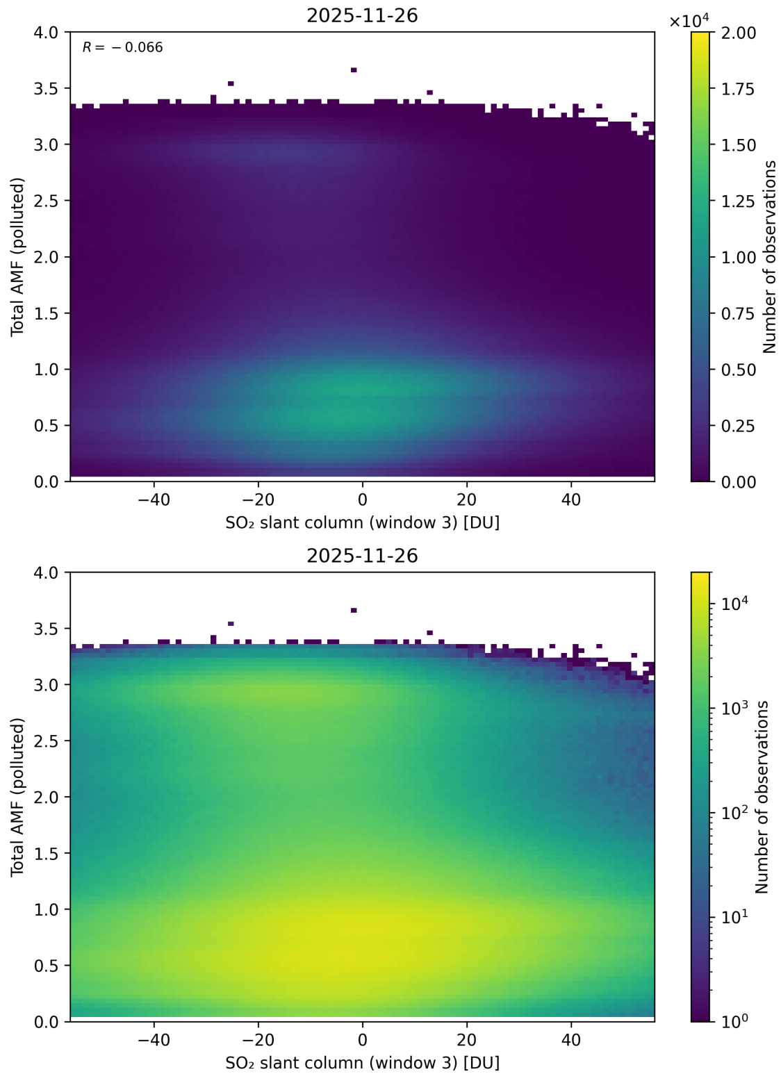
Figure 318: Scatter density plot of “SO 2 slant column (window 3)” against “Total AMF (polluted)” for 2025-11-25 to 2025-11-27.
