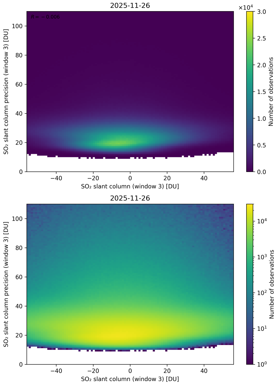
Figure 317: Scatter density plot of “SO 2 slant column (window 3)” against “SO 2 slant column precision (window 3)” for 2025-11-25 to 2025-11-27.
