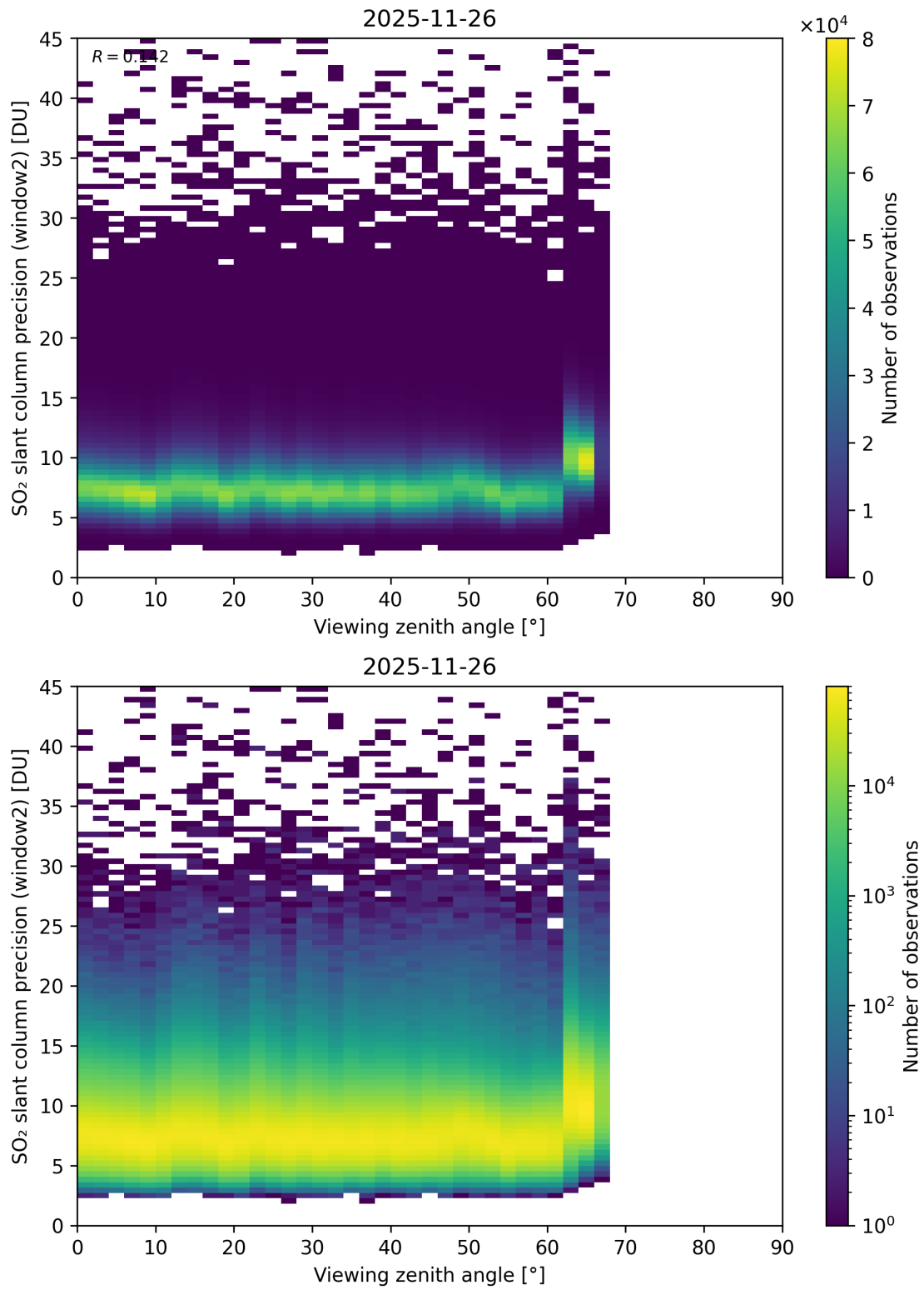
Figure 378: Scatter density plot of “Viewing zenith angle” against “SO 2 slant column precision (window2)” for 2025-11-25 to 2025-11-27.
