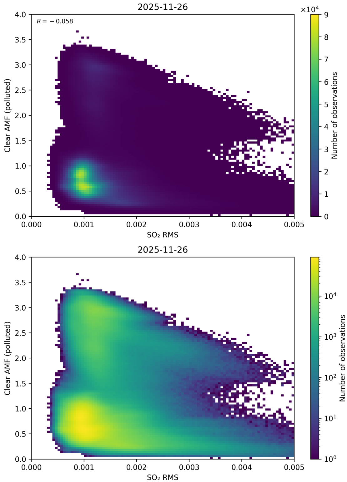
Figure 147: Scatter density plot of “SO 2 RMS” against “Clear AMF (polluted)” for 2025-11-25 to 2025-11-27.
