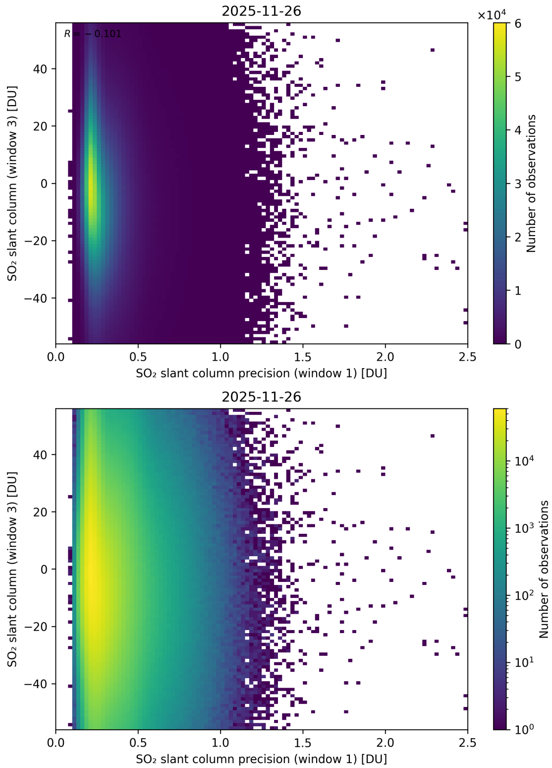
Figure 278: Scatter density plot of “SO 2 slant column precision (window 1)” against “SO 2 slant column (window 3)” for 2025-11-25 to 2025-11-27.
