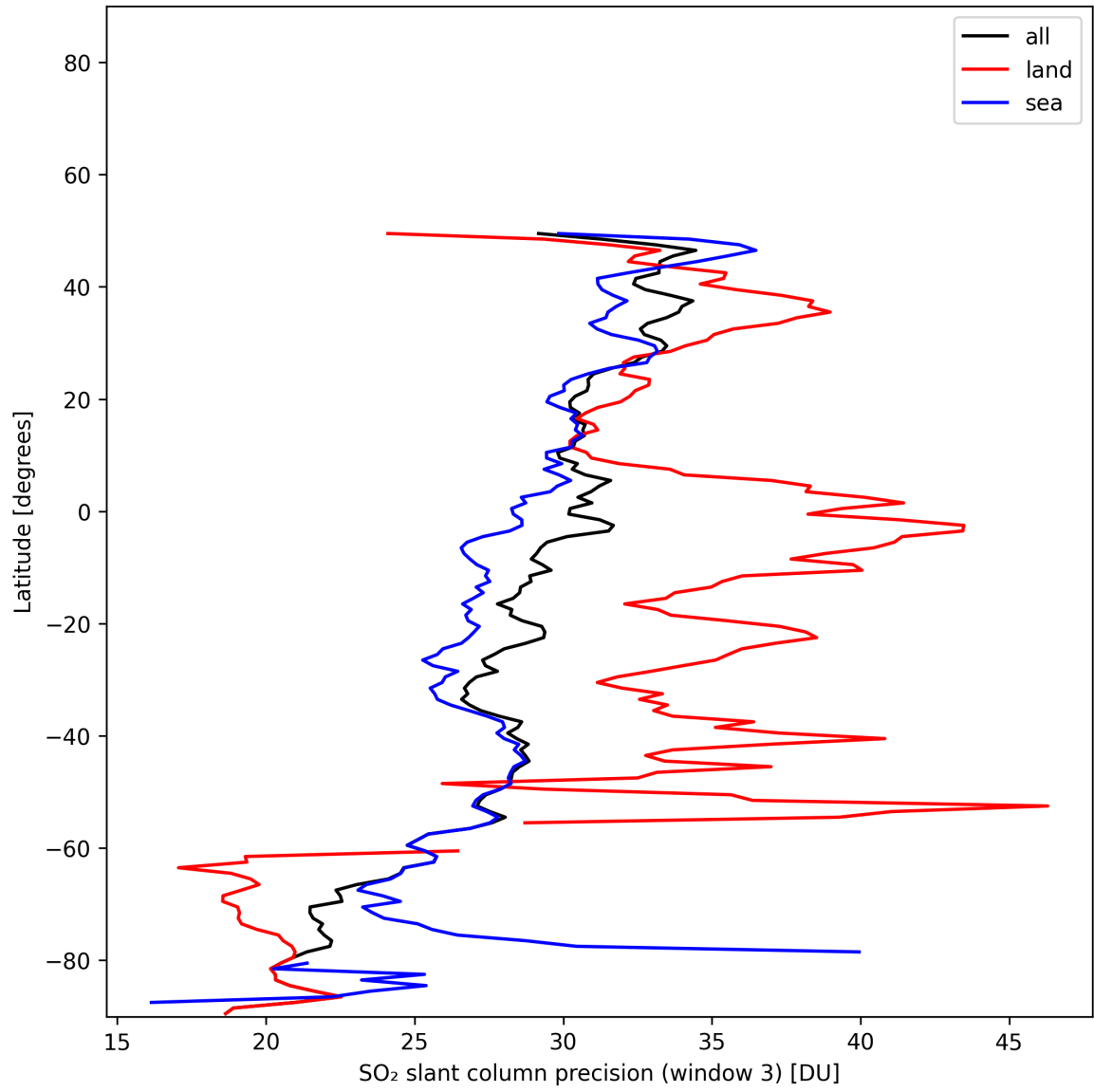
Figure 46: Zonal average of “SO 2 slant column precision (window 3)” for 2025-11-25 to 2025-11-27.
