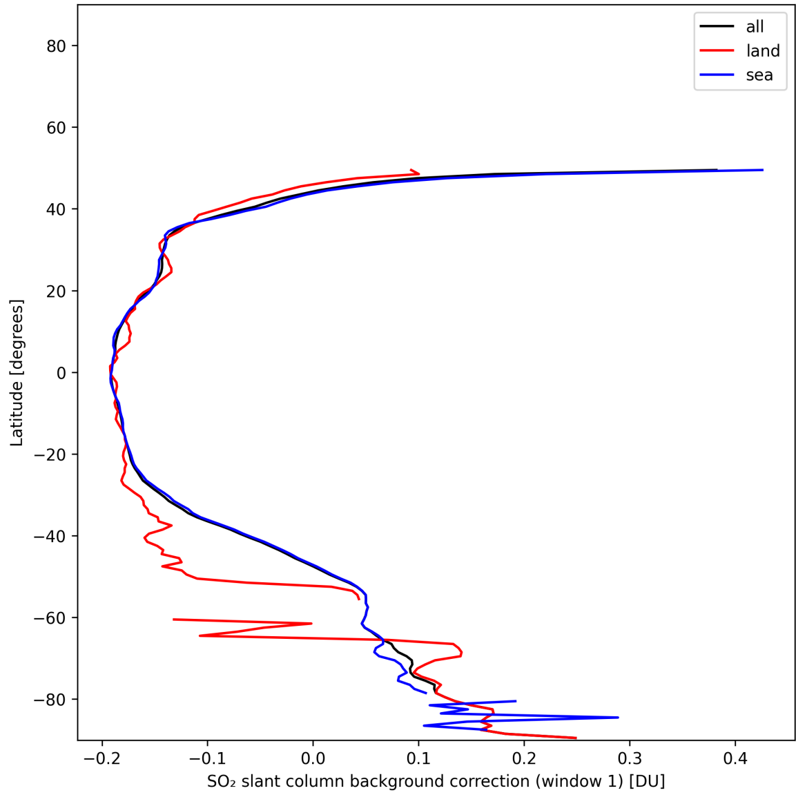
Figure 40: Zonal average of “SO 2 slant column background correction (window 1)” for 2025-11-25 to 2025-11-27.
