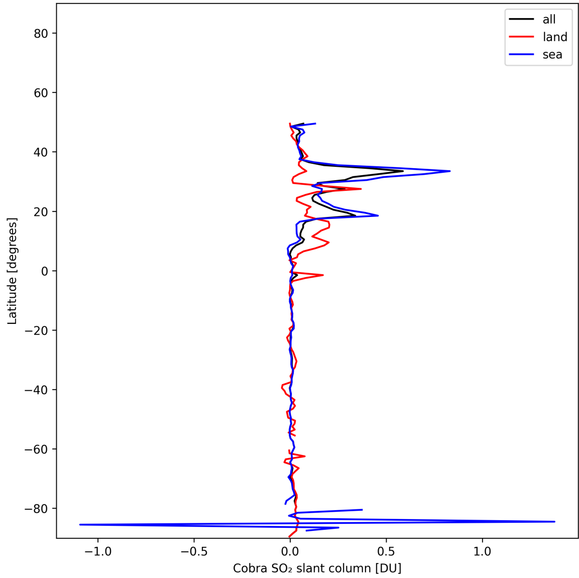
Figure 35: Zonal average of “Cobra SO 2 slant column” for 2025-11-25 to 2025-11-27.
