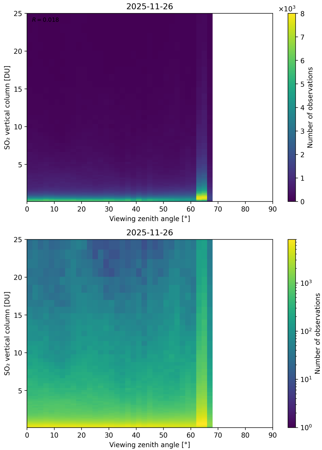
Figure 383: Scatter density plot of “Viewing zenith angle” against “SO 2 vertical column” for 2025-11-25 to 2025-11-27.
