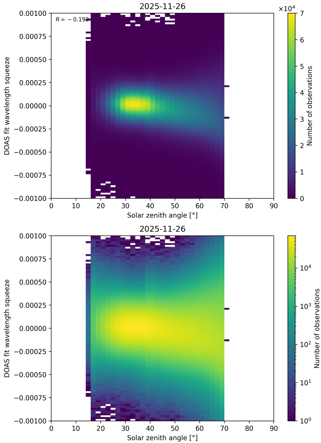
Figure 175: Scatter density plot of “Solar zenith angle” against “DOAS fit wavelength squeeze” for 2025-11-25 to 2025-11-27.
