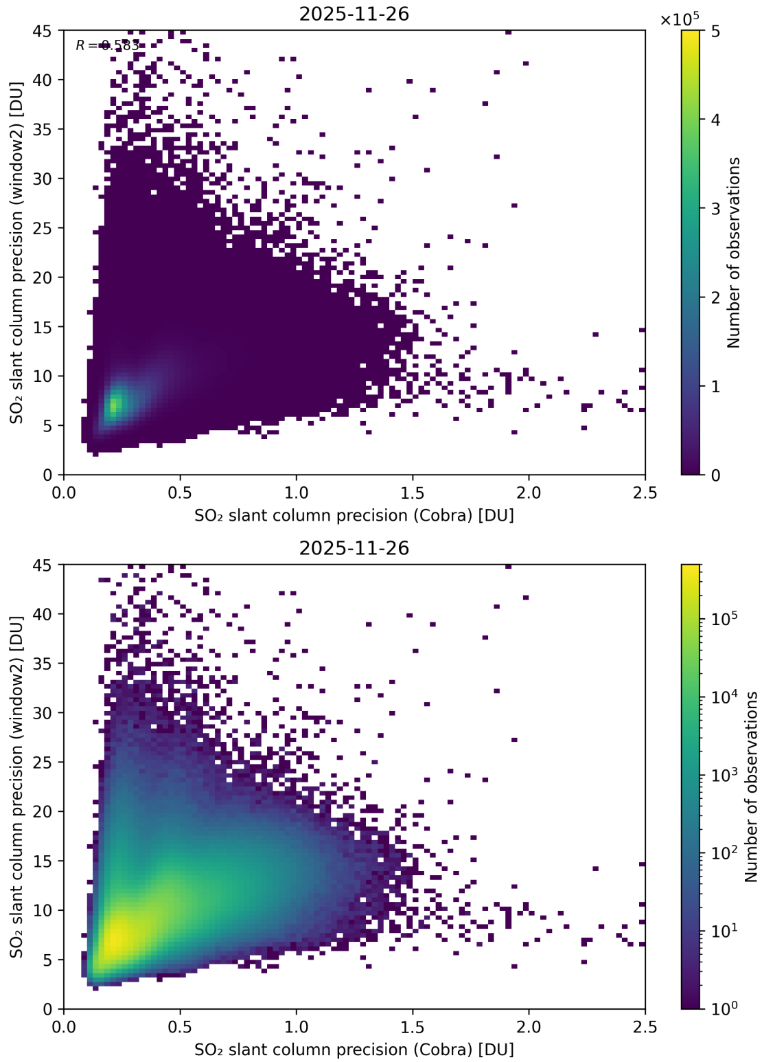
Figure 210: Scatter density plot of “SO 2 slant column precision (Cobra)” against “SO 2 slant column precision (window2)” for 2025-11-25 to 2025-11-27.
