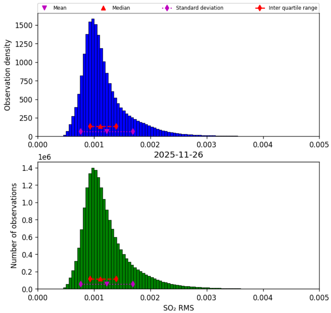
Figure 78: Histogram of “SO 2 RMS” for 2025-11-25 to 2025-11-27
