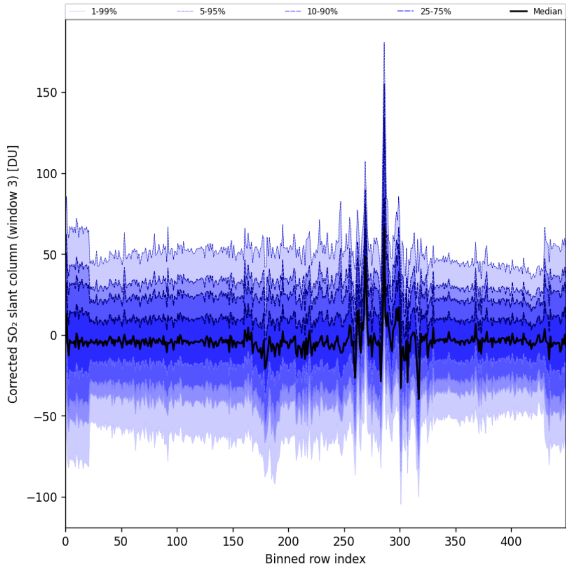
Figure 99: Along track statistics of "Corrected SO 2 slant column (window 3)" for 2025-11-25 to 2025-11-27
