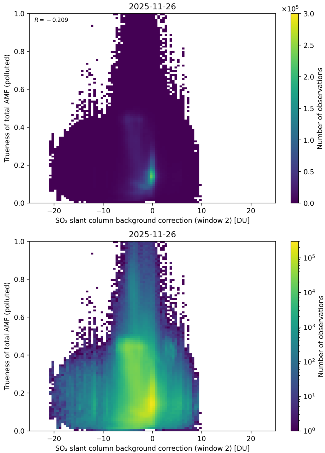
Figure 131: Scatter density plot of “SO 2 slant column background correction (window 2)” against “Trueness of total AMF (polluted)” for 2025-11-25 to 2025-11-27.
