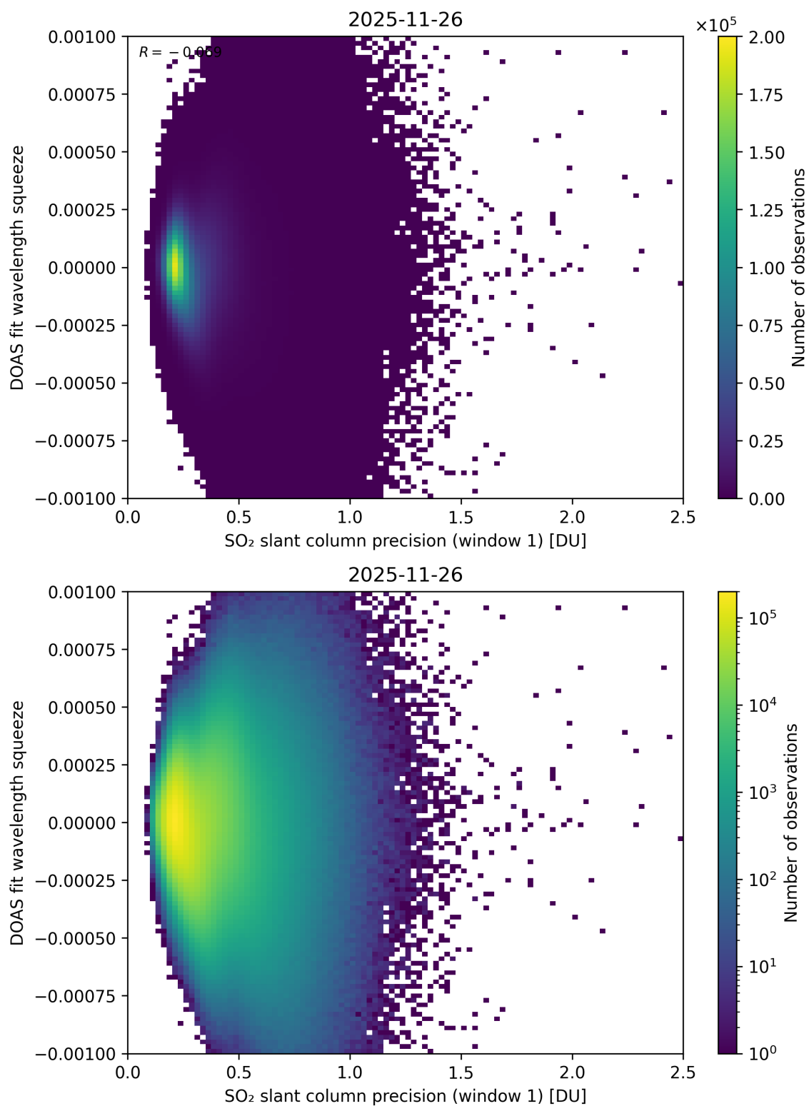
Figure 272: Scatter density plot of “SO 2 slant column precision (window 1)” against “DOAS fit wavelength squeeze” for 2025-11-25 to 2025-11-27.
