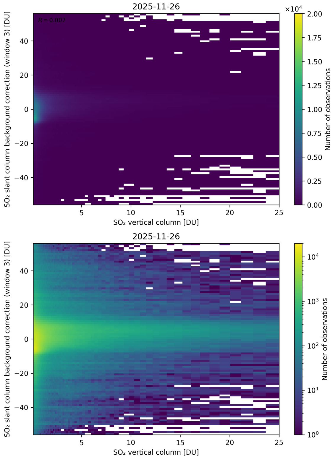
Figure 325: Scatter density plot of “SO 2 vertical column” against “SO 2 slant column background correction (window 3)” for 2025-11-25 to 2025-11-27.
