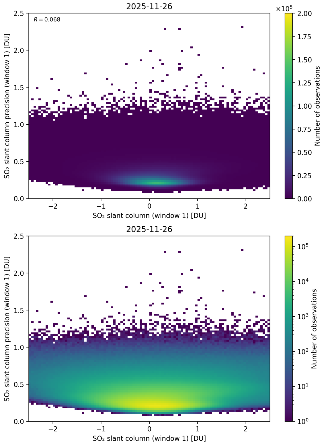
Figure 285: Scatter density plot of “SO 2 slant column (window 1)” against “SO 2 slant column precision (window 1)” for 2025-11-25 to 2025-11-27.
