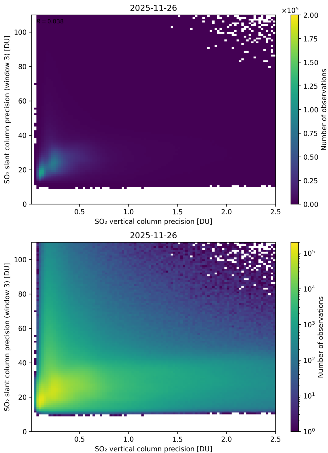
Figure 345: Scatter density plot of “SO 2 vertical column precision” against “SO 2 slant column precision (window 3)” for 2025-11-25 to 2025-11-27.
