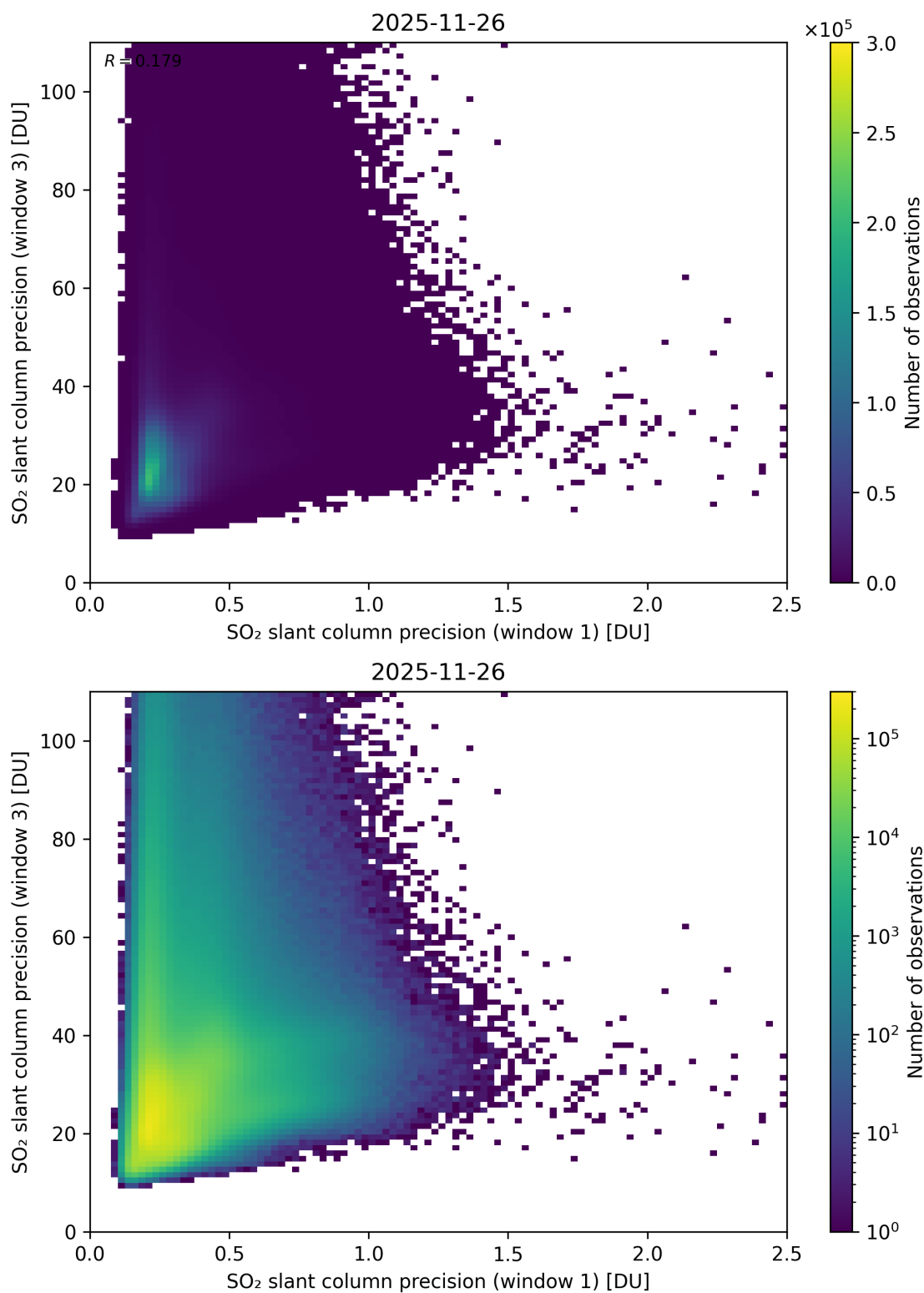
Figure 279: Scatter density plot of “SO 2 slant column precision (window 1)” against “SO 2 slant column precision (window 3)” for 2025-11-25 to 2025-11-27.
