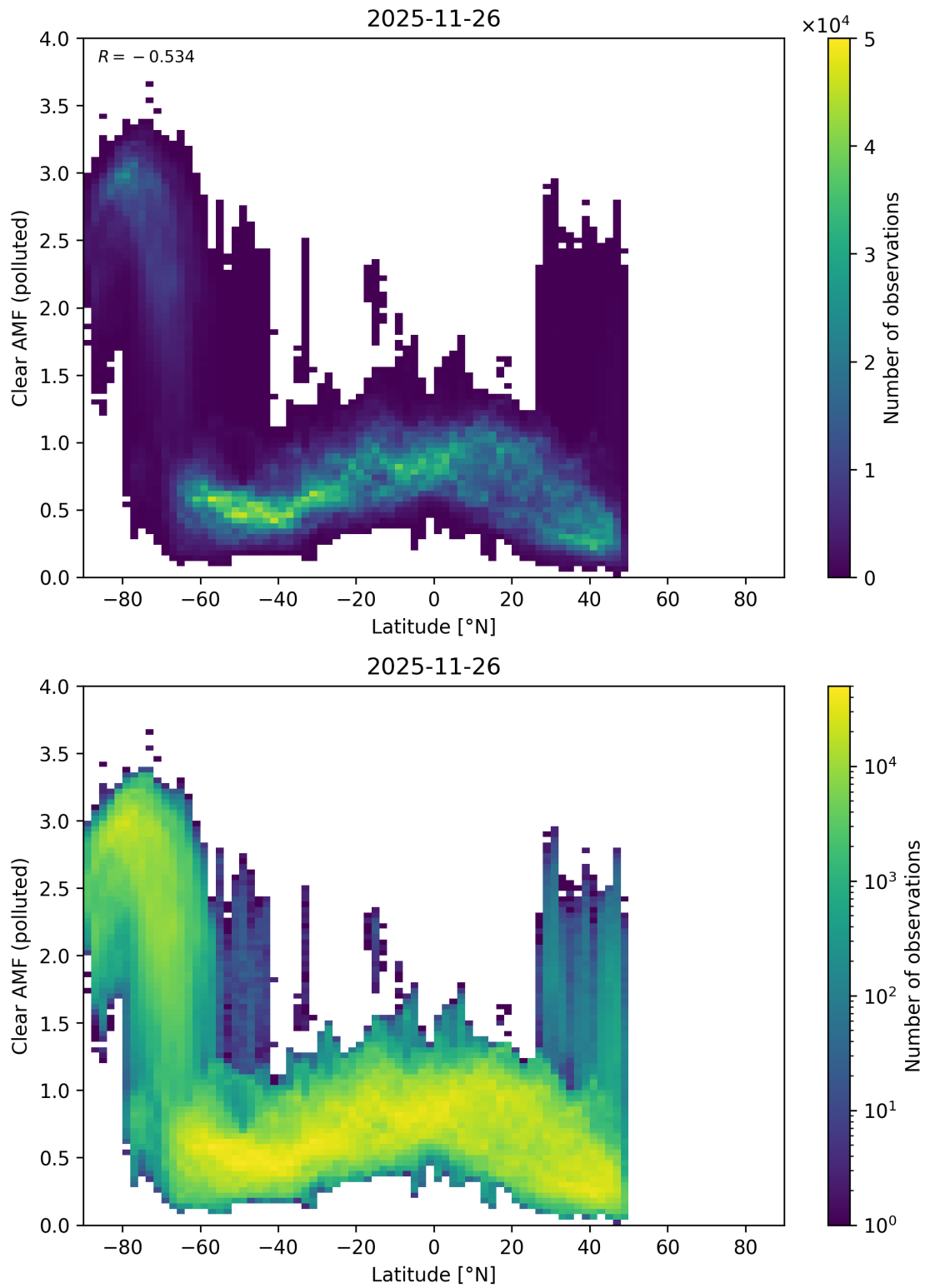
Figure 156: Scatter density plot of “Latitude” against “Clear AMF (polluted)” for 2025-11-25 to 2025-11-27.
