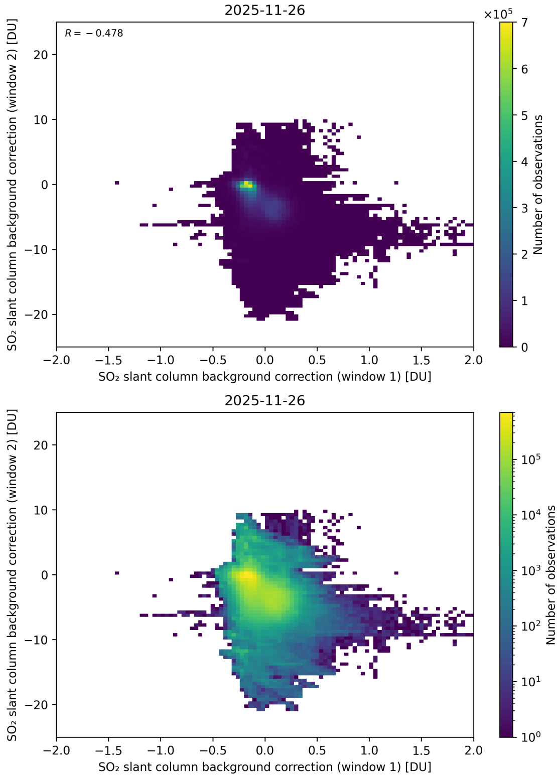
Figure 109: Scatter density plot of “SO 2 slant column background correction (window 1)” against “SO 2 slant column background correction (window 2)” for 2025-11-25 to 2025-11-27.
