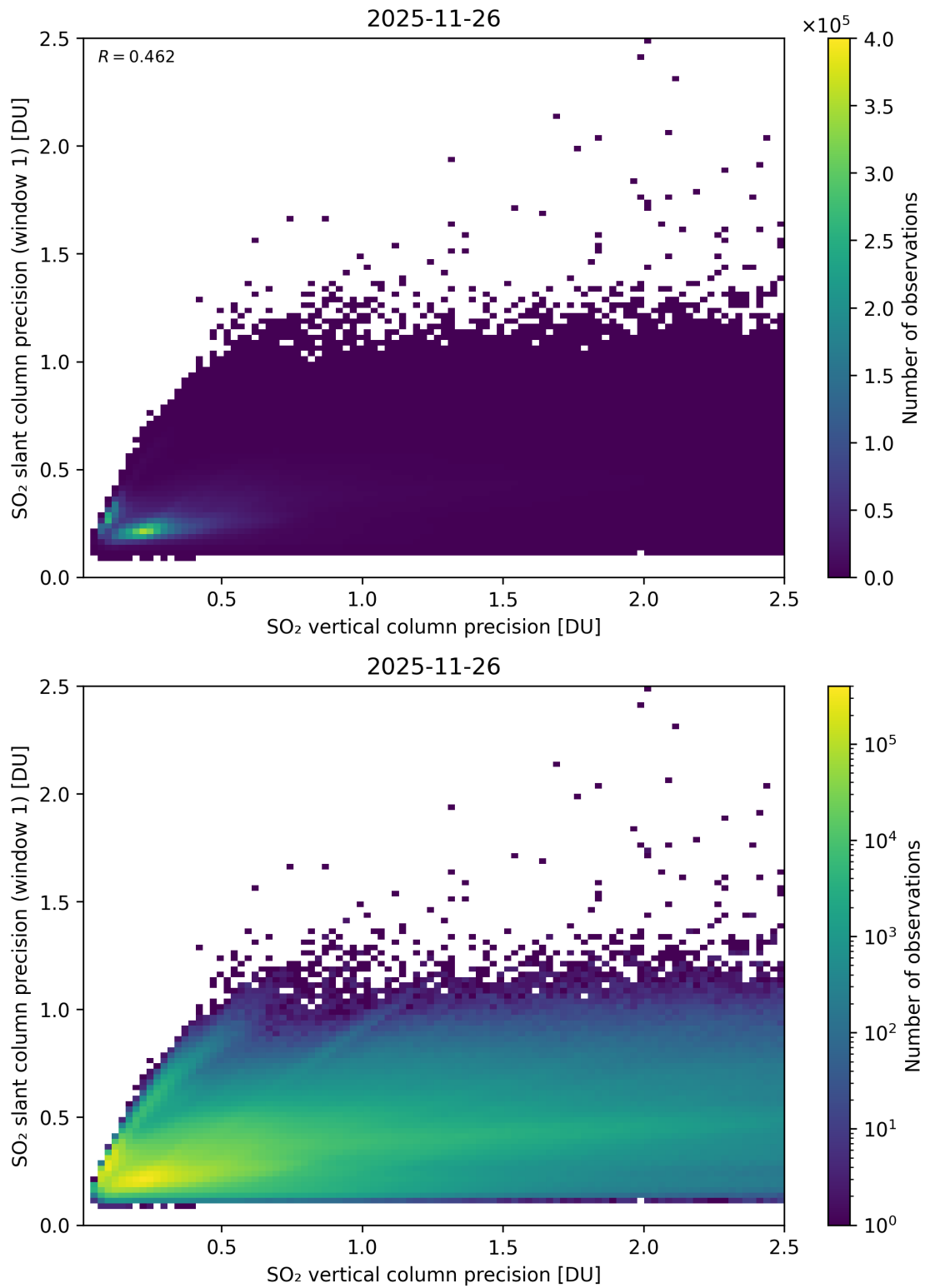
Figure 342: Scatter density plot of “SO 2 vertical column precision” against “SO 2 slant column precision (window 1)” for 2025-11-25 to 2025-11-27.
