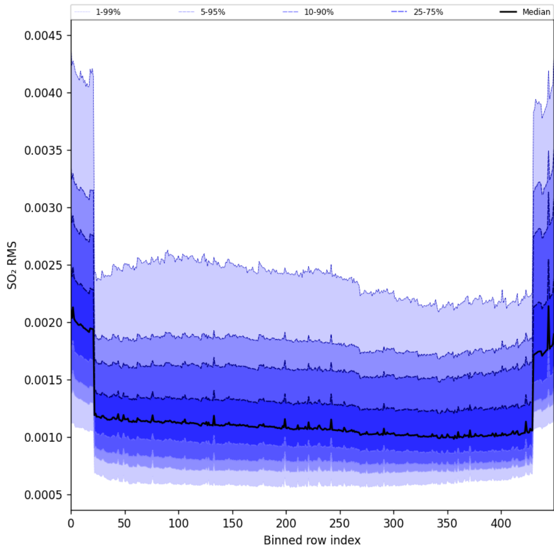
Figure 104: Along track statistics of “SO 2 RMS” for 2025-11-25 to 2025-11-27
