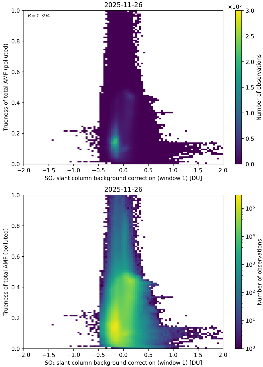
Figure 121: Scatter density plot of “SO 2 slant column background correction (window 1)” against “Trueness of total AMF (polluted)” for 2025-11-25 to 2025-11-27.
