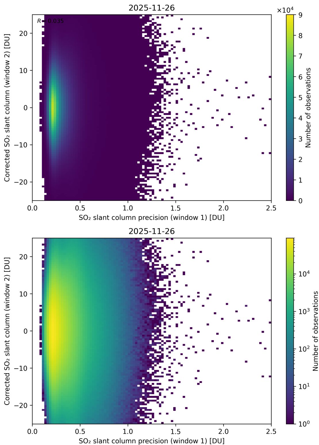
Figure 275: Scatter density plot of “SO 2 slant column precision (window 1)” against “Corrected SO 2 slant column (window 2)” for 2025-11-25 to 2025-11-27.
