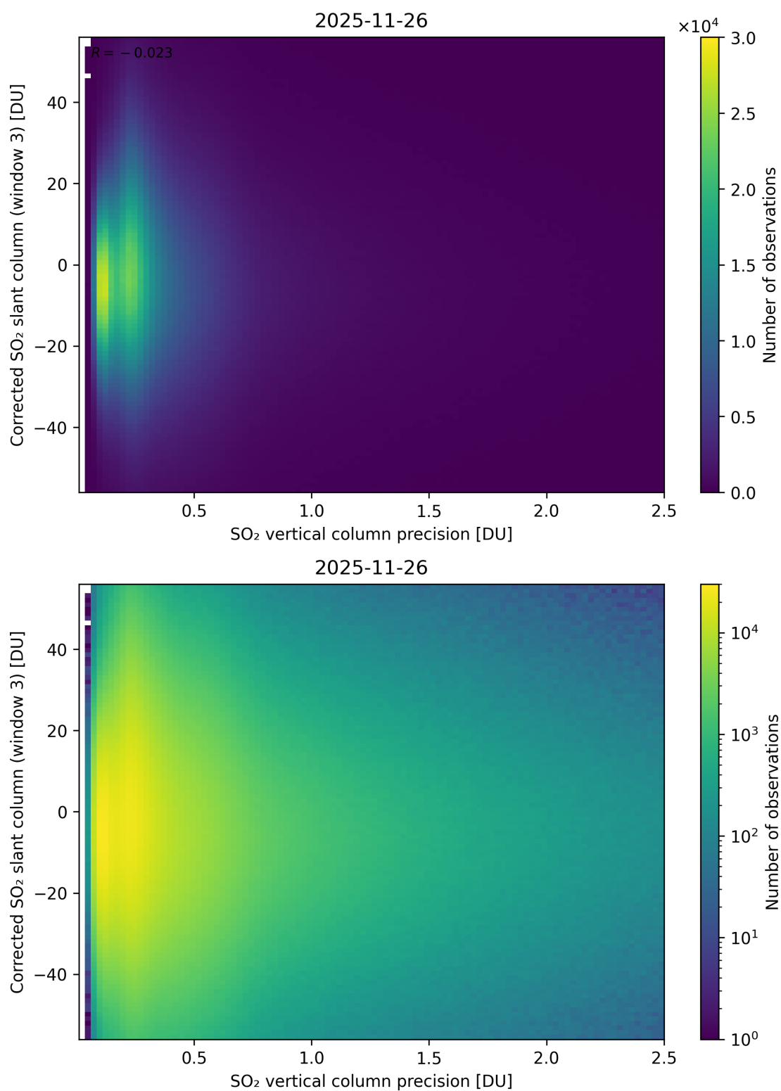
Figure 340: Scatter density plot of “SO 2 vertical column precision” against “Corrected SO 2 slant column (window 3)” for 2025-11-25 to 2025-11-27.
