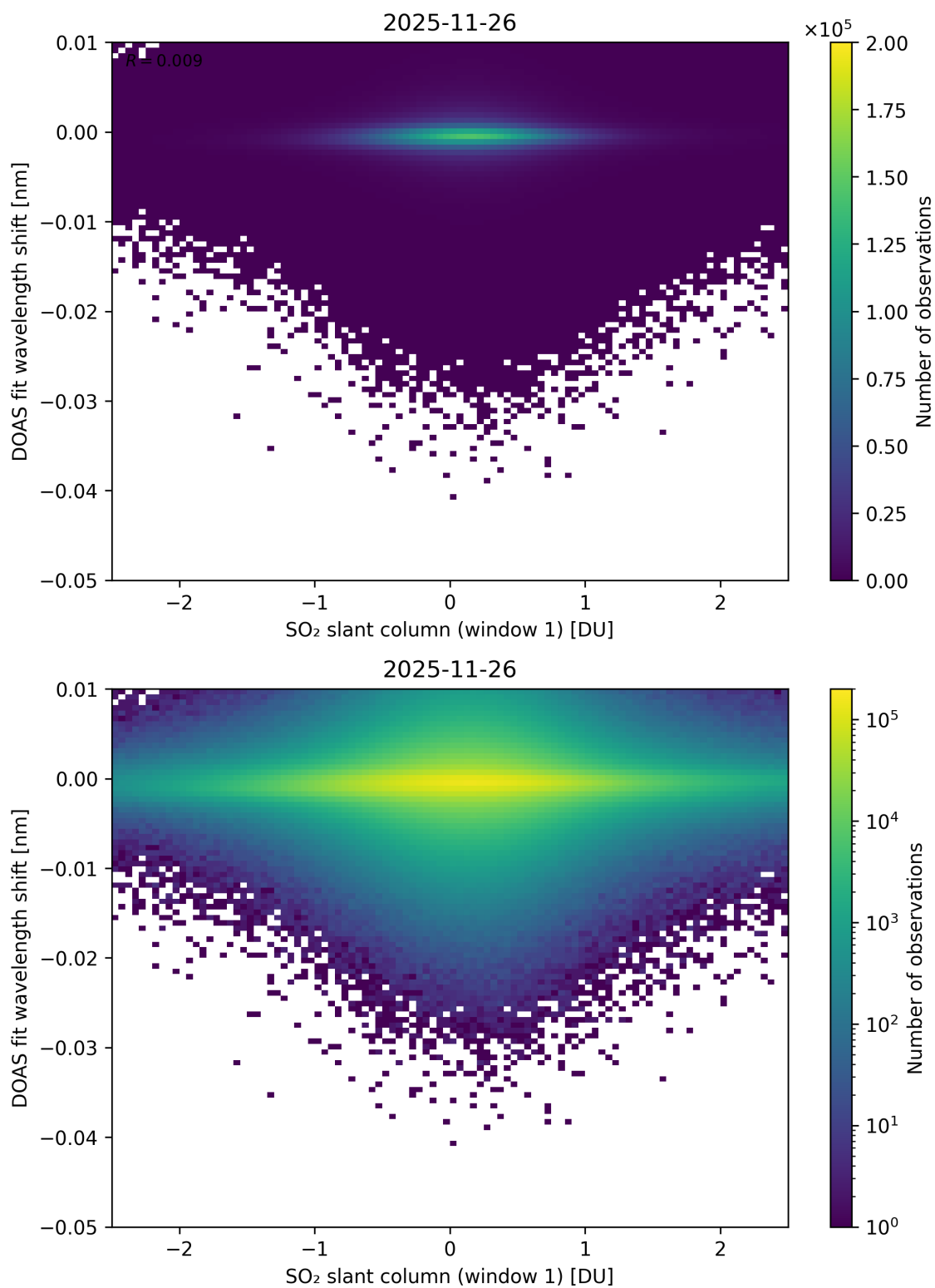
Figure 265: Scatter density plot of “SO 2 slant column (window 1)” against “DOAS fit wavelength shift” for 2025-11-25 to 2025-11-27.
