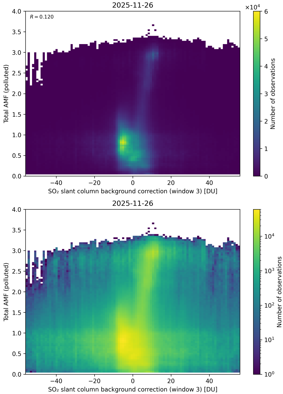
Figure 136: Scatter density plot of “SO 2 slant column background correction (window 3)” against “Total AMF (polluted)” for 2025-11-25 to 2025-11-27.
