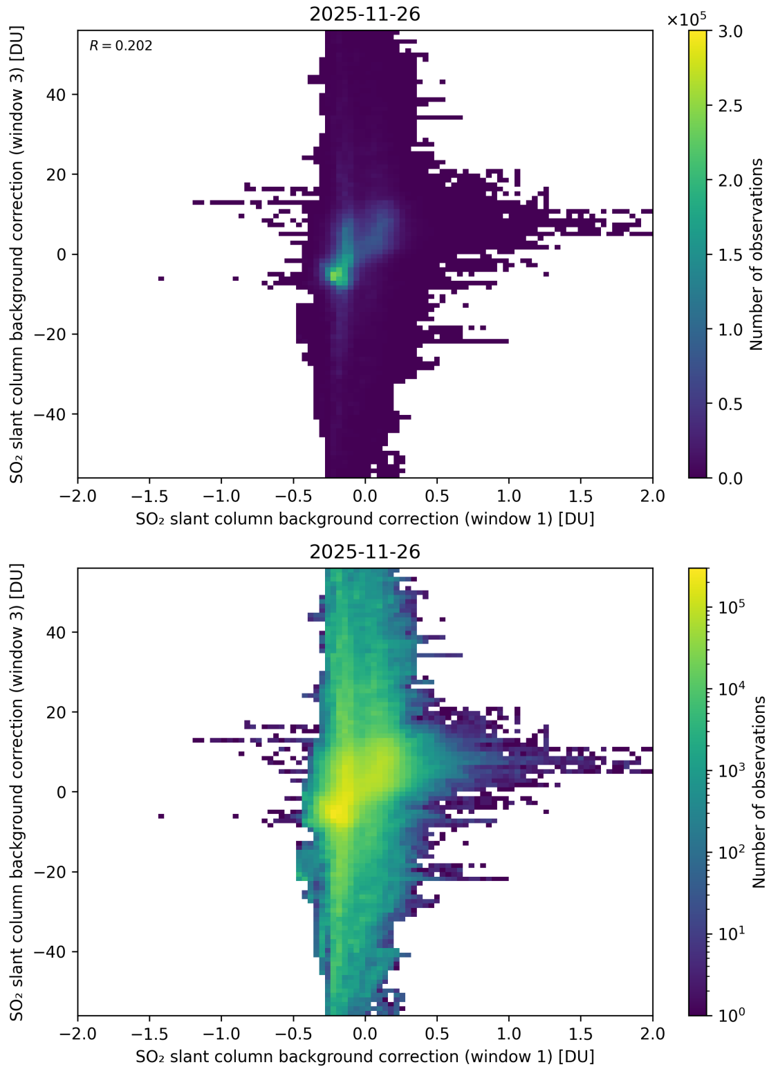
Figure 110: Scatter density plot of “SO 2 slant column background correction (window 1)” against “SO 2 slant column background correction (window 3)” for 2025-11-25 to 2025-11-27.
