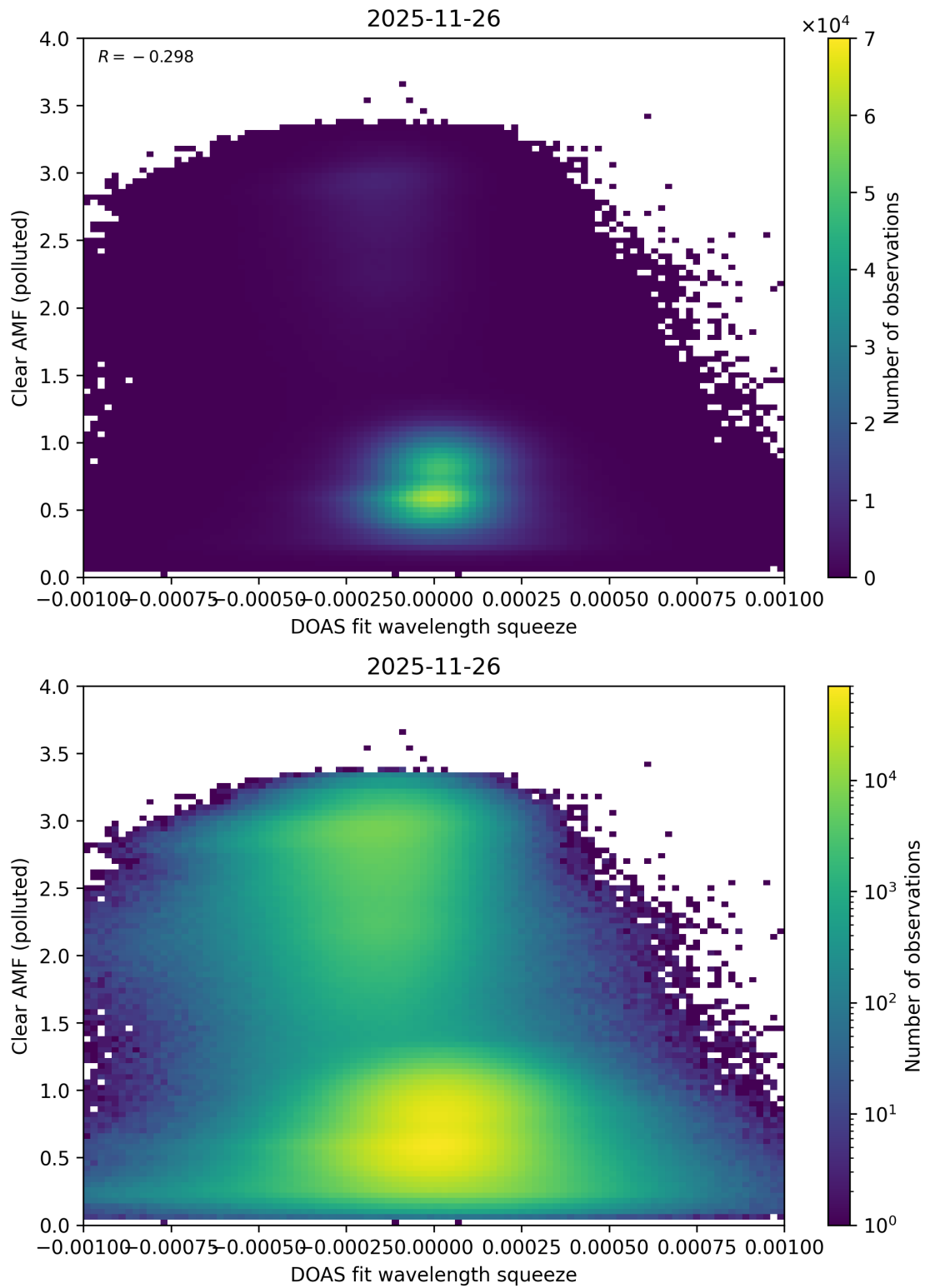
Figure 144: Scatter density plot of “DOAS fit wavelength squeeze” against “Clear AMF (polluted)” for 2025-11-25 to 2025-11-27.
