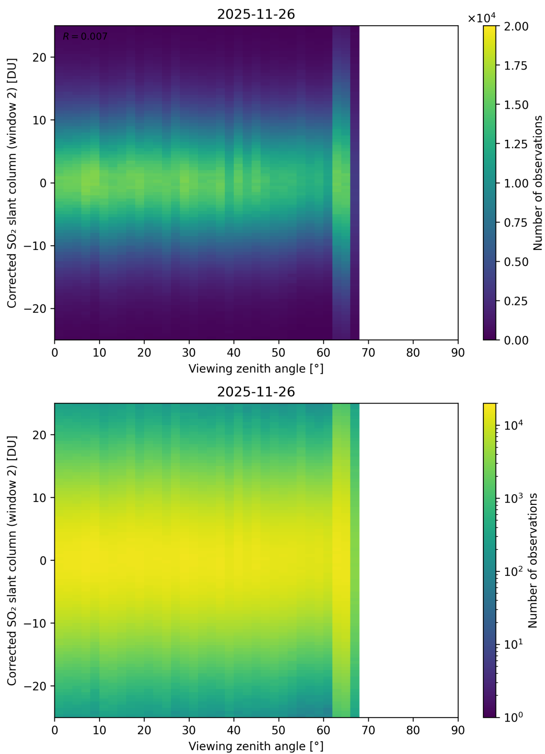
Figure 374: Scatter density plot of “Viewing zenith angle” against “Corrected SO 2 slant column (window 2)” for 2025-11-25 to 2025-11-27.
