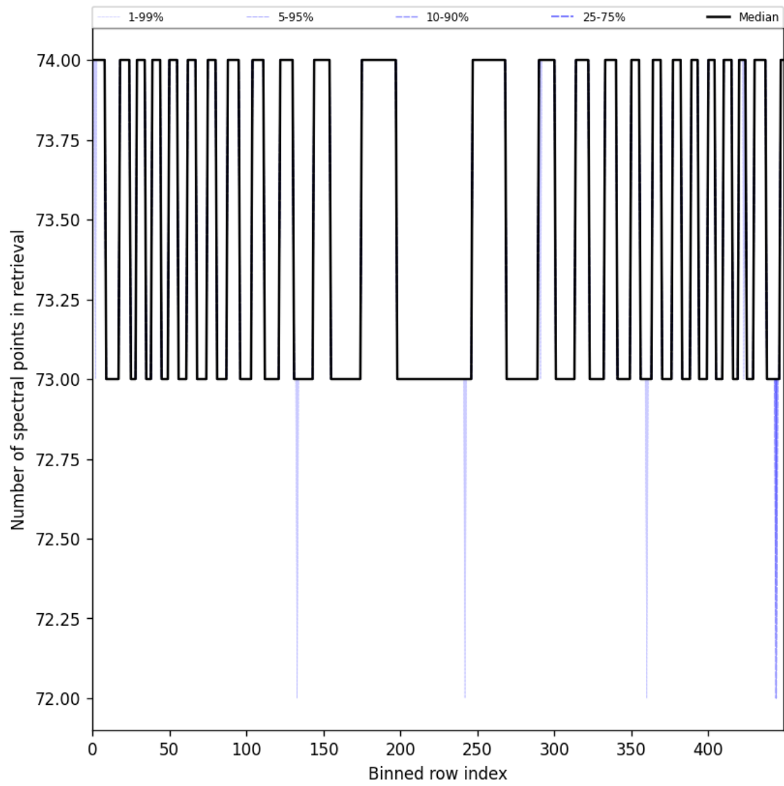
Figure 108: Along track statistics of “Number of spectral points in retrieval” for 2025-11-25 to 2025-11-27
