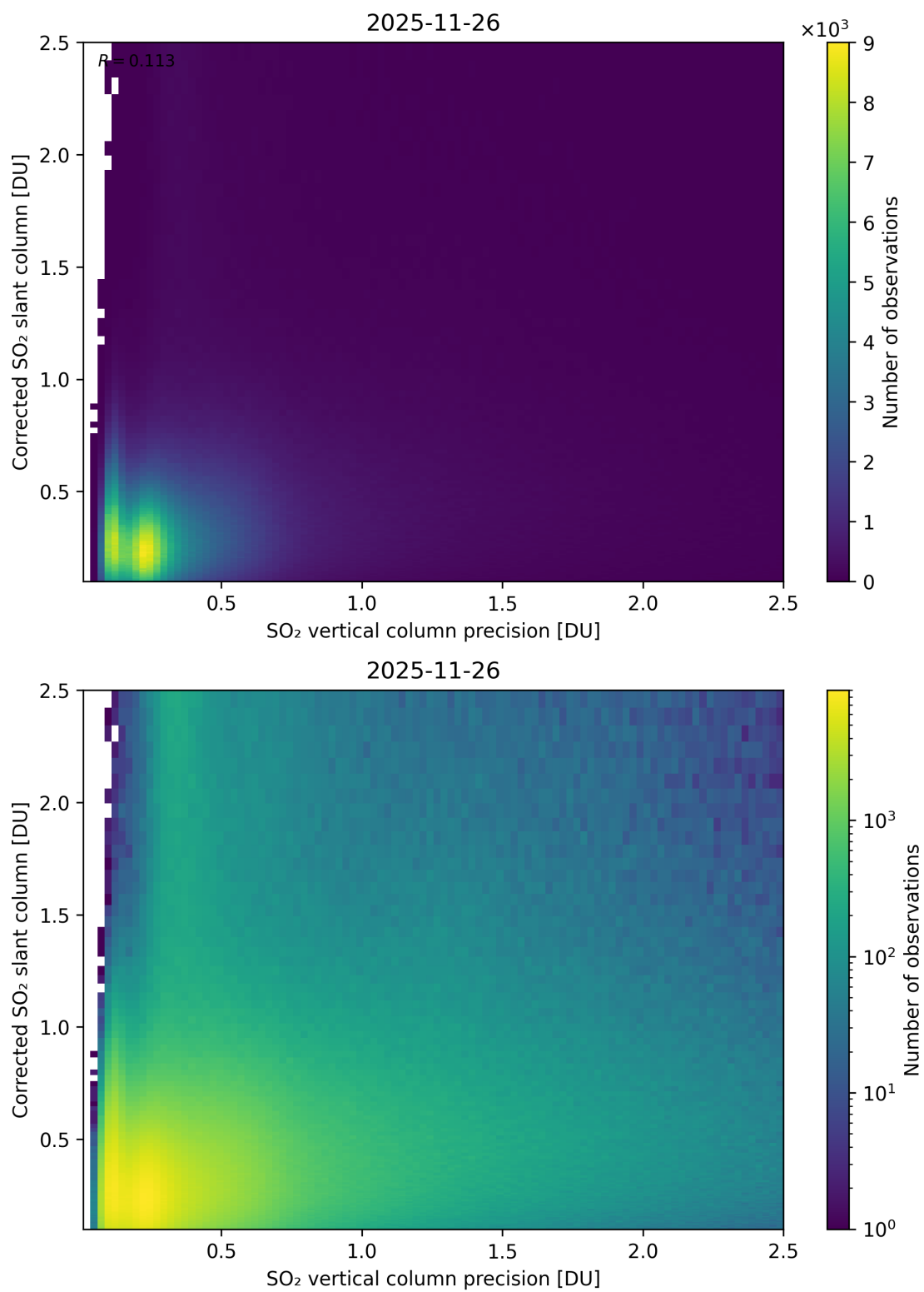
Figure 338: Scatter density plot of “SO 2 vertical column precision” against “Corrected SO 2 slant column” for 2025-11-25 to 2025-11-27.
