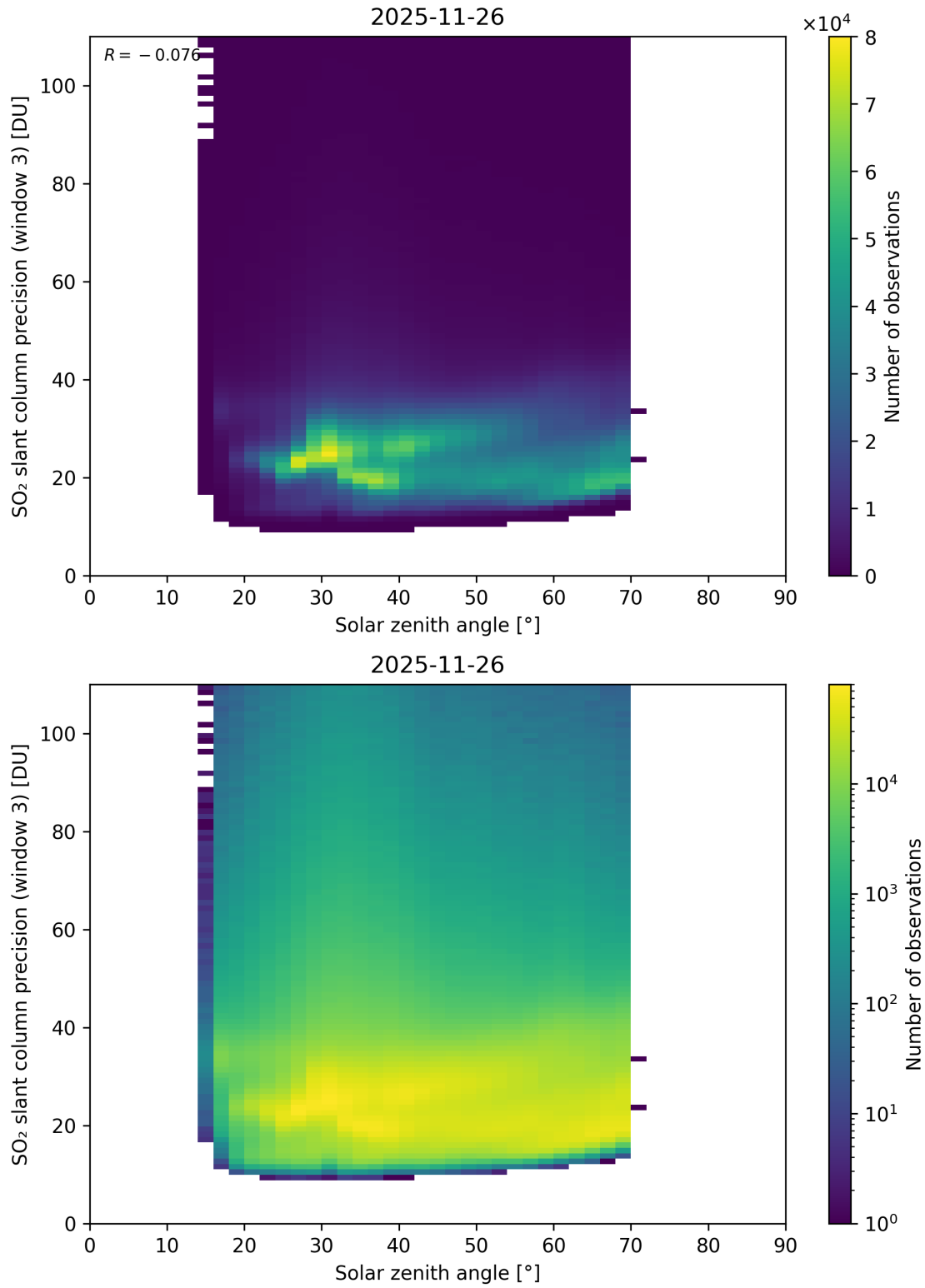
Figure 188: Scatter density plot of “Solar zenith angle” against “SO 2 slant column precision (window 3)” for 2025-11-25 to 2025-11-27.
