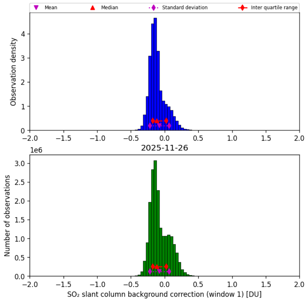
Figure 66: Histogram of “SO 2 slant column background correction (window 1)” for 2025-11-25 to 2025-11-27
