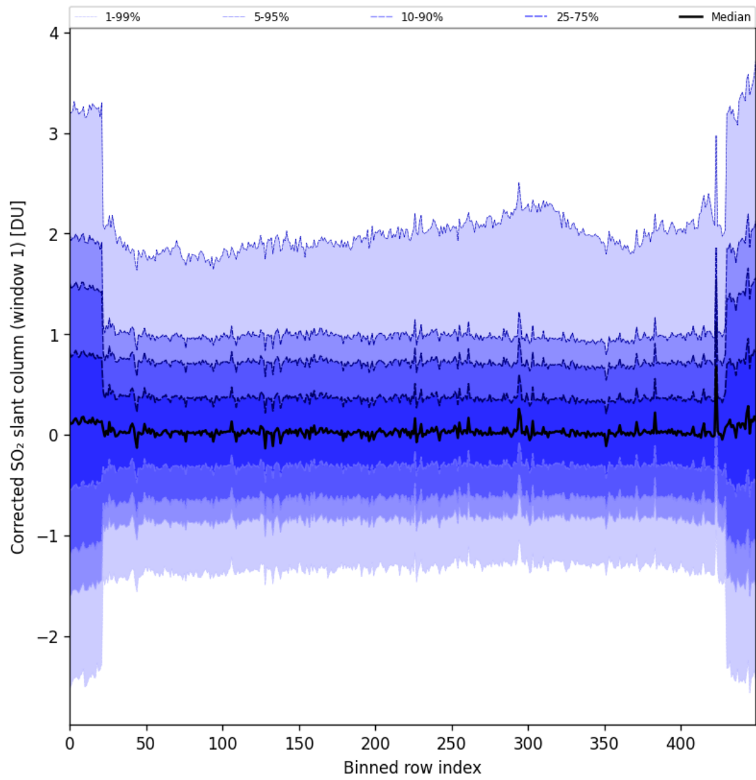
Figure 91: Along track statistics of “Corrected SO 2 slant column (window 1)” for 2025-11-25 to 2025-11-27
