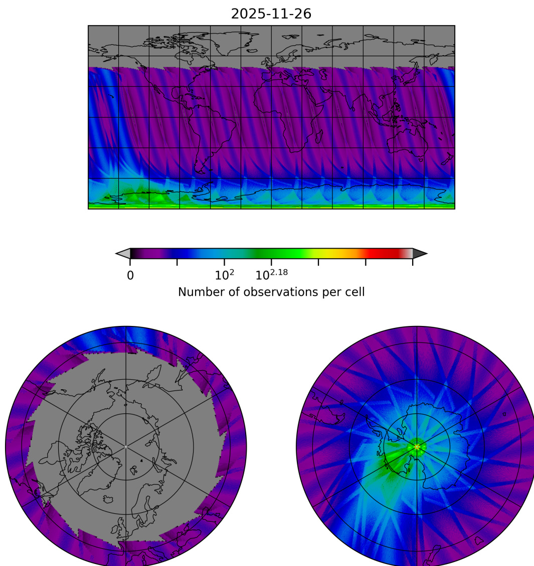
Figure 30: Map of the number of observations for 2025-11-25 to 2025-11-27
