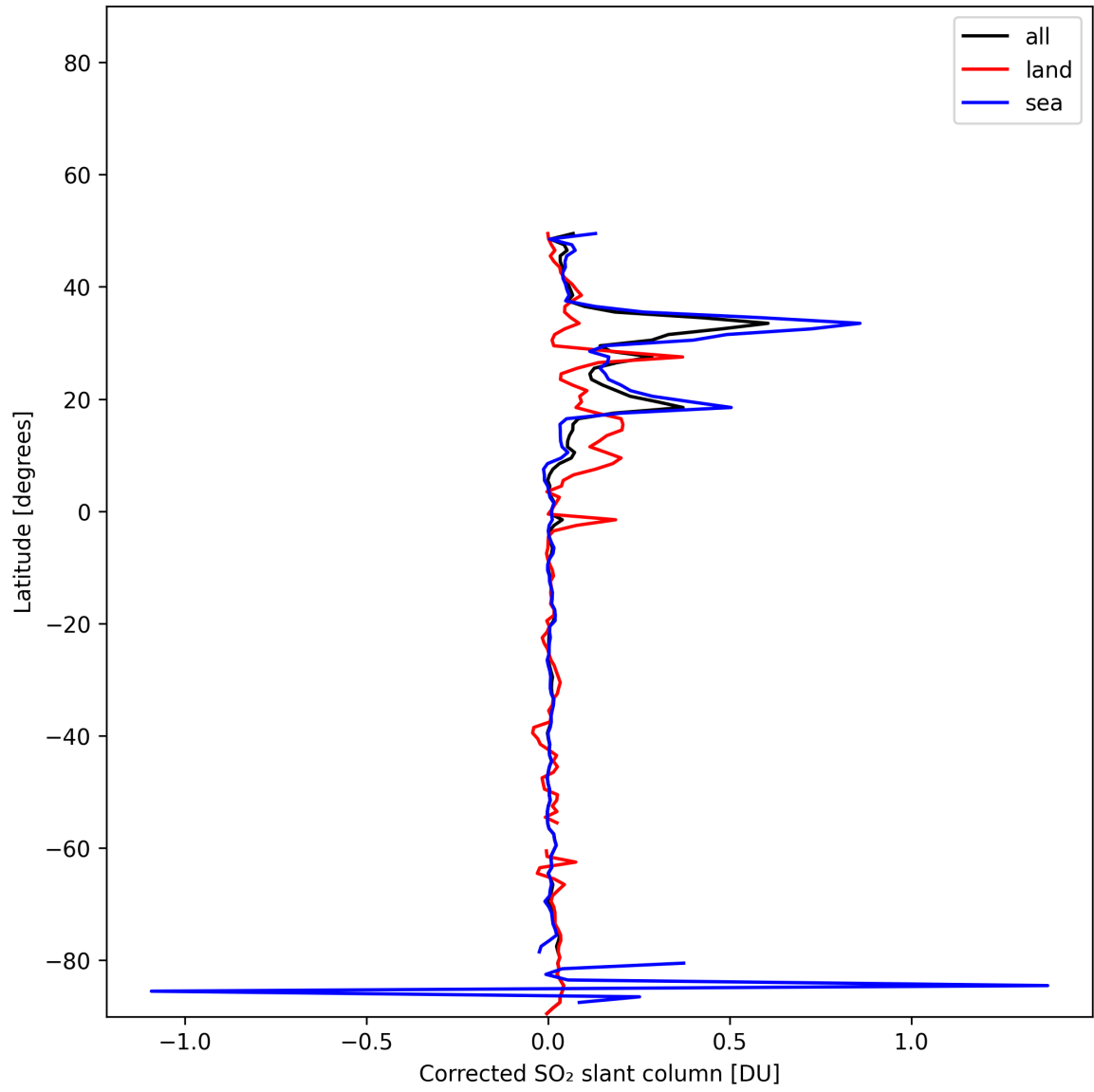
Figure 34: Zonal average of “Corrected SO 2 slant column” for 2025-11-25 to 2025-11-27.
