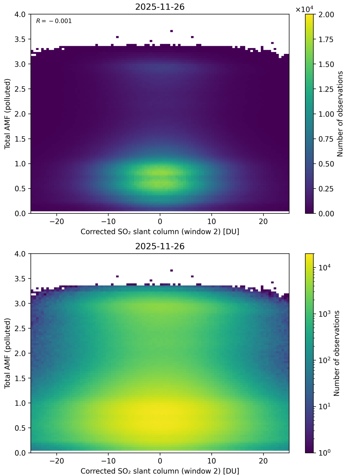
Figure 253: Scatter density plot of “Corrected SO 2 slant column (window 2)” against “Total AMF (polluted)” for 2025-11-25 to 2025-11-27.
