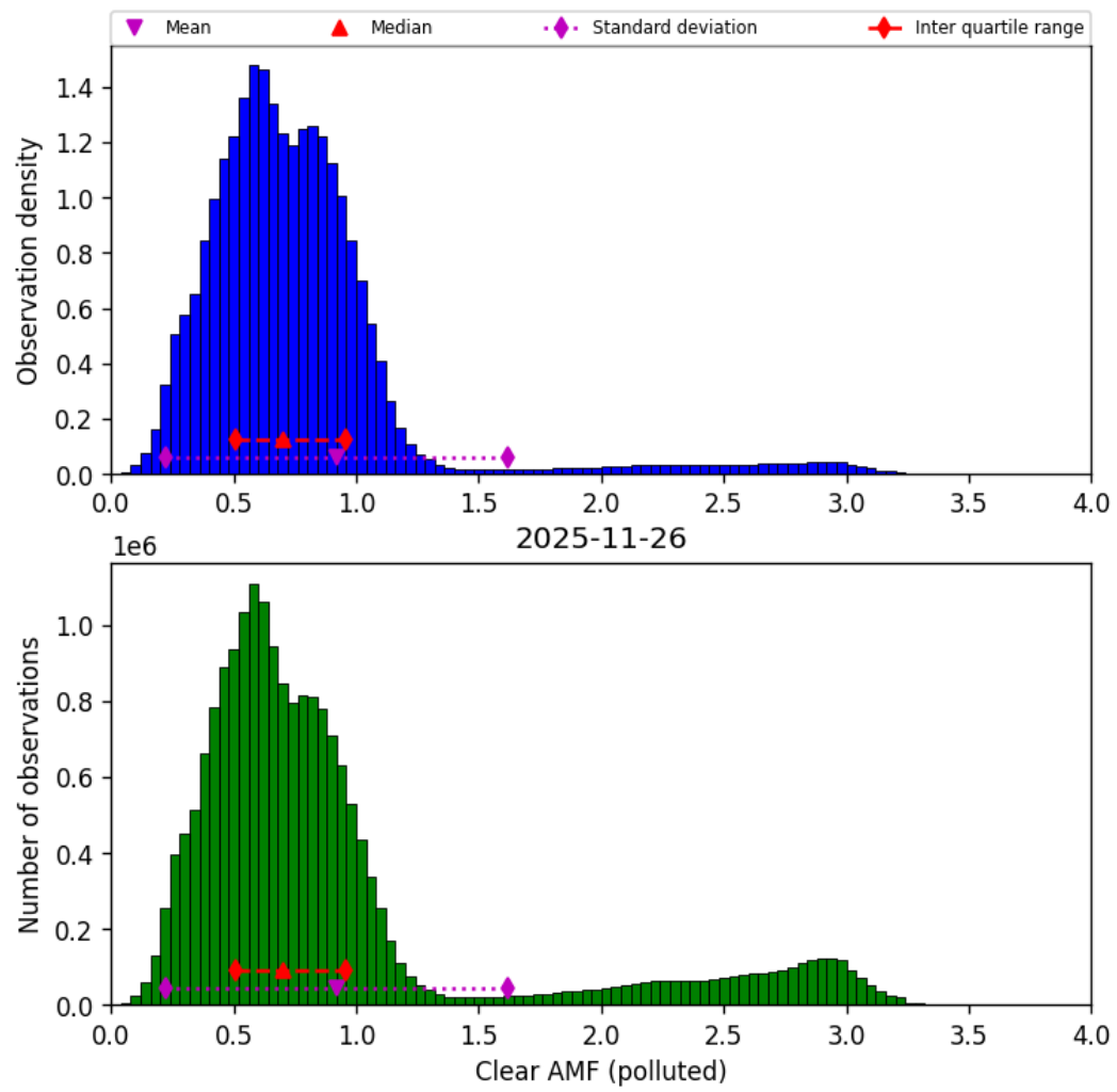
Figure 81: Histogram of “Clear AMF (polluted)” for 2025-11-25 to 2025-11-27
