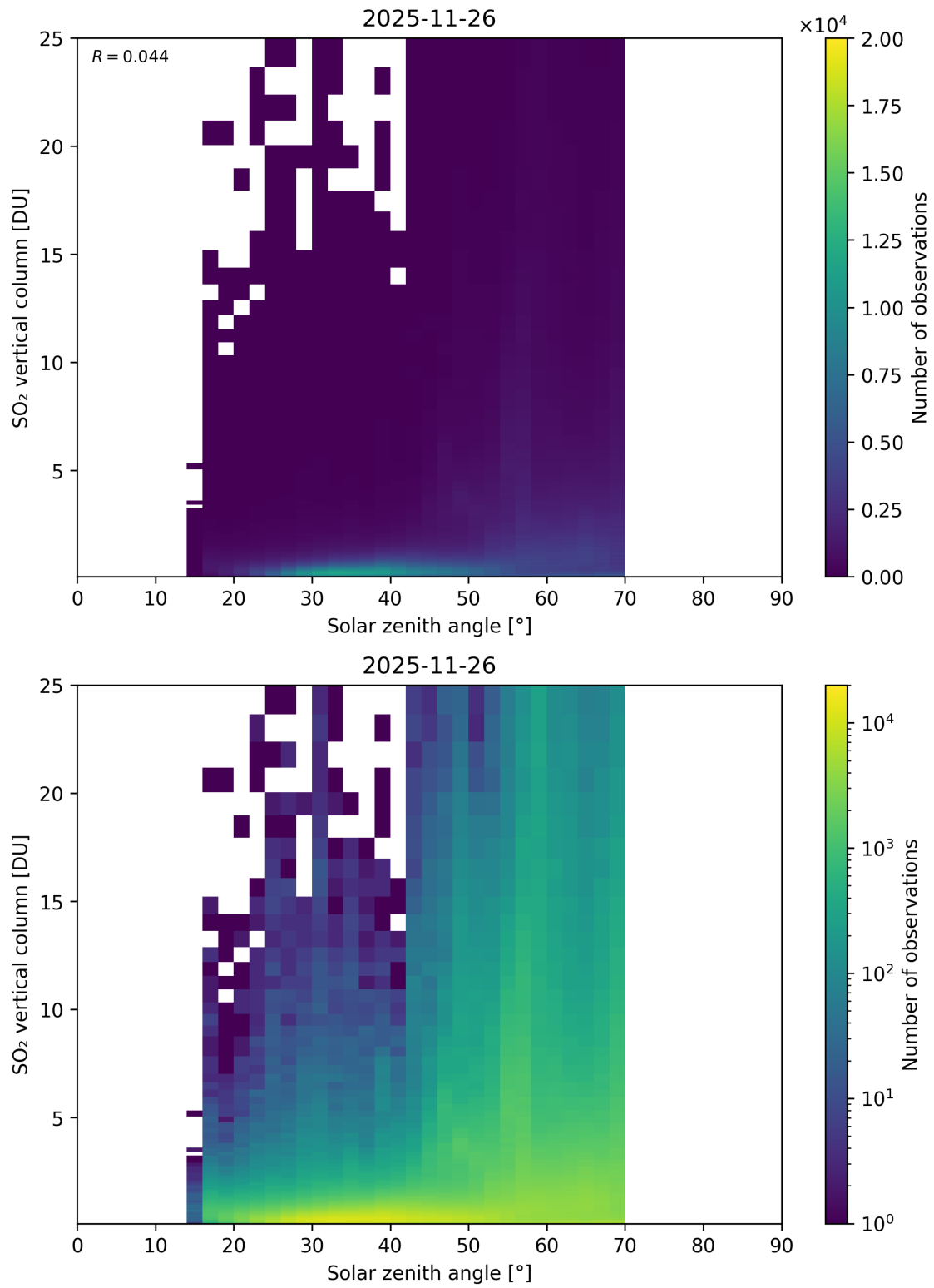
Figure 191: Scatter density plot of “Solar zenith angle” against “SO 2 vertical column” for 2025-11-25 to 2025-11-27.
