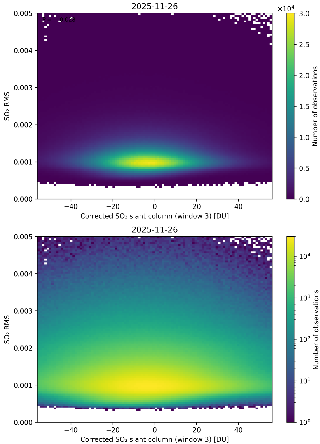
Figure 258: Scatter density plot of “Corrected SO 2 slant column (window 3)” against “SO 2 RMS” for 2025-11-25 to 2025-11-27.
