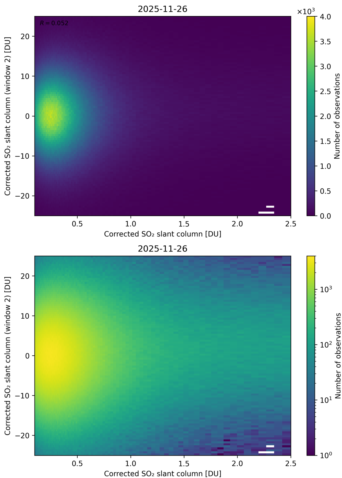
Figure 235: Scatter density plot of “Corrected SO 2 slant column” against “Corrected SO 2 slant column (window 2)” for 2025-11-25 to 2025-11-27.
