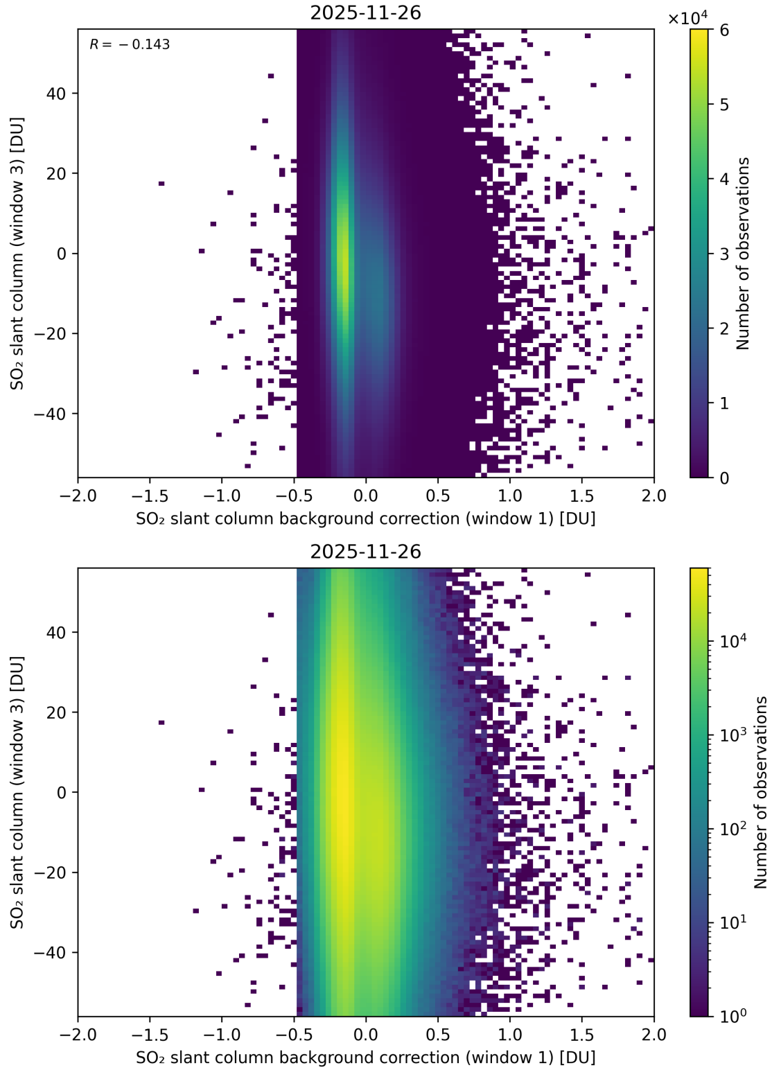
Figure 118: Scatter density plot of “SO 2 slant column background correction (window 1)” against “SO 2 slant column (window 3)” for 2025-11-25 to 2025-11-27.
