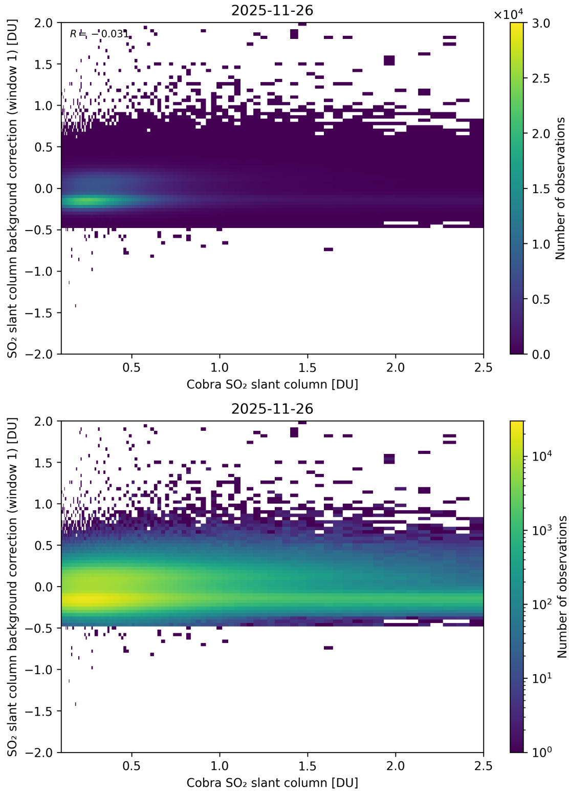
Figure 193: Scatter density plot of “Cobra SO 2 slant column” against “SO 2 slant column background correction (window 1)” for 2025-11-25 to 2025-11-27.
