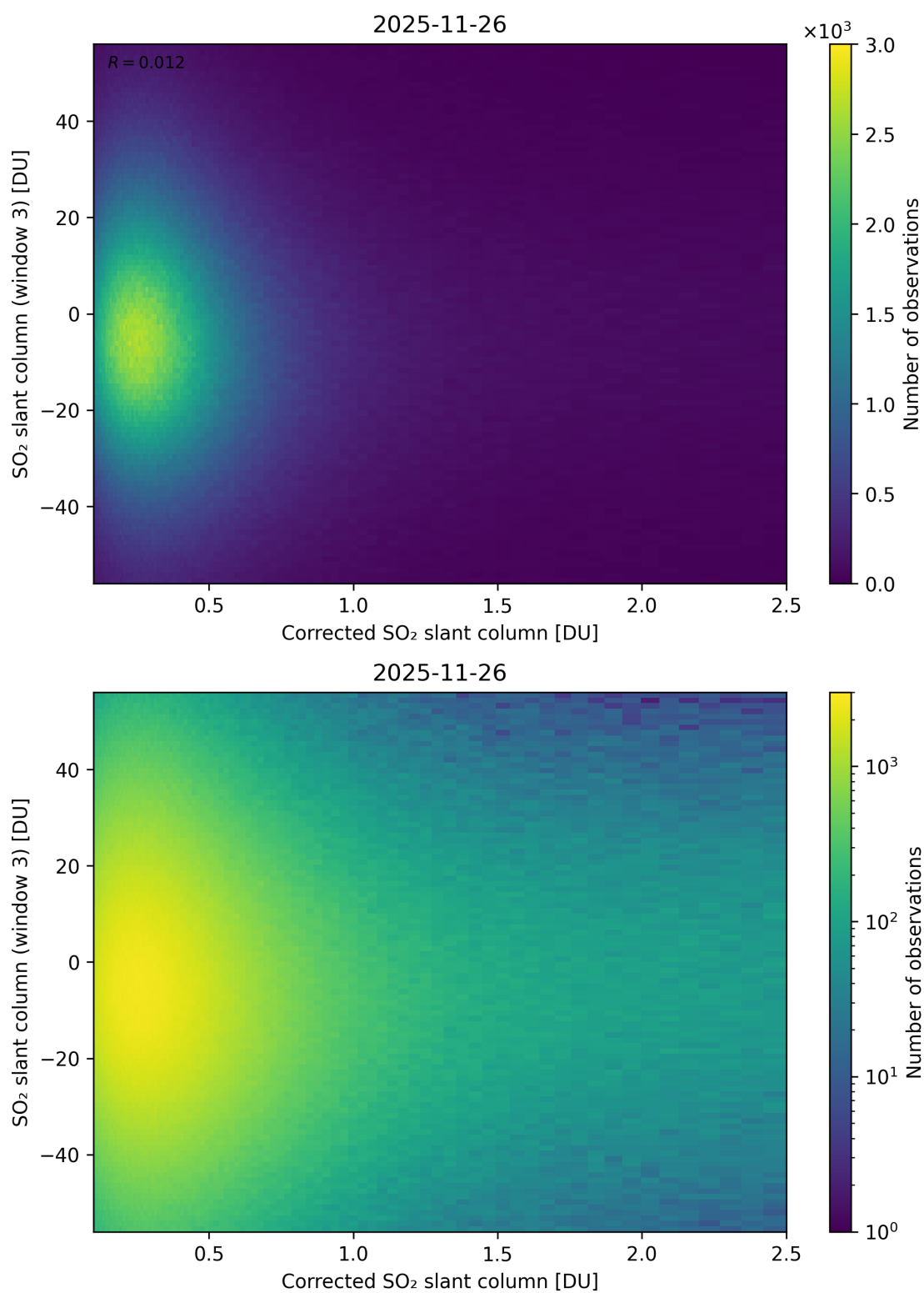
Figure 240: Scatter density plot of “Corrected SO 2 slant column” against “SO 2 slant column (window 3)” for 2025-11-25 to 2025-11-27.
