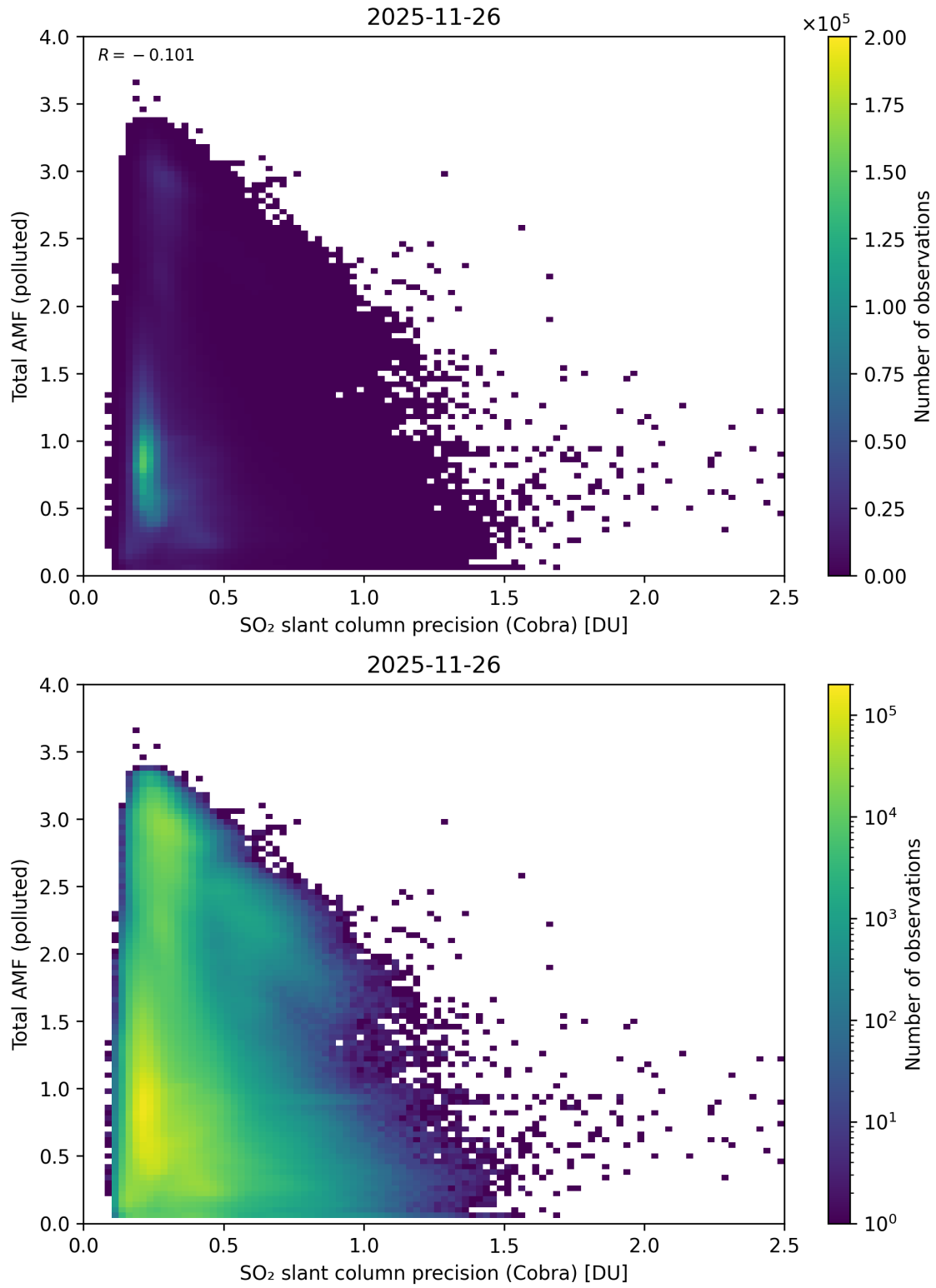
Figure 213: Scatter density plot of “SO 2 slant column precision (Cobra)” against “Total AMF (polluted)” for 2025-11-25 to 2025-11-27.
