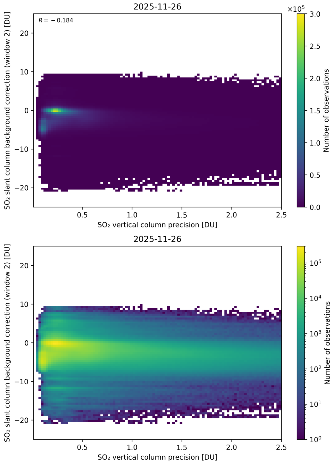
Figure 330: Scatter density plot of “SO 2 vertical column precision” against “SO 2 slant column background correction (window 2)” for 2025-11-25 to 2025-11-27.
