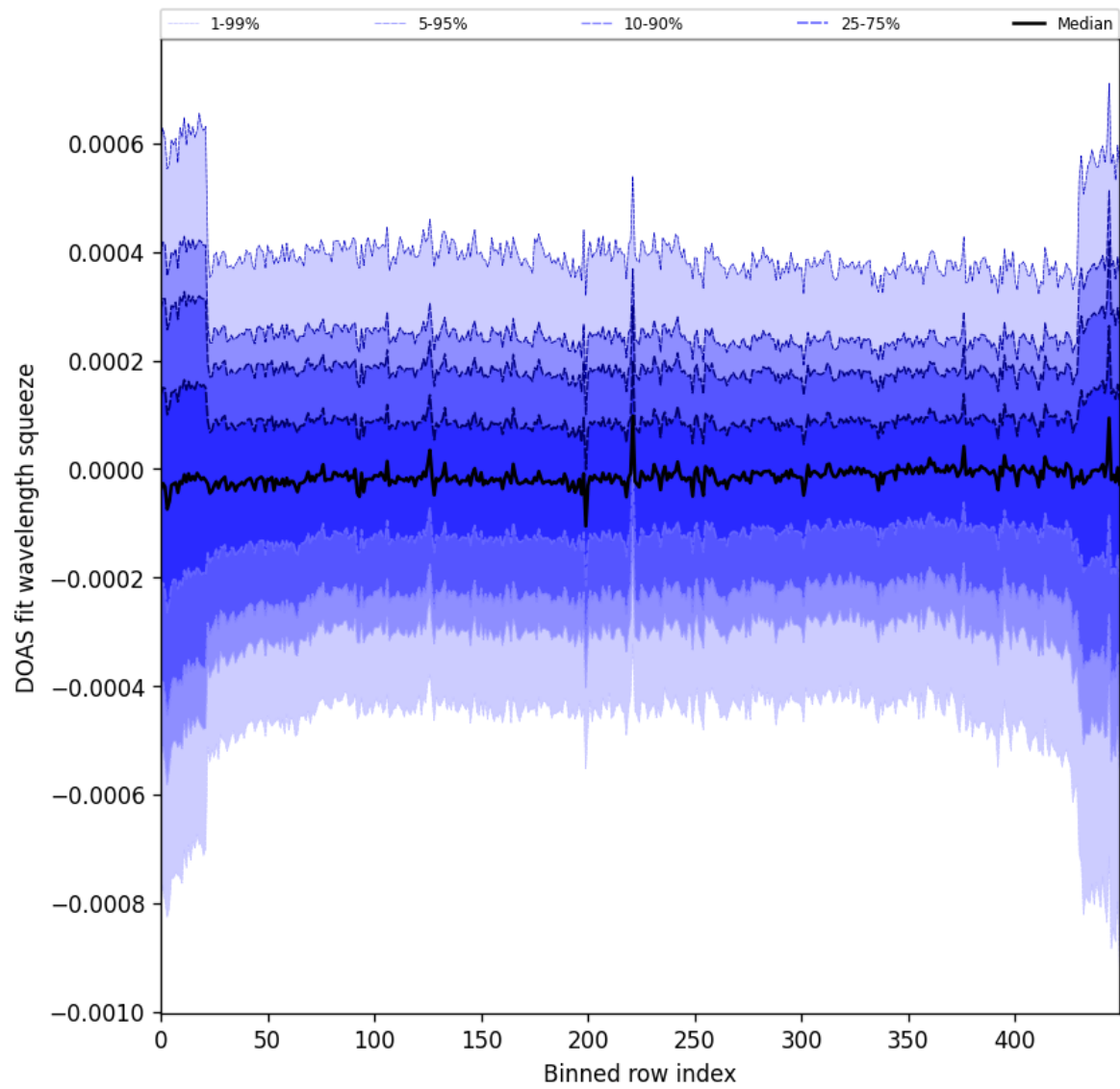
Figure 103: Along track statistics of “DOAS fit wavelength squeeze” for 2025-11-25 to 2025-11-27
