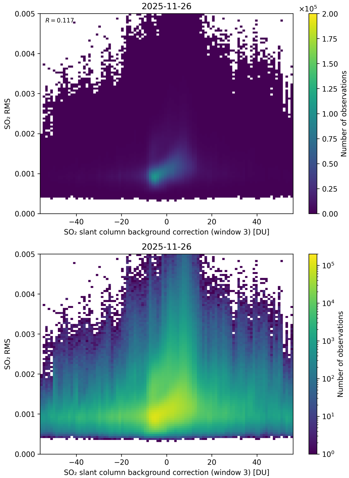
Figure 134: Scatter density plot of “SO 2 slant column background correction (window 3)” against “SO 2 RMS” for 2025-11-25 to 2025-11-27.
