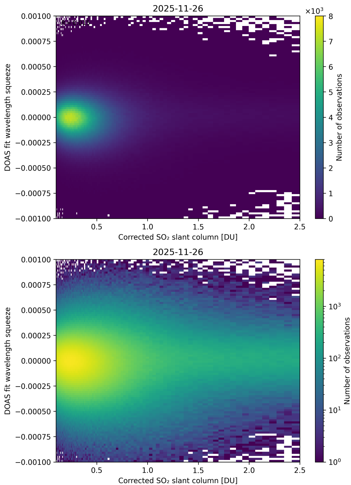
Figure 230: Scatter density plot of “Corrected SO 2 slant column” against “DOAS fit wavelength squeeze” for 2025-11-25 to 2025-11-27.
