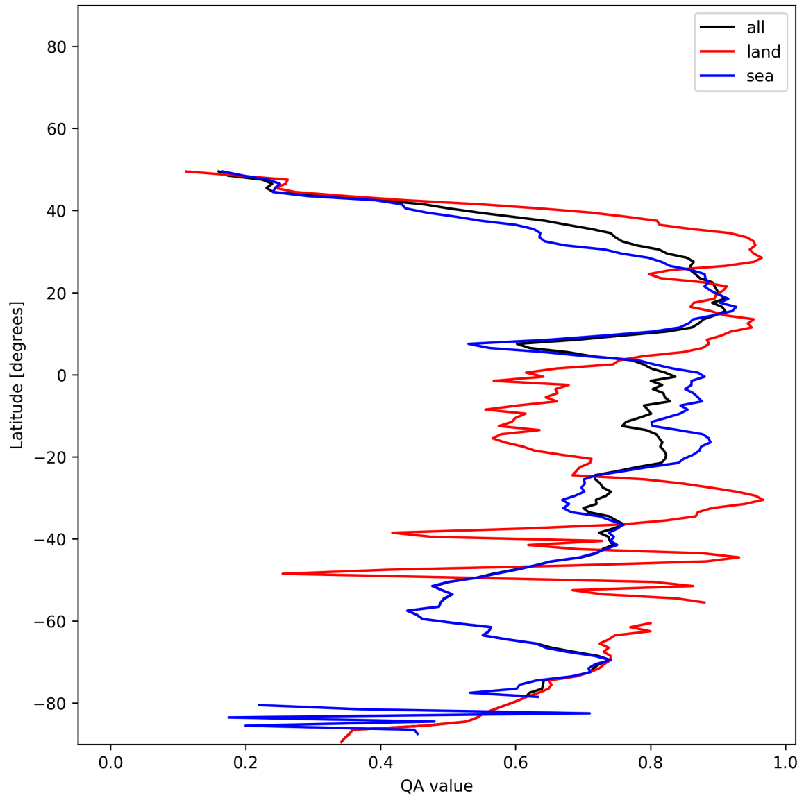
Figure 31: Zonal average of “QA value” for 2025-11-25 to 2025-11-27.
