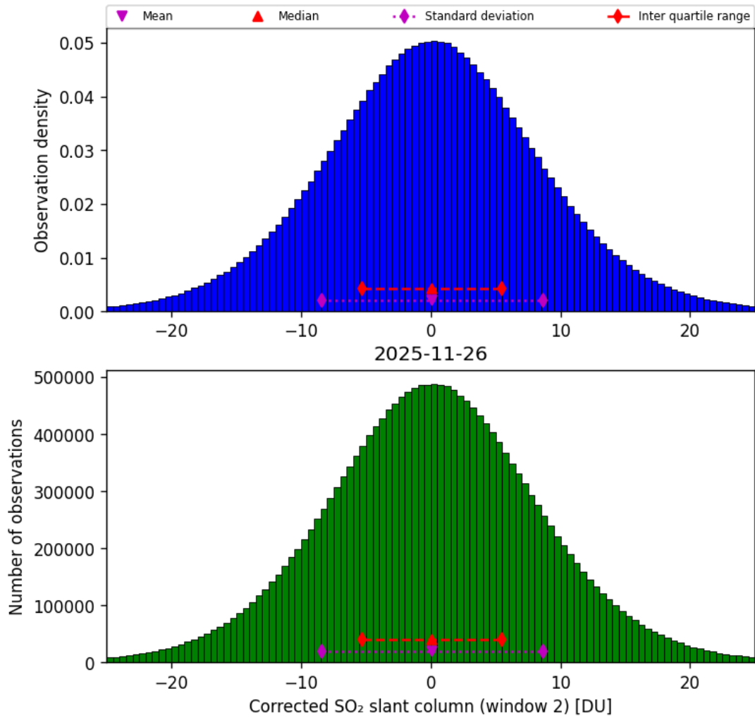
Figure 69: Histogram of “Corrected SO 2 slant column (window 2)” for 2025-11-25 to 2025-11-27
