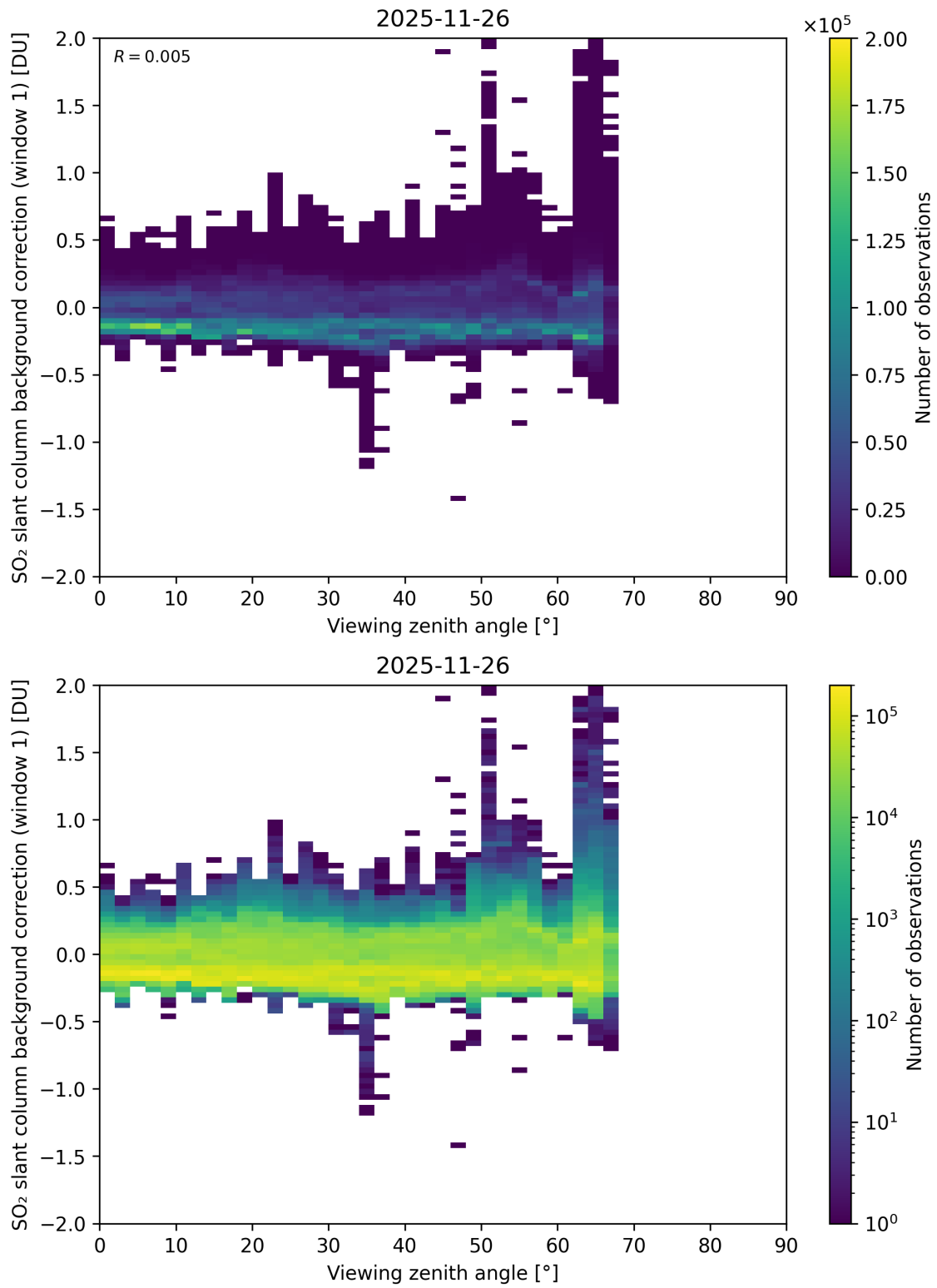
Figure 362: Scatter density plot of “Viewing zenith angle” against “SO 2 slant column background correction (window 1)” for 2025-11-25 to 2025-11-27.
