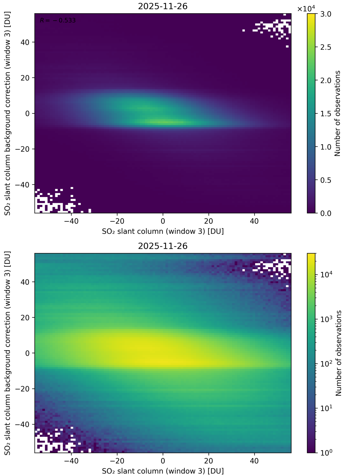
Figure 303: Scatter density plot of “SO 2 slant column (window 3)” against “SO 2 slant column background correction (window 3)” for 2025-11-25 to 2025-11-27.
