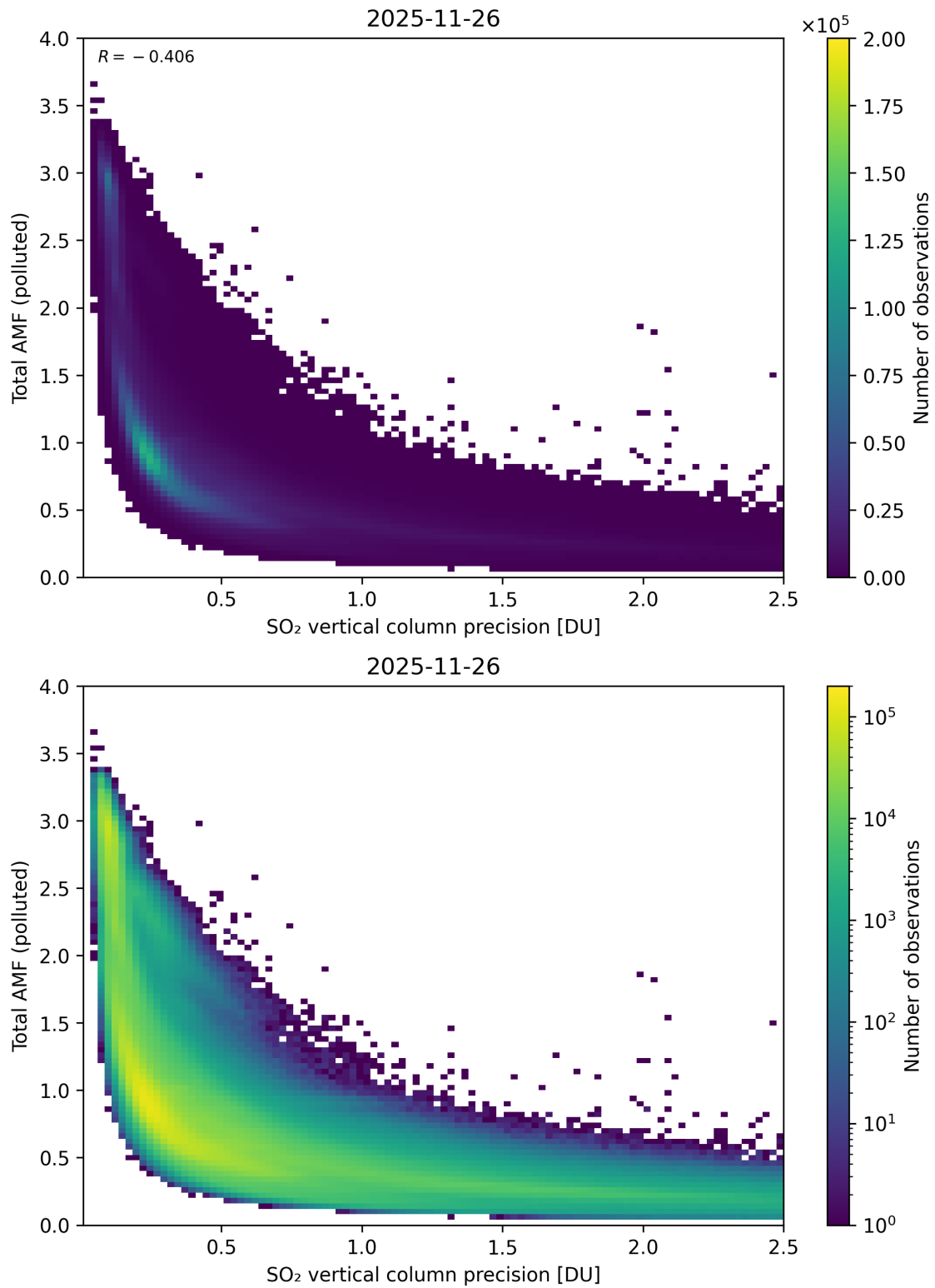
Figure 346: Scatter density plot of “SO 2 vertical column precision” against “Total AMF (polluted)” for 2025-11-25 to 2025-11-27.
