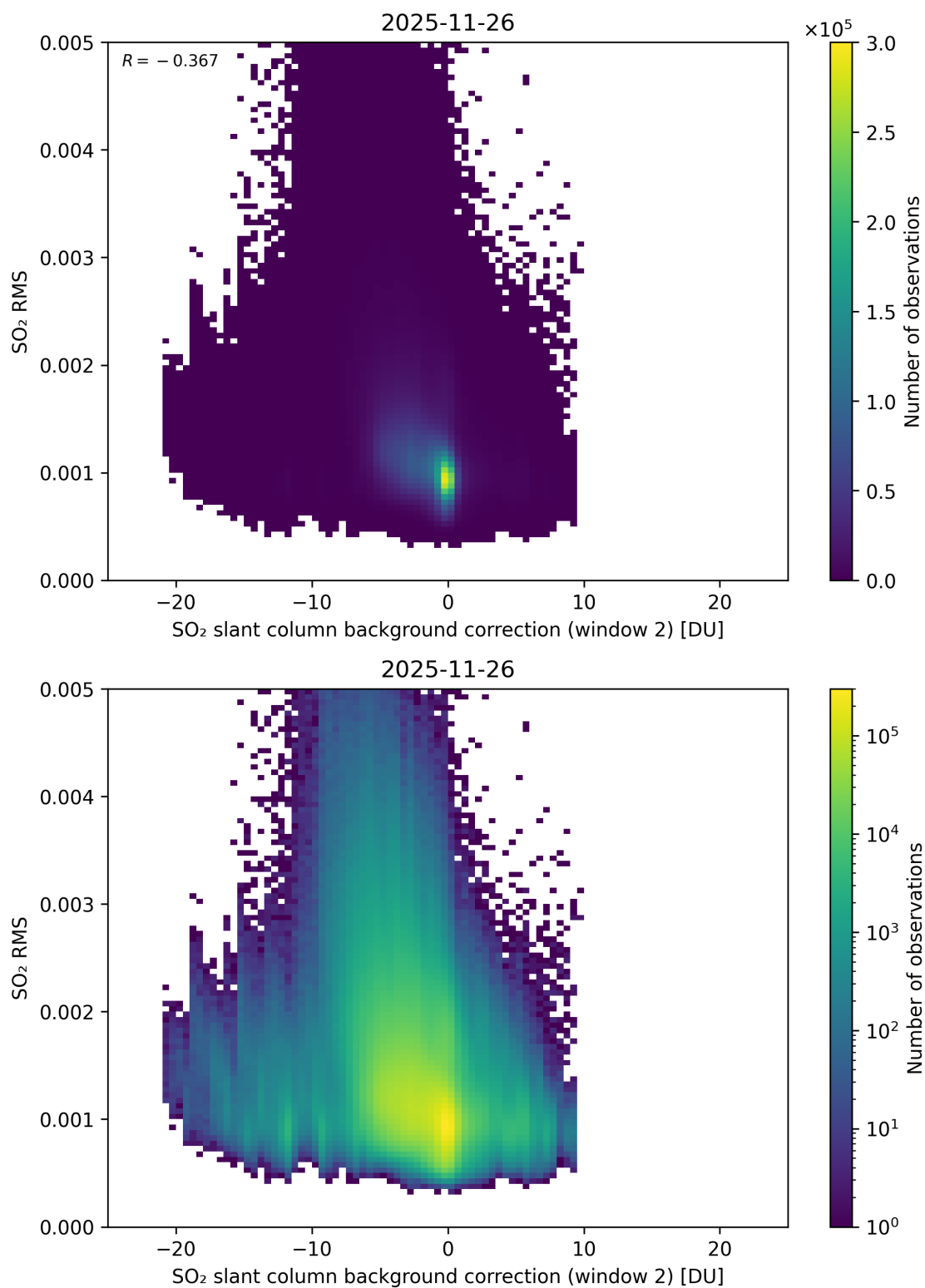
Figure 125: Scatter density plot of “SO 2 slant column background correction (window 2)” against “SO 2 RMS” for 2025-11-25 to 2025-11-27.
