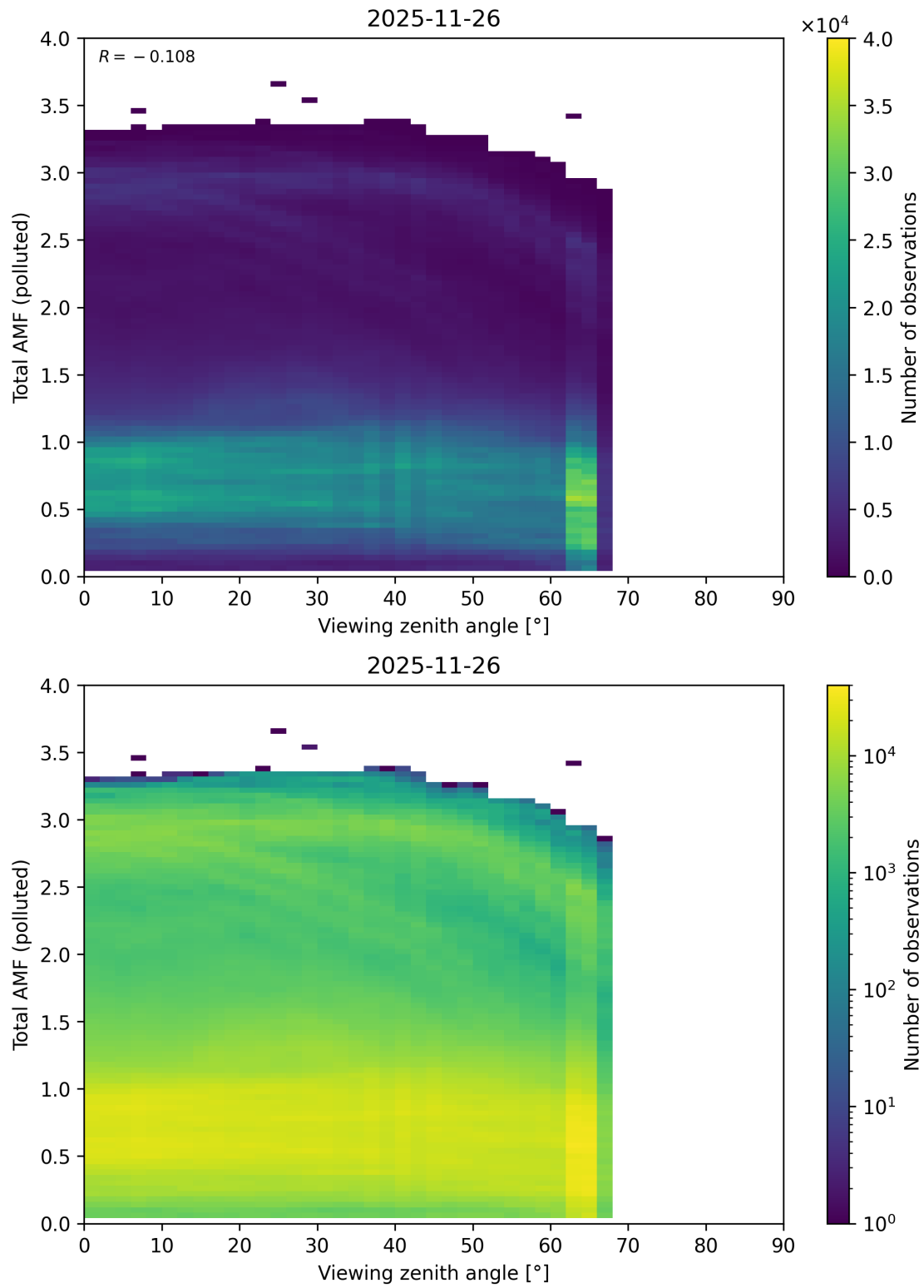
Figure 381: Scatter density plot of “Viewing zenith angle” against “Total AMF (polluted)” for 2025-11-25 to 2025-11-27.
