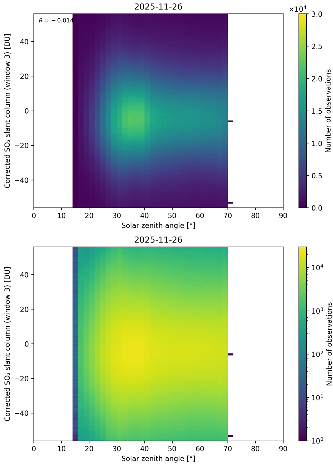
Figure 183: Scatter density plot of “Solar zenith angle” against “Corrected SO 2 slant column (window 3)” for 2025-11-25 to 2025-11-27.
