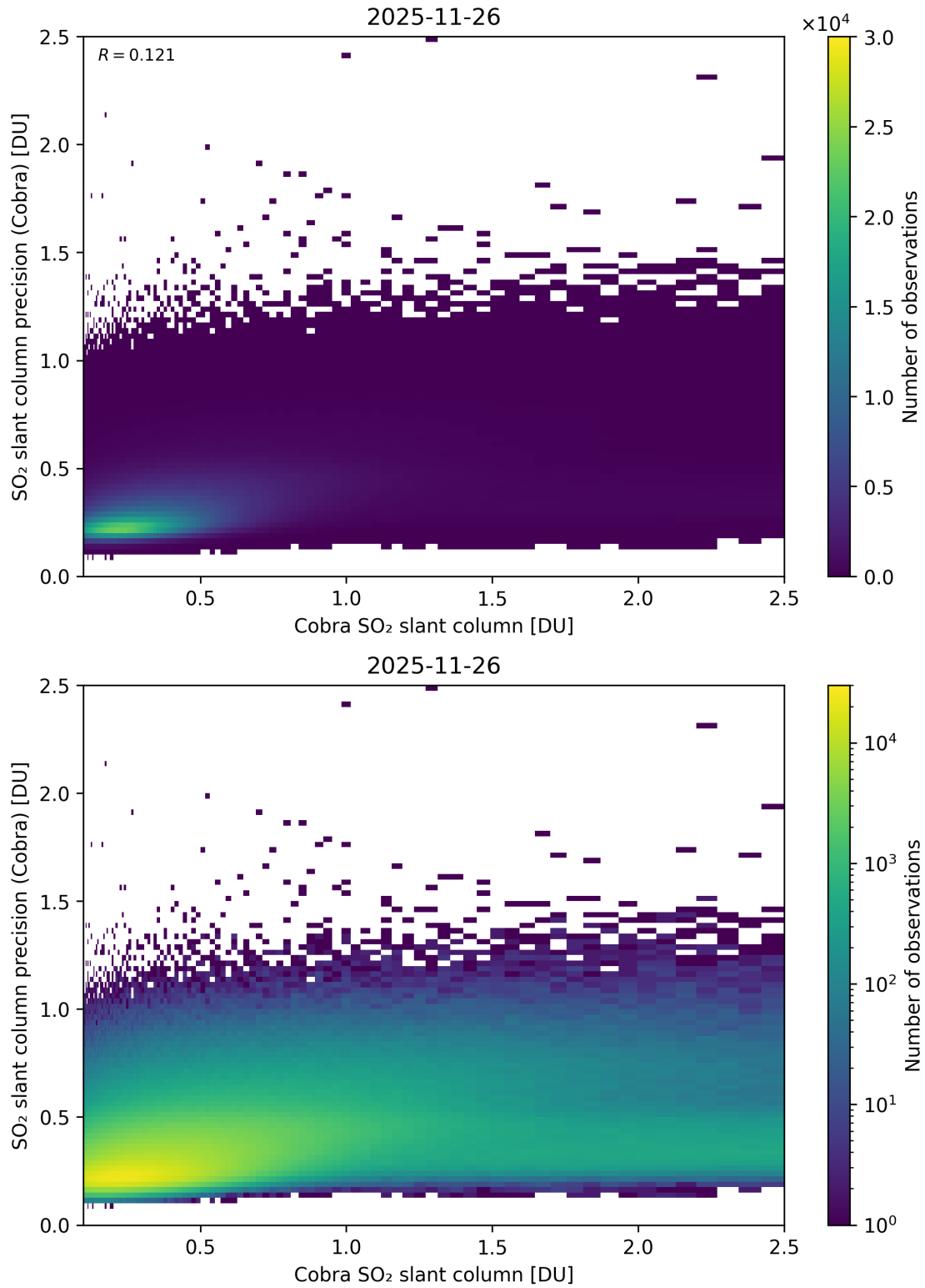
Figure 216: Scatter density plot of “Cobra SO 2 slant column” against “SO 2 slant column precision (Cobra)” for 2025-11-25 to 2025-11-27.
