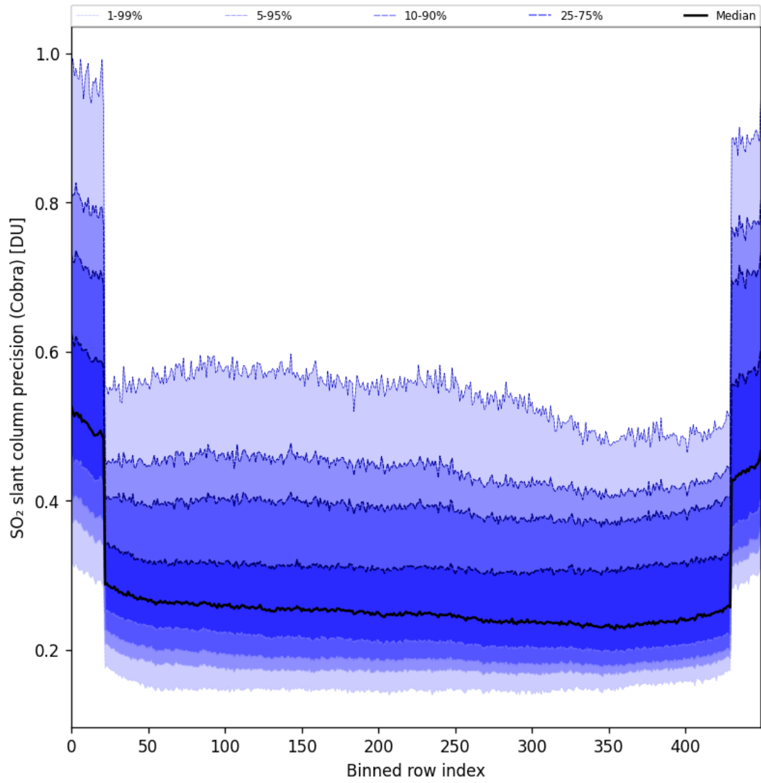
Figure 88: Along track statistics of “SO 2 slant column precision (Cobra)” for 2025-11-25 to 2025-11-27
