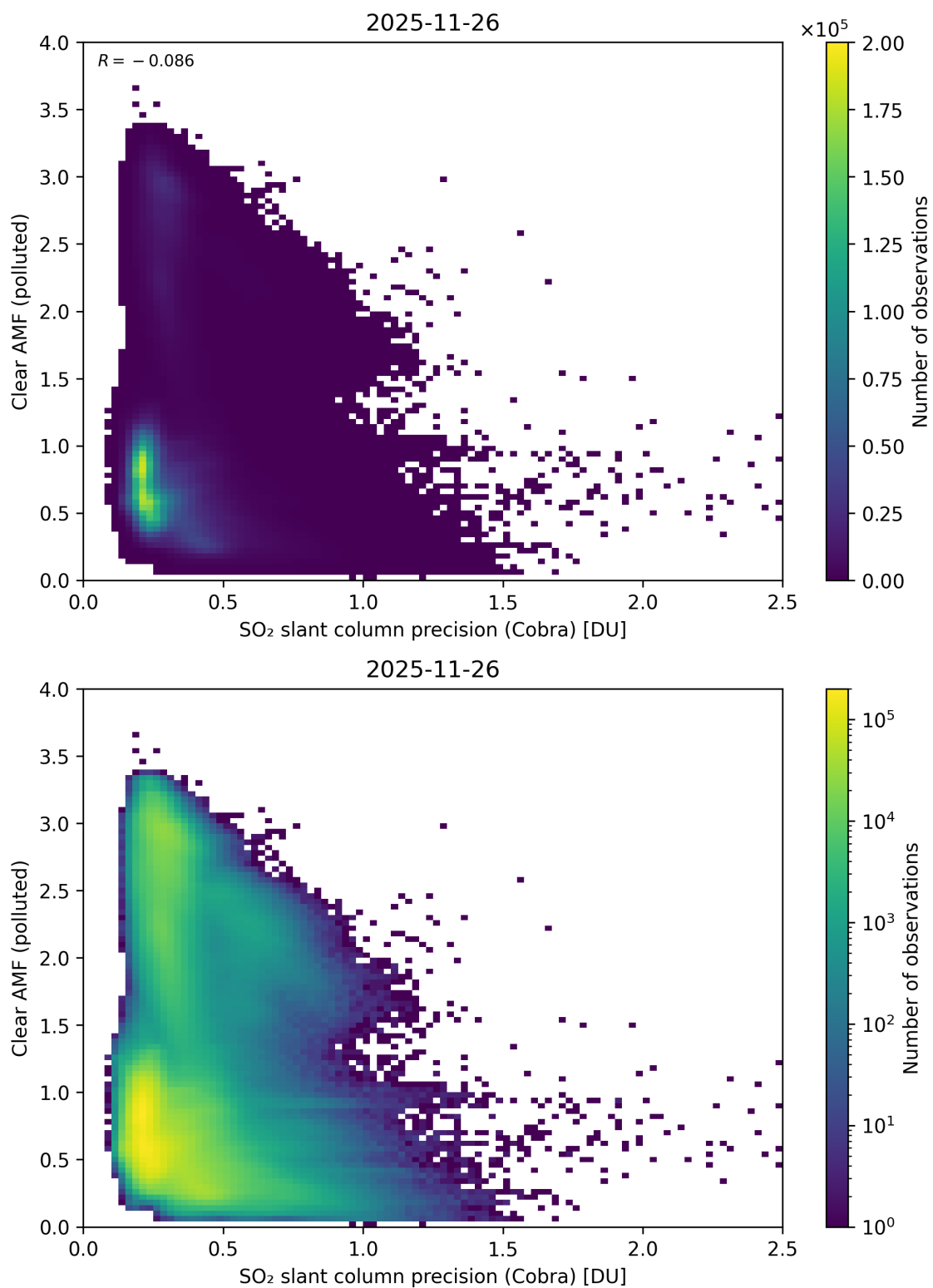
Figure 205: Scatter density plot of “SO 2 slant column precision (Cobra)” against “Clear AMF (polluted)” for 2025-11-25 to 2025-11-27.
