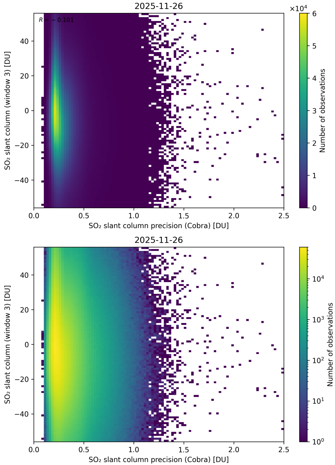
Figure 211: Scatter density plot of “SO 2 slant column precision (Cobra)” against “SO 2 slant column (window 3)” for 2025-11-25 to 2025-11-27.
