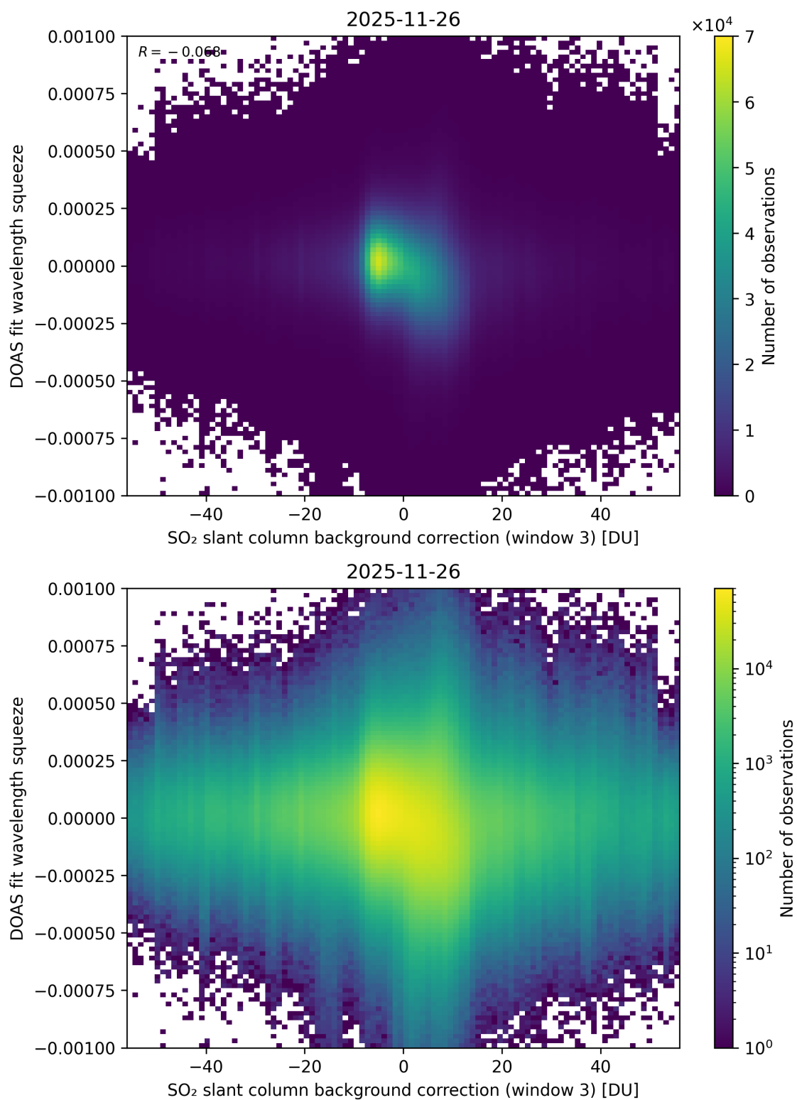
Figure 133: Scatter density plot of “SO 2 slant column background correction (window 3)” against “DOAS fit wavelength squeeze” for 2025-11-25 to 2025-11-27.
