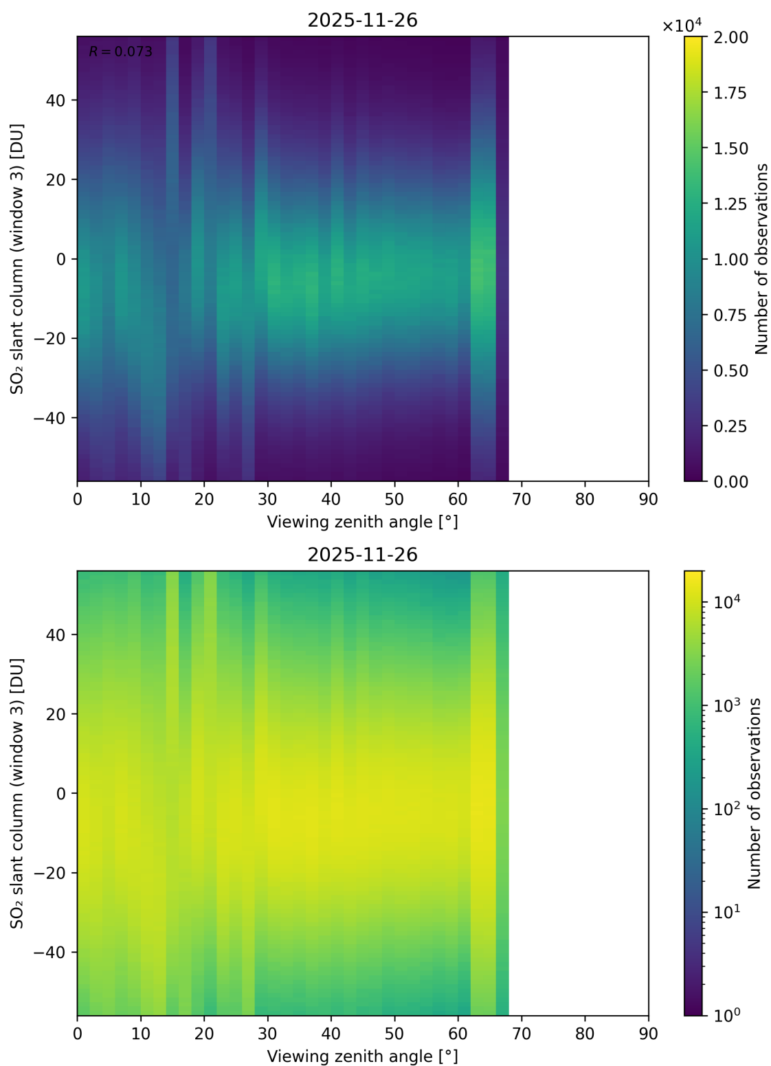
Figure 379: Scatter density plot of “Viewing zenith angle” against “SO 2 slant column (window 3)” for 2025-11-25 to 2025-11-27.
