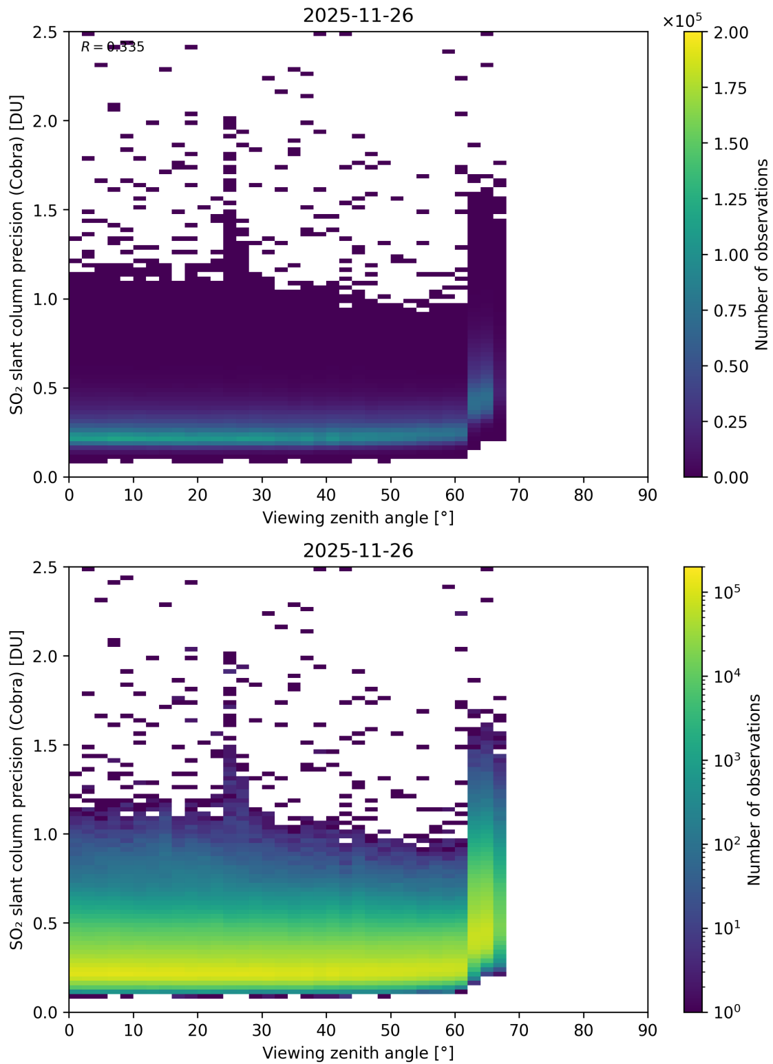
Figure 372: Scatter density plot of “Viewing zenith angle” against “SO 2 slant column precision (Cobra)” for 2025-11-25 to 2025-11-27.
