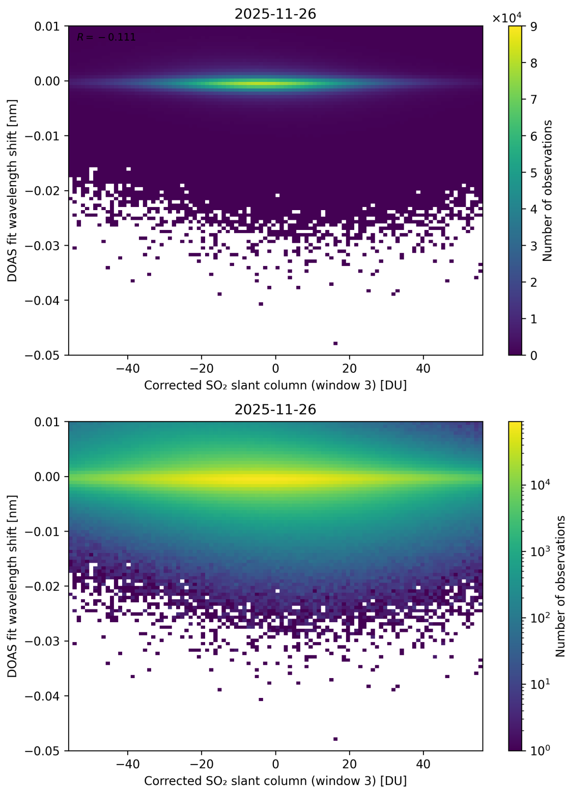
Figure 256: Scatter density plot of “Corrected SO 2 slant column (window 3)” against “DOAS fit wavelength shift” for 2025-11-25 to 2025-11-27.
