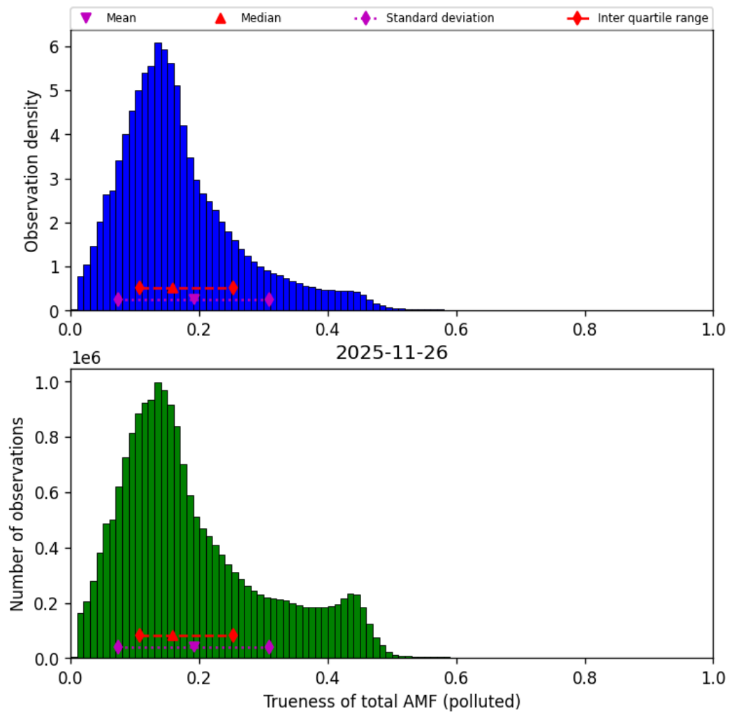
Figure 80: Histogram of “Trueness of total AMF (polluted)” for 2025-11-25 to 2025-11-27
