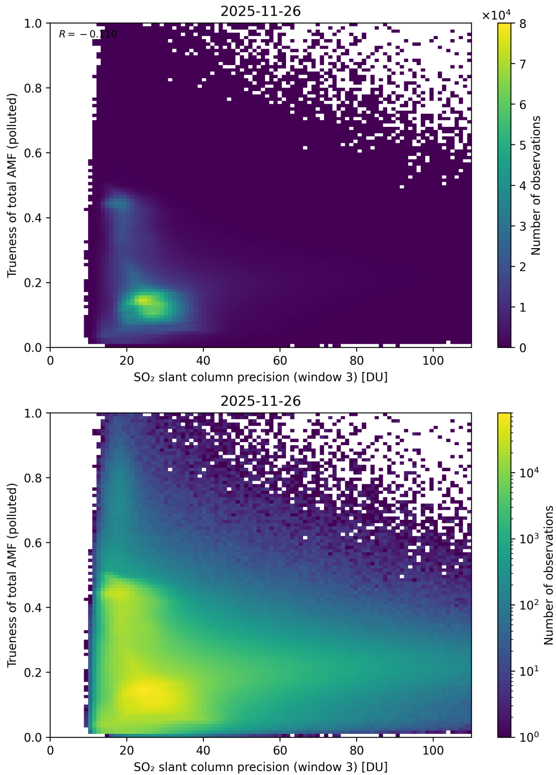
Figure 314: Scatter density plot of “SO 2 slant column precision (window 3)” against “Trueness of total AMF (polluted)” for 2025-11-25 to 2025-11-27.
