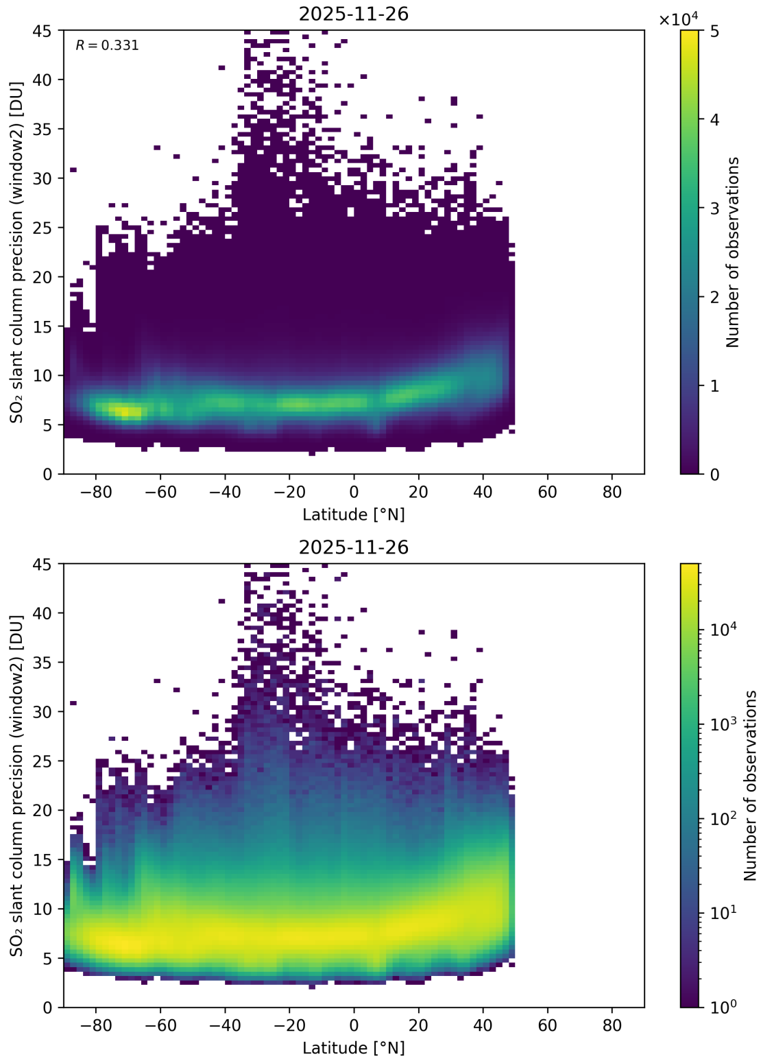
Figure 164: Scatter density plot of “Latitude” against “SO 2 slant column precision (window2)” for 2025-11-25 to 2025-11-27.
