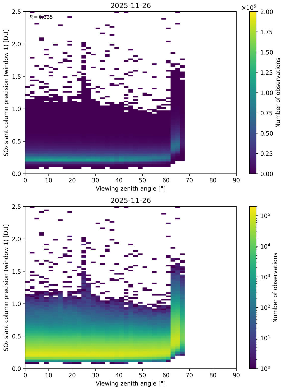
Figure 377: Scatter density plot of “Viewing zenith angle” against “SO 2 slant column precision (window 1)” for 2025-11-25 to 2025-11-27.
