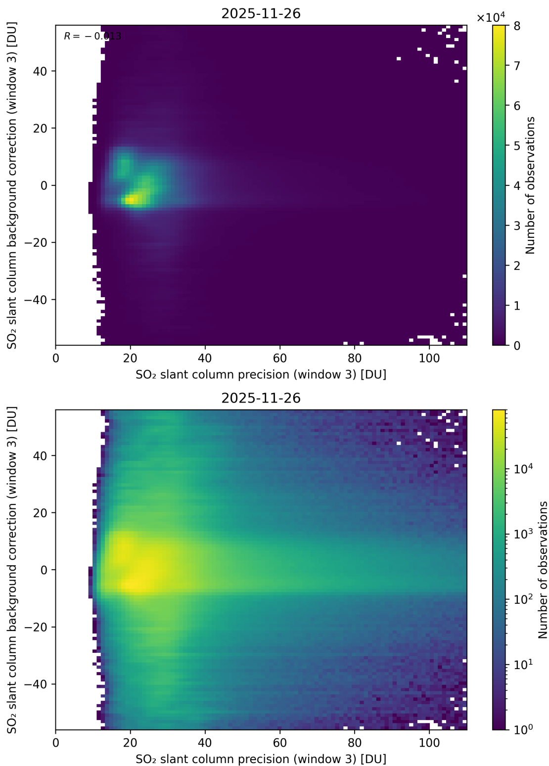
Figure 307: Scatter density plot of “SO 2 slant column precision (window 3)” against “SO 2 slant column background correction (window 3)” for 2025-11-25 to 2025-11-27.
