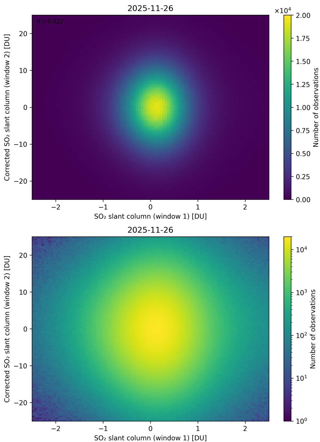
Figure 283: Scatter density plot of “SO 2 slant column (window 1)” against “Corrected SO 2 slant column (window 2)” for 2025-11-25 to 2025-11-27.
