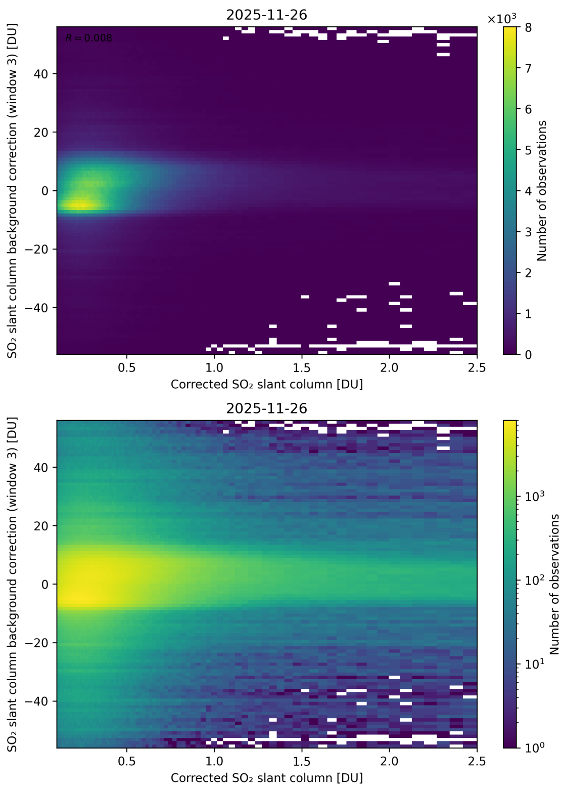
Figure 228: Scatter density plot of “Corrected SO 2 slant column” against “SO 2 slant column background correction (window 3)” for 2025-11-25 to 2025-11-27.
