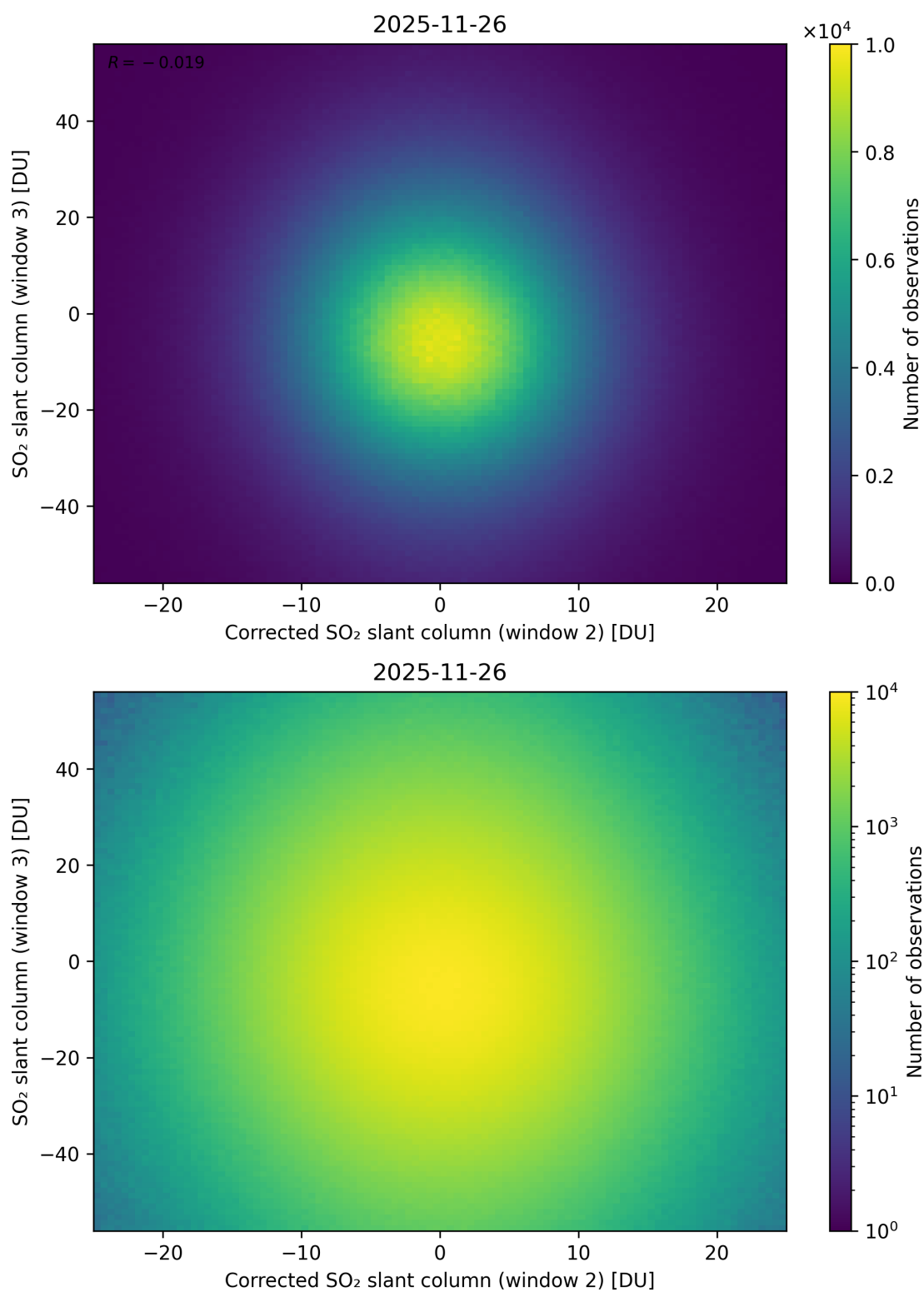
Figure 251: Scatter density plot of “Corrected SO 2 slant column (window 2)” against “SO 2 slant column (window 3)” for 2025-11-25 to 2025-11-27.
