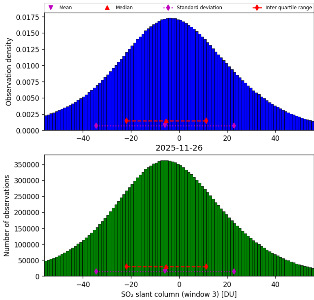
Figure 71: Histogram of “SO 2 slant column (window 3)” for 2025-11-25 to 2025-11-27
