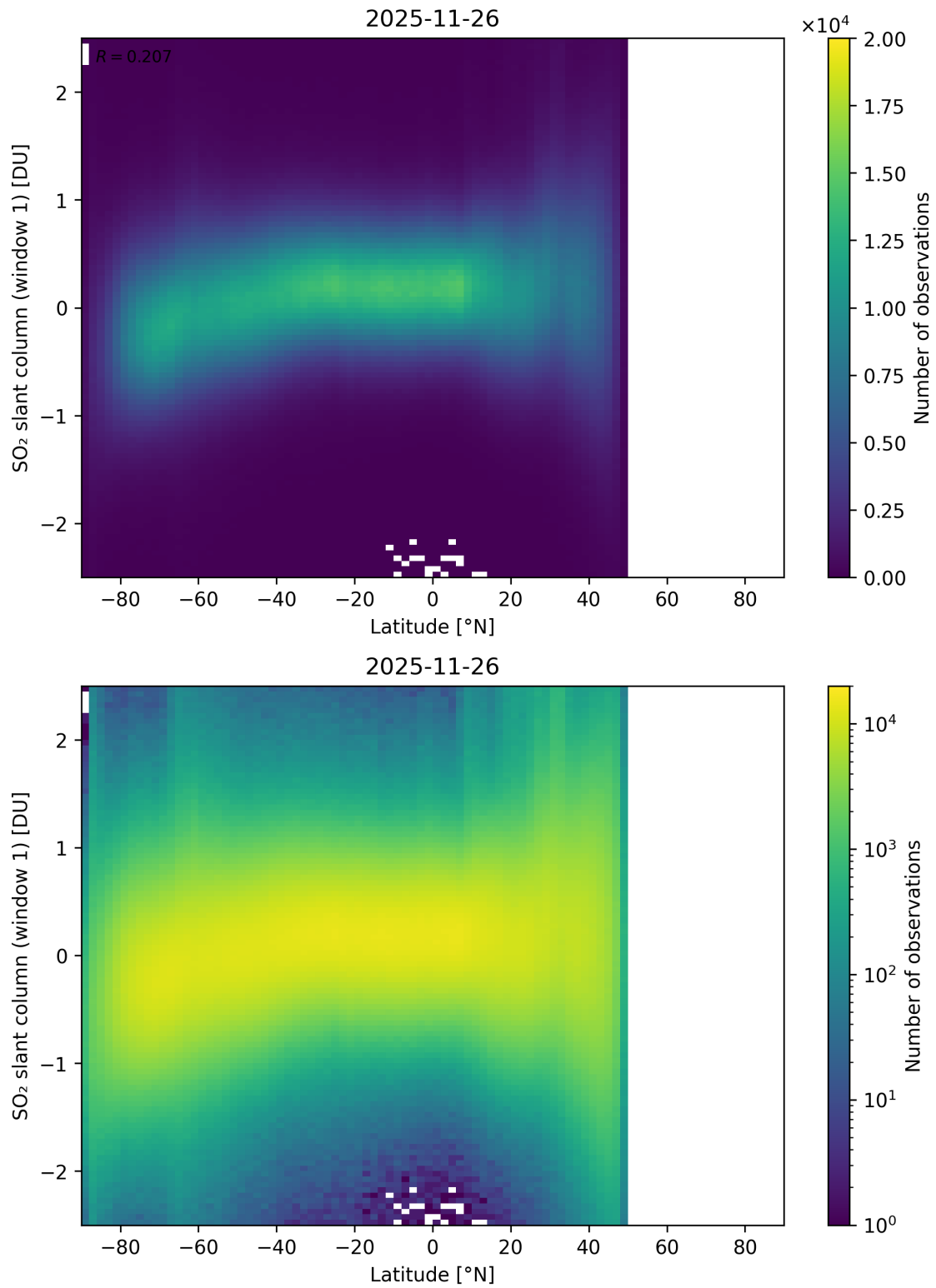
Figure 162: Scatter density plot of “Latitude” against “SO 2 slant column (window 1)” for 2025-11-25 to 2025-11-27.
