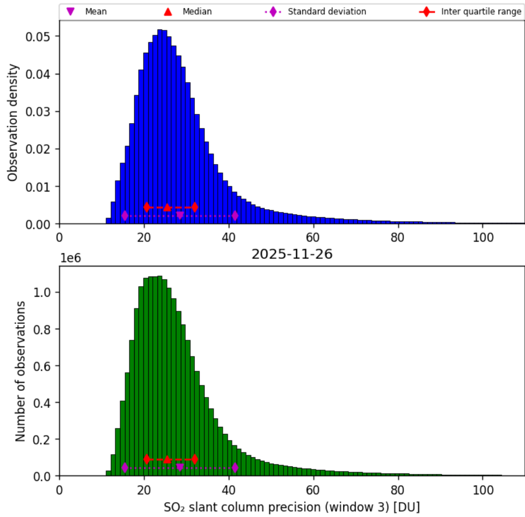
Figure 72: Histogram of “SO 2 slant column precision (window 3)” for 2025-11-25 to 2025-11-27
