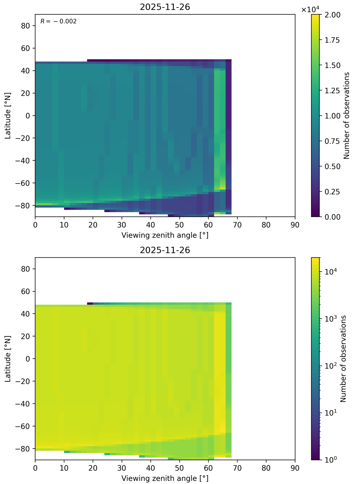
Figure 368: Scatter density plot of “Viewing zenith angle” against “Latitude” for 2025-11-25 to 2025-11-27.
