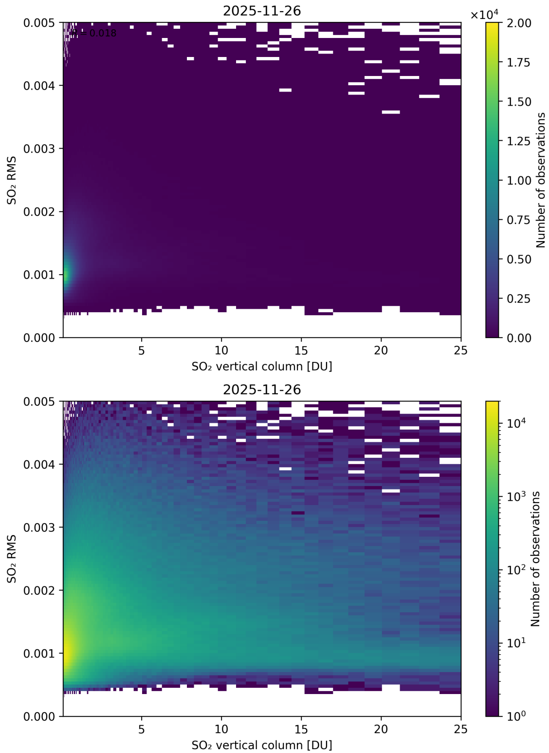
Figure 328: Scatter density plot of “SO 2 vertical column” against “SO 2 RMS” for 2025-11-25 to 2025-11-27.
