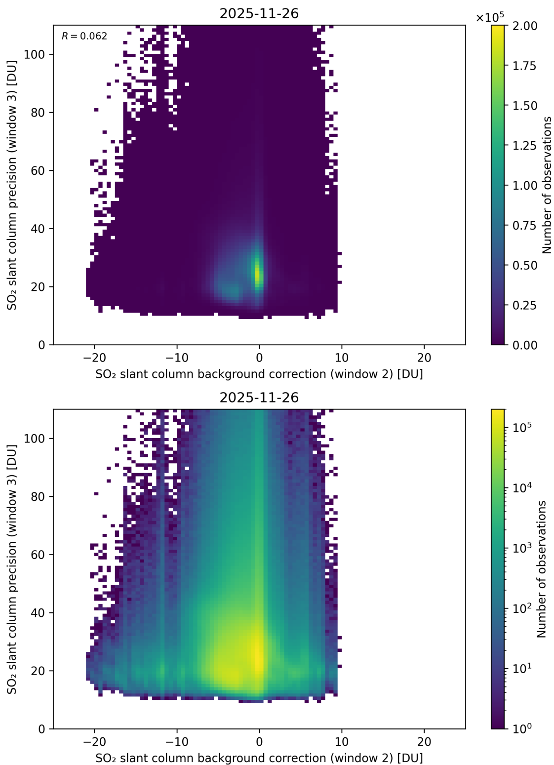
Figure 129: Scatter density plot of “SO 2 slant column background correction (window 2)” against “SO 2 slant column precision (window 3)” for 2025-11-25 to 2025-11-27.
