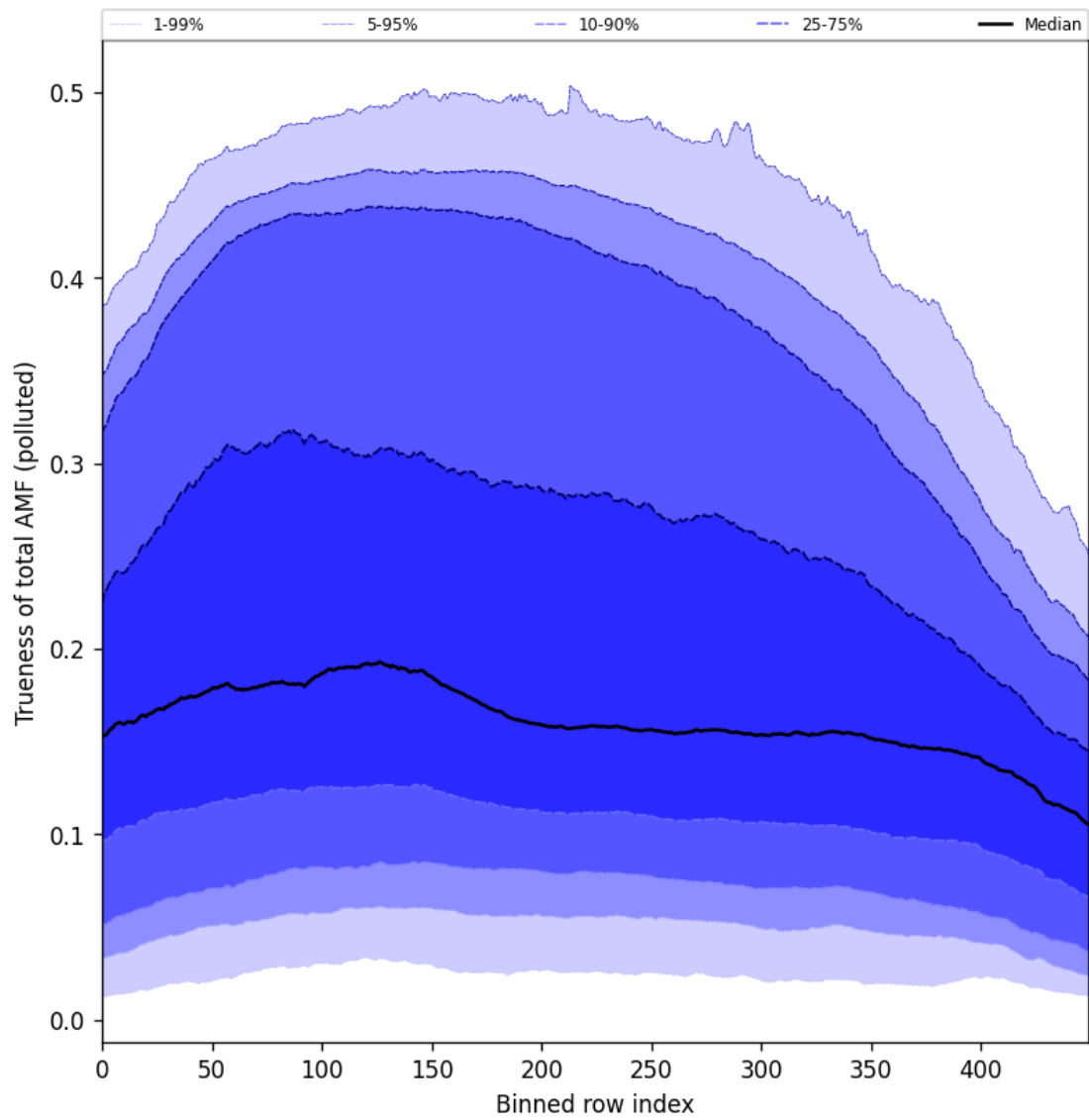
Figure 106: Along track statistics of “Trueness of total AMF (polluted)” for 2025-11-25 to 2025-11-27
