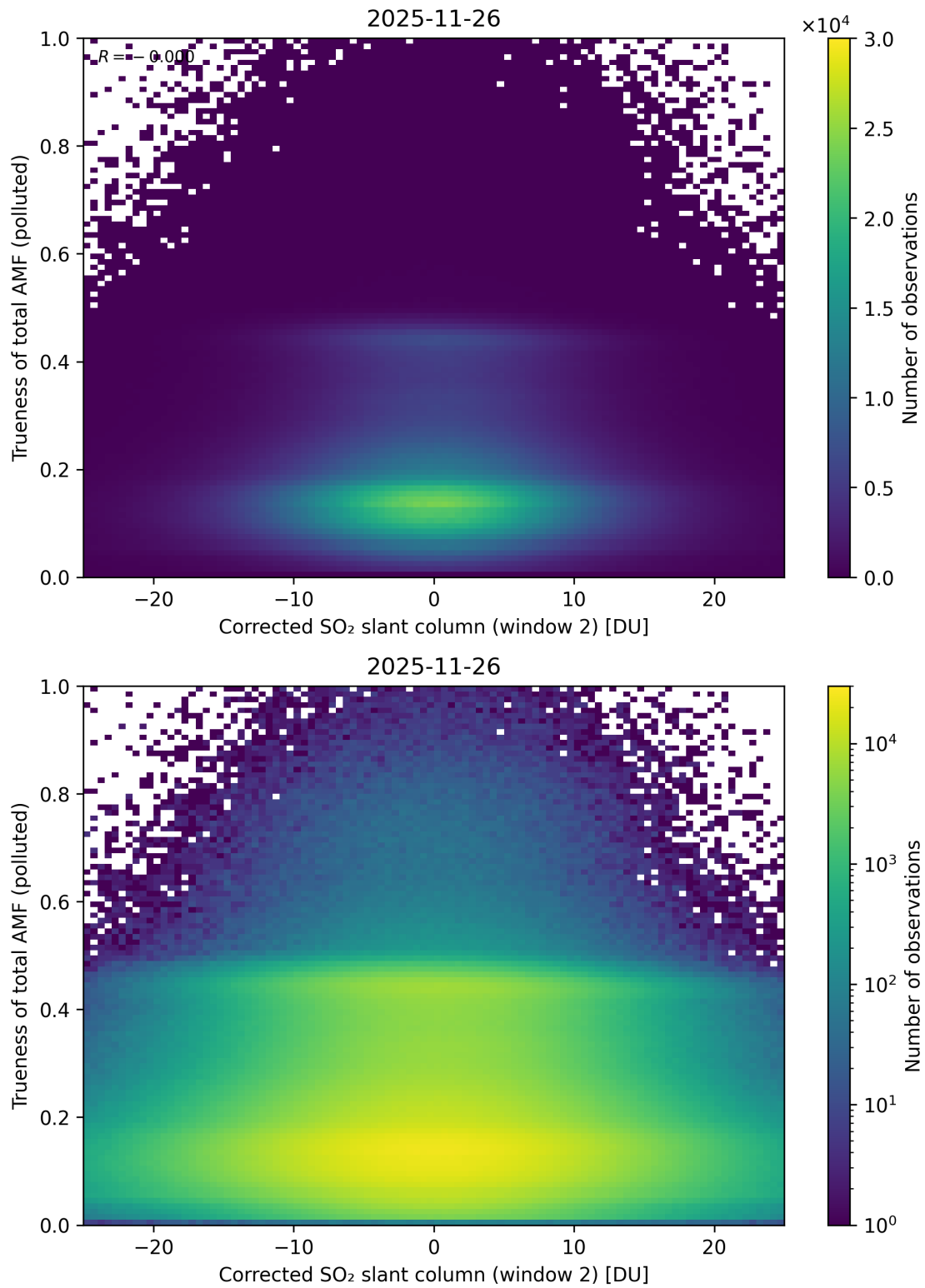
Figure 254: Scatter density plot of “Corrected SO 2 slant column (window 2)” against “Trueness of total AMF (polluted)” for 2025-11-25 to 2025-11-27.
