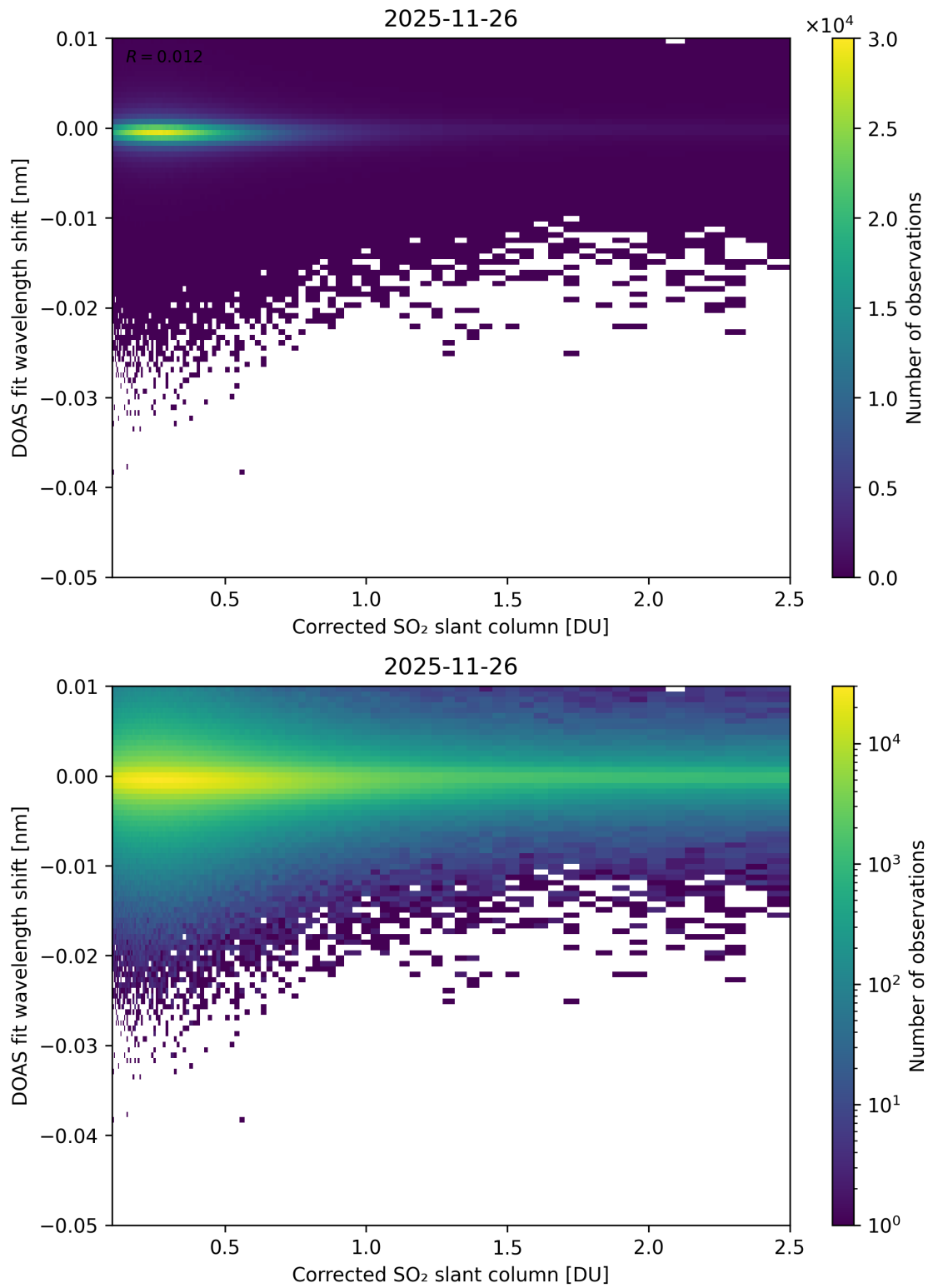
Figure 229: Scatter density plot of “Corrected SO 2 slant column” against “DOAS fit wavelength shift” for 2025-11-25 to 2025-11-27.
