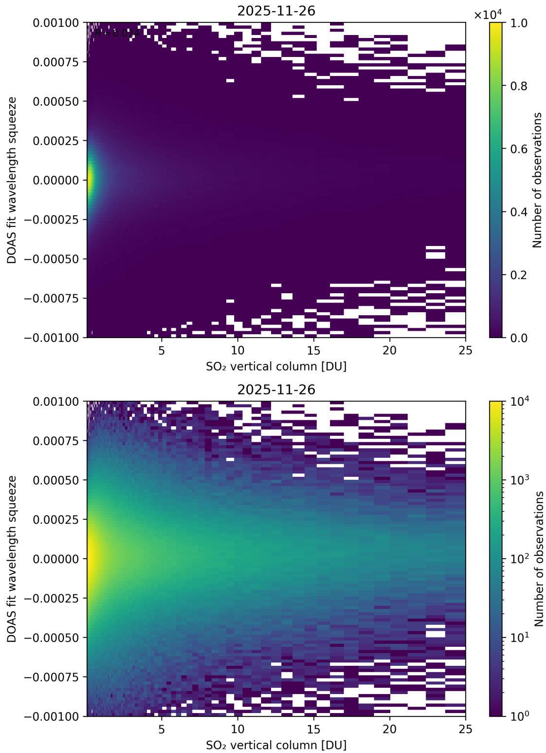
Figure 327: Scatter density plot of “SO 2 vertical column” against “DOAS fit wavelength squeeze” for 2025-11-25 to 2025-11-27.
