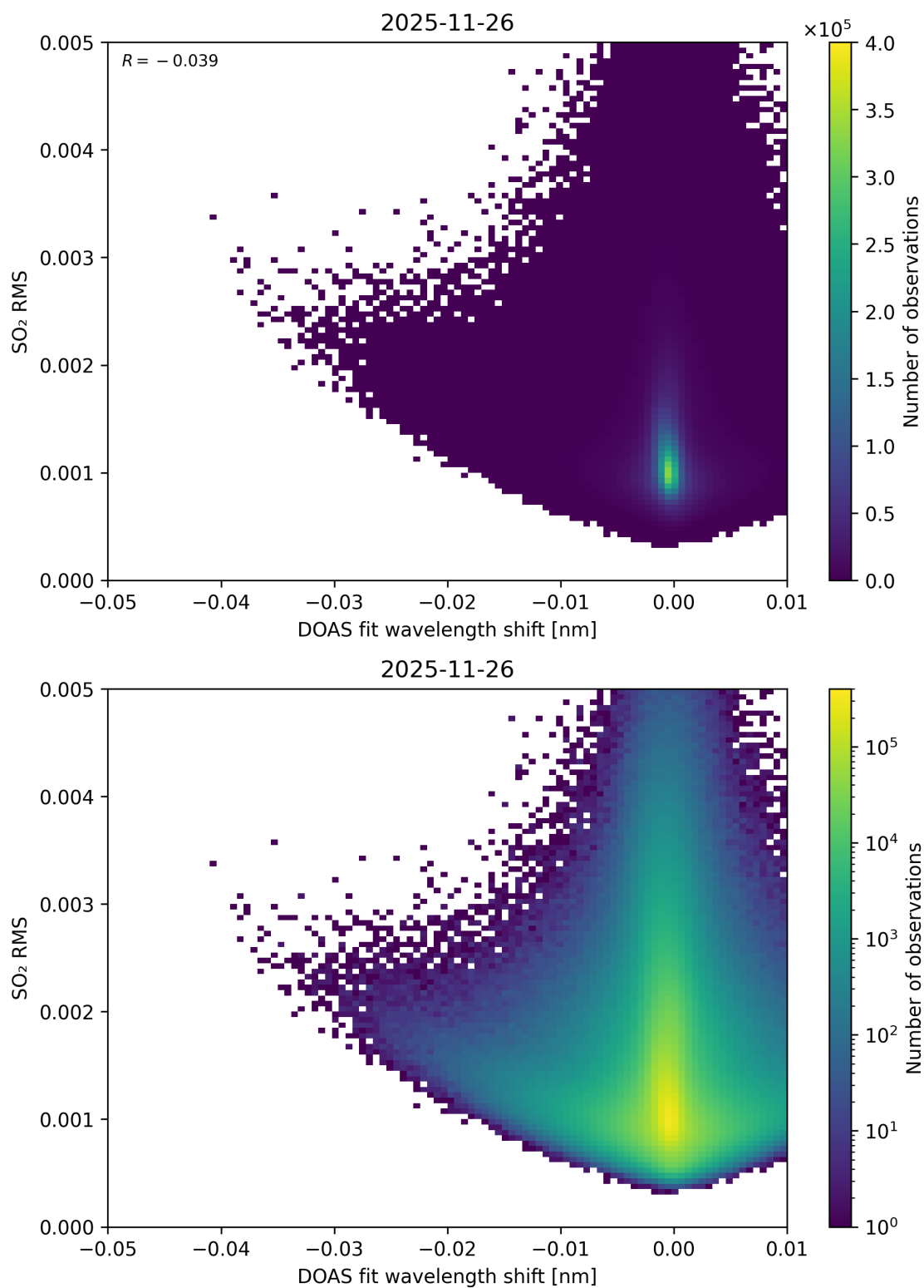
Figure 139: Scatter density plot of “DOAS fit wavelength shift” against “SO 2 RMS” for 2025-11-25 to 2025-11-27.
