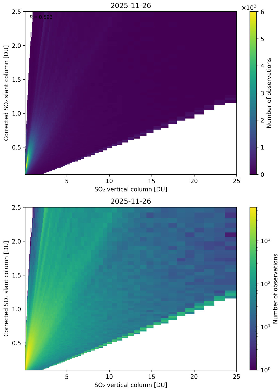
Figure 351: Scatter density plot of “SO 2 vertical column” against “Corrected SO 2 slant column” for 2025-11-25 to 2025-11-27.
