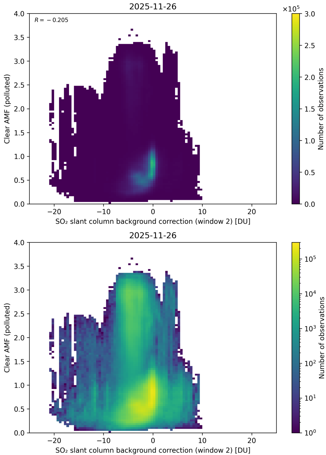
Figure 126: Scatter density plot of “SO 2 slant column background correction (window 2)” against “Clear AMF (polluted)” for 2025-11-25 to 2025-11-27.
