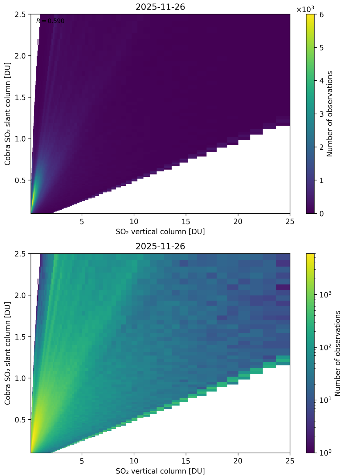
Figure 349: Scatter density plot of “SO 2 vertical column” against “Cobra SO 2 slant column” for 2025-11-25 to 2025-11-27.
