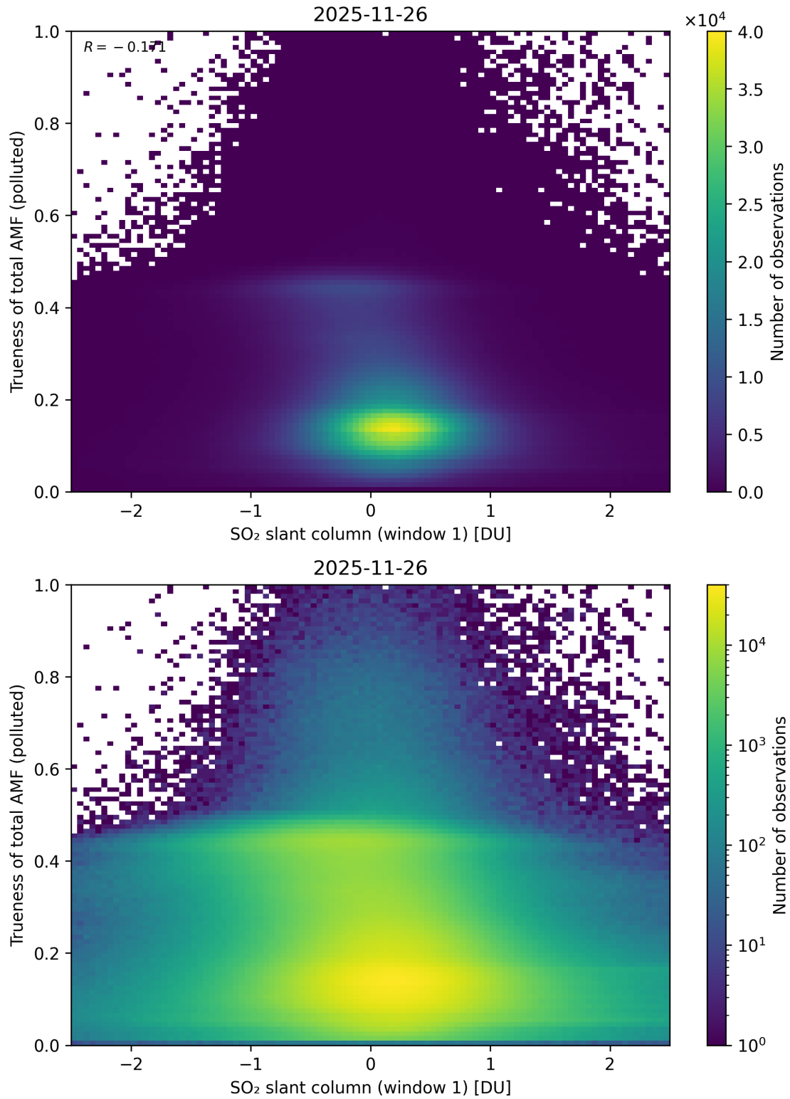
Figure 290: Scatter density plot of “SO 2 slant column (window 1)” against “Trueness of total AMF (polluted)” for 2025-11-25 to 2025-11-27.
