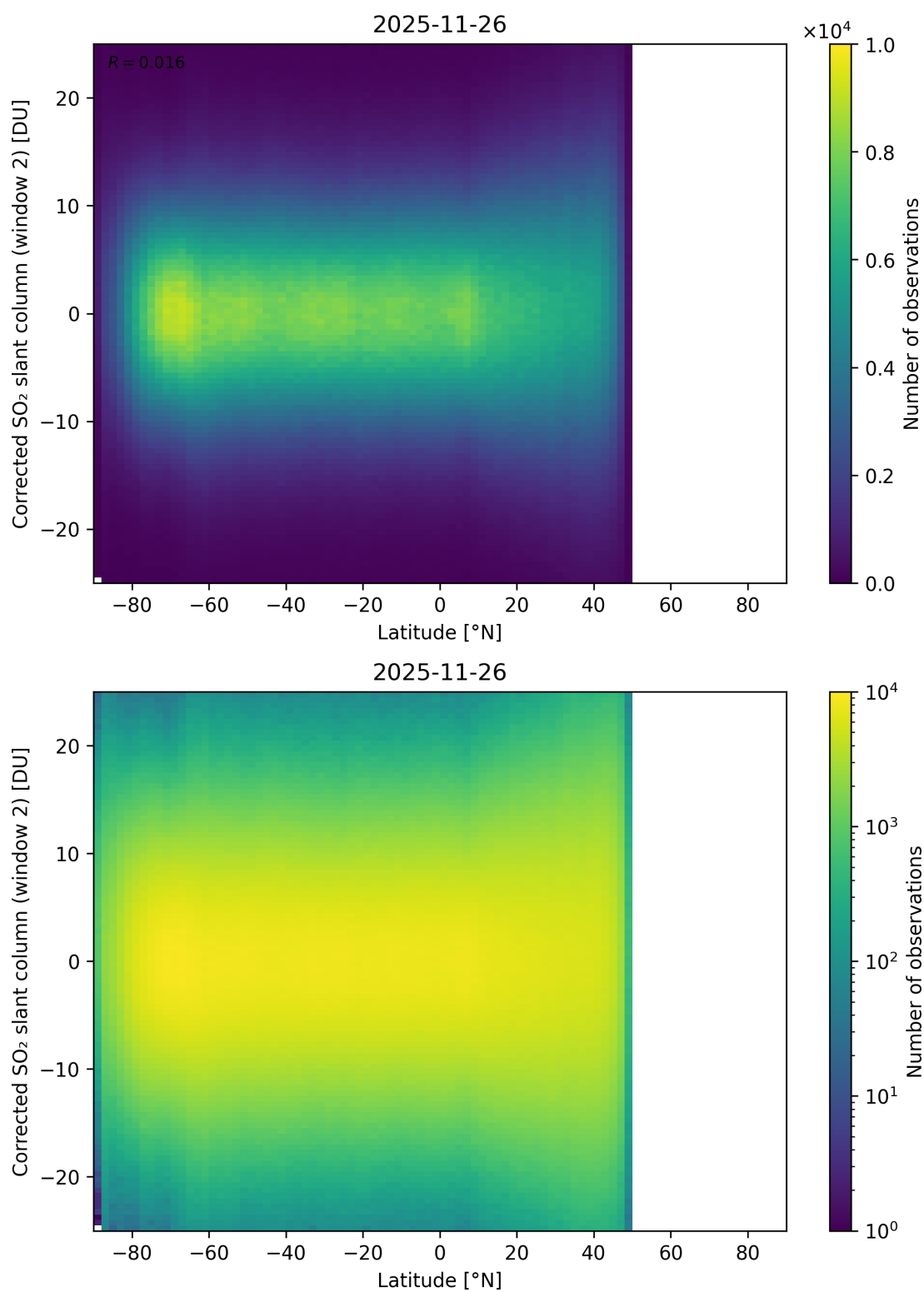
Figure 160: Scatter density plot of “Latitude” against “Corrected SO 2 slant column (window 2)” for 2025-11-25 to 2025-11-27.
