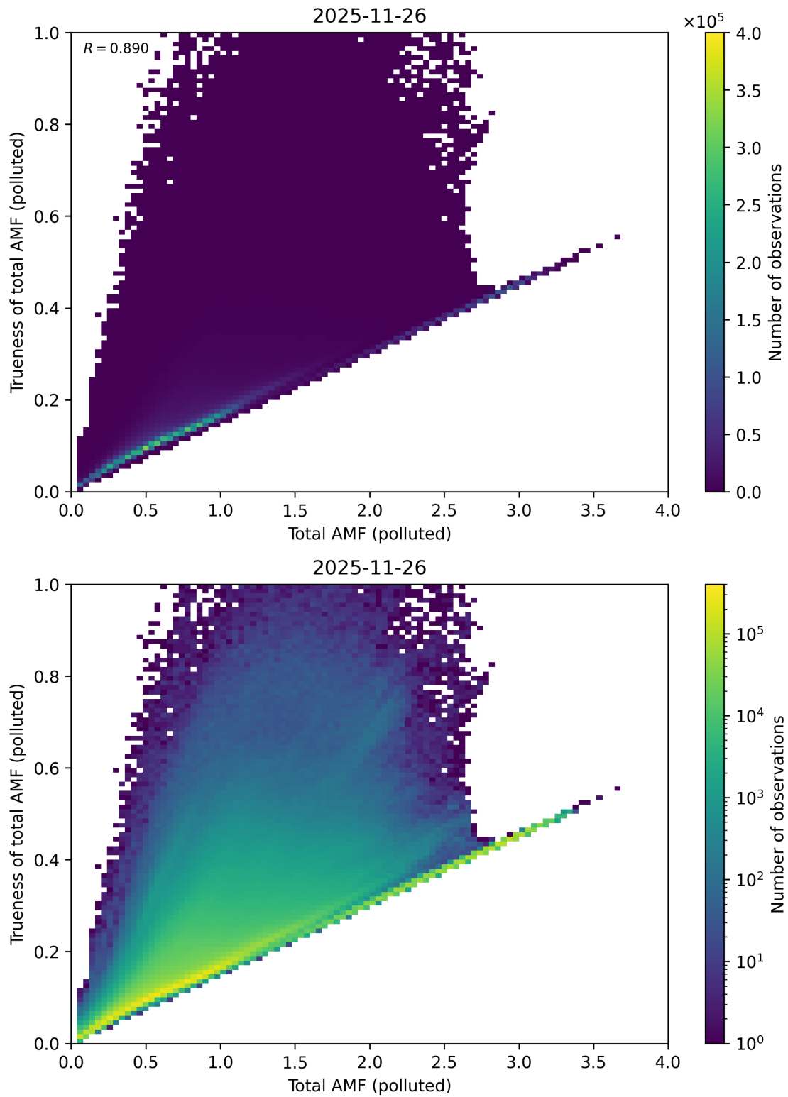
Figure 321: Scatter density plot of “Total AMF (polluted)” against “Trueness of total AMF (polluted)” for 2025-11-25 to 2025-11-27.
