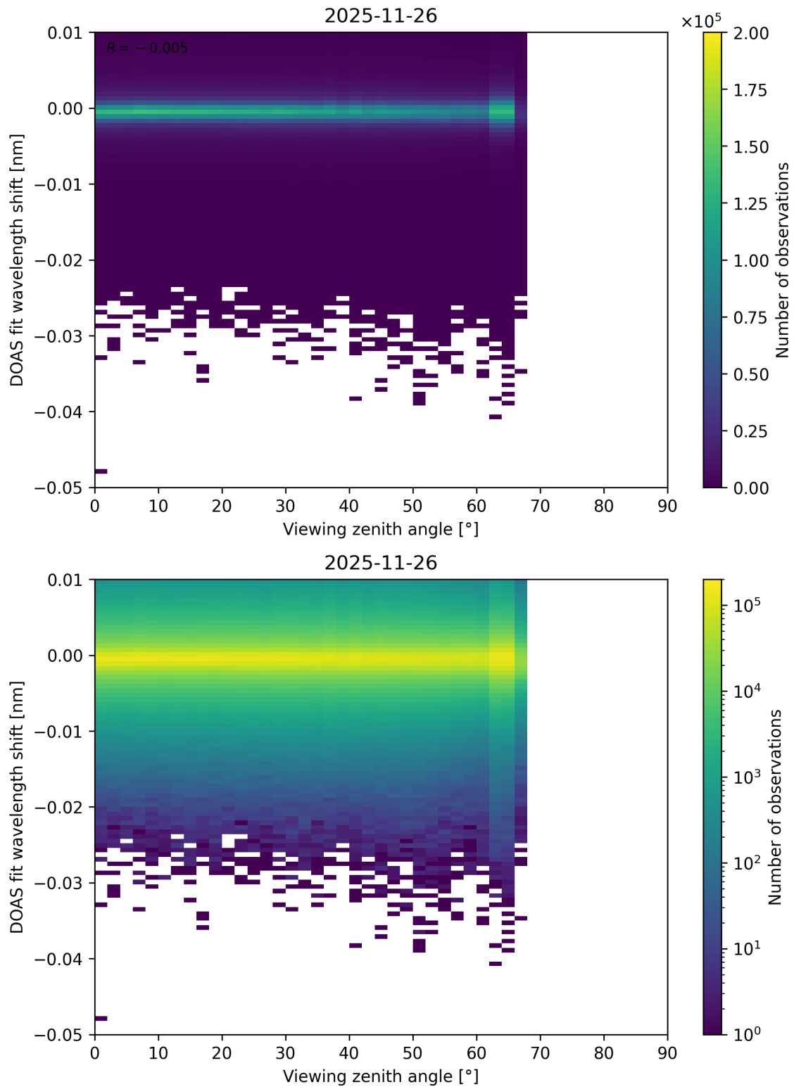
Figure 365: Scatter density plot of “Viewing zenith angle” against “DOAS fit wavelength shift” for 2025-11-25 to 2025-11-27.
