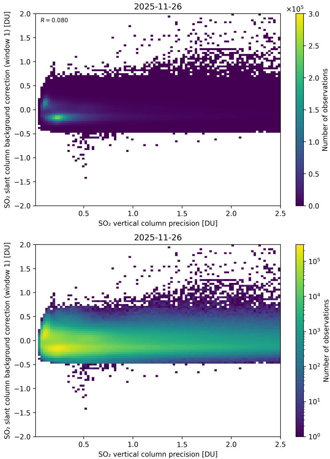
Figure 329: Scatter density plot of “SO 2 vertical column precision” against “SO 2 slant column background correction (window 1)” for 2025-11-25 to 2025-11-27.
