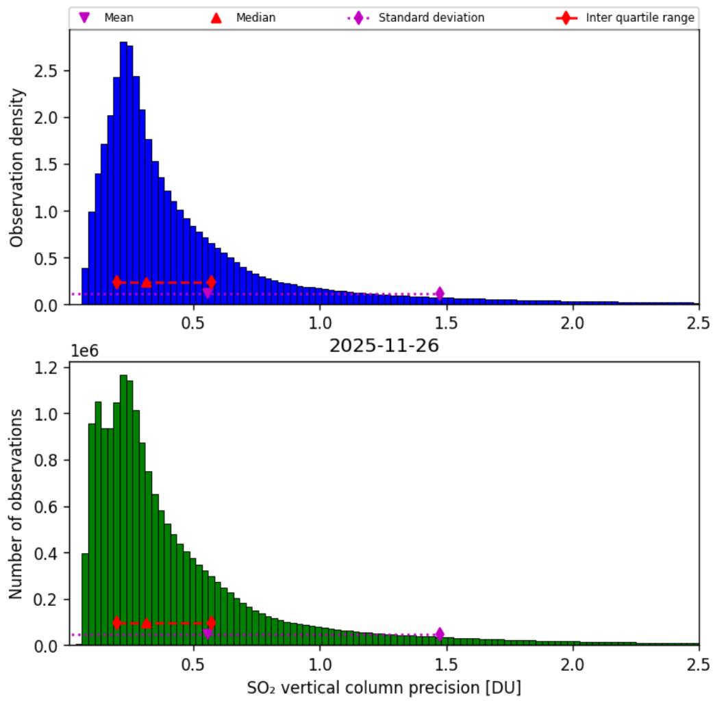
Figure 59: Histogram of “SO 2 vertical column precision” for 2025-11-25 to 2025-11-27
