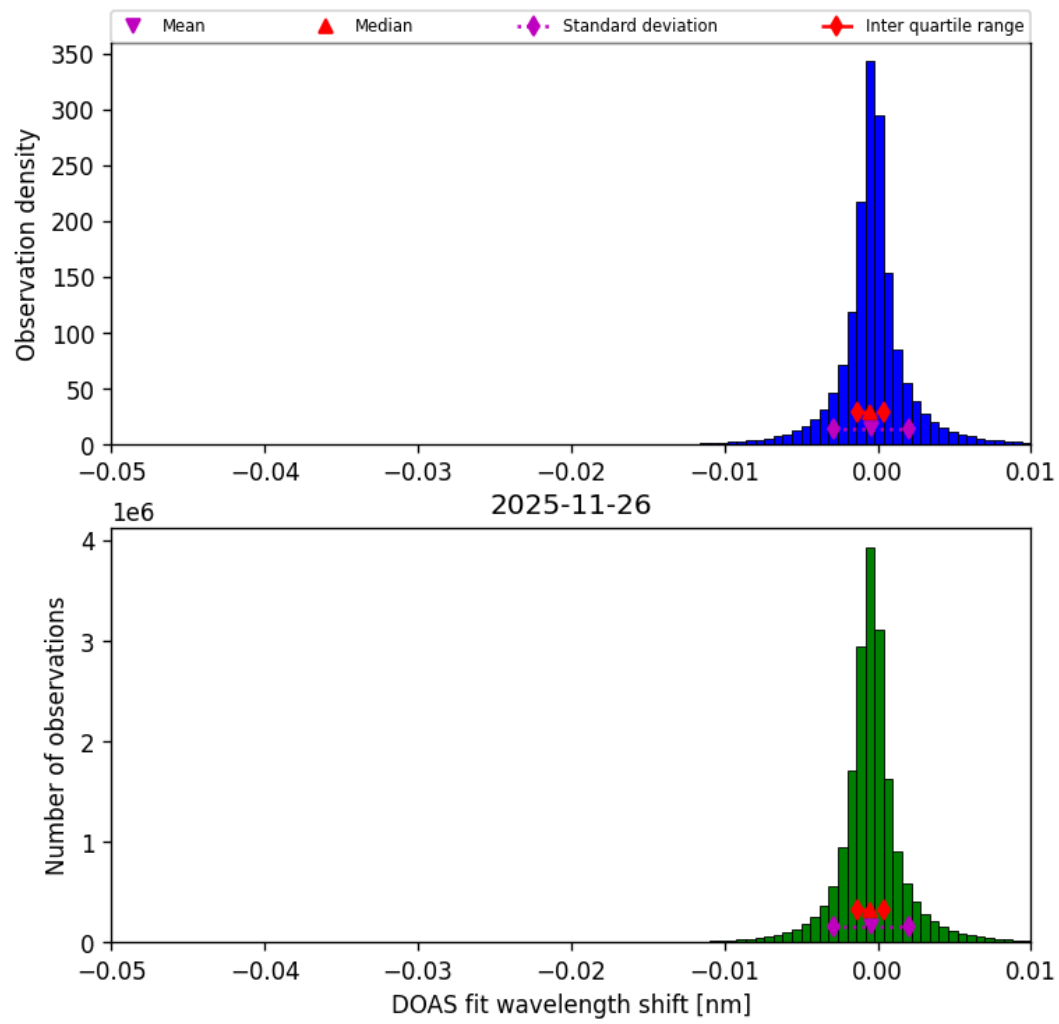
Figure 76: Histogram of “DOAS fit wavelength shift” for 2025-11-25 to 2025-11-27
