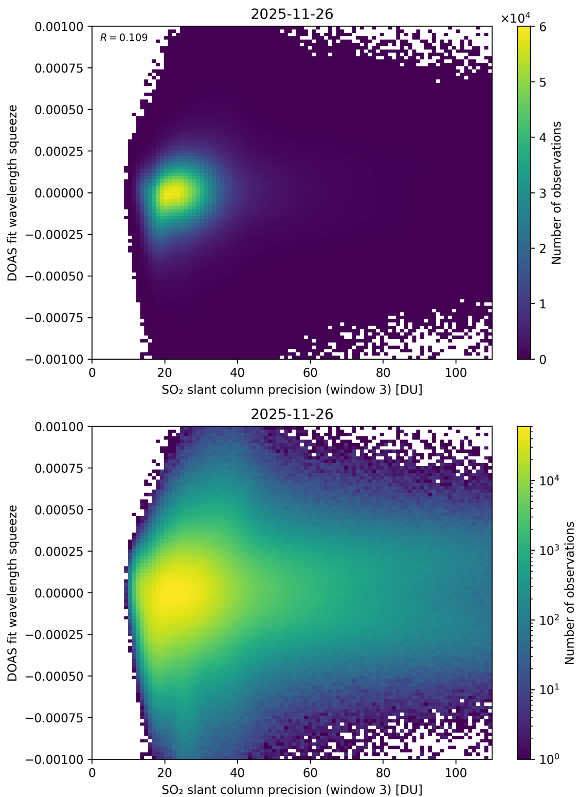
Figure 309: Scatter density plot of “SO 2 slant column precision (window 3)” against “DOAS fit wavelength squeeze” for 2025-11-25 to 2025-11-27.
