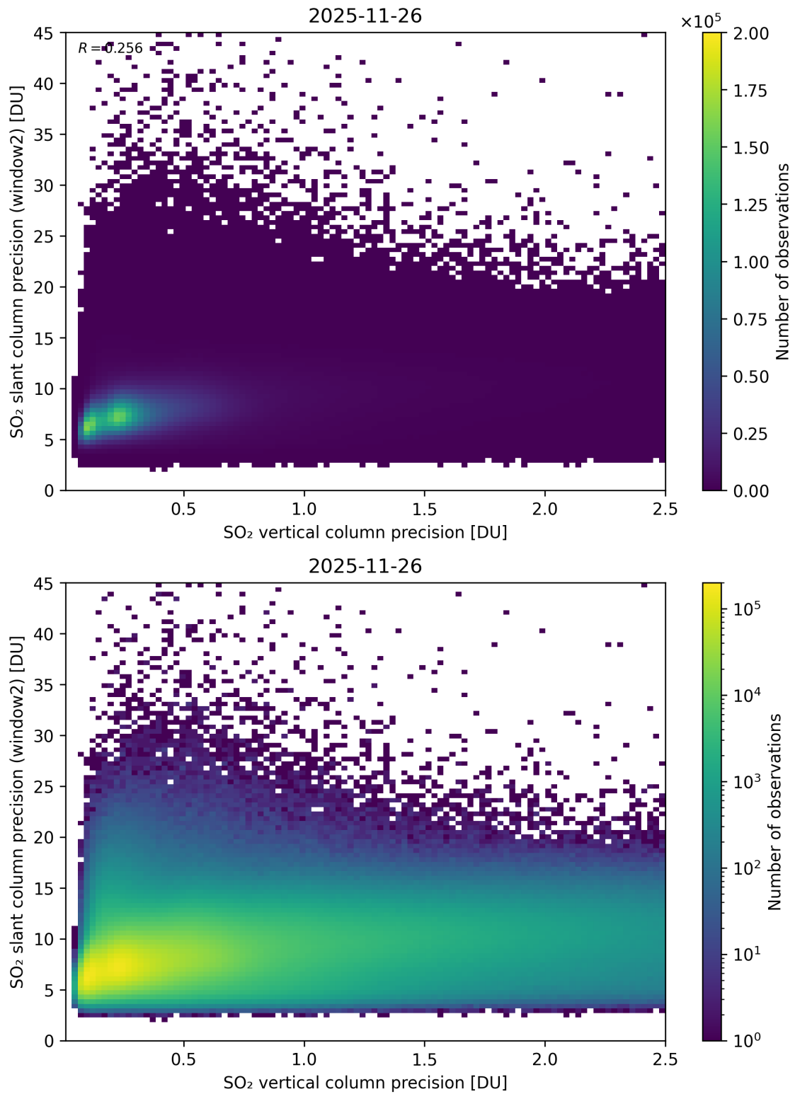
Figure 343: Scatter density plot of “SO 2 vertical column precision” against “SO 2 slant column precision (window2)” for 2025-11-25 to 2025-11-27.
