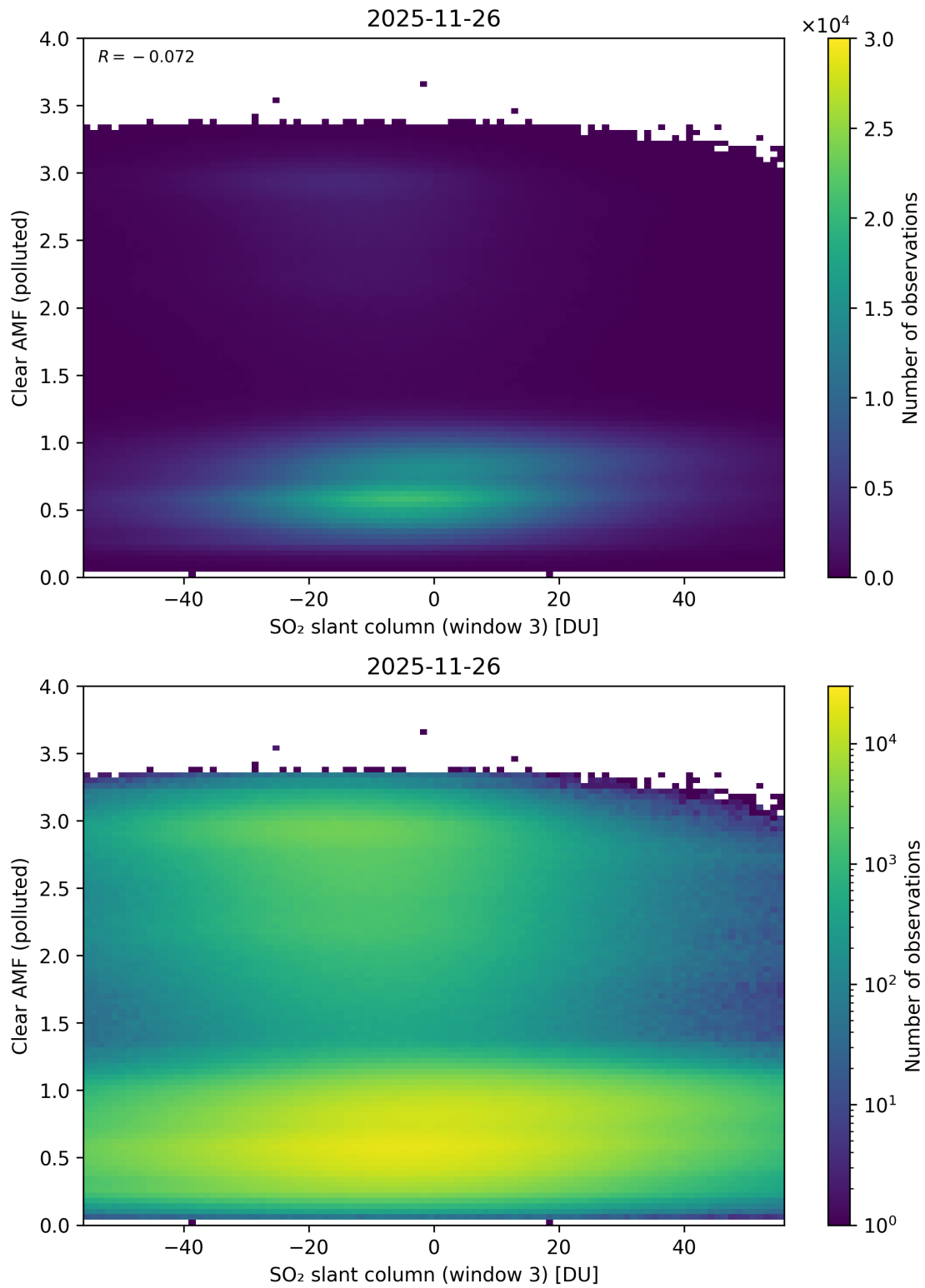
Figure 315: Scatter density plot of “SO 2 slant column (window 3)” against “Clear AMF (polluted)” for 2025-11-25 to 2025-11-27.
