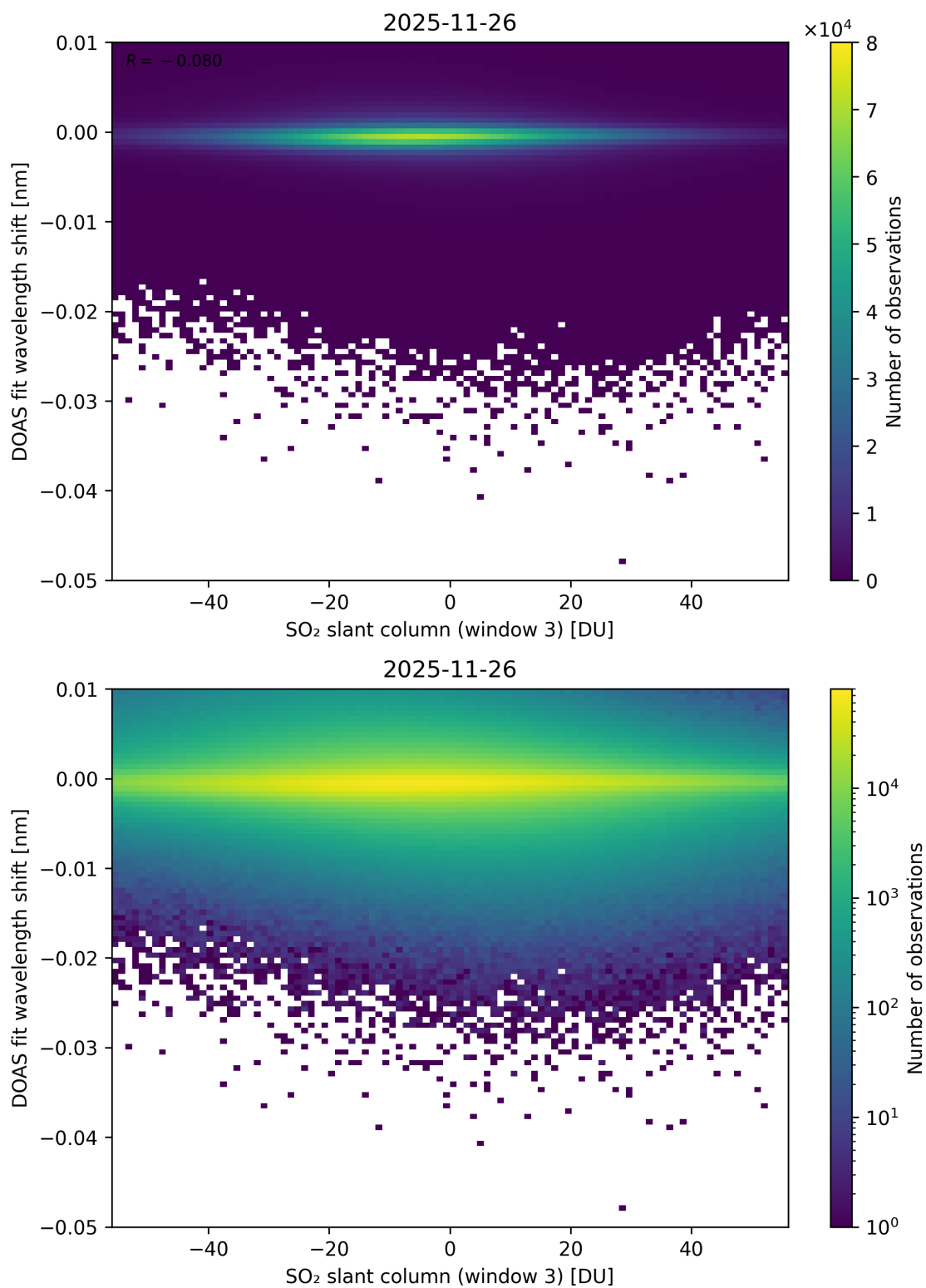
Figure 304: Scatter density plot of “SO 2 slant column (window 3)” against “DOAS fit wavelength shift” for 2025-11-25 to 2025-11-27.
