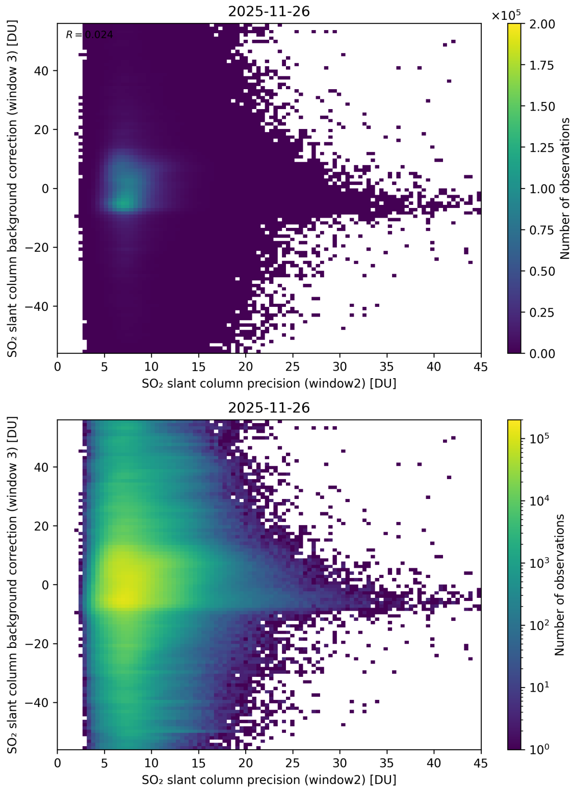
Figure 292: Scatter density plot of “SO 2 slant column precision (window2)” against “SO 2 slant column background correction (window 3)” for 2025-11-25 to 2025-11-27.
