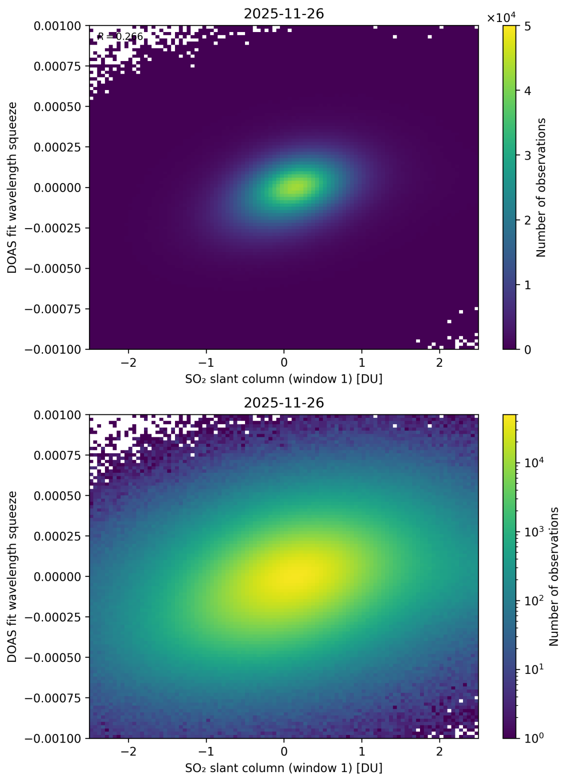
Figure 266: Scatter density plot of “SO 2 slant column (window 1)” against “DOAS fit wavelength squeeze” for 2025-11-25 to 2025-11-27.
