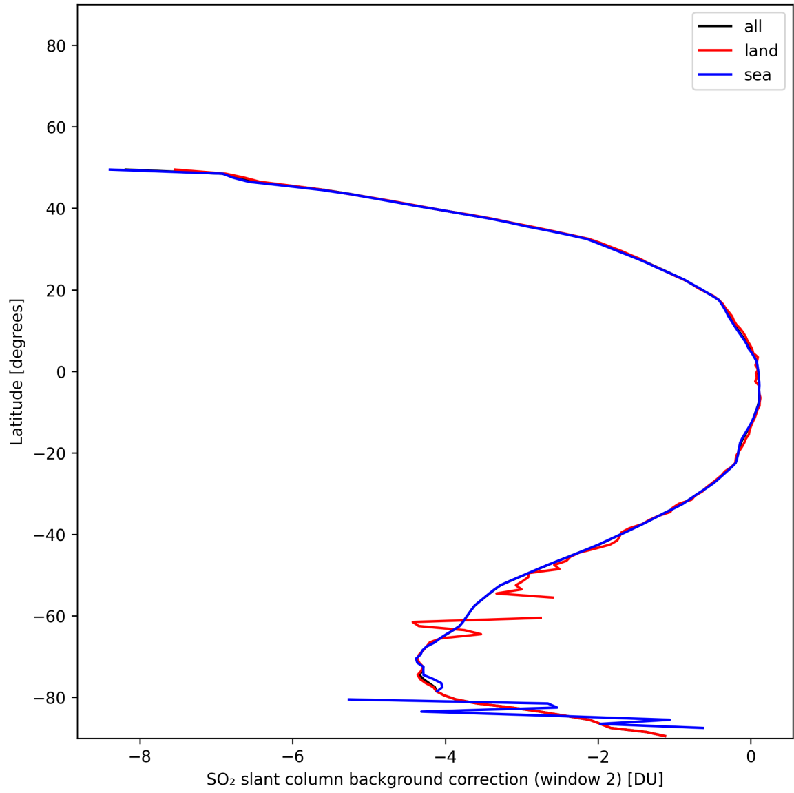
Figure 44: Zonal average of “SO 2 slant column background correction (window 2)” for 2025-11-25 to 2025-11-27.
