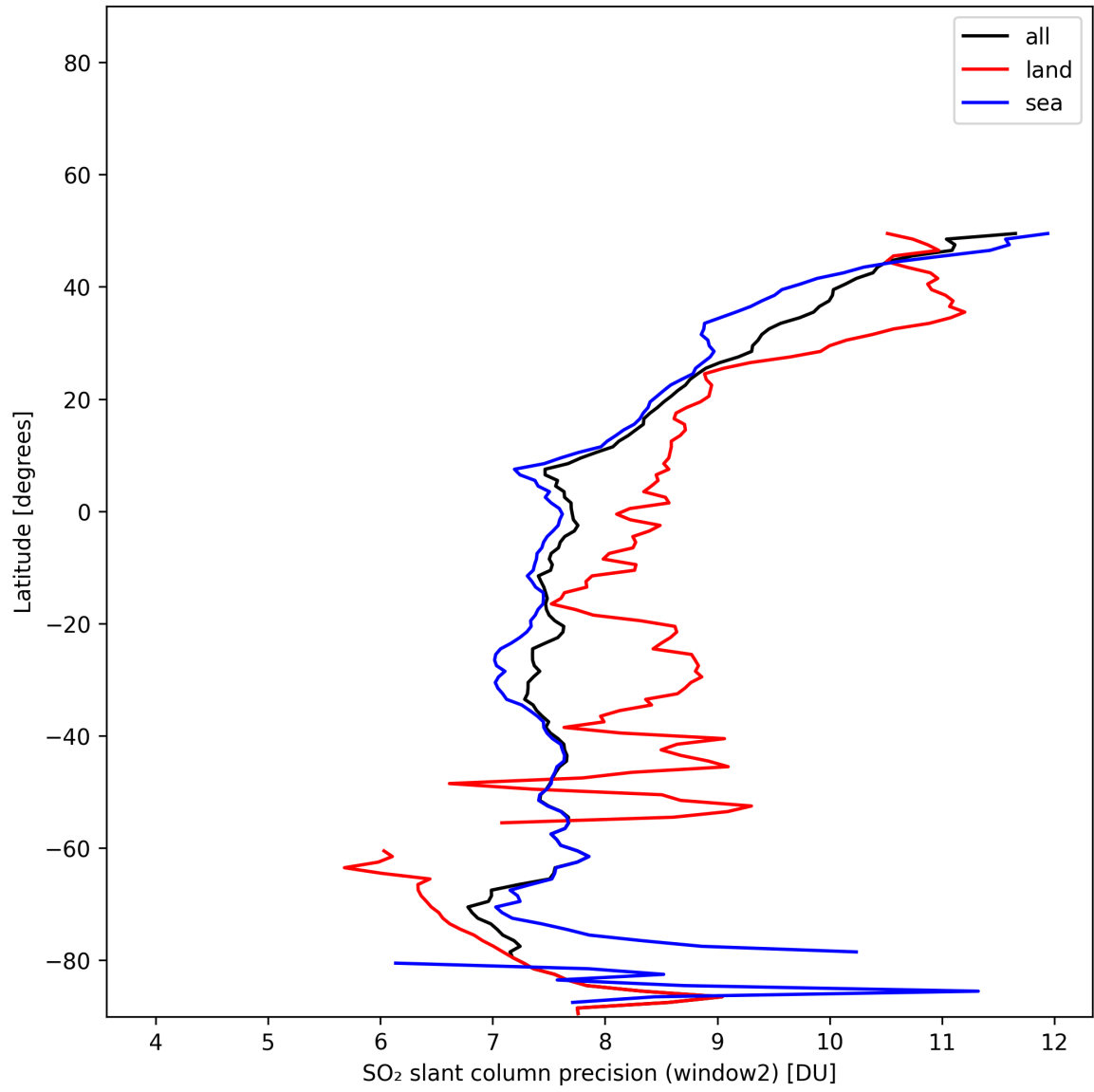
Figure 42: Zonal average of “SO 2 slant column precision (window2)” for 2025-11-25 to 2025-11-27.
