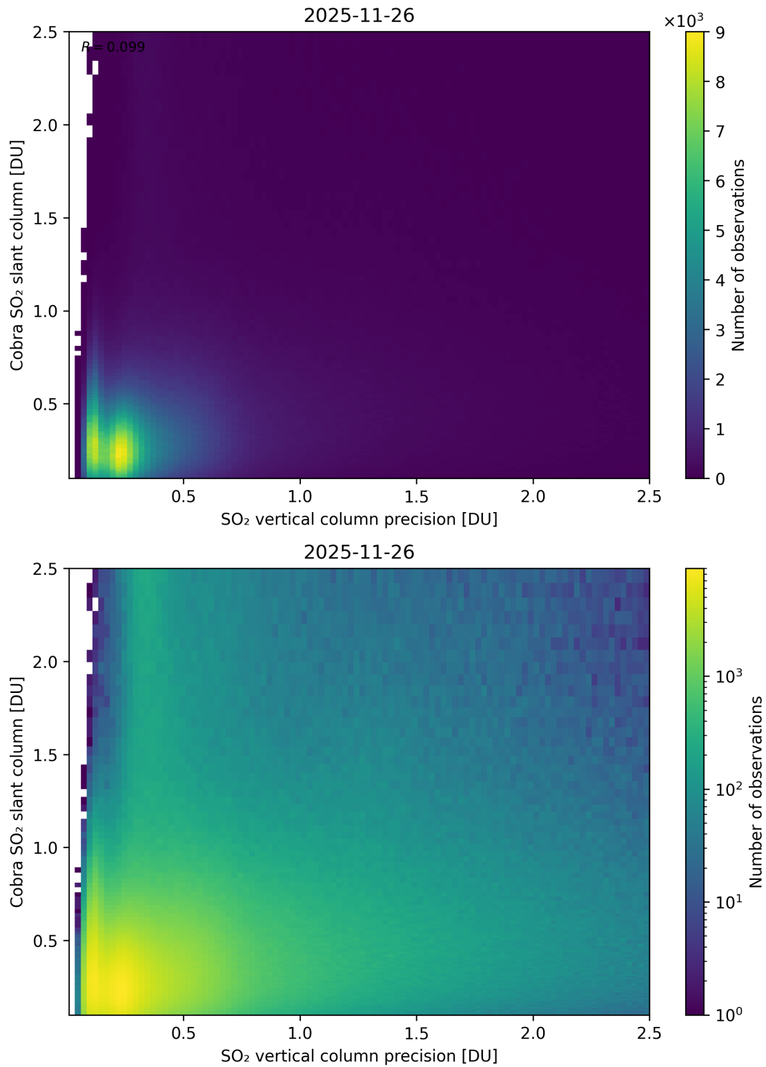
Figure 336: Scatter density plot of “SO 2 vertical column precision” against “Cobra SO 2 slant column” for 2025-11-25 to 2025-11-27.
