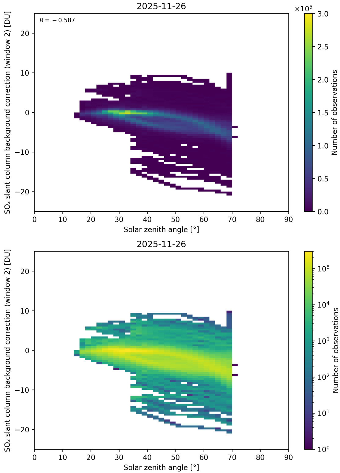
Figure 172: Scatter density plot of “Solar zenith angle” against “SO 2 slant column background correction (window 2)” for 2025-11-25 to 2025-11-27.
