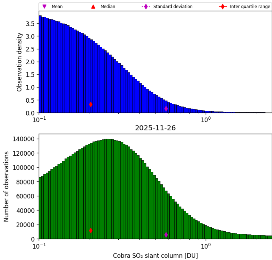
Figure 61: Histogram of “Cobra SO 2 slant column” for 2025-11-25 to 2025-11-27
