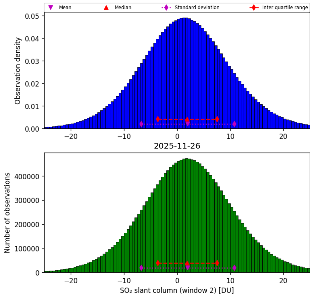
Figure 67: Histogram of “SO 2 slant column (window 2)” for 2025-11-25 to 2025-11-27
