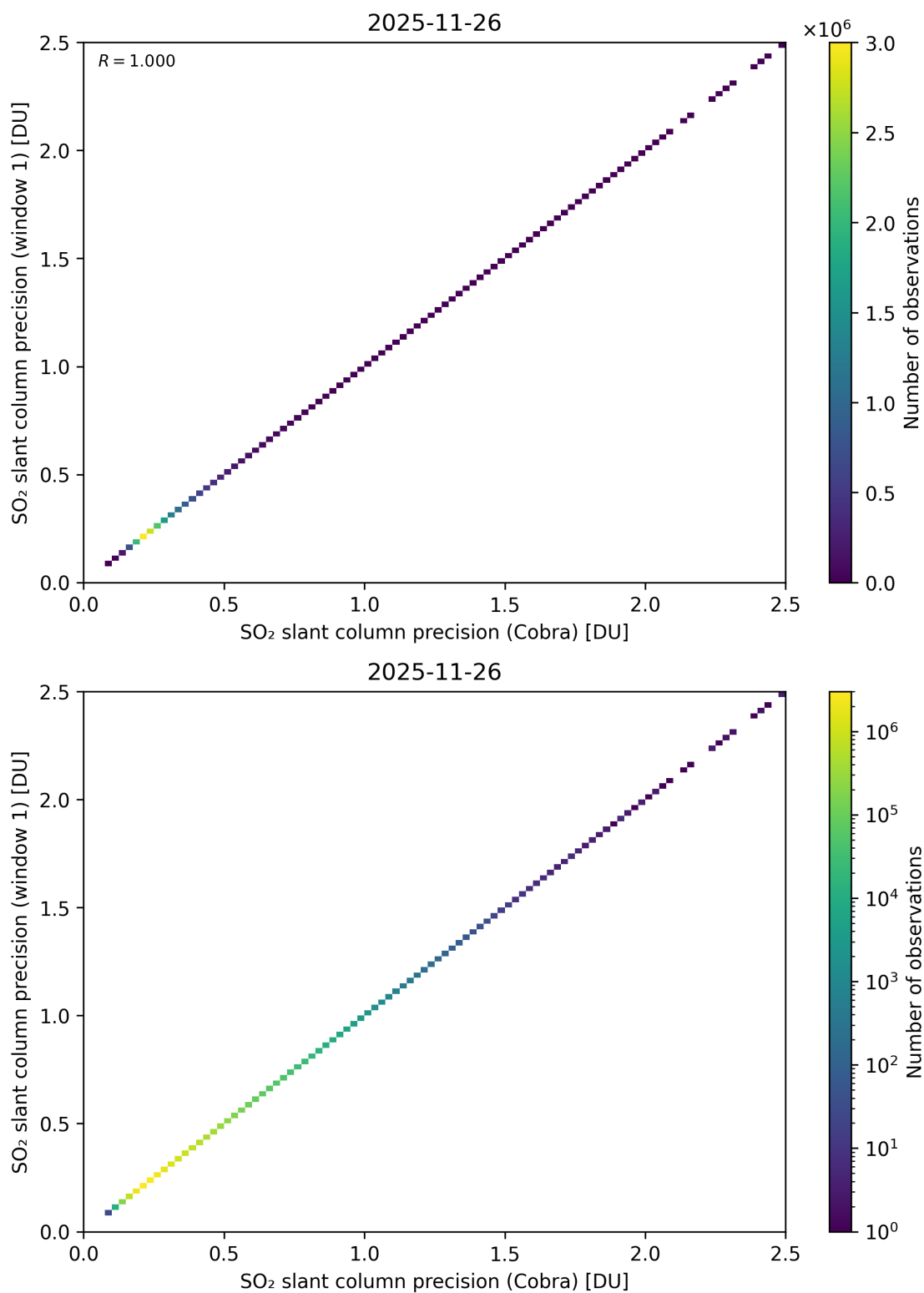
Figure 209: Scatter density plot of “SO 2 slant column precision (Cobra)” against “SO 2 slant column precision (window 1)” for 2025-11-25 to 2025-11-27.
