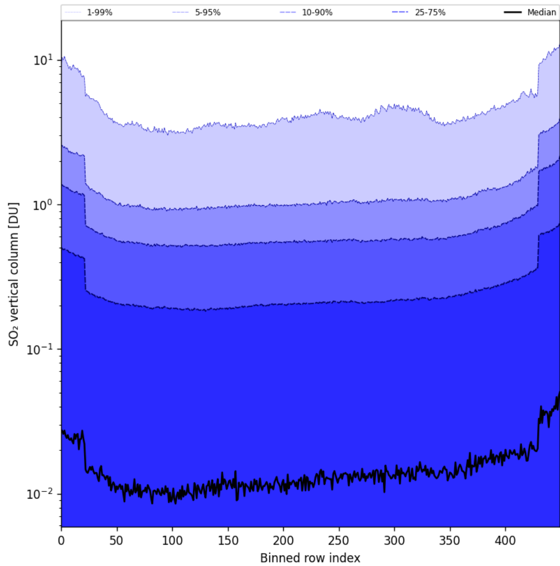
Figure 84: Along track statistics of “SO 2 vertical column” for 2025-11-25 to 2025-11-27
