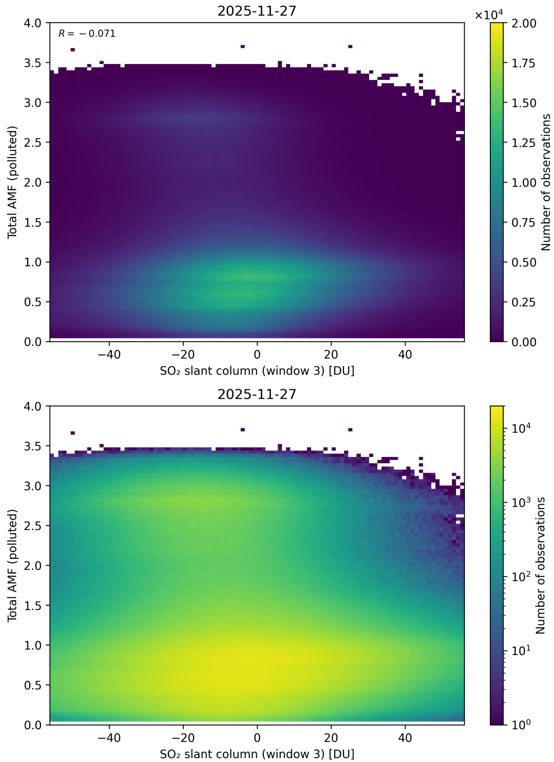
Figure 318: Scatter density plot of “SO 2 slant column (window 3)” against “Total AMF (polluted)” for 2025-11-26 to 2025-11-28.
