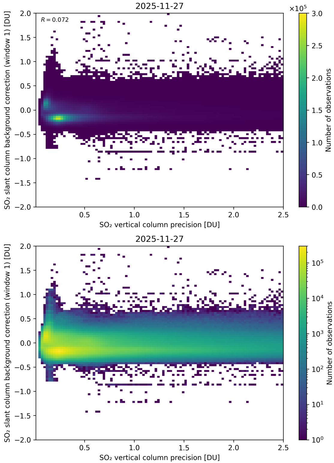
Figure 329: Scatter density plot of “SO 2 vertical column precision” against “SO 2 slant column background correction (window 1)” for 2025-11-26 to 2025-11-28.
