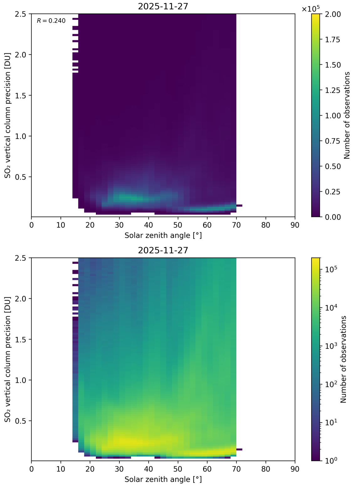
Figure 192: Scatter density plot of “Solar zenith angle” against “SO 2 vertical column precision” for 2025-11-26 to 2025-11-28.
