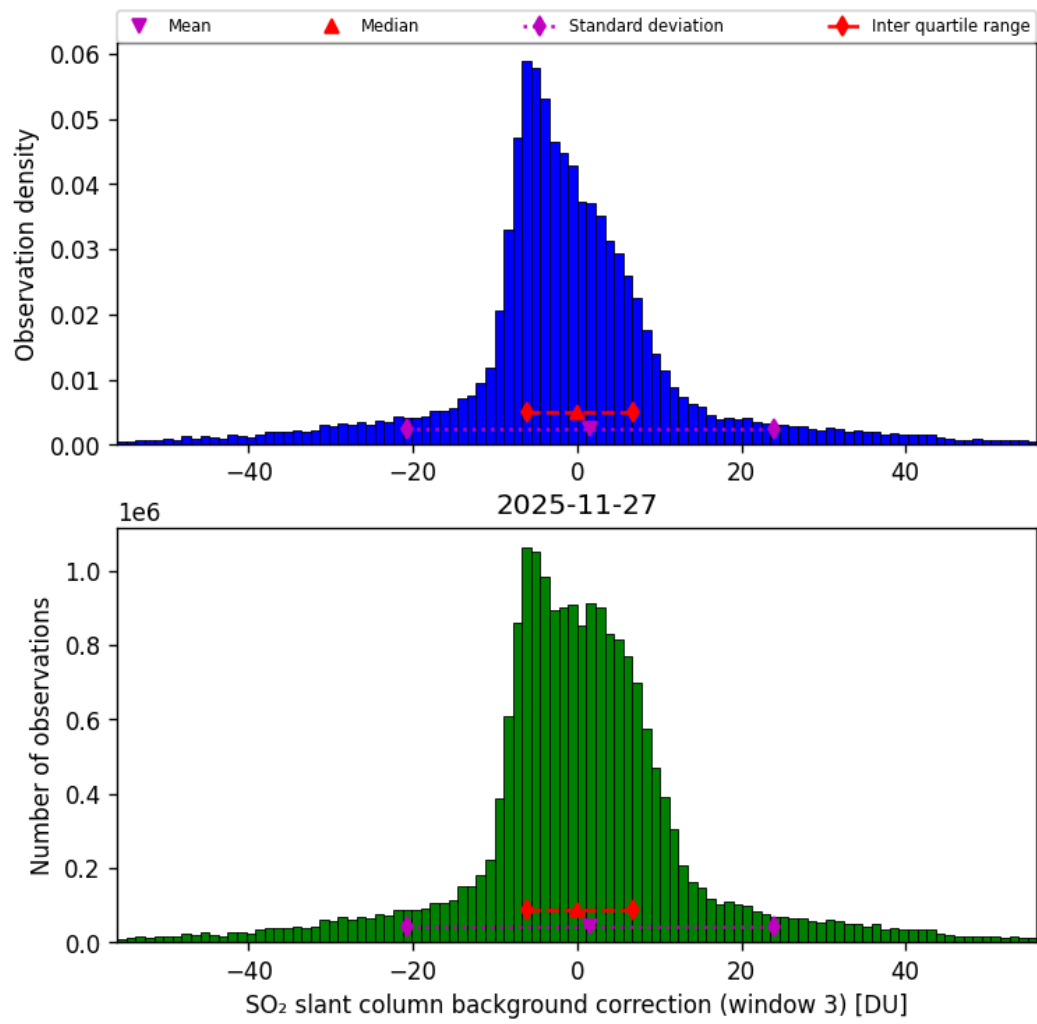
Figure 74: Histogram of “SO 2 slant column background correction (window 3)” for 2025-11-26 to 2025-11-28
