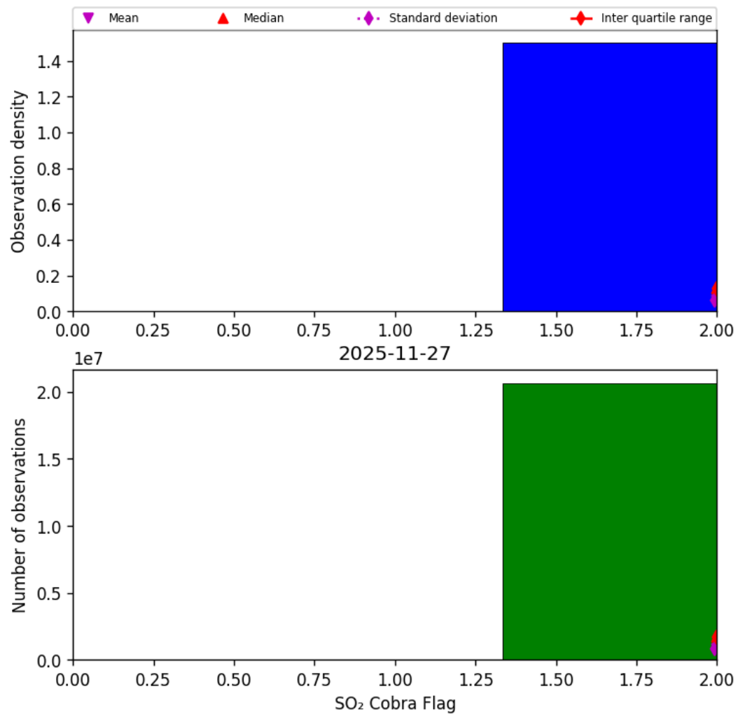
Figure 75: Histogram of “SO 2 Cobra Flag” for 2025-11-26 to 2025-11-28
