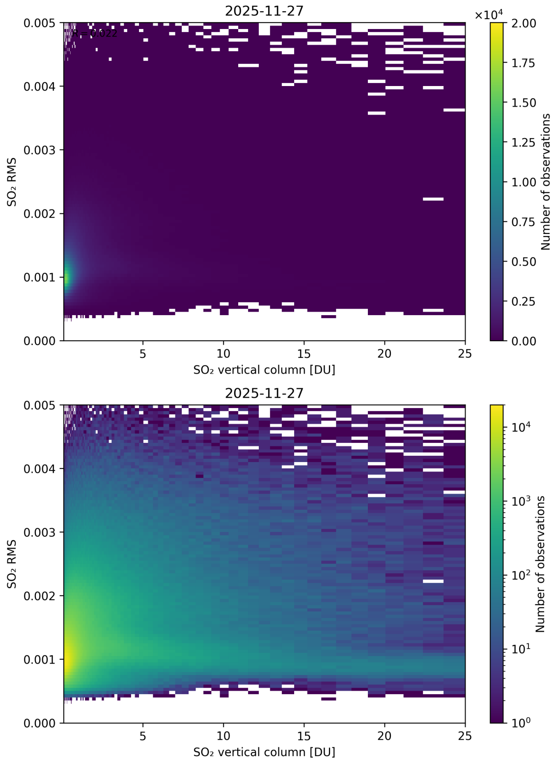
Figure 328: Scatter density plot of “SO 2 vertical column” against “SO 2 RMS” for 2025-11-26 to 2025-11-28.
