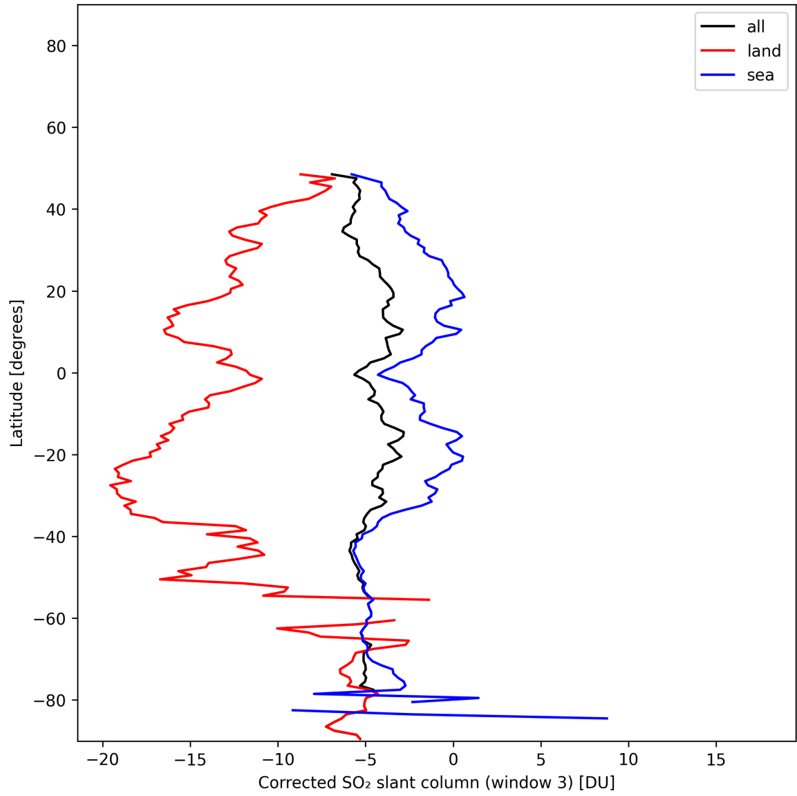
Figure 47: Zonal average of “Corrected SO 2 slant column (window 3)” for 2025-11-26 to 2025-11-28.
