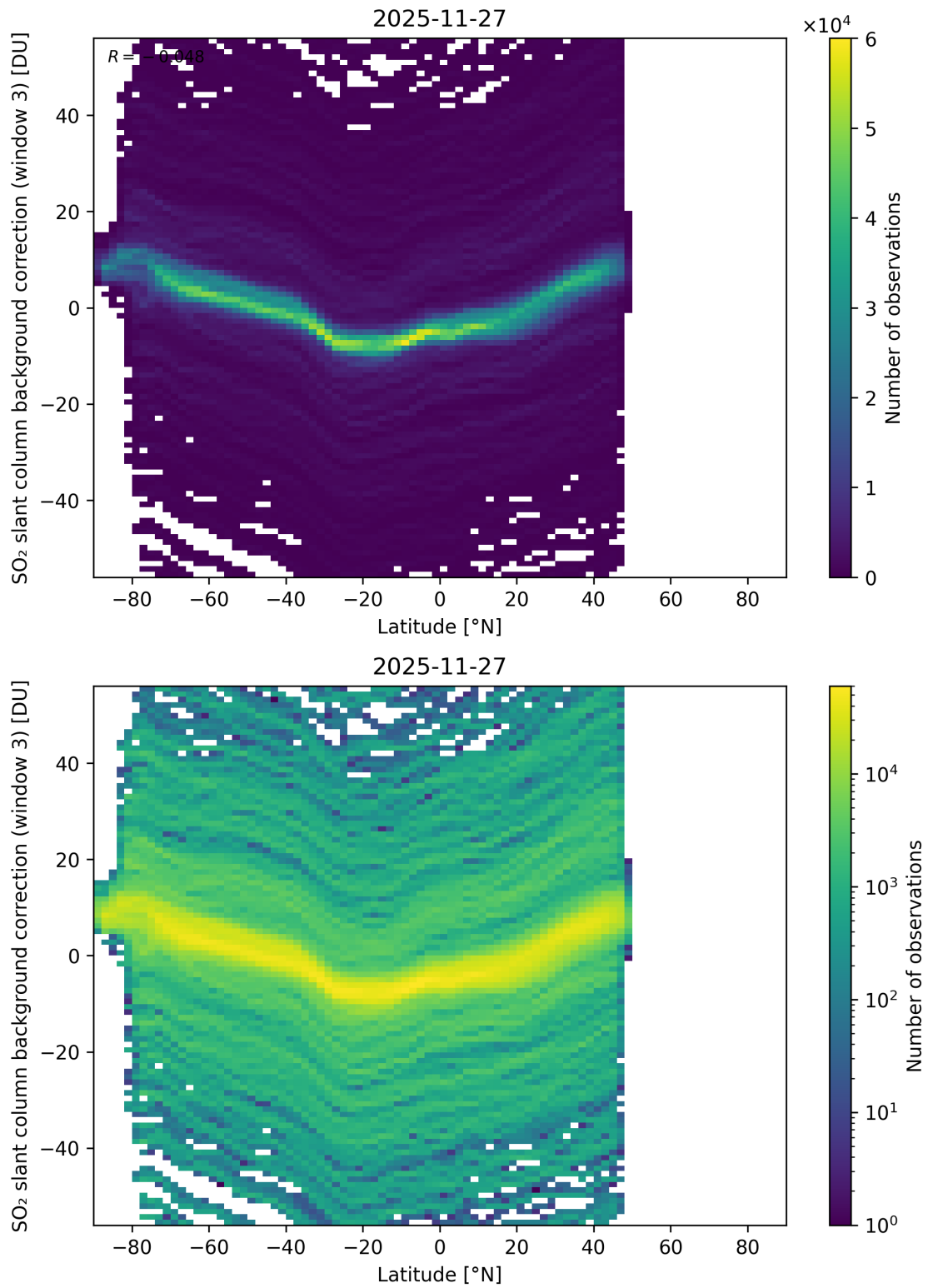
Figure 152: Scatter density plot of “Latitude” against “SO 2 slant column background correction (window 3)” for 2025-11-26 to 2025-11-28.
