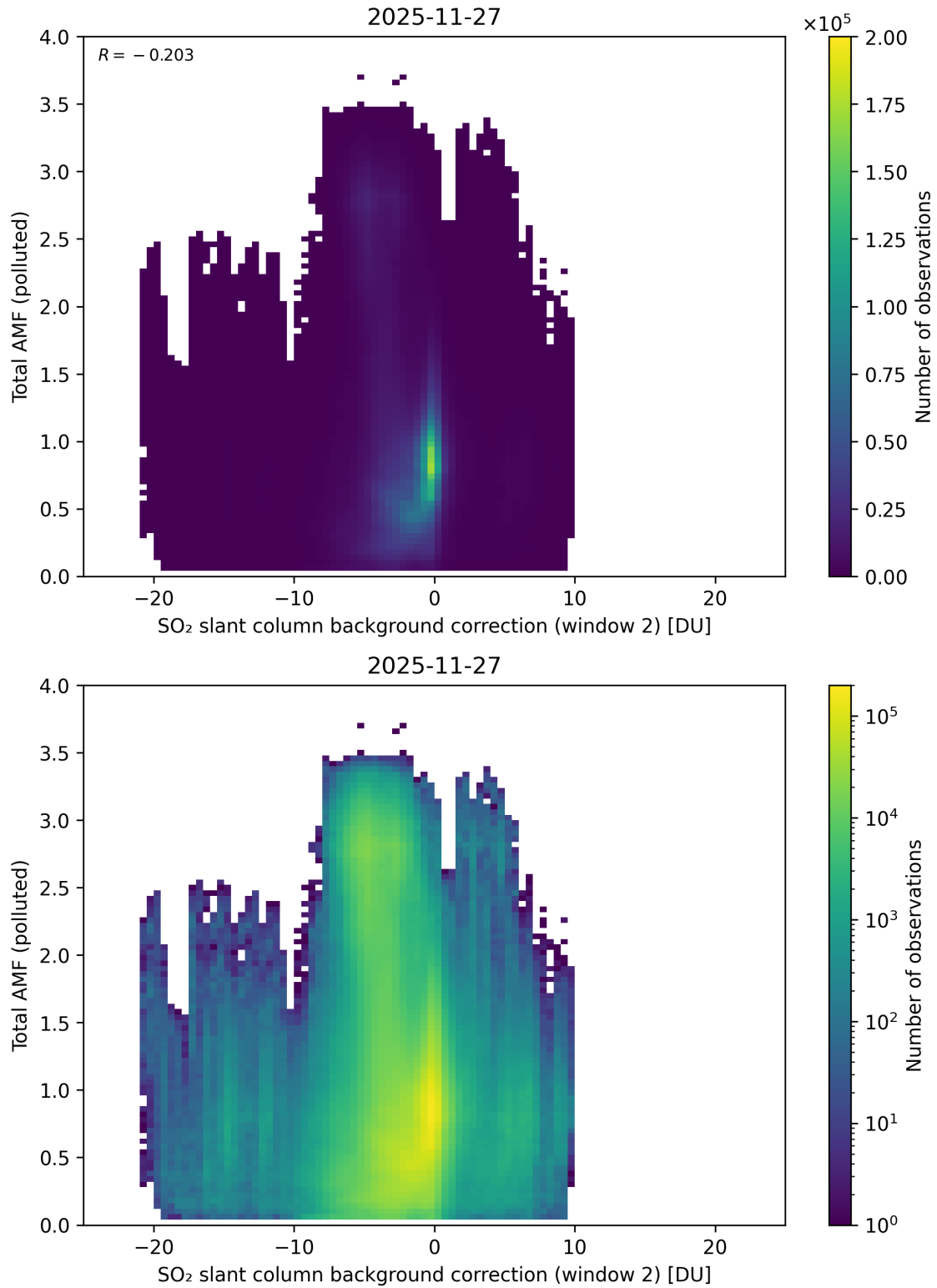
Figure 130: Scatter density plot of “SO 2 slant column background correction (window 2)” against “Total AMF (polluted)” for 2025-11-26 to 2025-11-28.
