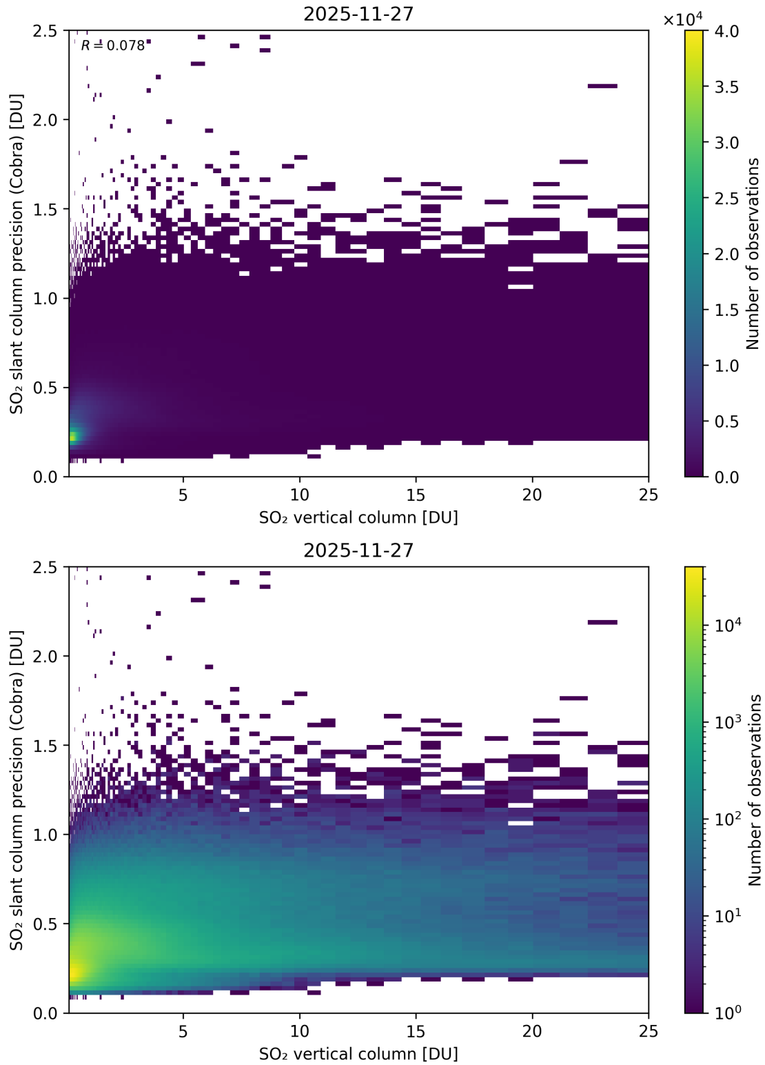
Figure 350: Scatter density plot of “SO 2 vertical column” against “SO 2 slant column precision (Cobra)” for 2025-11-26 to 2025-11-28.
