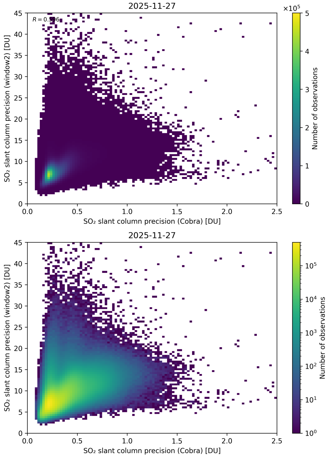
Figure 210: Scatter density plot of “SO 2 slant column precision (Cobra)” against “SO 2 slant column precision (window2)” for 2025-11-26 to 2025-11-28.
