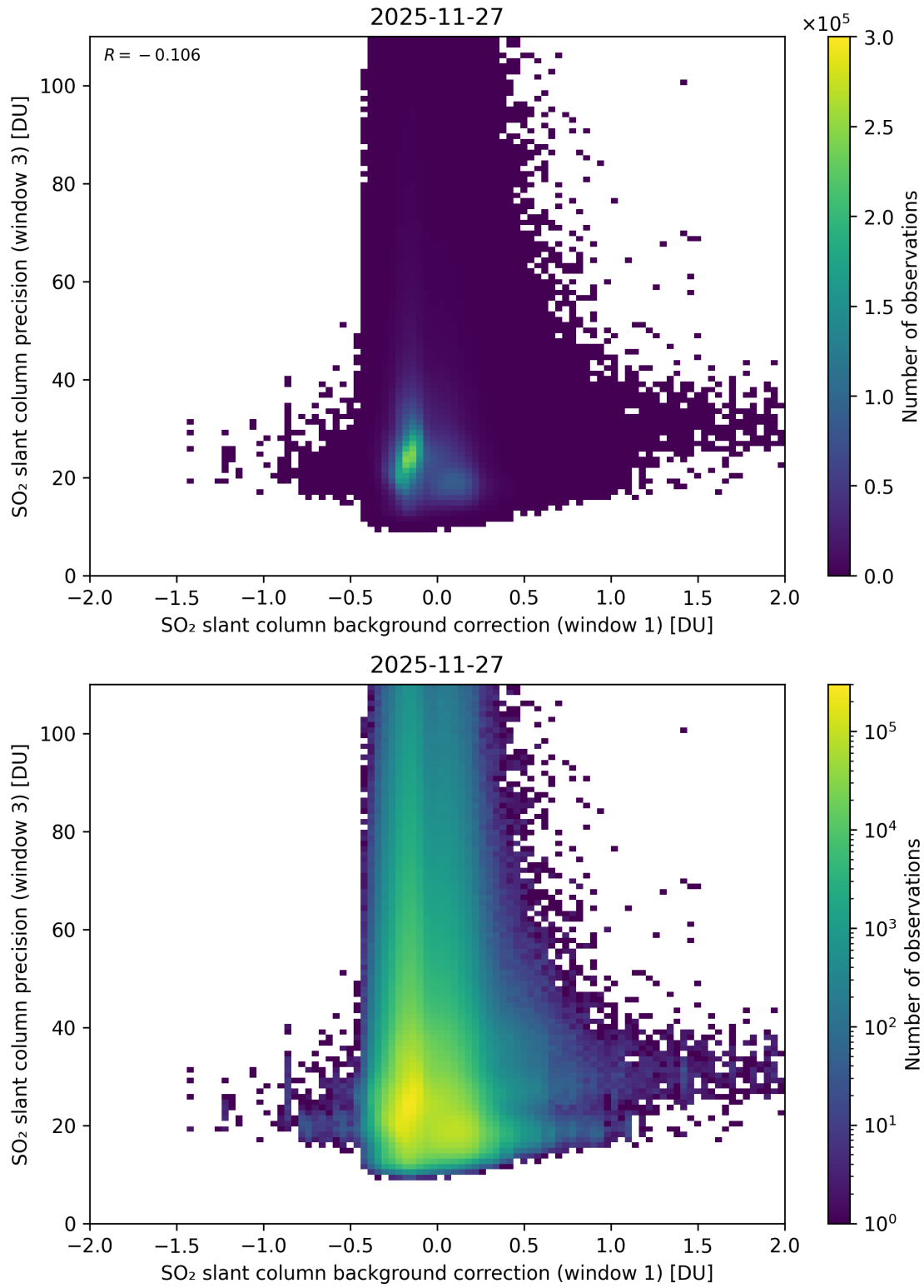
Figure 119: Scatter density plot of “SO 2 slant column background correction (window 1)” against “SO 2 slant column precision (window 3)” for 2025-11-26 to 2025-11-28.
