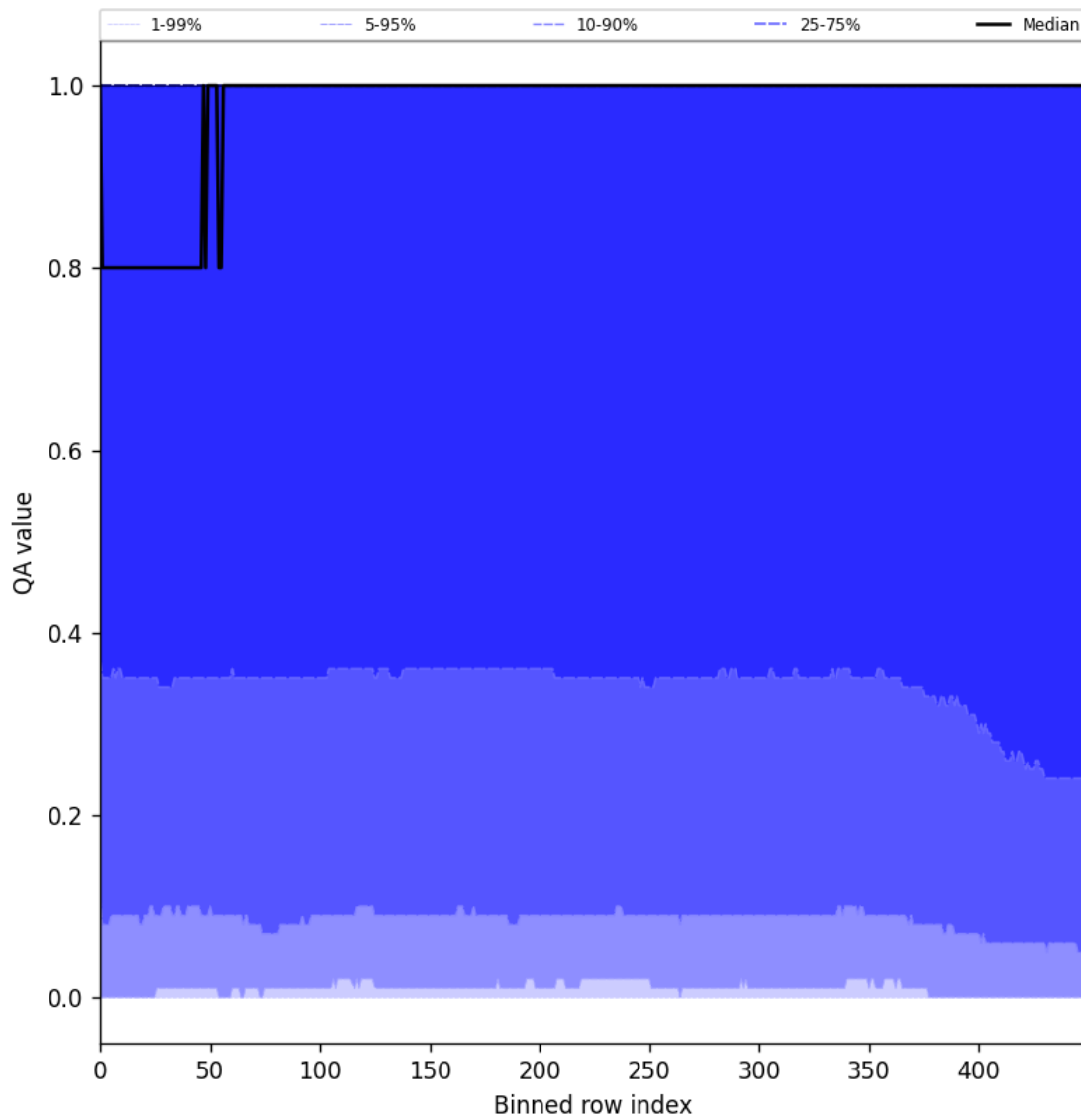
Figure 83: Along track statistics of “QA value” for 2025-11-26 to 2025-11-28
