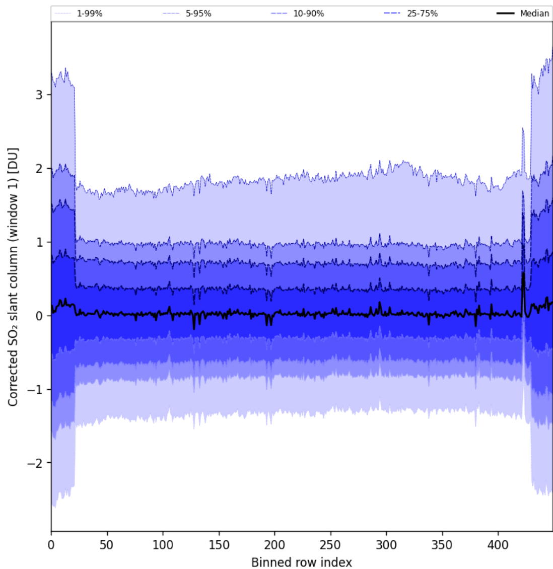
Figure 91: Along track statistics of “Corrected SO 2 slant column (window 1)” for 2025-11-26 to 2025-11-28
