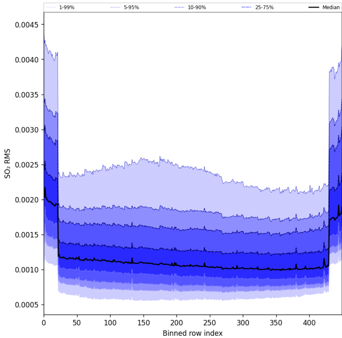
Figure 104: Along track statistics of “SO 2 RMS” for 2025-11-26 to 2025-11-28
