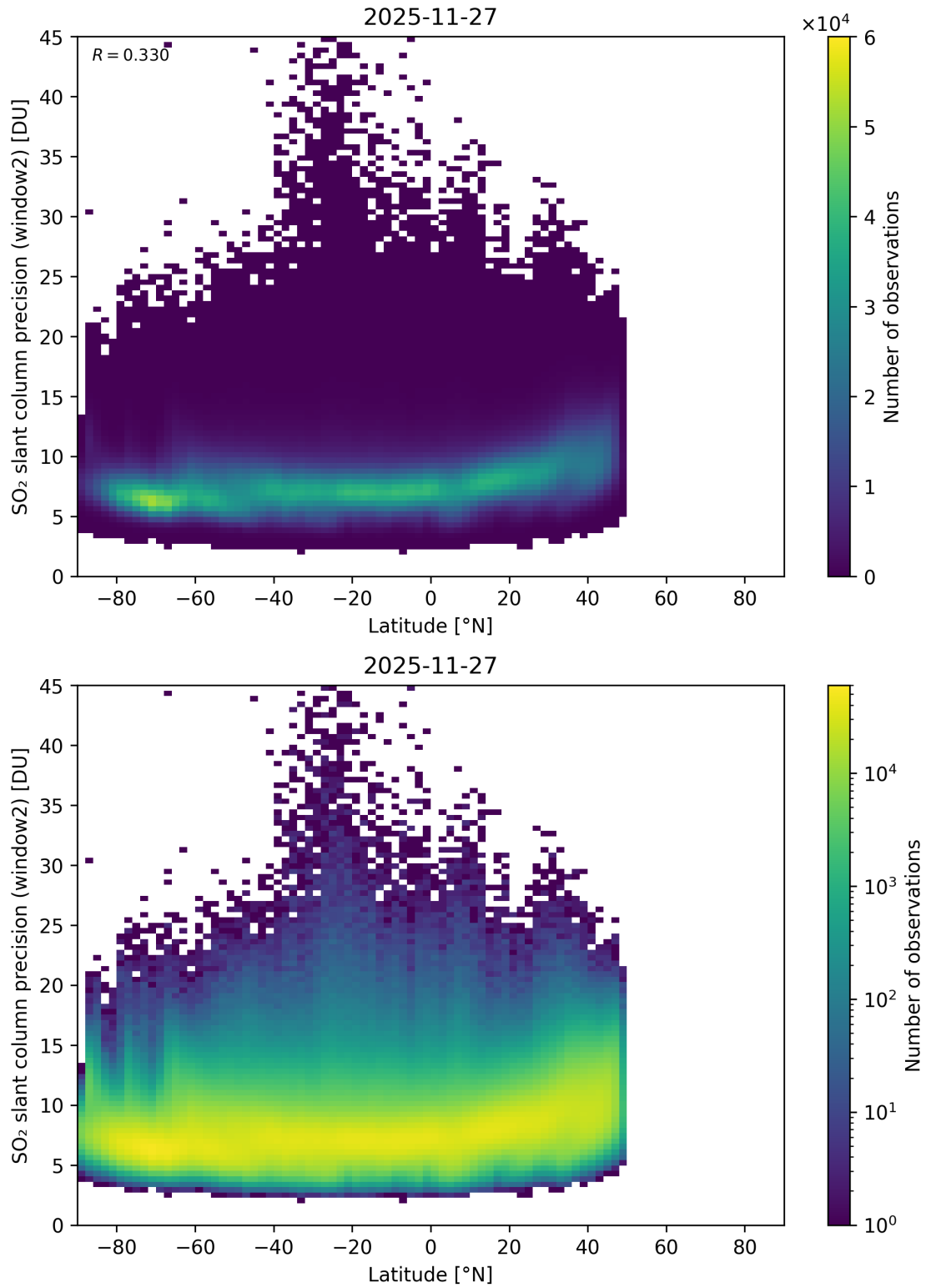
Figure 164: Scatter density plot of “Latitude” against “SO 2 slant column precision (window2)” for 2025-11-26 to 2025-11-28.
