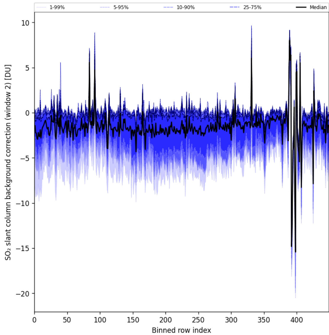
Figure 96: Along track statistics of “SO 2 slant column background correction (window 2)” for 2025-11-26 to 2025-11-28
