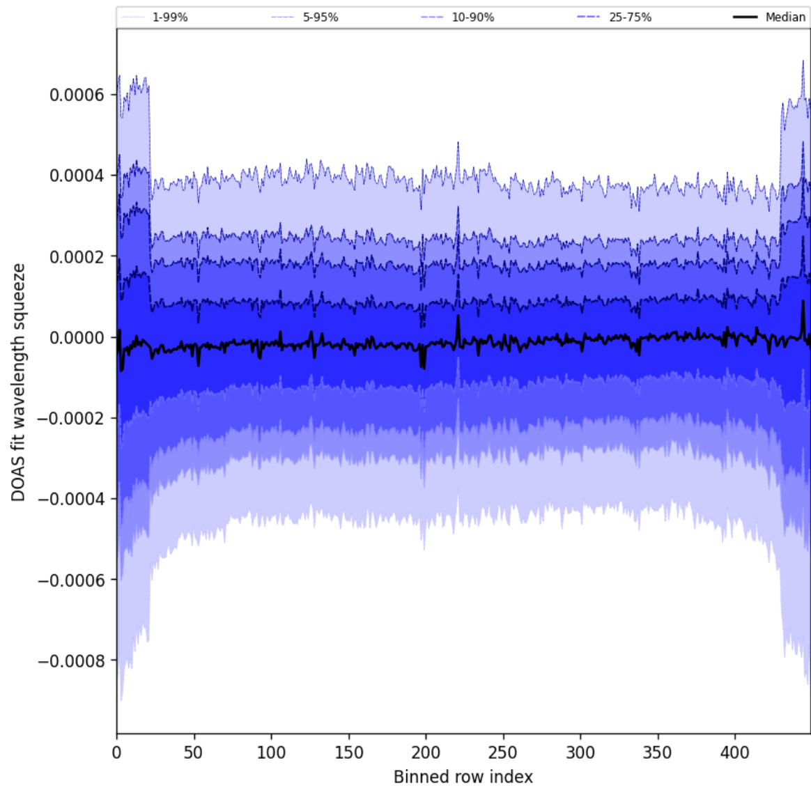
Figure 103: Along track statistics of “DOAS fit wavelength squeeze” for 2025-11-26 to 2025-11-28
