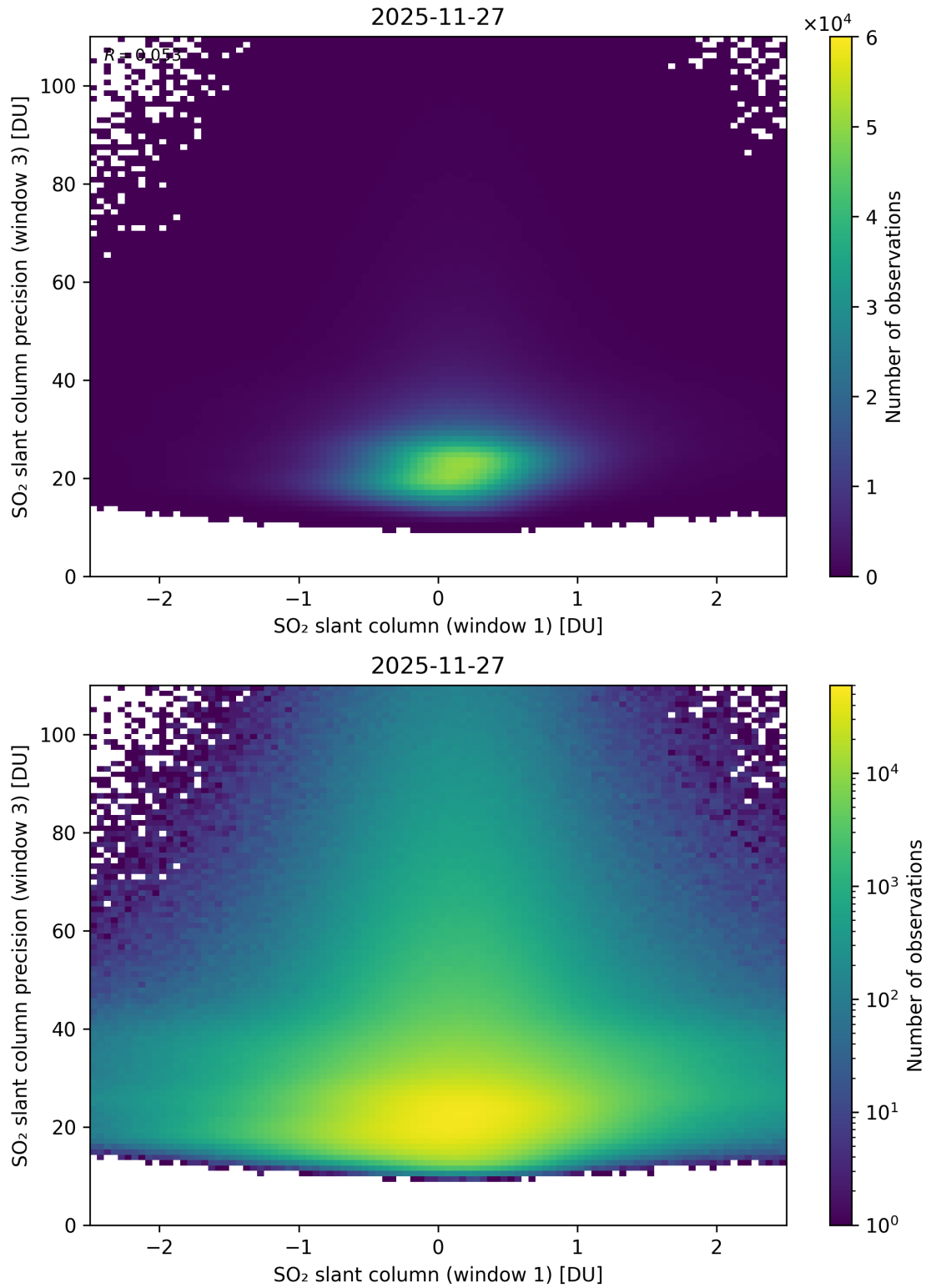
Figure 288: Scatter density plot of “SO 2 slant column (window 1)” against “SO 2 slant column precision (window 3)” for 2025-11-26 to 2025-11-28.
