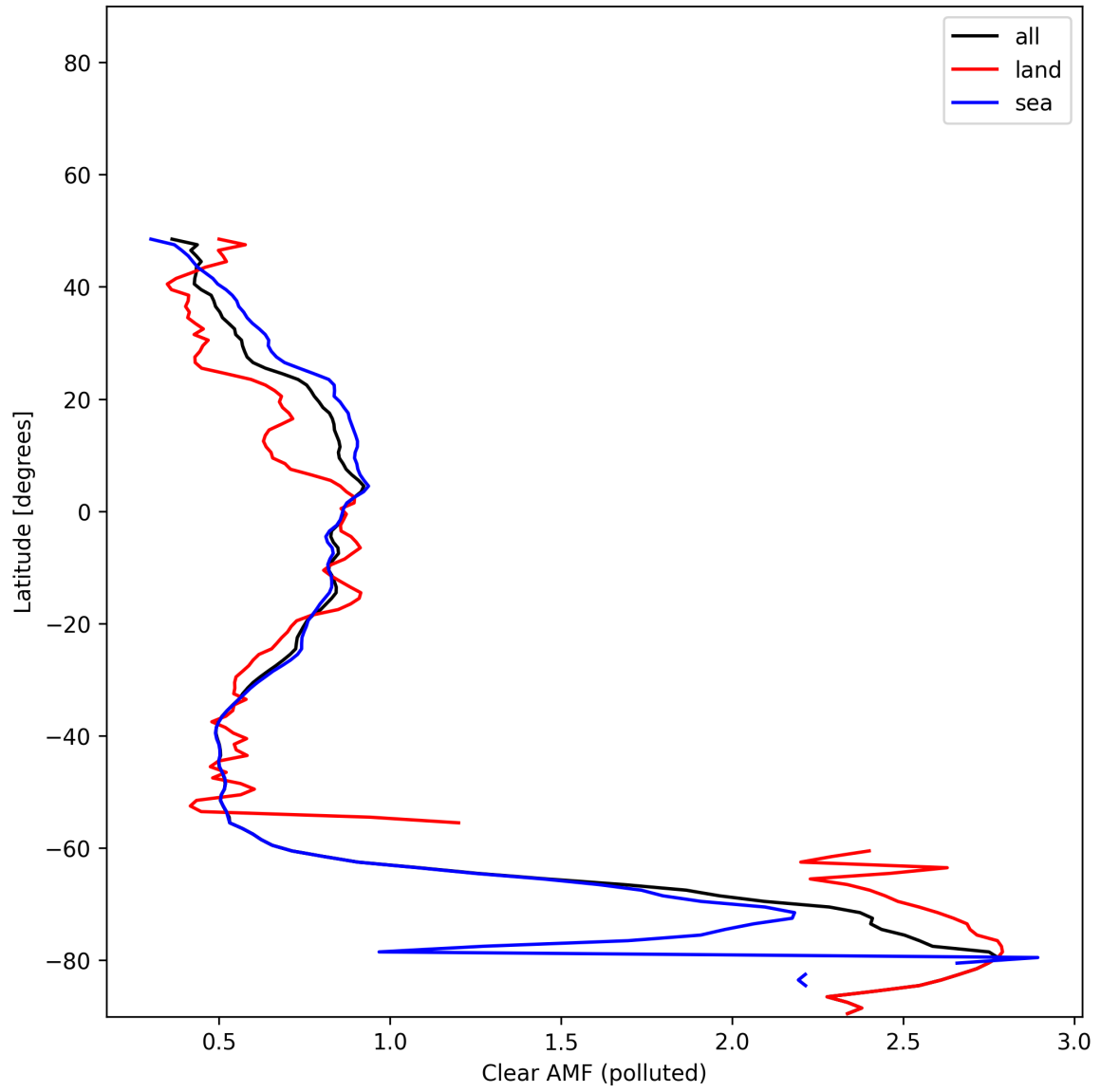
Figure 55: Zonal average of “Clear AMF (polluted)” for 2025-11-26 to 2025-11-28.
