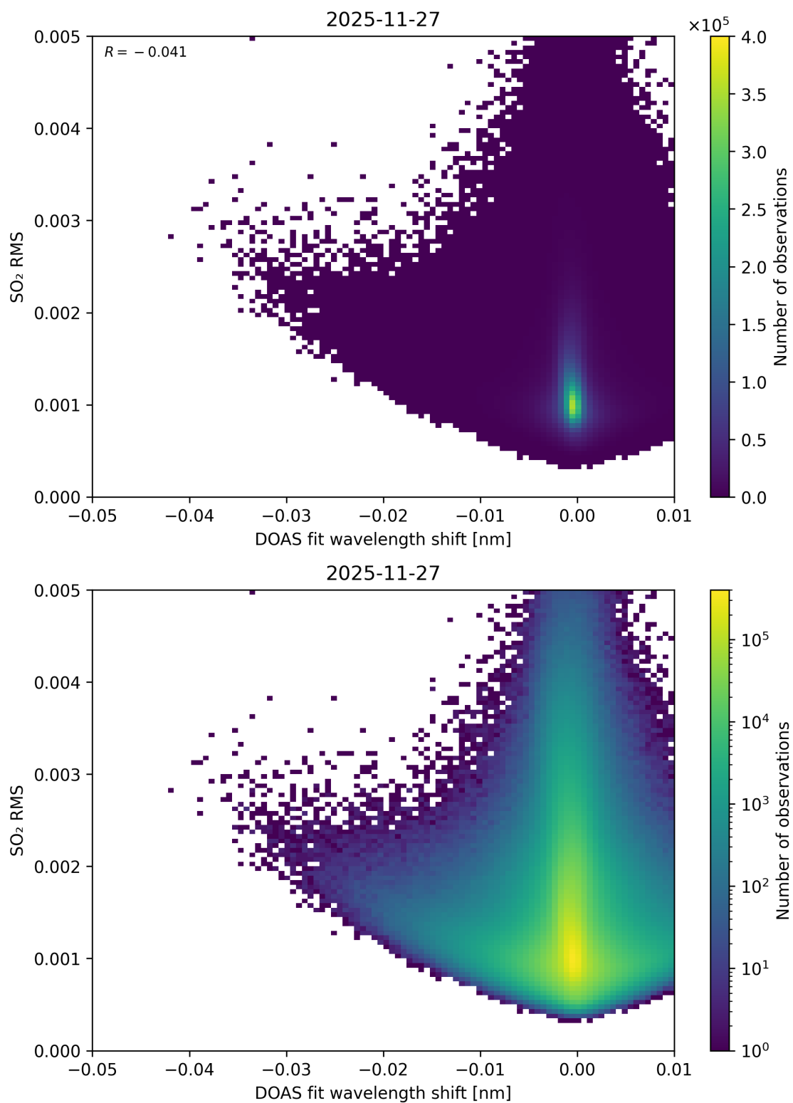
Figure 139: Scatter density plot of “DOAS fit wavelength shift” against “SO 2 RMS” for 2025-11-26 to 2025-11-28.
