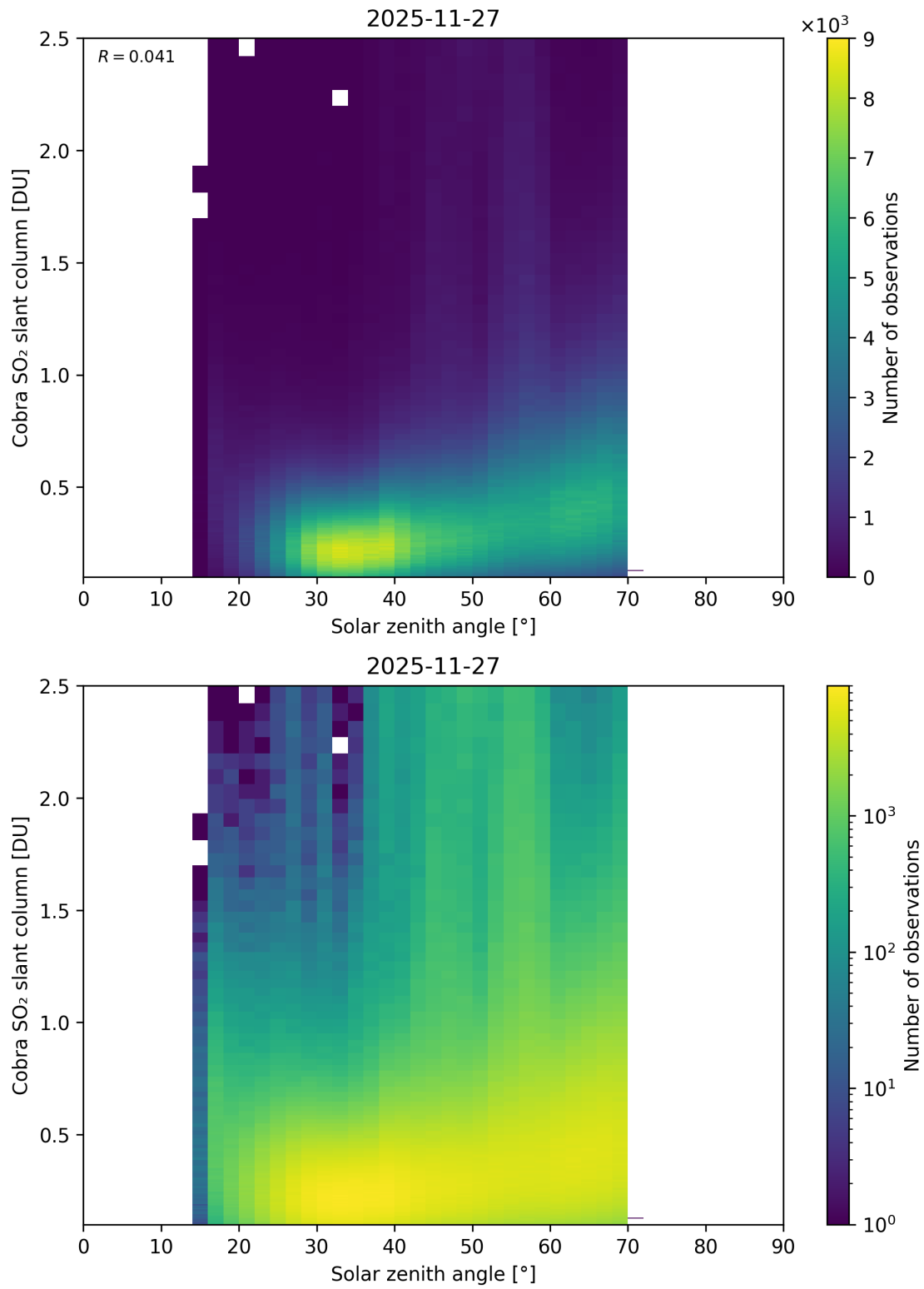
Figure 179: Scatter density plot of “Solar zenith angle” against “Cobra SO 2 slant column” for 2025-11-26 to 2025-11-28.
