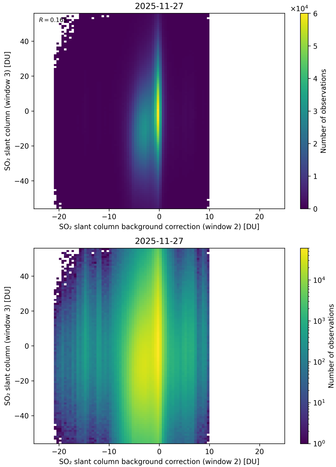
Figure 128: Scatter density plot of “SO 2 slant column background correction (window 2)” against “SO 2 slant column (window 3)” for 2025-11-26 to 2025-11-28.
