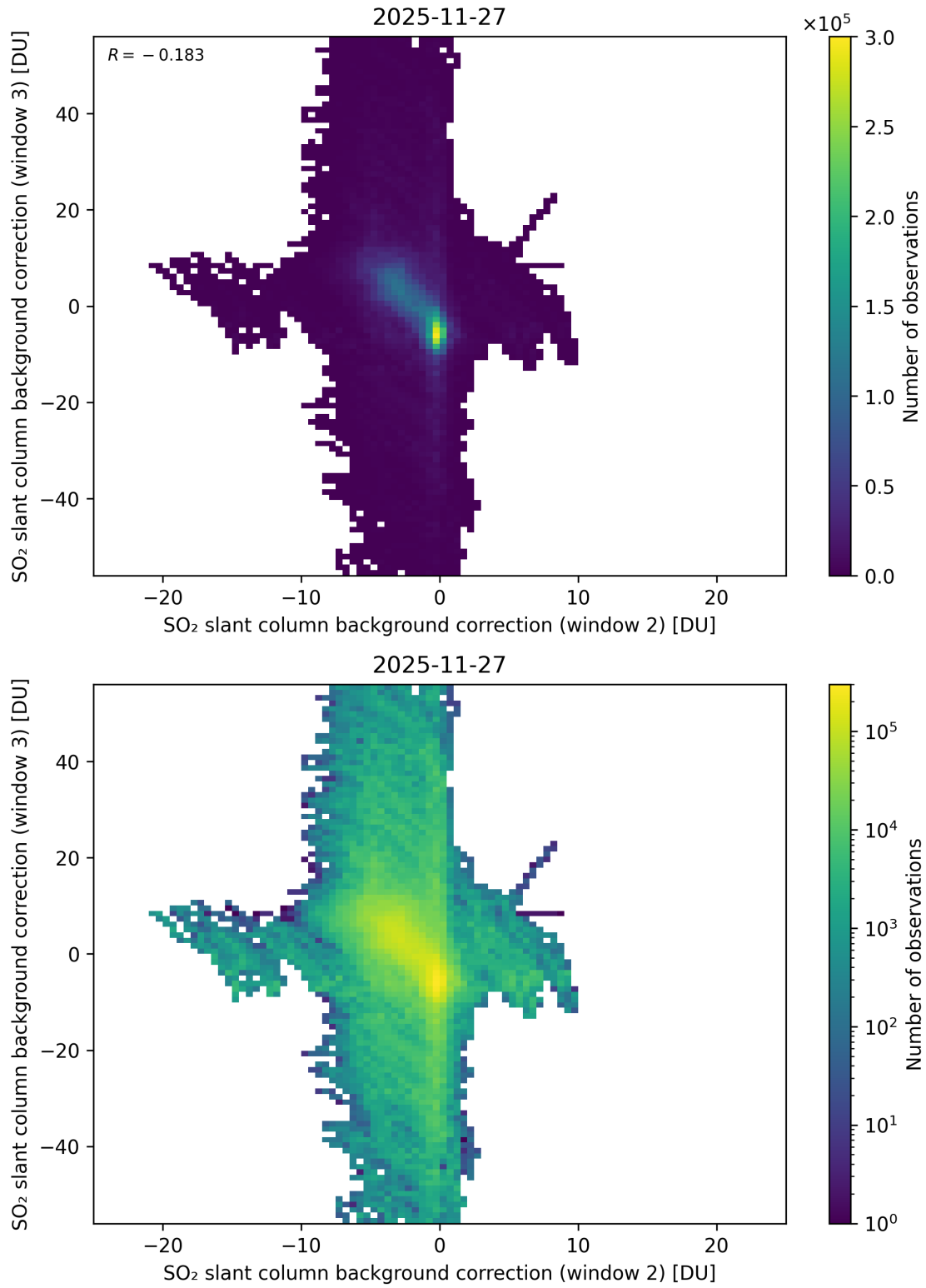
Figure 122: Scatter density plot of “SO 2 slant column background correction (window 2)” against “SO 2 slant column background correction (window 3)” for 2025-11-26 to 2025-11-28.
