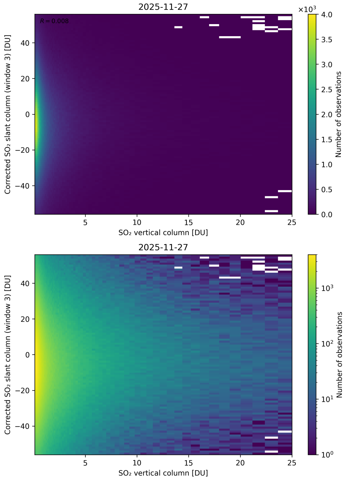
Figure 353: Scatter density plot of “SO 2 vertical column” against “Corrected SO 2 slant column (window 3)” for 2025-11-26 to 2025-11-28.
