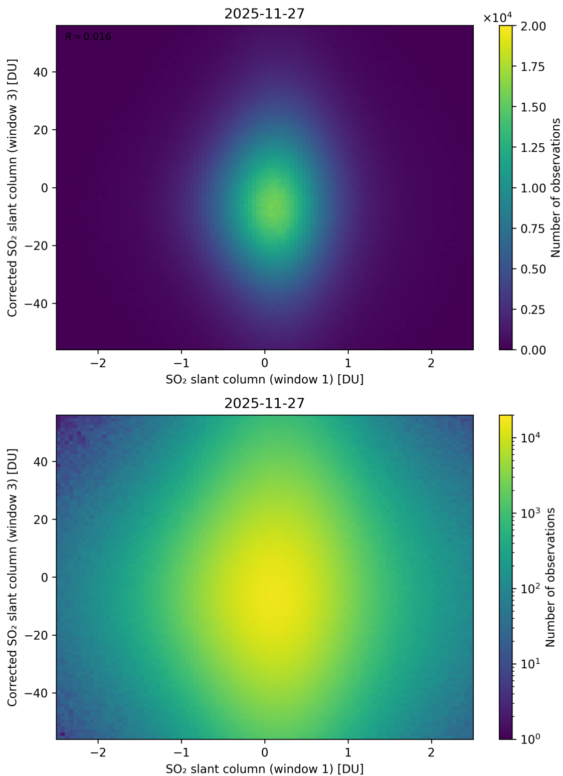
Figure 284: Scatter density plot of “SO 2 slant column (window 1)” against “Corrected SO 2 slant column (window 3)” for 2025-11-26 to 2025-11-28.
