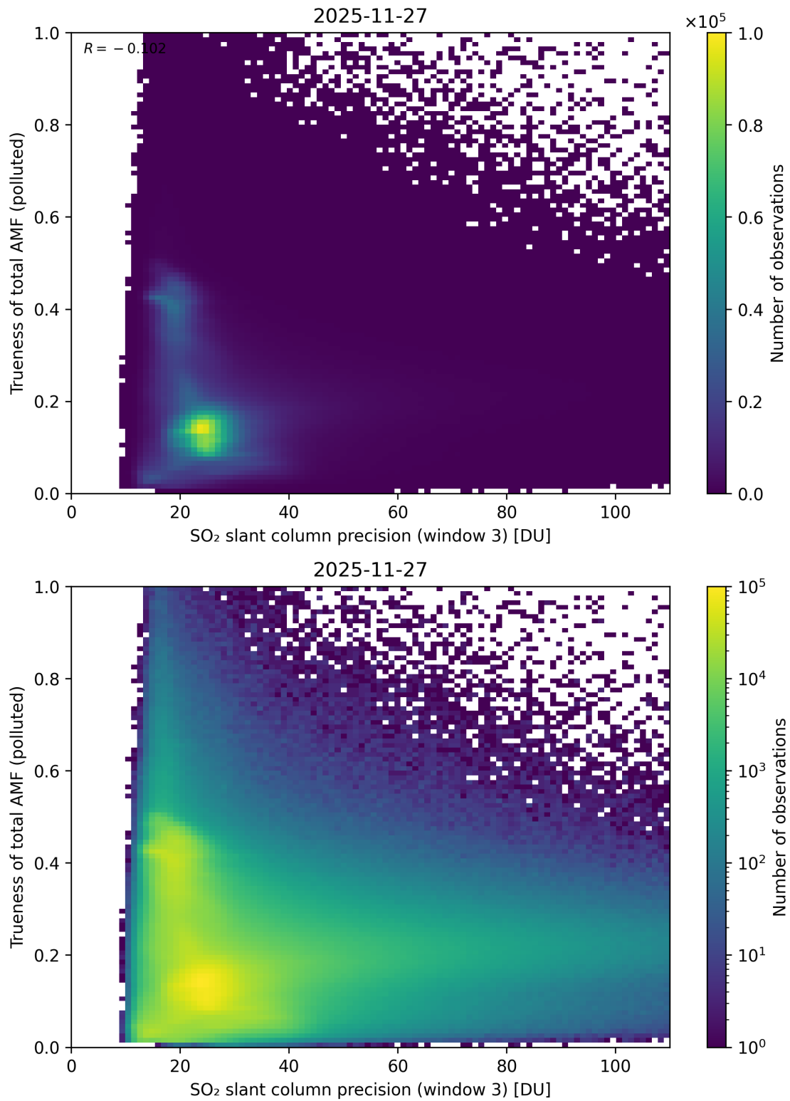
Figure 314: Scatter density plot of “SO 2 slant column precision (window 3)” against “Trueness of total AMF (polluted)” for 2025-11-26 to 2025-11-28.
