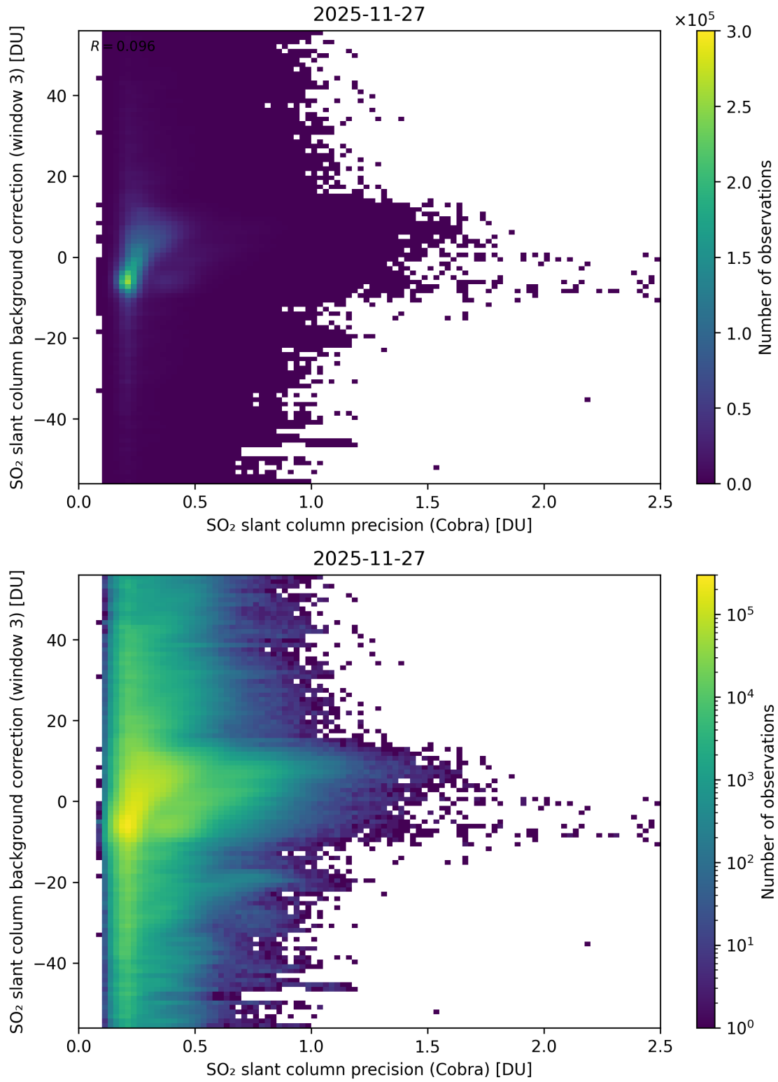
Figure 201: Scatter density plot of “SO 2 slant column precision (Cobra)” against “SO 2 slant column background correction (window 3)” for 2025-11-26 to 2025-11-28.
