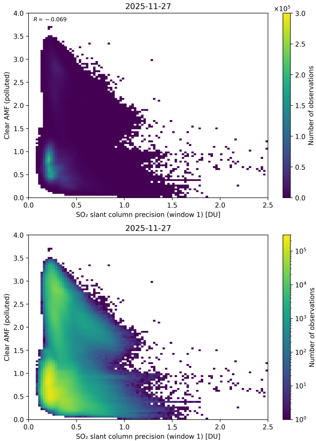
Figure 274: Scatter density plot of “SO 2 slant column precision (window 1)” against “Clear AMF (polluted)” for 2025-11-26 to 2025-11-28.
