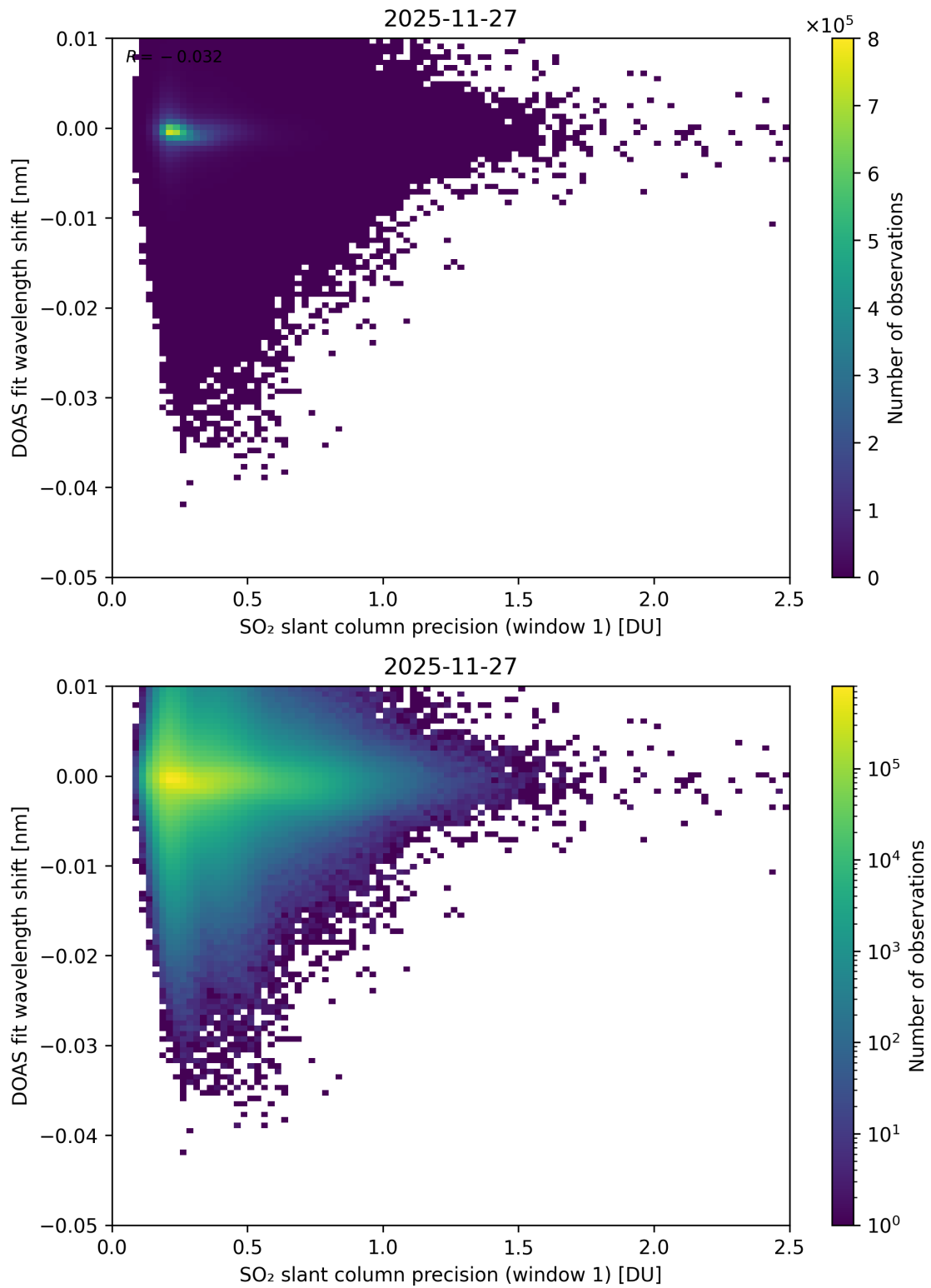
Figure 271: Scatter density plot of “SO 2 slant column precision (window 1)” against “DOAS fit wavelength shift” for 2025-11-26 to 2025-11-28.
