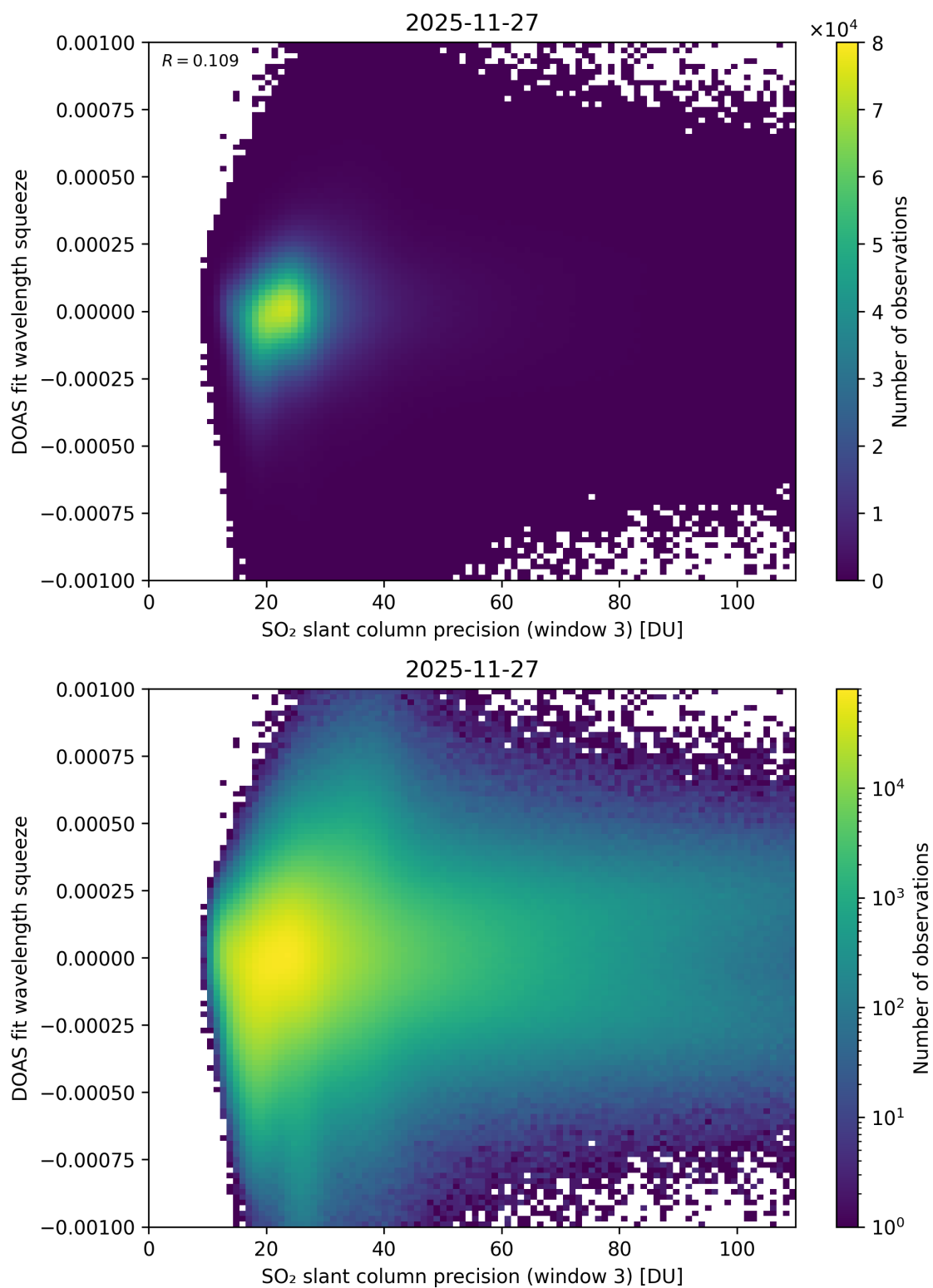
Figure 309: Scatter density plot of “SO 2 slant column precision (window 3)” against “DOAS fit wavelength squeeze” for 2025-11-26 to 2025-11-28.
