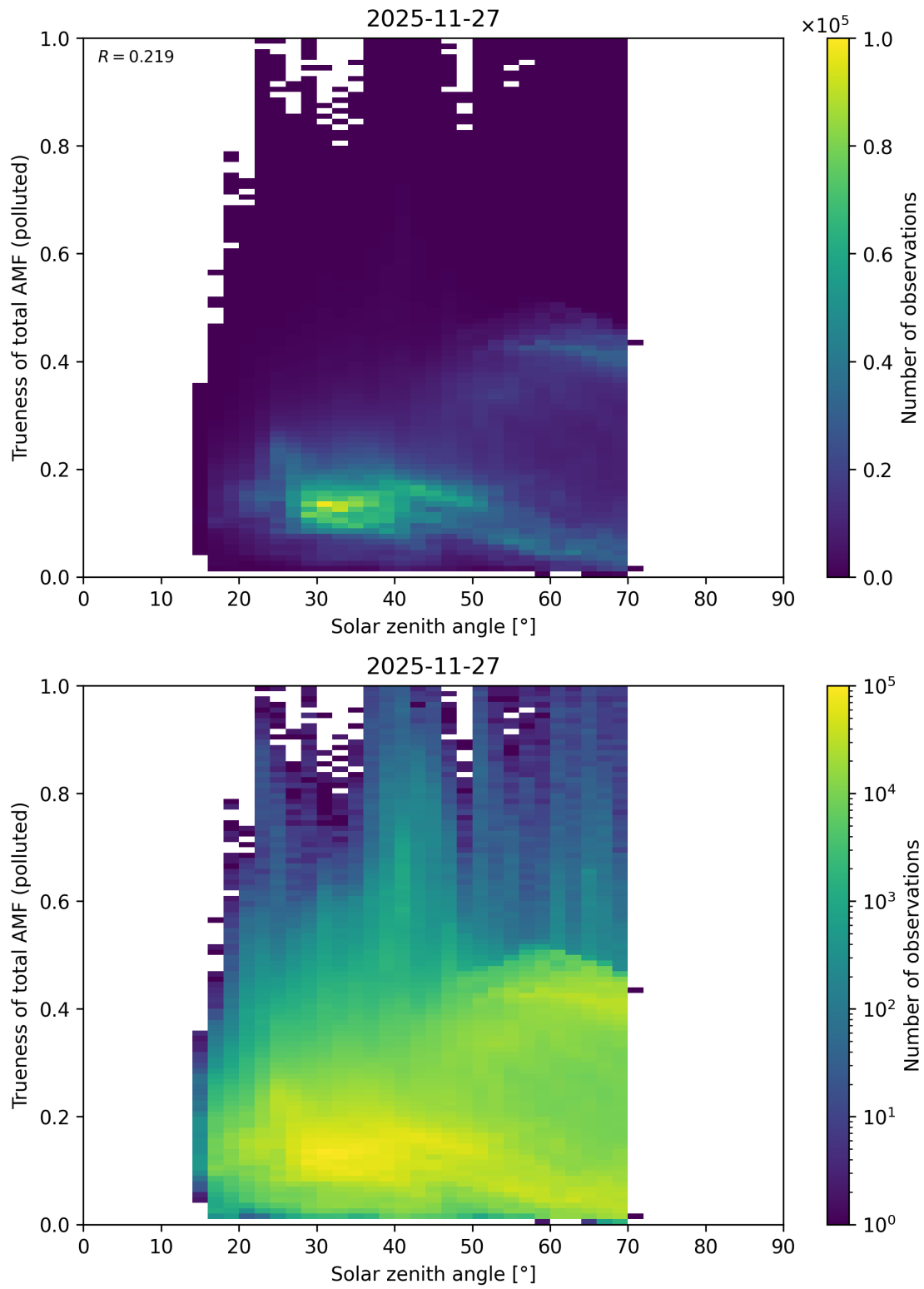
Figure 190: Scatter density plot of “Solar zenith angle” against “Trueness of total AMF (polluted)” for 2025-11-26 to 2025-11-28.
