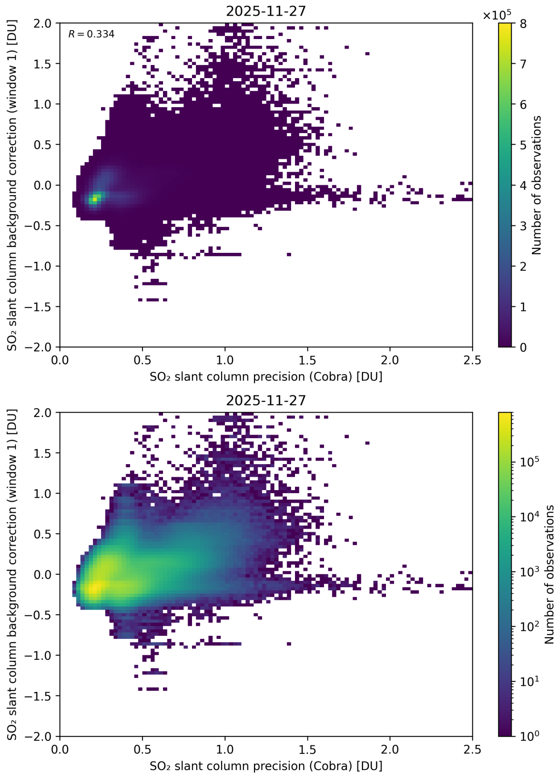
Figure 199: Scatter density plot of “SO 2 slant column precision (Cobra)” against “SO 2 slant column background correction (window 1)” for 2025-11-26 to 2025-11-28.
