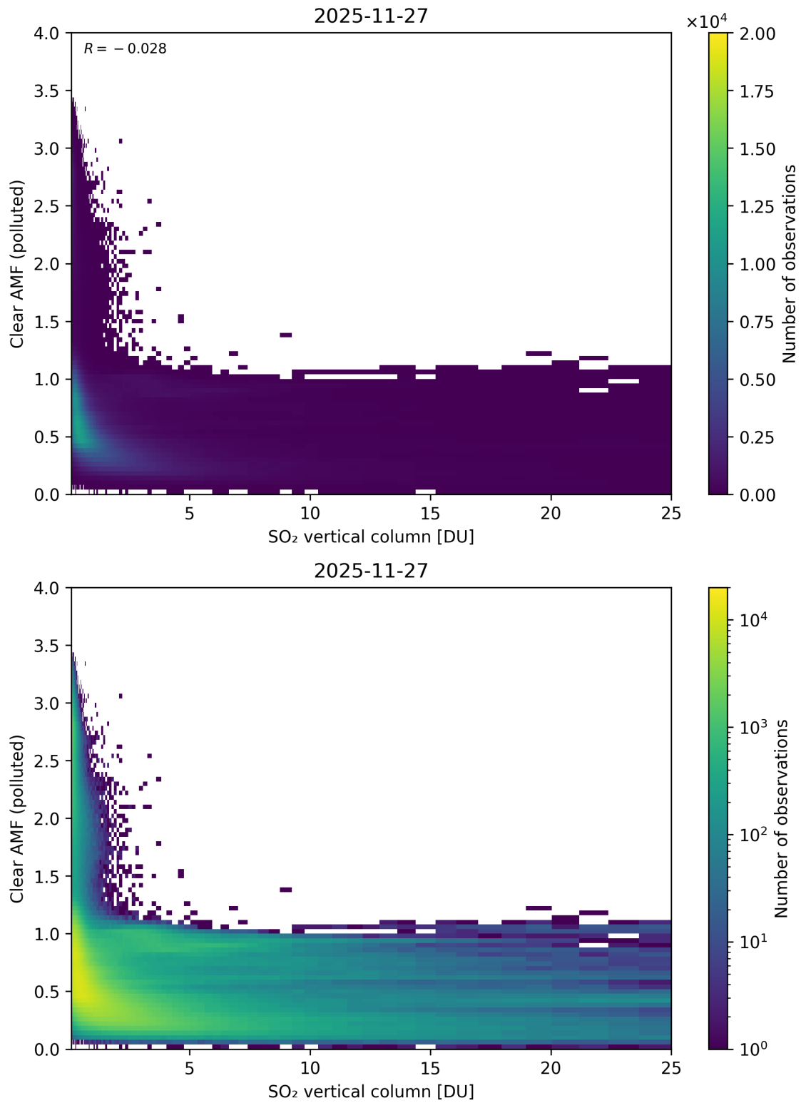
Figure 348: Scatter density plot of “SO 2 vertical column” against “Clear AMF (polluted)” for 2025-11-26 to 2025-11-28.
