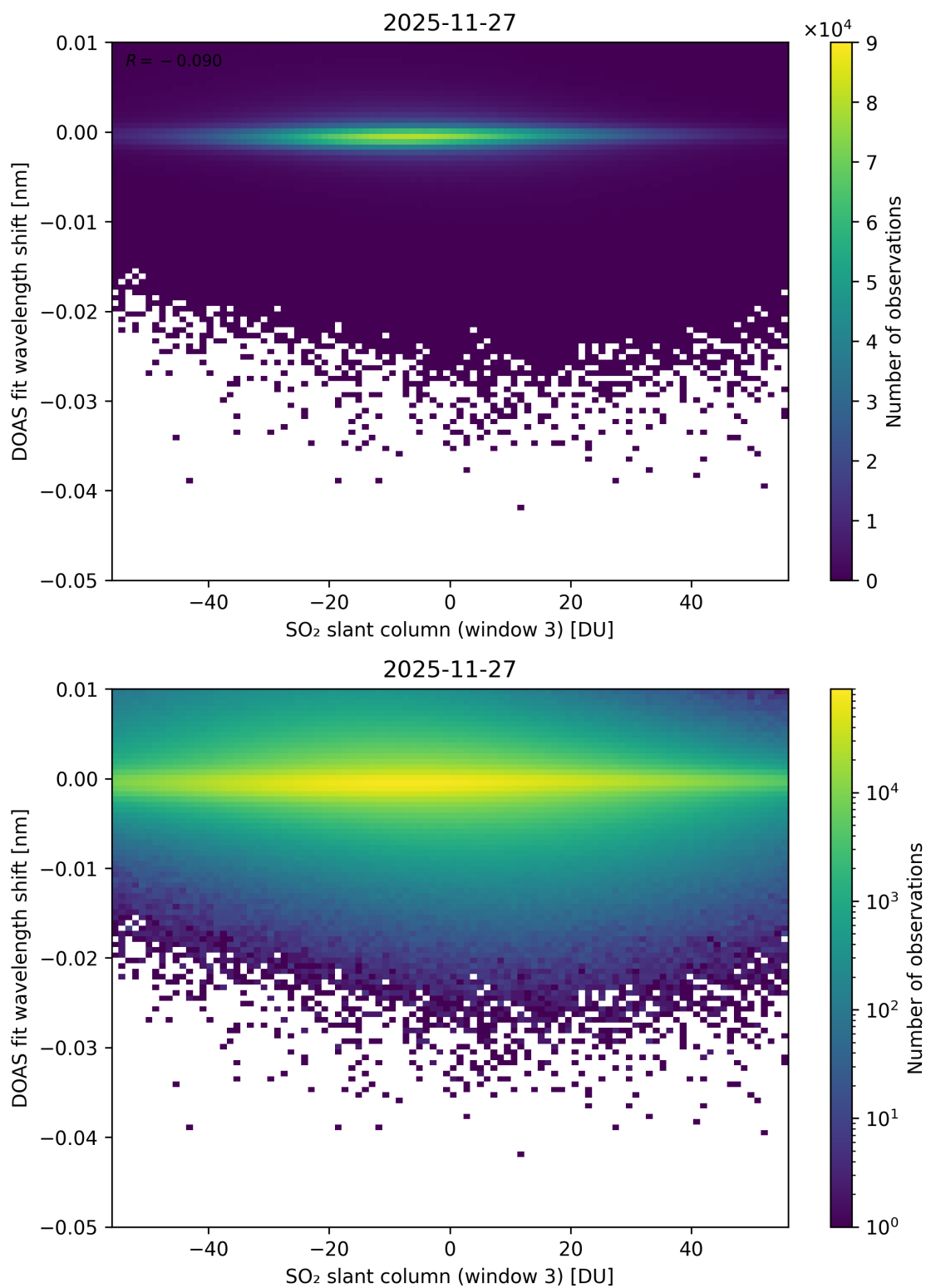
Figure 304: Scatter density plot of “SO 2 slant column (window 3)” against “DOAS fit wavelength shift” for 2025-11-26 to 2025-11-28.
