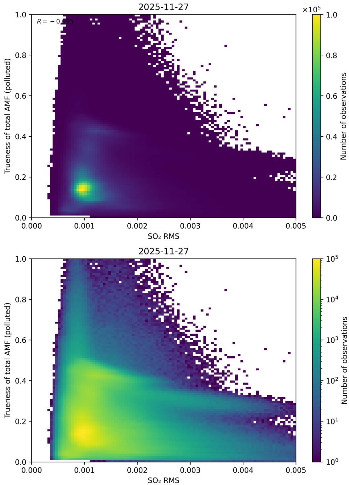
Figure 149: Scatter density plot of “SO 2 RMS” against “Trueness of total AMF (polluted)” for 2025-11-26 to 2025-11-28.
