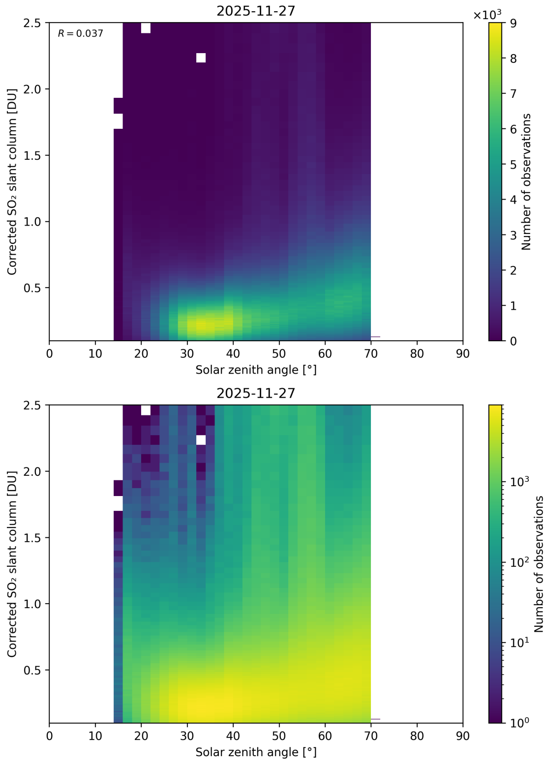
Figure 181: Scatter density plot of “Solar zenith angle” against “Corrected SO 2 slant column” for 2025-11-26 to 2025-11-28.
