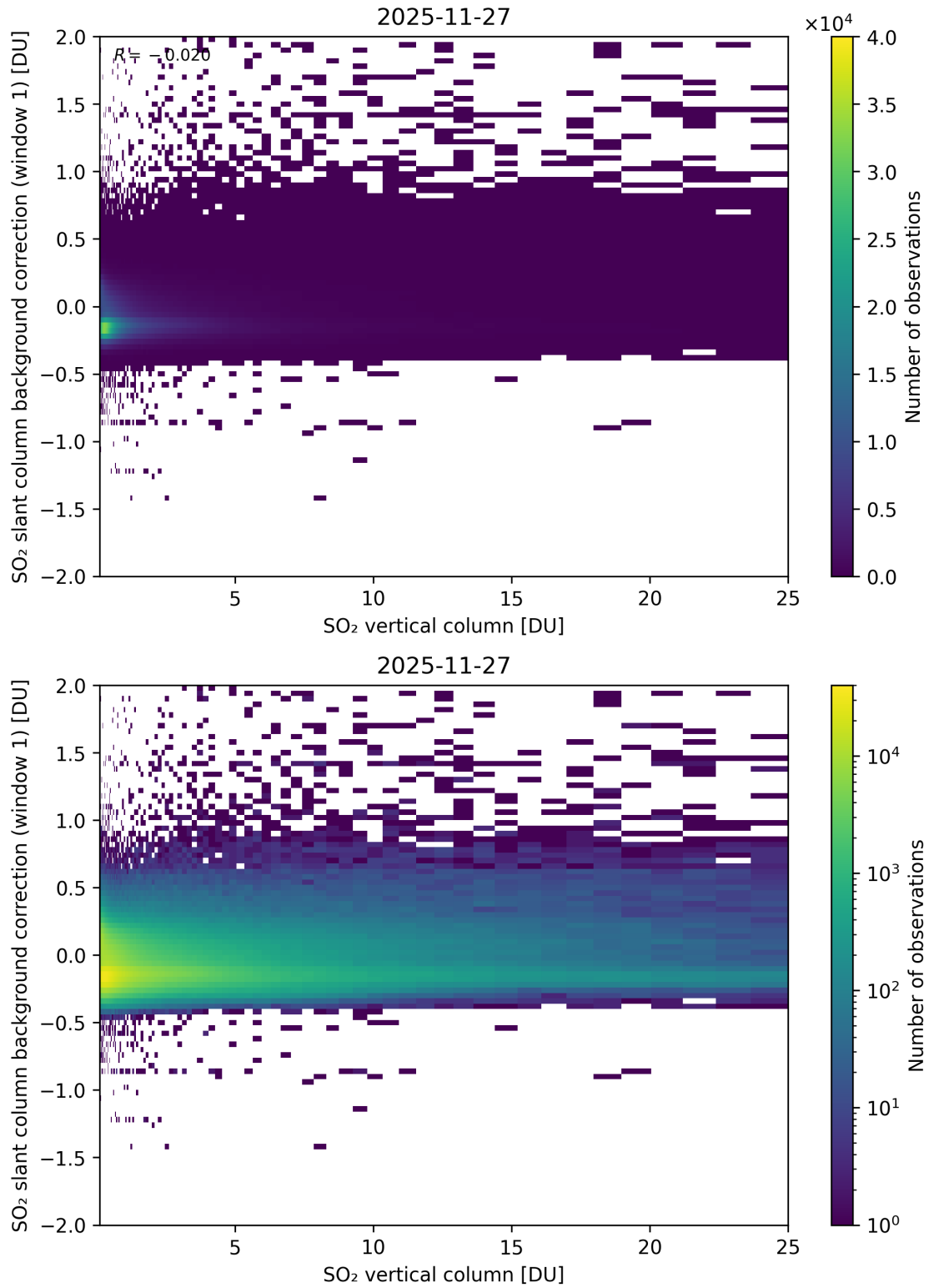
Figure 323: Scatter density plot of “SO 2 vertical column” against “SO 2 slant column background correction (window 1)” for 2025-11-26 to 2025-11-28.
