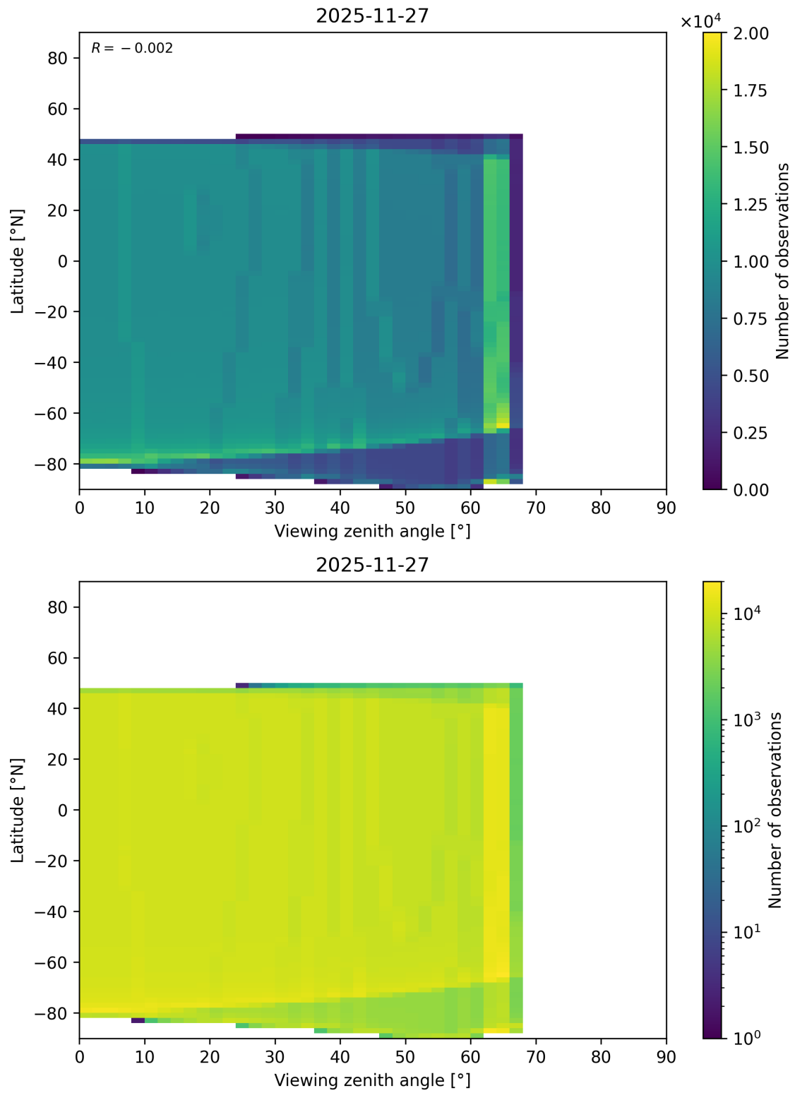
Figure 368: Scatter density plot of “Viewing zenith angle” against “Latitude” for 2025-11-26 to 2025-11-28.
