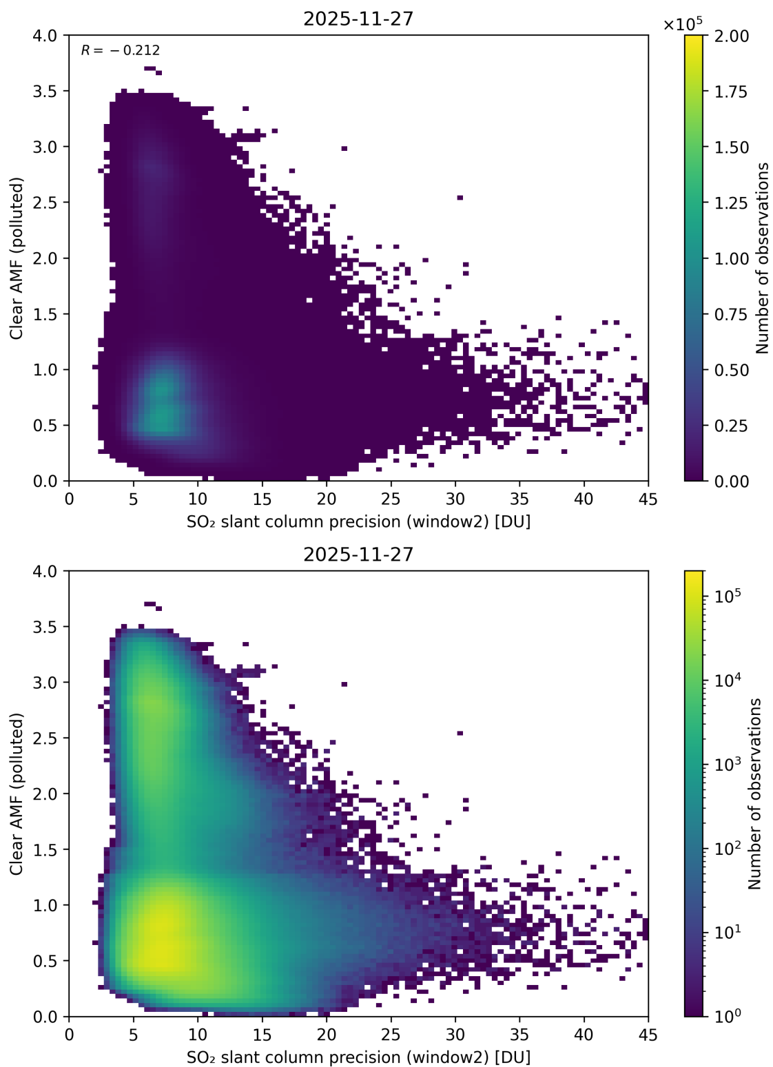
Figure 296: Scatter density plot of “SO 2 slant column precision (window2)” against “Clear AMF (polluted)” for 2025-11-26 to 2025-11-28.
