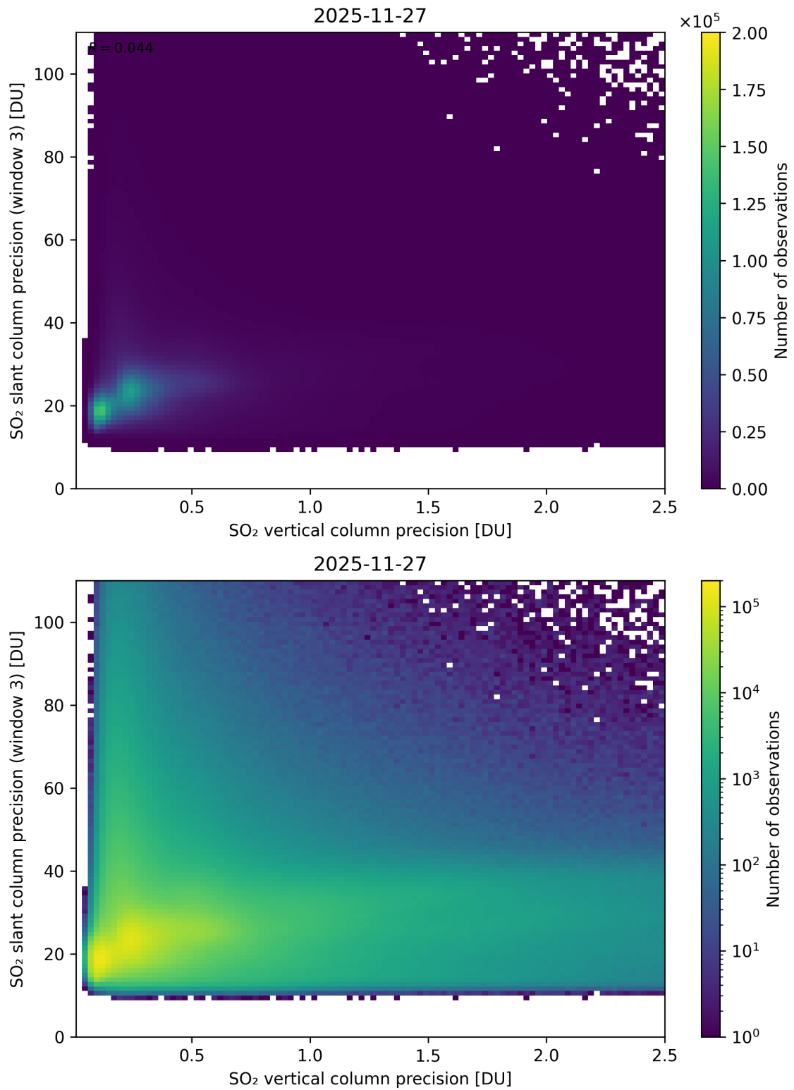
Figure 345: Scatter density plot of “SO 2 vertical column precision” against “SO 2 slant column precision (window 3)” for 2025-11-26 to 2025-11-28.
