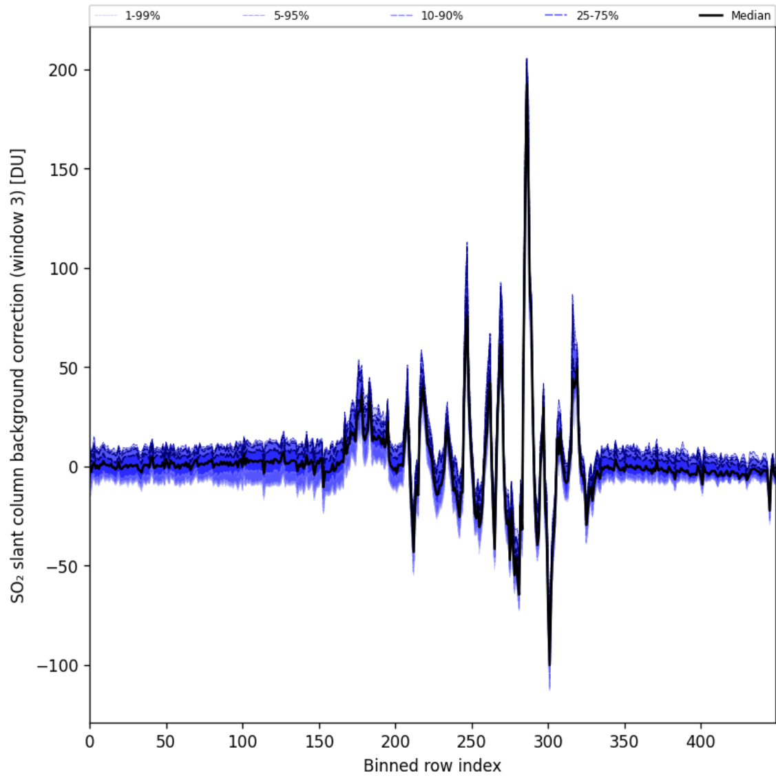
Figure 100: Along track statistics of “SO 2 slant column background correction (window 3)” for 2025-11-26 to 2025-11-28
