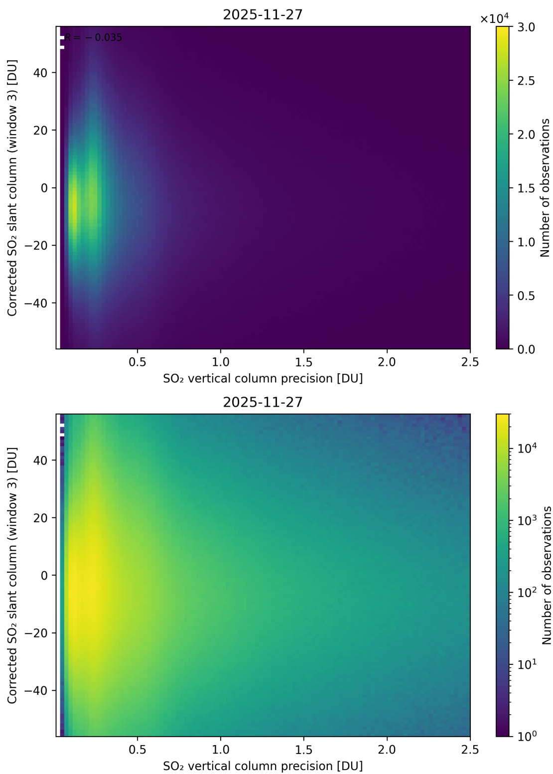
Figure 340: Scatter density plot of “SO 2 vertical column precision” against “Corrected SO 2 slant column (window 3)” for 2025-11-26 to 2025-11-28.
