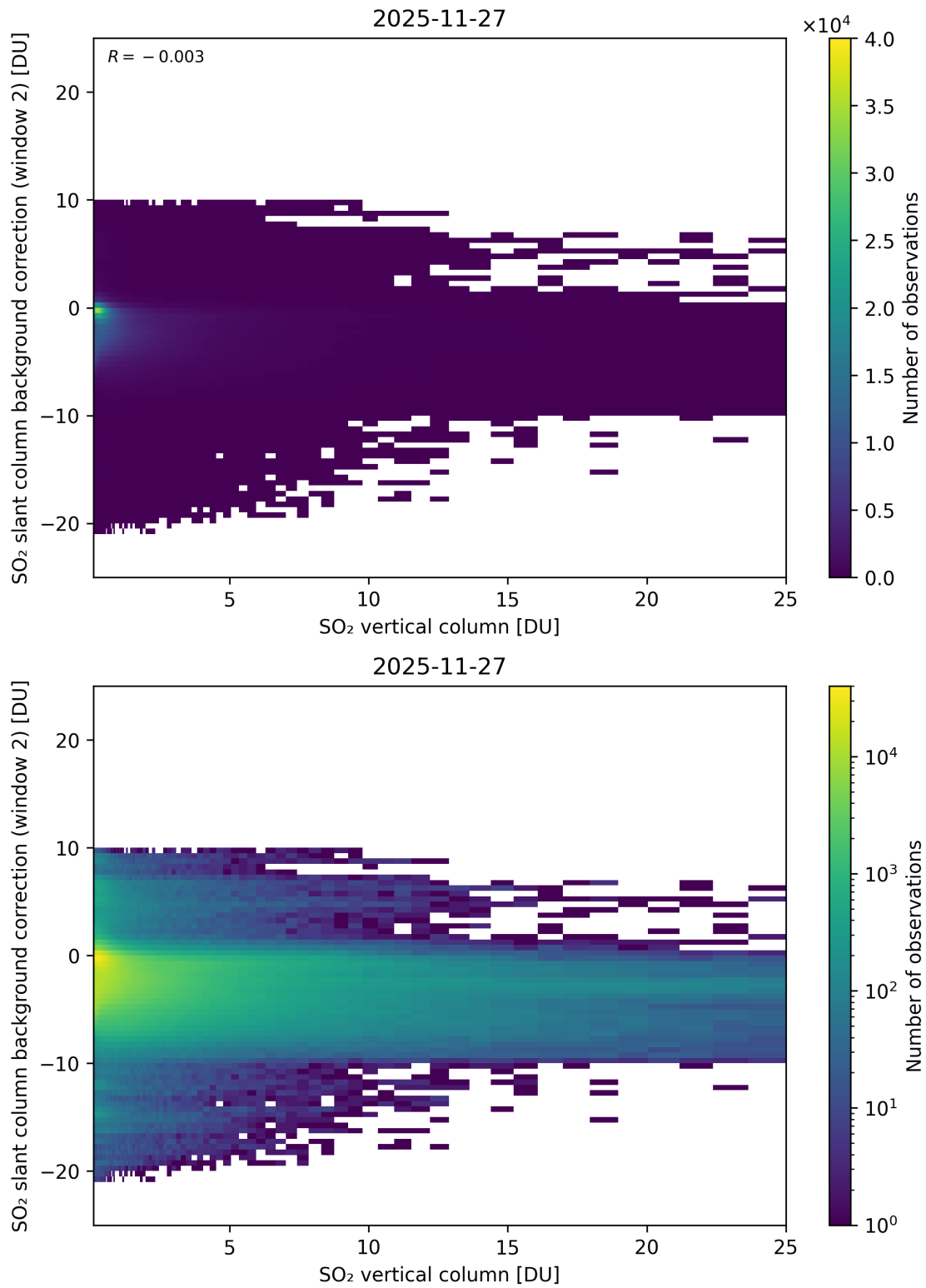
Figure 324: Scatter density plot of “SO 2 vertical column” against “SO 2 slant column background correction (window 2)” for 2025-11-26 to 2025-11-28.
