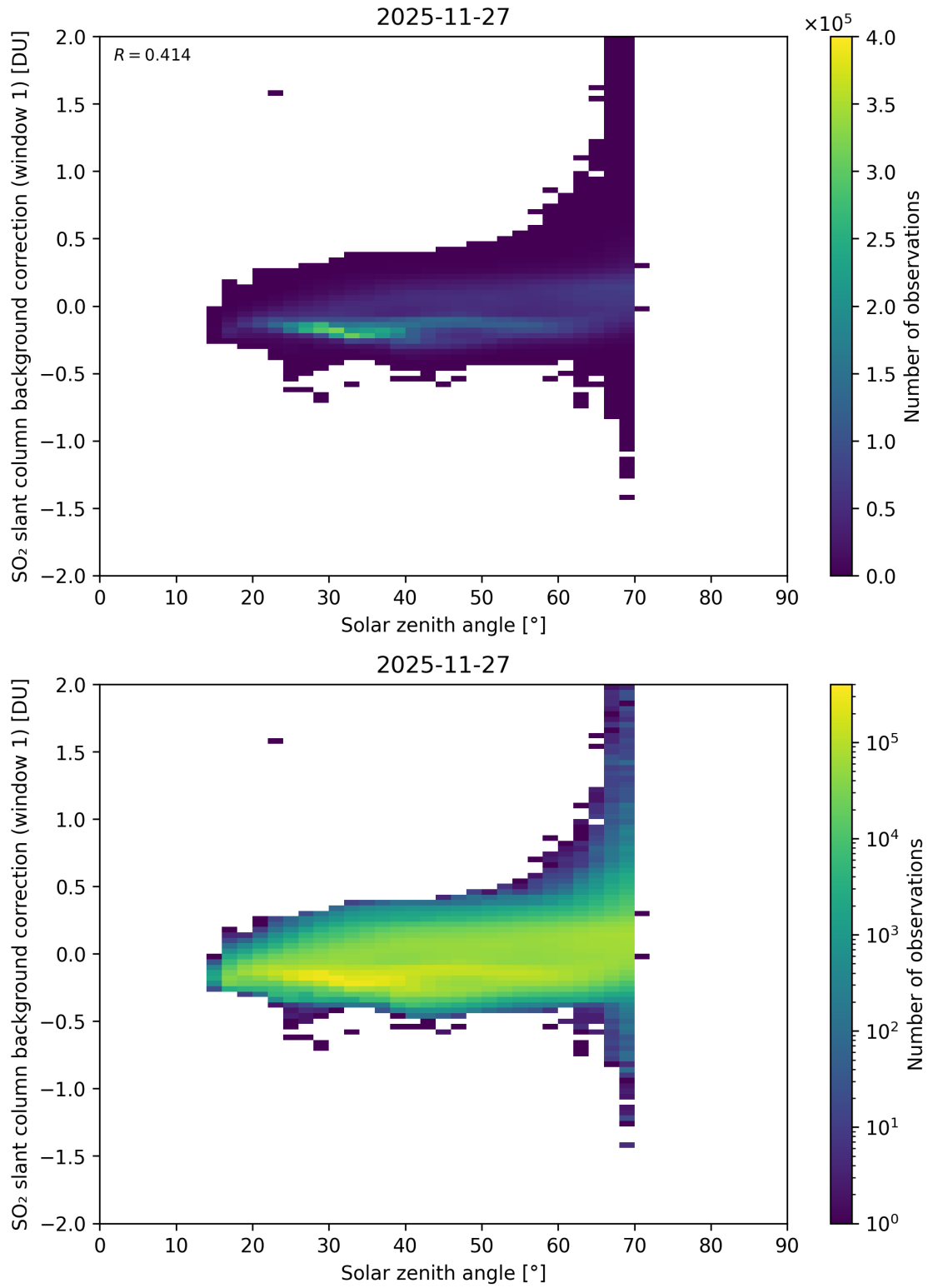
Figure 171: Scatter density plot of “Solar zenith angle” against “SO 2 slant column background correction (window 1)” for 2025-11-26 to 2025-11-28.
