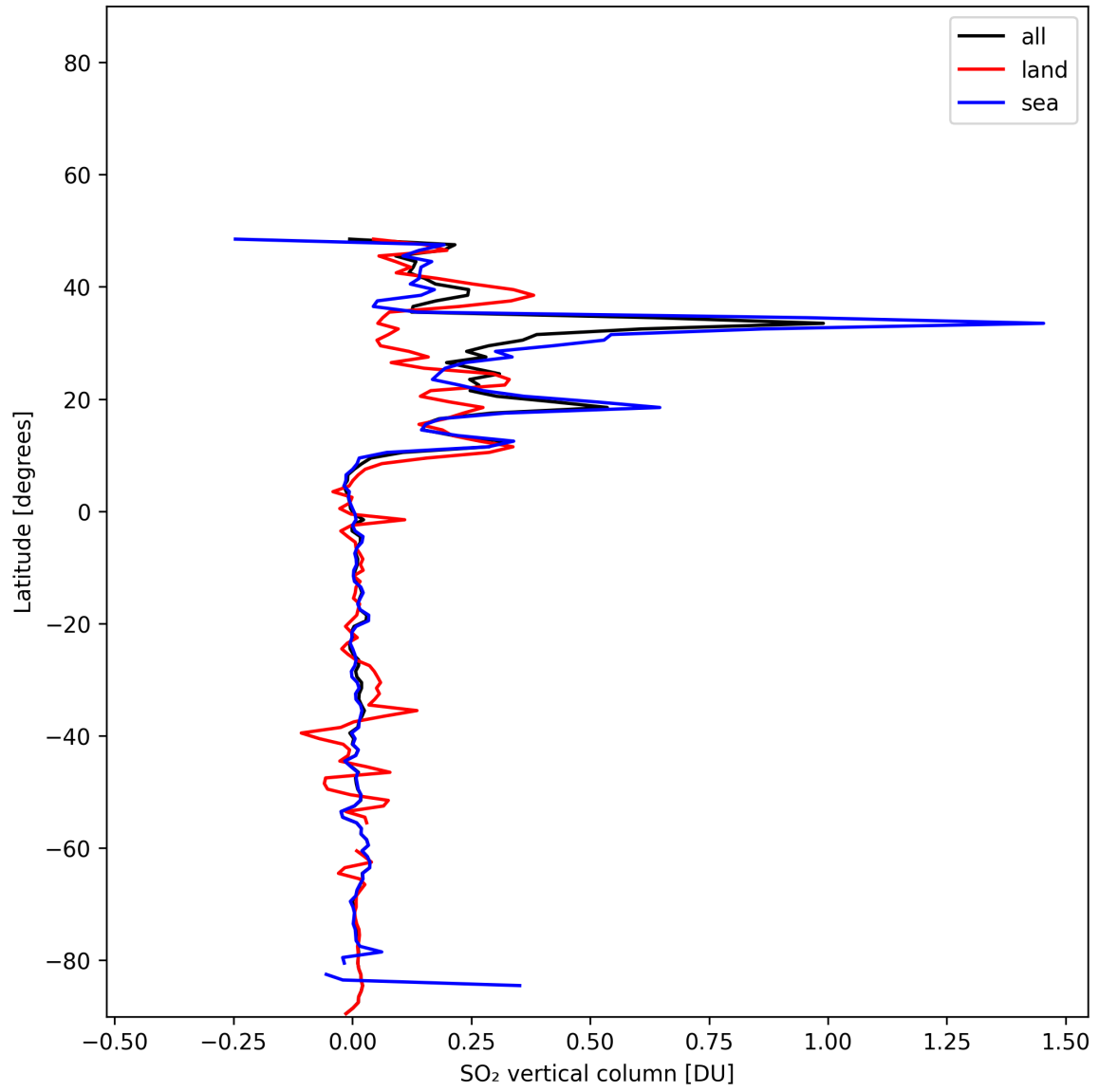
Figure 32: Zonal average of “SO 2 vertical column” for 2025-11-26 to 2025-11-28.
