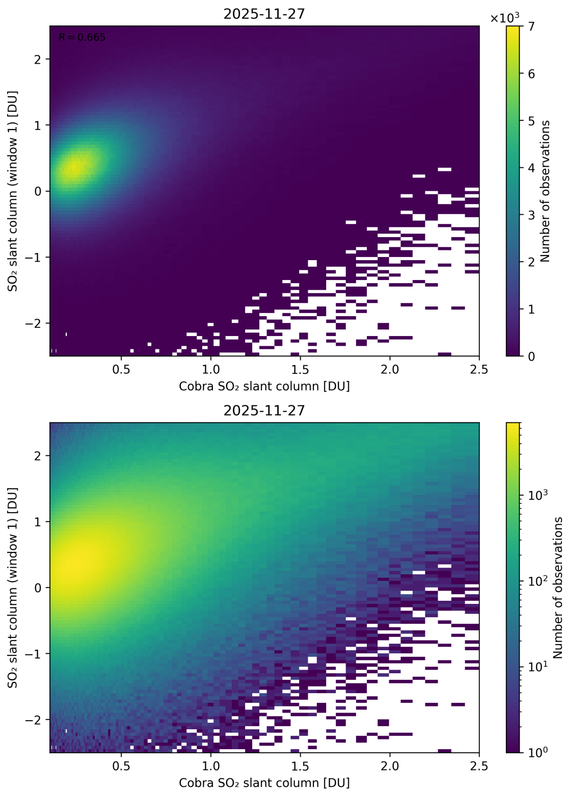
Figure 219: Scatter density plot of “Cobra SO 2 slant column” against “SO 2 slant column (window 1)” for 2025-11-26 to 2025-11-28.
