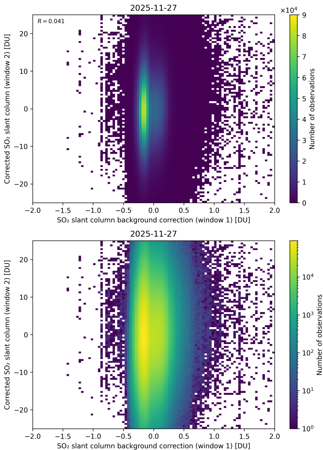
Figure 115: Scatter density plot of “SO 2 slant column background correction (window 1)” against “Corrected SO 2 slant column (window 2)” for 2025-11-26 to 2025-11-28.
