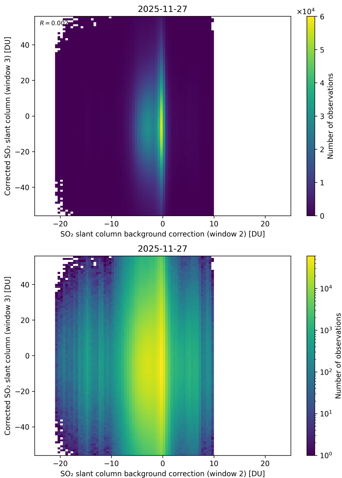
Figure 127: Scatter density plot of “SO 2 slant column background correction (window 2)” against “Corrected SO 2 slant column (window 3)” for 2025-11-26 to 2025-11-28.
