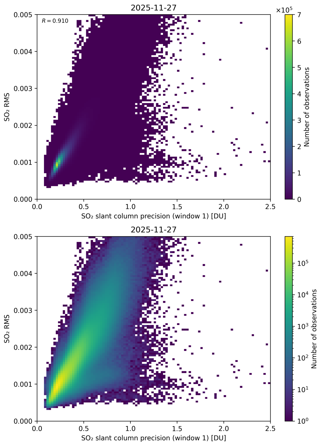
Figure 273: Scatter density plot of “SO 2 slant column precision (window 1)” against “SO 2 RMS” for 2025-11-26 to 2025-11-28.
