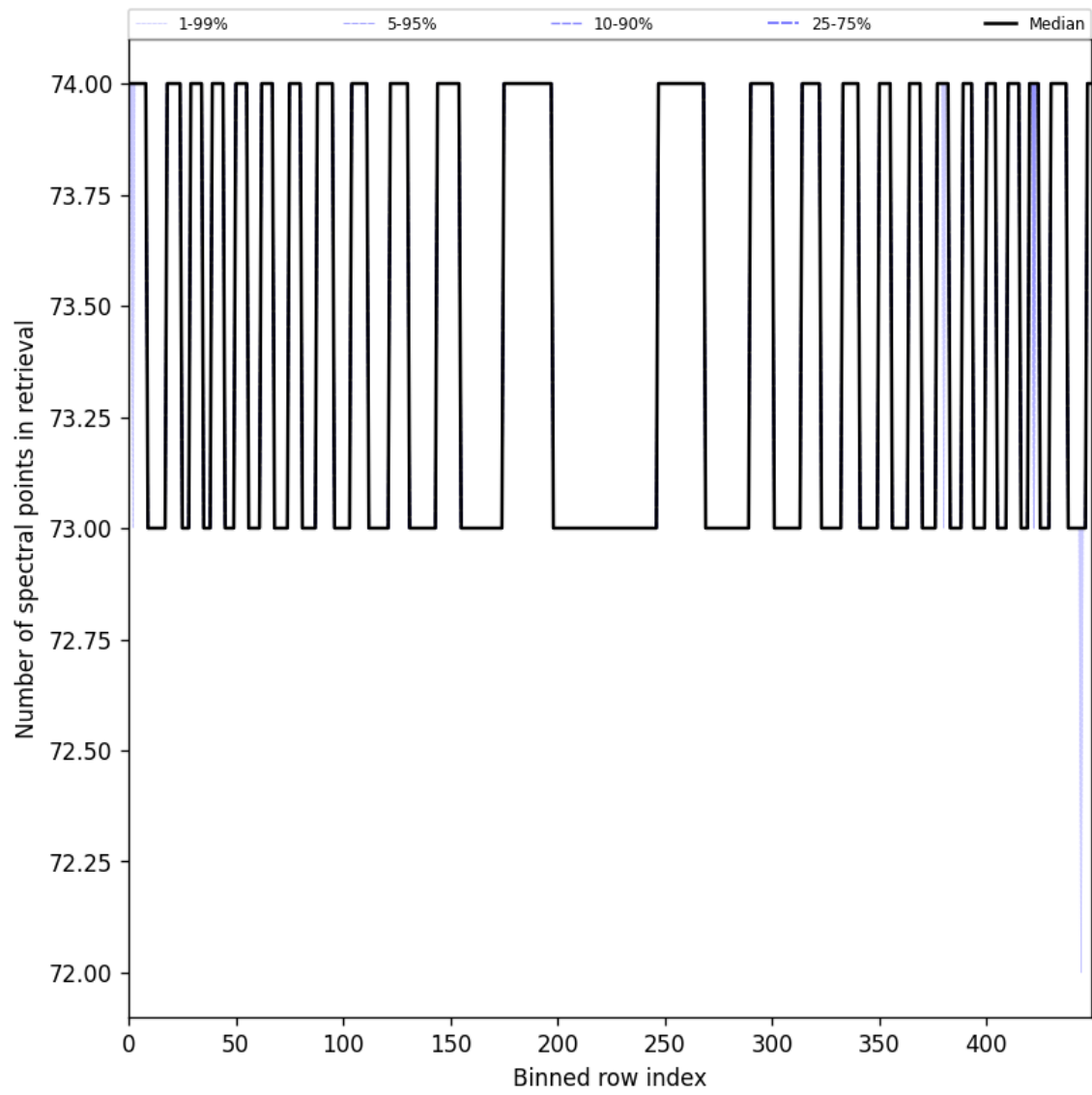
Figure 108: Along track statistics of “Number of spectral points in retrieval” for 2025-11-26 to 2025-11-28
