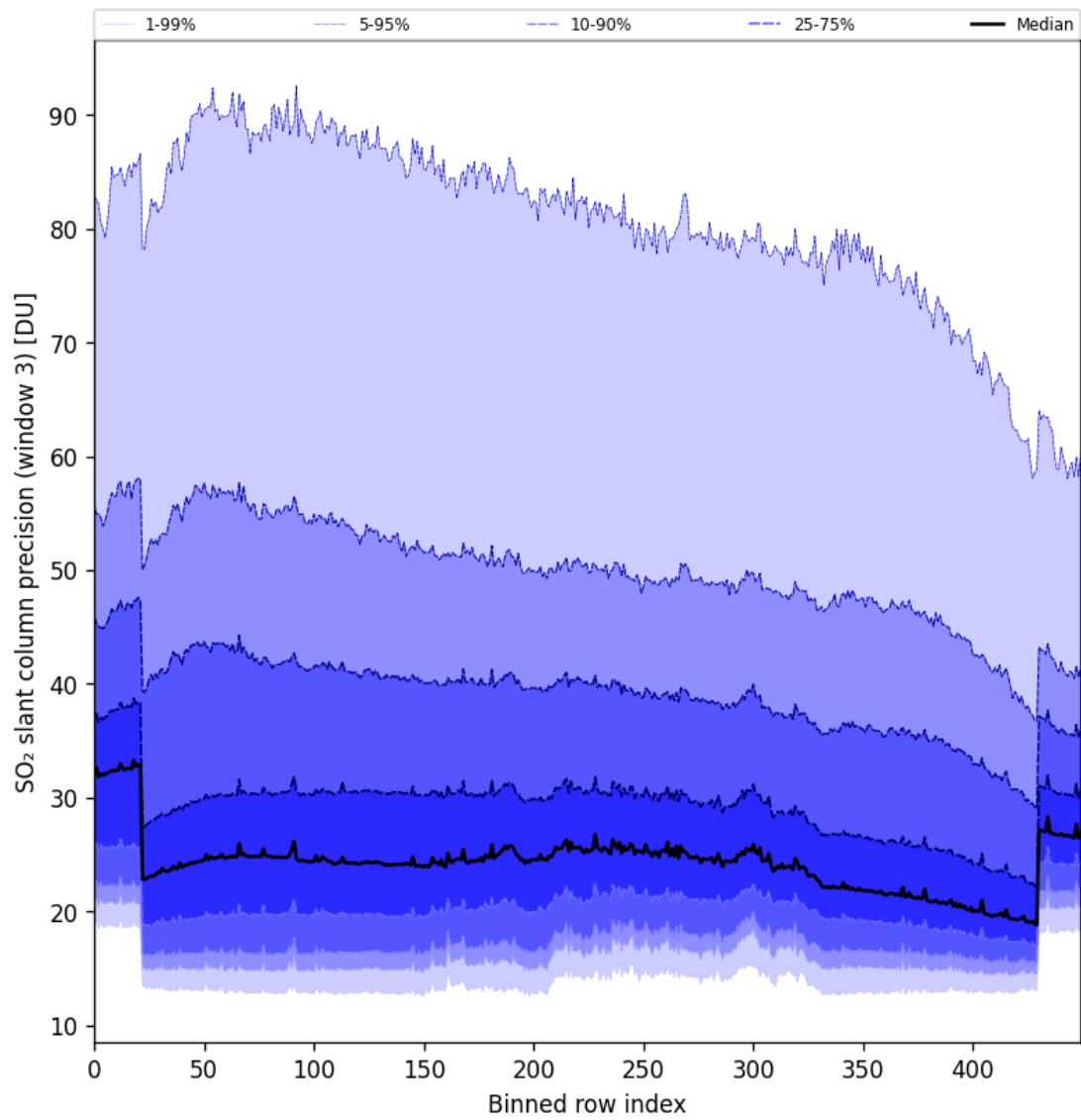
Figure 98: Along track statistics of “SO 2 slant column precision (window 3)” for 2025-11-26 to 2025-11-28
