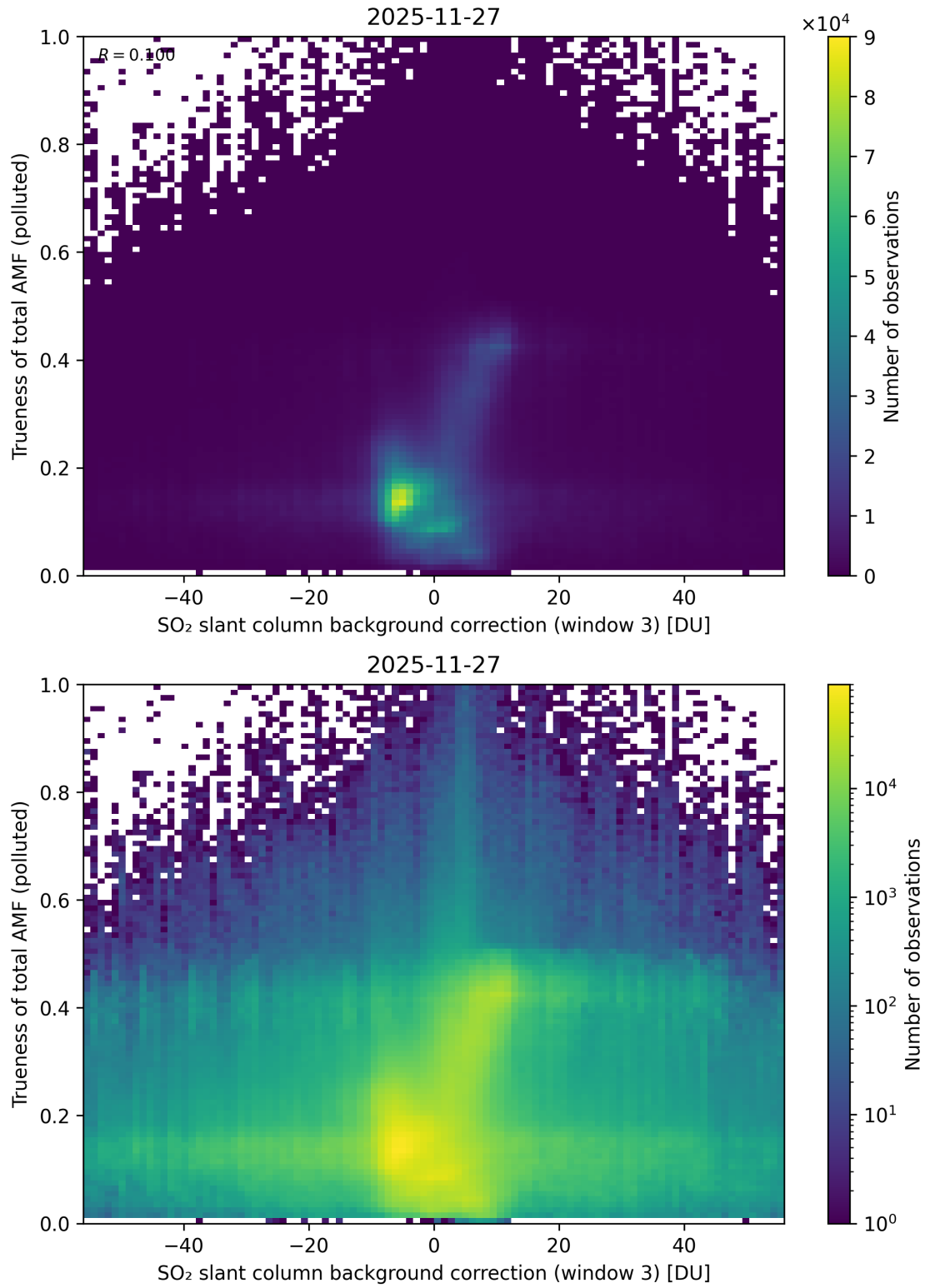
Figure 137: Scatter density plot of “SO 2 slant column background correction (window 3)” against “Trueness of total AMF (polluted)” for 2025-11-26 to 2025-11-28.
