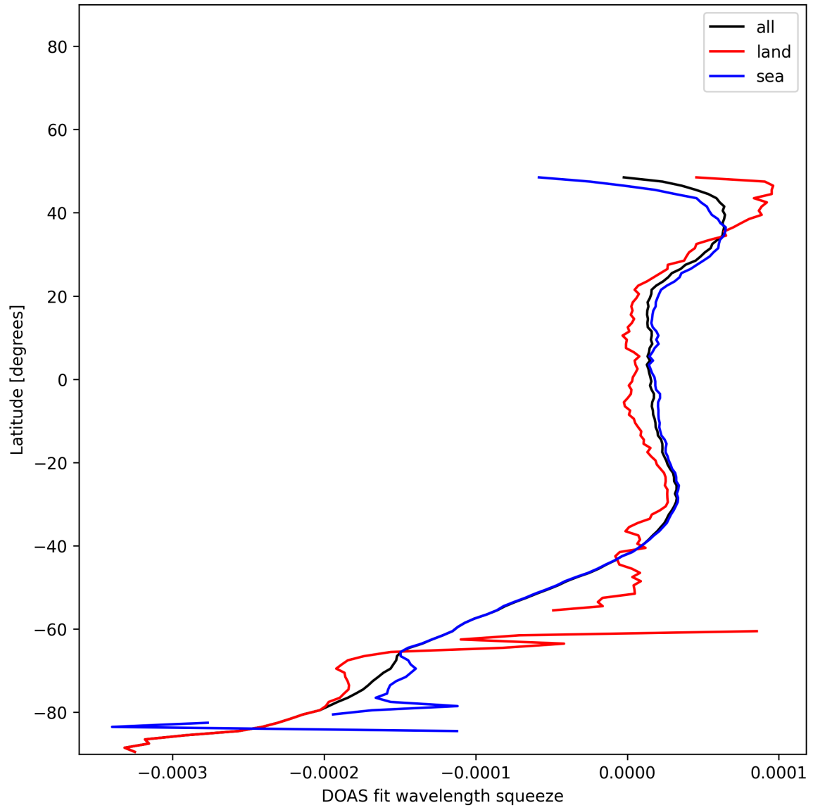
Figure 51: Zonal average of “DOAS fit wavelength squeeze” for 2025-11-26 to 2025-11-28.
