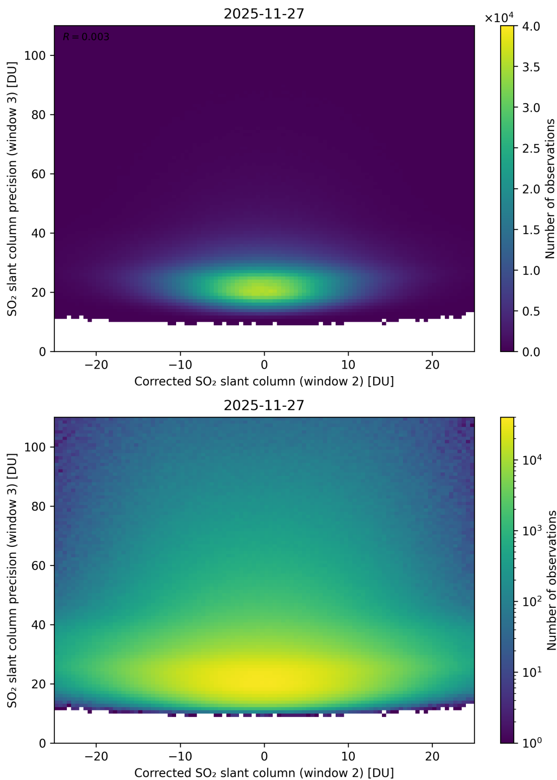
Figure 252: Scatter density plot of “Corrected SO 2 slant column (window 2)” against “SO 2 slant column precision (window 3)” for 2025-11-26 to 2025-11-28.
