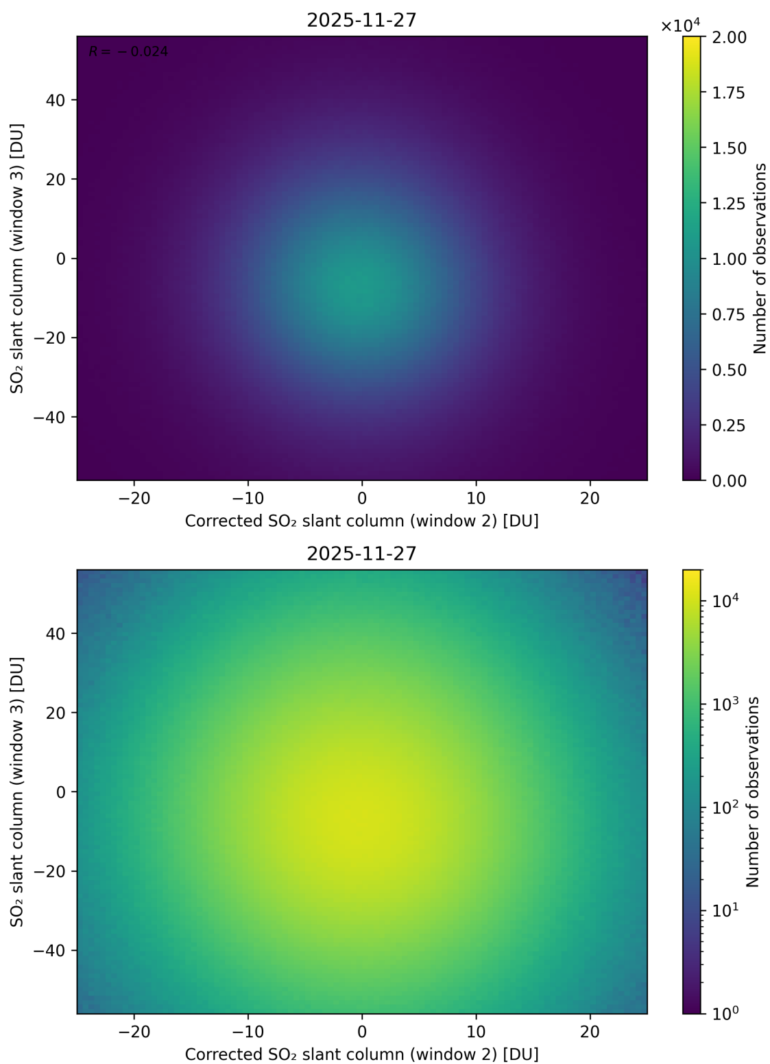
Figure 251: Scatter density plot of “Corrected SO 2 slant column (window 2)” against “SO 2 slant column (window 3)” for 2025-11-26 to 2025-11-28.
