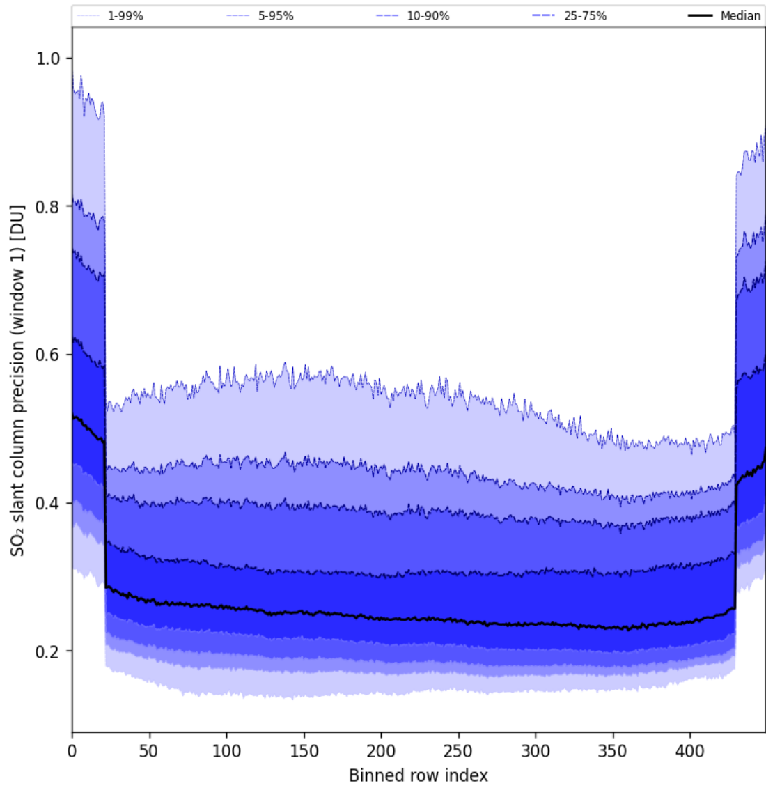
Figure 90: Along track statistics of “SO 2 slant column precision (window 1)” for 2025-11-26 to 2025-11-28
