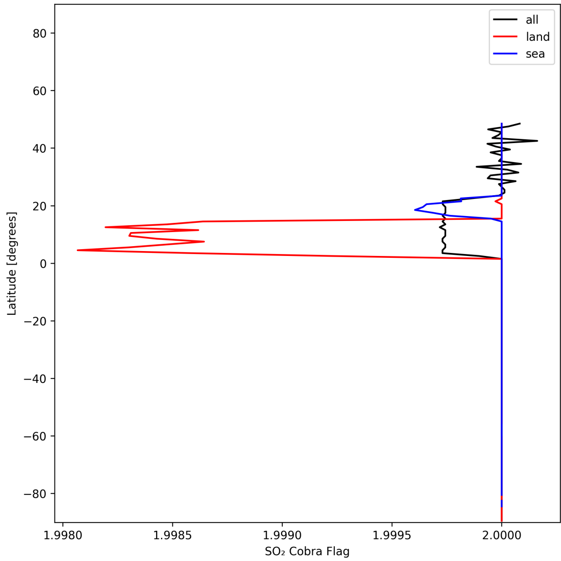
Figure 49: Zonal average of “SO 2 Cobra Flag” for 2025-11-26 to 2025-11-28.
