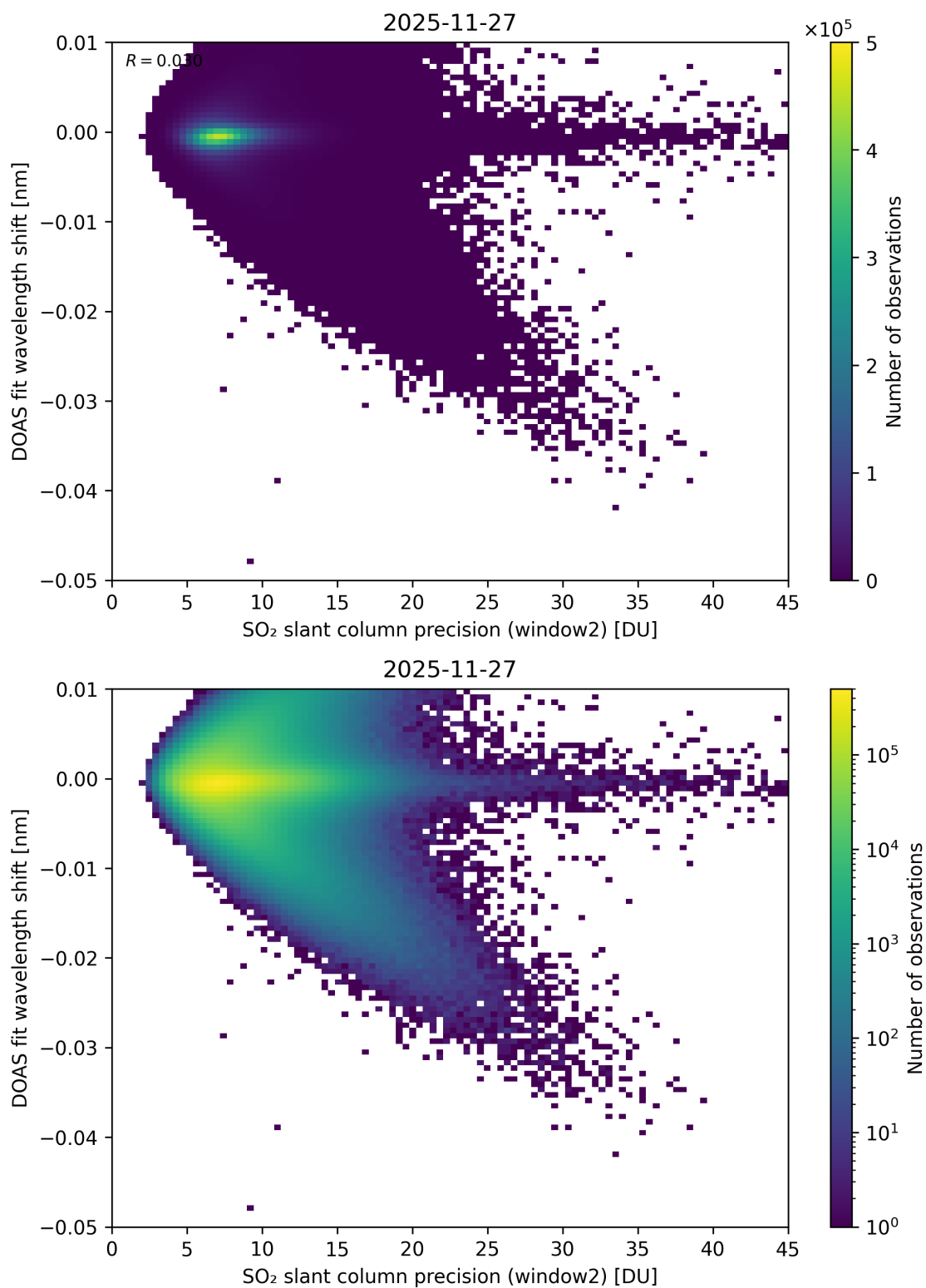
Figure 293: Scatter density plot of “SO 2 slant column precision (window2)” against “DOAS fit wavelength shift” for 2025-11-26 to 2025-11-28.
