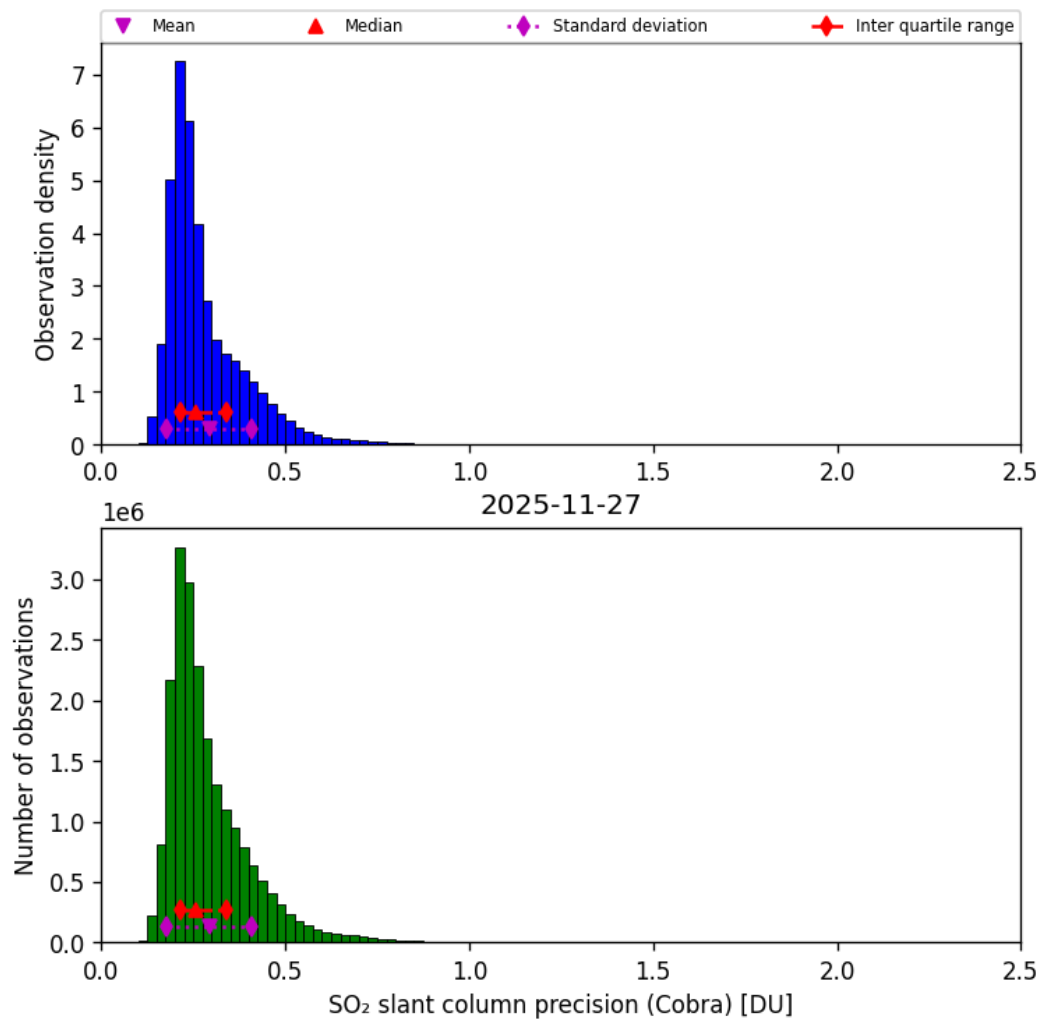
Figure 62: Histogram of “SO 2 slant column precision (Cobra)” for 2025-11-26 to 2025-11-28
