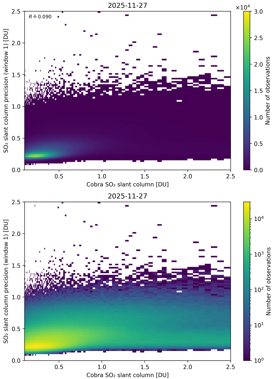
Figure 220: Scatter density plot of “Cobra SO 2 slant column” against “SO 2 slant column precision (window 1)” for 2025-11-26 to 2025-11-28.
