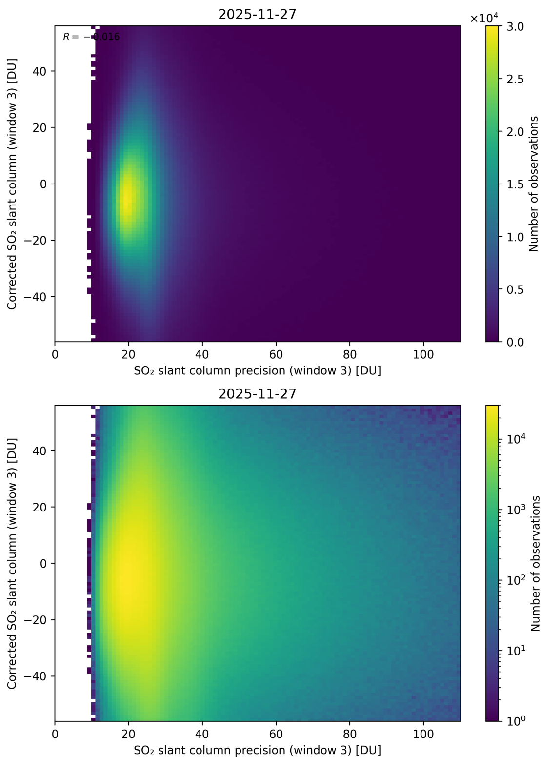
Figure 312: Scatter density plot of “SO 2 slant column precision (window 3)” against “Corrected SO 2 slant column (window 3)” for 2025-11-26 to 2025-11-28.
