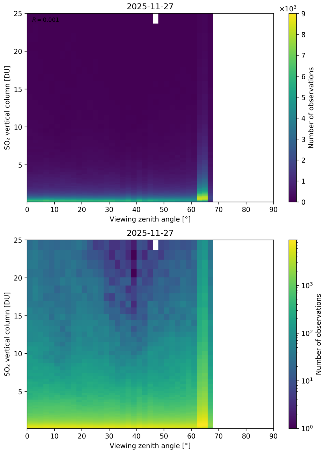
Figure 383: Scatter density plot of “Viewing zenith angle” against “SO 2 vertical column” for 2025-11-26 to 2025-11-28.
