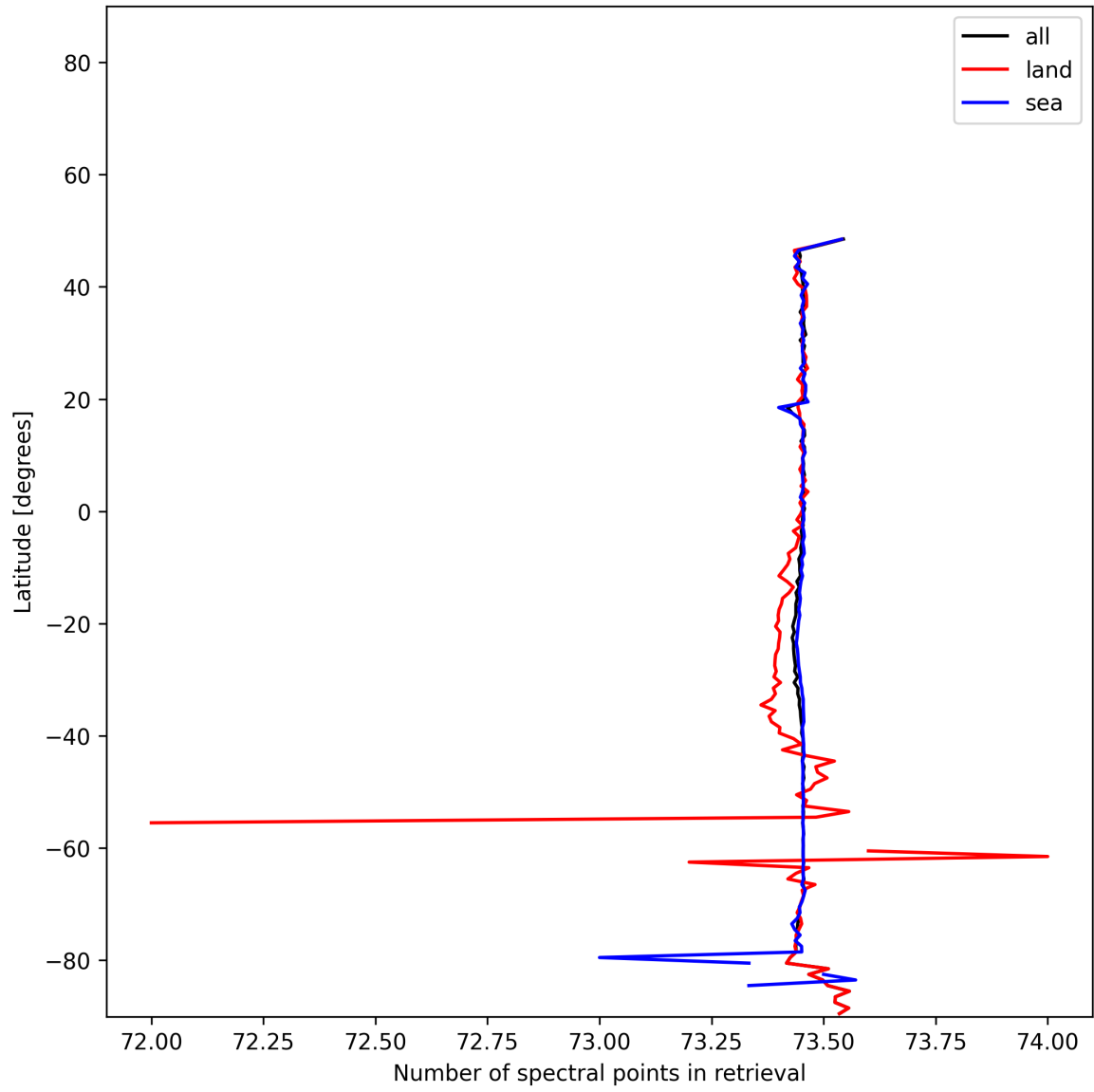
Figure 56: Zonal average of “Number of spectral points in retrieval” for 2025-11-26 to 2025-11-28.
