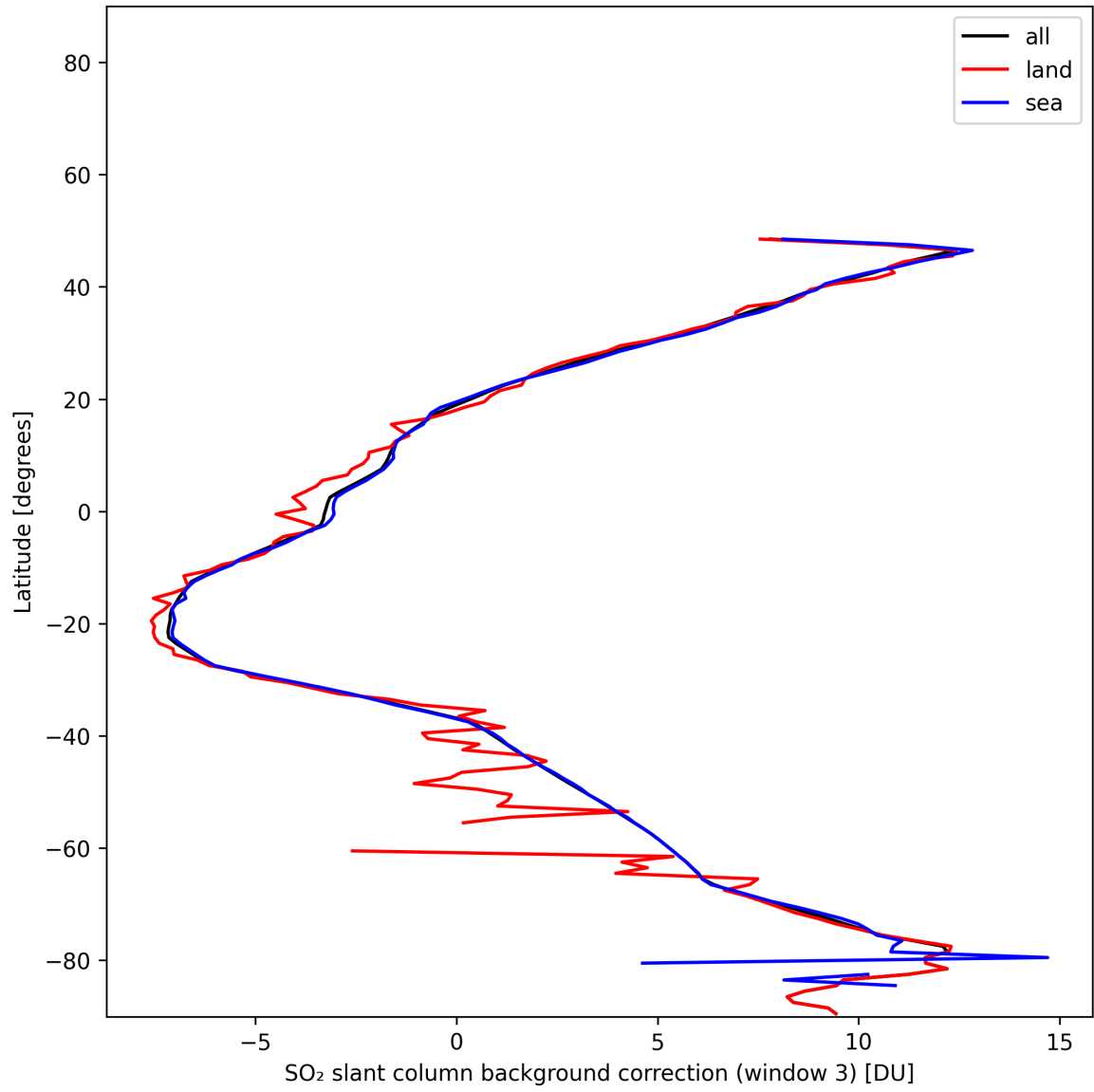
Figure 48: Zonal average of “SO 2 slant column background correction (window 3)” for 2025-11-26 to 2025-11-28.
