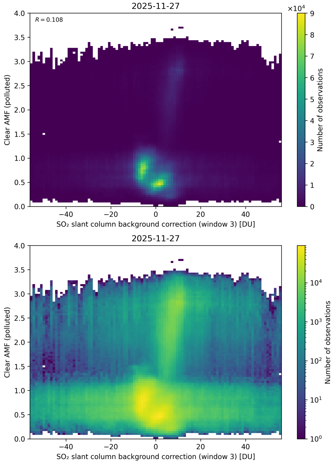
Figure 135: Scatter density plot of “SO 2 slant column background correction (window 3)” against “Clear AMF (polluted)” for 2025-11-26 to 2025-11-28.
