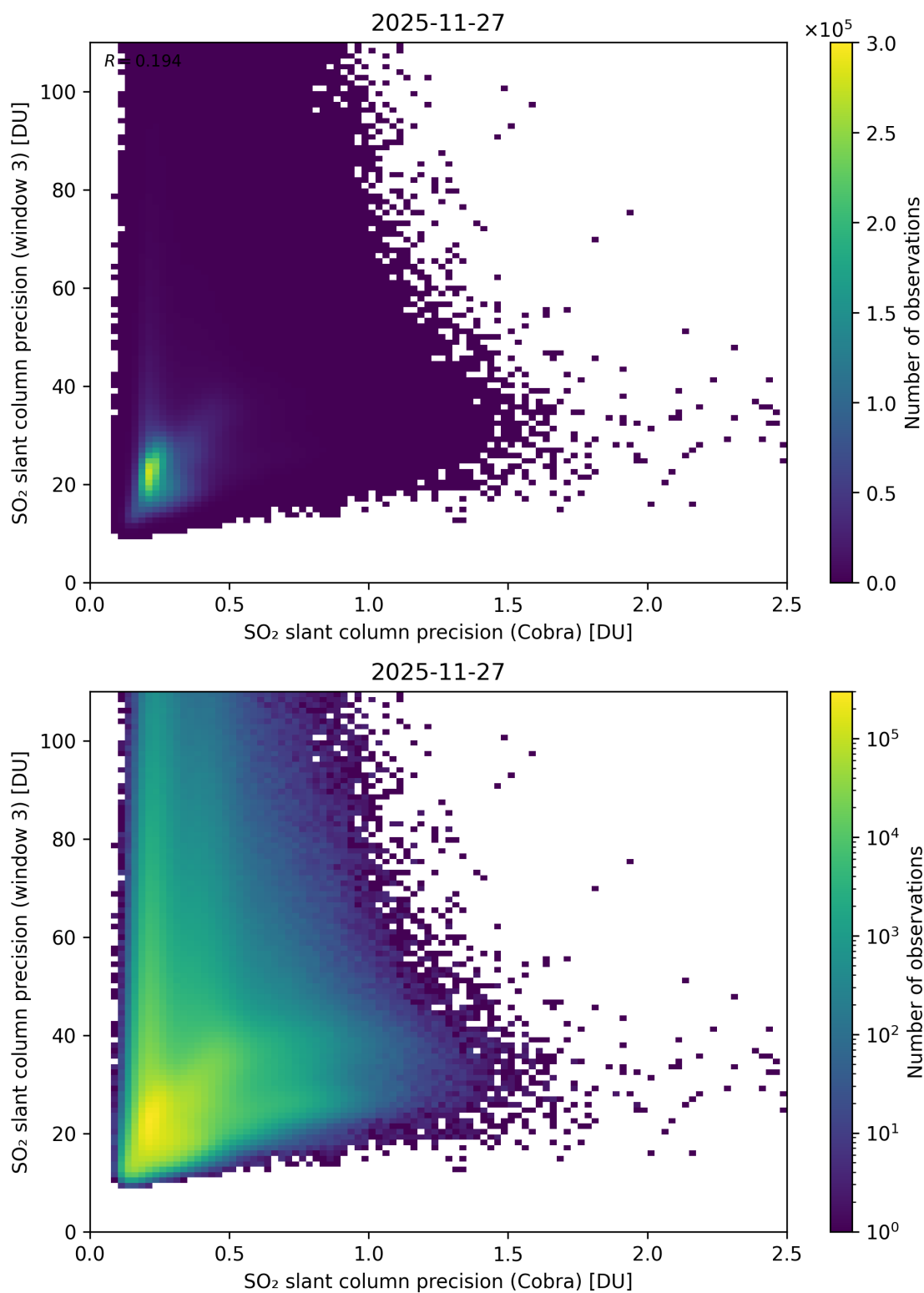
Figure 212: Scatter density plot of “SO 2 slant column precision (Cobra)” against “SO 2 slant column precision (window 3)” for 2025-11-26 to 2025-11-28.
