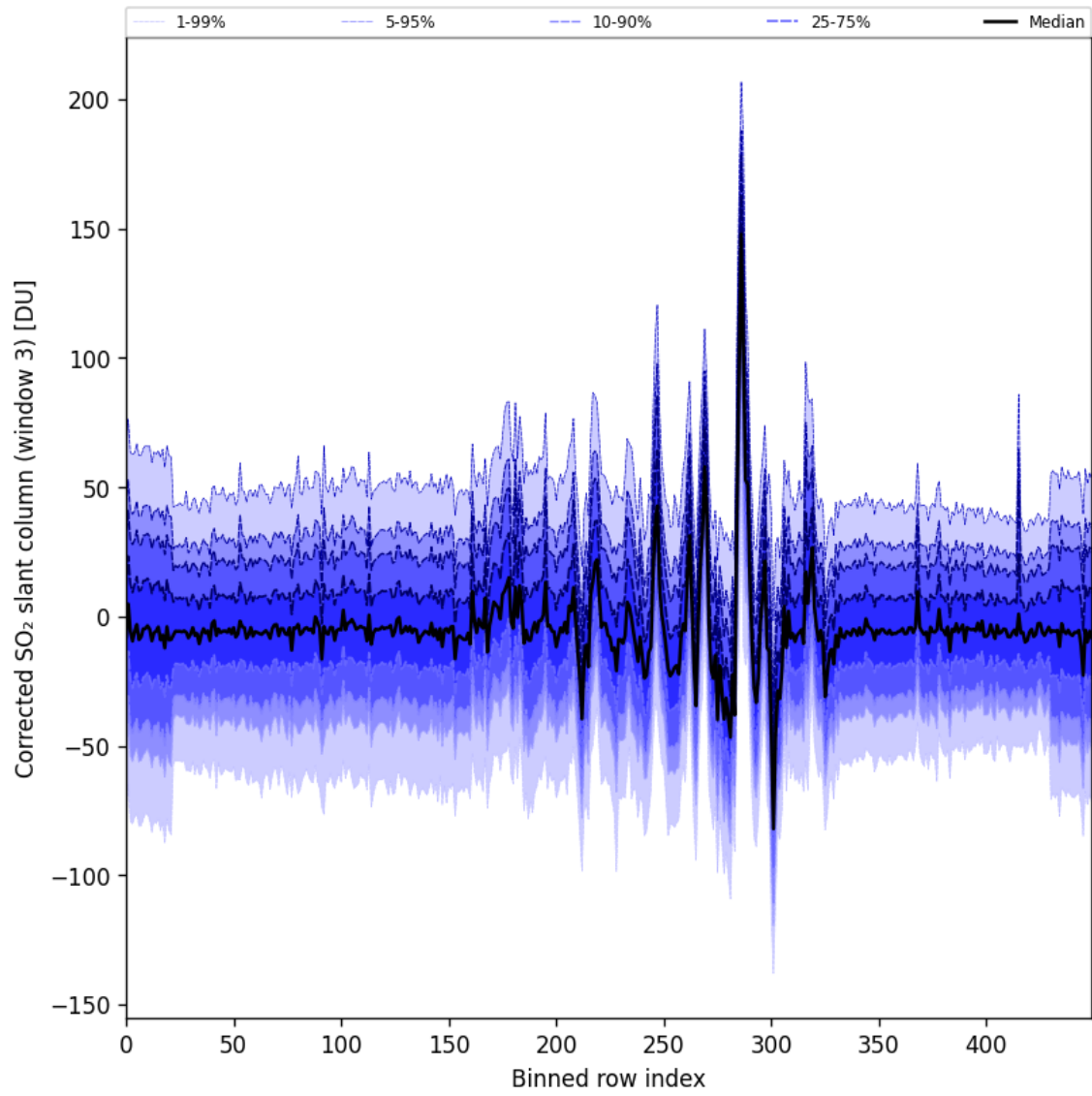
Figure 99: Along track statistics of “Corrected SO 2 slant column (window 3)” for 2025-11-26 to 2025-11-28
