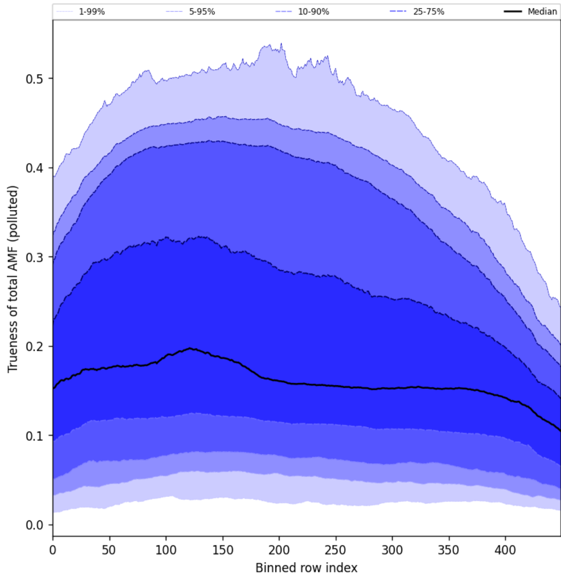
Figure 106: Along track statistics of “Trueness of total AMF (polluted)” for 2025-11-26 to 2025-11-28
