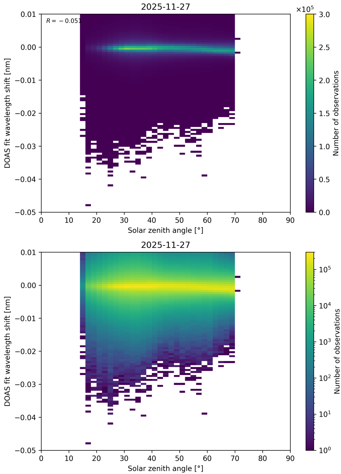
Figure 174: Scatter density plot of “Solar zenith angle” against “DOAS fit wavelength shift” for 2025-11-26 to 2025-11-28.
