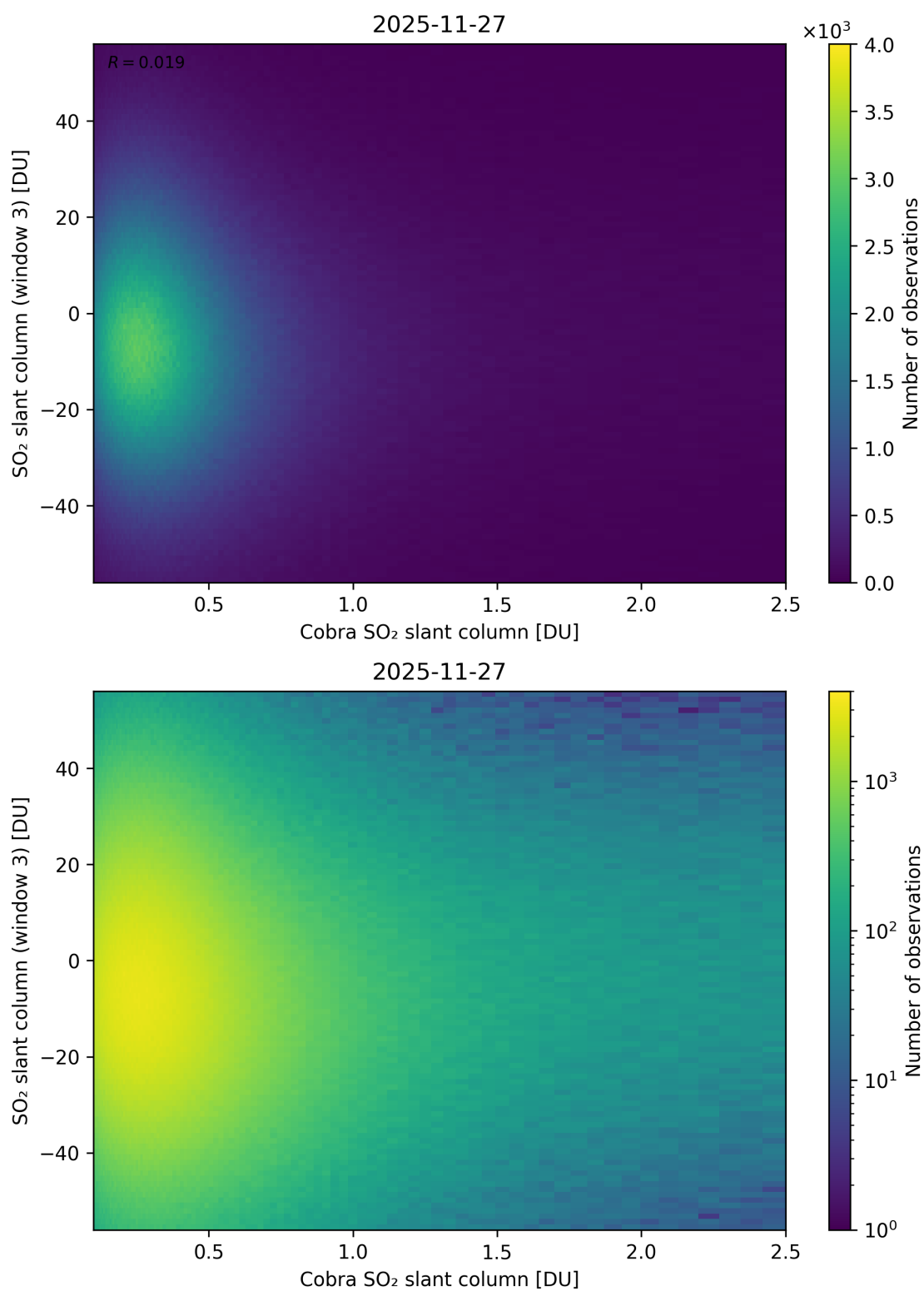
Figure 222: Scatter density plot of “Cobra SO 2 slant column” against “SO 2 slant column (window 3)” for 2025-11-26 to 2025-11-28.
