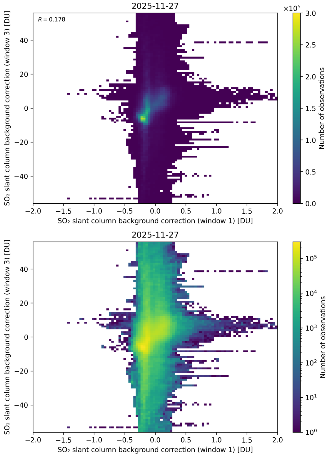
Figure 110: Scatter density plot of “SO 2 slant column background correction (window 1)” against “SO 2 slant column background correction (window 3)” for 2025-11-26 to 2025-11-28.
