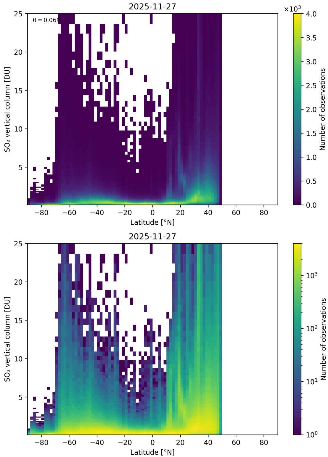
Figure 169: Scatter density plot of “Latitude” against “SO 2 vertical column” for 2025-11-26 to 2025-11-28.
