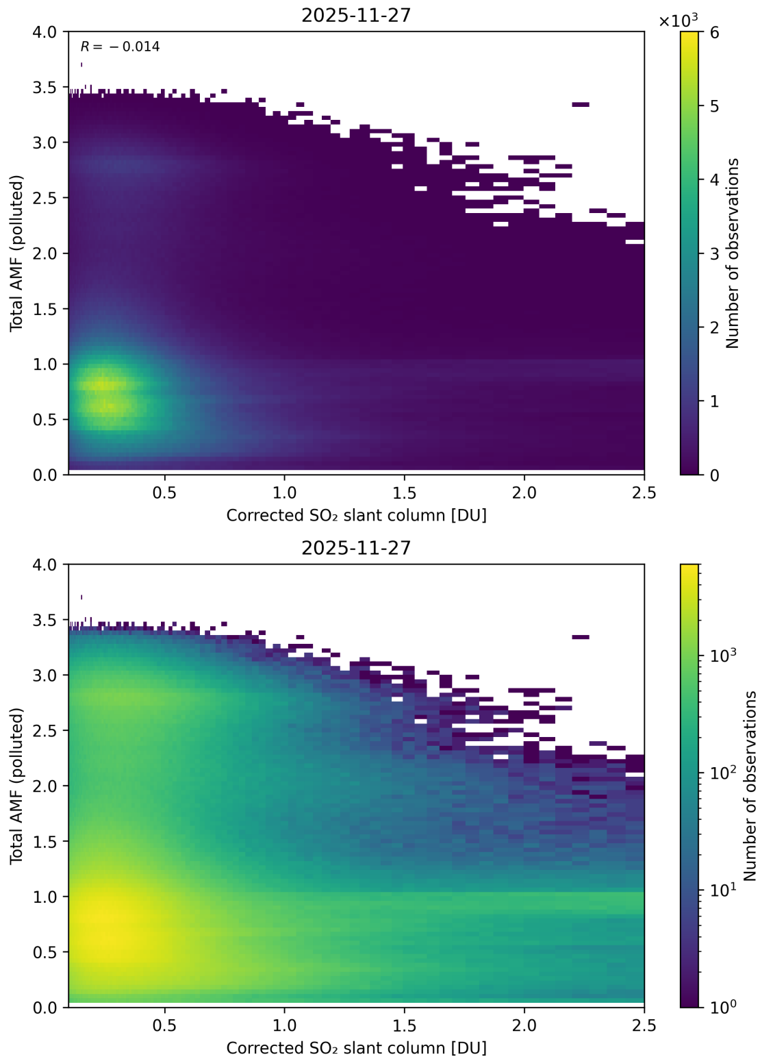
Figure 242: Scatter density plot of “Corrected SO 2 slant column” against “Total AMF (polluted)” for 2025-11-26 to 2025-11-28.
