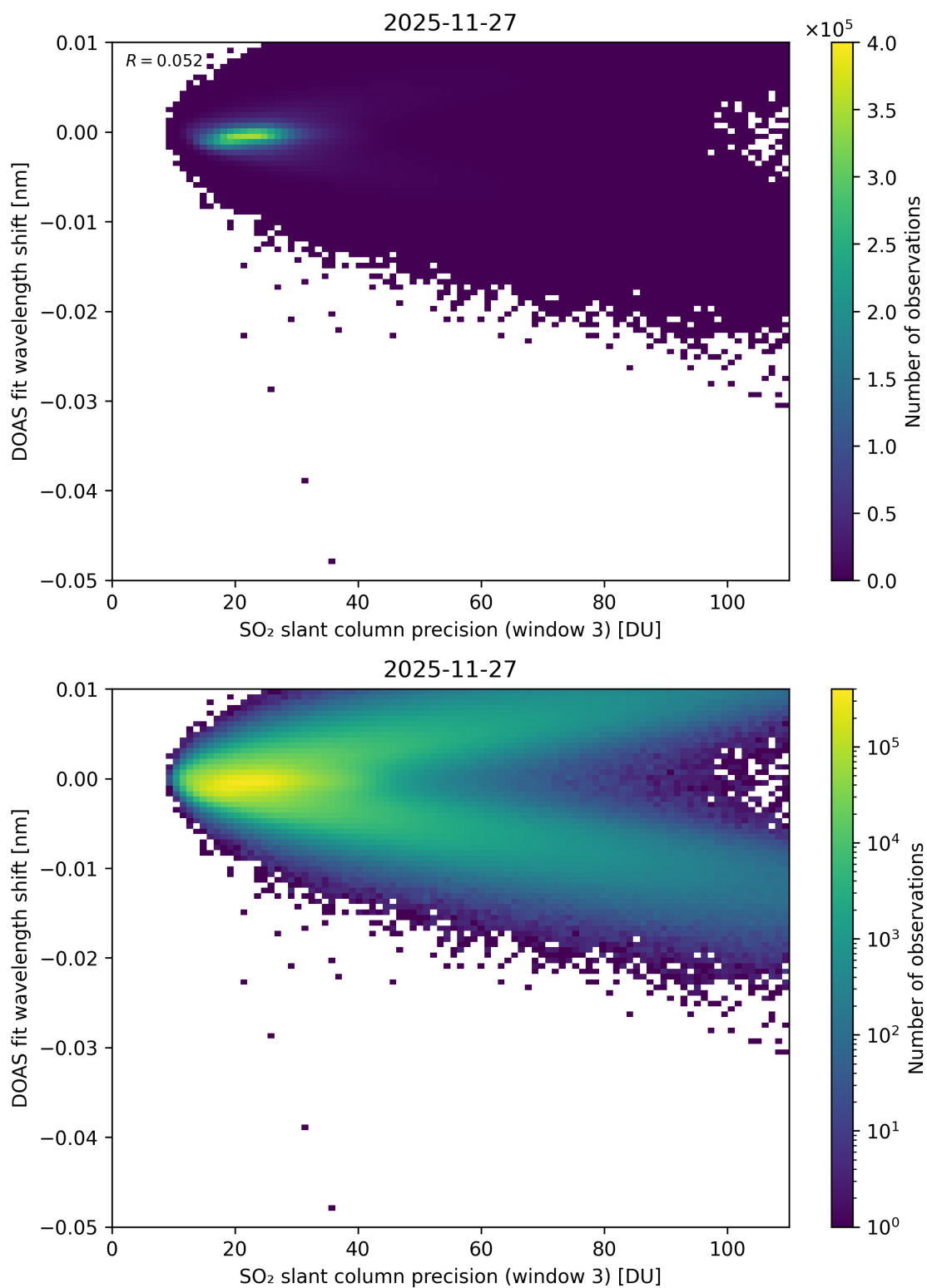
Figure 308: Scatter density plot of “SO 2 slant column precision (window 3)” against “DOAS fit wavelength shift” for 2025-11-26 to 2025-11-28.
