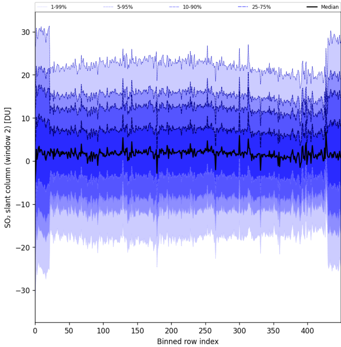
Figure 93: Along track statistics of “SO 2 slant column (window 2)” for 2025-11-26 to 2025-11-28
