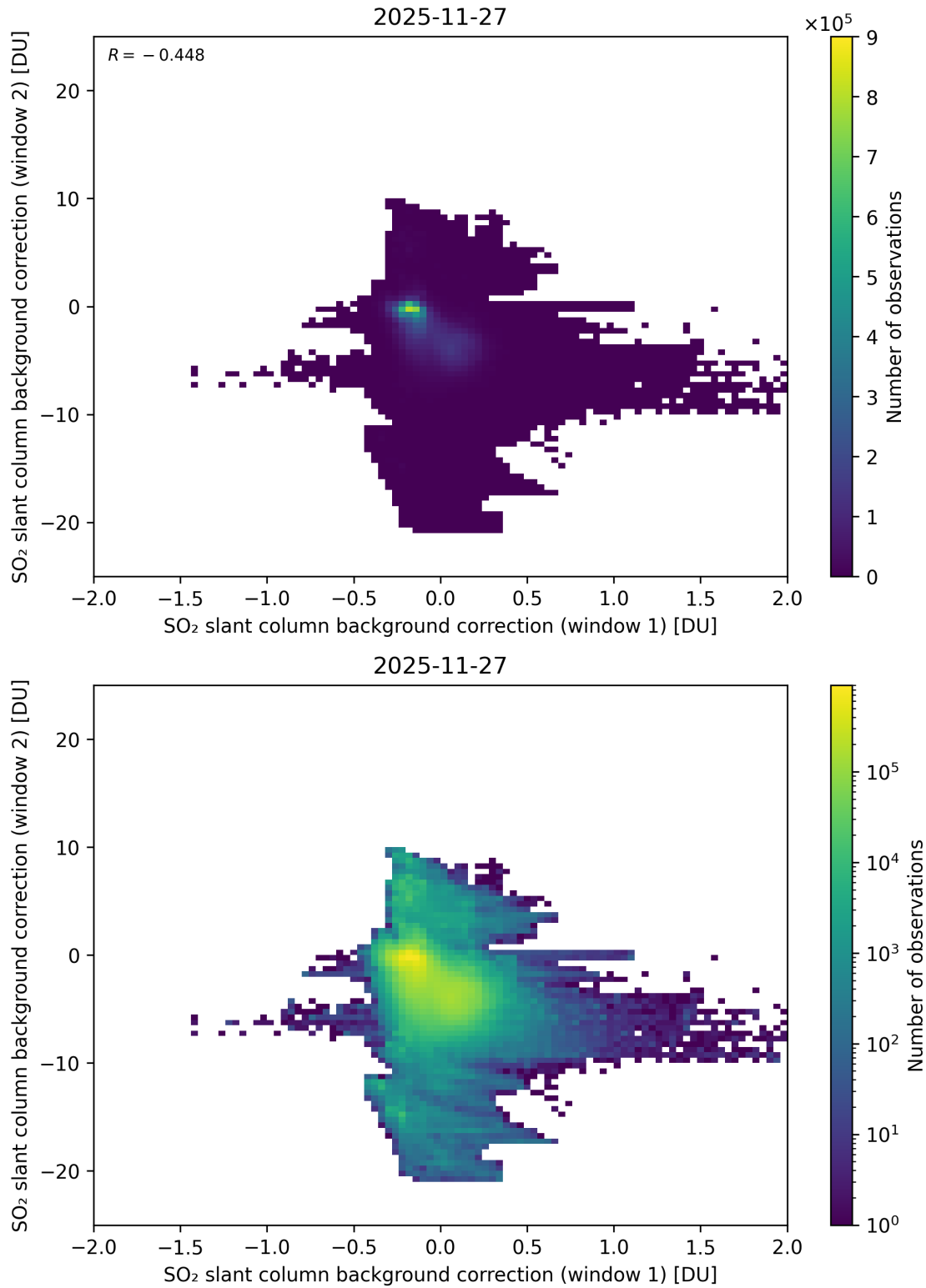
Figure 109: Scatter density plot of “SO 2 slant column background correction (window 1)” against “SO 2 slant column background correction (window 2)” for 2025-11-26 to 2025-11-28.
