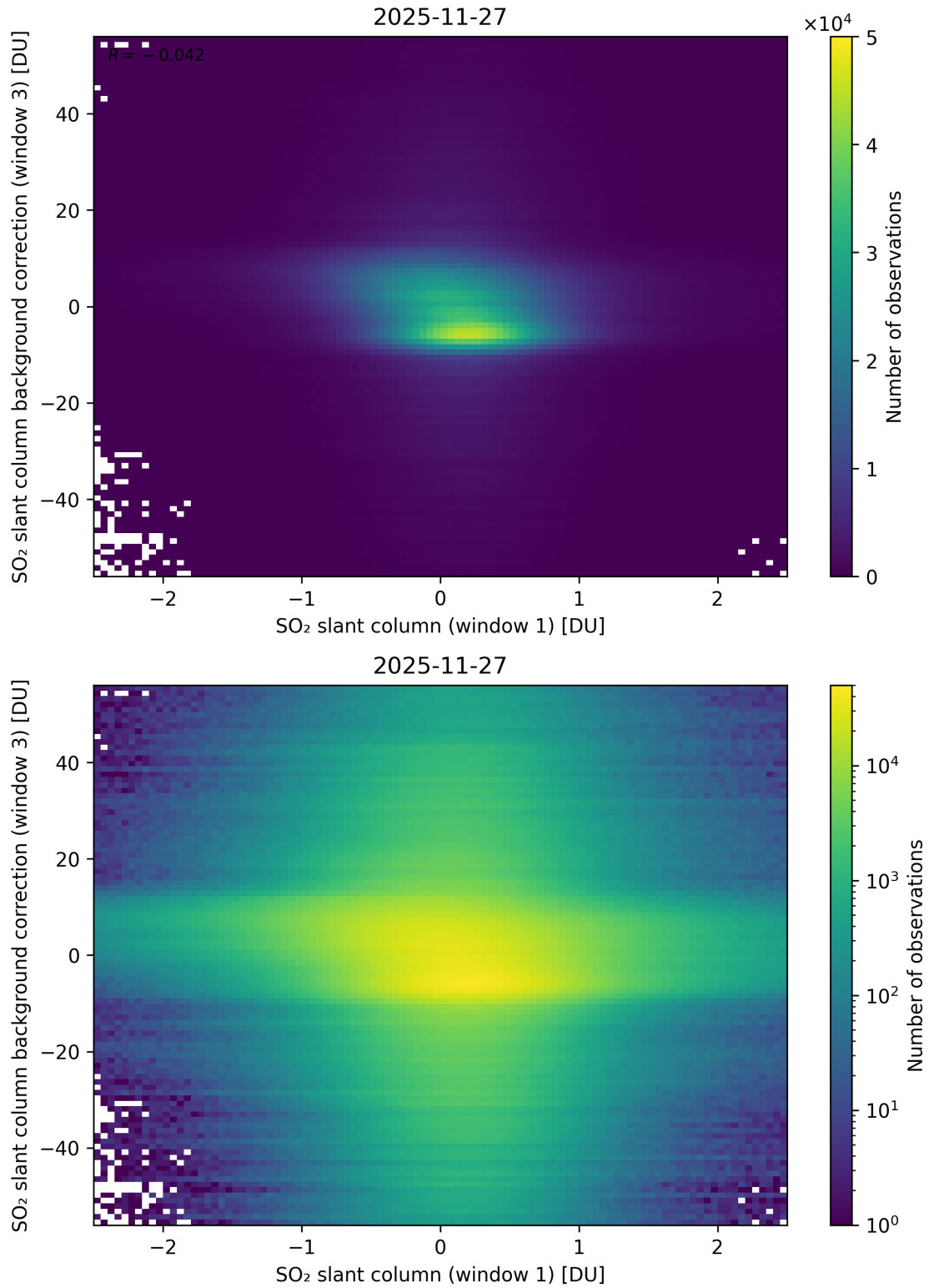
Figure 264: Scatter density plot of “SO 2 slant column (window 1)” against “SO 2 slant column background correction (window 3)” for 2025-11-26 to 2025-11-28.
