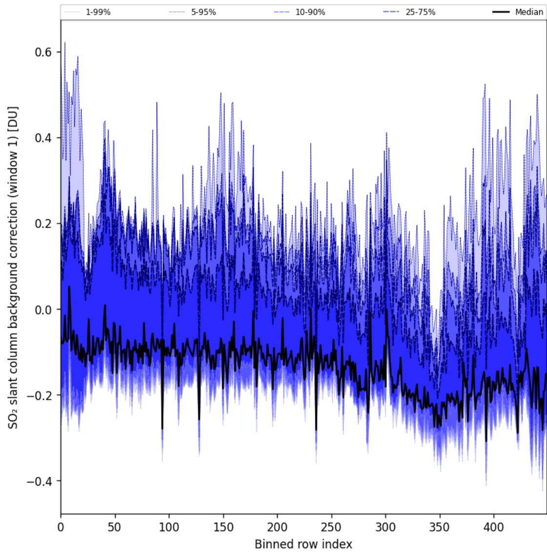
Figure 92: Along track statistics of “SO 2 slant column background correction (window 1)” for 2025-11-26 to 2025-11-28
