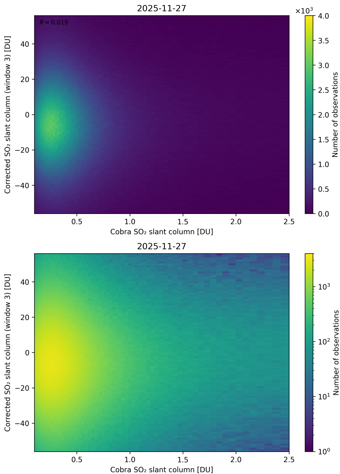
Figure 218: Scatter density plot of “Cobra SO 2 slant column” against “Corrected SO 2 slant column (window 3)” for 2025-11-26 to 2025-11-28.
