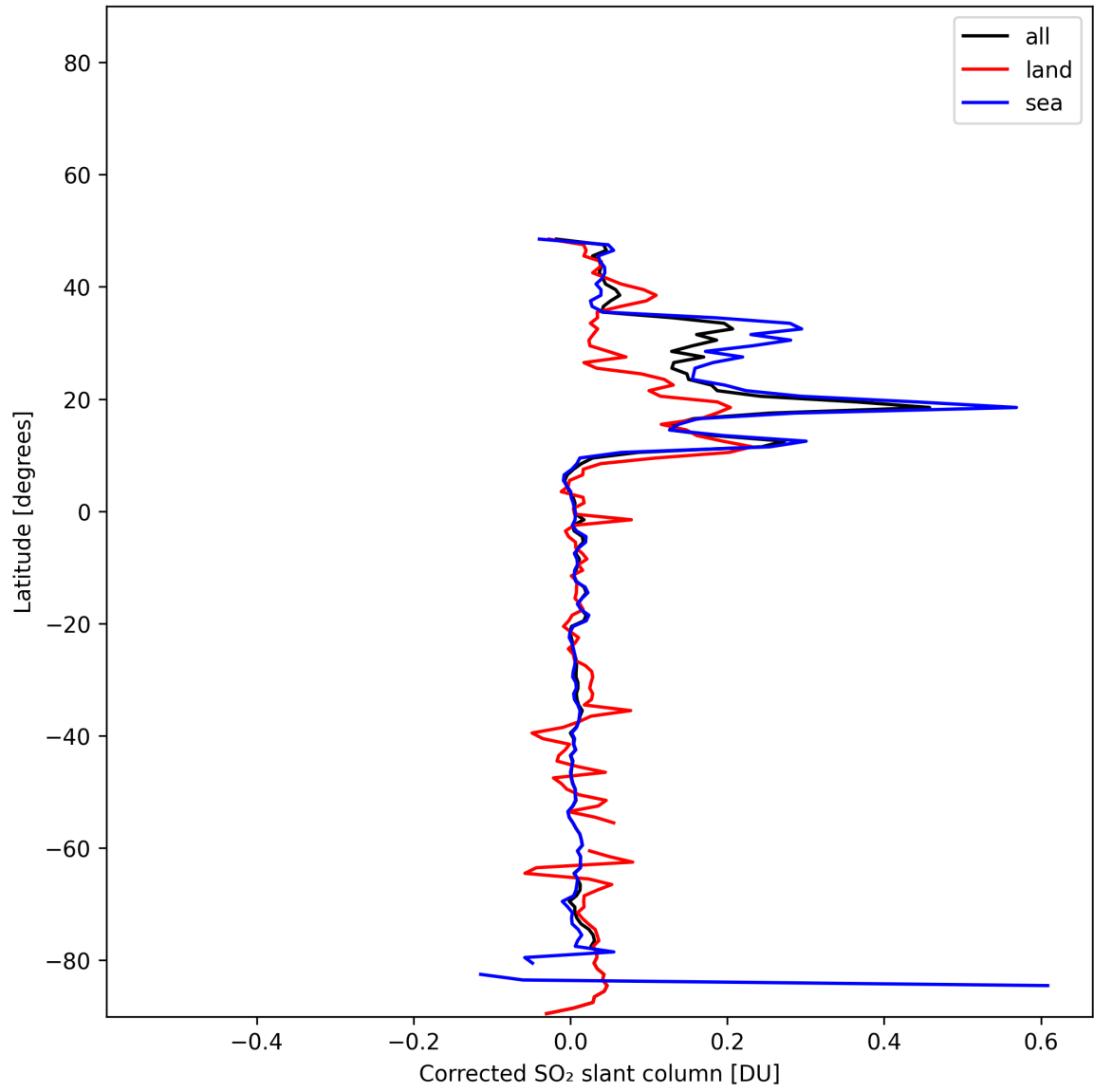
Figure 34: Zonal average of “Corrected SO 2 slant column” for 2025-11-26 to 2025-11-28.
