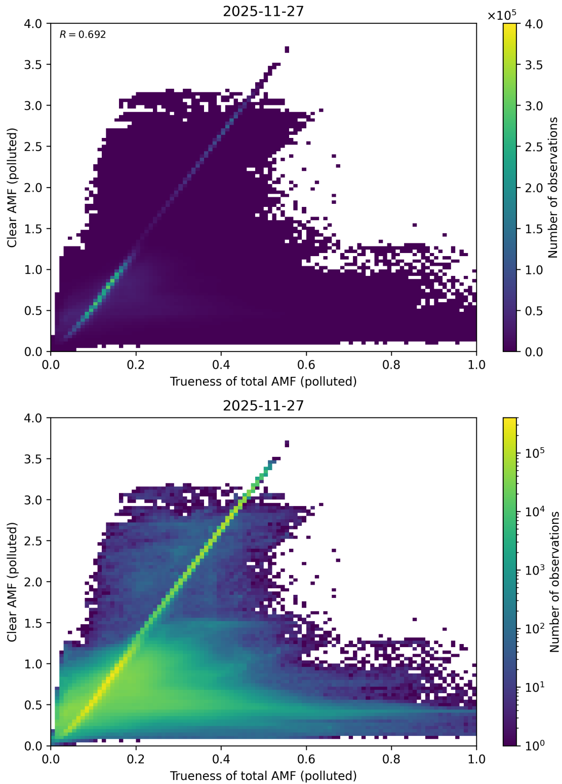
Figure 322: Scatter density plot of “Trueness of total AMF (polluted)” against “Clear AMF (polluted)” for 2025-11-26 to 2025-11-28.
