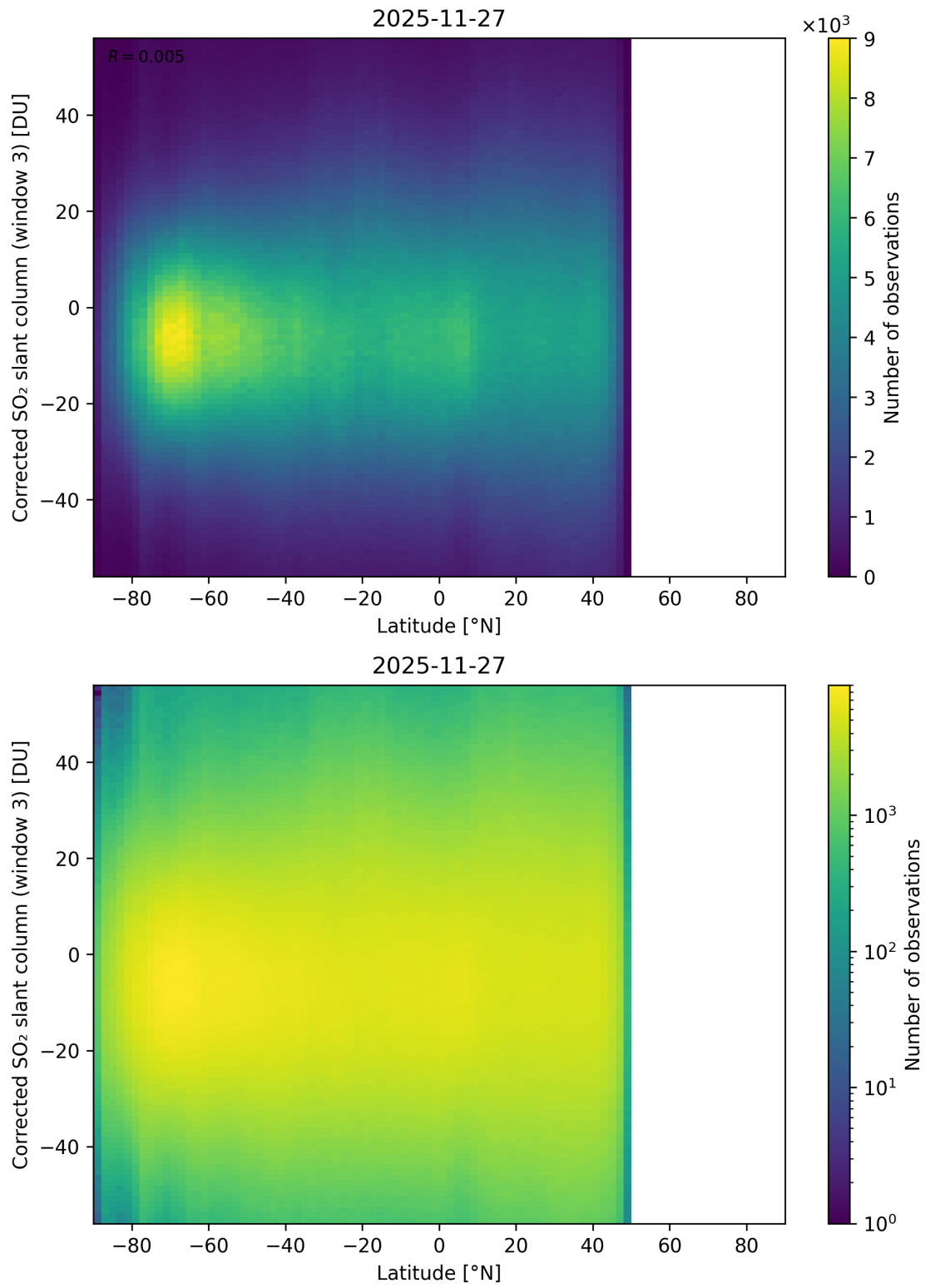
Figure 161: Scatter density plot of “Latitude” against “Corrected SO 2 slant column (window 3)” for 2025-11-26 to 2025-11-28.
