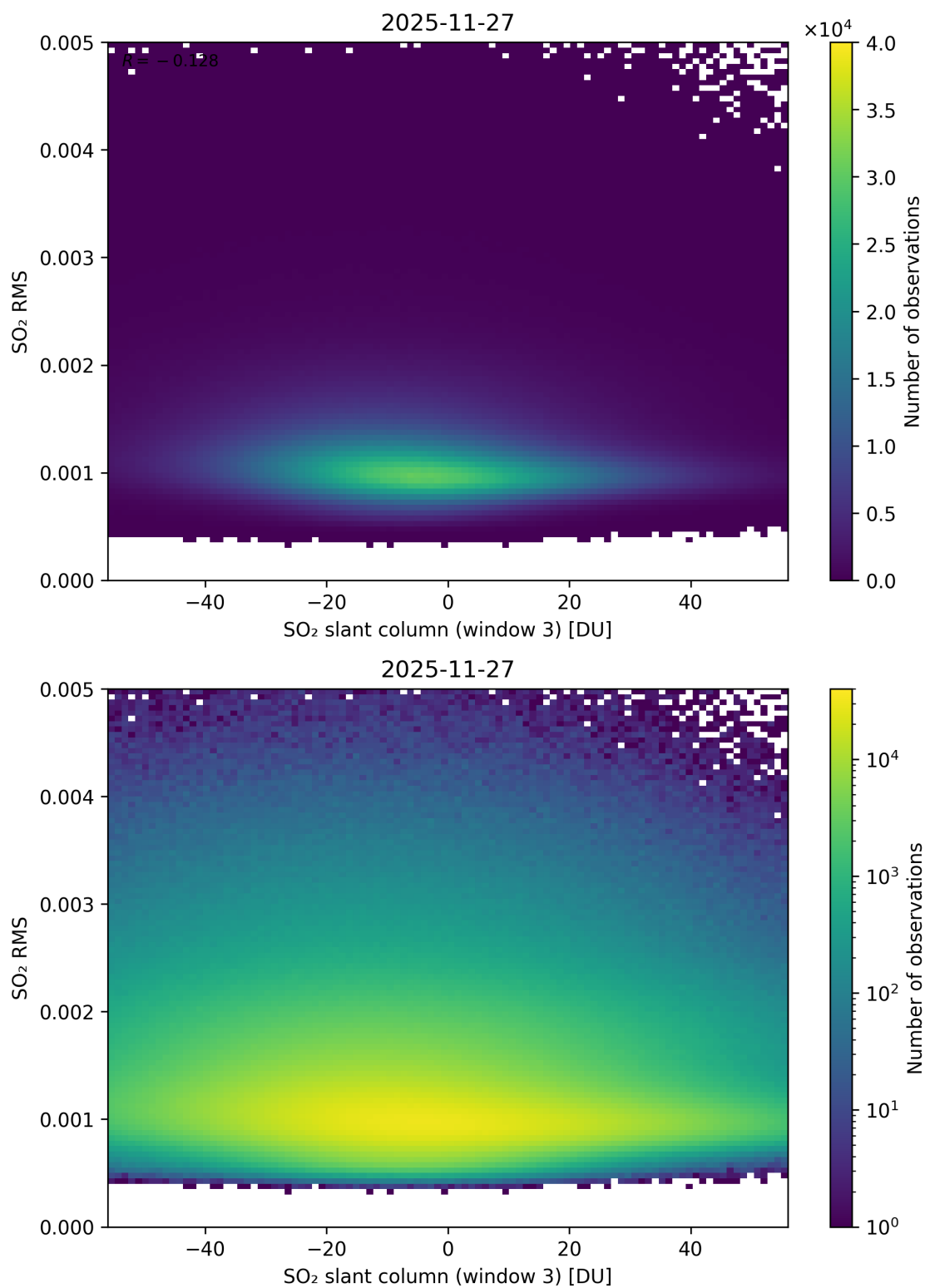
Figure 306: Scatter density plot of “SO 2 slant column (window 3)” against “SO 2 RMS” for 2025-11-26 to 2025-11-28.
