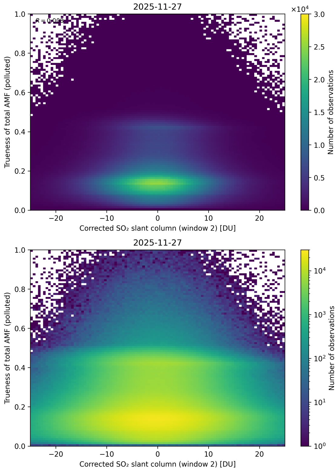
Figure 254: Scatter density plot of “Corrected SO 2 slant column (window 2)” against “Trueness of total AMF (polluted)” for 2025-11-26 to 2025-11-28.
