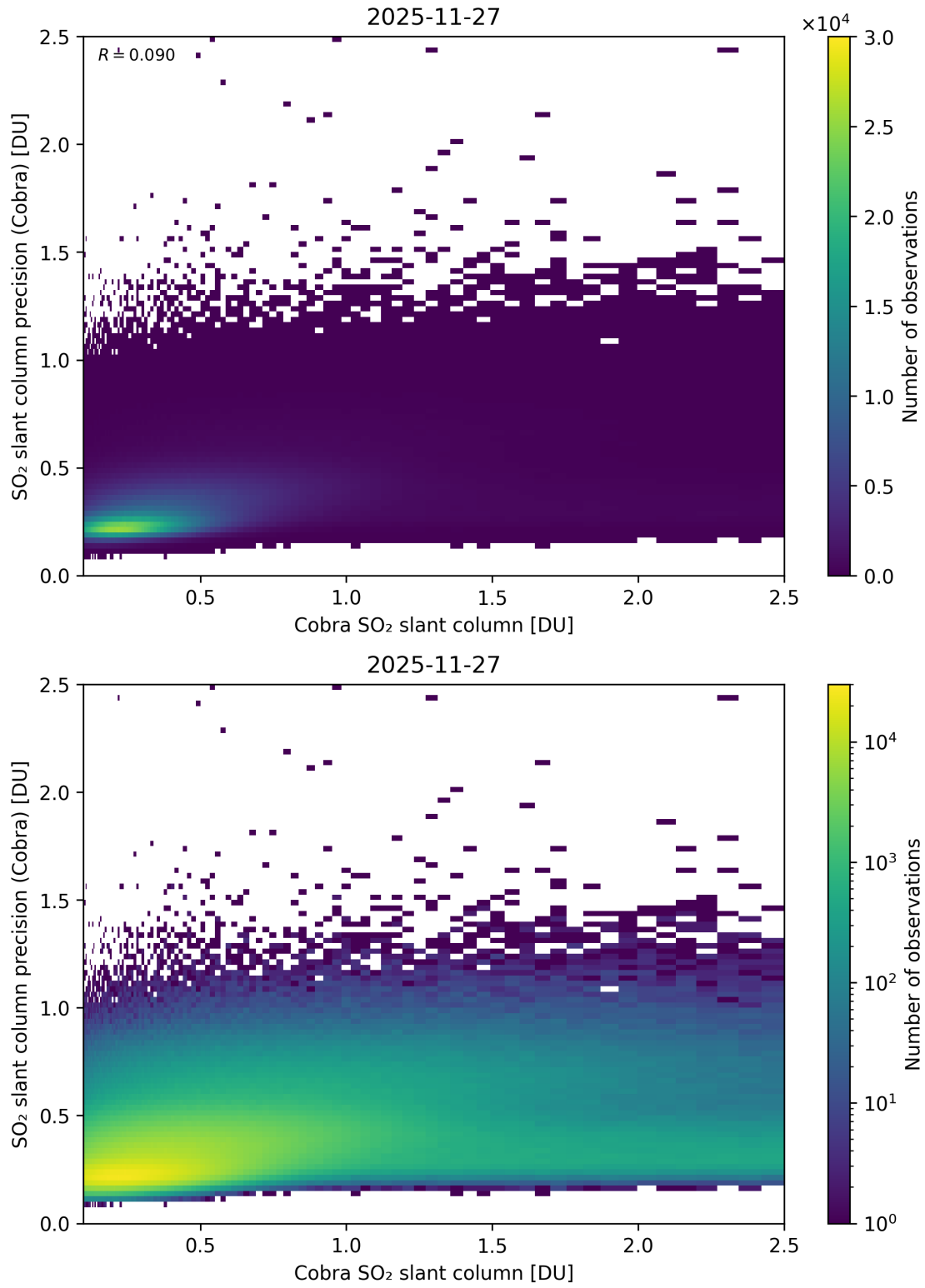
Figure 216: Scatter density plot of “Cobra SO 2 slant column” against “SO 2 slant column precision (Cobra)” for 2025-11-26 to 2025-11-28.
