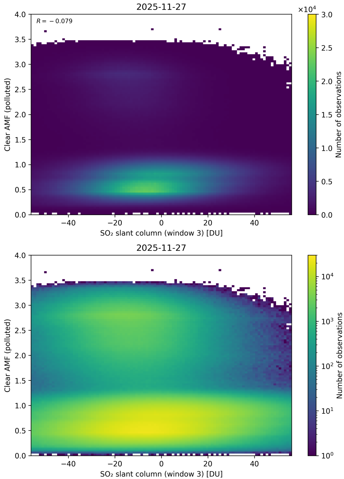
Figure 315: Scatter density plot of “SO 2 slant column (window 3)” against “Clear AMF (polluted)” for 2025-11-26 to 2025-11-28.
