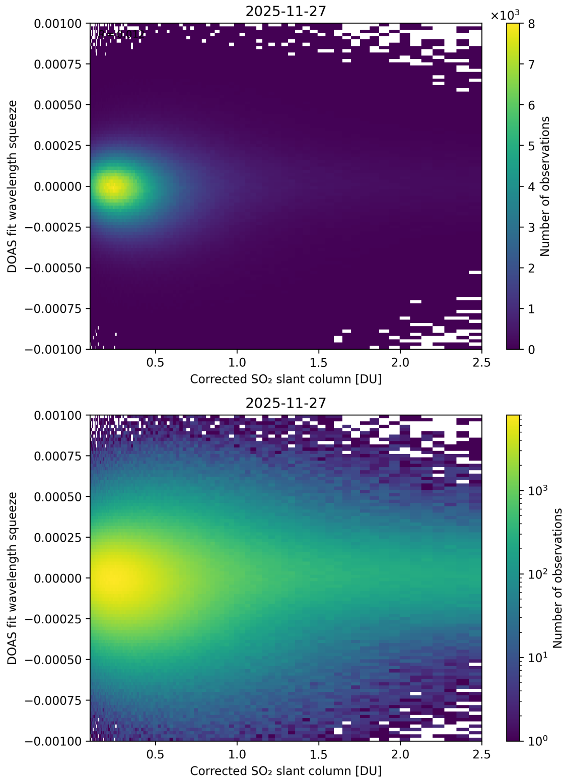
Figure 230: Scatter density plot of "Corrected SO 2 slant column" against "DOAS fit wavelength squeeze" for 2025-11-26 to 2025-11-28.
