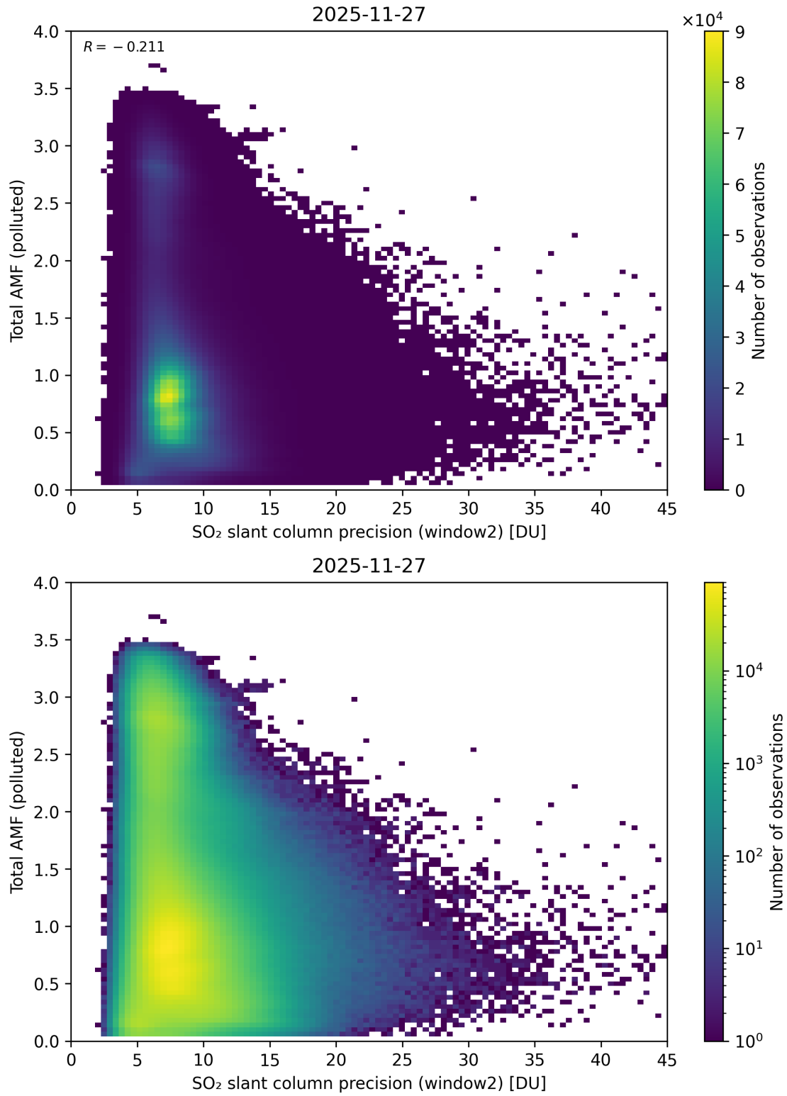
Figure 301: Scatter density plot of “SO 2 slant column precision (window2)” against “Total AMF (polluted)” for 2025-11-26 to 2025-11-28.
