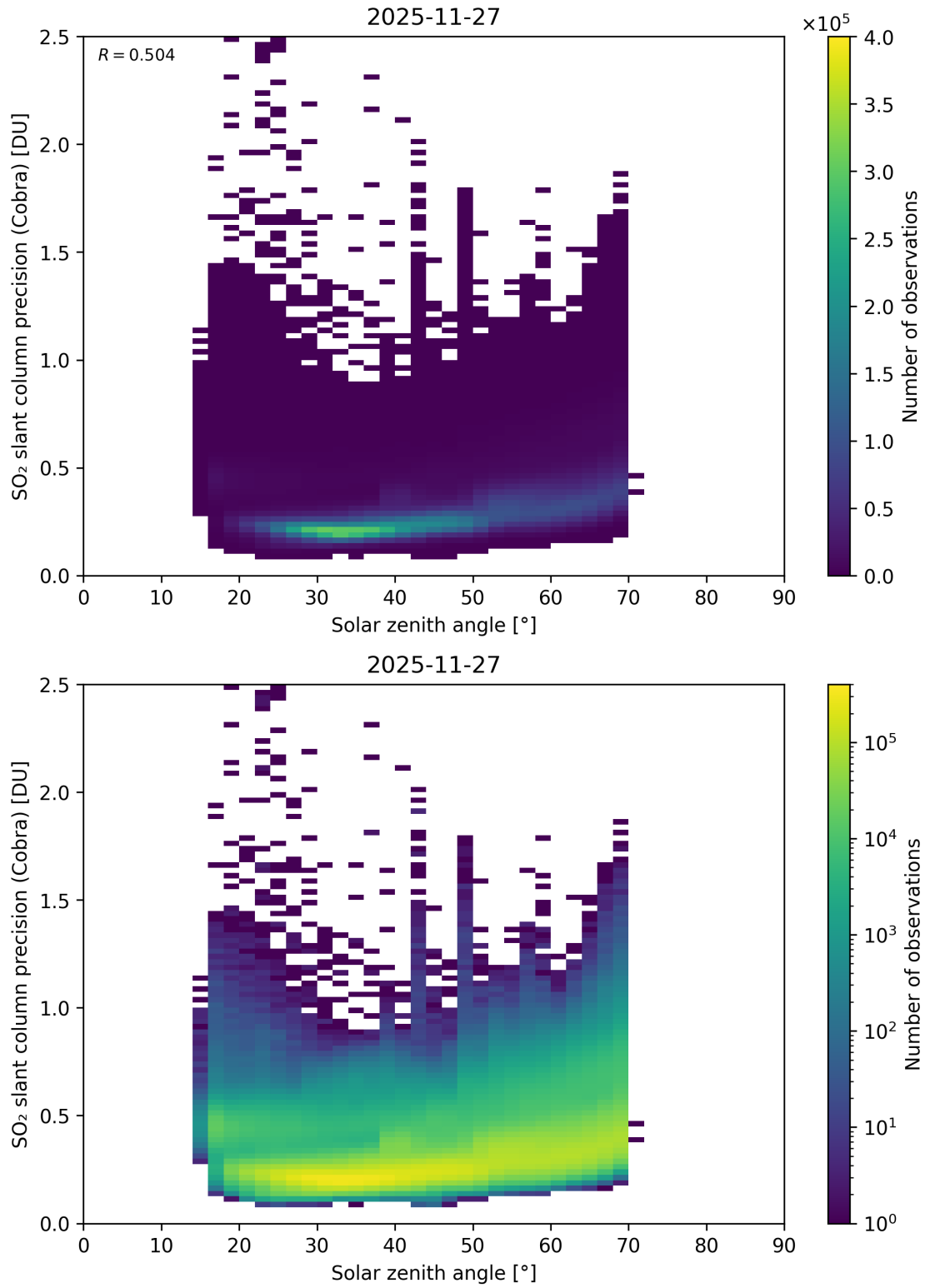
Figure 180: Scatter density plot of “Solar zenith angle” against “SO 2 slant column precision (Cobra)” for 2025-11-26 to 2025-11-28.
