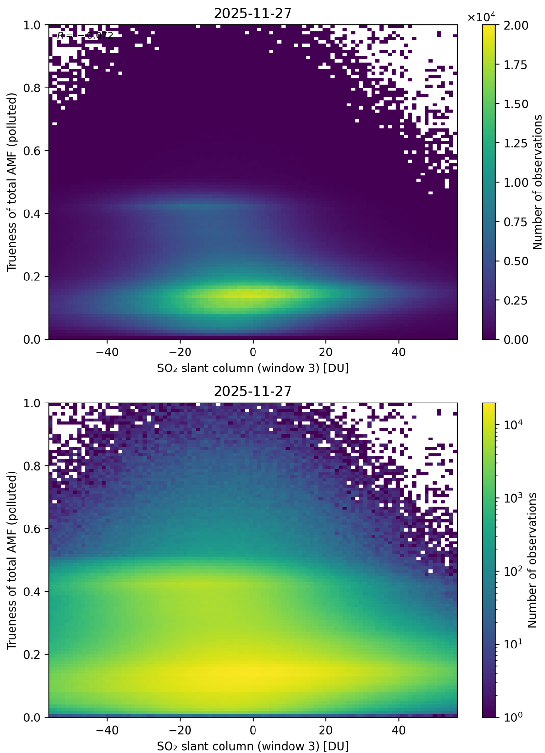
Figure 319: Scatter density plot of “SO 2 slant column (window 3)” against “Trueness of total AMF (polluted)” for 2025-11-26 to 2025-11-28.
