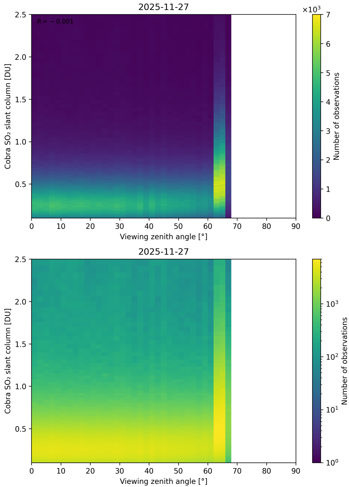
Figure 371: Scatter density plot of “Viewing zenith angle” against “Cobra SO 2 slant column” for 2025-11-26 to 2025-11-28.
