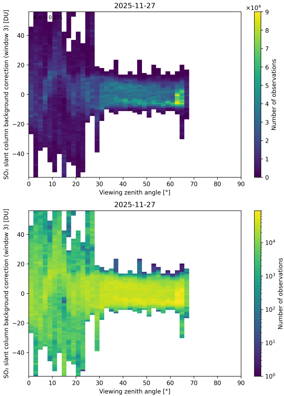
Figure 364: Scatter density plot of “Viewing zenith angle” against “SO 2 slant column background correction (window 3)” for 2025-11-26 to 2025-11-28.
