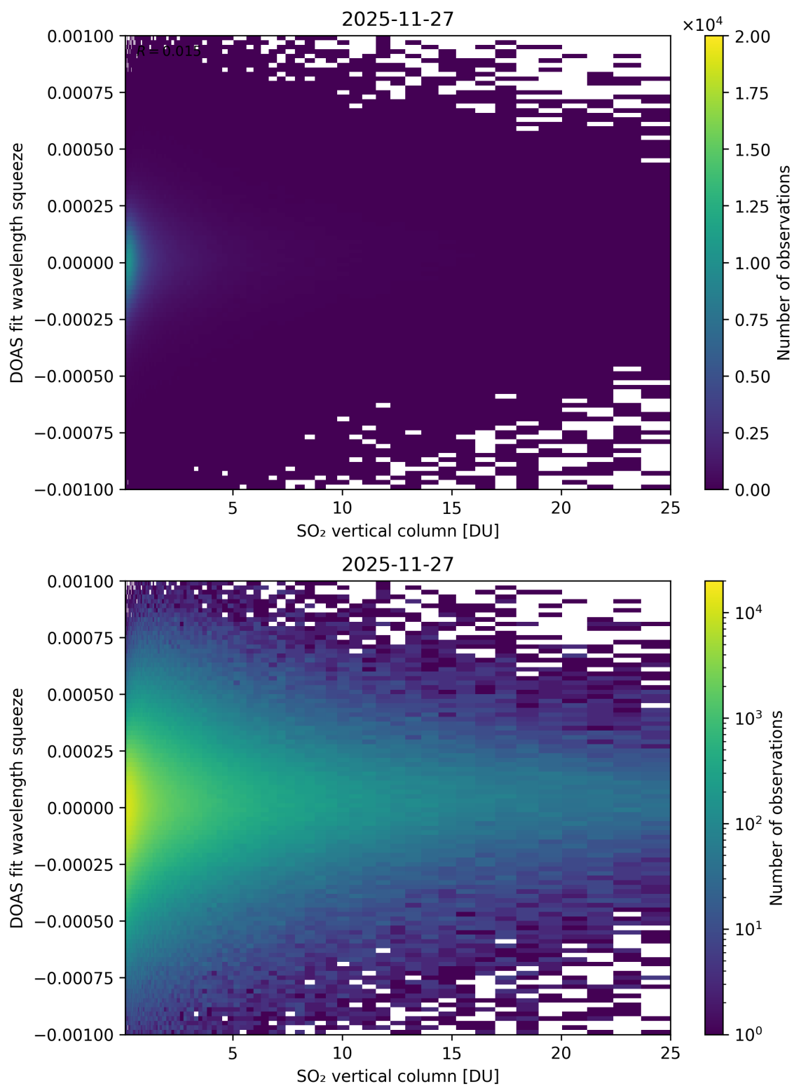
Figure 327: Scatter density plot of “SO 2 vertical column” against “DOAS fit wavelength squeeze” for 2025-11-26 to 2025-11-28.
