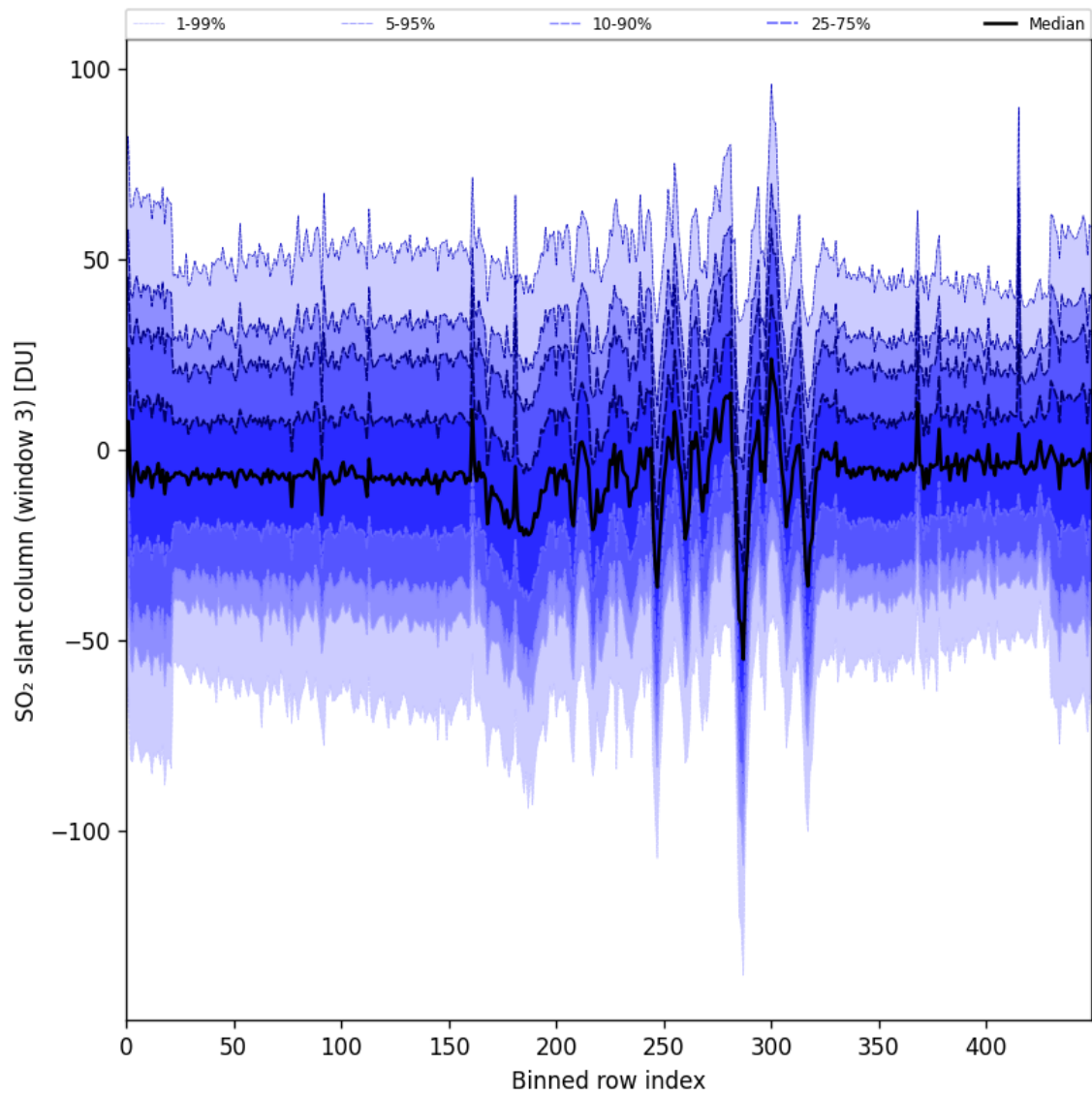
Figure 97: Along track statistics of “SO 2 slant column (window 3)” for 2025-11-26 to 2025-11-28
