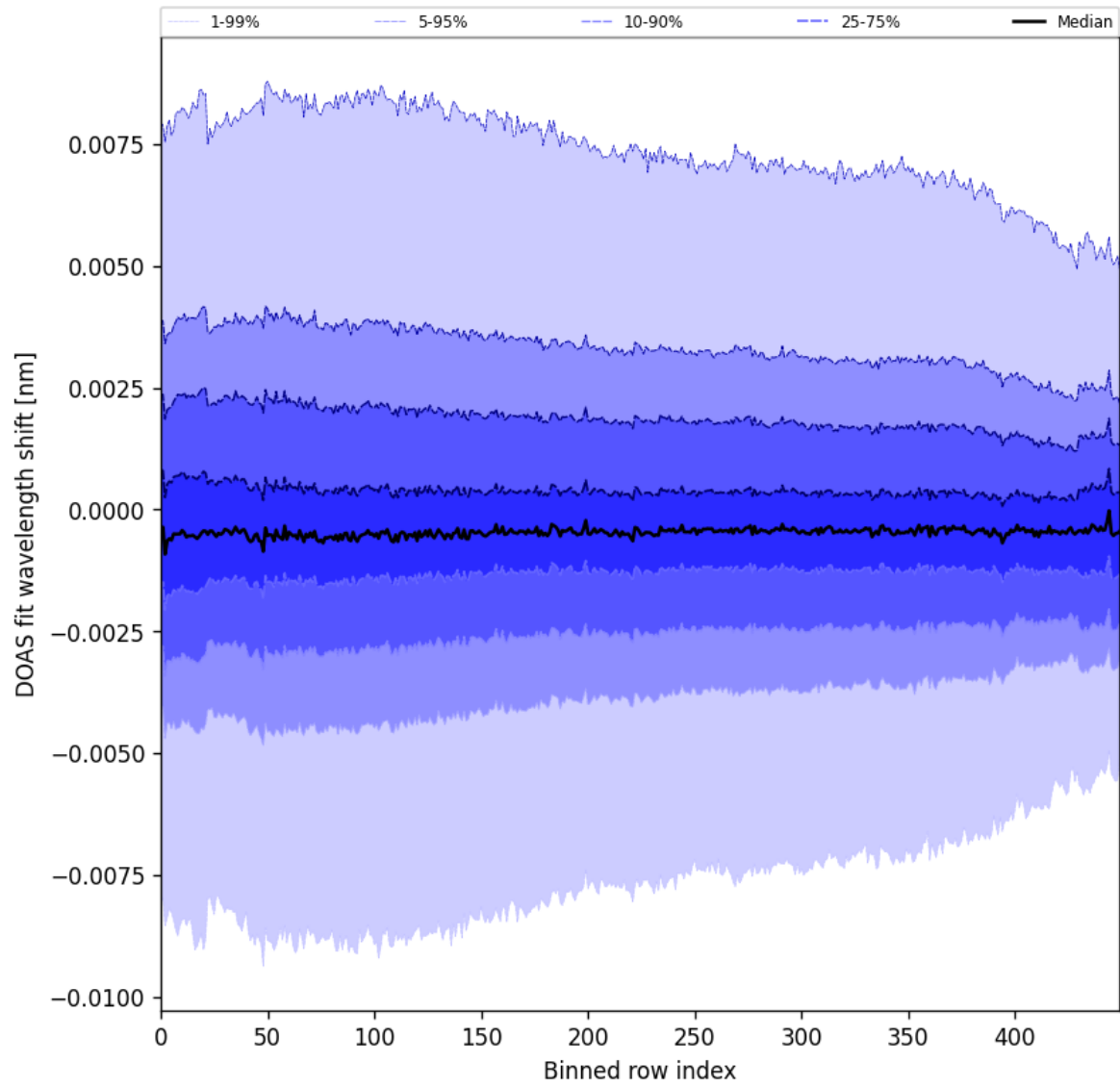
Figure 102: Along track statistics of “DOAS fit wavelength shift” for 2025-11-26 to 2025-11-28
