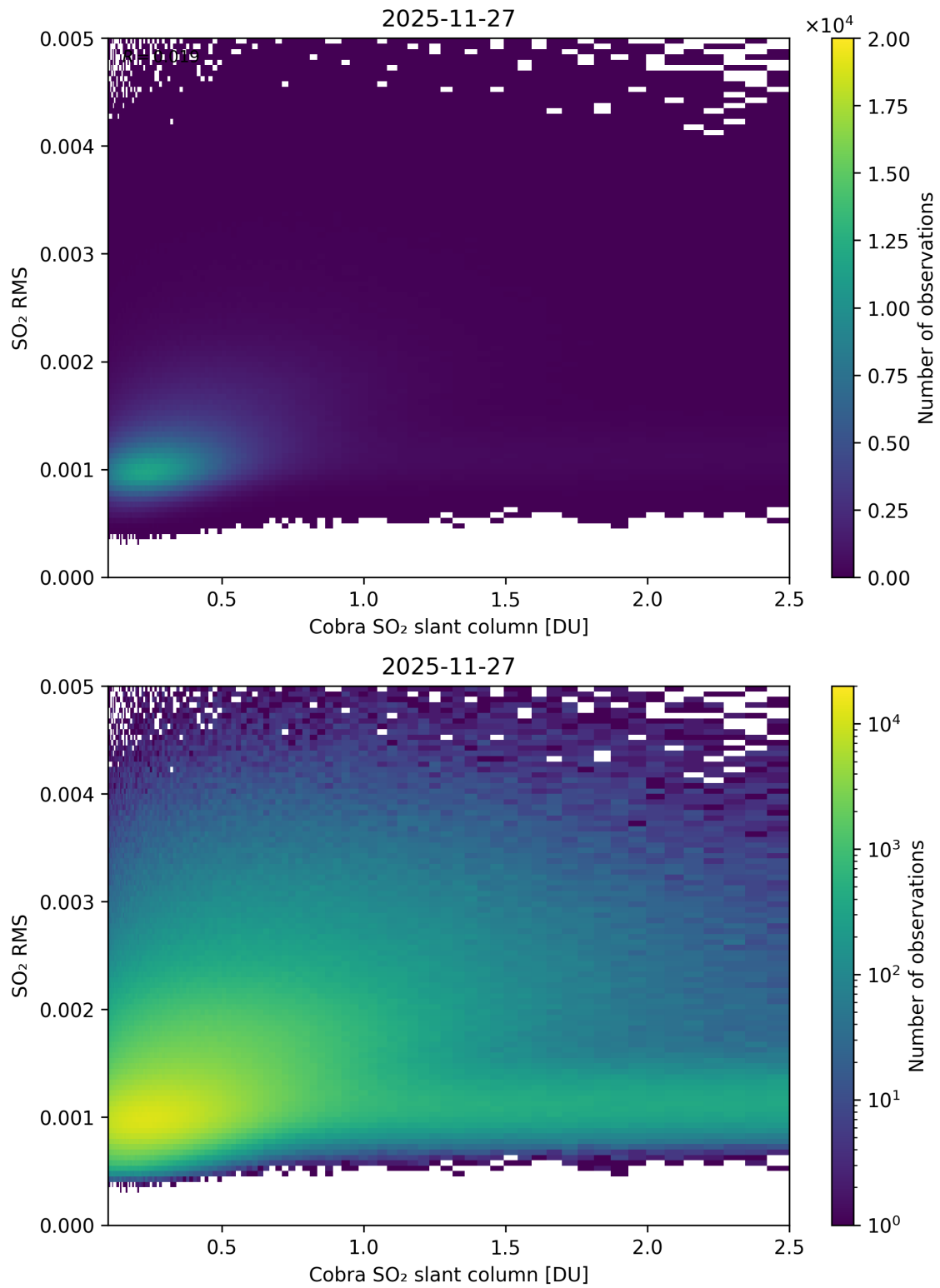
Figure 198: Scatter density plot of “Cobra SO 2 slant column” against “SO 2 RMS” for 2025-11-26 to 2025-11-28.
