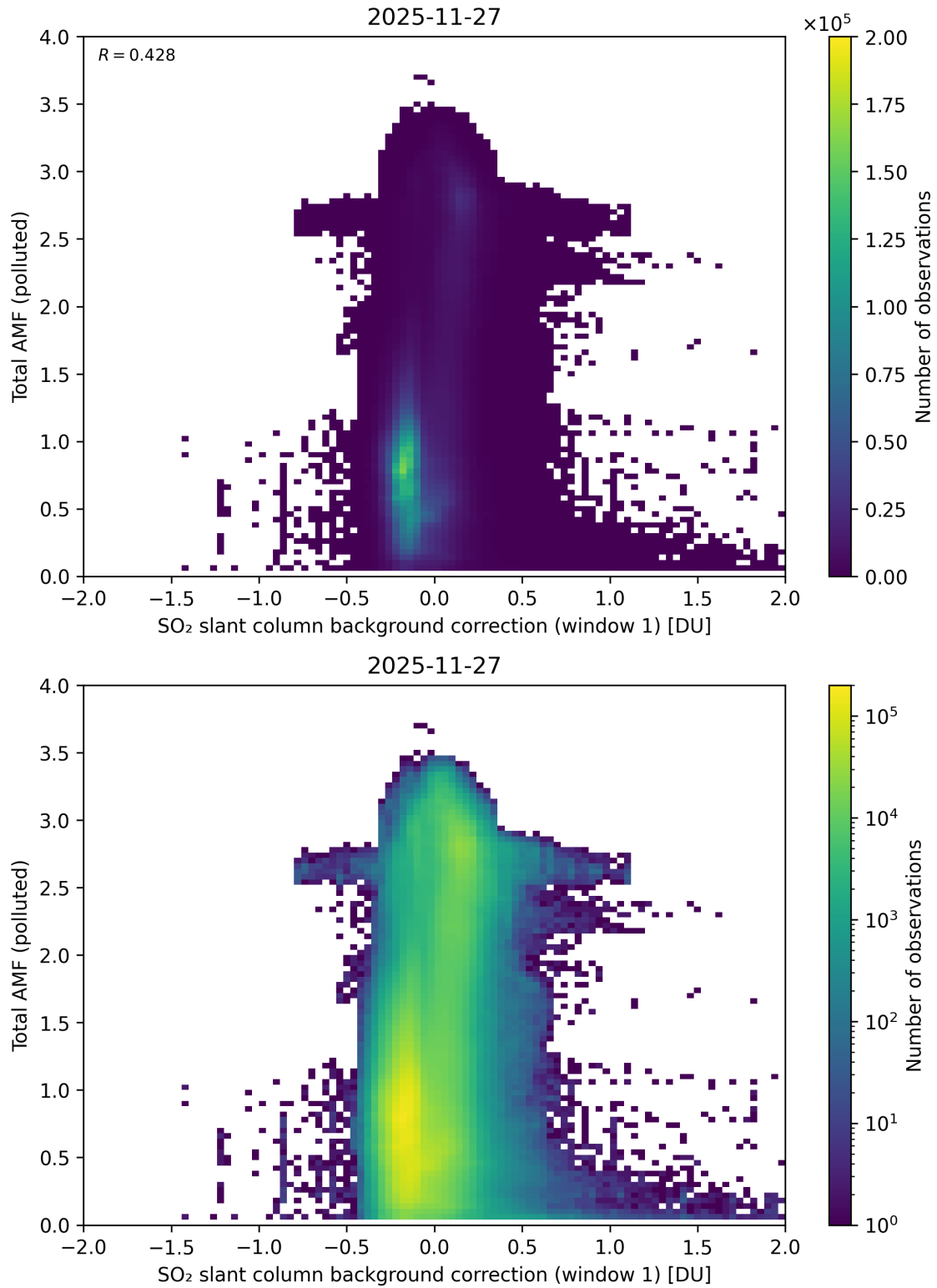
Figure 120: Scatter density plot of “SO 2 slant column background correction (window 1)” against “Total AMF (polluted)” for 2025-11-26 to 2025-11-28.
