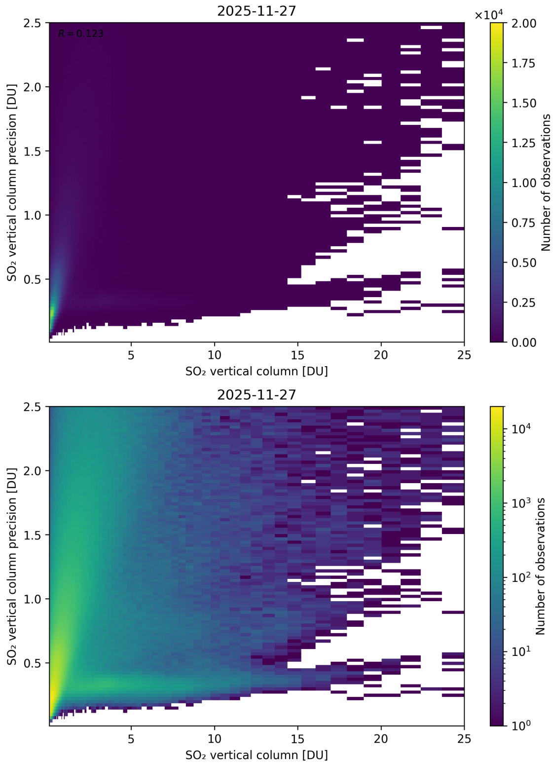
Figure 361: Scatter density plot of “SO 2 vertical column” against “SO 2 vertical column precision” for 2025-11-26 to 2025-11-28.
