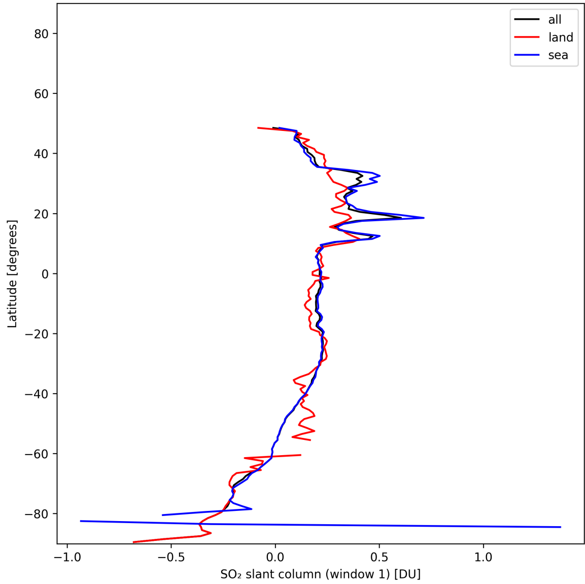
Figure 37: Zonal average of “SO 2 slant column (window 1)” for 2025-11-26 to 2025-11-28.
