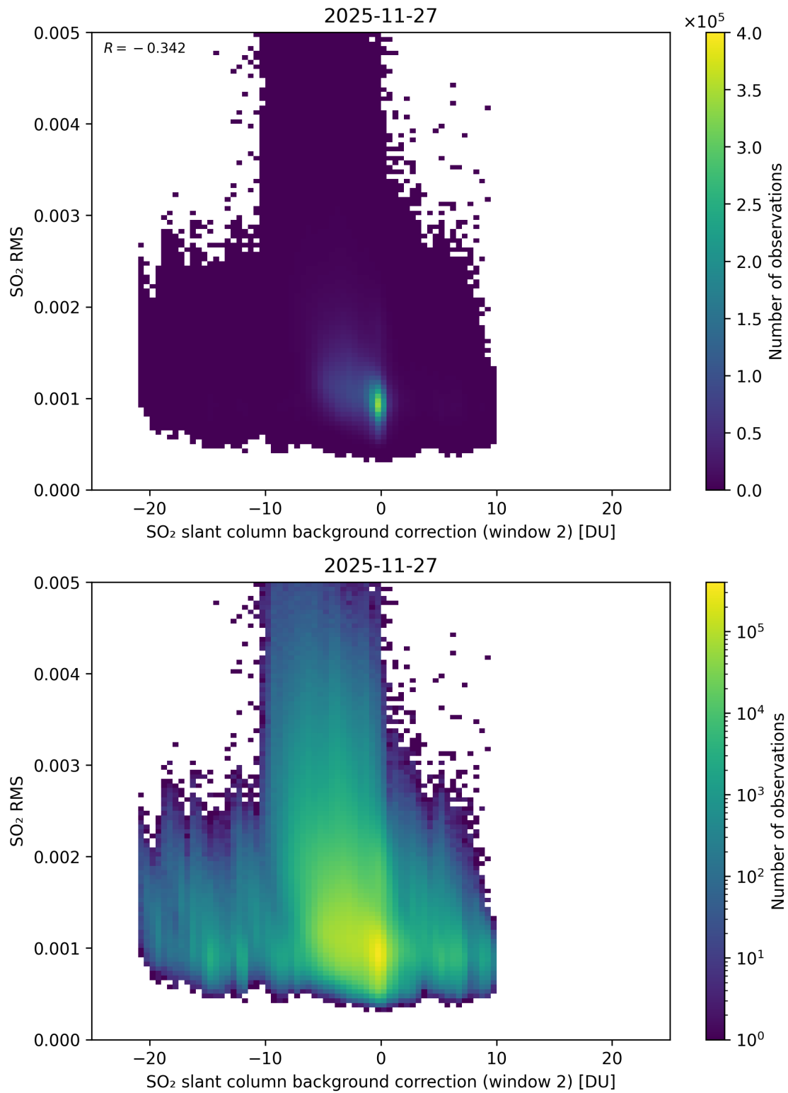
Figure 125: Scatter density plot of “SO 2 slant column background correction (window 2)” against “SO 2 RMS” for 2025-11-26 to 2025-11-28.
