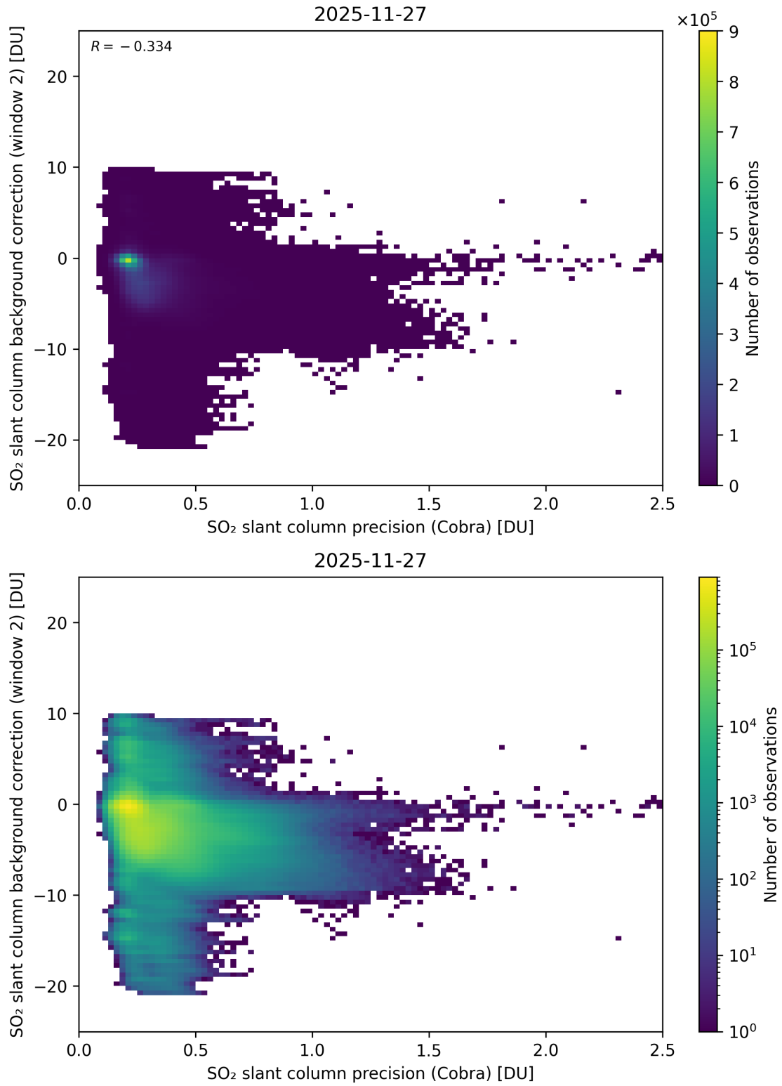
Figure 200: Scatter density plot of “SO 2 slant column precision (Cobra)” against “SO 2 slant column background correction (window 2)” for 2025-11-26 to 2025-11-28.
