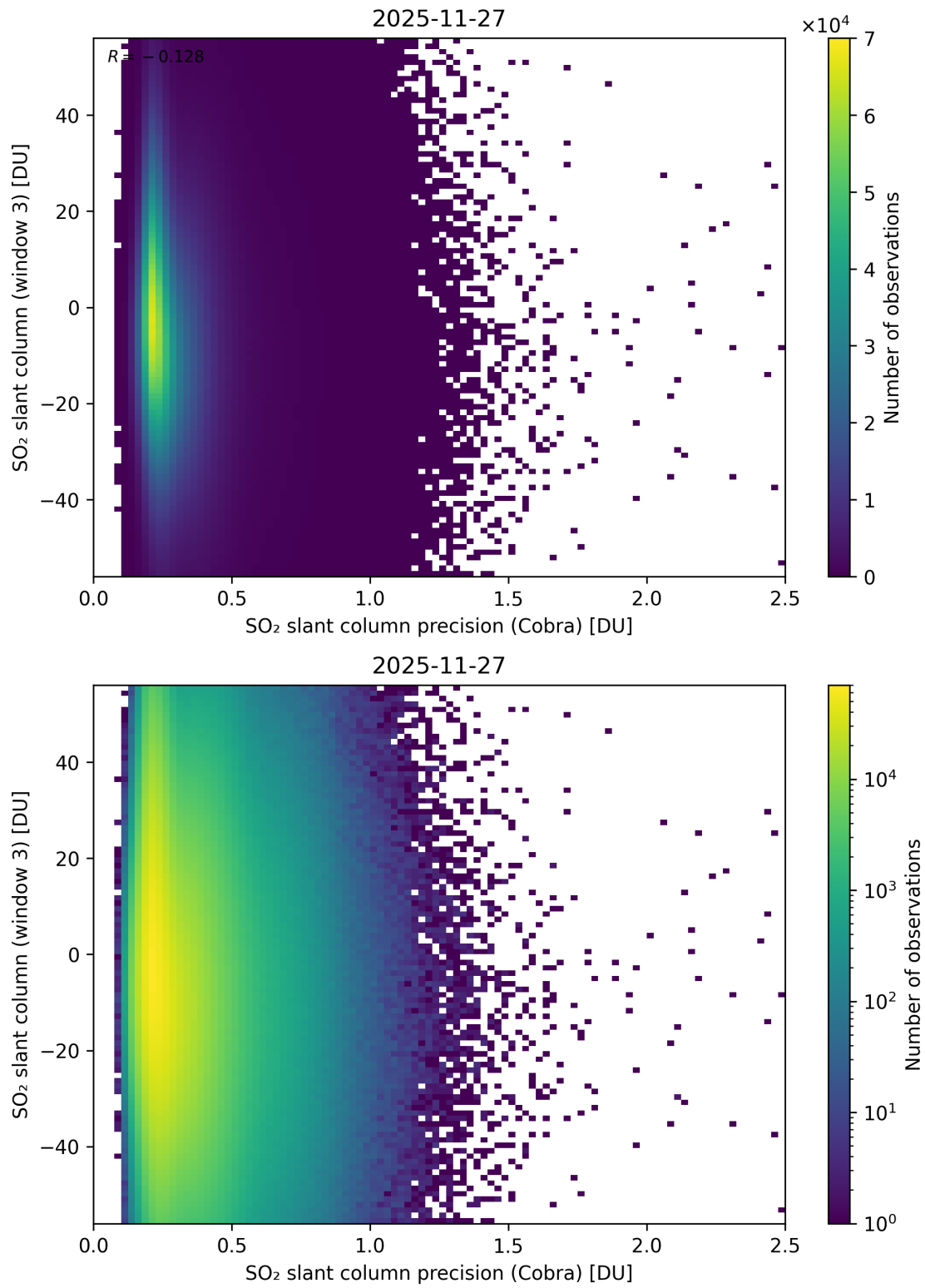
Figure 211: Scatter density plot of “SO 2 slant column precision (Cobra)” against “SO 2 slant column (window 3)” for 2025-11-26 to 2025-11-28.
