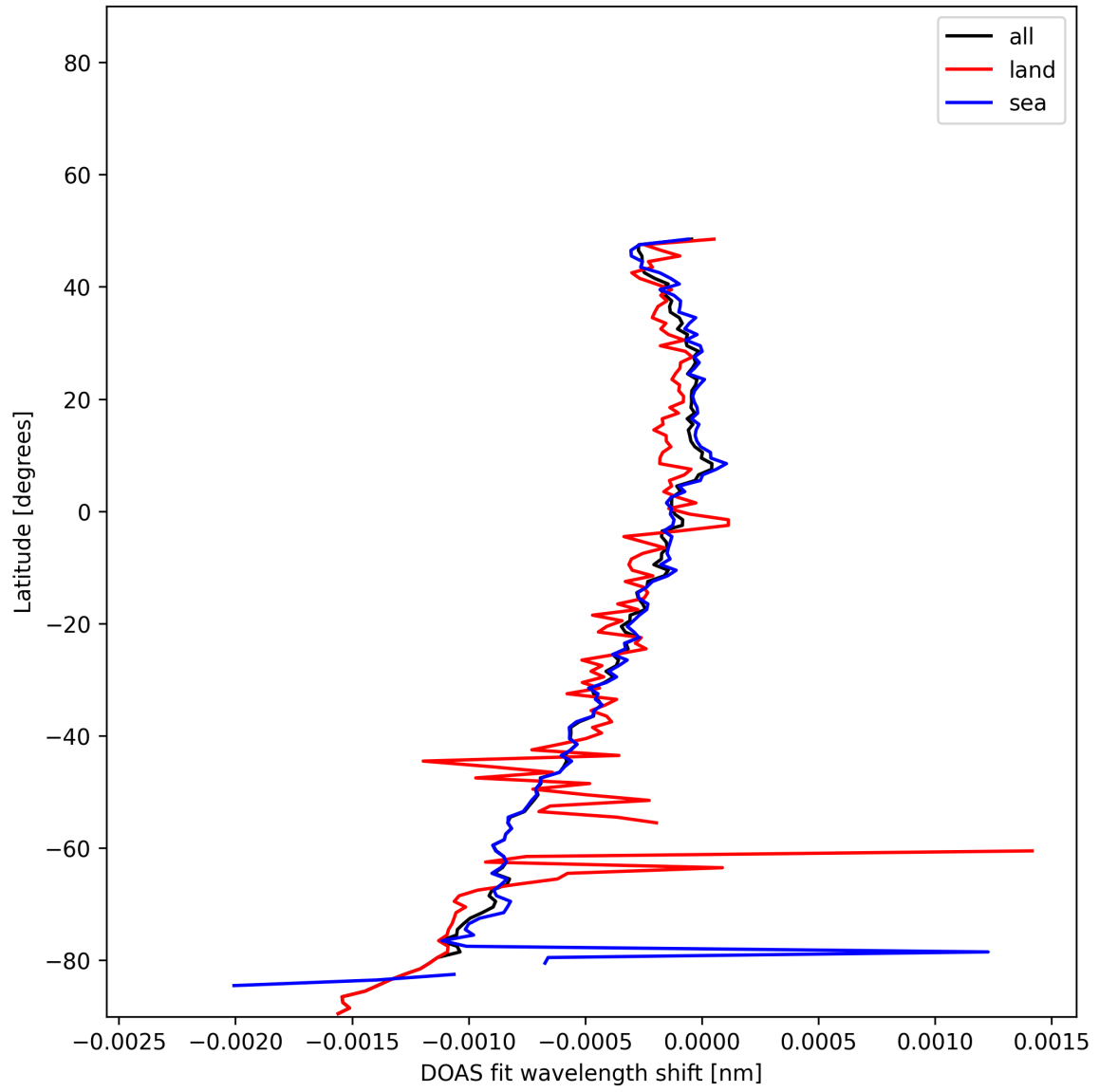
Figure 50: Zonal average of "DOAS fit wavelength shift" for 2025-11-26 to 2025-11-28.
