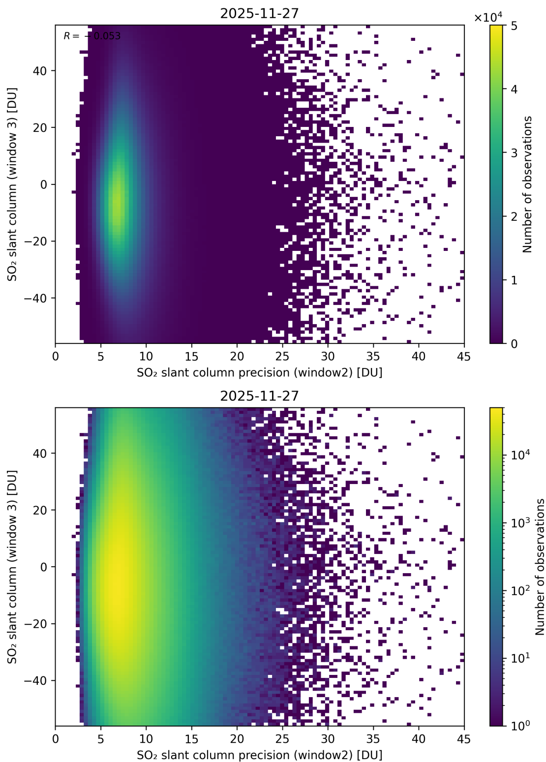
Figure 299: Scatter density plot of “SO 2 slant column precision (window2)” against “SO 2 slant column (window 3)” for 2025-11-26 to 2025-11-28.
