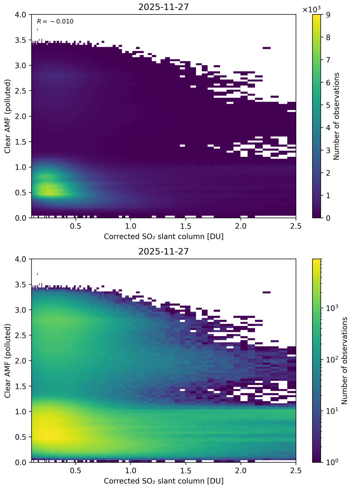
Figure 232: Scatter density plot of “Corrected SO 2 slant column” against “Clear AMF (polluted)” for 2025-11-26 to 2025-11-28.
