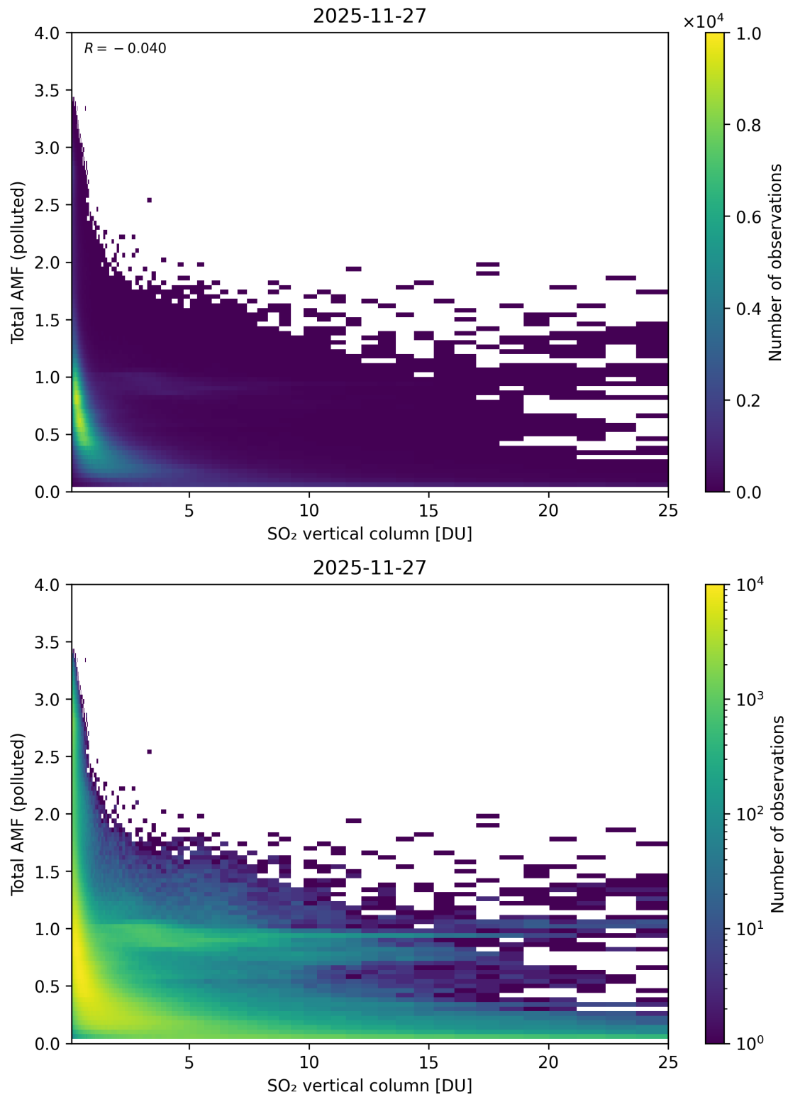
Figure 359: Scatter density plot of “SO 2 vertical column” against “Total AMF (polluted)” for 2025-11-26 to 2025-11-28.
