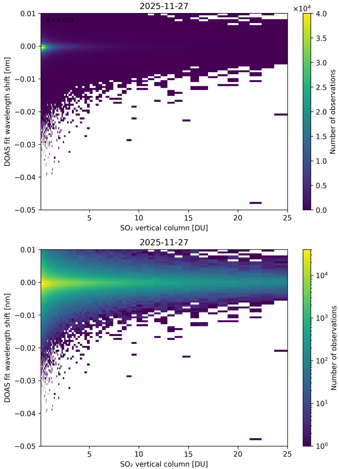
Figure 326: Scatter density plot of “SO 2 vertical column” against “DOAS fit wavelength shift” for 2025-11-26 to 2025-11-28.
