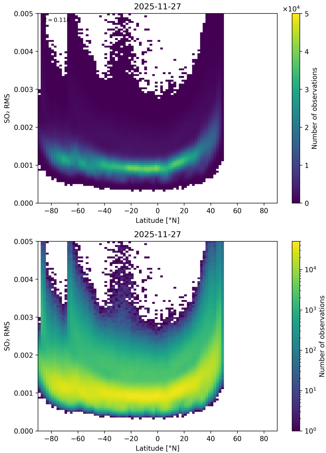
Figure 155: Scatter density plot of “Latitude” against “SO 2 RMS” for 2025-11-26 to 2025-11-28.
