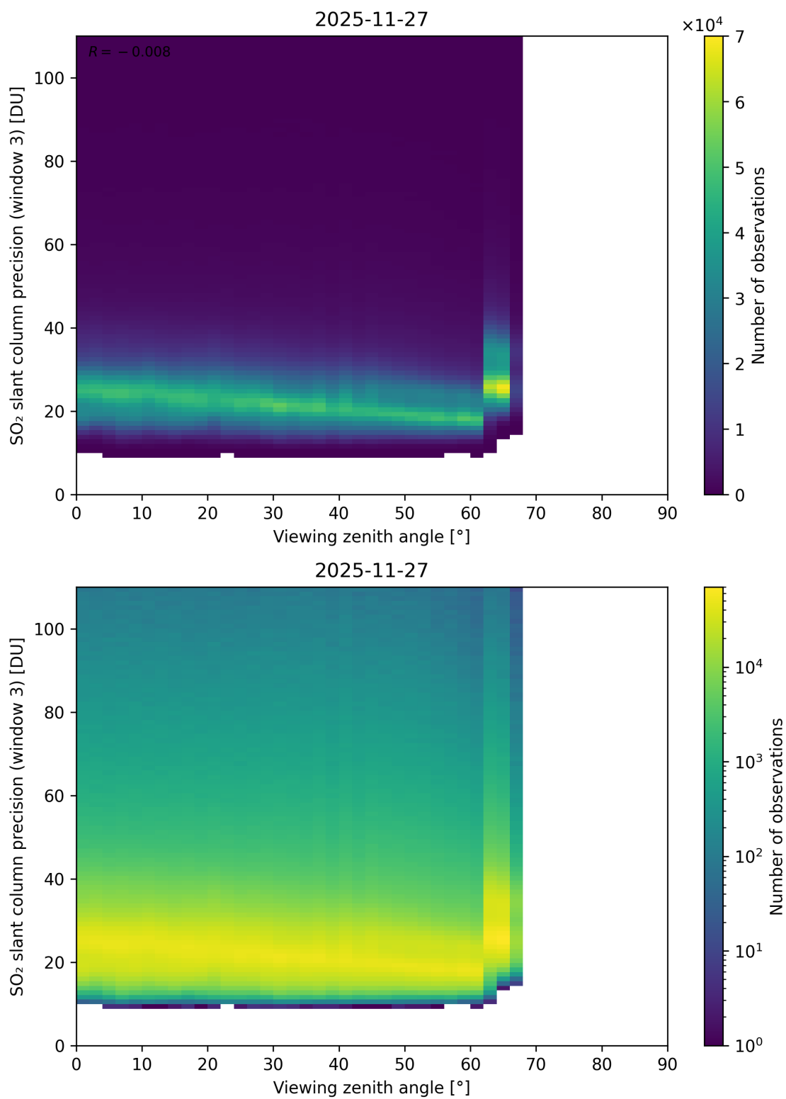
Figure 380: Scatter density plot of “Viewing zenith angle” against “SO 2 slant column precision (window 3)” for 2025-11-26 to 2025-11-28.
