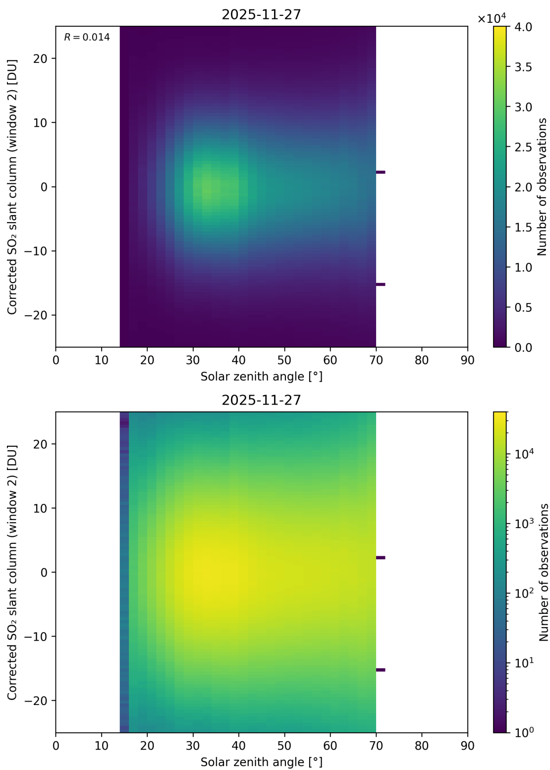
Figure 182: Scatter density plot of “Solar zenith angle” against “Corrected SO 2 slant column (window 2)” for 2025-11-26 to 2025-11-28.
