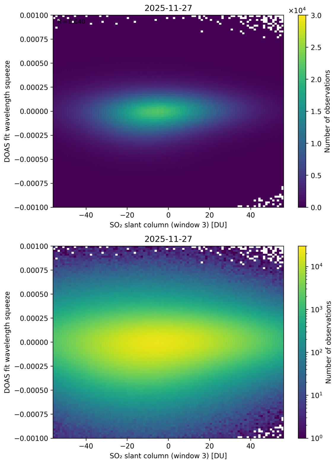
Figure 305: Scatter density plot of “SO 2 slant column (window 3)” against “DOAS fit wavelength squeeze” for 2025-11-26 to 2025-11-28.
