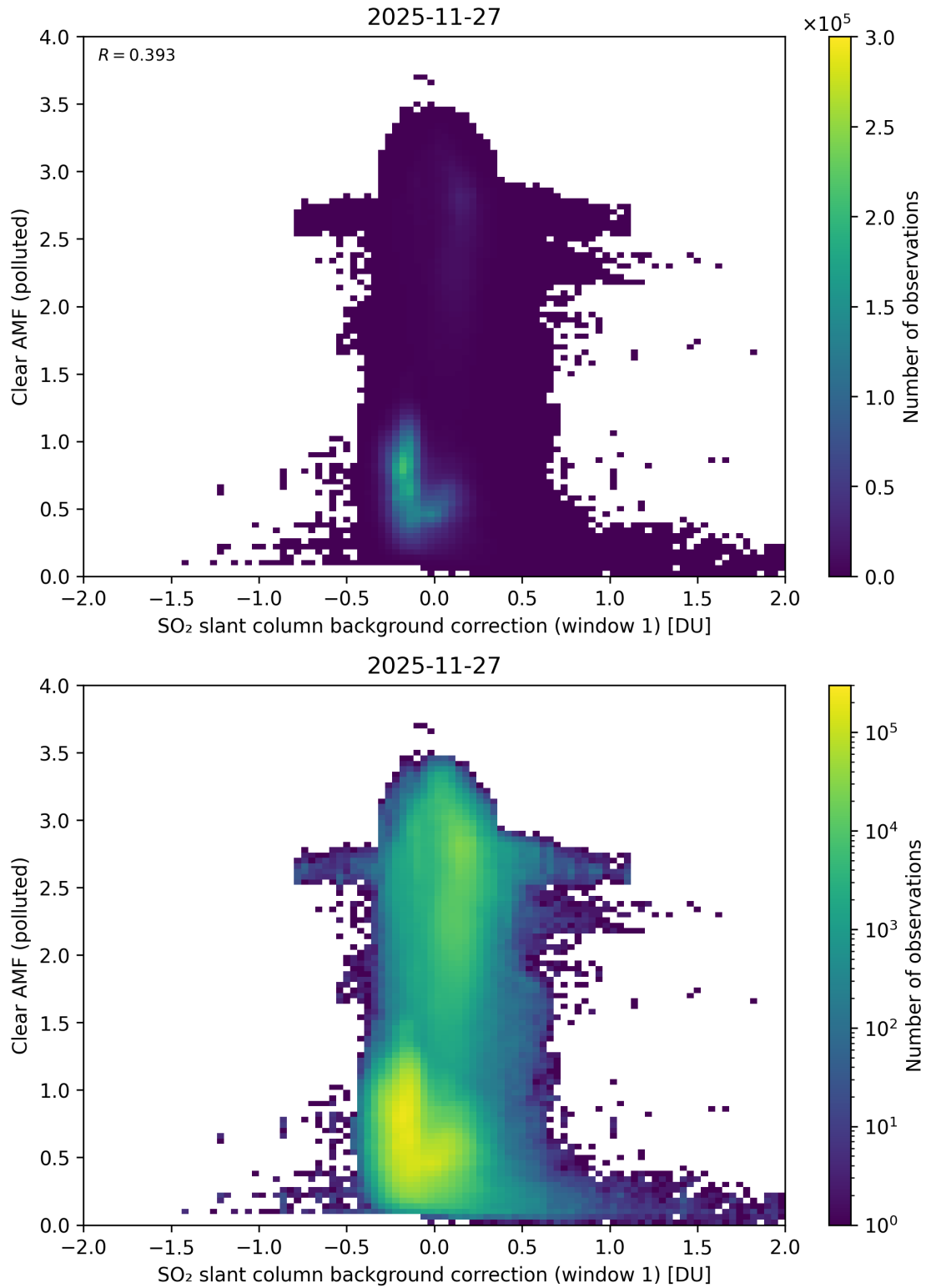
Figure 114: Scatter density plot of “SO 2 slant column background correction (window 1)” against “Clear AMF (polluted)” for 2025-11-26 to 2025-11-28.
