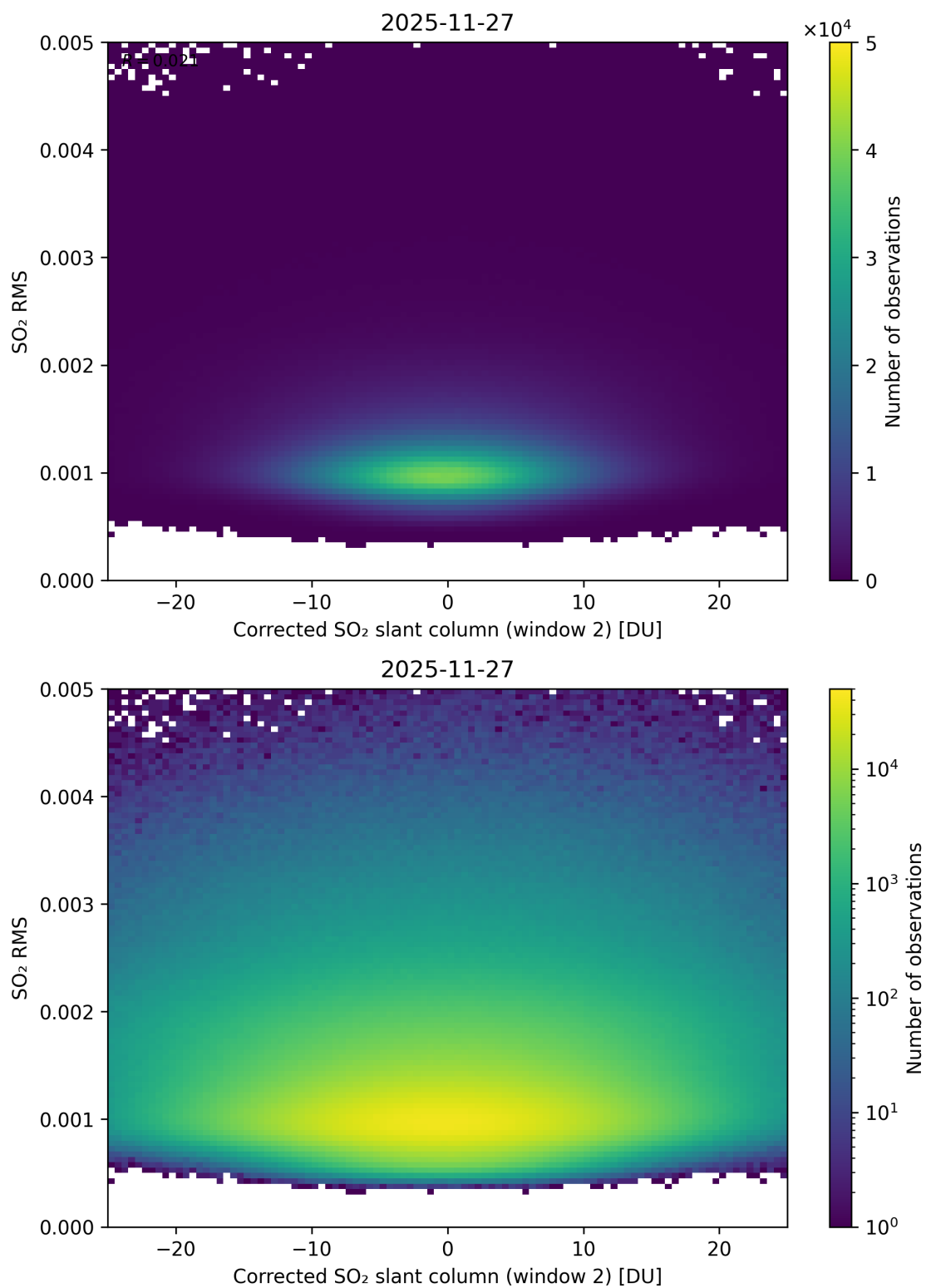
Figure 248: Scatter density plot of “Corrected SO 2 slant column (window 2)” against “SO 2 RMS” for 2025-11-26 to 2025-11-28.
