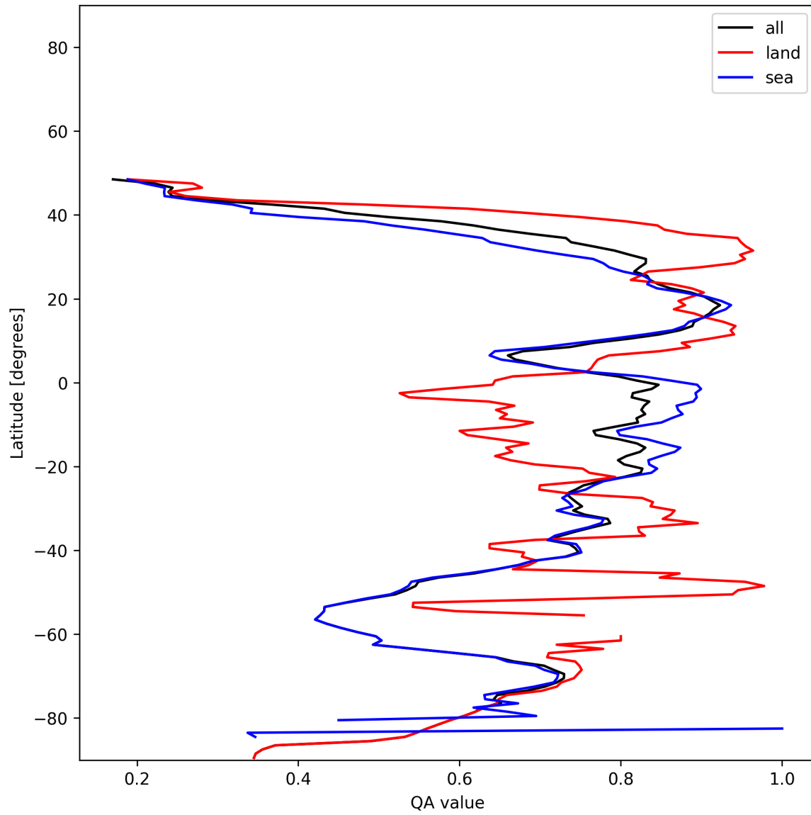
Figure 31: Zonal average of “QA value” for 2025-11-26 to 2025-11-28.
