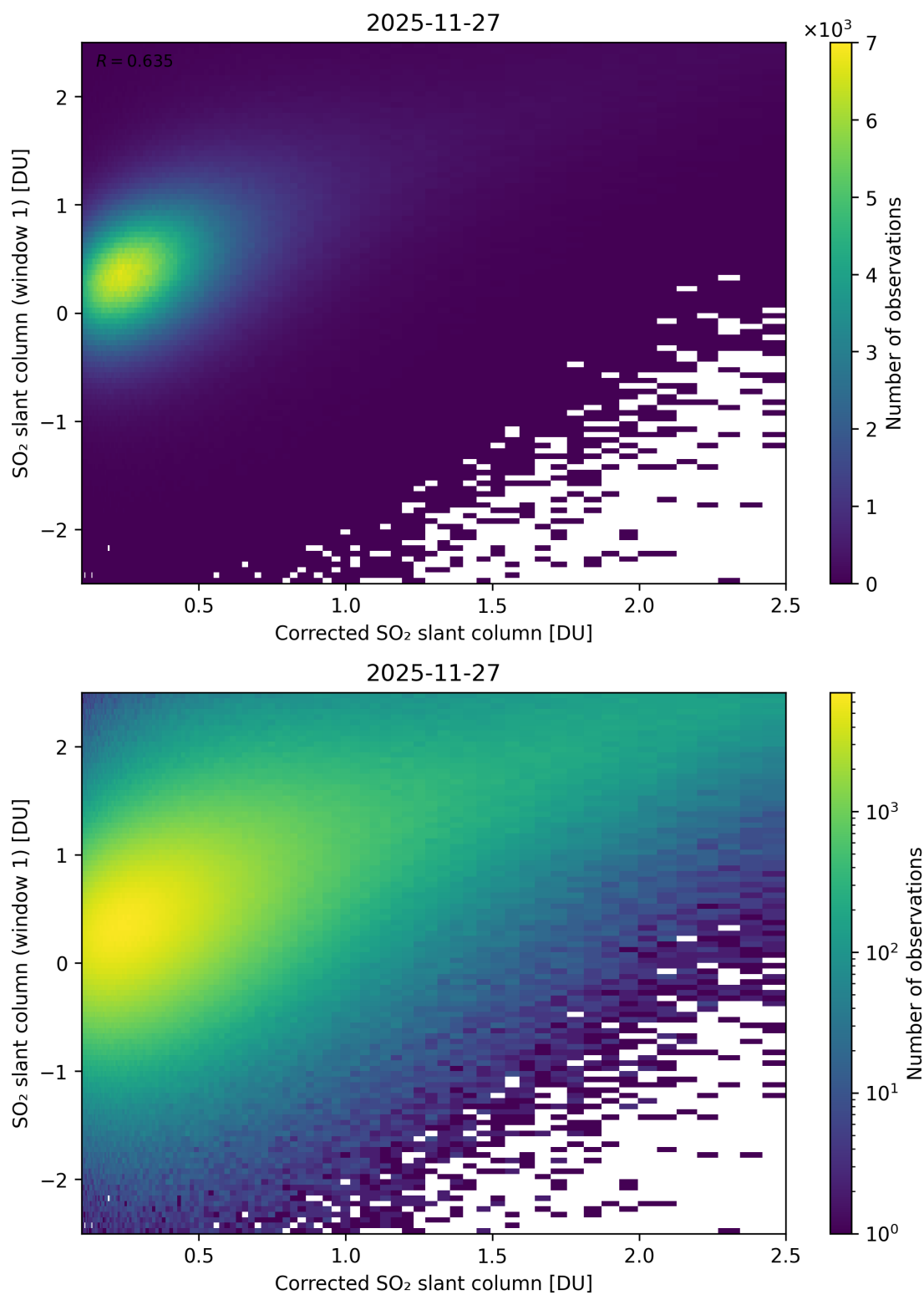
Figure 237: Scatter density plot of “Corrected SO 2 slant column” against “SO 2 slant column (window 1)” for 2025-11-26 to 2025-11-28.
