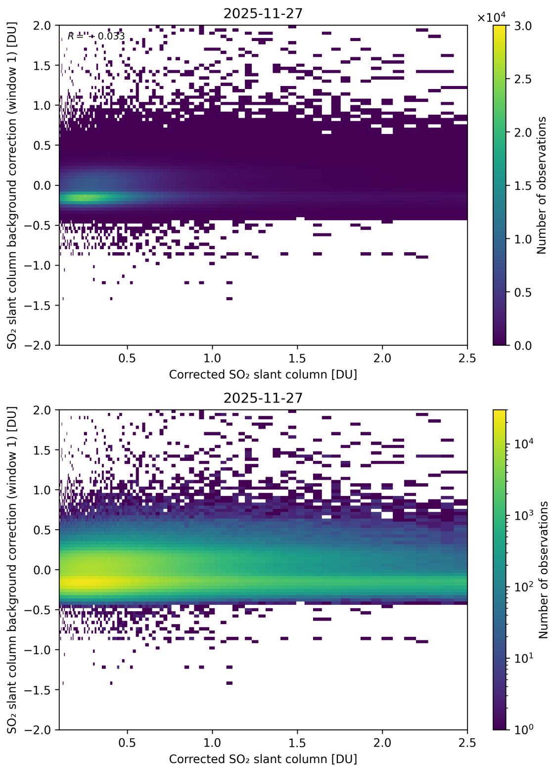
Figure 226: Scatter density plot of “Corrected SO 2 slant column” against “SO 2 slant column background correction (window 1)” for 2025-11-26 to 2025-11-28.
