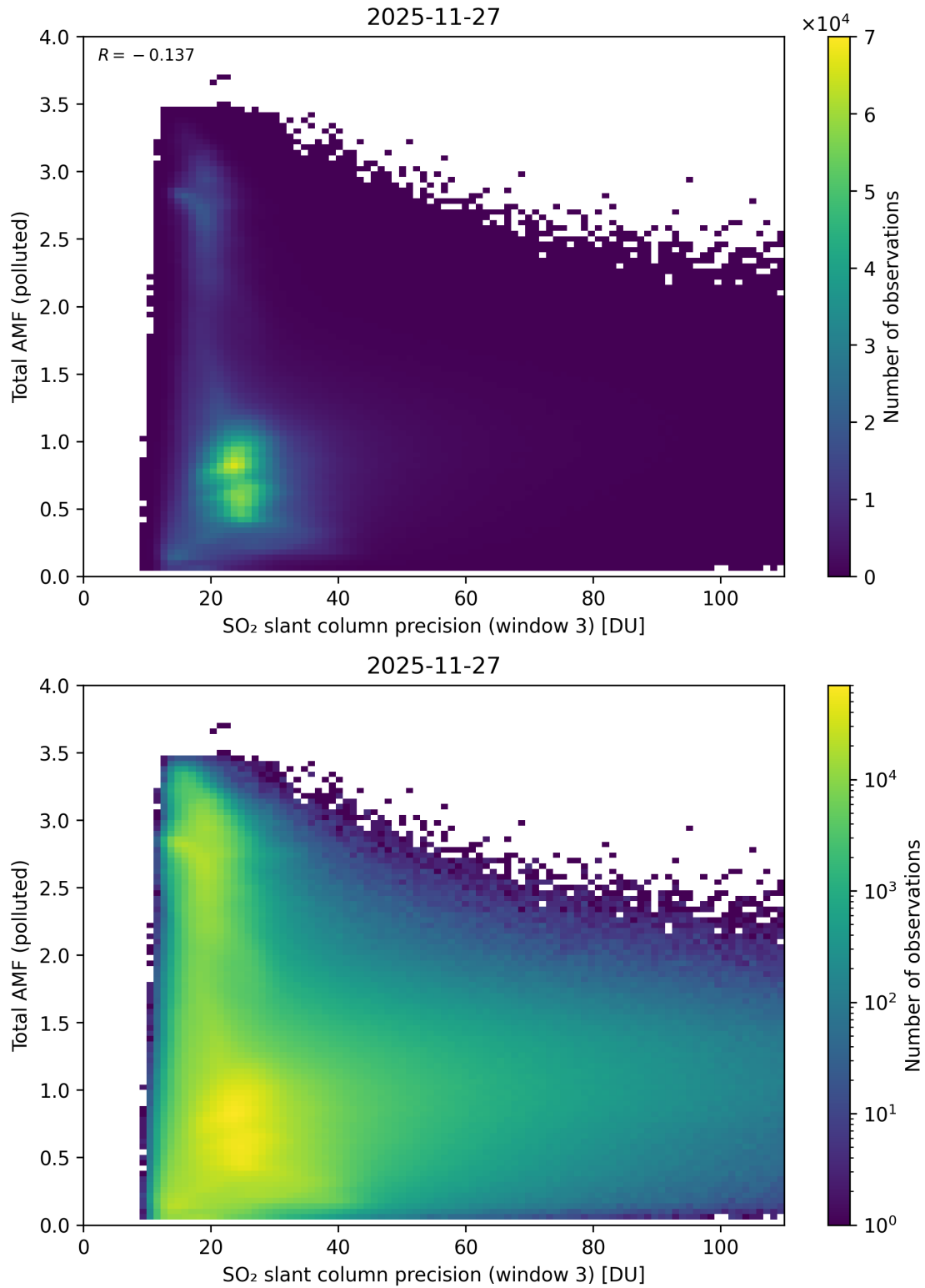
Figure 313: Scatter density plot of “SO 2 slant column precision (window 3)” against “Total AMF (polluted)” for 2025-11-26 to 2025-11-28.
