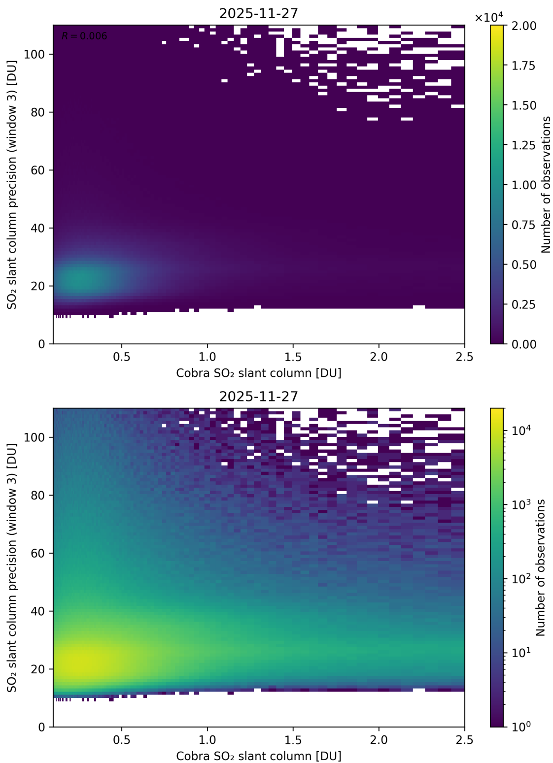
Figure 223: Scatter density plot of “Cobra SO 2 slant column” against “SO 2 slant column precision (window 3)” for 2025-11-26 to 2025-11-28.
