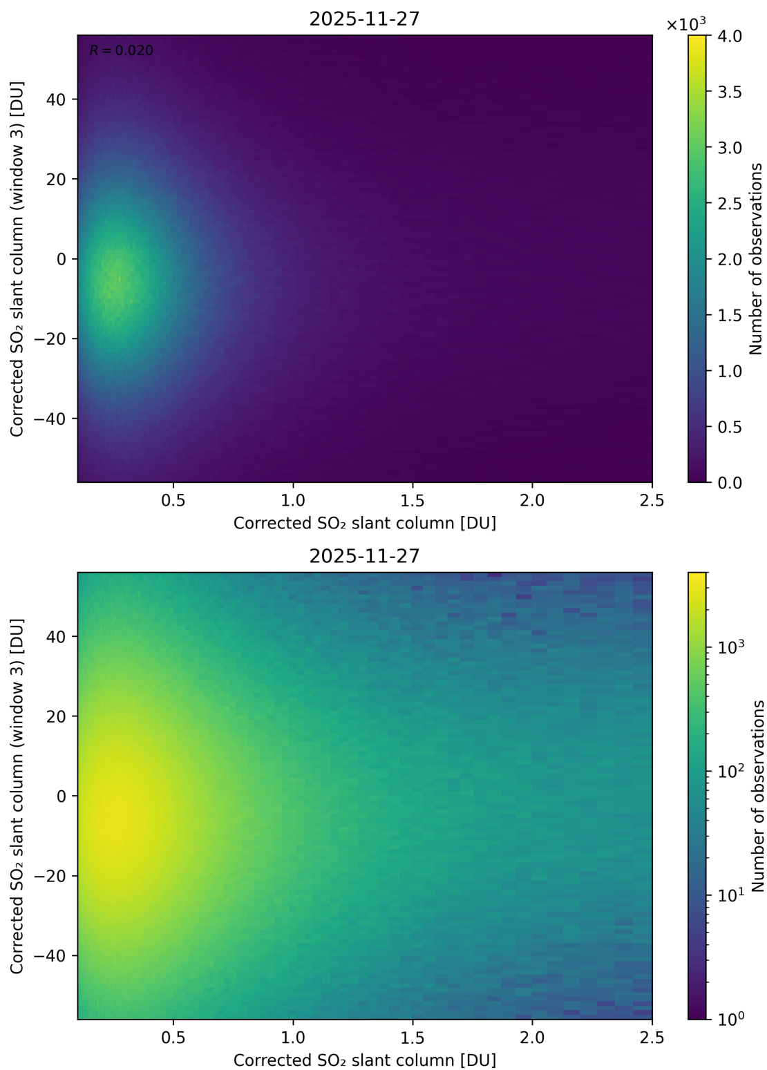
Figure 236: Scatter density plot of “Corrected SO 2 slant column” against “Corrected SO 2 slant column (window 3)” for 2025-11-26 to 2025-11-28.
