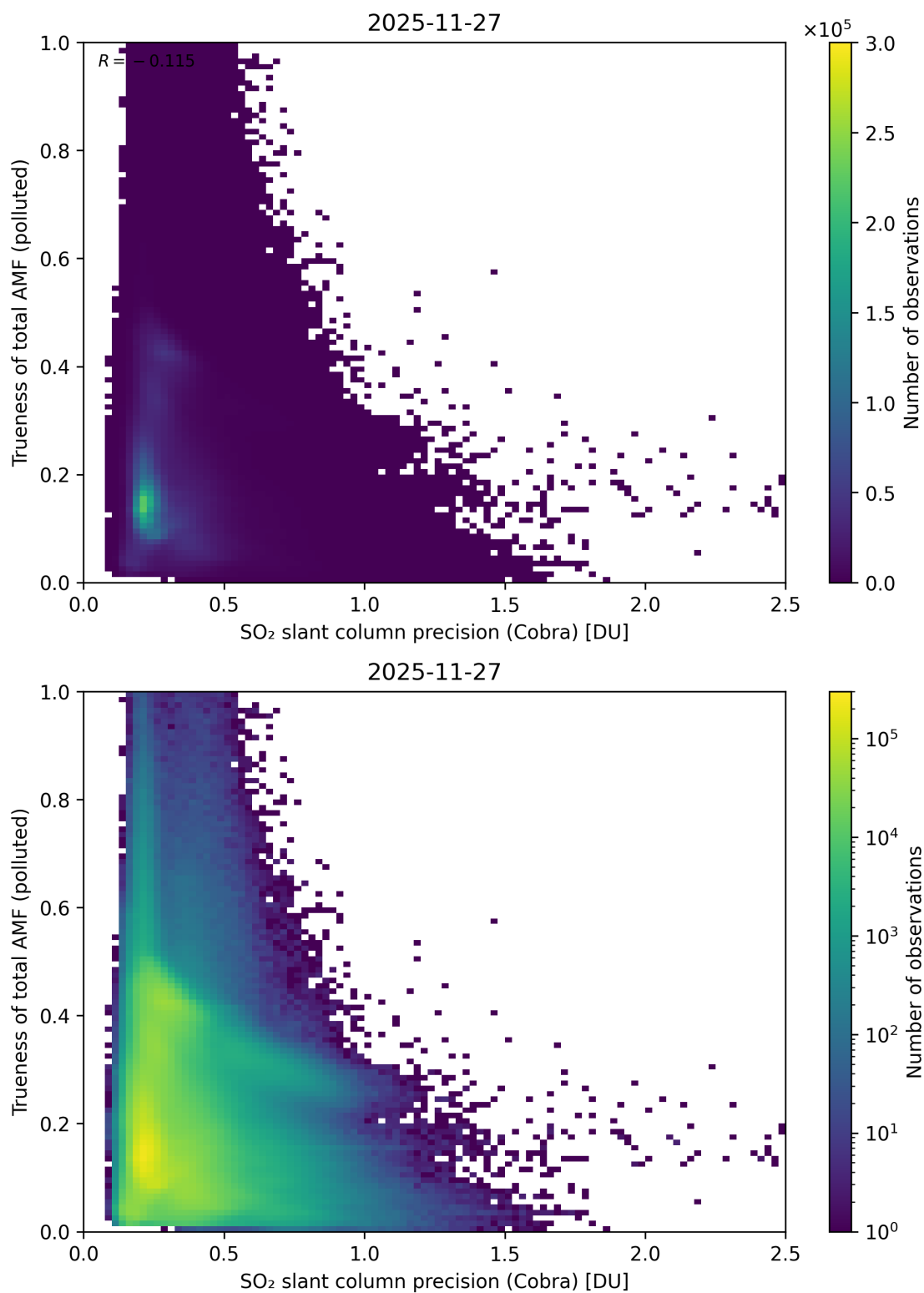
Figure 214: Scatter density plot of “SO 2 slant column precision (Cobra)” against “Trueness of total AMF (polluted)” for 2025-11-26 to 2025-11-28.
