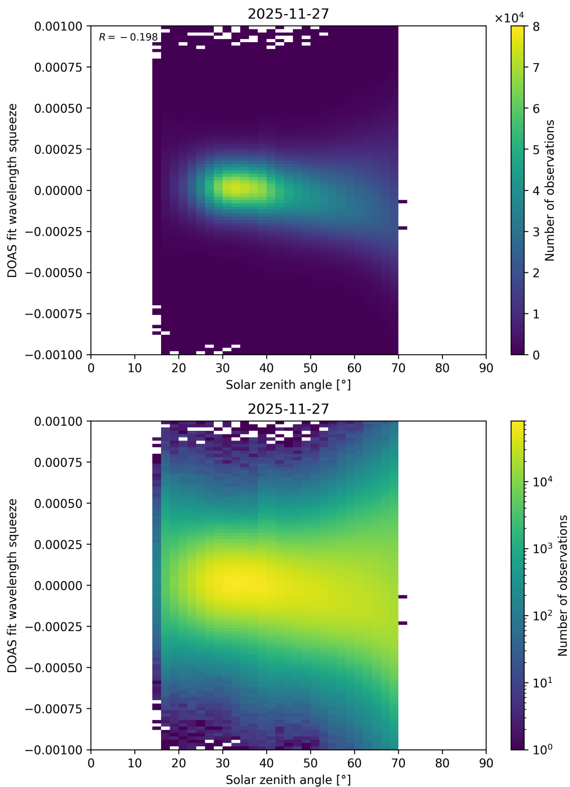
Figure 175: Scatter density plot of “Solar zenith angle” against “DOAS fit wavelength squeeze” for 2025-11-26 to 2025-11-28.
