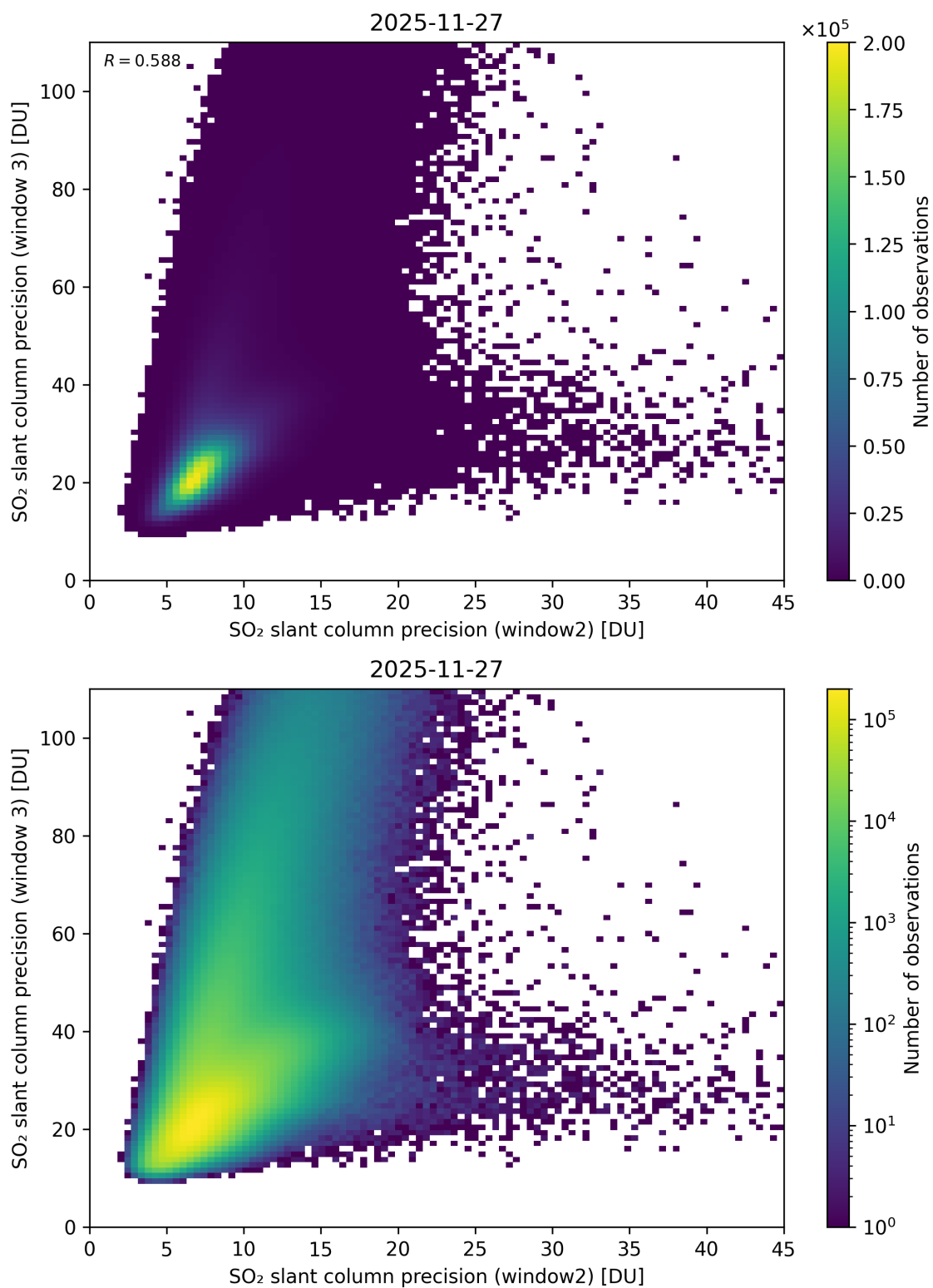
Figure 300: Scatter density plot of “SO 2 slant column precision (window2)” against “SO 2 slant column precision (window 3)” for 2025-11-26 to 2025-11-28.
