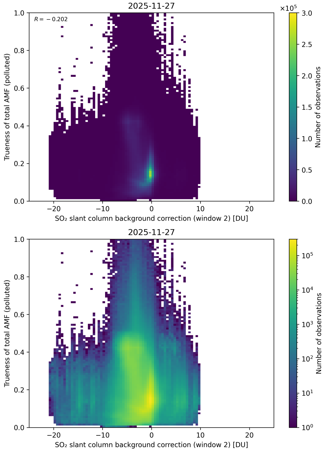
Figure 131: Scatter density plot of “SO 2 slant column background correction (window 2)” against “Trueness of total AMF (polluted)” for 2025-11-26 to 2025-11-28.
