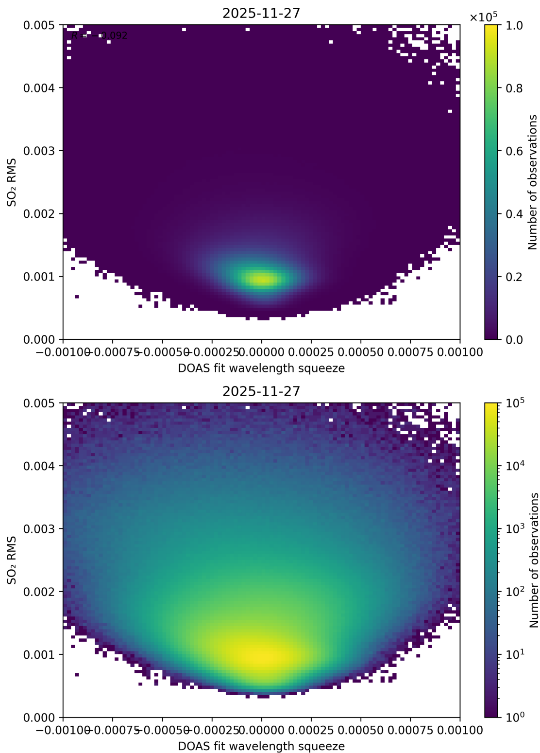
Figure 143: Scatter density plot of “DOAS fit wavelength squeeze” against “SO 2 RMS” for 2025-11-26 to 2025-11-28.
