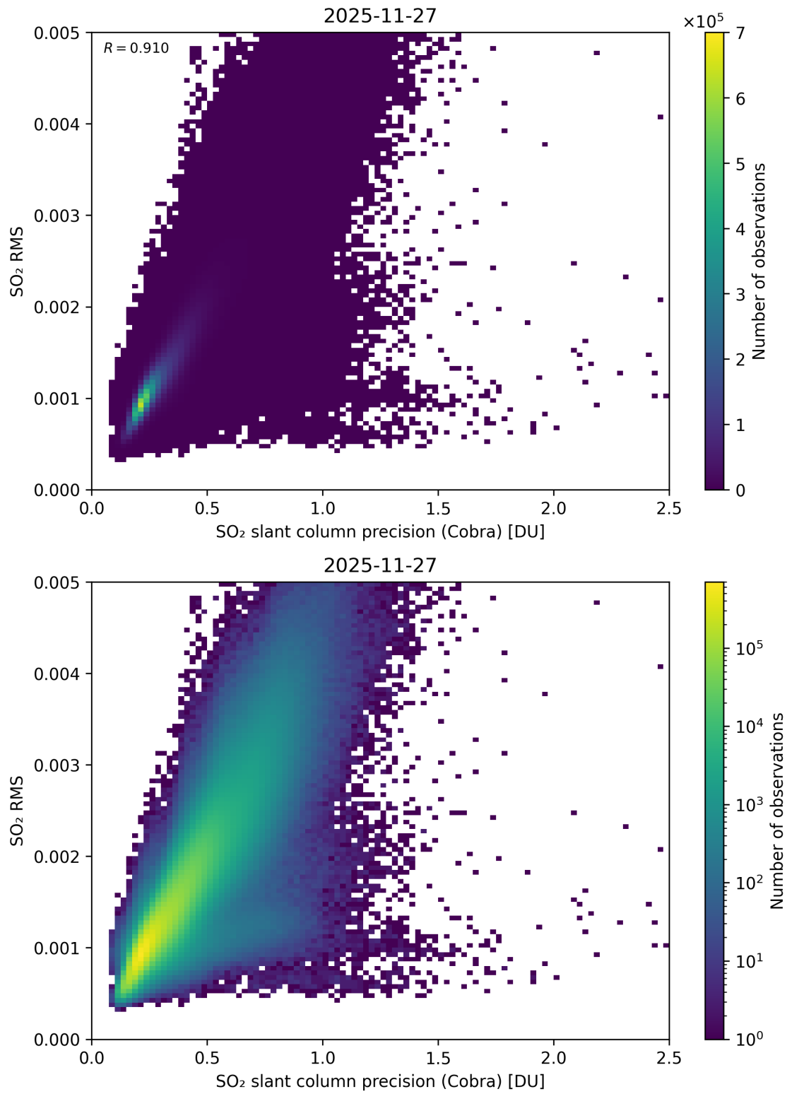
Figure 204: Scatter density plot of “SO 2 slant column precision (Cobra)” against “SO 2 RMS” for 2025-11-26 to 2025-11-28.
