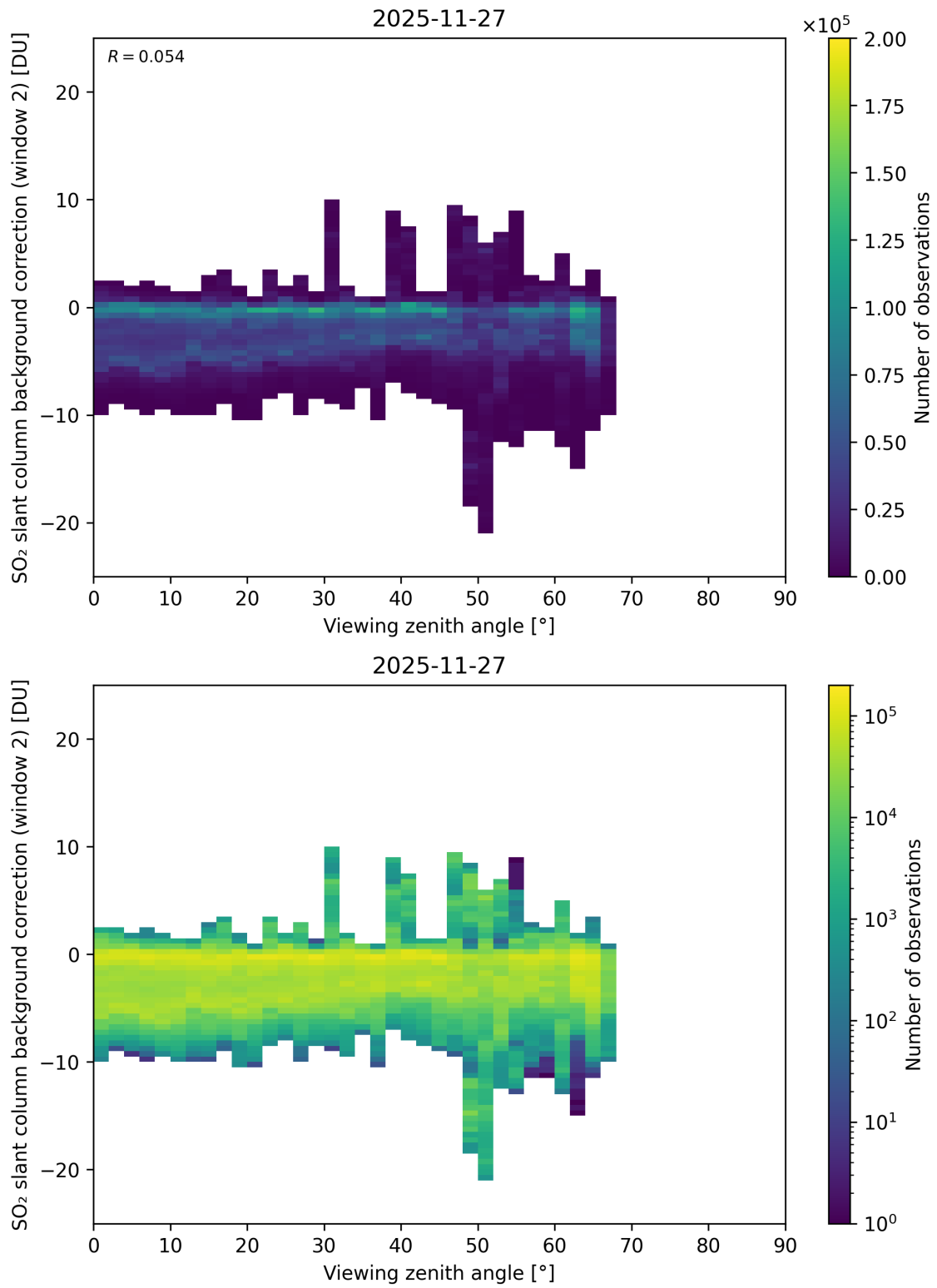
Figure 363: Scatter density plot of “Viewing zenith angle” against “SO 2 slant column background correction (window 2)” for 2025-11-26 to 2025-11-28.
