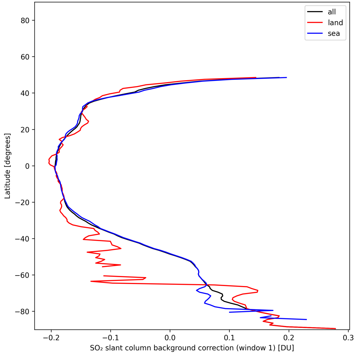
Figure 40: Zonal average of “SO 2 slant column background correction (window 1)” for 2025-11-26 to 2025-11-28.
