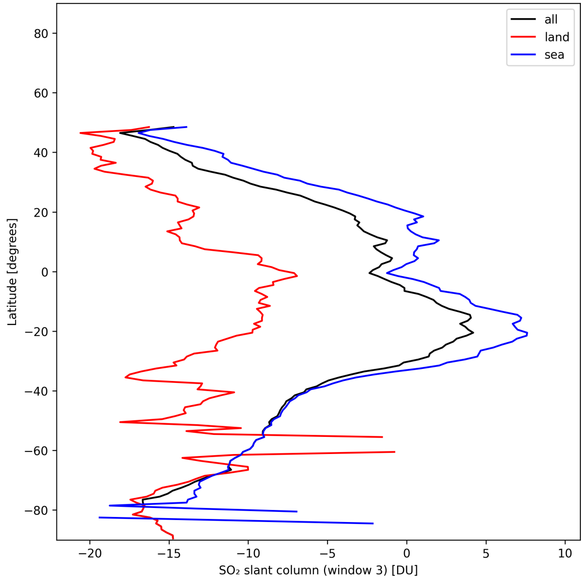
Figure 45: Zonal average of “SO 2 slant column (window 3)” for 2025-11-26 to 2025-11-28.
