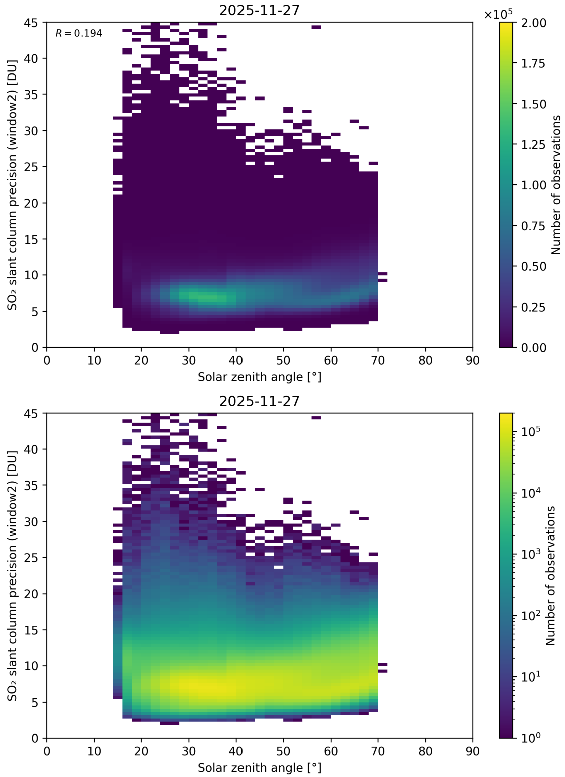
Figure 186: Scatter density plot of “Solar zenith angle” against “SO 2 slant column precision (window2)” for 2025-11-26 to 2025-11-28.
