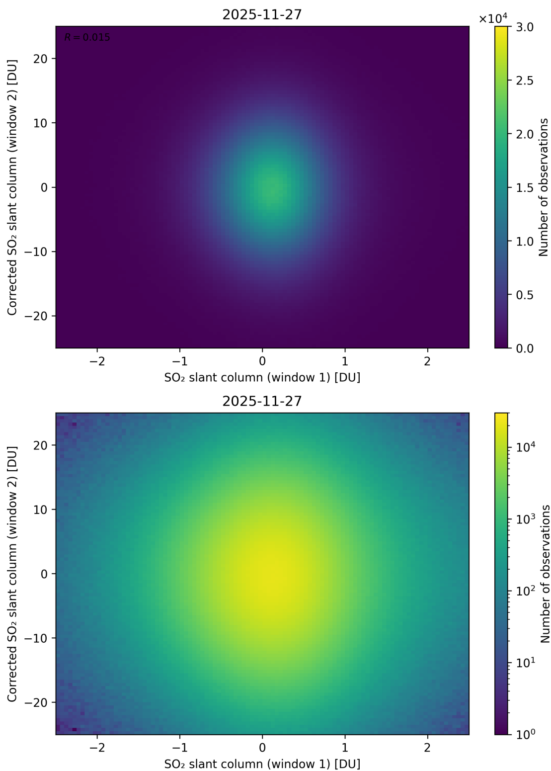
Figure 283: Scatter density plot of “SO 2 slant column (window 1)” against “Corrected SO 2 slant column (window 2)” for 2025-11-26 to 2025-11-28.
