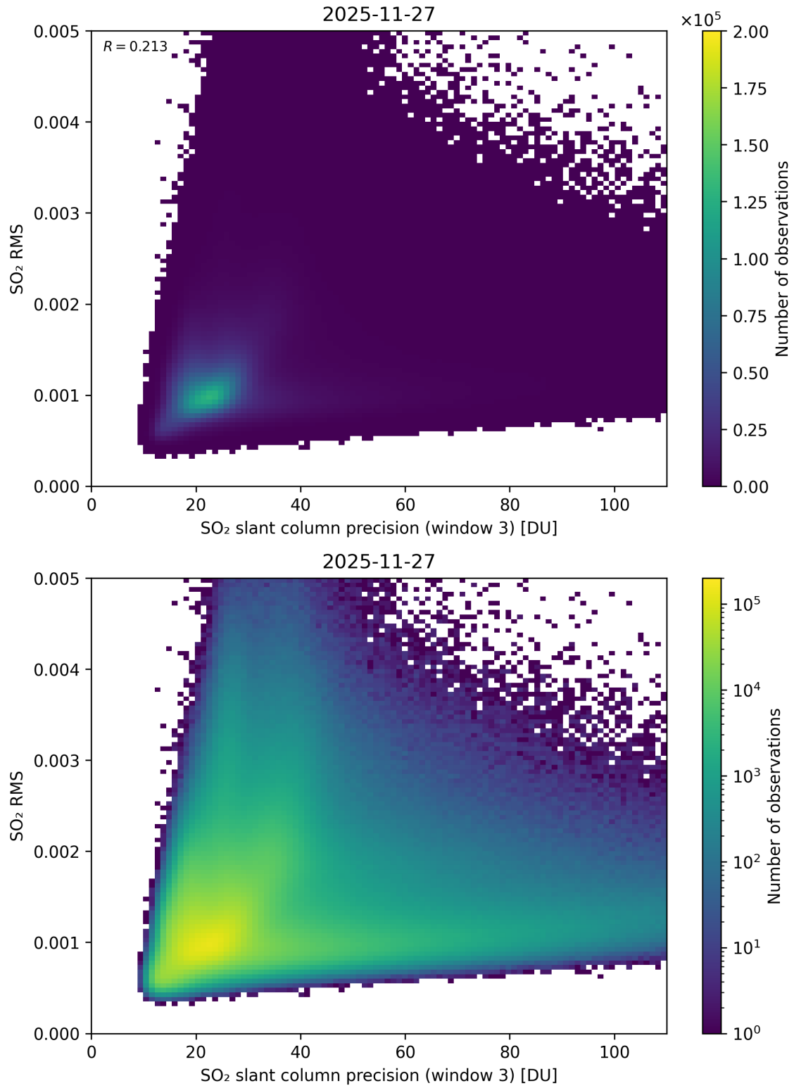
Figure 310: Scatter density plot of “SO 2 slant column precision (window 3)” against “SO 2 RMS” for 2025-11-26 to 2025-11-28.
