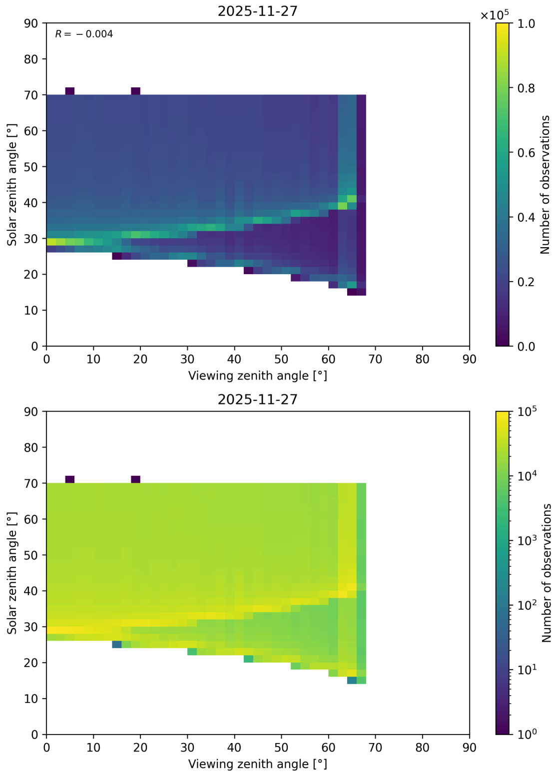
Figure 369: Scatter density plot of “Viewing zenith angle” against “Solar zenith angle” for 2025-11-26 to 2025-11-28.
