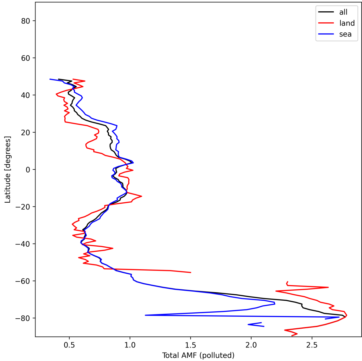
Figure 53: Zonal average of “Total AMF (polluted)” for 2025-11-26 to 2025-11-28.
