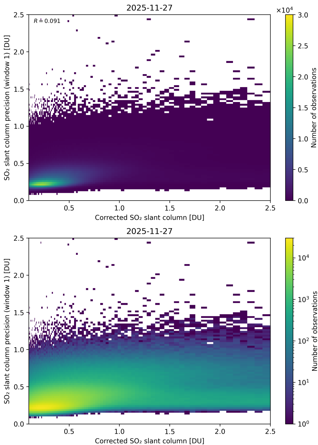
Figure 238: Scatter density plot of “Corrected SO 2 slant column” against “SO 2 slant column precision (window 1)” for 2025-11-26 to 2025-11-28.
