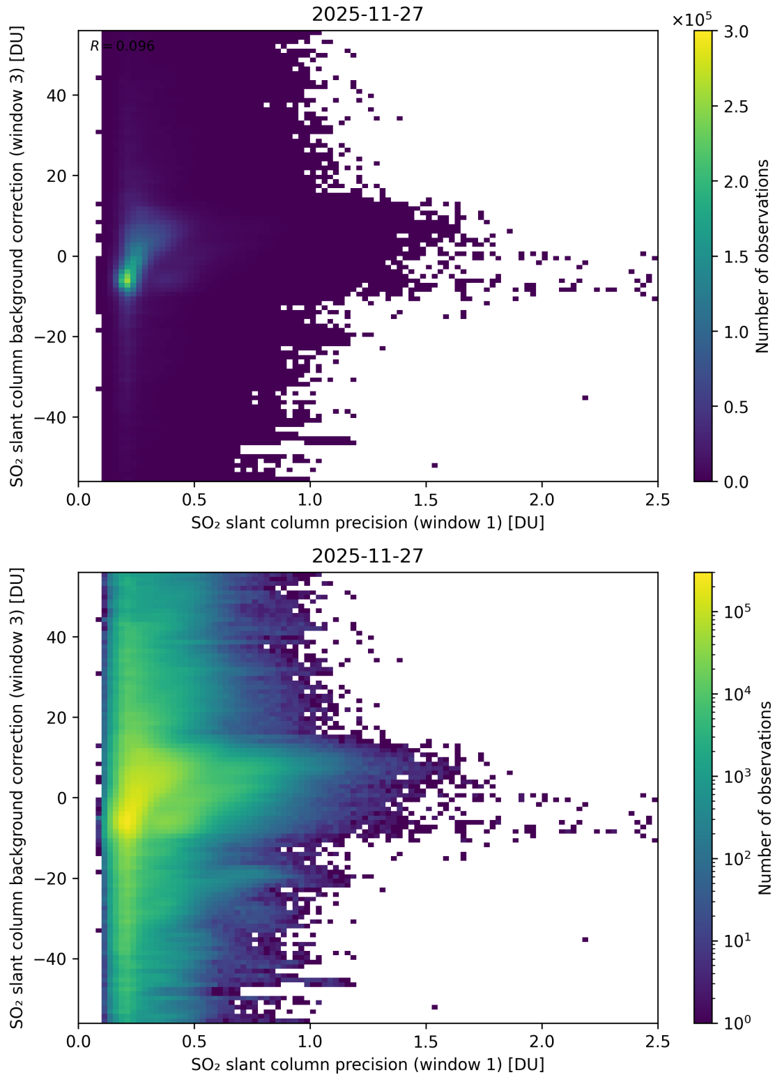
Figure 270: Scatter density plot of “SO 2 slant column precision (window 1)” against “SO 2 slant column background correction (window 3)” for 2025-11-26 to 2025-11-28.
