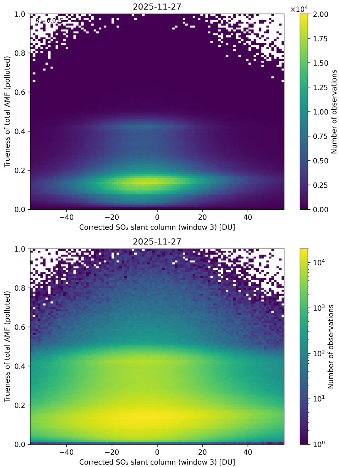
Figure 261: Scatter density plot of “Corrected SO 2 slant column (window 3)” against “Trueness of total AMF (polluted)” for 2025-11-26 to 2025-11-28.
