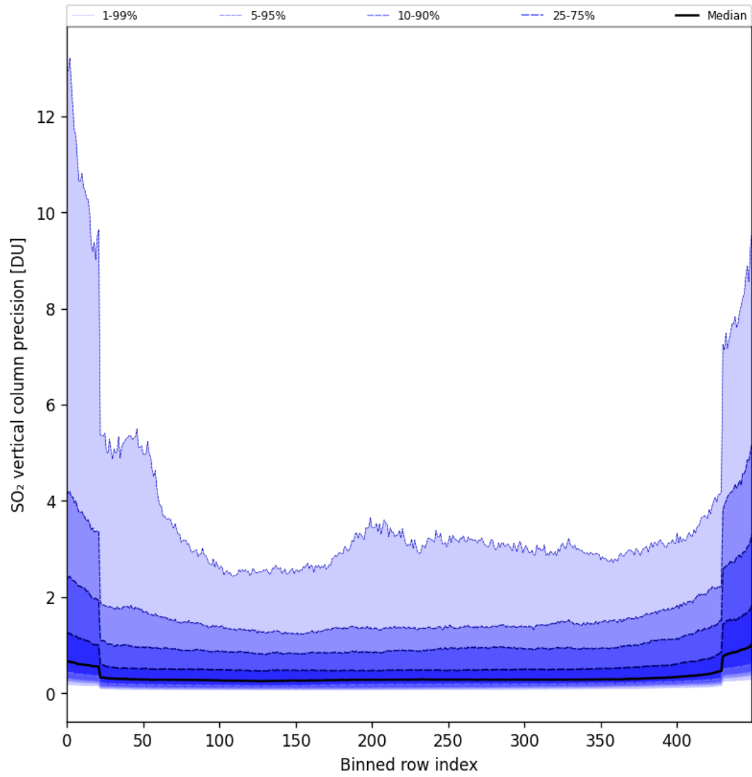
Figure 85: Along track statistics of “SO 2 vertical column precision” for 2025-11-26 to 2025-11-28
