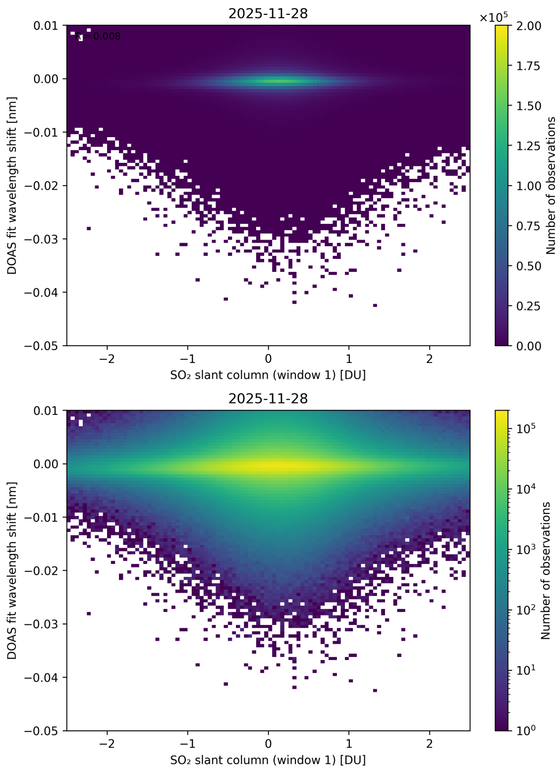
Figure 265: Scatter density plot of “SO 2 slant column (window 1)” against “DOAS fit wavelength shift” for 2025-11-28 to 2025-11-29.
