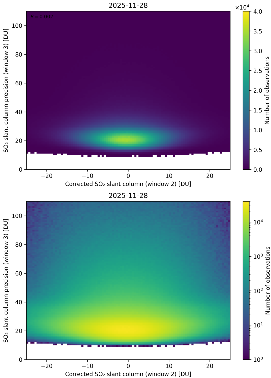
Figure 252: Scatter density plot of “Corrected SO 2 slant column (window 2)” against “SO 2 slant column precision (window 3)” for 2025-11-28 to 2025-11-29.
