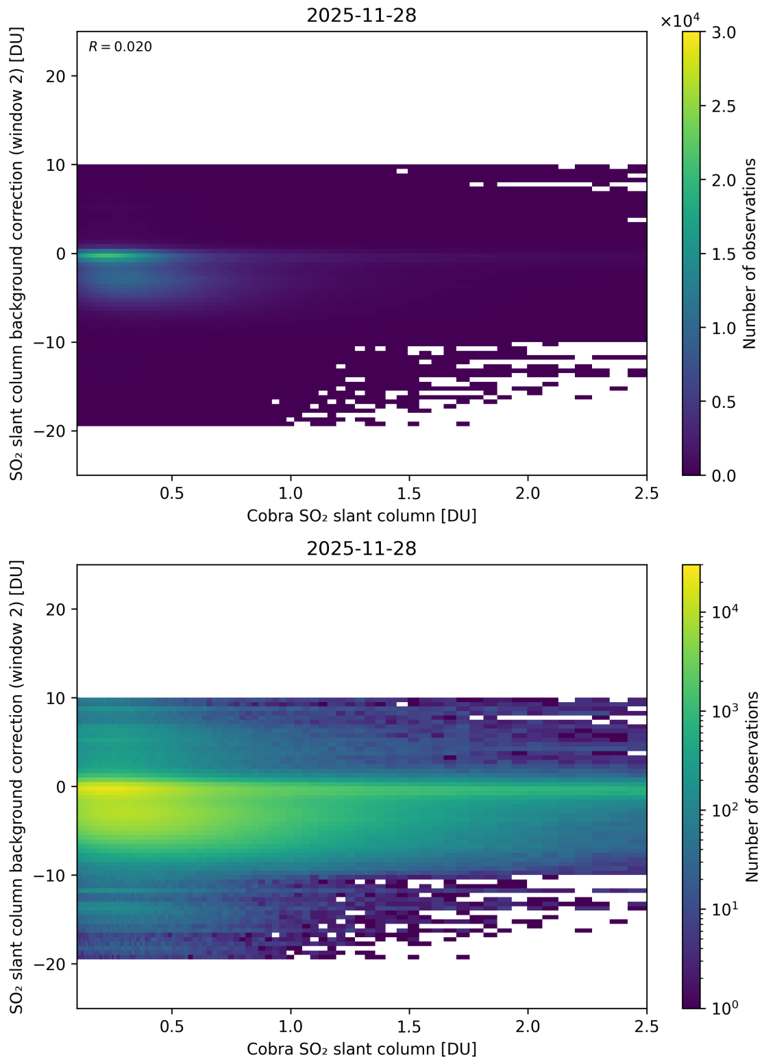
Figure 194: Scatter density plot of “Cobra SO 2 slant column” against “SO 2 slant column background correction (window 2)” for 2025-11-28 to 2025-11-29.
