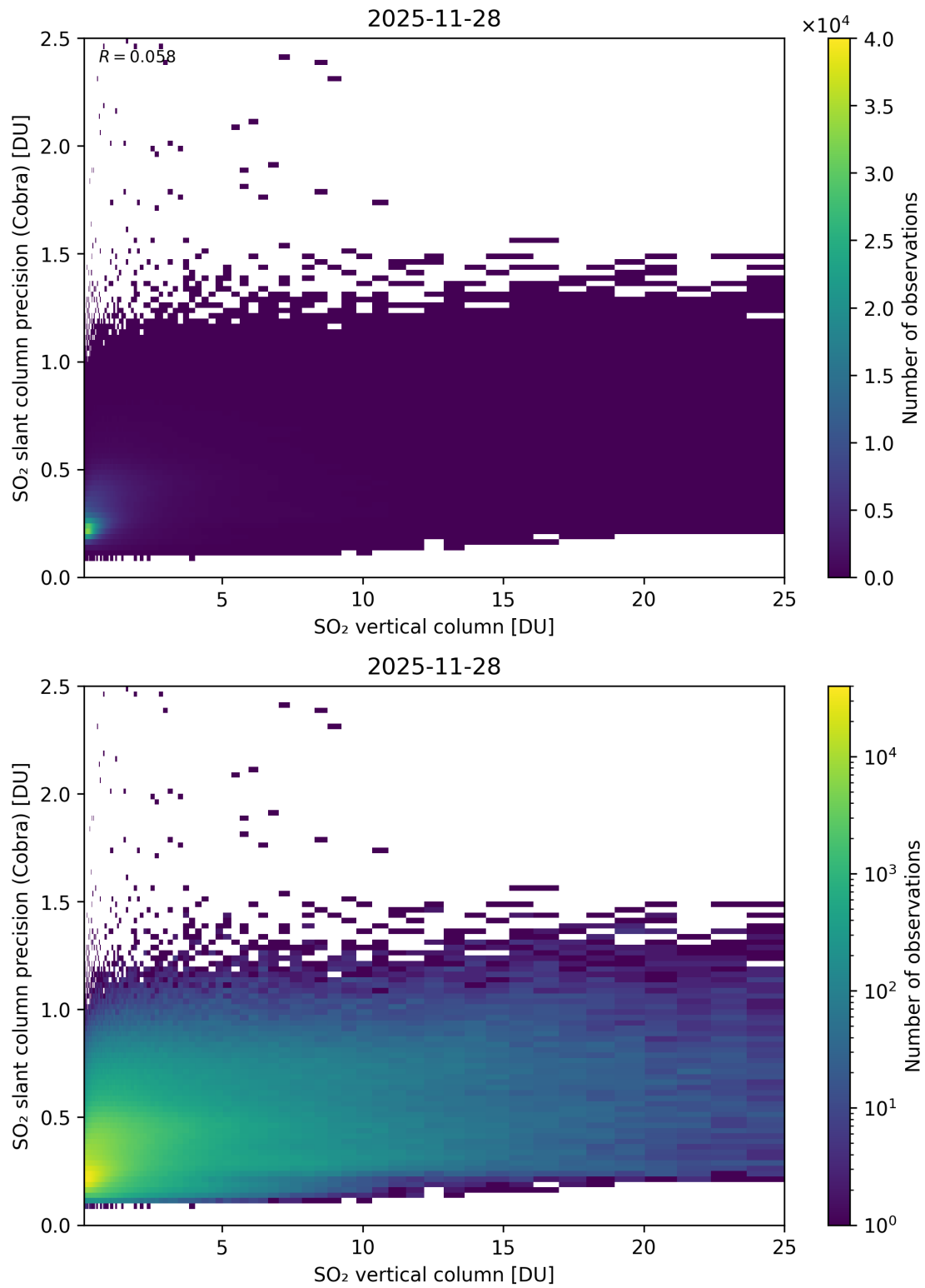
Figure 350: Scatter density plot of “SO 2 vertical column” against “SO 2 slant column precision (Cobra)” for 2025-11-28 to 2025-11-29.
