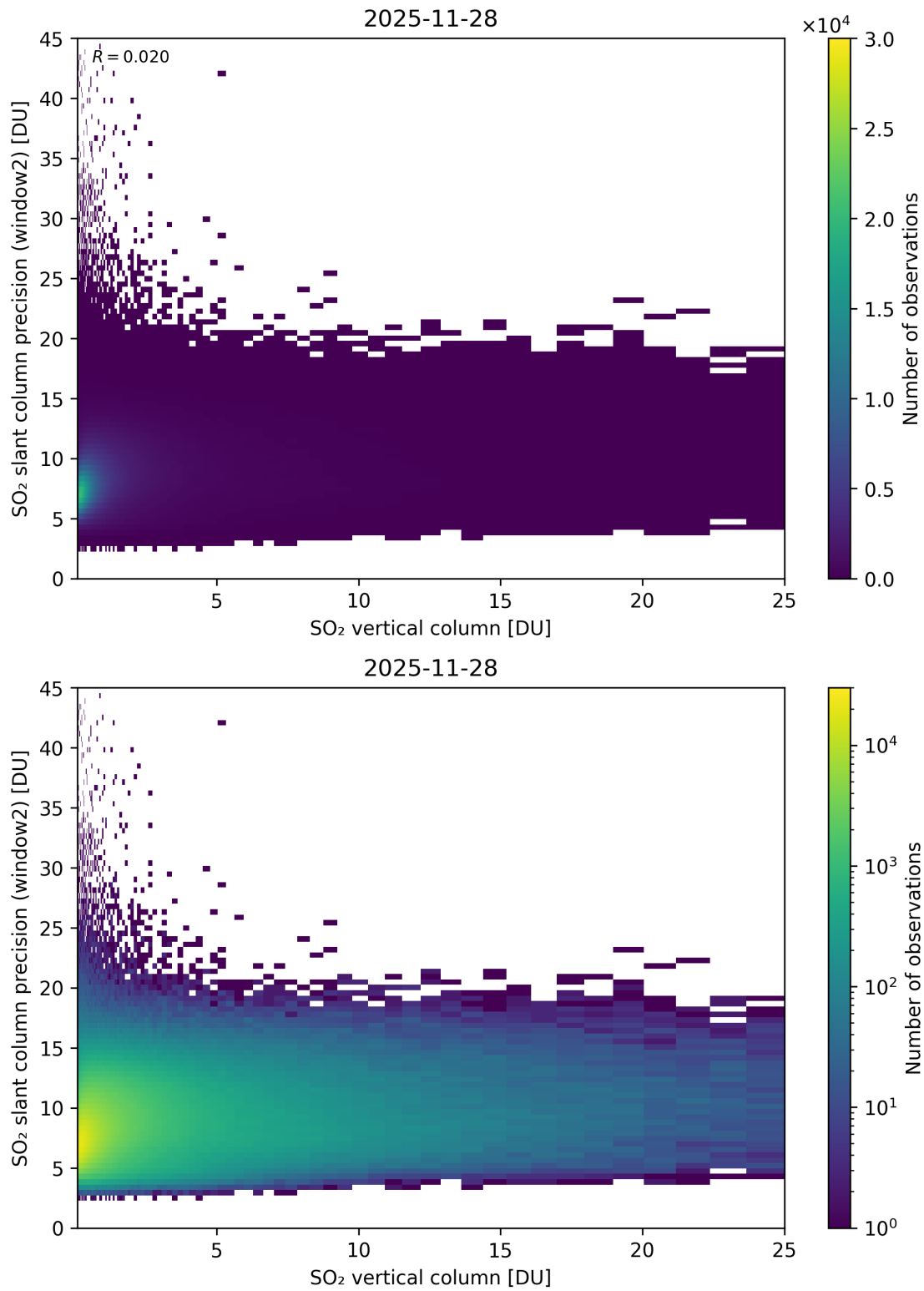
Figure 356: Scatter density plot of “SO 2 vertical column” against “SO 2 slant column precision (window2)” for 2025-11-28 to 2025-11-29.
