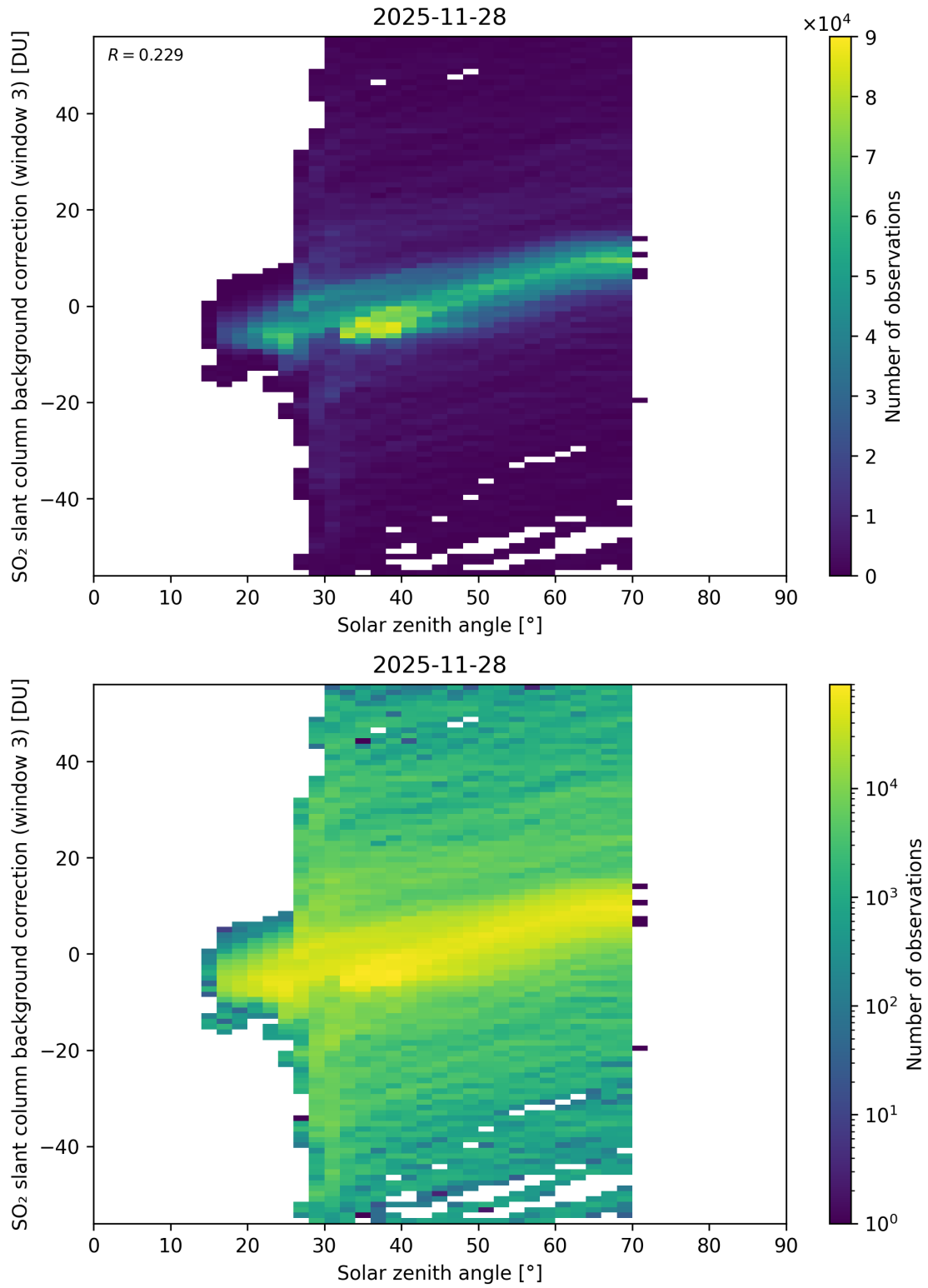
Figure 173: Scatter density plot of “Solar zenith angle” against “SO 2 slant column background correction (window 3)” for 2025-11-28 to 2025-11-29.
