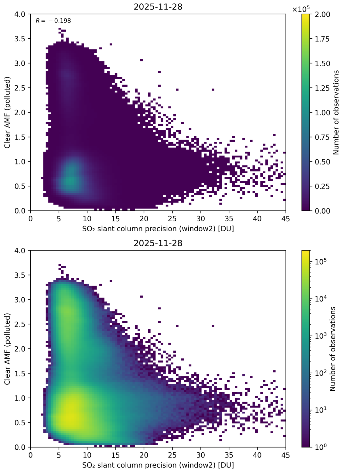
Figure 296: Scatter density plot of “SO 2 slant column precision (window2)” against “Clear AMF (polluted)” for 2025-11-28 to 2025-11-29.
