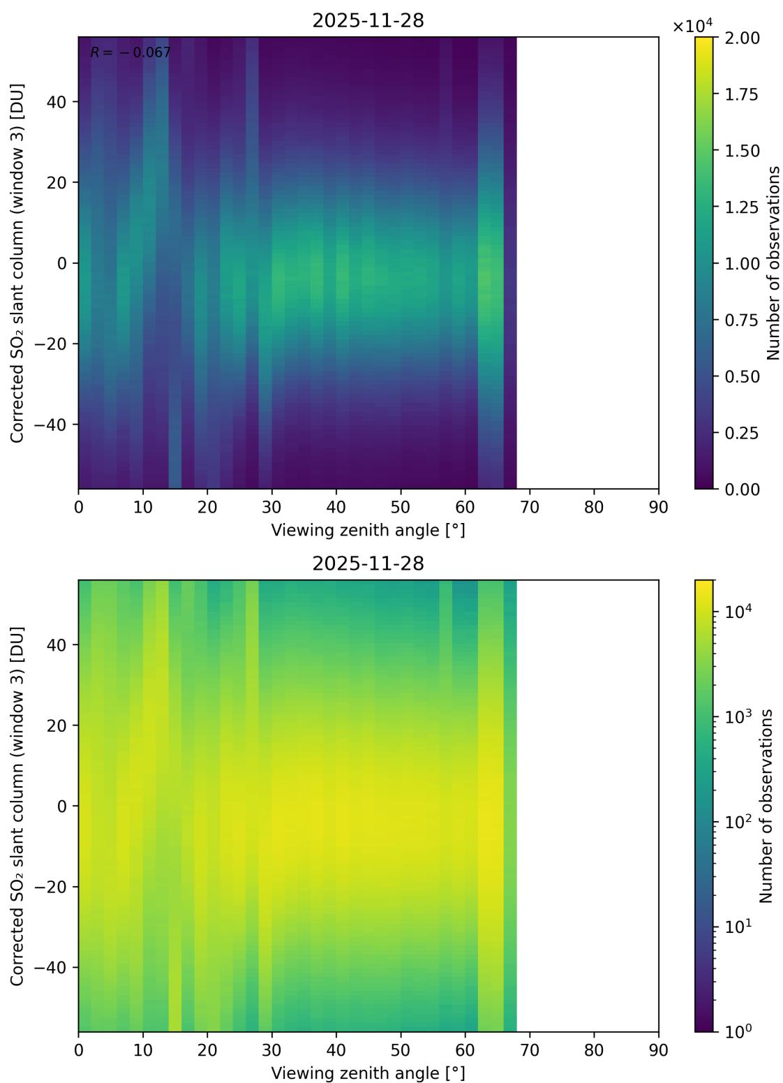
Figure 375: Scatter density plot of “Viewing zenith angle” against “Corrected SO 2 slant column (window 3)” for 2025-11-28 to 2025-11-29.
