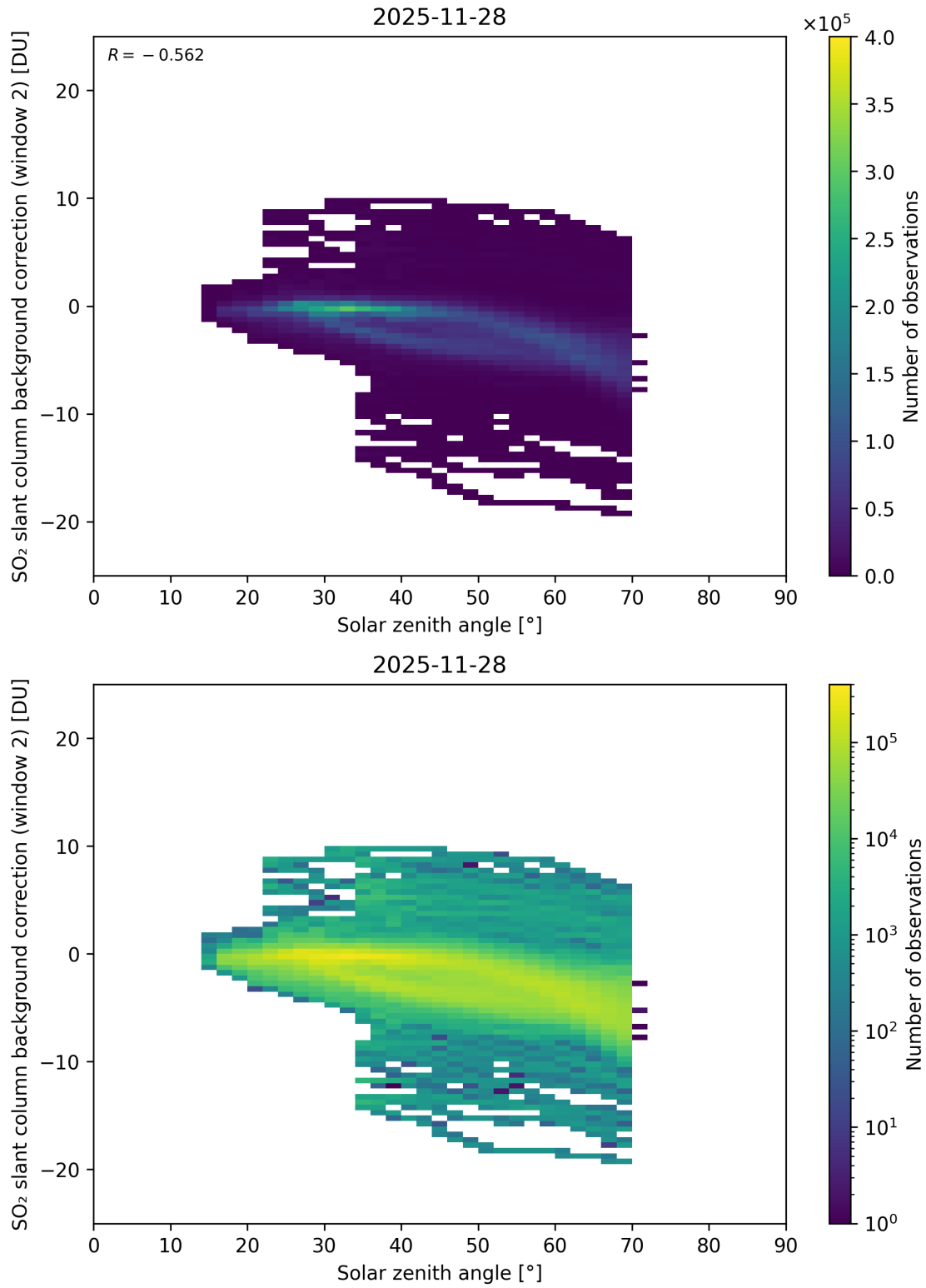
Figure 172: Scatter density plot of “Solar zenith angle” against “SO 2 slant column background correction (window 2)” for 2025-11-28 to 2025-11-29.
