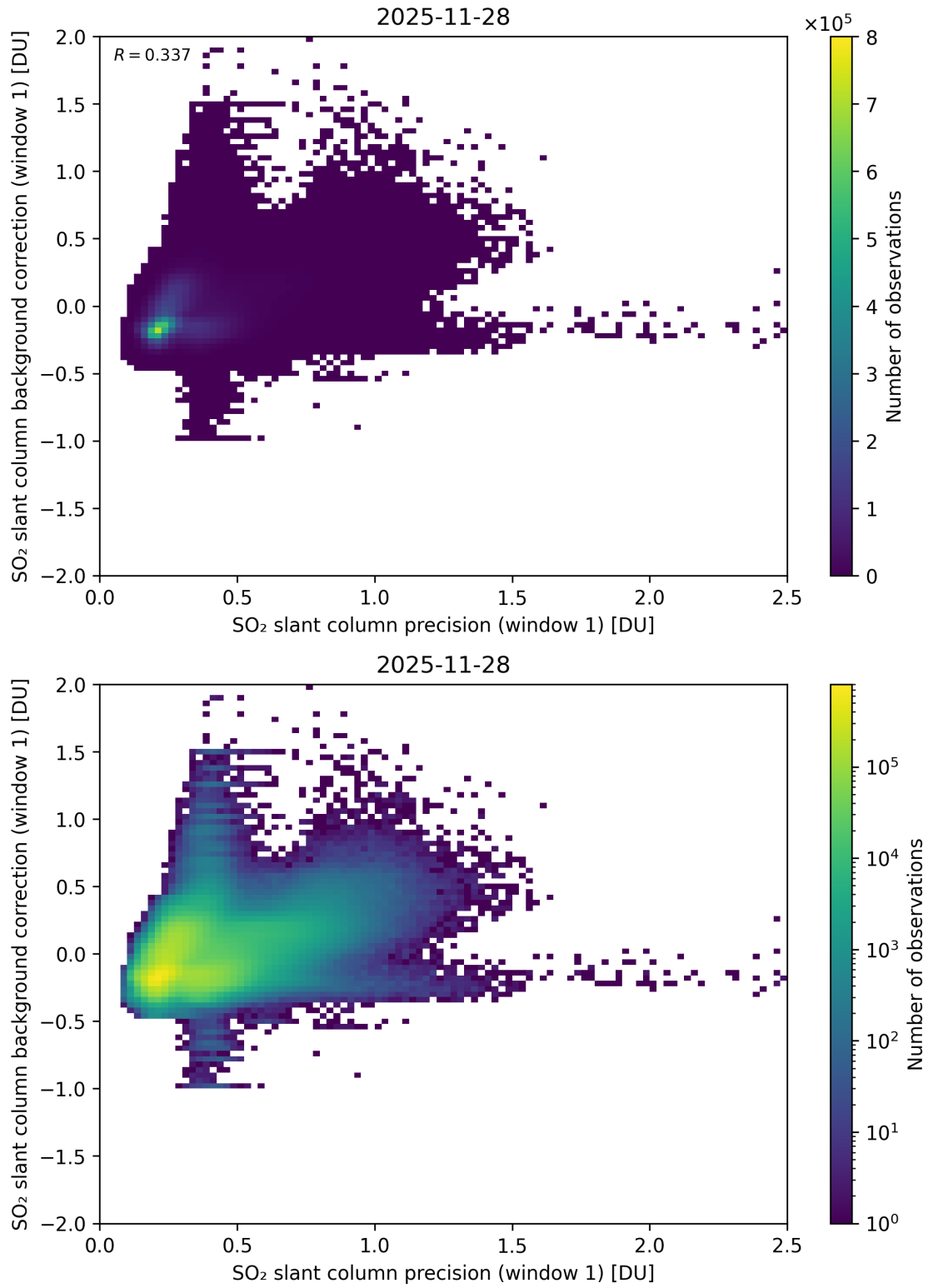
Figure 268: Scatter density plot of “SO 2 slant column precision (window 1)” against “SO 2 slant column background correction (window 1)” for 2025-11-28 to 2025-11-29.
