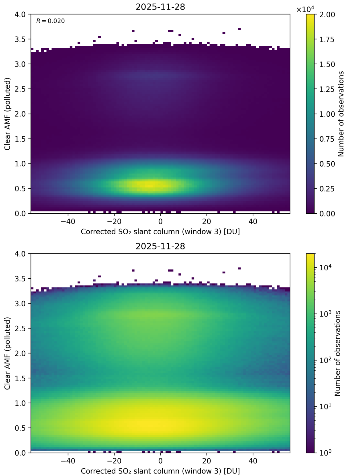
Figure 259: Scatter density plot of “Corrected SO 2 slant column (window 3)” against “Clear AMF (polluted)” for 2025-11-28 to 2025-11-29.
