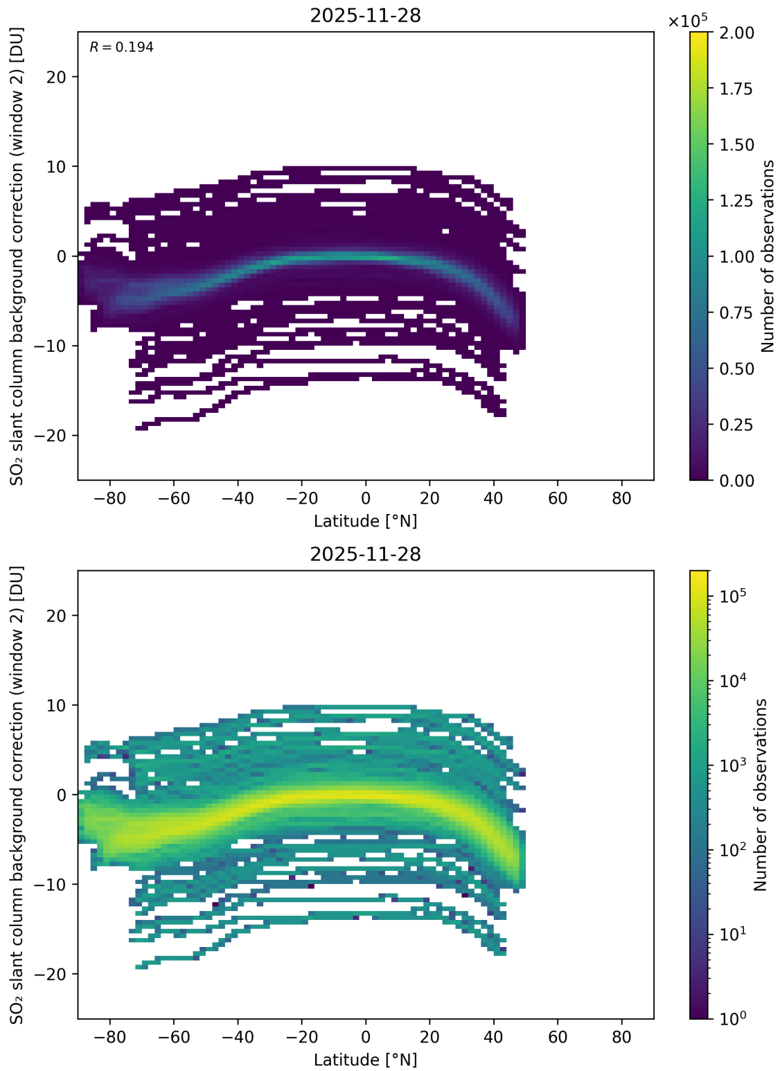
Figure 151: Scatter density plot of “Latitude” against “SO 2 slant column background correction (window 2)” for 2025-11-28 to 2025-11-29.
