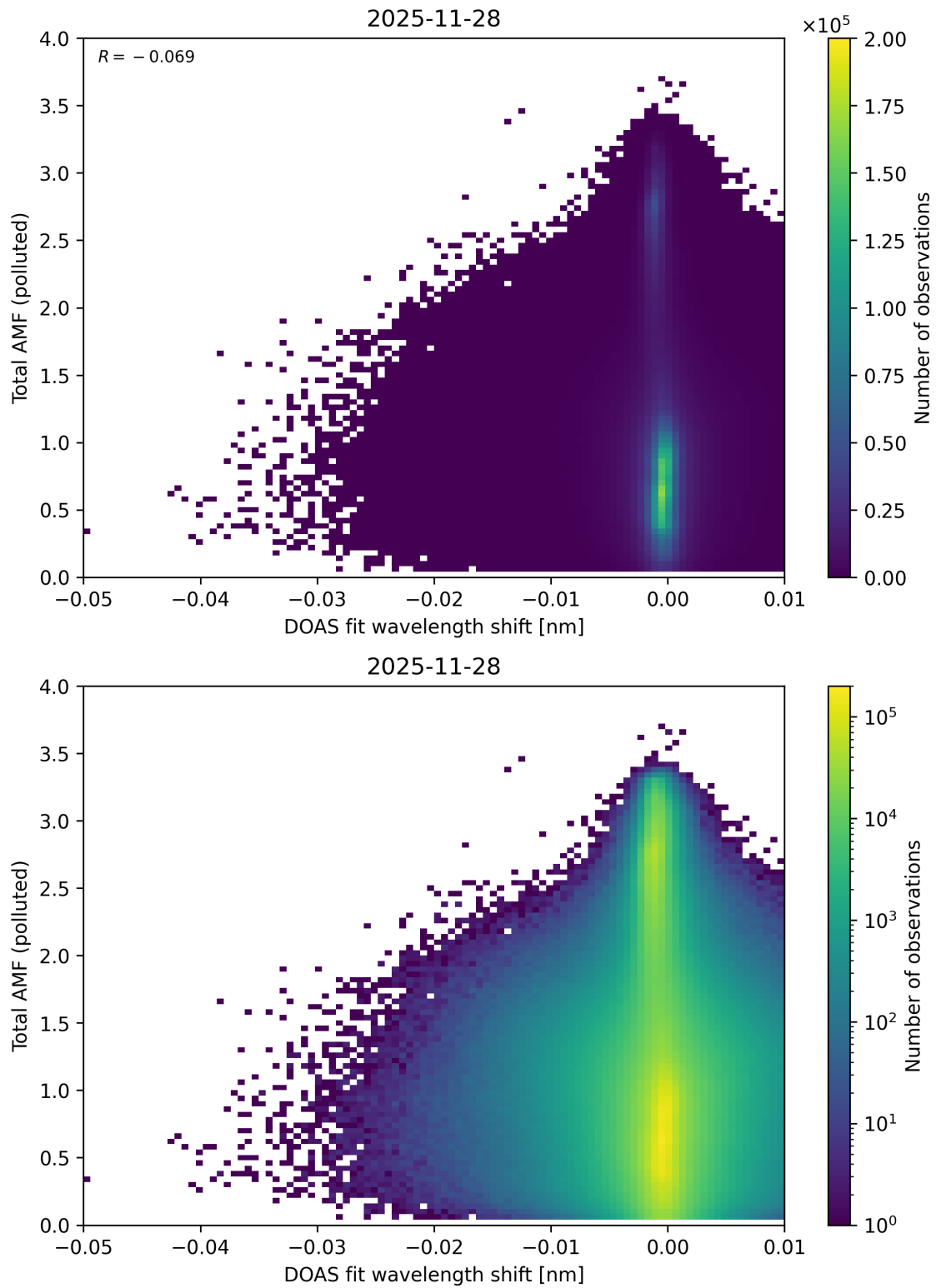
Figure 141: Scatter density plot of “DOAS fit wavelength shift” against “Total AMF (polluted)” for 2025-11-28 to 2025-11-29.
