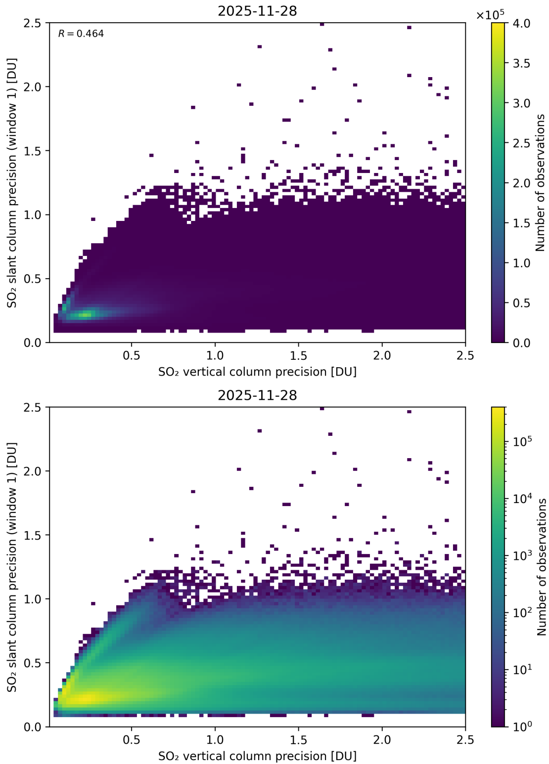
Figure 342: Scatter density plot of “SO 2 vertical column precision” against “SO 2 slant column precision (window 1)” for 2025-11-28 to 2025-11-29.
