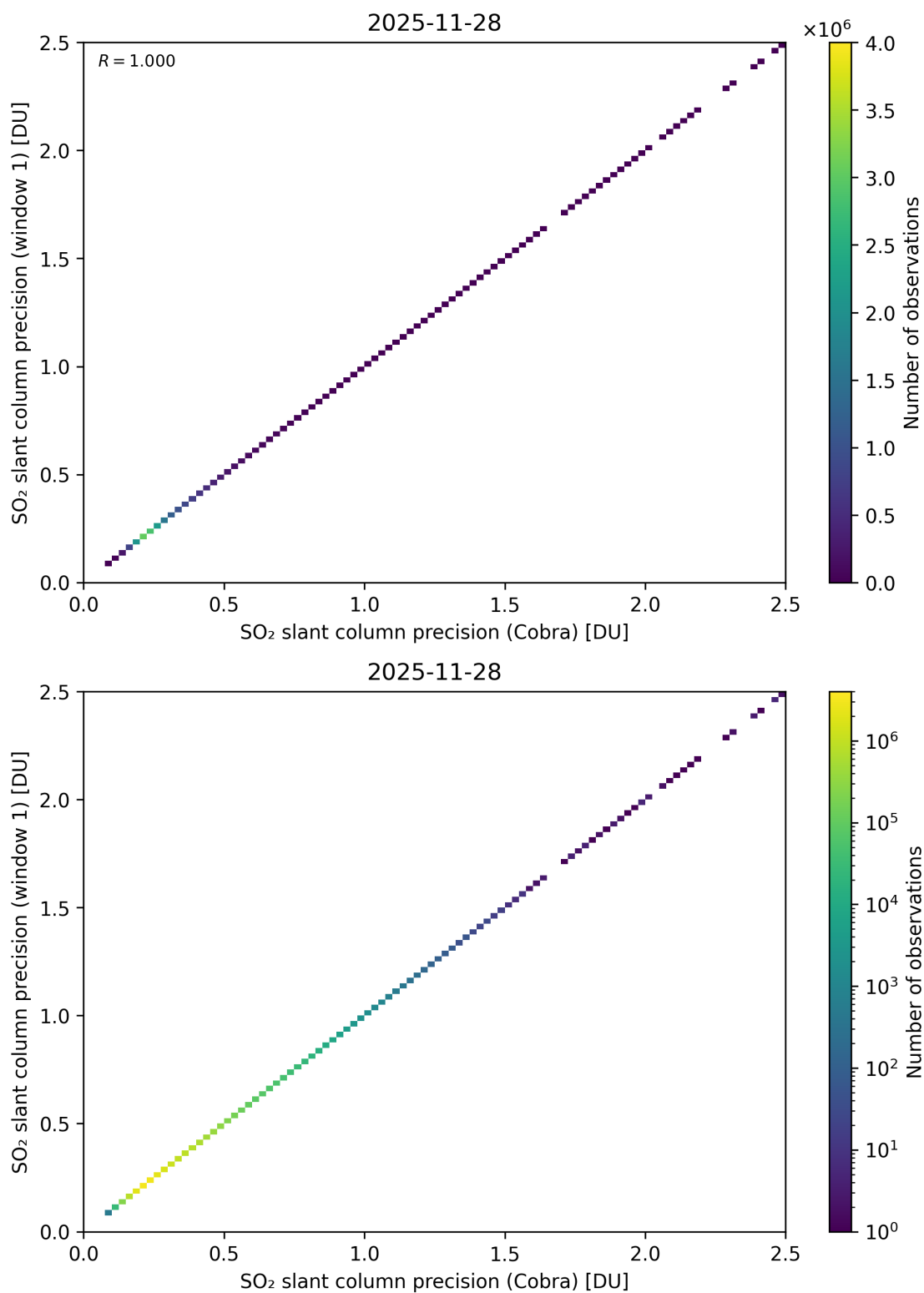
Figure 209: Scatter density plot of “SO 2 slant column precision (Cobra)” against “SO 2 slant column precision (window 1)” for 2025-11-28 to 2025-11-29.
