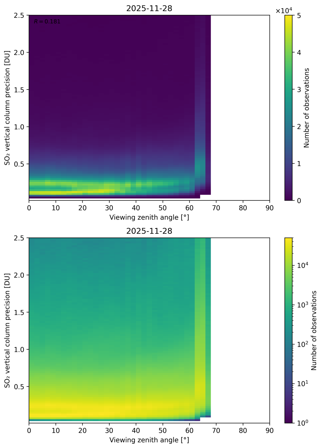
Figure 384: Scatter density plot of “Viewing zenith angle” against “SO 2 vertical column precision” for 2025-11-28 to 2025-11-29.
