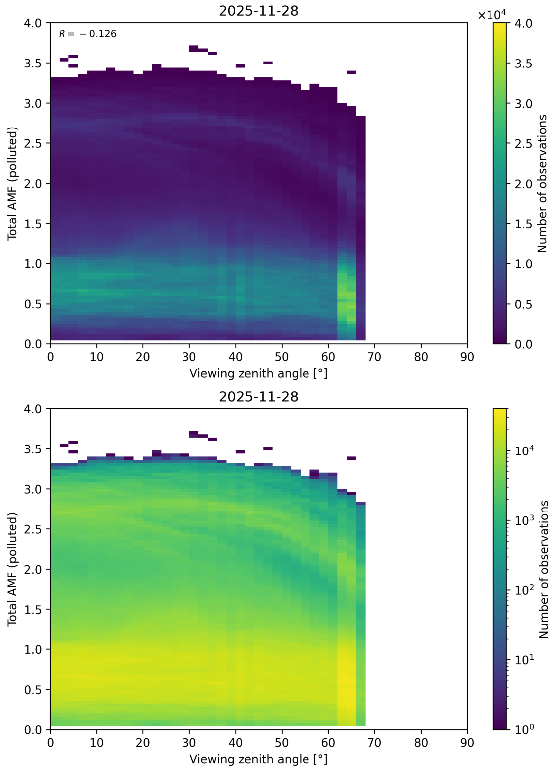
Figure 381: Scatter density plot of “Viewing zenith angle” against “Total AMF (polluted)” for 2025-11-28 to 2025-11-29.
