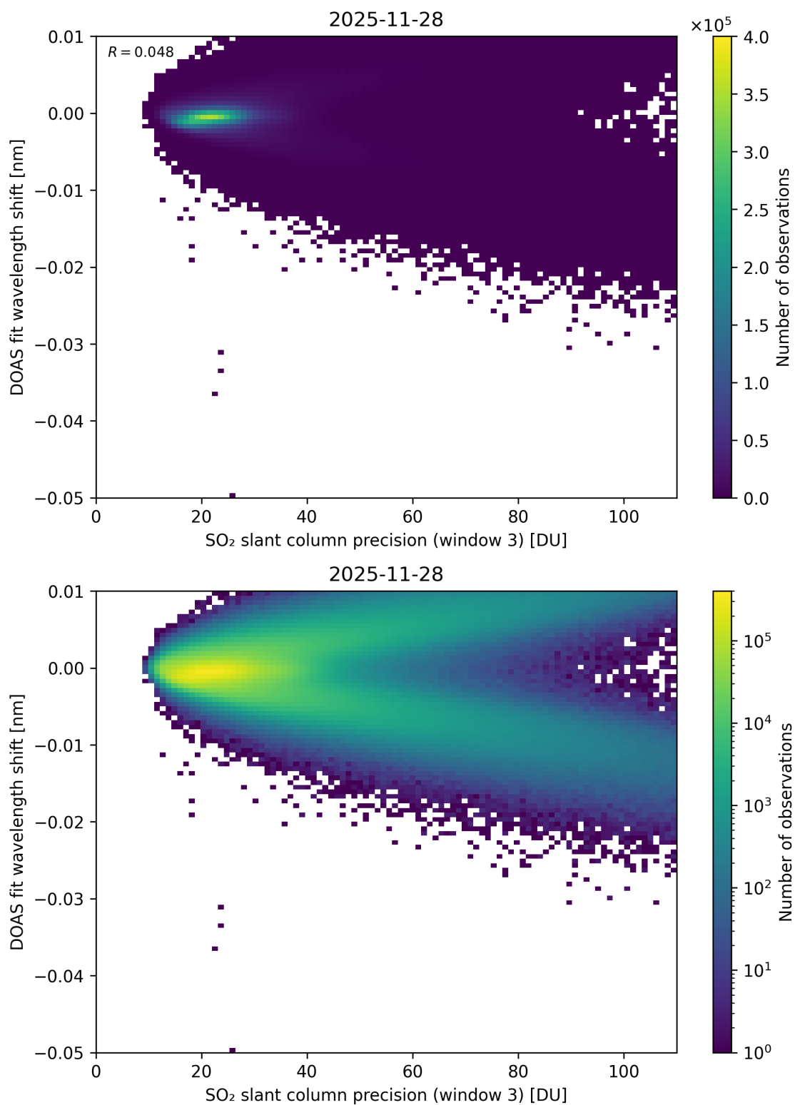
Figure 308: Scatter density plot of “SO 2 slant column precision (window 3)” against “DOAS fit wavelength shift” for 2025-11-28 to 2025-11-29.
