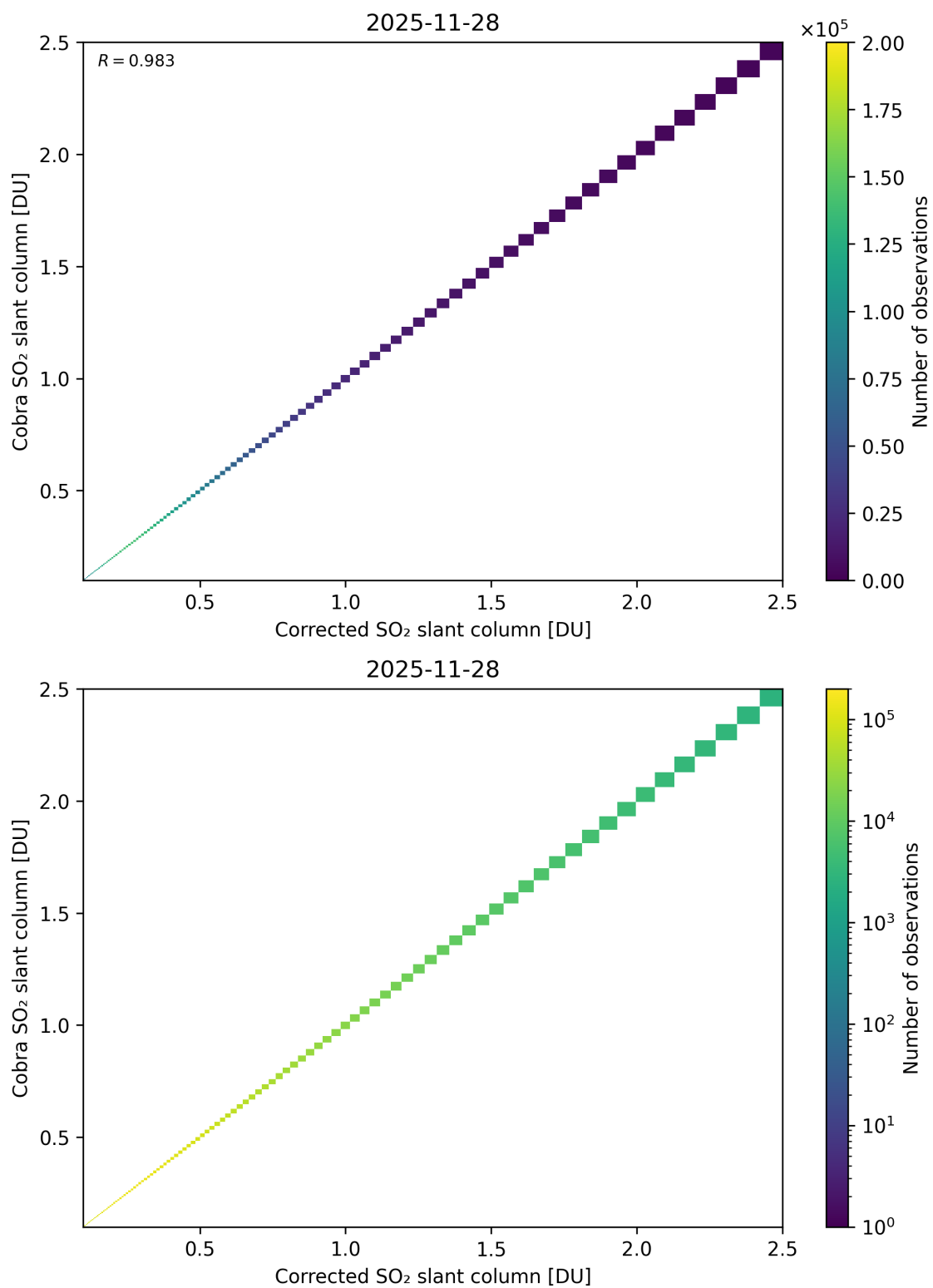
Figure 233: Scatter density plot of “Corrected SO 2 slant column” against “Cobra SO 2 slant column” for 2025-11-28 to 2025-11-29.
