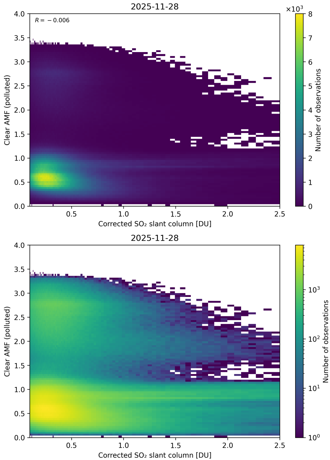
Figure 232: Scatter density plot of “Corrected SO 2 slant column” against “Clear AMF (polluted)” for 2025-11-28 to 2025-11-29.
