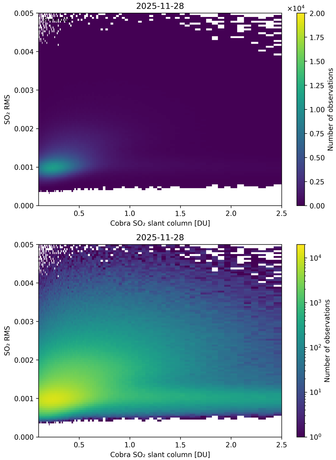
Figure 198: Scatter density plot of “Cobra SO 2 slant column” against “SO 2 RMS” for 2025-11-28 to 2025-11-29.
