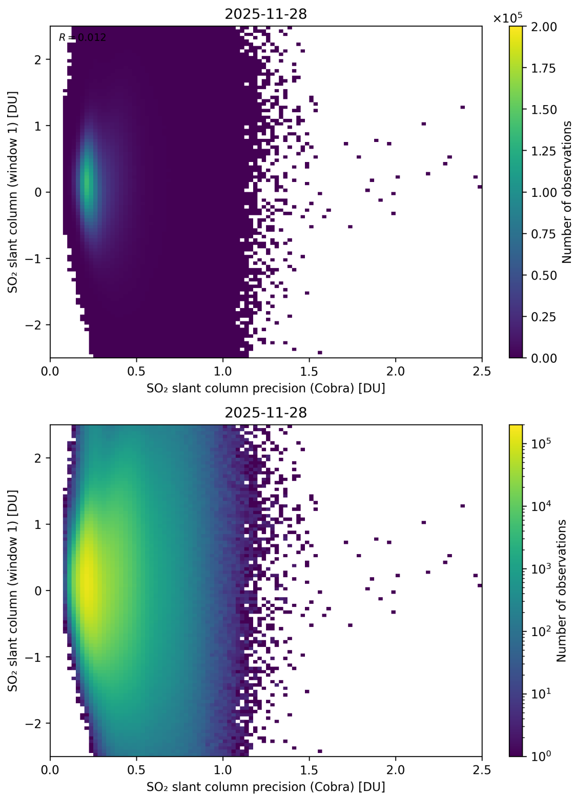
Figure 208: Scatter density plot of “SO 2 slant column precision (Cobra)” against “SO 2 slant column (window 1)” for 2025-11-28 to 2025-11-29.
