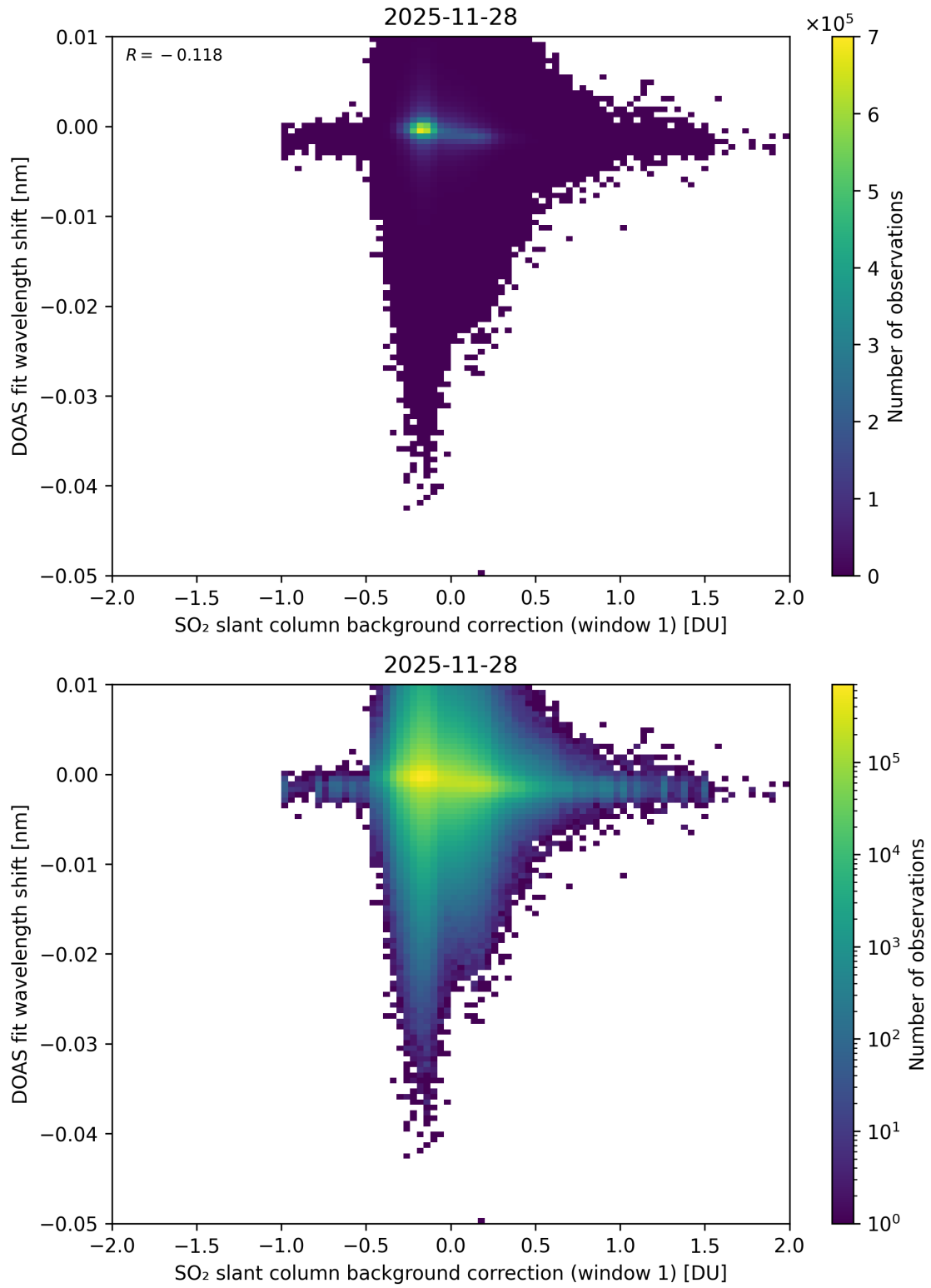
Figure 111: Scatter density plot of “SO 2 slant column background correction (window 1)” against “DOAS fit wavelength shift” for 2025-11-28 to 2025-11-29.
