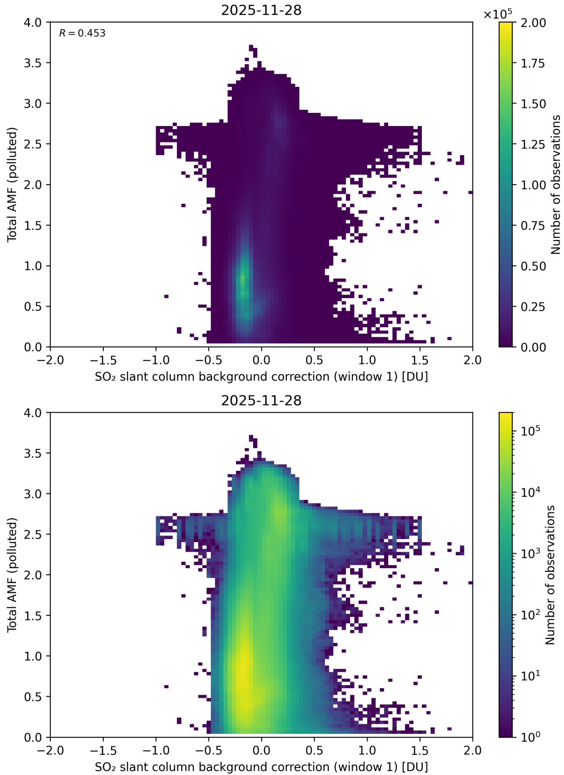
Figure 120: Scatter density plot of “SO 2 slant column background correction (window 1)” against “Total AMF (polluted)” for 2025-11-28 to 2025-11-29.
