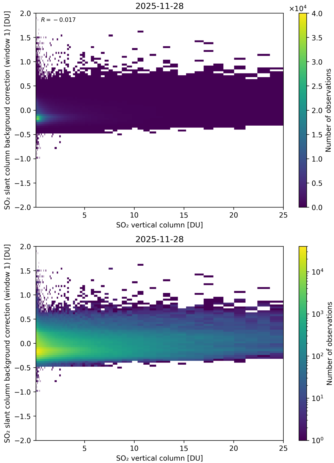
Figure 323: Scatter density plot of “SO 2 vertical column” against “SO 2 slant column background correction (window 1)” for 2025-11-28 to 2025-11-29.
