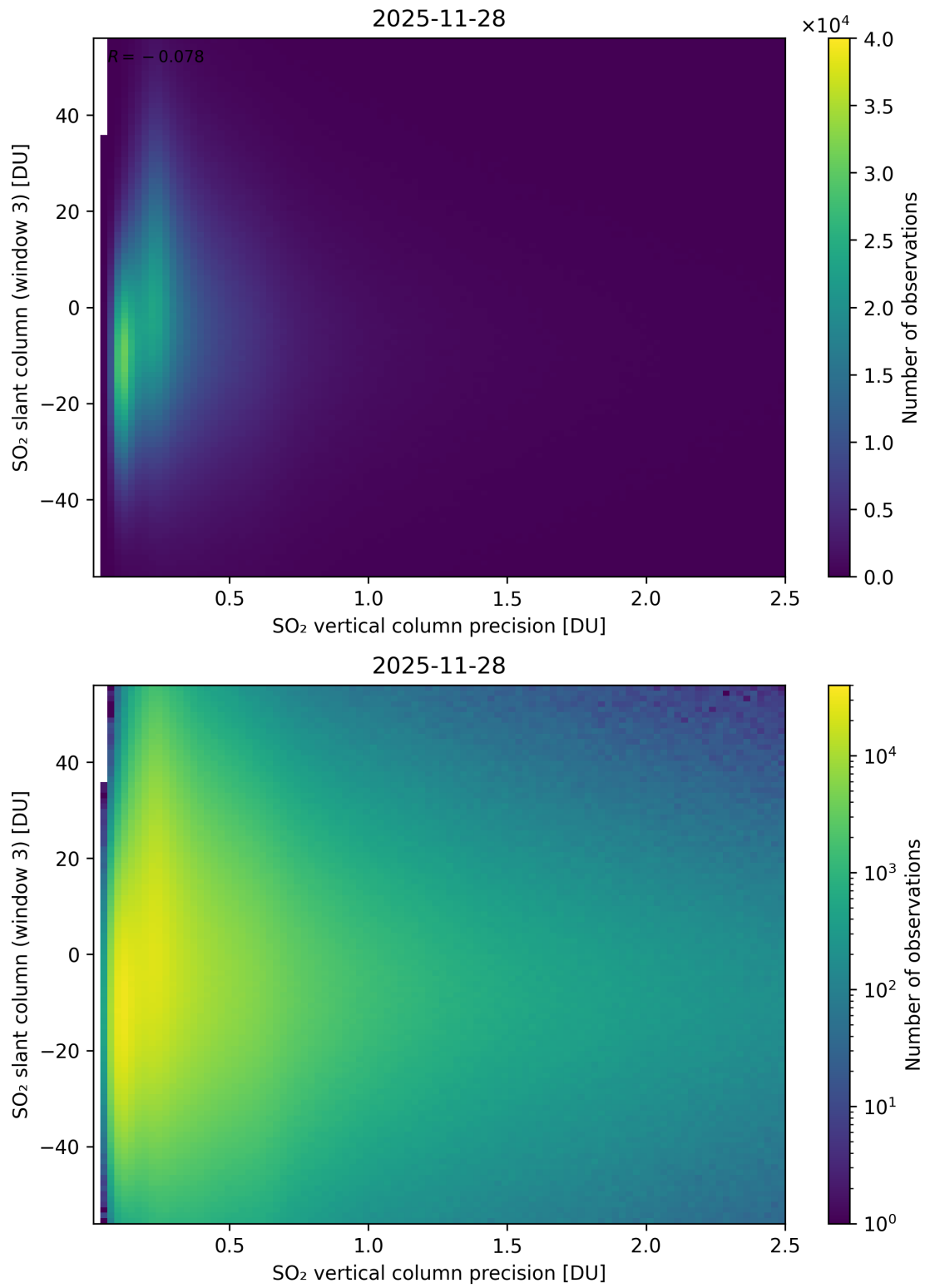
Figure 344: Scatter density plot of “SO 2 vertical column precision” against “SO 2 slant column (window 3)” for 2025-11-28 to 2025-11-29.
