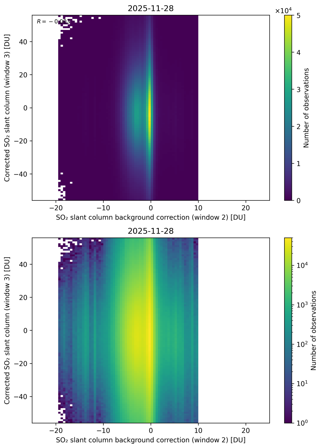
Figure 127: Scatter density plot of “SO 2 slant column background correction (window 2)” against “Corrected SO 2 slant column (window 3)” for 2025-11-28 to 2025-11-29.
