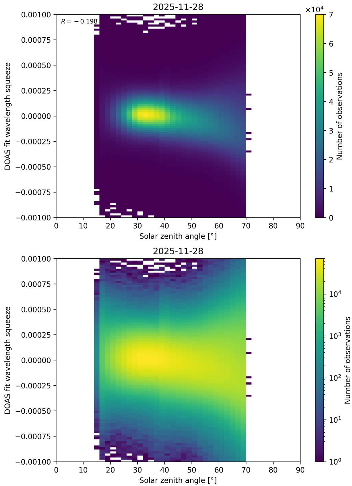
Figure 175: Scatter density plot of “Solar zenith angle” against “DOAS fit wavelength squeeze” for 2025-11-28 to 2025-11-29.
