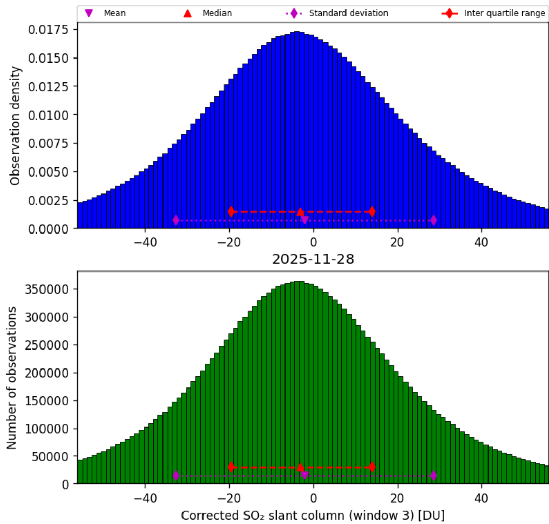
Figure 73: Histogram of “Corrected SO 2 slant column (window 3)” for 2025-11-28 to 2025-11-29
