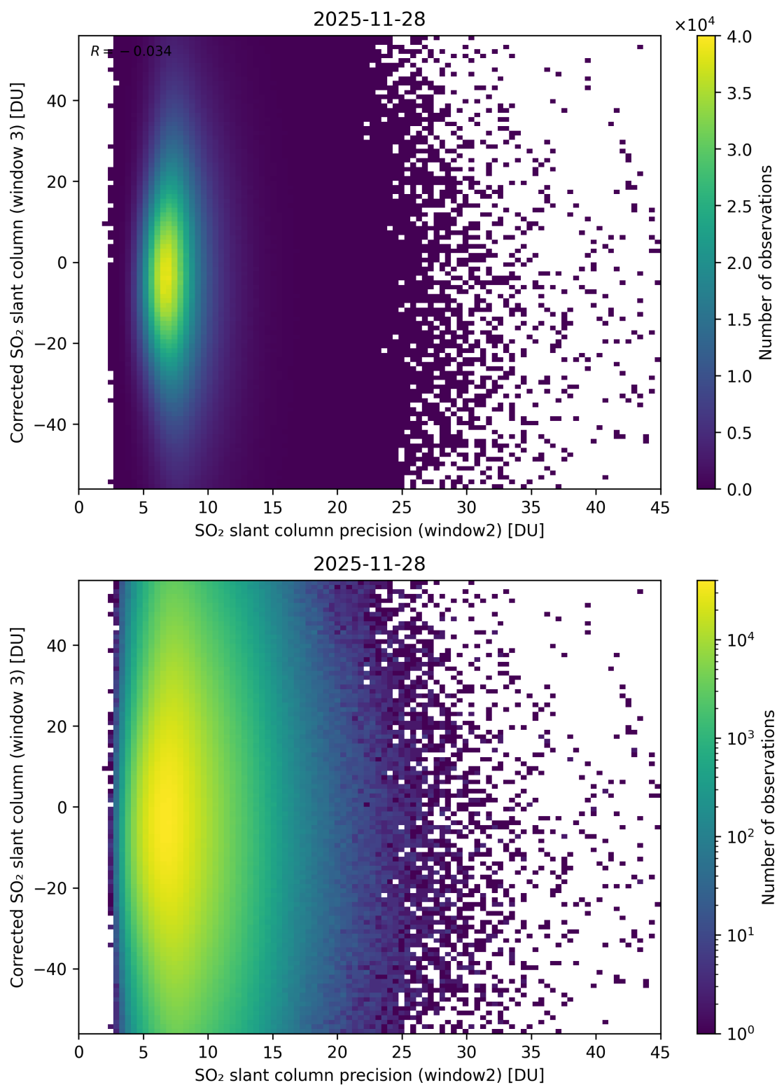
Figure 298: Scatter density plot of “SO 2 slant column precision (window2)” against “Corrected SO 2 slant column (window 3)” for 2025-11-28 to 2025-11-29.
