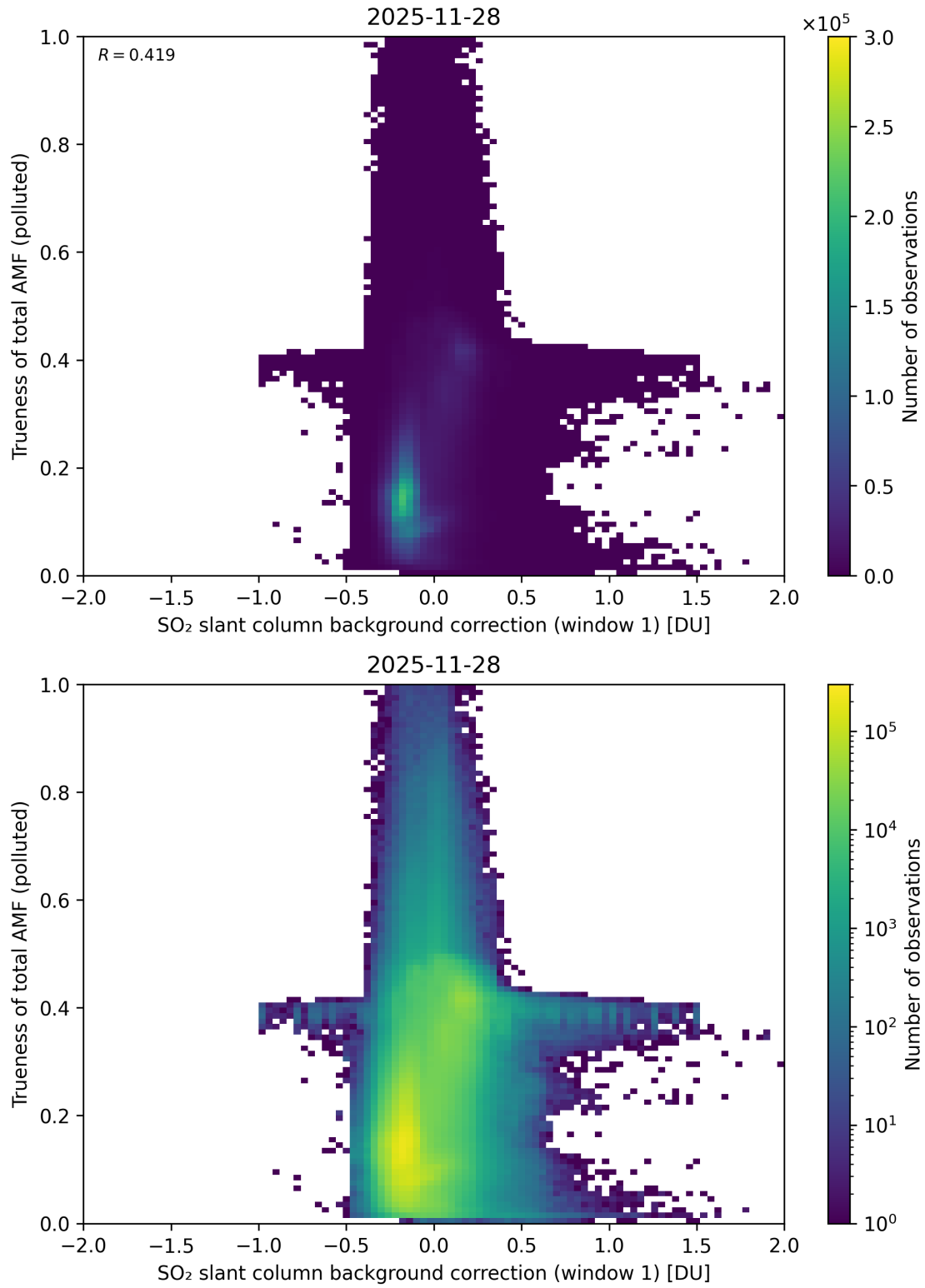
Figure 121: Scatter density plot of “SO 2 slant column background correction (window 1)” against “Trueness of total AMF (polluted)” for 2025-11-28 to 2025-11-29.
