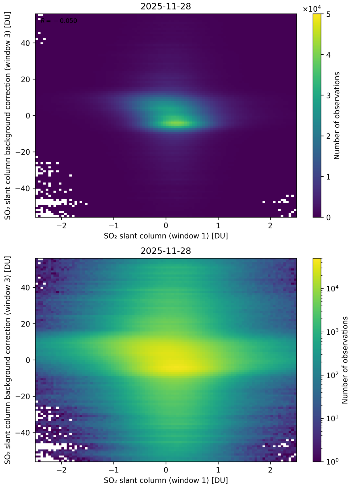
Figure 264: Scatter density plot of “SO 2 slant column (window 1)” against “SO 2 slant column background correction (window 3)” for 2025-11-28 to 2025-11-29.
