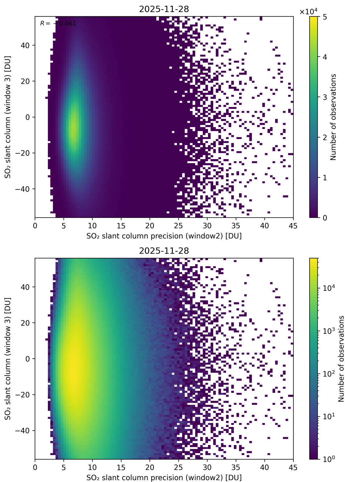
Figure 299: Scatter density plot of “SO 2 slant column precision (window2)” against “SO 2 slant column (window 3)” for 2025-11-28 to 2025-11-29.
