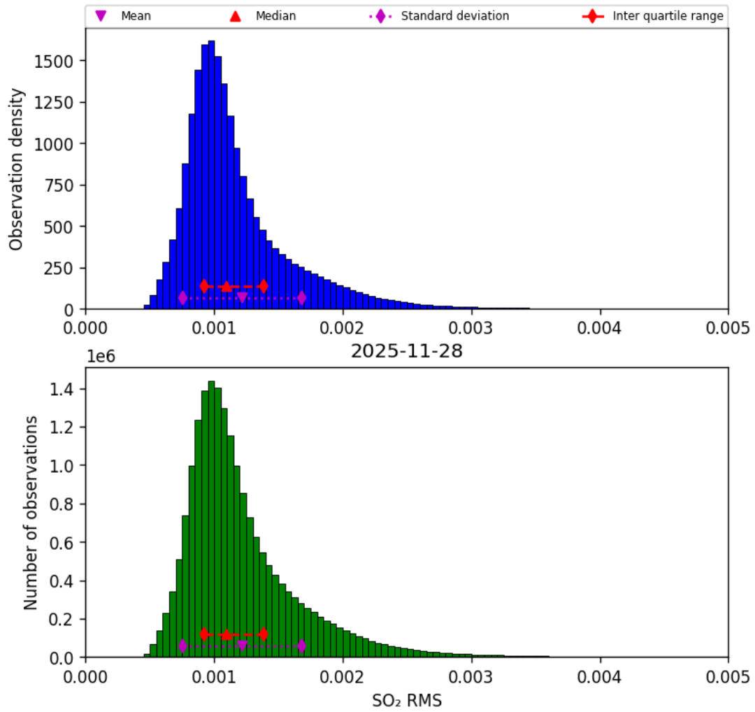
Figure 78: Histogram of “SO 2 RMS” for 2025-11-28 to 2025-11-29
