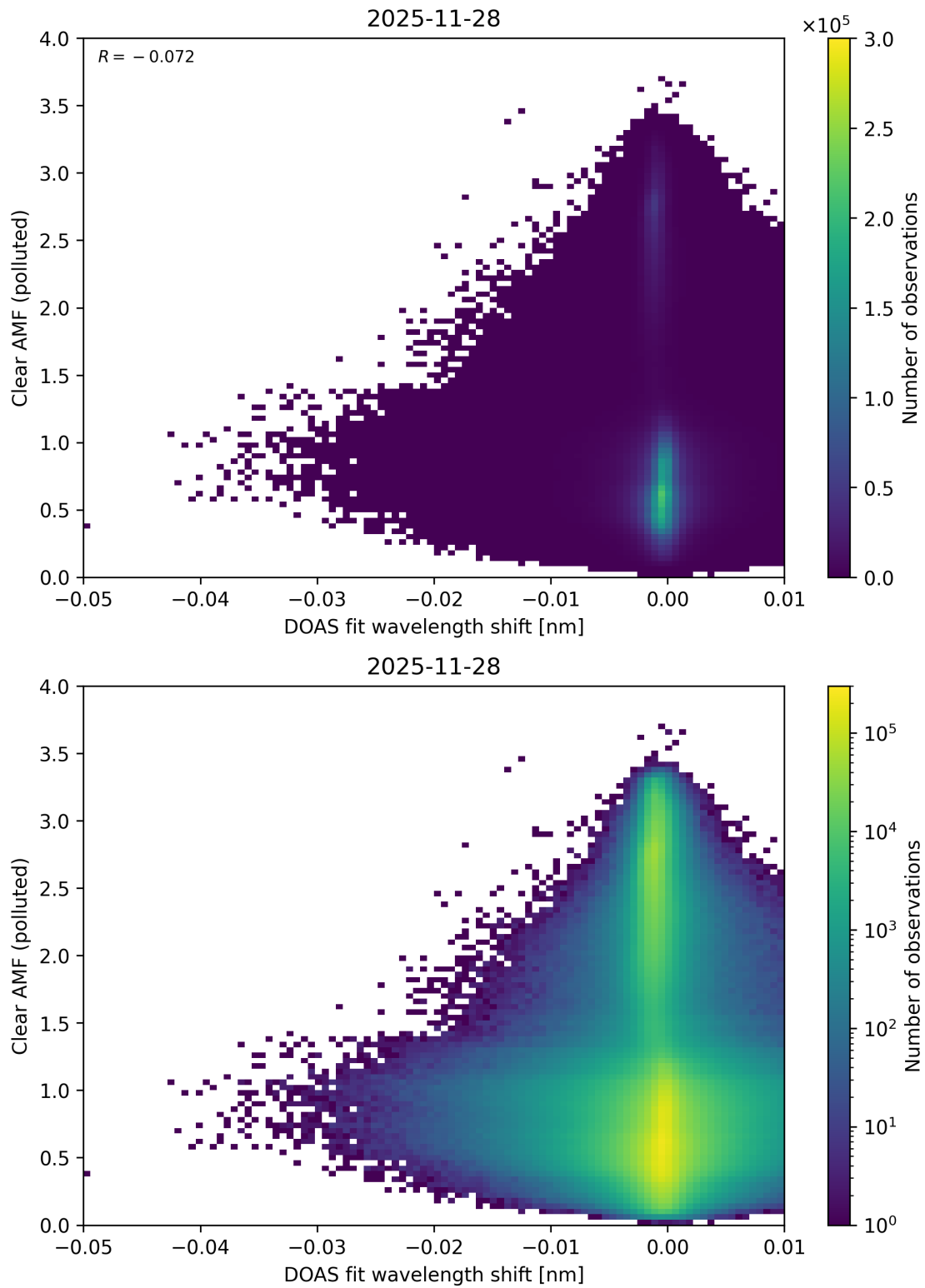
Figure 140: Scatter density plot of “DOAS fit wavelength shift” against “Clear AMF (polluted)” for 2025-11-28 to 2025-11-29.
