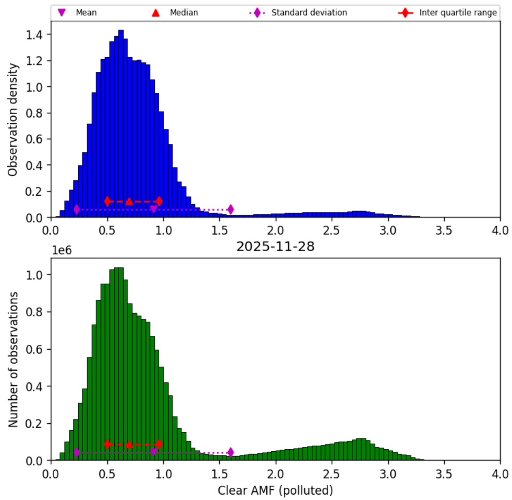
Figure 81: Histogram of “Clear AMF (polluted)” for 2025-11-28 to 2025-11-29
