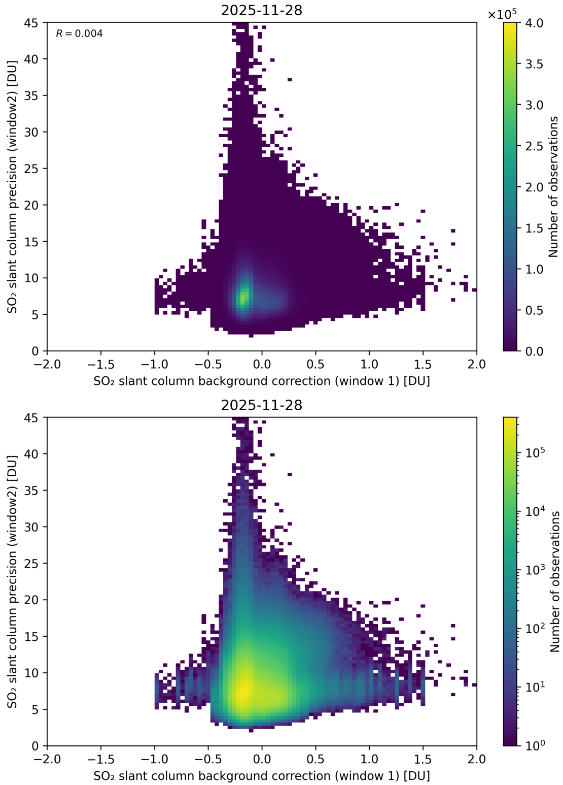
Figure 117: Scatter density plot of “SO 2 slant column background correction (window 1)” against “SO 2 slant column precision (window2)” for 2025-11-28 to 2025-11-29.
