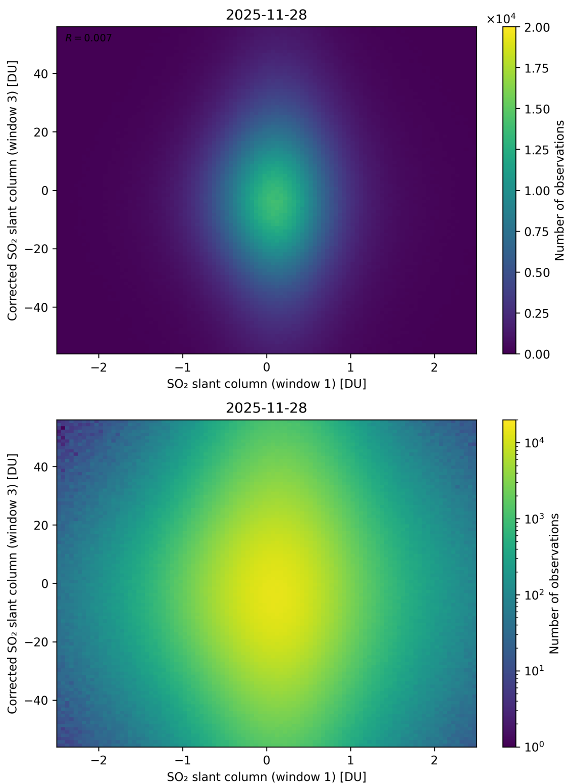
Figure 284: Scatter density plot of “SO 2 slant column (window 1)” against “Corrected SO 2 slant column (window 3)” for 2025-11-28 to 2025-11-29.
