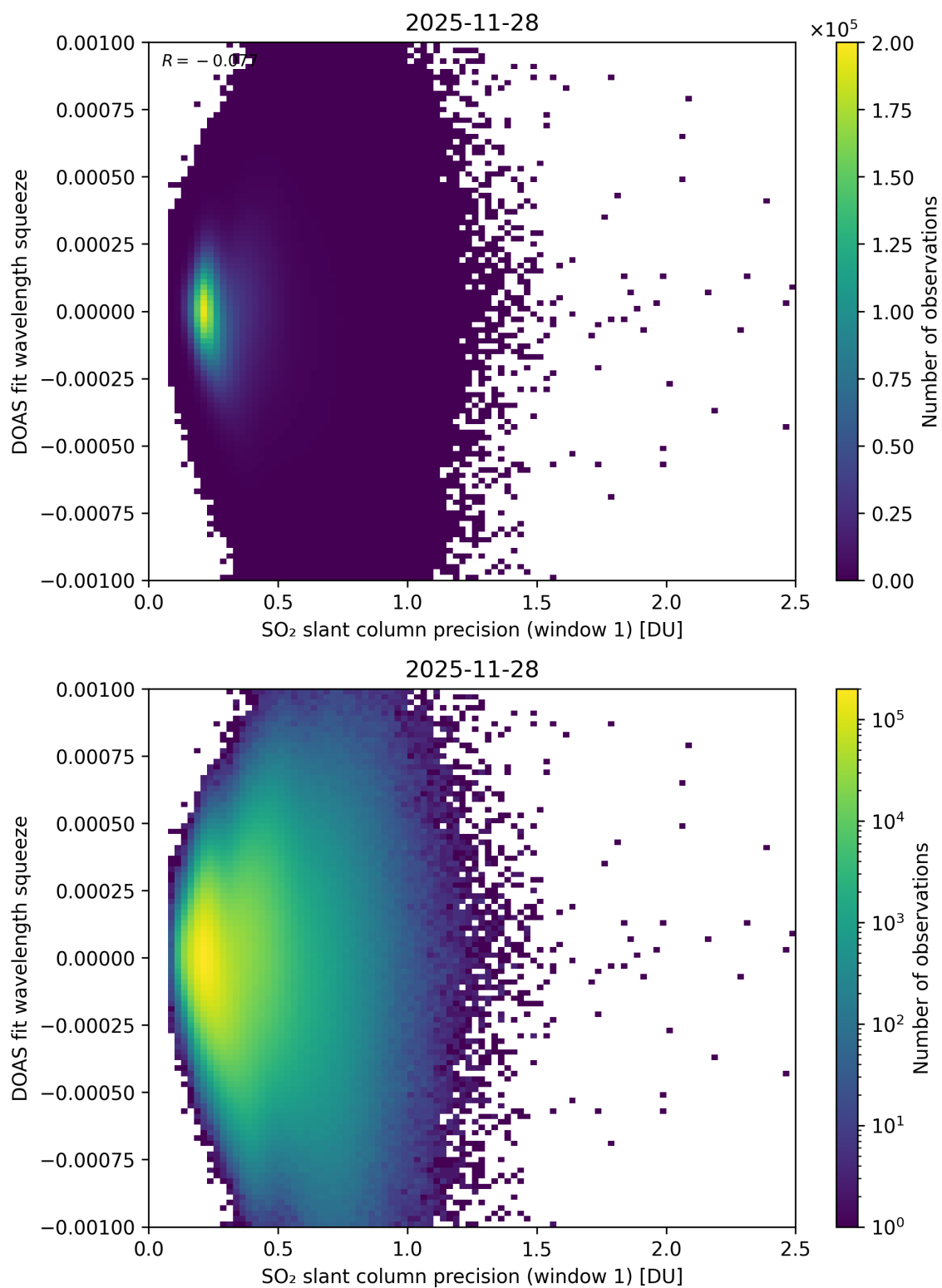
Figure 272: Scatter density plot of “SO 2 slant column precision (window 1)” against “DOAS fit wavelength squeeze” for 2025-11-28 to 2025-11-29.
