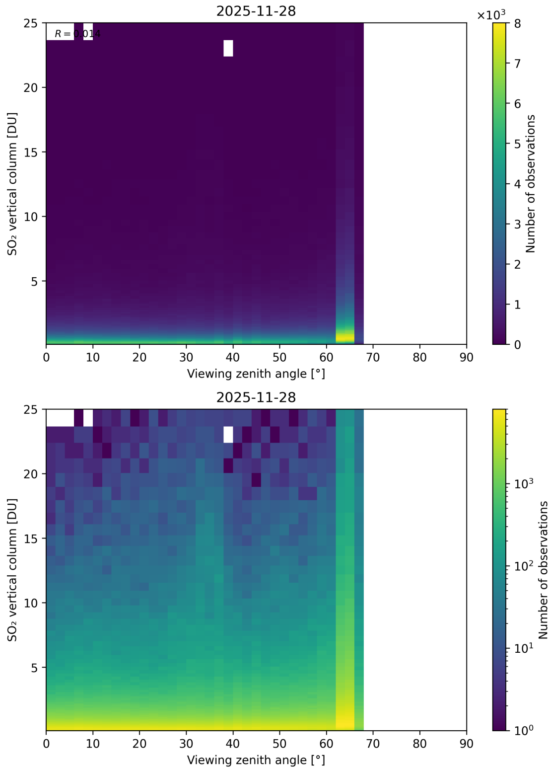
Figure 383: Scatter density plot of “Viewing zenith angle” against “SO 2 vertical column” for 2025-11-28 to 2025-11-29.
