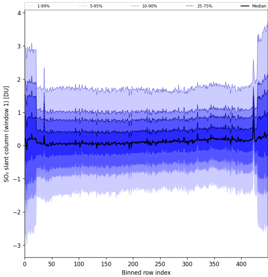
Figure 89: Along track statistics of “SO 2 slant column (window 1)” for 2025-11-28 to 2025-11-29
