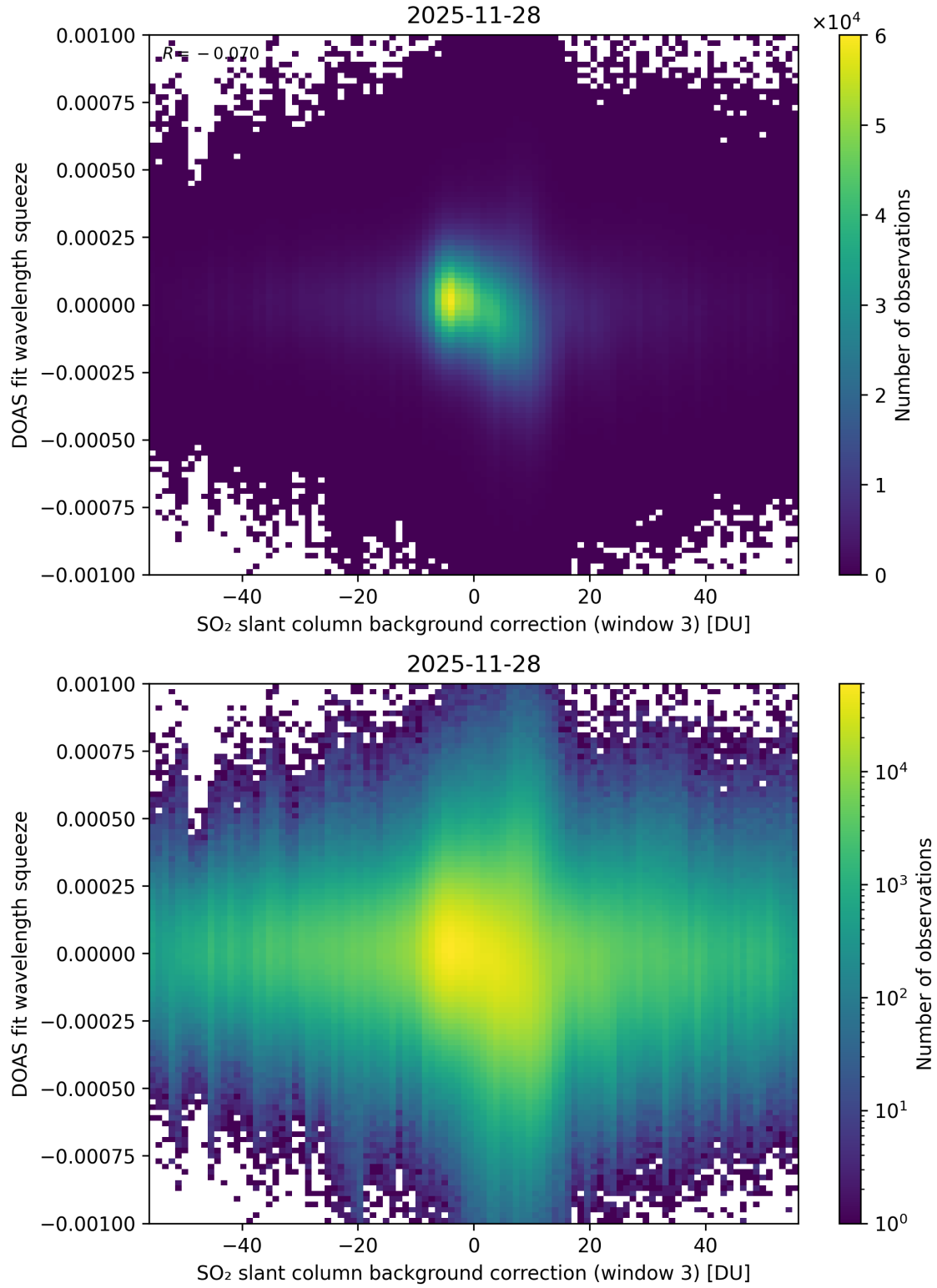
Figure 133: Scatter density plot of “SO 2 slant column background correction (window 3)” against “DOAS fit wavelength squeeze” for 2025-11-28 to 2025-11-29.
