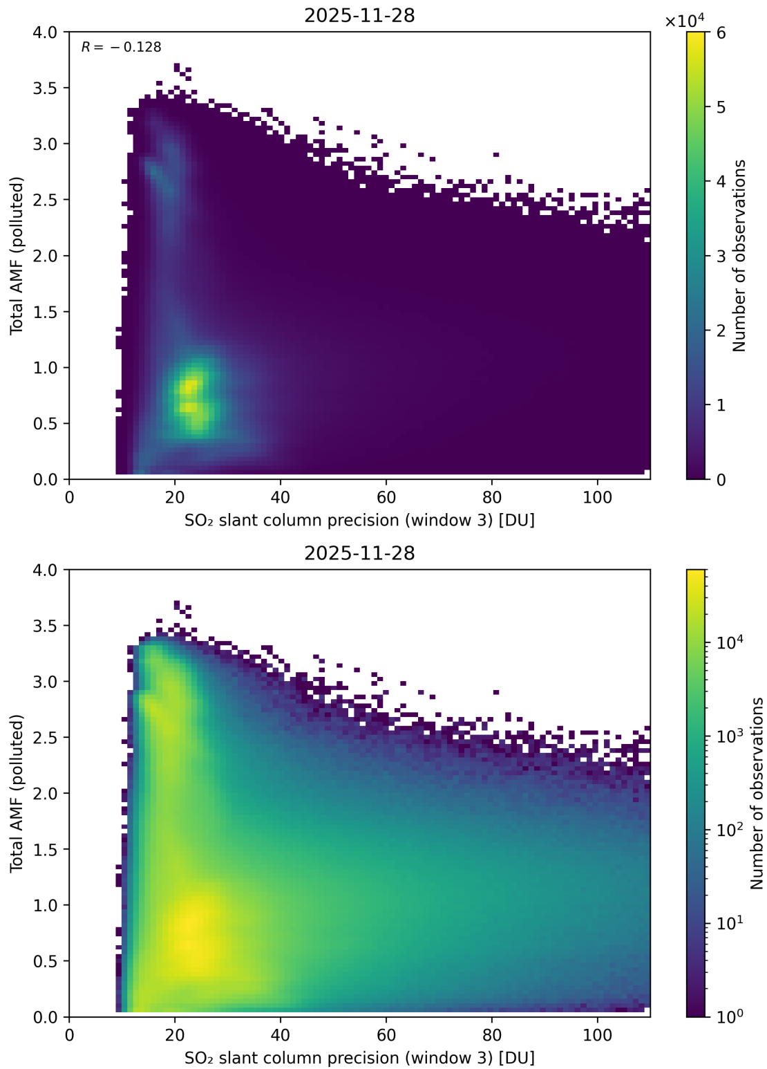
Figure 313: Scatter density plot of “SO 2 slant column precision (window 3)” against “Total AMF (polluted)” for 2025-11-28 to 2025-11-29.
