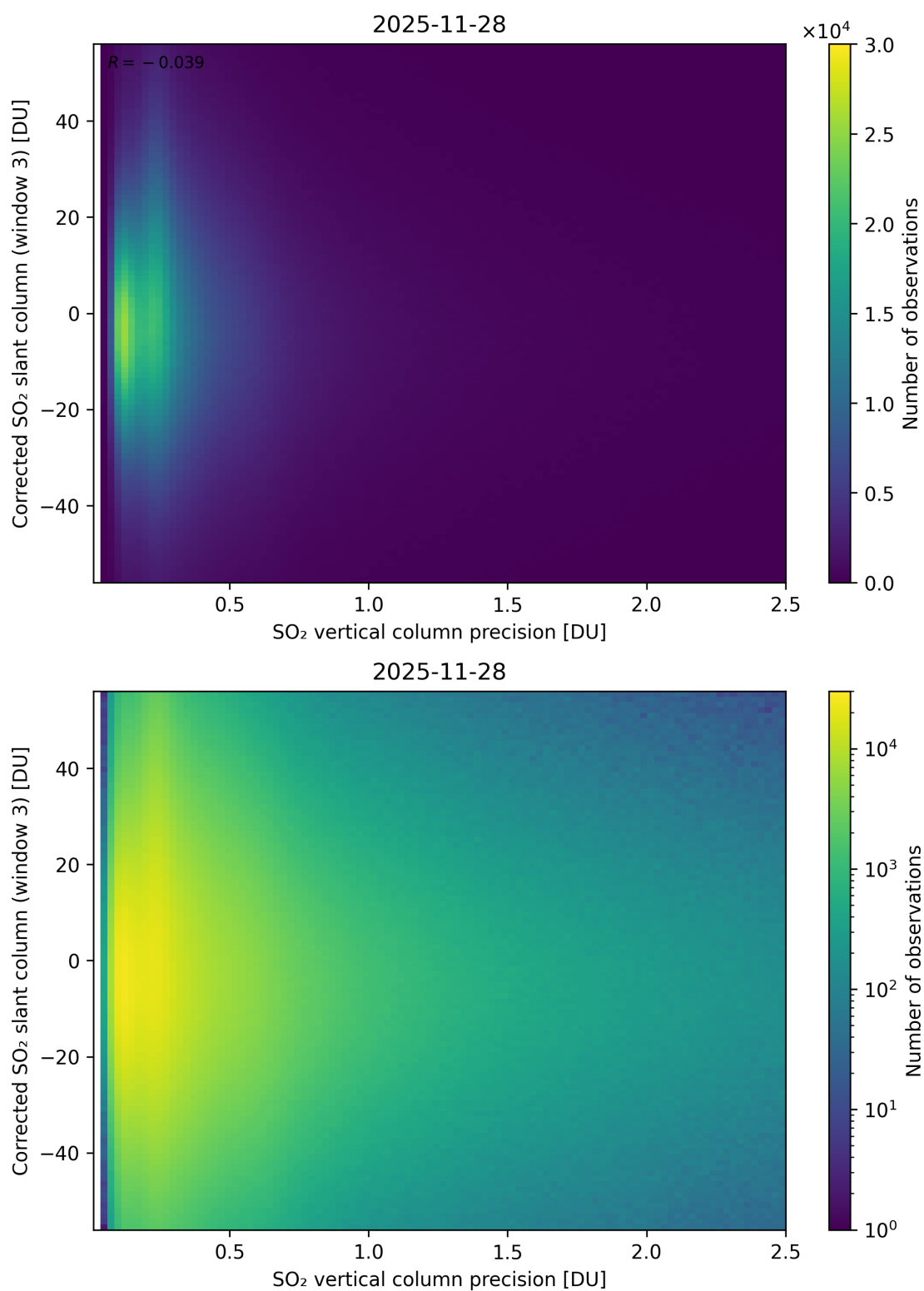
Figure 340: Scatter density plot of “SO 2 vertical column precision” against “Corrected SO 2 slant column (window 3)” for 2025-11-28 to 2025-11-29.
