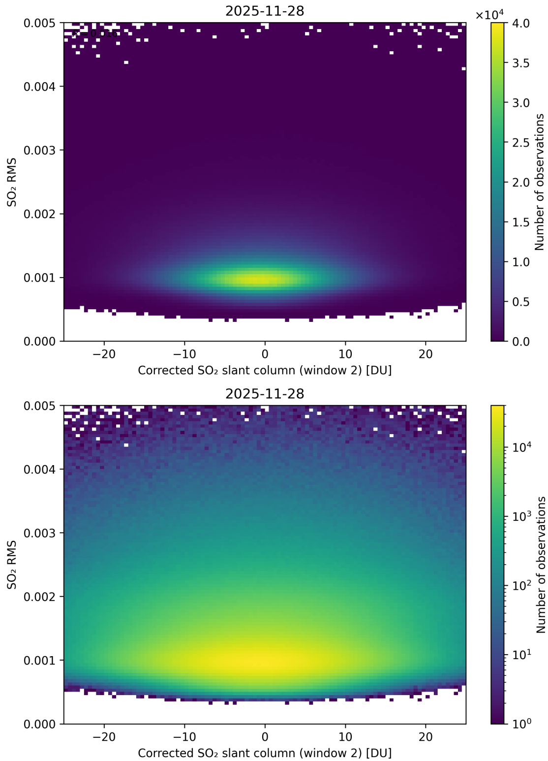
Figure 248: Scatter density plot of “Corrected SO 2 slant column (window 2)” against “SO 2 RMS” for 2025-11-28 to 2025-11-29.
