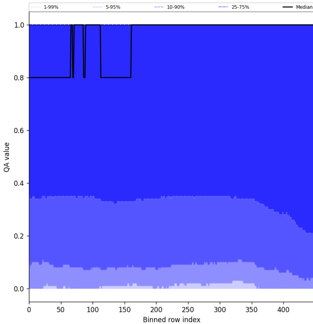
Figure 83: Along track statistics of “QA value” for 2025-11-28 to 2025-11-29
