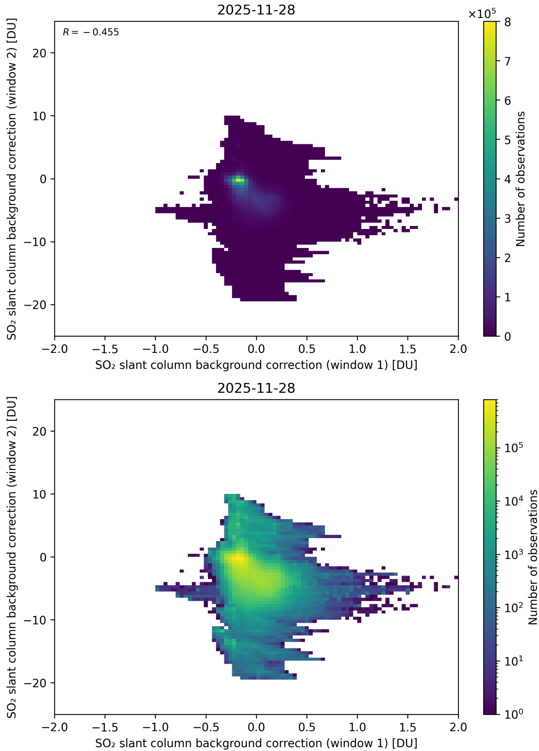
Figure 109: Scatter density plot of “SO 2 slant column background correction (window 1)” against “SO 2 slant column background correction (window 2)” for 2025-11-28 to 2025-11-29.
