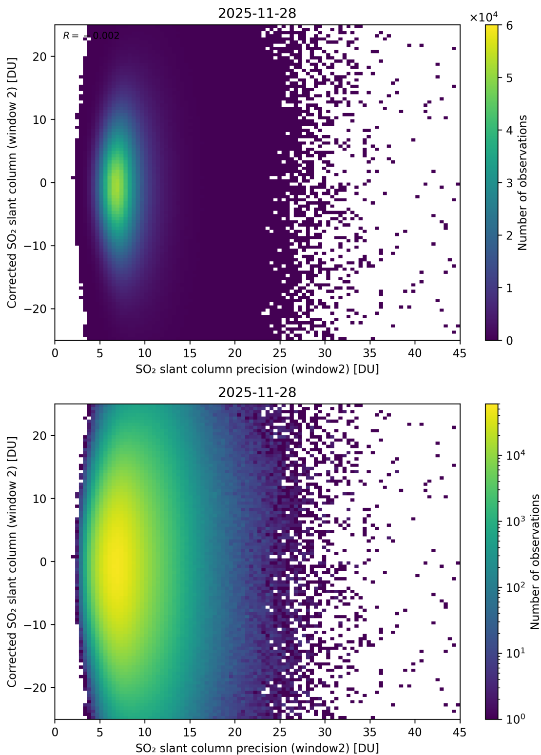
Figure 297: Scatter density plot of “SO 2 slant column precision (window2)” against “Corrected SO 2 slant column (window 2)” for 2025-11-28 to 2025-11-29.
