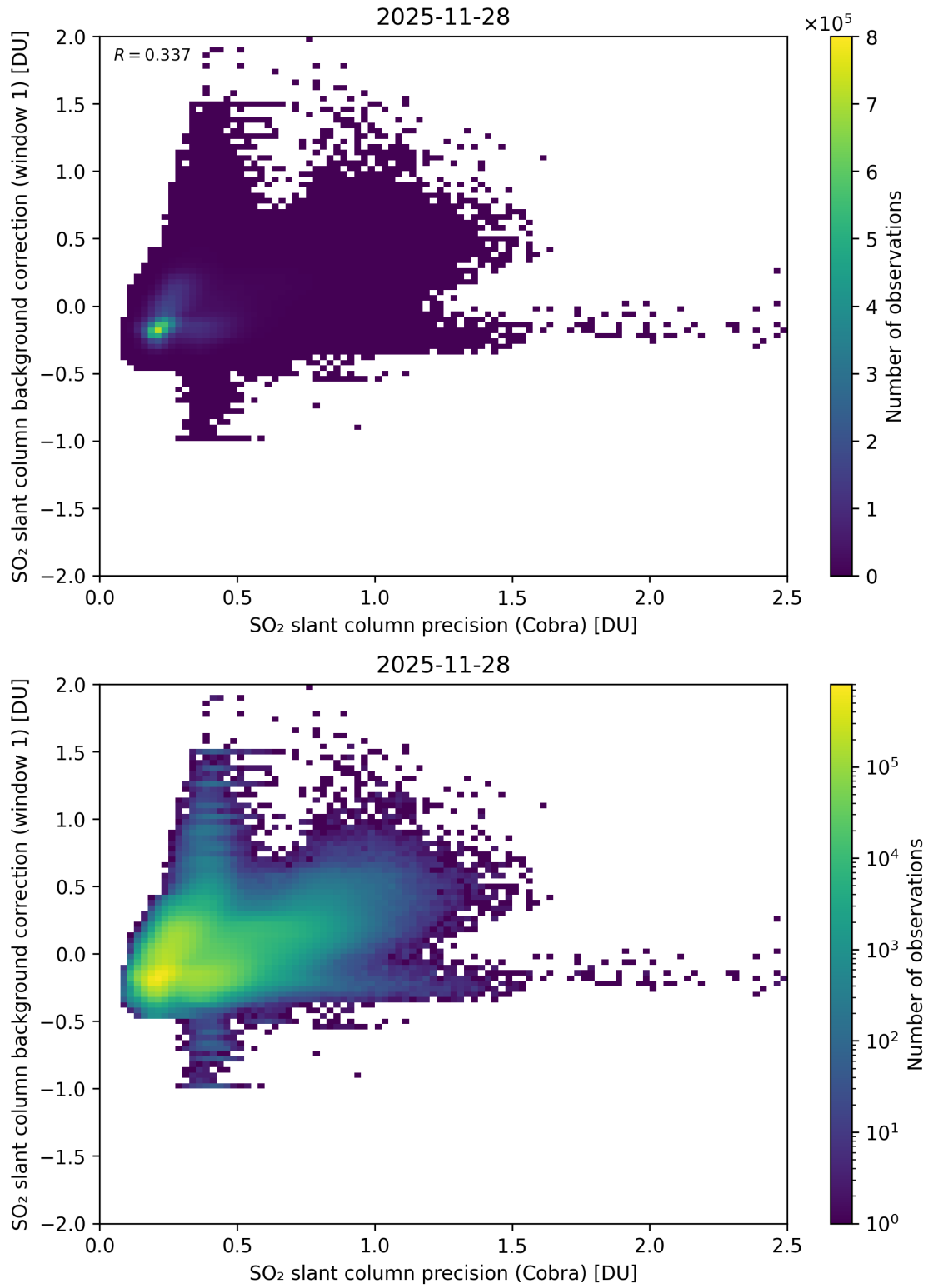
Figure 199: Scatter density plot of “SO 2 slant column precision (Cobra)” against “SO 2 slant column background correction (window 1)” for 2025-11-28 to 2025-11-29.
