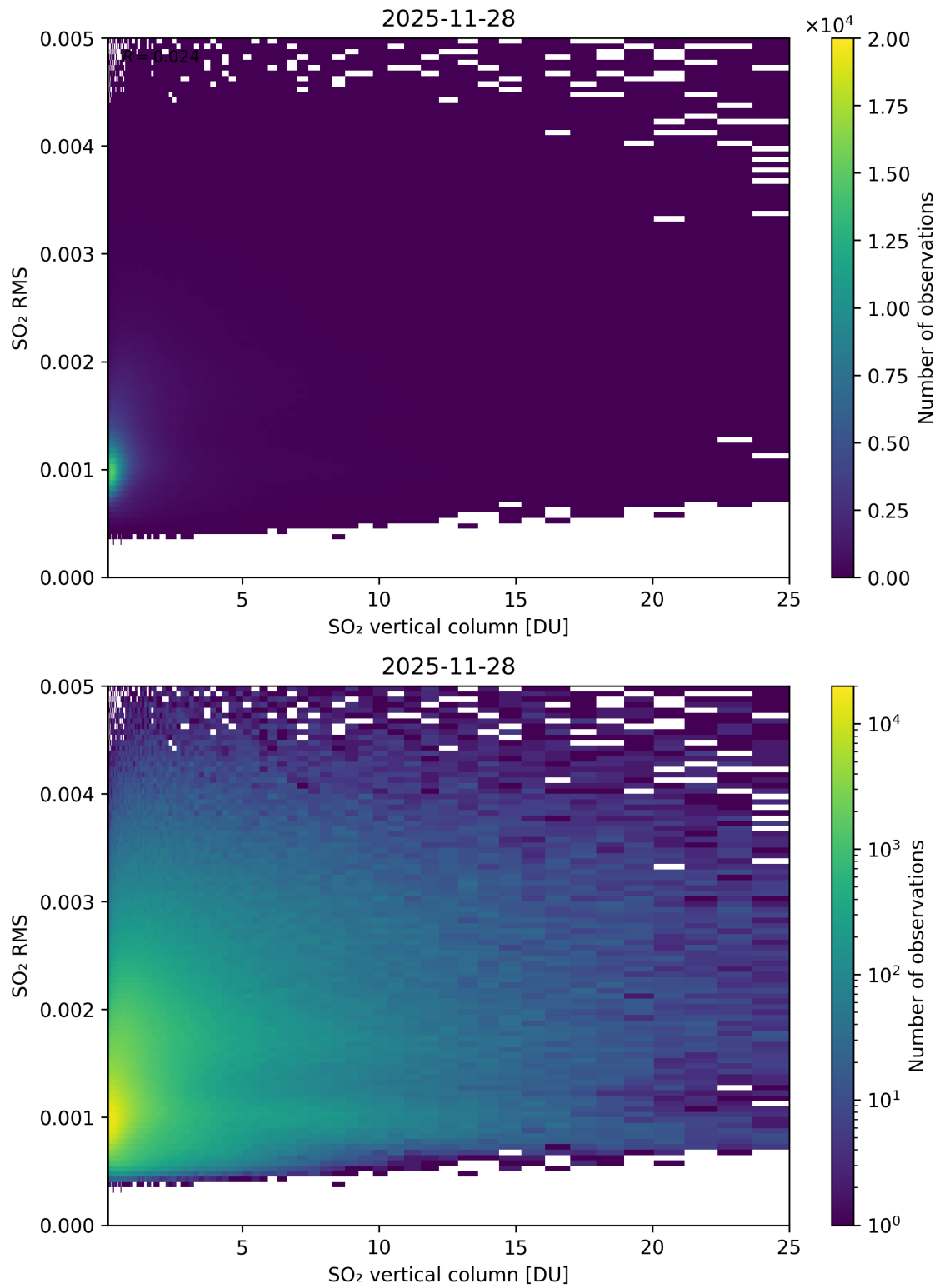
Figure 328: Scatter density plot of “SO 2 vertical column” against “SO 2 RMS” for 2025-11-28 to 2025-11-29.
