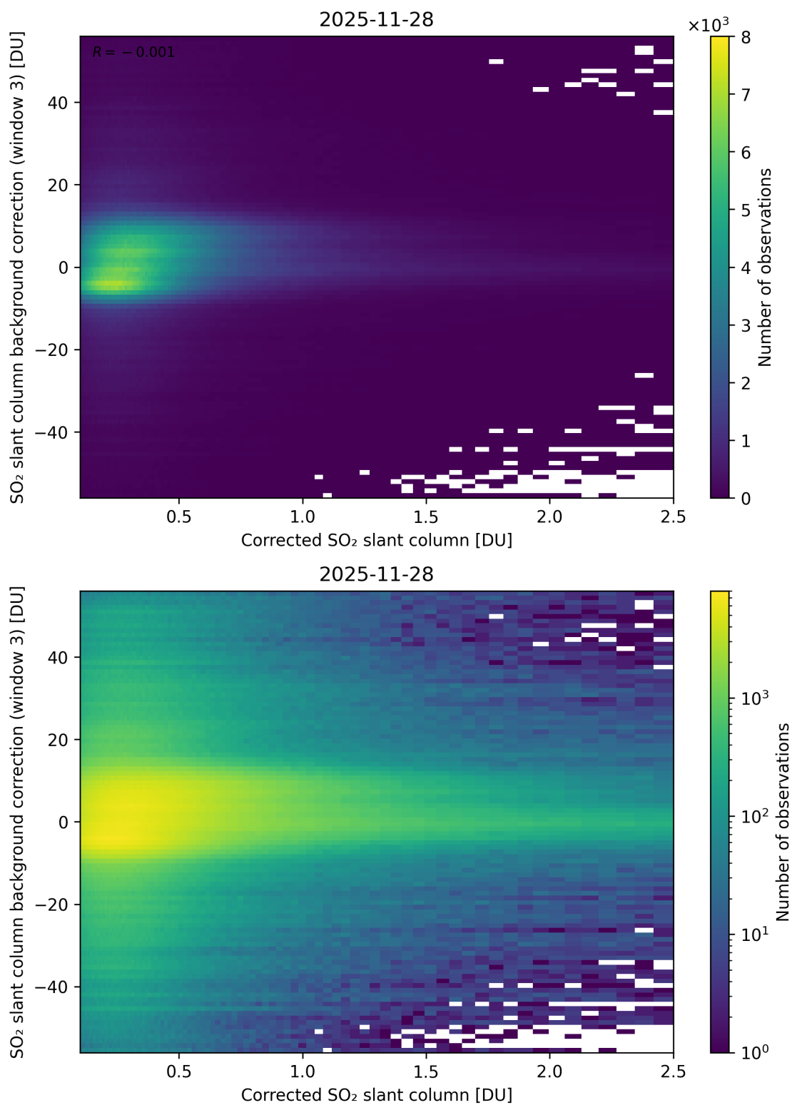
Figure 228: Scatter density plot of “Corrected SO 2 slant column” against “SO 2 slant column background correction (window 3)” for 2025-11-28 to 2025-11-29.
