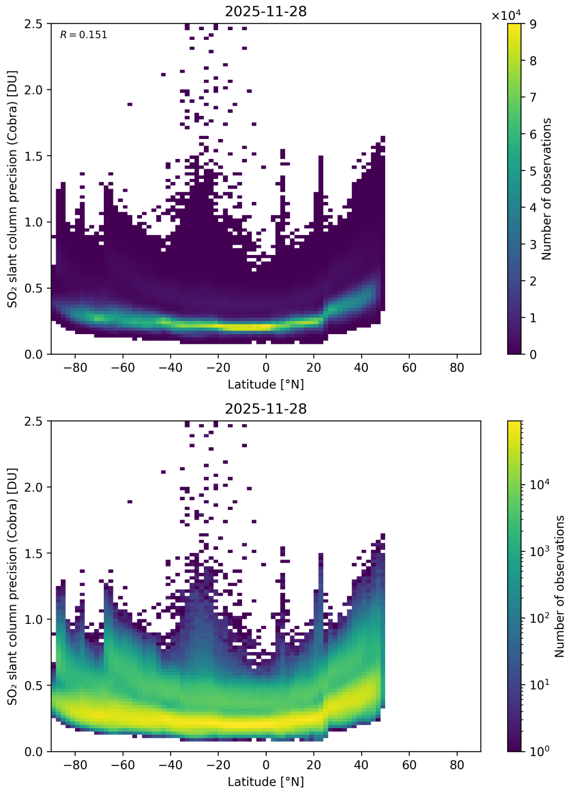
Figure 158: Scatter density plot of “Latitude” against “SO 2 slant column precision (Cobra)” for 2025-11-28 to 2025-11-29.
