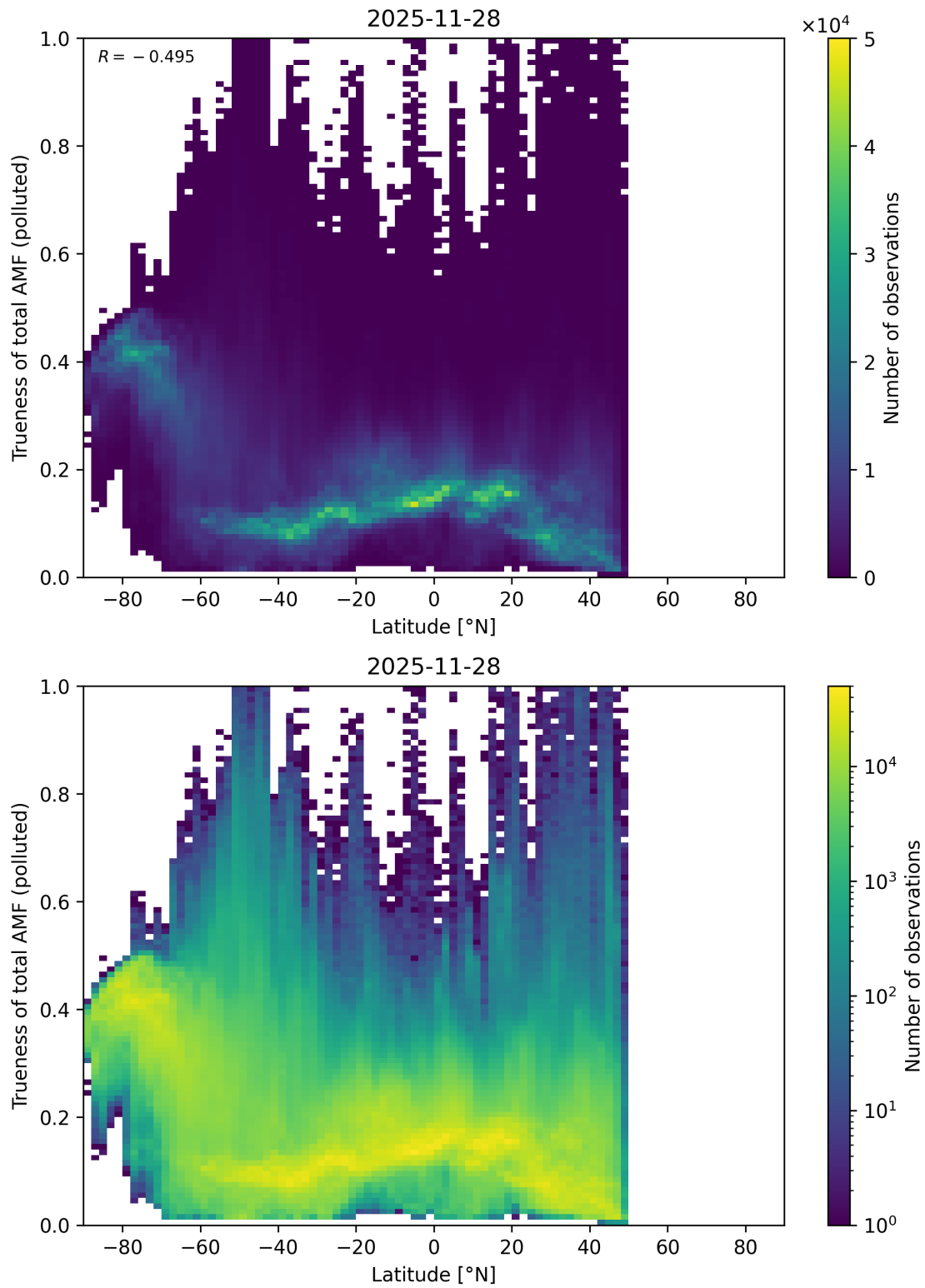
Figure 168: Scatter density plot of “Latitude” against “Trueness of total AMF (polluted)” for 2025-11-28 to 2025-11-29.
