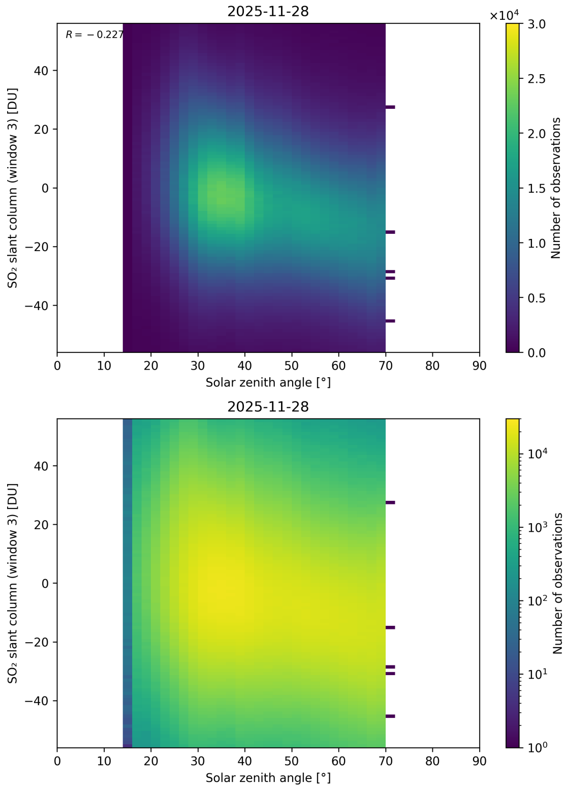
Figure 187: Scatter density plot of “Solar zenith angle” against “SO 2 slant column (window 3)” for 2025-11-28 to 2025-11-29.
