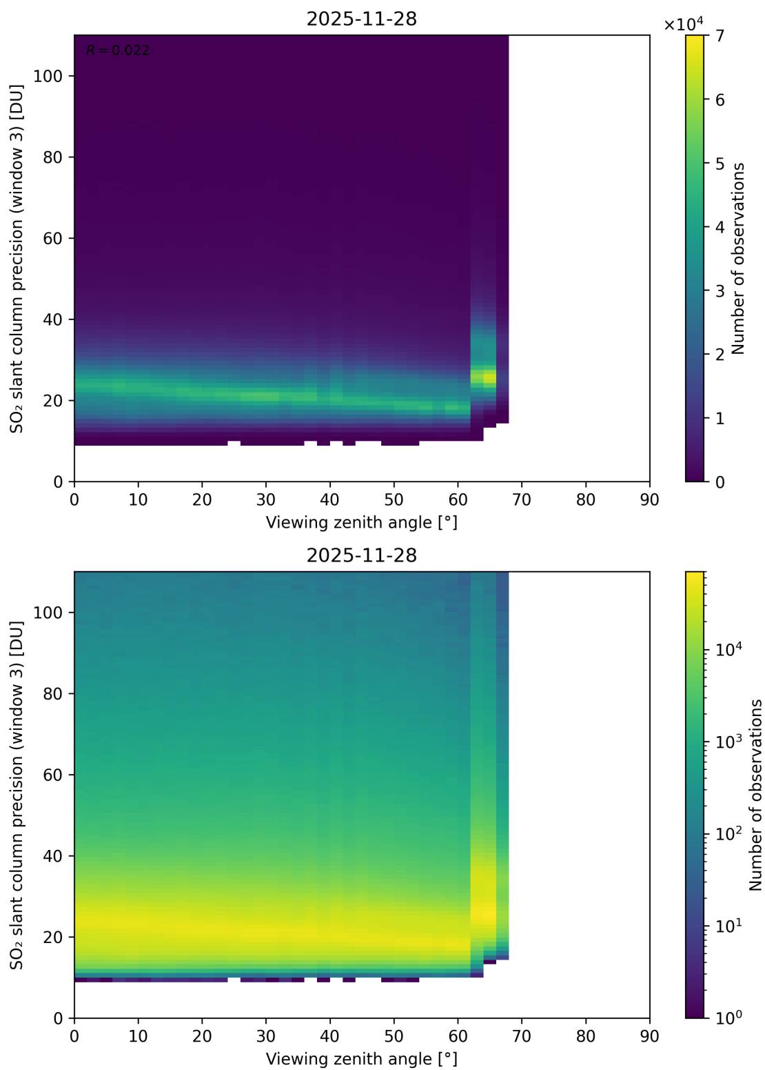
Figure 380: Scatter density plot of “Viewing zenith angle” against “SO 2 slant column precision (window 3)” for 2025-11-28 to 2025-11-29.
