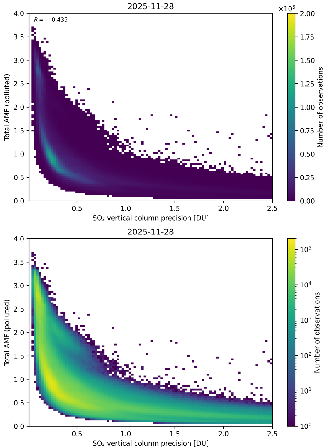
Figure 346: Scatter density plot of “SO 2 vertical column precision” against “Total AMF (polluted)” for 2025-11-28 to 2025-11-29.
