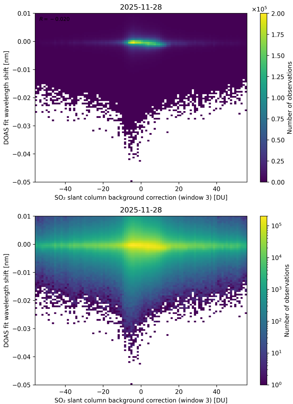
Figure 132: Scatter density plot of “SO 2 slant column background correction (window 3)” against “DOAS fit wavelength shift” for 2025-11-28 to 2025-11-29.
