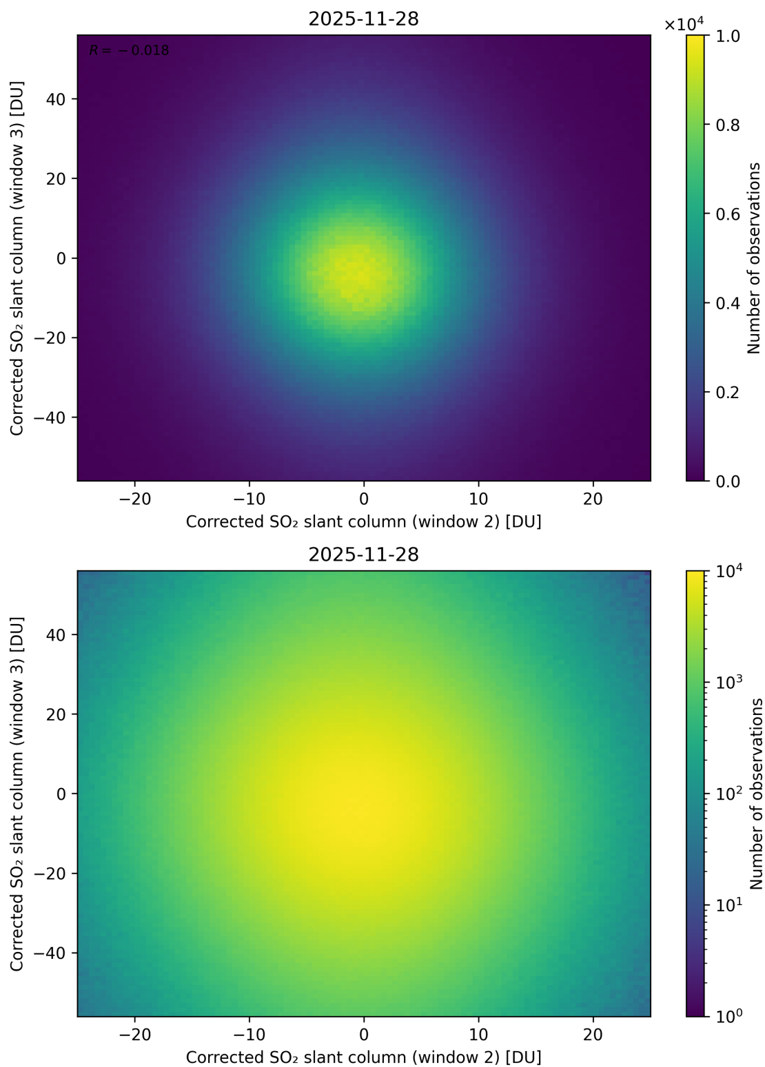
Figure 250: Scatter density plot of “Corrected SO 2 slant column (window 2)” against “Corrected SO 2 slant column (window 3)” for 2025-11-28 to 2025-11-29.
