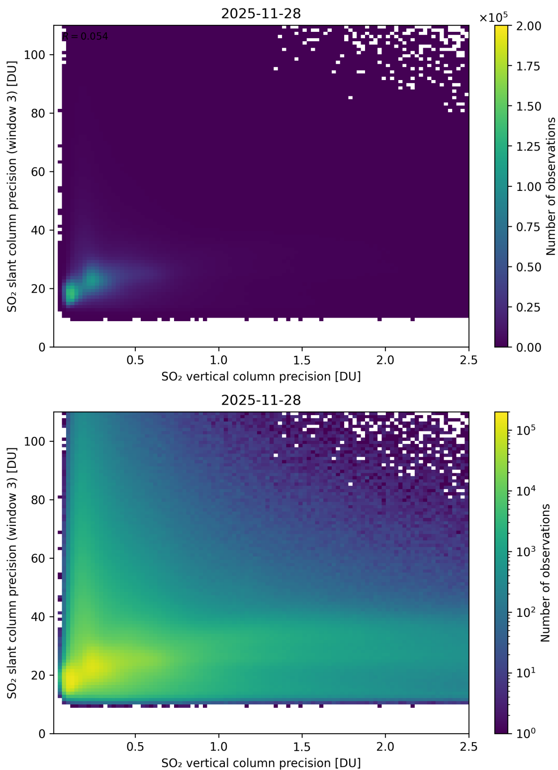
Figure 345: Scatter density plot of “SO 2 vertical column precision” against “SO 2 slant column precision (window 3)” for 2025-11-28 to 2025-11-29.
