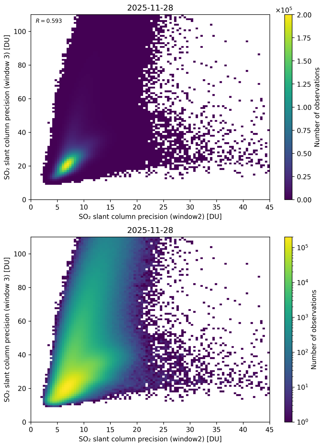
Figure 300: Scatter density plot of “SO 2 slant column precision (window2)” against “SO 2 slant column precision (window 3)” for 2025-11-28 to 2025-11-29.
