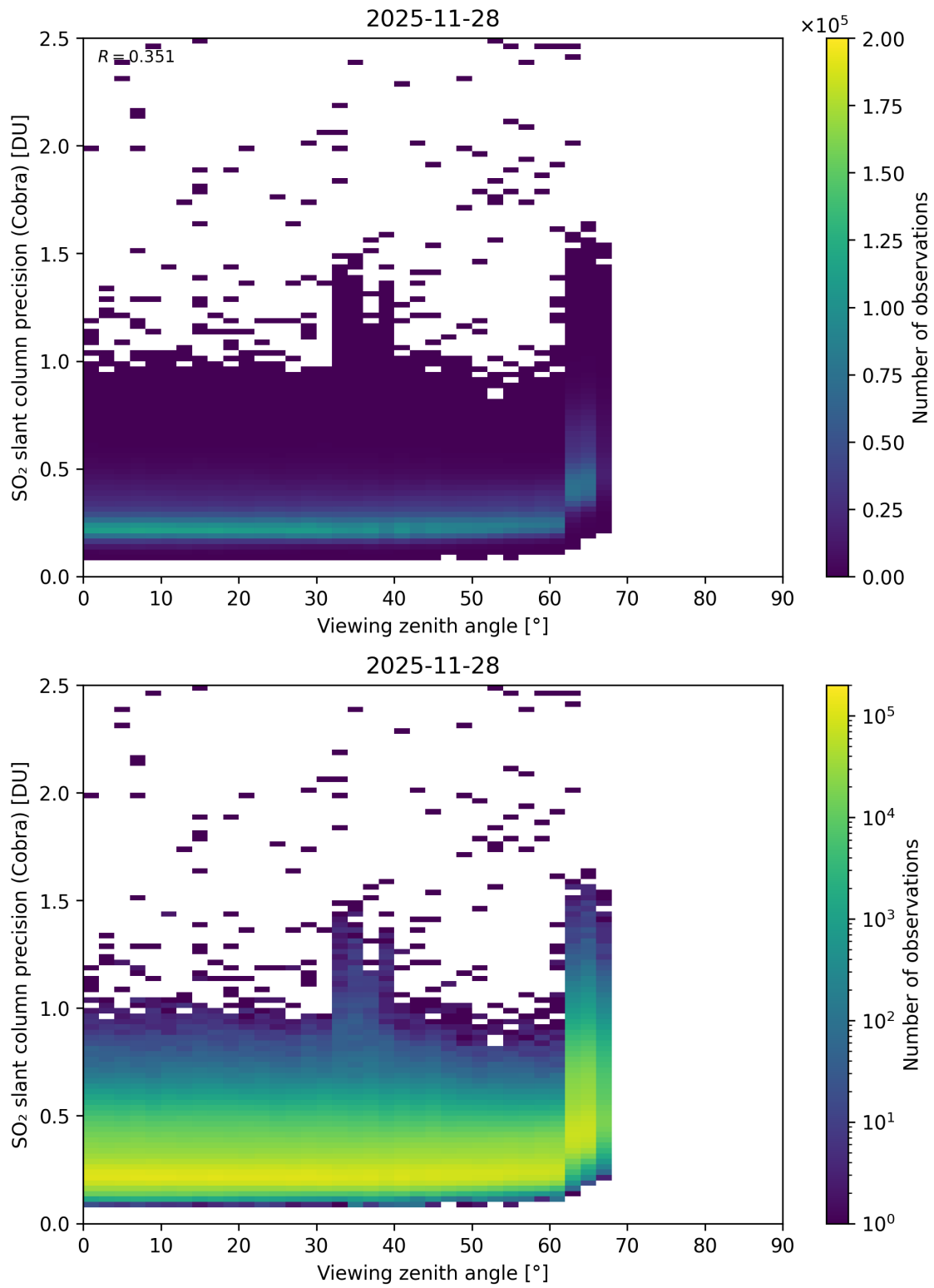
Figure 372: Scatter density plot of “Viewing zenith angle” against “SO 2 slant column precision (Cobra)” for 2025-11-28 to 2025-11-29.
