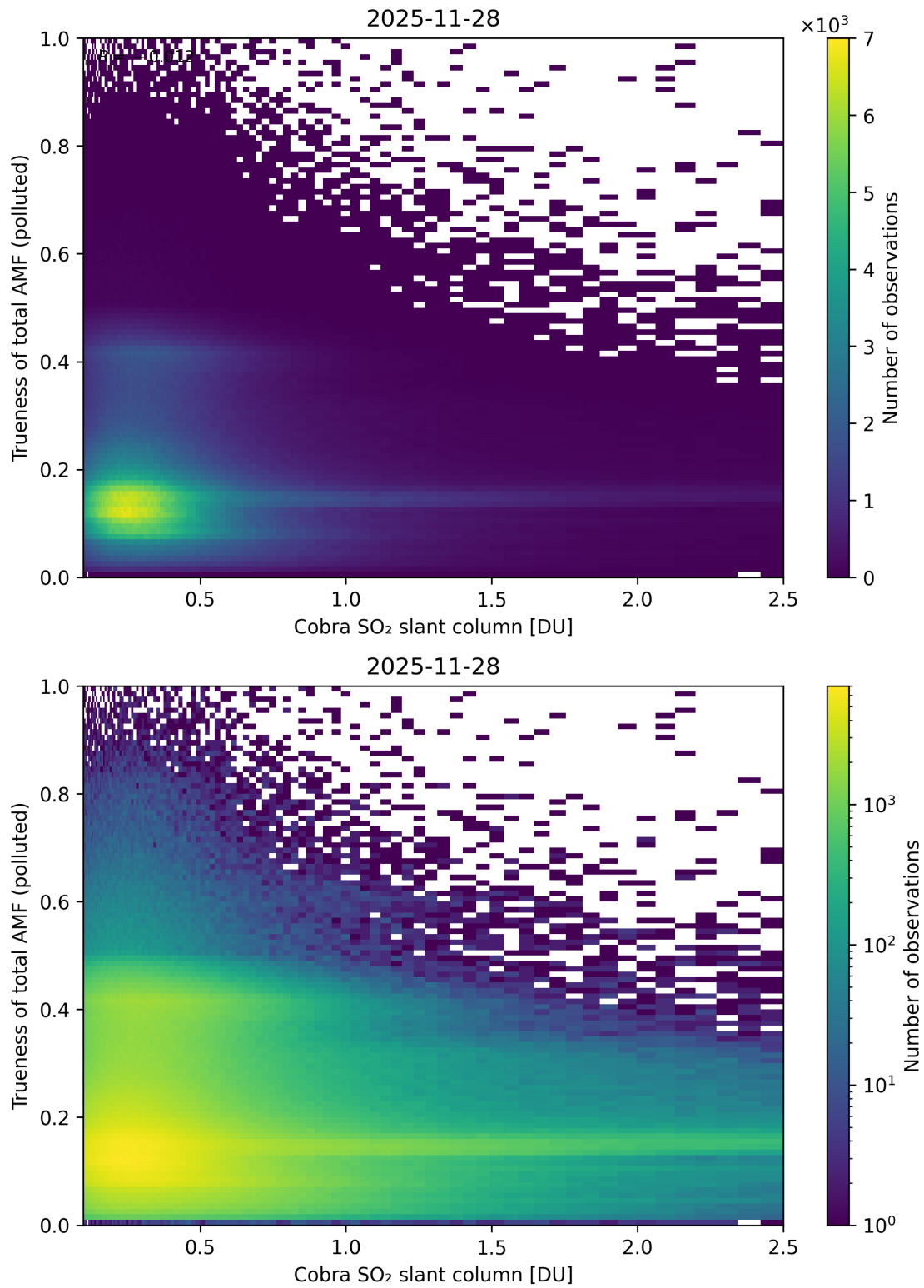
Figure 225: Scatter density plot of “Cobra SO 2 slant column” against “Trueness of total AMF (polluted)” for 2025-11-28 to 2025-11-29.
