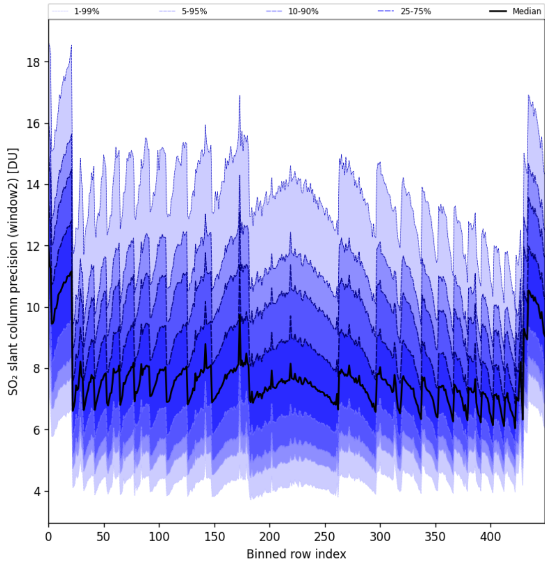
Figure 94: Along track statistics of “SO 2 slant column precision (window2)” for 2025-11-28 to 2025-11-29
