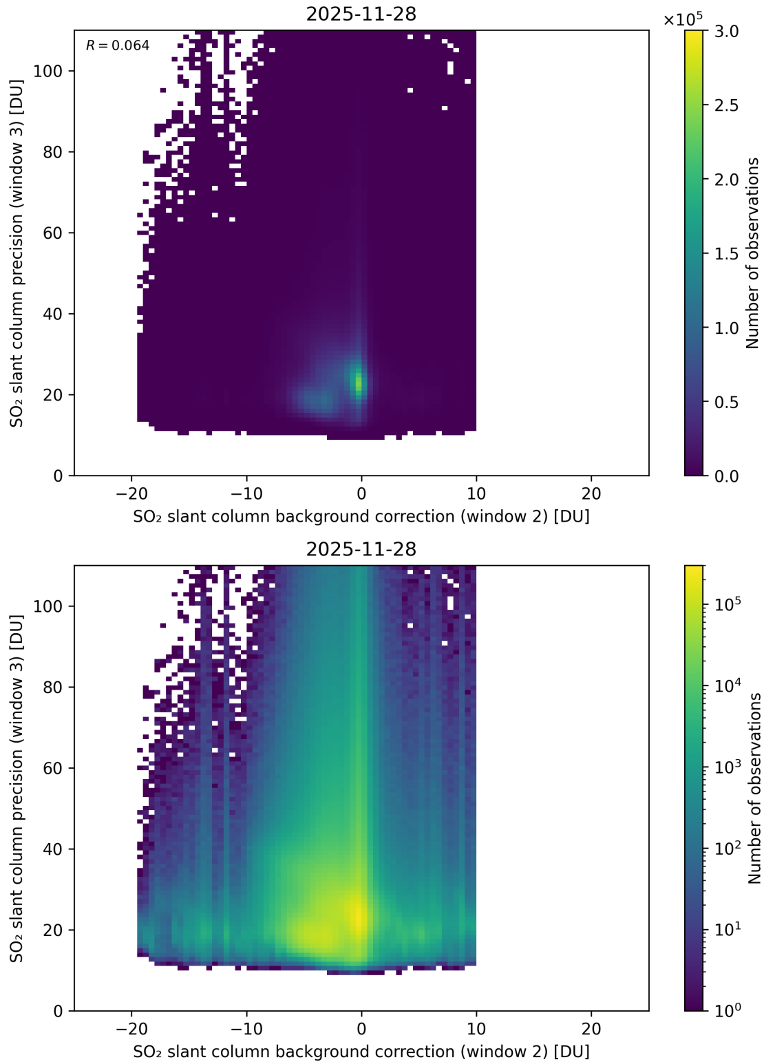
Figure 129: Scatter density plot of “SO 2 slant column background correction (window 2)” against “SO 2 slant column precision (window 3)” for 2025-11-28 to 2025-11-29.
