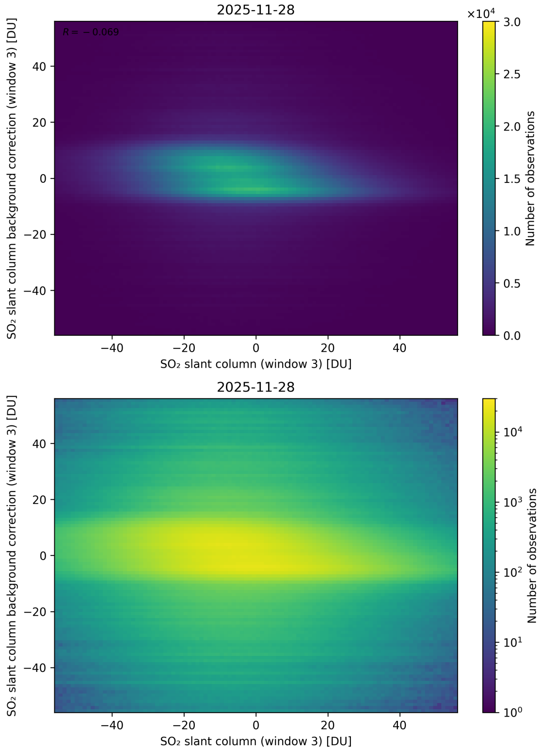
Figure 303: Scatter density plot of “SO 2 slant column (window 3)” against “SO 2 slant column background correction (window 3)” for 2025-11-28 to 2025-11-29.
