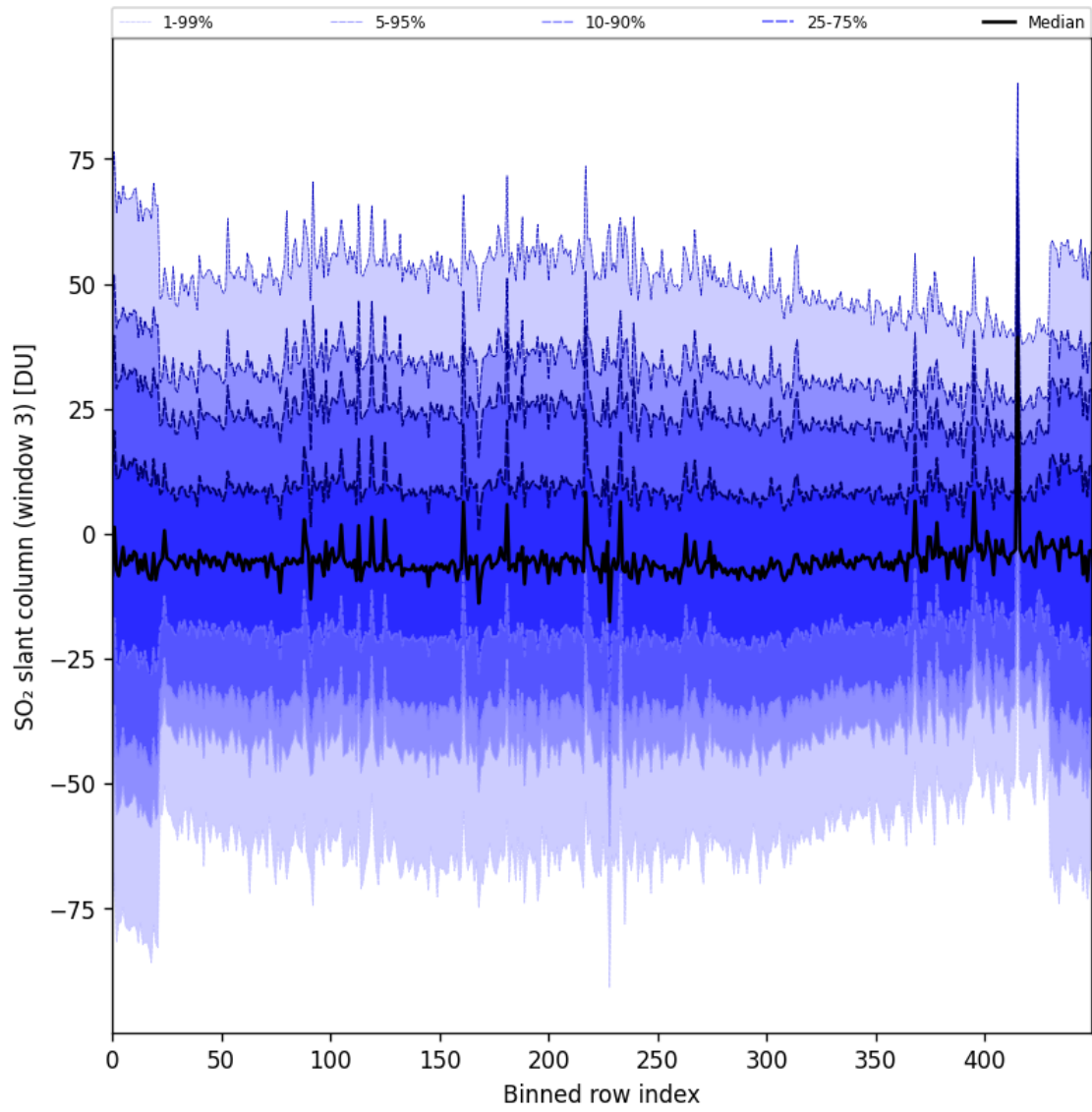
Figure 97: Along track statistics of “SO 2 slant column (window 3)” for 2025-11-28 to 2025-11-29
