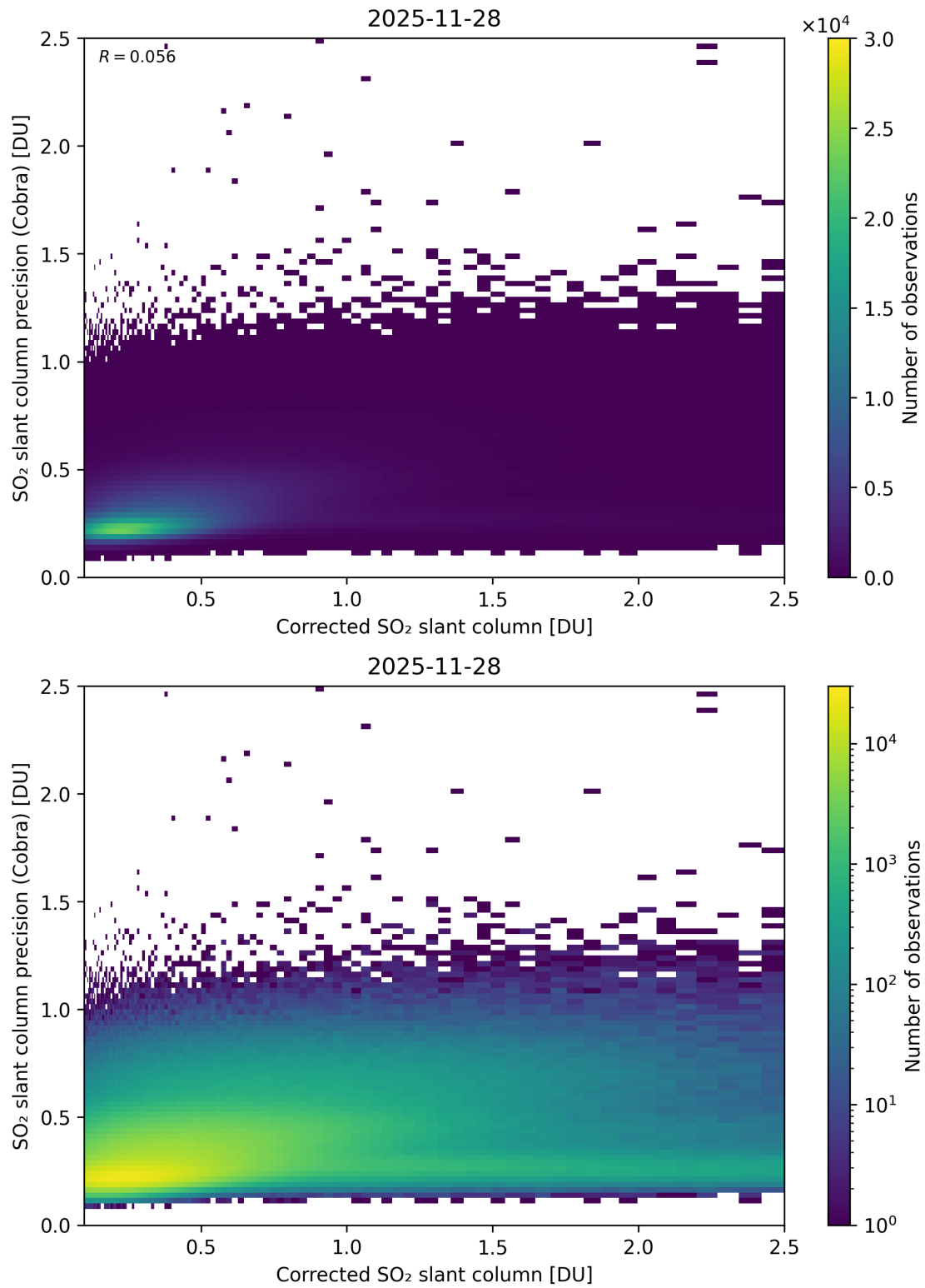
Figure 234: Scatter density plot of “Corrected SO 2 slant column” against “SO 2 slant column precision (Cobra)” for 2025-11-28 to 2025-11-29.
