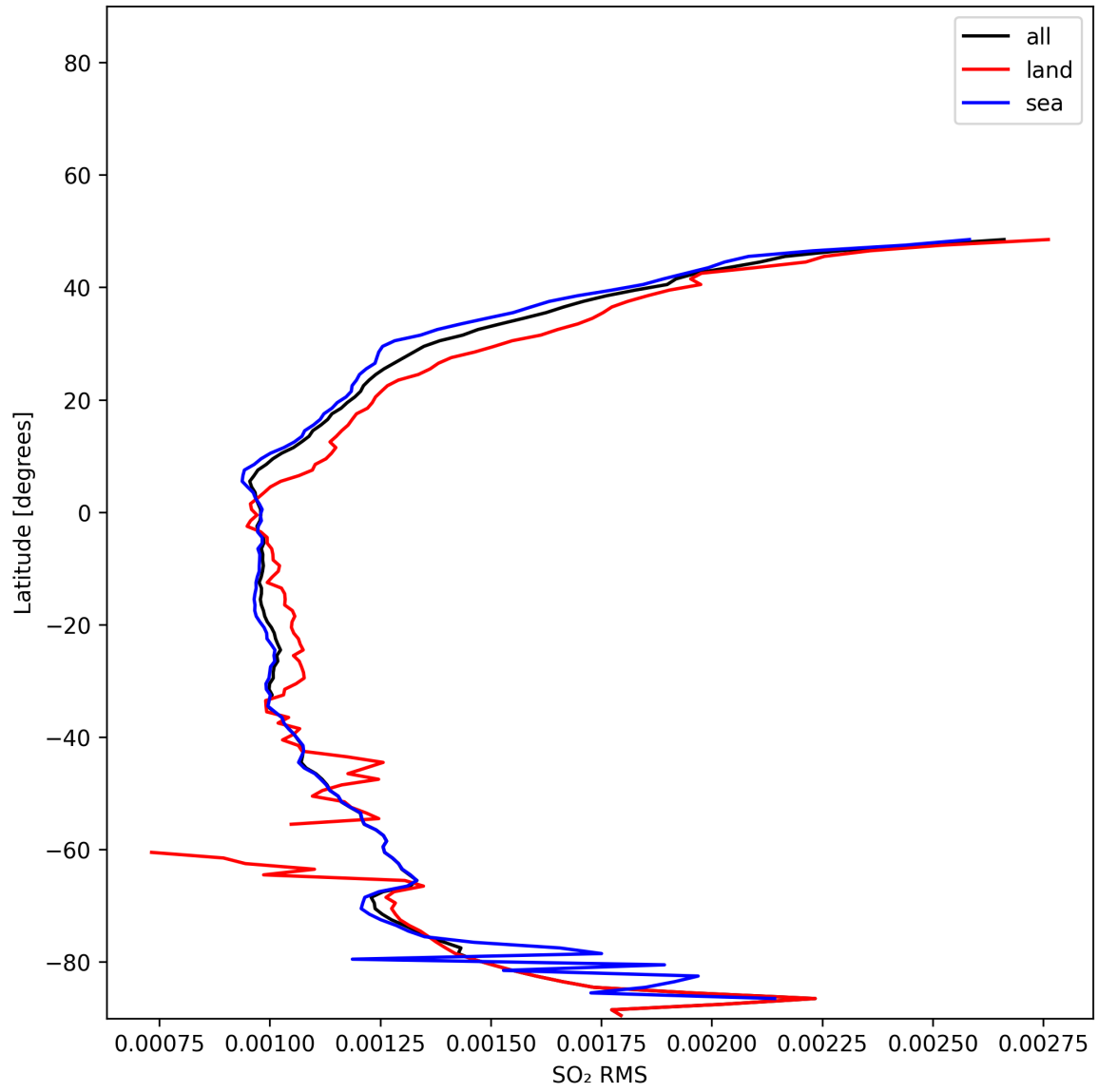
Figure 52: Zonal average of “SO 2 RMS” for 2025-11-28 to 2025-11-29.
