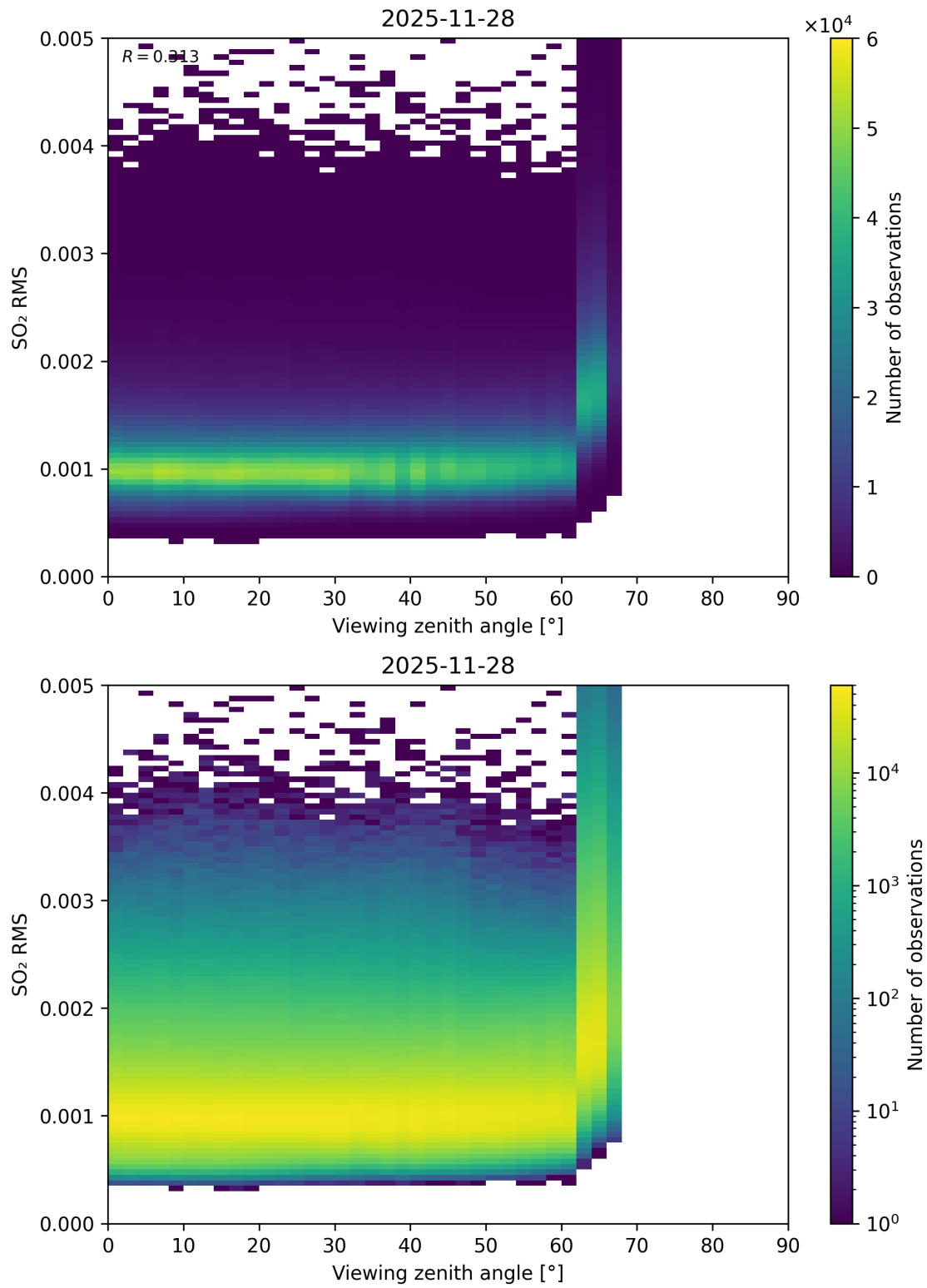
Figure 367: Scatter density plot of “Viewing zenith angle” against “SO 2 RMS” for 2025-11-28 to 2025-11-29.
