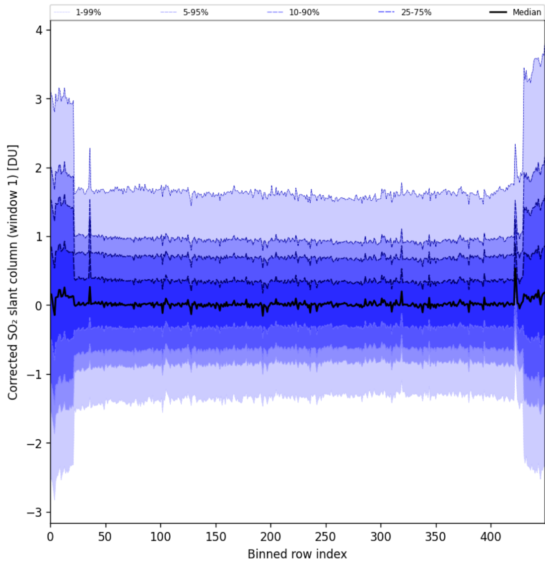
Figure 91: Along track statistics of “Corrected SO 2 slant column (window 1)” for 2025-11-28 to 2025-11-29
