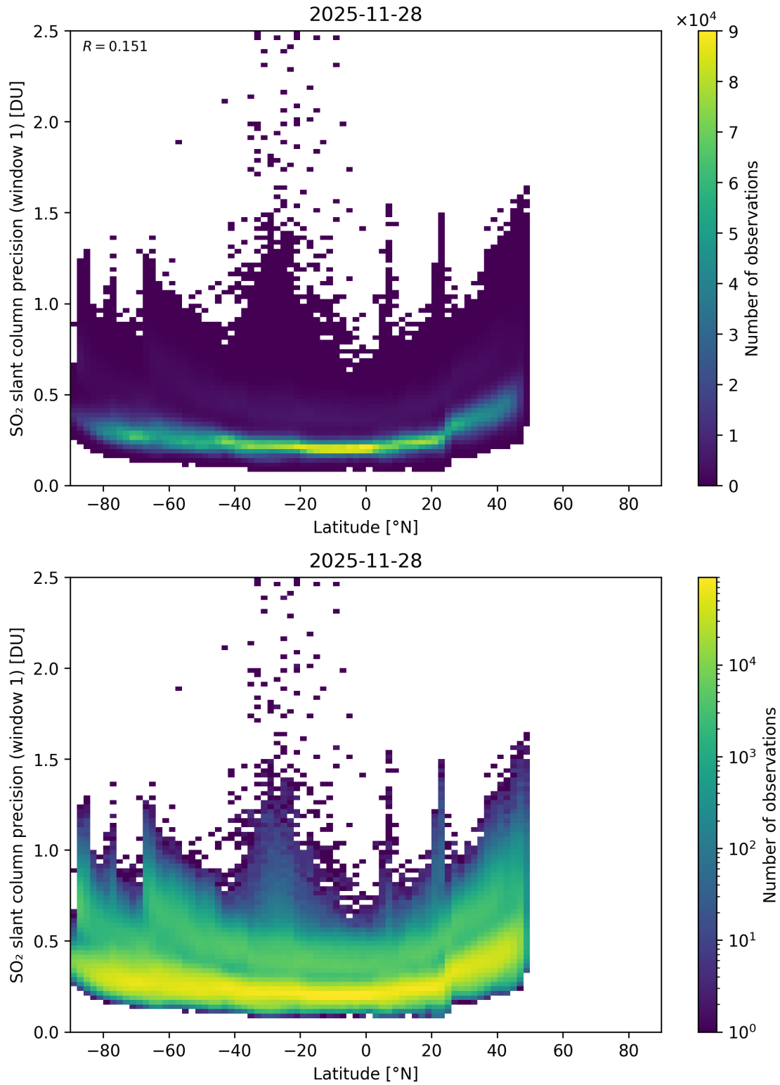
Figure 163: Scatter density plot of “Latitude” against “SO 2 slant column precision (window 1)” for 2025-11-28 to 2025-11-29.
