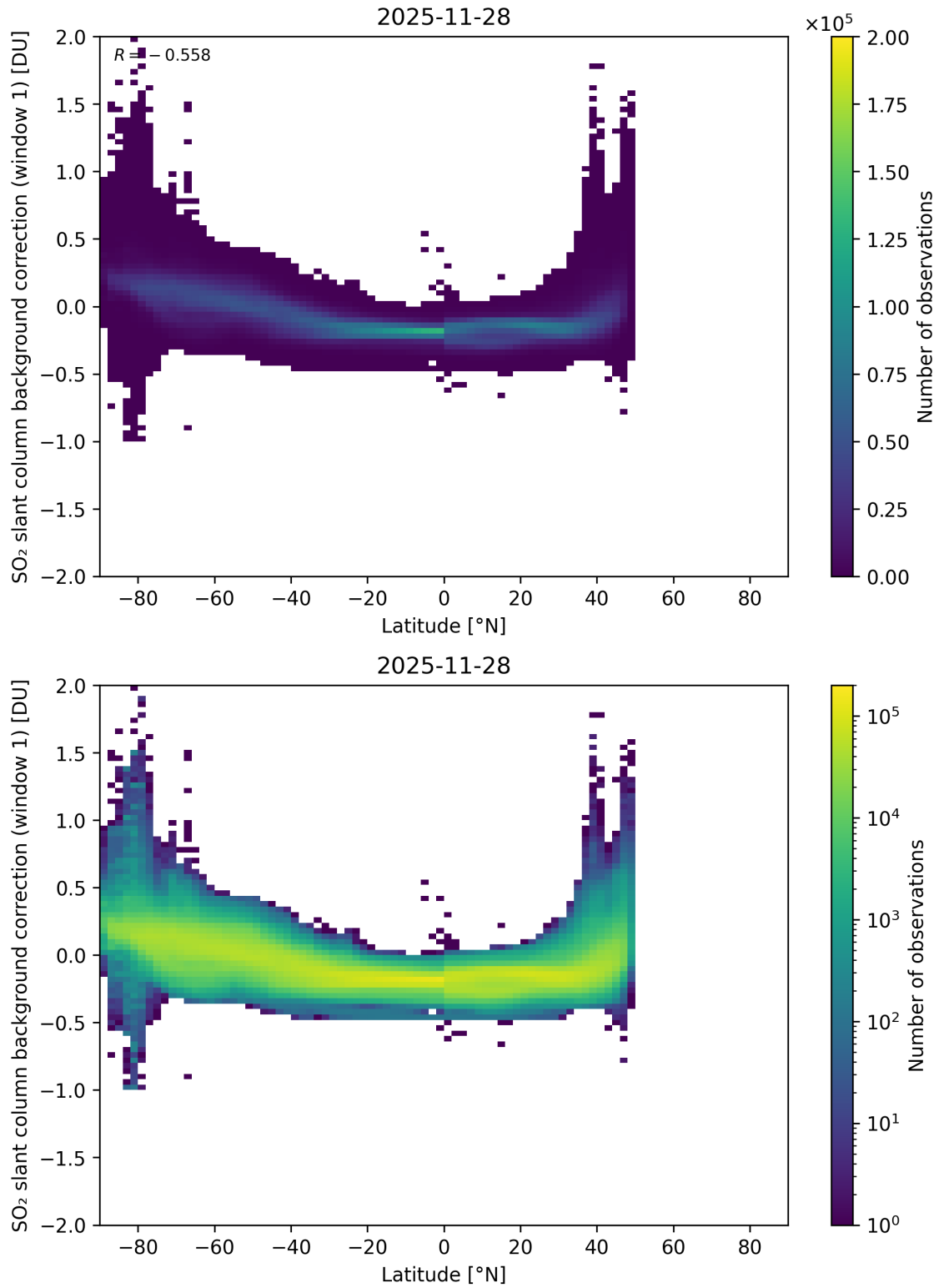
Figure 150: Scatter density plot of “Latitude” against “SO 2 slant column background correction (window 1)” for 2025-11-28 to 2025-11-29.
