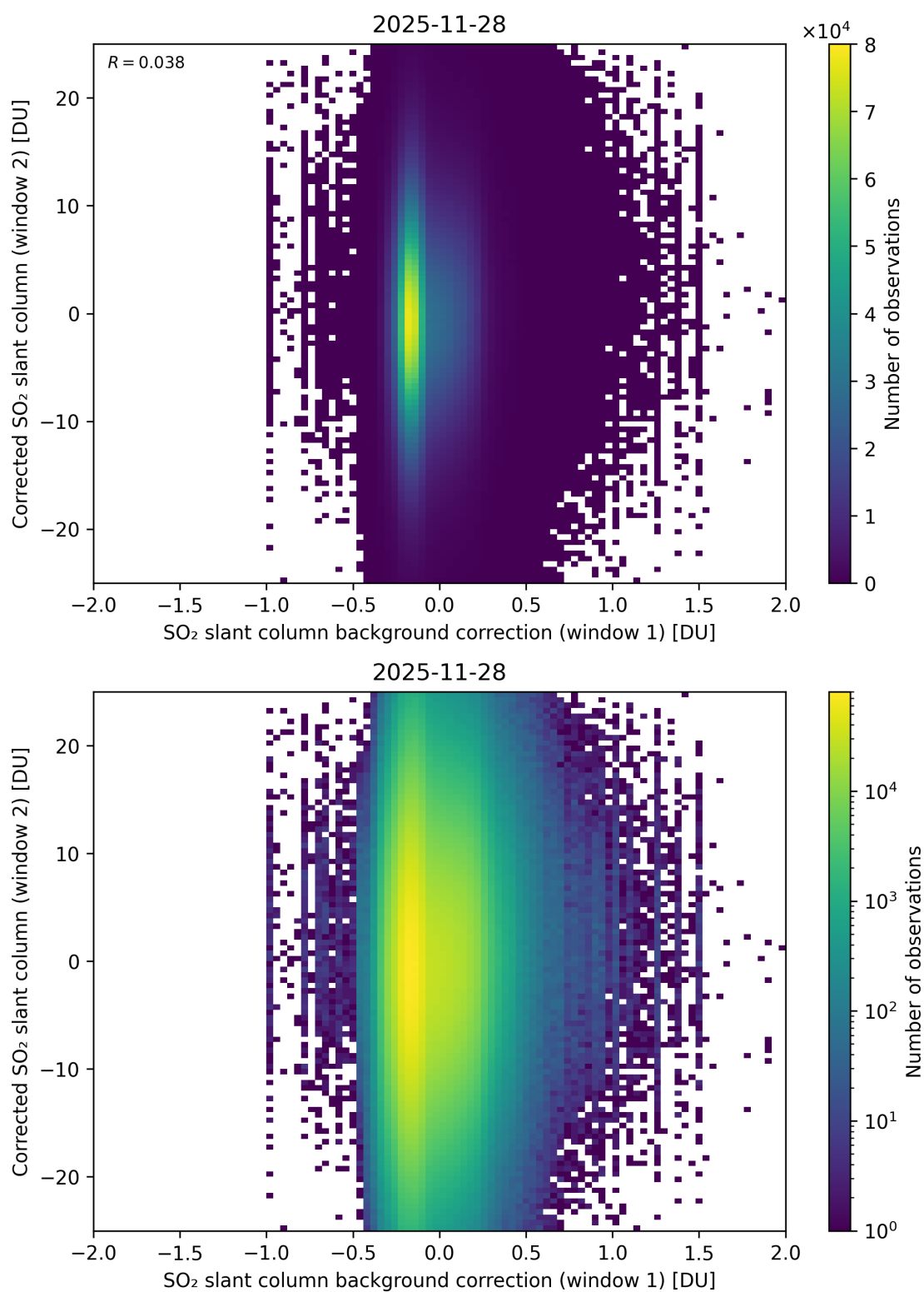
Figure 115: Scatter density plot of “SO 2 slant column background correction (window 1)” against “Corrected SO 2 slant column (window 2)” for 2025-11-28 to 2025-11-29.
