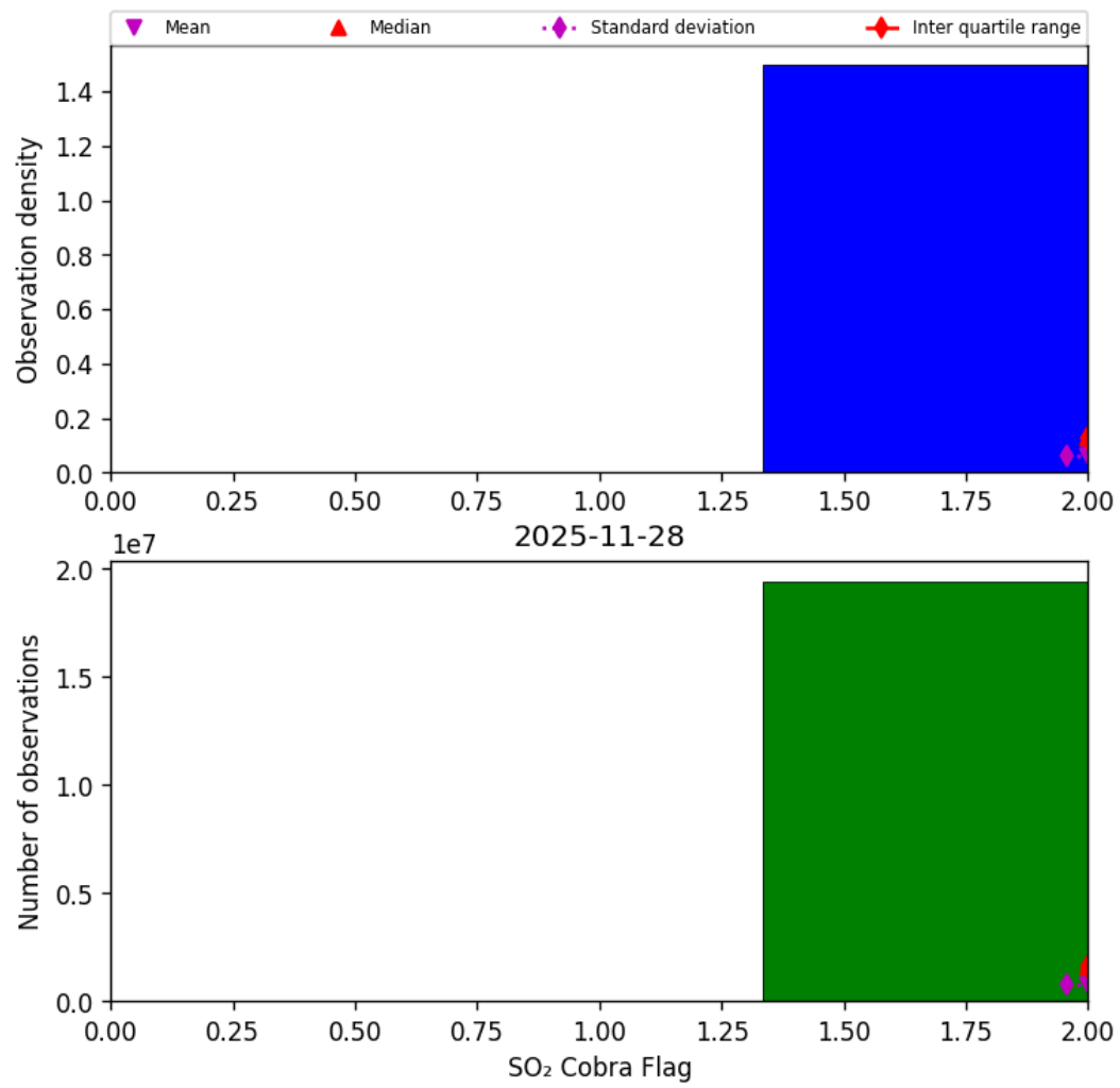
Figure 75: Histogram of "SO 2 Cobra Flag" for 2025-11-28 to 2025-11-29
