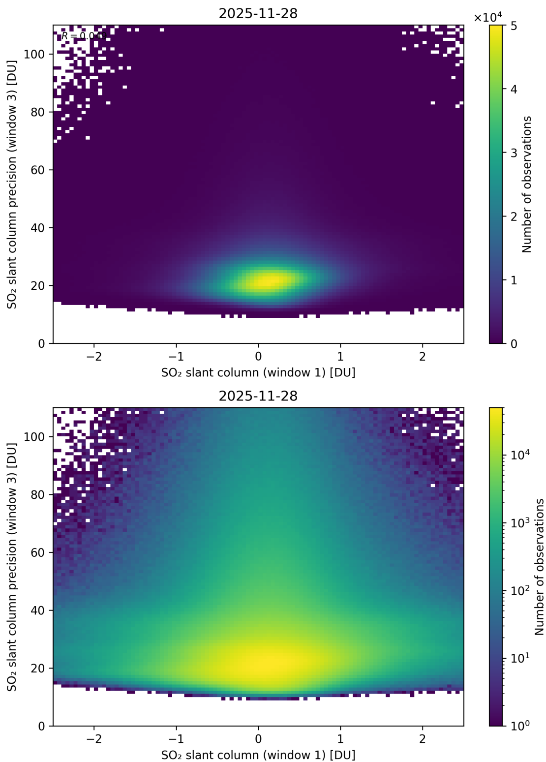
Figure 288: Scatter density plot of “SO 2 slant column (window 1)” against “SO 2 slant column precision (window 3)” for 2025-11-28 to 2025-11-29.
