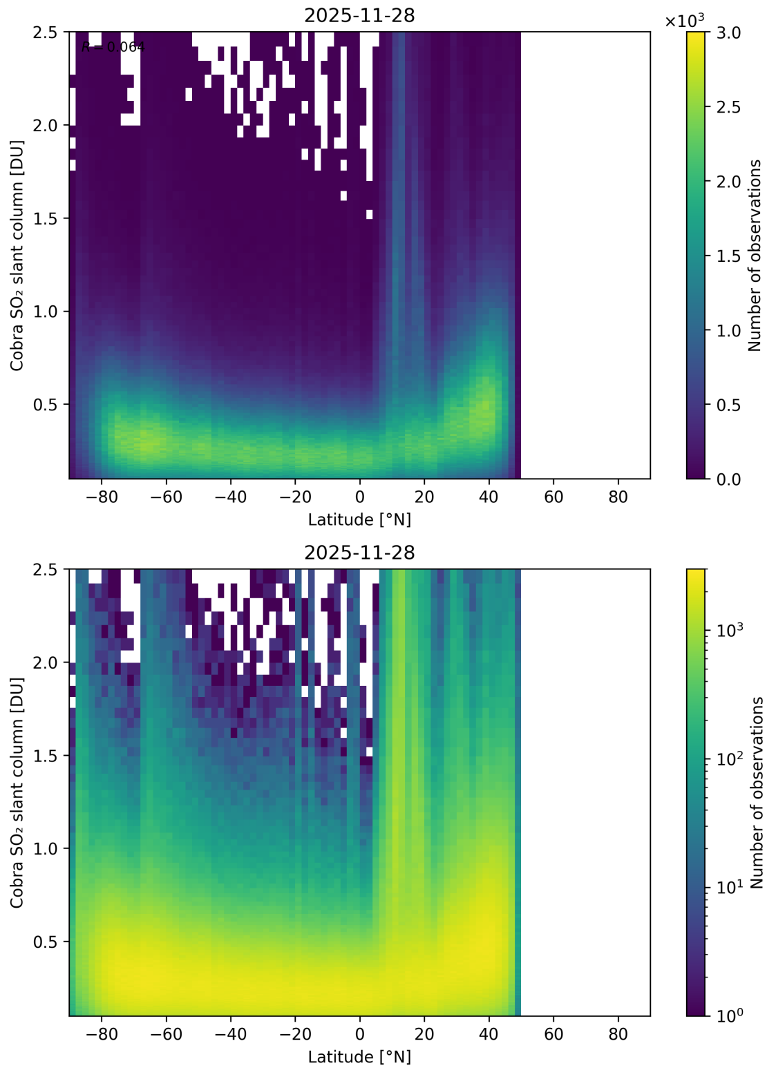
Figure 157: Scatter density plot of “Latitude” against “Cobra SO 2 slant column” for 2025-11-28 to 2025-11-29.
