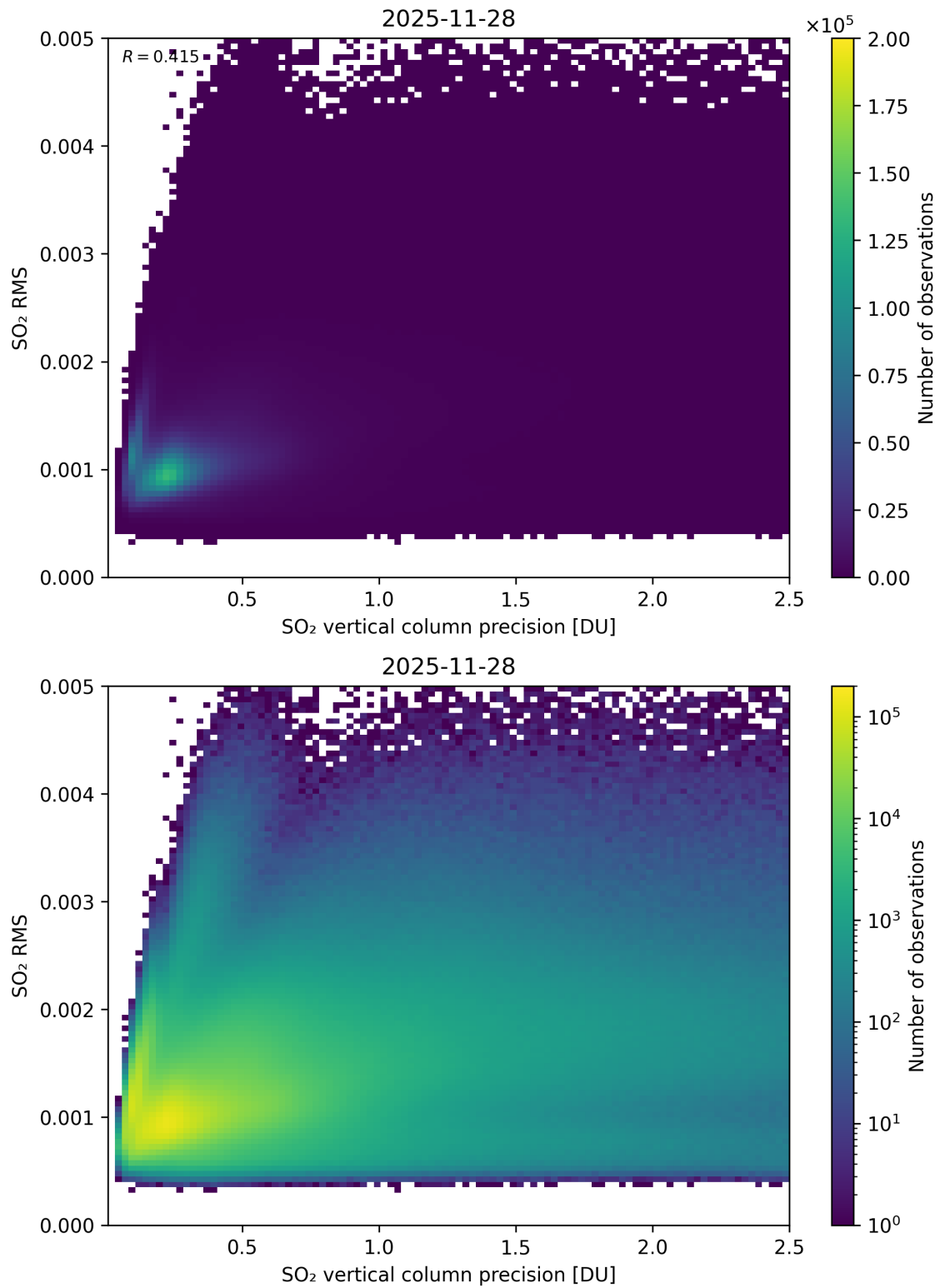
Figure 334: Scatter density plot of “SO 2 vertical column precision” against “SO 2 RMS” for 2025-11-28 to 2025-11-29.
