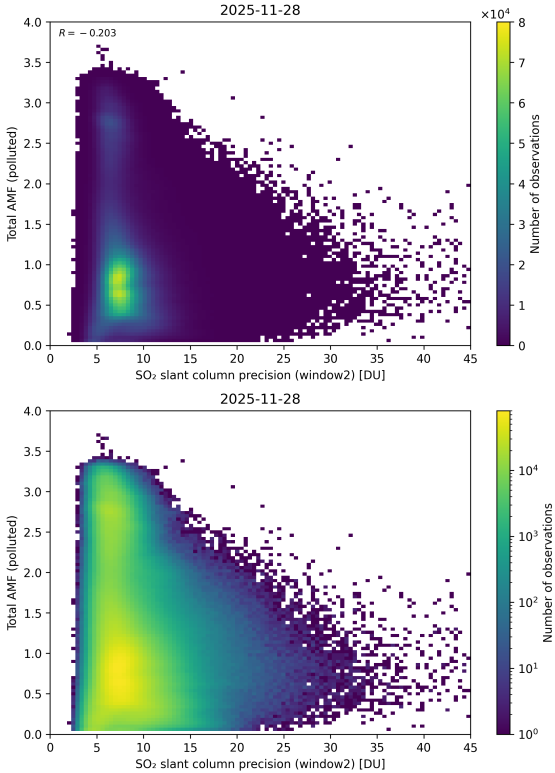
Figure 301: Scatter density plot of “SO 2 slant column precision (window2)” against “Total AMF (polluted)” for 2025-11-28 to 2025-11-29.
