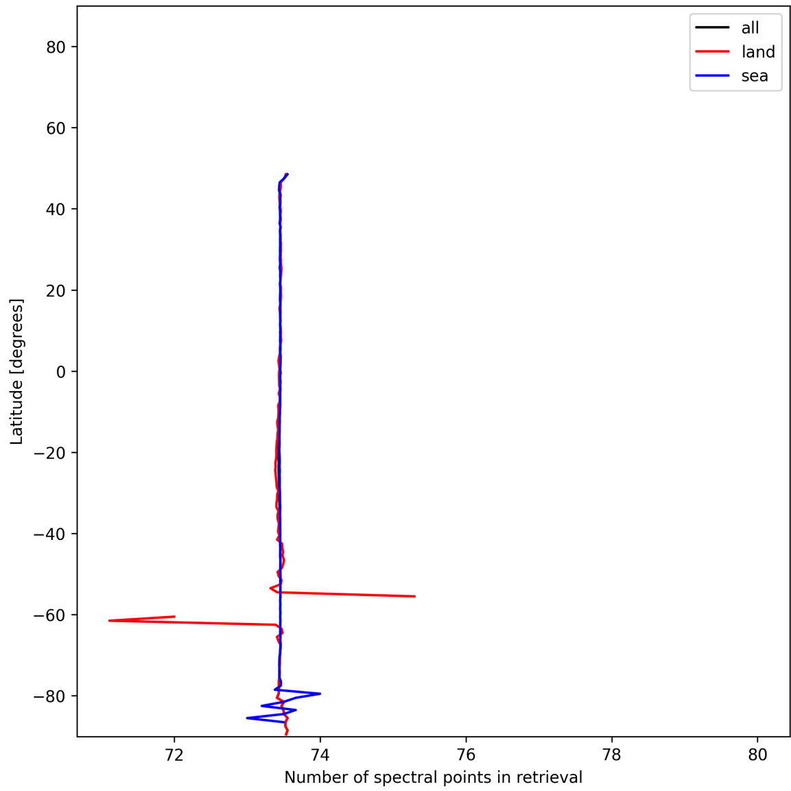
Figure 56: Zonal average of “Number of spectral points in retrieval” for 2025-11-28 to 2025-11-29.
