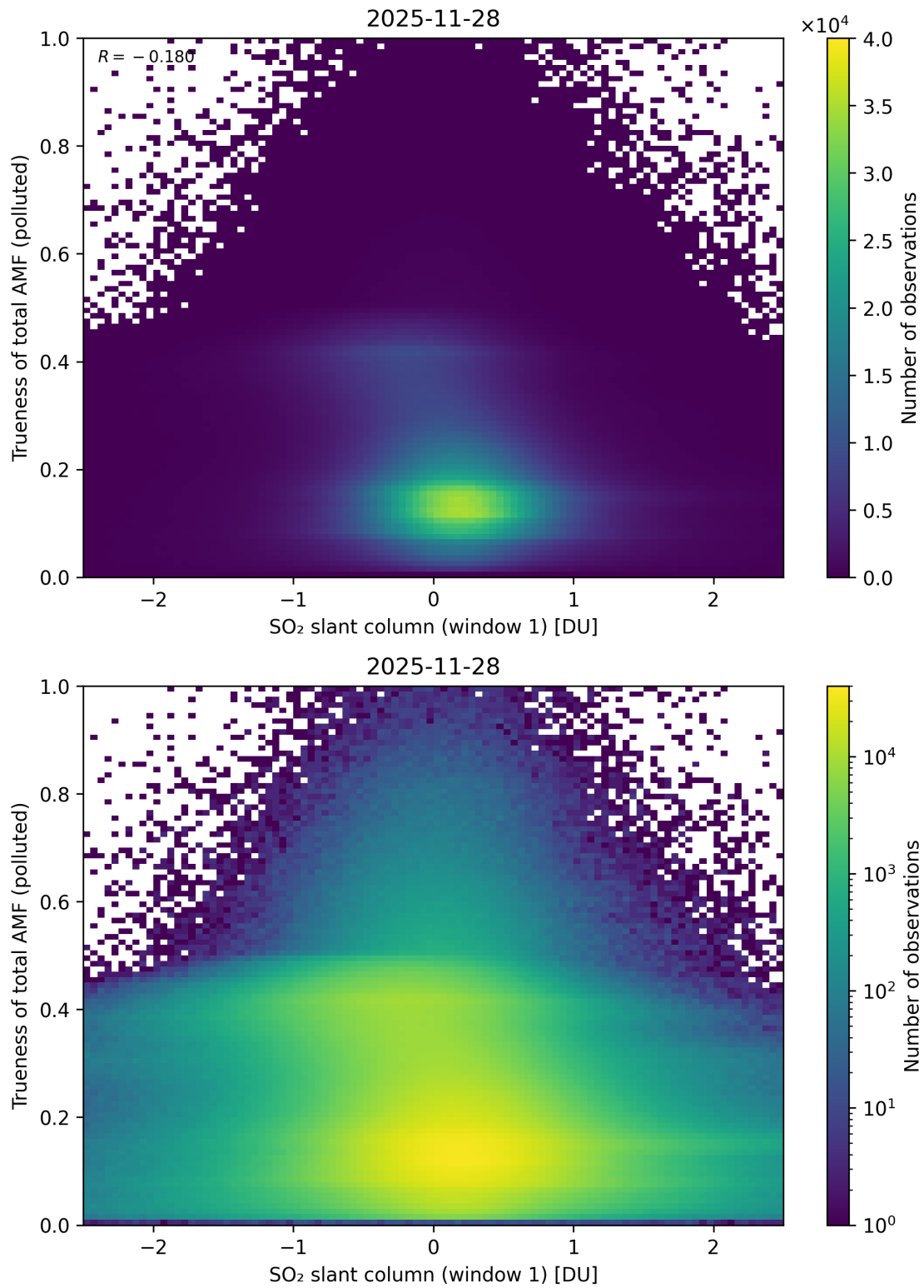
Figure 290: Scatter density plot of “SO 2 slant column (window 1)” against “Trueness of total AMF (polluted)” for 2025-11-28 to 2025-11-29.
