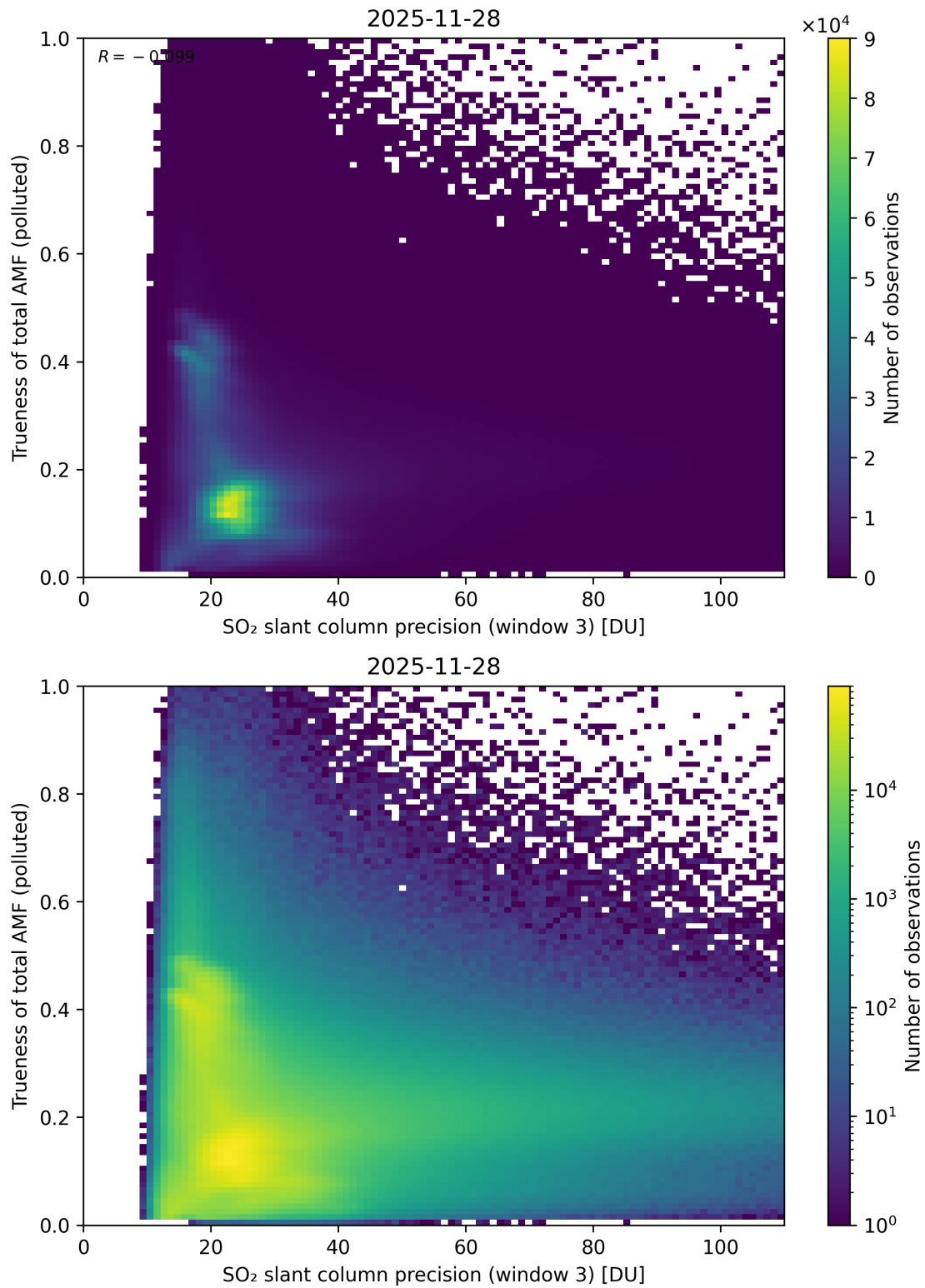
Figure 314: Scatter density plot of “SO 2 slant column precision (window 3)” against “Trueness of total AMF (polluted)” for 2025-11-28 to 2025-11-29.
