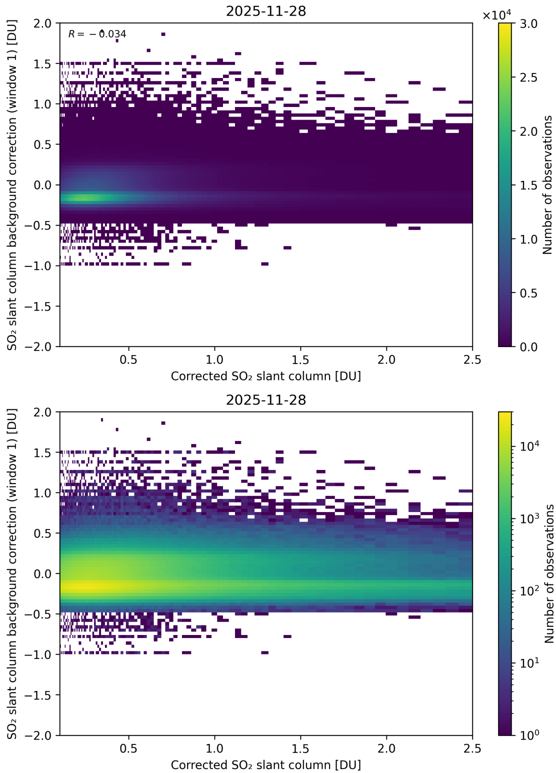
Figure 226: Scatter density plot of “Corrected SO 2 slant column” against “SO 2 slant column background correction (window 1)” for 2025-11-28 to 2025-11-29.
