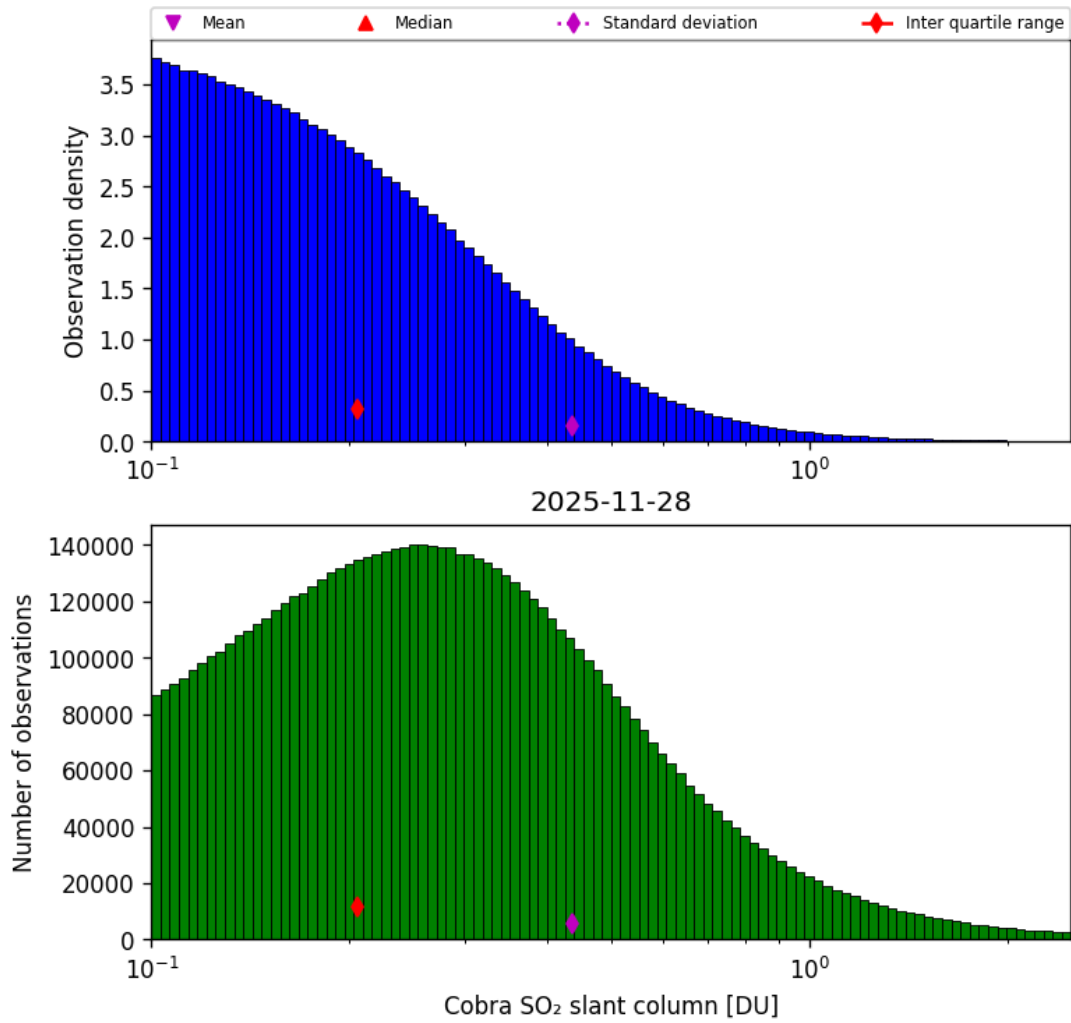
Figure 61: Histogram of “Cobra SO 2 slant column” for 2025-11-28 to 2025-11-29
