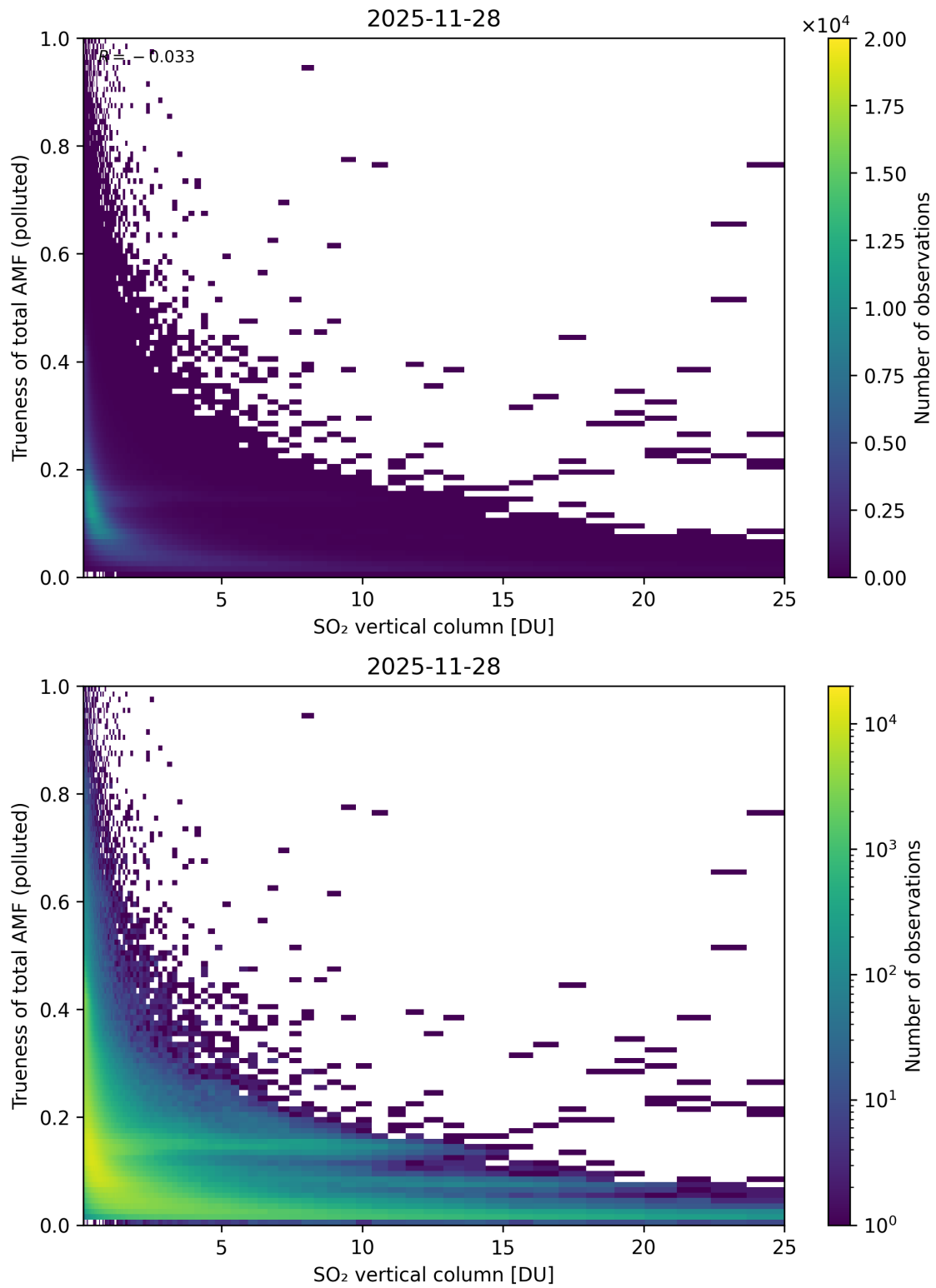
Figure 360: Scatter density plot of “SO 2 vertical column” against “Truthness of total AMF (polluted)” for 2025-11-28 to 2025-11-29.
