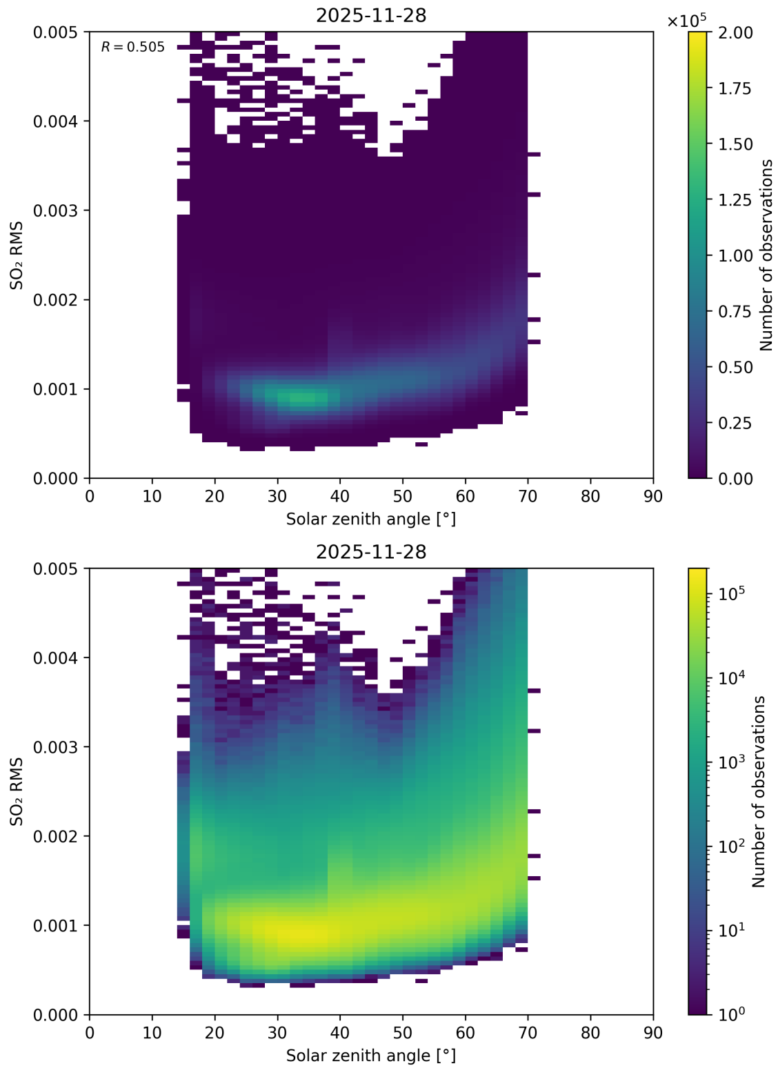
Figure 176: Scatter density plot of “Solar zenith angle” against “SO 2 RMS” for 2025-11-28 to 2025-11-29.
