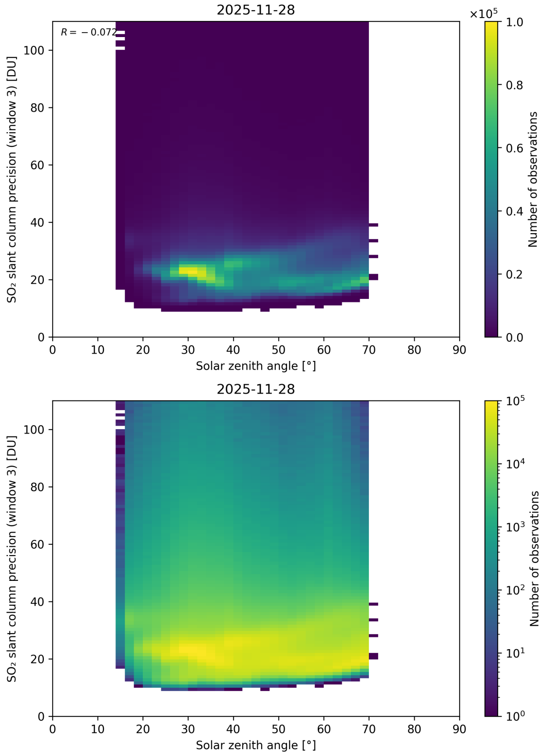
Figure 188: Scatter density plot of “Solar zenith angle” against “SO 2 slant column precision (window 3)” for 2025-11-28 to 2025-11-29.
