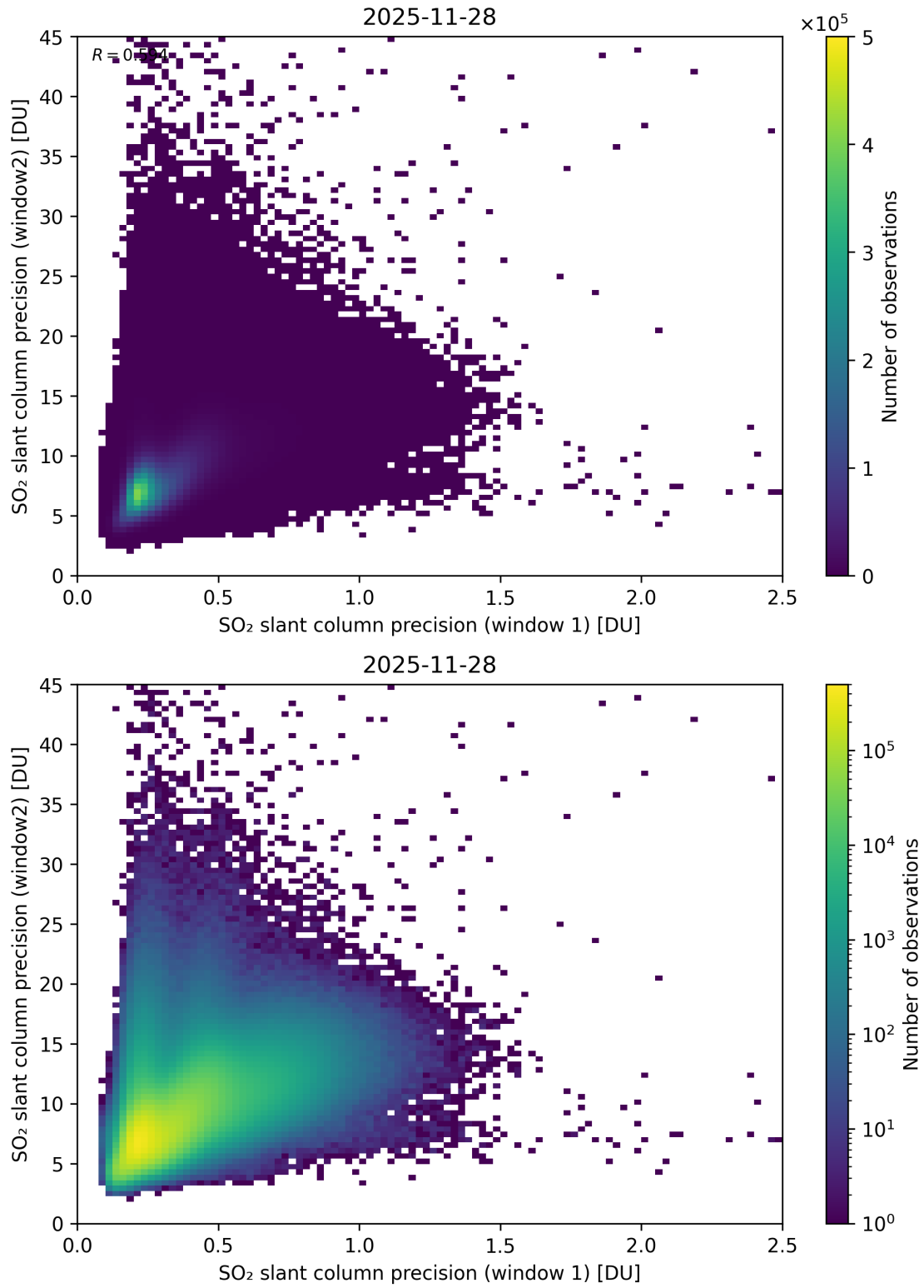
Figure 277: Scatter density plot of “SO 2 slant column precision (window 1)” against “SO 2 slant column precision (window2)” for 2025-11-28 to 2025-11-29.
