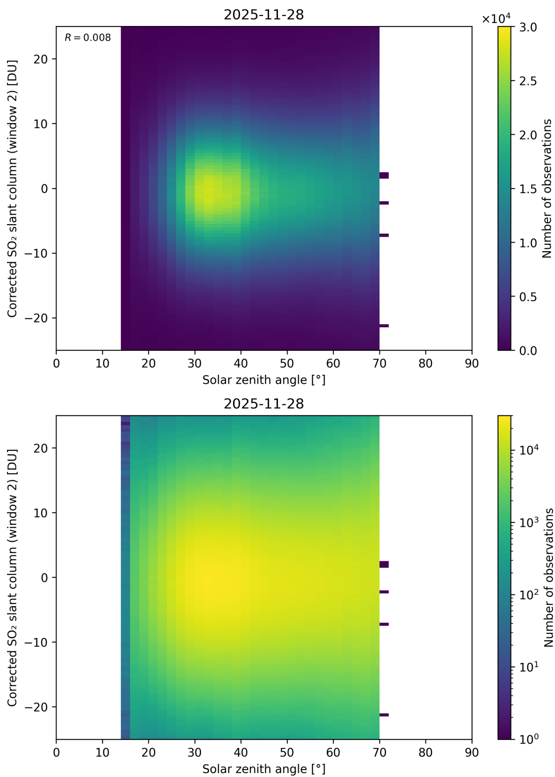
Figure 182: Scatter density plot of “Solar zenith angle” against “Corrected SO 2 slant column (window 2)” for 2025-11-28 to 2025-11-29.
