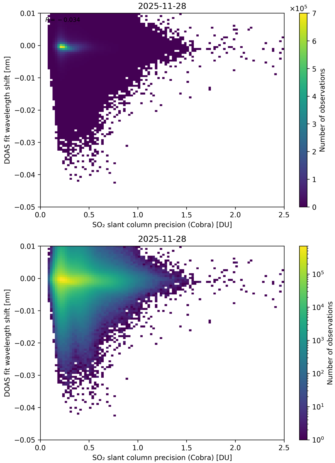
Figure 202: Scatter density plot of “SO 2 slant column precision (Cobra)” against “DOAS fit wavelength shift” for 2025-11-28 to 2025-11-29.
