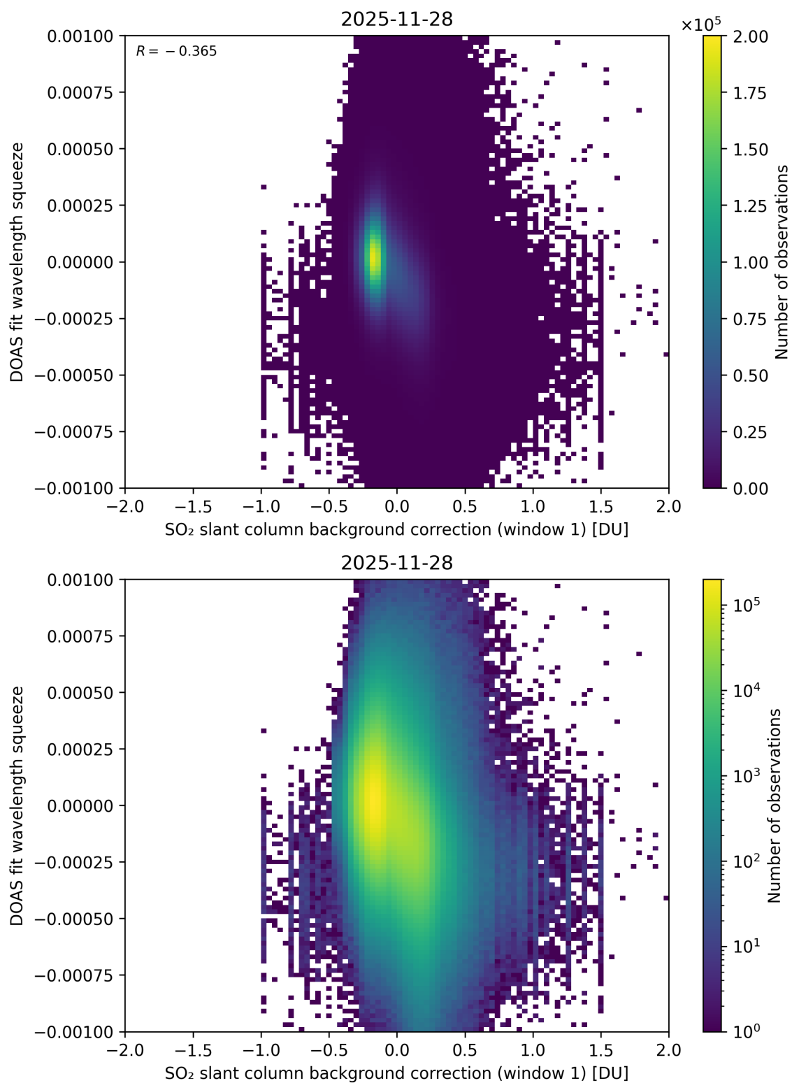
Figure 112: Scatter density plot of “SO 2 slant column background correction (window 1)” against “DOAS fit wavelength squeeze” for 2025-11-28 to 2025-11-29.
