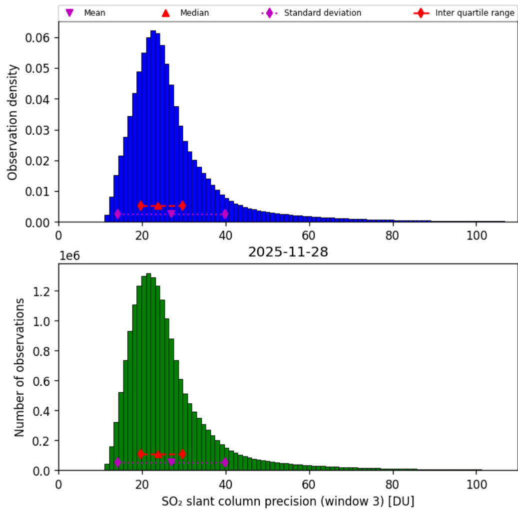
Figure 72: Histogram of “SO 2 slant column precision (window 3)” for 2025-11-28 to 2025-11-29
