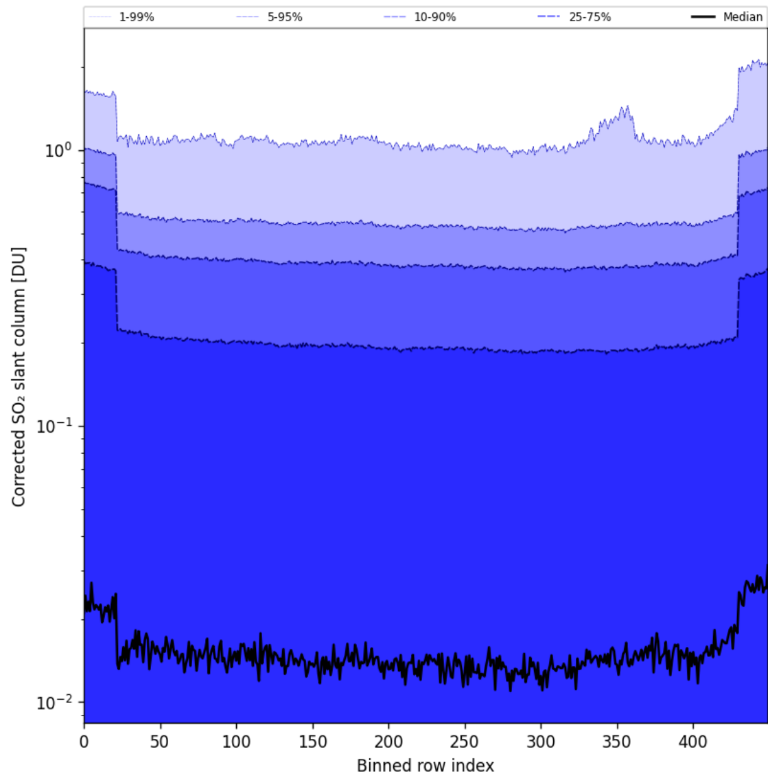
Figure 86: Along track statistics of "Corrected SO 2 slant column" for 2025-11-28 to 2025-11-29
