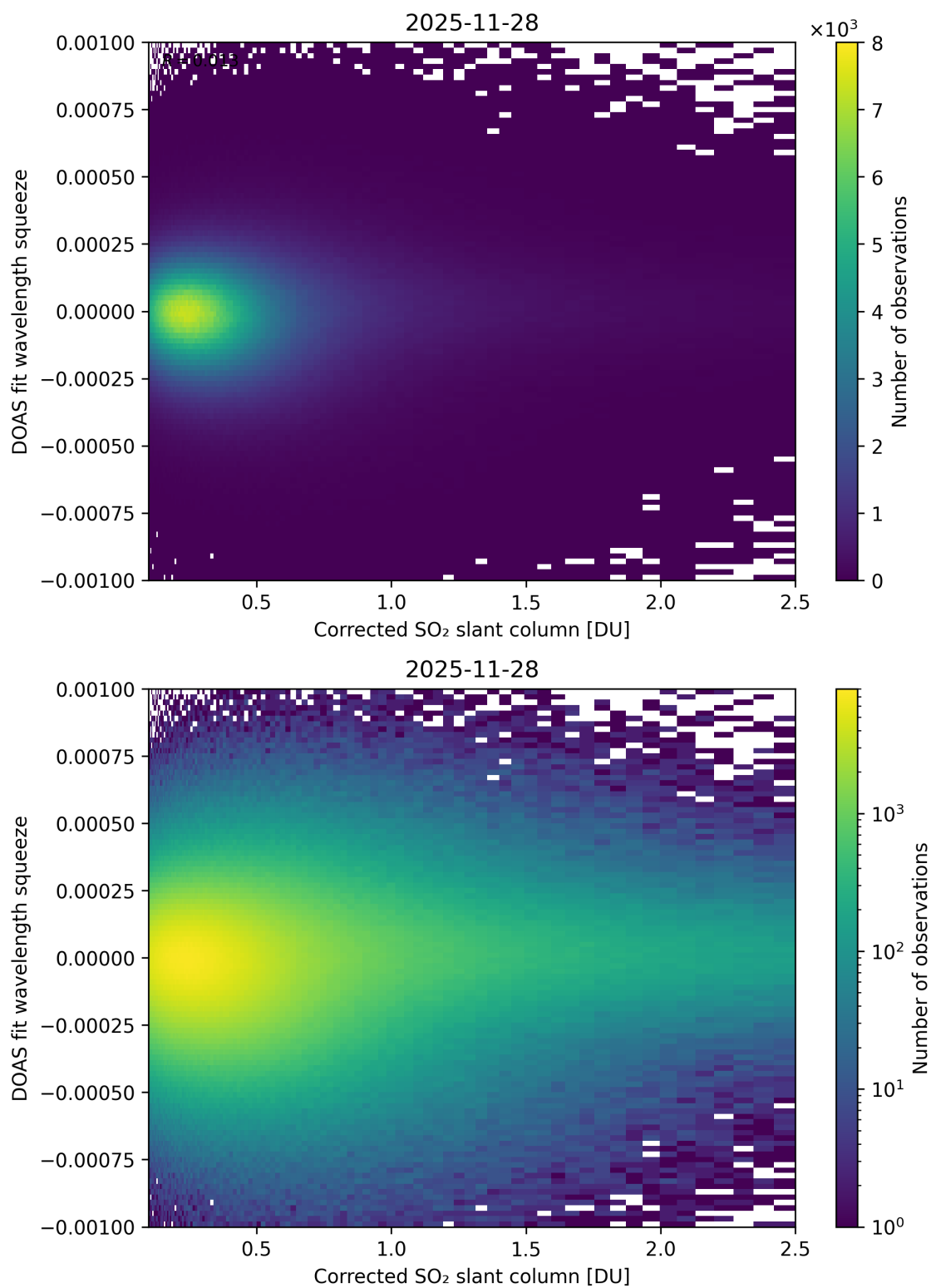
Figure 230: Scatter density plot of "Corrected SO 2 slant column" against "DOAS fit wavelength squeeze" for 2025-11-28 to 2025-11-29.
