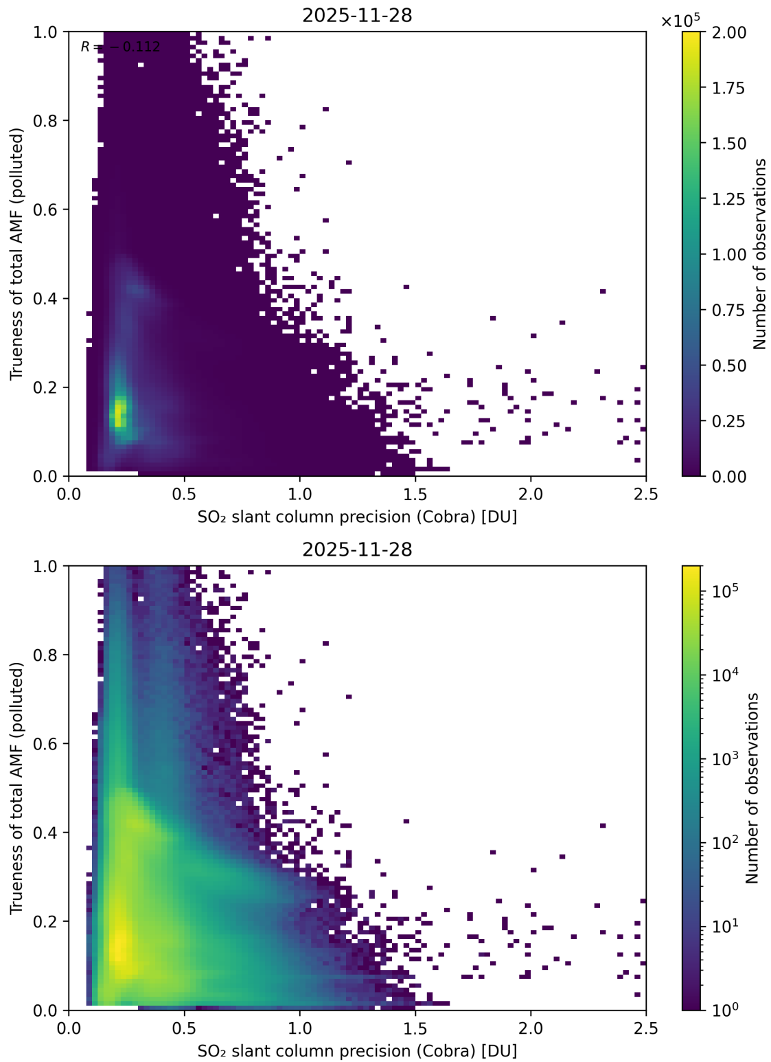
Figure 214: Scatter density plot of “SO 2 slant column precision (Cobra)” against “Trueness of total AMF (polluted)” for 2025-11-28 to 2025-11-29.
