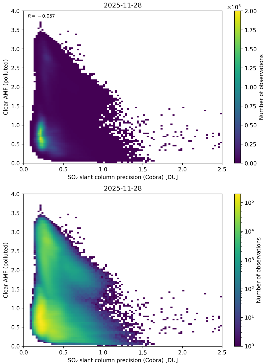
Figure 205: Scatter density plot of “SO 2 slant column precision (Cobra)” against “Clear AMF (polluted)” for 2025-11-28 to 2025-11-29.
