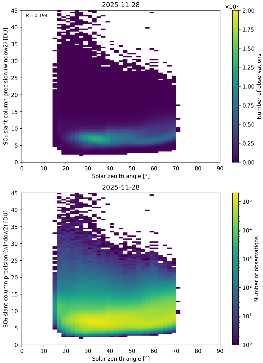
Figure 186: Scatter density plot of “Solar zenith angle” against “SO 2 slant column precision (window2)” for 2025-11-28 to 2025-11-29.
