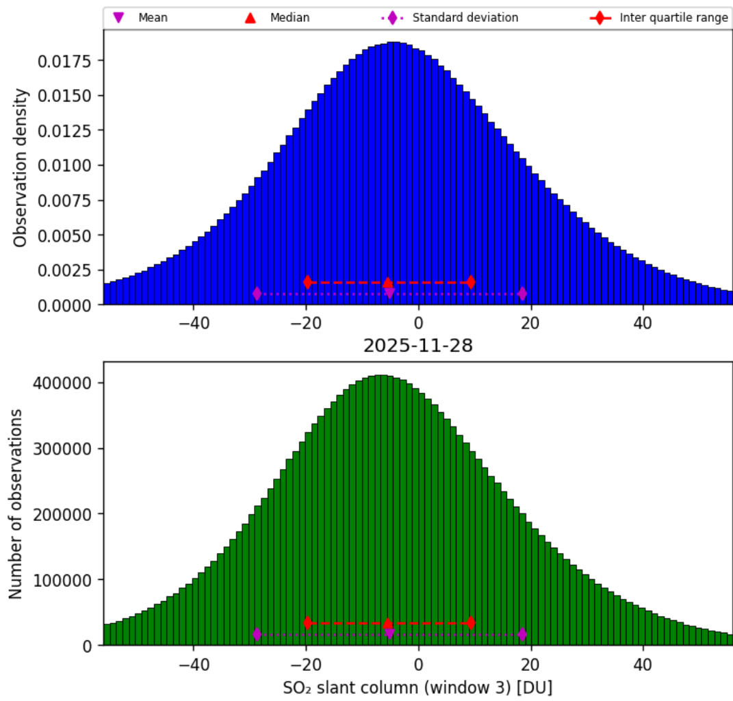
Figure 71: Histogram of “SO 2 slant column (window 3)” for 2025-11-28 to 2025-11-29
