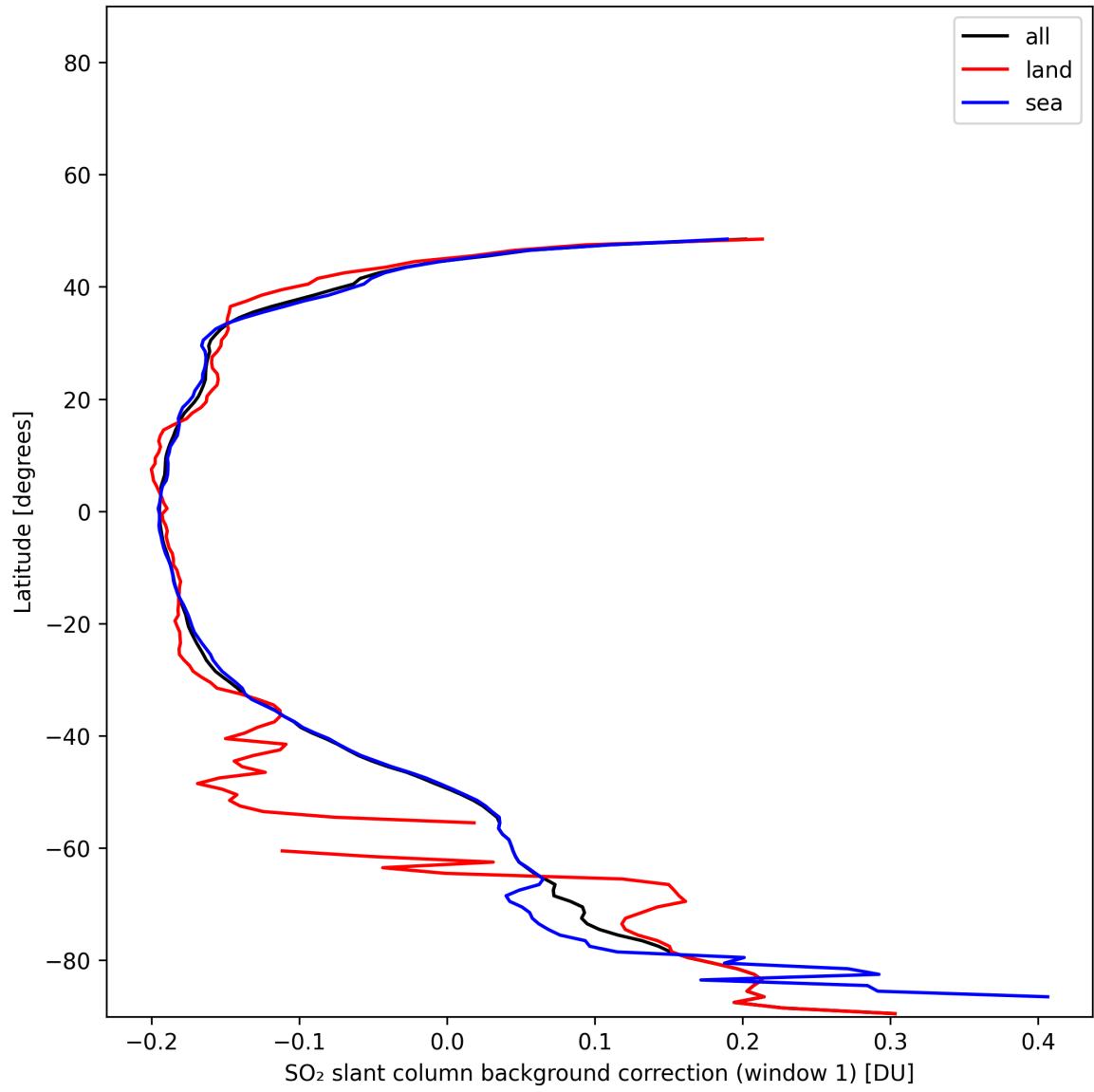
Figure 40: Zonal average of “SO 2 slant column background correction (window 1)” for 2025-11-28 to 2025-11-29.
