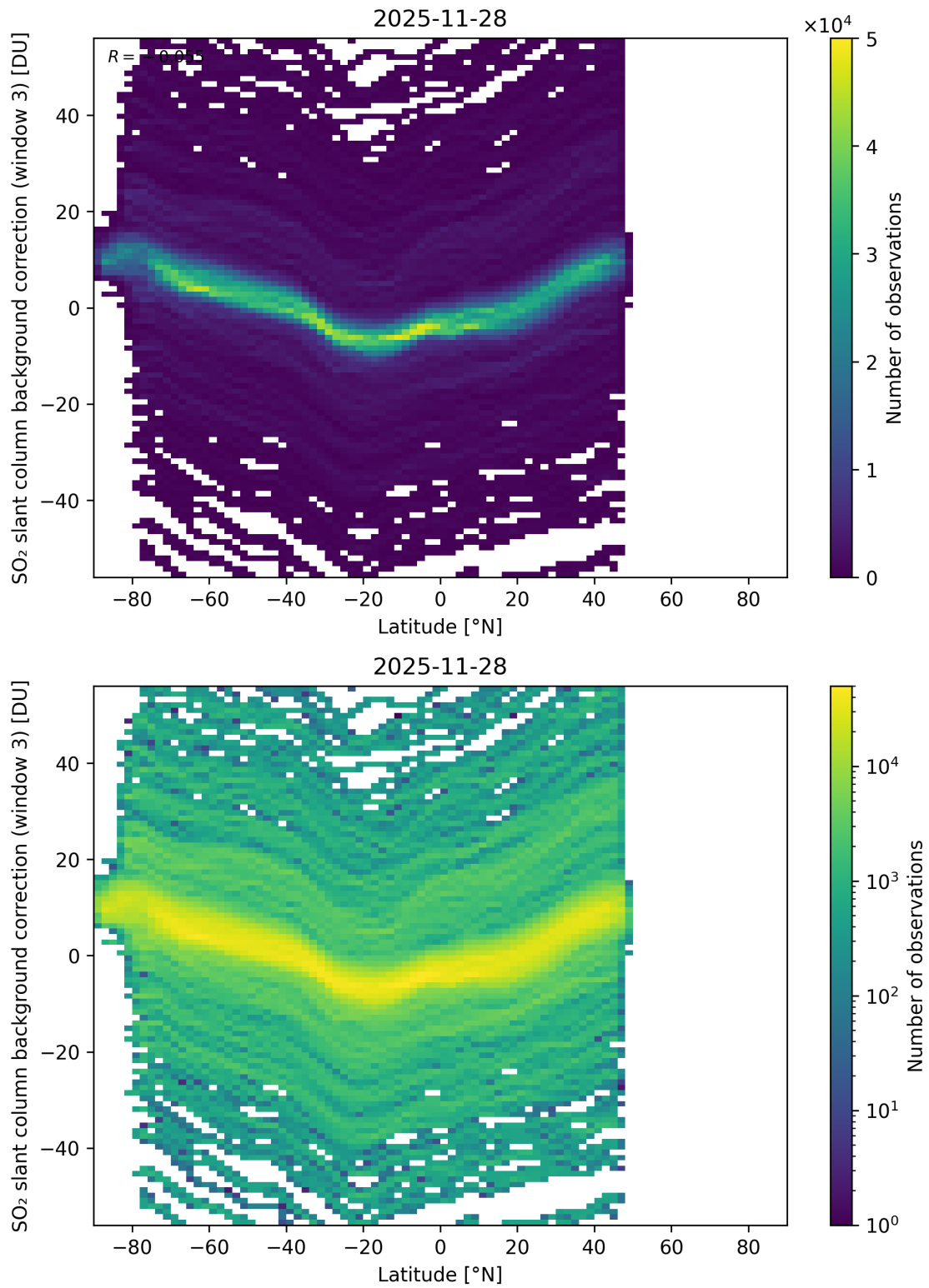
Figure 152: Scatter density plot of “Latitude” against “SO 2 slant column background correction (window 3)” for 2025-11-28 to 2025-11-29.
