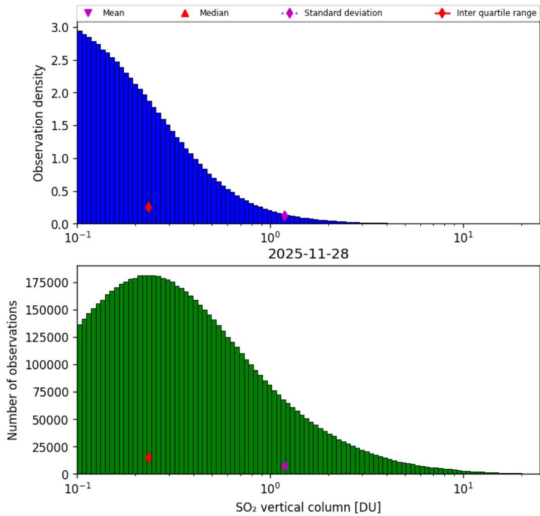
Figure 58: Histogram of “SO 2 vertical column” for 2025-11-28 to 2025-11-29
