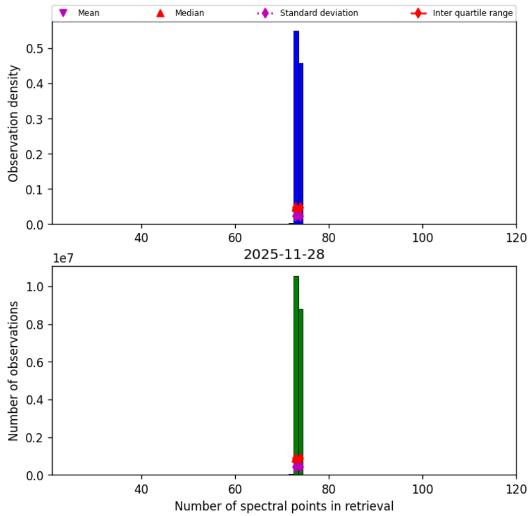
Figure 82: Histogram of “Number of spectral points in retrieval” for 2025-11-28 to 2025-11-29
