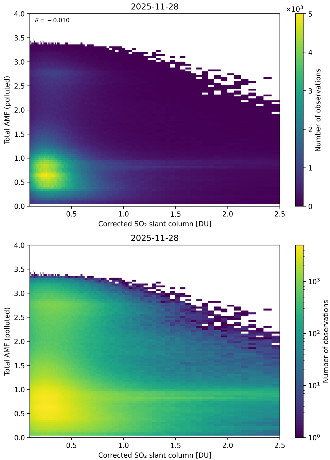
Figure 242: Scatter density plot of “Corrected SO 2 slant column” against “Total AMF (polluted)” for 2025-11-28 to 2025-11-29.
