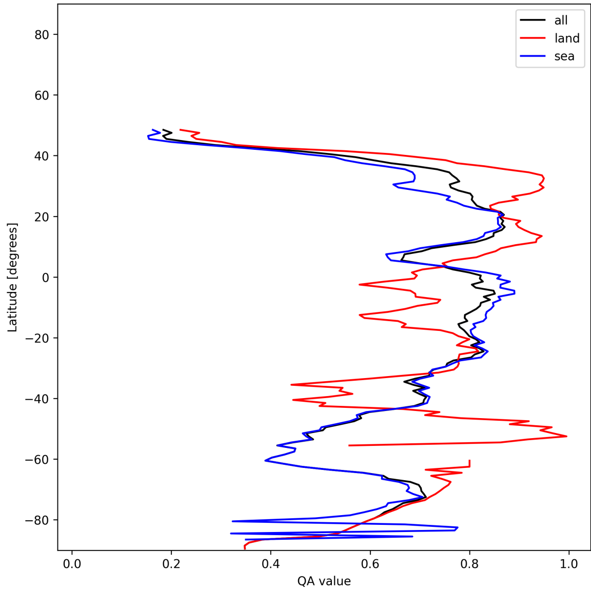
Figure 31: Zonal average of “QA value” for 2025-11-28 to 2025-11-29.
