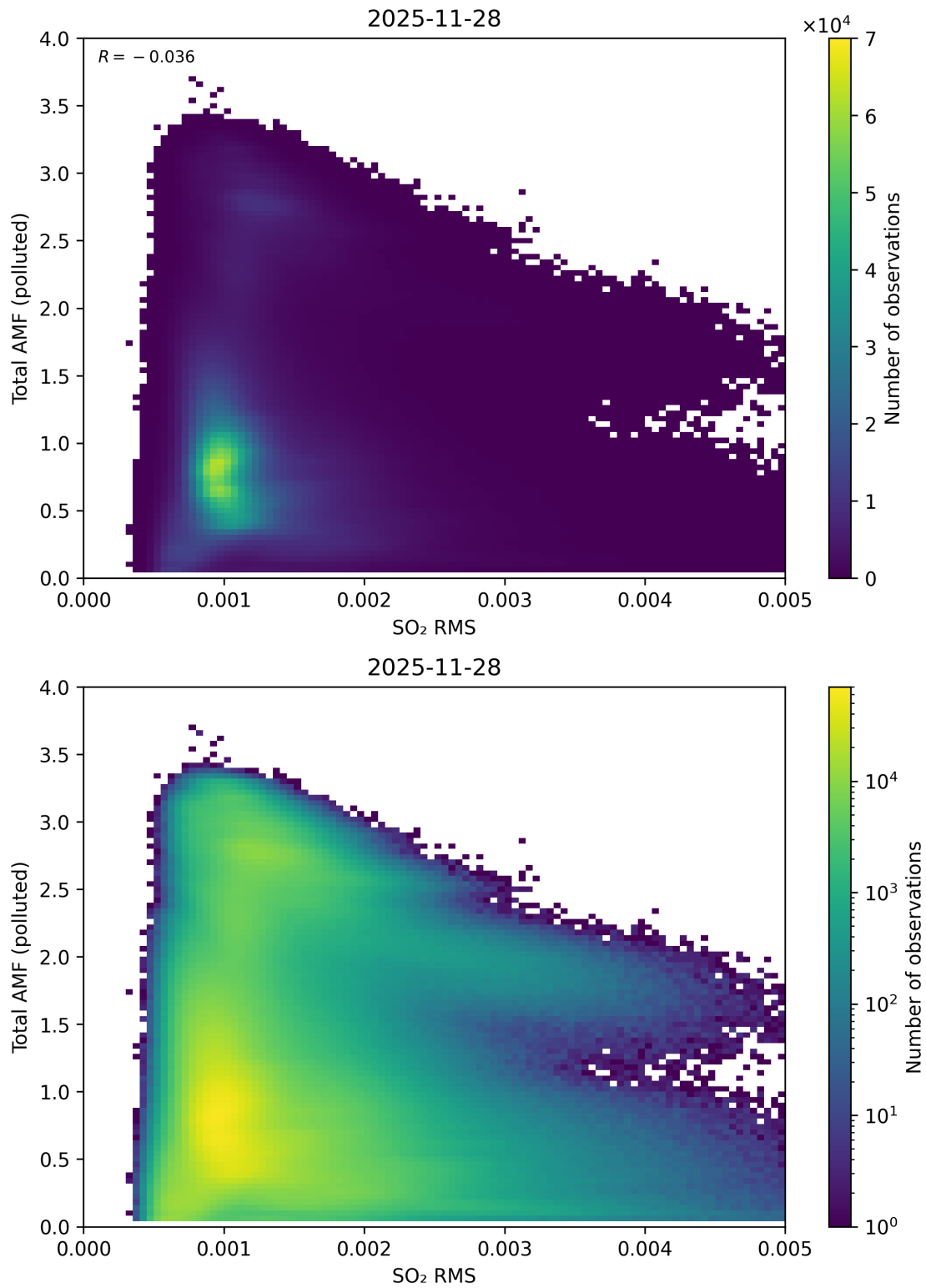
Figure 148: Scatter density plot of “SO 2 RMS” against “Total AMF (polluted)” for 2025-11-28 to 2025-11-29.
