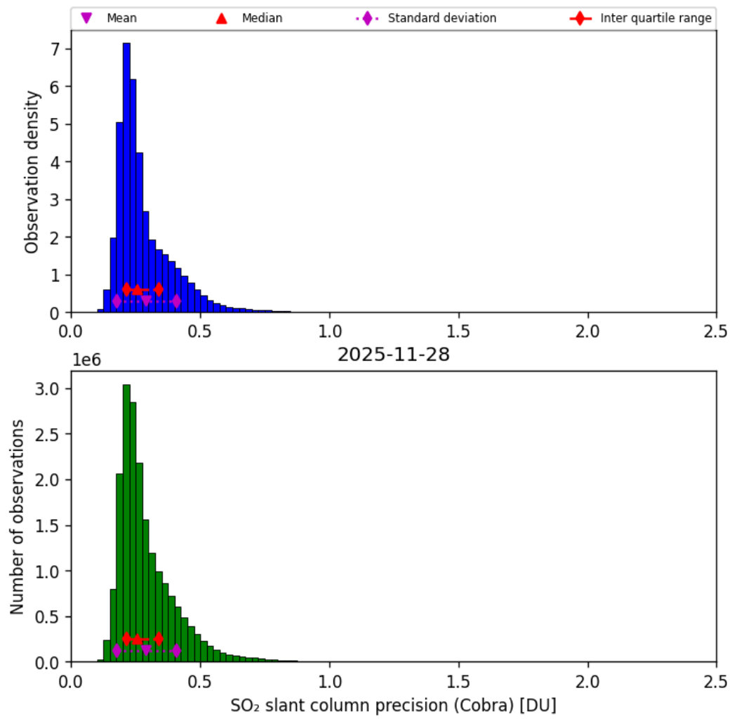
Figure 62: Histogram of “SO 2 slant column precision (Cobra)” for 2025-11-28 to 2025-11-29
