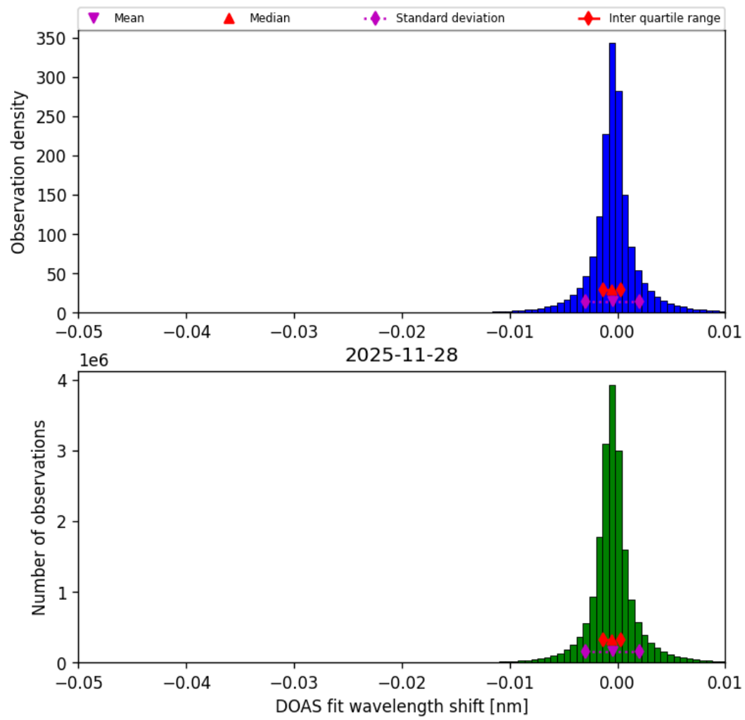
Figure 76: Histogram of “DOAS fit wavelength shift” for 2025-11-28 to 2025-11-29
