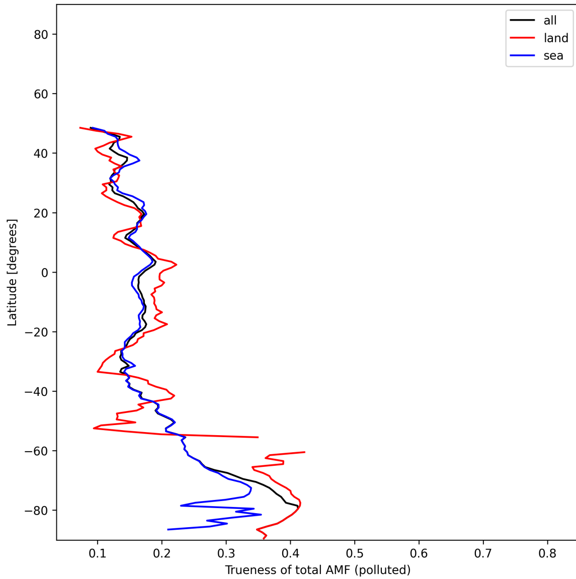
Figure 54: Zonal average of “Trueness of total AMF (polluted)” for 2025-11-28 to 2025-11-29.
