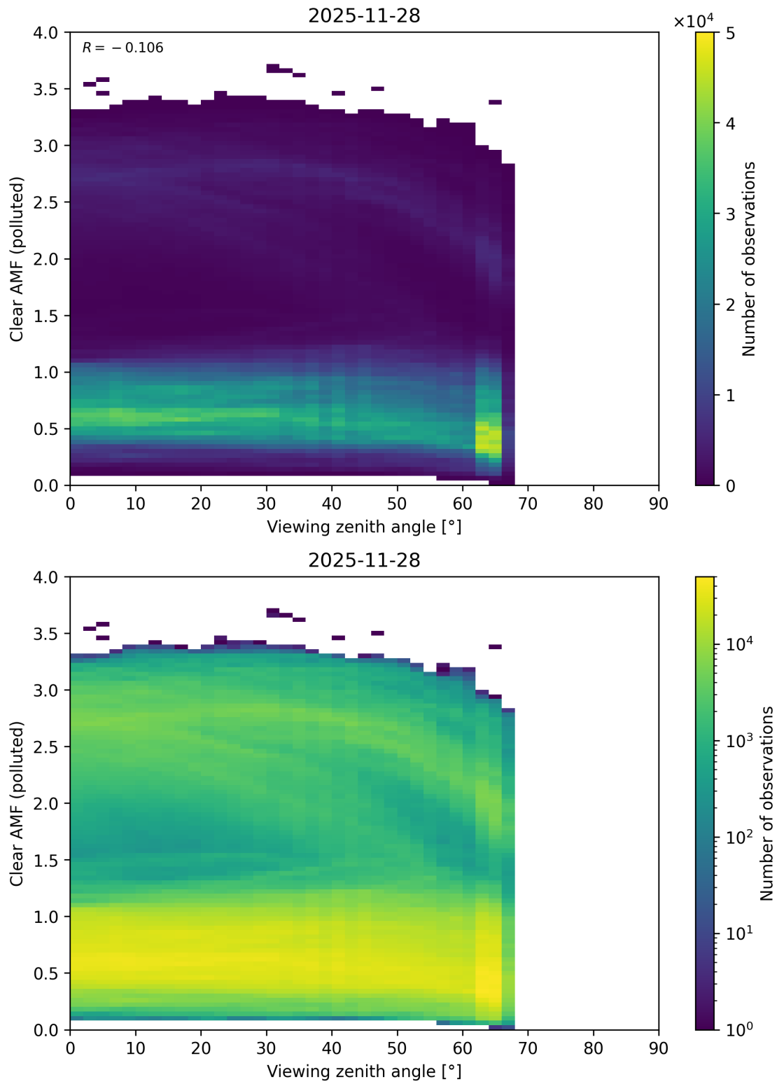
Figure 370: Scatter density plot of “Viewing zenith angle” against “Clear AMF (polluted)” for 2025-11-28 to 2025-11-29.
