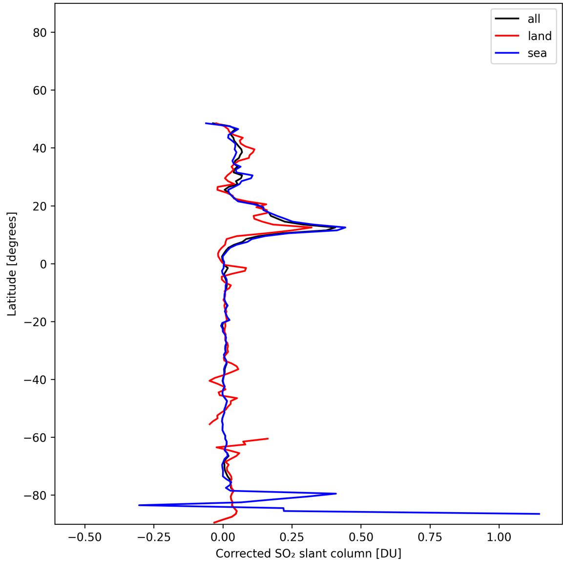
Figure 34: Zonal average of “Corrected SO 2 slant column” for 2025-11-28 to 2025-11-29.
