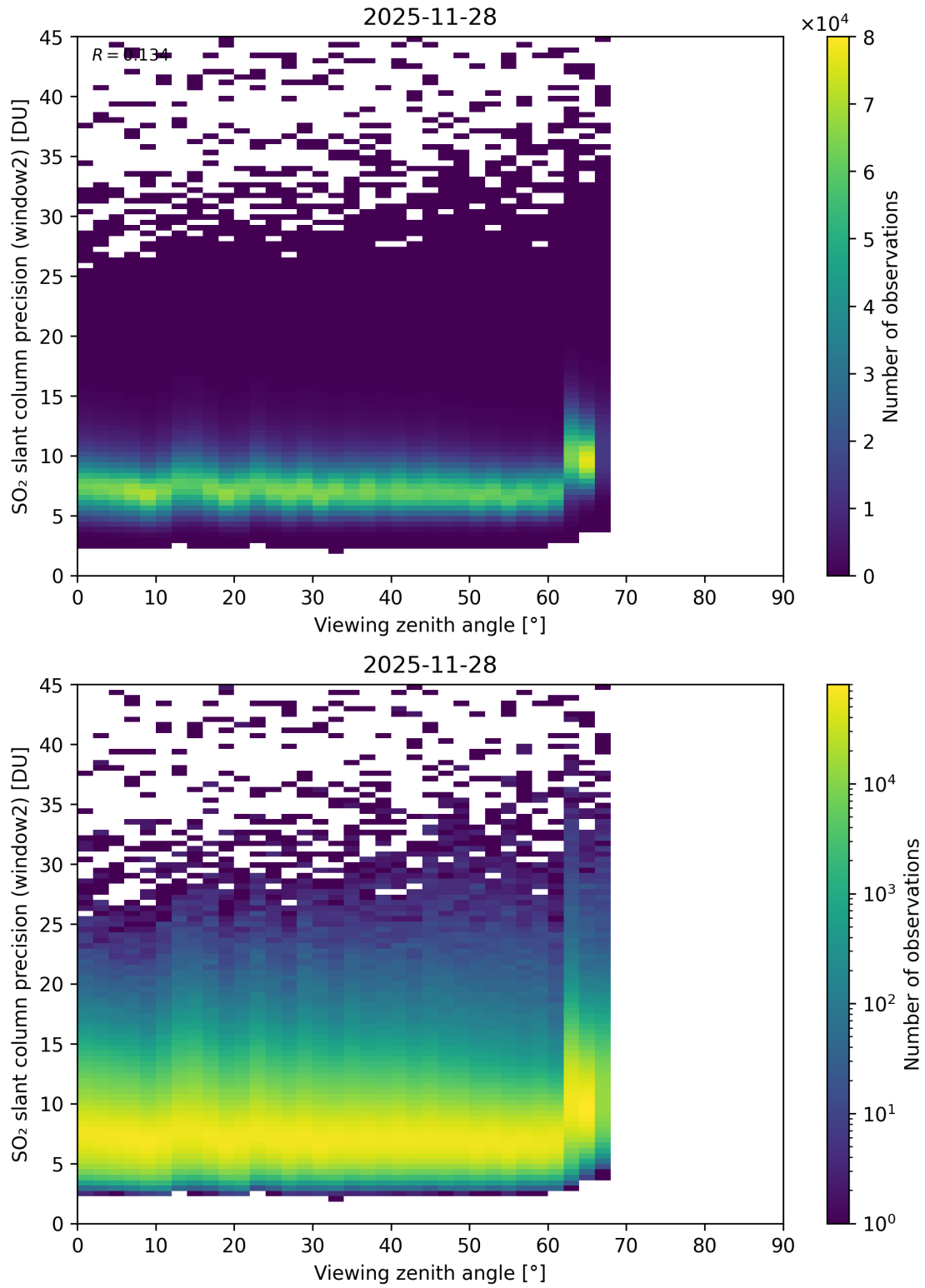
Figure 378: Scatter density plot of “Viewing zenith angle” against “SO 2 slant column precision (window2)” for 2025-11-28 to 2025-11-29.
