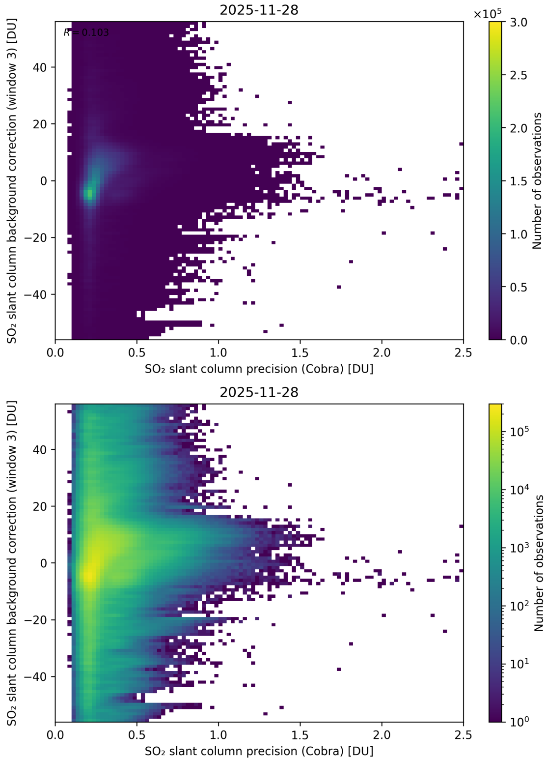
Figure 201: Scatter density plot of “SO 2 slant column precision (Cobra)” against “SO 2 slant column background correction (window 3)” for 2025-11-28 to 2025-11-29.
