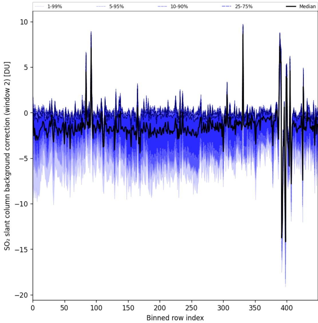
Figure 96: Along track statistics of "SO 2 slant column background correction (window 2)" for 2025-11-28 to 2025-11-29
