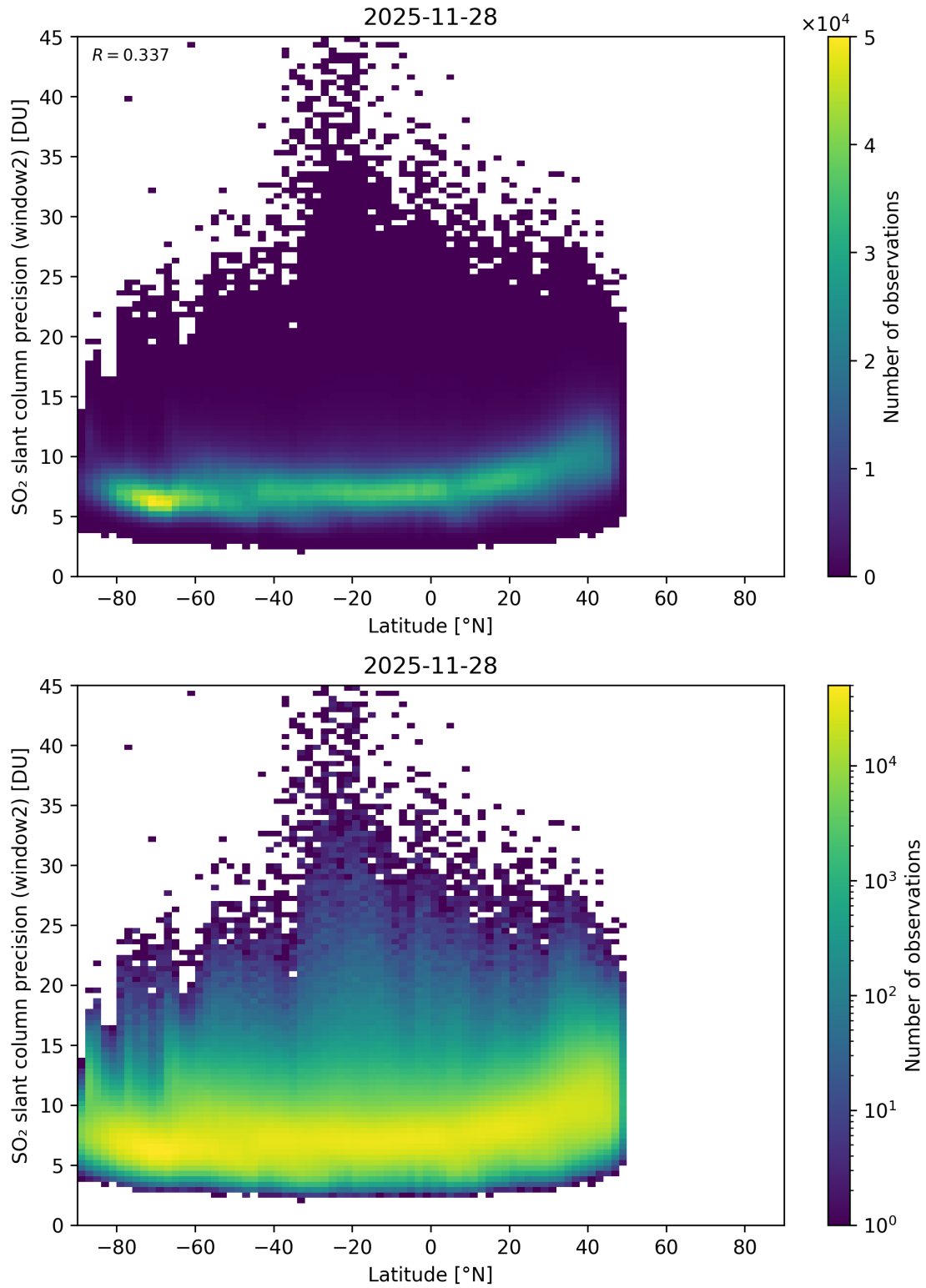
Figure 164: Scatter density plot of “Latitude” against “SO 2 slant column precision (window2)” for 2025-11-28 to 2025-11-29.
