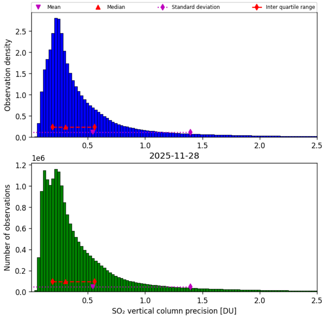
Figure 59: Histogram of “SO 2 vertical column precision” for 2025-11-28 to 2025-11-29
