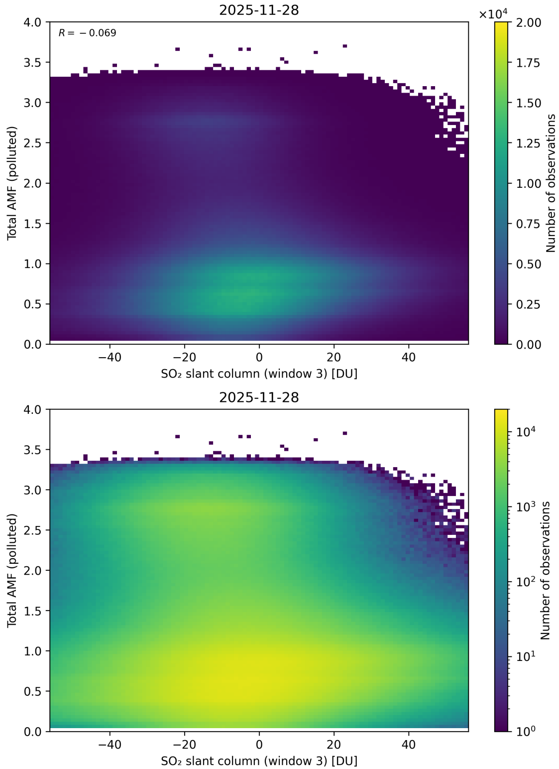
Figure 318: Scatter density plot of “SO 2 slant column (window 3)” against “Total AMF (polluted)” for 2025-11-28 to 2025-11-29.
