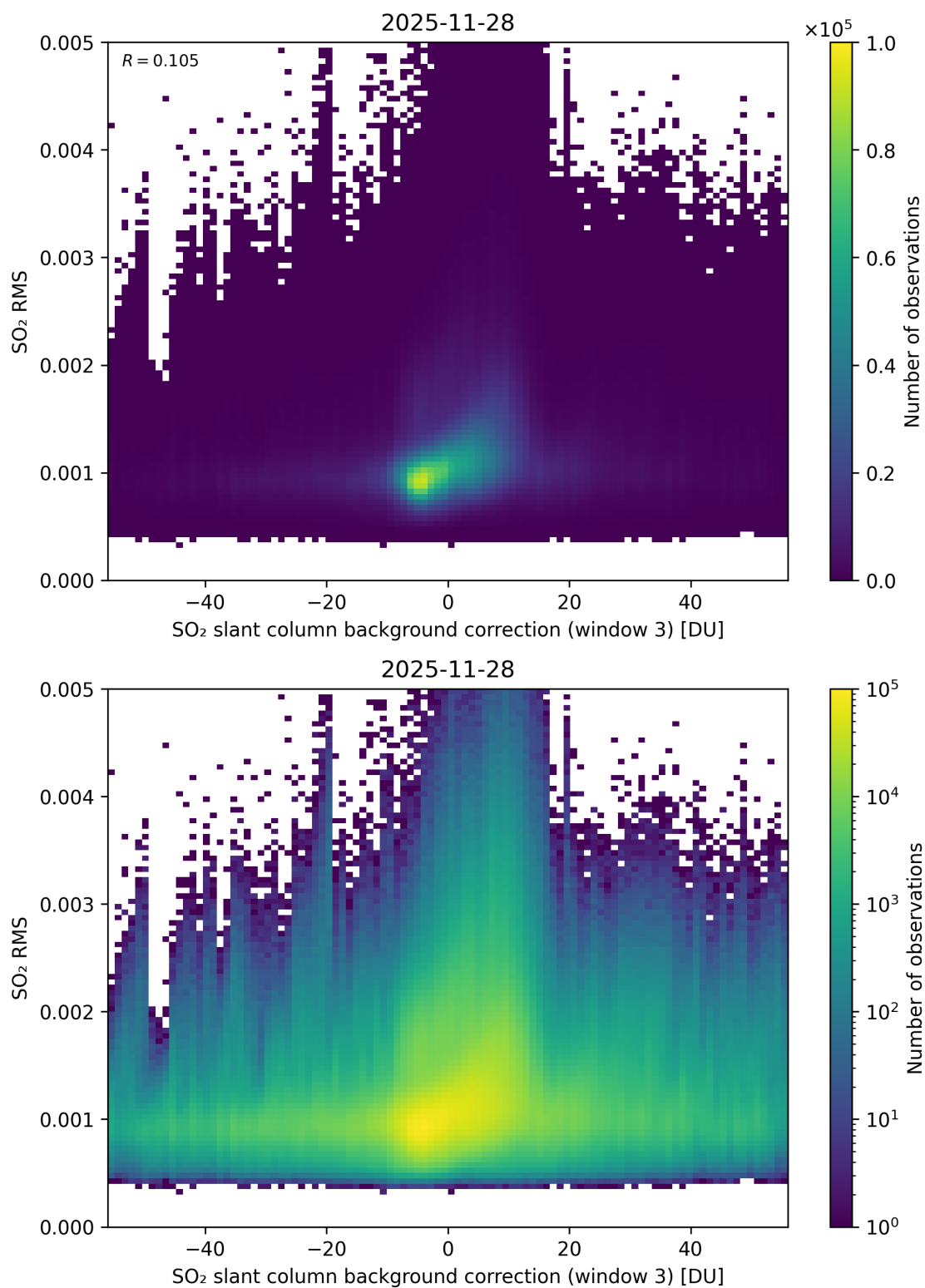
Figure 134: Scatter density plot of “SO 2 slant column background correction (window 3)” against “SO 2 RMS” for 2025-11-28 to 2025-11-29.
