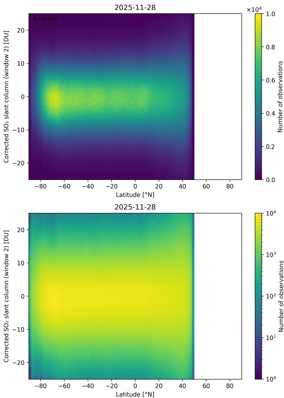
Figure 160: Scatter density plot of “Latitude” against “Corrected SO 2 slant column (window 2)” for 2025-11-28 to 2025-11-29.
