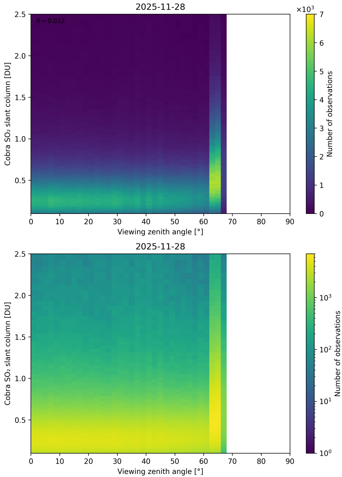
Figure 371: Scatter density plot of “Viewing zenith angle” against “Cobra SO 2 slant column” for 2025-11-28 to 2025-11-29.
