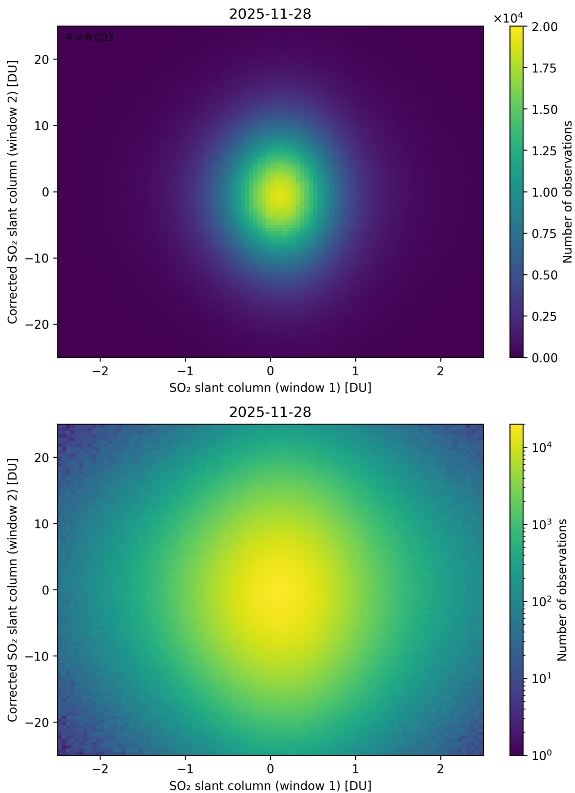
Figure 283: Scatter density plot of “SO 2 slant column (window 1)” against “Corrected SO 2 slant column (window 2)” for 2025-11-28 to 2025-11-29.
