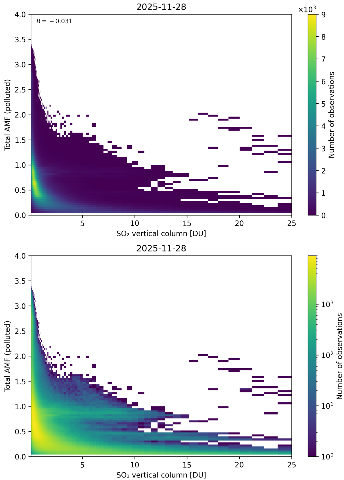
Figure 359: Scatter density plot of “SO 2 vertical column” against “Total AMF (polluted)” for 2025-11-28 to 2025-11-29.
