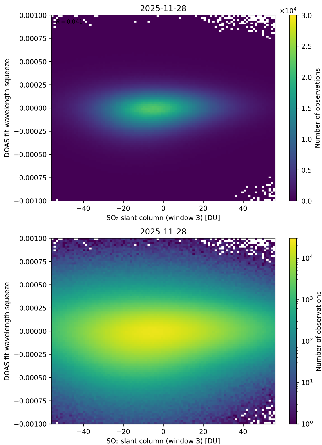
Figure 305: Scatter density plot of “SO 2 slant column (window 3)” against “DOAS fit wavelength squeeze” for 2025-11-28 to 2025-11-29.
