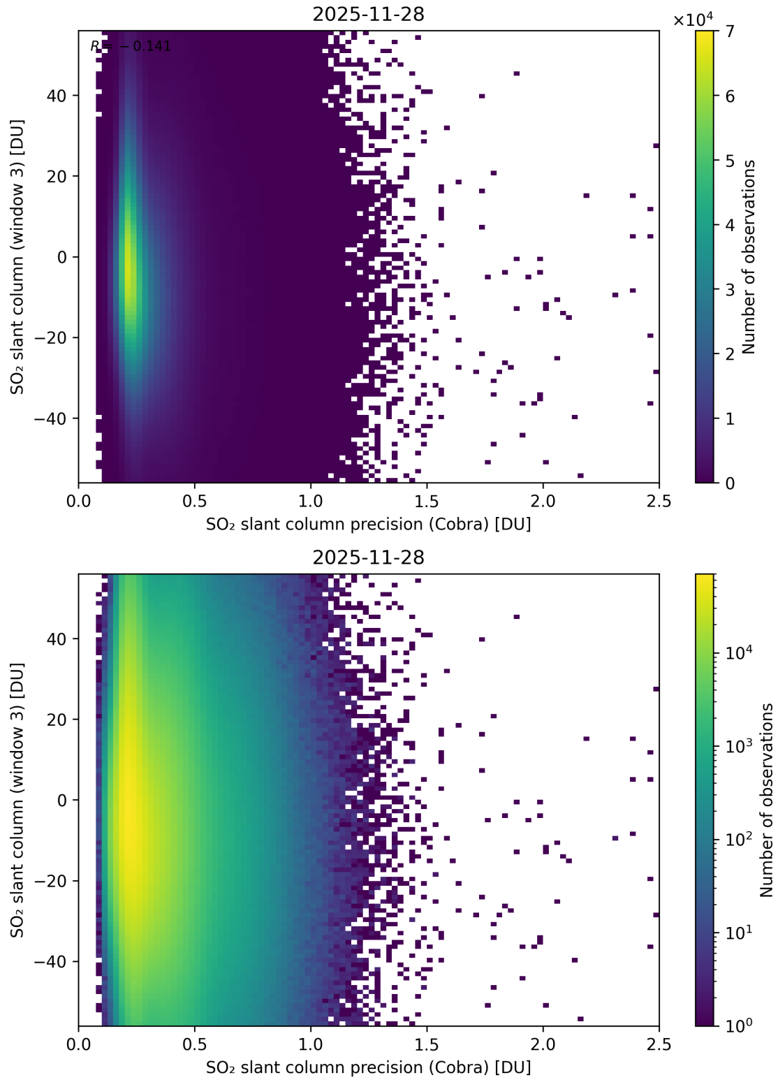
Figure 211: Scatter density plot of “SO 2 slant column precision (Cobra)” against “SO 2 slant column (window 3)” for 2025-11-28 to 2025-11-29.
