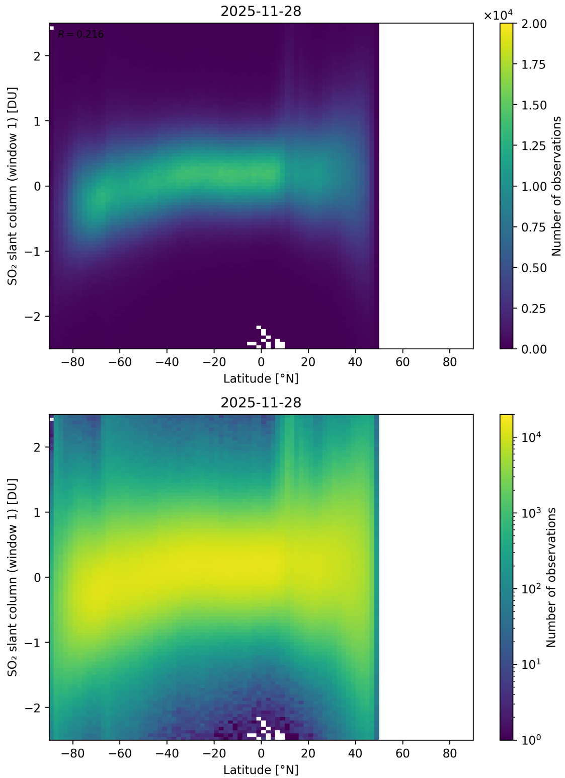
Figure 162: Scatter density plot of “Latitude” against “SO 2 slant column (window 1)” for 2025-11-28 to 2025-11-29.
