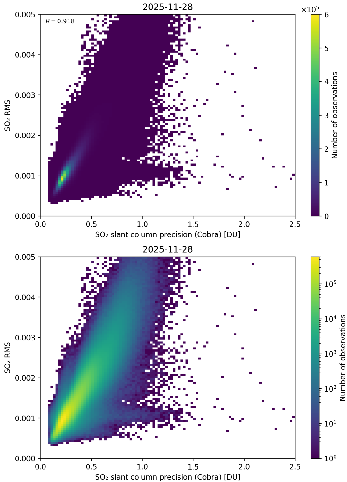
Figure 204: Scatter density plot of “SO 2 slant column precision (Cobra)” against “SO 2 RMS” for 2025-11-28 to 2025-11-29.
