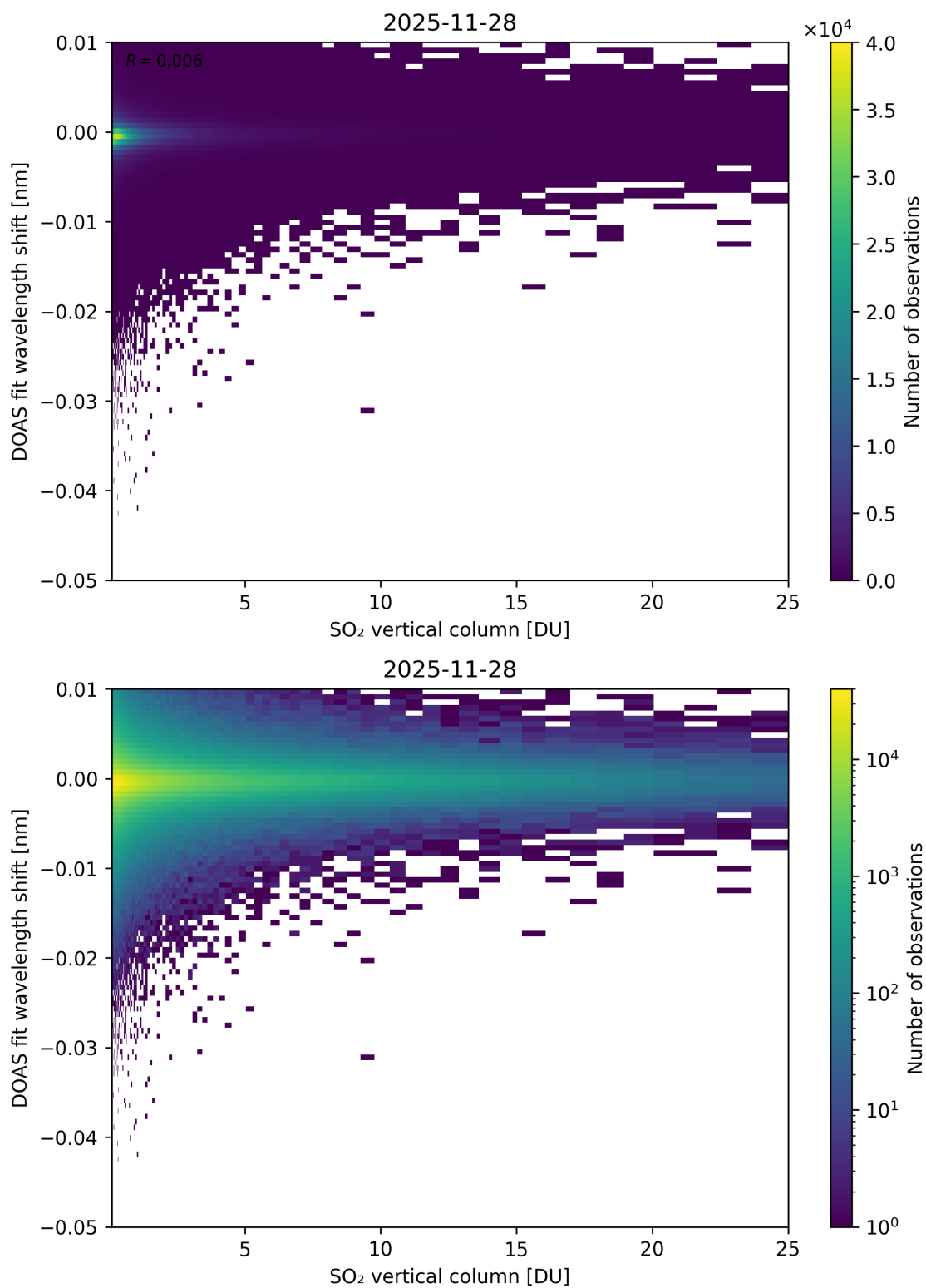
Figure 326: Scatter density plot of “SO 2 vertical column” against “DOAS fit wavelength shift” for 2025-11-28 to 2025-11-29.
