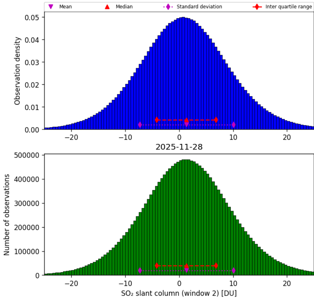
Figure 67: Histogram of “SO 2 slant column (window 2)” for 2025-11-28 to 2025-11-29
