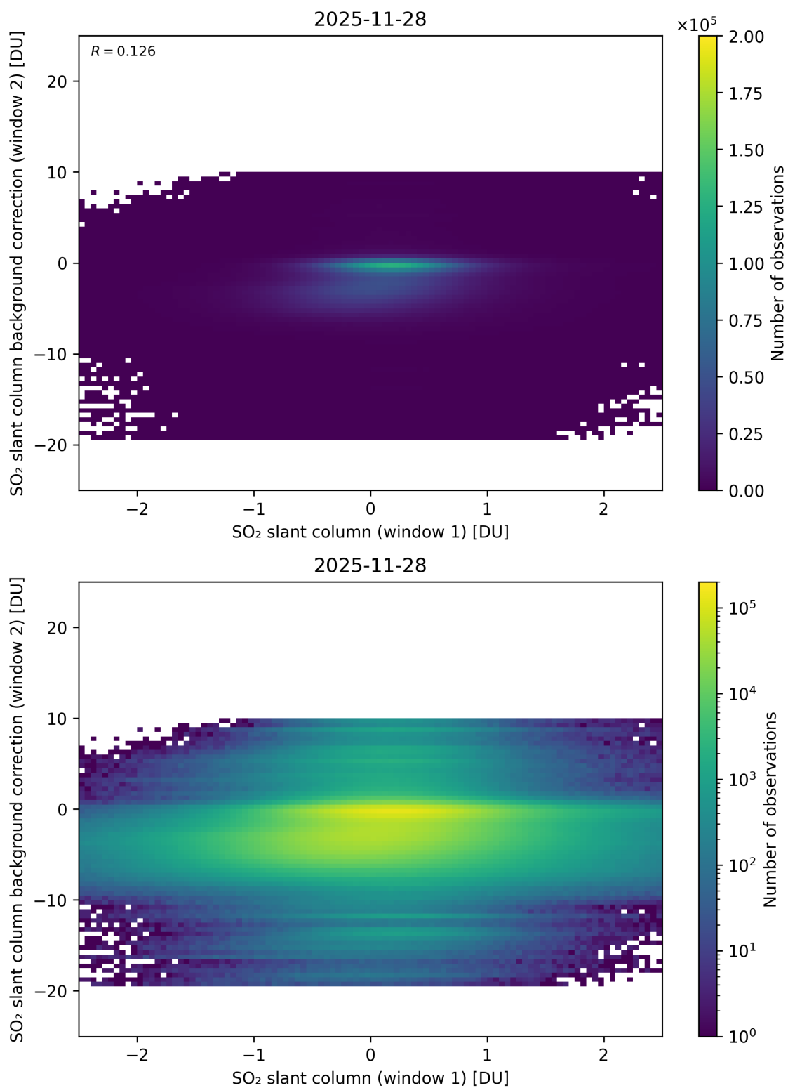
Figure 263: Scatter density plot of “SO 2 slant column (window 1)” against “SO 2 slant column background correction (window 2)” for 2025-11-28 to 2025-11-29.
