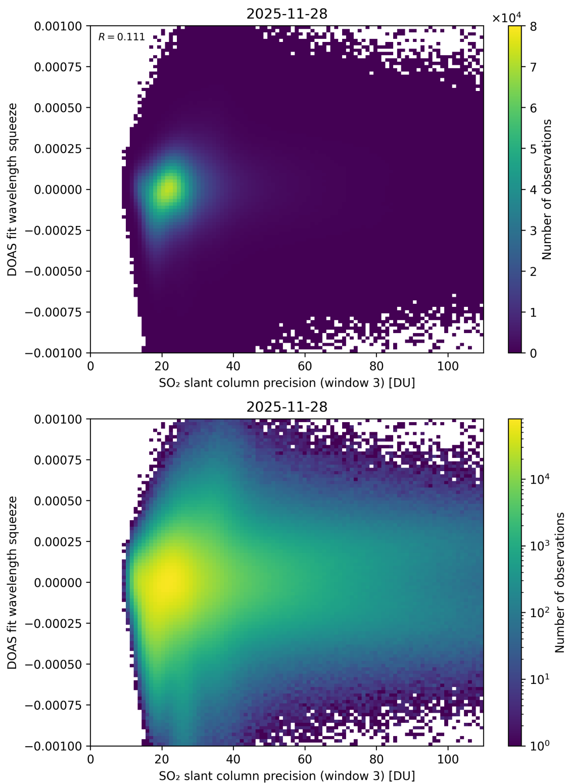
Figure 309: Scatter density plot of “SO 2 slant column precision (window 3)” against “DOAS fit wavelength squeeze” for 2025-11-28 to 2025-11-29.
