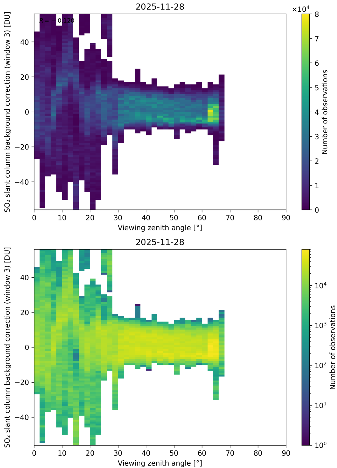
Figure 364: Scatter density plot of “Viewing zenith angle” against “SO 2 slant column background correction (window 3)” for 2025-11-28 to 2025-11-29.
