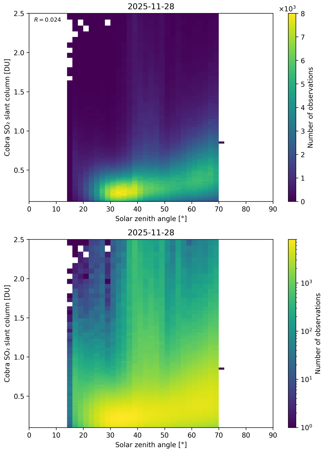
Figure 179: Scatter density plot of “Solar zenith angle” against “Cobra SO 2 slant column” for 2025-11-28 to 2025-11-29.
