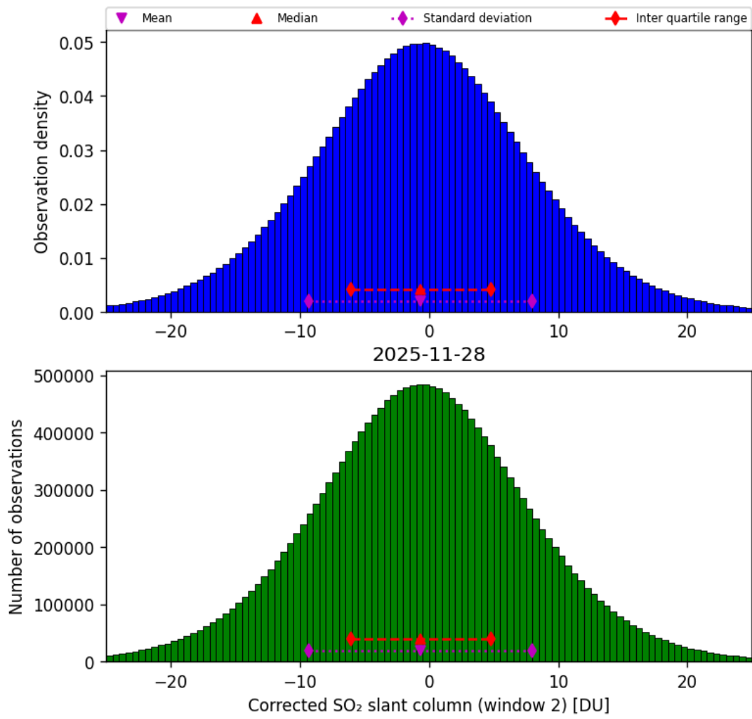
Figure 69: Histogram of “Corrected SO 2 slant column (window 2)” for 2025-11-28 to 2025-11-29
