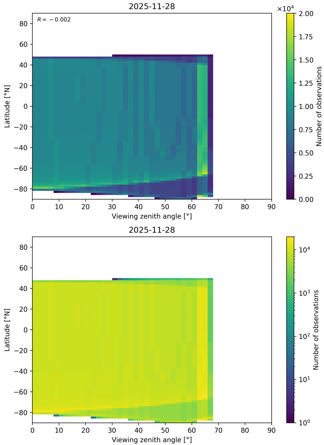
Figure 368: Scatter density plot of “Viewing zenith angle” against “Latitude” for 2025-11-28 to 2025-11-29.
