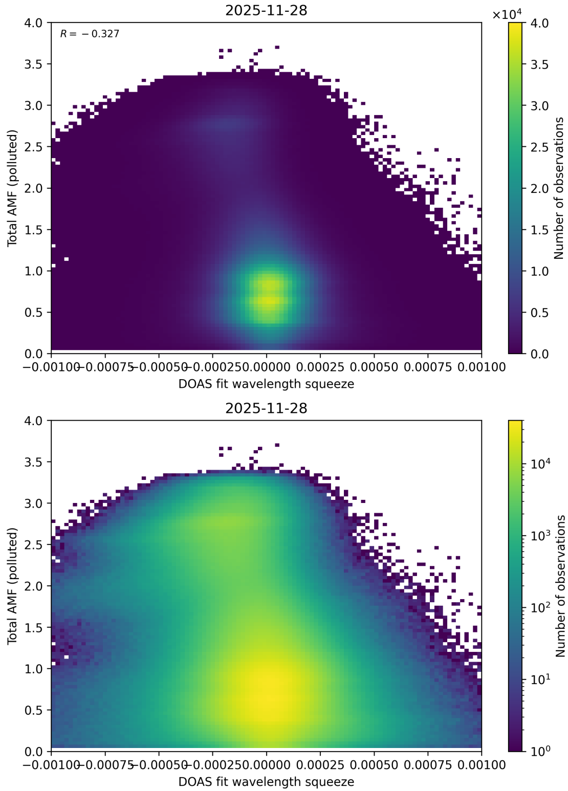
Figure 145: Scatter density plot of “DOAS fit wavelength squeeze” against “Total AMF (polluted)” for 2025-11-28 to 2025-11-29.
