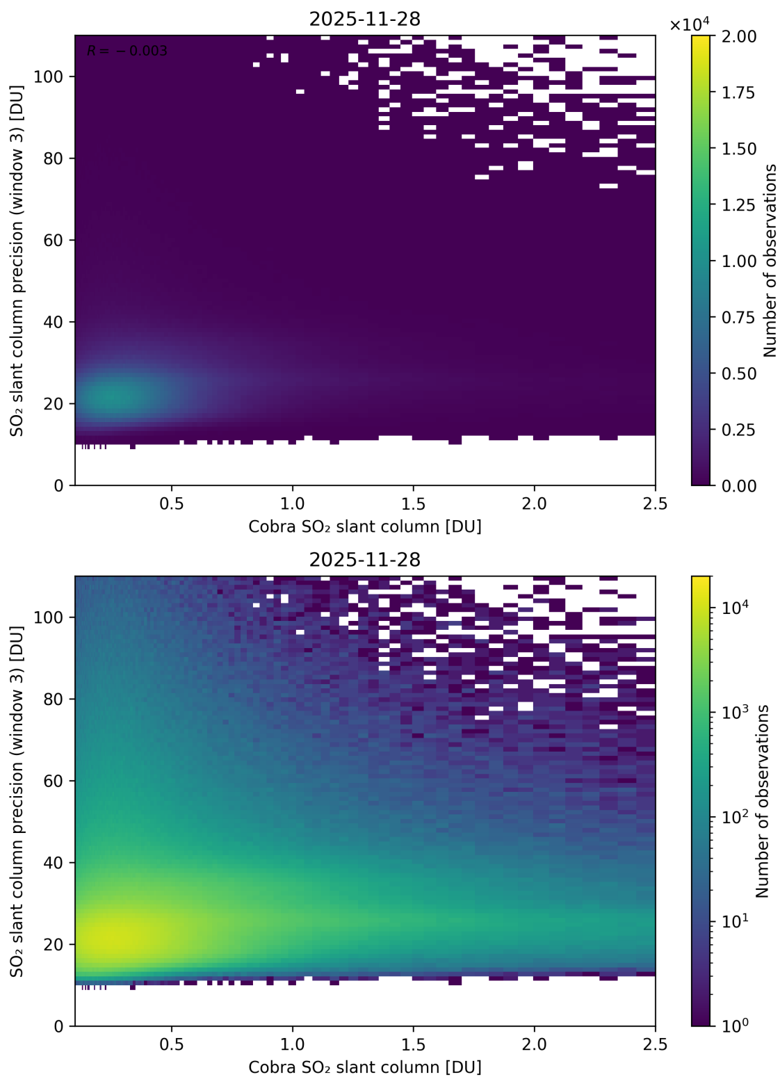
Figure 223: Scatter density plot of “Cobra SO 2 slant column” against “SO 2 slant column precision (window 3)” for 2025-11-28 to 2025-11-29.
