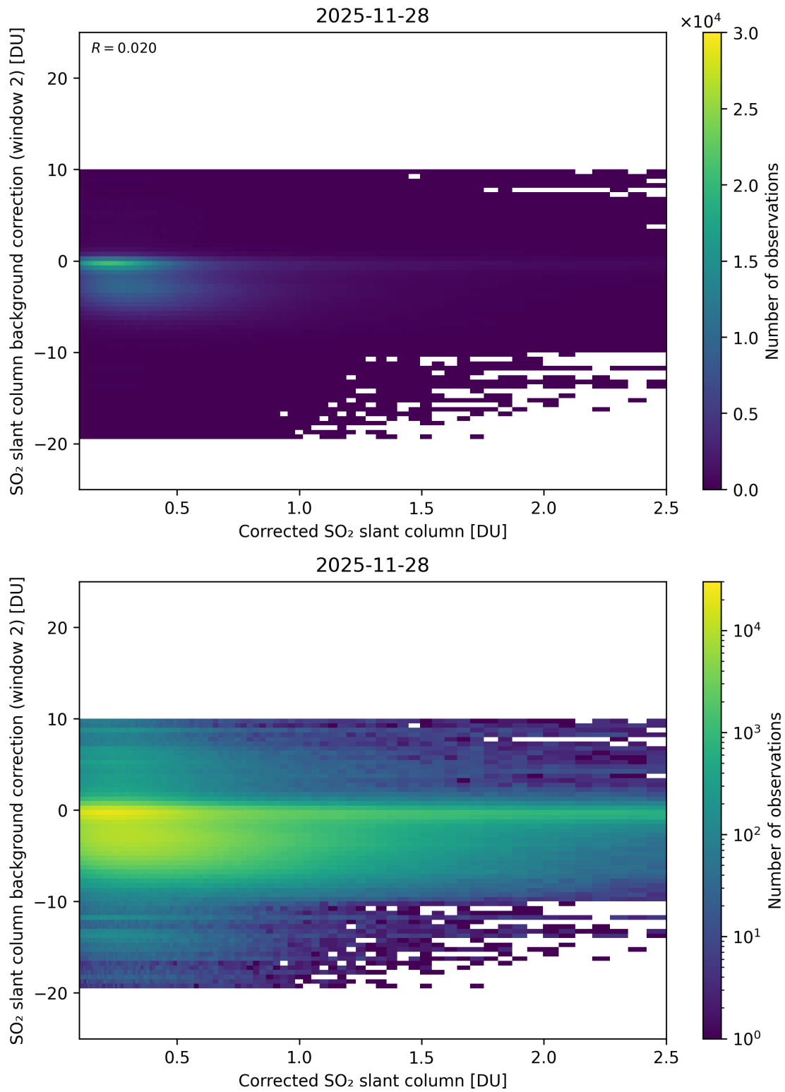
Figure 227: Scatter density plot of “Corrected SO 2 slant column” against “SO 2 slant column background correction (window 2)” for 2025-11-28 to 2025-11-29.
