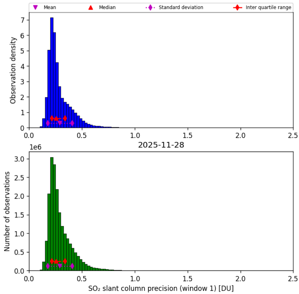
Figure 64: Histogram of “SO 2 slant column precision (window 1)” for 2025-11-28 to 2025-11-29
