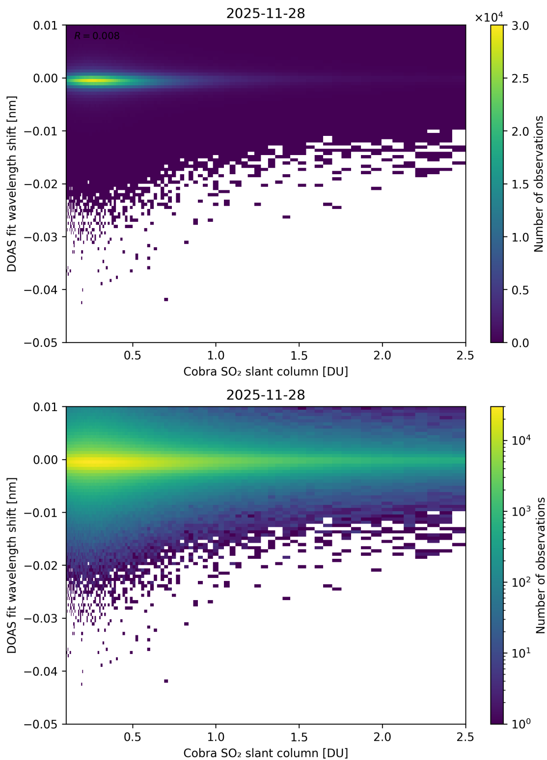
Figure 196: Scatter density plot of “Cobra SO 2 slant column” against “DOAS fit wavelength shift” for 2025-11-28 to 2025-11-29.
