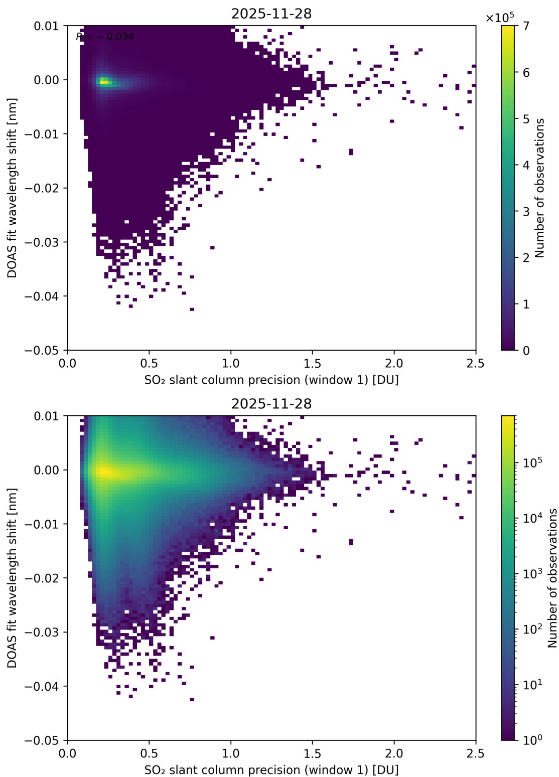
Figure 271: Scatter density plot of “SO 2 slant column precision (window 1)” against “DOAS fit wavelength shift” for 2025-11-28 to 2025-11-29.
