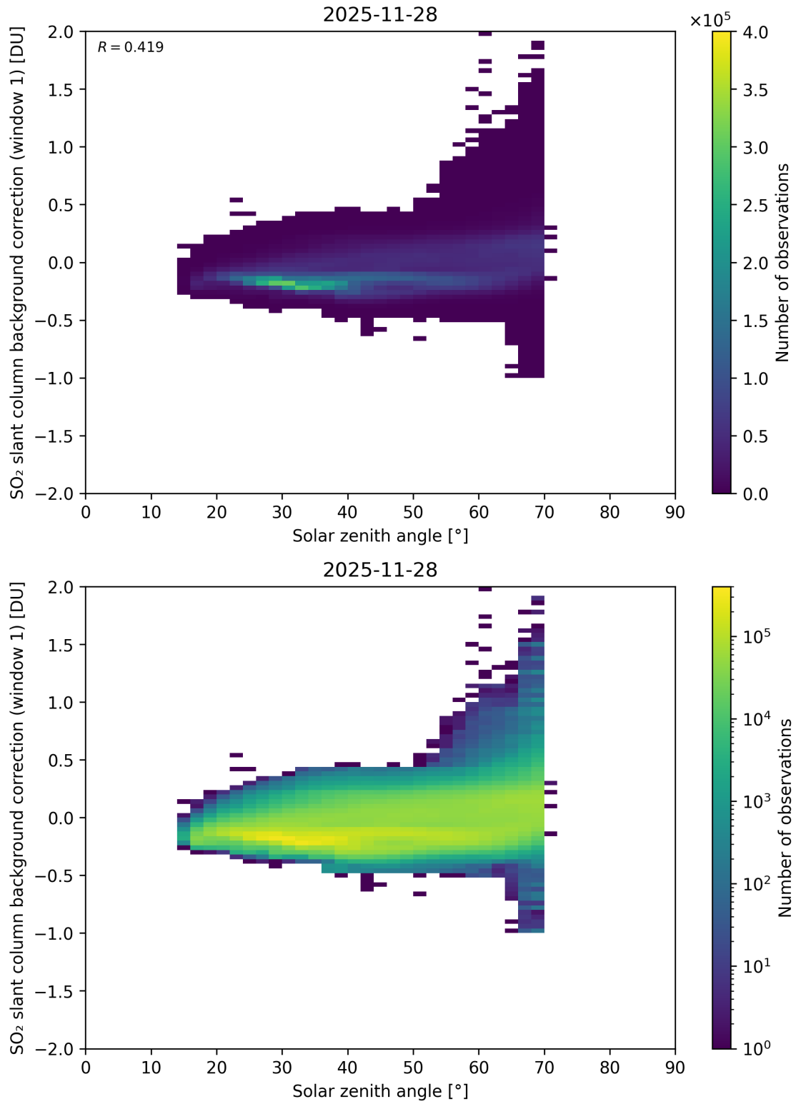
Figure 171: Scatter density plot of “Solar zenith angle” against “SO 2 slant column background correction (window 1)” for 2025-11-28 to 2025-11-29.
