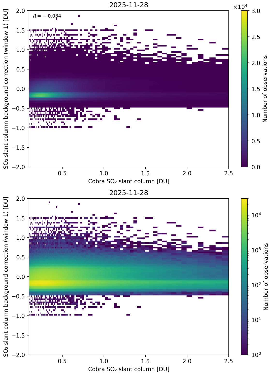
Figure 193: Scatter density plot of “Cobra SO 2 slant column” against “SO 2 slant column background correction (window 1)” for 2025-11-28 to 2025-11-29.
