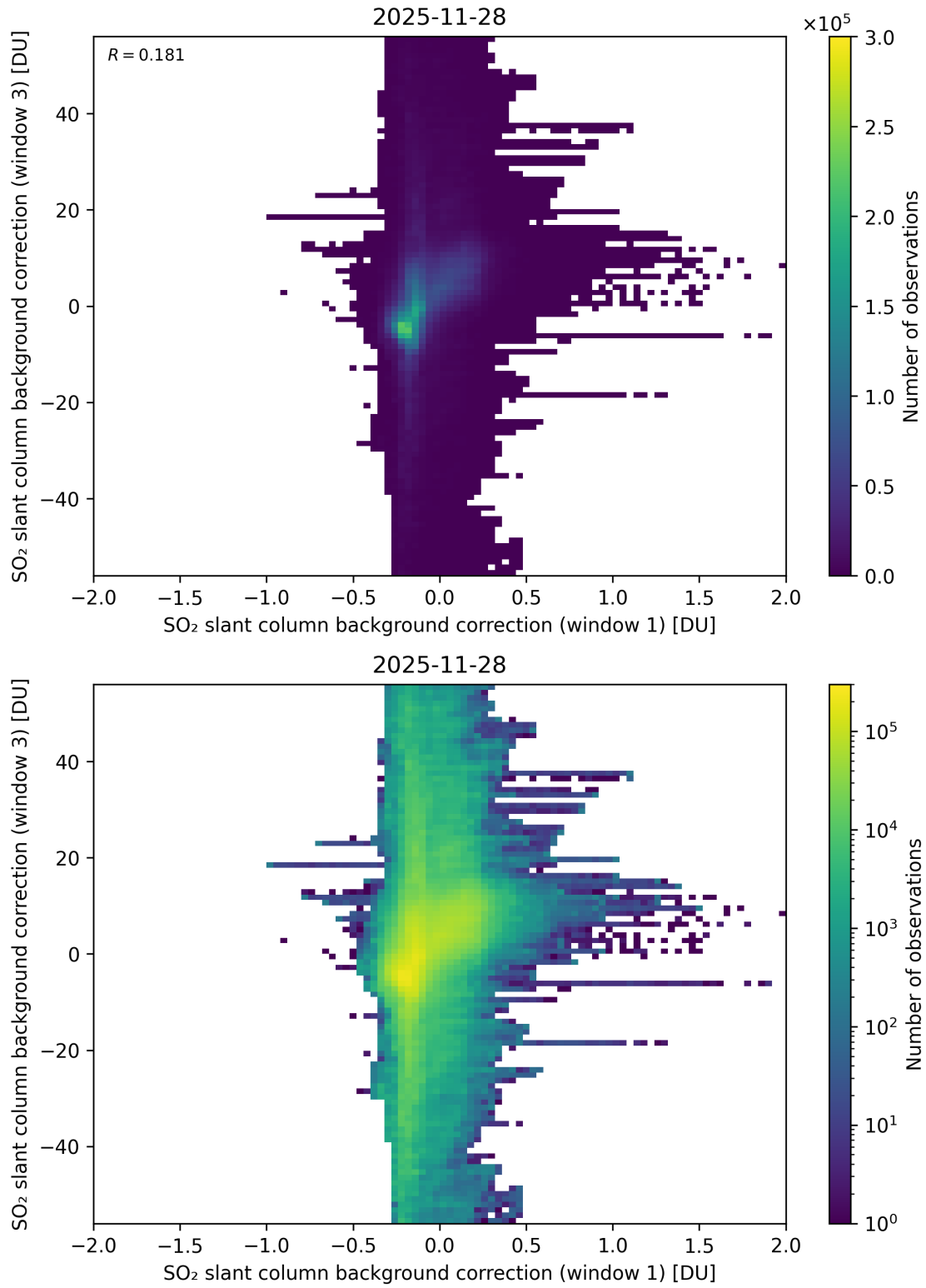
Figure 110: Scatter density plot of “SO 2 slant column background correction (window 1)” against “SO 2 slant column background correction (window 3)” for 2025-11-28 to 2025-11-29.
