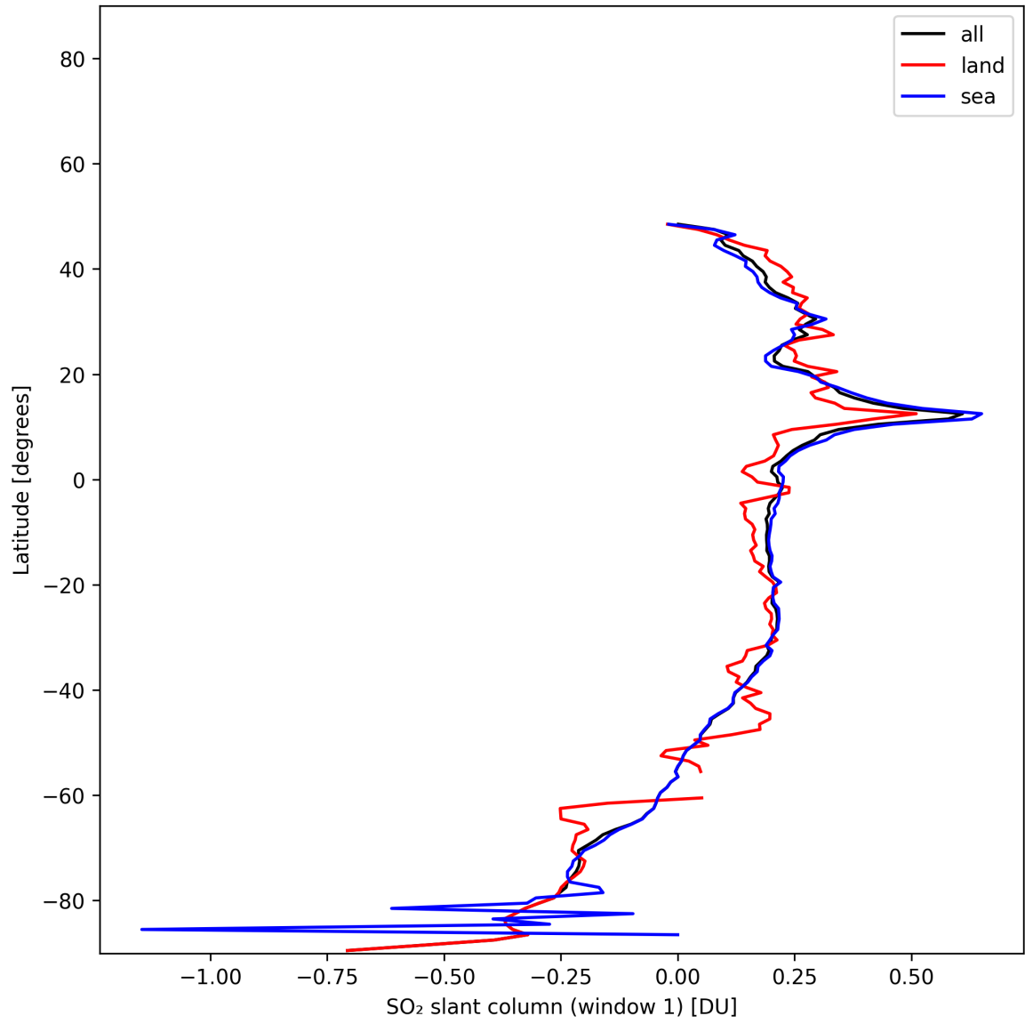
Figure 37: Zonal average of “SO 2 slant column (window 1)” for 2025-11-28 to 2025-11-29.
