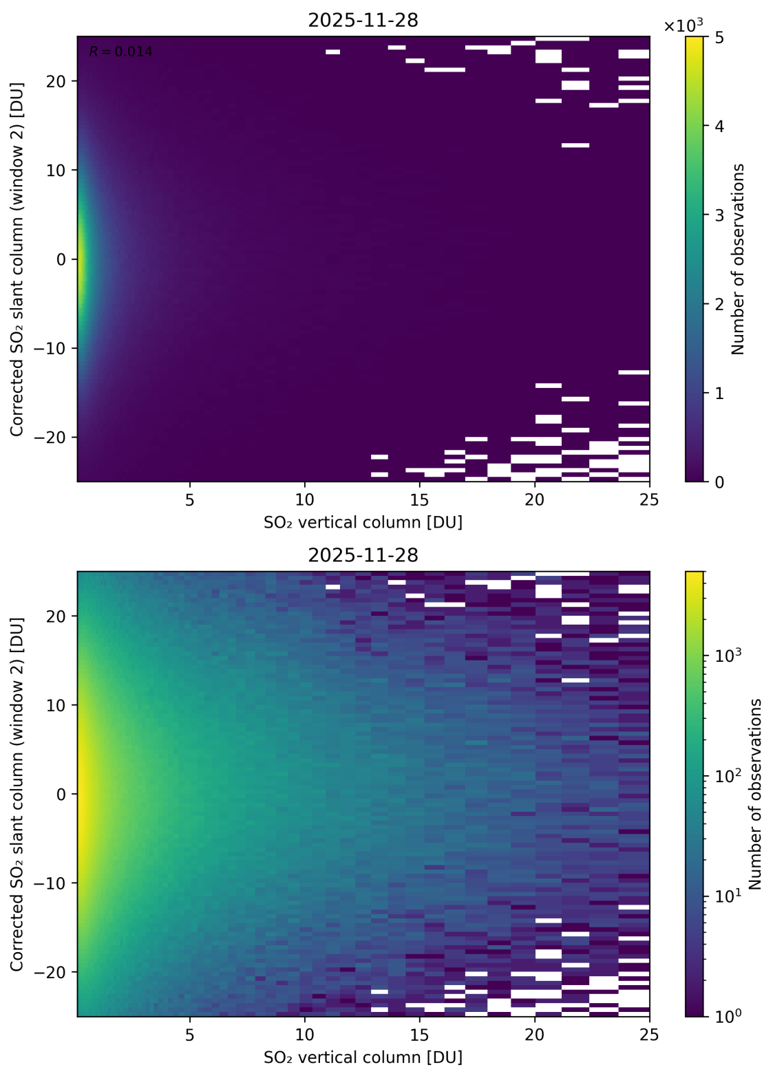
Figure 352: Scatter density plot of “SO 2 vertical column” against “Corrected SO 2 slant column (window 2)” for 2025-11-28 to 2025-11-29.
