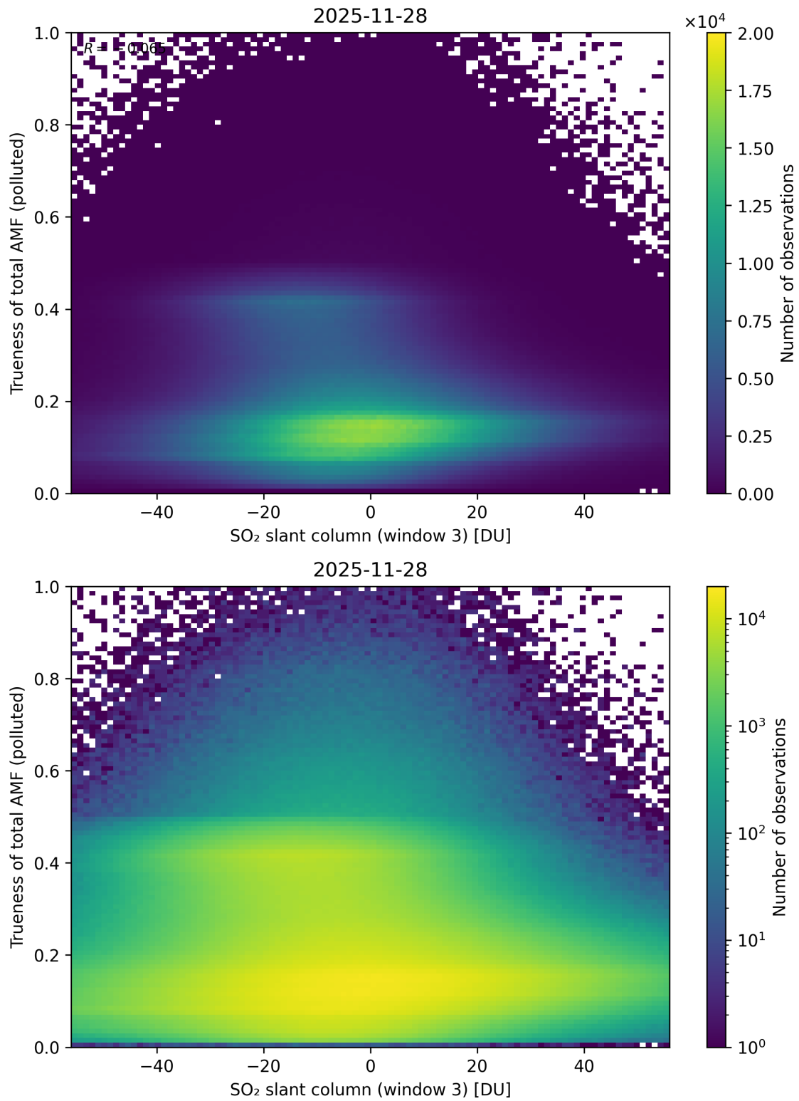
Figure 319: Scatter density plot of “SO 2 slant column (window 3)” against “Trueness of total AMF (polluted)” for 2025-11-28 to 2025-11-29.
