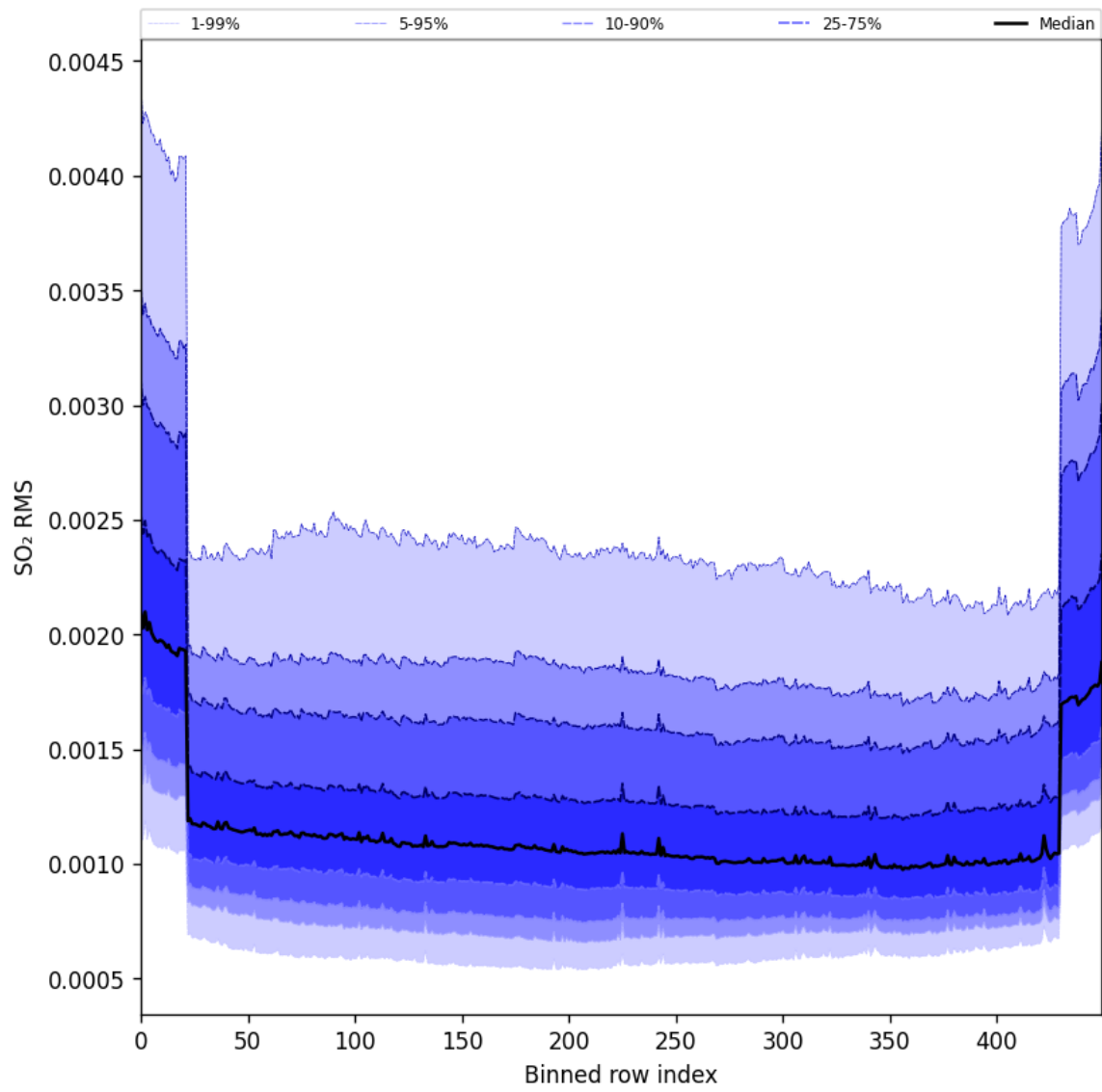
Figure 104: Along track statistics of “SO 2 RMS” for 2025-11-28 to 2025-11-29
