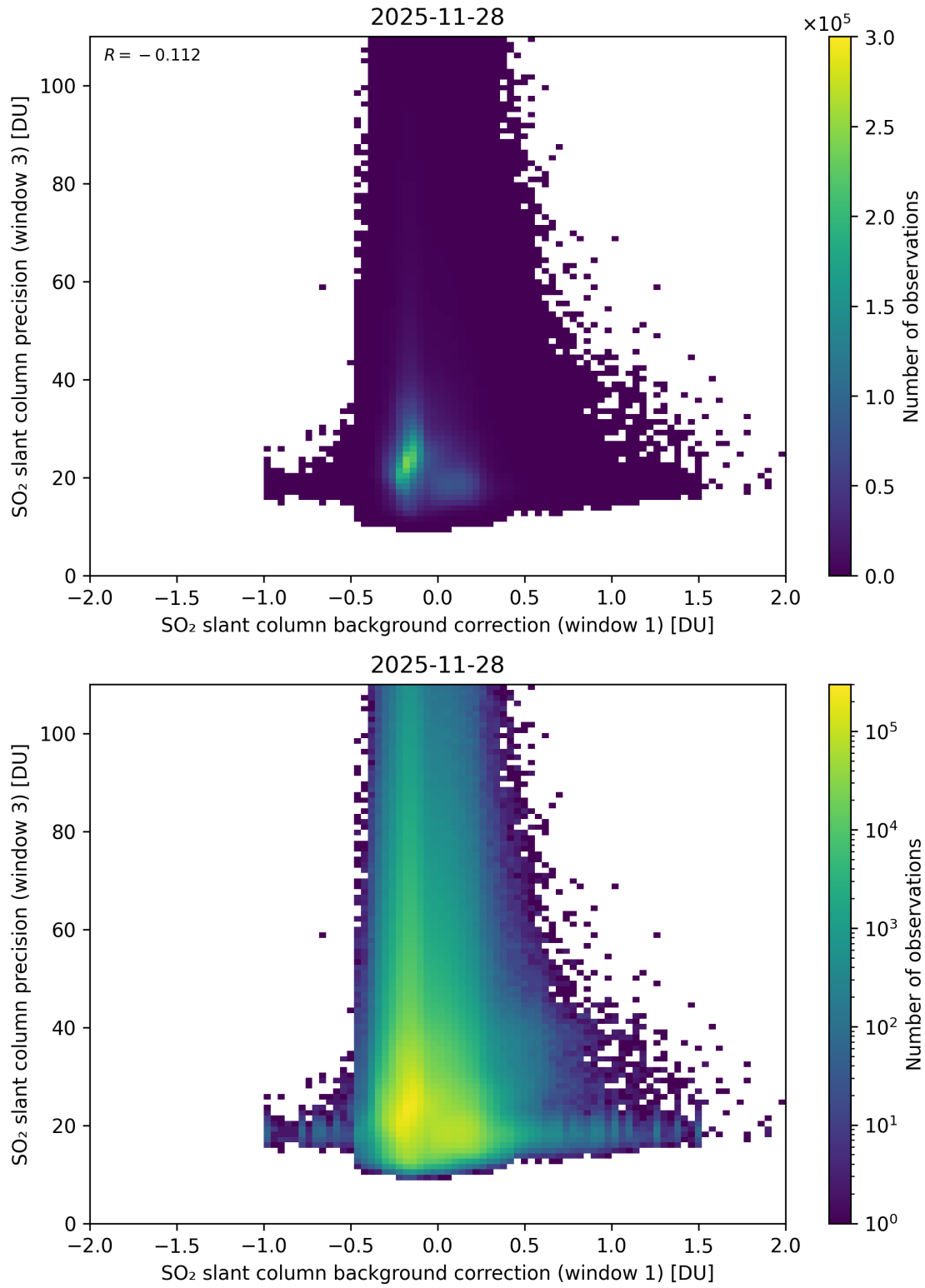
Figure 119: Scatter density plot of “SO 2 slant column background correction (window 1)” against “SO 2 slant column precision (window 3)” for 2025-11-28 to 2025-11-29.
