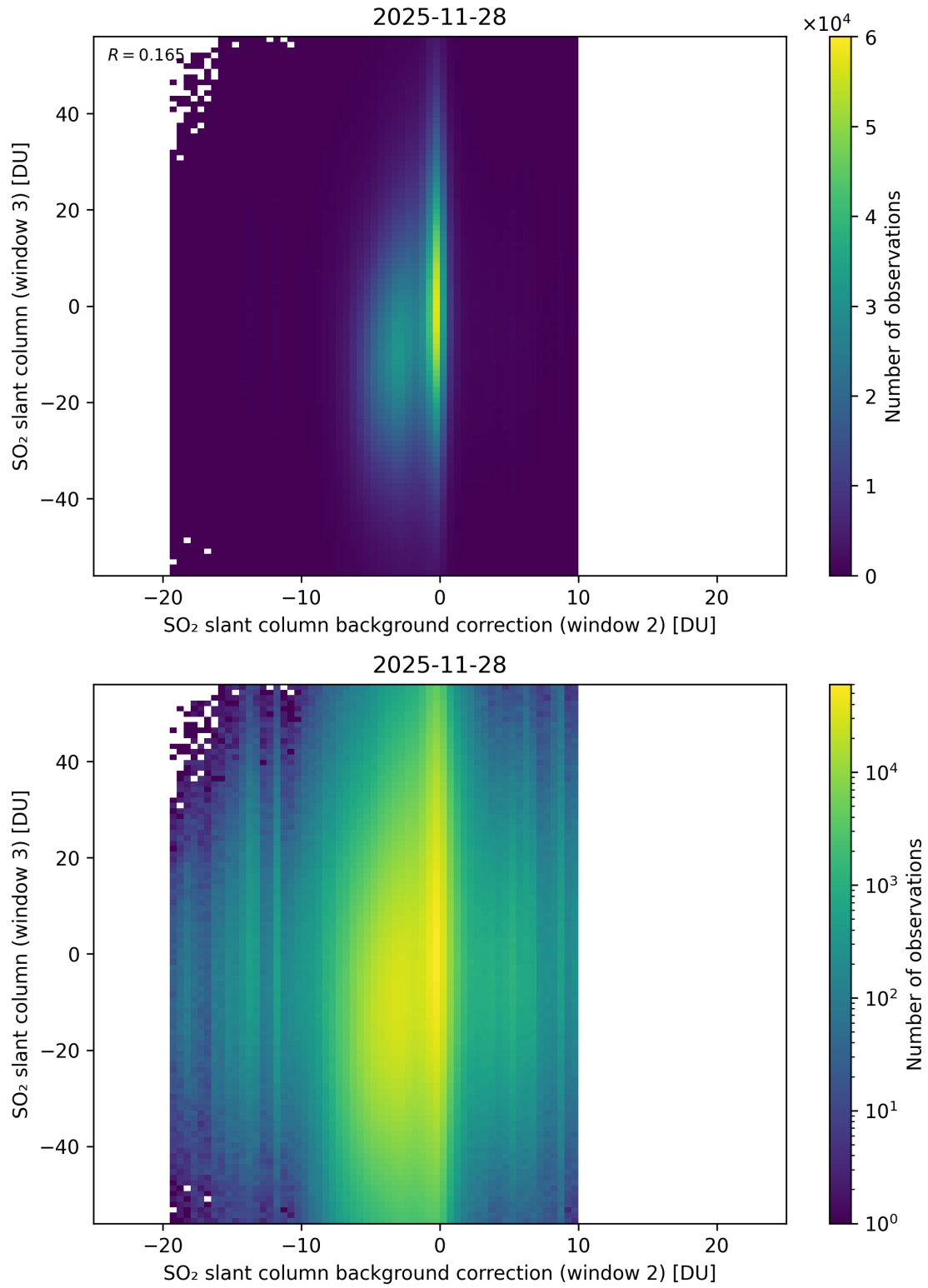
Figure 128: Scatter density plot of “SO 2 slant column background correction (window 2)” against “SO 2 slant column (window 3)” for 2025-11-28 to 2025-11-29.
