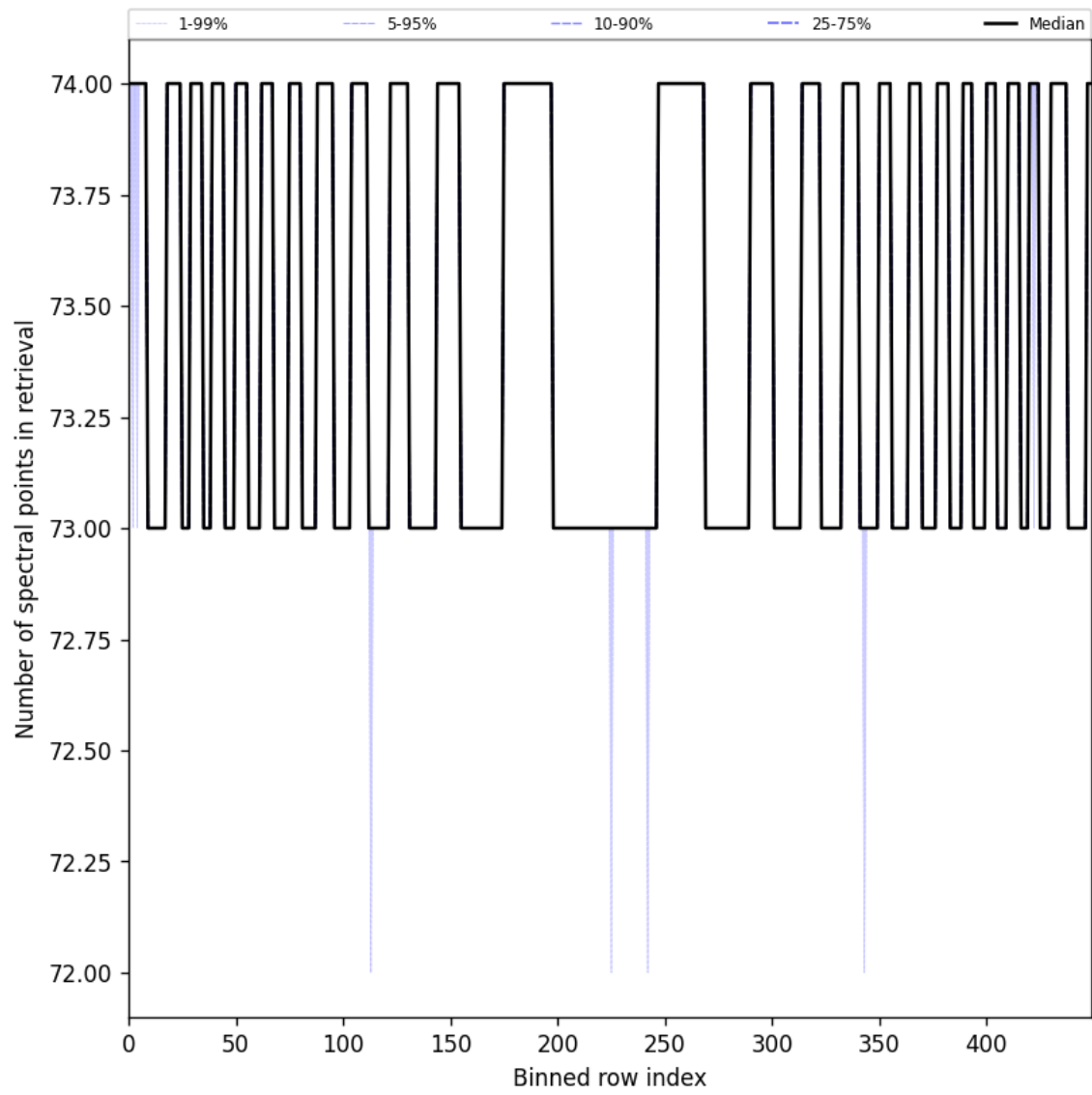
Figure 108: Along track statistics of “Number of spectral points in retrieval” for 2025-11-28 to 2025-11-29
