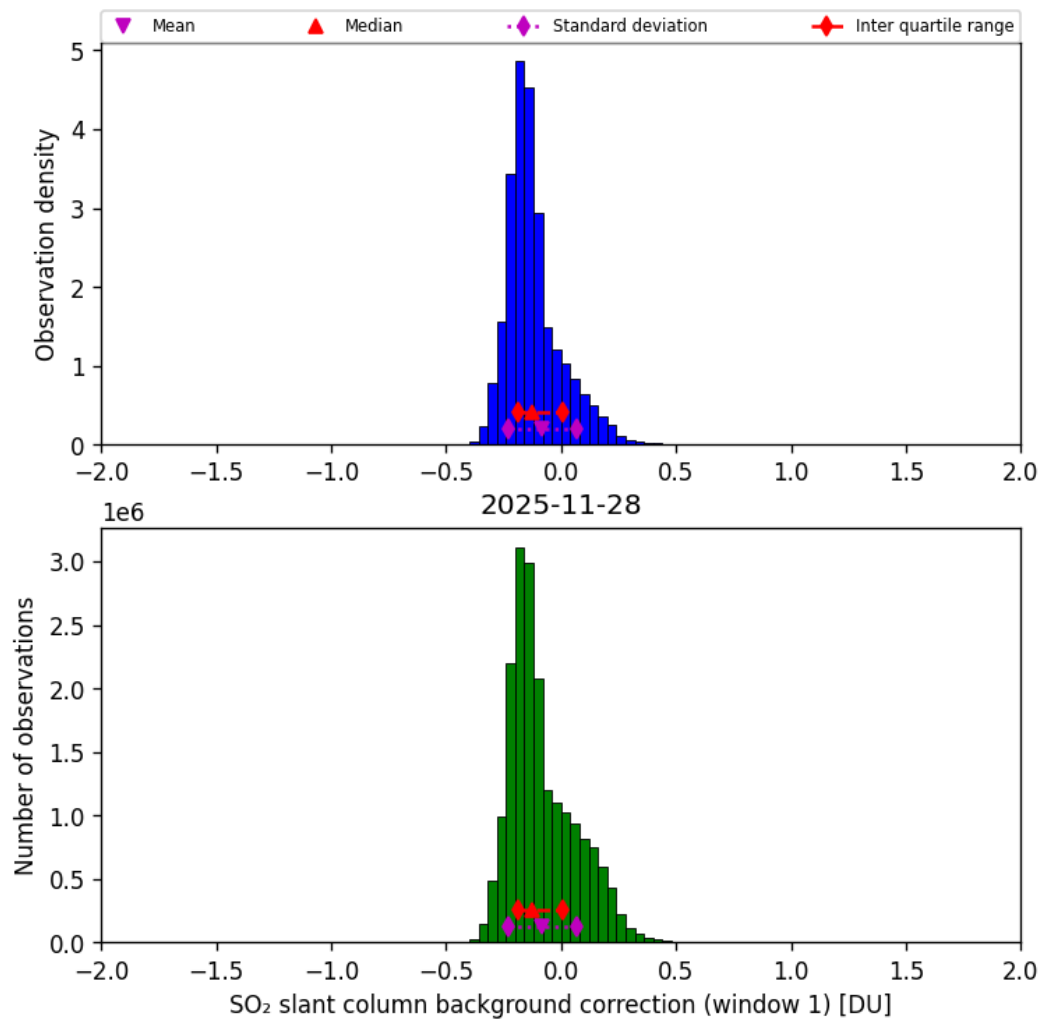
Figure 66: Histogram of “SO 2 slant column background correction (window 1)” for 2025-11-28 to 2025-11-29
