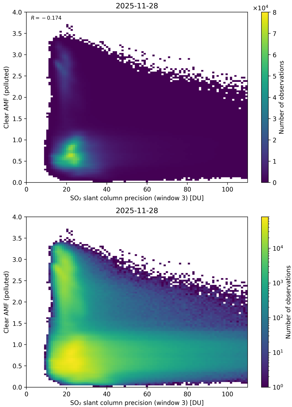
Figure 311: Scatter density plot of “SO 2 slant column precision (window 3)” against “Clear AMF (polluted)” for 2025-11-28 to 2025-11-29.
