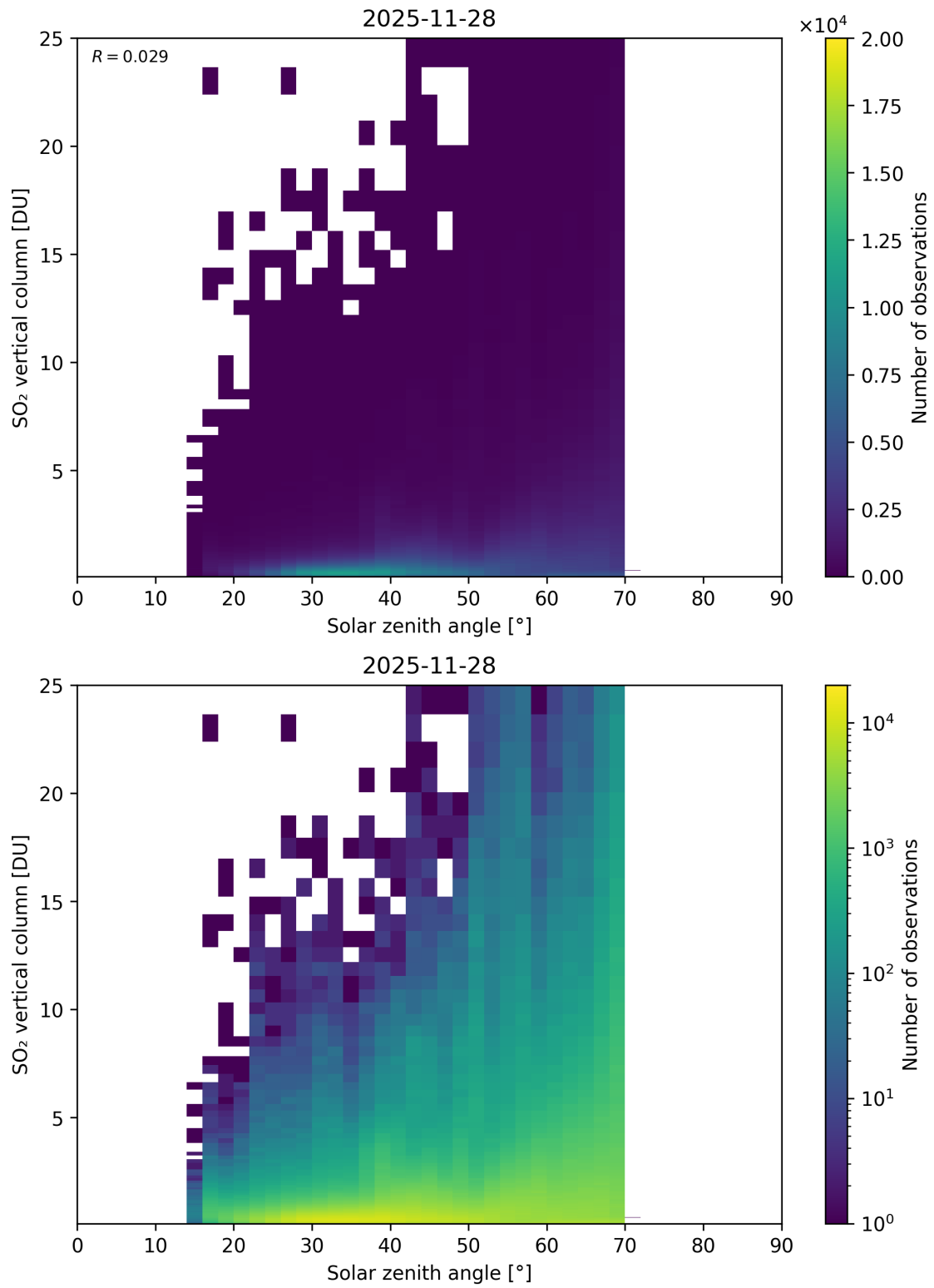
Figure 191: Scatter density plot of “Solar zenith angle” against “SO 2 vertical column” for 2025-11-28 to 2025-11-29.
