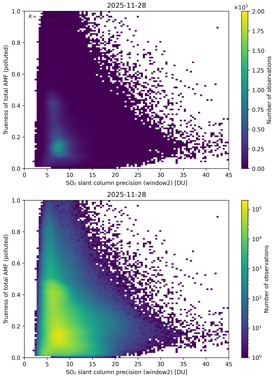
Figure 302: Scatter density plot of “SO 2 slant column precision (window2)” against “Trueness of total AMF (polluted)” for 2025-11-28 to 2025-11-29.
