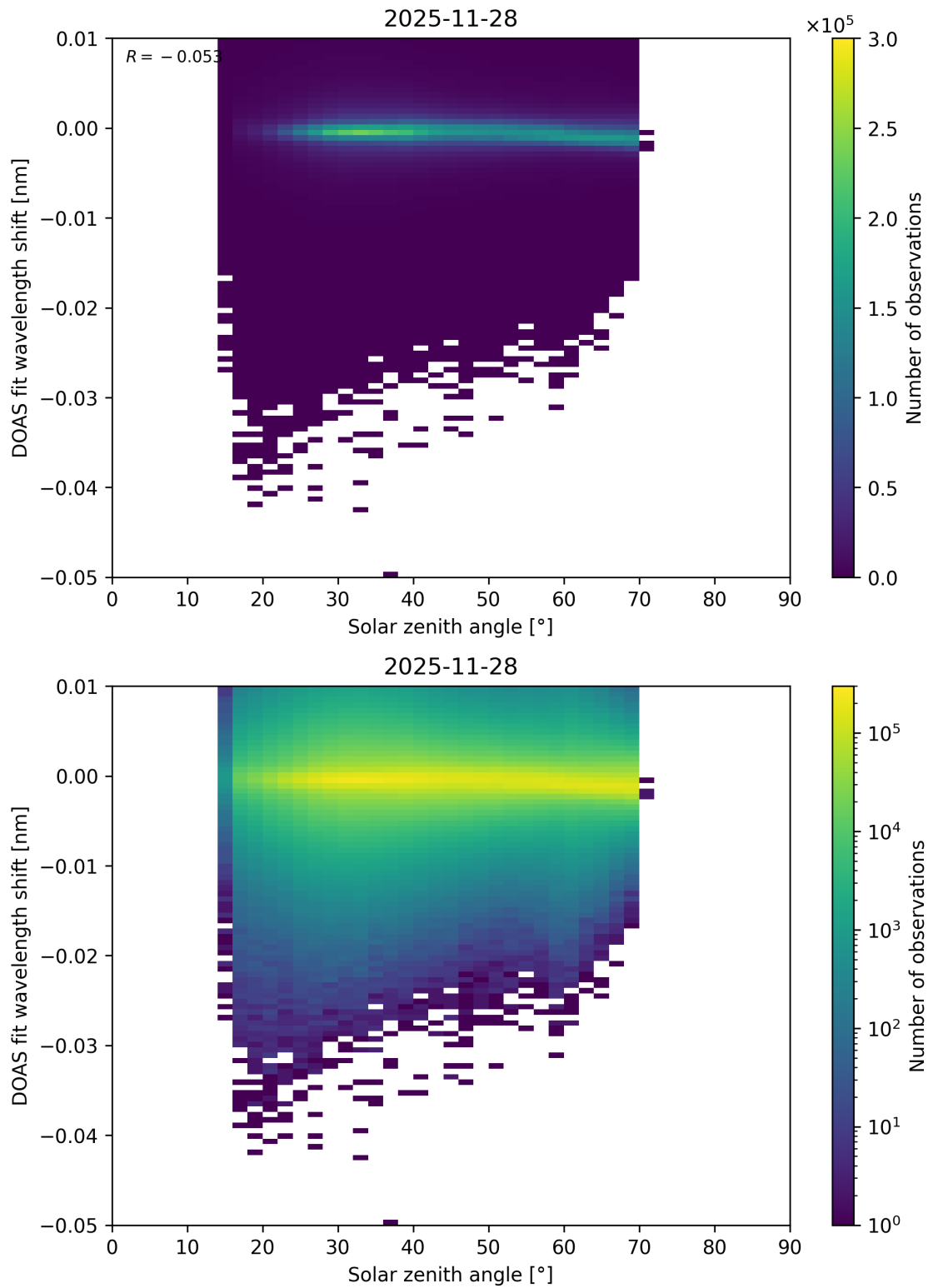
Figure 174: Scatter density plot of “Solar zenith angle” against “DOAS fit wavelength shift” for 2025-11-28 to 2025-11-29.
