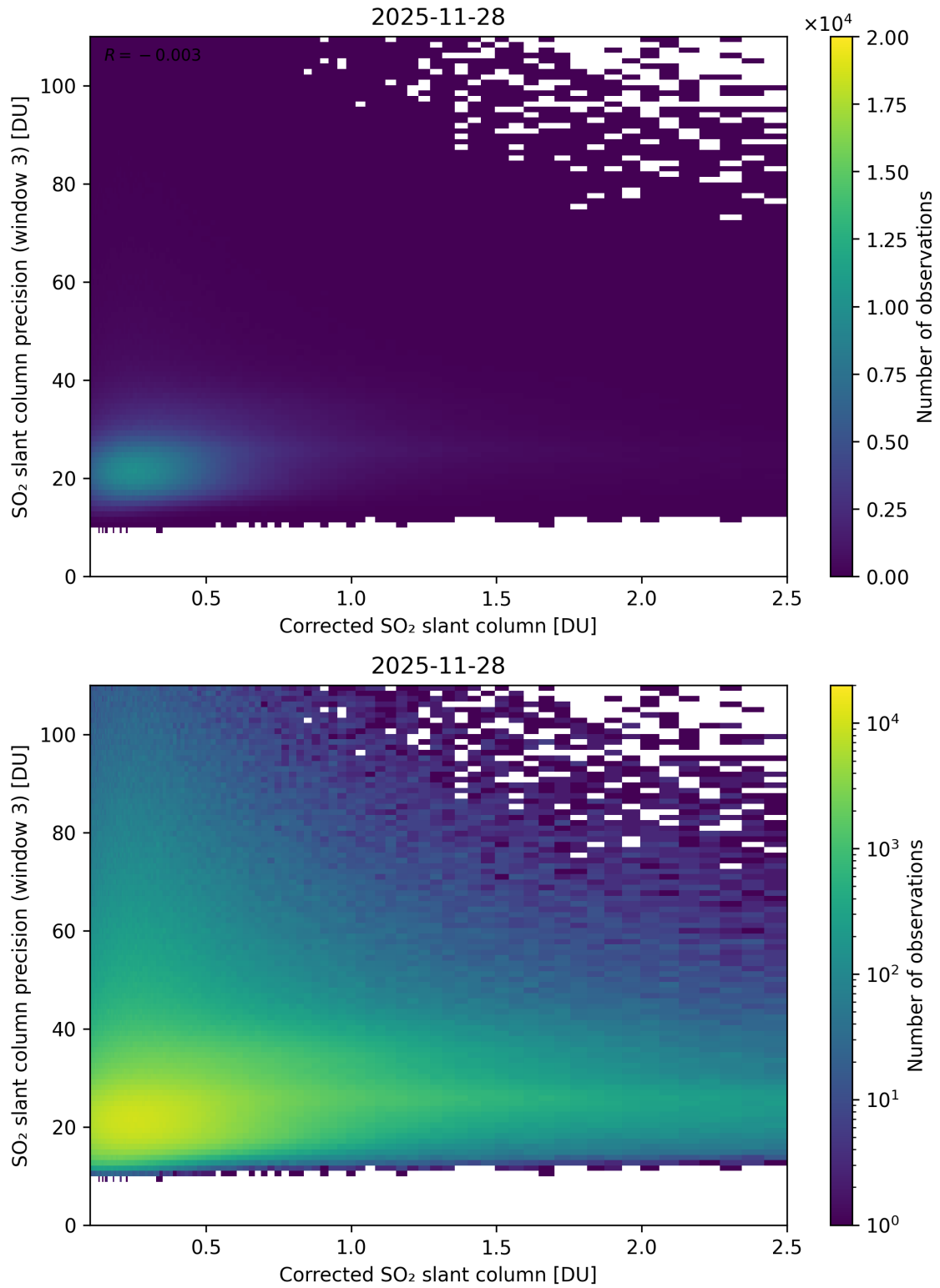
Figure 241: Scatter density plot of “Corrected SO 2 slant column” against “SO 2 slant column precision (window 3)” for 2025-11-28 to 2025-11-29.
