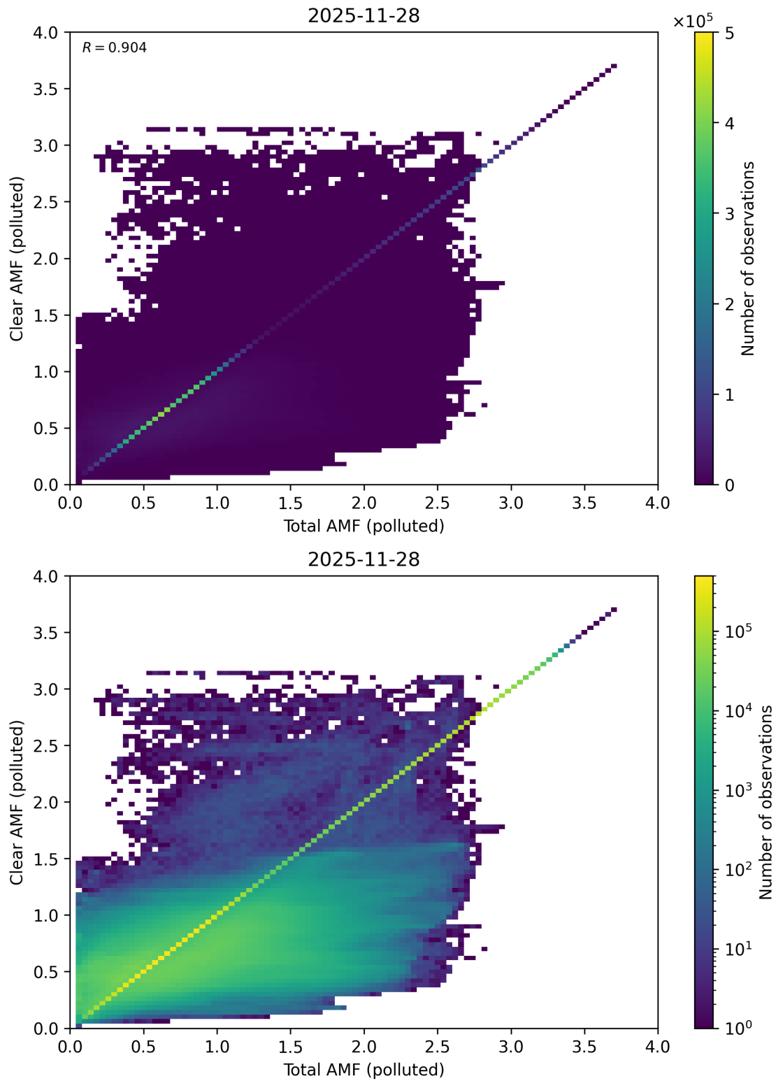
Figure 320: Scatter density plot of “Total AMF (polluted)” against “Clear AMF (polluted)” for 2025-11-28 to 2025-11-29.
