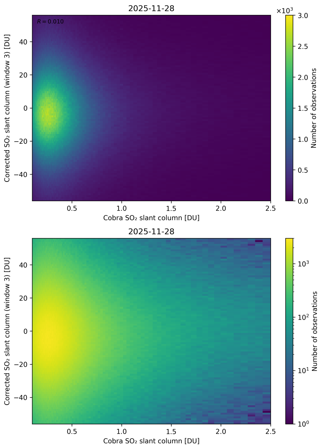
Figure 218: Scatter density plot of “Cobra SO 2 slant column” against “Corrected SO 2 slant column (window 3)” for 2025-11-28 to 2025-11-29.
