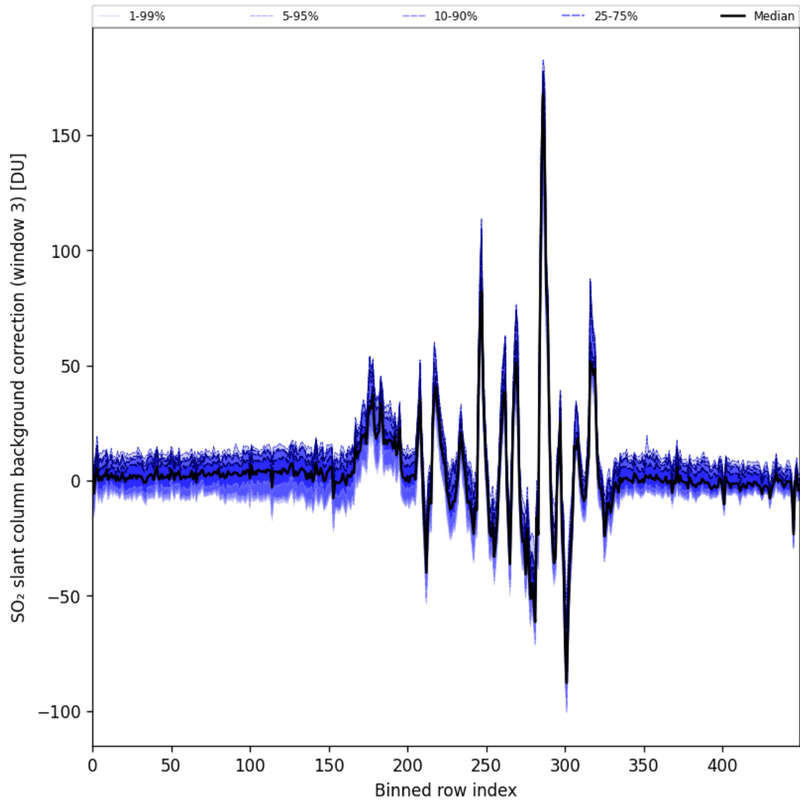
Figure 100: Along track statistics of “SO 2 slant column background correction (window 3)” for 2025-11-28 to 2025-11-29
