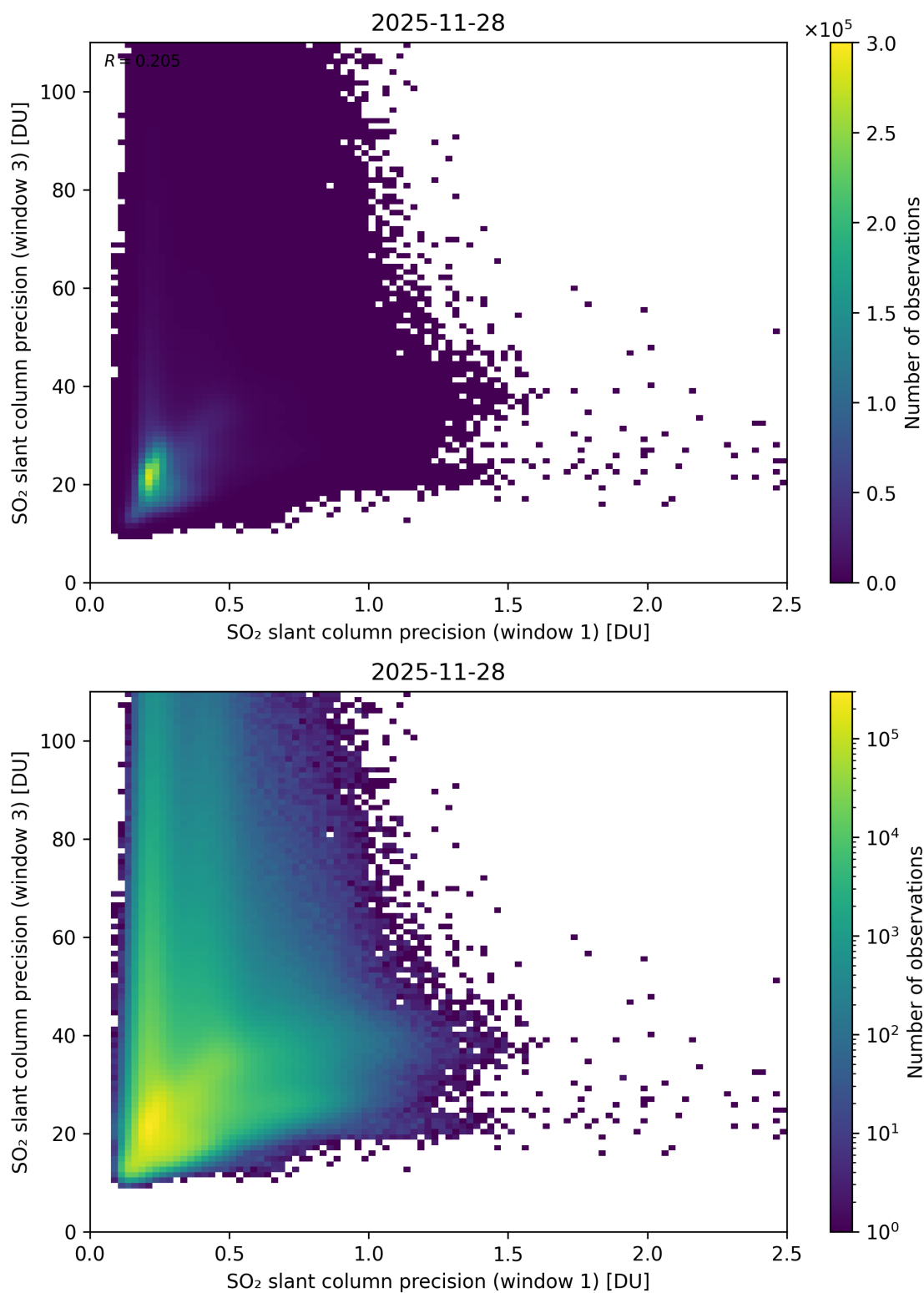
Figure 279: Scatter density plot of “SO 2 slant column precision (window 1)” against “SO 2 slant column precision (window 3)” for 2025-11-28 to 2025-11-29.
