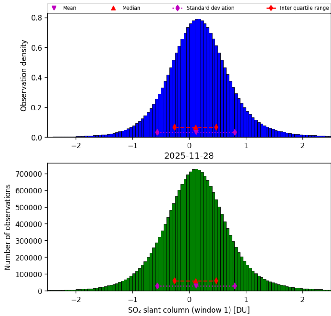
Figure 63: Histogram of “SO 2 slant column (window 1)” for 2025-11-28 to 2025-11-29
