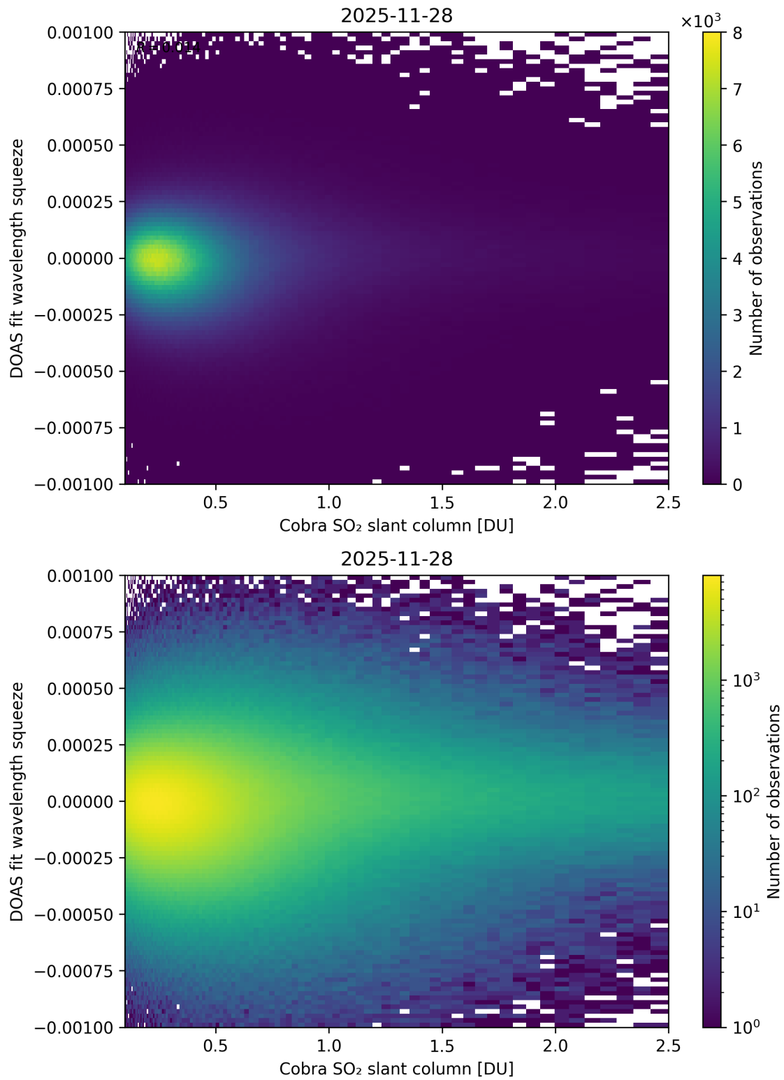
Figure 197: Scatter density plot of “Cobra SO 2 slant column” against “DOAS fit wavelength squeeze” for 2025-11-28 to 2025-11-29.
