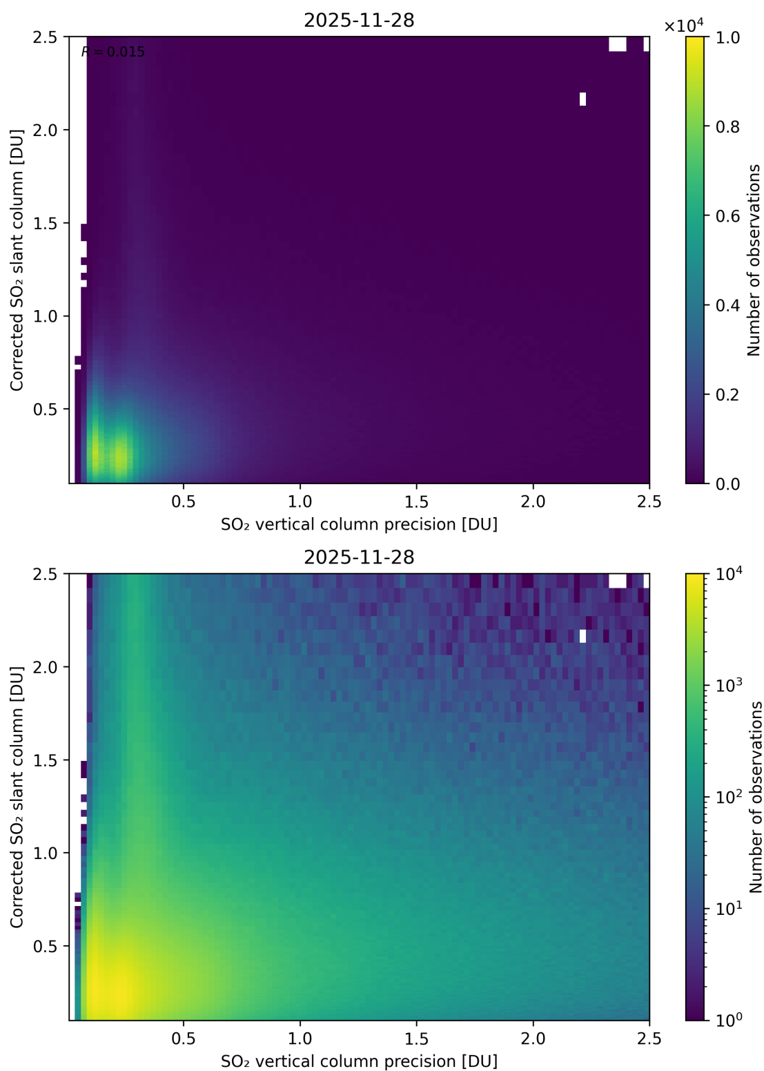
Figure 338: Scatter density plot of “SO 2 vertical column precision” against “Corrected SO 2 slant column” for 2025-11-28 to 2025-11-29.
