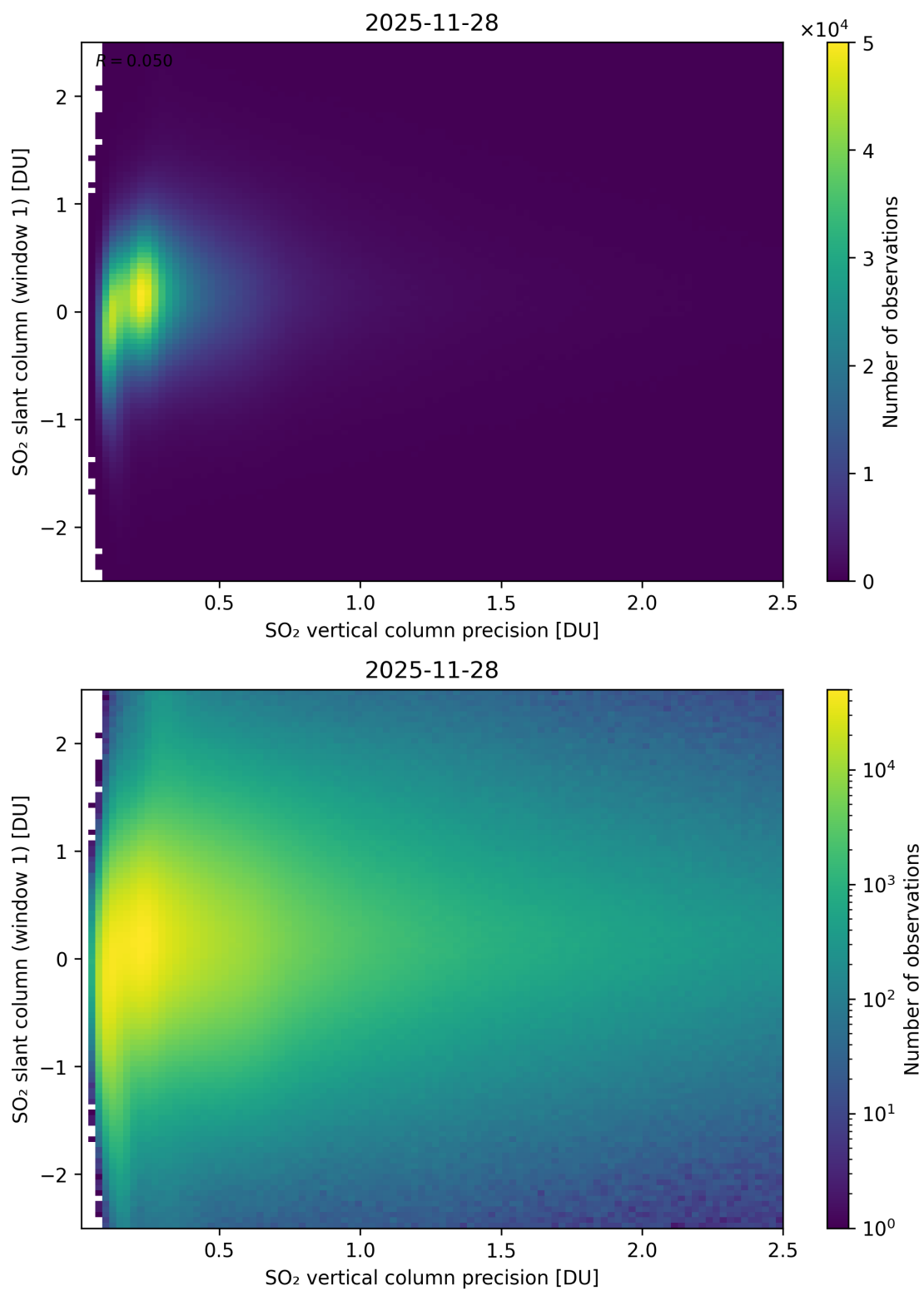
Figure 341: Scatter density plot of “SO 2 vertical column precision” against “SO 2 slant column (window 1)” for 2025-11-28 to 2025-11-29.
