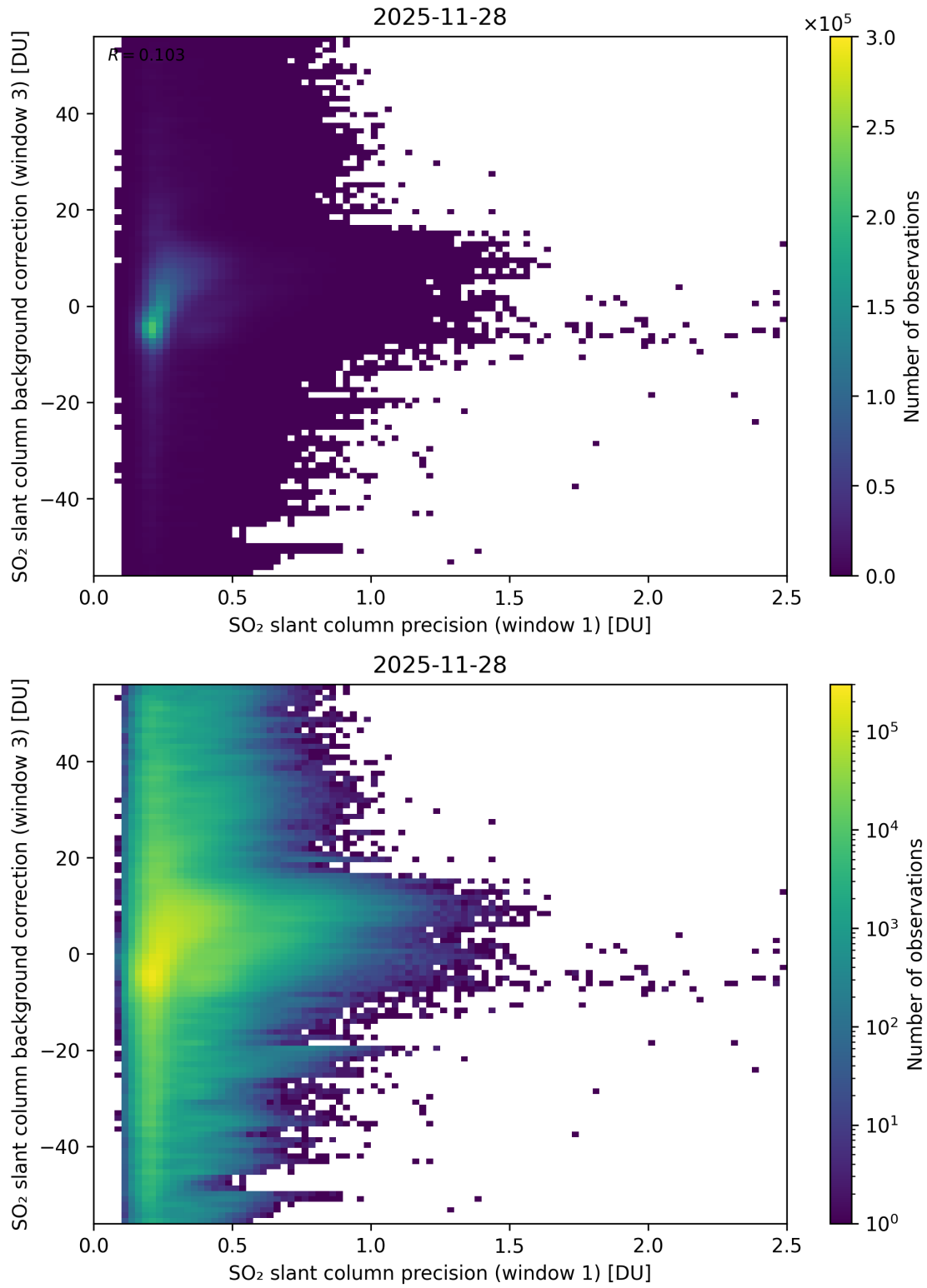
Figure 270: Scatter density plot of “SO 2 slant column precision (window 1)” against “SO 2 slant column background correction (window 3)” for 2025-11-28 to 2025-11-29.
