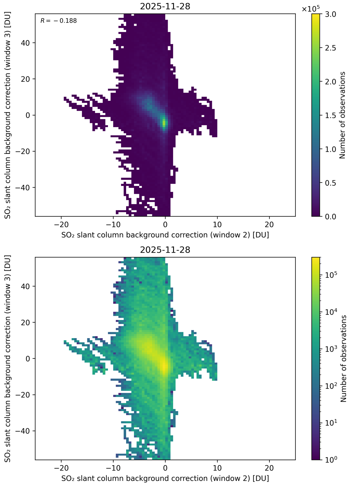
Figure 122: Scatter density plot of “SO 2 slant column background correction (window 2)” against “SO 2 slant column background correction (window 3)” for 2025-11-28 to 2025-11-29.
