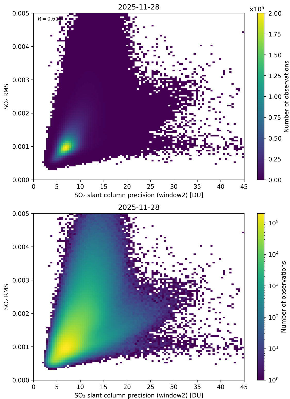
Figure 295: Scatter density plot of “SO 2 slant column precision (window2)” against “SO 2 RMS” for 2025-11-28 to 2025-11-29.
