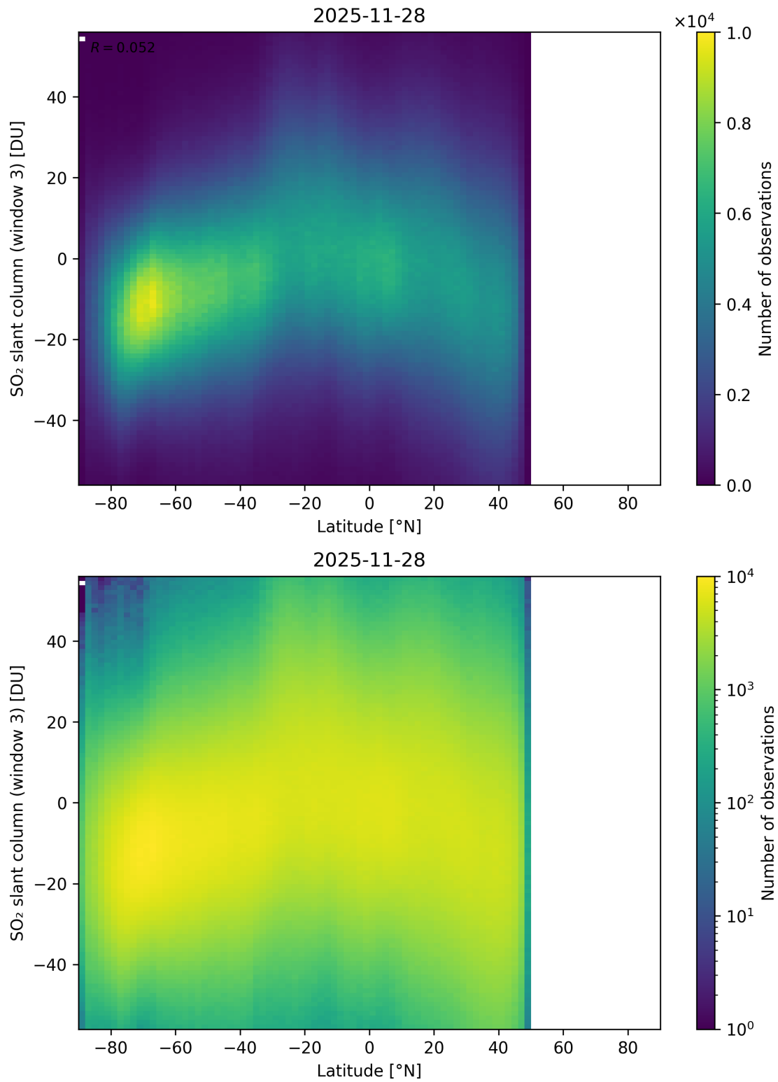
Figure 165: Scatter density plot of “Latitude” against “SO 2 slant column (window 3)” for 2025-11-28 to 2025-11-29.
