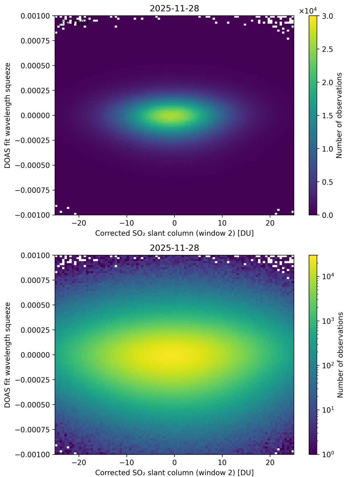
Figure 247: Scatter density plot of “Corrected SO 2 slant column (window 2)” against “DOAS fit wavelength squeeze” for 2025-11-28 to 2025-11-29.
