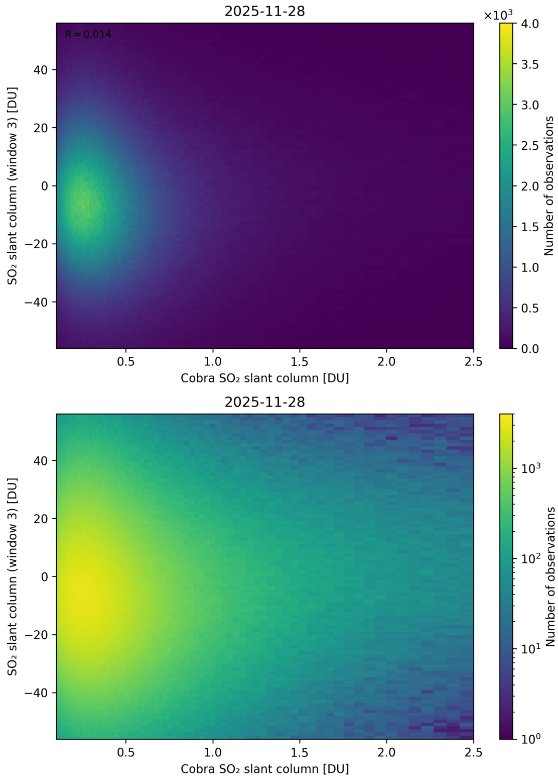
Figure 222: Scatter density plot of “Cobra SO 2 slant column” against “SO 2 slant column (window 3)” for 2025-11-28 to 2025-11-29.
