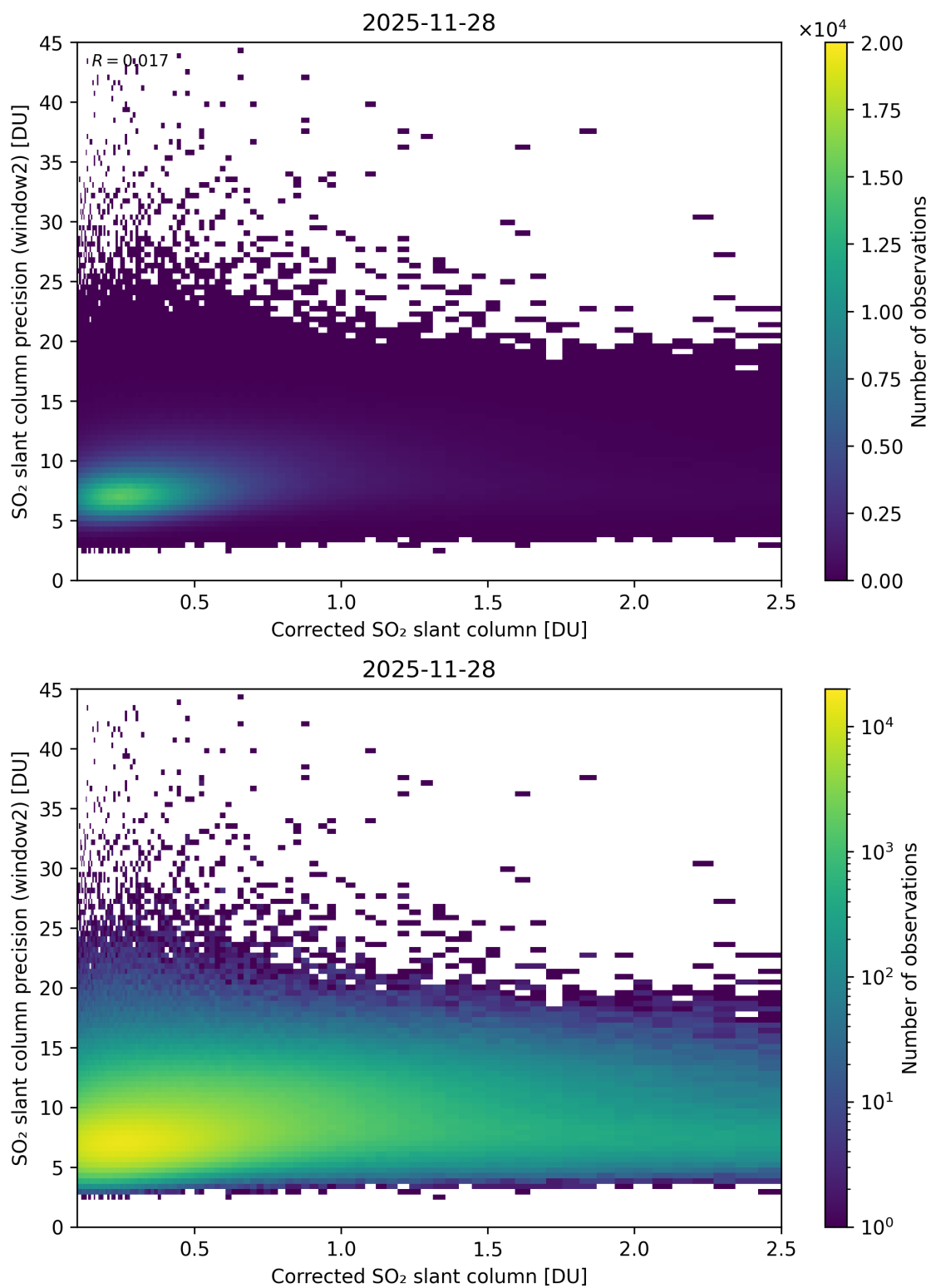
Figure 239: Scatter density plot of “Corrected SO 2 slant column” against “SO 2 slant column precision (window2)” for 2025-11-28 to 2025-11-29.
