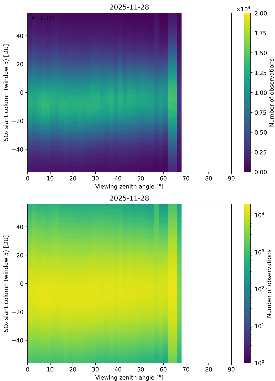
Figure 379: Scatter density plot of “Viewing zenith angle” against “SO 2 slant column (window 3)” for 2025-11-28 to 2025-11-29.
