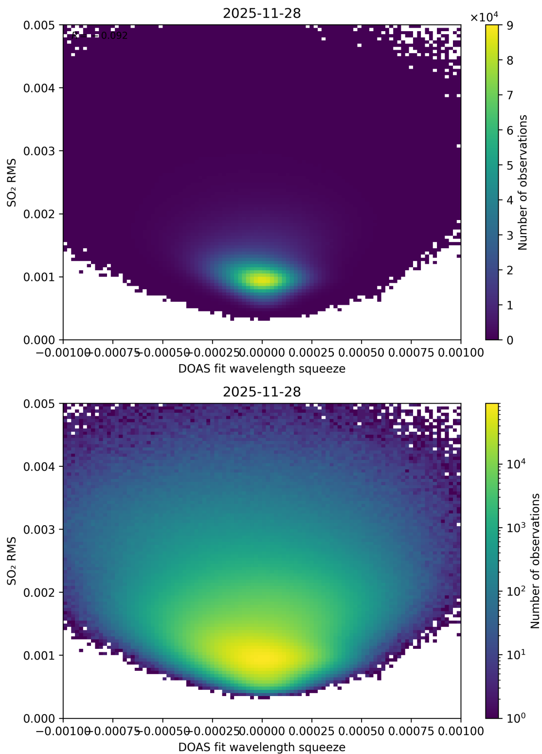
Figure 143: Scatter density plot of “DOAS fit wavelength squeeze” against “SO 2 RMS” for 2025-11-28 to 2025-11-29.
