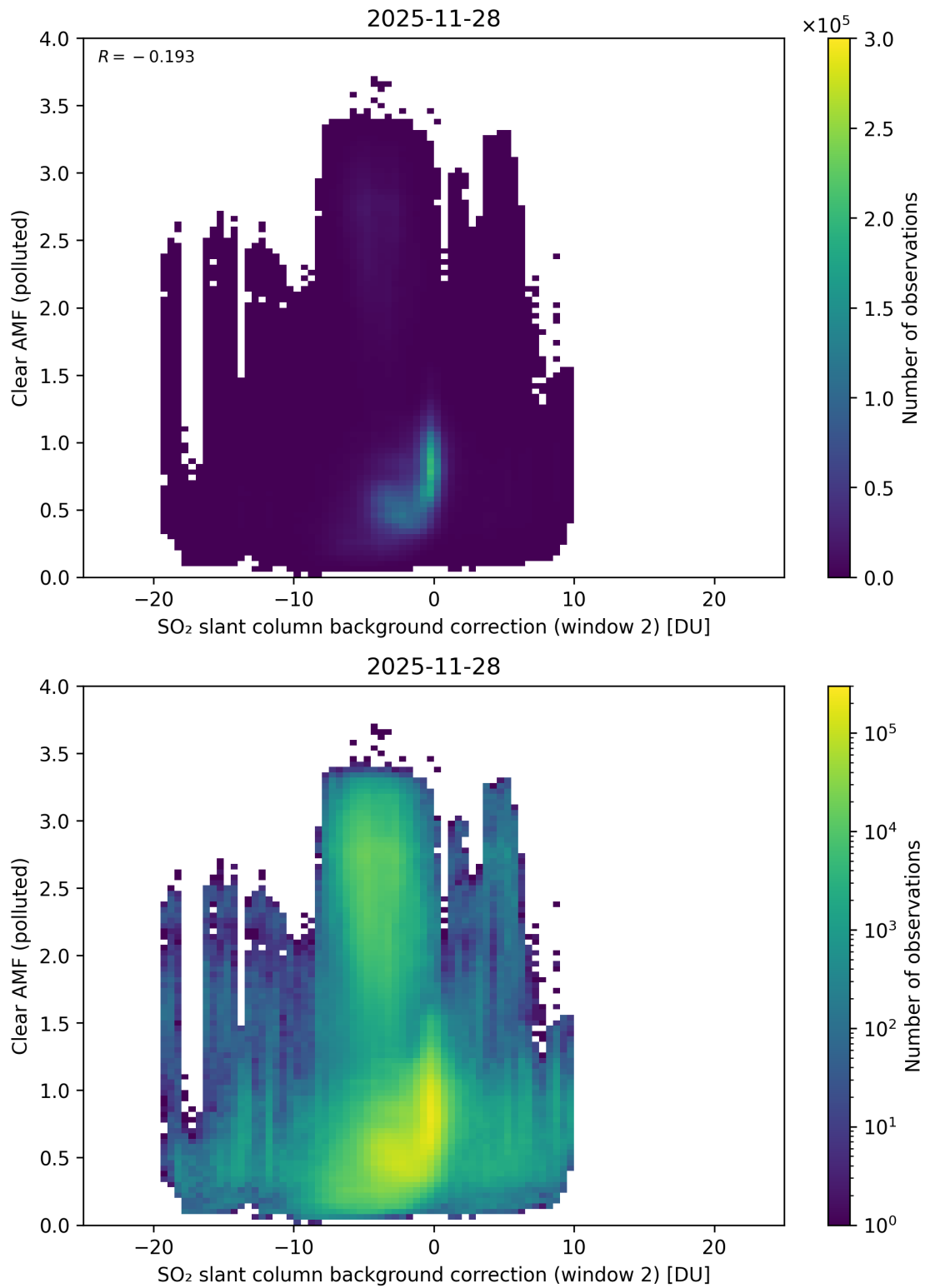
Figure 126: Scatter density plot of “SO 2 slant column background correction (window 2)” against “Clear AMF (polluted)” for 2025-11-28 to 2025-11-29.
