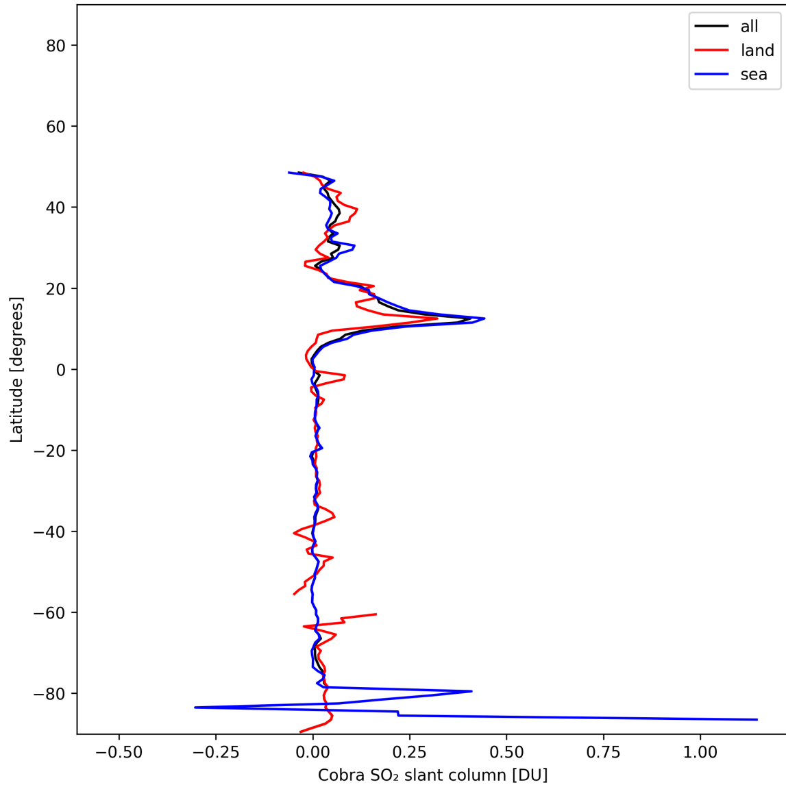
Figure 35: Zonal average of “Cobra SO 2 slant column” for 2025-11-28 to 2025-11-29.
