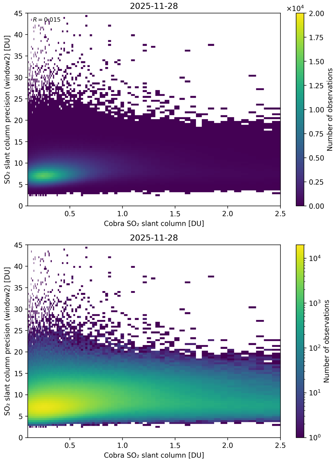
Figure 221: Scatter density plot of “Cobra SO 2 slant column” against “SO 2 slant column precision (window2)” for 2025-11-28 to 2025-11-29.
