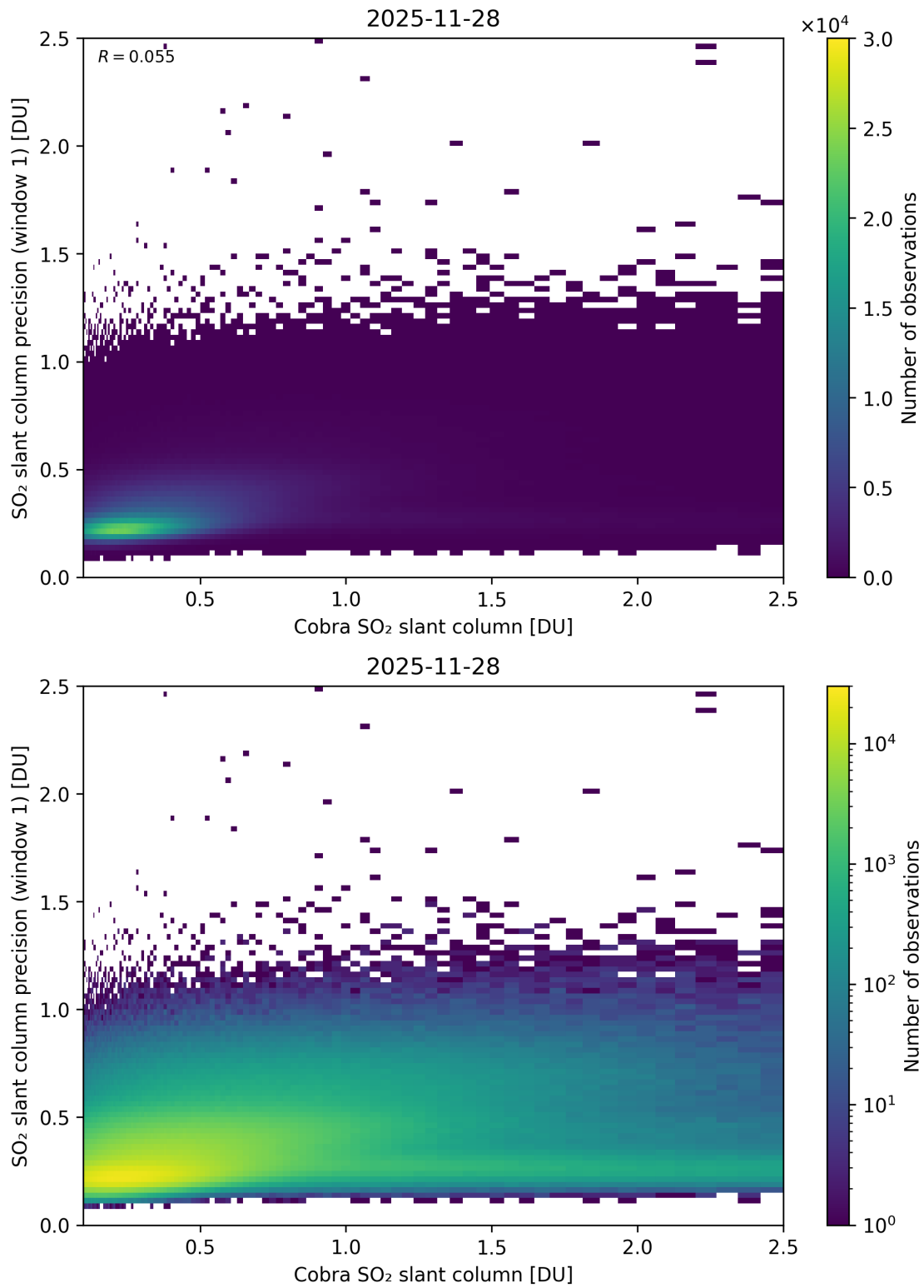
Figure 220: Scatter density plot of “Cobra SO 2 slant column” against “SO 2 slant column precision (window 1)” for 2025-11-28 to 2025-11-29.
