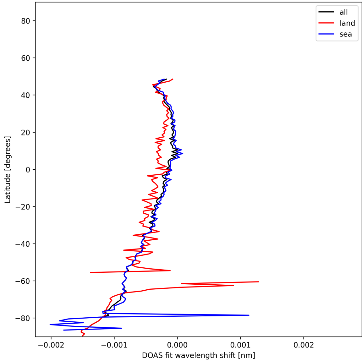
Figure 50: Zonal average of “DOAS fit wavelength shift” for 2025-11-28 to 2025-11-29.
