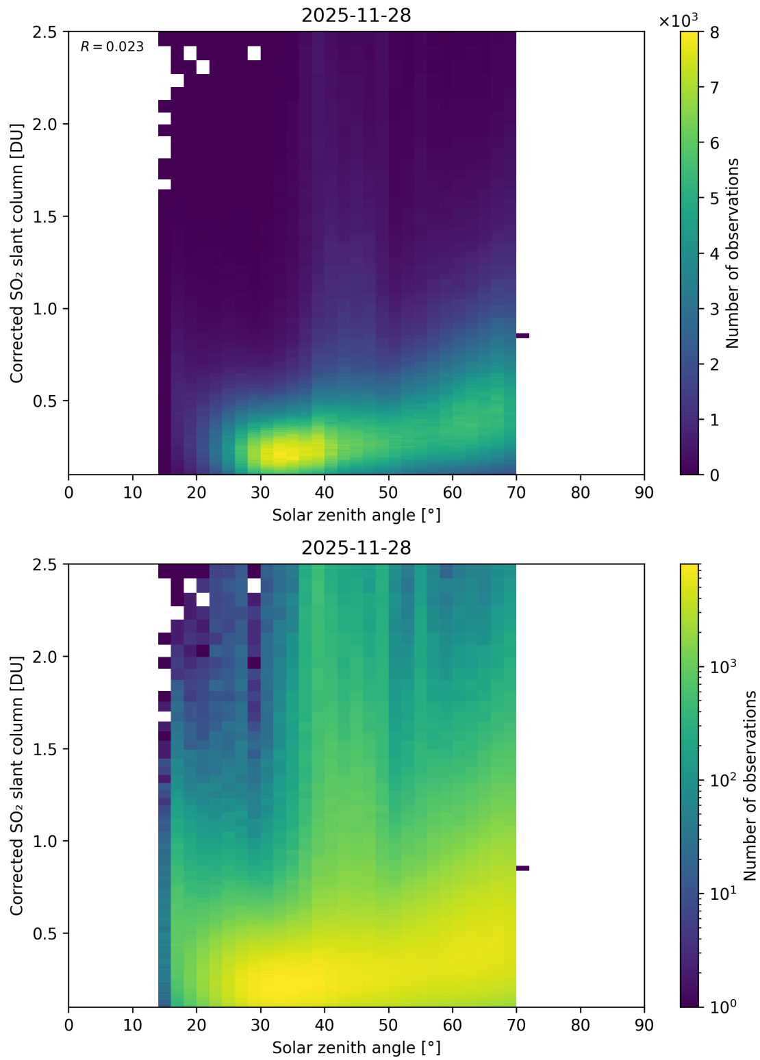
Figure 181: Scatter density plot of “Solar zenith angle” against “Corrected SO 2 slant column” for 2025-11-28 to 2025-11-29.
