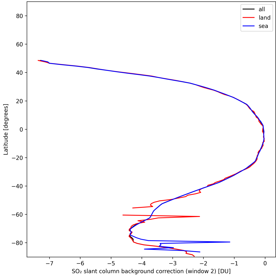
Figure 44: Zonal average of “SO 2 slant column background correction (window 2)” for 2025-11-28 to 2025-11-29.
