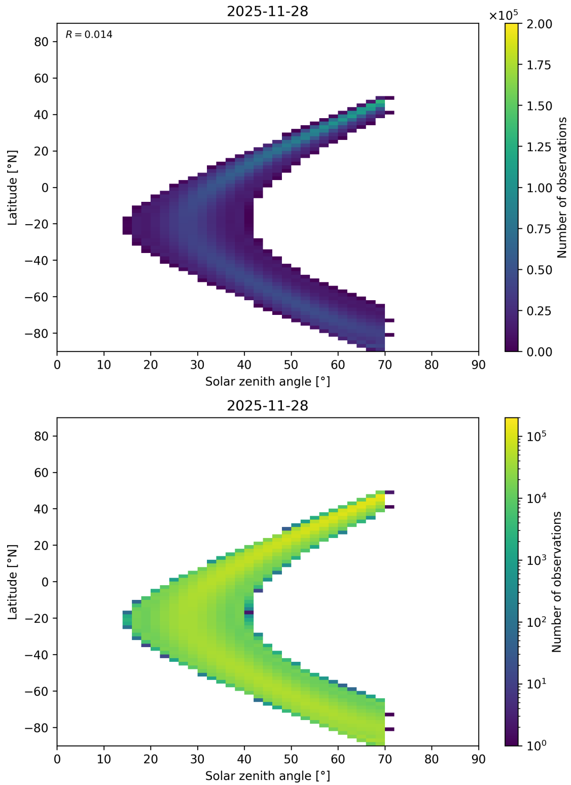
Figure 177: Scatter density plot of “Solar zenith angle” against “Latitude” for 2025-11-28 to 2025-11-29.
