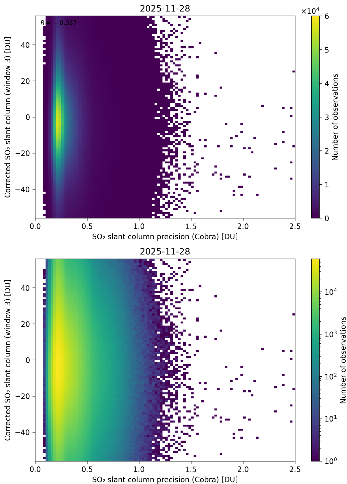
Figure 207: Scatter density plot of “SO 2 slant column precision (Cobra)” against “Corrected SO 2 slant column (window 3)” for 2025-11-28 to 2025-11-29.
