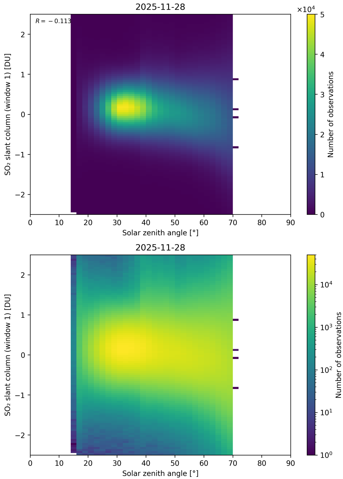
Figure 184: Scatter density plot of “Solar zenith angle” against “SO 2 slant column (window 1)” for 2025-11-28 to 2025-11-29.
