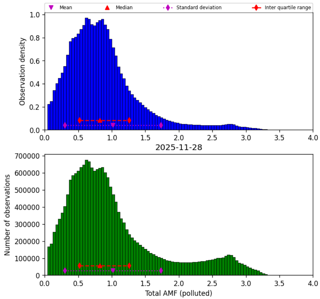
Figure 79: Histogram of “Total AMF (polluted)” for 2025-11-28 to 2025-11-29
