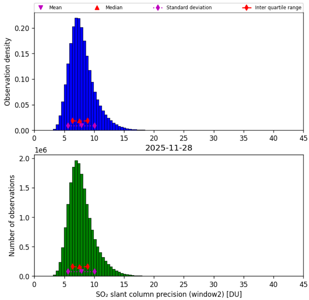
Figure 68: Histogram of “SO 2 slant column precision (window2)” for 2025-11-28 to 2025-11-29
