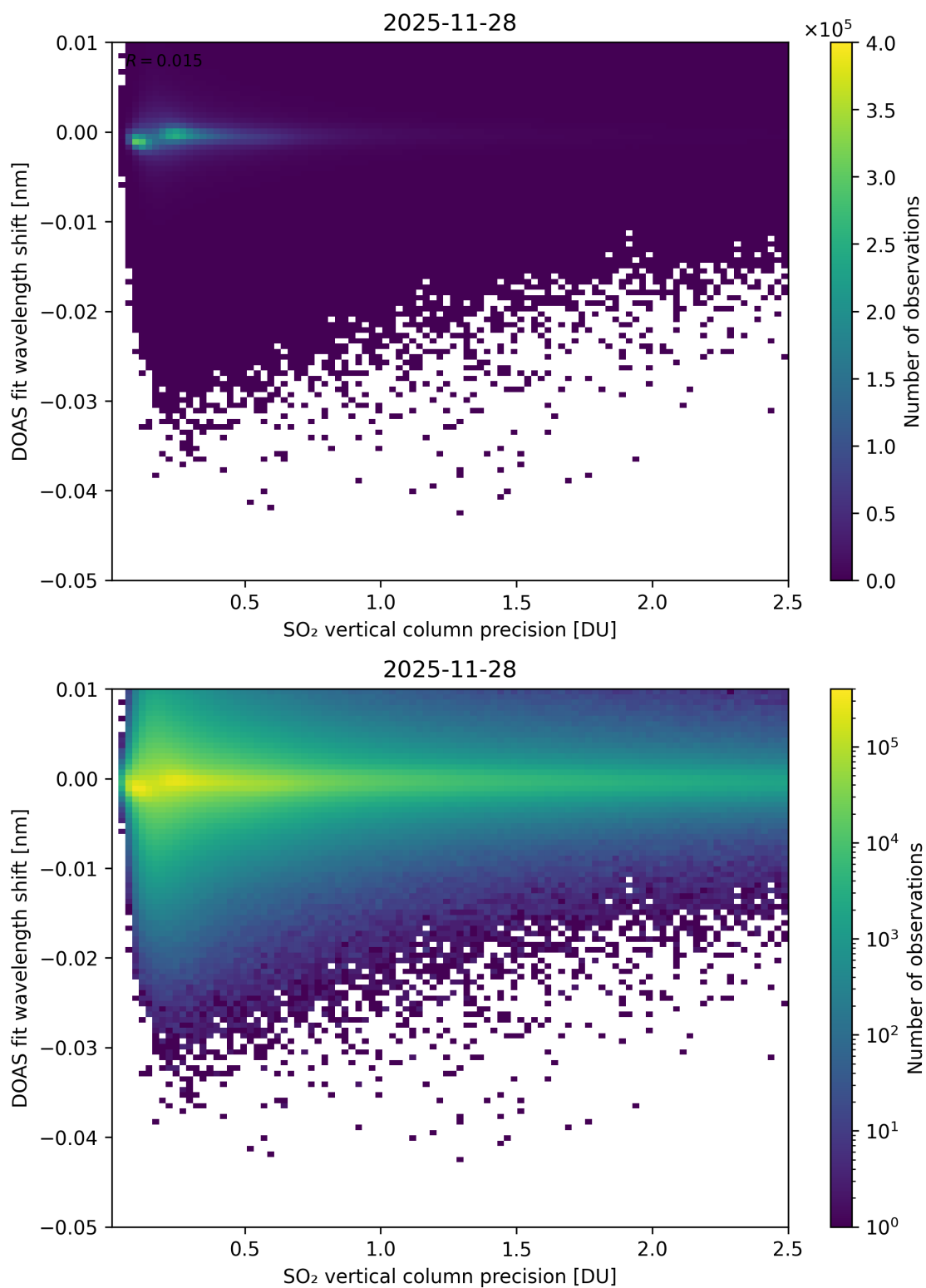
Figure 332: Scatter density plot of “SO 2 vertical column precision” against “DOAS fit wavelength shift” for 2025-11-28 to 2025-11-29.
