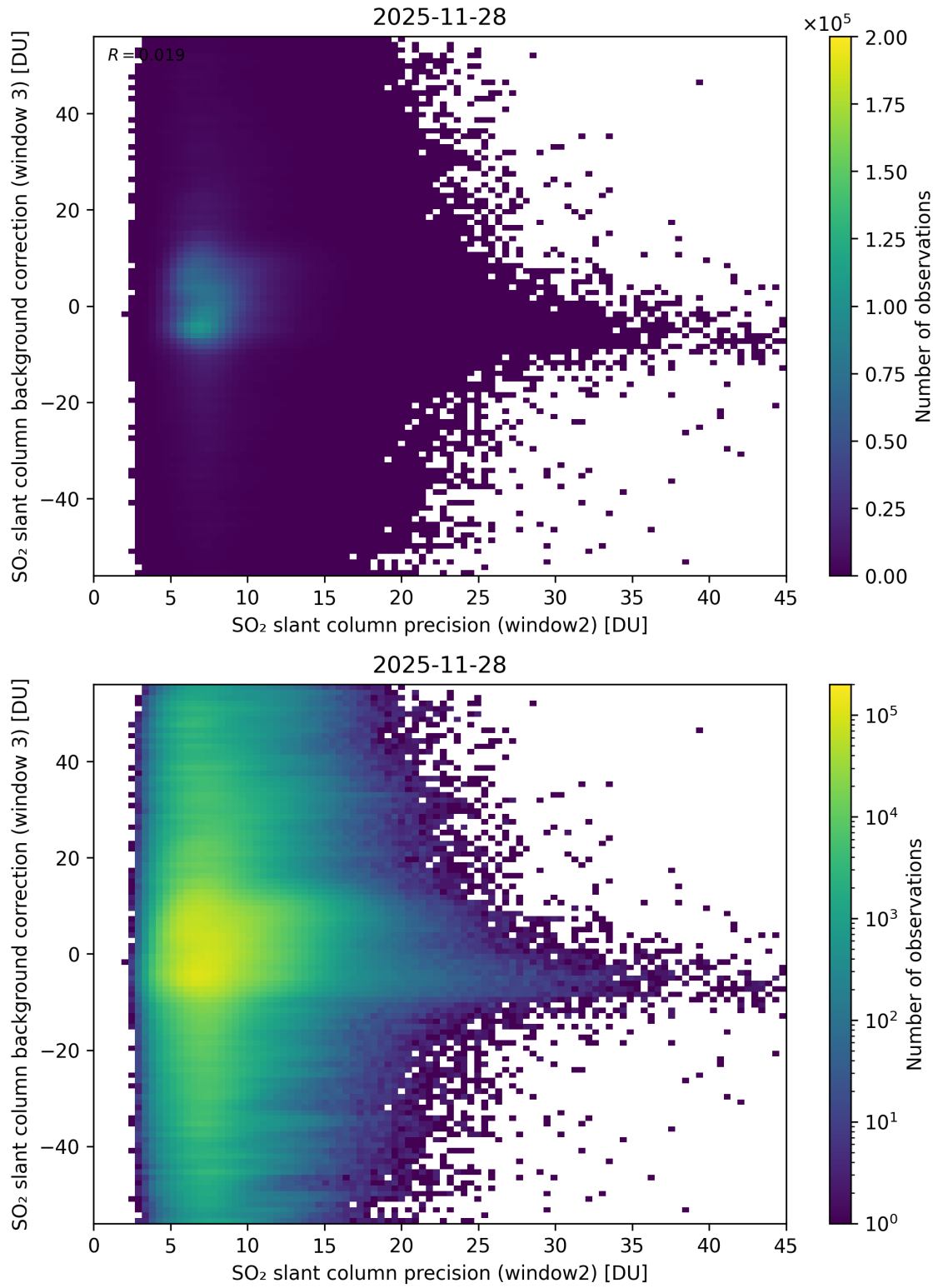
Figure 292: Scatter density plot of “SO 2 slant column precision (window2)” against “SO 2 slant column background correction (window 3)” for 2025-11-28 to 2025-11-29.
