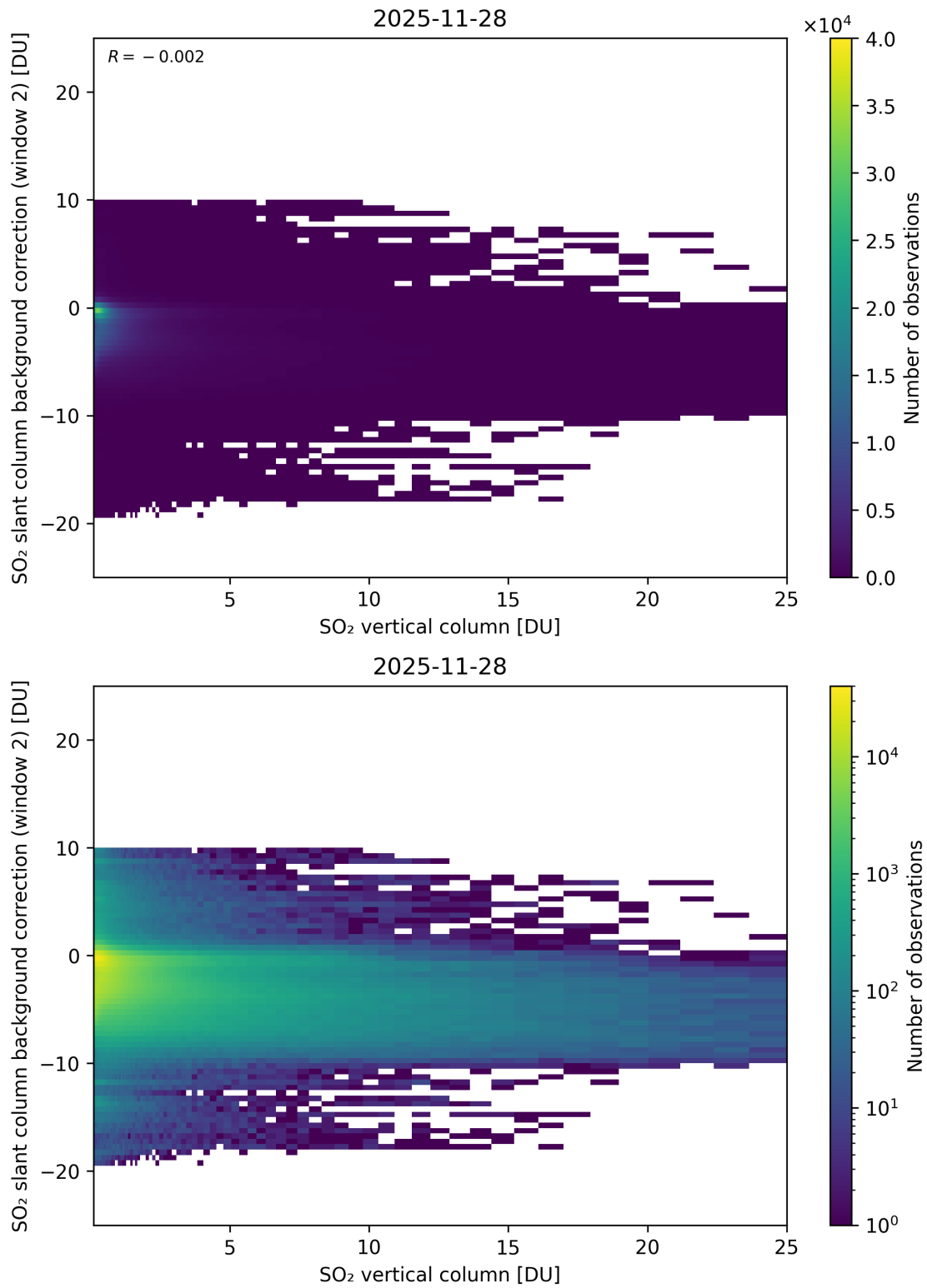
Figure 324: Scatter density plot of “SO 2 vertical column” against “SO 2 slant column background correction (window 2)” for 2025-11-28 to 2025-11-29.
