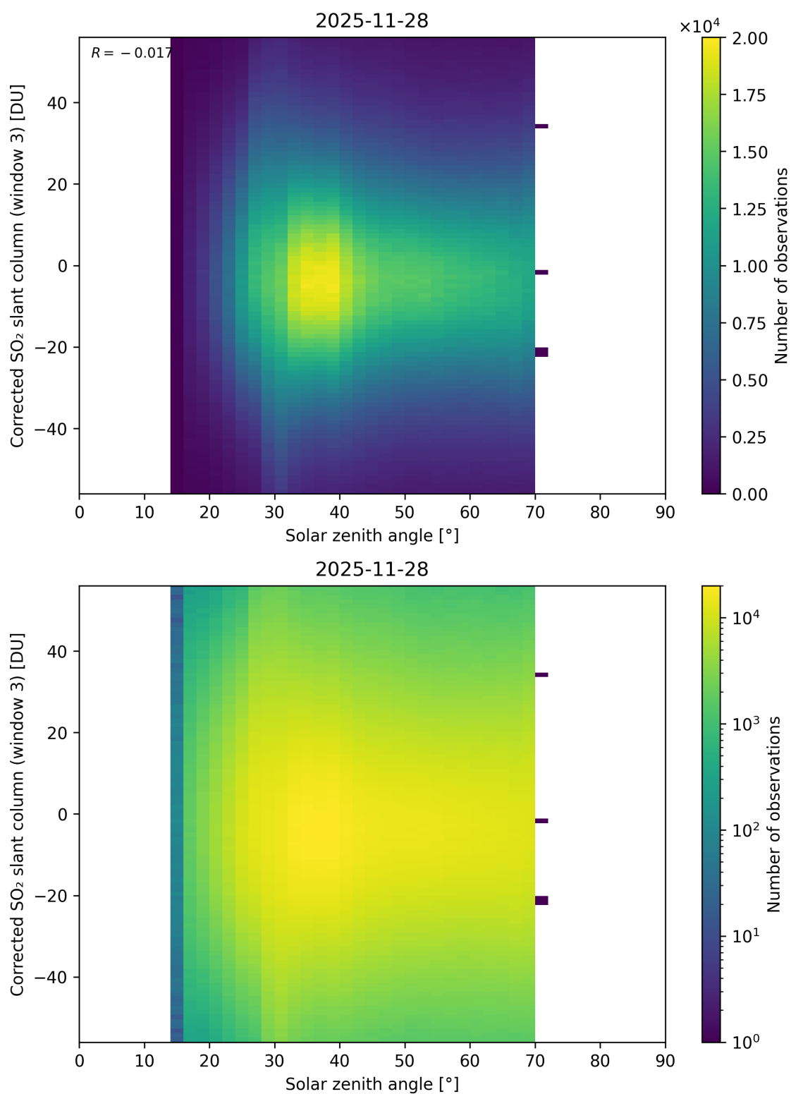
Figure 183: Scatter density plot of “Solar zenith angle” against “Corrected SO 2 slant column (window 3)” for 2025-11-28 to 2025-11-29.
