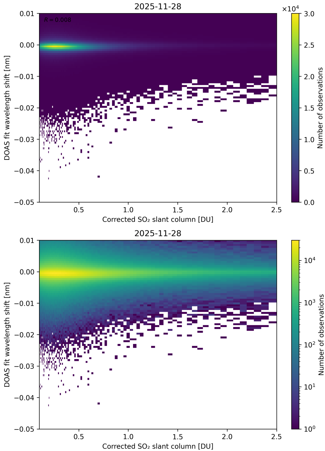
Figure 229: Scatter density plot of “Corrected SO 2 slant column” against “DOAS fit wavelength shift” for 2025-11-28 to 2025-11-29.
