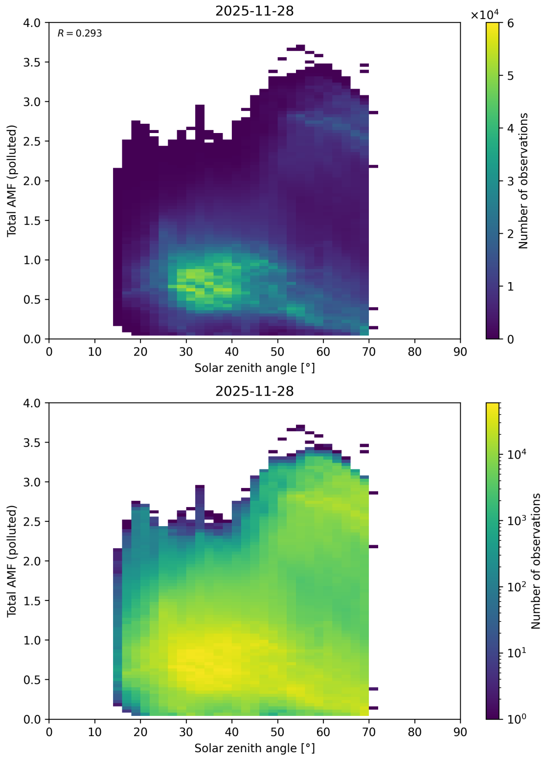
Figure 189: Scatter density plot of “Solar zenith angle” against “Total AMF (polluted)” for 2025-11-28 to 2025-11-29.
