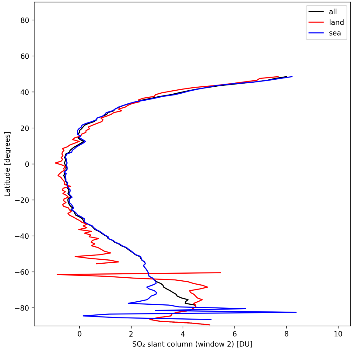
Figure 41: Zonal average of “SO 2 slant column (window 2)” for 2025-11-28 to 2025-11-29.
