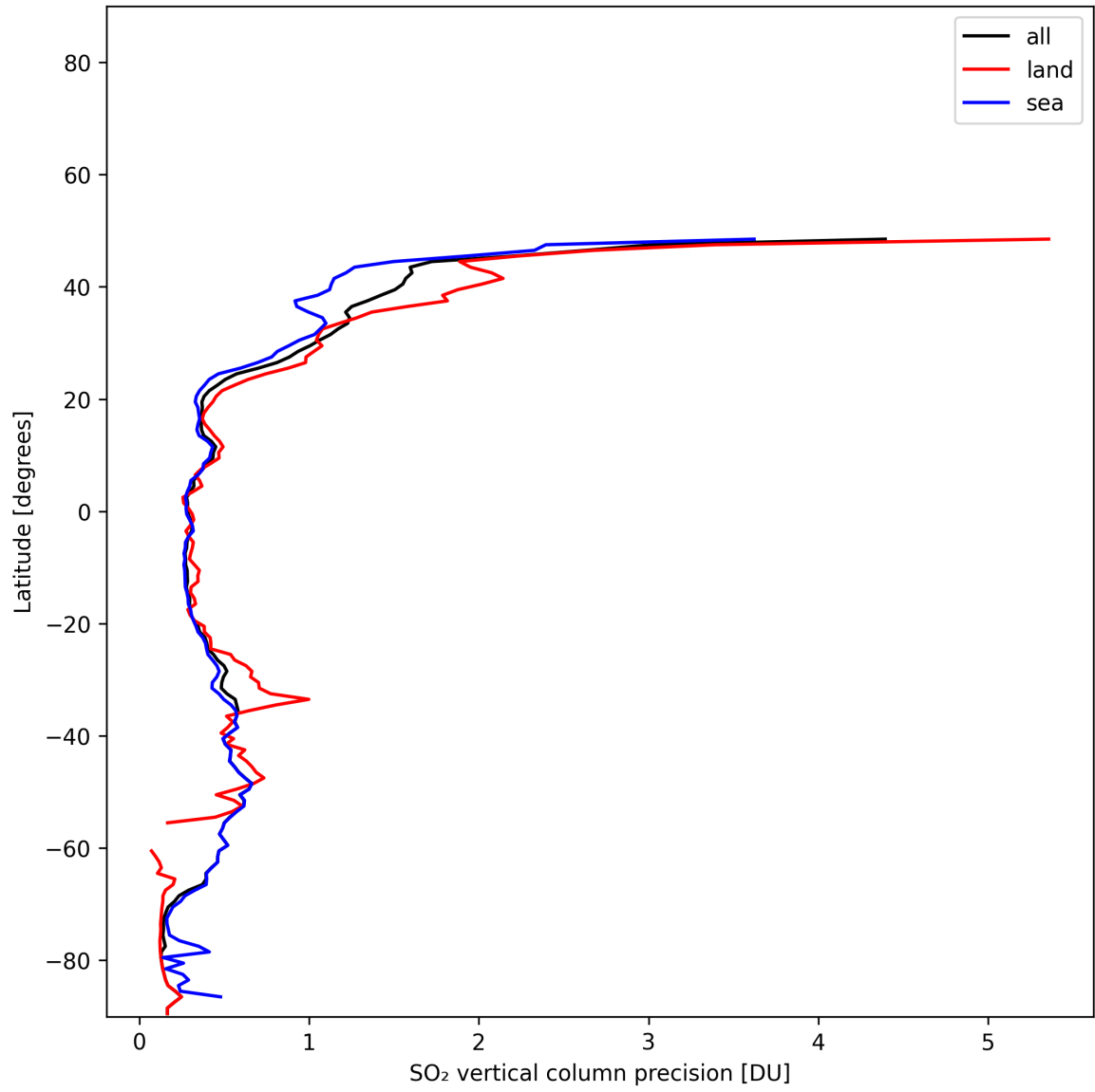
Figure 33: Zonal average of “SO 2 vertical column precision” for 2025-11-28 to 2025-11-29.
