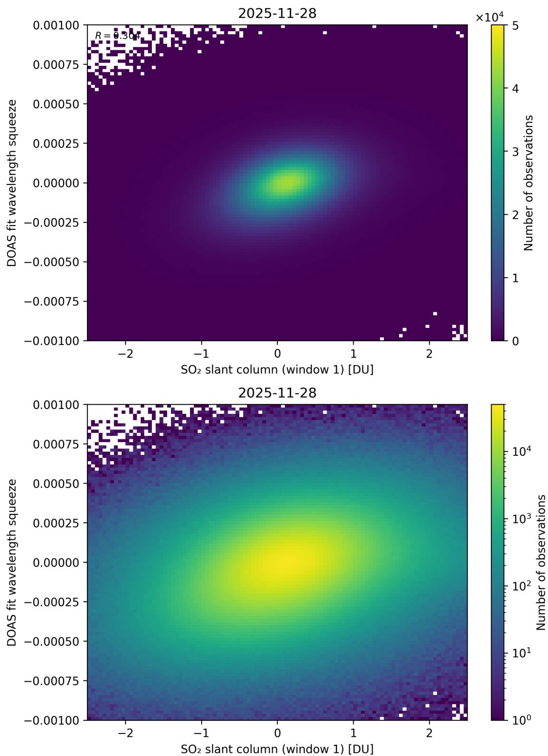
Figure 266: Scatter density plot of “SO 2 slant column (window 1)” against “DOAS fit wavelength squeeze” for 2025-11-28 to 2025-11-29.
