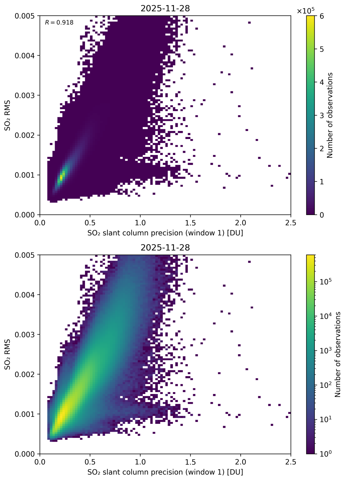
Figure 273: Scatter density plot of “SO 2 slant column precision (window 1)” against “SO 2 RMS” for 2025-11-28 to 2025-11-29.
