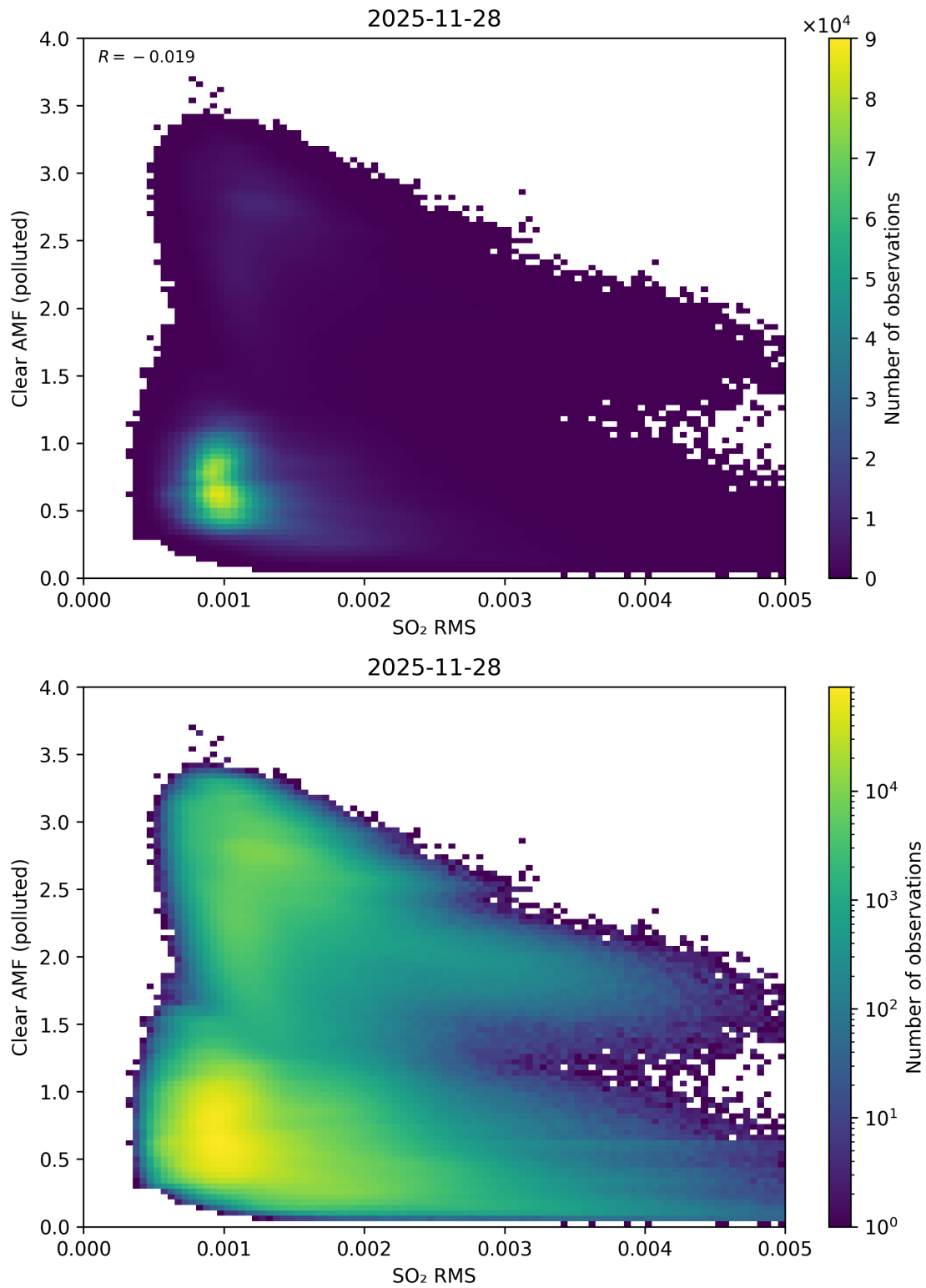
Figure 147: Scatter density plot of “SO 2 RMS” against “Clear AMF (polluted)” for 2025-11-28 to 2025-11-29.
