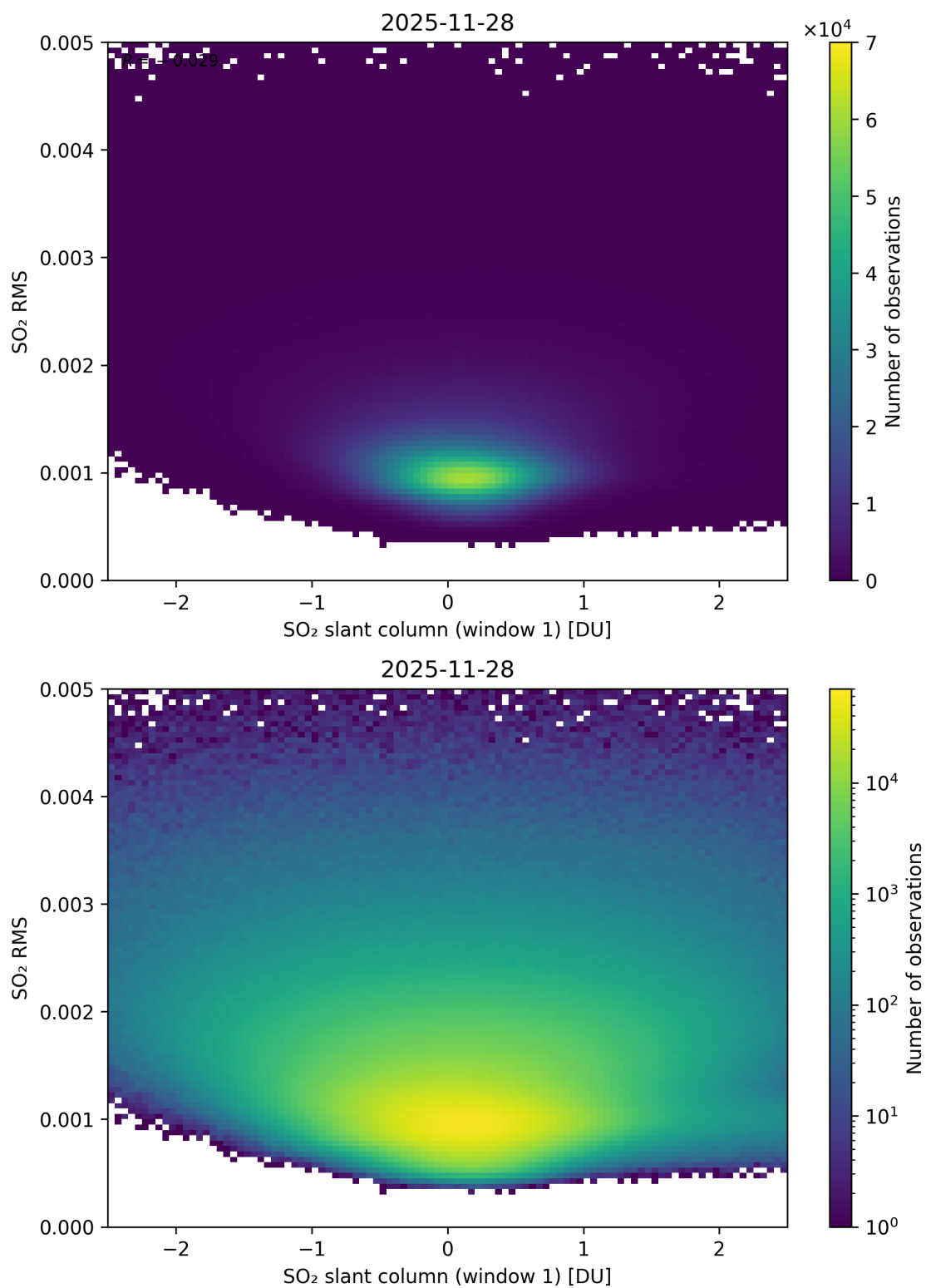
Figure 267: Scatter density plot of “SO 2 slant column (window 1)” against “SO 2 RMS” for 2025-11-28 to 2025-11-29.
