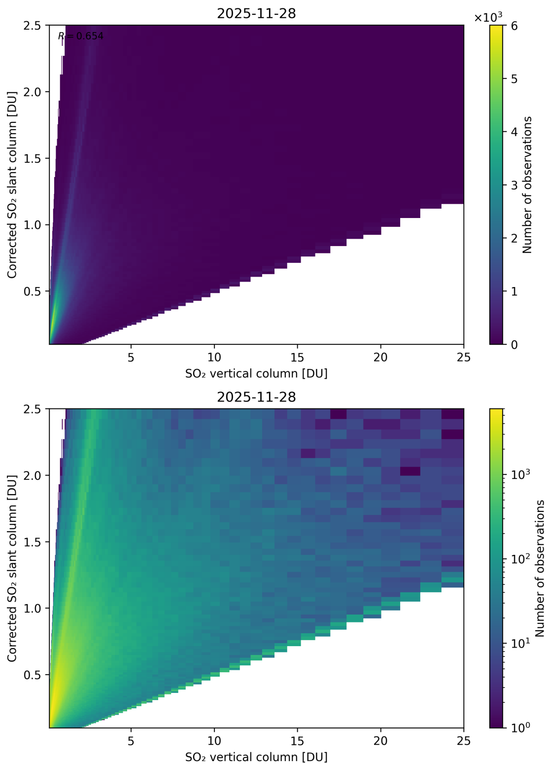
Figure 351: Scatter density plot of “SO 2 vertical column” against “Corrected SO 2 slant column” for 2025-11-28 to 2025-11-29.
