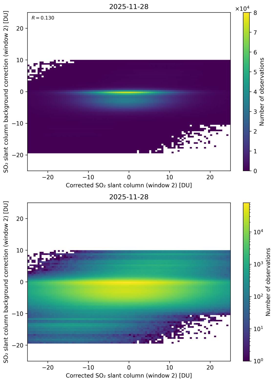
Figure 244: Scatter density plot of “Corrected SO 2 slant column (window 2)” against “SO 2 slant column background correction (window 2)” for 2025-11-28 to 2025-11-29.
