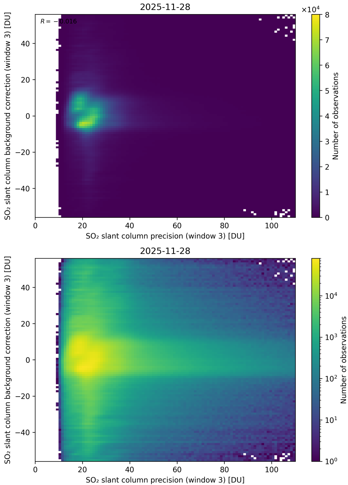
Figure 307: Scatter density plot of “SO 2 slant column precision (window 3)” against “SO 2 slant column background correction (window 3)” for 2025-11-28 to 2025-11-29.
