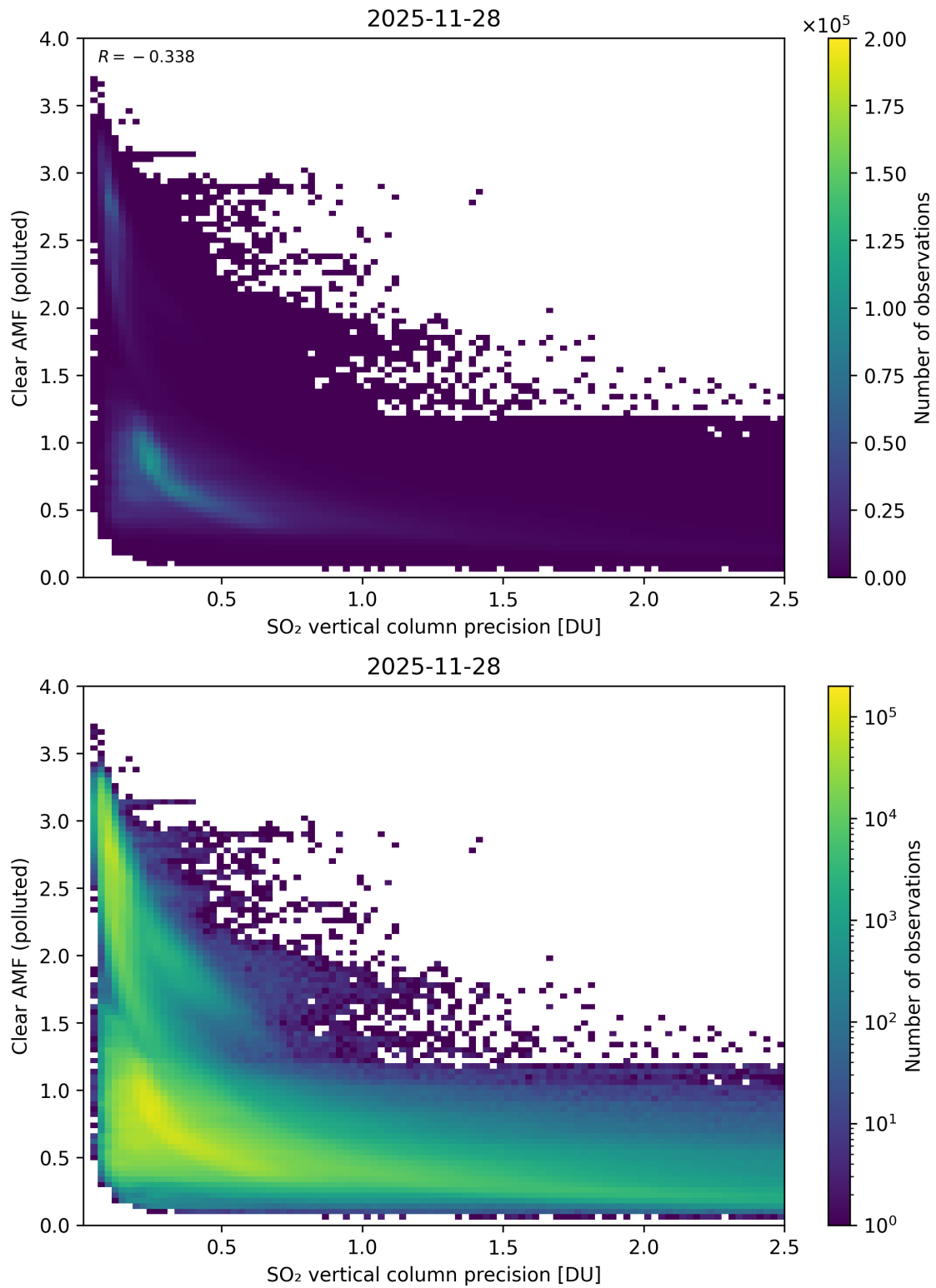
Figure 335: Scatter density plot of “SO 2 vertical column precision” against “Clear AMF (polluted)” for 2025-11-28 to 2025-11-29.
