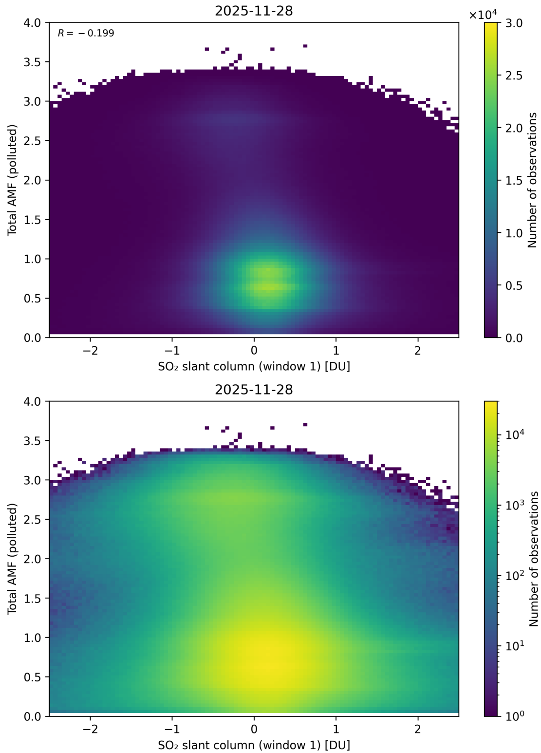
Figure 289: Scatter density plot of “SO 2 slant column (window 1)” against “Total AMF (polluted)” for 2025-11-28 to 2025-11-29.
