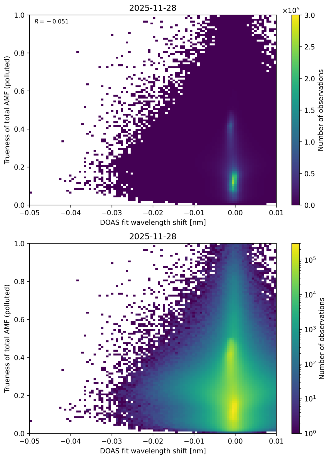
Figure 142: Scatter density plot of “DOAS fit wavelength shift” against “Trueness of total AMF (polluted)” for 2025-11-28 to 2025-11-29.
