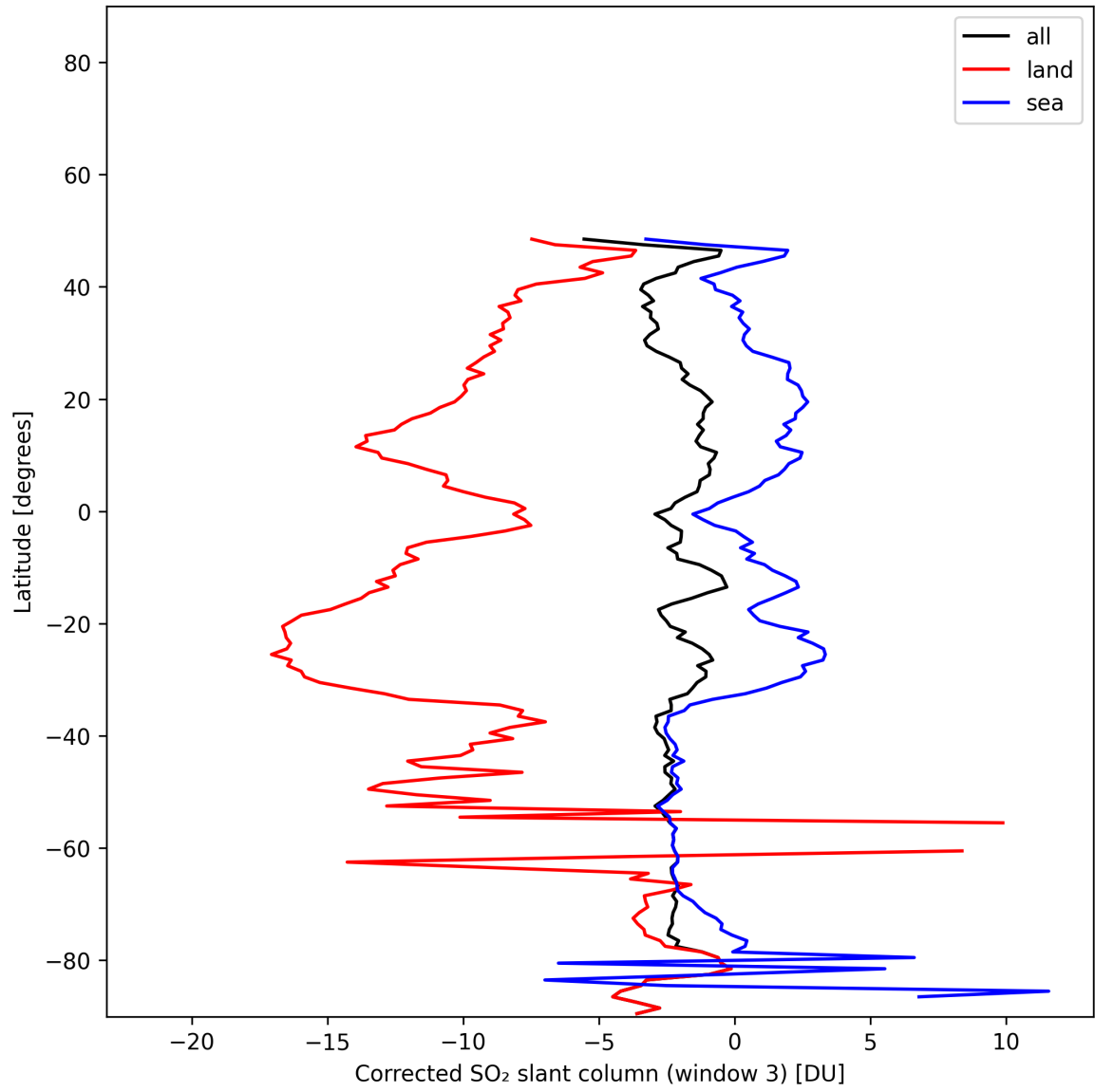
Figure 47: Zonal average of “Corrected SO 2 slant column (window 3)” for 2025-11-28 to 2025-11-29.
