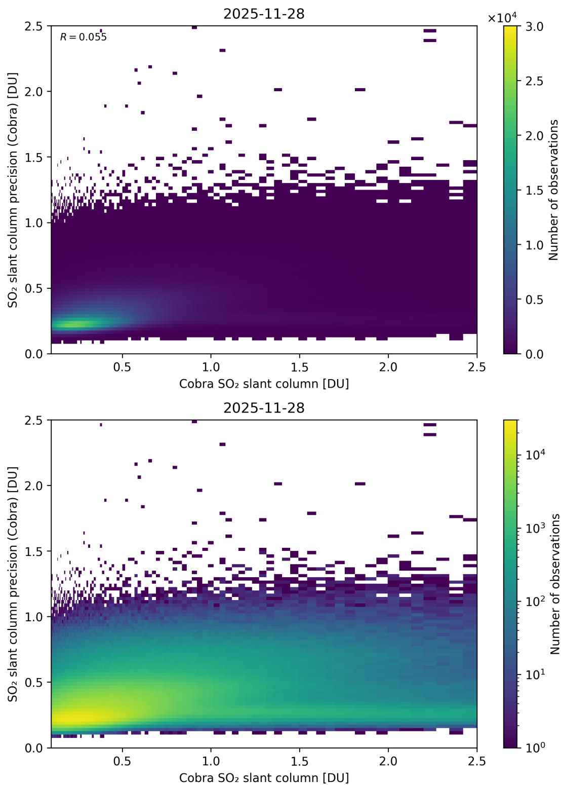
Figure 216: Scatter density plot of “Cobra SO 2 slant column” against “SO 2 slant column precision (Cobra)” for 2025-11-28 to 2025-11-29.
