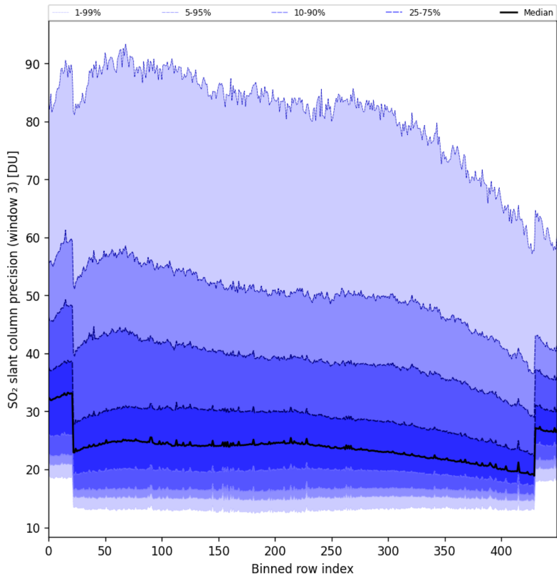
Figure 98: Along track statistics of “SO 2 slant column precision (window 3)” for 2025-11-28 to 2025-11-29
