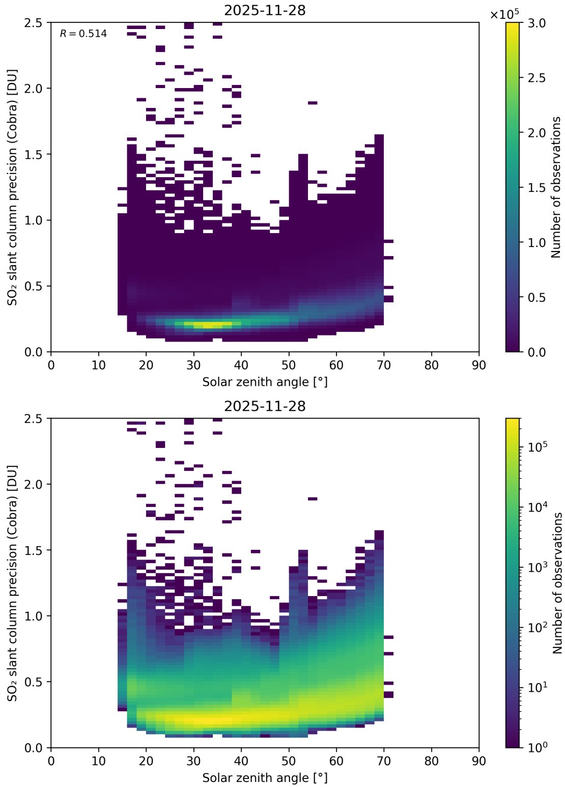
Figure 180: Scatter density plot of “Solar zenith angle” against “SO 2 slant column precision (Cobra)” for 2025-11-28 to 2025-11-29.
