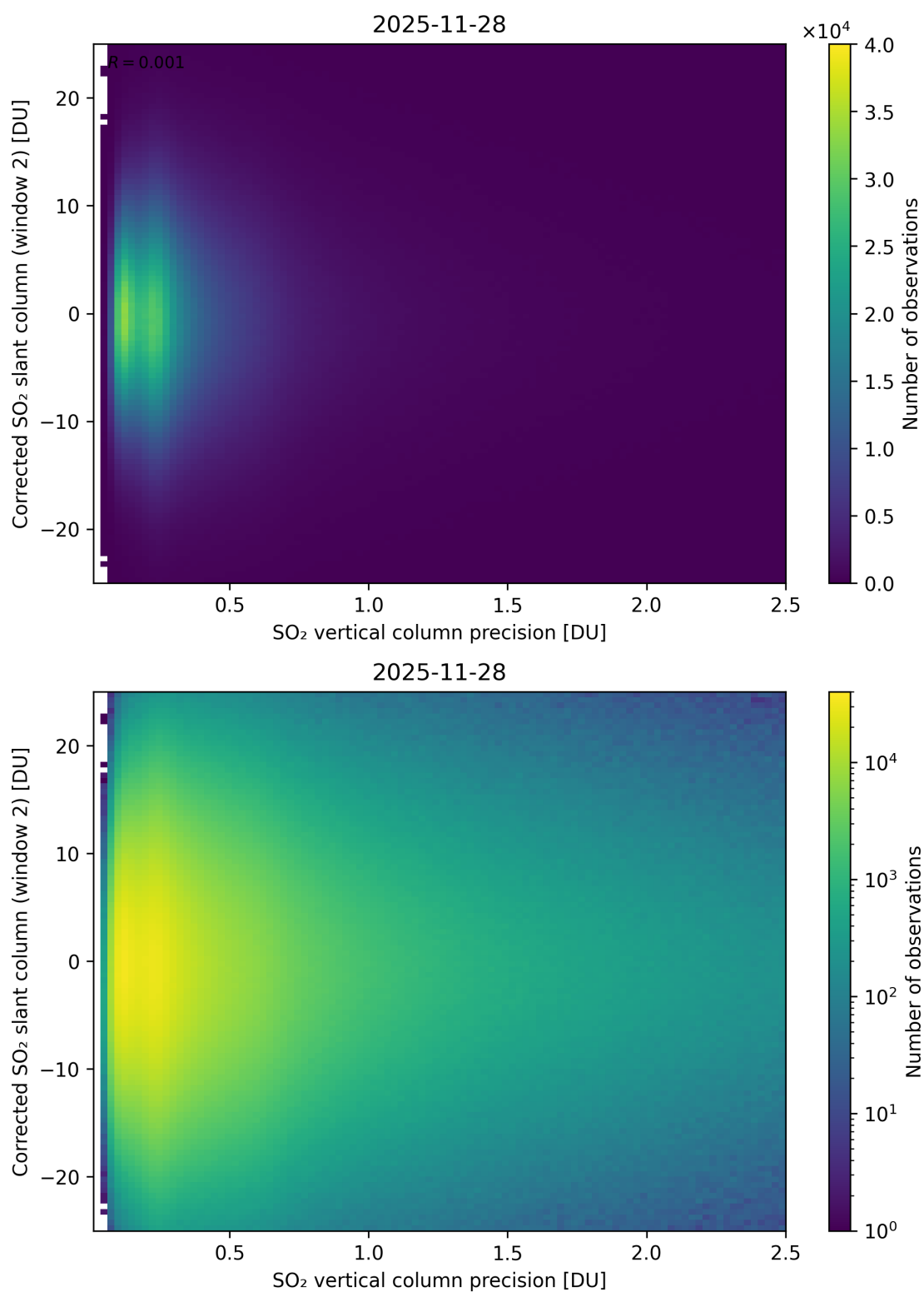
Figure 339: Scatter density plot of “SO 2 vertical column precision” against “Corrected SO 2 slant column (window 2)” for 2025-11-28 to 2025-11-29.
