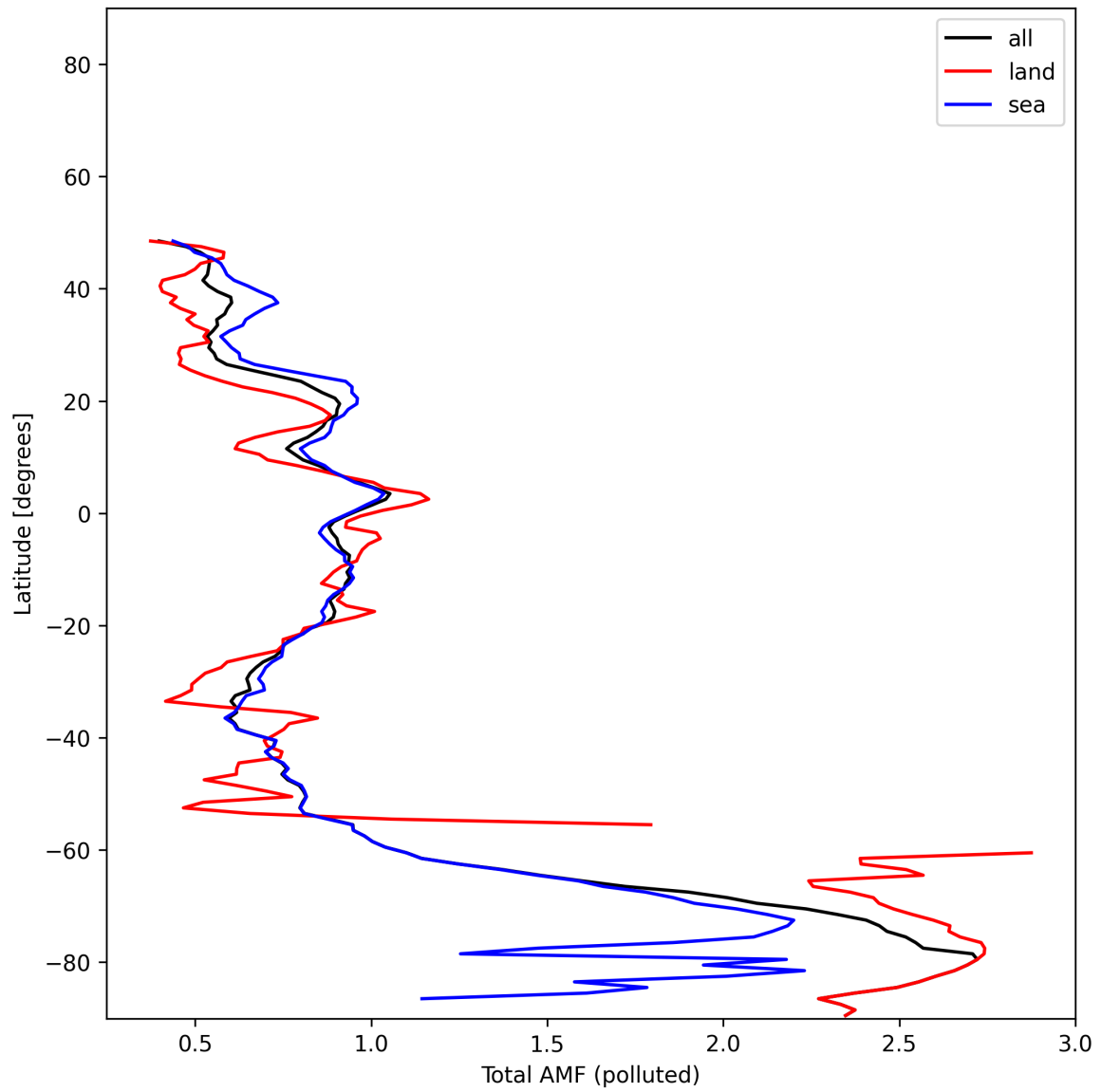
Figure 53: Zonal average of “Total AMF (polluted)” for 2025-11-28 to 2025-11-29.
