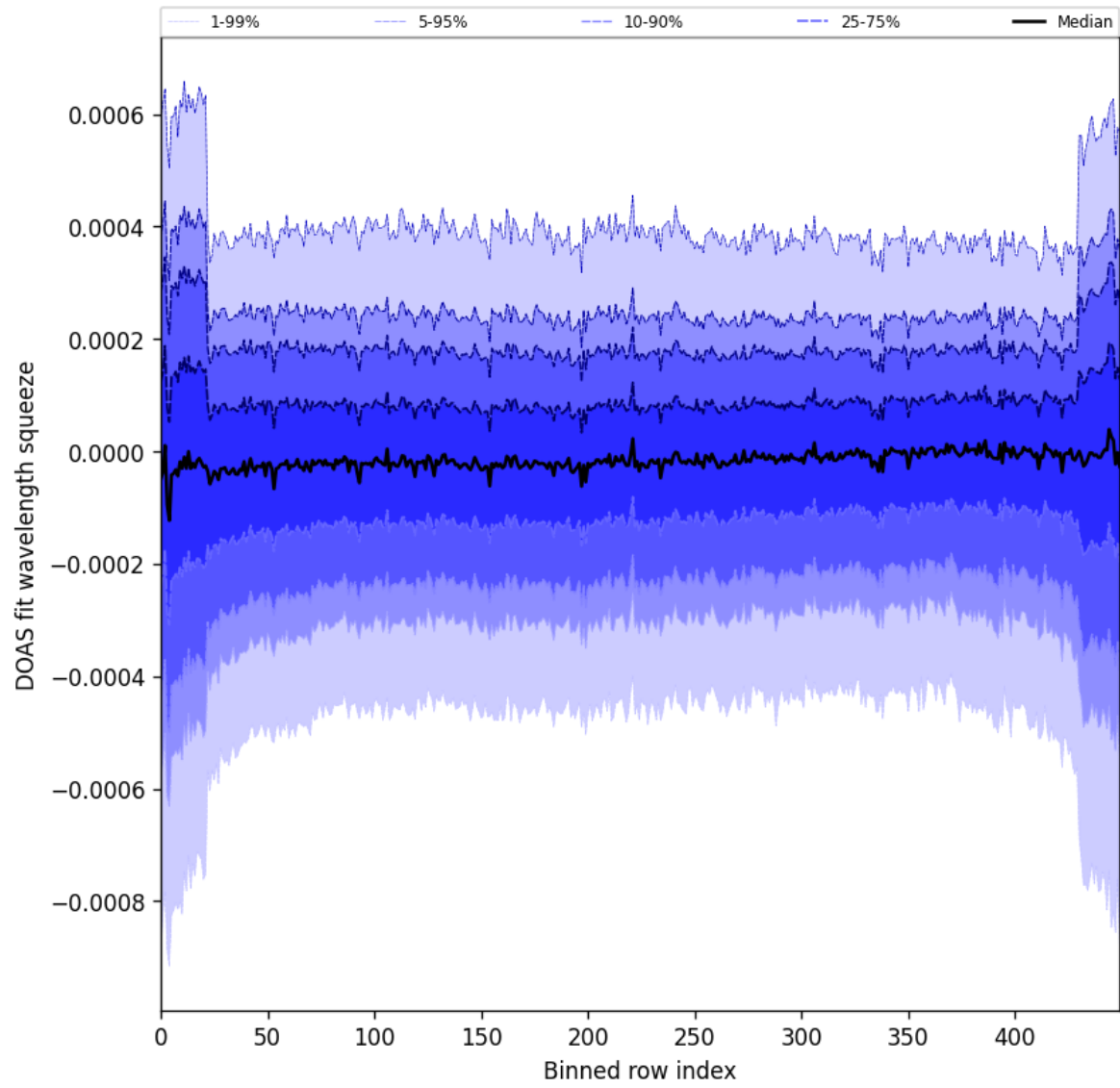
Figure 103: Along track statistics of “DOAS fit wavelength squeeze” for 2025-11-28 to 2025-11-29
