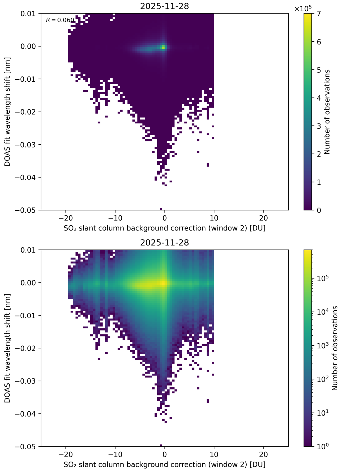
Figure 123: Scatter density plot of “SO 2 slant column background correction (window 2)” against “DOAS fit wavelength shift” for 2025-11-28 to 2025-11-29.
