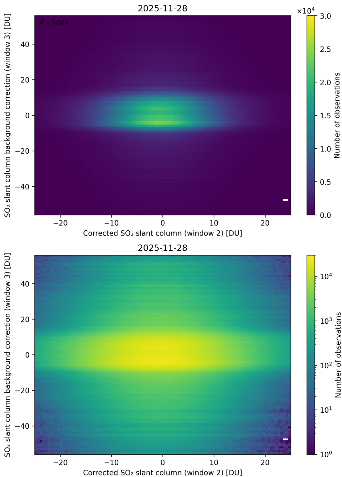
Figure 245: Scatter density plot of “Corrected SO 2 slant column (window 2)” against “SO 2 slant column background correction (window 3)” for 2025-11-28 to 2025-11-29.
