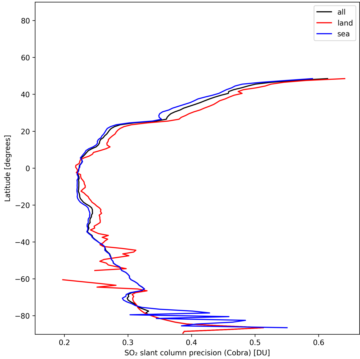
Figure 36: Zonal average of “SO 2 slant column precision (Cobra)” for 2025-11-28 to 2025-11-29.
