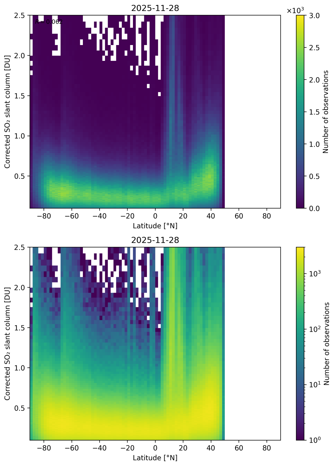
Figure 159: Scatter density plot of “Latitude” against “Corrected SO 2 slant column” for 2025-11-28 to 2025-11-29.
