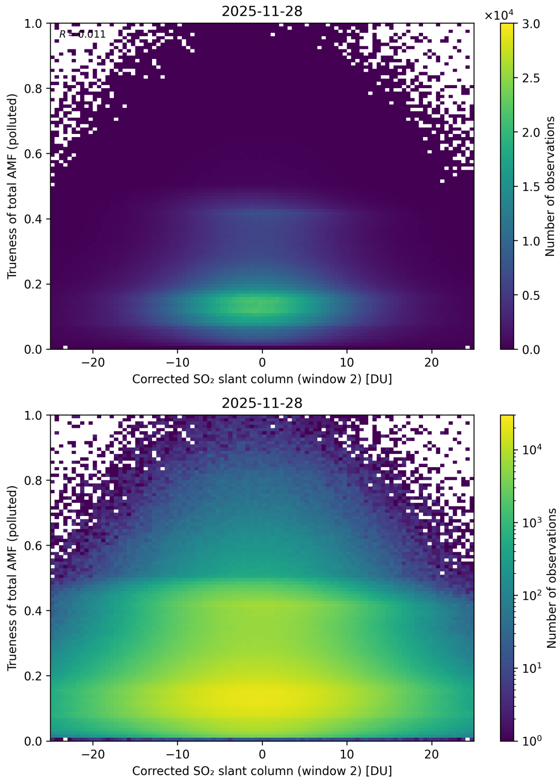
Figure 254: Scatter density plot of “Corrected SO 2 slant column (window 2)” against “Trueness of total AMF (polluted)” for 2025-11-28 to 2025-11-29.
