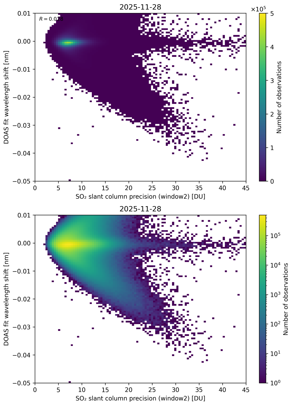
Figure 293: Scatter density plot of “SO 2 slant column precision (window2)” against “DOAS fit wavelength shift” for 2025-11-28 to 2025-11-29.
