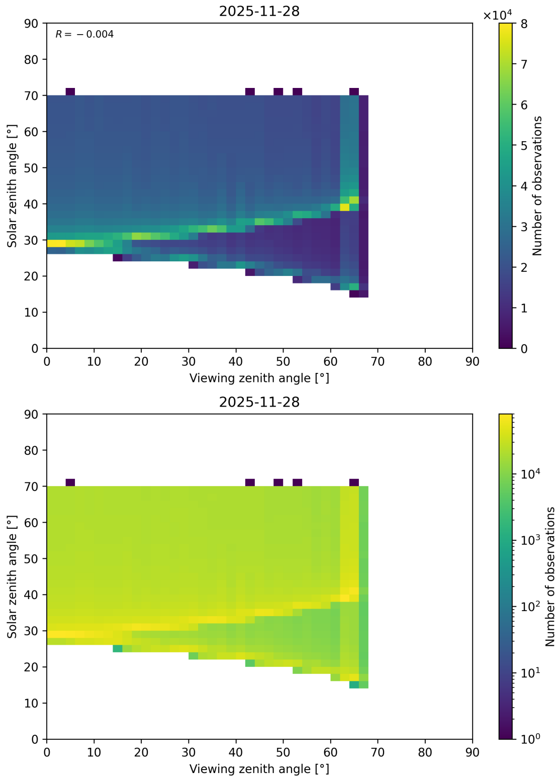
Figure 369: Scatter density plot of “Viewing zenith angle” against “Solar zenith angle” for 2025-11-28 to 2025-11-29.
