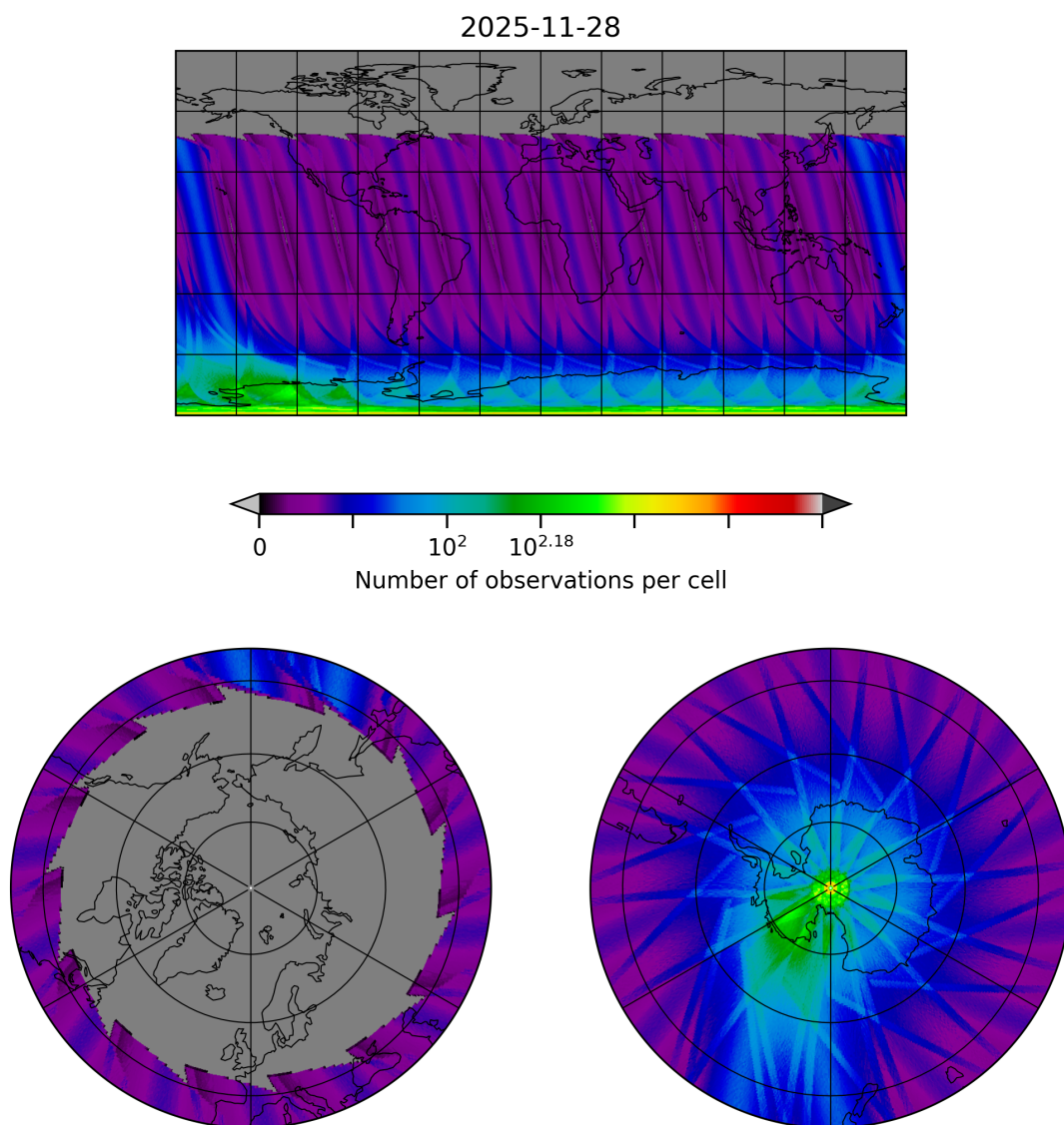
Figure 30: Map of the number of observations for 2025-11-28 to 2025-11-29
