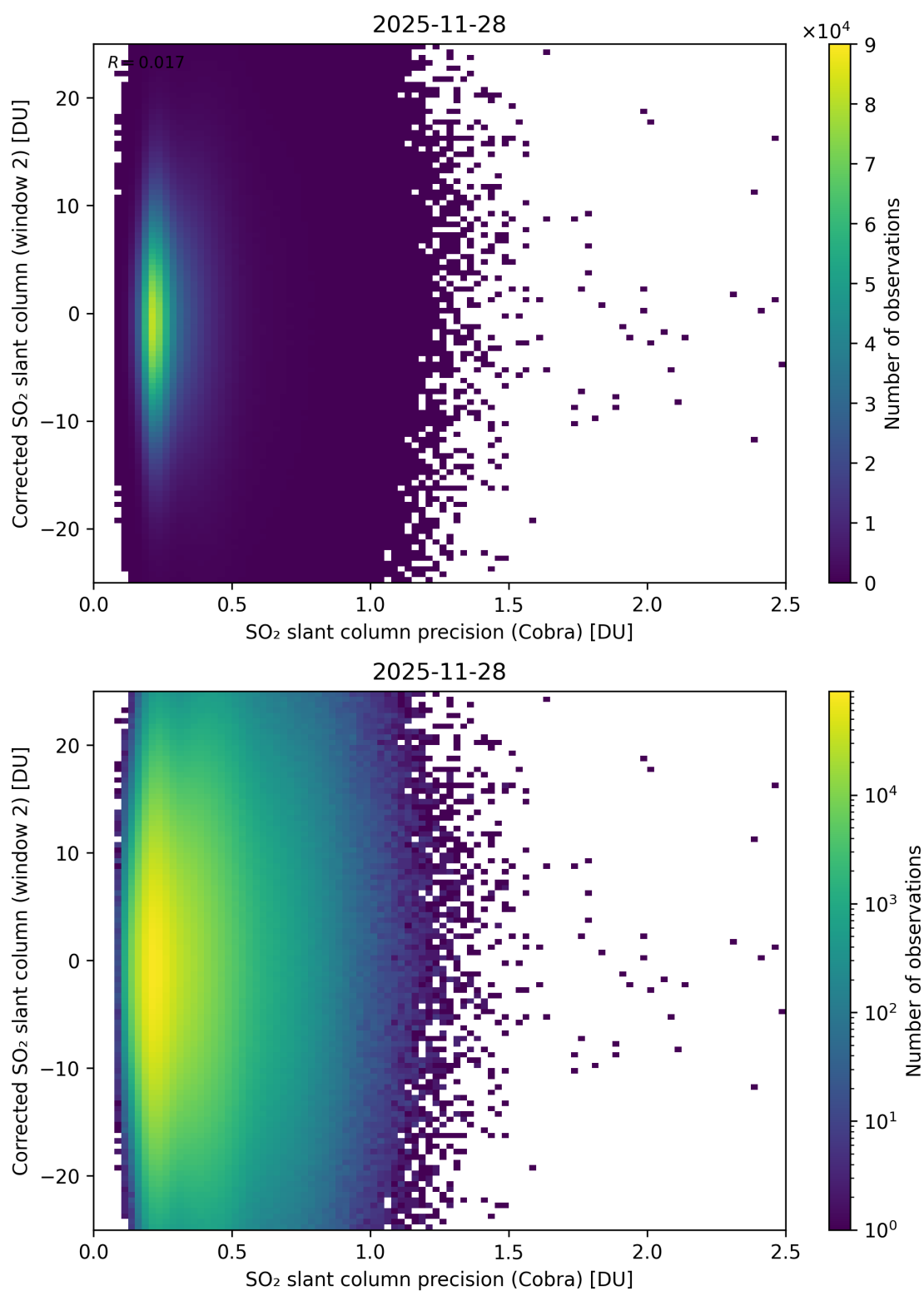
Figure 206: Scatter density plot of “SO 2 slant column precision (Cobra)” against “Corrected SO 2 slant column (window 2)” for 2025-11-28 to 2025-11-29.
