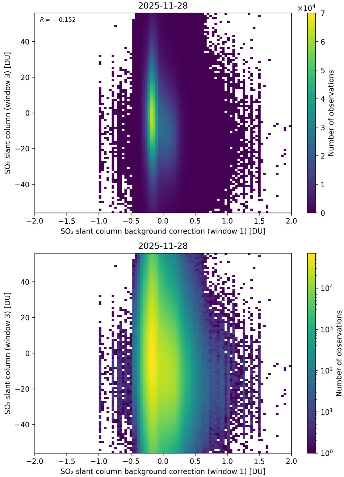
Figure 118: Scatter density plot of “SO 2 slant column background correction (window 1)” against “SO 2 slant column (window 3)” for 2025-11-28 to 2025-11-29.
