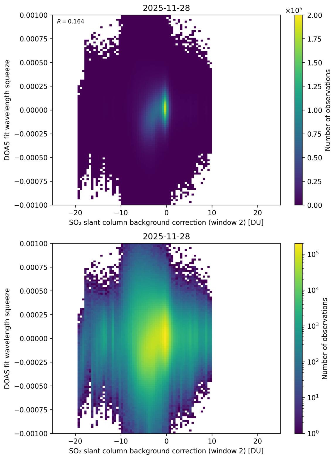
Figure 124: Scatter density plot of “SO 2 slant column background correction (window 2)” against “DOAS fit wavelength squeeze” for 2025-11-28 to 2025-11-29.
