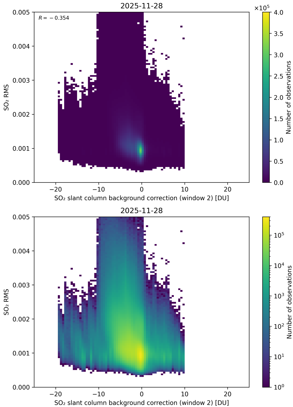
Figure 125: Scatter density plot of “SO 2 slant column background correction (window 2)” against “SO 2 RMS” for 2025-11-28 to 2025-11-29.
