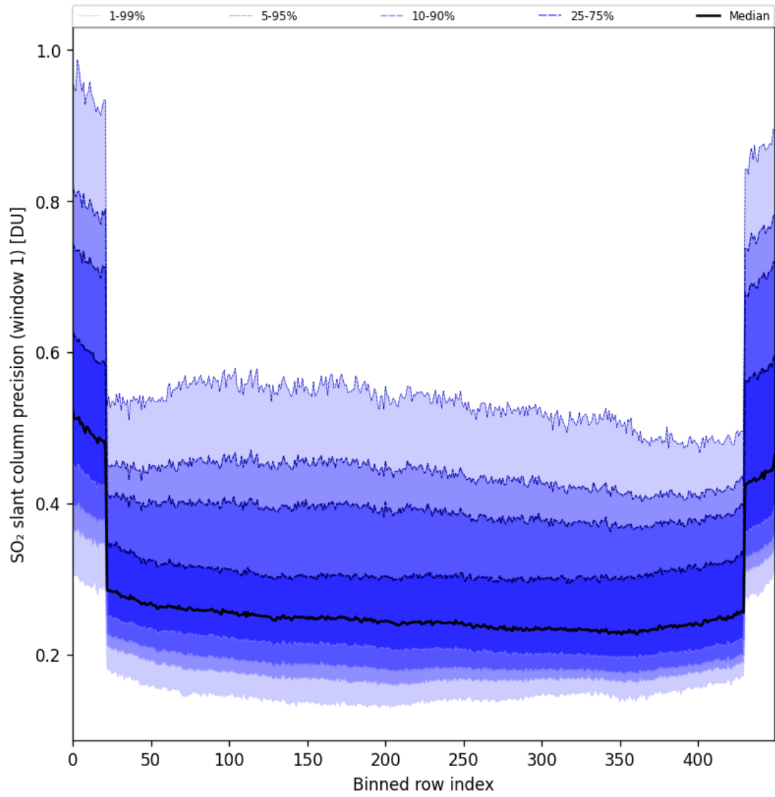
Figure 90: Along track statistics of “SO 2 slant column precision (window 1)” for 2025-11-28 to 2025-11-29
