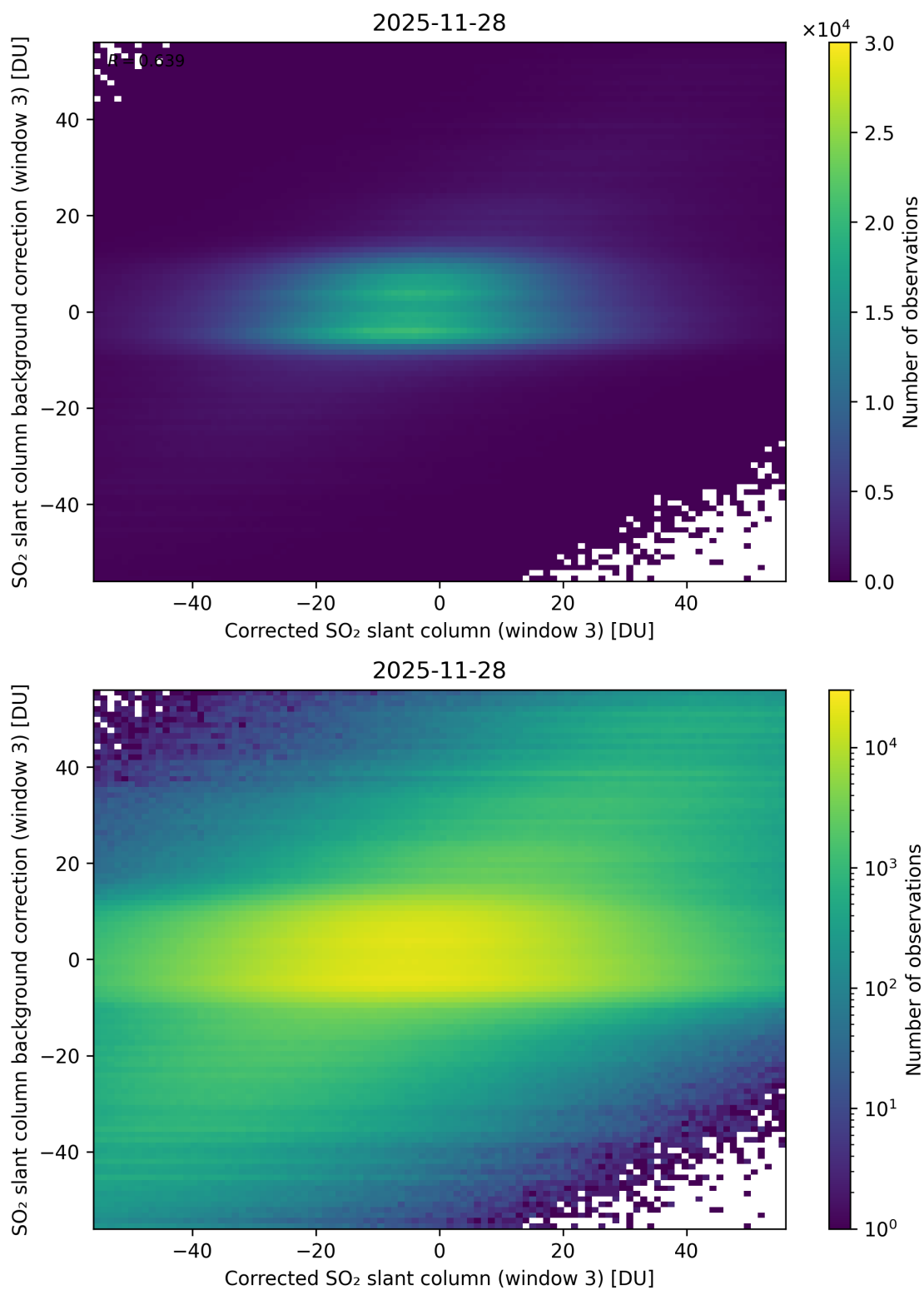
Figure 255: Scatter density plot of “Corrected SO 2 slant column (window 3)” against “SO 2 slant column background correction (window 3)” for 2025-11-28 to 2025-11-29.
