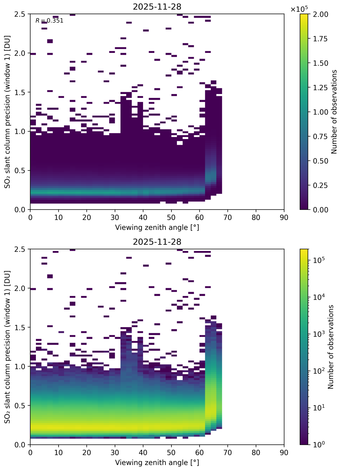
Figure 377: Scatter density plot of “Viewing zenith angle” against “SO 2 slant column precision (window 1)” for 2025-11-28 to 2025-11-29.
