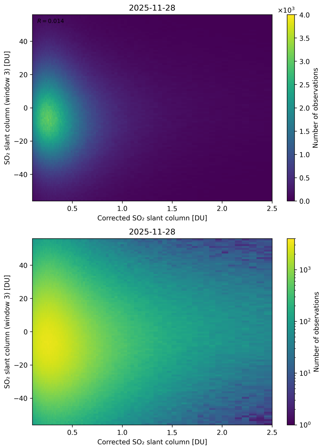
Figure 240: Scatter density plot of “Corrected SO 2 slant column” against “SO 2 slant column (window 3)” for 2025-11-28 to 2025-11-29.
