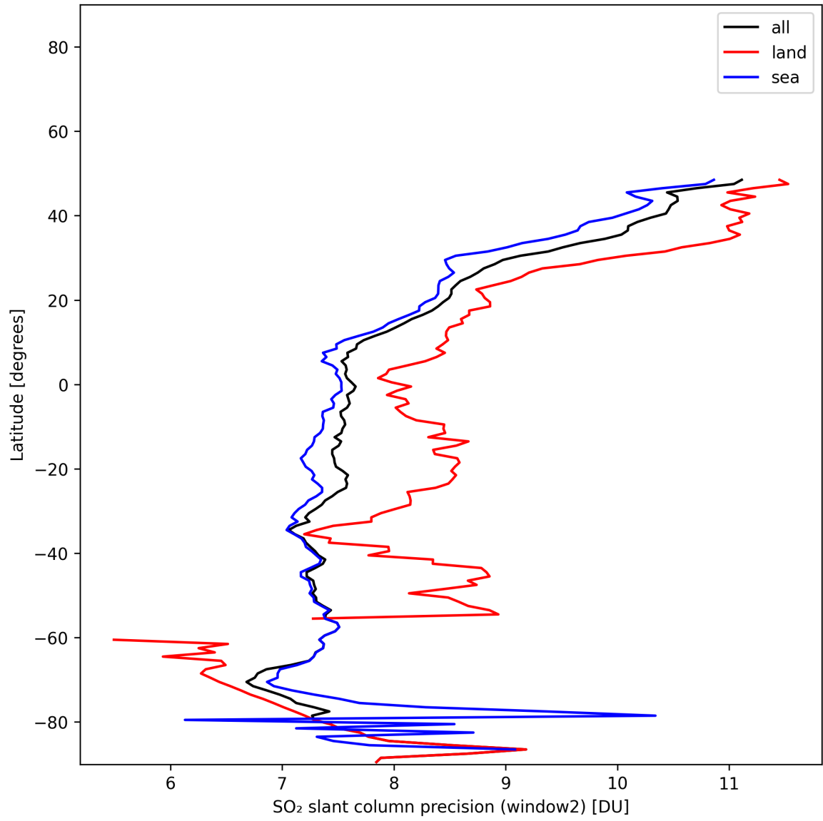
Figure 42: Zonal average of "SO 2 slant column precision (window2)" for 2025-11-28 to 2025-11-29.
