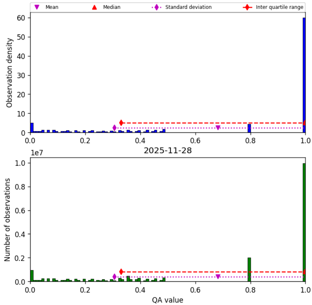
Figure 57: Histogram of “QA value” for 2025-11-28 to 2025-11-29
