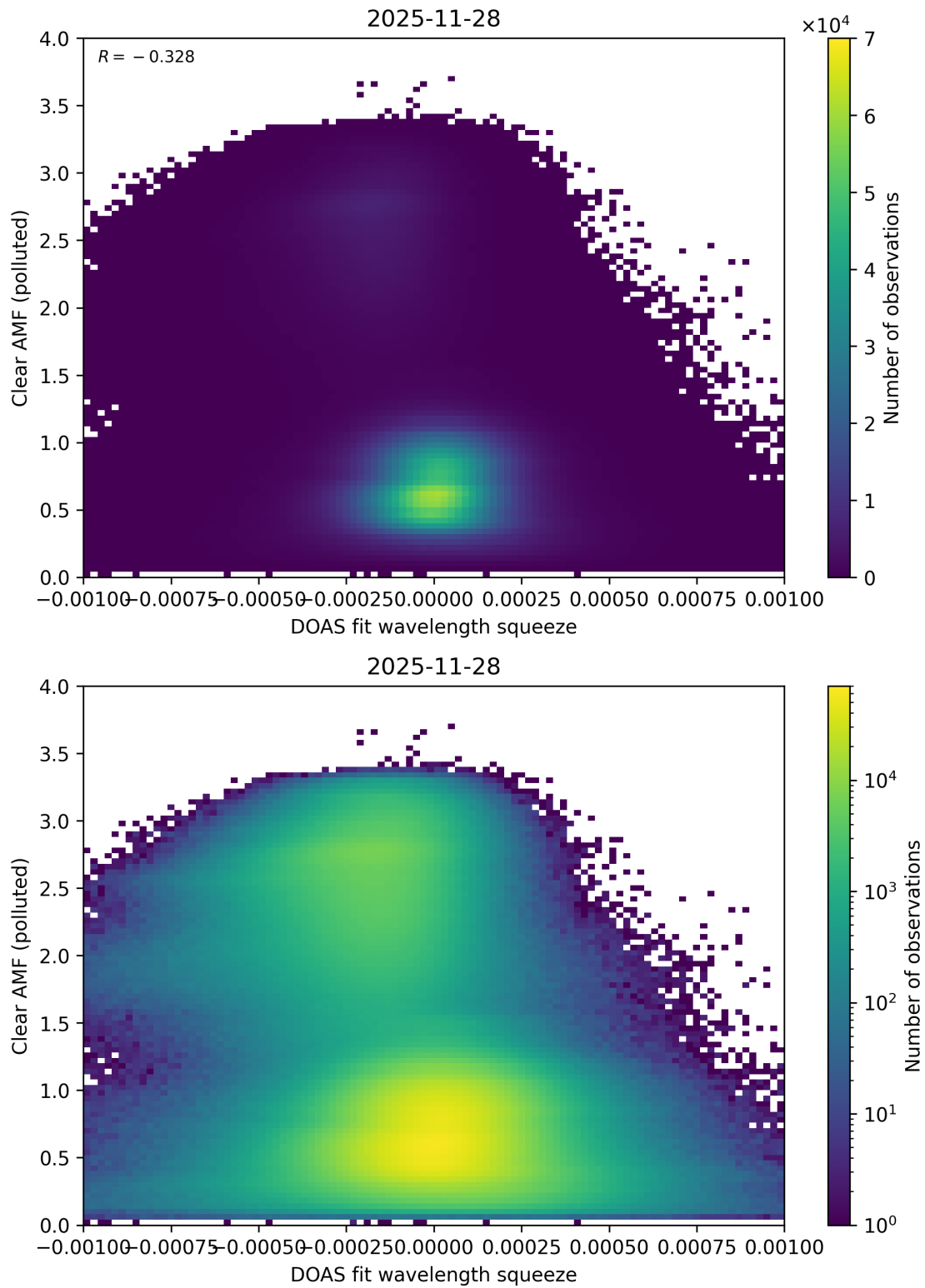
Figure 144: Scatter density plot of “DOAS fit wavelength squeeze” against “Clear AMF (polluted)” for 2025-11-28 to 2025-11-29.
