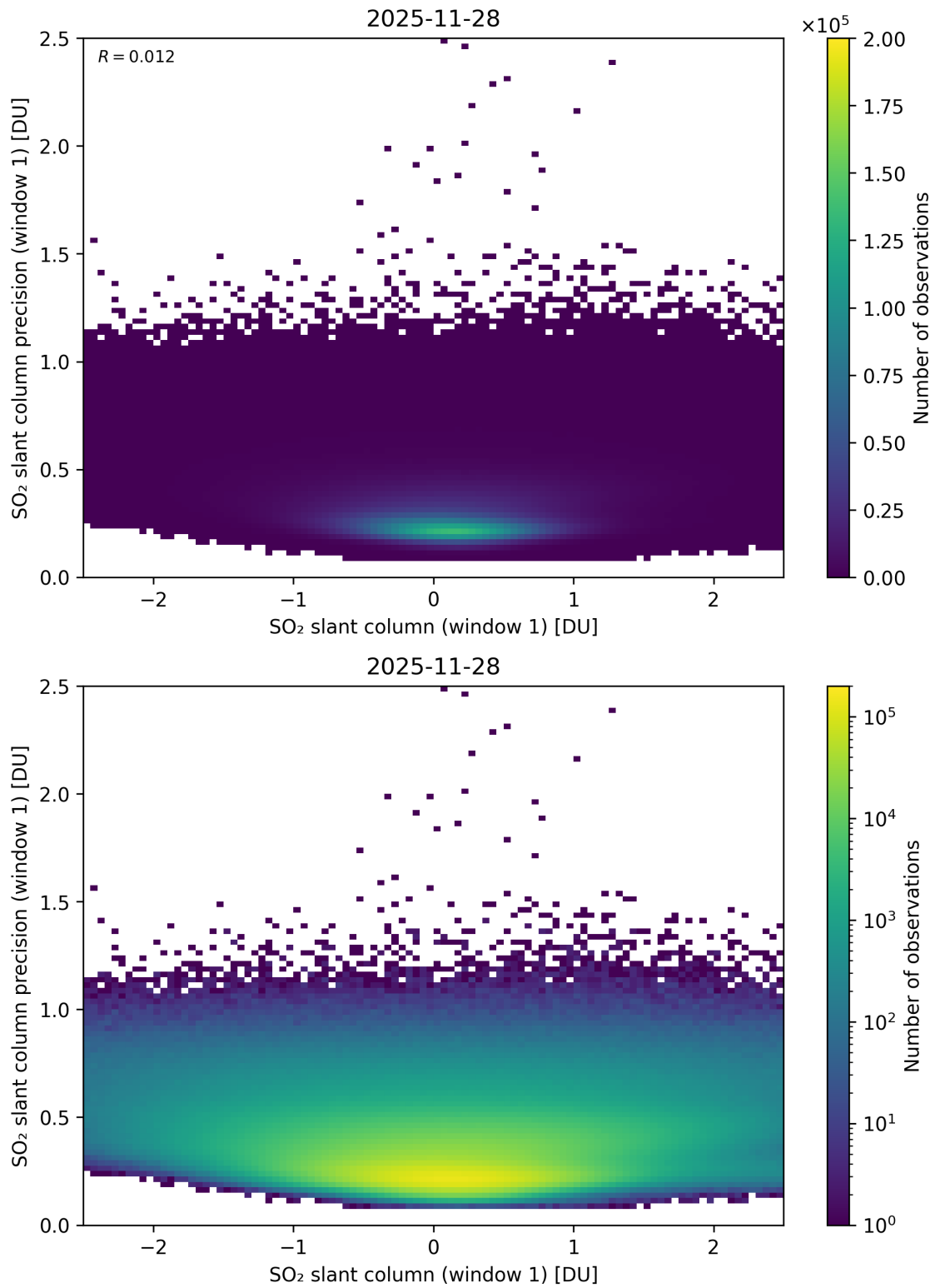
Figure 285: Scatter density plot of “SO 2 slant column (window 1)” against “SO 2 slant column precision (window 1)” for 2025-11-28 to 2025-11-29.
