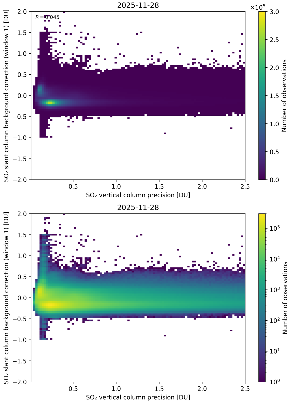
Figure 329: Scatter density plot of “SO 2 vertical column precision” against “SO 2 slant column background correction (window 1)” for 2025-11-28 to 2025-11-29.
