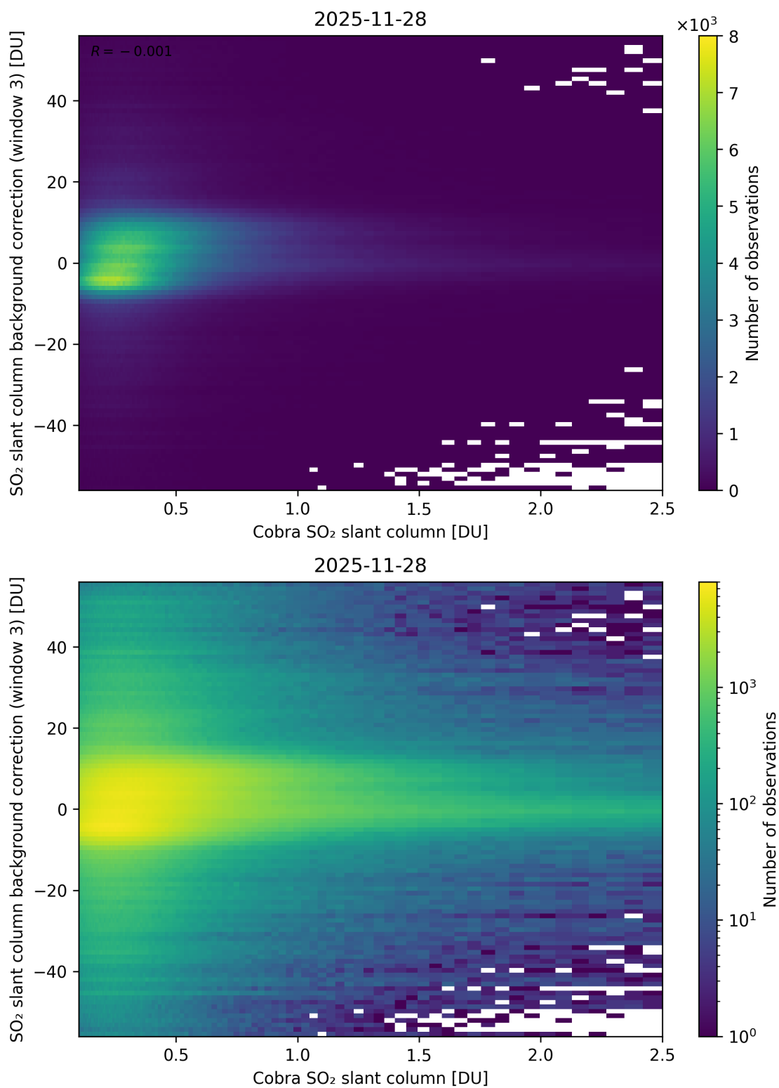
Figure 195: Scatter density plot of “Cobra SO 2 slant column” against “SO 2 slant column background correction (window 3)” for 2025-11-28 to 2025-11-29.
