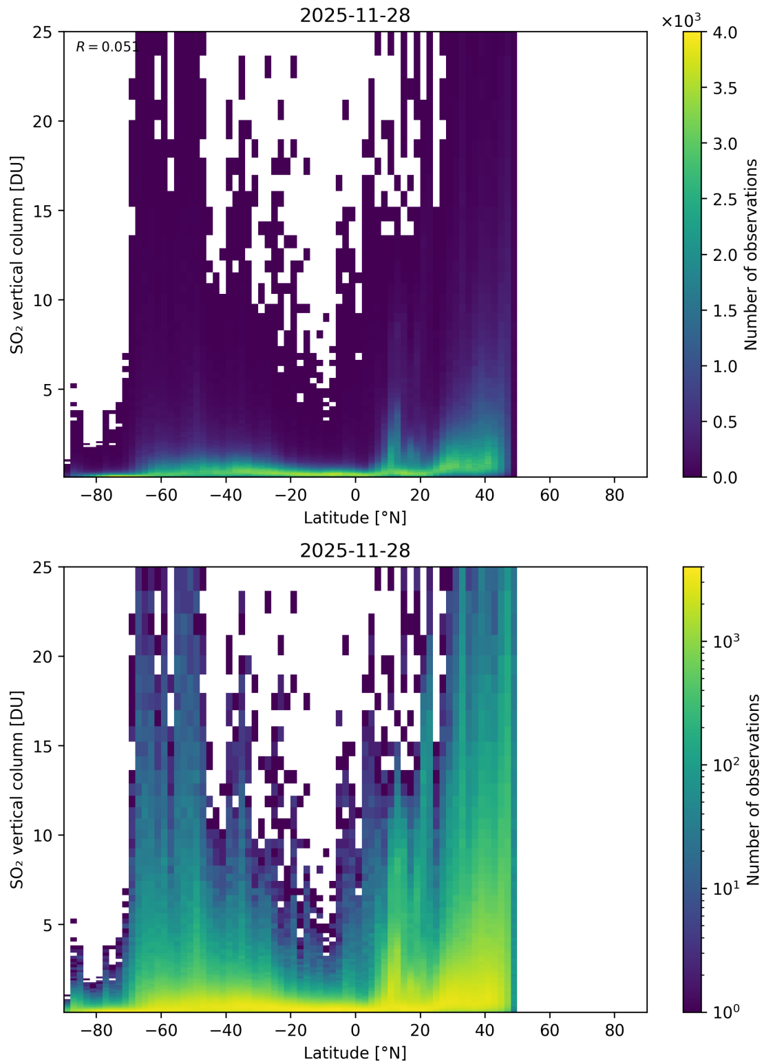
Figure 169: Scatter density plot of “Latitude” against “SO 2 vertical column” for 2025-11-28 to 2025-11-29.
