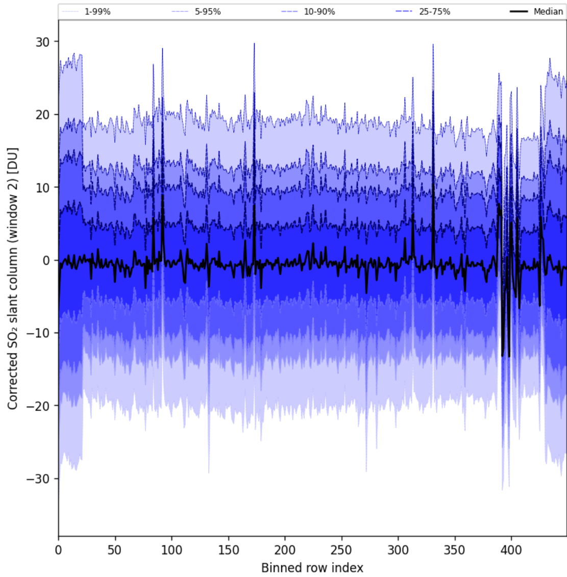
Figure 95: Along track statistics of “Corrected SO 2 slant column (window 2)” for 2025-11-28 to 2025-11-29
