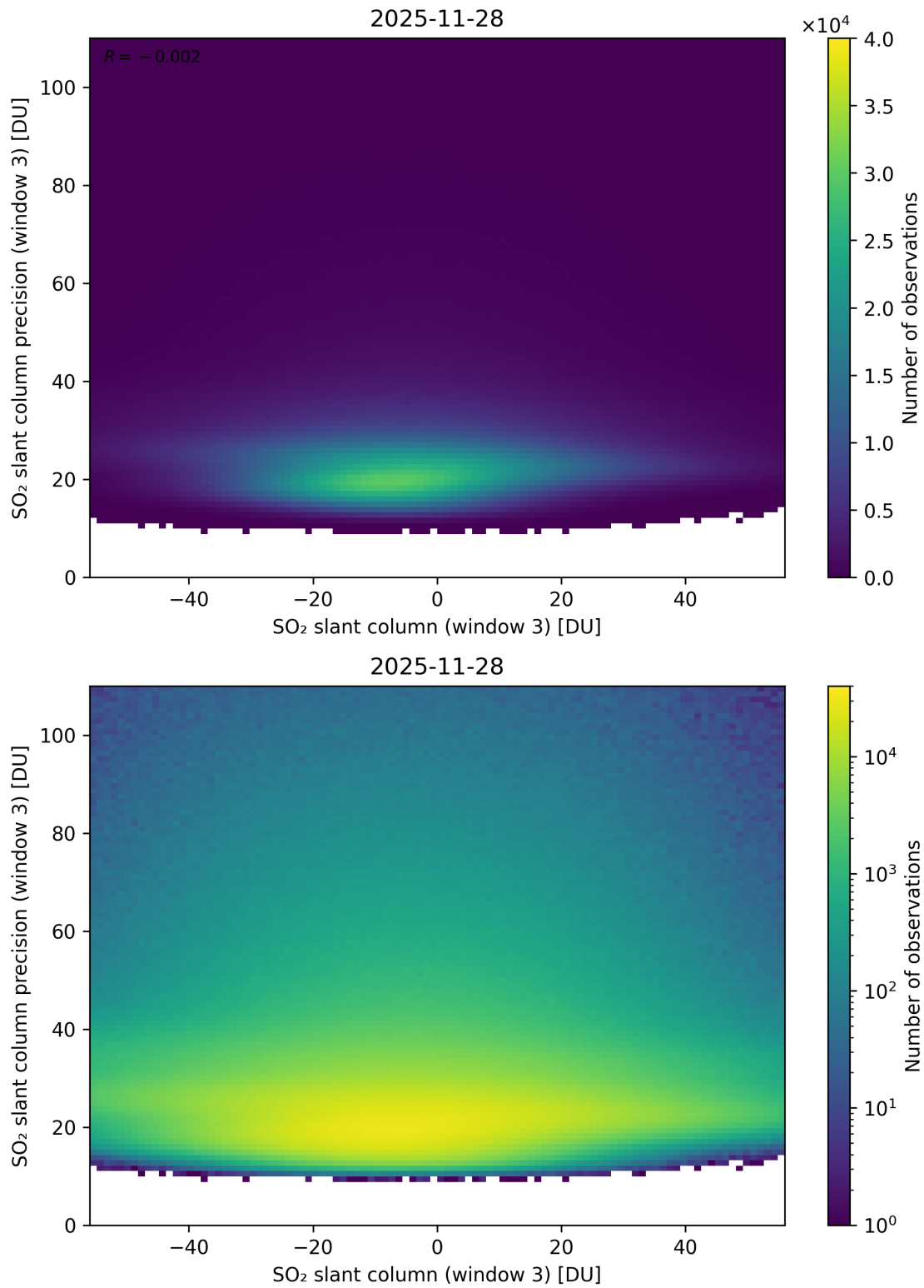
Figure 317: Scatter density plot of “SO 2 slant column (window 3)” against “SO 2 slant column precision (window 3)” for 2025-11-28 to 2025-11-29.
