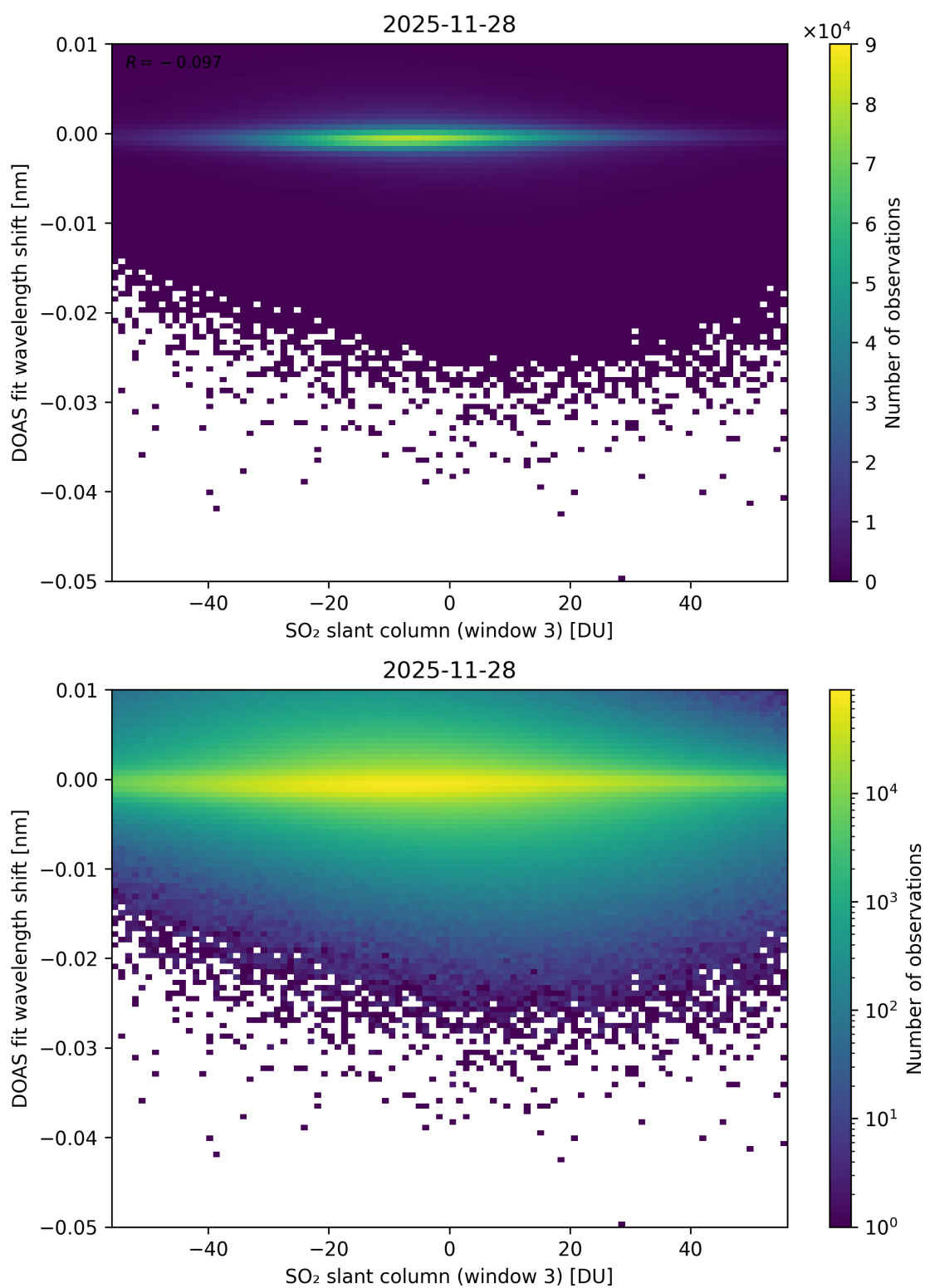
Figure 304: Scatter density plot of “SO 2 slant column (window 3)” against “DOAS fit wavelength shift” for 2025-11-28 to 2025-11-29.
