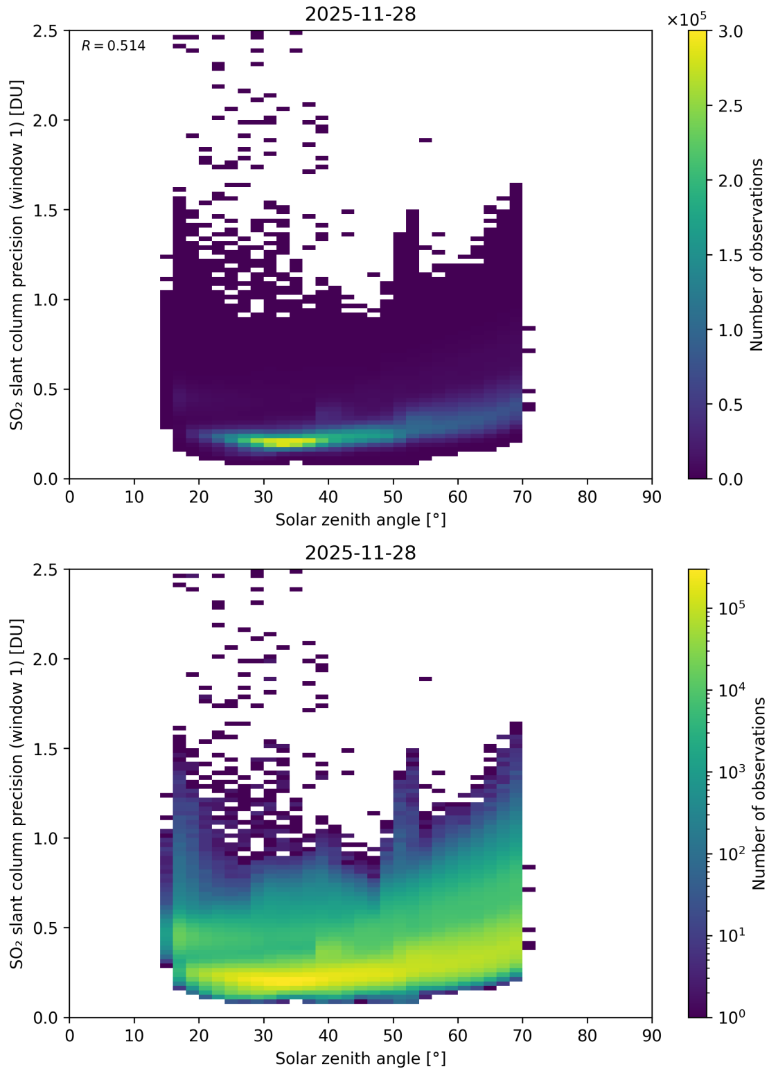
Figure 185: Scatter density plot of “Solar zenith angle” against “SO 2 slant column precision (window 1)” for 2025-11-28 to 2025-11-29.
