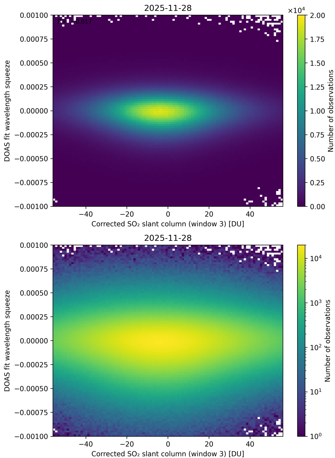
Figure 257: Scatter density plot of “Corrected SO 2 slant column (window 3)” against “DOAS fit wavelength squeeze” for 2025-11-28 to 2025-11-29.
