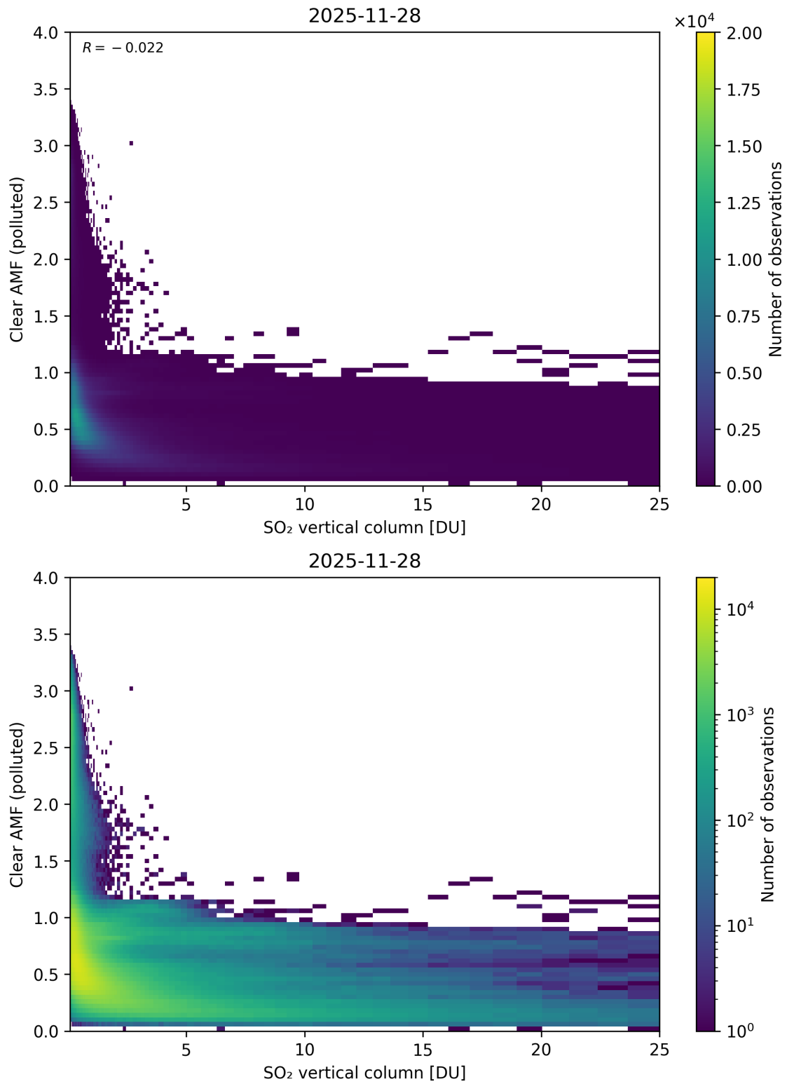
Figure 348: Scatter density plot of “SO 2 vertical column” against “Clear AMF (polluted)” for 2025-11-28 to 2025-11-29.
