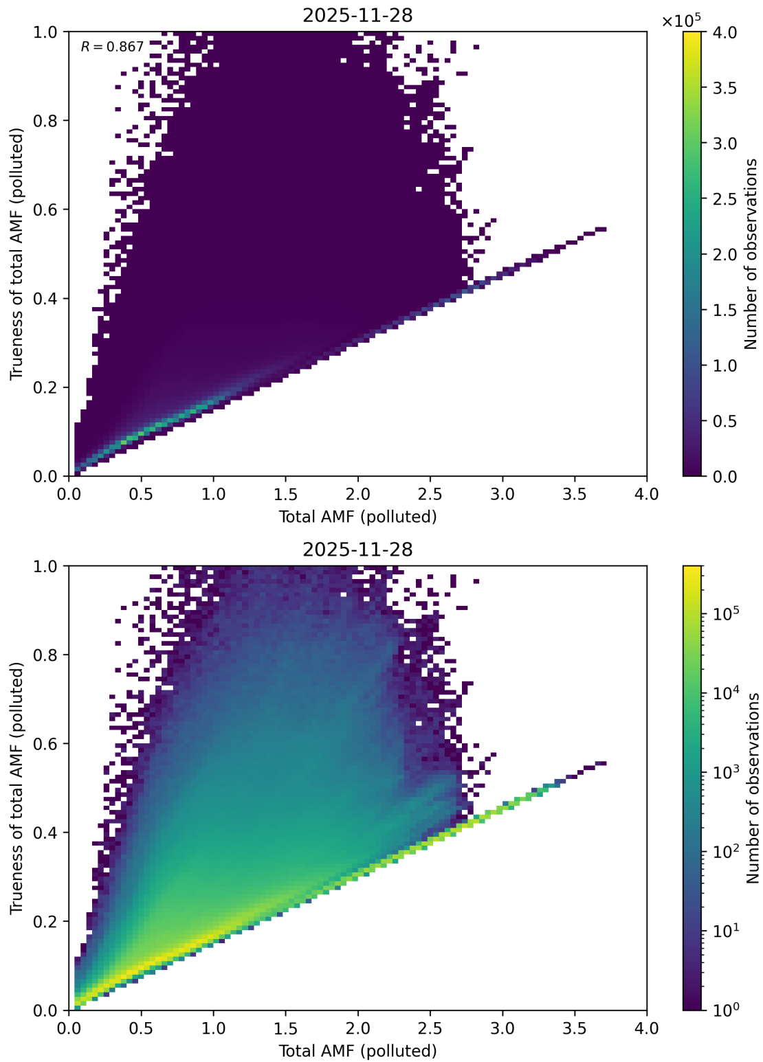
Figure 321: Scatter density plot of “Total AMF (polluted)” against “Trueness of total AMF (polluted)” for 2025-11-28 to 2025-11-29.
