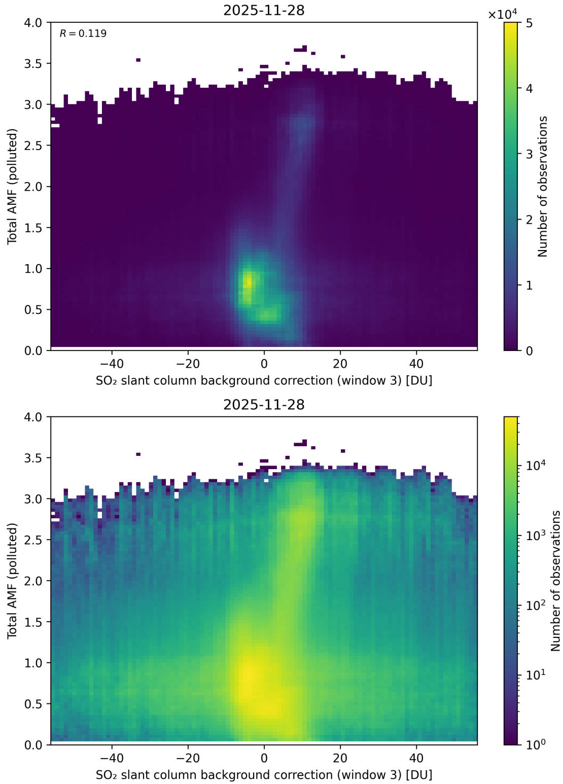
Figure 136: Scatter density plot of “SO 2 slant column background correction (window 3)” against “Total AMF (polluted)” for 2025-11-28 to 2025-11-29.
