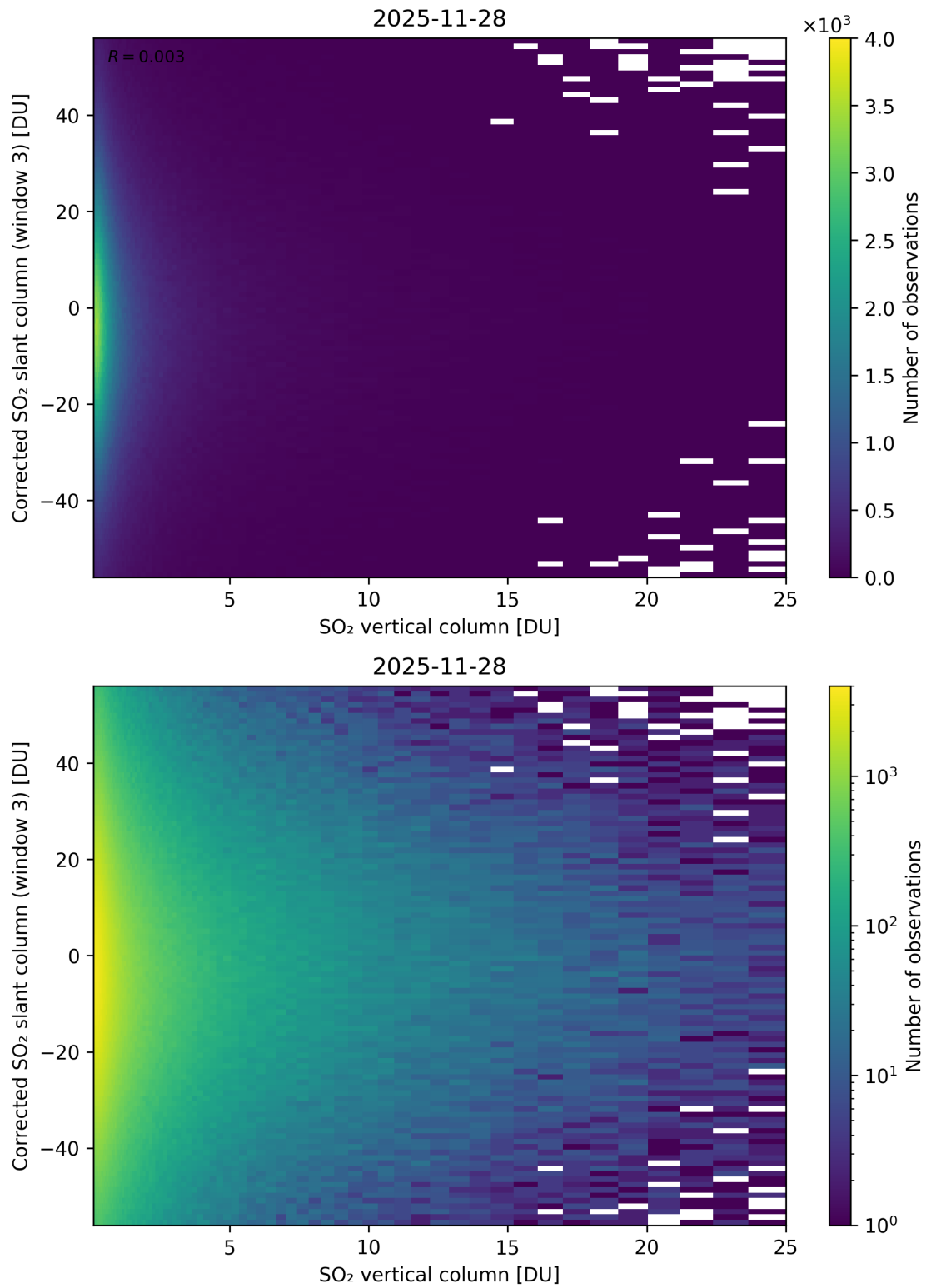
Figure 353: Scatter density plot of “SO 2 vertical column” against “Corrected SO 2 slant column (window 3)” for 2025-11-28 to 2025-11-29.
