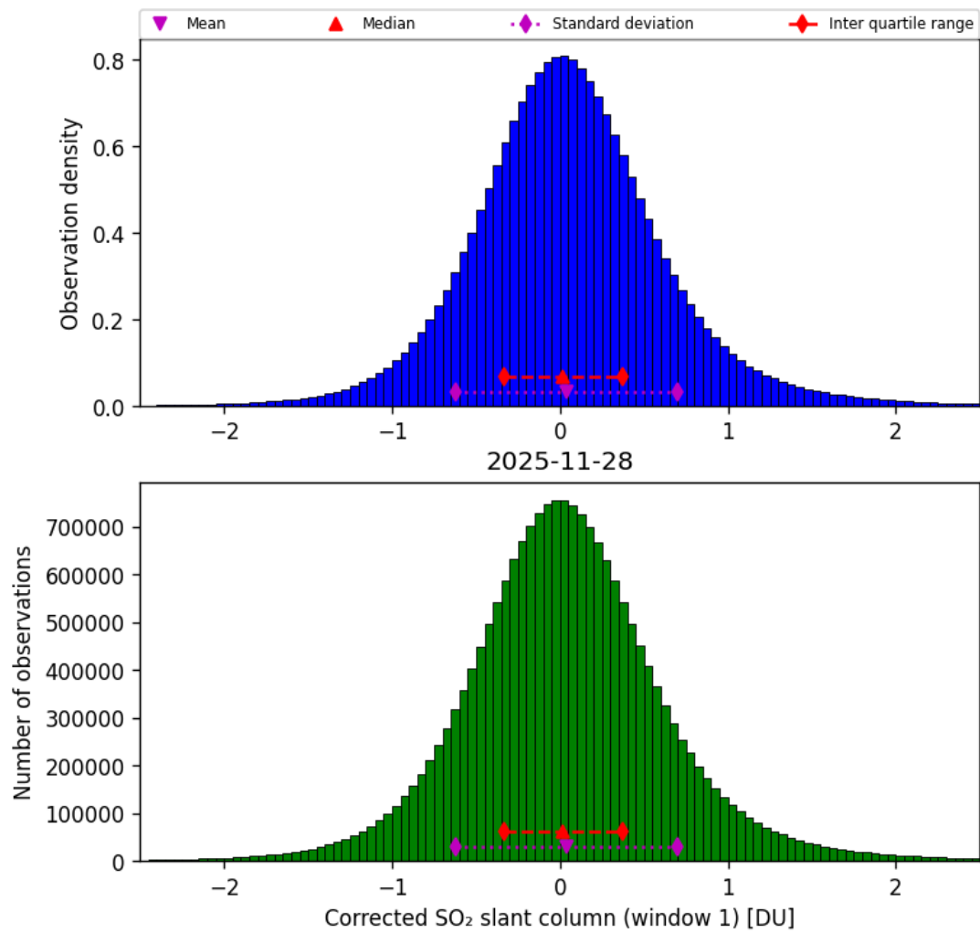
Figure 65: Histogram of “Corrected SO 2 slant column (window 1)” for 2025-11-28 to 2025-11-29
