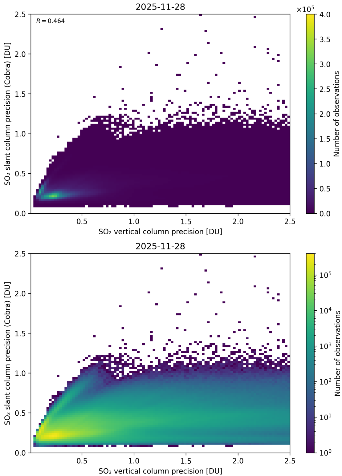
Figure 337: Scatter density plot of “SO 2 vertical column precision” against “SO 2 slant column precision (Cobra)” for 2025-11-28 to 2025-11-29.
