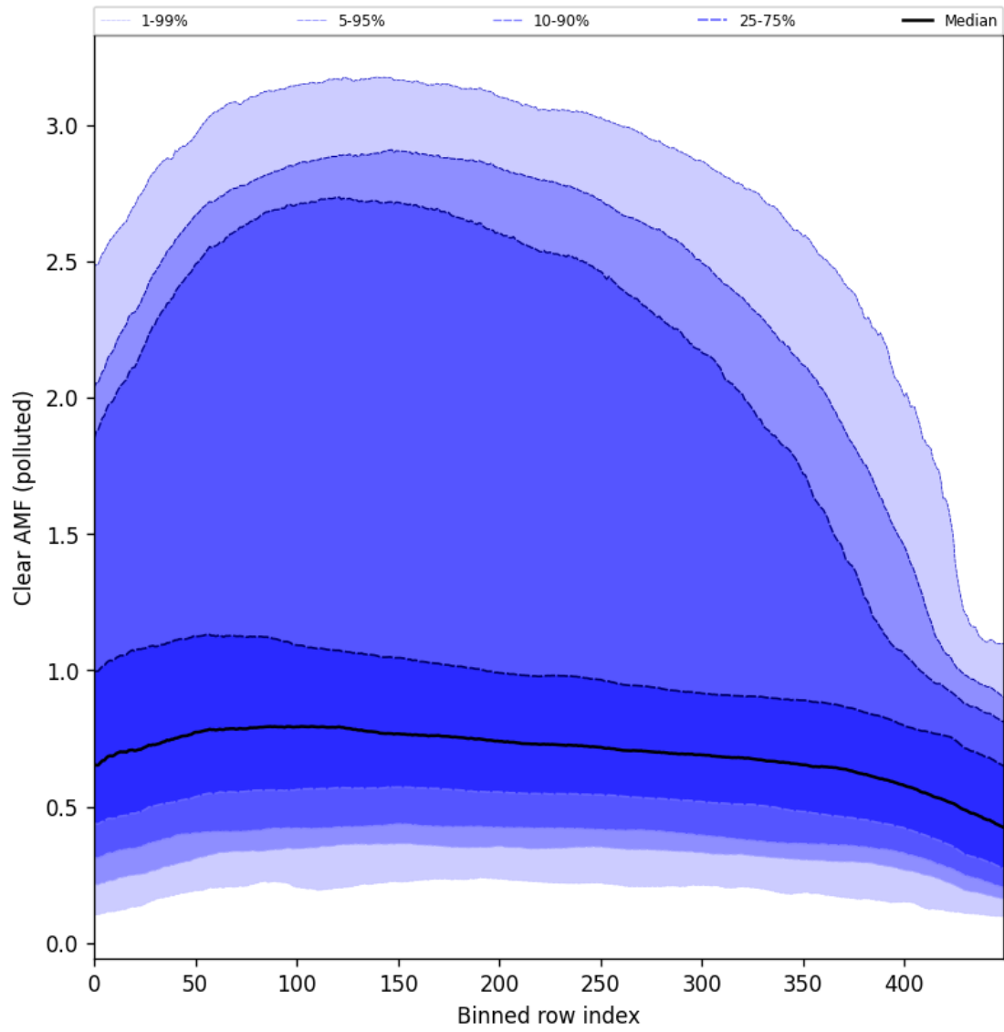
Figure 107: Along track statistics of “Clear AMF (polluted)” for 2025-11-28 to 2025-11-29
