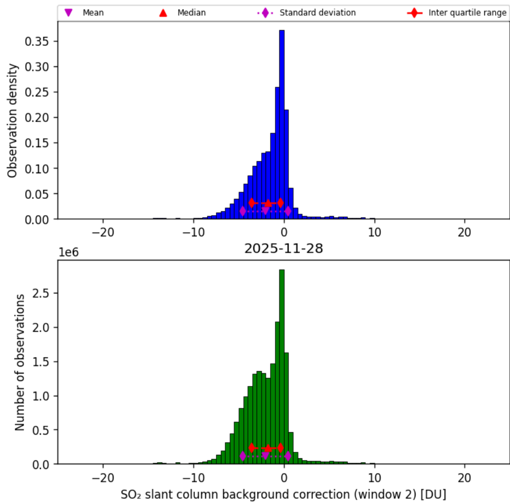
Figure 70: Histogram of “SO 2 slant column background correction (window 2)” for 2025-11-28 to 2025-11-29
