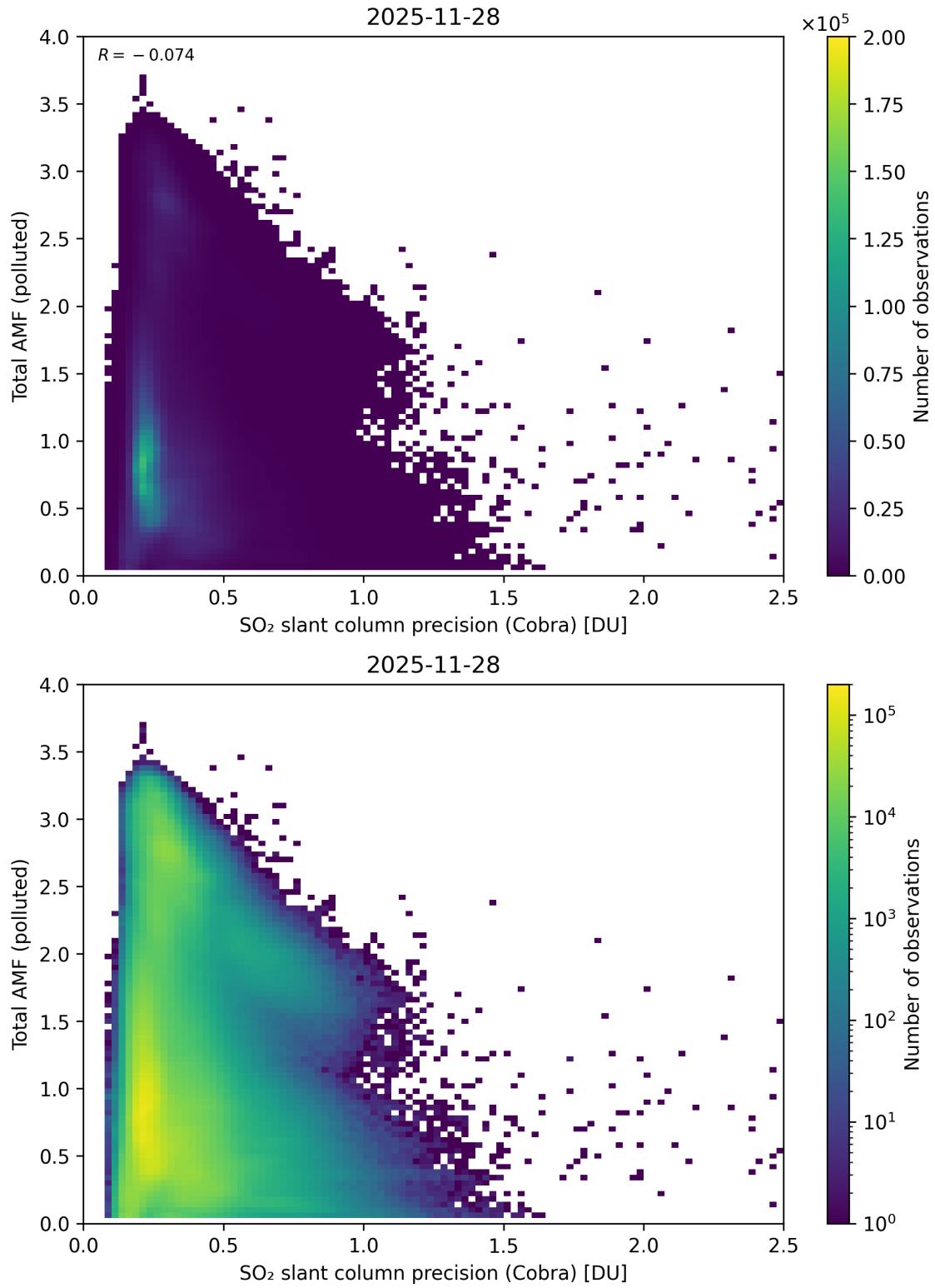
Figure 213: Scatter density plot of “SO 2 slant column precision (Cobra)” against “Total AMF (polluted)” for 2025-11-28 to 2025-11-29.
