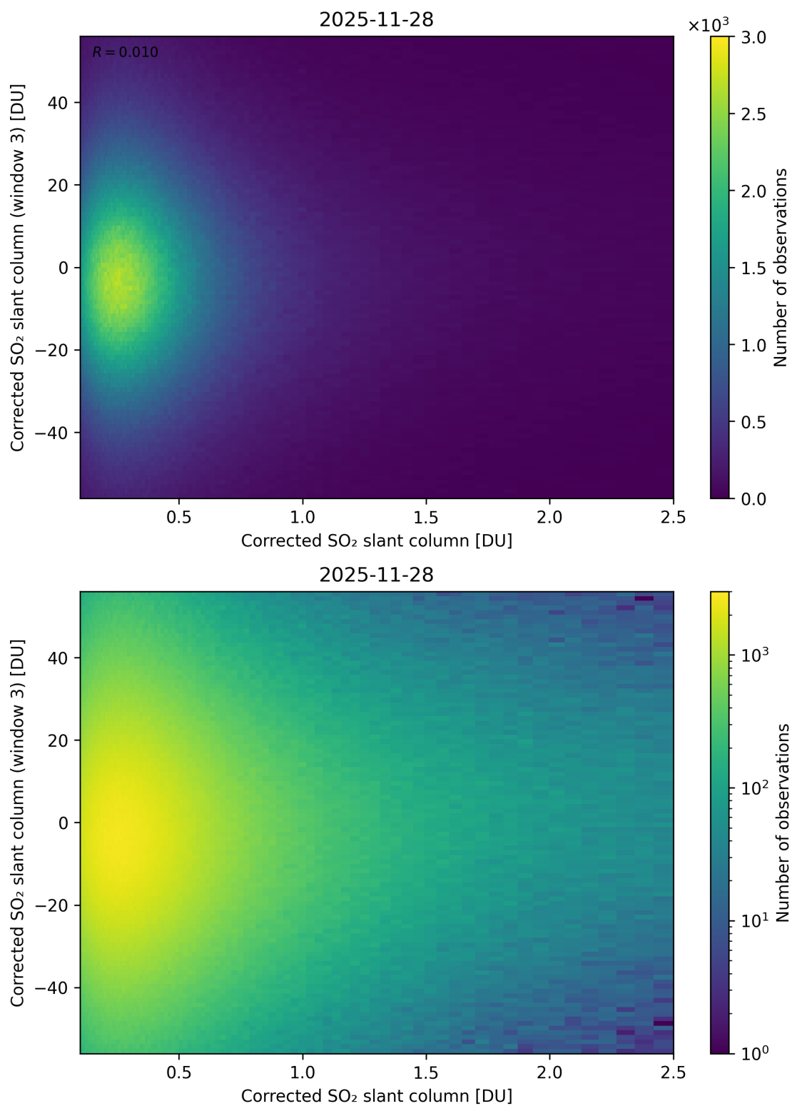
Figure 236: Scatter density plot of “Corrected SO 2 slant column” against “Corrected SO 2 slant column (window 3)” for 2025-11-28 to 2025-11-29.
