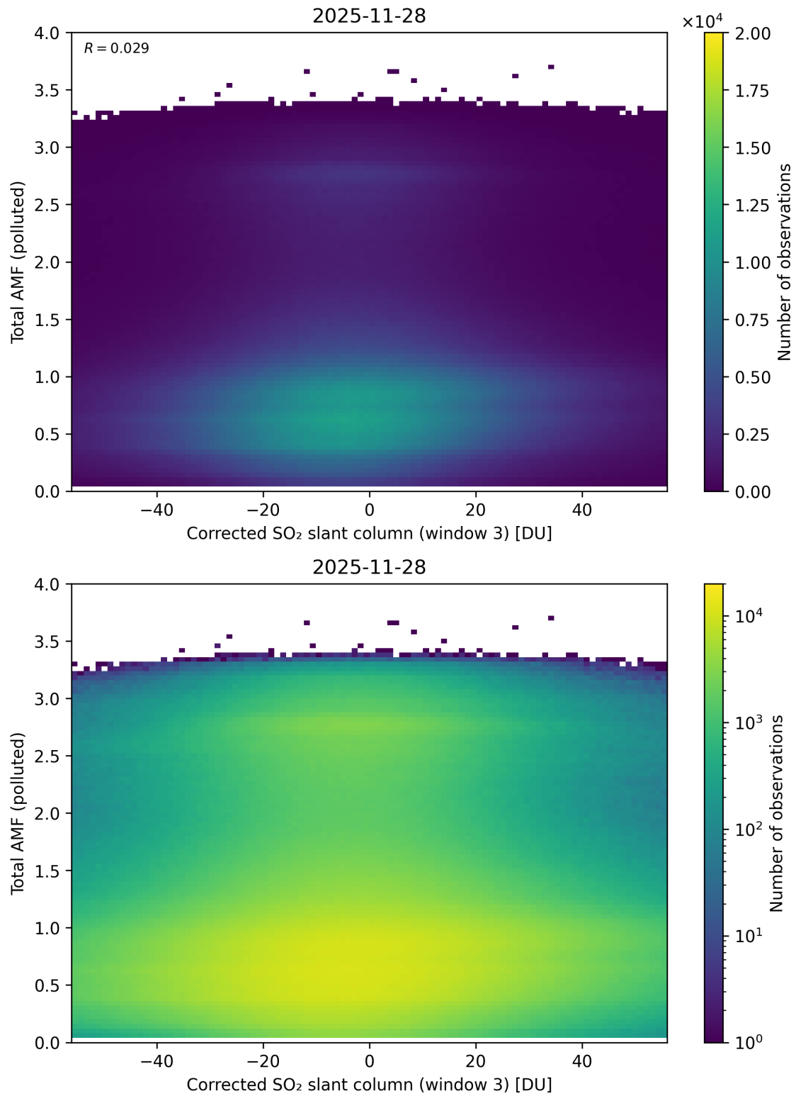
Figure 260: Scatter density plot of “Corrected SO 2 slant column (window 3)” against “Total AMF (polluted)” for 2025-11-28 to 2025-11-29.
