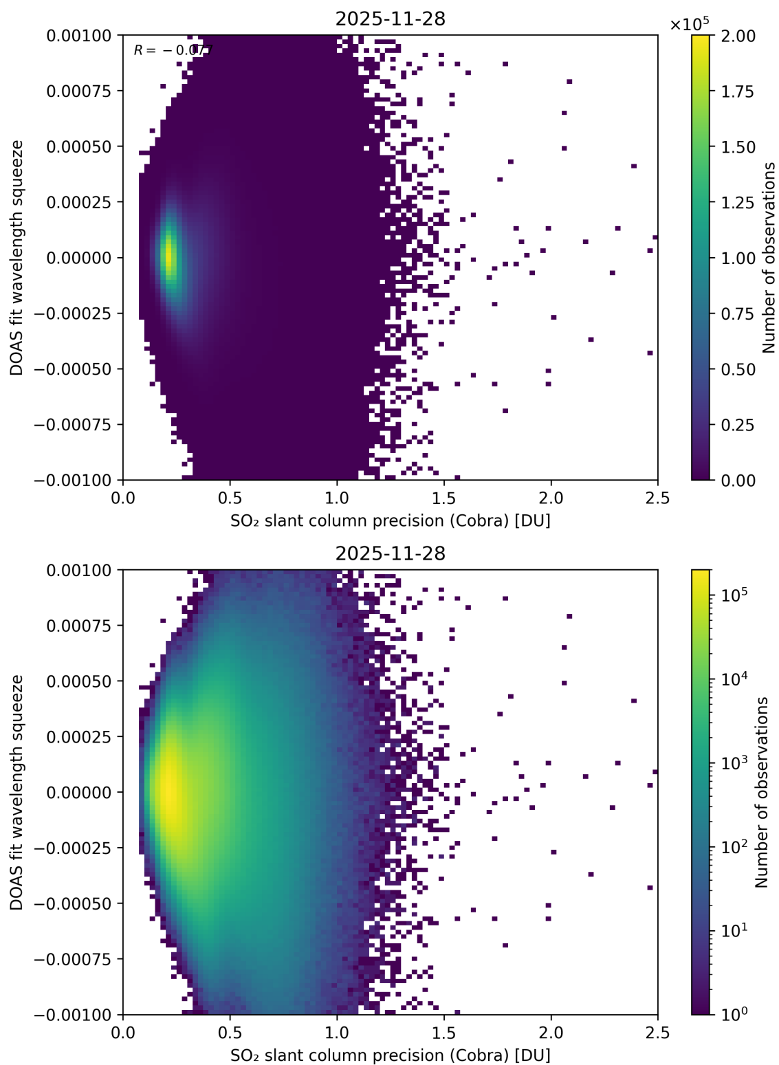
Figure 203: Scatter density plot of “SO 2 slant column precision (Cobra)” against “DOAS fit wavelength squeeze” for 2025-11-28 to 2025-11-29.
