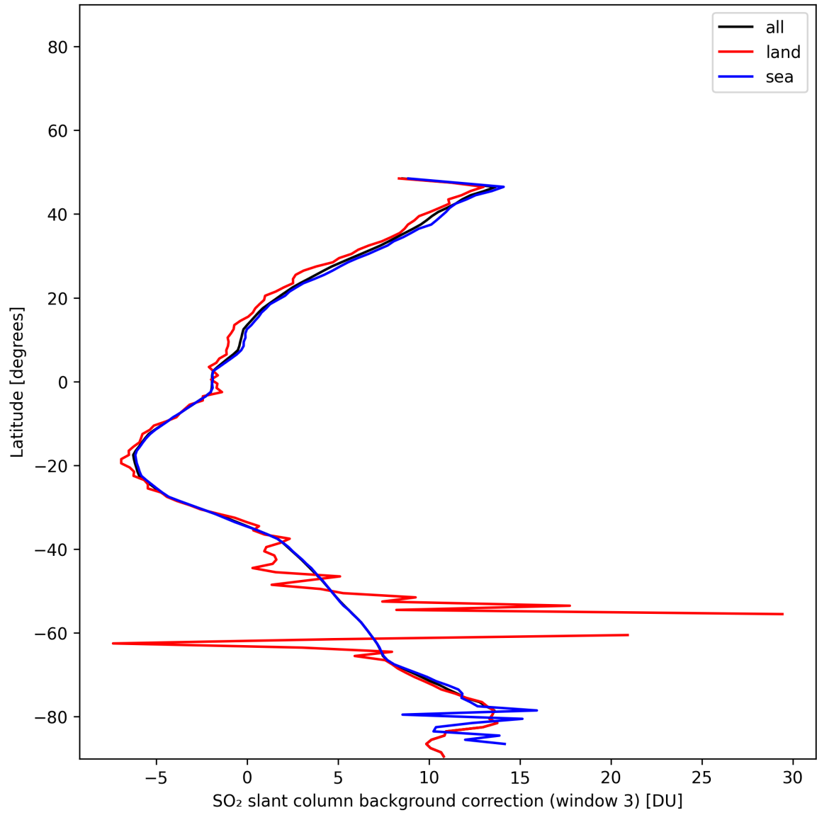
Figure 48: Zonal average of “SO 2 slant column background correction (window 3)” for 2025-11-28 to 2025-11-29.
