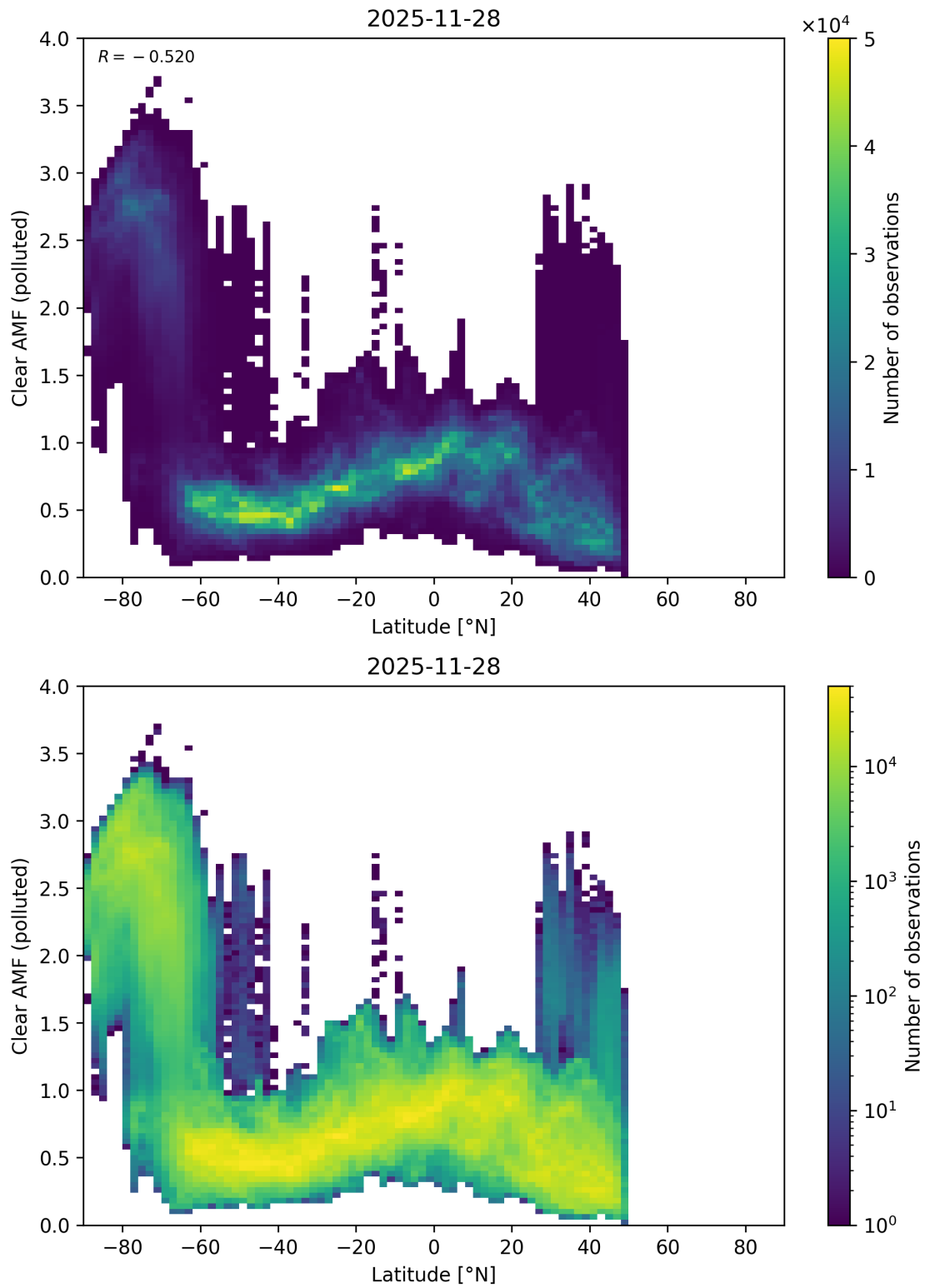
Figure 156: Scatter density plot of “Latitude” against “Clear AMF (polluted)” for 2025-11-28 to 2025-11-29.
