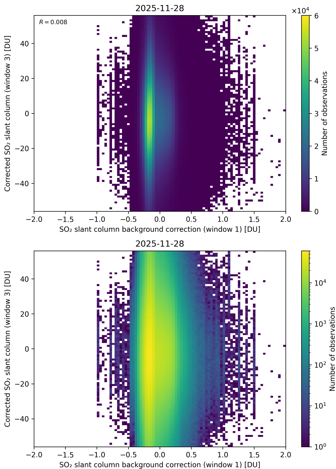
Figure 116: Scatter density plot of “SO 2 slant column background correction (window 1)” against “Corrected SO 2 slant column (window 3)” for 2025-11-28 to 2025-11-29.
