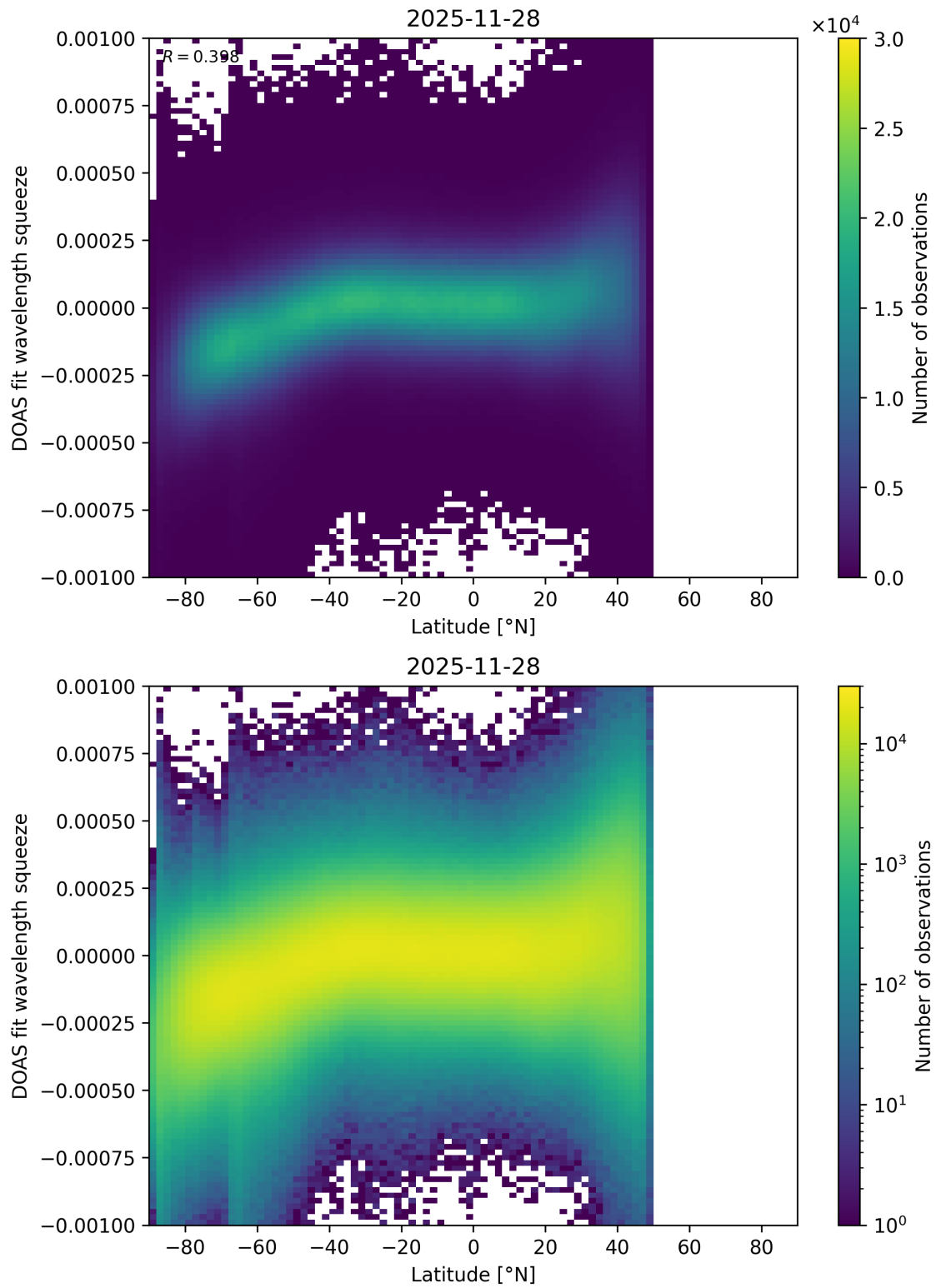
Figure 154: Scatter density plot of “Latitude” against “DOAS fit wavelength squeeze” for 2025-11-28 to 2025-11-29.
