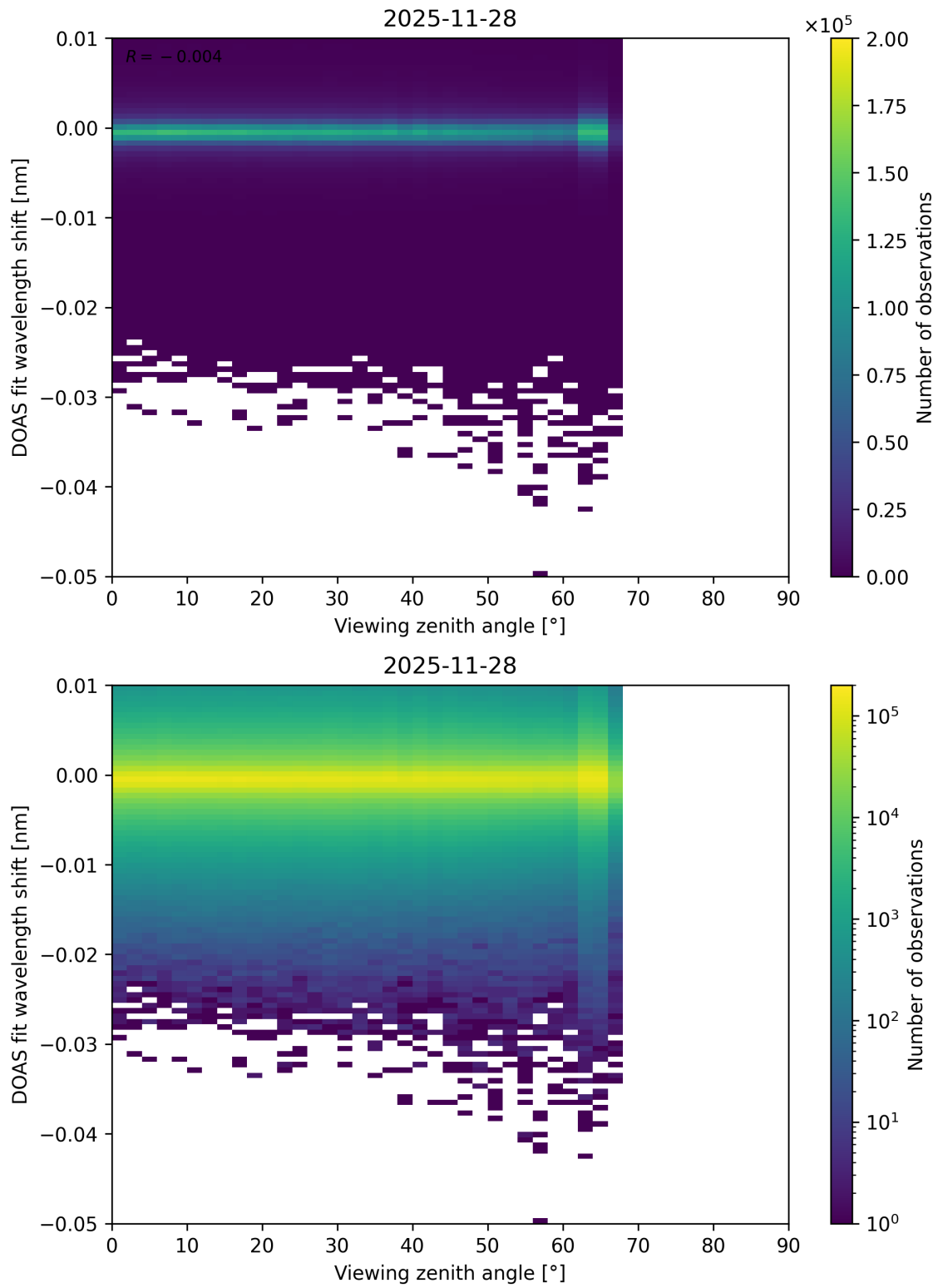
Figure 365: Scatter density plot of “Viewing zenith angle” against “DOAS fit wavelength shift” for 2025-11-28 to 2025-11-29.
