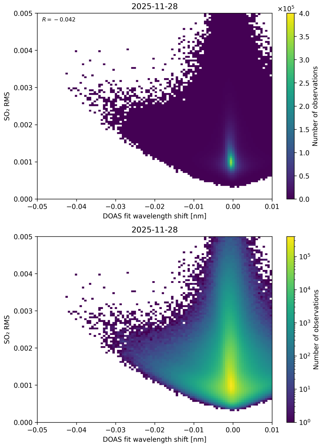
Figure 139: Scatter density plot of “DOAS fit wavelength shift” against “SO 2 RMS” for 2025-11-28 to 2025-11-29.
