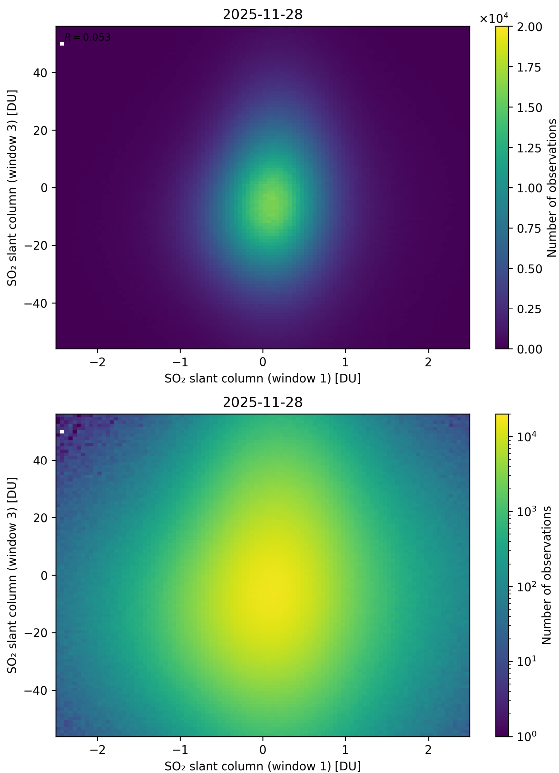
Figure 287: Scatter density plot of “SO 2 slant column (window 1)” against “SO 2 slant column (window 3)” for 2025-11-28 to 2025-11-29.
