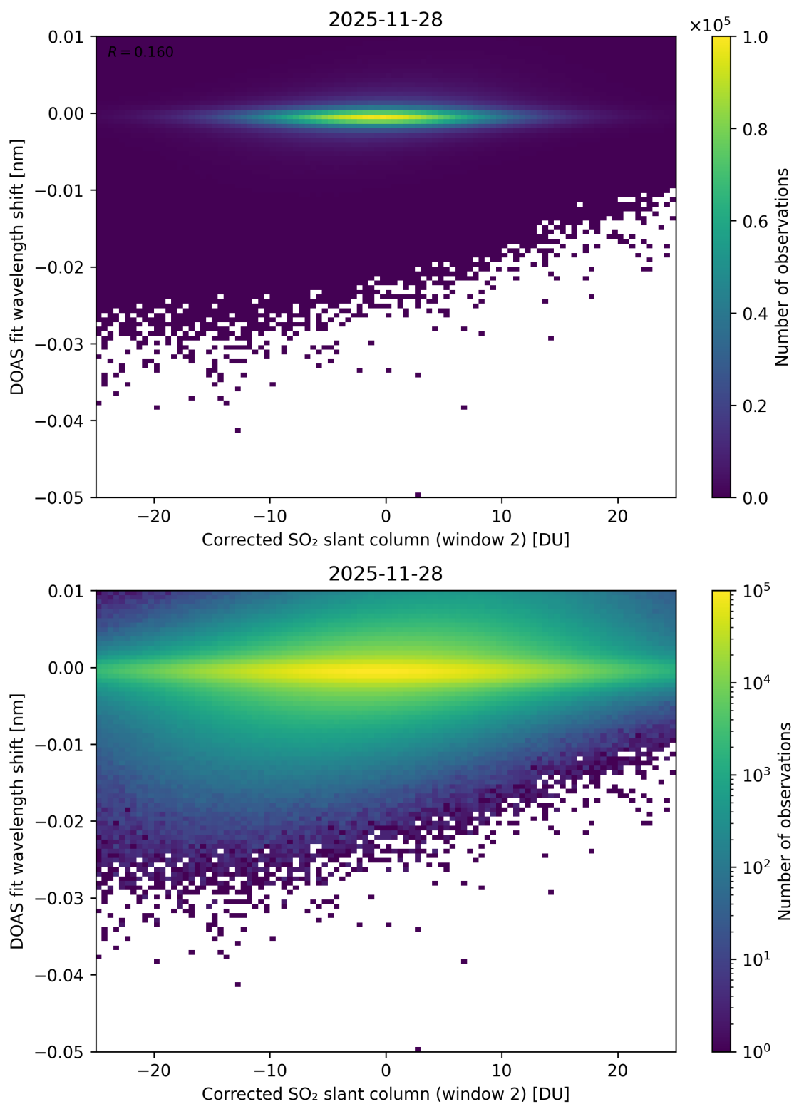
Figure 246: Scatter density plot of “Corrected SO 2 slant column (window 2)” against “DOAS fit wavelength shift” for 2025-11-28 to 2025-11-29.
