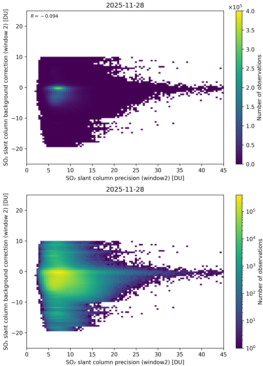
Figure 291: Scatter density plot of “SO 2 slant column precision (window2)” against “SO 2 slant column background correction (window 2)” for 2025-11-28 to 2025-11-29.
