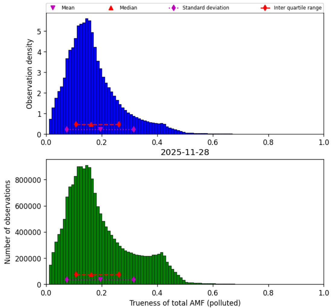
Figure 80: Histogram of “Trueness of total AMF (polluted)” for 2025-11-28 to 2025-11-29
