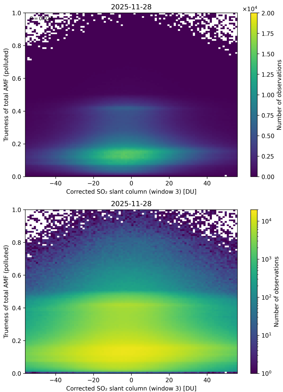
Figure 261: Scatter density plot of “Corrected SO 2 slant column (window 3)” against “Trueness of total AMF (polluted)” for 2025-11-28 to 2025-11-29.
