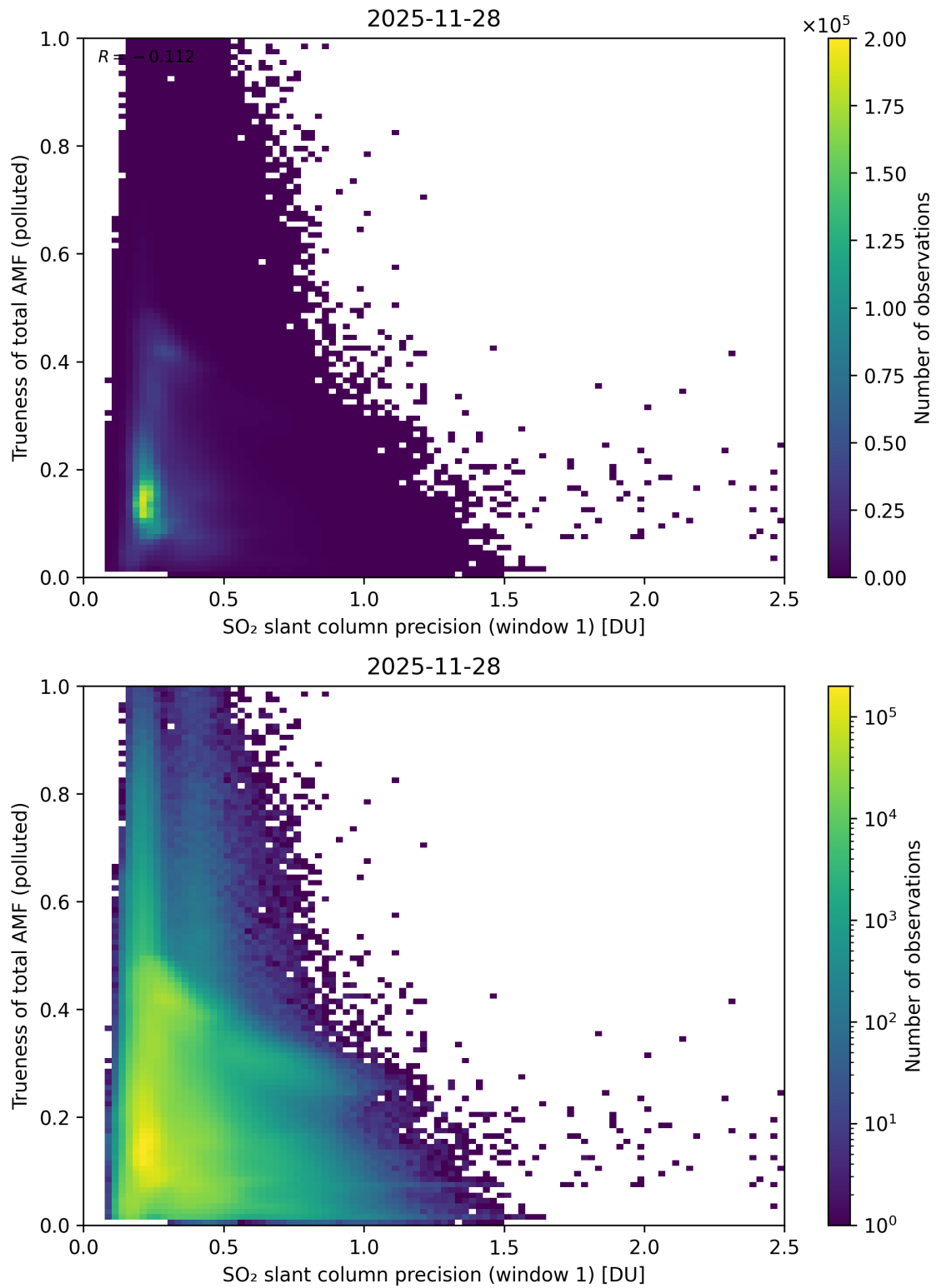
Figure 281: Scatter density plot of “SO 2 slant column precision (window 1)” against “Trueness of total AMF (polluted)” for 2025-11-28 to 2025-11-29.
