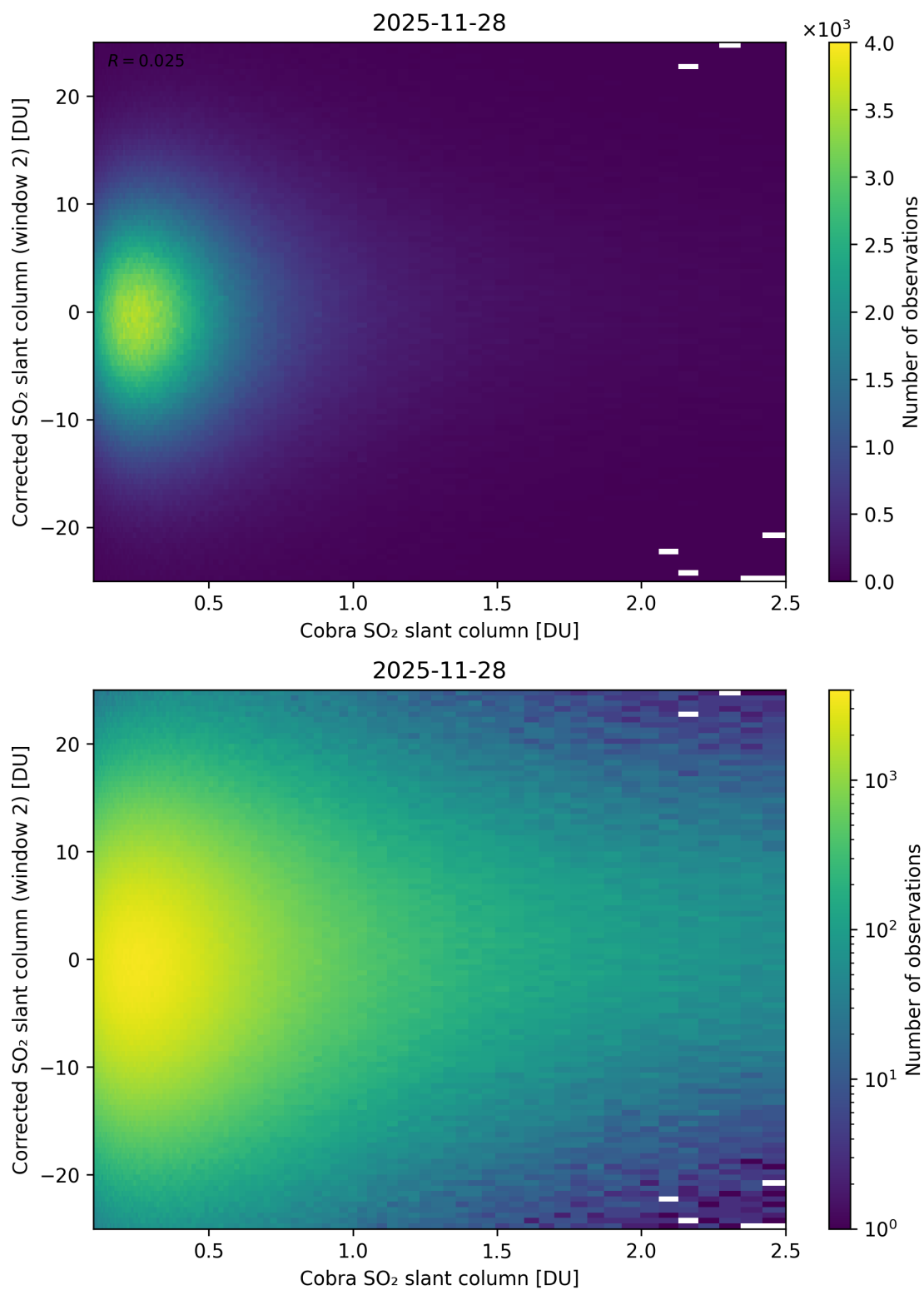
Figure 217: Scatter density plot of “Cobra SO 2 slant column” against “Corrected SO 2 slant column (window 2)” for 2025-11-28 to 2025-11-29.
