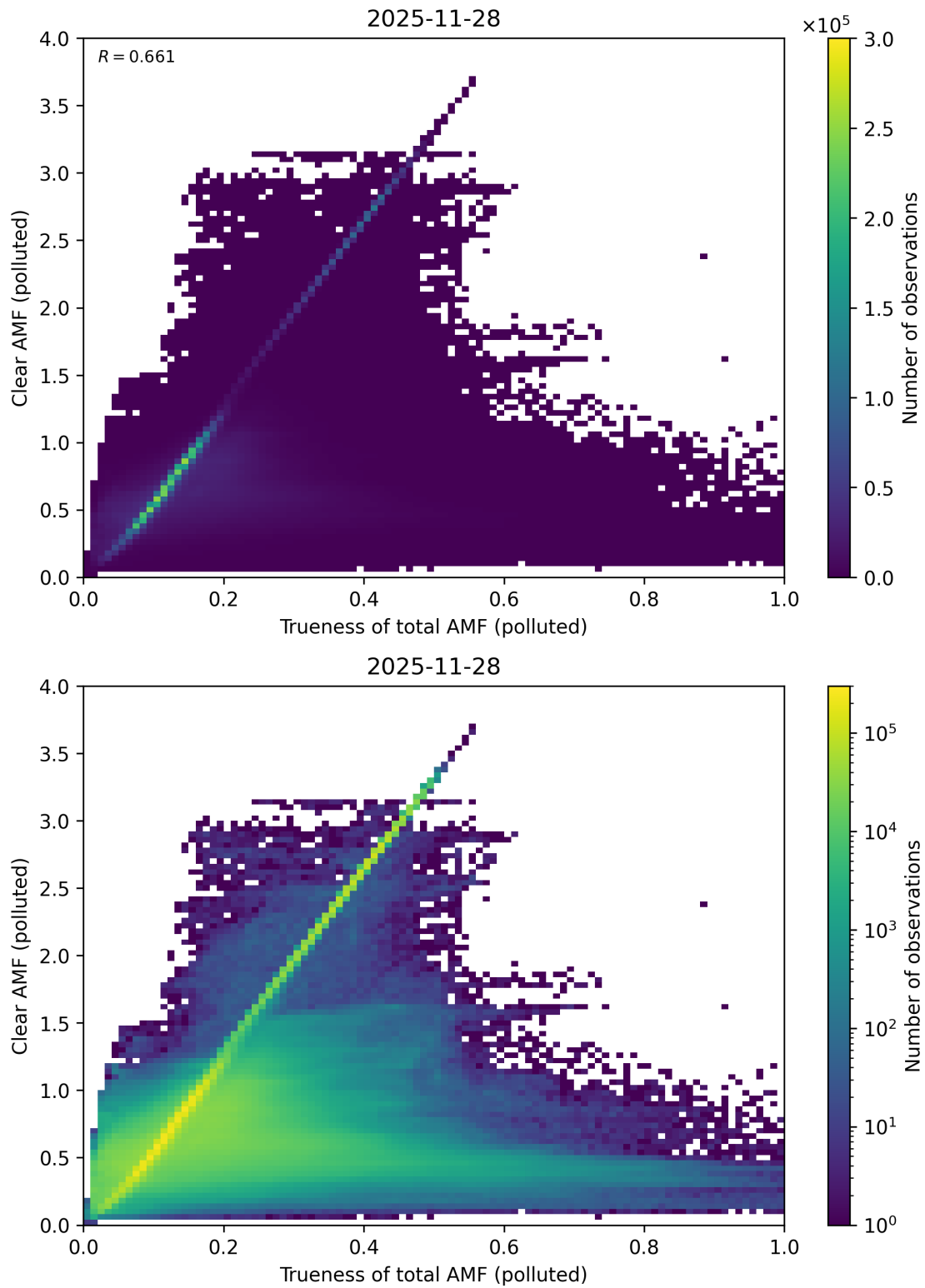
Figure 322: Scatter density plot of “Trueness of total AMF (polluted)” against “Clear AMF (polluted)” for 2025-11-28 to 2025-11-29.
