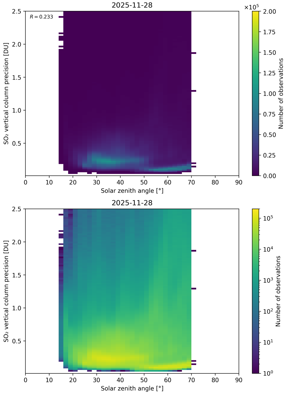
Figure 192: Scatter density plot of “Solar zenith angle” against “SO 2 vertical column precision” for 2025-11-28 to 2025-11-29.
