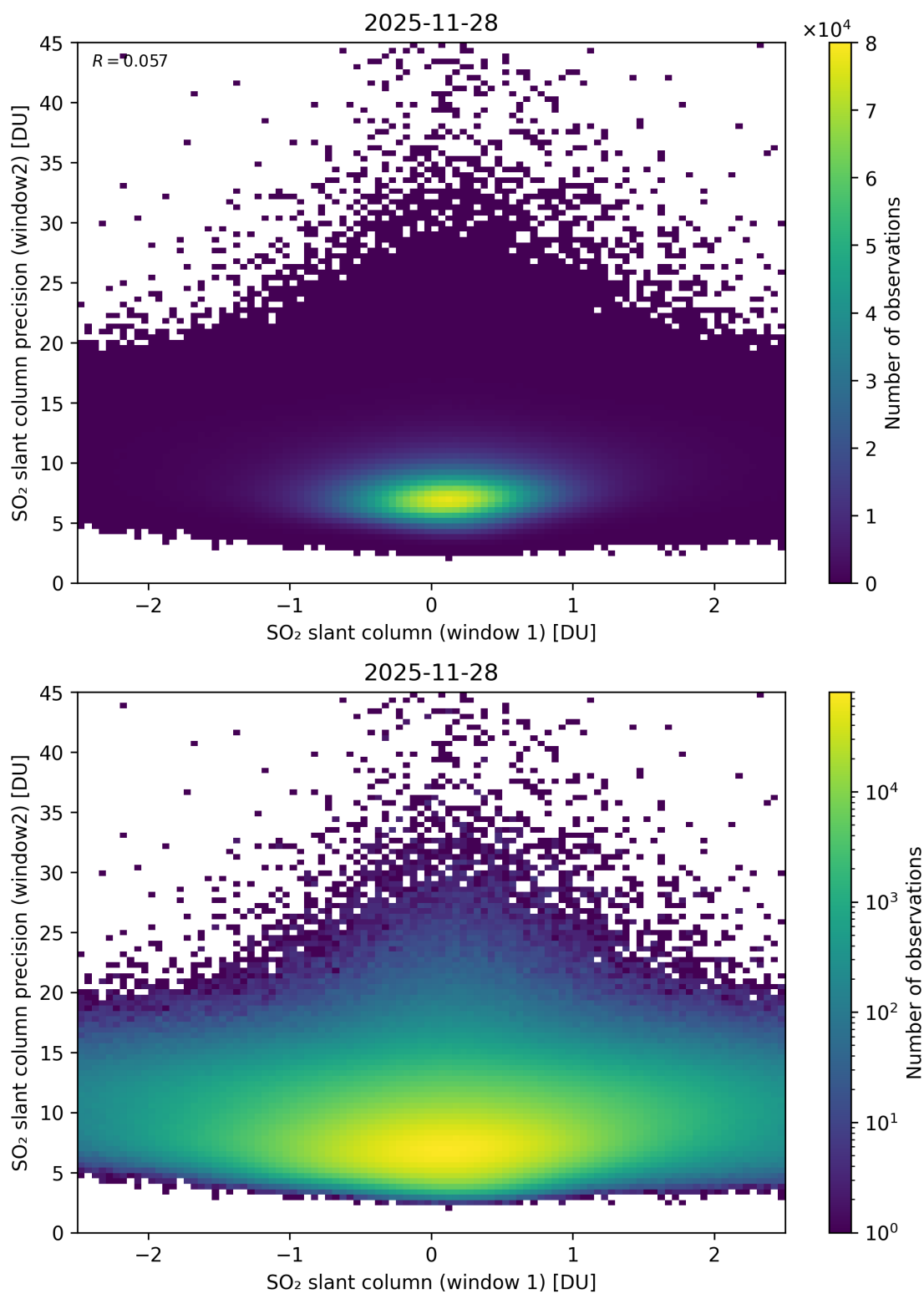
Figure 286: Scatter density plot of “SO 2 slant column (window 1)” against “SO 2 slant column precision (window2)” for 2025-11-28 to 2025-11-29.
