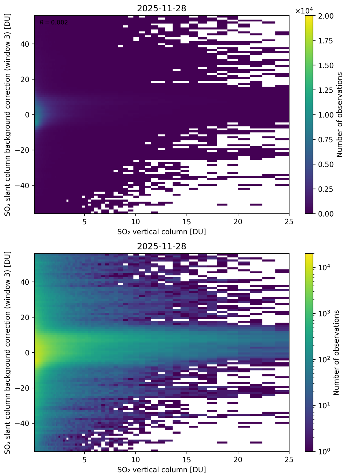
Figure 325: Scatter density plot of “SO 2 vertical column” against “SO 2 slant column background correction (window 3)” for 2025-11-28 to 2025-11-29.
