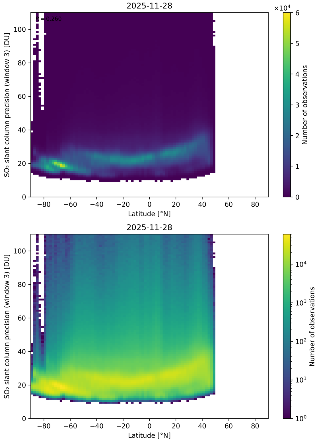
Figure 166: Scatter density plot of “Latitude” against “SO 2 slant column precision (window 3)” for 2025-11-28 to 2025-11-29.
