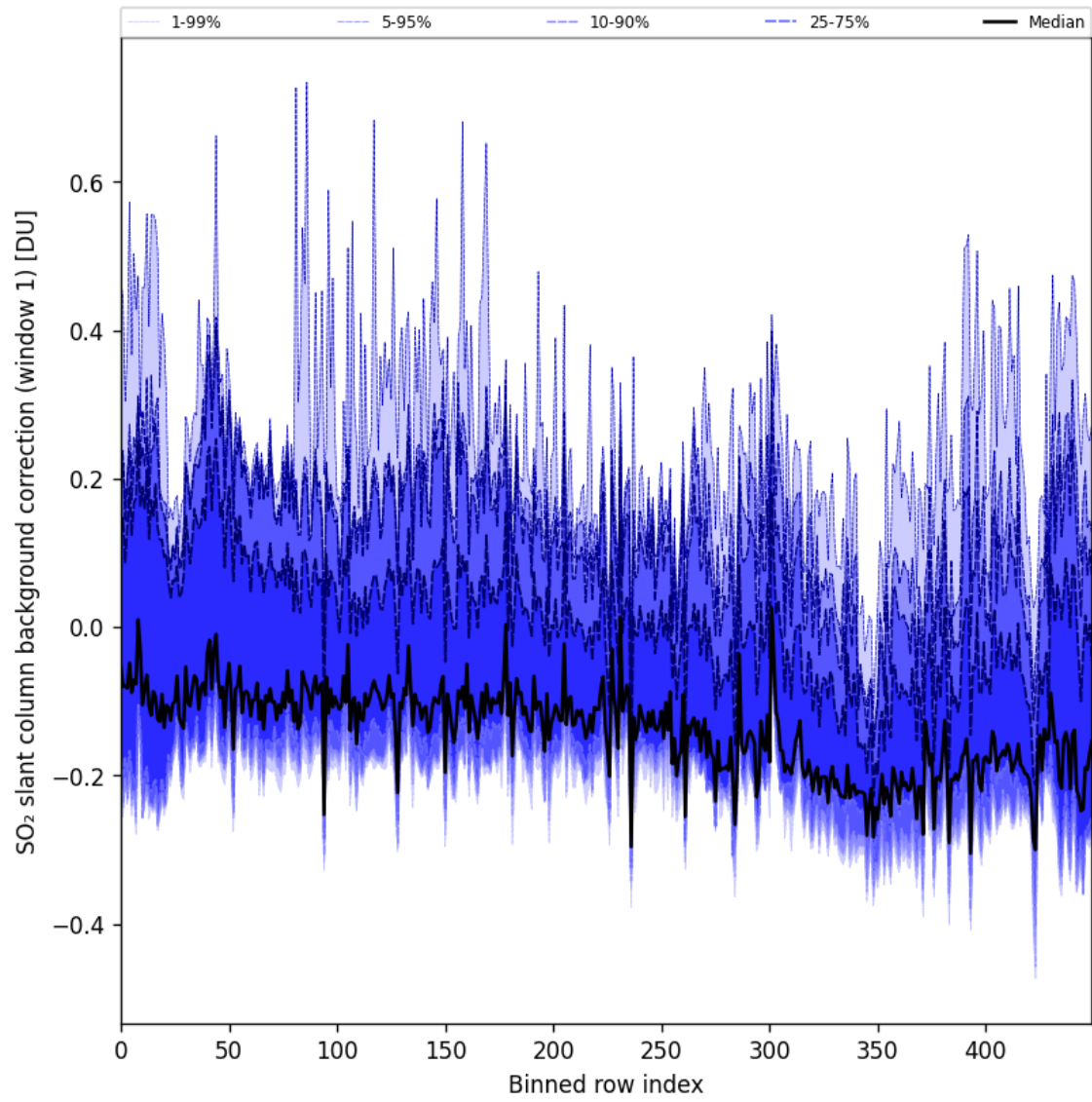
Figure 92: Along track statistics of “SO 2 slant column background correction (window 1)” for 2025-11-28 to 2025-11-29
