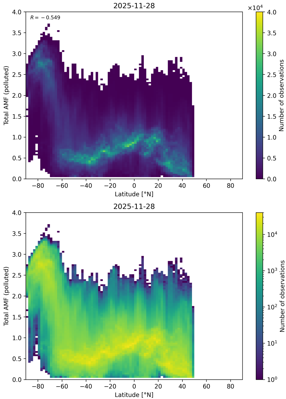
Figure 167: Scatter density plot of “Latitude” against “Total AMF (polluted)” for 2025-11-28 to 2025-11-29.
