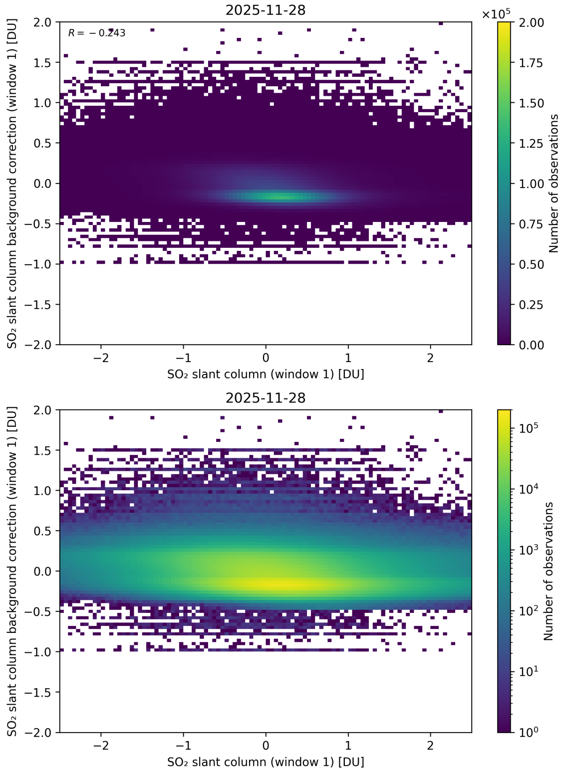
Figure 262: Scatter density plot of “SO 2 slant column (window 1)” against “SO 2 slant column background correction (window 1)” for 2025-11-28 to 2025-11-29.
