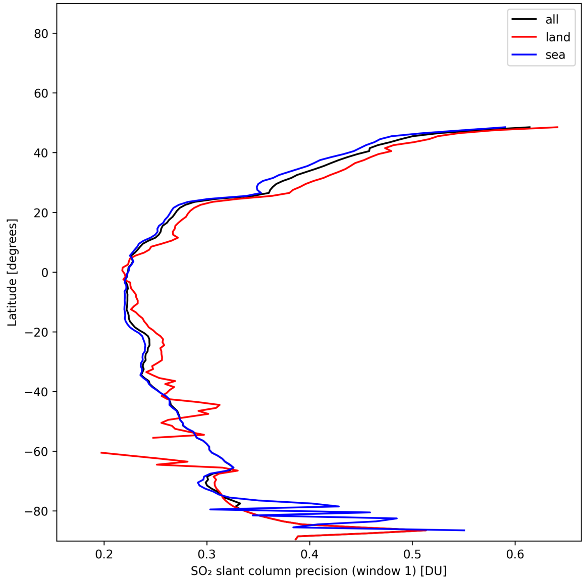
Figure 38: Zonal average of “SO 2 slant column precision (window 1)” for 2025-11-28 to 2025-11-29.
