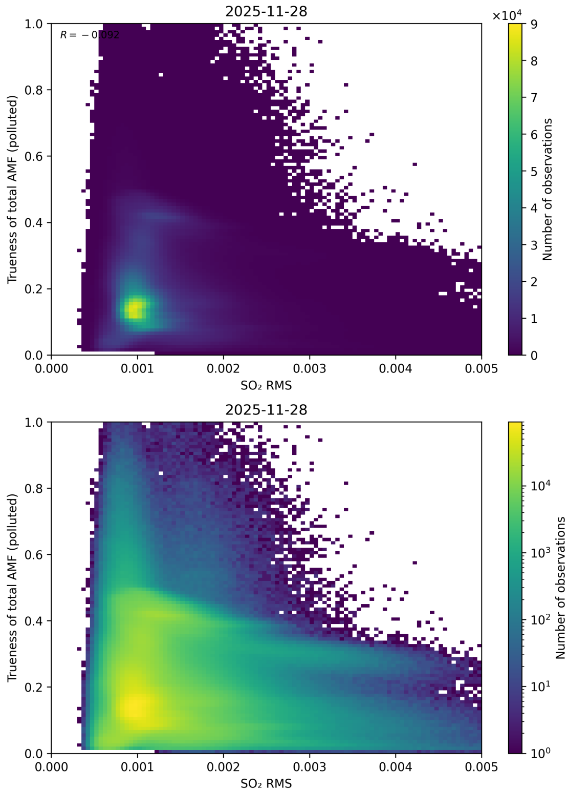
Figure 149: Scatter density plot of “SO 2 RMS” against “Trueness of total AMF (polluted)” for 2025-11-28 to 2025-11-29.
