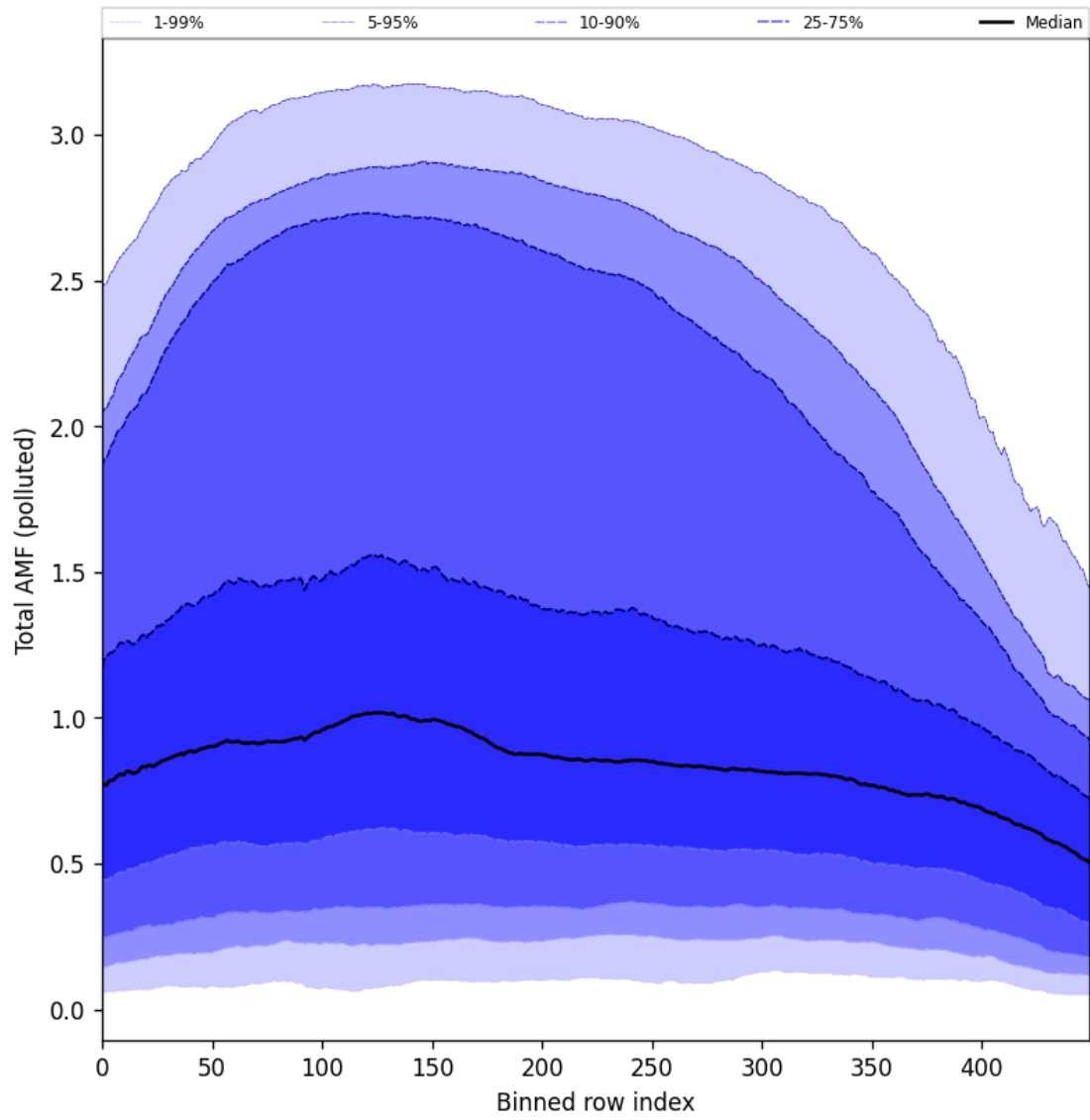
Figure 105: Along track statistics of “Total AMF (polluted)” for 2025-11-28 to 2025-11-29
