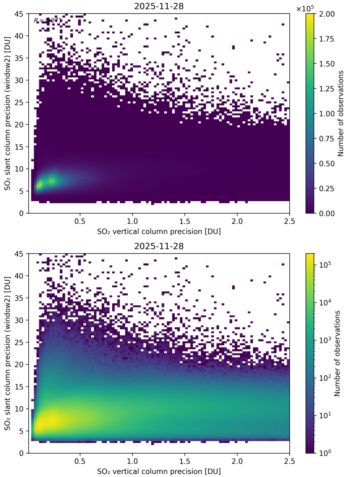
Figure 343: Scatter density plot of “SO 2 vertical column precision” against “SO 2 slant column precision (window2)” for 2025-11-28 to 2025-11-29.
