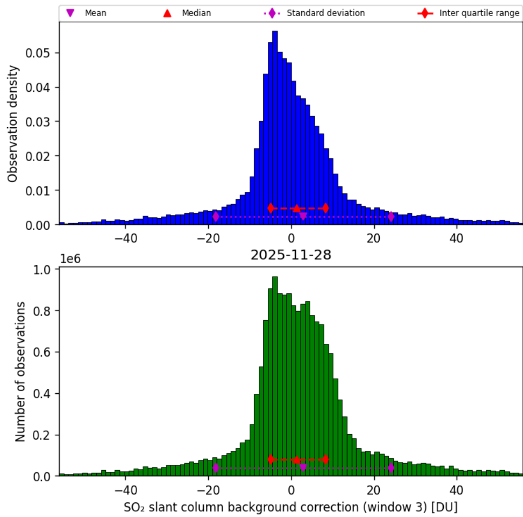
Figure 74: Histogram of “SO 2 slant column background correction (window 3)” for 2025-11-28 to 2025-11-29
