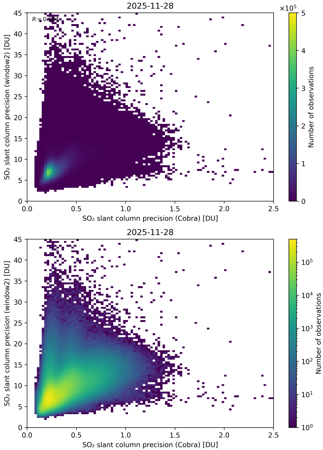
Figure 210: Scatter density plot of “SO 2 slant column precision (Cobra)” against “SO 2 slant column precision (window2)” for 2025-11-28 to 2025-11-29.
