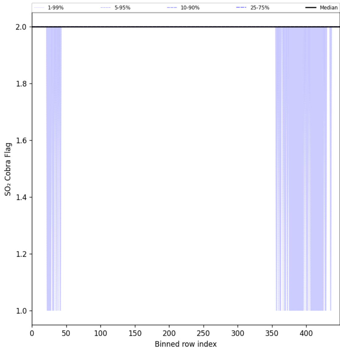
Figure 101: Along track statistics of “SO 2 Cobra Flag” for 2025-11-28 to 2025-11-29
