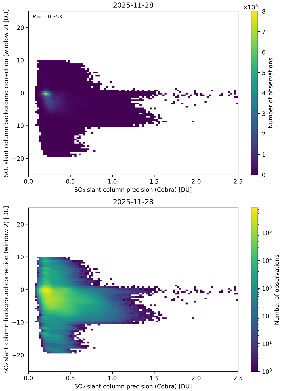
Figure 200: Scatter density plot of “SO 2 slant column precision (Cobra)” against “SO 2 slant column background correction (window 2)” for 2025-11-28 to 2025-11-29.
