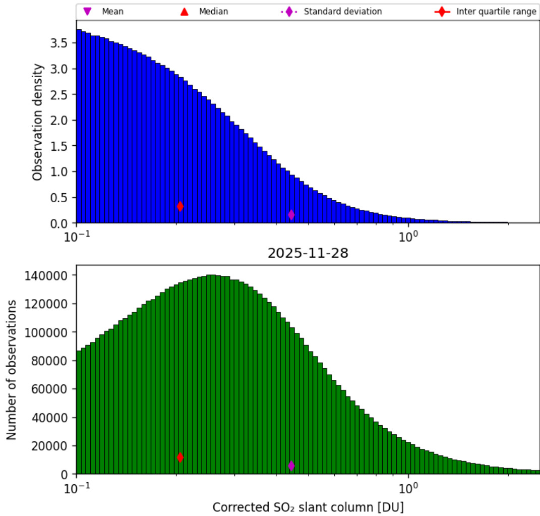
Figure 60: Histogram of “Corrected SO 2 slant column” for 2025-11-28 to 2025-11-29
