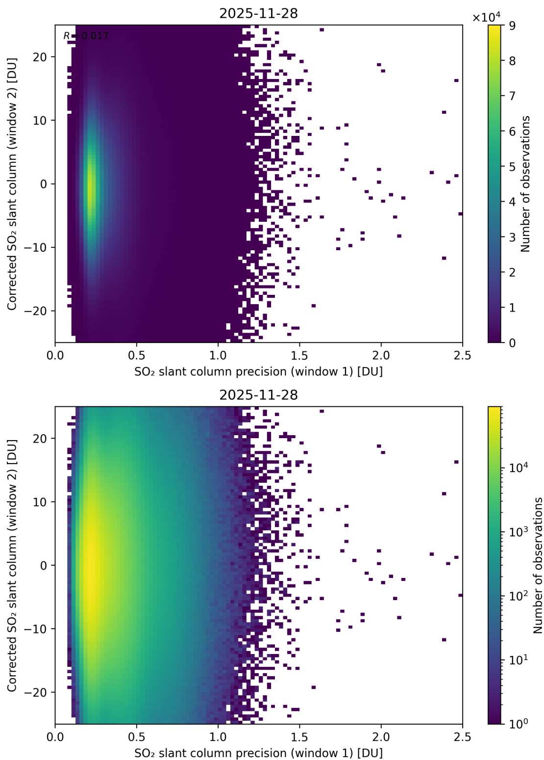
Figure 275: Scatter density plot of “SO 2 slant column precision (window 1)” against “Corrected SO 2 slant column (window 2)” for 2025-11-28 to 2025-11-29.
