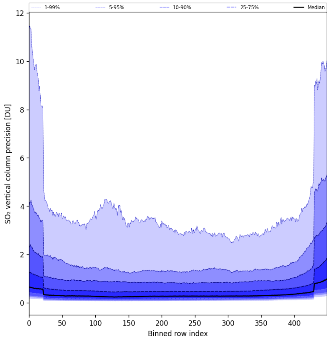
Figure 85: Along track statistics of “SO 2 vertical column precision” for 2025-11-28 to 2025-11-29
