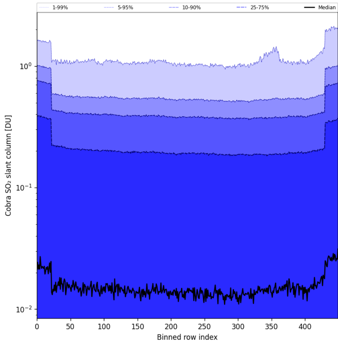
Figure 87: Along track statistics of “Cobra SO 2 slant column” for 2025-11-28 to 2025-11-29
