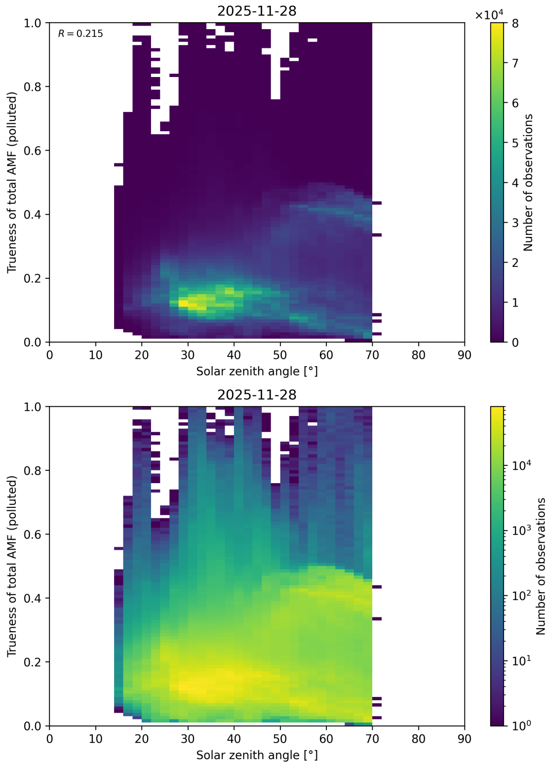
Figure 190: Scatter density plot of “Solar zenith angle” against “Trueness of total AMF (polluted)” for 2025-11-28 to 2025-11-29.
