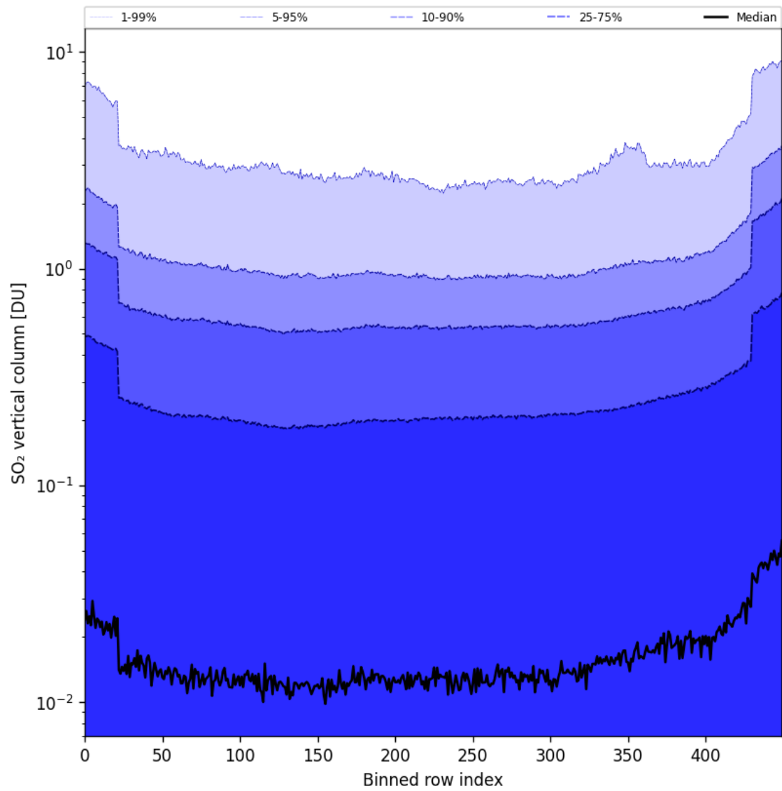
Figure 84: Along track statistics of “SO 2 vertical column” for 2025-11-28 to 2025-11-29
