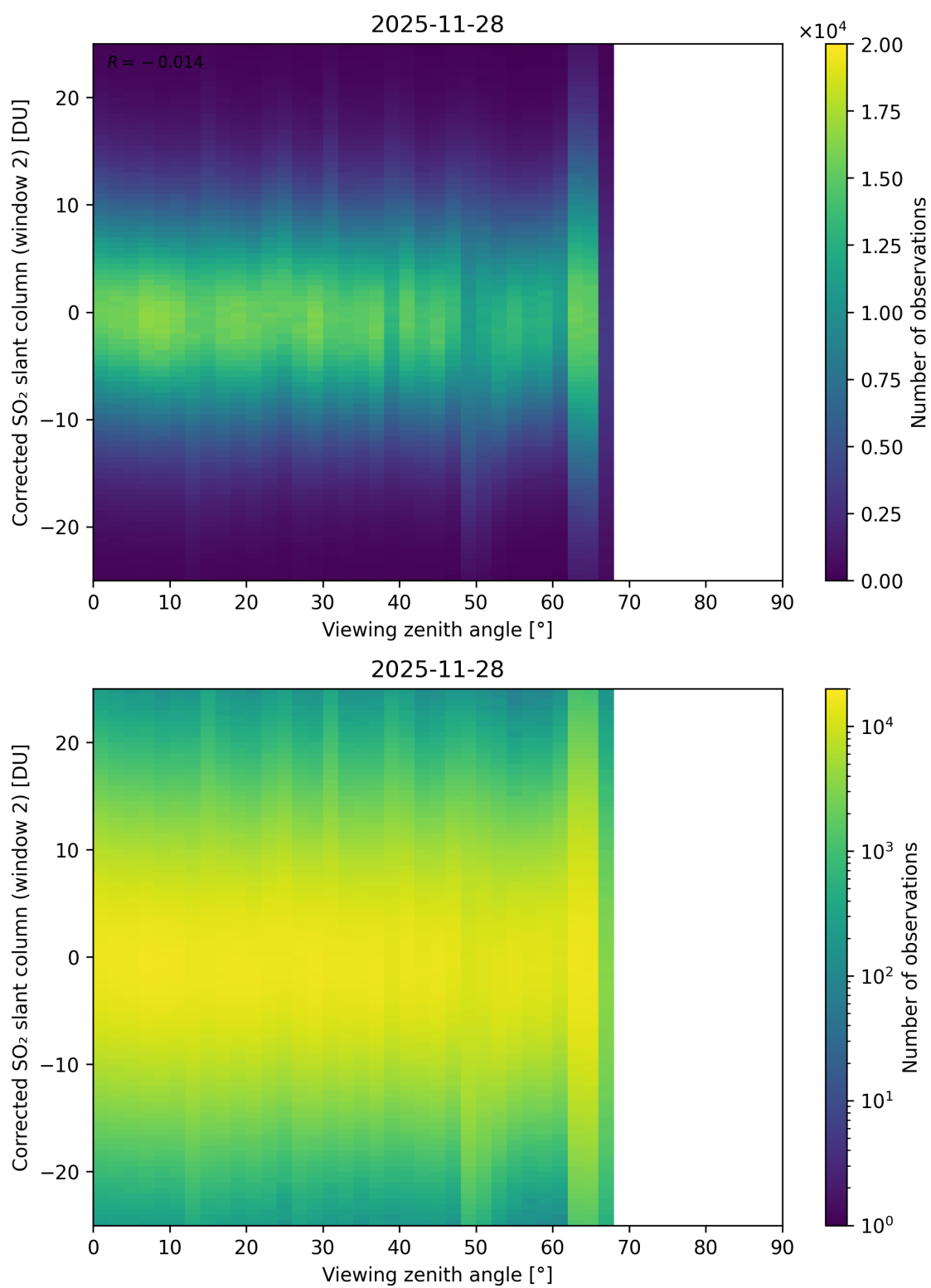
Figure 374: Scatter density plot of “Viewing zenith angle” against “Corrected SO 2 slant column (window 2)” for 2025-11-28 to 2025-11-29.
