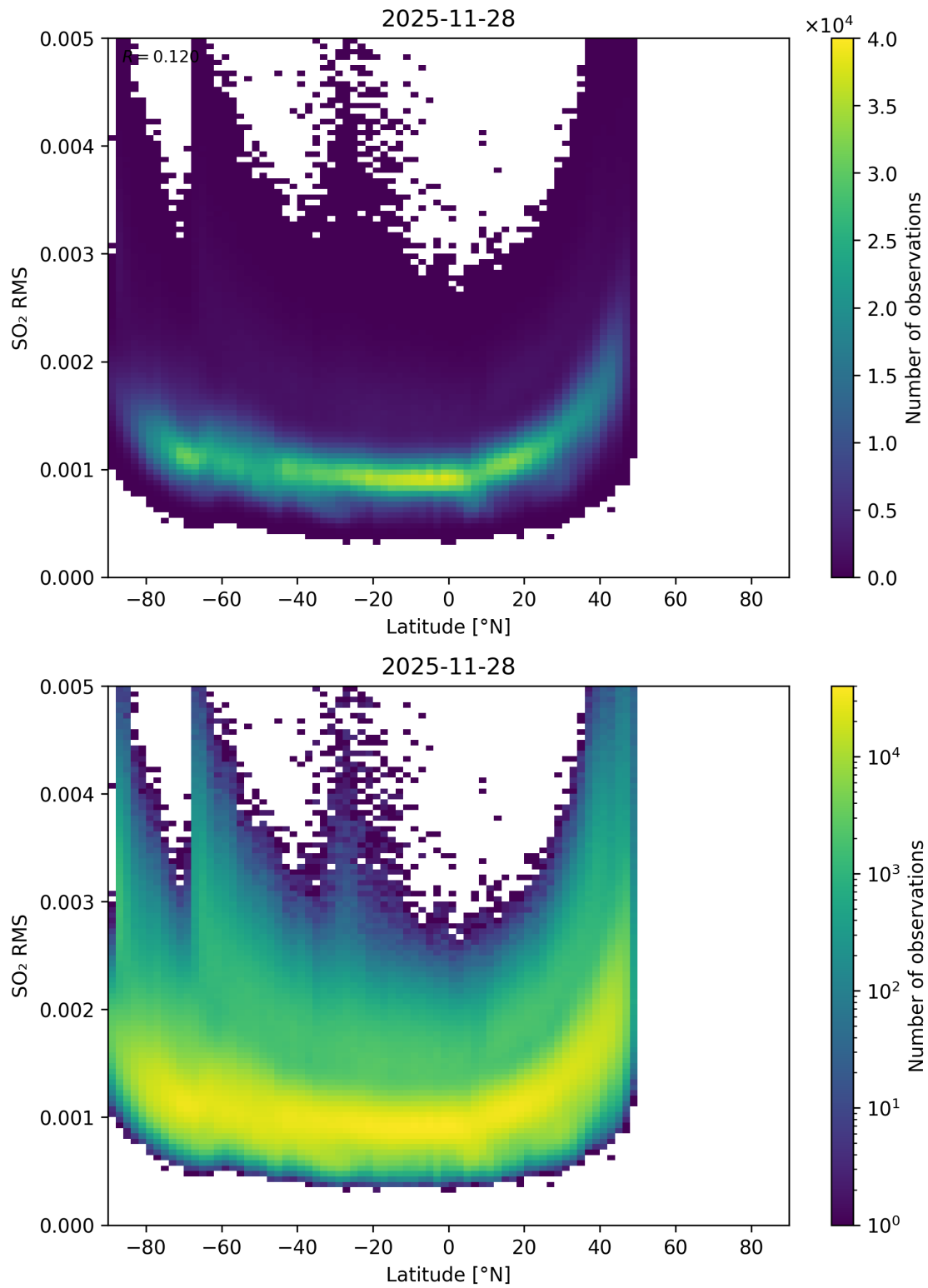
Figure 155: Scatter density plot of “Latitude” against “SO 2 RMS” for 2025-11-28 to 2025-11-29.
