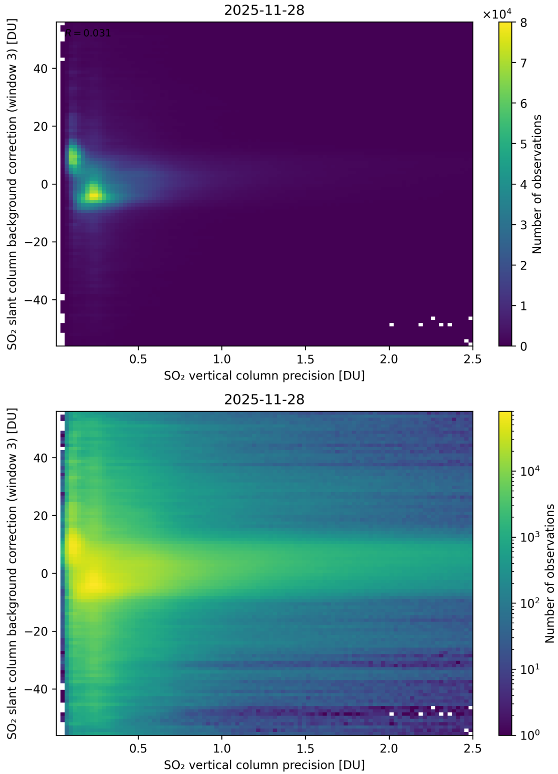
Figure 331: Scatter density plot of “SO 2 vertical column precision” against “SO 2 slant column background correction (window 3)” for 2025-11-28 to 2025-11-29.
