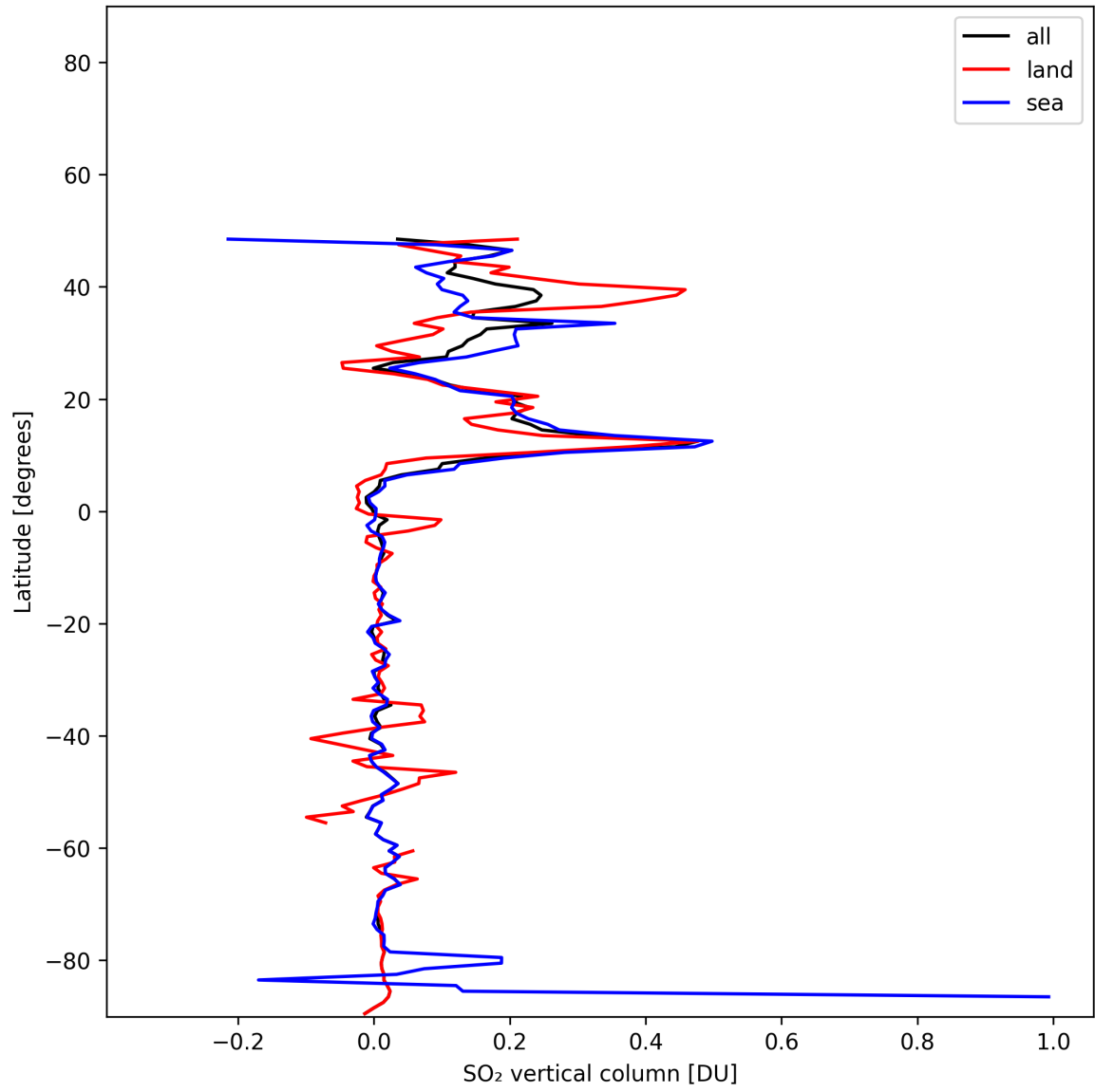
Figure 32: Zonal average of “SO 2 vertical column” for 2025-11-28 to 2025-11-29.
