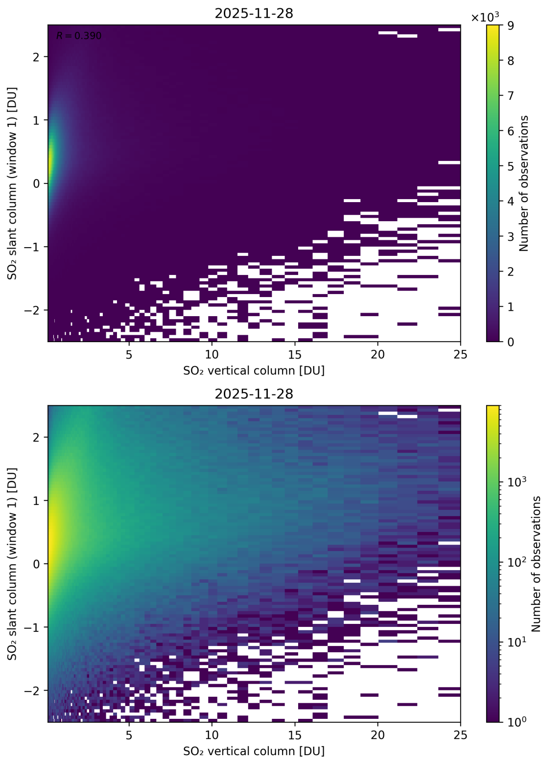
Figure 354: Scatter density plot of “SO 2 vertical column” against “SO 2 slant column (window 1)” for 2025-11-28 to 2025-11-29.
