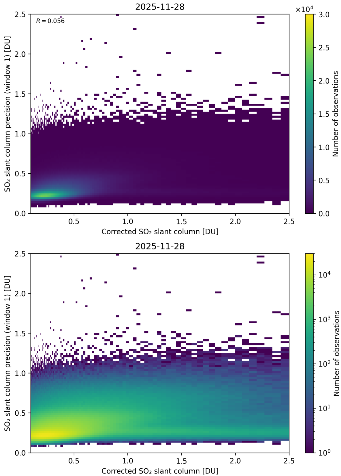
Figure 238: Scatter density plot of “Corrected SO 2 slant column” against “SO 2 slant column precision (window 1)” for 2025-11-28 to 2025-11-29.
