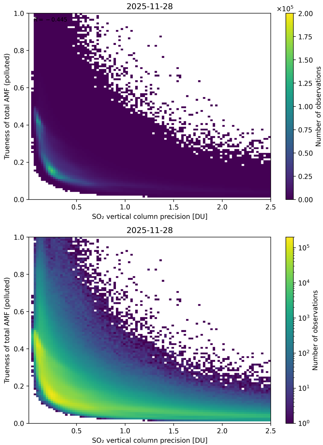
Figure 347: Scatter density plot of “SO 2 vertical column precision” against “Trueness of total AMF (polluted)” for 2025-11-28 to 2025-11-29.
