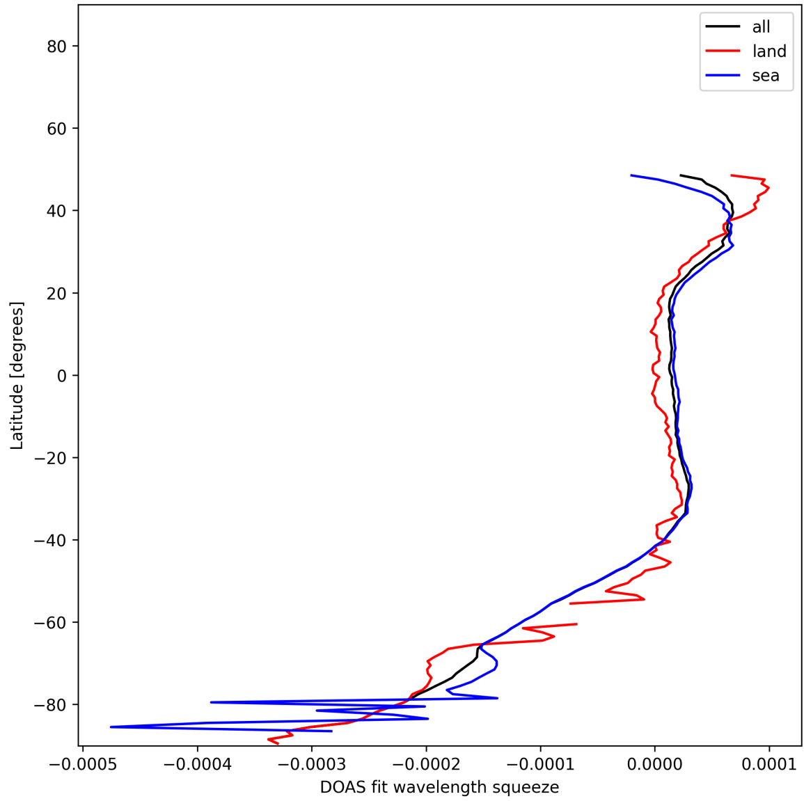
Figure 51: Zonal average of “DOAS fit wavelength squeeze” for 2025-11-28 to 2025-11-29.
