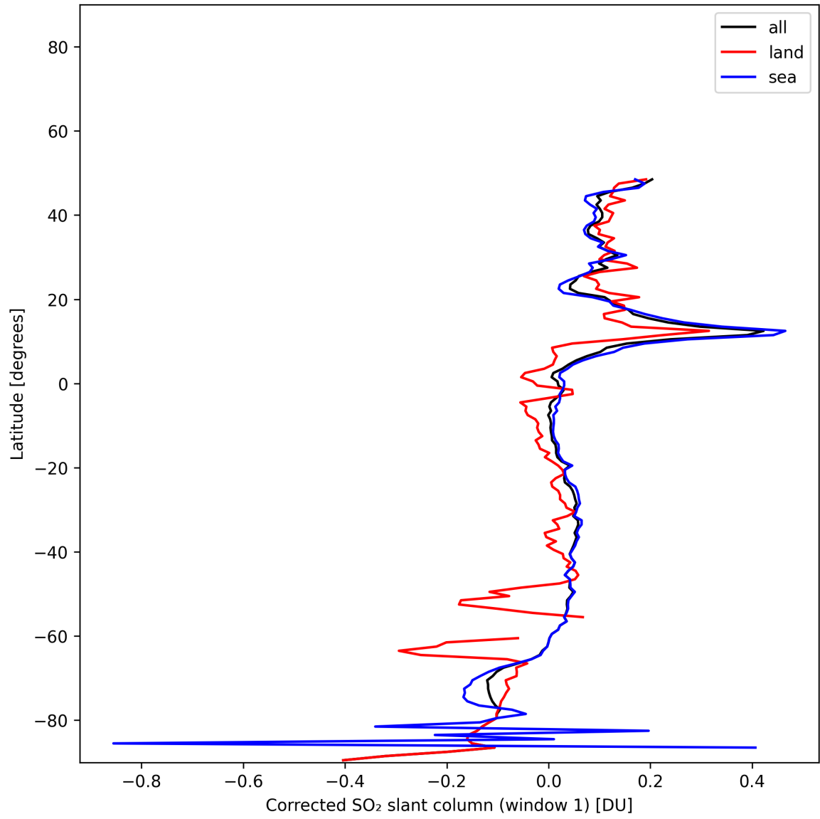
Figure 39: Zonal average of “Corrected SO 2 slant column (window 1)” for 2025-11-28 to 2025-11-29.
