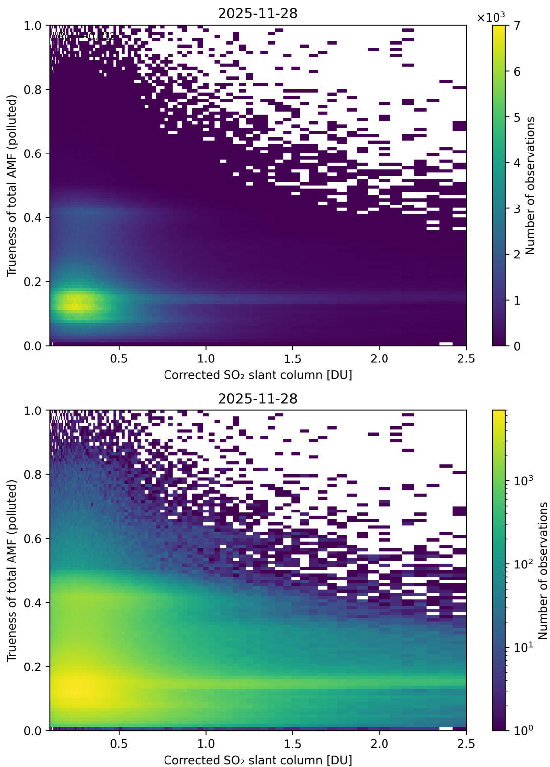
Figure 243: Scatter density plot of “Corrected SO 2 slant column” against “Trueness of total AMF (polluted)” for 2025-11-28 to 2025-11-29.
