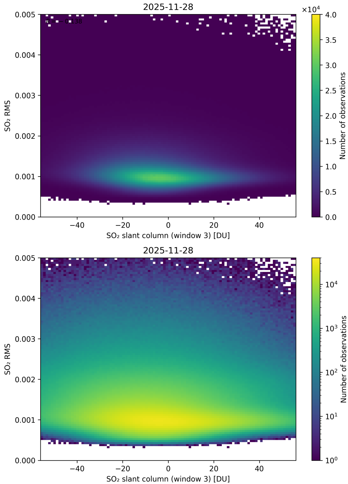
Figure 306: Scatter density plot of “SO 2 slant column (window 3)” against “SO 2 RMS” for 2025-11-28 to 2025-11-29.
