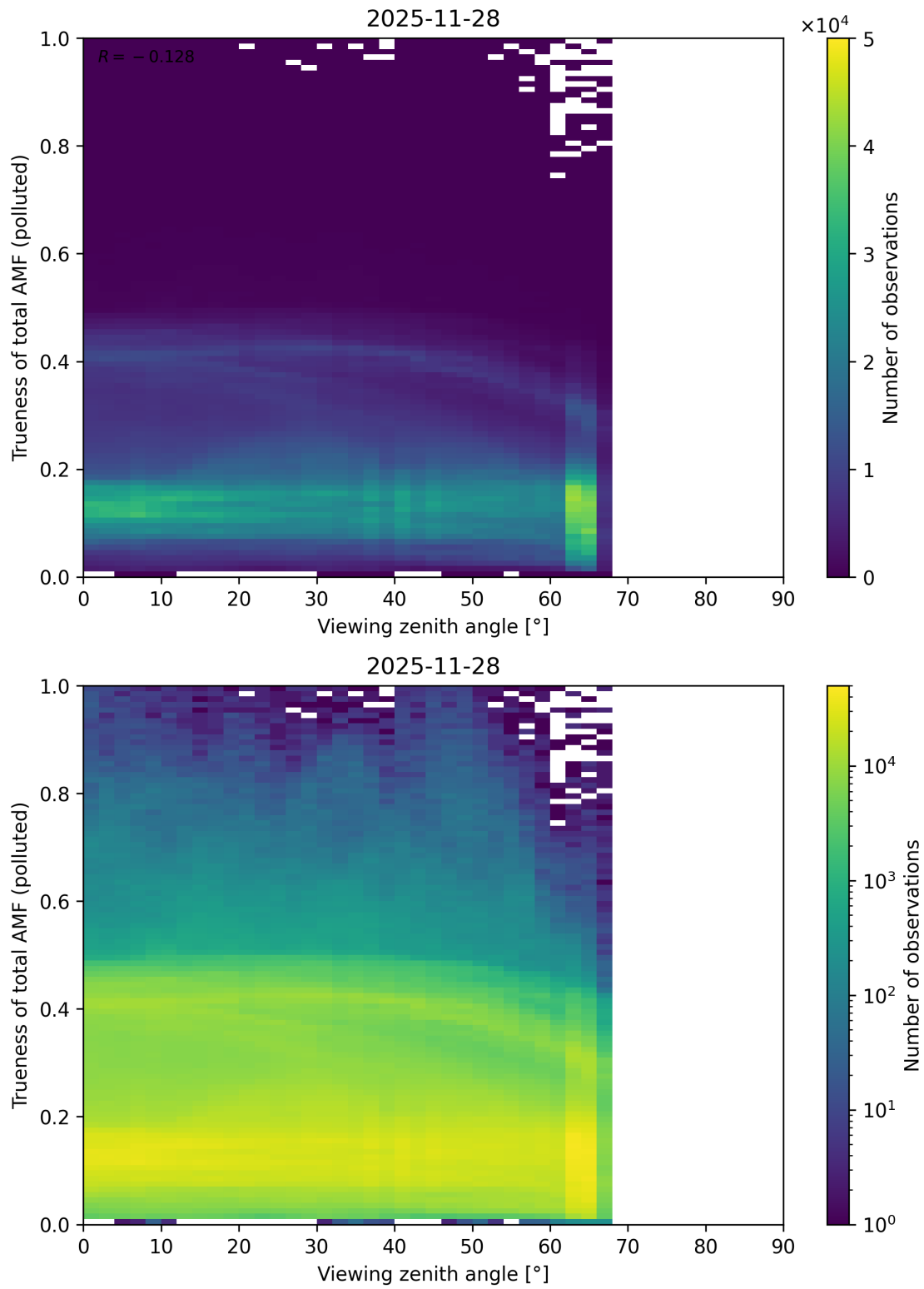
Figure 382: Scatter density plot of “Viewing zenith angle” against “Trueness of total AMF (polluted)” for 2025-11-28 to 2025-11-29.
