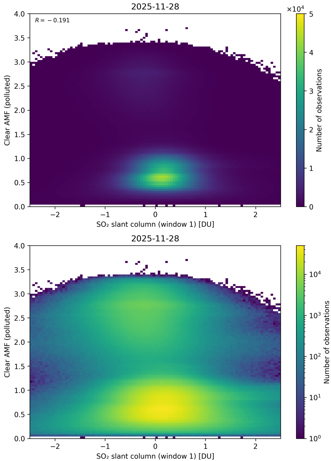
Figure 282: Scatter density plot of “SO 2 slant column (window 1)” against “Clear AMF (polluted)” for 2025-11-28 to 2025-11-29.
