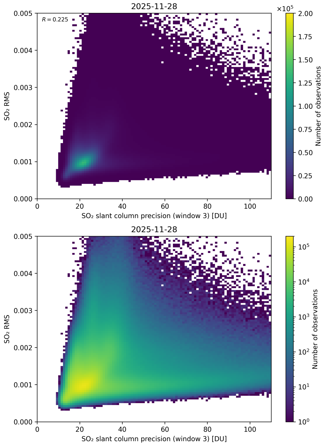
Figure 310: Scatter density plot of “SO 2 slant column precision (window 3)” against “SO 2 RMS” for 2025-11-28 to 2025-11-29.
