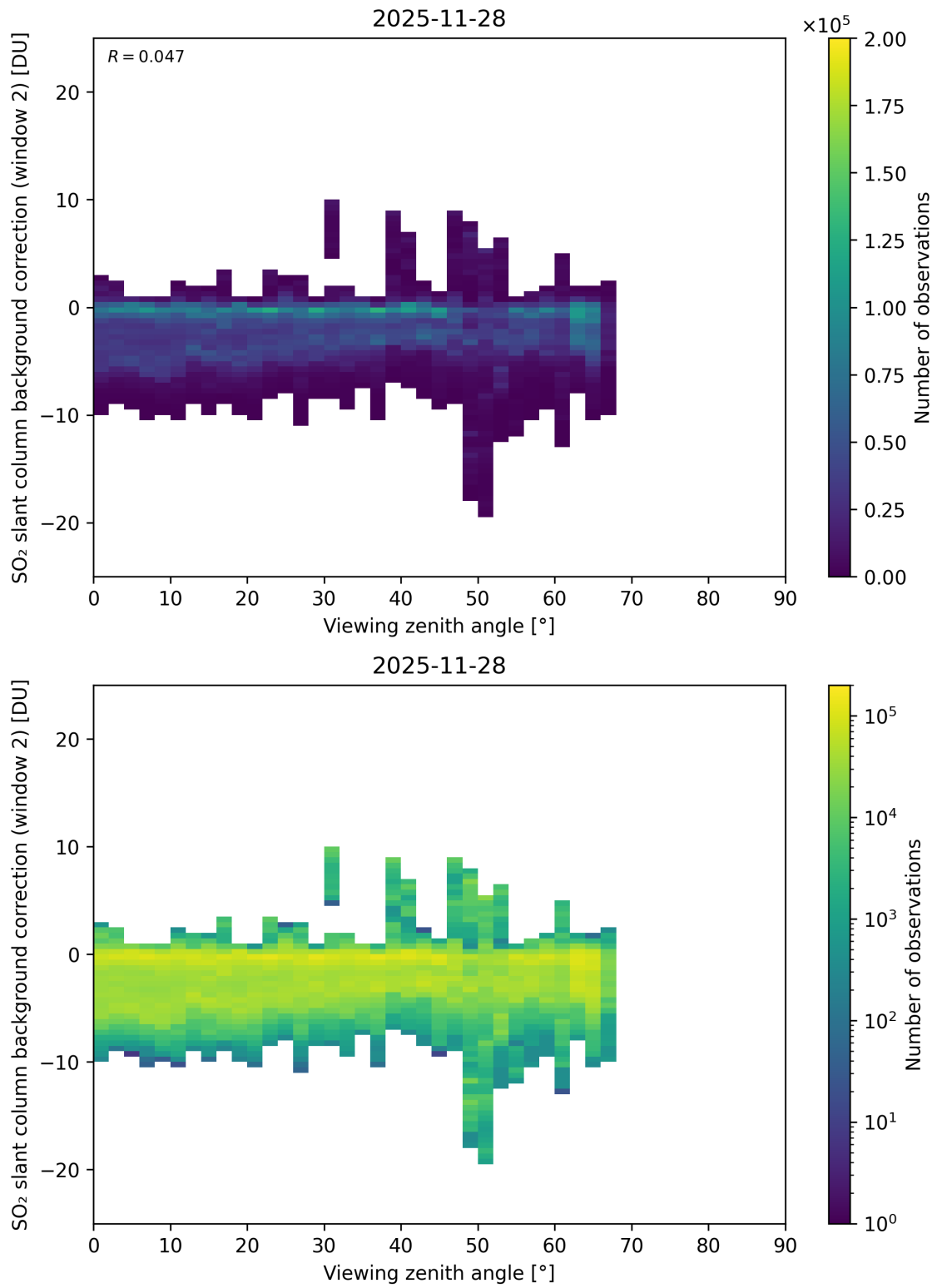
Figure 363: Scatter density plot of “Viewing zenith angle” against “SO 2 slant column background correction (window 2)” for 2025-11-28 to 2025-11-29.
