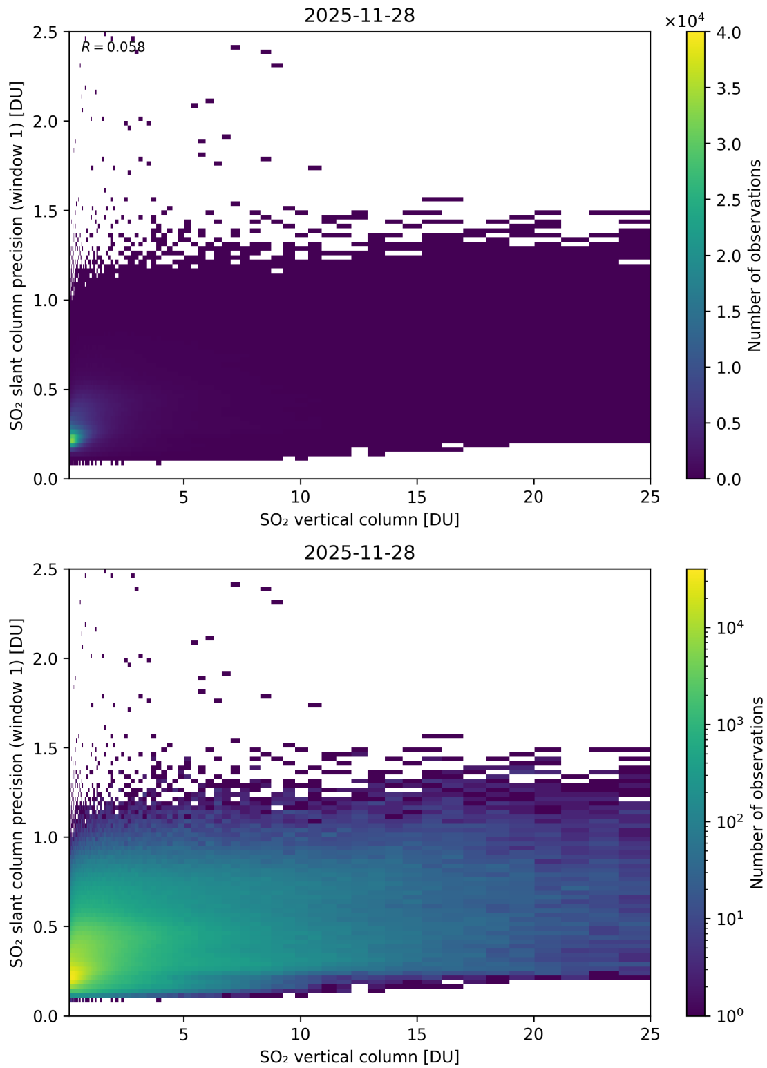
Figure 355: Scatter density plot of “SO 2 vertical column” against “SO 2 slant column precision (window 1)” for 2025-11-28 to 2025-11-29.
