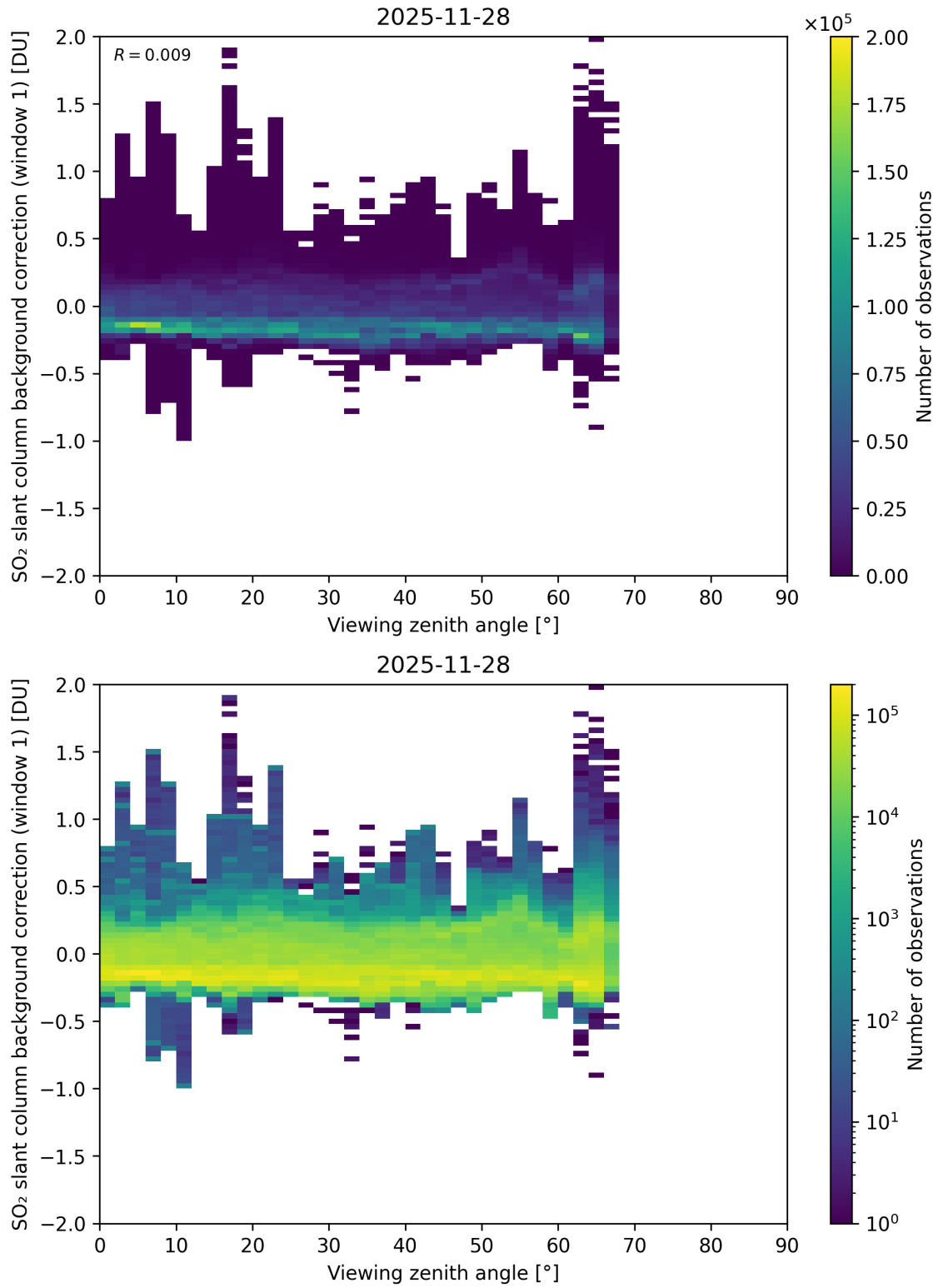
Figure 362: Scatter density plot of “Viewing zenith angle” against “SO 2 slant column background correction (window 1)” for 2025-11-28 to 2025-11-29.
