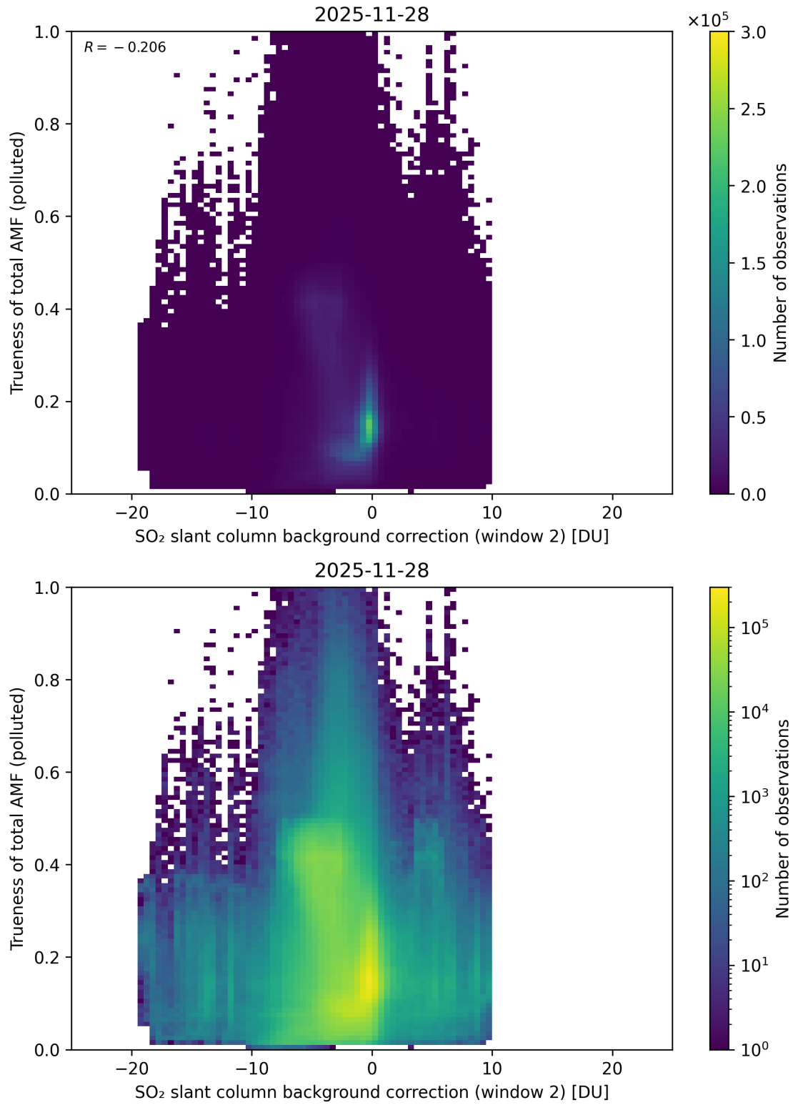
Figure 131: Scatter density plot of “SO 2 slant column background correction (window 2)” against “Trueness of total AMF (polluted)” for 2025-11-28 to 2025-11-29.
