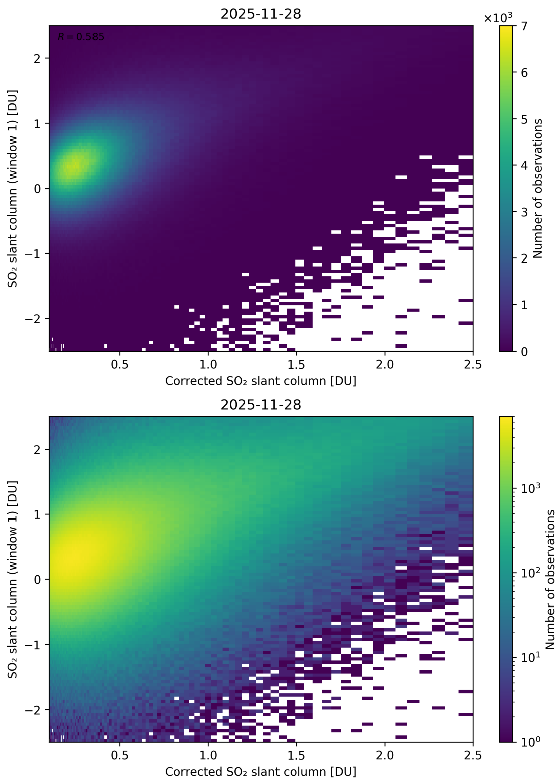
Figure 237: Scatter density plot of “Corrected SO 2 slant column” against “SO 2 slant column (window 1)” for 2025-11-28 to 2025-11-29.
