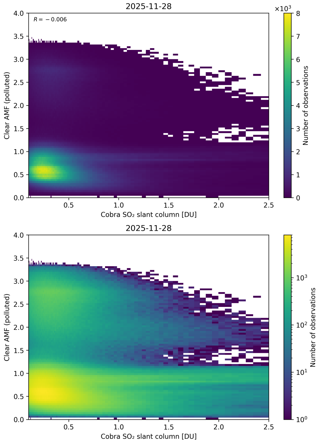
Figure 215: Scatter density plot of “Cobra SO 2 slant column” against “Clear AMF (polluted)” for 2025-11-28 to 2025-11-29.
