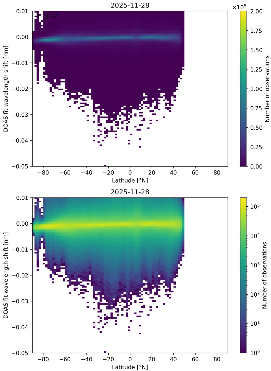
Figure 153: Scatter density plot of “Latitude” against “DOAS fit wavelength shift” for 2025-11-28 to 2025-11-29.
