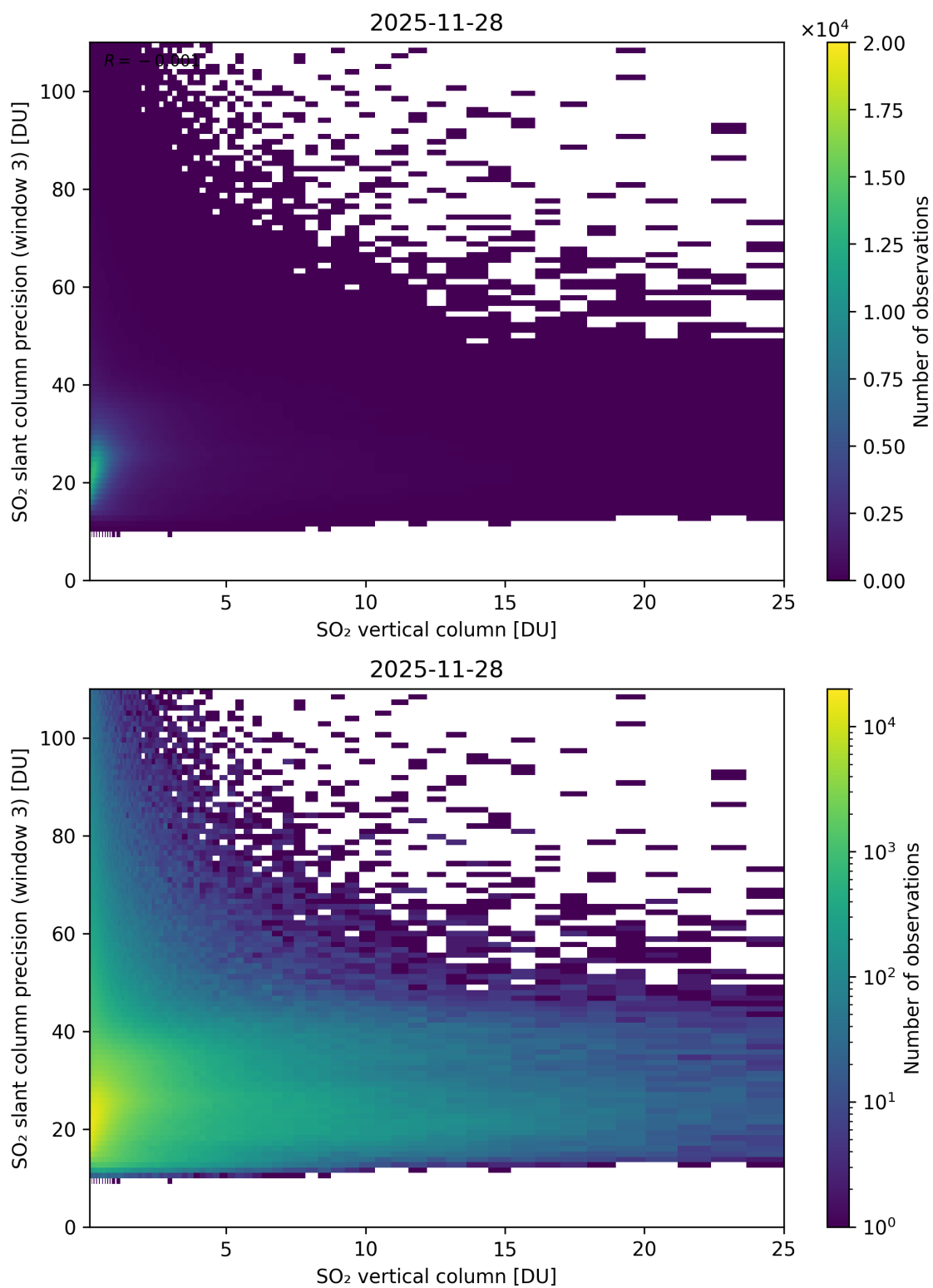
Figure 358: Scatter density plot of “SO 2 vertical column” against “SO 2 slant column precision (window 3)” for 2025-11-28 to 2025-11-29.
