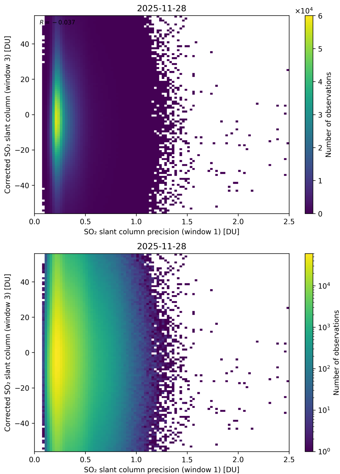
Figure 276: Scatter density plot of “SO 2 slant column precision (window 1)” against “Corrected SO 2 slant column (window 3)” for 2025-11-28 to 2025-11-29.
