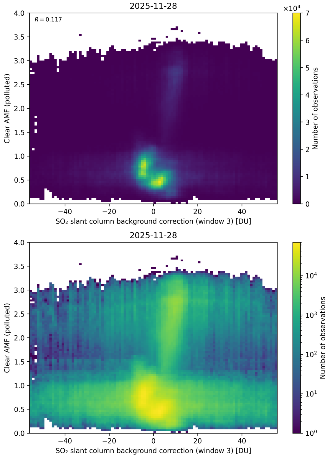
Figure 135: Scatter density plot of “SO 2 slant column background correction (window 3)” against “Clear AMF (polluted)” for 2025-11-28 to 2025-11-29.
