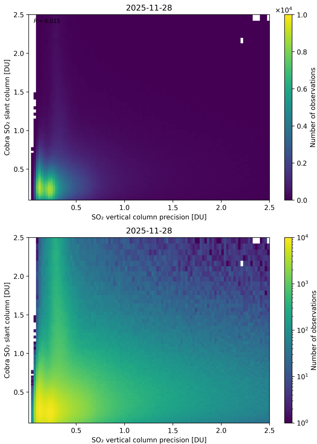
Figure 336: Scatter density plot of “SO 2 vertical column precision” against “Cobra SO 2 slant column” for 2025-11-28 to 2025-11-29.
