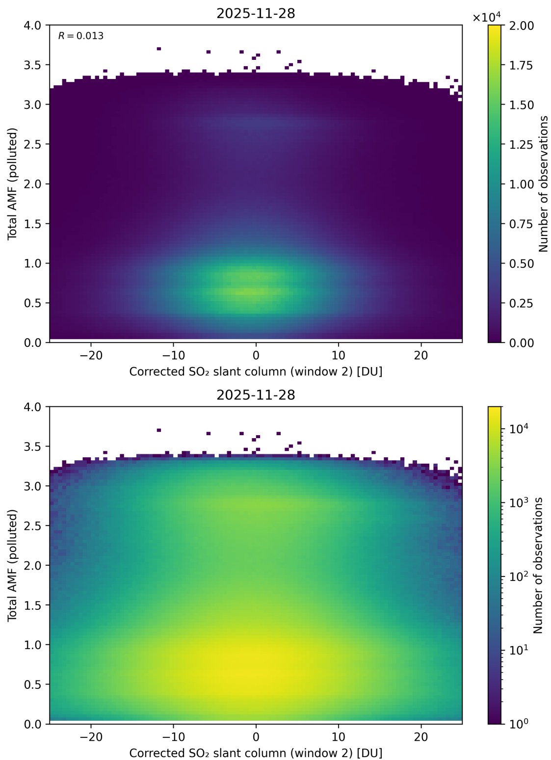
Figure 253: Scatter density plot of “Corrected SO 2 slant column (window 2)” against “Total AMF (polluted)” for 2025-11-28 to 2025-11-29.
