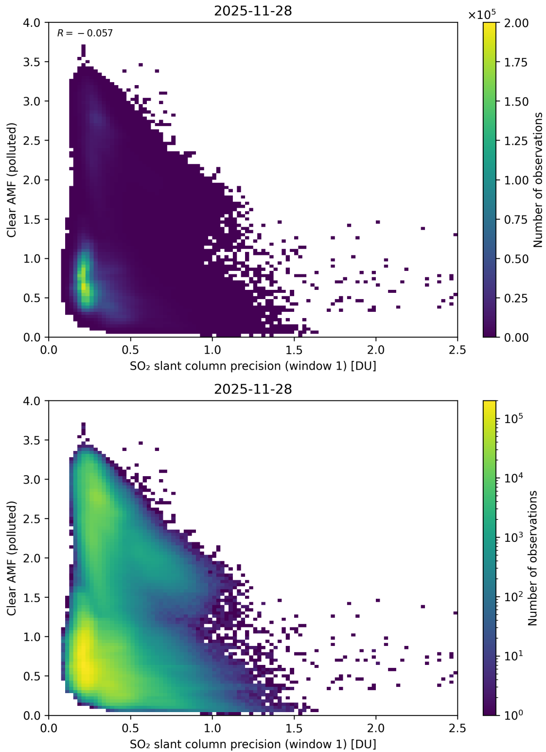
Figure 274: Scatter density plot of “SO 2 slant column precision (window 1)” against “Clear AMF (polluted)” for 2025-11-28 to 2025-11-29.
