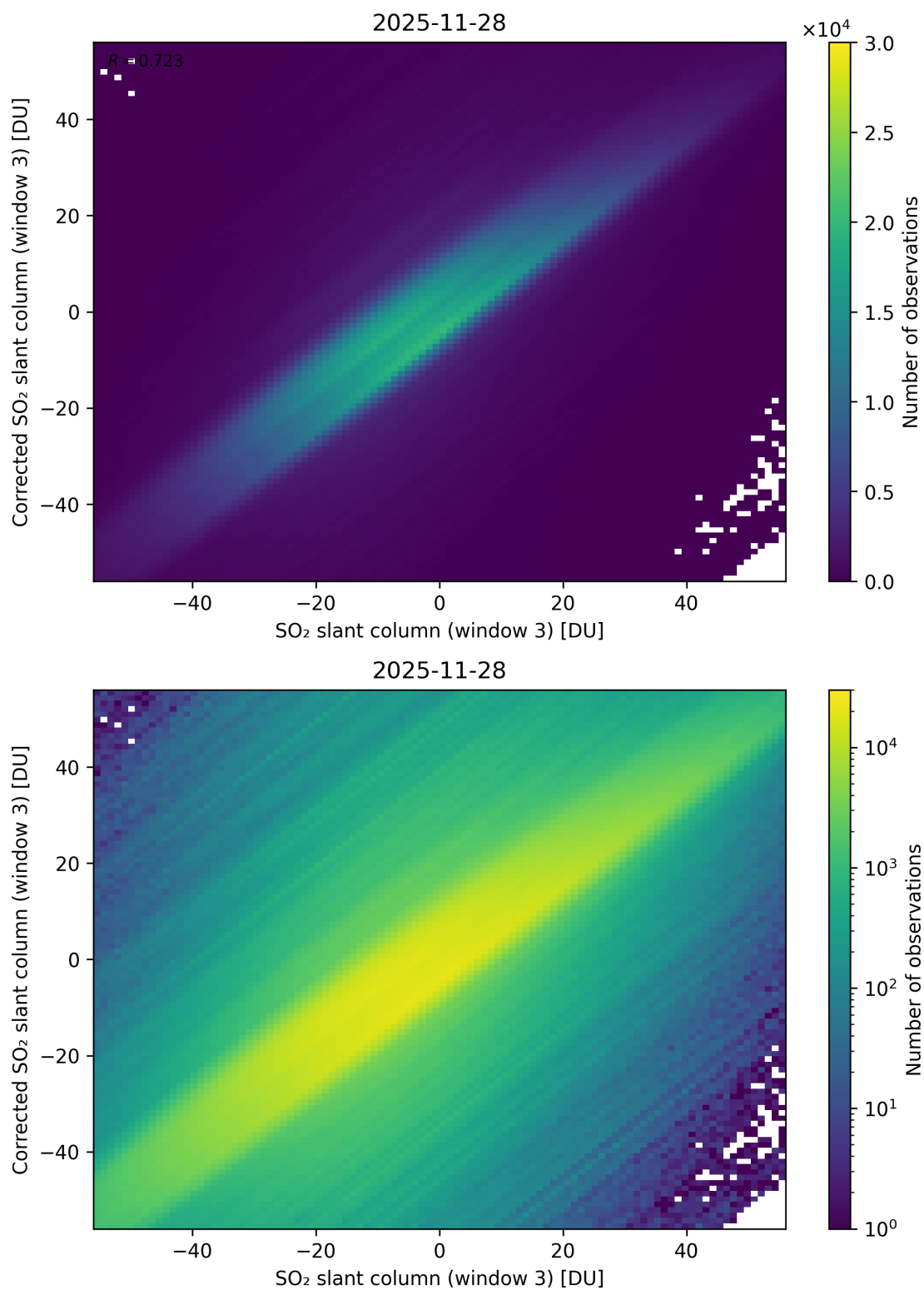
Figure 316: Scatter density plot of “SO 2 slant column (window 3)” against “Corrected SO 2 slant column (window 3)” for 2025-11-28 to 2025-11-29.
