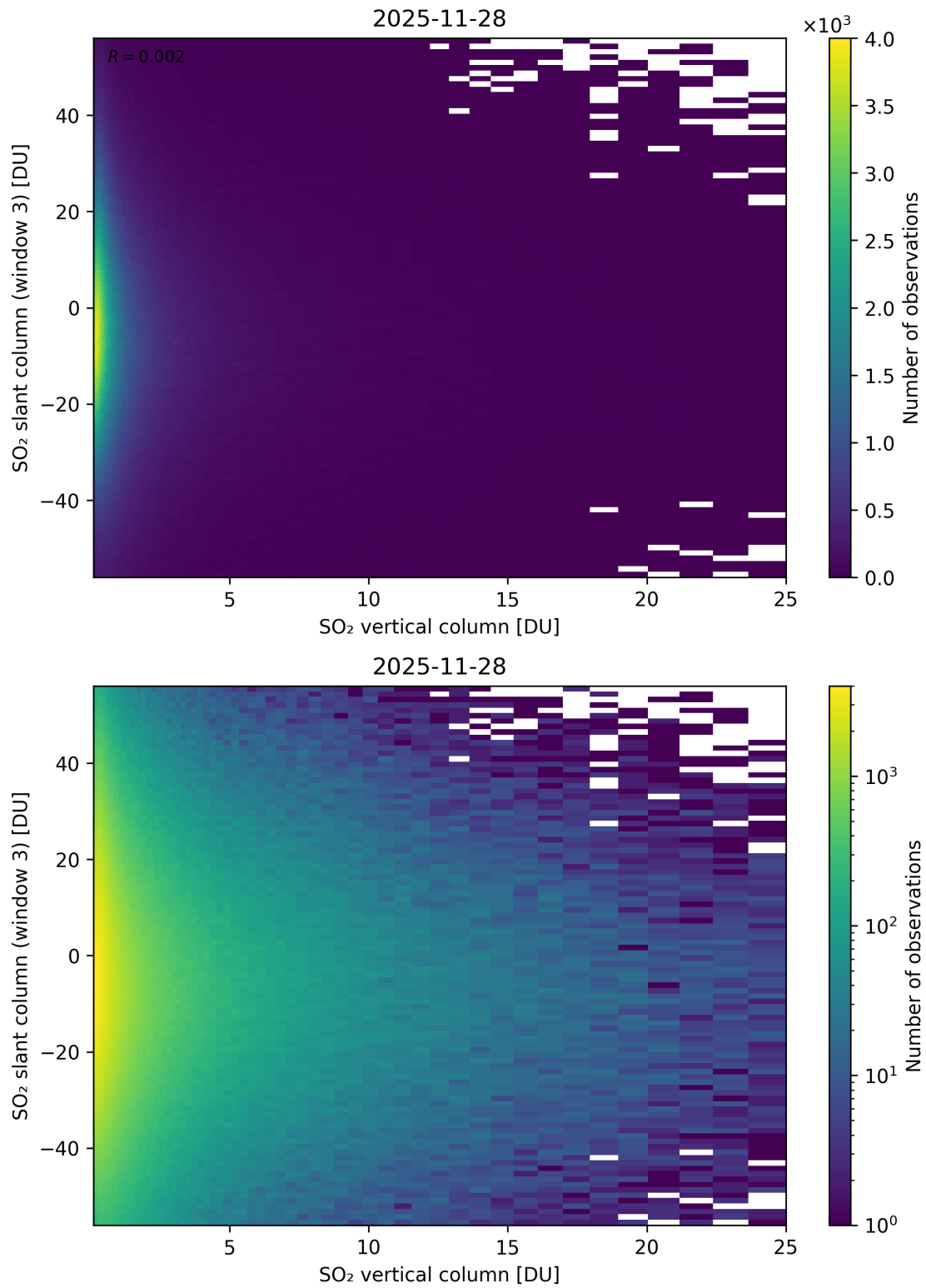
Figure 357: Scatter density plot of “SO 2 vertical column” against “SO 2 slant column (window 3)” for 2025-11-28 to 2025-11-29.
