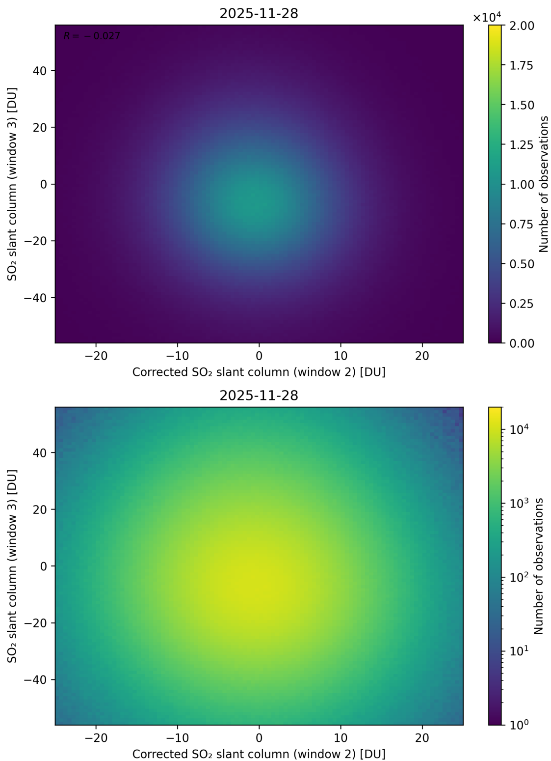
Figure 251: Scatter density plot of “Corrected SO 2 slant column (window 2)” against “SO 2 slant column (window 3)” for 2025-11-28 to 2025-11-29.
