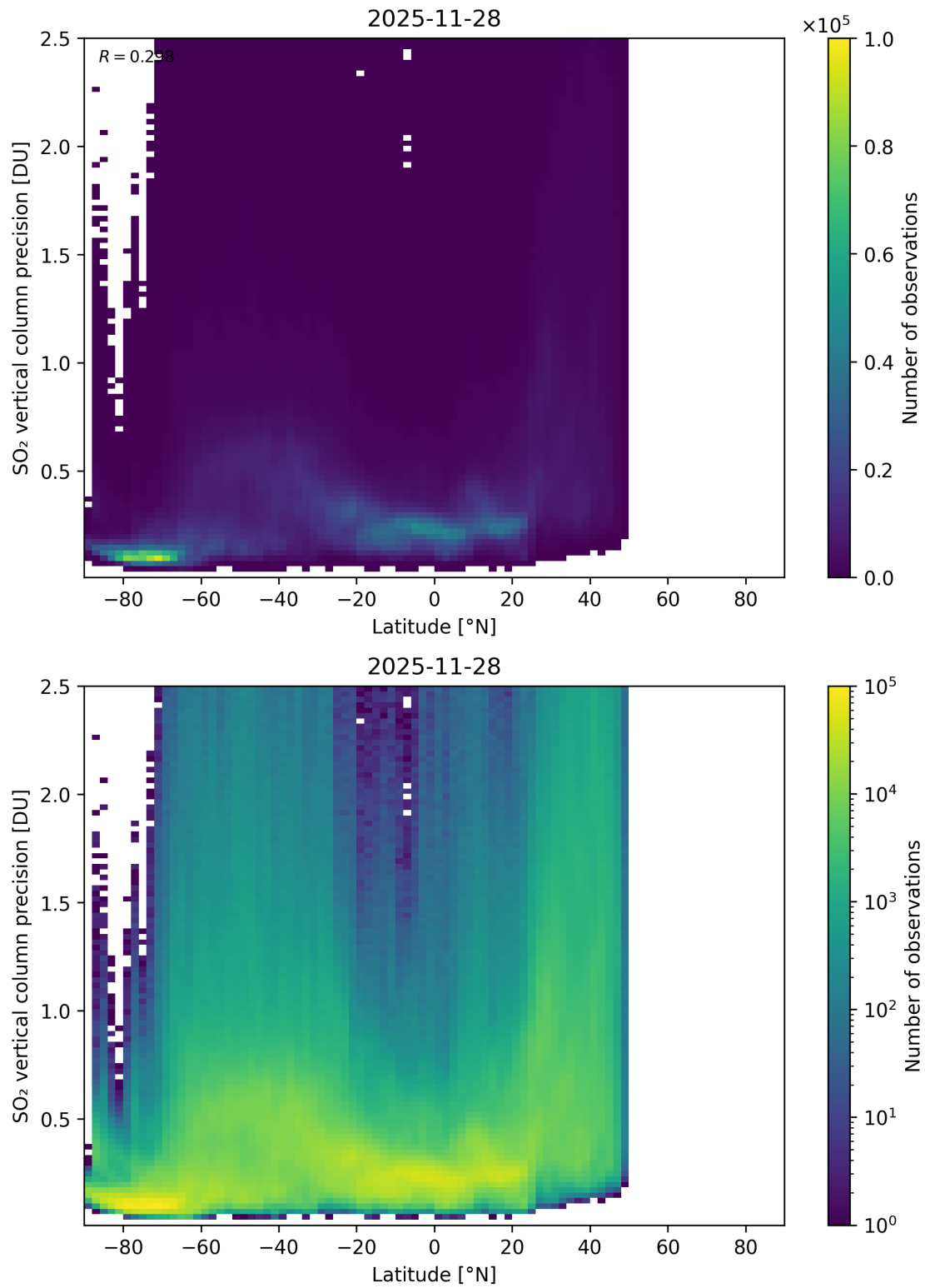
Figure 170: Scatter density plot of “Latitude” against “SO 2 vertical column precision” for 2025-11-28 to 2025-11-29.
