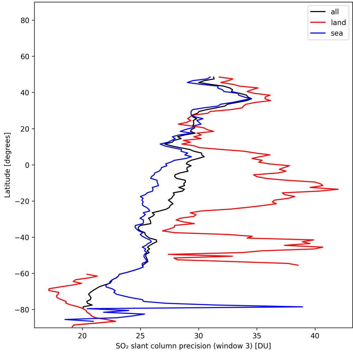
Figure 46: Zonal average of “SO 2 slant column precision (window 3)” for 2025-11-28 to 2025-11-29.
