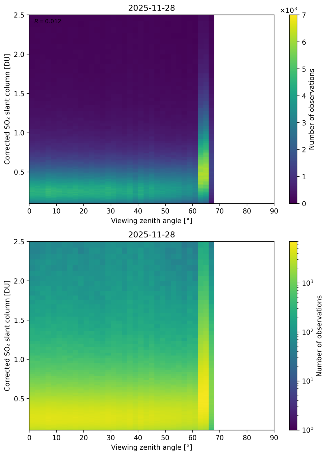
Figure 373: Scatter density plot of “Viewing zenith angle” against “Corrected SO 2 slant column” for 2025-11-28 to 2025-11-29.
