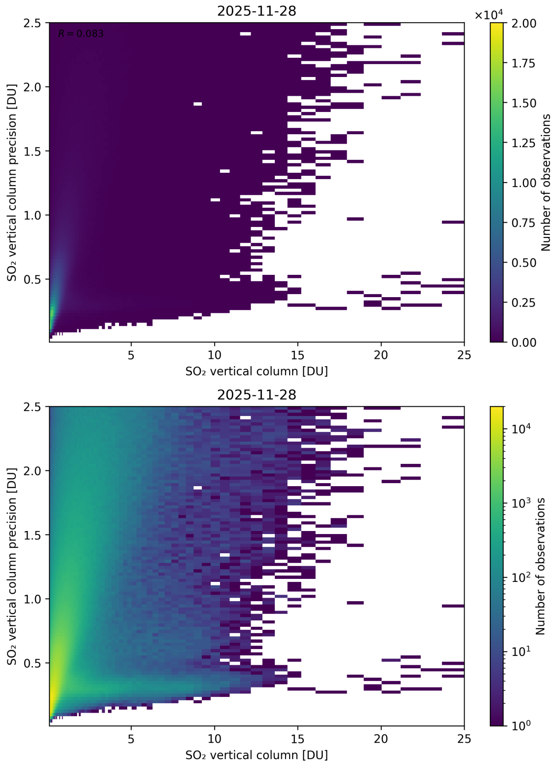
Figure 361: Scatter density plot of “SO 2 vertical column” against “SO 2 vertical column precision” for 2025-11-28 to 2025-11-29.
