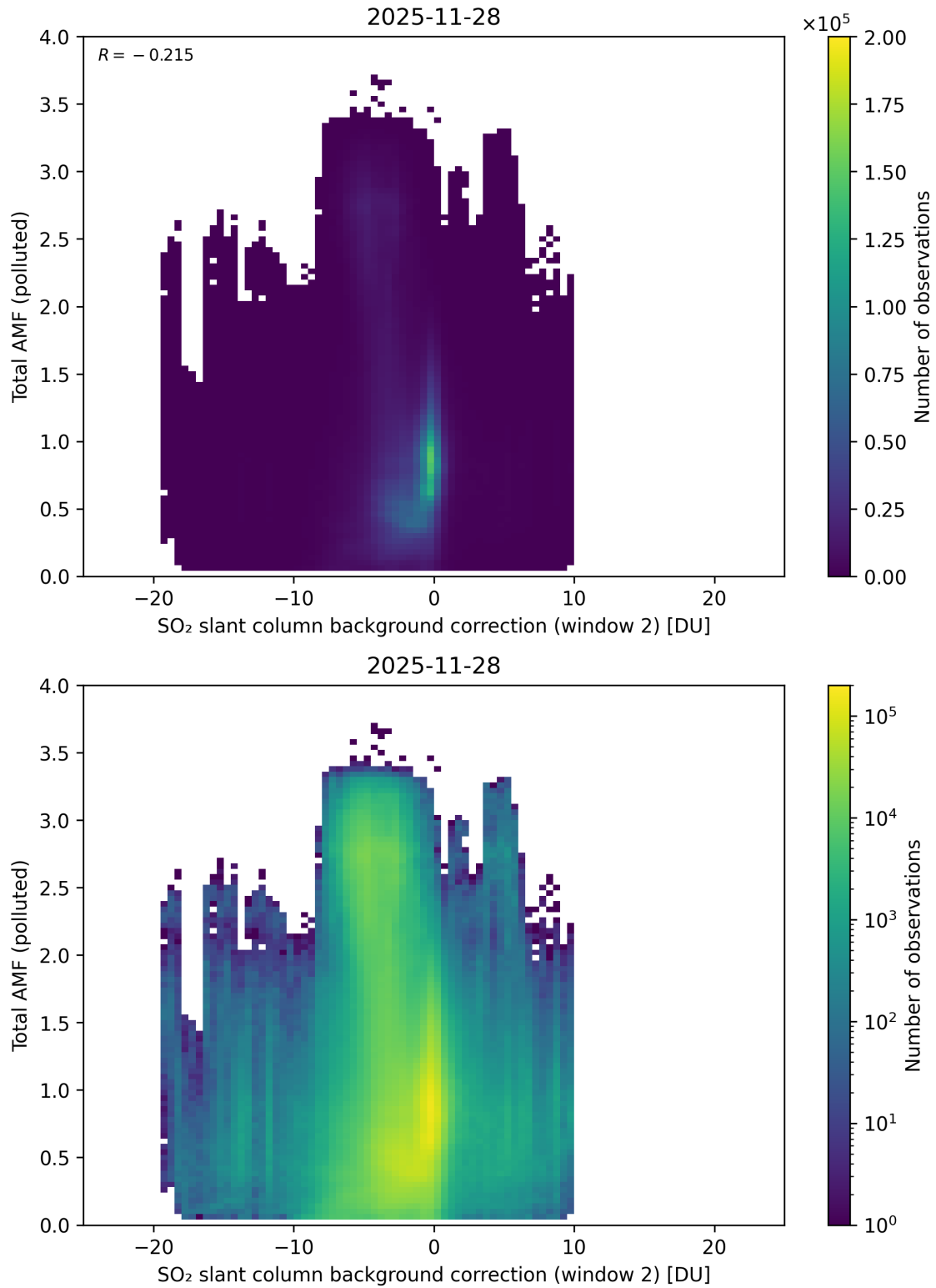
Figure 130: Scatter density plot of “SO 2 slant column background correction (window 2)” against “Total AMF (polluted)” for 2025-11-28 to 2025-11-29.
