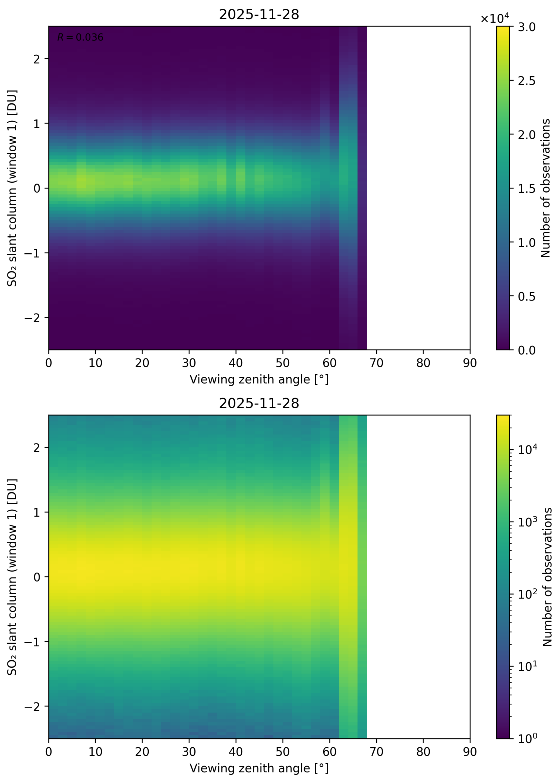
Figure 376: Scatter density plot of “Viewing zenith angle” against “SO 2 slant column (window 1)” for 2025-11-28 to 2025-11-29.
