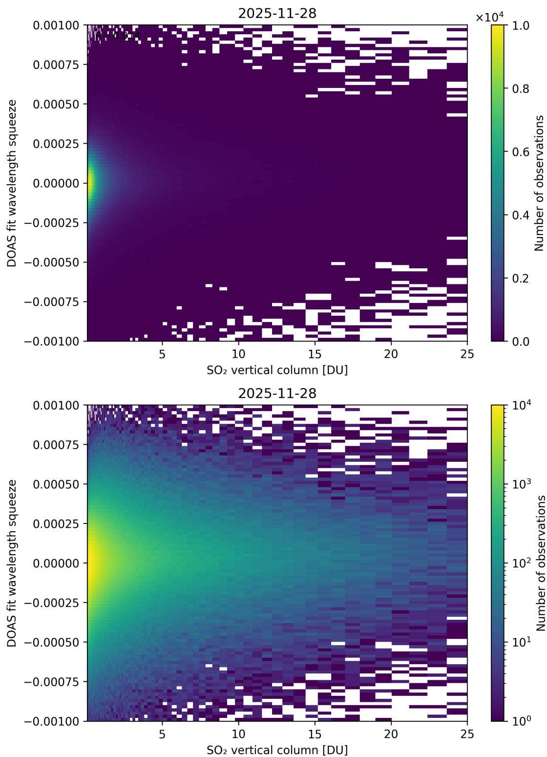
Figure 327: Scatter density plot of “SO 2 vertical column” against “DOAS fit wavelength squeeze” for 2025-11-28 to 2025-11-29.
