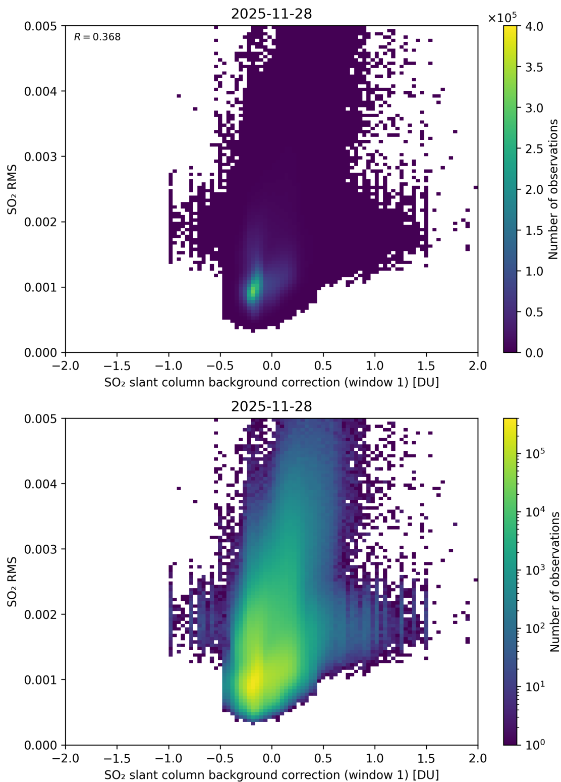
Figure 113: Scatter density plot of “SO 2 slant column background correction (window 1)” against “SO 2 RMS” for 2025-11-28 to 2025-11-29.
