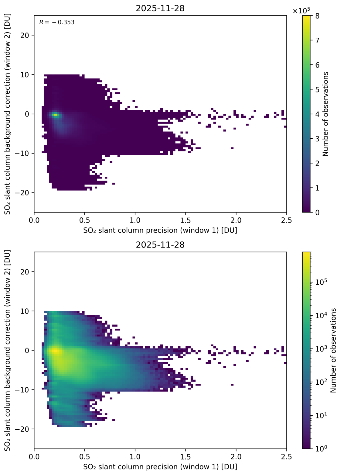
Figure 269: Scatter density plot of “SO 2 slant column precision (window 1)” against “SO 2 slant column background correction (window 2)” for 2025-11-28 to 2025-11-29.
