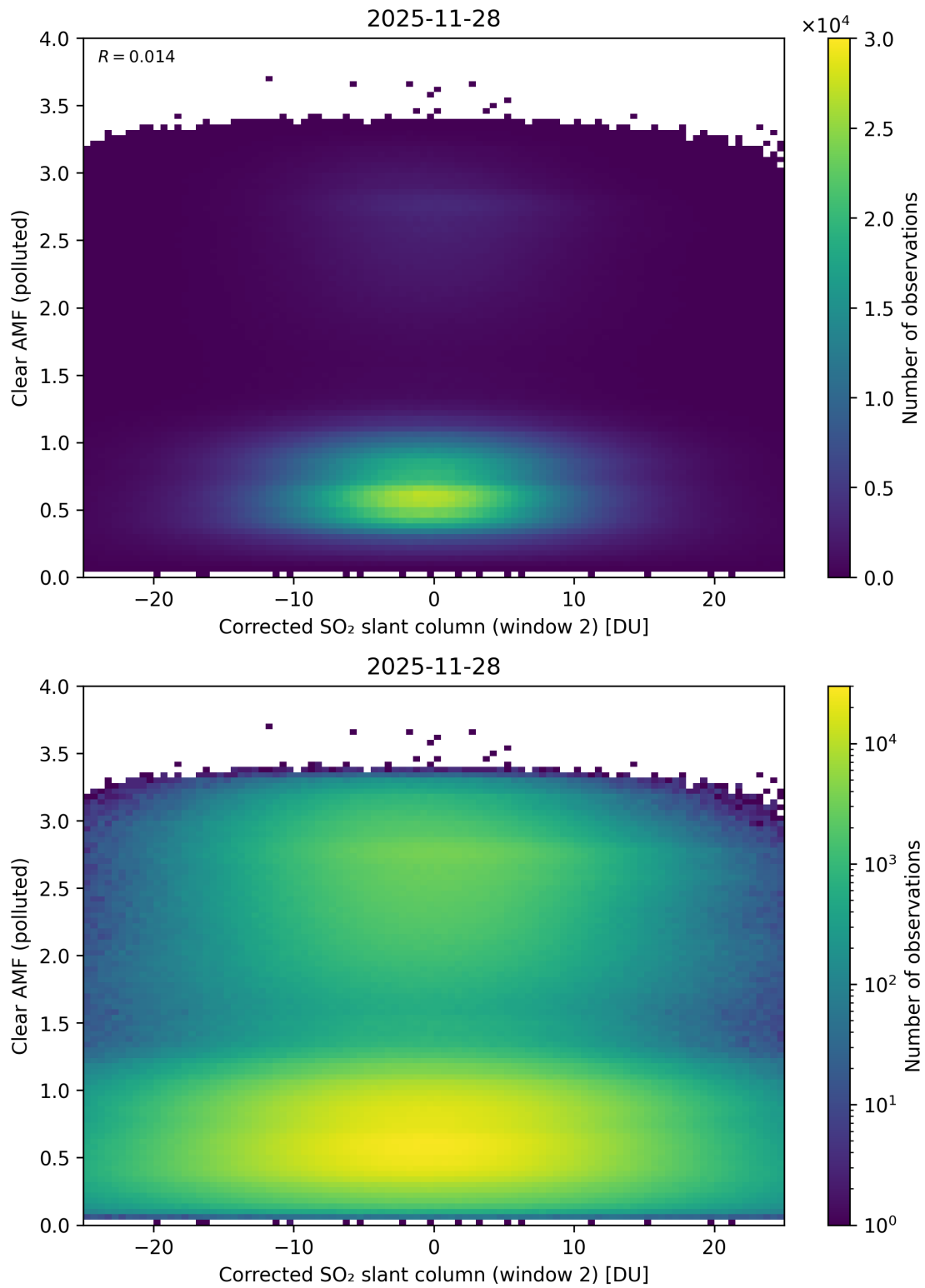
Figure 249: Scatter density plot of “Corrected SO 2 slant column (window 2)” against “Clear AMF (polluted)” for 2025-11-28 to 2025-11-29.
