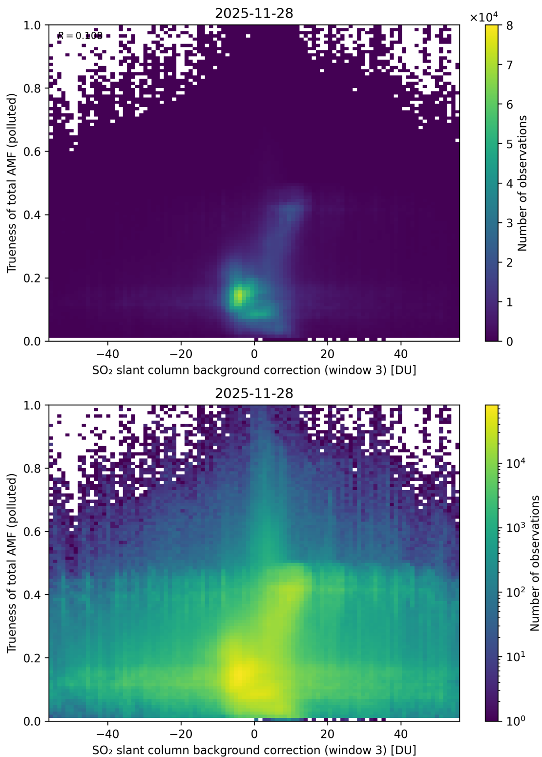
Figure 137: Scatter density plot of “SO 2 slant column background correction (window 3)” against “Trueness of total AMF (polluted)” for 2025-11-28 to 2025-11-29.
