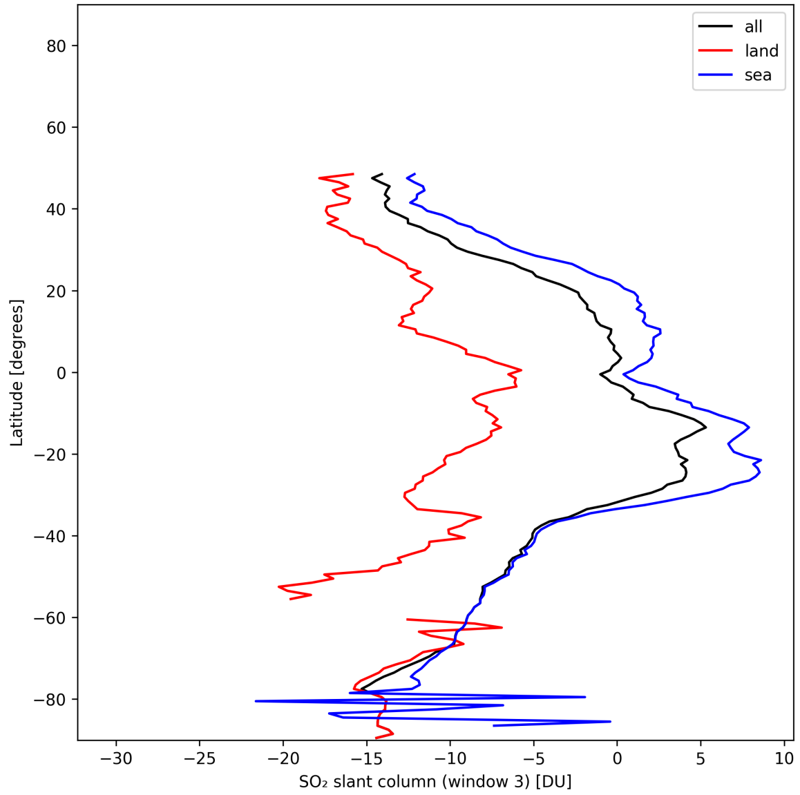
Figure 45: Zonal average of “SO 2 slant column (window 3)” for 2025-11-28 to 2025-11-29.
