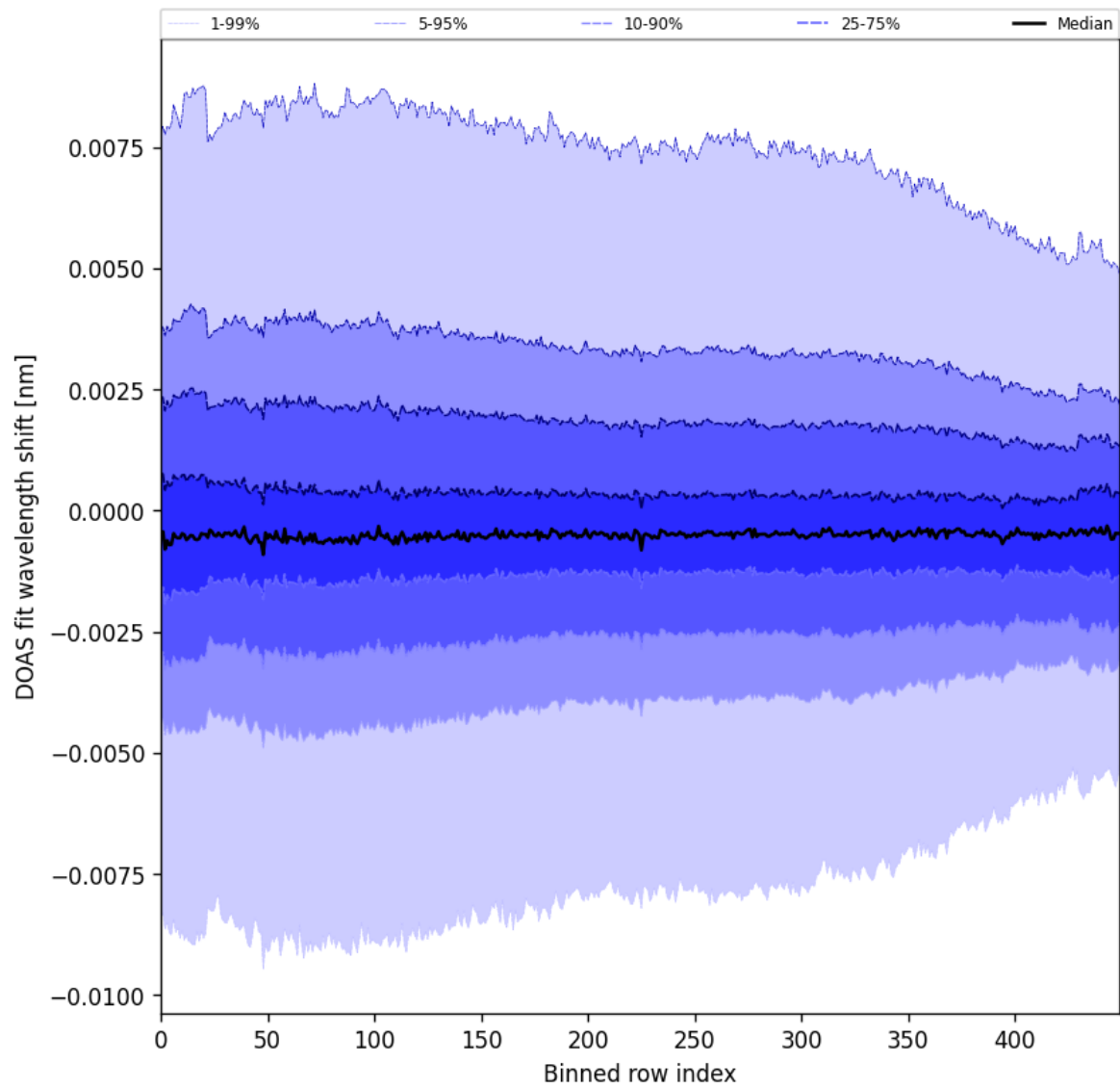
Figure 102: Along track statistics of “DOAS fit wavelength shift” for 2025-11-28 to 2025-11-29
