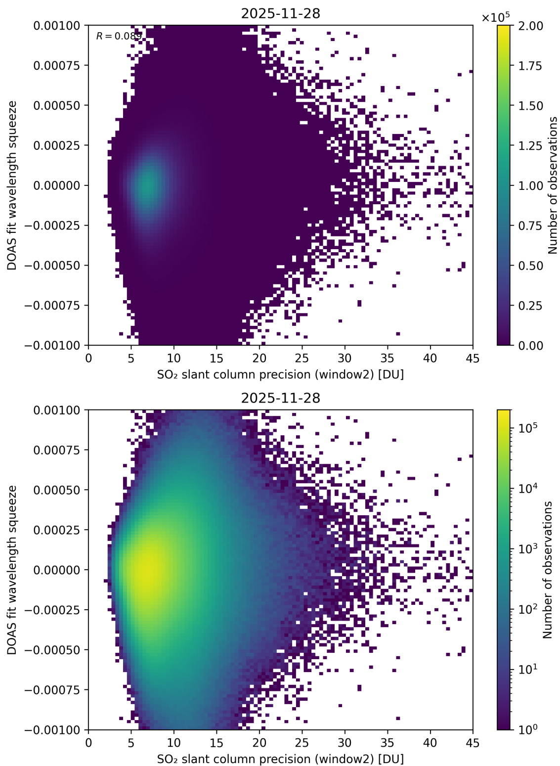
Figure 294: Scatter density plot of “SO 2 slant column precision (window2)” against “DOAS fit wavelength squeeze” for 2025-11-28 to 2025-11-29.
