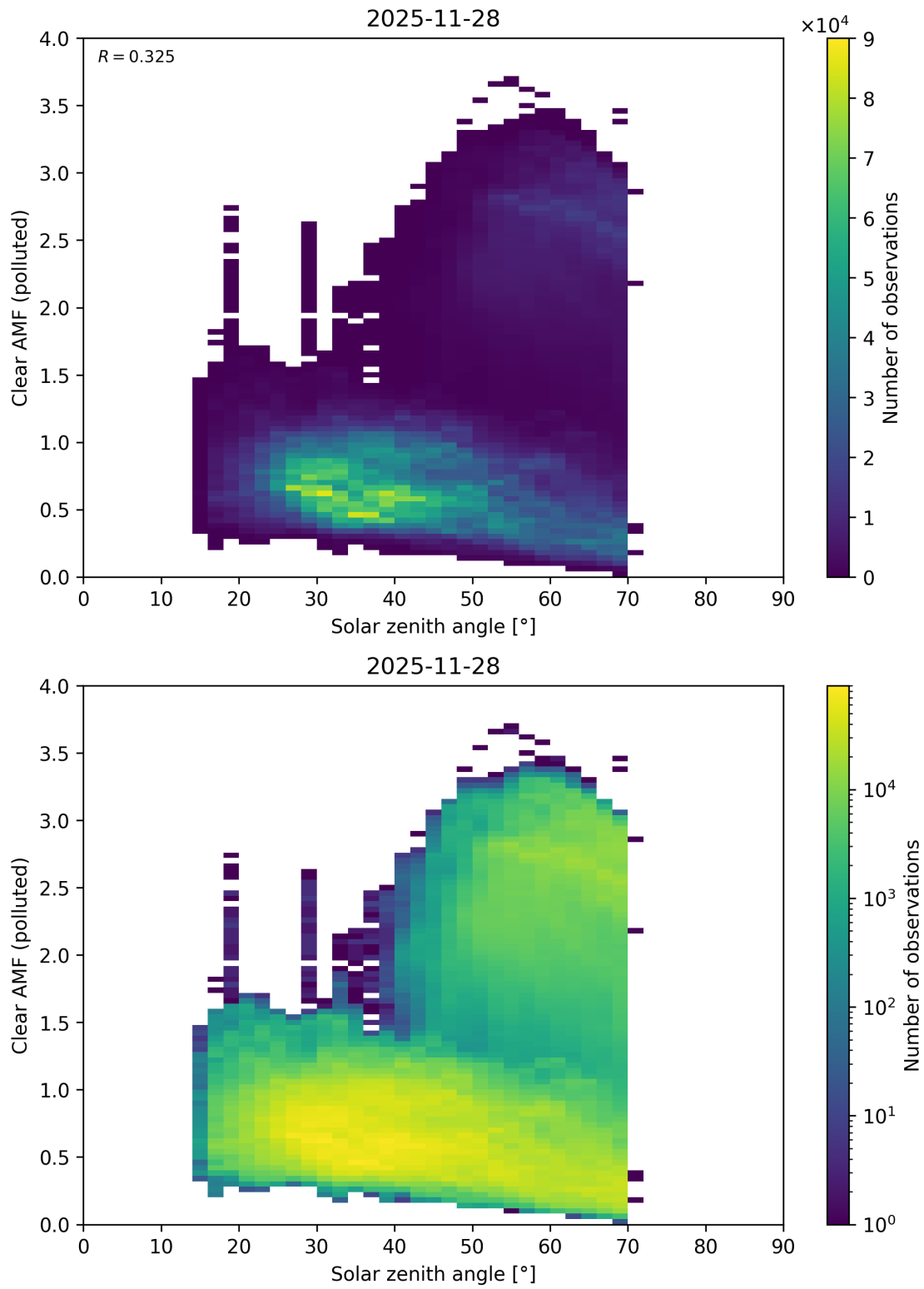
Figure 178: Scatter density plot of “Solar zenith angle” against “Clear AMF (polluted)” for 2025-11-28 to 2025-11-29.
