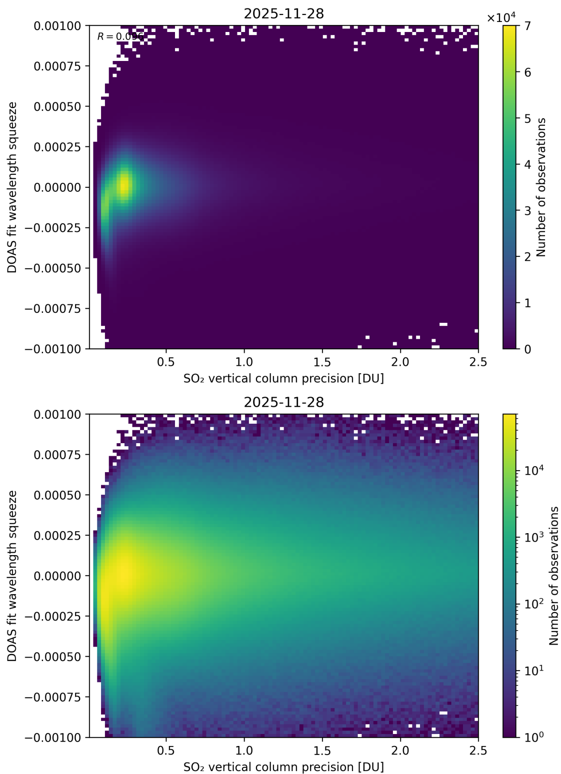
Figure 333: Scatter density plot of “SO 2 vertical column precision” against “DOAS fit wavelength squeeze” for 2025-11-28 to 2025-11-29.
