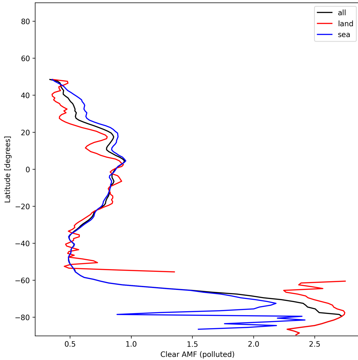
Figure 55: Zonal average of “Clear AMF (polluted)” for 2025-11-28 to 2025-11-29.
