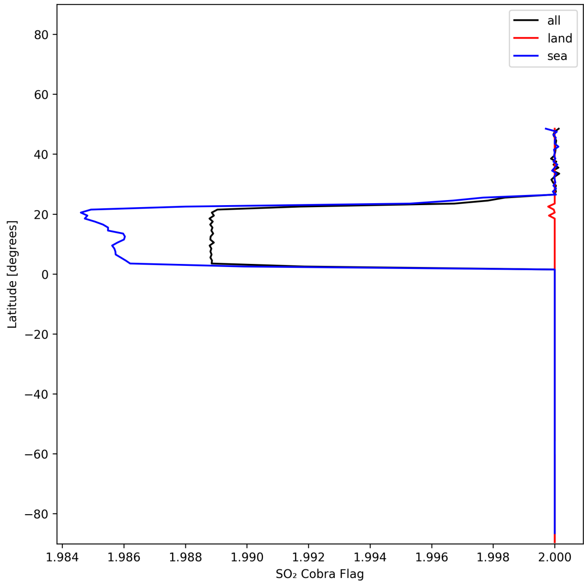
Figure 49: Zonal average of “SO 2 Cobra Flag” for 2025-11-28 to 2025-11-29.
