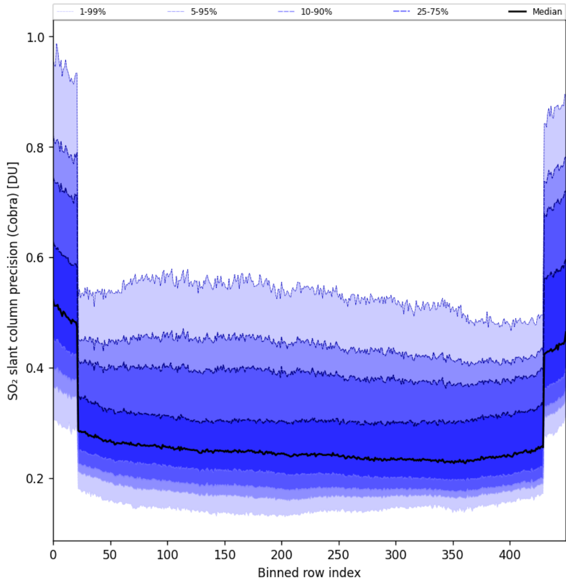
Figure 88: Along track statistics of “SO 2 slant column precision (Cobra)” for 2025-11-28 to 2025-11-29
