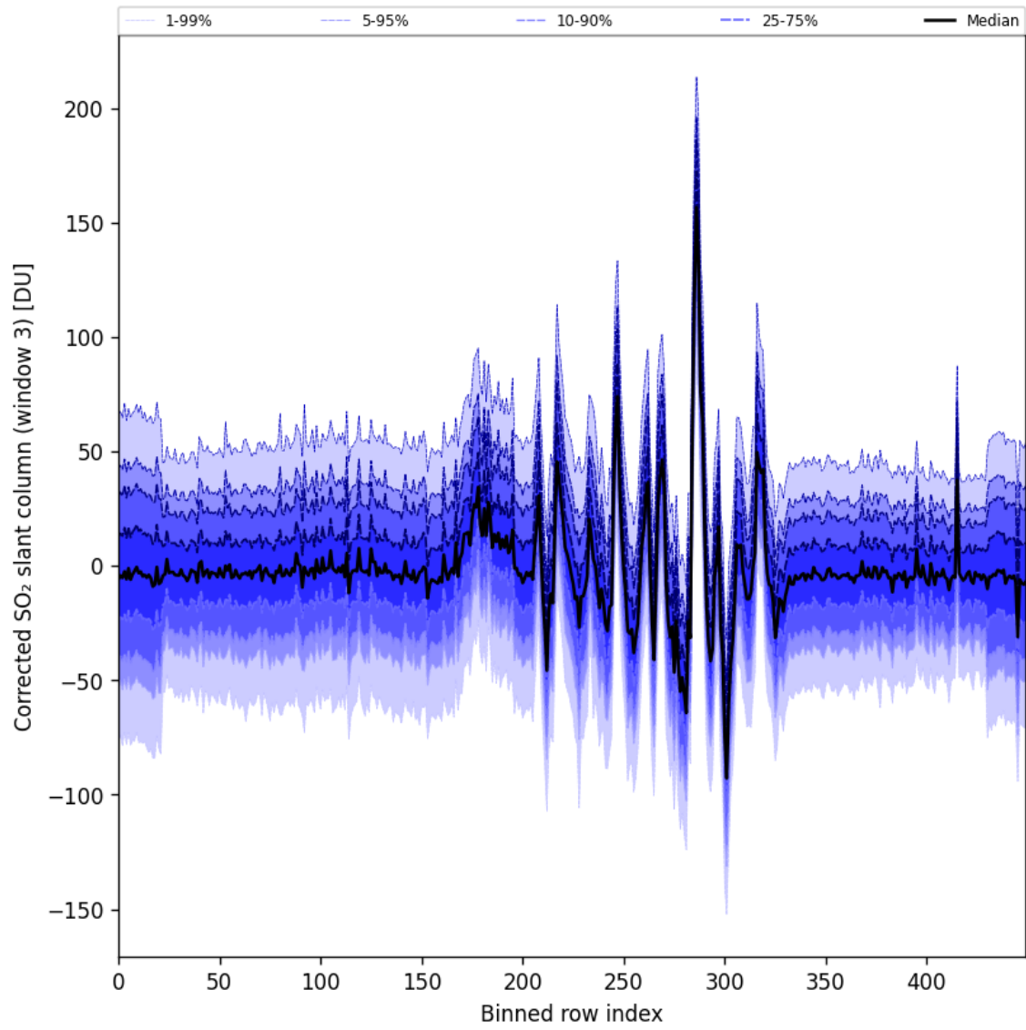
Figure 99: Along track statistics of “Corrected SO 2 slant column (window 3)” for 2025-11-28 to 2025-11-29
