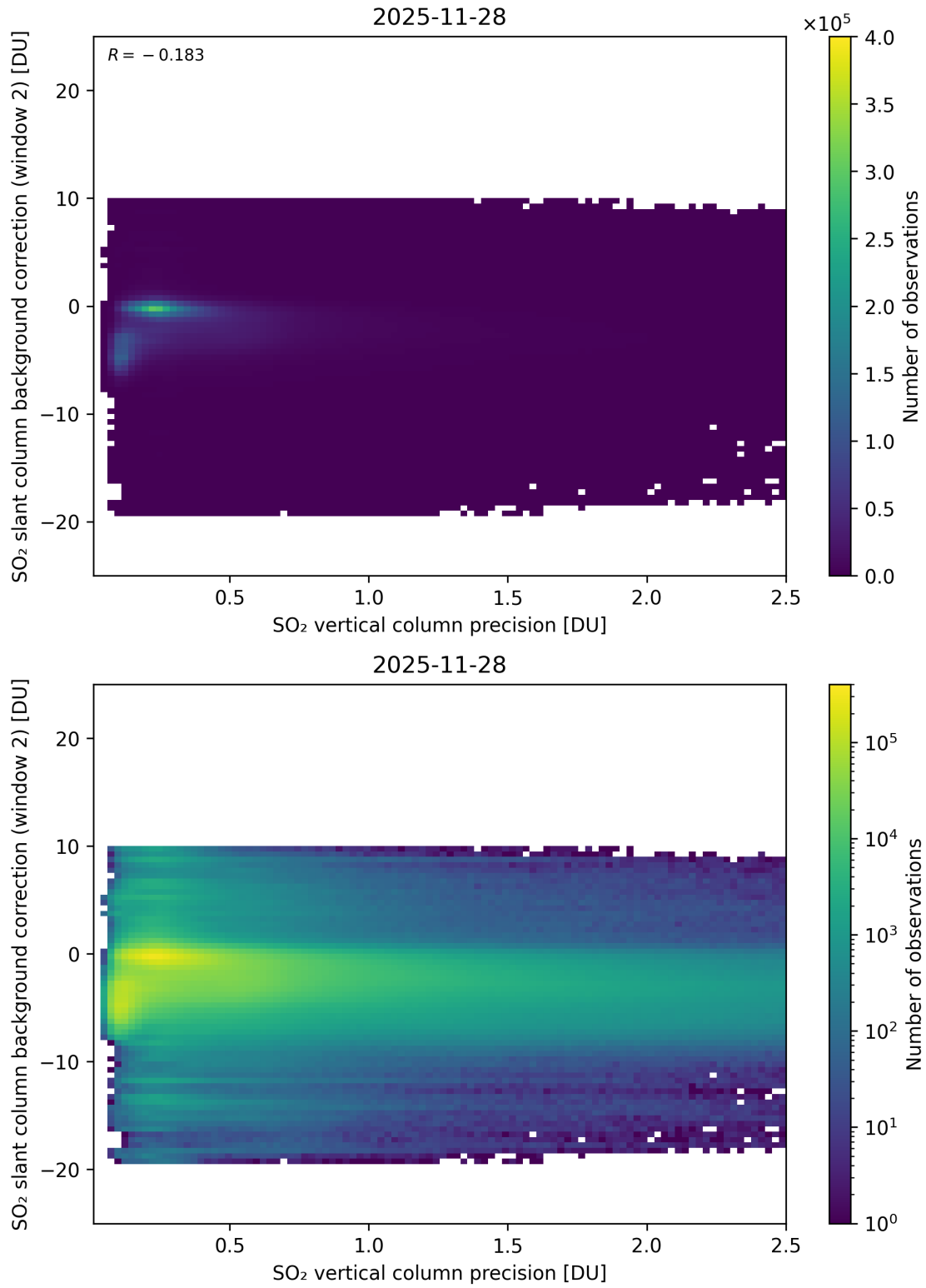
Figure 330: Scatter density plot of “SO 2 vertical column precision” against “SO 2 slant column background correction (window 2)” for 2025-11-28 to 2025-11-29.
