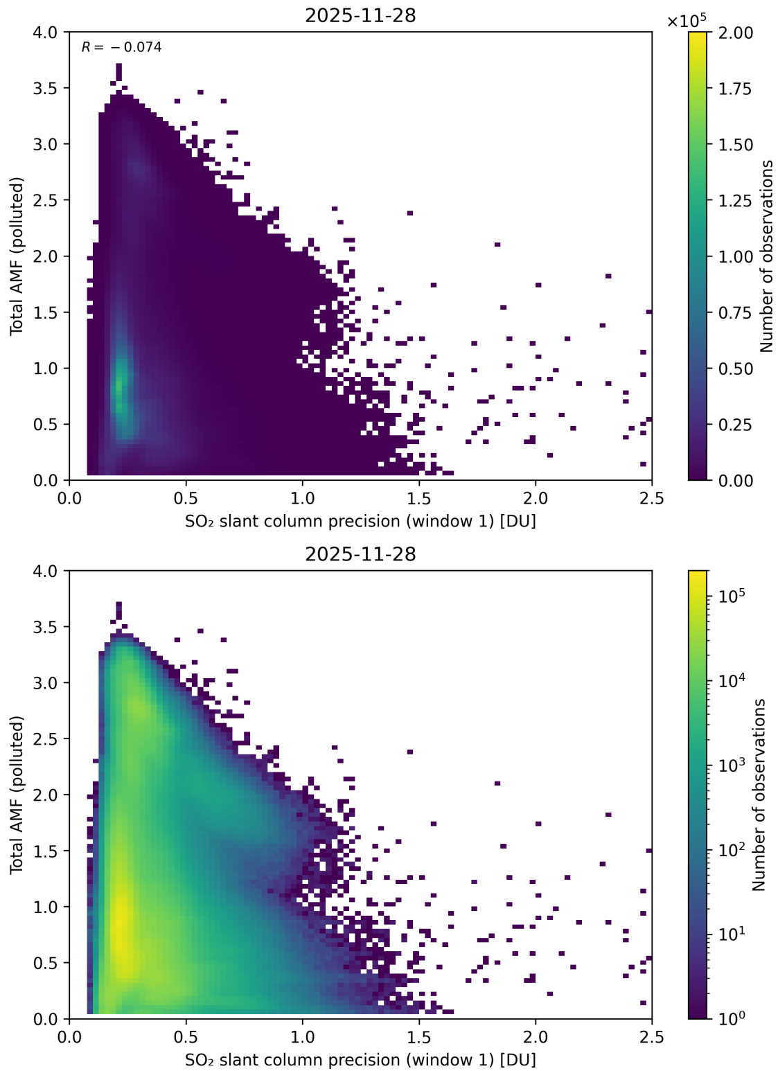
Figure 280: Scatter density plot of “SO 2 slant column precision (window 1)” against “Total AMF (polluted)” for 2025-11-28 to 2025-11-29.
