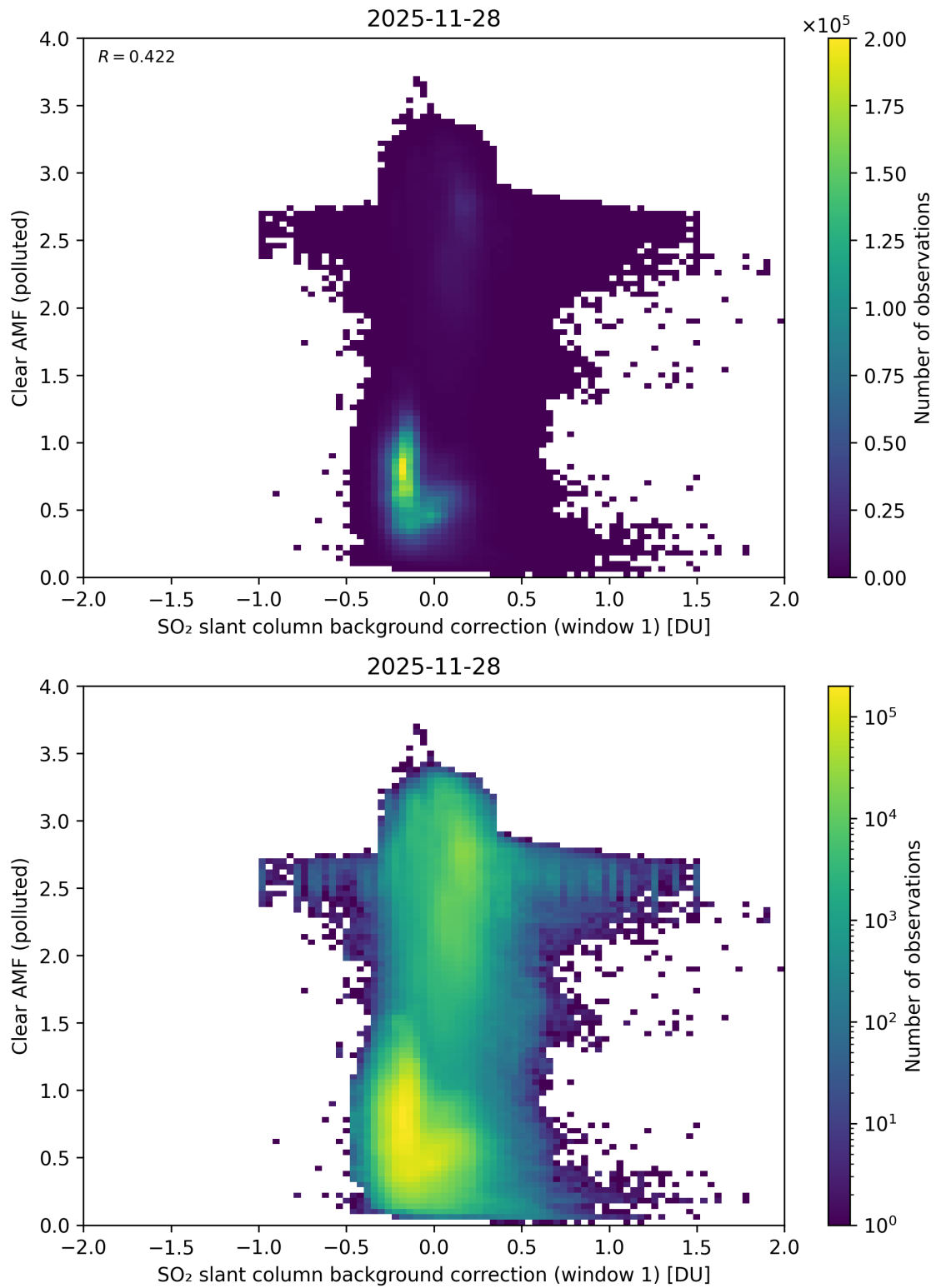
Figure 114: Scatter density plot of “SO 2 slant column background correction (window 1)” against “Clear AMF (polluted)” for 2025-11-28 to 2025-11-29.
