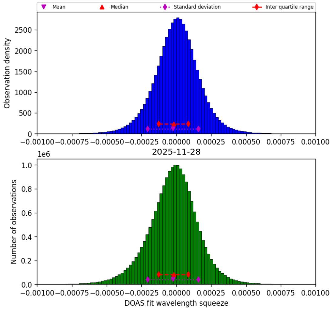
Figure 77: Histogram of “DOAS fit wavelength squeeze” for 2025-11-28 to 2025-11-29
