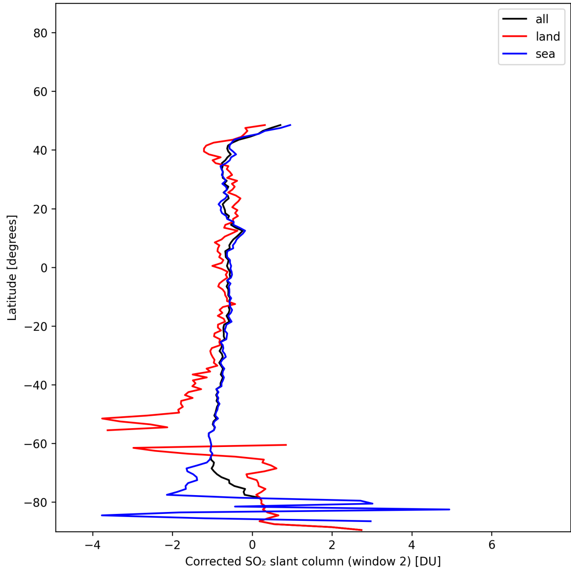
Figure 43: Zonal average of “Corrected SO 2 slant column (window 2)” for 2025-11-28 to 2025-11-29.
