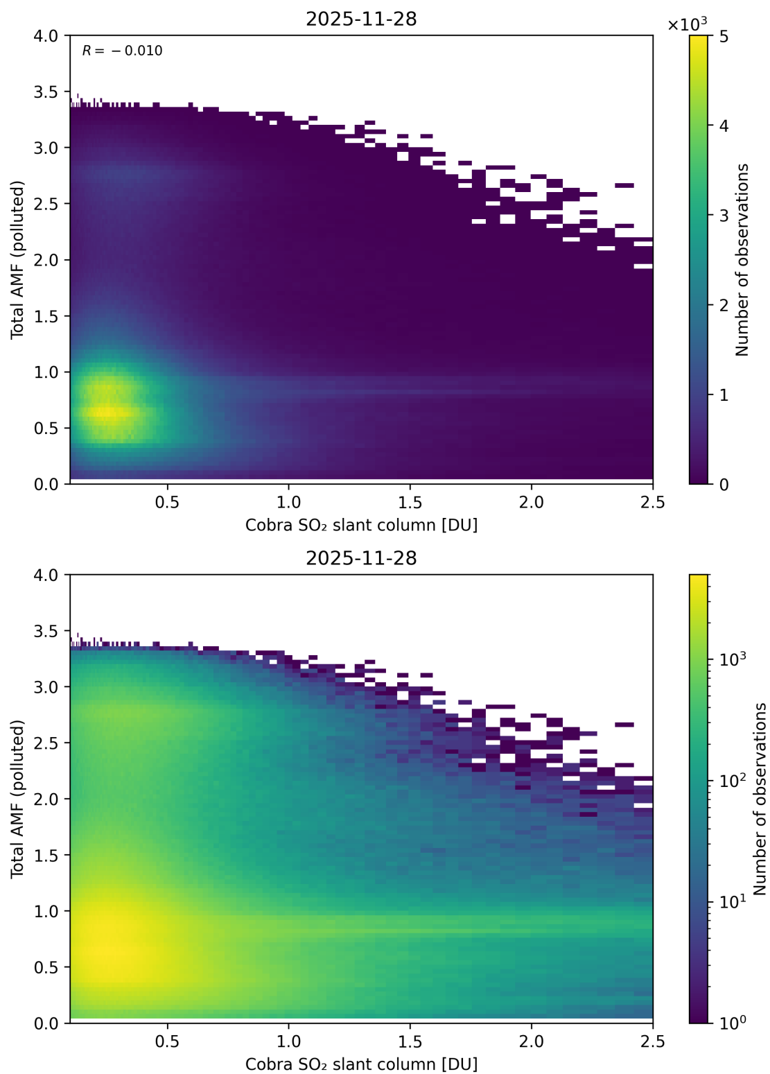
Figure 224: Scatter density plot of “Cobra SO 2 slant column” against “Total AMF (polluted)” for 2025-11-28 to 2025-11-29.
