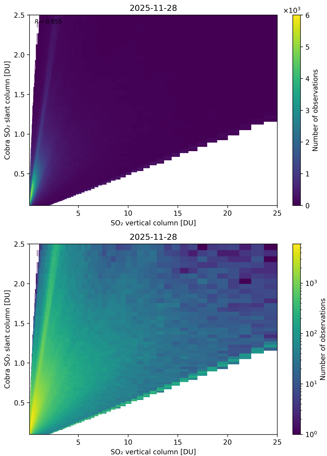
Figure 349: Scatter density plot of “SO 2 vertical column” against “Cobra SO 2 slant column” for 2025-11-28 to 2025-11-29.
