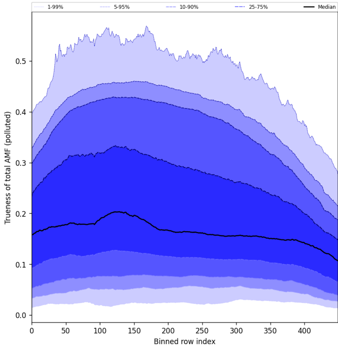
Figure 106: Along track statistics of “Trueness of total AMF (polluted)” for 2025-11-28 to 2025-11-29
