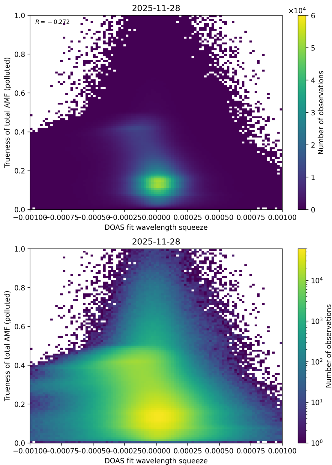
Figure 146: Scatter density plot of “DOAS fit wavelength squeeze” against “Trueness of total AMF (polluted)” for 2025-11-28 to 2025-11-29.
