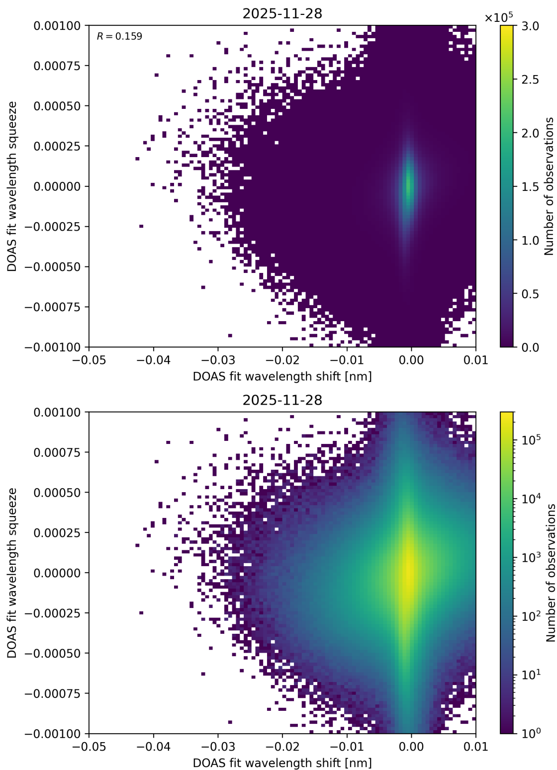
Figure 138: Scatter density plot of “DOAS fit wavelength shift” against “DOAS fit wavelength squeeze” for 2025-11-28 to 2025-11-29.
