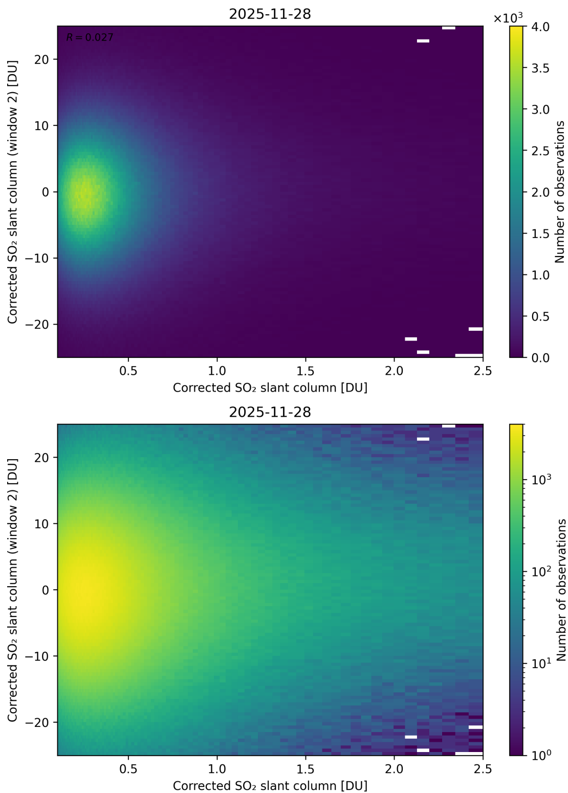
Figure 235: Scatter density plot of “Corrected SO 2 slant column” against “Corrected SO 2 slant column (window 2)” for 2025-11-28 to 2025-11-29.
