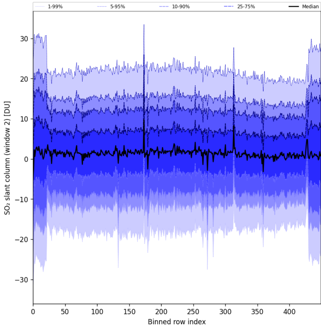
Figure 93: Along track statistics of “SO 2 slant column (window 2)” for 2025-11-28 to 2025-11-29
