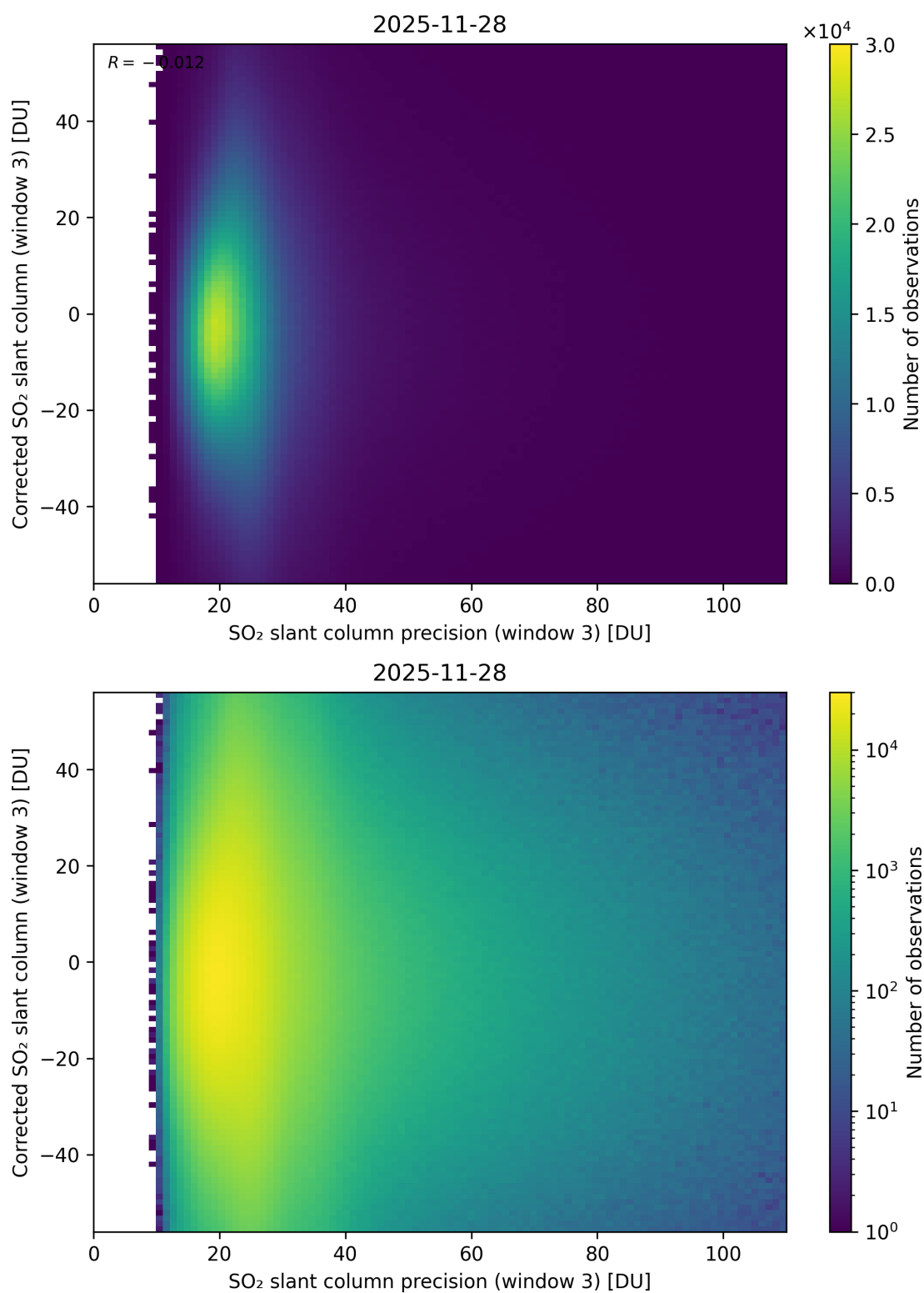
Figure 312: Scatter density plot of “SO 2 slant column precision (window 3)” against “Corrected SO 2 slant column (window 3)” for 2025-11-28 to 2025-11-29.
