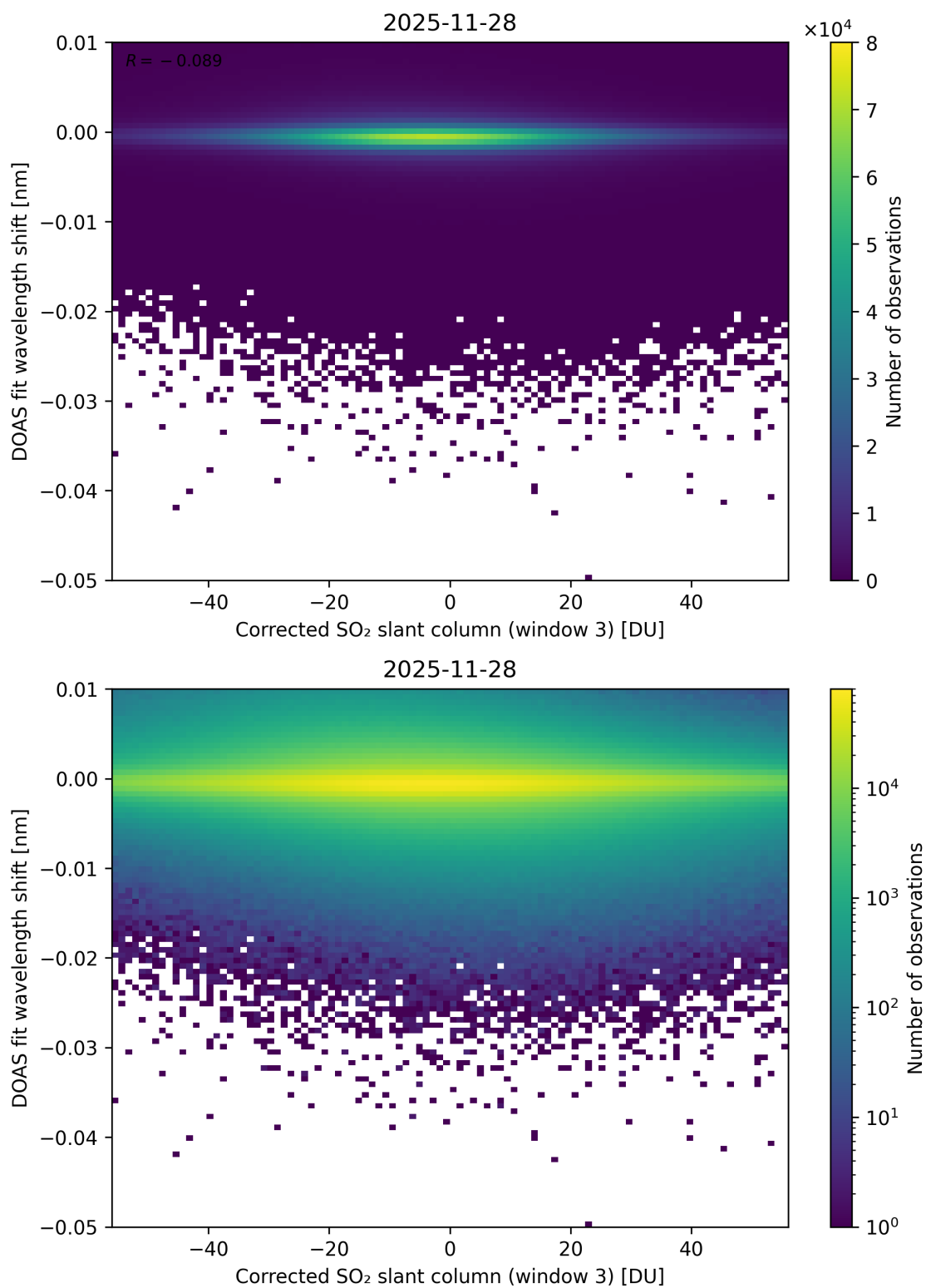
Figure 256: Scatter density plot of “Corrected SO 2 slant column (window 3)” against “DOAS fit wavelength shift” for 2025-11-28 to 2025-11-29.
