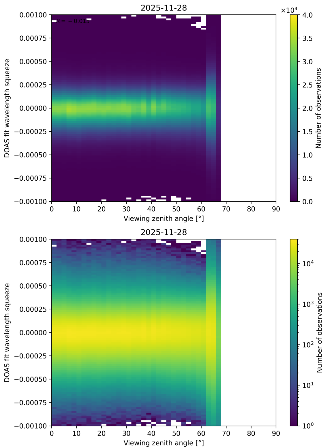
Figure 366: Scatter density plot of “Viewing zenith angle” against “DOAS fit wavelength squeeze” for 2025-11-28 to 2025-11-29.
