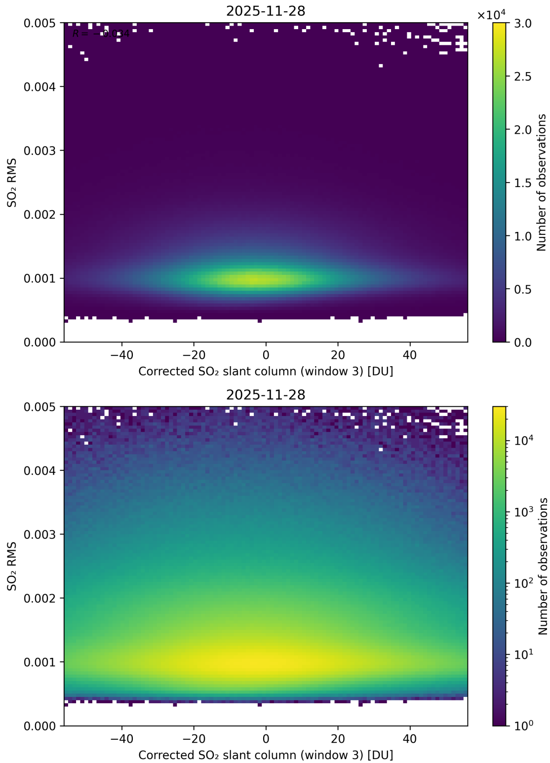
Figure 258: Scatter density plot of “Corrected SO 2 slant column (window 3)” against “SO 2 RMS” for 2025-11-28 to 2025-11-29.
