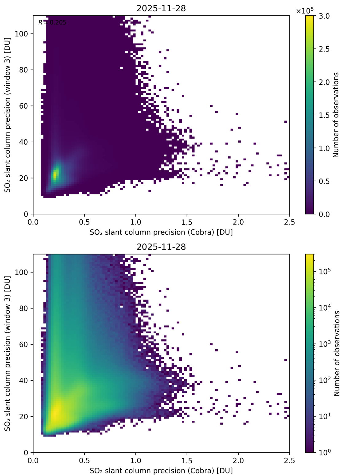
Figure 212: Scatter density plot of “SO 2 slant column precision (Cobra)” against “SO 2 slant column precision (window 3)” for 2025-11-28 to 2025-11-29.
