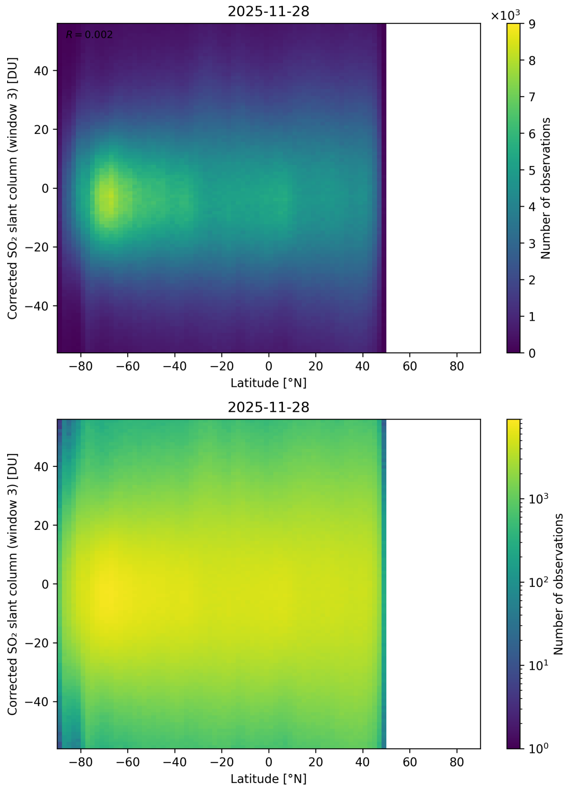
Figure 161: Scatter density plot of “Latitude” against “Corrected SO 2 slant column (window 3)” for 2025-11-28 to 2025-11-29.
