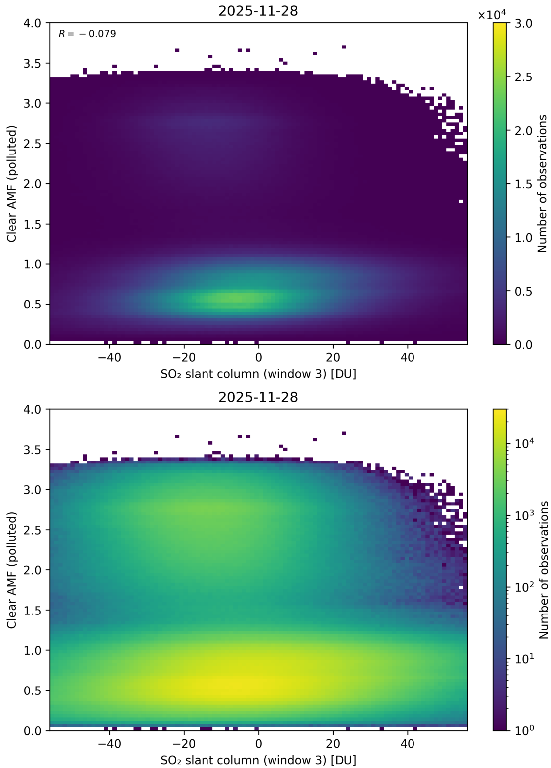
Figure 315: Scatter density plot of “SO 2 slant column (window 3)” against “Clear AMF (polluted)” for 2025-11-28 to 2025-11-29.
