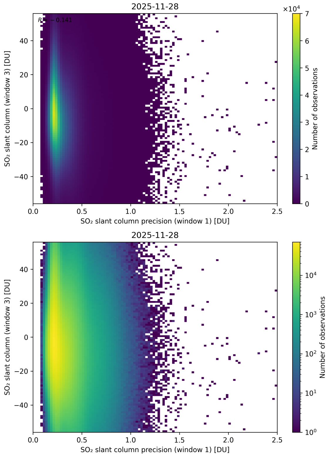
Figure 278: Scatter density plot of “SO 2 slant column precision (window 1)” against “SO 2 slant column (window 3)” for 2025-11-28 to 2025-11-29.
