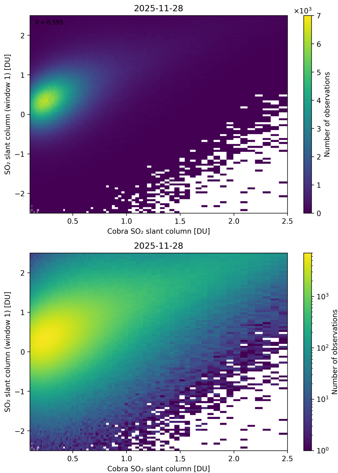
Figure 219: Scatter density plot of “Cobra SO 2 slant column” against “SO 2 slant column (window 1)” for 2025-11-28 to 2025-11-29.
