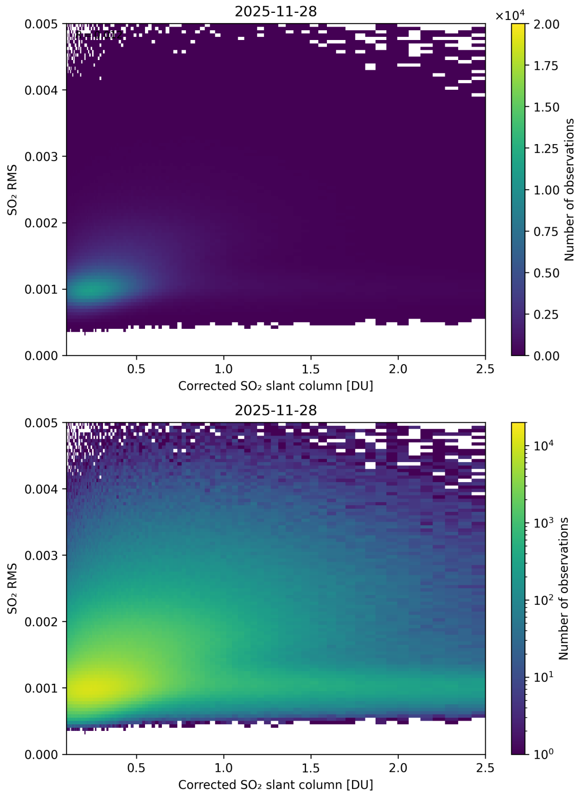
Figure 231: Scatter density plot of “Corrected SO 2 slant column” against “SO 2 RMS” for 2025-11-28 to 2025-11-29.
