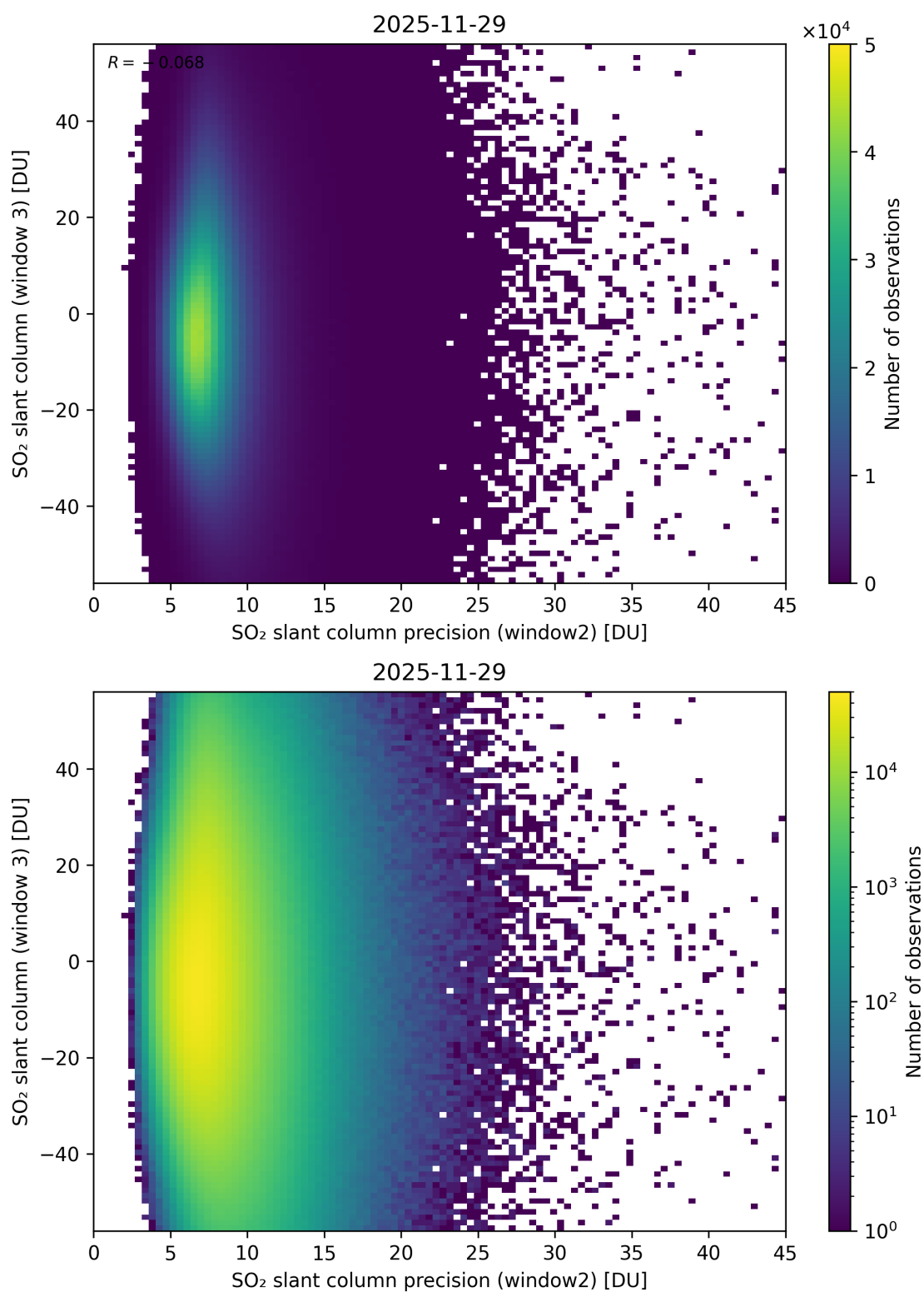
Figure 299: Scatter density plot of “SO 2 slant column precision (window2)” against “SO 2 slant column (window 3)” for 2025-11-28 to 2025-11-30.
