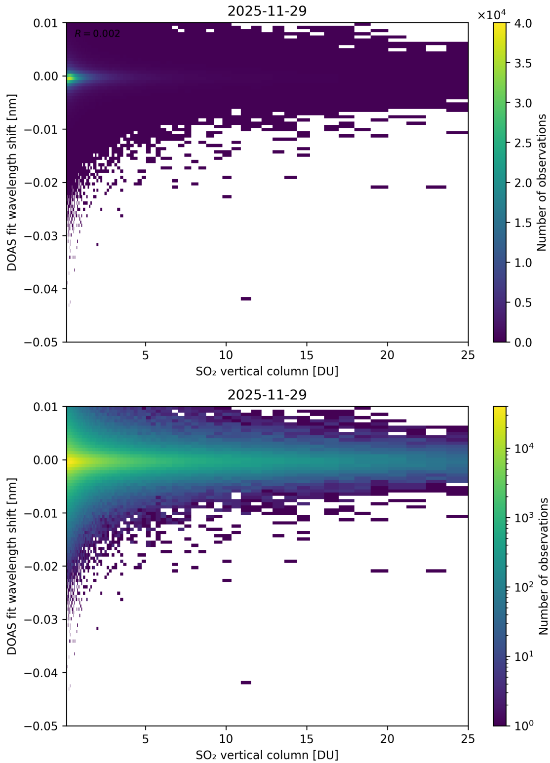
Figure 326: Scatter density plot of “SO 2 vertical column” against “DOAS fit wavelength shift” for 2025-11-28 to 2025-11-30.
