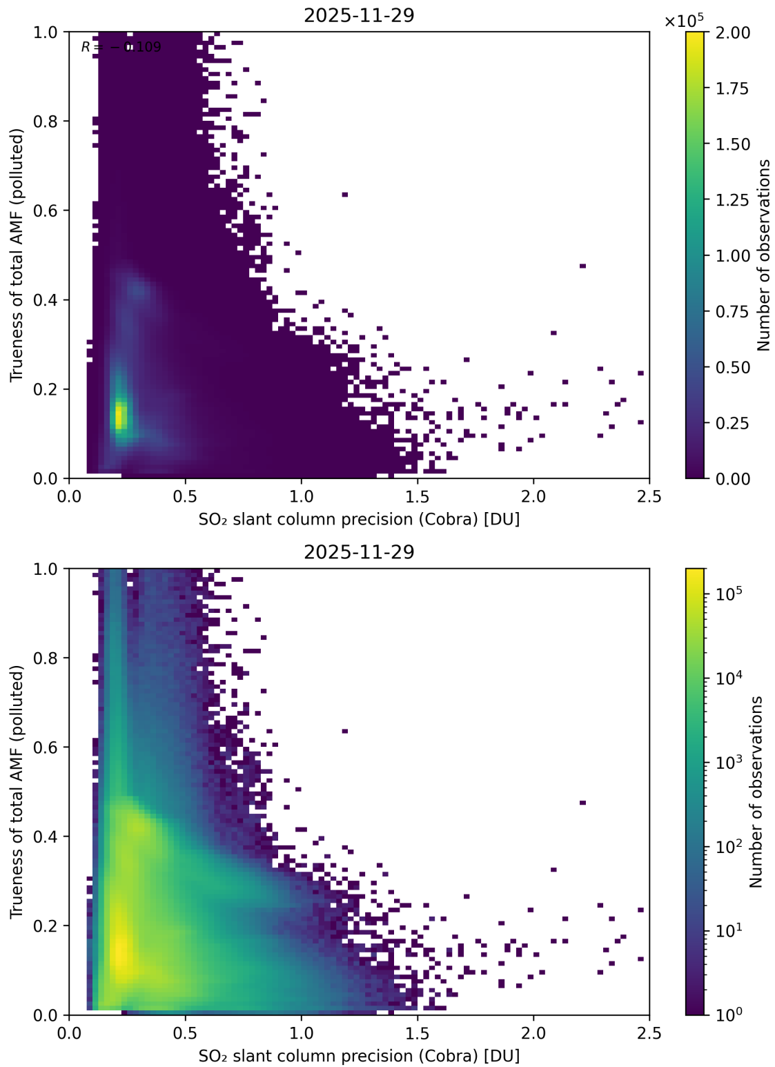
Figure 214: Scatter density plot of “SO 2 slant column precision (Cobra)” against “Trueness of total AMF (polluted)” for 2025-11-28 to 2025-11-30.
