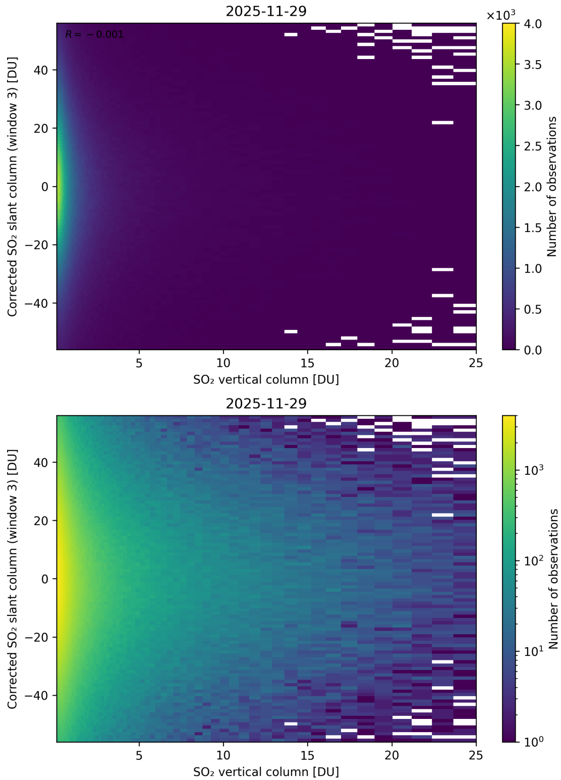
Figure 353: Scatter density plot of “SO 2 vertical column” against “Corrected SO 2 slant column (window 3)” for 2025-11-28 to 2025-11-30.
