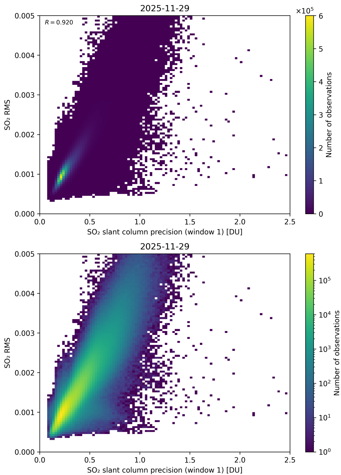
Figure 273: Scatter density plot of “SO 2 slant column precision (window 1)” against “SO 2 RMS” for 2025-11-28 to 2025-11-30.
