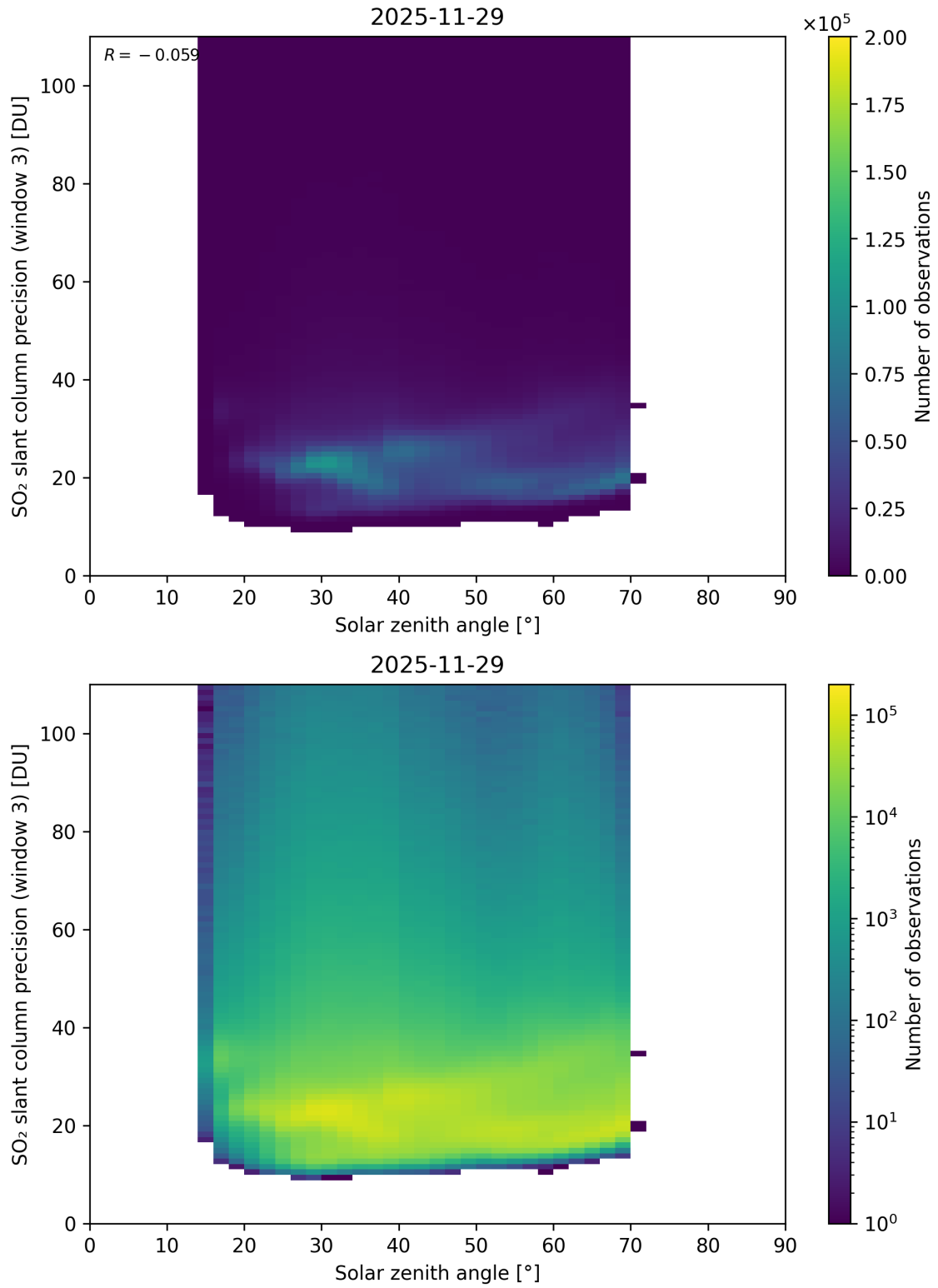
Figure 188: Scatter density plot of “Solar zenith angle” against “SO 2 slant column precision (window 3)” for 2025-11-28 to 2025-11-30.
