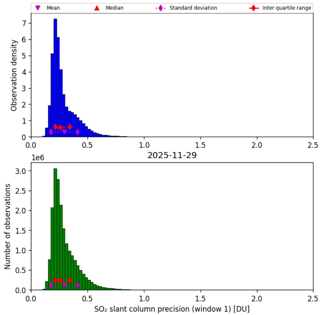
Figure 64: Histogram of “SO 2 slant column precision (window 1)” for 2025-11-28 to 2025-11-30
