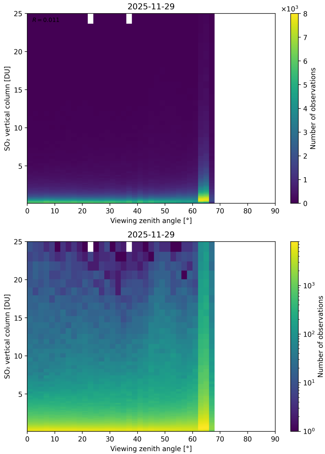
Figure 383: Scatter density plot of “Viewing zenith angle” against “SO 2 vertical column” for 2025-11-28 to 2025-11-30.
