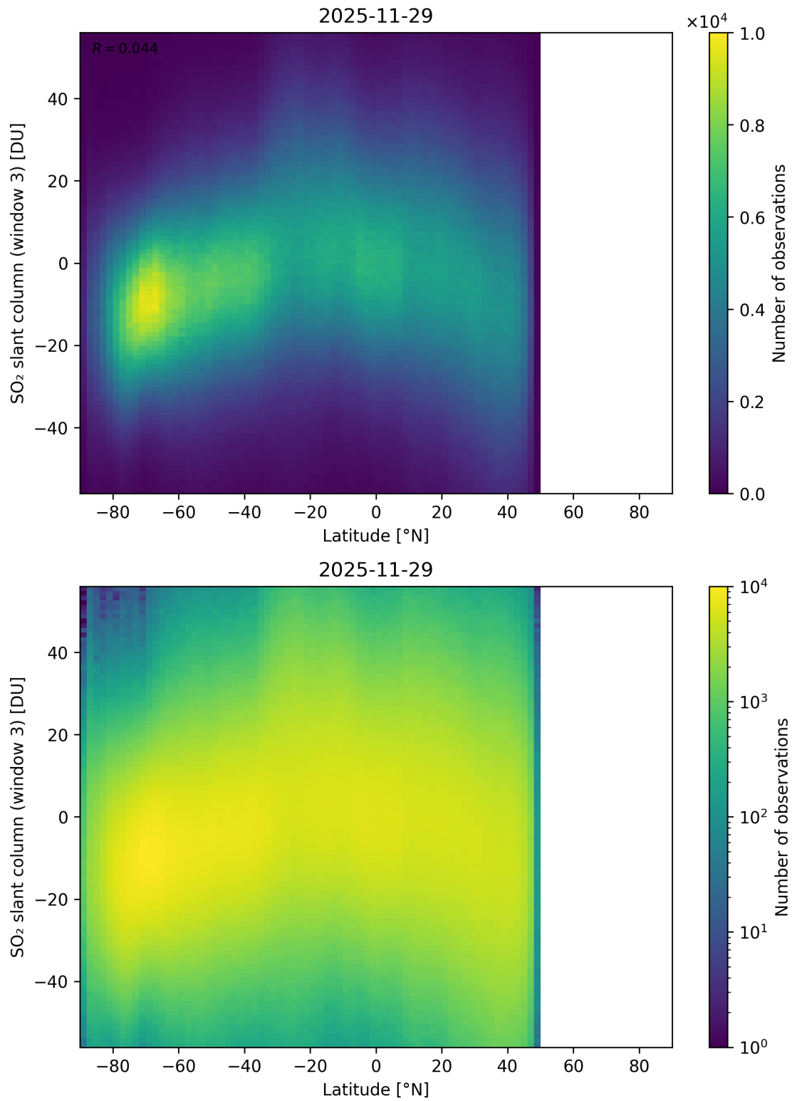
Figure 165: Scatter density plot of “Latitude” against “SO 2 slant column (window 3)” for 2025-11-28 to 2025-11-30.
