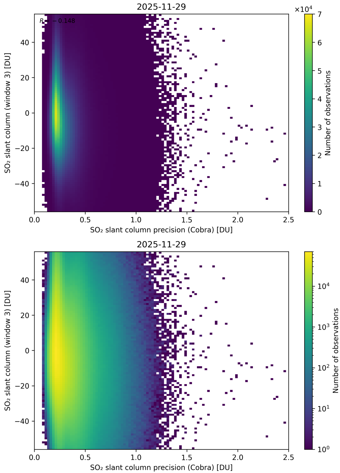
Figure 211: Scatter density plot of “SO 2 slant column precision (Cobra)” against “SO 2 slant column (window 3)” for 2025-11-28 to 2025-11-30.
