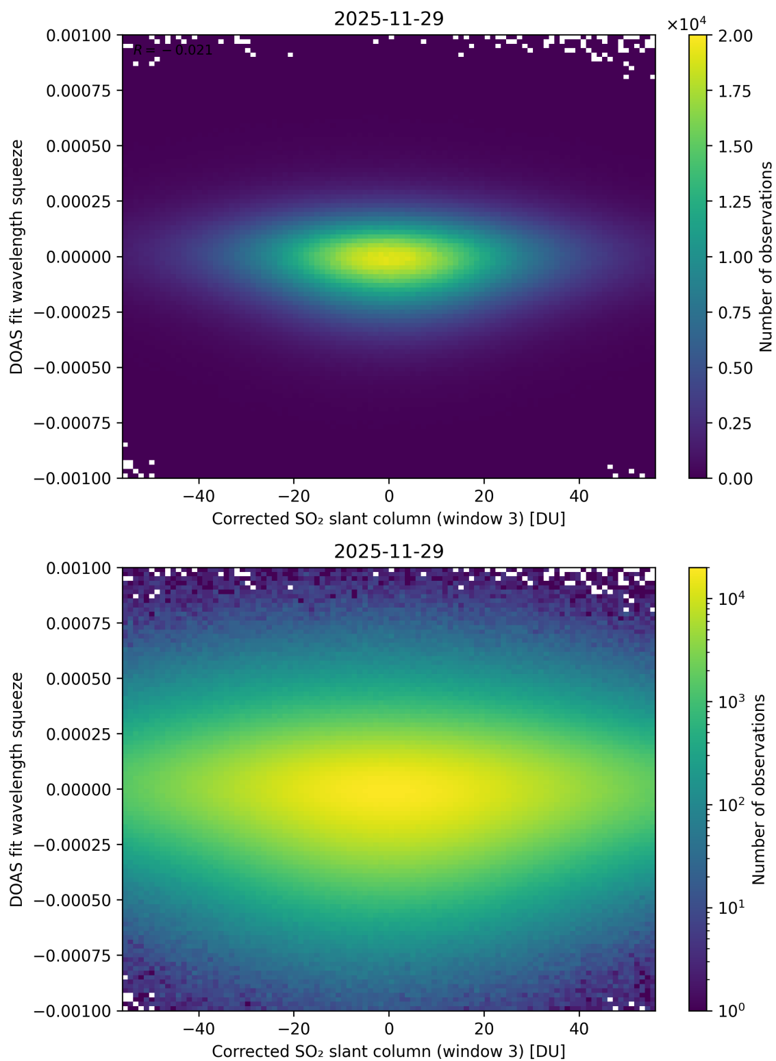
Figure 257: Scatter density plot of “Corrected SO 2 slant column (window 3)” against “DOAS fit wavelength squeeze” for 2025-11-28 to 2025-11-30.
