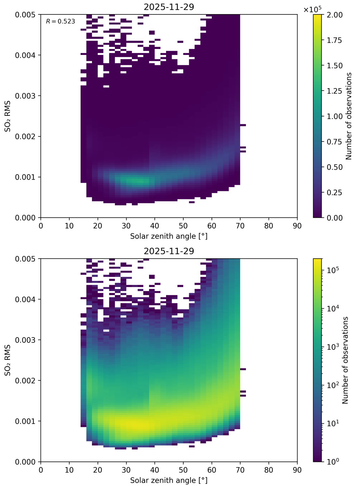
Figure 176: Scatter density plot of “Solar zenith angle” against “SO 2 RMS” for 2025-11-28 to 2025-11-30.
