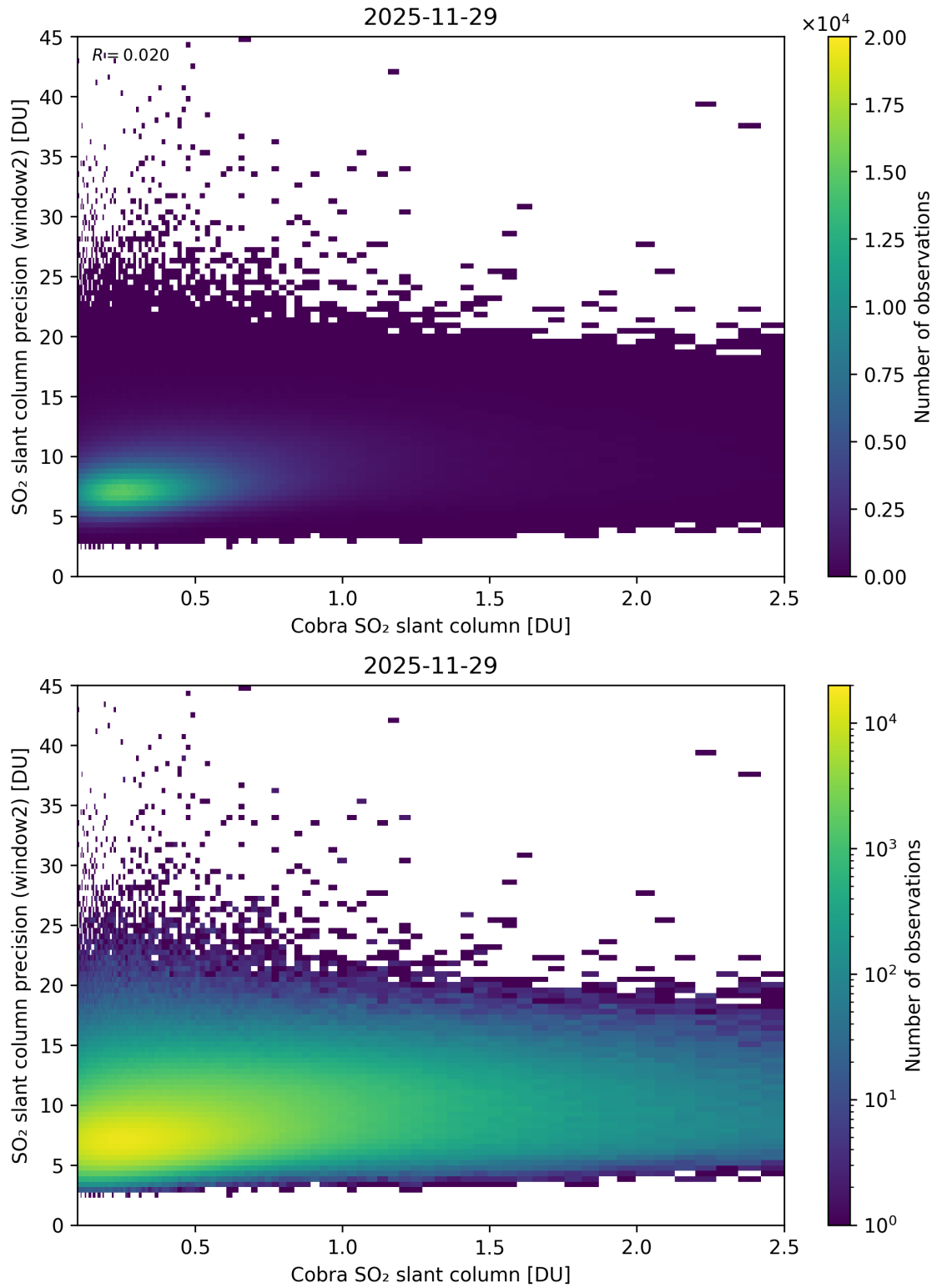
Figure 221: Scatter density plot of “Cobra SO 2 slant column” against “SO 2 slant column precision (window2)” for 2025-11-28 to 2025-11-30.
