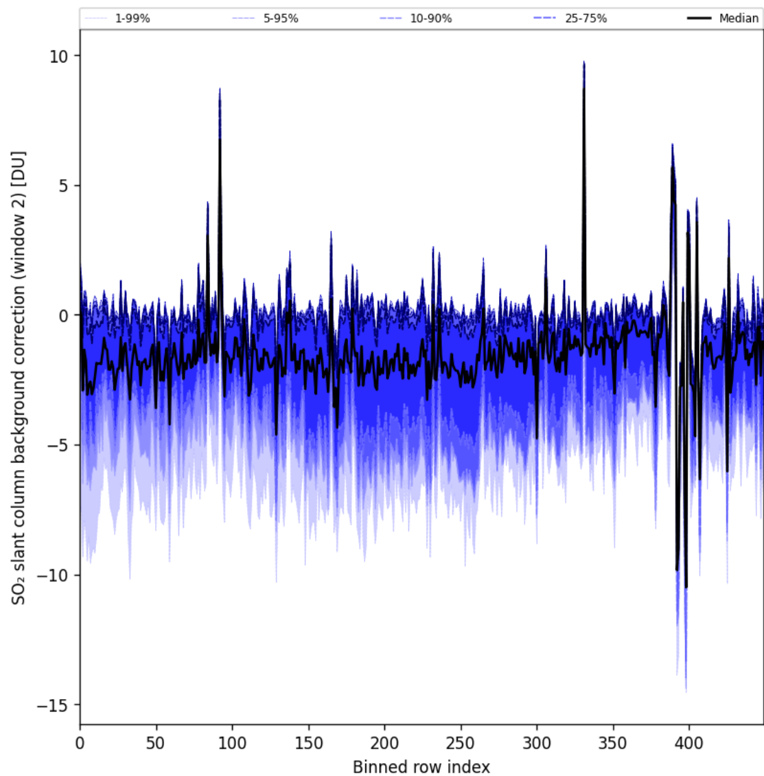
Figure 96: Along track statistics of “SO 2 slant column background correction (window 2)” for 2025-11-28 to 2025-11-30
