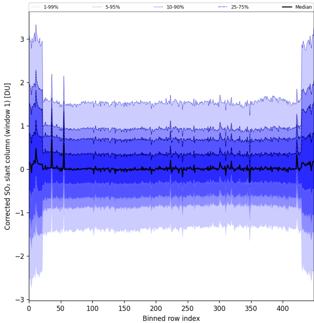
Figure 91: Along track statistics of “Corrected SO 2 slant column (window 1)” for 2025-11-28 to 2025-11-30
