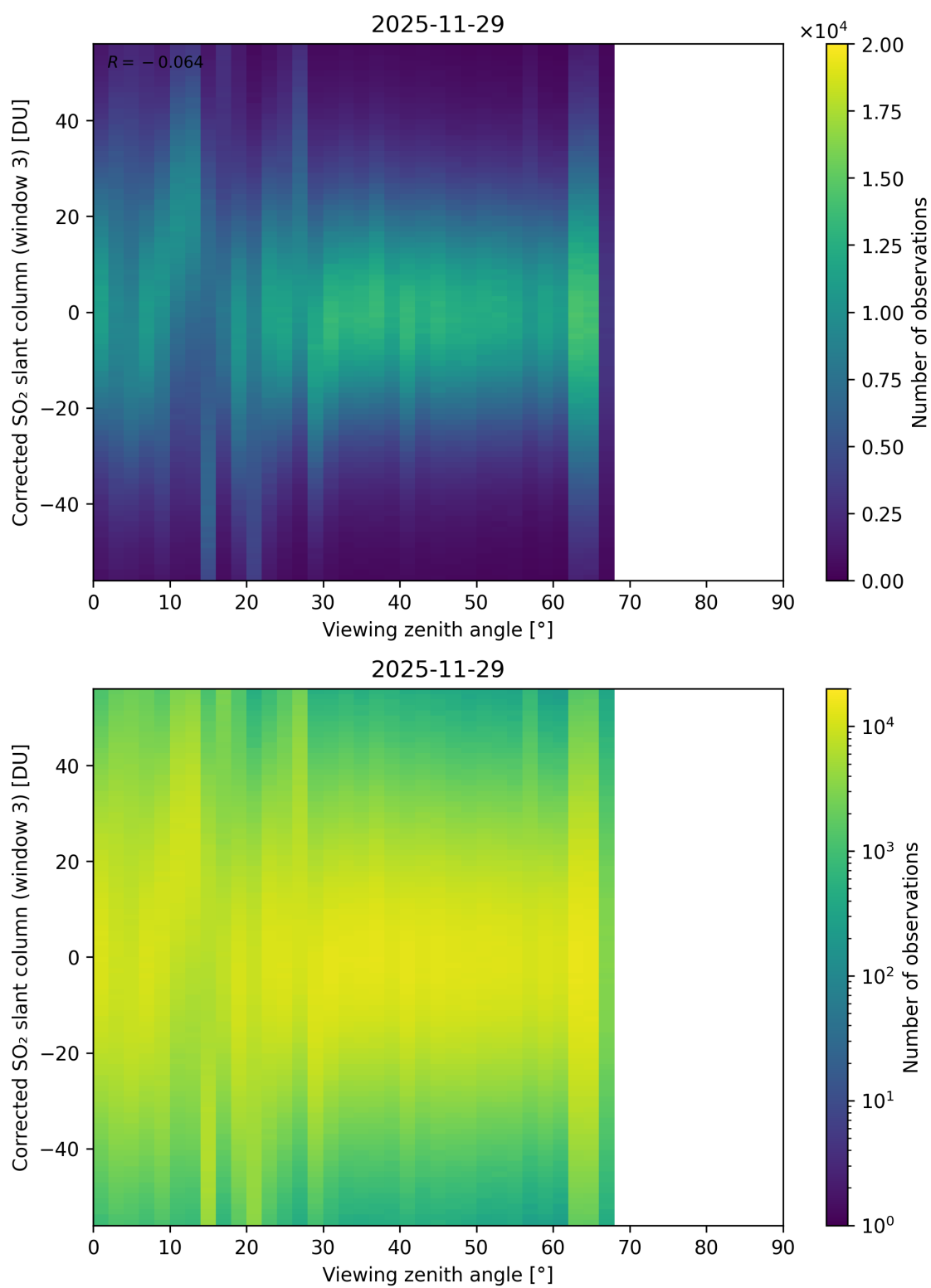
Figure 375: Scatter density plot of “Viewing zenith angle” against “Corrected SO 2 slant column (window 3)” for 2025-11-28 to 2025-11-30.
