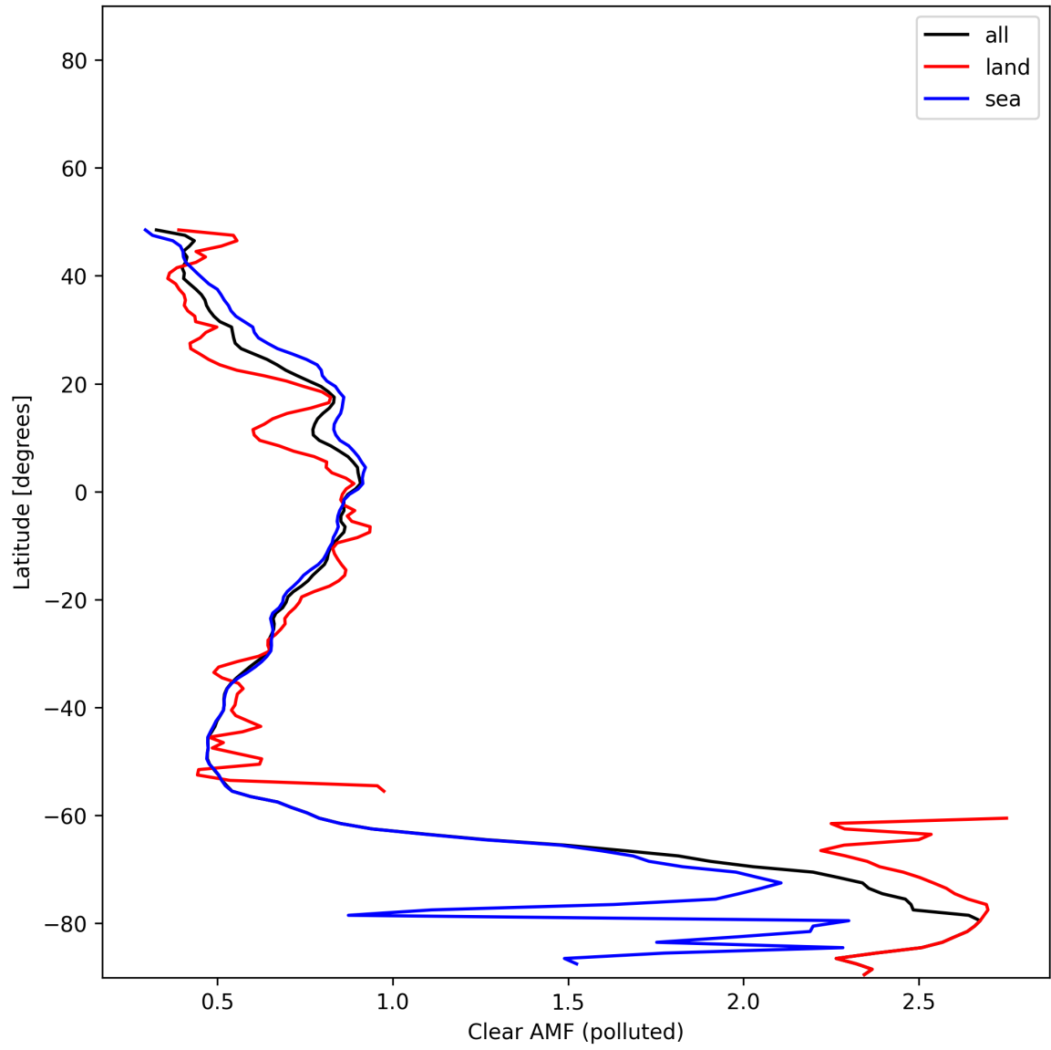
Figure 55: Zonal average of “Clear AMF (polluted)” for 2025-11-28 to 2025-11-30.
