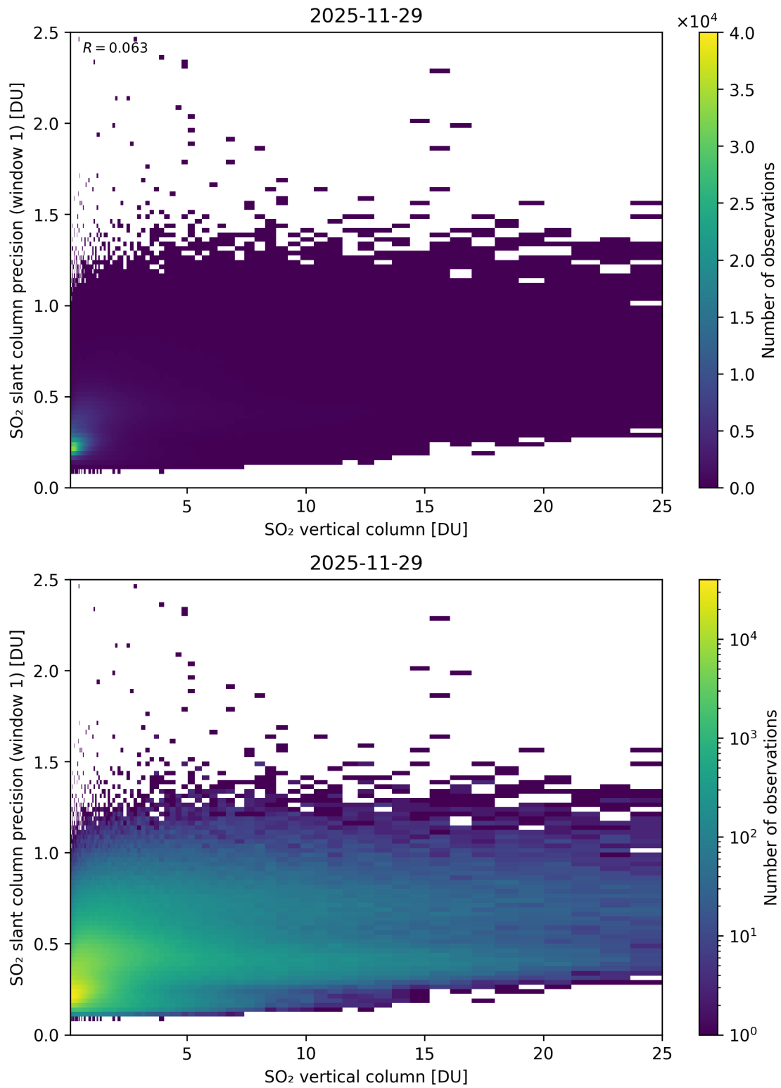
Figure 355: Scatter density plot of “SO 2 vertical column” against “SO 2 slant column precision (window 1)” for 2025-11-28 to 2025-11-30.
