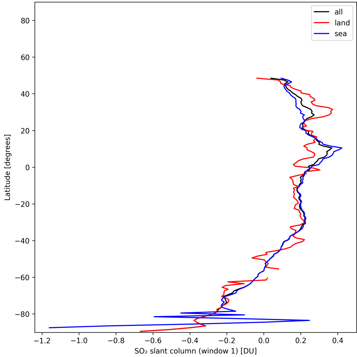
Figure 37: Zonal average of “SO 2 slant column (window 1)” for 2025-11-28 to 2025-11-30.
