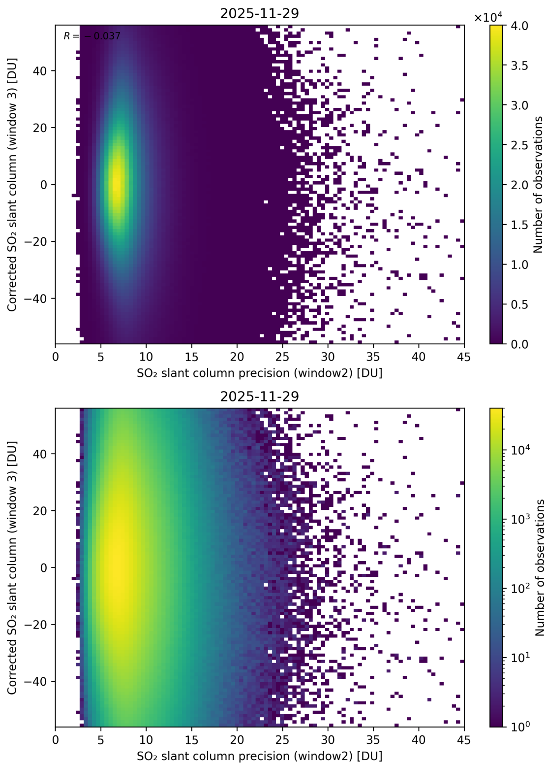
Figure 298: Scatter density plot of “SO 2 slant column precision (window2)” against “Corrected SO 2 slant column (window 3)” for 2025-11-28 to 2025-11-30.
