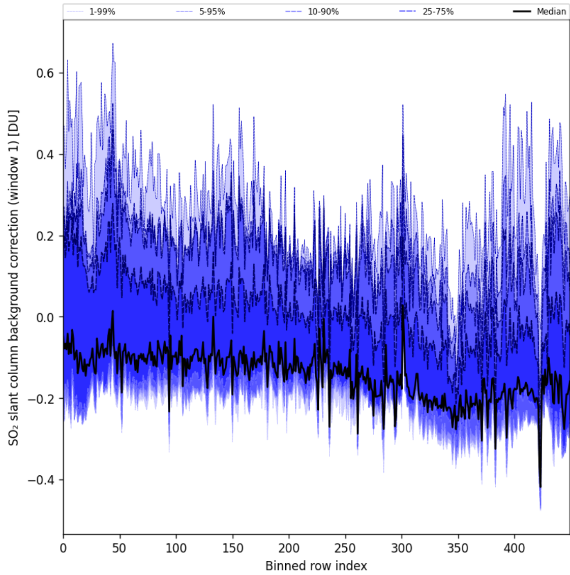
Figure 92: Along track statistics of “SO 2 slant column background correction (window 1)” for 2025-11-28 to 2025-11-30
