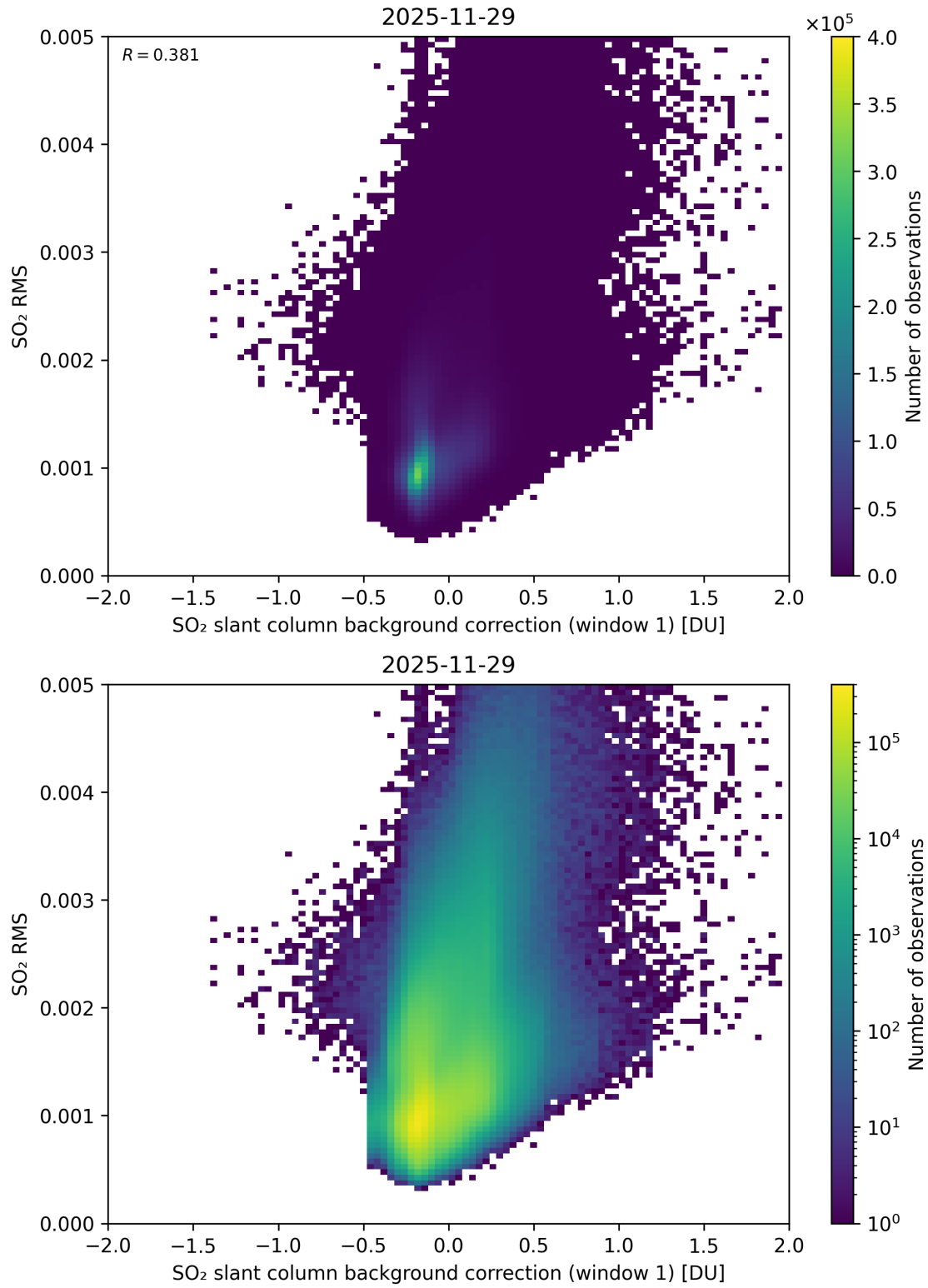
Figure 113: Scatter density plot of “SO 2 slant column background correction (window 1)” against “SO 2 RMS” for 2025-11-28 to 2025-11-30.
