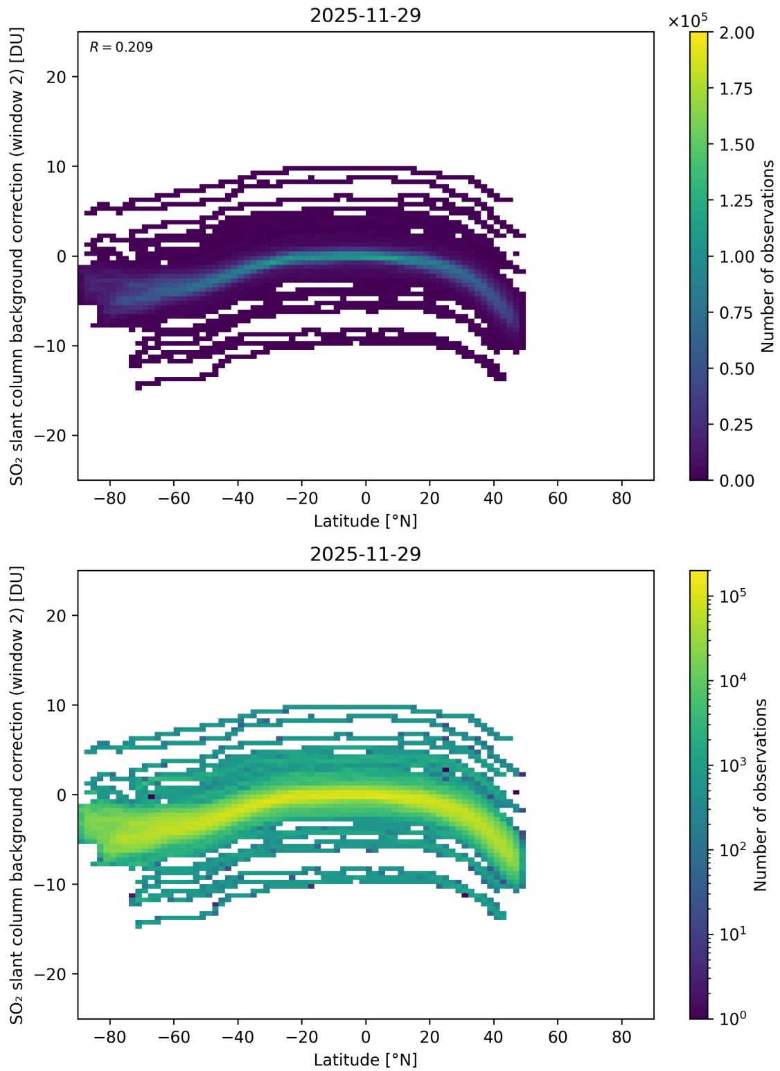
Figure 151: Scatter density plot of “Latitude” against “SO 2 slant column background correction (window 2)” for 2025-11-28 to 2025-11-30.
