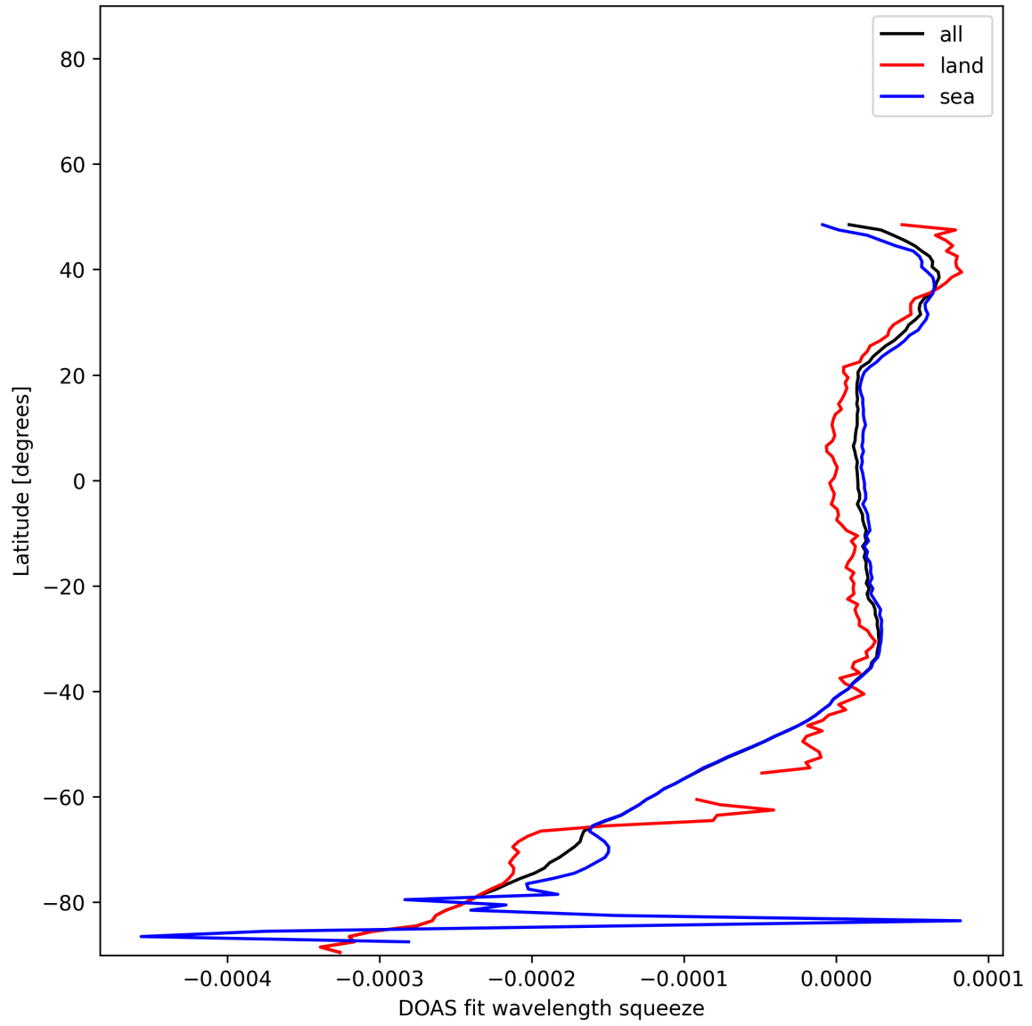
Figure 51: Zonal average of “DOAS fit wavelength squeeze” for 2025-11-28 to 2025-11-30.
