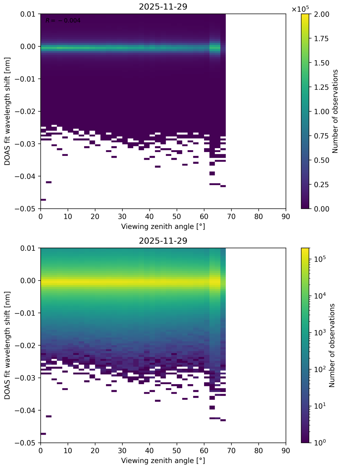
Figure 365: Scatter density plot of “Viewing zenith angle” against “DOAS fit wavelength shift” for 2025-11-28 to 2025-11-30.
