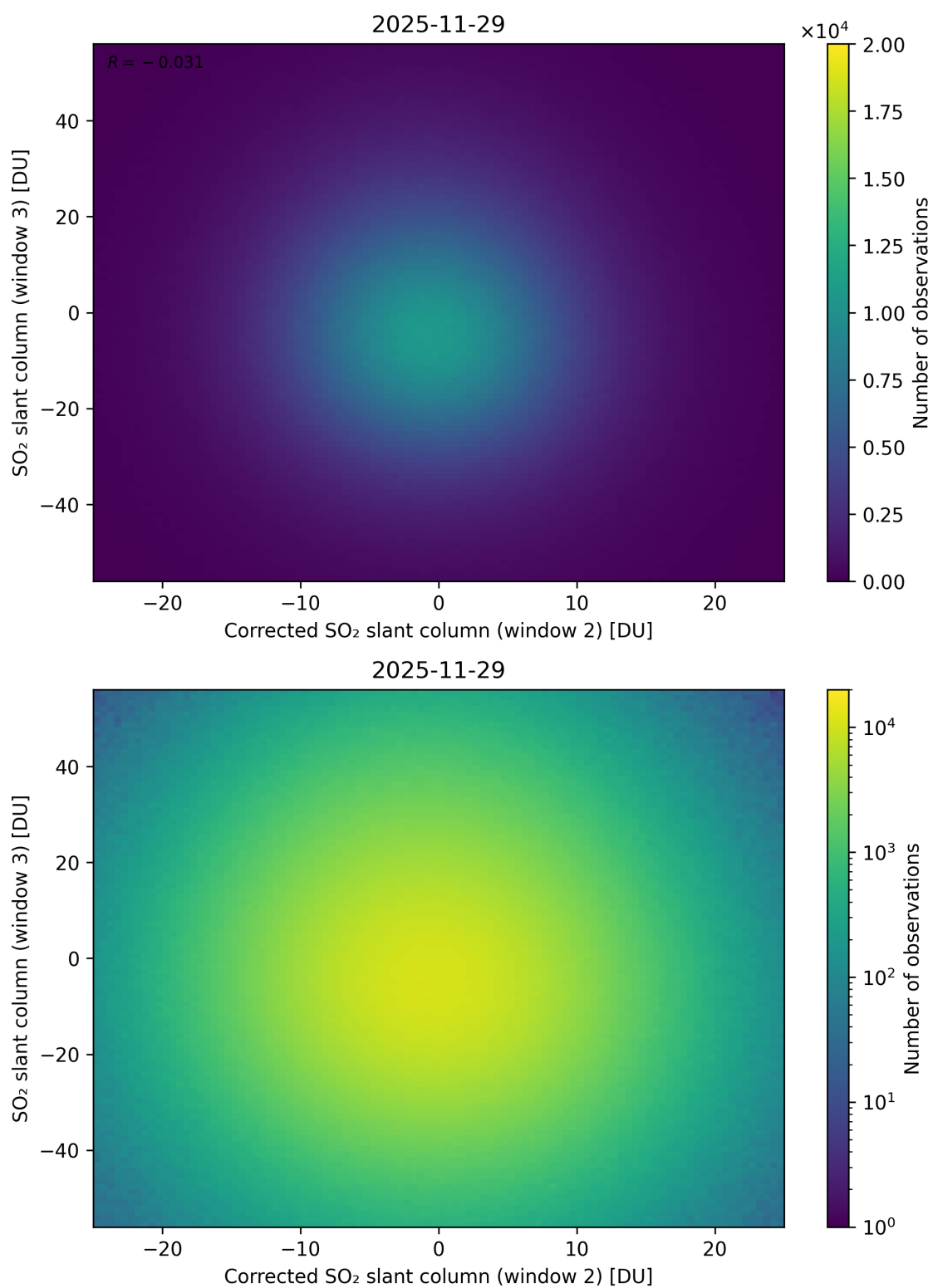
Figure 251: Scatter density plot of “Corrected SO 2 slant column (window 2)” against “SO 2 slant column (window 3)” for 2025-11-28 to 2025-11-30.
