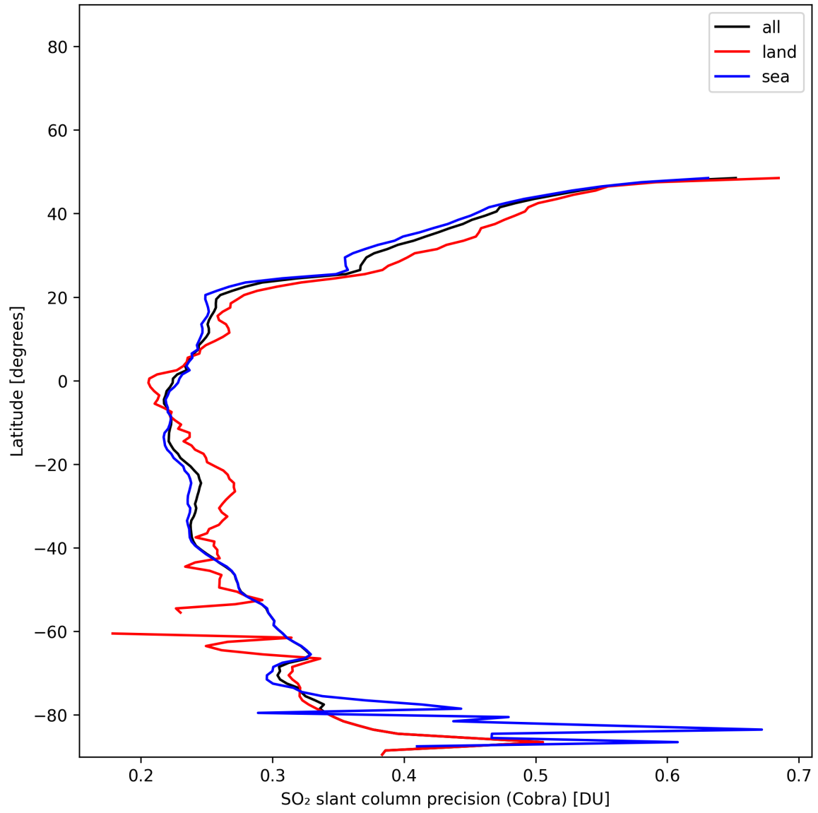
Figure 36: Zonal average of “SO 2 slant column precision (Cobra)” for 2025-11-28 to 2025-11-30.
