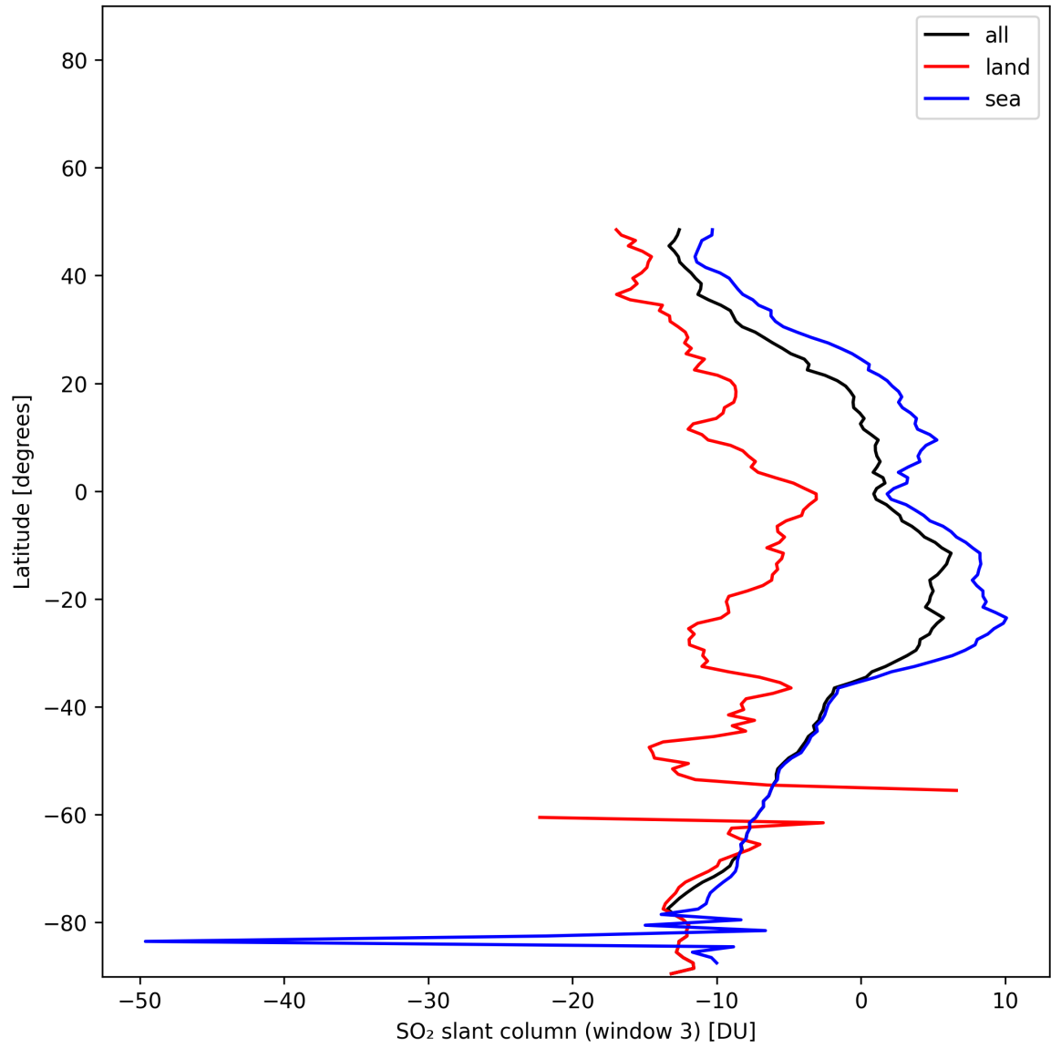
Figure 45: Zonal average of “SO 2 slant column (window 3)” for 2025-11-28 to 2025-11-30.
