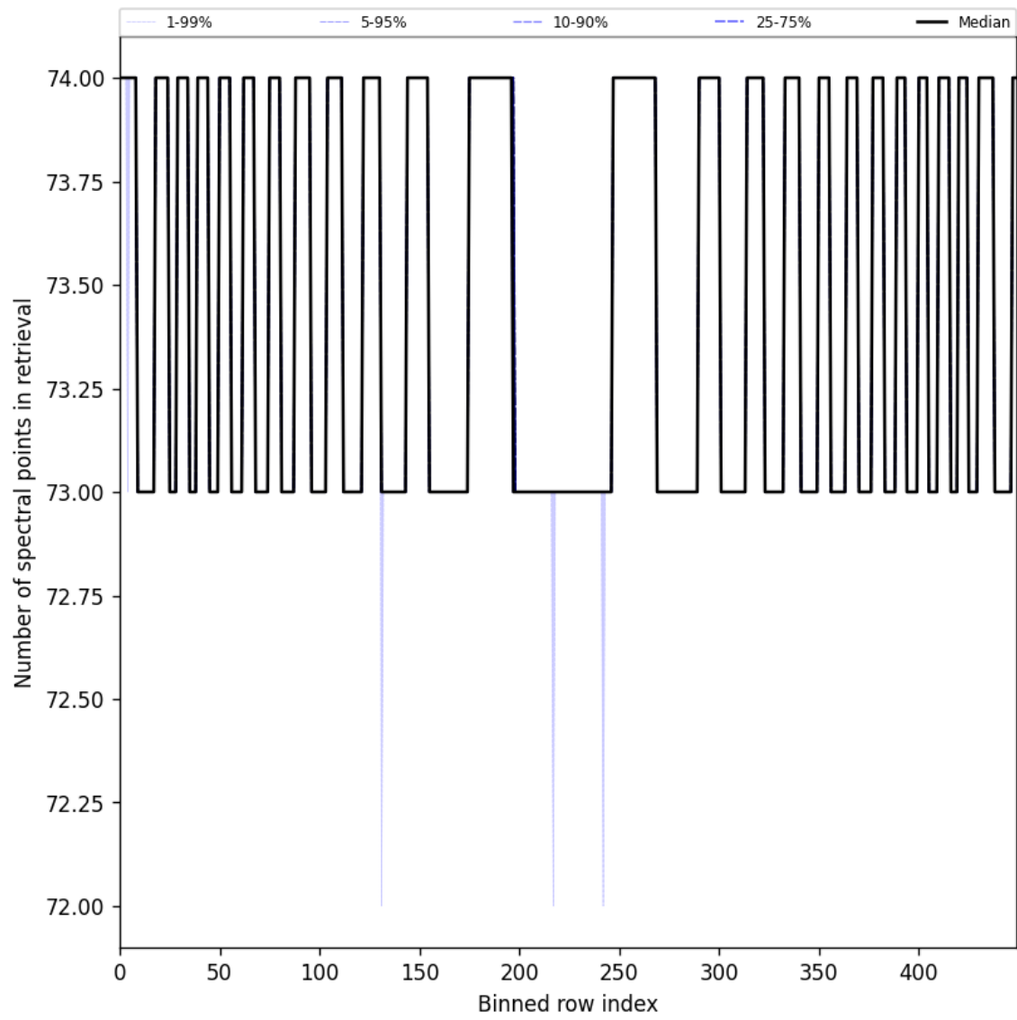
Figure 108: Along track statistics of “Number of spectral points in retrieval” for 2025-11-28 to 2025-11-30
