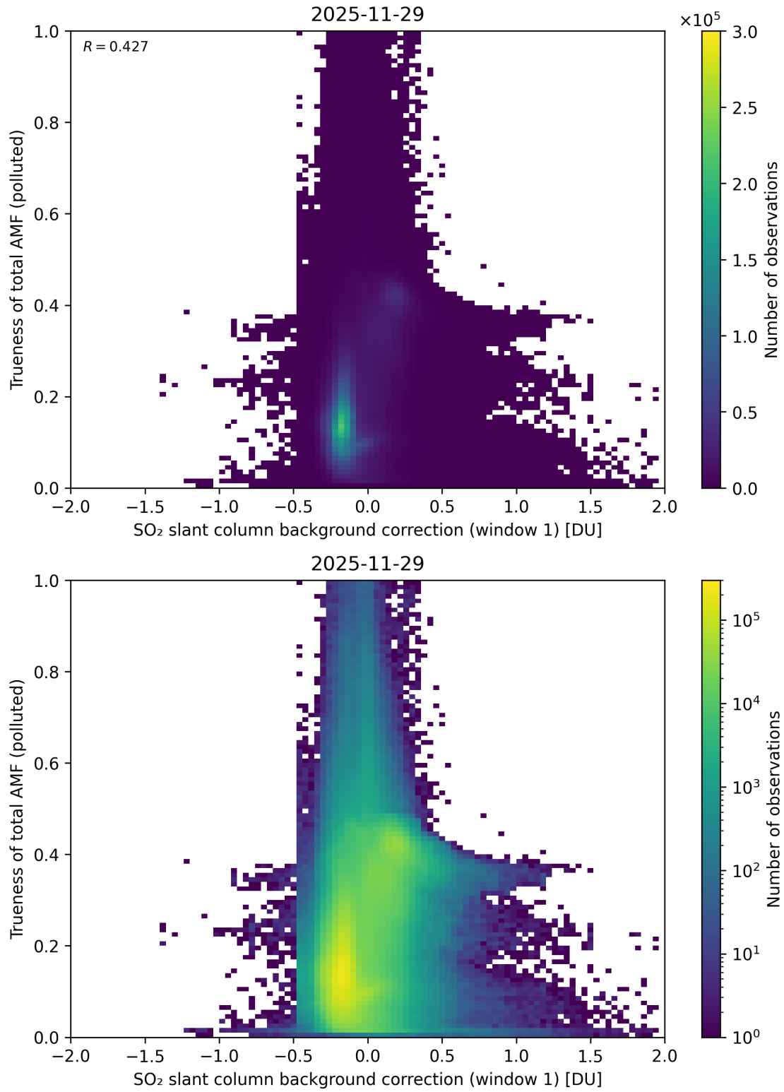
Figure 121: Scatter density plot of “SO 2 slant column background correction (window 1)” against “Trueness of total AMF (polluted)” for 2025-11-28 to 2025-11-30.
