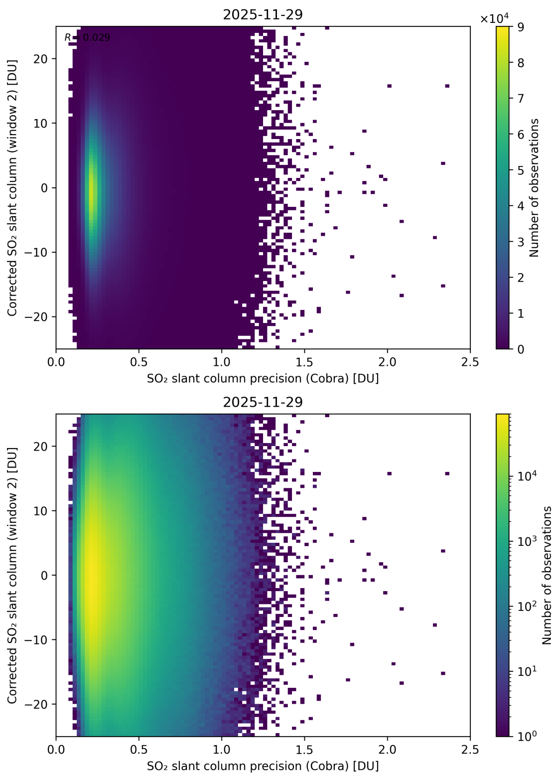
Figure 206: Scatter density plot of “SO 2 slant column precision (Cobra)” against “Corrected SO 2 slant column (window 2)” for 2025-11-28 to 2025-11-30.
