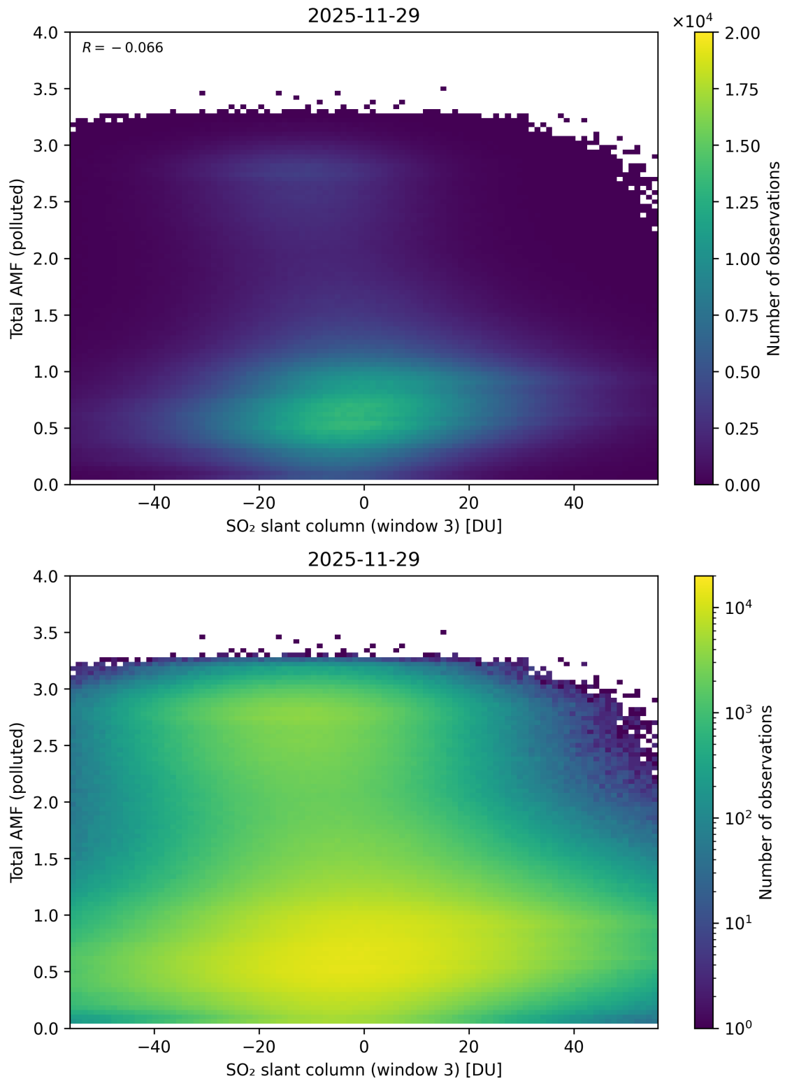
Figure 318: Scatter density plot of “SO 2 slant column (window 3)” against “Total AMF (polluted)” for 2025-11-28 to 2025-11-30.
