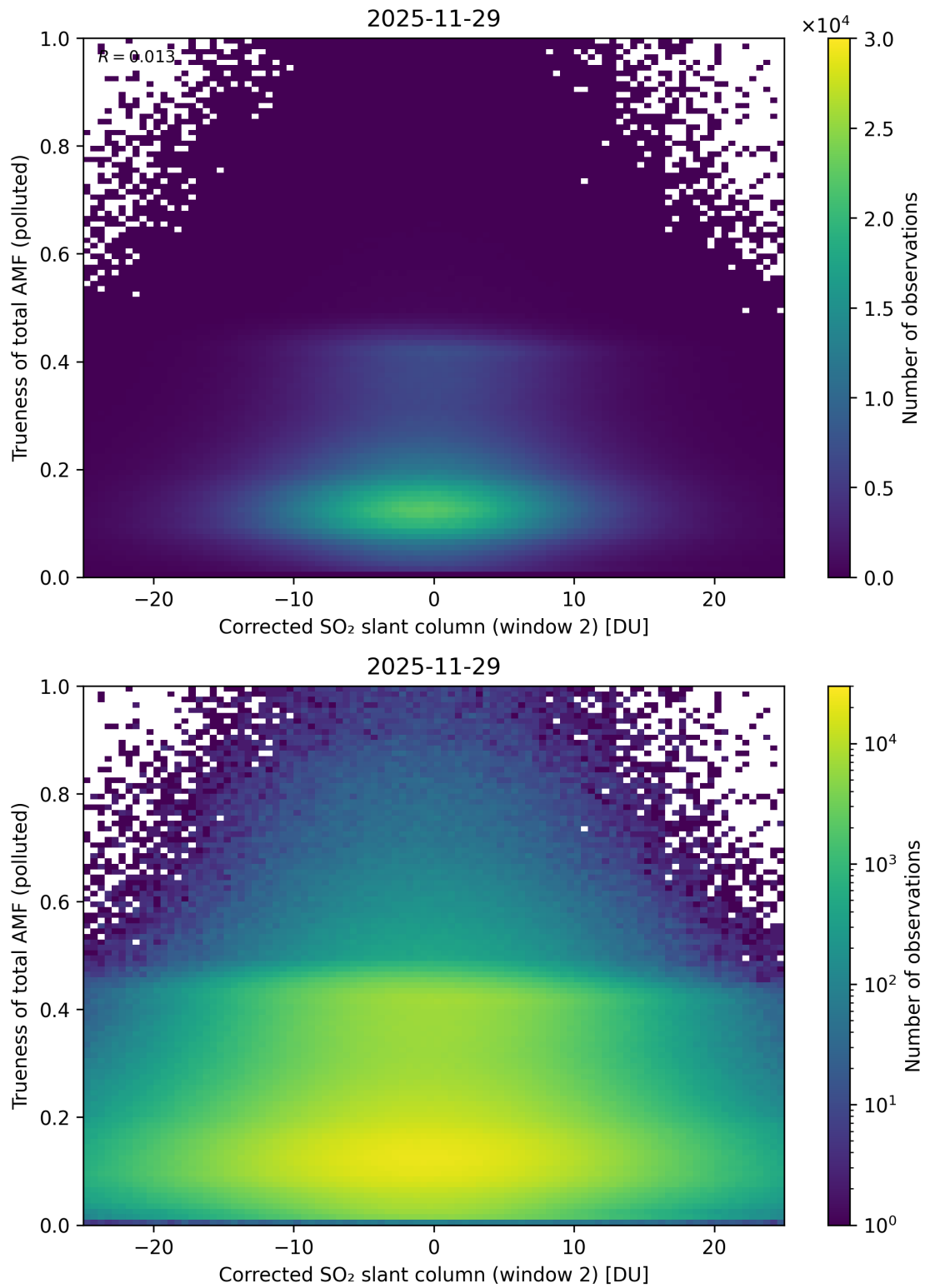
Figure 254: Scatter density plot of “Corrected SO 2 slant column (window 2)” against “Trueness of total AMF (polluted)” for 2025-11-28 to 2025-11-30.
