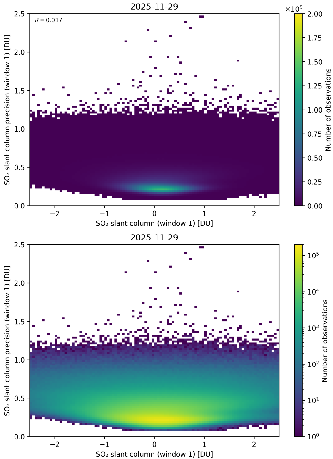
Figure 285: Scatter density plot of “SO 2 slant column (window 1)” against “SO 2 slant column precision (window 1)” for 2025-11-28 to 2025-11-30.
