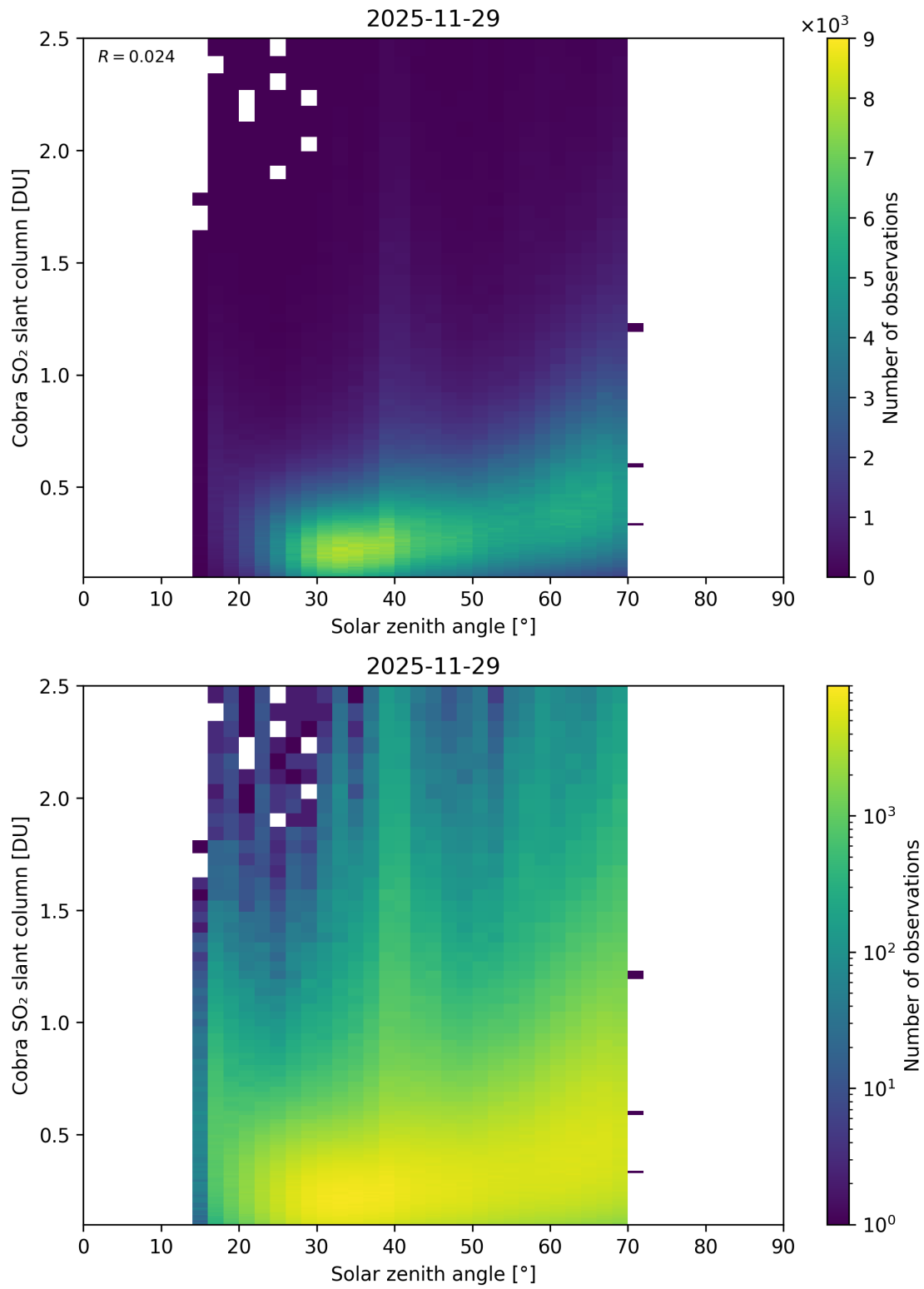
Figure 179: Scatter density plot of “Solar zenith angle” against “Cobra SO 2 slant column” for 2025-11-28 to 2025-11-30.
