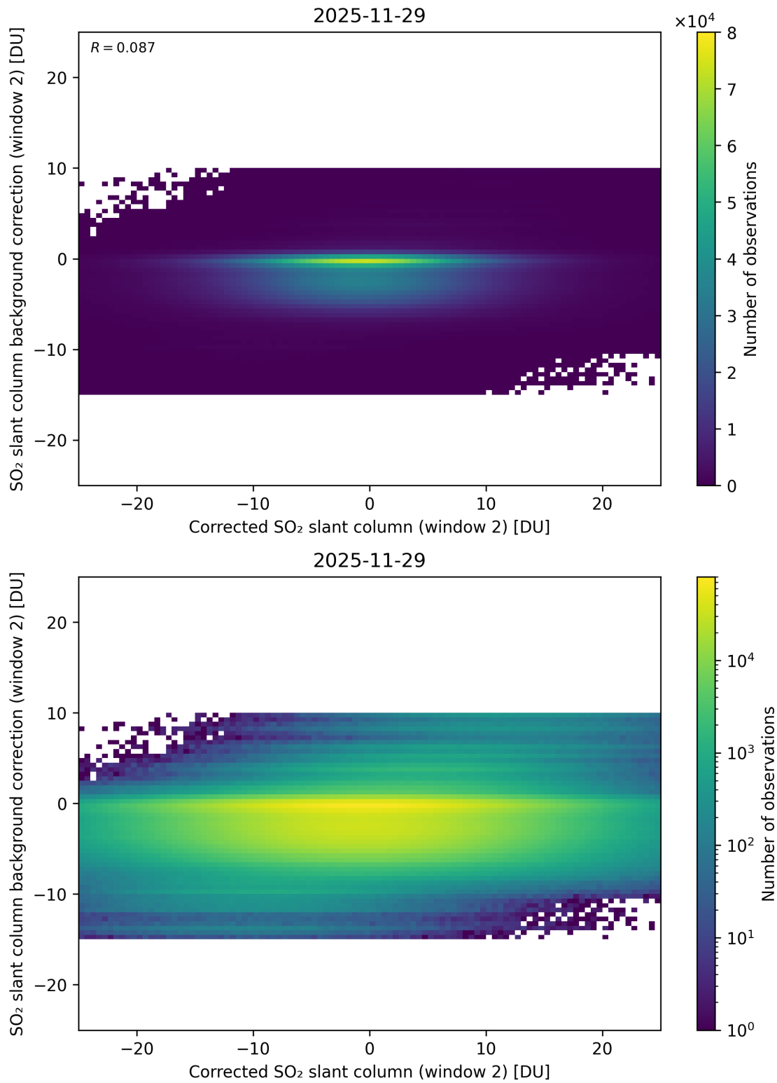
Figure 244: Scatter density plot of “Corrected SO 2 slant column (window 2)” against “SO 2 slant column background correction (window 2)” for 2025-11-28 to 2025-11-30.
