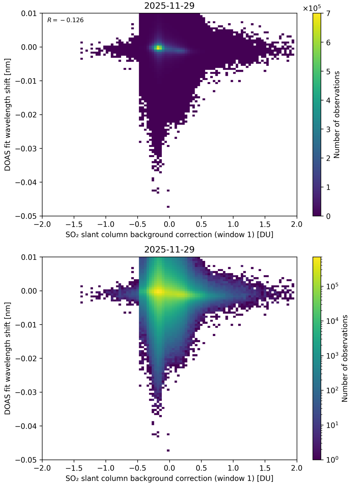
Figure 111: Scatter density plot of “SO 2 slant column background correction (window 1)” against “DOAS fit wavelength shift” for 2025-11-28 to 2025-11-30.
