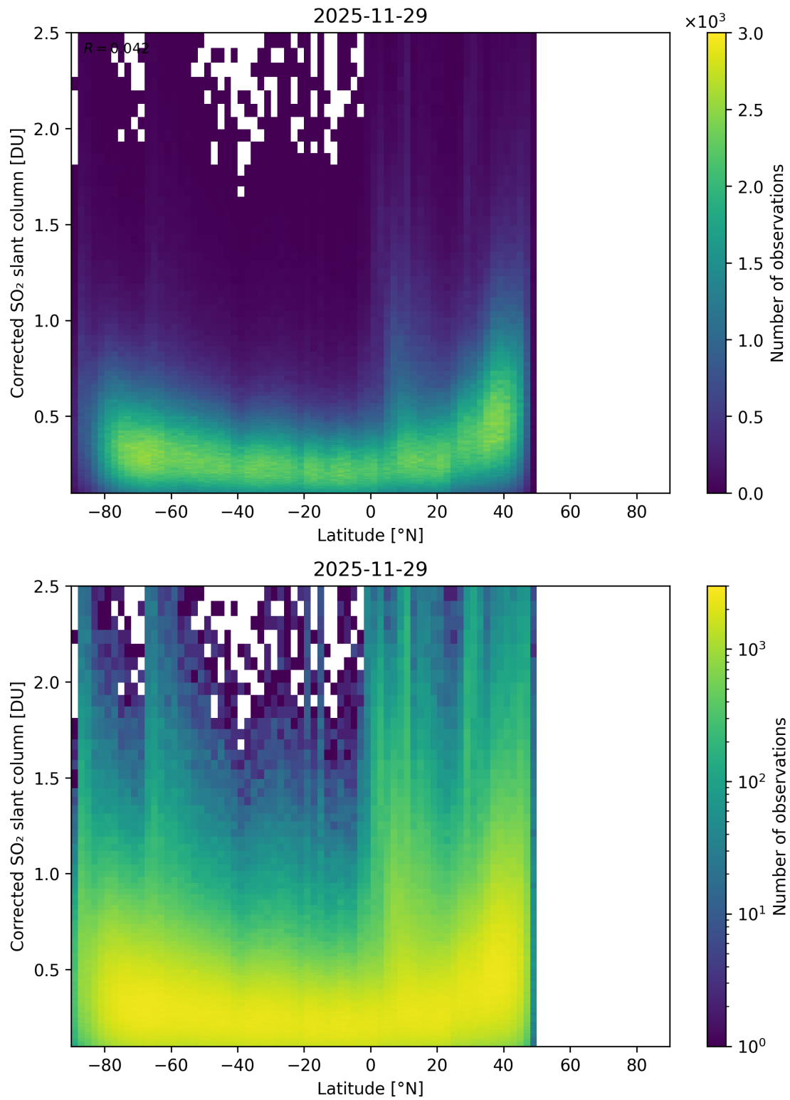
Figure 159: Scatter density plot of “Latitude” against “Corrected SO 2 slant column” for 2025-11-28 to 2025-11-30.
