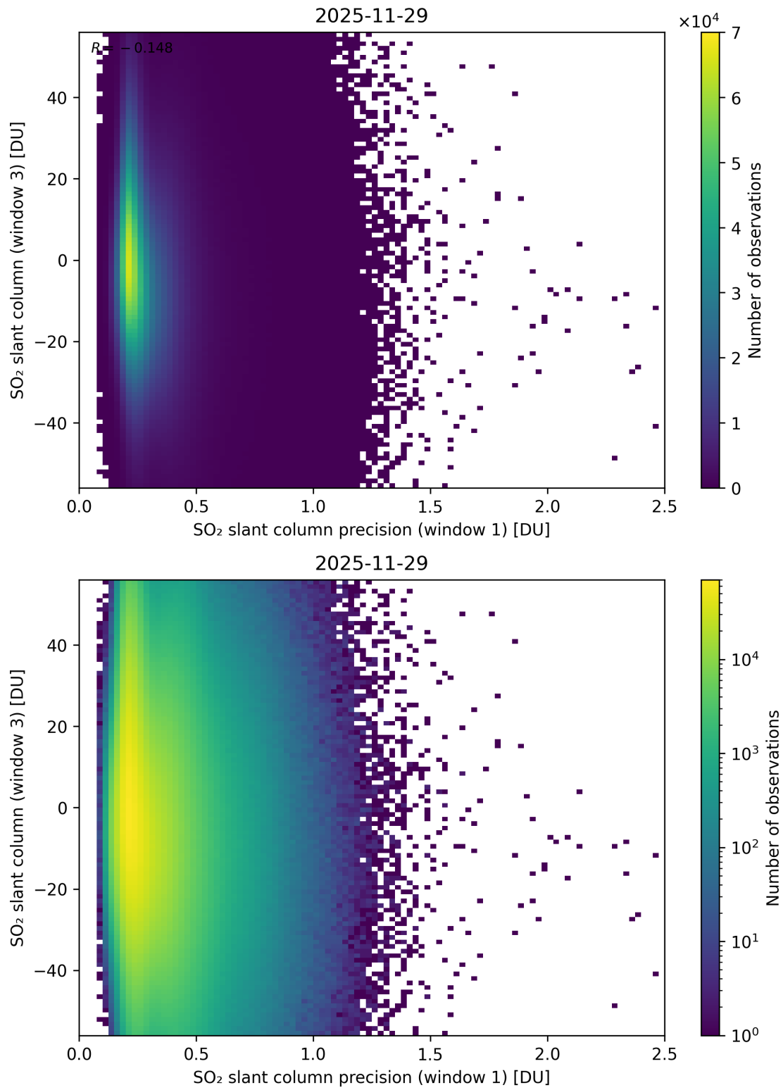
Figure 278: Scatter density plot of “SO 2 slant column precision (window 1)” against “SO 2 slant column (window 3)” for 2025-11-28 to 2025-11-30.
