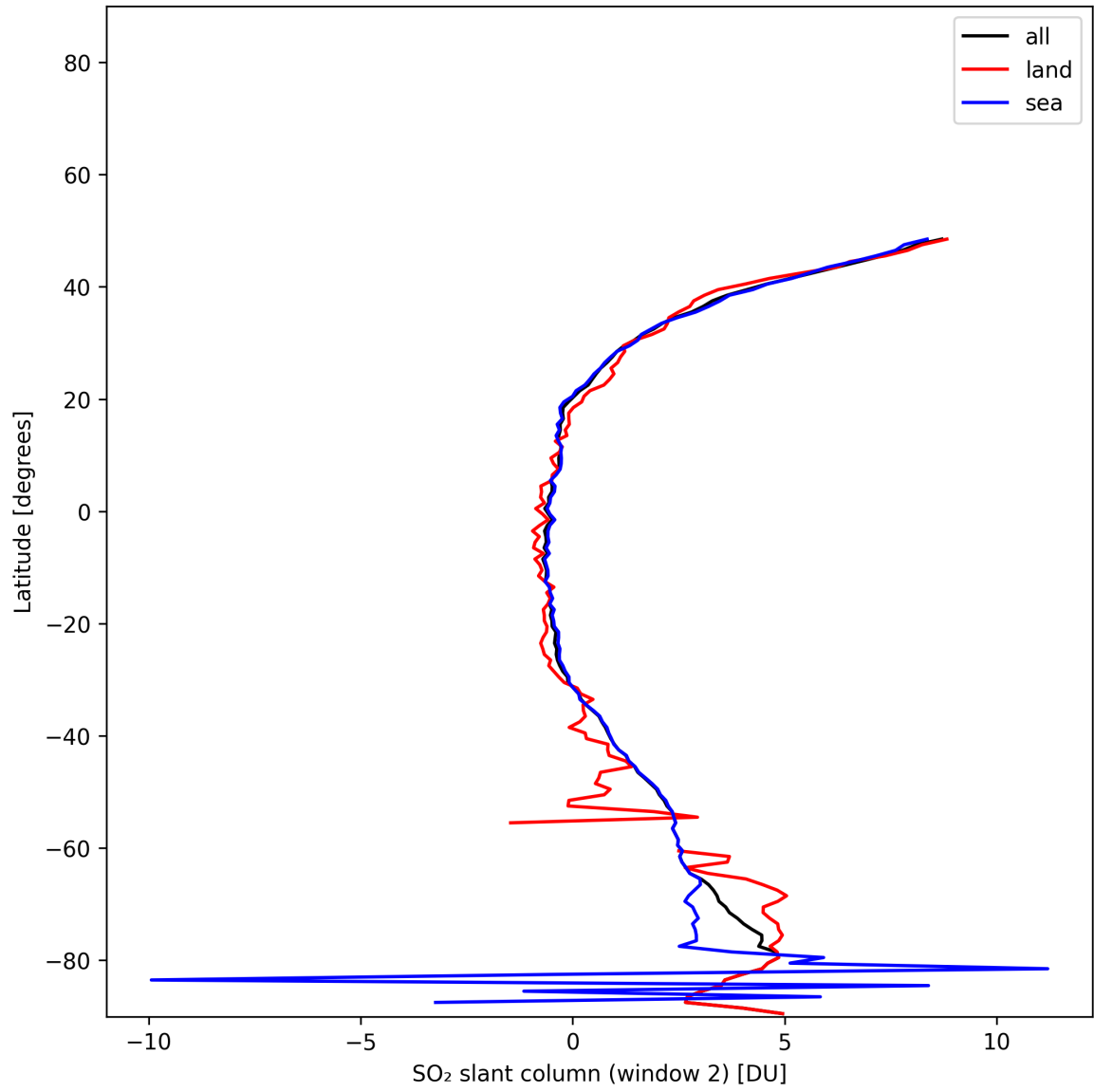
Figure 41: Zonal average of “SO 2 slant column (window 2)” for 2025-11-28 to 2025-11-30.
