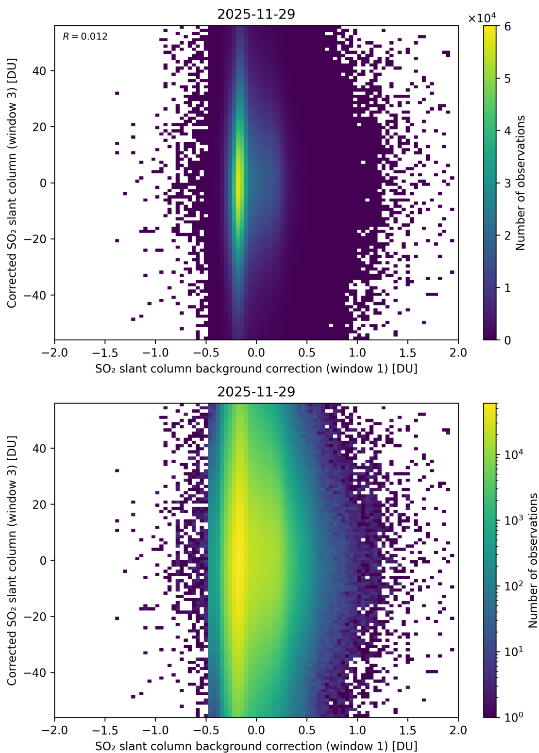
Figure 116: Scatter density plot of “SO 2 slant column background correction (window 1)” against “Corrected SO 2 slant column (window 3)” for 2025-11-28 to 2025-11-30.
