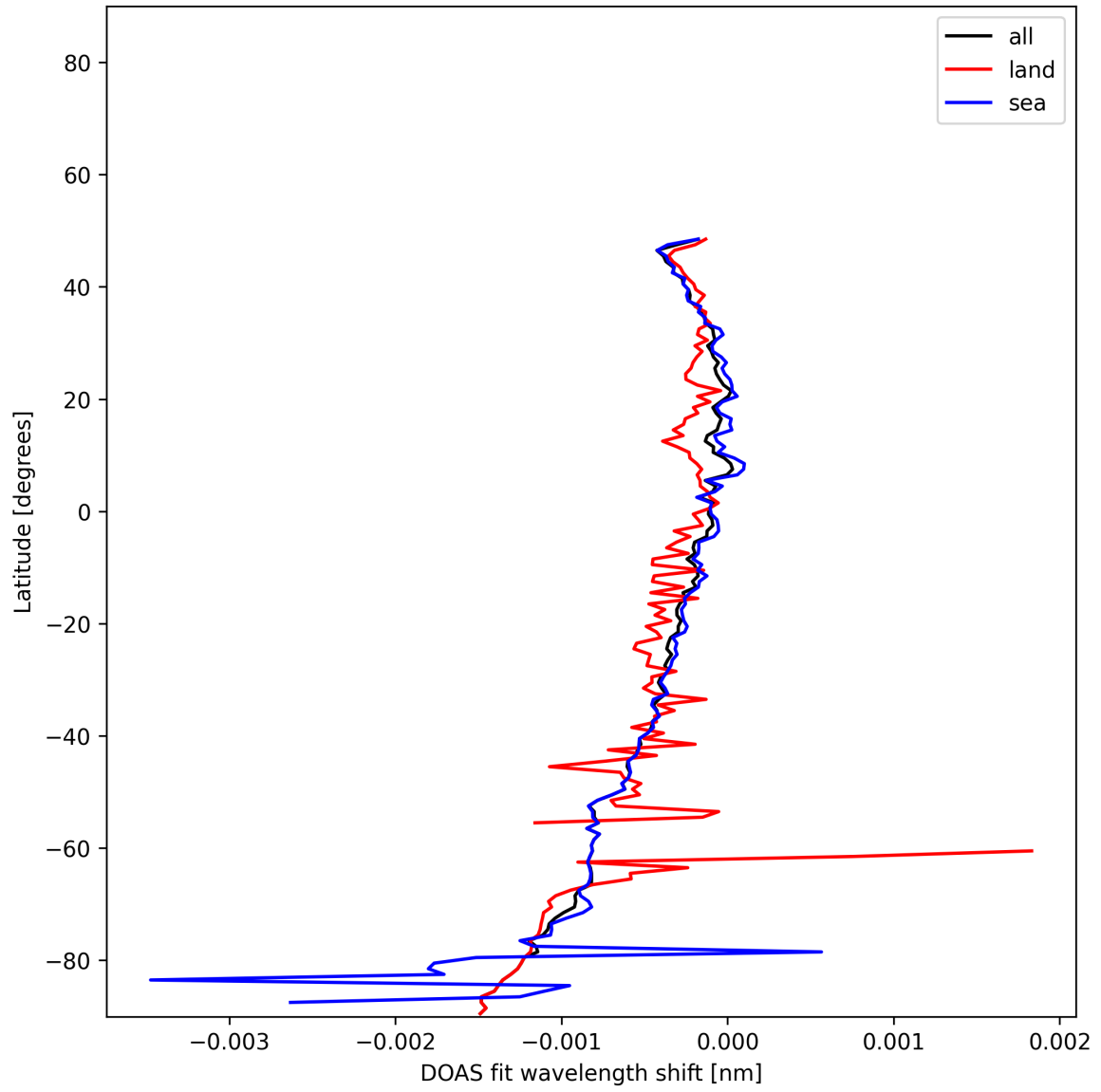
Figure 50: Zonal average of "DOAS fit wavelength shift" for 2025-11-28 to 2025-11-30.
