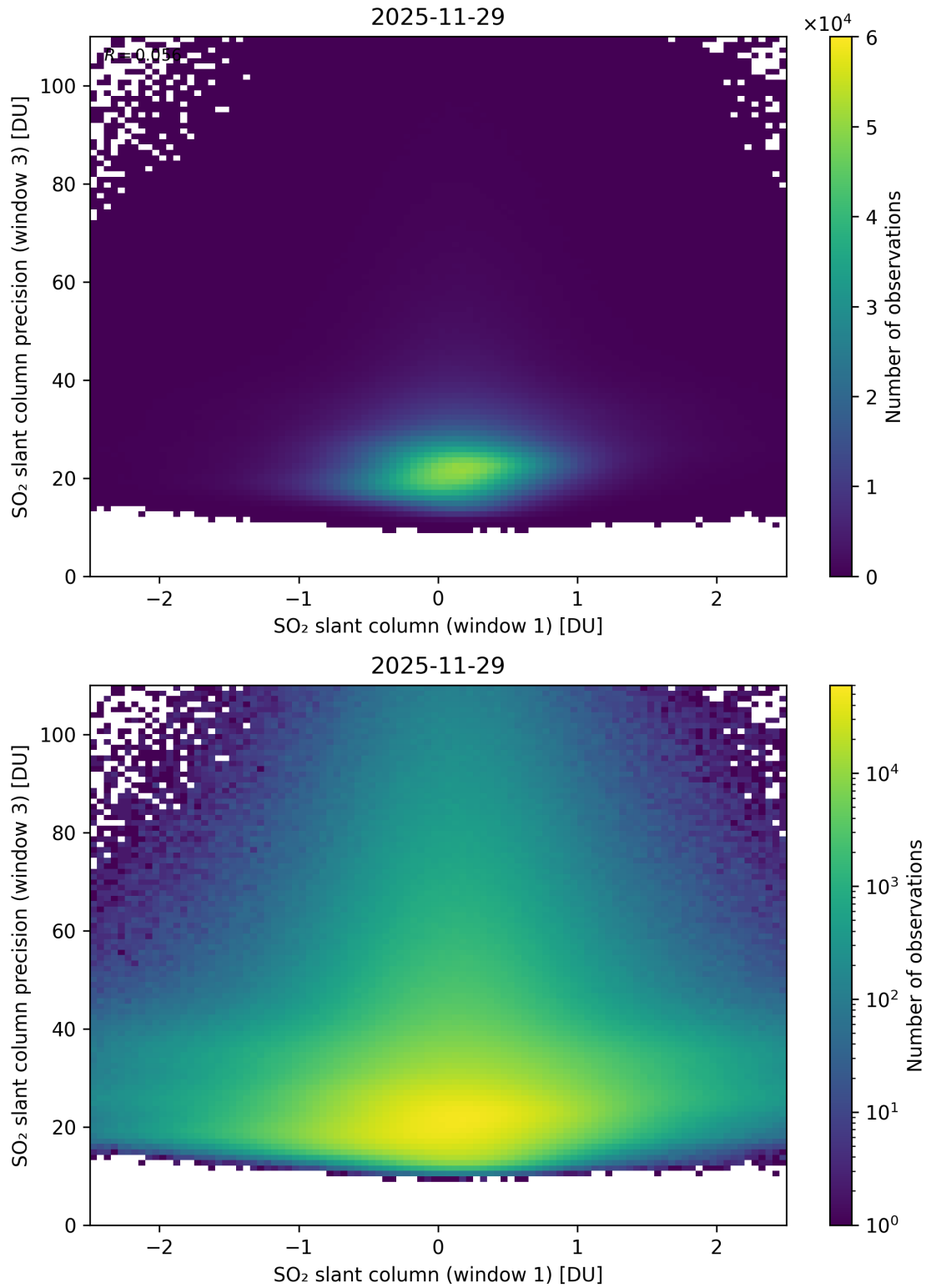
Figure 288: Scatter density plot of “SO 2 slant column (window 1)” against “SO 2 slant column precision (window 3)” for 2025-11-28 to 2025-11-30.
