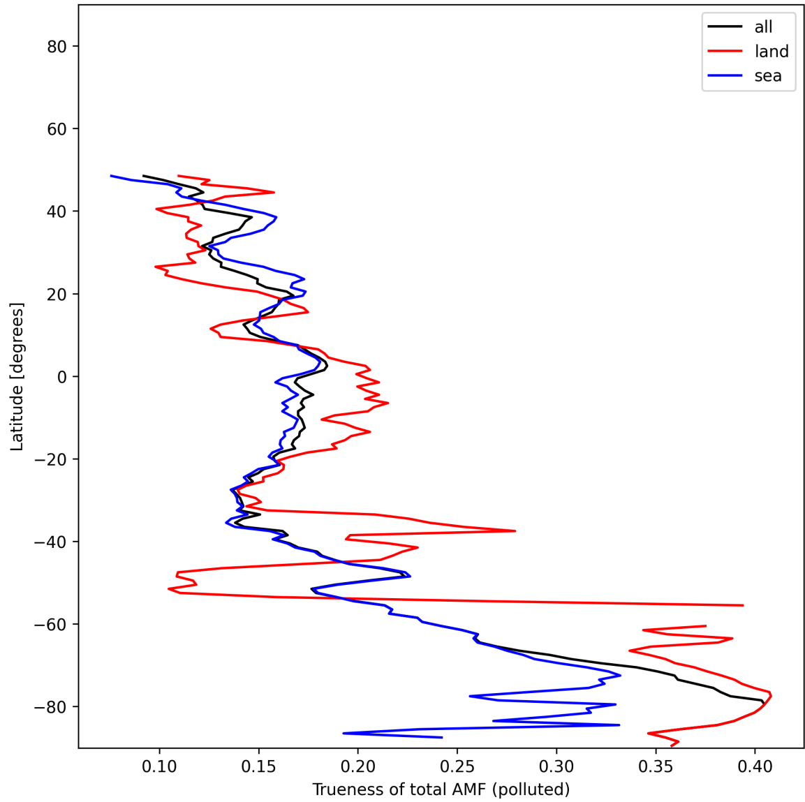
Figure 54: Zonal average of “Trueness of total AMF (polluted)” for 2025-11-28 to 2025-11-30.
