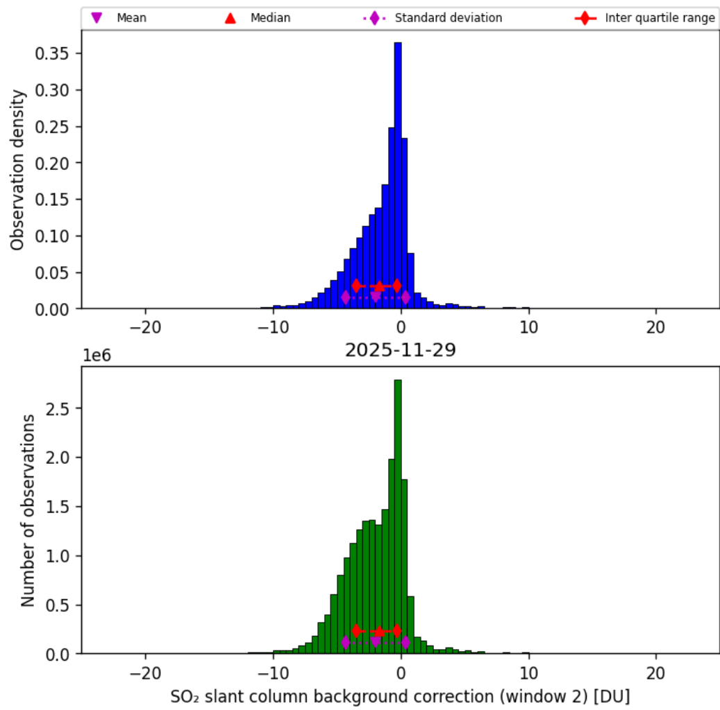
Figure 70: Histogram of “SO 2 slant column background correction (window 2)” for 2025-11-28 to 2025-11-30
