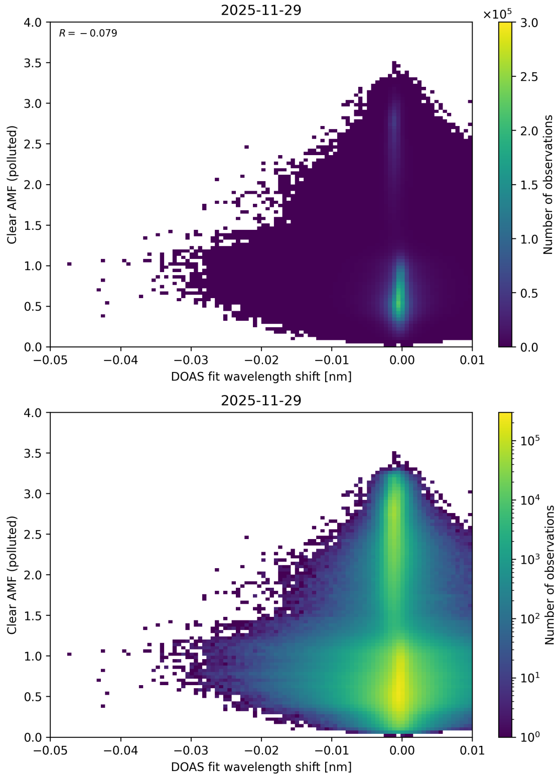
Figure 140: Scatter density plot of “DOAS fit wavelength shift” against “Clear AMF (polluted)” for 2025-11-28 to 2025-11-30.
