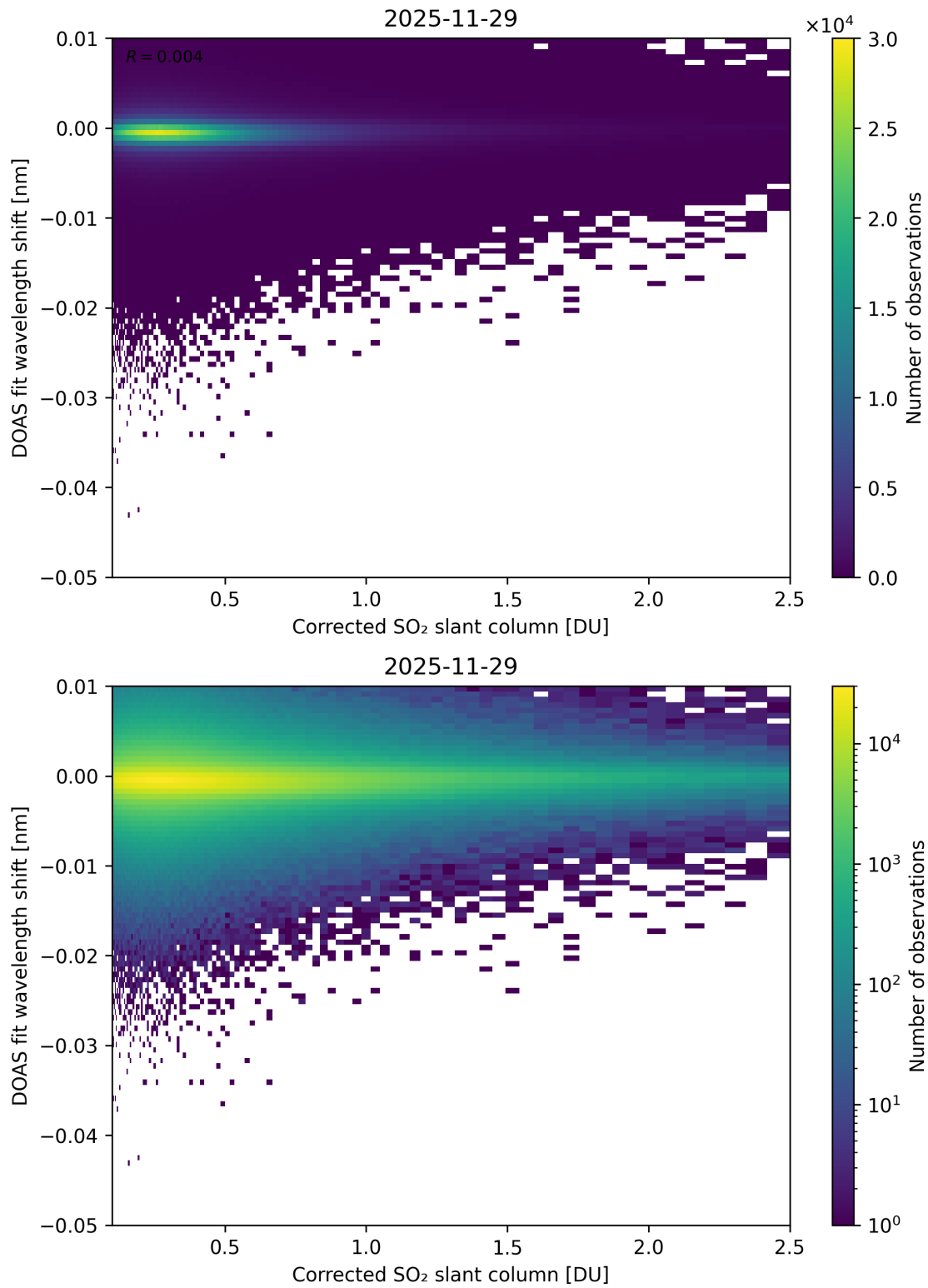
Figure 229: Scatter density plot of “Corrected SO 2 slant column” against “DOAS fit wavelength shift” for 2025-11-28 to 2025-11-30.
