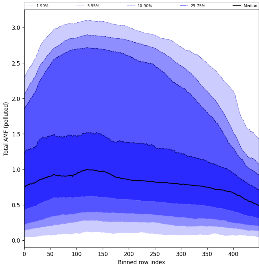
Figure 105: Along track statistics of “Total AMF (polluted)” for 2025-11-28 to 2025-11-30
