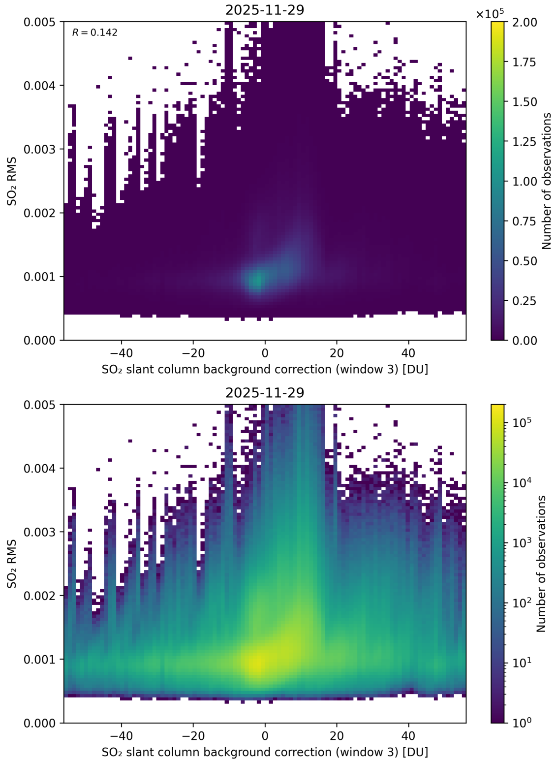
Figure 134: Scatter density plot of “SO 2 slant column background correction (window 3)” against “SO 2 RMS” for 2025-11-28 to 2025-11-30.
