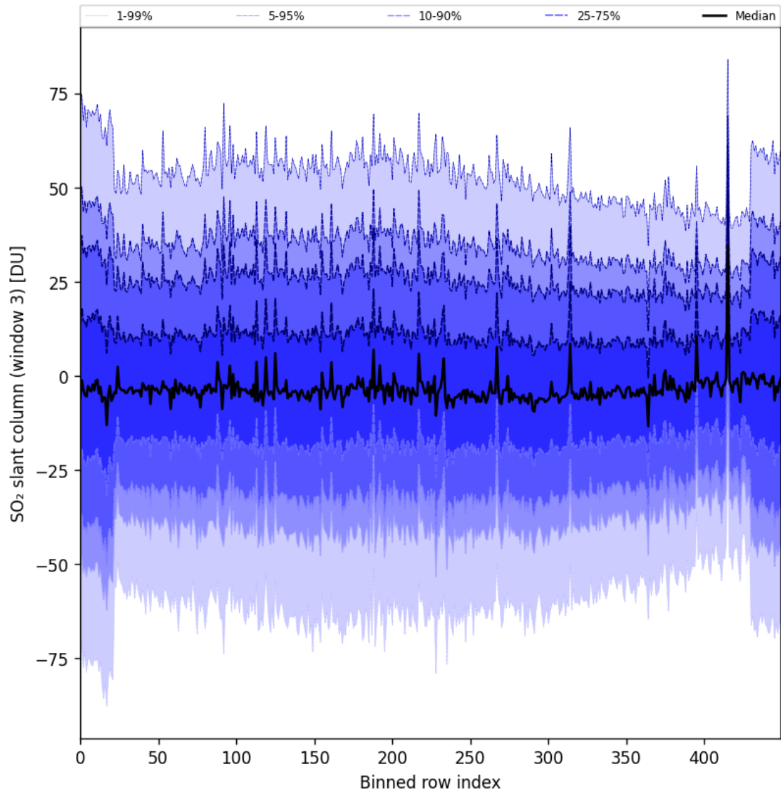
Figure 97: Along track statistics of “SO 2 slant column (window 3)” for 2025-11-28 to 2025-11-30
