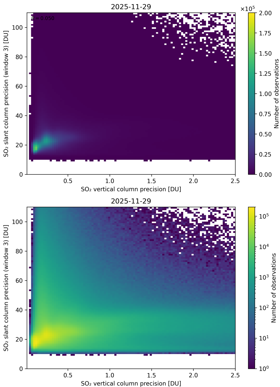
Figure 345: Scatter density plot of “SO 2 vertical column precision” against “SO 2 slant column precision (window 3)” for 2025-11-28 to 2025-11-30.
