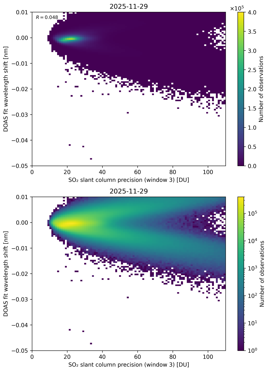
Figure 308: Scatter density plot of “SO 2 slant column precision (window 3)” against “DOAS fit wavelength shift” for 2025-11-28 to 2025-11-30.
