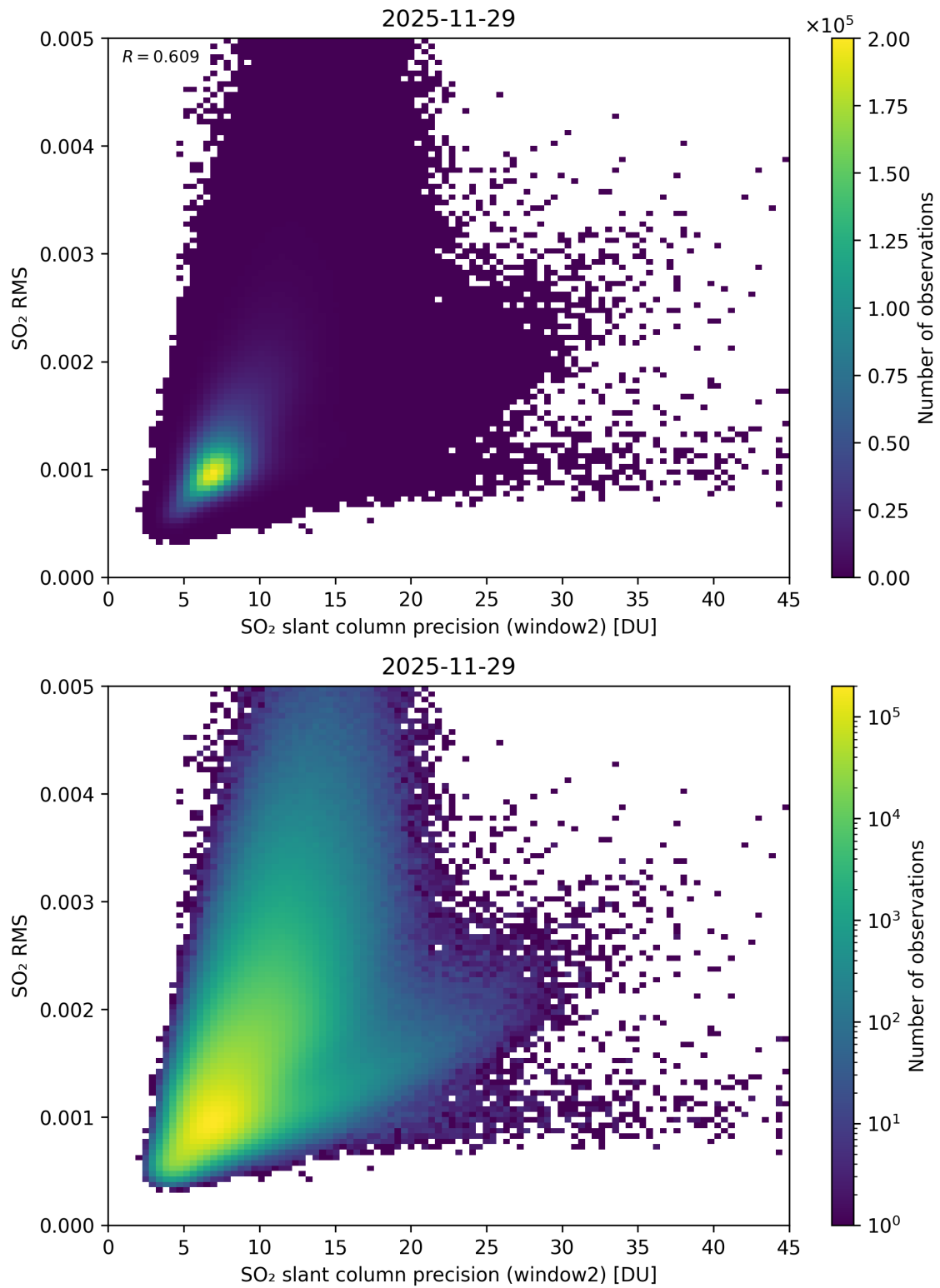
Figure 295: Scatter density plot of “SO 2 slant column precision (window2)” against “SO 2 RMS” for 2025-11-28 to 2025-11-30.
