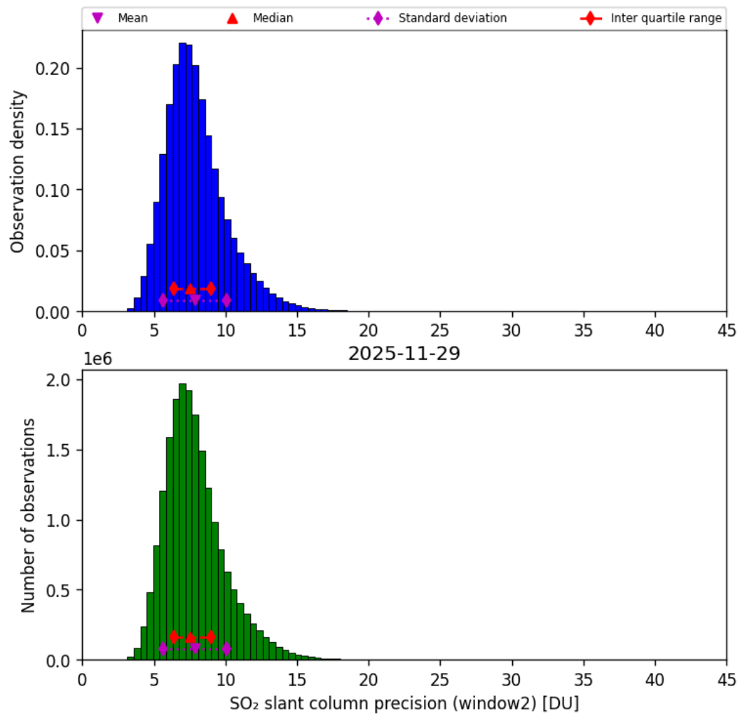
Figure 68: Histogram of “SO 2 slant column precision (window2)” for 2025-11-28 to 2025-11-30
