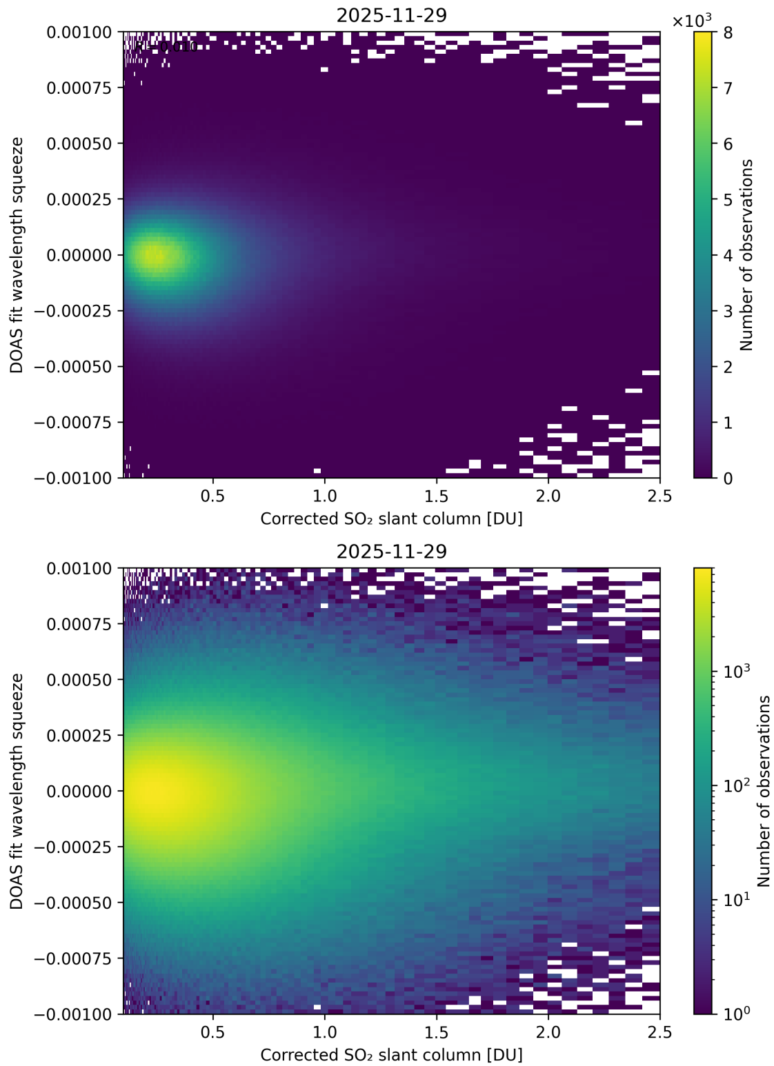
Figure 230: Scatter density plot of "Corrected SO 2 slant column" against "DOAS fit wavelength squeeze" for 2025-11-28 to 2025-11-30.
