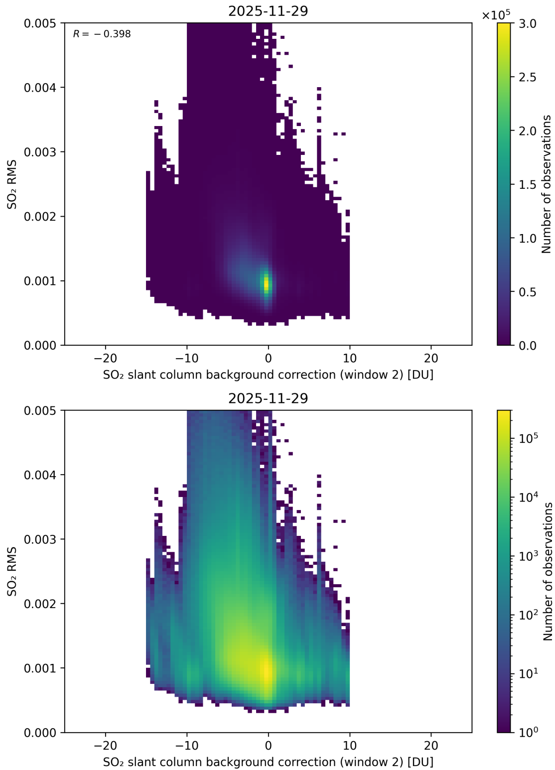
Figure 125: Scatter density plot of “SO 2 slant column background correction (window 2)” against “SO 2 RMS” for 2025-11-28 to 2025-11-30.
