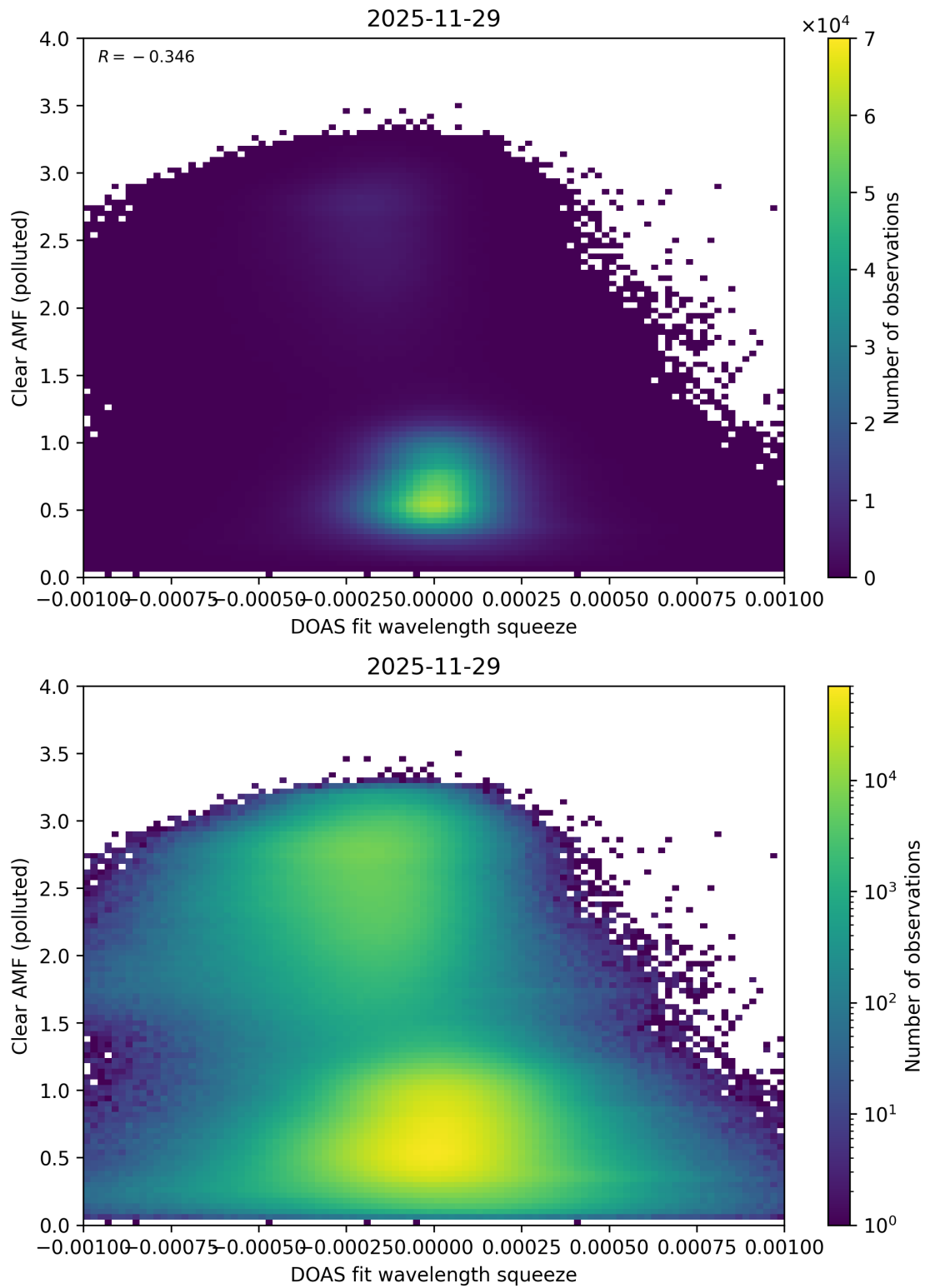
Figure 144: Scatter density plot of “DOAS fit wavelength squeeze” against “Clear AMF (polluted)” for 2025-11-28 to 2025-11-30.
