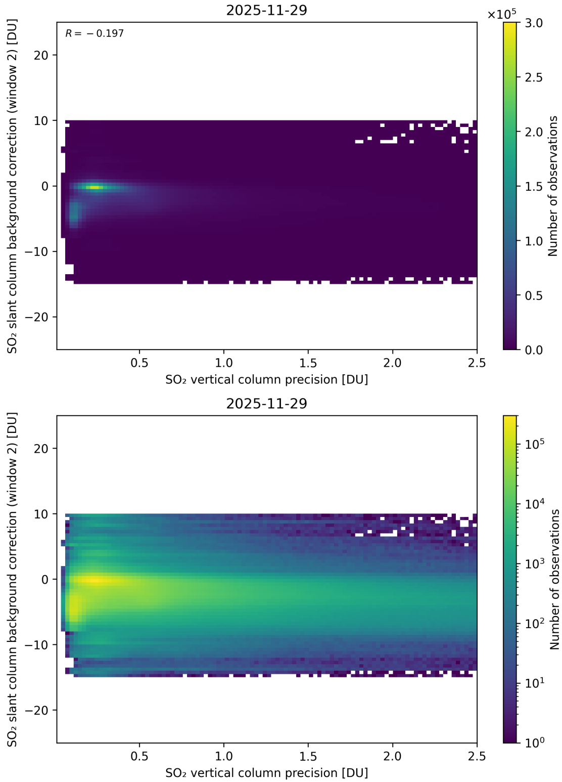
Figure 330: Scatter density plot of “SO 2 vertical column precision” against “SO 2 slant column background correction (window 2)” for 2025-11-28 to 2025-11-30.
