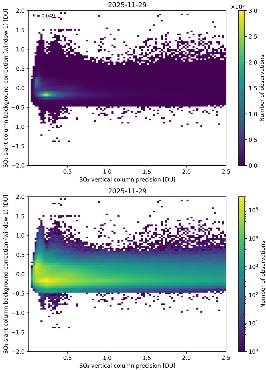
Figure 329: Scatter density plot of “SO 2 vertical column precision” against “SO 2 slant column background correction (window 1)” for 2025-11-28 to 2025-11-30.
