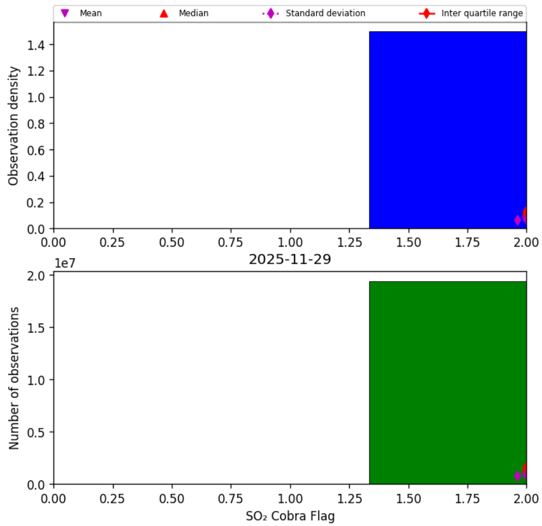
Figure 75: Histogram of “SO 2 Cobra Flag” for 2025-11-28 to 2025-11-30
