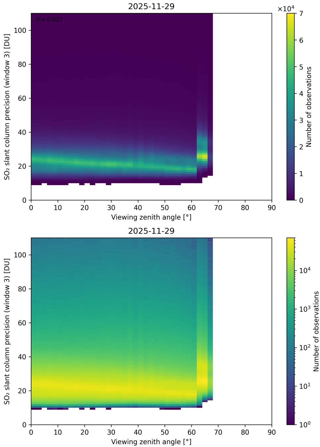
Figure 380: Scatter density plot of “Viewing zenith angle” against “SO 2 slant column precision (window 3)” for 2025-11-28 to 2025-11-30.
