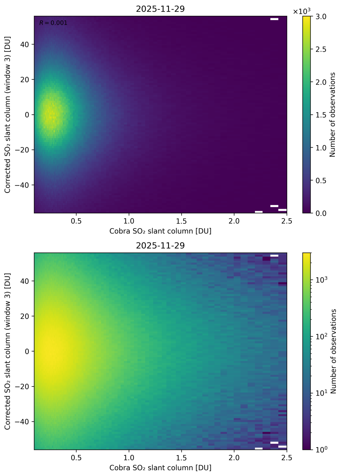
Figure 218: Scatter density plot of “Cobra SO 2 slant column” against “Corrected SO 2 slant column (window 3)” for 2025-11-28 to 2025-11-30.
