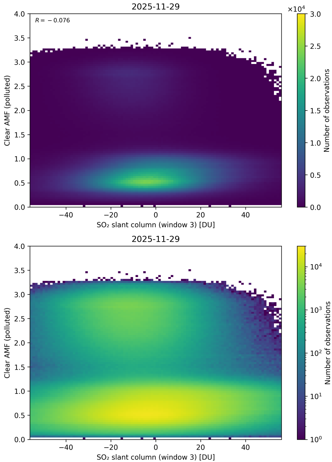
Figure 315: Scatter density plot of “SO 2 slant column (window 3)” against “Clear AMF (polluted)” for 2025-11-28 to 2025-11-30.
