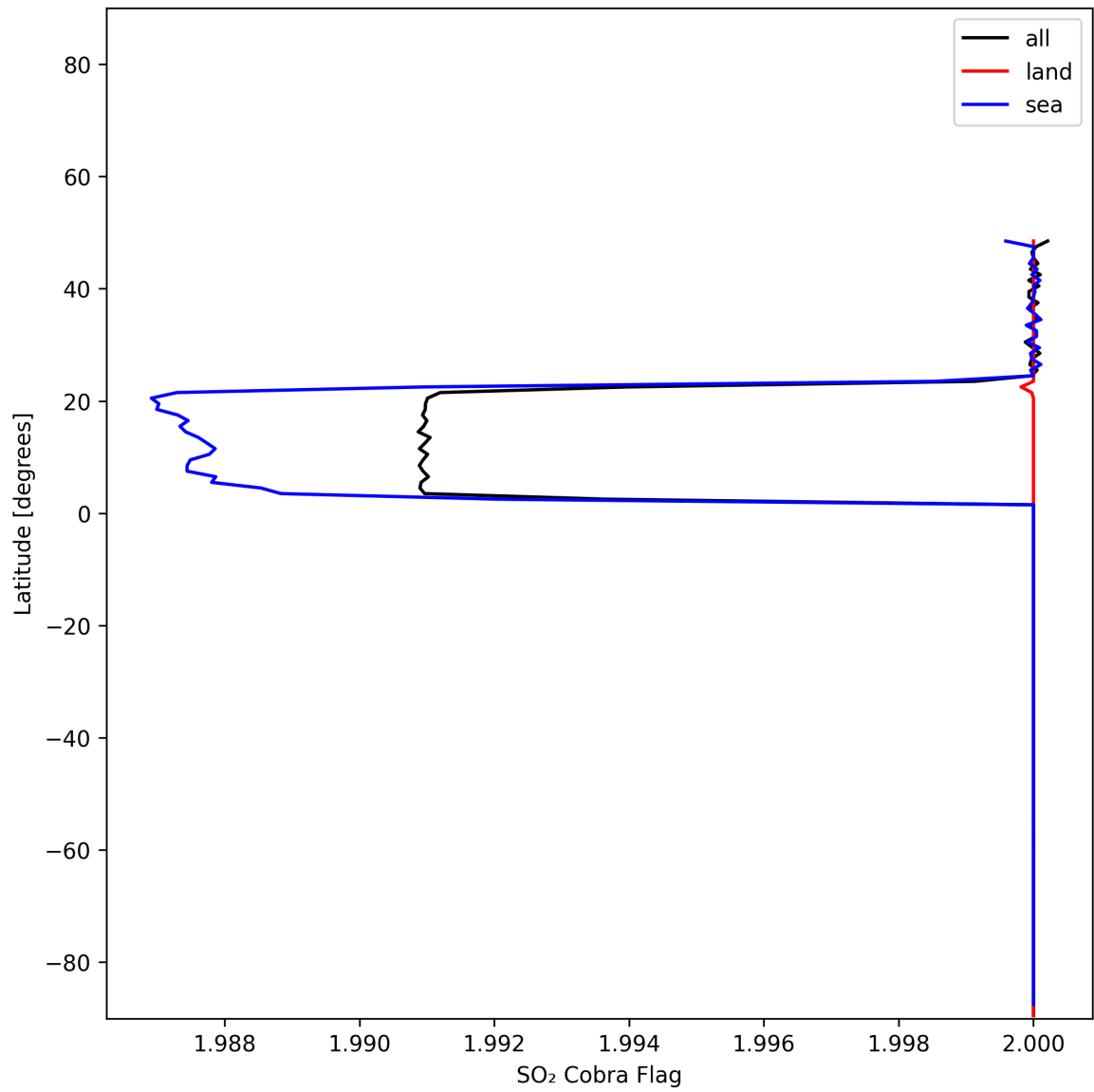
Figure 49: Zonal average of “SO 2 Cobra Flag” for 2025-11-28 to 2025-11-30.
