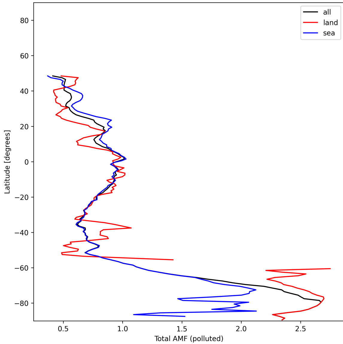
Figure 53: Zonal average of “Total AMF (polluted)” for 2025-11-28 to 2025-11-30.
