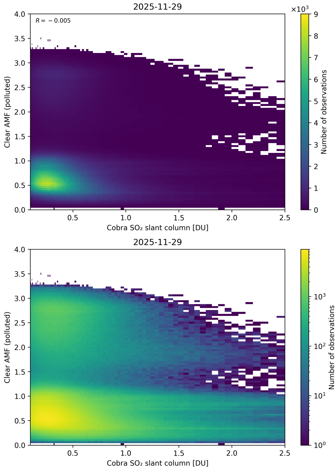
Figure 215: Scatter density plot of “Cobra SO 2 slant column” against “Clear AMF (polluted)” for 2025-11-28 to 2025-11-30.
