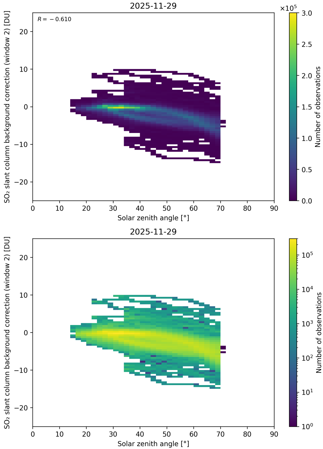
Figure 172: Scatter density plot of “Solar zenith angle” against “SO 2 slant column background correction (window 2)” for 2025-11-28 to 2025-11-30.
