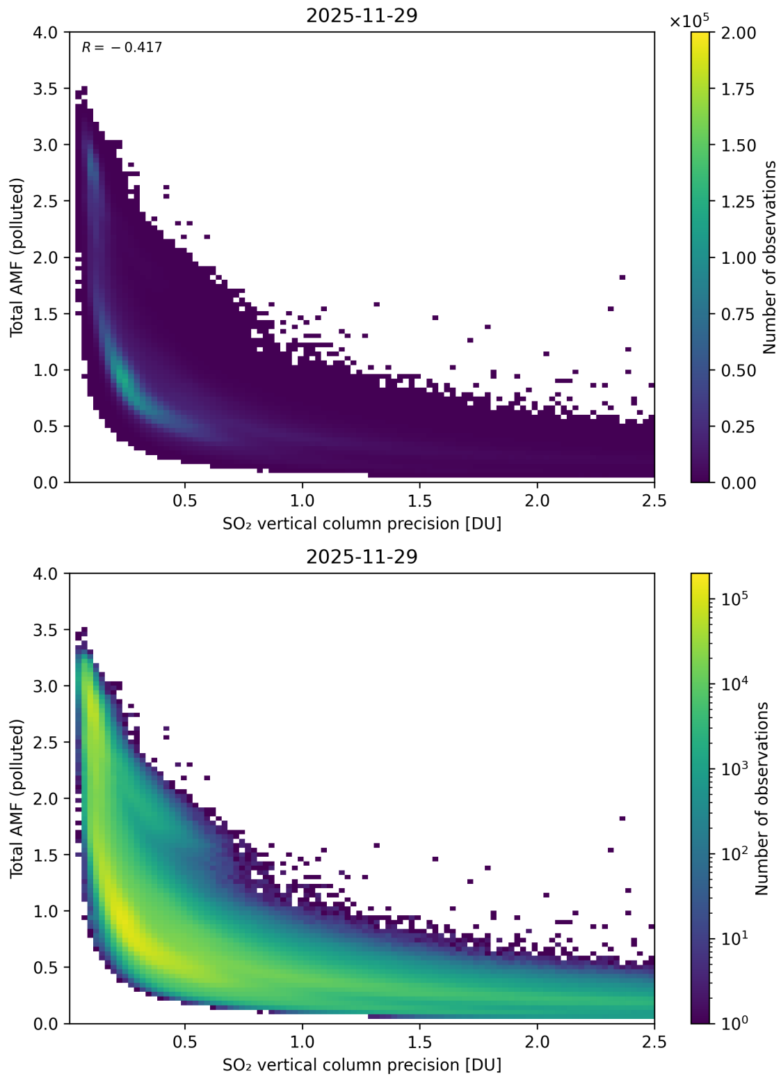
Figure 346: Scatter density plot of “SO 2 vertical column precision” against “Total AMF (polluted)” for 2025-11-28 to 2025-11-30.
