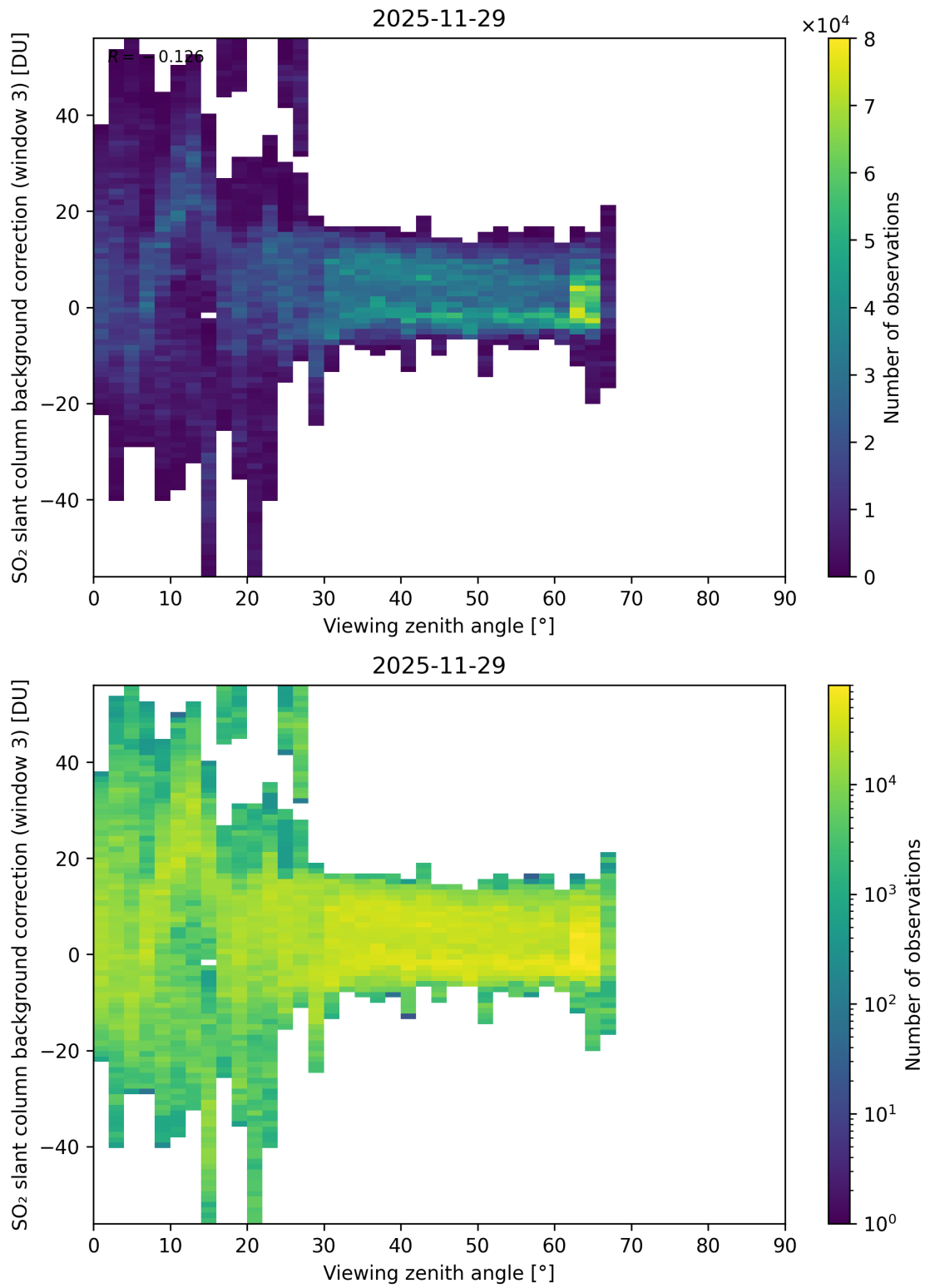
Figure 364: Scatter density plot of “Viewing zenith angle” against “SO 2 slant column background correction (window 3)” for 2025-11-28 to 2025-11-30.
