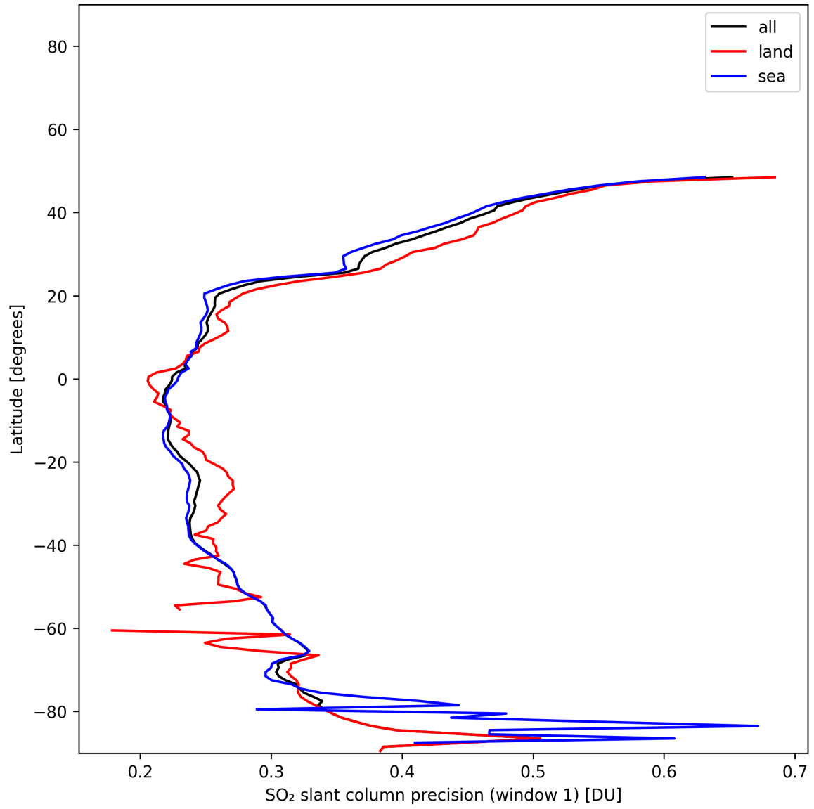
Figure 38: Zonal average of “SO 2 slant column precision (window 1)” for 2025-11-28 to 2025-11-30.
