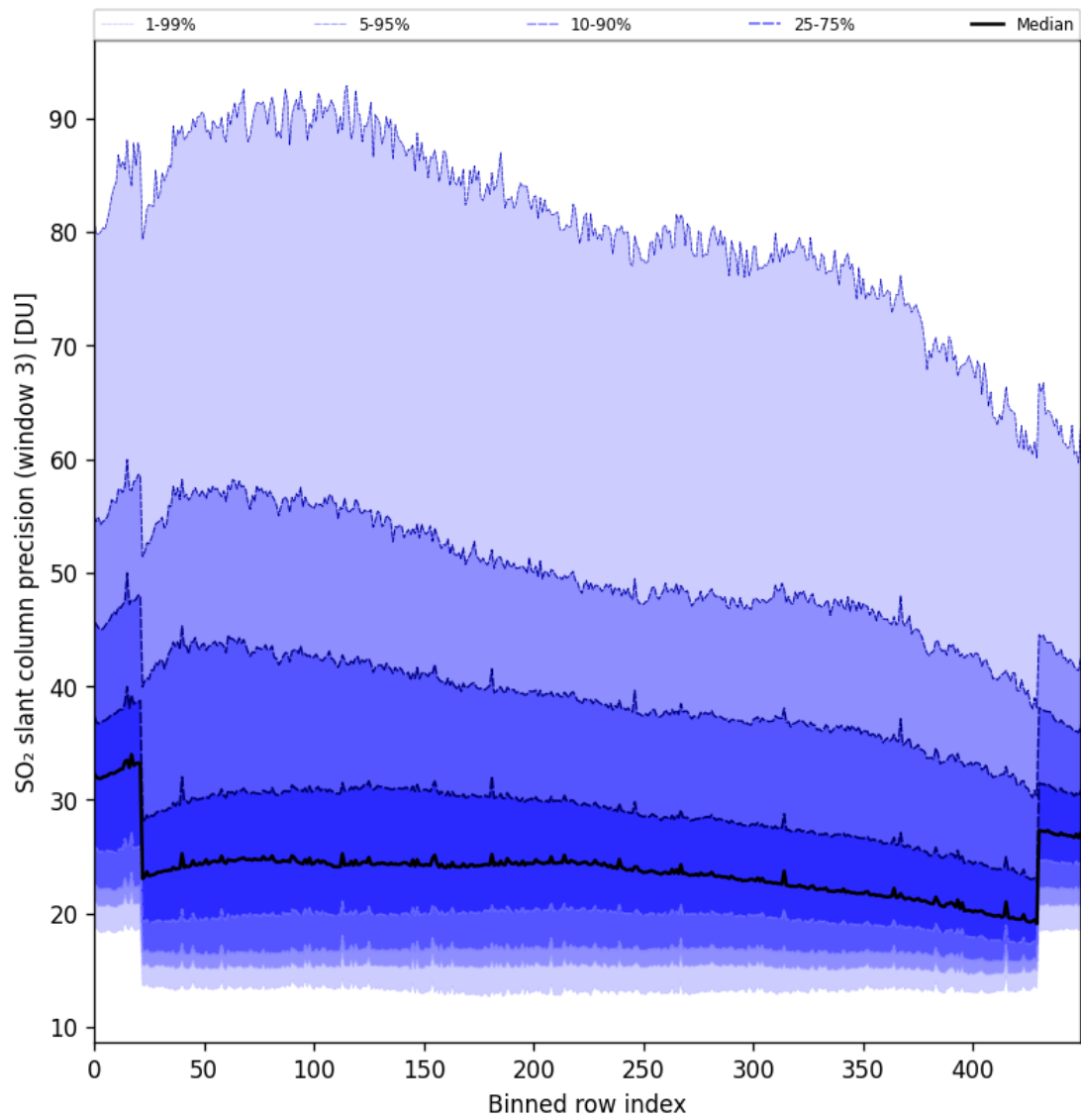
Figure 98: Along track statistics of “SO 2 slant column precision (window 3)” for 2025-11-28 to 2025-11-30
