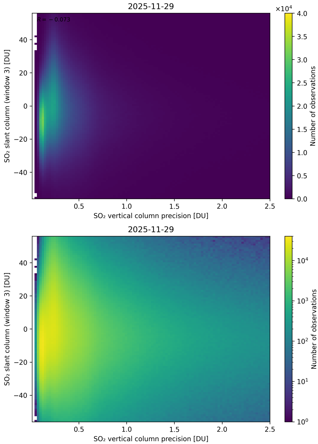
Figure 344: Scatter density plot of “SO 2 vertical column precision” against “SO 2 slant column (window 3)” for 2025-11-28 to 2025-11-30.
