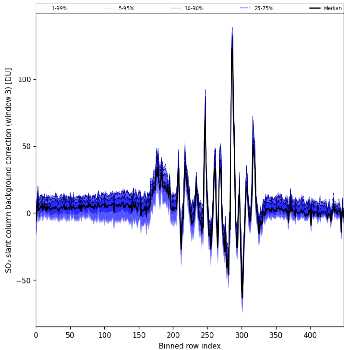
Figure 100: Along track statistics of “SO 2 slant column background correction (window 3)” for 2025-11-28 to 2025-11-30
