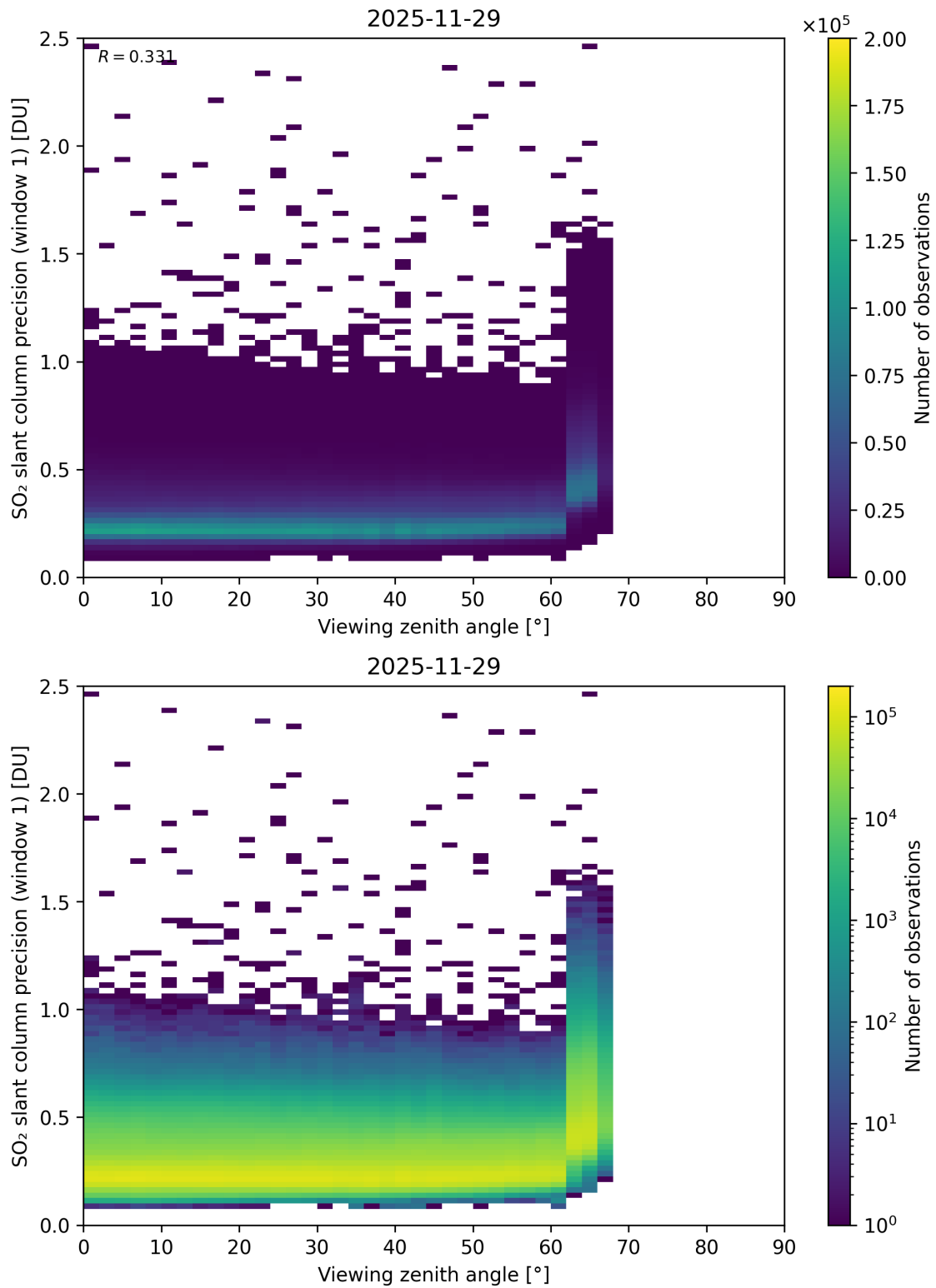
Figure 377: Scatter density plot of “Viewing zenith angle” against “SO 2 slant column precision (window 1)” for 2025-11-28 to 2025-11-30.
