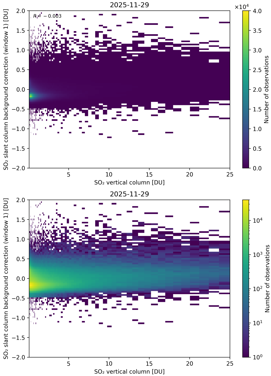
Figure 323: Scatter density plot of “SO 2 vertical column” against “SO 2 slant column background correction (window 1)” for 2025-11-28 to 2025-11-30.
