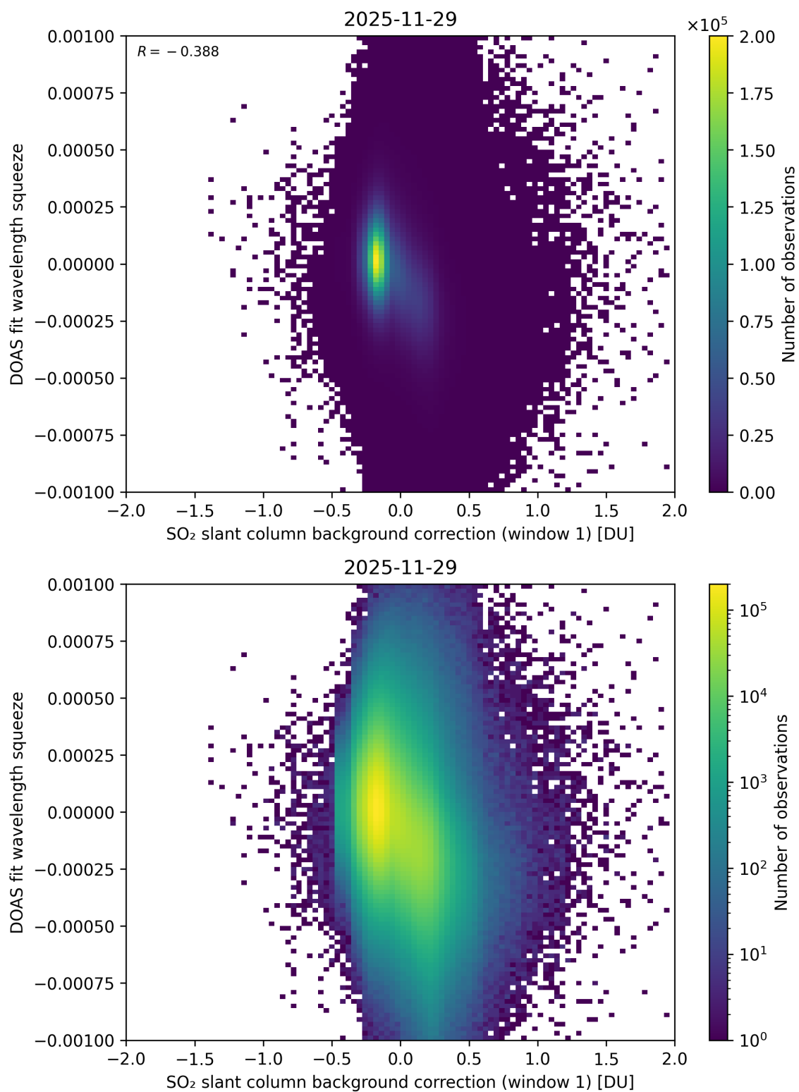
Figure 112: Scatter density plot of “SO 2 slant column background correction (window 1)” against “DOAS fit wavelength squeeze” for 2025-11-28 to 2025-11-30.
