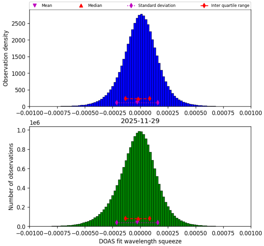
Figure 77: Histogram of "DOAS fit wavelength squeeze" for 2025-11-28 to 2025-11-30
