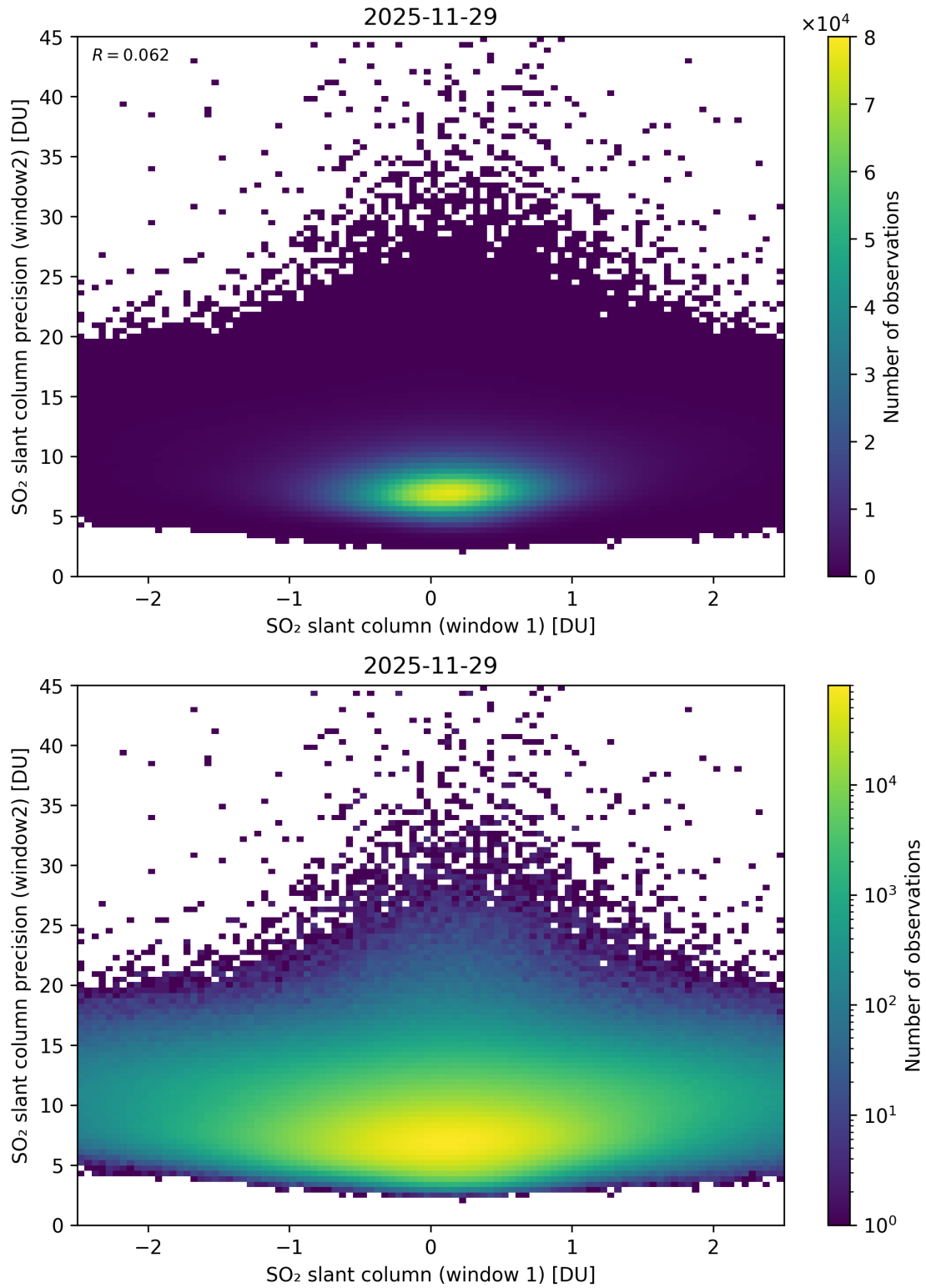
Figure 286: Scatter density plot of “SO 2 slant column (window 1)” against “SO 2 slant column precision (window2)” for 2025-11-28 to 2025-11-30.
