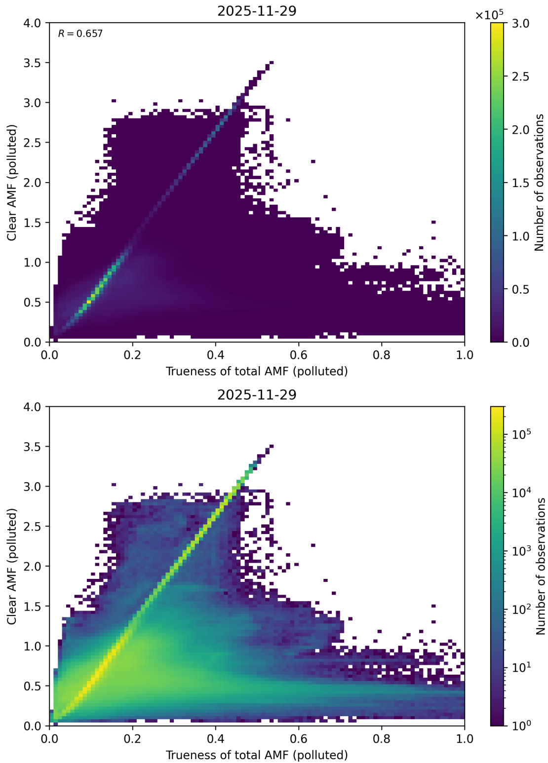
Figure 322: Scatter density plot of “Trueness of total AMF (polluted)” against “Clear AMF (polluted)” for 2025-11-28 to 2025-11-30.
