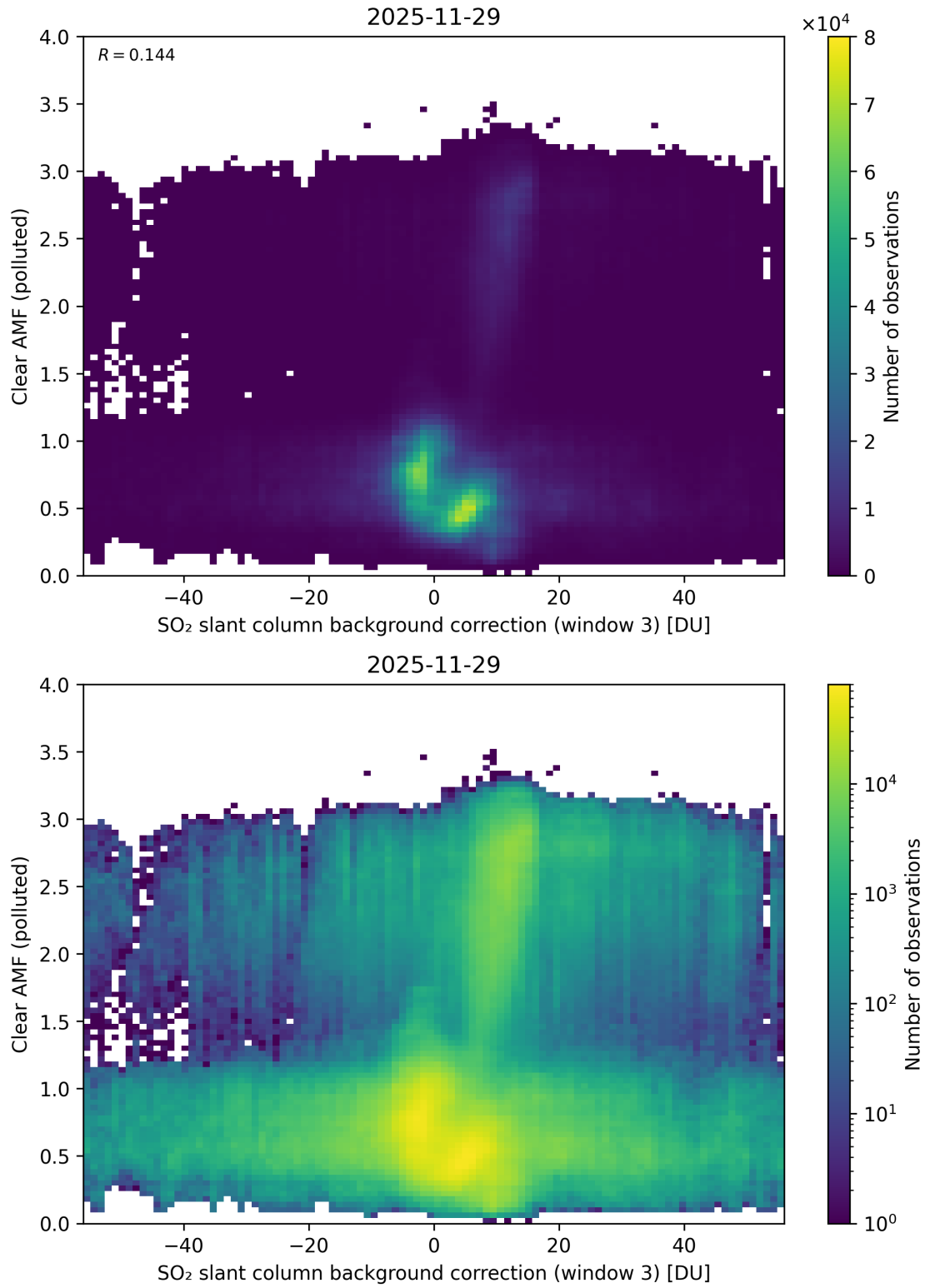
Figure 135: Scatter density plot of “SO 2 slant column background correction (window 3)” against “Clear AMF (polluted)” for 2025-11-28 to 2025-11-30.
