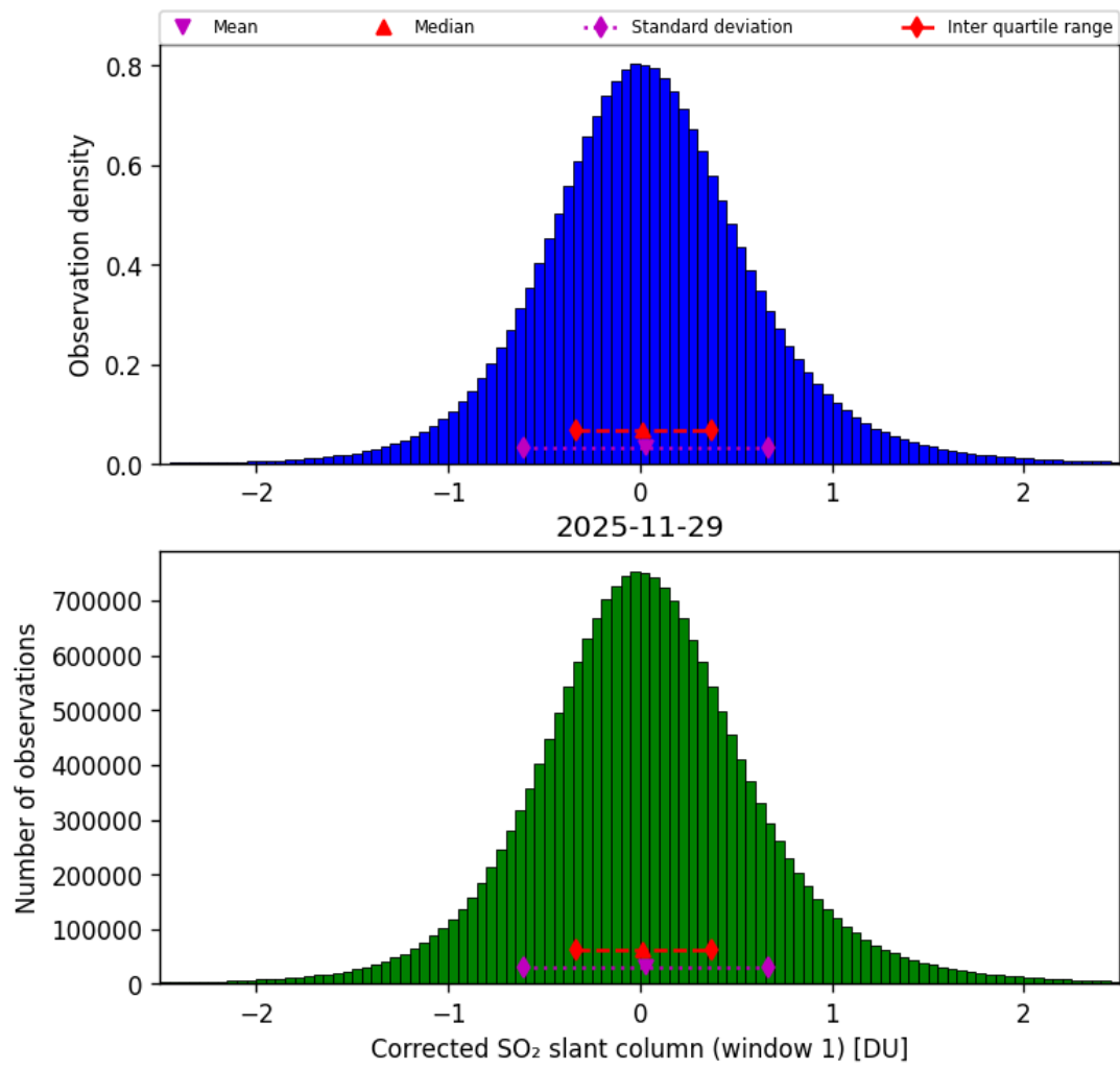
Figure 65: Histogram of “Corrected SO 2 slant column (window 1)” for 2025-11-28 to 2025-11-30
