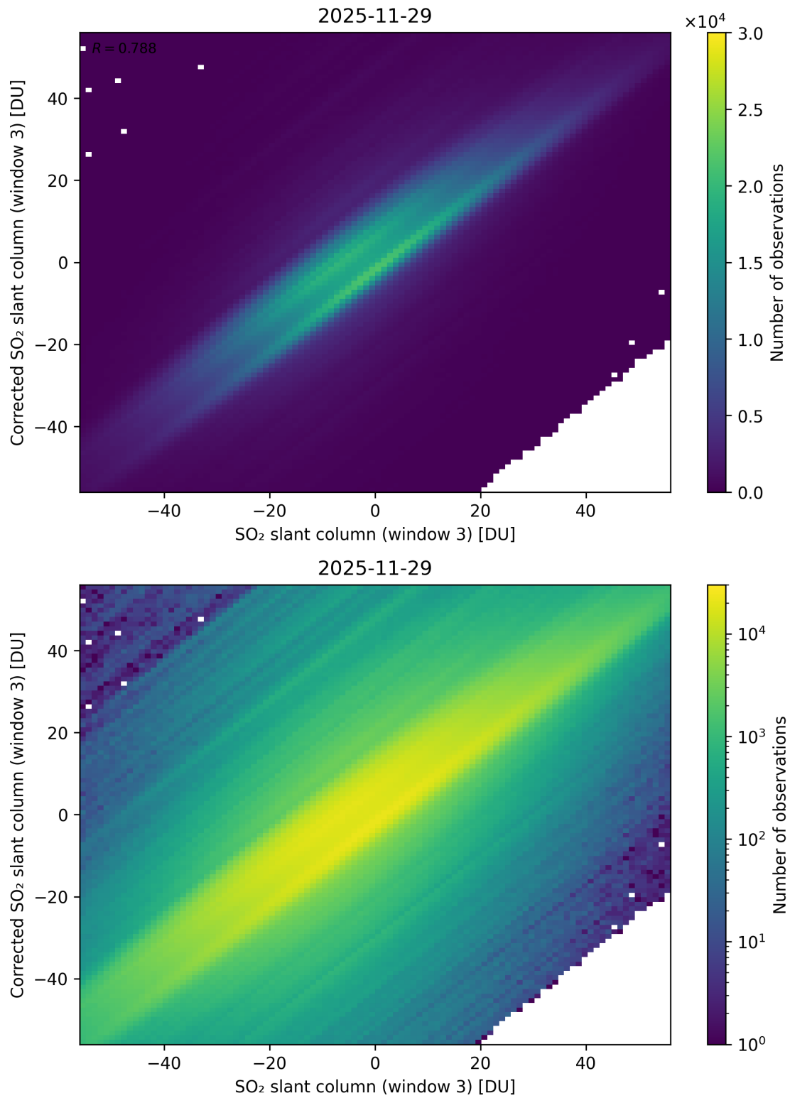
Figure 316: Scatter density plot of “SO 2 slant column (window 3)” against “Corrected SO 2 slant column (window 3)” for 2025-11-28 to 2025-11-30.
