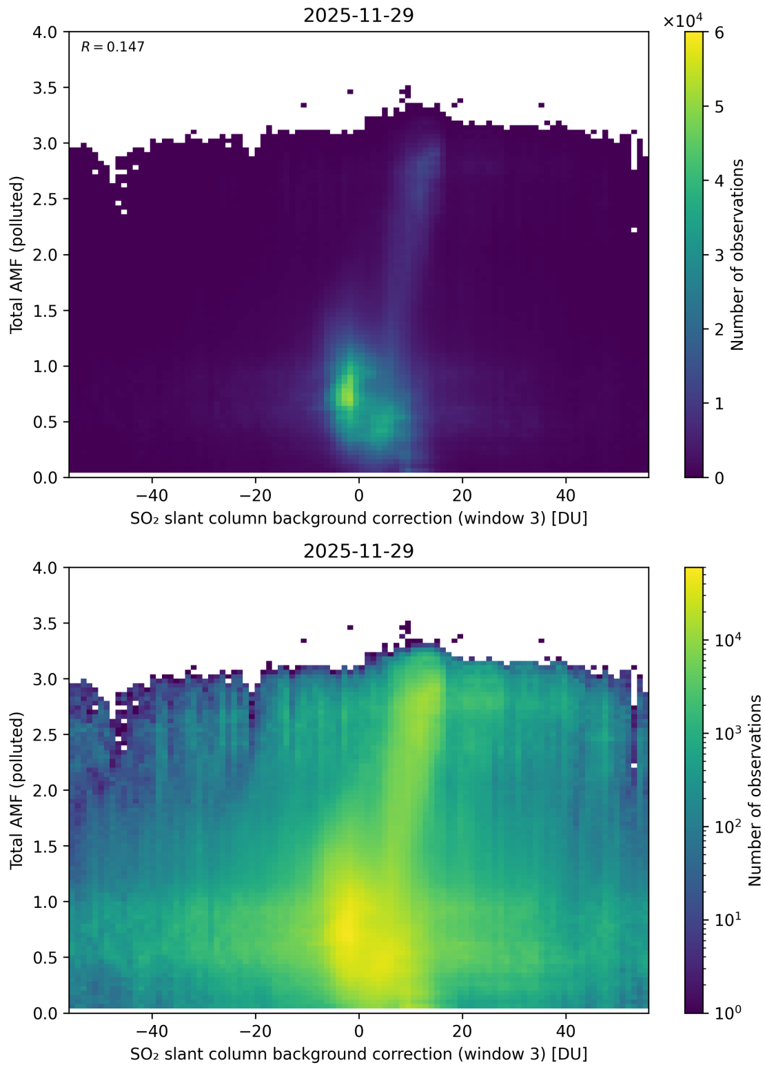
Figure 136: Scatter density plot of “SO 2 slant column background correction (window 3)” against “Total AMF (polluted)” for 2025-11-28 to 2025-11-30.
