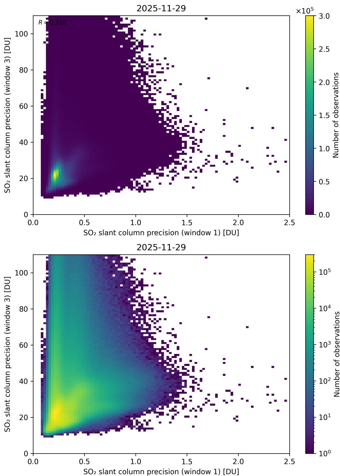
Figure 279: Scatter density plot of “SO 2 slant column precision (window 1)” against “SO 2 slant column precision (window 3)” for 2025-11-28 to 2025-11-30.
