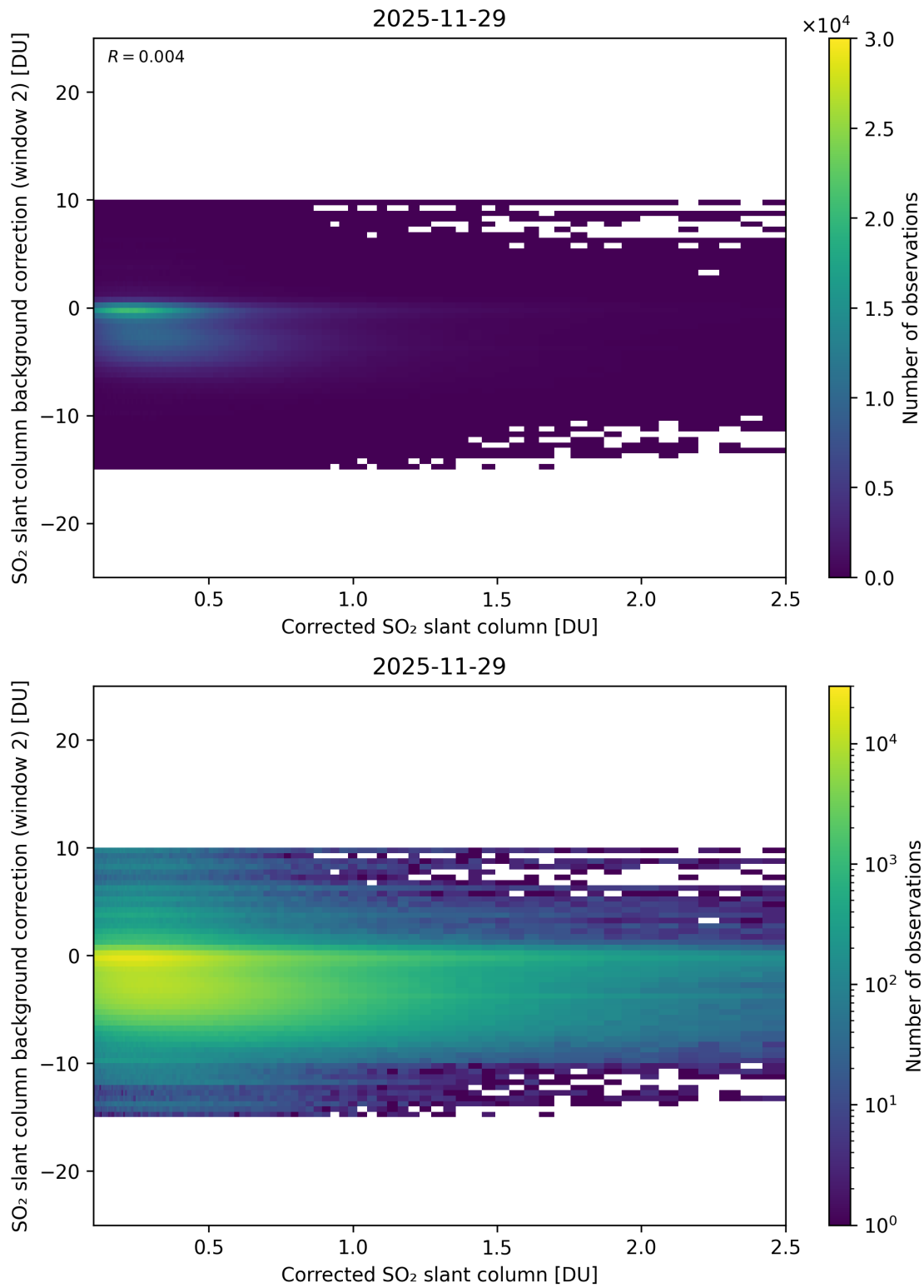
Figure 227: Scatter density plot of “Corrected SO 2 slant column” against “SO 2 slant column background correction (window 2)” for 2025-11-28 to 2025-11-30.
