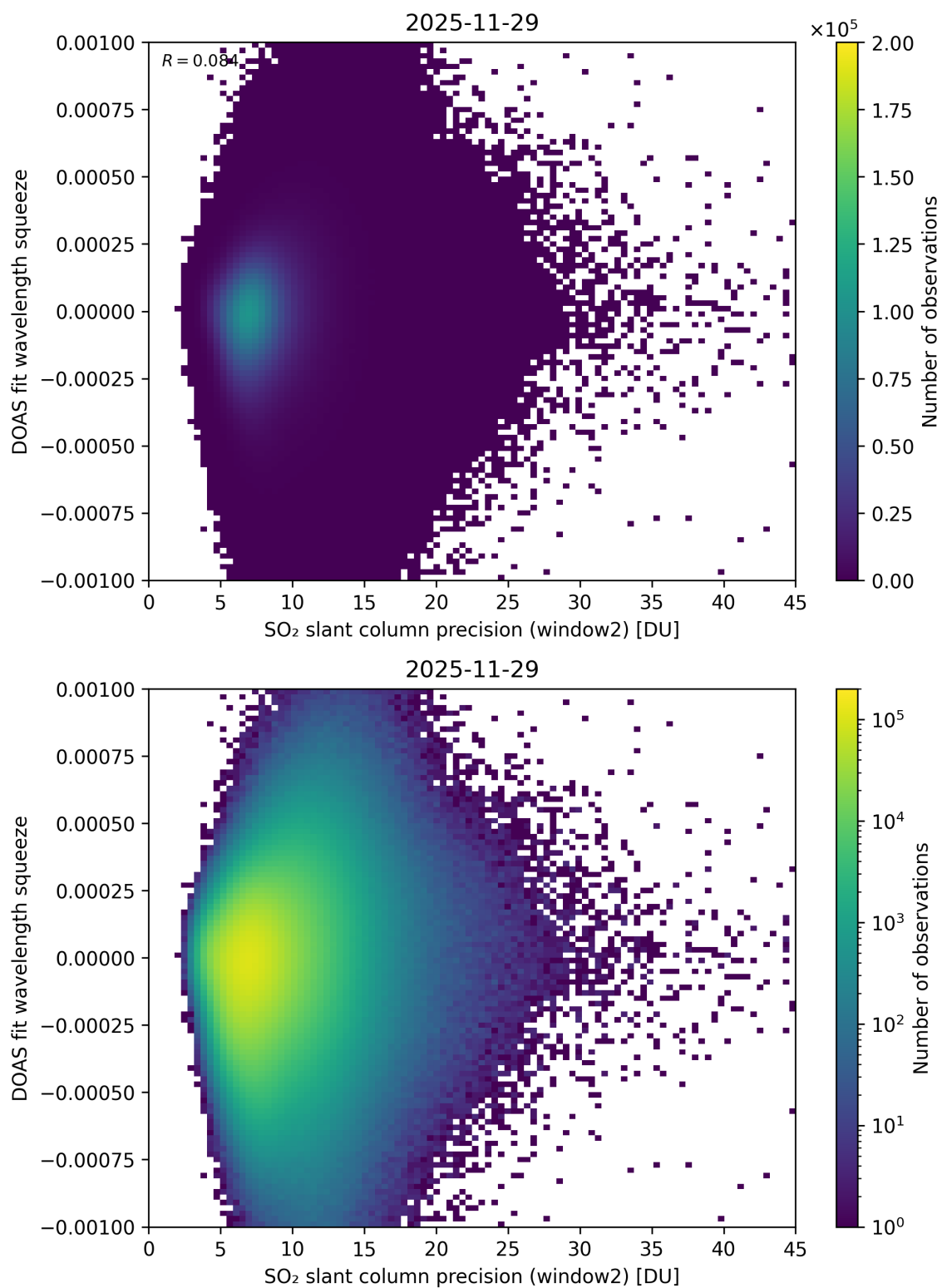
Figure 294: Scatter density plot of “SO 2 slant column precision (window2)” against “DOAS fit wavelength squeeze” for 2025-11-28 to 2025-11-30.
