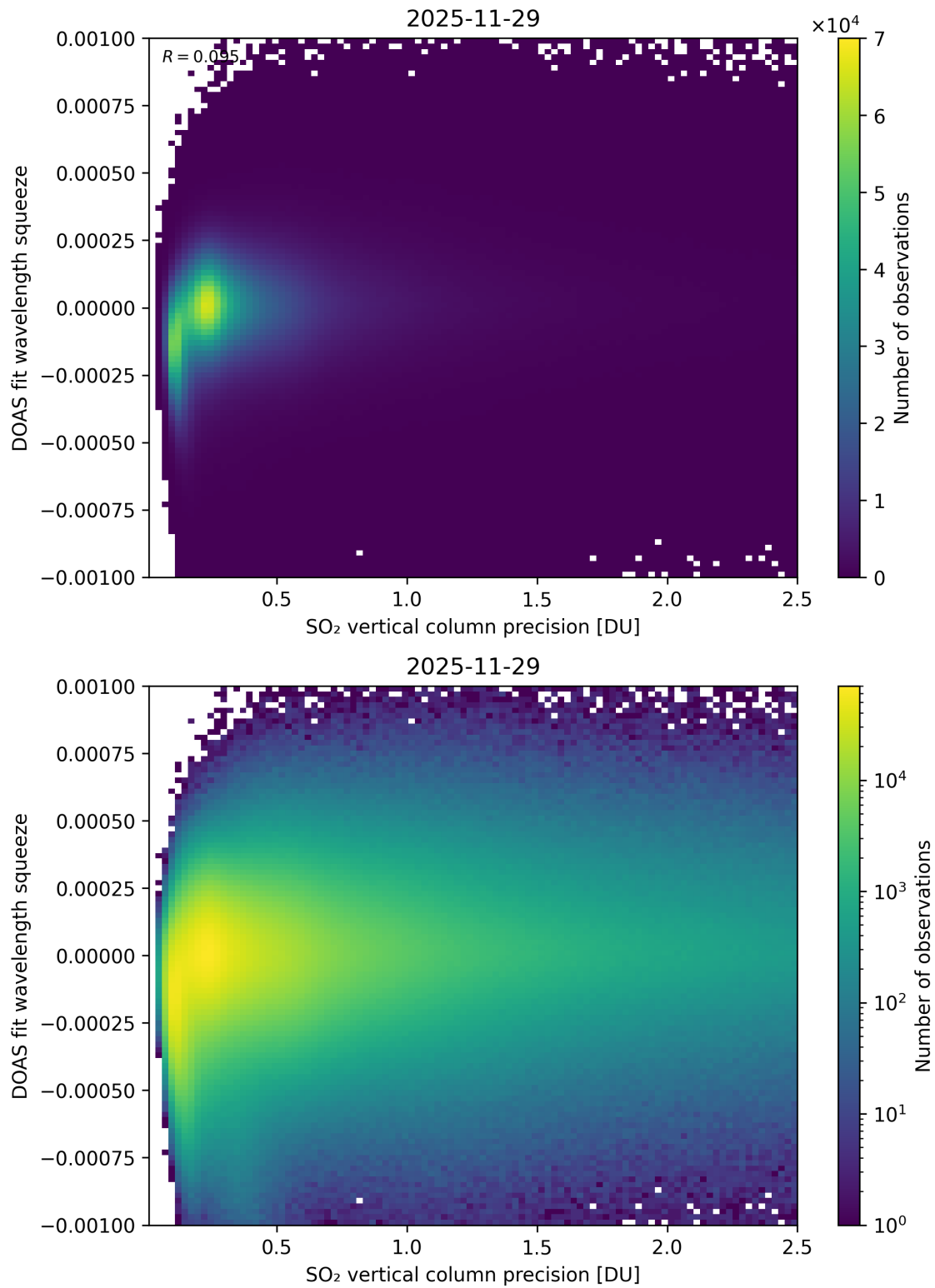
Figure 333: Scatter density plot of “SO 2 vertical column precision” against “DOAS fit wavelength squeeze” for 2025-11-28 to 2025-11-30.
