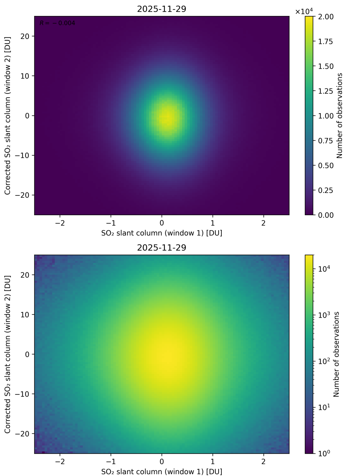
Figure 283: Scatter density plot of “SO 2 slant column (window 1)” against “Corrected SO 2 slant column (window 2)” for 2025-11-28 to 2025-11-30.
