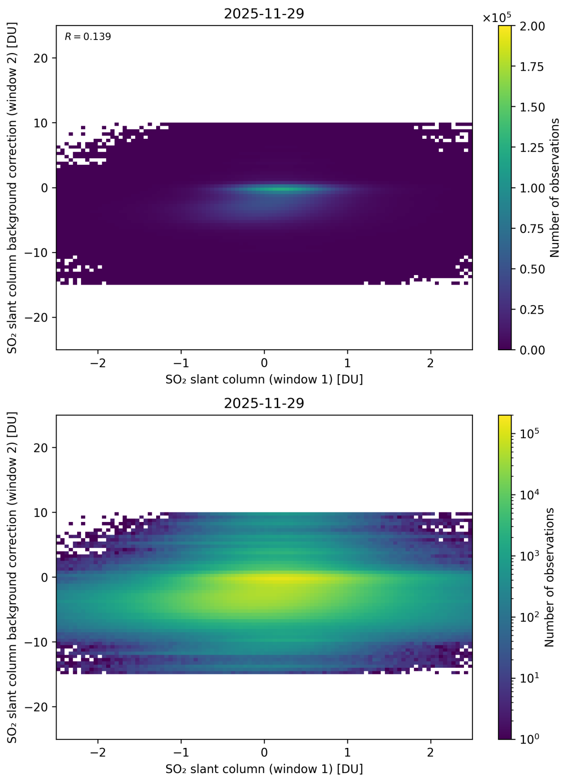
Figure 263: Scatter density plot of “SO 2 slant column (window 1)” against “SO 2 slant column background correction (window 2)” for 2025-11-28 to 2025-11-30.
