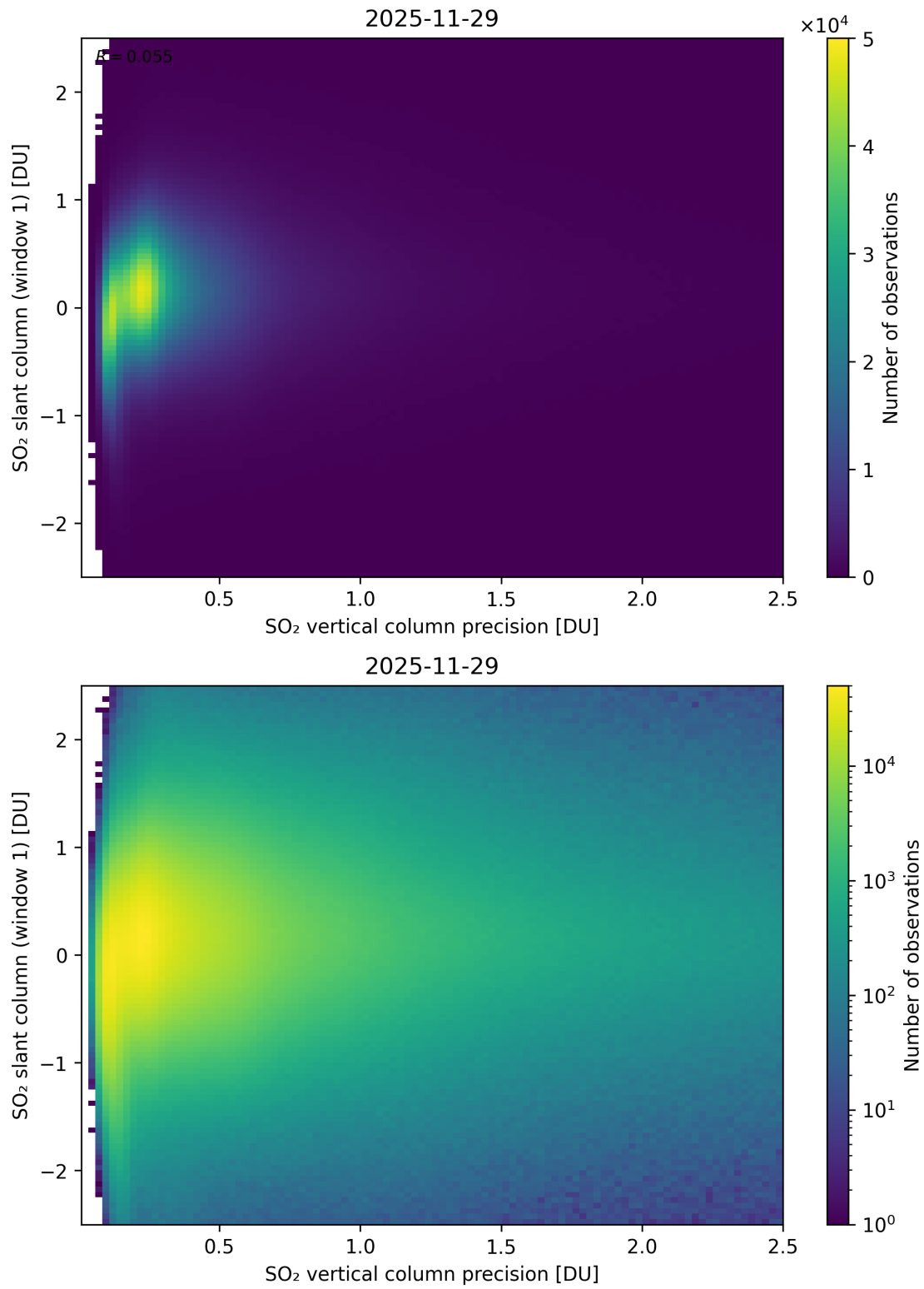
Figure 341: Scatter density plot of “SO 2 vertical column precision” against “SO 2 slant column (window 1)” for 2025-11-28 to 2025-11-30.
