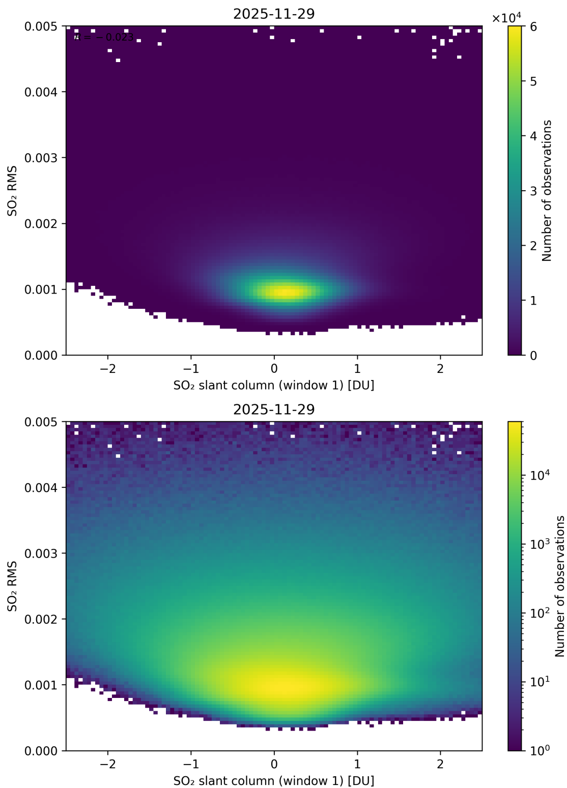
Figure 267: Scatter density plot of “SO 2 slant column (window 1)” against “SO 2 RMS” for 2025-11-28 to 2025-11-30.
