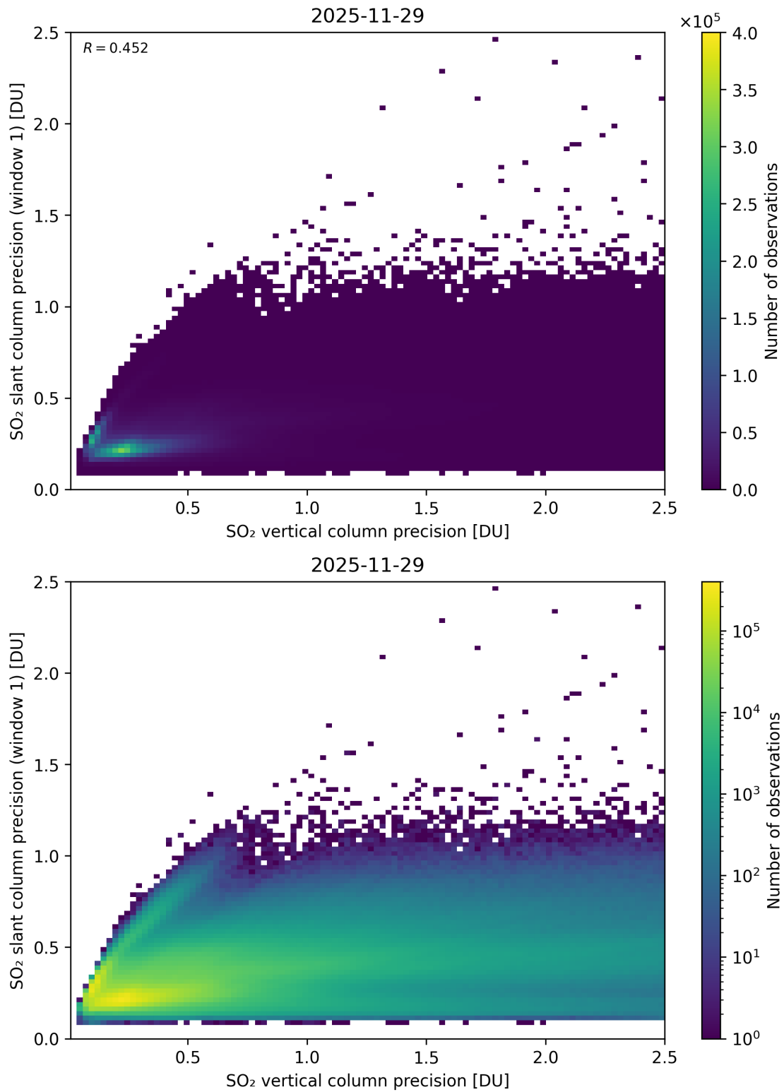
Figure 342: Scatter density plot of “SO 2 vertical column precision” against “SO 2 slant column precision (window 1)” for 2025-11-28 to 2025-11-30.
