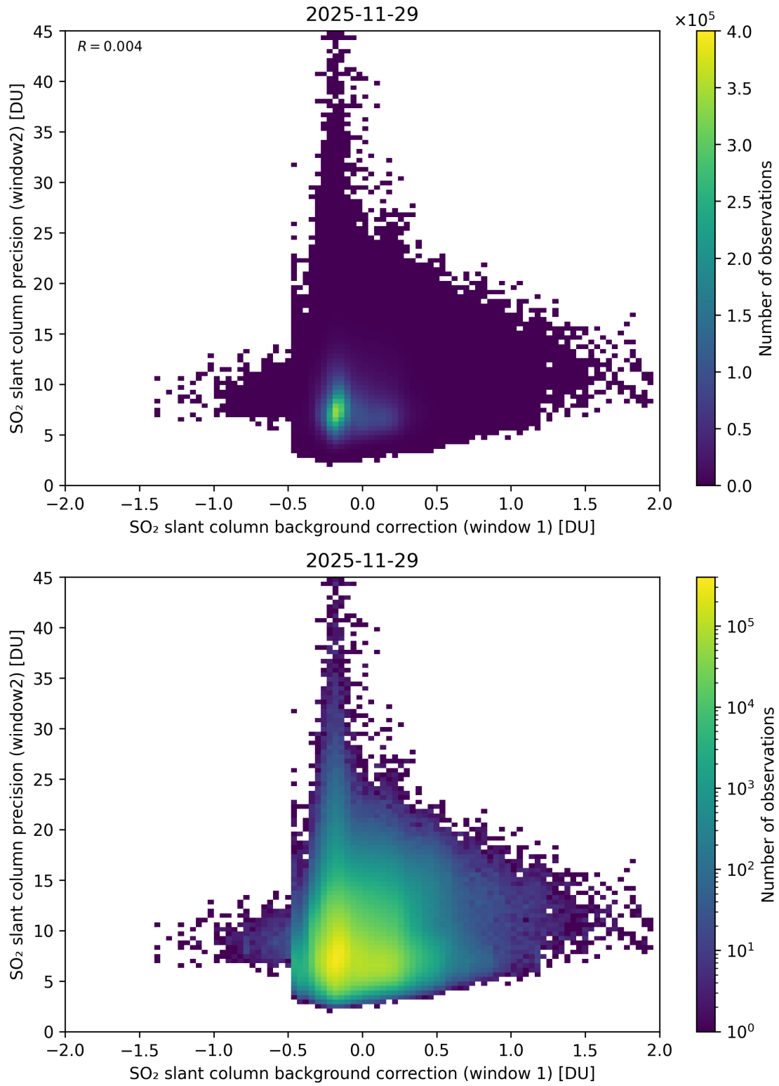
Figure 117: Scatter density plot of “SO 2 slant column background correction (window 1)” against “SO 2 slant column precision (window2)” for 2025-11-28 to 2025-11-30.
