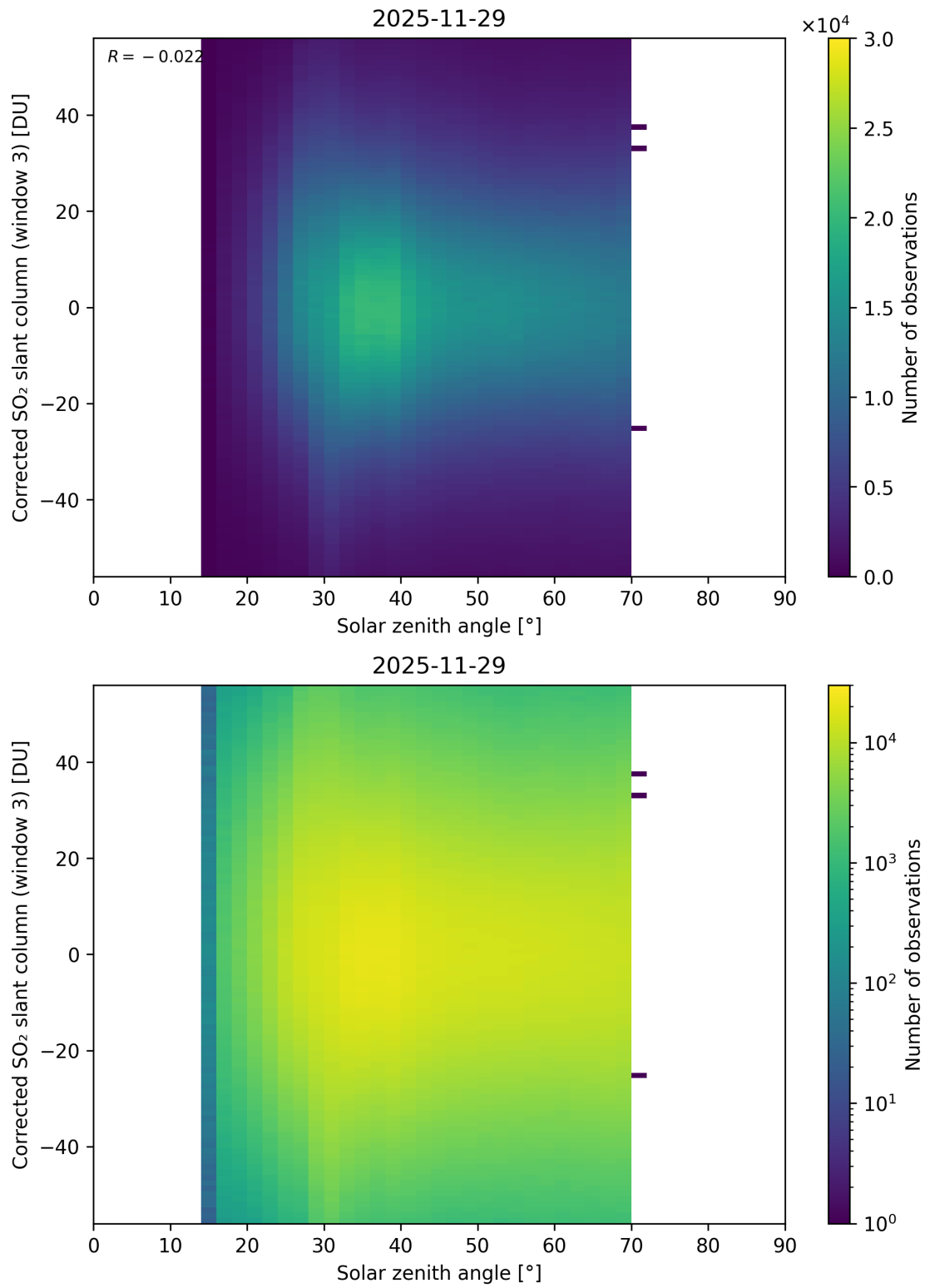
Figure 183: Scatter density plot of “Solar zenith angle” against “Corrected SO 2 slant column (window 3)” for 2025-11-28 to 2025-11-30.
