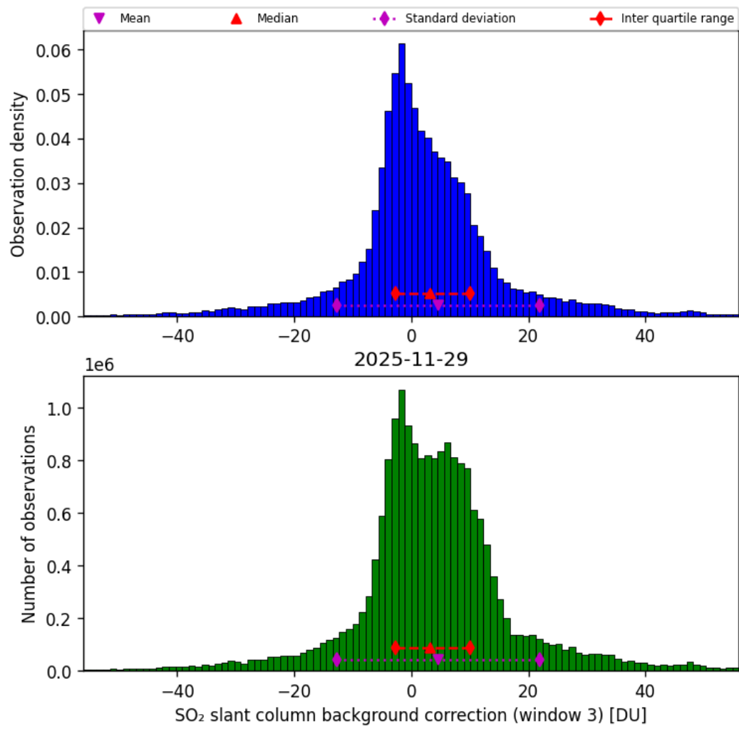
Figure 74: Histogram of “SO 2 slant column background correction (window 3)” for 2025-11-28 to 2025-11-30
