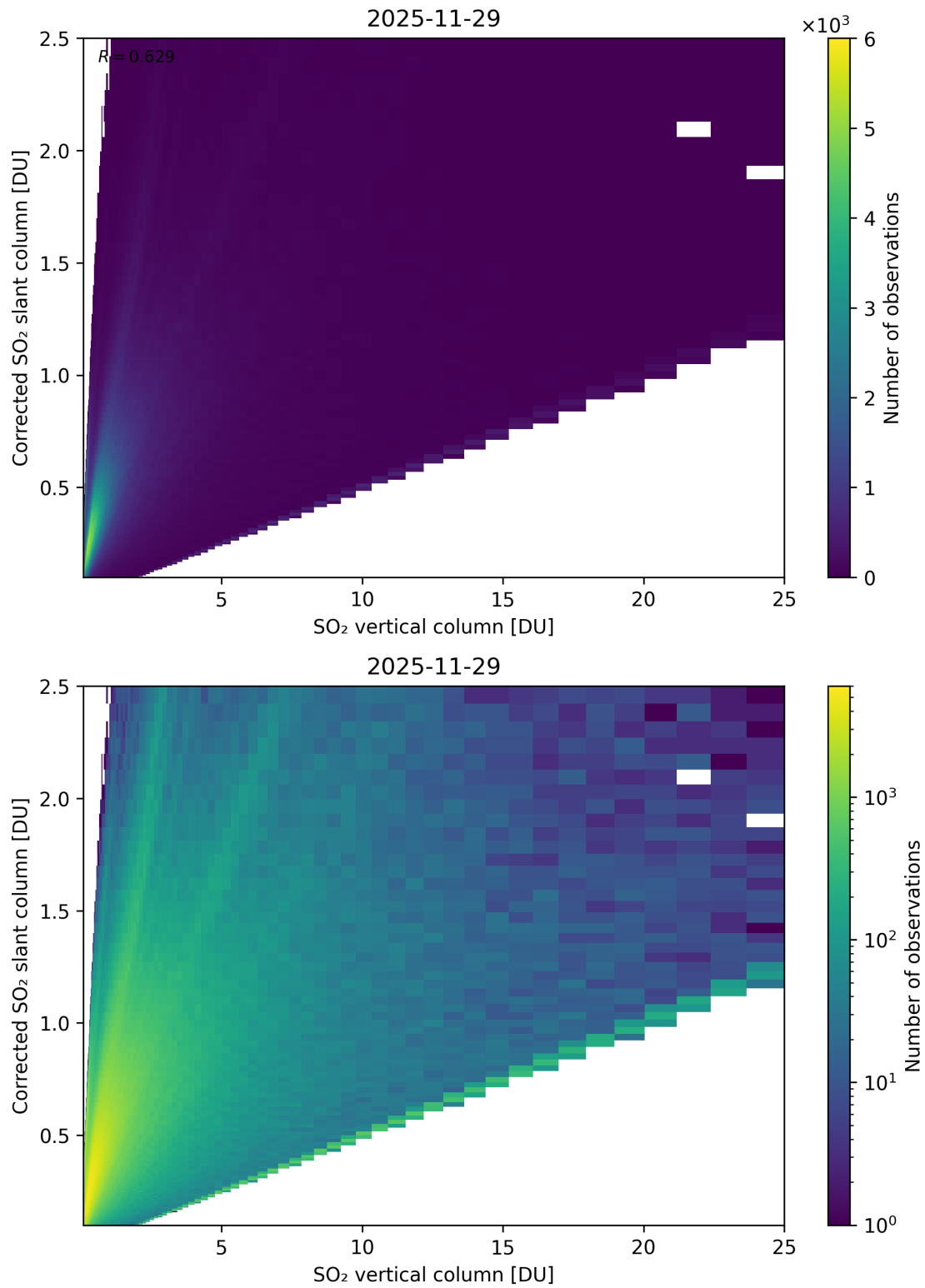
Figure 351: Scatter density plot of “SO 2 vertical column” against “Corrected SO 2 slant column” for 2025-11-28 to 2025-11-30.
