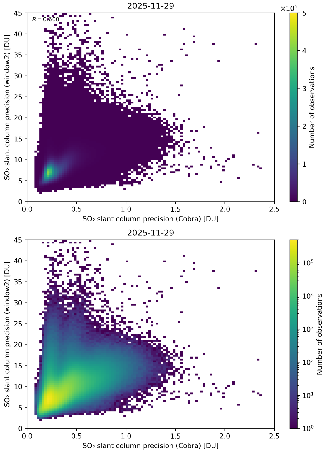
Figure 210: Scatter density plot of “SO 2 slant column precision (Cobra)” against “SO 2 slant column precision (window2)” for 2025-11-28 to 2025-11-30.
