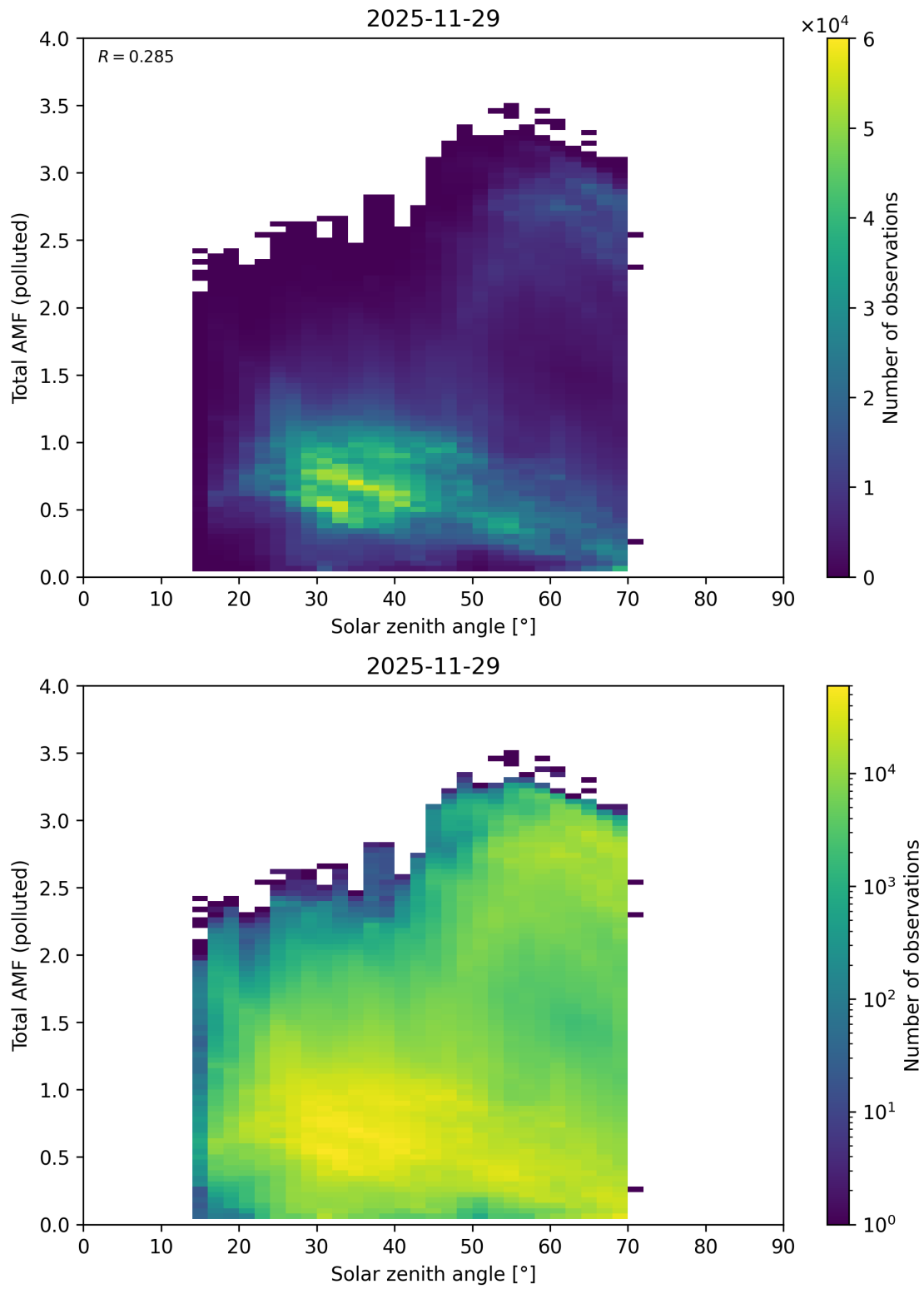
Figure 189: Scatter density plot of “Solar zenith angle” against “Total AMF (polluted)” for 2025-11-28 to 2025-11-30.
