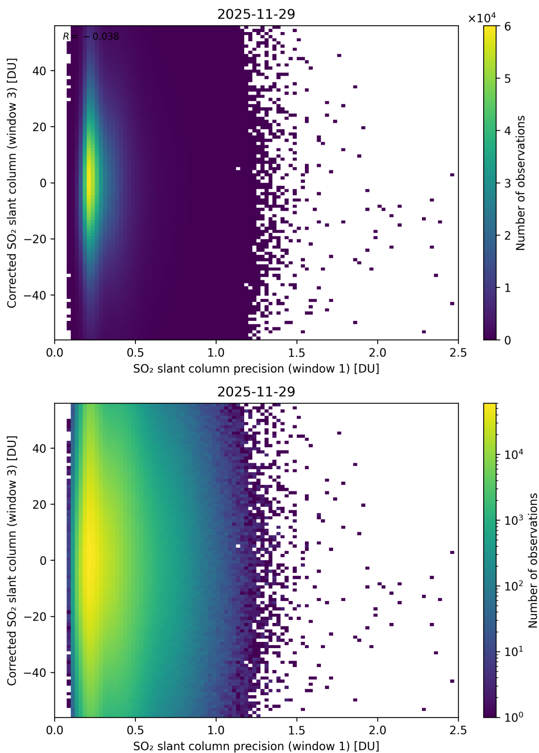
Figure 276: Scatter density plot of “SO 2 slant column precision (window 1)” against “Corrected SO 2 slant column (window 3)” for 2025-11-28 to 2025-11-30.
