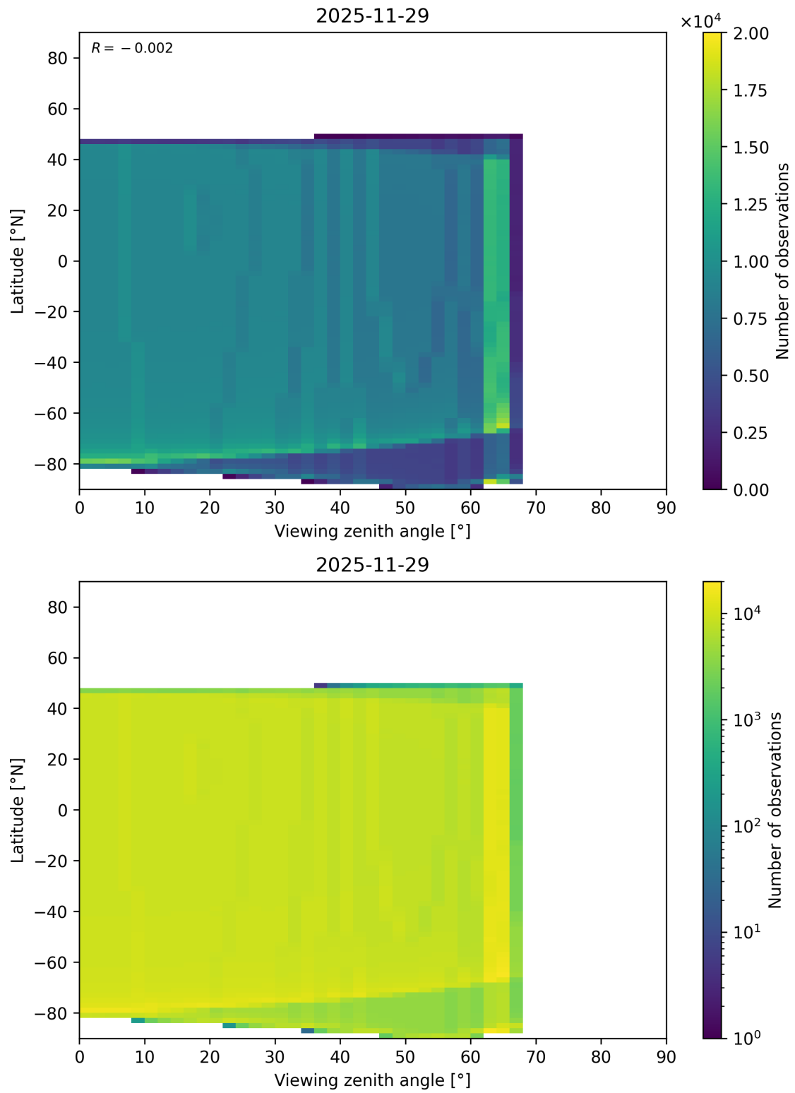
Figure 368: Scatter density plot of “Viewing zenith angle” against “Latitude” for 2025-11-28 to 2025-11-30.
