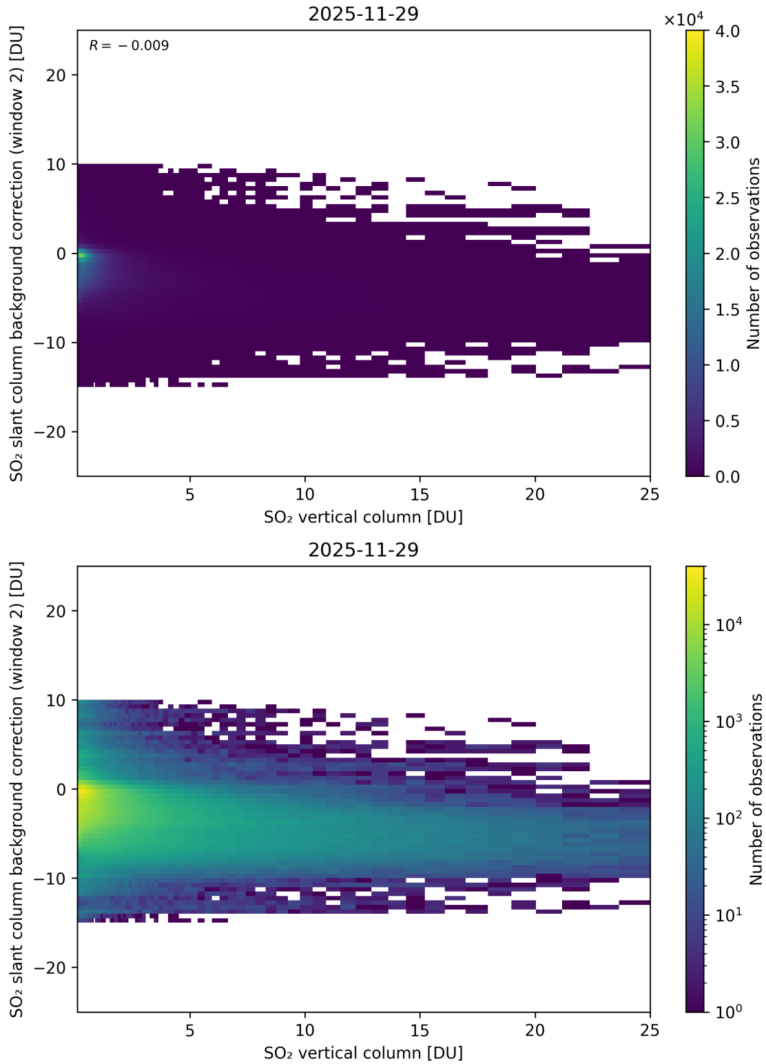
Figure 324: Scatter density plot of “SO 2 vertical column” against “SO 2 slant column background correction (window 2)” for 2025-11-28 to 2025-11-30.
