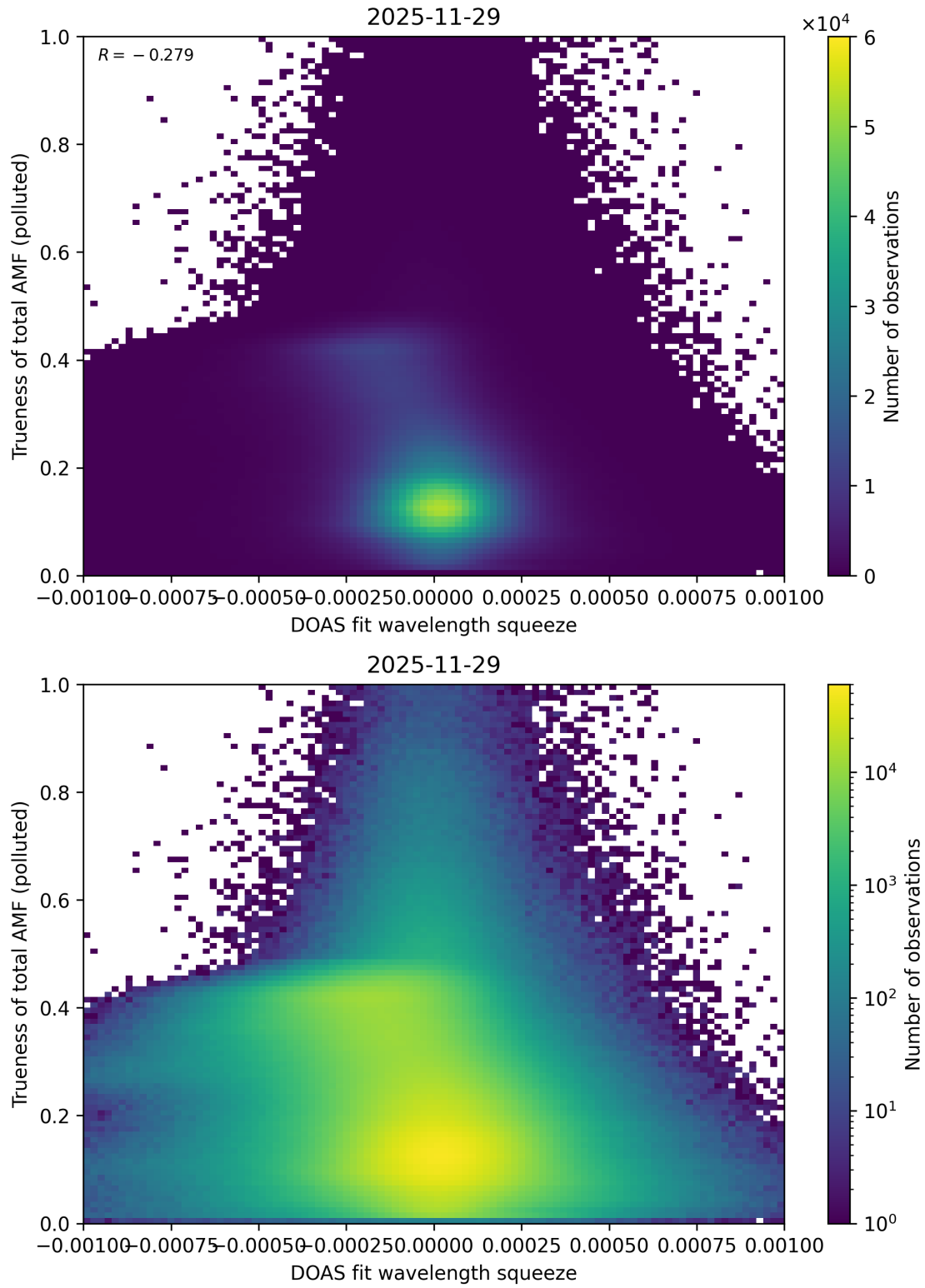
Figure 146: Scatter density plot of “DOAS fit wavelength squeeze” against “Trueness of total AMF (polluted)” for 2025-11-28 to 2025-11-30.
