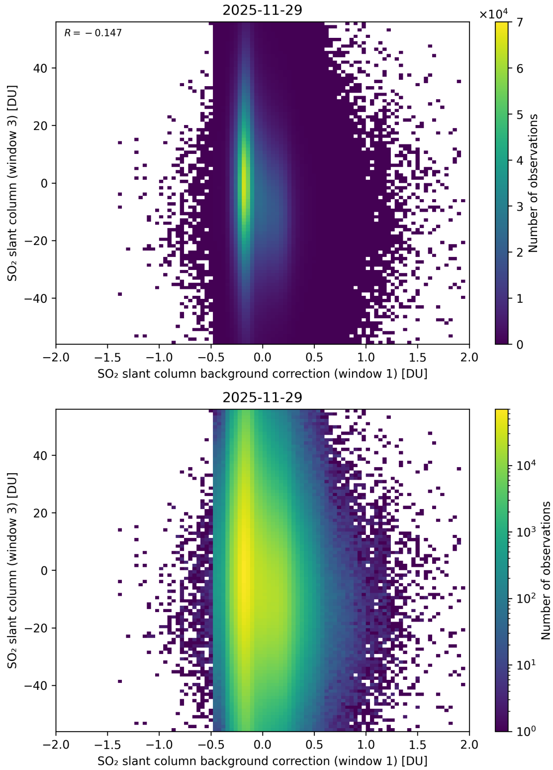
Figure 118: Scatter density plot of “SO 2 slant column background correction (window 1)” against “SO 2 slant column (window 3)” for 2025-11-28 to 2025-11-30.
