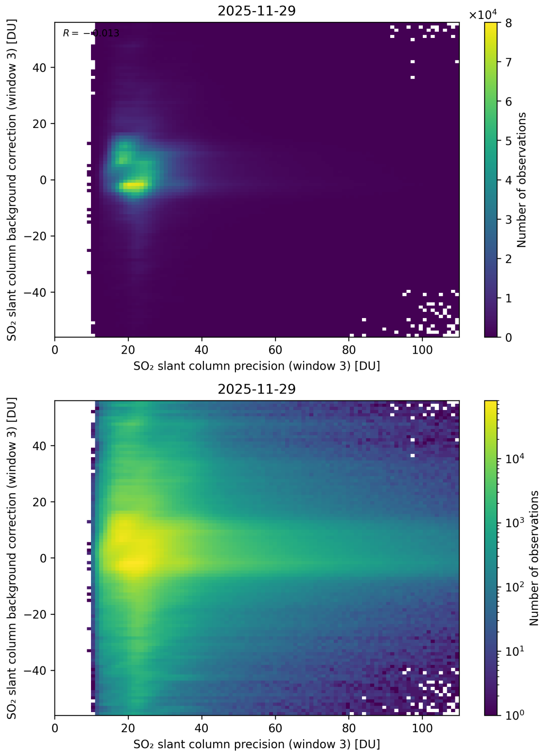
Figure 307: Scatter density plot of “SO 2 slant column precision (window 3)” against “SO 2 slant column background correction (window 3)” for 2025-11-28 to 2025-11-30.
