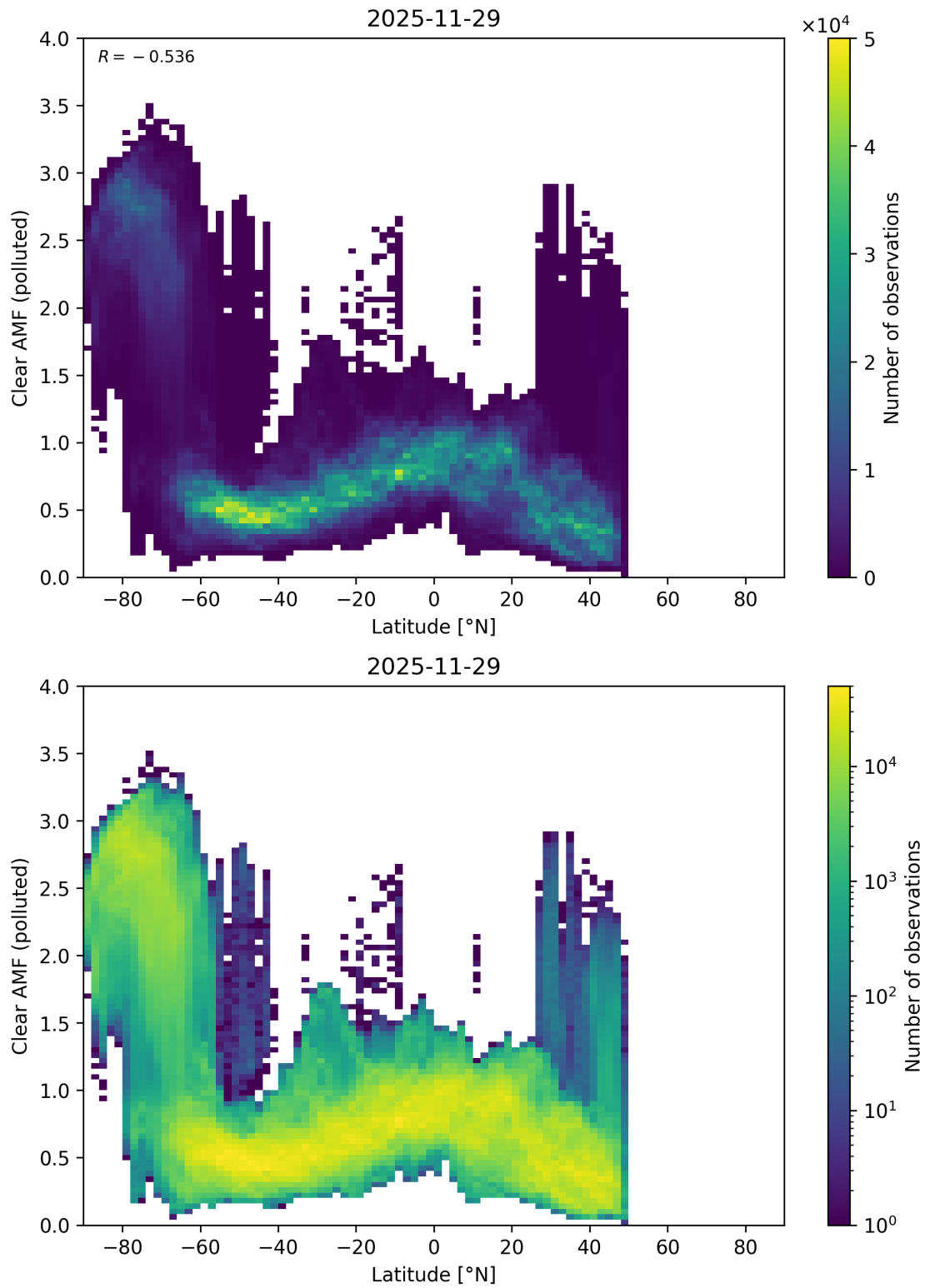
Figure 156: Scatter density plot of “Latitude” against “Clear AMF (polluted)” for 2025-11-28 to 2025-11-30.
