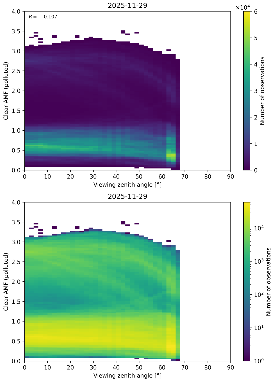
Figure 370: Scatter density plot of “Viewing zenith angle” against “Clear AMF (polluted)” for 2025-11-28 to 2025-11-30.
