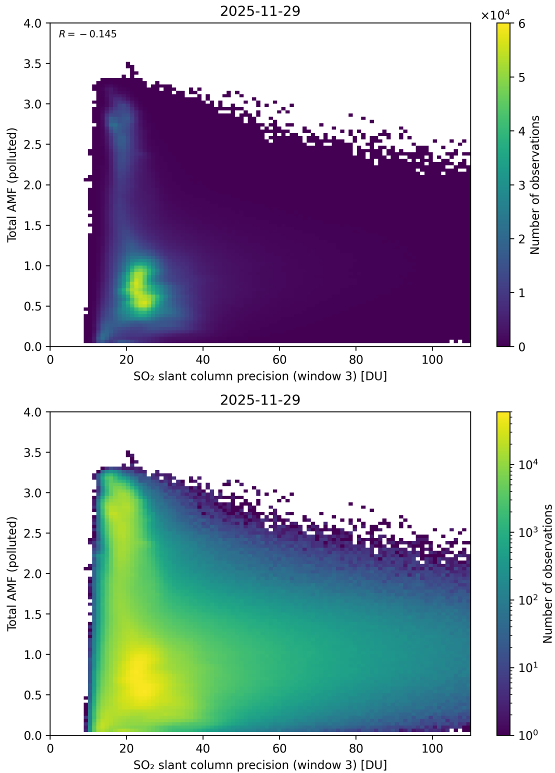
Figure 313: Scatter density plot of “SO 2 slant column precision (window 3)” against “Total AMF (polluted)” for 2025-11-28 to 2025-11-30.
