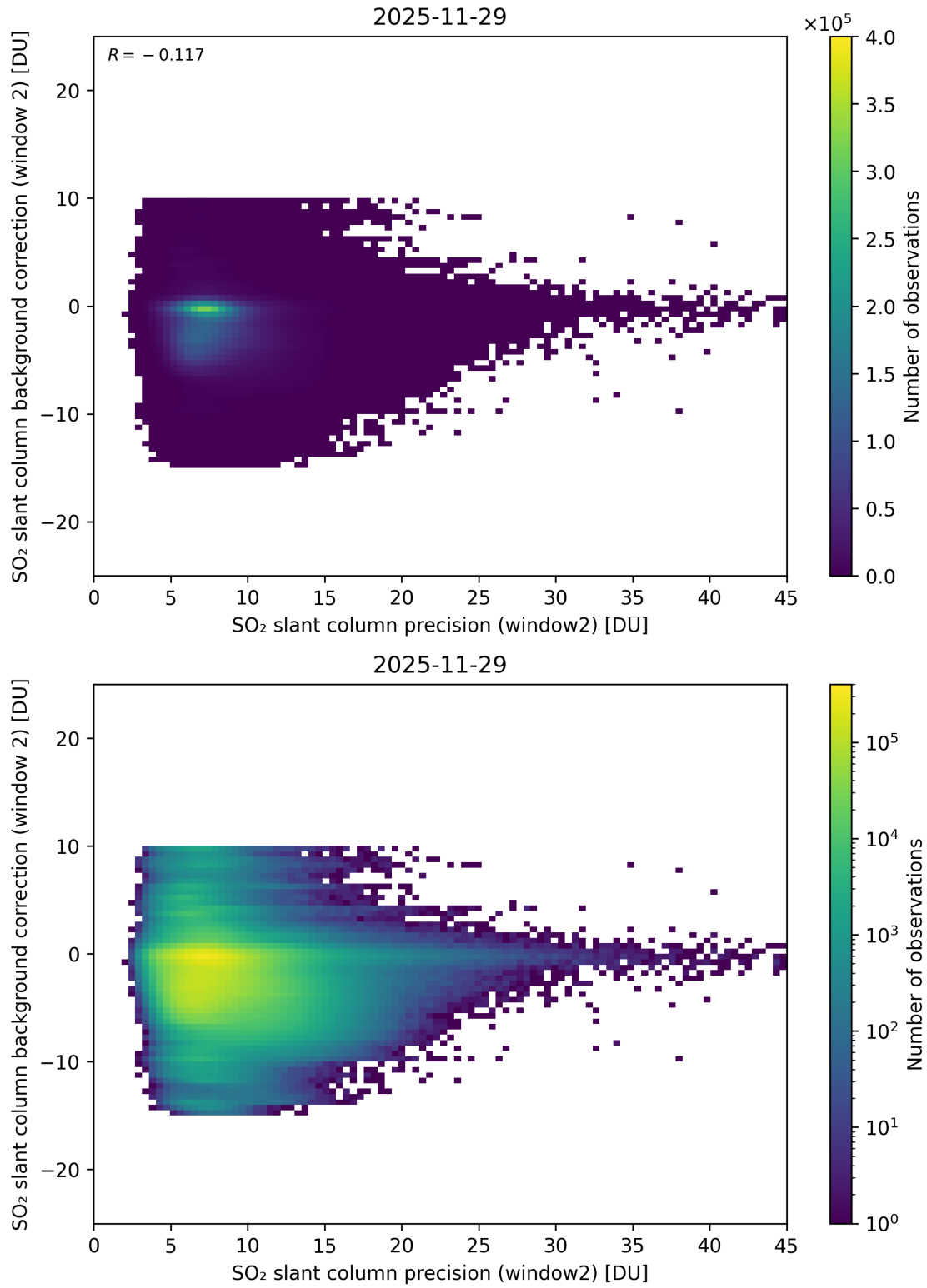
Figure 291: Scatter density plot of “SO 2 slant column precision (window2)” against “SO 2 slant column background correction (window 2)” for 2025-11-28 to 2025-11-30.
