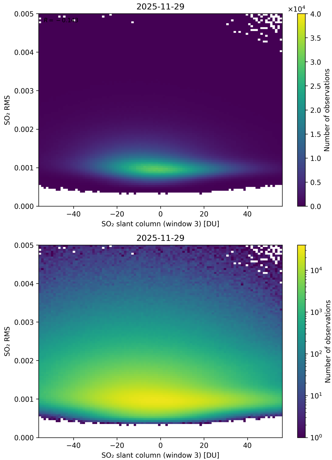
Figure 306: Scatter density plot of “SO 2 slant column (window 3)” against “SO 2 RMS” for 2025-11-28 to 2025-11-30.
