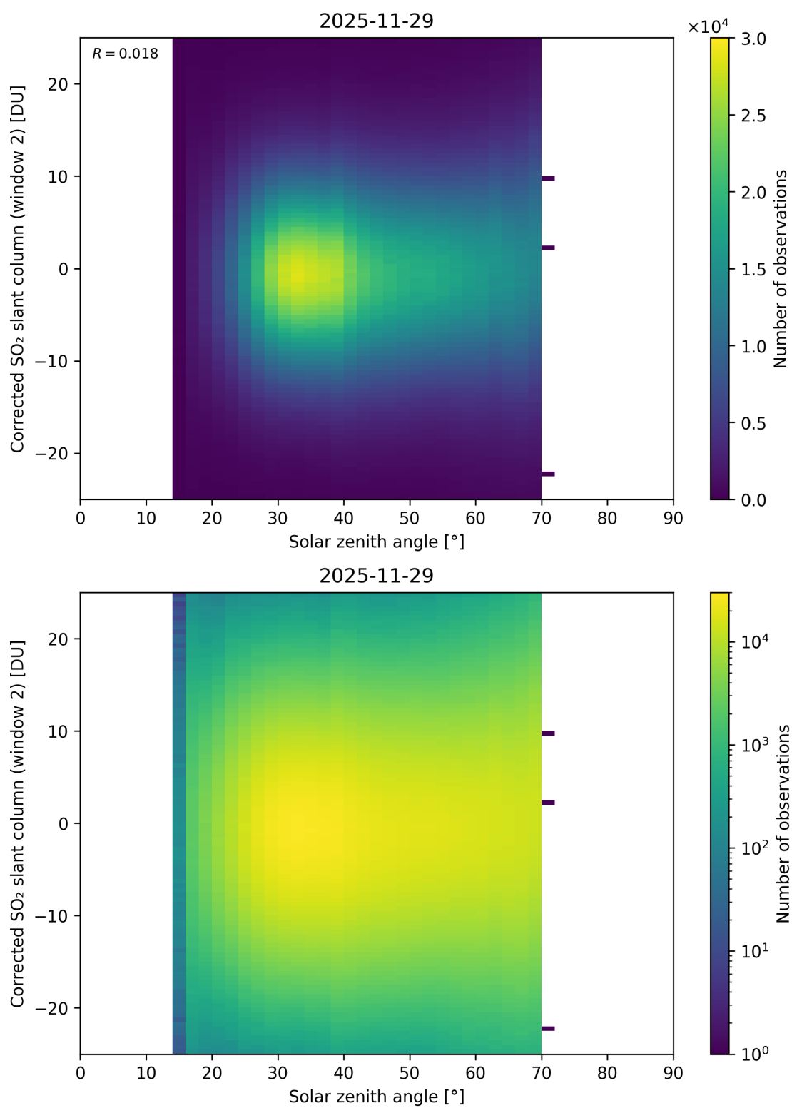
Figure 182: Scatter density plot of “Solar zenith angle” against “Corrected SO 2 slant column (window 2)” for 2025-11-28 to 2025-11-30.
