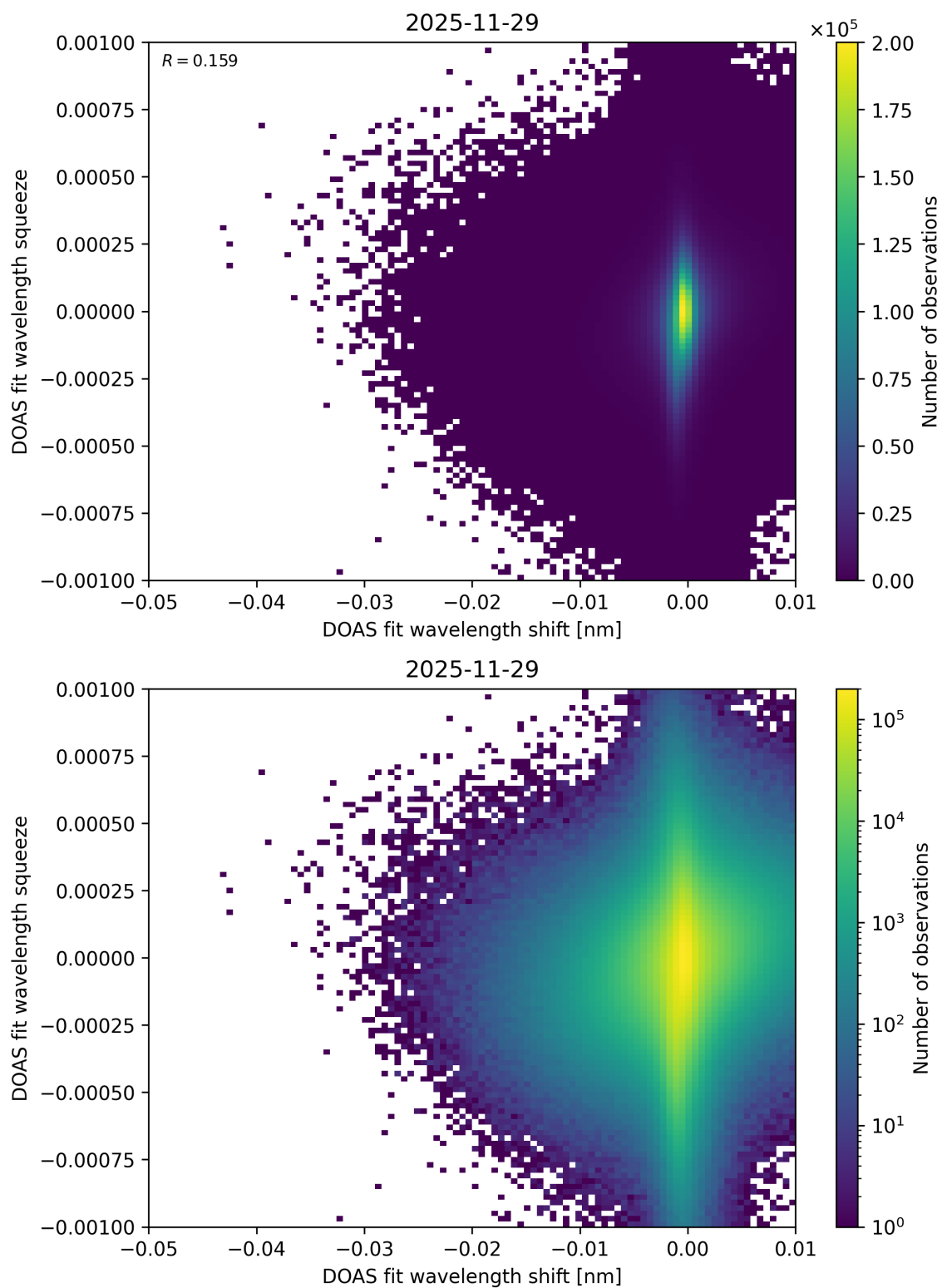
Figure 138: Scatter density plot of “DOAS fit wavelength shift” against “DOAS fit wavelength squeeze” for 2025-11-28 to 2025-11-30.
