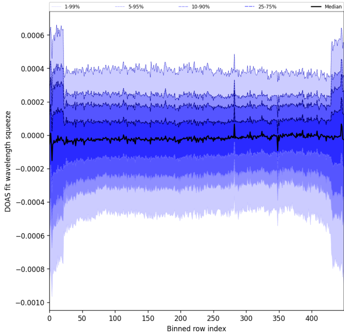
Figure 103: Along track statistics of “DOAS fit wavelength squeeze” for 2025-11-28 to 2025-11-30
