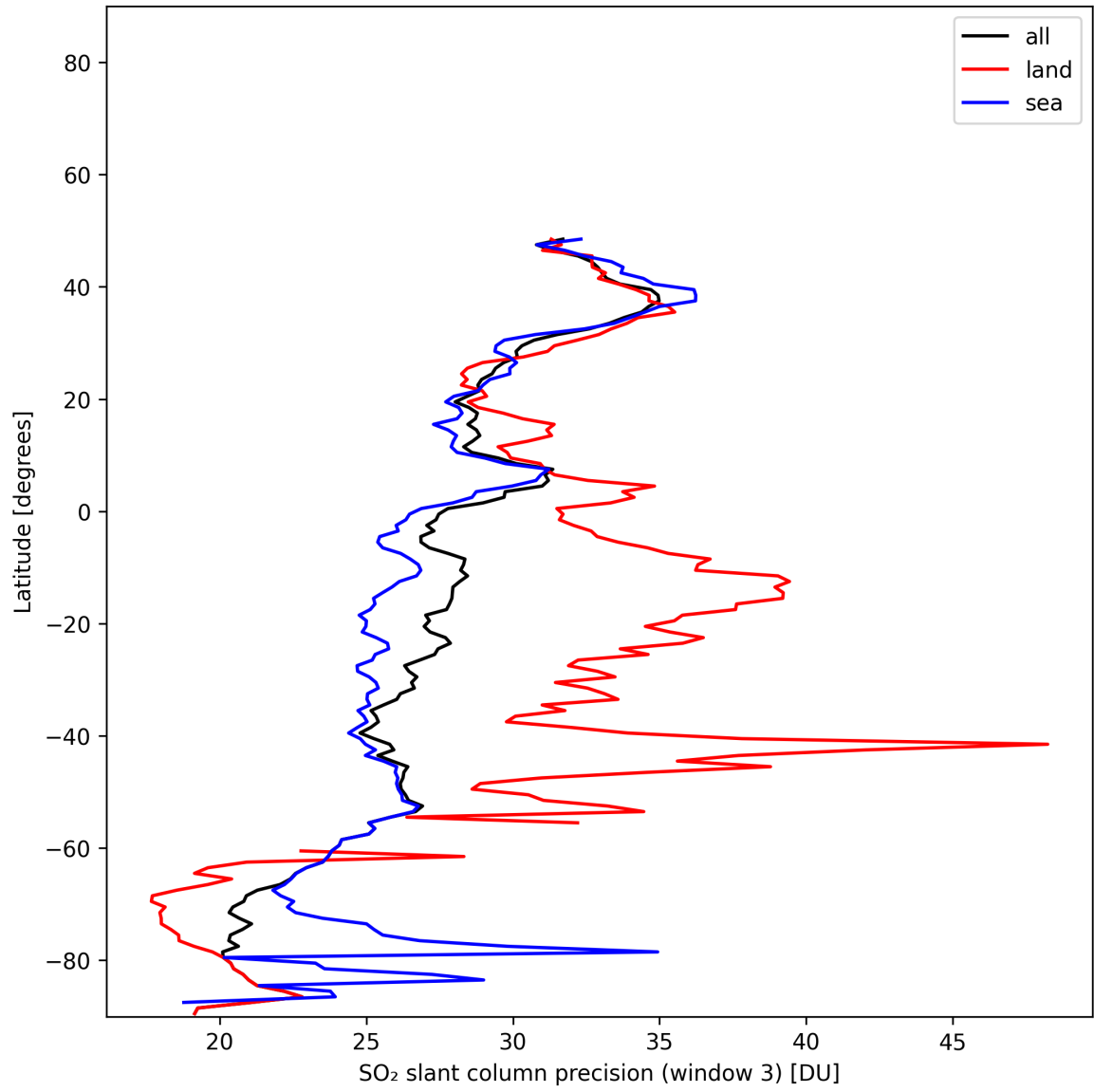
Figure 46: Zonal average of “SO 2 slant column precision (window 3)” for 2025-11-28 to 2025-11-30.
