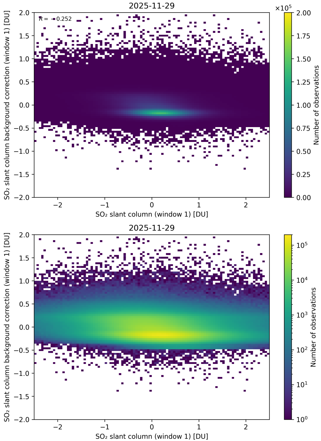
Figure 262: Scatter density plot of “SO 2 slant column (window 1)” against “SO 2 slant column background correction (window 1)” for 2025-11-28 to 2025-11-30.
