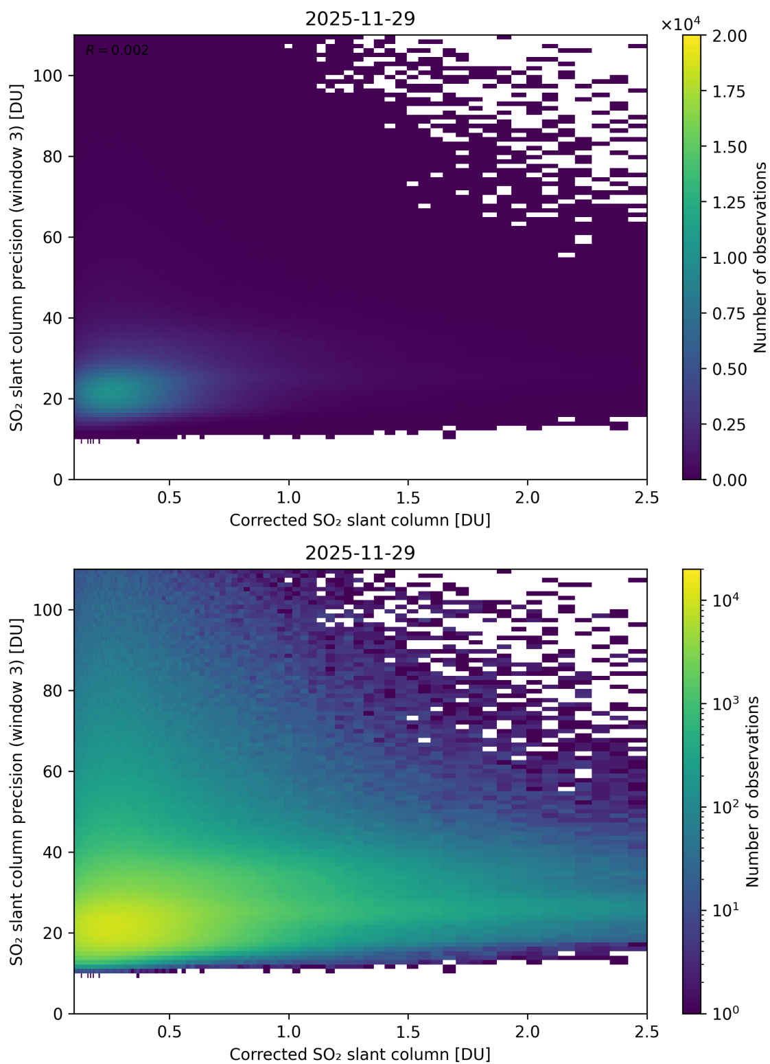
Figure 241: Scatter density plot of “Corrected SO 2 slant column” against “SO 2 slant column precision (window 3)” for 2025-11-28 to 2025-11-30.
