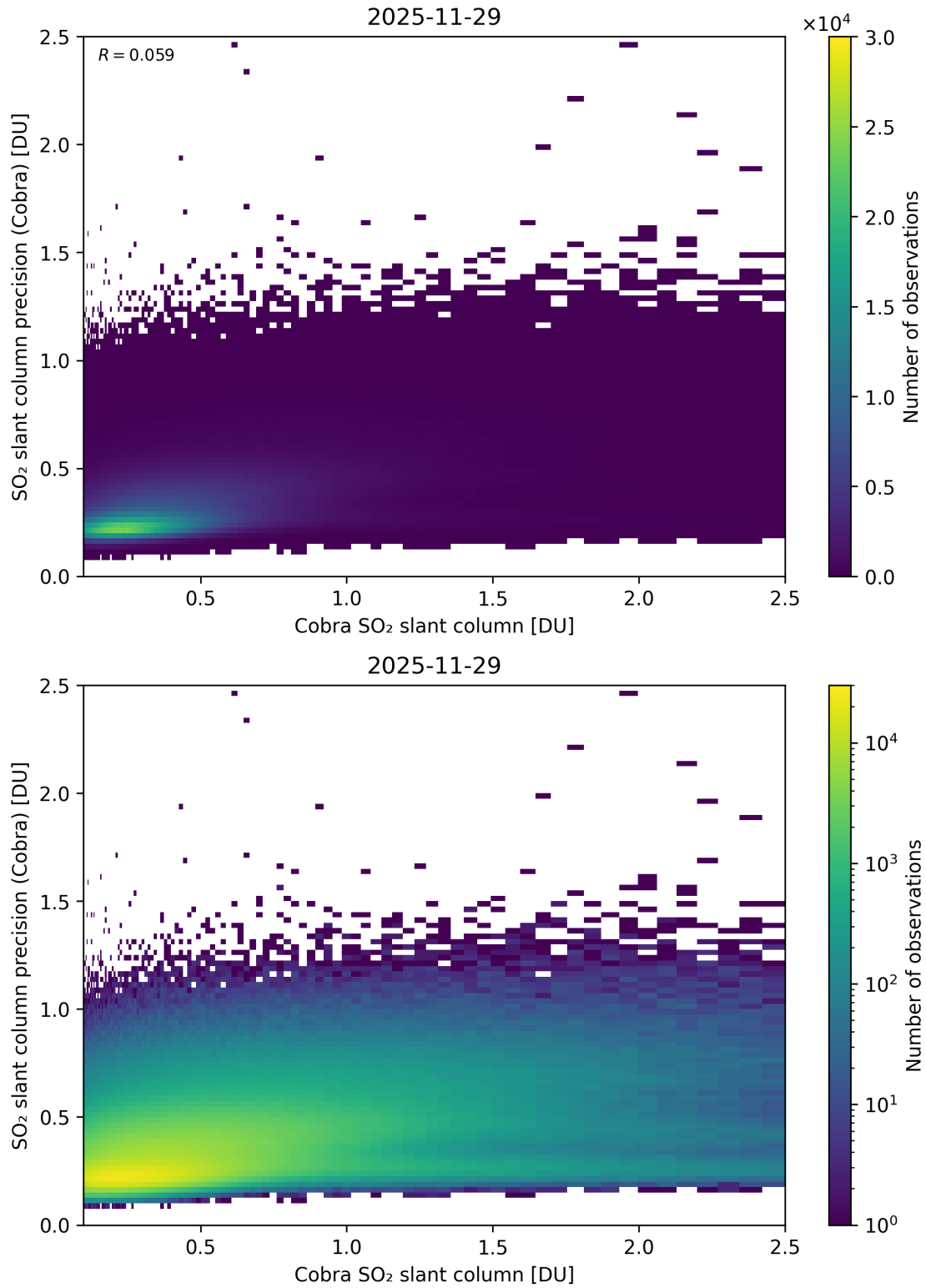
Figure 216: Scatter density plot of “Cobra SO 2 slant column” against “SO 2 slant column precision (Cobra)” for 2025-11-28 to 2025-11-30.
