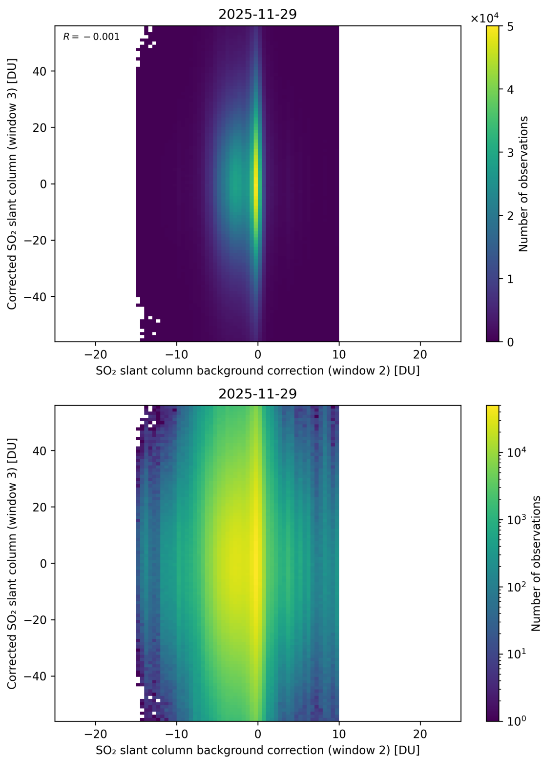
Figure 127: Scatter density plot of “SO 2 slant column background correction (window 2)” against “Corrected SO 2 slant column (window 3)” for 2025-11-28 to 2025-11-30.
