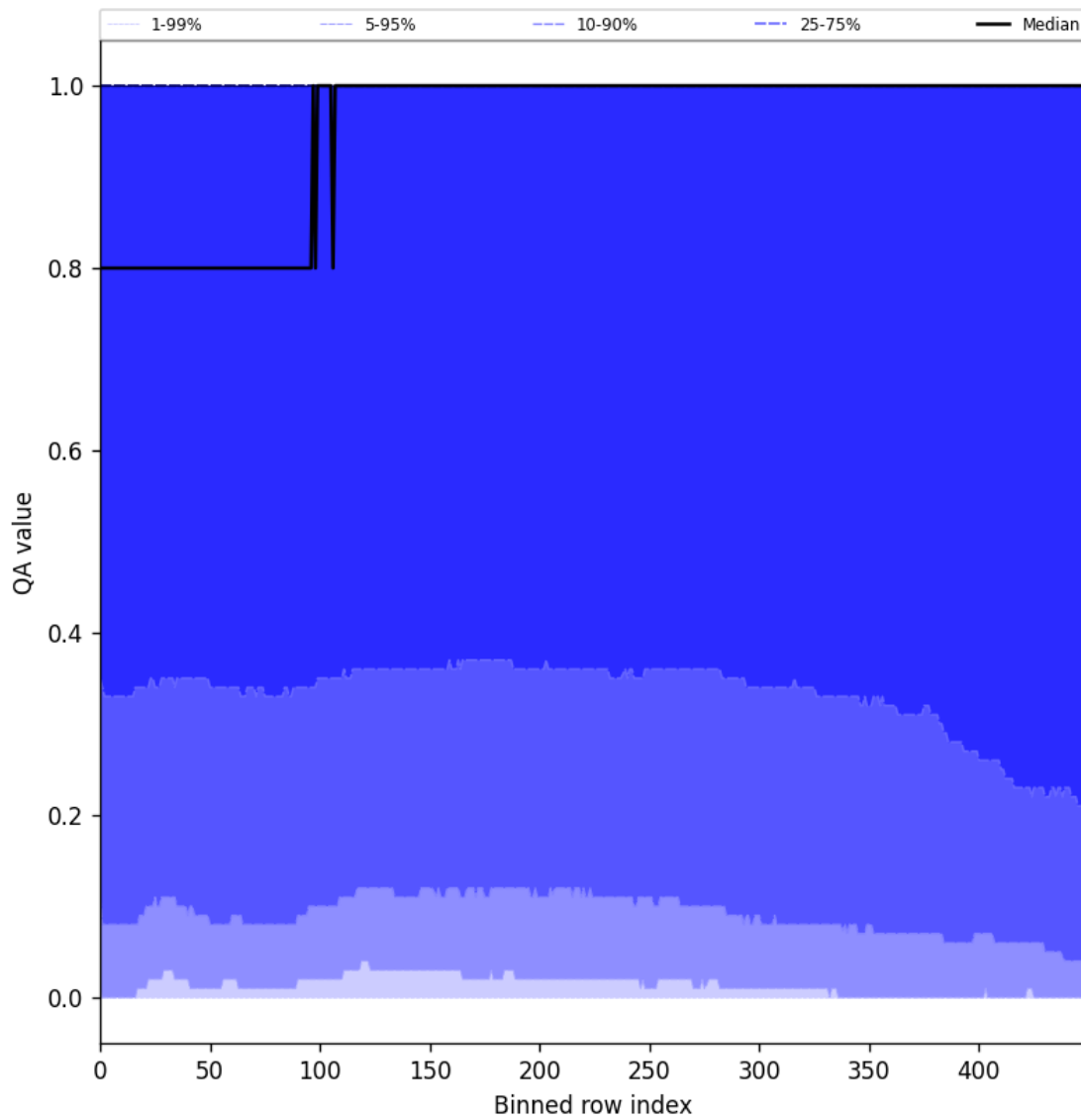
Figure 83: Along track statistics of “QA value” for 2025-11-28 to 2025-11-30
