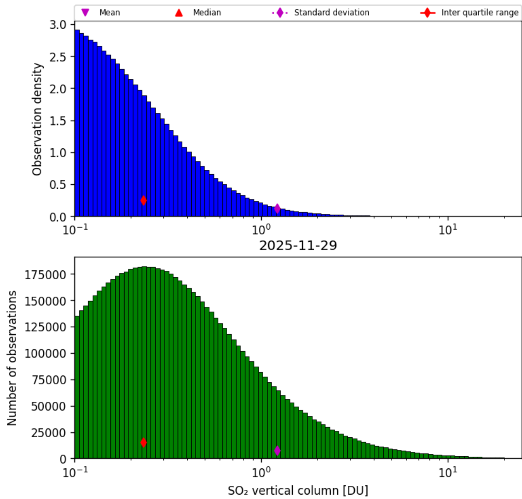
Figure 58: Histogram of “SO 2 vertical column” for 2025-11-28 to 2025-11-30
