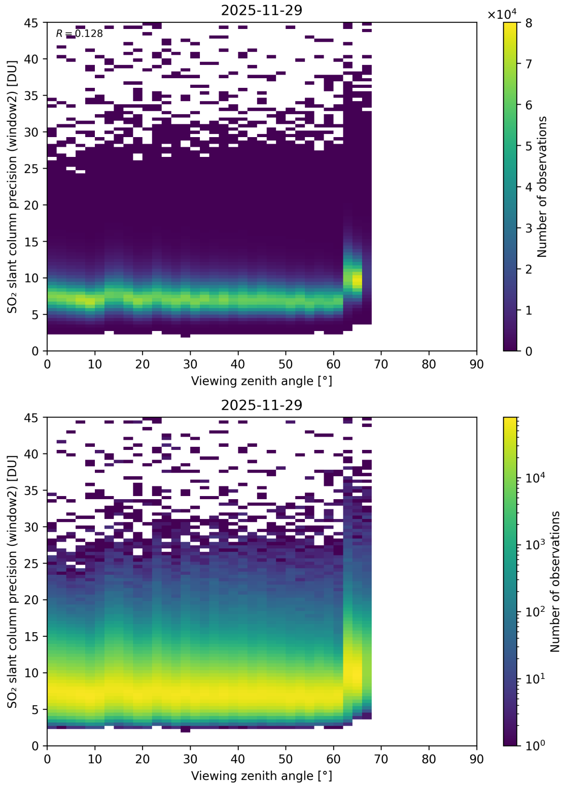
Figure 378: Scatter density plot of “Viewing zenith angle” against “SO 2 slant column precision (window2)” for 2025-11-28 to 2025-11-30.
