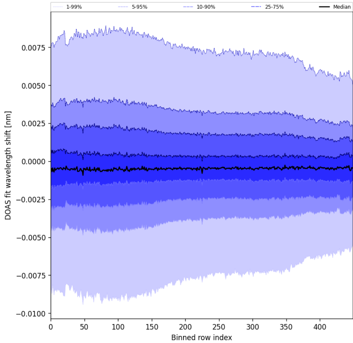
Figure 102: Along track statistics of “DOAS fit wavelength shift” for 2025-11-28 to 2025-11-30
