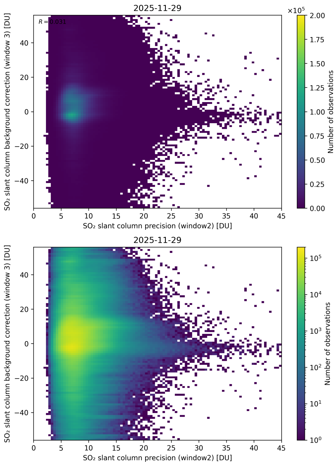
Figure 292: Scatter density plot of “SO 2 slant column precision (window2)” against “SO 2 slant column background correction (window 3)” for 2025-11-28 to 2025-11-30.
