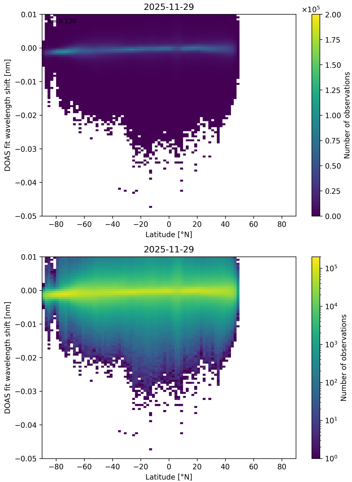
Figure 153: Scatter density plot of “Latitude” against “DOAS fit wavelength shift” for 2025-11-28 to 2025-11-30.
