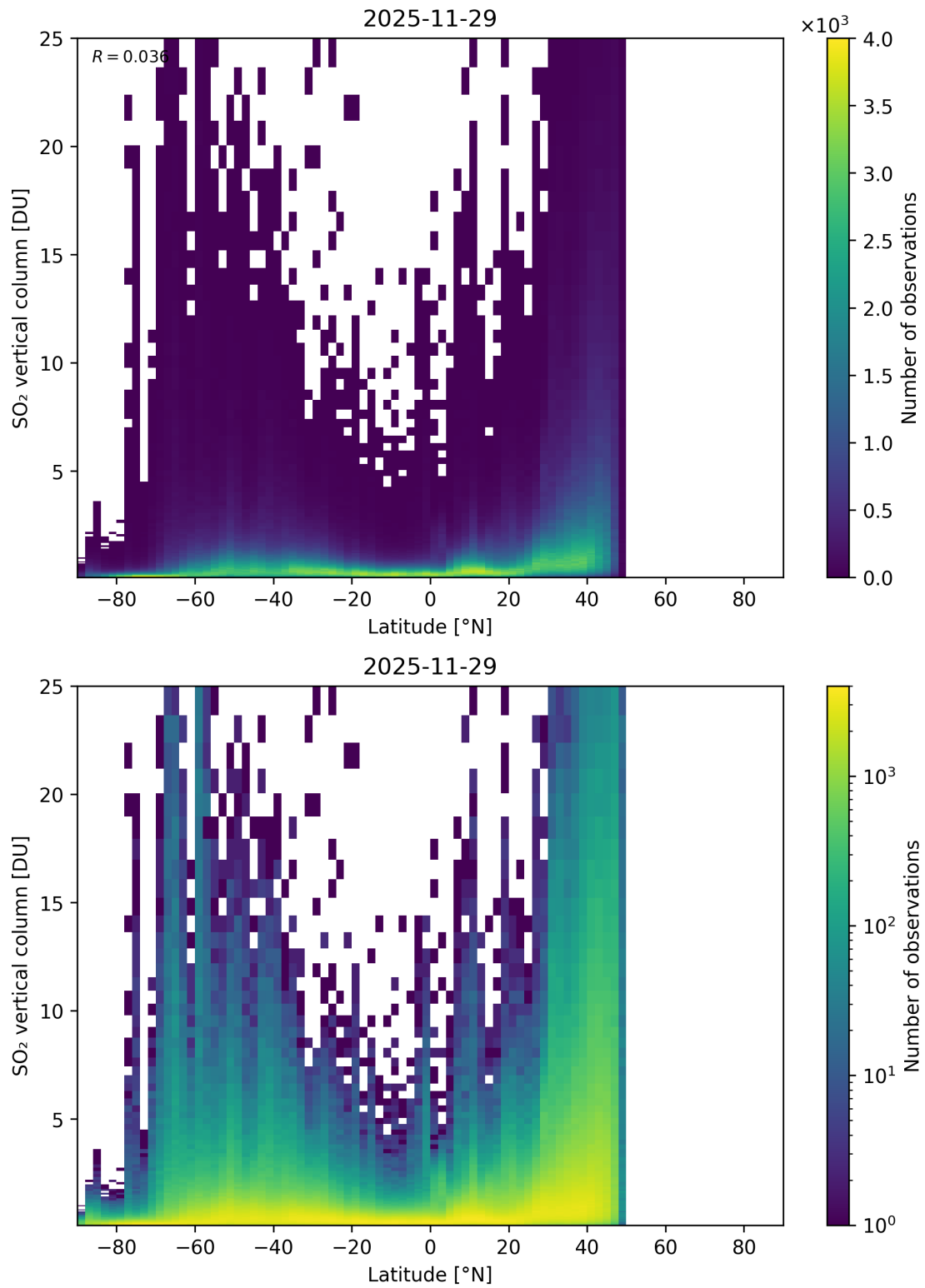
Figure 169: Scatter density plot of “Latitude” against “SO 2 vertical column” for 2025-11-28 to 2025-11-30.
