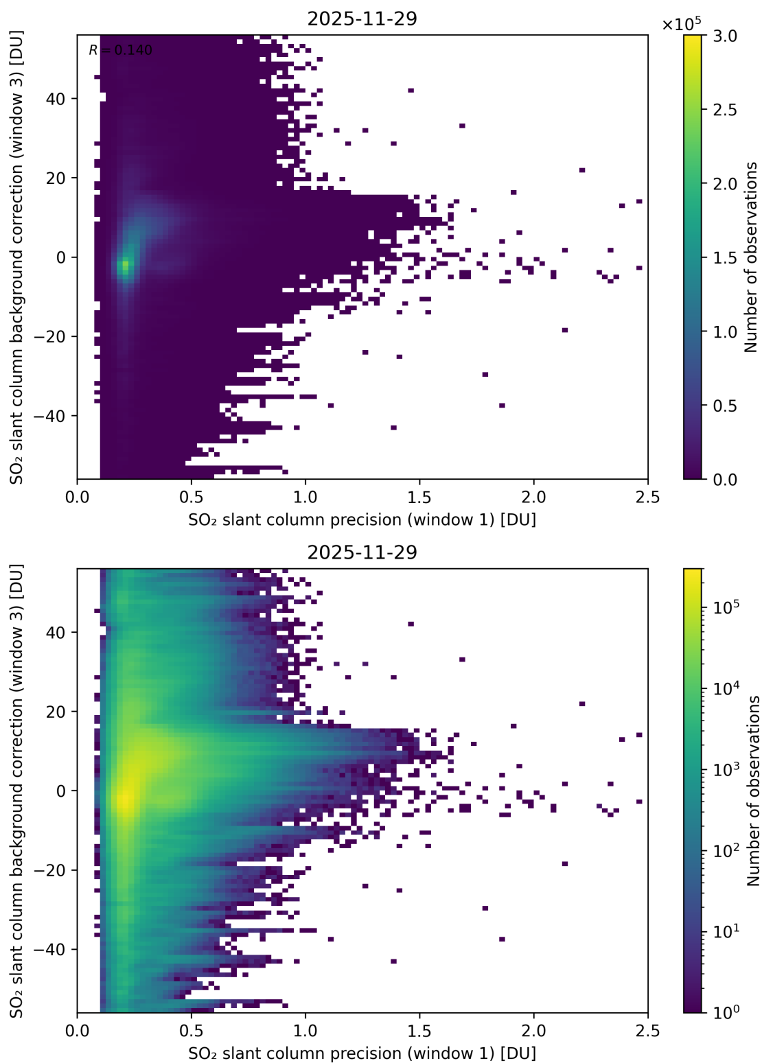
Figure 270: Scatter density plot of “SO 2 slant column precision (window 1)” against “SO 2 slant column background correction (window 3)” for 2025-11-28 to 2025-11-30.
