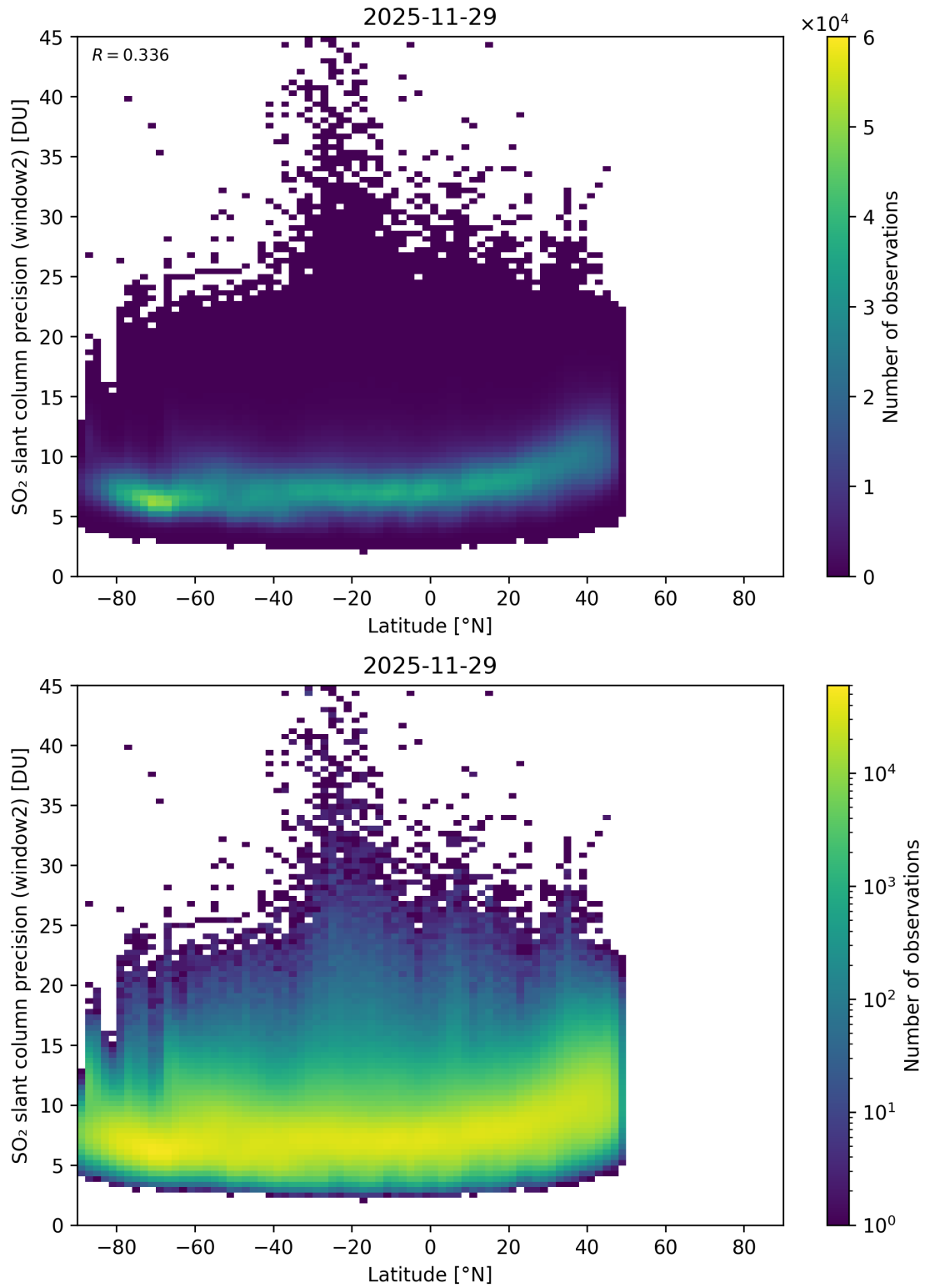
Figure 164: Scatter density plot of “Latitude” against “SO 2 slant column precision (window2)” for 2025-11-28 to 2025-11-30.
