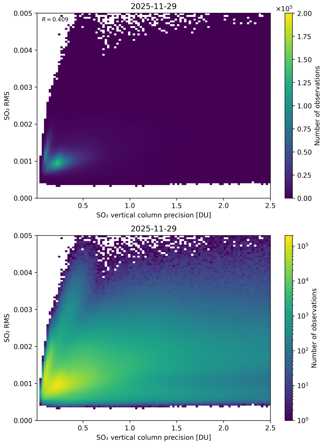
Figure 334: Scatter density plot of “SO 2 vertical column precision” against “SO 2 RMS” for 2025-11-28 to 2025-11-30.
