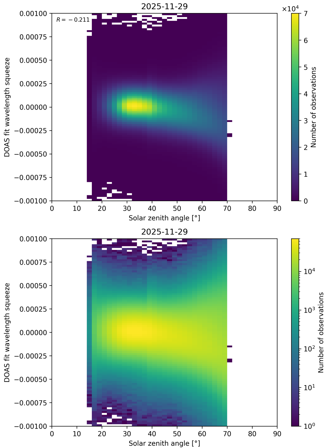
Figure 175: Scatter density plot of “Solar zenith angle” against “DOAS fit wavelength squeeze” for 2025-11-28 to 2025-11-30.
