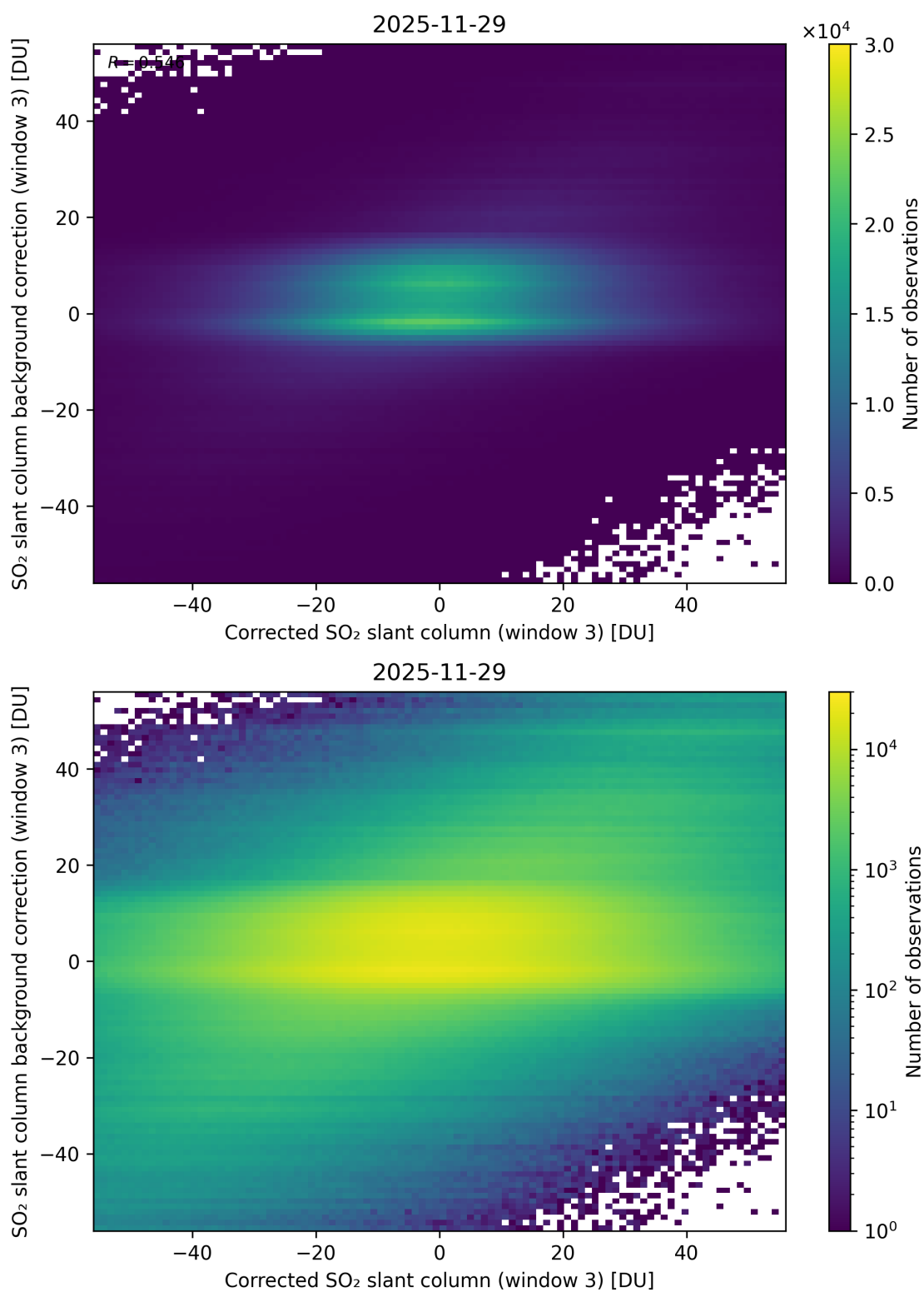
Figure 255: Scatter density plot of “Corrected SO 2 slant column (window 3)” against “SO 2 slant column background correction (window 3)” for 2025-11-28 to 2025-11-30.
