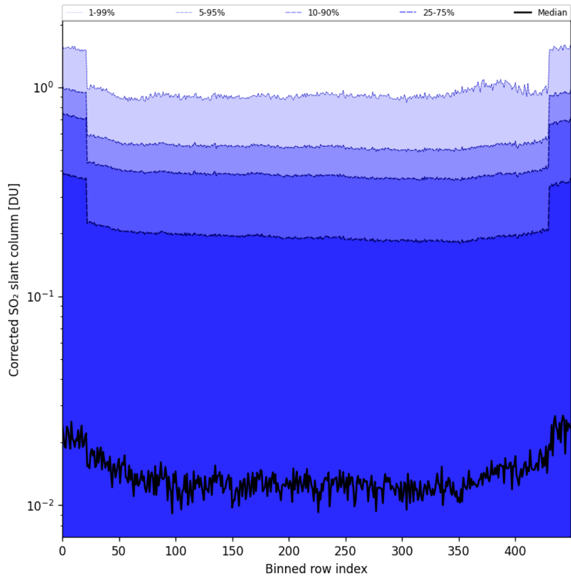
Figure 86: Along track statistics of "Corrected SO 2 slant column" for 2025-11-28 to 2025-11-30
