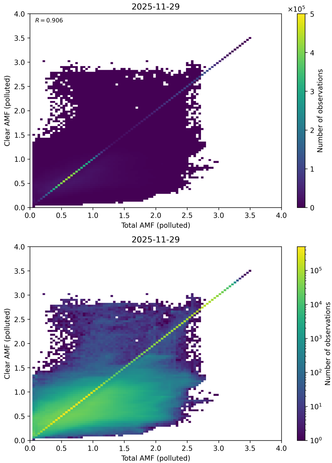
Figure 320: Scatter density plot of “Total AMF (polluted)” against “Clear AMF (polluted)” for 2025-11-28 to 2025-11-30.
