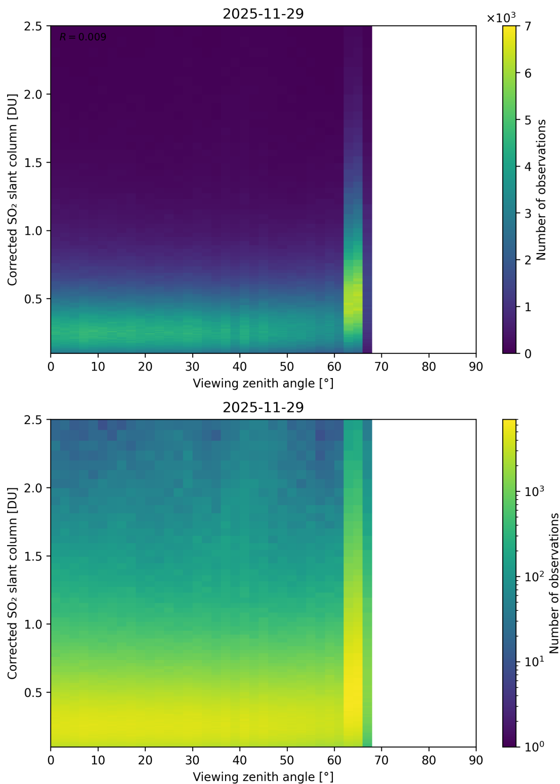
Figure 373: Scatter density plot of “Viewing zenith angle” against “Corrected SO 2 slant column” for 2025-11-28 to 2025-11-30.
