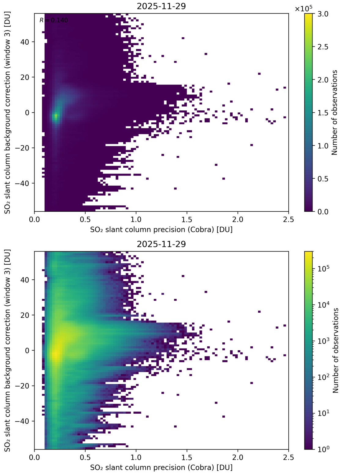
Figure 201: Scatter density plot of “SO 2 slant column precision (Cobra)” against “SO 2 slant column background correction (window 3)” for 2025-11-28 to 2025-11-30.
