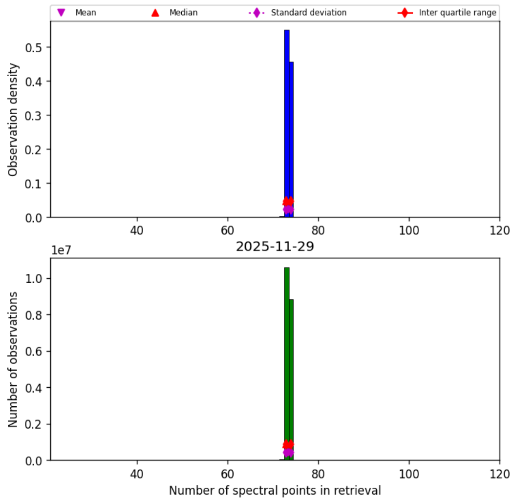
Figure 82: Histogram of “Number of spectral points in retrieval” for 2025-11-28 to 2025-11-30
