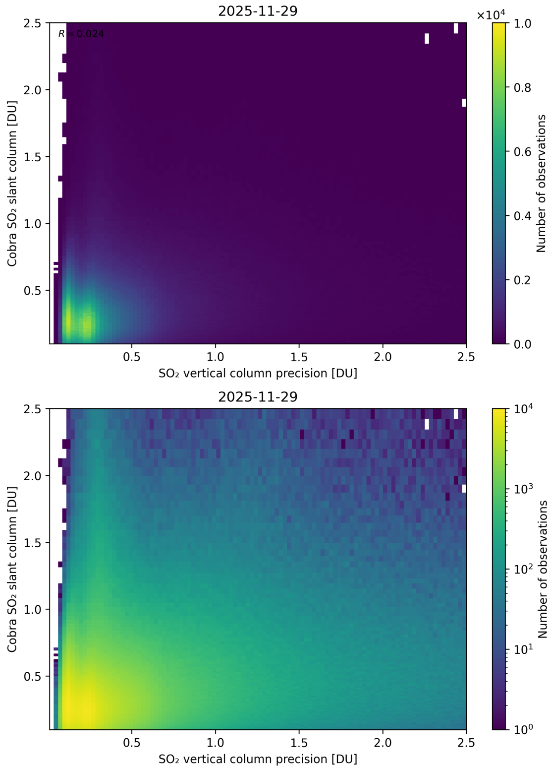
Figure 336: Scatter density plot of “SO 2 vertical column precision” against “Cobra SO 2 slant column” for 2025-11-28 to 2025-11-30.
