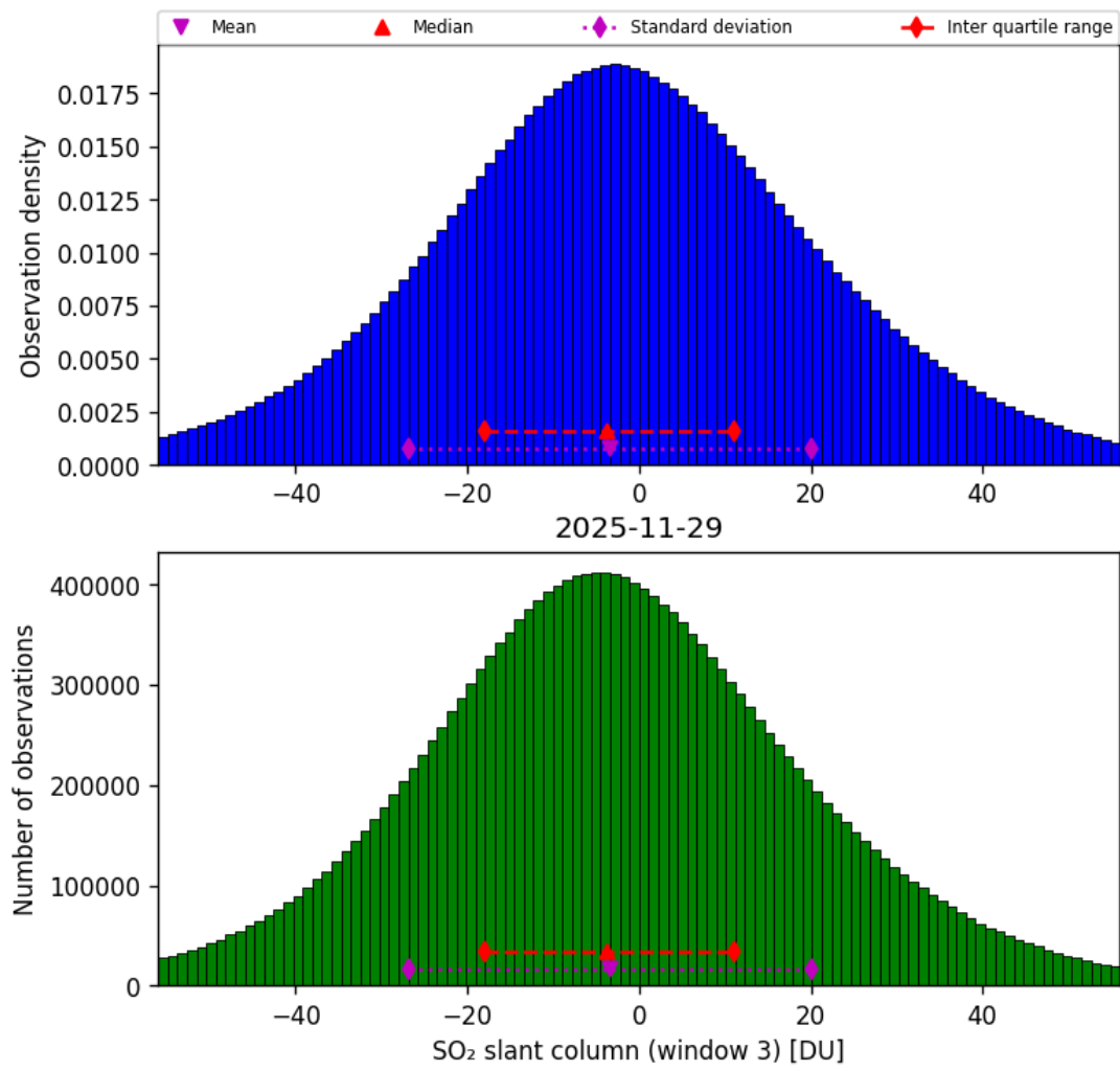
Figure 71: Histogram of “SO 2 slant column (window 3)” for 2025-11-28 to 2025-11-30
