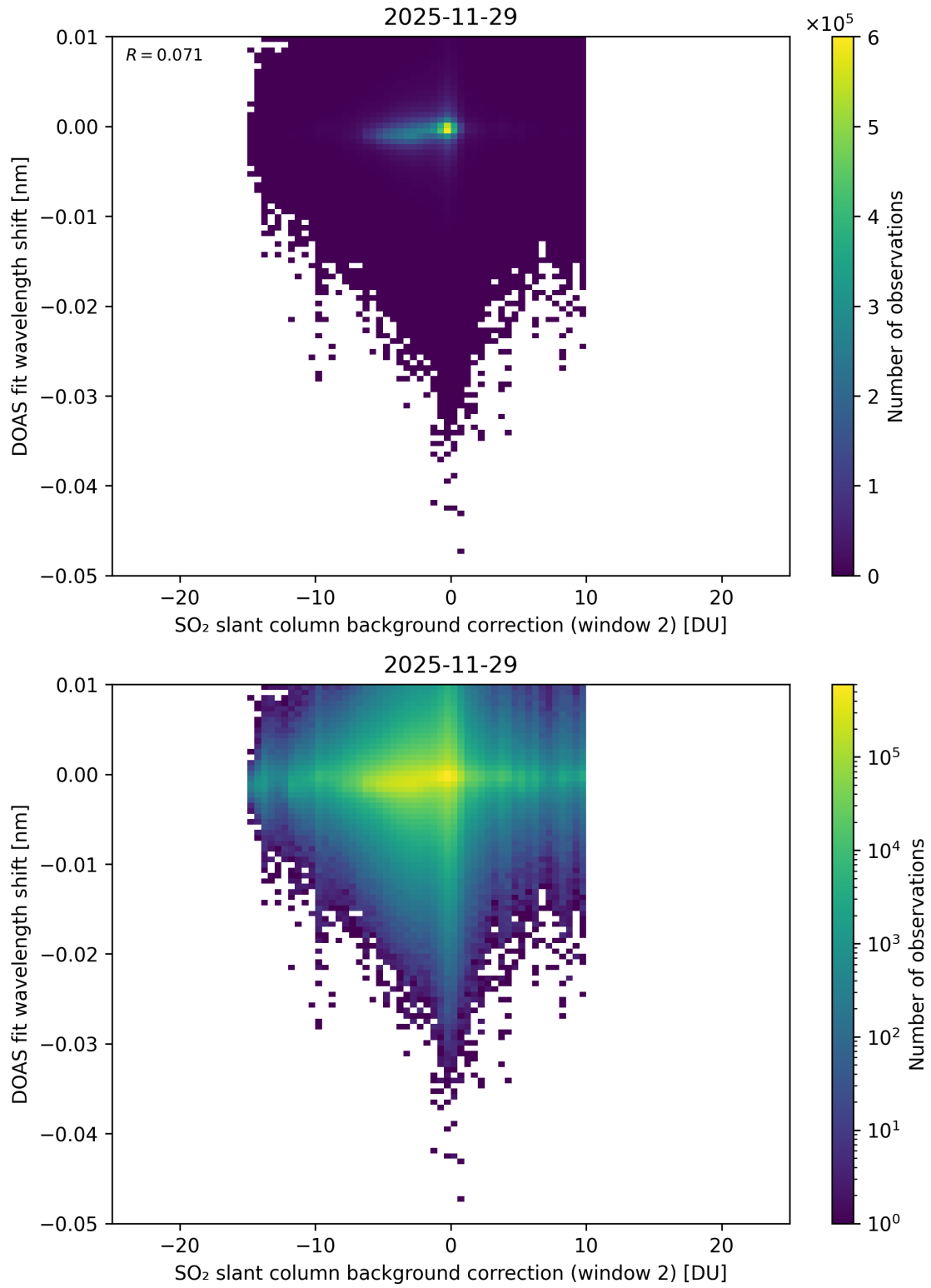
Figure 123: Scatter density plot of “SO 2 slant column background correction (window 2)” against “DOAS fit wavelength shift” for 2025-11-28 to 2025-11-30.
