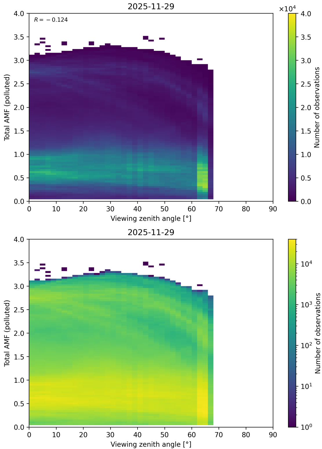
Figure 381: Scatter density plot of “Viewing zenith angle” against “Total AMF (polluted)” for 2025-11-28 to 2025-11-30.
