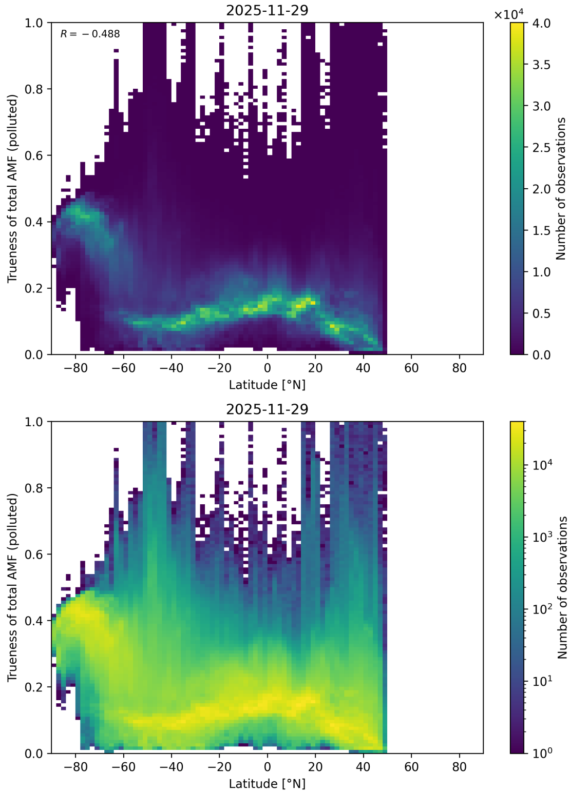
Figure 168: Scatter density plot of “Latitude” against “Trueness of total AMF (polluted)” for 2025-11-28 to 2025-11-30.
