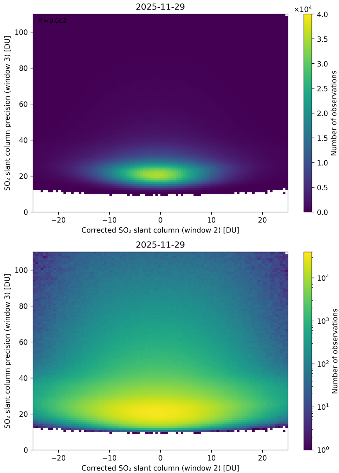
Figure 252: Scatter density plot of “Corrected SO 2 slant column (window 2)” against “SO 2 slant column precision (window 3)” for 2025-11-28 to 2025-11-30.
