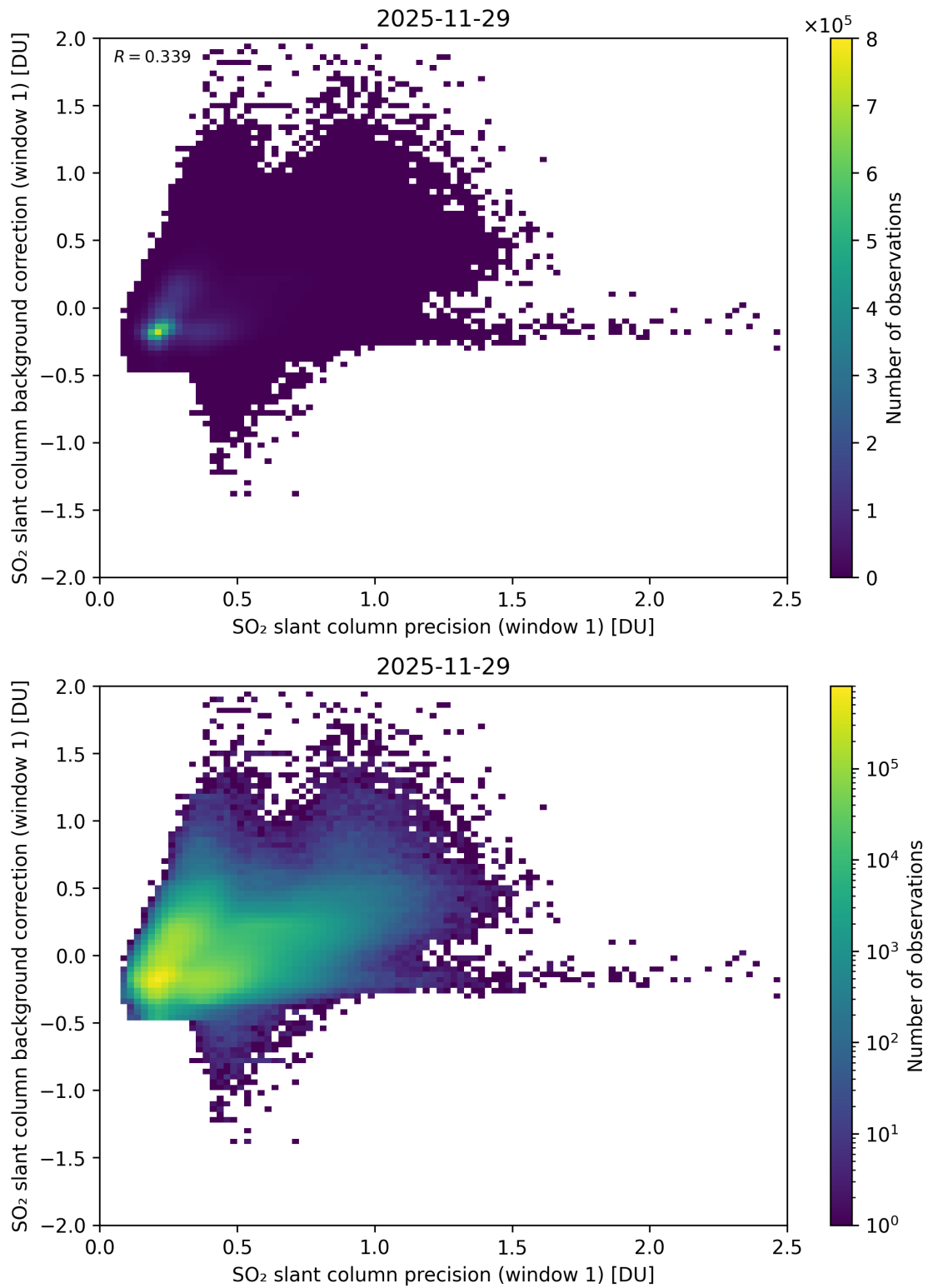
Figure 268: Scatter density plot of “SO 2 slant column precision (window 1)” against “SO 2 slant column background correction (window 1)” for 2025-11-28 to 2025-11-30.
