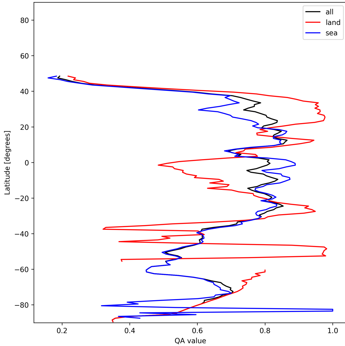
Figure 31: Zonal average of “QA value” for 2025-11-28 to 2025-11-30.
