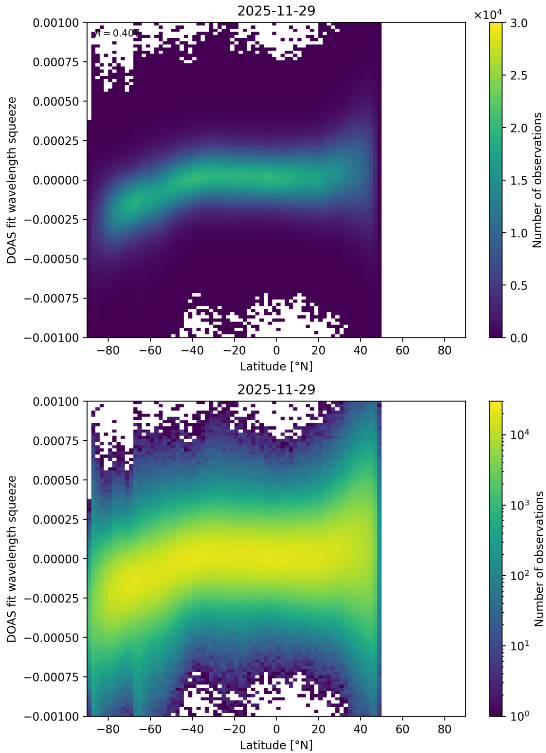
Figure 154: Scatter density plot of “Latitude” against “DOAS fit wavelength squeeze” for 2025-11-28 to 2025-11-30.
