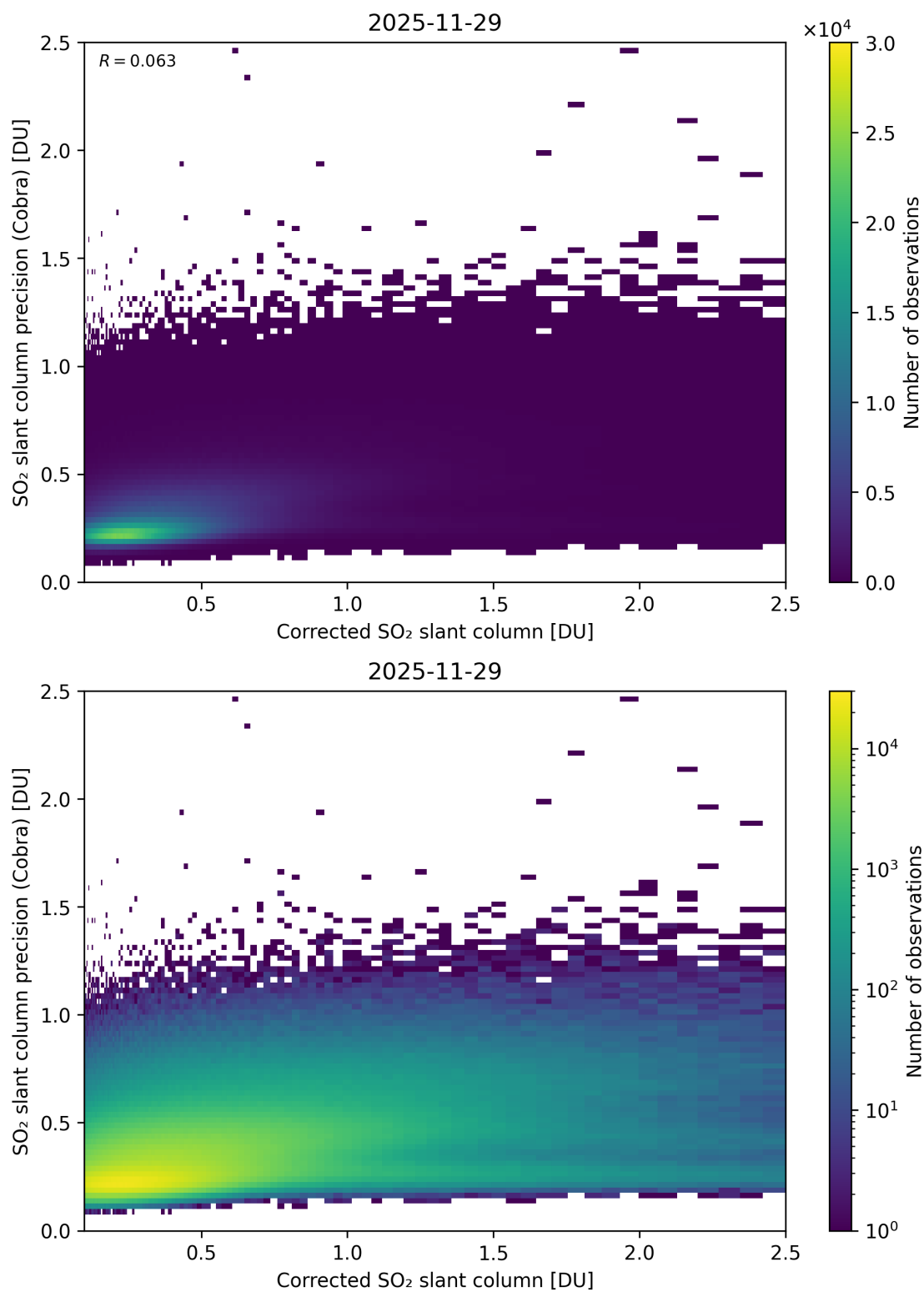
Figure 234: Scatter density plot of “Corrected SO 2 slant column” against “SO 2 slant column precision (Cobra)” for 2025-11-28 to 2025-11-30.
