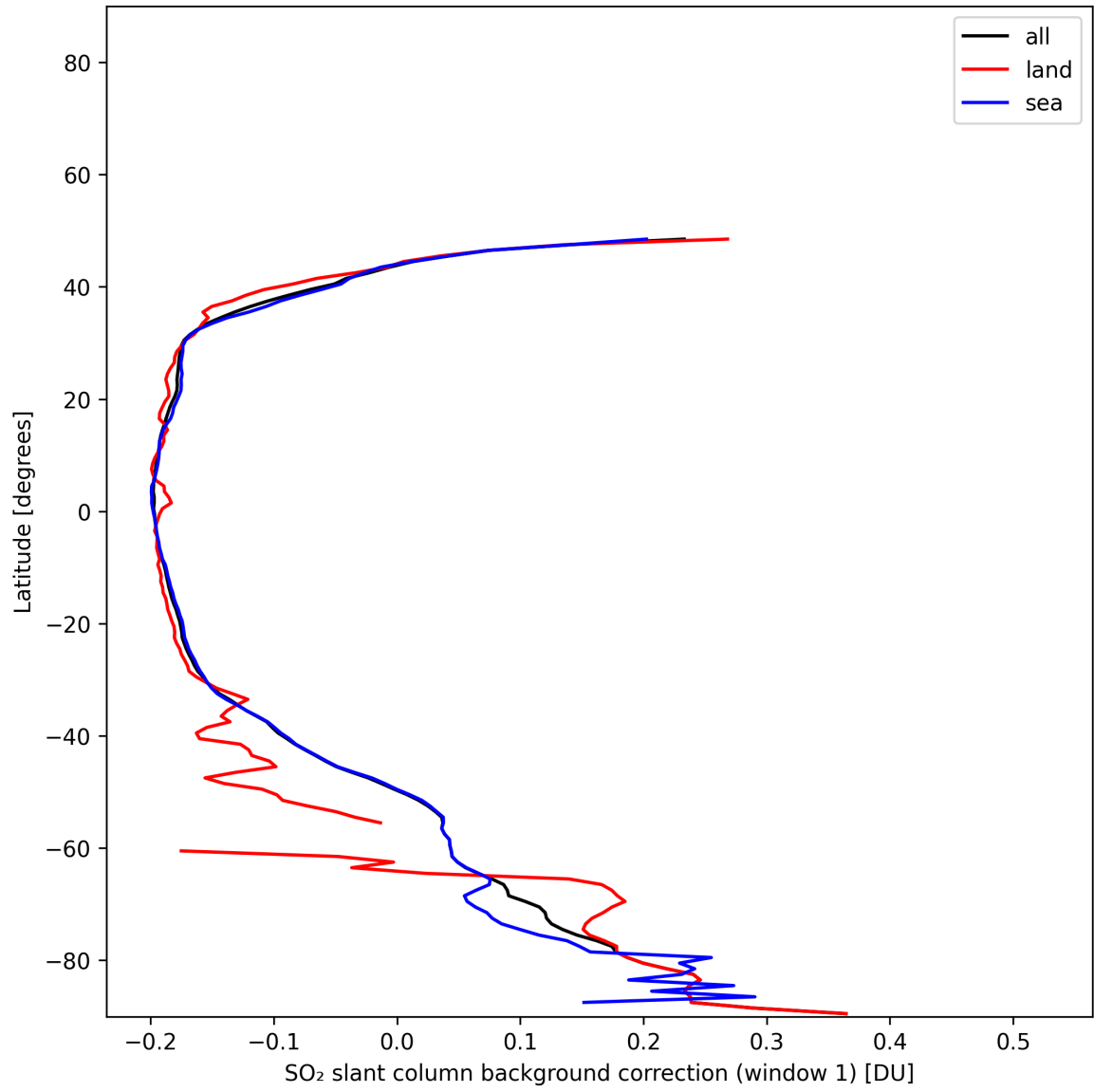
Figure 40: Zonal average of “SO 2 slant column background correction (window 1)” for 2025-11-28 to 2025-11-30.
