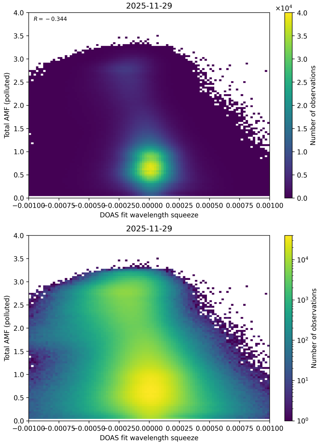
Figure 145: Scatter density plot of “DOAS fit wavelength squeeze” against “Total AMF (polluted)” for 2025-11-28 to 2025-11-30.
