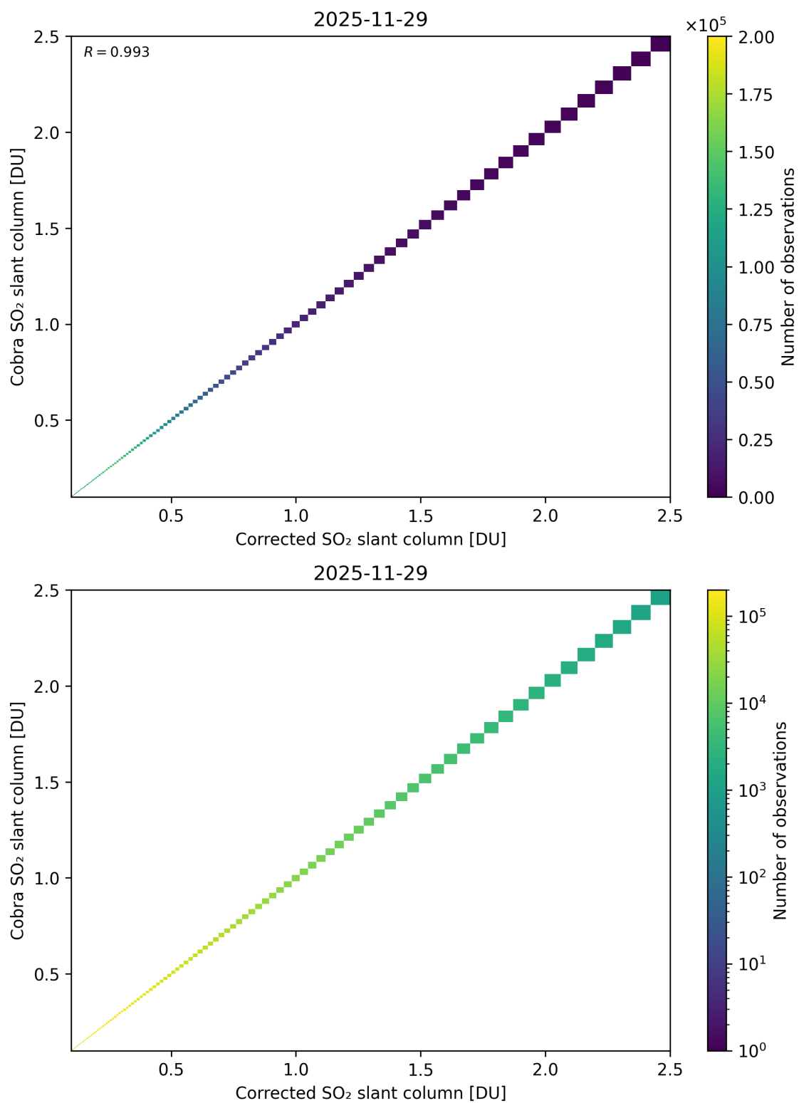
Figure 233: Scatter density plot of “Corrected SO 2 slant column” against “Cobra SO 2 slant column” for 2025-11-28 to 2025-11-30.
