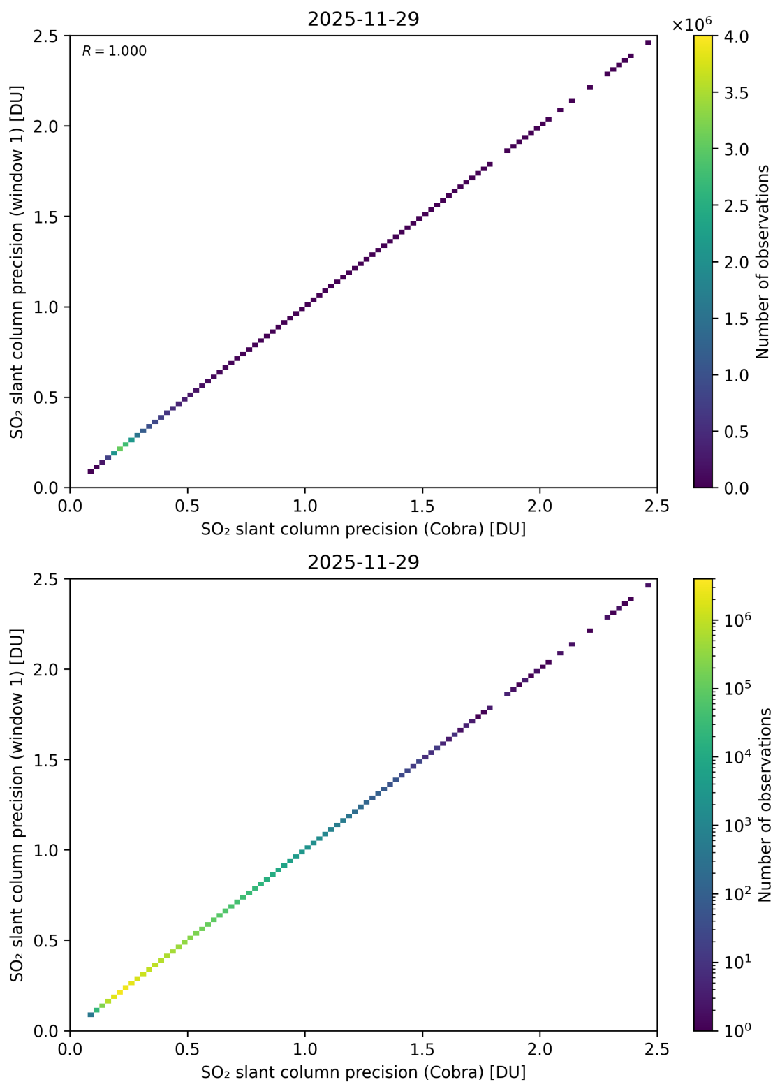
Figure 209: Scatter density plot of “SO 2 slant column precision (Cobra)” against “SO 2 slant column precision (window 1)” for 2025-11-28 to 2025-11-30.
