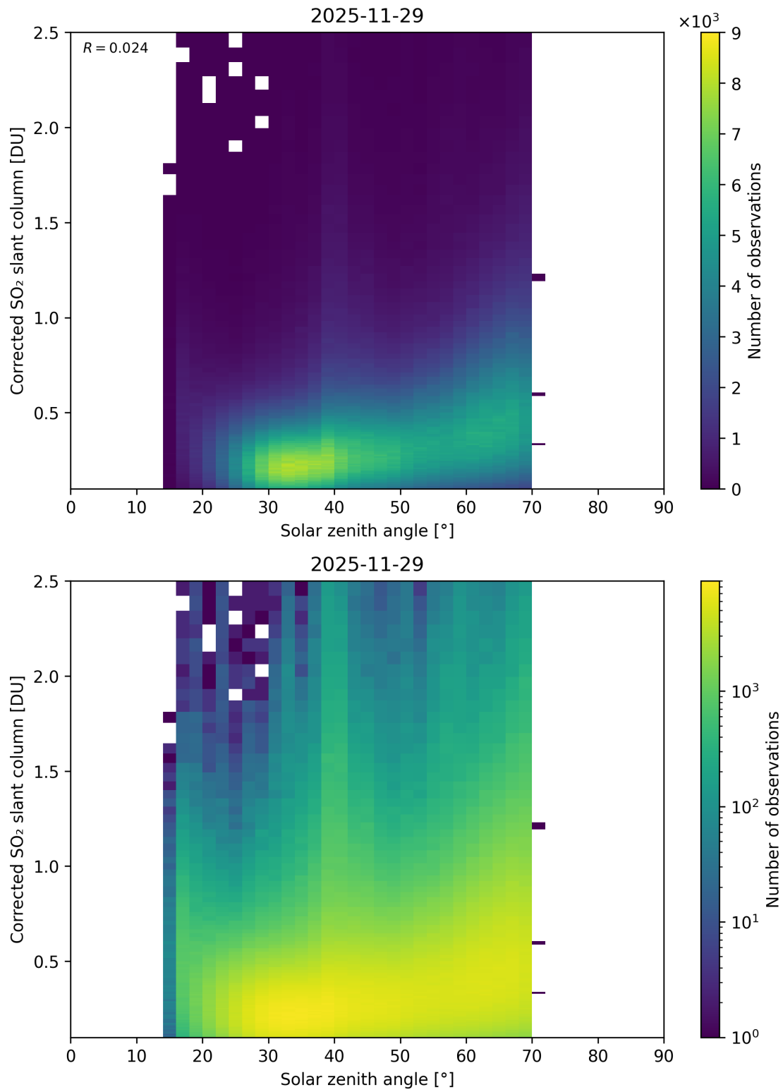
Figure 181: Scatter density plot of “Solar zenith angle” against “Corrected SO 2 slant column” for 2025-11-28 to 2025-11-30.
