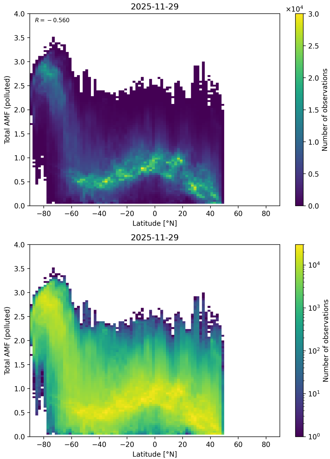
Figure 167: Scatter density plot of “Latitude” against “Total AMF (polluted)” for 2025-11-28 to 2025-11-30.
