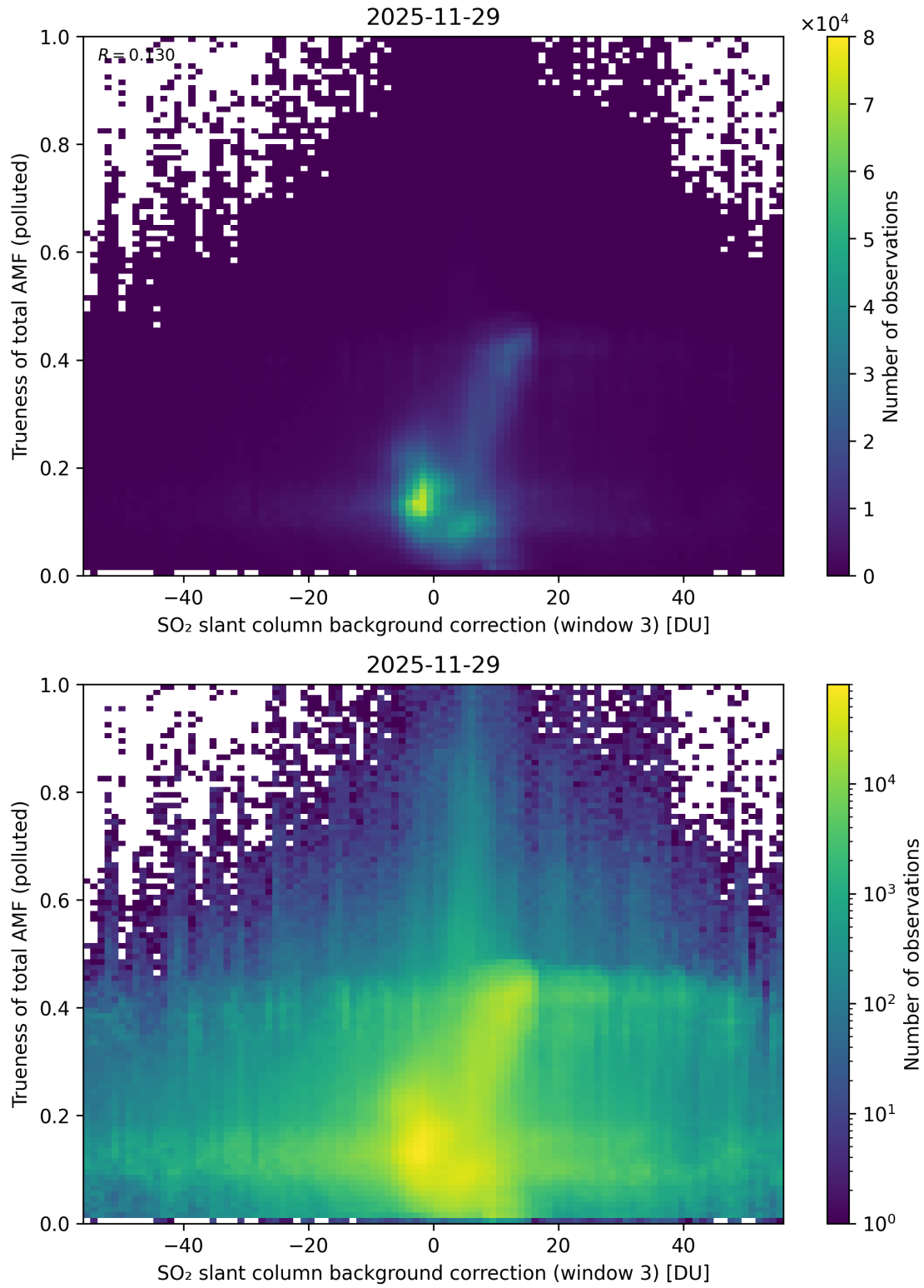
Figure 137: Scatter density plot of “SO 2 slant column background correction (window 3)” against “Trueness of total AMF (polluted)” for 2025-11-28 to 2025-11-30.
