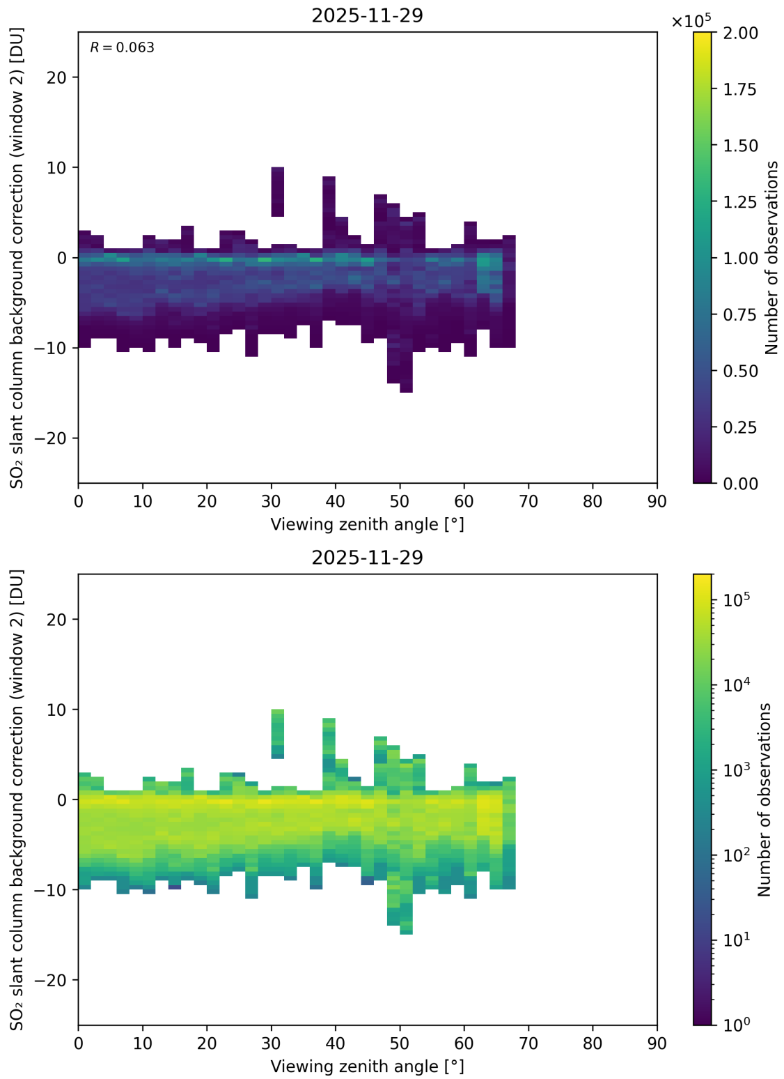
Figure 363: Scatter density plot of “Viewing zenith angle” against “SO 2 slant column background correction (window 2)” for 2025-11-28 to 2025-11-30.
