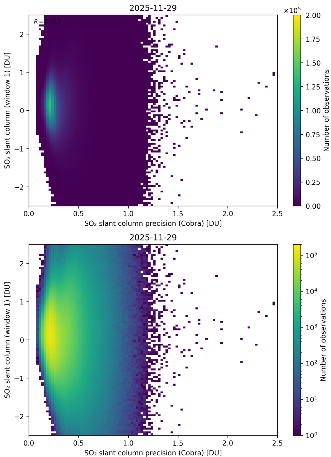
Figure 208: Scatter density plot of “SO 2 slant column precision (Cobra)” against “SO 2 slant column (window 1)” for 2025-11-28 to 2025-11-30.
