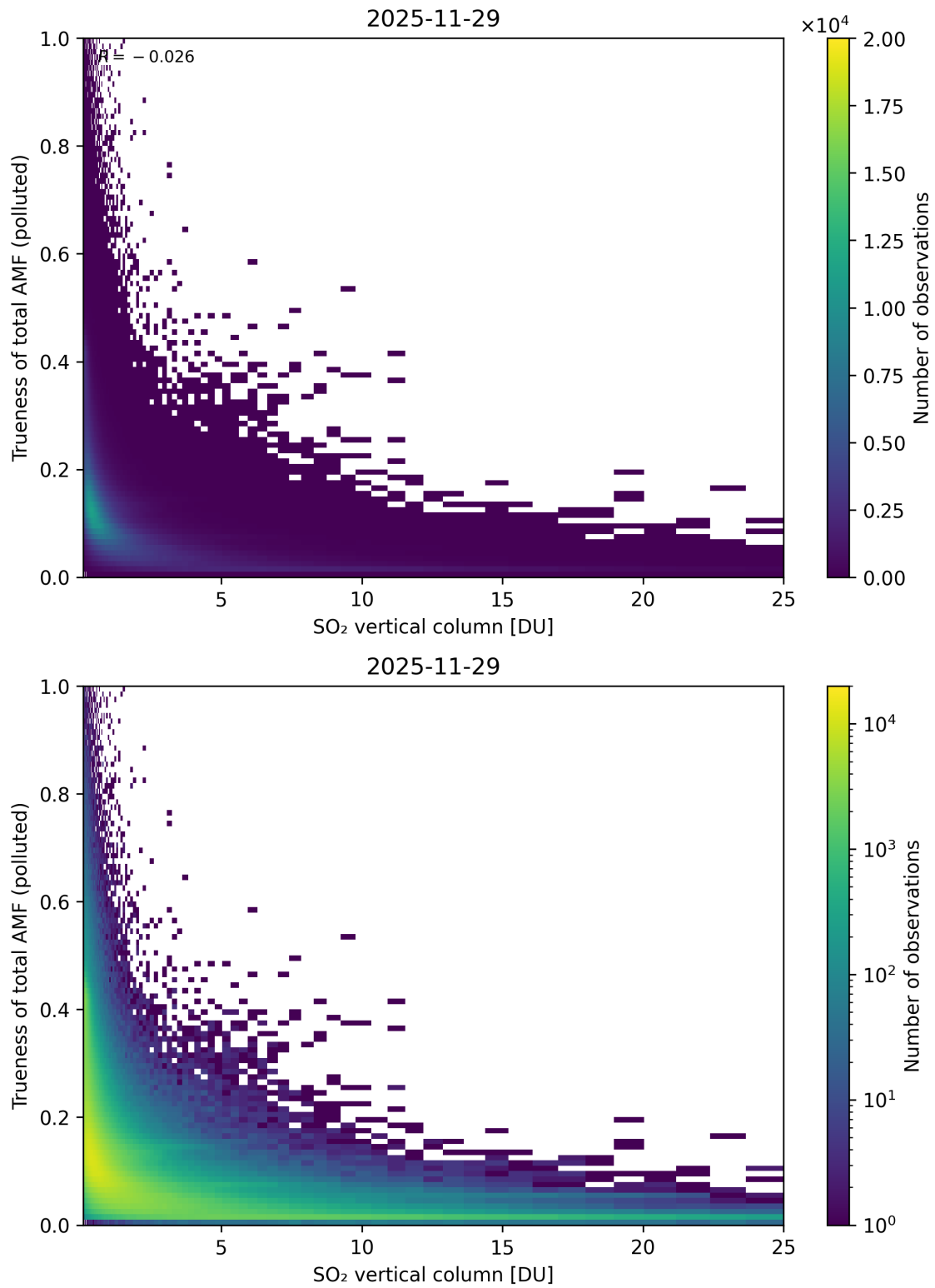
Figure 360: Scatter density plot of “SO 2 vertical column” against “Trueness of total AMF (polluted)” for 2025-11-28 to 2025-11-30.
