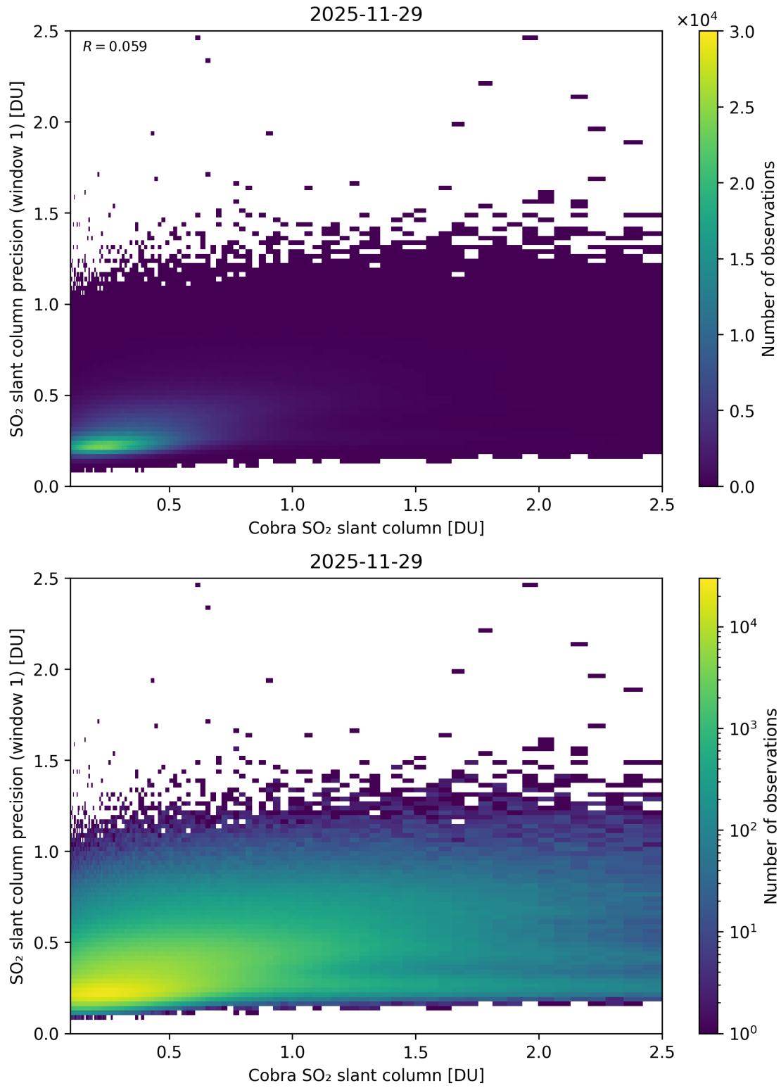
Figure 220: Scatter density plot of “Cobra SO 2 slant column” against “SO 2 slant column precision (window 1)” for 2025-11-28 to 2025-11-30.
