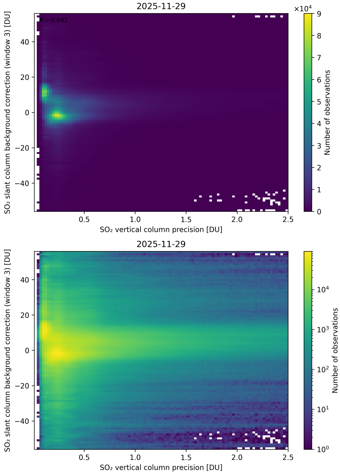
Figure 331: Scatter density plot of “SO 2 vertical column precision” against “SO 2 slant column background correction (window 3)” for 2025-11-28 to 2025-11-30.
