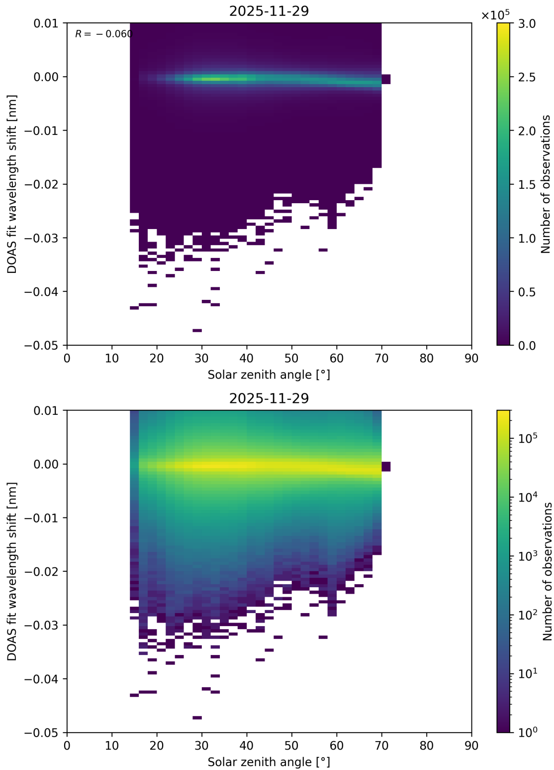
Figure 174: Scatter density plot of “Solar zenith angle” against “DOAS fit wavelength shift” for 2025-11-28 to 2025-11-30.
