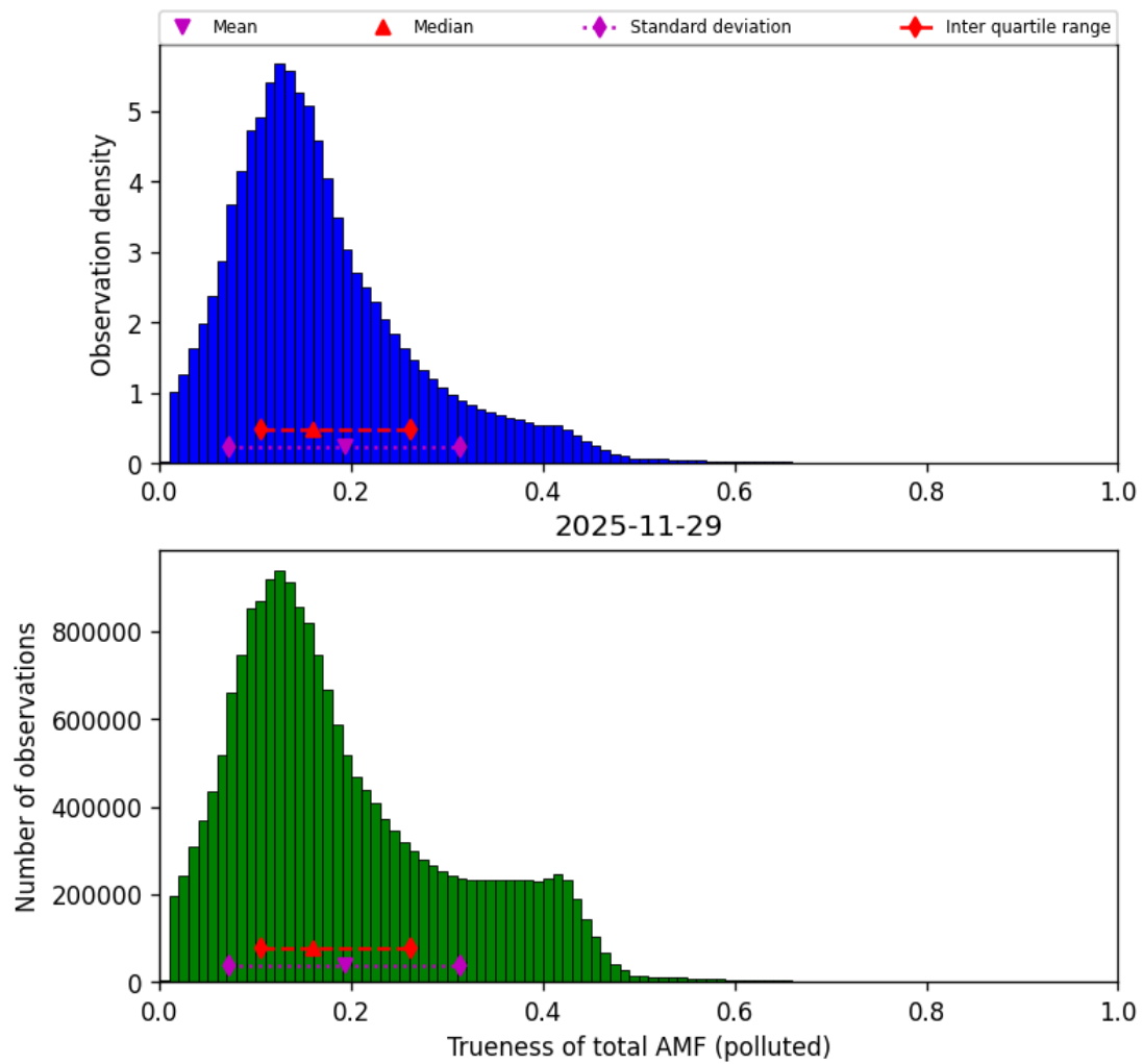
Figure 80: Histogram of “Trueness of total AMF (polluted)” for 2025-11-28 to 2025-11-30
