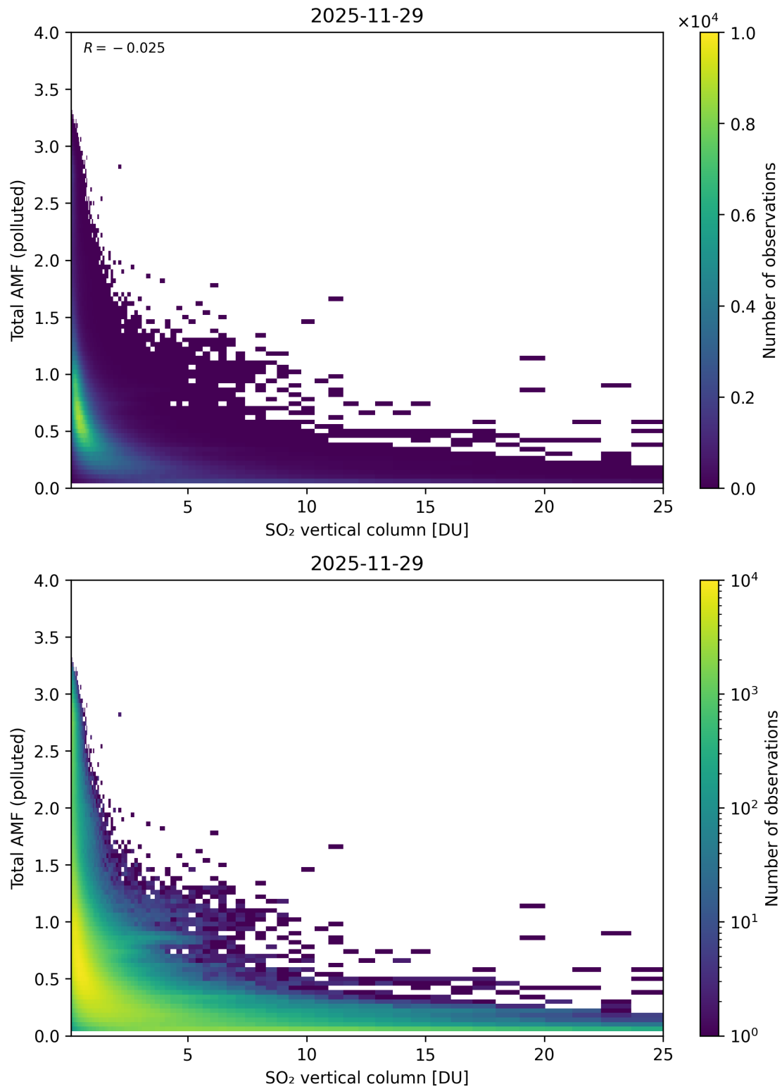
Figure 359: Scatter density plot of “SO 2 vertical column” against “Total AMF (polluted)” for 2025-11-28 to 2025-11-30.
