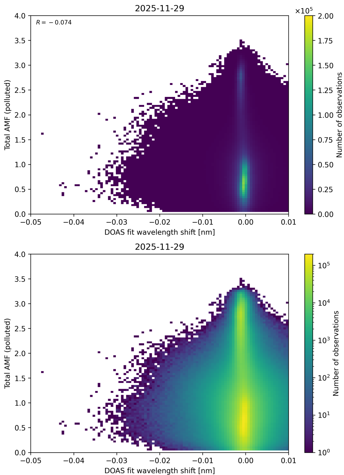
Figure 141: Scatter density plot of “DOAS fit wavelength shift” against “Total AMF (polluted)” for 2025-11-28 to 2025-11-30.
