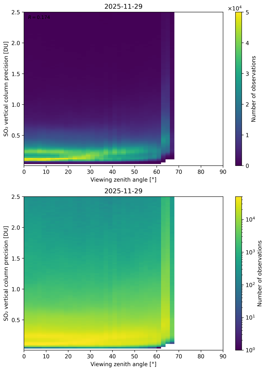
Figure 384: Scatter density plot of “Viewing zenith angle” against “SO 2 vertical column precision” for 2025-11-28 to 2025-11-30.
