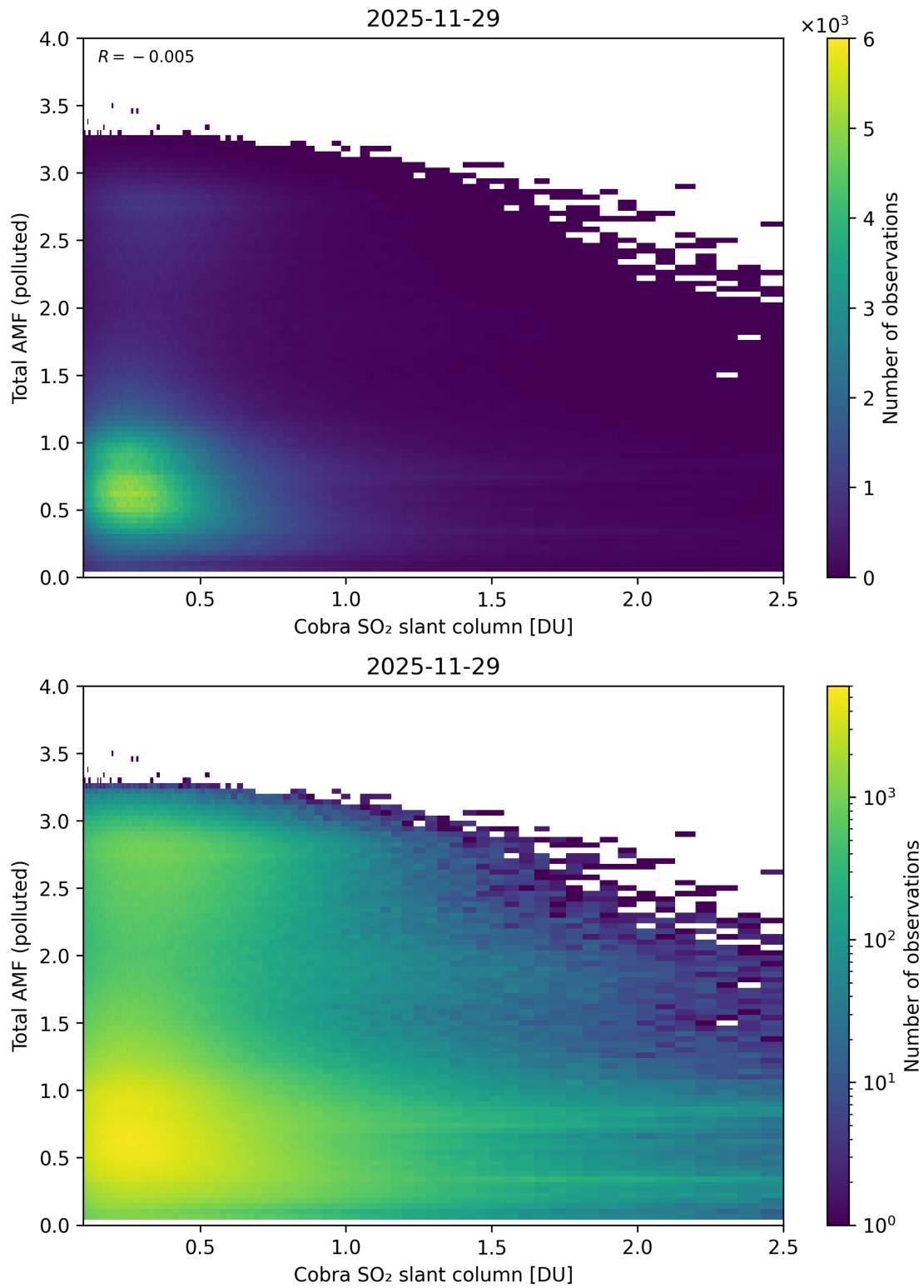
Figure 224: Scatter density plot of “Cobra SO 2 slant column” against “Total AMF (polluted)” for 2025-11-28 to 2025-11-30.
