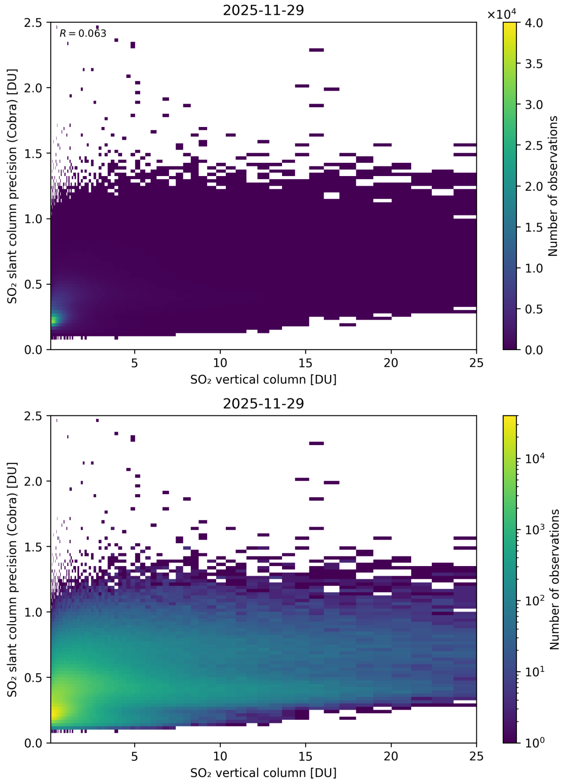
Figure 350: Scatter density plot of “SO 2 vertical column” against “SO 2 slant column precision (Cobra)” for 2025-11-28 to 2025-11-30.
