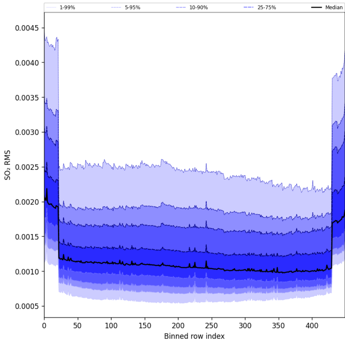
Figure 104: Along track statistics of “SO 2 RMS” for 2025-11-28 to 2025-11-30
