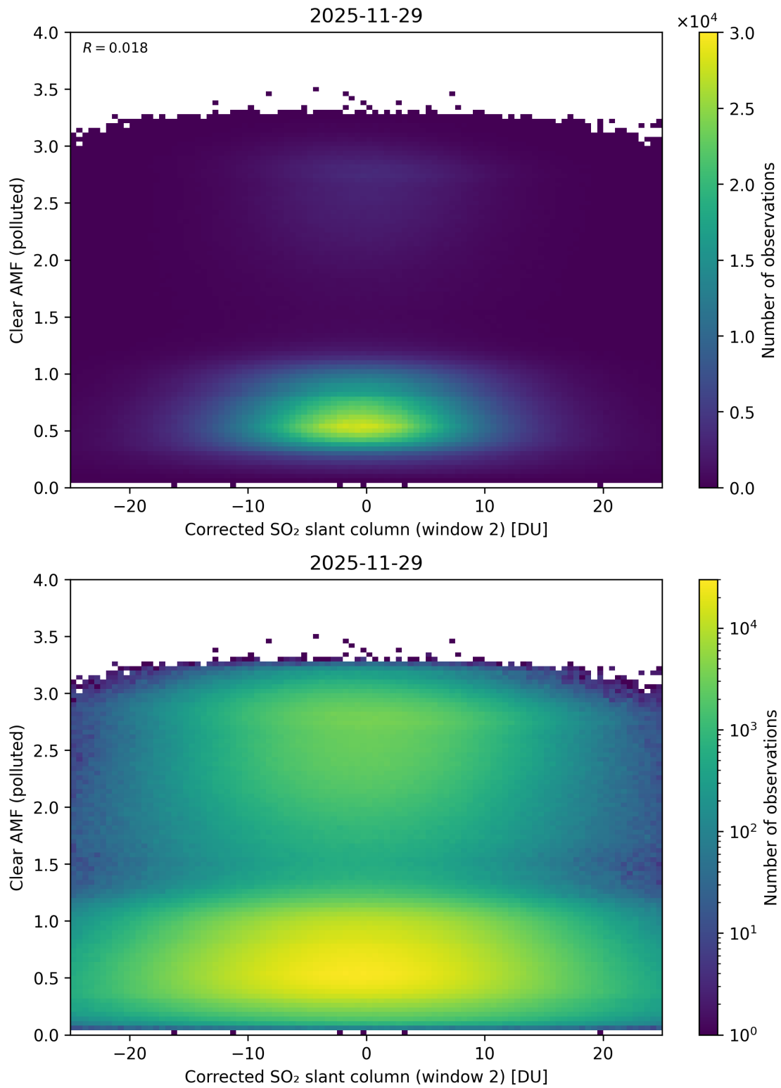
Figure 249: Scatter density plot of “Corrected SO 2 slant column (window 2)” against “Clear AMF (polluted)” for 2025-11-28 to 2025-11-30.
