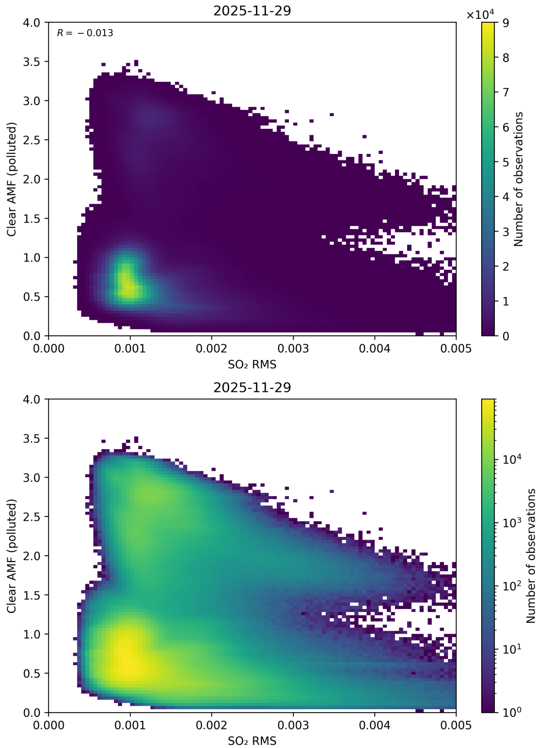
Figure 147: Scatter density plot of “SO 2 RMS” against “Clear AMF (polluted)” for 2025-11-28 to 2025-11-30.
