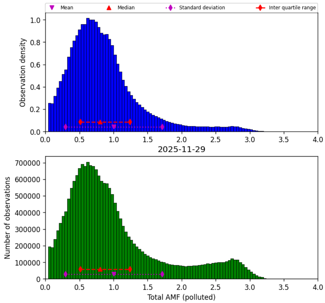
Figure 79: Histogram of “Total AMF (polluted)” for 2025-11-28 to 2025-11-30
