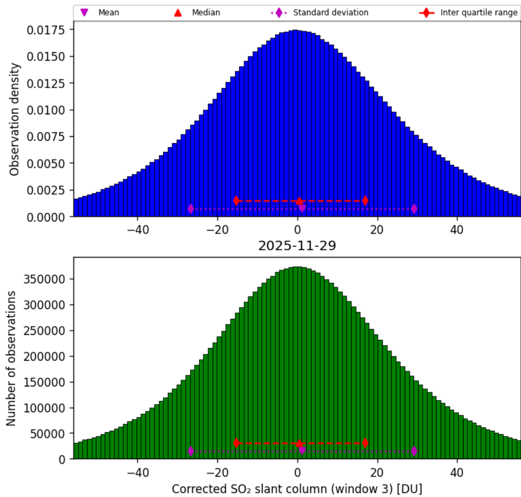
Figure 73: Histogram of “Corrected SO 2 slant column (window 3)” for 2025-11-28 to 2025-11-30
