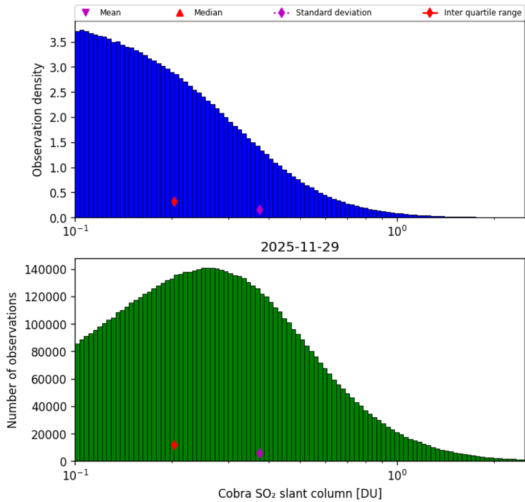
Figure 61: Histogram of “Cobra SO 2 slant column” for 2025-11-28 to 2025-11-30
