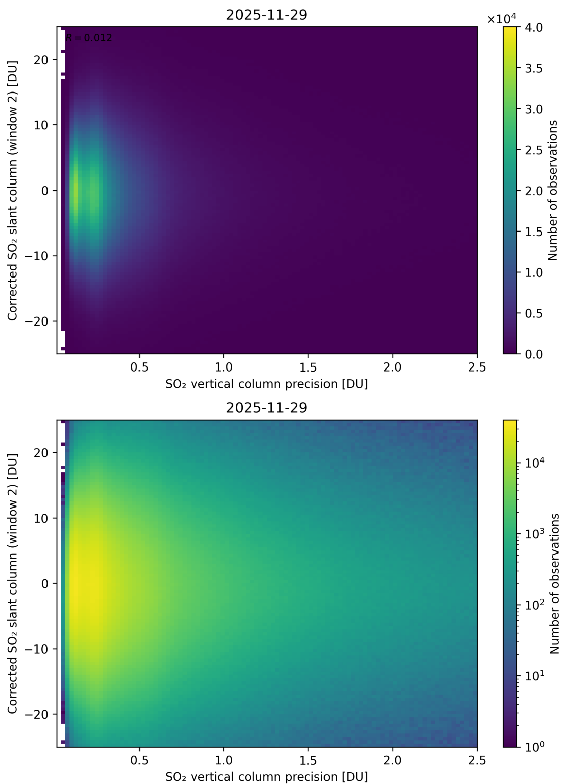
Figure 339: Scatter density plot of “SO 2 vertical column precision” against “Corrected SO 2 slant column (window 2)” for 2025-11-28 to 2025-11-30.
