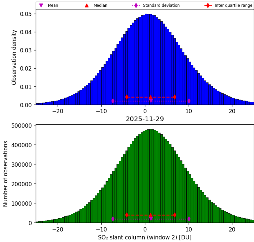
Figure 67: Histogram of “SO 2 slant column (window 2)” for 2025-11-28 to 2025-11-30
