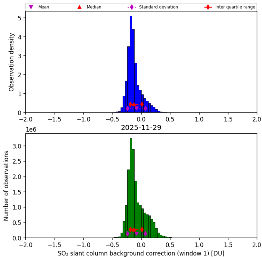
Figure 66: Histogram of “SO 2 slant column background correction (window 1)” for 2025-11-28 to 2025-11-30
