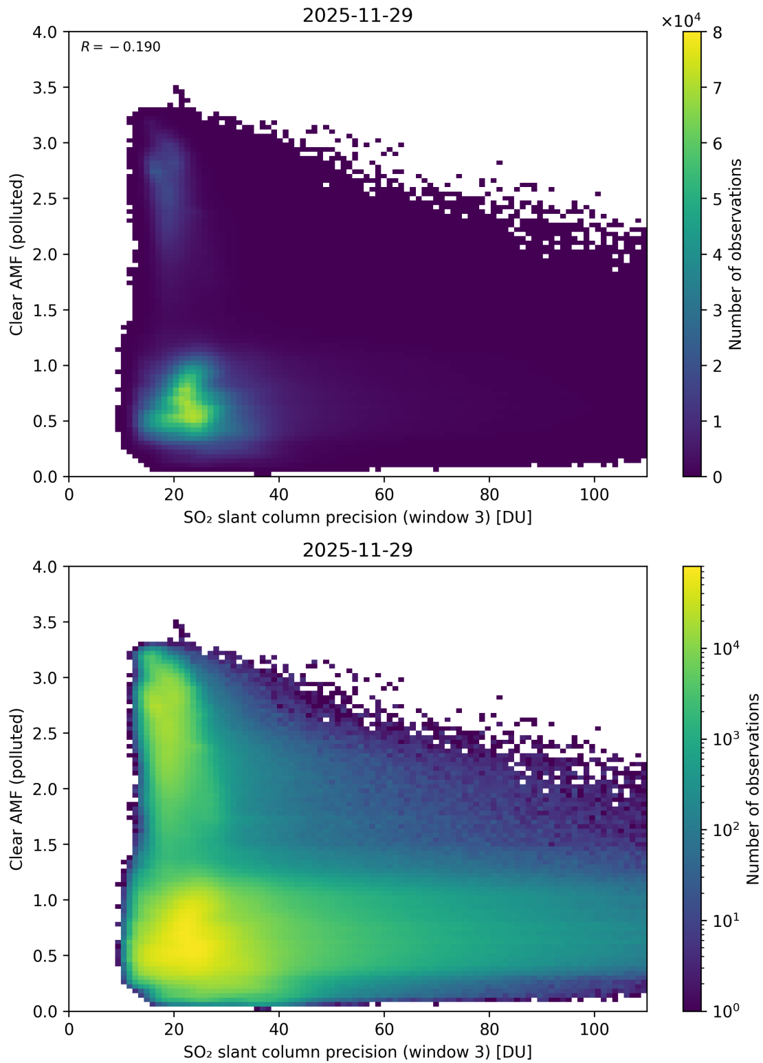
Figure 311: Scatter density plot of “SO 2 slant column precision (window 3)” against “Clear AMF (polluted)” for 2025-11-28 to 2025-11-30.
