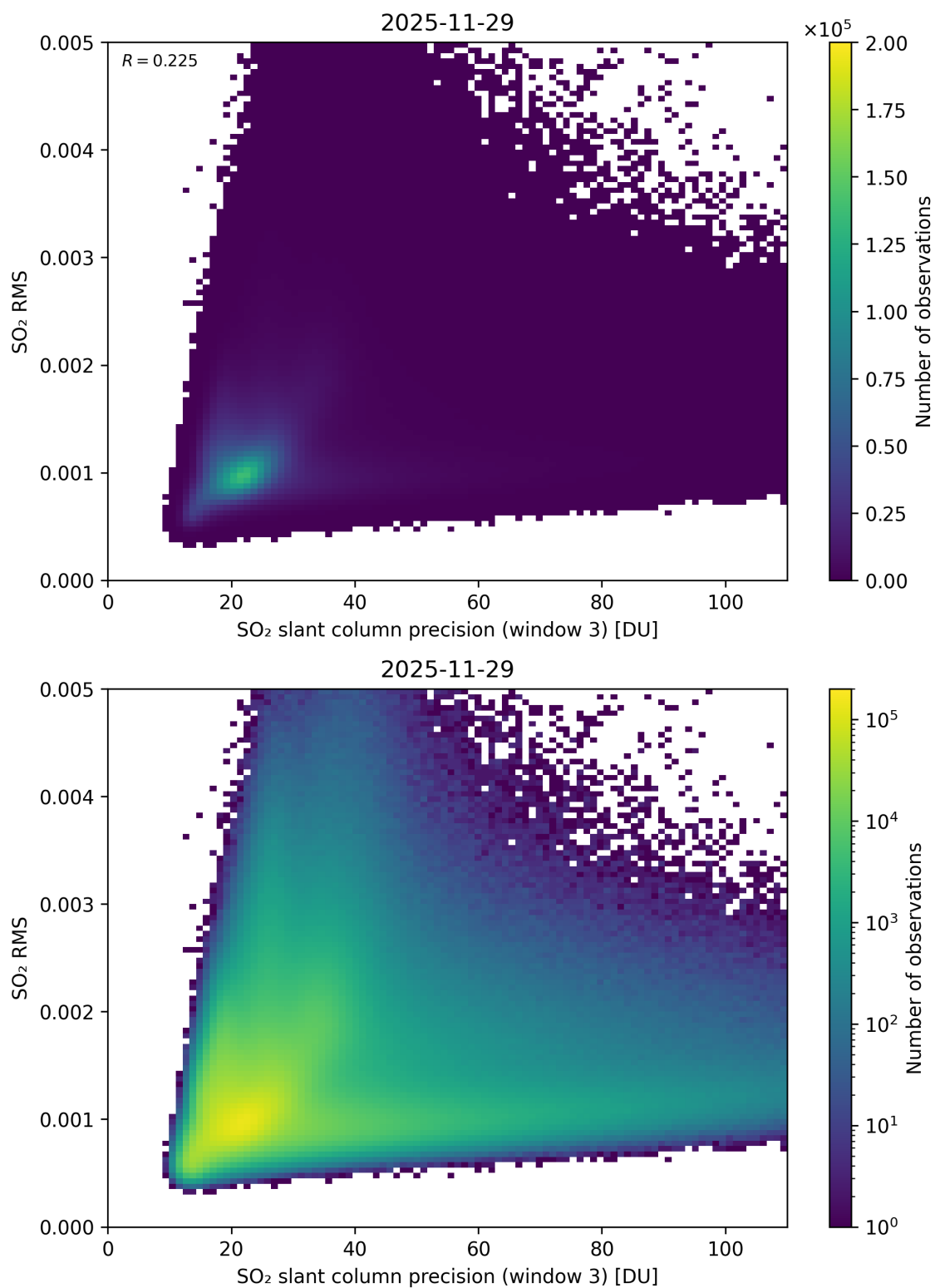
Figure 310: Scatter density plot of “SO 2 slant column precision (window 3)” against “SO 2 RMS” for 2025-11-28 to 2025-11-30.
