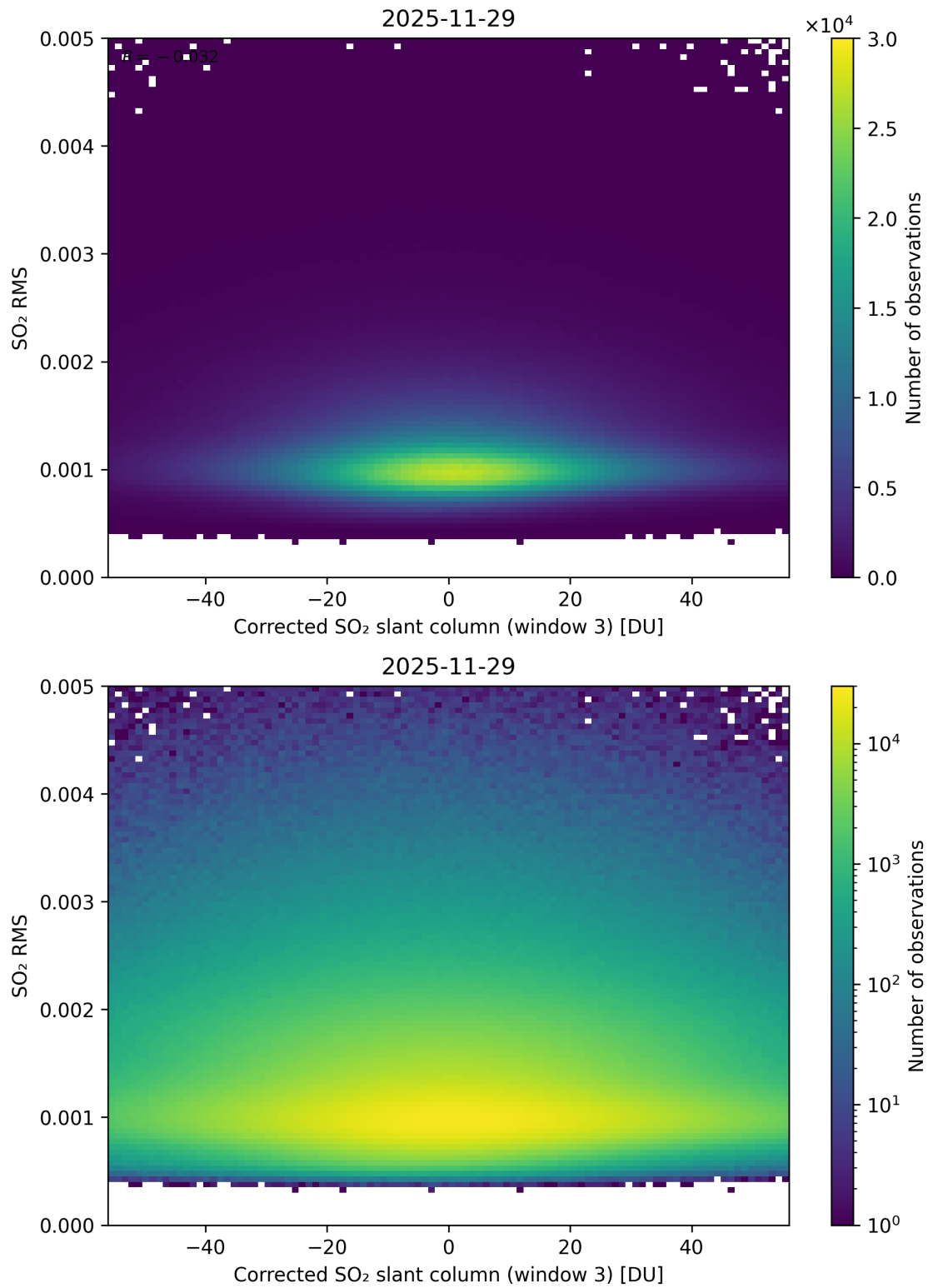
Figure 258: Scatter density plot of “Corrected SO 2 slant column (window 3)” against “SO 2 RMS” for 2025-11-28 to 2025-11-30.
