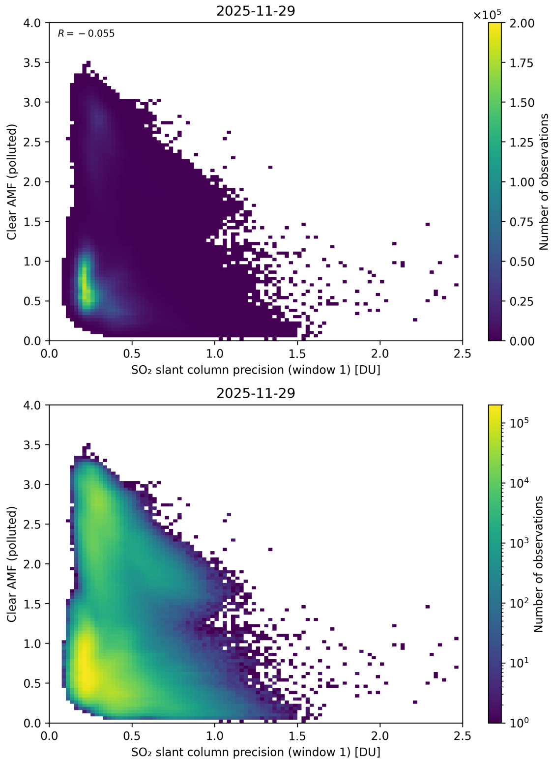
Figure 274: Scatter density plot of “SO 2 slant column precision (window 1)” against “Clear AMF (polluted)” for 2025-11-28 to 2025-11-30.
