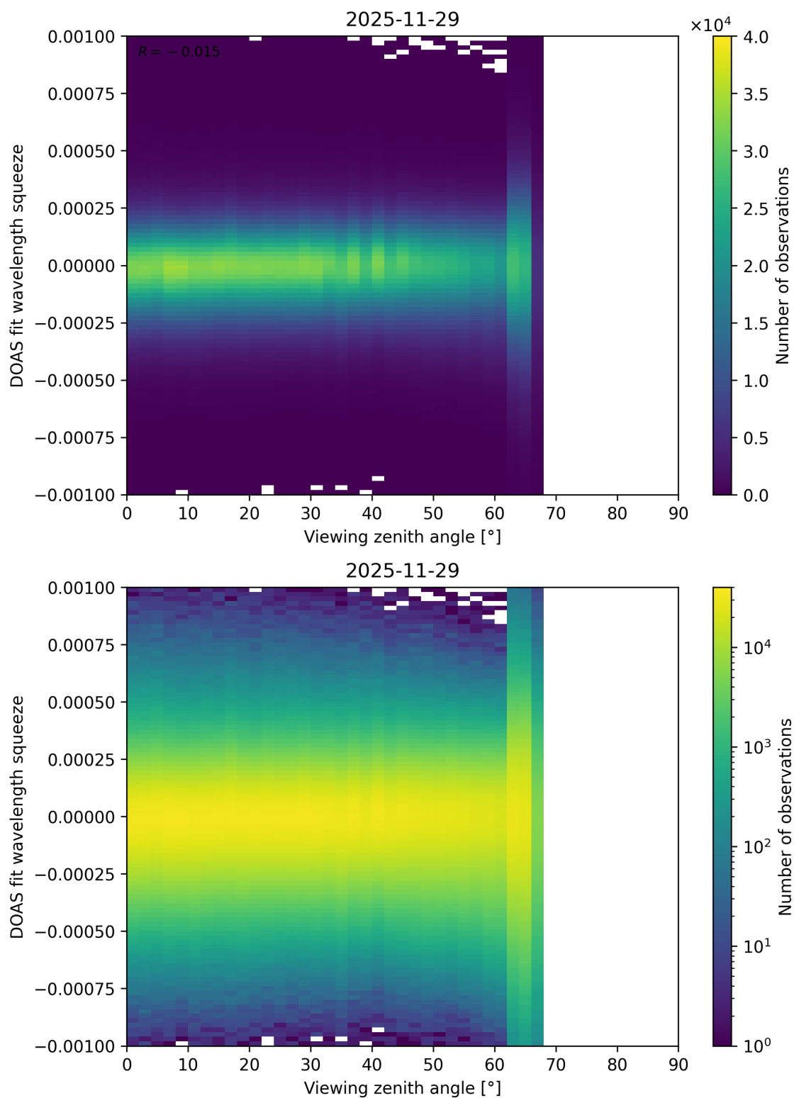
Figure 366: Scatter density plot of “Viewing zenith angle” against “DOAS fit wavelength squeeze” for 2025-11-28 to 2025-11-30.
