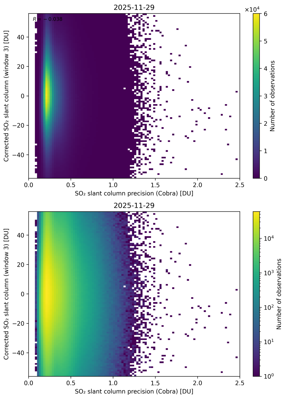
Figure 207: Scatter density plot of “SO 2 slant column precision (Cobra)” against “Corrected SO 2 slant column (window 3)” for 2025-11-28 to 2025-11-30.
