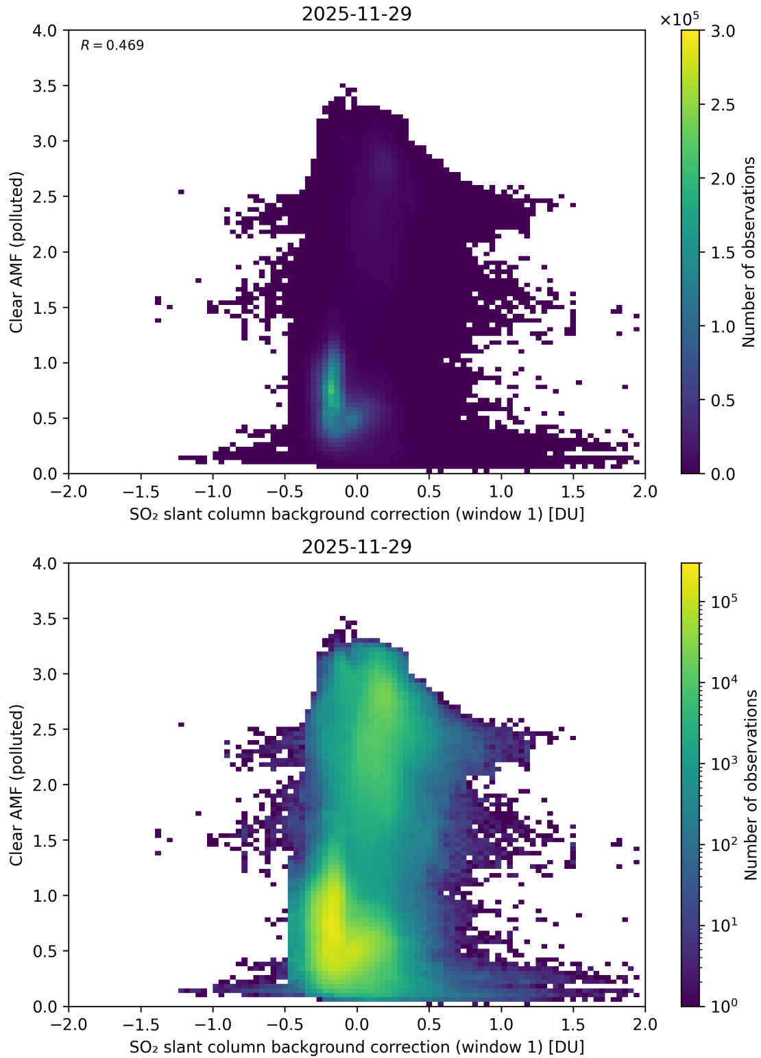
Figure 114: Scatter density plot of “SO 2 slant column background correction (window 1)” against “Clear AMF (polluted)” for 2025-11-28 to 2025-11-30.
