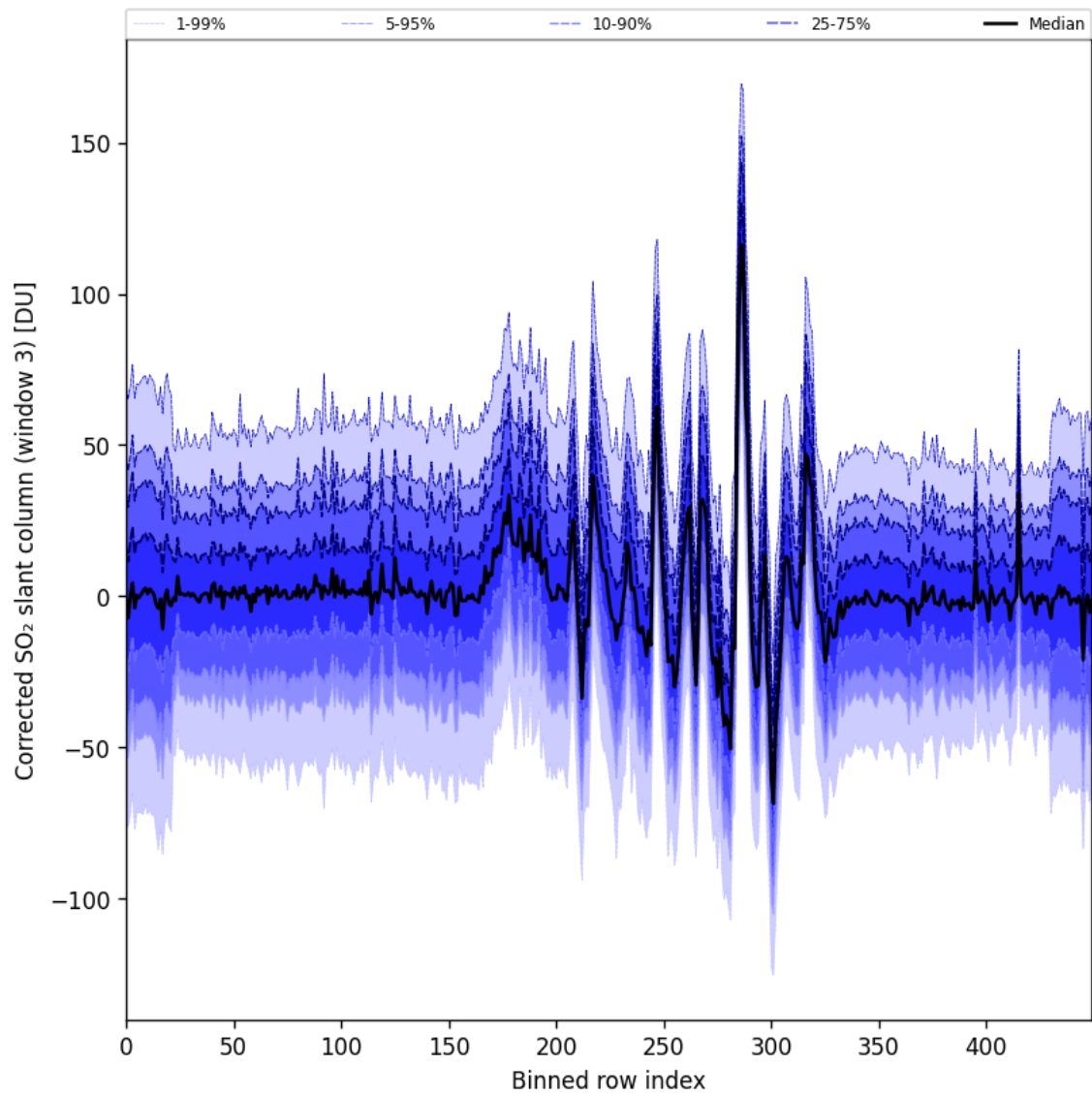
Figure 99: Along track statistics of “Corrected SO 2 slant column (window 3)” for 2025-11-28 to 2025-11-30
