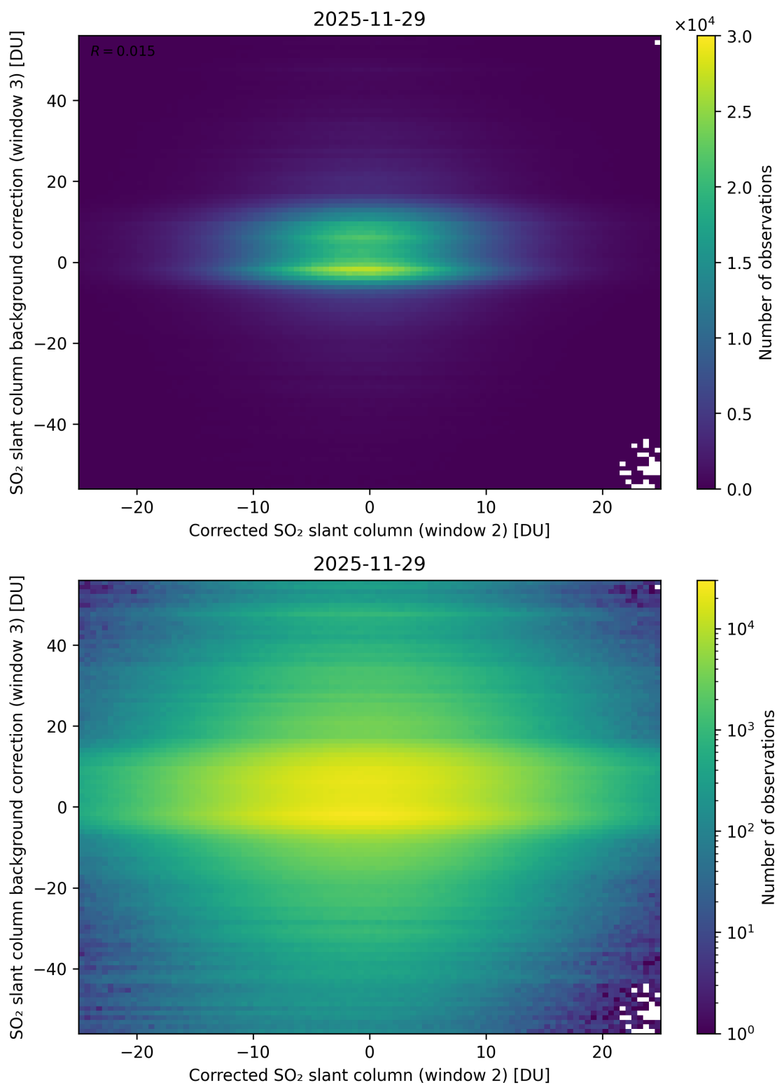
Figure 245: Scatter density plot of “Corrected SO 2 slant column (window 2)” against “SO 2 slant column background correction (window 3)” for 2025-11-28 to 2025-11-30.
