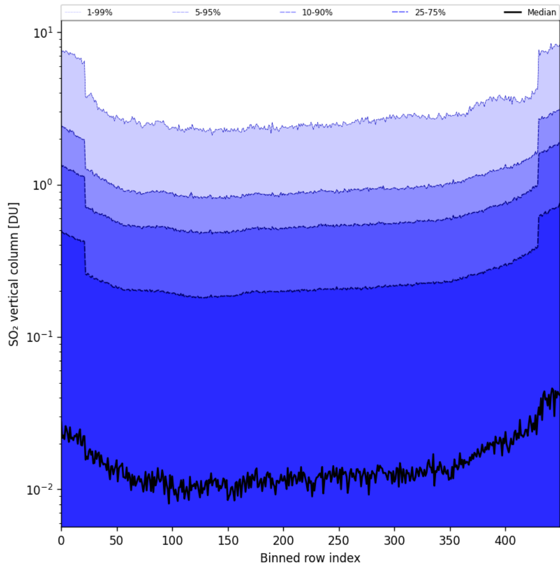
Figure 84: Along track statistics of “SO 2 vertical column” for 2025-11-28 to 2025-11-30
