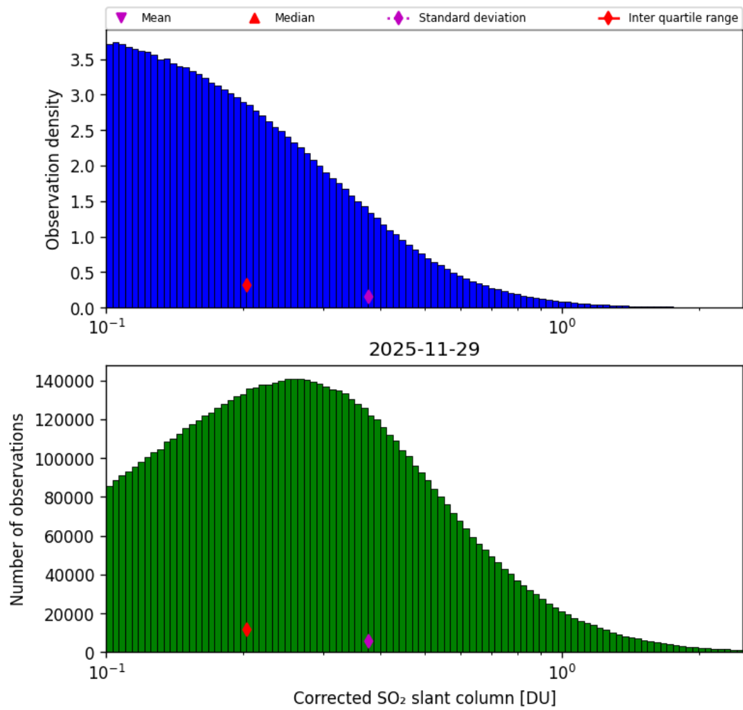
Figure 60: Histogram of "Corrected SO 2 slant column" for 2025-11-28 to 2025-11-30
