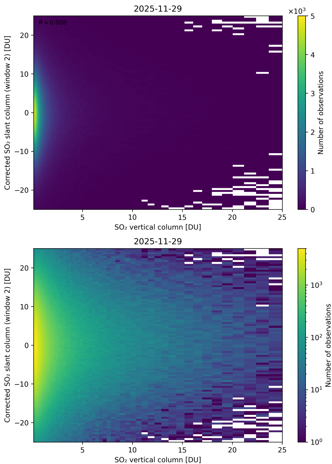
Figure 352: Scatter density plot of “SO 2 vertical column” against “Corrected SO 2 slant column (window 2)” for 2025-11-28 to 2025-11-30.
