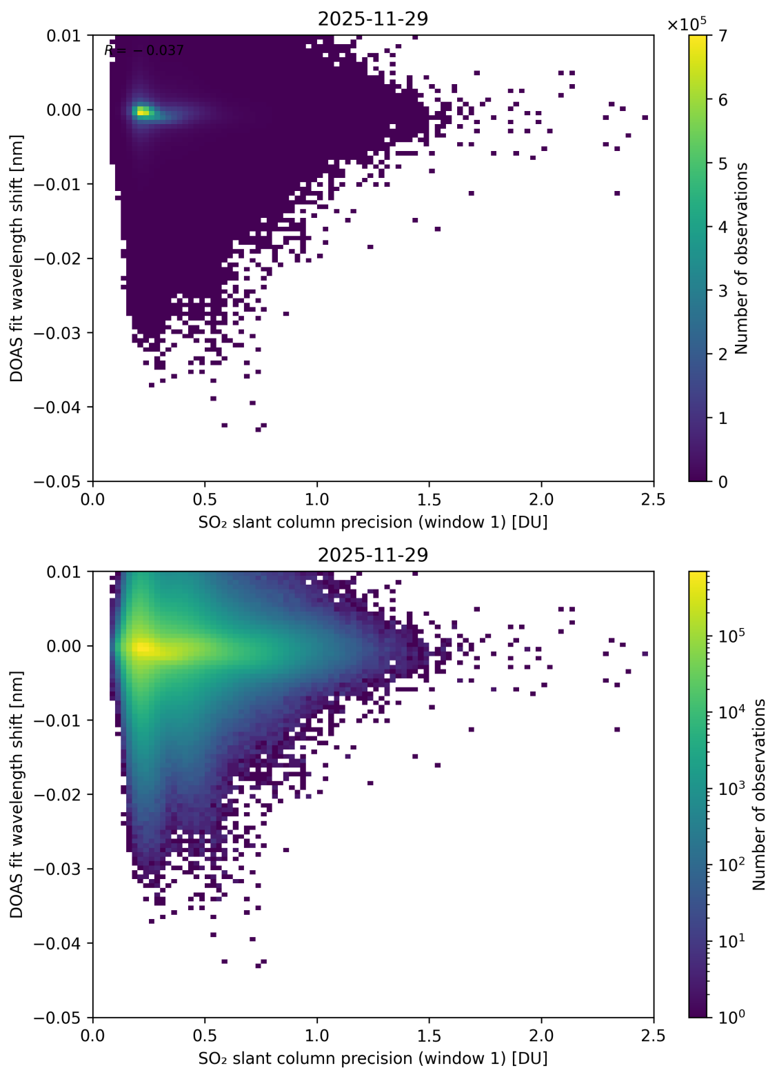
Figure 271: Scatter density plot of “SO 2 slant column precision (window 1)” against “DOAS fit wavelength shift” for 2025-11-28 to 2025-11-30.
