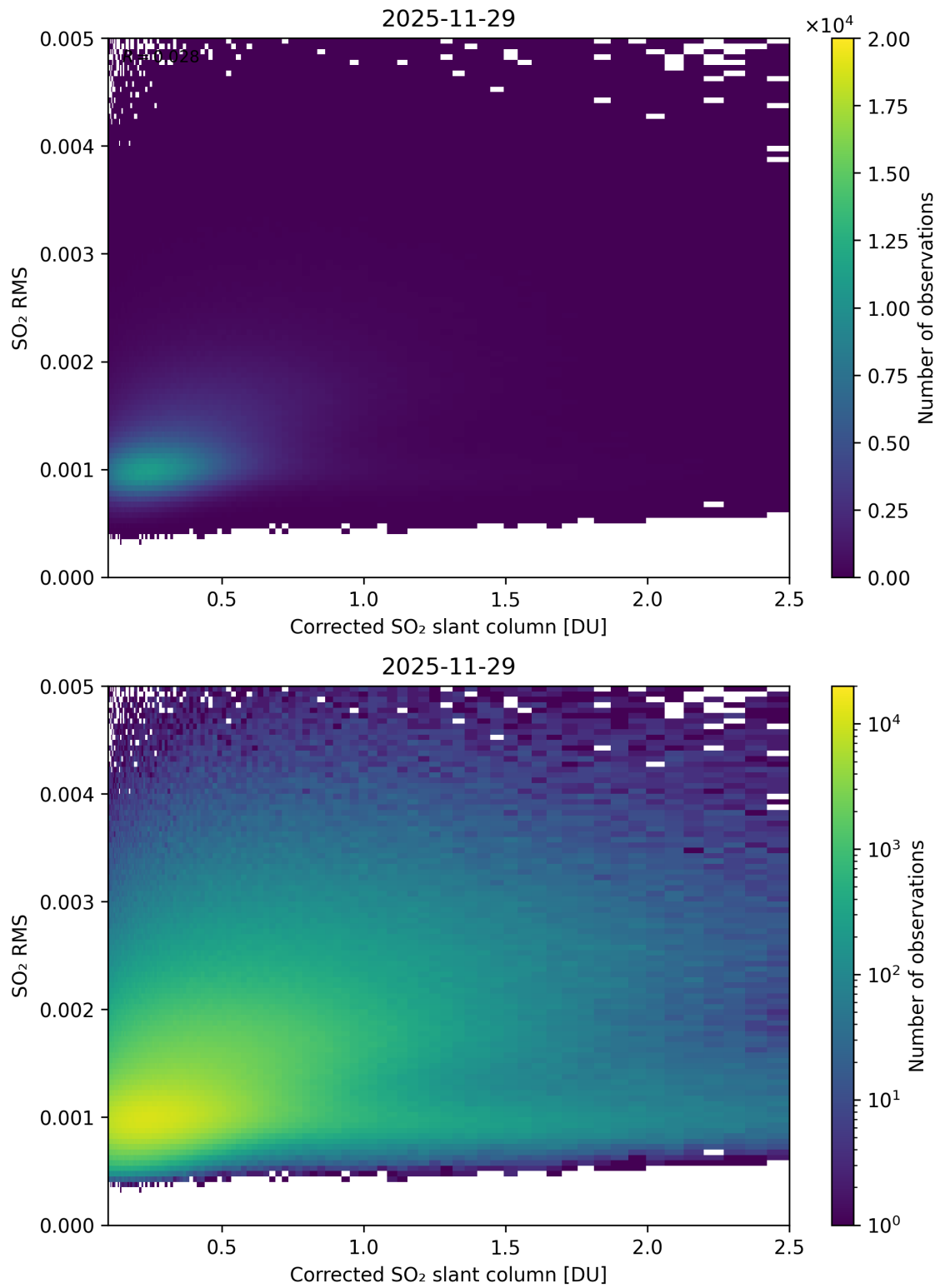
Figure 231: Scatter density plot of “Corrected SO 2 slant column” against “SO 2 RMS” for 2025-11-28 to 2025-11-30.
