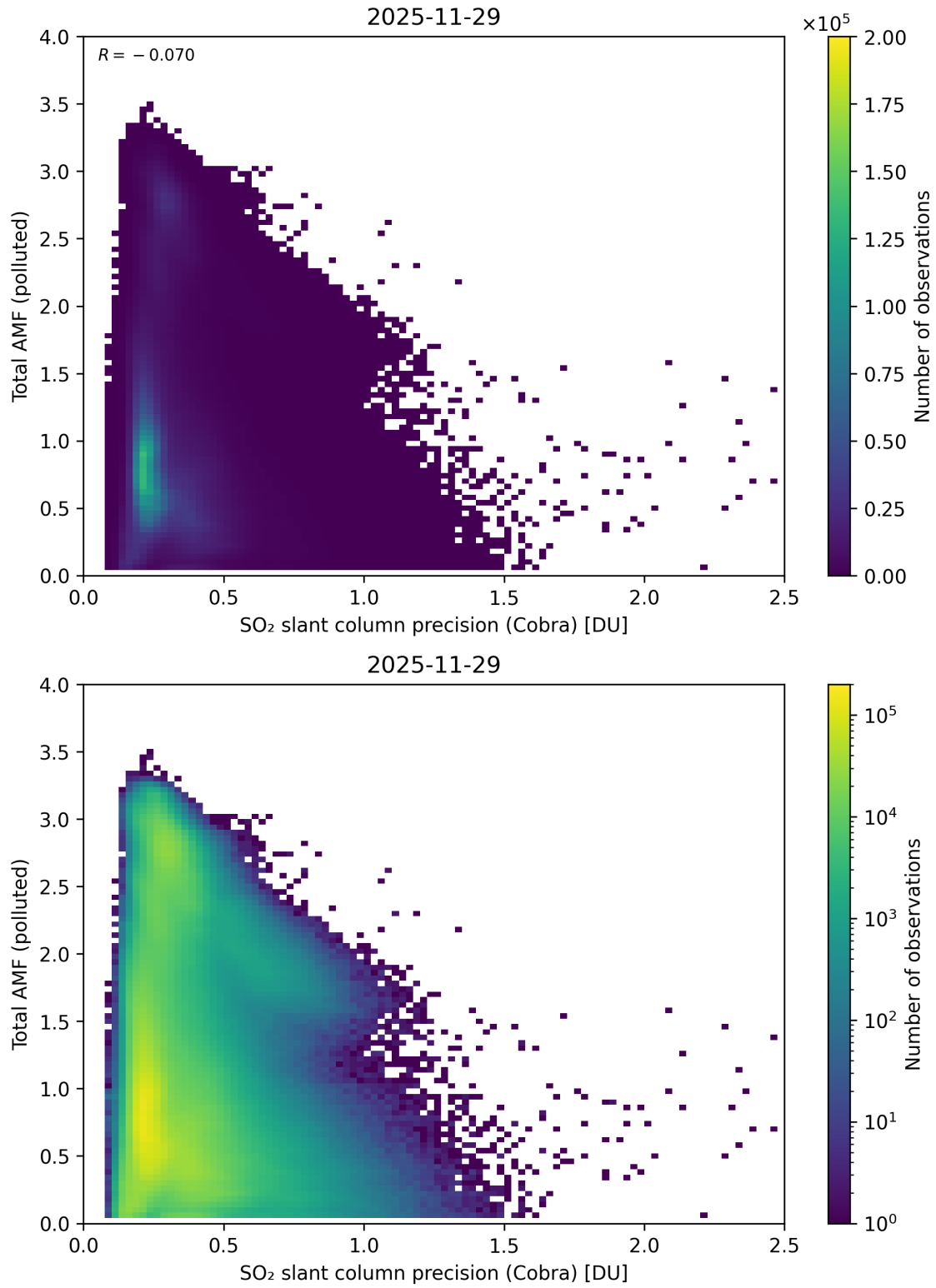
Figure 213: Scatter density plot of “SO 2 slant column precision (Cobra)” against “Total AMF (polluted)” for 2025-11-28 to 2025-11-30.
