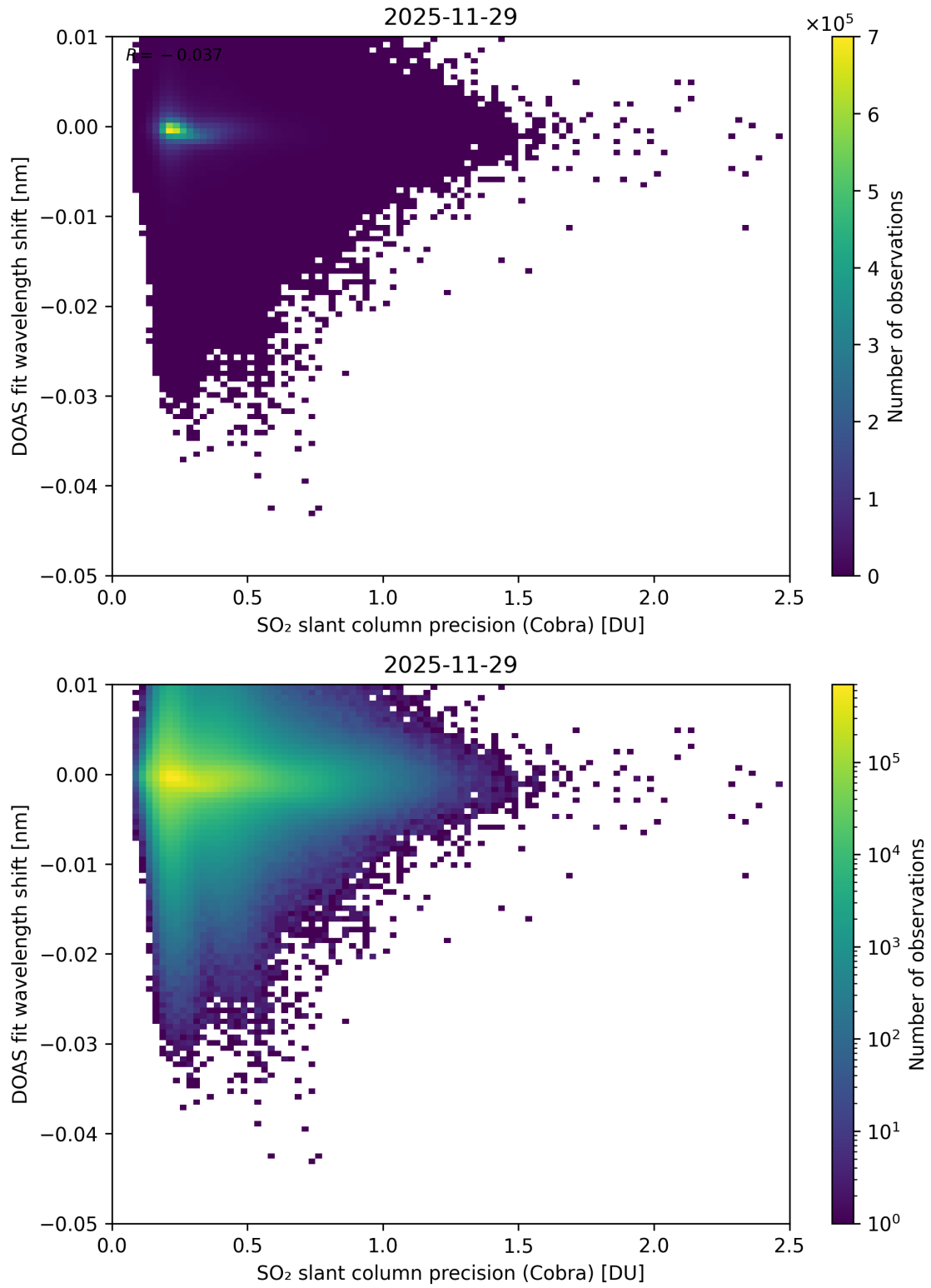
Figure 202: Scatter density plot of “SO 2 slant column precision (Cobra)” against “DOAS fit wavelength shift” for 2025-11-28 to 2025-11-30.
