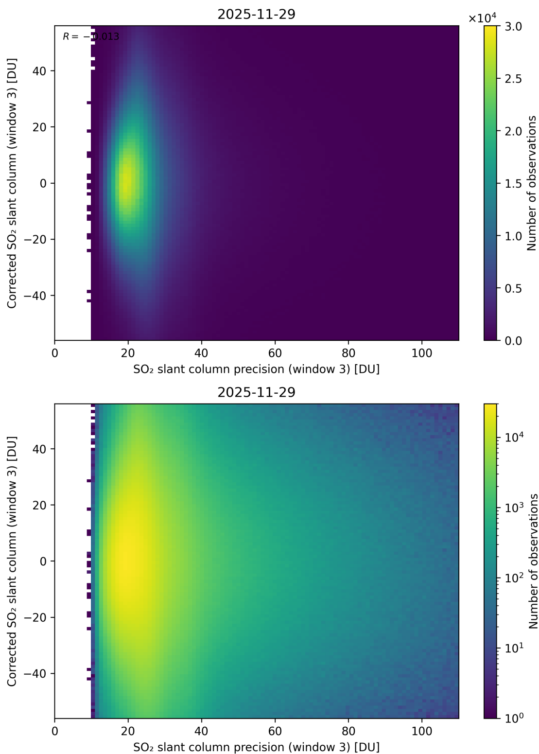
Figure 312: Scatter density plot of “SO 2 slant column precision (window 3)” against “Corrected SO 2 slant column (window 3)” for 2025-11-28 to 2025-11-30.
