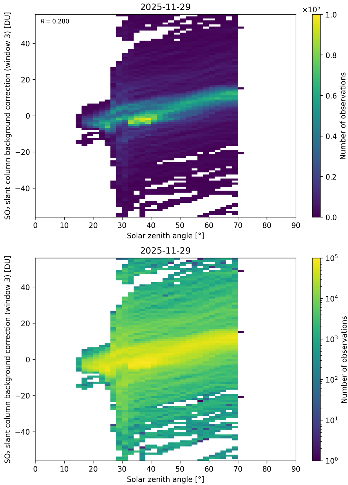
Figure 173: Scatter density plot of “Solar zenith angle” against “SO 2 slant column background correction (window 3)” for 2025-11-28 to 2025-11-30.
