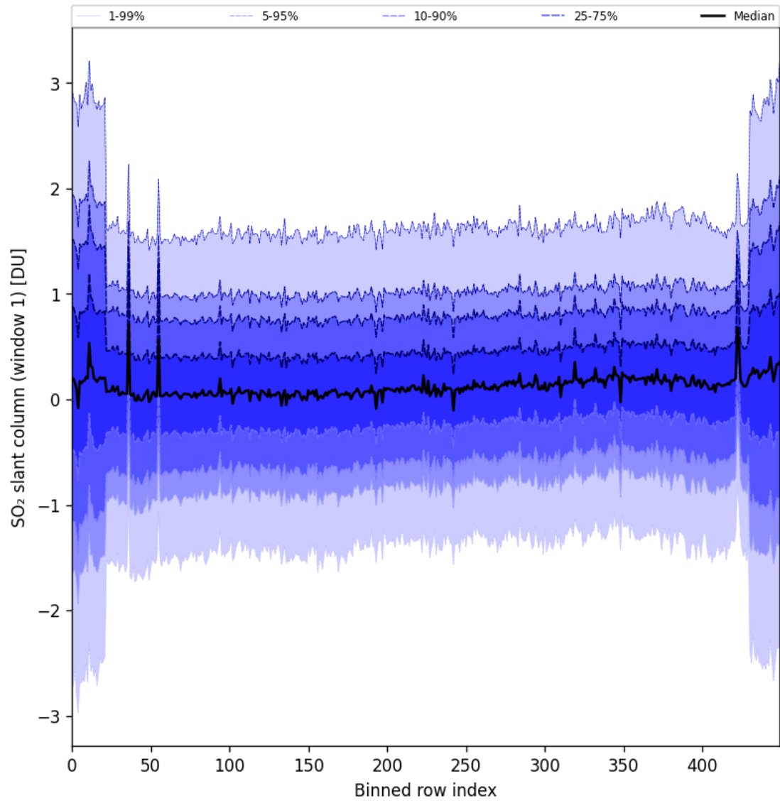
Figure 89: Along track statistics of “SO 2 slant column (window 1)” for 2025-11-28 to 2025-11-30
