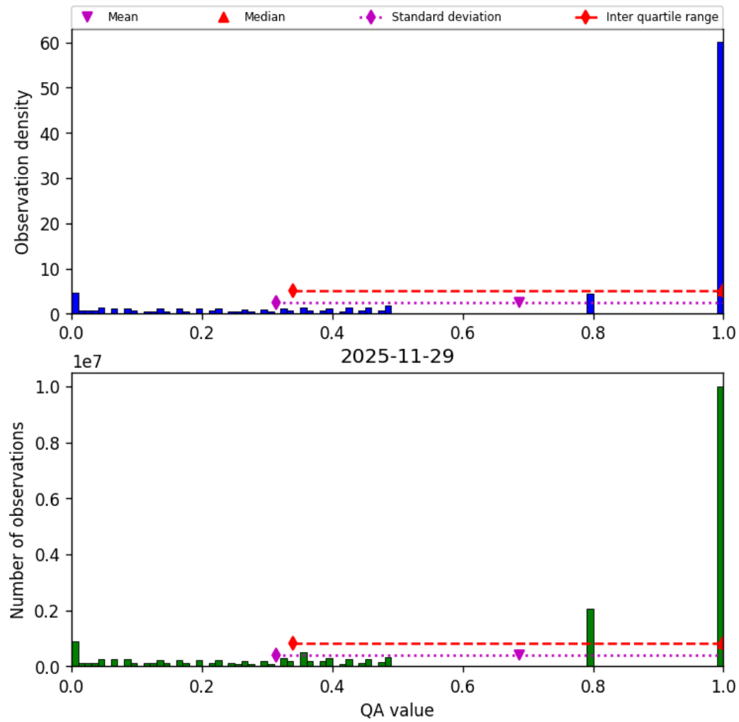
Figure 57: Histogram of “QA value” for 2025-11-28 to 2025-11-30
