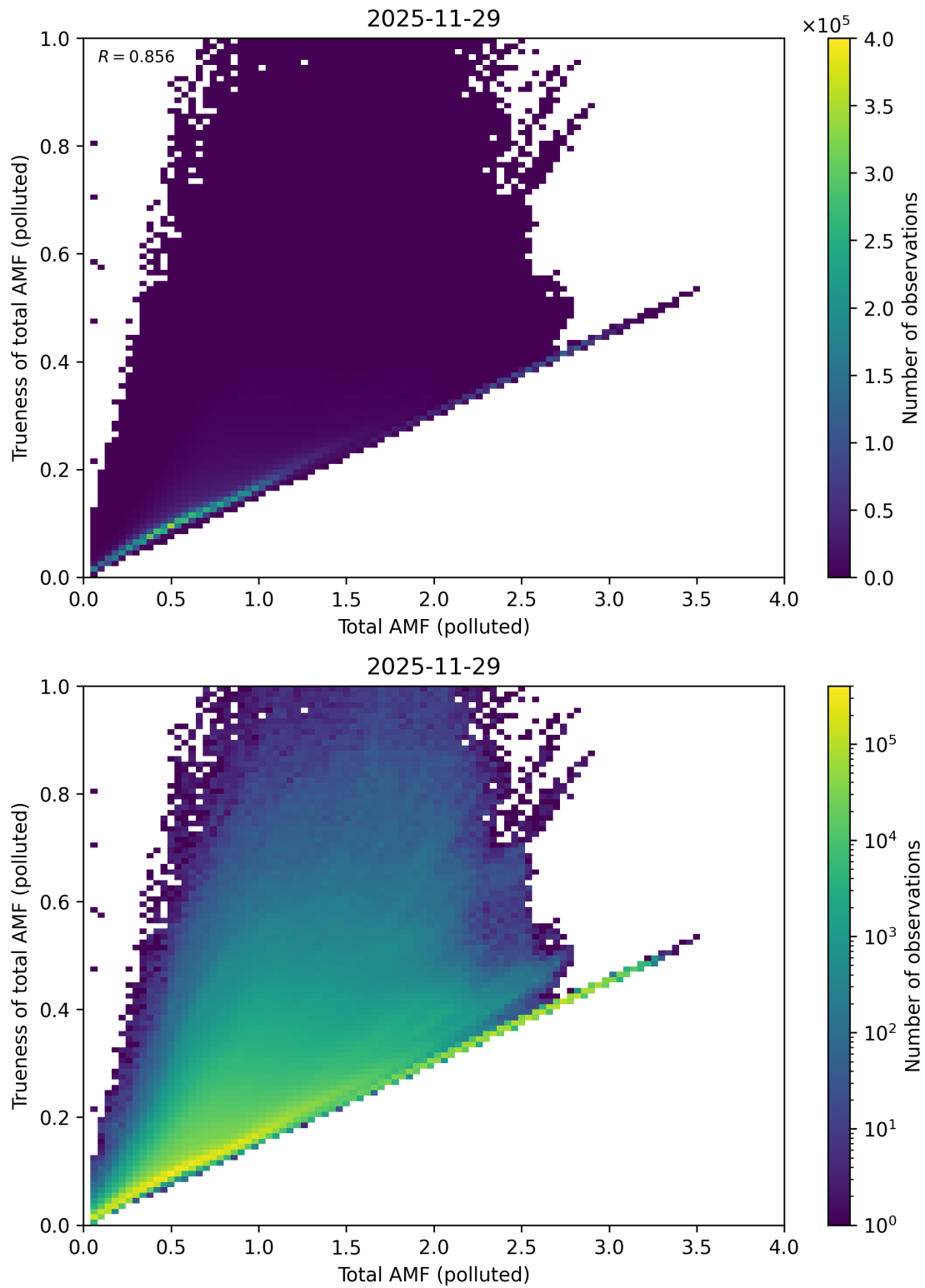
Figure 321: Scatter density plot of “Total AMF (polluted)” against “Trueness of total AMF (polluted)” for 2025-11-28 to 2025-11-30.
