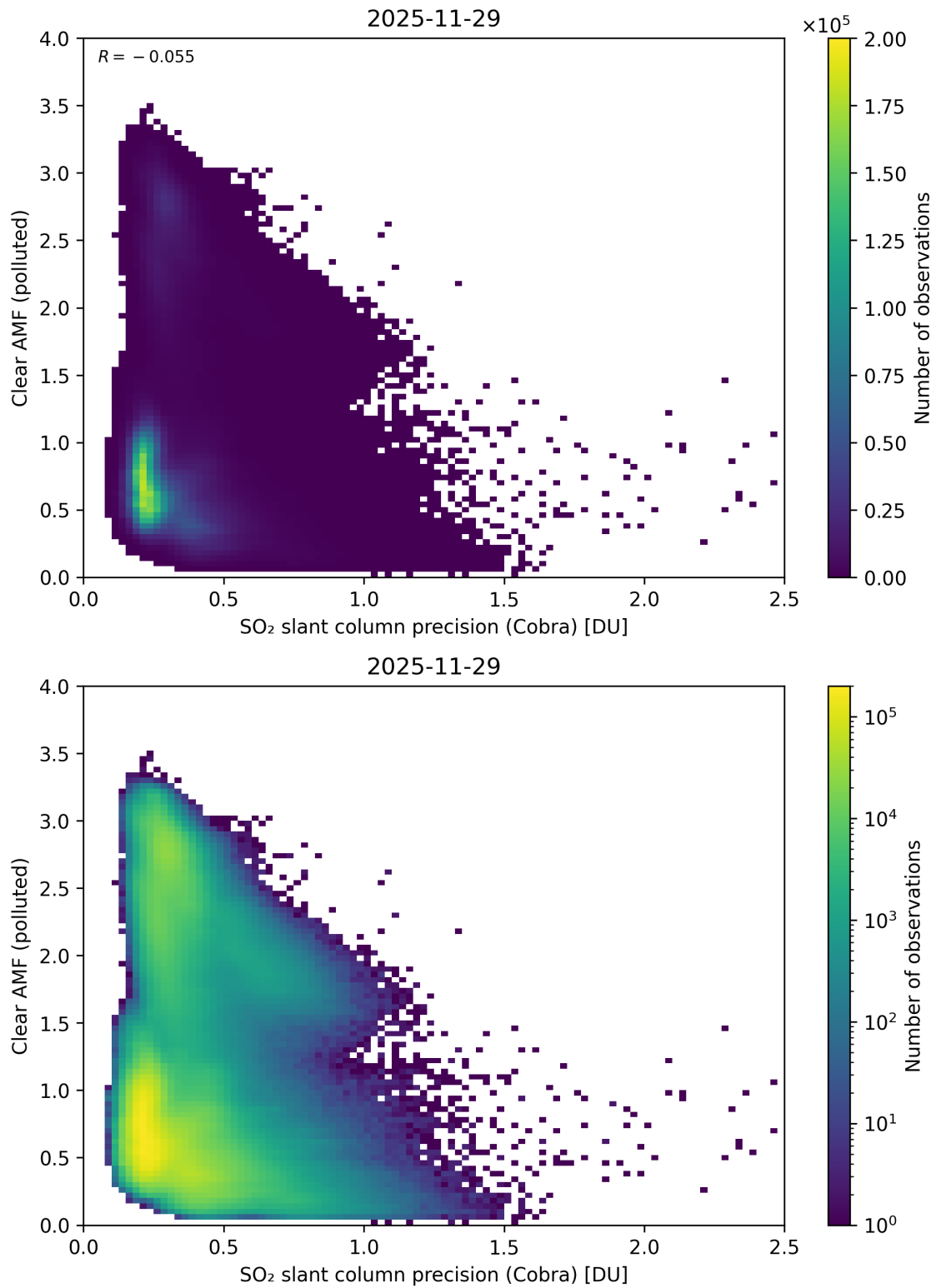
Figure 205: Scatter density plot of “SO 2 slant column precision (Cobra)” against “Clear AMF (polluted)” for 2025-11-28 to 2025-11-30.
