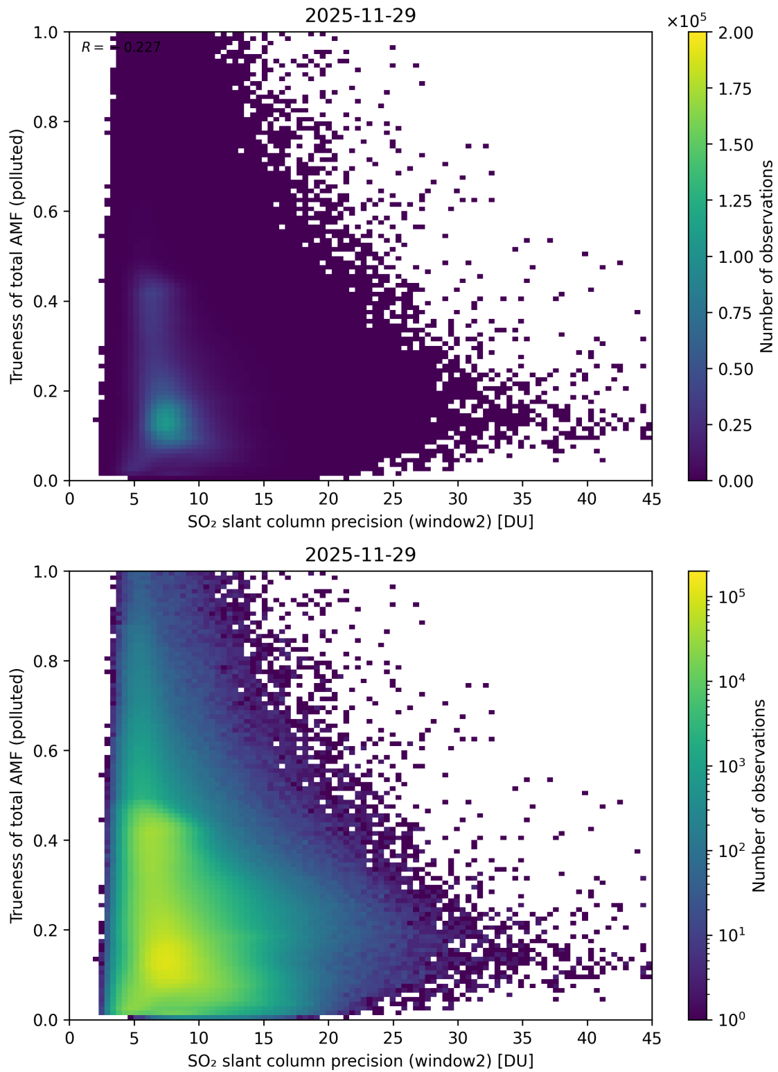
Figure 302: Scatter density plot of “SO 2 slant column precision (window2)” against “Trueness of total AMF (polluted)” for 2025-11-28 to 2025-11-30.
