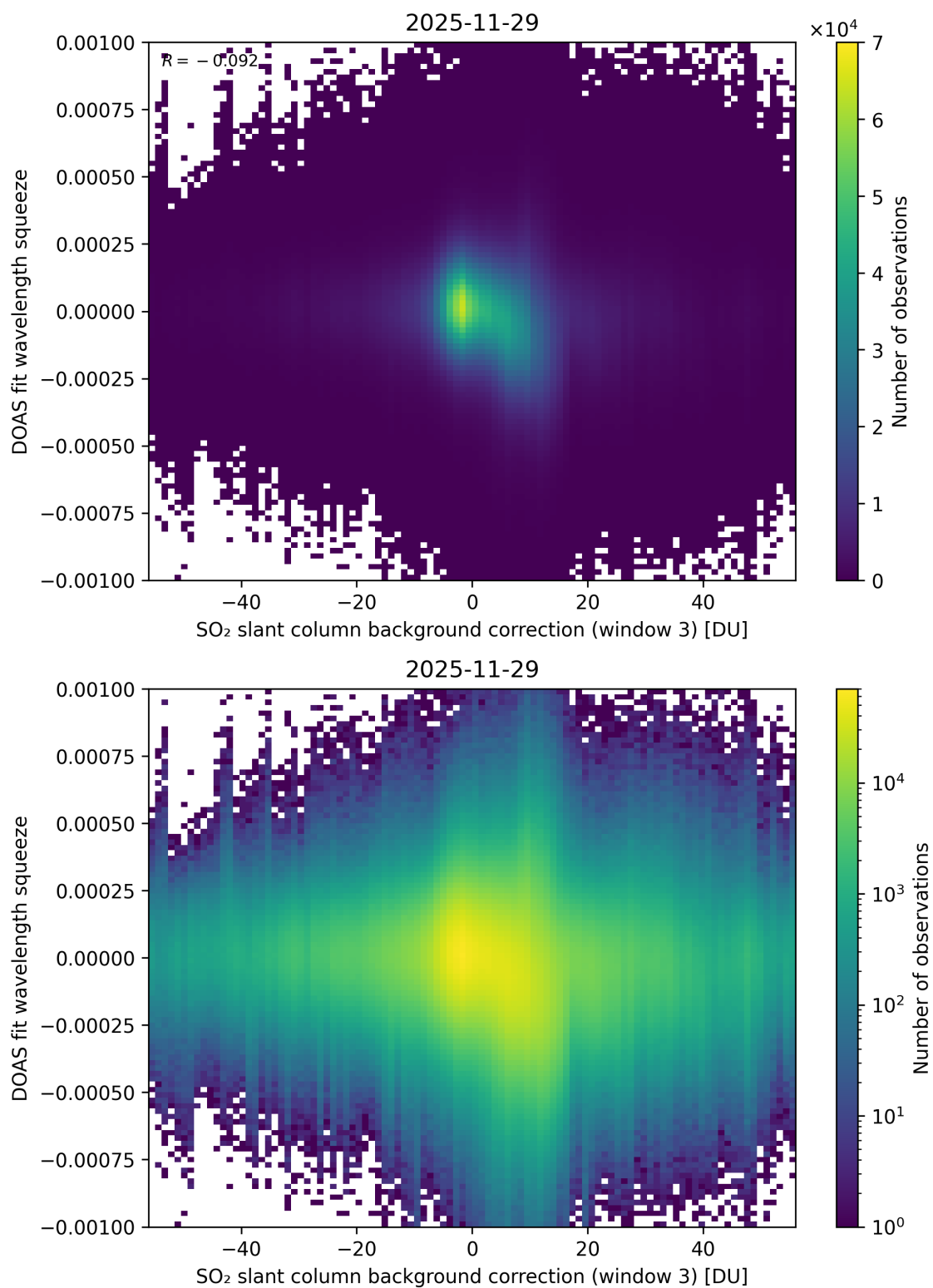
Figure 133: Scatter density plot of “SO 2 slant column background correction (window 3)” against “DOAS fit wavelength squeeze” for 2025-11-28 to 2025-11-30.
