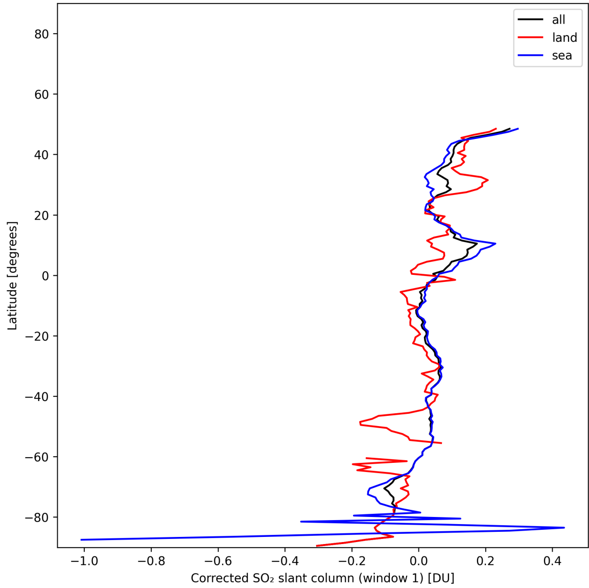
Figure 39: Zonal average of “Corrected SO 2 slant column (window 1)” for 2025-11-28 to 2025-11-30.
