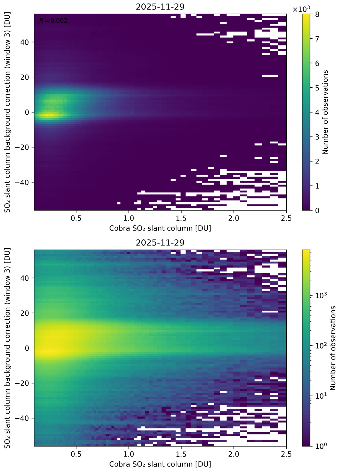
Figure 195: Scatter density plot of “Cobra SO 2 slant column” against “SO 2 slant column background correction (window 3)” for 2025-11-28 to 2025-11-30.
