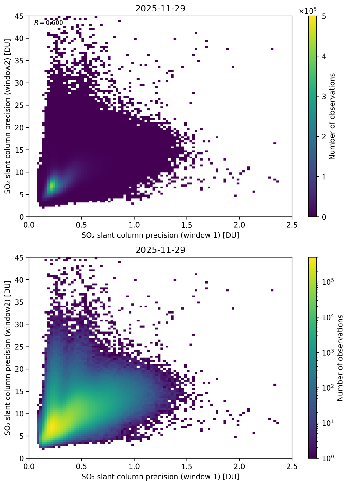
Figure 277: Scatter density plot of “SO 2 slant column precision (window 1)” against “SO 2 slant column precision (window 2)” for 2025-11-28 to 2025-11-30.
