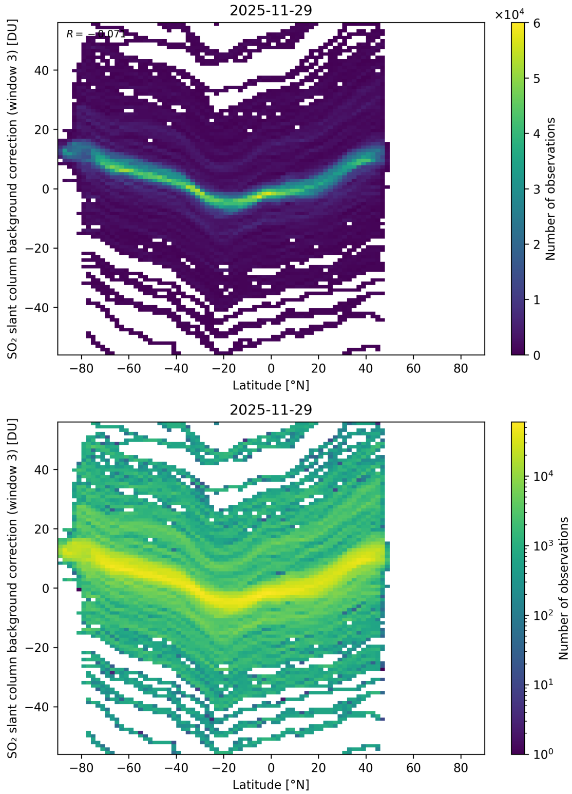
Figure 152: Scatter density plot of “Latitude” against “SO 2 slant column background correction (window 3)” for 2025-11-28 to 2025-11-30.
