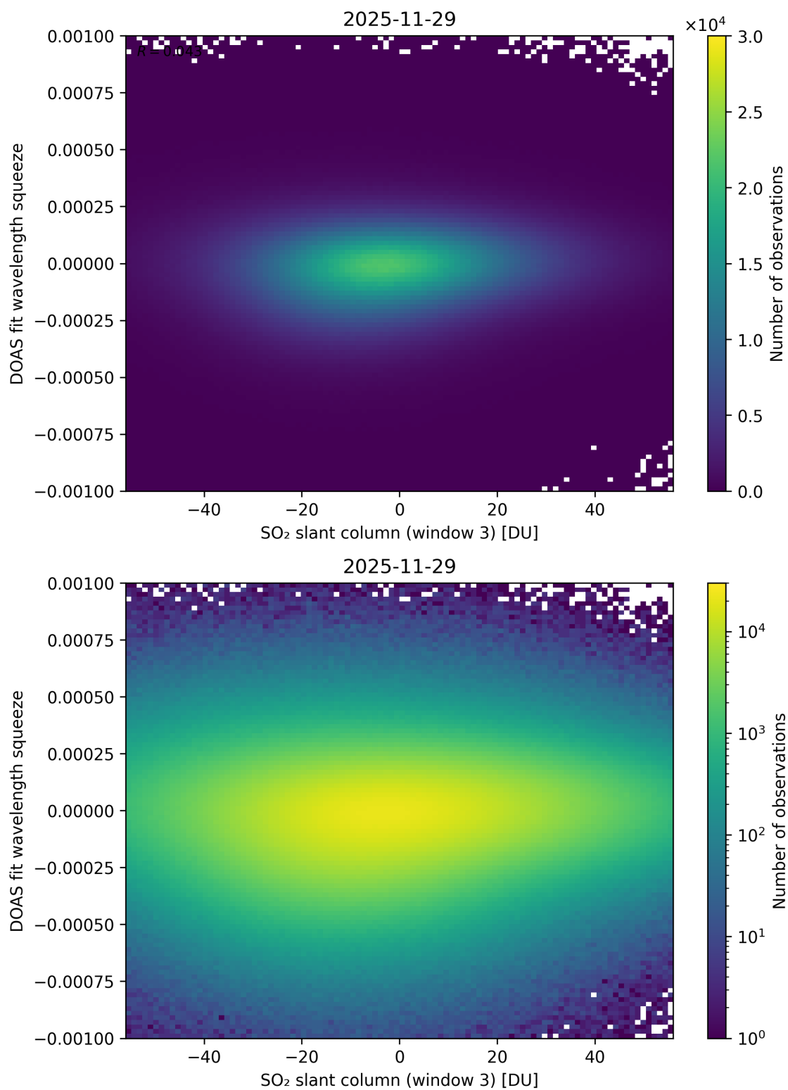
Figure 305: Scatter density plot of “SO 2 slant column (window 3)” against “DOAS fit wavelength squeeze” for 2025-11-28 to 2025-11-30.
