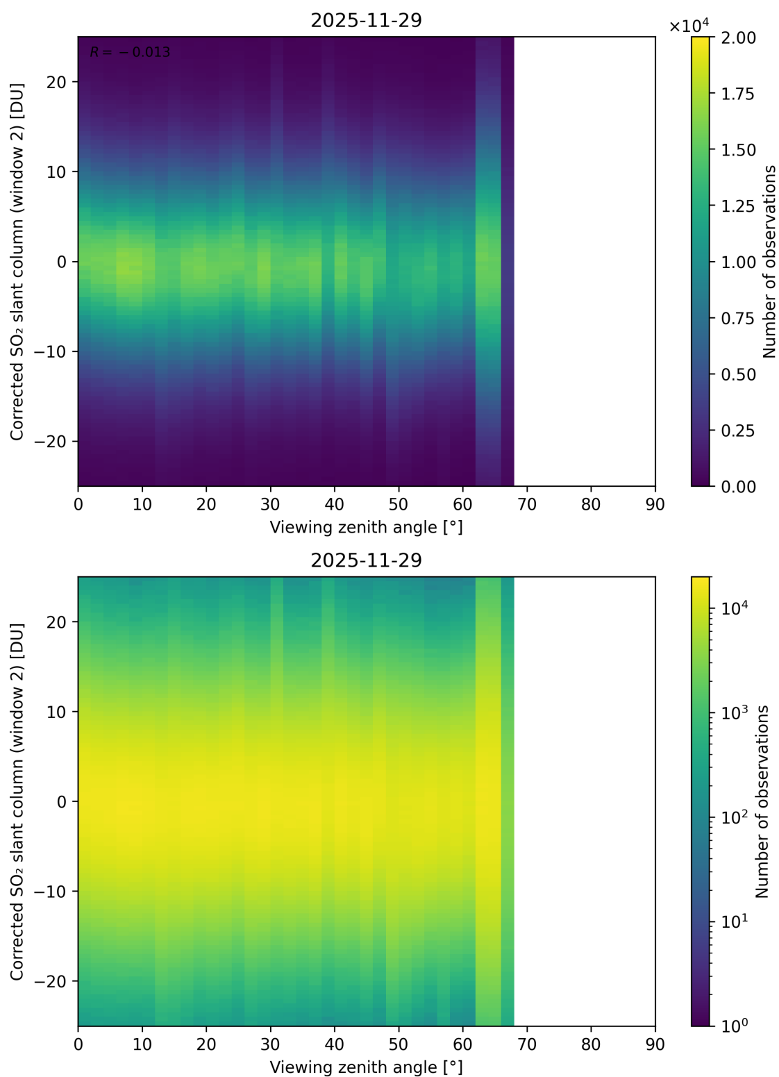
Figure 374: Scatter density plot of “Viewing zenith angle” against “Corrected SO 2 slant column (window 2)” for 2025-11-28 to 2025-11-30.
