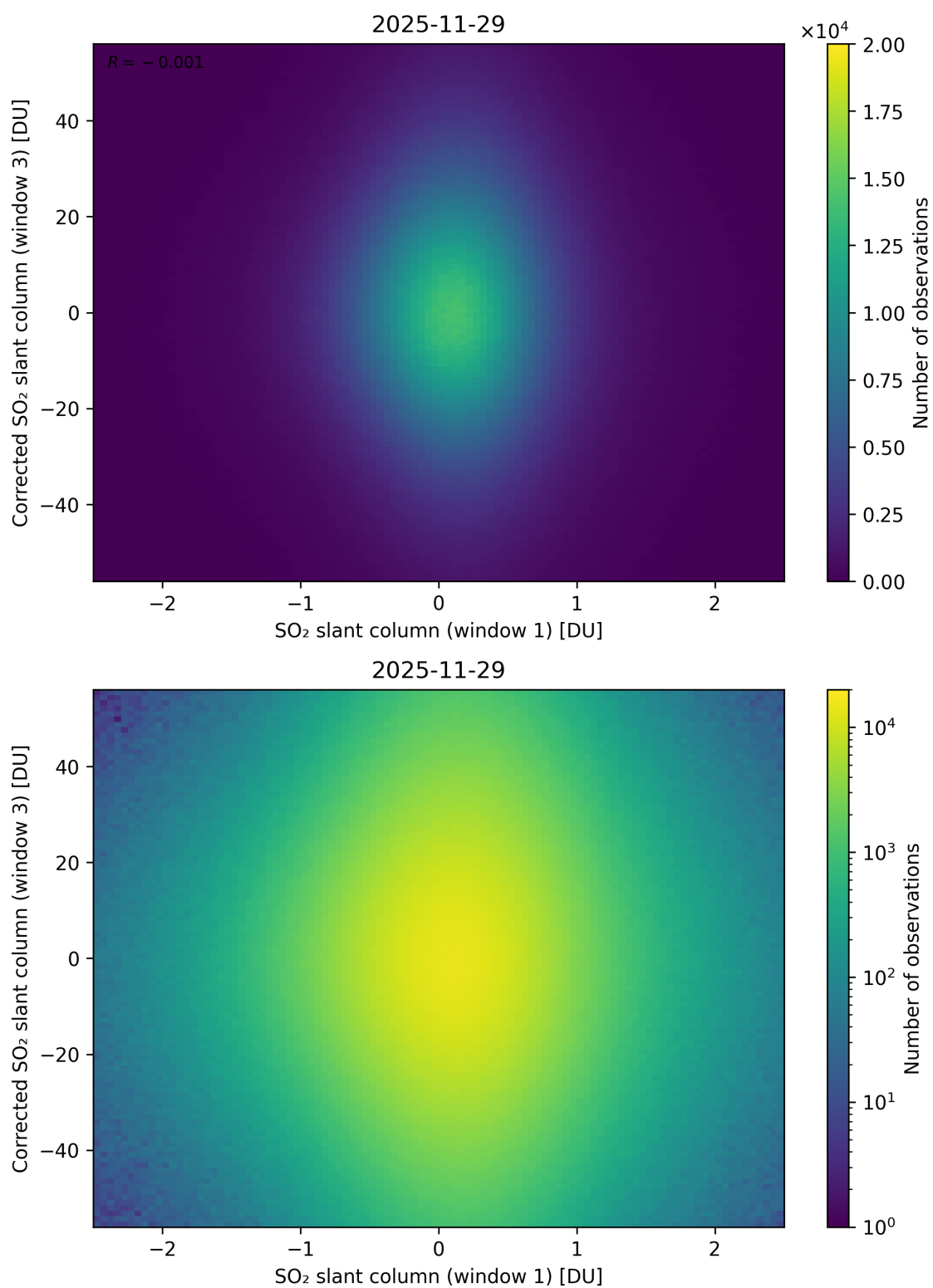
Figure 284: Scatter density plot of “SO 2 slant column (window 1)” against “Corrected SO 2 slant column (window 3)” for 2025-11-28 to 2025-11-30.
