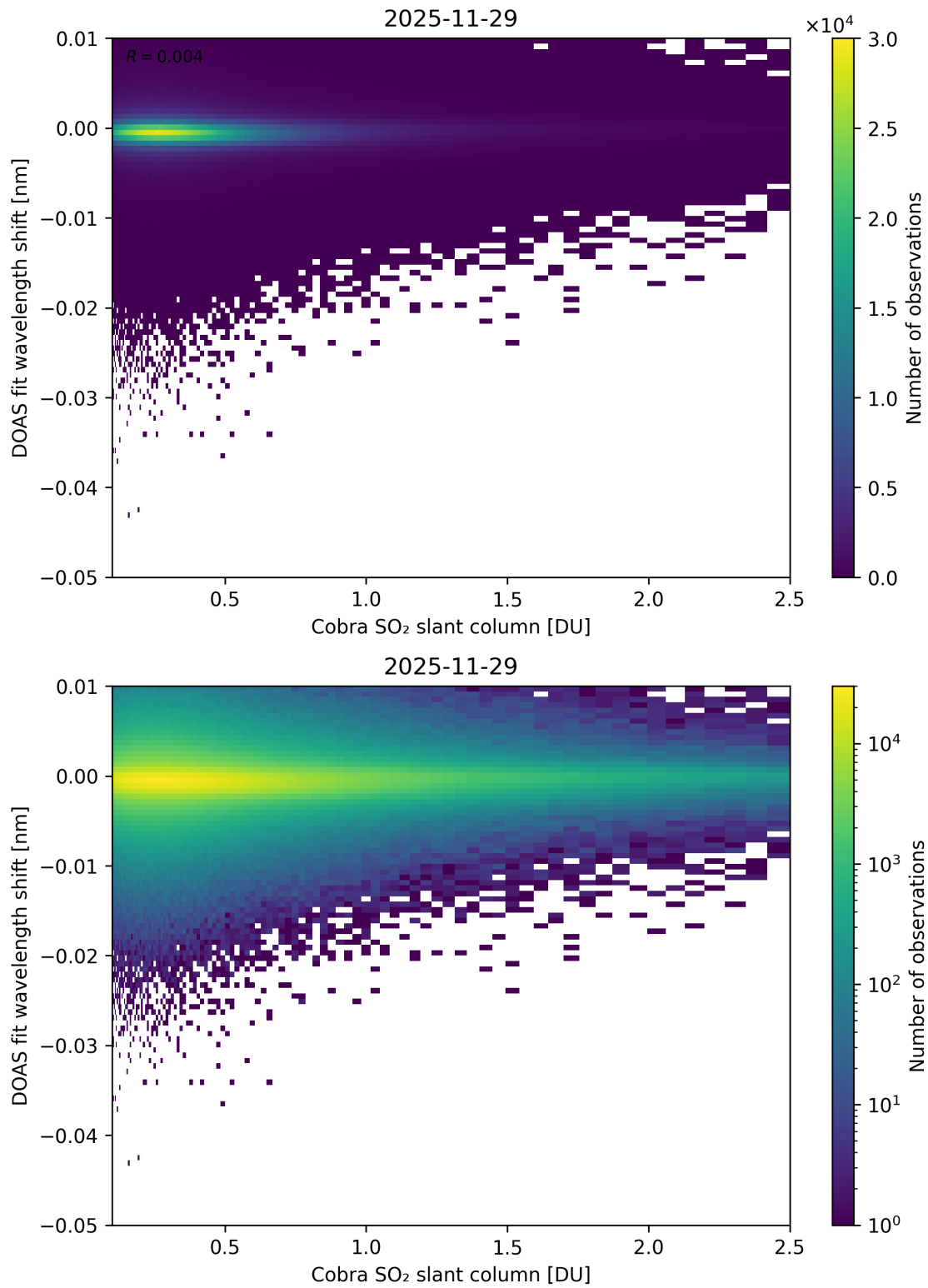
Figure 196: Scatter density plot of “Cobra SO 2 slant column” against “DOAS fit wavelength shift” for 2025-11-28 to 2025-11-30.
