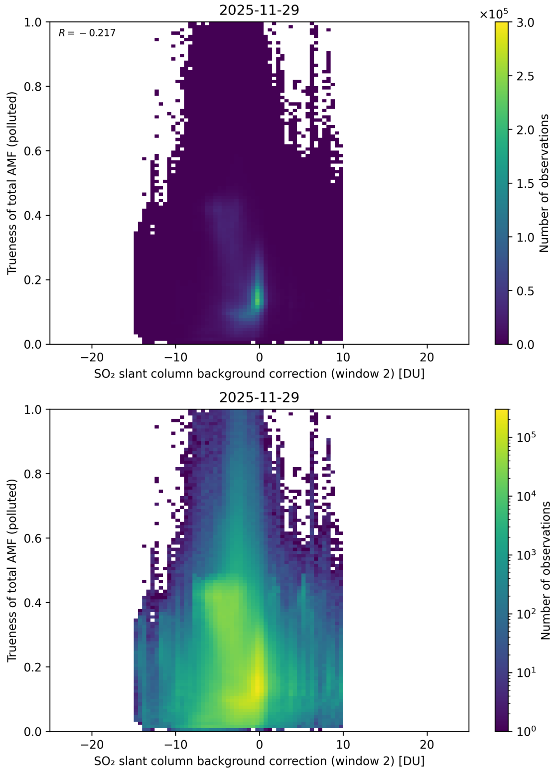
Figure 131: Scatter density plot of “SO 2 slant column background correction (window 2)” against “Trueness of total AMF (polluted)” for 2025-11-28 to 2025-11-30.
