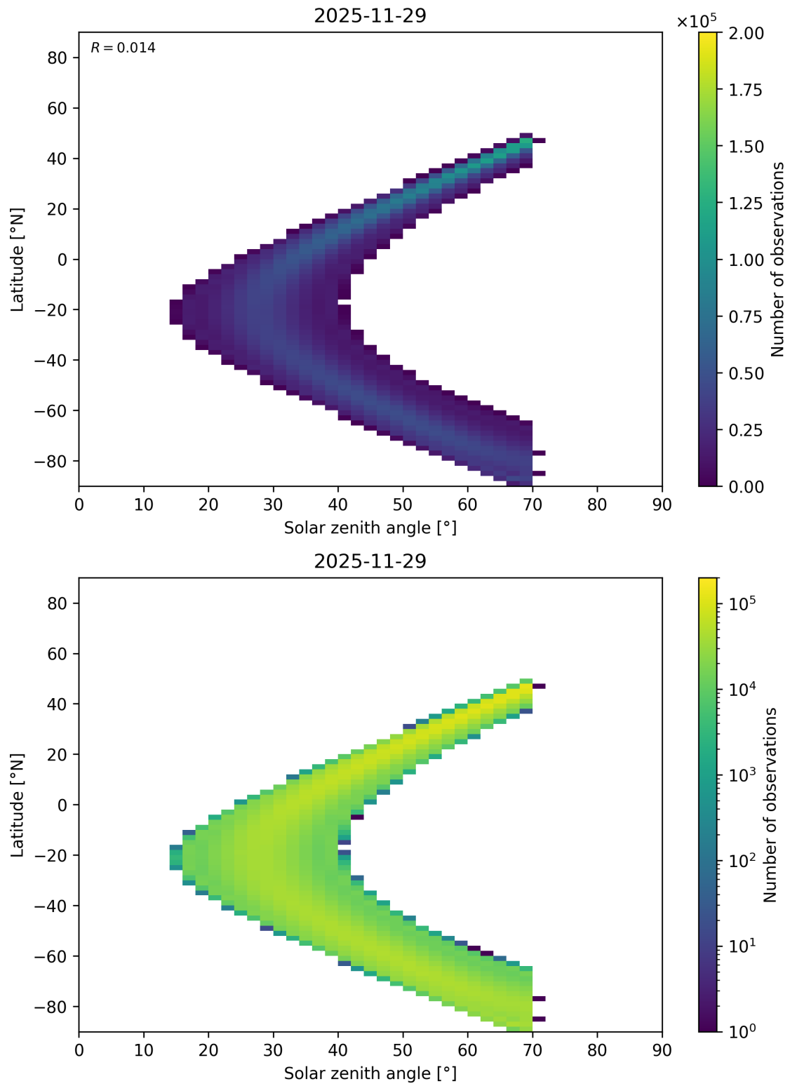
Figure 177: Scatter density plot of “Solar zenith angle” against “Latitude” for 2025-11-28 to 2025-11-30.
