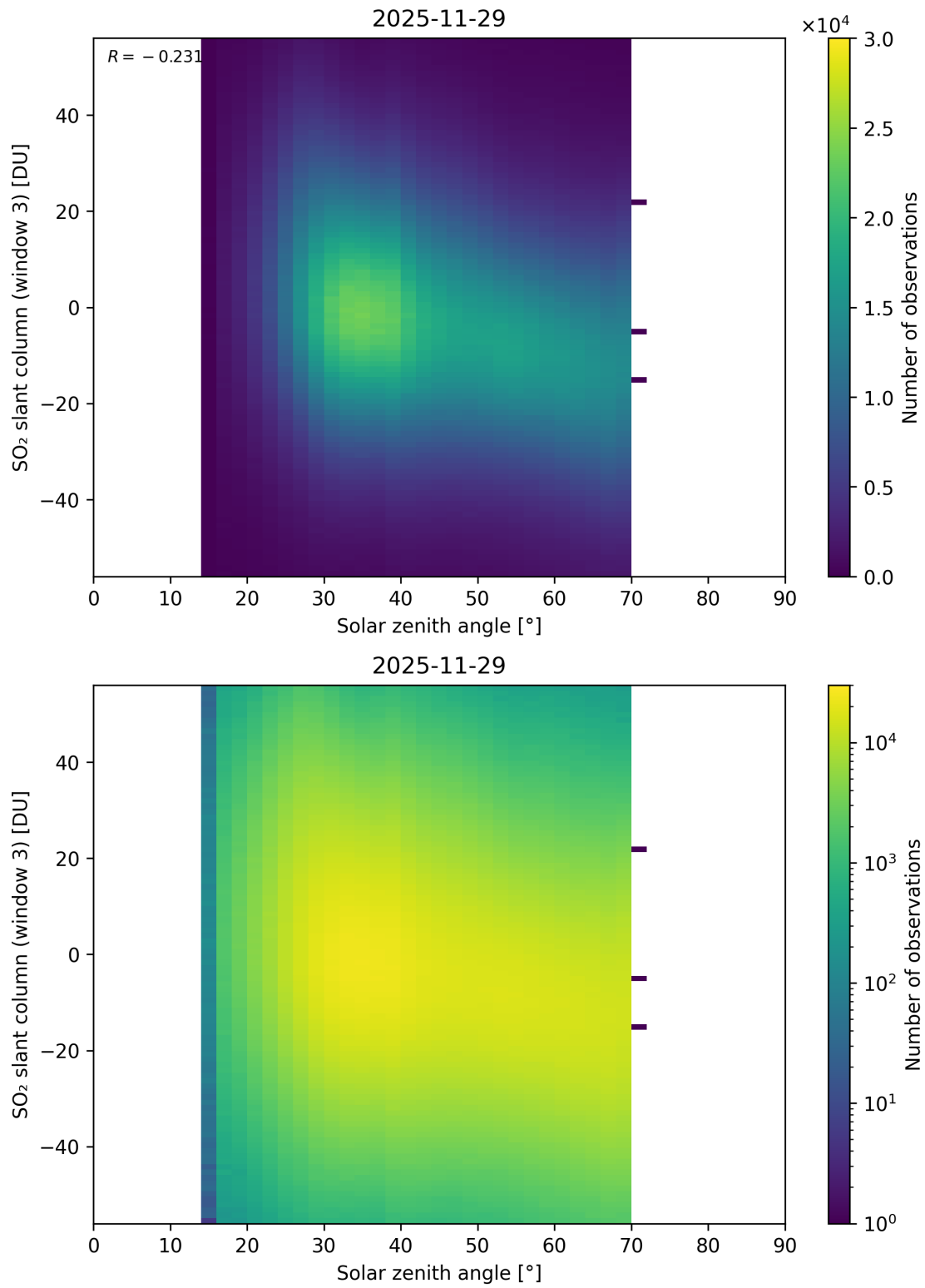
Figure 187: Scatter density plot of “Solar zenith angle” against “SO 2 slant column (window 3)” for 2025-11-28 to 2025-11-30.
