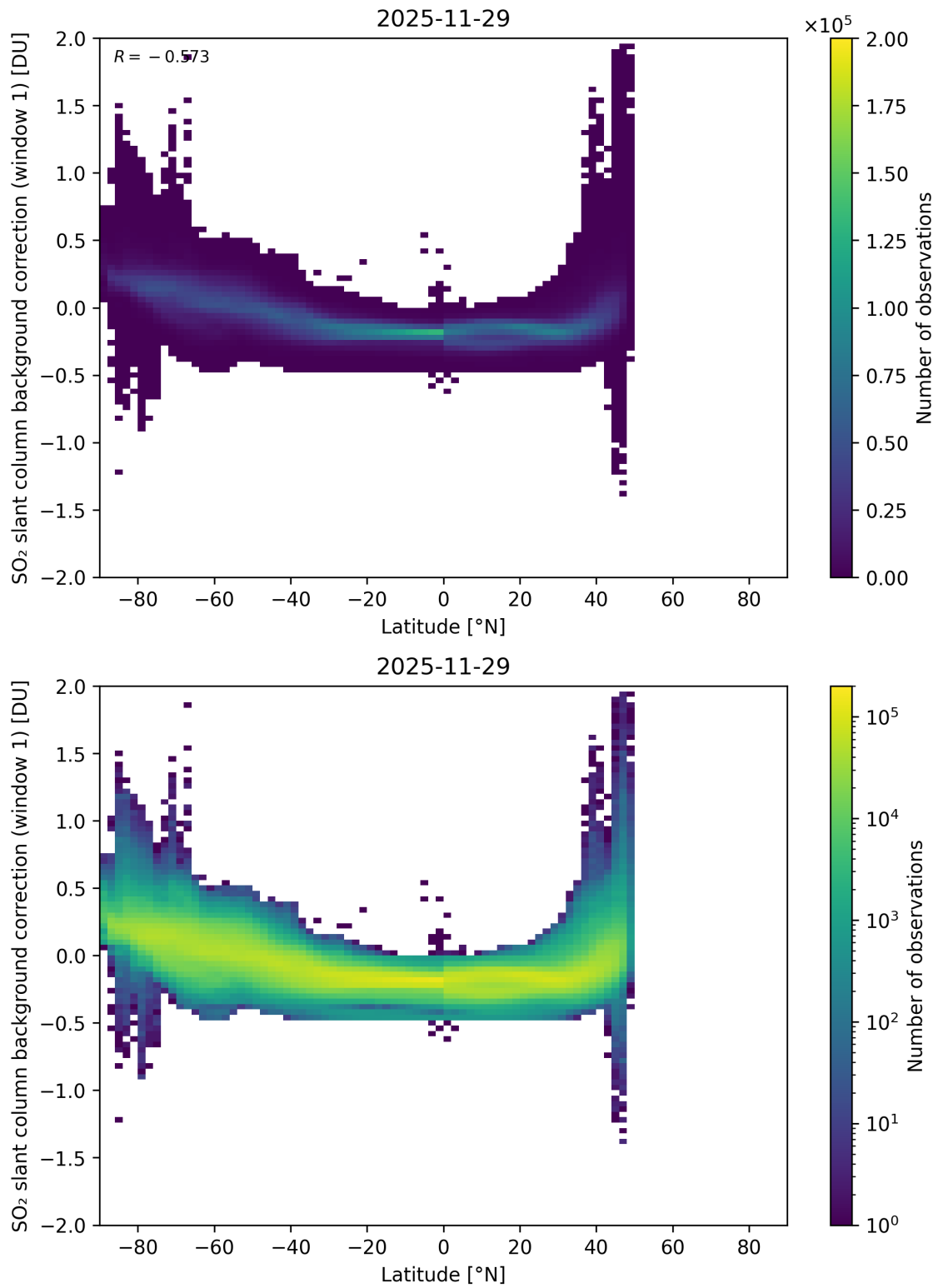
Figure 150: Scatter density plot of “Latitude” against “SO 2 slant column background correction (window 1)” for 2025-11-28 to 2025-11-30.
