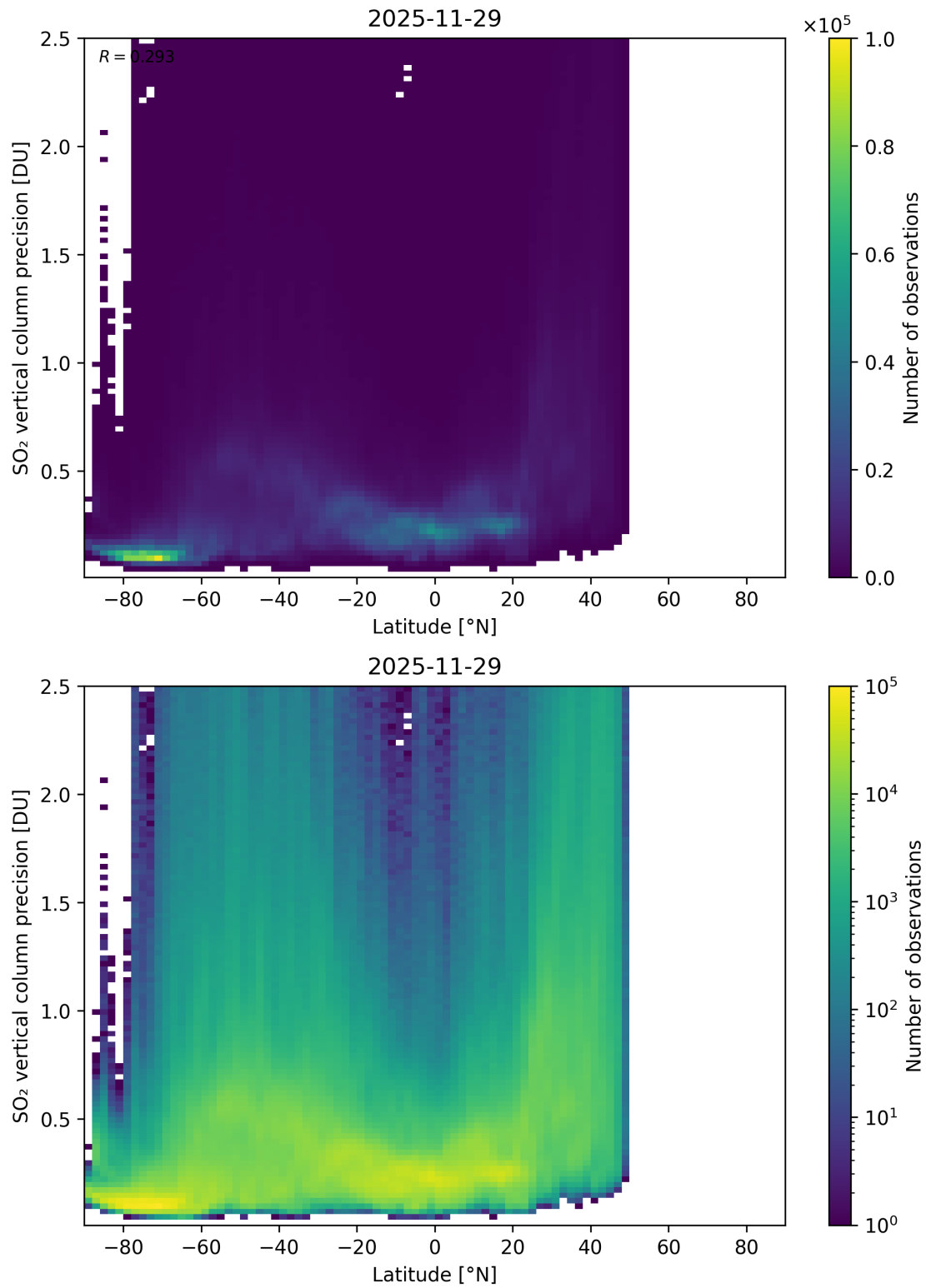
Figure 170: Scatter density plot of “Latitude” against “SO 2 vertical column precision” for 2025-11-28 to 2025-11-30.
