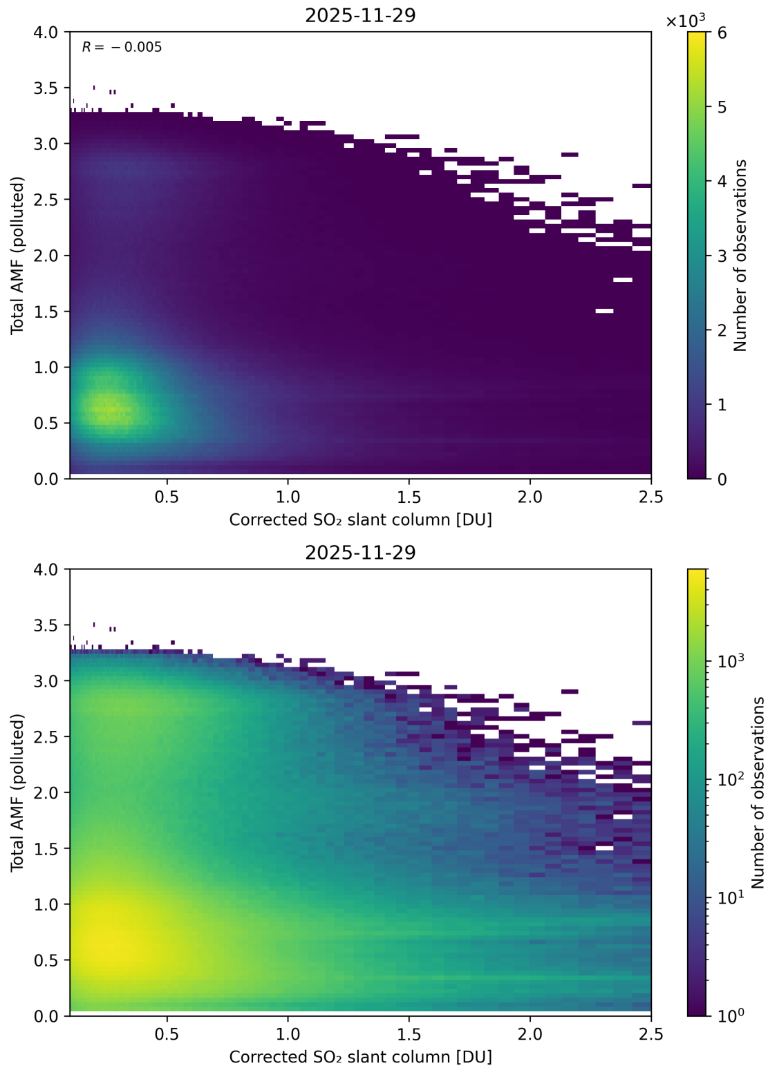
Figure 242: Scatter density plot of “Corrected SO 2 slant column” against “Total AMF (polluted)” for 2025-11-28 to 2025-11-30.
