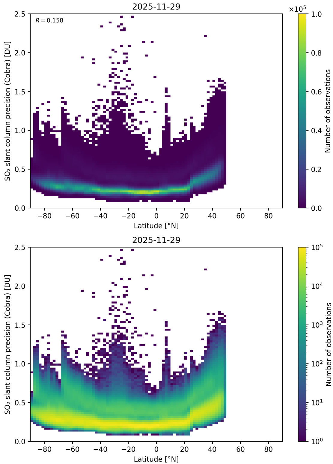
Figure 158: Scatter density plot of “Latitude” against “SO 2 slant column precision (Cobra)” for 2025-11-28 to 2025-11-30.
