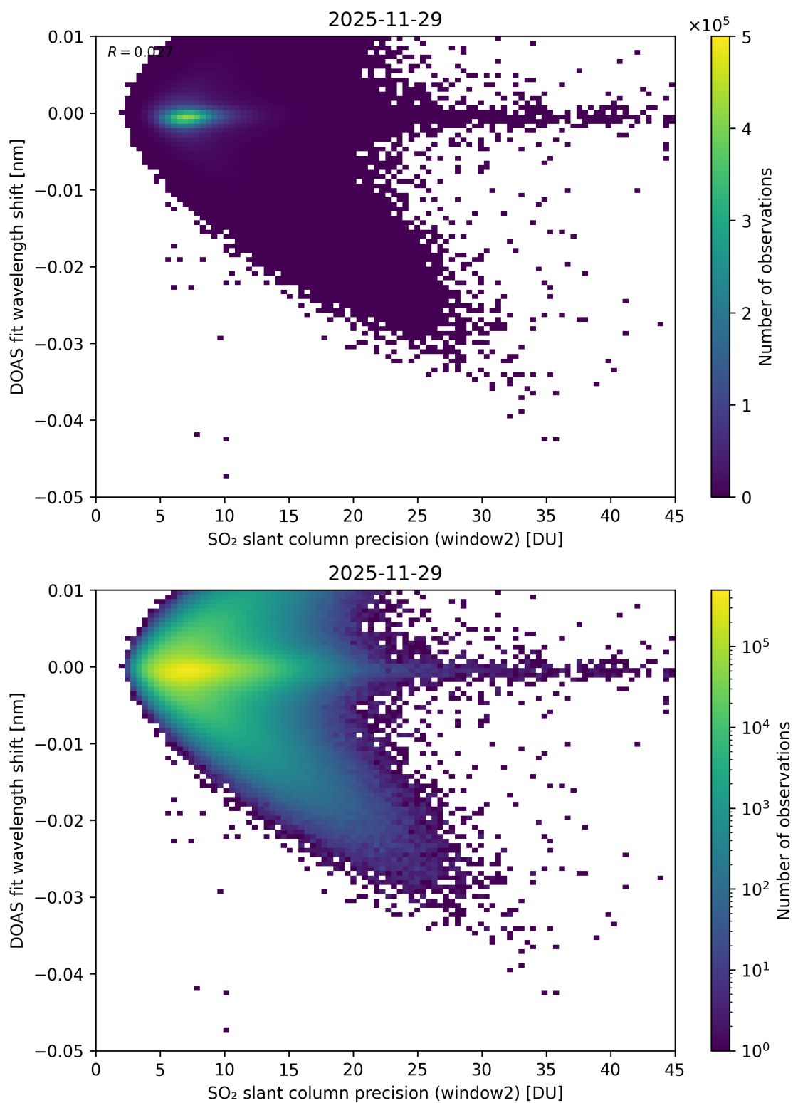
Figure 293: Scatter density plot of “SO 2 slant column precision (window2)” against “DOAS fit wavelength shift” for 2025-11-28 to 2025-11-30.
