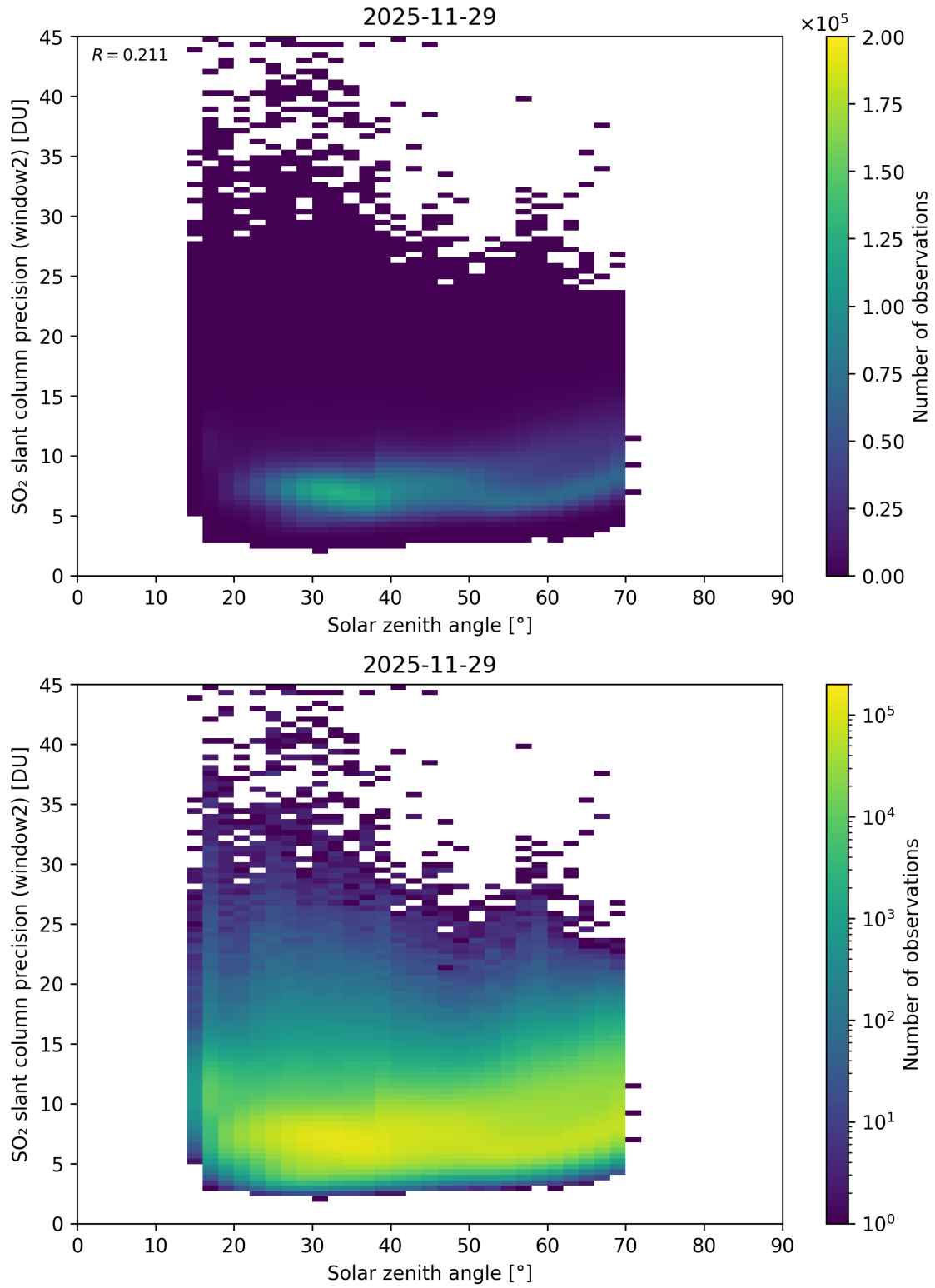
Figure 186: Scatter density plot of “Solar zenith angle” against “SO 2 slant column precision (window2)” for 2025-11-28 to 2025-11-30.
