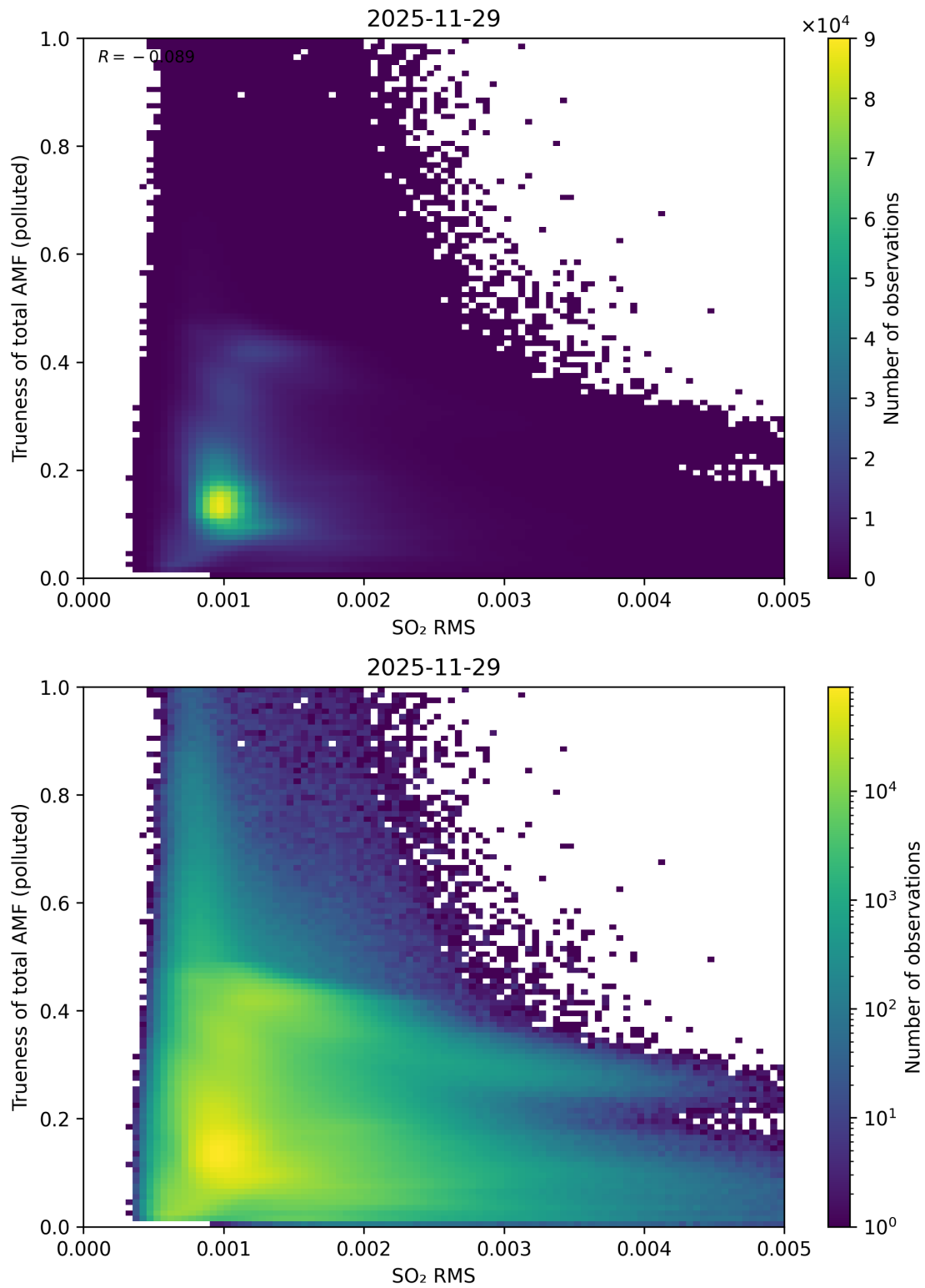
Figure 149: Scatter density plot of “SO 2 RMS” against “Trueness of total AMF (polluted)” for 2025-11-28 to 2025-11-30.
