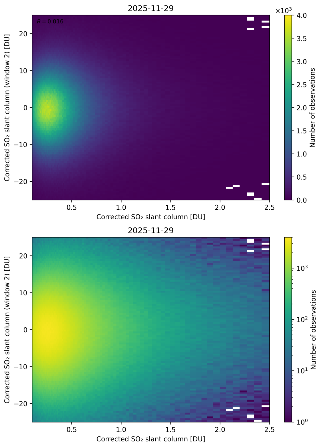
Figure 235: Scatter density plot of “Corrected SO 2 slant column” against “Corrected SO 2 slant column (window 2)” for 2025-11-28 to 2025-11-30.
