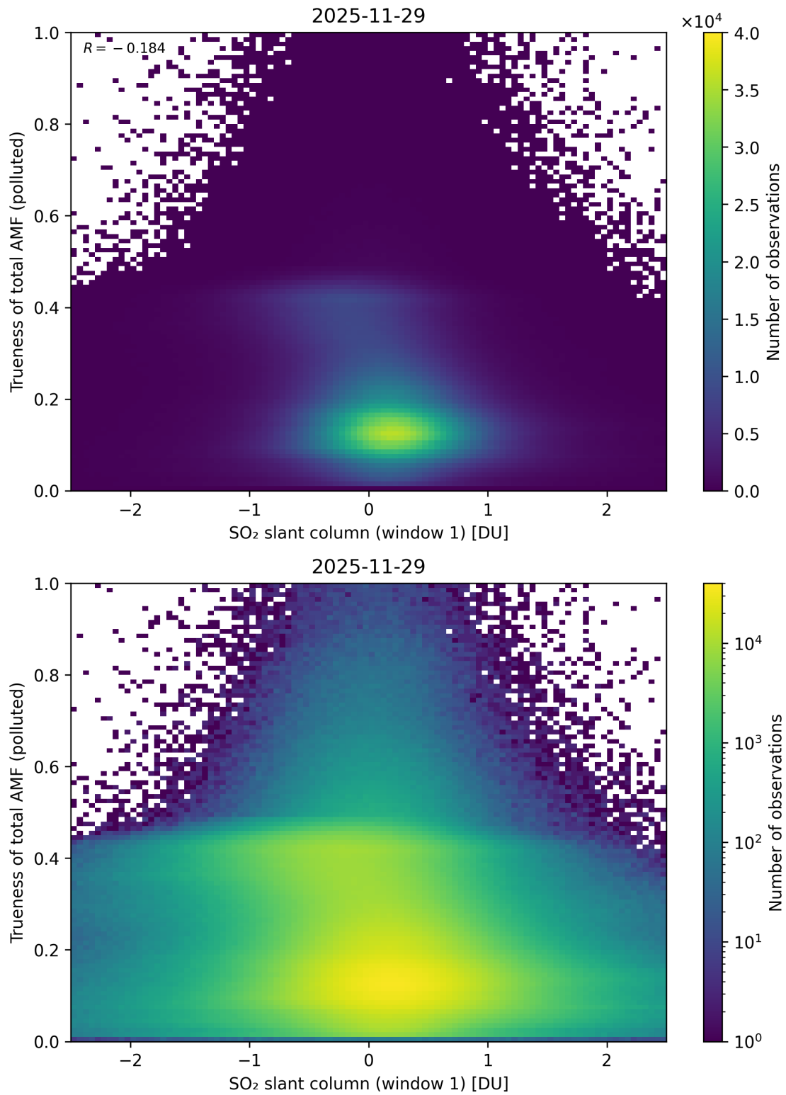
Figure 290: Scatter density plot of “SO 2 slant column (window 1)” against “Trueness of total AMF (polluted)” for 2025-11-28 to 2025-11-30.
