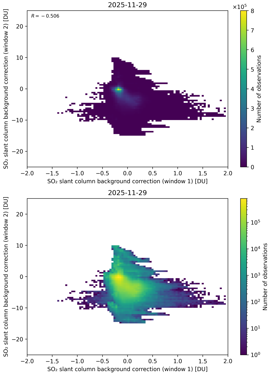
Figure 109: Scatter density plot of “SO 2 slant column background correction (window 1)” against “SO 2 slant column background correction (window 2)” for 2025-11-28 to 2025-11-30.
