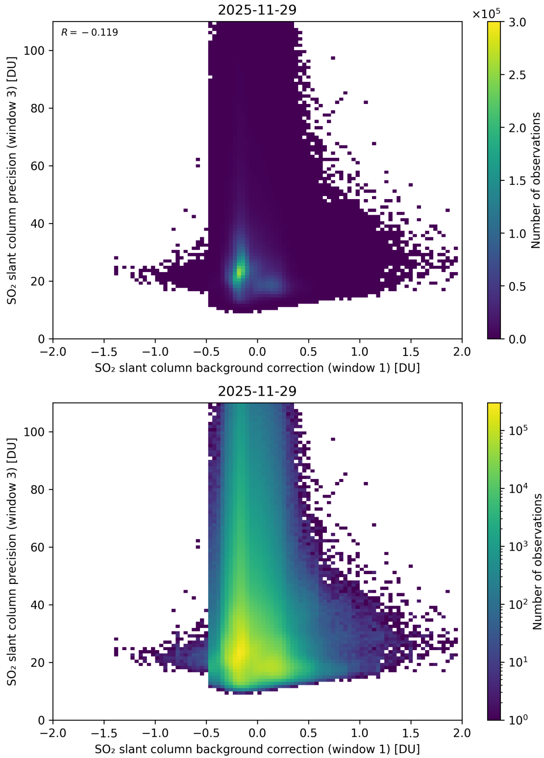
Figure 119: Scatter density plot of “SO 2 slant column background correction (window 1)” against “SO 2 slant column precision (window 3)” for 2025-11-28 to 2025-11-30.
