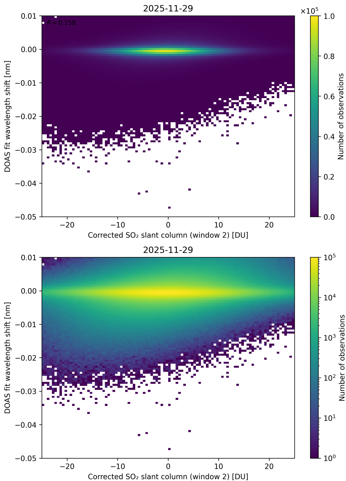
Figure 246: Scatter density plot of “Corrected SO 2 slant column (window 2)” against “DOAS fit wavelength shift” for 2025-11-28 to 2025-11-30.
