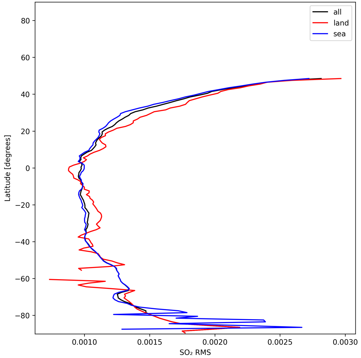
Figure 52: Zonal average of “SO 2 RMS” for 2025-11-28 to 2025-11-30.
