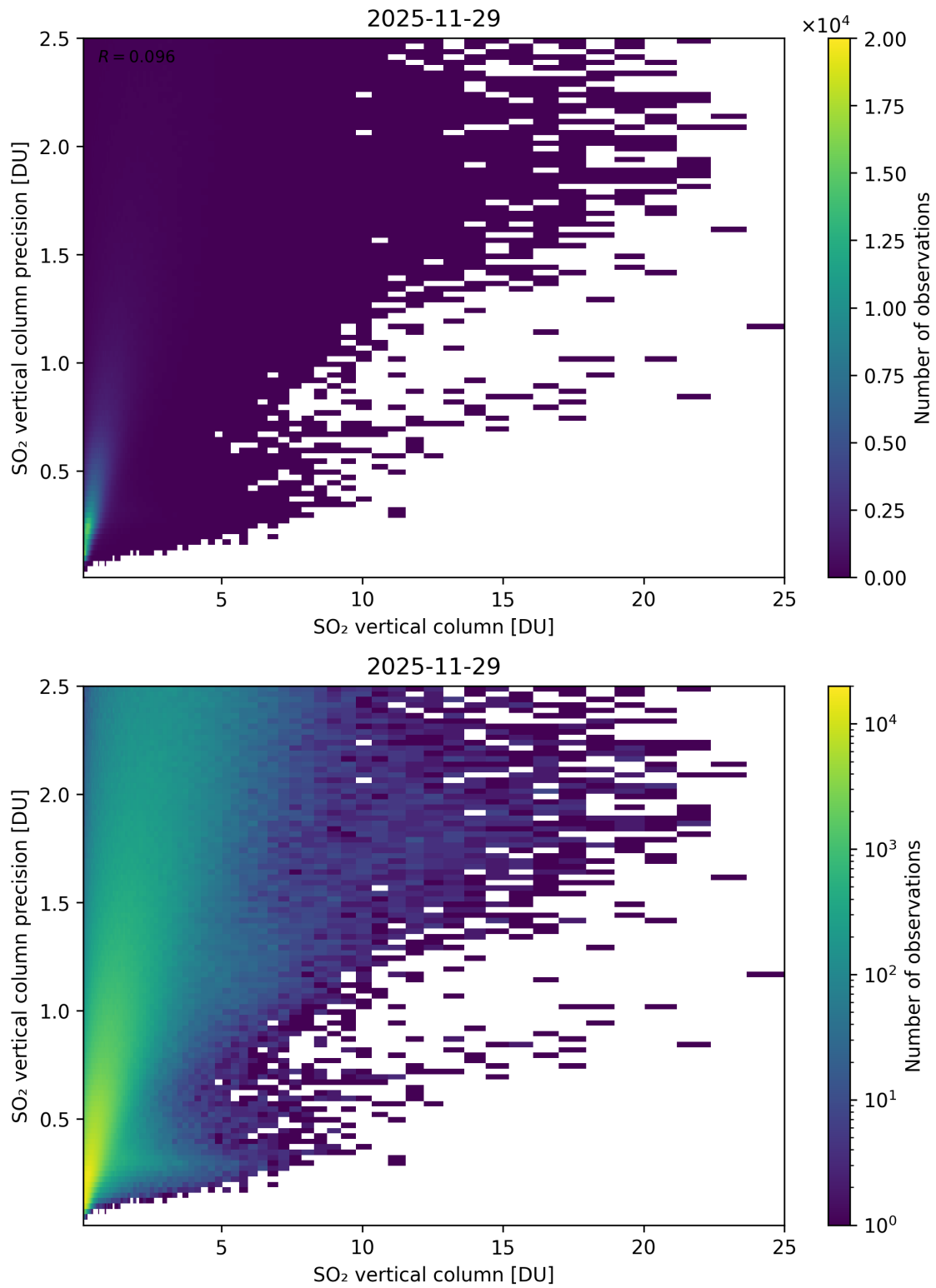
Figure 361: Scatter density plot of “SO 2 vertical column” against “SO 2 vertical column precision” for 2025-11-28 to 2025-11-30.
