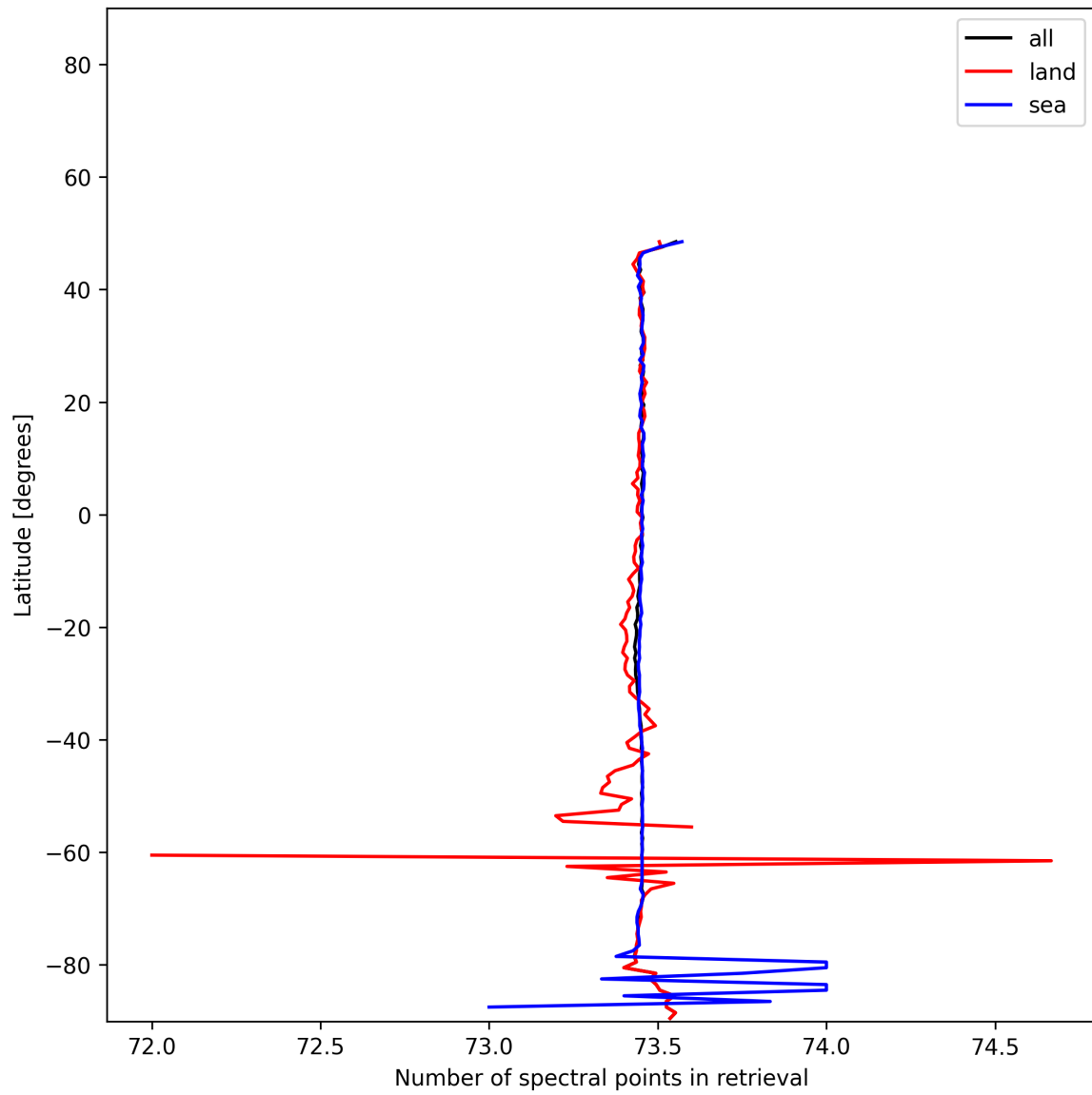
Figure 56: Zonal average of “Number of spectral points in retrieval” for 2025-11-28 to 2025-11-30.
