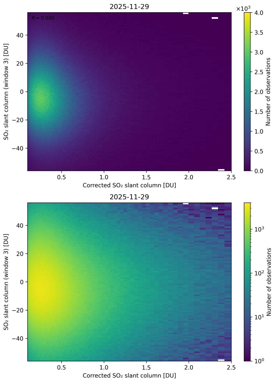
Figure 240: Scatter density plot of “Corrected SO 2 slant column” against “SO 2 slant column (window 3)” for 2025-11-28 to 2025-11-30.
