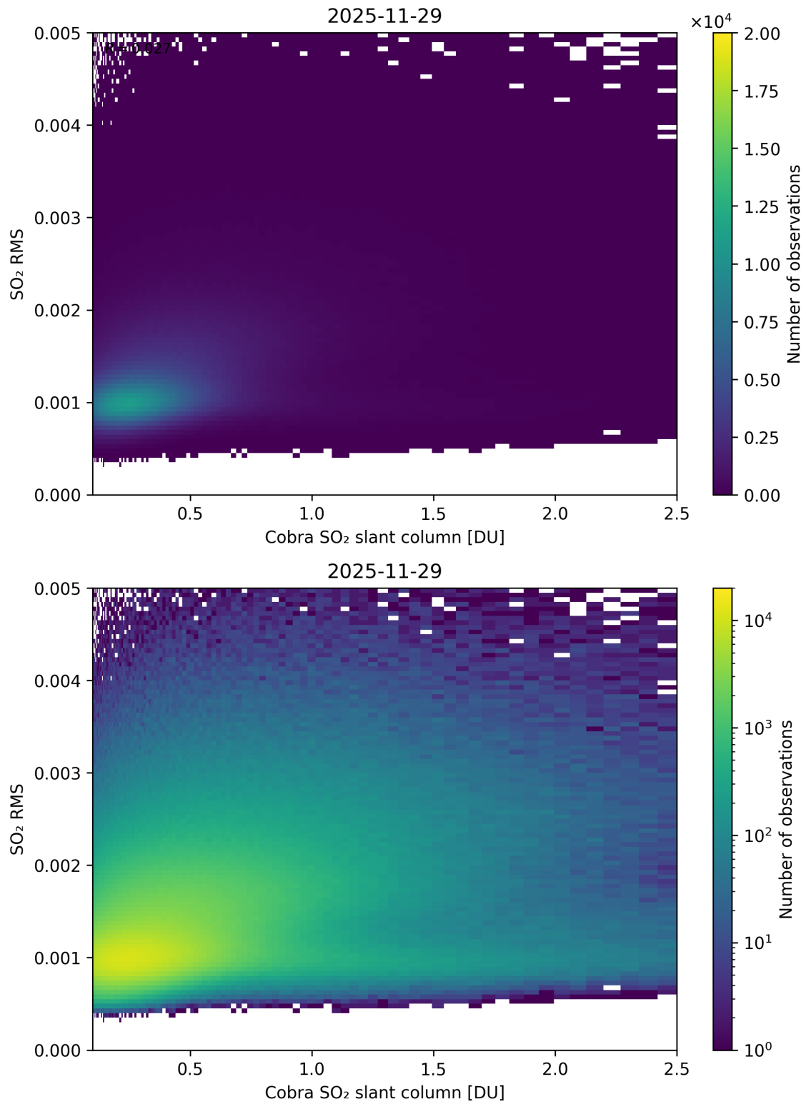
Figure 198: Scatter density plot of “Cobra SO 2 slant column” against “SO 2 RMS” for 2025-11-28 to 2025-11-30.
