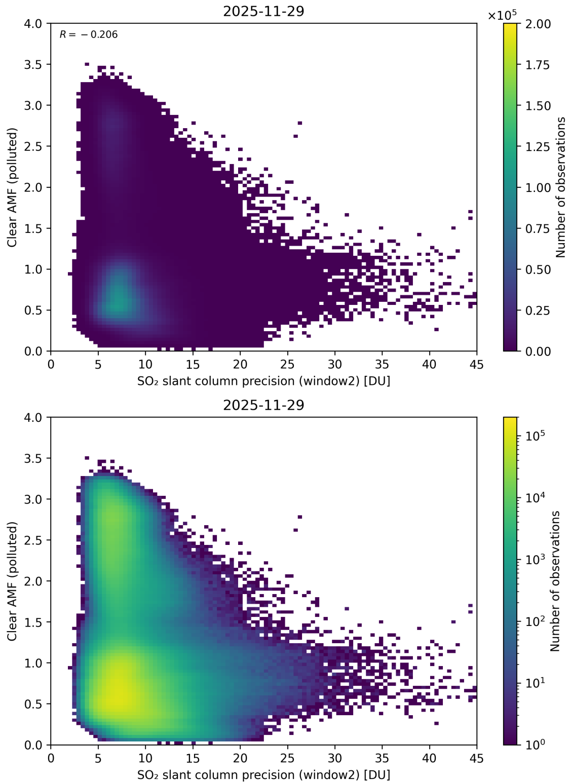
Figure 296: Scatter density plot of “SO 2 slant column precision (window2)” against “Clear AMF (polluted)” for 2025-11-28 to 2025-11-30.
