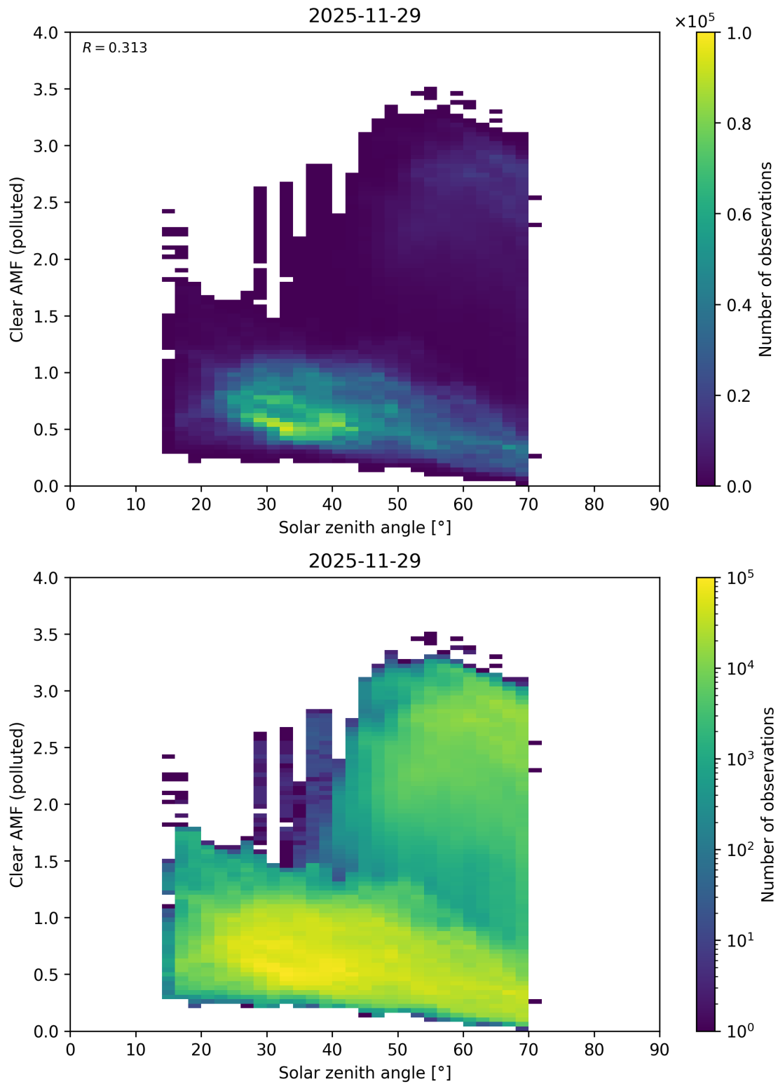
Figure 178: Scatter density plot of “Solar zenith angle” against “Clear AMF (polluted)” for 2025-11-28 to 2025-11-30.
