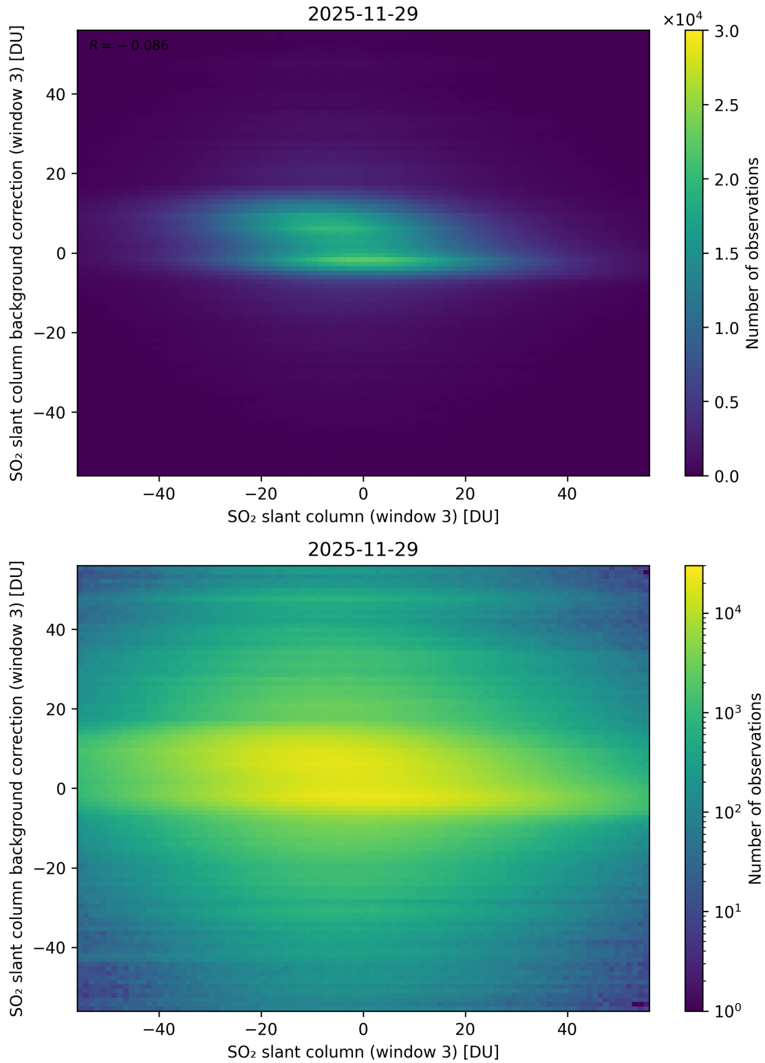
Figure 303: Scatter density plot of “SO 2 slant column (window 3)” against “SO 2 slant column background correction (window 3)” for 2025-11-28 to 2025-11-30.
