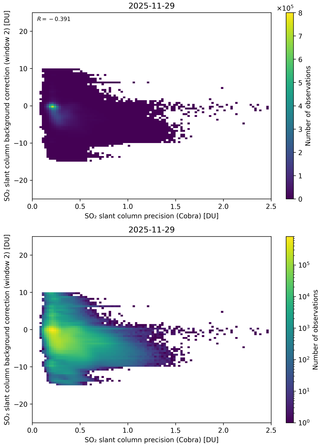
Figure 200: Scatter density plot of “SO 2 slant column precision (Cobra)” against “SO 2 slant column background correction (window 2)” for 2025-11-28 to 2025-11-30.
