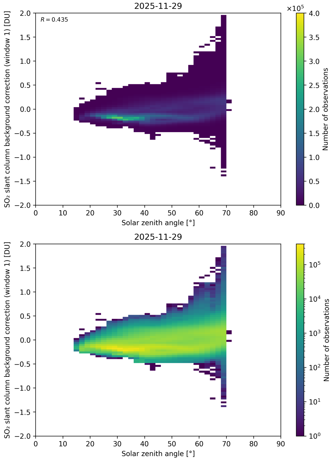
Figure 171: Scatter density plot of “Solar zenith angle” against “SO 2 slant column background correction (window 1)” for 2025-11-28 to 2025-11-30.
