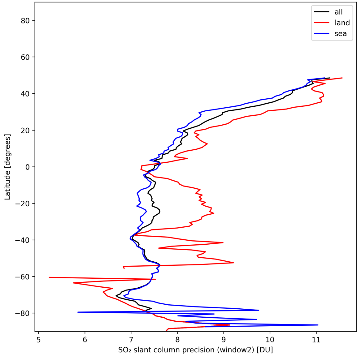
Figure 42: Zonal average of “SO 2 slant column precision (window2)” for 2025-11-28 to 2025-11-30.
