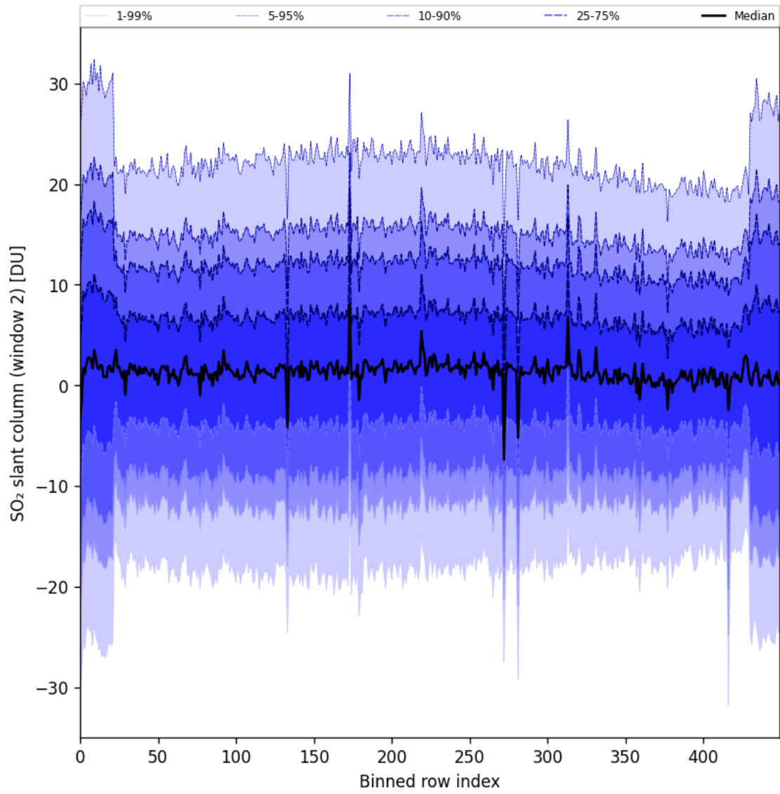
Figure 93: Along track statistics of “SO 2 slant column (window 2)” for 2025-11-28 to 2025-11-30
