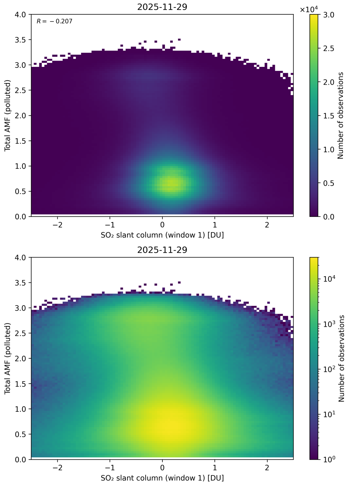
Figure 289: Scatter density plot of “SO 2 slant column (window 1)” against “Total AMF (polluted)” for 2025-11-28 to 2025-11-30.
