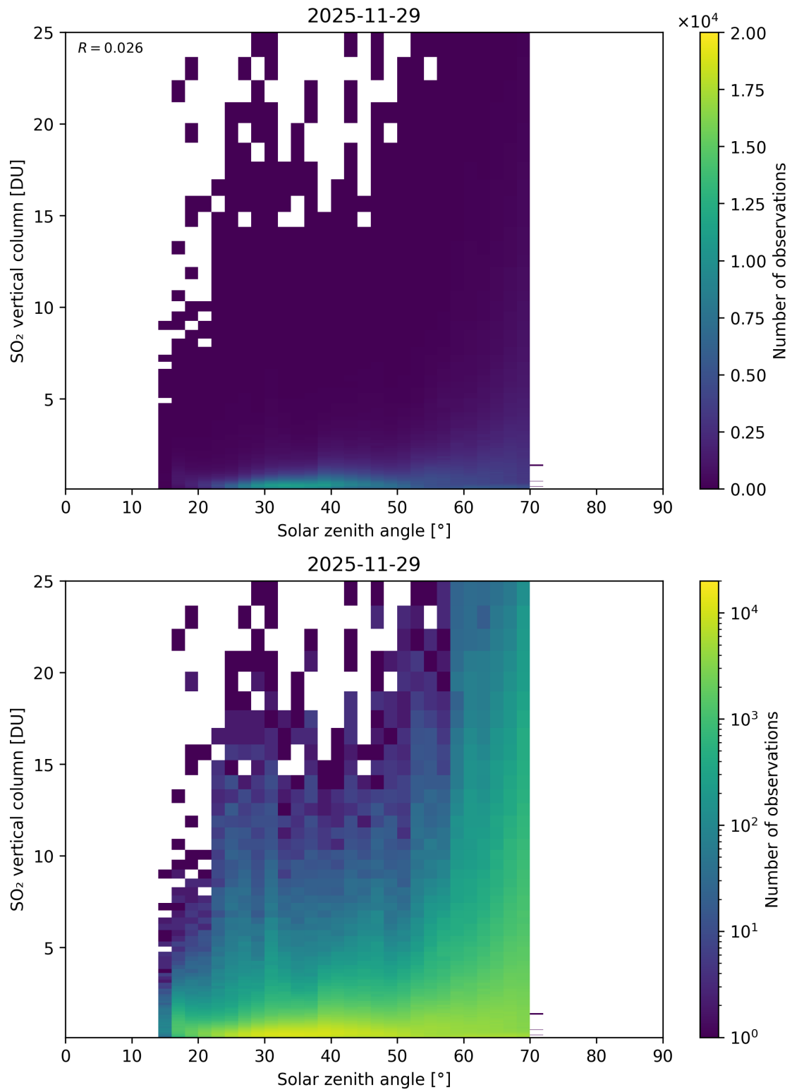
Figure 191: Scatter density plot of “Solar zenith angle” against “SO 2 vertical column” for 2025-11-28 to 2025-11-30.
