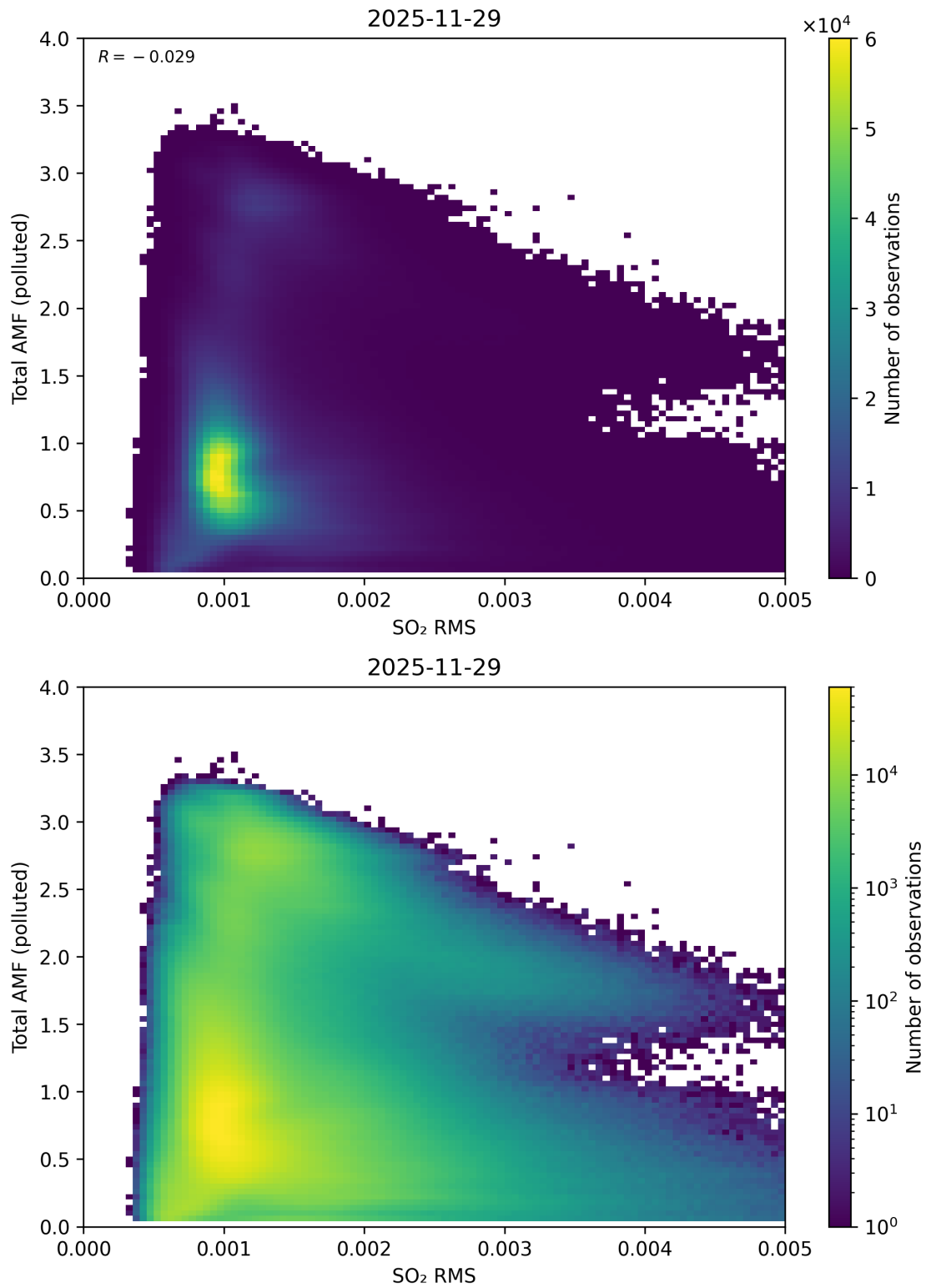
Figure 148: Scatter density plot of “SO 2 RMS” against “Total AMF (polluted)” for 2025-11-28 to 2025-11-30.
