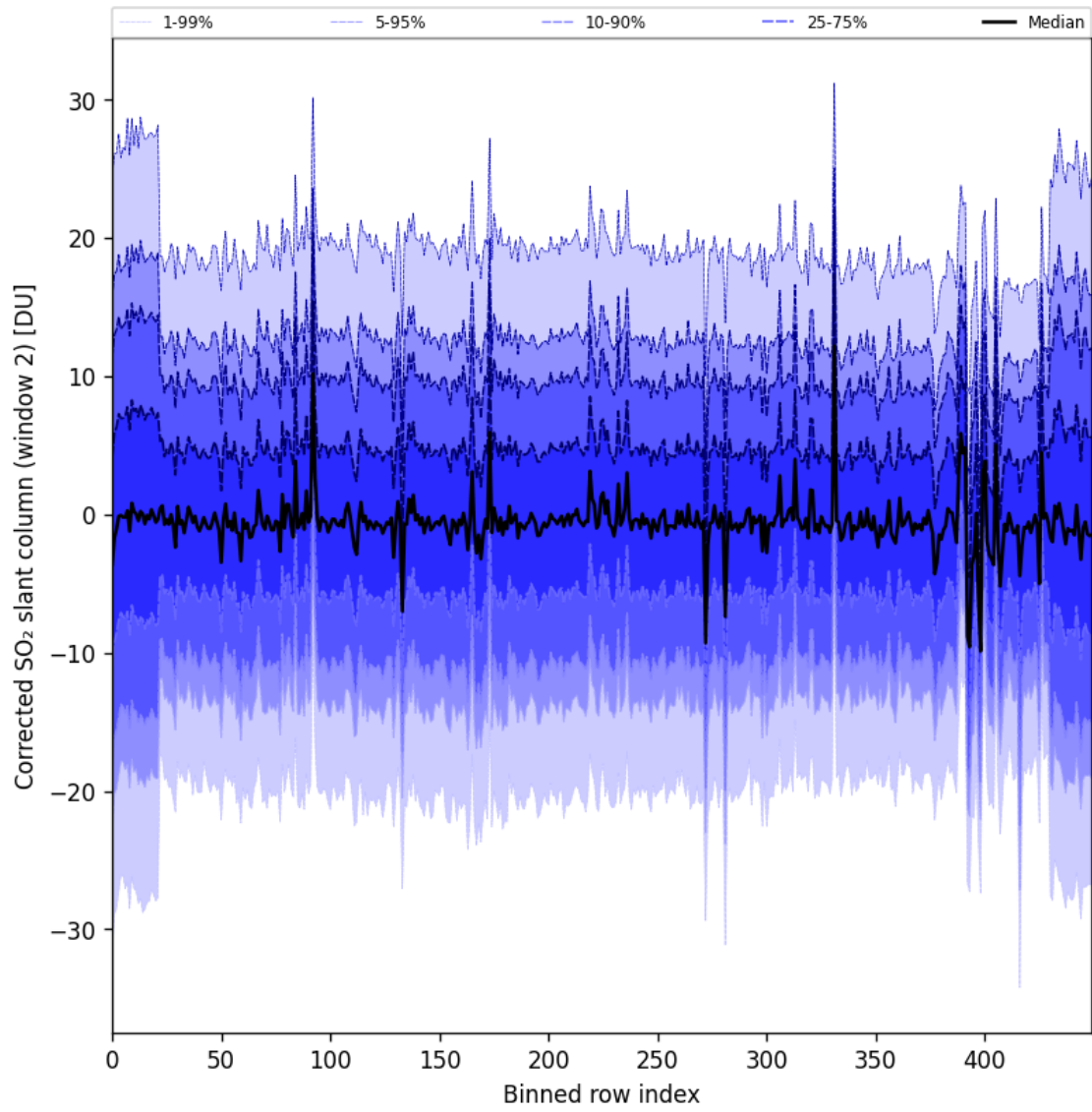
Figure 95: Along track statistics of “Corrected SO 2 slant column (window 2)” for 2025-11-28 to 2025-11-30
