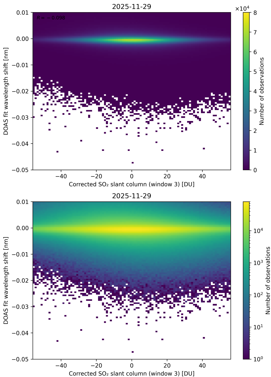
Figure 256: Scatter density plot of “Corrected SO 2 slant column (window 3)” against “DOAS fit wavelength shift” for 2025-11-28 to 2025-11-30.
