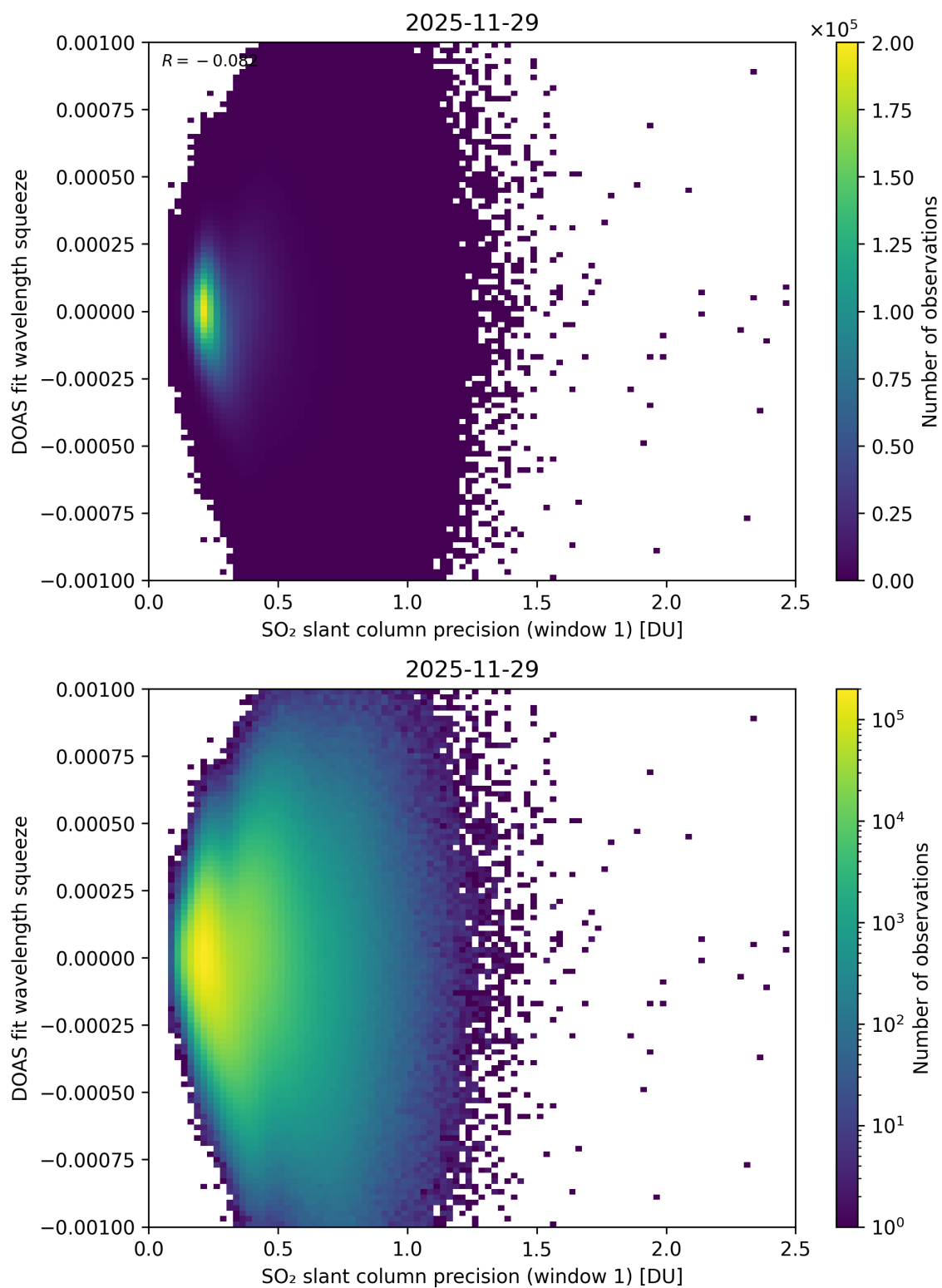
Figure 272: Scatter density plot of “SO 2 slant column precision (window 1)” against “DOAS fit wavelength squeeze” for 2025-11-28 to 2025-11-30.
