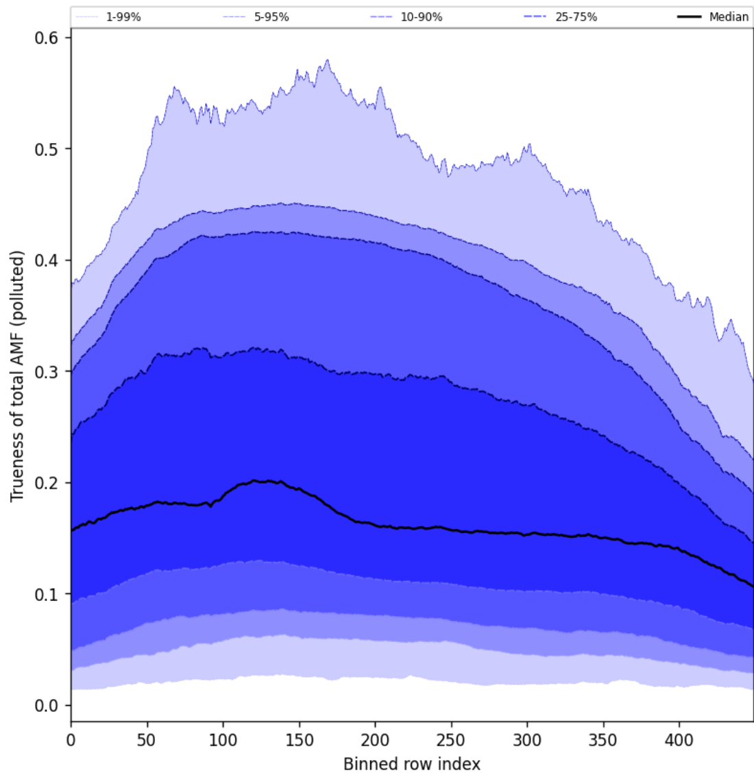
Figure 106: Along track statistics of “Trueness of total AMF (polluted)” for 2025-11-28 to 2025-11-30
