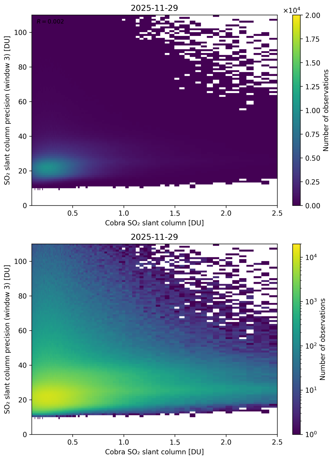
Figure 223: Scatter density plot of “Cobra SO 2 slant column” against “SO 2 slant column precision (window 3)” for 2025-11-28 to 2025-11-30.
