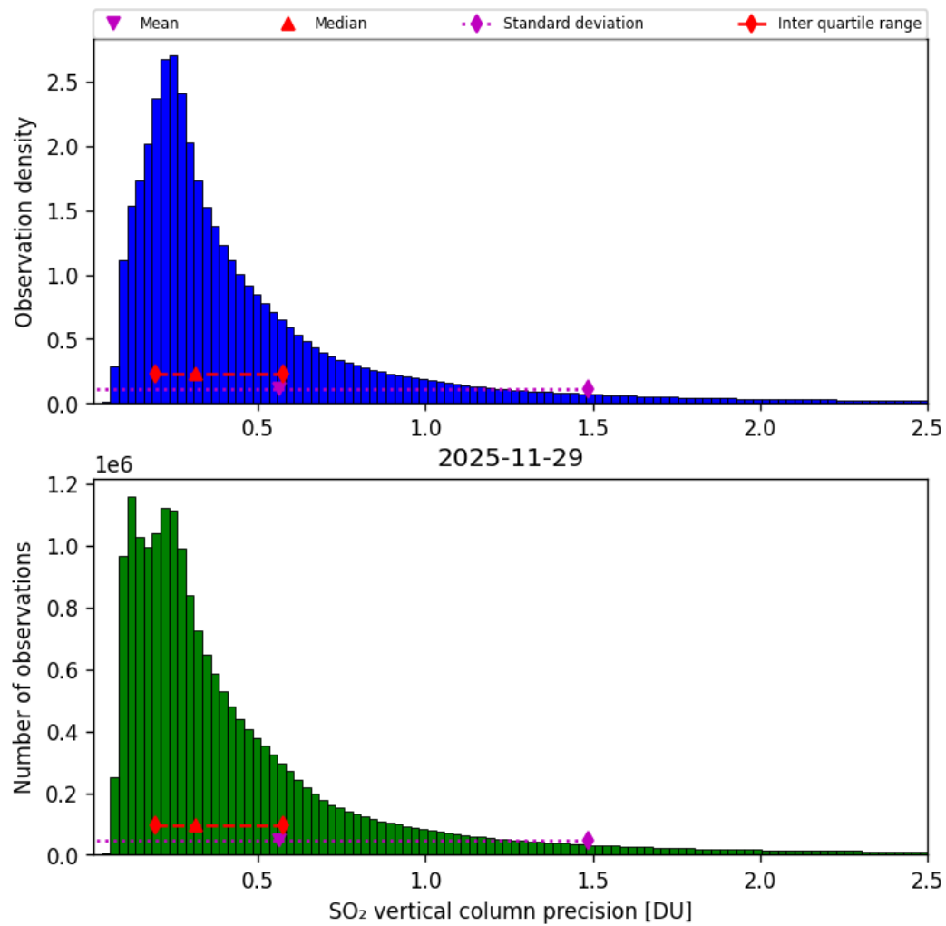
Figure 59: Histogram of “SO 2 vertical column precision” for 2025-11-28 to 2025-11-30
