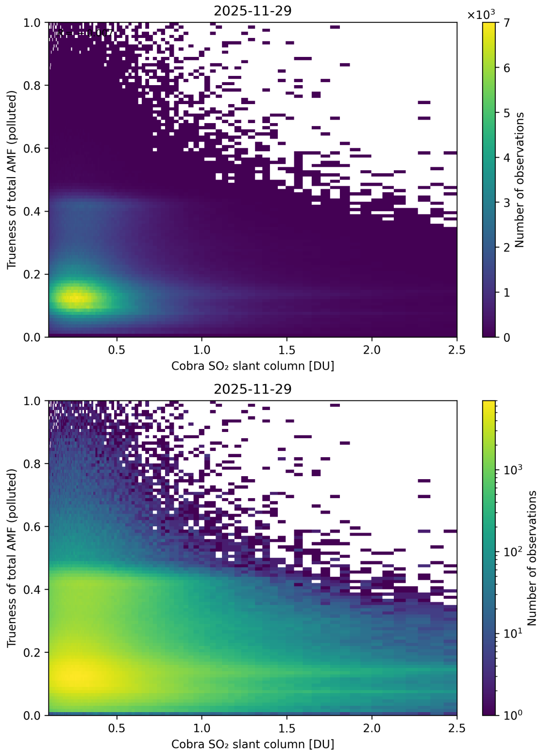
Figure 225: Scatter density plot of “Cobra SO 2 slant column” against “Trueness of total AMF (polluted)” for 2025-11-28 to 2025-11-30.
