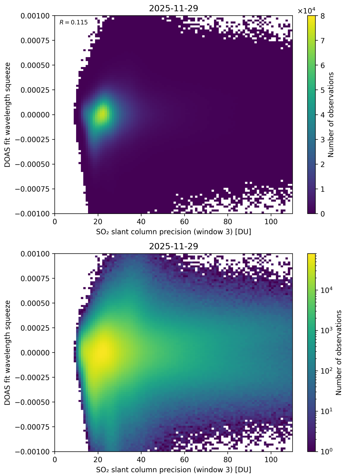
Figure 309: Scatter density plot of “SO 2 slant column precision (window 3)” against “DOAS fit wavelength squeeze” for 2025-11-28 to 2025-11-30.
