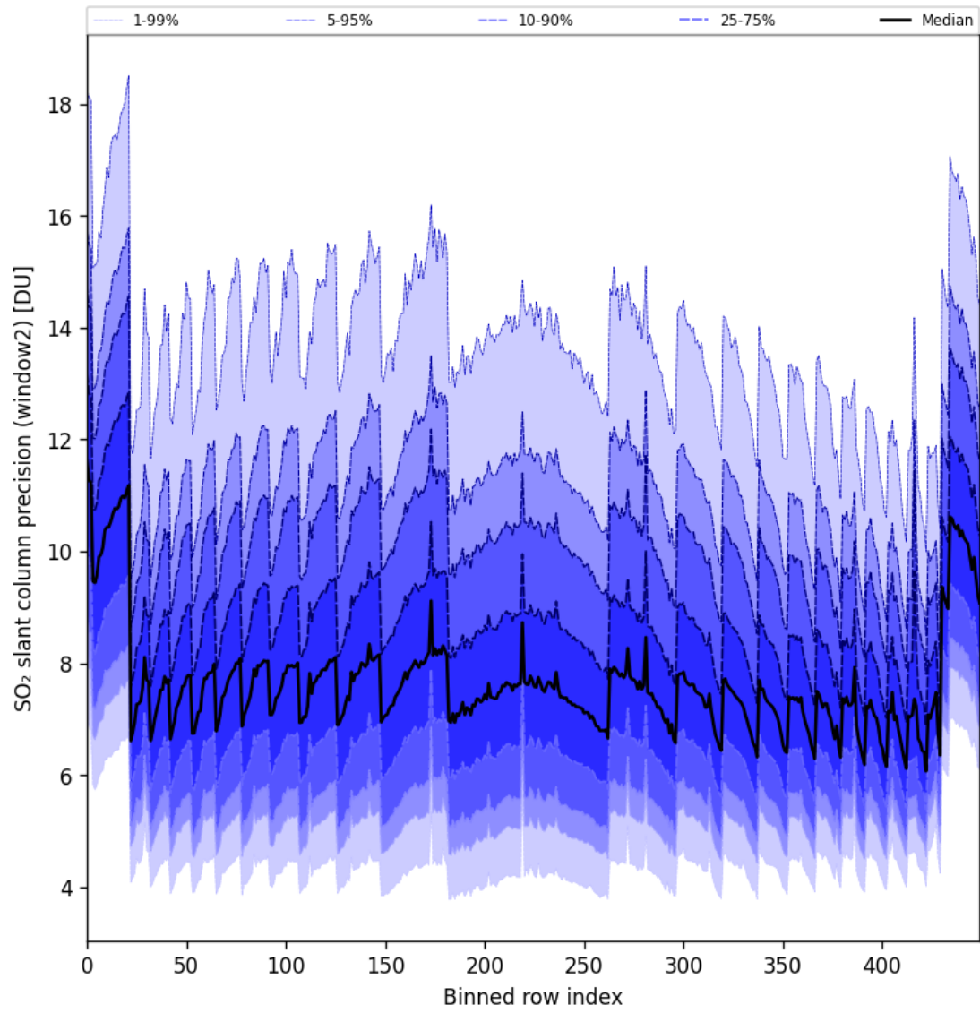
Figure 94: Along track statistics of “SO 2 slant column precision (window2)” for 2025-11-28 to 2025-11-30
