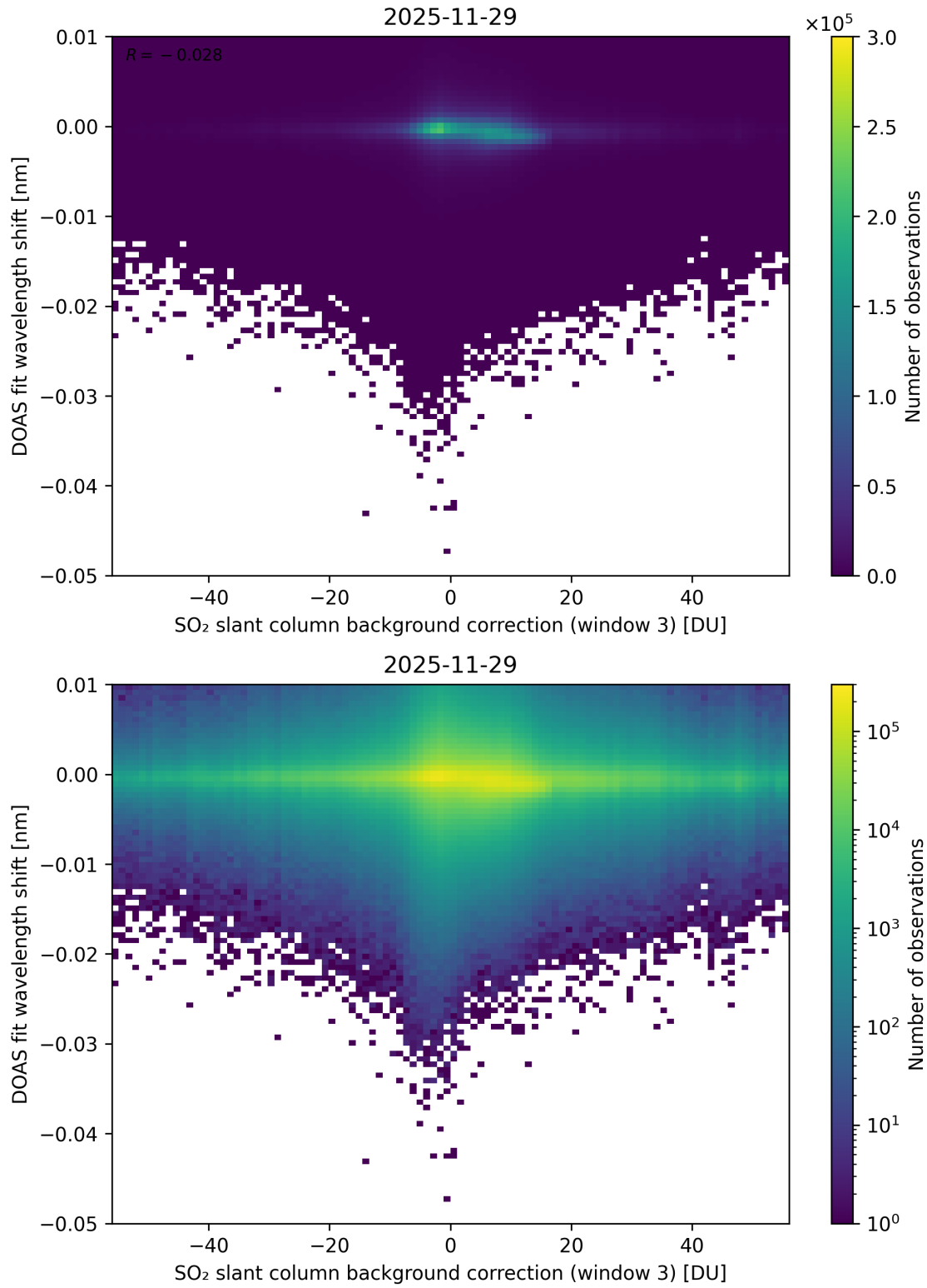
Figure 132: Scatter density plot of “SO 2 slant column background correction (window 3)” against “DOAS fit wavelength shift” for 2025-11-28 to 2025-11-30.
