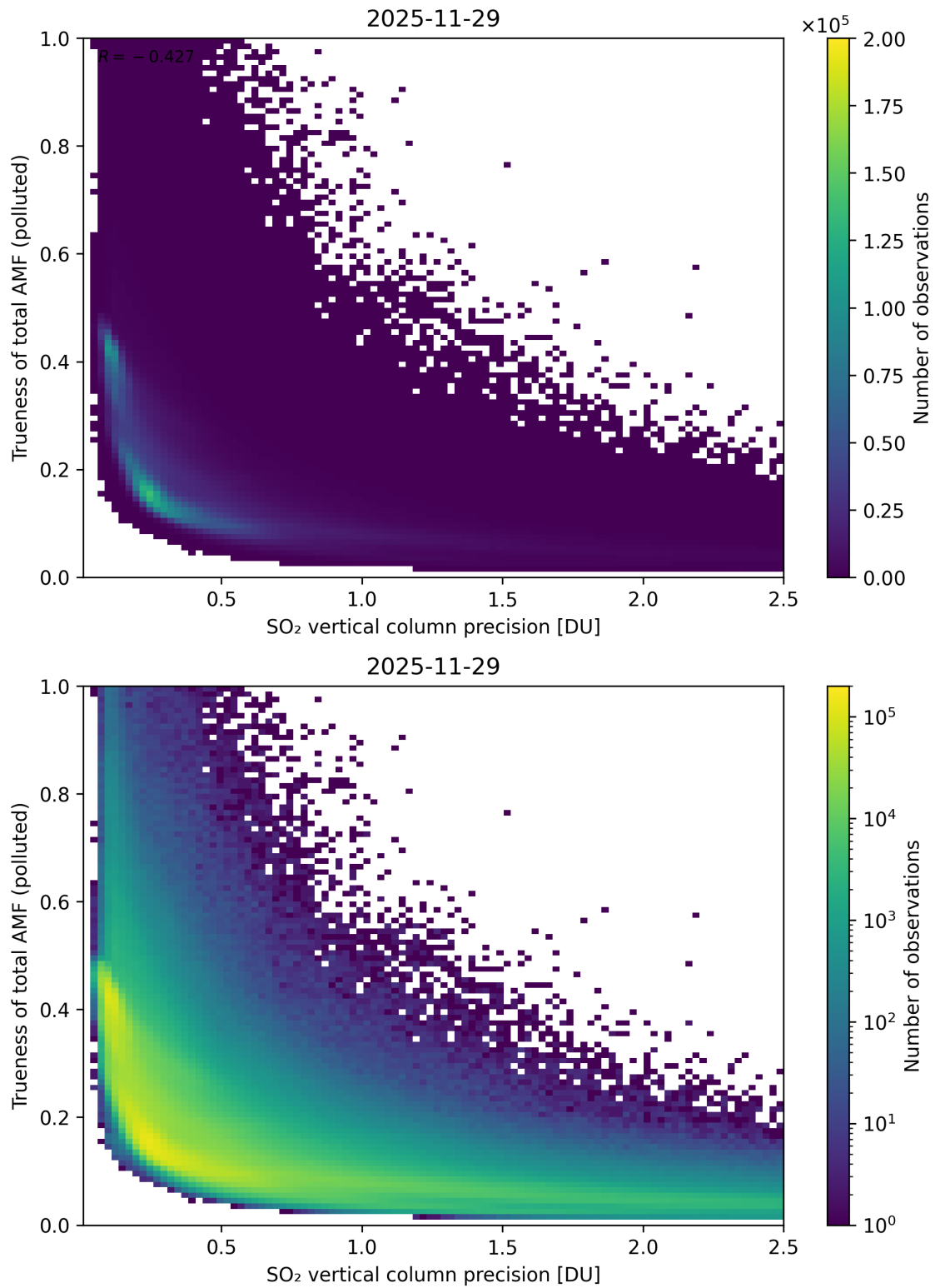
Figure 347: Scatter density plot of “SO 2 vertical column precision” against “Trueness of total AMF (polluted)” for 2025-11-28 to 2025-11-30.
