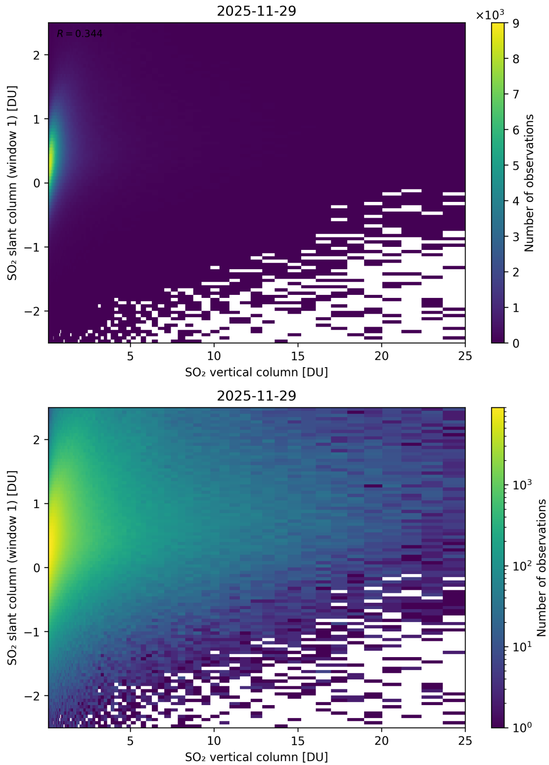
Figure 354: Scatter density plot of “SO 2 vertical column” against “SO 2 slant column (window 1)” for 2025-11-28 to 2025-11-30.
