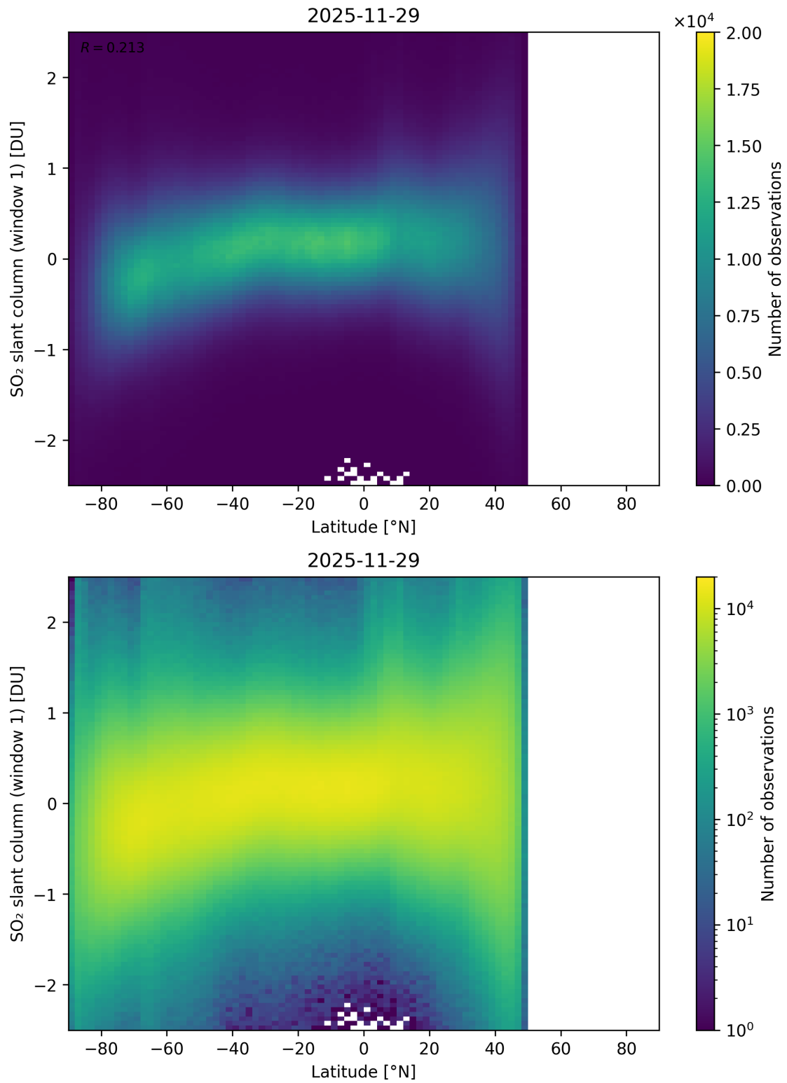
Figure 162: Scatter density plot of “Latitude” against “SO 2 slant column (window 1)” for 2025-11-28 to 2025-11-30.
