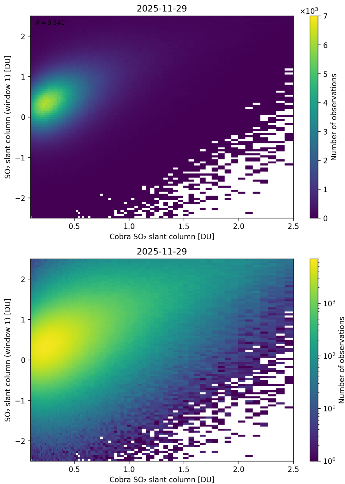
Figure 219: Scatter density plot of “Cobra SO 2 slant column” against “SO 2 slant column (window 1)” for 2025-11-28 to 2025-11-30.
