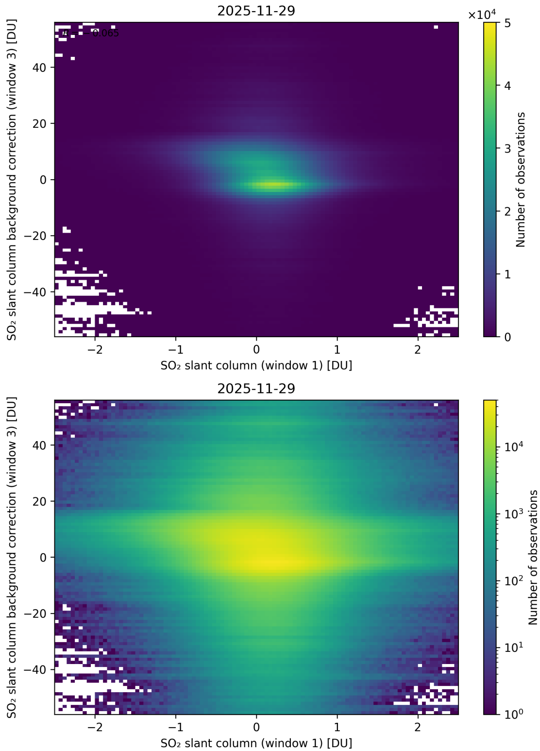
Figure 264: Scatter density plot of “SO 2 slant column (window 1)” against “SO 2 slant column background correction (window 3)” for 2025-11-28 to 2025-11-30.
