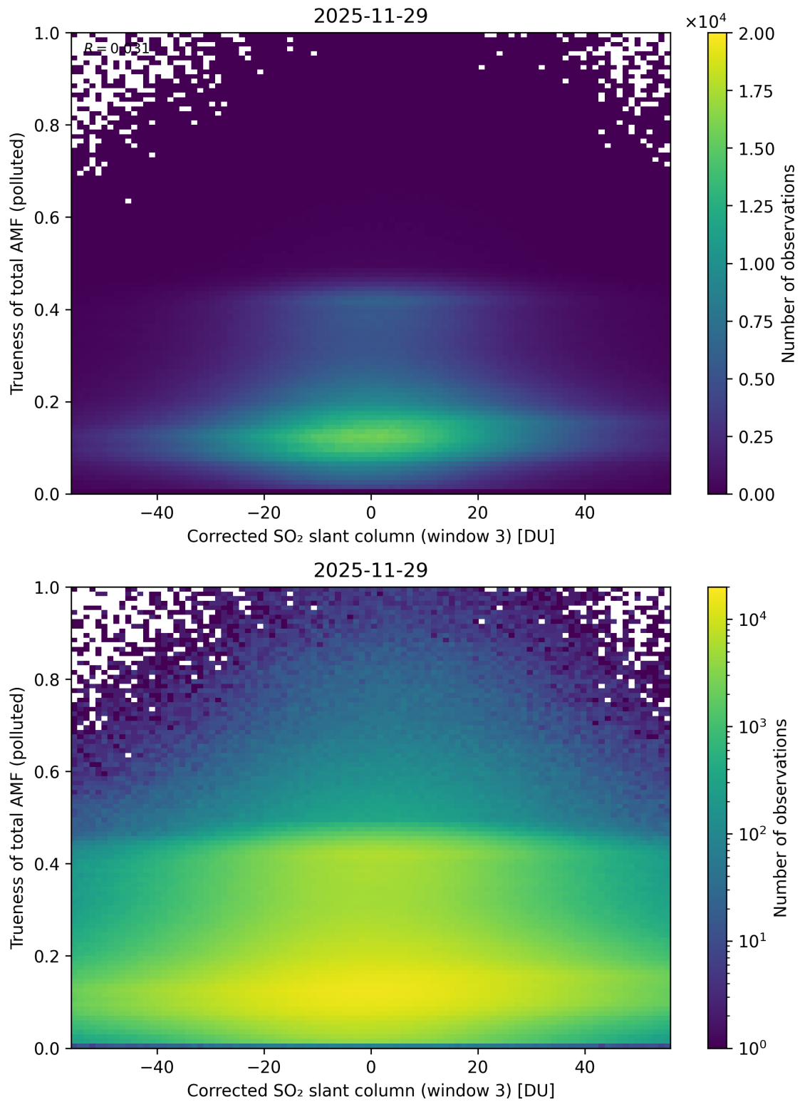
Figure 261: Scatter density plot of “Corrected SO 2 slant column (window 3)” against “Trueness of total AMF (polluted)” for 2025-11-28 to 2025-11-30.
