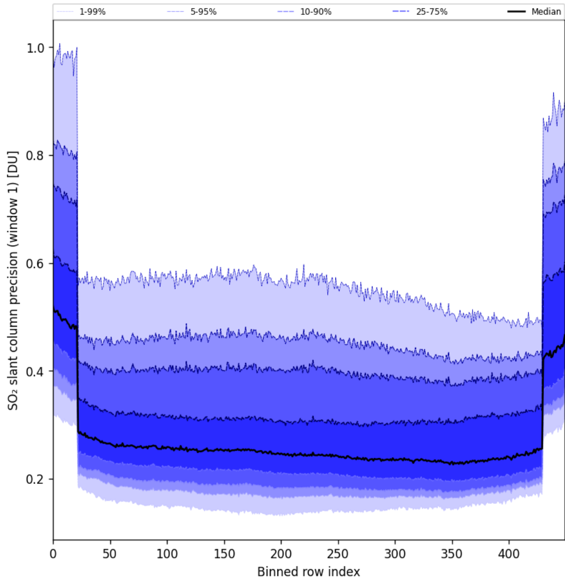
Figure 90: Along track statistics of “SO 2 slant column precision (window 1)” for 2025-11-28 to 2025-11-30
