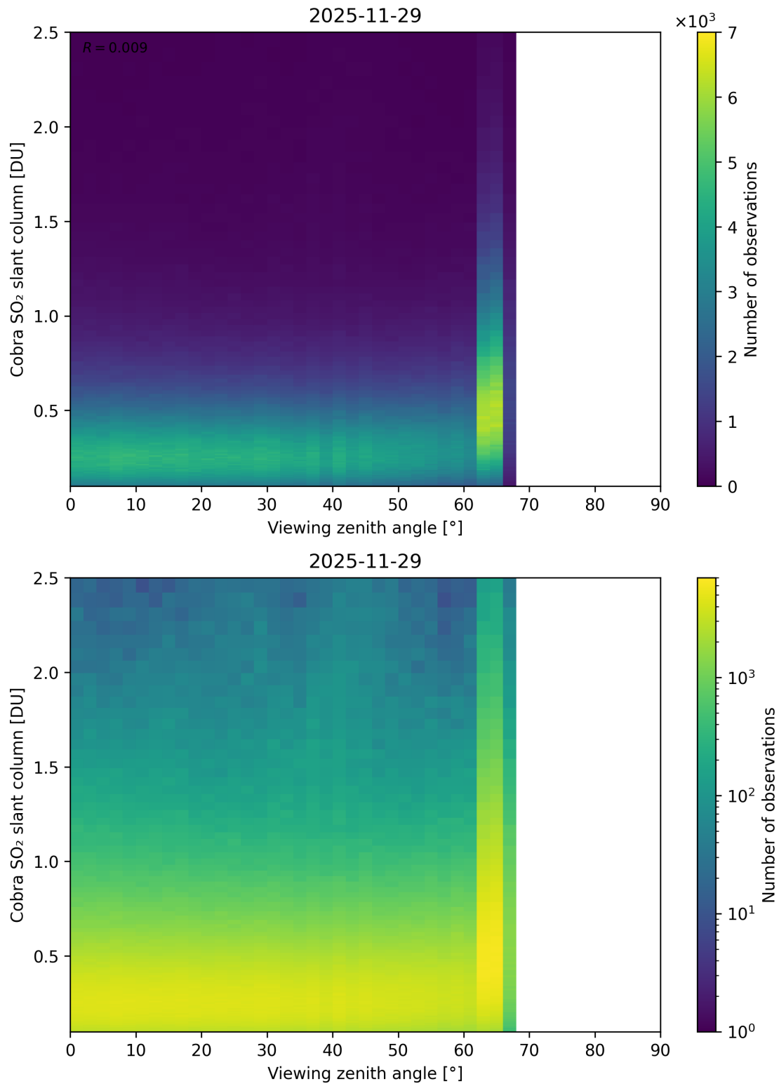
Figure 371: Scatter density plot of “Viewing zenith angle” against “Cobra SO 2 slant column” for 2025-11-28 to 2025-11-30.
