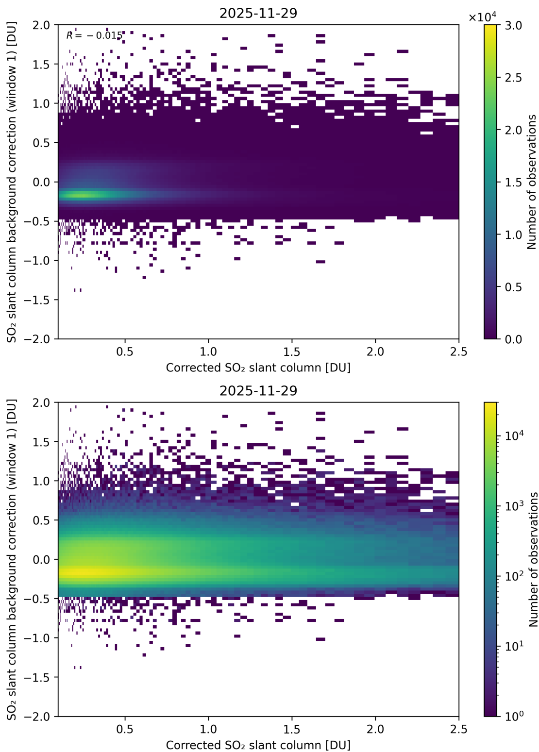
Figure 226: Scatter density plot of “Corrected SO 2 slant column” against “SO 2 slant column background correction (window 1)” for 2025-11-28 to 2025-11-30.
