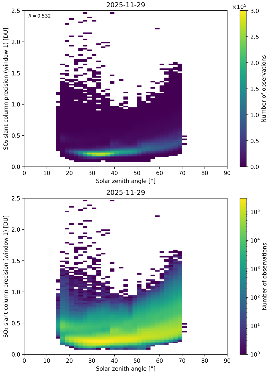
Figure 185: Scatter density plot of “Solar zenith angle” against “SO 2 slant column precision (window 1)” for 2025-11-28 to 2025-11-30.
