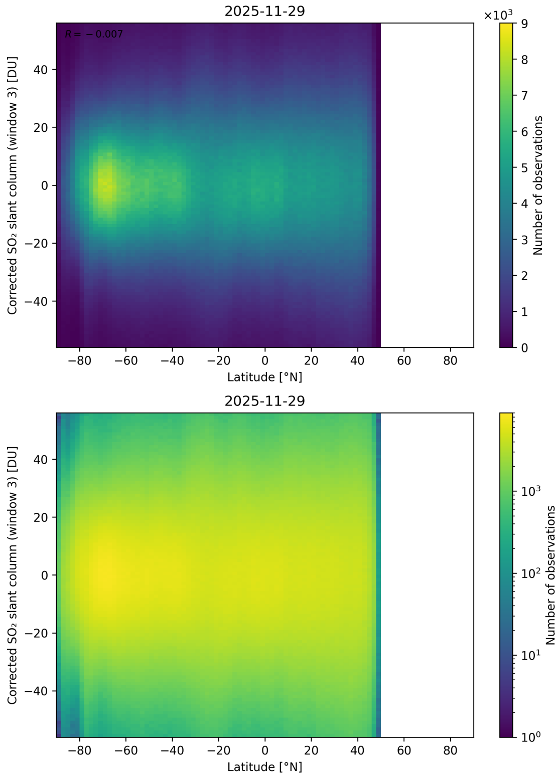
Figure 161: Scatter density plot of “Latitude” against “Corrected SO 2 slant column (window 3)” for 2025-11-28 to 2025-11-30.
