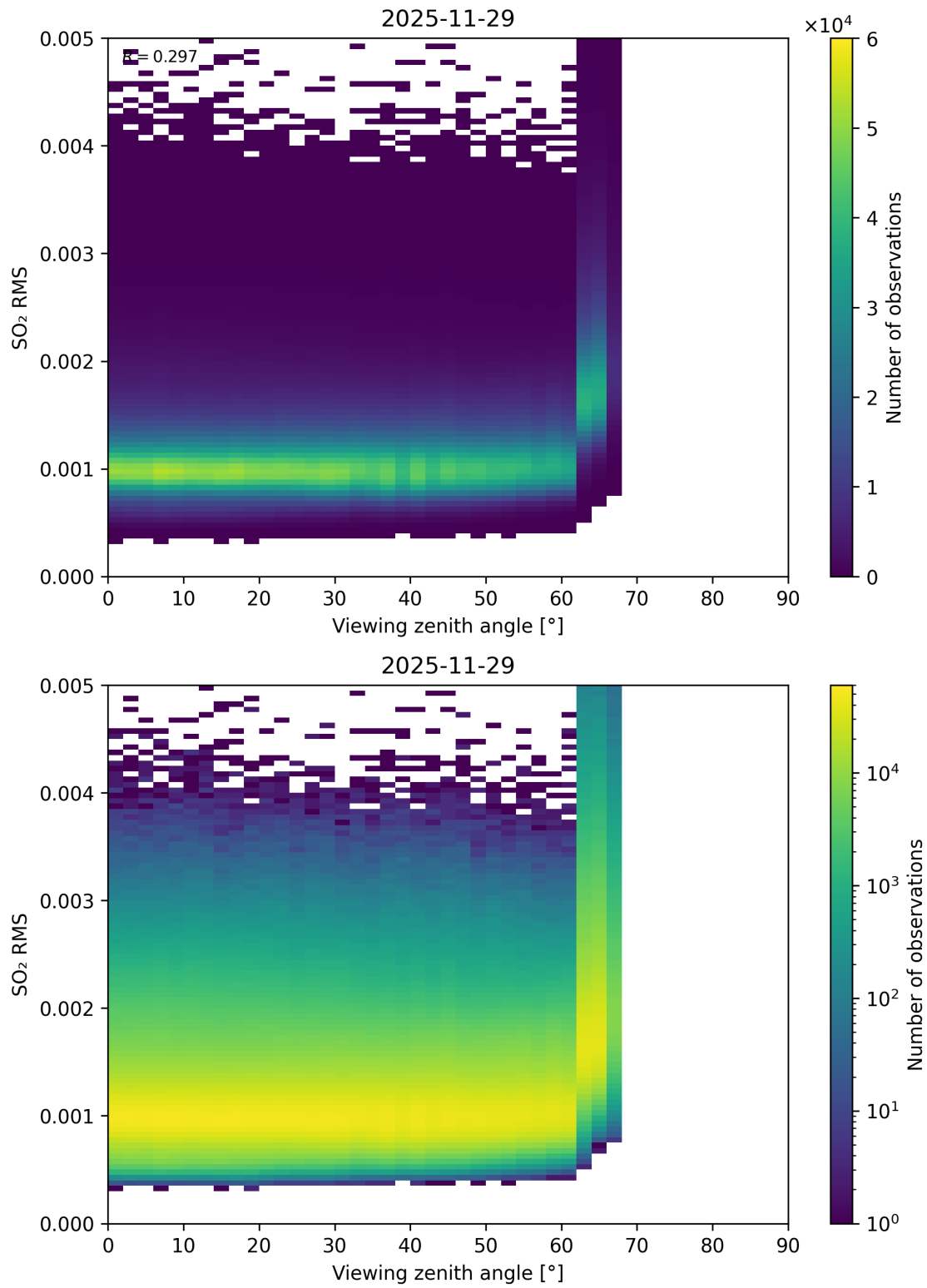
Figure 367: Scatter density plot of “Viewing zenith angle” against “SO 2 RMS” for 2025-11-28 to 2025-11-30.
