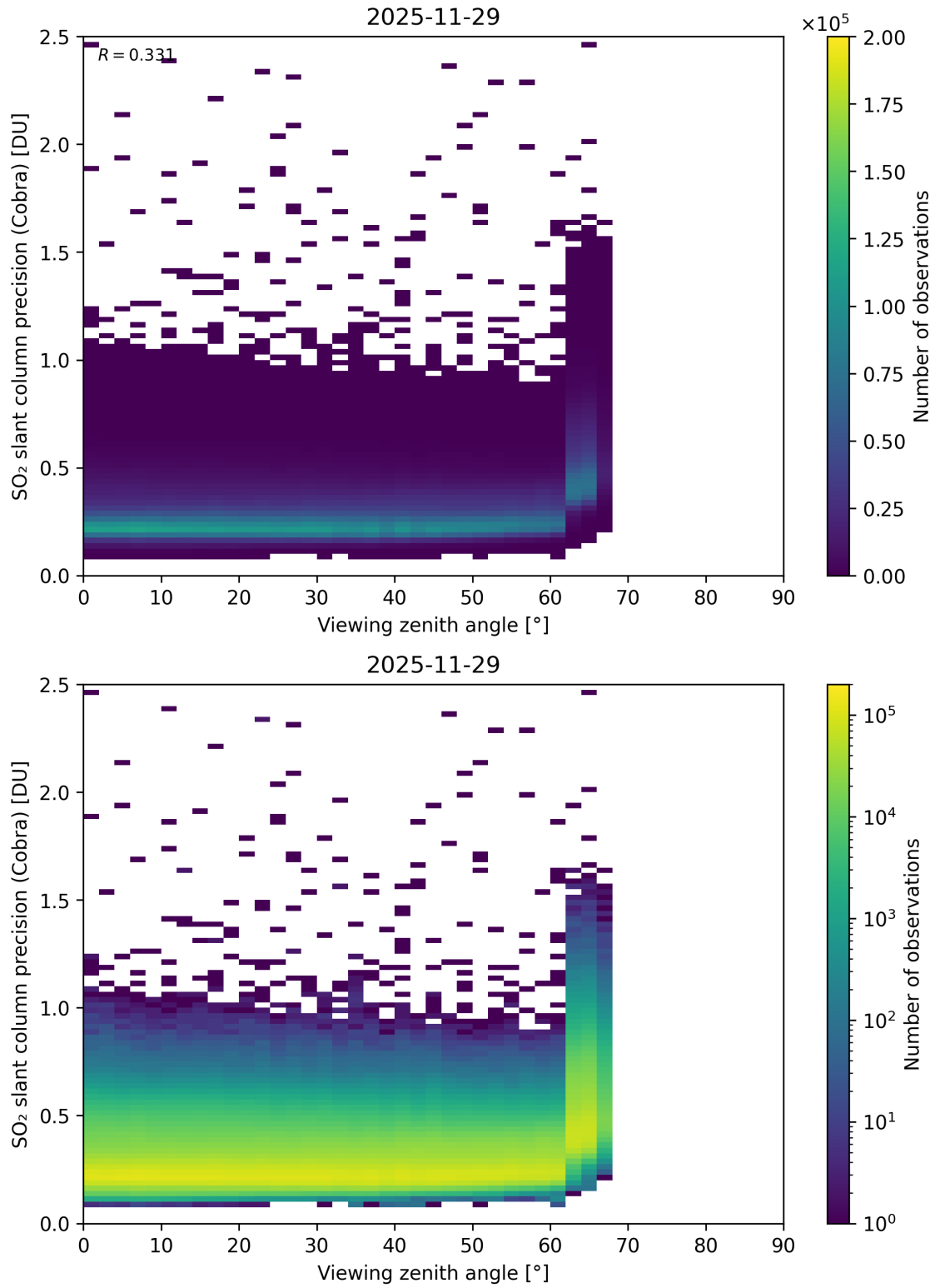
Figure 372: Scatter density plot of “Viewing zenith angle” against “SO 2 slant column precision (Cobra)” for 2025-11-28 to 2025-11-30.
