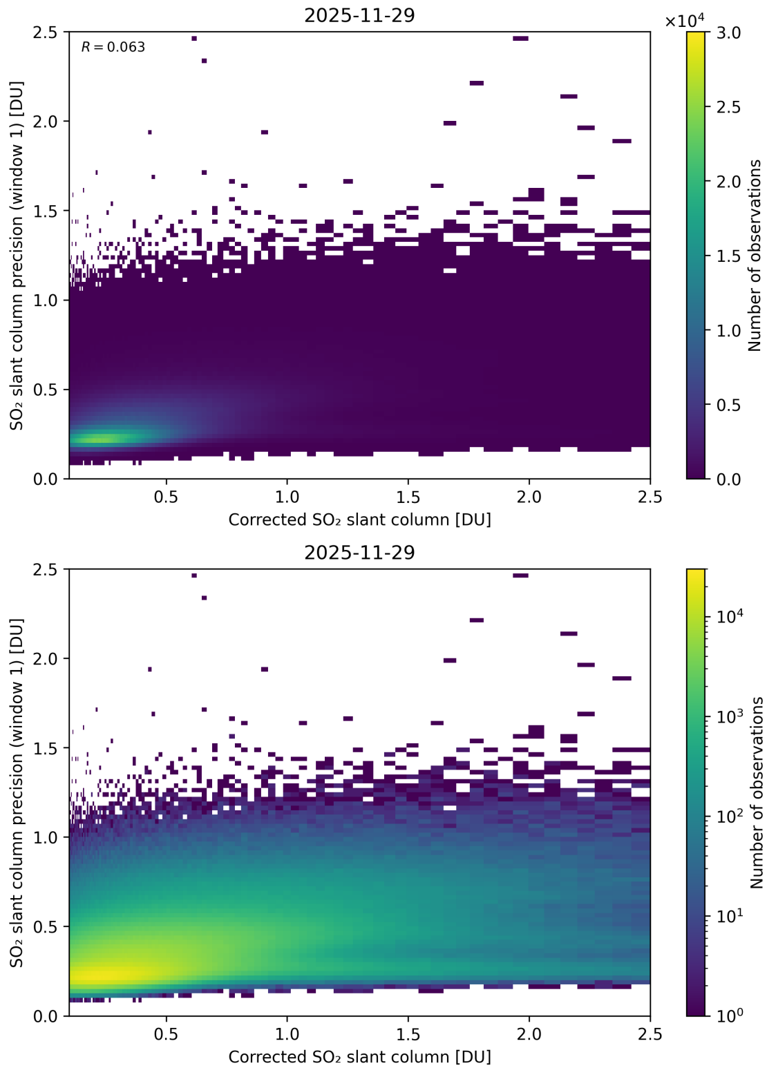
Figure 238: Scatter density plot of “Corrected SO 2 slant column” against “SO 2 slant column precision (window 1)” for 2025-11-28 to 2025-11-30.
