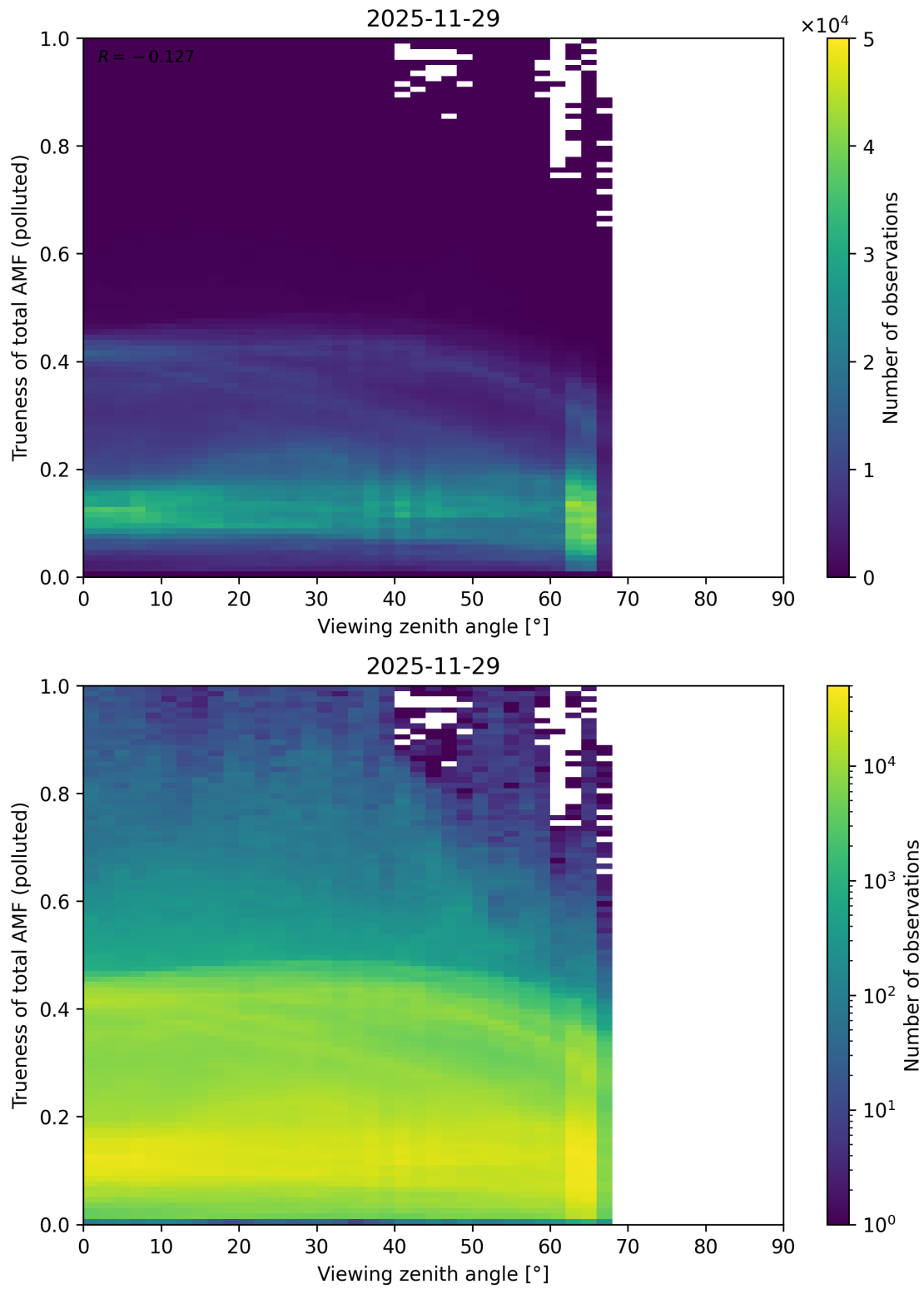
Figure 382: Scatter density plot of “Viewing zenith angle” against “Trueness of total AMF (polluted)” for 2025-11-28 to 2025-11-30.
