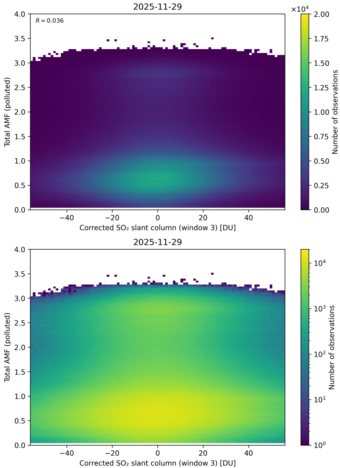
Figure 260: Scatter density plot of “Corrected SO 2 slant column (window 3)” against “Total AMF (polluted)” for 2025-11-28 to 2025-11-30.
