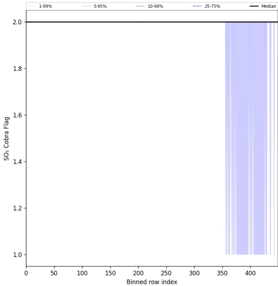
Figure 101: Along track statistics of “SO 2 Cobra Flag” for 2025-11-28 to 2025-11-30
