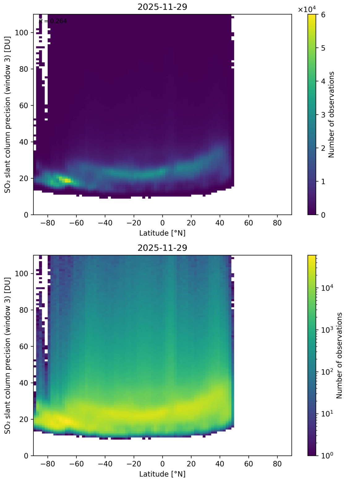
Figure 166: Scatter density plot of “Latitude” against “SO 2 slant column precision (window 3)” for 2025-11-28 to 2025-11-30.
