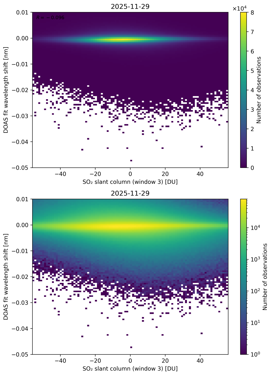
Figure 304: Scatter density plot of “SO 2 slant column (window 3)” against “DOAS fit wavelength shift” for 2025-11-28 to 2025-11-30.
