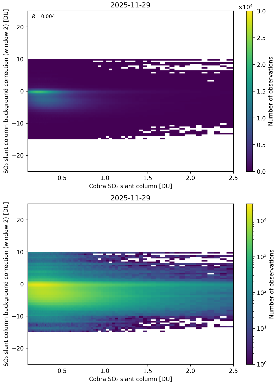
Figure 194: Scatter density plot of “Cobra SO 2 slant column” against “SO 2 slant column background correction (window 2)” for 2025-11-28 to 2025-11-30.
