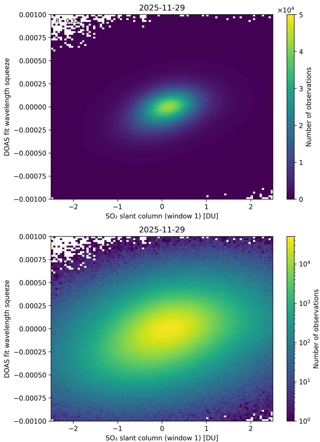
Figure 266: Scatter density plot of “SO 2 slant column (window 1)” against “DOAS fit wavelength squeeze” for 2025-11-28 to 2025-11-30.
