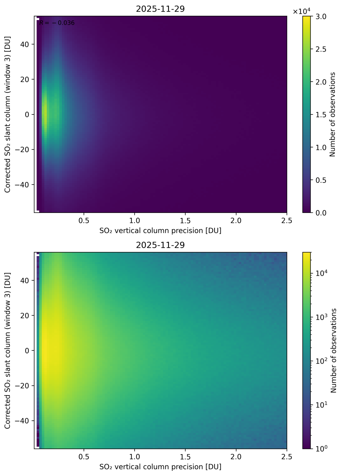
Figure 340: Scatter density plot of “SO 2 vertical column precision” against “Corrected SO 2 slant column (window 3)” for 2025-11-28 to 2025-11-30.
