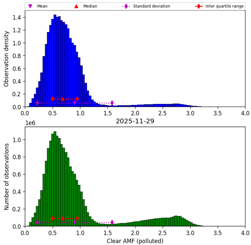
Figure 81: Histogram of “Clear AMF (polluted)” for 2025-11-28 to 2025-11-30
