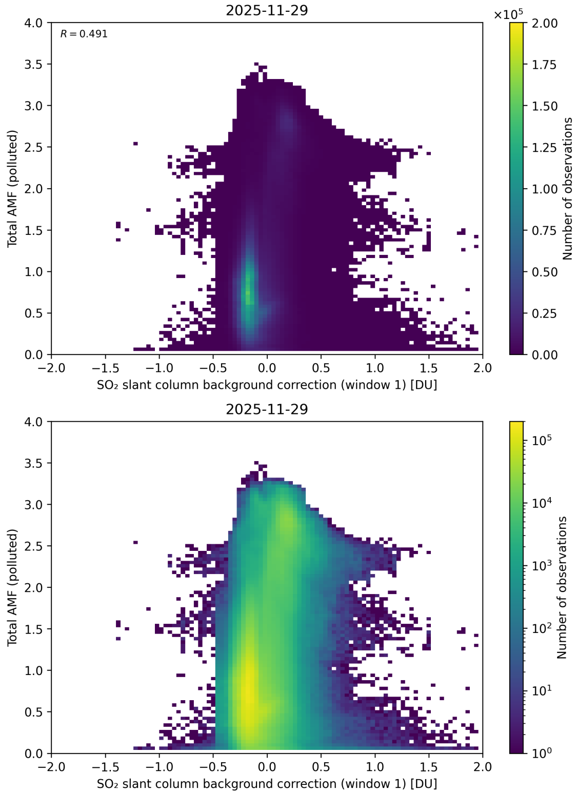
Figure 120: Scatter density plot of “SO 2 slant column background correction (window 1)” against “Total AMF (polluted)” for 2025-11-28 to 2025-11-30.
