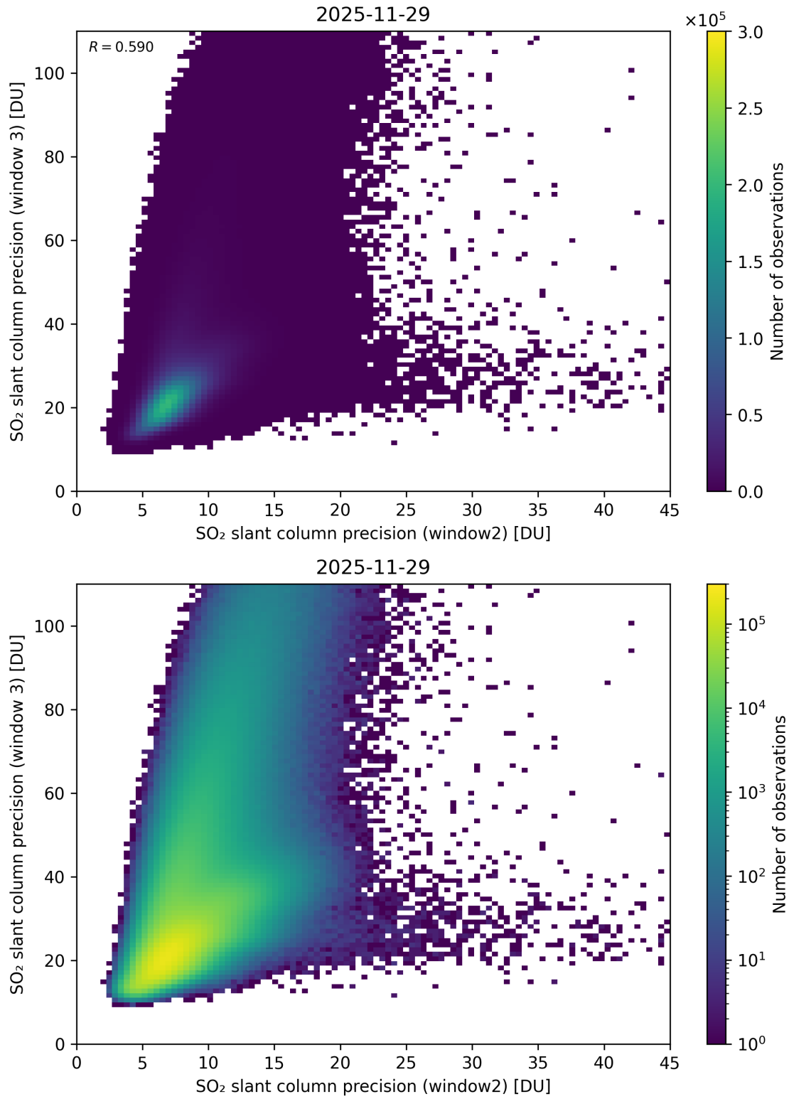
Figure 300: Scatter density plot of “SO 2 slant column precision (window2)” against “SO 2 slant column precision (window 3)” for 2025-11-28 to 2025-11-30.
