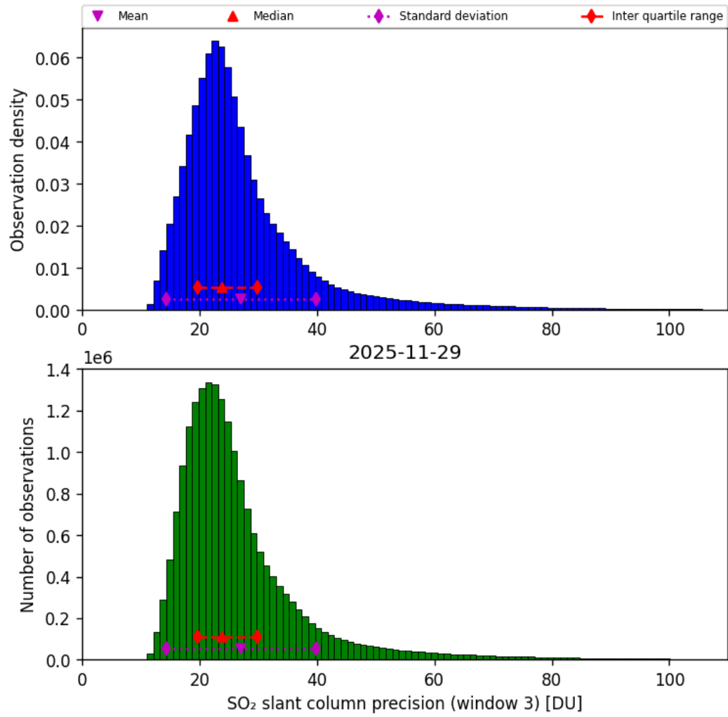
Figure 72: Histogram of “SO 2 slant column precision (window 3)” for 2025-11-28 to 2025-11-30
