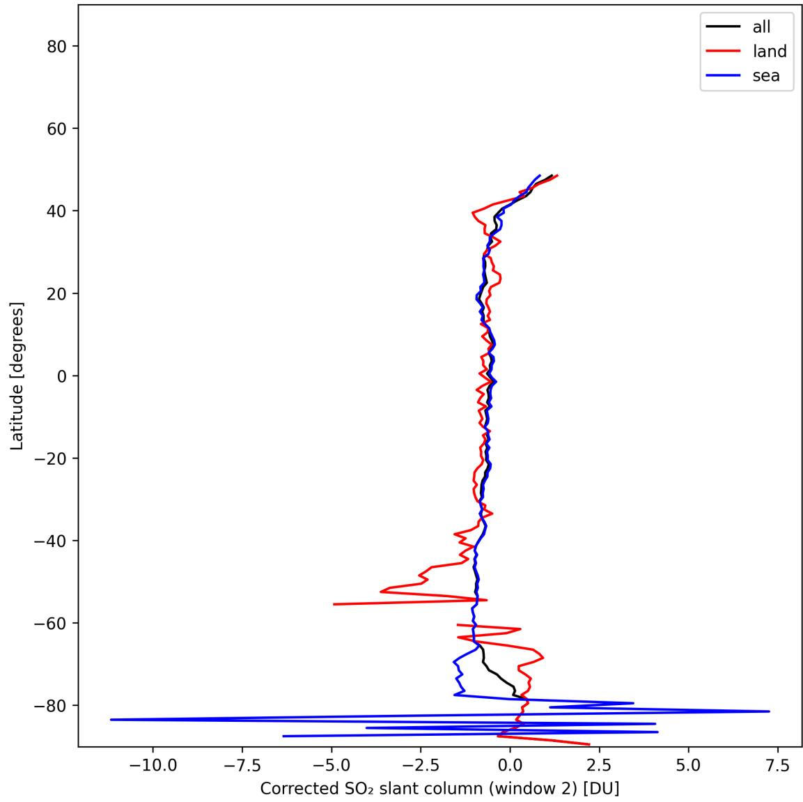
Figure 43: Zonal average of “Corrected SO 2 slant column (window 2)” for 2025-11-28 to 2025-11-30.
