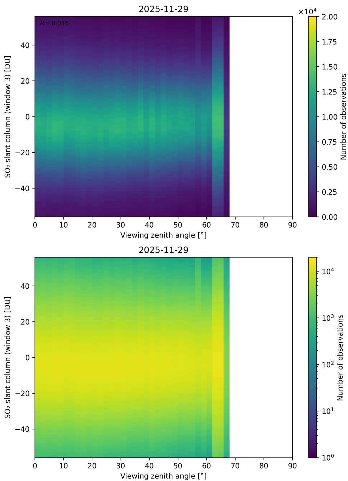
Figure 379: Scatter density plot of “Viewing zenith angle” against “SO 2 slant column (window 3)” for 2025-11-28 to 2025-11-30.
