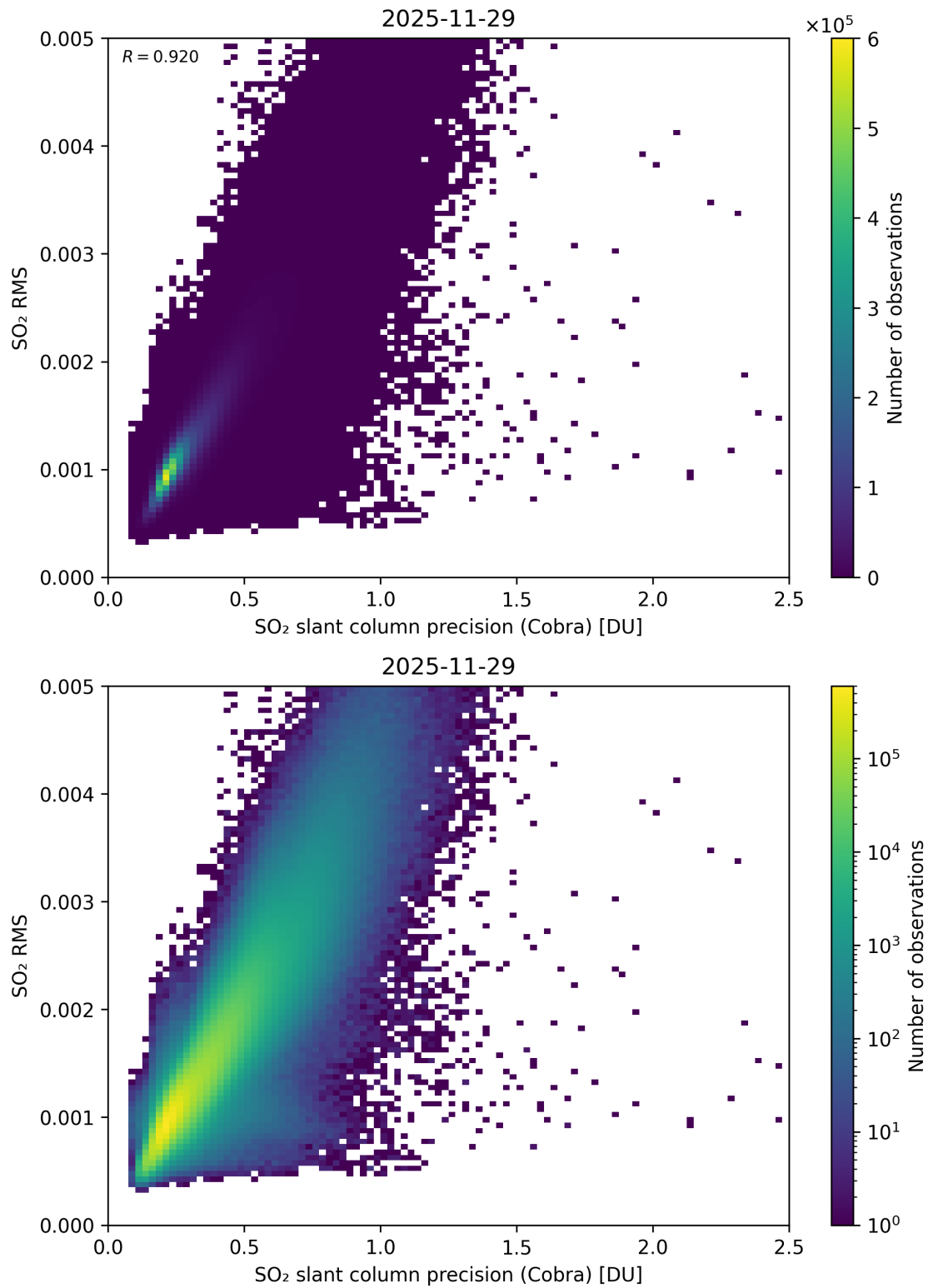
Figure 204: Scatter density plot of “SO 2 slant column precision (Cobra)” against “SO 2 RMS” for 2025-11-28 to 2025-11-30.
