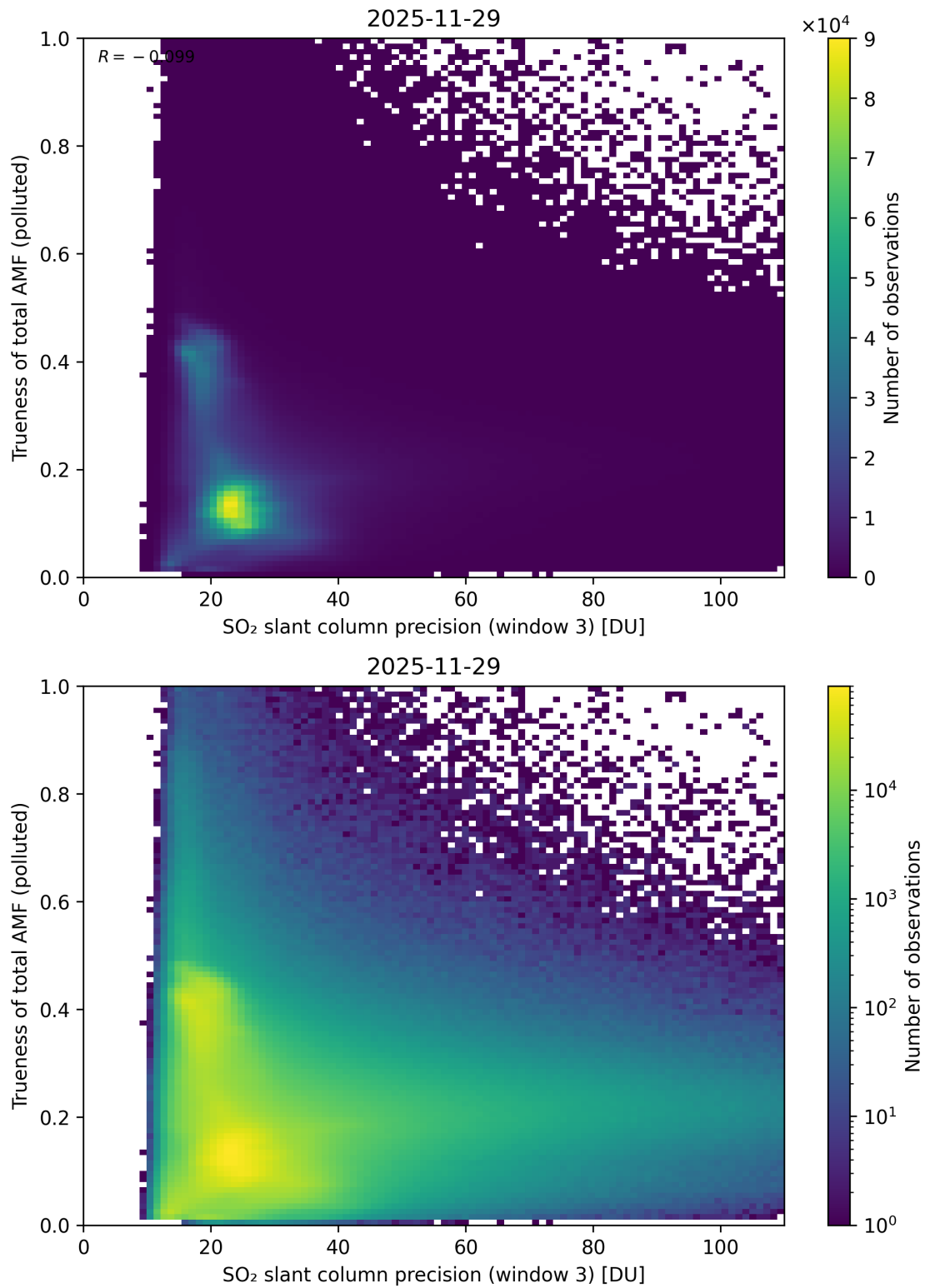
Figure 314: Scatter density plot of “SO 2 slant column precision (window 3)” against “Trueness of total AMF (polluted)” for 2025-11-28 to 2025-11-30.
