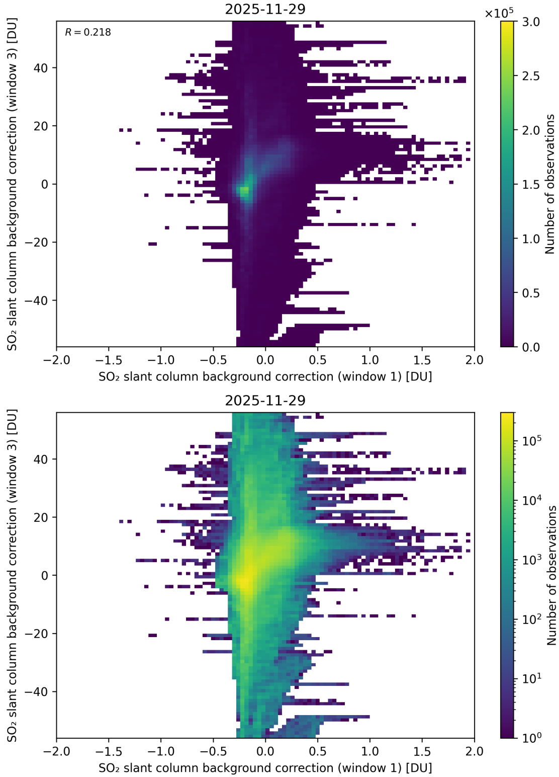
Figure 110: Scatter density plot of “SO 2 slant column background correction (window 1)” against “SO 2 slant column background correction (window 3)” for 2025-11-28 to 2025-11-30.
