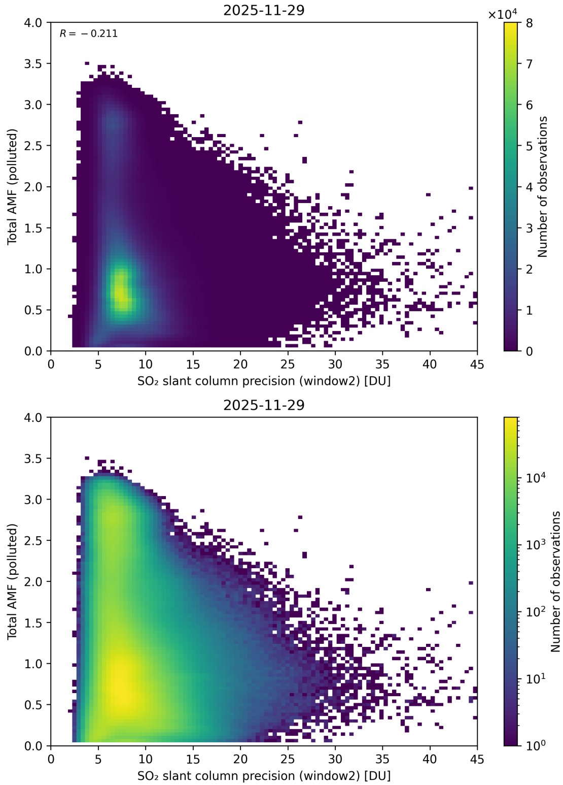
Figure 301: Scatter density plot of “SO 2 slant column precision (window2)” against “Total AMF (polluted)” for 2025-11-28 to 2025-11-30.
