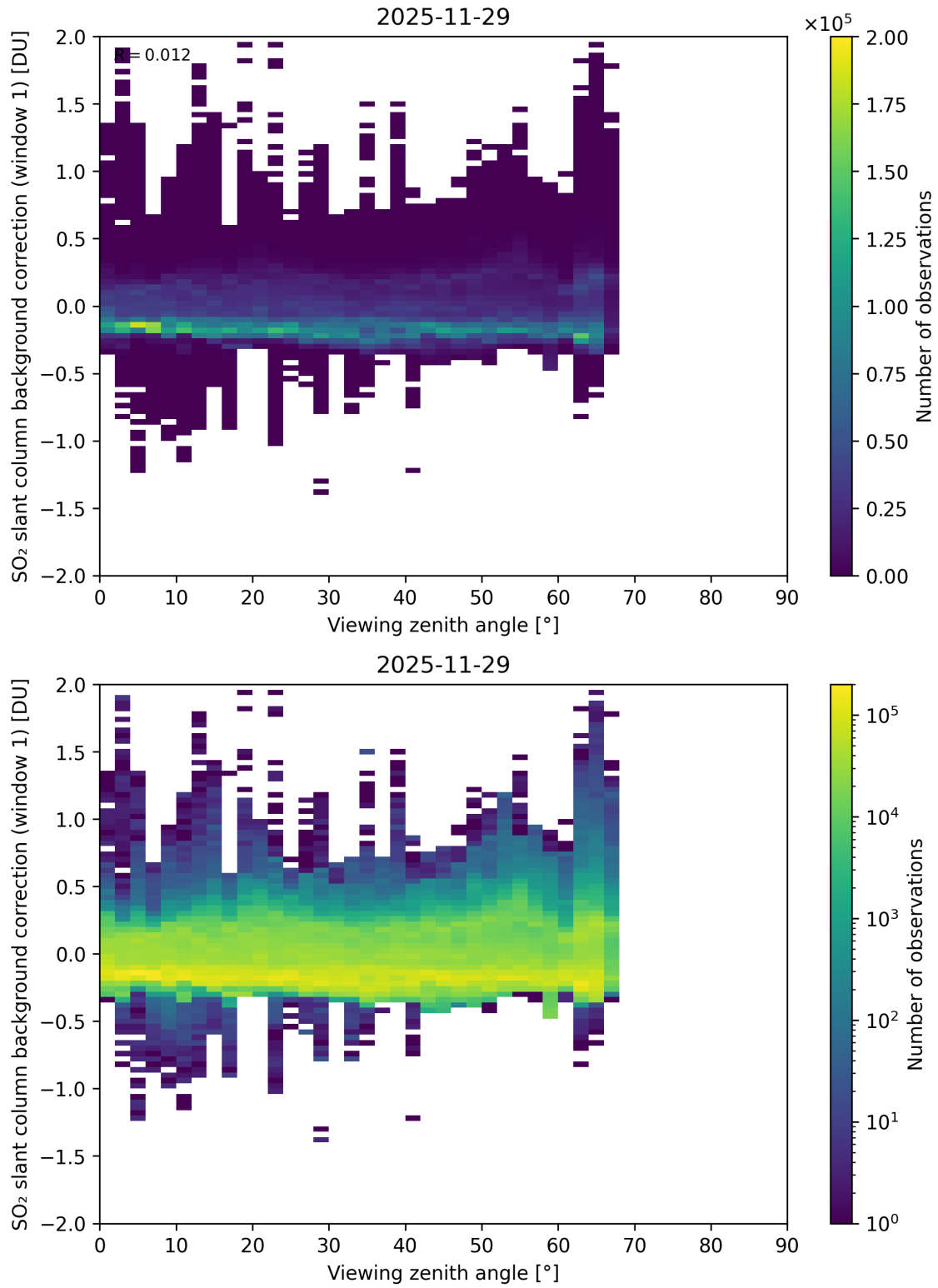
Figure 362: Scatter density plot of “Viewing zenith angle” against “SO 2 slant column background correction (window 1)” for 2025-11-28 to 2025-11-30.
