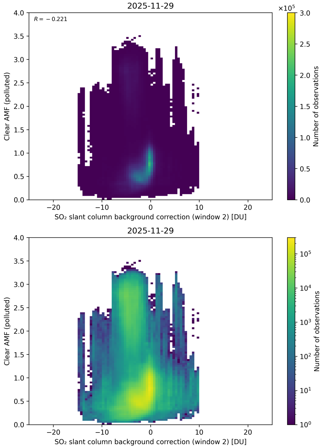
Figure 126: Scatter density plot of “SO 2 slant column background correction (window 2)” against “Clear AMF (polluted)” for 2025-11-28 to 2025-11-30.
