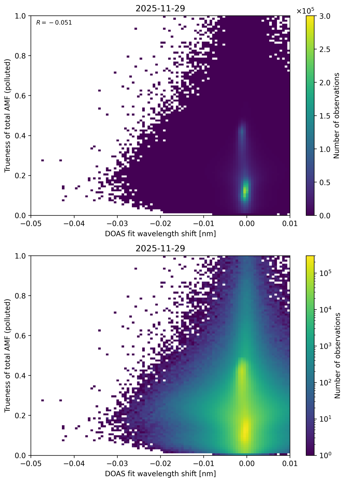
Figure 142: Scatter density plot of “DOAS fit wavelength shift” against “Trueness of total AMF (polluted)” for 2025-11-28 to 2025-11-30.
