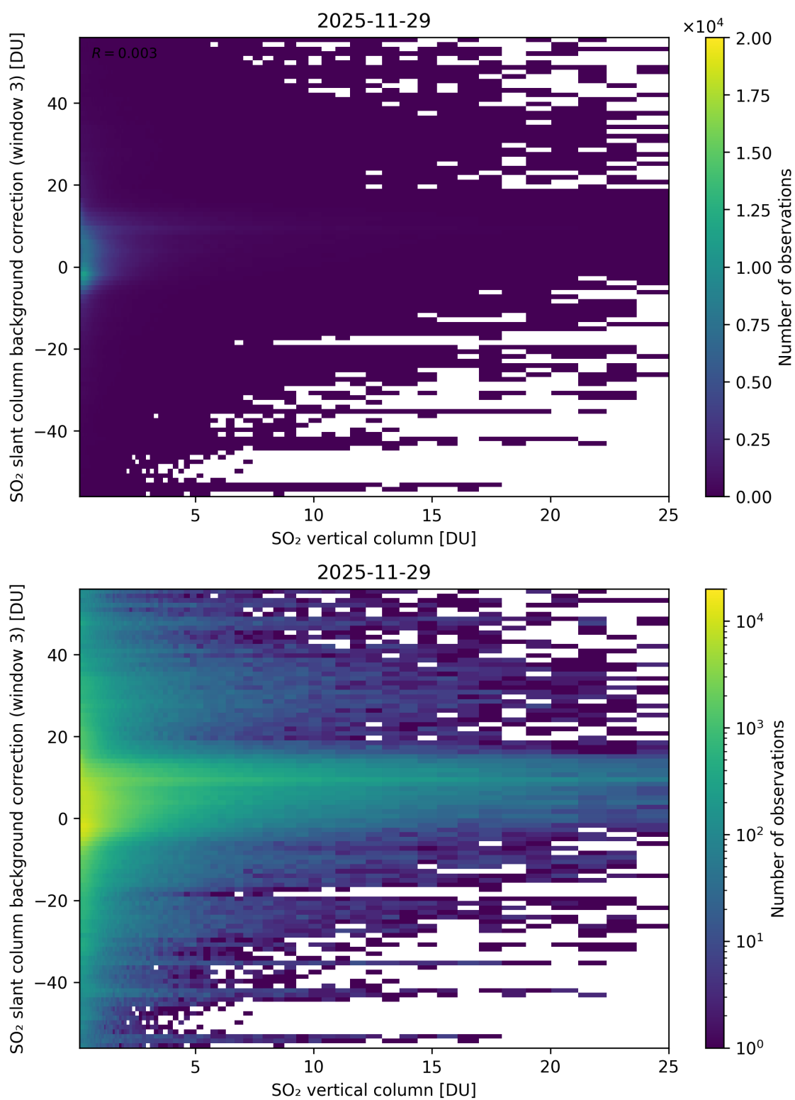
Figure 325: Scatter density plot of “SO 2 vertical column” against “SO 2 slant column background correction (window 3)” for 2025-11-28 to 2025-11-30.
