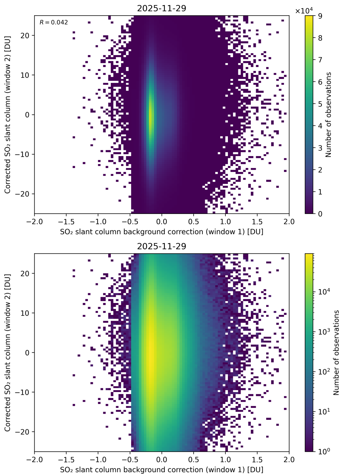
Figure 115: Scatter density plot of “SO 2 slant column background correction (window 1)” against “Corrected SO 2 slant column (window 2)” for 2025-11-28 to 2025-11-30.
