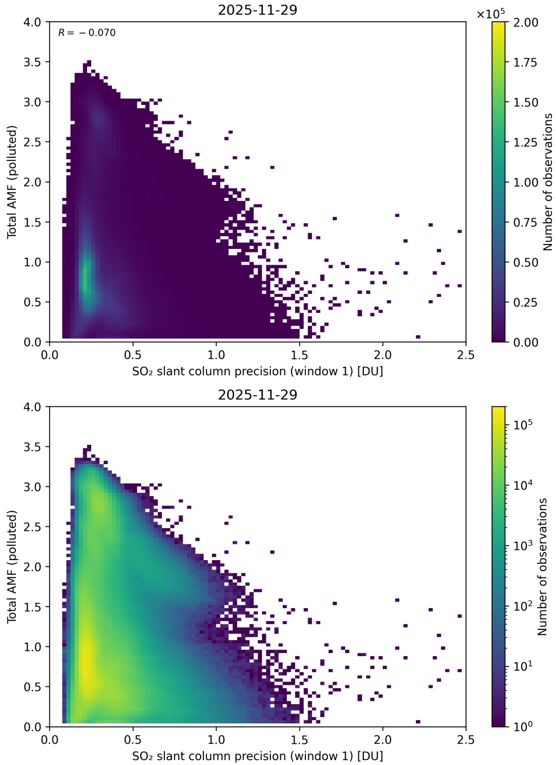
Figure 280: Scatter density plot of “SO 2 slant column precision (window 1)” against “Total AMF (polluted)” for 2025-11-28 to 2025-11-30.
