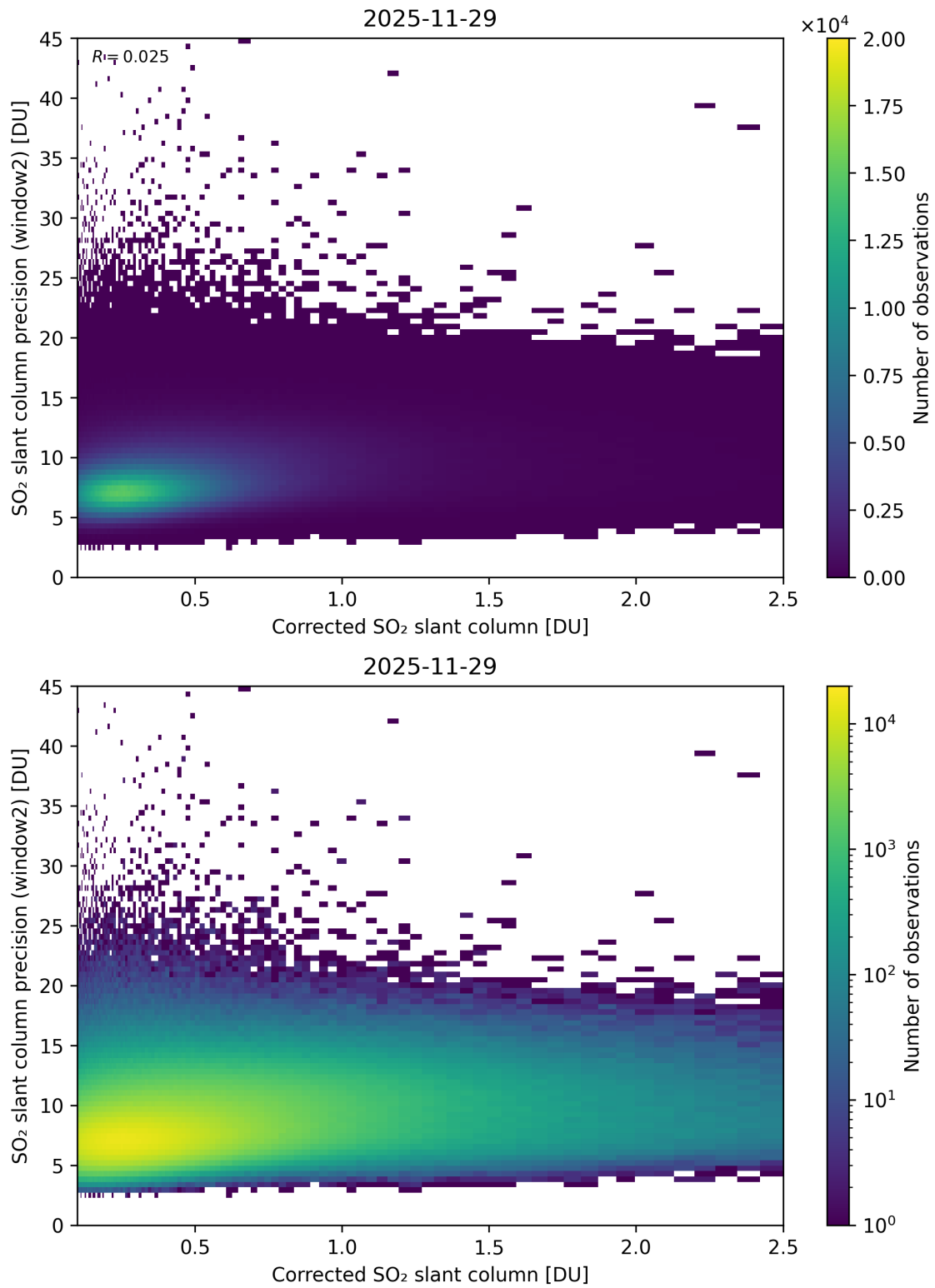
Figure 239: Scatter density plot of “Corrected SO 2 slant column” against “SO 2 slant column precision (window2)” for 2025-11-28 to 2025-11-30.
