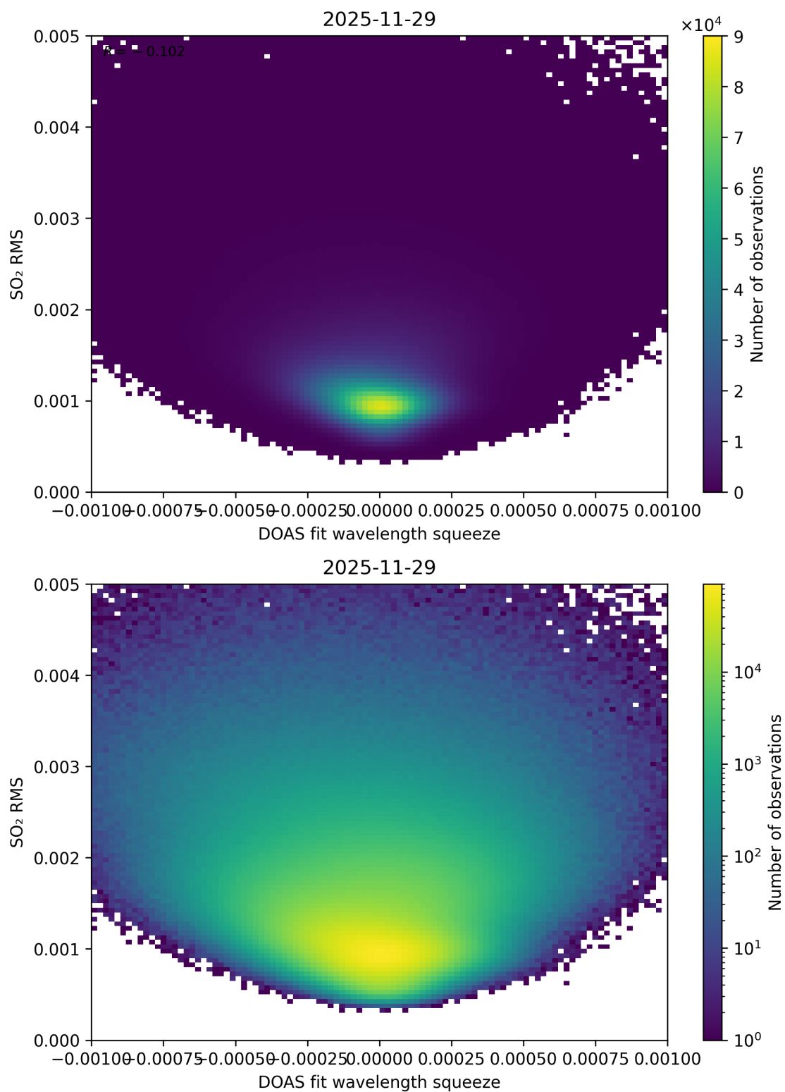
Figure 143: Scatter density plot of “DOAS fit wavelength squeeze” against “SO 2 RMS” for 2025-11-28 to 2025-11-30.
