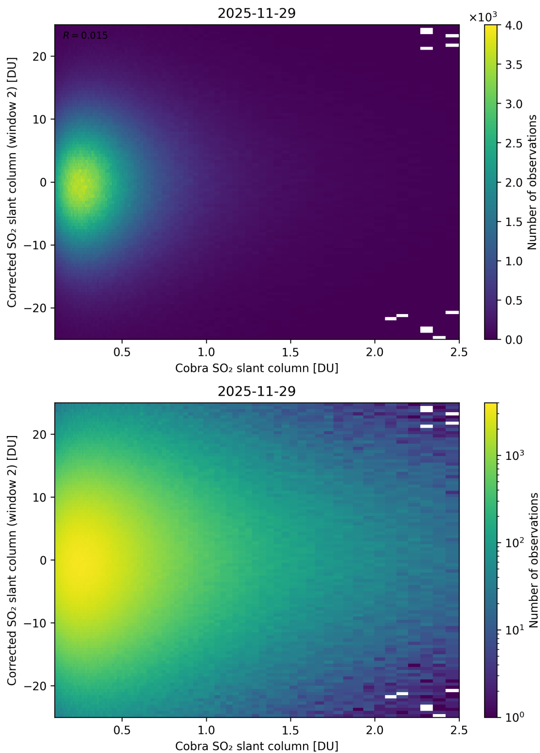
Figure 217: Scatter density plot of “Cobra SO 2 slant column” against “Corrected SO 2 slant column (window 2)” for 2025-11-28 to 2025-11-30.
