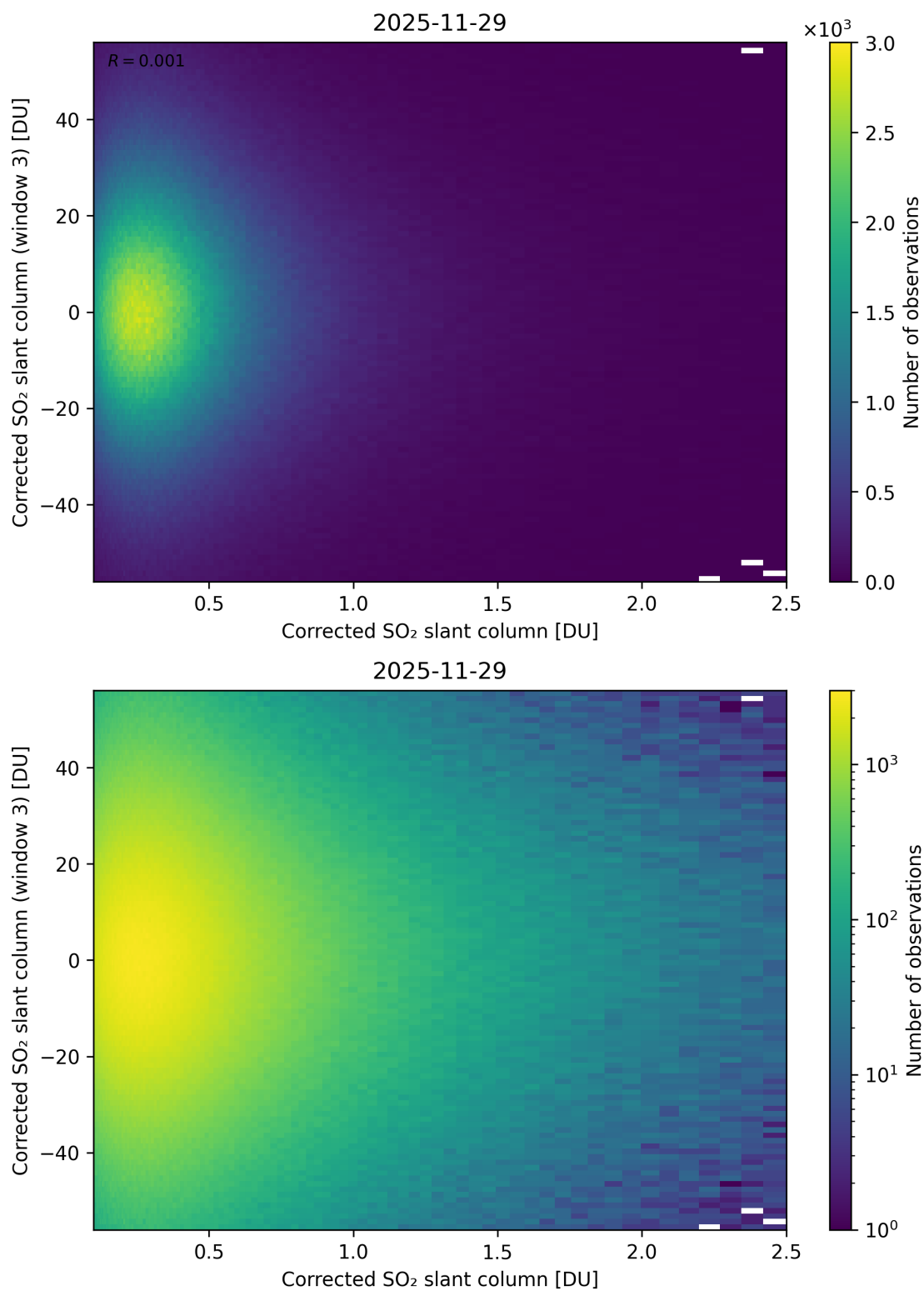
Figure 236: Scatter density plot of “Corrected SO 2 slant column” against “Corrected SO 2 slant column (window 3)” for 2025-11-28 to 2025-11-30.
