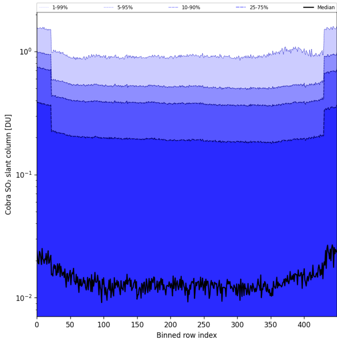
Figure 87: Along track statistics of “Cobra SO 2 slant column” for 2025-11-28 to 2025-11-30
