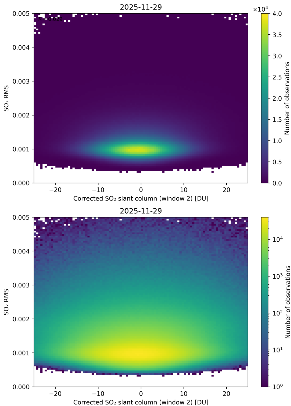
Figure 248: Scatter density plot of “Corrected SO 2 slant column (window 2)” against “SO 2 RMS” for 2025-11-28 to 2025-11-30.
