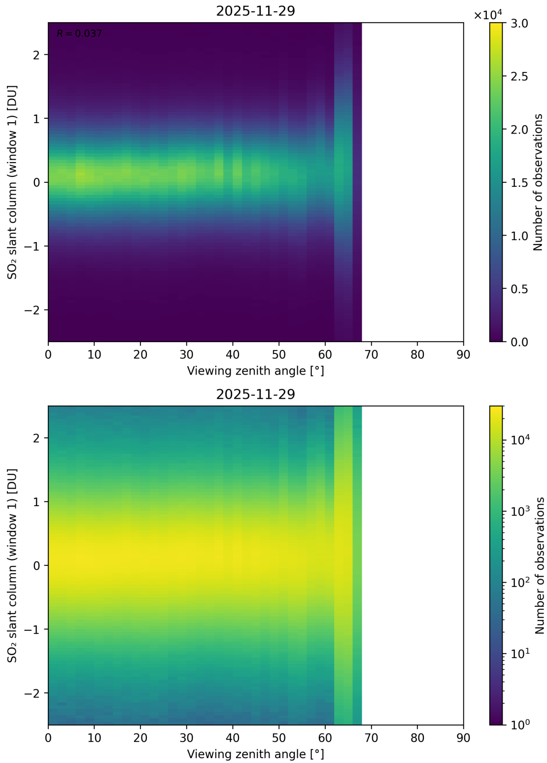
Figure 376: Scatter density plot of “Viewing zenith angle” against “SO 2 slant column (window 1)” for 2025-11-28 to 2025-11-30.
