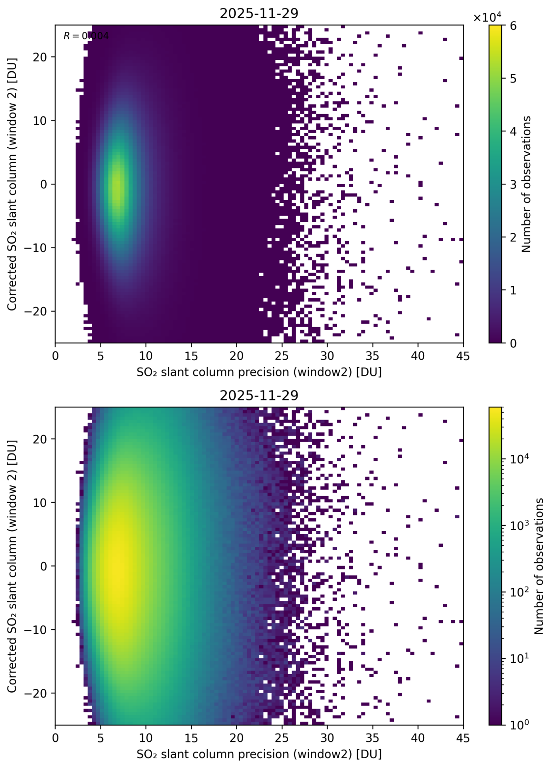
Figure 297: Scatter density plot of “SO 2 slant column precision (window2)” against “Corrected SO 2 slant column (window 2)” for 2025-11-28 to 2025-11-30.
