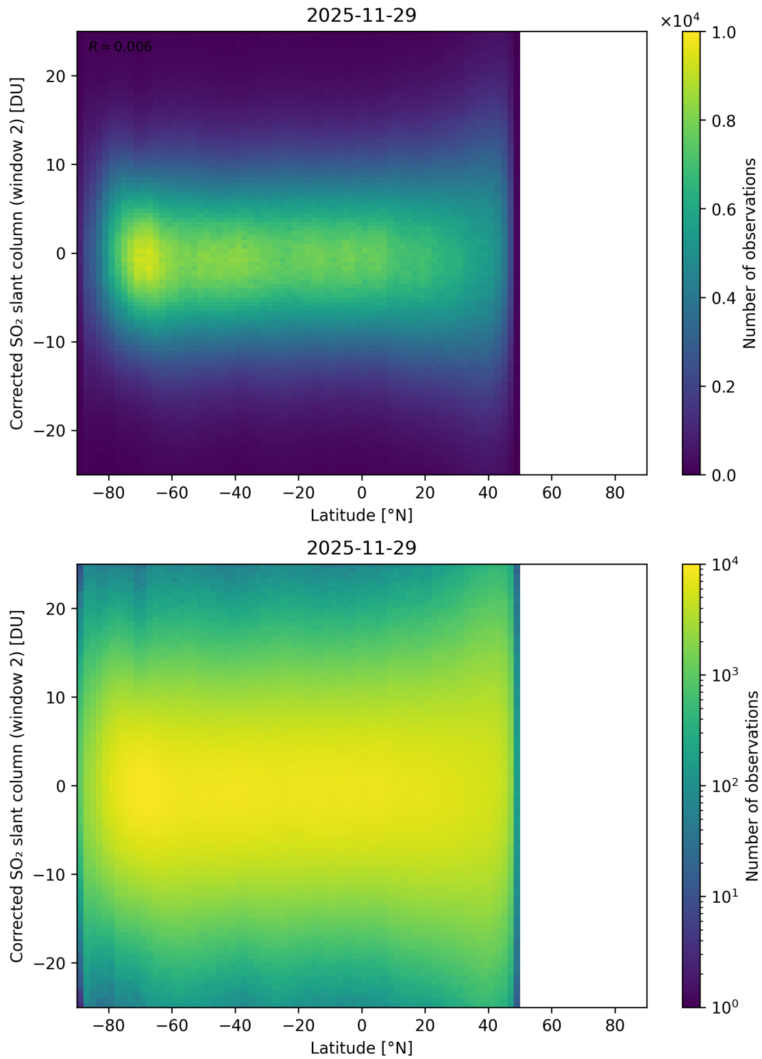
Figure 160: Scatter density plot of “Latitude” against “Corrected SO 2 slant column (window 2)” for 2025-11-28 to 2025-11-30.
