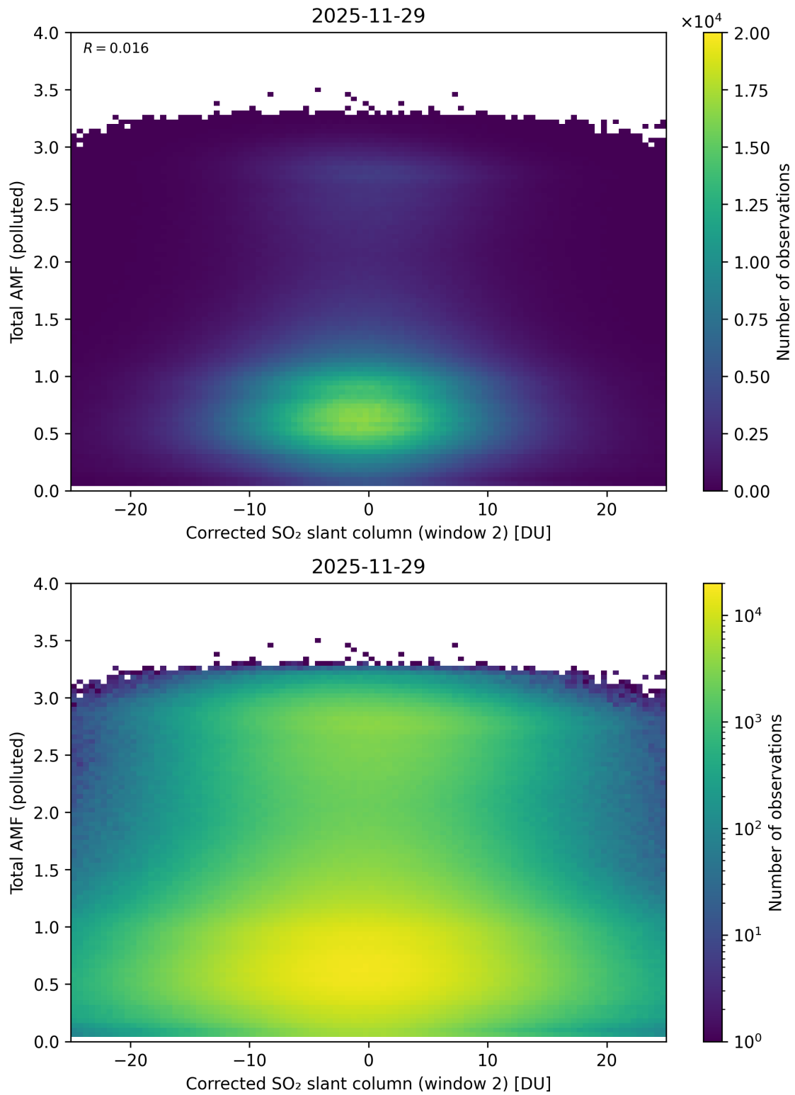
Figure 253: Scatter density plot of “Corrected SO 2 slant column (window 2)” against “Total AMF (polluted)” for 2025-11-28 to 2025-11-30.
