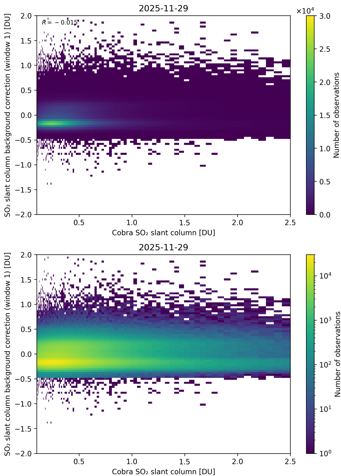
Figure 193: Scatter density plot of “Cobra SO 2 slant column” against “SO 2 slant column background correction (window 1)” for 2025-11-28 to 2025-11-30.
