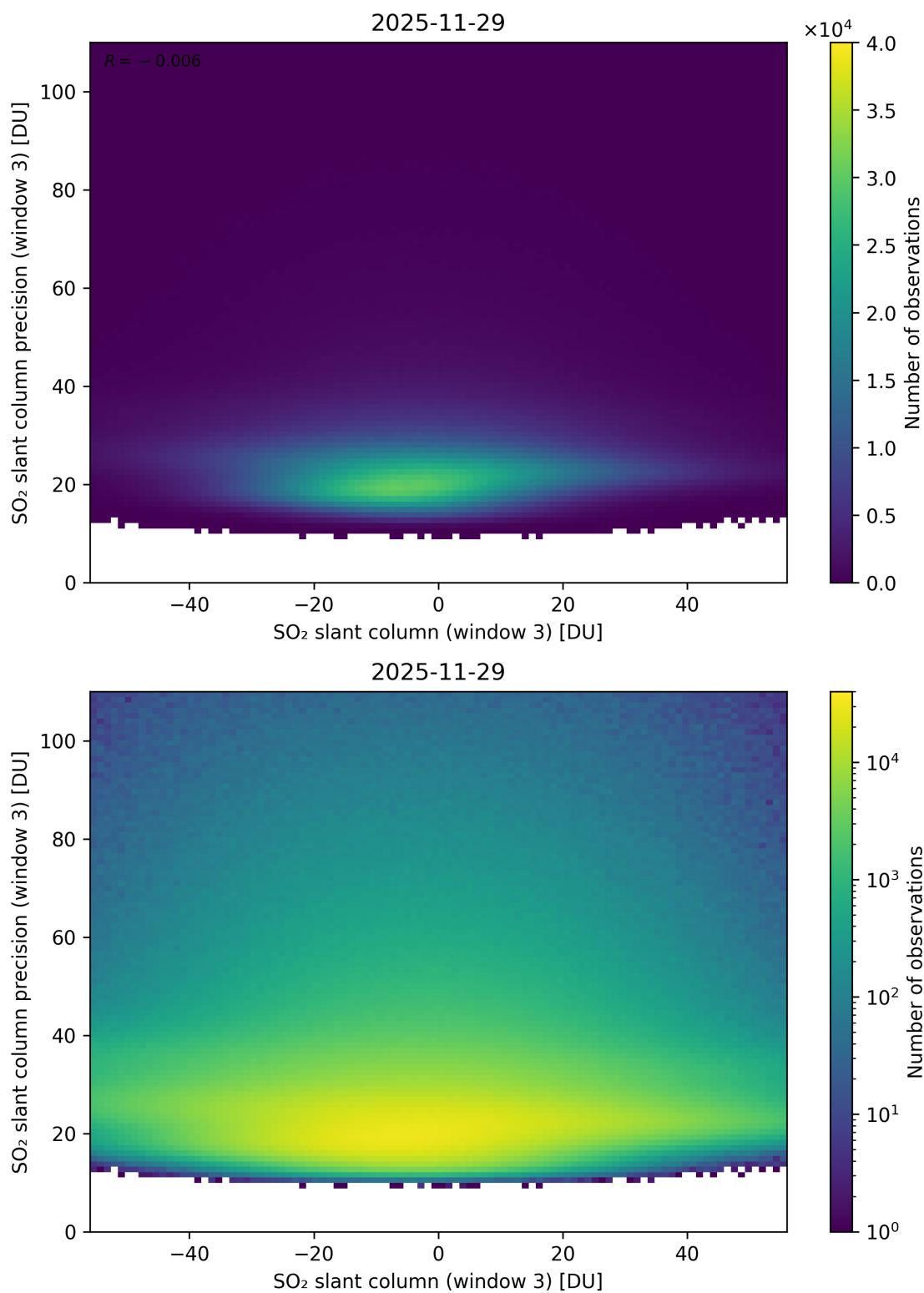
Figure 317: Scatter density plot of “SO 2 slant column (window 3)” against “SO 2 slant column precision (window 3)” for 2025-11-28 to 2025-11-30.
