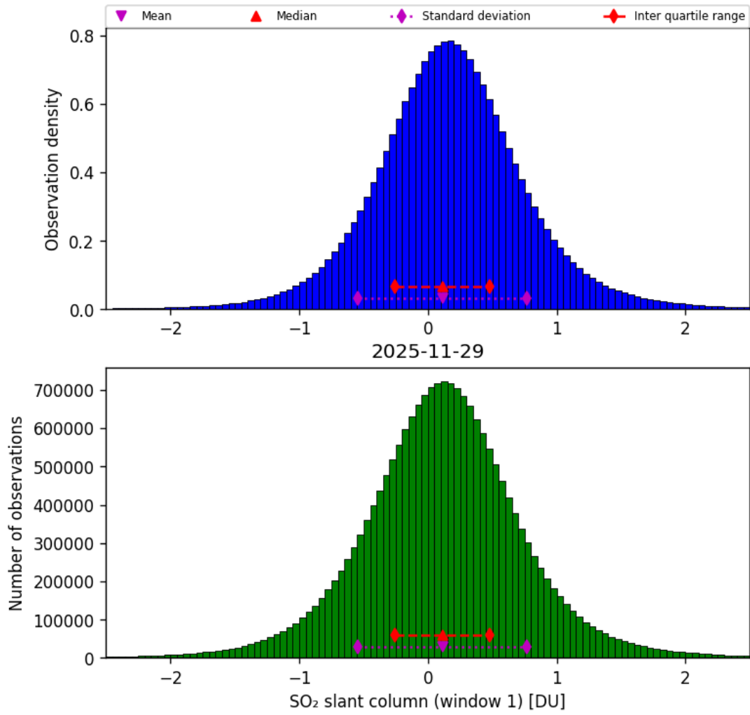
Figure 63: Histogram of “SO 2 slant column (window 1)” for 2025-11-28 to 2025-11-30
