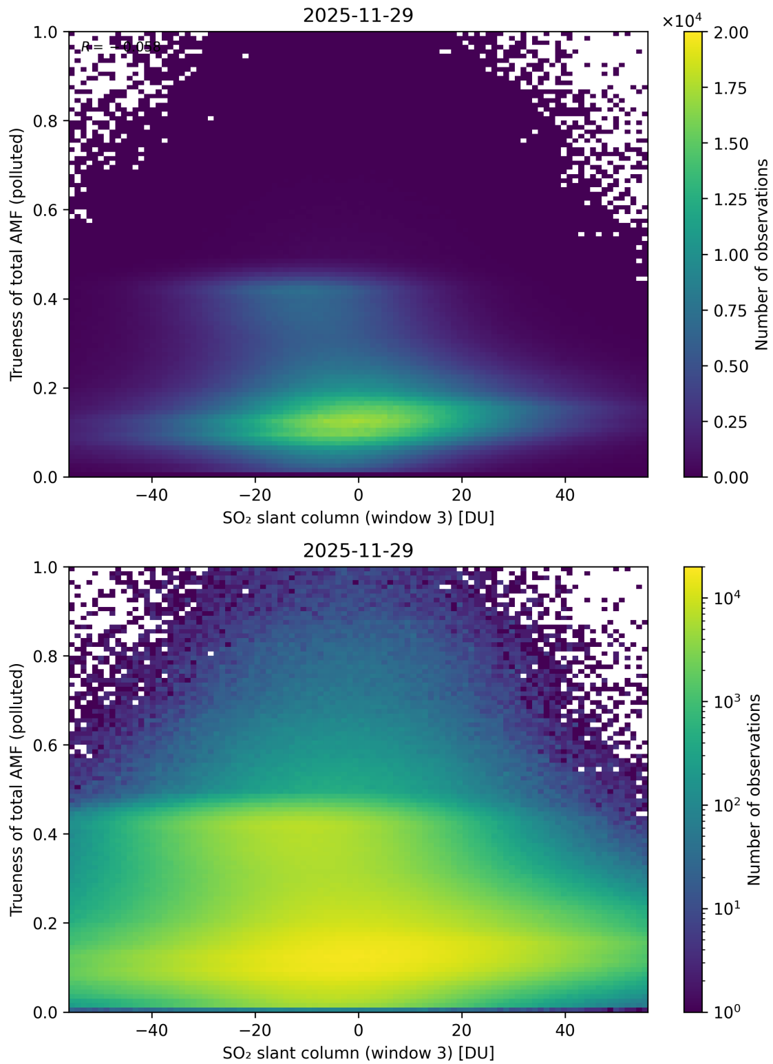
Figure 319: Scatter density plot of “SO 2 slant column (window 3)” against “Trueness of total AMF (polluted)” for 2025-11-28 to 2025-11-30.
