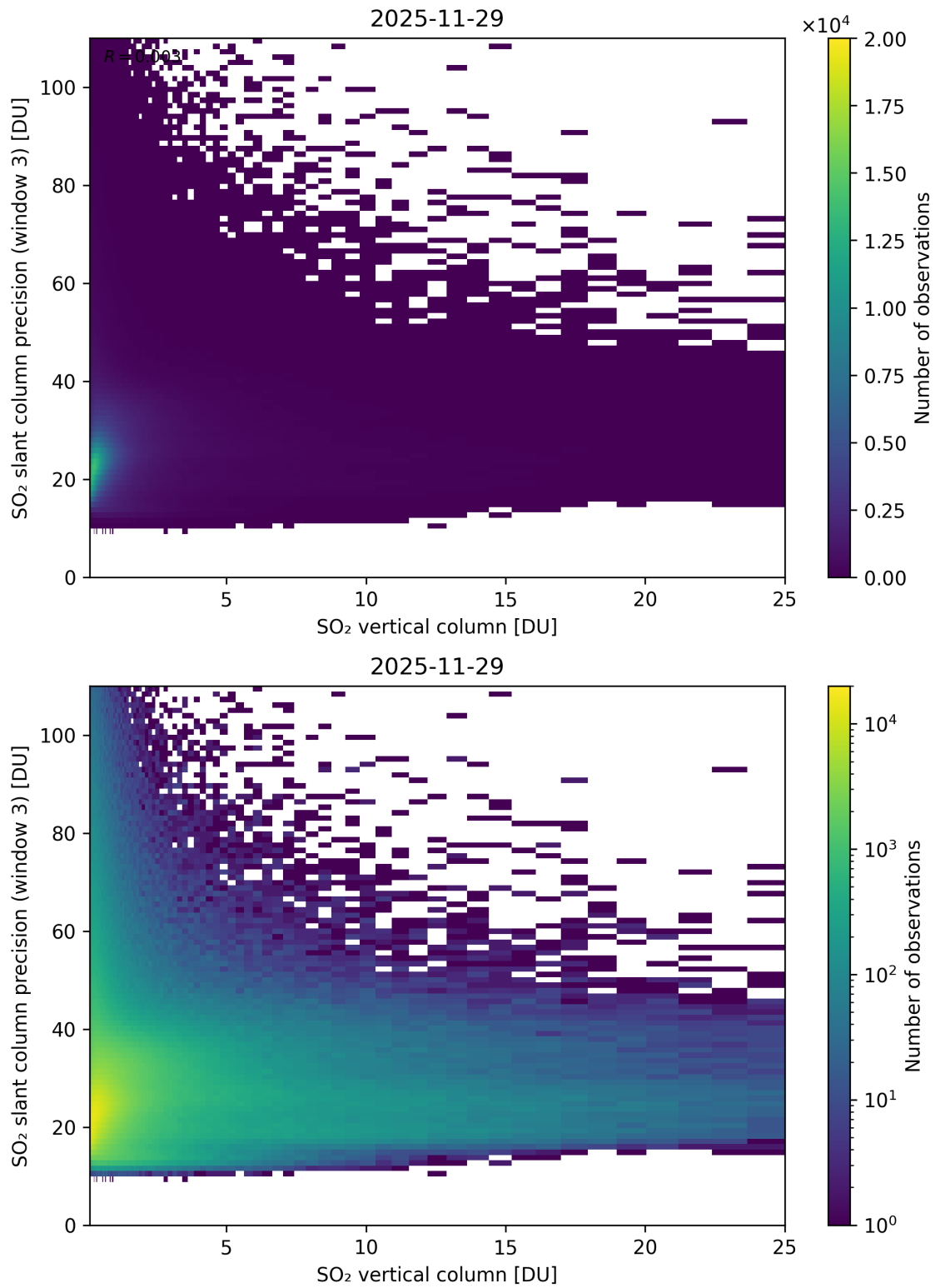
Figure 358: Scatter density plot of “SO 2 vertical column” against “SO 2 slant column precision (window 3)” for 2025-11-28 to 2025-11-30.
