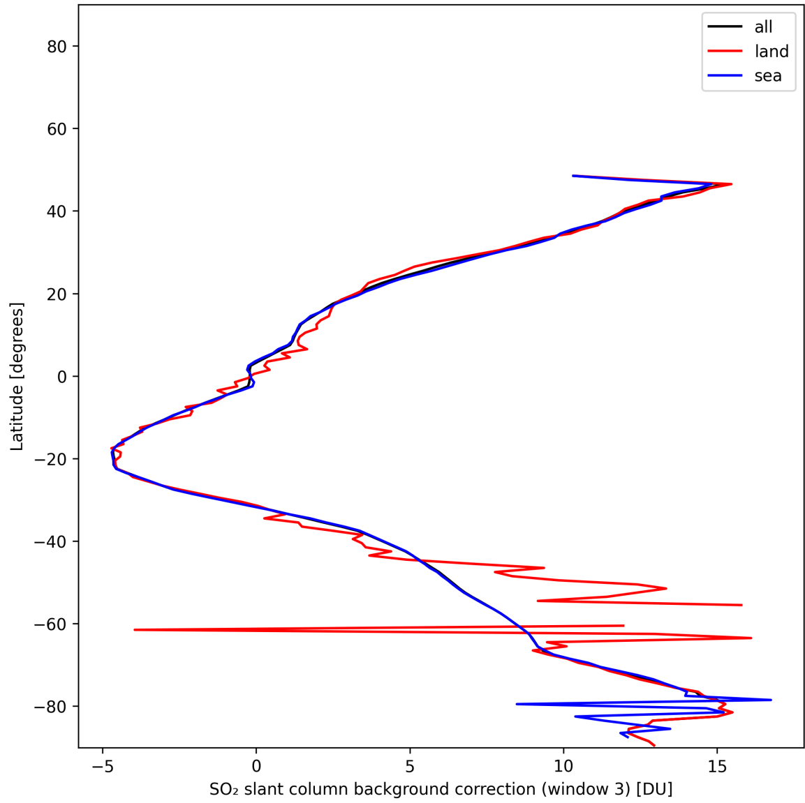
Figure 48: Zonal average of “SO 2 slant column background correction (window 3)” for 2025-11-28 to 2025-11-30.
