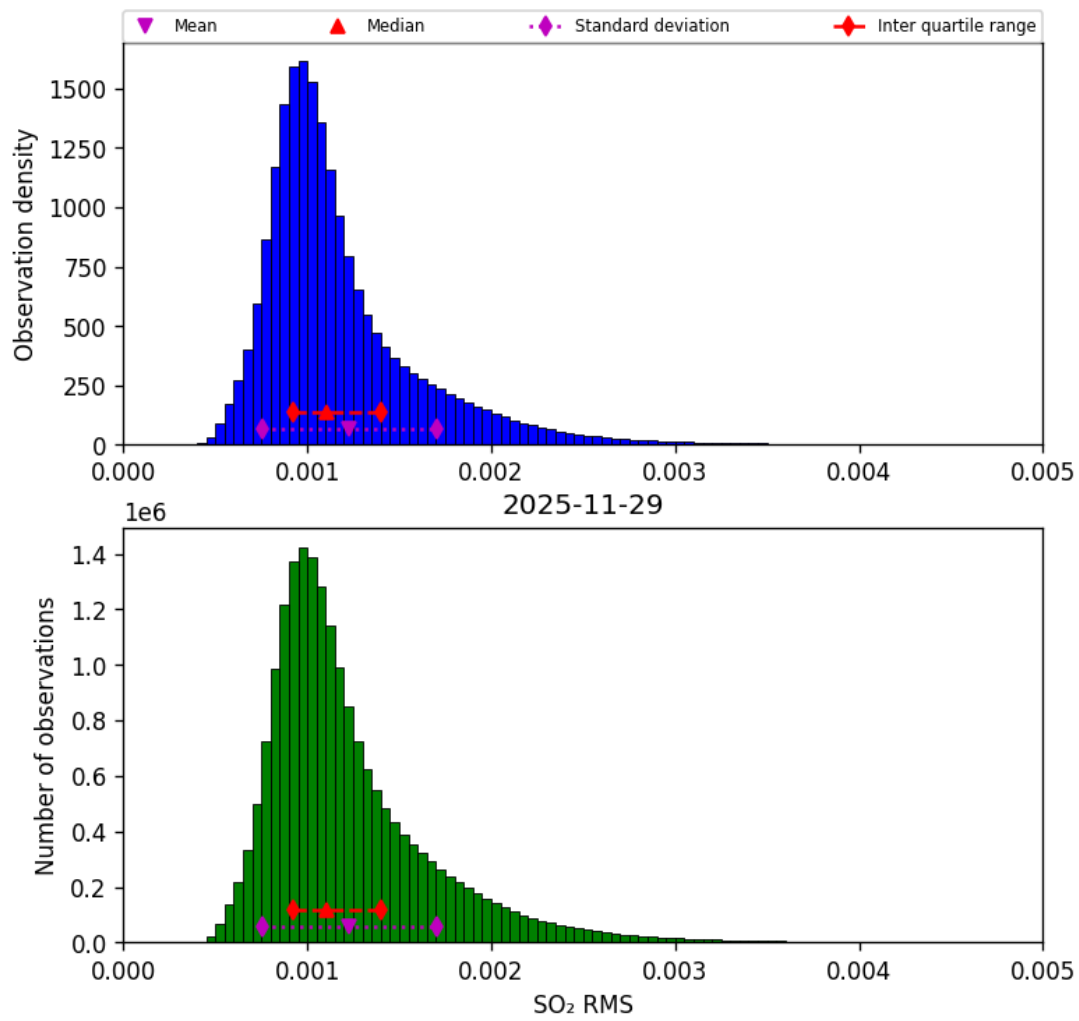
Figure 78: Histogram of “SO 2 RMS” for 2025-11-28 to 2025-11-30
