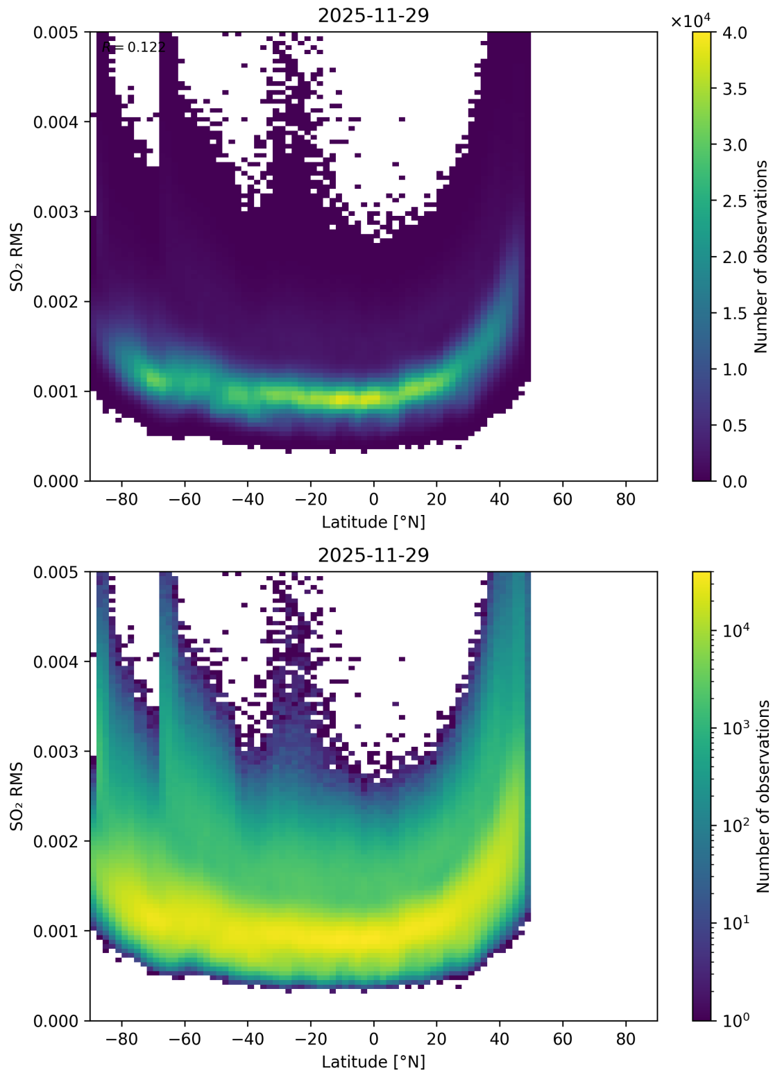
Figure 155: Scatter density plot of “Latitude” against “SO 2 RMS” for 2025-11-28 to 2025-11-30.
