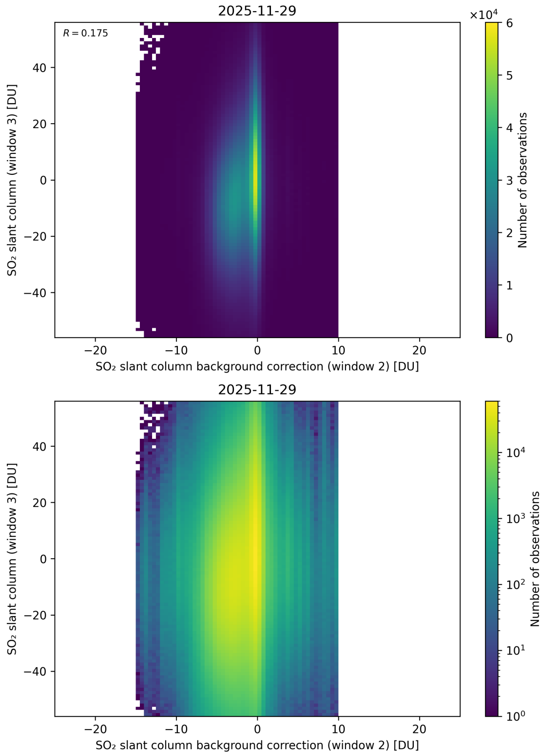
Figure 128: Scatter density plot of “SO 2 slant column background correction (window 2)” against “SO 2 slant column (window 3)” for 2025-11-28 to 2025-11-30.
