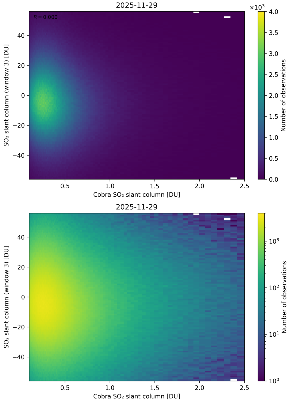
Figure 222: Scatter density plot of “Cobra SO 2 slant column” against “SO 2 slant column (window 3)” for 2025-11-28 to 2025-11-30.
