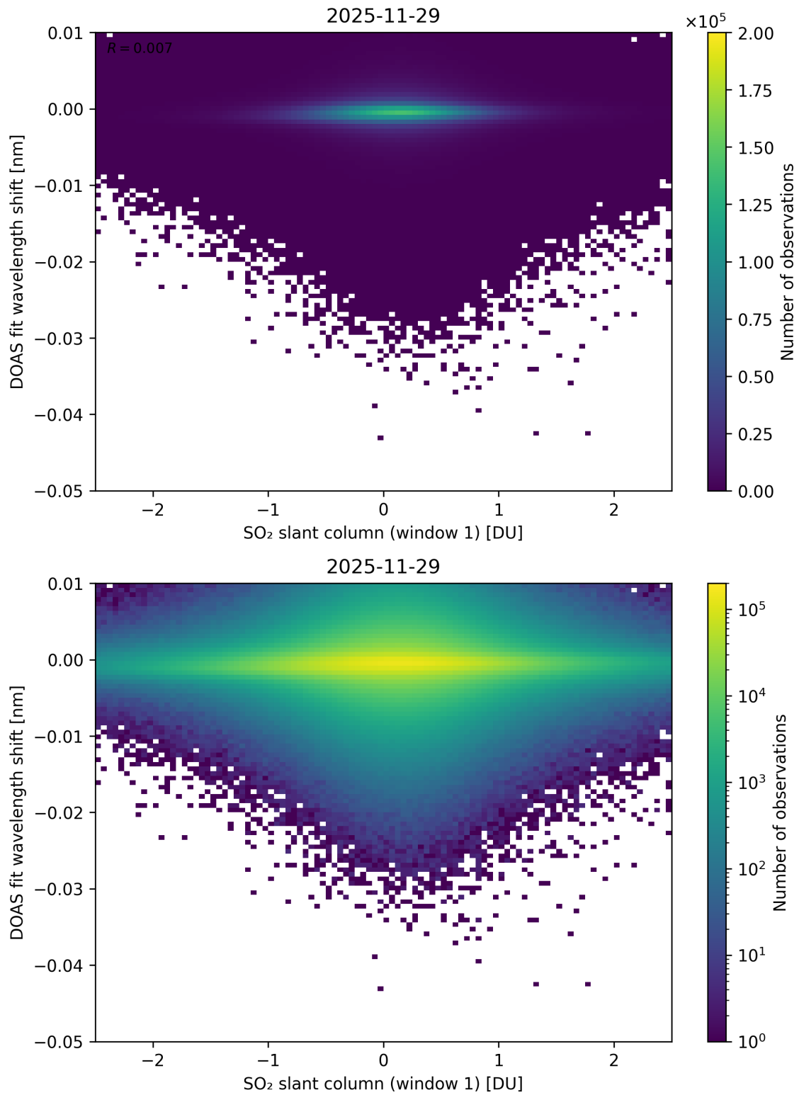
Figure 265: Scatter density plot of “SO 2 slant column (window 1)” against “DOAS fit wavelength shift” for 2025-11-28 to 2025-11-30.
