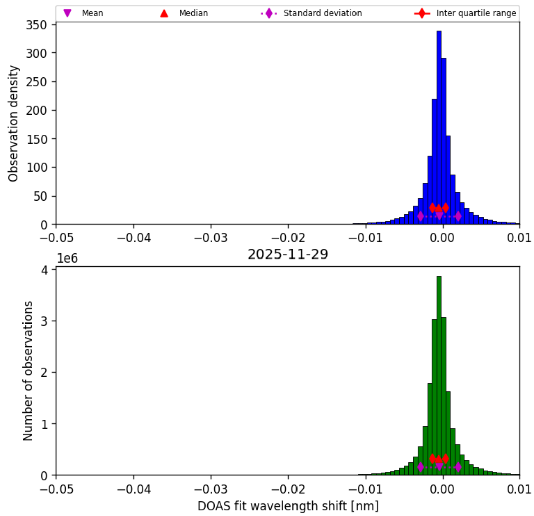
Figure 76: Histogram of “DOAS fit wavelength shift” for 2025-11-28 to 2025-11-30
