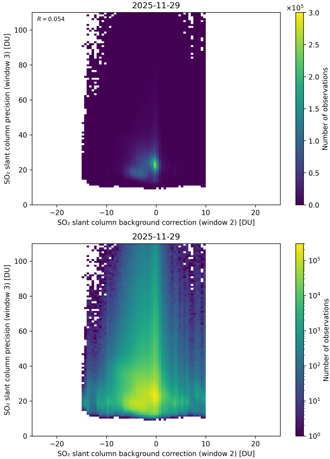
Figure 129: Scatter density plot of “SO 2 slant column background correction (window 2)” against “SO 2 slant column precision (window 3)” for 2025-11-28 to 2025-11-30.
