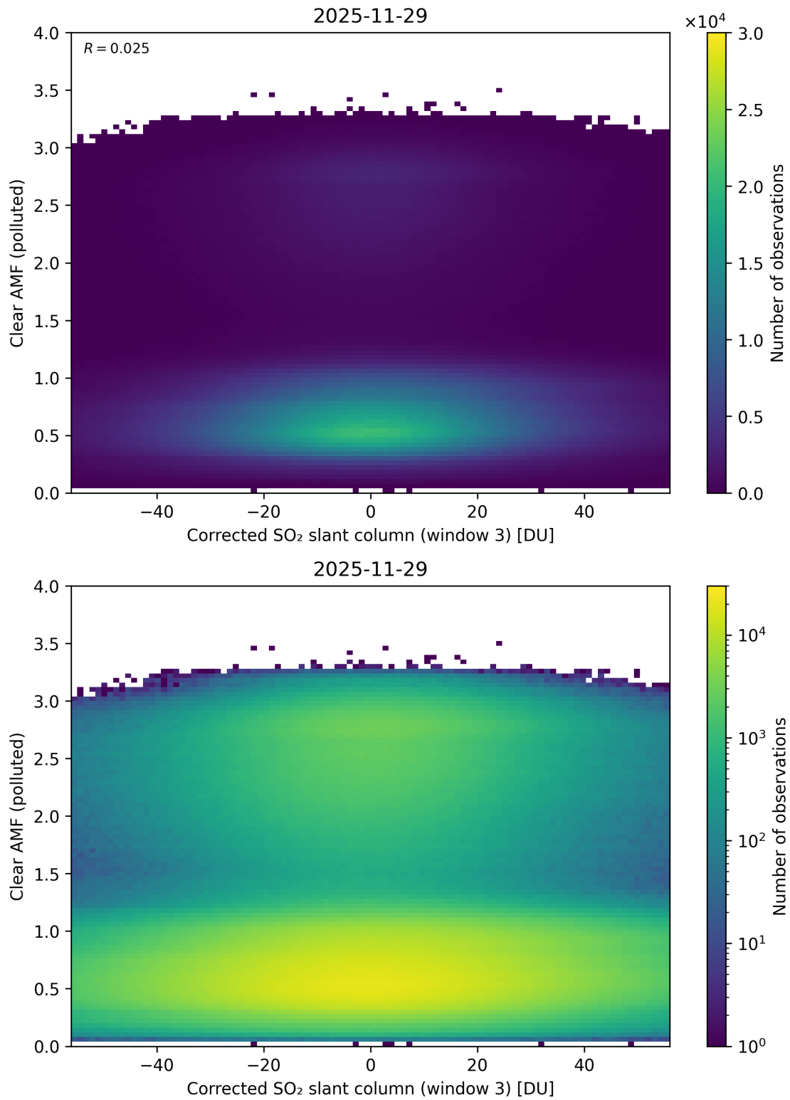
Figure 259: Scatter density plot of “Corrected SO 2 slant column (window 3)” against “Clear AMF (polluted)” for 2025-11-28 to 2025-11-30.
