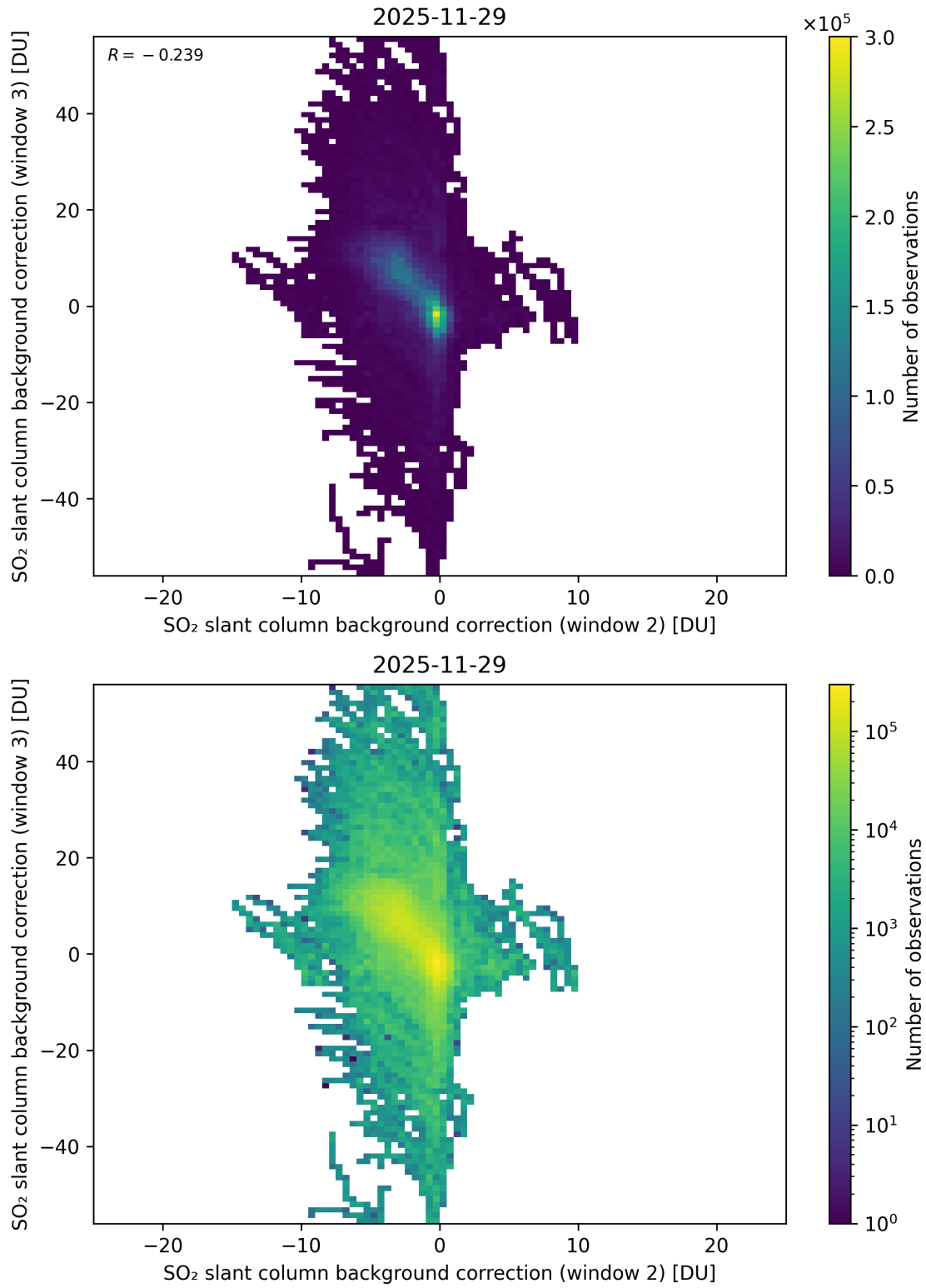
Figure 122: Scatter density plot of “SO 2 slant column background correction (window 2)” against “SO 2 slant column background correction (window 3)” for 2025-11-28 to 2025-11-30.
