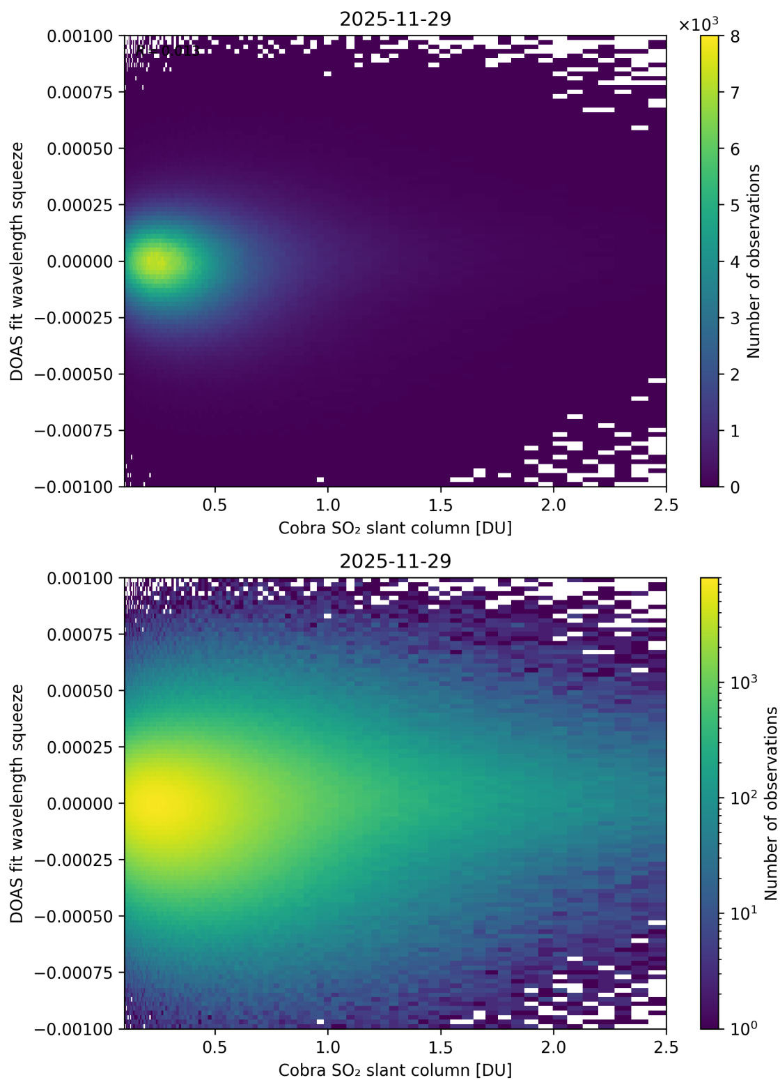
Figure 197: Scatter density plot of “Cobra SO 2 slant column” against “DOAS fit wavelength squeeze” for 2025-11-28 to 2025-11-30.
