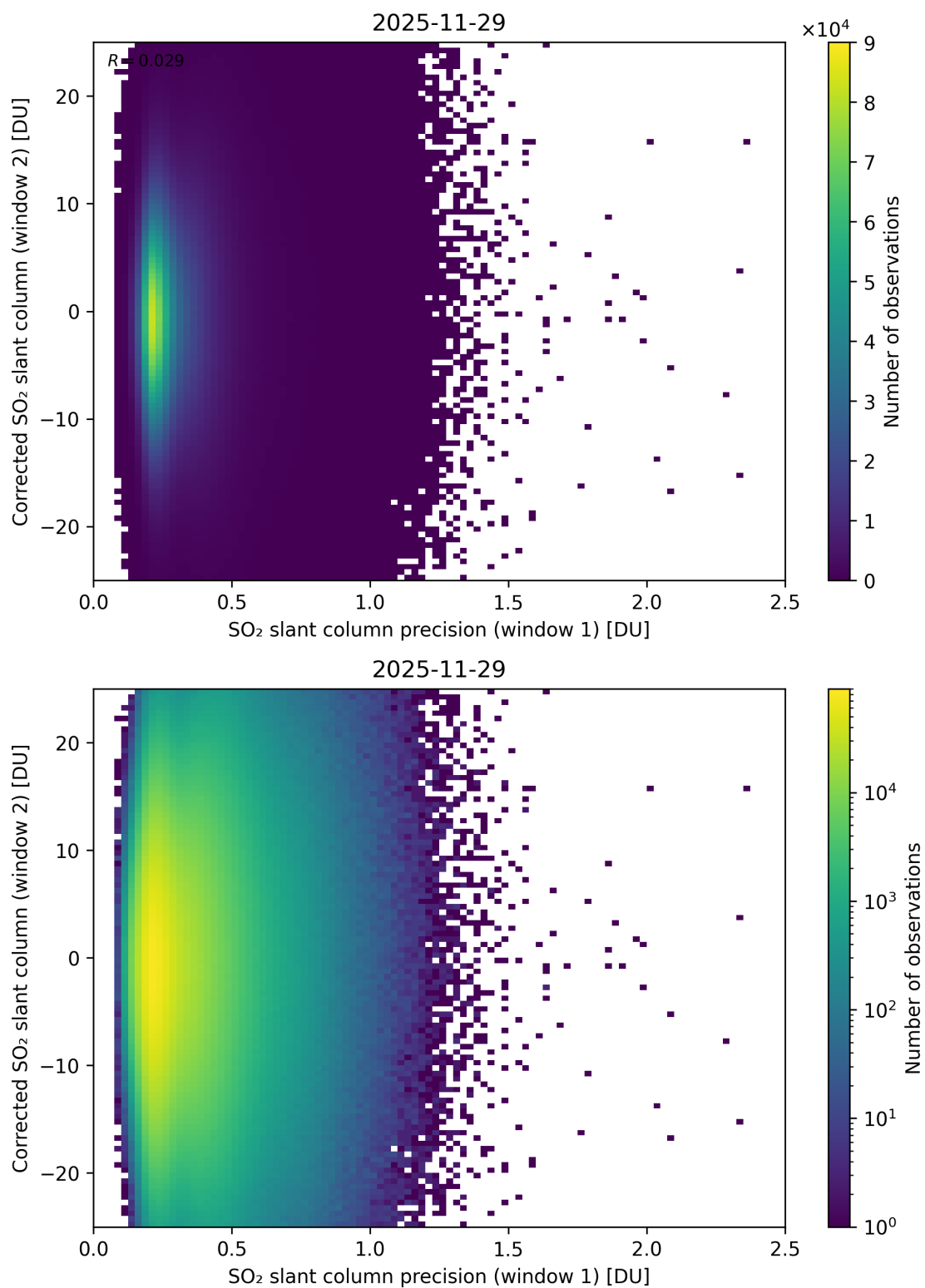
Figure 275: Scatter density plot of “SO 2 slant column precision (window 1)” against “Corrected SO 2 slant column (window 2)” for 2025-11-28 to 2025-11-30.
