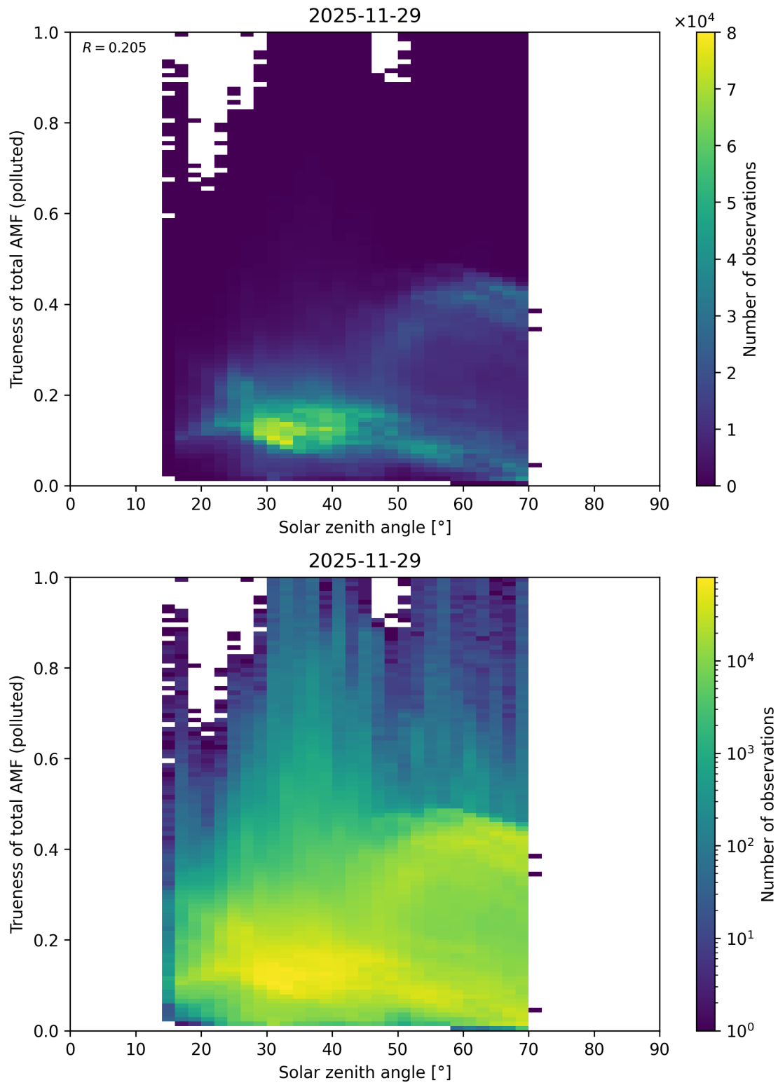
Figure 190: Scatter density plot of “Solar zenith angle” against “Trueness of total AMF (polluted)” for 2025-11-28 to 2025-11-30.
