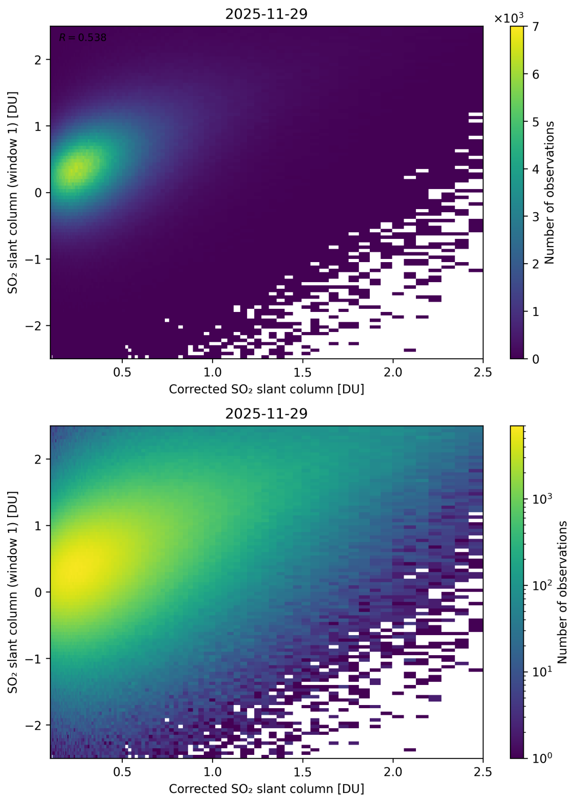
Figure 237: Scatter density plot of “Corrected SO 2 slant column” against “SO 2 slant column (window 1)” for 2025-11-28 to 2025-11-30.
