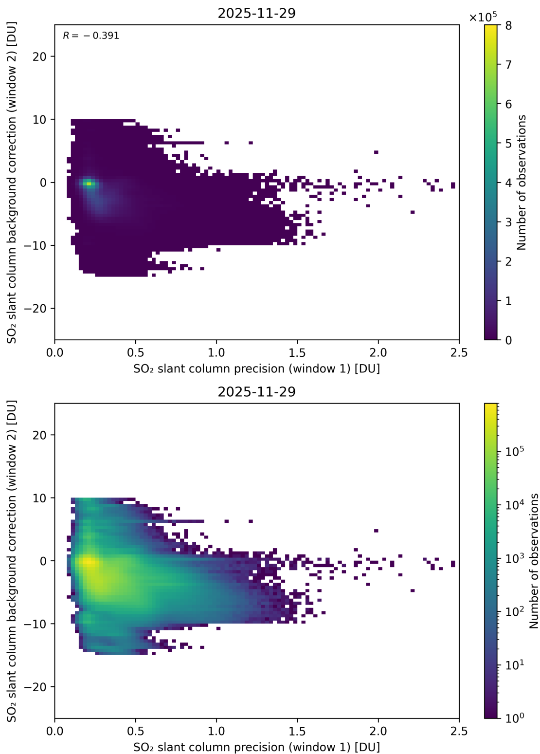
Figure 269: Scatter density plot of “SO 2 slant column precision (window 1)” against “SO 2 slant column background correction (window 2)” for 2025-11-28 to 2025-11-30.
