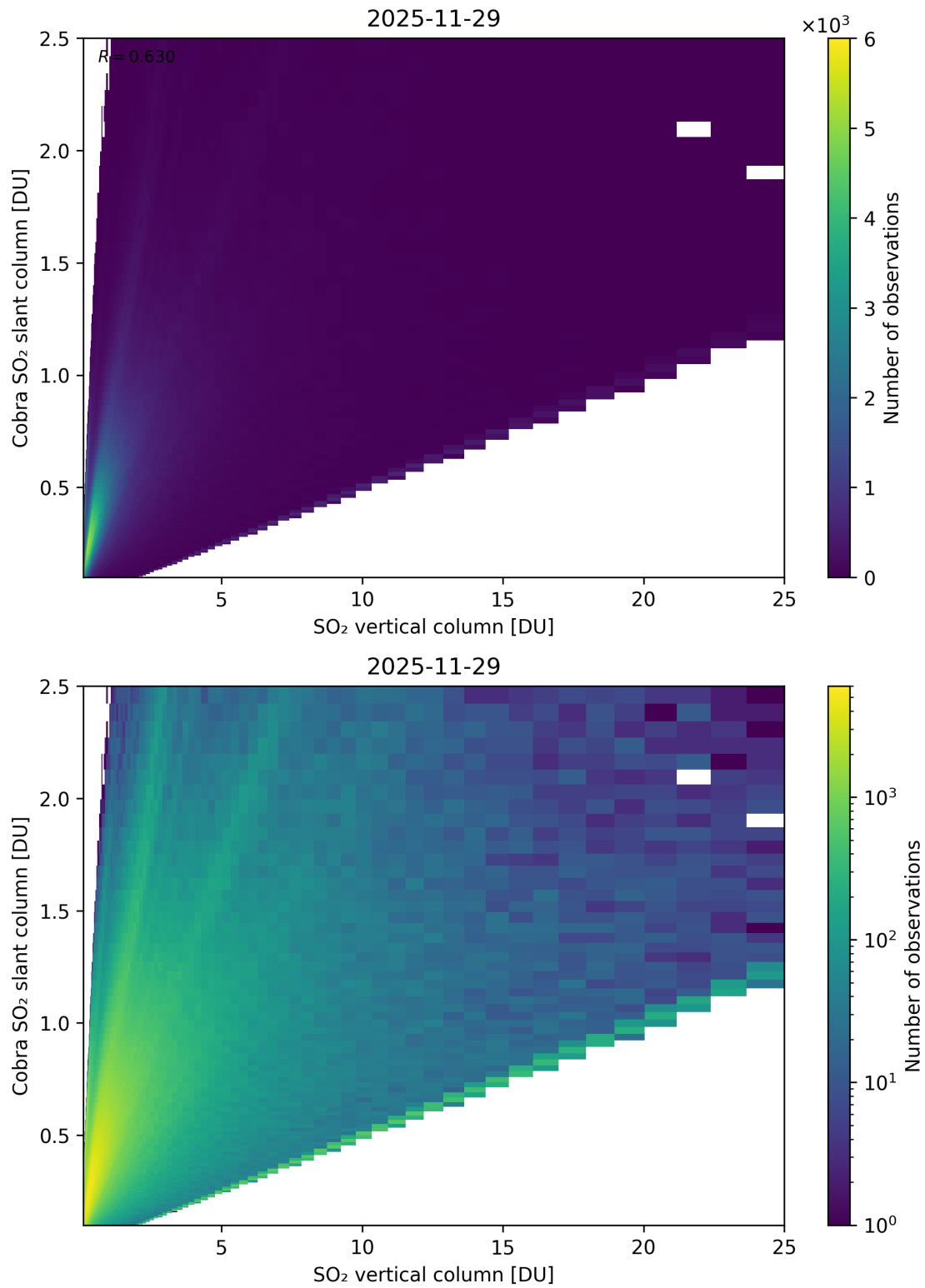
Figure 349: Scatter density plot of “SO 2 vertical column” against “Cobra SO 2 slant column” for 2025-11-28 to 2025-11-30.
