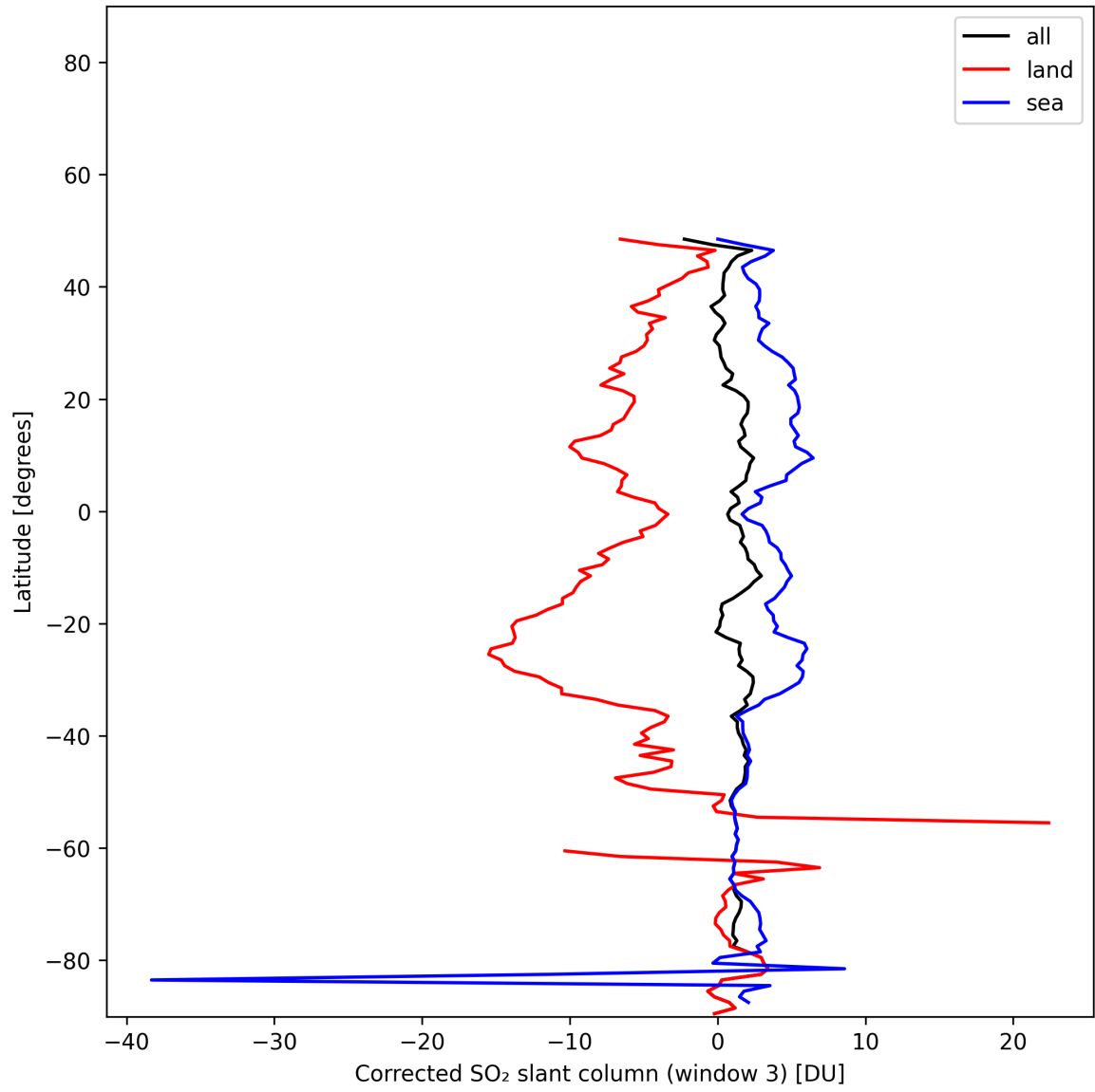
Figure 47: Zonal average of “Corrected SO 2 slant column (window 3)” for 2025-11-28 to 2025-11-30.
