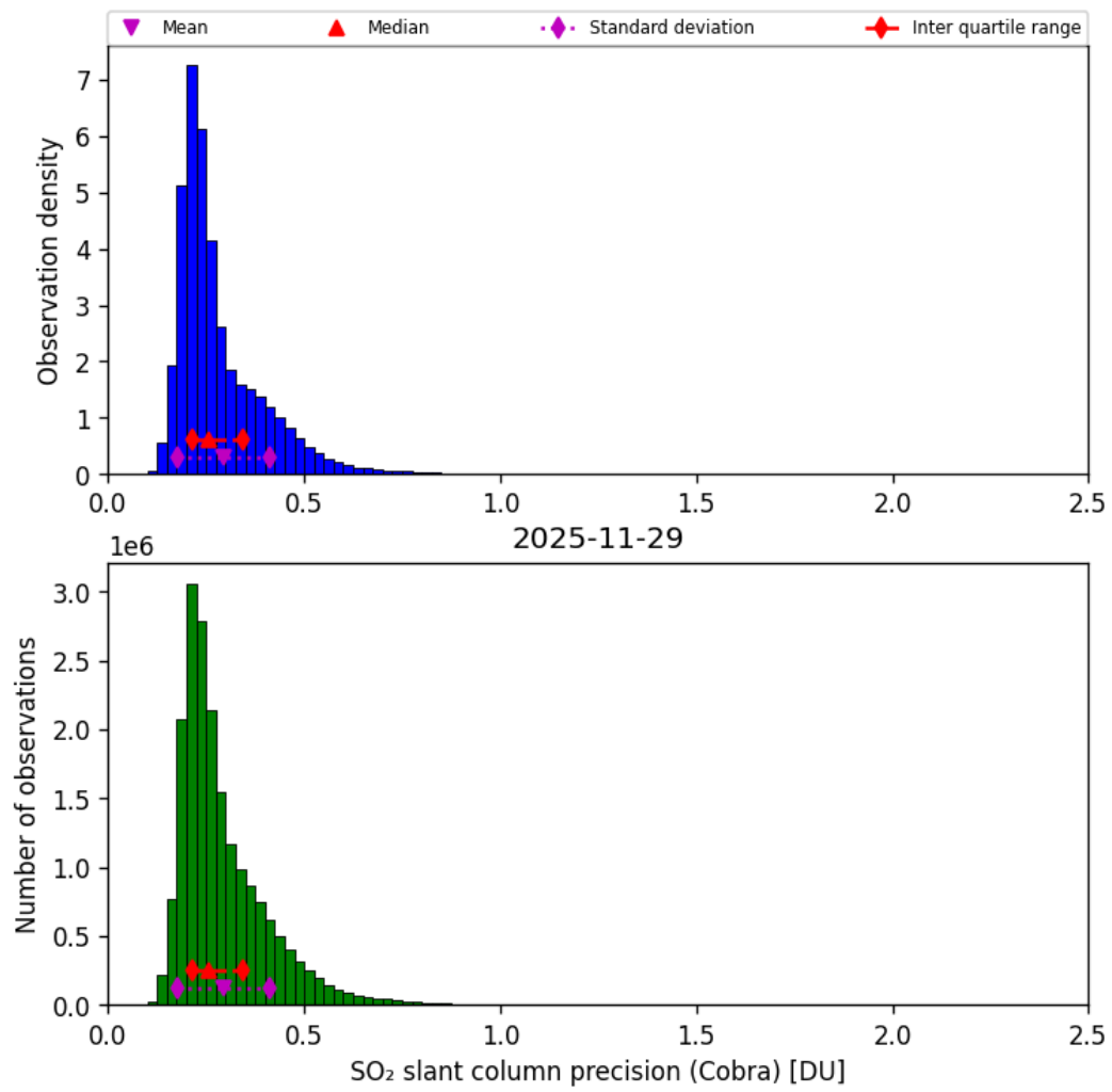
Figure 62: Histogram of “SO 2 slant column precision (Cobra)” for 2025-11-28 to 2025-11-30
