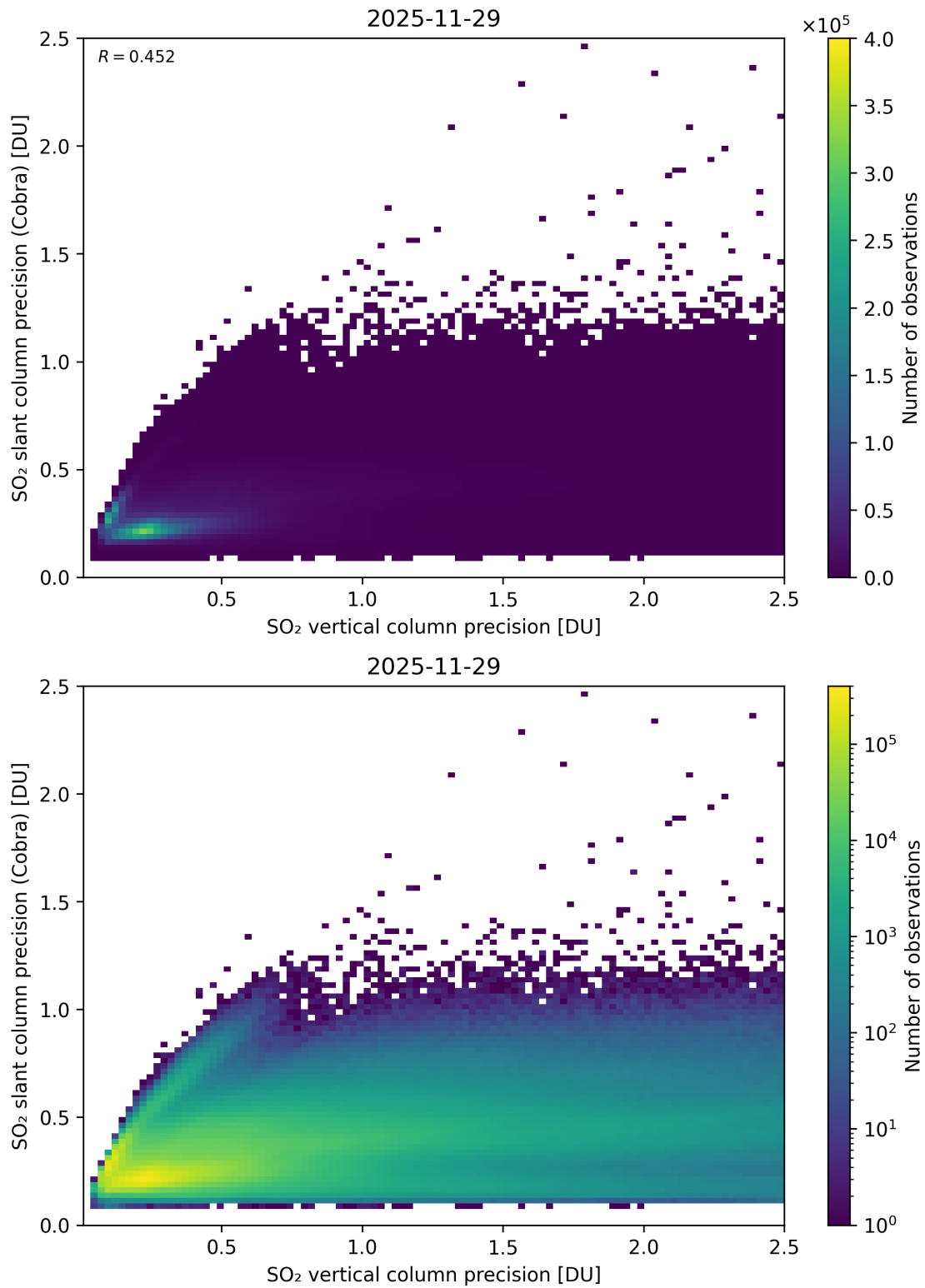
Figure 337: Scatter density plot of “SO 2 vertical column precision” against “SO 2 slant column precision (Cobra)” for 2025-11-28 to 2025-11-30.
