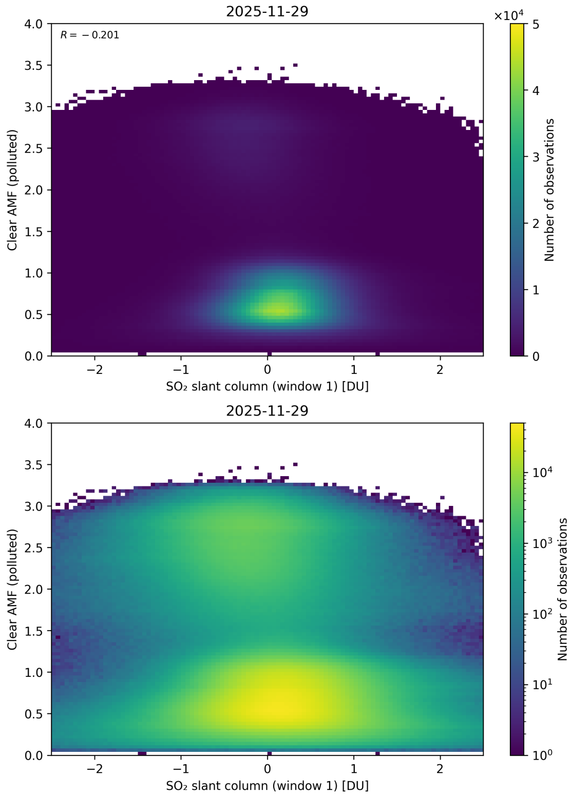
Figure 282: Scatter density plot of “SO 2 slant column (window 1)” against “Clear AMF (polluted)” for 2025-11-28 to 2025-11-30.
