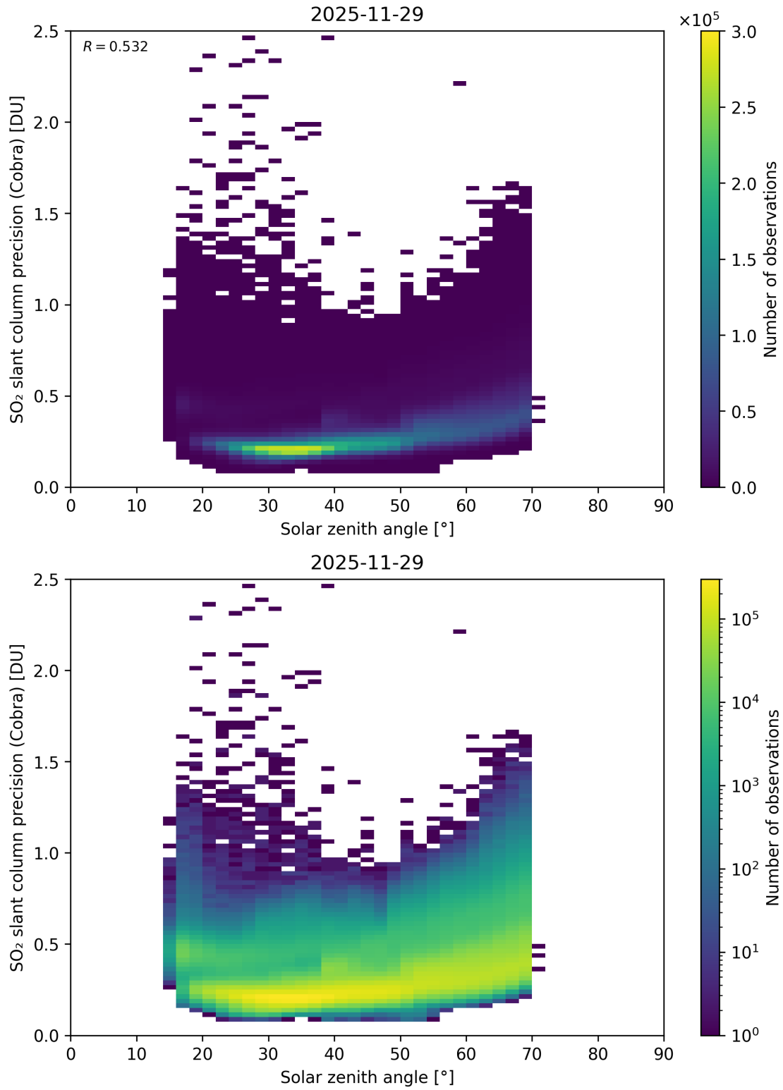
Figure 180: Scatter density plot of “Solar zenith angle” against “SO 2 slant column precision (Cobra)” for 2025-11-28 to 2025-11-30.
